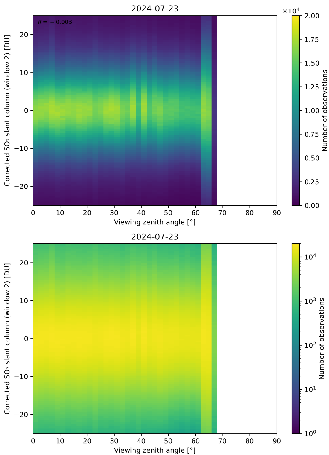
Figure 318: Scatter density plot of “Viewing zenith angle” against “Corrected SO 2 slant column (window 2)” for 2024-07-22 to 2024-07-24.
