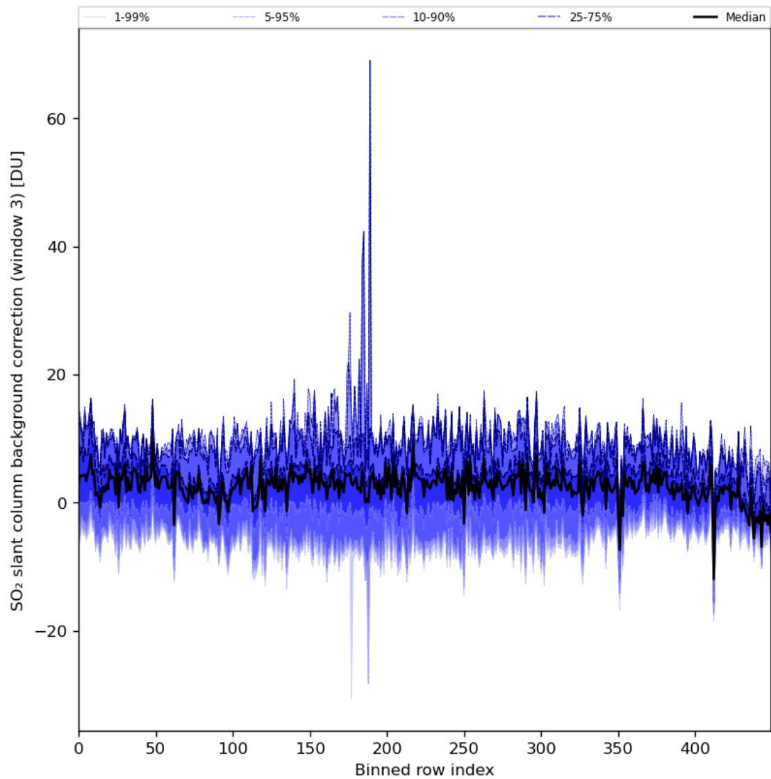
Figure 90: Along track statistics of “SO 2 slant column background correction (window 3)” for 2024-07-22 to 2024-07-24
