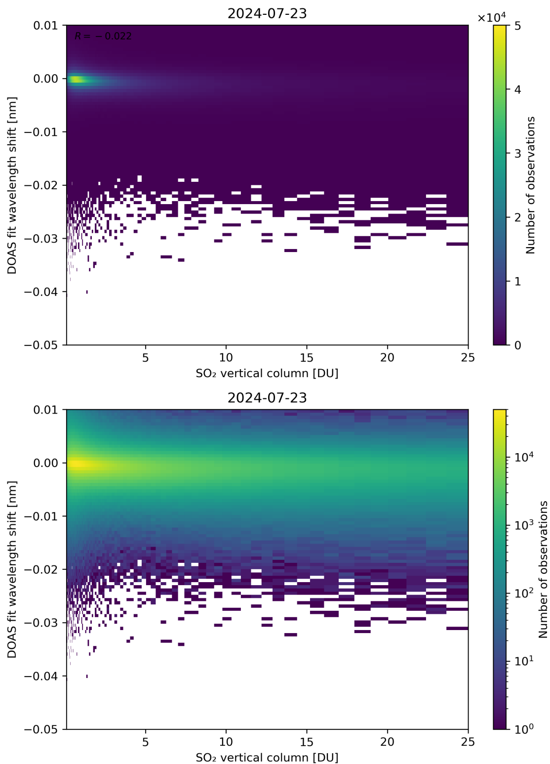
Figure 276: Scatter density plot of “SO 2 vertical column” against “DOAS fit wavelength shift” for 2024-07-22 to 2024-07-24.
