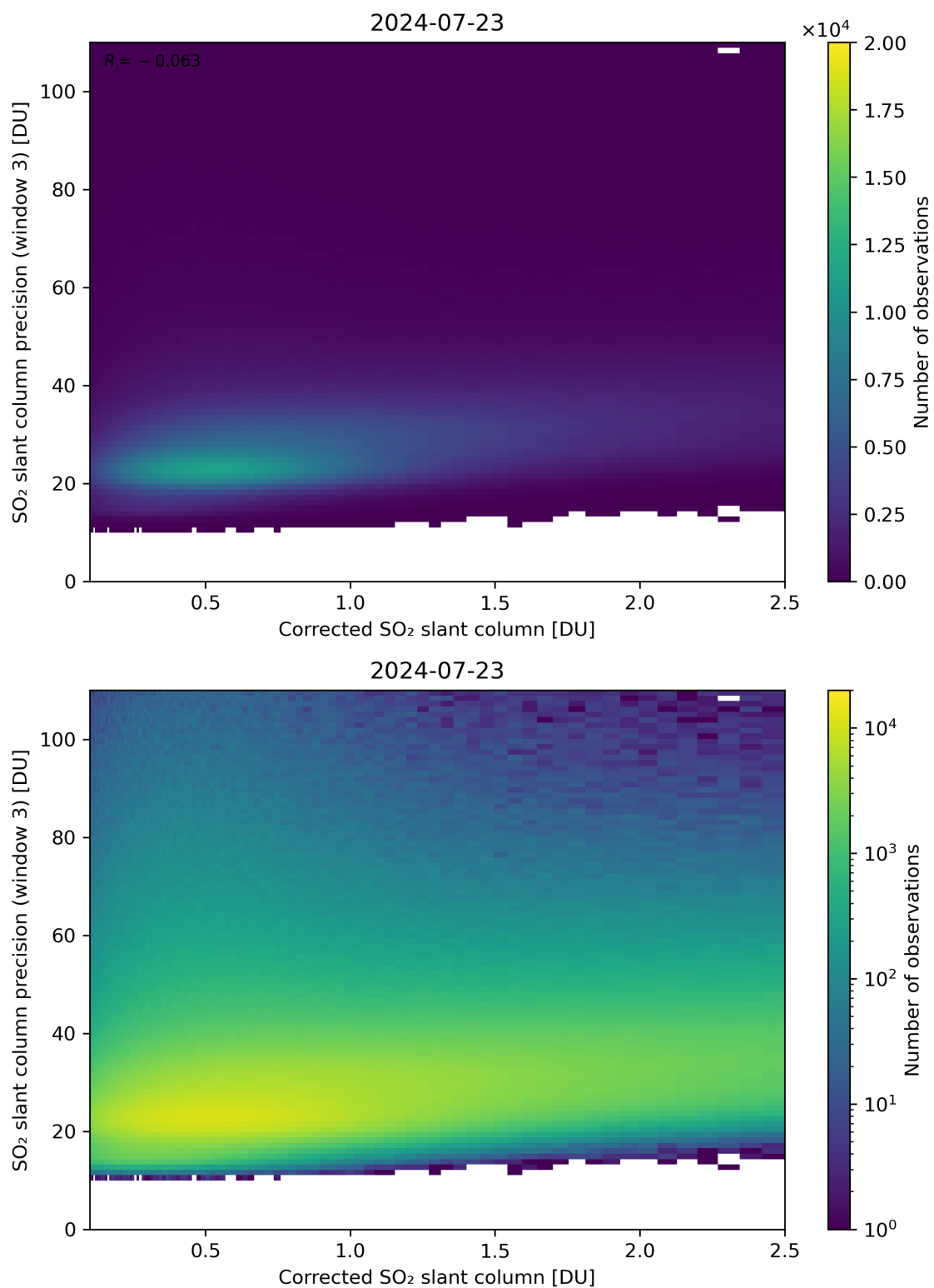
Figure 191: Scatter density plot of “Corrected SO 2 slant column” against “SO 2 slant column precision (window 3)” for 2024-07-22 to 2024-07-24.
