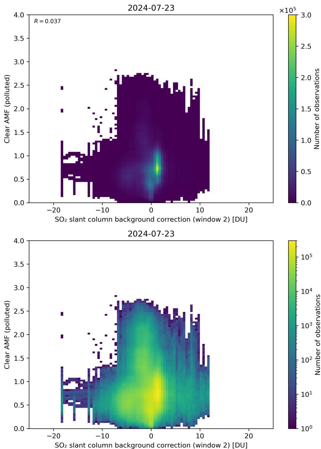
Figure 115: Scatter density plot of “SO 2 slant column background correction (window 2)” against “Clear AMF (polluted)” for 2024-07-22 to 2024-07-24.
