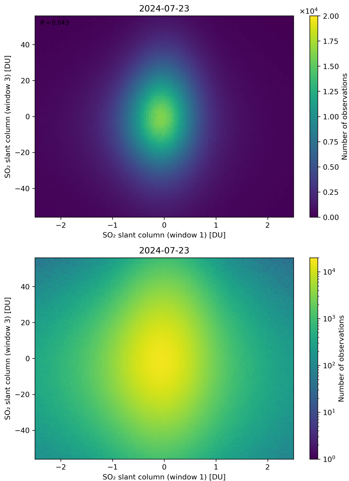
Figure 237: Scatter density plot of “SO 2 slant column (window 1)” against “SO 2 slant column (window 3)” for 2024-07-22 to 2024-07-24.
