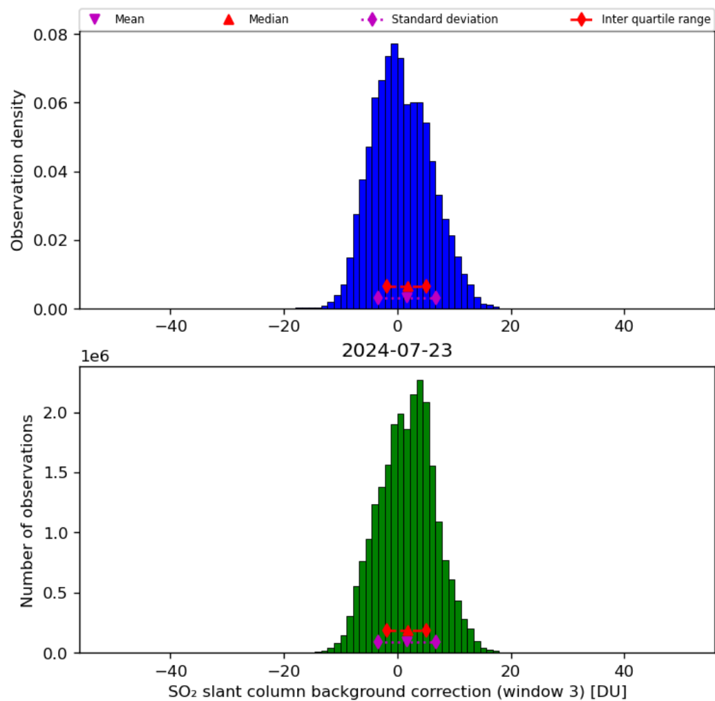
Figure 67: Histogram of “SO 2 slant column background correction (window 3)” for 2024-07-22 to 2024-07-24
