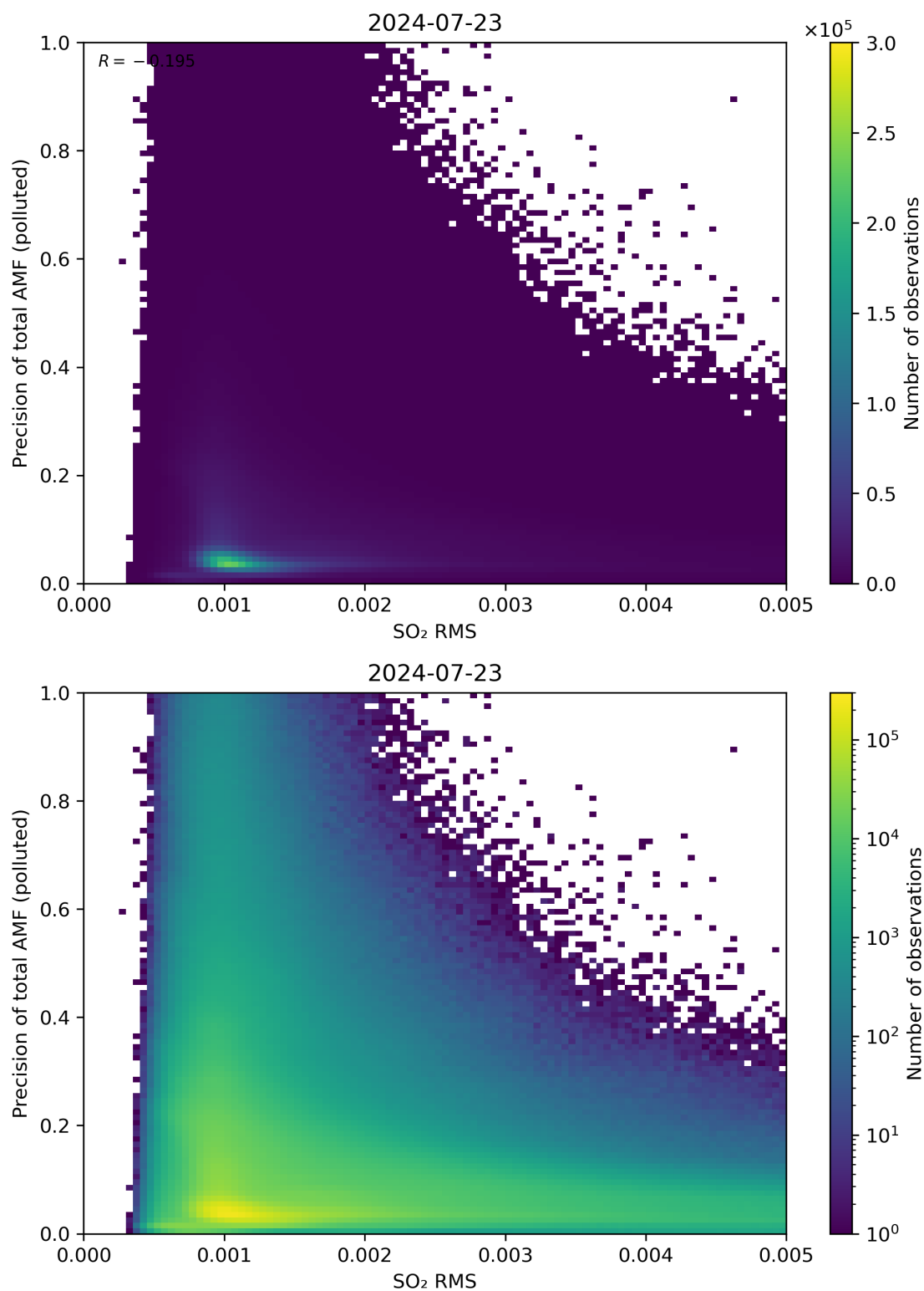
Figure 138: Scatter density plot of “SO 2 RMS” against “Precision of total AMF (polluted)” for 2024-07-22 to 2024-07-24.
