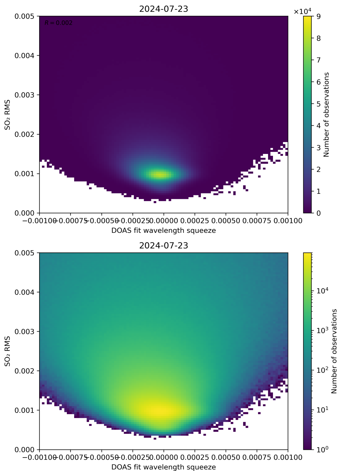
Figure 132: Scatter density plot of “DOAS fit wavelength squeeze” against “SO 2 RMS” for 2024-07-22 to 2024-07-24.
