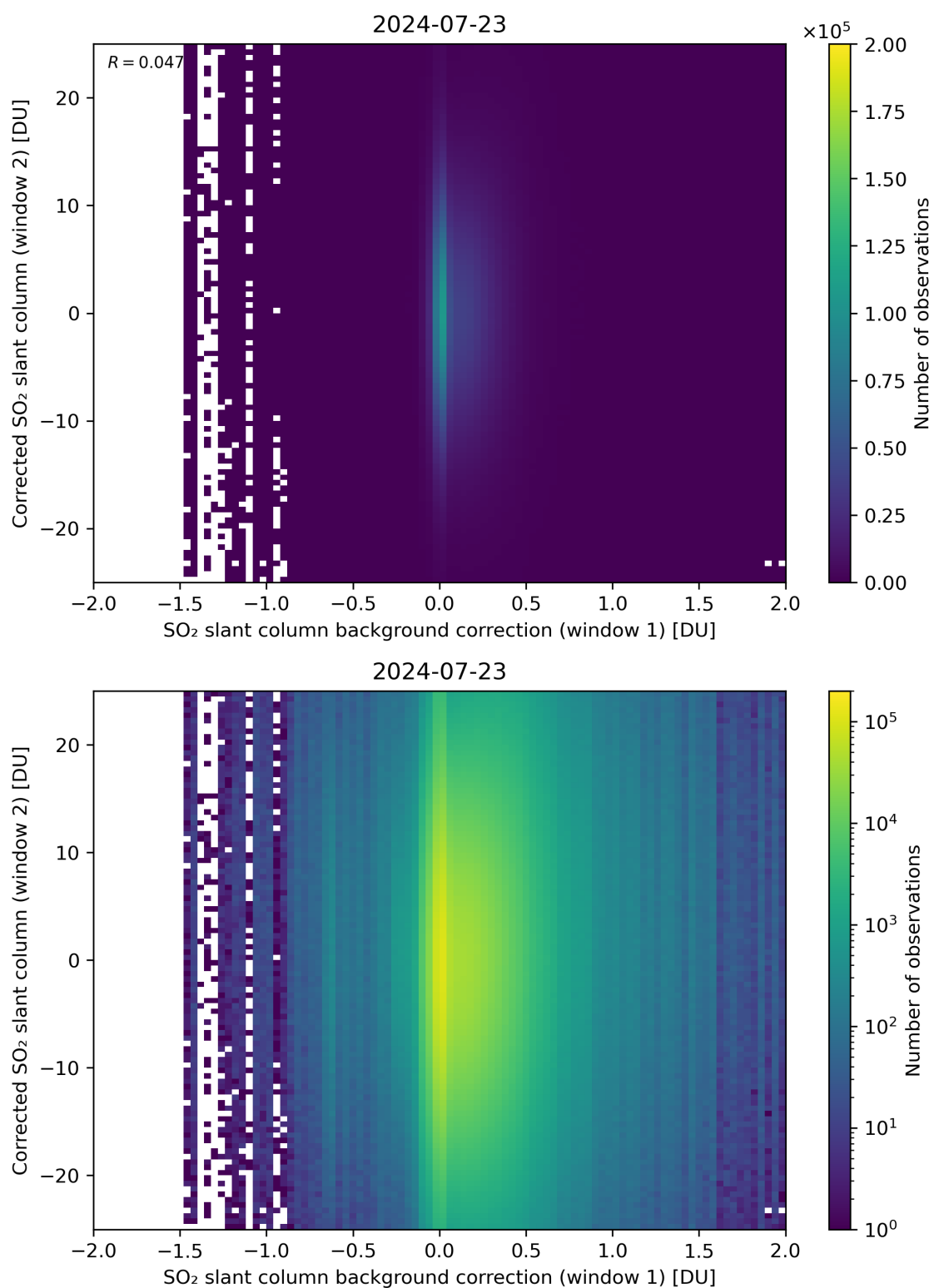
Figure 104: Scatter density plot of “SO 2 slant column background correction (window 1)” against “Corrected SO 2 slant column (window 2)” for 2024-07-22 to 2024-07-24.
