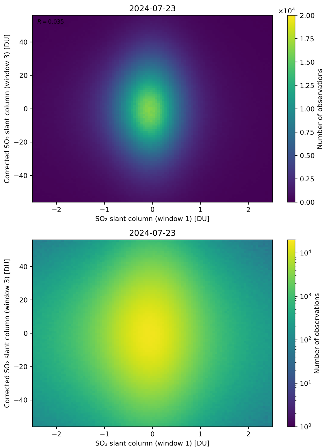
Figure 234: Scatter density plot of “SO 2 slant column (window 1)” against “Corrected SO 2 slant column (window 3)” for 2024-07-22 to 2024-07-24.
