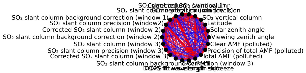
Figure 1: Map of correlation graph for 2024-07-22 to 2024-07-24.
