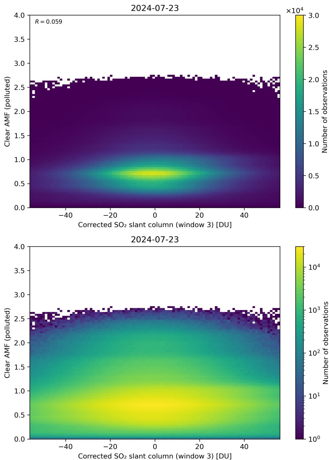
Figure 209: Scatter density plot of “Corrected SO 2 slant column (window 3)” against “Clear AMF (polluted)” for 2024-07-22 to 2024-07-24.
