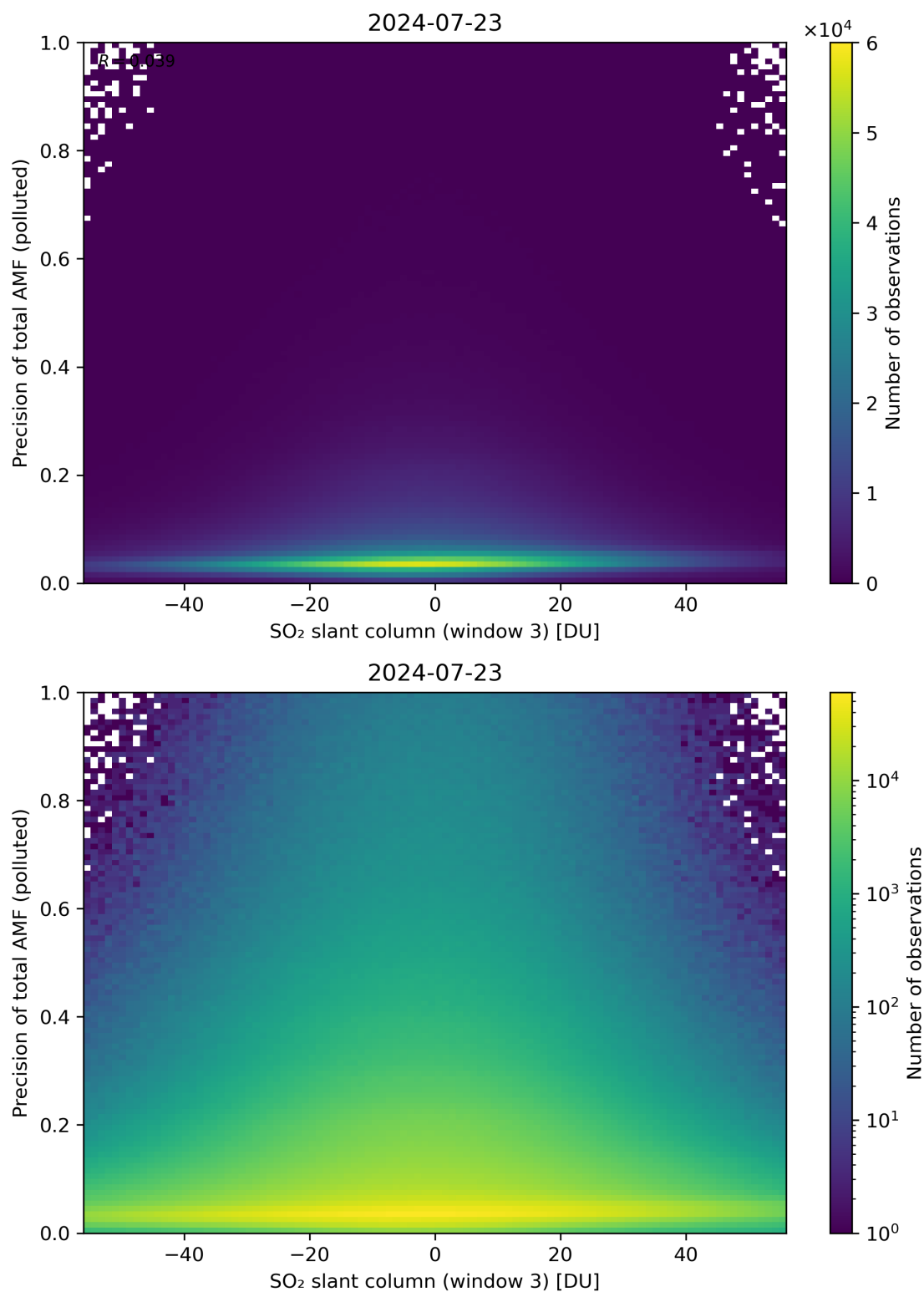
Figure 269: Scatter density plot of “SO 2 slant column (window 3)” against “Precision of total AMF (polluted)” for 2024-07-22 to 2024-07-24.
