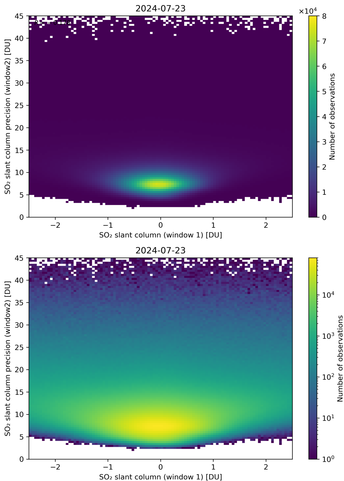
Figure 236: Scatter density plot of “SO 2 slant column (window 1)” against “SO 2 slant column precision (window2)” for 2024-07-22 to 2024-07-24.
