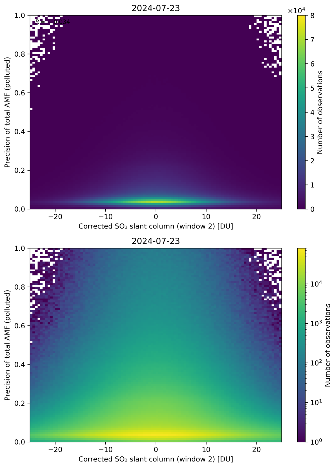
Figure 204: Scatter density plot of “Corrected SO 2 slant column (window 2)” against “Precision of total AMF (polluted)” for 2024-07-22 to 2024-07-24.
