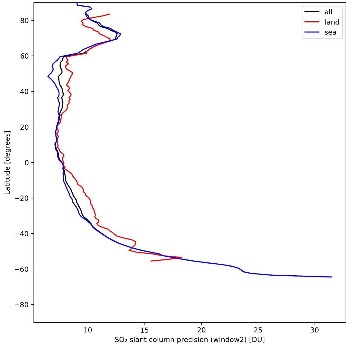
Figure 38: Zonal average of “SO 2 slant column precision (window2)” for 2024-07-22 to 2024-07-24.
