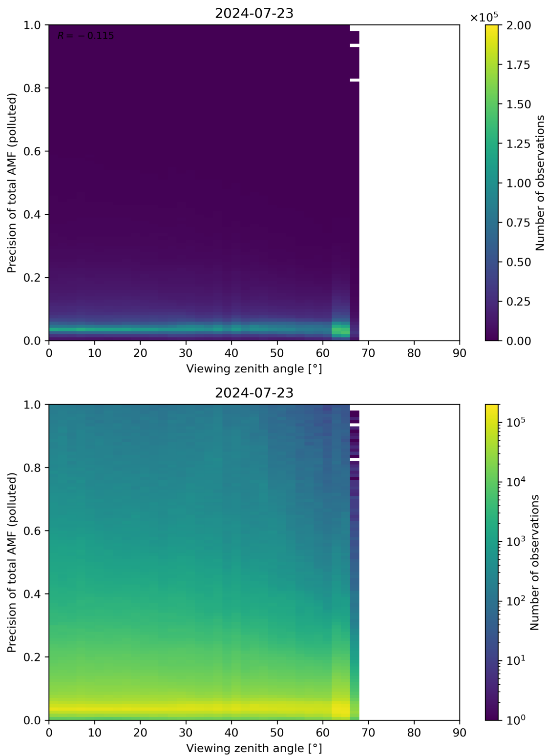
Figure 326: Scatter density plot of “Viewing zenith angle” against “Precision of total AMF (polluted)” for 2024-07-22 to 2024-07-24.
