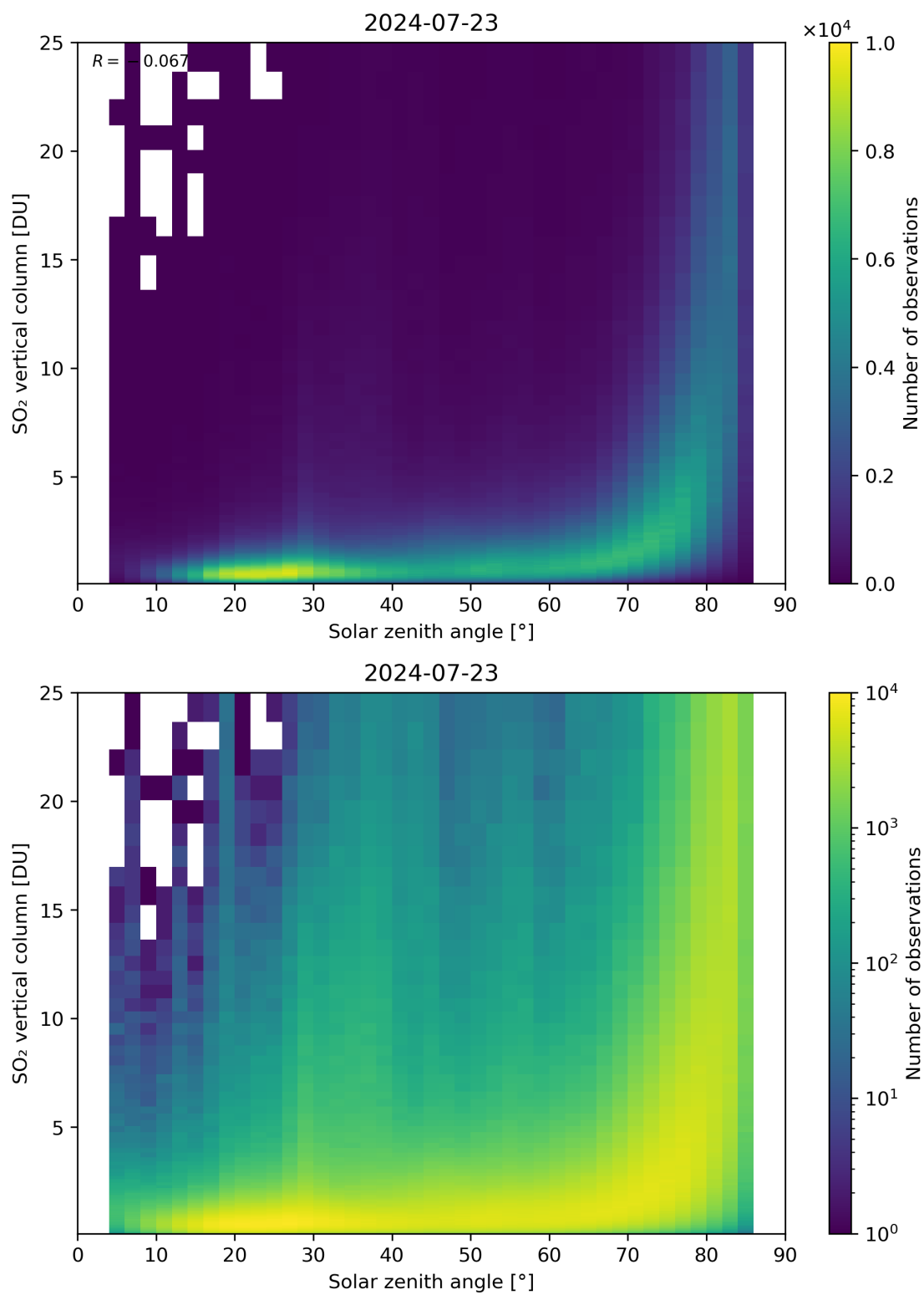
Figure 176: Scatter density plot of “Solar zenith angle” against “SO 2 vertical column” for 2024-07-22 to 2024-07-24.
