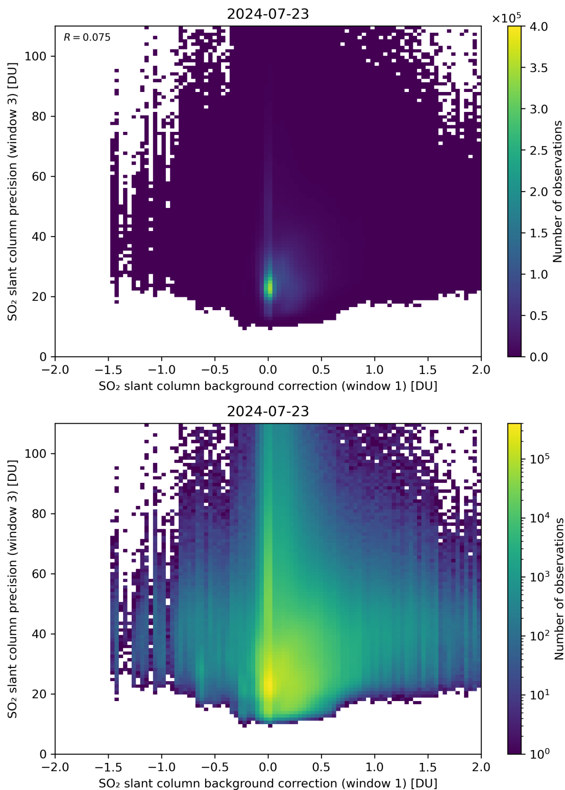
Figure 108: Scatter density plot of “SO 2 slant column background correction (window 1)” against “SO 2 slant column precision (window 3)” for 2024-07-22 to 2024-07-24.
