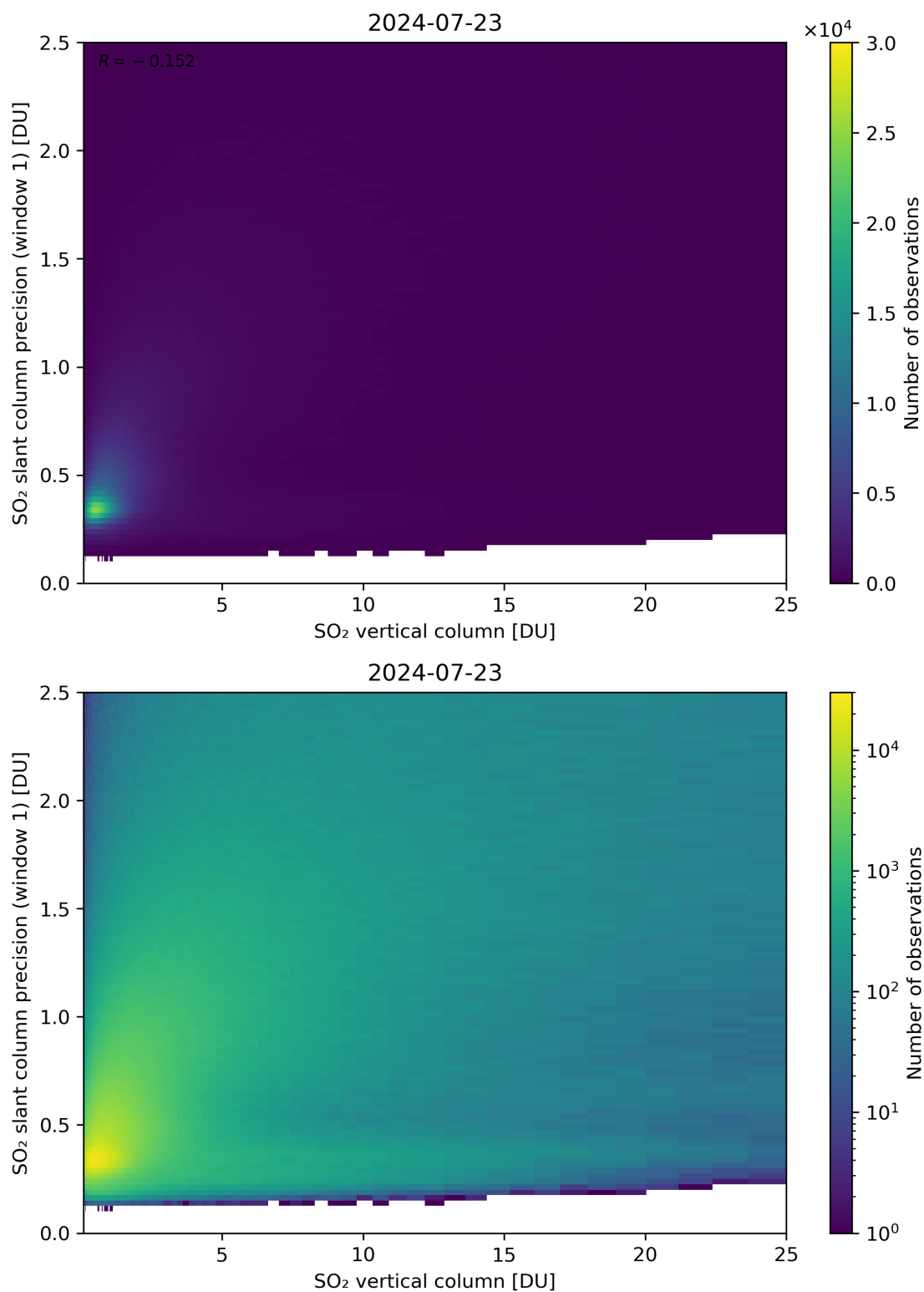
Figure 301: Scatter density plot of “SO 2 vertical column” against “SO 2 slant column precision (window 1)” for 2024-07-22 to 2024-07-24.
