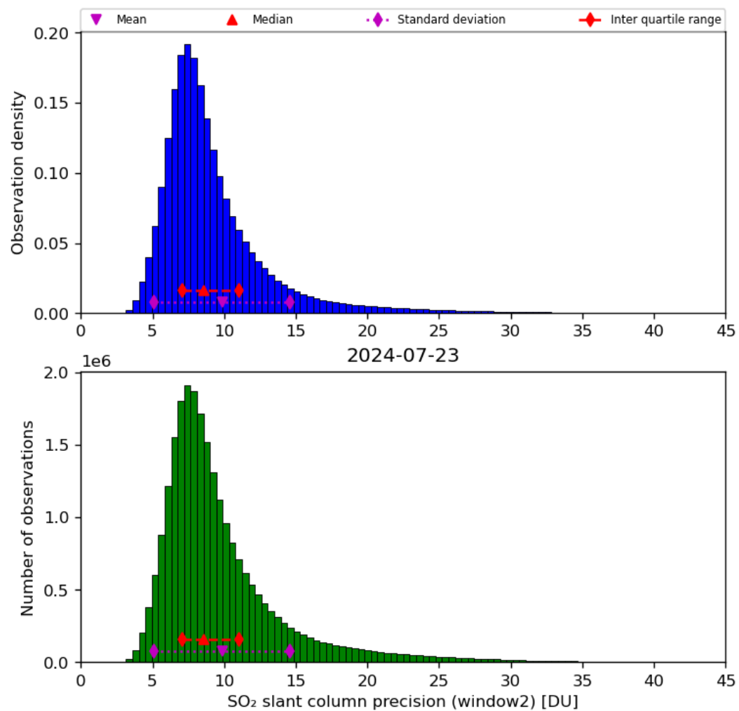
Figure 61: Histogram of “SO 2 slant column precision (window2)” for 2024-07-22 to 2024-07-24
