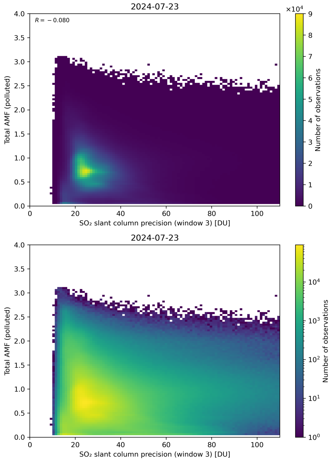
Figure 263: Scatter density plot of “SO 2 slant column precision (window 3)” against “Total AMF (polluted)” for 2024-07-22 to 2024-07-24.
