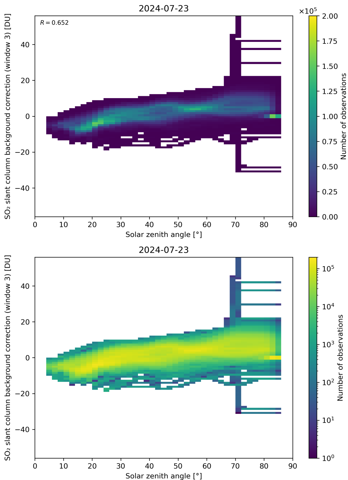
Figure 160: Scatter density plot of “Solar zenith angle” against “SO 2 slant column background correction (window 3)” for 2024-07-22 to 2024-07-24.
