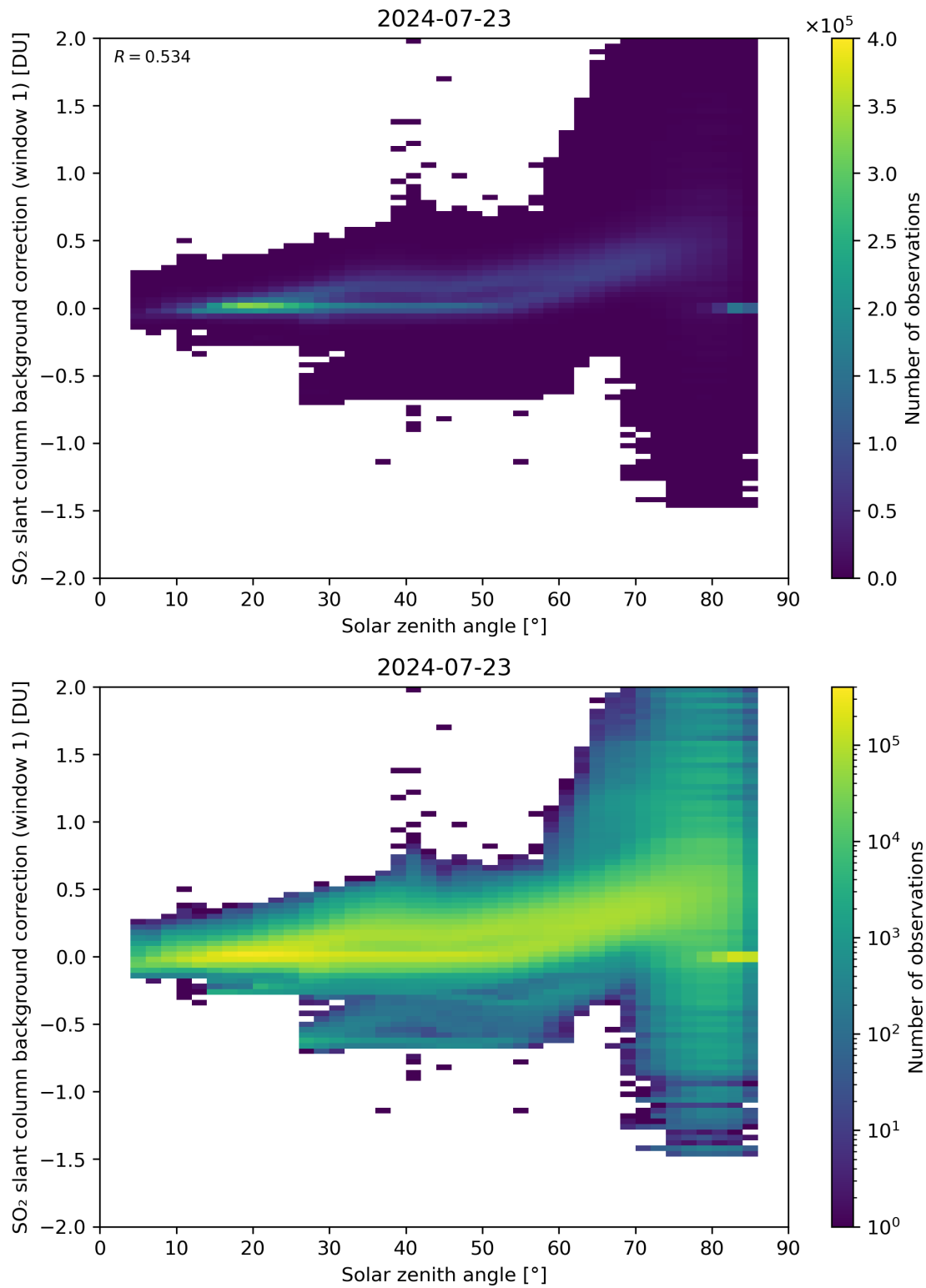
Figure 158: Scatter density plot of “Solar zenith angle” against “SO 2 slant column background correction (window 1)” for 2024-07-22 to 2024-07-24.
