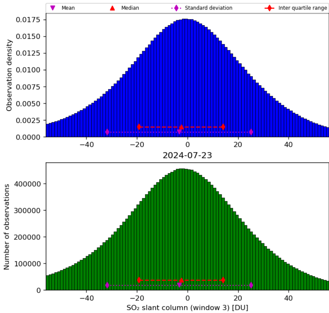
Figure 64: Histogram of “SO 2 slant column (window 3)” for 2024-07-22 to 2024-07-24
