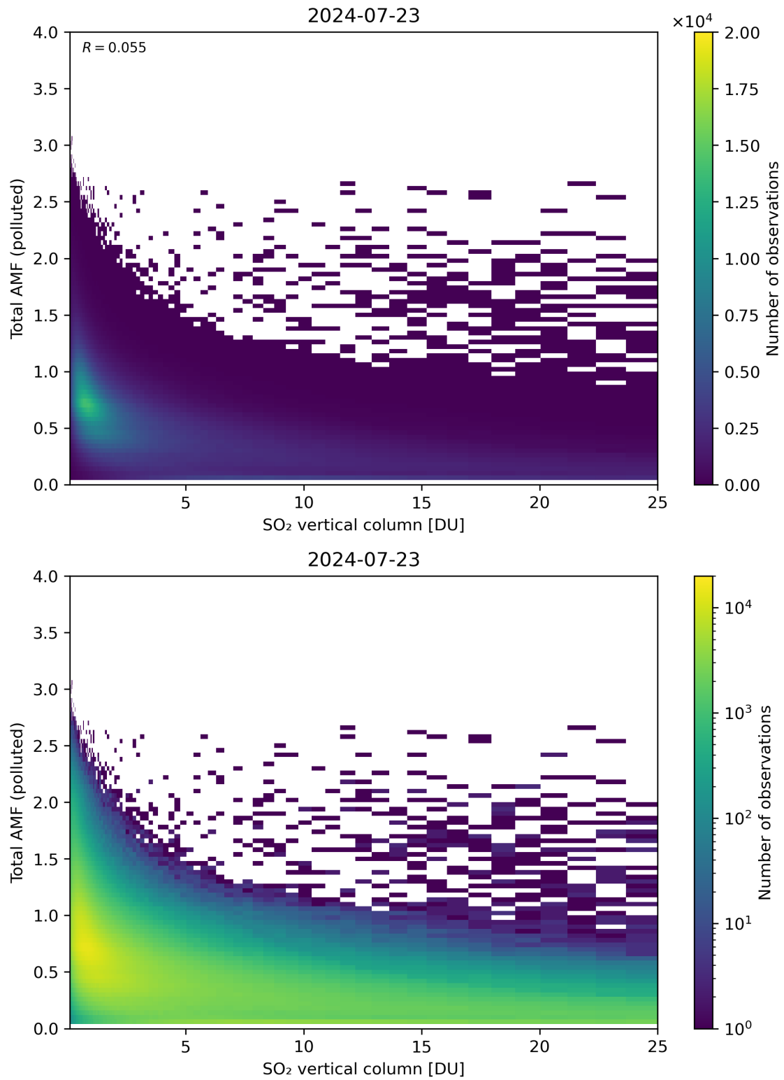
Figure 305: Scatter density plot of “SO 2 vertical column” against “Total AMF (polluted)” for 2024-07-22 to 2024-07-24.
