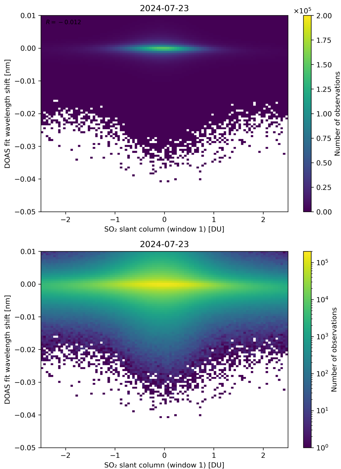
Figure 215: Scatter density plot of “SO 2 slant column (window 1)” against “DOAS fit wavelength shift” for 2024-07-22 to 2024-07-24.
