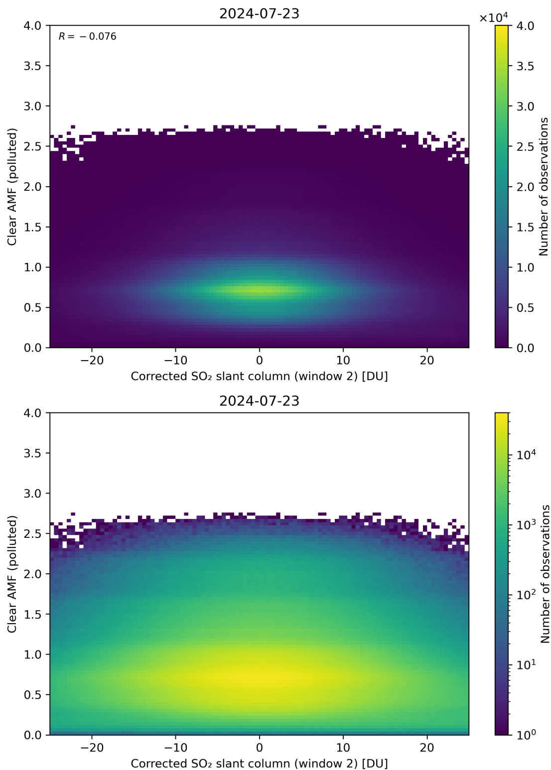
Figure 199: Scatter density plot of “Corrected SO 2 slant column (window 2)” against “Clear AMF (polluted)” for 2024-07-22 to 2024-07-24.
