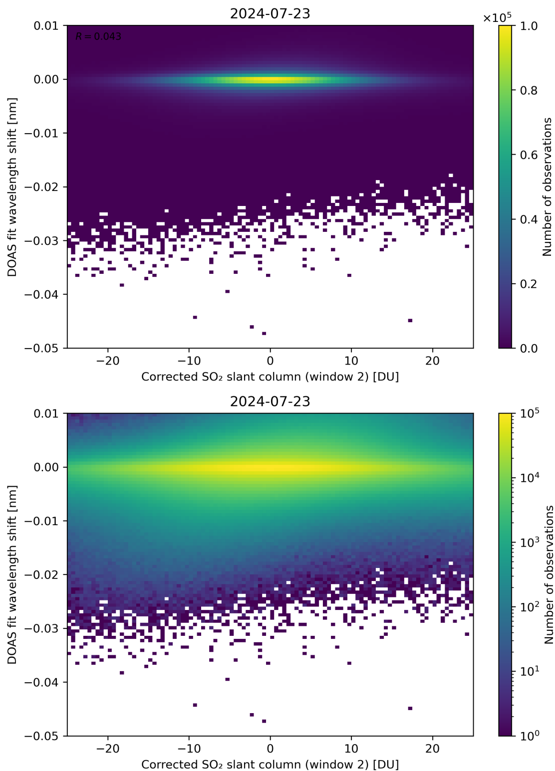
Figure 196: Scatter density plot of “Corrected SO 2 slant column (window 2)” against “DOAS fit wavelength shift” for 2024-07-22 to 2024-07-24.
