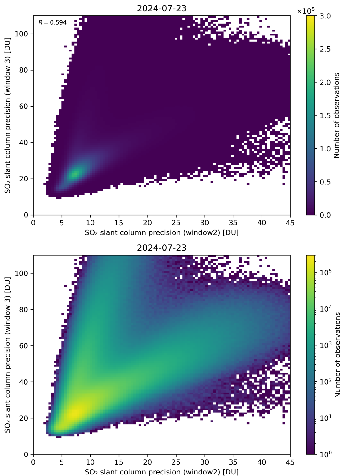
Figure 250: Scatter density plot of “SO 2 slant column precision (window2)” against “SO 2 slant column precision (window 3)” for 2024-07-22 to 2024-07-24.
