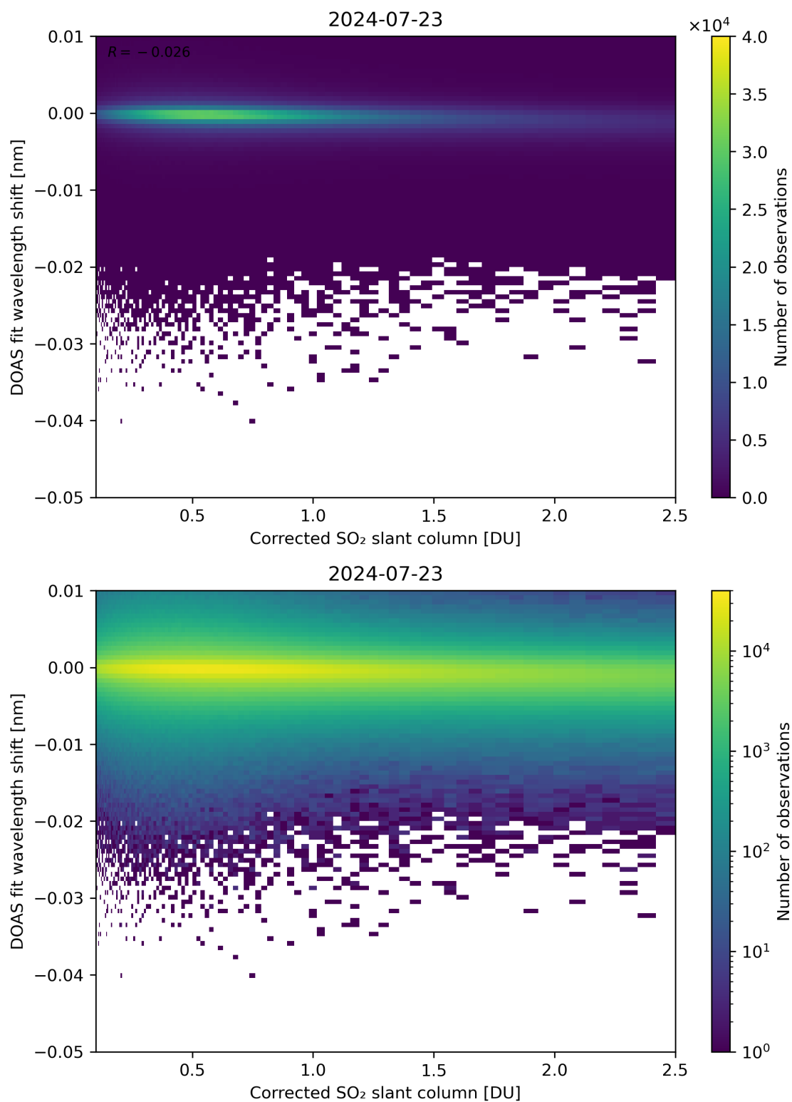
Figure 181: Scatter density plot of “Corrected SO 2 slant column” against “DOAS fit wavelength shift” for 2024-07-22 to 2024-07-24.
