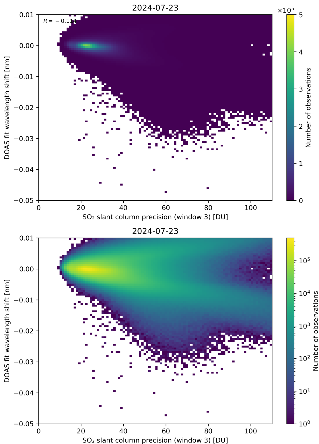
Figure 258: Scatter density plot of “SO 2 slant column precision (window 3)” against “DOAS fit wavelength shift” for 2024-07-22 to 2024-07-24.
