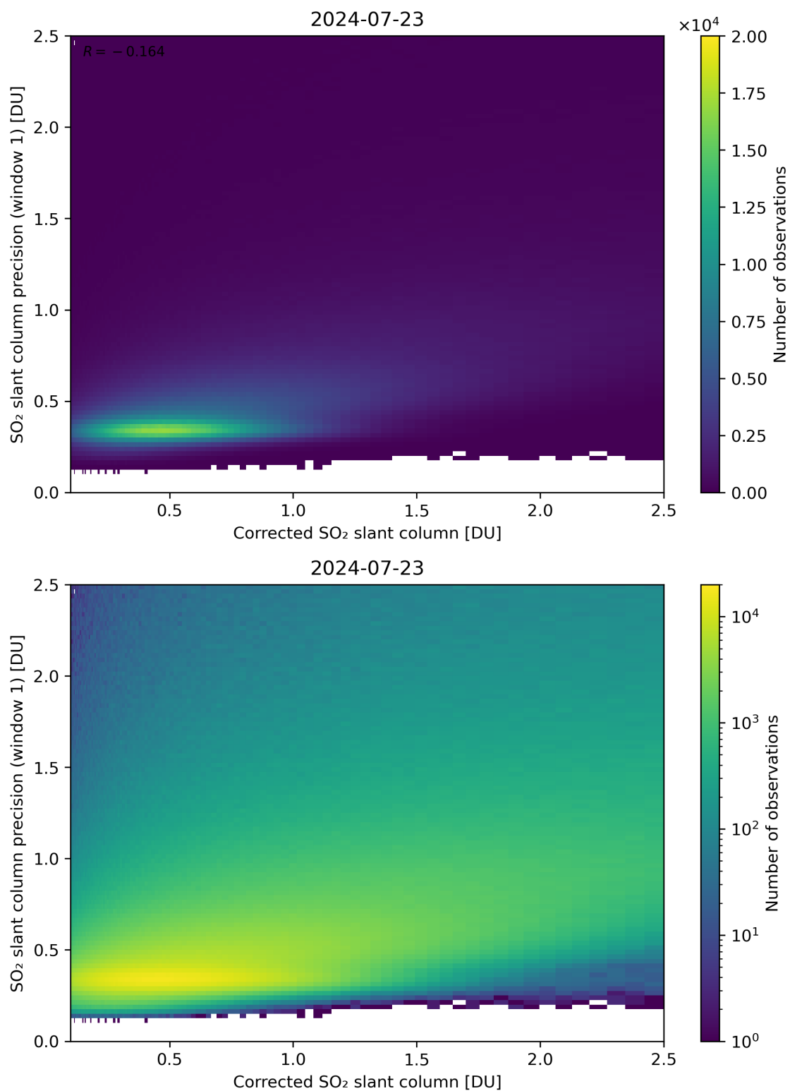
Figure 188: Scatter density plot of “Corrected SO 2 slant column” against “SO 2 slant column precision (window 1)” for 2024-07-22 to 2024-07-24.
