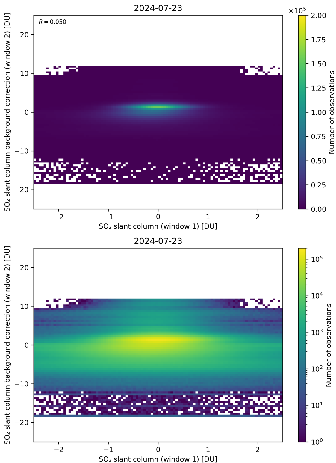
Figure 213: Scatter density plot of “SO 2 slant column (window 1)” against “SO 2 slant column background correction (window 2)” for 2024-07-22 to 2024-07-24.
