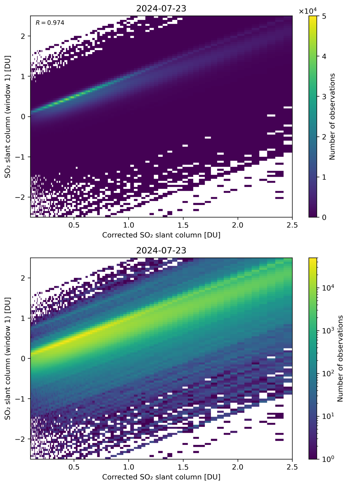
Figure 187: Scatter density plot of “Corrected SO 2 slant column” against “SO 2 slant column (window 1)” for 2024-07-22 to 2024-07-24.
