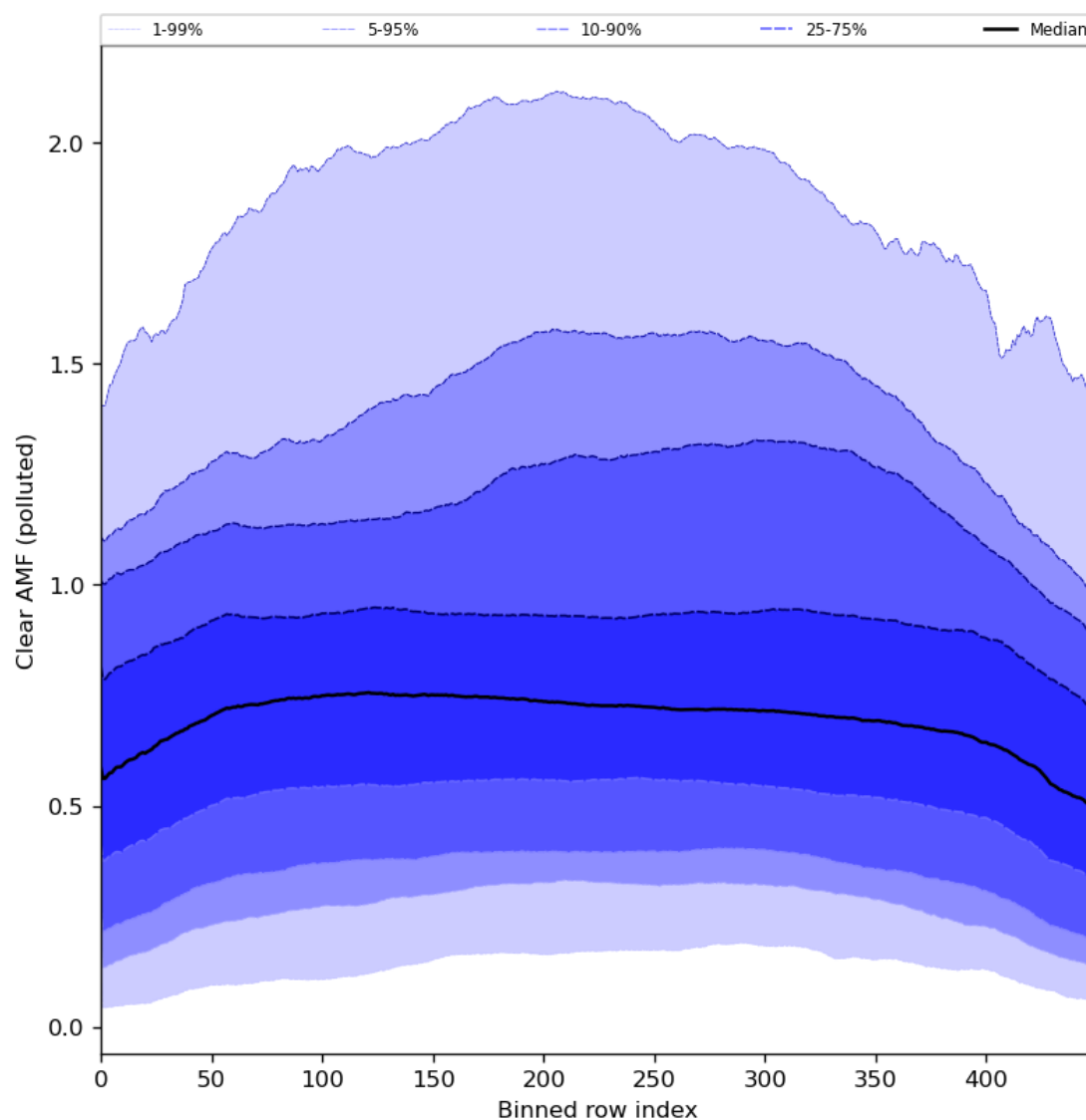
Figure 96: Along track statistics of “Clear AMF (polluted)” for 2024-07-22 to 2024-07-24
