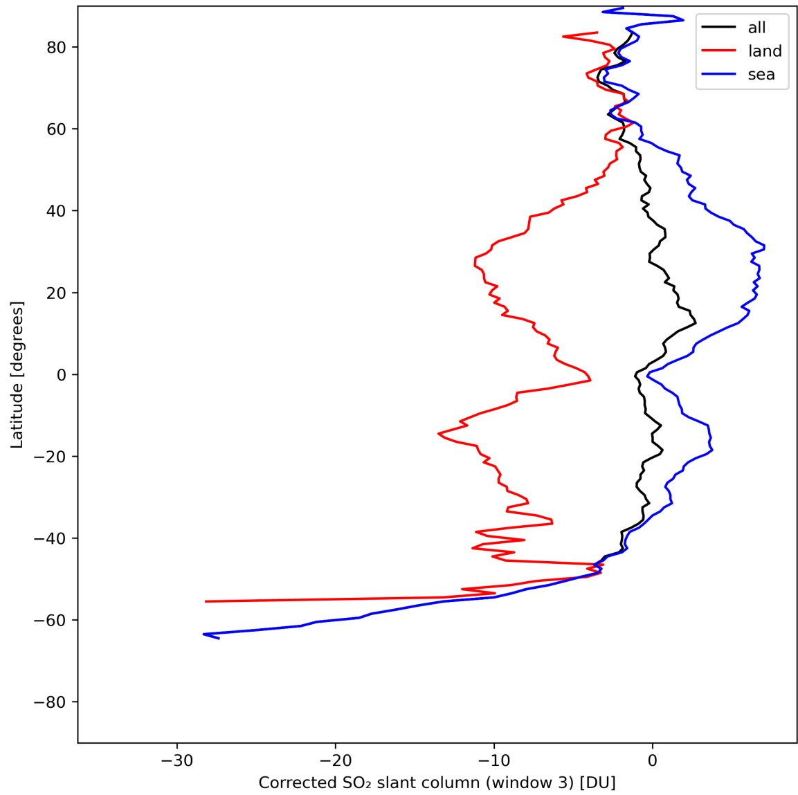
Figure 43: Zonal average of “Corrected SO 2 slant column (window 3)” for 2024-07-22 to 2024-07-24.
