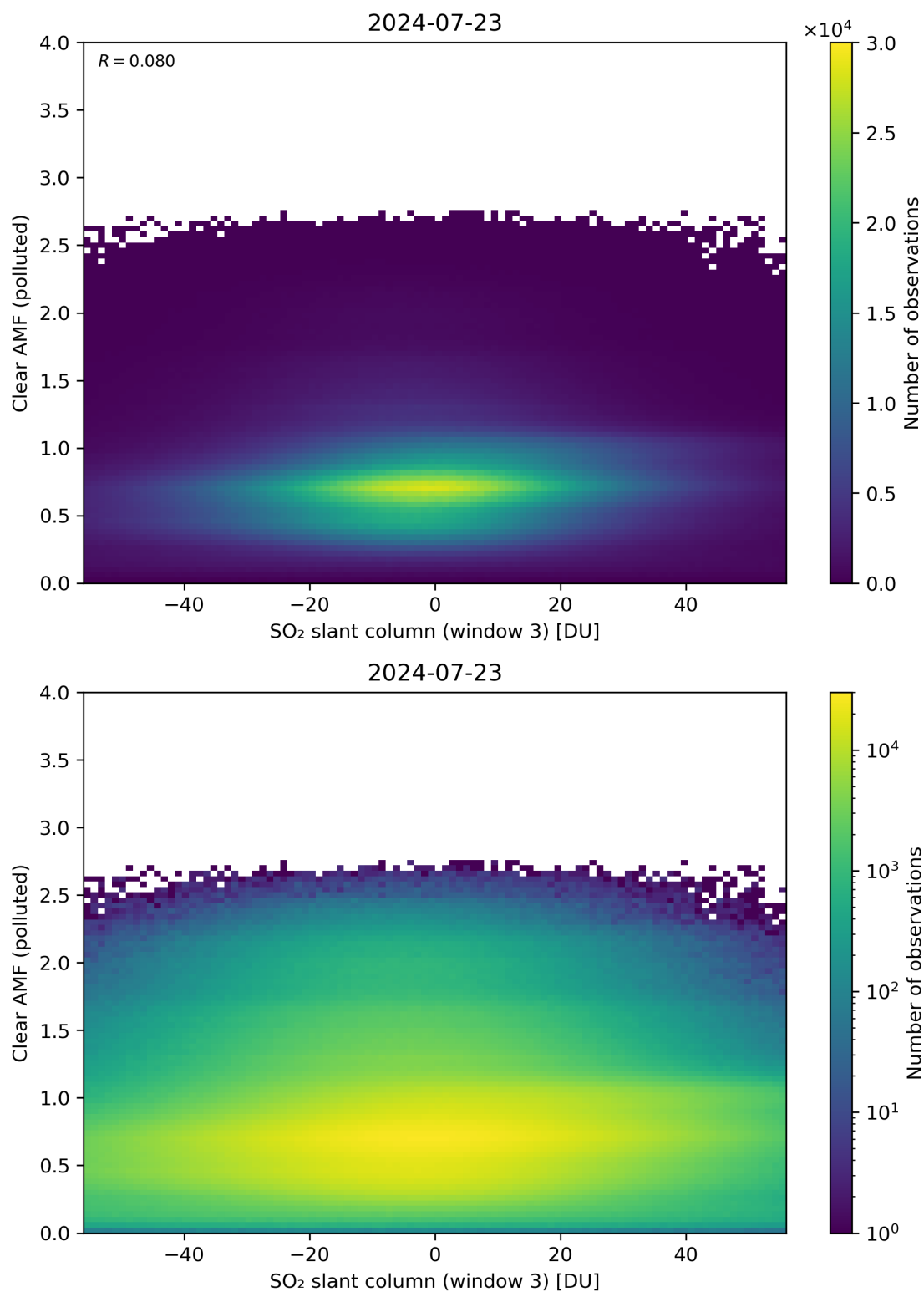
Figure 265: Scatter density plot of “SO 2 slant column (window 3)” against “Clear AMF (polluted)” for 2024-07-22 to 2024-07-24.
