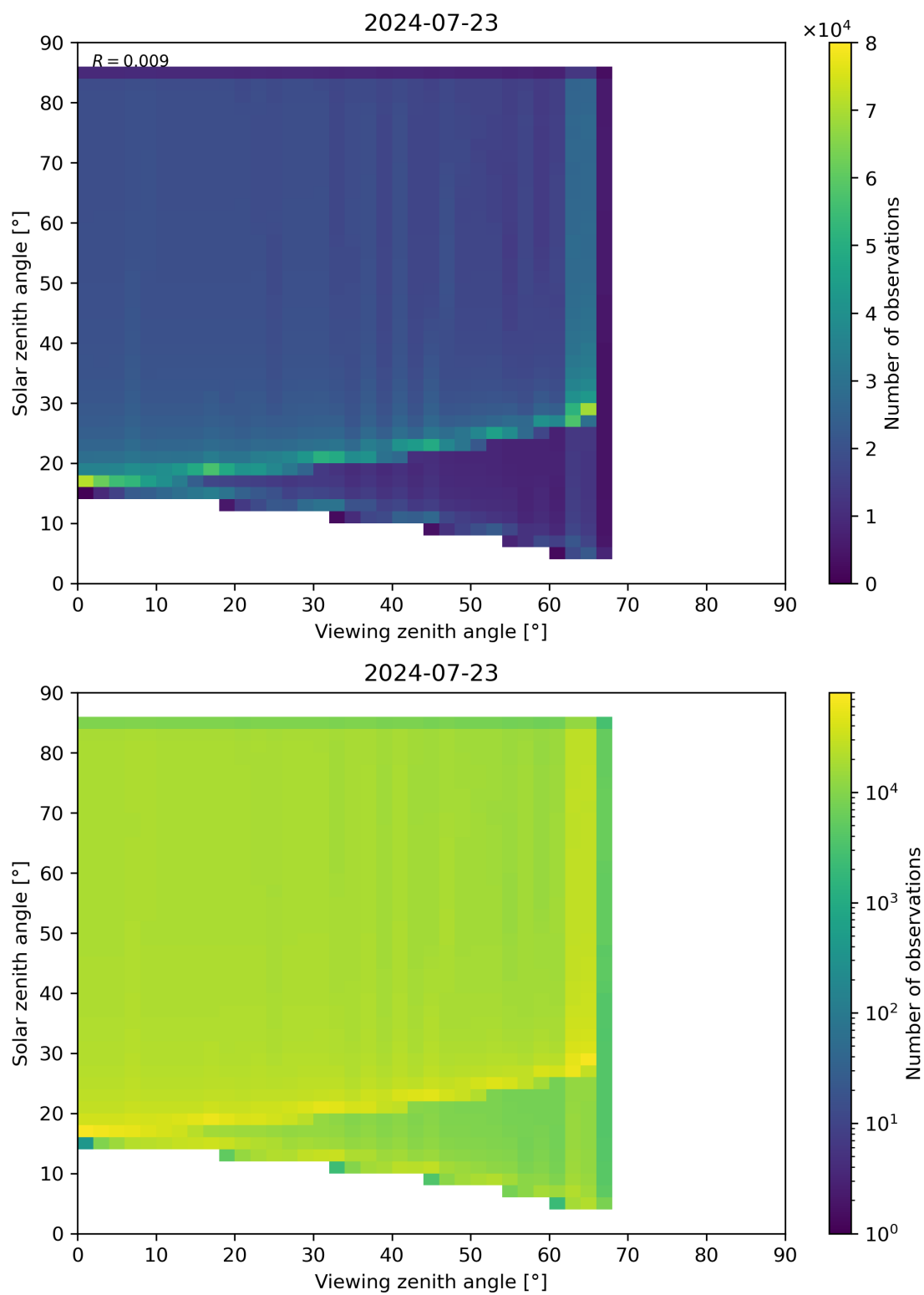
Figure 315: Scatter density plot of “Viewing zenith angle” against “Solar zenith angle” for 2024-07-22 to 2024-07-24.
