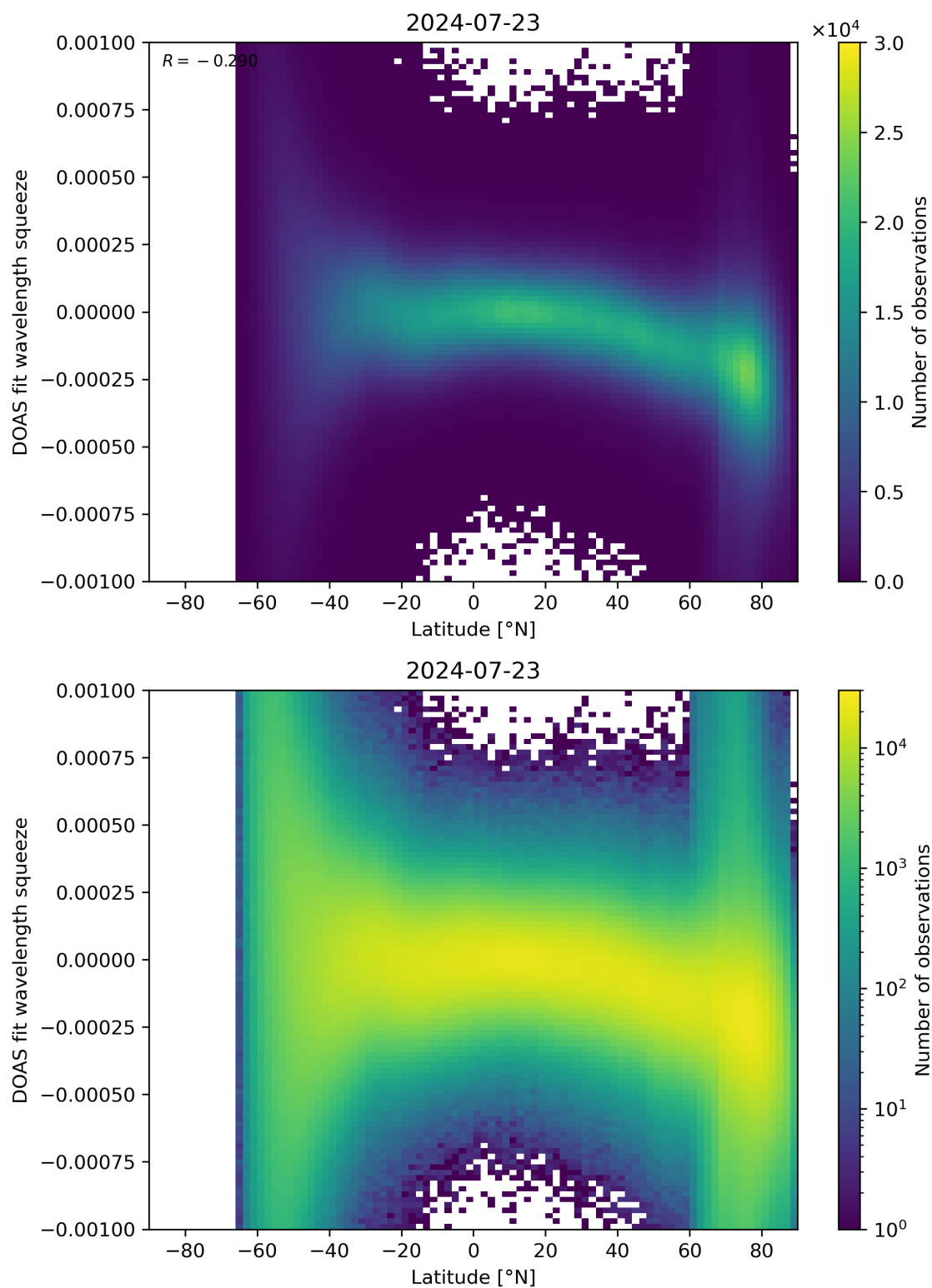
Figure 143: Scatter density plot of “Latitude” against “DOAS fit wavelength squeeze” for 2024-07-22 to 2024-07-24.
