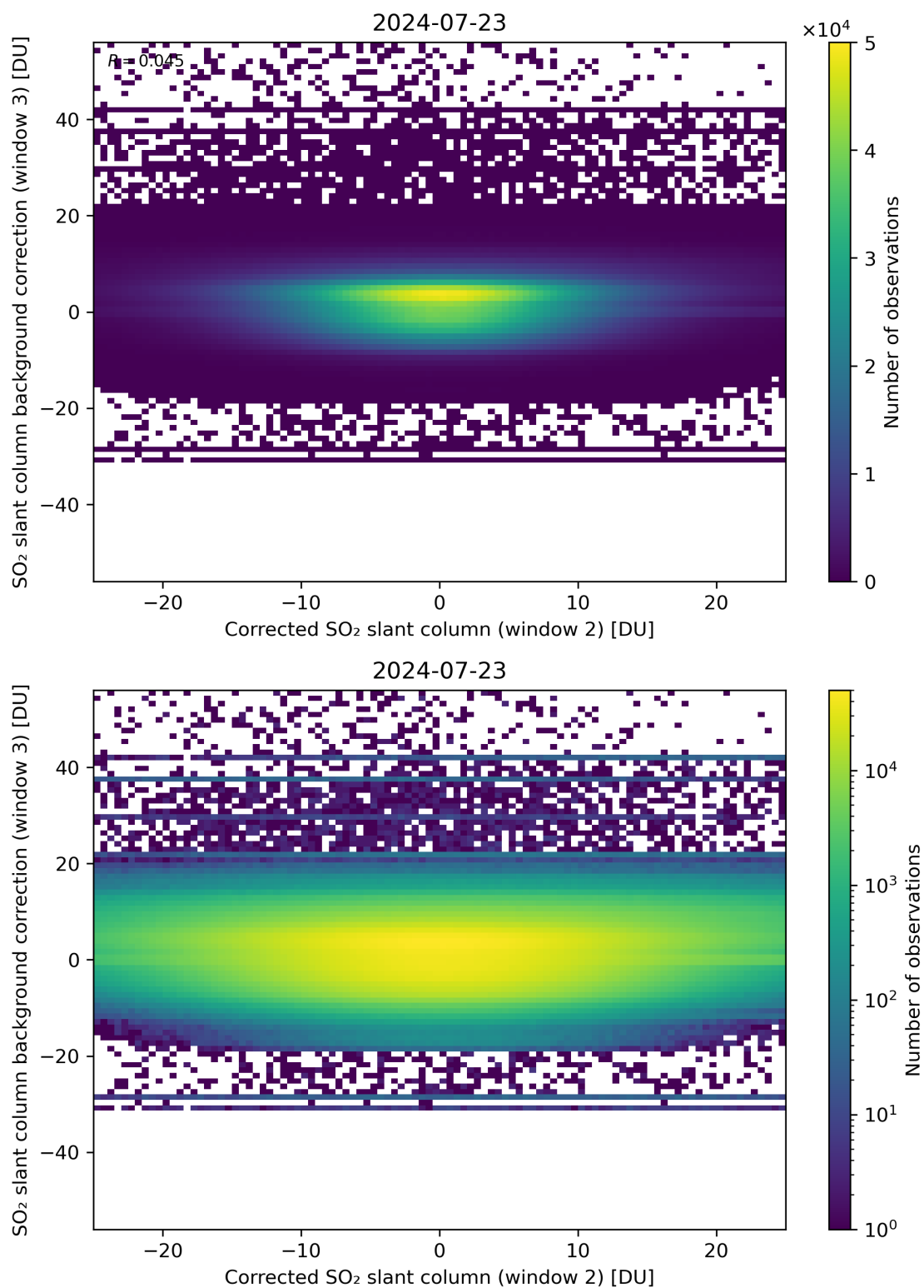
Figure 195: Scatter density plot of “Corrected SO 2 slant column (window 2)” against “SO 2 slant column background correction (window 3)” for 2024-07-22 to 2024-07-24.
