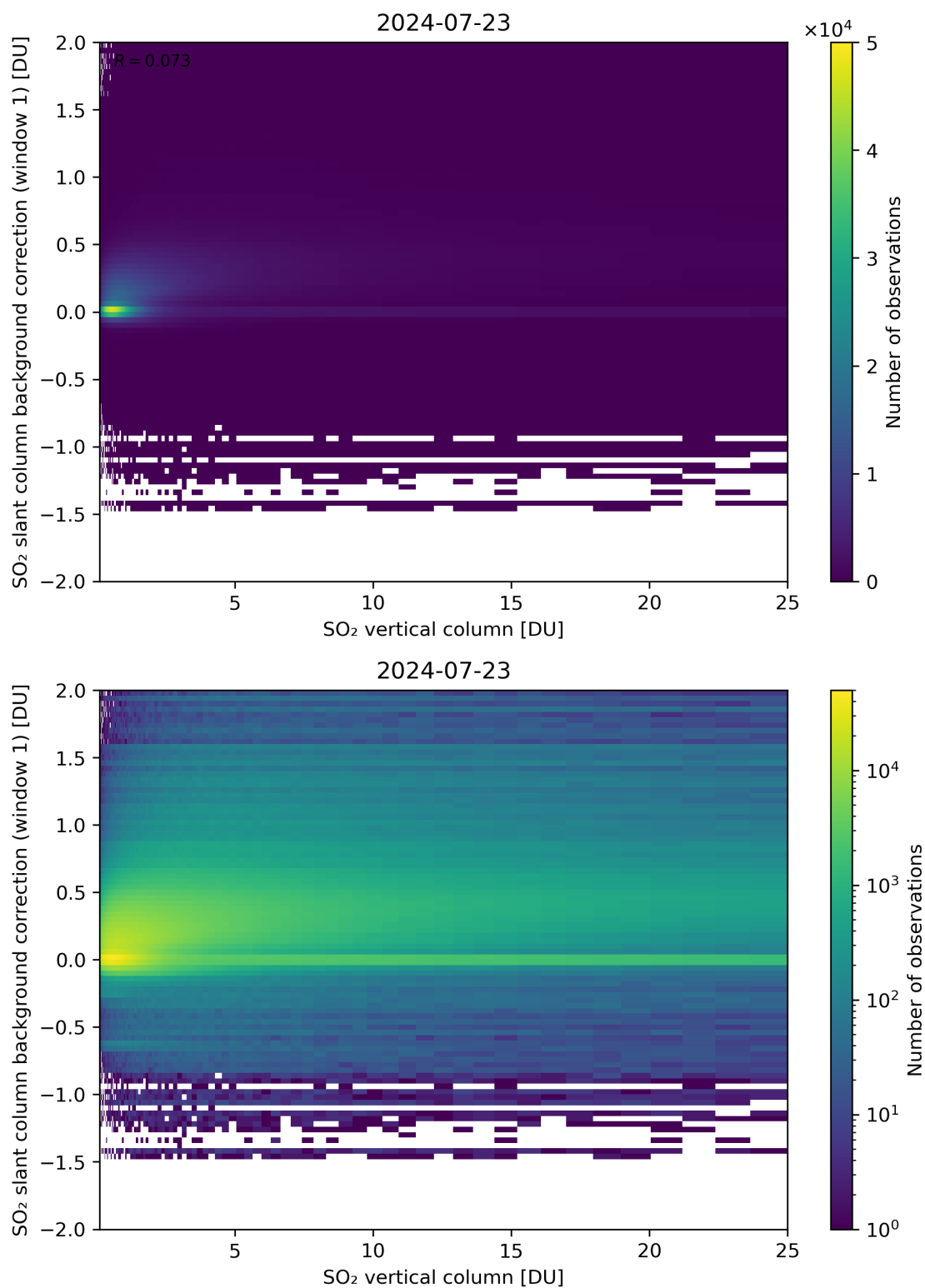
Figure 273: Scatter density plot of “SO 2 vertical column” against “SO 2 slant column background correction (window 1)” for 2024-07-22 to 2024-07-24.
