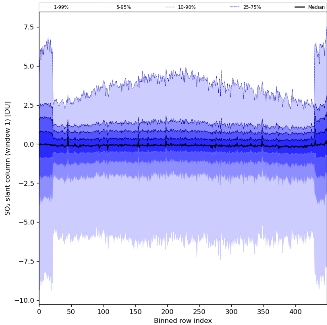
Figure 79: Along track statistics of “SO 2 slant column (window 1)” for 2024-07-22 to 2024-07-24
