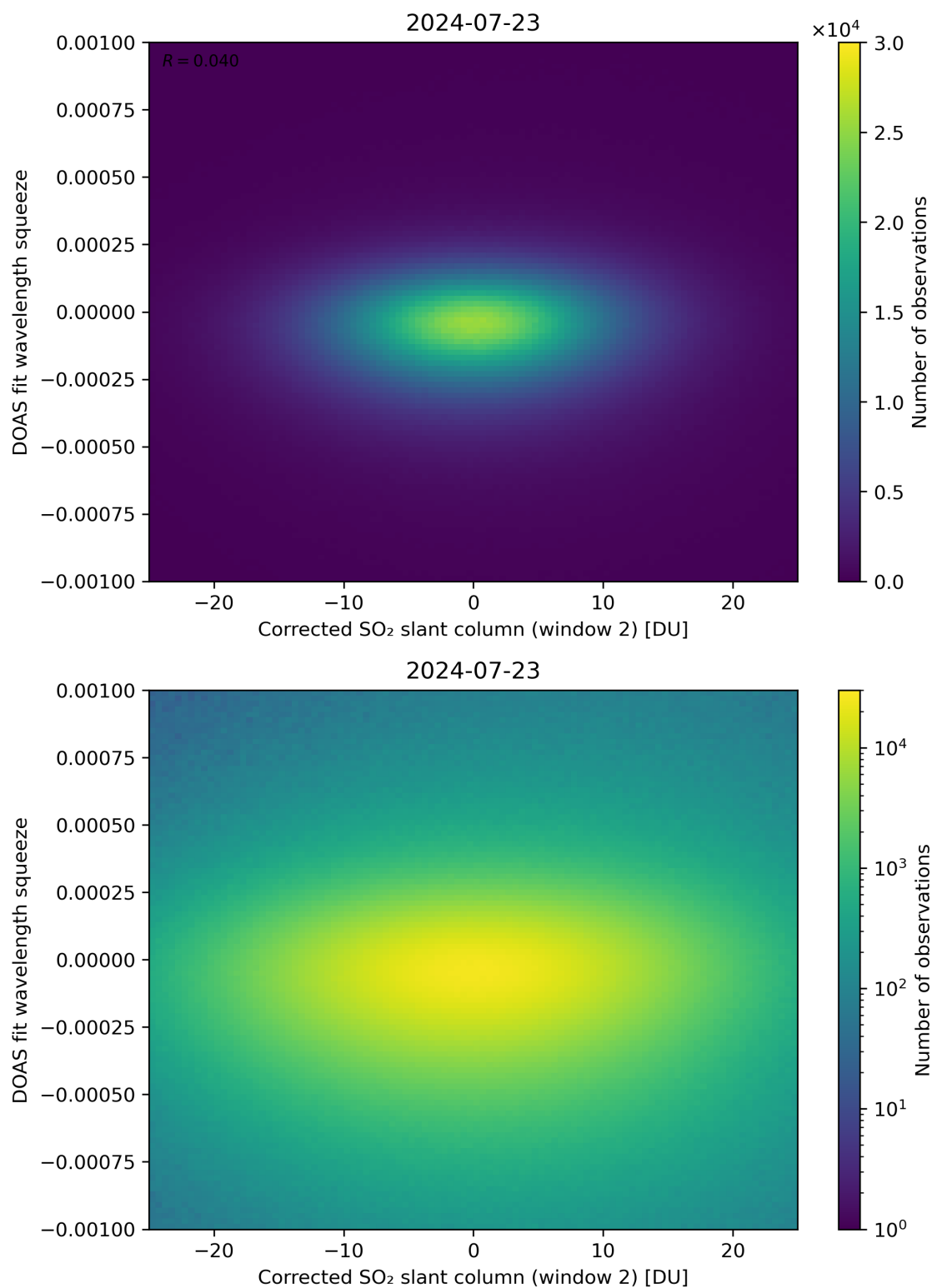
Figure 197: Scatter density plot of “Corrected SO 2 slant column (window 2)” against “DOAS fit wavelength squeeze” for 2024-07-22 to 2024-07-24.
