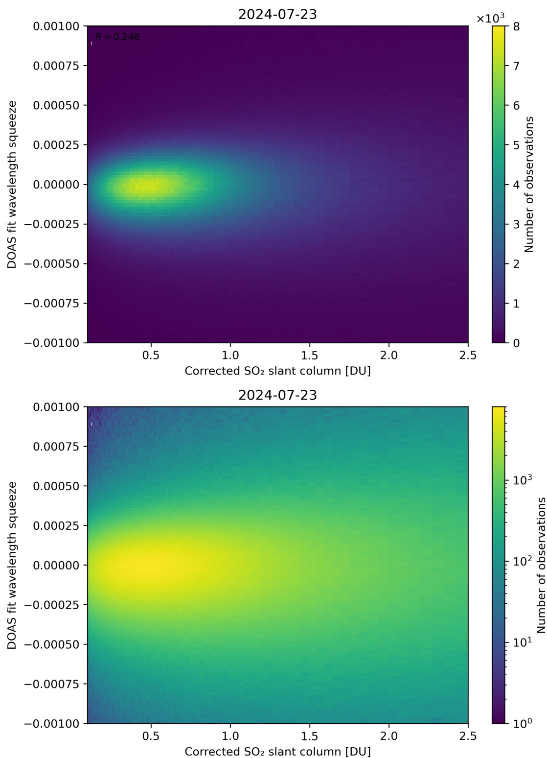
Figure 182: Scatter density plot of “Corrected SO 2 slant column” against “DOAS fit wavelength squeeze” for 2024-07-22 to 2024-07-24.
