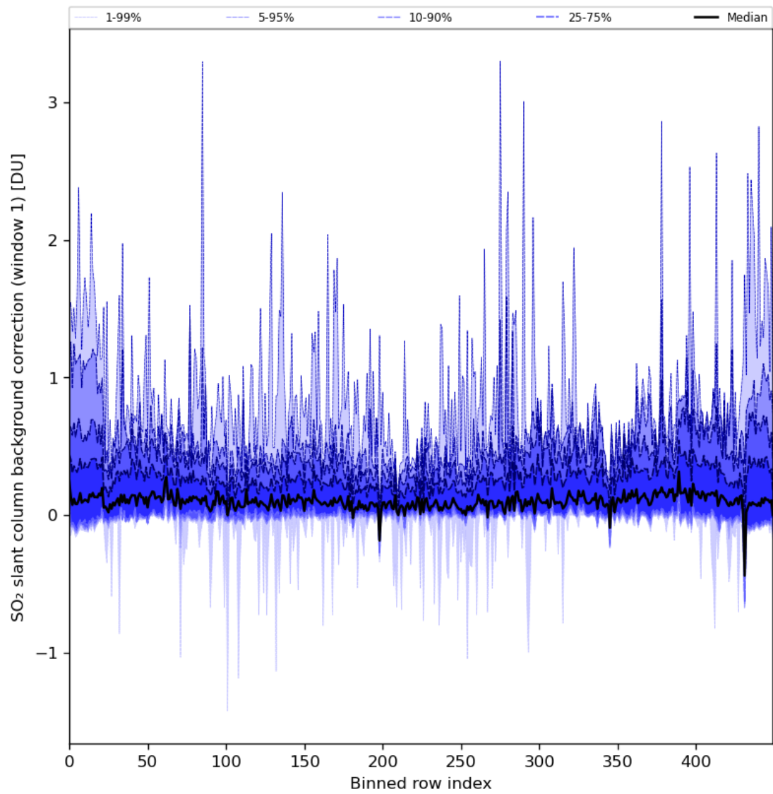
Figure 82: Along track statistics of "SO 2 slant column background correction (window 1)" for 2024-07-22 to 2024-07-24
