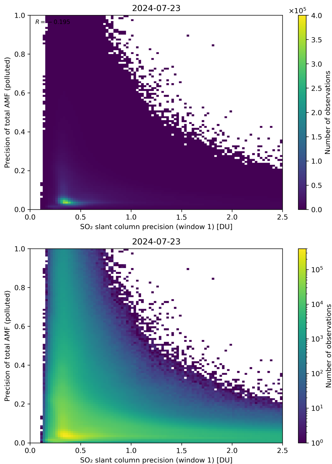
Figure 231: Scatter density plot of “SO 2 slant column precision (window 1)” against “Precision of total AMF (polluted)” for 2024-07-22 to 2024-07-24.
