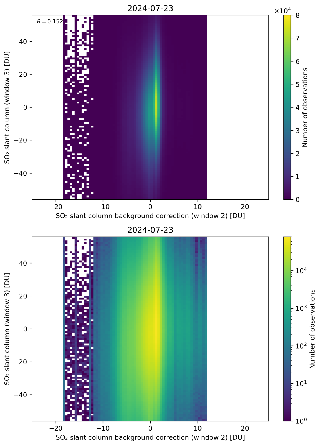
Figure 117: Scatter density plot of “SO 2 slant column background correction (window 2)” against “SO 2 slant column (window 3)” for 2024-07-22 to 2024-07-24.
