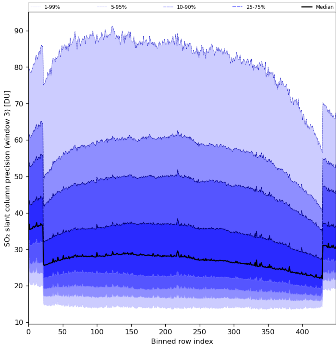
Figure 88: Along track statistics of “SO 2 slant column precision (window 3)” for 2024-07-22 to 2024-07-24
