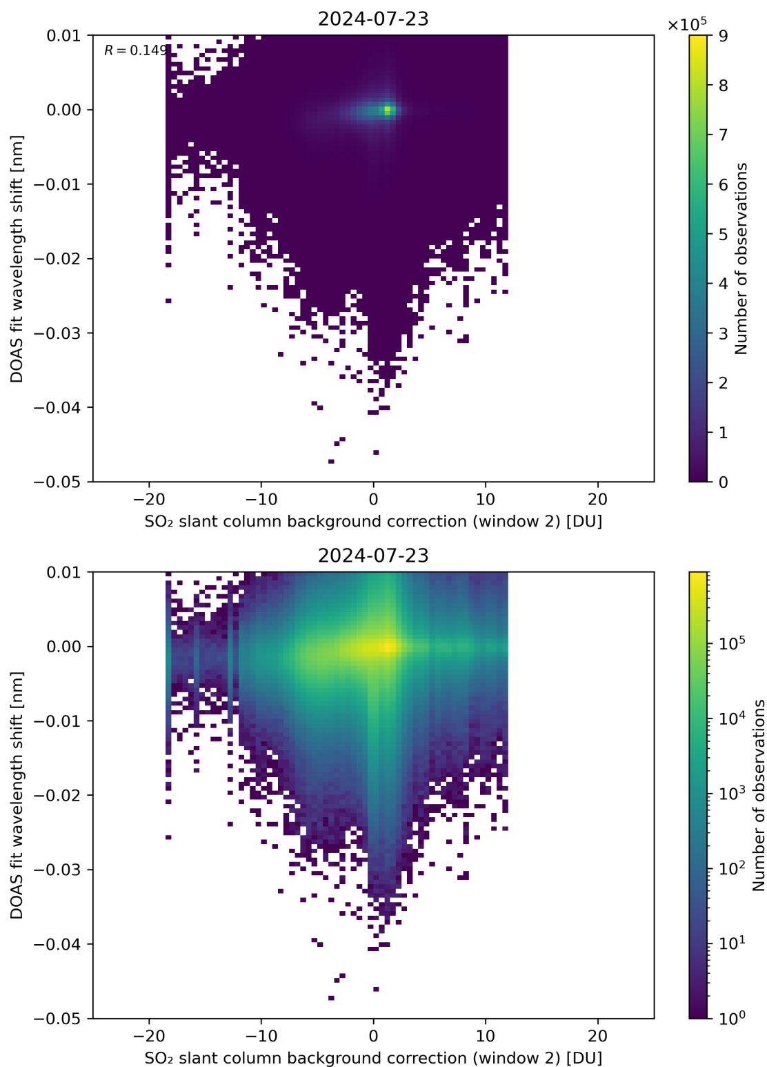
Figure 112: Scatter density plot of “SO 2 slant column background correction (window 2)” against “DOAS fit wavelength shift” for 2024-07-22 to 2024-07-24.
