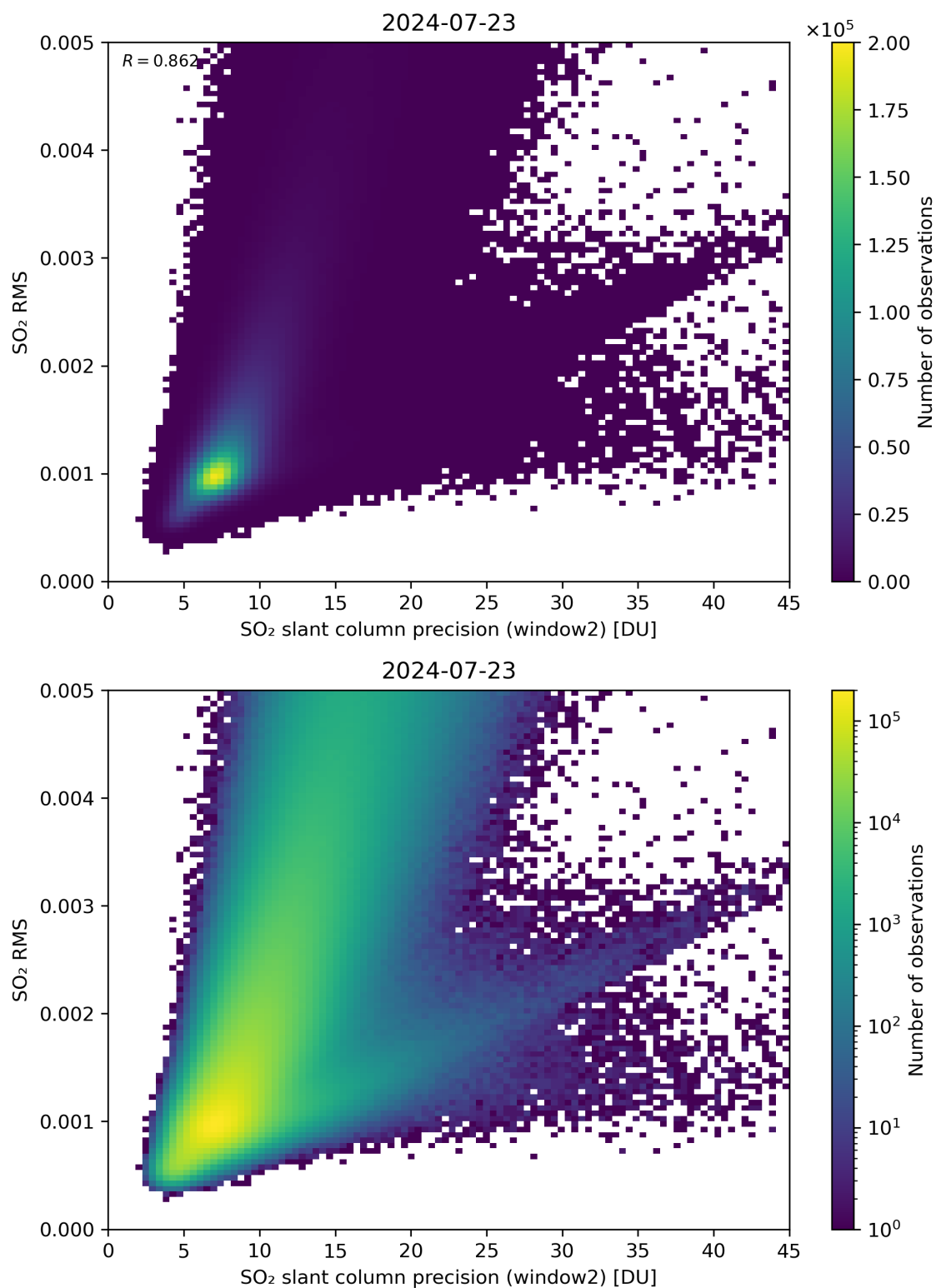
Figure 245: Scatter density plot of “SO 2 slant column precision (window2)” against “SO 2 RMS” for 2024-07-22 to 2024-07-24.
