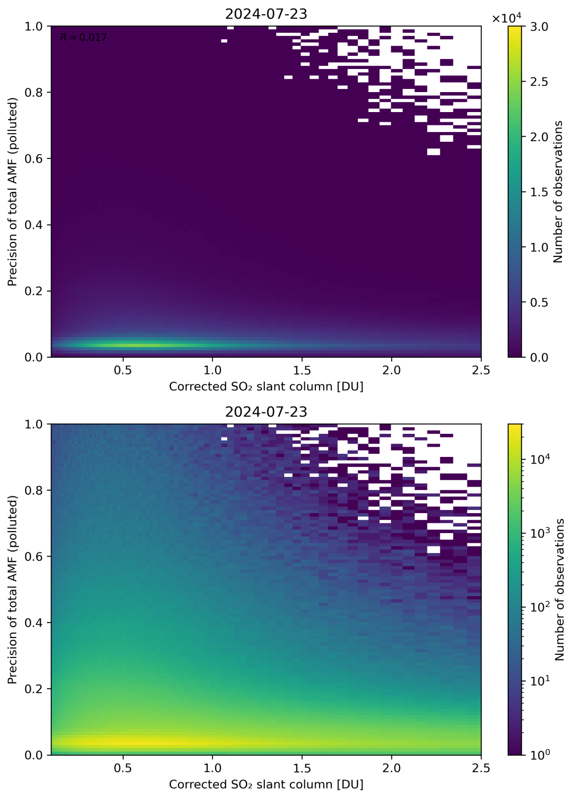
Figure 193: Scatter density plot of “Corrected SO 2 slant column” against “Precision of total AMF (polluted)” for 2024-07-22 to 2024-07-24.
