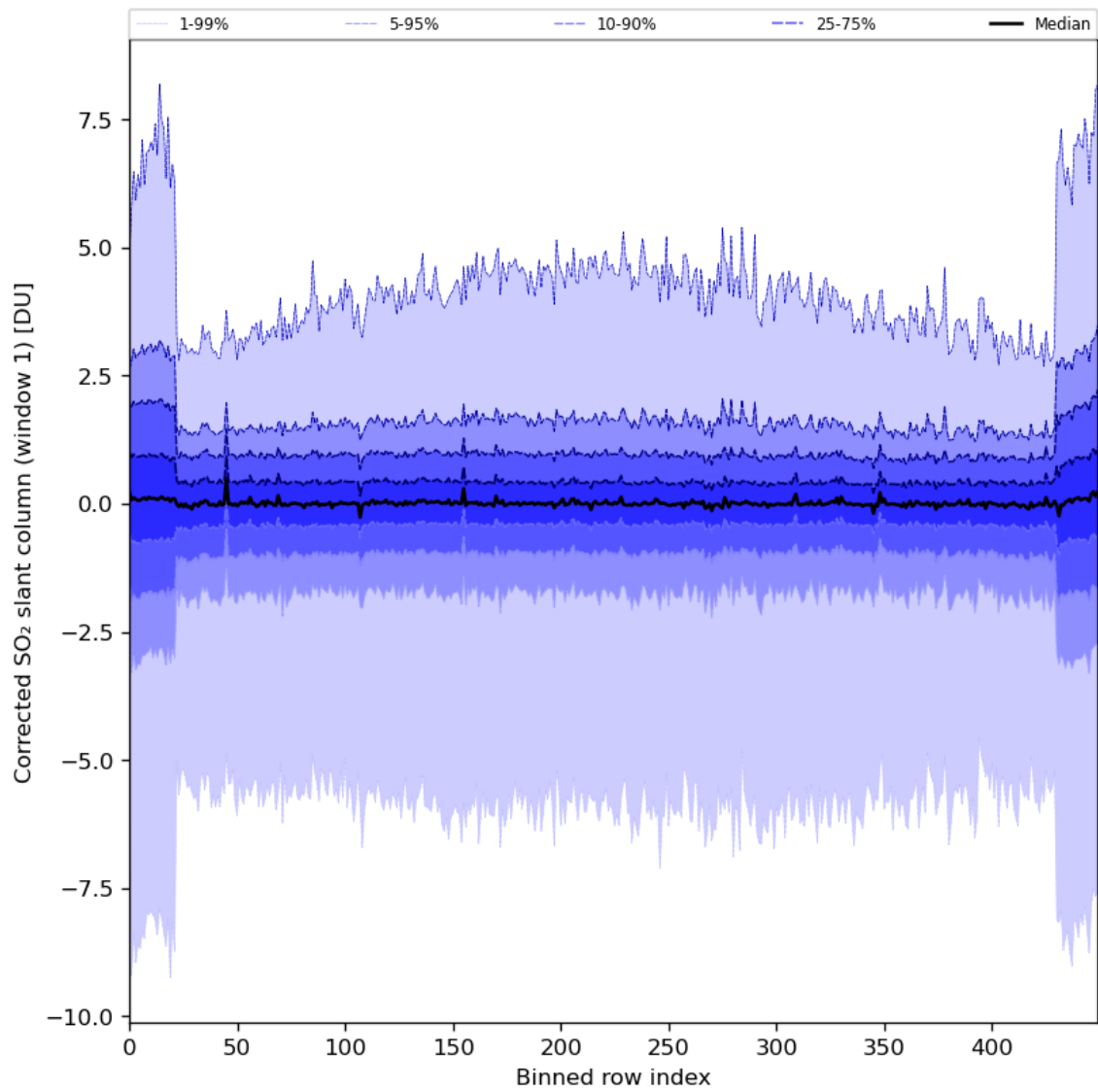
Figure 81: Along track statistics of “Corrected SO 2 slant column (window 1)” for 2024-07-22 to 2024-07-24
