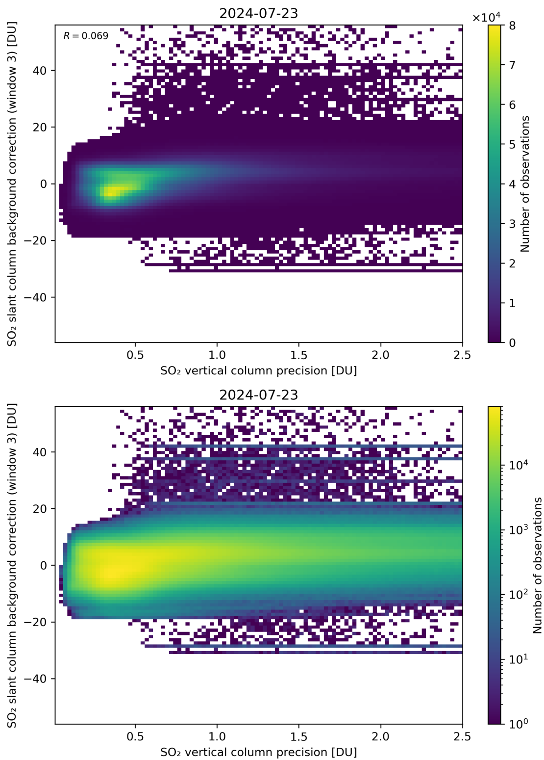
Figure 281: Scatter density plot of “SO 2 vertical column precision” against “SO 2 slant column background correction (window 3)” for 2024-07-22 to 2024-07-24.
