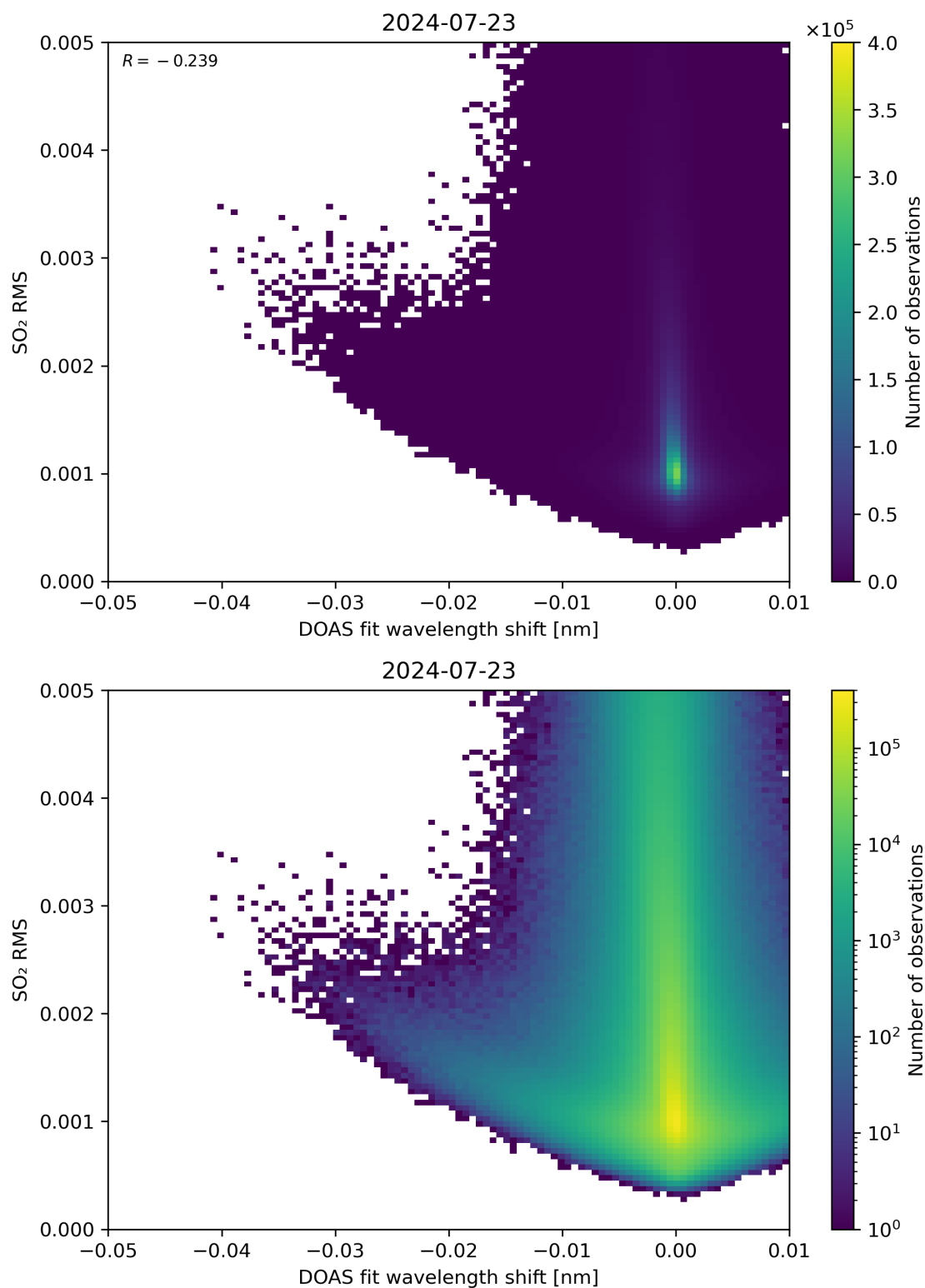
Figure 128: Scatter density plot of “DOAS fit wavelength shift” against “SO 2 RMS” for 2024-07-22 to 2024-07-24.
