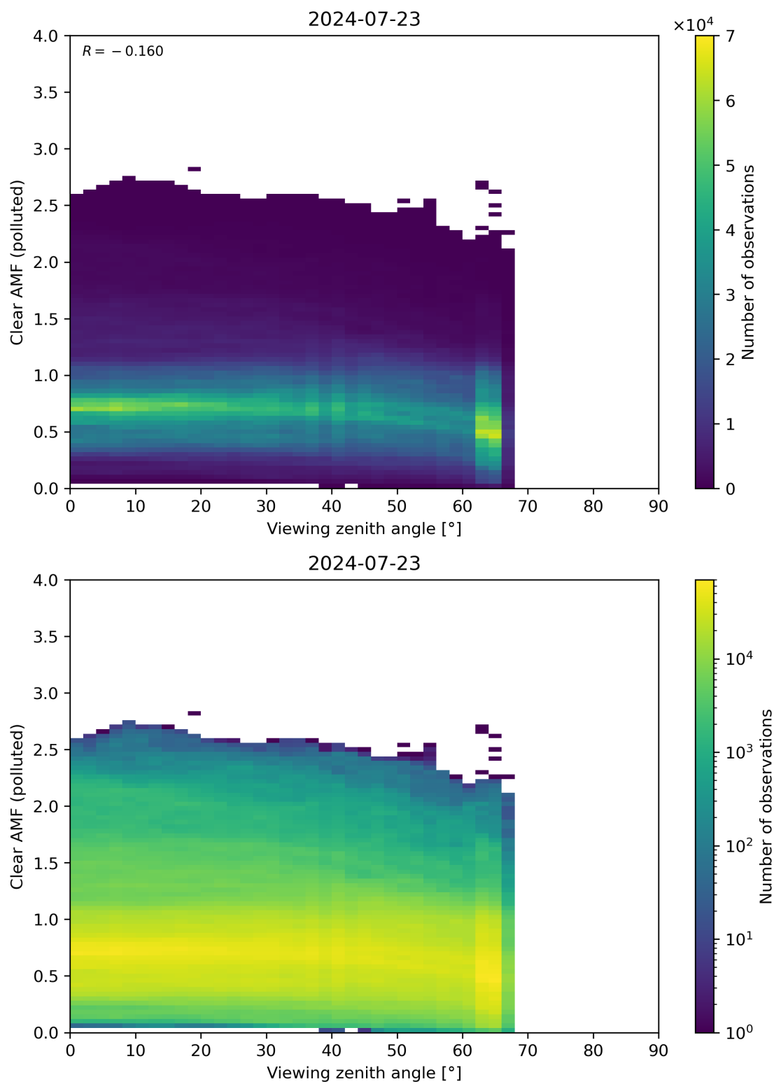
Figure 316: Scatter density plot of “Viewing zenith angle” against “Clear AMF (polluted)” for 2024-07-22 to 2024-07-24.
