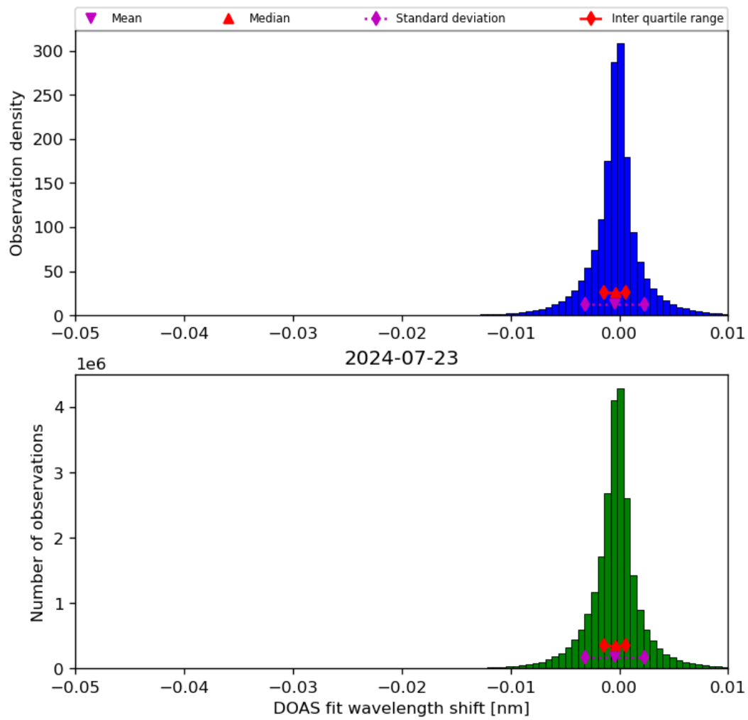
Figure 68: Histogram of “DOAS fit wavelength shift” for 2024-07-22 to 2024-07-24
