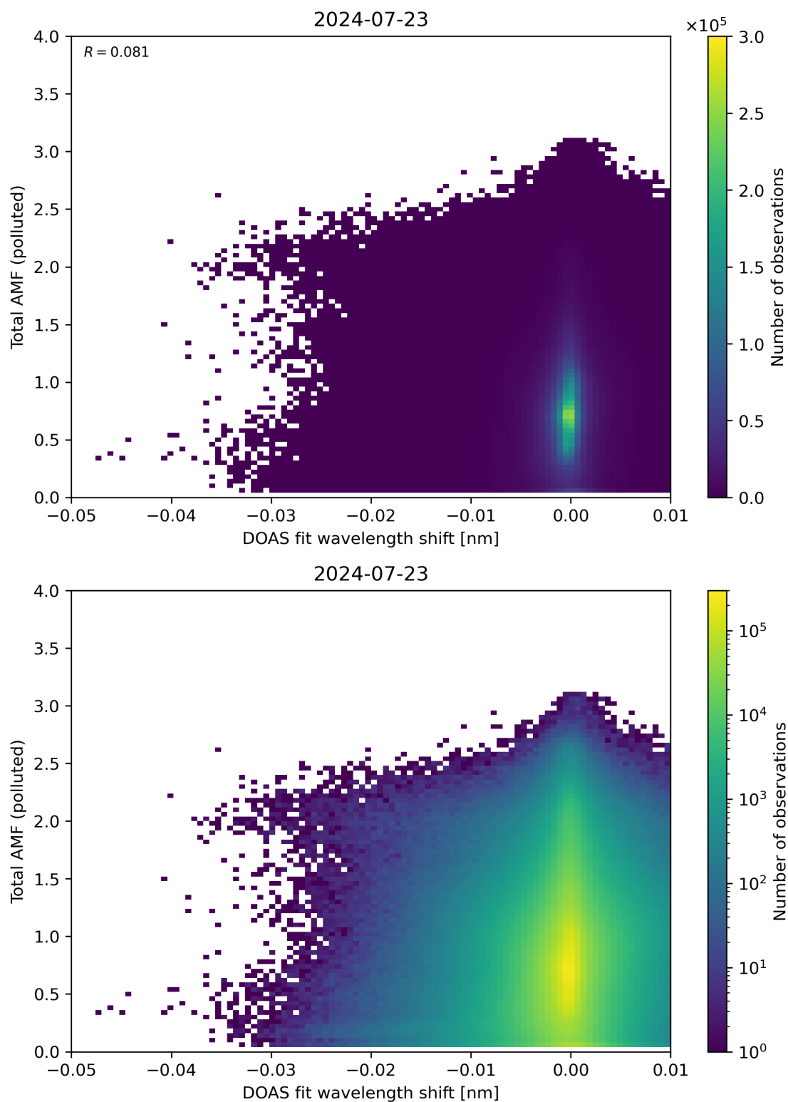
Figure 130: Scatter density plot of “DOAS fit wavelength shift” against “Total AMF (polluted)” for 2024-07-22 to 2024-07-24.
