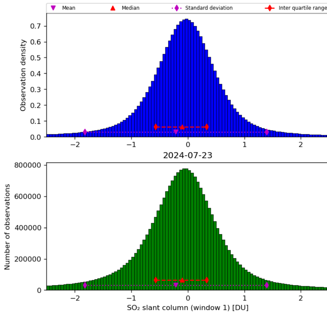
Figure 56: Histogram of “SO 2 slant column (window 1)” for 2024-07-22 to 2024-07-24
