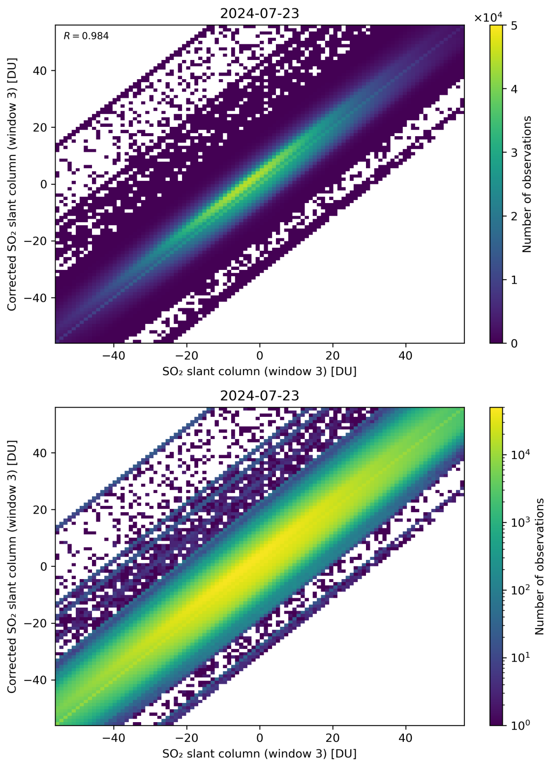
Figure 266: Scatter density plot of “SO 2 slant column (window 3)” against “Corrected SO 2 slant column (window 3)” for 2024-07-22 to 2024-07-24.
