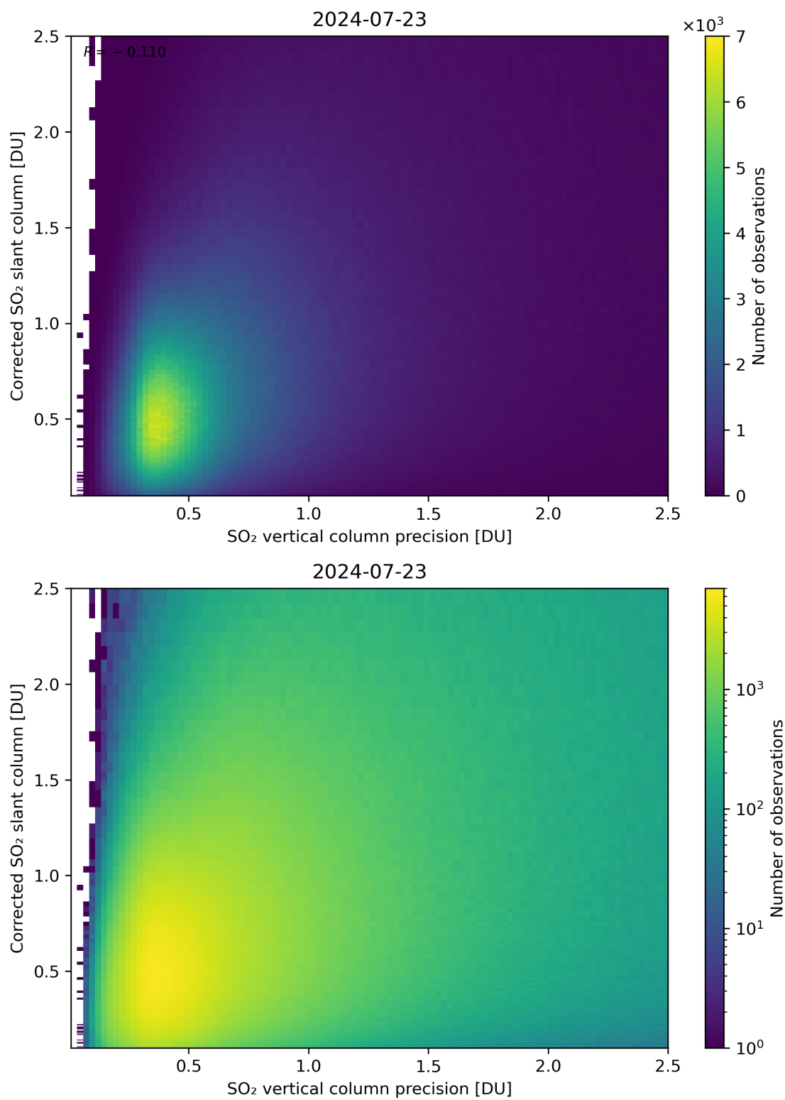
Figure 286: Scatter density plot of “SO 2 vertical column precision” against “Corrected SO 2 slant column” for 2024-07-22 to 2024-07-24.
