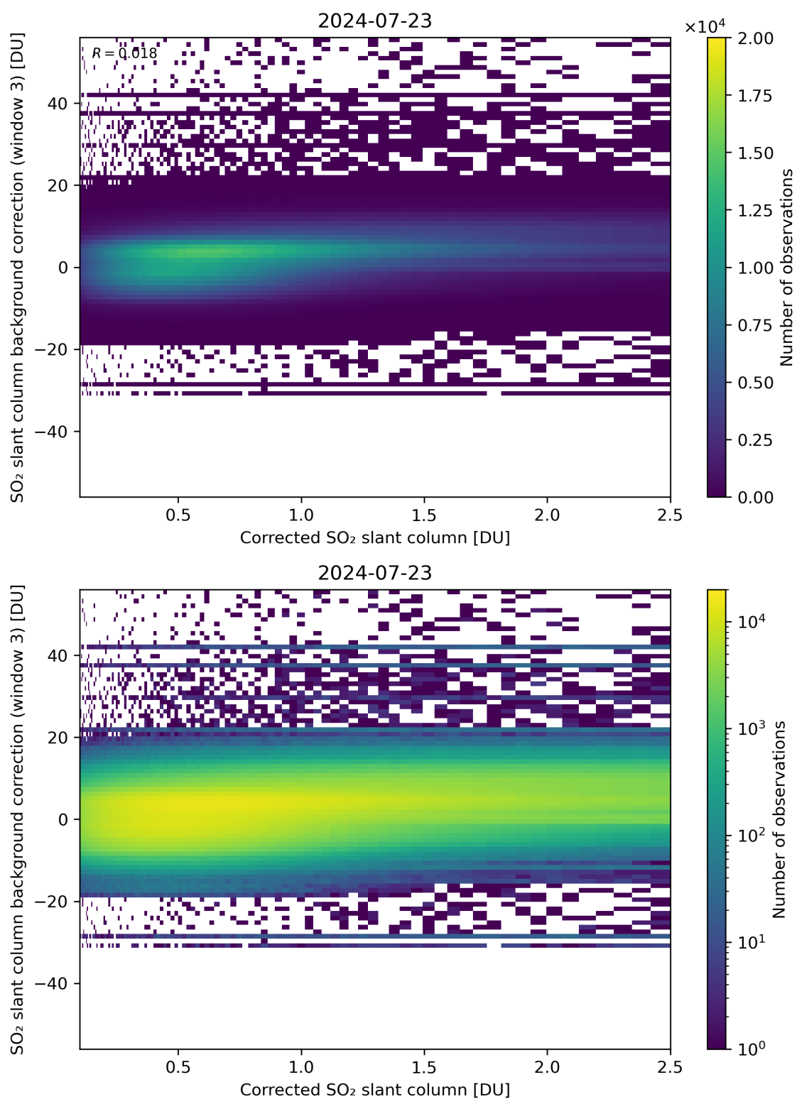
Figure 180: Scatter density plot of “Corrected SO 2 slant column” against “SO 2 slant column background correction (window 3)” for 2024-07-22 to 2024-07-24.
