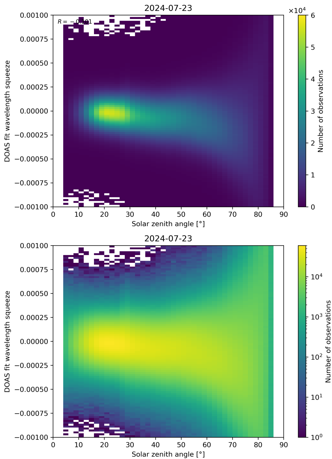
Figure 162: Scatter density plot of “Solar zenith angle” against “DOAS fit wavelength squeeze” for 2024-07-22 to 2024-07-24.
