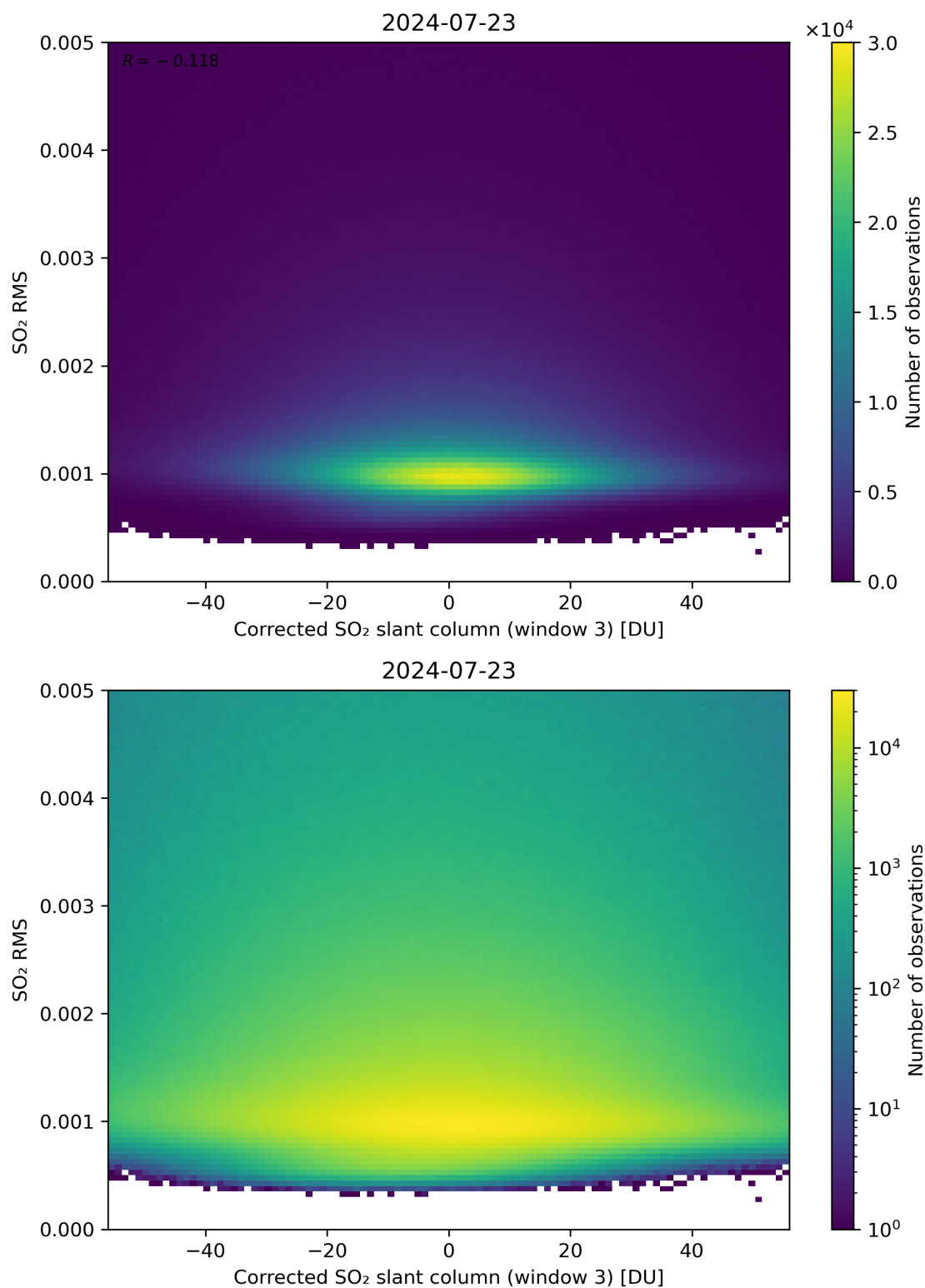
Figure 208: Scatter density plot of “Corrected SO 2 slant column (window 3)” against “SO 2 RMS” for 2024-07-22 to 2024-07-24.
