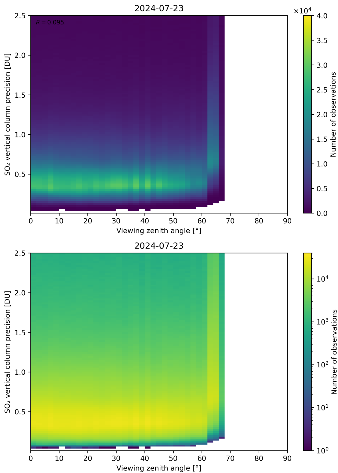
Figure 328: Scatter density plot of “Viewing zenith angle” against “SO 2 vertical column precision” for 2024-07-22 to 2024-07-24.
