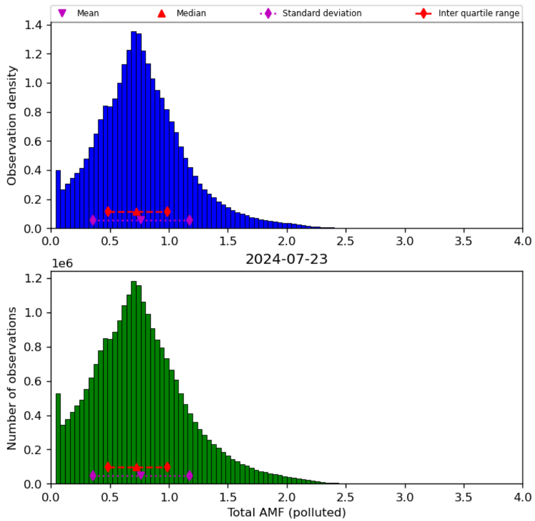
Figure 71: Histogram of “Total AMF (polluted)” for 2024-07-22 to 2024-07-24
