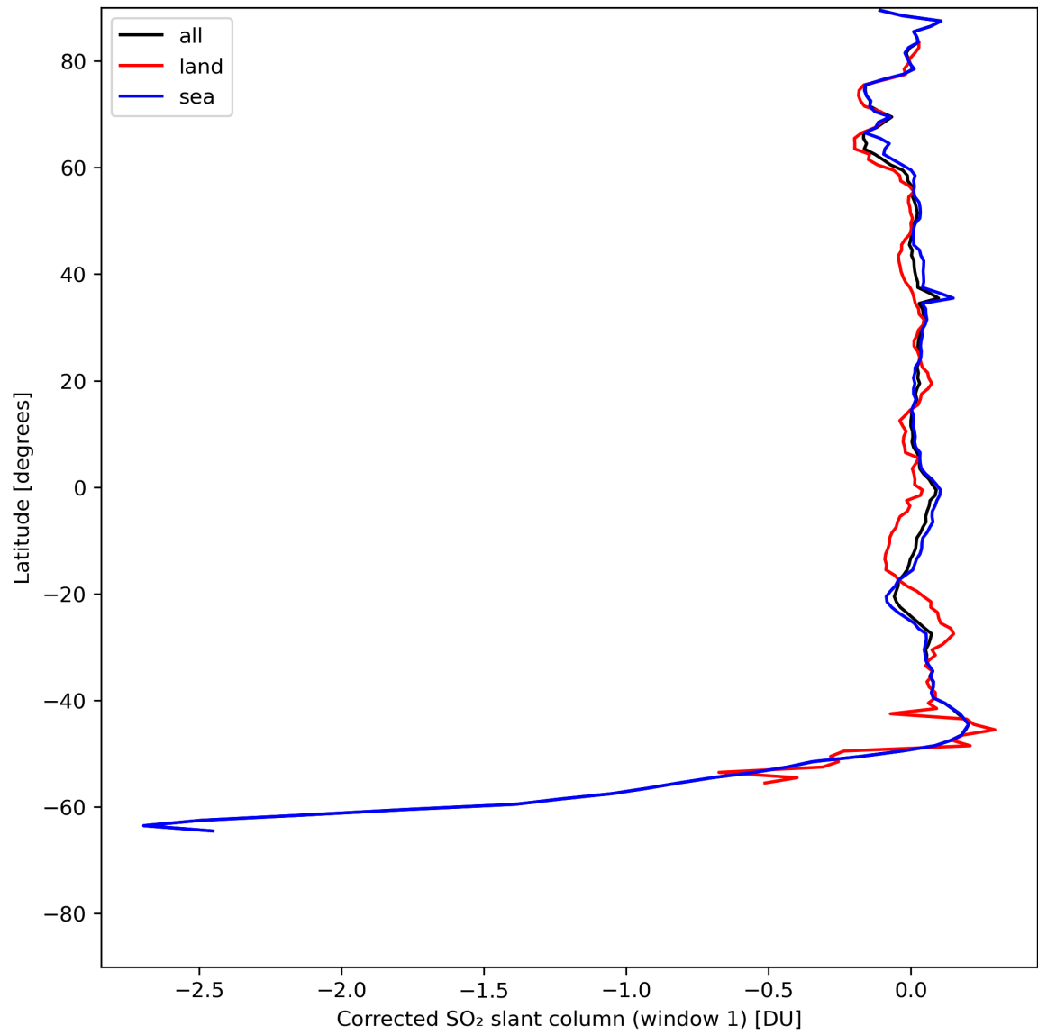
Figure 35: Zonal average of “Corrected SO 2 slant column (window 1)” for 2024-07-22 to 2024-07-24.
