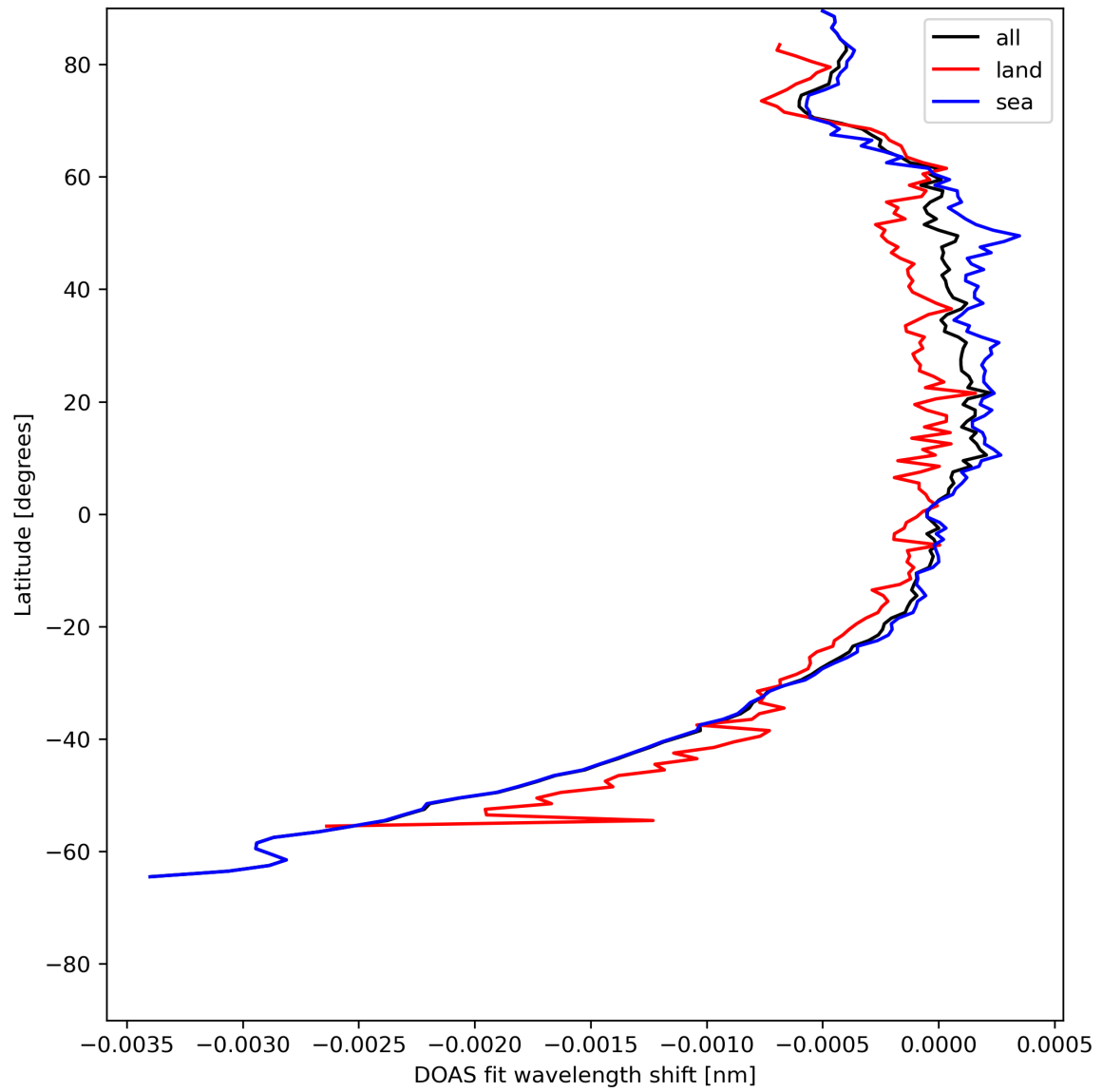
Figure 45: Zonal average of “DOAS fit wavelength shift” for 2024-07-22 to 2024-07-24.
