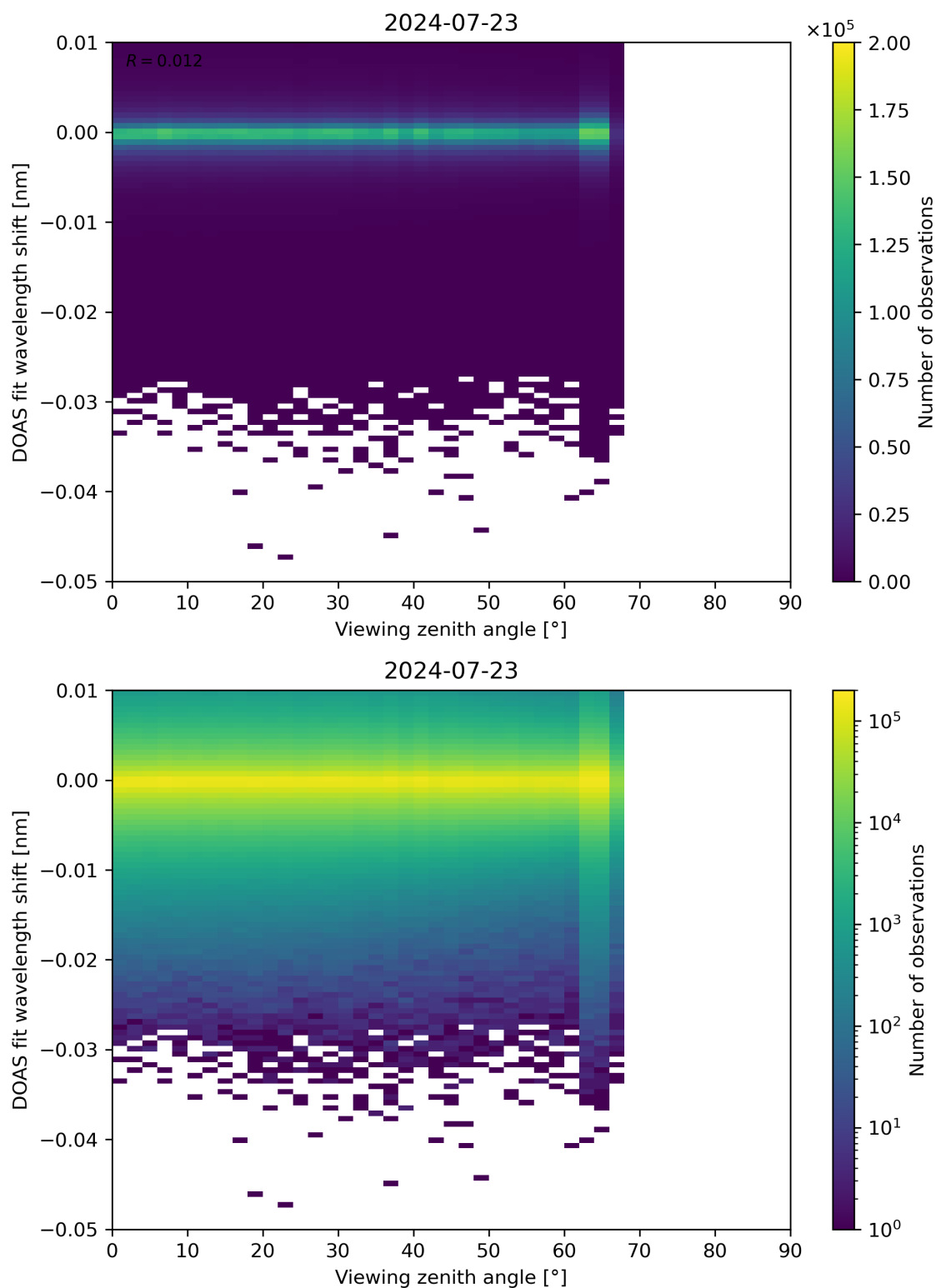
Figure 311: Scatter density plot of “Viewing zenith angle” against “DOAS fit wavelength shift” for 2024-07-22 to 2024-07-24.
