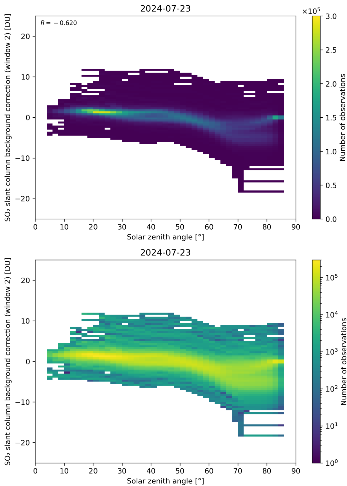
Figure 159: Scatter density plot of “Solar zenith angle” against “SO 2 slant column background correction (window 2)” for 2024-07-22 to 2024-07-24.
