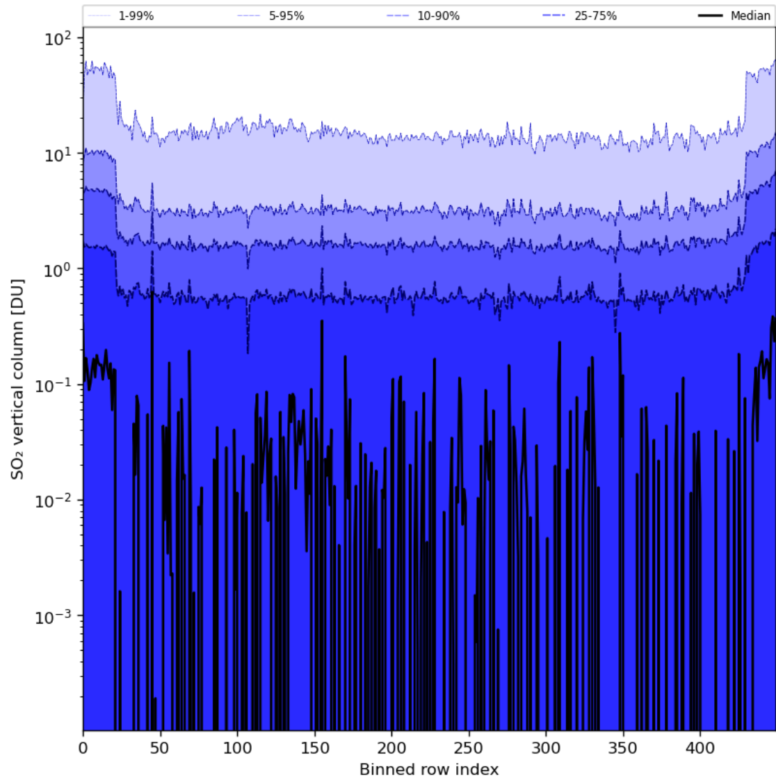
Figure 76: Along track statistics of “SO 2 vertical column” for 2024-07-22 to 2024-07-24
