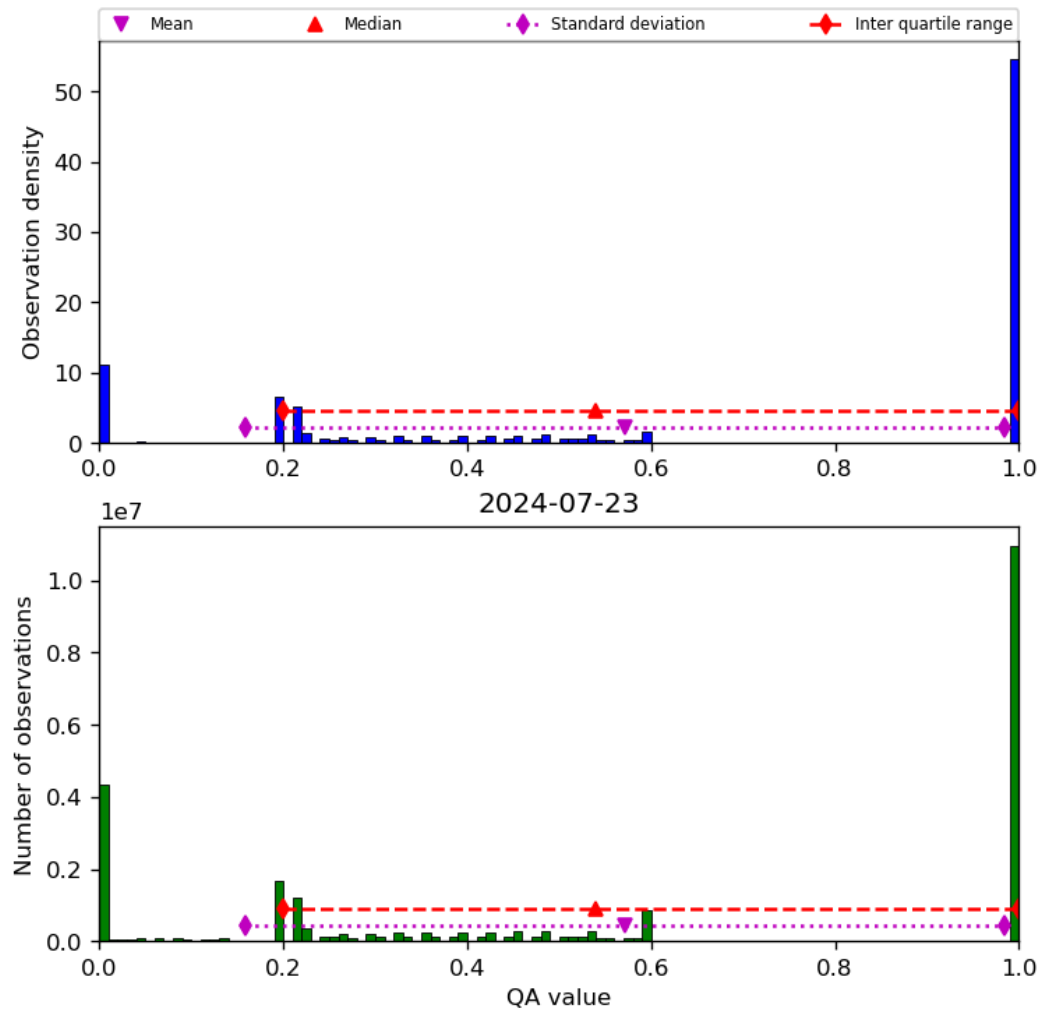
Figure 52: Histogram of “QA value” for 2024-07-22 to 2024-07-24
