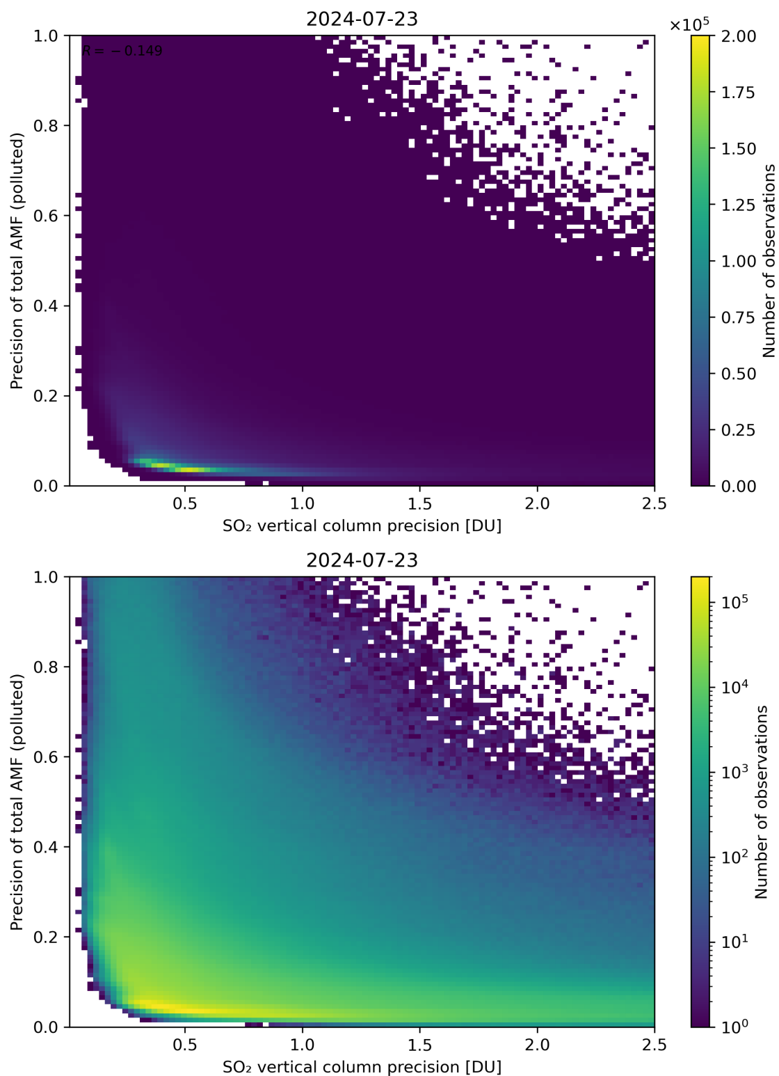
Figure 295: Scatter density plot of “SO 2 vertical column precision” against “Precision of total AMF (polluted)” for 2024-07-22 to 2024-07-24.
