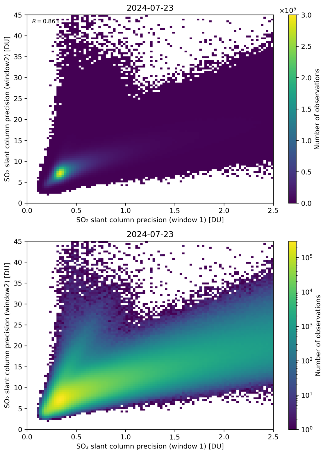
Figure 227: Scatter density plot of “SO 2 slant column precision (window 1)” against “SO 2 slant column precision (window2)” for 2024-07-22 to 2024-07-24.
