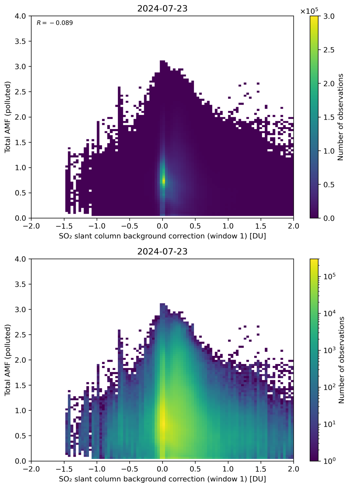
Figure 109: Scatter density plot of “SO 2 slant column background correction (window 1)” against “Total AMF (polluted)” for 2024-07-22 to 2024-07-24.
