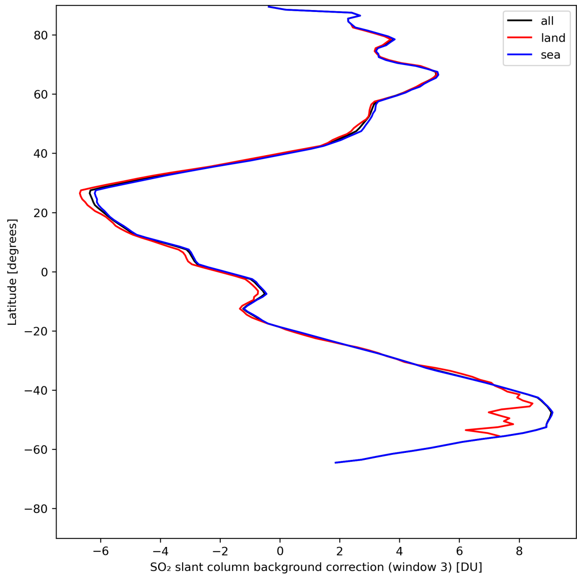
Figure 44: Zonal average of “SO 2 slant column background correction (window 3)” for 2024-07-22 to 2024-07-24.
