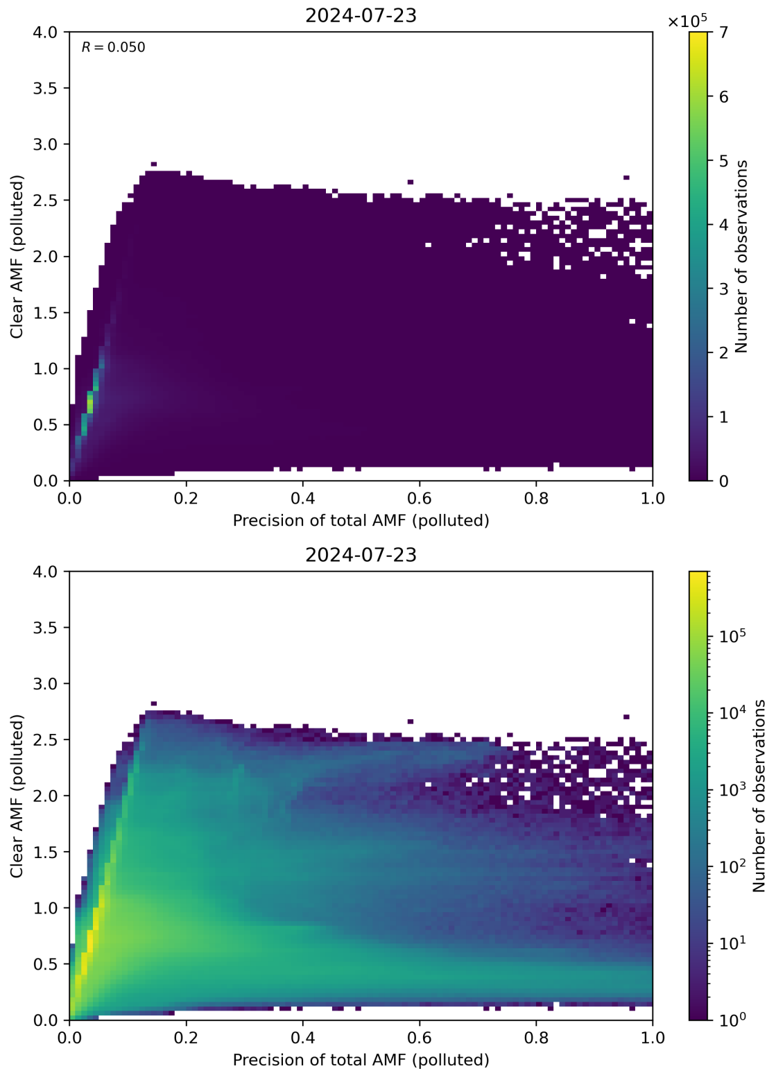
Figure 270: Scatter density plot of “Precision of total AMF (polluted)” against “Clear AMF (polluted)” for 2024-07-22 to 2024-07-24.
