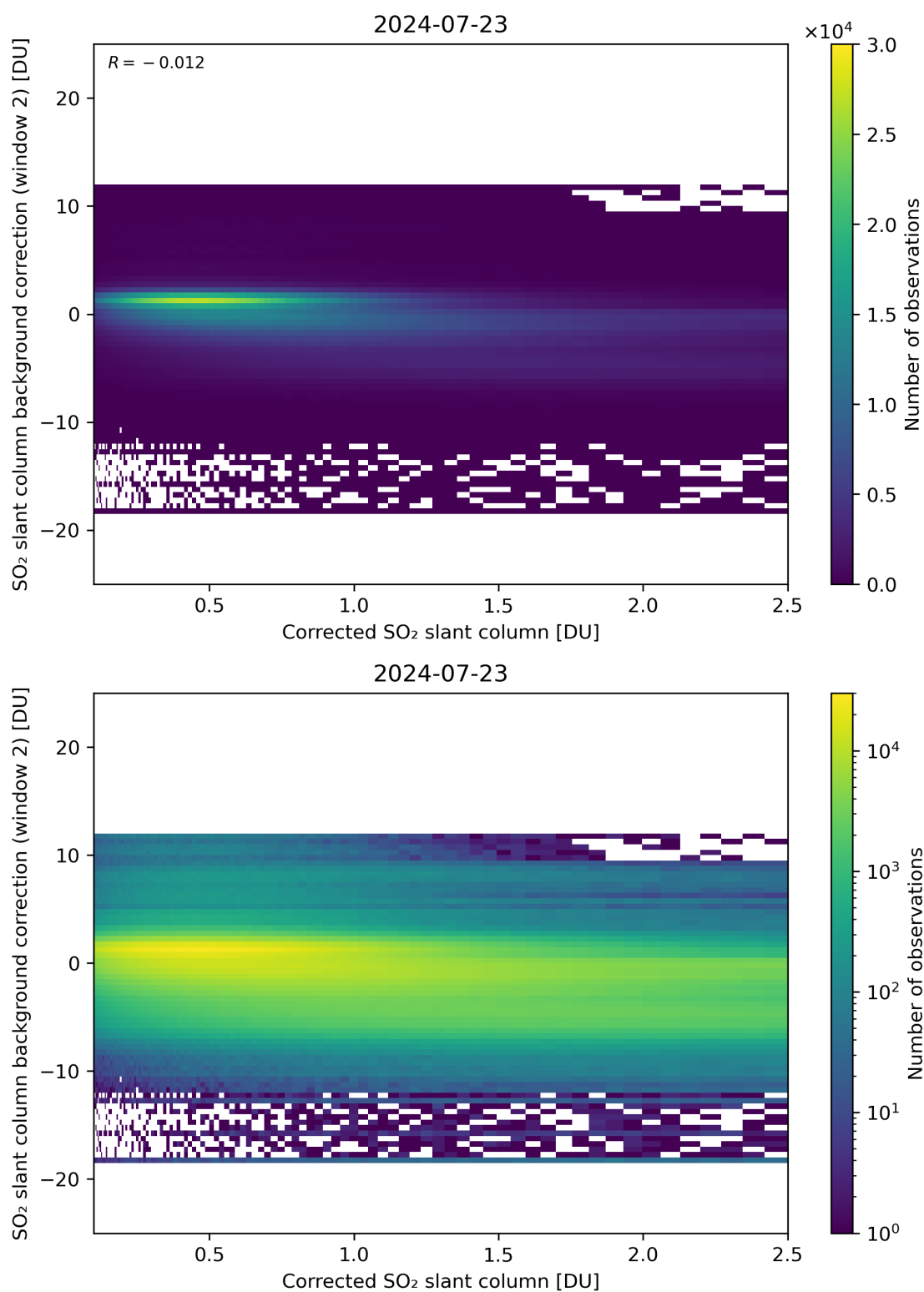
Figure 179: Scatter density plot of “Corrected SO 2 slant column” against “SO 2 slant column background correction (window 2)” for 2024-07-22 to 2024-07-24.
