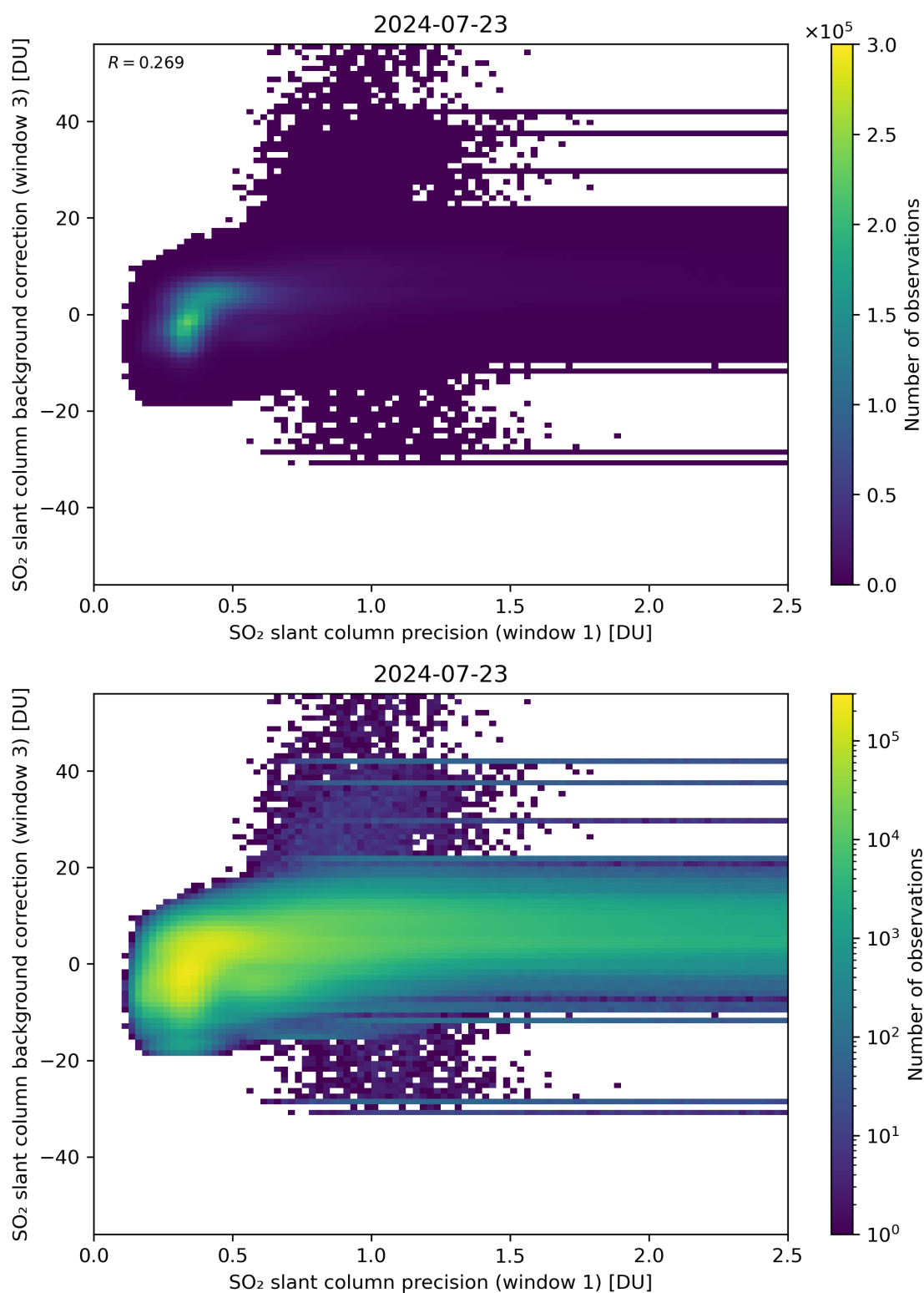
Figure 220: Scatter density plot of “SO 2 slant column precision (window 1)” against “SO 2 slant column background correction (window 3)” for 2024-07-22 to 2024-07-24.
