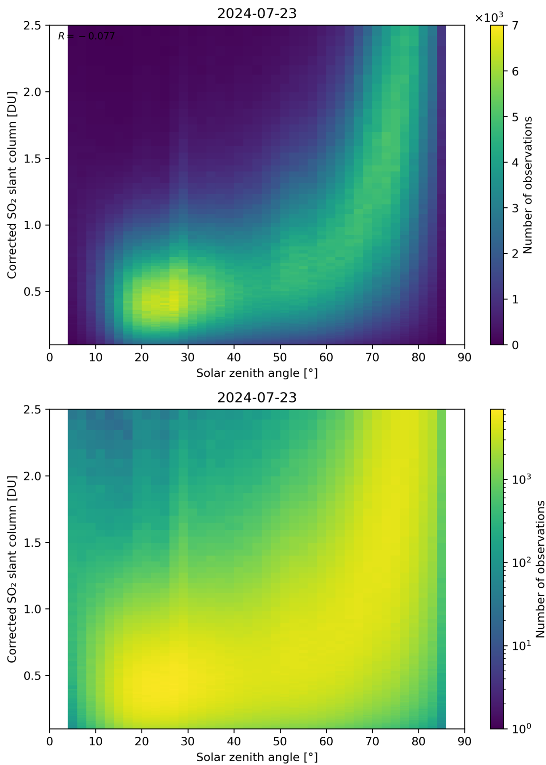
Figure 166: Scatter density plot of “Solar zenith angle” against “Corrected SO 2 slant column” for 2024-07-22 to 2024-07-24.
