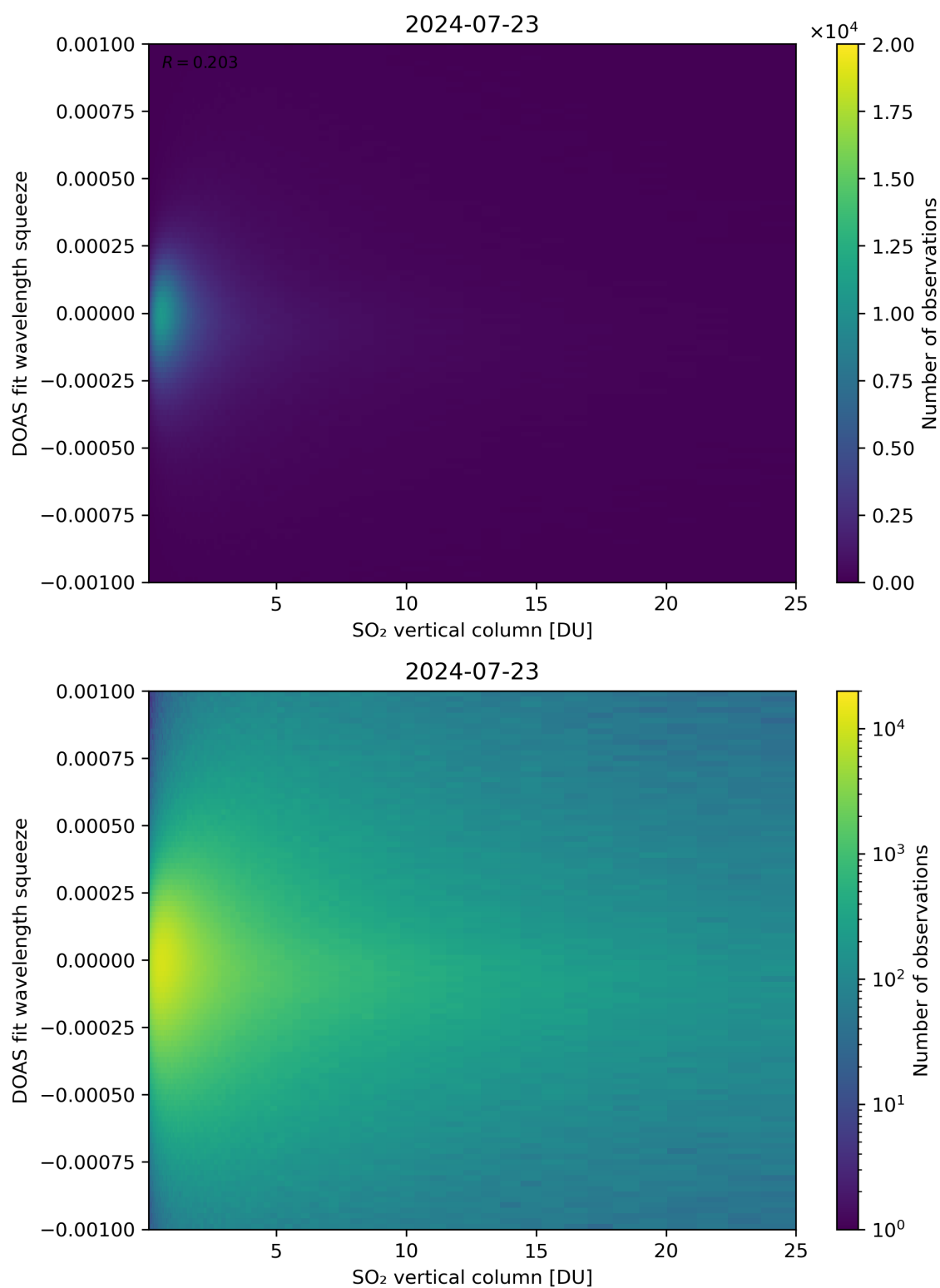
Figure 277: Scatter density plot of “SO 2 vertical column” against “DOAS fit wavelength squeeze” for 2024-07-22 to 2024-07-24.
