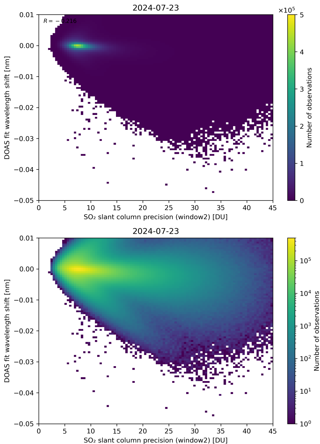
Figure 243: Scatter density plot of “SO 2 slant column precision (window2)” against “DOAS fit wavelength shift” for 2024-07-22 to 2024-07-24.
