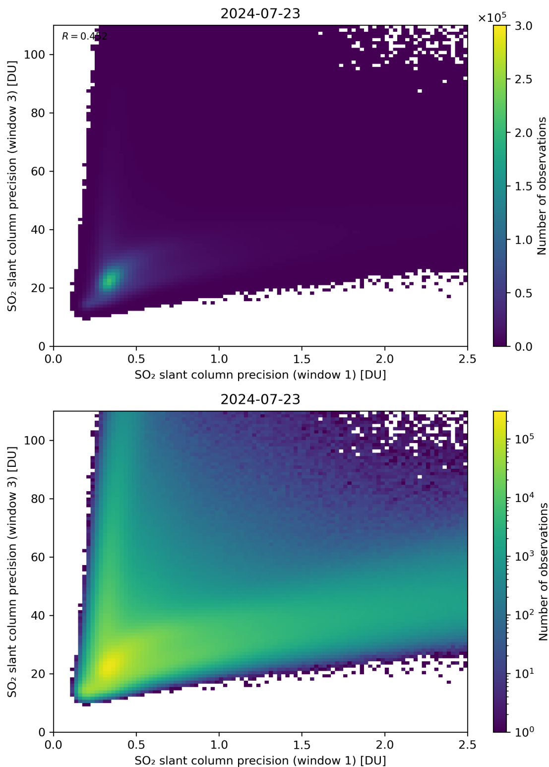
Figure 229: Scatter density plot of “SO 2 slant column precision (window 1)” against “SO 2 slant column precision (window 3)” for 2024-07-22 to 2024-07-24.
