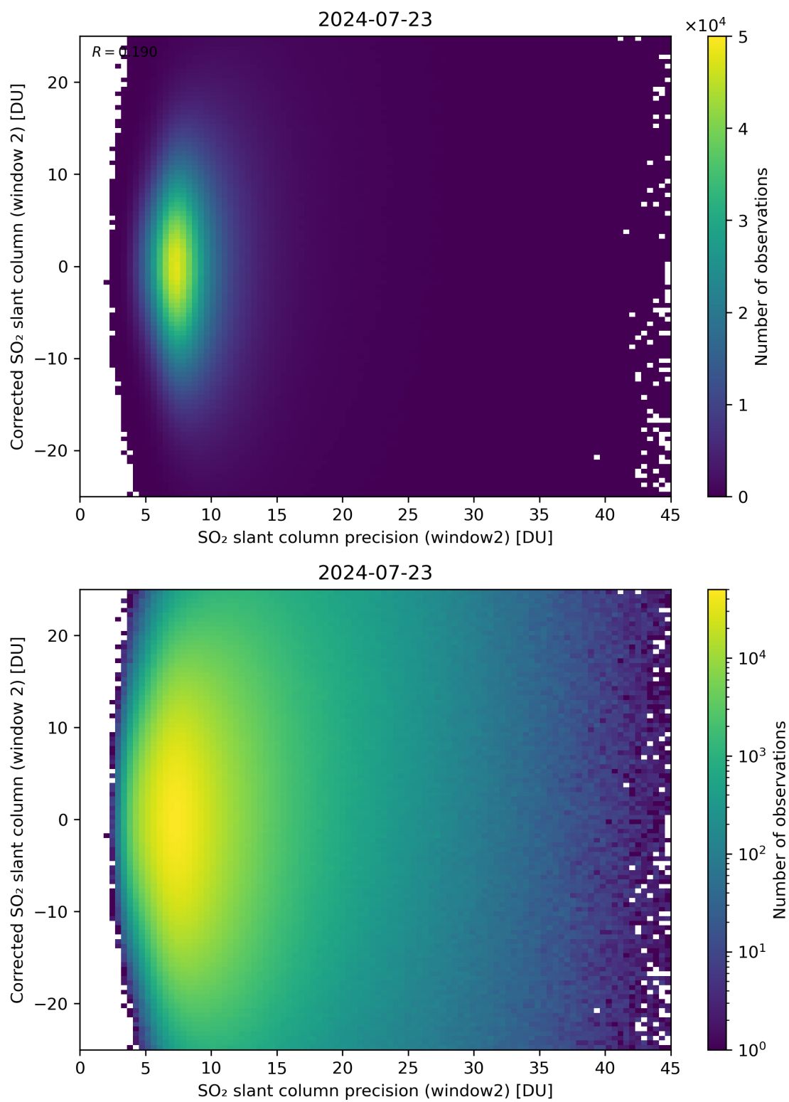
Figure 247: Scatter density plot of “SO 2 slant column precision (window2)” against “Corrected SO 2 slant column (window 2)” for 2024-07-22 to 2024-07-24.
