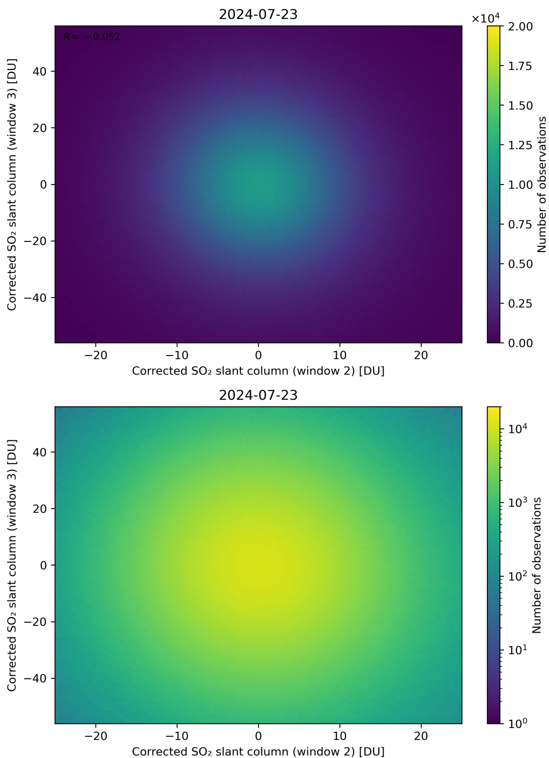
Figure 200: Scatter density plot of “Corrected SO 2 slant column (window 2)” against “Corrected SO 2 slant column (window 3)” for 2024-07-22 to 2024-07-24.
