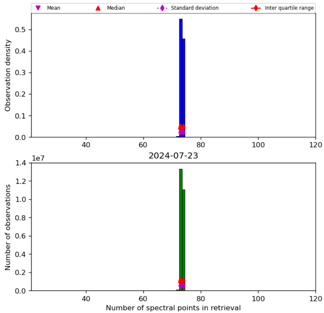
Figure 74: Histogram of “Number of spectral points in retrieval” for 2024-07-22 to 2024-07-24
