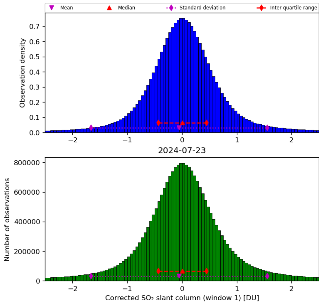
Figure 58: Histogram of “Corrected SO 2 slant column (window 1)” for 2024-07-22 to 2024-07-24
