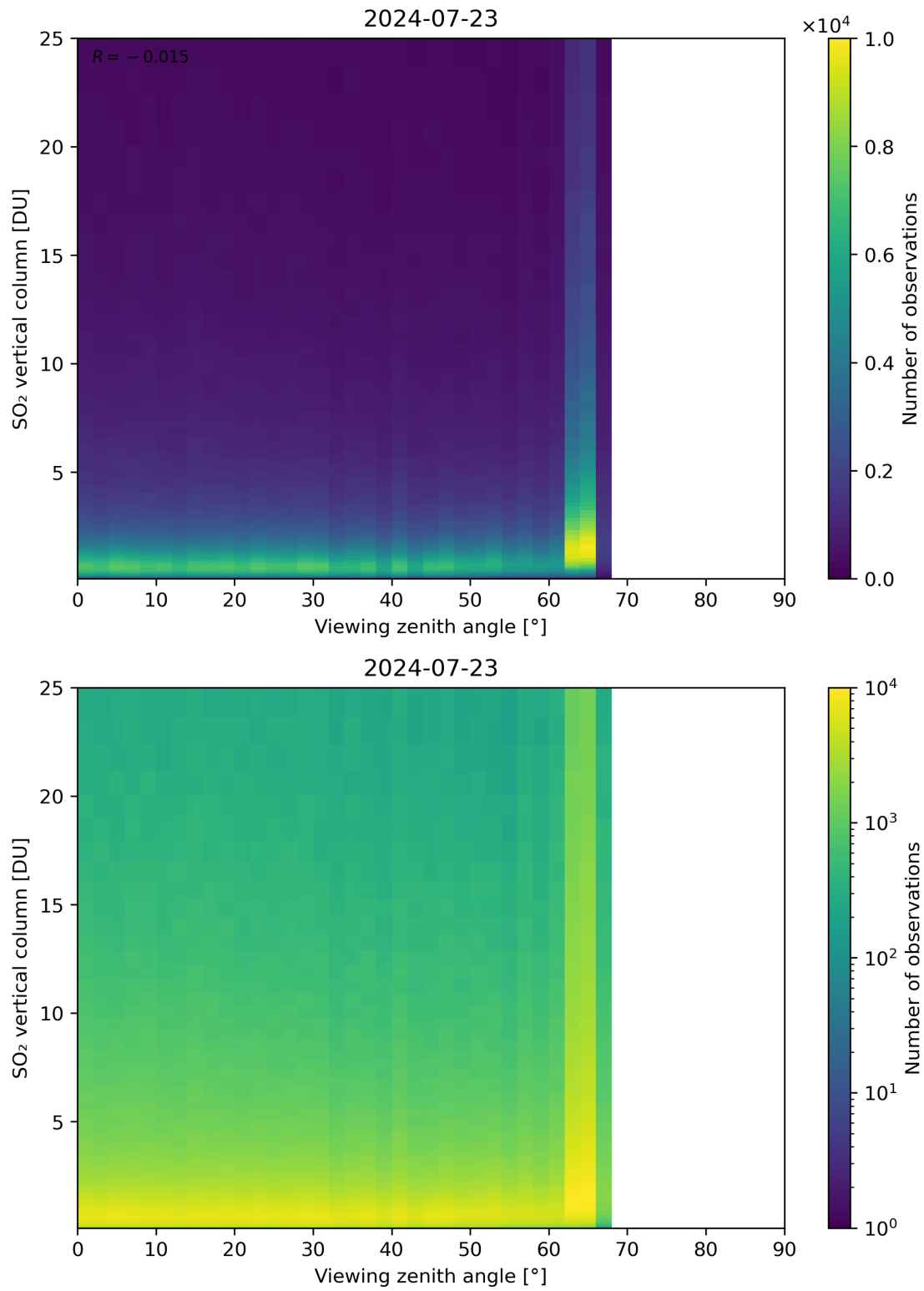
Figure 327: Scatter density plot of “Viewing zenith angle” against “SO 2 vertical column” for 2024-07-22 to 2024-07-24.
