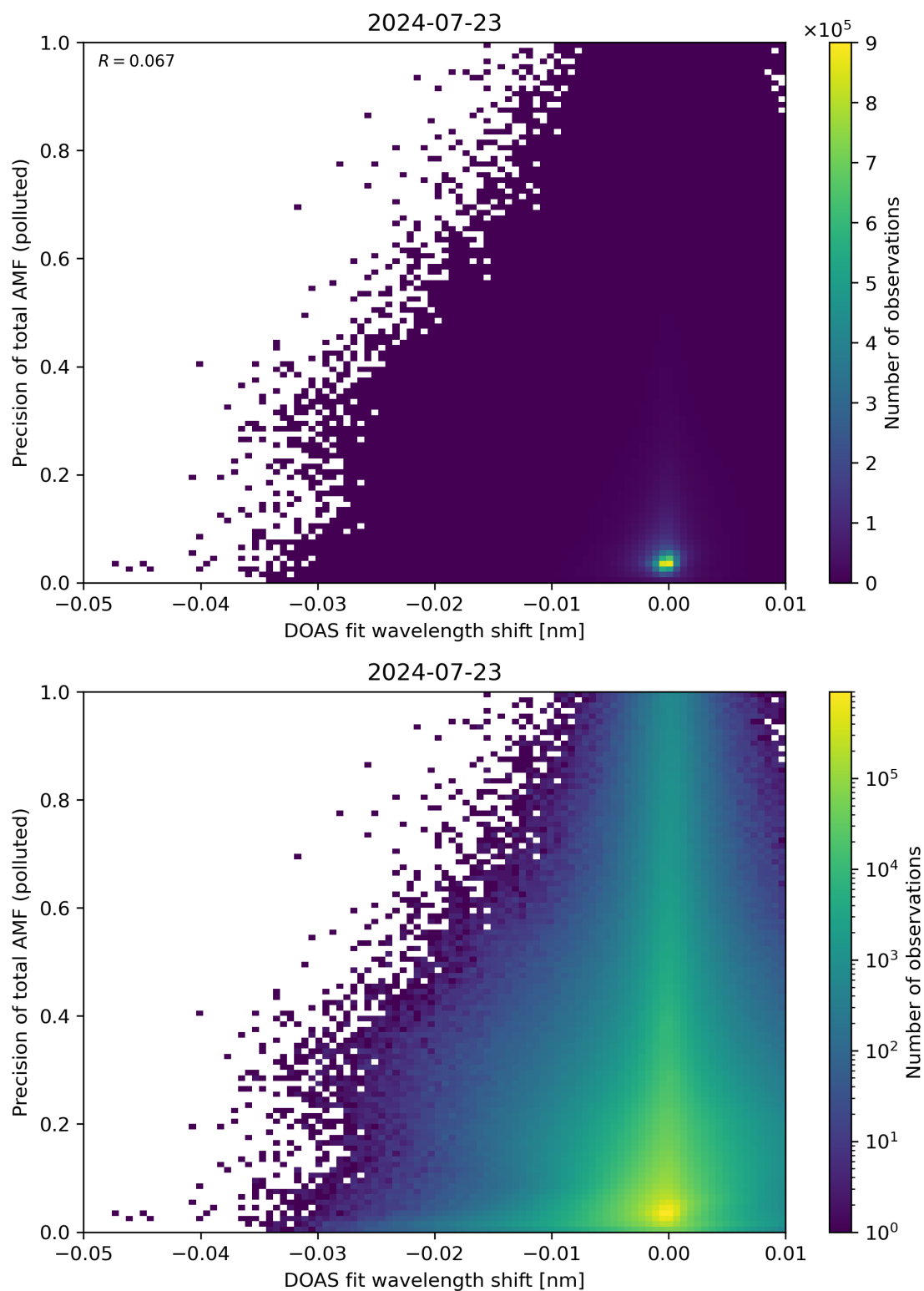
Figure 131: Scatter density plot of “DOAS fit wavelength shift” against “Precision of total AMF (polluted)” for 2024-07-22 to 2024-07-24.
