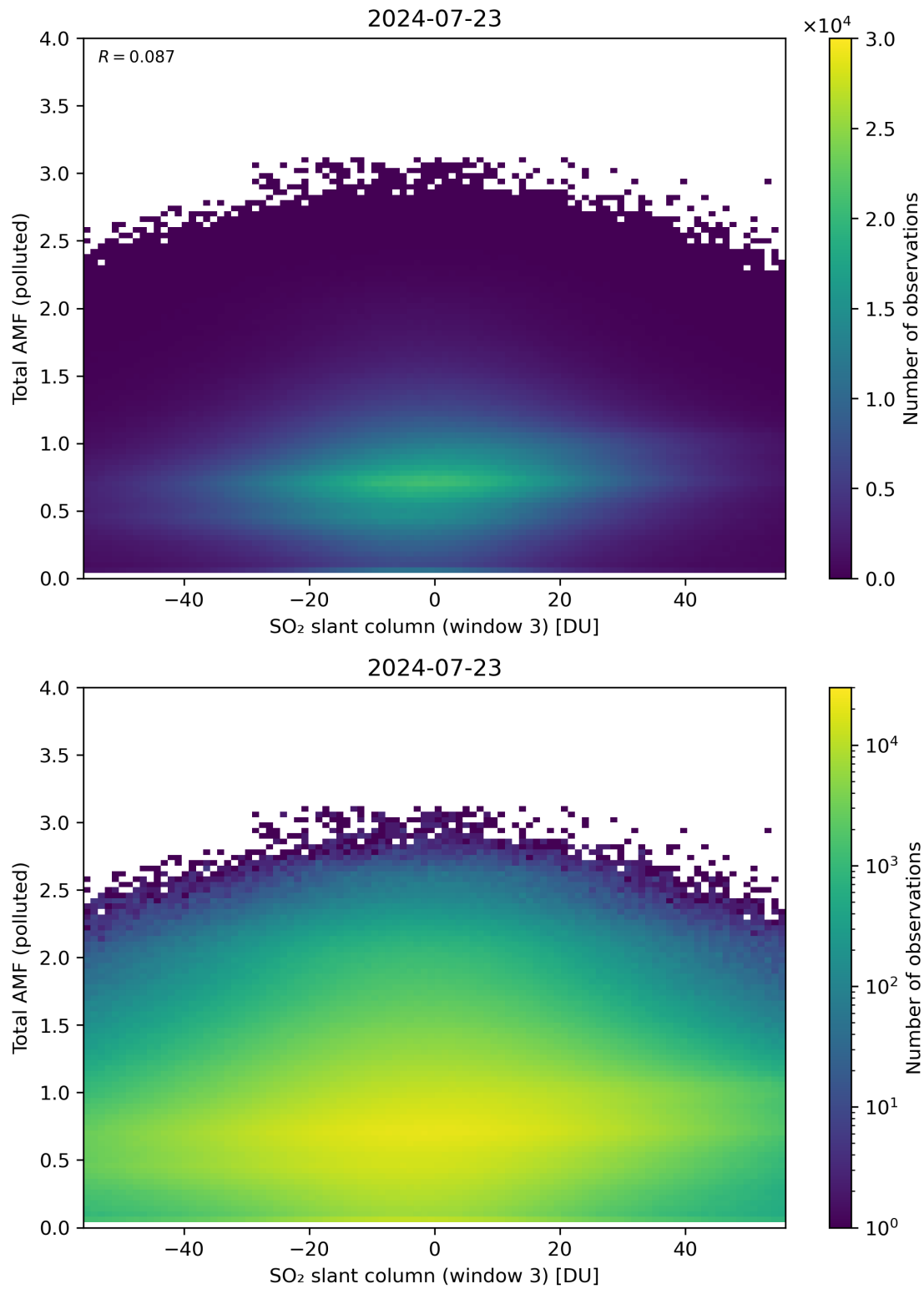
Figure 268: Scatter density plot of “SO 2 slant column (window 3)” against “Total AMF (polluted)” for 2024-07-22 to 2024-07-24.
