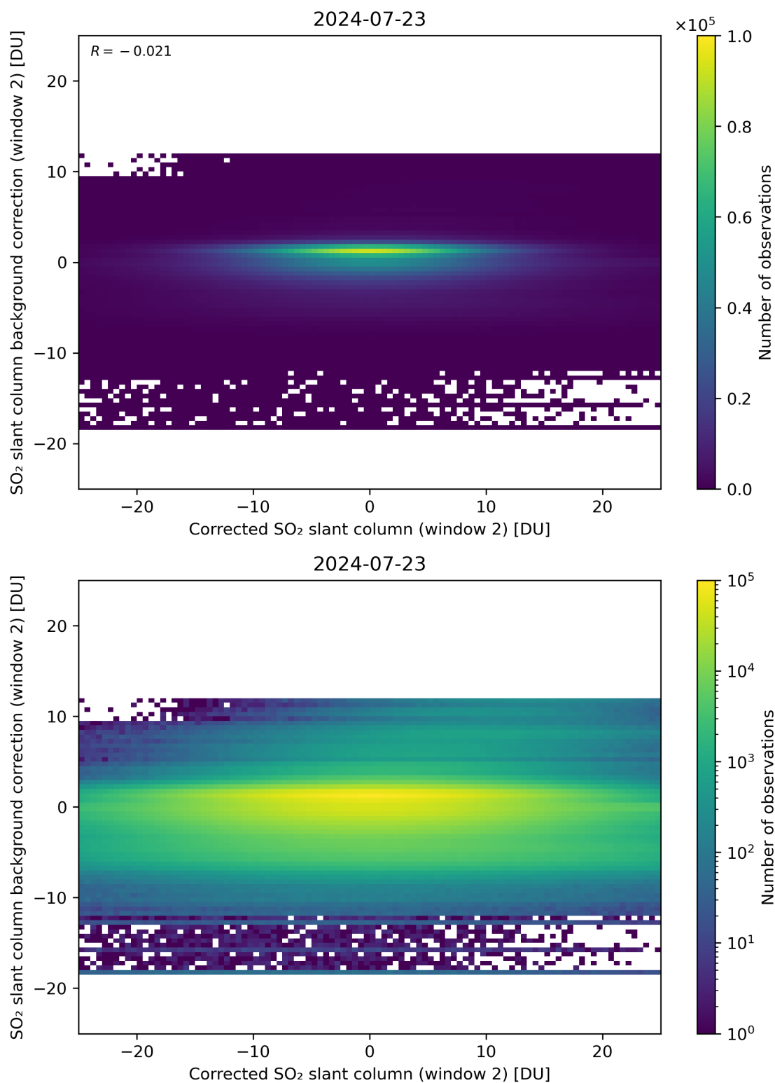
Figure 194: Scatter density plot of “Corrected SO 2 slant column (window 2)” against “SO 2 slant column background correction (window 2)” for 2024-07-22 to 2024-07-24.
