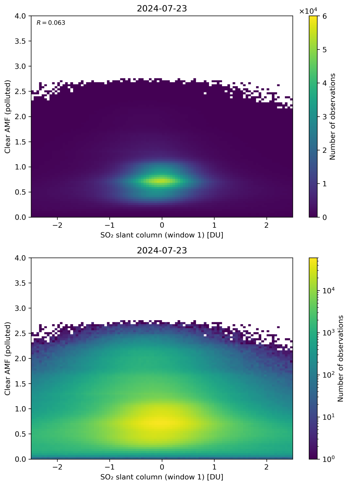
Figure 232: Scatter density plot of “SO 2 slant column (window 1)” against “Clear AMF (polluted)” for 2024-07-22 to 2024-07-24.
