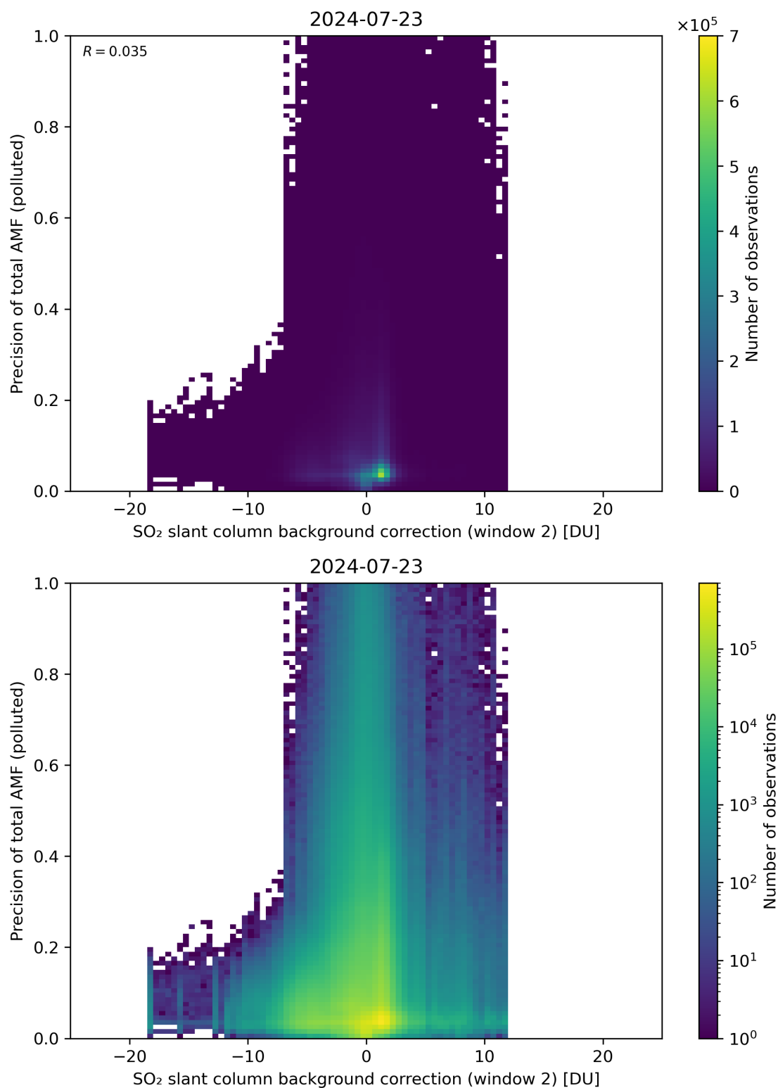
Figure 120: Scatter density plot of “SO 2 slant column background correction (window 2)” against “Precision of total AMF (polluted)” for 2024-07-22 to 2024-07-24.
