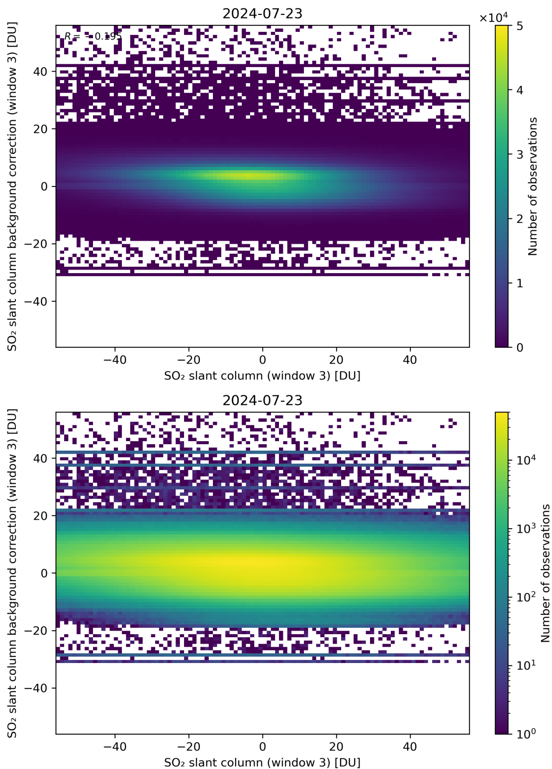
Figure 253: Scatter density plot of “SO 2 slant column (window 3)” against “SO 2 slant column background correction (window 3)” for 2024-07-22 to 2024-07-24.
