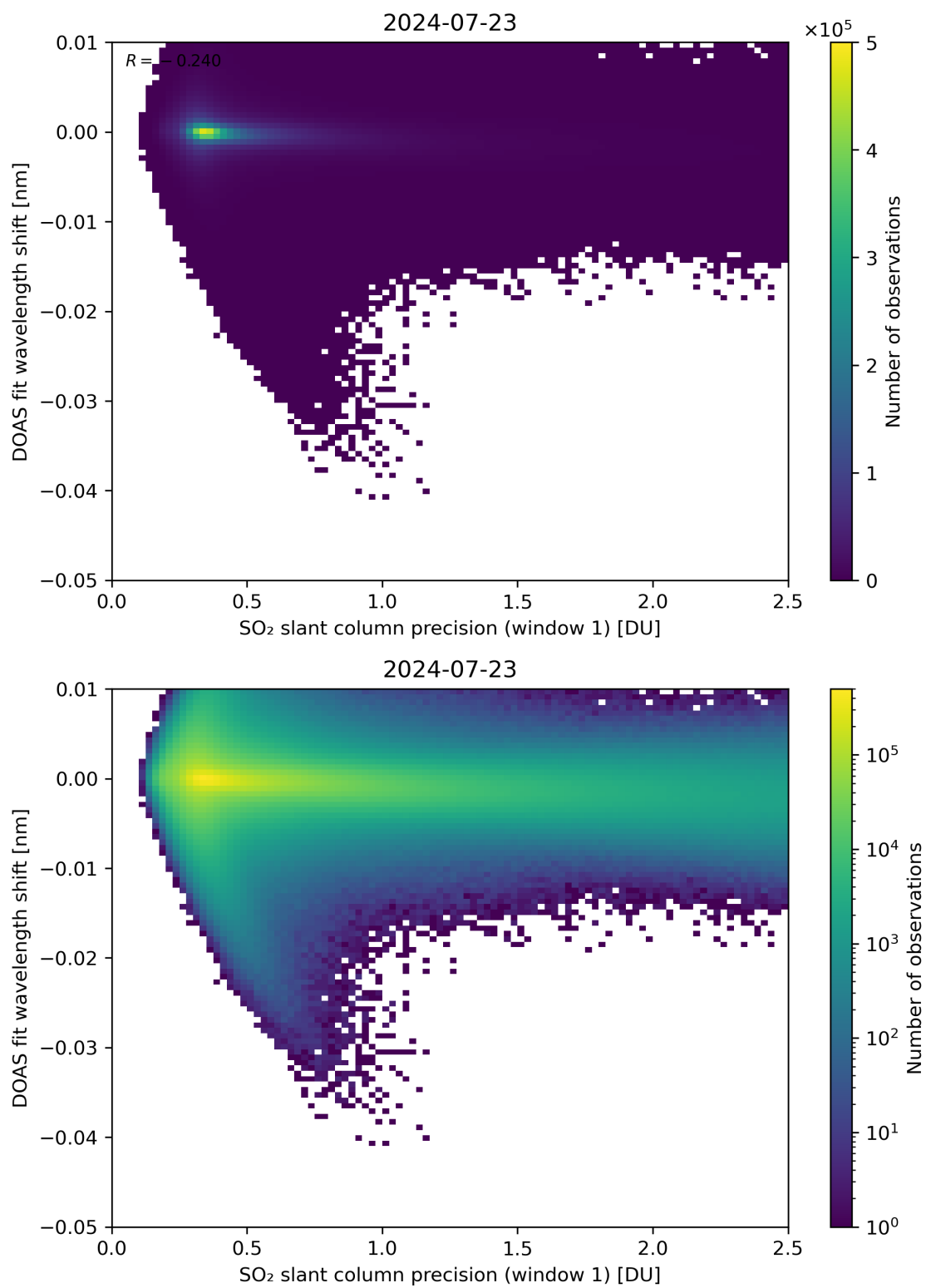
Figure 221: Scatter density plot of “SO 2 slant column precision (window 1)” against “DOAS fit wavelength shift” for 2024-07-22 to 2024-07-24.
