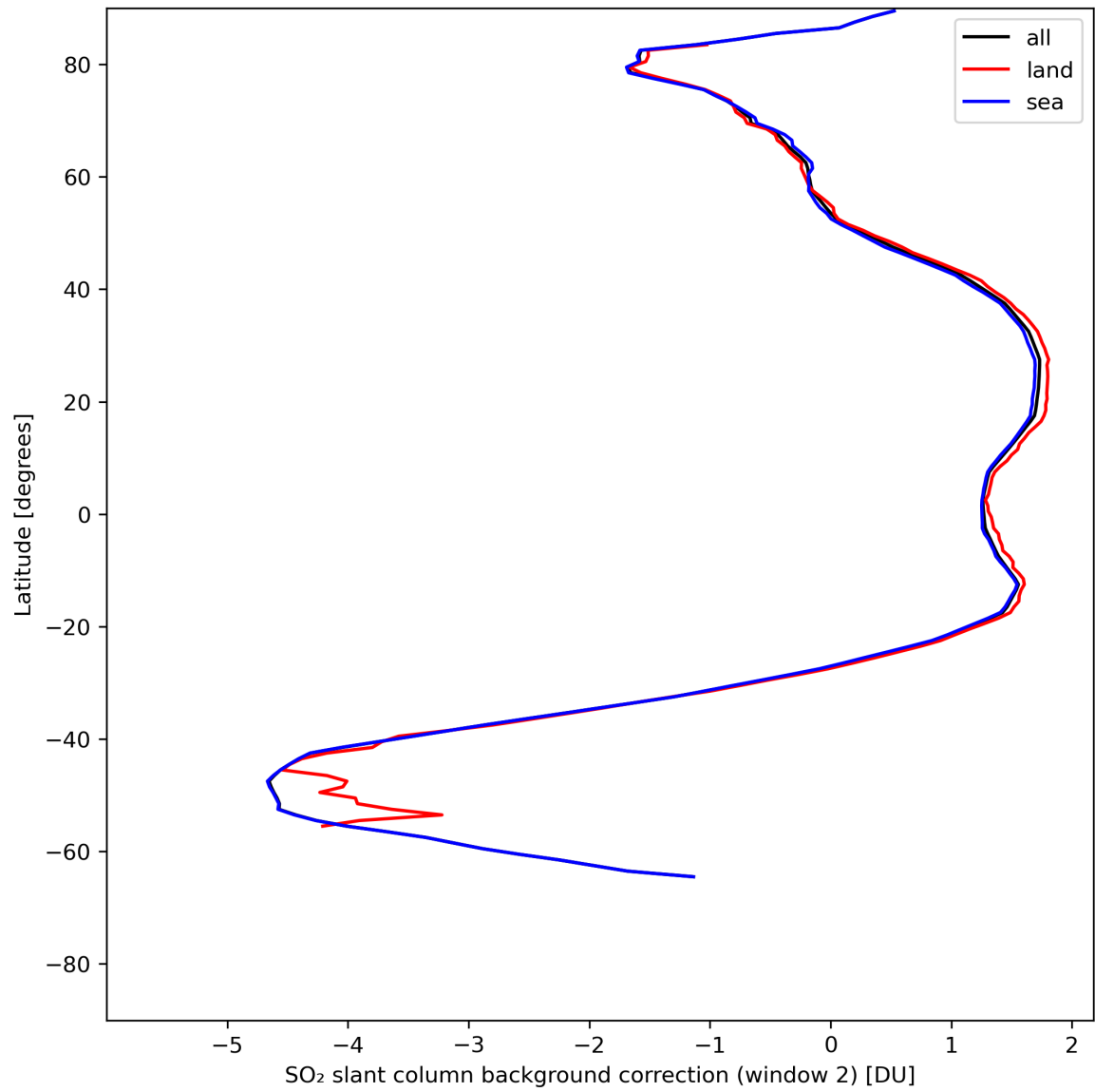
Figure 40: Zonal average of “SO 2 slant column background correction (window 2)” for 2024-07-22 to 2024-07-24.
