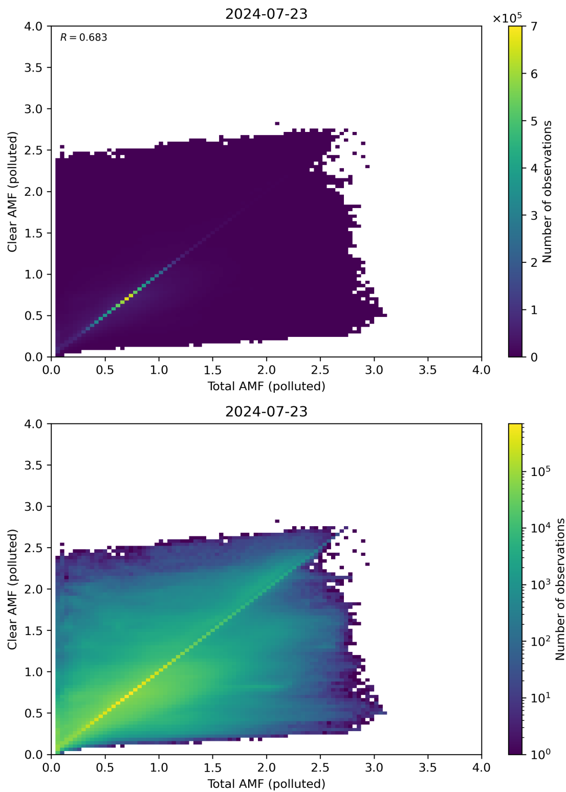
Figure 271: Scatter density plot of “Total AMF (polluted)” against “Clear AMF (polluted)” for 2024-07-22 to 2024-07-24.
