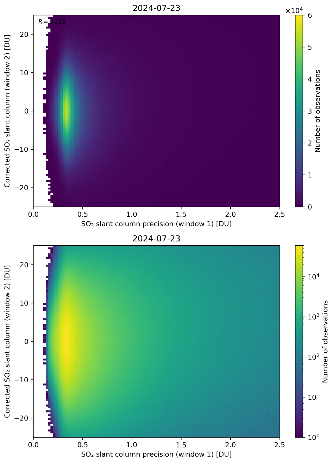
Figure 225: Scatter density plot of “SO 2 slant column precision (window 1)” against “Corrected SO 2 slant column (window 2)” for 2024-07-22 to 2024-07-24.
