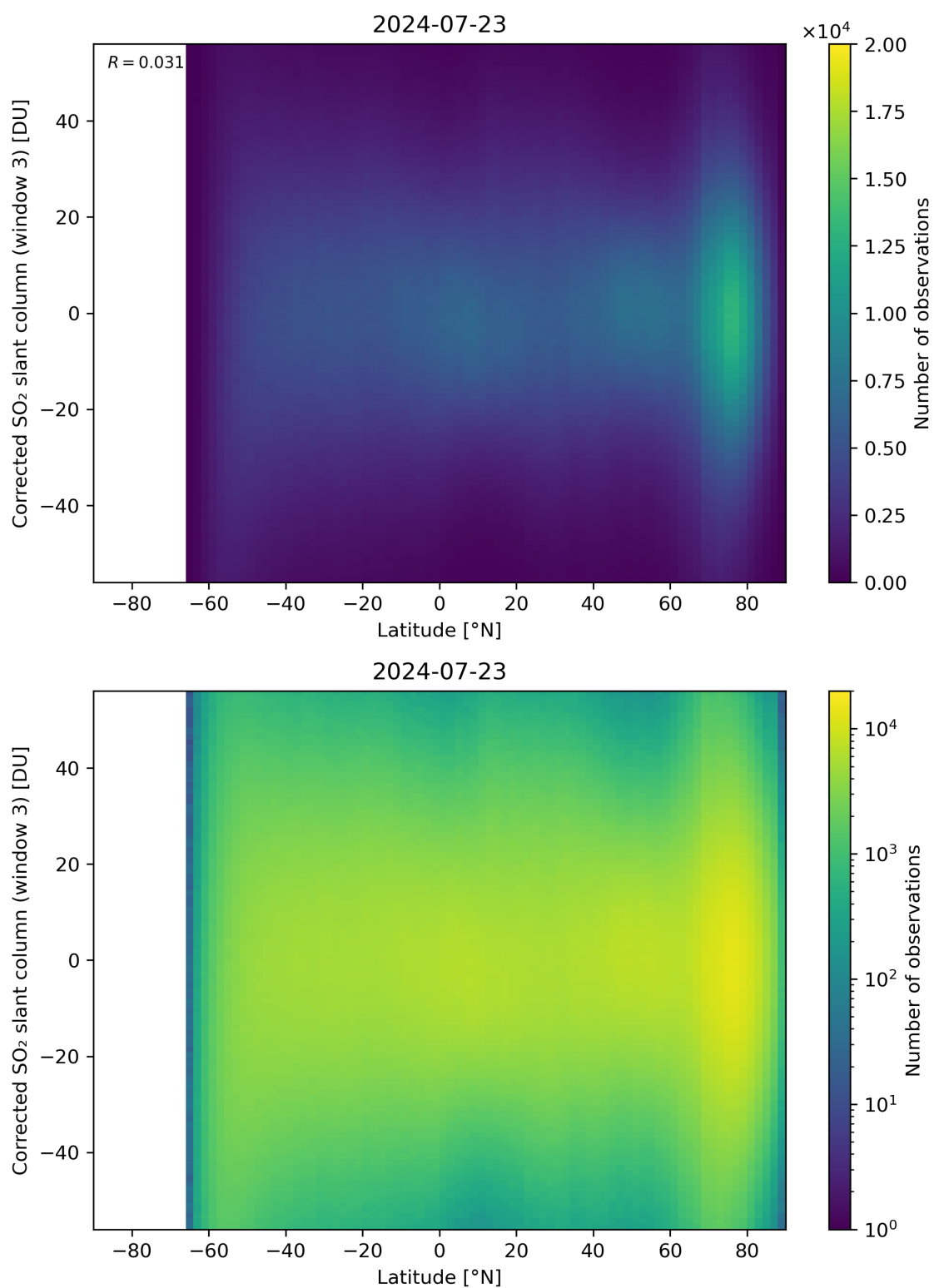
Figure 148: Scatter density plot of “Latitude” against “Corrected SO 2 slant column (window 3)” for 2024-07-22 to 2024-07-24.
