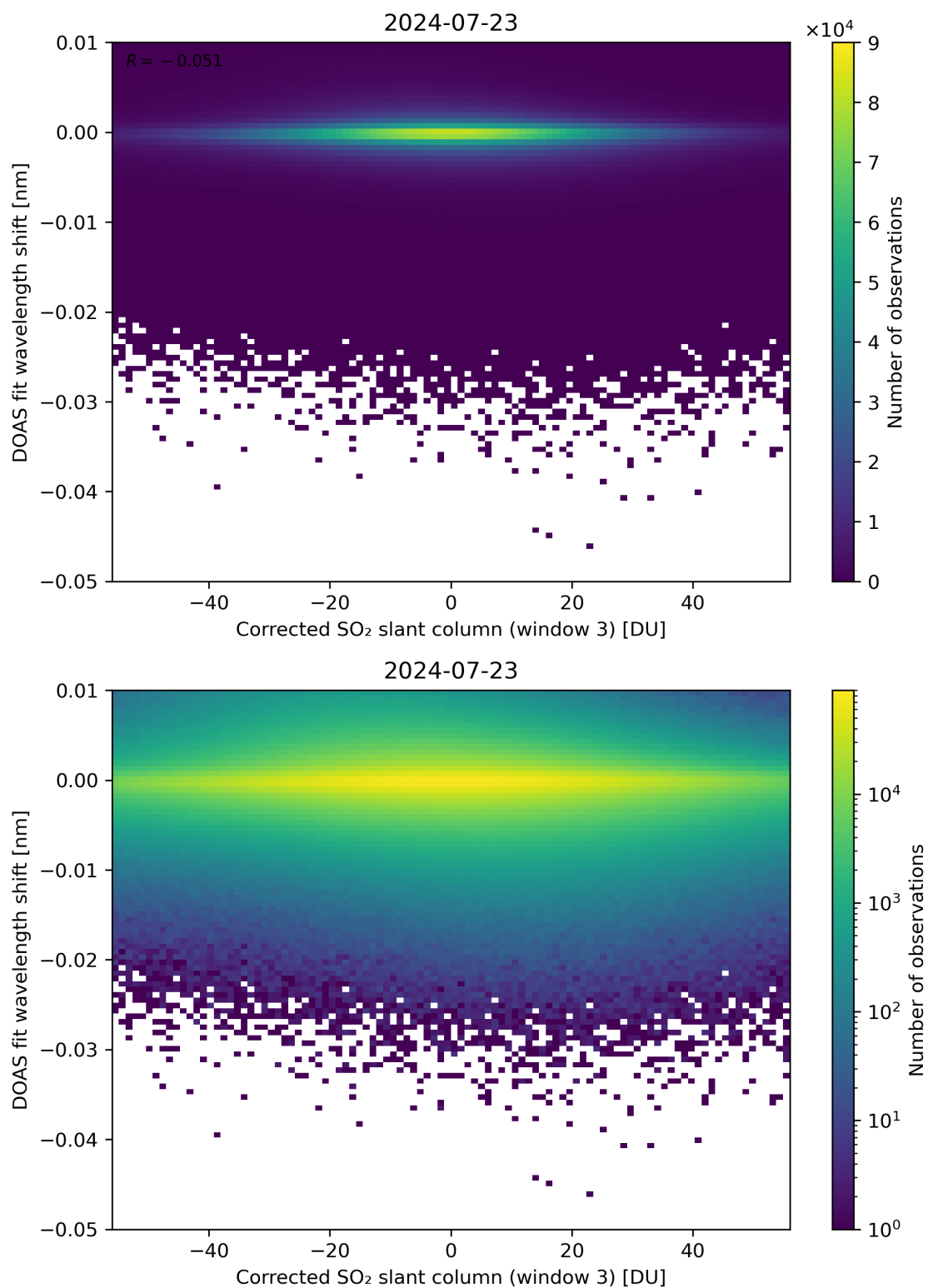
Figure 206: Scatter density plot of “Corrected SO 2 slant column (window 3)” against “DOAS fit wavelength shift” for 2024-07-22 to 2024-07-24.
