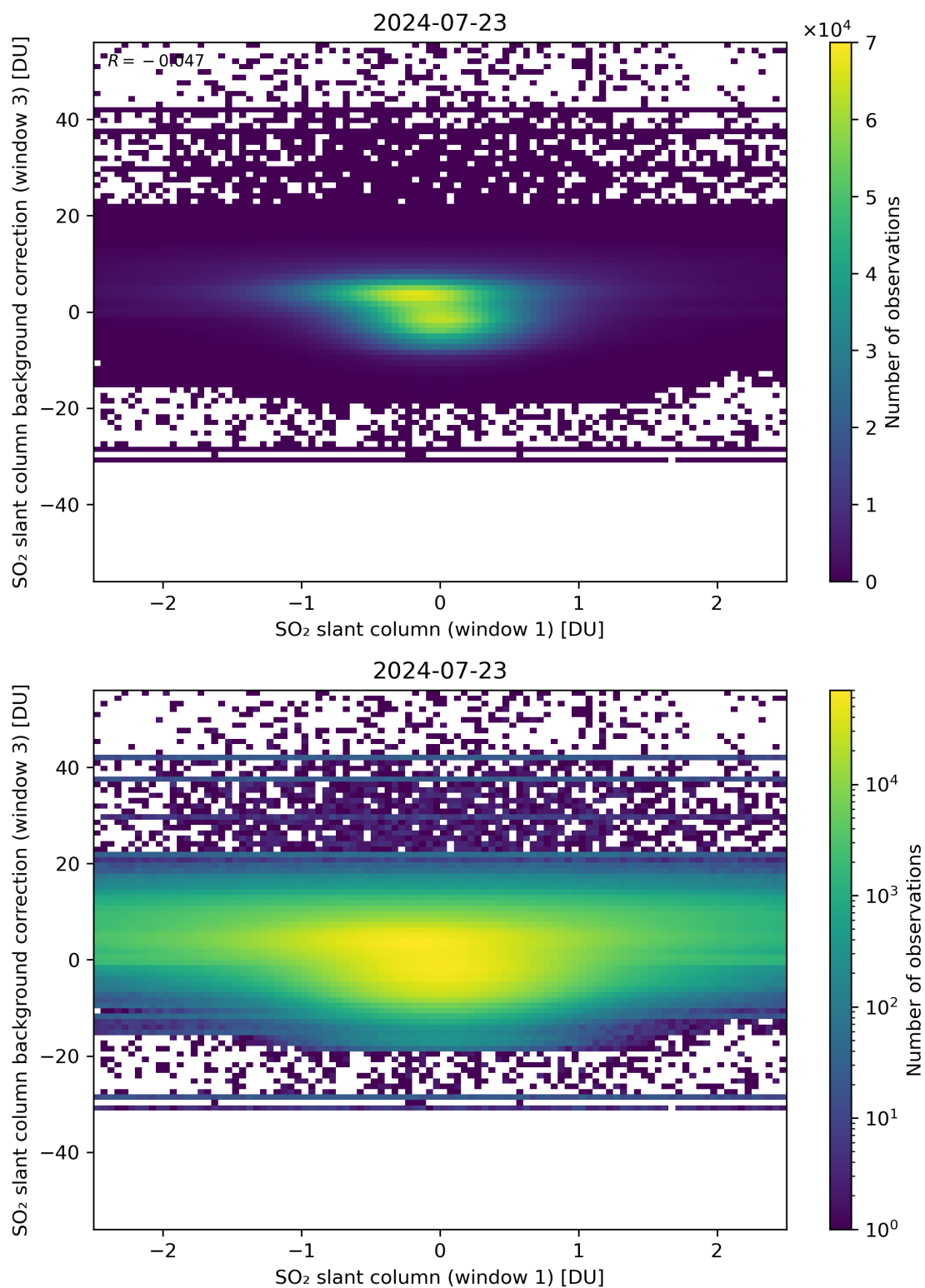
Figure 214: Scatter density plot of “SO 2 slant column (window 1)” against “SO 2 slant column background correction (window 3)” for 2024-07-22 to 2024-07-24.
