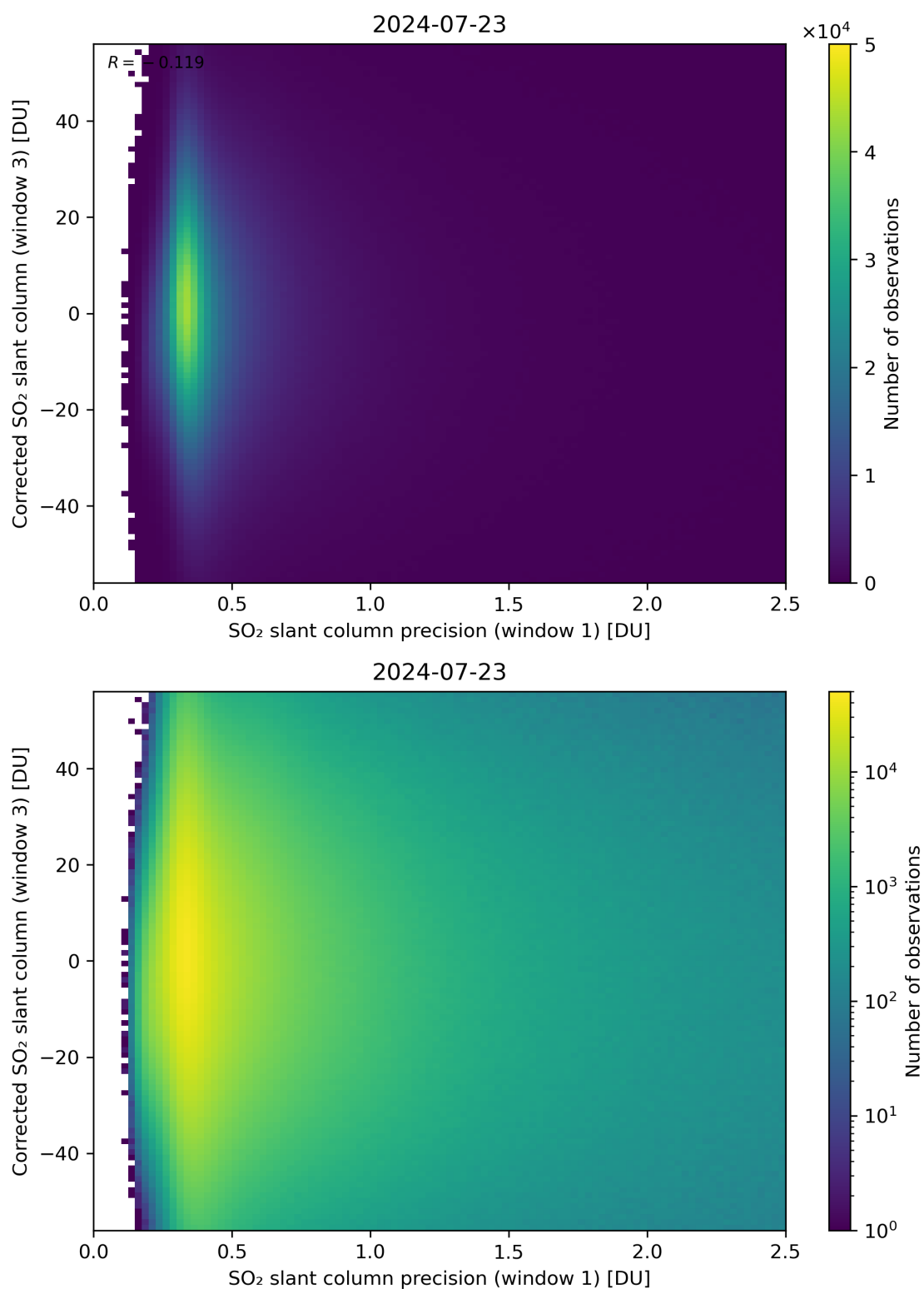
Figure 226: Scatter density plot of “SO 2 slant column precision (window 1)” against “Corrected SO 2 slant column (window 3)” for 2024-07-22 to 2024-07-24.
