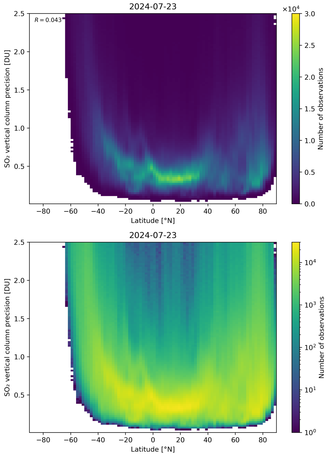
Figure 157: Scatter density plot of “Latitude” against “SO 2 vertical column precision” for 2024-07-22 to 2024-07-24.
