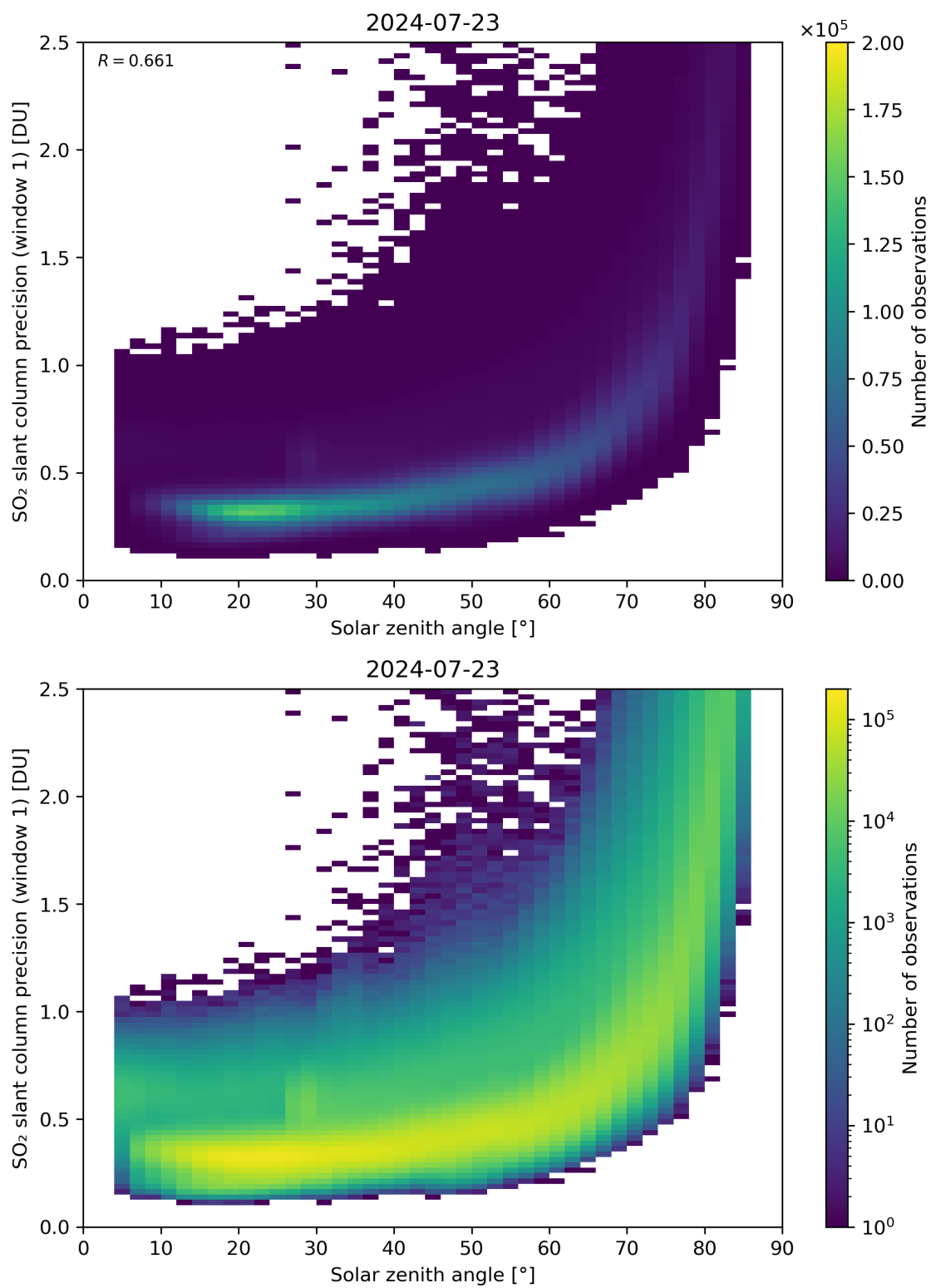
Figure 170: Scatter density plot of “Solar zenith angle” against “SO 2 slant column precision (window 1)” for 2024-07-22 to 2024-07-24.
