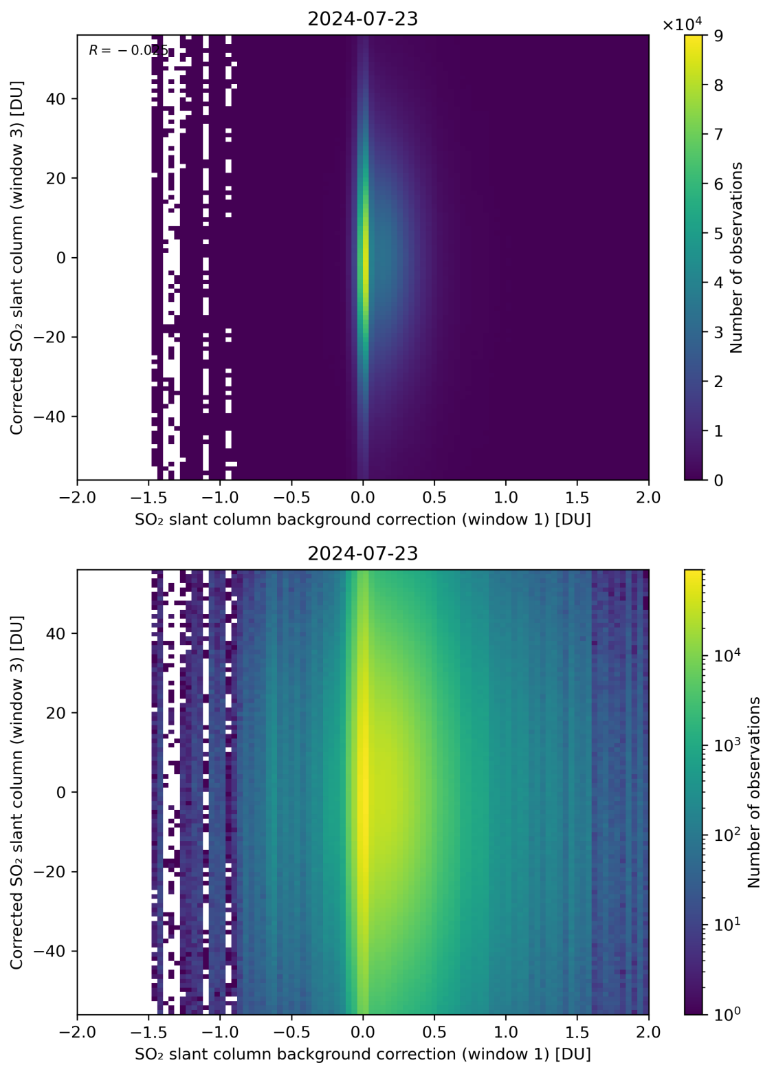
Figure 105: Scatter density plot of “SO 2 slant column background correction (window 1)” against “Corrected SO 2 slant column (window 3)” for 2024-07-22 to 2024-07-24.
