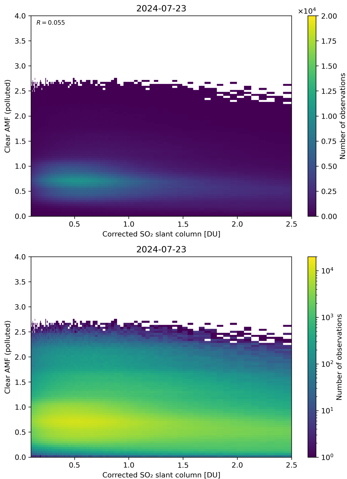
Figure 184: Scatter density plot of “Corrected SO 2 slant column” against “Clear AMF (polluted)” for 2024-07-22 to 2024-07-24.
