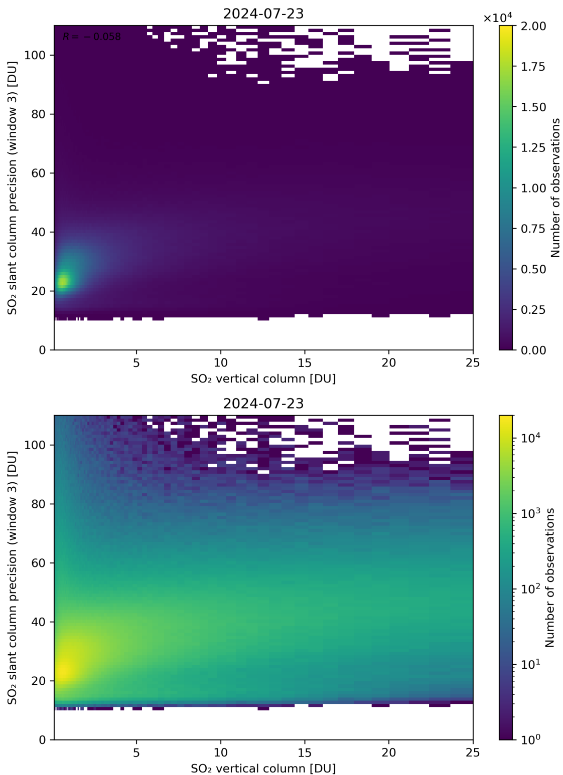
Figure 304: Scatter density plot of “SO 2 vertical column” against “SO 2 slant column precision (window 3)” for 2024-07-22 to 2024-07-24.
