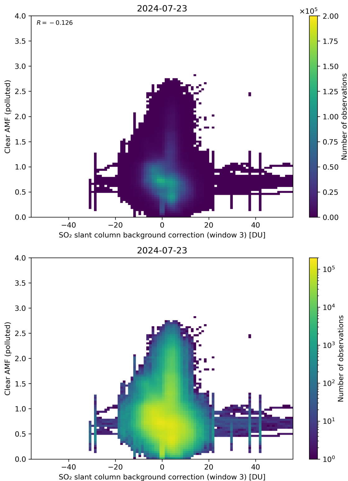
Figure 124: Scatter density plot of “SO 2 slant column background correction (window 3)” against “Clear AMF (polluted)” for 2024-07-22 to 2024-07-24.
