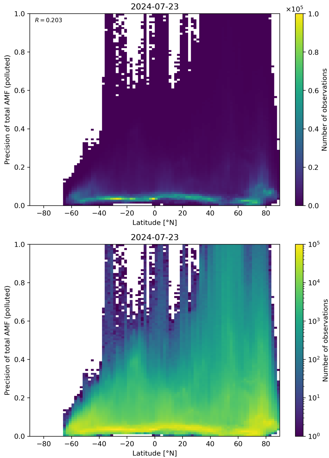
Figure 155: Scatter density plot of “Latitude” against “Precision of total AMF (polluted)” for 2024-07-22 to 2024-07-24.
