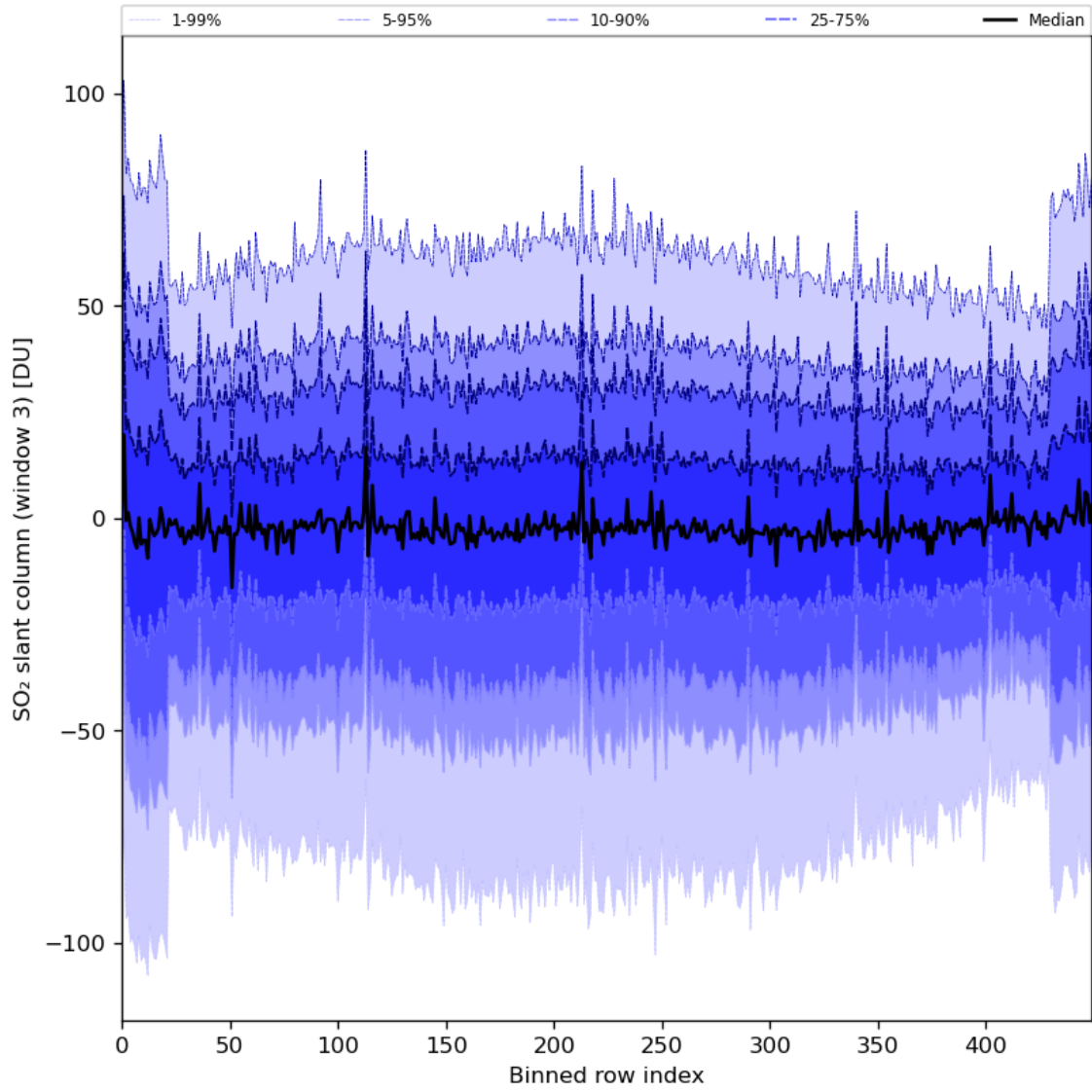
Figure 87: Along track statistics of “SO 2 slant column (window 3)” for 2024-07-22 to 2024-07-24
