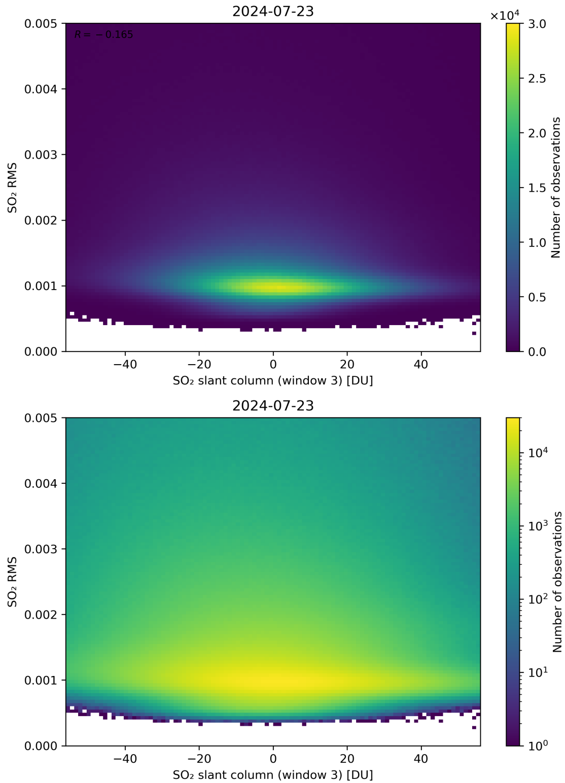
Figure 256: Scatter density plot of “SO 2 slant column (window 3)” against “SO 2 RMS” for 2024-07-22 to 2024-07-24.
