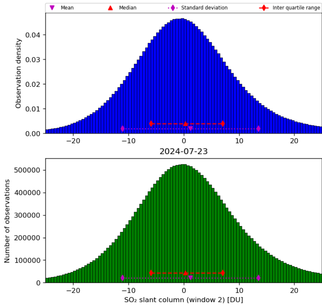
Figure 60: Histogram of “SO 2 slant column (window 2)” for 2024-07-22 to 2024-07-24
