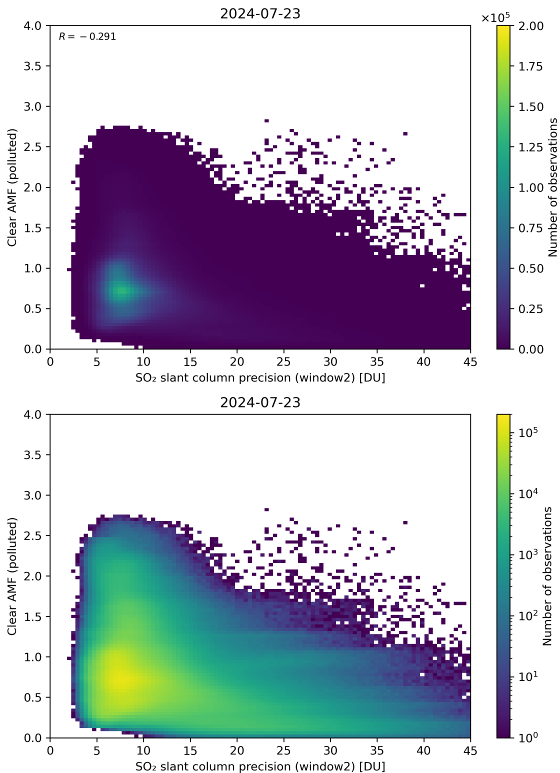
Figure 246: Scatter density plot of “SO 2 slant column precision (window2)” against “Clear AMF (polluted)” for 2024-07-22 to 2024-07-24.
