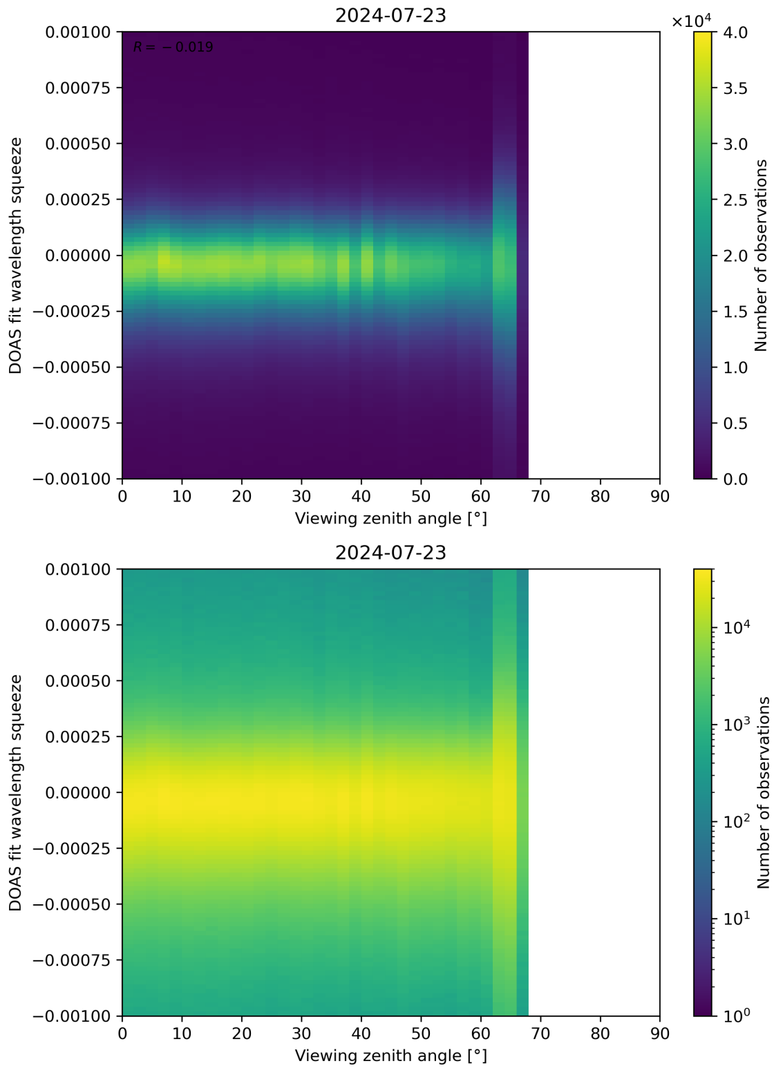
Figure 312: Scatter density plot of “Viewing zenith angle” against “DOAS fit wavelength squeeze” for 2024-07-22 to 2024-07-24.
