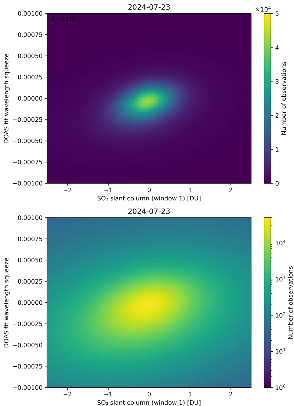
Figure 216: Scatter density plot of “SO 2 slant column (window 1)” against “DOAS fit wavelength squeeze” for 2024-07-22 to 2024-07-24.
