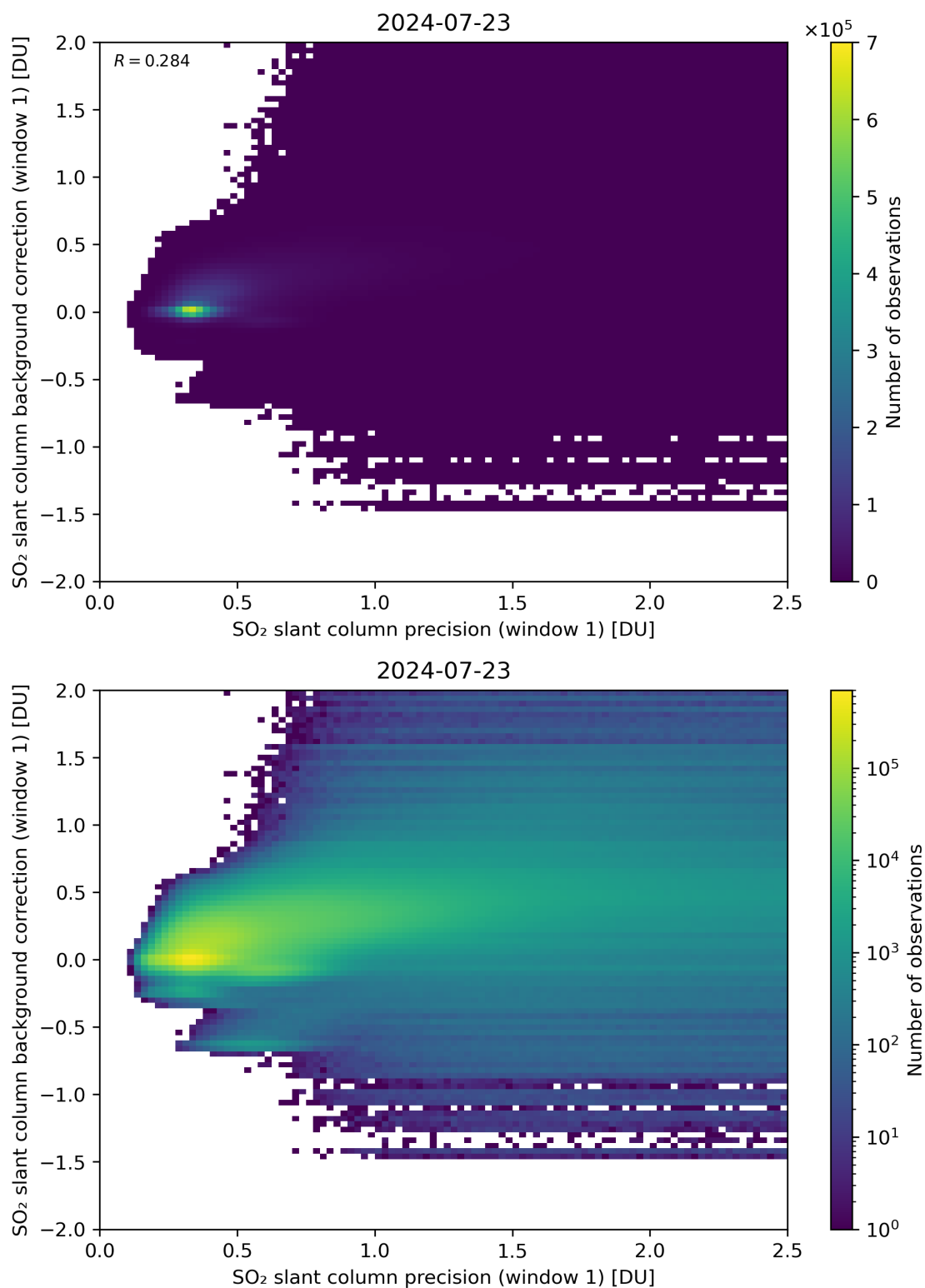
Figure 218: Scatter density plot of “SO 2 slant column precision (window 1)” against “SO 2 slant column background correction (window 1)” for 2024-07-22 to 2024-07-24.
