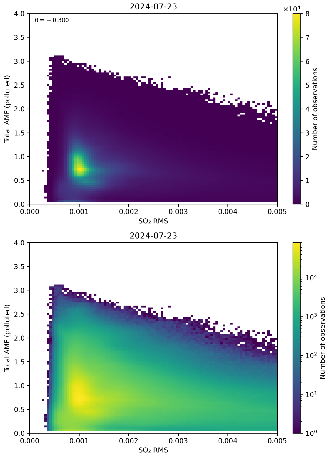
Figure 137: Scatter density plot of “SO 2 RMS” against “Total AMF (polluted)” for 2024-07-22 to 2024-07-24.
