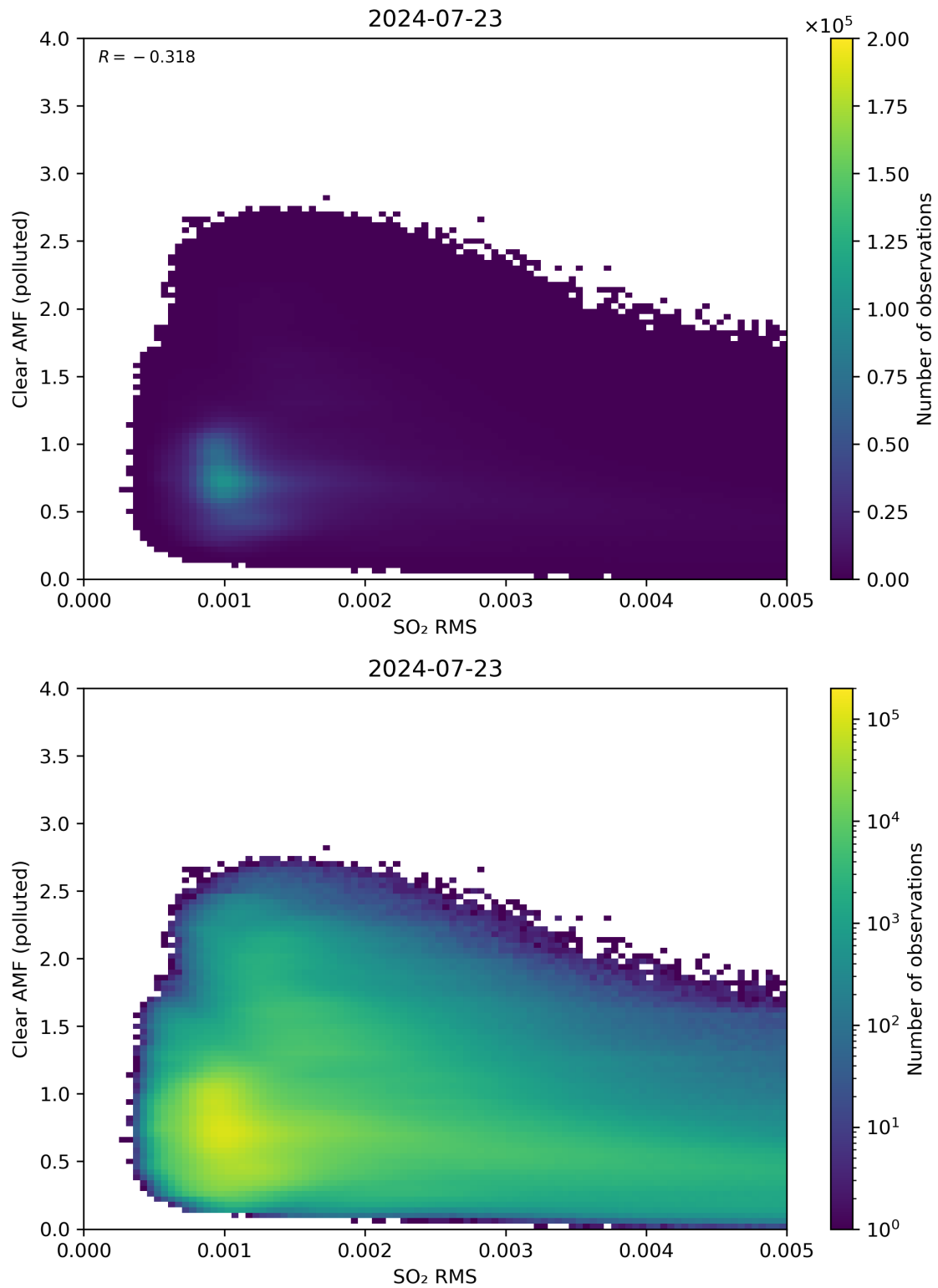
Figure 136: Scatter density plot of “SO 2 RMS” against “Clear AMF (polluted)” for 2024-07-22 to 2024-07-24.
