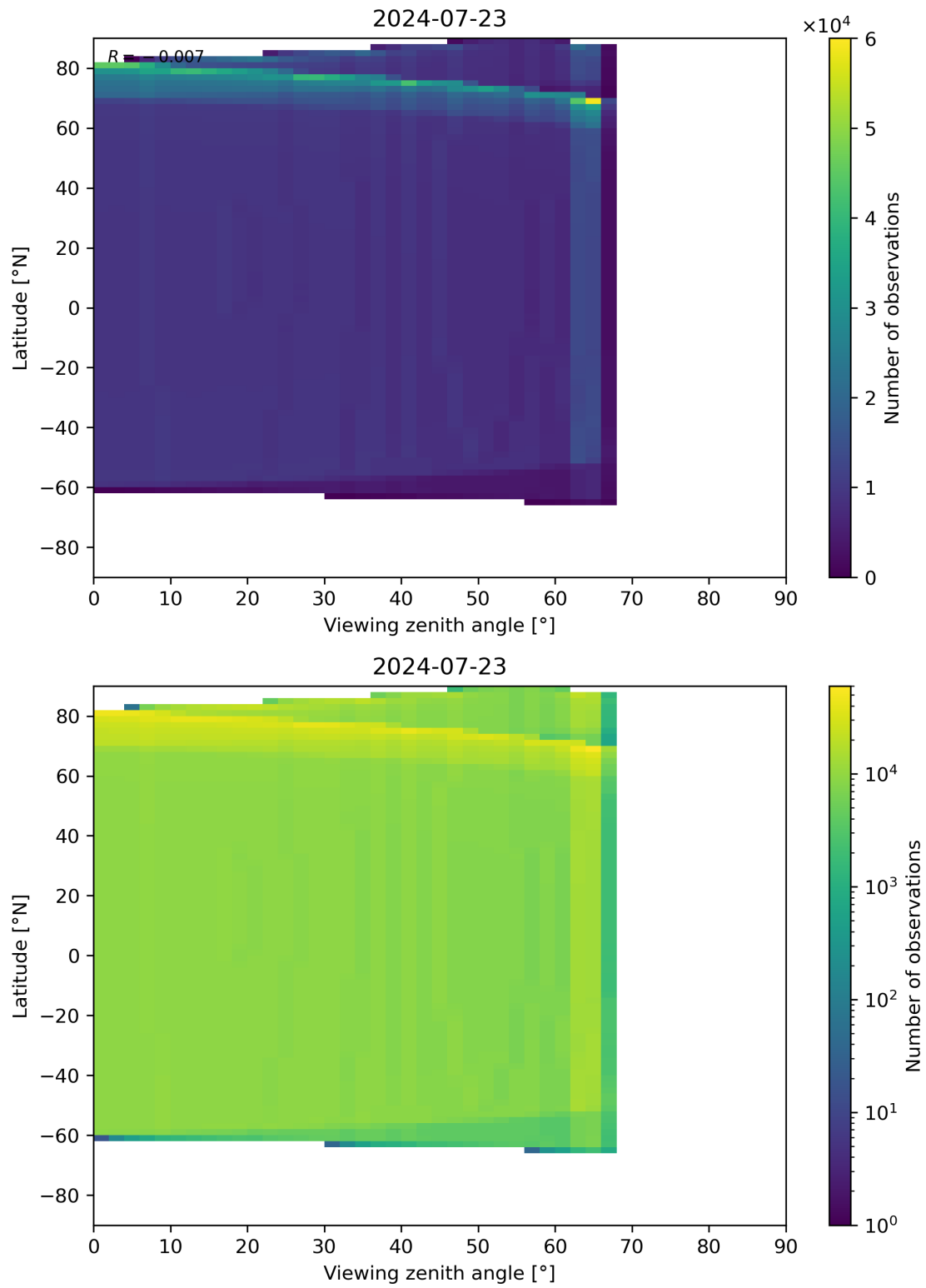
Figure 314: Scatter density plot of “Viewing zenith angle” against “Latitude” for 2024-07-22 to 2024-07-24.
