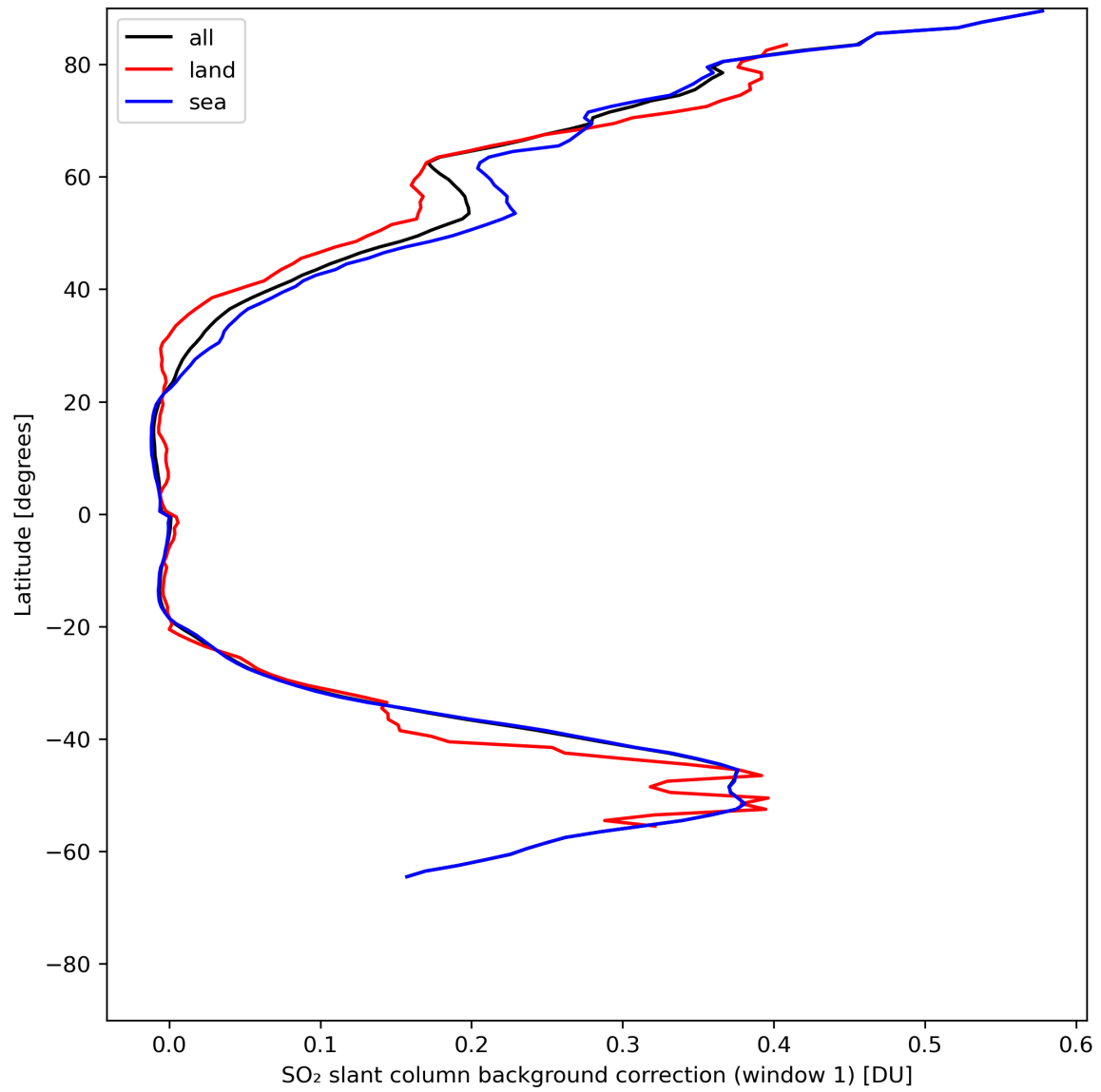
Figure 36: Zonal average of “SO 2 slant column background correction (window 1)” for 2024-07-22 to 2024-07-24.
