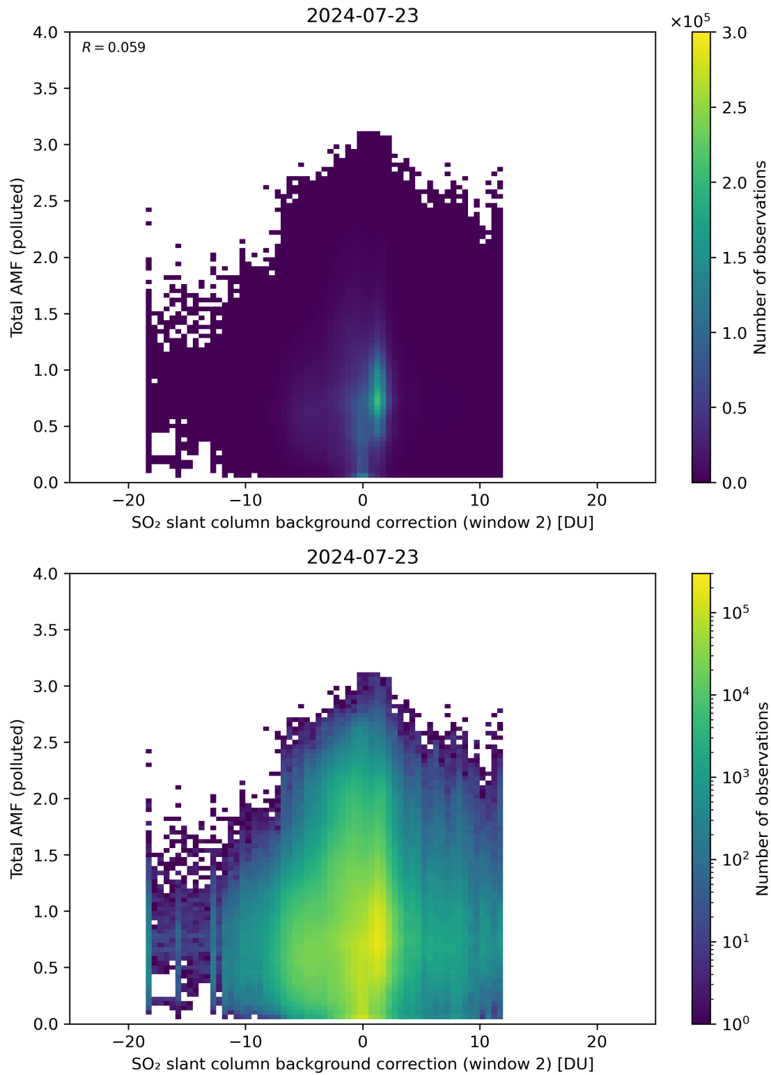
Figure 119: Scatter density plot of “SO 2 slant column background correction (window 2)” against “Total AMF (polluted)” for 2024-07-22 to 2024-07-24.
