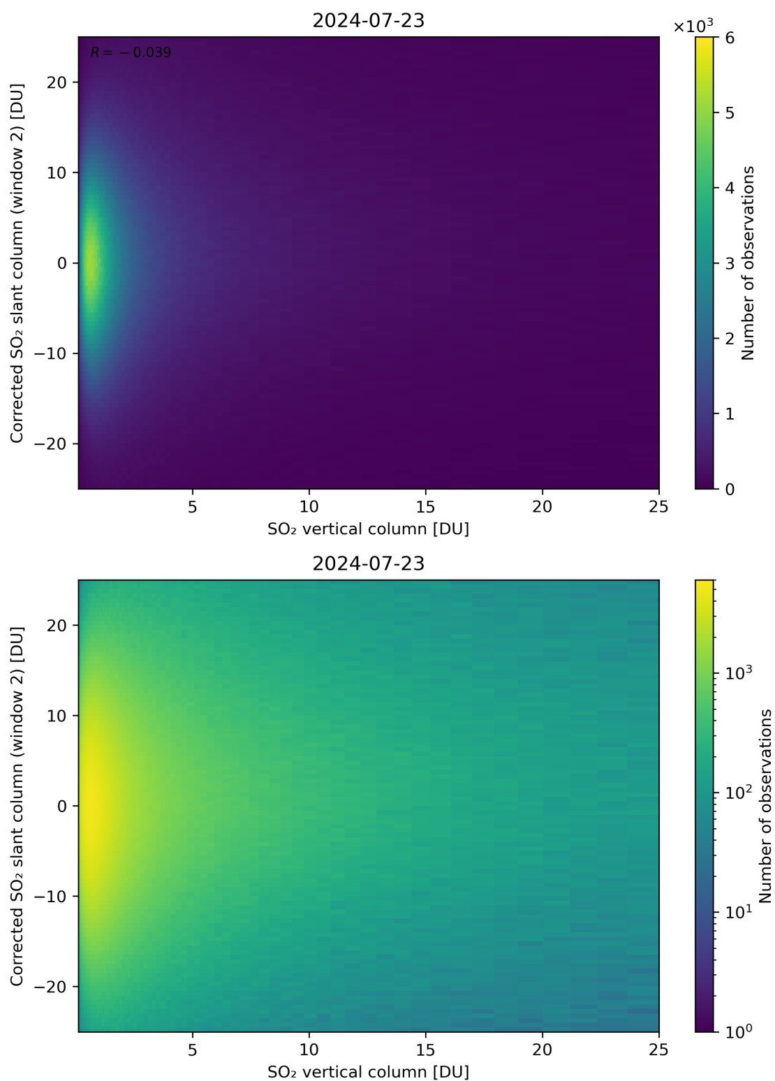
Figure 298: Scatter density plot of “SO 2 vertical column” against “Corrected SO 2 slant column (window 2)” for 2024-07-22 to 2024-07-24.
