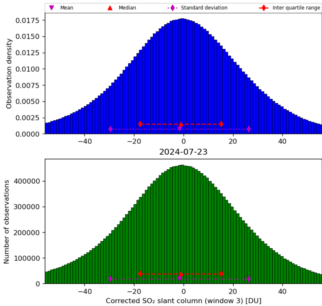
Figure 66: Histogram of “Corrected SO 2 slant column (window 3)” for 2024-07-22 to 2024-07-24
