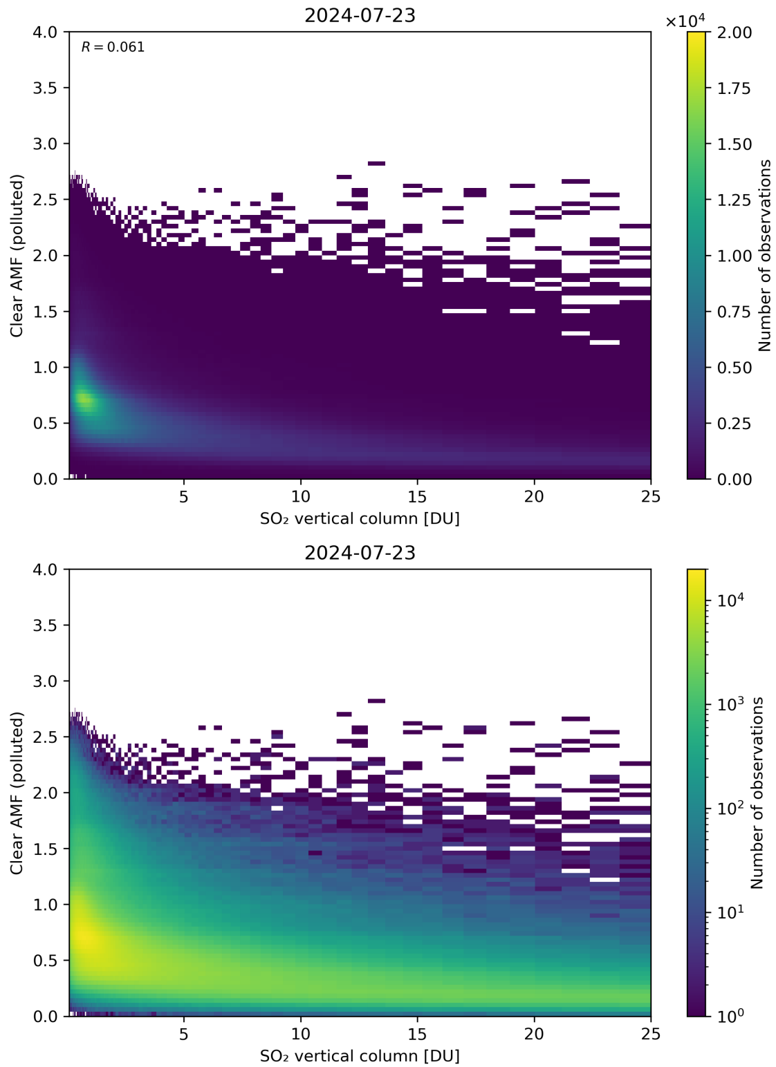
Figure 296: Scatter density plot of “SO 2 vertical column” against “Clear AMF (polluted)” for 2024-07-22 to 2024-07-24.
