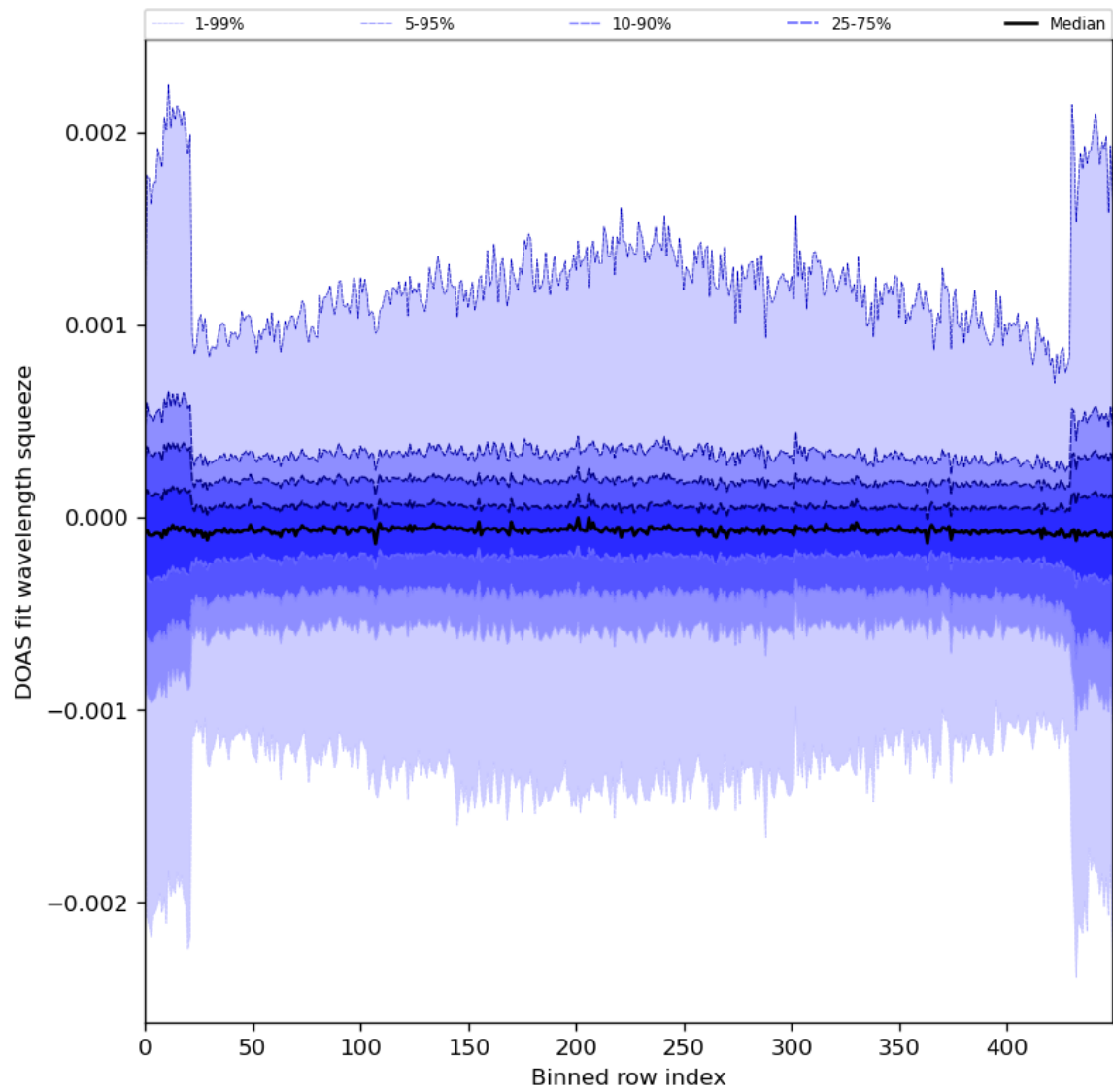
Figure 92: Along track statistics of “DOAS fit wavelength squeeze” for 2024-07-22 to 2024-07-24
