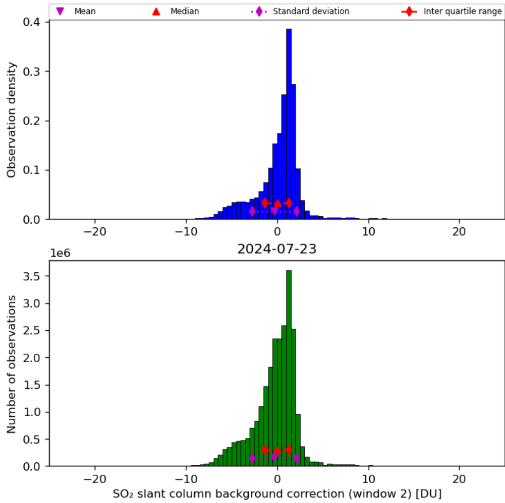
Figure 63: Histogram of “SO 2 slant column background correction (window 2)” for 2024-07-22 to 2024-07-24
