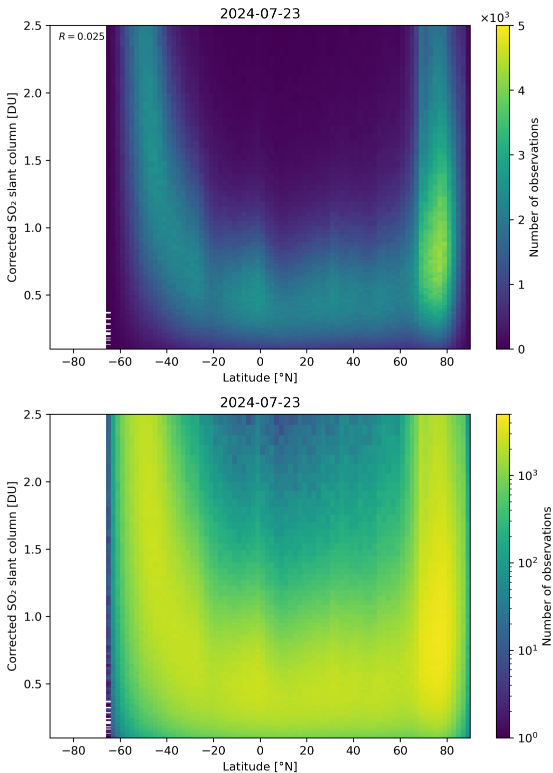
Figure 146: Scatter density plot of “Latitude” against “Corrected SO 2 slant column” for 2024-07-22 to 2024-07-24.
