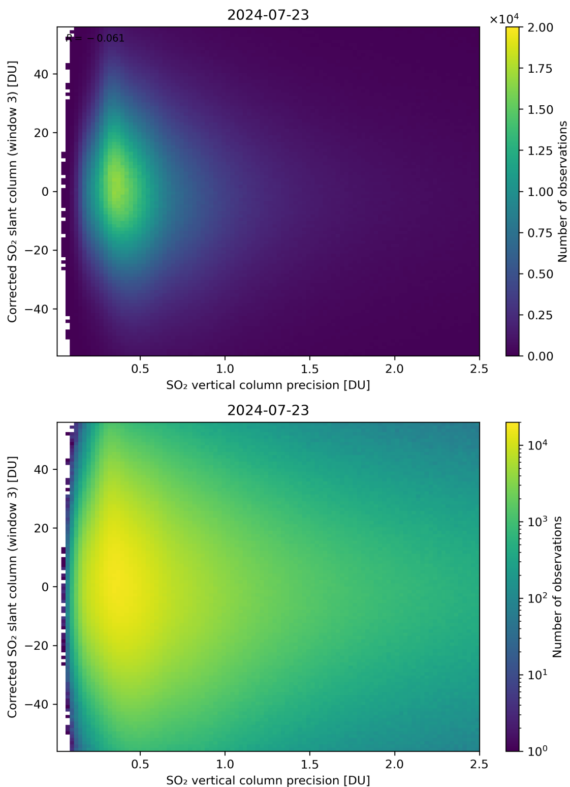
Figure 288: Scatter density plot of “SO 2 vertical column precision” against “Corrected SO 2 slant column (window 3)” for 2024-07-22 to 2024-07-24.
