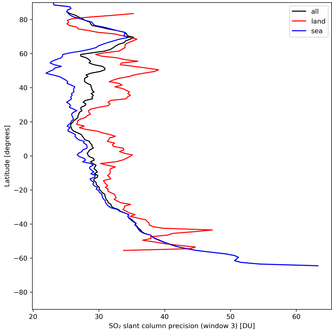
Figure 42: Zonal average of “SO 2 slant column precision (window 3)” for 2024-07-22 to 2024-07-24.
