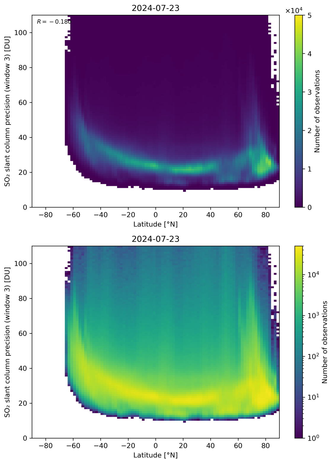
Figure 153: Scatter density plot of “Latitude” against “SO 2 slant column precision (window 3)” for 2024-07-22 to 2024-07-24.
