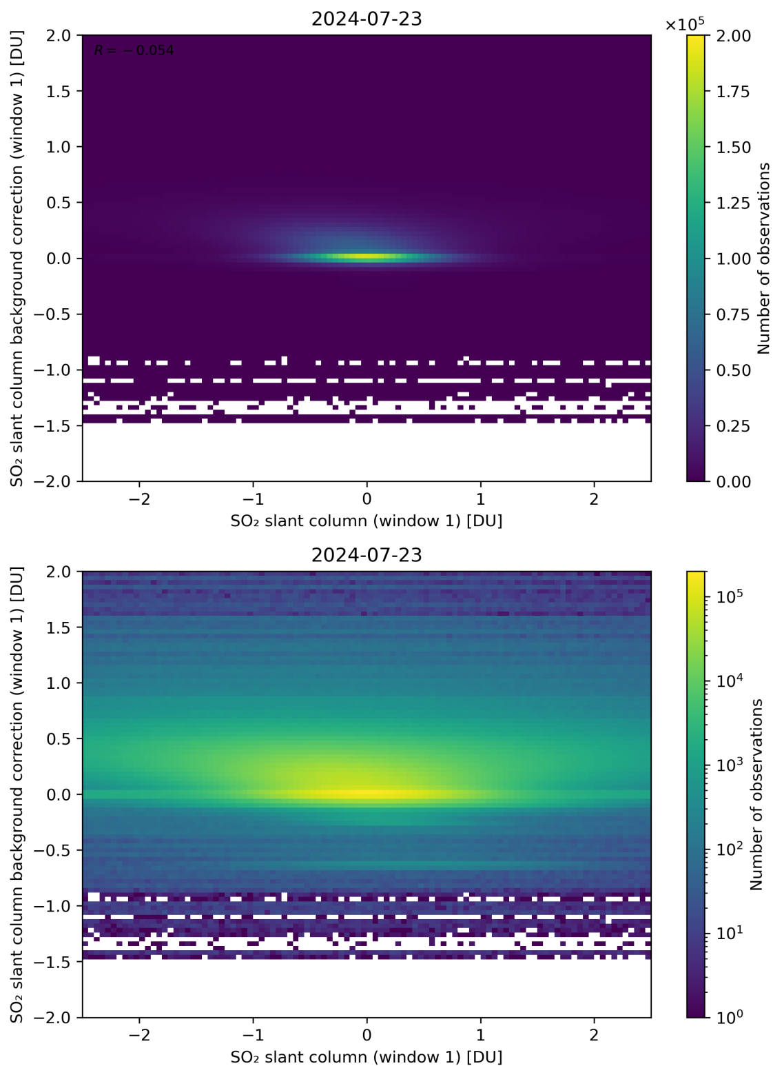
Figure 212: Scatter density plot of “SO 2 slant column (window 1)” against “SO 2 slant column background correction (window 1)” for 2024-07-22 to 2024-07-24.
