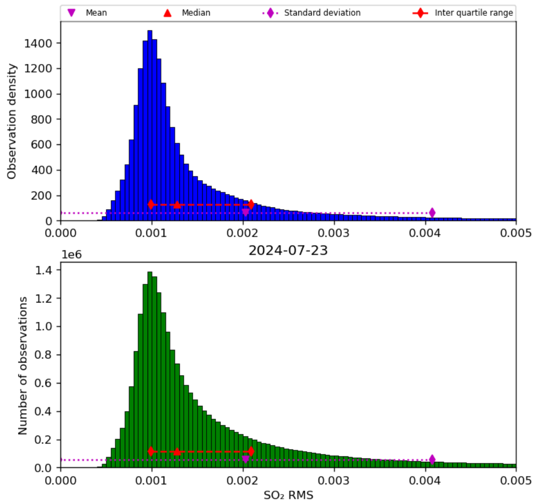
Figure 70: Histogram of “SO 2 RMS” for 2024-07-22 to 2024-07-24
