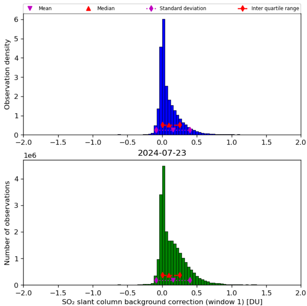
Figure 59: Histogram of “SO 2 slant column background correction (window 1)” for 2024-07-22 to 2024-07-24
