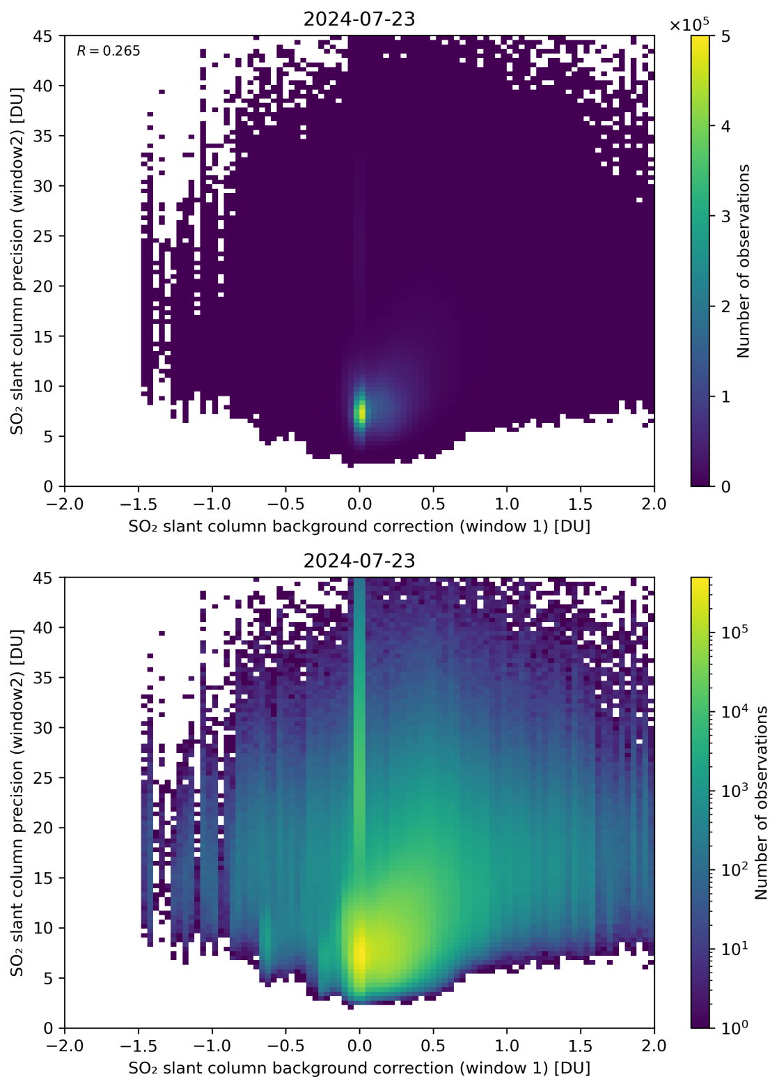
Figure 106: Scatter density plot of “SO 2 slant column background correction (window 1)” against “SO 2 slant column precision (window2)” for 2024-07-22 to 2024-07-24.
