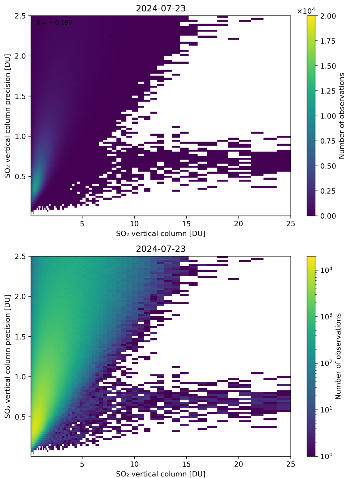
Figure 307: Scatter density plot of “SO 2 vertical column” against “SO 2 vertical column precision” for 2024-07-22 to 2024-07-24.
