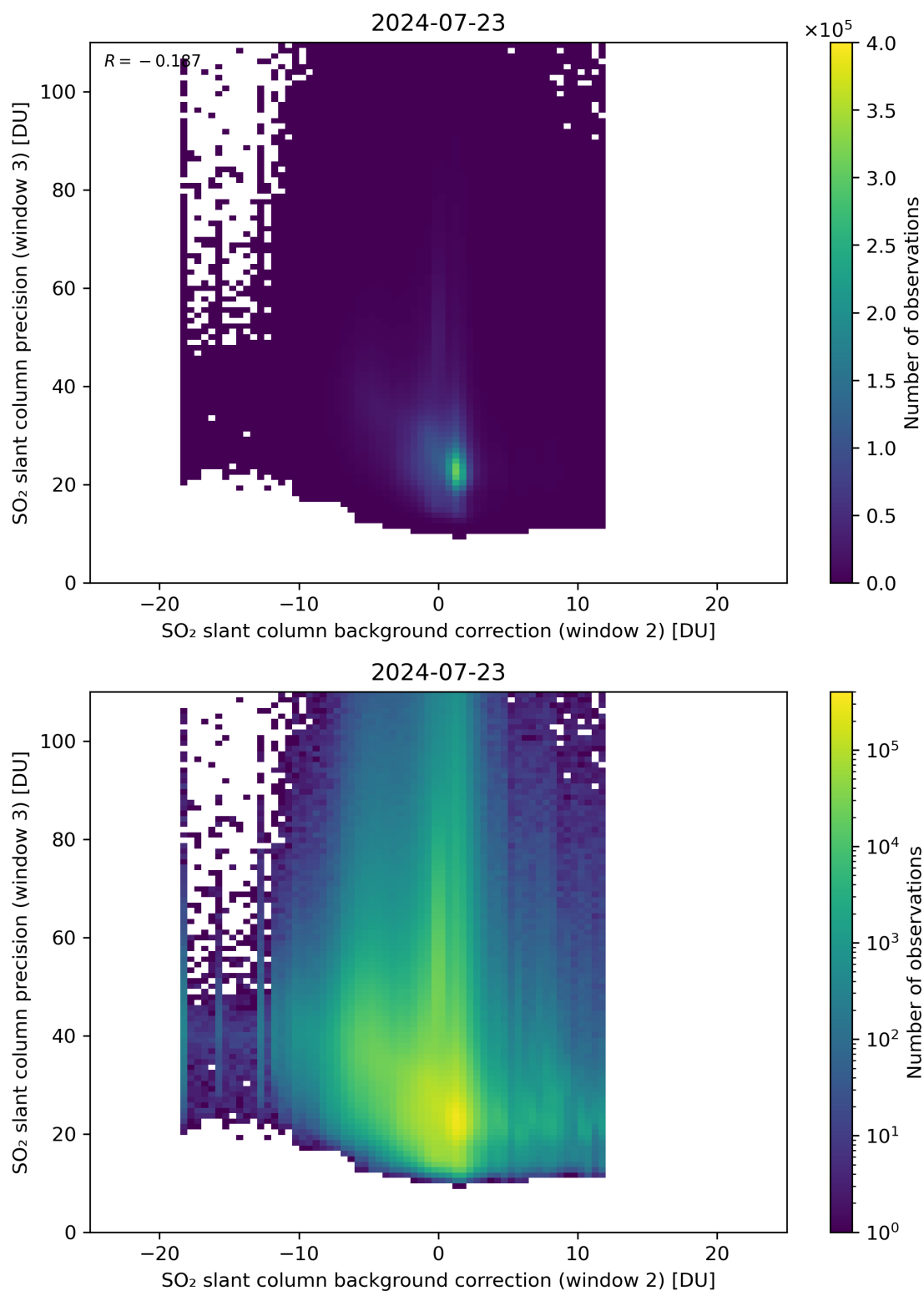
Figure 118: Scatter density plot of “SO 2 slant column background correction (window 2)” against “SO 2 slant column precision (window 3)” for 2024-07-22 to 2024-07-24.
