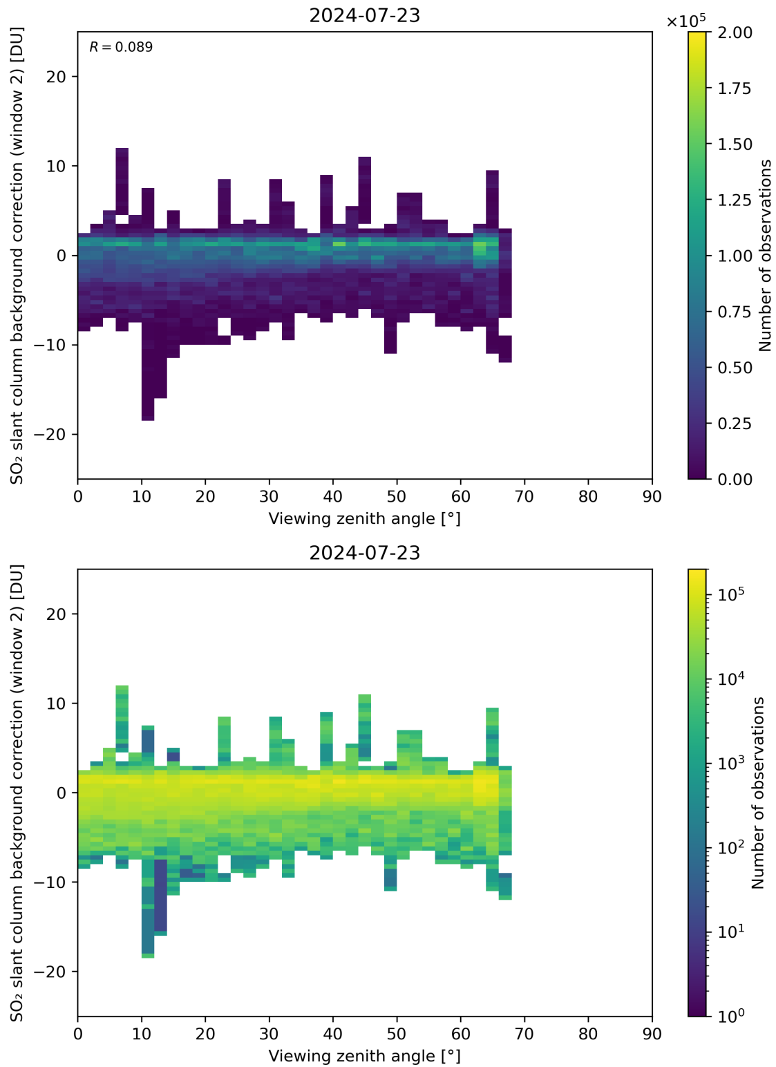
Figure 309: Scatter density plot of “Viewing zenith angle” against “SO 2 slant column background correction (window 2)” for 2024-07-22 to 2024-07-24.
