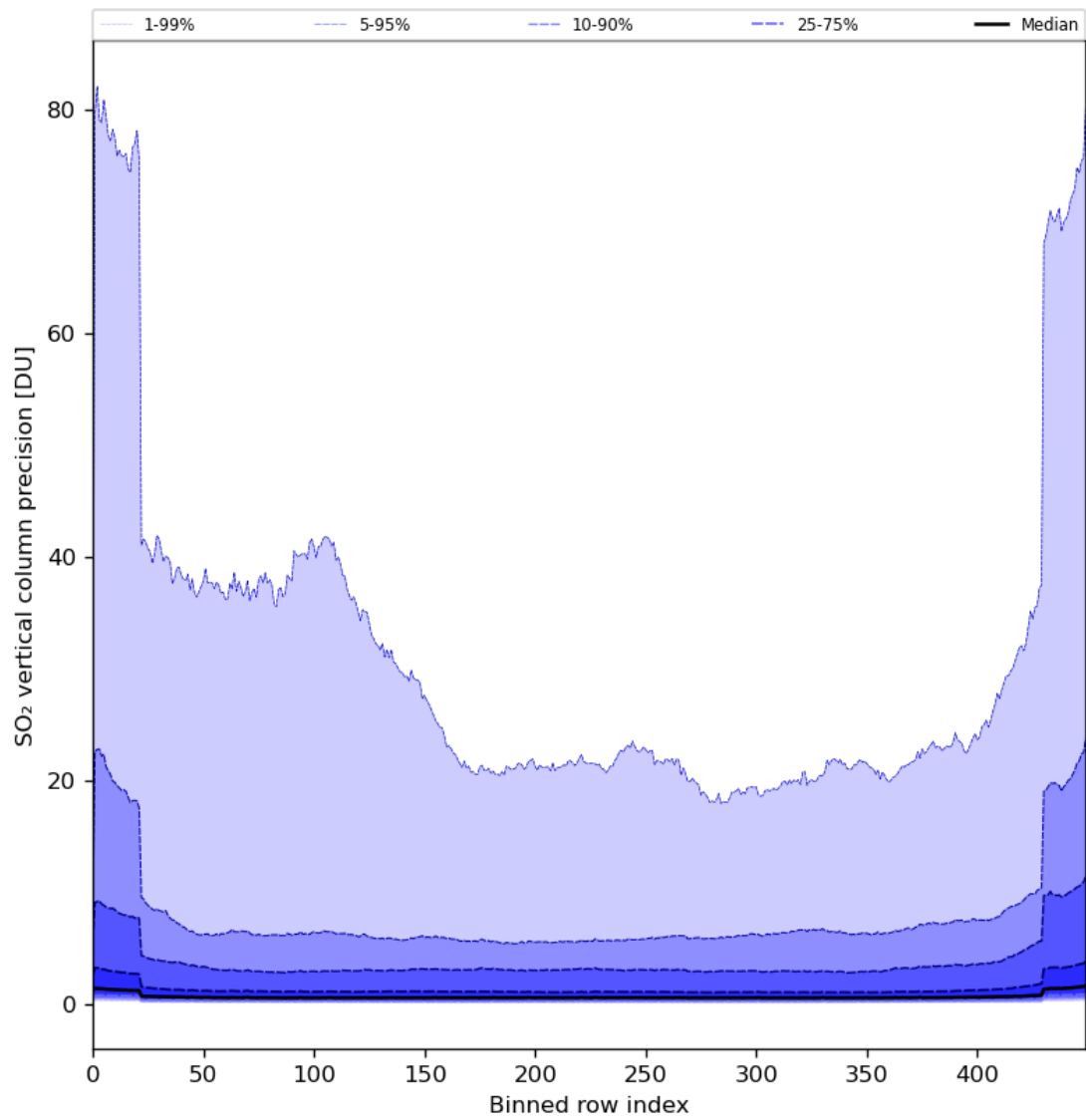
Figure 77: Along track statistics of “SO 2 vertical column precision” for 2024-07-22 to 2024-07-24
