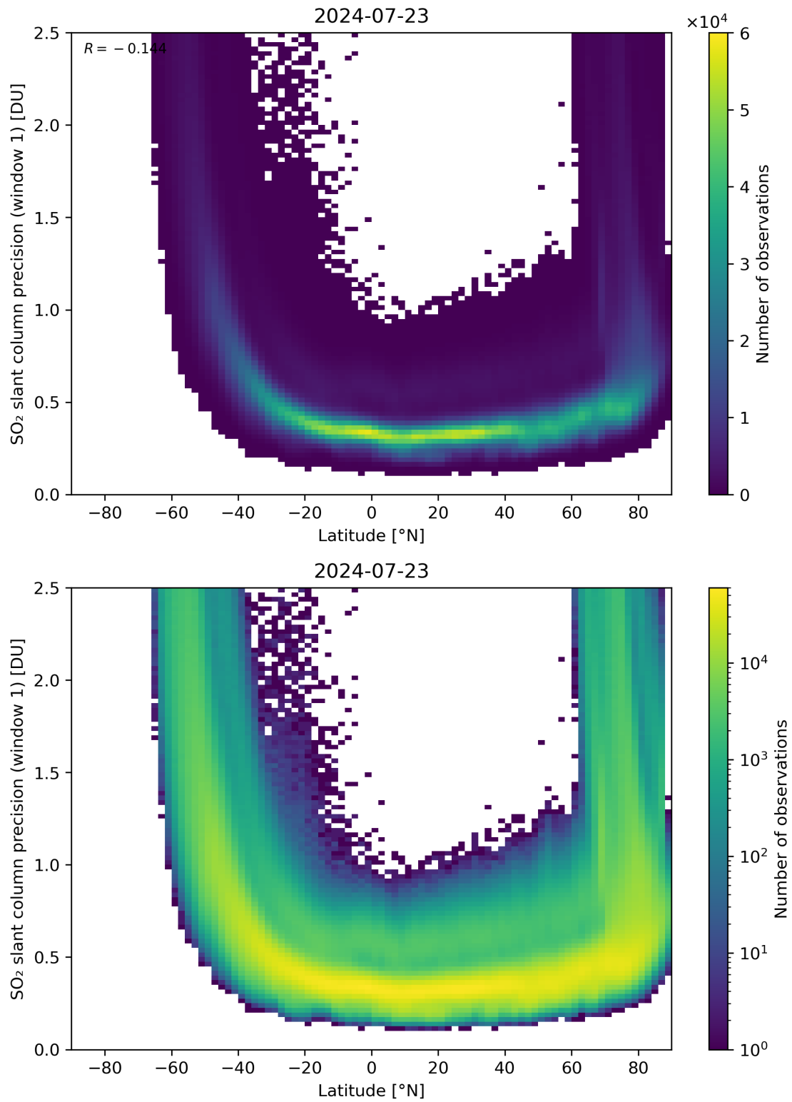
Figure 150: Scatter density plot of “Latitude” against “SO 2 slant column precision (window 1)” for 2024-07-22 to 2024-07-24.
