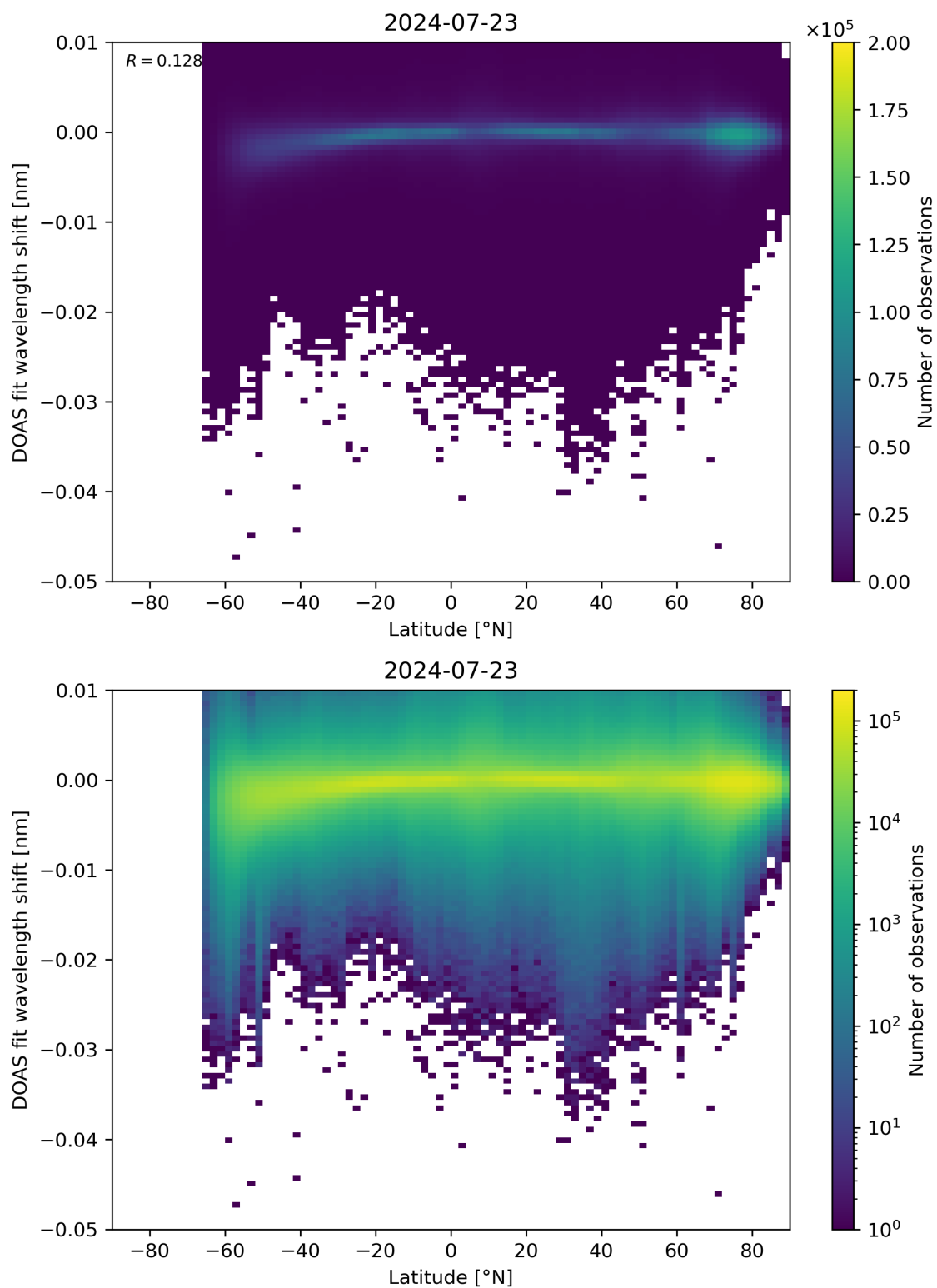
Figure 142: Scatter density plot of “Latitude” against “DOAS fit wavelength shift” for 2024-07-22 to 2024-07-24.
