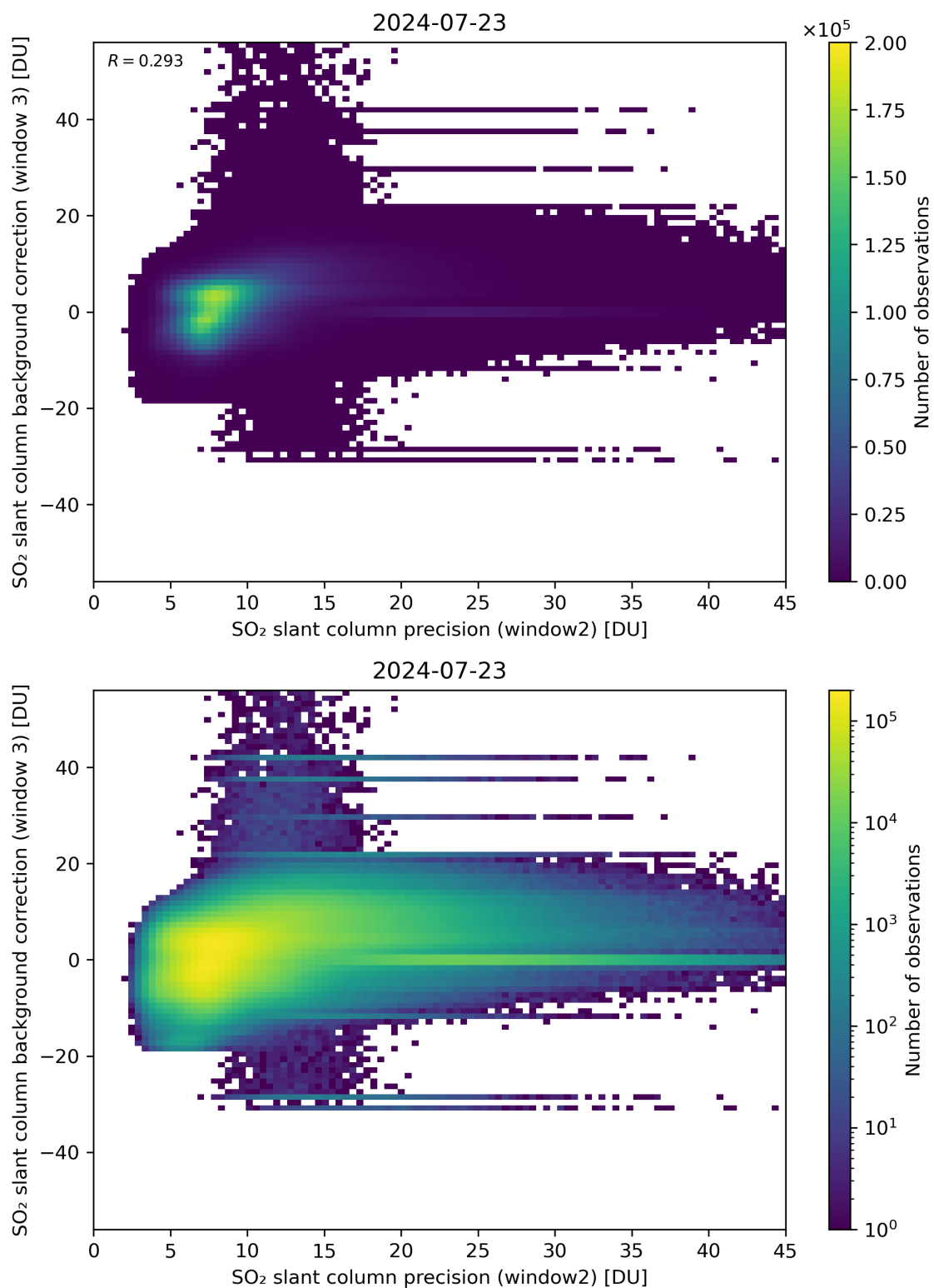
Figure 242: Scatter density plot of “SO 2 slant column precision (window2)” against “SO 2 slant column background correction (window 3)” for 2024-07-22 to 2024-07-24.
