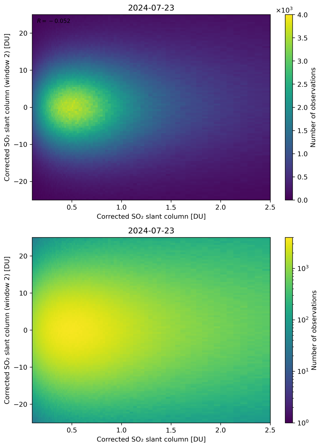
Figure 185: Scatter density plot of “Corrected SO 2 slant column” against “Corrected SO 2 slant column (window 2)” for 2024-07-22 to 2024-07-24.
