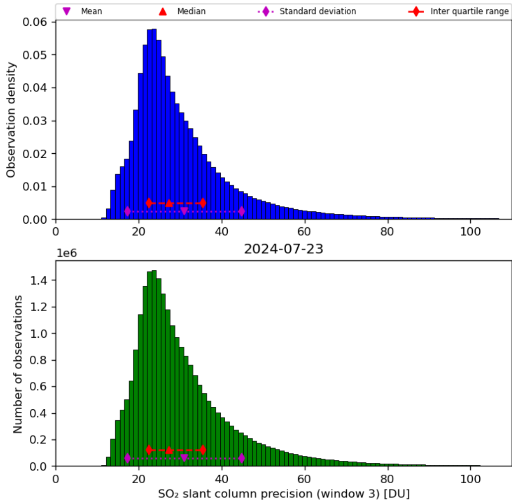
Figure 65: Histogram of “SO 2 slant column precision (window 3)” for 2024-07-22 to 2024-07-24
