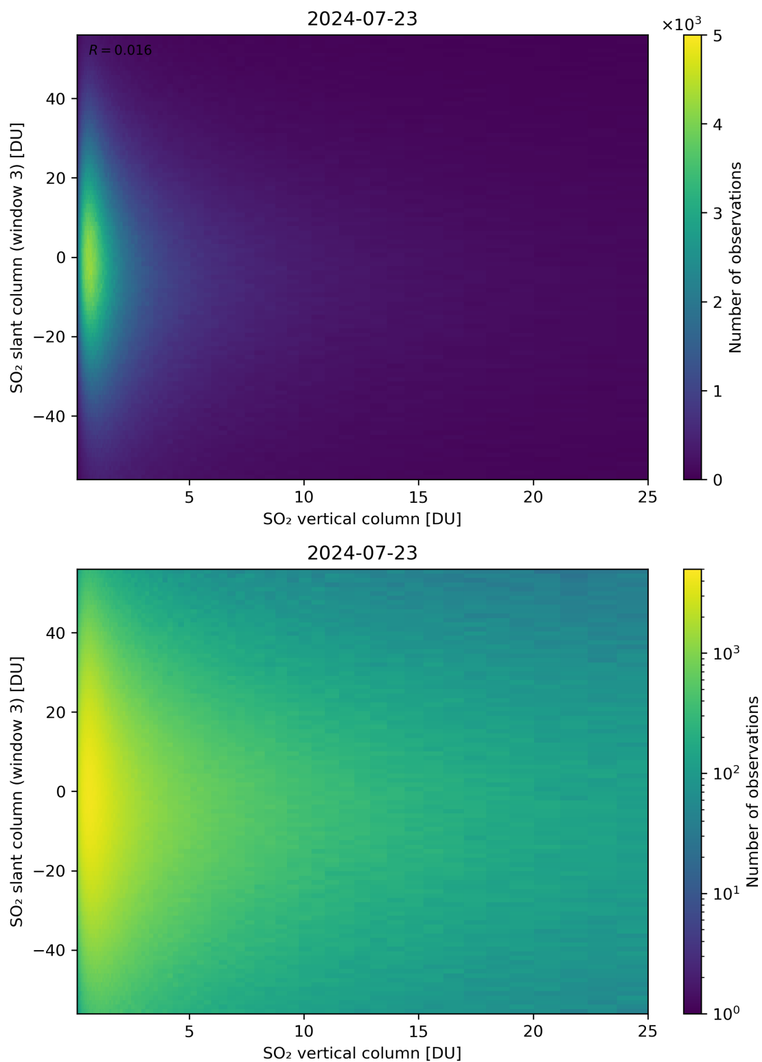
Figure 303: Scatter density plot of “SO 2 vertical column” against “SO 2 slant column (window 3)” for 2024-07-22 to 2024-07-24.
