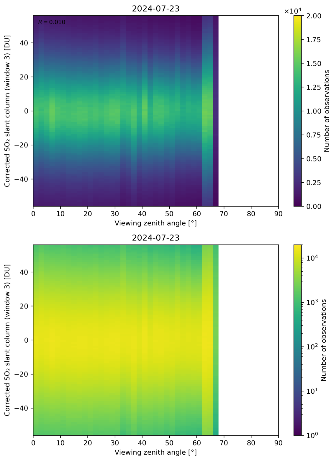
Figure 319: Scatter density plot of “Viewing zenith angle” against “Corrected SO 2 slant column (window 3)” for 2024-07-22 to 2024-07-24.
