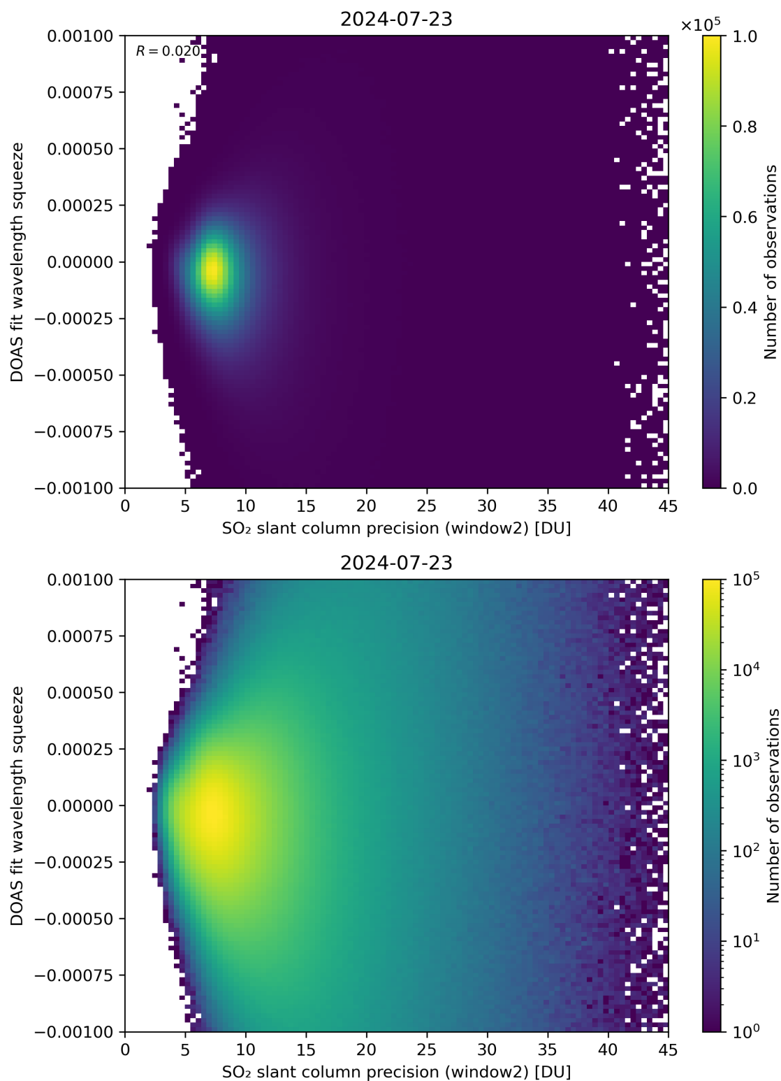
Figure 244: Scatter density plot of “SO 2 slant column precision (window2)” against “DOAS fit wavelength squeeze” for 2024-07-22 to 2024-07-24.
