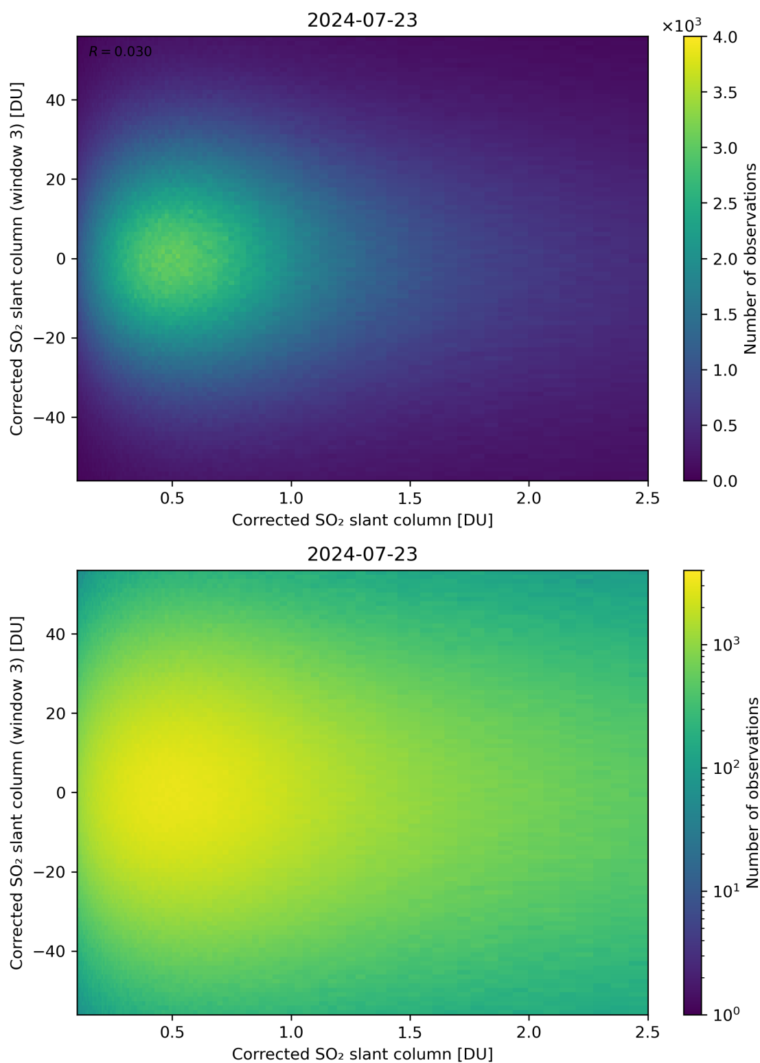
Figure 186: Scatter density plot of “Corrected SO 2 slant column” against “Corrected SO 2 slant column (window 3)” for 2024-07-22 to 2024-07-24.
