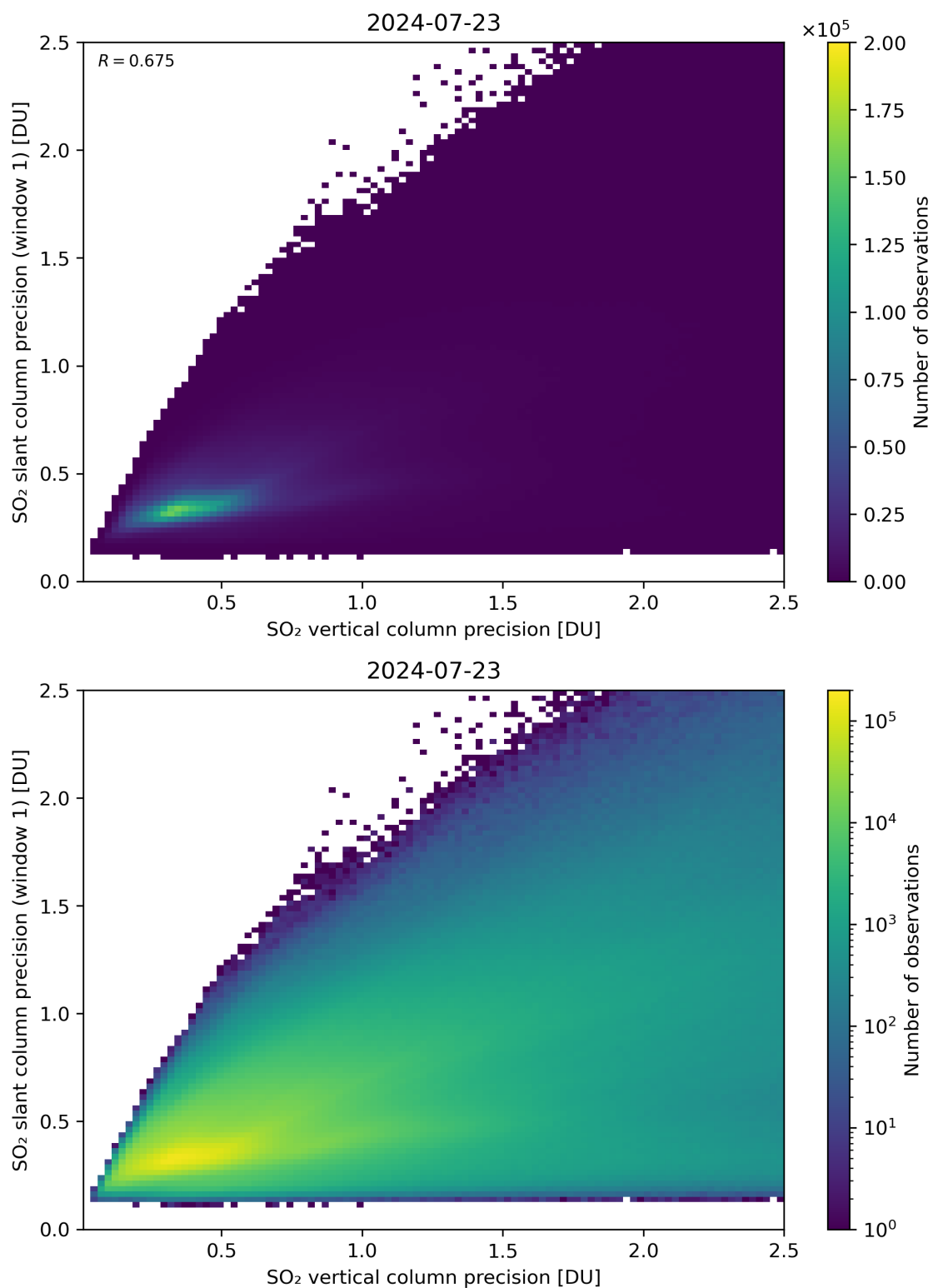
Figure 290: Scatter density plot of “SO 2 vertical column precision” against “SO 2 slant column precision (window 1)” for 2024-07-22 to 2024-07-24.
