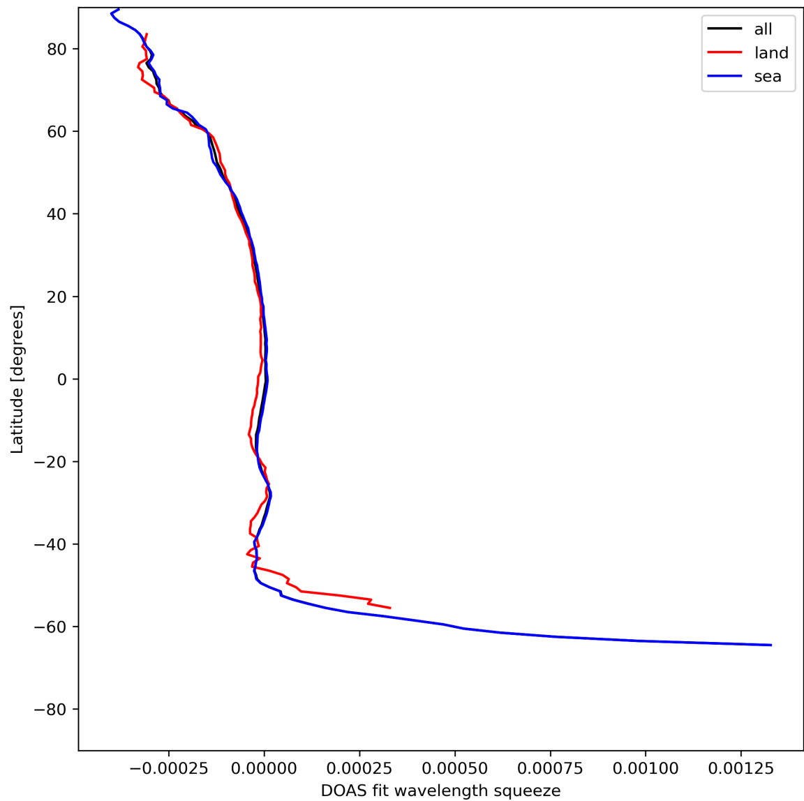
Figure 46: Zonal average of “DOAS fit wavelength squeeze” for 2024-07-22 to 2024-07-24.
