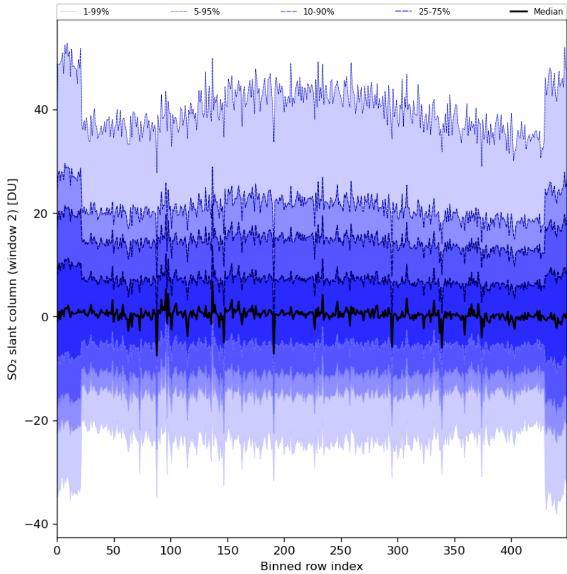
Figure 83: Along track statistics of “SO 2 slant column (window 2)” for 2024-07-22 to 2024-07-24
