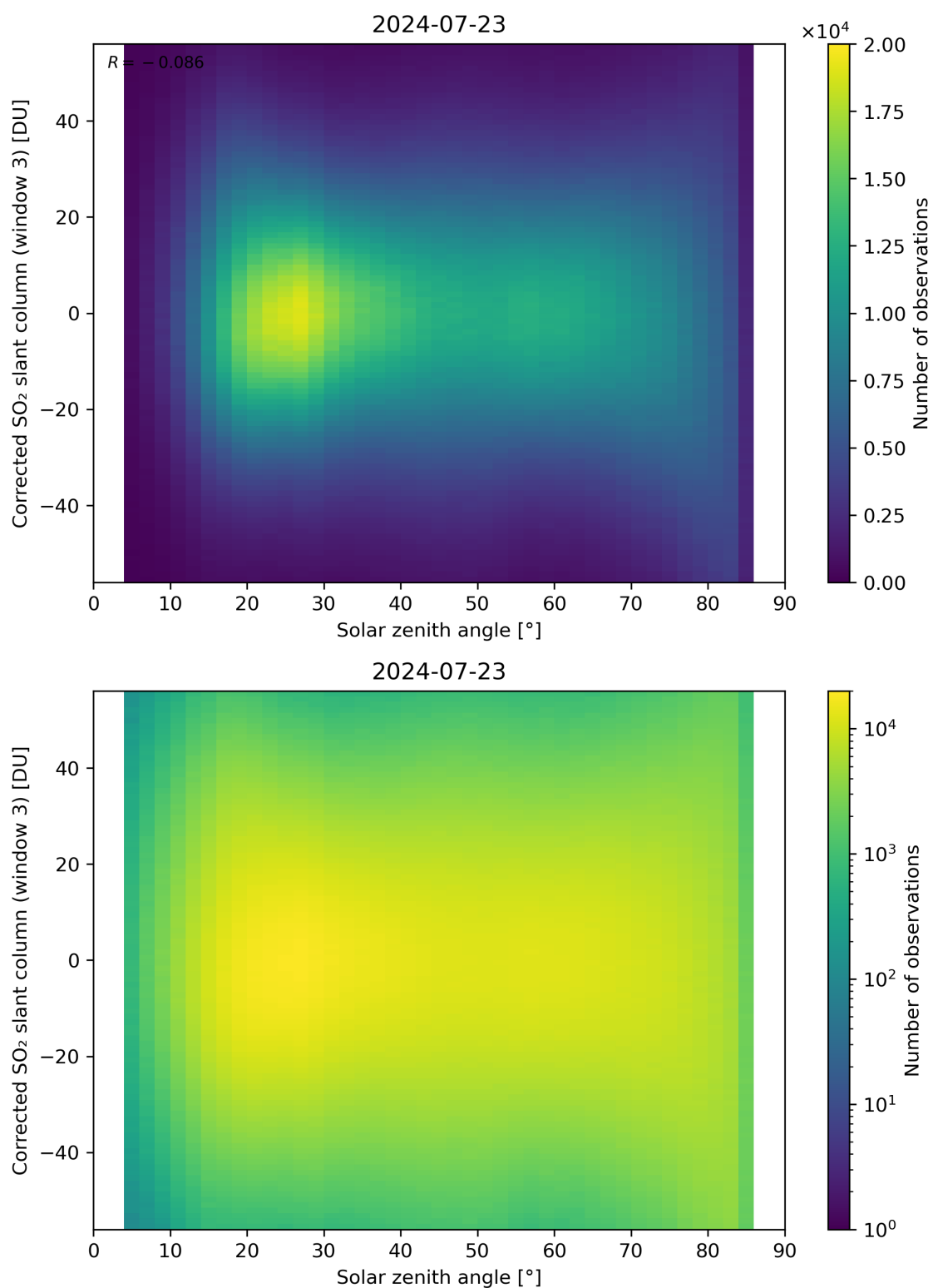
Figure 168: Scatter density plot of “Solar zenith angle” against “Corrected SO 2 slant column (window 3)” for 2024-07-22 to 2024-07-24.
