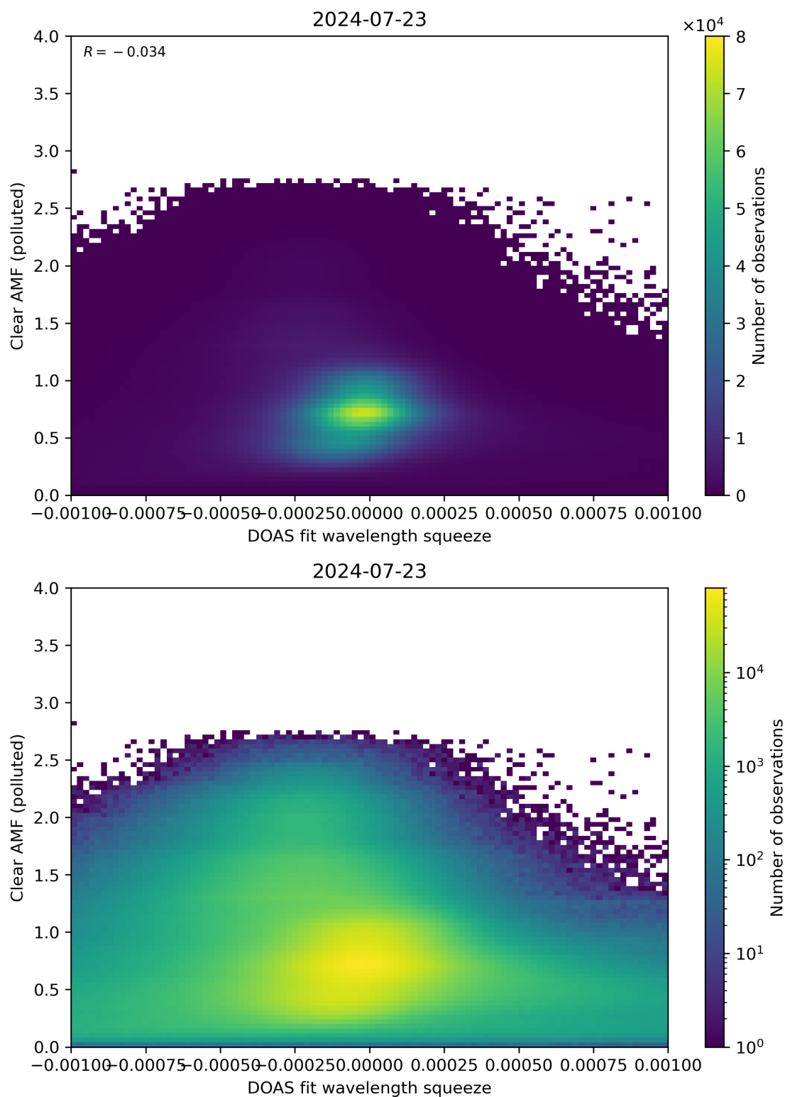
Figure 133: Scatter density plot of “DOAS fit wavelength squeeze” against “Clear AMF (polluted)” for 2024-07-22 to 2024-07-24.
