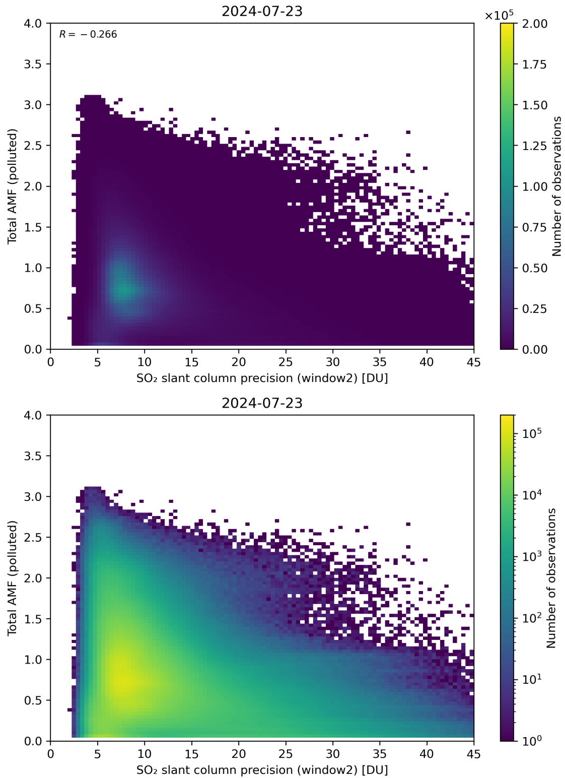
Figure 251: Scatter density plot of “SO 2 slant column precision (window2)” against “Total AMF (polluted)” for 2024-07-22 to 2024-07-24.
