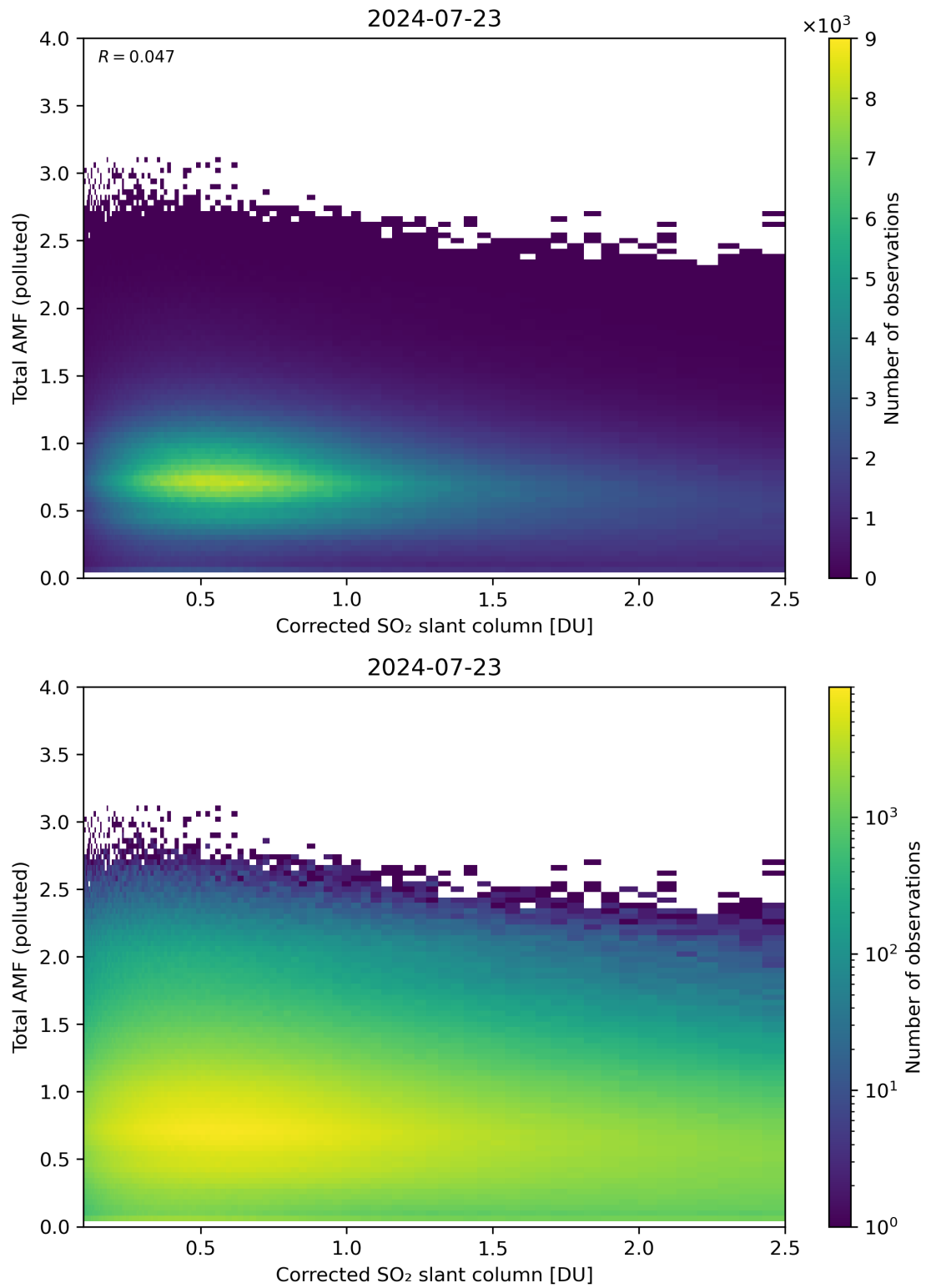
Figure 192: Scatter density plot of “Corrected SO 2 slant column” against “Total AMF (polluted)” for 2024-07-22 to 2024-07-24.
