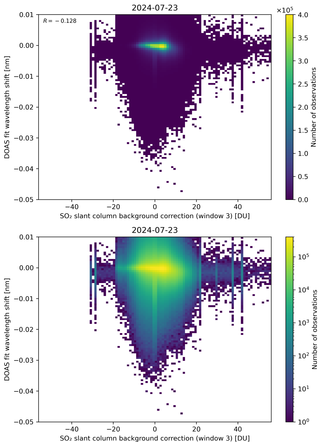
Figure 121: Scatter density plot of “SO 2 slant column background correction (window 3)” against “DOAS fit wavelength shift” for 2024-07-22 to 2024-07-24.
