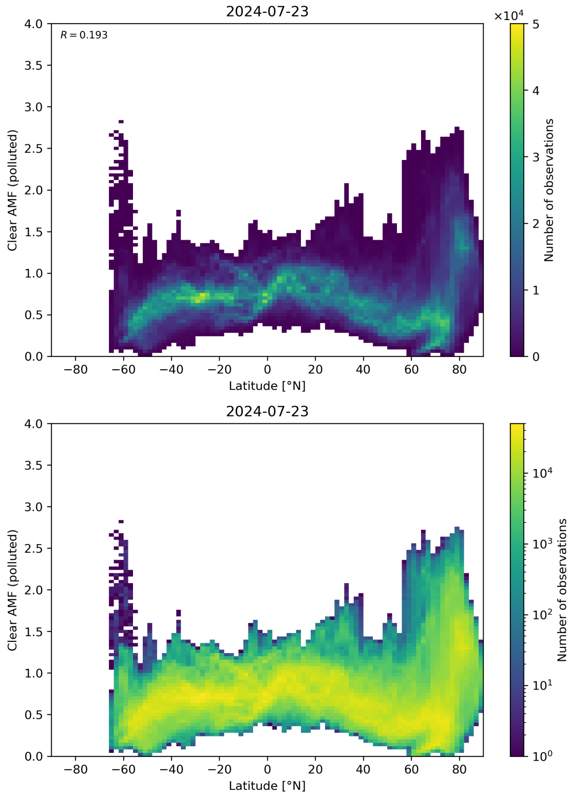
Figure 145: Scatter density plot of “Latitude” against “Clear AMF (polluted)” for 2024-07-22 to 2024-07-24.
