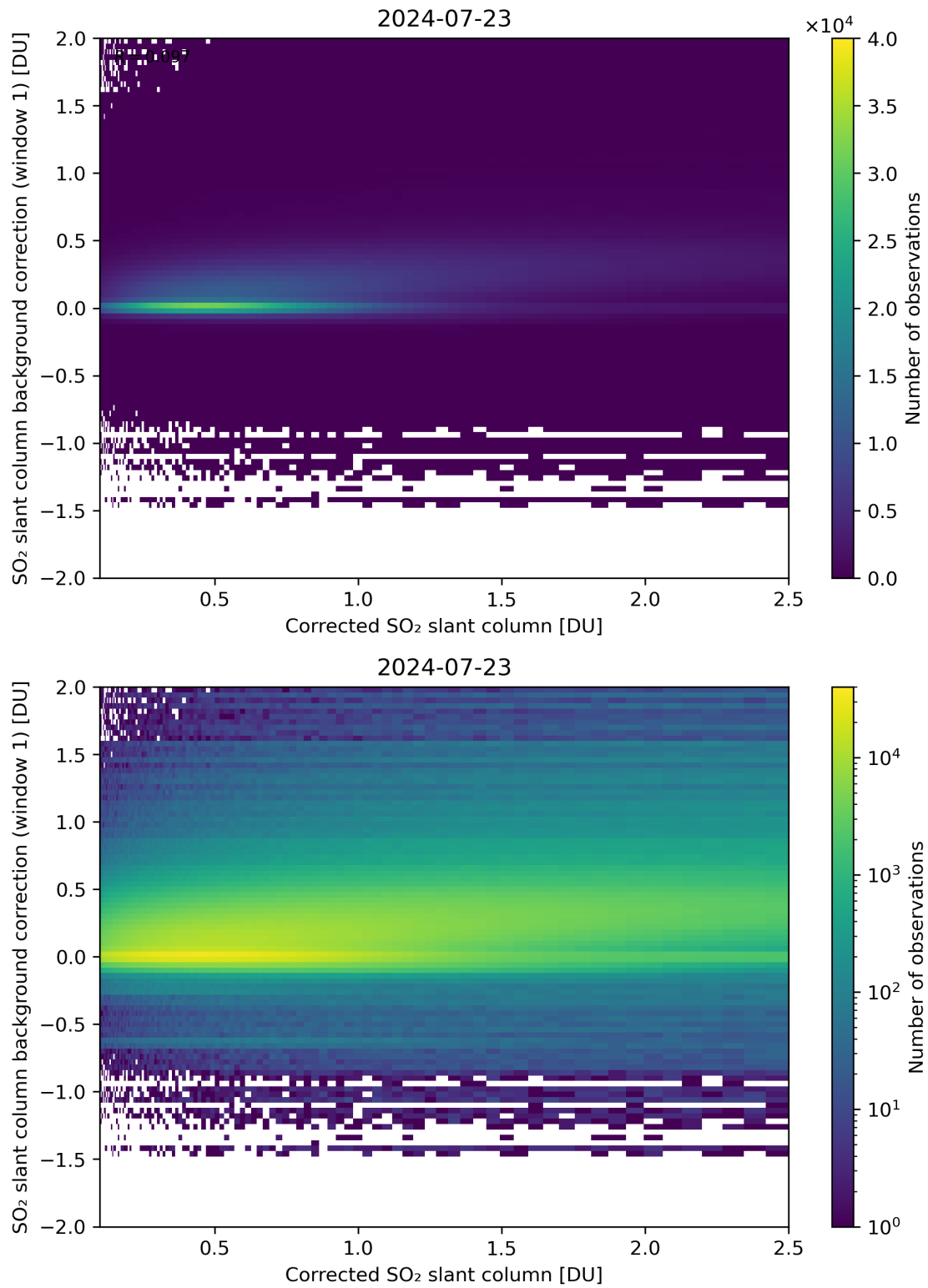
Figure 178: Scatter density plot of “Corrected SO 2 slant column” against “SO 2 slant column background correction (window 1)” for 2024-07-22 to 2024-07-24.
