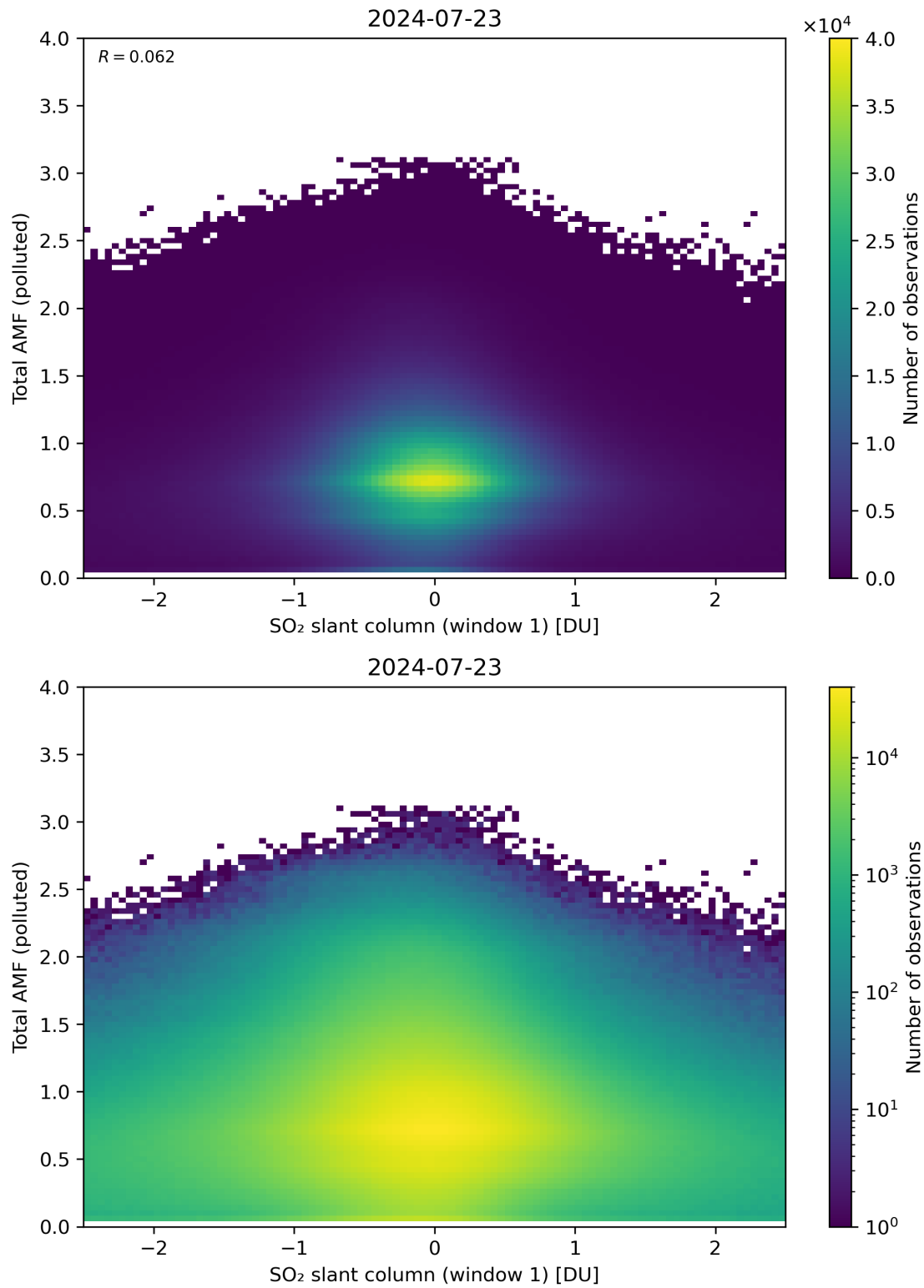
Figure 239: Scatter density plot of “SO 2 slant column (window 1)” against “Total AMF (polluted)” for 2024-07-22 to 2024-07-24.
