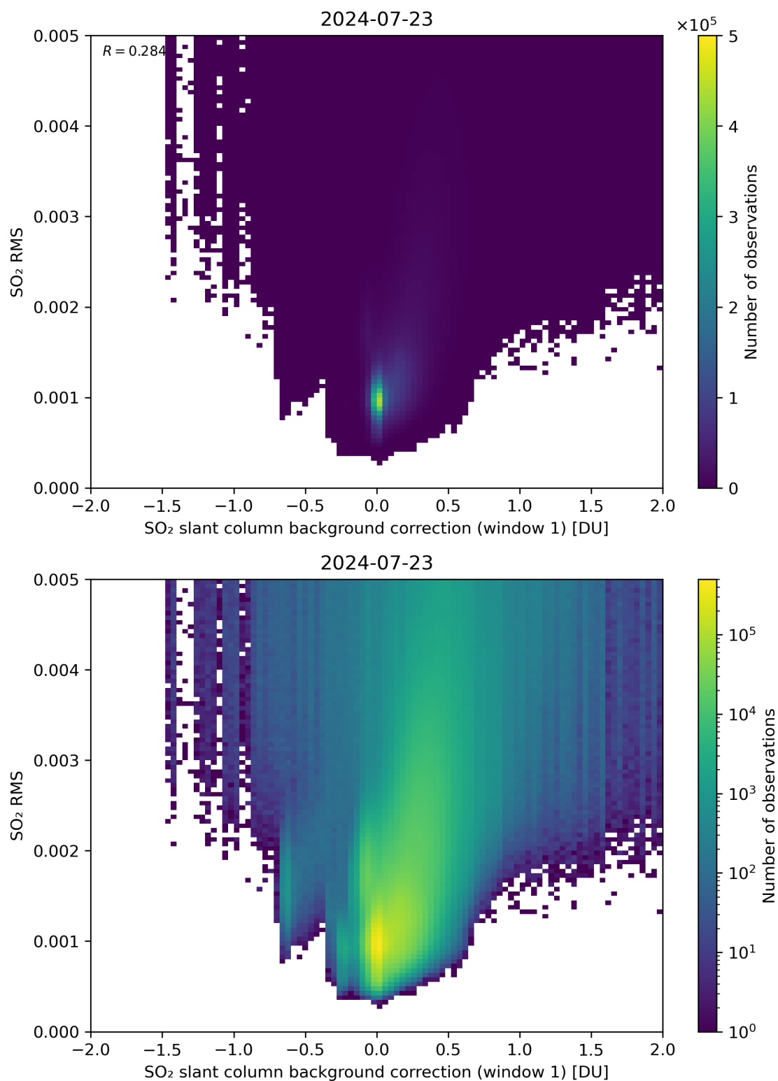
Figure 102: Scatter density plot of “SO 2 slant column background correction (window 1)” against “SO 2 RMS” for 2024-07-22 to 2024-07-24.
