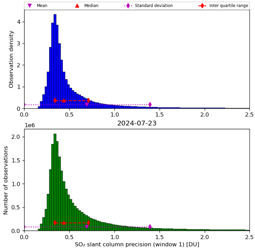
Figure 57: Histogram of “SO 2 slant column precision (window 1)” for 2024-07-22 to 2024-07-24
