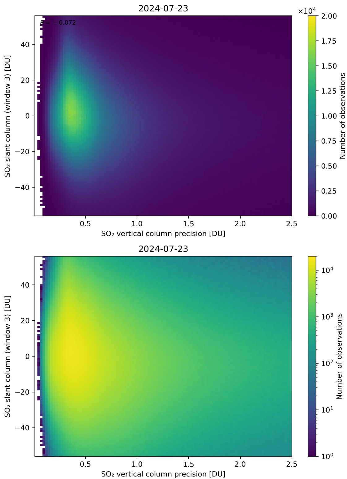
Figure 292: Scatter density plot of “SO 2 vertical column precision” against “SO 2 slant column (window 3)” for 2024-07-22 to 2024-07-24.
