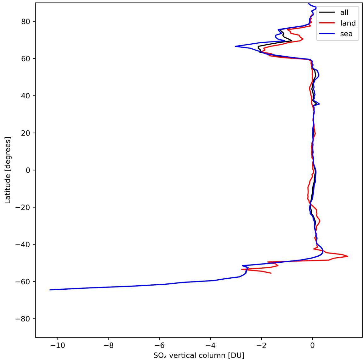
Figure 30: Zonal average of “SO 2 vertical column” for 2024-07-22 to 2024-07-24.
