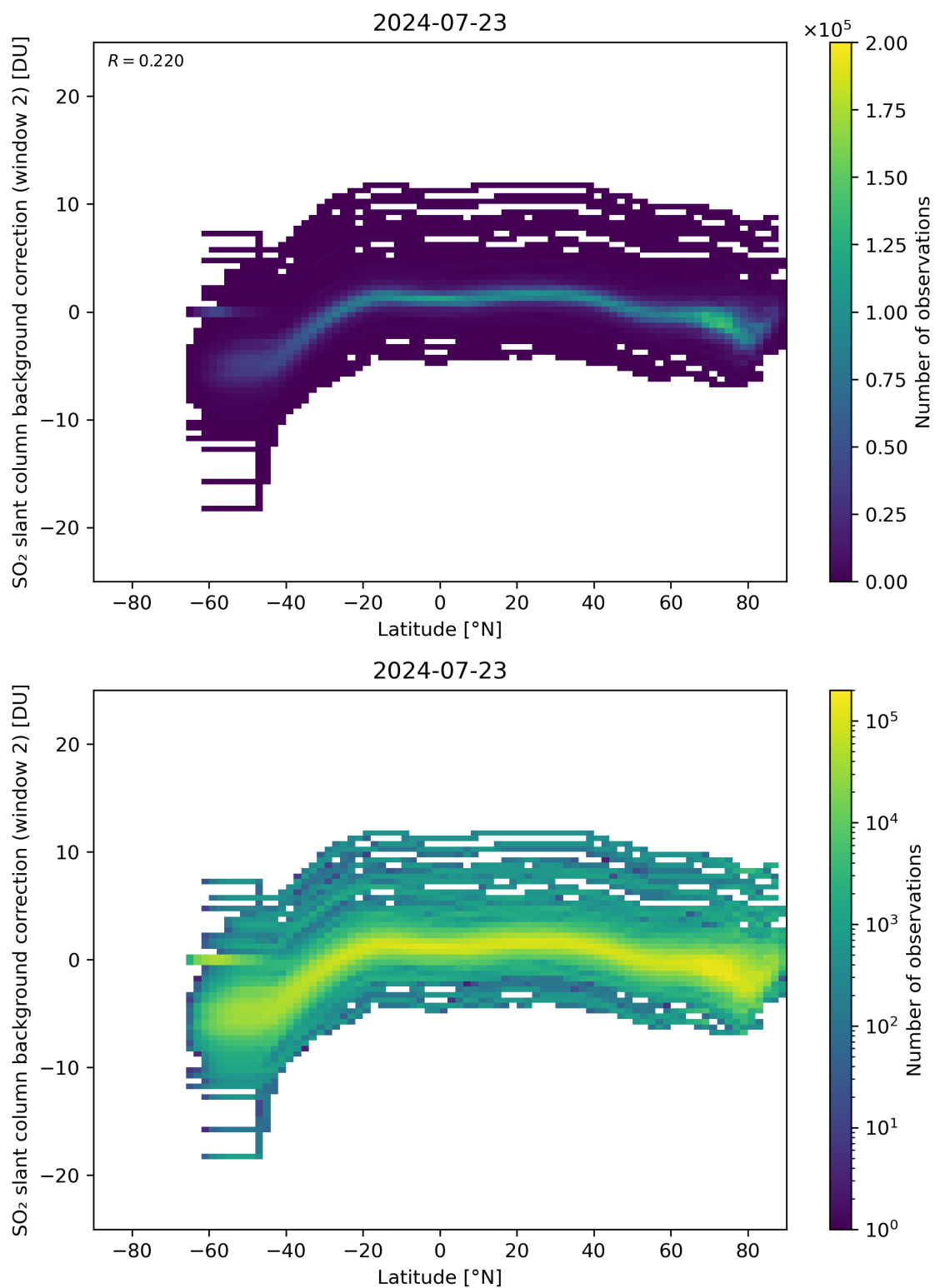
Figure 140: Scatter density plot of “Latitude” against “SO 2 slant column background correction (window 2)” for 2024-07-22 to 2024-07-24.
