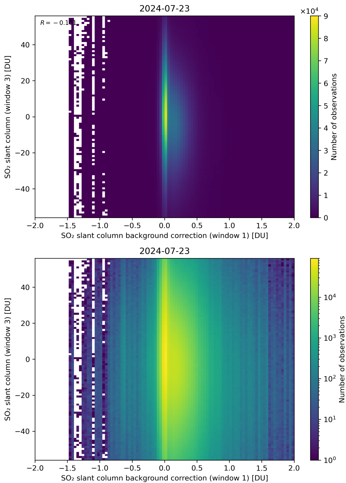
Figure 107: Scatter density plot of “SO 2 slant column background correction (window 1)” against “SO 2 slant column (window 3)” for 2024-07-22 to 2024-07-24.
