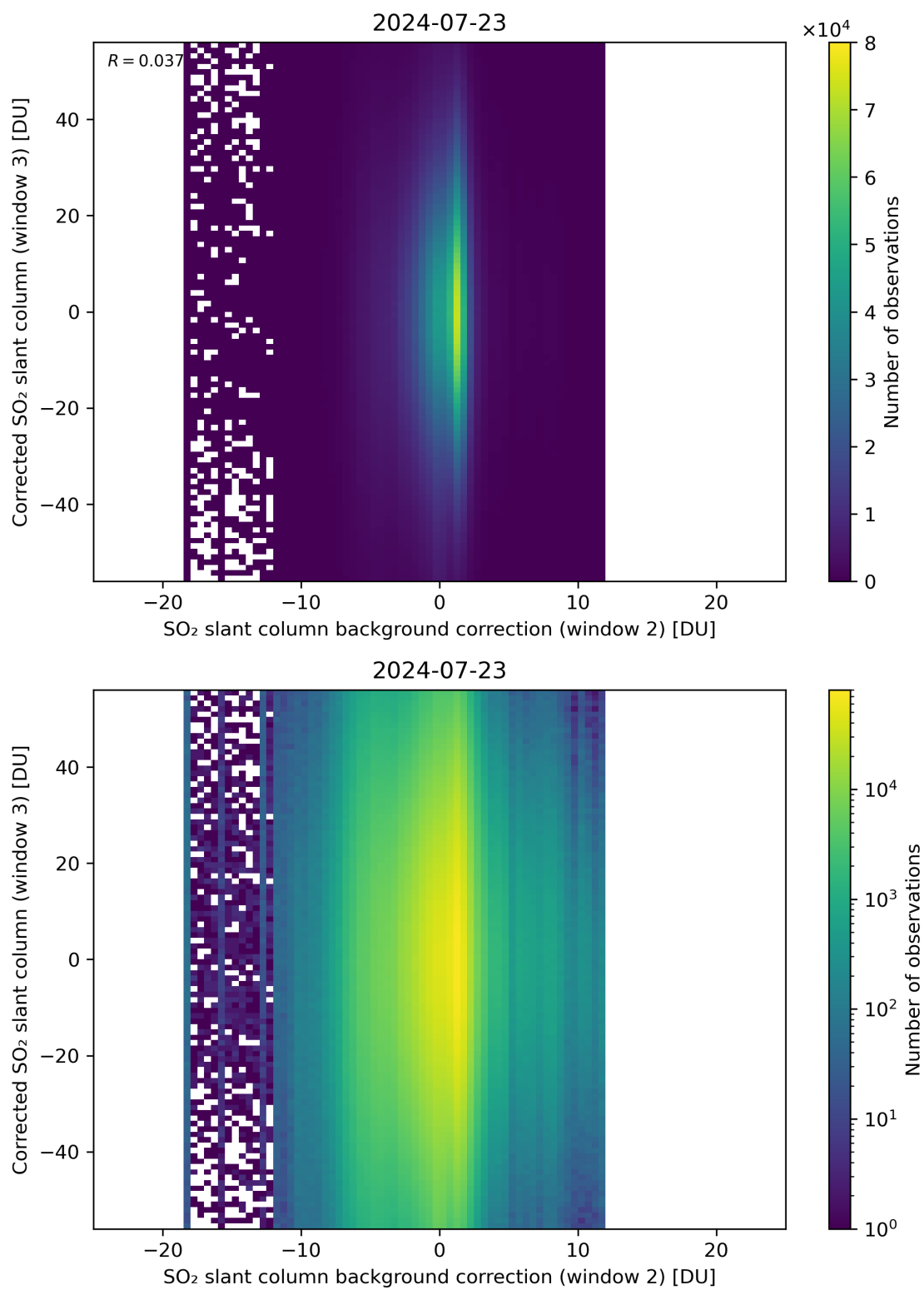
Figure 116: Scatter density plot of “SO 2 slant column background correction (window 2)” against “Corrected SO 2 slant column (window 3)” for 2024-07-22 to 2024-07-24.
