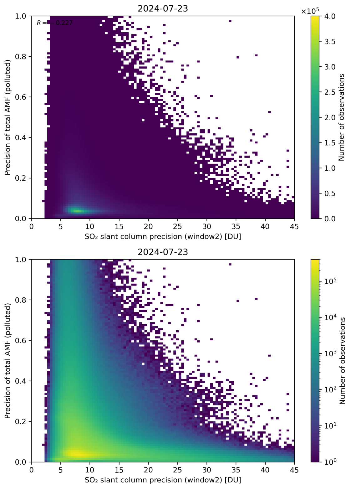
Figure 252: Scatter density plot of “SO 2 slant column precision (window2)” against “Precision of total AMF (polluted)” for 2024-07-22 to 2024-07-24.
