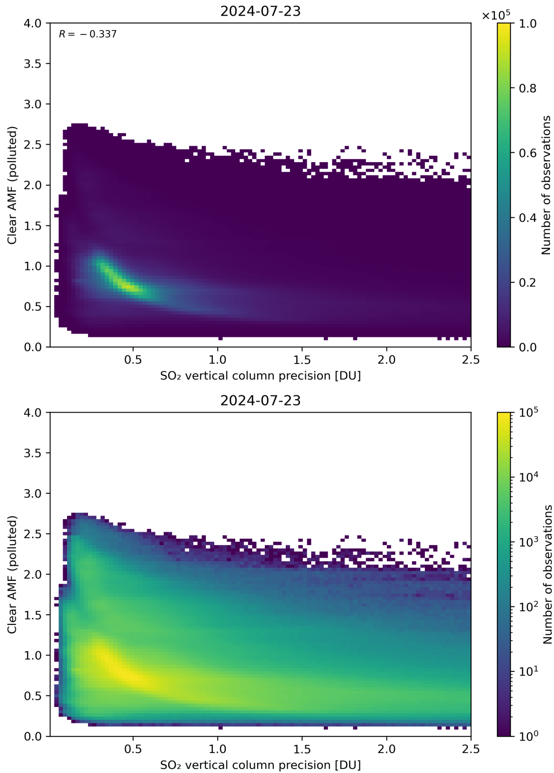
Figure 285: Scatter density plot of “SO 2 vertical column precision” against “Clear AMF (polluted)” for 2024-07-22 to 2024-07-24.
