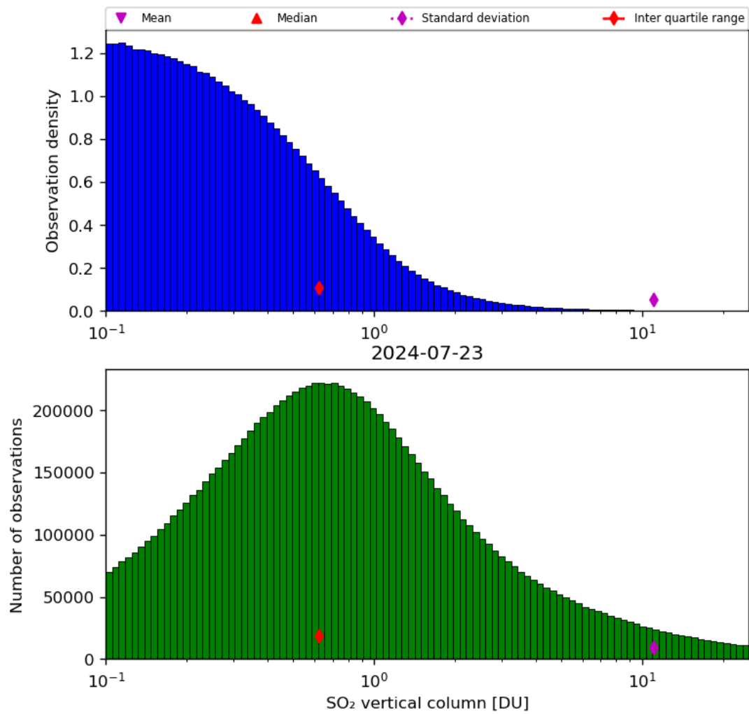
Figure 53: Histogram of “SO 2 vertical column” for 2024-07-22 to 2024-07-24
