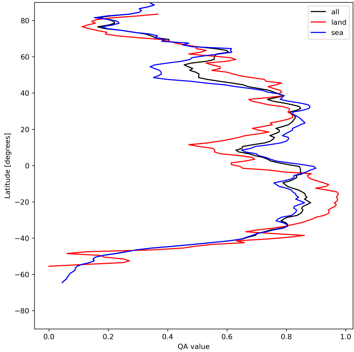
Figure 29: Zonal average of “QA value” for 2024-07-22 to 2024-07-24.
