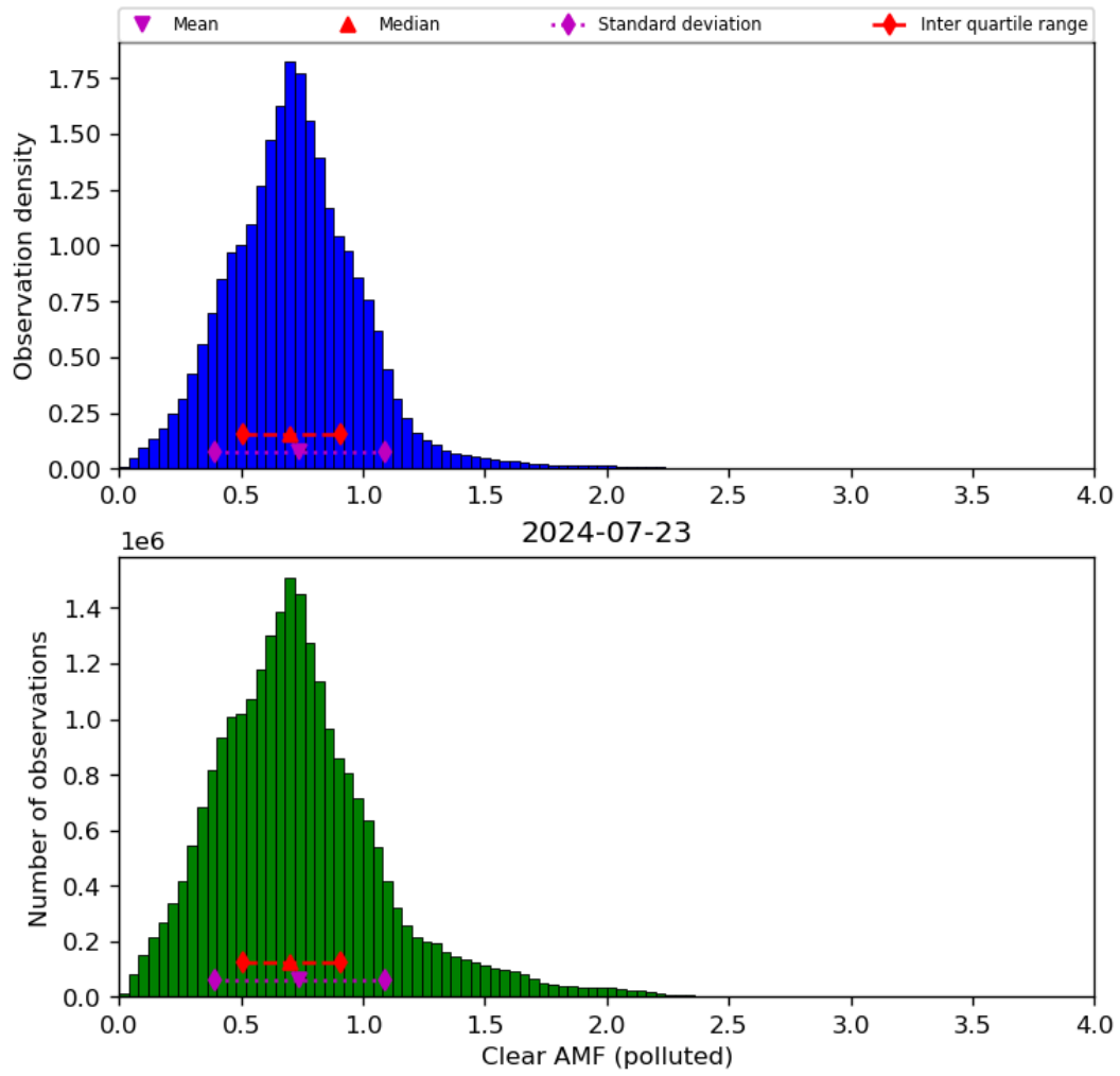
Figure 73: Histogram of “Clear AMF (polluted)” for 2024-07-22 to 2024-07-24
