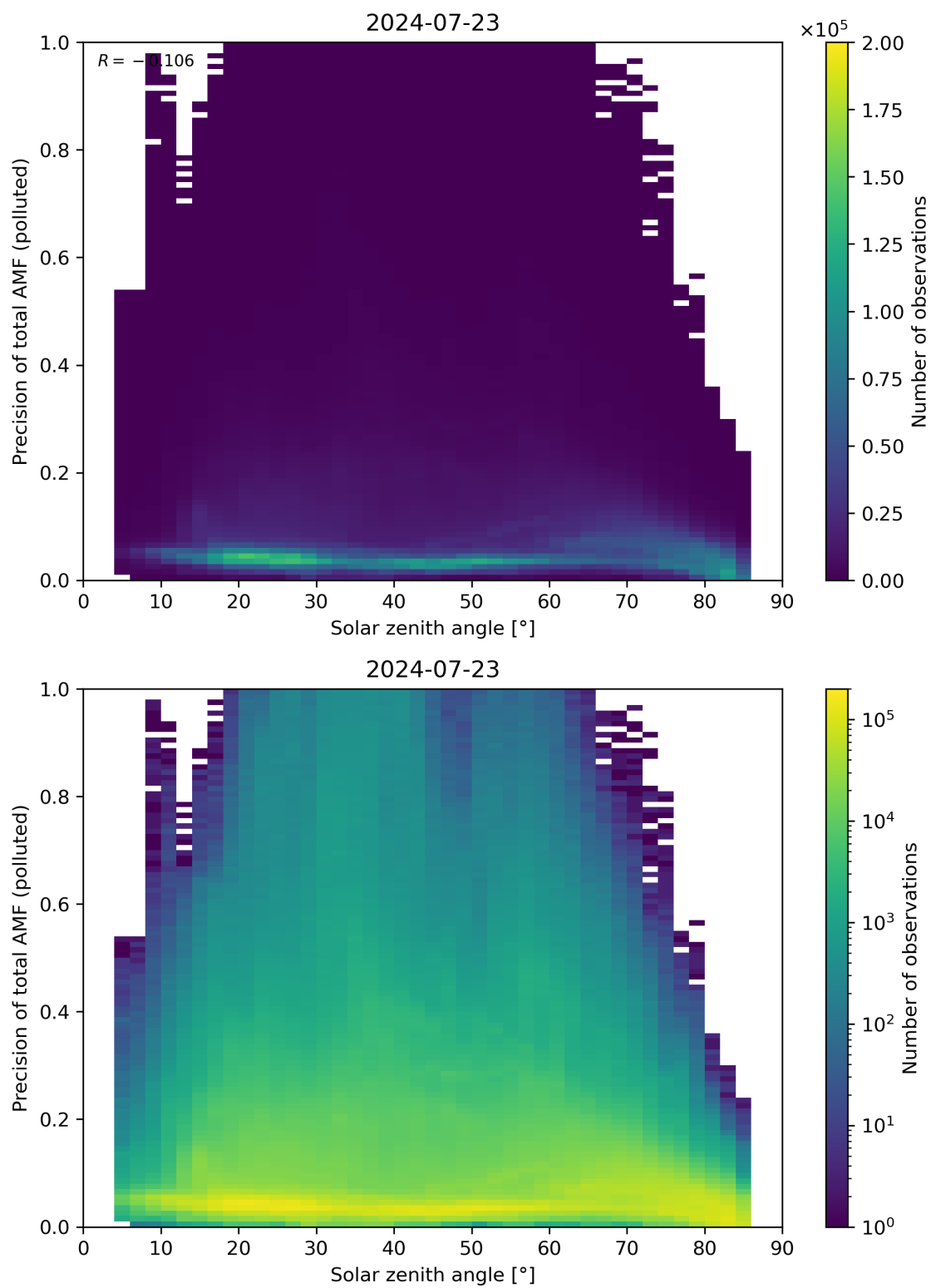
Figure 175: Scatter density plot of “Solar zenith angle” against “Precision of total AMF (polluted)” for 2024-07-22 to 2024-07-24.
