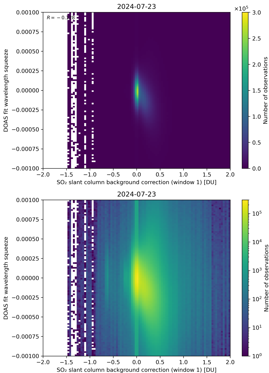
Figure 101: Scatter density plot of “SO 2 slant column background correction (window 1)” against “DOAS fit wavelength squeeze” for 2024-07-22 to 2024-07-24.
