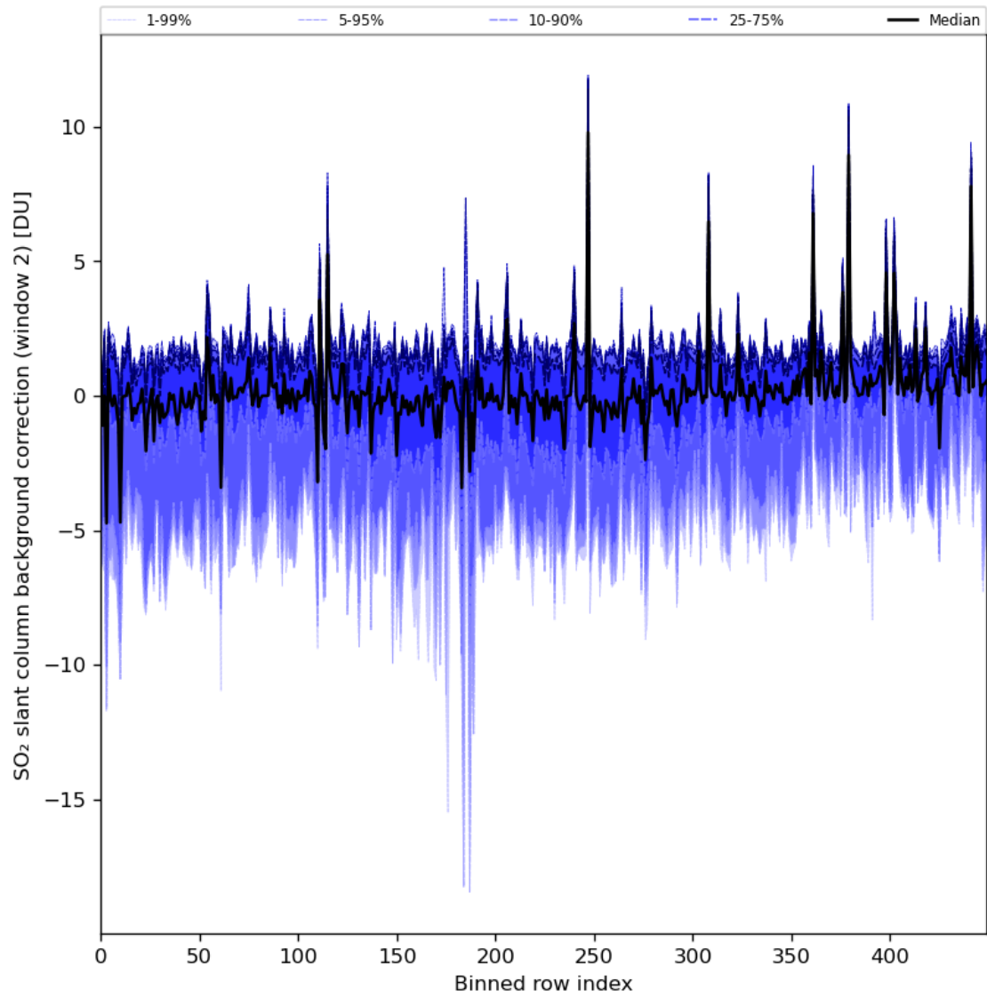
Figure 86: Along track statistics of “SO 2 slant column background correction (window 2)” for 2024-07-22 to 2024-07-24
