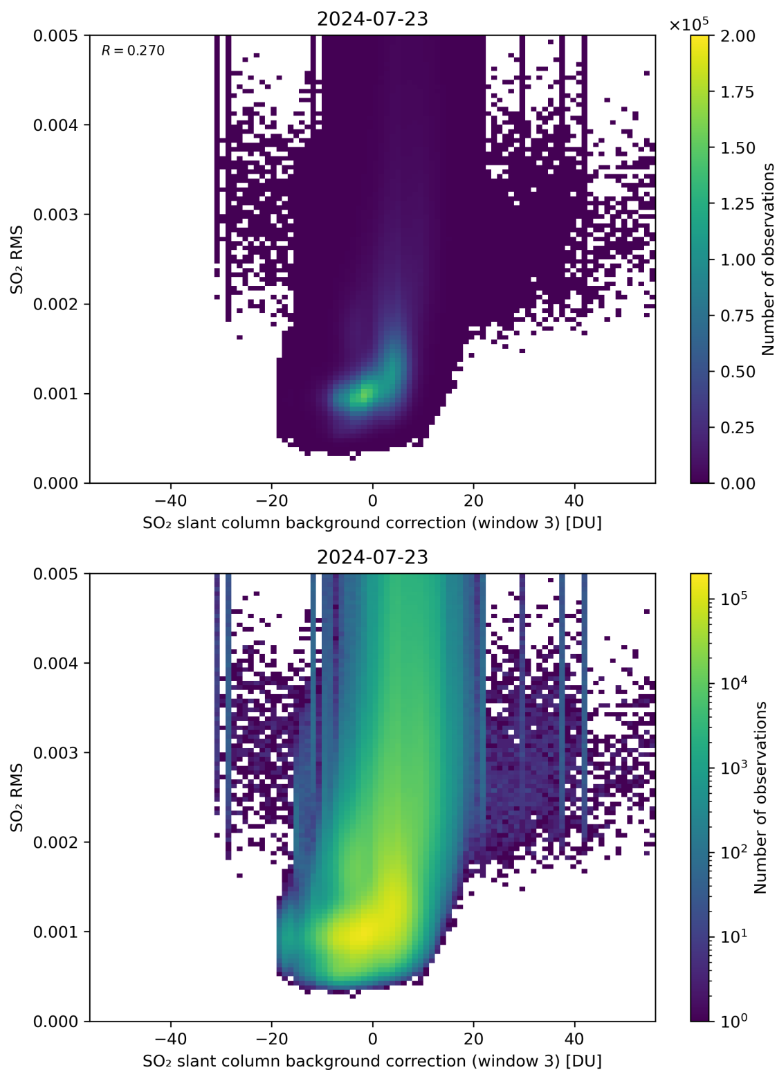
Figure 123: Scatter density plot of “SO 2 slant column background correction (window 3)” against “SO 2 RMS” for 2024-07-22 to 2024-07-24.
