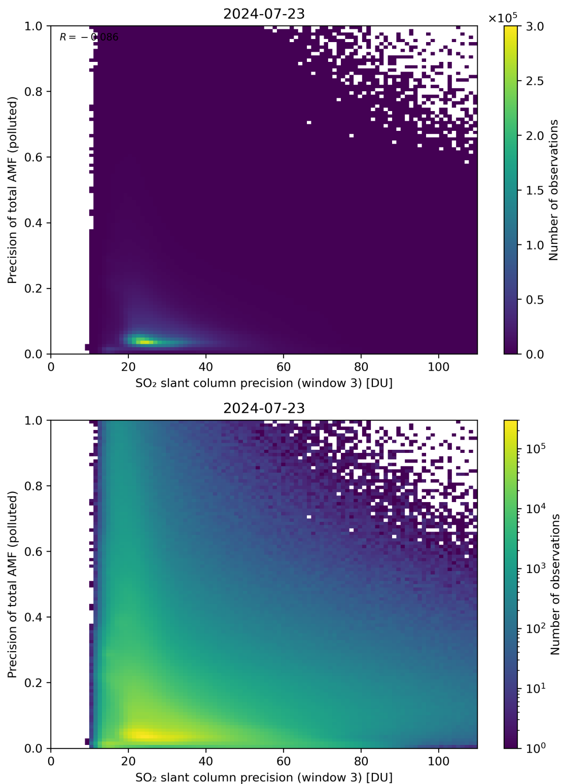
Figure 264: Scatter density plot of “SO 2 slant column precision (window 3)” against “Precision of total AMF (polluted)” for 2024-07-22 to 2024-07-24.
