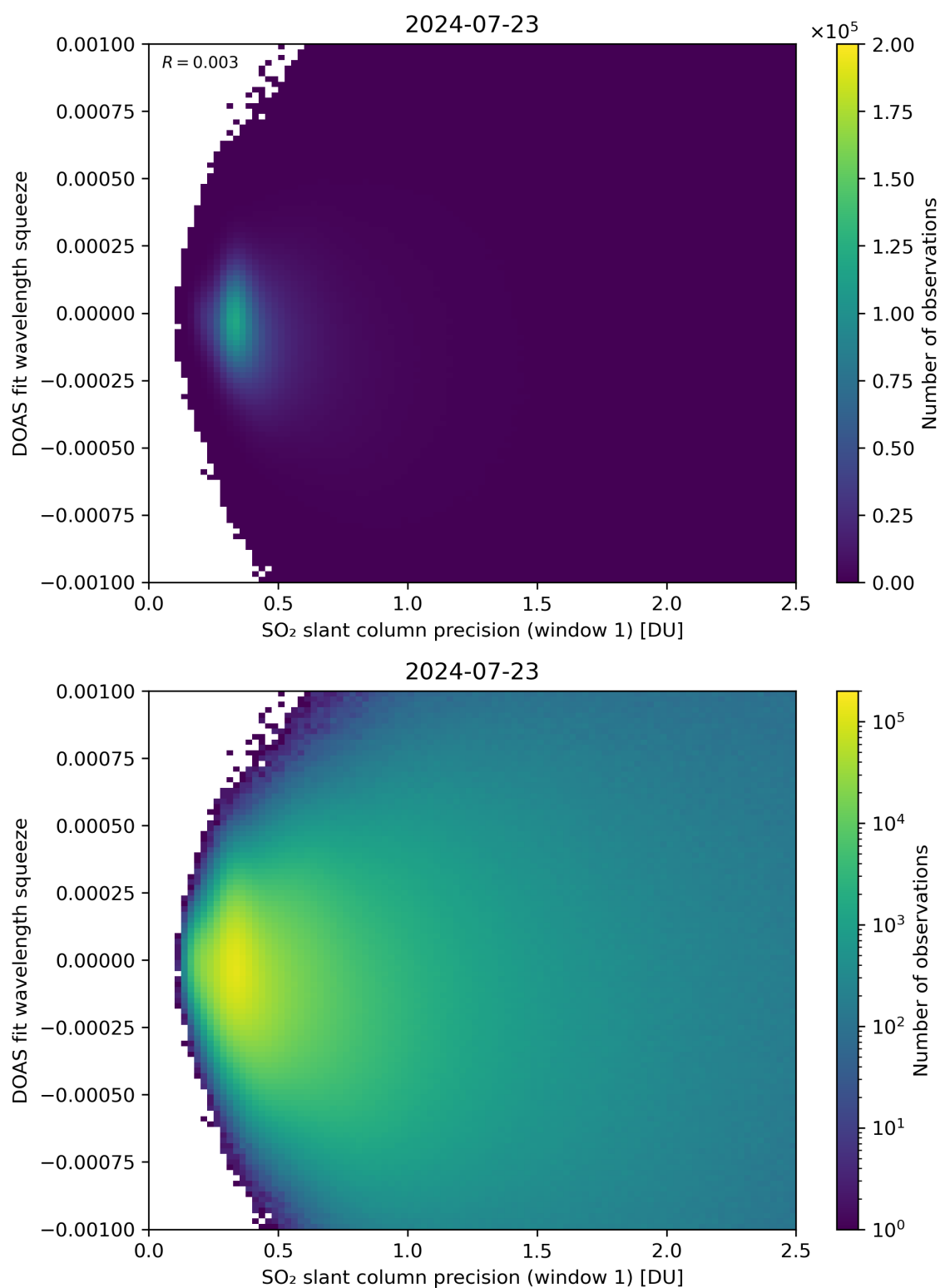
Figure 222: Scatter density plot of “SO 2 slant column precision (window 1)” against “DOAS fit wavelength squeeze” for 2024-07-22 to 2024-07-24.
