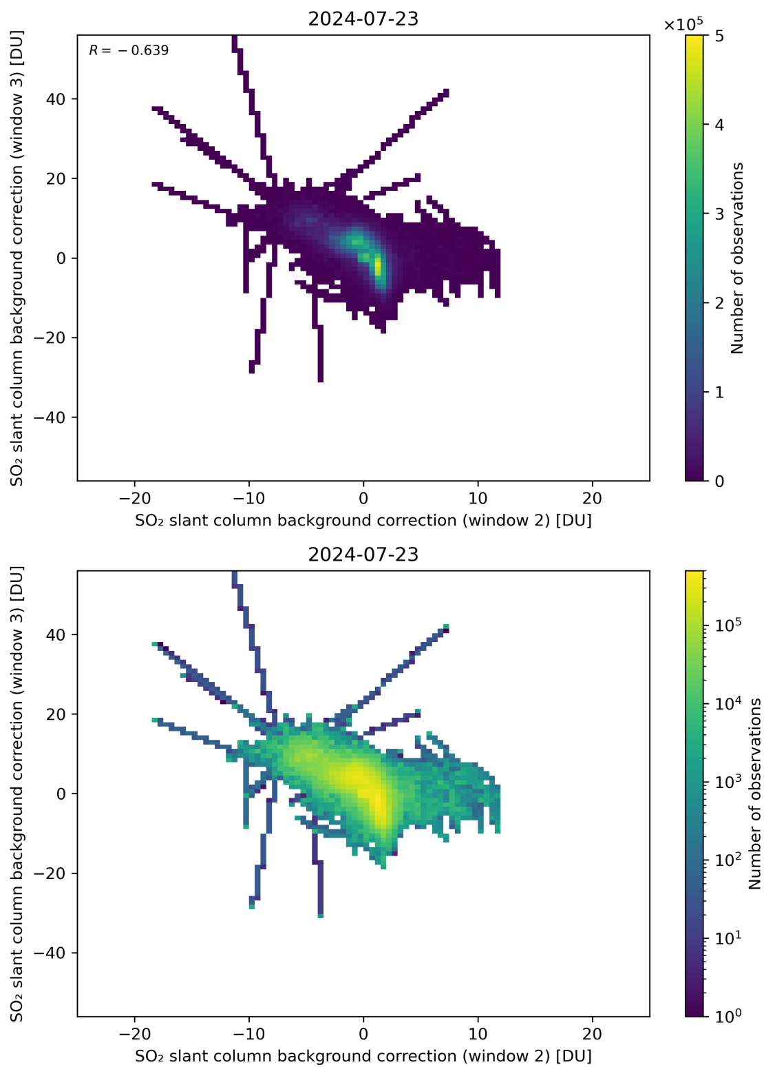
Figure 111: Scatter density plot of “SO 2 slant column background correction (window 2)” against “SO 2 slant column background correction (window 3)” for 2024-07-22 to 2024-07-24.
