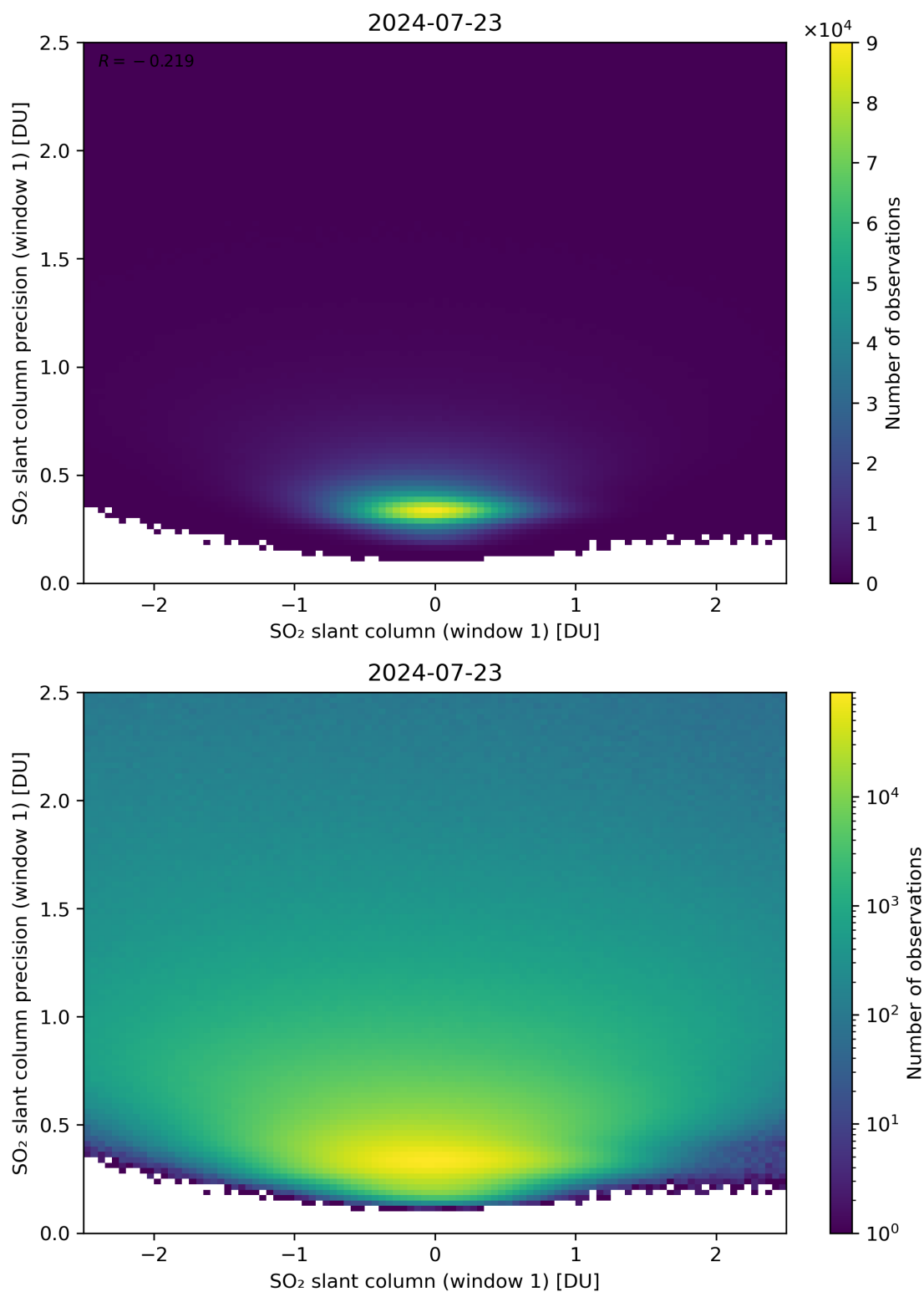
Figure 235: Scatter density plot of “SO 2 slant column (window 1)” against “SO 2 slant column precision (window 1)” for 2024-07-22 to 2024-07-24.
