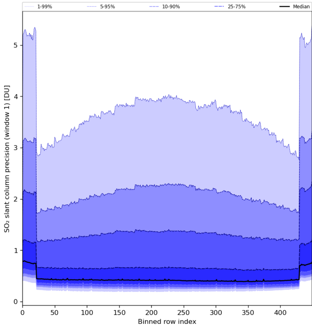
Figure 80: Along track statistics of “SO 2 slant column precision (window 1)” for 2024-07-22 to 2024-07-24
