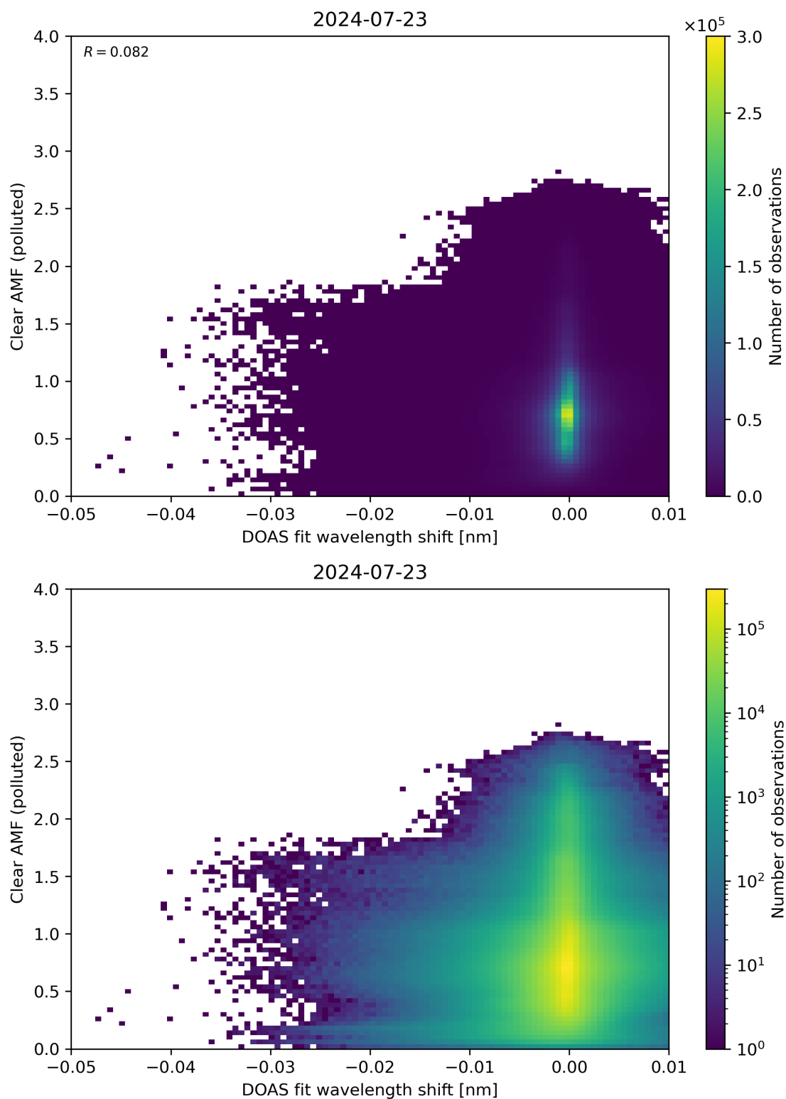
Figure 129: Scatter density plot of “DOAS fit wavelength shift” against “Clear AMF (polluted)” for 2024-07-22 to 2024-07-24.
