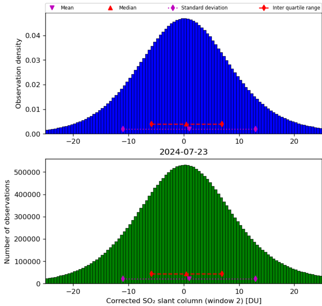
Figure 62: Histogram of “Corrected SO 2 slant column (window 2)” for 2024-07-22 to 2024-07-24
