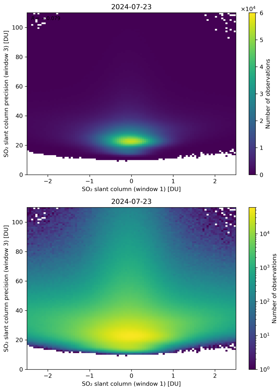
Figure 238: Scatter density plot of “SO 2 slant column (window 1)” against “SO 2 slant column precision (window 3)” for 2024-07-22 to 2024-07-24.
