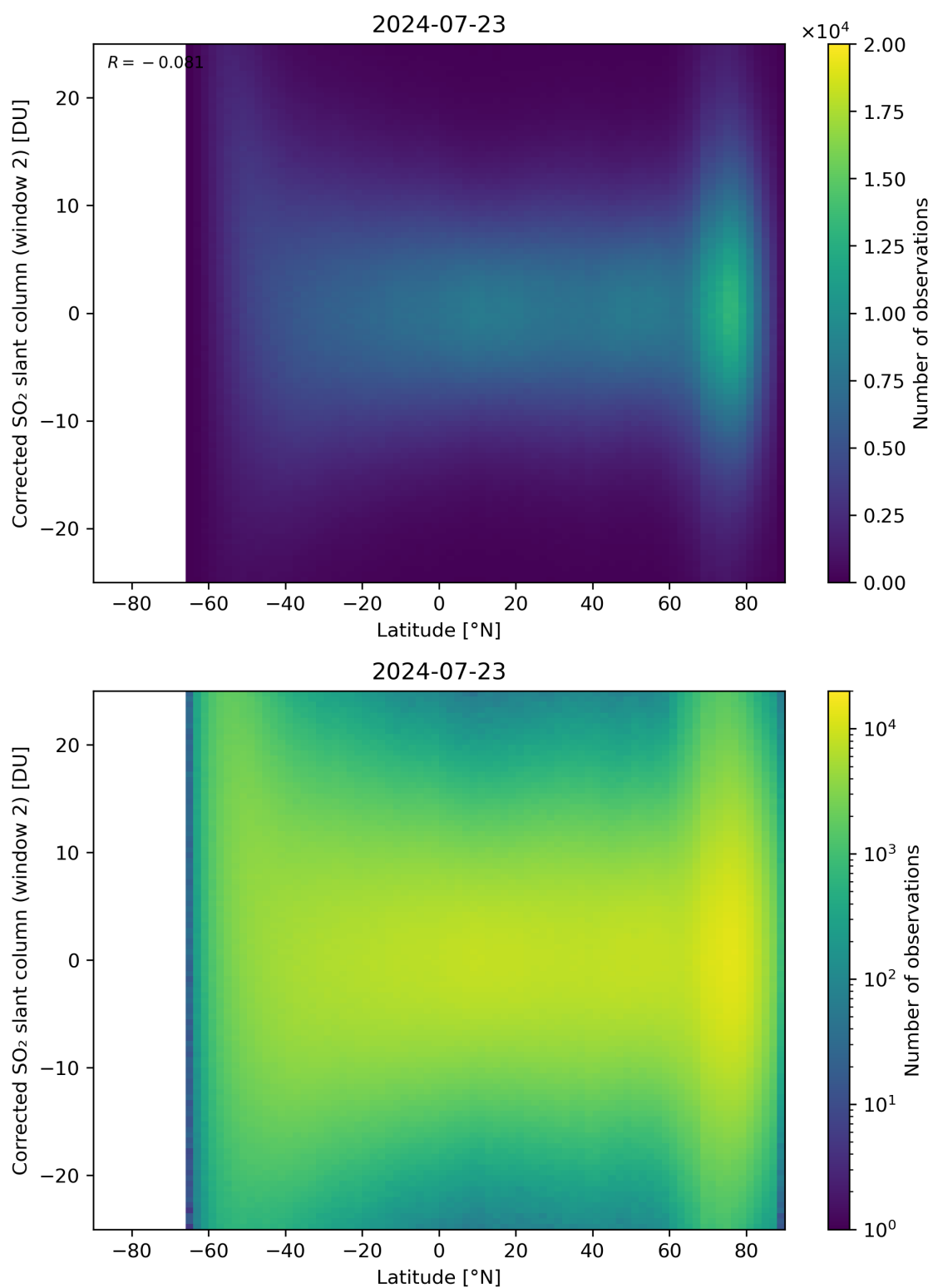
Figure 147: Scatter density plot of “Latitude” against “Corrected SO 2 slant column (window 2)” for 2024-07-22 to 2024-07-24.
