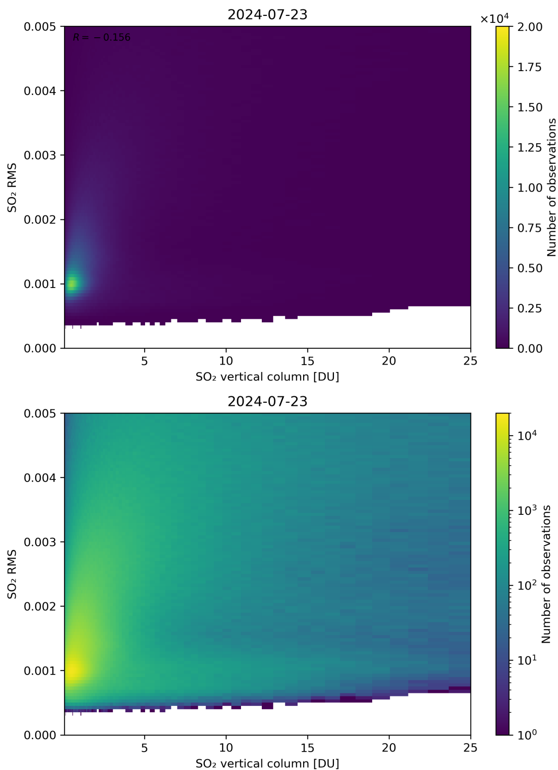
Figure 278: Scatter density plot of “SO 2 vertical column” against “SO 2 RMS” for 2024-07-22 to 2024-07-24.
