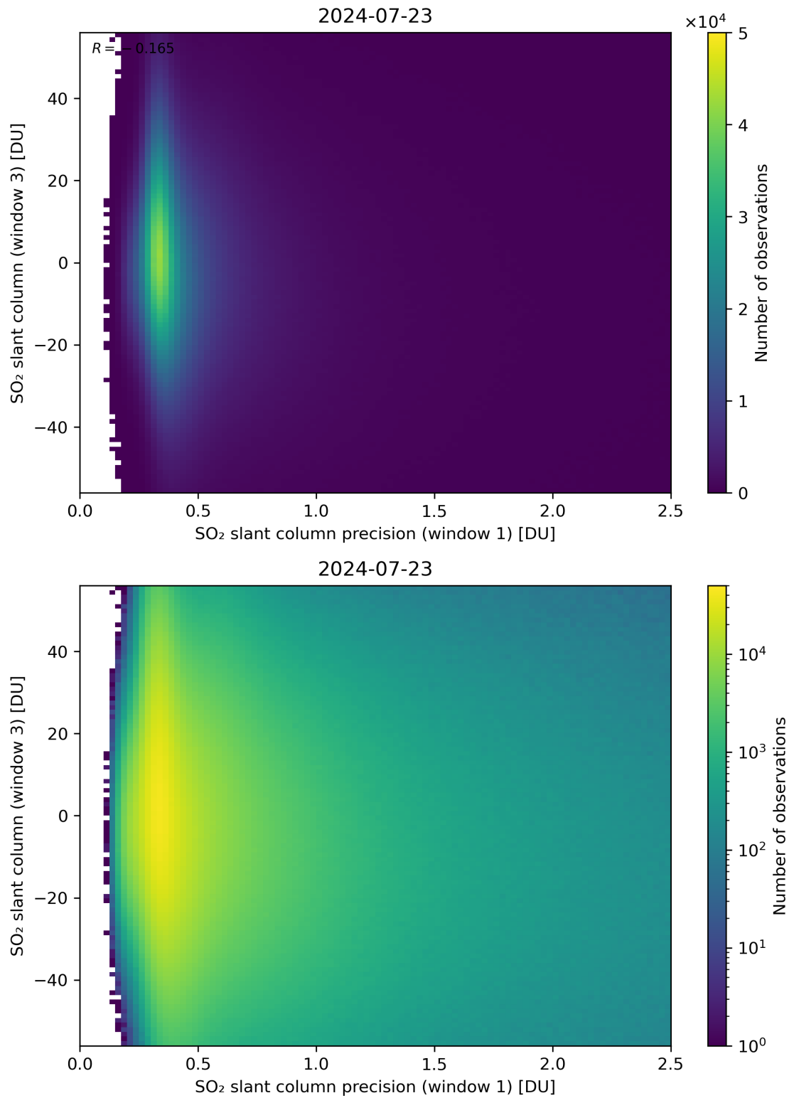
Figure 228: Scatter density plot of “SO 2 slant column precision (window 1)” against “SO 2 slant column (window 3)” for 2024-07-22 to 2024-07-24.
