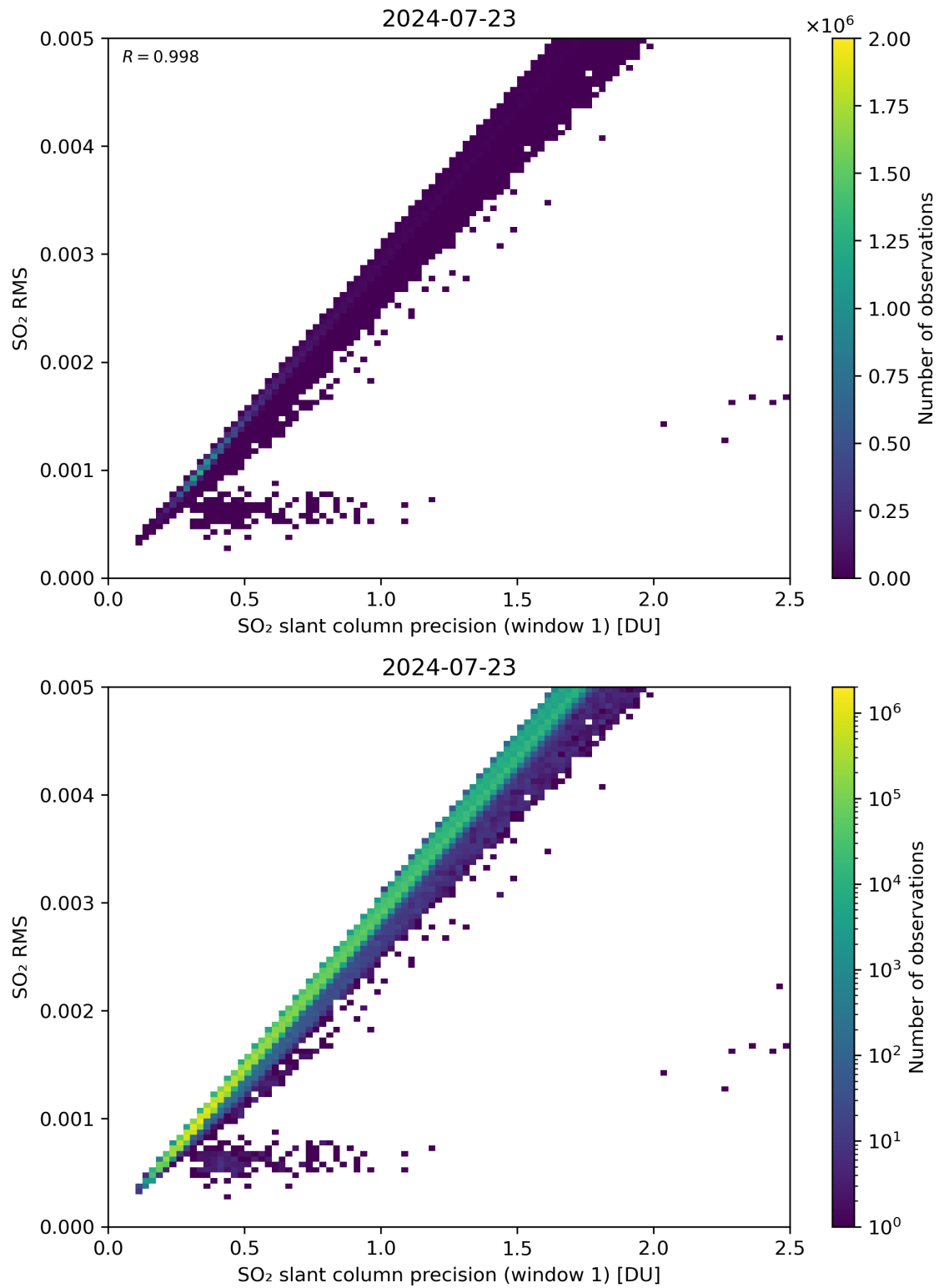
Figure 223: Scatter density plot of “SO 2 slant column precision (window 1)” against “SO 2 RMS” for 2024-07-22 to 2024-07-24.
