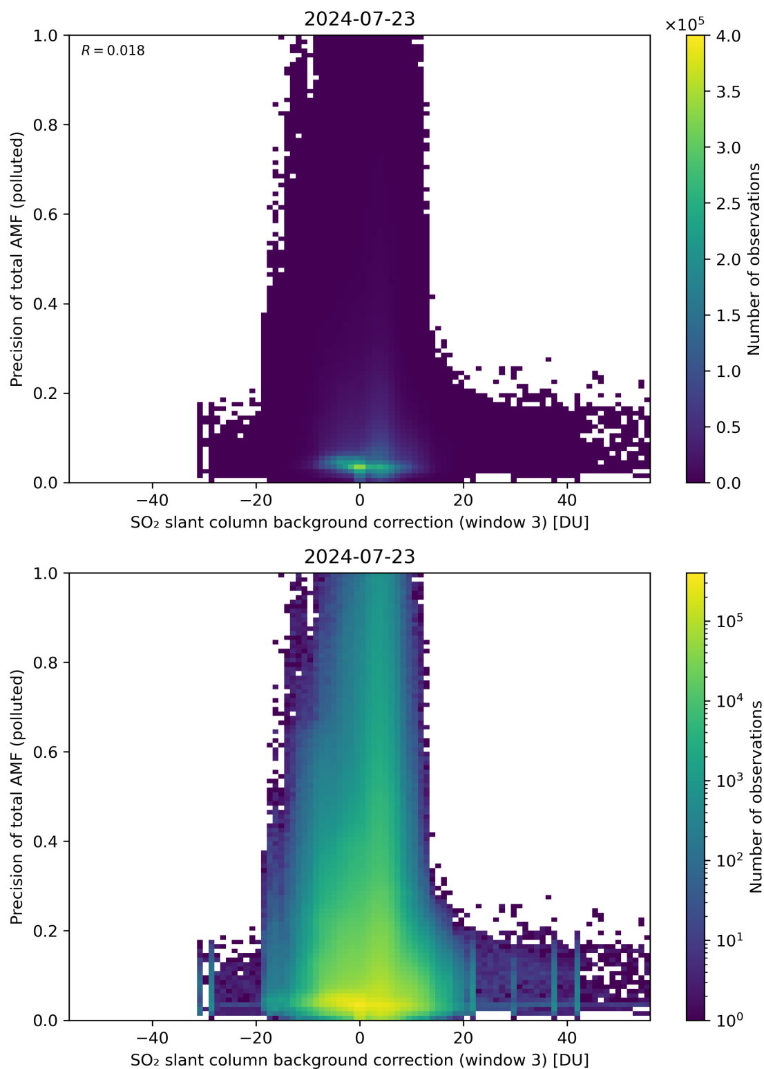
Figure 126: Scatter density plot of “SO 2 slant column background correction (window 3)” against “Precision of total AMF (polluted)” for 2024-07-22 to 2024-07-24.
