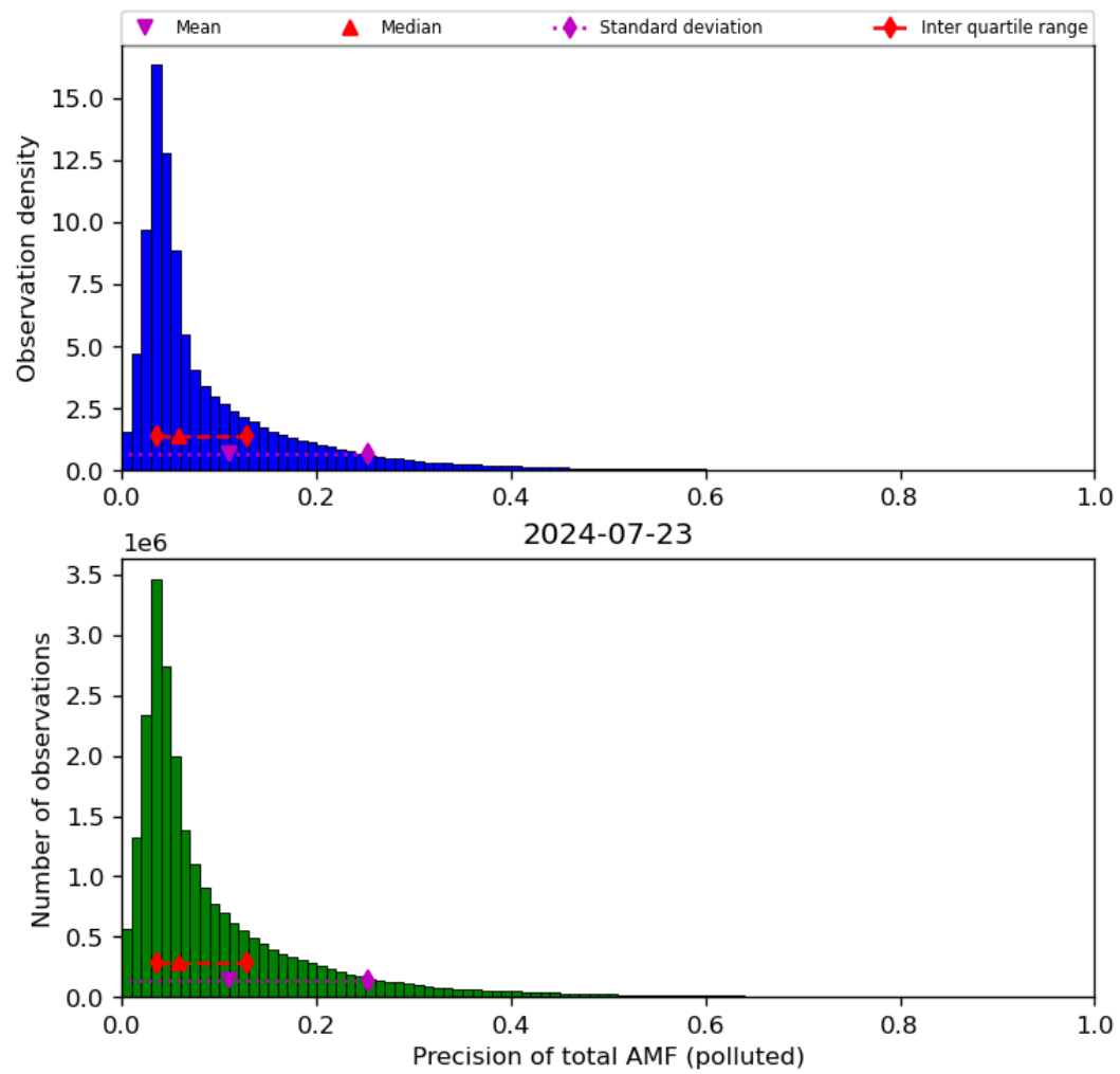
Figure 72: Histogram of “Precision of total AMF (polluted)” for 2024-07-22 to 2024-07-24
