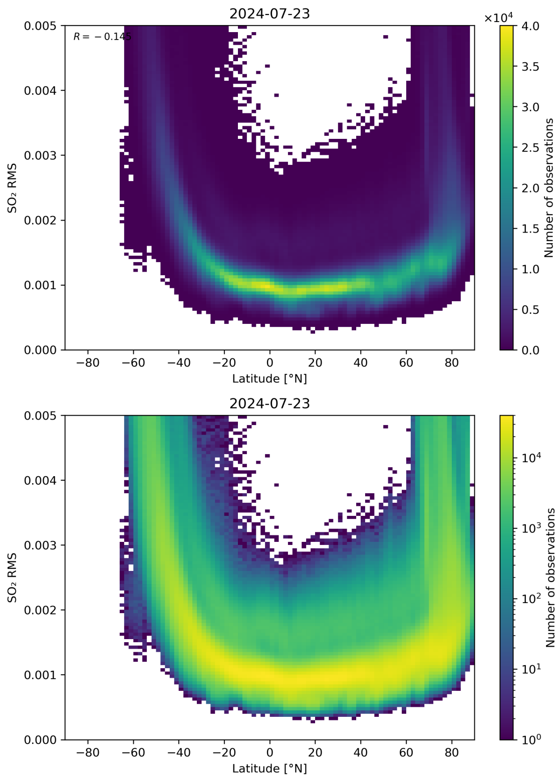
Figure 144: Scatter density plot of “Latitude” against “SO 2 RMS” for 2024-07-22 to 2024-07-24.
