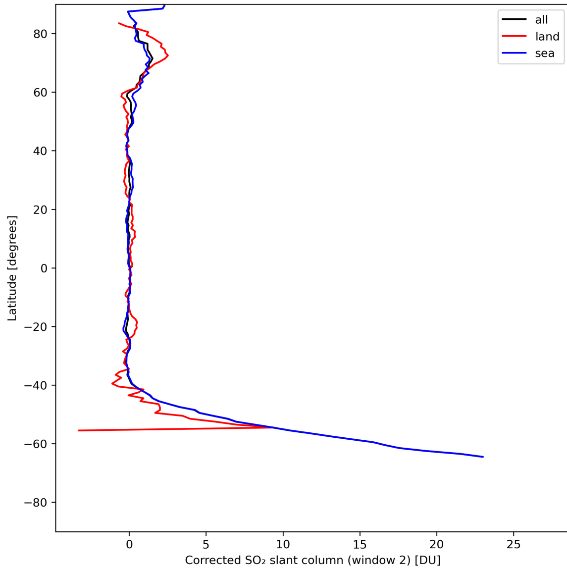
Figure 39: Zonal average of “Corrected SO 2 slant column (window 2)” for 2024-07-22 to 2024-07-24.
