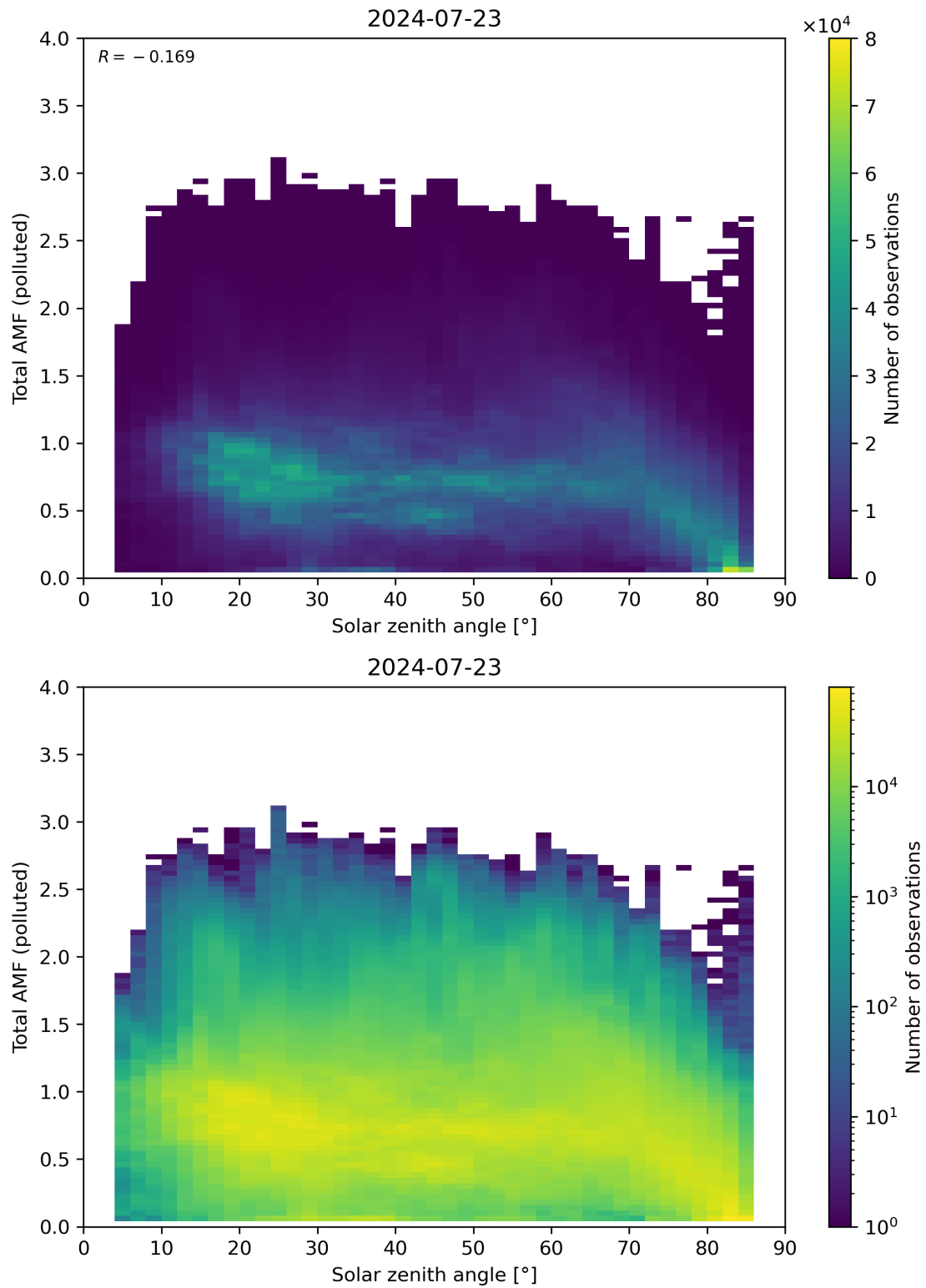
Figure 174: Scatter density plot of “Solar zenith angle” against “Total AMF (polluted)” for 2024-07-22 to 2024-07-24.
