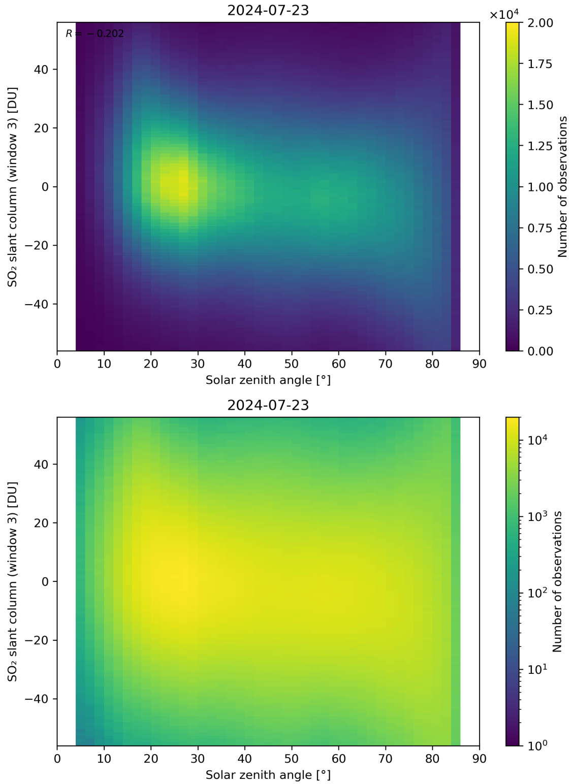
Figure 172: Scatter density plot of “Solar zenith angle” against “SO 2 slant column (window 3)” for 2024-07-22 to 2024-07-24.
