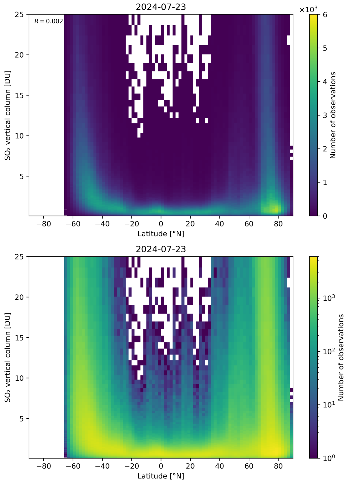
Figure 156: Scatter density plot of “Latitude” against “SO 2 vertical column” for 2024-07-22 to 2024-07-24.
