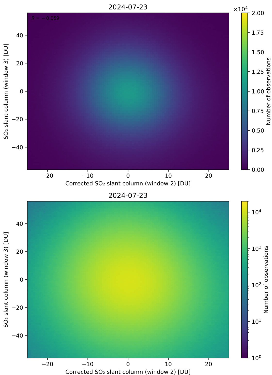
Figure 201: Scatter density plot of “Corrected SO 2 slant column (window 2)” against “SO 2 slant column (window 3)” for 2024-07-22 to 2024-07-24.
