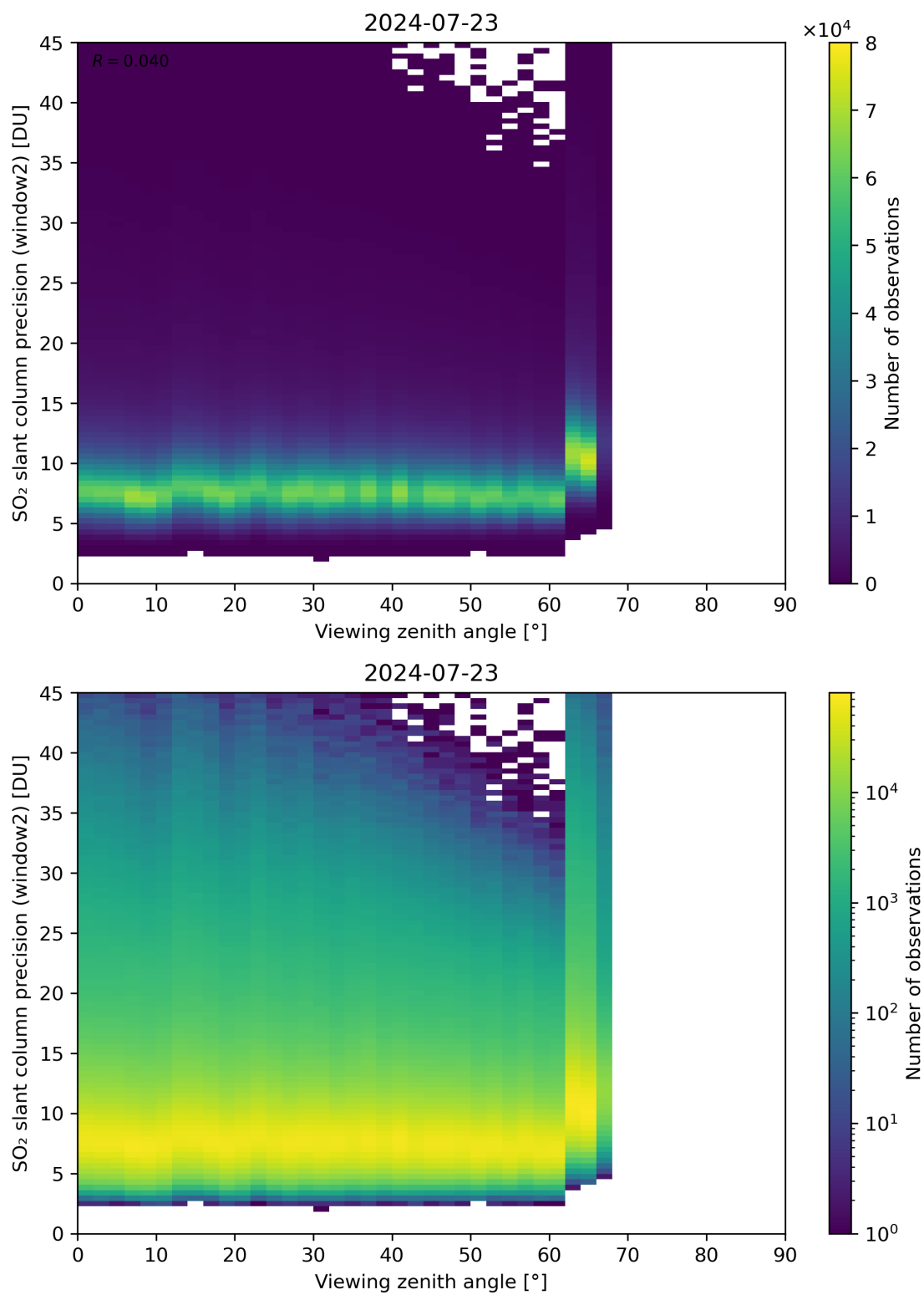
Figure 322: Scatter density plot of “Viewing zenith angle” against “SO 2 slant column precision (window2)” for 2024-07-22 to 2024-07-24.
