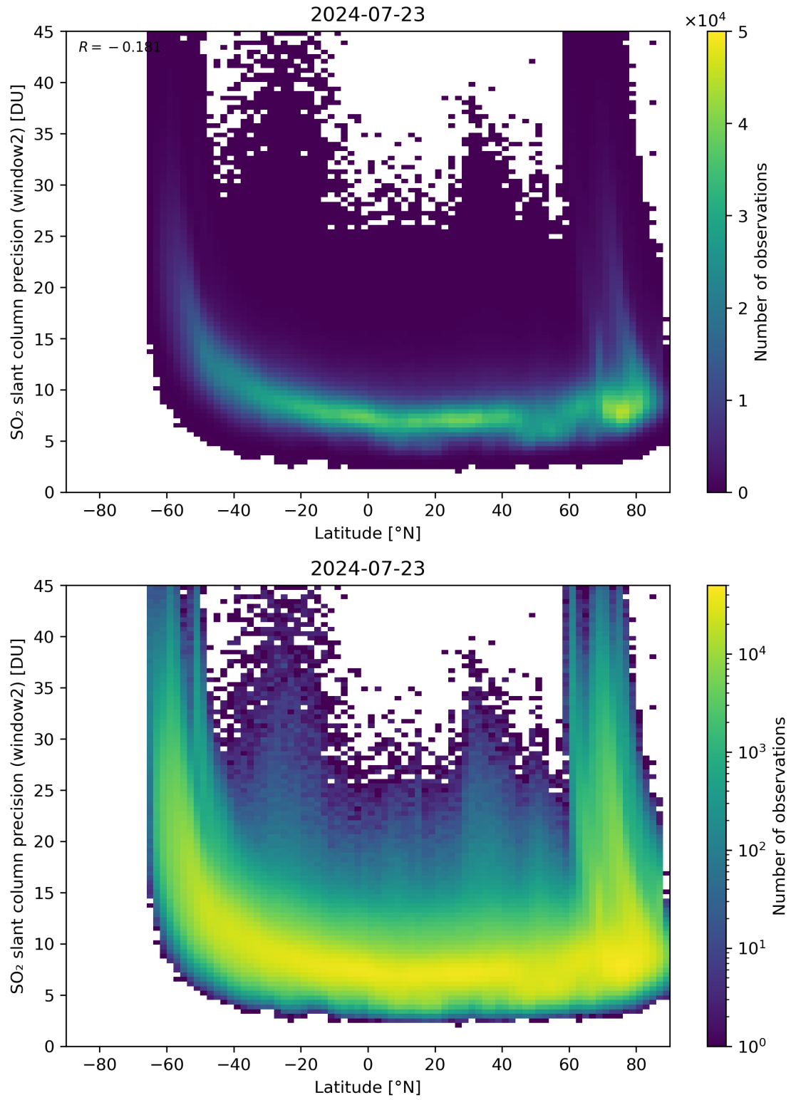
Figure 151: Scatter density plot of “Latitude” against “SO 2 slant column precision (window2)” for 2024-07-22 to 2024-07-24.
