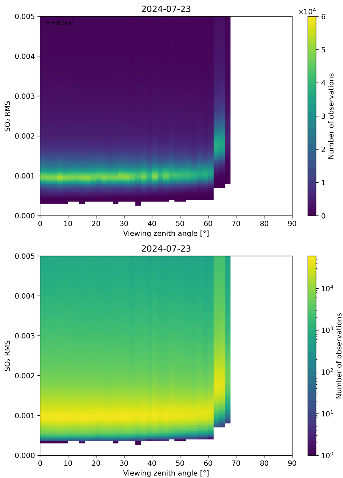
Figure 313: Scatter density plot of “Viewing zenith angle” against “SO 2 RMS” for 2024-07-22 to 2024-07-24.
