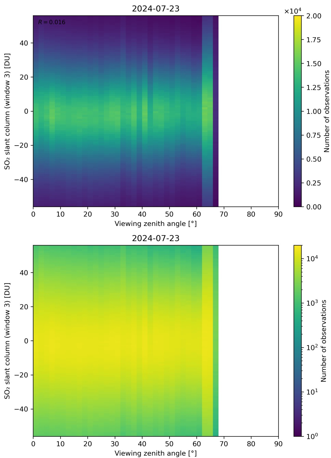
Figure 323: Scatter density plot of “Viewing zenith angle” against “SO 2 slant column (window 3)” for 2024-07-22 to 2024-07-24.
