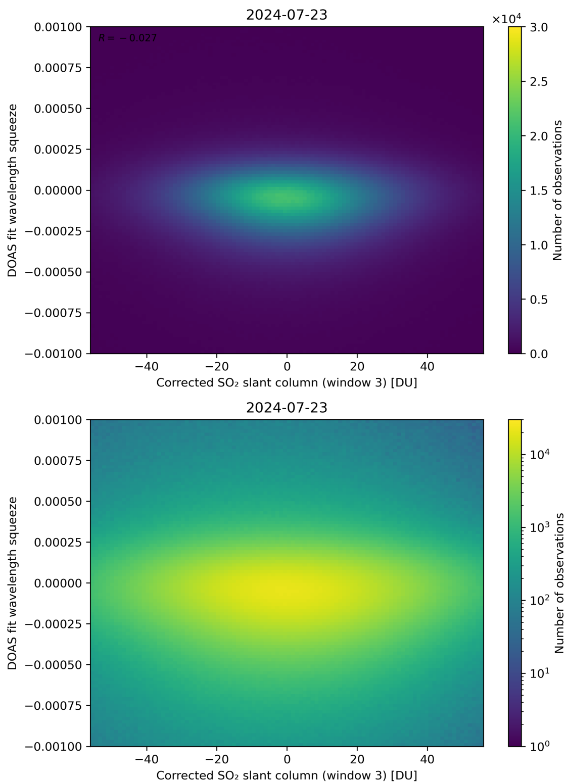
Figure 207: Scatter density plot of “Corrected SO 2 slant column (window 3)” against “DOAS fit wavelength squeeze” for 2024-07-22 to 2024-07-24.
