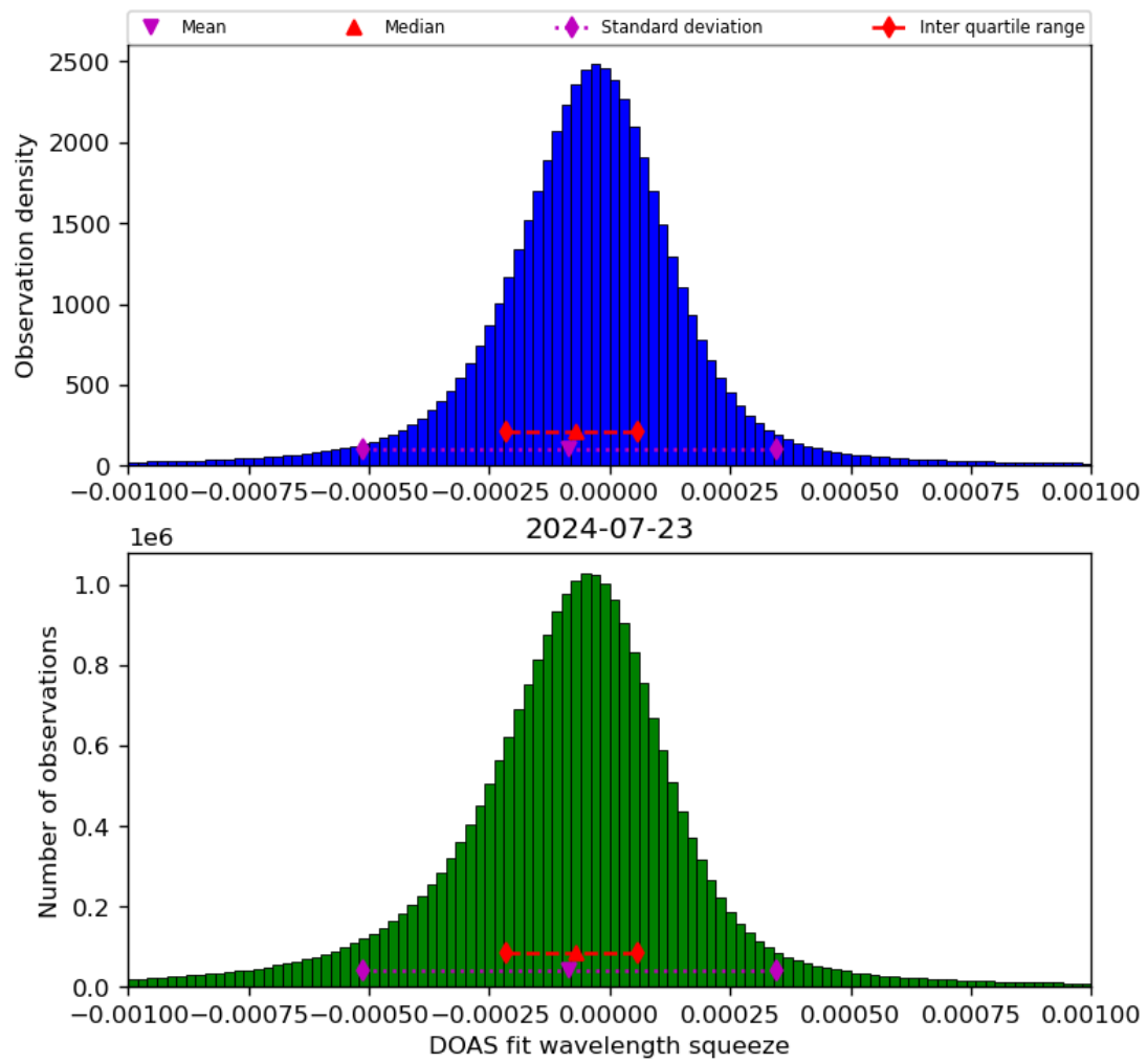
Figure 69: Histogram of “DOAS fit wavelength squeeze” for 2024-07-22 to 2024-07-24
