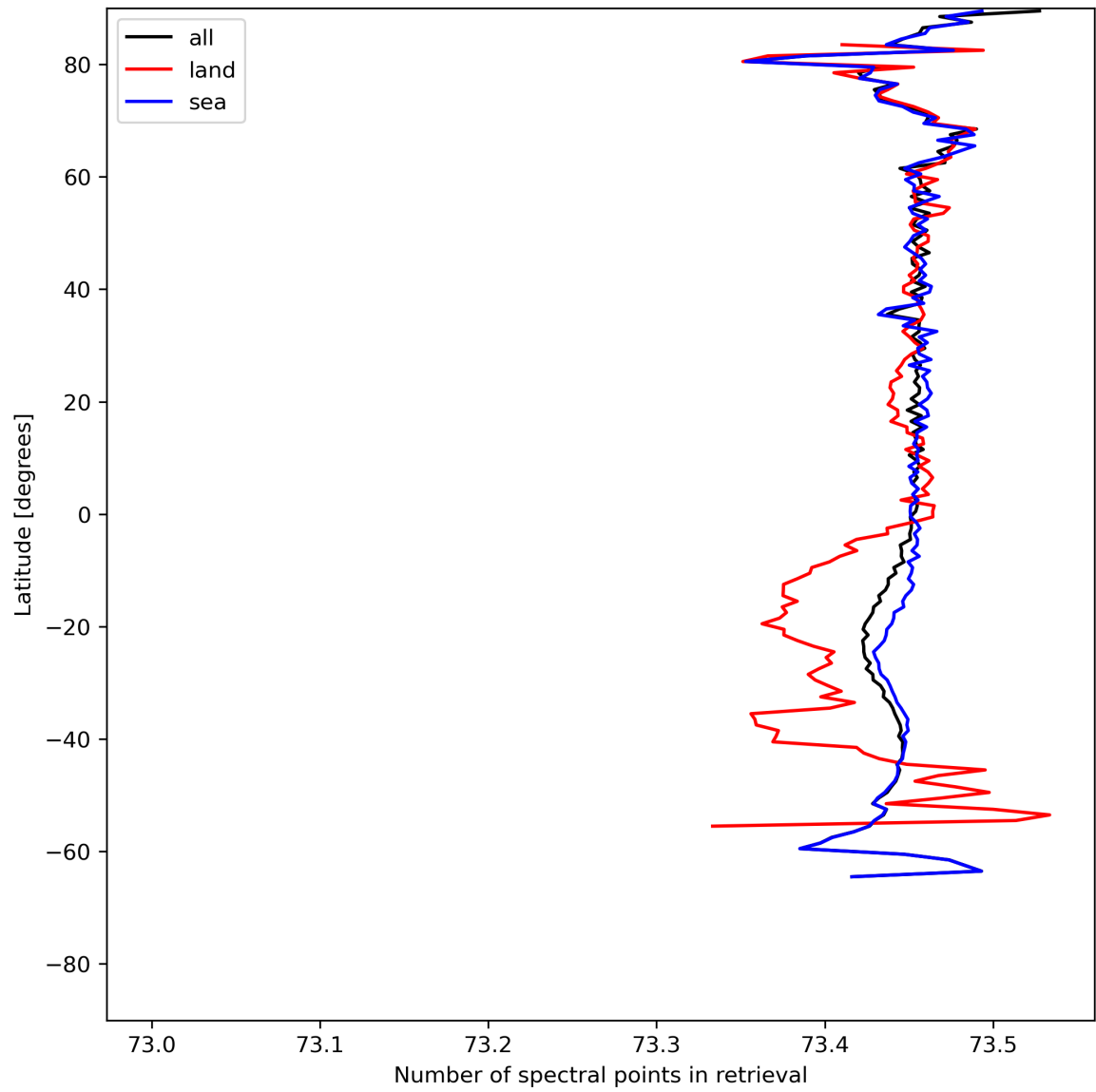
Figure 51: Zonal average of “Number of spectral points in retrieval” for 2024-07-22 to 2024-07-24.
