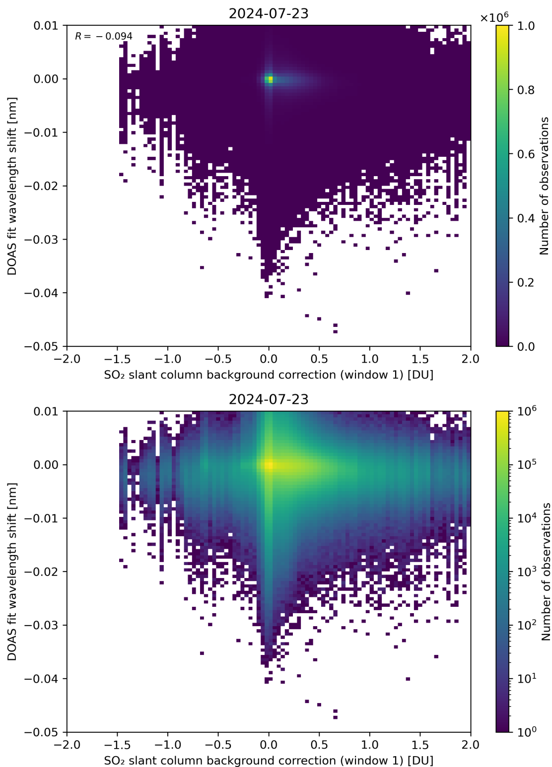
Figure 100: Scatter density plot of “SO 2 slant column background correction (window 1)” against “DOAS fit wavelength shift” for 2024-07-22 to 2024-07-24.
