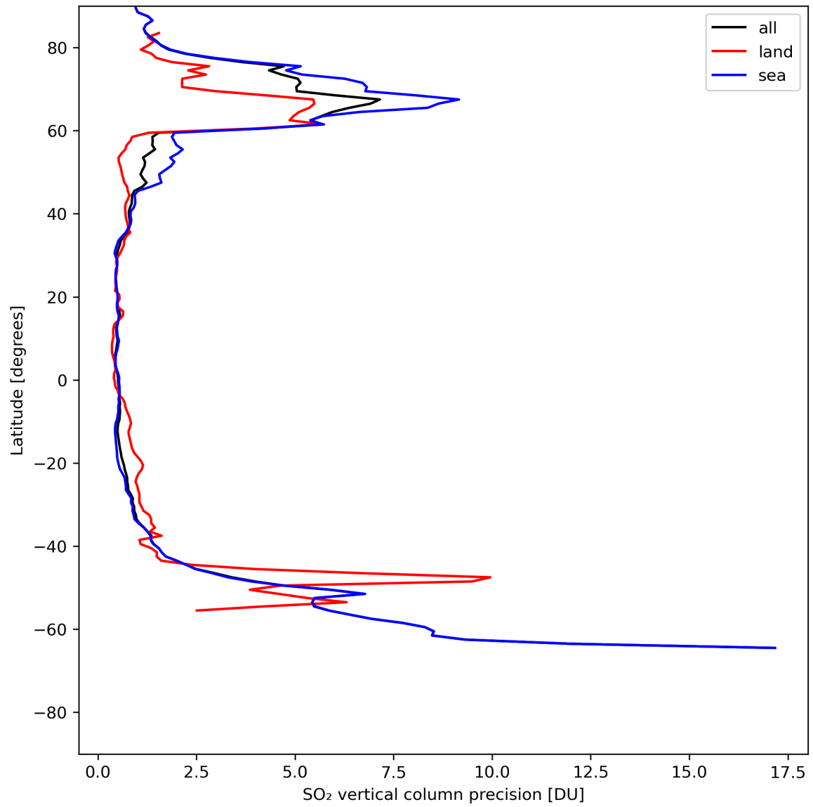
Figure 31: Zonal average of “SO 2 vertical column precision” for 2024-07-22 to 2024-07-24.
