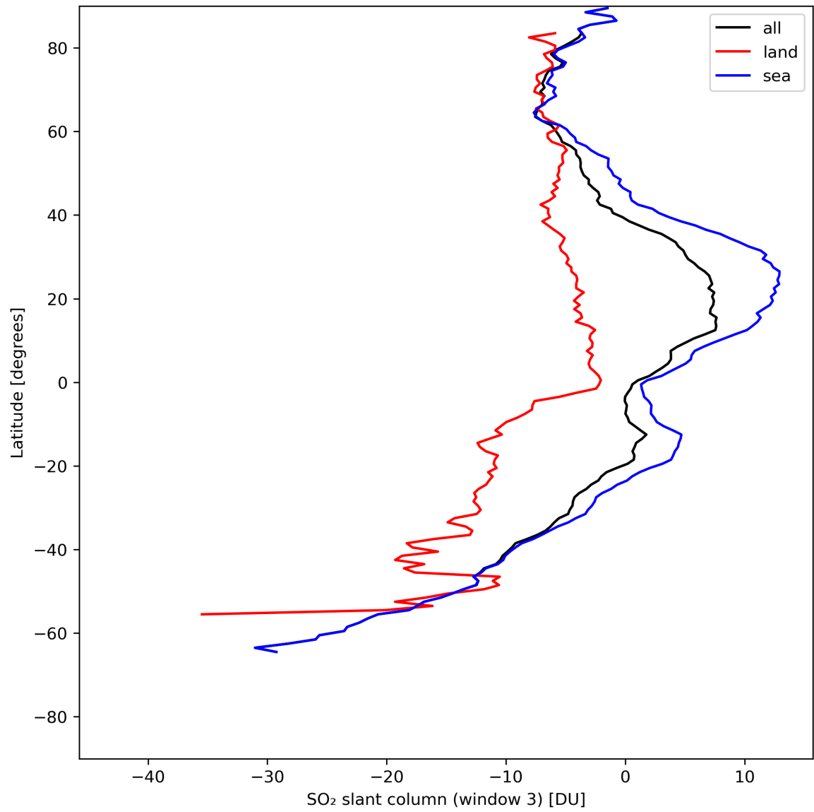
Figure 41: Zonal average of “SO 2 slant column (window 3)” for 2024-07-22 to 2024-07-24.
