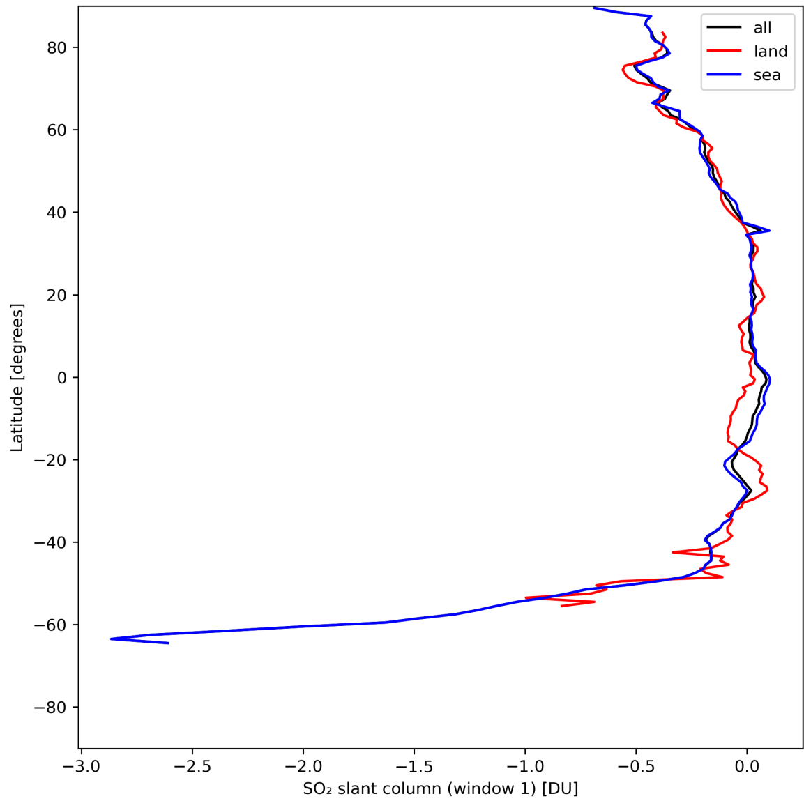
Figure 33: Zonal average of “SO 2 slant column (window 1)” for 2024-07-22 to 2024-07-24.
