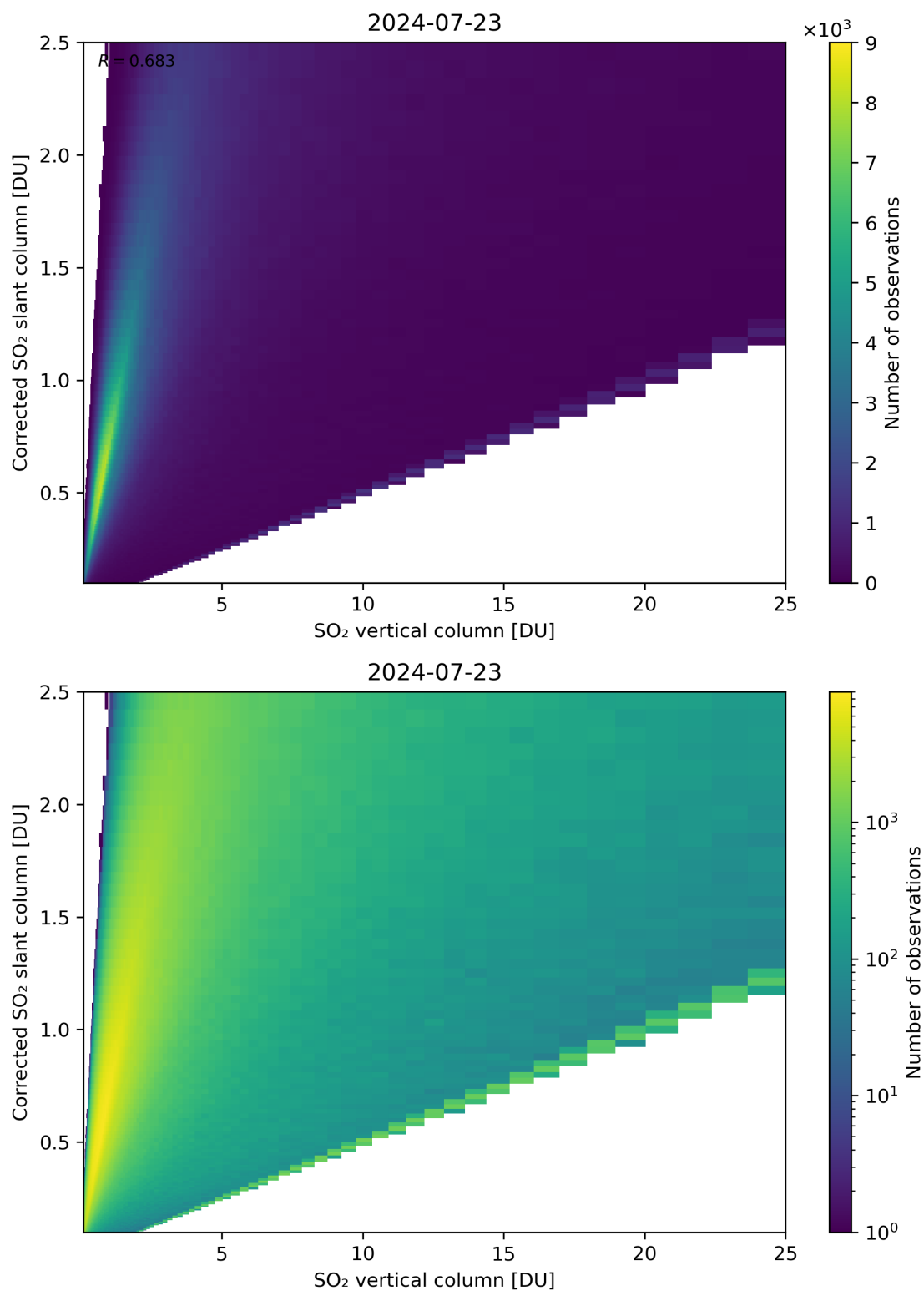
Figure 297: Scatter density plot of “SO 2 vertical column” against “Corrected SO 2 slant column” for 2024-07-22 to 2024-07-24.
