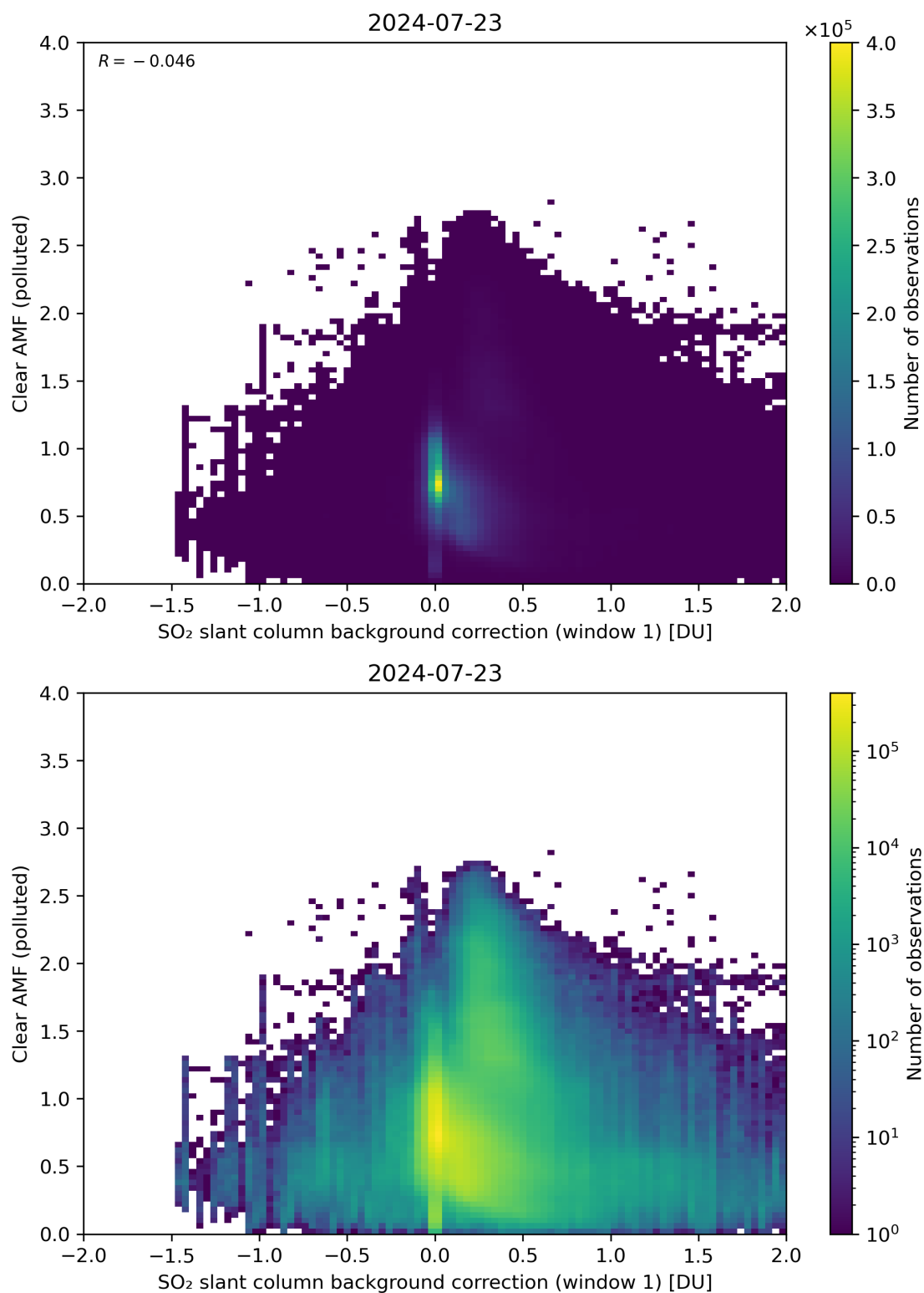
Figure 103: Scatter density plot of “SO 2 slant column background correction (window 1)” against “Clear AMF (polluted)” for 2024-07-22 to 2024-07-24.
