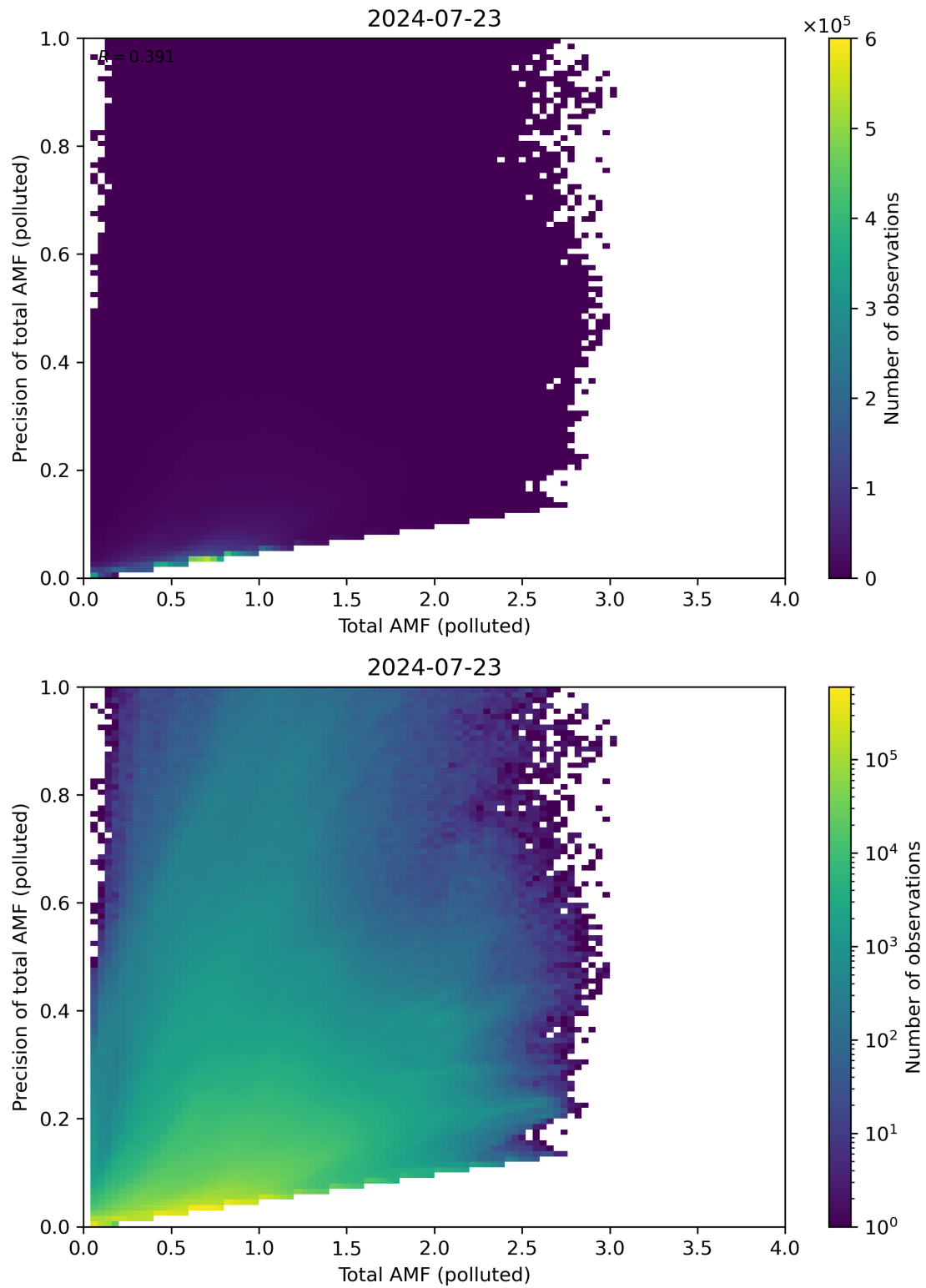
Figure 272: Scatter density plot of “Total AMF (polluted)” against “Precision of total AMF (polluted)” for 2024-07-22 to 2024-07-24.
