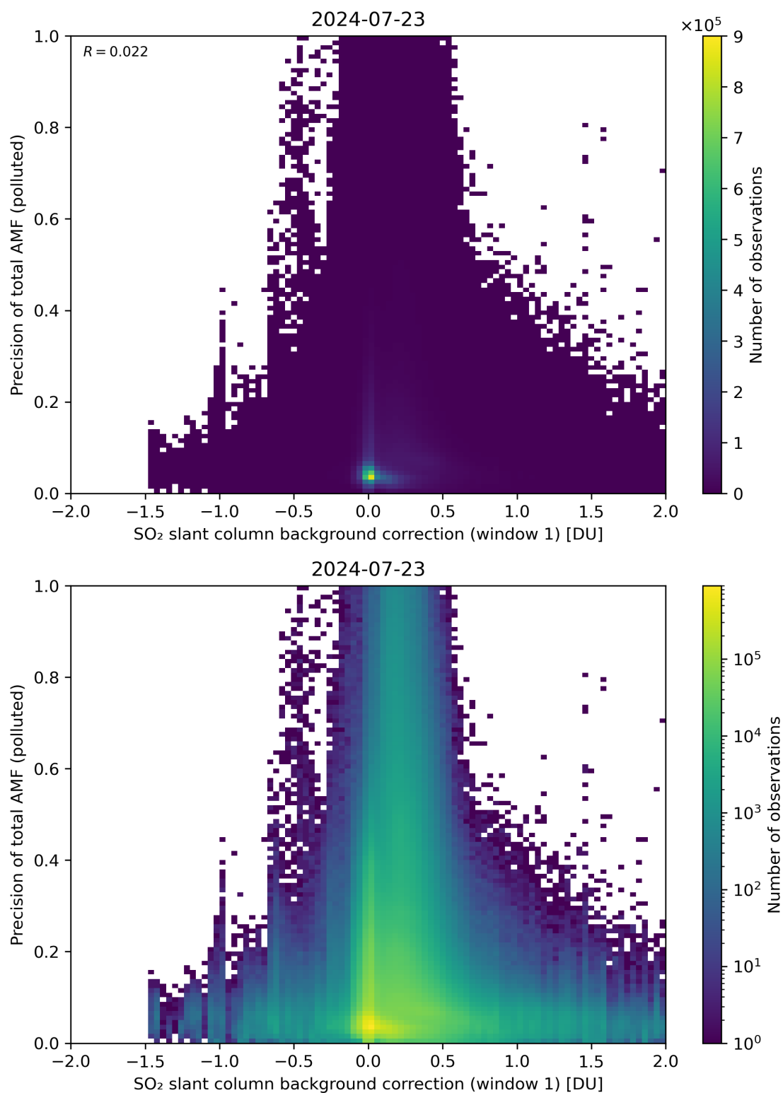
Figure 110: Scatter density plot of “SO 2 slant column background correction (window 1)” against “Precision of total AMF (polluted)” for 2024-07-22 to 2024-07-24.
