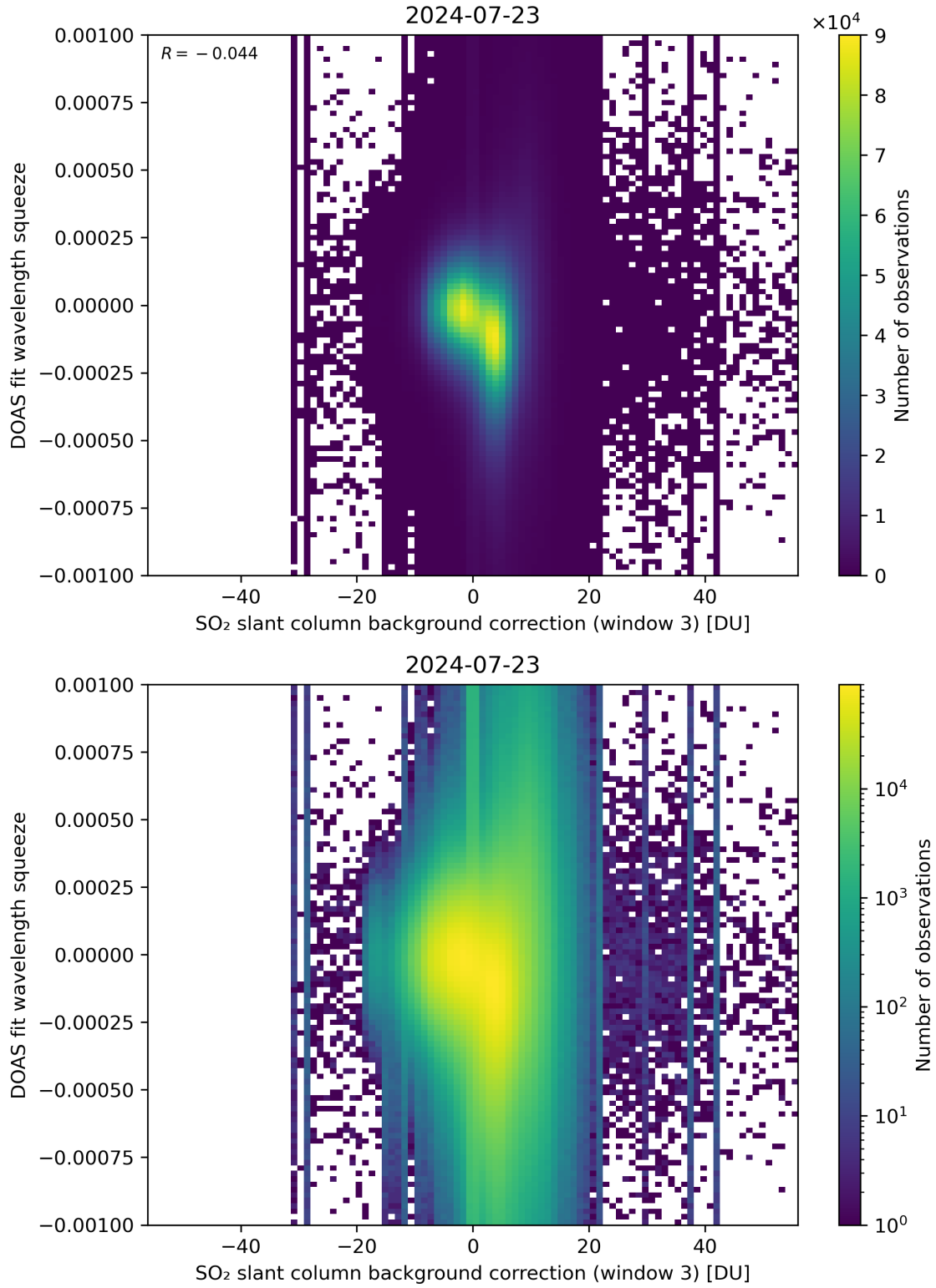
Figure 122: Scatter density plot of “SO 2 slant column background correction (window 3)” against “DOAS fit wavelength squeeze” for 2024-07-22 to 2024-07-24.
