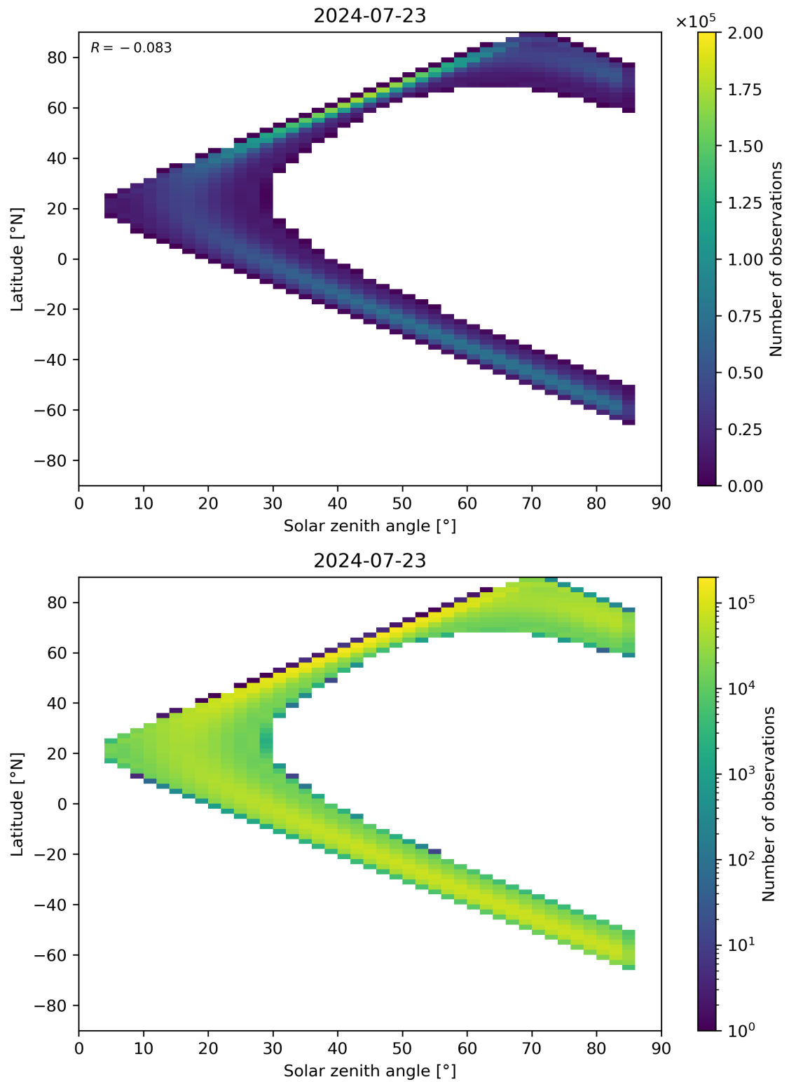
Figure 164: Scatter density plot of “Solar zenith angle” against “Latitude” for 2024-07-22 to 2024-07-24.
