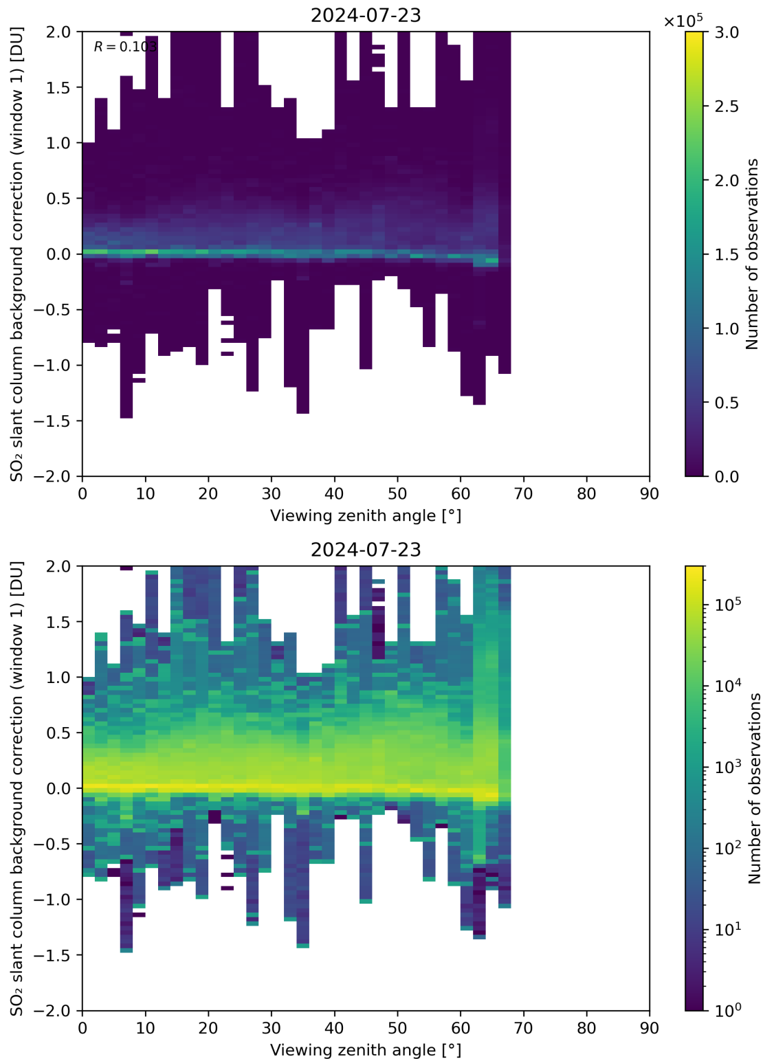
Figure 308: Scatter density plot of “Viewing zenith angle” against “SO 2 slant column background correction (window 1)” for 2024-07-22 to 2024-07-24.
