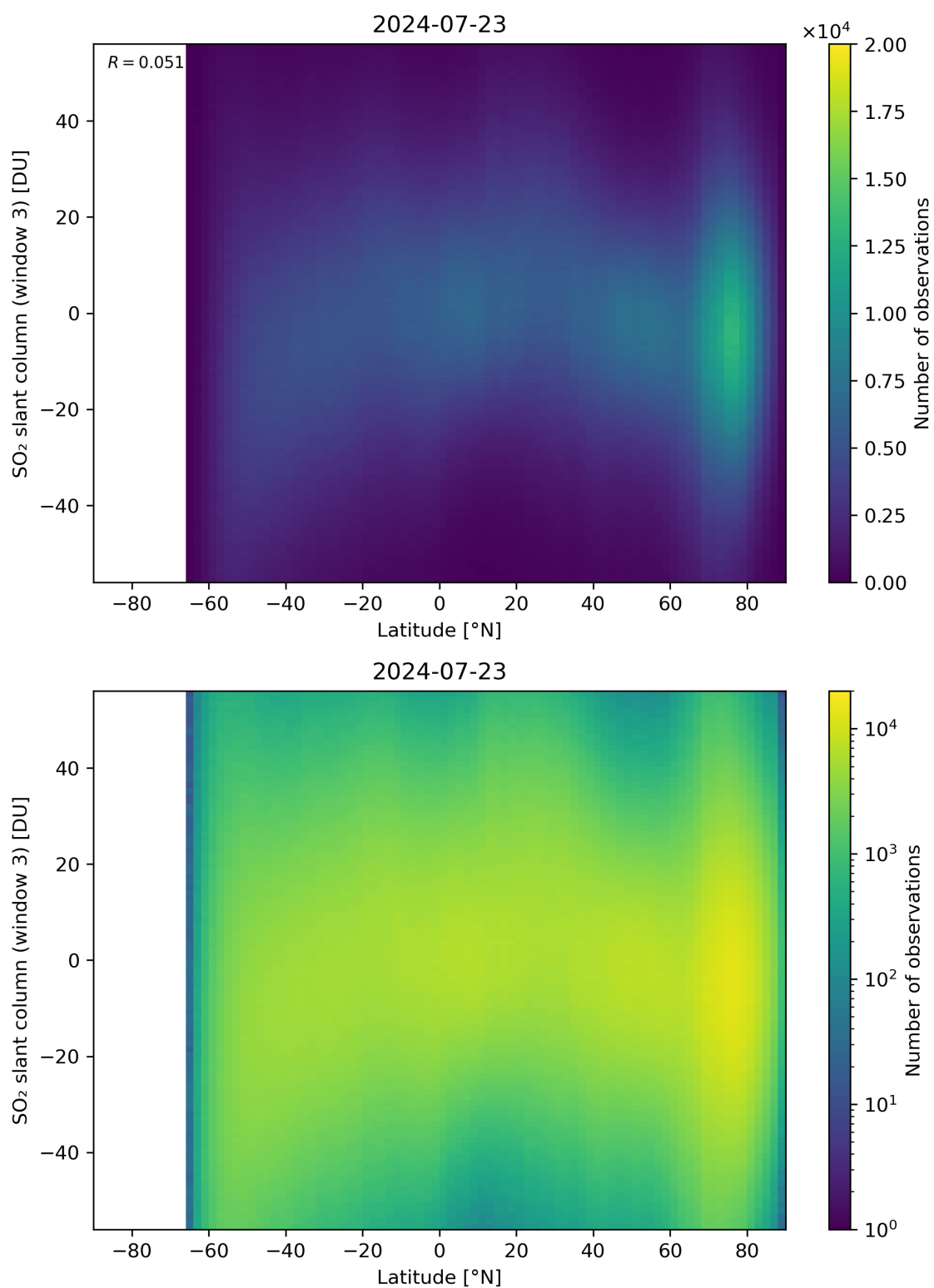
Figure 152: Scatter density plot of “Latitude” against “SO 2 slant column (window 3)” for 2024-07-22 to 2024-07-24.
