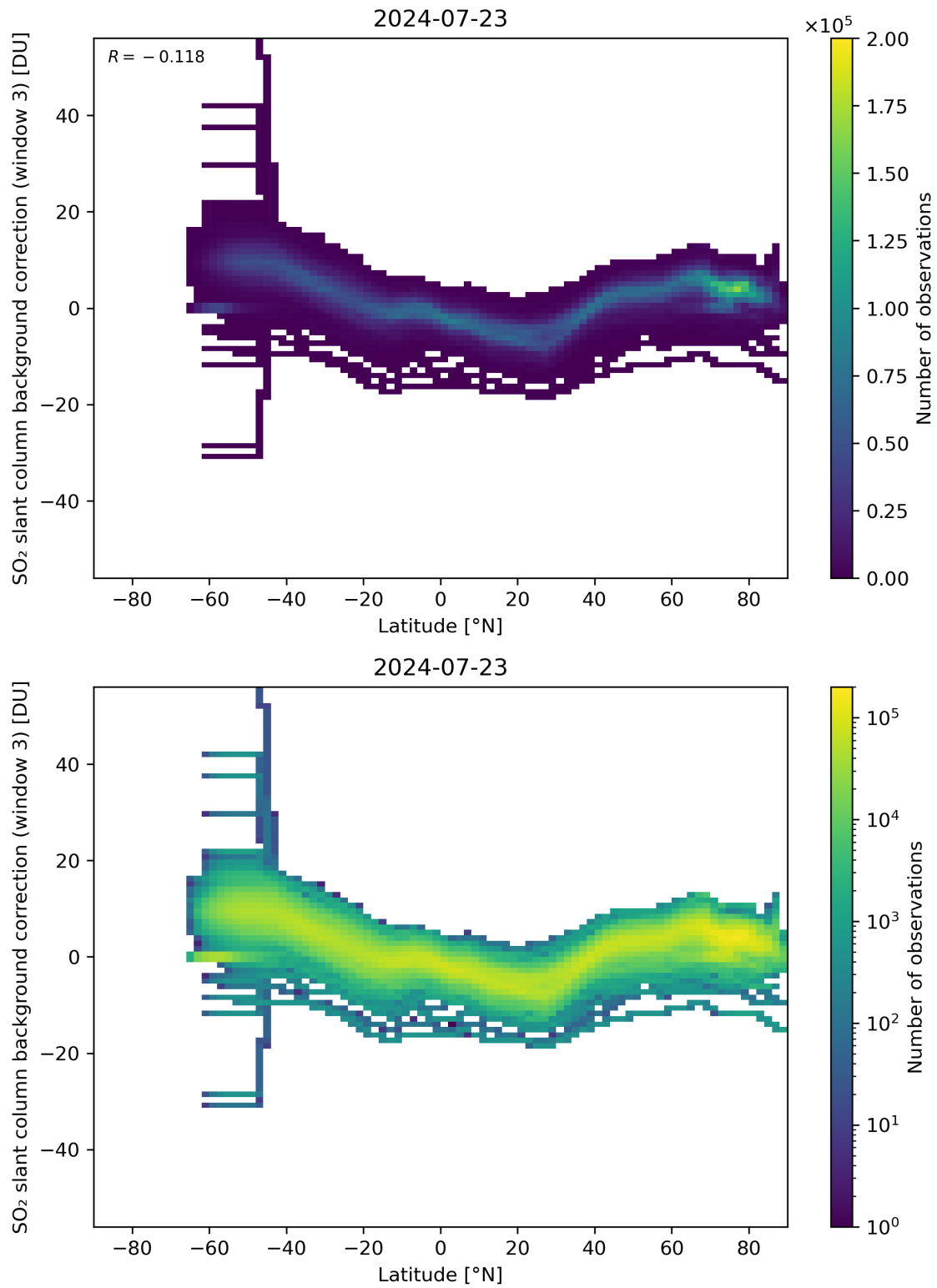
Figure 141: Scatter density plot of “Latitude” against “SO 2 slant column background correction (window 3)” for 2024-07-22 to 2024-07-24.
