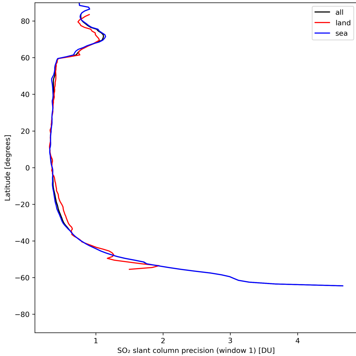
Figure 34: Zonal average of “SO 2 slant column precision (window 1)” for 2024-07-22 to 2024-07-24.
