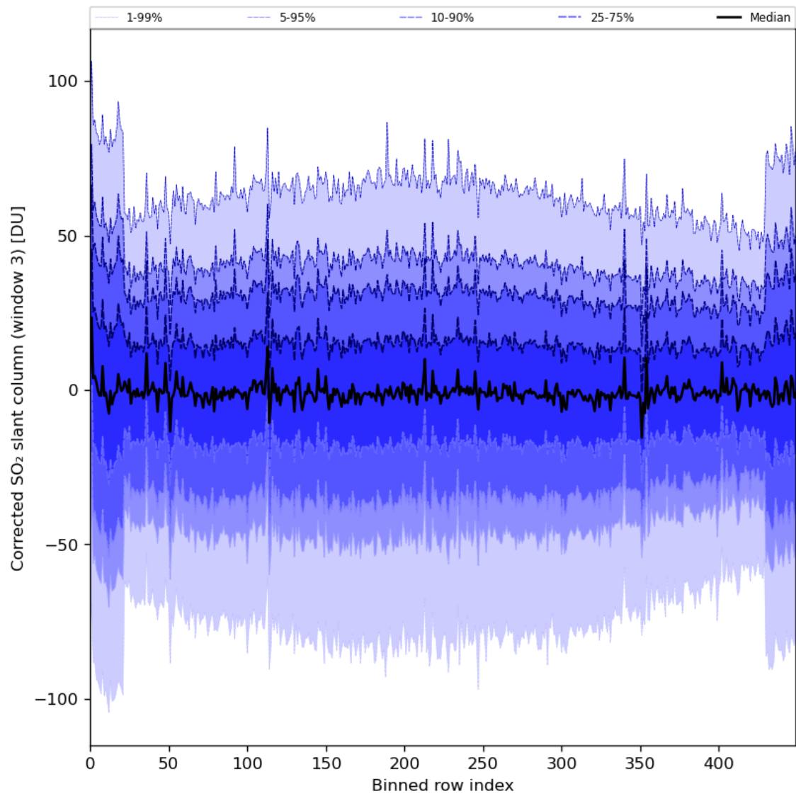
Figure 89: Along track statistics of “Corrected SO 2 slant column (window 3)” for 2024-07-22 to 2024-07-24
