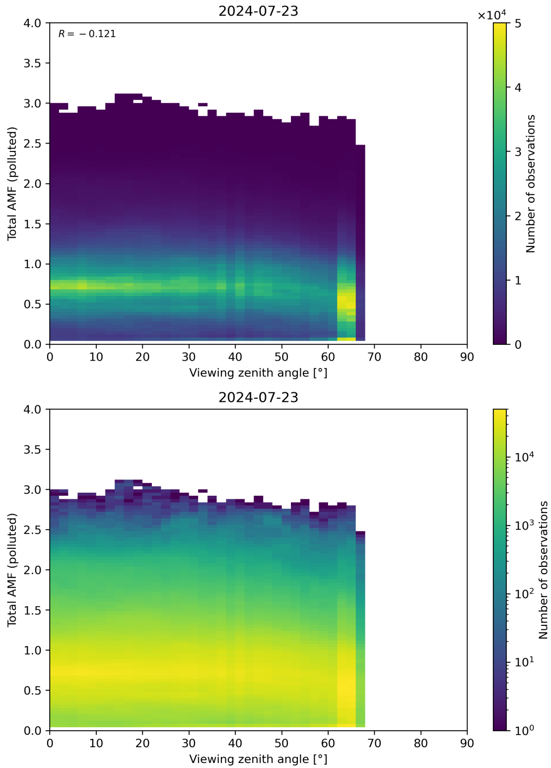
Figure 325: Scatter density plot of “Viewing zenith angle” against “Total AMF (polluted)” for 2024-07-22 to 2024-07-24.
