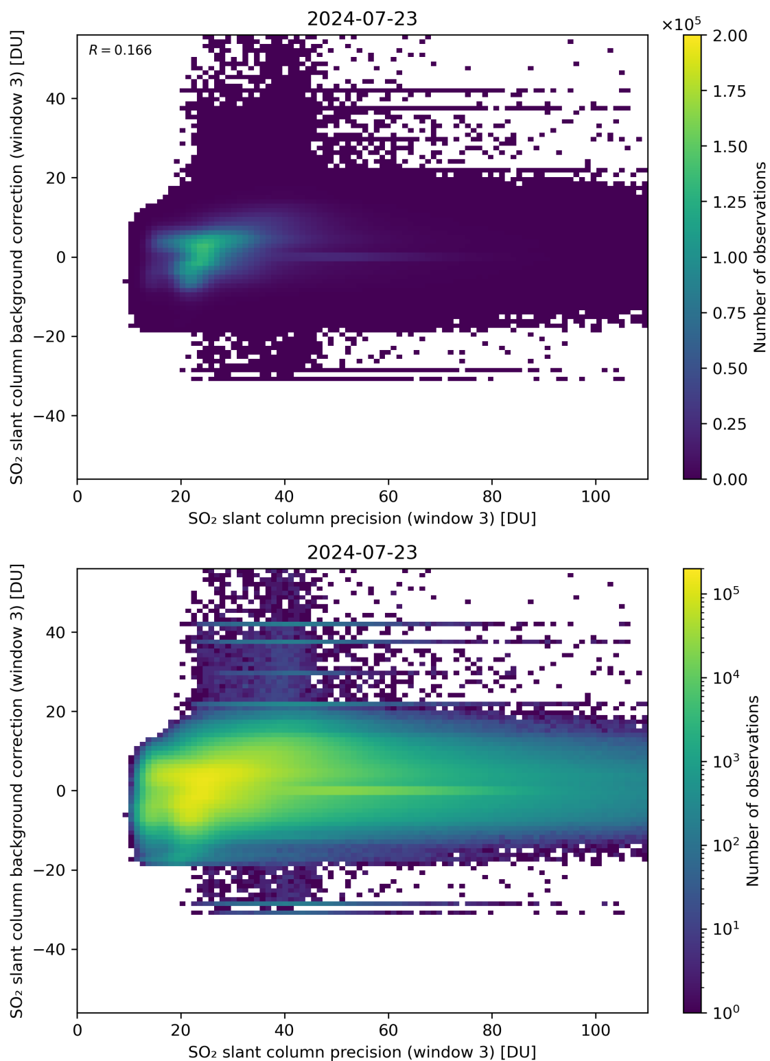
Figure 257: Scatter density plot of “SO 2 slant column precision (window 3)” against “SO 2 slant column background correction (window 3)” for 2024-07-22 to 2024-07-24.
