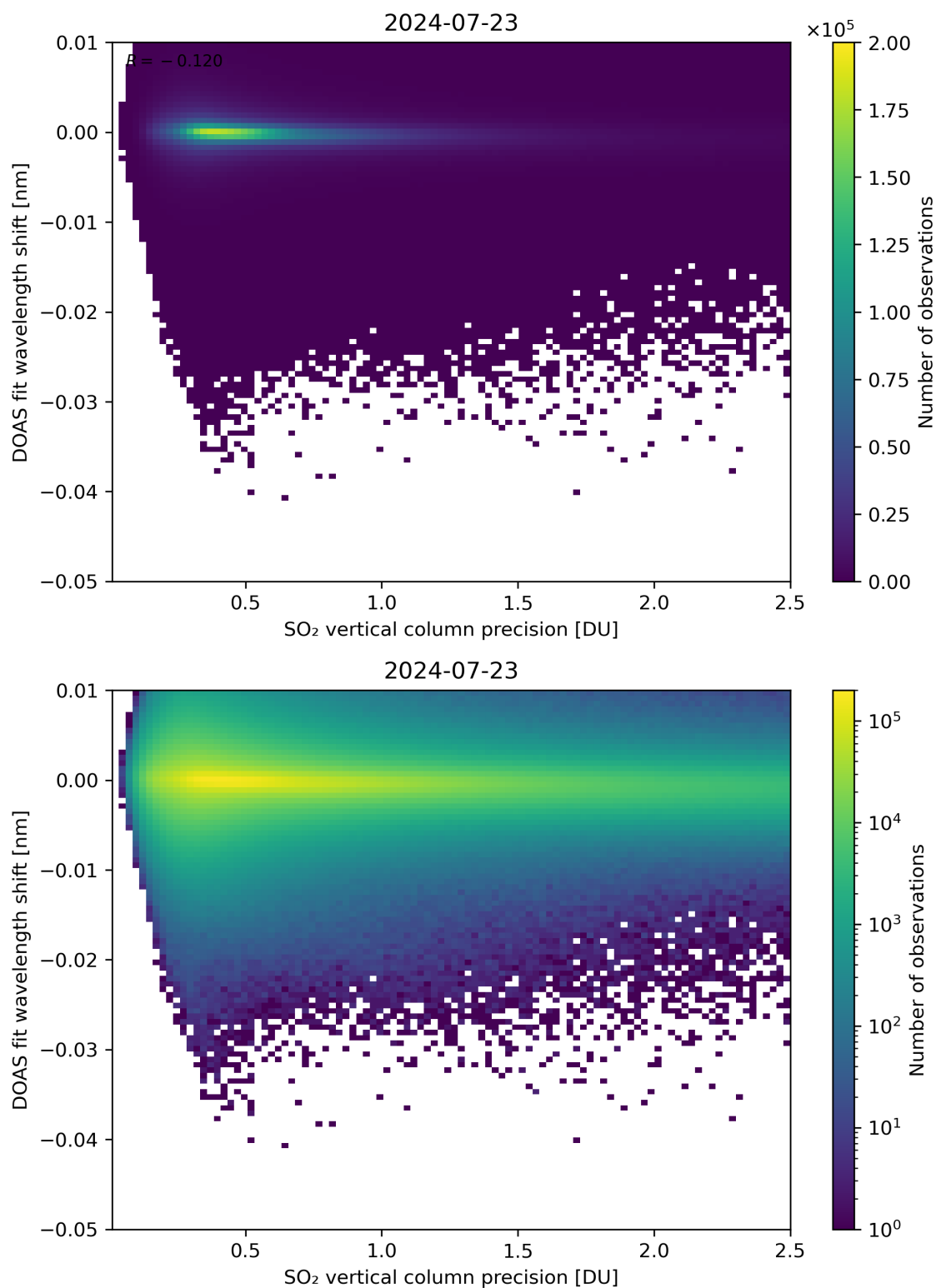
Figure 282: Scatter density plot of “SO 2 vertical column precision” against “DOAS fit wavelength shift” for 2024-07-22 to 2024-07-24.
