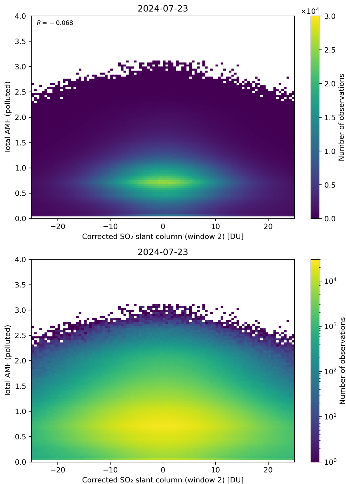
Figure 203: Scatter density plot of “Corrected SO 2 slant column (window 2)” against “Total AMF (polluted)” for 2024-07-22 to 2024-07-24.
