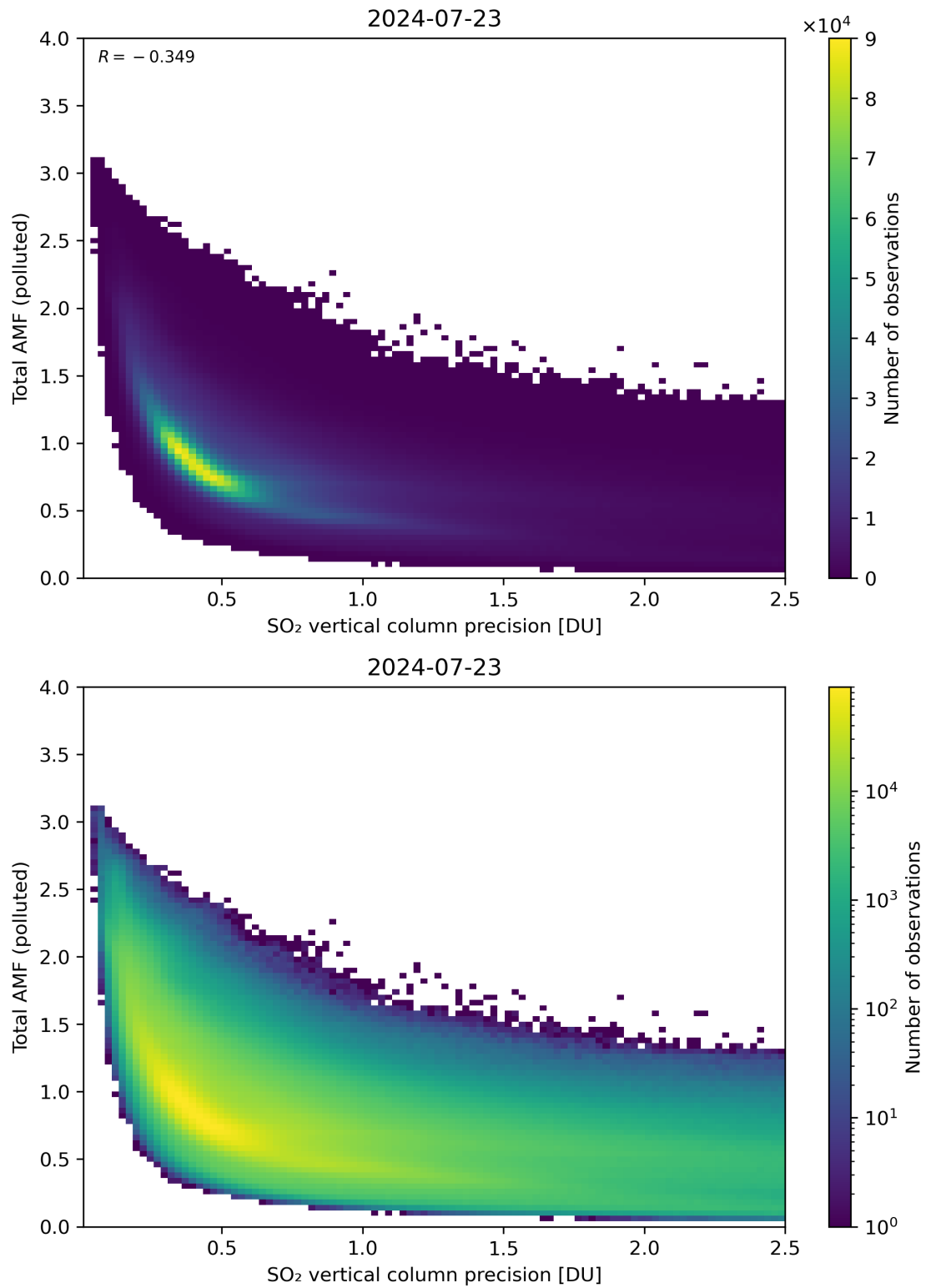
Figure 294: Scatter density plot of “SO 2 vertical column precision” against “Total AMF (polluted)” for 2024-07-22 to 2024-07-24.
