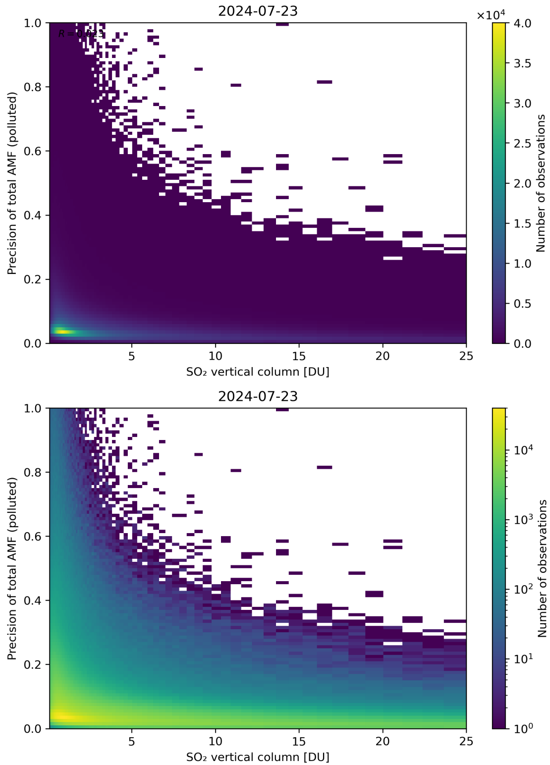
Figure 306: Scatter density plot of “SO 2 vertical column” against “Precision of total AMF (polluted)” for 2024-07-22 to 2024-07-24.
