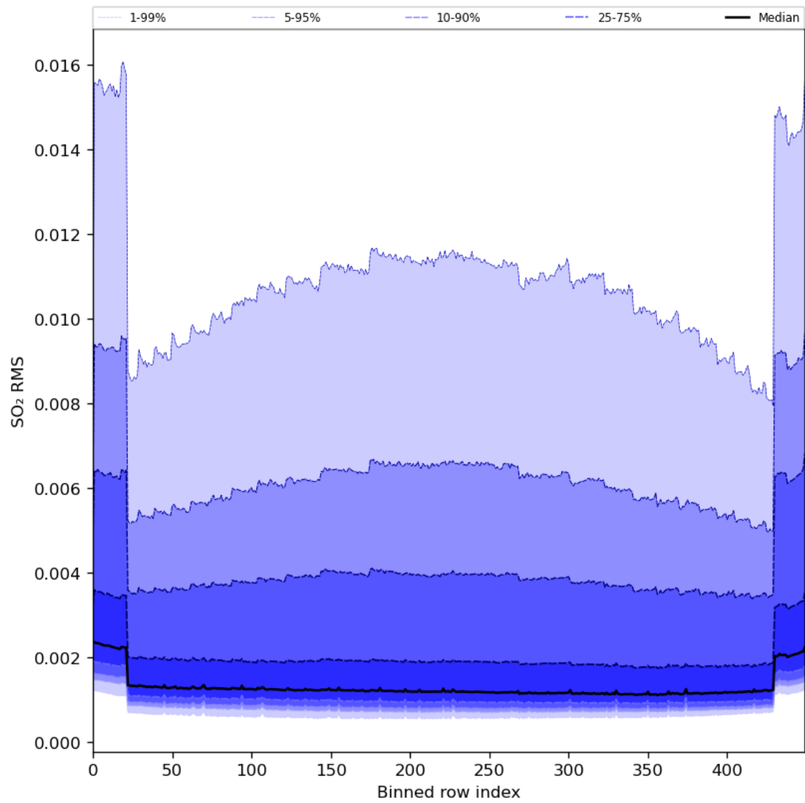
Figure 93: Along track statistics of “SO 2 RMS” for 2024-07-22 to 2024-07-24
