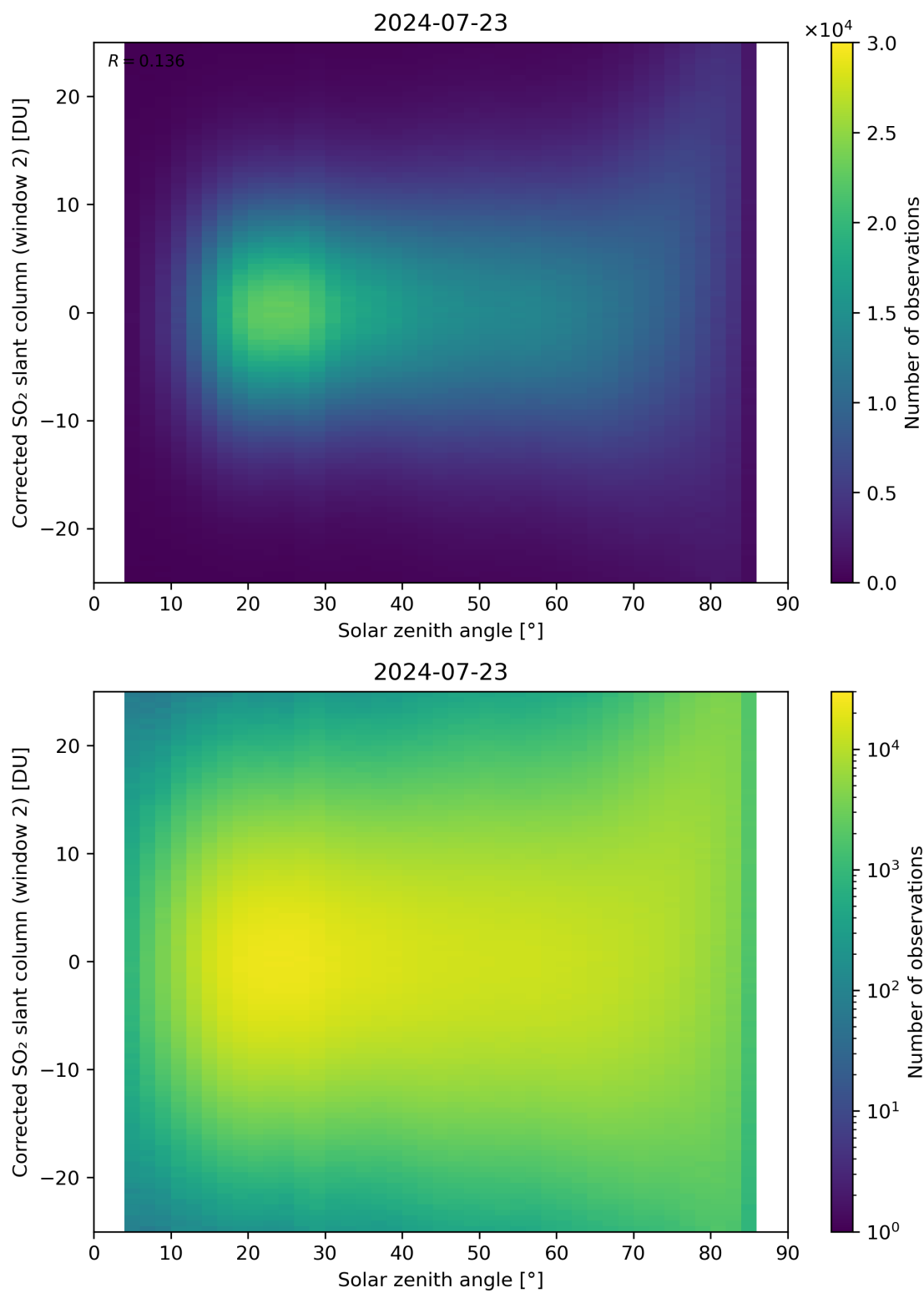
Figure 167: Scatter density plot of “Solar zenith angle” against “Corrected SO 2 slant column (window 2)” for 2024-07-22 to 2024-07-24.
