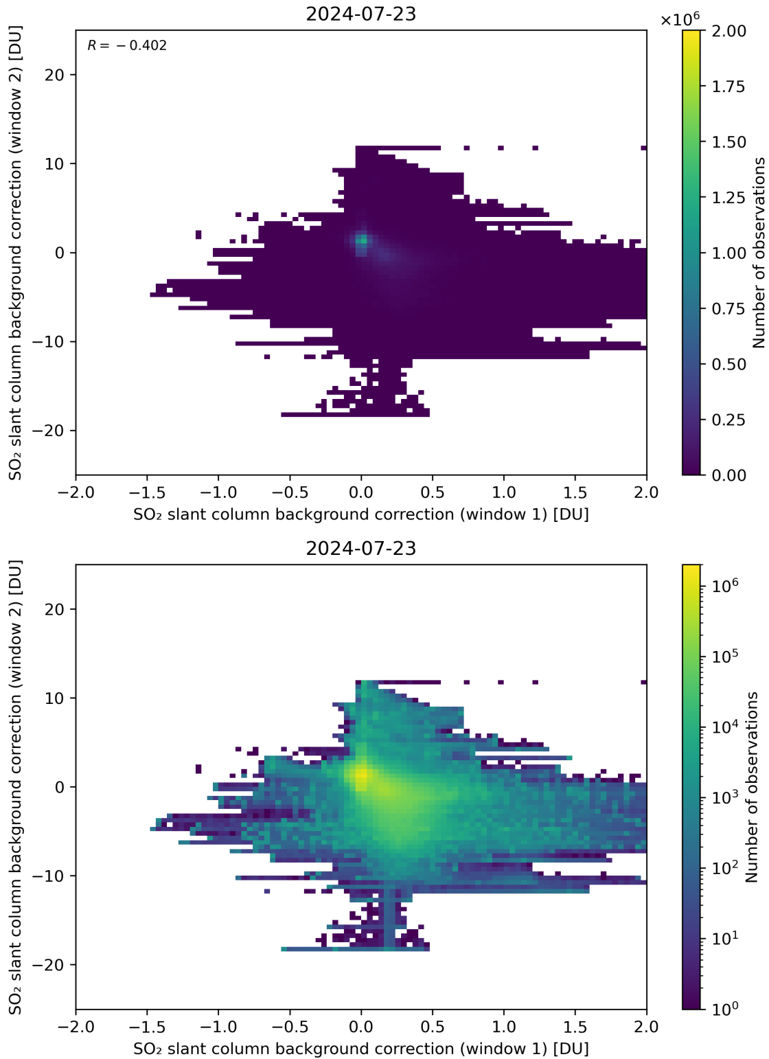
Figure 98: Scatter density plot of “SO 2 slant column background correction (window 1)” against “SO 2 slant column background correction (window 2)” for 2024-07-22 to 2024-07-24.
