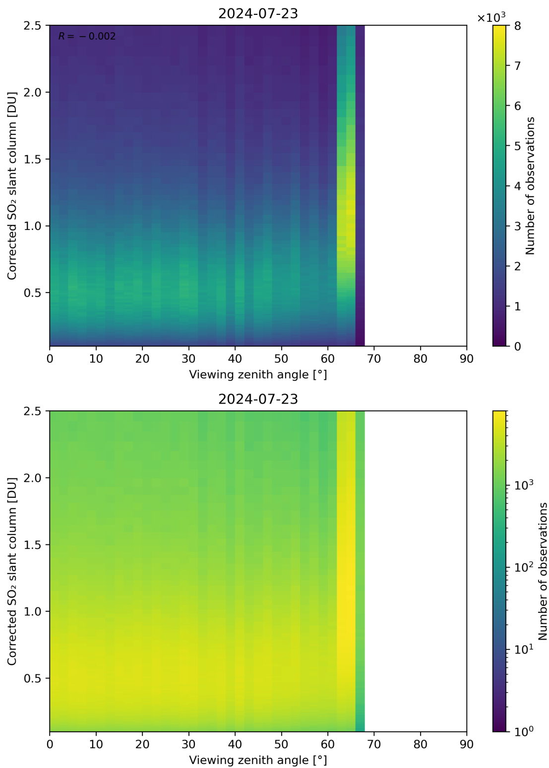
Figure 317: Scatter density plot of “Viewing zenith angle” against “Corrected SO 2 slant column” for 2024-07-22 to 2024-07-24.
