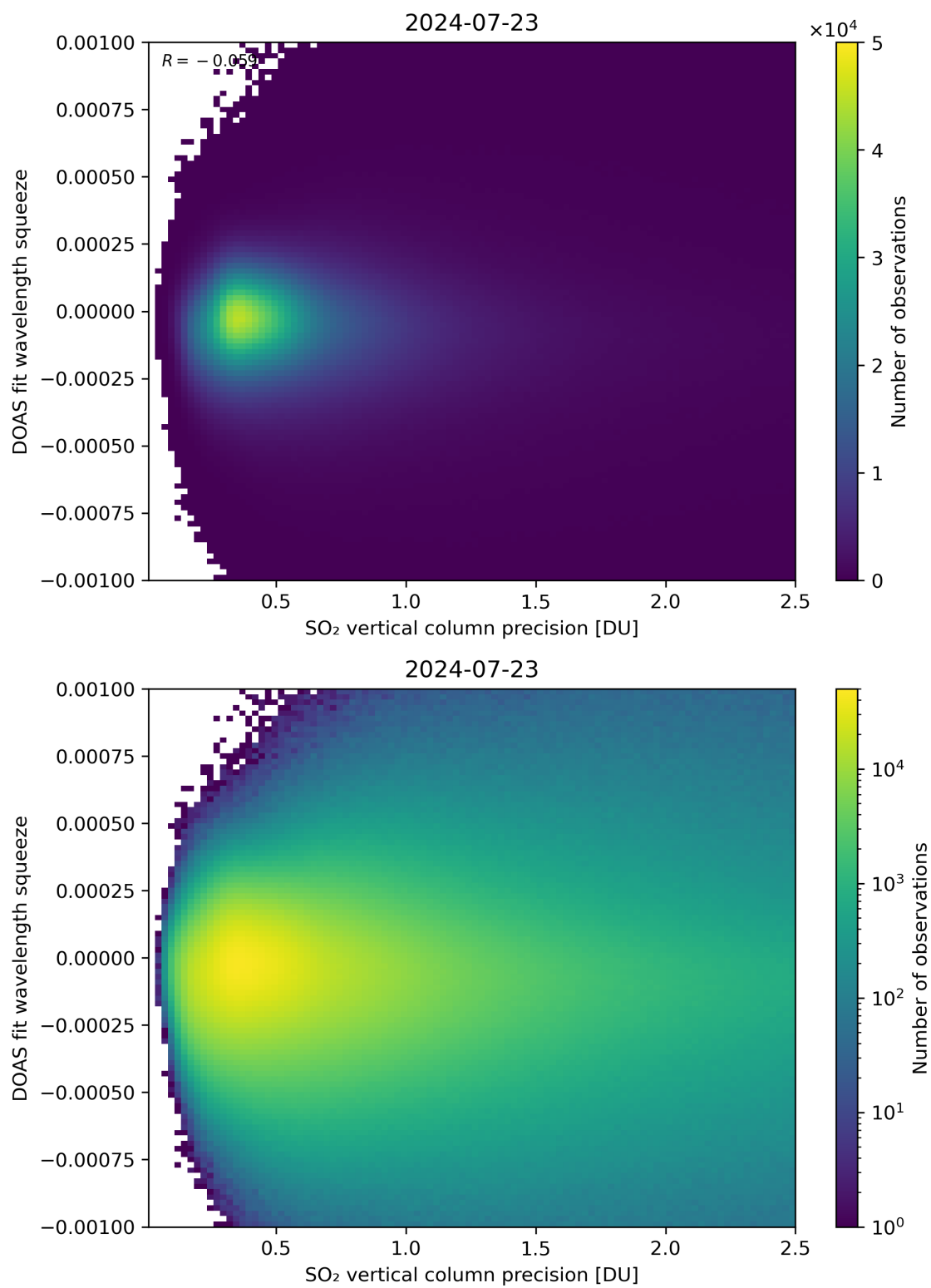
Figure 283: Scatter density plot of “SO 2 vertical column precision” against “DOAS fit wavelength squeeze” for 2024-07-22 to 2024-07-24.
