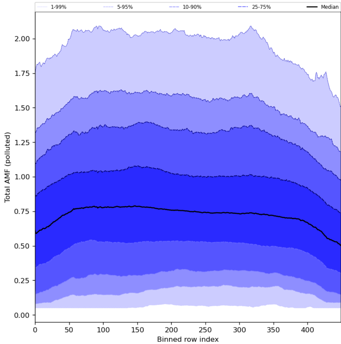
Figure 94: Along track statistics of “Total AMF (polluted)” for 2024-07-22 to 2024-07-24
