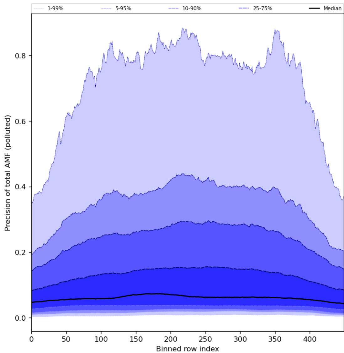
Figure 95: Along track statistics of “Precision of total AMF (polluted)” for 2024-07-22 to 2024-07-24
