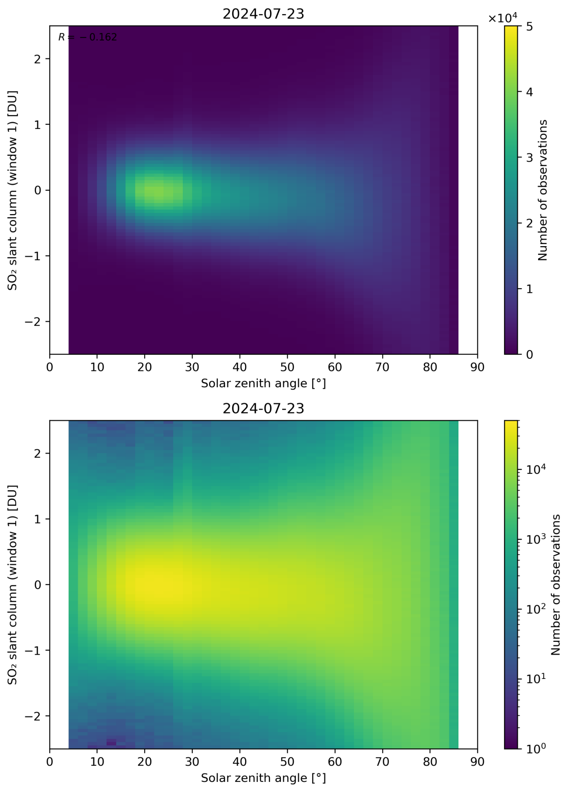
Figure 169: Scatter density plot of “Solar zenith angle” against “SO 2 slant column (window 1)” for 2024-07-22 to 2024-07-24.
