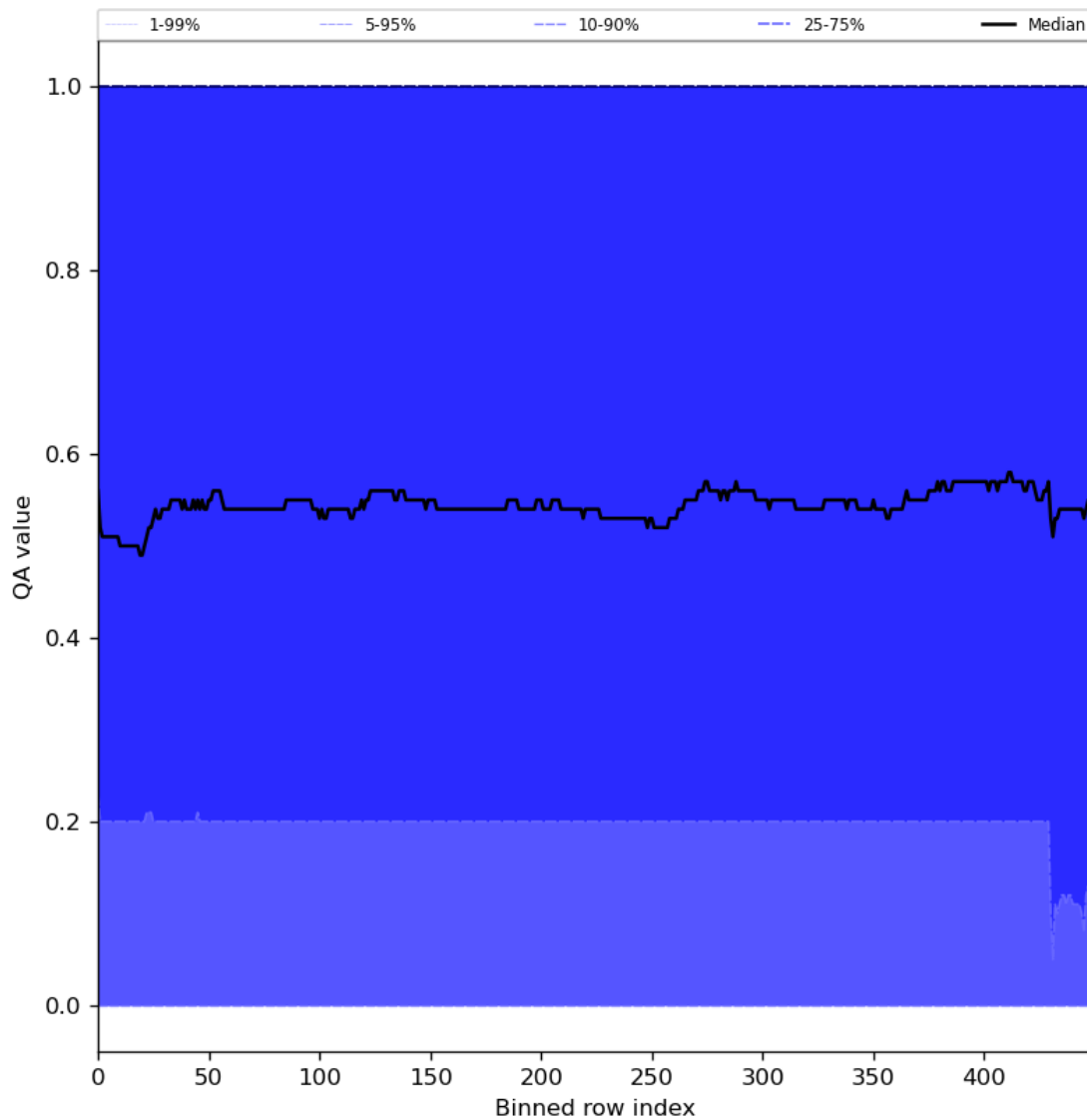
Figure 75: Along track statistics of “QA value” for 2024-07-22 to 2024-07-24
