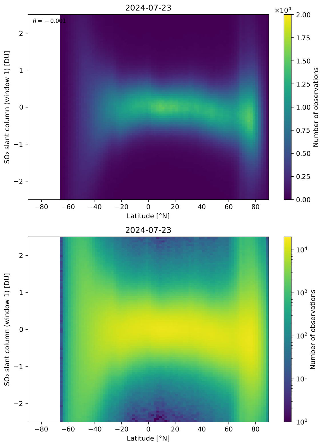
Figure 149: Scatter density plot of “Latitude” against “SO 2 slant column (window 1)” for 2024-07-22 to 2024-07-24.
