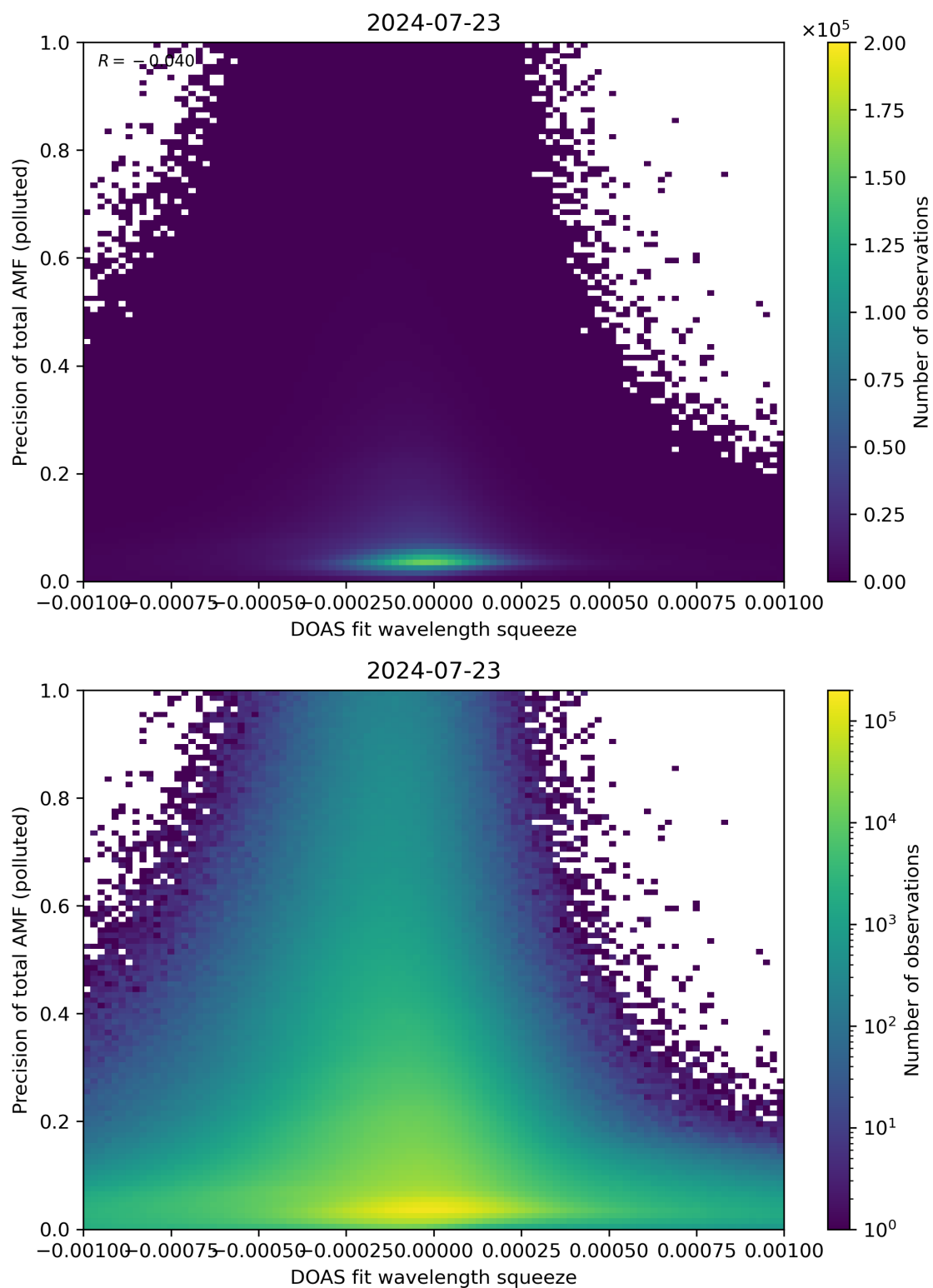
Figure 135: Scatter density plot of “DOAS fit wavelength squeeze” against “Precision of total AMF (polluted)” for 2024-07-22 to 2024-07-24.
