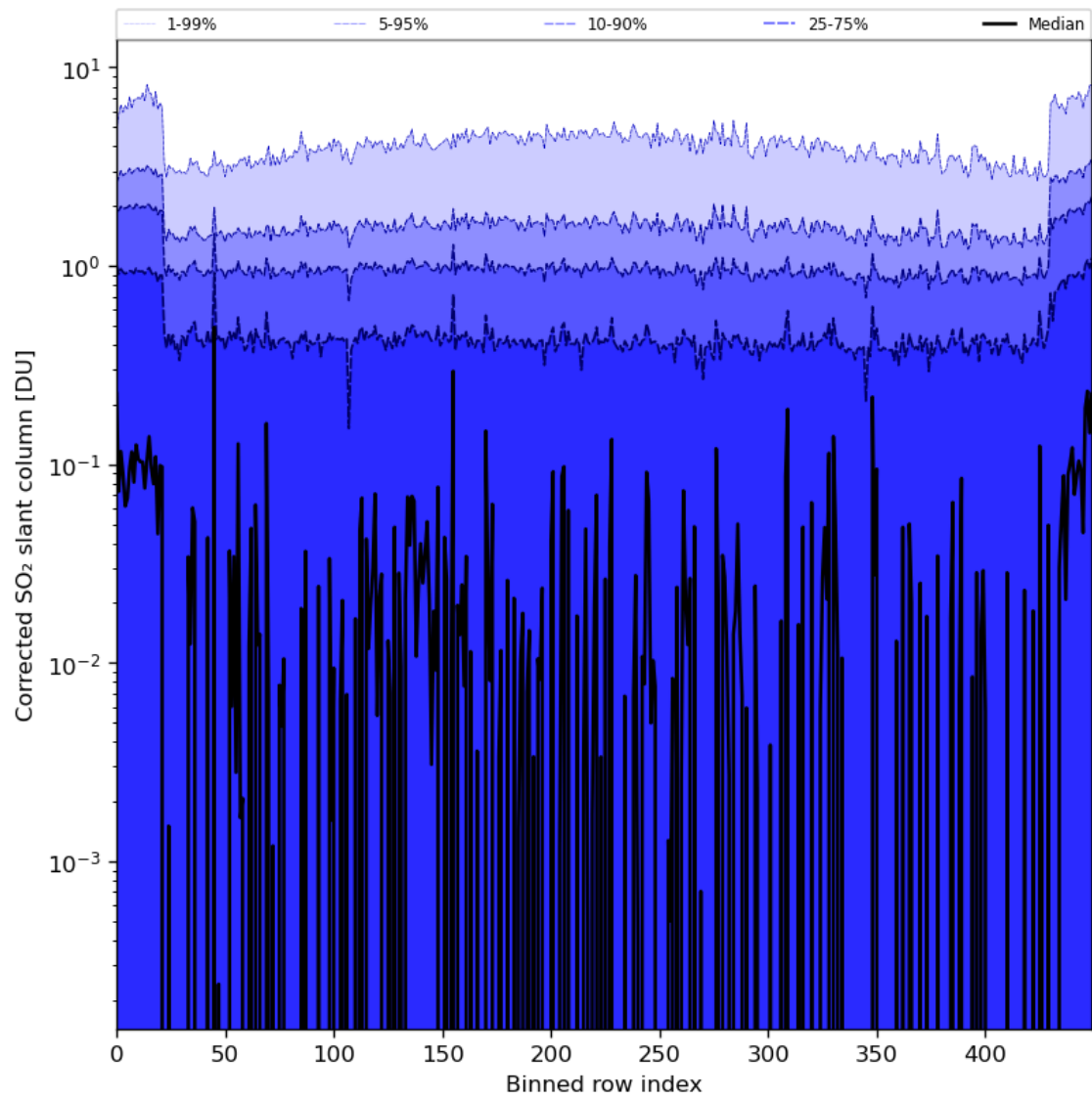
Figure 78: Along track statistics of “Corrected SO 2 slant column” for 2024-07-22 to 2024-07-24
