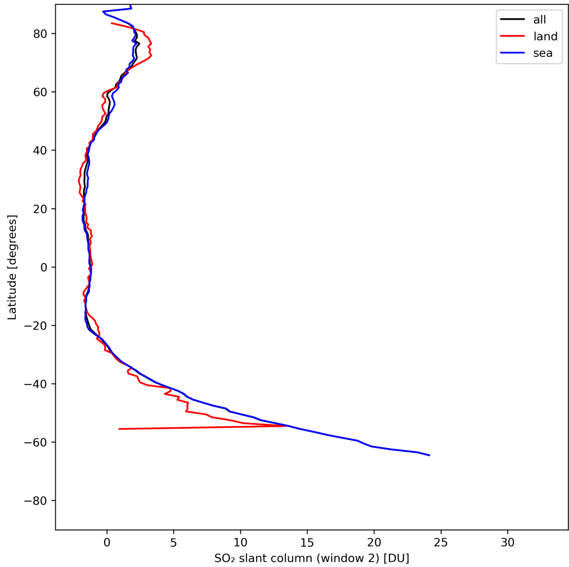
Figure 37: Zonal average of “SO 2 slant column (window 2)” for 2024-07-22 to 2024-07-24.
