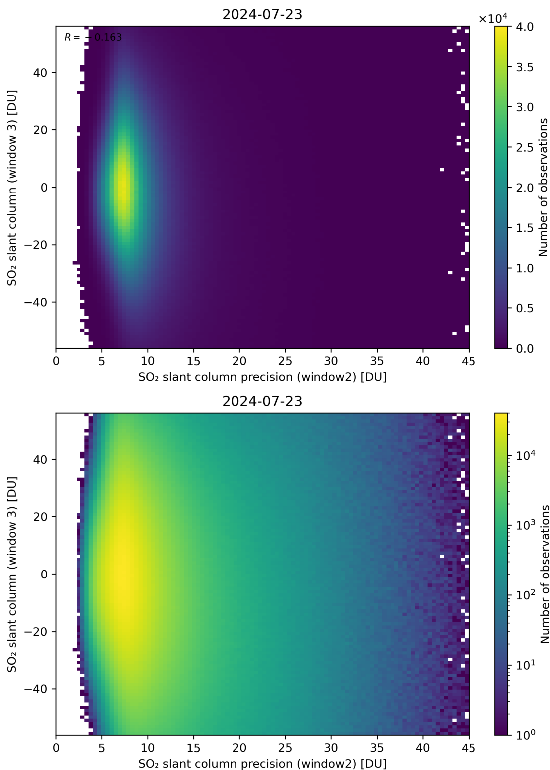
Figure 249: Scatter density plot of “SO 2 slant column precision (window2)” against “SO 2 slant column (window 3)” for 2024-07-22 to 2024-07-24.
