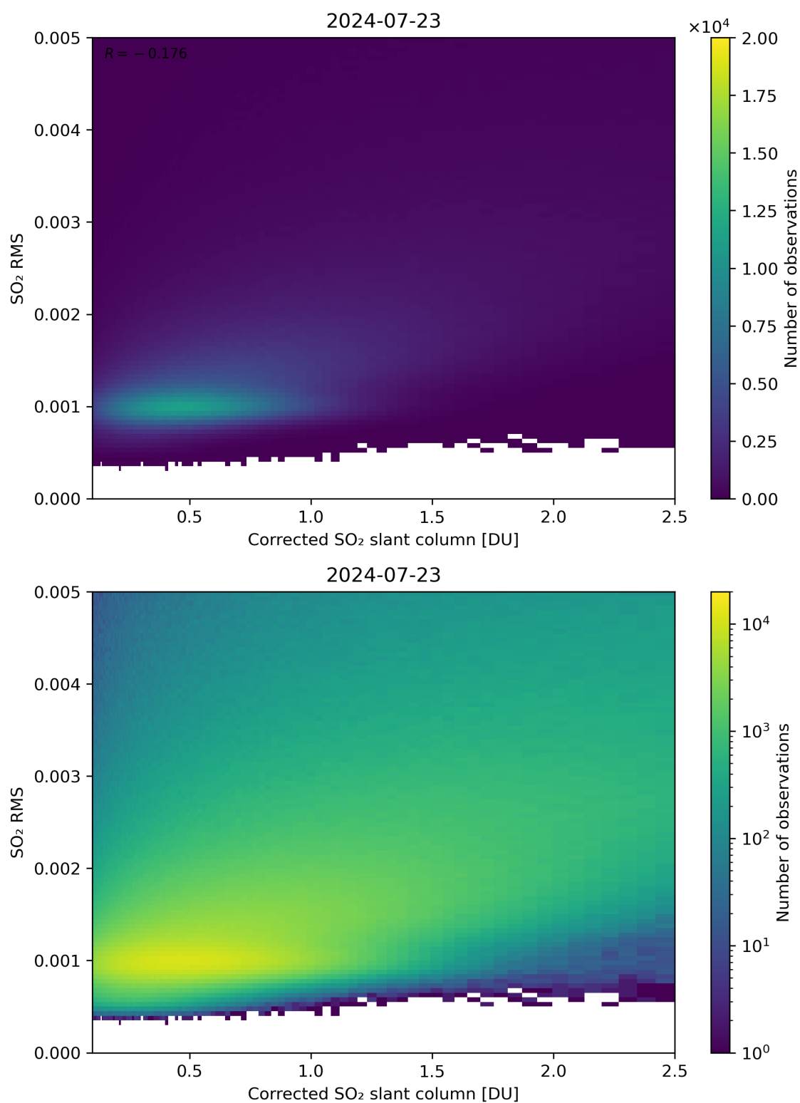
Figure 183: Scatter density plot of “Corrected SO 2 slant column” against “SO 2 RMS” for 2024-07-22 to 2024-07-24.
