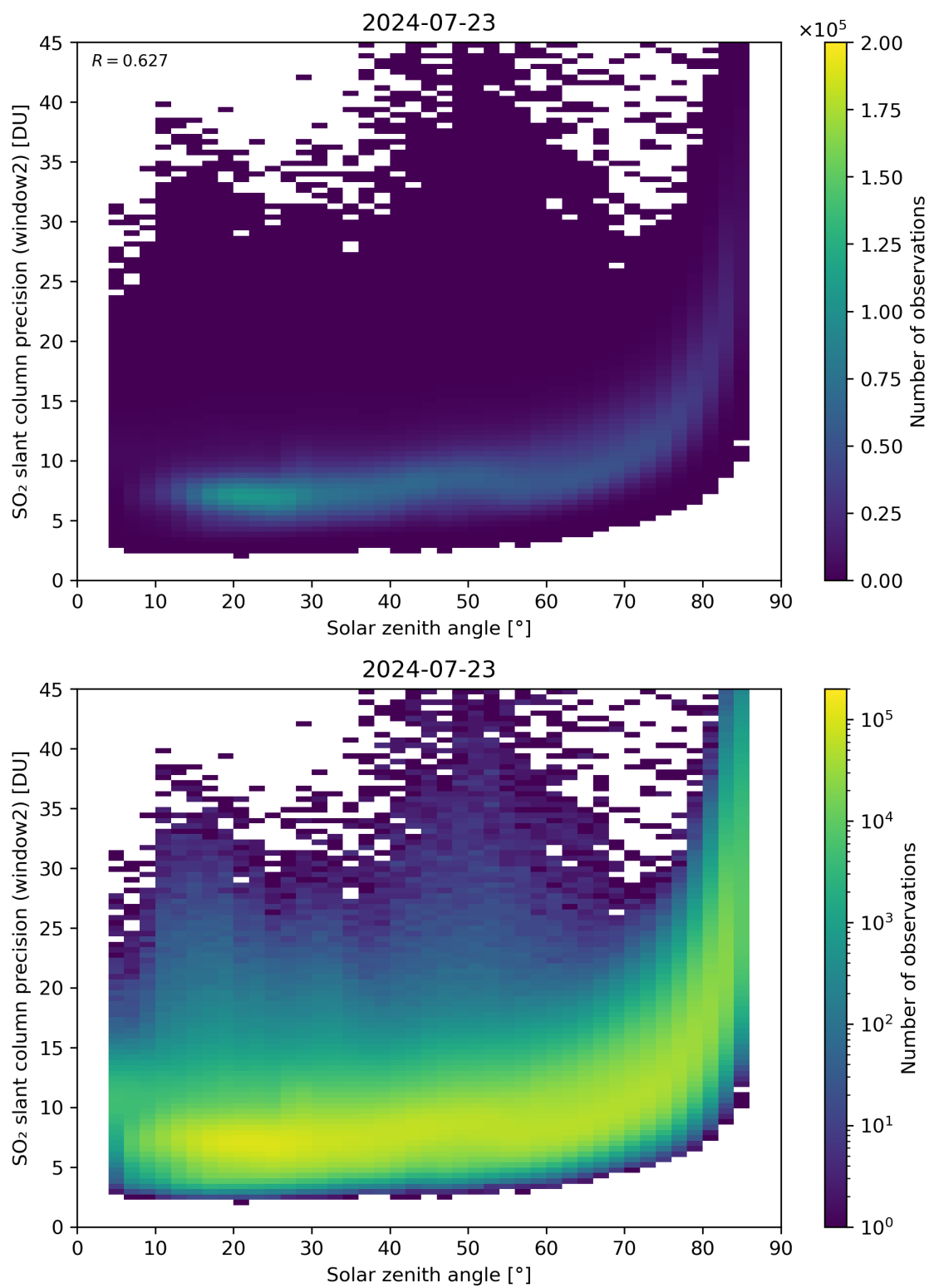
Figure 171: Scatter density plot of “Solar zenith angle” against “SO 2 slant column precision (window2)” for 2024-07-22 to 2024-07-24.
