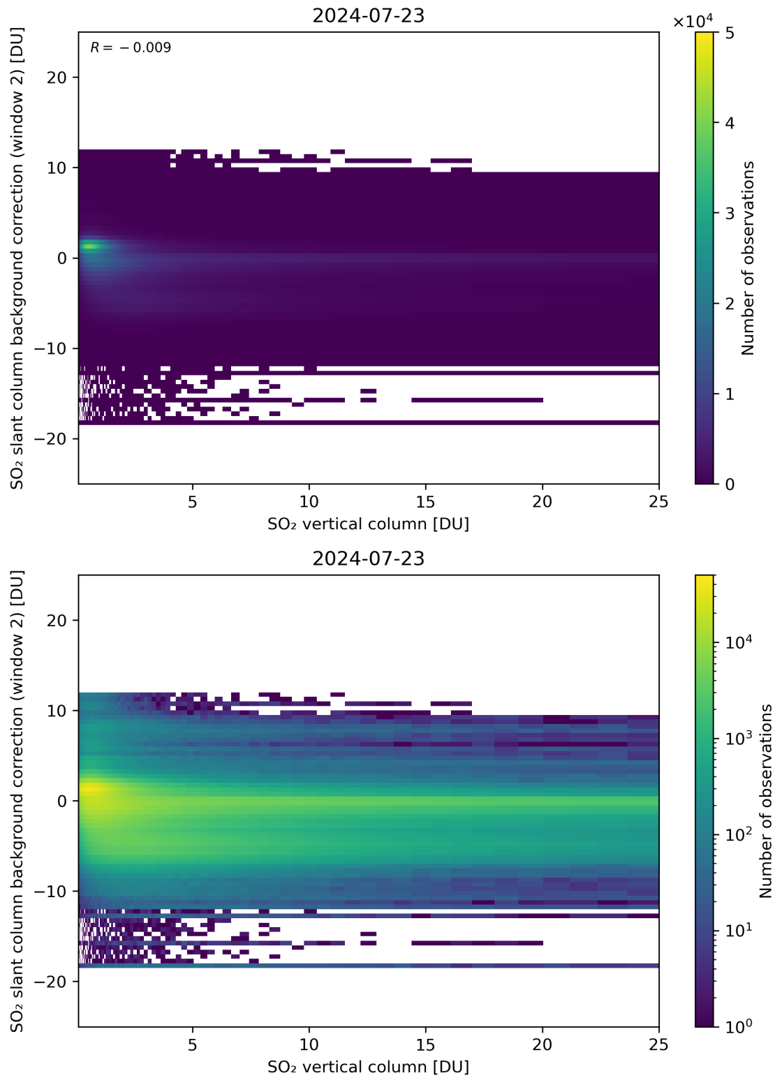
Figure 274: Scatter density plot of “SO 2 vertical column” against “SO 2 slant column background correction (window 2)” for 2024-07-22 to 2024-07-24.
