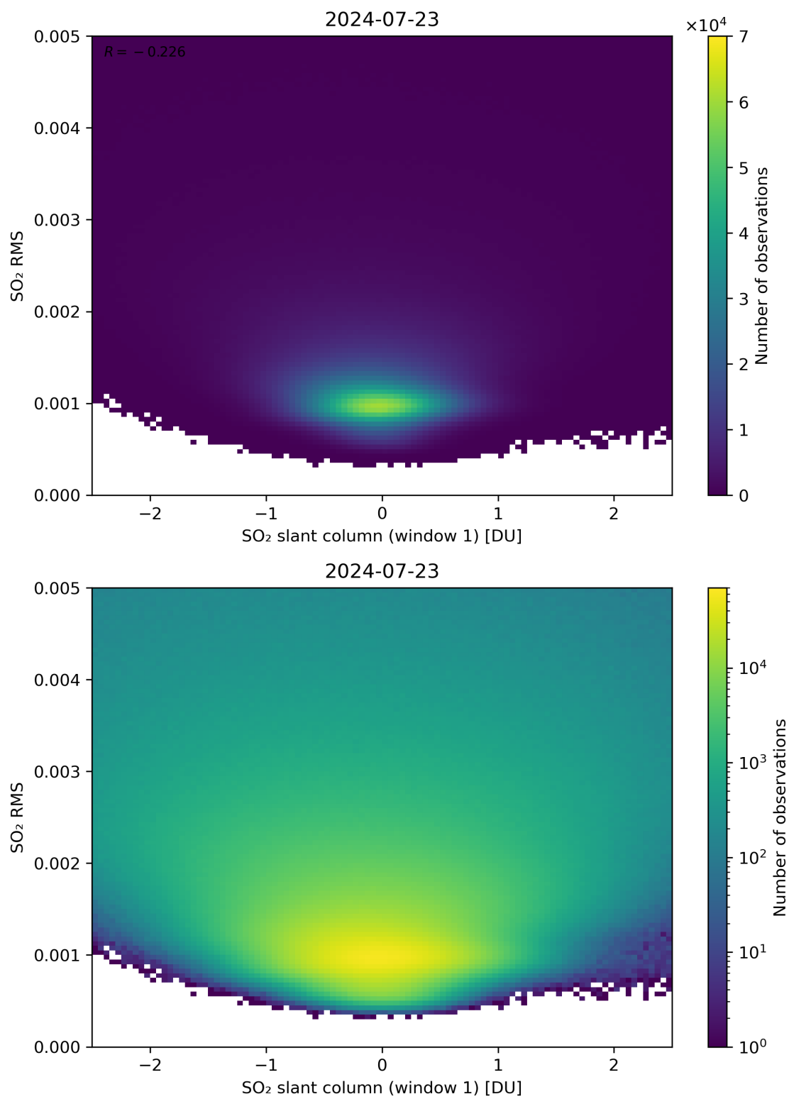
Figure 217: Scatter density plot of “SO 2 slant column (window 1)” against “SO 2 RMS” for 2024-07-22 to 2024-07-24.
