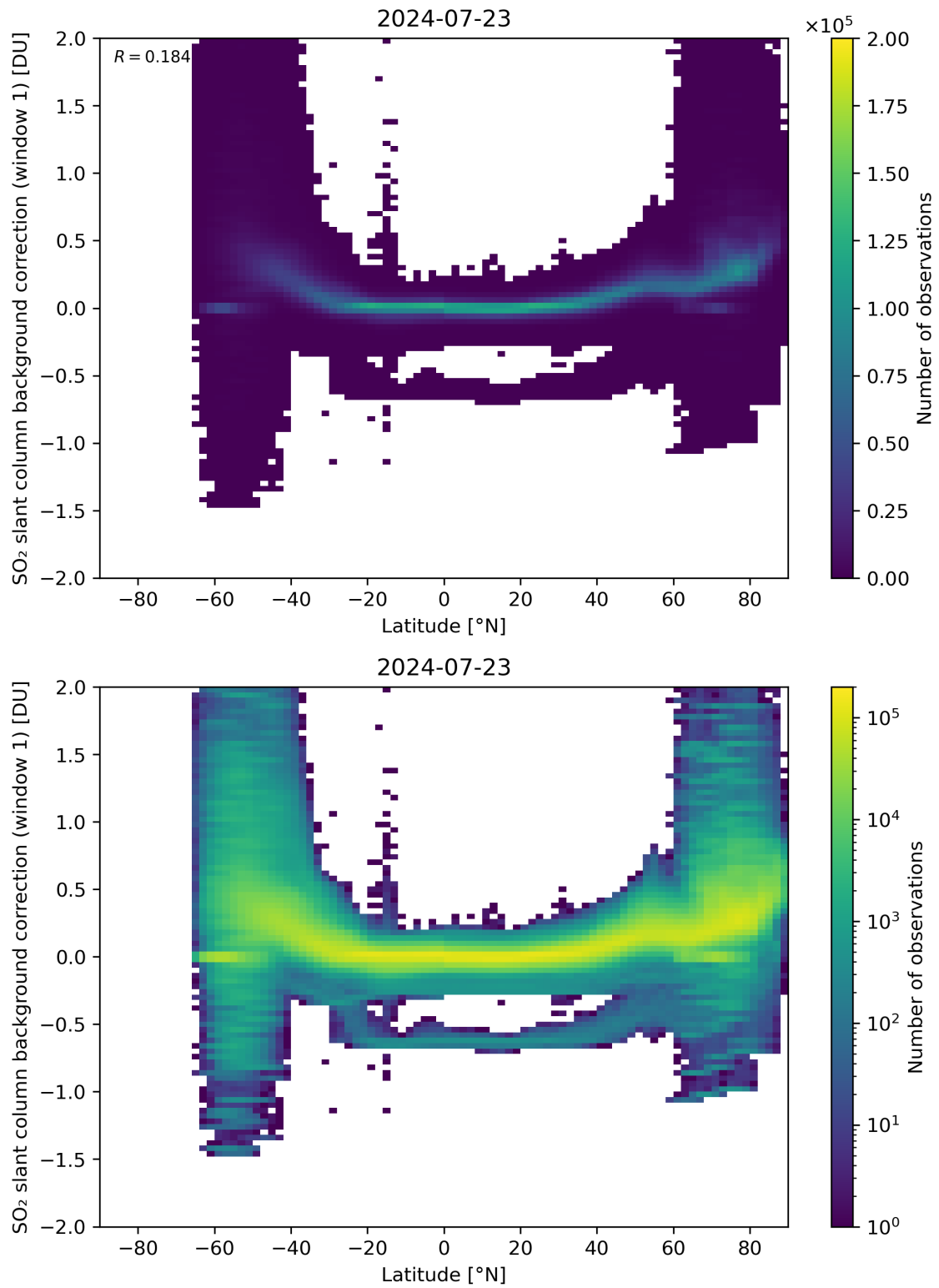
Figure 139: Scatter density plot of “Latitude” against “SO 2 slant column background correction (window 1)” for 2024-07-22 to 2024-07-24.
