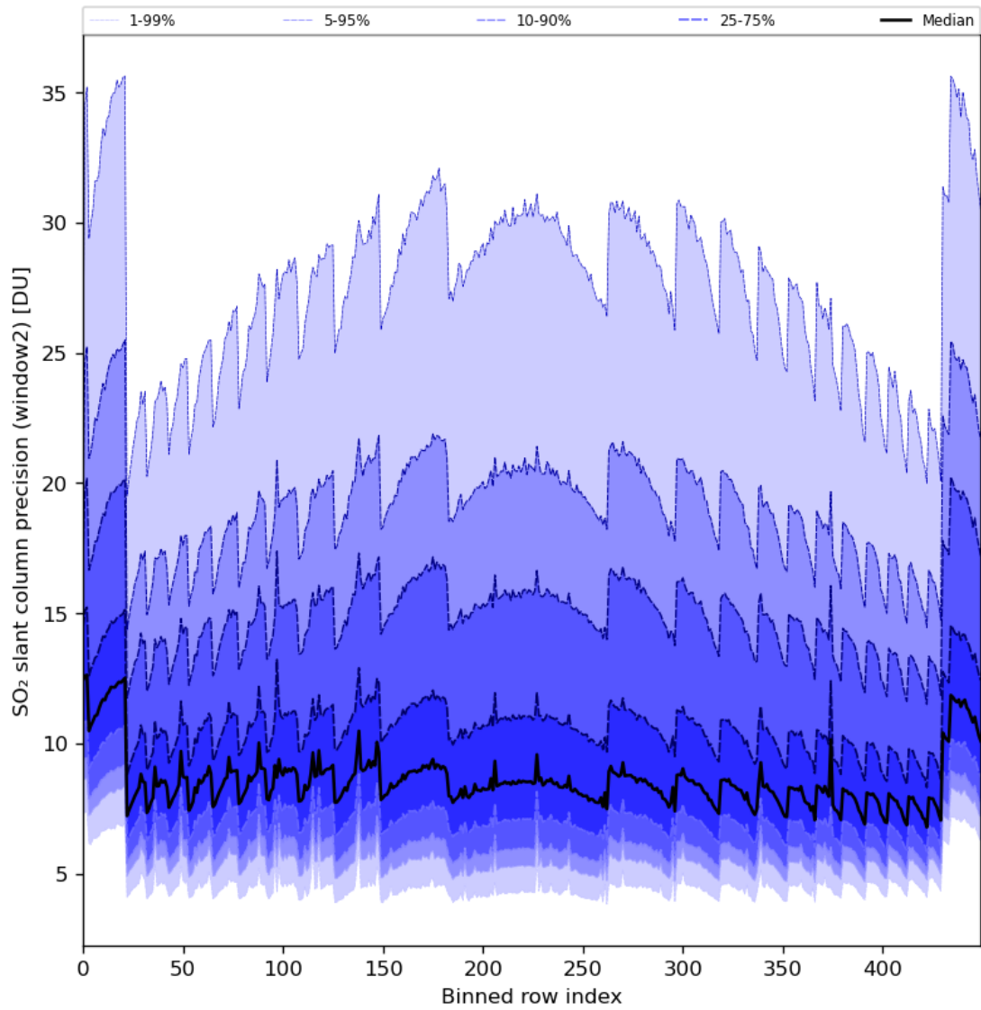
Figure 84: Along track statistics of “SO 2 slant column precision (window2)” for 2024-07-22 to 2024-07-24
