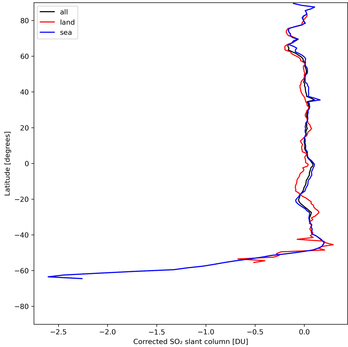
Figure 32: Zonal average of “Corrected SO 2 slant column” for 2024-07-22 to 2024-07-24.
