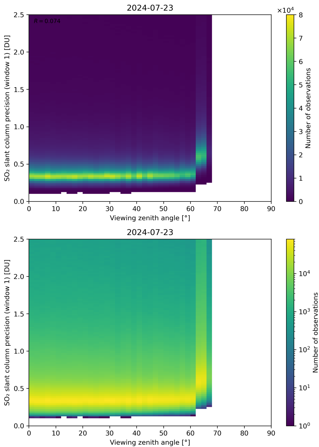
Figure 321: Scatter density plot of “Viewing zenith angle” against “SO 2 slant column precision (window 1)” for 2024-07-22 to 2024-07-24.
