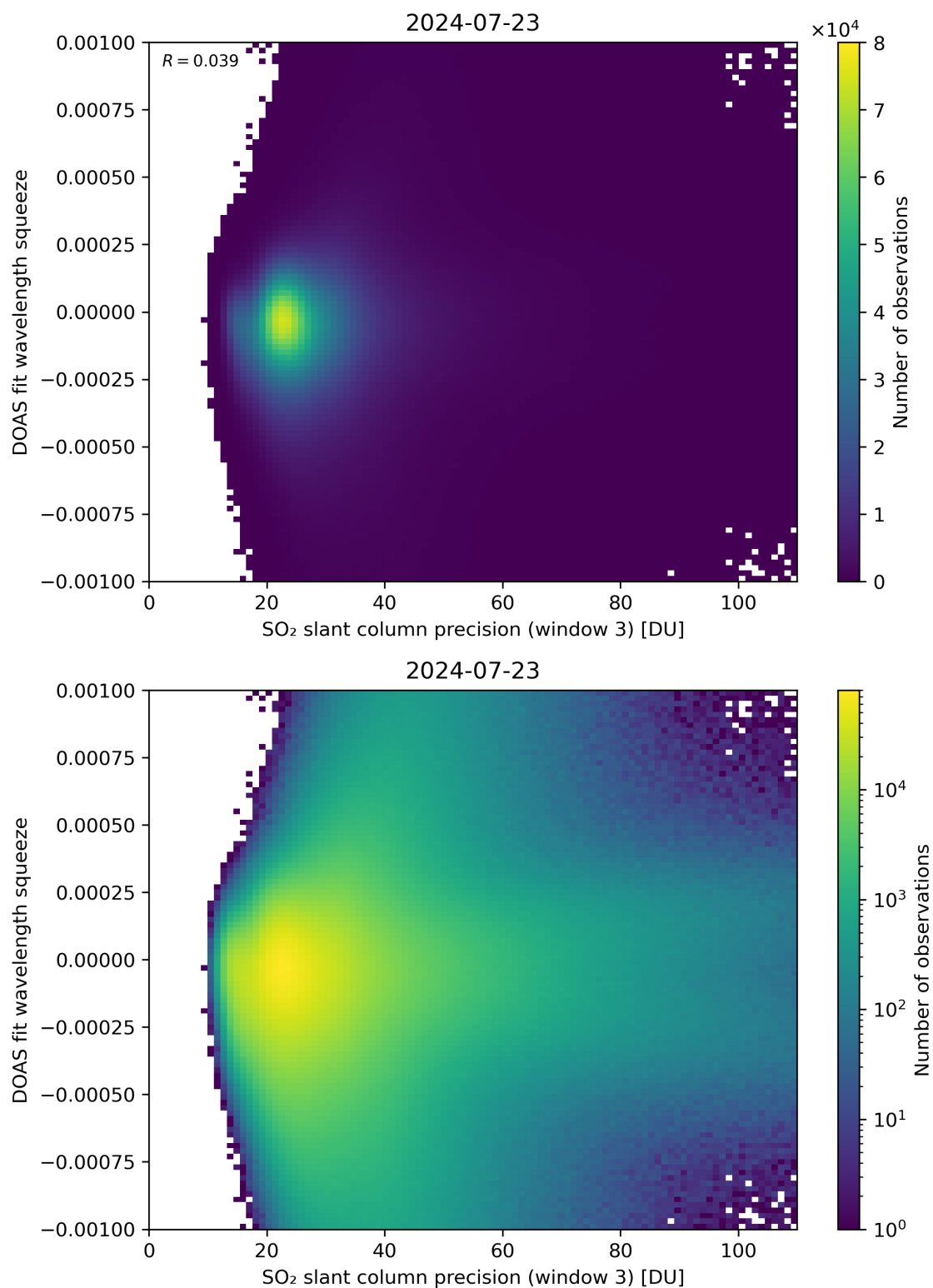
Figure 259: Scatter density plot of “SO 2 slant column precision (window 3)” against “DOAS fit wavelength squeeze” for 2024-07-22 to 2024-07-24.
