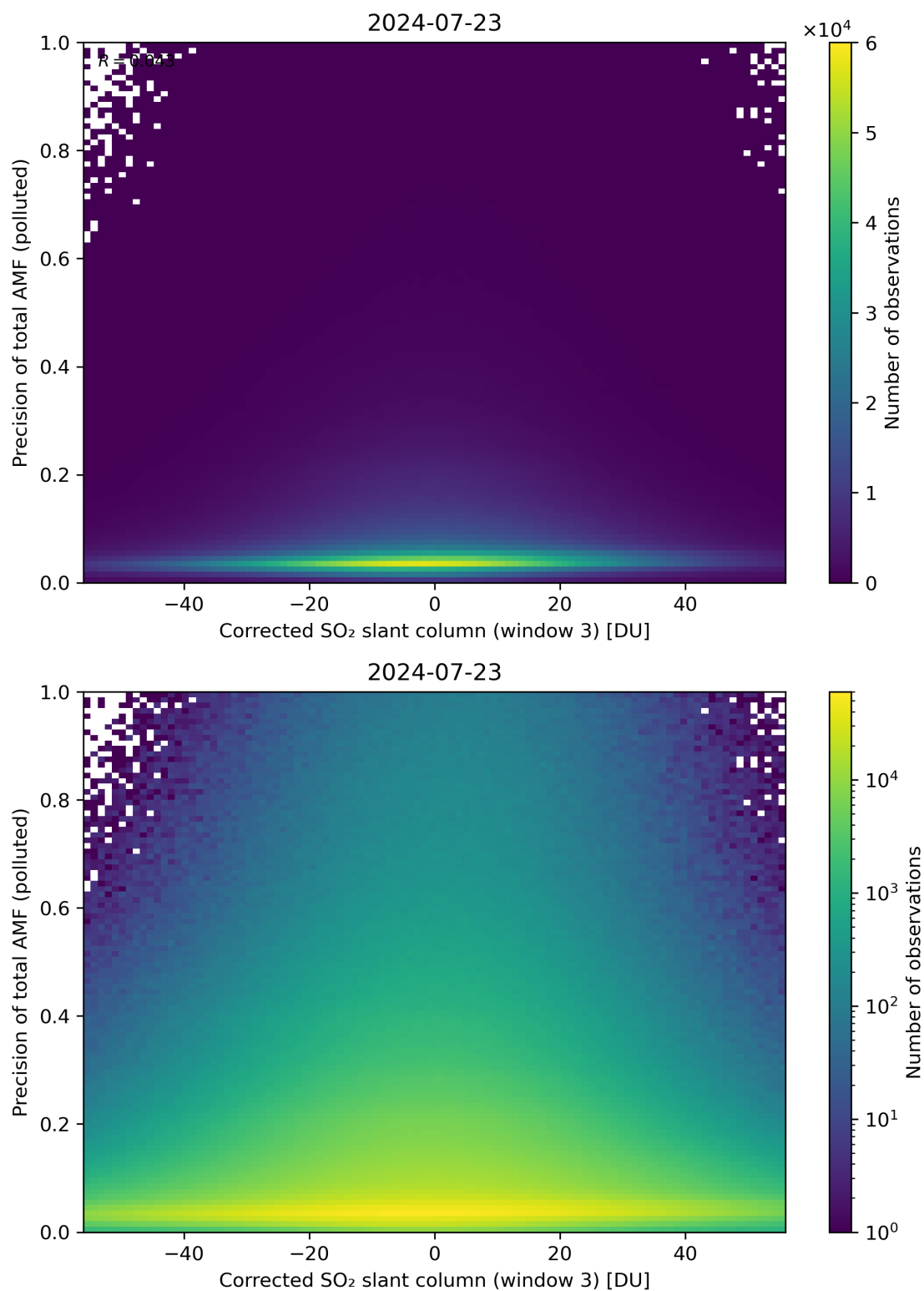
Figure 211: Scatter density plot of “Corrected SO 2 slant column (window 3)” against “Precision of total AMF (polluted)” for 2024-07-22 to 2024-07-24.
