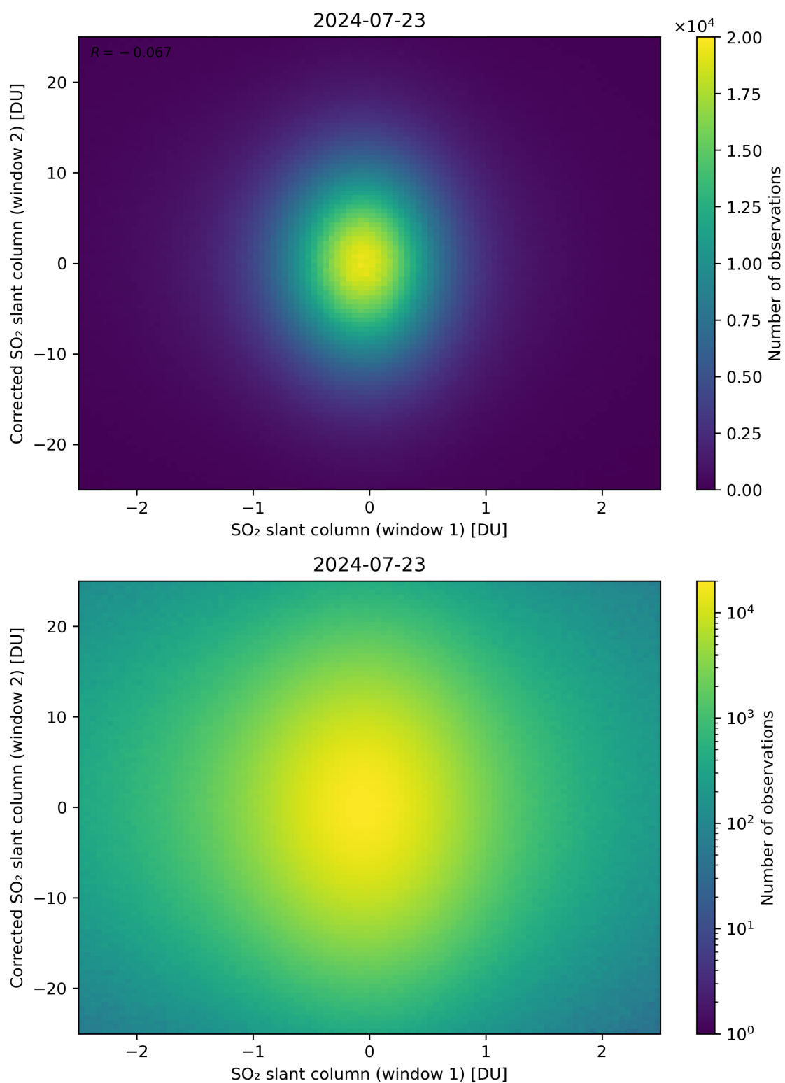
Figure 233: Scatter density plot of “SO 2 slant column (window 1)” against “Corrected SO 2 slant column (window 2)” for 2024-07-22 to 2024-07-24.
