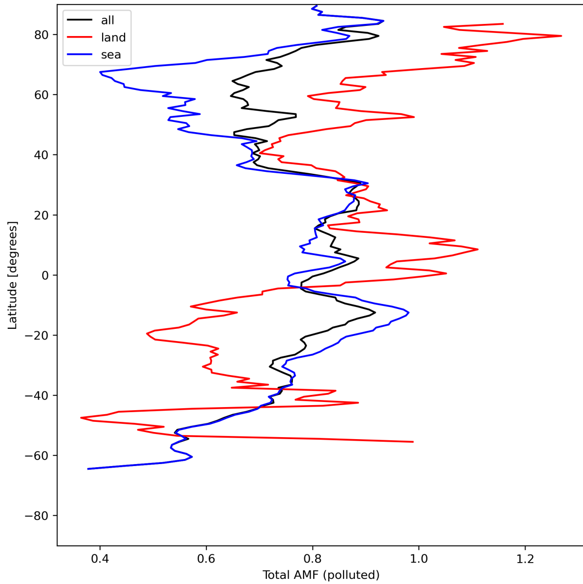
Figure 48: Zonal average of “Total AMF (polluted)” for 2024-07-22 to 2024-07-24.
