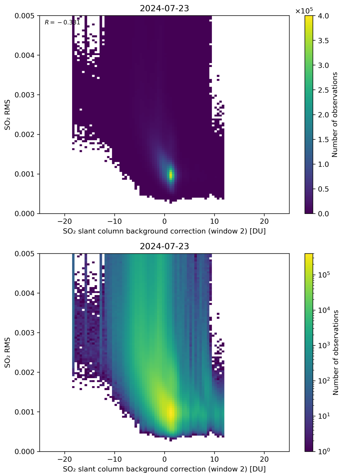
Figure 114: Scatter density plot of “SO 2 slant column background correction (window 2)” against “SO 2 RMS” for 2024-07-22 to 2024-07-24.
