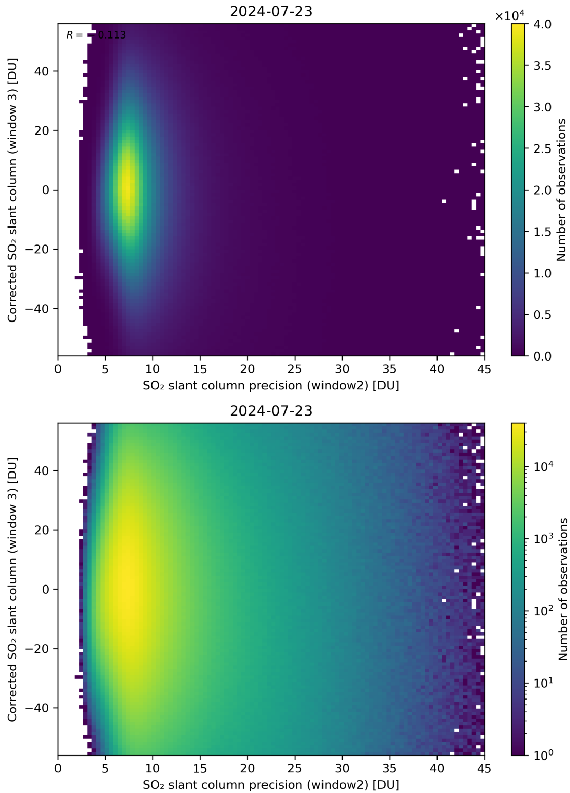
Figure 248: Scatter density plot of “SO 2 slant column precision (window2)” against “Corrected SO 2 slant column (window 3)” for 2024-07-22 to 2024-07-24.
