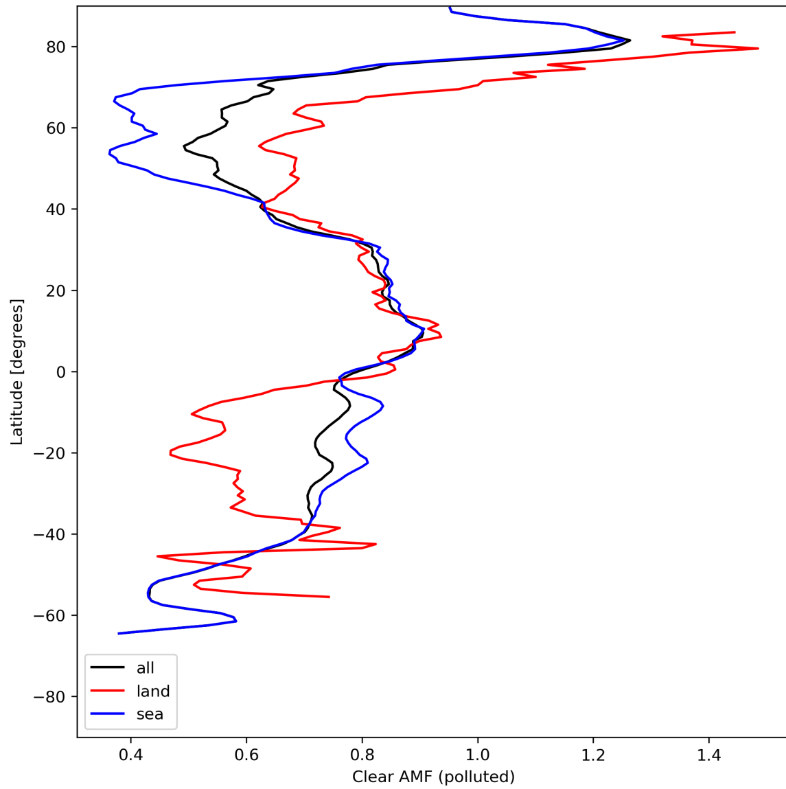
Figure 50: Zonal average of “Clear AMF (polluted)” for 2024-07-22 to 2024-07-24.
