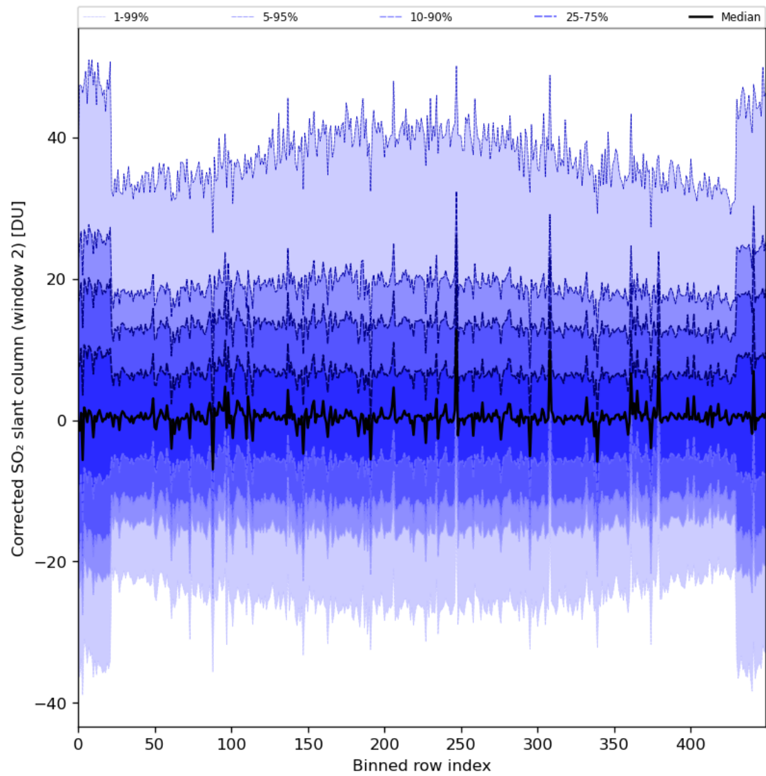
Figure 85: Along track statistics of “Corrected SO 2 slant column (window 2)” for 2024-07-22 to 2024-07-24
