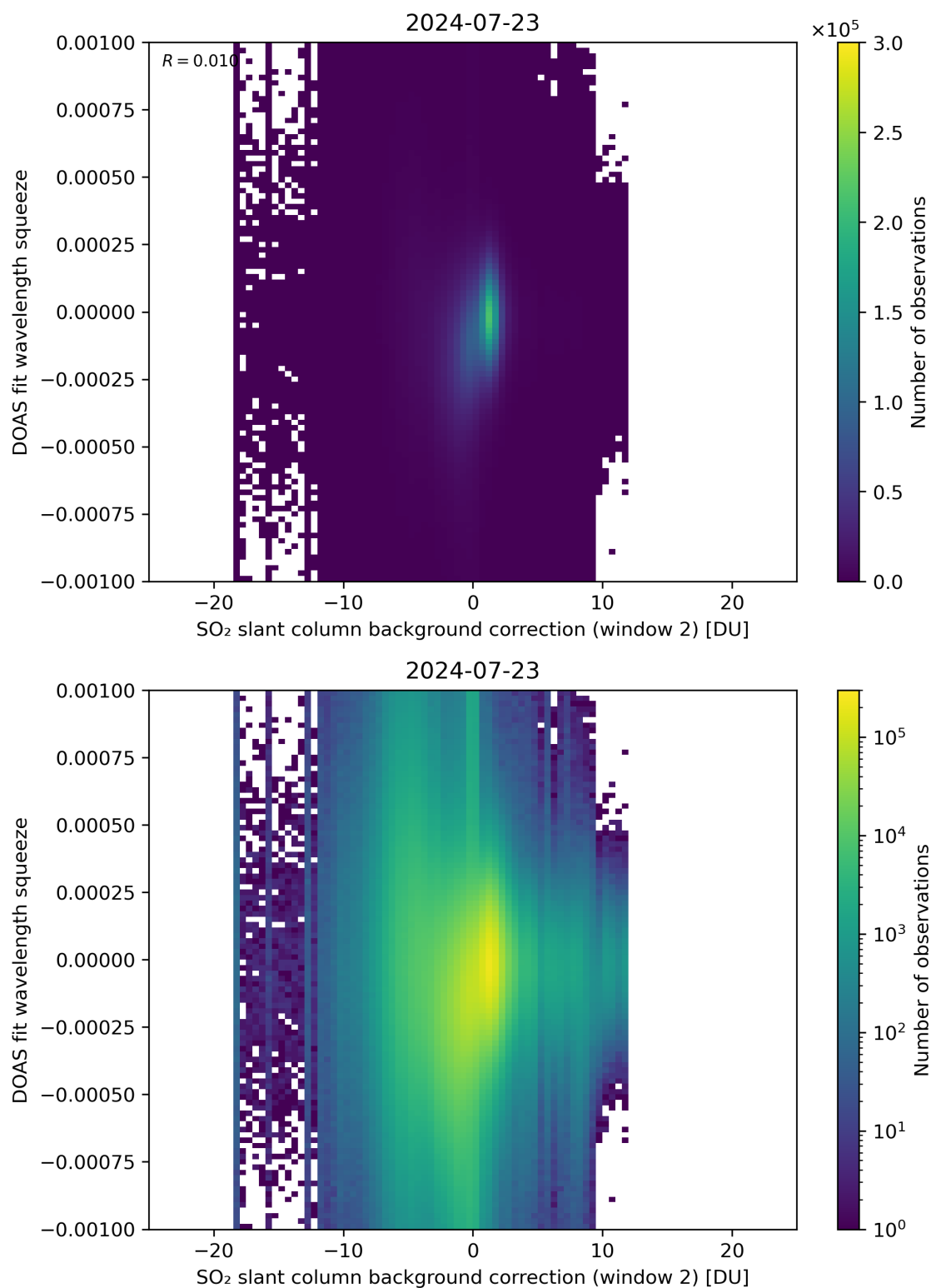
Figure 113: Scatter density plot of “SO 2 slant column background correction (window 2)” against “DOAS fit wavelength squeeze” for 2024-07-22 to 2024-07-24.
