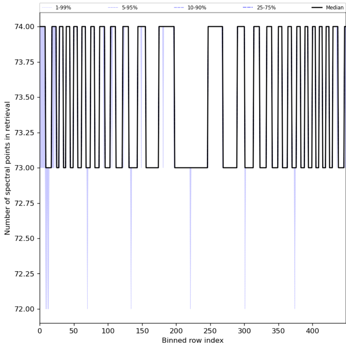
Figure 97: Along track statistics of “Number of spectral points in retrieval” for 2024-07-22 to 2024-07-24
