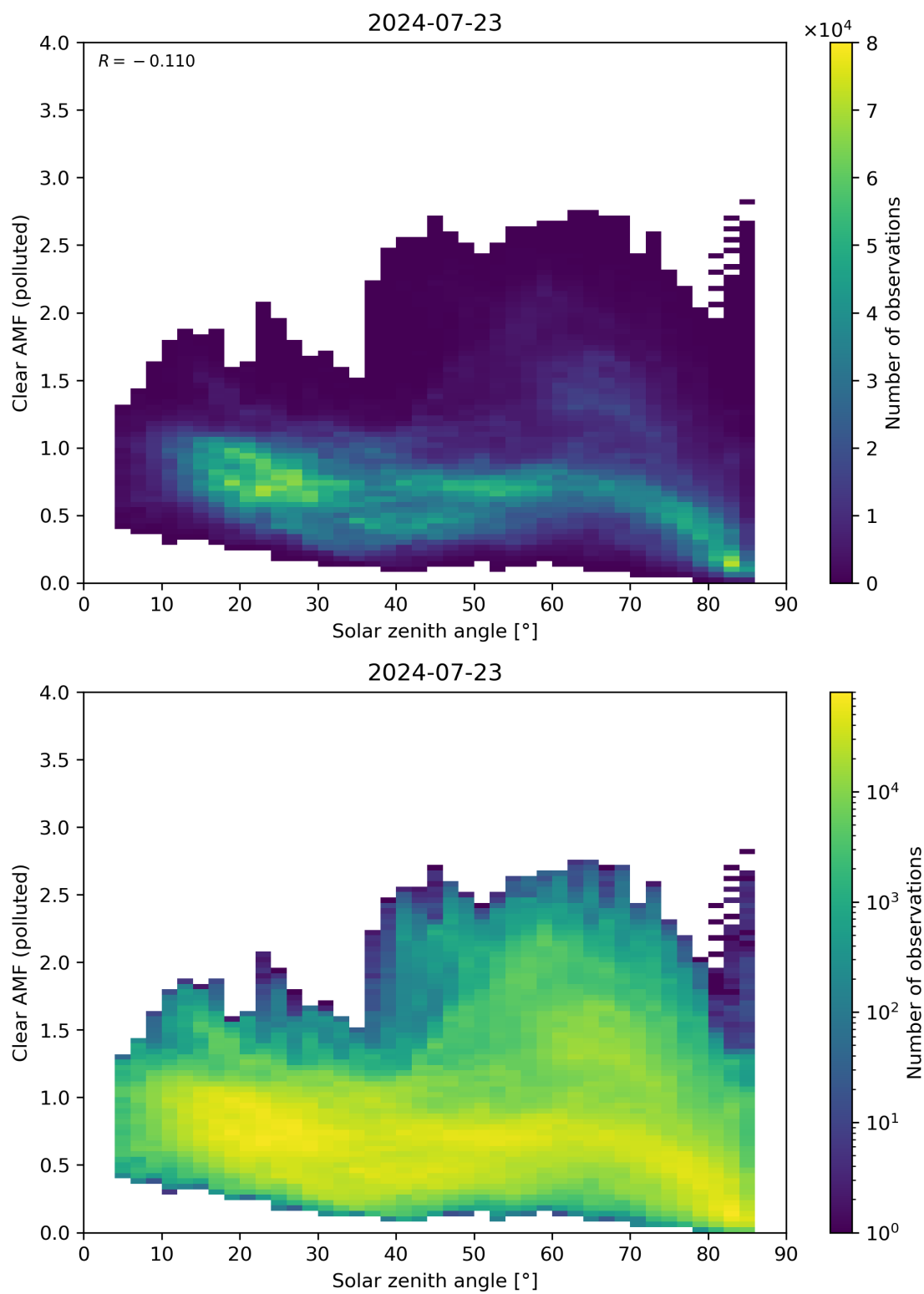
Figure 165: Scatter density plot of “Solar zenith angle” against “Clear AMF (polluted)” for 2024-07-22 to 2024-07-24.
