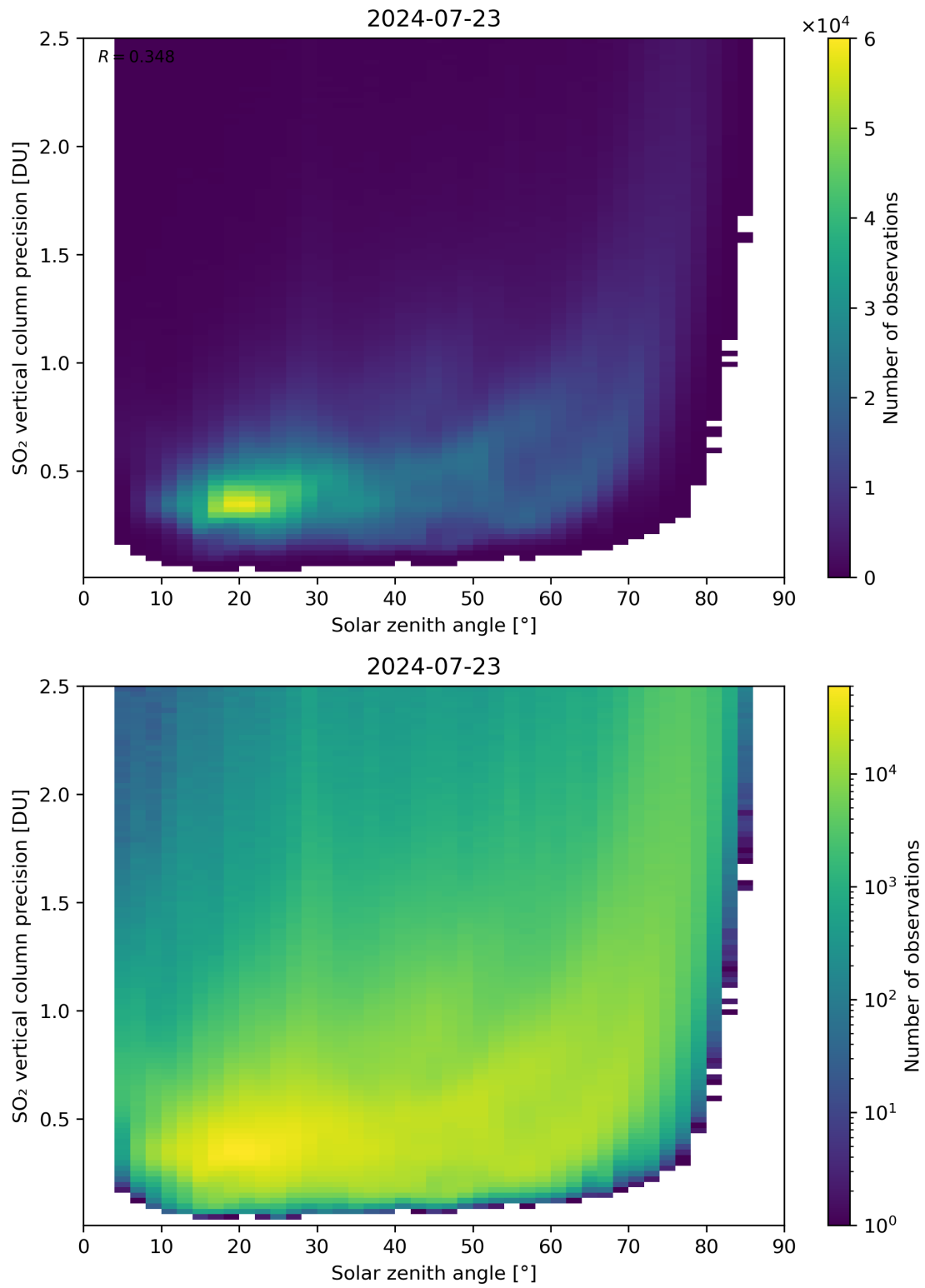
Figure 177: Scatter density plot of “Solar zenith angle” against “SO 2 vertical column precision” for 2024-07-22 to 2024-07-24.
