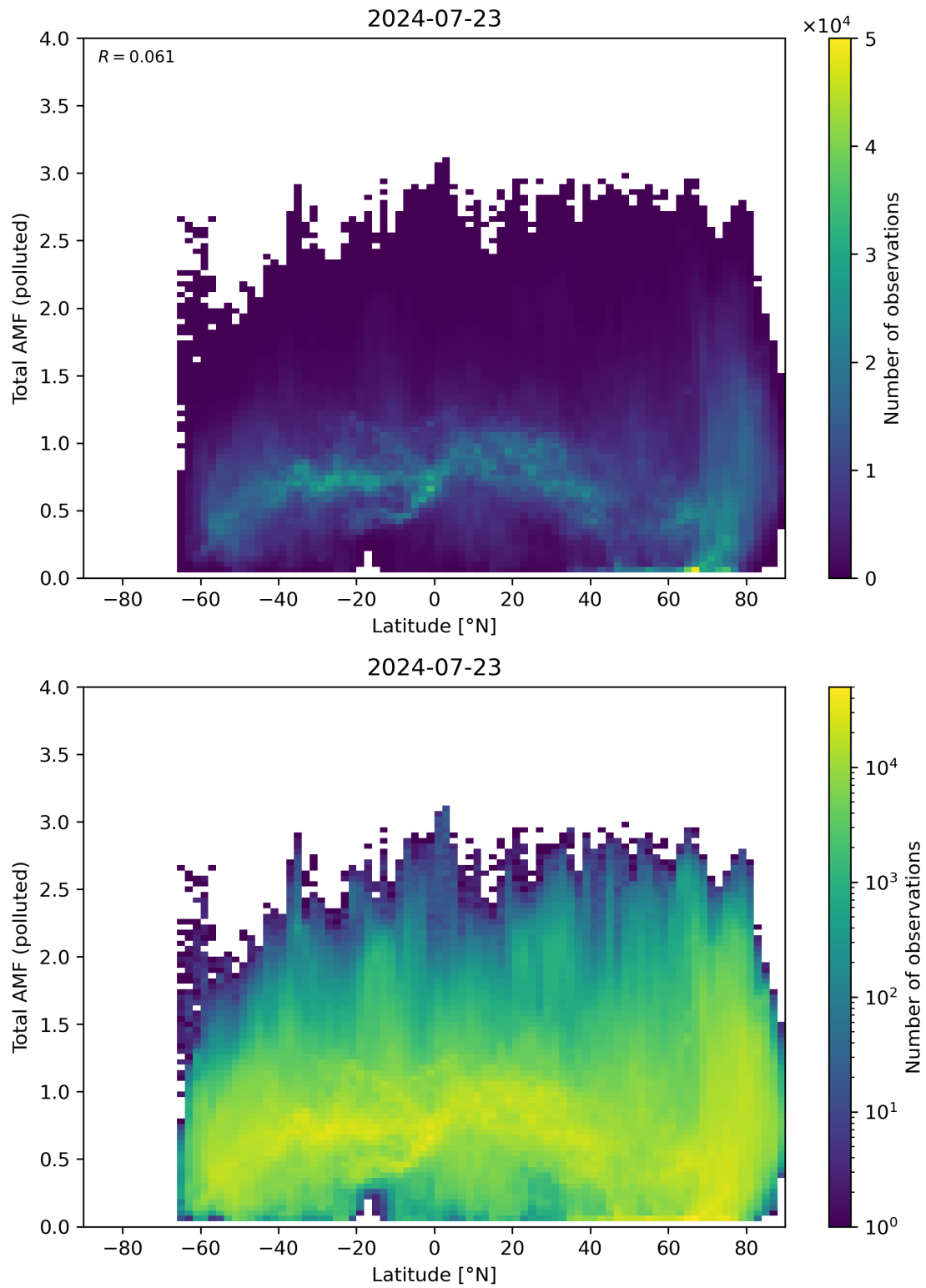
Figure 154: Scatter density plot of “Latitude” against “Total AMF (polluted)” for 2024-07-22 to 2024-07-24.
