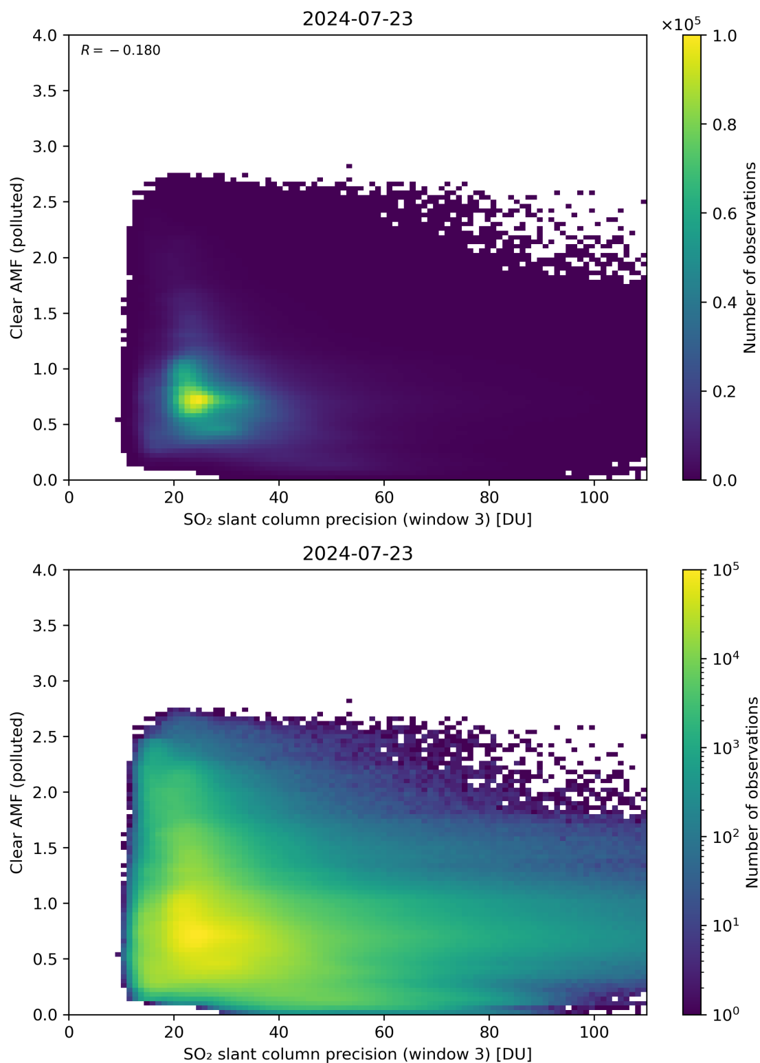
Figure 261: Scatter density plot of “SO 2 slant column precision (window 3)” against “Clear AMF (polluted)” for 2024-07-22 to 2024-07-24.
