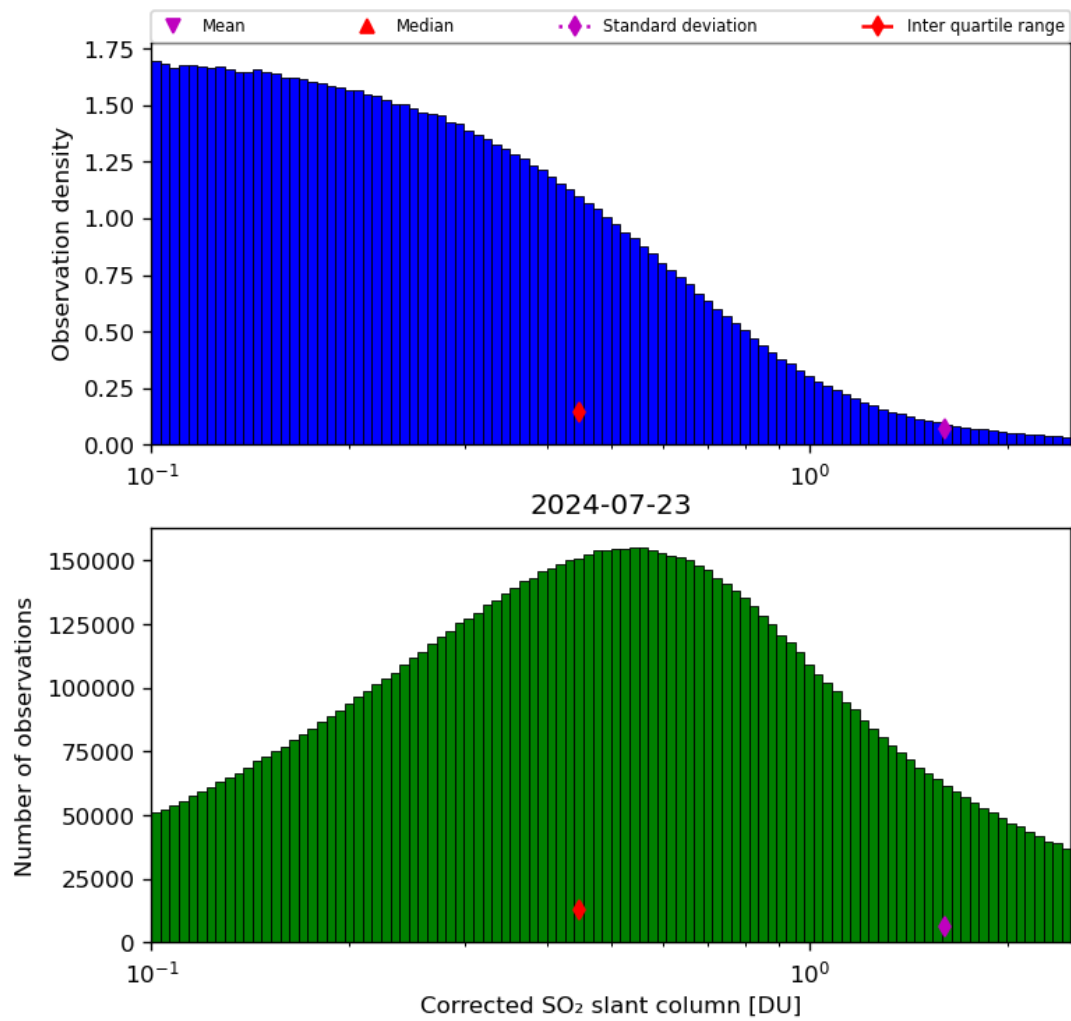
Figure 55: Histogram of “Corrected SO 2 slant column” for 2024-07-22 to 2024-07-24
