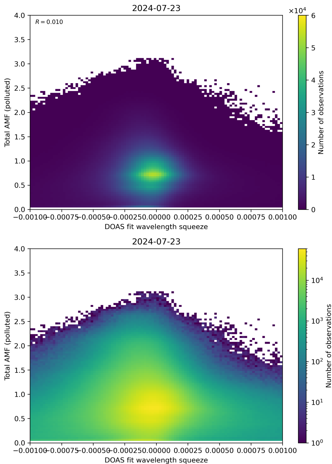
Figure 134: Scatter density plot of “DOAS fit wavelength squeeze” against “Total AMF (polluted)” for 2024-07-22 to 2024-07-24.
