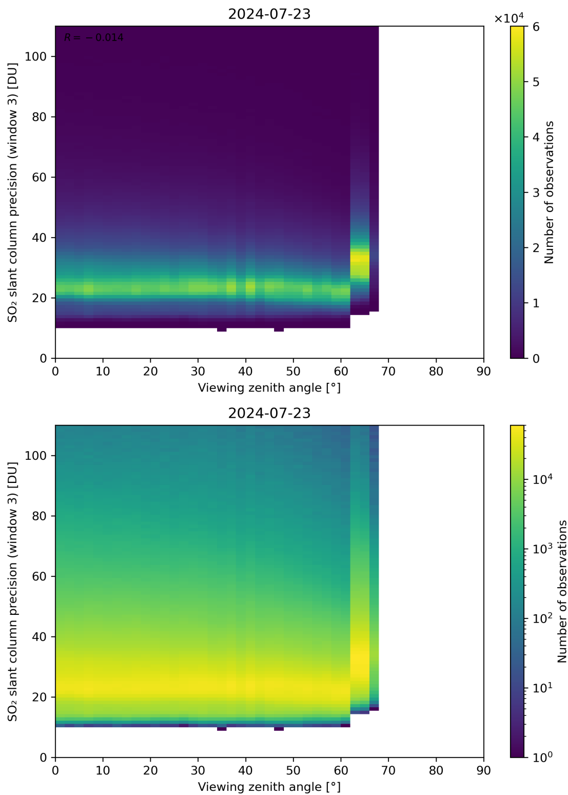
Figure 324: Scatter density plot of “Viewing zenith angle” against “SO 2 slant column precision (window 3)” for 2024-07-22 to 2024-07-24.
