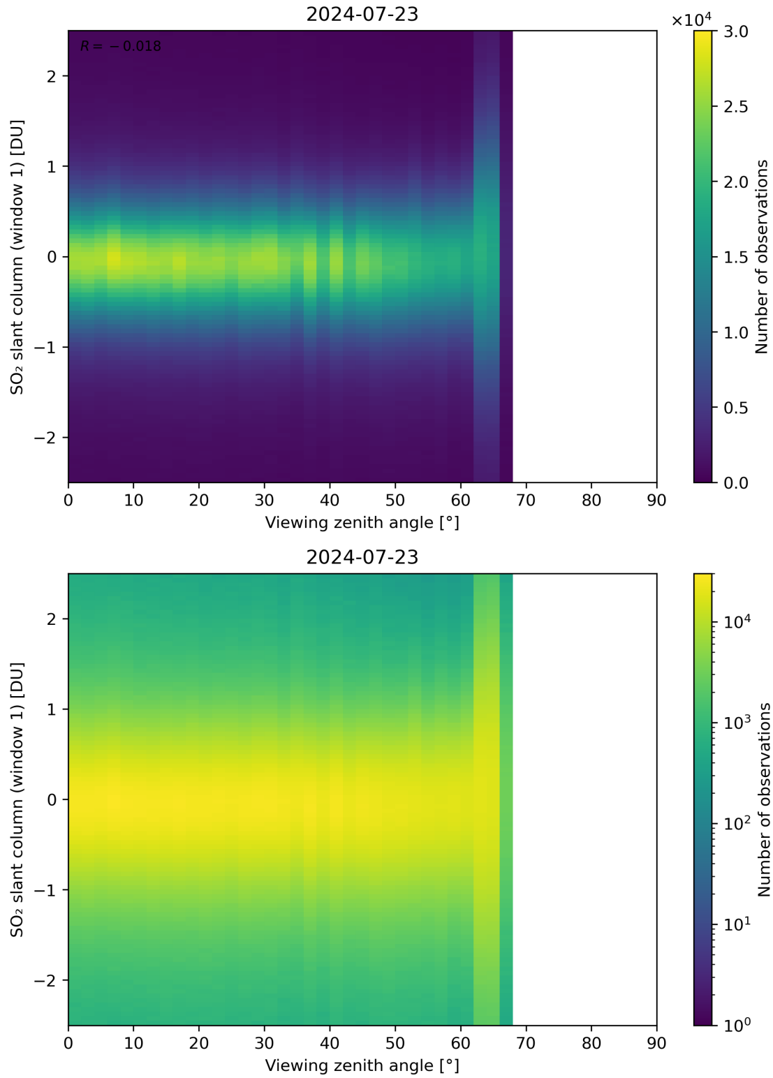
Figure 320: Scatter density plot of “Viewing zenith angle” against “SO 2 slant column (window 1)” for 2024-07-22 to 2024-07-24.
