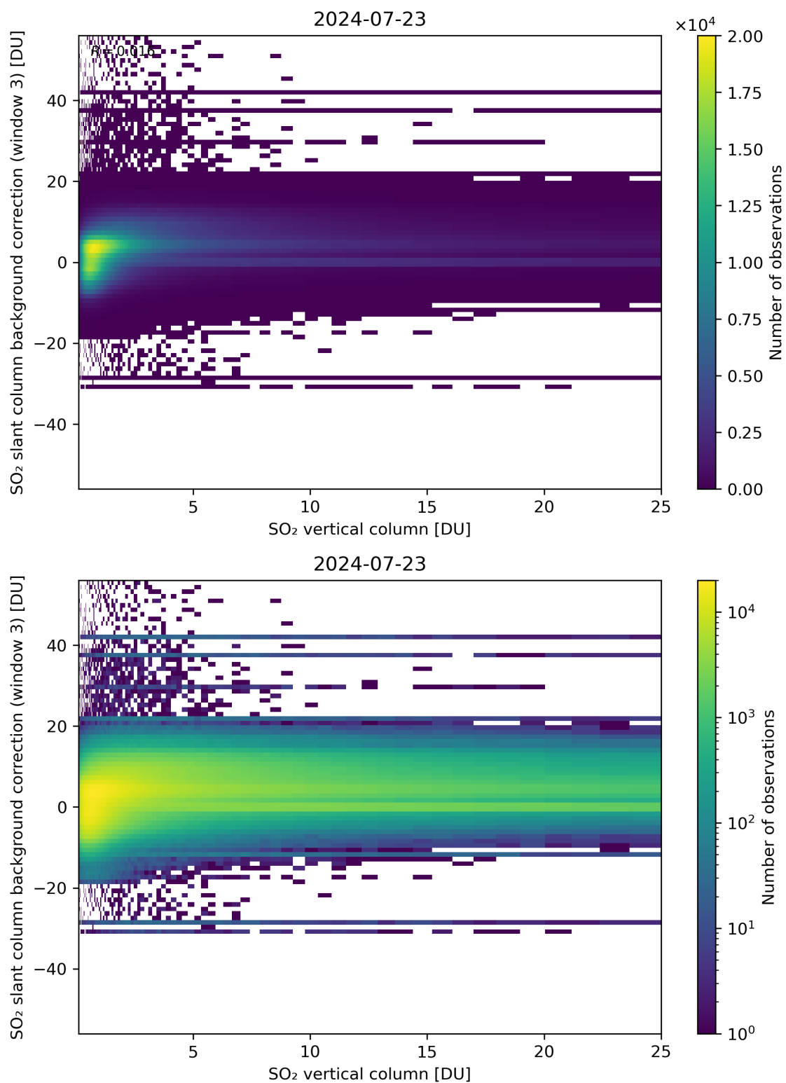
Figure 275: Scatter density plot of “SO 2 vertical column” against “SO 2 slant column background correction (window 3)” for 2024-07-22 to 2024-07-24.
