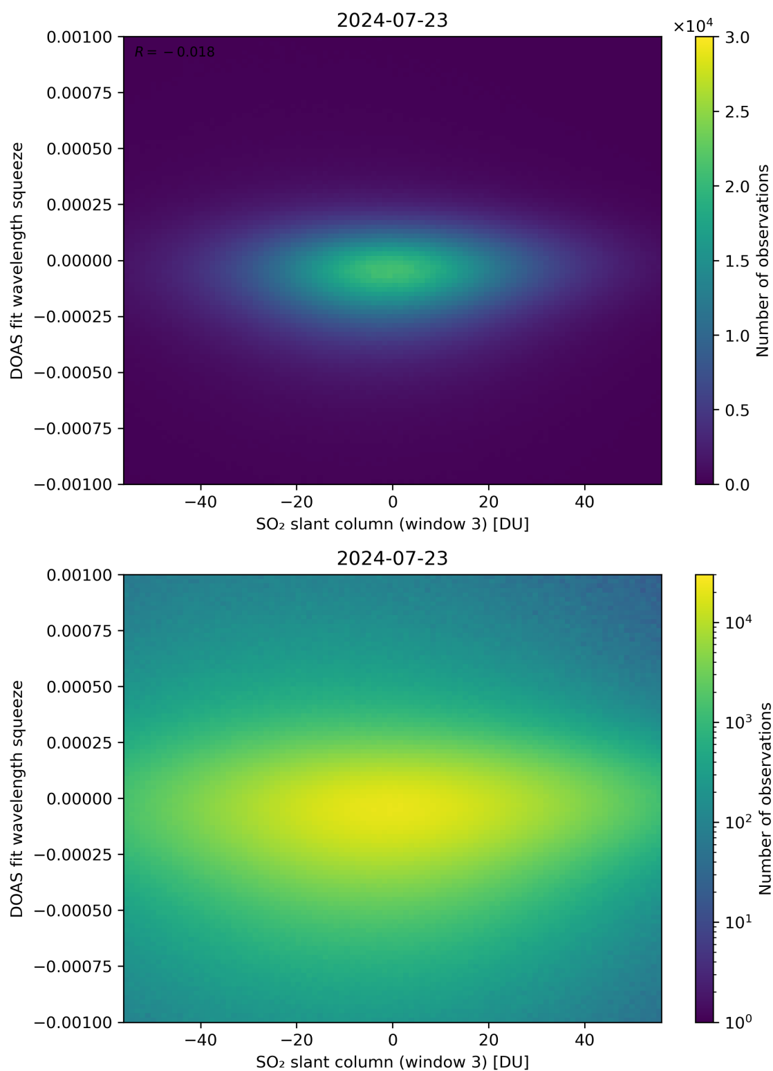
Figure 255: Scatter density plot of “SO 2 slant column (window 3)” against “DOAS fit wavelength squeeze” for 2024-07-22 to 2024-07-24.
