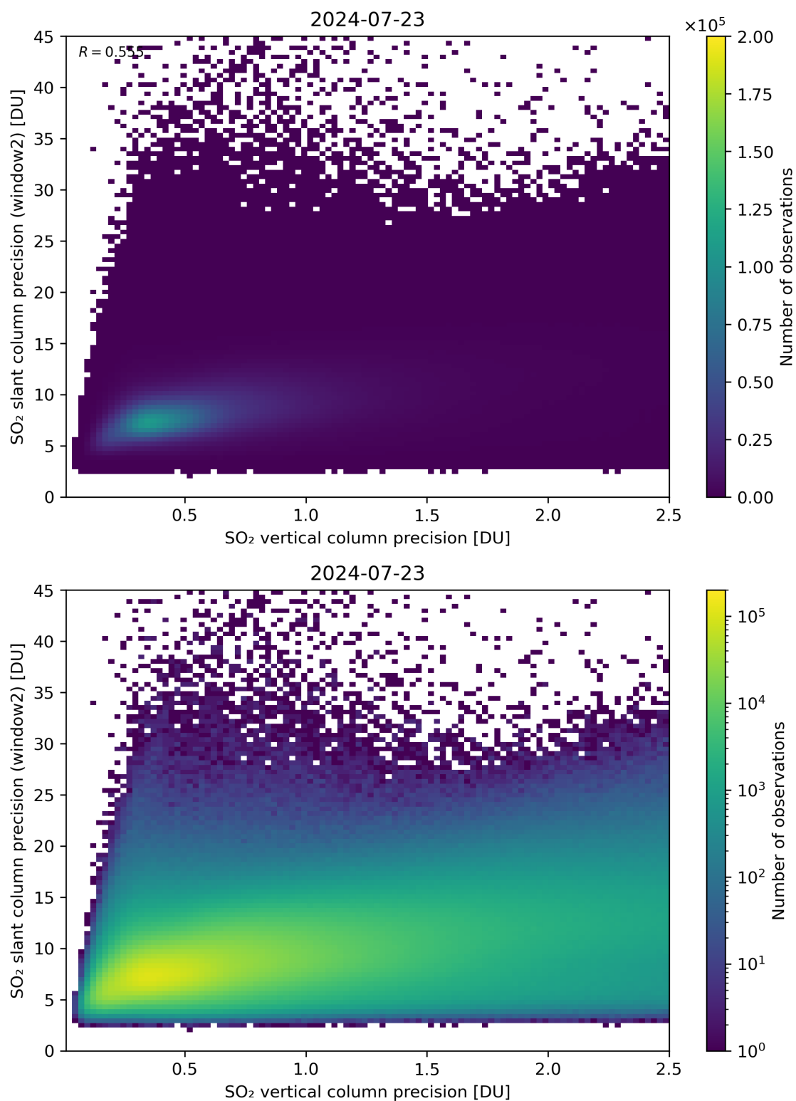
Figure 291: Scatter density plot of “SO 2 vertical column precision” against “SO 2 slant column precision (window2)” for 2024-07-22 to 2024-07-24.
