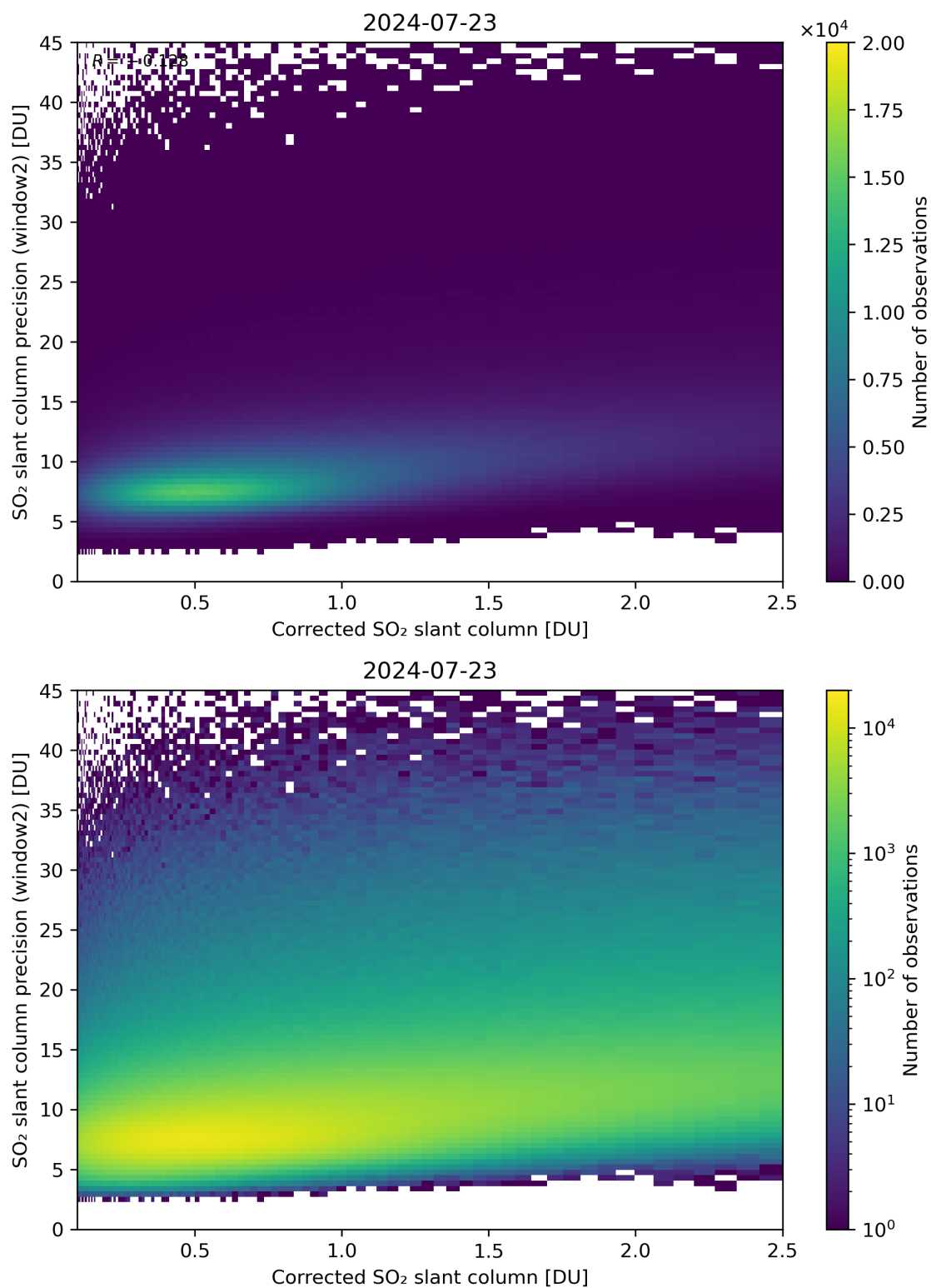
Figure 189: Scatter density plot of “Corrected SO 2 slant column” against “SO 2 slant column precision (window2)” for 2024-07-22 to 2024-07-24.
