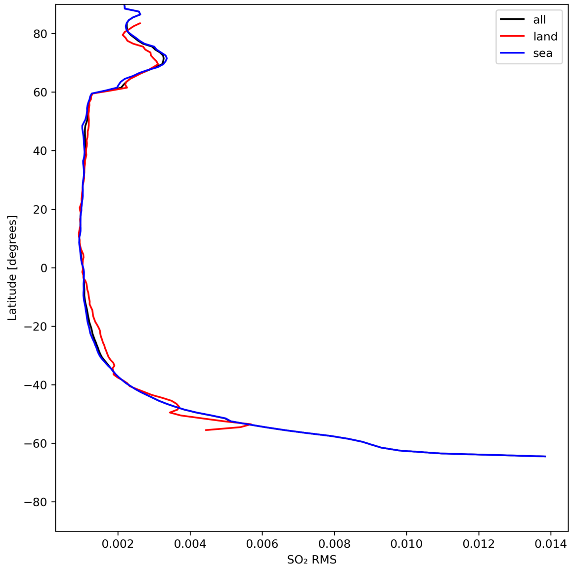
Figure 47: Zonal average of “SO 2 RMS” for 2024-07-22 to 2024-07-24.
