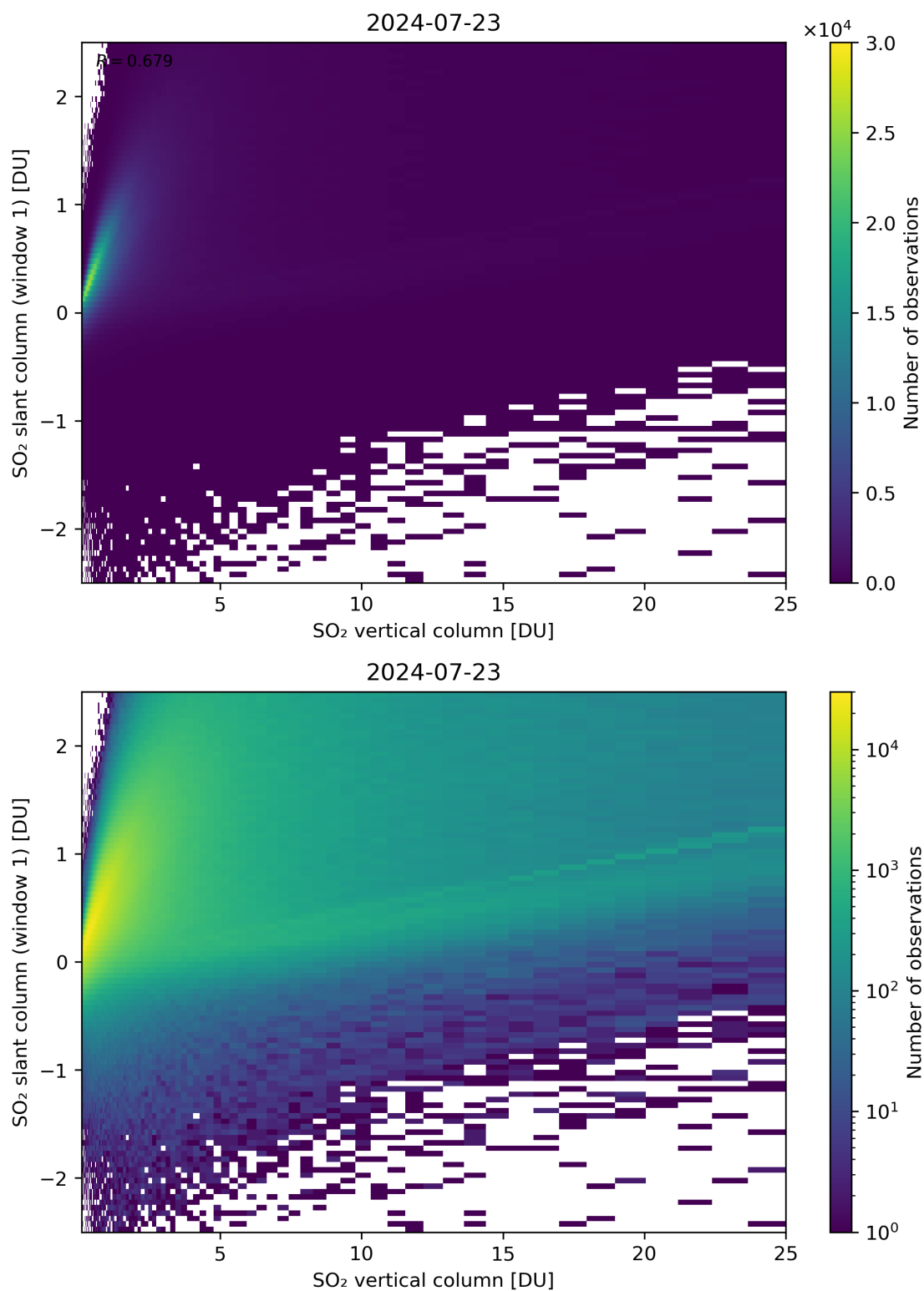
Figure 300: Scatter density plot of “SO 2 vertical column” against “SO 2 slant column (window 1)” for 2024-07-22 to 2024-07-24.
