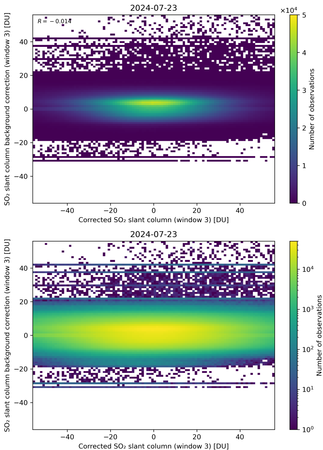
Figure 205: Scatter density plot of “Corrected SO 2 slant column (window 3)” against “SO 2 slant column background correction (window 3)” for 2024-07-22 to 2024-07-24.
