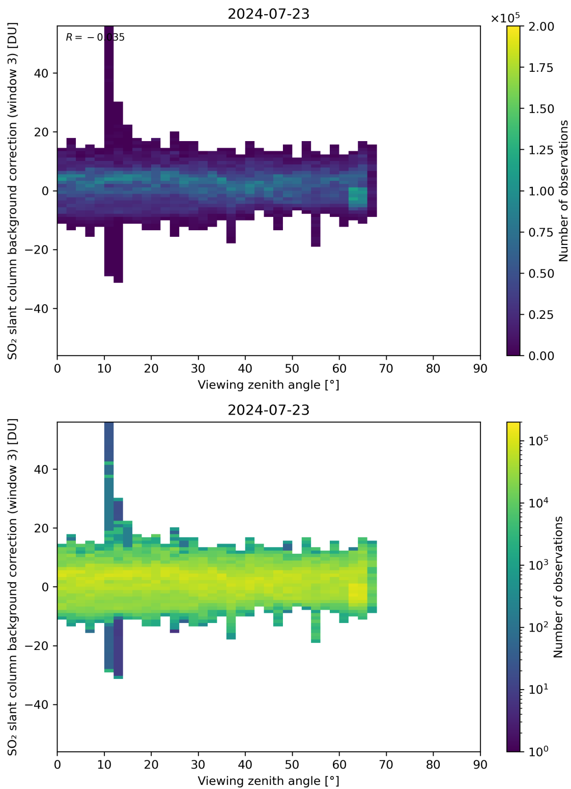
Figure 310: Scatter density plot of “Viewing zenith angle” against “SO 2 slant column background correction (window 3)” for 2024-07-22 to 2024-07-24.
