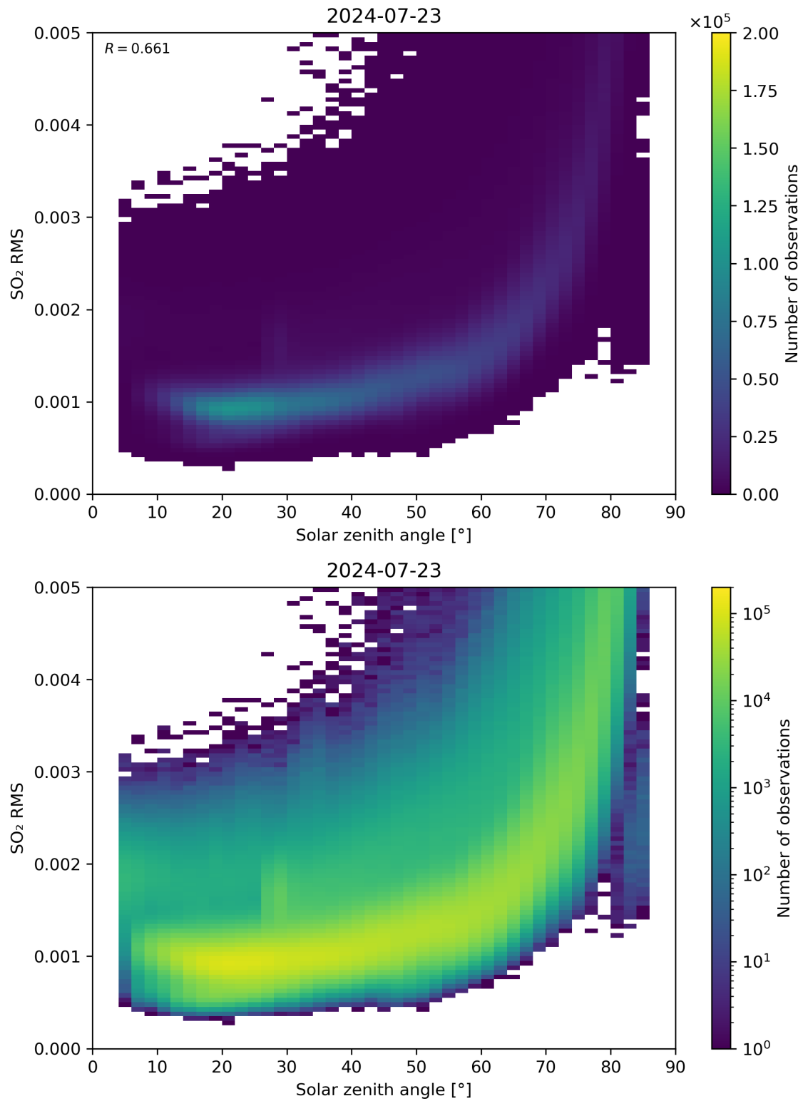
Figure 163: Scatter density plot of “Solar zenith angle” against “SO 2 RMS” for 2024-07-22 to 2024-07-24.
