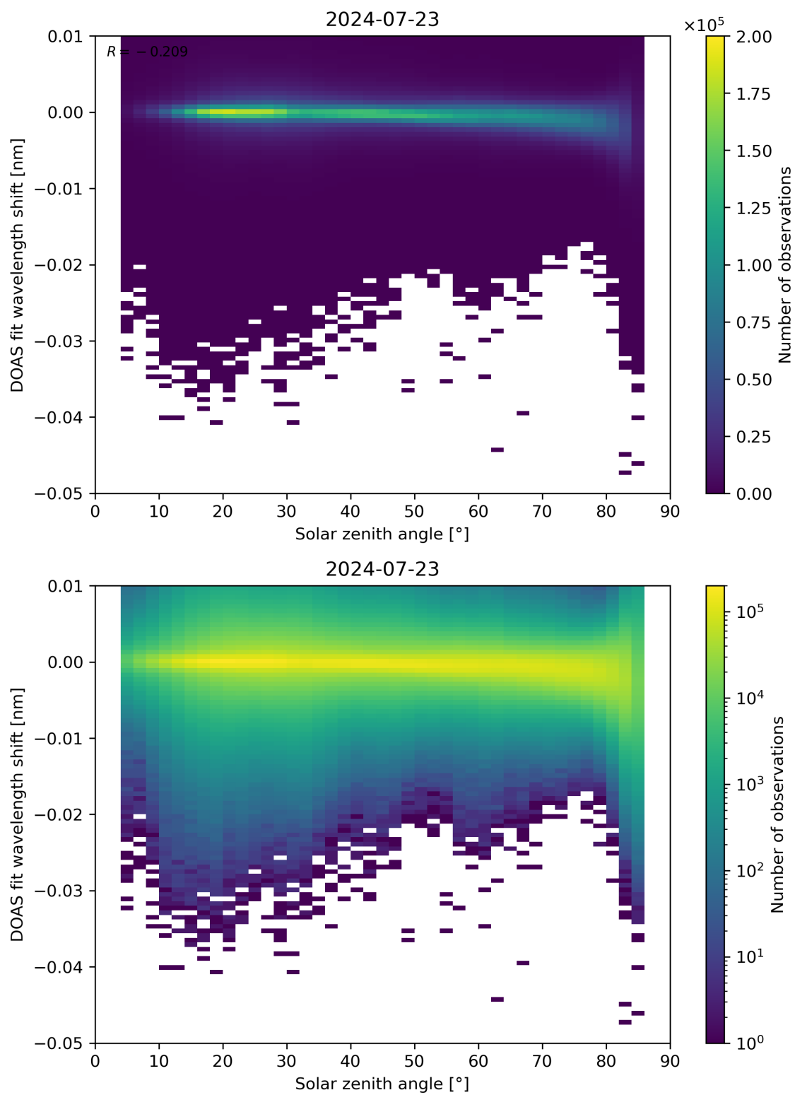
Figure 161: Scatter density plot of “Solar zenith angle” against “DOAS fit wavelength shift” for 2024-07-22 to 2024-07-24.
