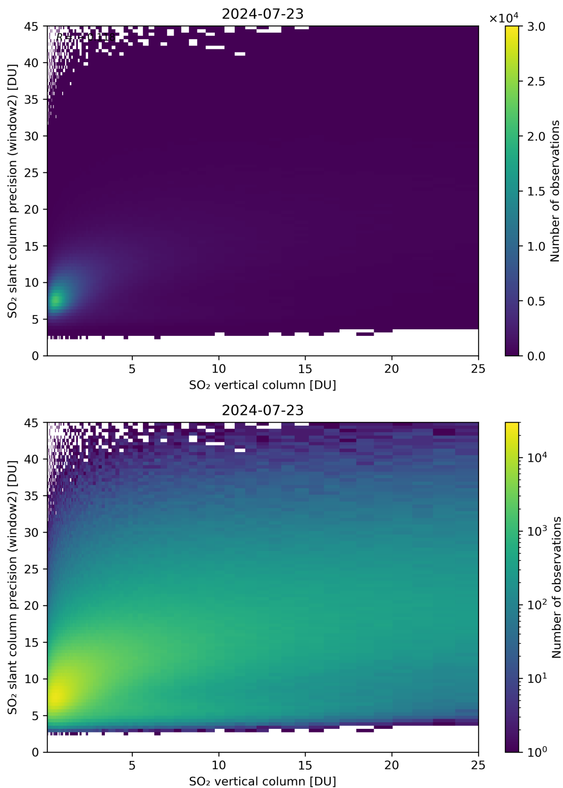
Figure 302: Scatter density plot of “SO 2 vertical column” against “SO 2 slant column precision (window2)” for 2024-07-22 to 2024-07-24.
