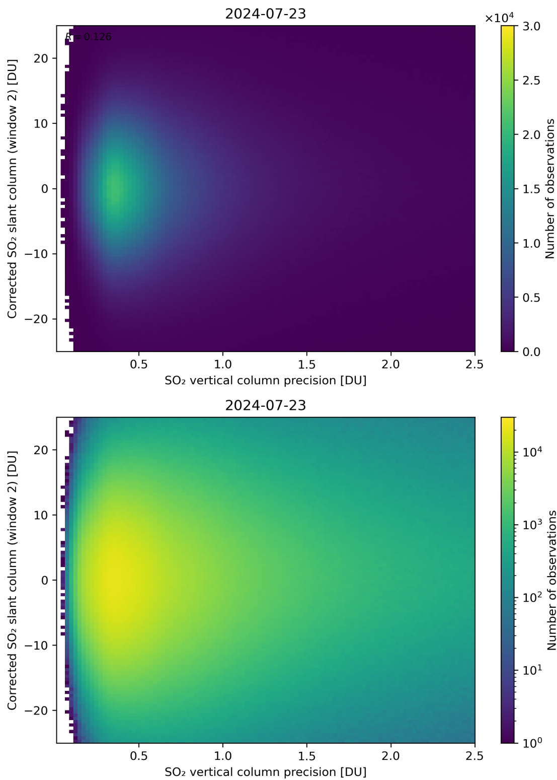
Figure 287: Scatter density plot of “SO 2 vertical column precision” against “Corrected SO 2 slant column (window 2)” for 2024-07-22 to 2024-07-24.
