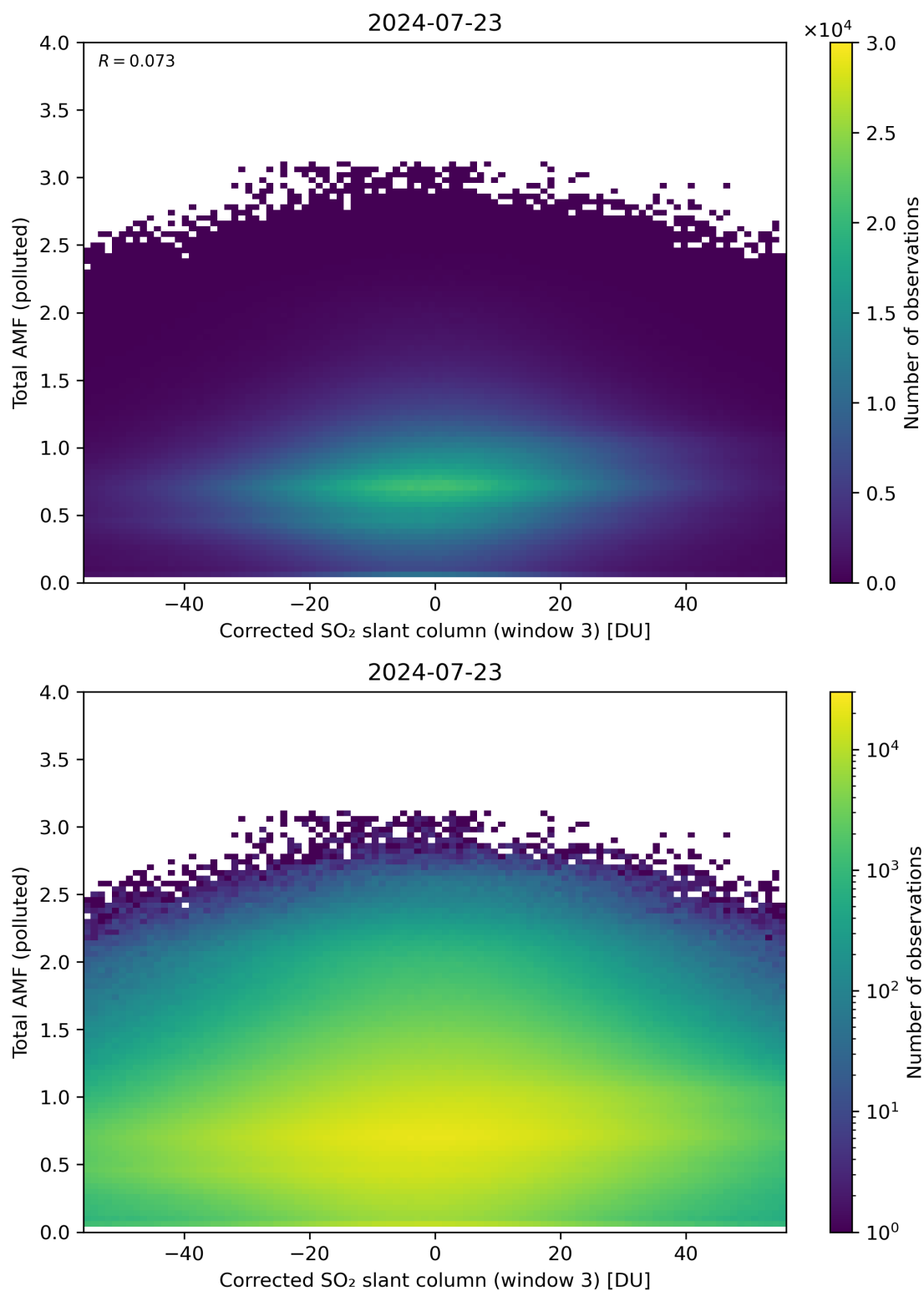
Figure 210: Scatter density plot of “Corrected SO 2 slant column (window 3)” against “Total AMF (polluted)” for 2024-07-22 to 2024-07-24.
