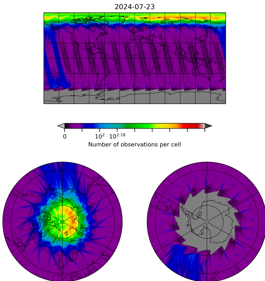
Figure 28: Map of the number of observations for 2024-07-22 to 2024-07-24
