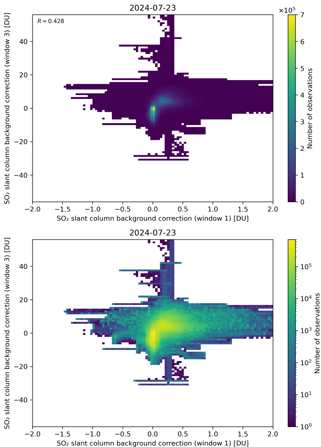
Figure 99: Scatter density plot of “SO 2 slant column background correction (window 1)” against “SO 2 slant column background correction (window 3)” for 2024-07-22 to 2024-07-24.
