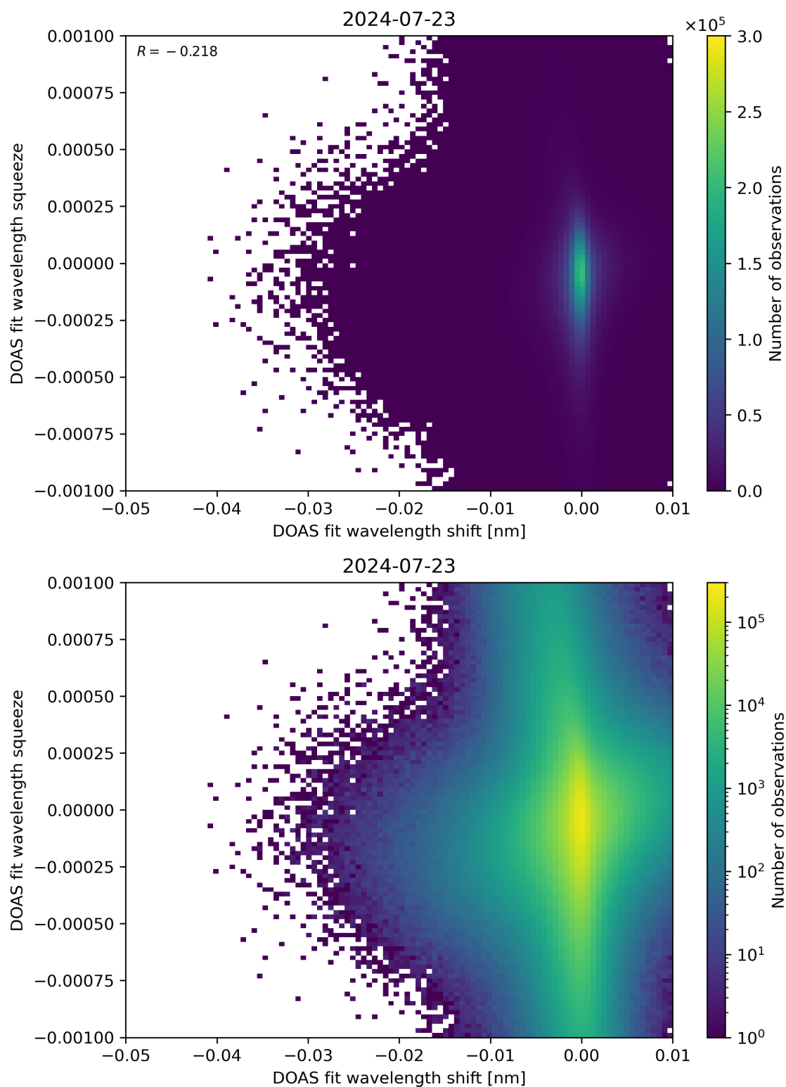
Figure 127: Scatter density plot of “DOAS fit wavelength shift” against “DOAS fit wavelength squeeze” for 2024-07-22 to 2024-07-24.
