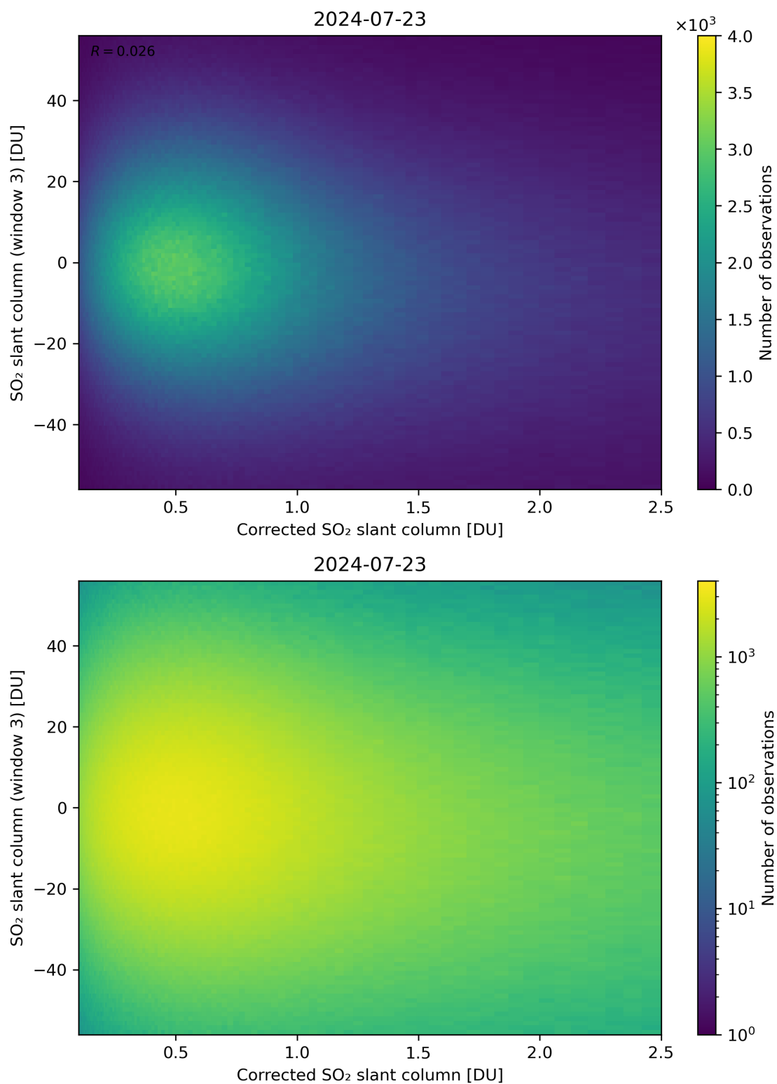
Figure 190: Scatter density plot of “Corrected SO 2 slant column” against “SO 2 slant column (window 3)” for 2024-07-22 to 2024-07-24.
