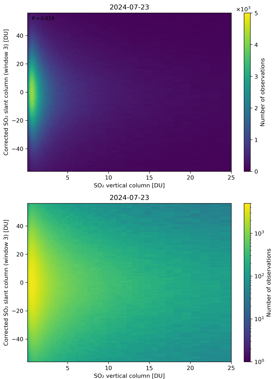
Figure 299: Scatter density plot of “SO 2 vertical column” against “Corrected SO 2 slant column (window 3)” for 2024-07-22 to 2024-07-24.
