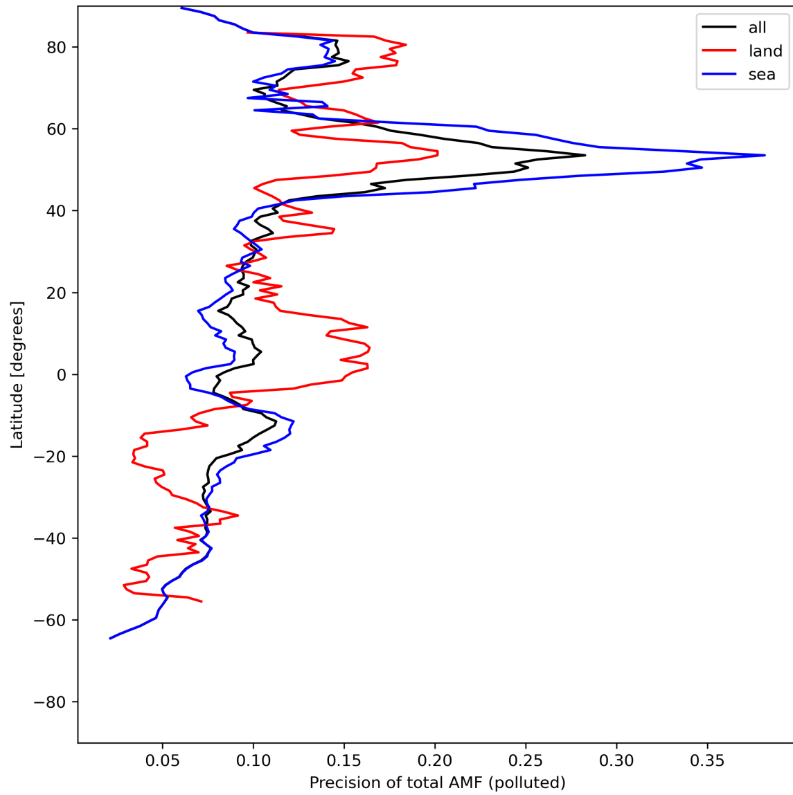
Figure 49: Zonal average of “Precision of total AMF (polluted)” for 2024-07-22 to 2024-07-24.
