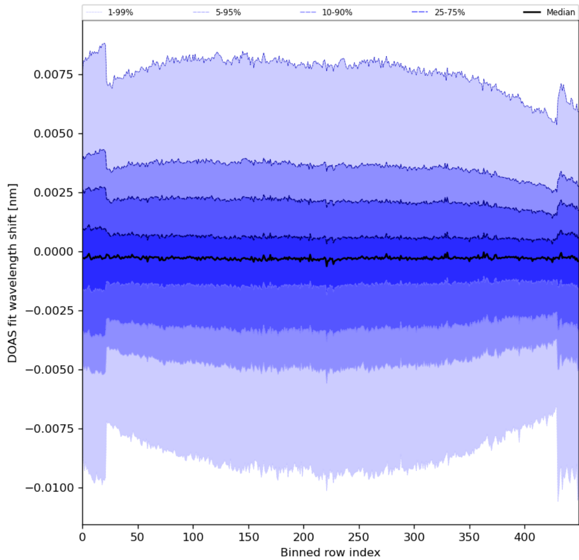
Figure 91: Along track statistics of “DOAS fit wavelength shift” for 2024-07-22 to 2024-07-24
