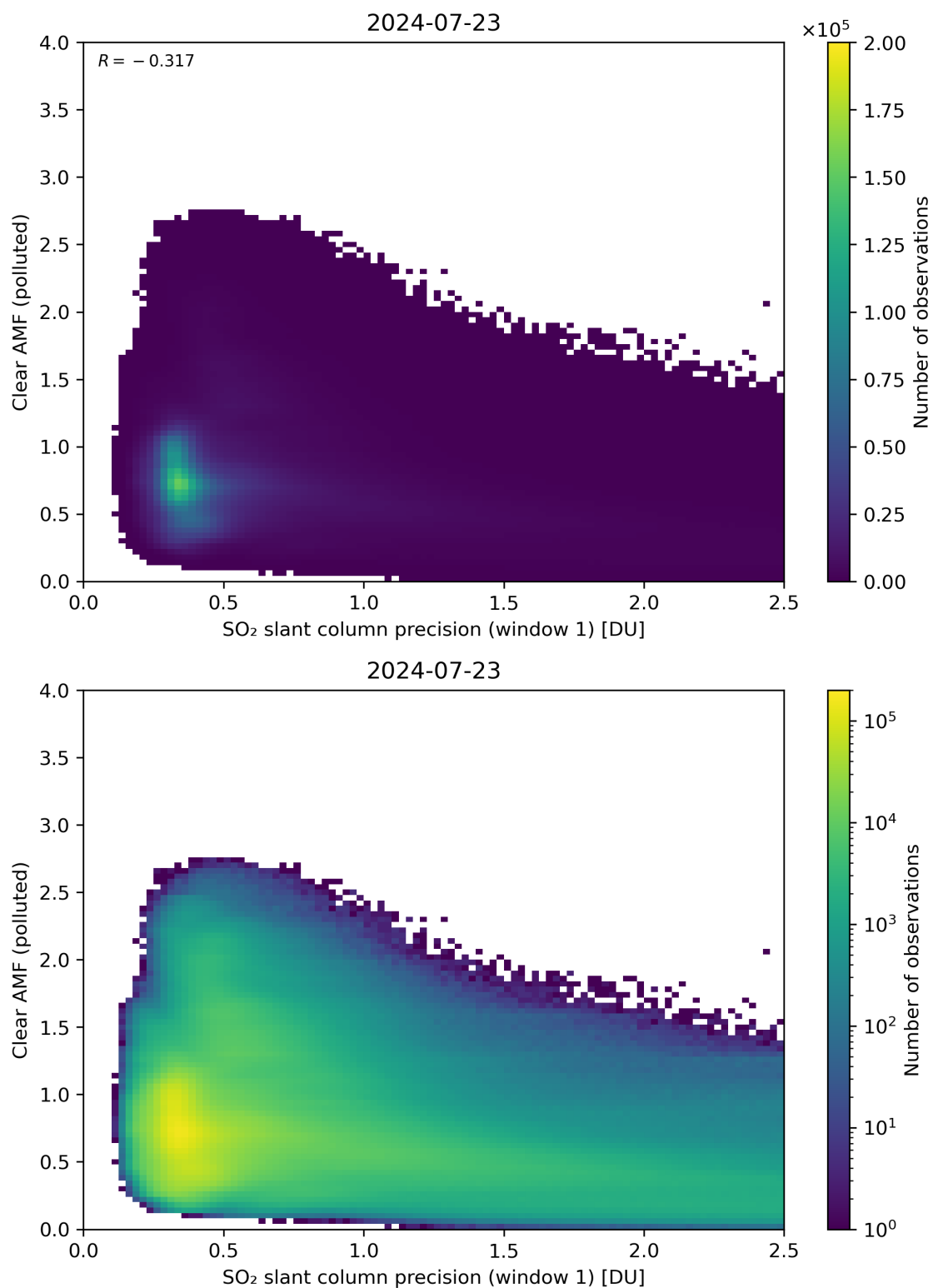
Figure 224: Scatter density plot of “SO 2 slant column precision (window 1)” against “Clear AMF (polluted)” for 2024-07-22 to 2024-07-24.
