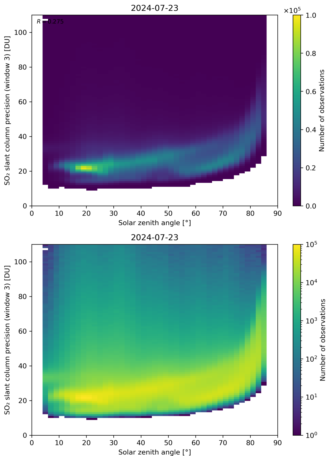
Figure 173: Scatter density plot of “Solar zenith angle” against “SO 2 slant column precision (window 3)” for 2024-07-22 to 2024-07-24.
