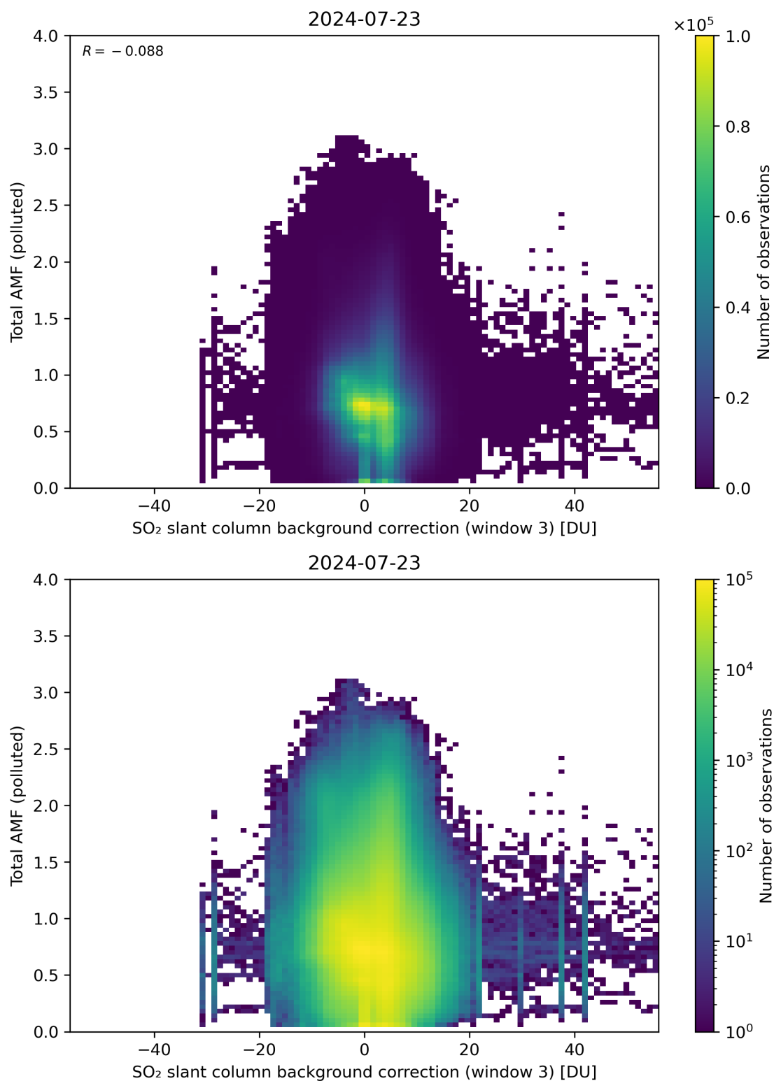
Figure 125: Scatter density plot of “SO 2 slant column background correction (window 3)” against “Total AMF (polluted)” for 2024-07-22 to 2024-07-24.
