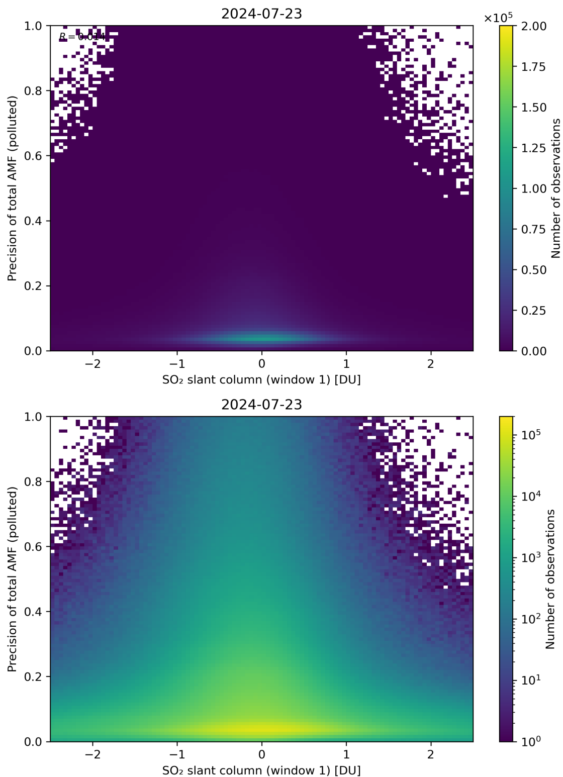
Figure 240: Scatter density plot of “SO 2 slant column (window 1)” against “Precision of total AMF (polluted)” for 2024-07-22 to 2024-07-24.
