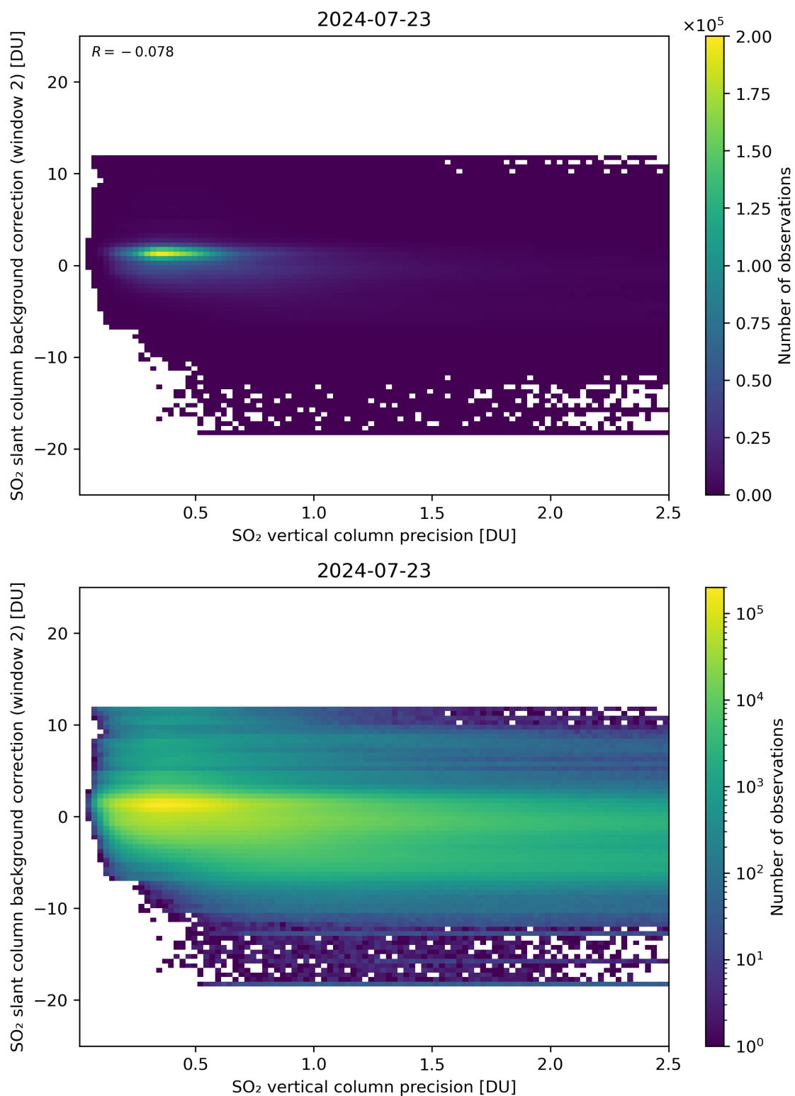
Figure 280: Scatter density plot of “SO 2 vertical column precision” against “SO 2 slant column background correction (window 2)” for 2024-07-22 to 2024-07-24.
