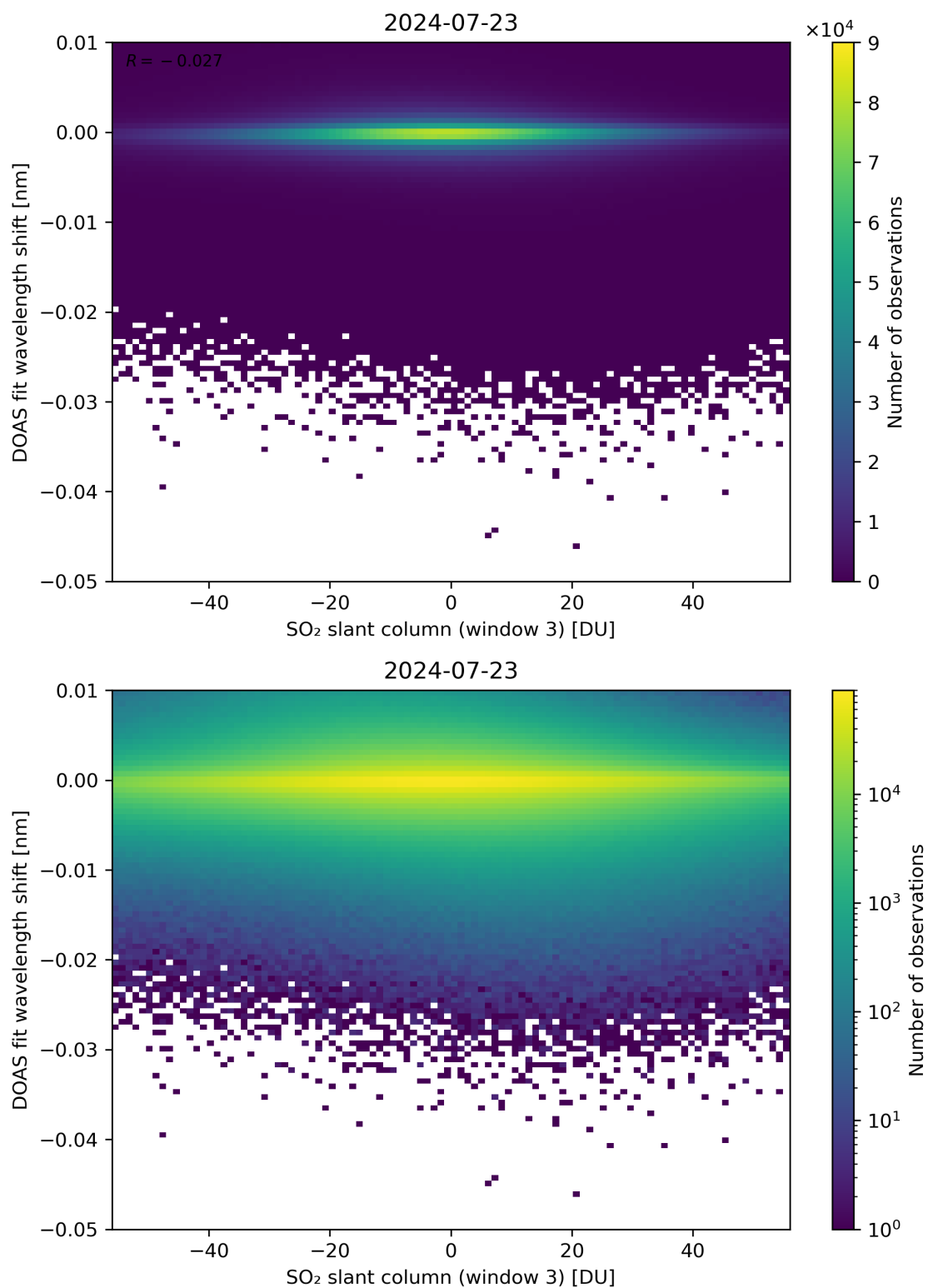
Figure 254: Scatter density plot of “SO 2 slant column (window 3)” against “DOAS fit wavelength shift” for 2024-07-22 to 2024-07-24.
