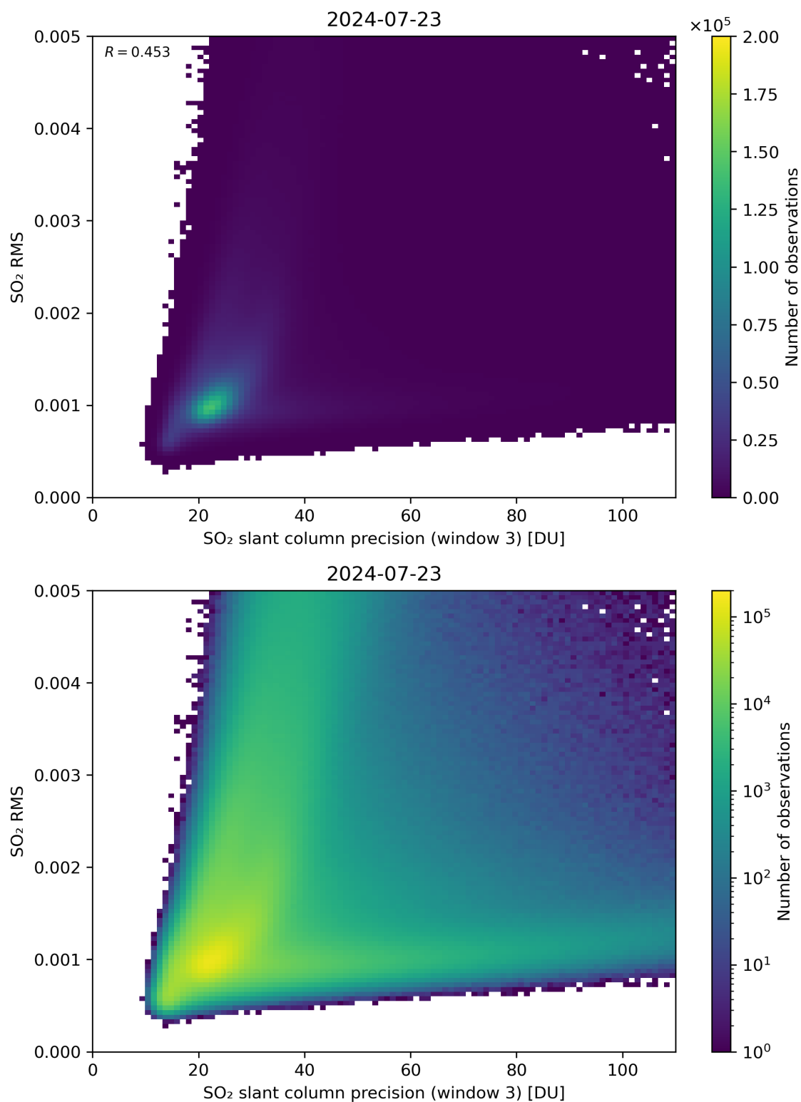
Figure 260: Scatter density plot of “SO 2 slant column precision (window 3)” against “SO 2 RMS” for 2024-07-22 to 2024-07-24.
