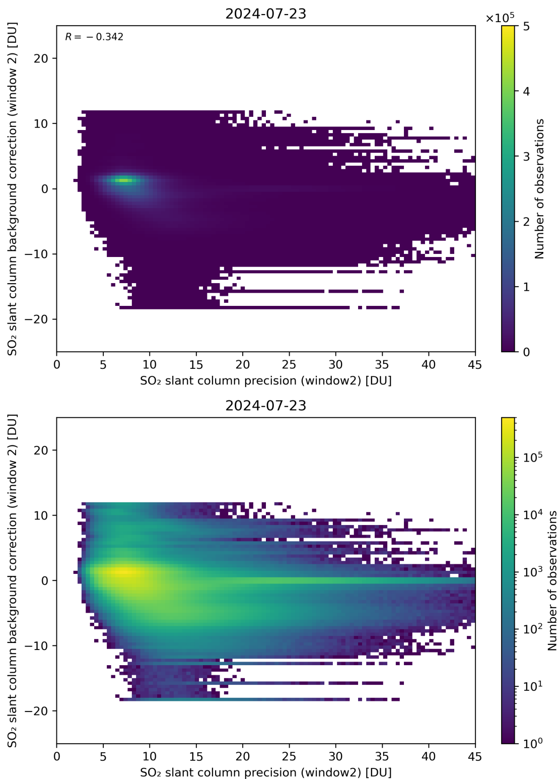
Figure 241: Scatter density plot of “SO 2 slant column precision (window2)” against “SO 2 slant column background correction (window 2)” for 2024-07-22 to 2024-07-24.
