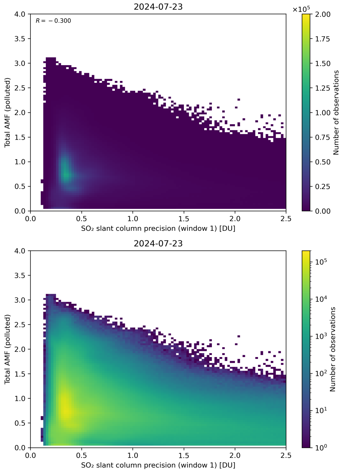
Figure 230: Scatter density plot of “SO 2 slant column precision (window 1)” against “Total AMF (polluted)” for 2024-07-22 to 2024-07-24.
