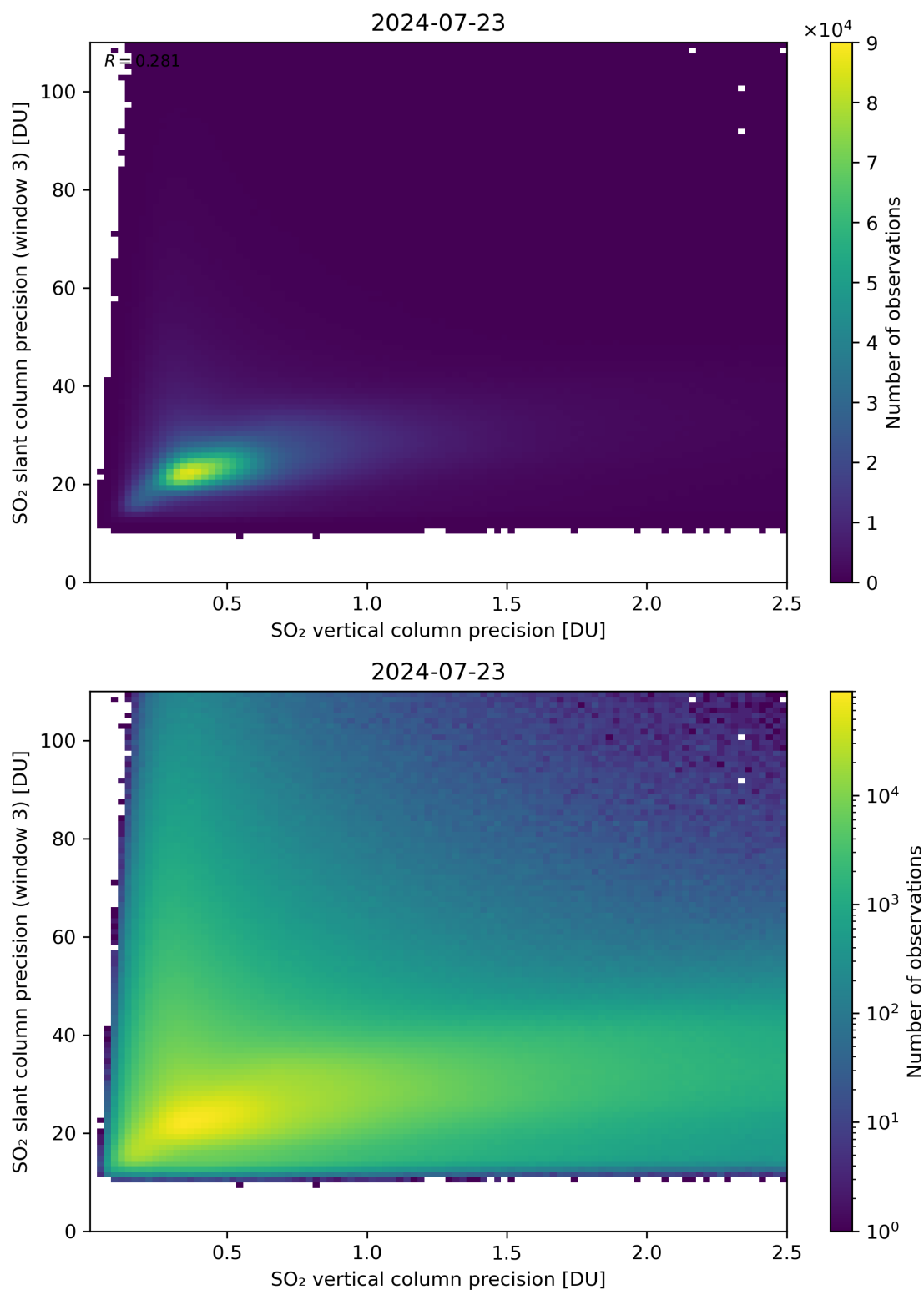
Figure 293: Scatter density plot of “SO 2 vertical column precision” against “SO 2 slant column precision (window 3)” for 2024-07-22 to 2024-07-24.
