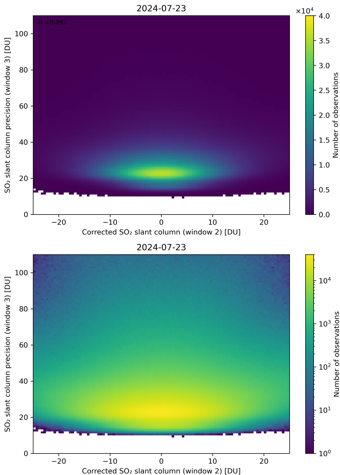
Figure 202: Scatter density plot of “Corrected SO 2 slant column (window 2)” against “SO 2 slant column precision (window 3)” for 2024-07-22 to 2024-07-24.
