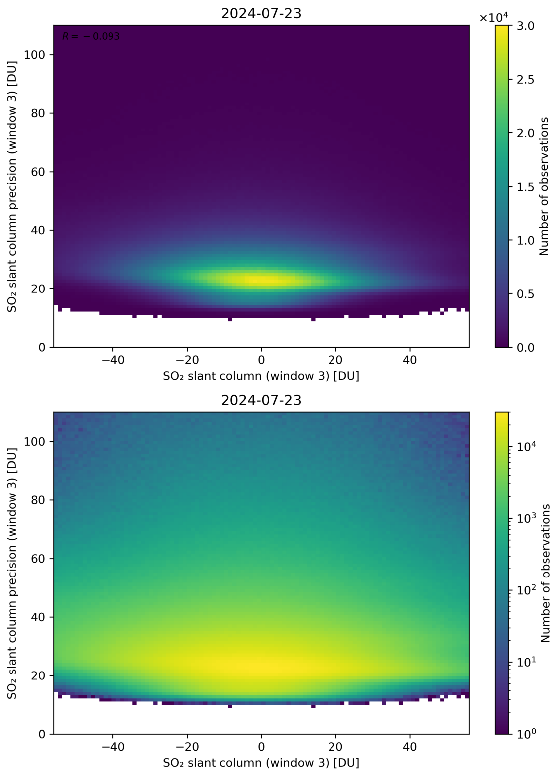
Figure 267: Scatter density plot of “SO 2 slant column (window 3)” against “SO 2 slant column precision (window 3)” for 2024-07-22 to 2024-07-24.
