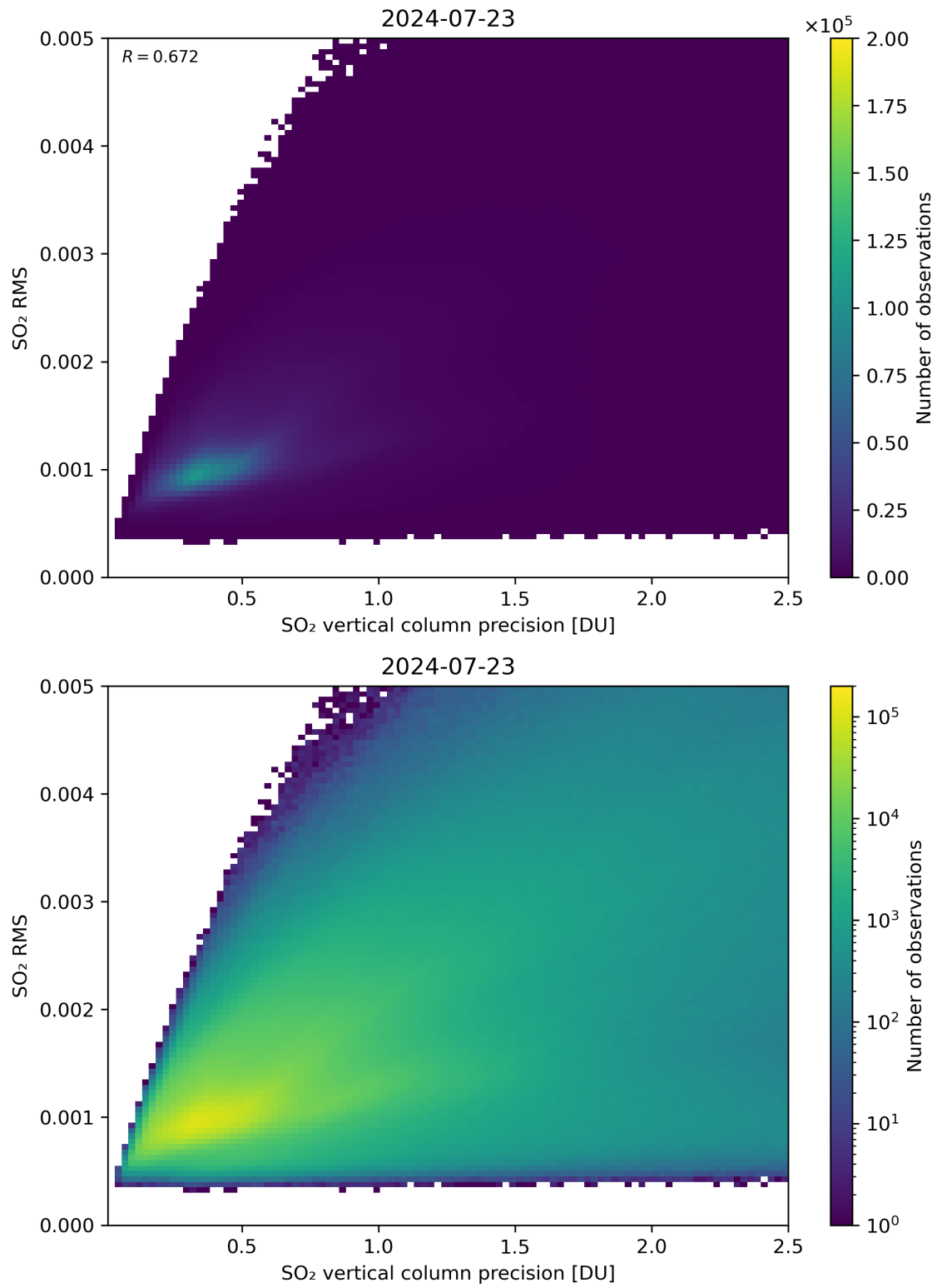
Figure 284: Scatter density plot of “SO 2 vertical column precision” against “SO 2 RMS” for 2024-07-22 to 2024-07-24.
