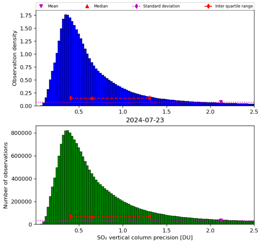
Figure 54: Histogram of “SO 2 vertical column precision” for 2024-07-22 to 2024-07-24
