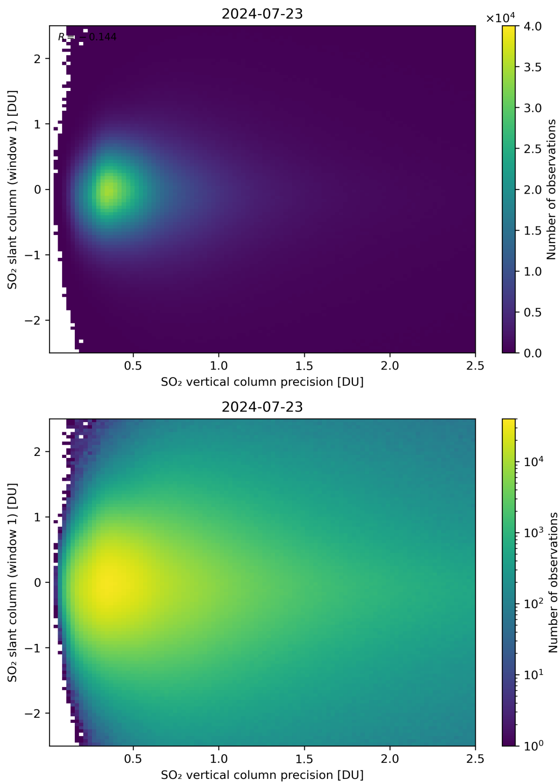
Figure 289: Scatter density plot of “SO 2 vertical column precision” against “SO 2 slant column (window 1)” for 2024-07-22 to 2024-07-24.
