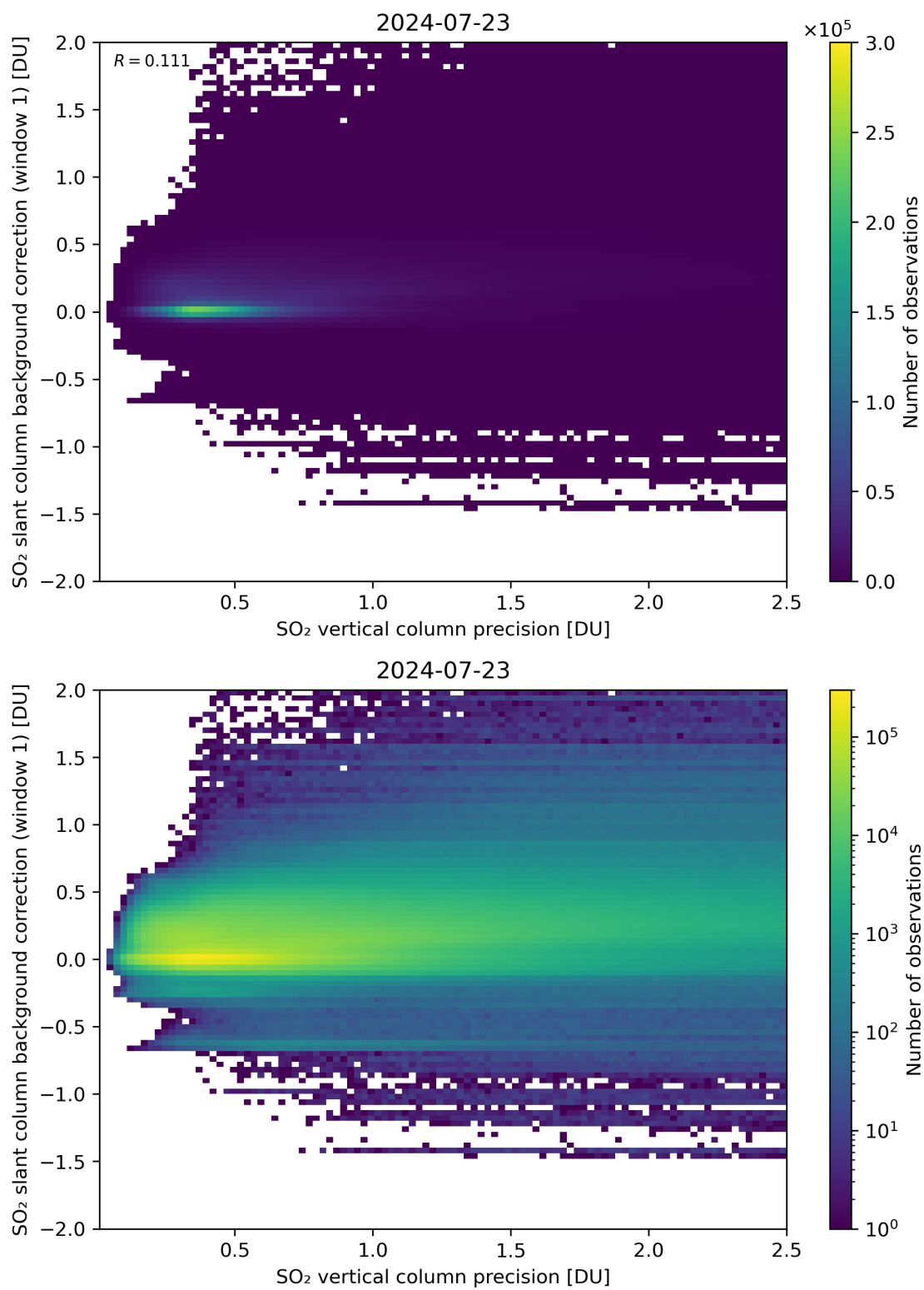
Figure 279: Scatter density plot of “SO 2 vertical column precision” against “SO 2 slant column background correction (window 1)” for 2024-07-22 to 2024-07-24.
