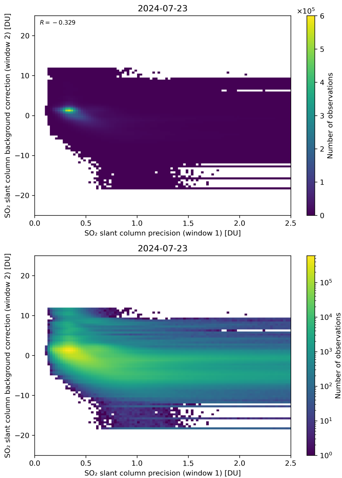
Figure 219: Scatter density plot of “SO 2 slant column precision (window 1)” against “SO 2 slant column background correction (window 2)” for 2024-07-22 to 2024-07-24.
