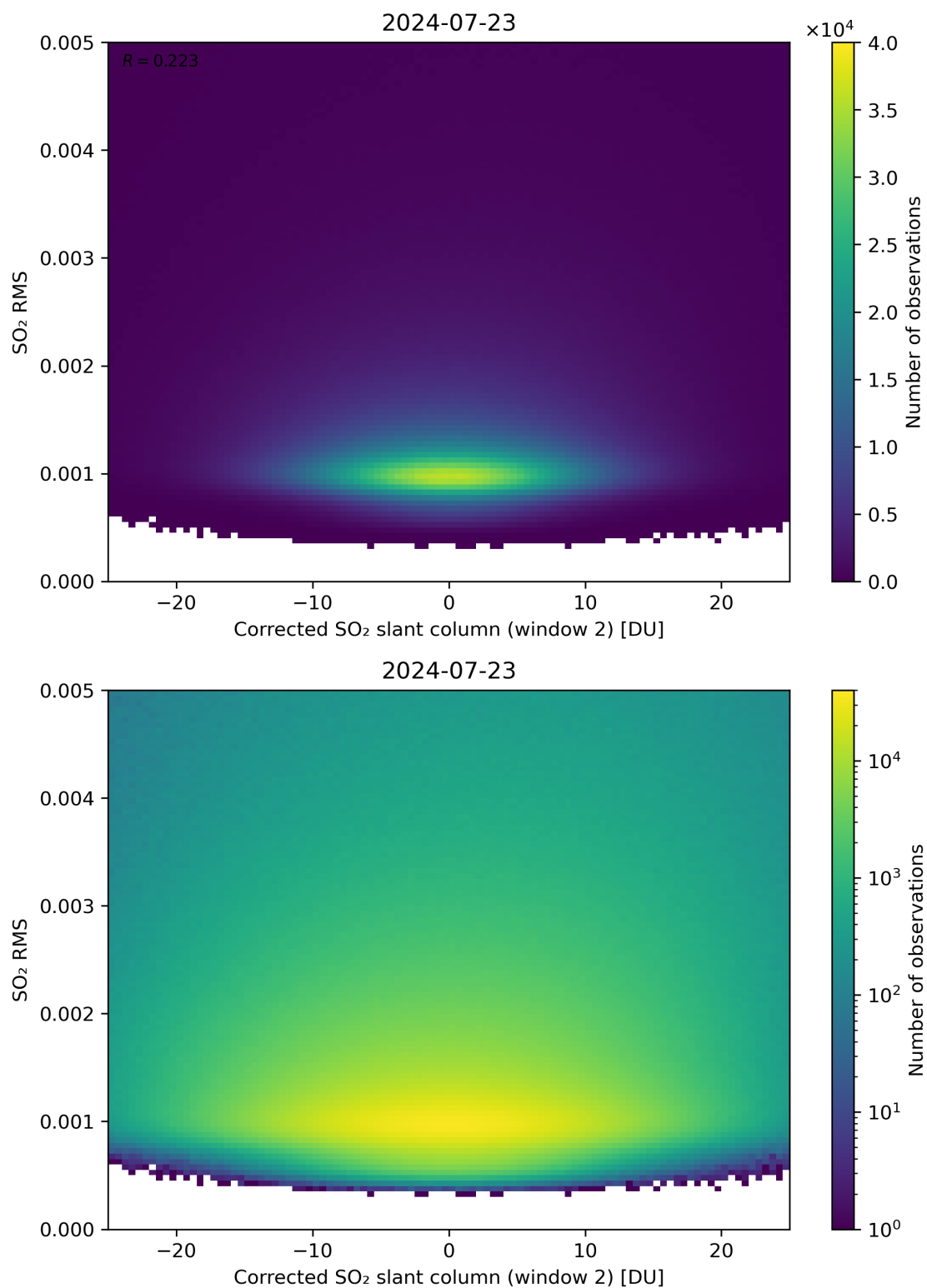
Figure 198: Scatter density plot of “Corrected SO 2 slant column (window 2)” against “SO 2 RMS” for 2024-07-22 to 2024-07-24.
