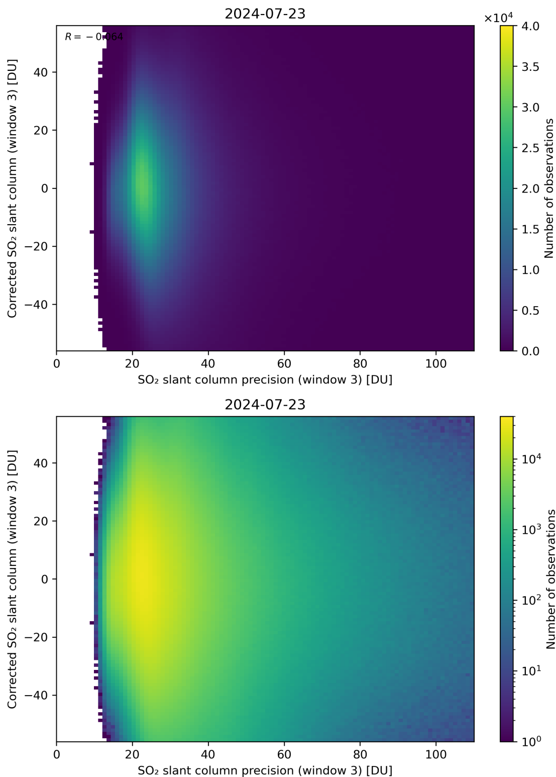
Figure 262: Scatter density plot of “SO 2 slant column precision (window 3)” against “Corrected SO 2 slant column (window 3)” for 2024-07-22 to 2024-07-24.
