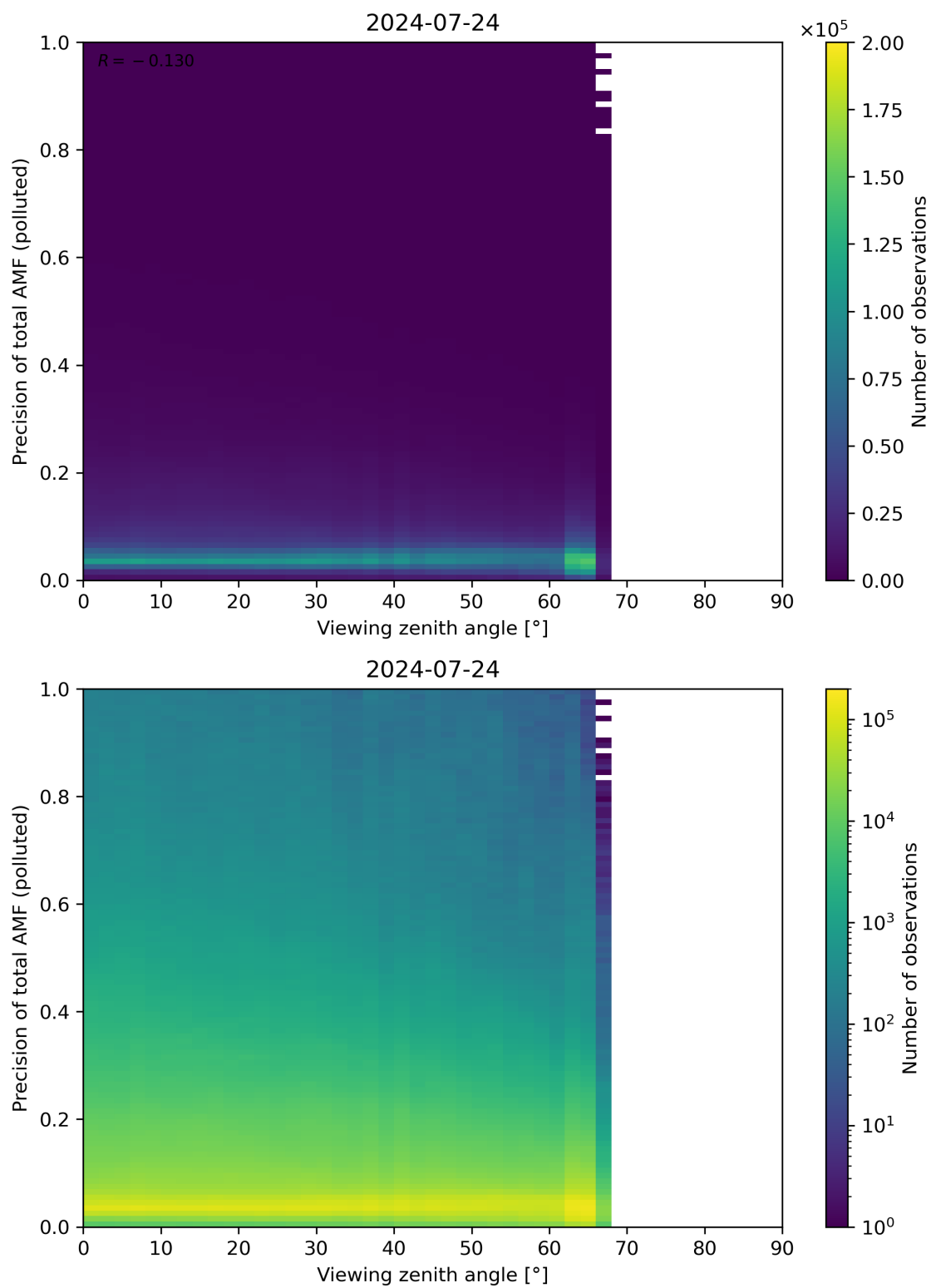
Figure 326: Scatter density plot of “Viewing zenith angle” against “Precision of total AMF (polluted)” for 2024-07-23 to 2024-07-25.
