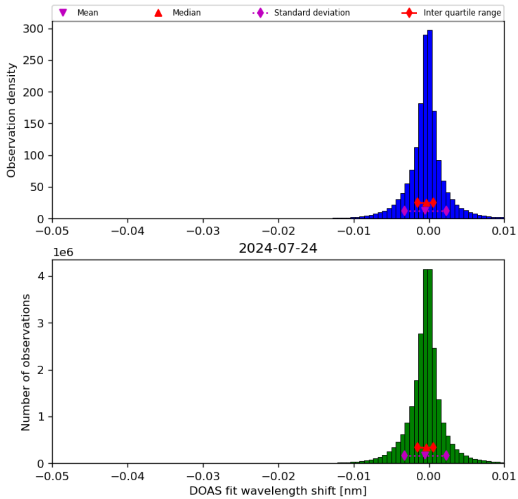
Figure 68: Histogram of “DOAS fit wavelength shift” for 2024-07-23 to 2024-07-25
