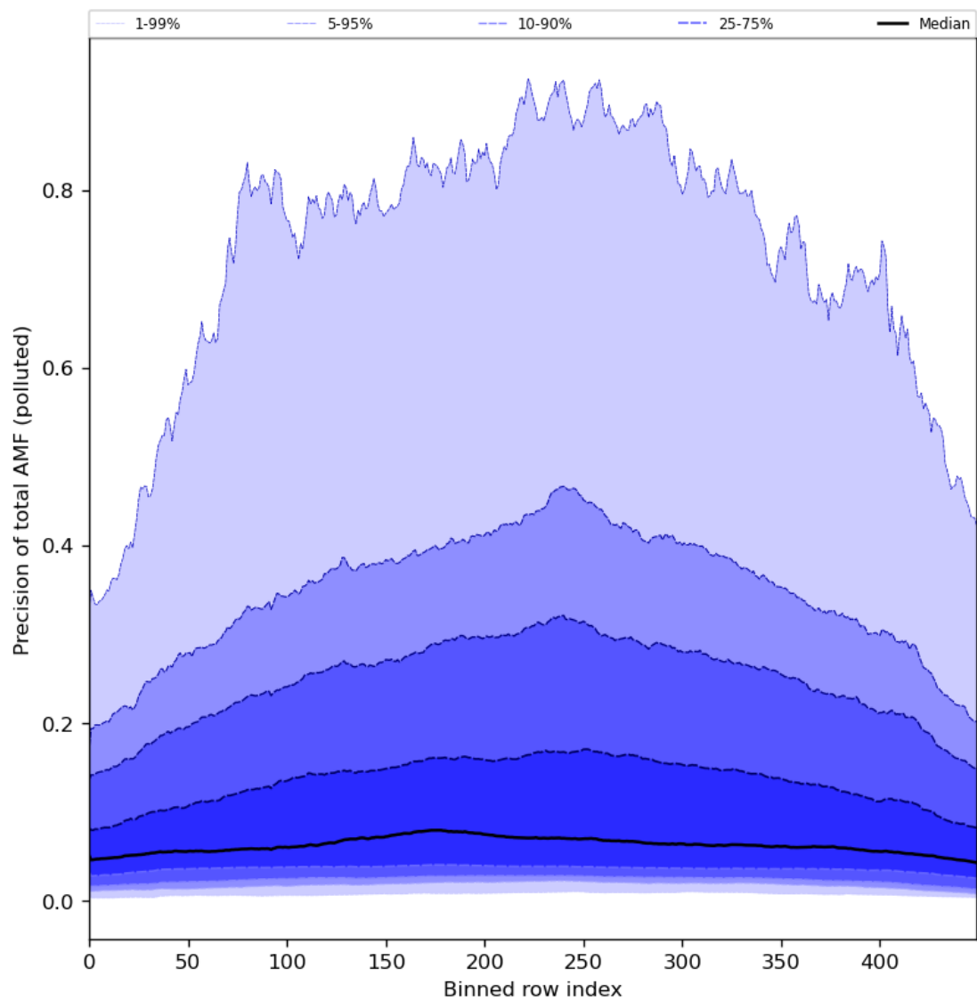
Figure 95: Along track statistics of “Precision of total AMF (polluted)” for 2024-07-23 to 2024-07-25
