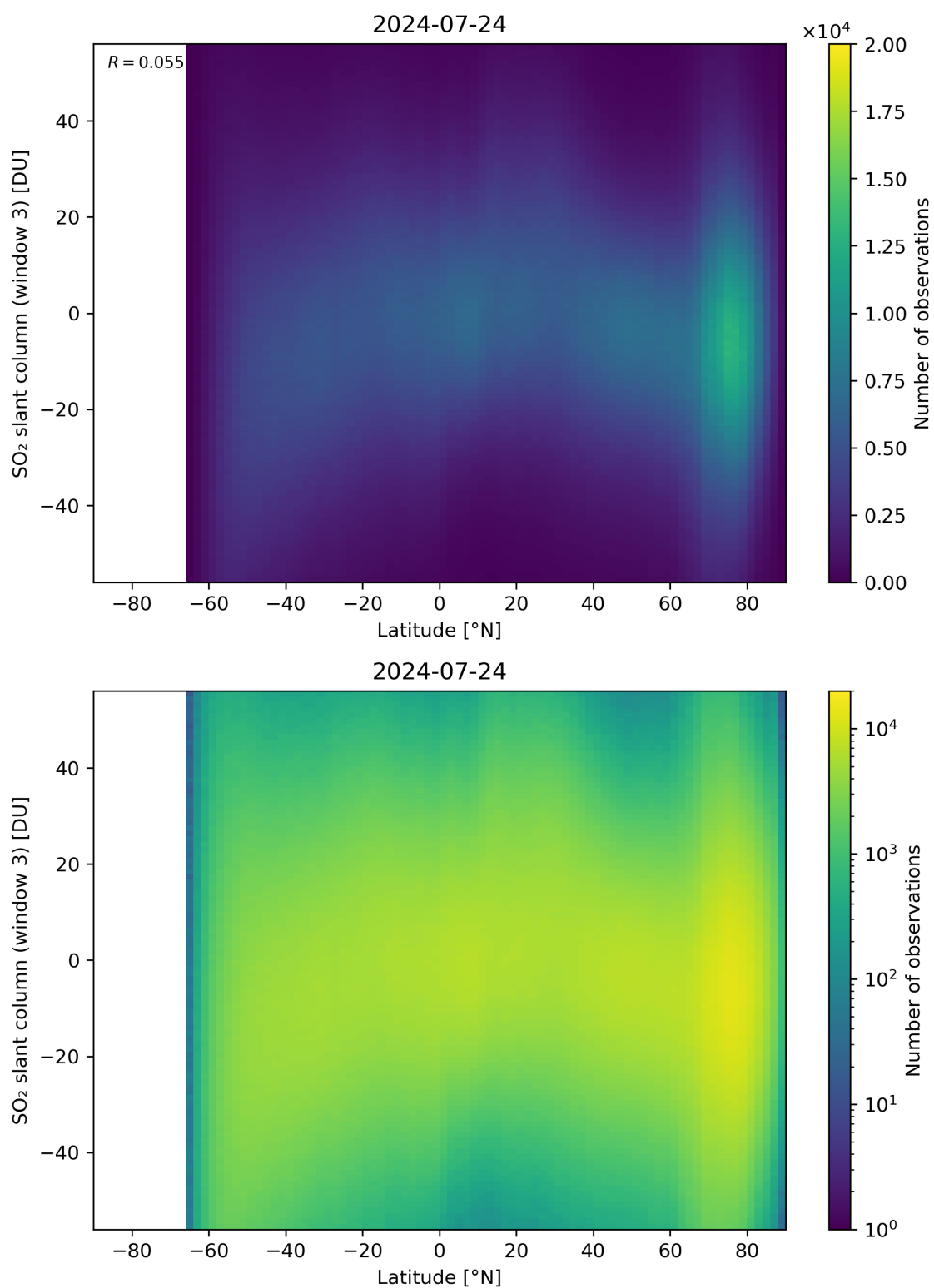
Figure 152: Scatter density plot of “Latitude” against “SO 2 slant column (window 3)” for 2024-07-23 to 2024-07-25.
