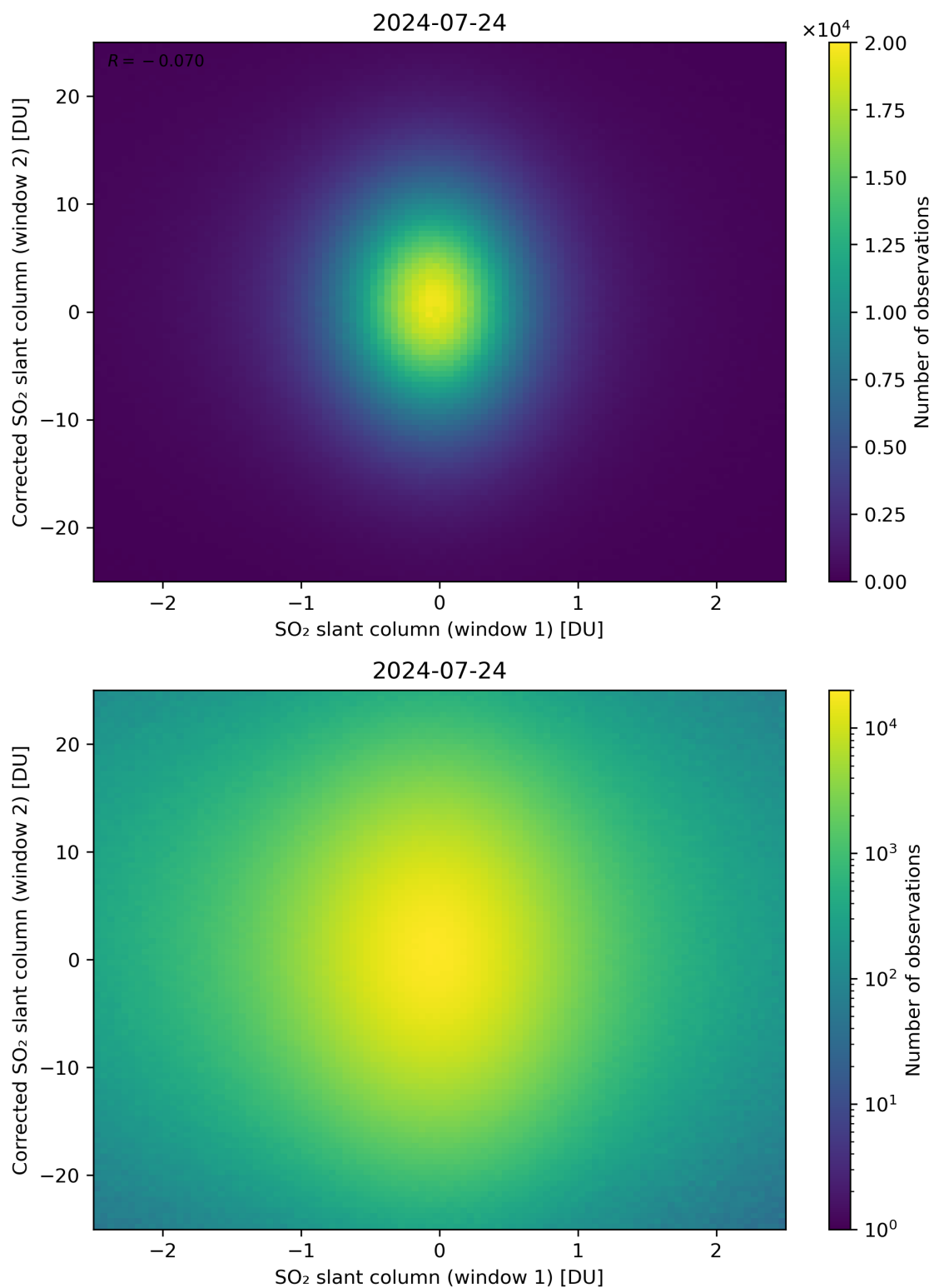
Figure 233: Scatter density plot of “SO 2 slant column (window 1)” against “Corrected SO 2 slant column (window 2)” for 2024-07-23 to 2024-07-25.
