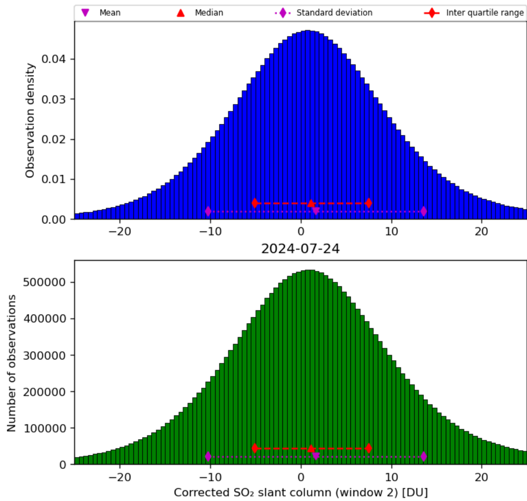
Figure 62: Histogram of “Corrected SO 2 slant column (window 2)” for 2024-07-23 to 2024-07-25
