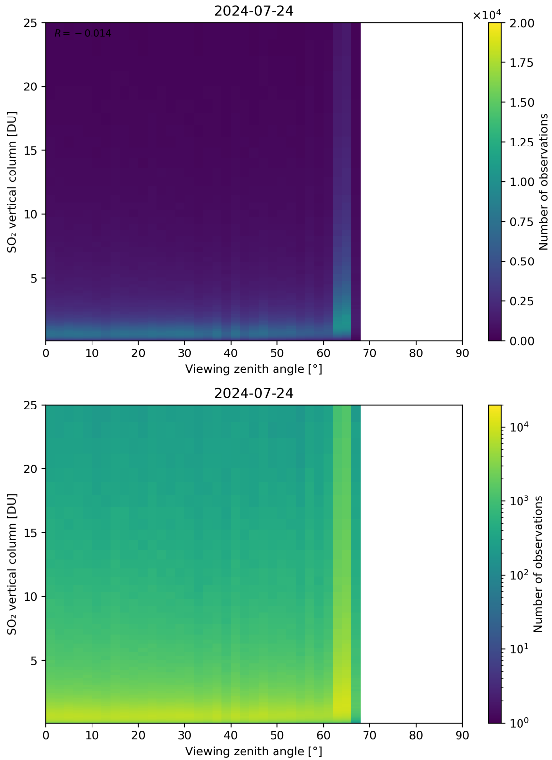
Figure 327: Scatter density plot of “Viewing zenith angle” against “SO 2 vertical column” for 2024-07-23 to 2024-07-25.
