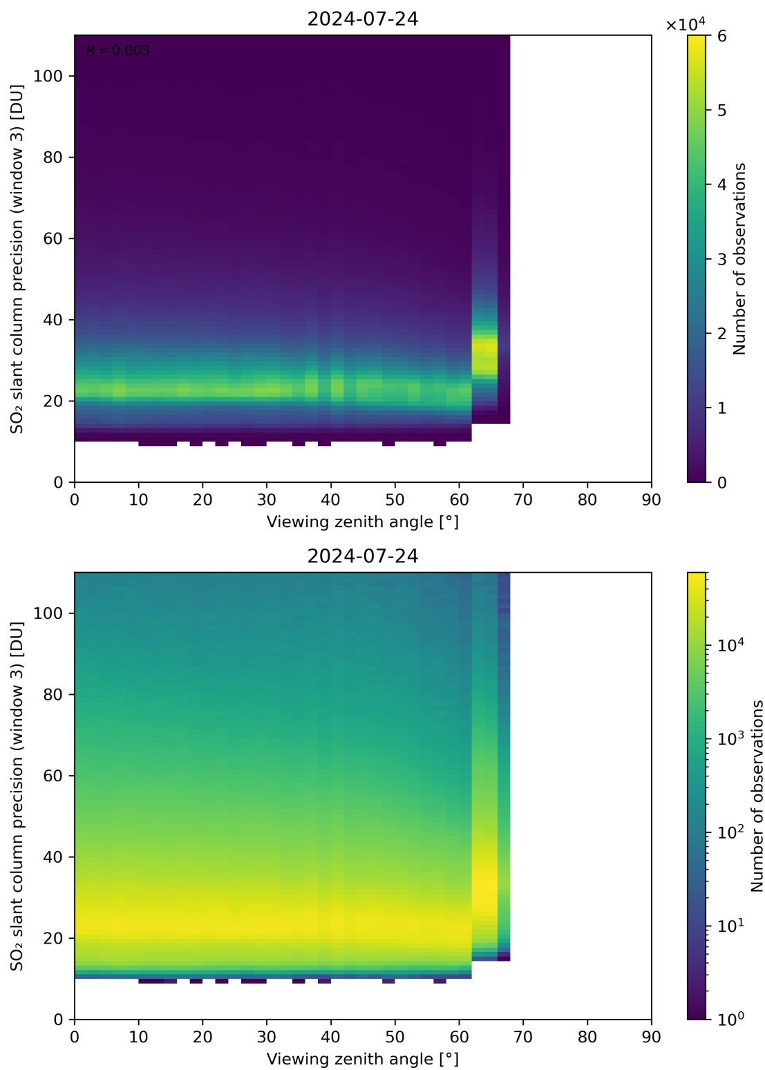
Figure 324: Scatter density plot of “Viewing zenith angle” against “SO 2 slant column precision (window 3)” for 2024-07-23 to 2024-07-25.
