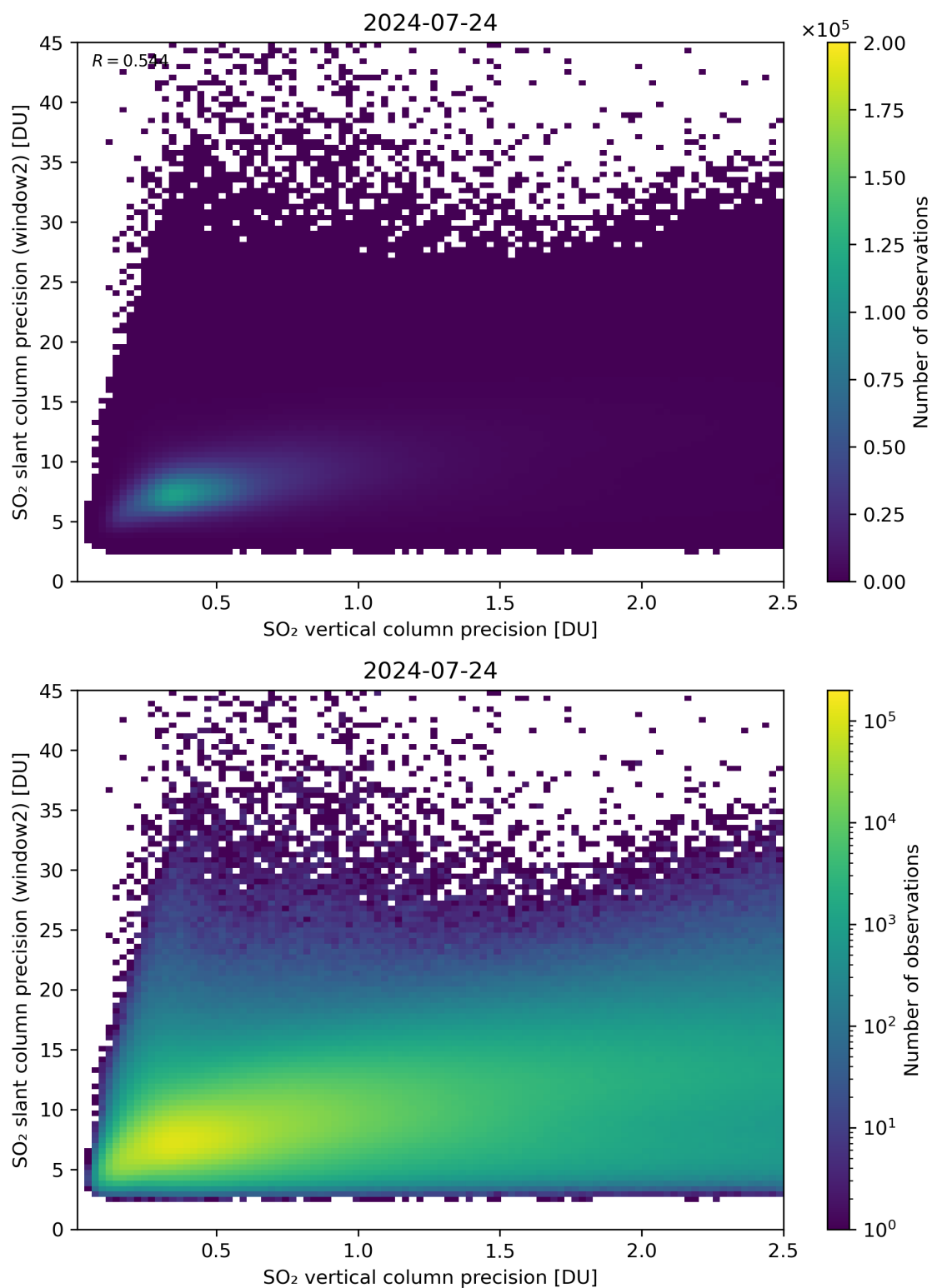
Figure 291: Scatter density plot of “SO 2 vertical column precision” against “SO 2 slant column precision (window2)” for 2024-07-23 to 2024-07-25.
