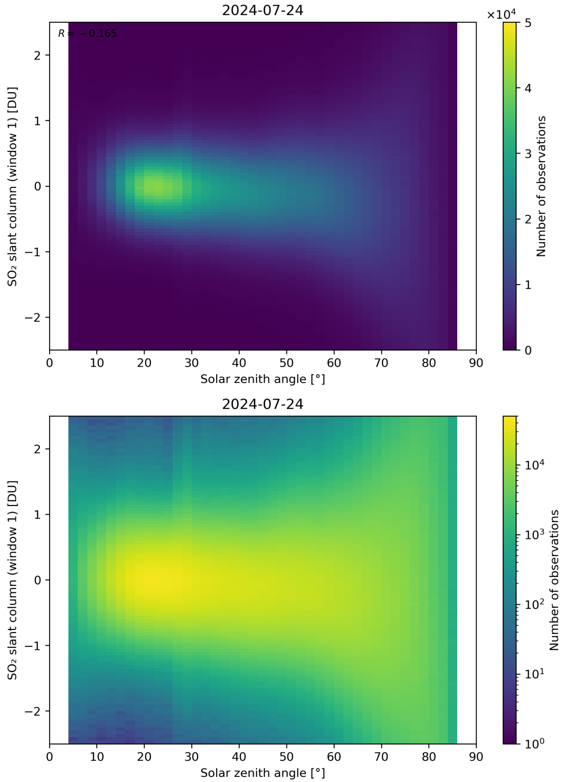
Figure 169: Scatter density plot of “Solar zenith angle” against “SO 2 slant column (window 1)” for 2024-07-23 to 2024-07-25.
