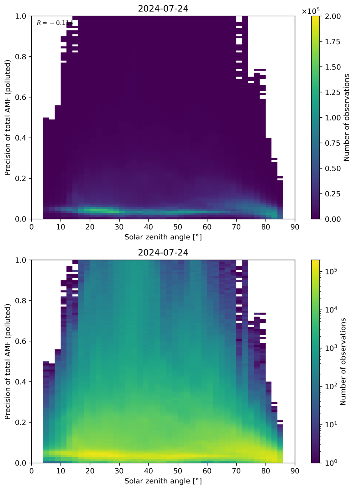
Figure 175: Scatter density plot of “Solar zenith angle” against “Precision of total AMF (polluted)” for 2024-07-23 to 2024-07-25.
