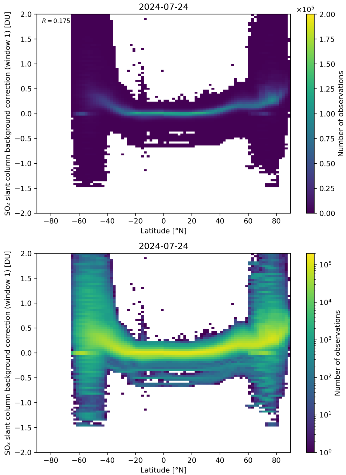
Figure 139: Scatter density plot of “Latitude” against “SO 2 slant column background correction (window 1)” for 2024-07-23 to 2024-07-25.
