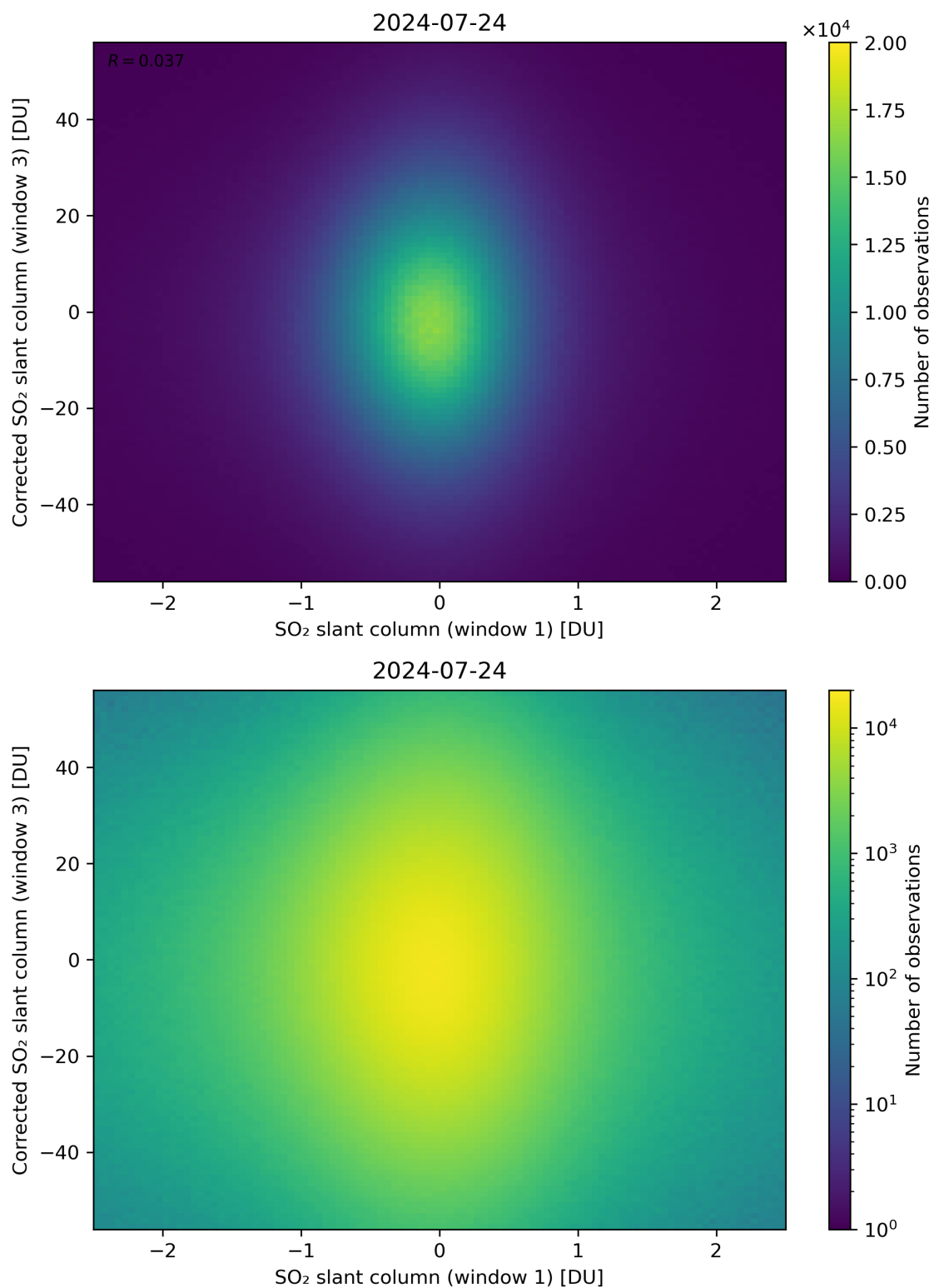
Figure 234: Scatter density plot of “SO 2 slant column (window 1)” against “Corrected SO 2 slant column (window 3)” for 2024-07-23 to 2024-07-25.
