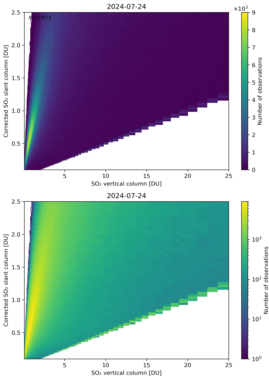
Figure 297: Scatter density plot of “SO 2 vertical column” against “Corrected SO 2 slant column” for 2024-07-23 to 2024-07-25.
