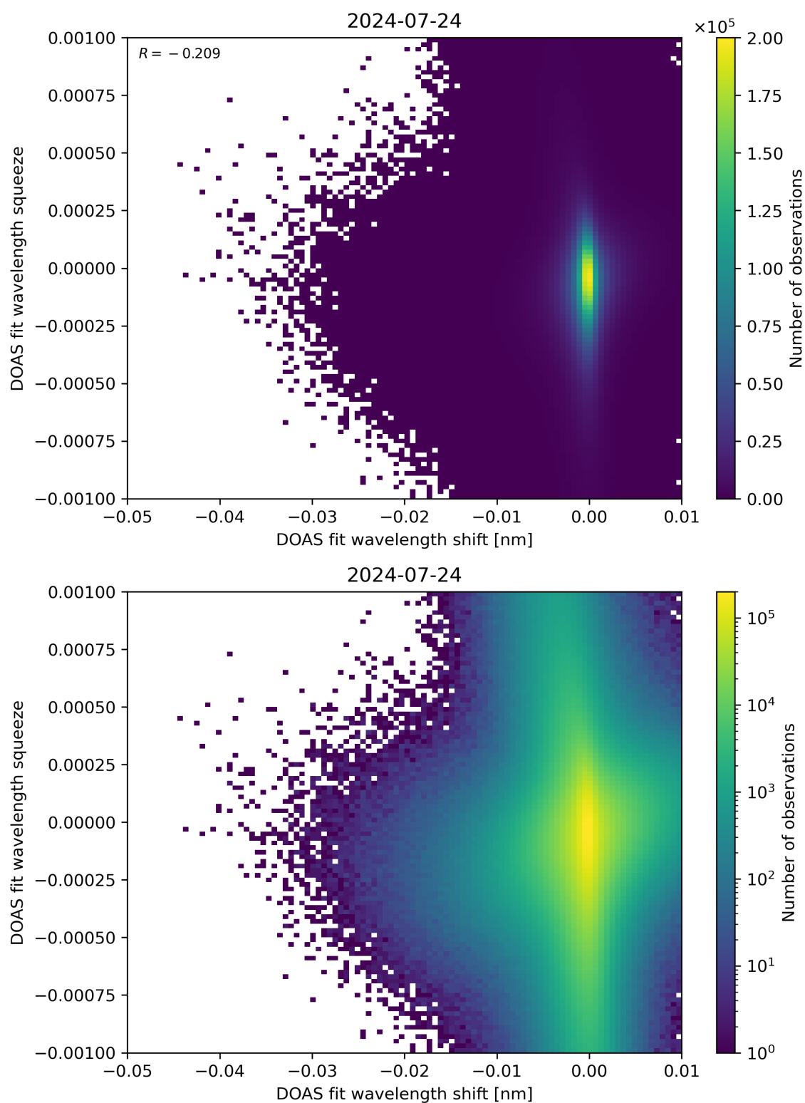
Figure 127: Scatter density plot of “DOAS fit wavelength shift” against “DOAS fit wavelength squeeze” for 2024-07-23 to 2024-07-25.
