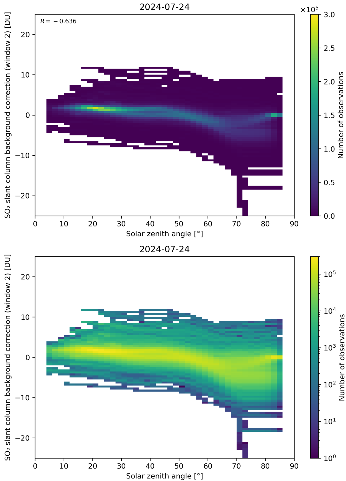
Figure 159: Scatter density plot of “Solar zenith angle” against “SO 2 slant column background correction (window 2)” for 2024-07-23 to 2024-07-25.
