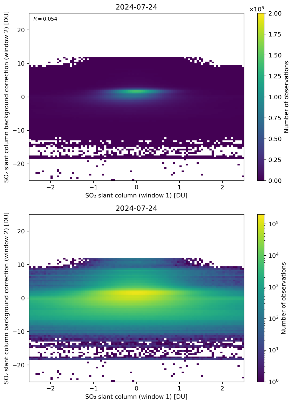
Figure 213: Scatter density plot of “SO 2 slant column (window 1)” against “SO 2 slant column background correction (window 2)” for 2024-07-23 to 2024-07-25.
