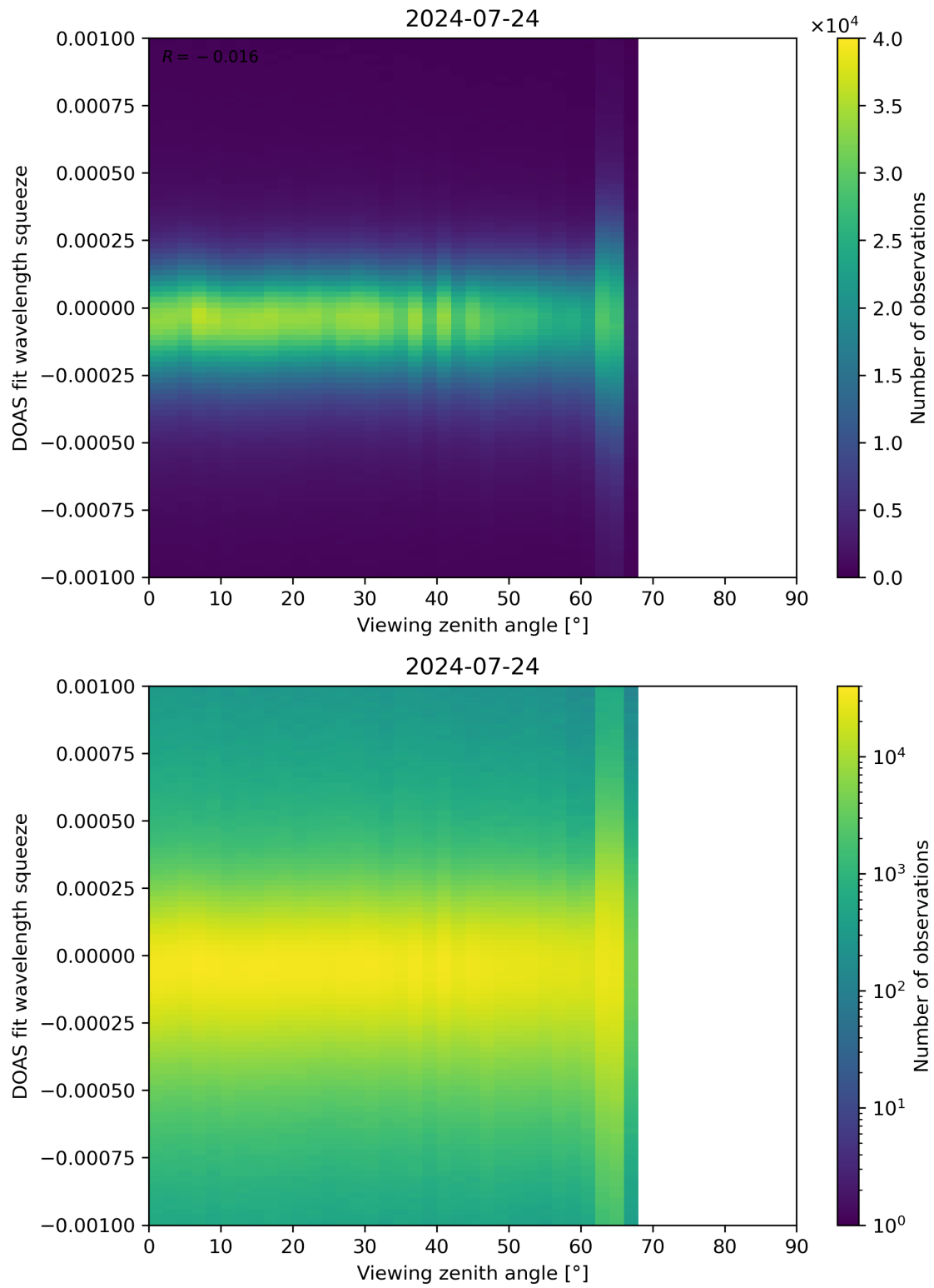
Figure 312: Scatter density plot of “Viewing zenith angle” against “DOAS fit wavelength squeeze” for 2024-07-23 to 2024-07-25.
