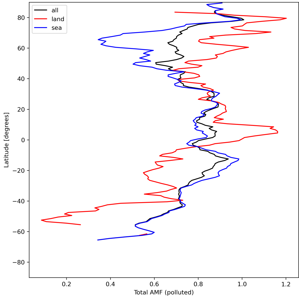
Figure 48: Zonal average of “Total AMF (polluted)” for 2024-07-23 to 2024-07-25.
