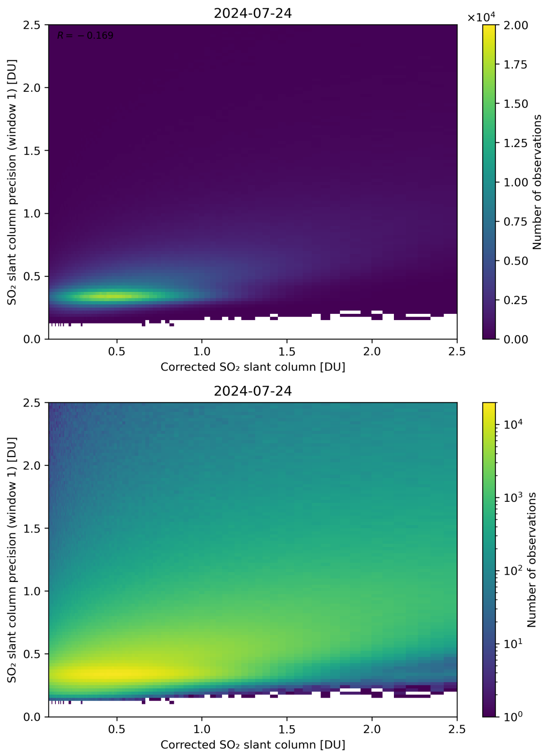
Figure 188: Scatter density plot of “Corrected SO 2 slant column” against “SO 2 slant column precision (window 1)” for 2024-07-23 to 2024-07-25.
