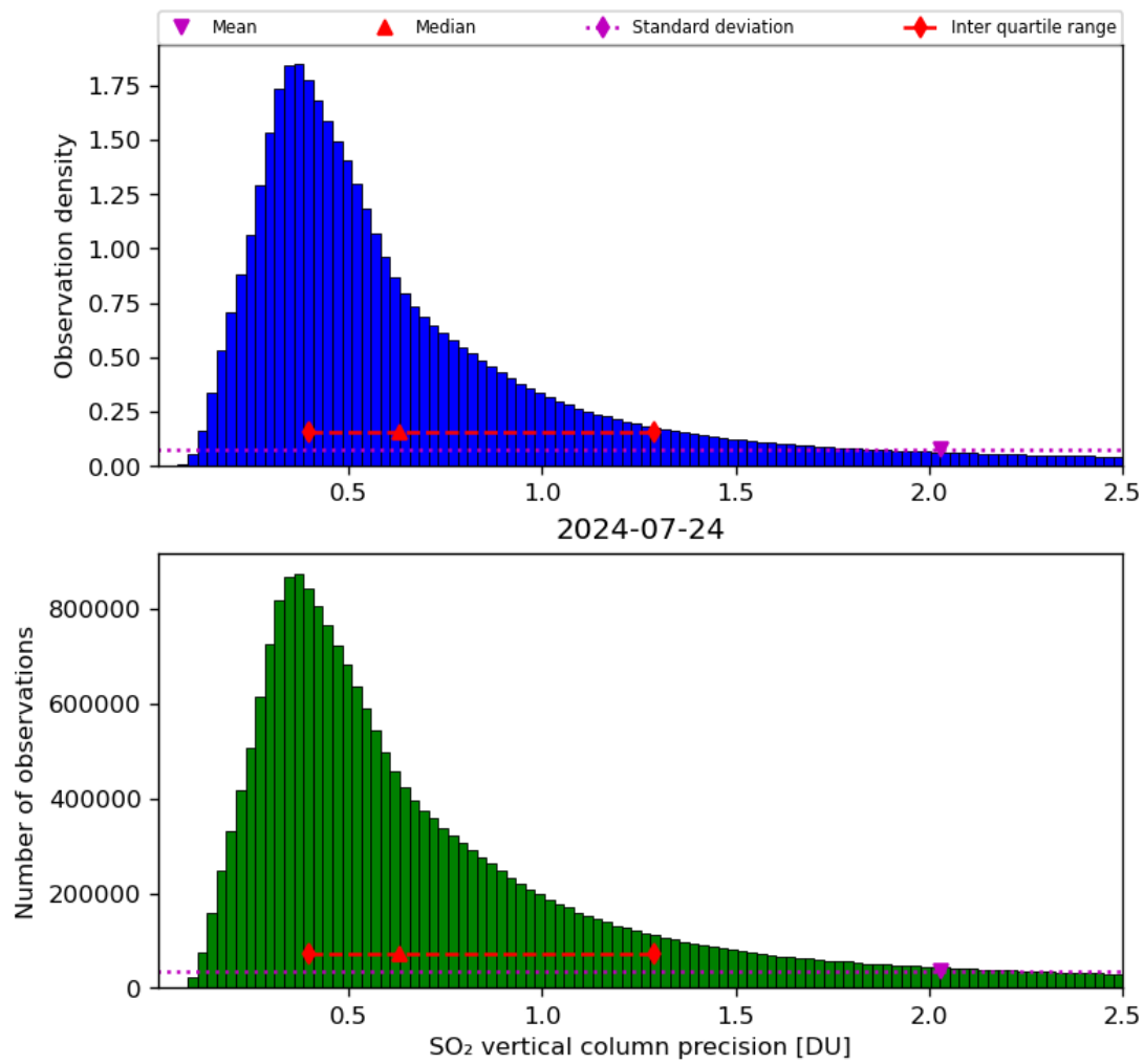
Figure 54: Histogram of “SO 2 vertical column precision” for 2024-07-23 to 2024-07-25
