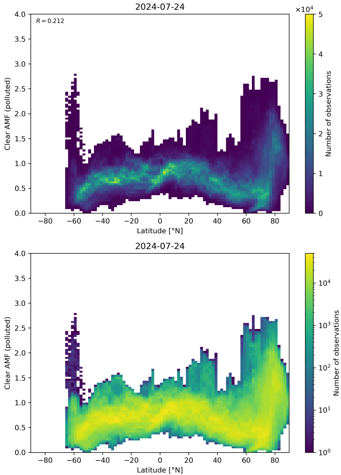
Figure 145: Scatter density plot of “Latitude” against “Clear AMF (polluted)” for 2024-07-23 to 2024-07-25.
