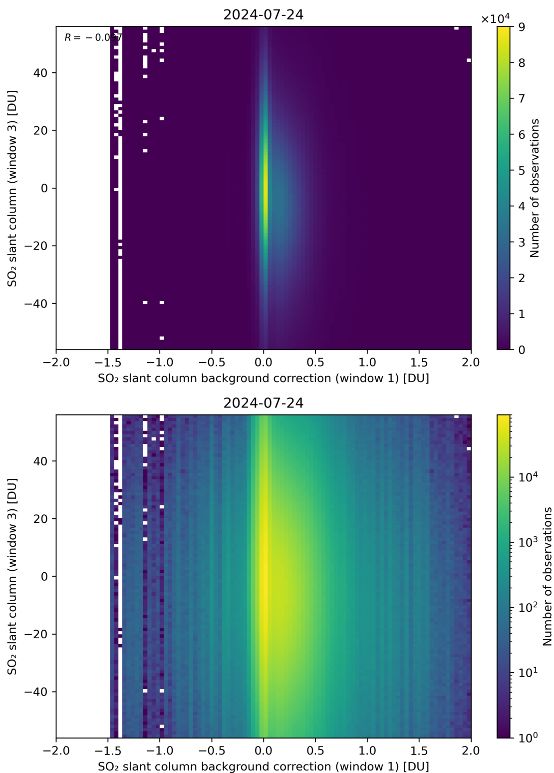
Figure 107: Scatter density plot of “SO 2 slant column background correction (window 1)” against “SO 2 slant column (window 3)” for 2024-07-23 to 2024-07-25.
