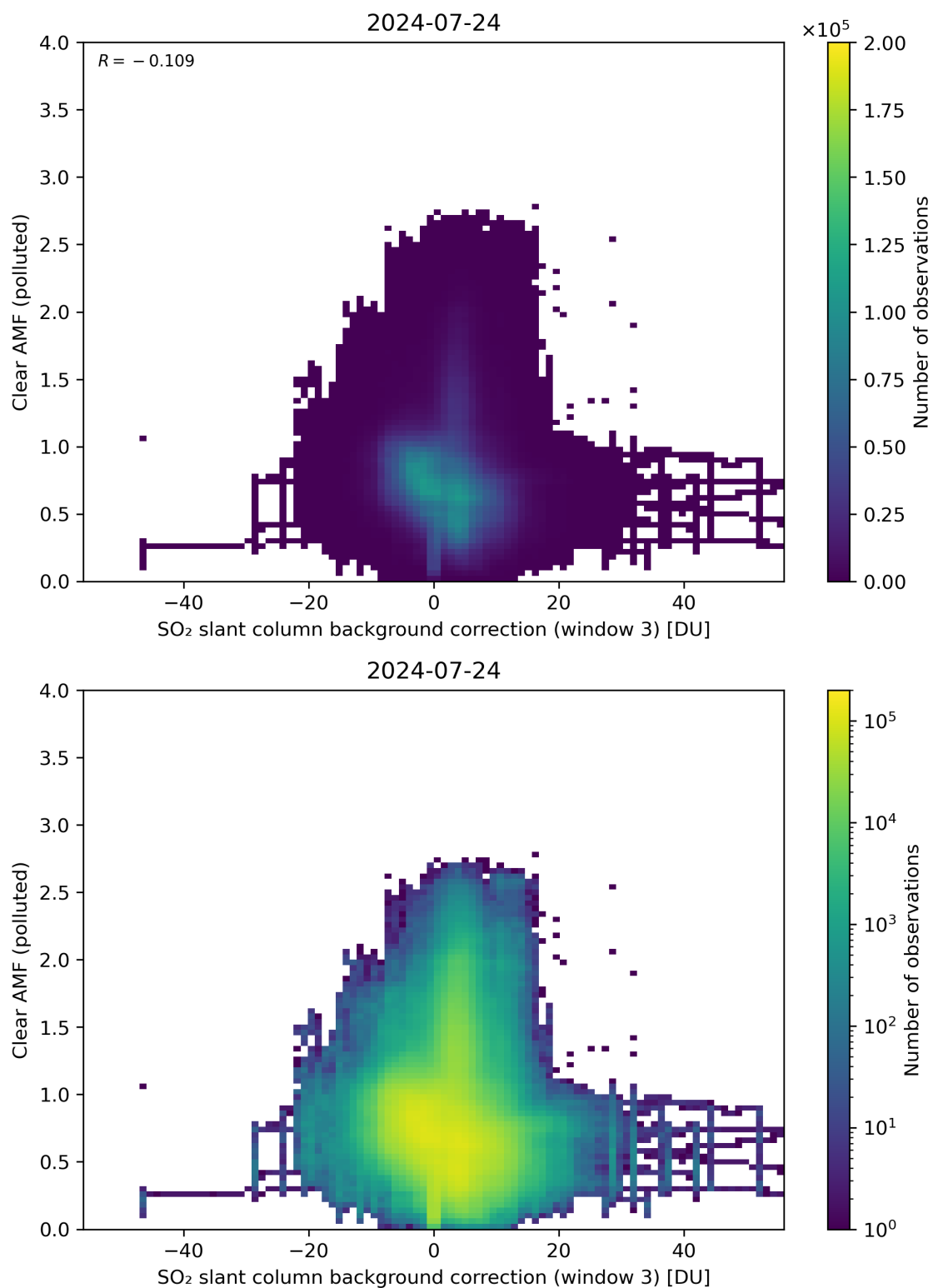
Figure 124: Scatter density plot of “SO 2 slant column background correction (window 3)” against “Clear AMF (polluted)” for 2024-07-23 to 2024-07-25.
