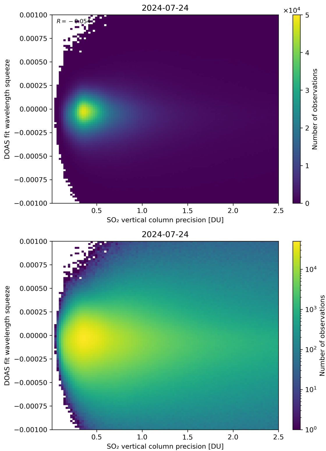
Figure 283: Scatter density plot of “SO 2 vertical column precision” against “DOAS fit wavelength squeeze” for 2024-07-23 to 2024-07-25.
