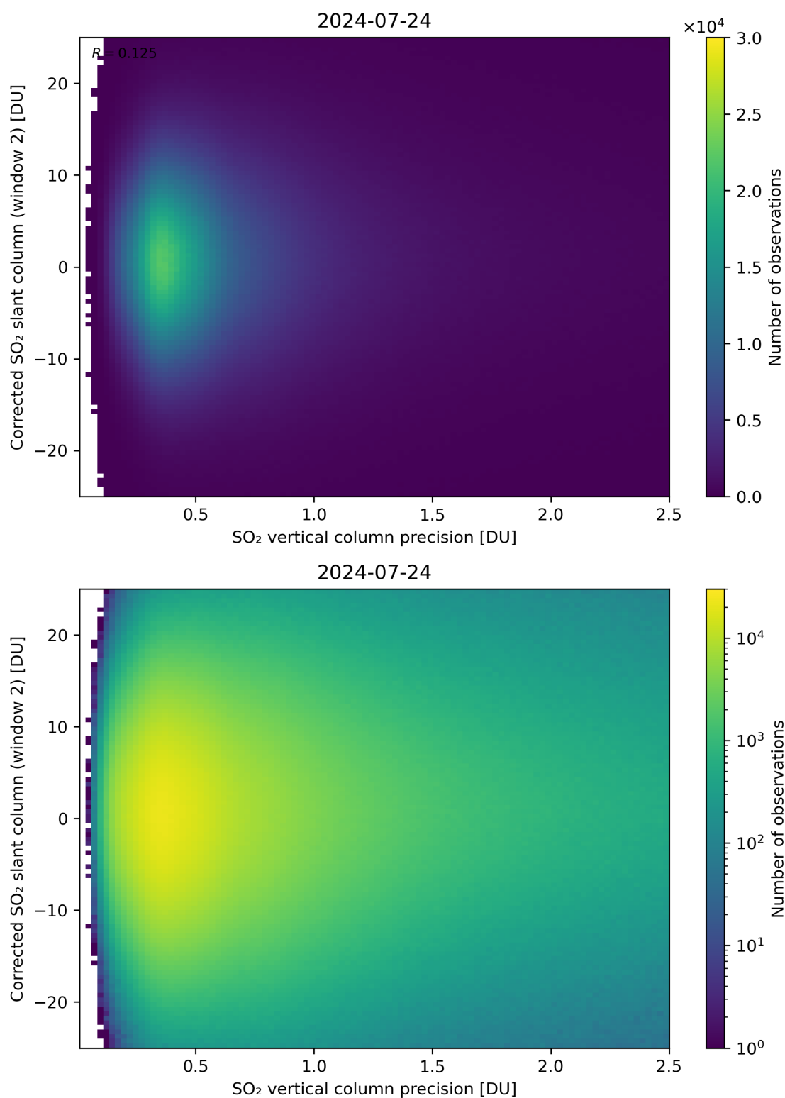
Figure 287: Scatter density plot of “SO 2 vertical column precision” against “Corrected SO 2 slant column (window 2)” for 2024-07-23 to 2024-07-25.
