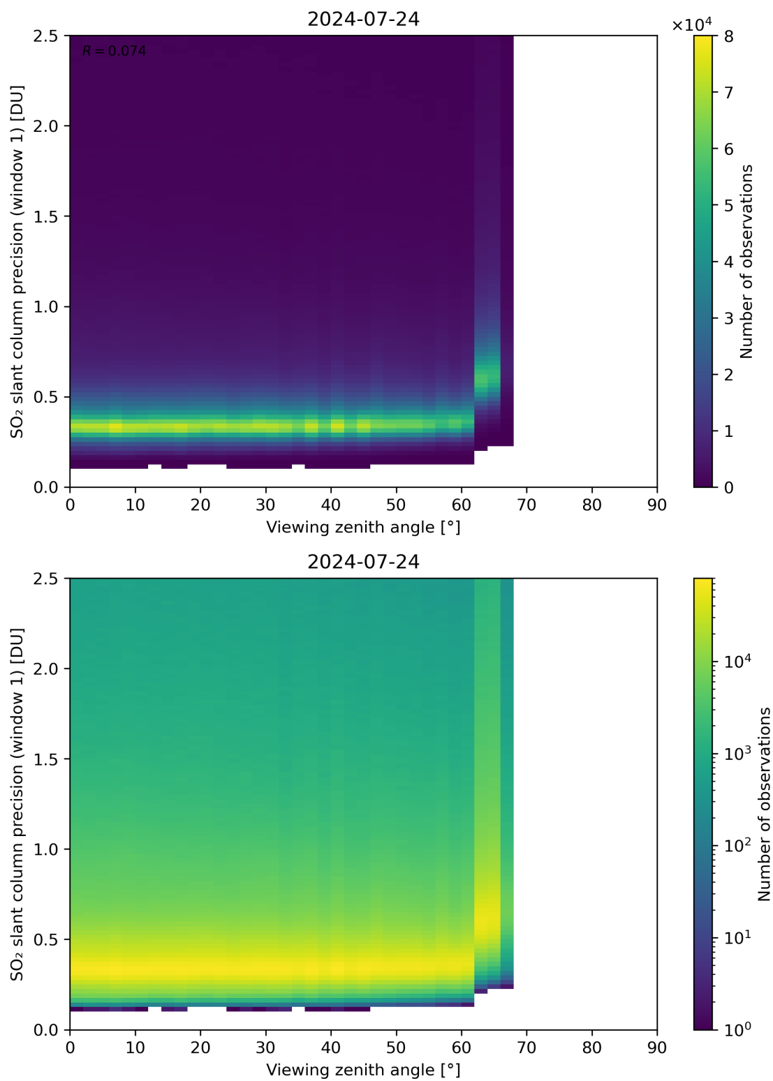
Figure 321: Scatter density plot of “Viewing zenith angle” against “SO 2 slant column precision (window 1)” for 2024-07-23 to 2024-07-25.
