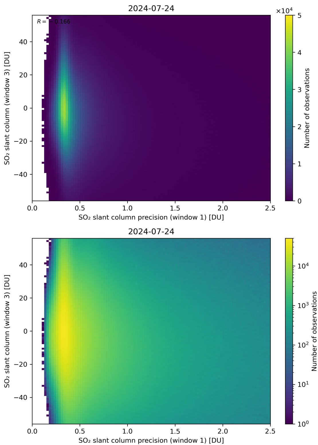
Figure 228: Scatter density plot of “SO 2 slant column precision (window 1)” against “SO 2 slant column (window 3)” for 2024-07-23 to 2024-07-25.
