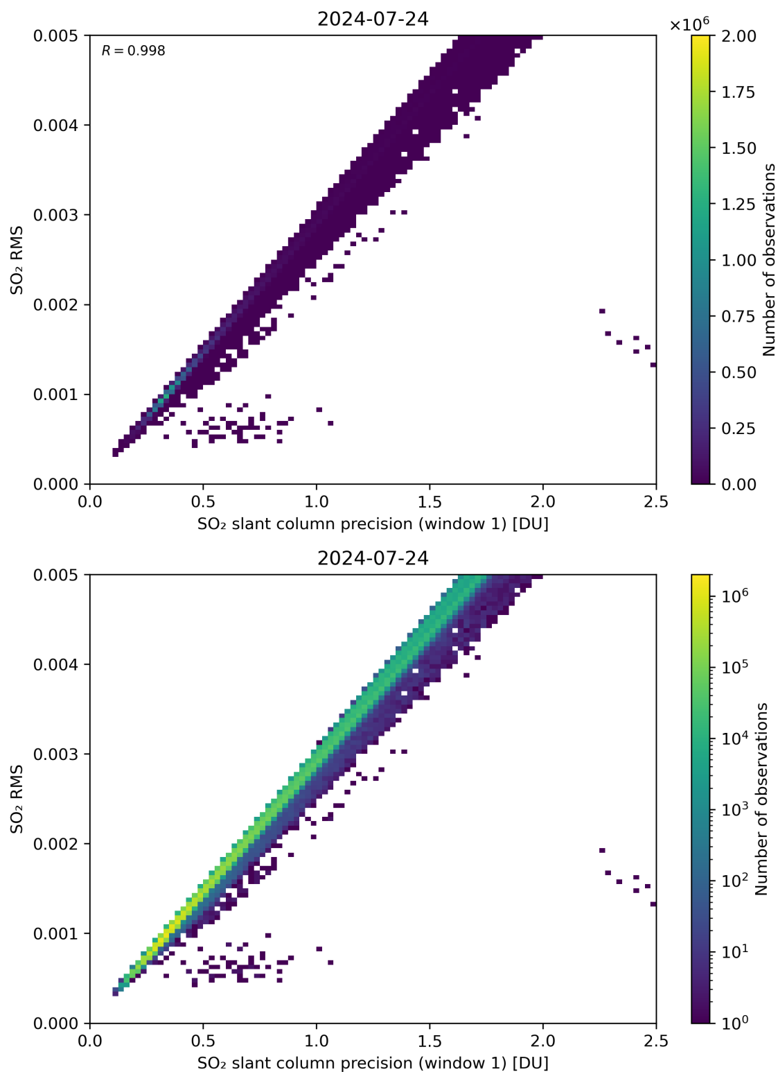
Figure 223: Scatter density plot of “SO 2 slant column precision (window 1)” against “SO 2 RMS” for 2024-07-23 to 2024-07-25.
