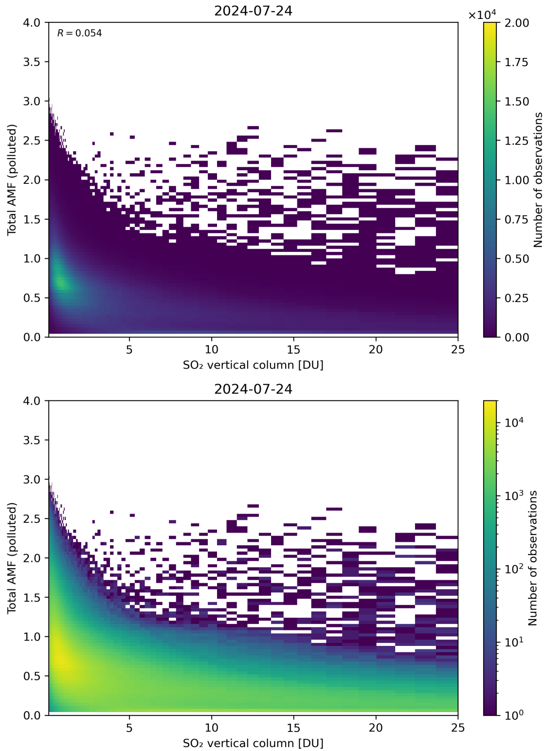
Figure 305: Scatter density plot of “SO 2 vertical column” against “Total AMF (polluted)” for 2024-07-23 to 2024-07-25.
