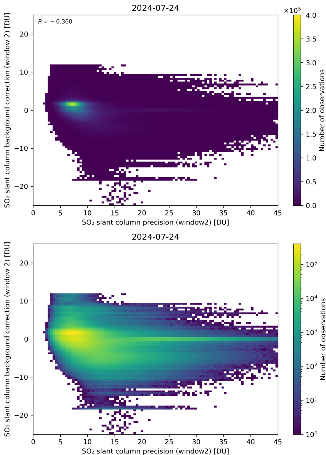
Figure 241: Scatter density plot of “SO 2 slant column precision (window2)” against “SO 2 slant column background correction (window 2)” for 2024-07-23 to 2024-07-25.
