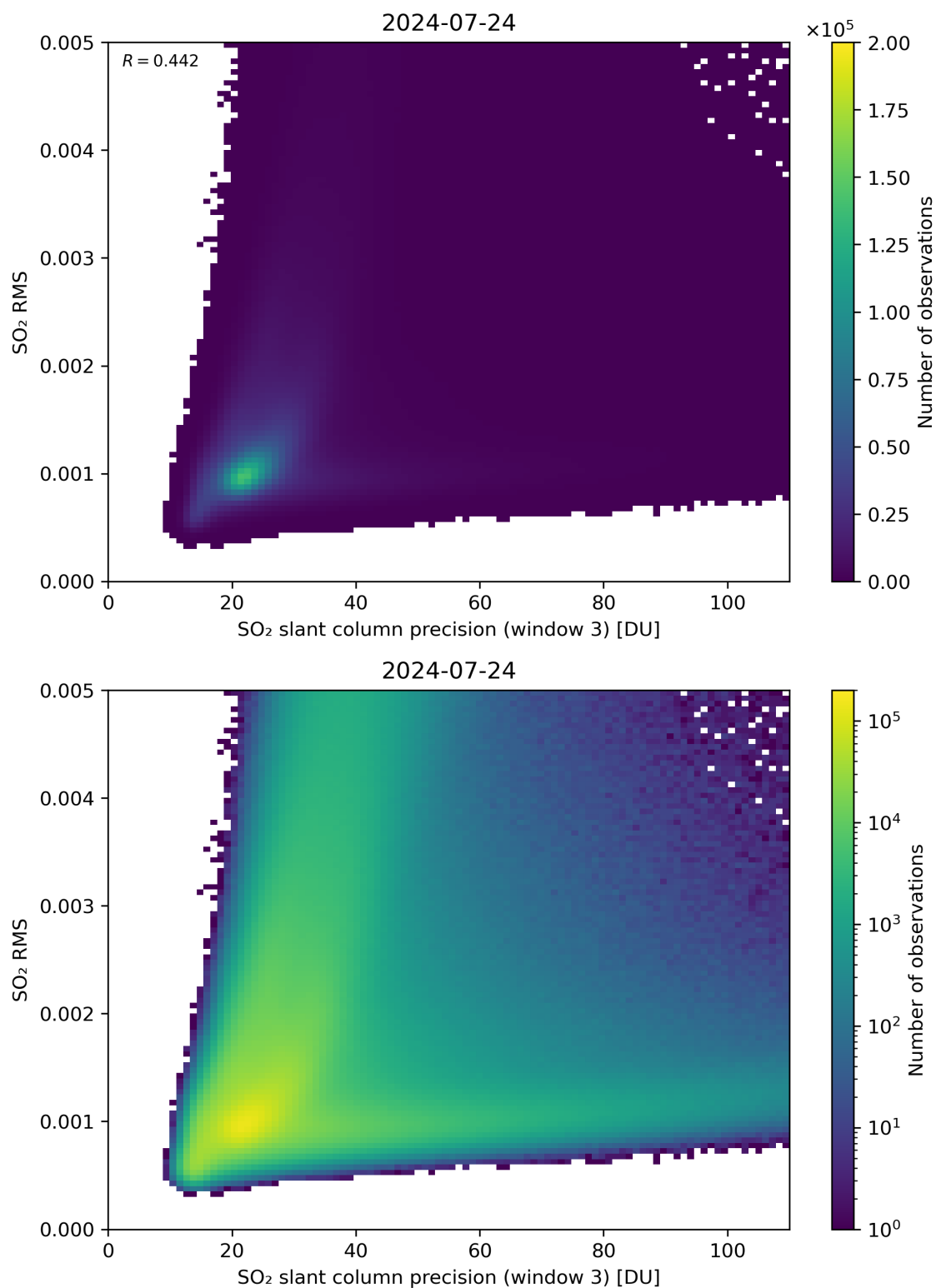
Figure 260: Scatter density plot of “SO 2 slant column precision (window 3)” against “SO 2 RMS” for 2024-07-23 to 2024-07-25.
