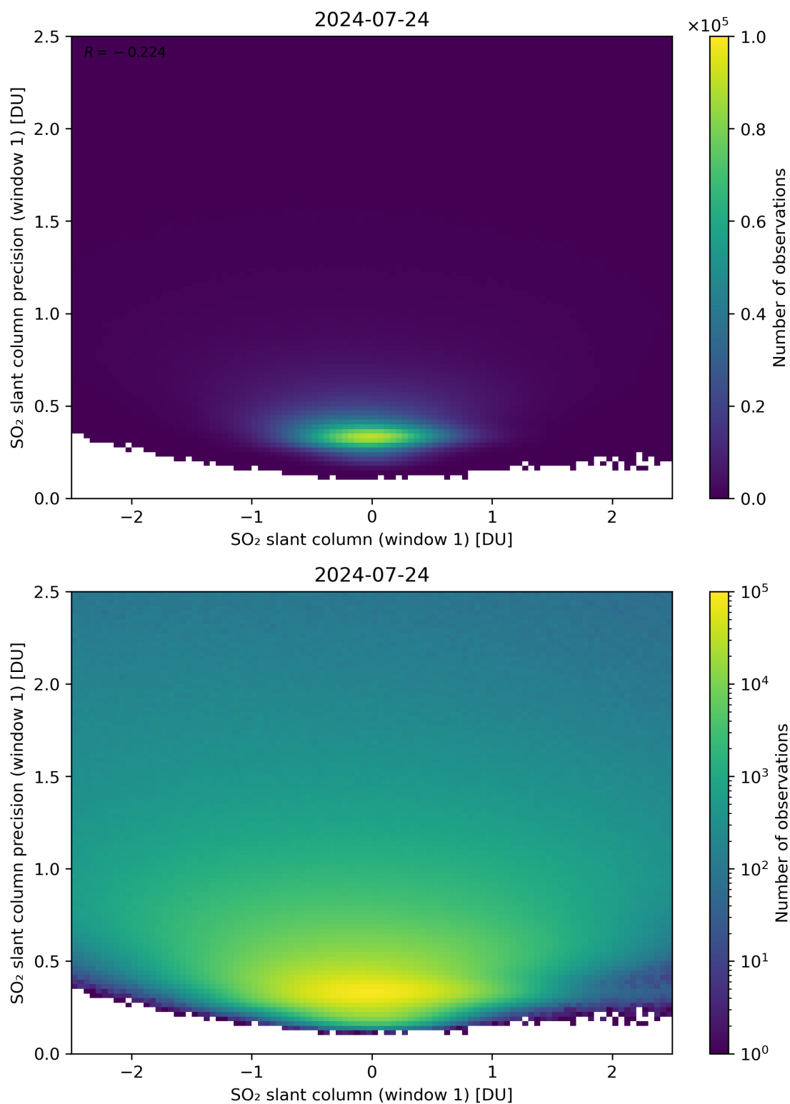
Figure 235: Scatter density plot of “SO 2 slant column (window 1)” against “SO 2 slant column precision (window 1)” for 2024-07-23 to 2024-07-25.
