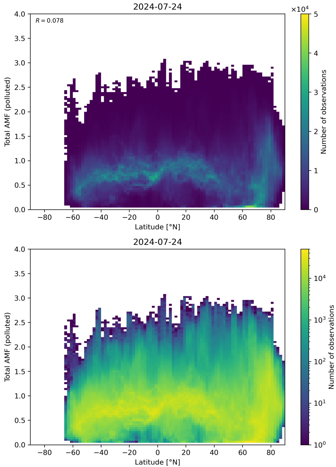
Figure 154: Scatter density plot of “Latitude” against “Total AMF (polluted)” for 2024-07-23 to 2024-07-25.
