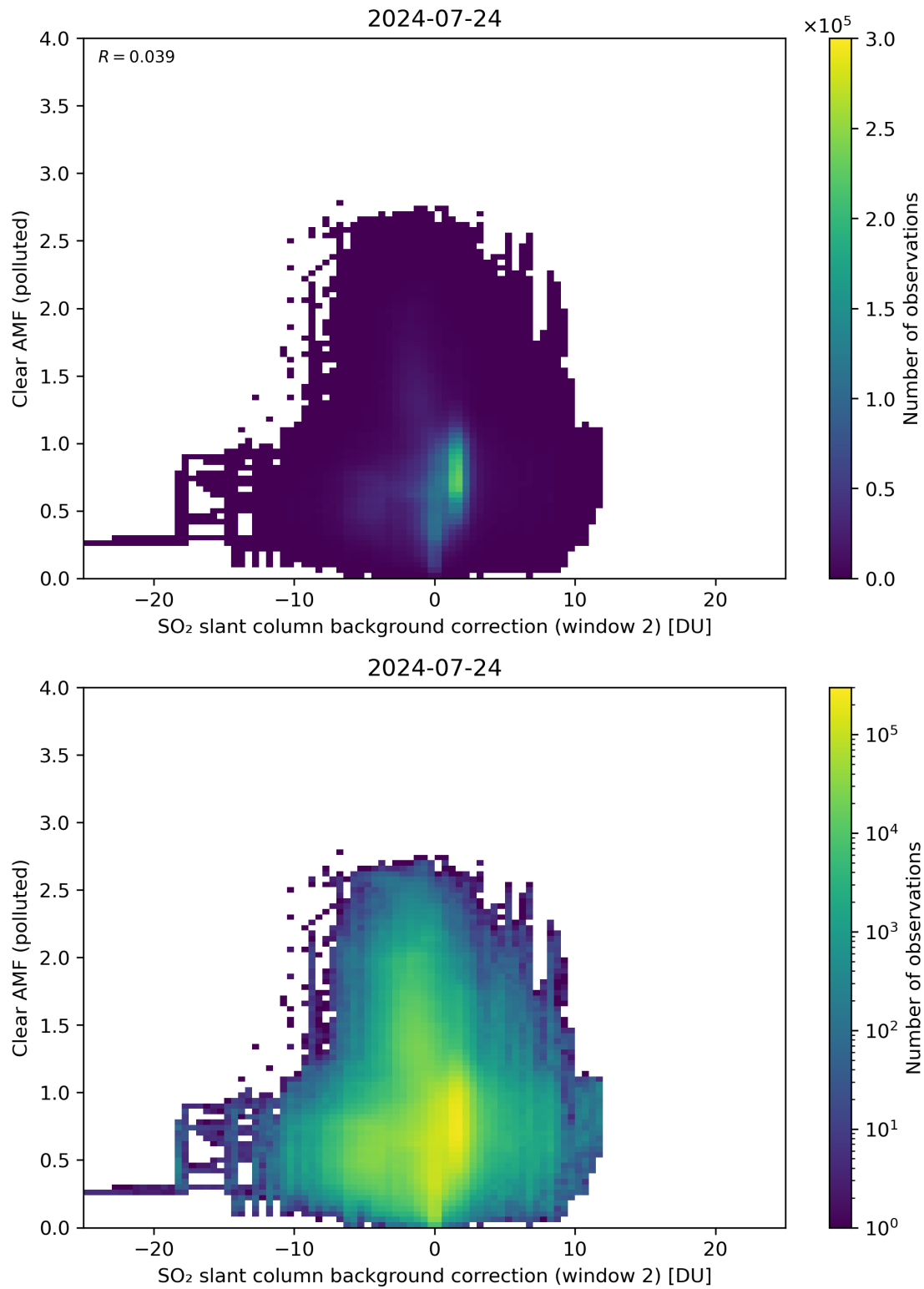
Figure 115: Scatter density plot of “SO 2 slant column background correction (window 2)” against “Clear AMF (polluted)” for 2024-07-23 to 2024-07-25.
