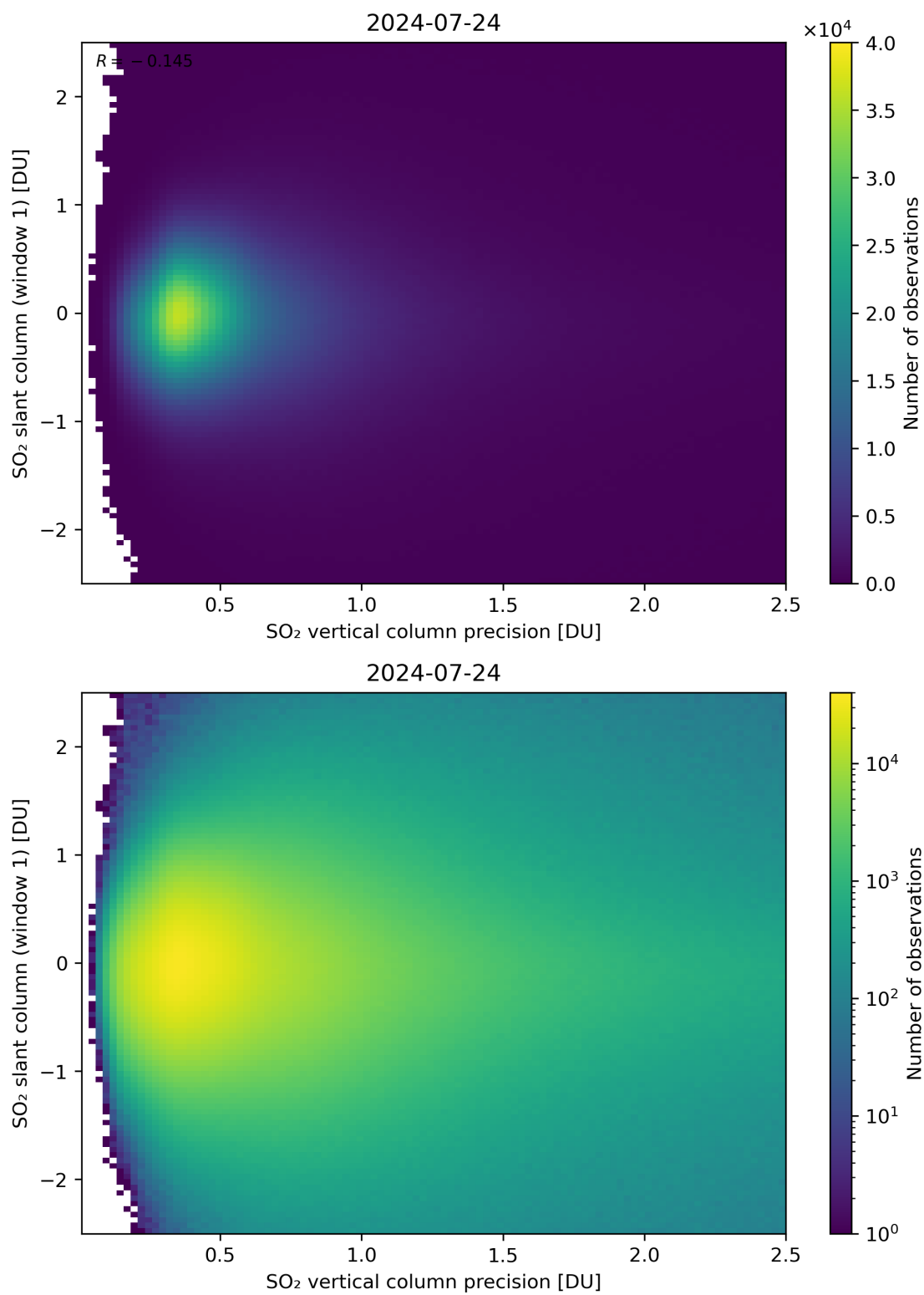
Figure 289: Scatter density plot of “SO 2 vertical column precision” against “SO 2 slant column (window 1)” for 2024-07-23 to 2024-07-25.
