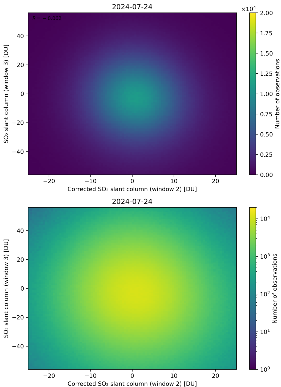
Figure 201: Scatter density plot of “Corrected SO 2 slant column (window 2)” against “SO 2 slant column (window 3)” for 2024-07-23 to 2024-07-25.
