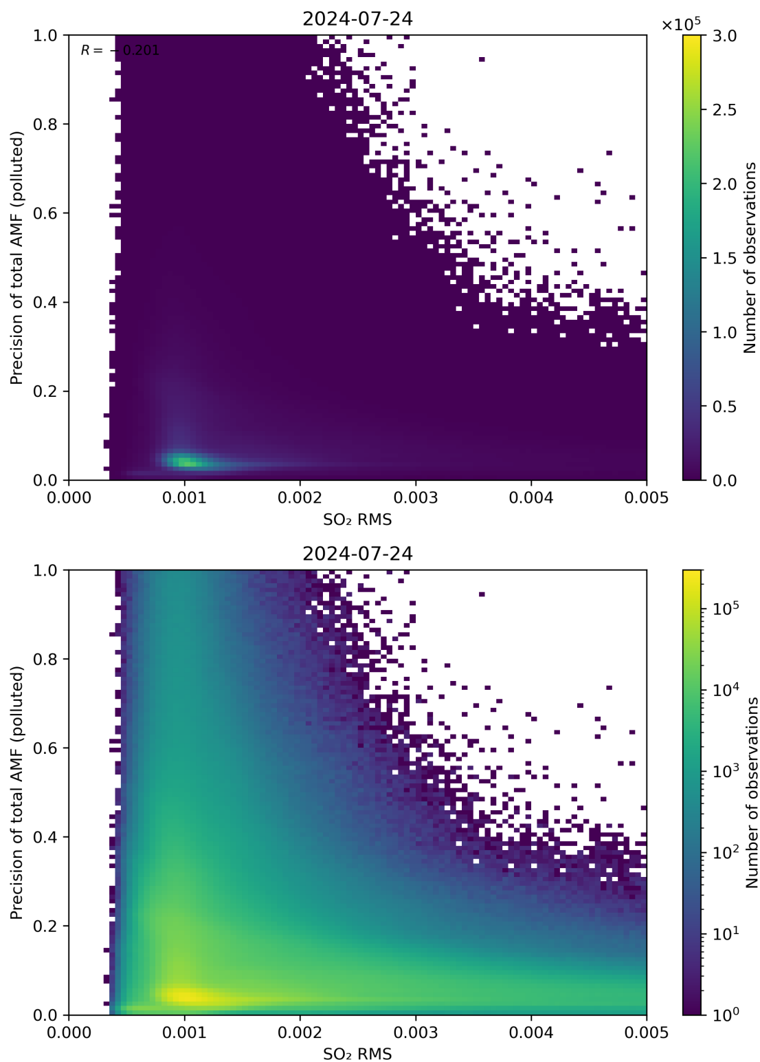
Figure 138: Scatter density plot of “SO 2 RMS” against “Precision of total AMF (polluted)” for 2024-07-23 to 2024-07-25.
