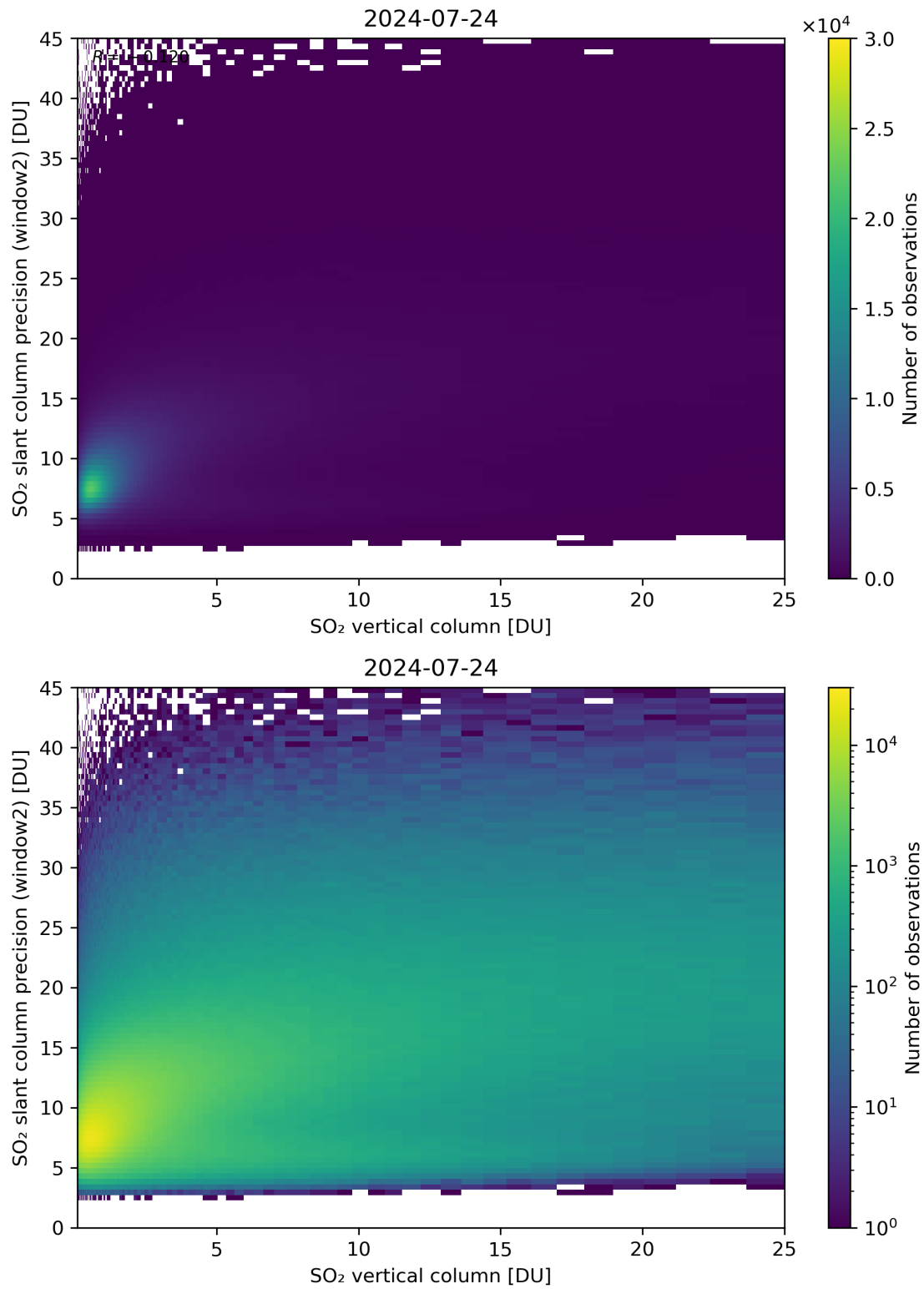
Figure 302: Scatter density plot of “SO 2 vertical column” against “SO 2 slant column precision (window2)” for 2024-07-23 to 2024-07-25.
