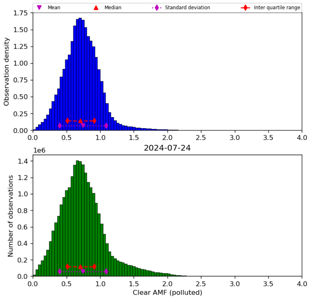
Figure 73: Histogram of “Clear AMF (polluted)” for 2024-07-23 to 2024-07-25
