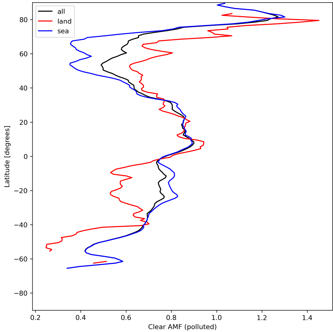
Figure 50: Zonal average of “Clear AMF (polluted)” for 2024-07-23 to 2024-07-25.
