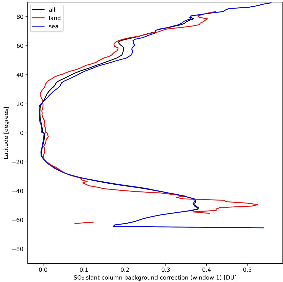
Figure 36: Zonal average of “SO 2 slant column background correction (window 1)” for 2024-07-23 to 2024-07-25.
