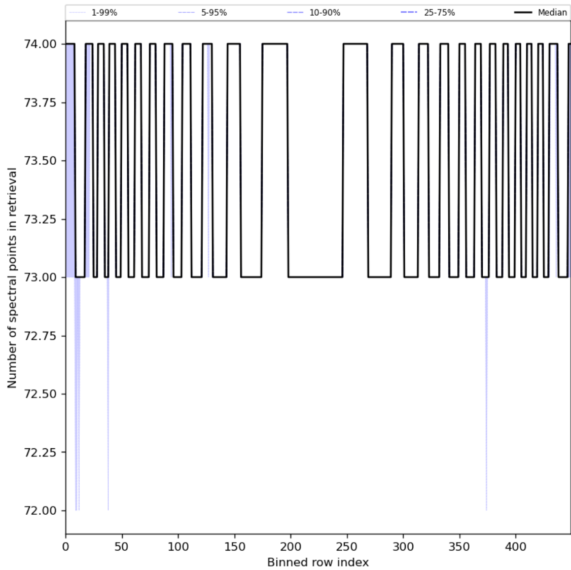
Figure 97: Along track statistics of “Number of spectral points in retrieval” for 2024-07-23 to 2024-07-25
