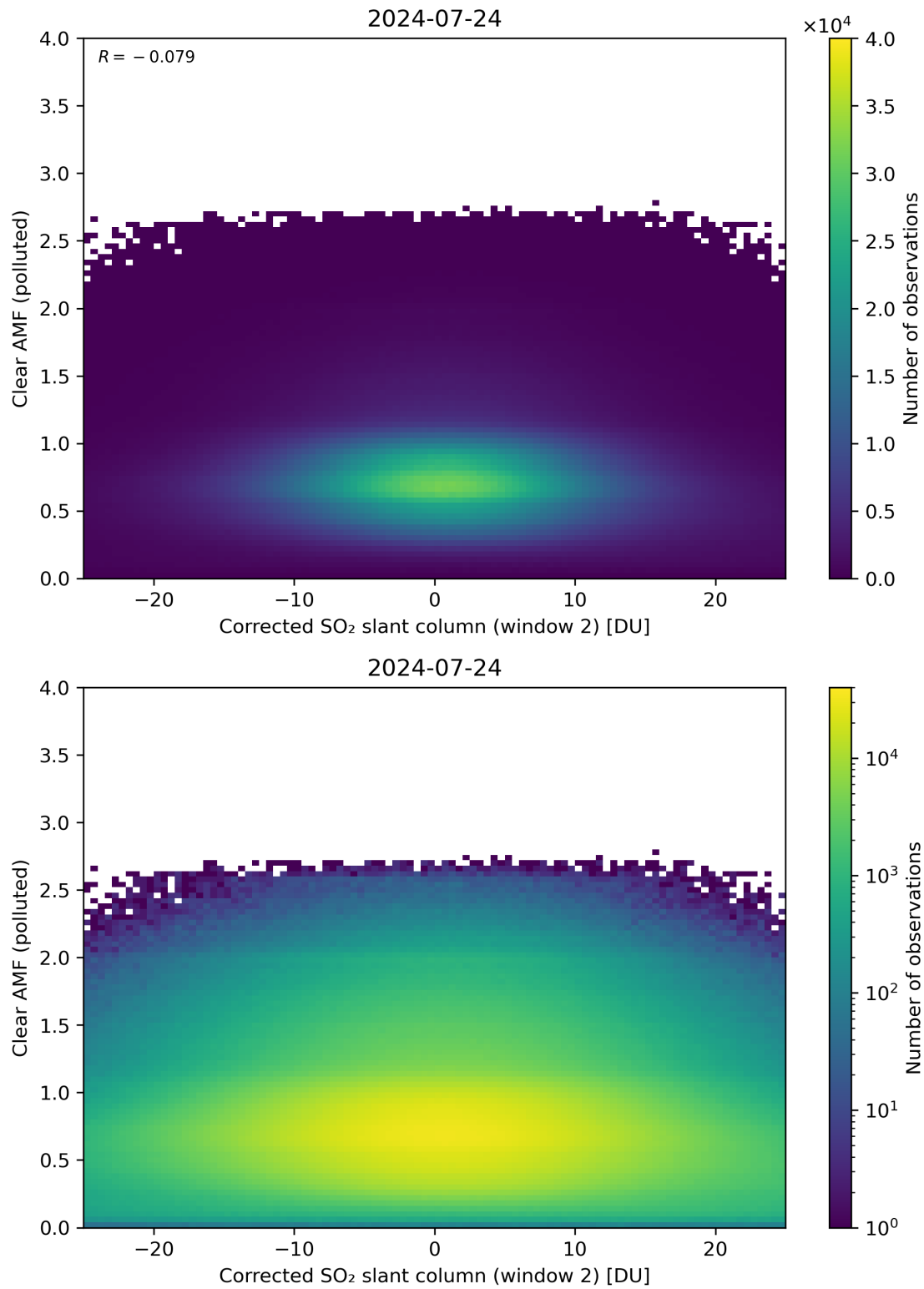
Figure 199: Scatter density plot of “Corrected SO 2 slant column (window 2)” against “Clear AMF (polluted)” for 2024-07-23 to 2024-07-25.
