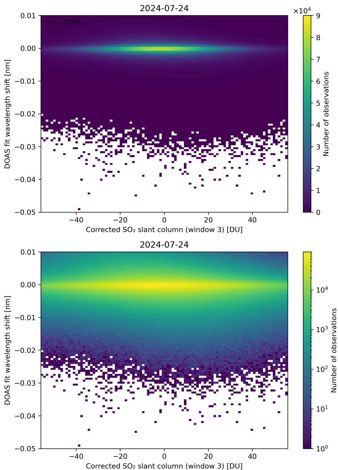
Figure 206: Scatter density plot of “Corrected SO 2 slant column (window 3)” against “DOAS fit wavelength shift” for 2024-07-23 to 2024-07-25.
