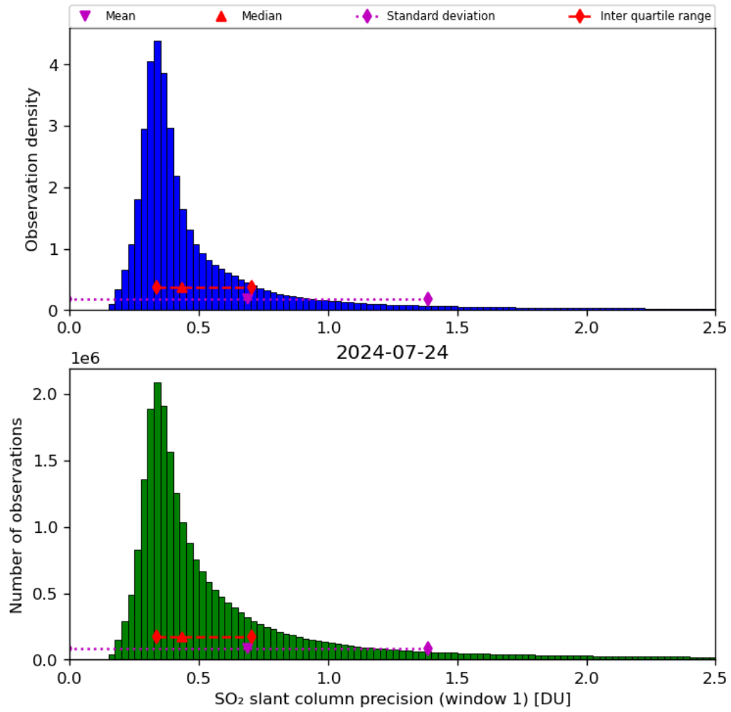
Figure 57: Histogram of “SO 2 slant column precision (window 1)” for 2024-07-23 to 2024-07-25
