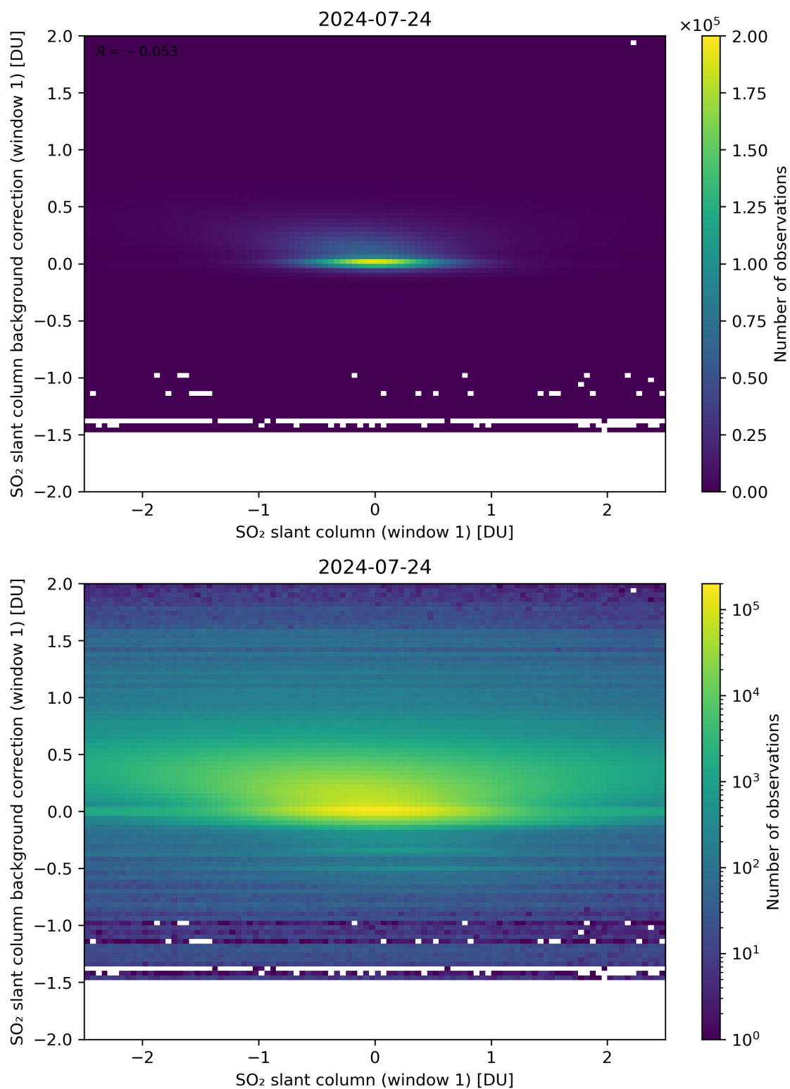
Figure 212: Scatter density plot of “SO 2 slant column (window 1)” against “SO 2 slant column background correction (window 1)” for 2024-07-23 to 2024-07-25.
