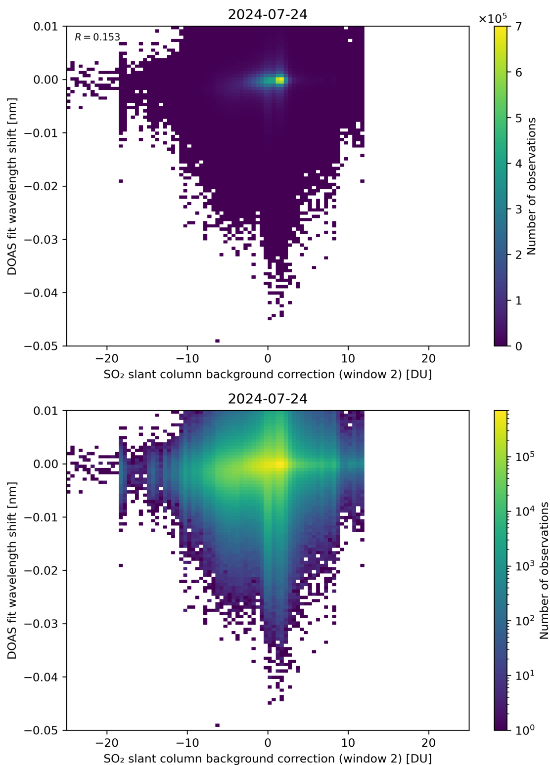
Figure 112: Scatter density plot of “SO 2 slant column background correction (window 2)” against “DOAS fit wavelength shift” for 2024-07-23 to 2024-07-25.
