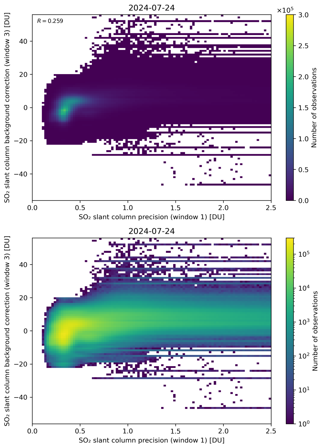
Figure 220: Scatter density plot of “SO 2 slant column precision (window 1)” against “SO 2 slant column background correction (window 3)” for 2024-07-23 to 2024-07-25.
