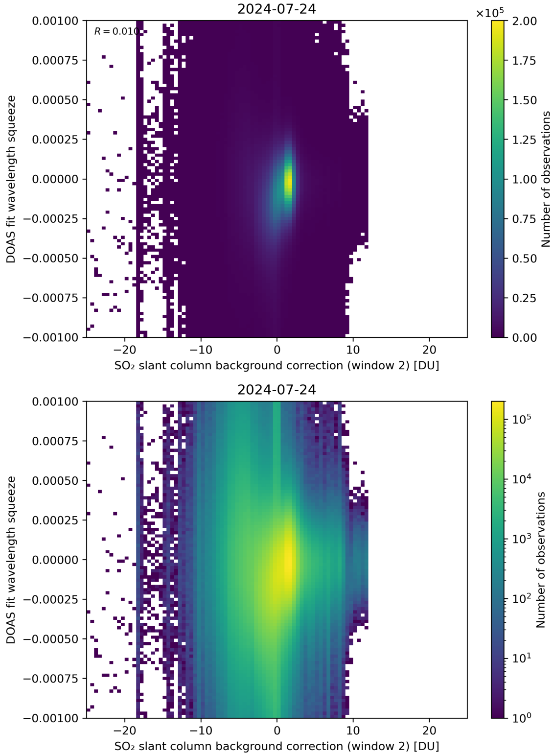
Figure 113: Scatter density plot of “SO 2 slant column background correction (window 2)” against “DOAS fit wavelength squeeze” for 2024-07-23 to 2024-07-25.
