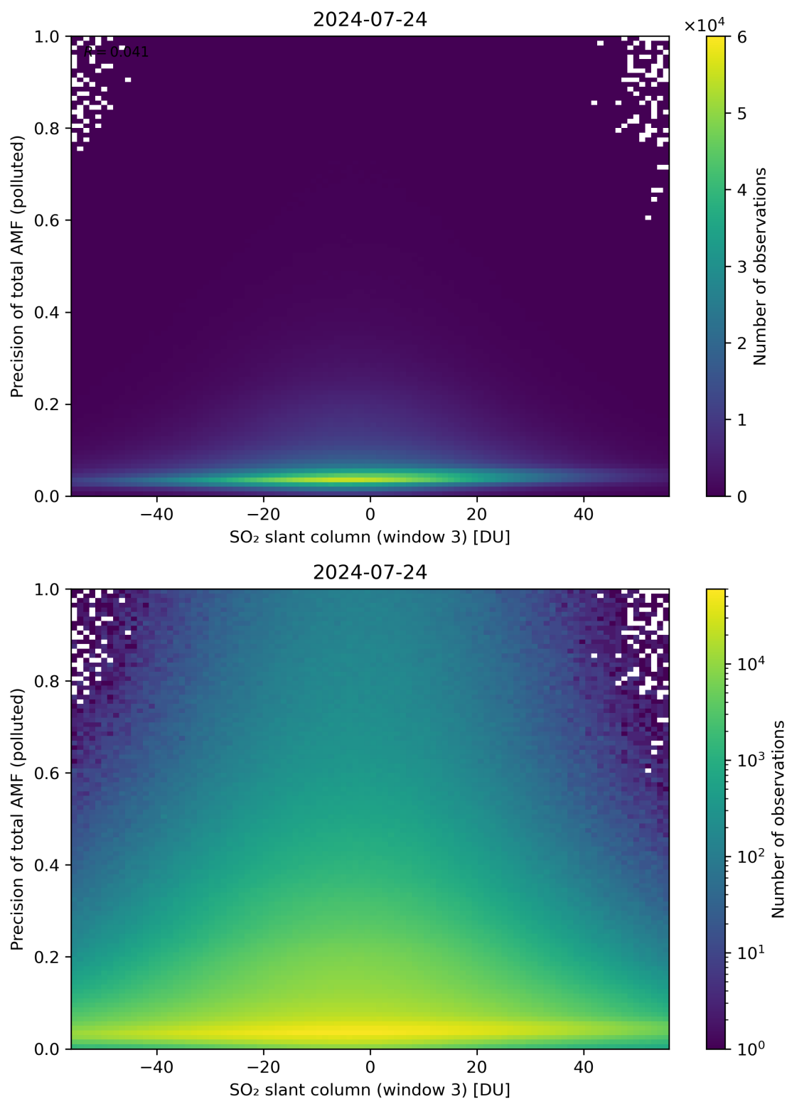
Figure 269: Scatter density plot of “SO 2 slant column (window 3)” against “Precision of total AMF (polluted)” for 2024-07-23 to 2024-07-25.
