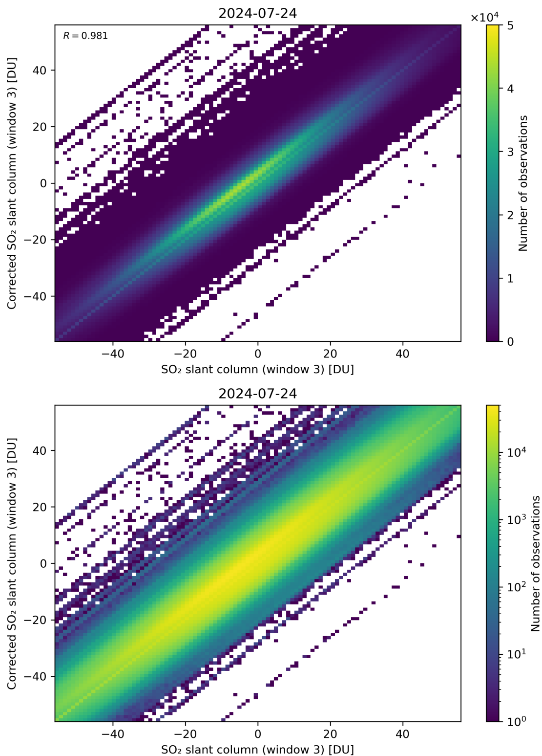
Figure 266: Scatter density plot of “SO 2 slant column (window 3)” against “Corrected SO 2 slant column (window 3)” for 2024-07-23 to 2024-07-25.
