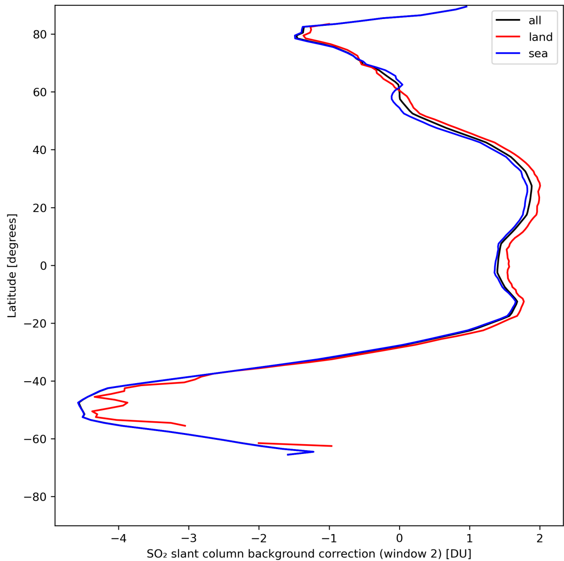
Figure 40: Zonal average of “SO 2 slant column background correction (window 2)” for 2024-07-23 to 2024-07-25.
