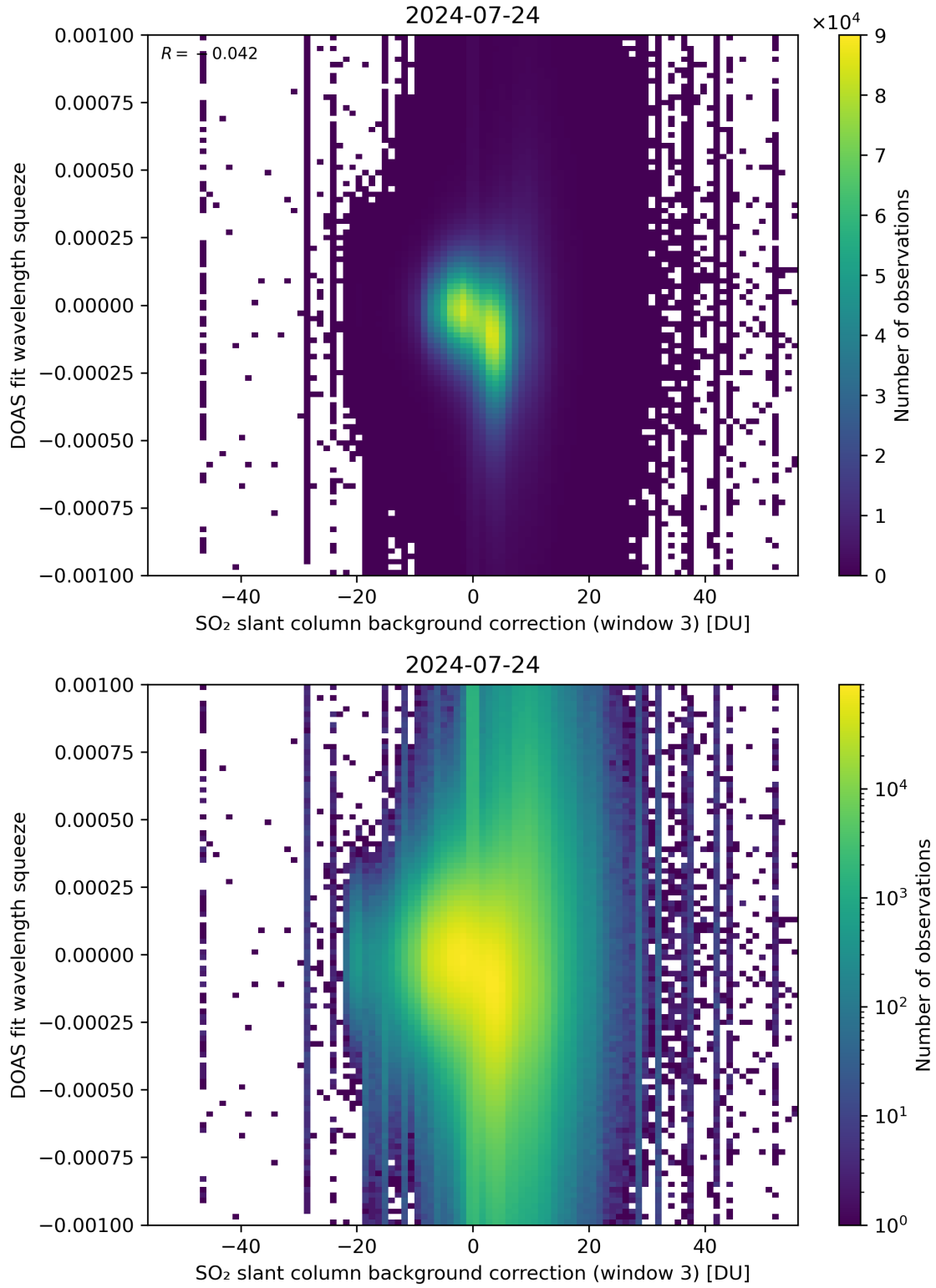
Figure 122: Scatter density plot of “SO 2 slant column background correction (window 3)” against “DOAS fit wavelength squeeze” for 2024-07-23 to 2024-07-25.
