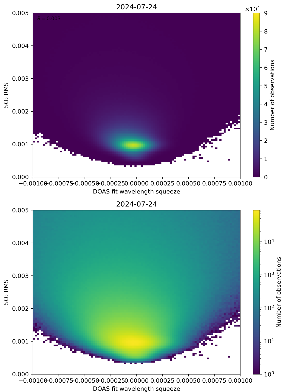
Figure 132: Scatter density plot of “DOAS fit wavelength squeeze” against “SO 2 RMS” for 2024-07-23 to 2024-07-25.
