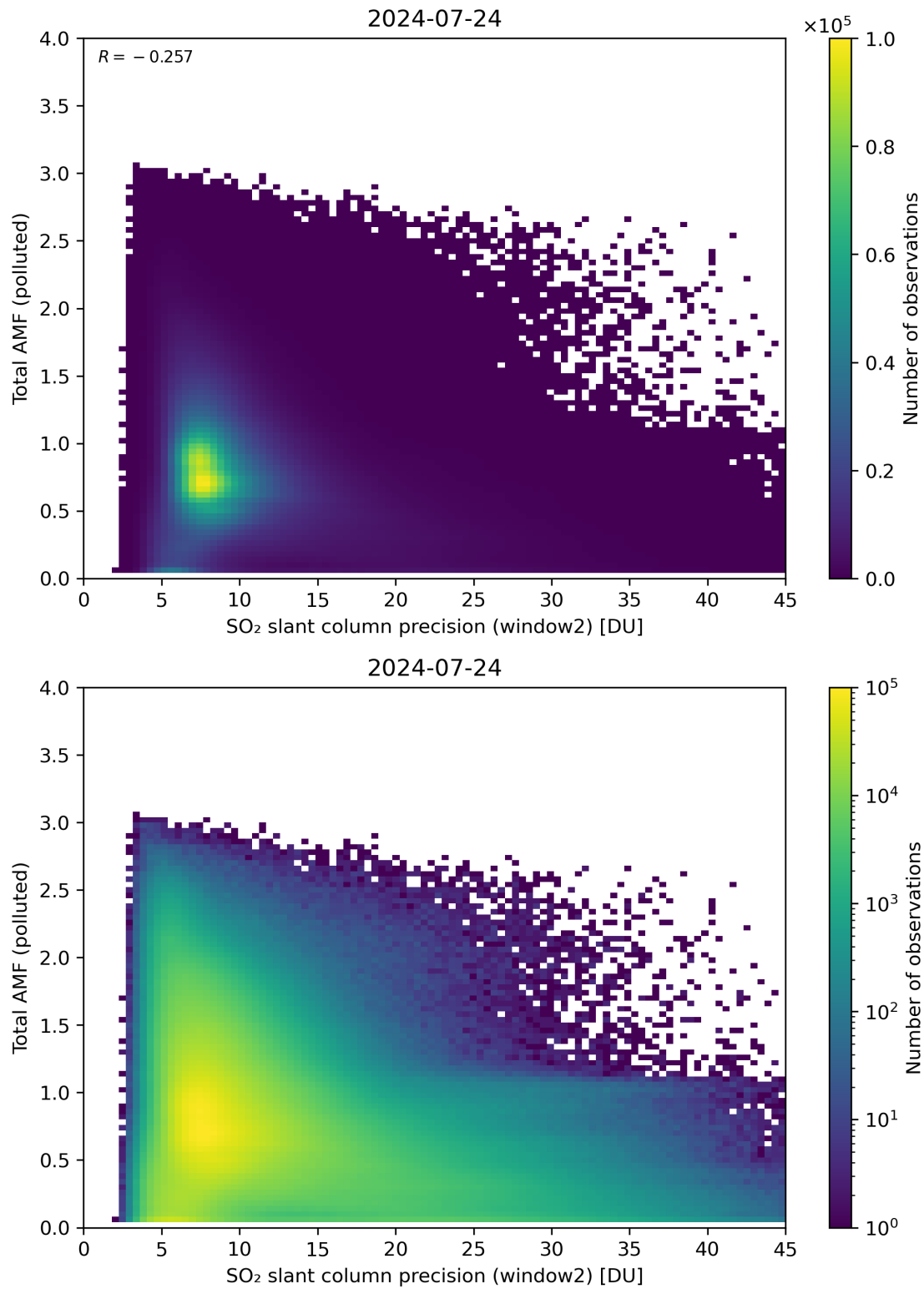
Figure 251: Scatter density plot of “SO 2 slant column precision (window2)” against “Total AMF (polluted)” for 2024-07-23 to 2024-07-25.
