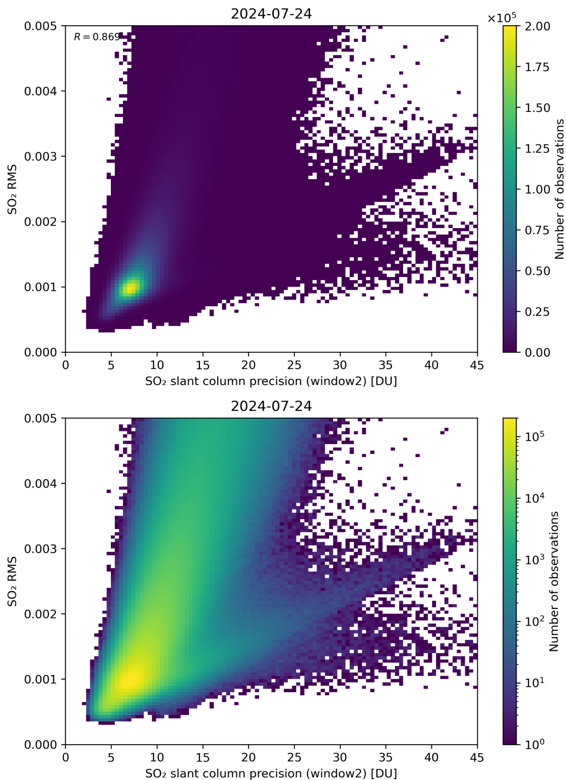
Figure 245: Scatter density plot of “SO 2 slant column precision (window2)” against “SO 2 RMS” for 2024-07-23 to 2024-07-25.
