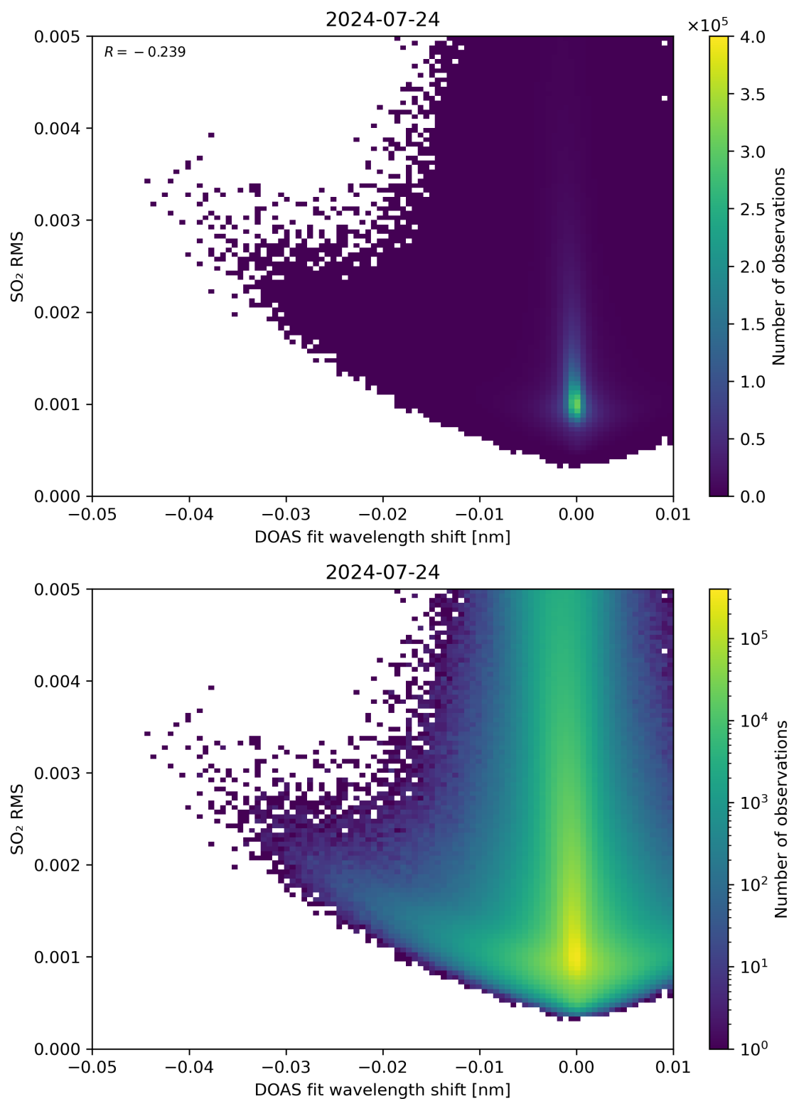
Figure 128: Scatter density plot of “DOAS fit wavelength shift” against “SO 2 RMS” for 2024-07-23 to 2024-07-25.
