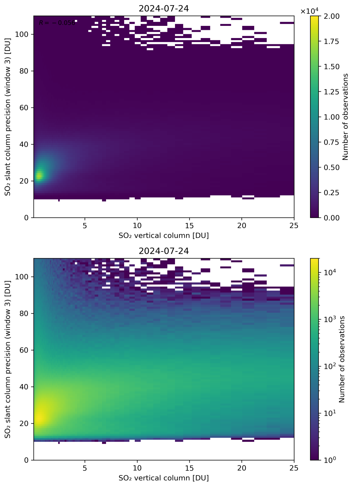
Figure 304: Scatter density plot of “SO 2 vertical column” against “SO 2 slant column precision (window 3)” for 2024-07-23 to 2024-07-25.
