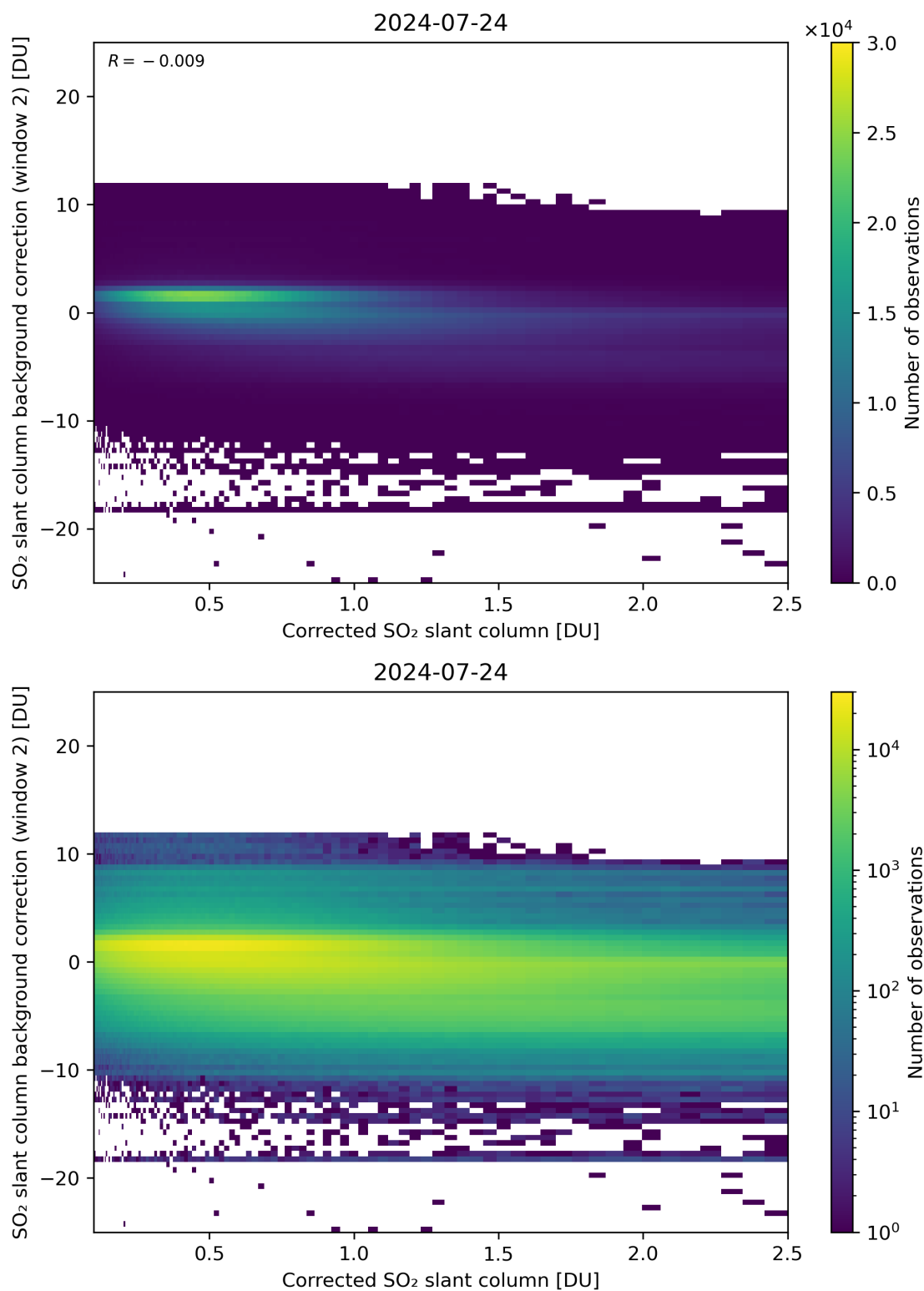
Figure 179: Scatter density plot of “Corrected SO 2 slant column” against “SO 2 slant column background correction (window 2)” for 2024-07-23 to 2024-07-25.
