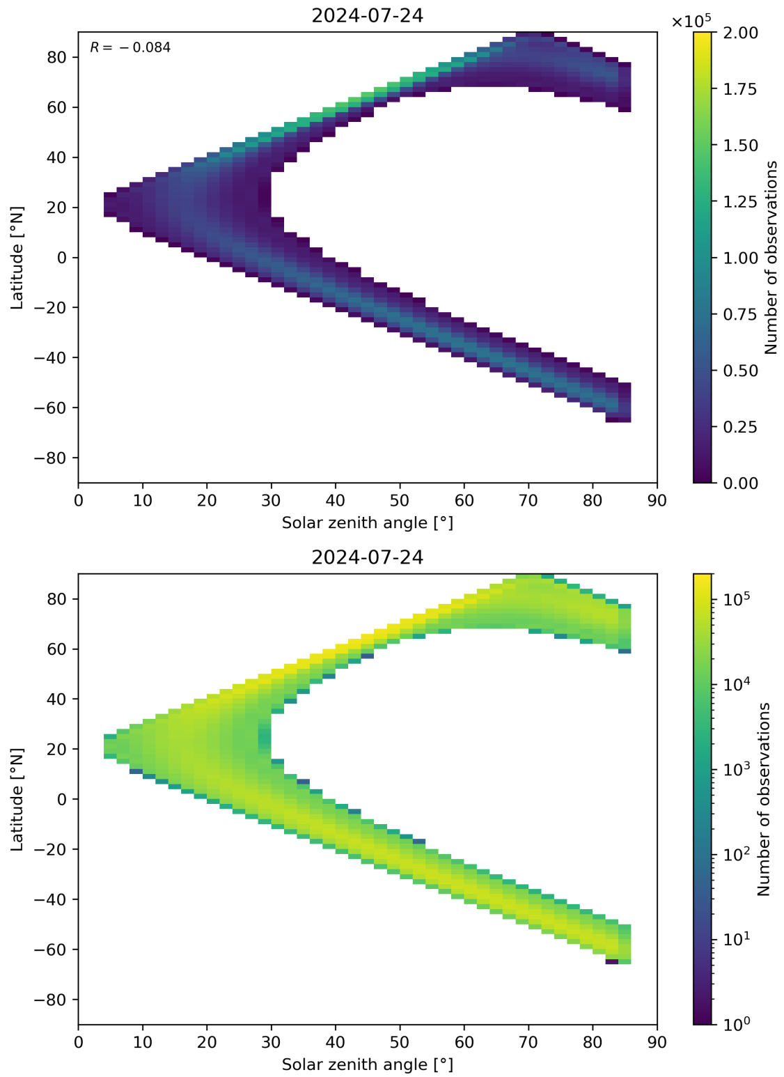
Figure 164: Scatter density plot of “Solar zenith angle” against “Latitude” for 2024-07-23 to 2024-07-25.
