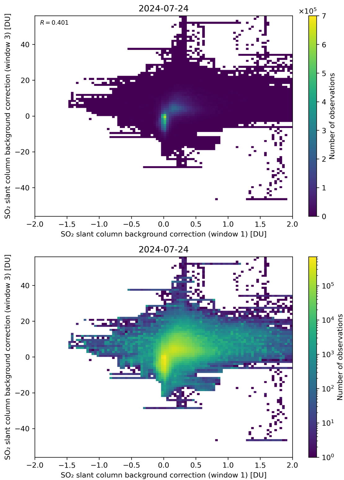
Figure 99: Scatter density plot of “SO 2 slant column background correction (window 1)” against “SO 2 slant column background correction (window 3)” for 2024-07-23 to 2024-07-25.
