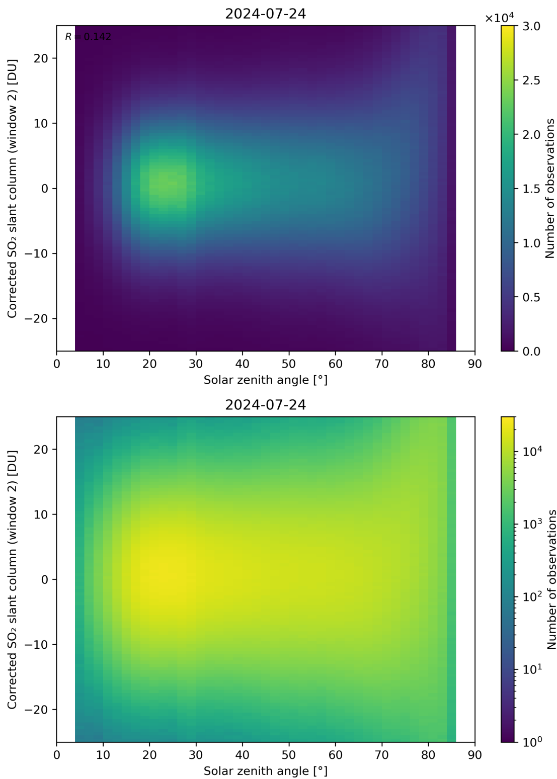
Figure 167: Scatter density plot of “Solar zenith angle” against “Corrected SO 2 slant column (window 2)” for 2024-07-23 to 2024-07-25.
