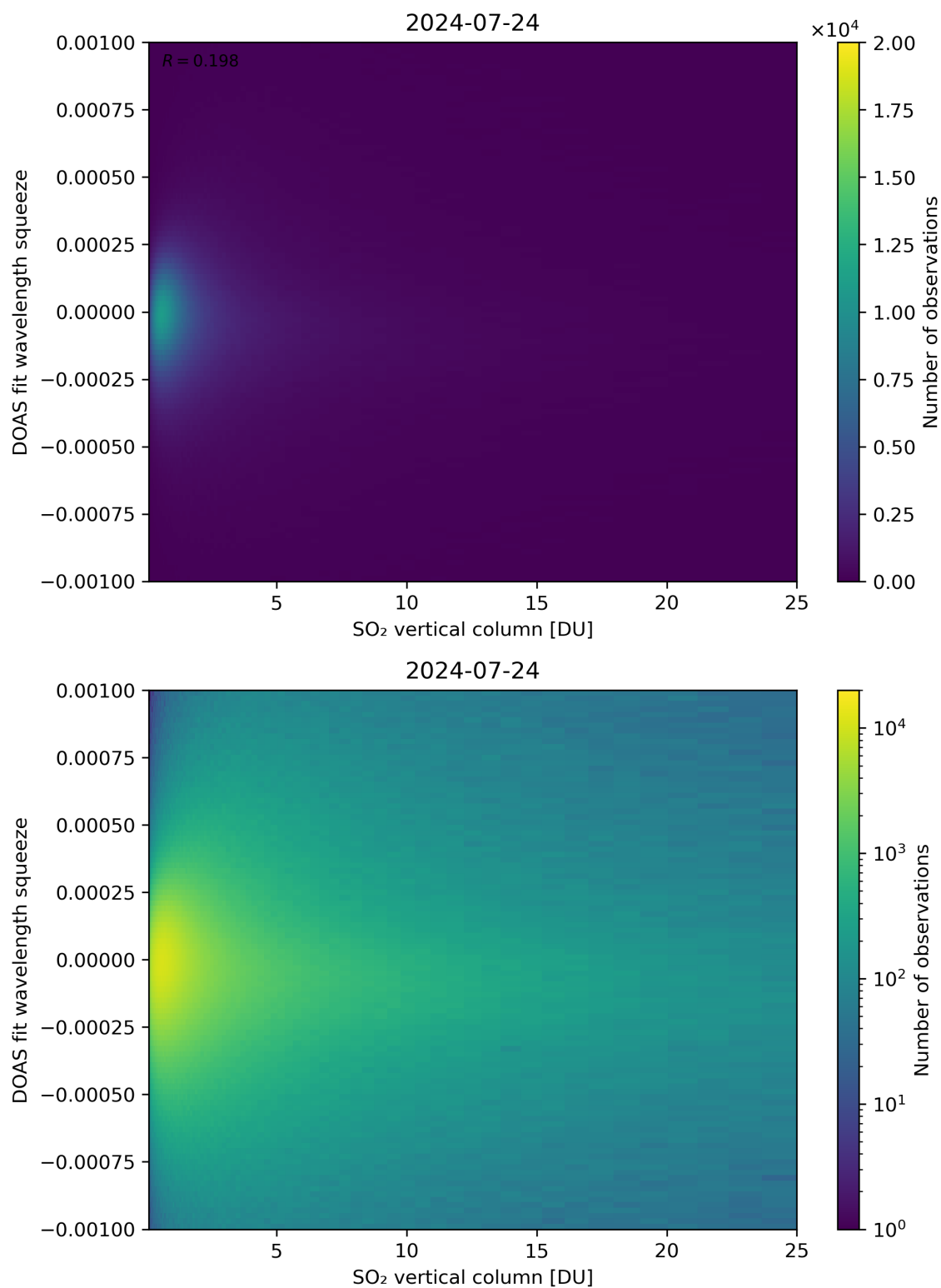
Figure 277: Scatter density plot of “SO 2 vertical column” against “DOAS fit wavelength squeeze” for 2024-07-23 to 2024-07-25.
