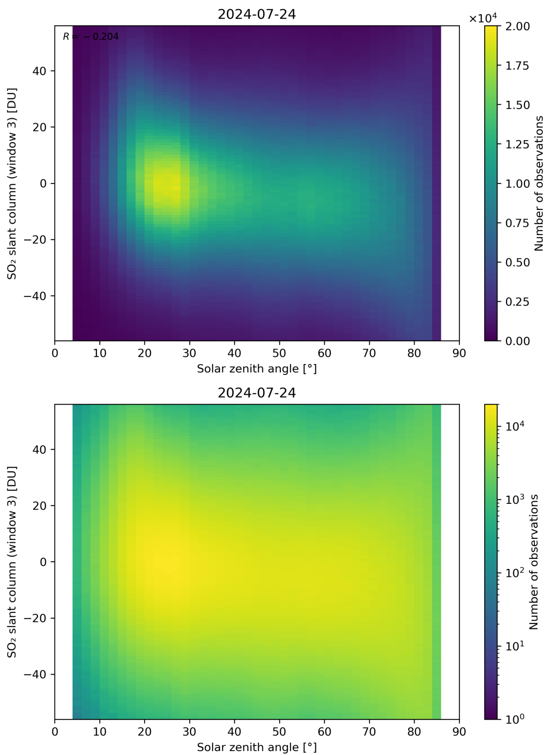
Figure 172: Scatter density plot of “Solar zenith angle” against “SO 2 slant column (window 3)” for 2024-07-23 to 2024-07-25.
