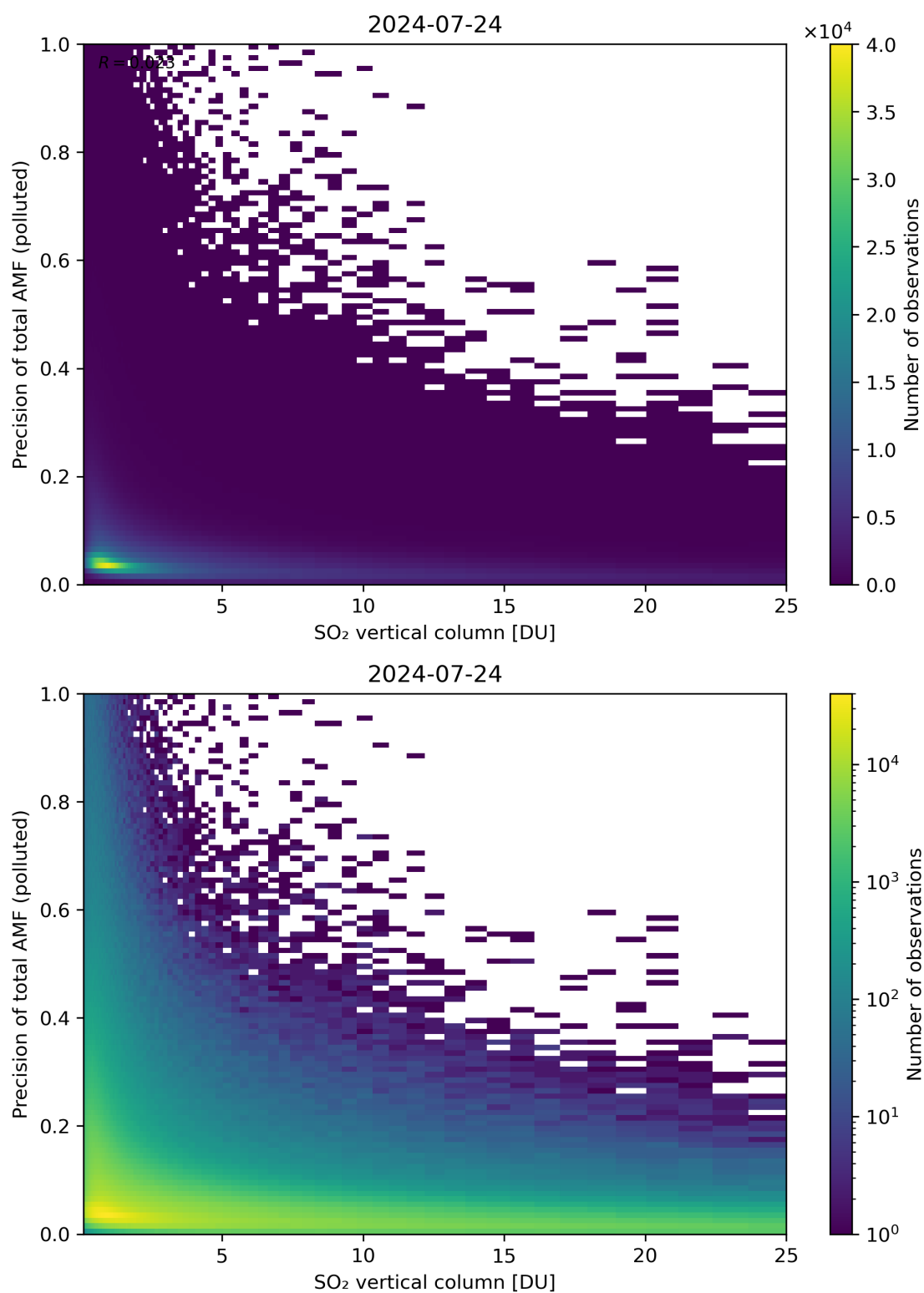
Figure 306: Scatter density plot of “SO 2 vertical column” against “Precision of total AMF (polluted)” for 2024-07-23 to 2024-07-25.
