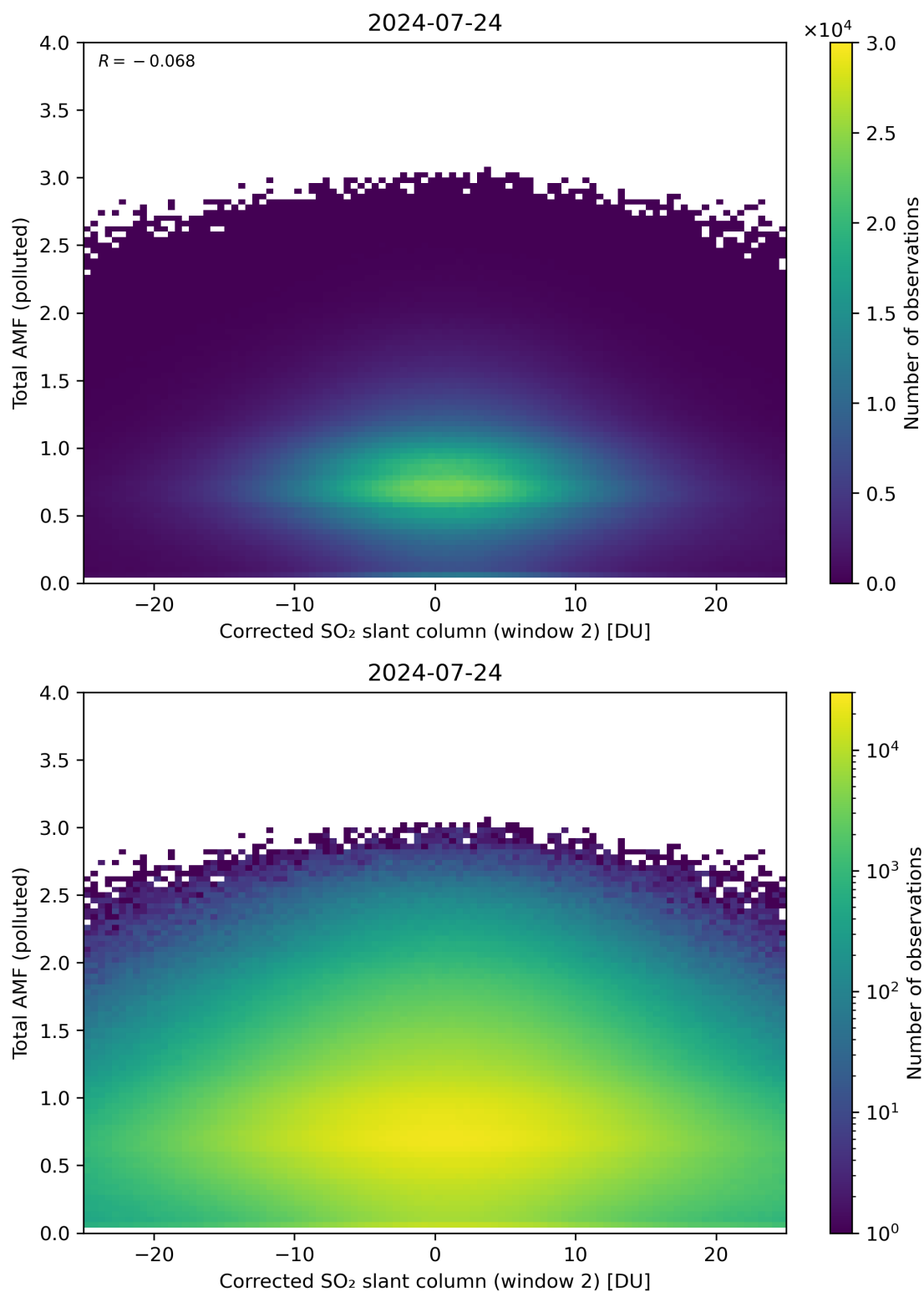
Figure 203: Scatter density plot of “Corrected SO 2 slant column (window 2)” against “Total AMF (polluted)” for 2024-07-23 to 2024-07-25.
