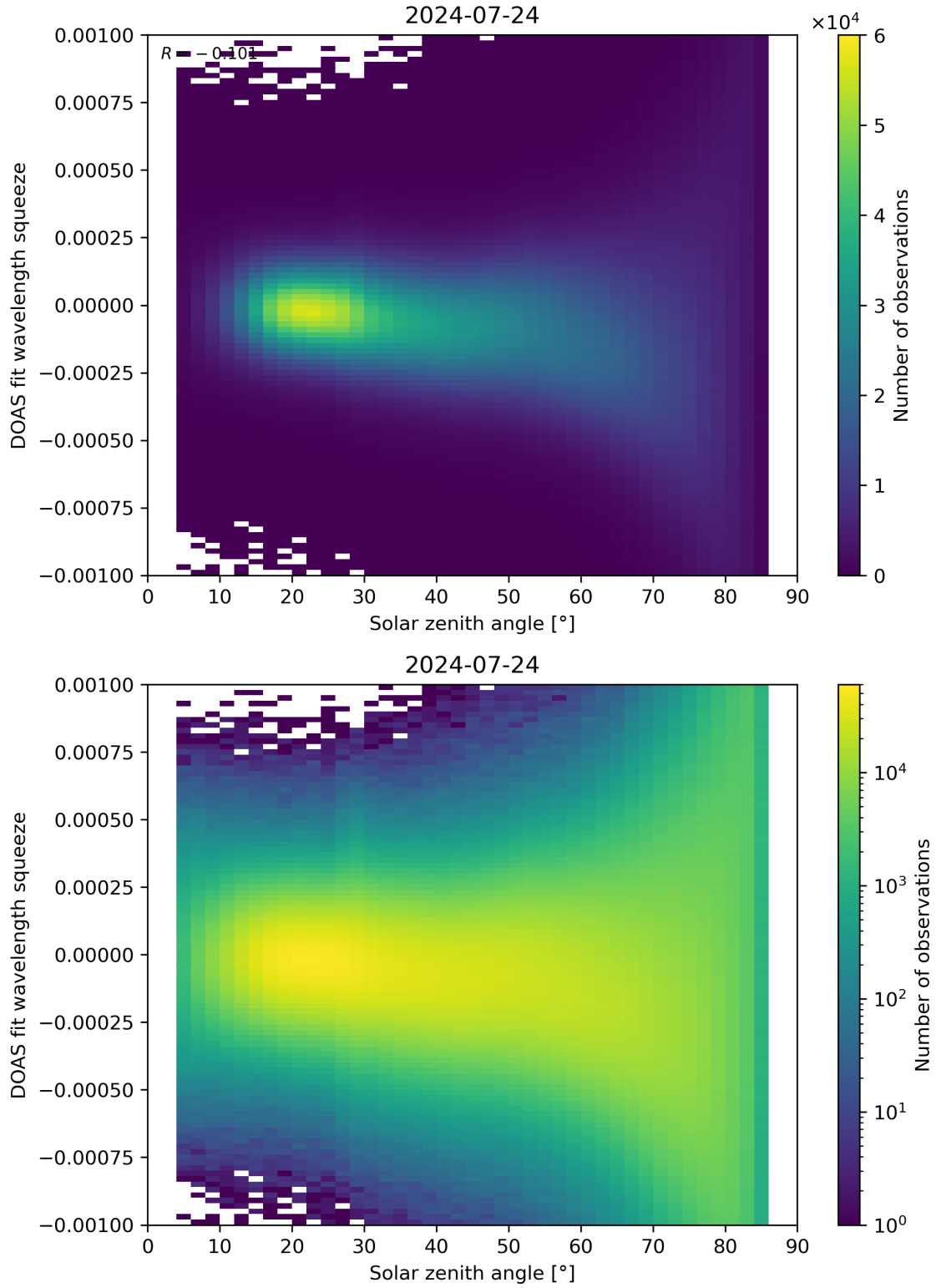
Figure 162: Scatter density plot of “Solar zenith angle” against “DOAS fit wavelength squeeze” for 2024-07-23 to 2024-07-25.
