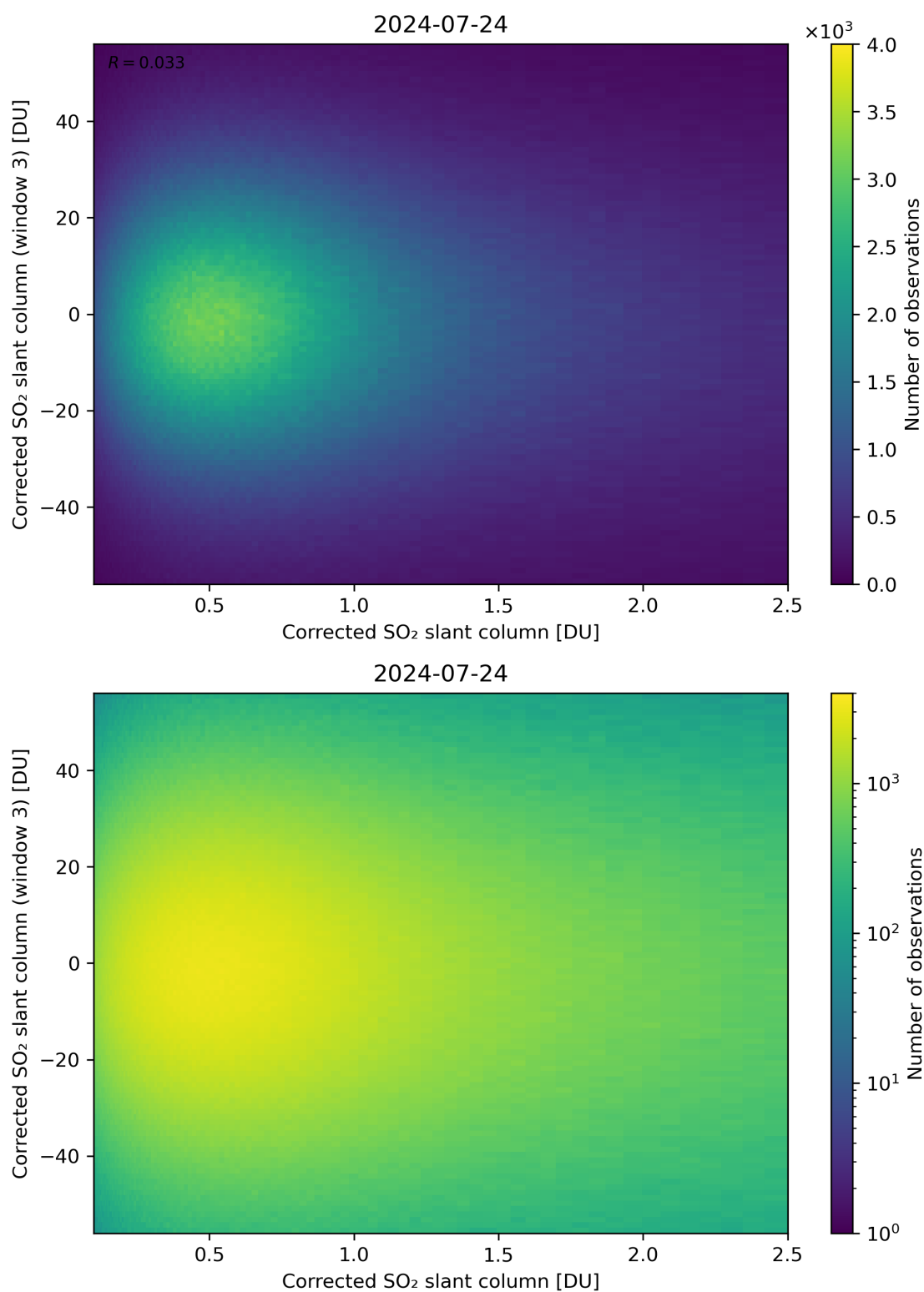
Figure 186: Scatter density plot of “Corrected SO 2 slant column” against “Corrected SO 2 slant column (window 3)” for 2024-07-23 to 2024-07-25.
