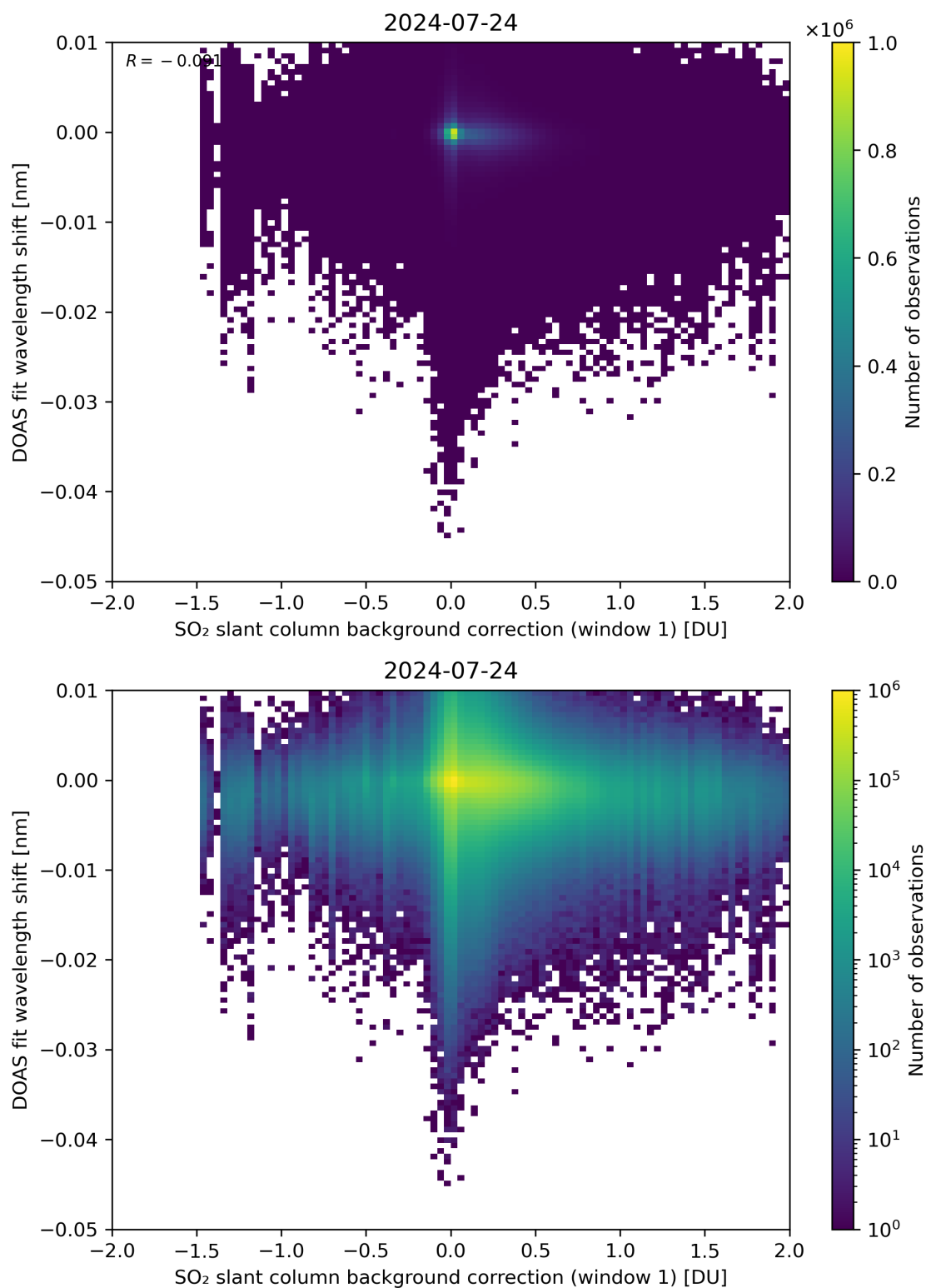
Figure 100: Scatter density plot of “SO 2 slant column background correction (window 1)” against “DOAS fit wavelength shift” for 2024-07-23 to 2024-07-25.
