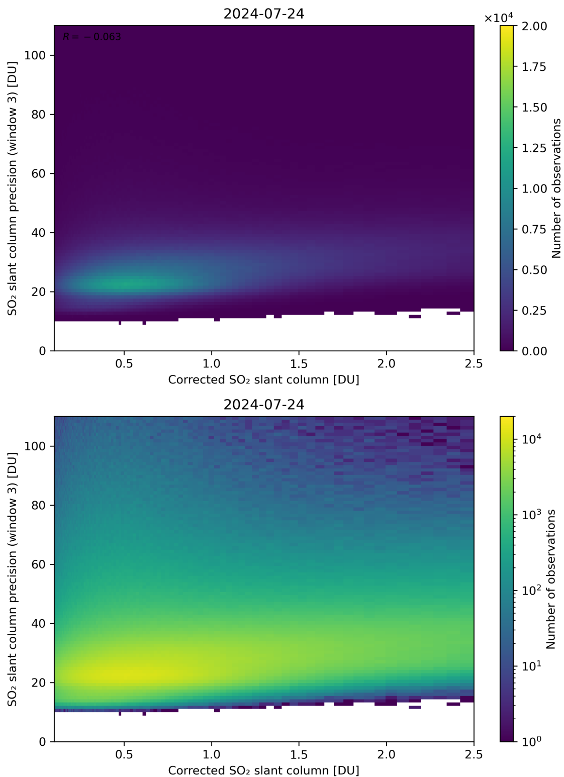
Figure 191: Scatter density plot of “Corrected SO 2 slant column” against “SO 2 slant column precision (window 3)” for 2024-07-23 to 2024-07-25.
