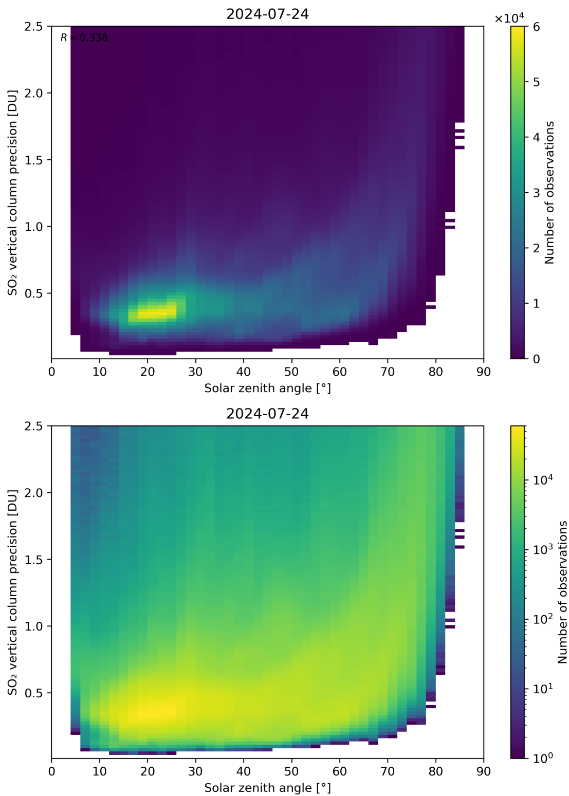
Figure 177: Scatter density plot of “Solar zenith angle” against “SO 2 vertical column precision” for 2024-07-23 to 2024-07-25.
