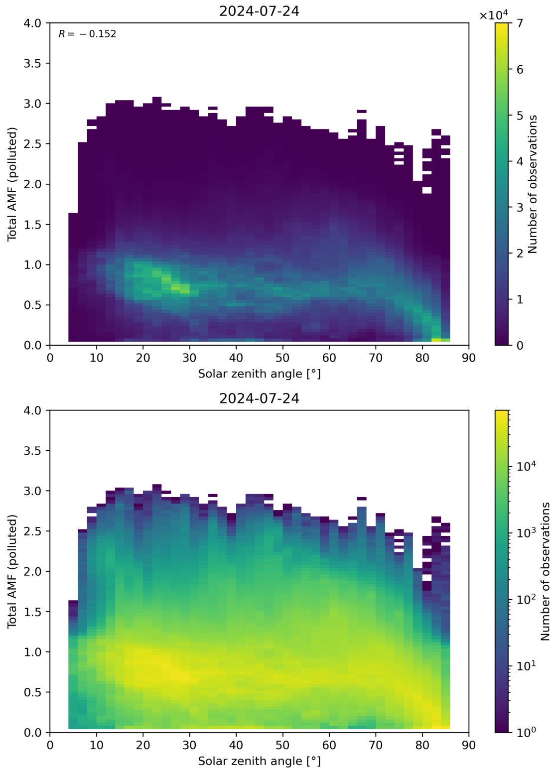
Figure 174: Scatter density plot of “Solar zenith angle” against “Total AMF (polluted)” for 2024-07-23 to 2024-07-25.
