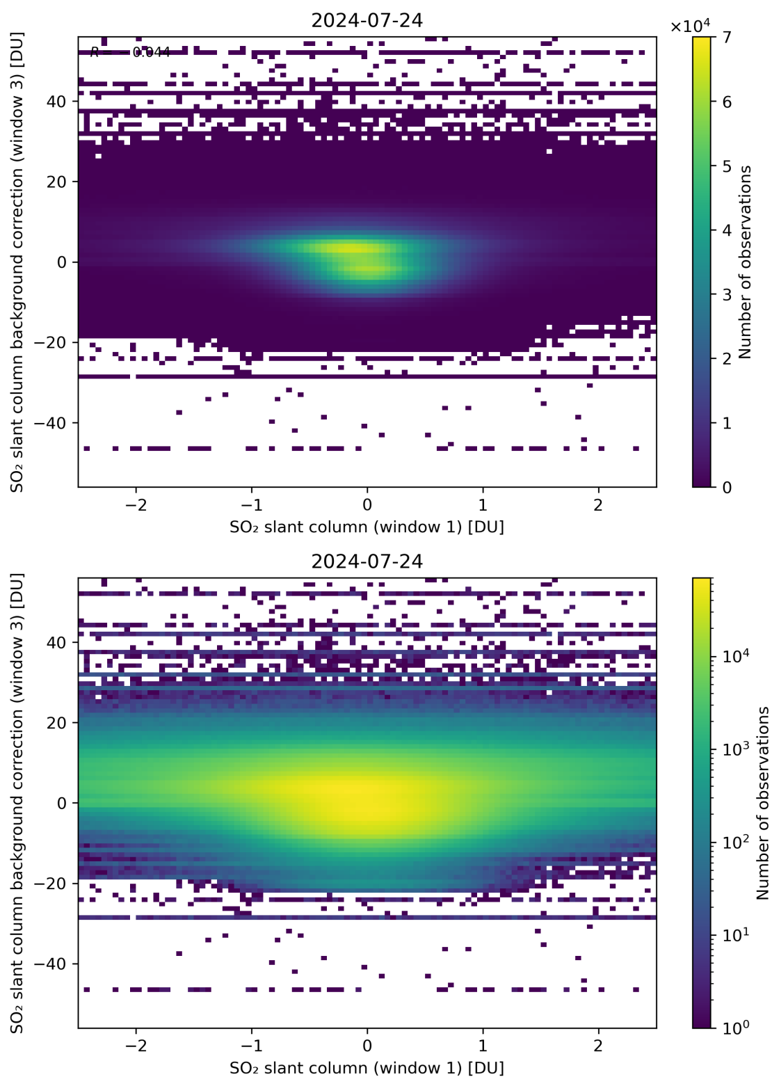
Figure 214: Scatter density plot of “SO 2 slant column (window 1)” against “SO 2 slant column background correction (window 3)” for 2024-07-23 to 2024-07-25.
