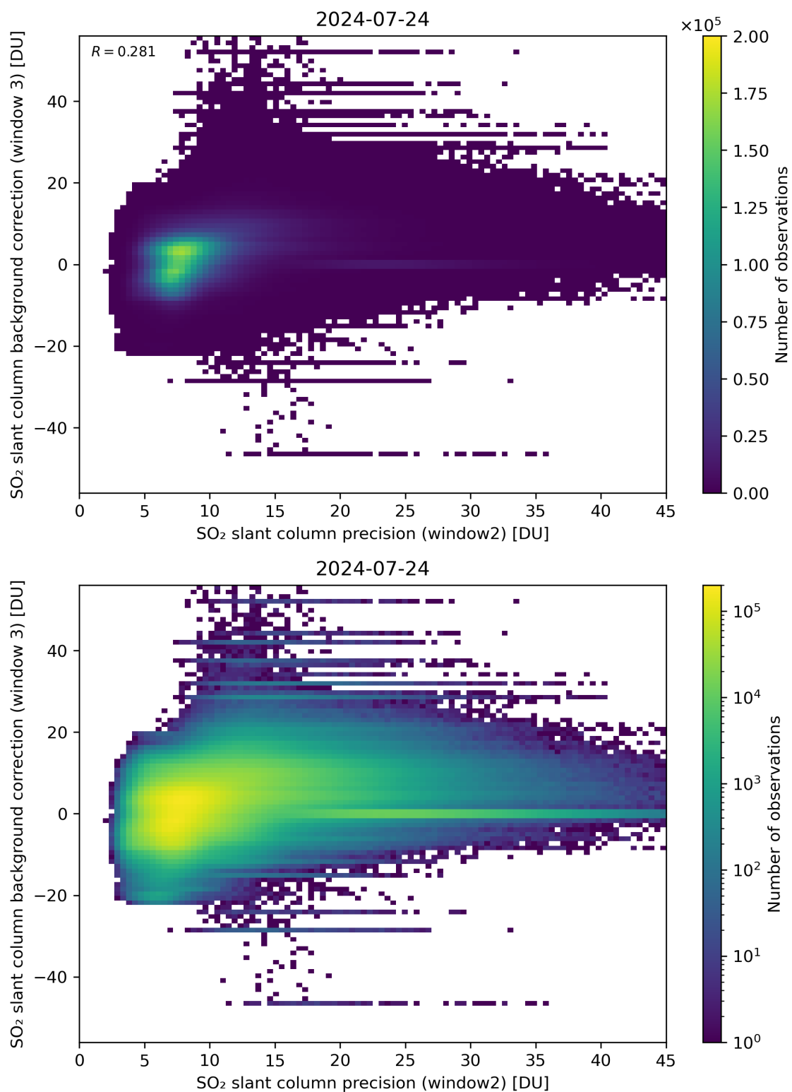
Figure 242: Scatter density plot of “SO 2 slant column precision (window2)” against “SO 2 slant column background correction (window 3)” for 2024-07-23 to 2024-07-25.
