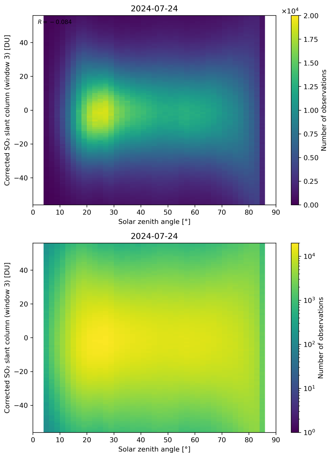
Figure 168: Scatter density plot of “Solar zenith angle” against “Corrected SO 2 slant column (window 3)” for 2024-07-23 to 2024-07-25.
