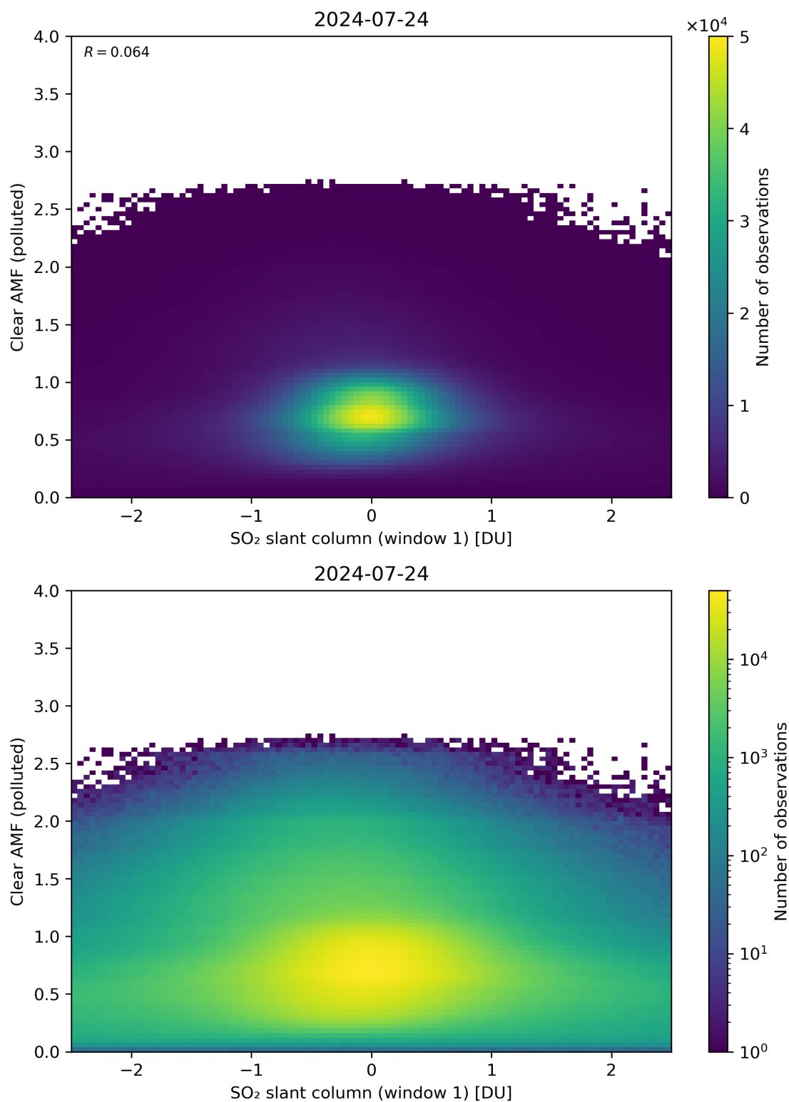
Figure 232: Scatter density plot of “SO 2 slant column (window 1)” against “Clear AMF (polluted)” for 2024-07-23 to 2024-07-25.
