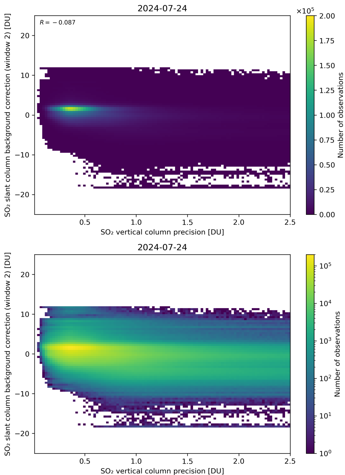
Figure 280: Scatter density plot of “SO 2 vertical column precision” against “SO 2 slant column background correction (window 2)” for 2024-07-23 to 2024-07-25.
