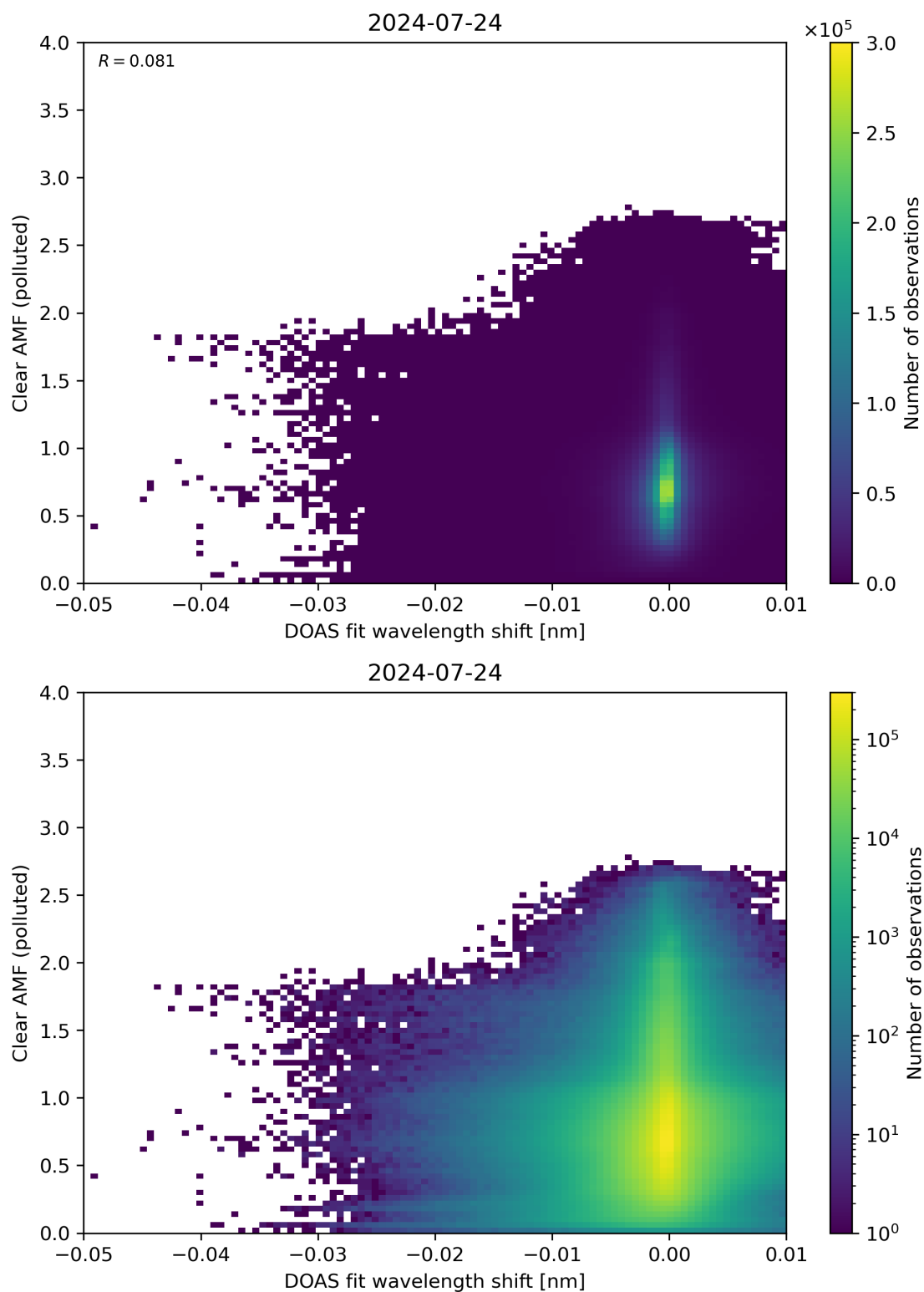
Figure 129: Scatter density plot of “DOAS fit wavelength shift” against “Clear AMF (polluted)” for 2024-07-23 to 2024-07-25.
