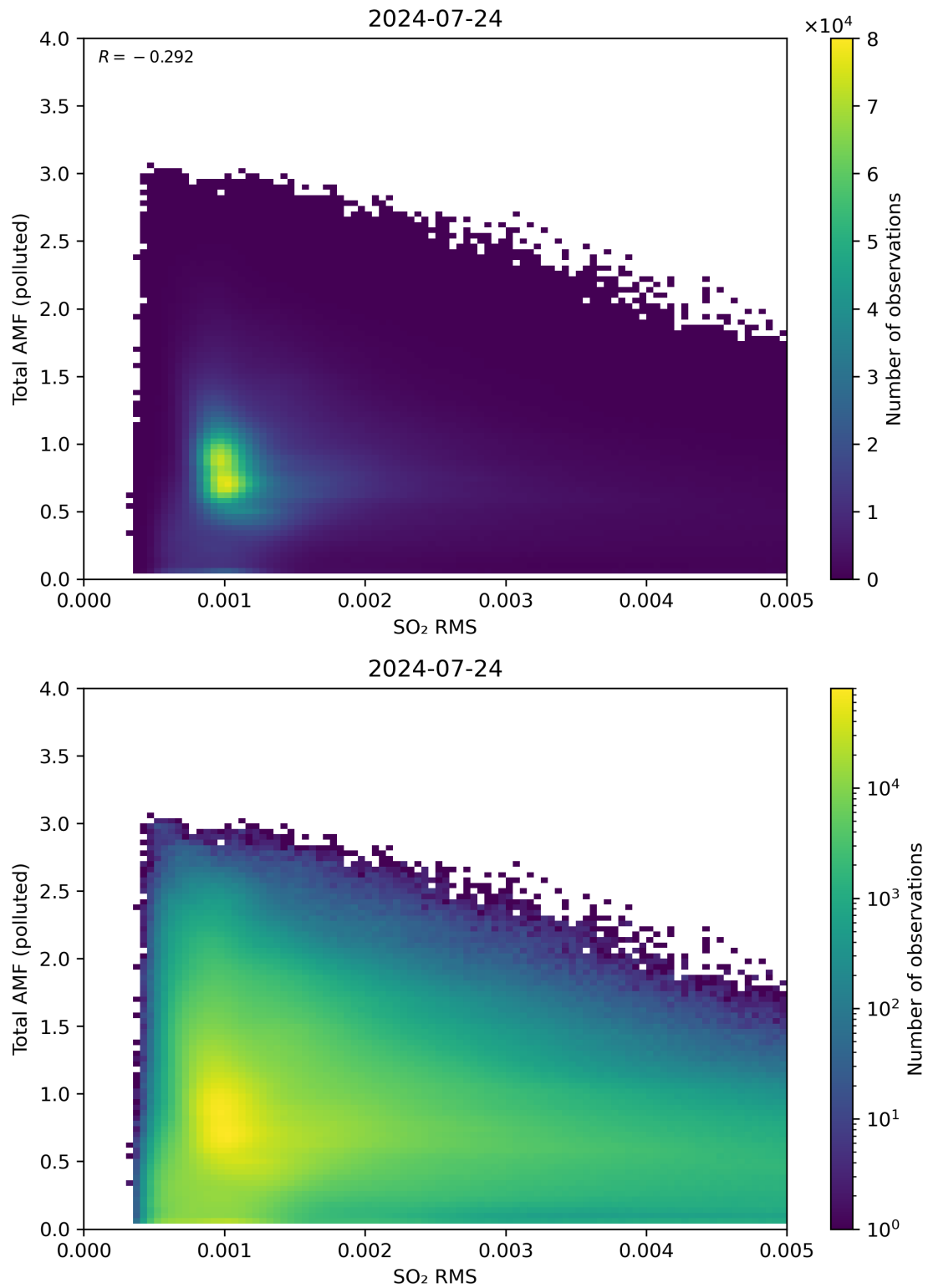
Figure 137: Scatter density plot of “SO 2 RMS” against “Total AMF (polluted)” for 2024-07-23 to 2024-07-25.
