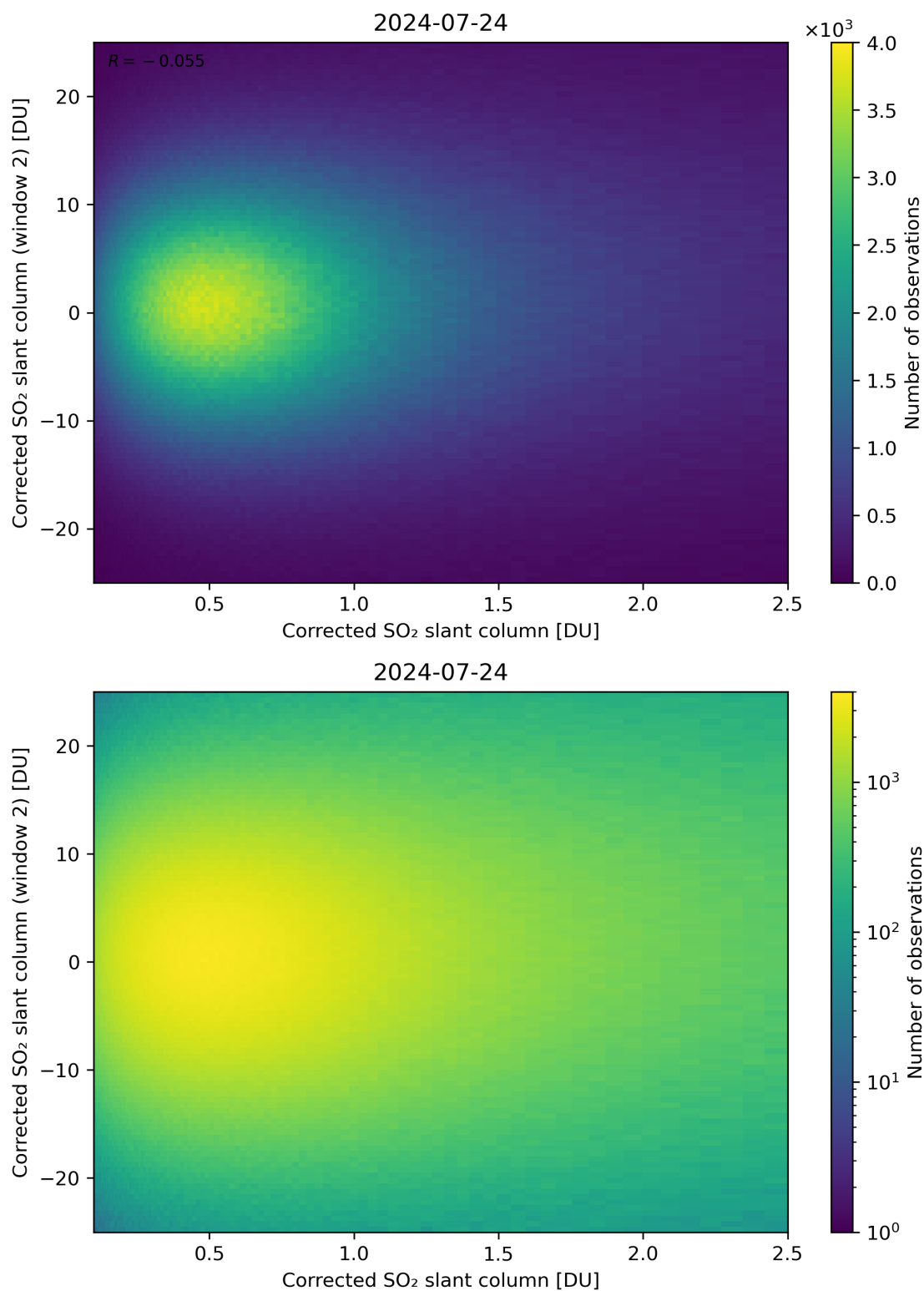
Figure 185: Scatter density plot of “Corrected SO 2 slant column” against “Corrected SO 2 slant column (window 2)” for 2024-07-23 to 2024-07-25.
