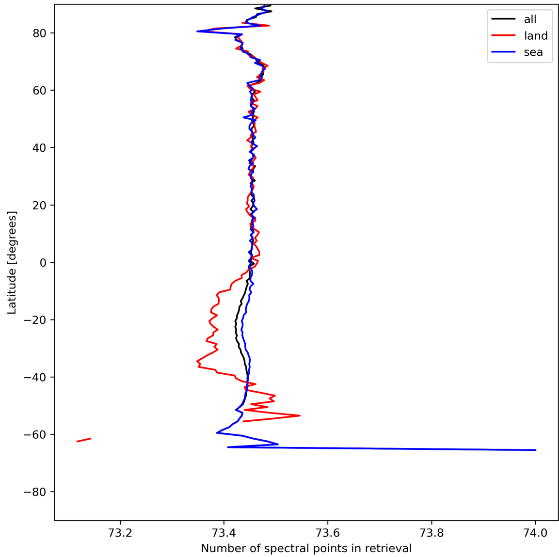
Figure 51: Zonal average of “Number of spectral points in retrieval” for 2024-07-23 to 2024-07-25.
