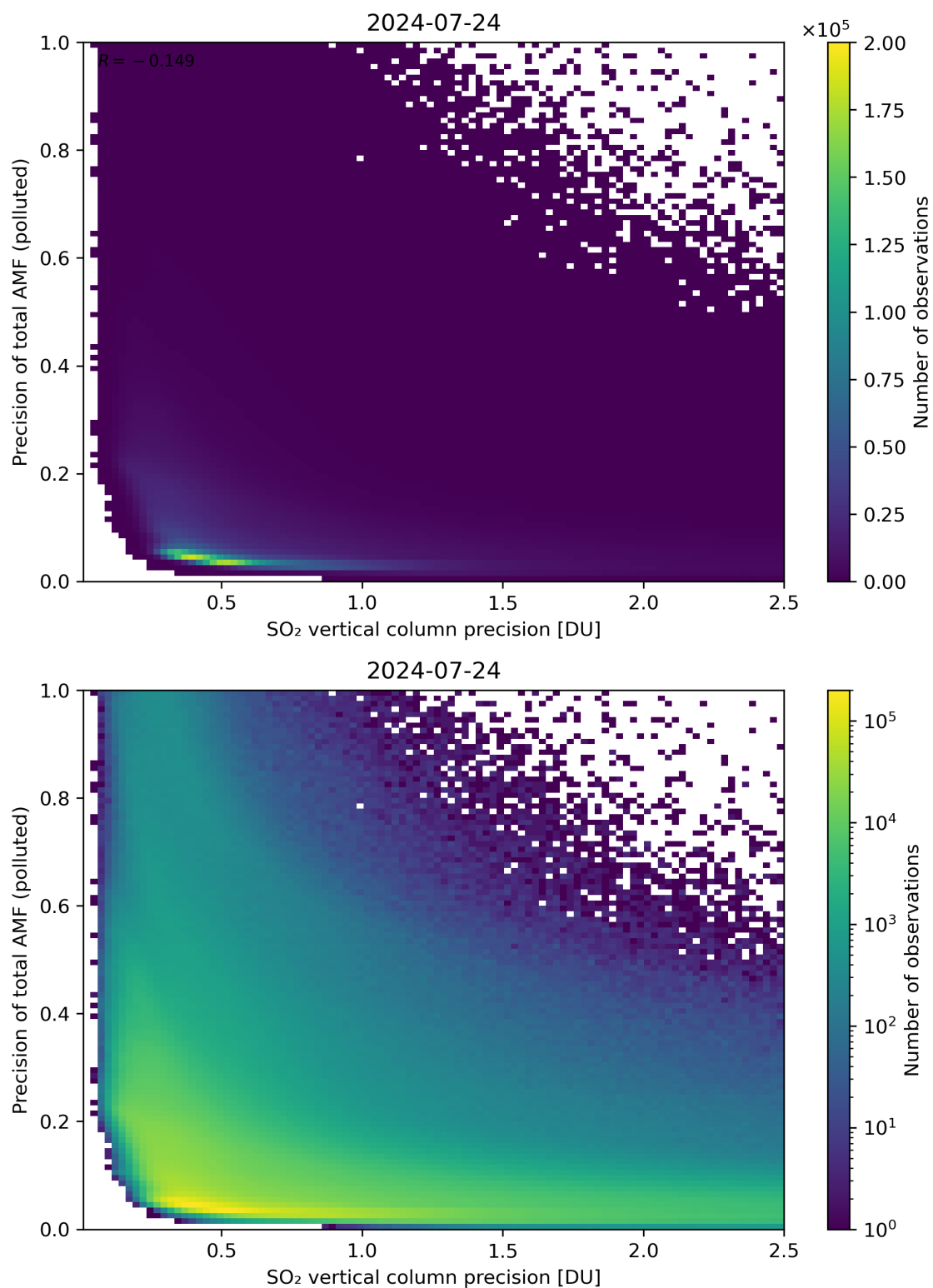
Figure 295: Scatter density plot of “SO 2 vertical column precision” against “Precision of total AMF (polluted)” for 2024-07-23 to 2024-07-25.
