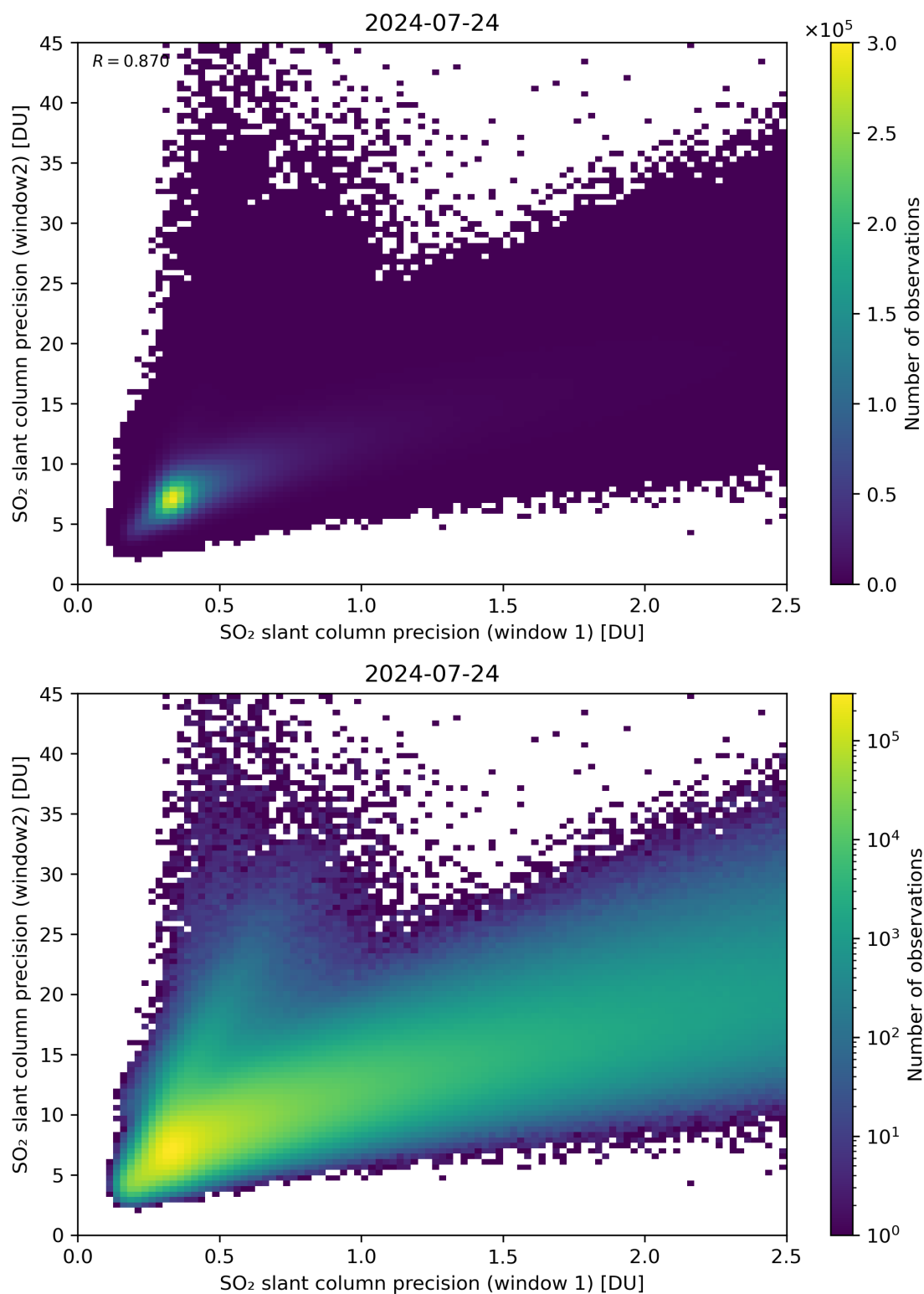
Figure 227: Scatter density plot of “SO 2 slant column precision (window 1)” against “SO 2 slant column precision (window2)” for 2024-07-23 to 2024-07-25.
