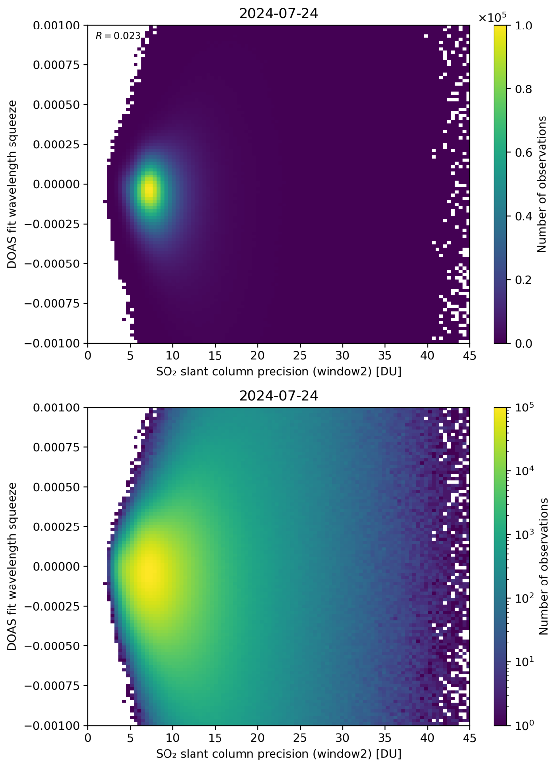
Figure 244: Scatter density plot of “SO 2 slant column precision (window2)” against “DOAS fit wavelength squeeze” for 2024-07-23 to 2024-07-25.
