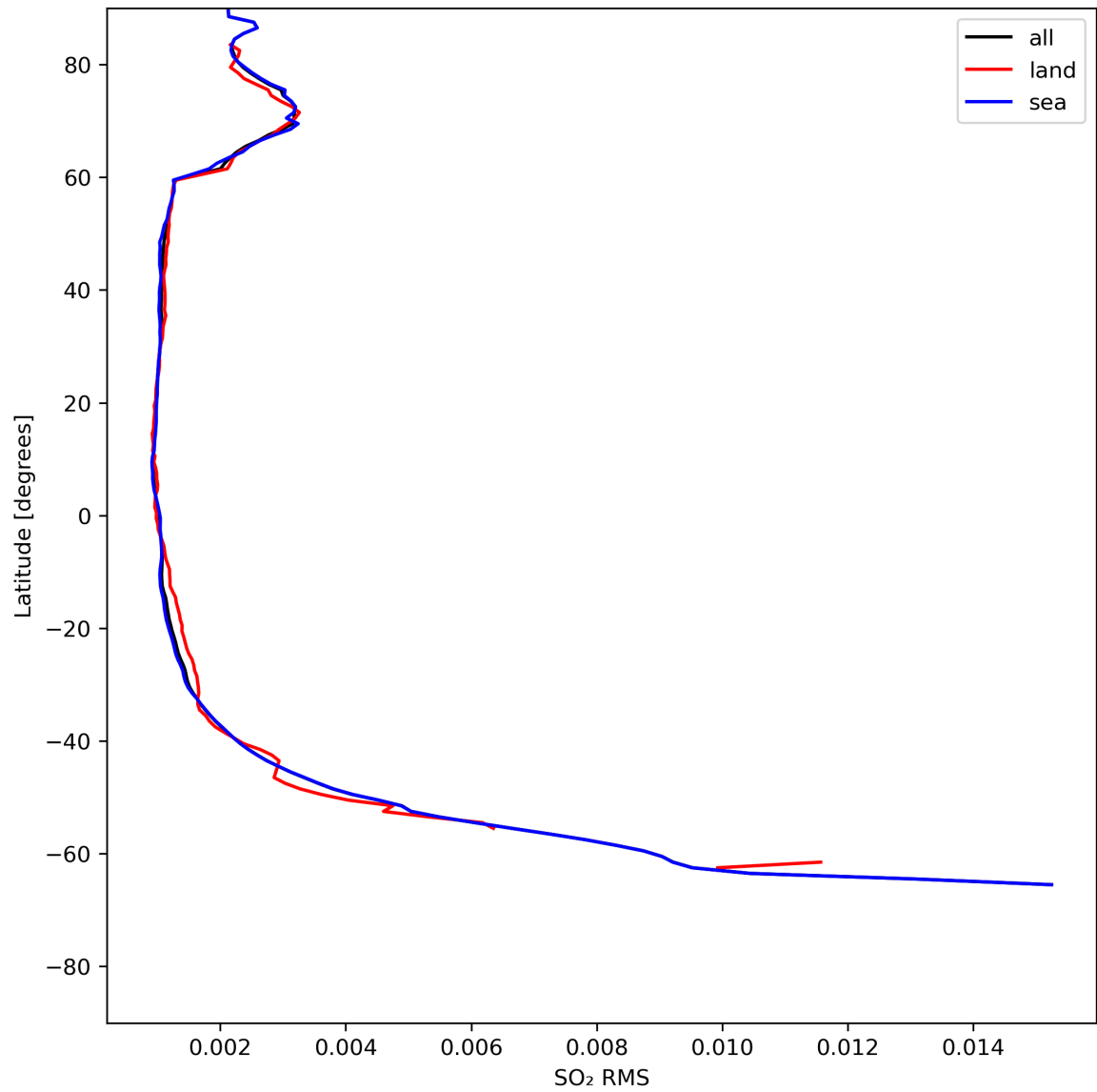
Figure 47: Zonal average of “SO 2 RMS” for 2024-07-23 to 2024-07-25.
