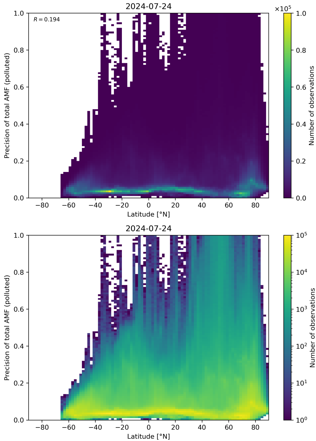
Figure 155: Scatter density plot of “Latitude” against “Precision of total AMF (polluted)” for 2024-07-23 to 2024-07-25.
