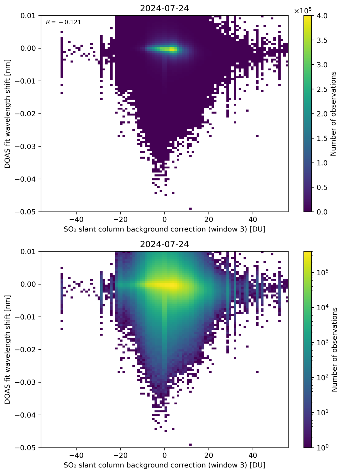
Figure 121: Scatter density plot of “SO 2 slant column background correction (window 3)” against “DOAS fit wavelength shift” for 2024-07-23 to 2024-07-25.
