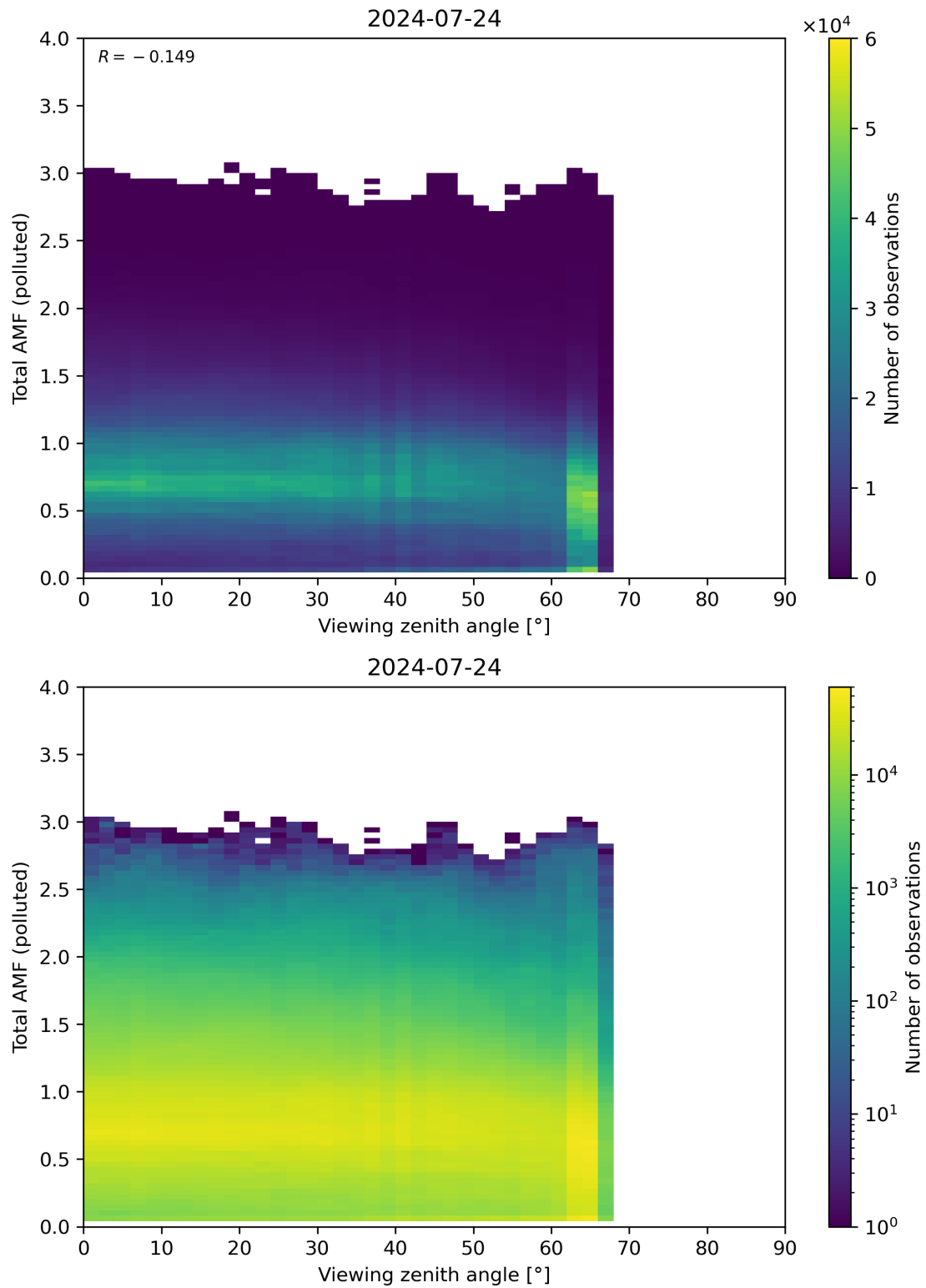
Figure 325: Scatter density plot of “Viewing zenith angle” against “Total AMF (polluted)” for 2024-07-23 to 2024-07-25.
