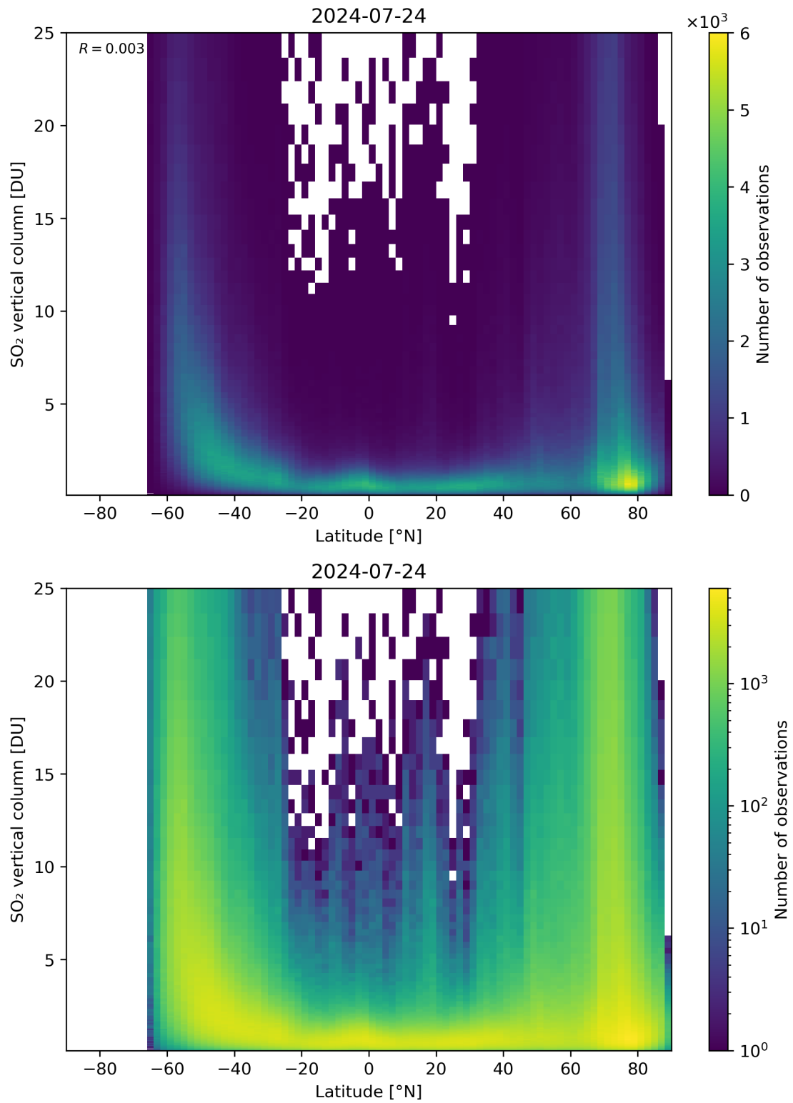
Figure 156: Scatter density plot of “Latitude” against “SO 2 vertical column” for 2024-07-23 to 2024-07-25.
