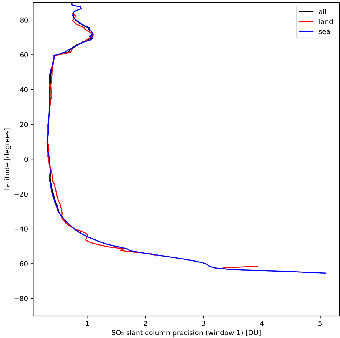
Figure 34: Zonal average of “SO 2 slant column precision (window 1)” for 2024-07-23 to 2024-07-25.
