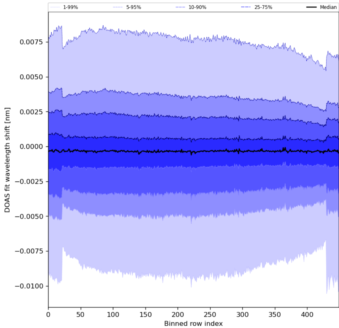
Figure 91: Along track statistics of “DOAS fit wavelength shift” for 2024-07-23 to 2024-07-25
