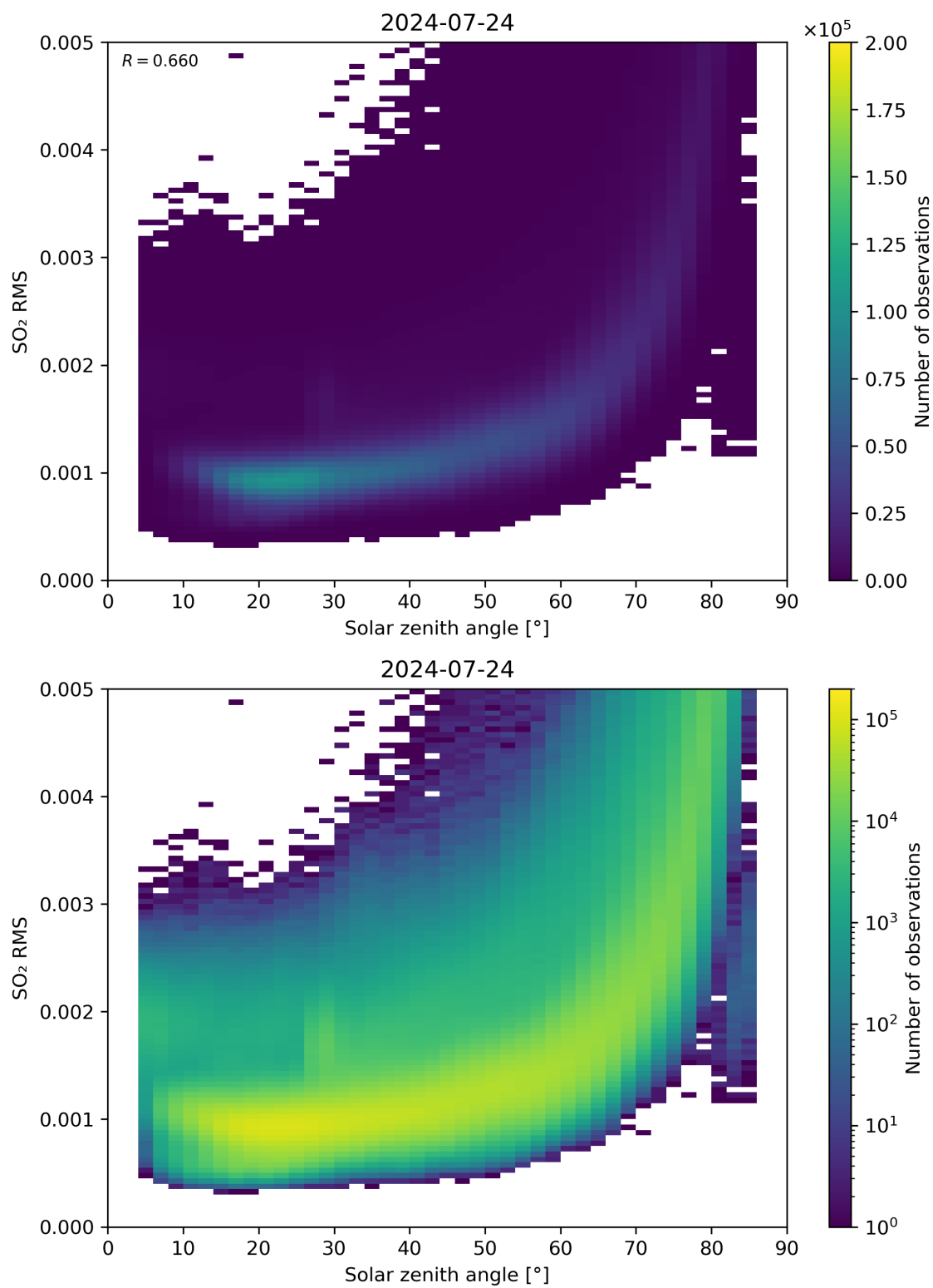
Figure 163: Scatter density plot of “Solar zenith angle” against “SO 2 RMS” for 2024-07-23 to 2024-07-25.
