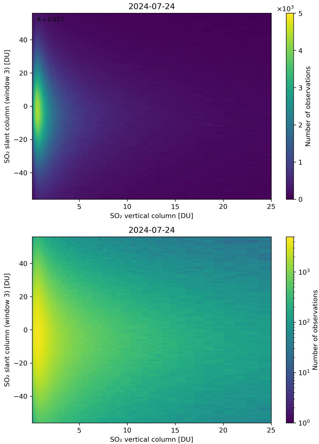
Figure 303: Scatter density plot of “SO 2 vertical column” against “SO 2 slant column (window 3)” for 2024-07-23 to 2024-07-25.
