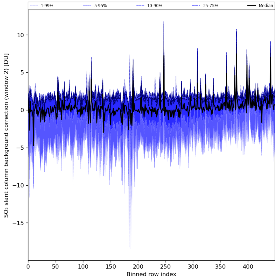
Figure 86: Along track statistics of “SO 2 slant column background correction (window 2)” for 2024-07-23 to 2024-07-25
