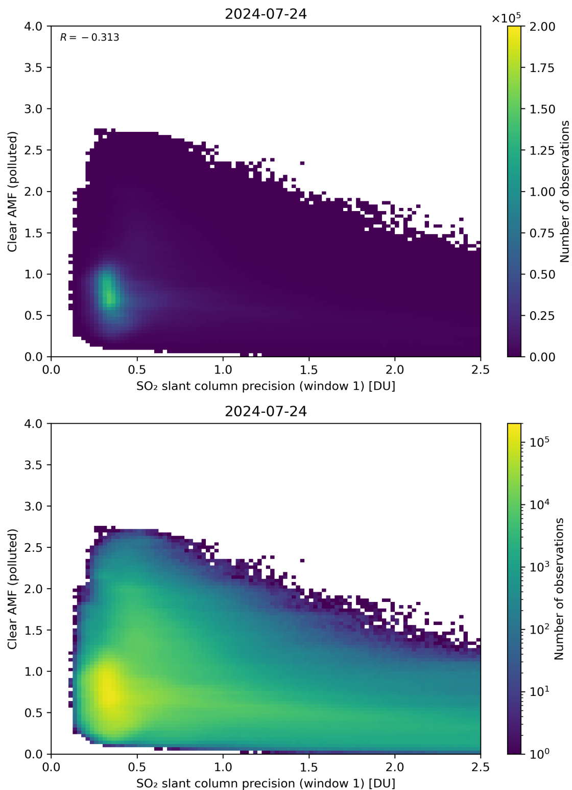
Figure 224: Scatter density plot of “SO 2 slant column precision (window 1)” against “Clear AMF (polluted)” for 2024-07-23 to 2024-07-25.
