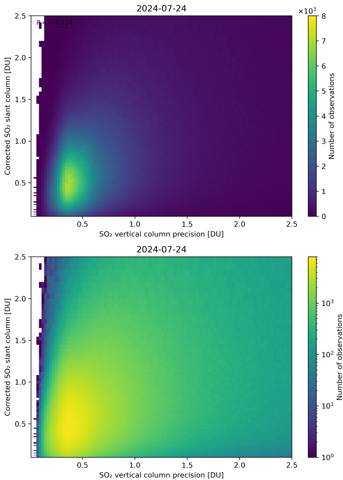
Figure 286: Scatter density plot of “SO 2 vertical column precision” against “Corrected SO 2 slant column” for 2024-07-23 to 2024-07-25.
