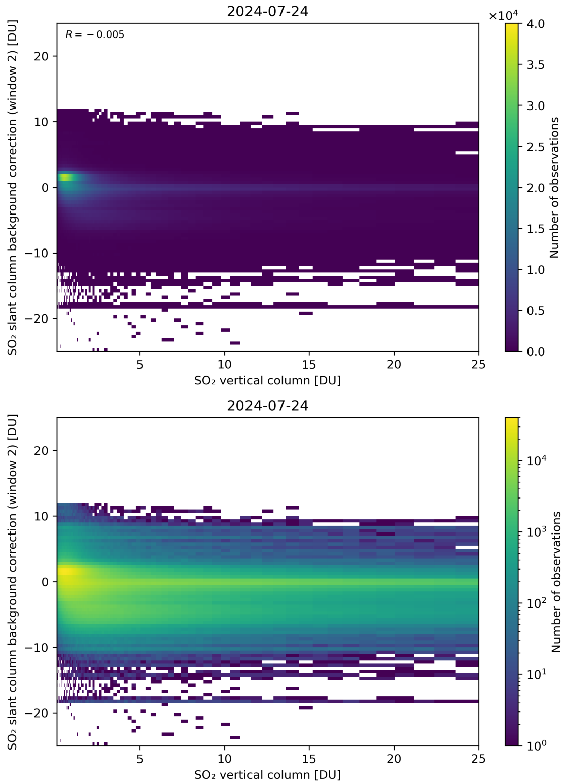
Figure 274: Scatter density plot of “SO 2 vertical column” against “SO 2 slant column background correction (window 2)” for 2024-07-23 to 2024-07-25.
