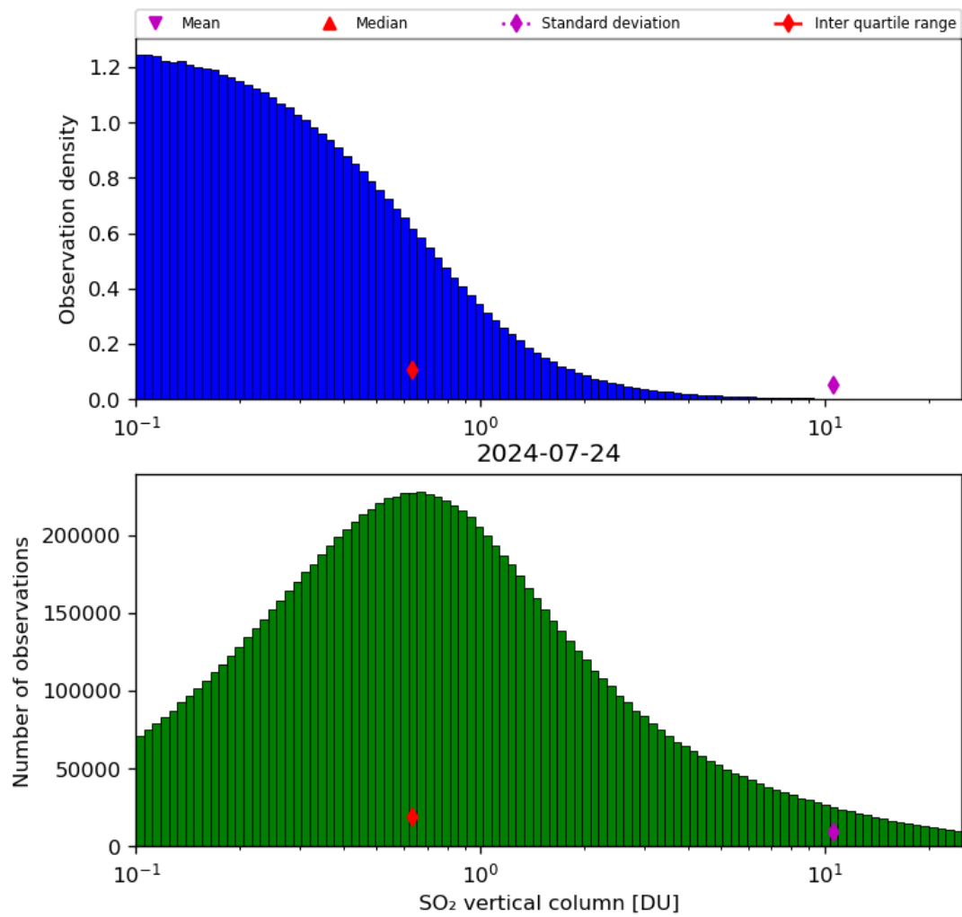
Figure 53: Histogram of “SO 2 vertical column” for 2024-07-23 to 2024-07-25
