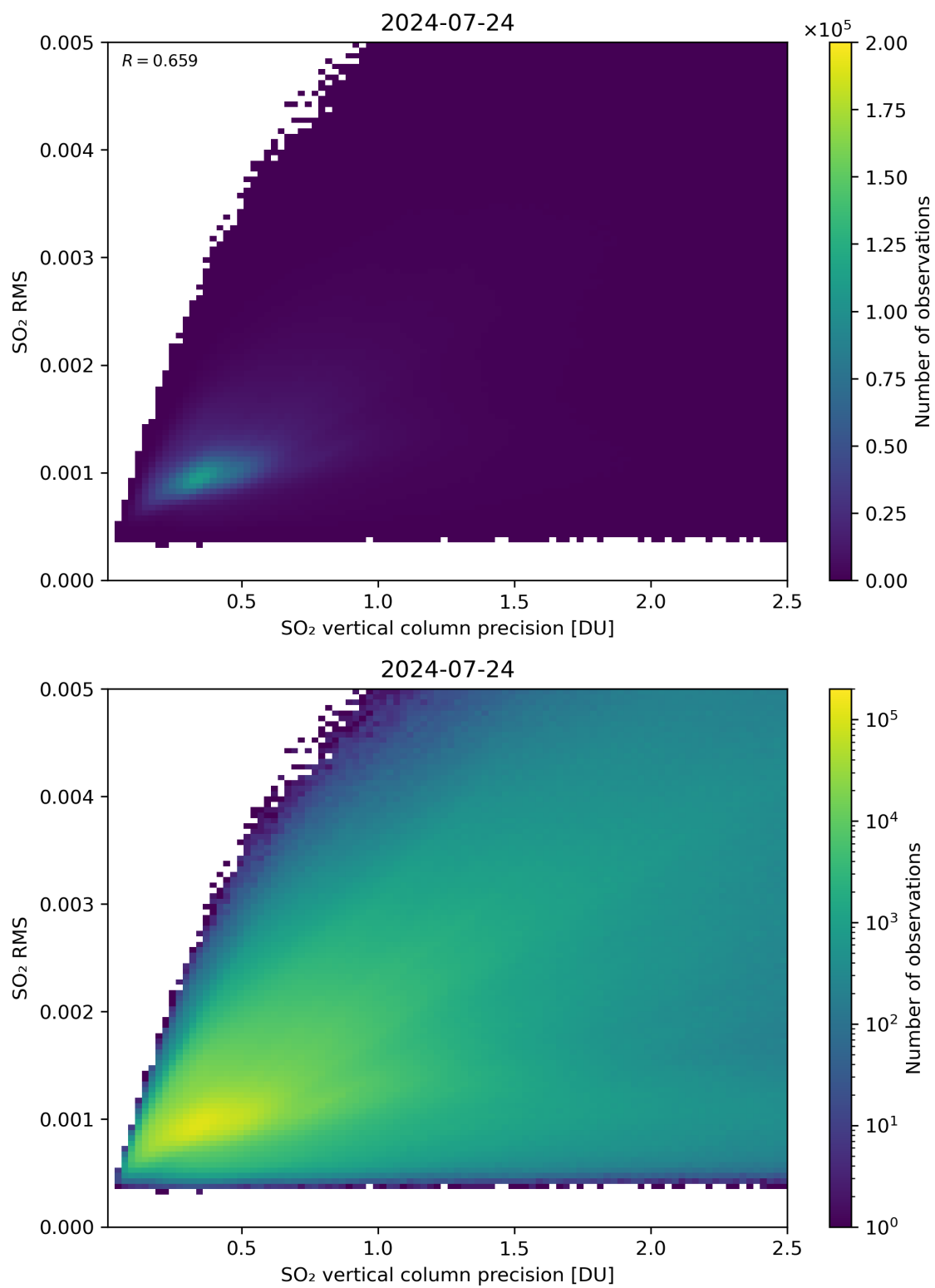
Figure 284: Scatter density plot of “SO 2 vertical column precision” against “SO 2 RMS” for 2024-07-23 to 2024-07-25.
