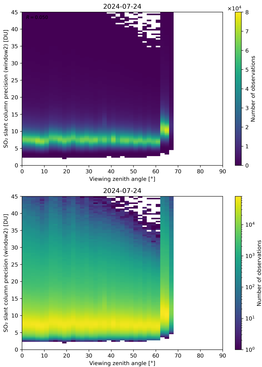
Figure 322: Scatter density plot of “Viewing zenith angle” against “SO 2 slant column precision (window2)” for 2024-07-23 to 2024-07-25.
