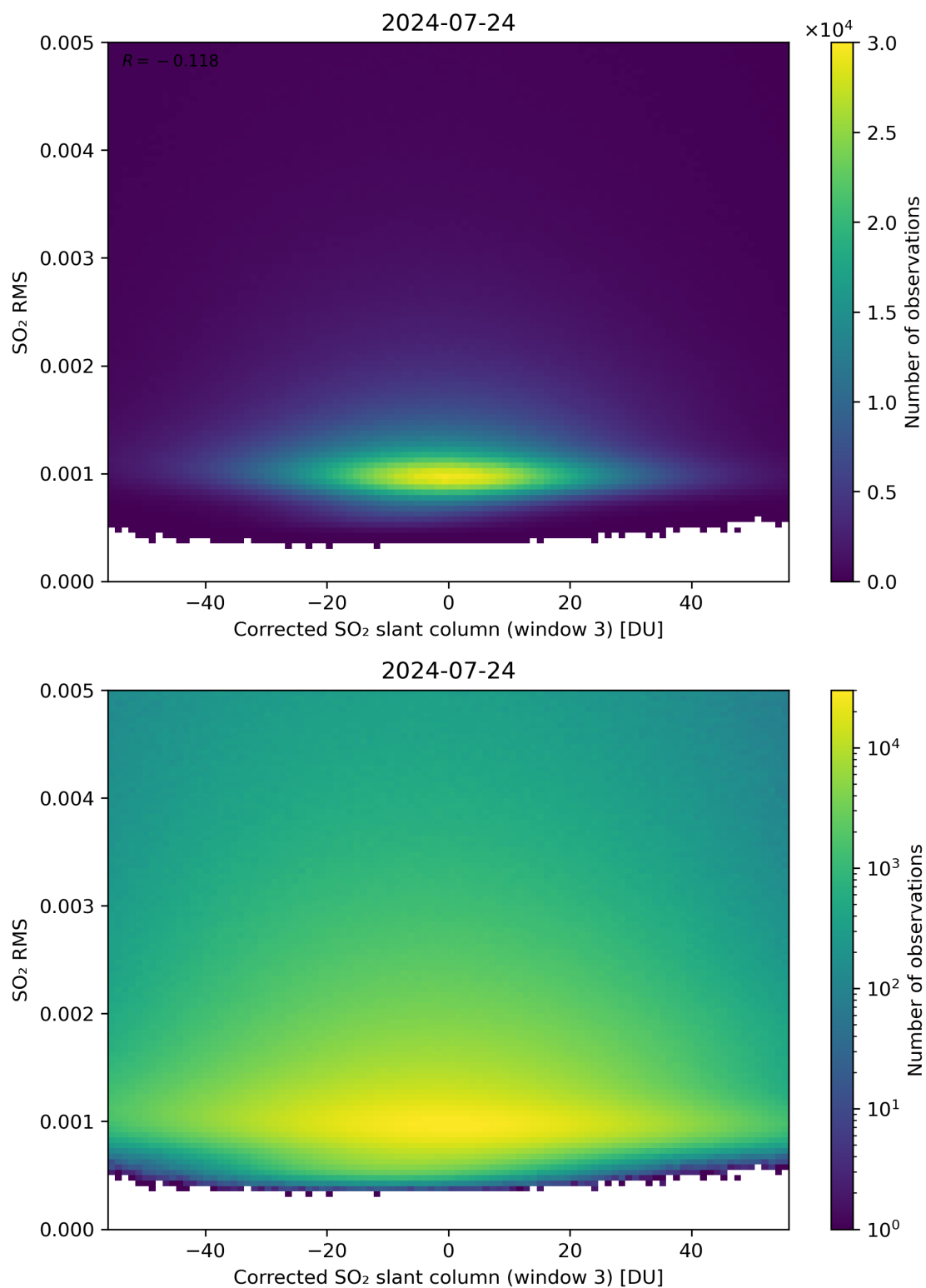
Figure 208: Scatter density plot of “Corrected SO 2 slant column (window 3)” against “SO 2 RMS” for 2024-07-23 to 2024-07-25.
