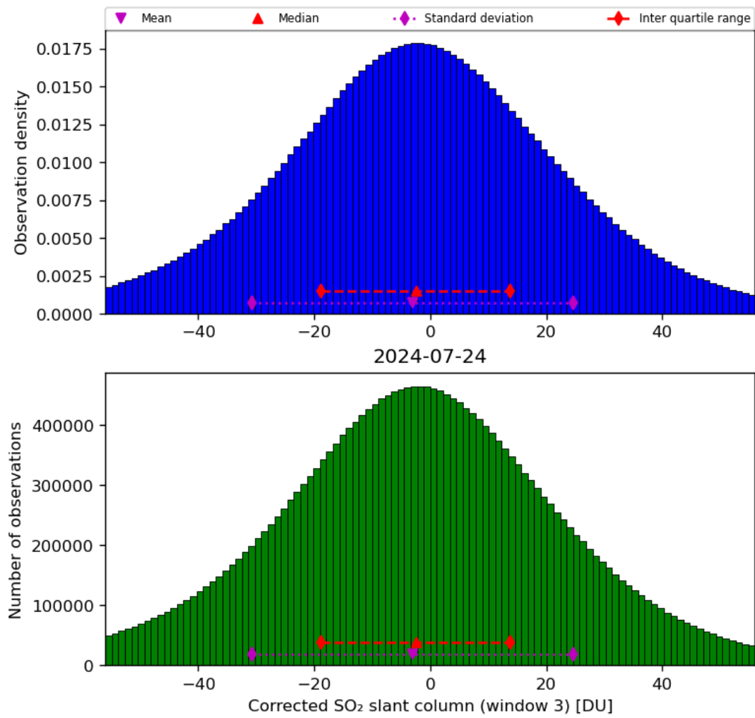
Figure 66: Histogram of “Corrected SO 2 slant column (window 3)” for 2024-07-23 to 2024-07-25
