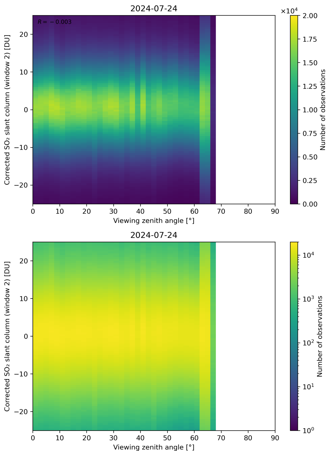
Figure 318: Scatter density plot of “Viewing zenith angle” against “Corrected SO 2 slant column (window 2)” for 2024-07-23 to 2024-07-25.
