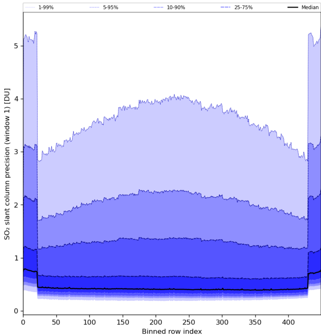
Figure 80: Along track statistics of “SO 2 slant column precision (window 1)” for 2024-07-23 to 2024-07-25
