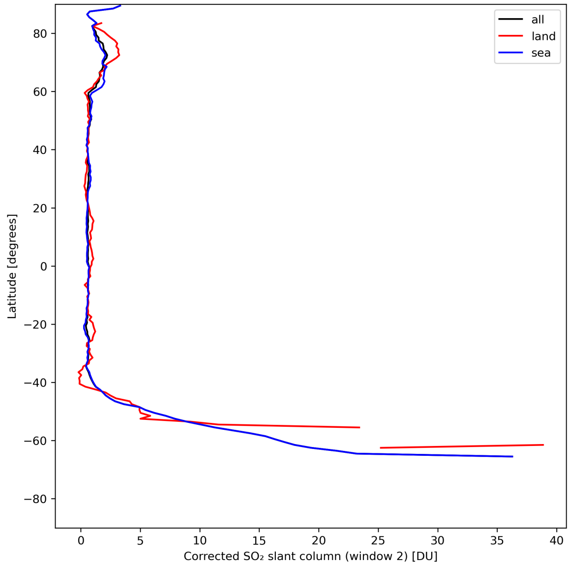
Figure 39: Zonal average of “Corrected SO 2 slant column (window 2)” for 2024-07-23 to 2024-07-25.
