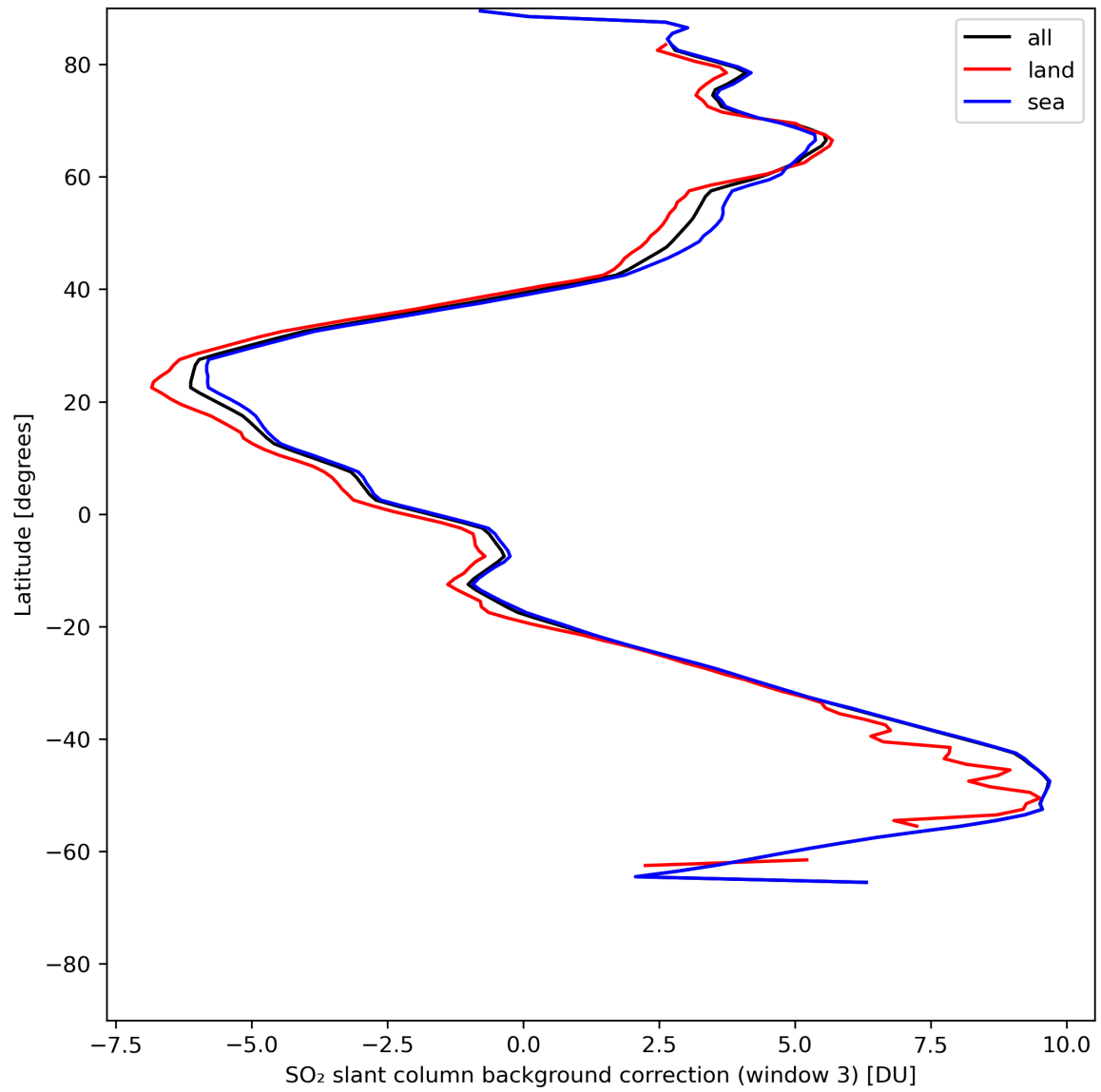
Figure 44: Zonal average of “SO 2 slant column background correction (window 3)” for 2024-07-23 to 2024-07-25.
