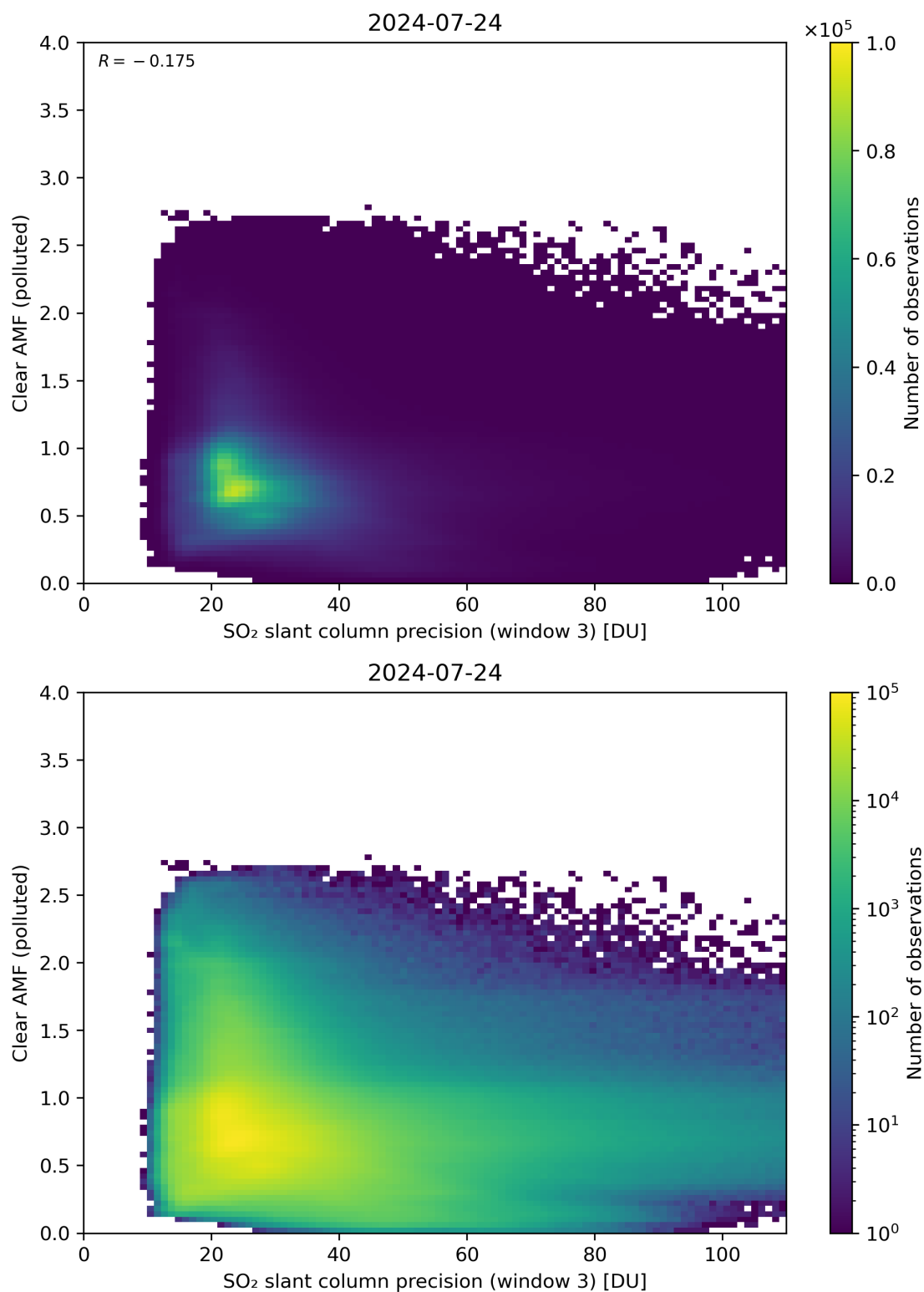
Figure 261: Scatter density plot of “SO 2 slant column precision (window 3)” against “Clear AMF (polluted)” for 2024-07-23 to 2024-07-25.
