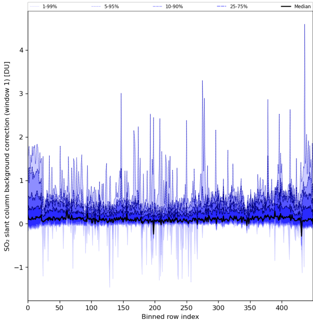
Figure 82: Along track statistics of “SO 2 slant column background correction (window 1)” for 2024-07-23 to 2024-07-25
