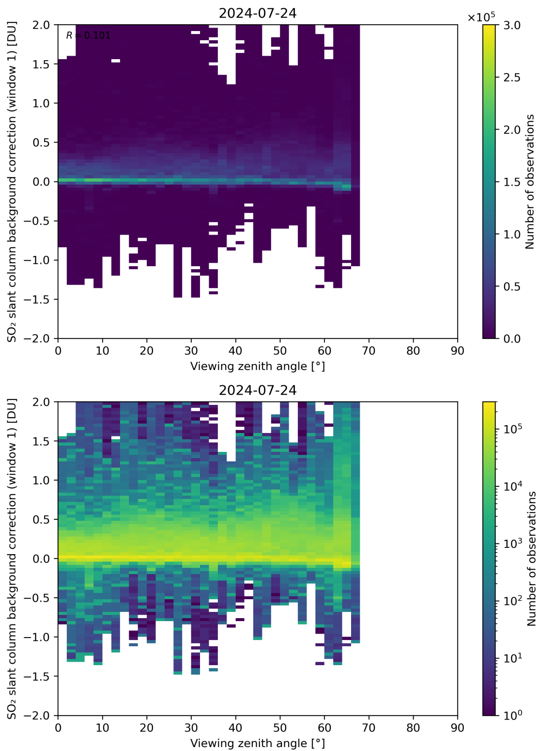
Figure 308: Scatter density plot of “Viewing zenith angle” against “SO 2 slant column background correction (window 1)” for 2024-07-23 to 2024-07-25.
