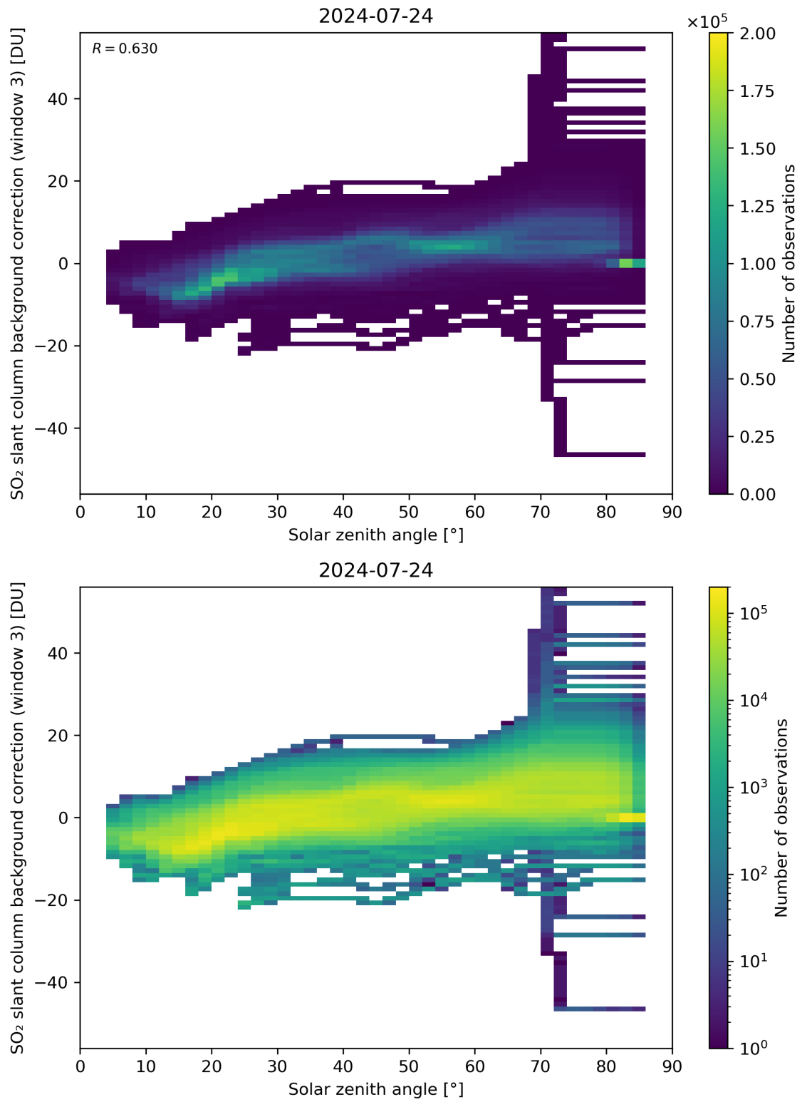
Figure 160: Scatter density plot of “Solar zenith angle” against “SO 2 slant column background correction (window 3)” for 2024-07-23 to 2024-07-25.
