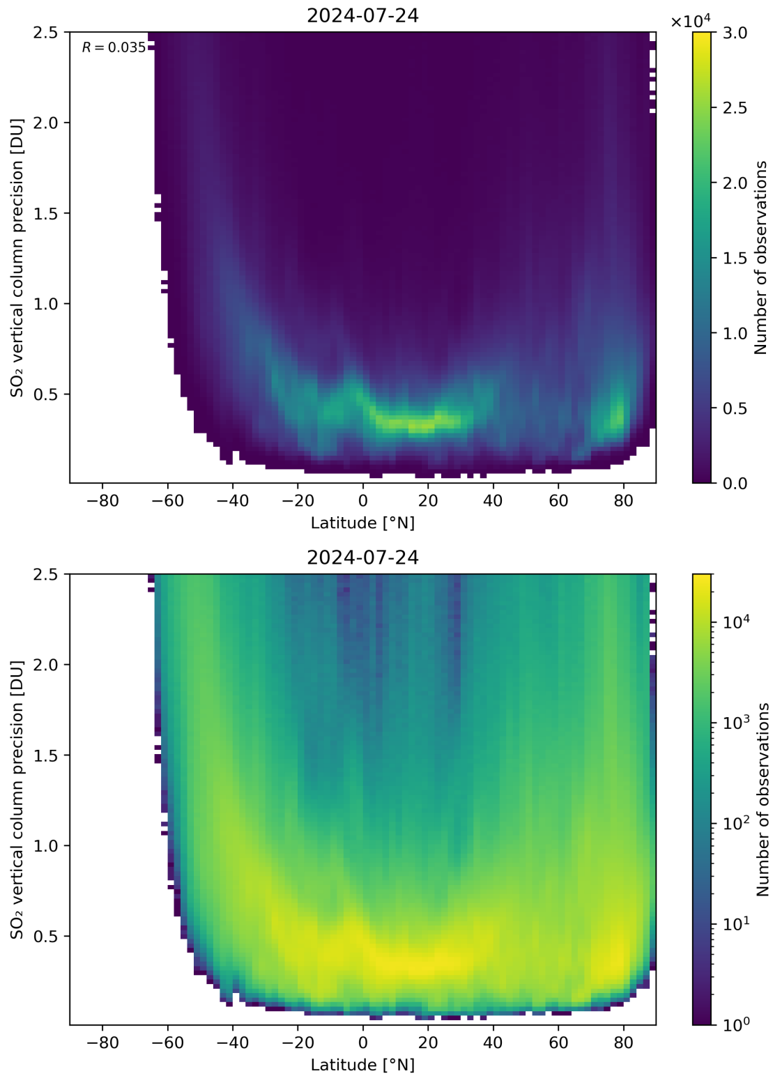
Figure 157: Scatter density plot of “Latitude” against “SO 2 vertical column precision” for 2024-07-23 to 2024-07-25.
