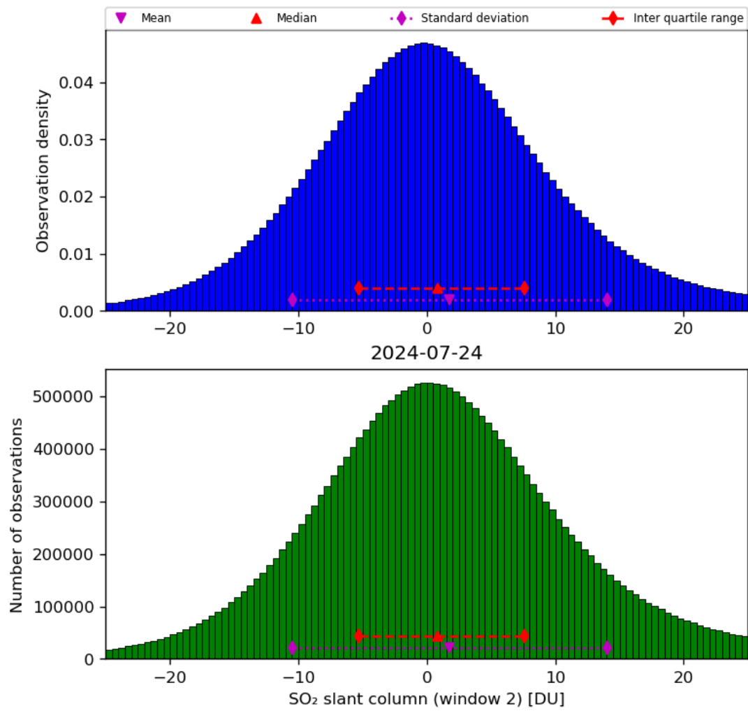
Figure 60: Histogram of “SO 2 slant column (window 2)” for 2024-07-23 to 2024-07-25
