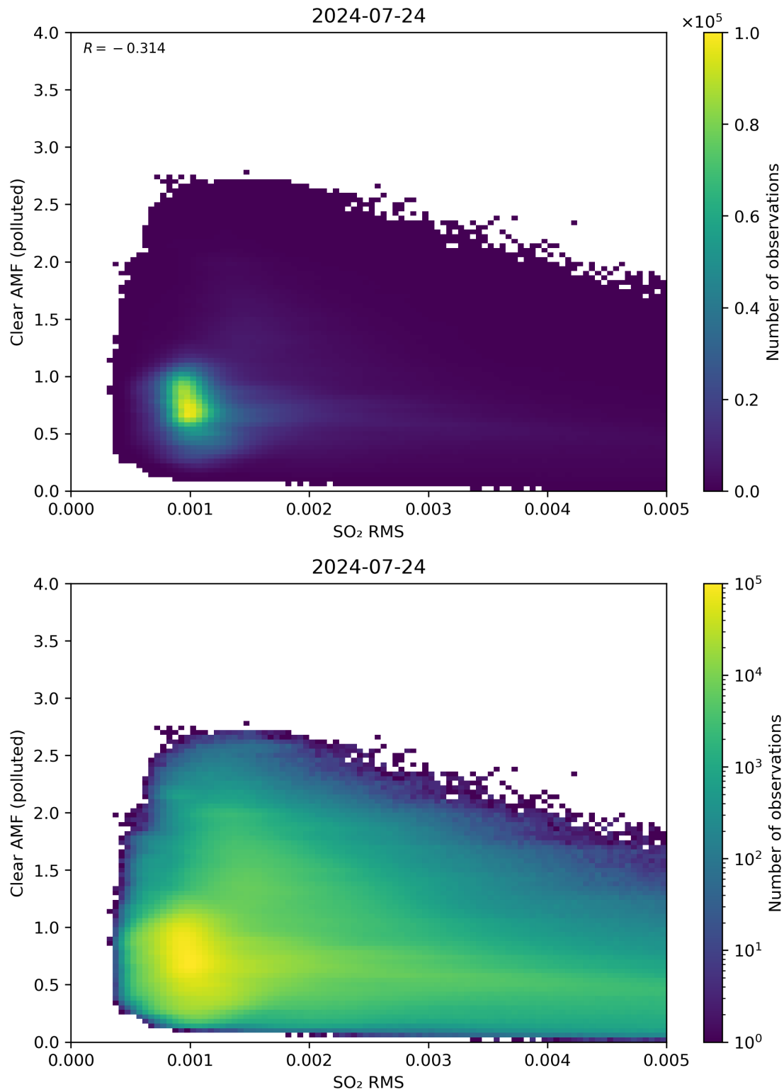
Figure 136: Scatter density plot of “SO 2 RMS” against “Clear AMF (polluted)” for 2024-07-23 to 2024-07-25.
