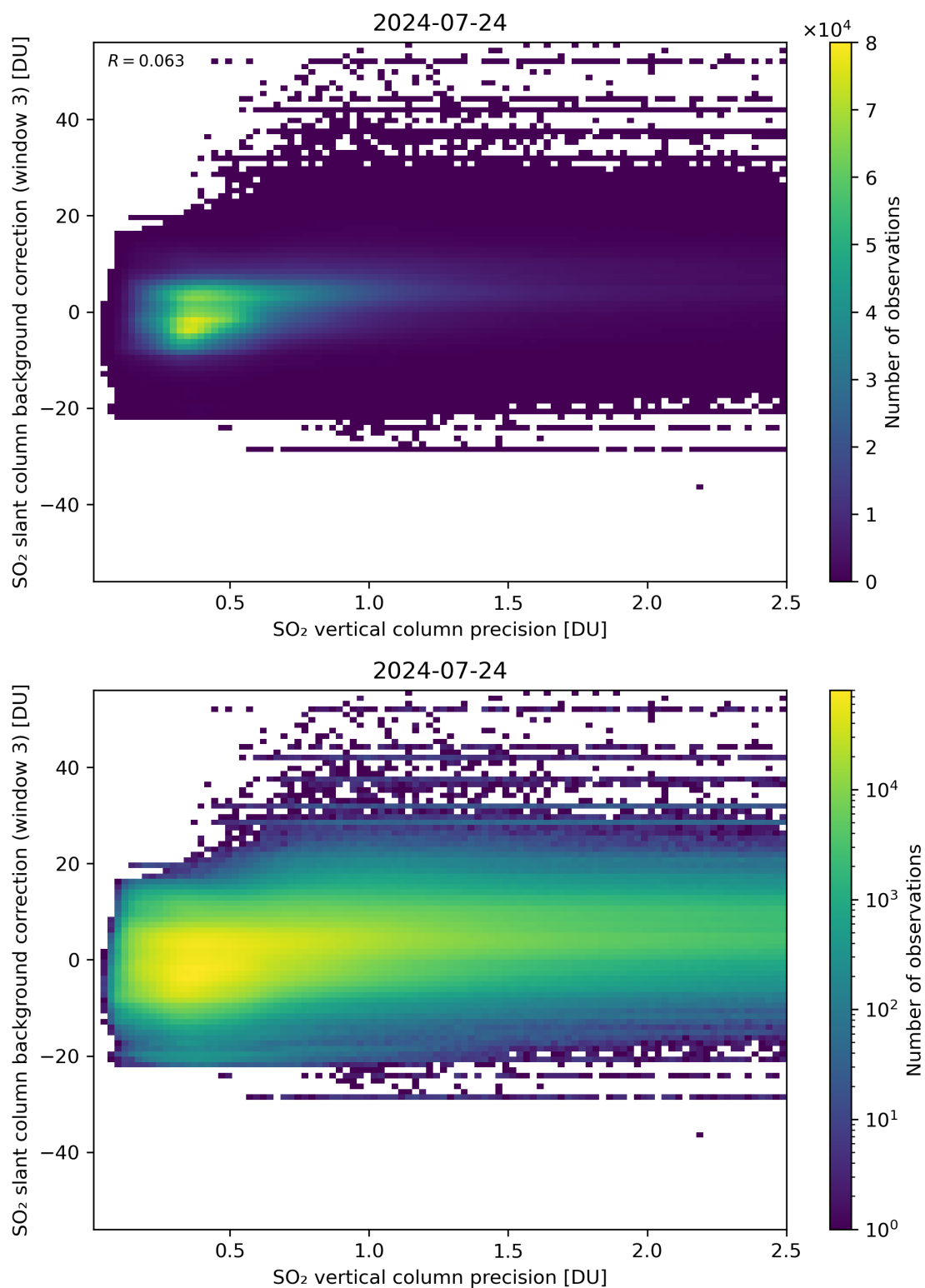
Figure 281: Scatter density plot of “SO 2 vertical column precision” against “SO 2 slant column background correction (window 3)” for 2024-07-23 to 2024-07-25.
