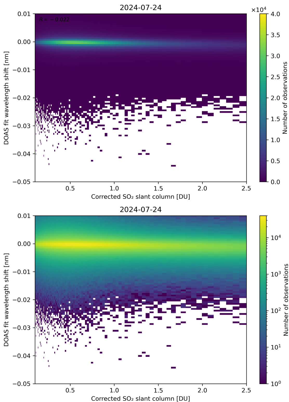
Figure 181: Scatter density plot of “Corrected SO 2 slant column” against “DOAS fit wavelength shift” for 2024-07-23 to 2024-07-25.
