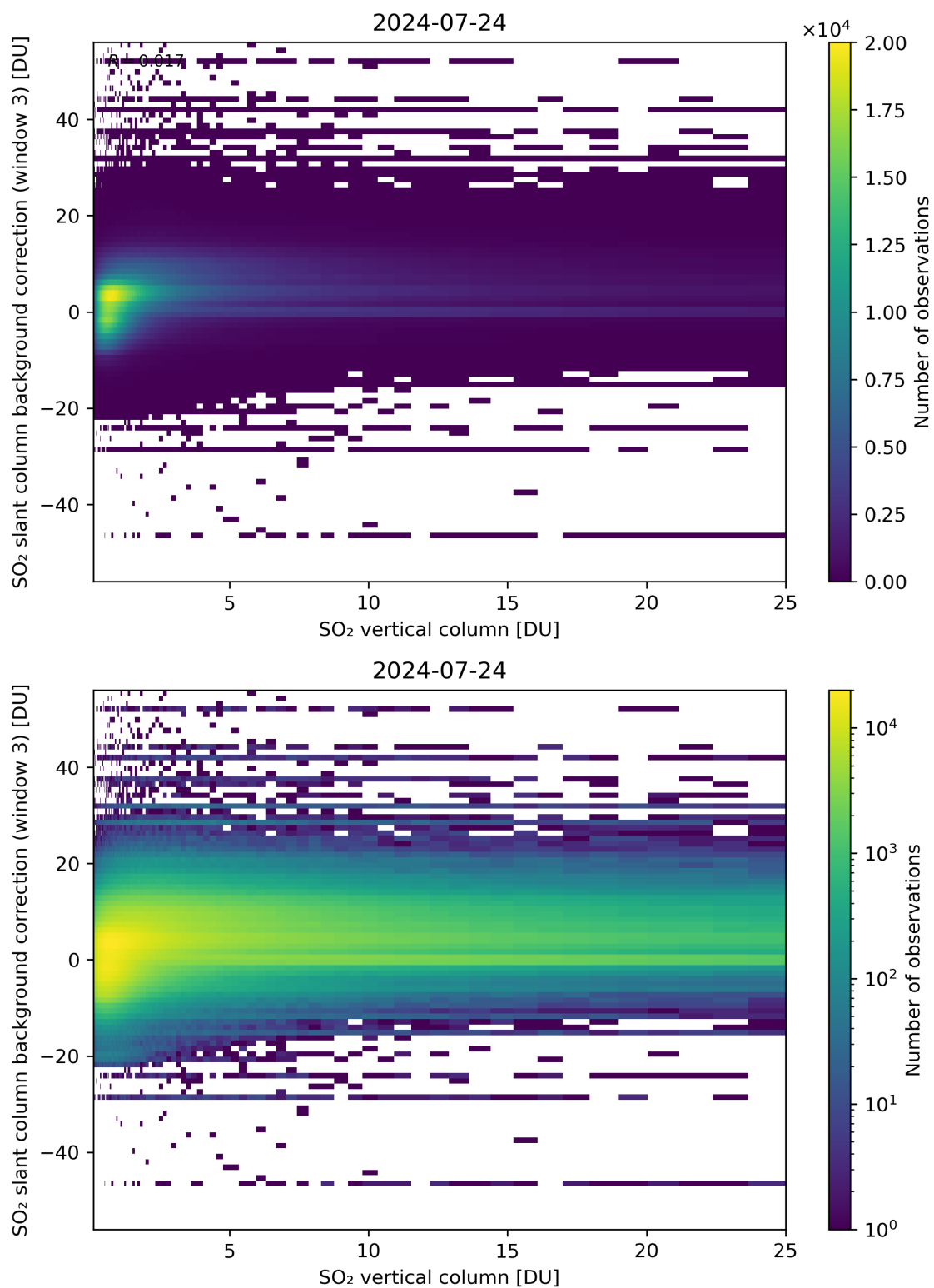
Figure 275: Scatter density plot of “SO 2 vertical column” against “SO 2 slant column background correction (window 3)” for 2024-07-23 to 2024-07-25.
