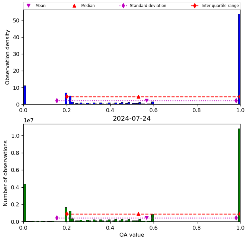
Figure 52: Histogram of “QA value” for 2024-07-23 to 2024-07-25
