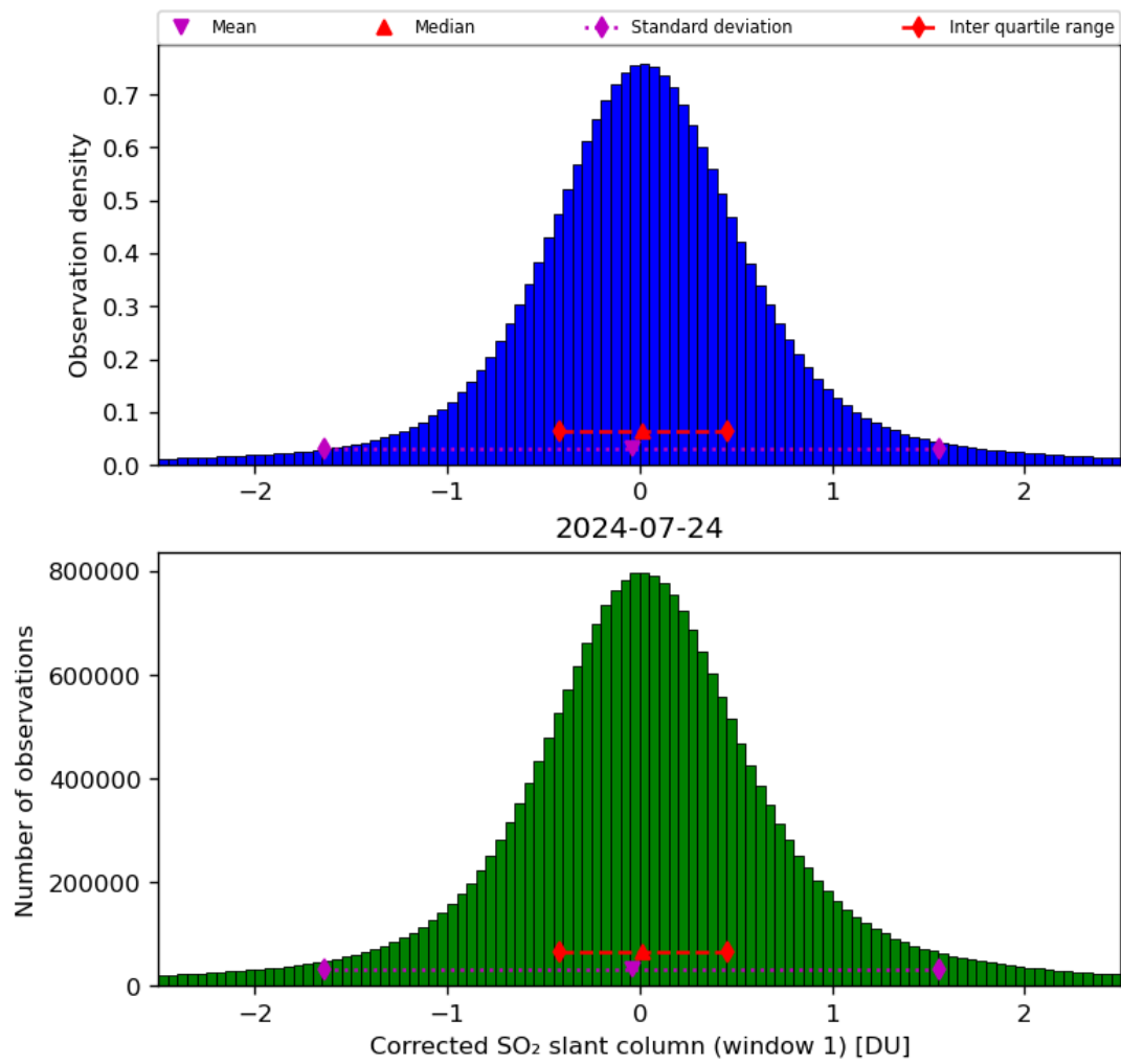
Figure 58: Histogram of “Corrected SO 2 slant column (window 1)” for 2024-07-23 to 2024-07-25
