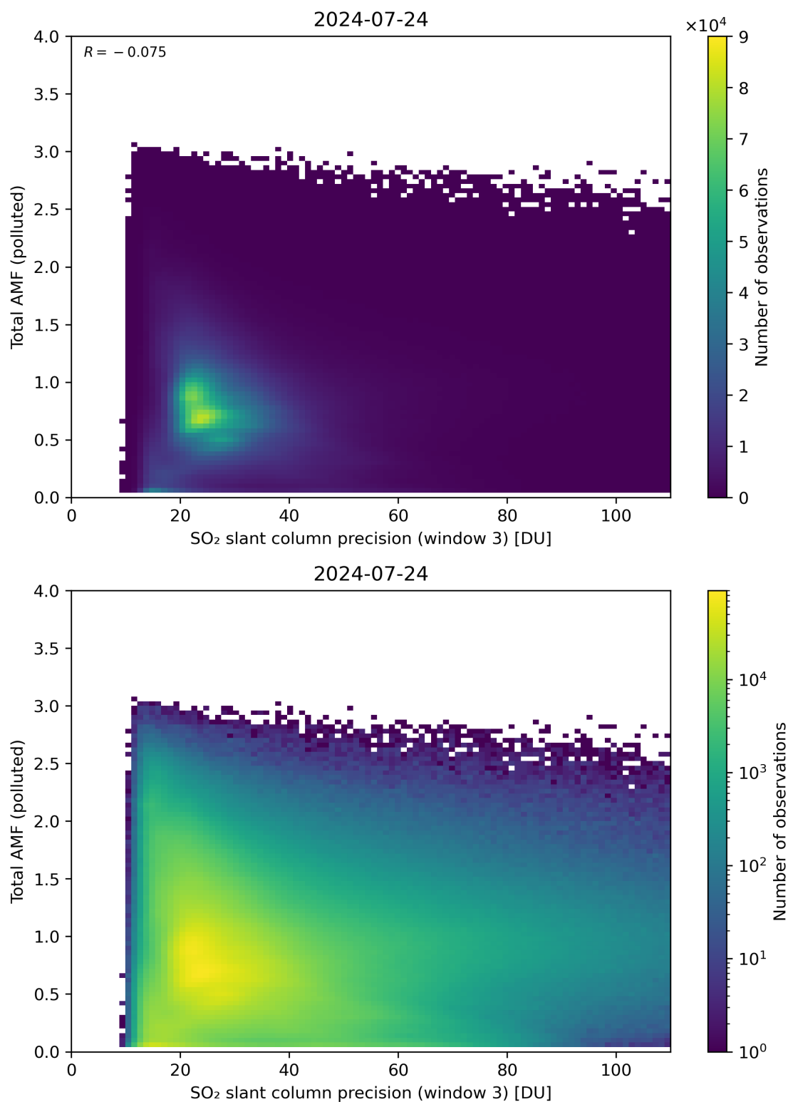
Figure 263: Scatter density plot of “SO 2 slant column precision (window 3)” against “Total AMF (polluted)” for 2024-07-23 to 2024-07-25.
