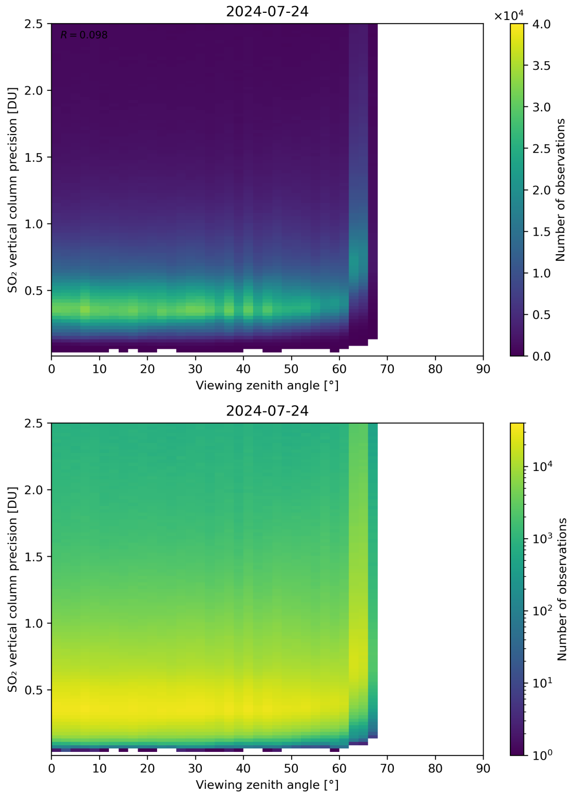
Figure 328: Scatter density plot of “Viewing zenith angle” against “SO 2 vertical column precision” for 2024-07-23 to 2024-07-25.
