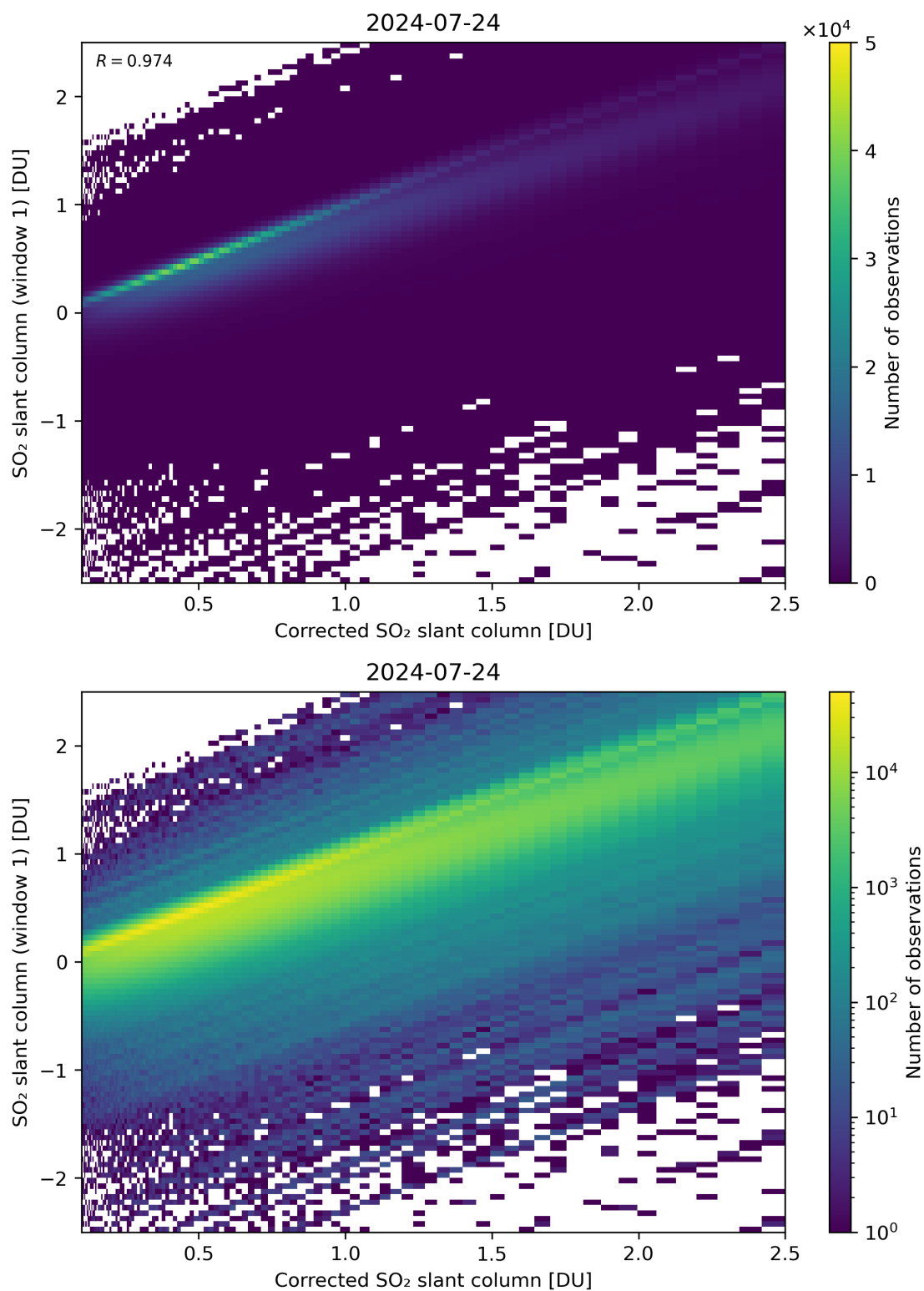
Figure 187: Scatter density plot of “Corrected SO 2 slant column” against “SO 2 slant column (window 1)” for 2024-07-23 to 2024-07-25.
