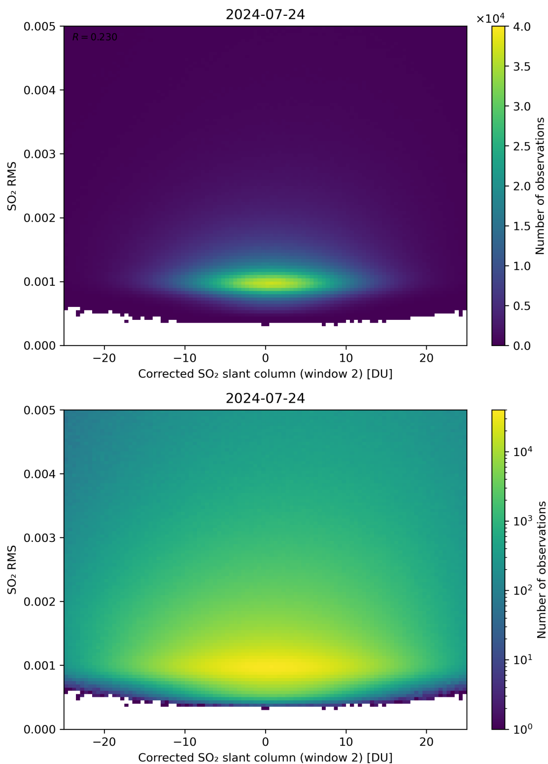
Figure 198: Scatter density plot of “Corrected SO 2 slant column (window 2)” against “SO 2 RMS” for 2024-07-23 to 2024-07-25.
