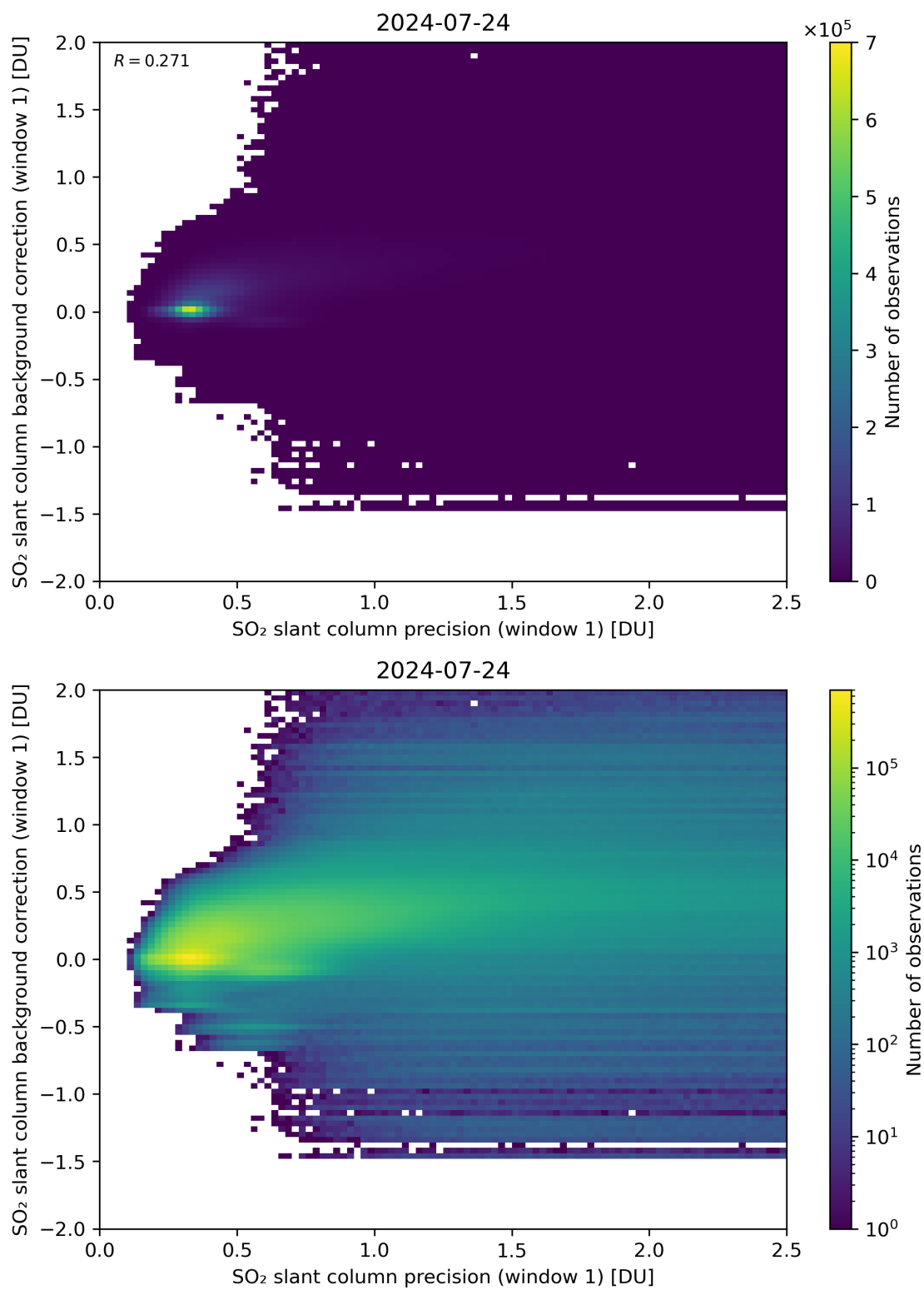
Figure 218: Scatter density plot of “SO 2 slant column precision (window 1)” against “SO 2 slant column background correction (window 1)” for 2024-07-23 to 2024-07-25.
