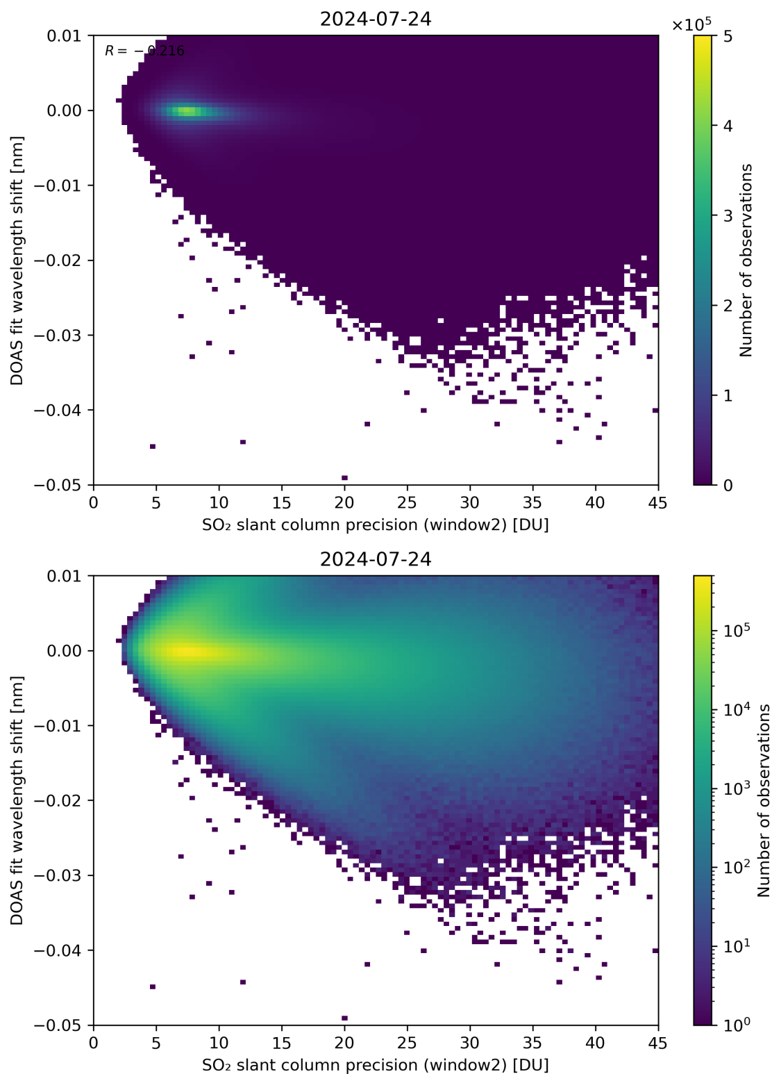
Figure 243: Scatter density plot of “SO 2 slant column precision (window2)” against “DOAS fit wavelength shift” for 2024-07-23 to 2024-07-25.
