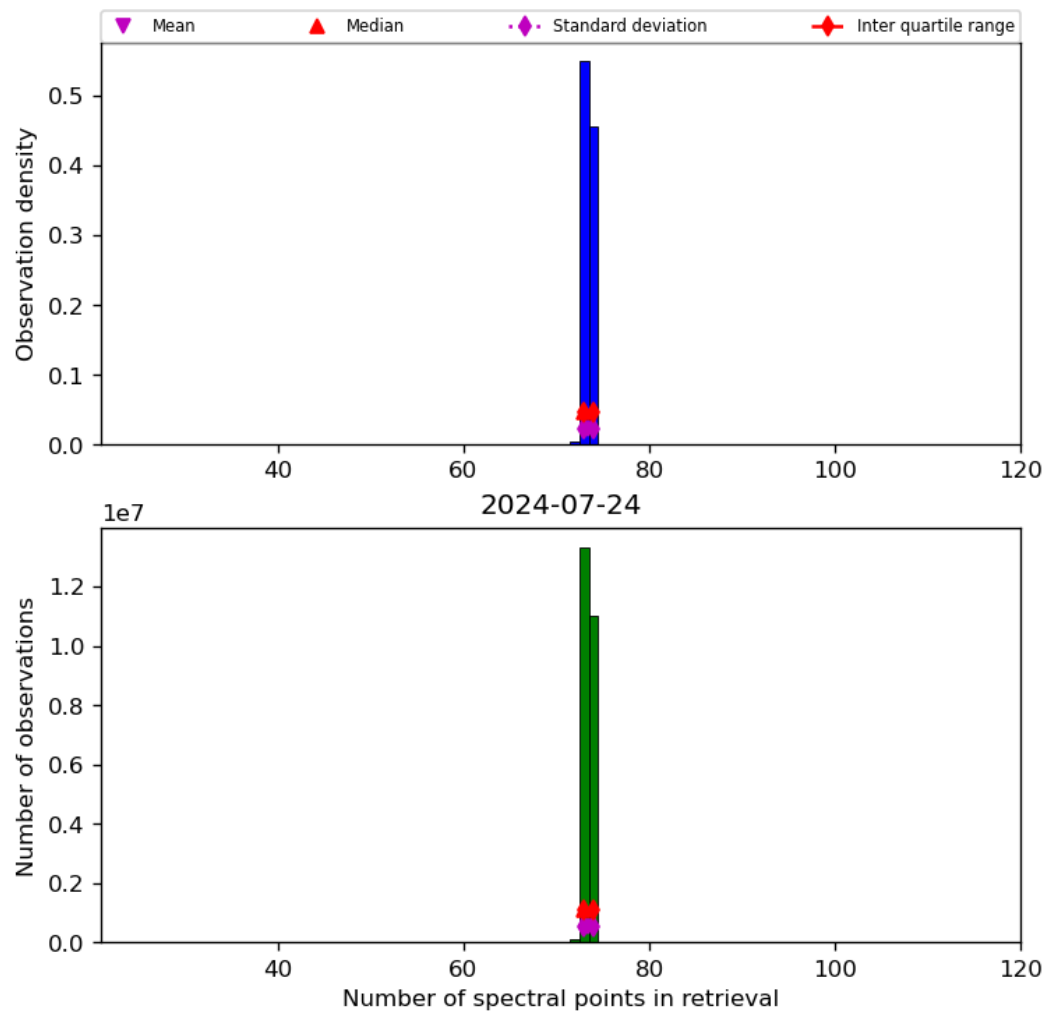
Figure 74: Histogram of “Number of spectral points in retrieval” for 2024-07-23 to 2024-07-25
