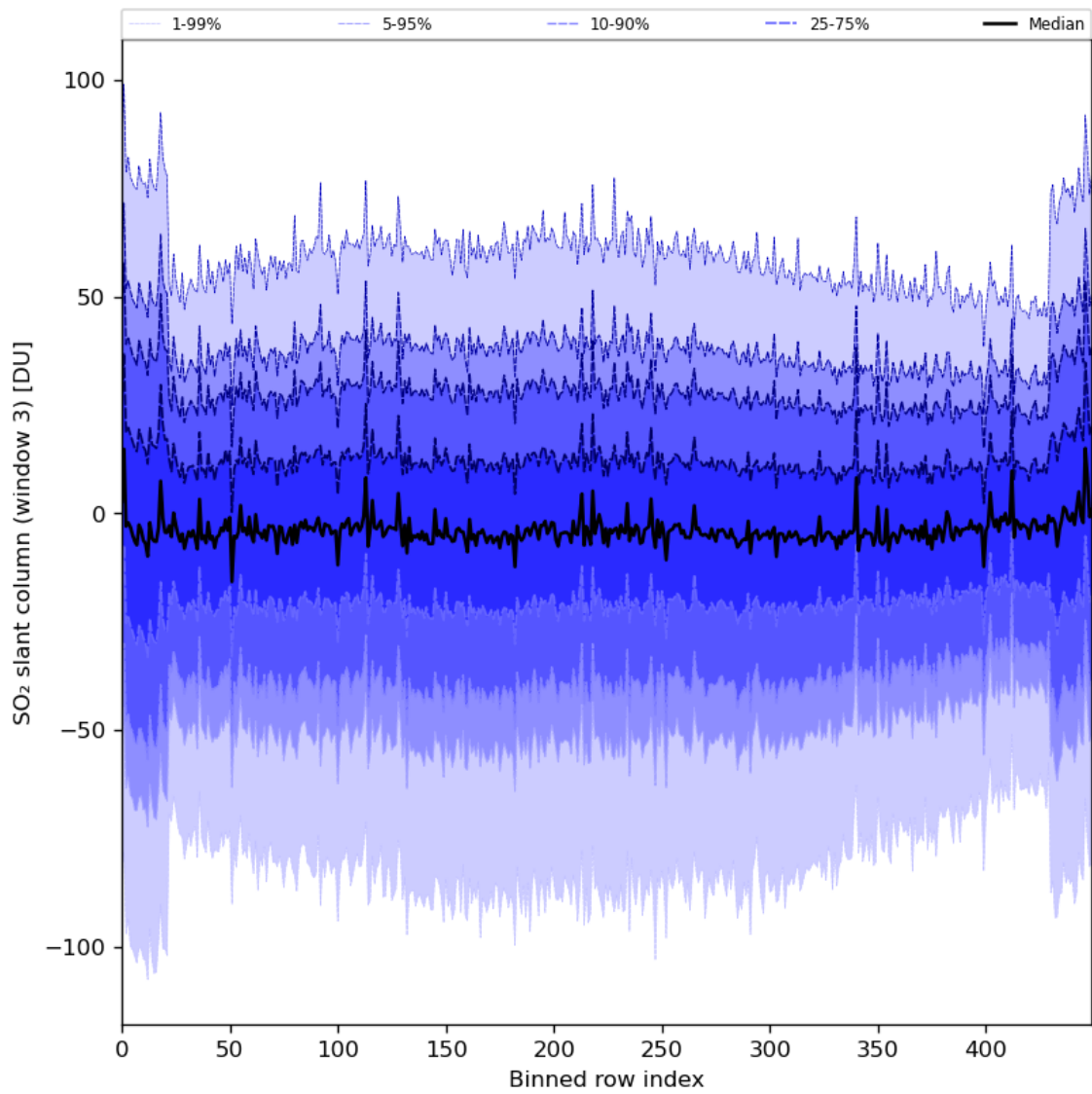
Figure 87: Along track statistics of “SO 2 slant column (window 3)” for 2024-07-23 to 2024-07-25
