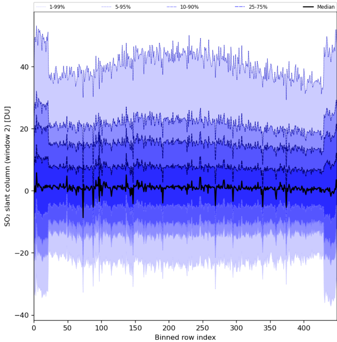
Figure 83: Along track statistics of “SO 2 slant column (window 2)” for 2024-07-23 to 2024-07-25
