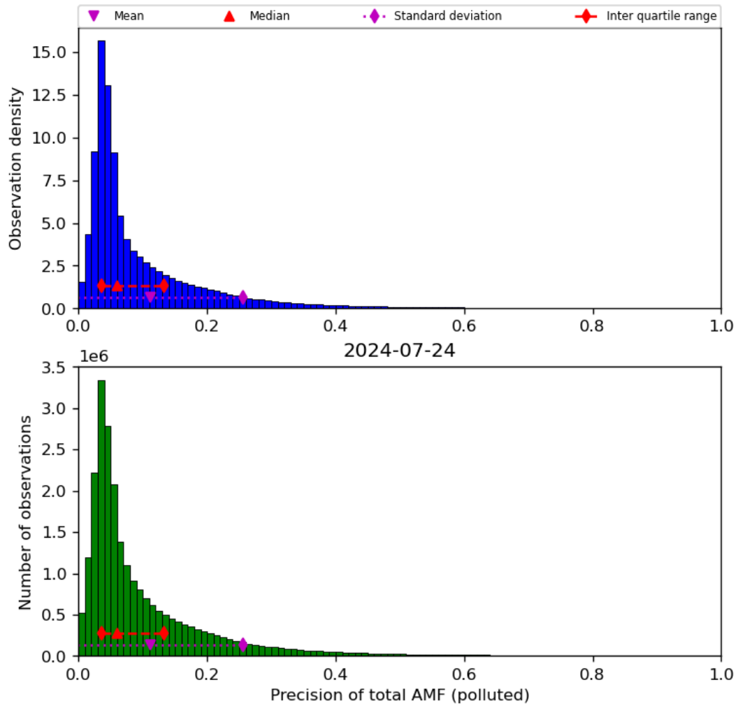
Figure 72: Histogram of “Precision of total AMF (polluted)” for 2024-07-23 to 2024-07-25
