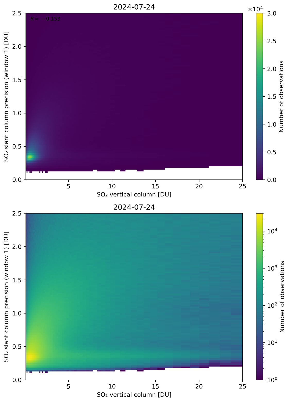
Figure 301: Scatter density plot of “SO 2 vertical column” against “SO 2 slant column precision (window 1)” for 2024-07-23 to 2024-07-25.
