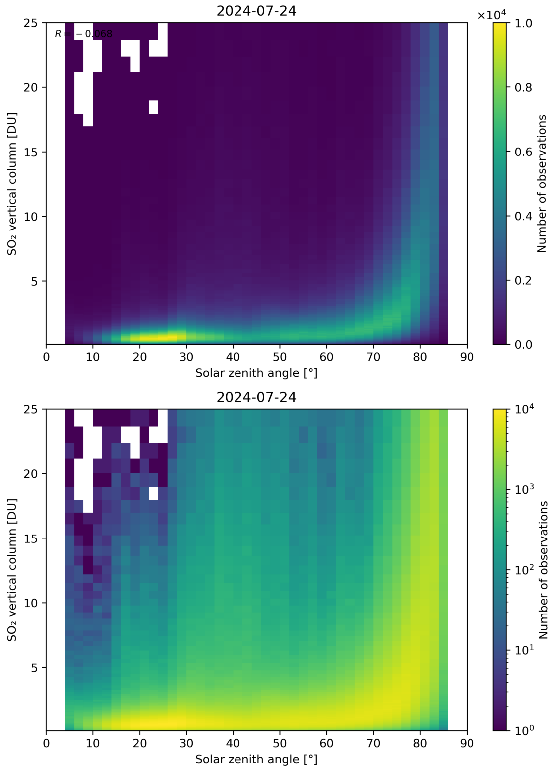
Figure 176: Scatter density plot of “Solar zenith angle” against “SO 2 vertical column” for 2024-07-23 to 2024-07-25.
