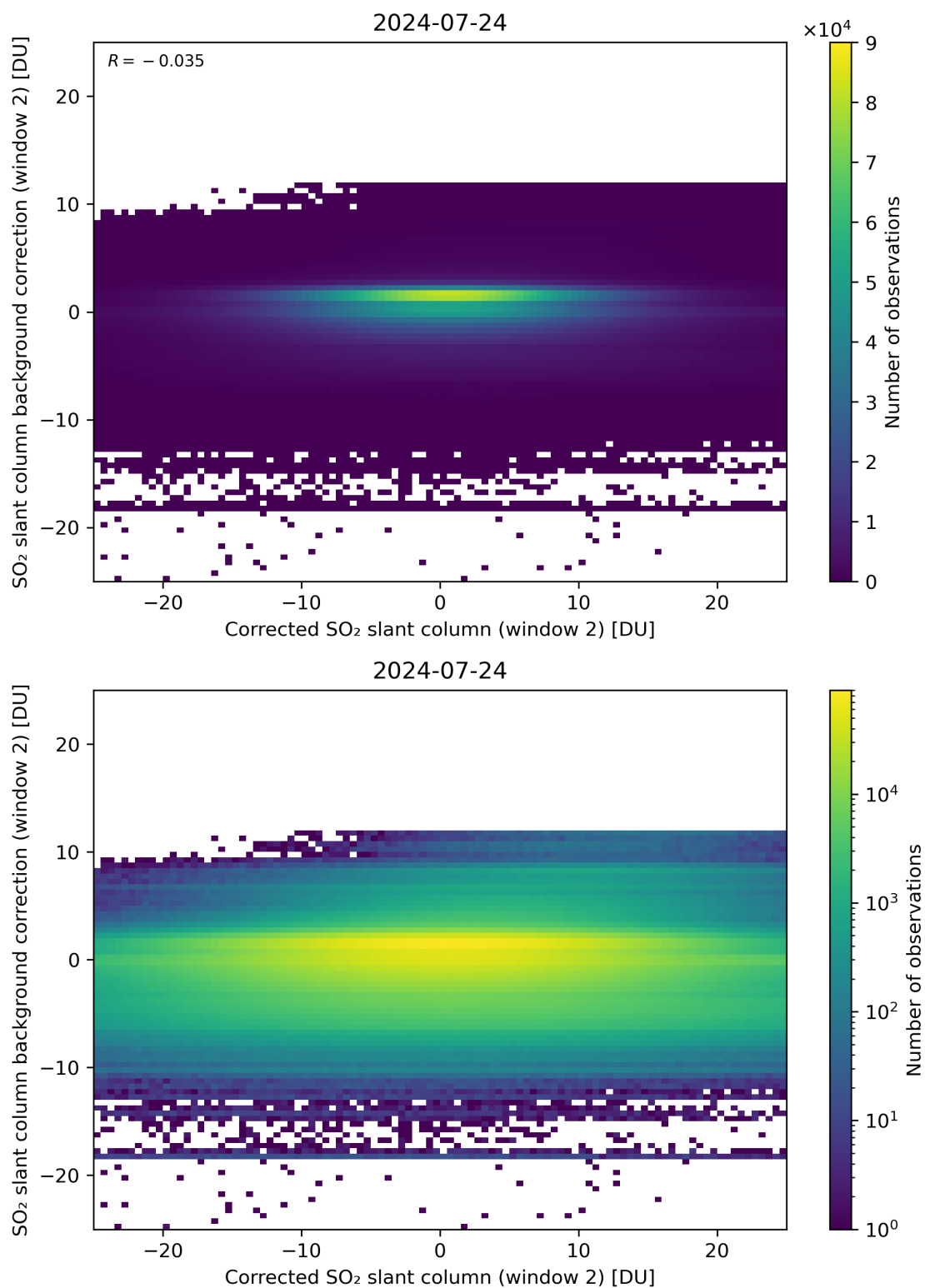
Figure 194: Scatter density plot of “Corrected SO 2 slant column (window 2)” against “SO 2 slant column background correction (window 2)” for 2024-07-23 to 2024-07-25.
