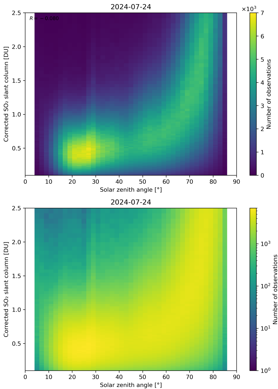
Figure 166: Scatter density plot of “Solar zenith angle” against “Corrected SO 2 slant column” for 2024-07-23 to 2024-07-25.
