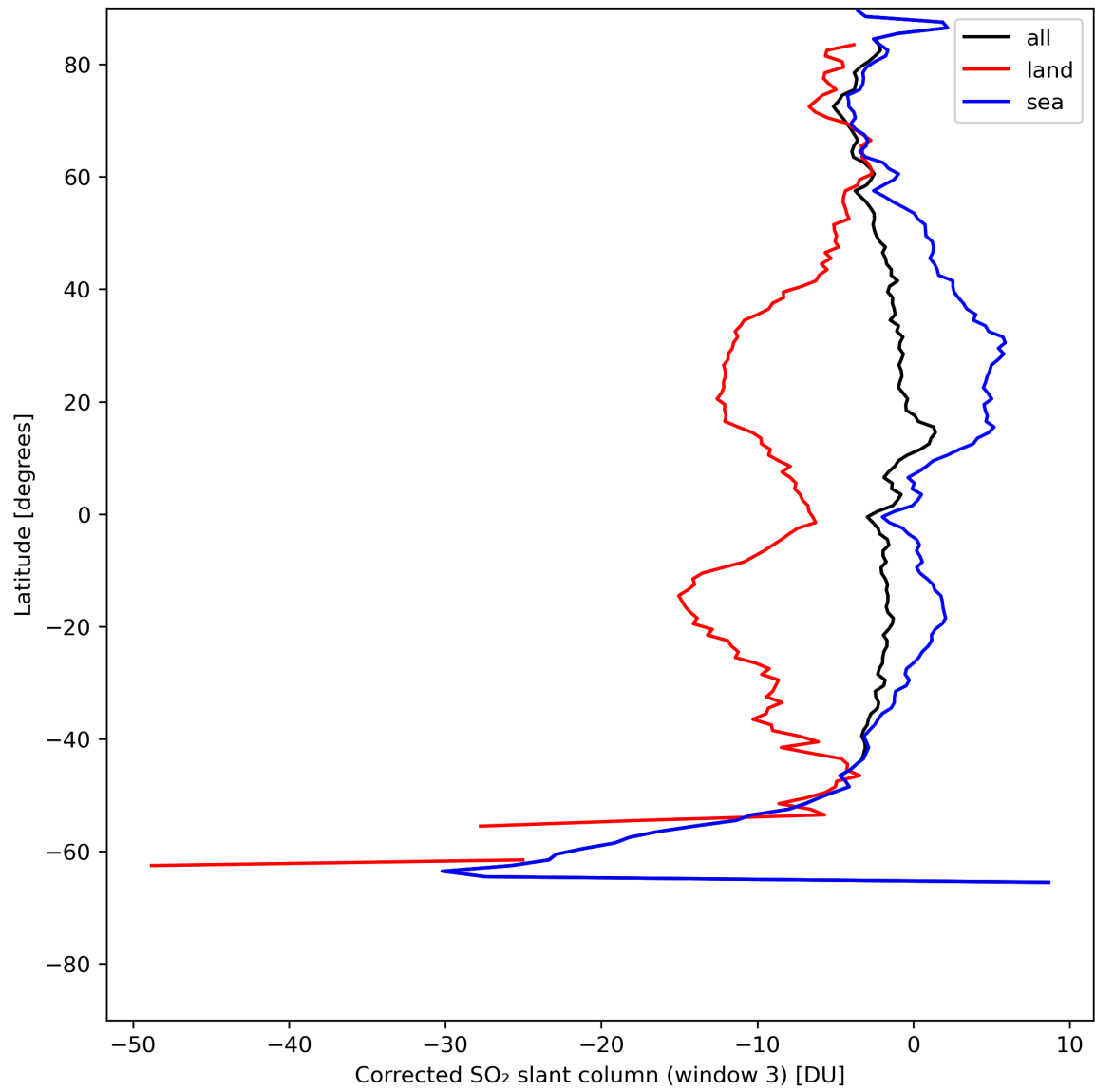
Figure 43: Zonal average of “Corrected SO 2 slant column (window 3)” for 2024-07-23 to 2024-07-25.
