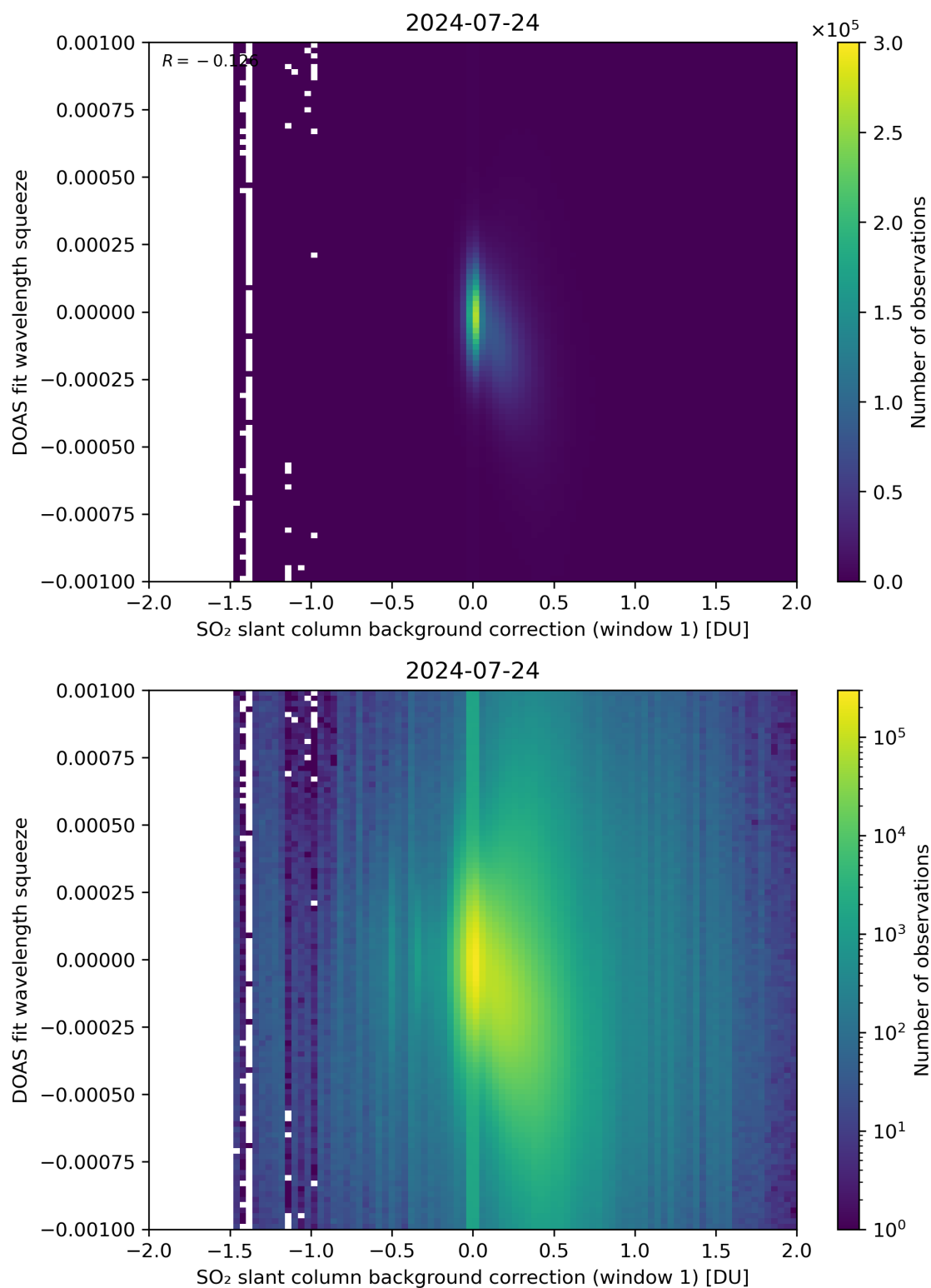
Figure 101: Scatter density plot of “SO 2 slant column background correction (window 1)” against “DOAS fit wavelength squeeze” for 2024-07-23 to 2024-07-25.
