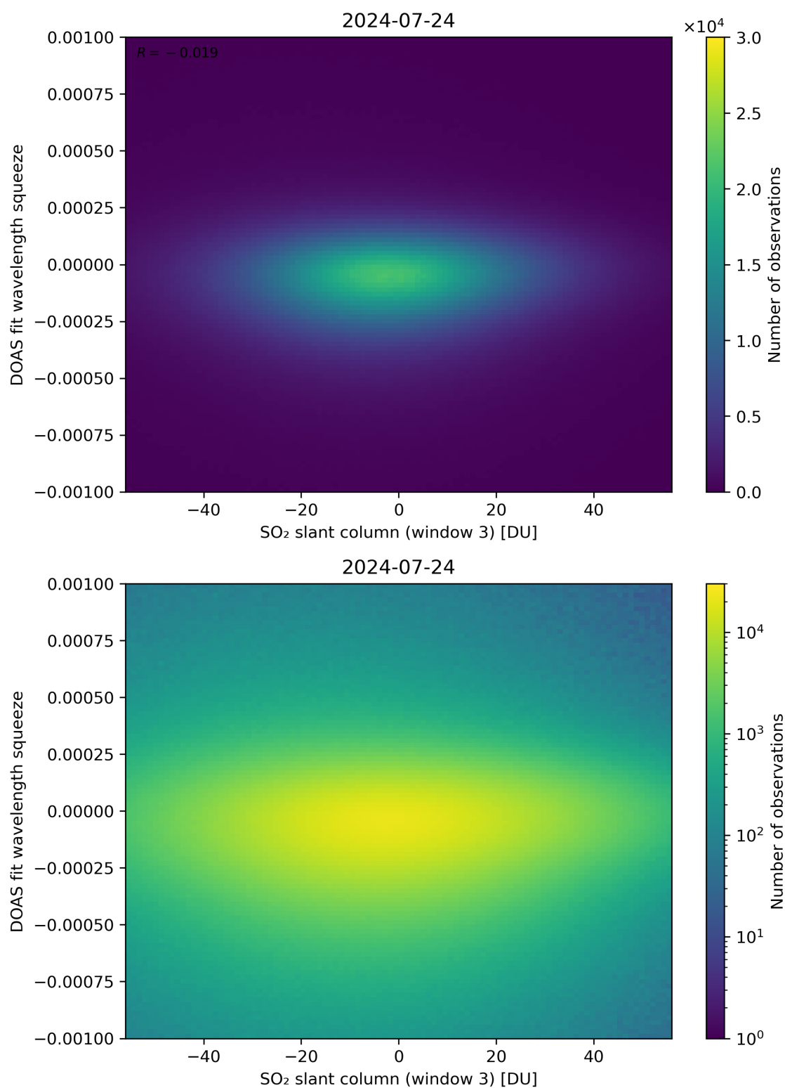
Figure 255: Scatter density plot of “SO 2 slant column (window 3)” against “DOAS fit wavelength squeeze” for 2024-07-23 to 2024-07-25.
