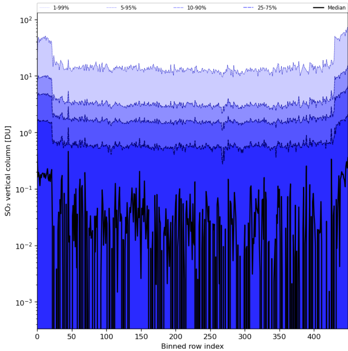
Figure 76: Along track statistics of “SO 2 vertical column” for 2024-07-23 to 2024-07-25
