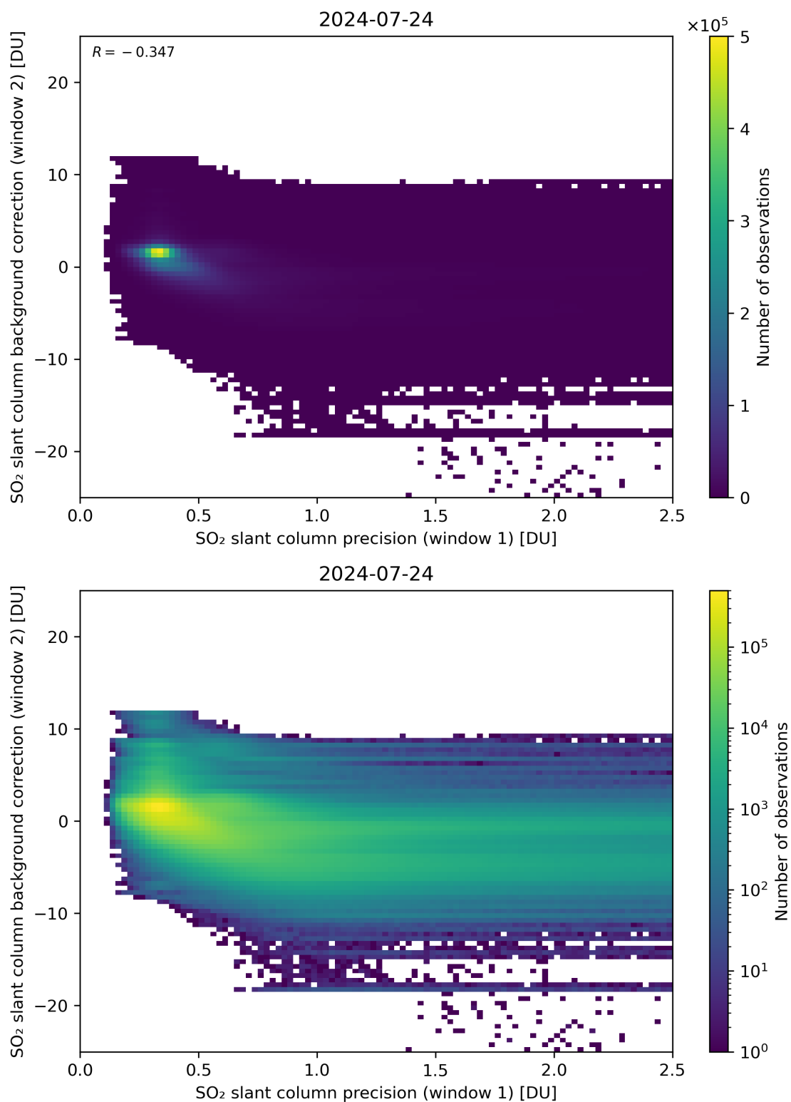
Figure 219: Scatter density plot of “SO 2 slant column precision (window 1)” against “SO 2 slant column background correction (window 2)” for 2024-07-23 to 2024-07-25.
