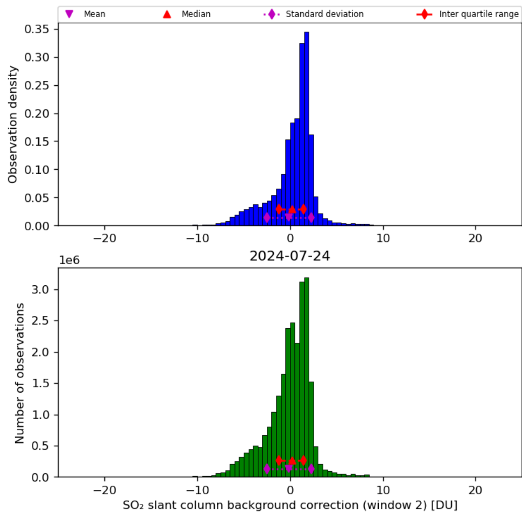
Figure 63: Histogram of “SO 2 slant column background correction (window 2)” for 2024-07-23 to 2024-07-25
