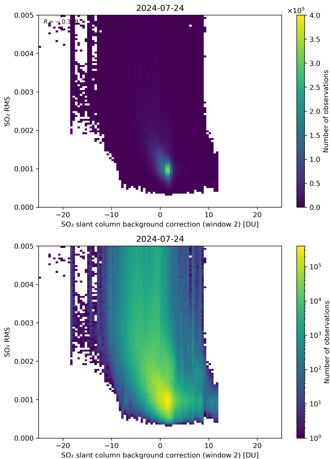
Figure 114: Scatter density plot of “SO 2 slant column background correction (window 2)” against “SO 2 RMS” for 2024-07-23 to 2024-07-25.
