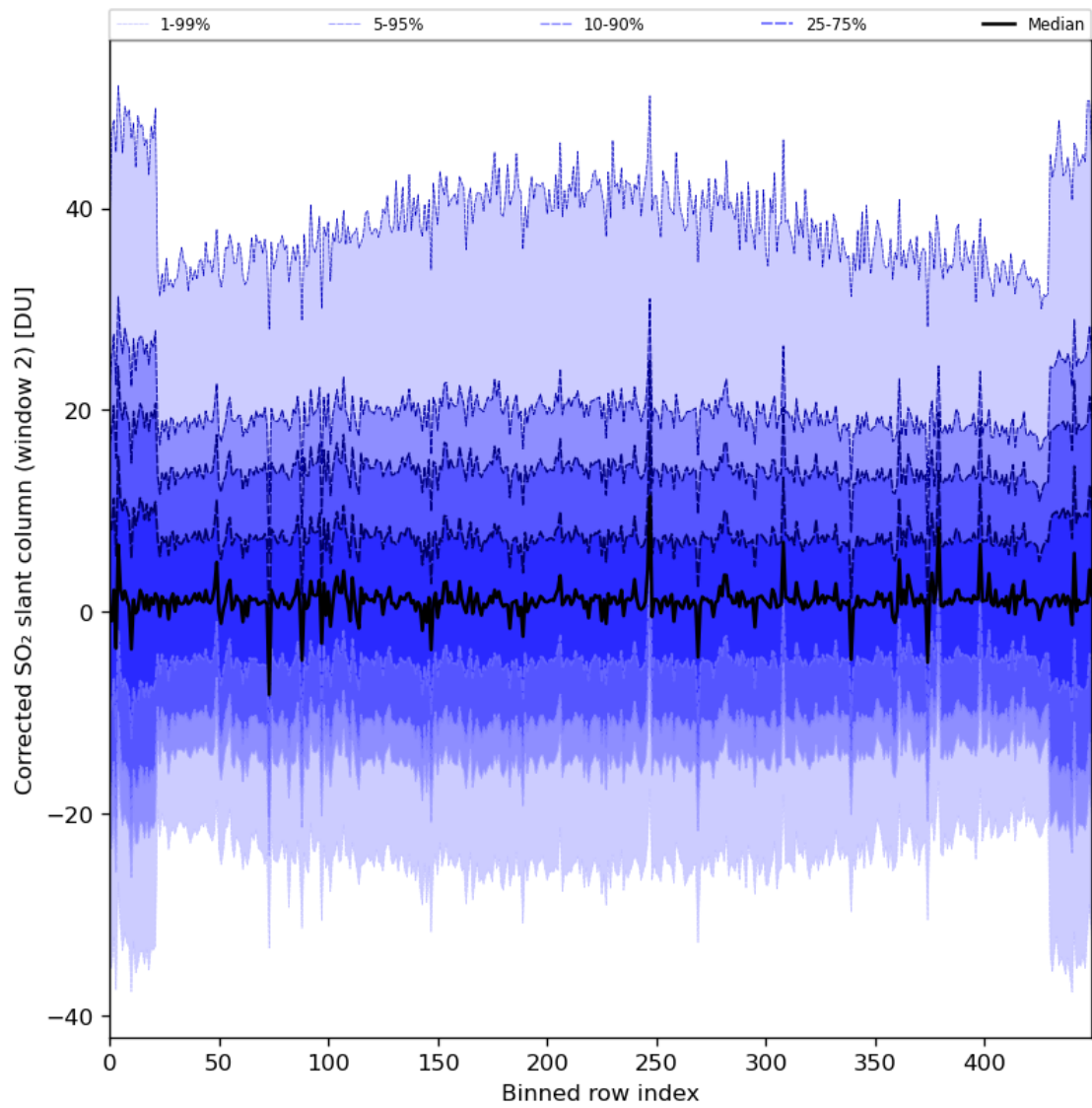
Figure 85: Along track statistics of “Corrected SO 2 slant column (window 2)” for 2024-07-23 to 2024-07-25
