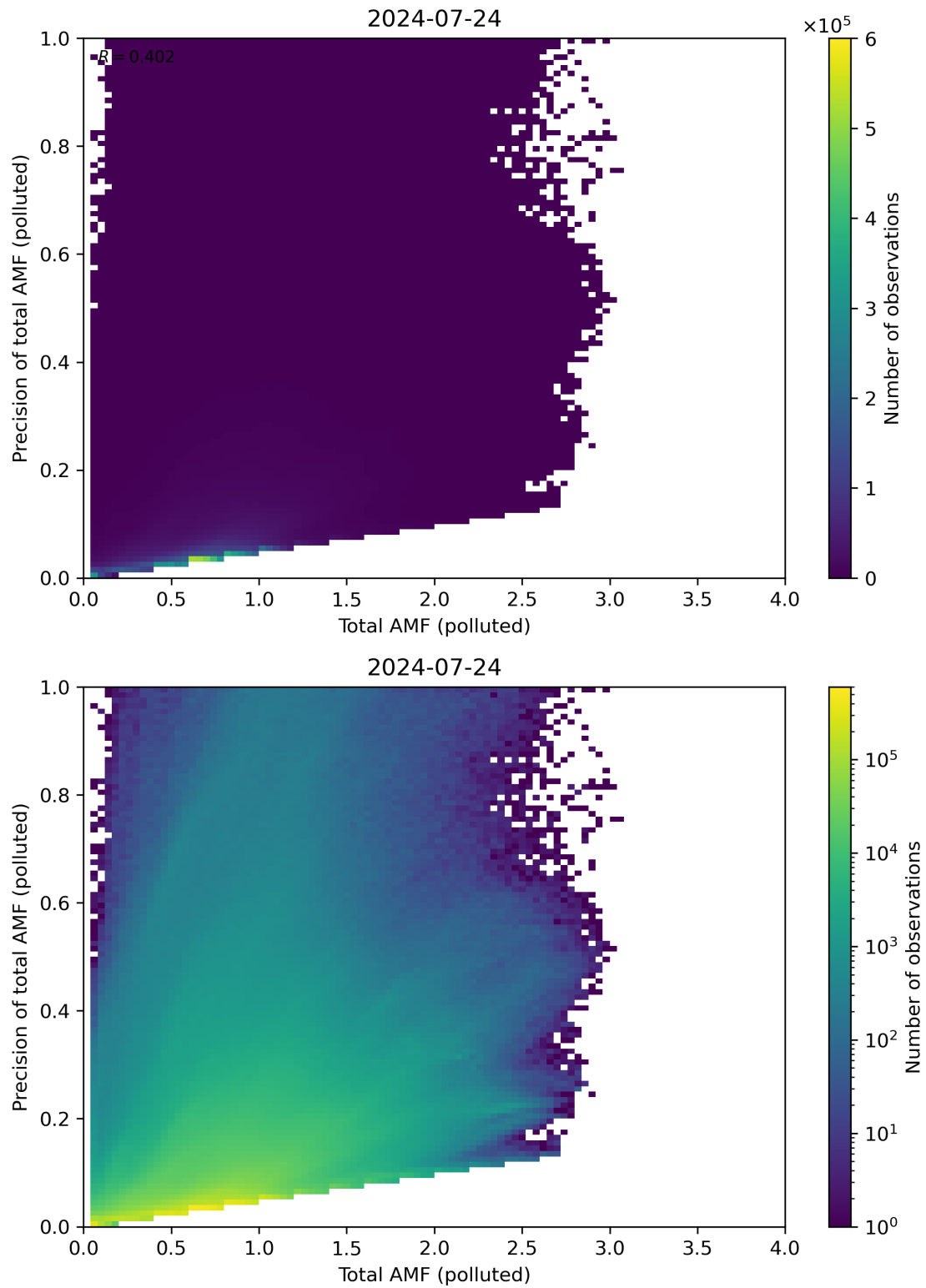
Figure 272: Scatter density plot of “Total AMF (polluted)” against “Precision of total AMF (polluted)” for 2024-07-23 to 2024-07-25.
