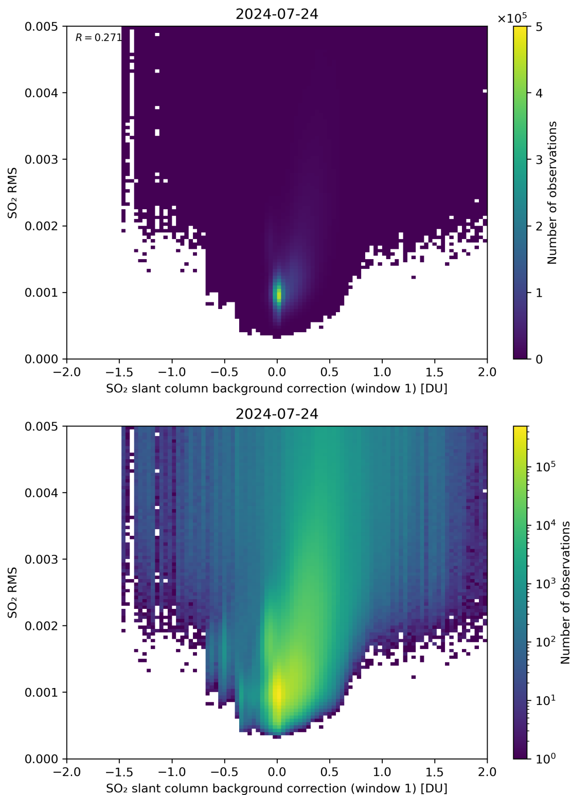
Figure 102: Scatter density plot of “SO 2 slant column background correction (window 1)” against “SO 2 RMS” for 2024-07-23 to 2024-07-25.
