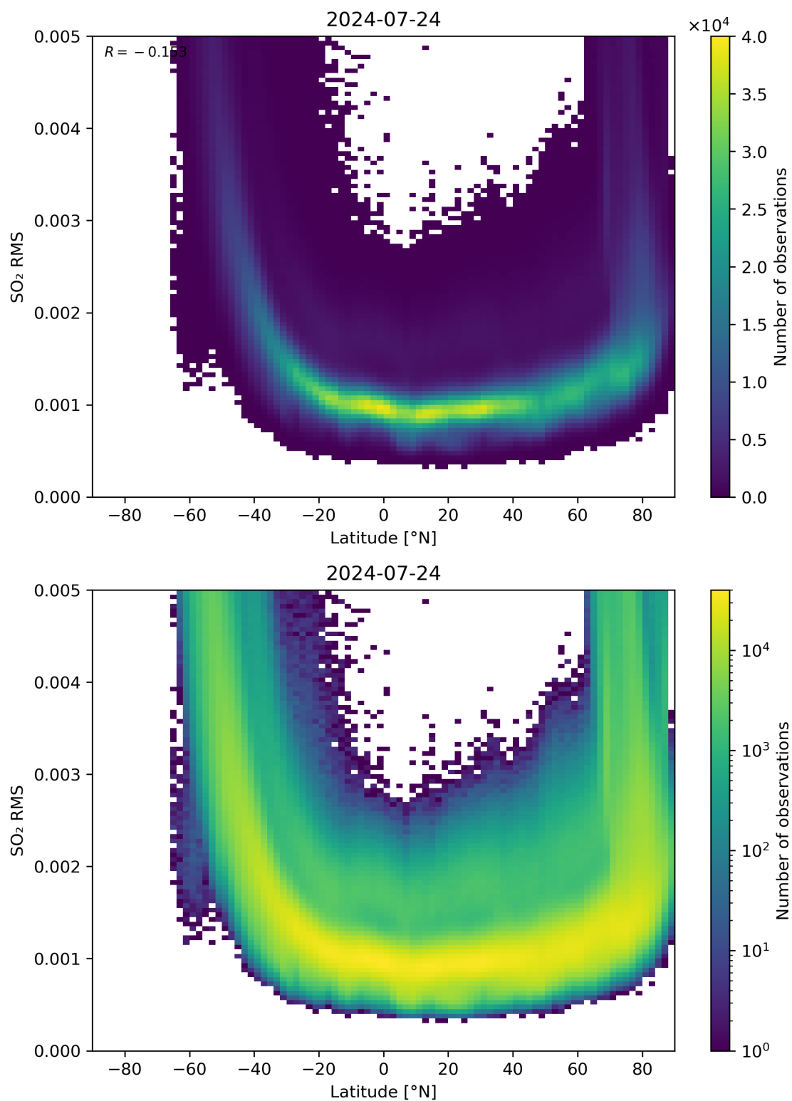
Figure 144: Scatter density plot of “Latitude” against “SO 2 RMS” for 2024-07-23 to 2024-07-25.
