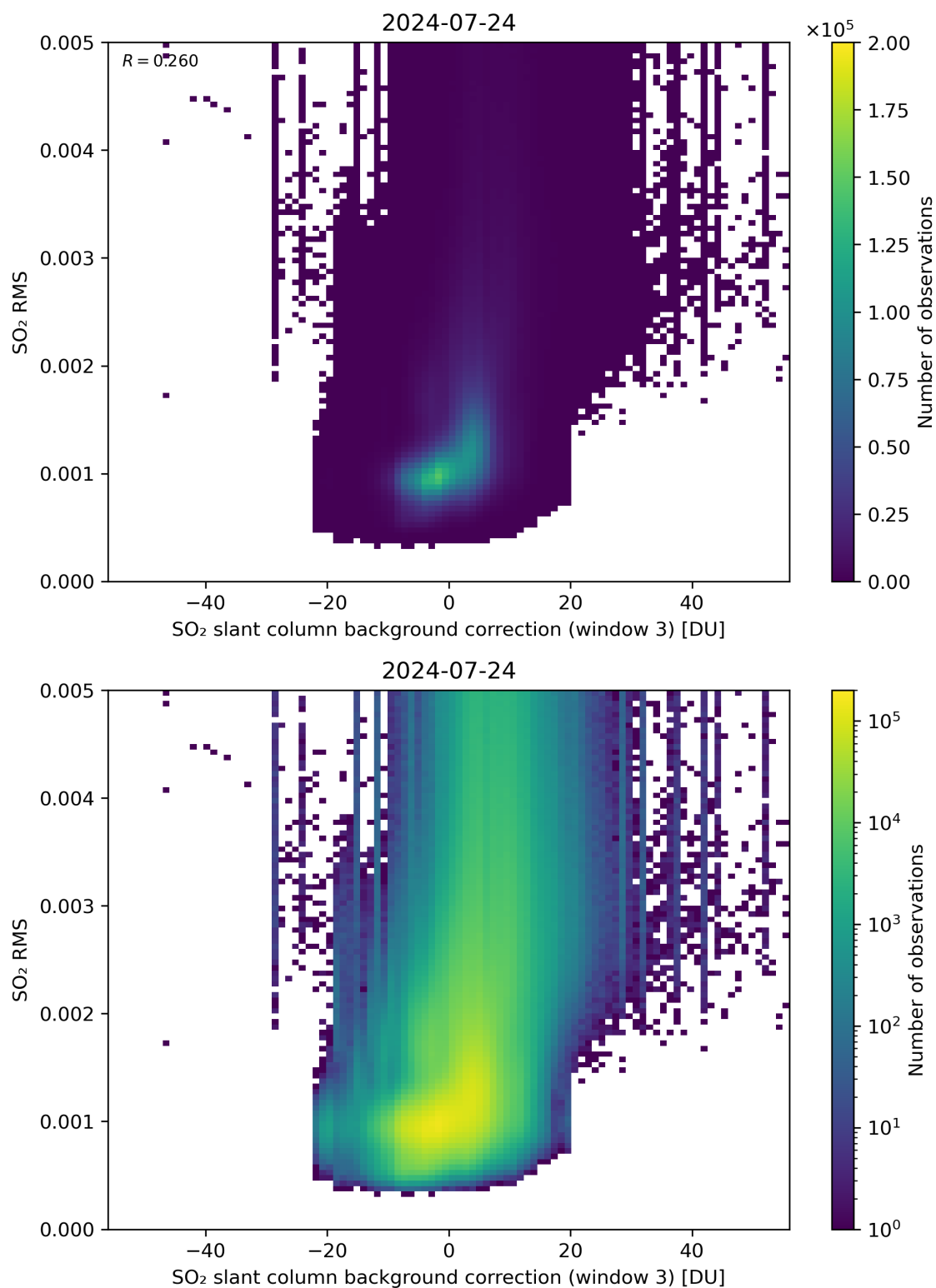
Figure 123: Scatter density plot of “SO 2 slant column background correction (window 3)” against “SO 2 RMS” for 2024-07-23 to 2024-07-25.
