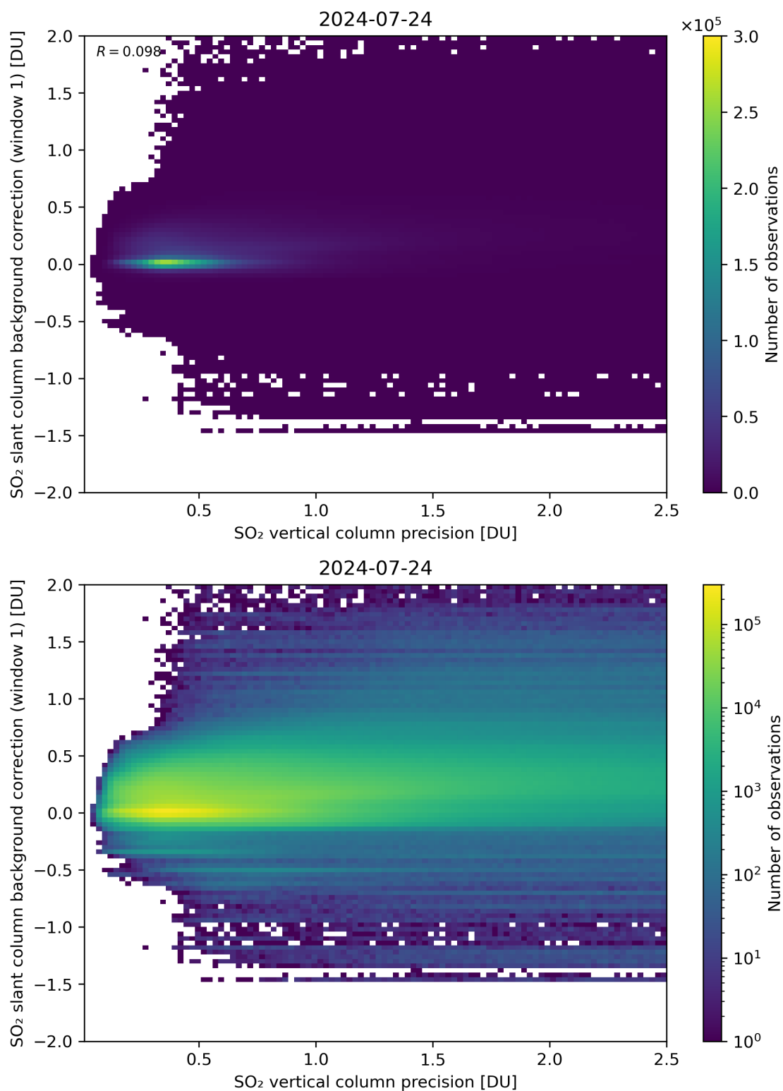
Figure 279: Scatter density plot of “SO 2 vertical column precision” against “SO 2 slant column background correction (window 1)” for 2024-07-23 to 2024-07-25.
