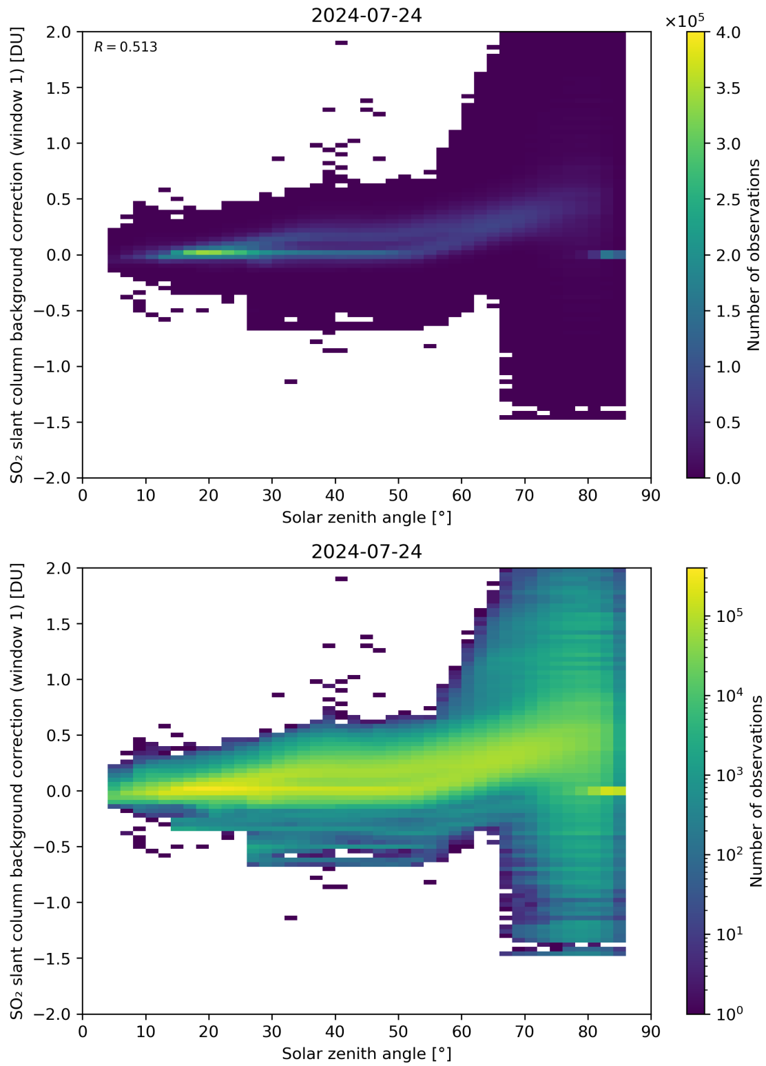
Figure 158: Scatter density plot of “Solar zenith angle” against “SO 2 slant column background correction (window 1)” for 2024-07-23 to 2024-07-25.
