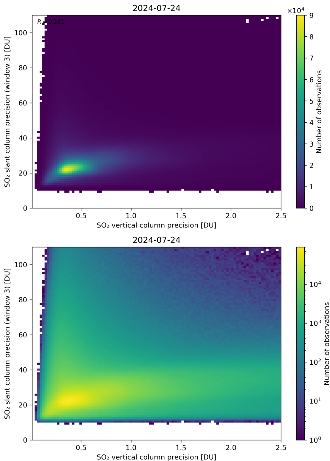
Figure 293: Scatter density plot of “SO 2 vertical column precision” against “SO 2 slant column precision (window 3)” for 2024-07-23 to 2024-07-25.
