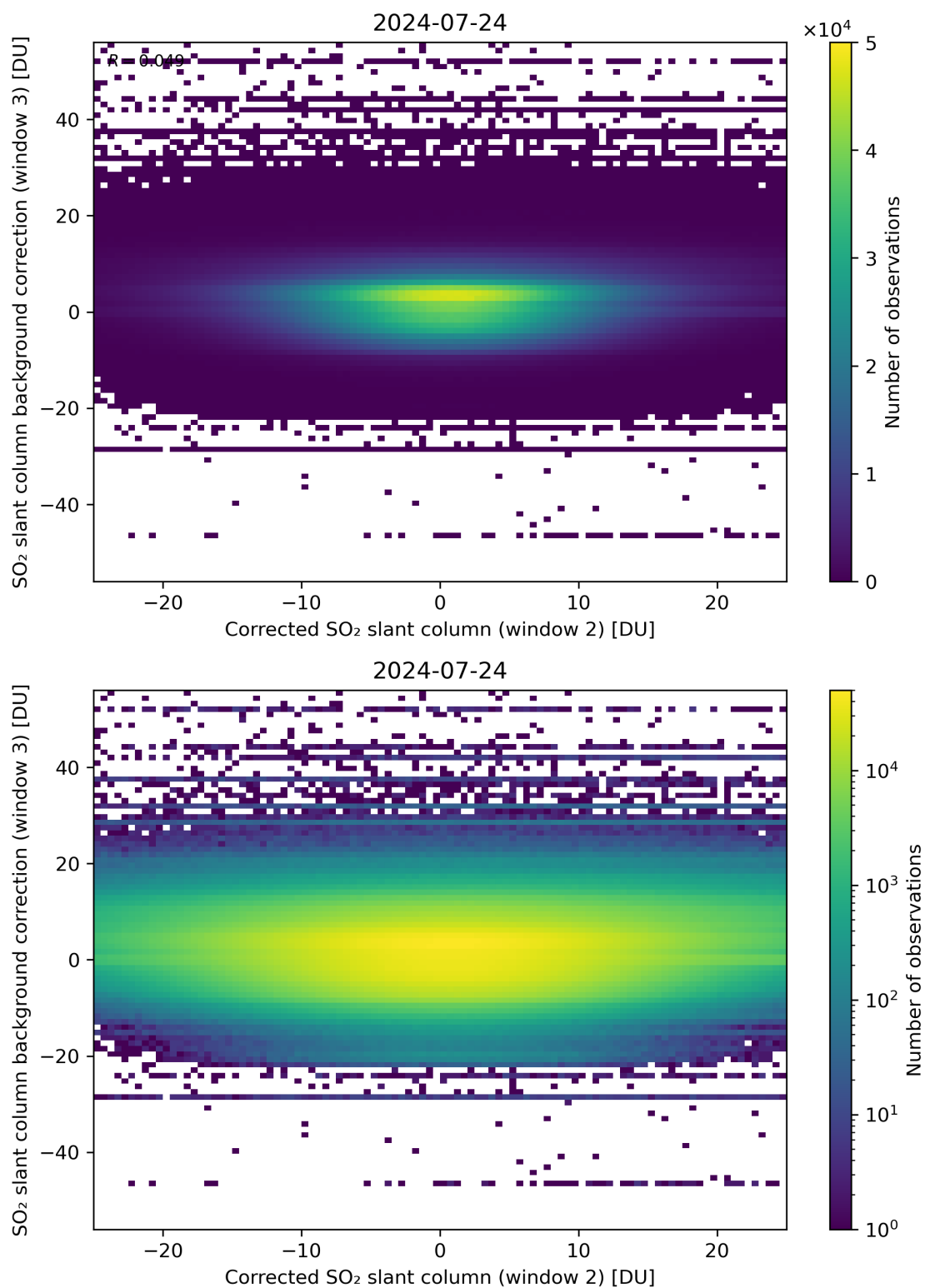
Figure 195: Scatter density plot of “Corrected SO 2 slant column (window 2)” against “SO 2 slant column background correction (window 3)” for 2024-07-23 to 2024-07-25.
