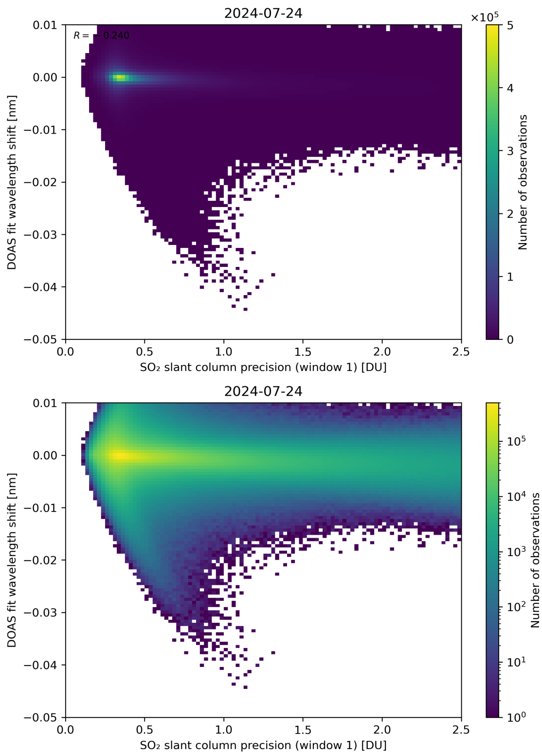
Figure 221: Scatter density plot of “SO 2 slant column precision (window 1)” against “DOAS fit wavelength shift” for 2024-07-23 to 2024-07-25.
