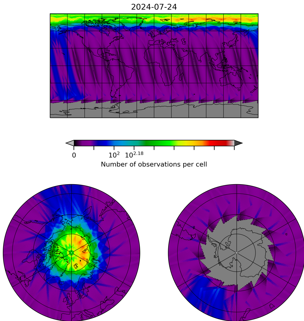
Figure 28: Map of the number of observations for 2024-07-23 to 2024-07-25
