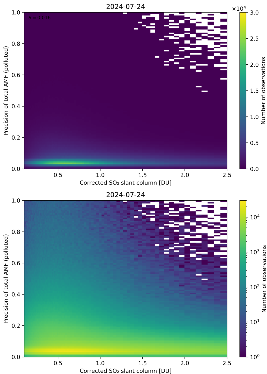
Figure 193: Scatter density plot of “Corrected SO 2 slant column” against “Precision of total AMF (polluted)” for 2024-07-23 to 2024-07-25.
