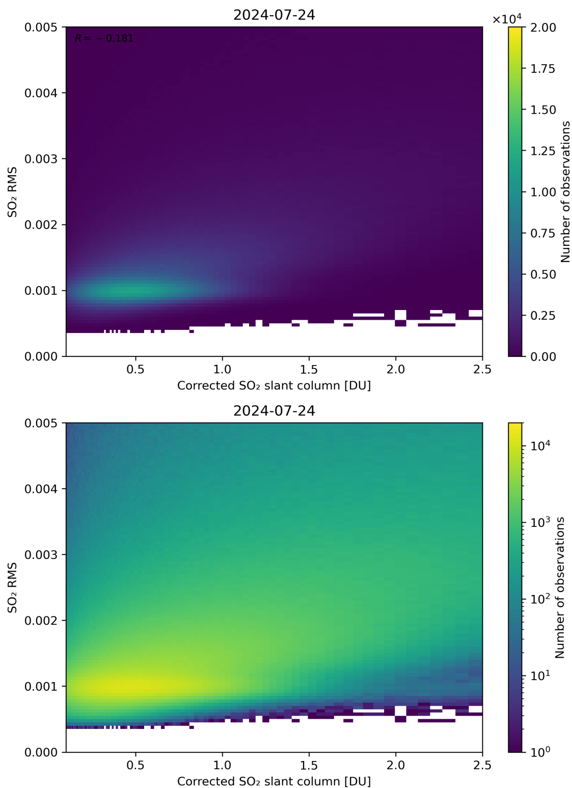
Figure 183: Scatter density plot of “Corrected SO 2 slant column” against “SO 2 RMS” for 2024-07-23 to 2024-07-25.
