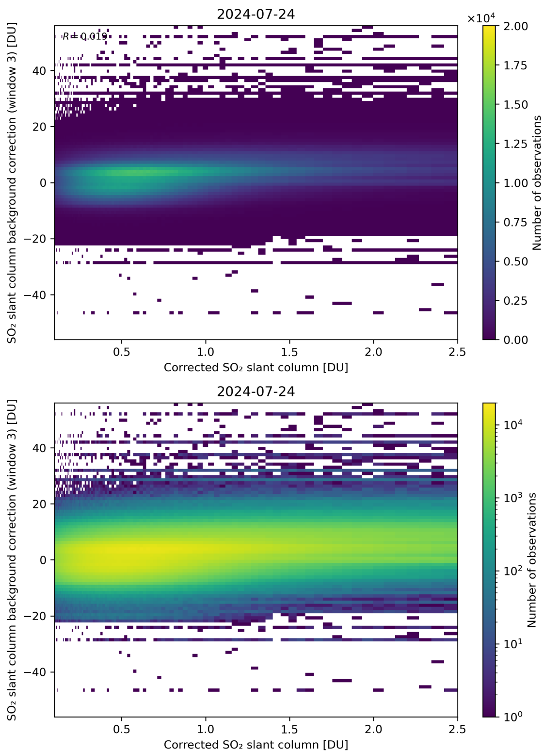
Figure 180: Scatter density plot of “Corrected SO 2 slant column” against “SO 2 slant column background correction (window 3)” for 2024-07-23 to 2024-07-25.
