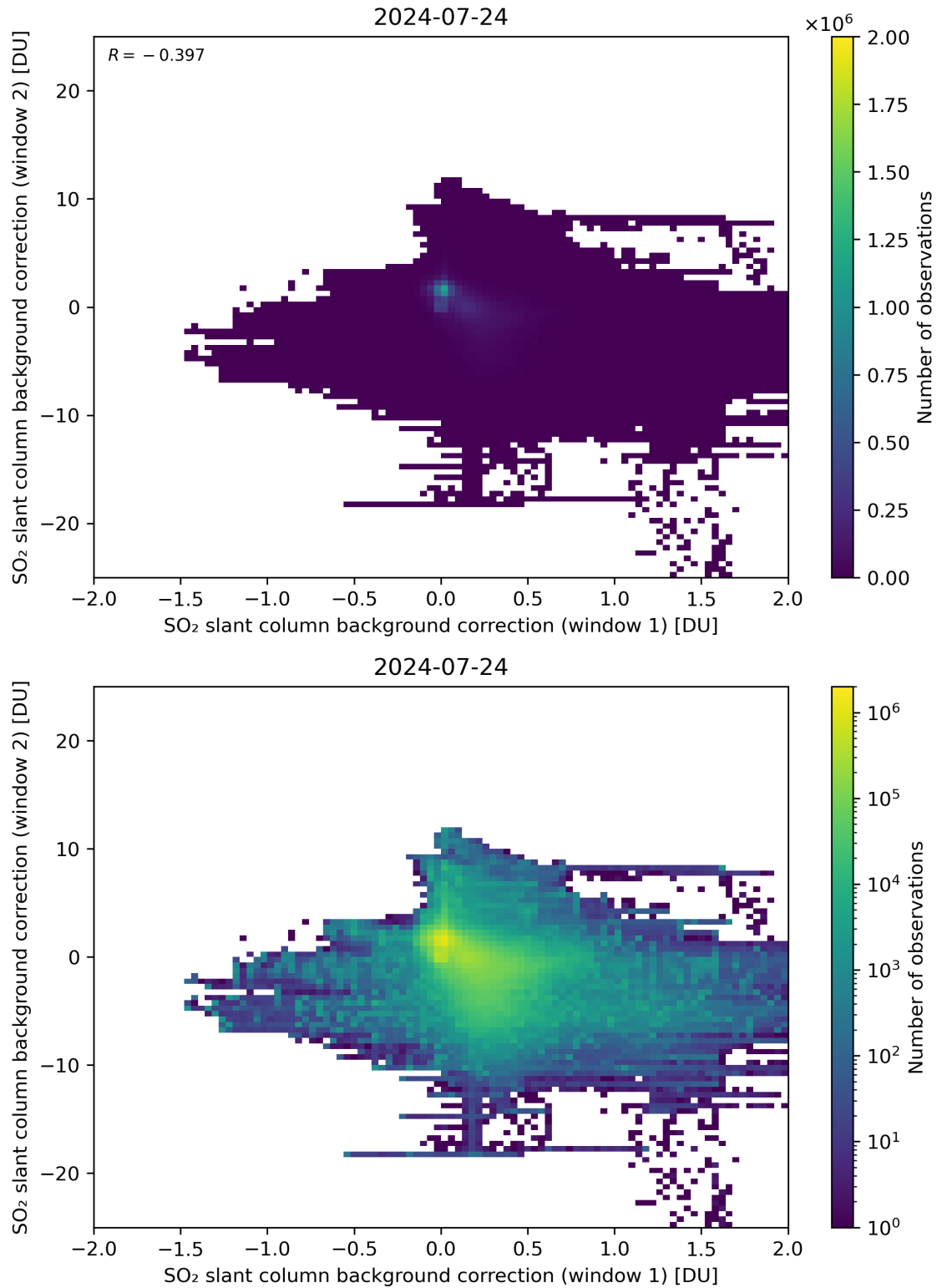
Figure 98: Scatter density plot of “SO 2 slant column background correction (window 1)” against “SO 2 slant column background correction (window 2)” for 2024-07-23 to 2024-07-25.
