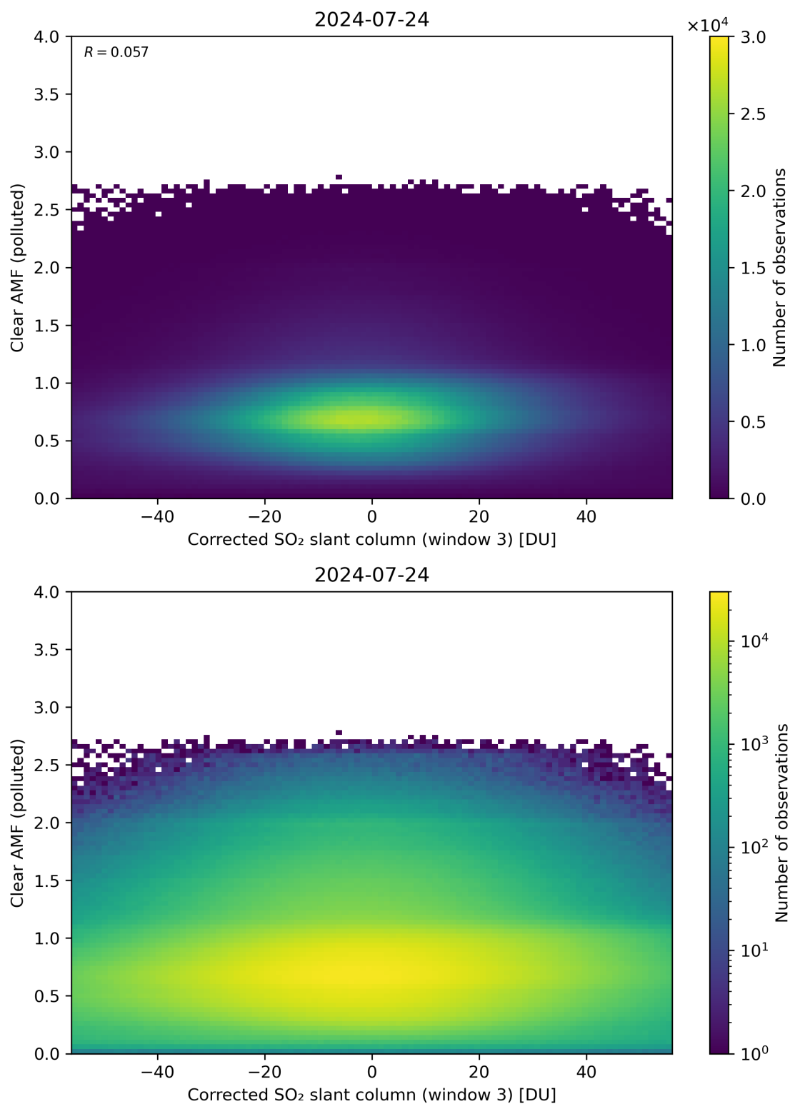
Figure 209: Scatter density plot of “Corrected SO 2 slant column (window 3)” against “Clear AMF (polluted)” for 2024-07-23 to 2024-07-25.
