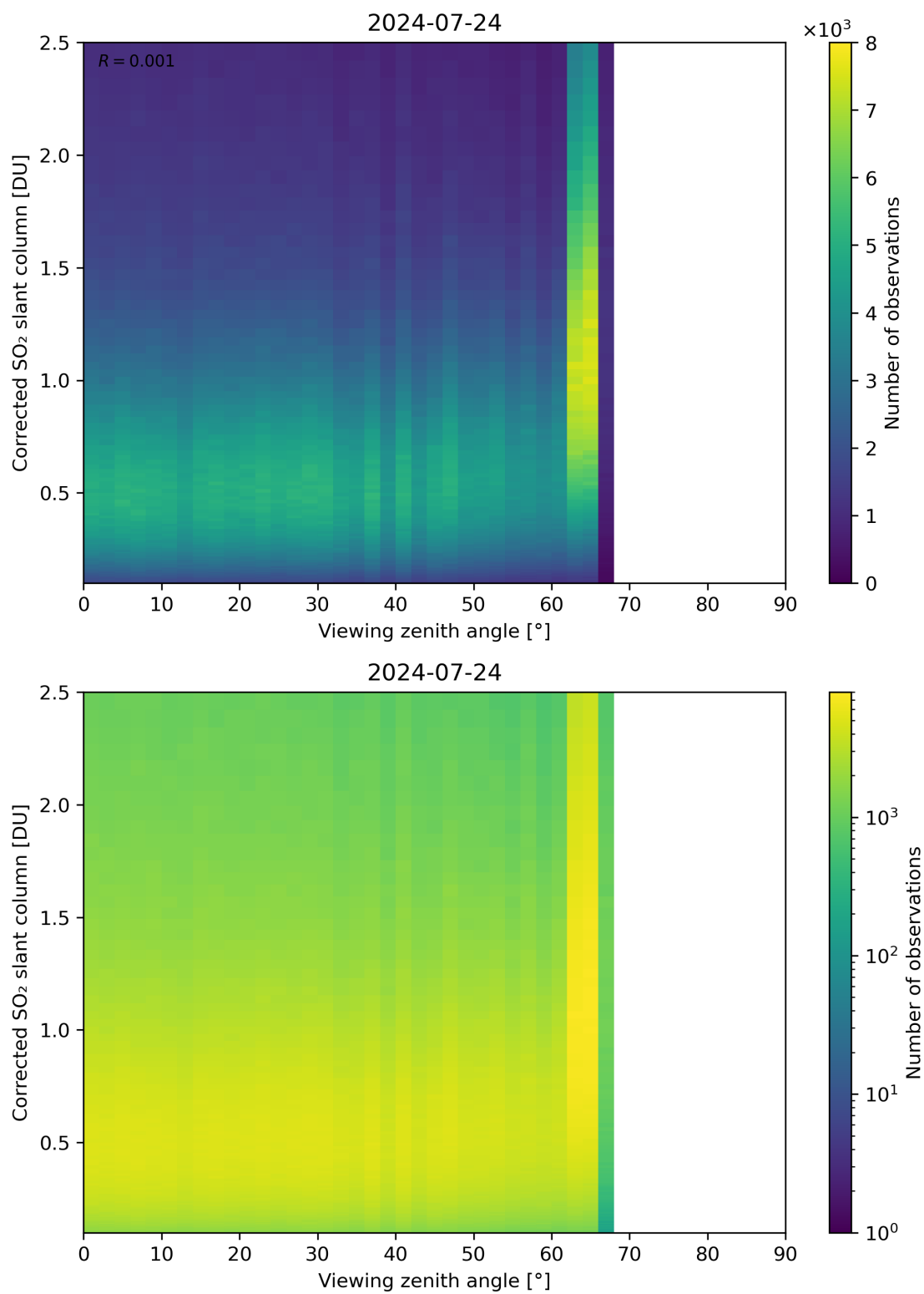
Figure 317: Scatter density plot of “Viewing zenith angle” against “Corrected SO 2 slant column” for 2024-07-23 to 2024-07-25.
