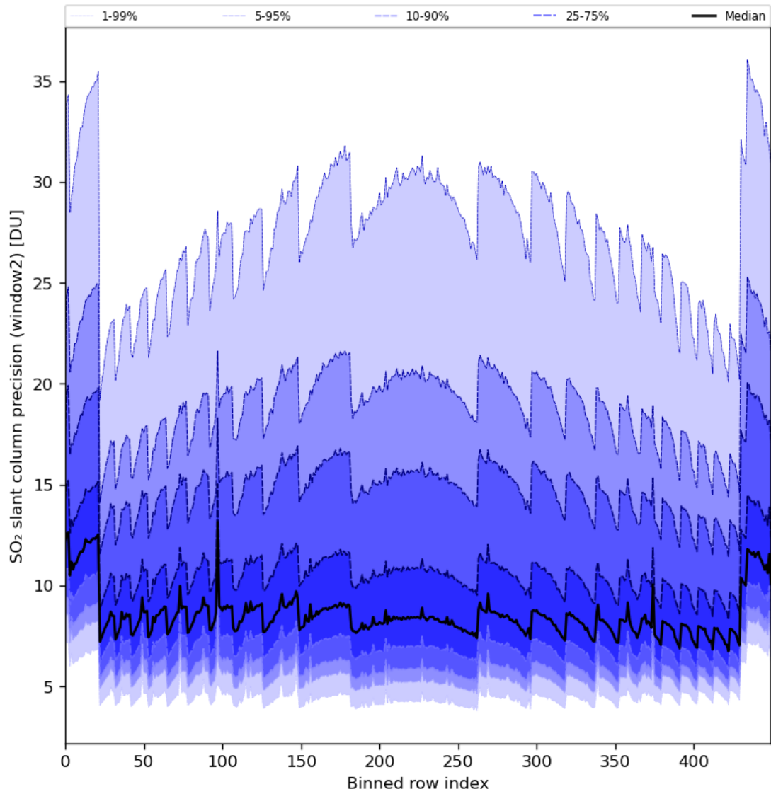
Figure 84: Along track statistics of "SO 2 slant column precision (window2)" for 2024-07-23 to 2024-07-25
