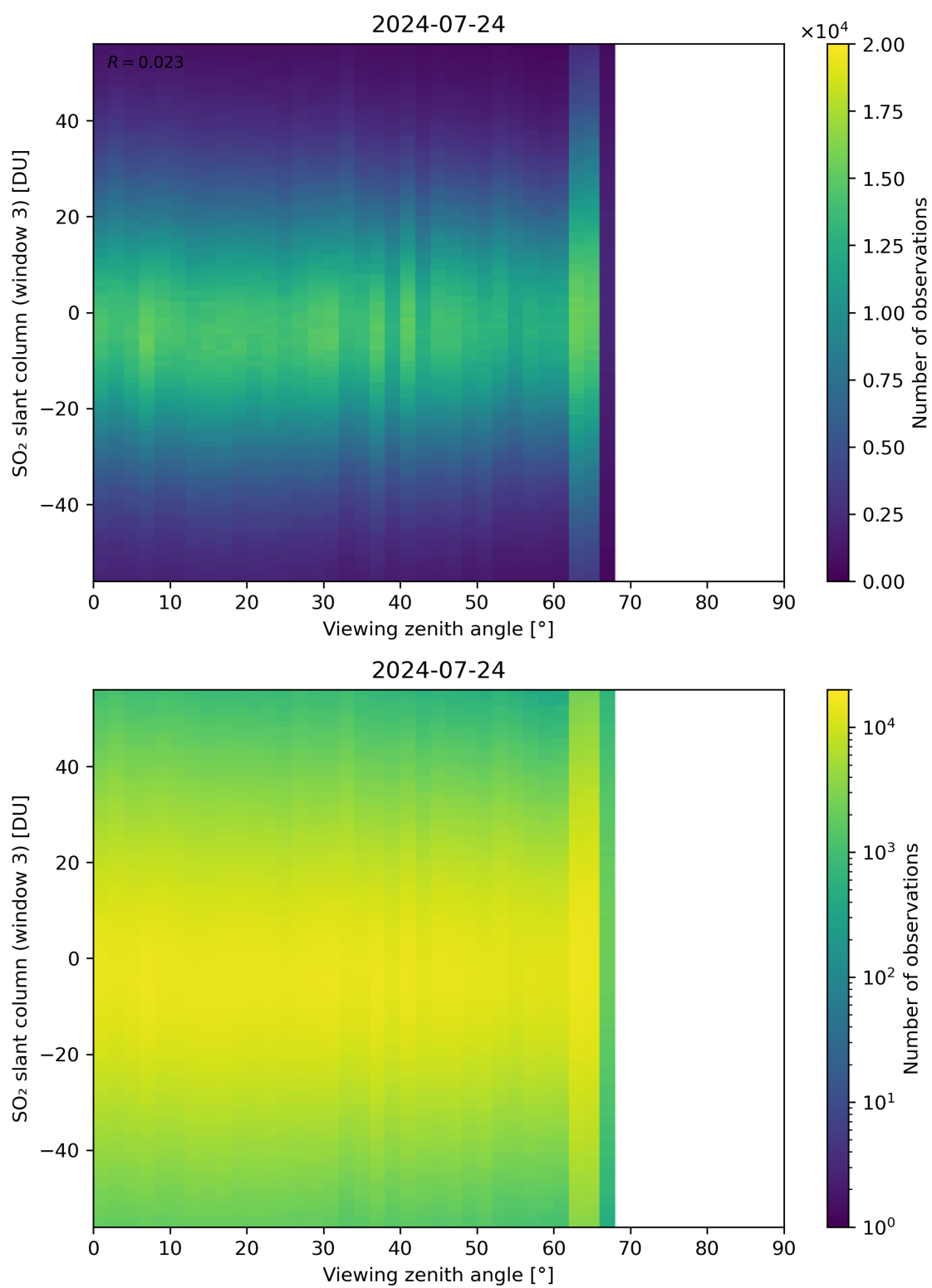
Figure 323: Scatter density plot of “Viewing zenith angle” against “SO 2 slant column (window 3)” for 2024-07-23 to 2024-07-25.
