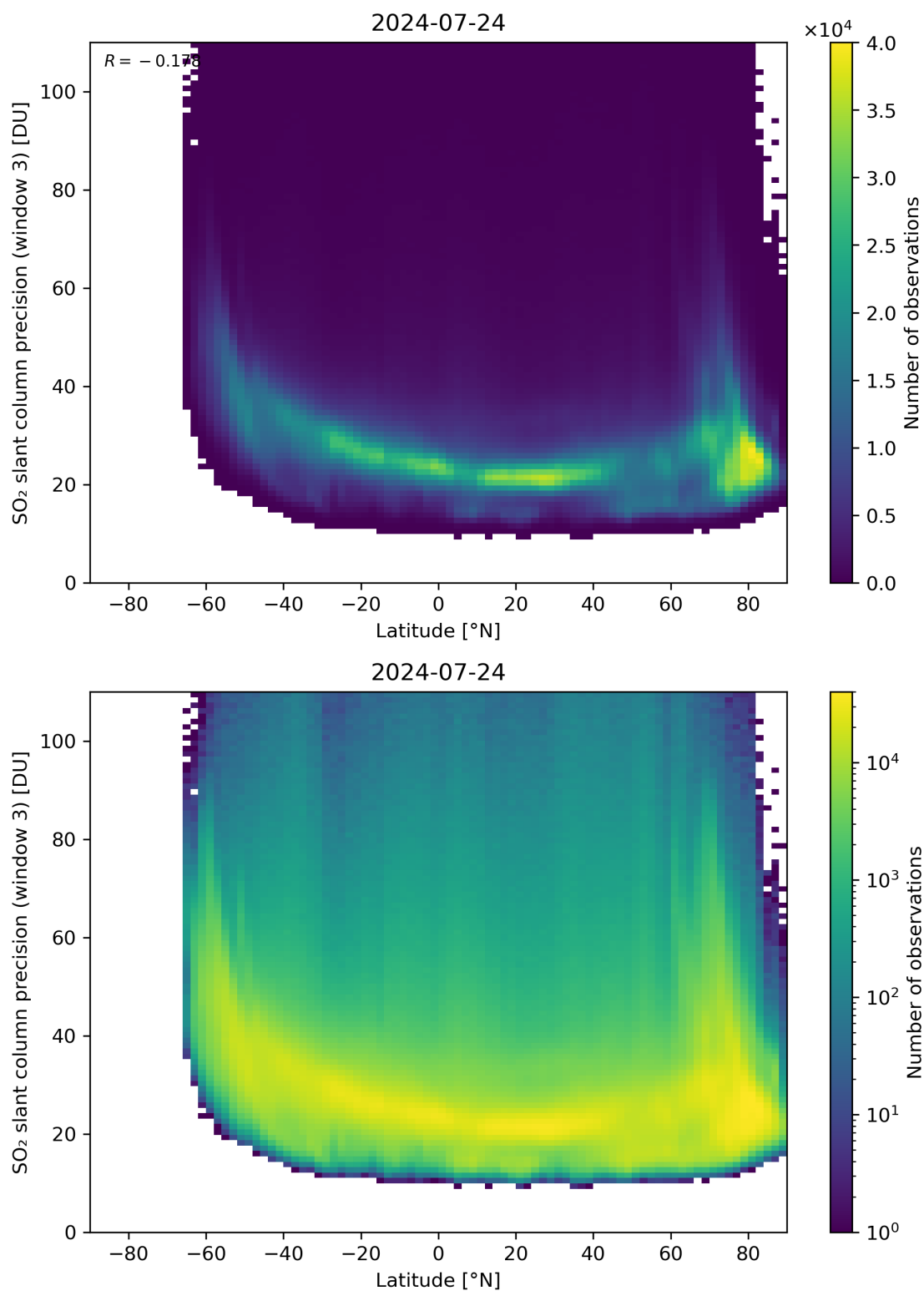
Figure 153: Scatter density plot of “Latitude” against “SO 2 slant column precision (window 3)” for 2024-07-23 to 2024-07-25.
