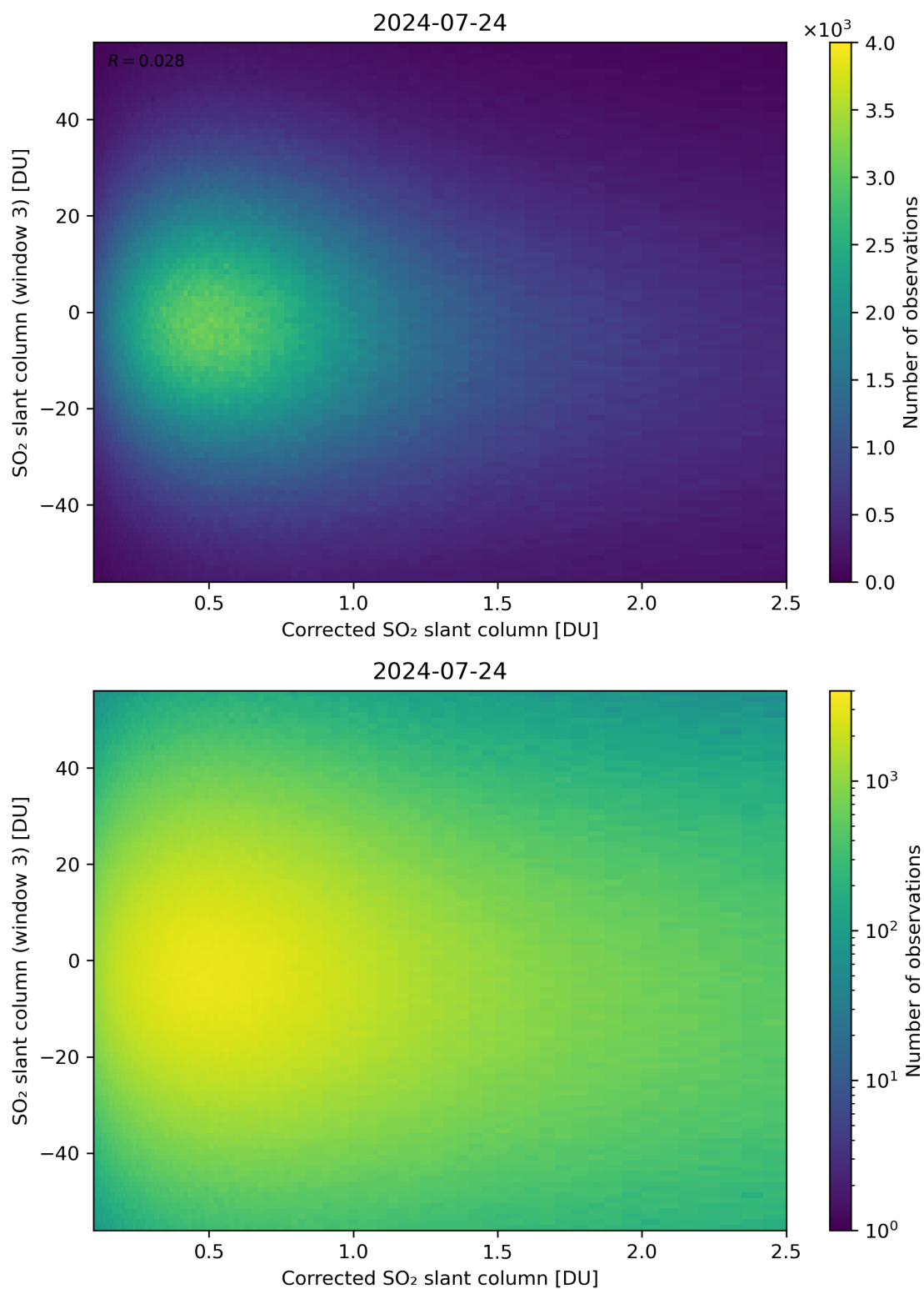
Figure 190: Scatter density plot of “Corrected SO 2 slant column” against “SO 2 slant column (window 3)” for 2024-07-23 to 2024-07-25.
