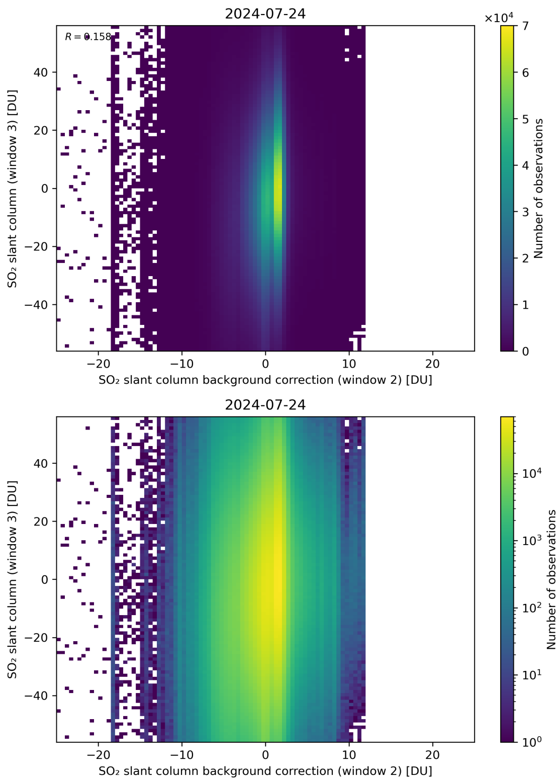
Figure 117: Scatter density plot of “SO 2 slant column background correction (window 2)” against “SO 2 slant column (window 3)” for 2024-07-23 to 2024-07-25.
