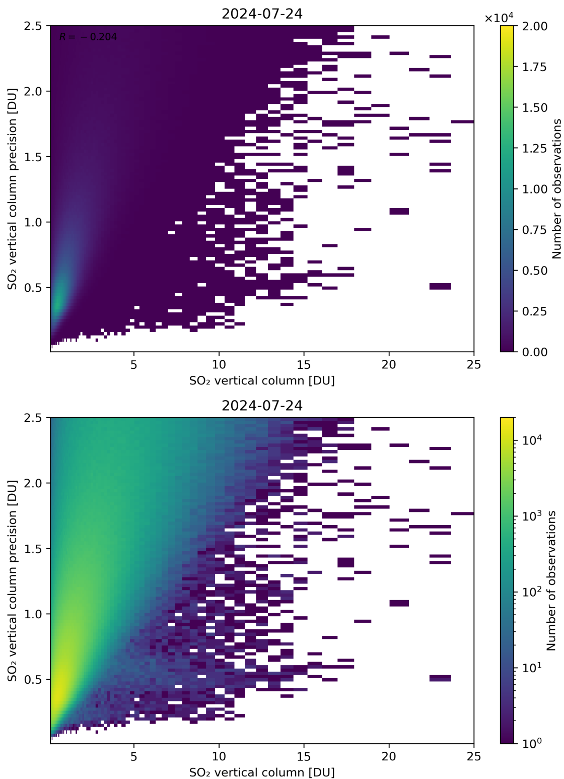
Figure 307: Scatter density plot of “SO 2 vertical column” against “SO 2 vertical column precision” for 2024-07-23 to 2024-07-25.
