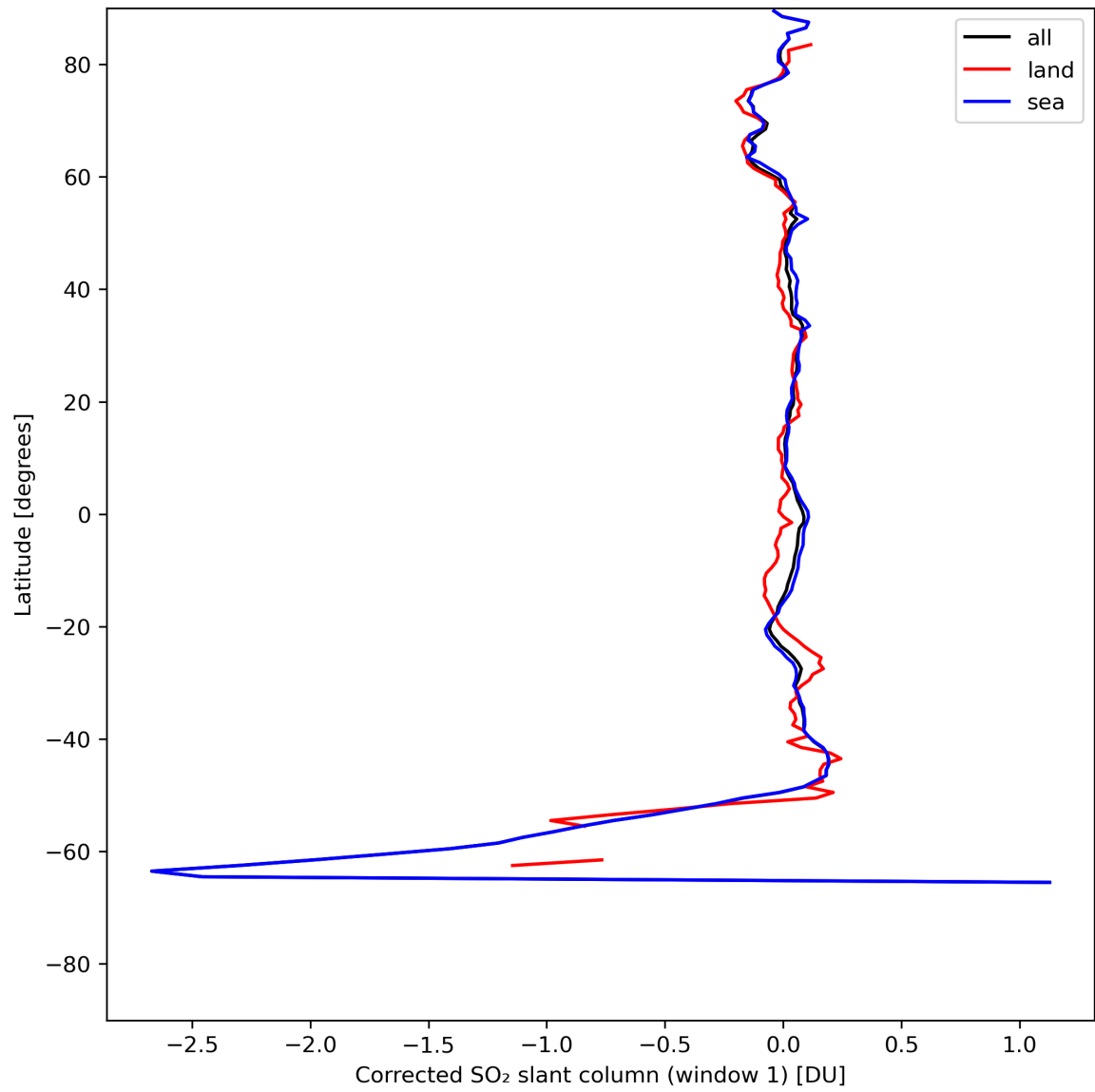
Figure 35: Zonal average of “Corrected SO 2 slant column (window 1)” for 2024-07-23 to 2024-07-25.
