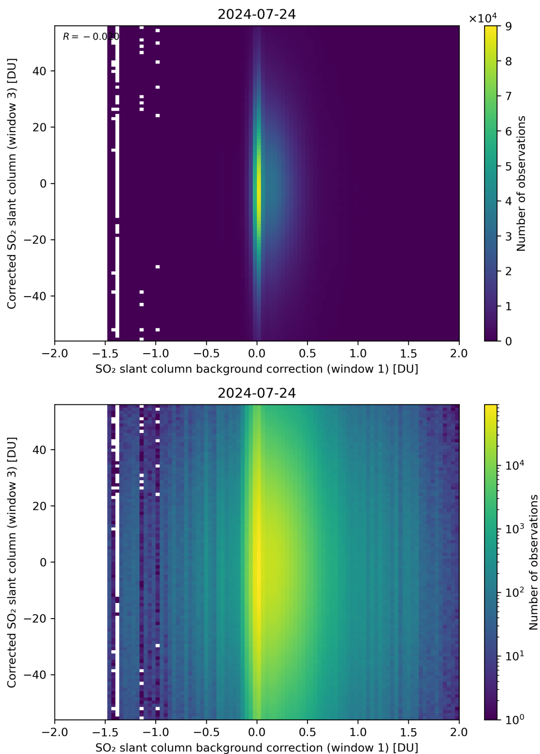
Figure 105: Scatter density plot of “SO 2 slant column background correction (window 1)” against “Corrected SO 2 slant column (window 3)” for 2024-07-23 to 2024-07-25.
