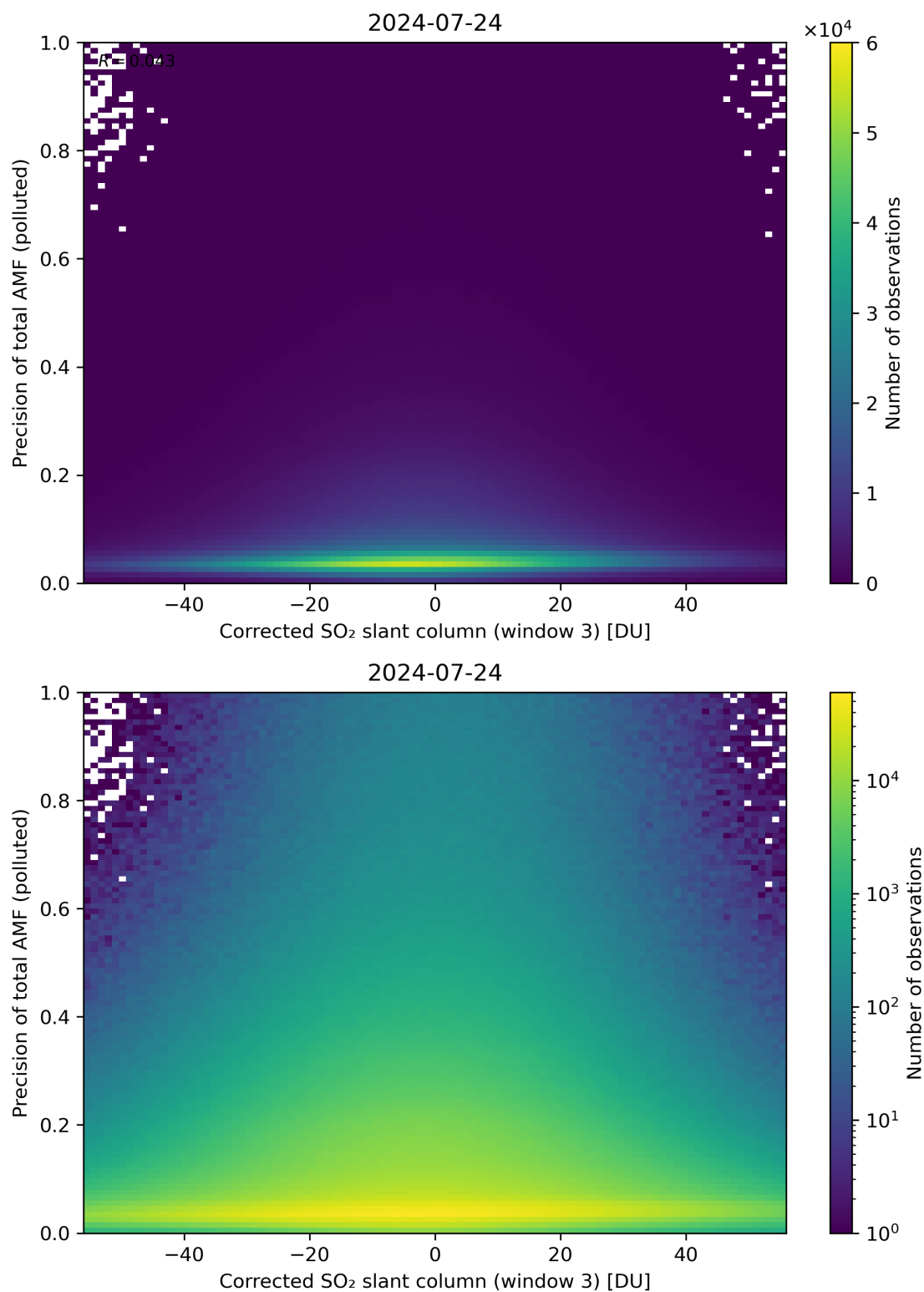
Figure 211: Scatter density plot of “Corrected SO 2 slant column (window 3)” against “Precision of total AMF (polluted)” for 2024-07-23 to 2024-07-25.
