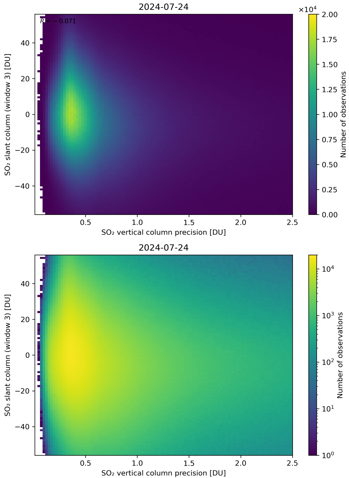
Figure 292: Scatter density plot of “SO 2 vertical column precision” against “SO 2 slant column (window 3)” for 2024-07-23 to 2024-07-25.
