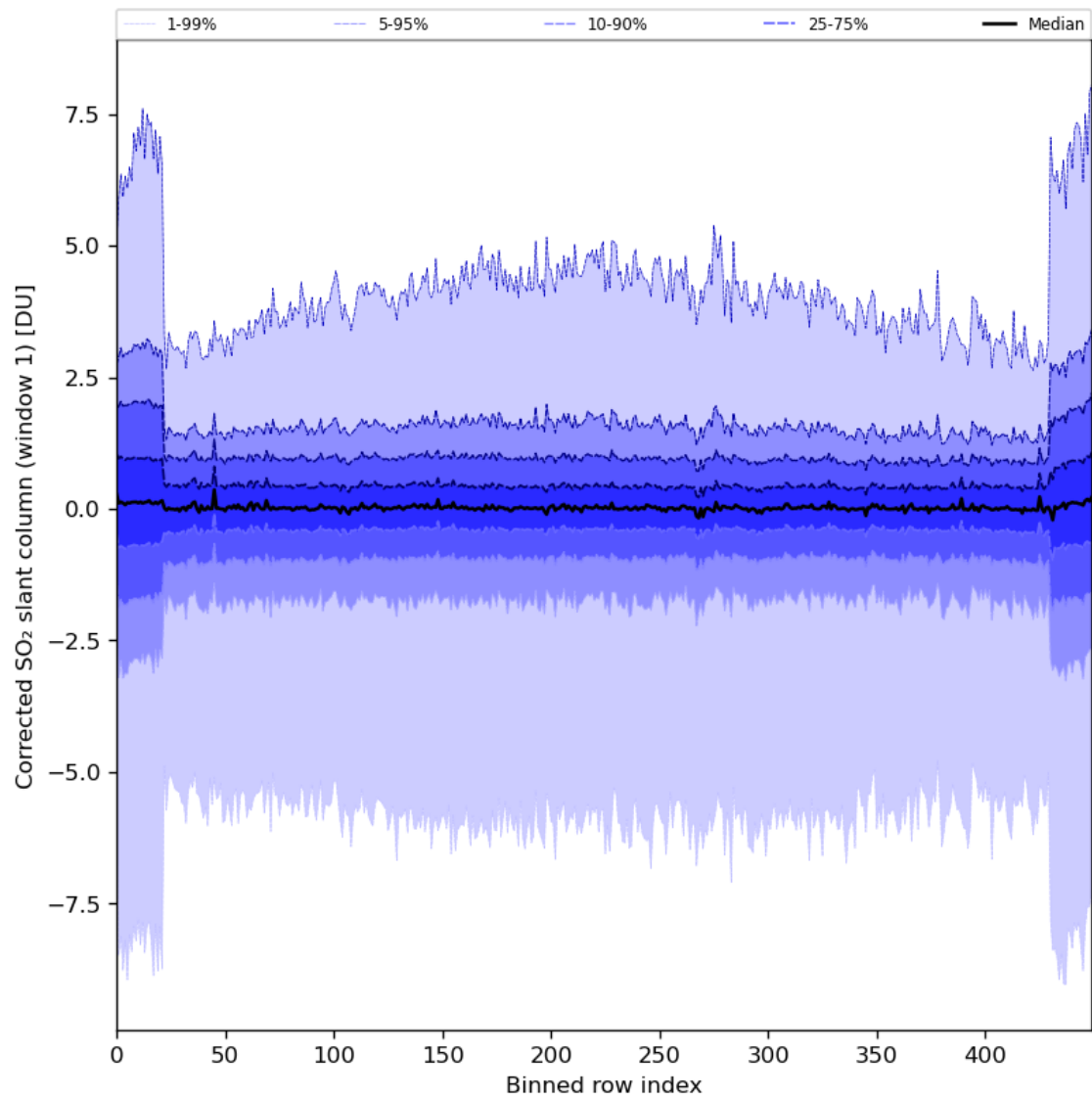
Figure 81: Along track statistics of "Corrected SO 2 slant column (window 1)" for 2024-07-23 to 2024-07-25
