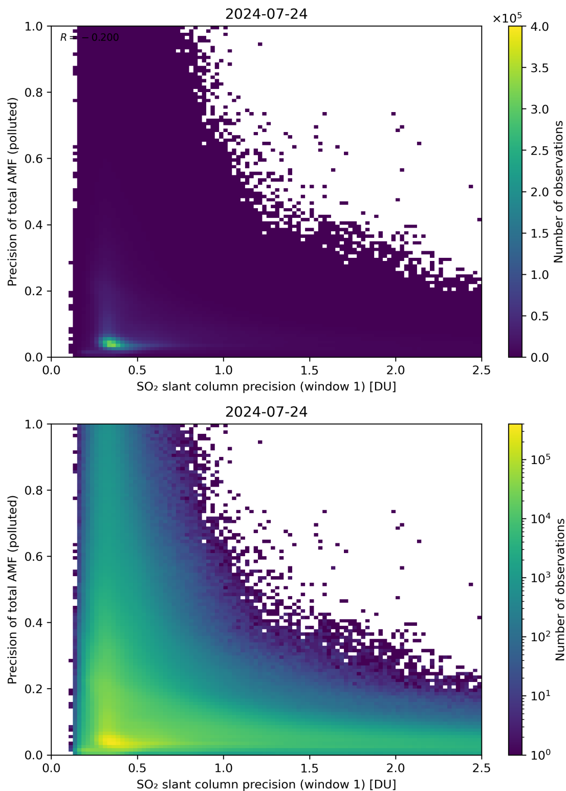
Figure 231: Scatter density plot of “SO 2 slant column precision (window 1)” against “Precision of total AMF (polluted)” for 2024-07-23 to 2024-07-25.
