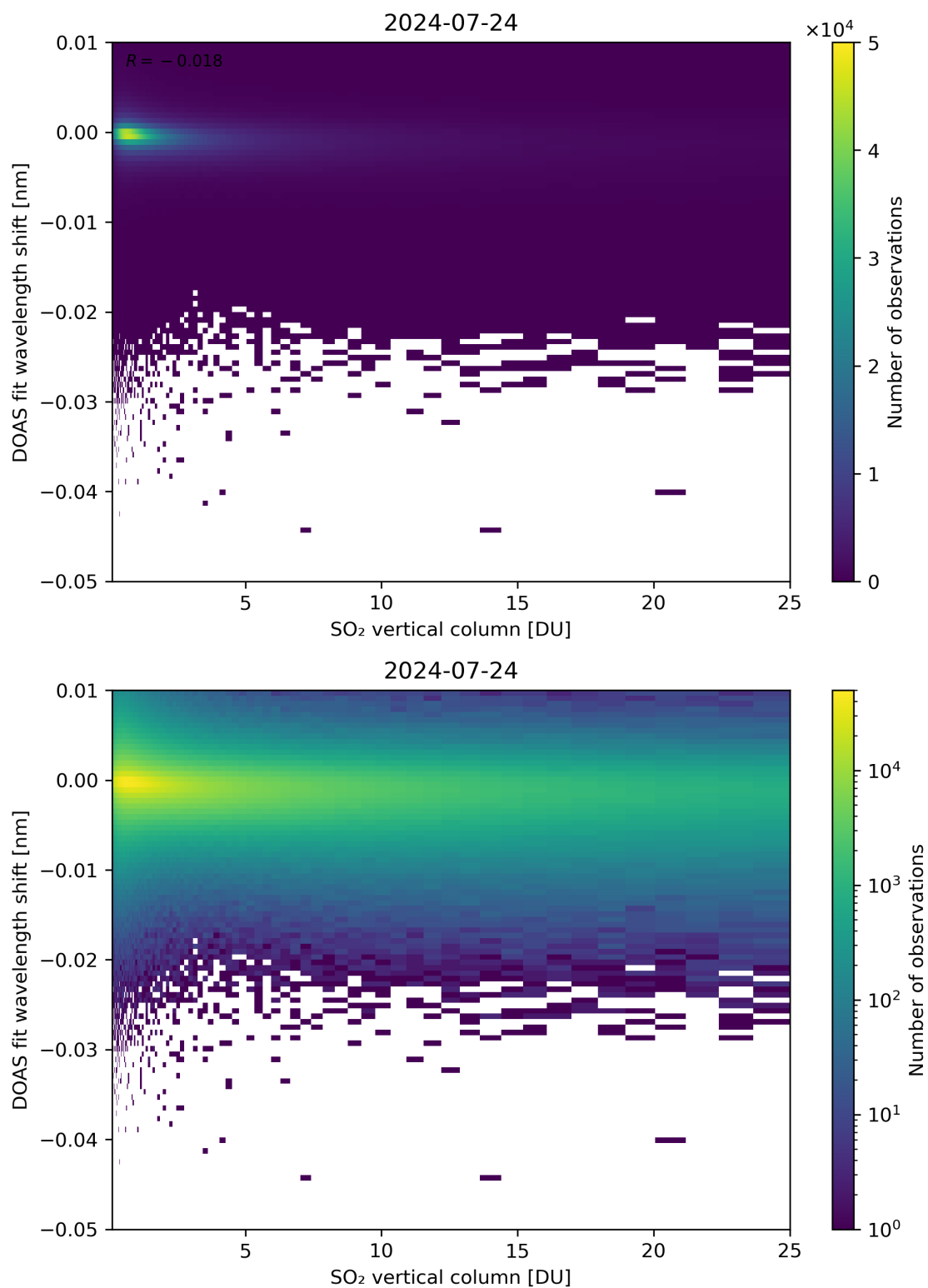
Figure 276: Scatter density plot of “SO 2 vertical column” against “DOAS fit wavelength shift” for 2024-07-23 to 2024-07-25.
