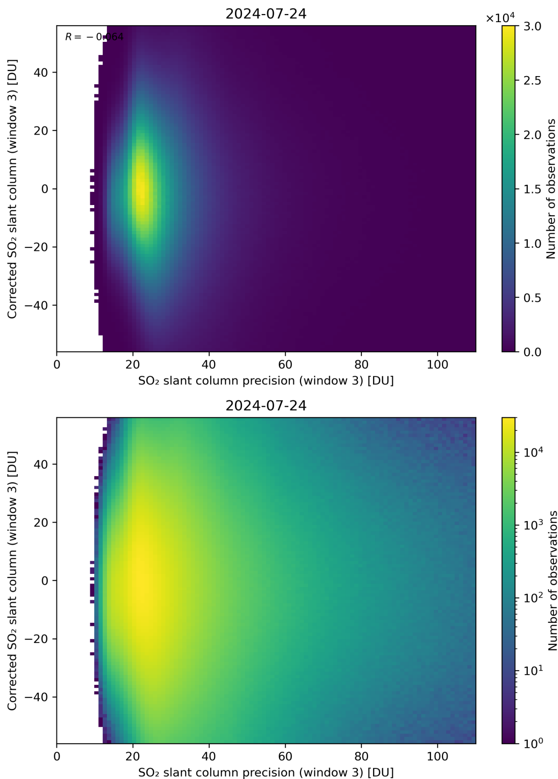
Figure 262: Scatter density plot of “SO 2 slant column precision (window 3)” against “Corrected SO 2 slant column (window 3)” for 2024-07-23 to 2024-07-25.
