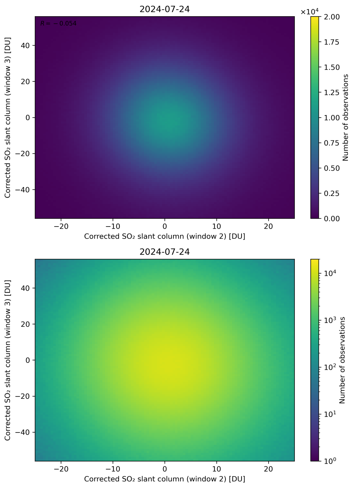
Figure 200: Scatter density plot of “Corrected SO 2 slant column (window 2)” against “Corrected SO 2 slant column (window 3)” for 2024-07-23 to 2024-07-25.
