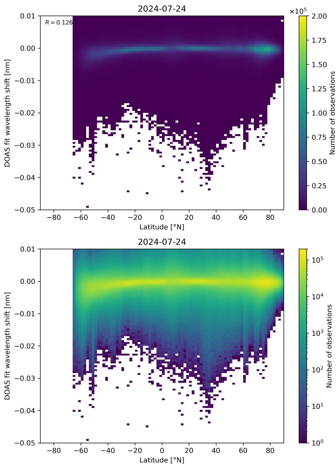
Figure 142: Scatter density plot of “Latitude” against “DOAS fit wavelength shift” for 2024-07-23 to 2024-07-25.
