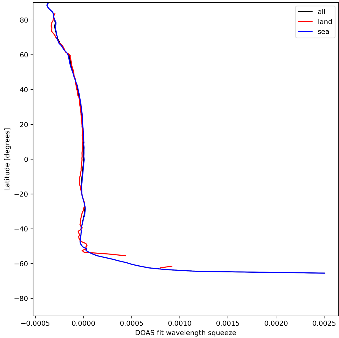
Figure 46: Zonal average of “DOAS fit wavelength squeeze” for 2024-07-23 to 2024-07-25.
