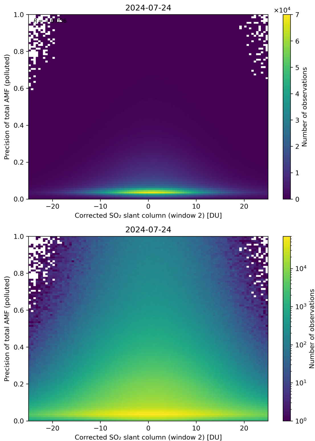
Figure 204: Scatter density plot of “Corrected SO 2 slant column (window 2)” against “Precision of total AMF (polluted)” for 2024-07-23 to 2024-07-25.
