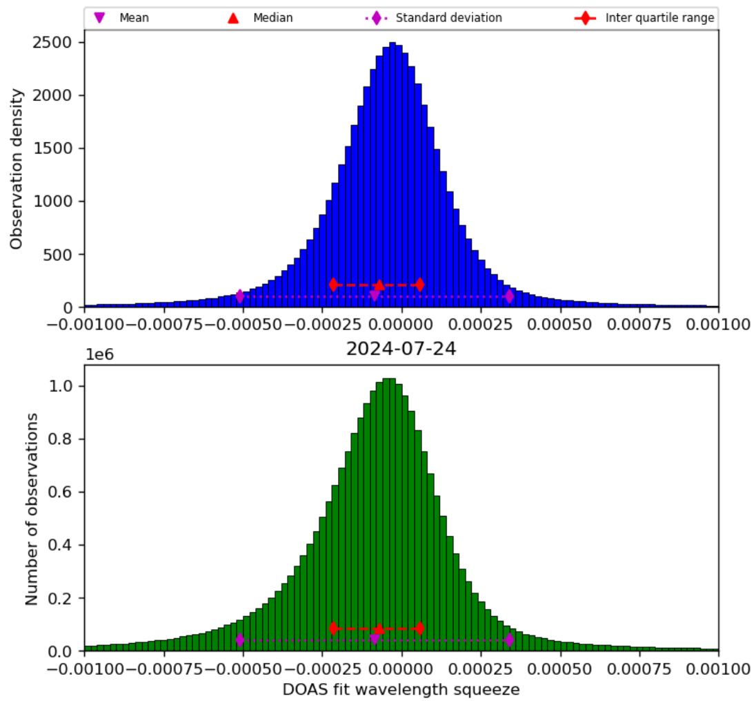
Figure 69: Histogram of “DOAS fit wavelength squeeze” for 2024-07-23 to 2024-07-25
