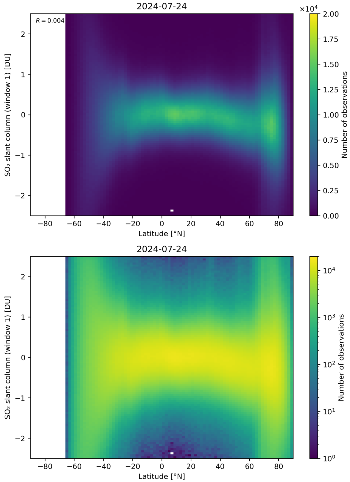
Figure 149: Scatter density plot of “Latitude” against “SO 2 slant column (window 1)” for 2024-07-23 to 2024-07-25.
