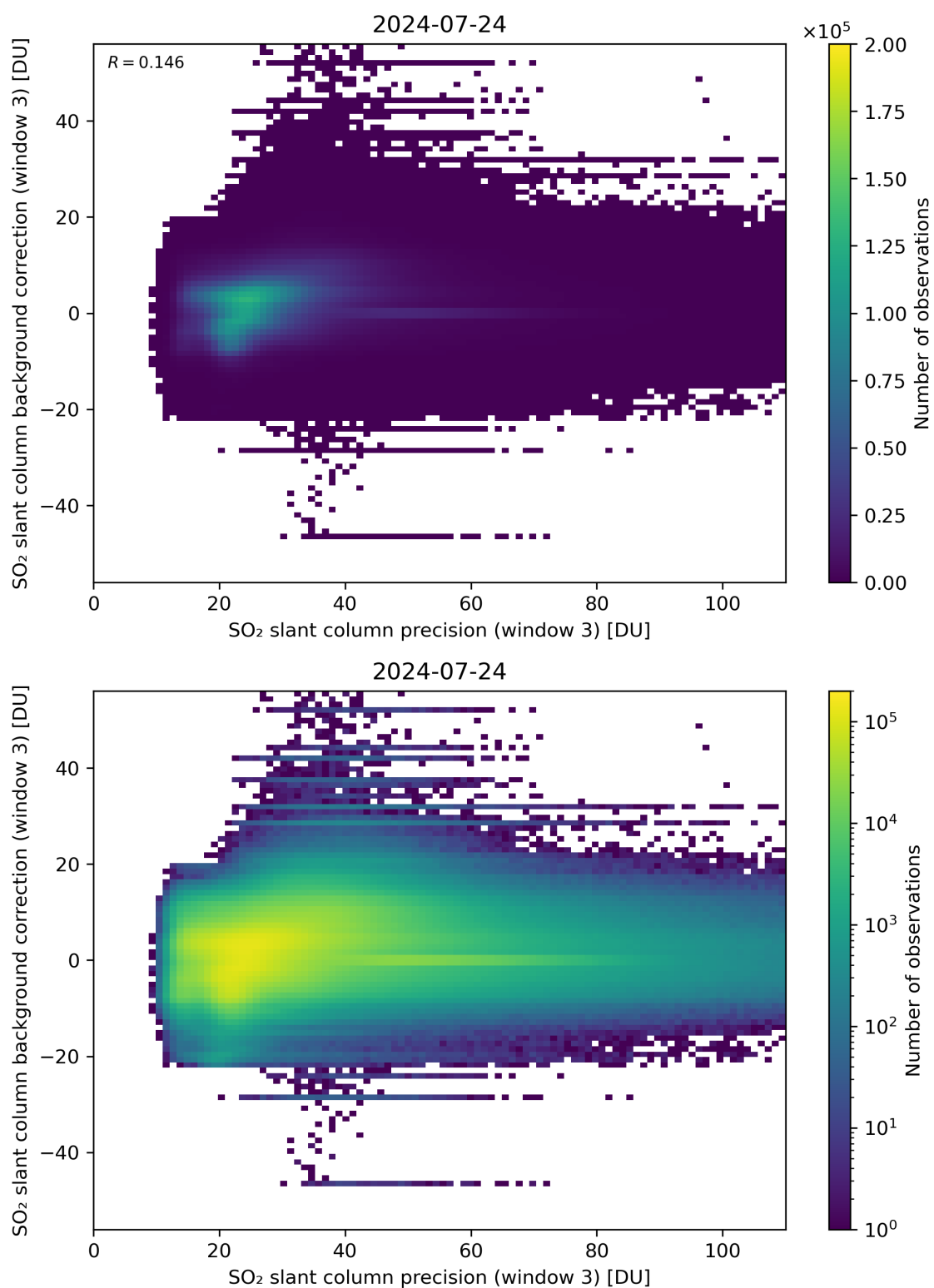
Figure 257: Scatter density plot of “SO 2 slant column precision (window 3)” against “SO 2 slant column background correction (window 3)” for 2024-07-23 to 2024-07-25.
