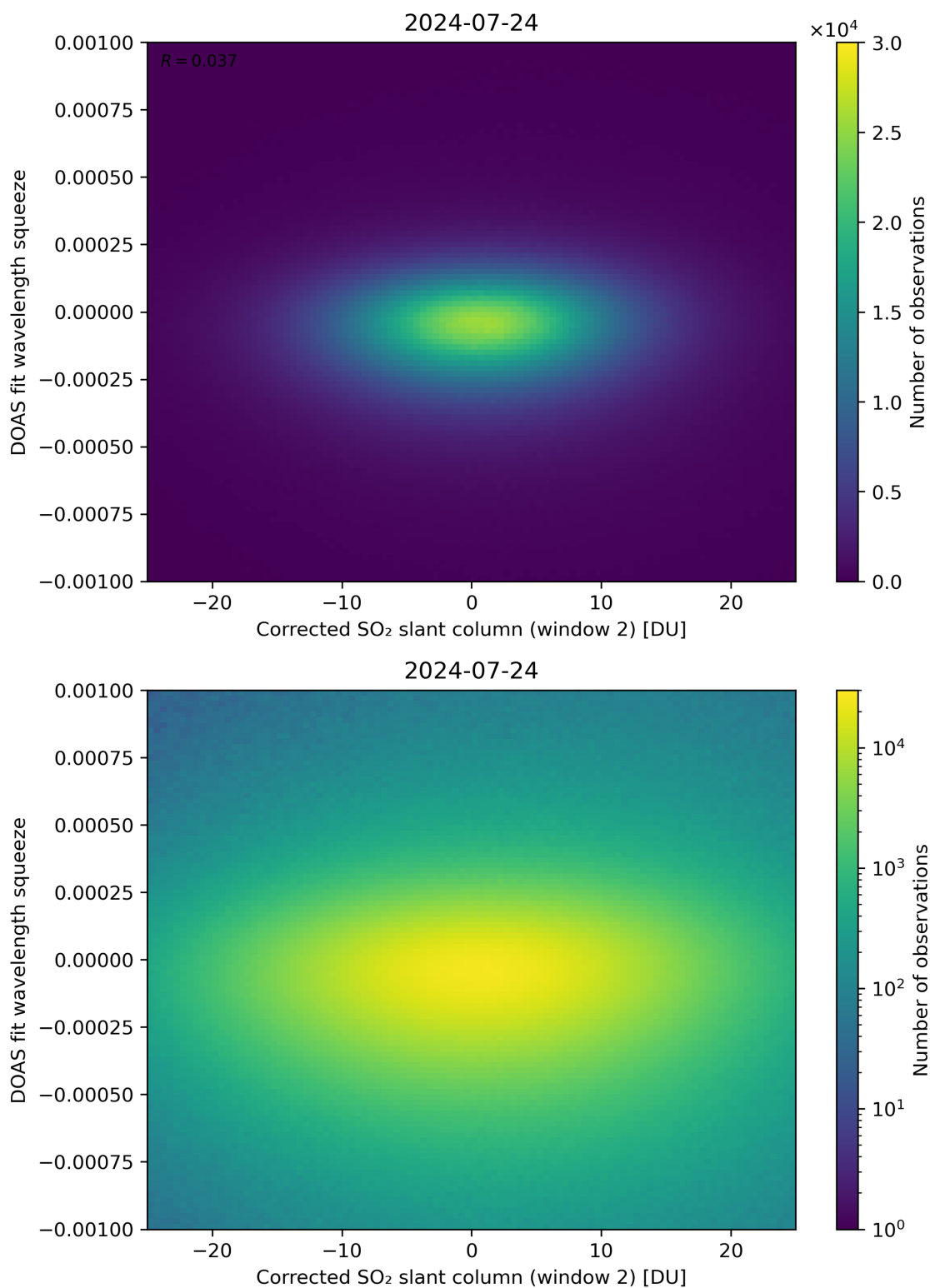
Figure 197: Scatter density plot of “Corrected SO 2 slant column (window 2)” against “DOAS fit wavelength squeeze” for 2024-07-23 to 2024-07-25.
