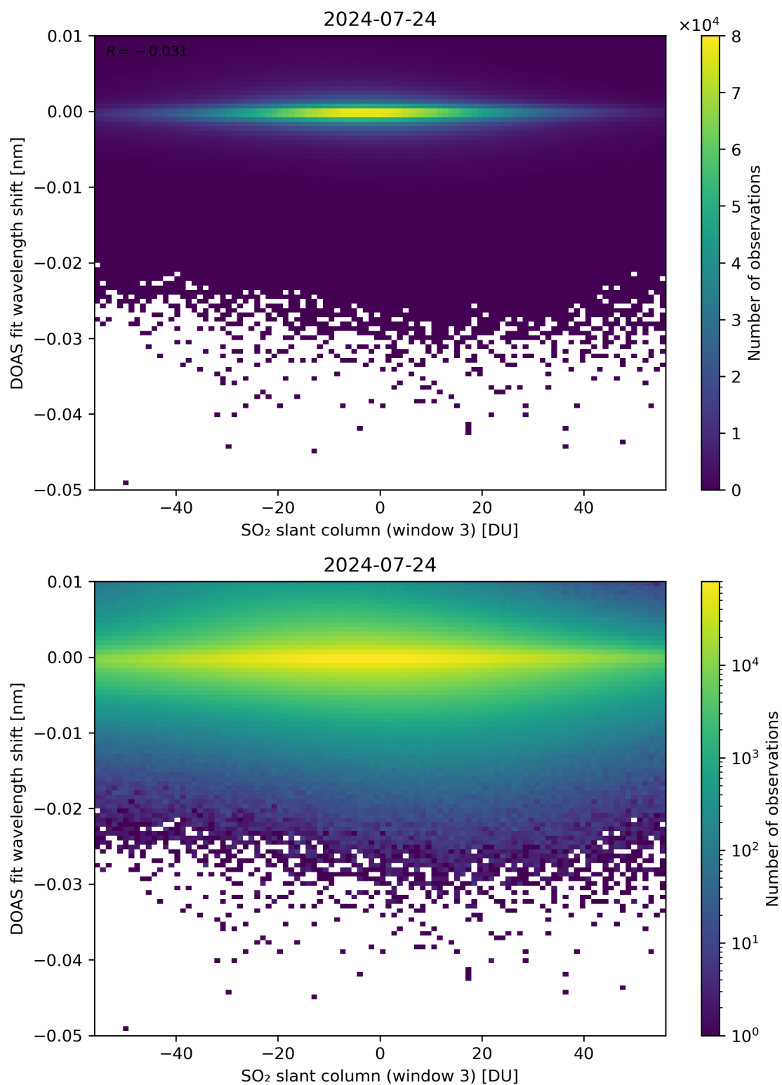
Figure 254: Scatter density plot of “SO 2 slant column (window 3)” against “DOAS fit wavelength shift” for 2024-07-23 to 2024-07-25.
