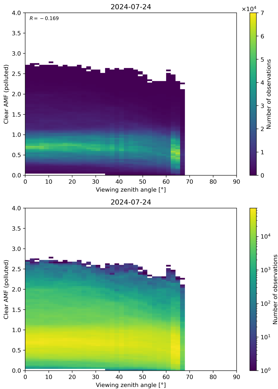
Figure 316: Scatter density plot of “Viewing zenith angle” against “Clear AMF (polluted)” for 2024-07-23 to 2024-07-25.
