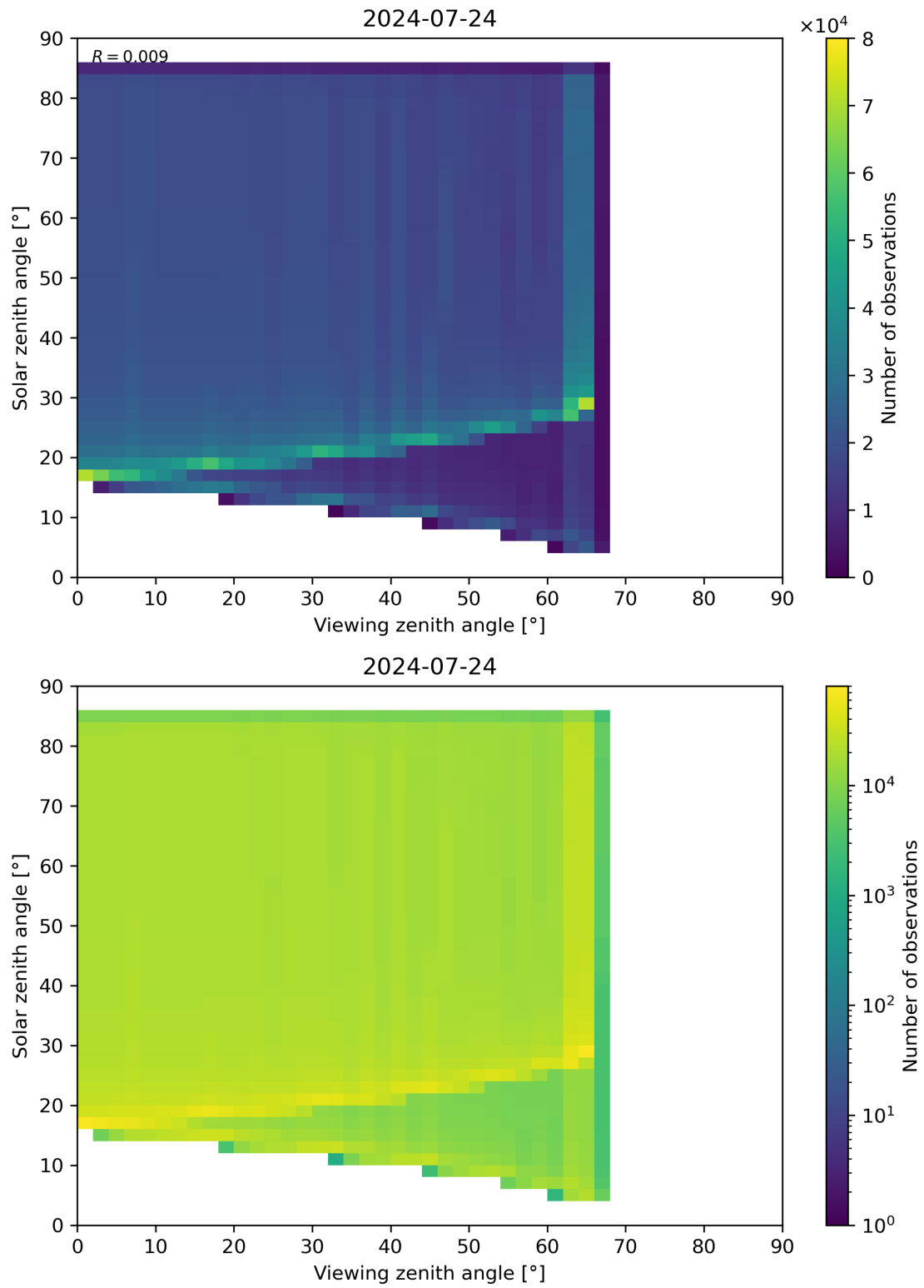
Figure 315: Scatter density plot of “Viewing zenith angle” against “Solar zenith angle” for 2024-07-23 to 2024-07-25.
