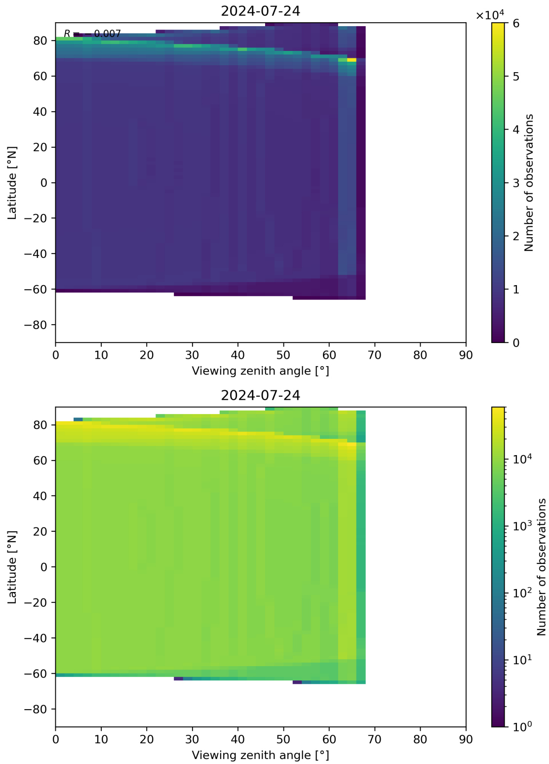
Figure 314: Scatter density plot of “Viewing zenith angle” against “Latitude” for 2024-07-23 to 2024-07-25.
