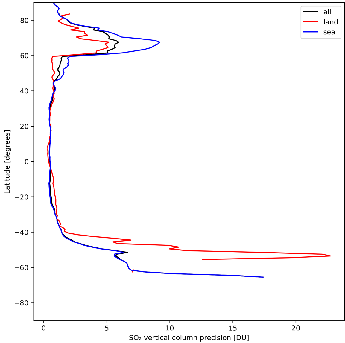
Figure 31: Zonal average of “SO 2 vertical column precision” for 2024-07-23 to 2024-07-25.
