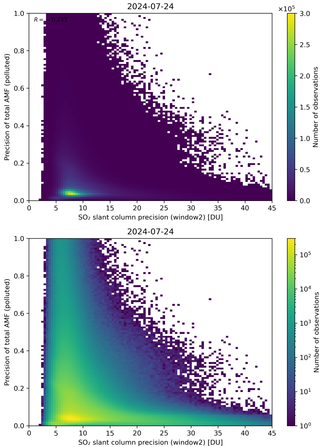
Figure 252: Scatter density plot of “SO 2 slant column precision (window2)” against “Precision of total AMF (polluted)” for 2024-07-23 to 2024-07-25.
