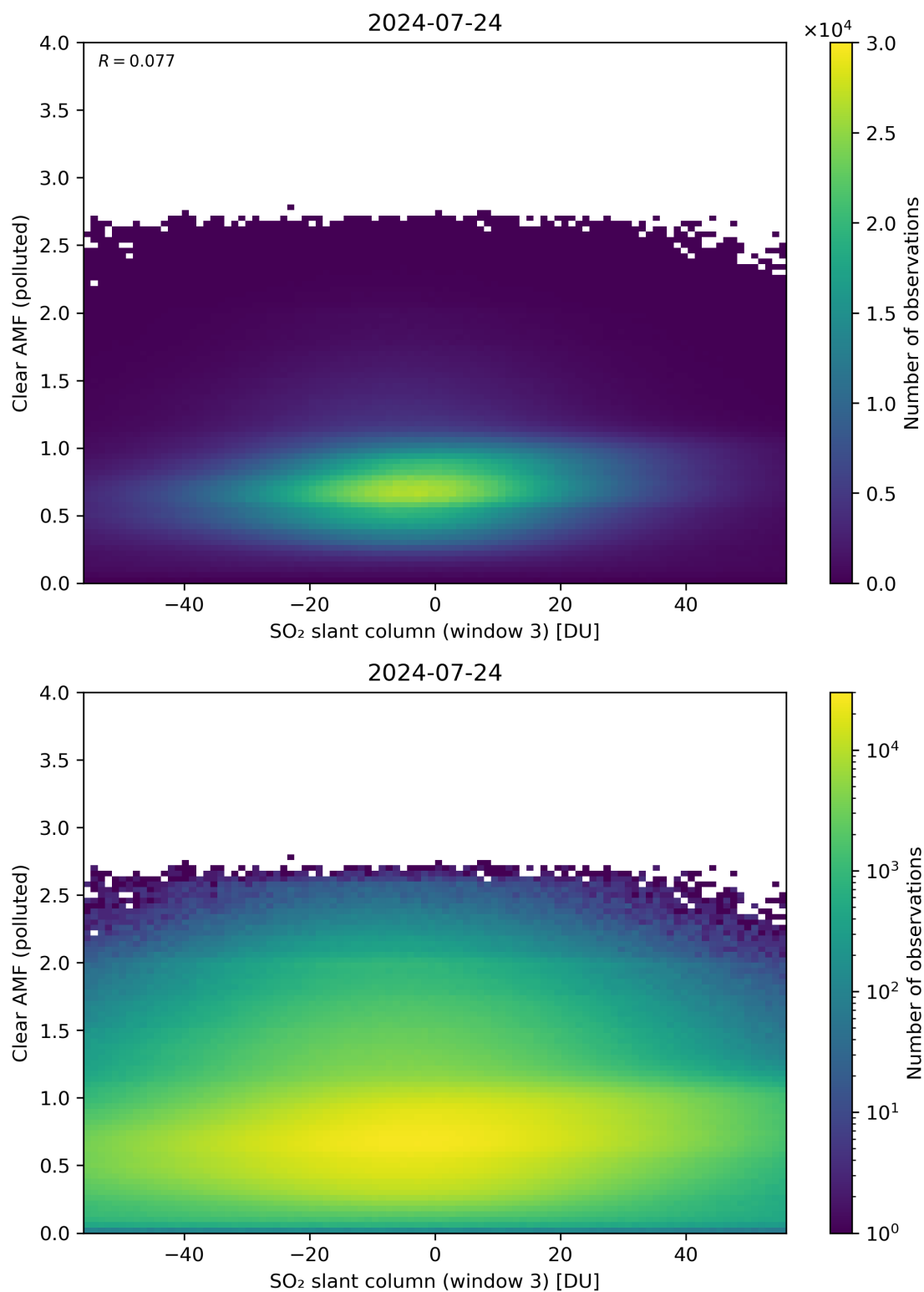
Figure 265: Scatter density plot of “SO 2 slant column (window 3)” against “Clear AMF (polluted)” for 2024-07-23 to 2024-07-25.
