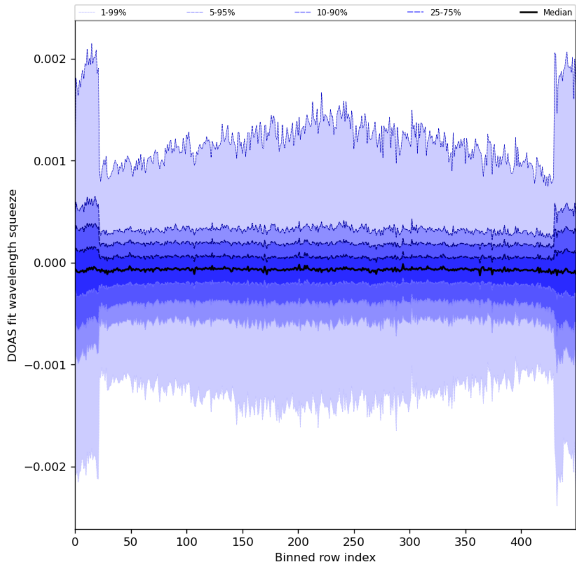
Figure 92: Along track statistics of “DOAS fit wavelength squeeze” for 2024-07-23 to 2024-07-25
