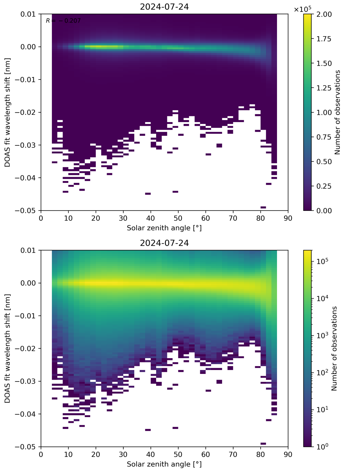
Figure 161: Scatter density plot of “Solar zenith angle” against “DOAS fit wavelength shift” for 2024-07-23 to 2024-07-25.
