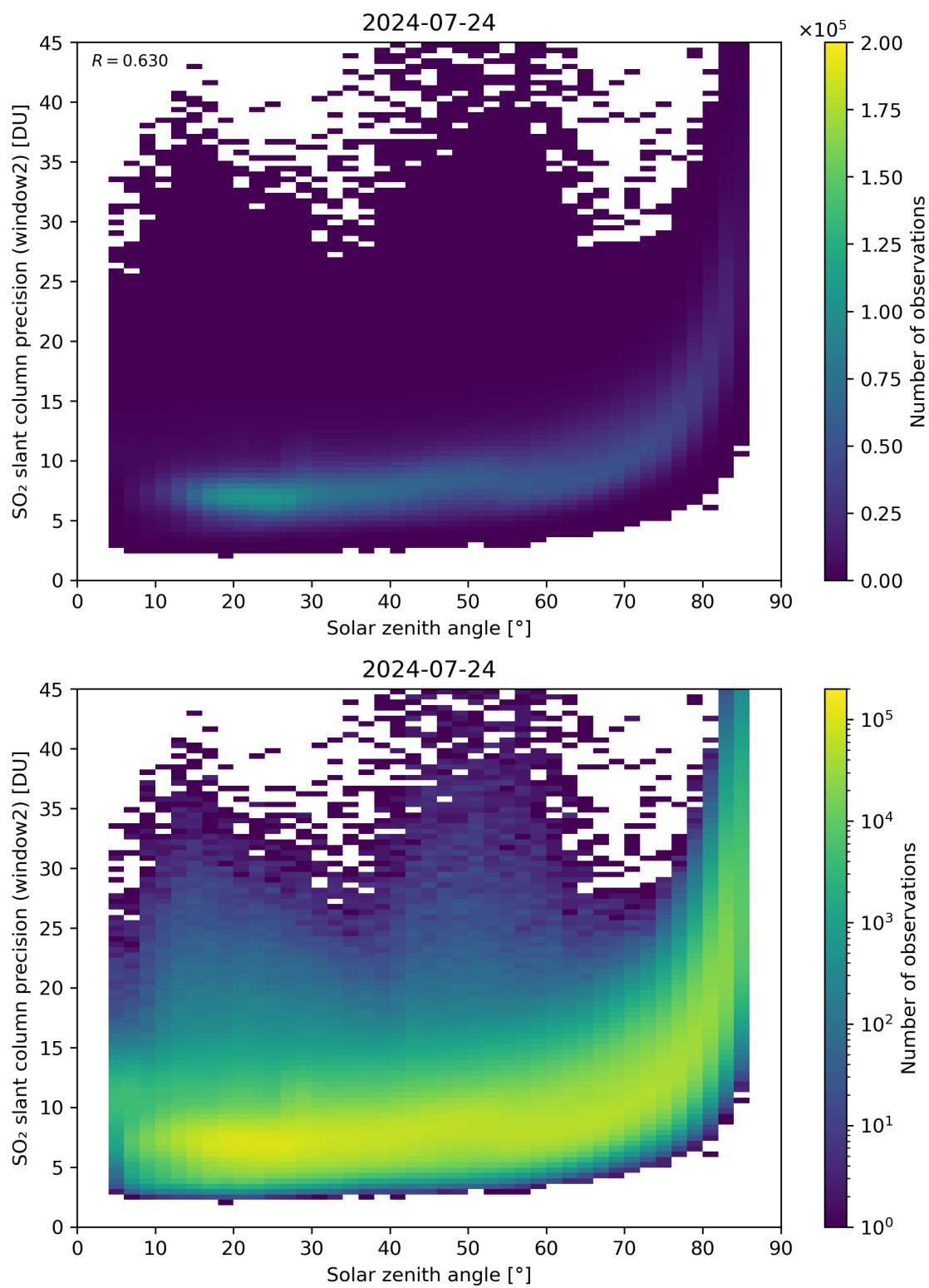
Figure 171: Scatter density plot of “Solar zenith angle” against “SO 2 slant column precision (window2)” for 2024-07-23 to 2024-07-25.
