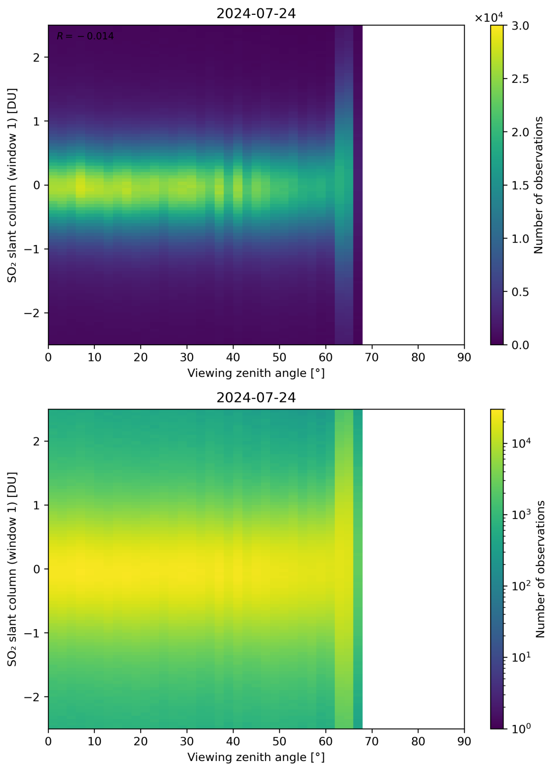
Figure 320: Scatter density plot of “Viewing zenith angle” against “SO 2 slant column (window 1)” for 2024-07-23 to 2024-07-25.
