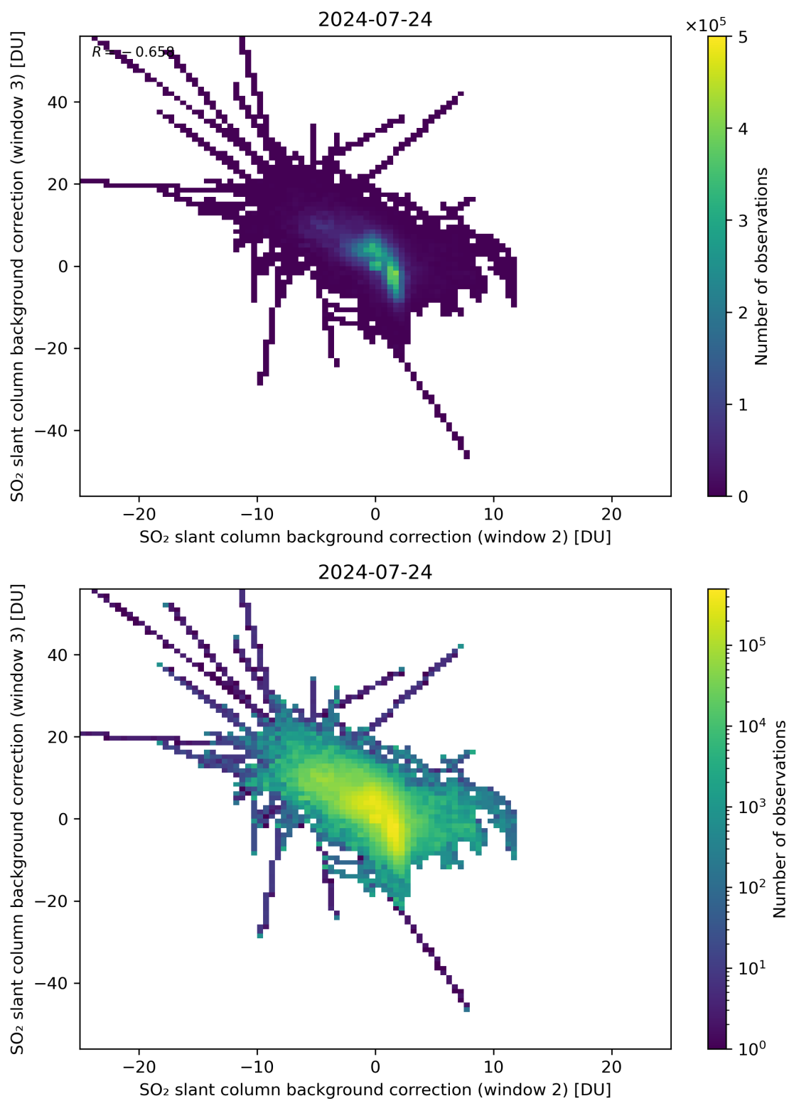
Figure 111: Scatter density plot of “SO 2 slant column background correction (window 2)” against “SO 2 slant column background correction (window 3)” for 2024-07-23 to 2024-07-25.
