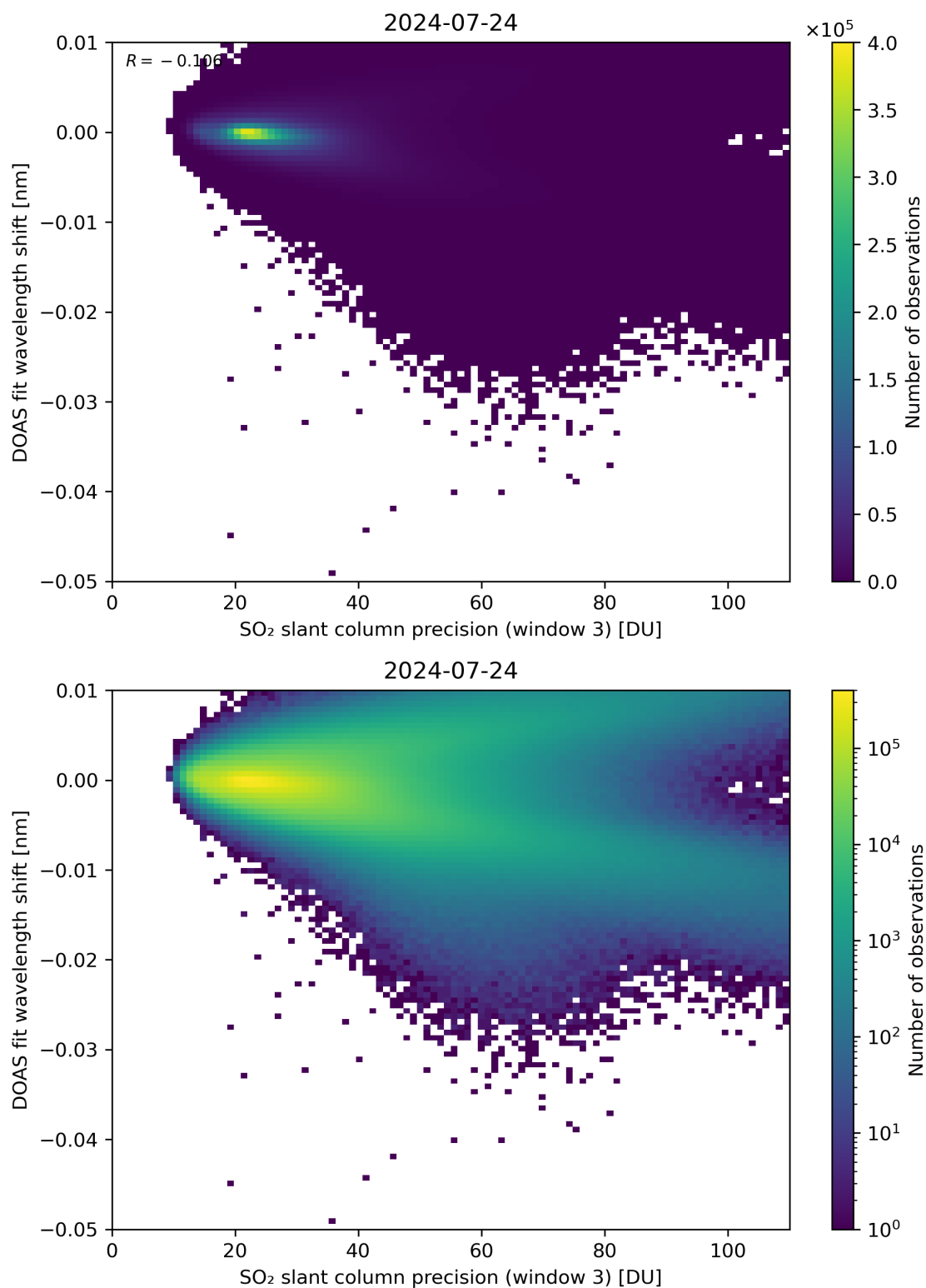
Figure 258: Scatter density plot of “SO 2 slant column precision (window 3)” against “DOAS fit wavelength shift” for 2024-07-23 to 2024-07-25.
