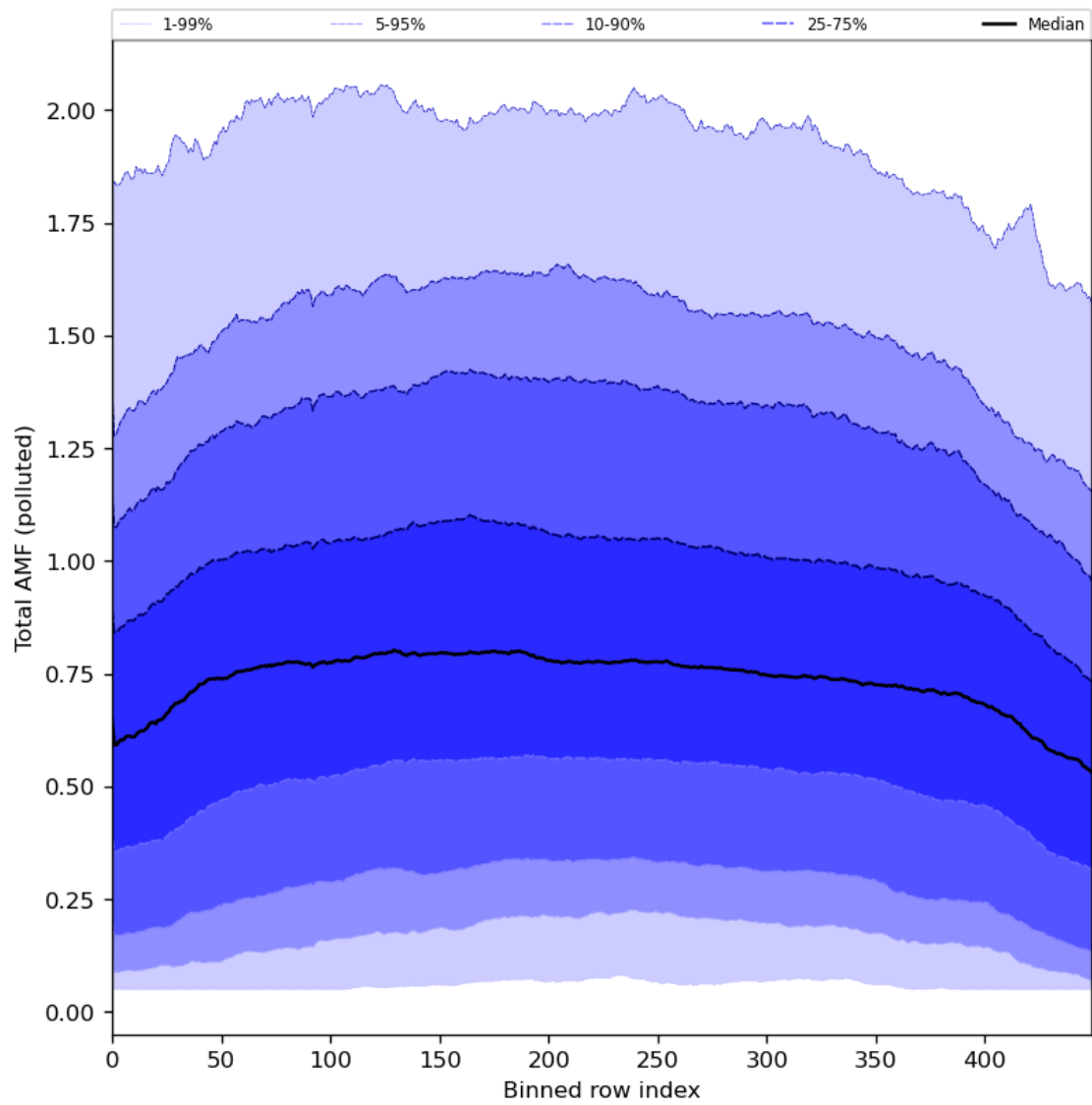
Figure 94: Along track statistics of “Total AMF (polluted)” for 2024-07-23 to 2024-07-25
