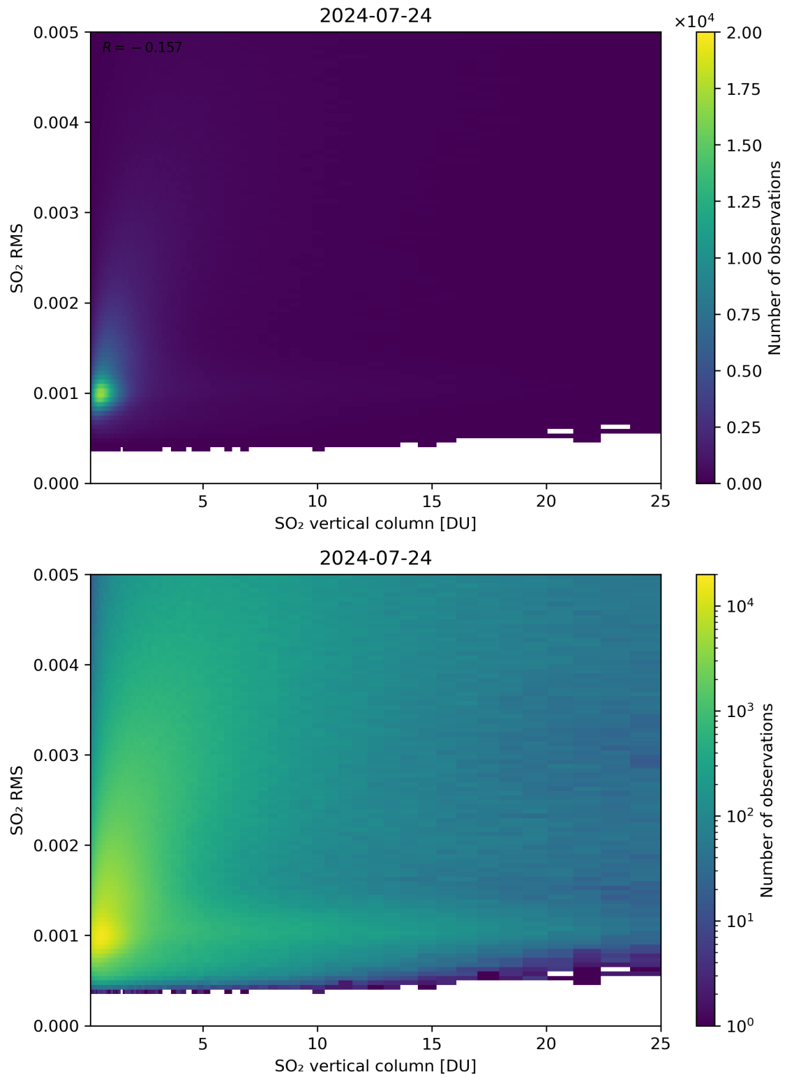
Figure 278: Scatter density plot of “SO 2 vertical column” against “SO 2 RMS” for 2024-07-23 to 2024-07-25.
