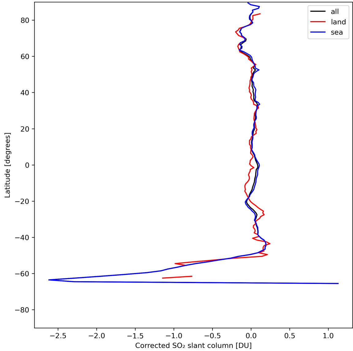
Figure 32: Zonal average of “Corrected SO 2 slant column” for 2024-07-23 to 2024-07-25.
