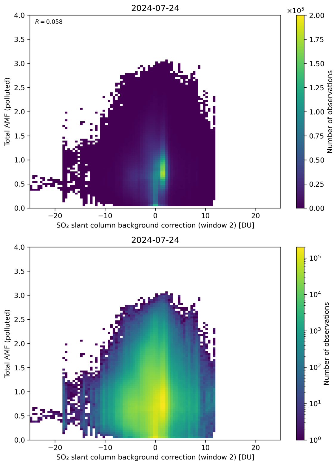
Figure 119: Scatter density plot of “SO 2 slant column background correction (window 2)” against “Total AMF (polluted)” for 2024-07-23 to 2024-07-25.
