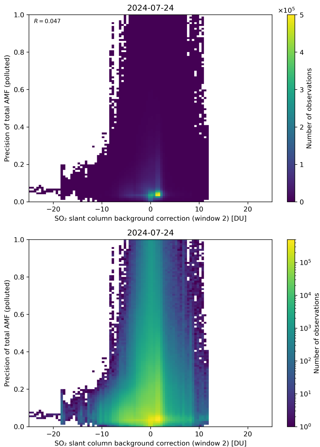
Figure 120: Scatter density plot of “SO 2 slant column background correction (window 2)” against “Precision of total AMF (polluted)” for 2024-07-23 to 2024-07-25.
