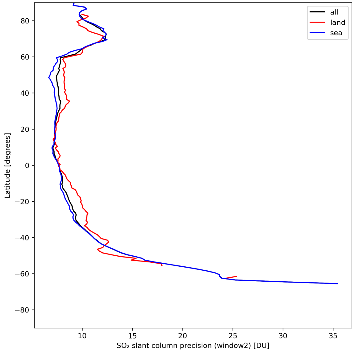
Figure 38: Zonal average of “SO 2 slant column precision (window2)” for 2024-07-23 to 2024-07-25.
