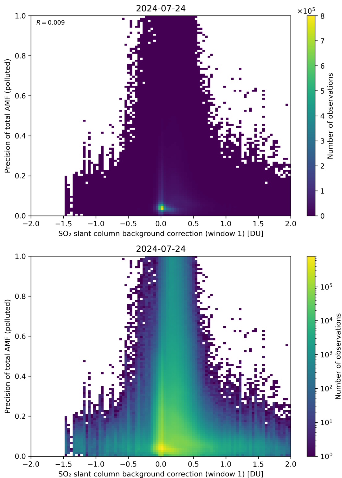
Figure 110: Scatter density plot of “SO 2 slant column background correction (window 1)” against “Precision of total AMF (polluted)” for 2024-07-23 to 2024-07-25.
