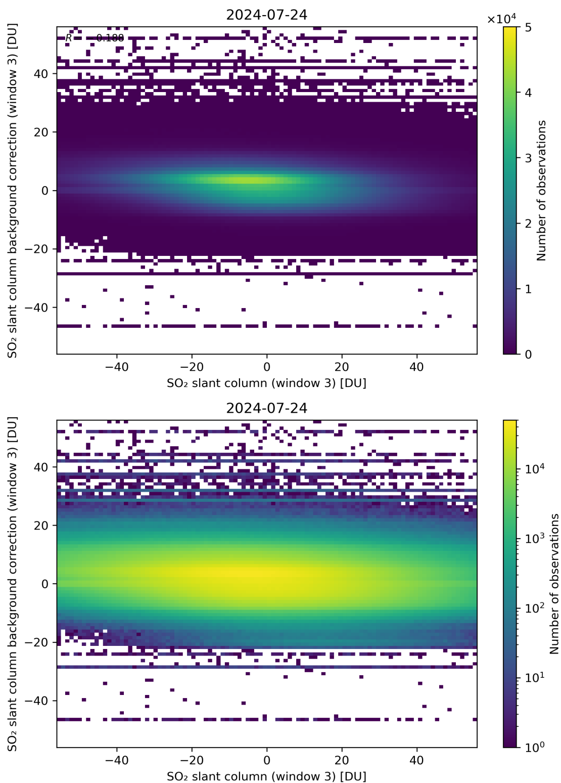
Figure 253: Scatter density plot of “SO 2 slant column (window 3)” against “SO 2 slant column background correction (window 3)” for 2024-07-23 to 2024-07-25.
