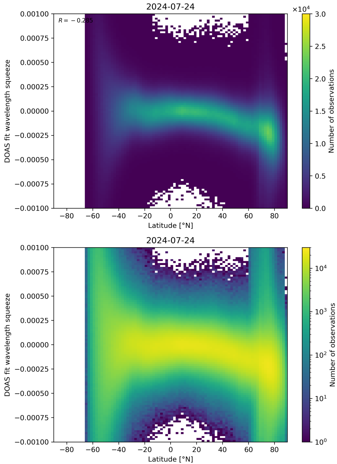
Figure 143: Scatter density plot of “Latitude” against “DOAS fit wavelength squeeze” for 2024-07-23 to 2024-07-25.
