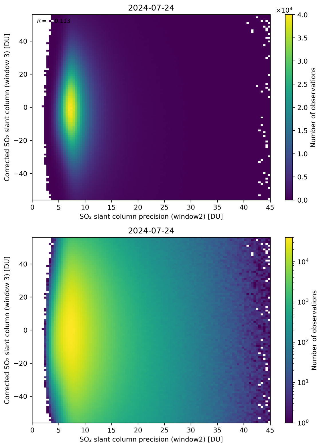
Figure 248: Scatter density plot of “SO 2 slant column precision (window2)” against “Corrected SO 2 slant column (window 3)” for 2024-07-23 to 2024-07-25.
