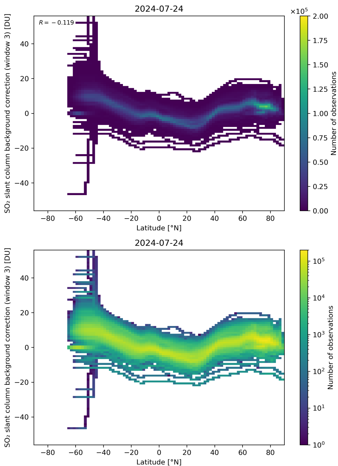
Figure 141: Scatter density plot of “Latitude” against “SO 2 slant column background correction (window 3)” for 2024-07-23 to 2024-07-25.
