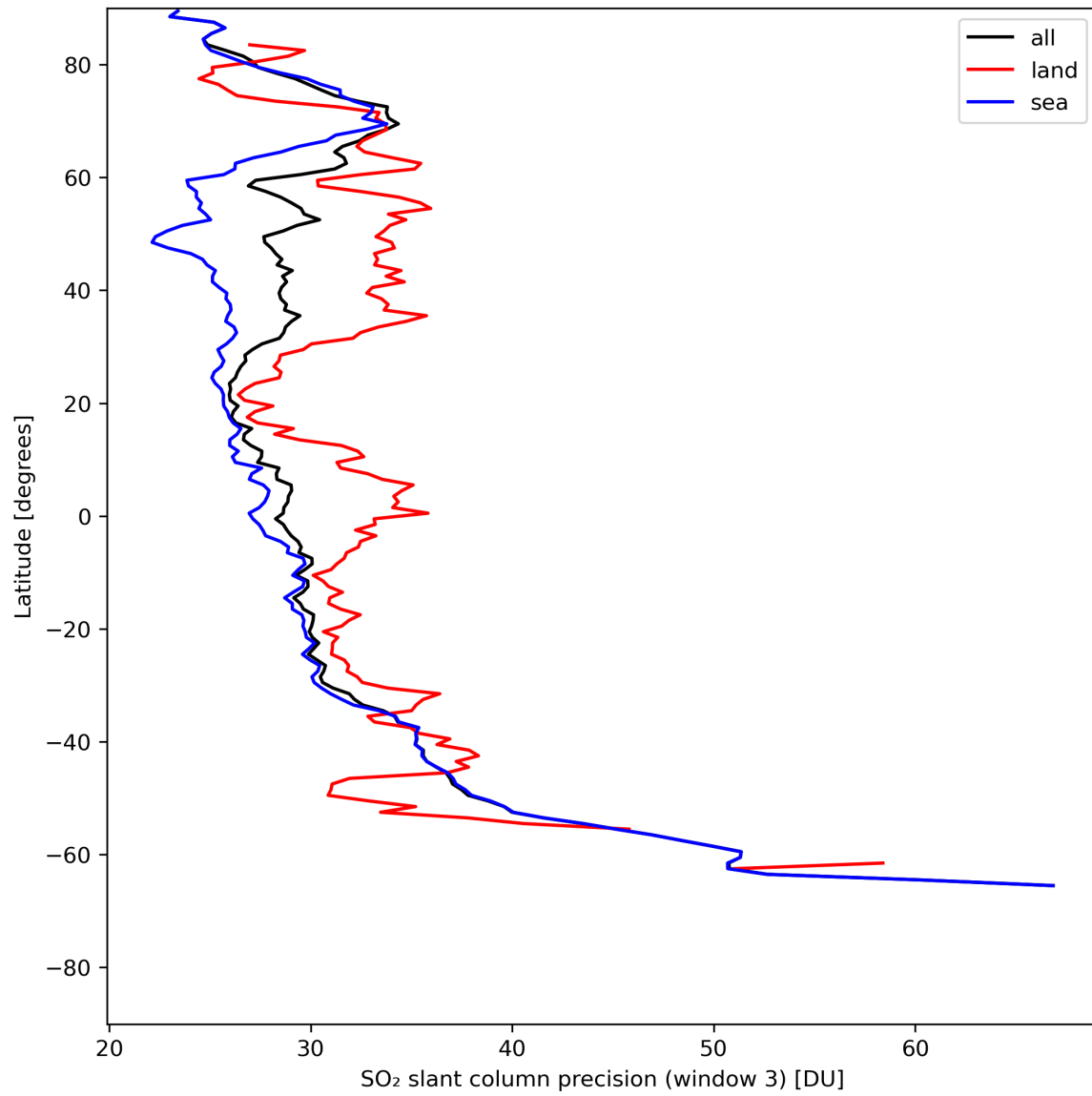
Figure 42: Zonal average of “SO 2 slant column precision (window 3)” for 2024-07-23 to 2024-07-25.
