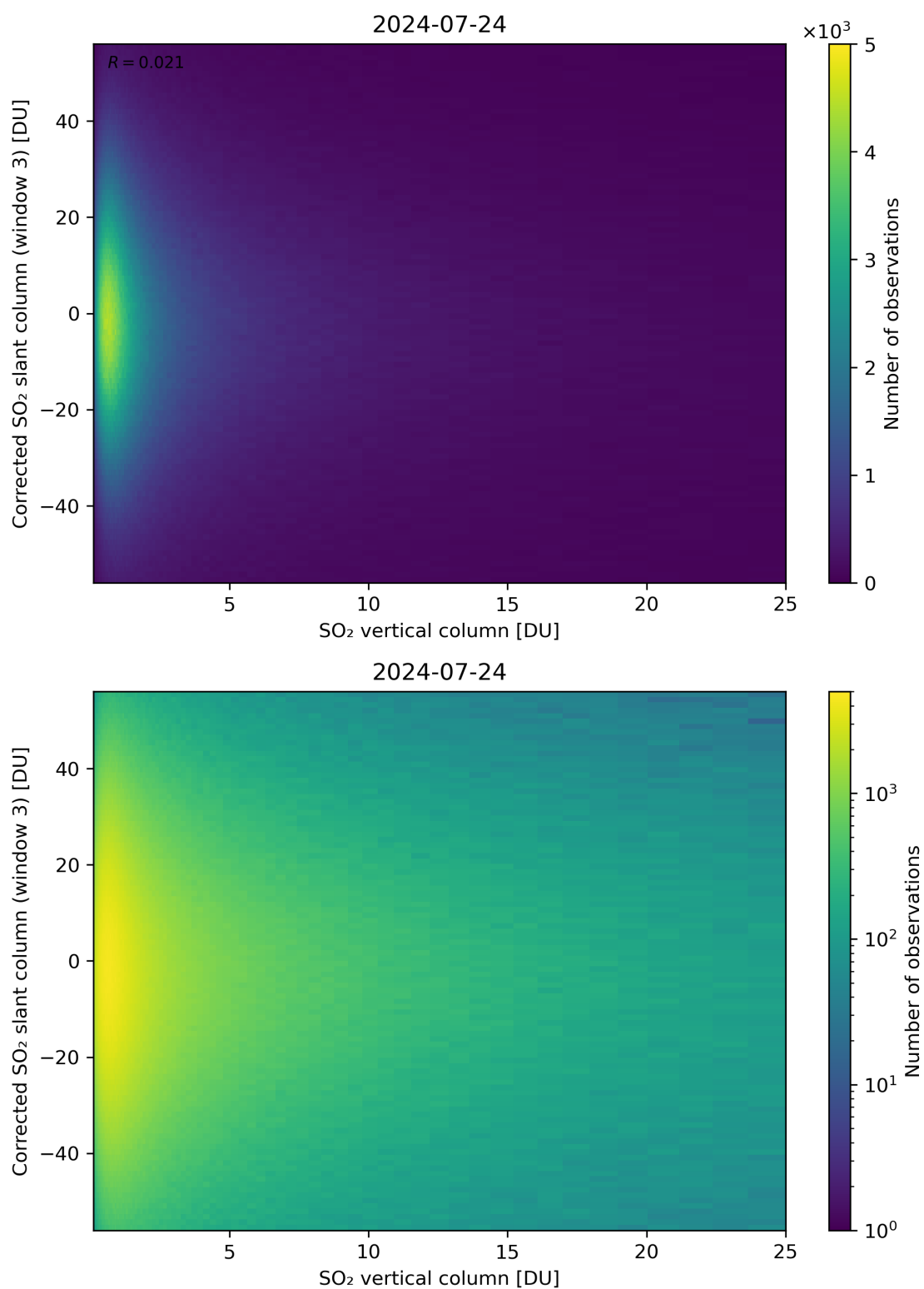
Figure 299: Scatter density plot of “SO 2 vertical column” against “Corrected SO 2 slant column (window 3)” for 2024-07-23 to 2024-07-25.
