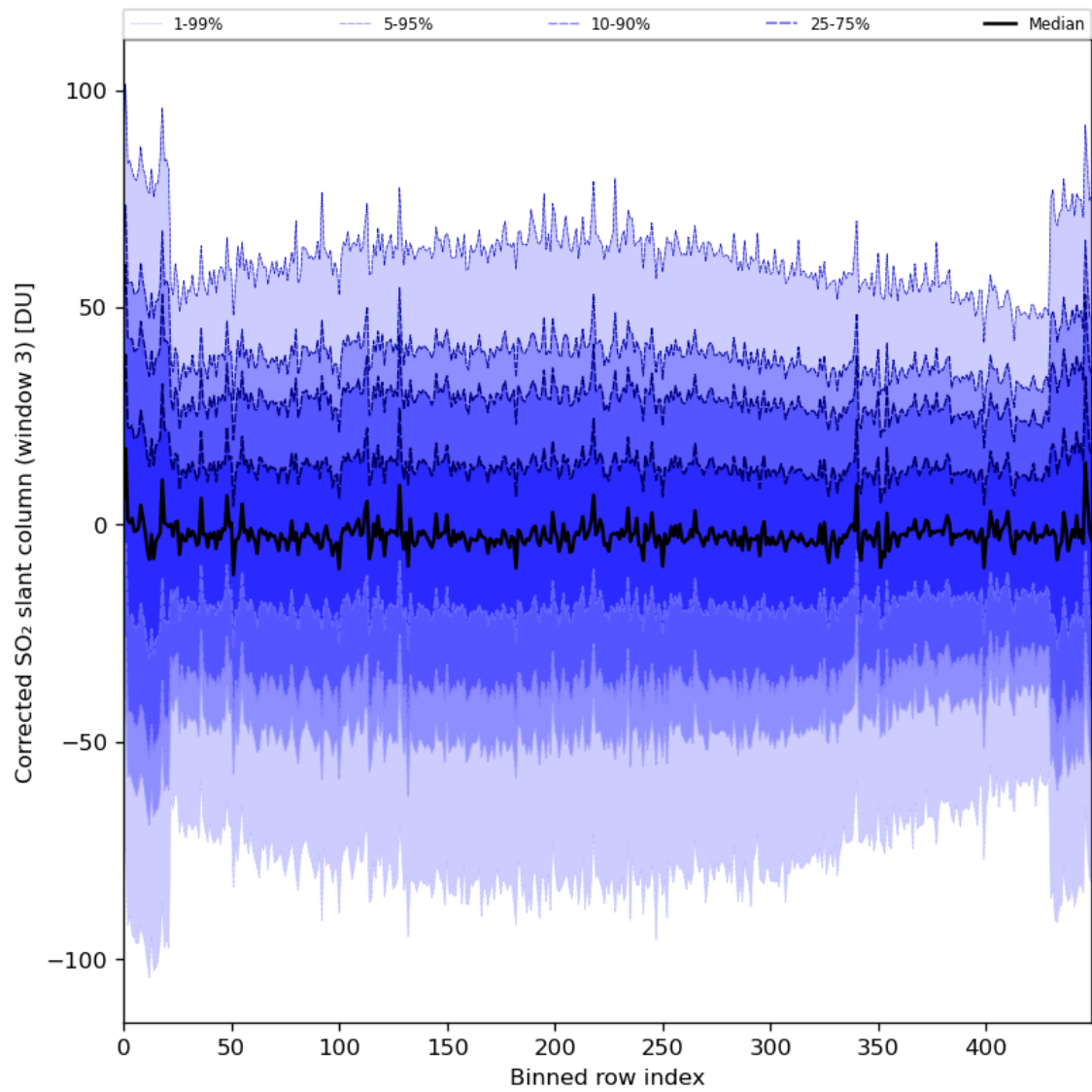
Figure 89: Along track statistics of “Corrected SO 2 slant column (window 3)” for 2024-07-23 to 2024-07-25
