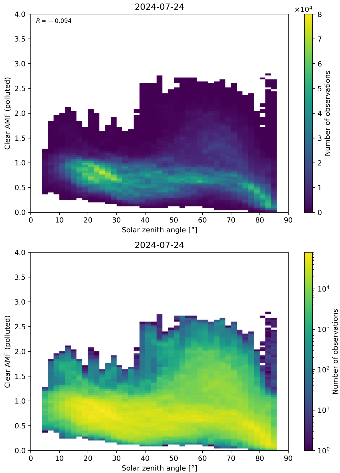
Figure 165: Scatter density plot of “Solar zenith angle” against “Clear AMF (polluted)” for 2024-07-23 to 2024-07-25.
