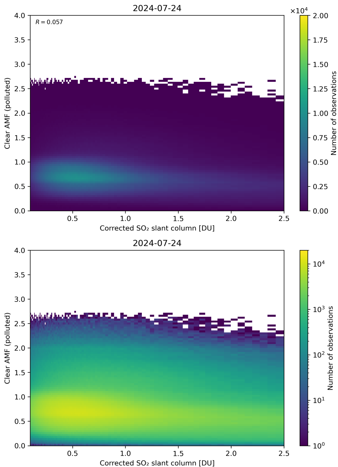
Figure 184: Scatter density plot of “Corrected SO 2 slant column” against “Clear AMF (polluted)” for 2024-07-23 to 2024-07-25.
