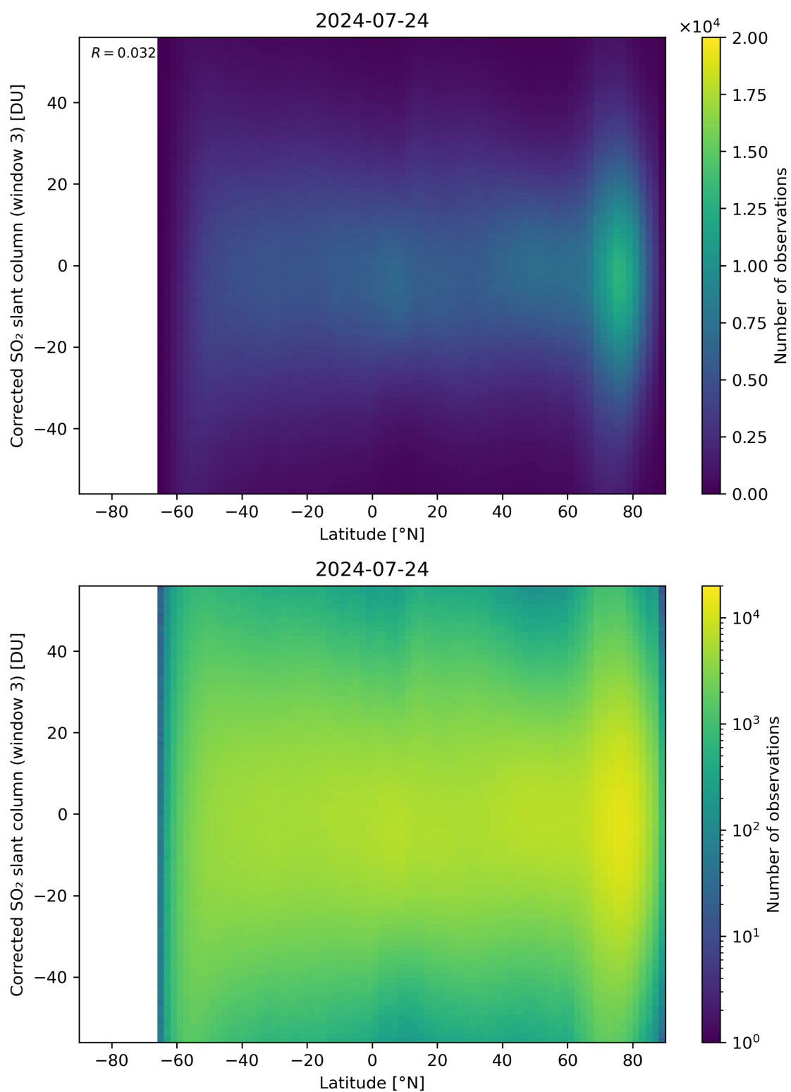
Figure 148: Scatter density plot of “Latitude” against “Corrected SO 2 slant column (window 3)” for 2024-07-23 to 2024-07-25.
