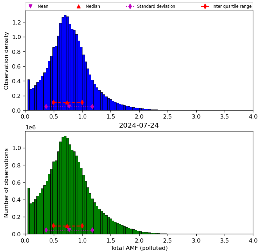
Figure 71: Histogram of “Total AMF (polluted)” for 2024-07-23 to 2024-07-25
