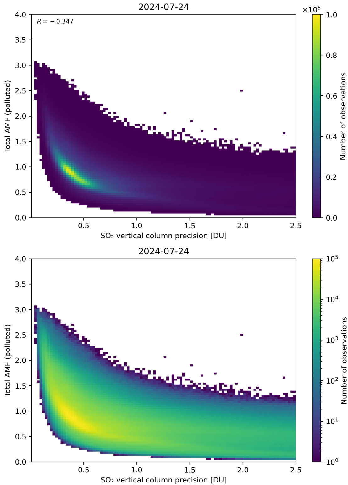
Figure 294: Scatter density plot of “SO 2 vertical column precision” against “Total AMF (polluted)” for 2024-07-23 to 2024-07-25.
