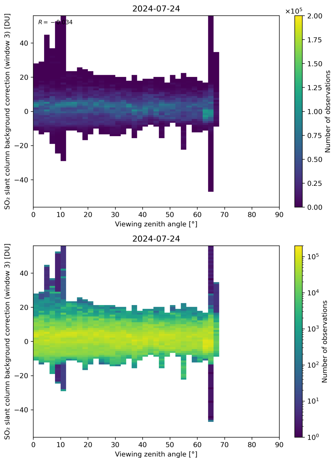
Figure 310: Scatter density plot of “Viewing zenith angle” against “SO 2 slant column background correction (window 3)” for 2024-07-23 to 2024-07-25.
