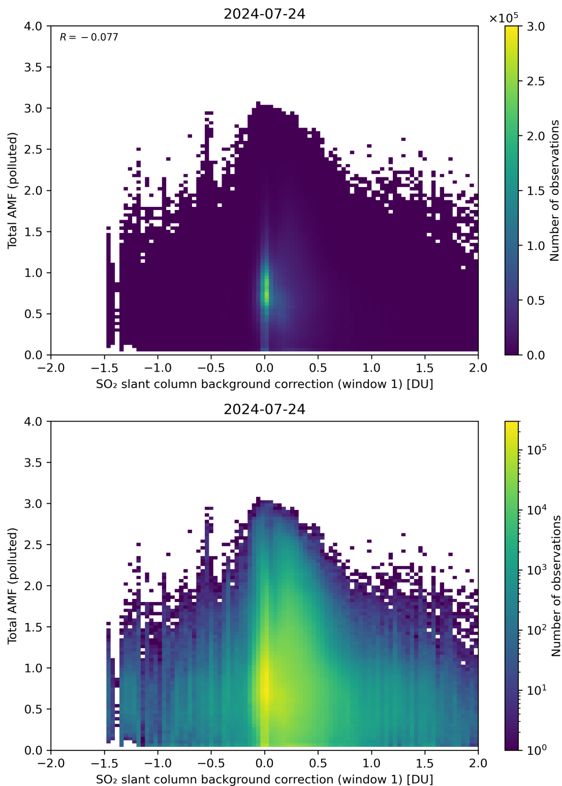
Figure 109: Scatter density plot of “SO 2 slant column background correction (window 1)” against “Total AMF (polluted)” for 2024-07-23 to 2024-07-25.
