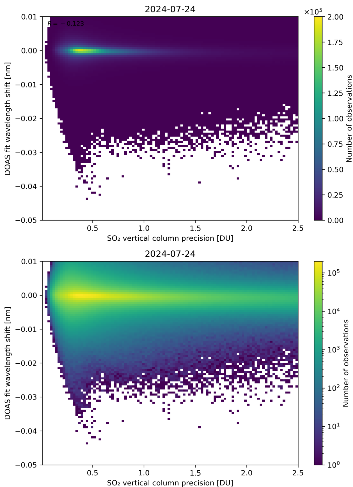
Figure 282: Scatter density plot of “SO 2 vertical column precision” against “DOAS fit wavelength shift” for 2024-07-23 to 2024-07-25.
