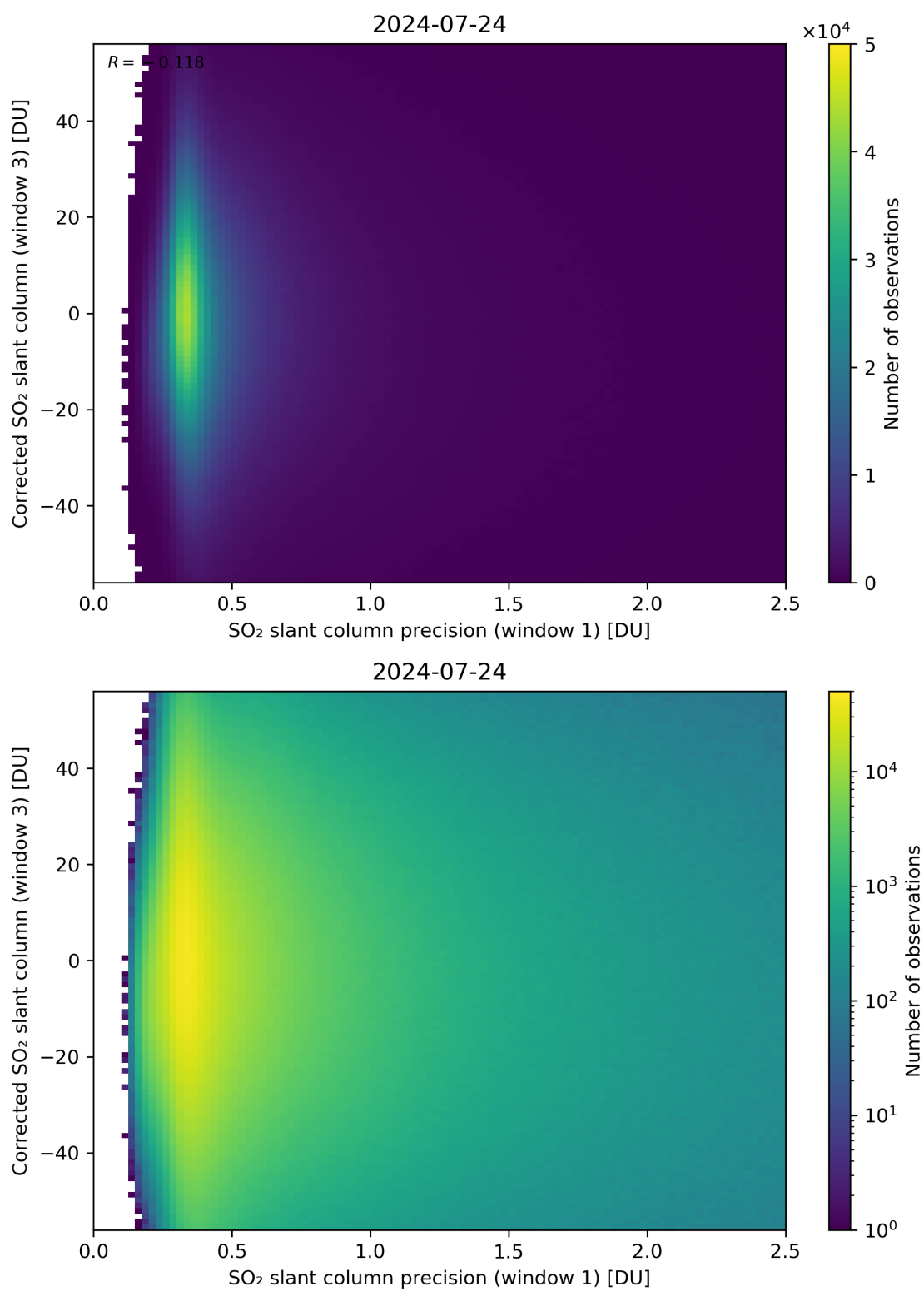
Figure 226: Scatter density plot of “SO 2 slant column precision (window 1)” against “Corrected SO 2 slant column (window 3)” for 2024-07-23 to 2024-07-25.
