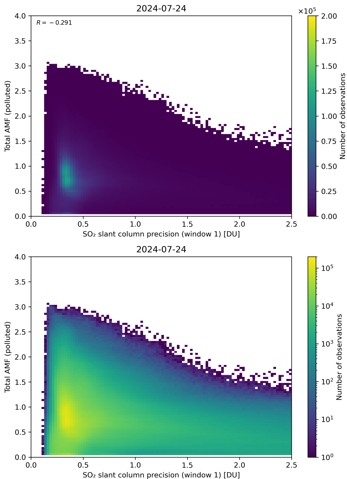
Figure 230: Scatter density plot of “SO 2 slant column precision (window 1)” against “Total AMF (polluted)” for 2024-07-23 to 2024-07-25.
