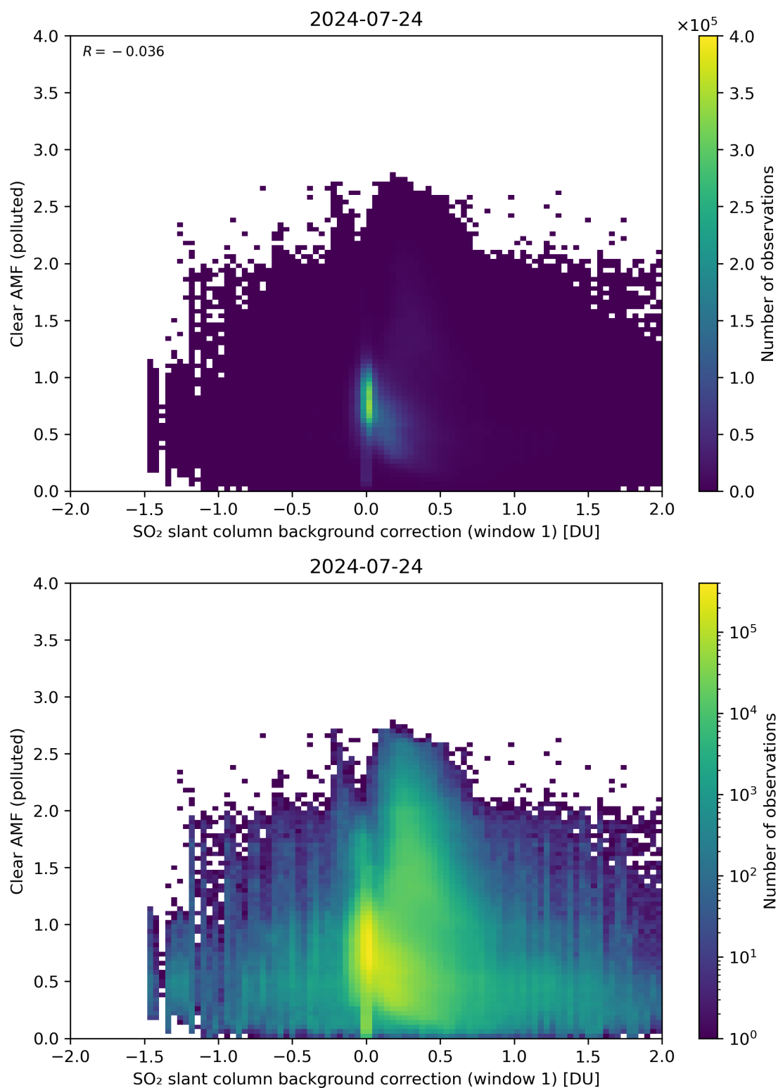
Figure 103: Scatter density plot of “SO 2 slant column background correction (window 1)” against “Clear AMF (polluted)” for 2024-07-23 to 2024-07-25.
