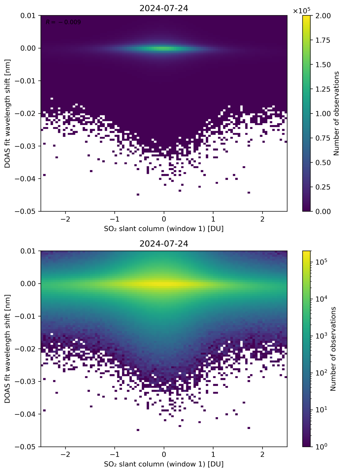
Figure 215: Scatter density plot of “SO 2 slant column (window 1)” against “DOAS fit wavelength shift” for 2024-07-23 to 2024-07-25.
