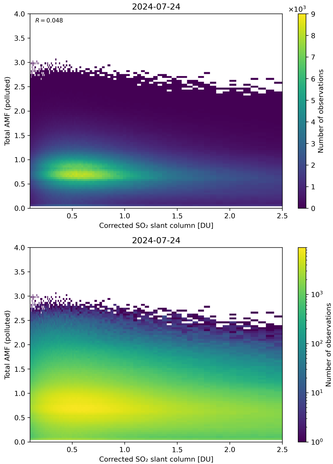
Figure 192: Scatter density plot of “Corrected SO 2 slant column” against “Total AMF (polluted)” for 2024-07-23 to 2024-07-25.
