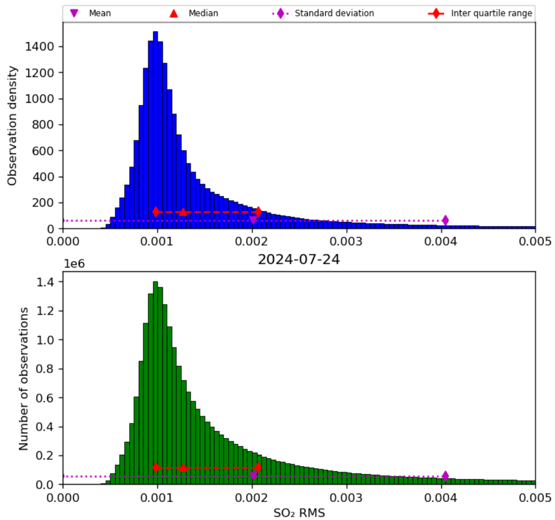
Figure 70: Histogram of “SO 2 RMS” for 2024-07-23 to 2024-07-25
