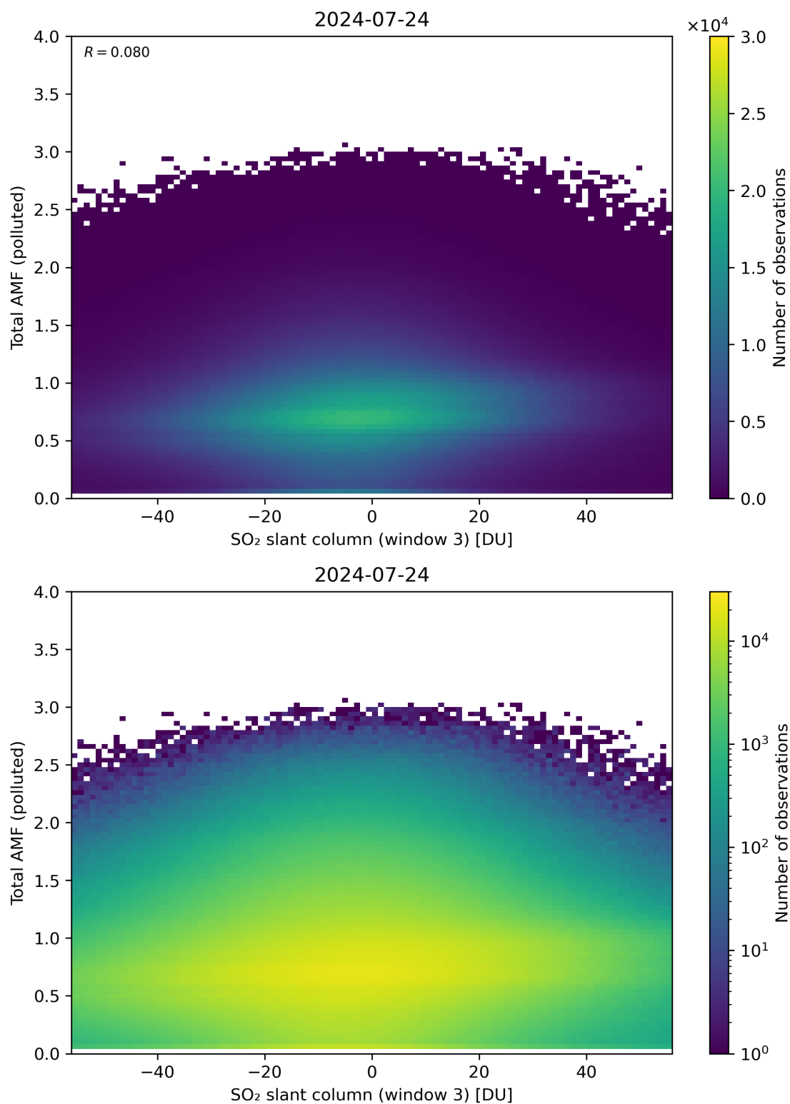
Figure 268: Scatter density plot of “SO 2 slant column (window 3)” against “Total AMF (polluted)” for 2024-07-23 to 2024-07-25.
