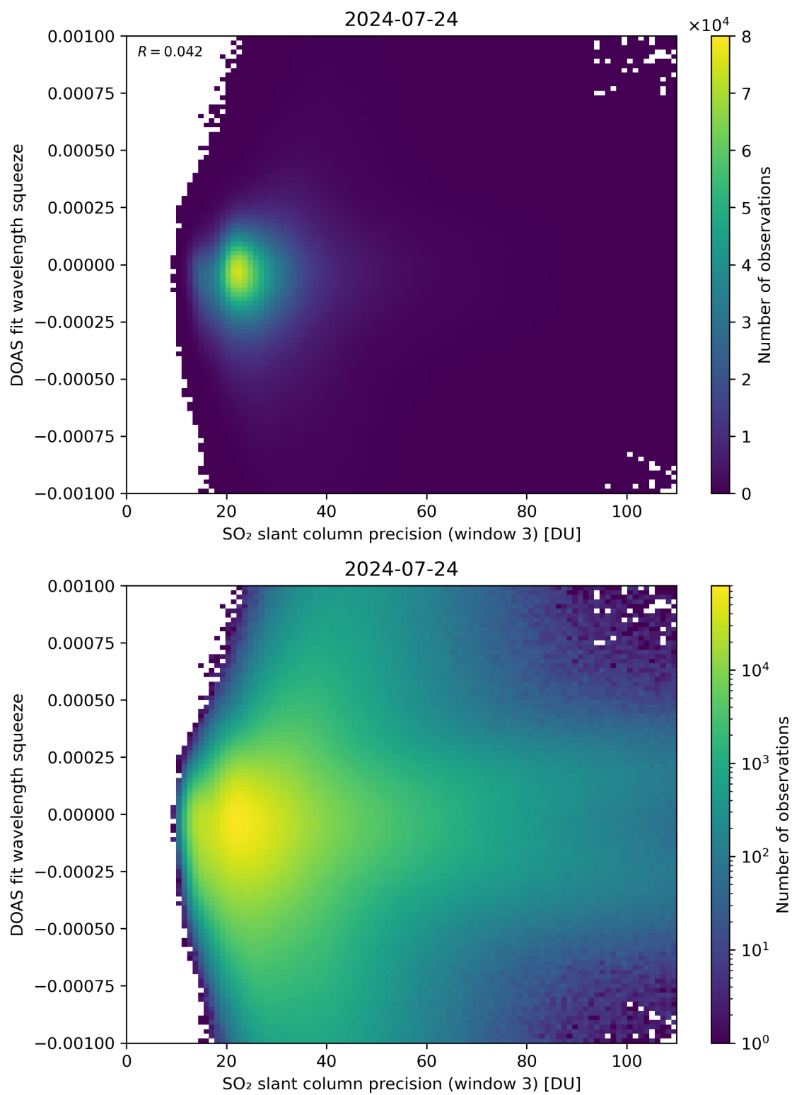
Figure 259: Scatter density plot of “SO 2 slant column precision (window 3)” against “DOAS fit wavelength squeeze” for 2024-07-23 to 2024-07-25.
