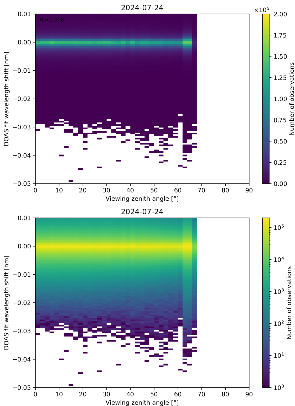
Figure 311: Scatter density plot of “Viewing zenith angle” against “DOAS fit wavelength shift” for 2024-07-23 to 2024-07-25.
