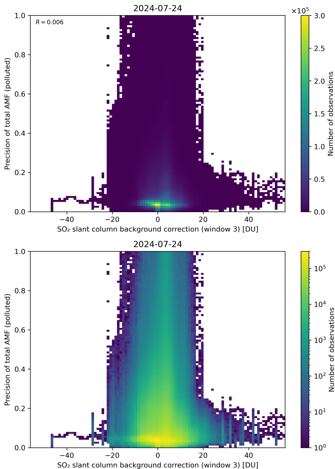
Figure 126: Scatter density plot of “SO 2 slant column background correction (window 3)” against “Precision of total AMF (polluted)” for 2024-07-23 to 2024-07-25.
