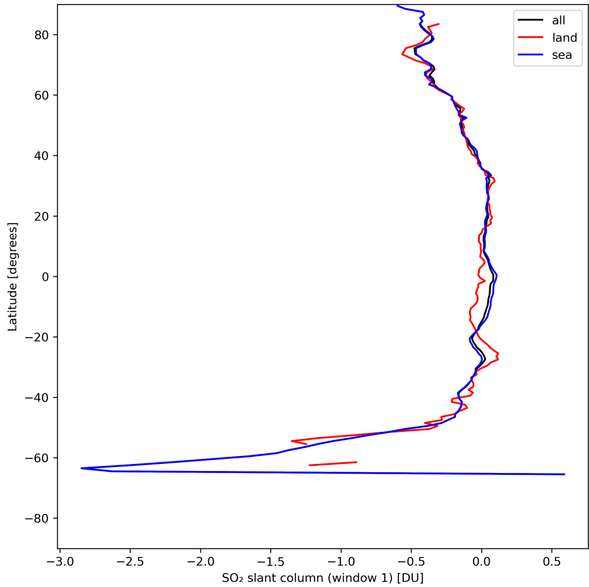
Figure 33: Zonal average of “SO 2 slant column (window 1)” for 2024-07-23 to 2024-07-25.
