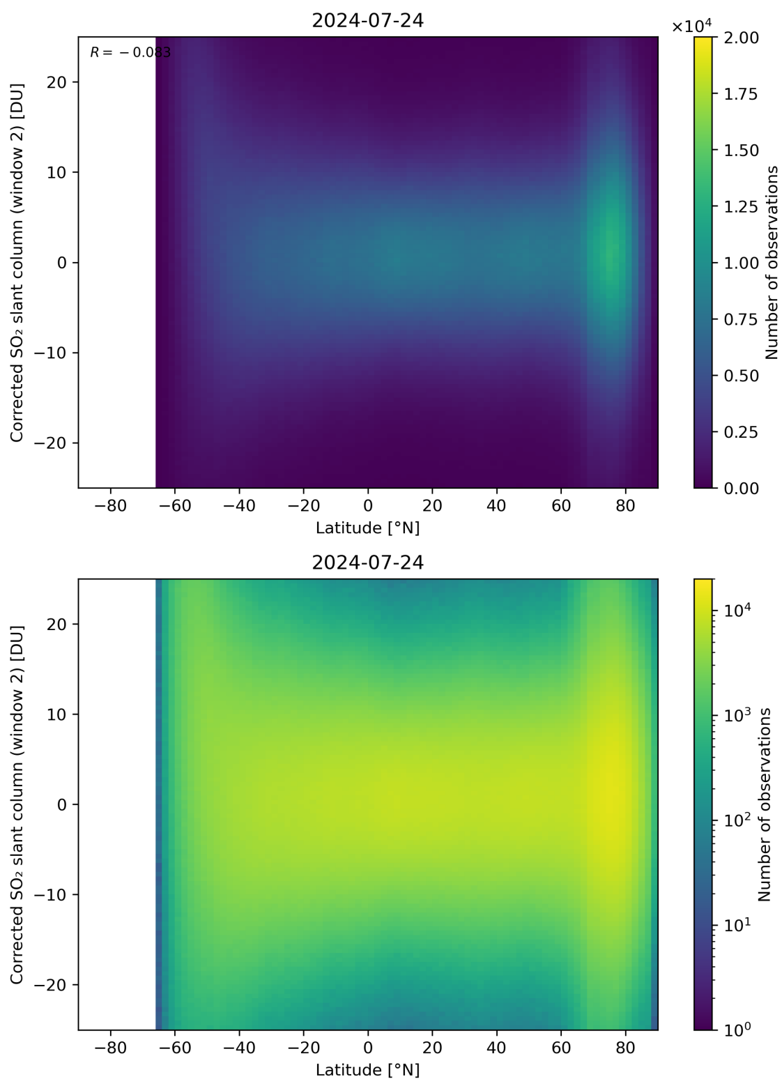
Figure 147: Scatter density plot of “Latitude” against “Corrected SO 2 slant column (window 2)” for 2024-07-23 to 2024-07-25.
