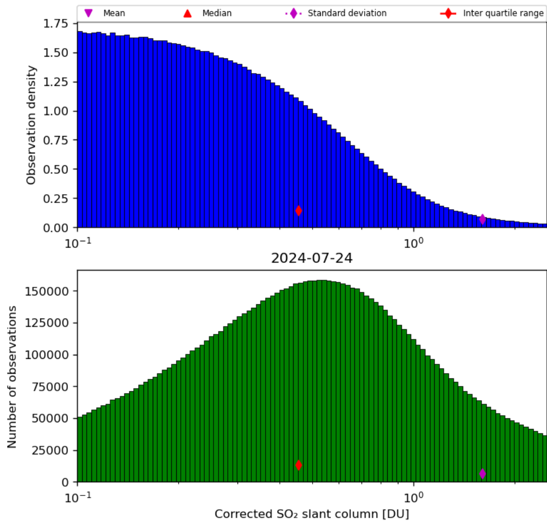
Figure 55: Histogram of “Corrected SO 2 slant column” for 2024-07-23 to 2024-07-25
