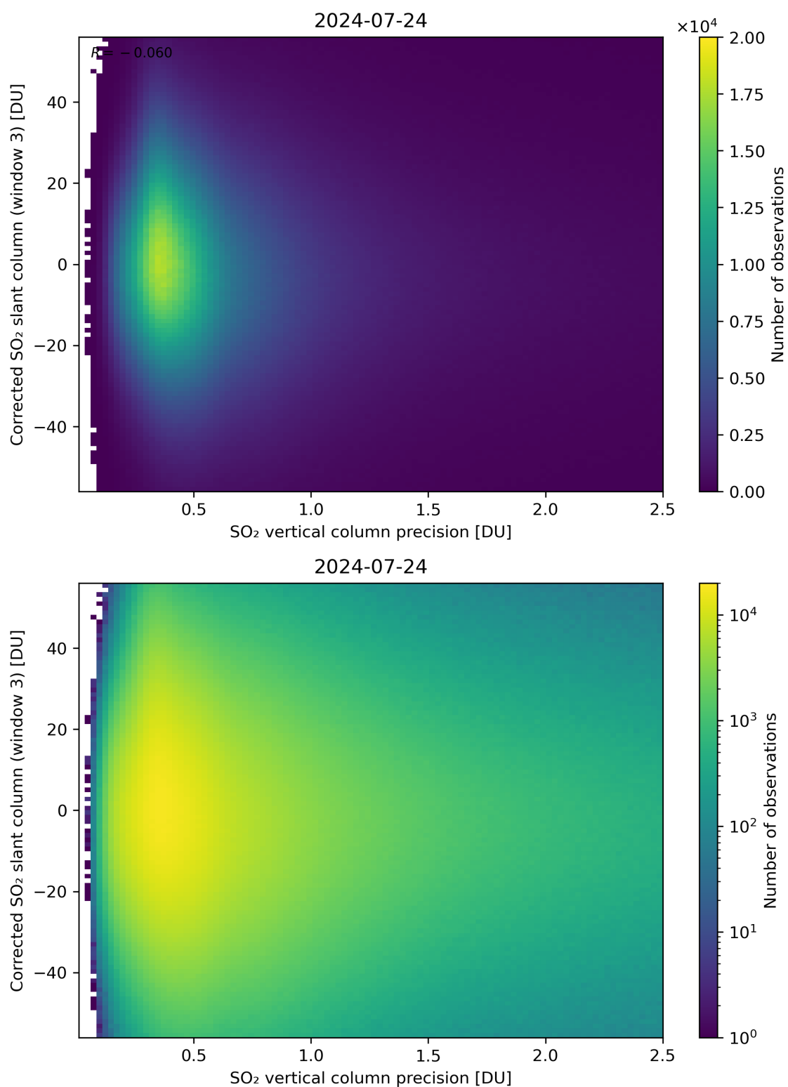
Figure 288: Scatter density plot of “SO 2 vertical column precision” against “Corrected SO 2 slant column (window 3)” for 2024-07-23 to 2024-07-25.
