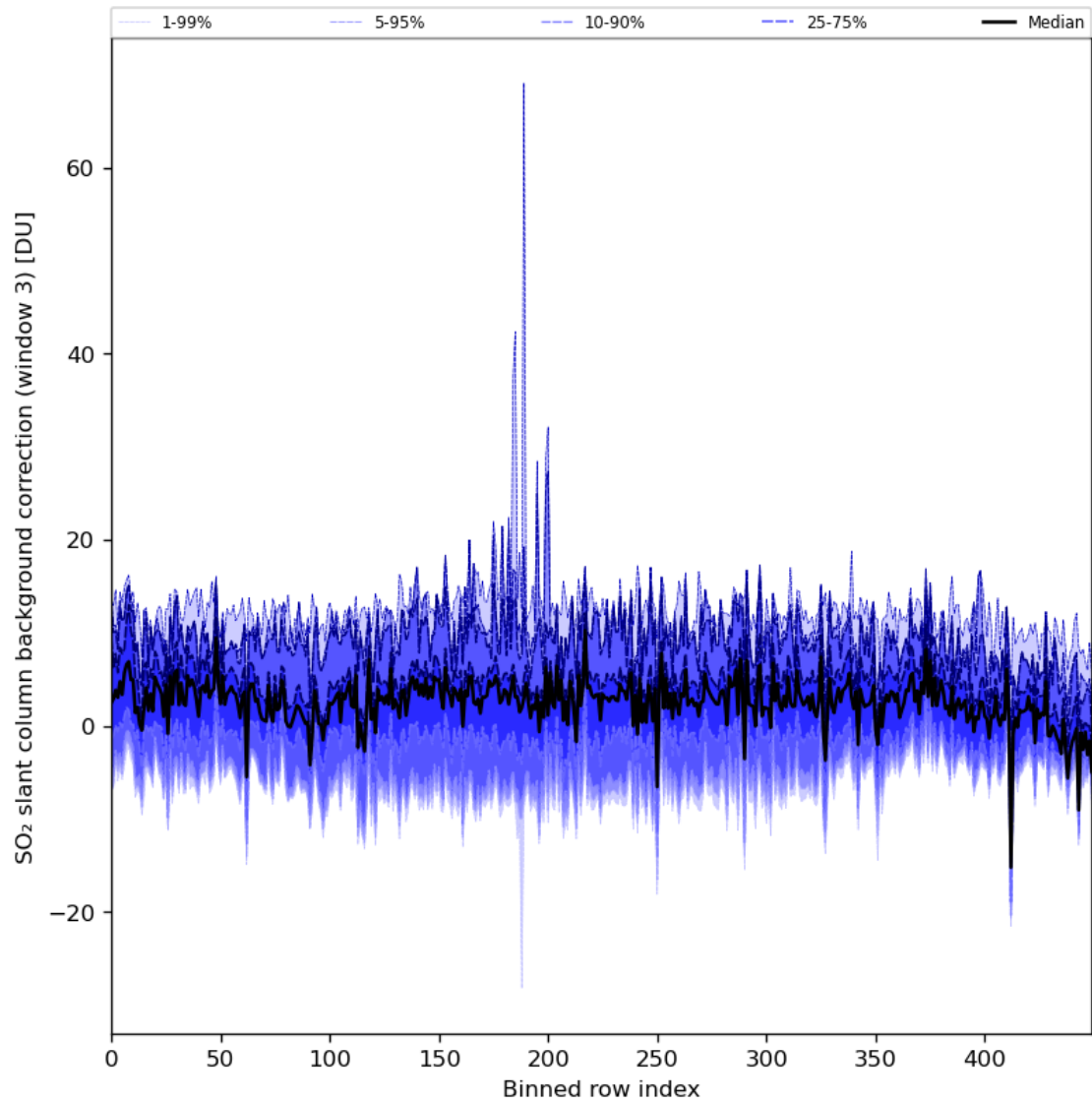
Figure 90: Along track statistics of “SO 2 slant column background correction (window 3)” for 2024-07-23 to 2024-07-25
