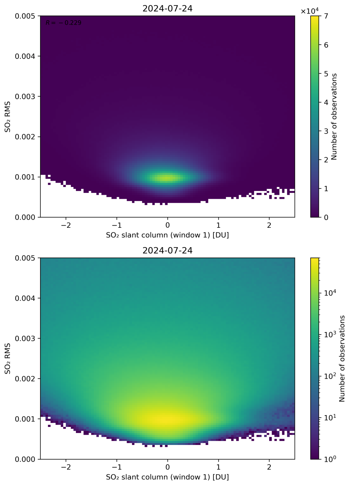
Figure 217: Scatter density plot of “SO 2 slant column (window 1)” against “SO 2 RMS” for 2024-07-23 to 2024-07-25.
