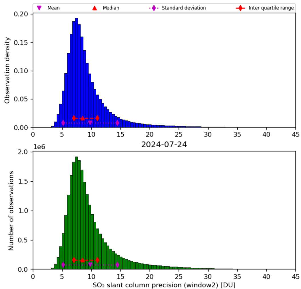
Figure 61: Histogram of “SO 2 slant column precision (window2)” for 2024-07-23 to 2024-07-25
