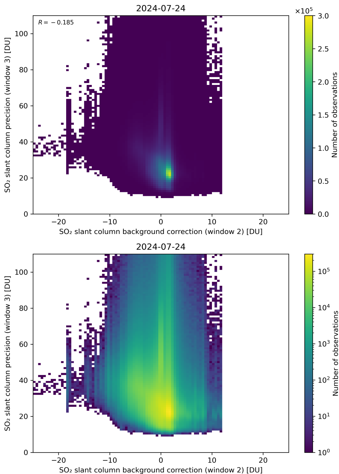
Figure 118: Scatter density plot of “SO 2 slant column background correction (window 2)” against “SO 2 slant column precision (window 3)” for 2024-07-23 to 2024-07-25.
