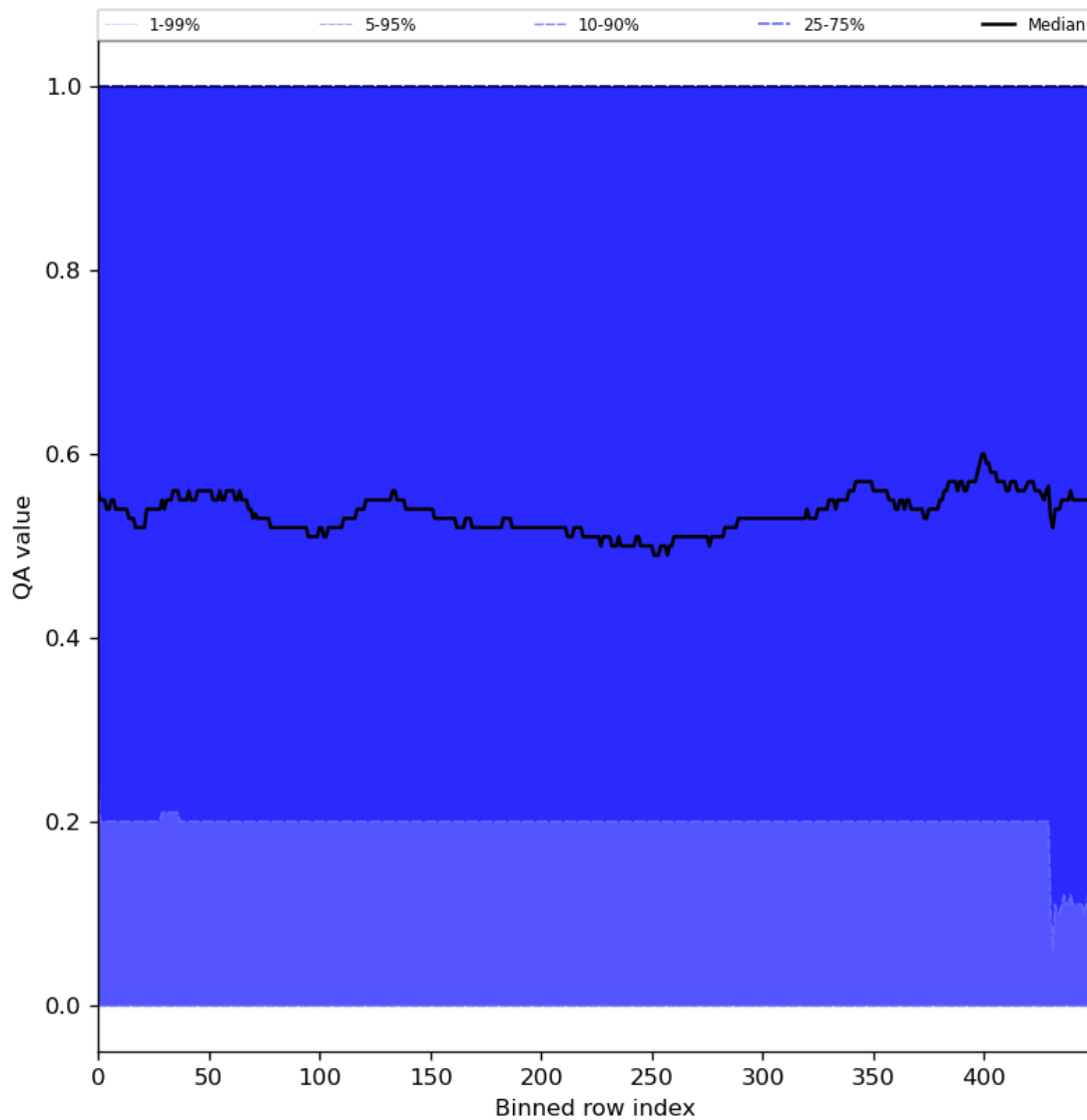
Figure 75: Along track statistics of “QA value” for 2024-07-23 to 2024-07-25
