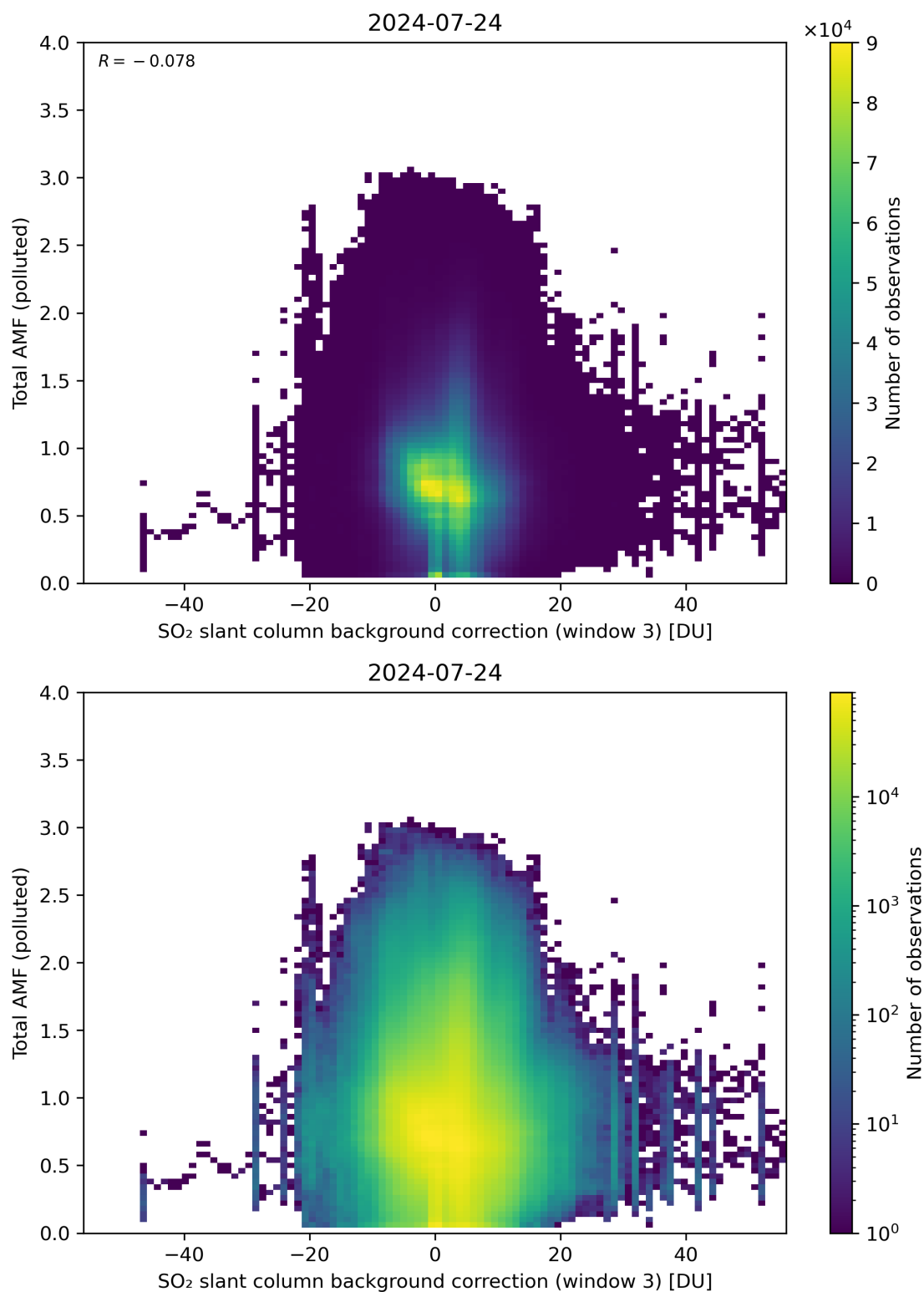
Figure 125: Scatter density plot of “SO 2 slant column background correction (window 3)” against “Total AMF (polluted)” for 2024-07-23 to 2024-07-25.
