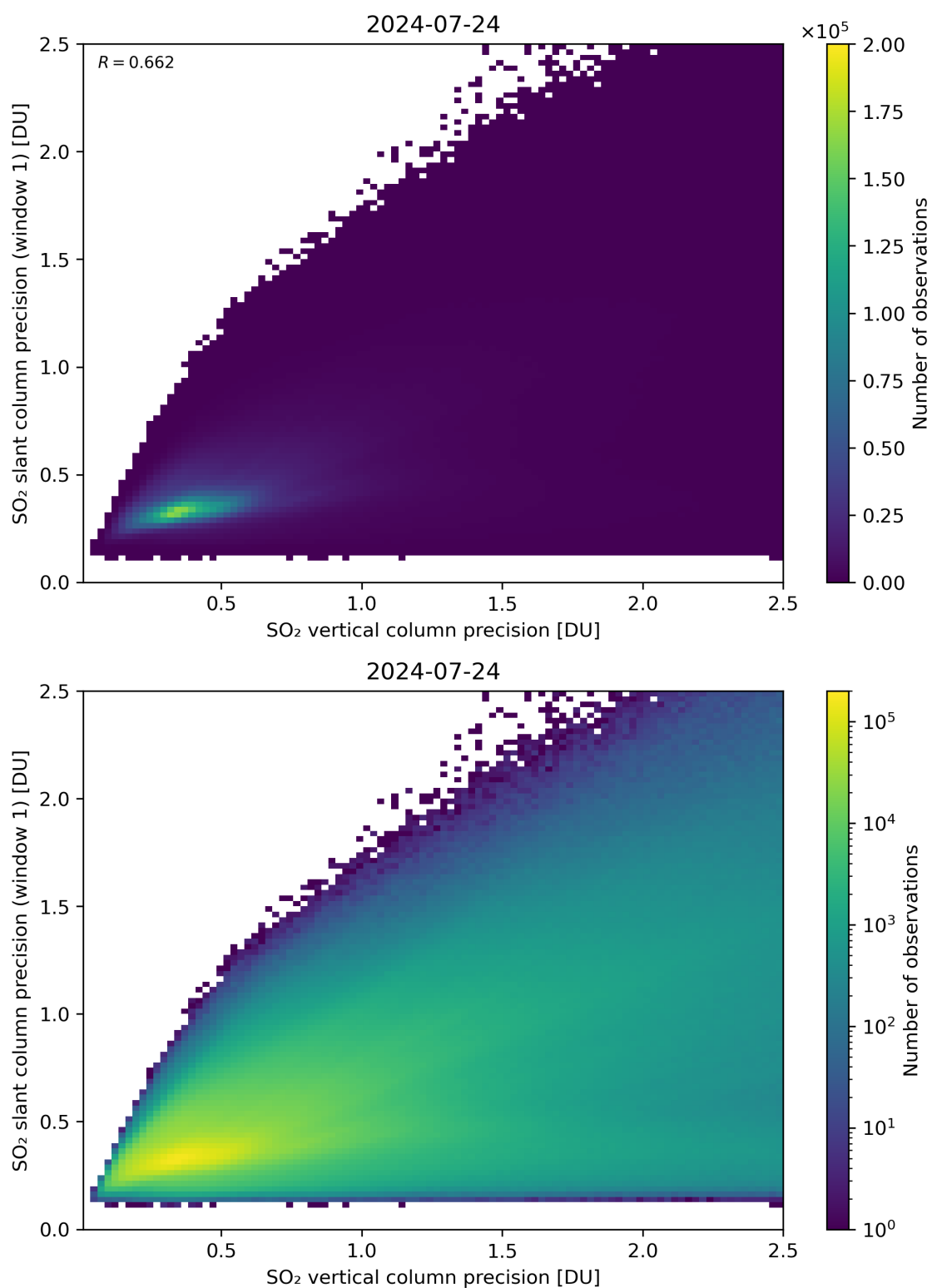
Figure 290: Scatter density plot of “SO 2 vertical column precision” against “SO 2 slant column precision (window 1)” for 2024-07-23 to 2024-07-25.
