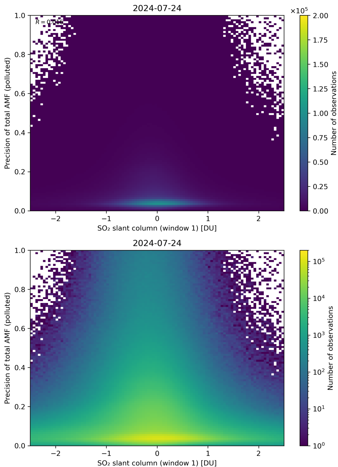
Figure 240: Scatter density plot of “SO 2 slant column (window 1)” against “Precision of total AMF (polluted)” for 2024-07-23 to 2024-07-25.
