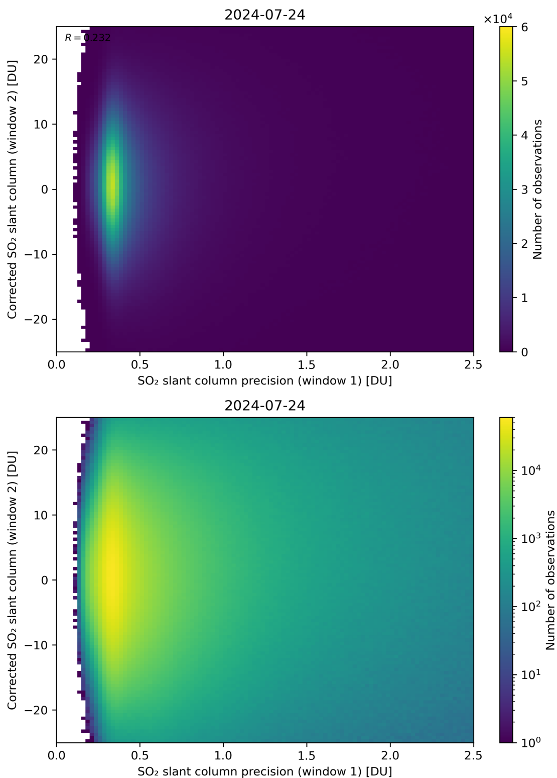
Figure 225: Scatter density plot of “SO 2 slant column precision (window 1)” against “Corrected SO 2 slant column (window 2)” for 2024-07-23 to 2024-07-25.
