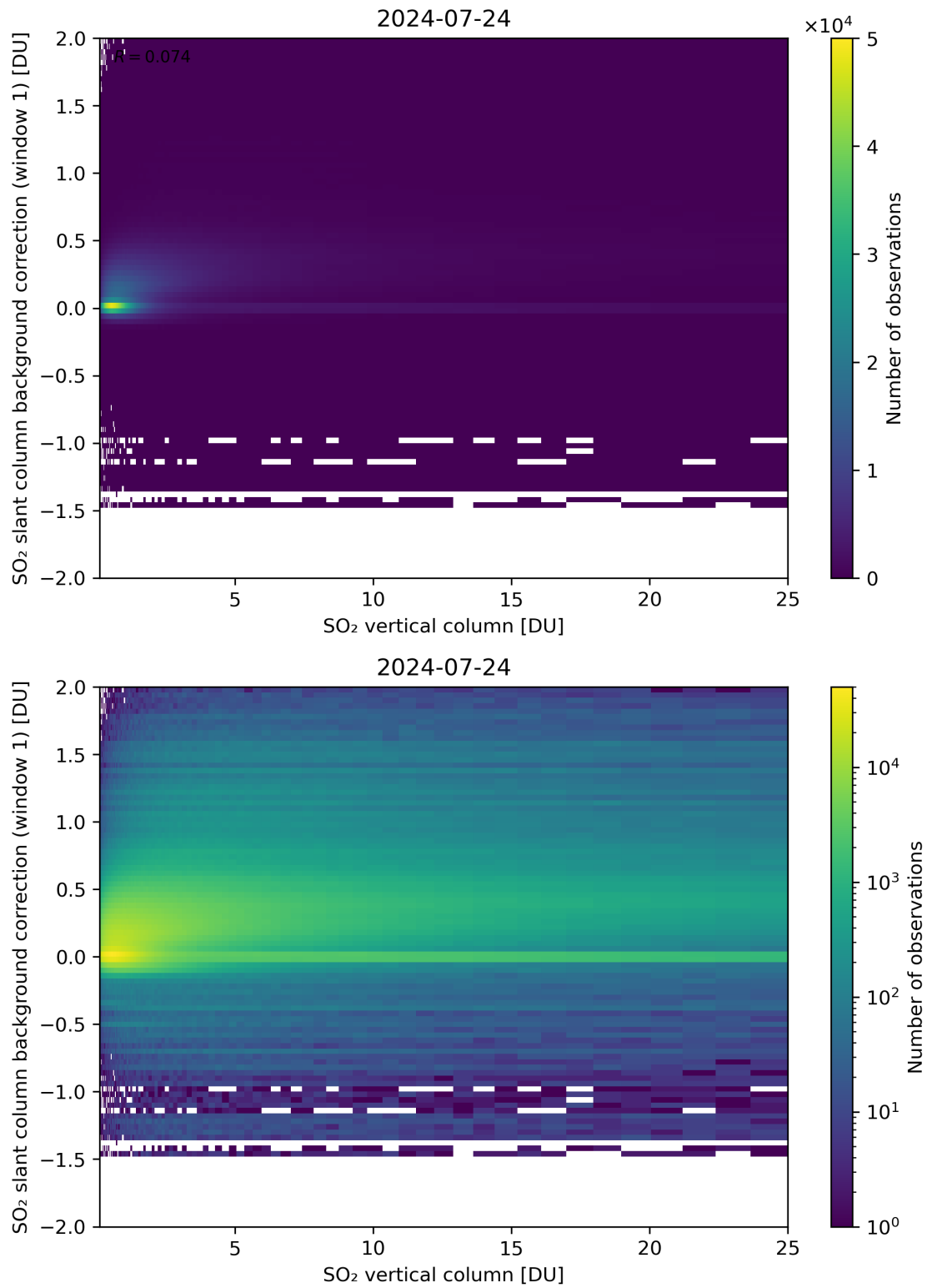
Figure 273: Scatter density plot of “SO 2 vertical column” against “SO 2 slant column background correction (window 1)” for 2024-07-23 to 2024-07-25.
