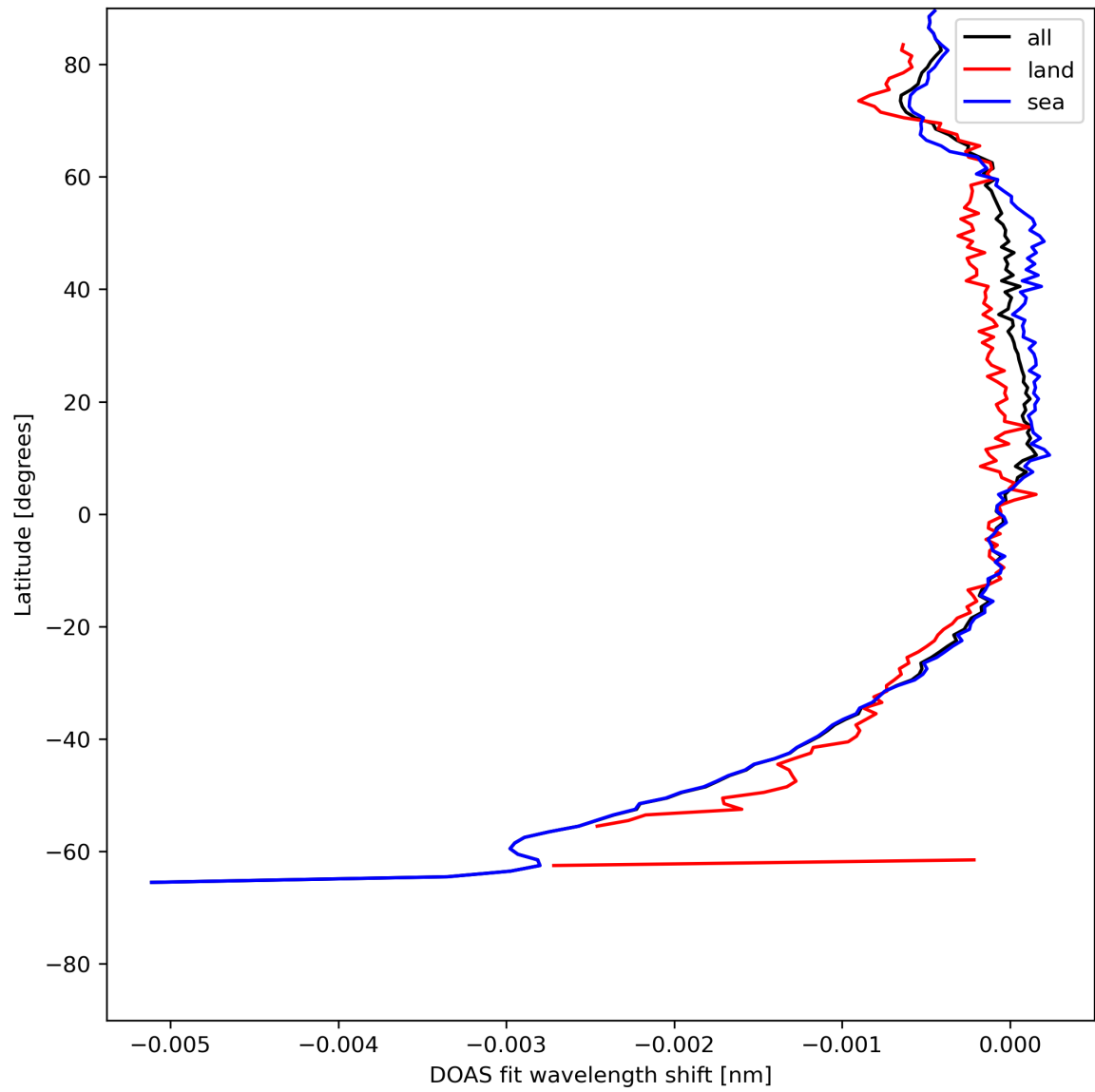
Figure 45: Zonal average of “DOAS fit wavelength shift” for 2024-07-23 to 2024-07-25.
