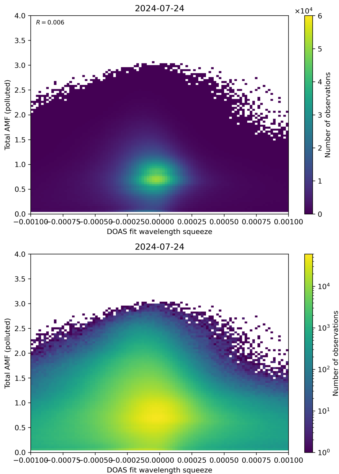
Figure 134: Scatter density plot of “DOAS fit wavelength squeeze” against “Total AMF (polluted)” for 2024-07-23 to 2024-07-25.
