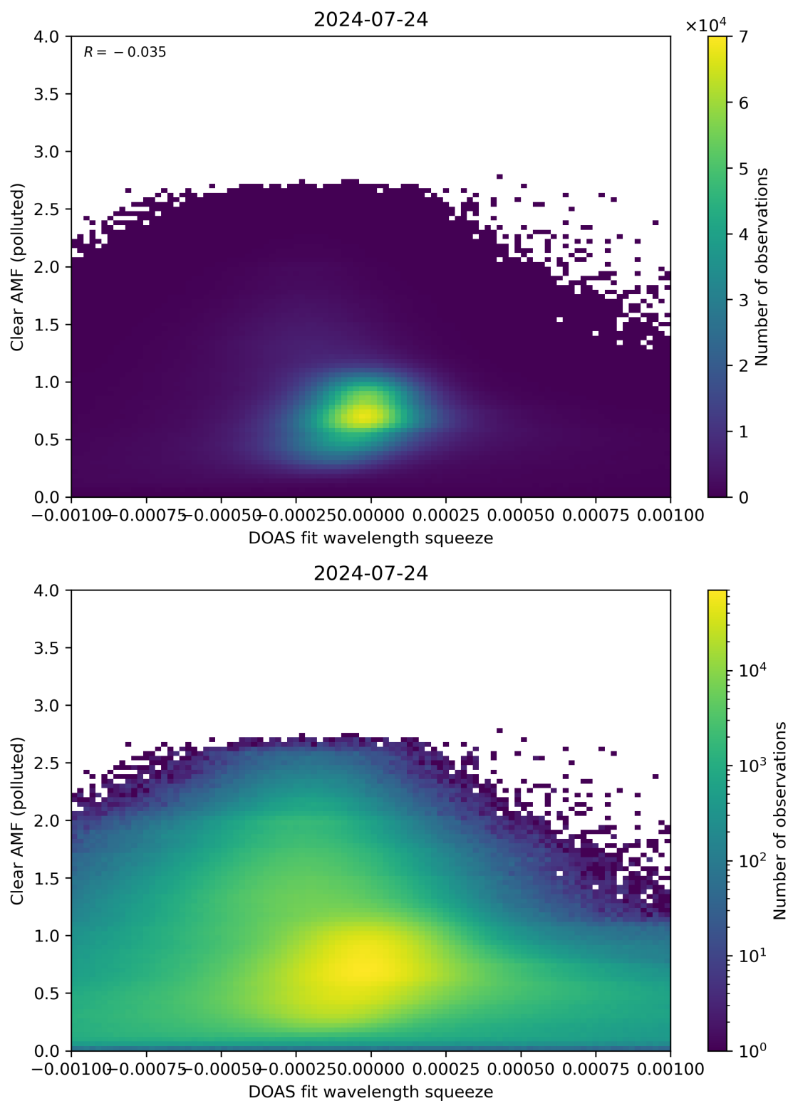
Figure 133: Scatter density plot of “DOAS fit wavelength squeeze” against “Clear AMF (polluted)” for 2024-07-23 to 2024-07-25.
