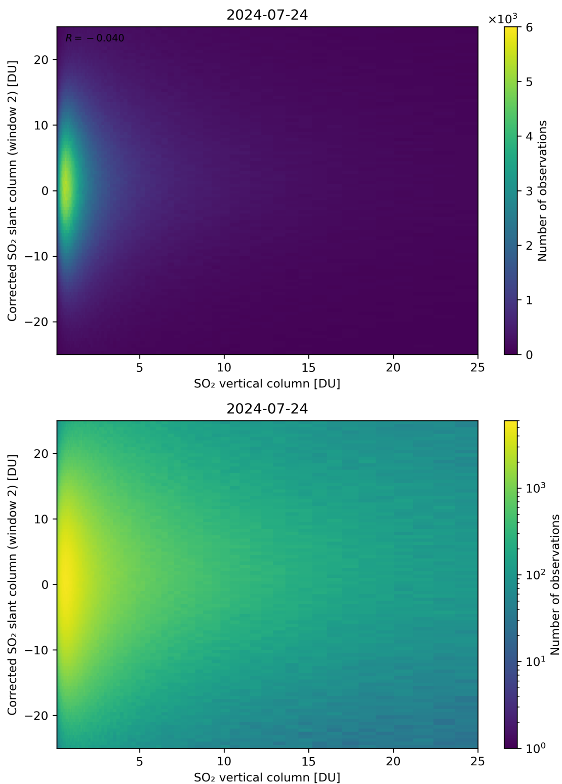
Figure 298: Scatter density plot of “SO 2 vertical column” against “Corrected SO 2 slant column (window 2)” for 2024-07-23 to 2024-07-25.
