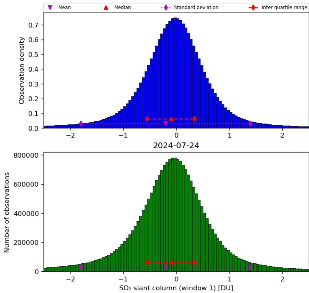
Figure 56: Histogram of “SO 2 slant column (window 1)” for 2024-07-23 to 2024-07-25
