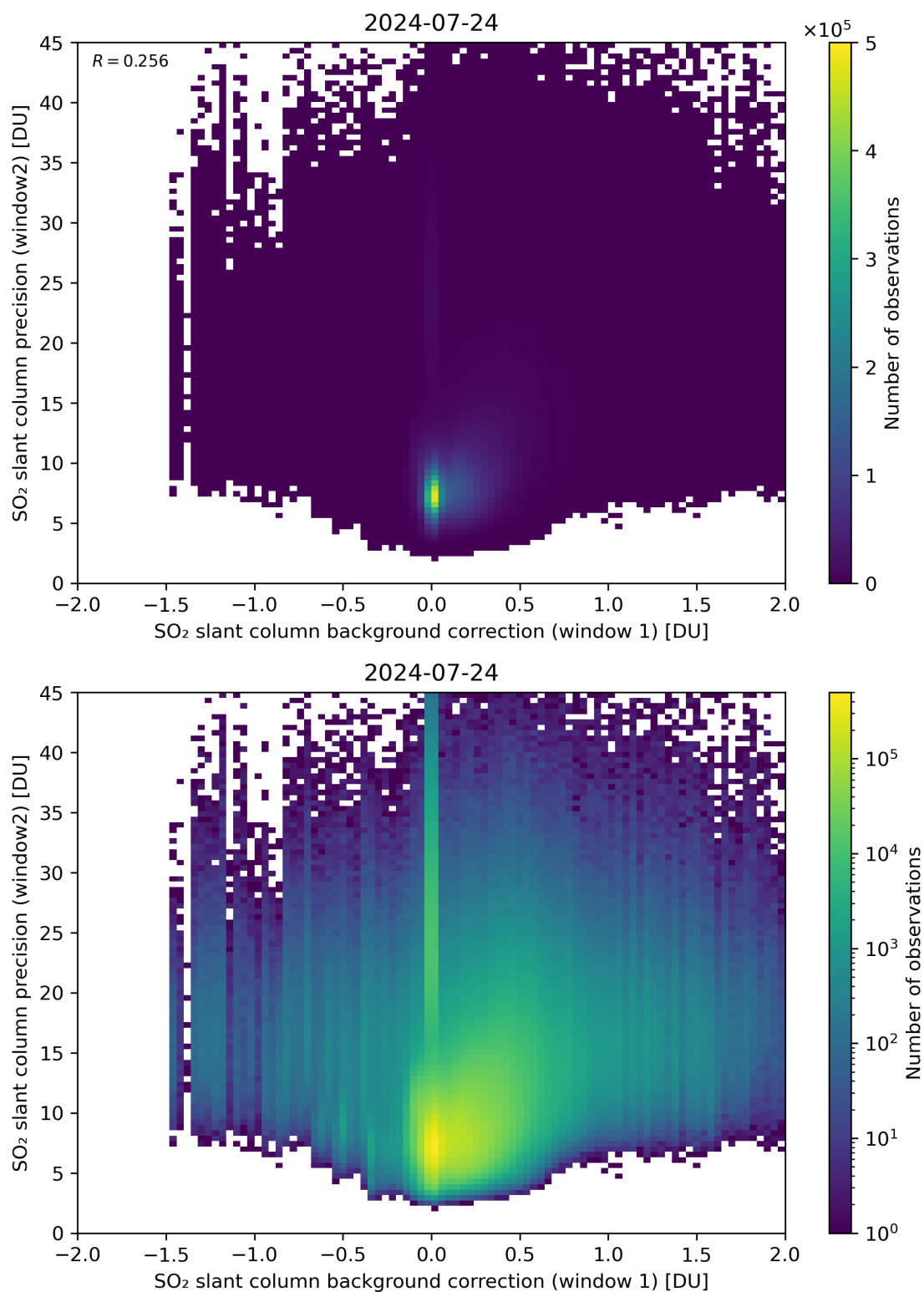
Figure 106: Scatter density plot of “SO 2 slant column background correction (window 1)” against “SO 2 slant column precision (window2)” for 2024-07-23 to 2024-07-25.
