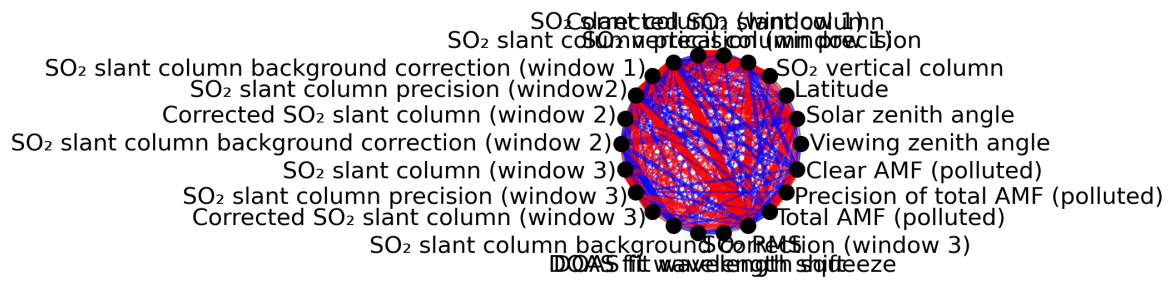
Figure 1: Map of correlation graph for 2024-07-23 to 2024-07-25.
