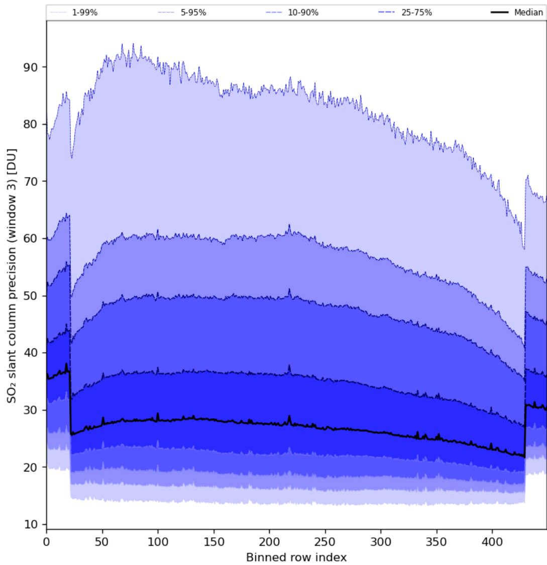
Figure 88: Along track statistics of “SO 2 slant column precision (window 3)” for 2024-07-23 to 2024-07-25
