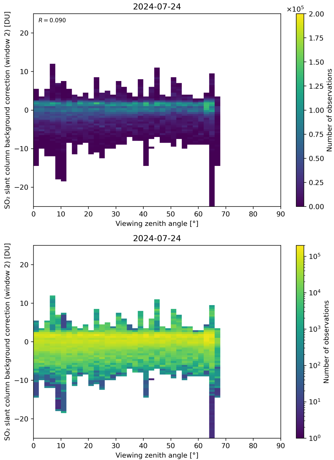
Figure 309: Scatter density plot of “Viewing zenith angle” against “SO 2 slant column background correction (window 2)” for 2024-07-23 to 2024-07-25.
