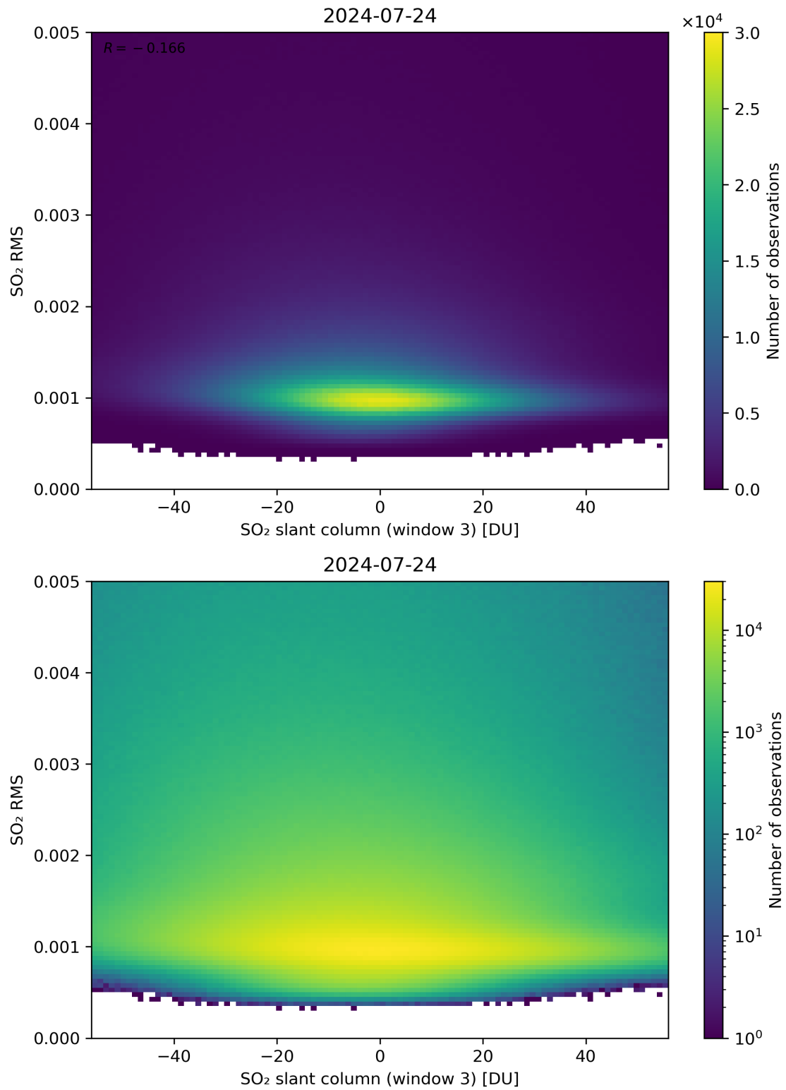
Figure 256: Scatter density plot of “SO 2 slant column (window 3)” against “SO 2 RMS” for 2024-07-23 to 2024-07-25.
