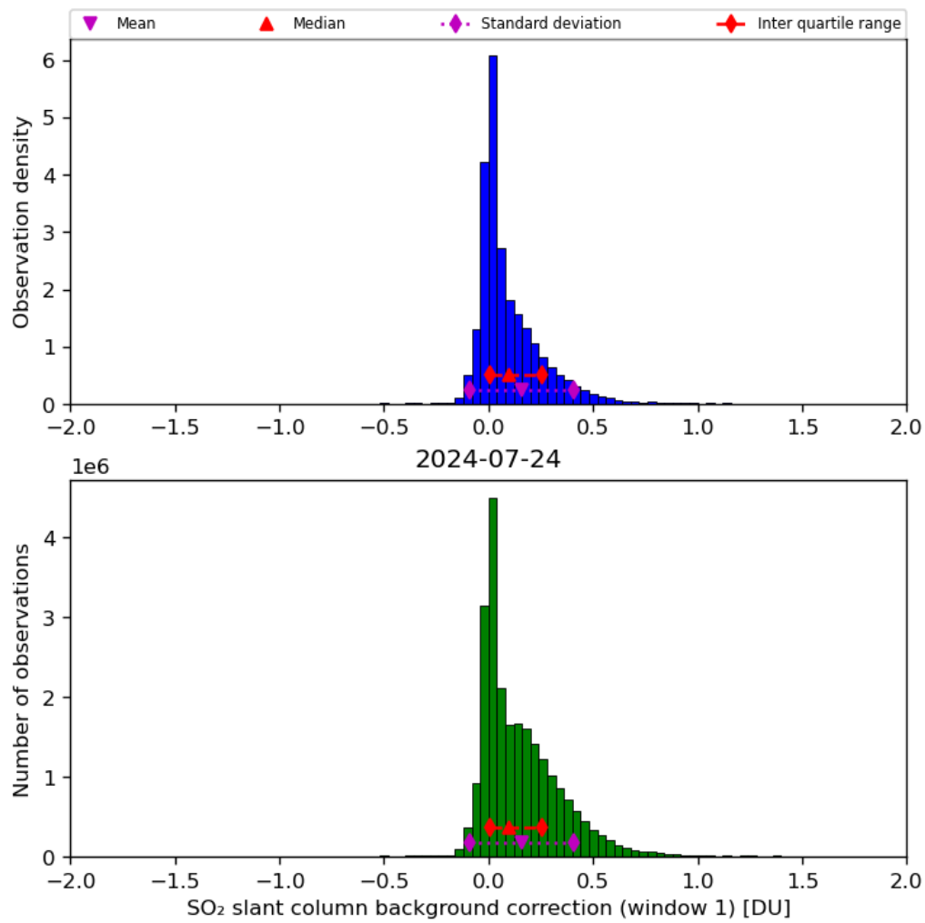
Figure 59: Histogram of “SO 2 slant column background correction (window 1)” for 2024-07-23 to 2024-07-25
