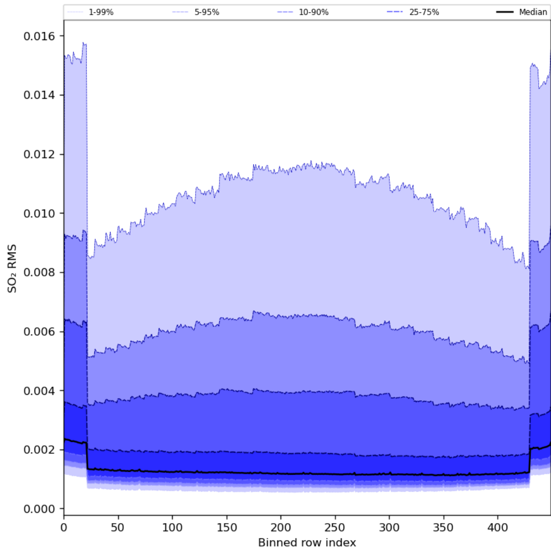
Figure 93: Along track statistics of “SO 2 RMS” for 2024-07-23 to 2024-07-25
