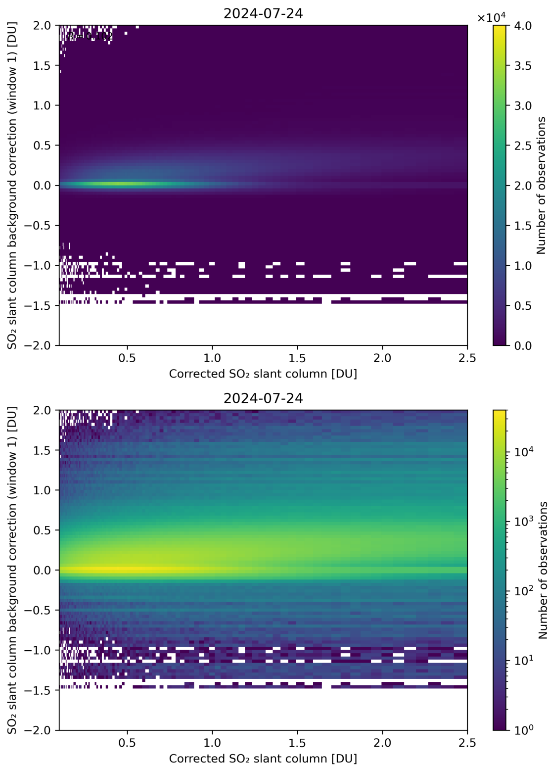
Figure 178: Scatter density plot of “Corrected SO 2 slant column” against “SO 2 slant column background correction (window 1)” for 2024-07-23 to 2024-07-25.
