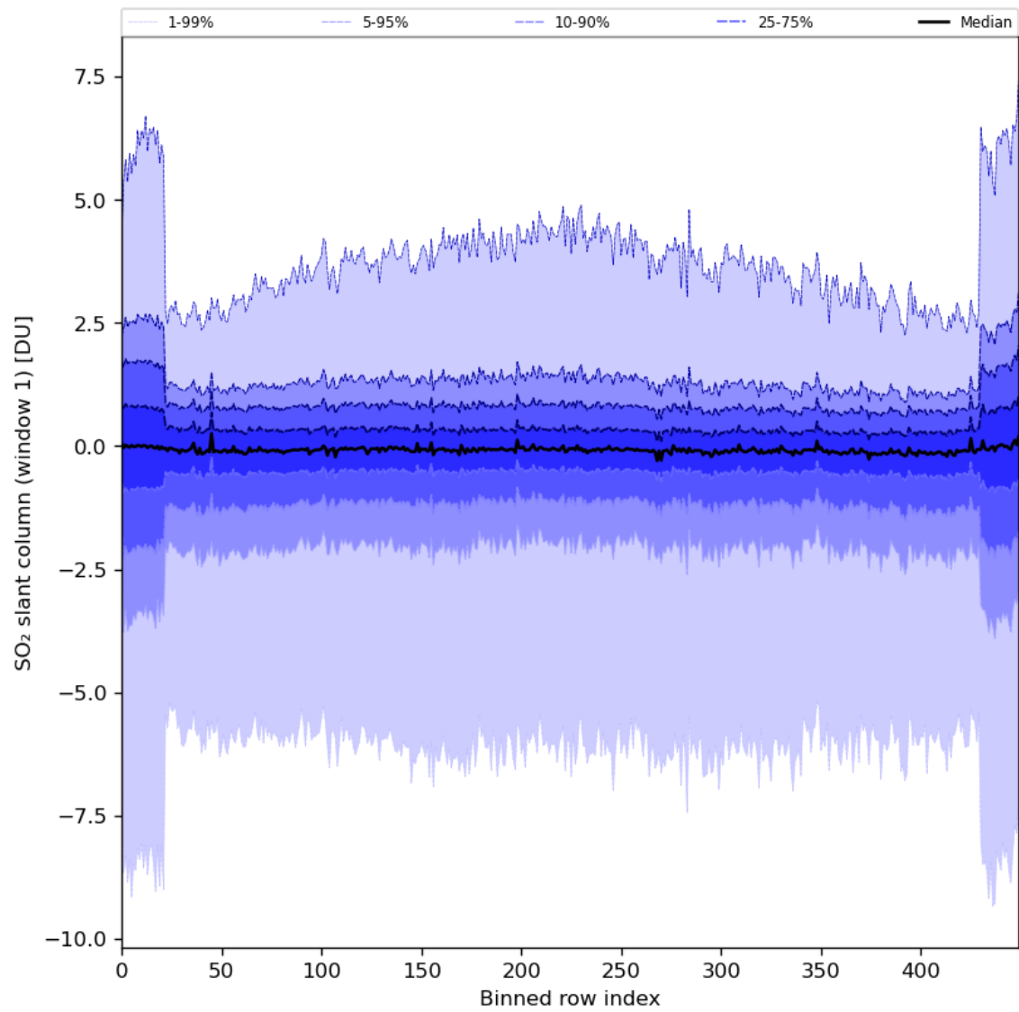
Figure 79: Along track statistics of “SO 2 slant column (window 1)” for 2024-07-23 to 2024-07-25
