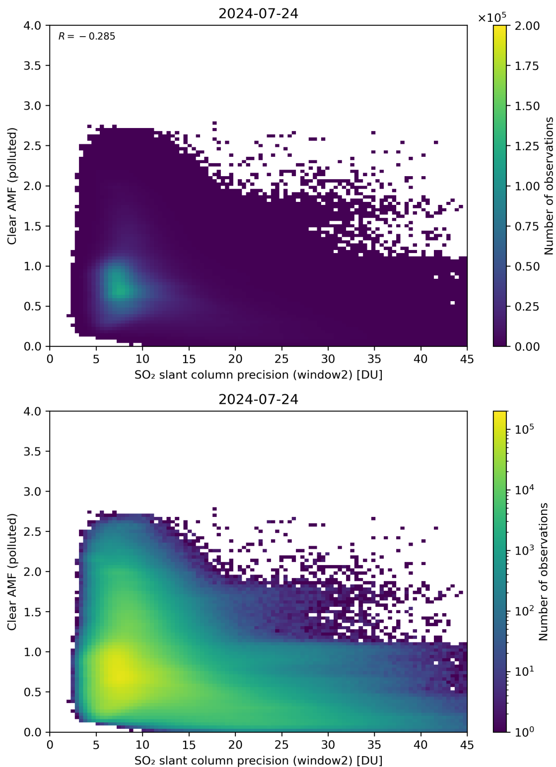
Figure 246: Scatter density plot of “SO 2 slant column precision (window2)” against “Clear AMF (polluted)” for 2024-07-23 to 2024-07-25.
