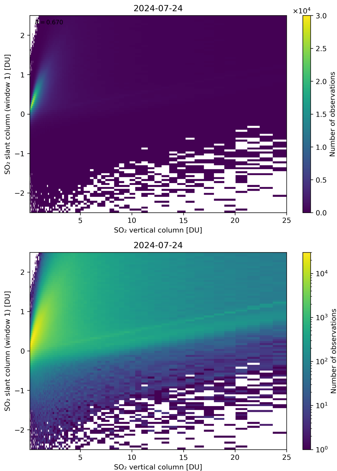
Figure 300: Scatter density plot of “SO 2 vertical column” against “SO 2 slant column (window 1)” for 2024-07-23 to 2024-07-25.
