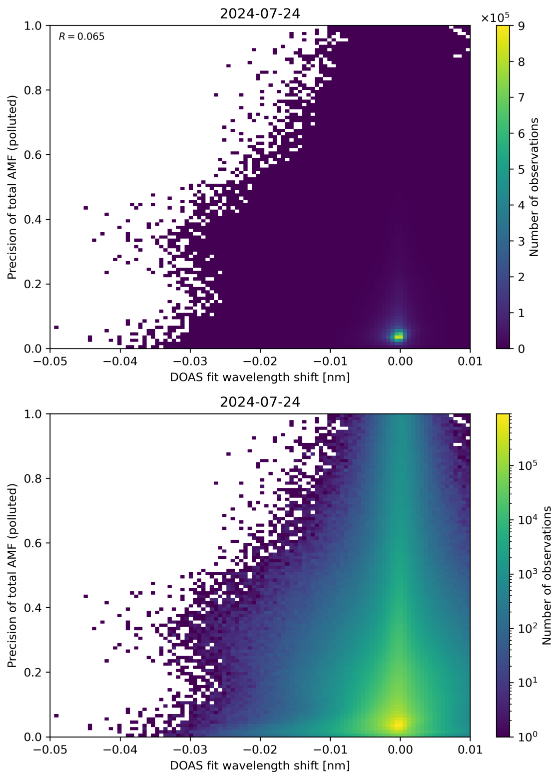
Figure 131: Scatter density plot of “DOAS fit wavelength shift” against “Precision of total AMF (polluted)” for 2024-07-23 to 2024-07-25.
