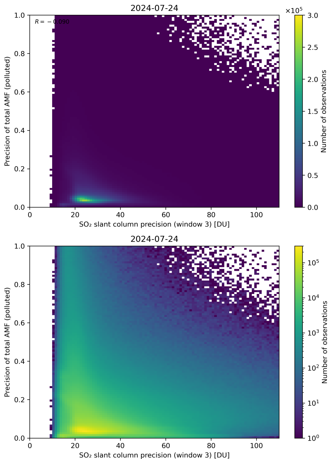
Figure 264: Scatter density plot of “SO 2 slant column precision (window 3)” against “Precision of total AMF (polluted)” for 2024-07-23 to 2024-07-25.
