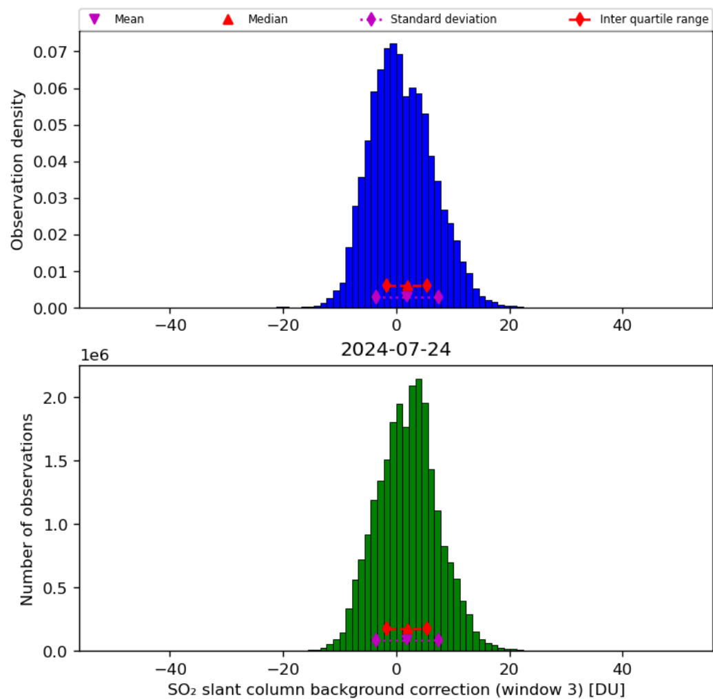
Figure 67: Histogram of “SO 2 slant column background correction (window 3)” for 2024-07-23 to 2024-07-25
