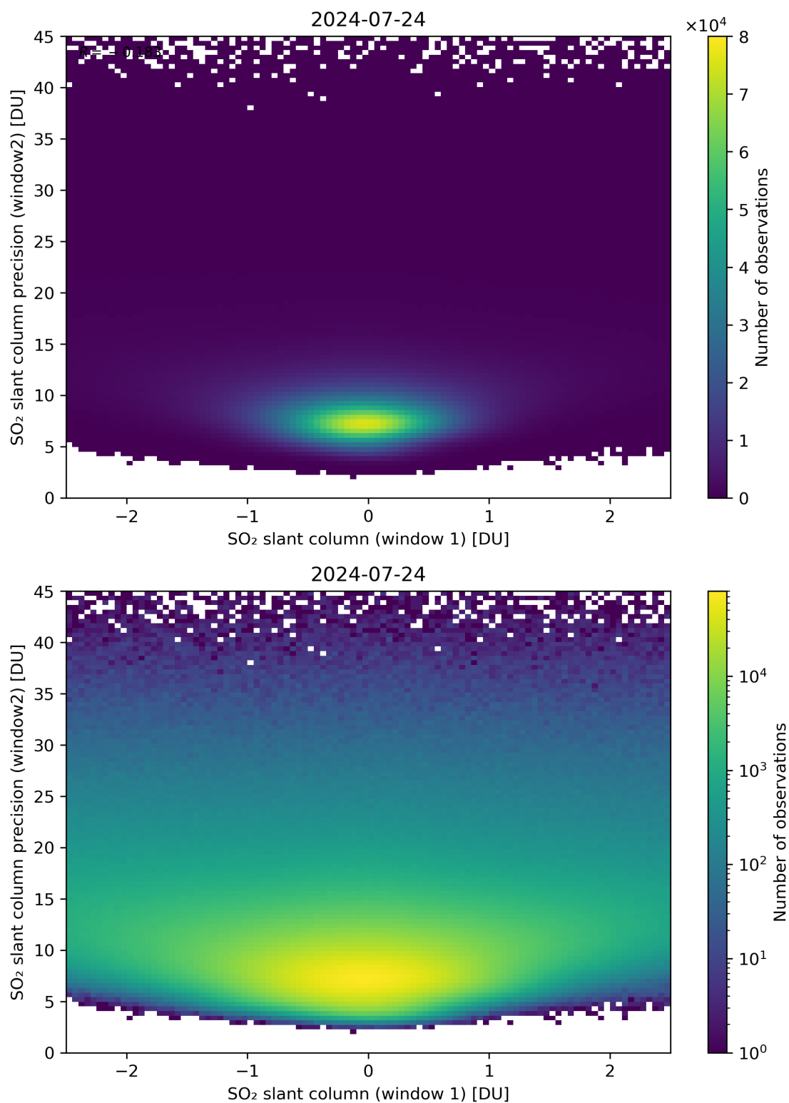
Figure 236: Scatter density plot of “SO 2 slant column (window 1)” against “SO 2 slant column precision (window2)” for 2024-07-23 to 2024-07-25.
