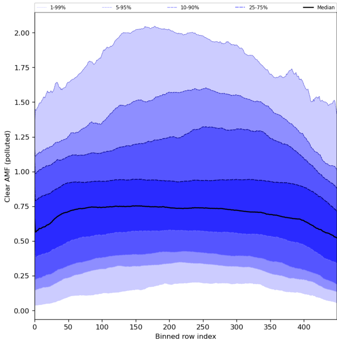
Figure 96: Along track statistics of “Clear AMF (polluted)” for 2024-07-23 to 2024-07-25
