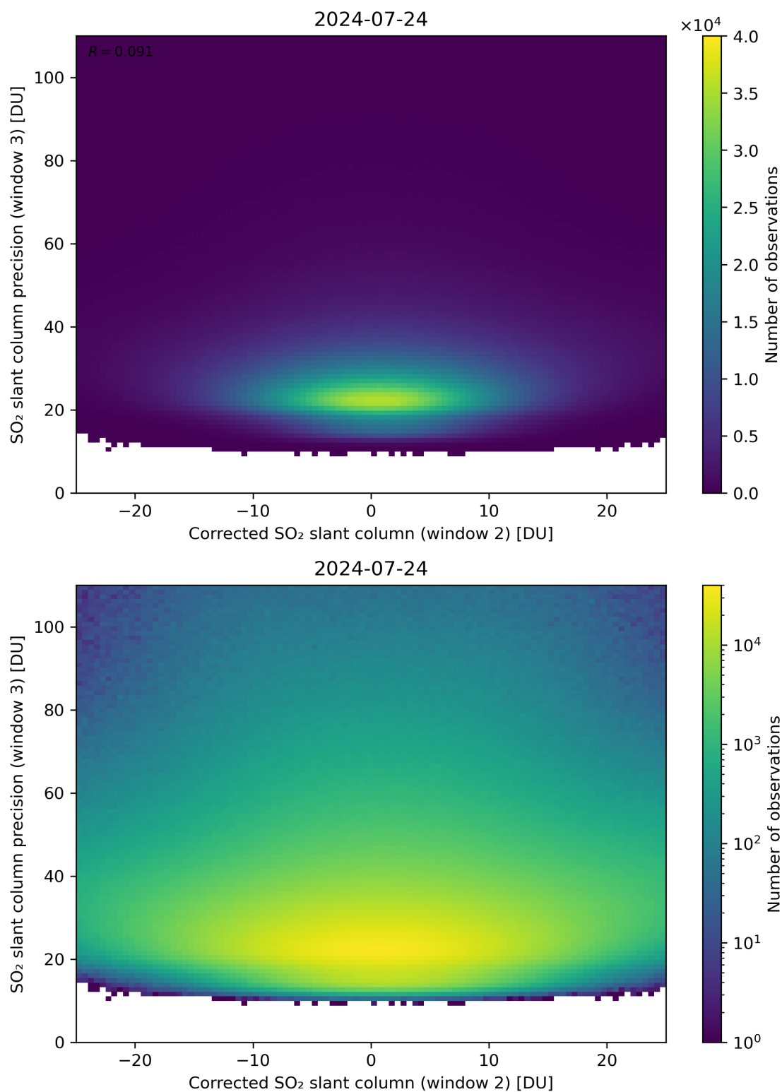
Figure 202: Scatter density plot of “Corrected SO 2 slant column (window 2)” against “SO 2 slant column precision (window 3)” for 2024-07-23 to 2024-07-25.
