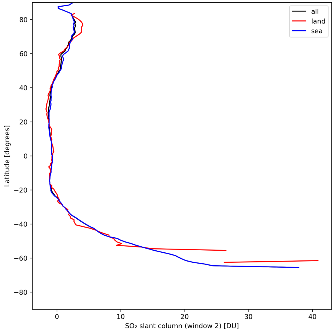
Figure 37: Zonal average of “SO 2 slant column (window 2)” for 2024-07-23 to 2024-07-25.
