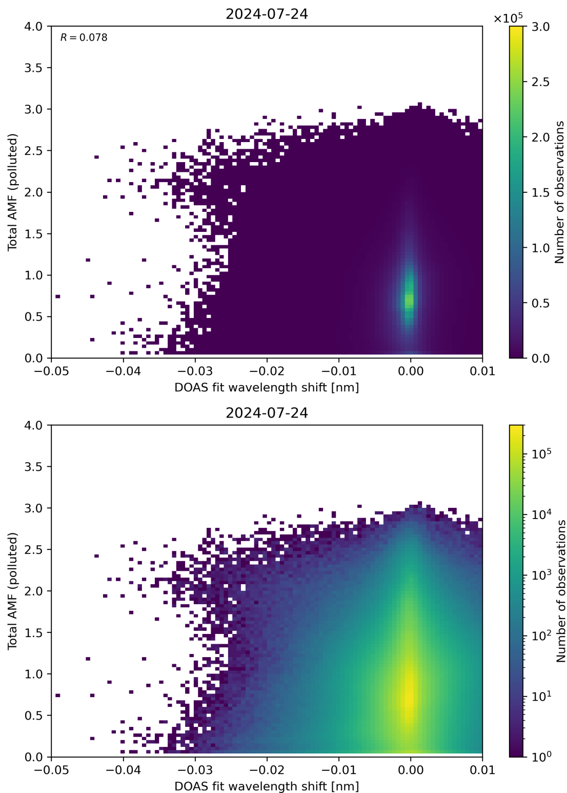
Figure 130: Scatter density plot of “DOAS fit wavelength shift” against “Total AMF (polluted)” for 2024-07-23 to 2024-07-25.
