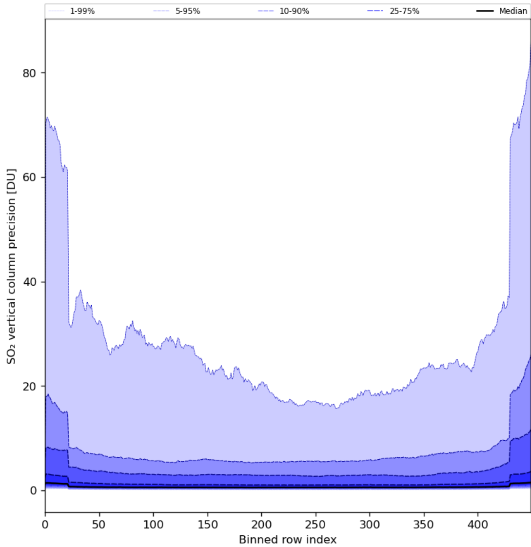
Figure 77: Along track statistics of “SO 2 vertical column precision” for 2024-07-23 to 2024-07-25
