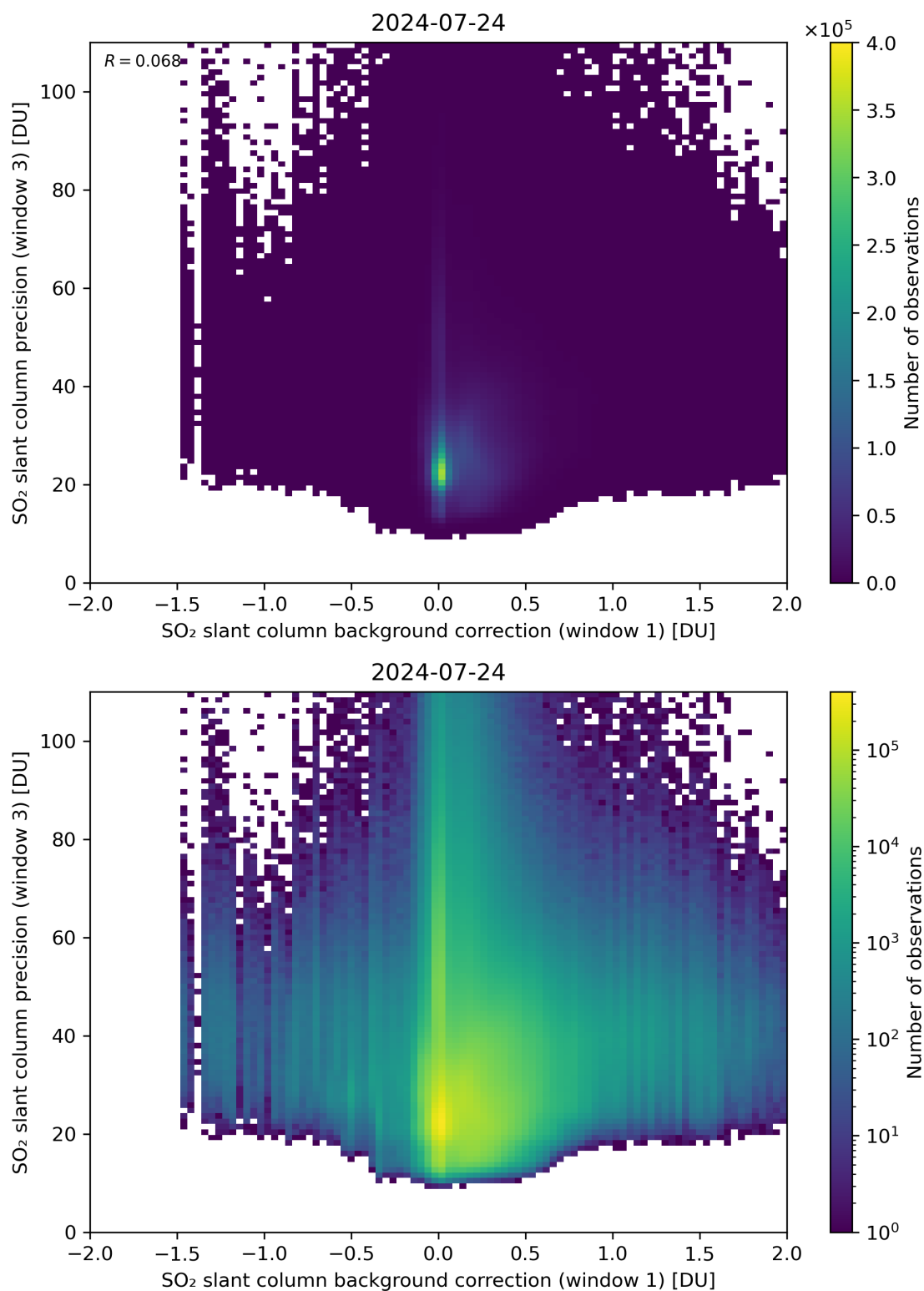
Figure 108: Scatter density plot of “SO 2 slant column background correction (window 1)” against “SO 2 slant column precision (window 3)” for 2024-07-23 to 2024-07-25.
