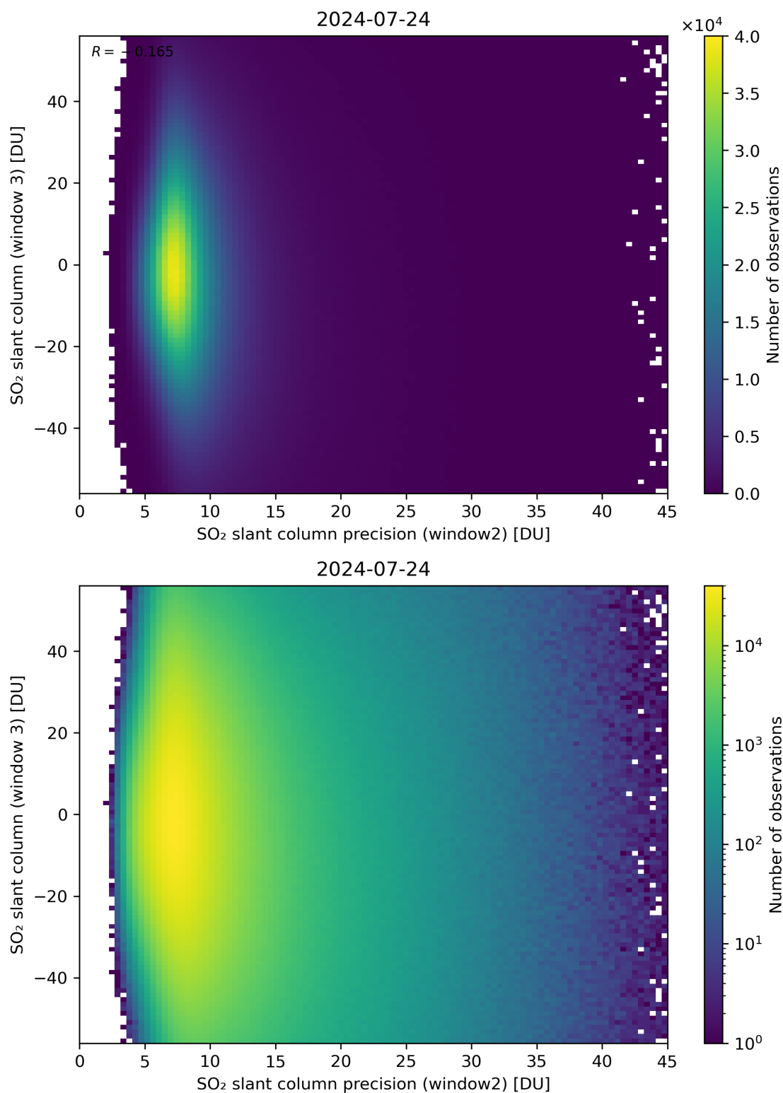
Figure 249: Scatter density plot of “SO 2 slant column precision (window2)” against “SO 2 slant column (window 3)” for 2024-07-23 to 2024-07-25.
