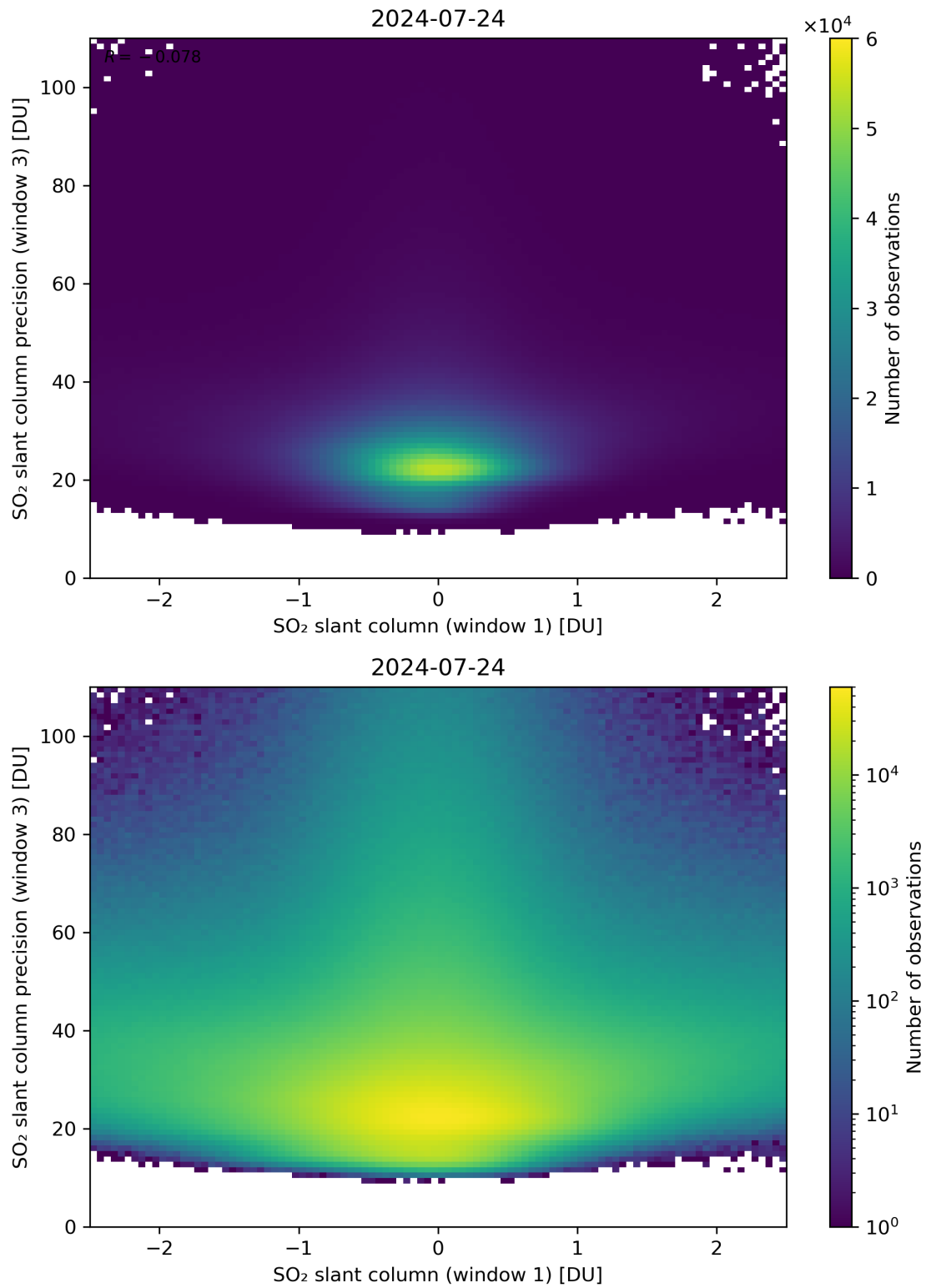
Figure 238: Scatter density plot of “SO 2 slant column (window 1)” against “SO 2 slant column precision (window 3)” for 2024-07-23 to 2024-07-25.
