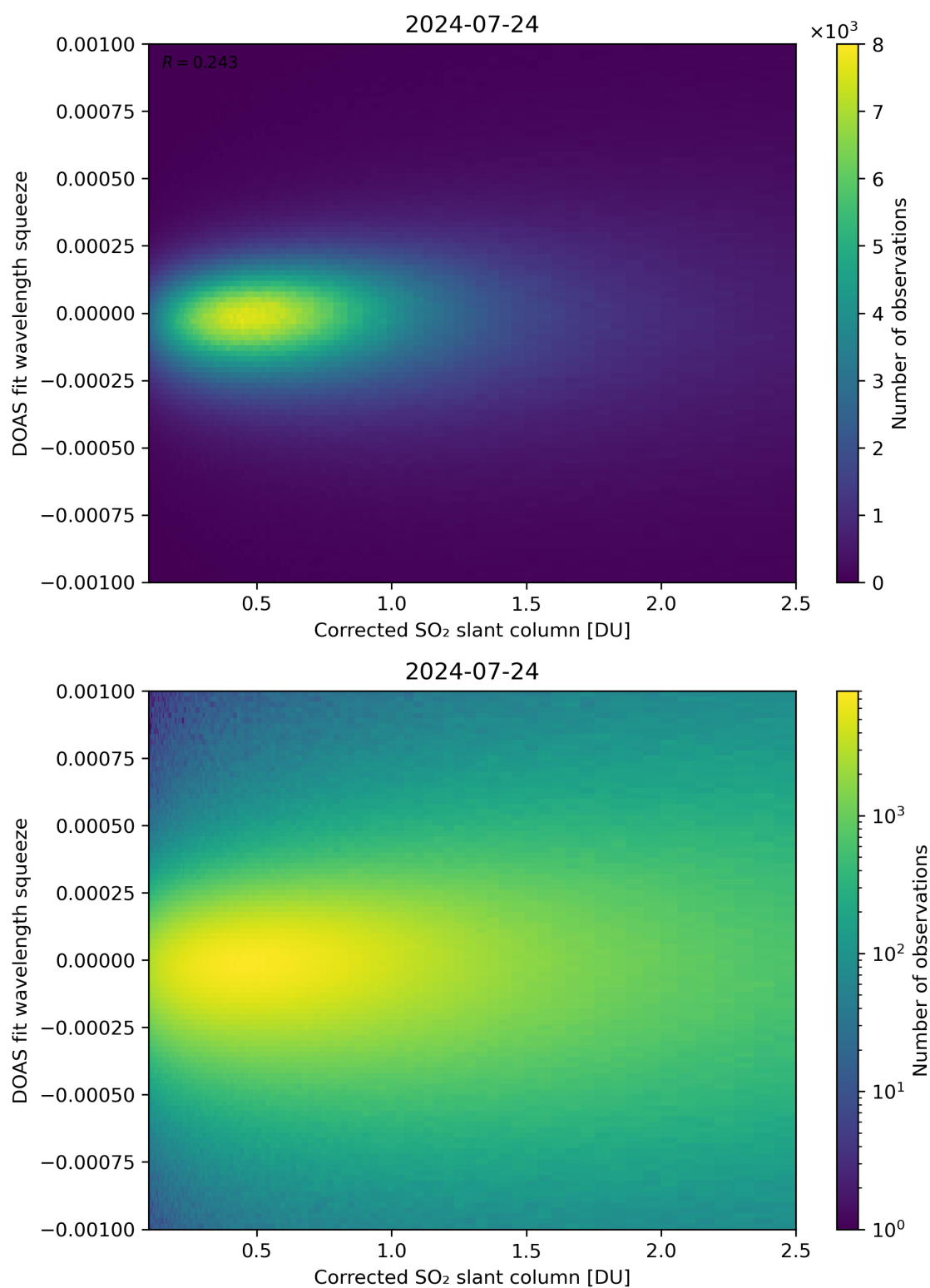
Figure 182: Scatter density plot of “Corrected SO 2 slant column” against “DOAS fit wavelength squeeze” for 2024-07-23 to 2024-07-25.
