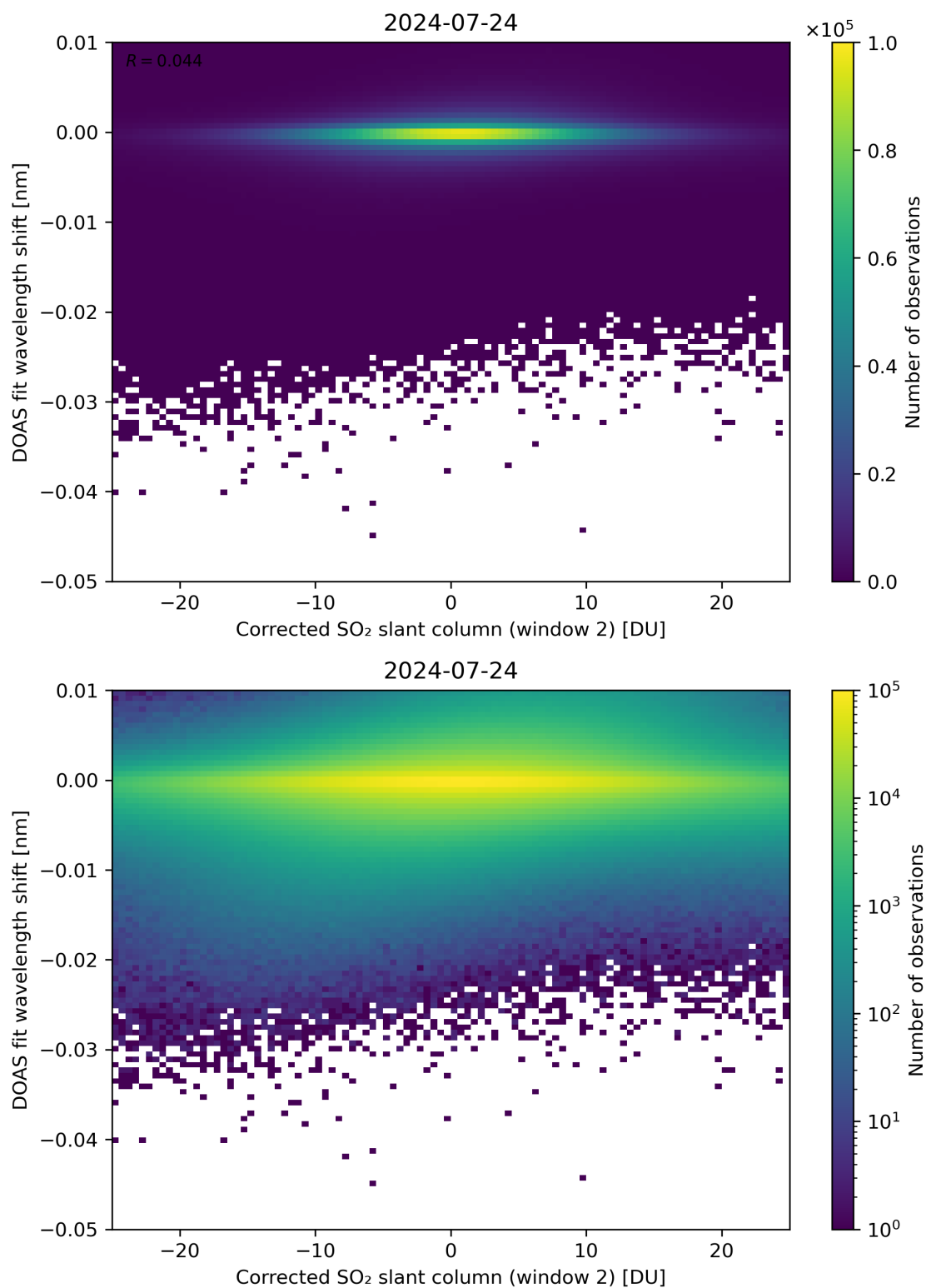
Figure 196: Scatter density plot of “Corrected SO 2 slant column (window 2)” against “DOAS fit wavelength shift” for 2024-07-23 to 2024-07-25.
