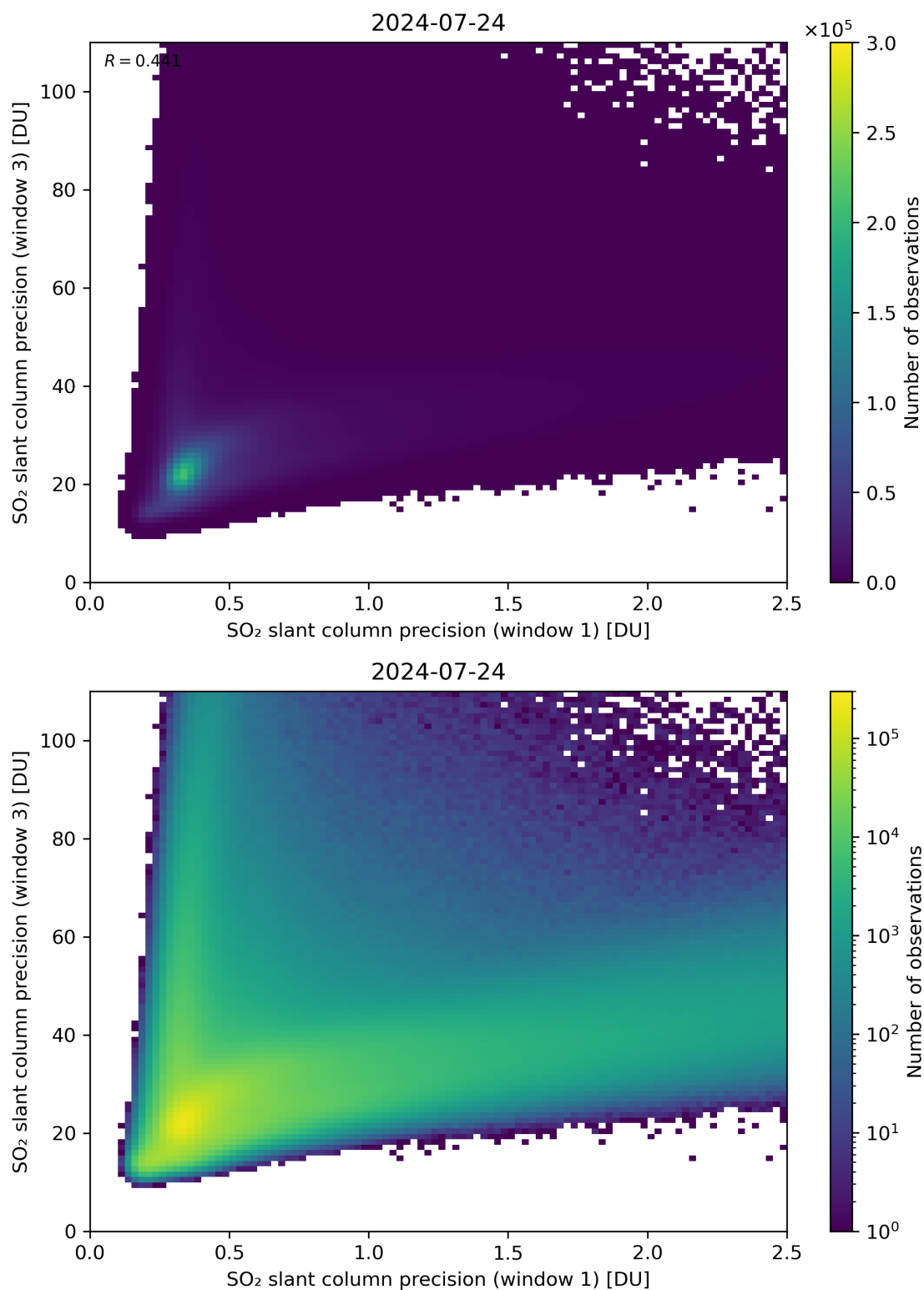
Figure 229: Scatter density plot of “SO 2 slant column precision (window 1)” against “SO 2 slant column precision (window 3)” for 2024-07-23 to 2024-07-25.
