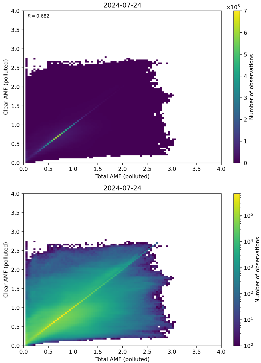
Figure 271: Scatter density plot of “Total AMF (polluted)” against “Clear AMF (polluted)” for 2024-07-23 to 2024-07-25.
