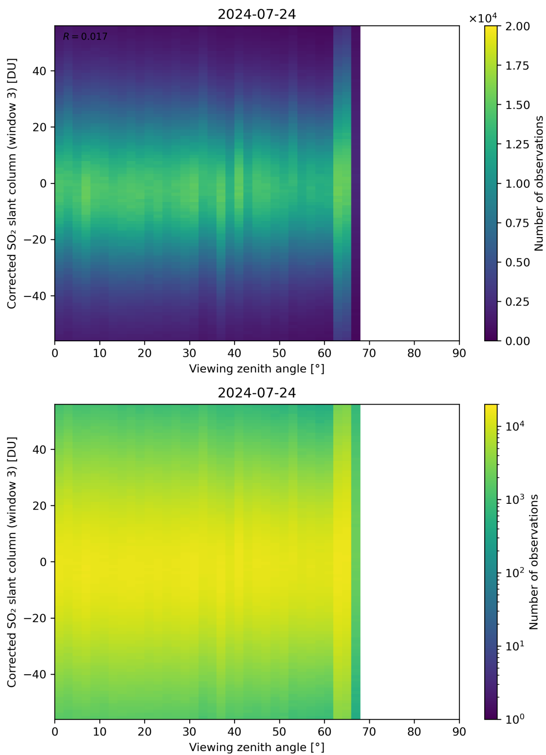
Figure 319: Scatter density plot of “Viewing zenith angle” against “Corrected SO 2 slant column (window 3)” for 2024-07-23 to 2024-07-25.
