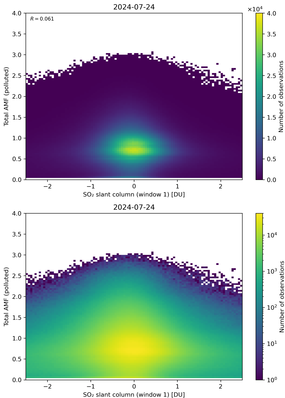
Figure 239: Scatter density plot of “SO 2 slant column (window 1)” against “Total AMF (polluted)” for 2024-07-23 to 2024-07-25.
