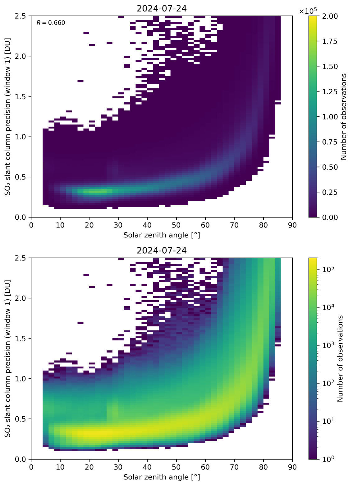
Figure 170: Scatter density plot of “Solar zenith angle” against “SO 2 slant column precision (window 1)” for 2024-07-23 to 2024-07-25.
