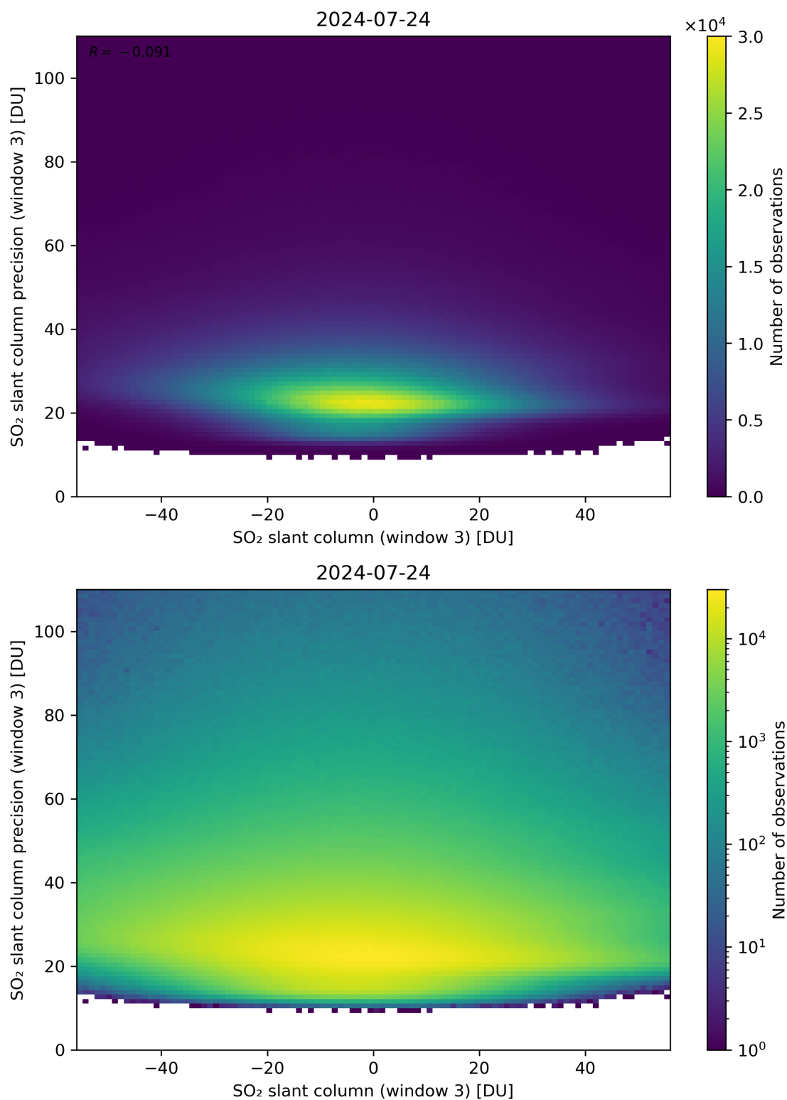
Figure 267: Scatter density plot of “SO 2 slant column (window 3)” against “SO 2 slant column precision (window 3)” for 2024-07-23 to 2024-07-25.
