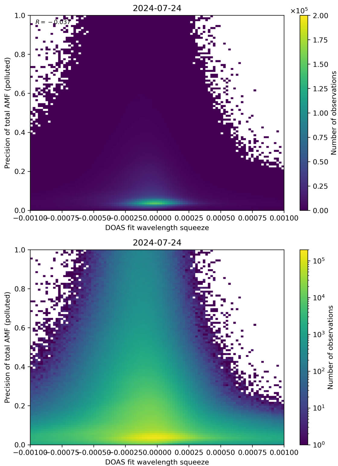
Figure 135: Scatter density plot of “DOAS fit wavelength squeeze” against “Precision of total AMF (polluted)” for 2024-07-23 to 2024-07-25.
