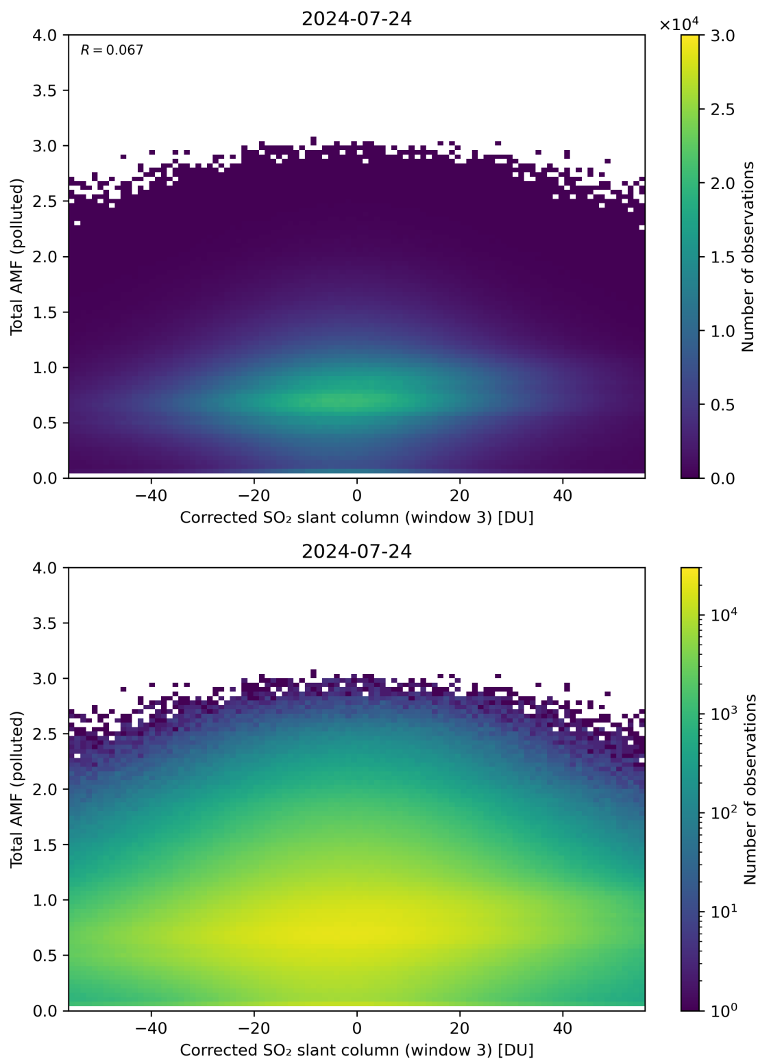
Figure 210: Scatter density plot of “Corrected SO 2 slant column (window 3)” against “Total AMF (polluted)” for 2024-07-23 to 2024-07-25.
