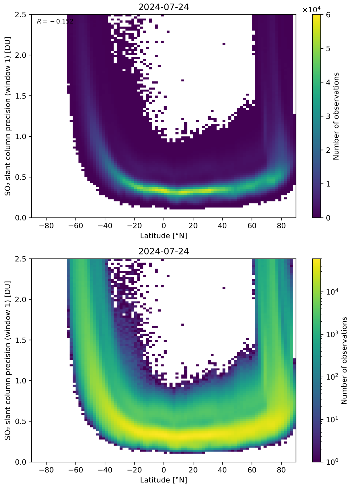
Figure 150: Scatter density plot of “Latitude” against “SO 2 slant column precision (window 1)” for 2024-07-23 to 2024-07-25.
