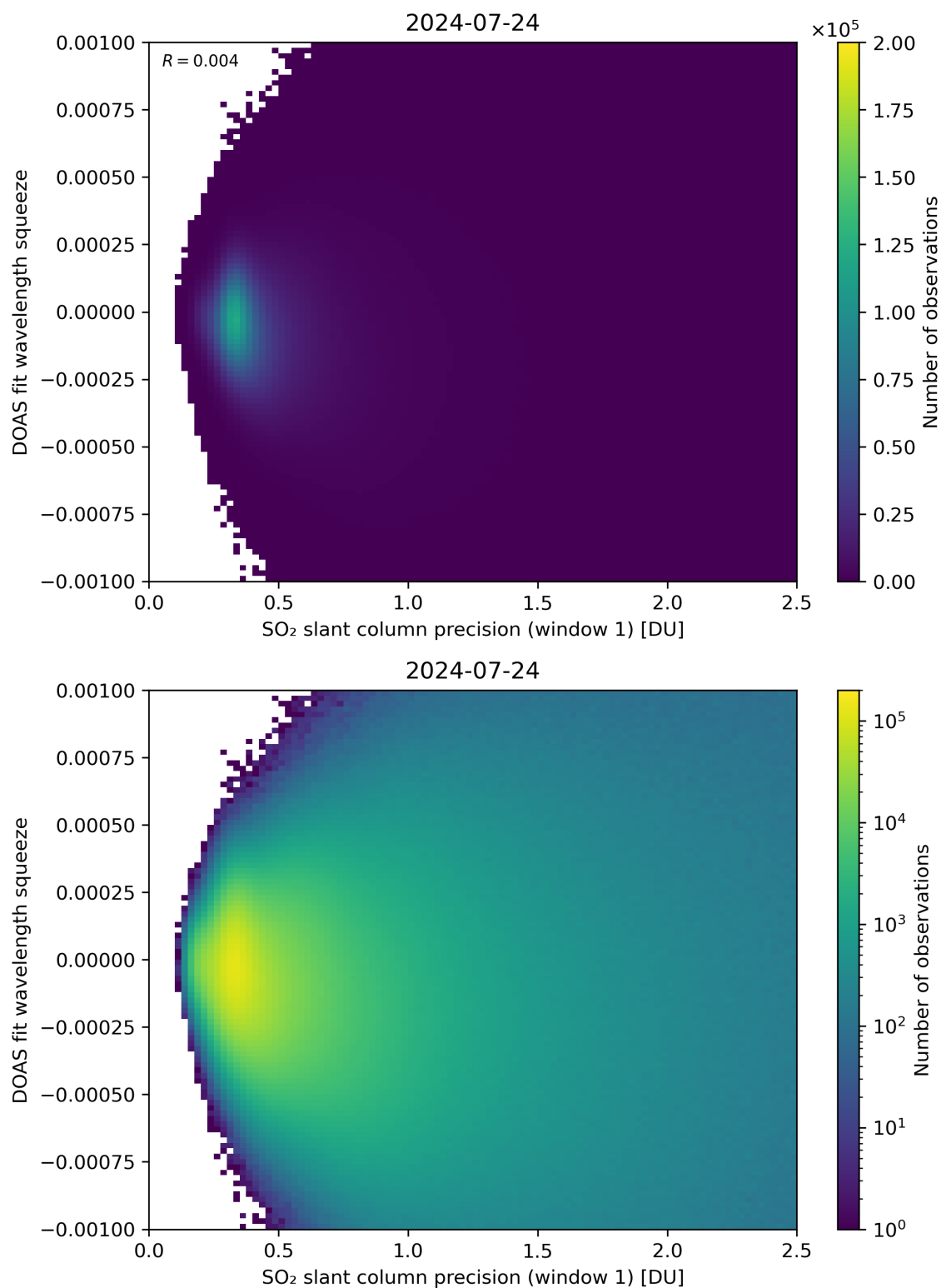
Figure 222: Scatter density plot of “SO 2 slant column precision (window 1)” against “DOAS fit wavelength squeeze” for 2024-07-23 to 2024-07-25.
