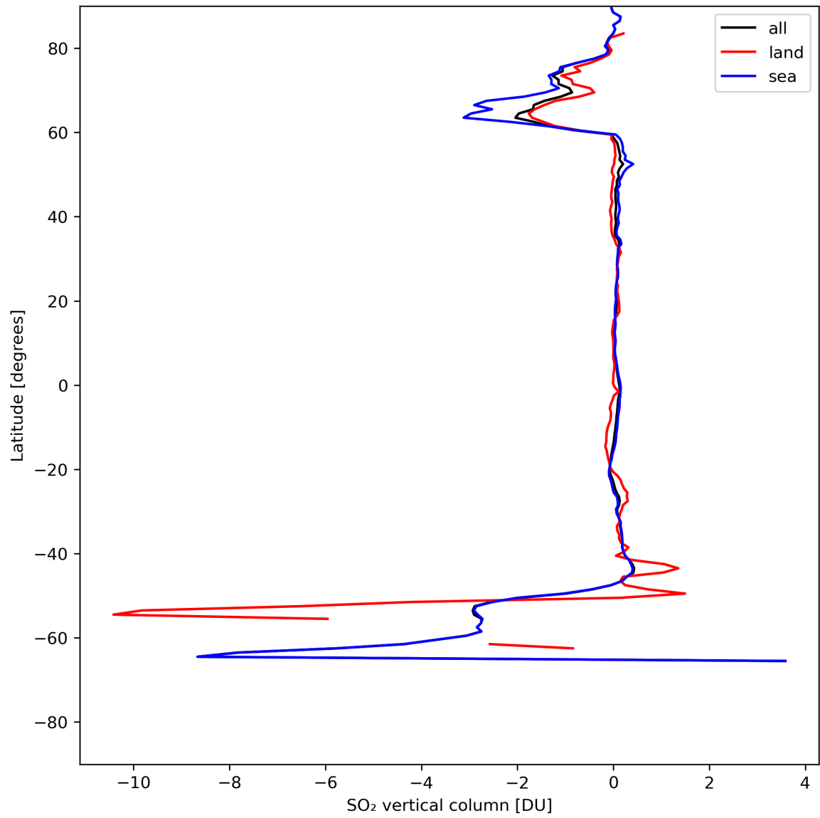
Figure 30: Zonal average of “SO 2 vertical column” for 2024-07-23 to 2024-07-25.
