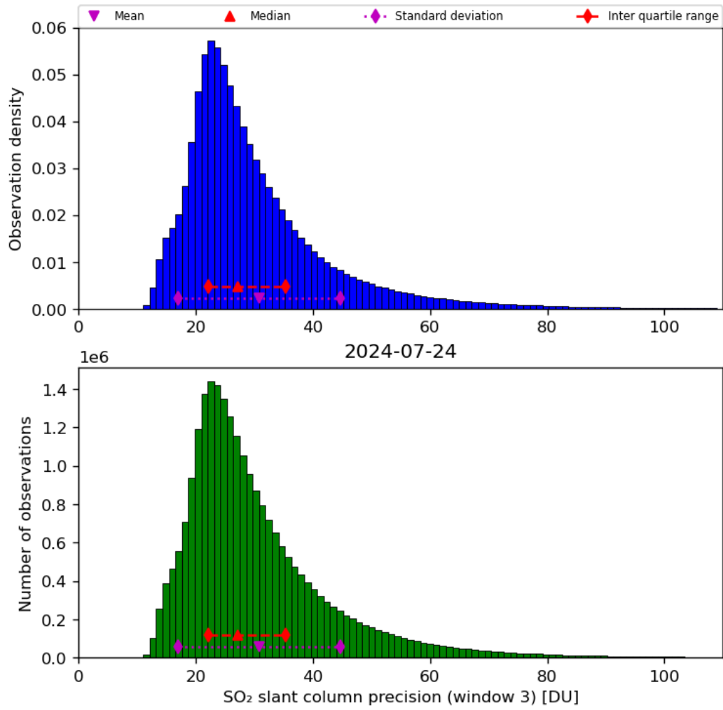
Figure 65: Histogram of “SO 2 slant column precision (window 3)” for 2024-07-23 to 2024-07-25
