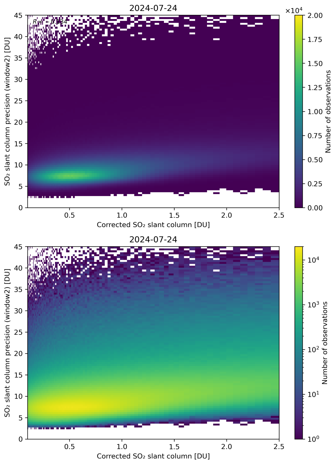
Figure 189: Scatter density plot of “Corrected SO 2 slant column” against “SO 2 slant column precision (window2)” for 2024-07-23 to 2024-07-25.
