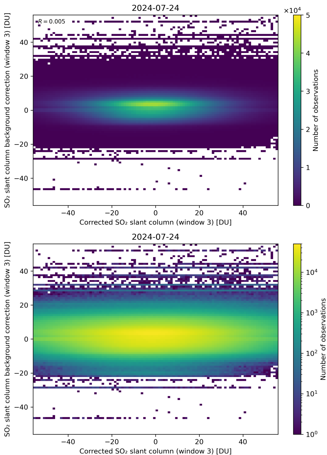
Figure 205: Scatter density plot of “Corrected SO 2 slant column (window 3)” against “SO 2 slant column background correction (window 3)” for 2024-07-23 to 2024-07-25.
