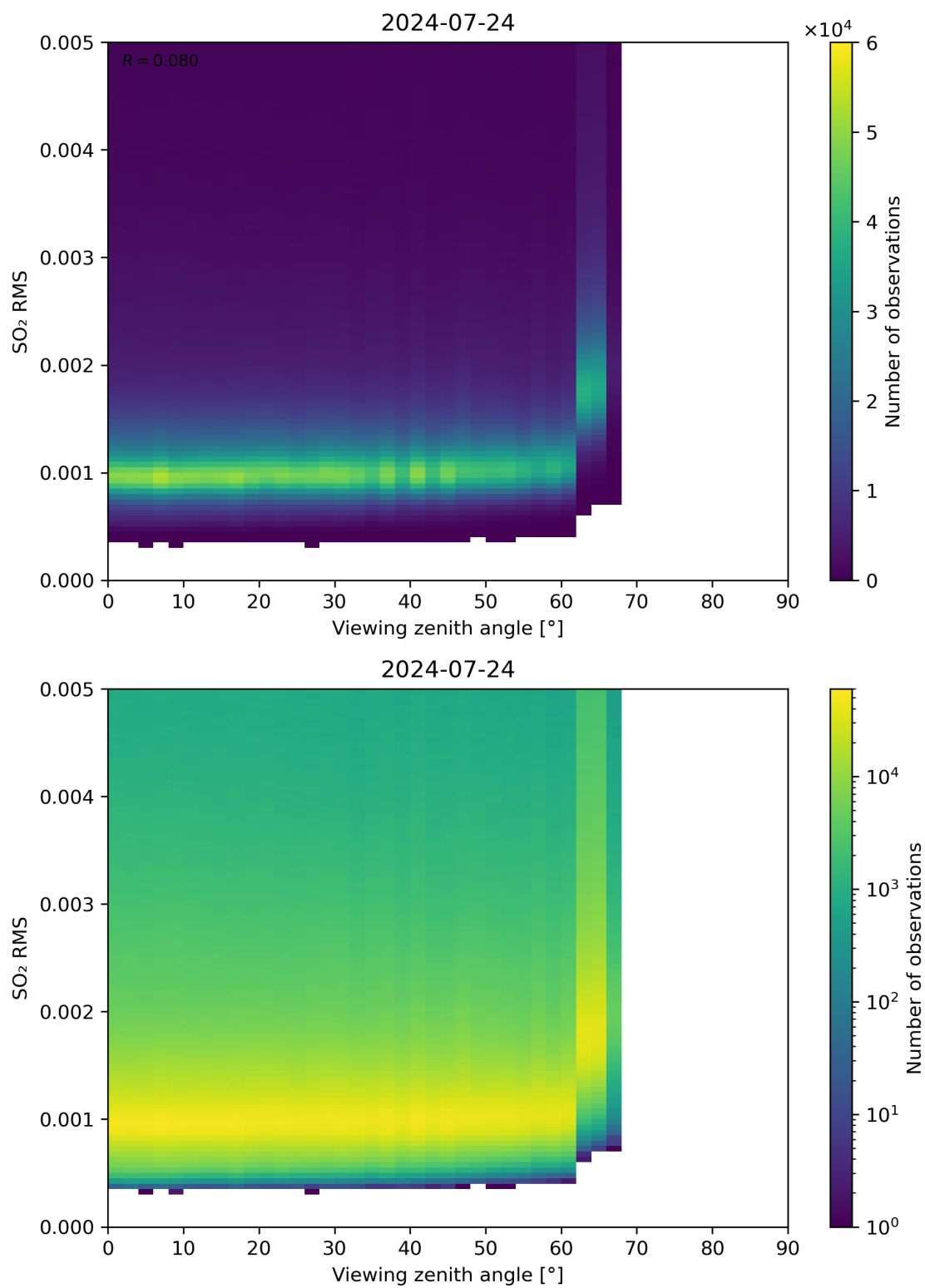
Figure 313: Scatter density plot of “Viewing zenith angle” against “SO 2 RMS” for 2024-07-23 to 2024-07-25.
