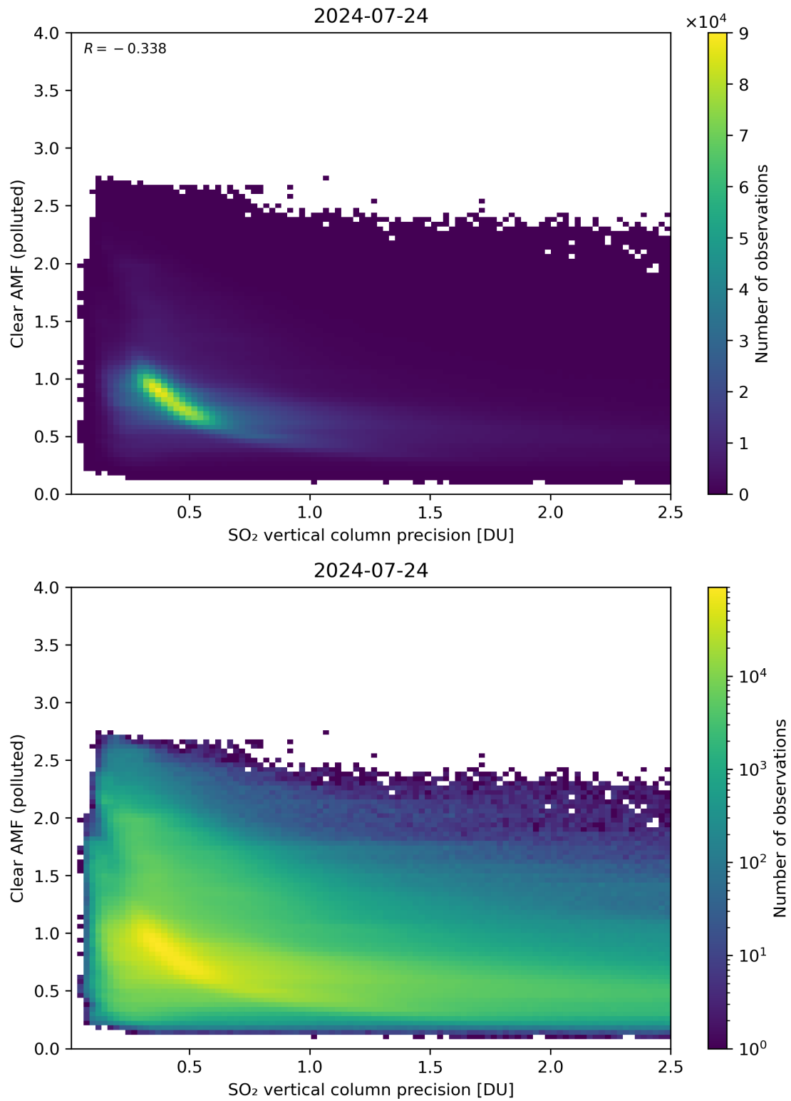
Figure 285: Scatter density plot of “SO 2 vertical column precision” against “Clear AMF (polluted)” for 2024-07-23 to 2024-07-25.
