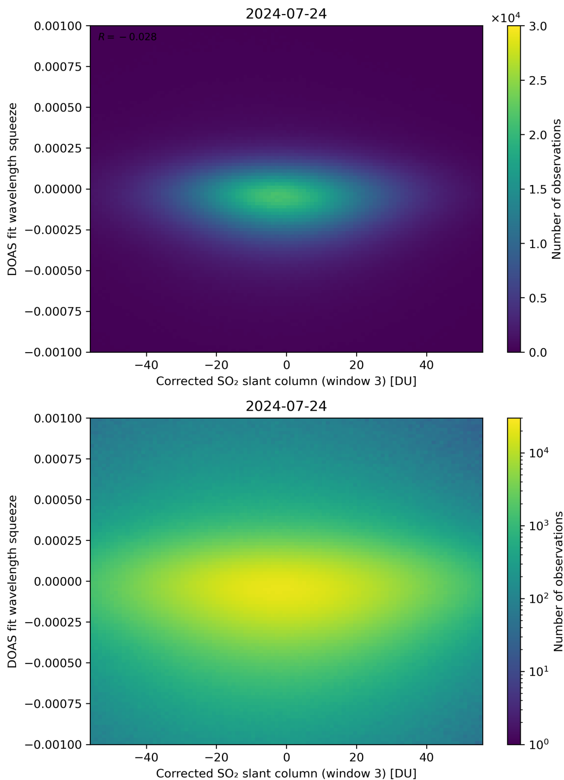
Figure 207: Scatter density plot of “Corrected SO 2 slant column (window 3)” against “DOAS fit wavelength squeeze” for 2024-07-23 to 2024-07-25.
