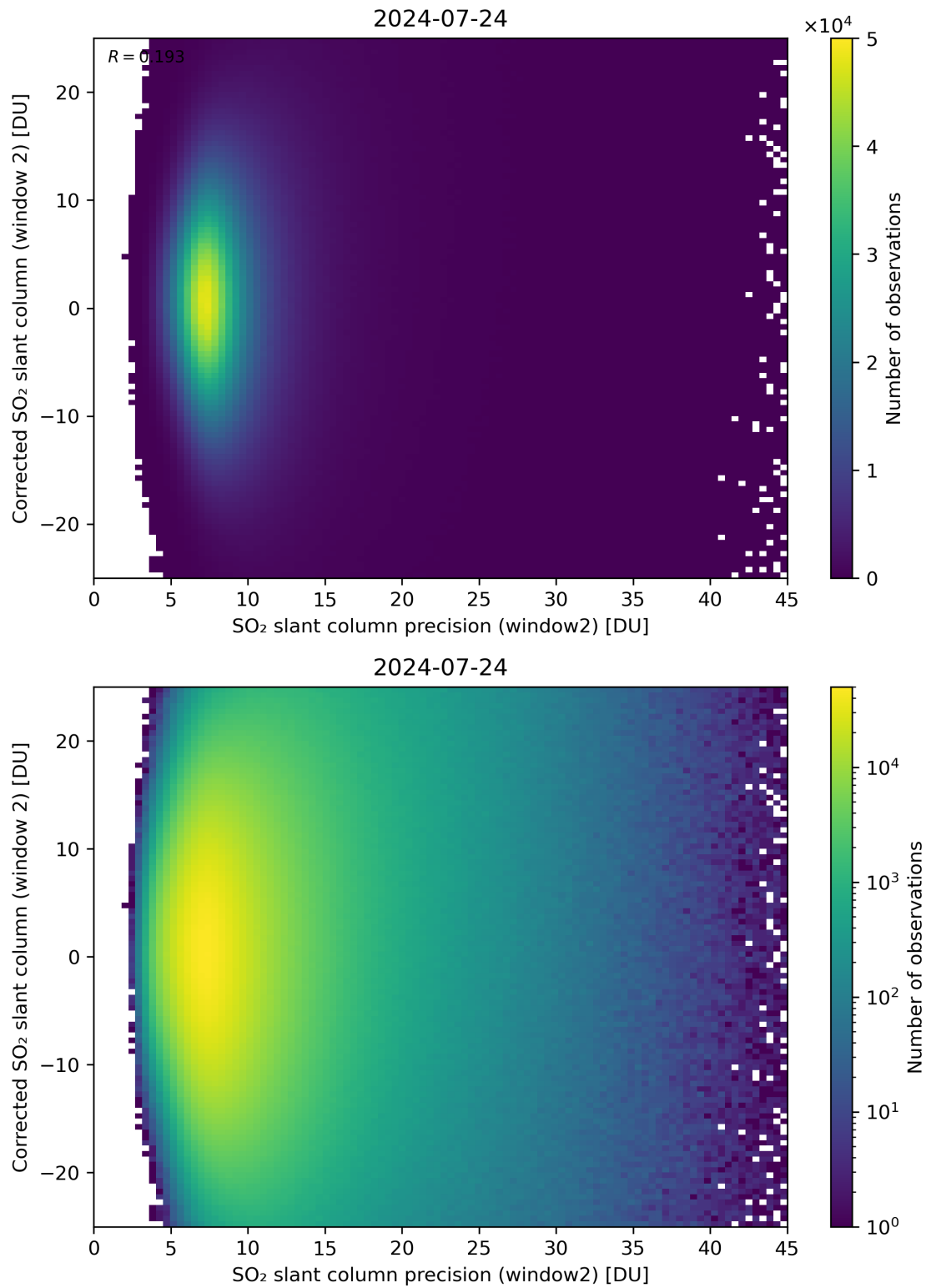
Figure 247: Scatter density plot of “SO 2 slant column precision (window2)” against “Corrected SO 2 slant column (window 2)” for 2024-07-23 to 2024-07-25.
