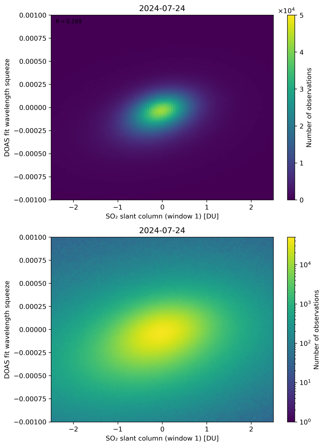
Figure 216: Scatter density plot of “SO 2 slant column (window 1)” against “DOAS fit wavelength squeeze” for 2024-07-23 to 2024-07-25.
