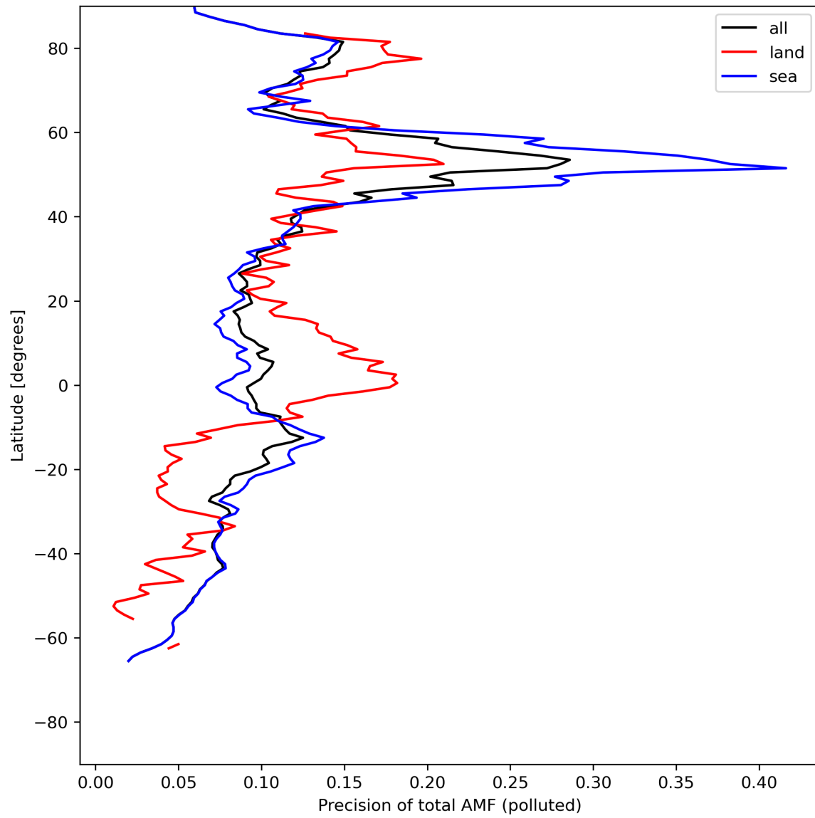
Figure 49: Zonal average of “Precision of total AMF (polluted)” for 2024-07-23 to 2024-07-25.
