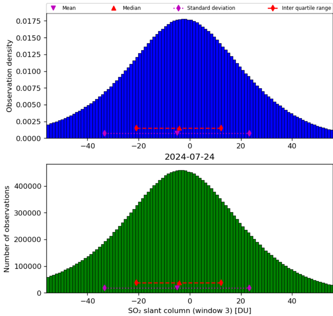
Figure 64: Histogram of “SO 2 slant column (window 3)” for 2024-07-23 to 2024-07-25
