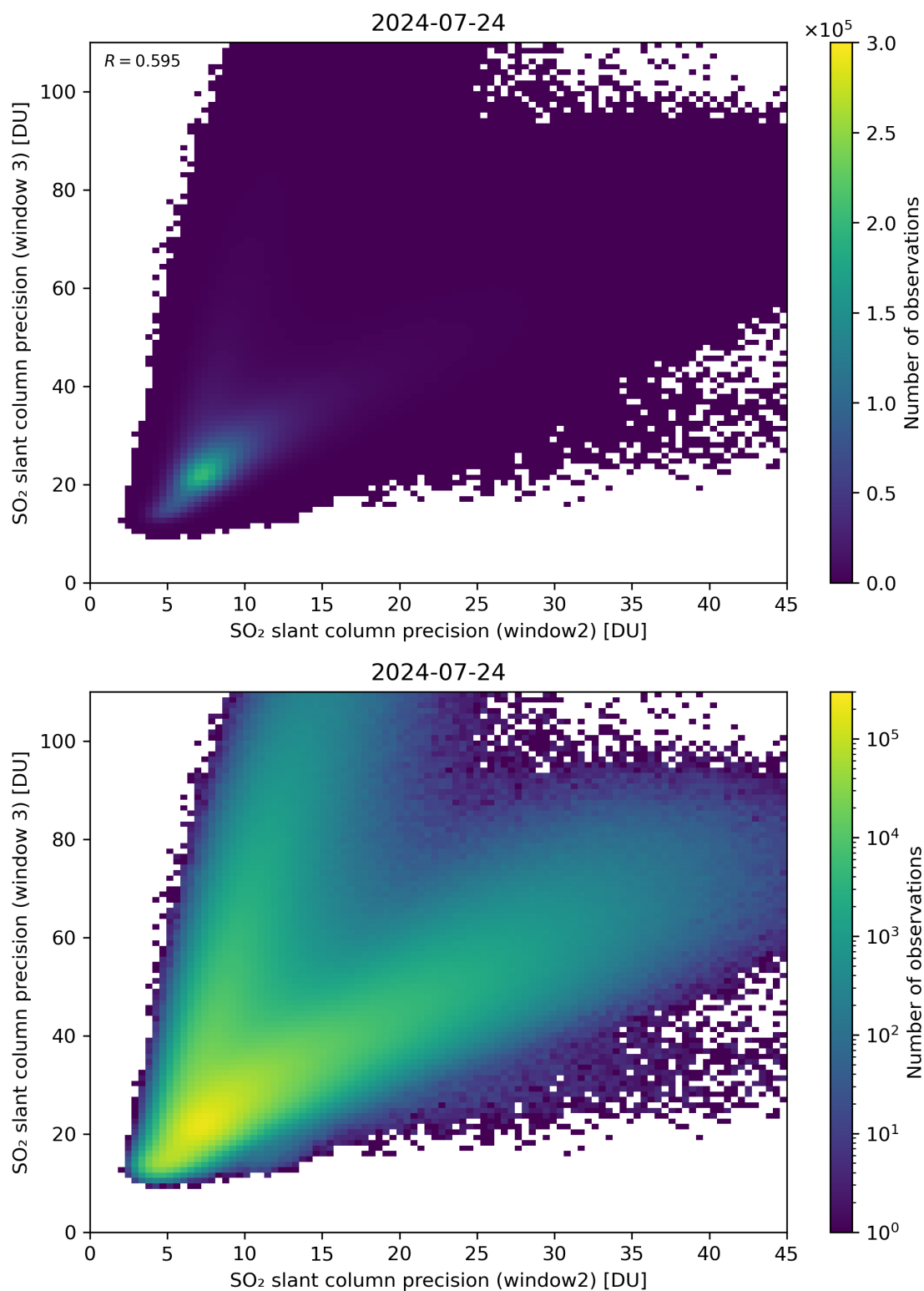
Figure 250: Scatter density plot of “SO 2 slant column precision (window2)” against “SO 2 slant column precision (window 3)” for 2024-07-23 to 2024-07-25.
