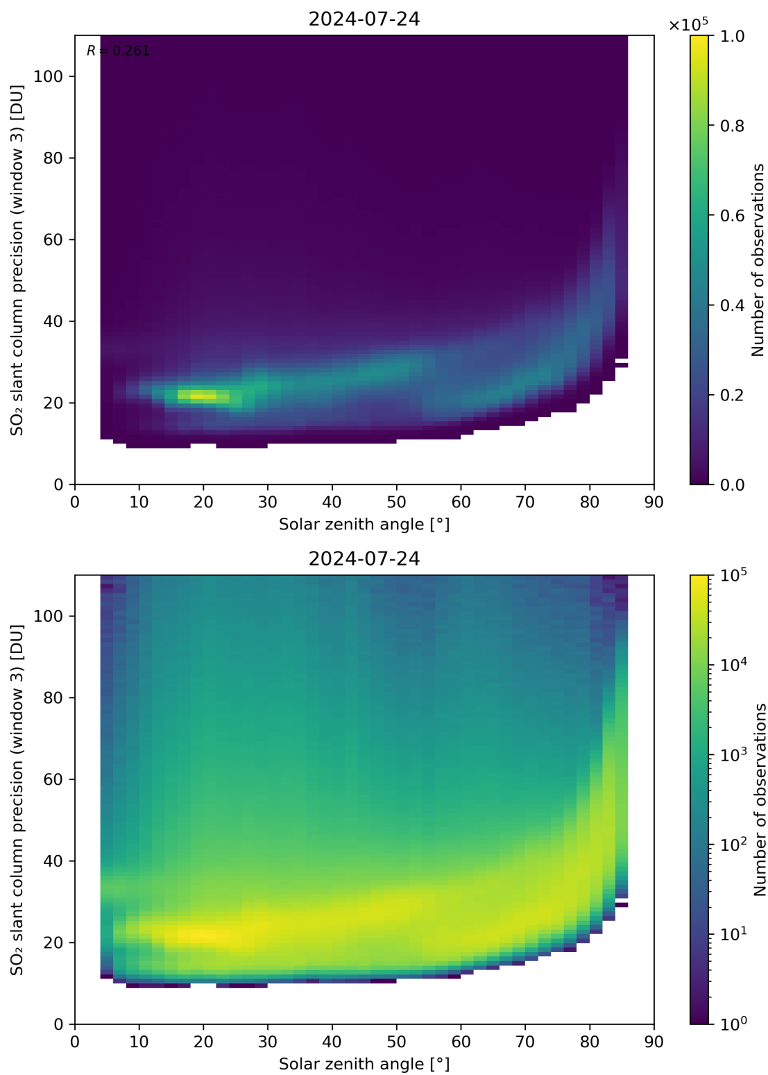
Figure 173: Scatter density plot of “Solar zenith angle” against “SO 2 slant column precision (window 3)” for 2024-07-23 to 2024-07-25.
