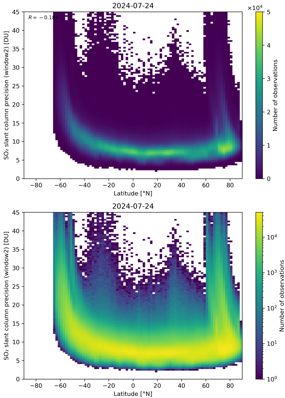
Figure 151: Scatter density plot of “Latitude” against “SO 2 slant column precision (window2)” for 2024-07-23 to 2024-07-25.
