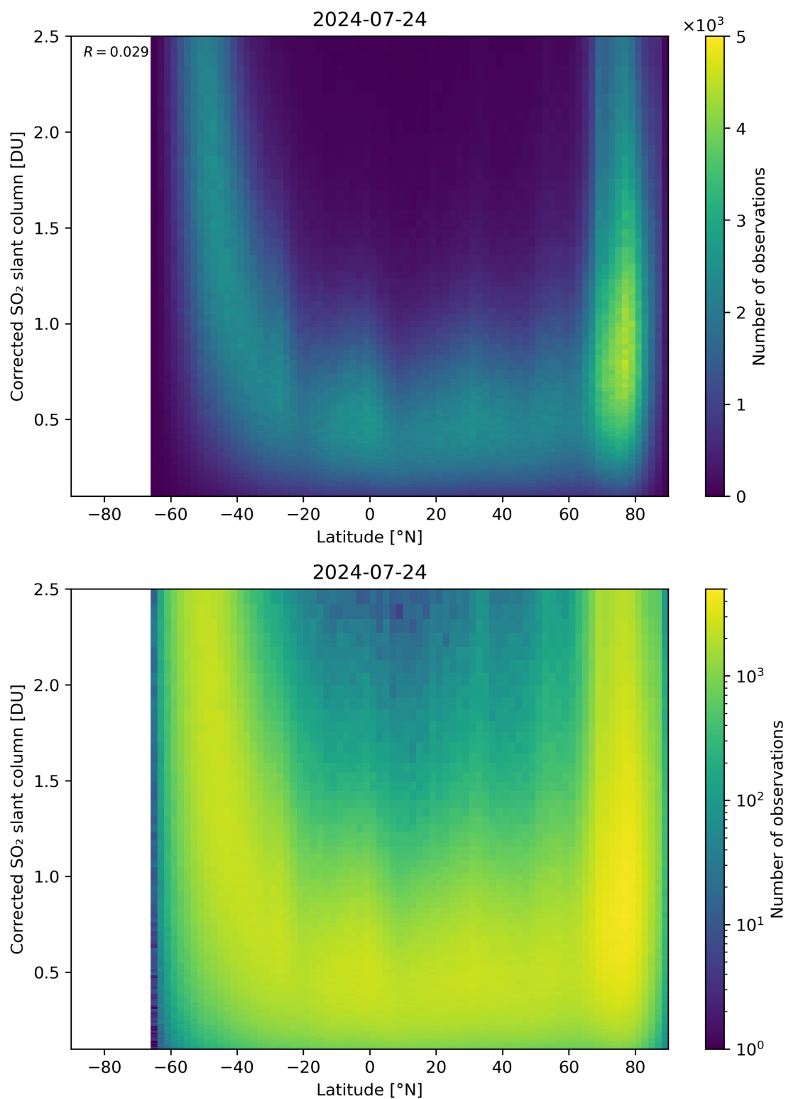
Figure 146: Scatter density plot of “Latitude” against “Corrected SO 2 slant column” for 2024-07-23 to 2024-07-25.
