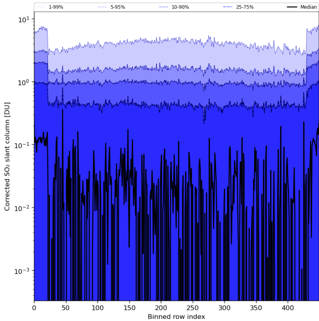
Figure 78: Along track statistics of “Corrected SO 2 slant column” for 2024-07-23 to 2024-07-25
