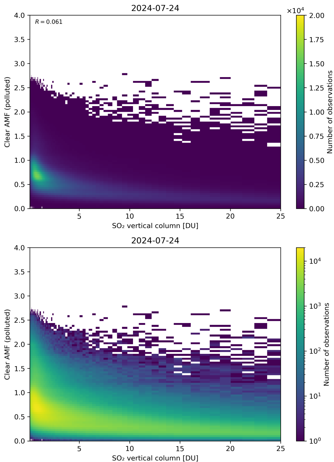
Figure 296: Scatter density plot of “SO 2 vertical column” against “Clear AMF (polluted)” for 2024-07-23 to 2024-07-25.
