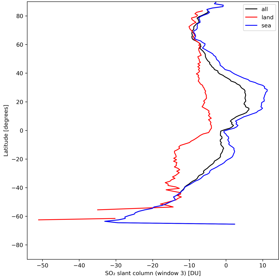
Figure 41: Zonal average of “SO 2 slant column (window 3)” for 2024-07-23 to 2024-07-25.
