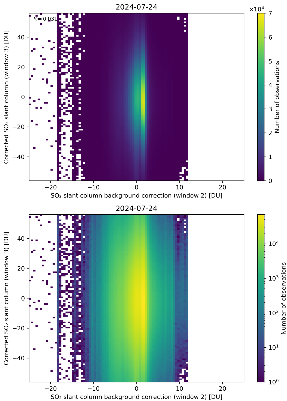
Figure 116: Scatter density plot of “SO 2 slant column background correction (window 2)” against “Corrected SO 2 slant column (window 3)” for 2024-07-23 to 2024-07-25.
