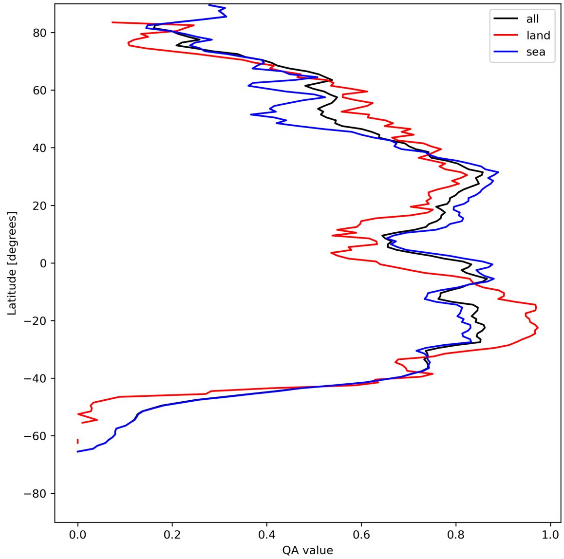
Figure 29: Zonal average of “QA value” for 2024-07-23 to 2024-07-25.
