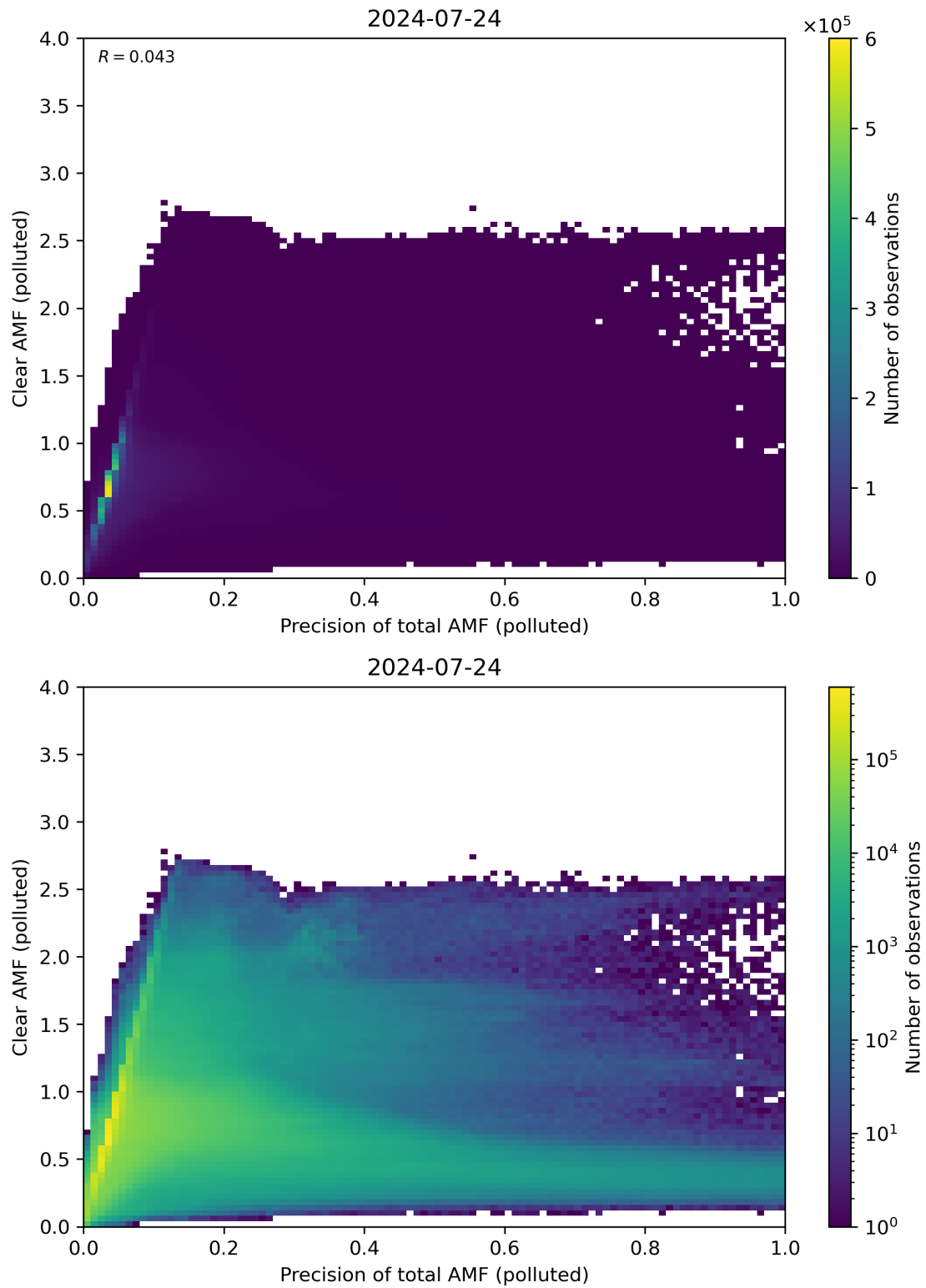
Figure 270: Scatter density plot of “Precision of total AMF (polluted)” against “Clear AMF (polluted)” for 2024-07-23 to 2024-07-25.
