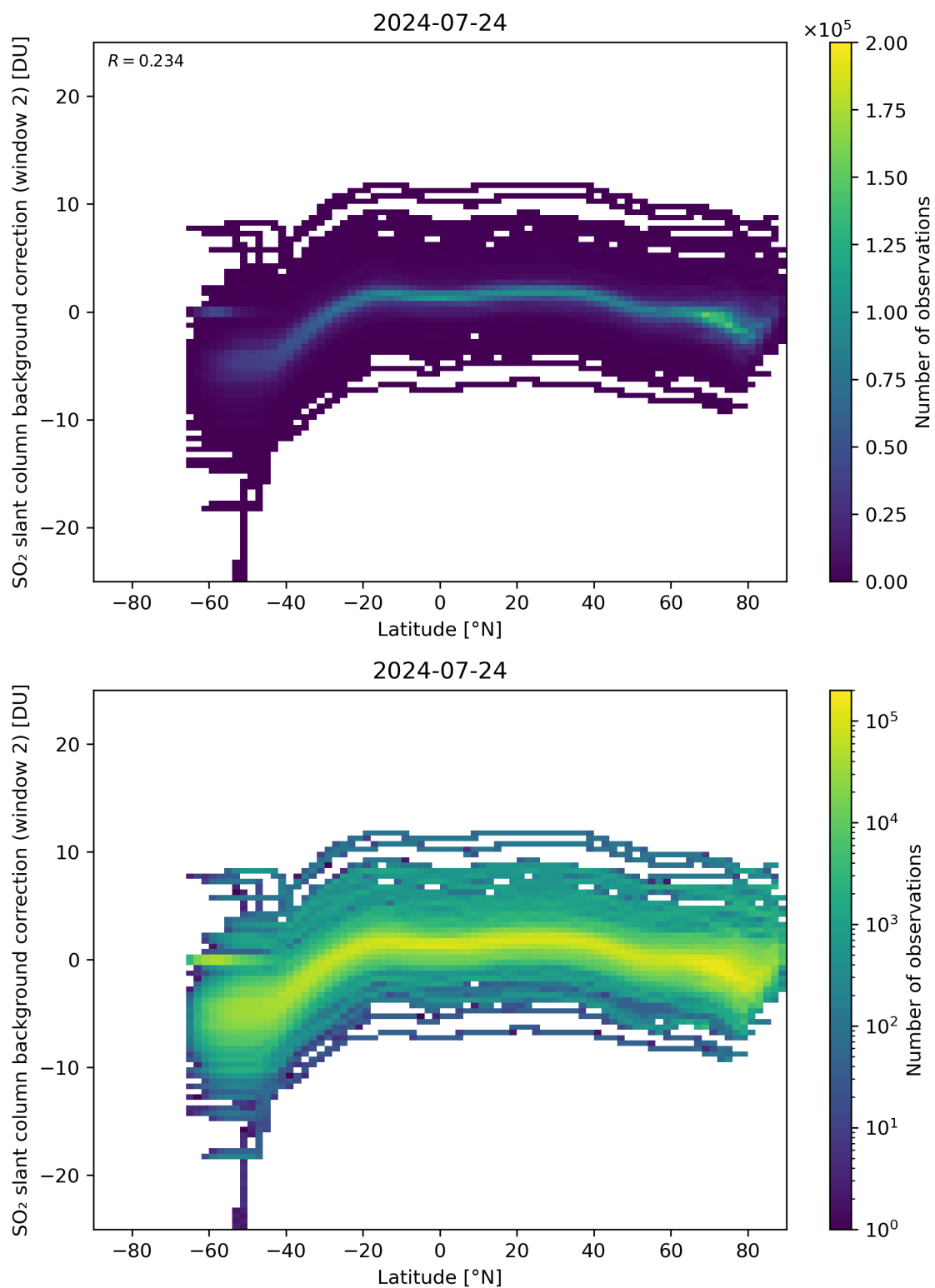
Figure 140: Scatter density plot of “Latitude” against “SO 2 slant column background correction (window 2)” for 2024-07-23 to 2024-07-25.
