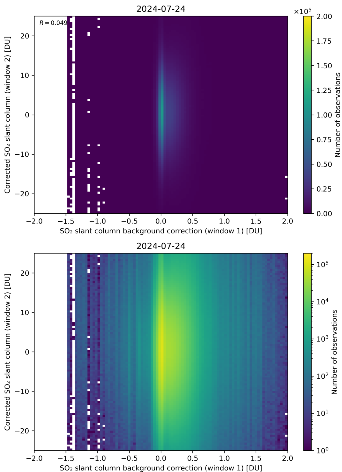
Figure 104: Scatter density plot of “SO 2 slant column background correction (window 1)” against “Corrected SO 2 slant column (window 2)” for 2024-07-23 to 2024-07-25.
