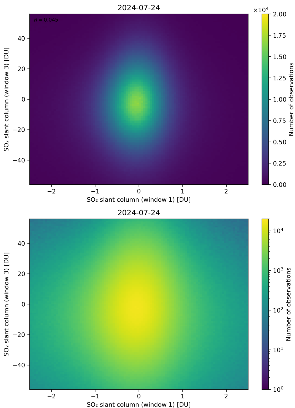
Figure 237: Scatter density plot of “SO 2 slant column (window 1)” against “SO 2 slant column (window 3)” for 2024-07-23 to 2024-07-25.
