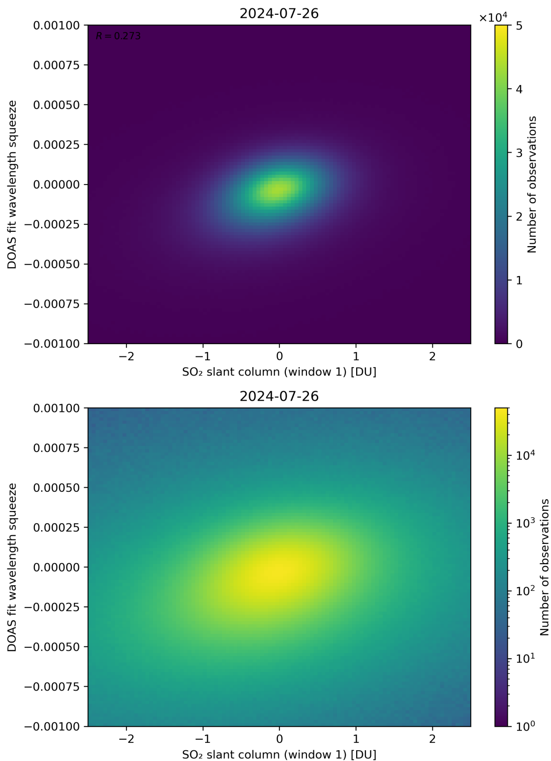
Figure 216: Scatter density plot of “SO 2 slant column (window 1)” against “DOAS fit wavelength squeeze” for 2024-07-26 to 2024-07-27.
