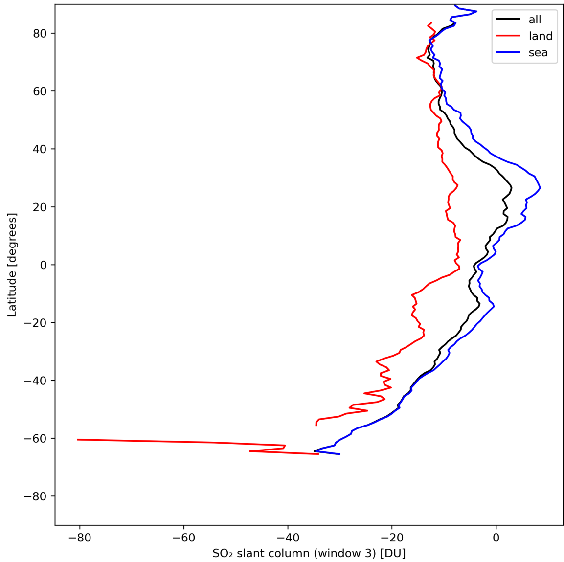
Figure 41: Zonal average of “SO 2 slant column (window 3)” for 2024-07-26 to 2024-07-27.
