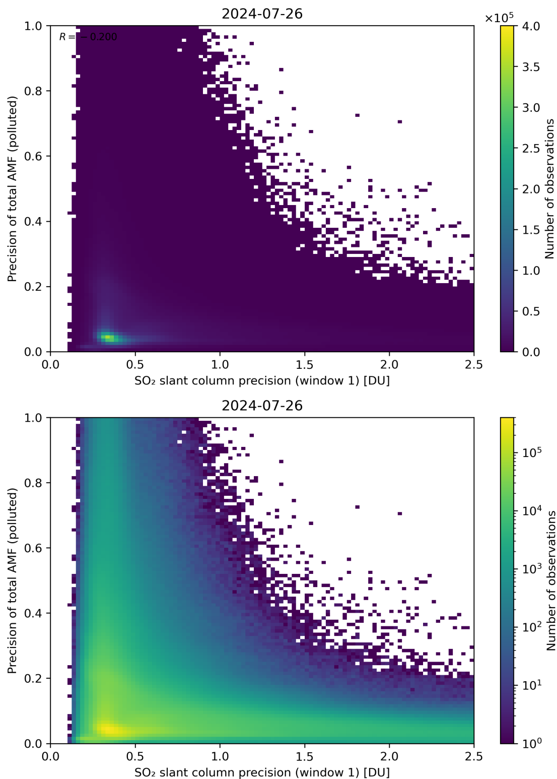
Figure 231: Scatter density plot of “SO 2 slant column precision (window 1)” against “Precision of total AMF (polluted)” for 2024-07-26 to 2024-07-27.
