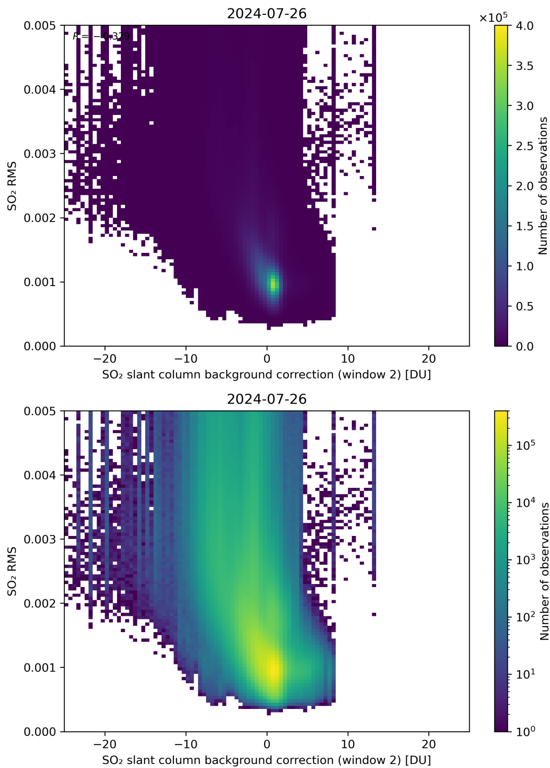
Figure 114: Scatter density plot of “SO 2 slant column background correction (window 2)” against “SO 2 RMS” for 2024-07-26 to 2024-07-27.
