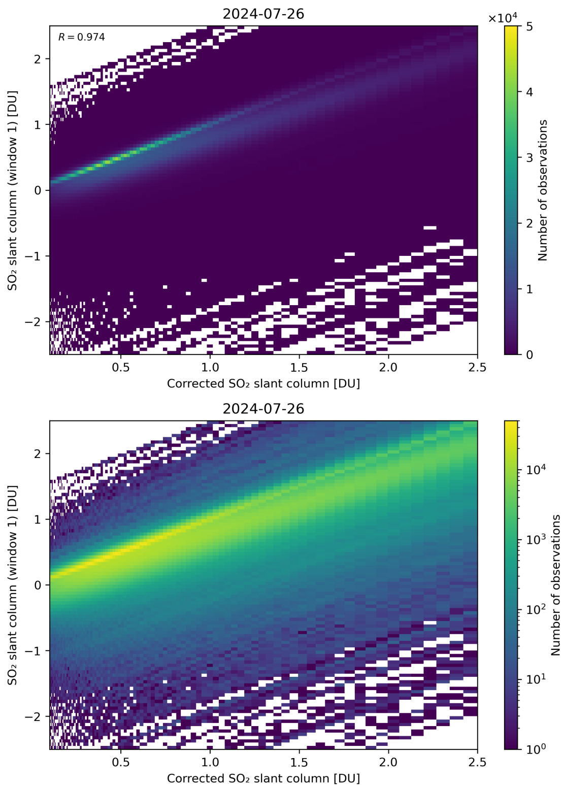
Figure 187: Scatter density plot of “Corrected SO 2 slant column” against “SO 2 slant column (window 1)” for 2024-07-26 to 2024-07-27.
