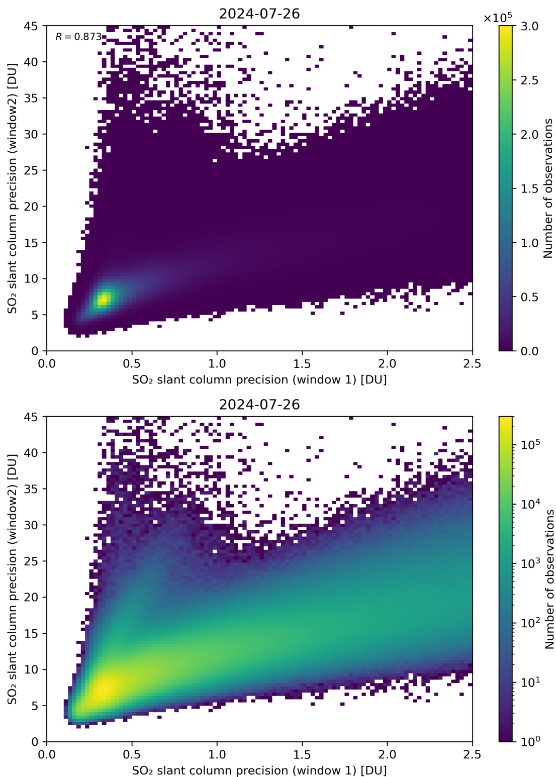
Figure 227: Scatter density plot of “SO 2 slant column precision (window 1)” against “SO 2 slant column precision (window2)” for 2024-07-26 to 2024-07-27.
