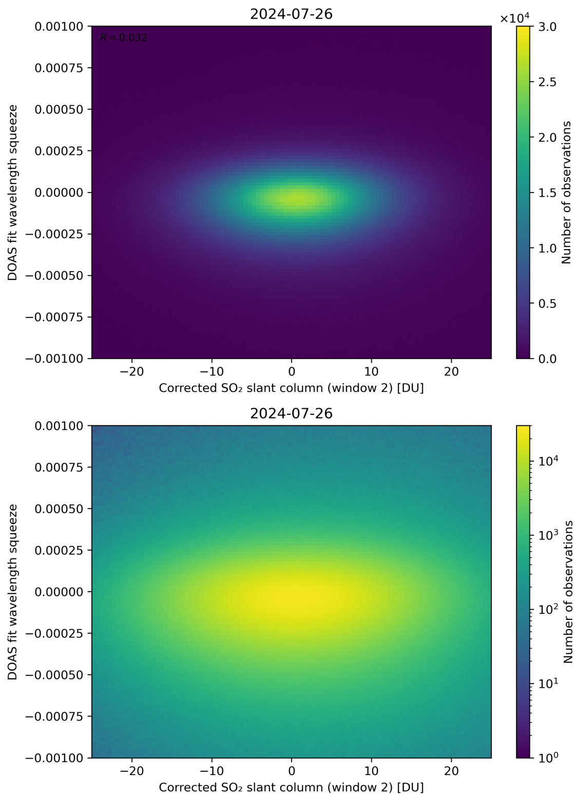
Figure 197: Scatter density plot of “Corrected SO 2 slant column (window 2)” against “DOAS fit wavelength squeeze” for 2024-07-26 to 2024-07-27.
