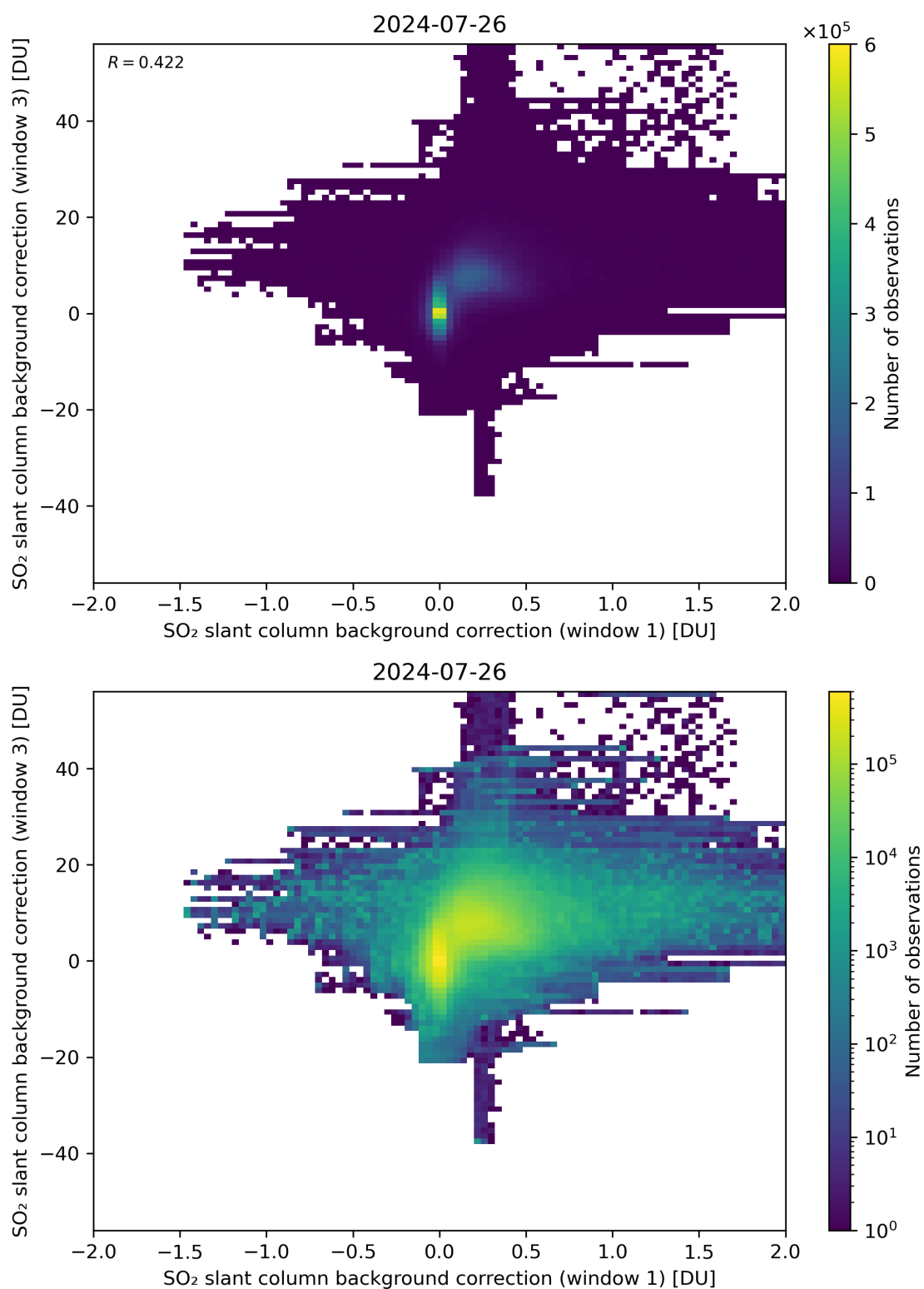
Figure 99: Scatter density plot of “SO 2 slant column background correction (window 1)” against “SO 2 slant column background correction (window 3)” for 2024-07-26 to 2024-07-27.
