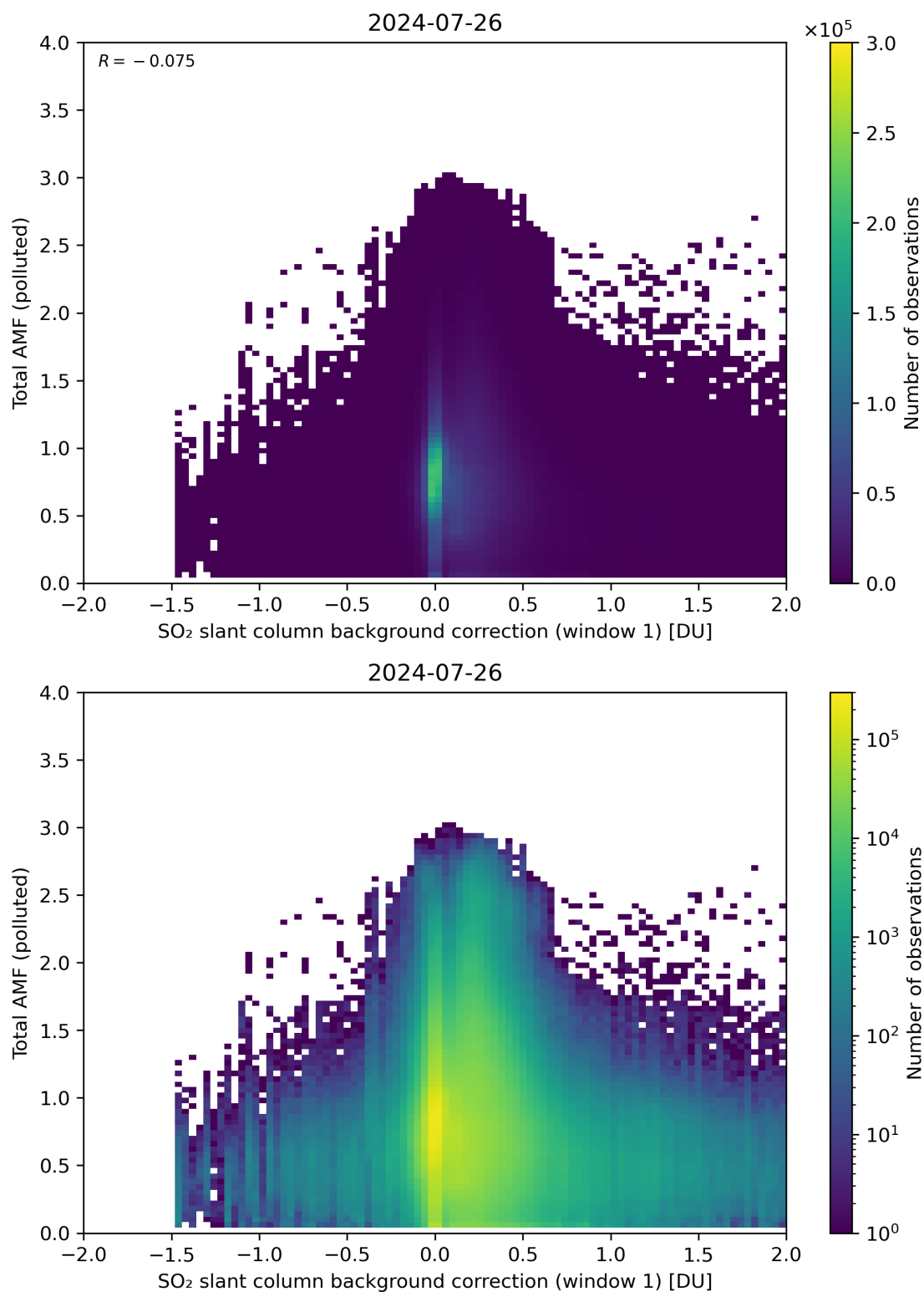
Figure 109: Scatter density plot of “SO 2 slant column background correction (window 1)” against “Total AMF (polluted)” for 2024-07-26 to 2024-07-27.
