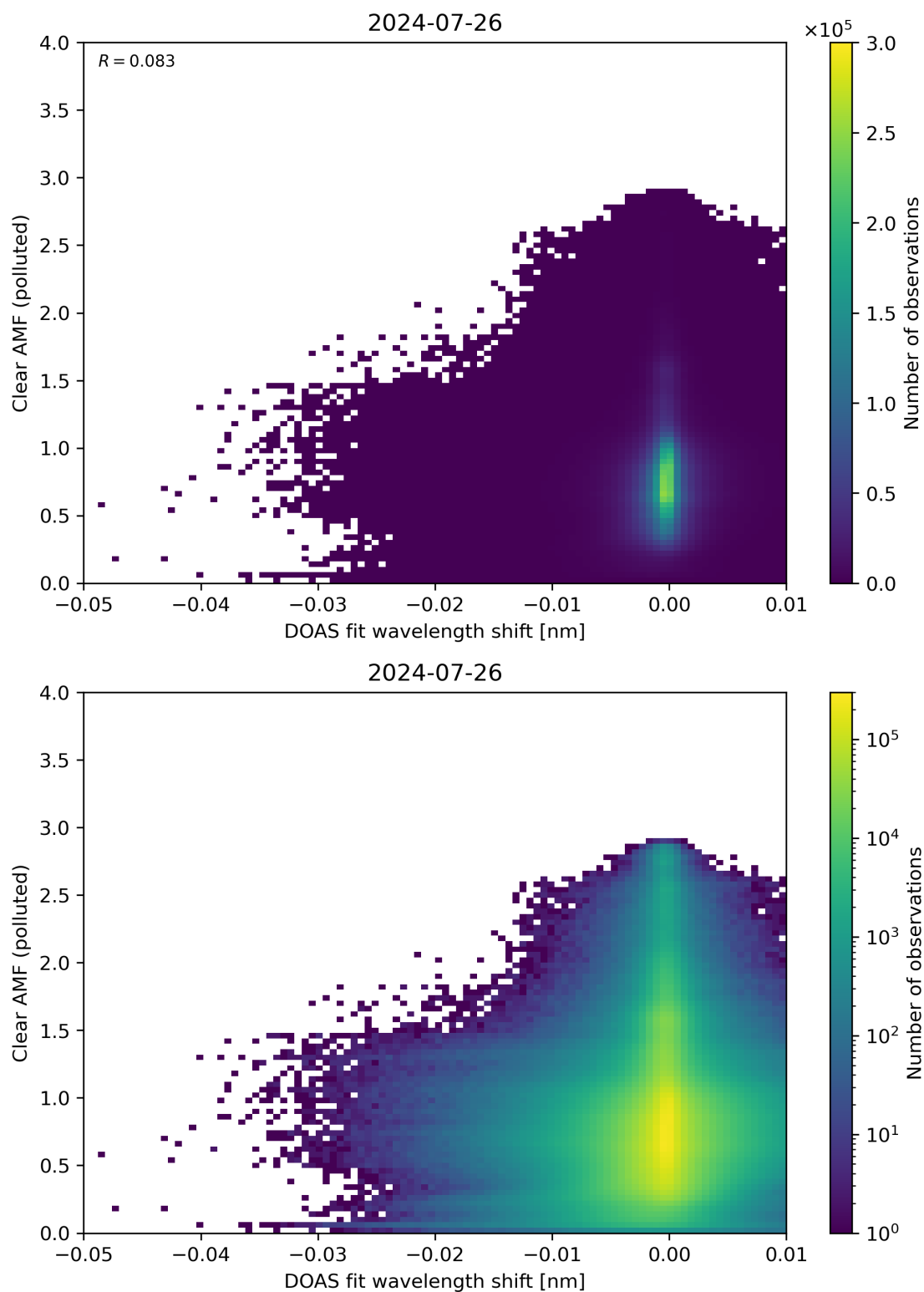
Figure 129: Scatter density plot of “DOAS fit wavelength shift” against “Clear AMF (polluted)” for 2024-07-26 to 2024-07-27.
