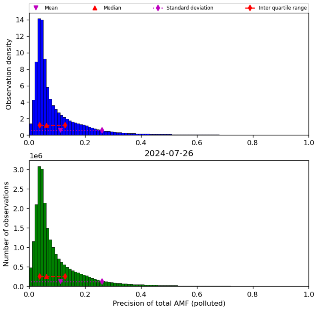
Figure 72: Histogram of “Precision of total AMF (polluted)” for 2024-07-26 to 2024-07-27
