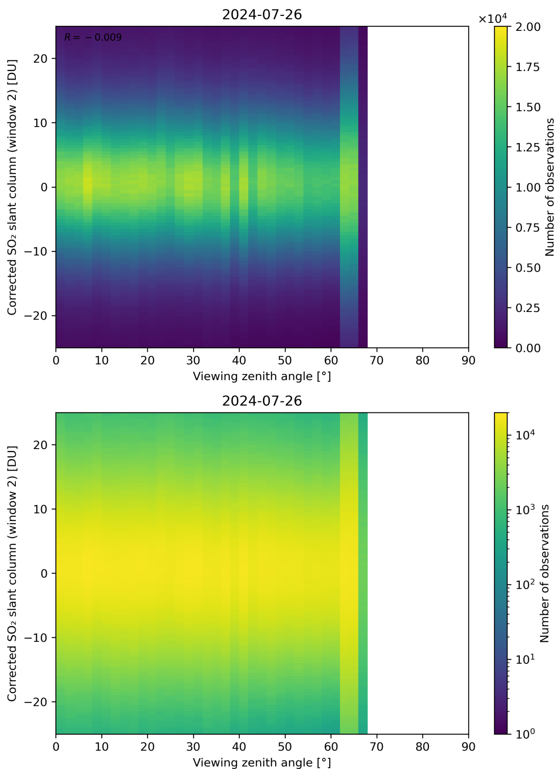
Figure 318: Scatter density plot of “Viewing zenith angle” against “Corrected SO 2 slant column (window 2)” for 2024-07-26 to 2024-07-27.
