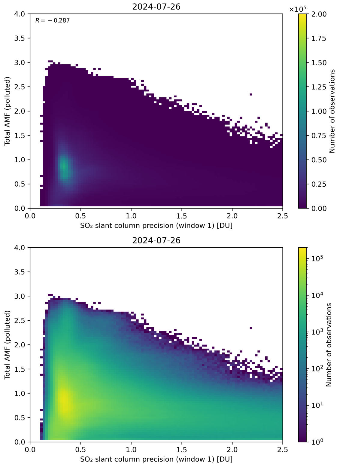
Figure 230: Scatter density plot of “SO 2 slant column precision (window 1)” against “Total AMF (polluted)” for 2024-07-26 to 2024-07-27.
