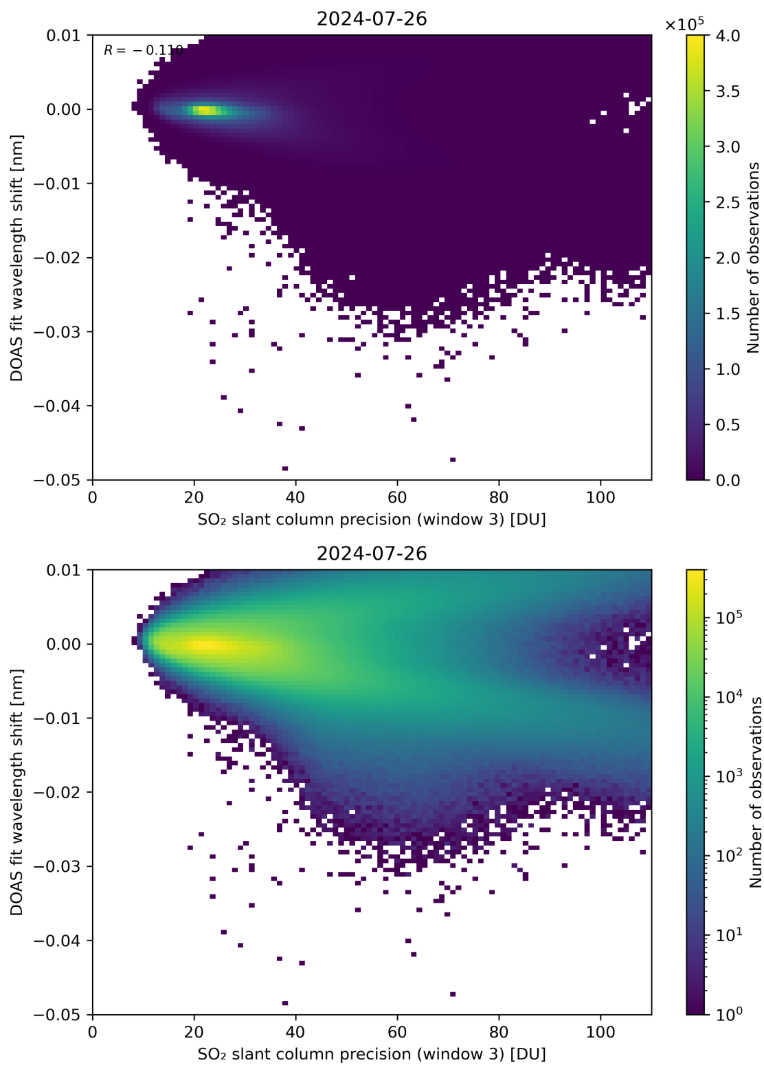
Figure 258: Scatter density plot of “SO 2 slant column precision (window 3)” against “DOAS fit wavelength shift” for 2024-07-26 to 2024-07-27.
