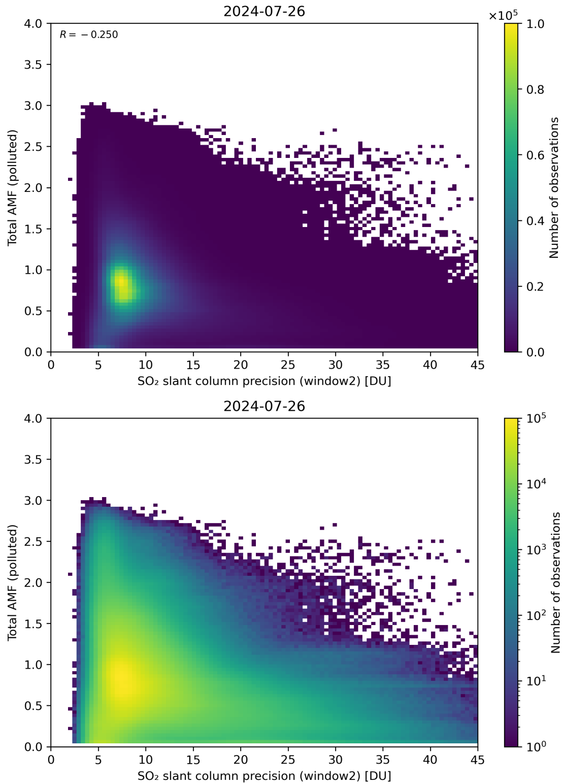
Figure 251: Scatter density plot of “SO 2 slant column precision (window2)” against “Total AMF (polluted)” for 2024-07-26 to 2024-07-27.
