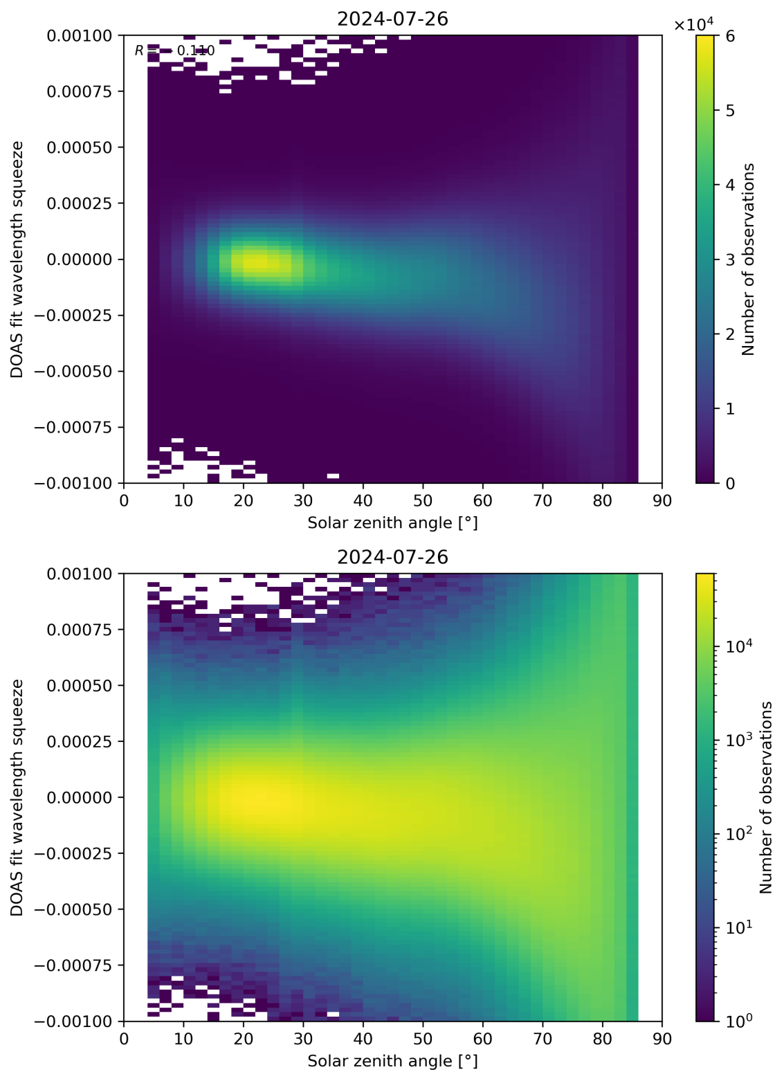
Figure 162: Scatter density plot of “Solar zenith angle” against “DOAS fit wavelength squeeze” for 2024-07-26 to 2024-07-27.
