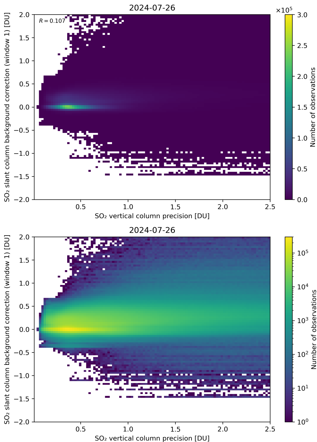
Figure 279: Scatter density plot of “SO 2 vertical column precision” against “SO 2 slant column background correction (window 1)” for 2024-07-26 to 2024-07-27.
