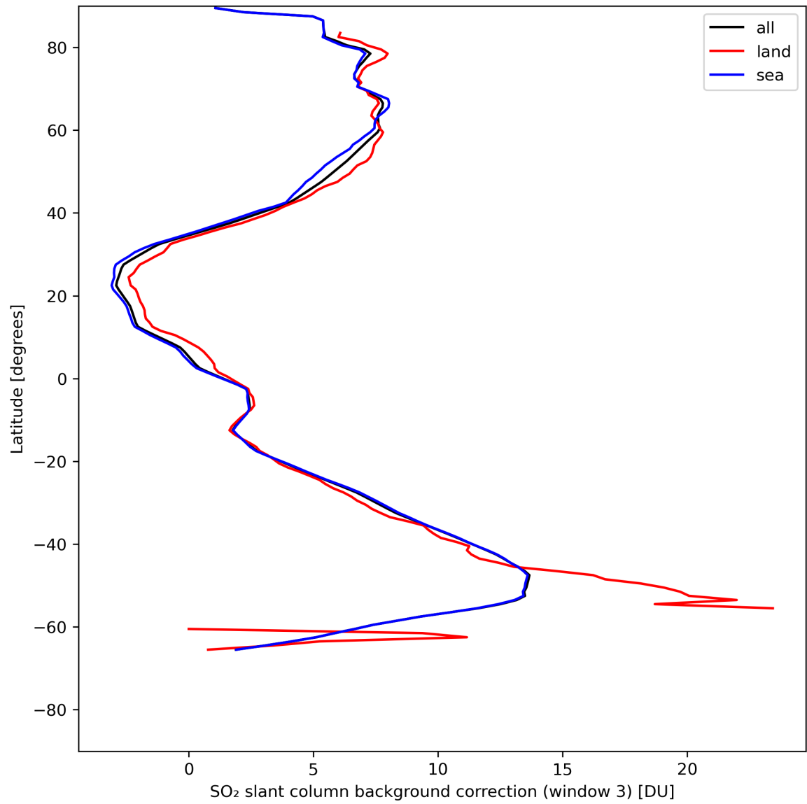
Figure 44: Zonal average of “SO 2 slant column background correction (window 3)” for 2024-07-26 to 2024-07-27.
