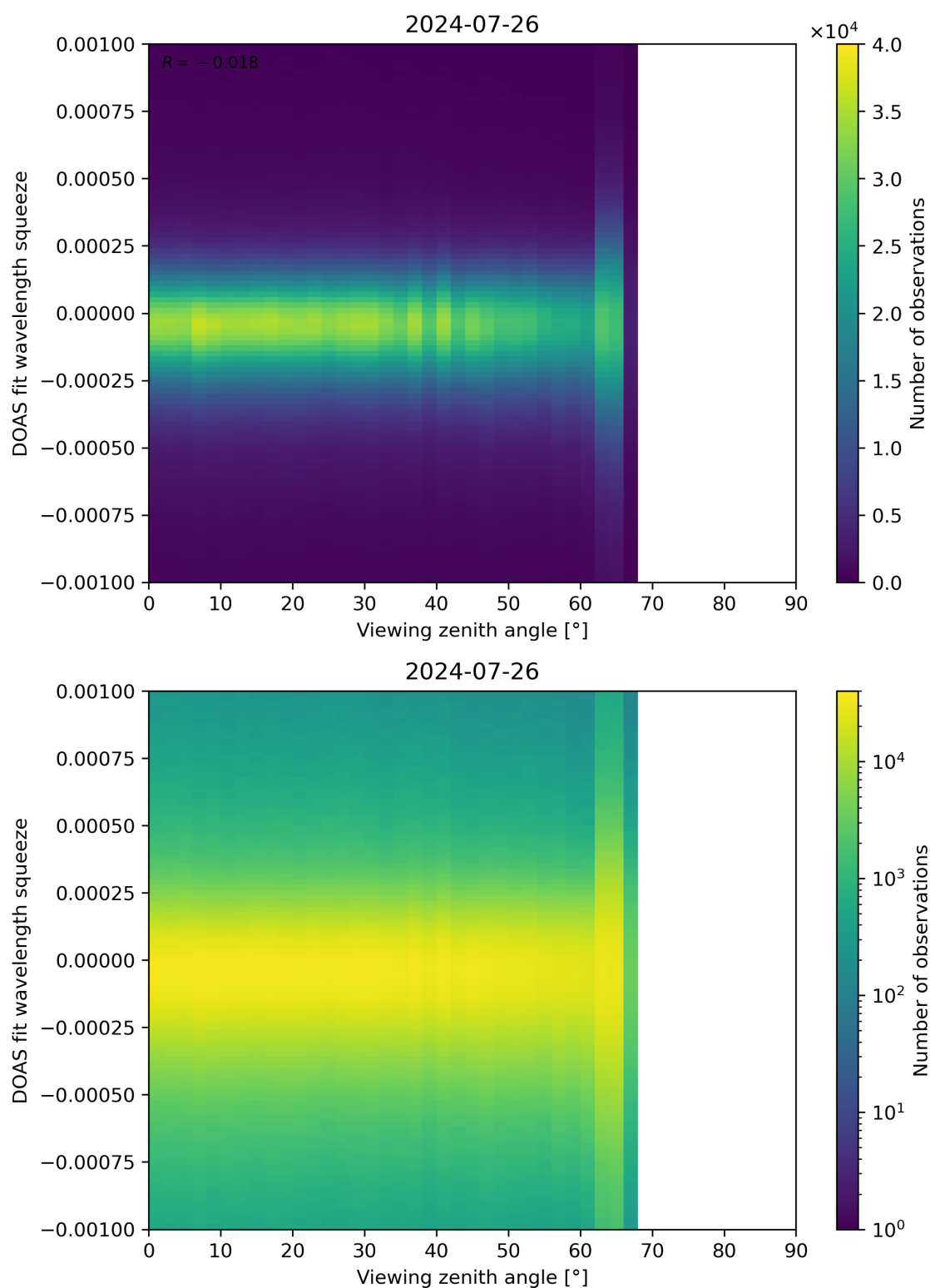
Figure 312: Scatter density plot of “Viewing zenith angle” against “DOAS fit wavelength squeeze” for 2024-07-26 to 2024-07-27.
