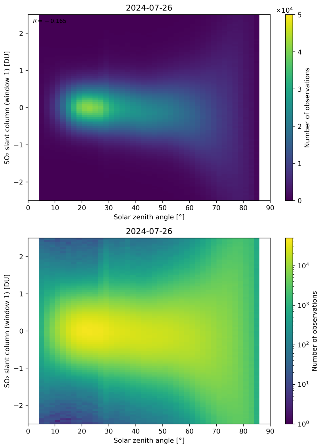
Figure 169: Scatter density plot of “Solar zenith angle” against “SO 2 slant column (window 1)” for 2024-07-26 to 2024-07-27.
