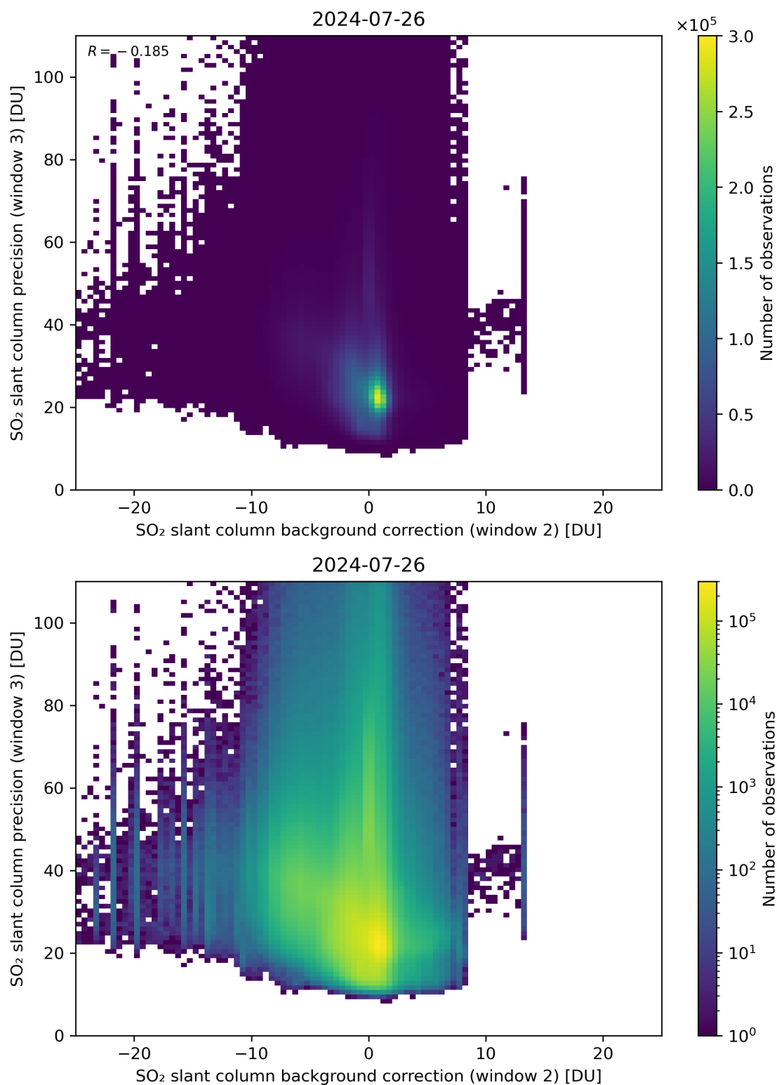
Figure 118: Scatter density plot of “SO 2 slant column background correction (window 2)” against “SO 2 slant column precision (window 3)” for 2024-07-26 to 2024-07-27.
