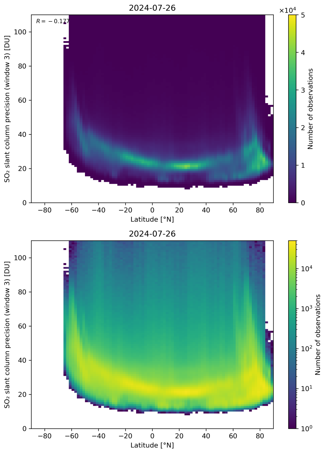
Figure 153: Scatter density plot of “Latitude” against “SO 2 slant column precision (window 3)” for 2024-07-26 to 2024-07-27.
