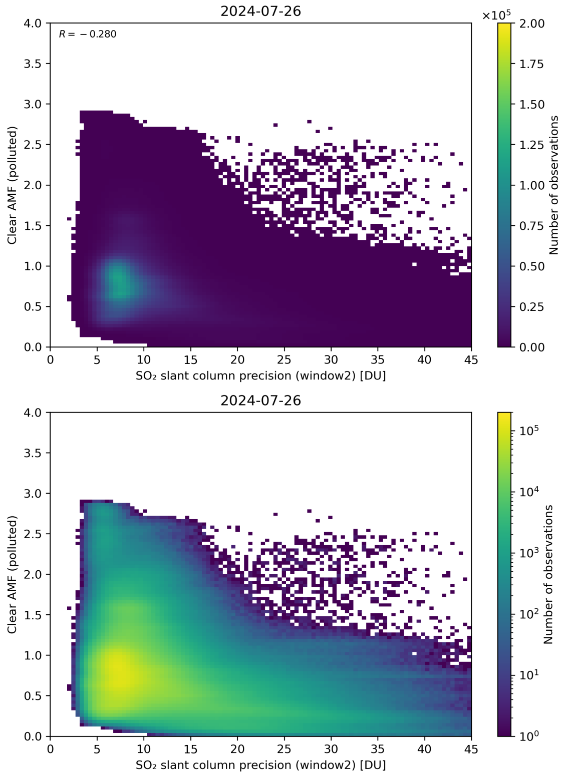
Figure 246: Scatter density plot of “SO 2 slant column precision (window2)” against “Clear AMF (polluted)” for 2024-07-26 to 2024-07-27.
