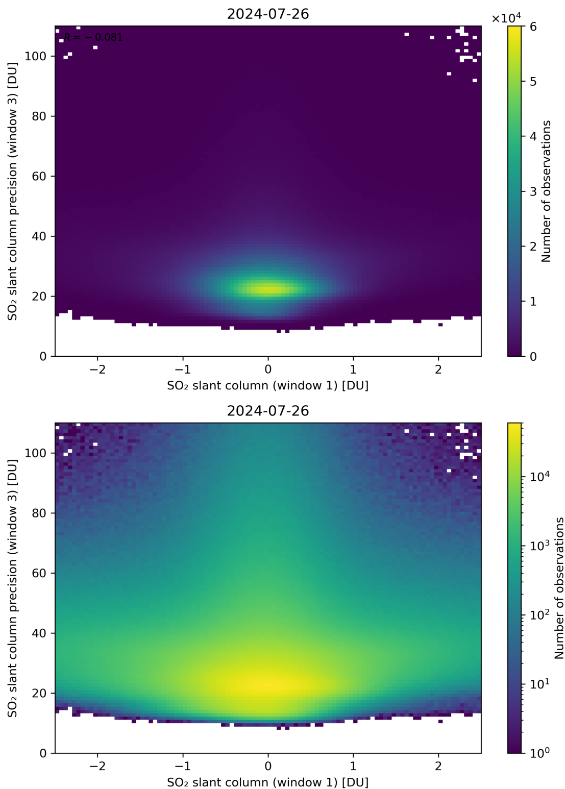
Figure 238: Scatter density plot of “SO 2 slant column (window 1)” against “SO 2 slant column precision (window 3)” for 2024-07-26 to 2024-07-27.
