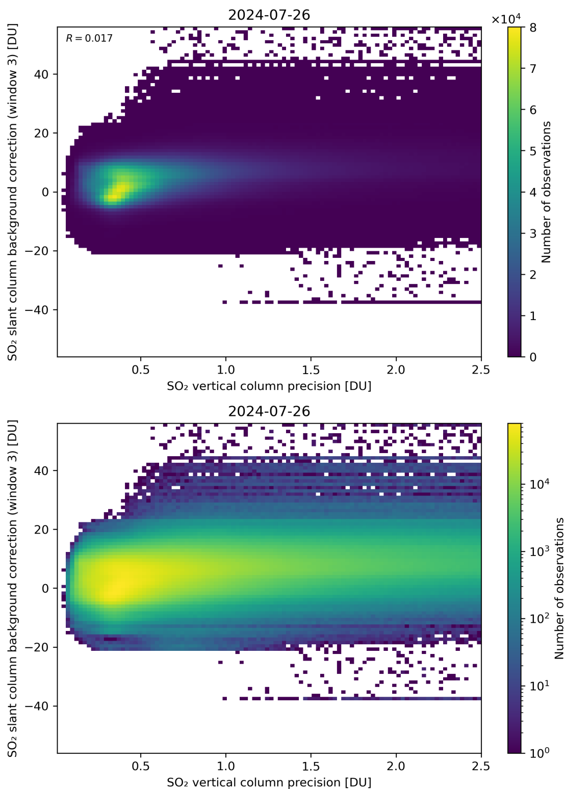
Figure 281: Scatter density plot of “SO 2 vertical column precision” against “SO 2 slant column background correction (window 3)” for 2024-07-26 to 2024-07-27.
