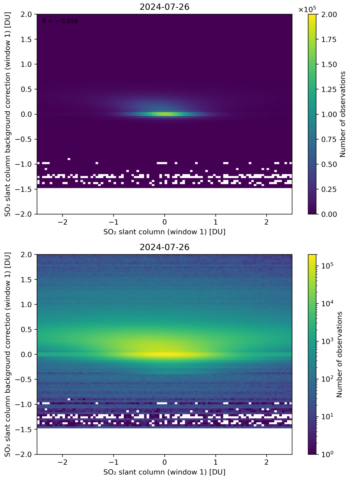
Figure 212: Scatter density plot of “SO 2 slant column (window 1)” against “SO 2 slant column background correction (window 1)” for 2024-07-26 to 2024-07-27.
