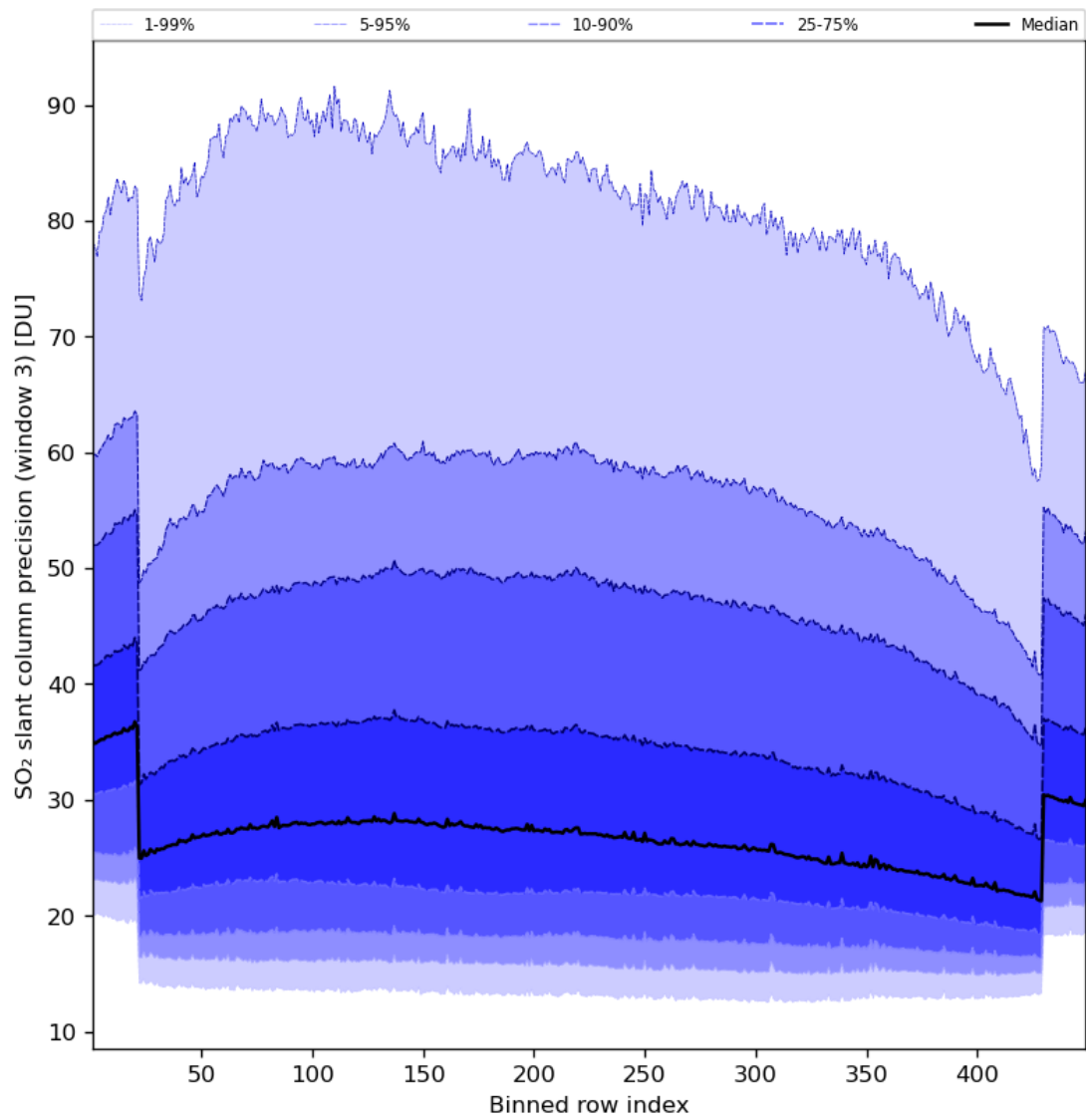
Figure 88: Along track statistics of “SO 2 slant column precision (window 3)” for 2024-07-26 to 2024-07-27
