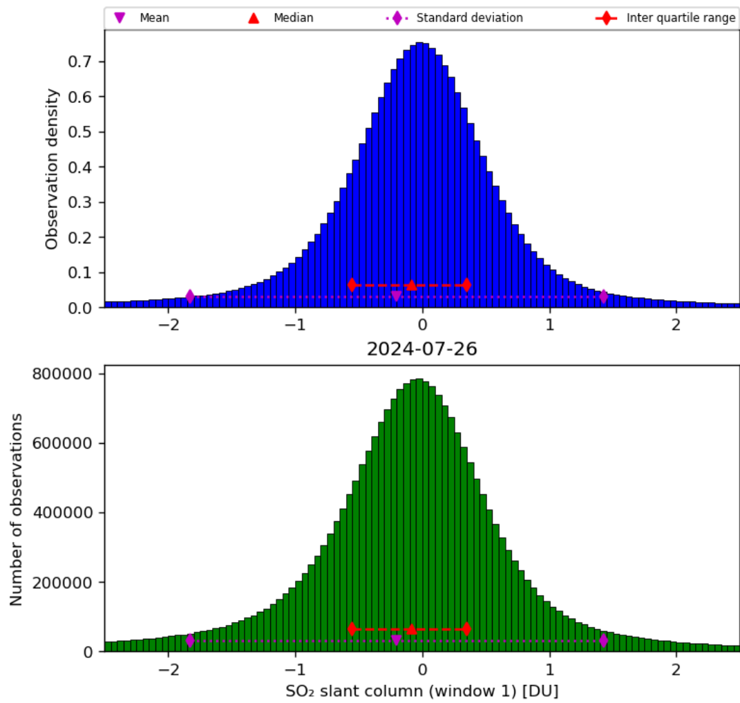
Figure 56: Histogram of “SO 2 slant column (window 1)” for 2024-07-26 to 2024-07-27
