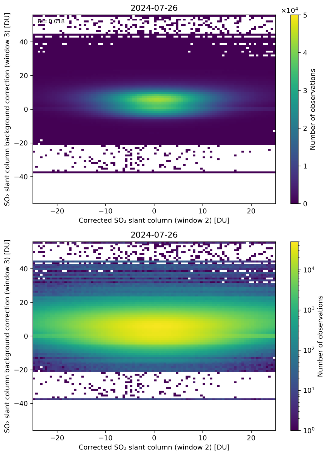
Figure 195: Scatter density plot of “Corrected SO 2 slant column (window 2)” against “SO 2 slant column background correction (window 3)” for 2024-07-26 to 2024-07-27.
