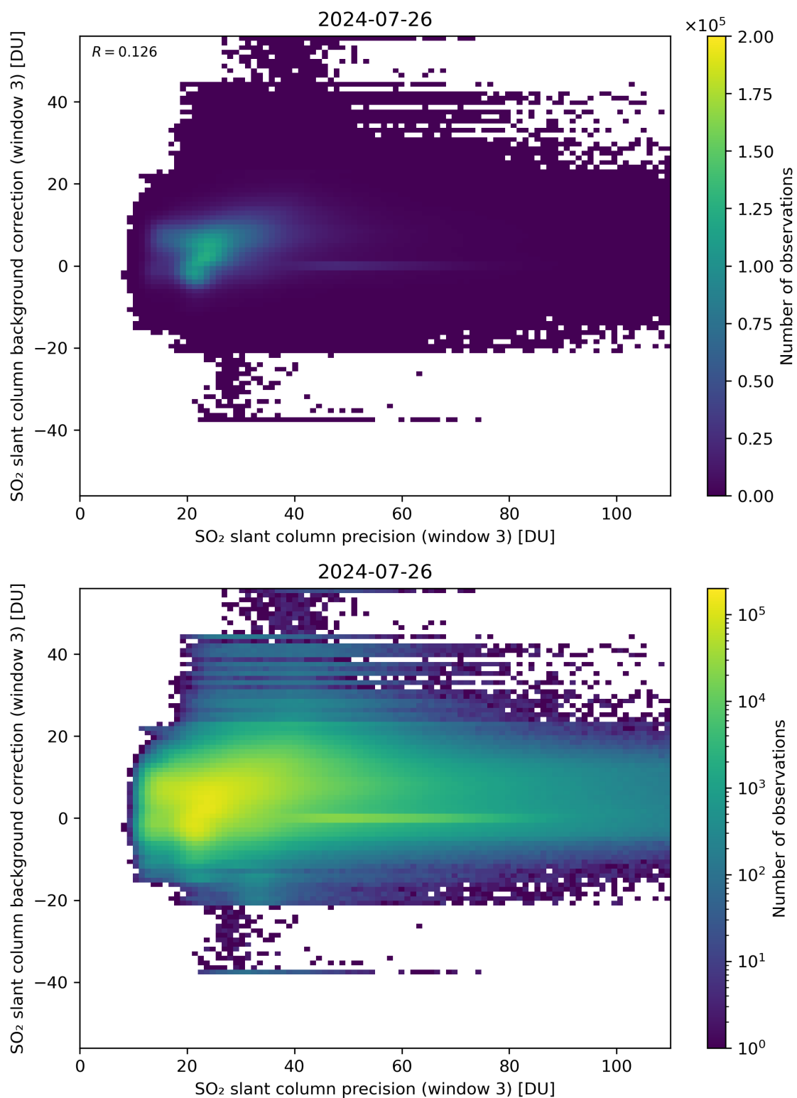
Figure 257: Scatter density plot of “SO 2 slant column precision (window 3)” against “SO 2 slant column background correction (window 3)” for 2024-07-26 to 2024-07-27.
