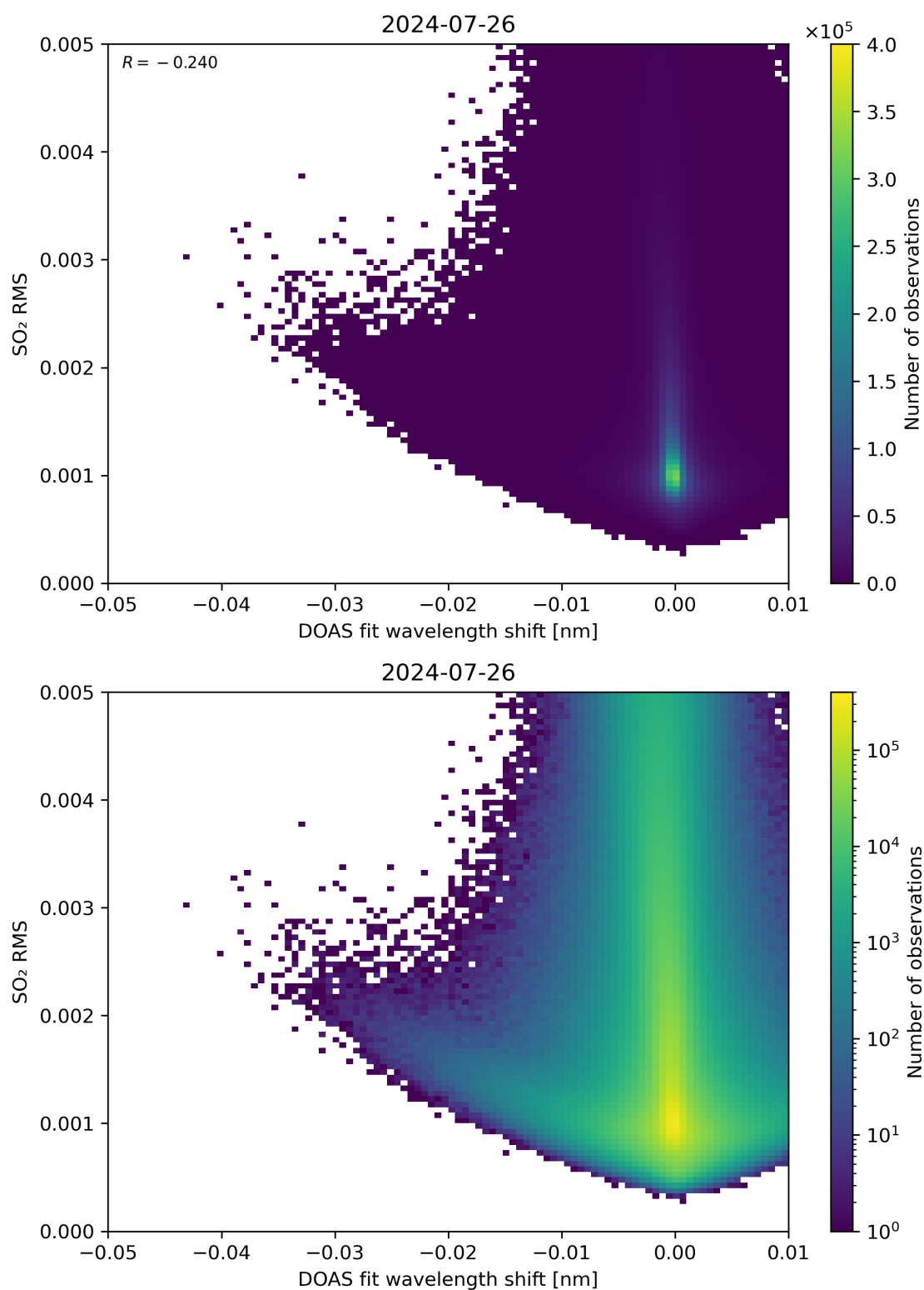
Figure 128: Scatter density plot of “DOAS fit wavelength shift” against “SO 2 RMS” for 2024-07-26 to 2024-07-27.
