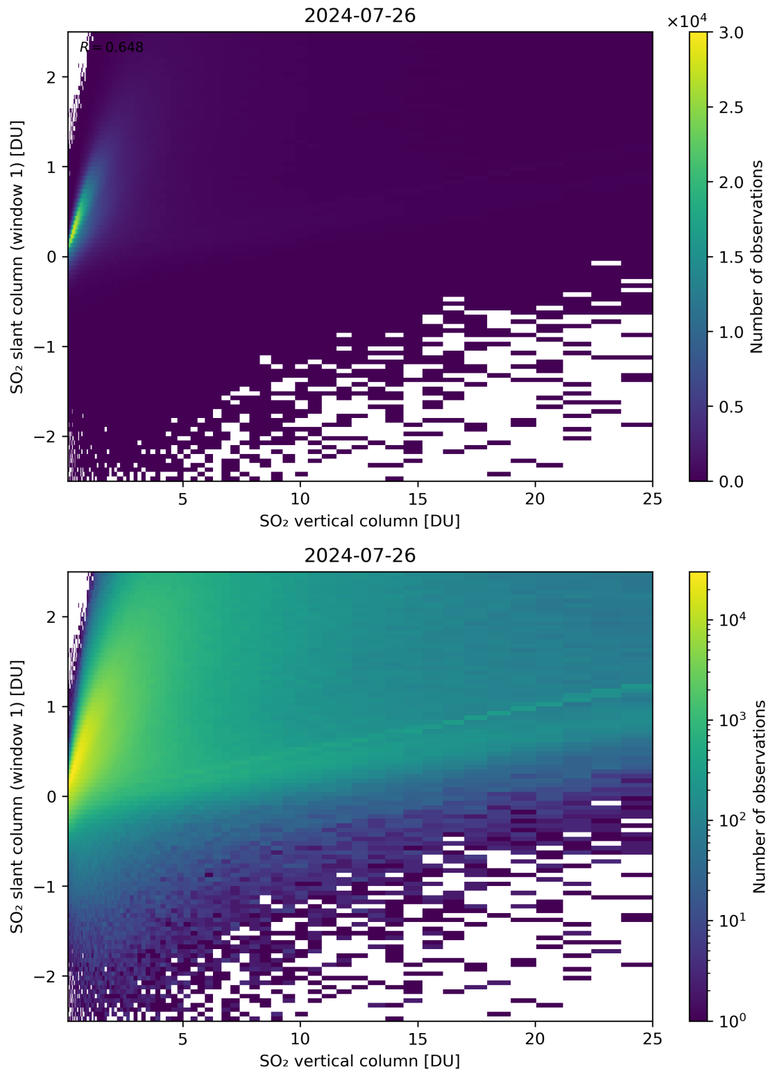
Figure 300: Scatter density plot of “SO 2 vertical column” against “SO 2 slant column (window 1)” for 2024-07-26 to 2024-07-27.
