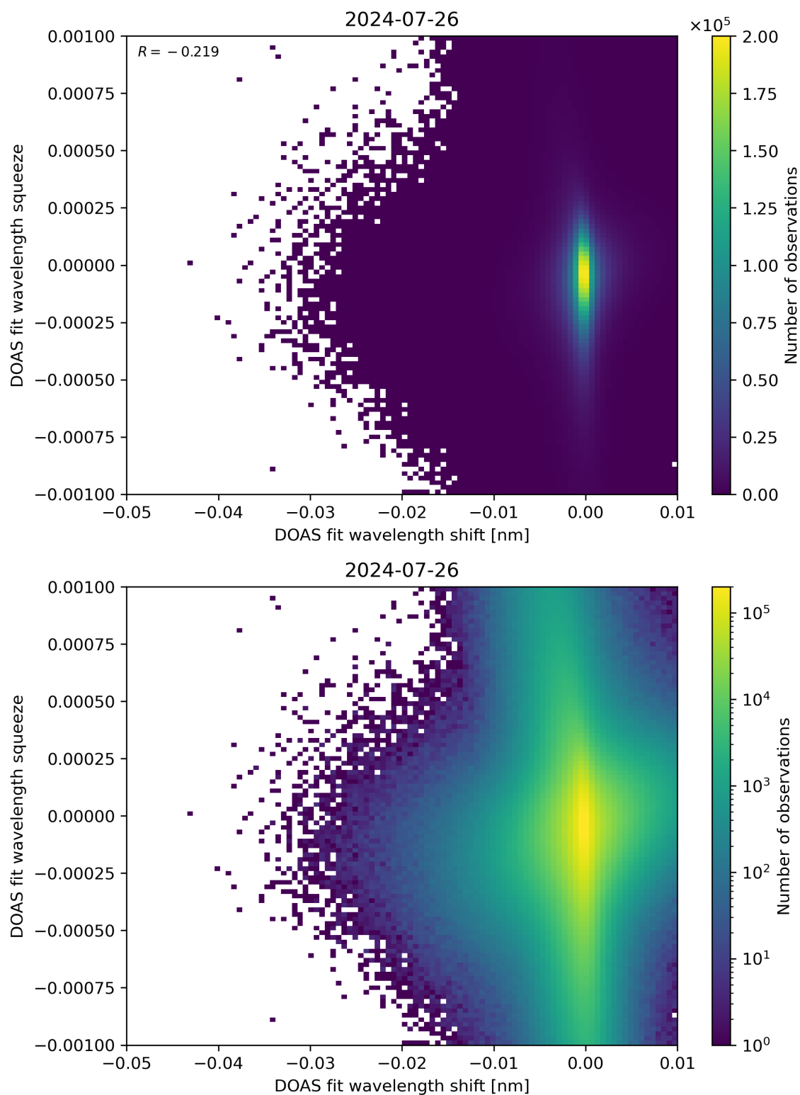
Figure 127: Scatter density plot of “DOAS fit wavelength shift” against “DOAS fit wavelength squeeze” for 2024-07-26 to 2024-07-27.
