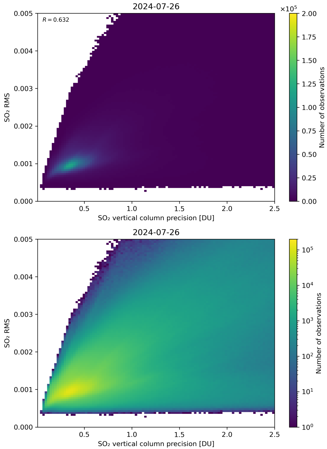
Figure 284: Scatter density plot of “SO 2 vertical column precision” against “SO 2 RMS” for 2024-07-26 to 2024-07-27.
