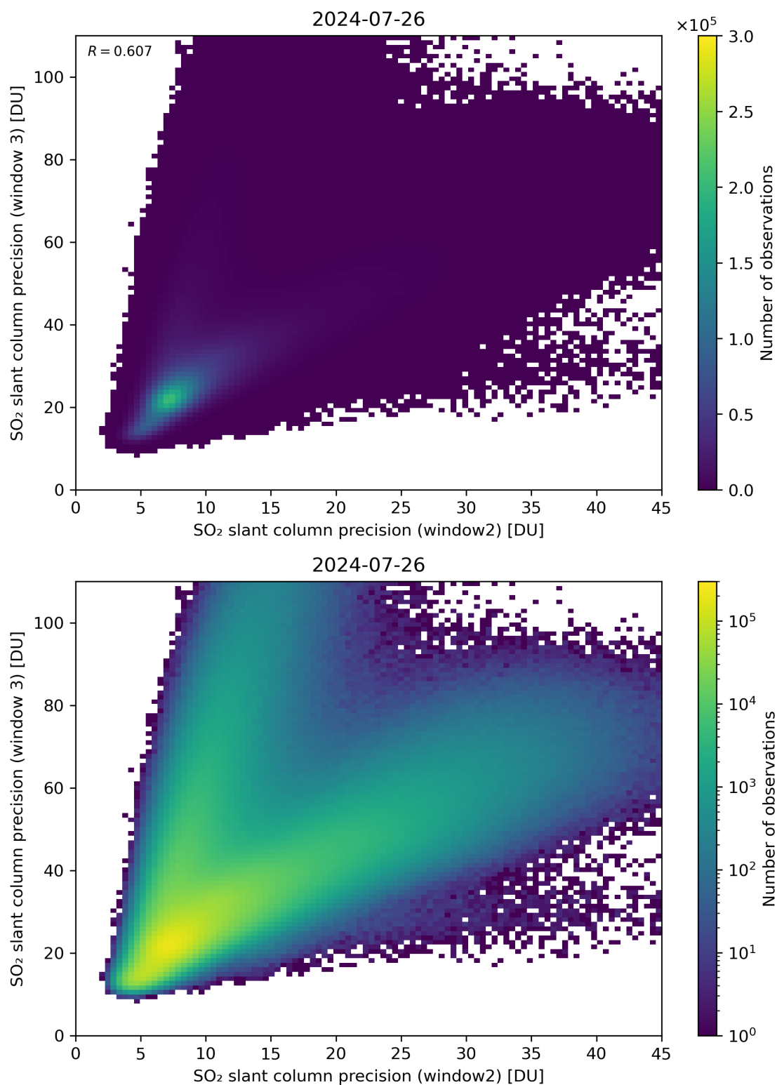
Figure 250: Scatter density plot of “SO 2 slant column precision (window2)” against “SO 2 slant column precision (window 3)” for 2024-07-26 to 2024-07-27.
