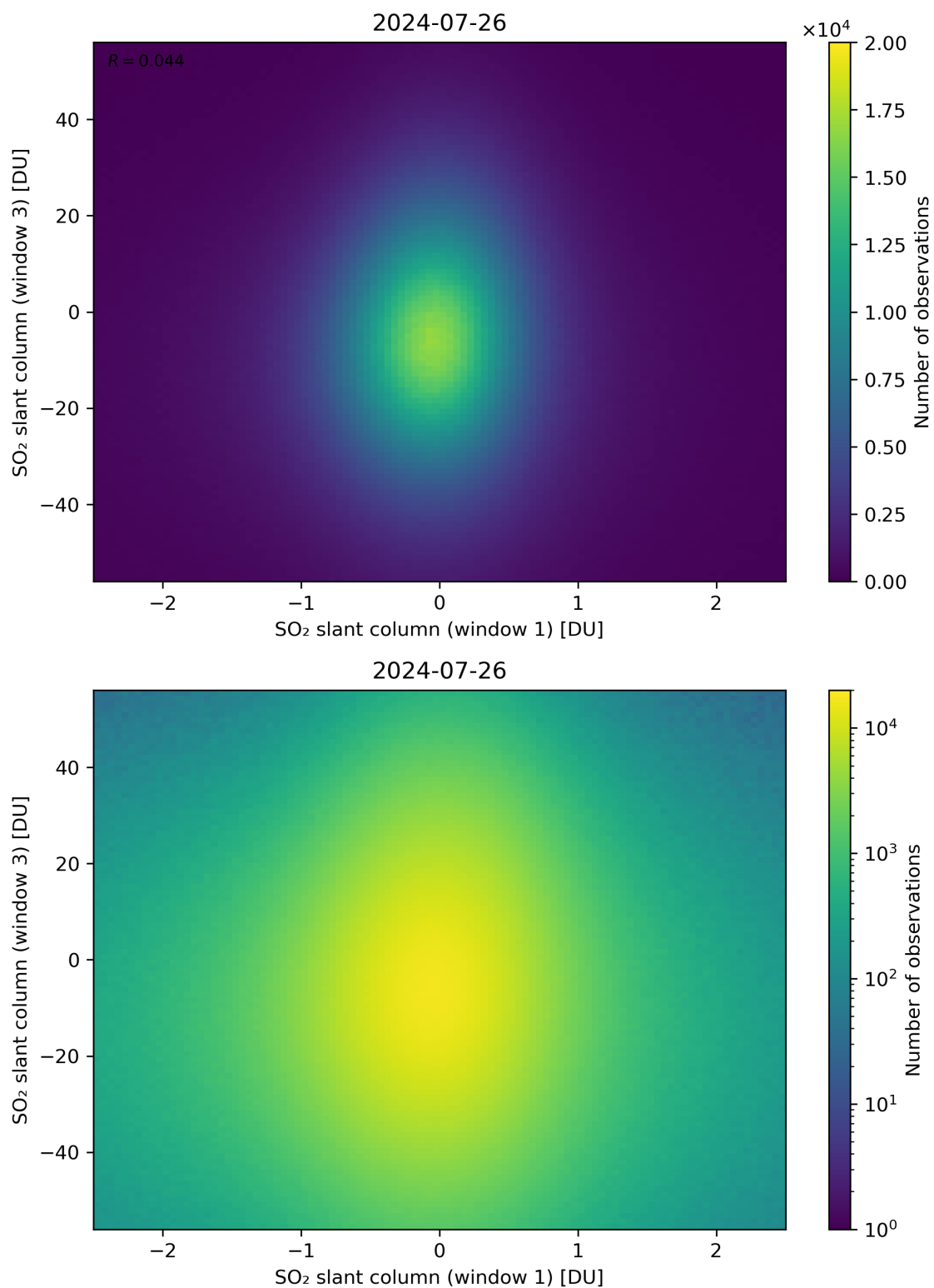
Figure 237: Scatter density plot of “SO 2 slant column (window 1)” against “SO 2 slant column (window 3)” for 2024-07-26 to 2024-07-27.
