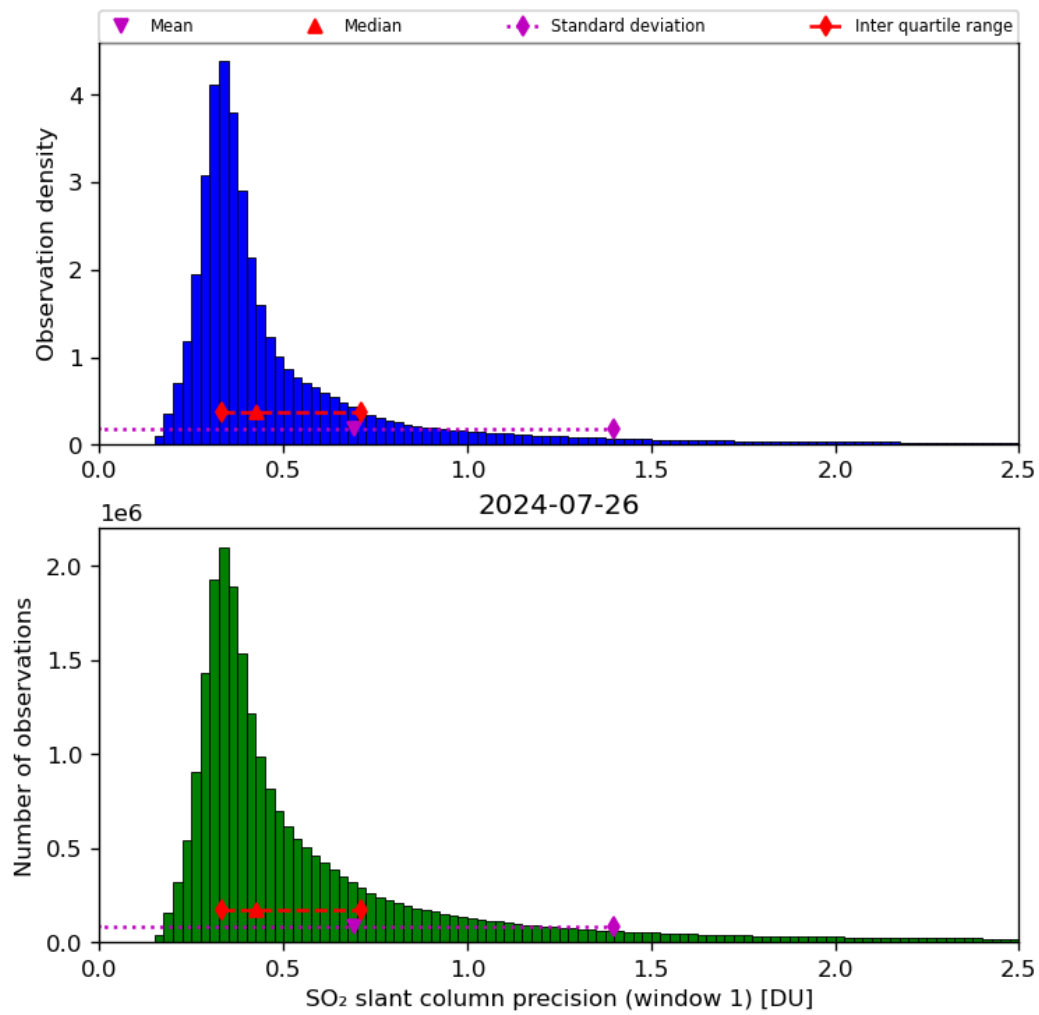
Figure 57: Histogram of “SO 2 slant column precision (window 1)” for 2024-07-26 to 2024-07-27
