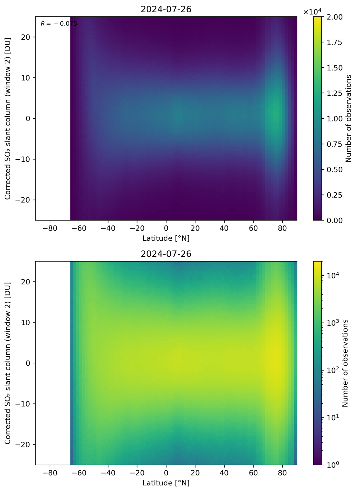
Figure 147: Scatter density plot of “Latitude” against “Corrected SO 2 slant column (window 2)” for 2024-07-26 to 2024-07-27.
