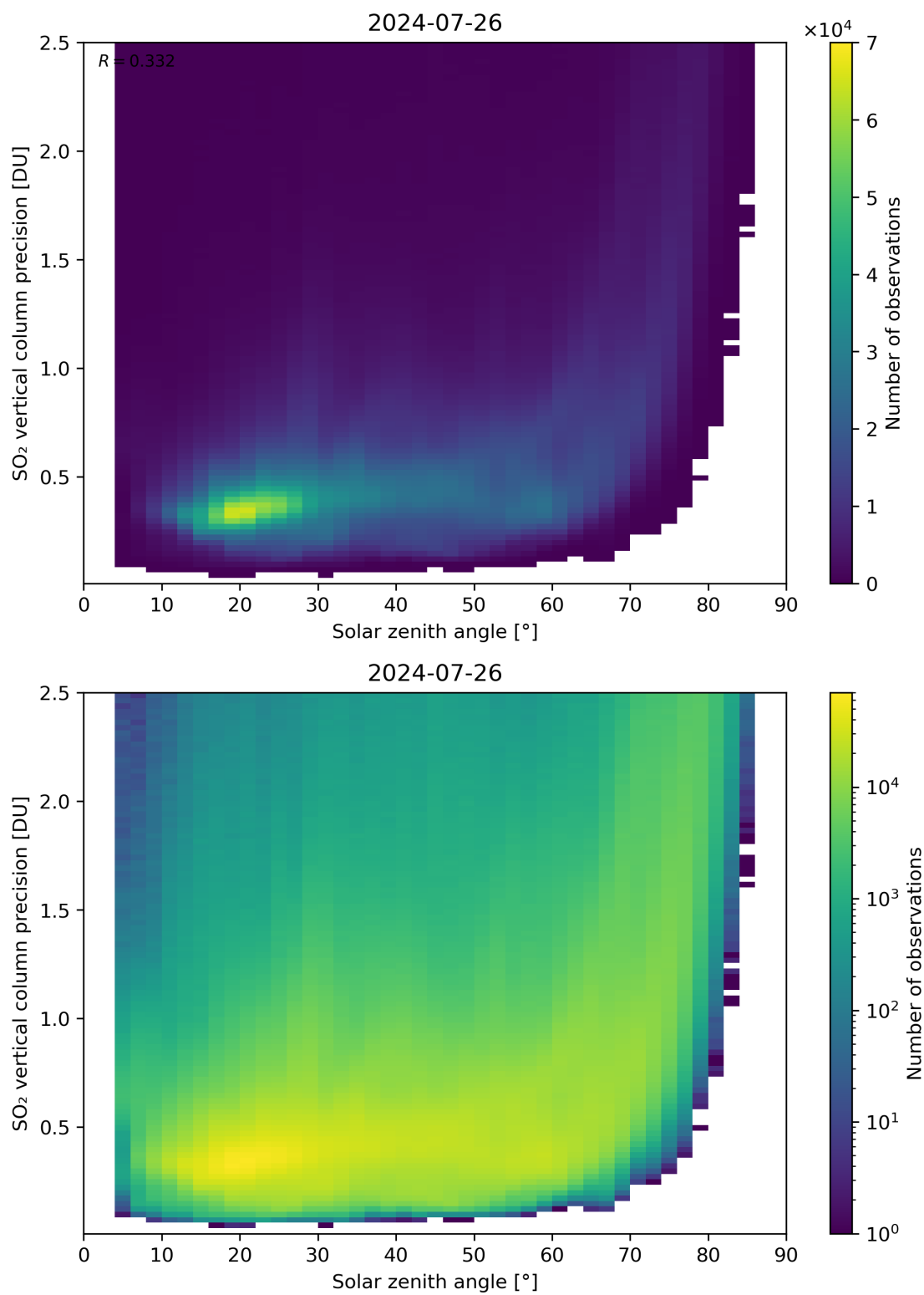
Figure 177: Scatter density plot of “Solar zenith angle” against “SO 2 vertical column precision” for 2024-07-26 to 2024-07-27.
