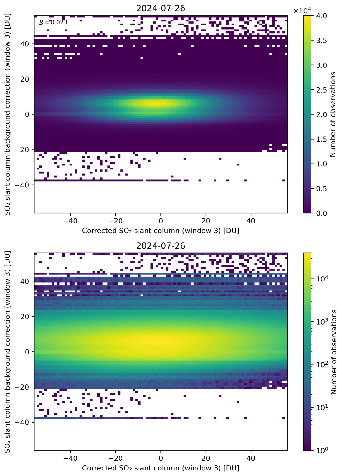
Figure 205: Scatter density plot of “Corrected SO 2 slant column (window 3)” against “SO 2 slant column background correction (window 3)” for 2024-07-26 to 2024-07-27.
