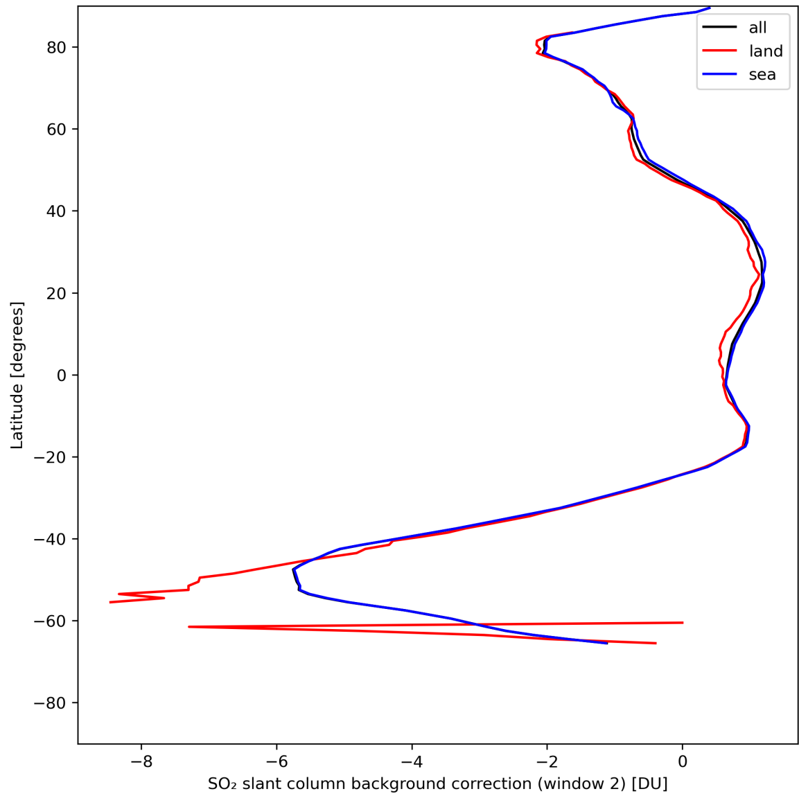
Figure 40: Zonal average of “SO 2 slant column background correction (window 2)” for 2024-07-26 to 2024-07-27.
