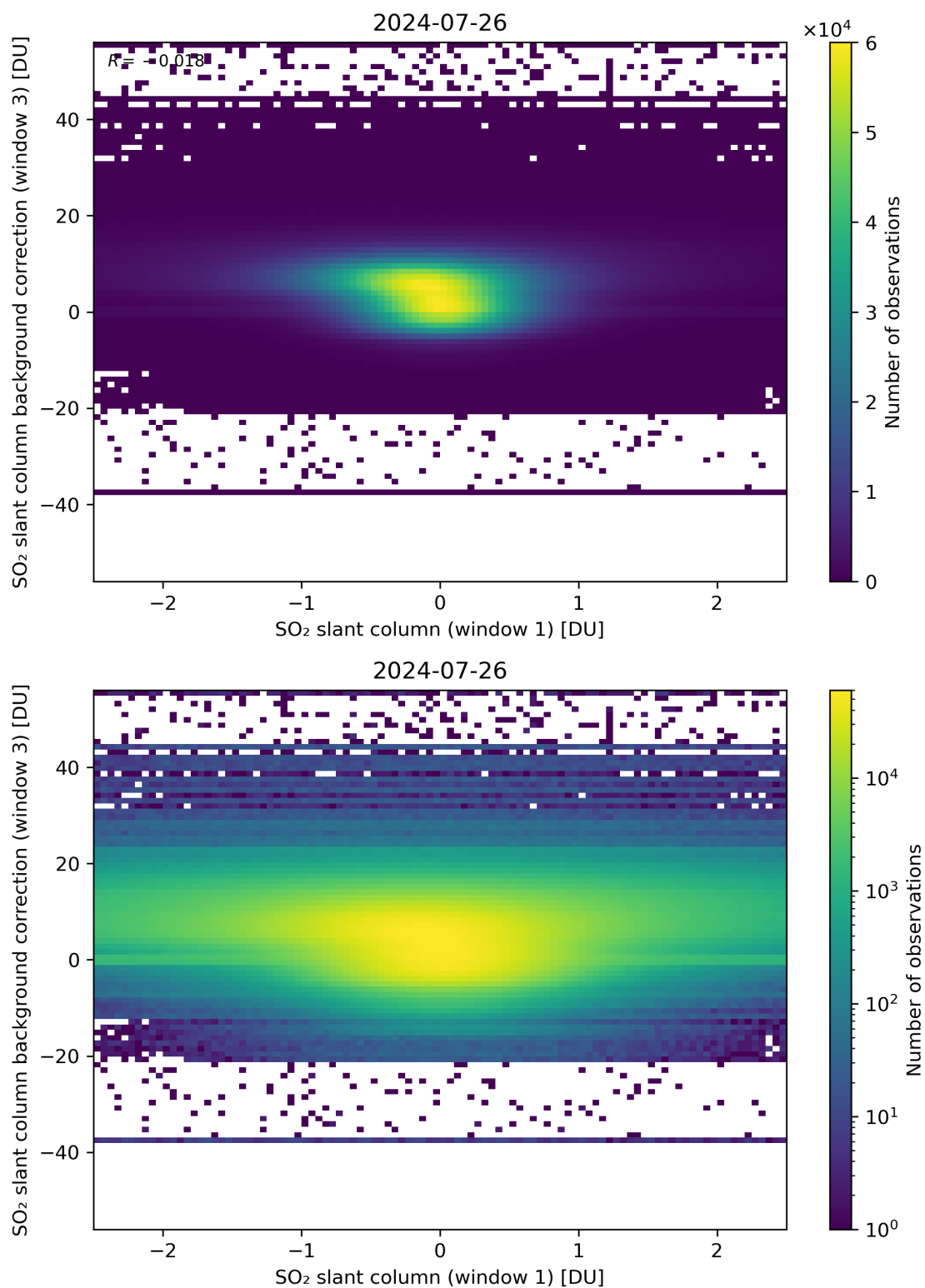
Figure 214: Scatter density plot of “SO 2 slant column (window 1)” against “SO 2 slant column background correction (window 3)” for 2024-07-26 to 2024-07-27.
