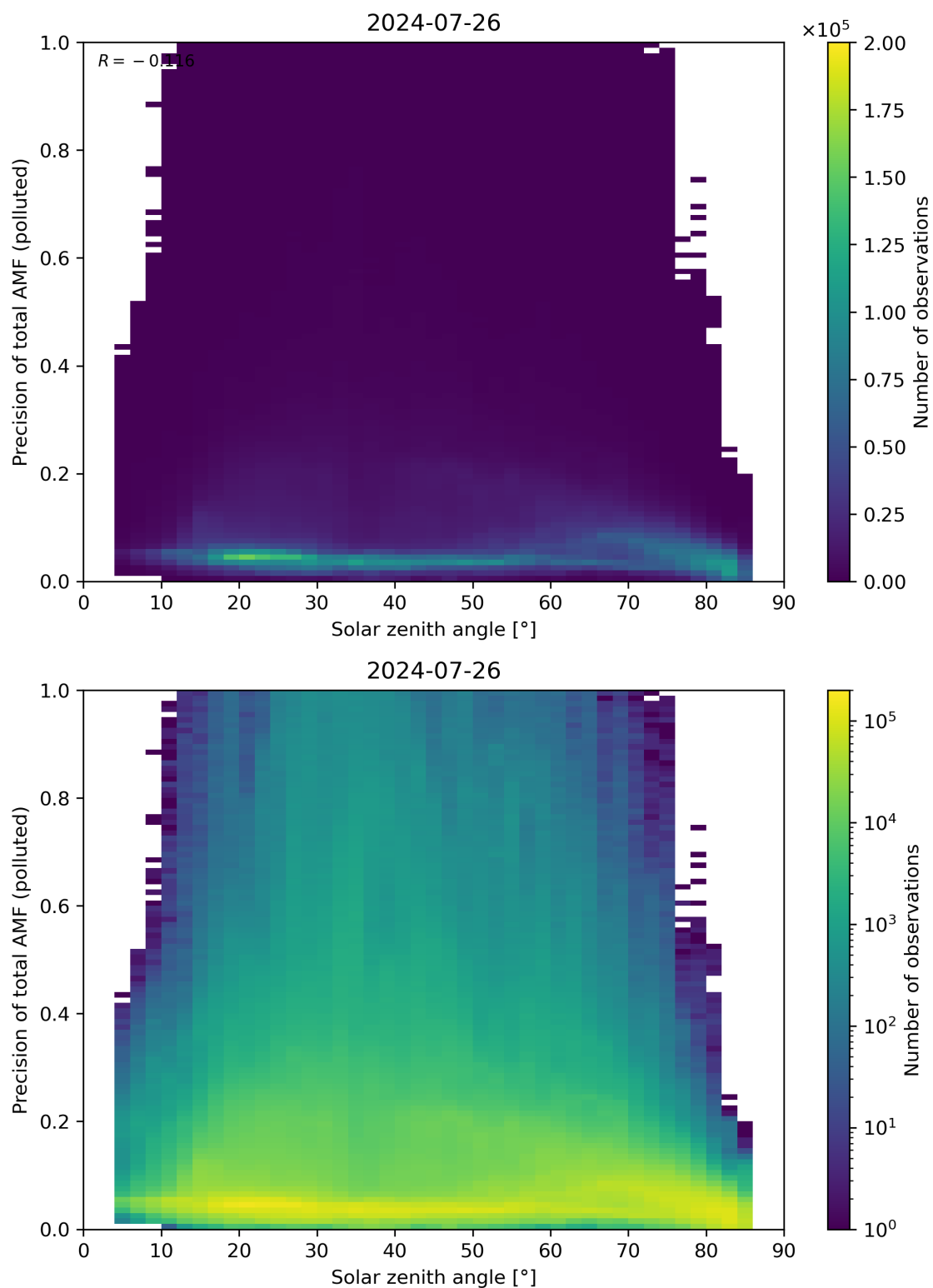
Figure 175: Scatter density plot of “Solar zenith angle” against “Precision of total AMF (polluted)” for 2024-07-26 to 2024-07-27.
