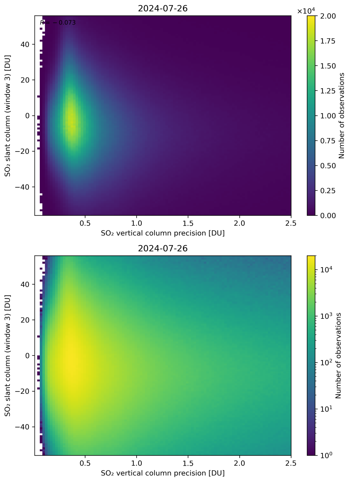
Figure 292: Scatter density plot of “SO 2 vertical column precision” against “SO 2 slant column (window 3)” for 2024-07-26 to 2024-07-27.
