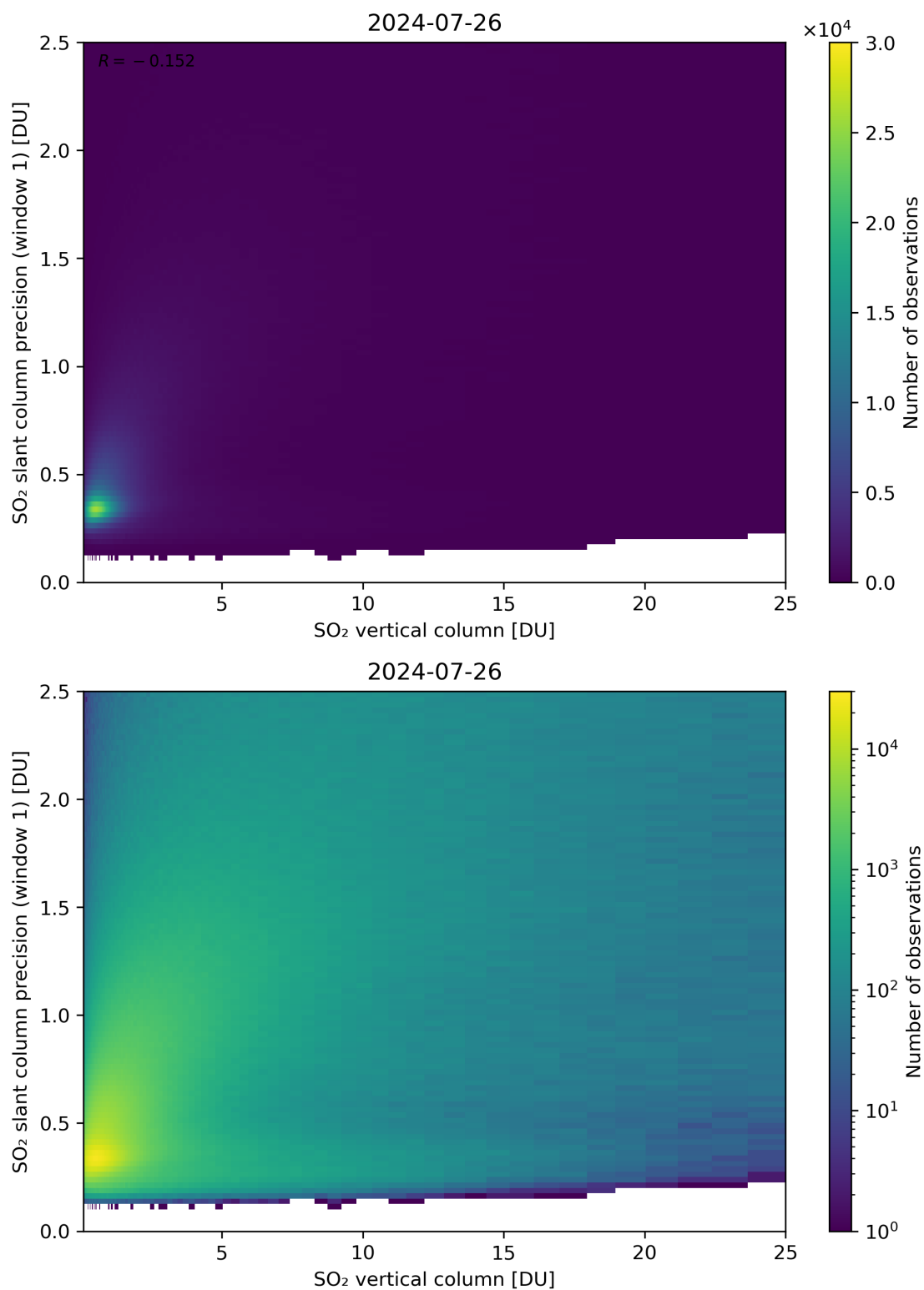
Figure 301: Scatter density plot of “SO 2 vertical column” against “SO 2 slant column precision (window 1)” for 2024-07-26 to 2024-07-27.
