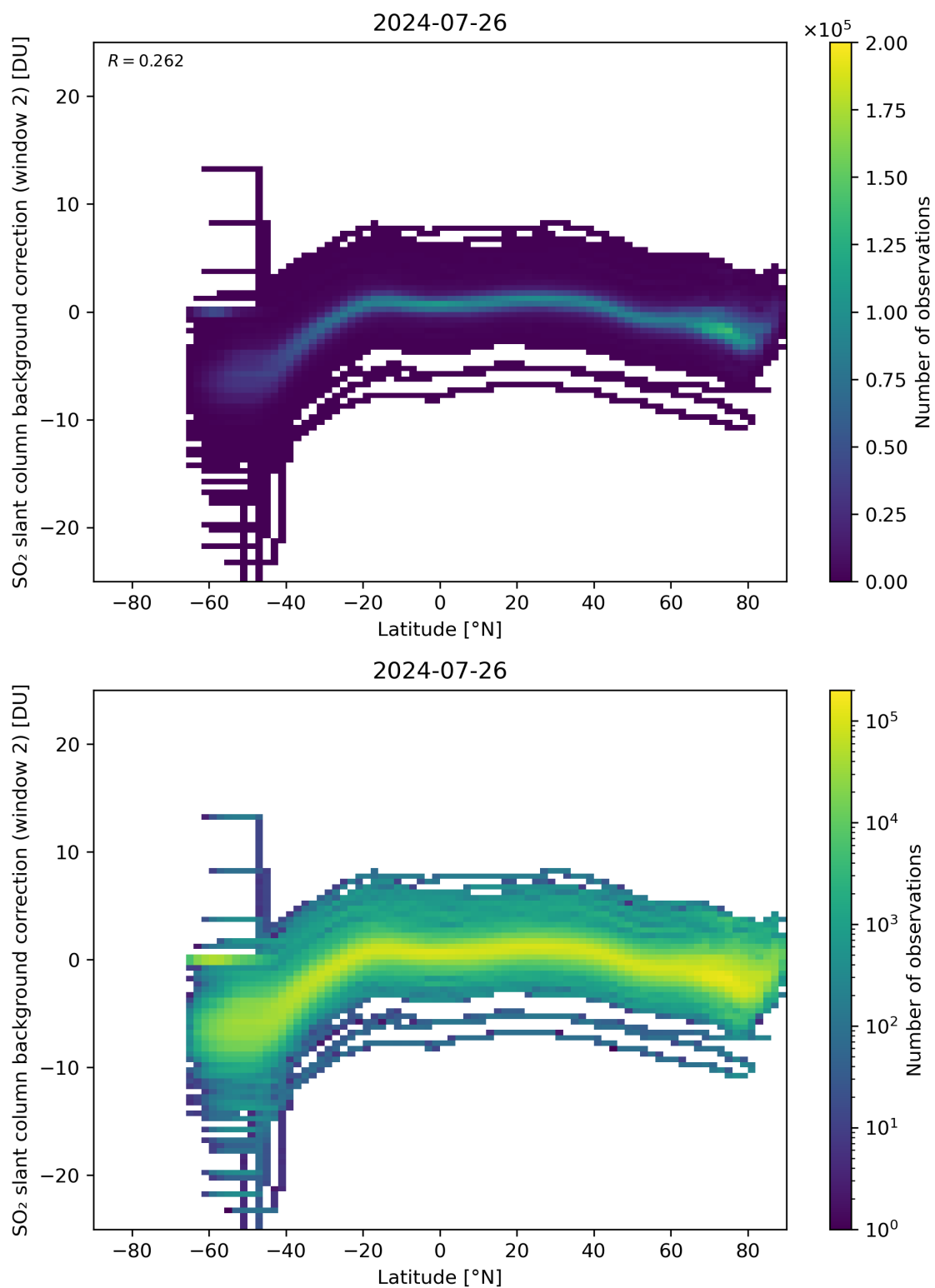
Figure 140: Scatter density plot of “Latitude” against “SO 2 slant column background correction (window 2)” for 2024-07-26 to 2024-07-27.
