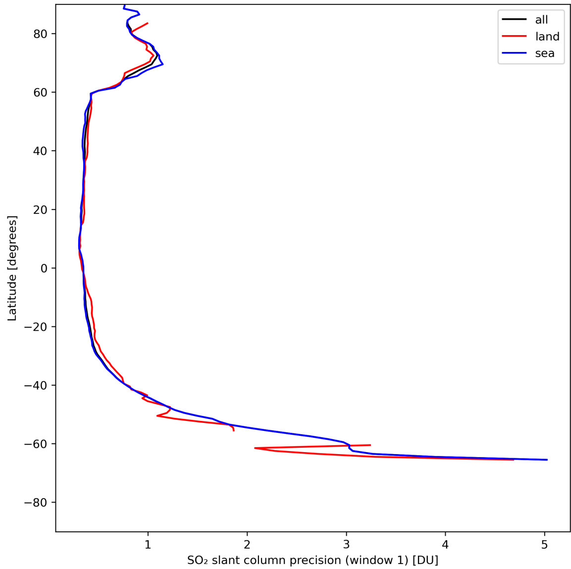
Figure 34: Zonal average of “SO 2 slant column precision (window 1)” for 2024-07-26 to 2024-07-27.
