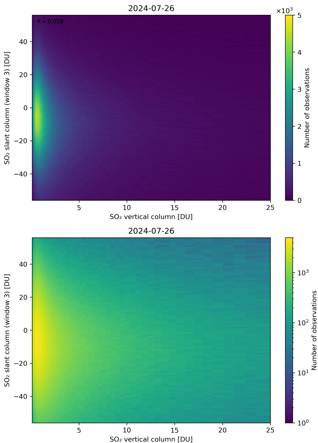
Figure 303: Scatter density plot of “SO 2 vertical column” against “SO 2 slant column (window 3)” for 2024-07-26 to 2024-07-27.
