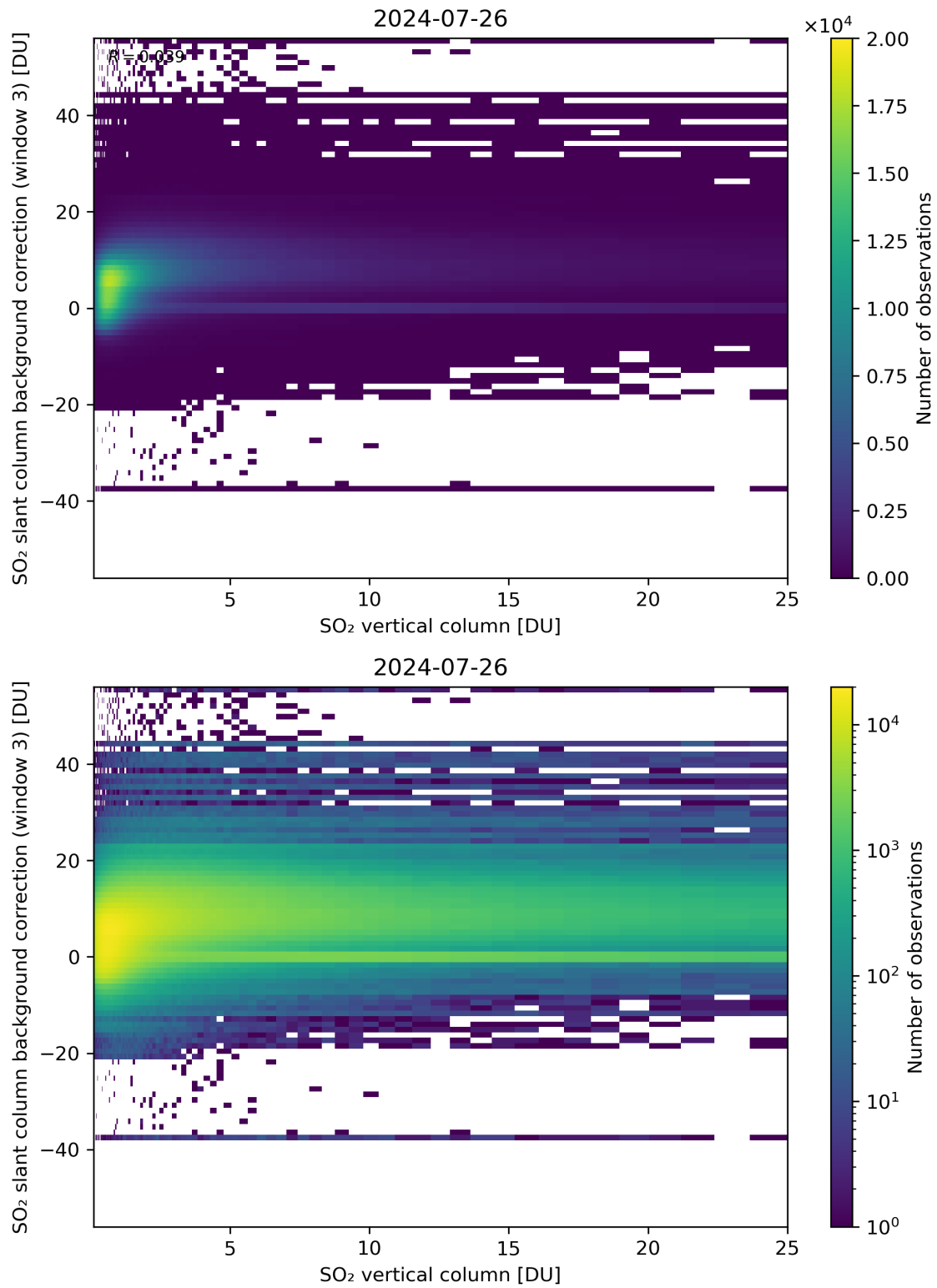
Figure 275: Scatter density plot of “SO 2 vertical column” against “SO 2 slant column background correction (window 3)” for 2024-07-26 to 2024-07-27.
