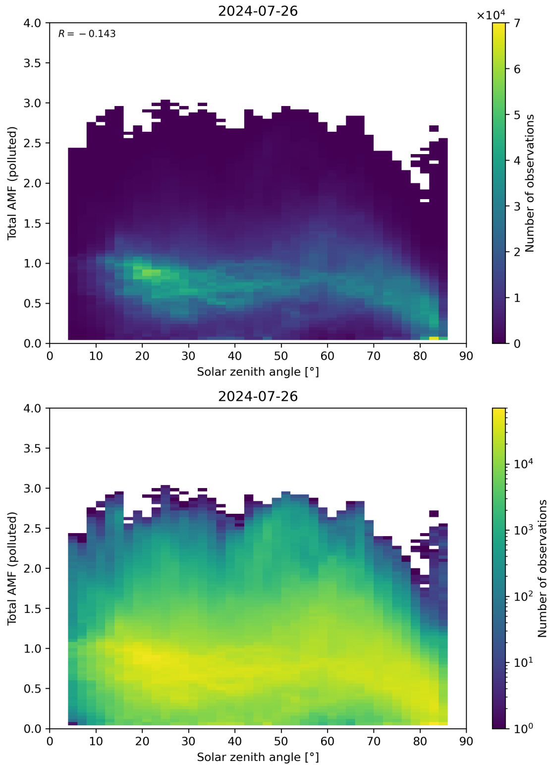
Figure 174: Scatter density plot of “Solar zenith angle” against “Total AMF (polluted)” for 2024-07-26 to 2024-07-27.
