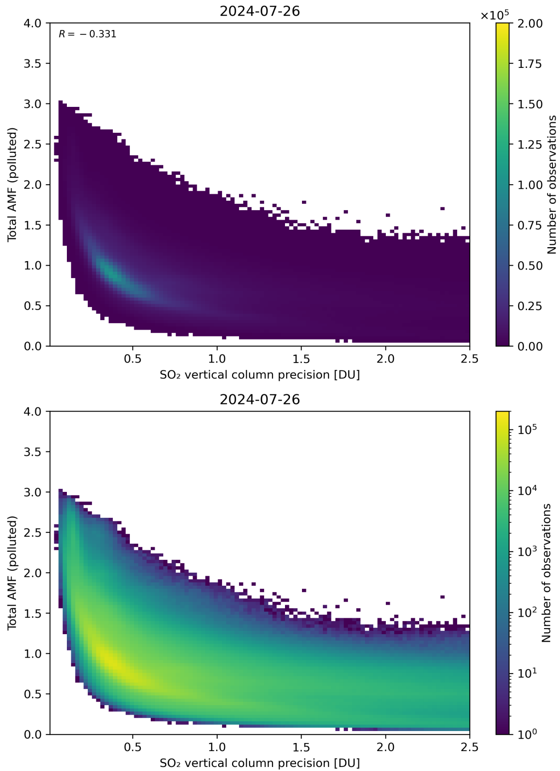
Figure 294: Scatter density plot of “SO 2 vertical column precision” against “Total AMF (polluted)” for 2024-07-26 to 2024-07-27.
