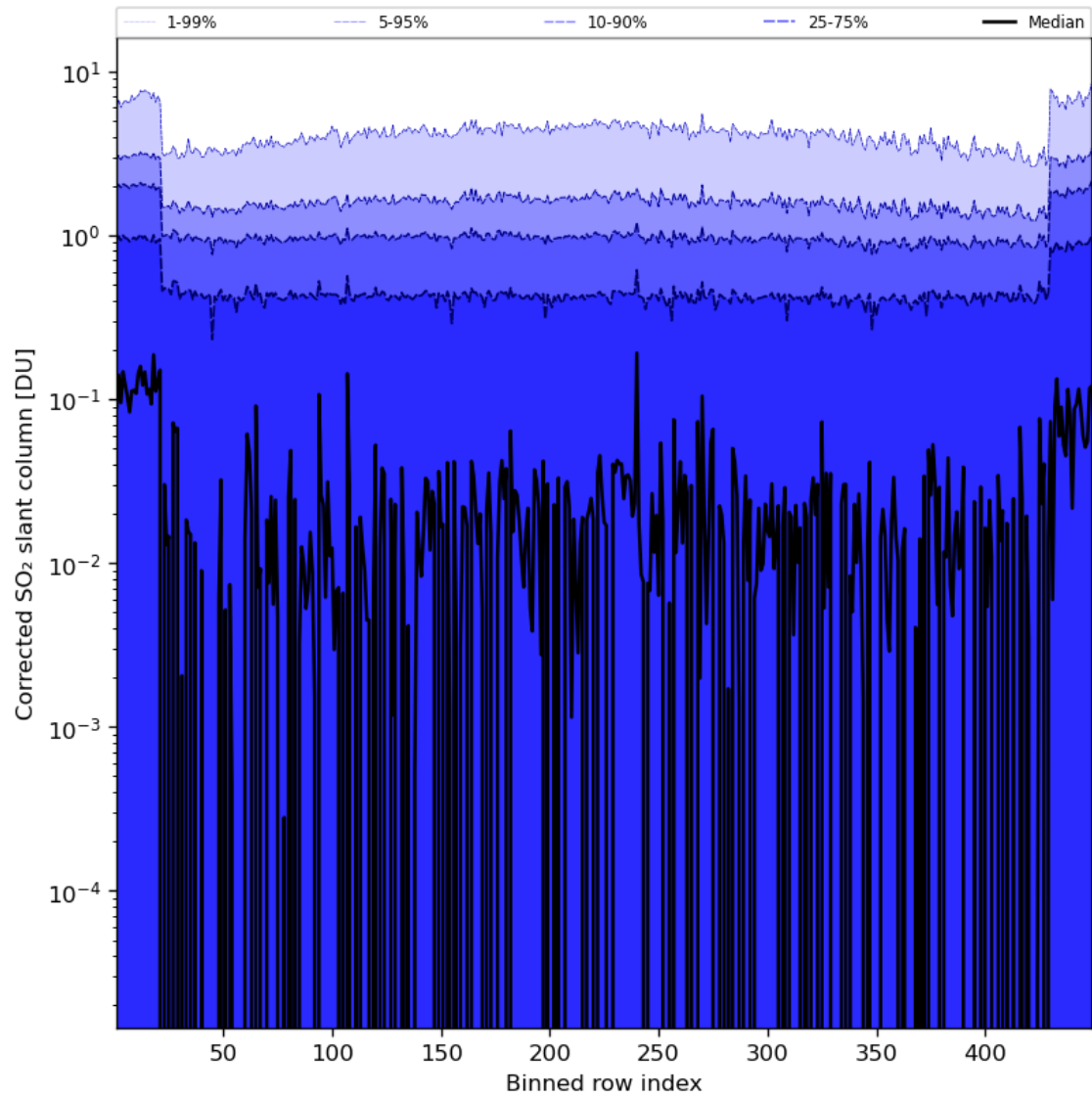
Figure 78: Along track statistics of “Corrected SO 2 slant column” for 2024-07-26 to 2024-07-27
