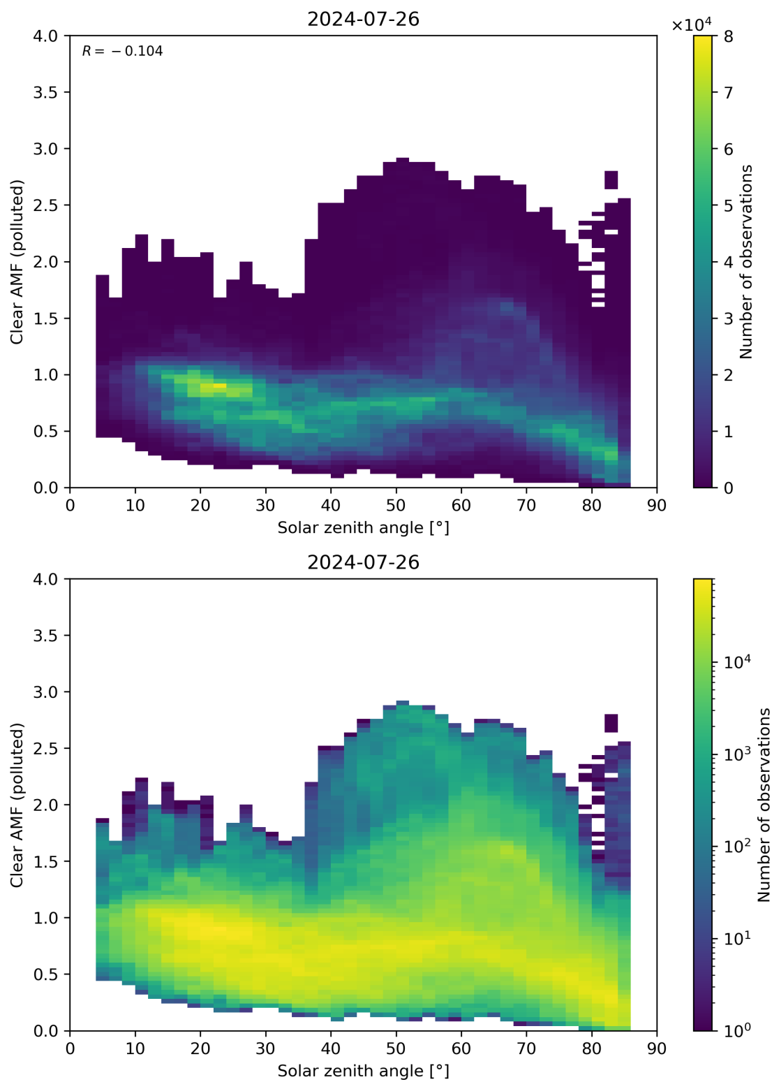
Figure 165: Scatter density plot of “Solar zenith angle” against “Clear AMF (polluted)” for 2024-07-26 to 2024-07-27.
