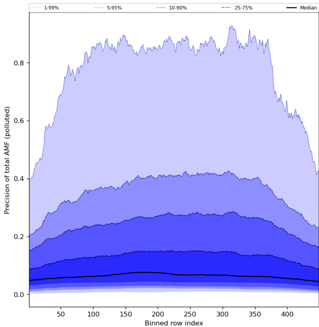
Figure 95: Along track statistics of “Precision of total AMF (polluted)” for 2024-07-26 to 2024-07-27
