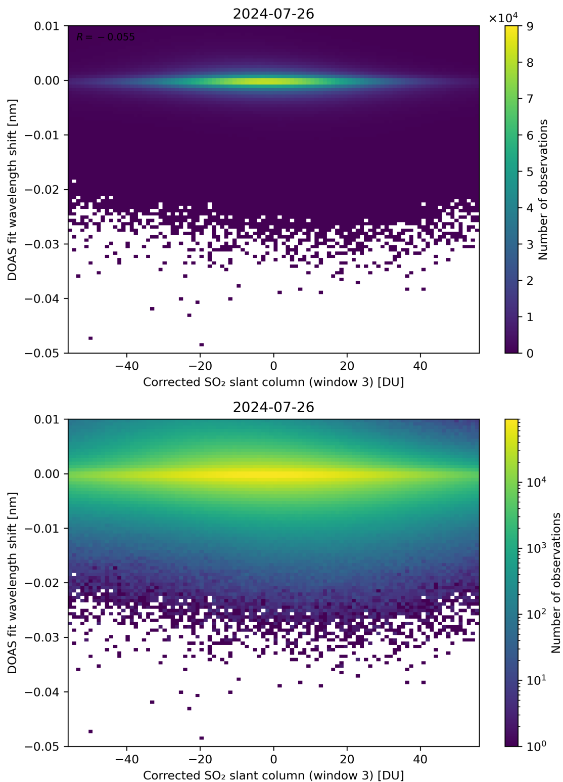
Figure 206: Scatter density plot of “Corrected SO 2 slant column (window 3)” against “DOAS fit wavelength shift” for 2024-07-26 to 2024-07-27.
