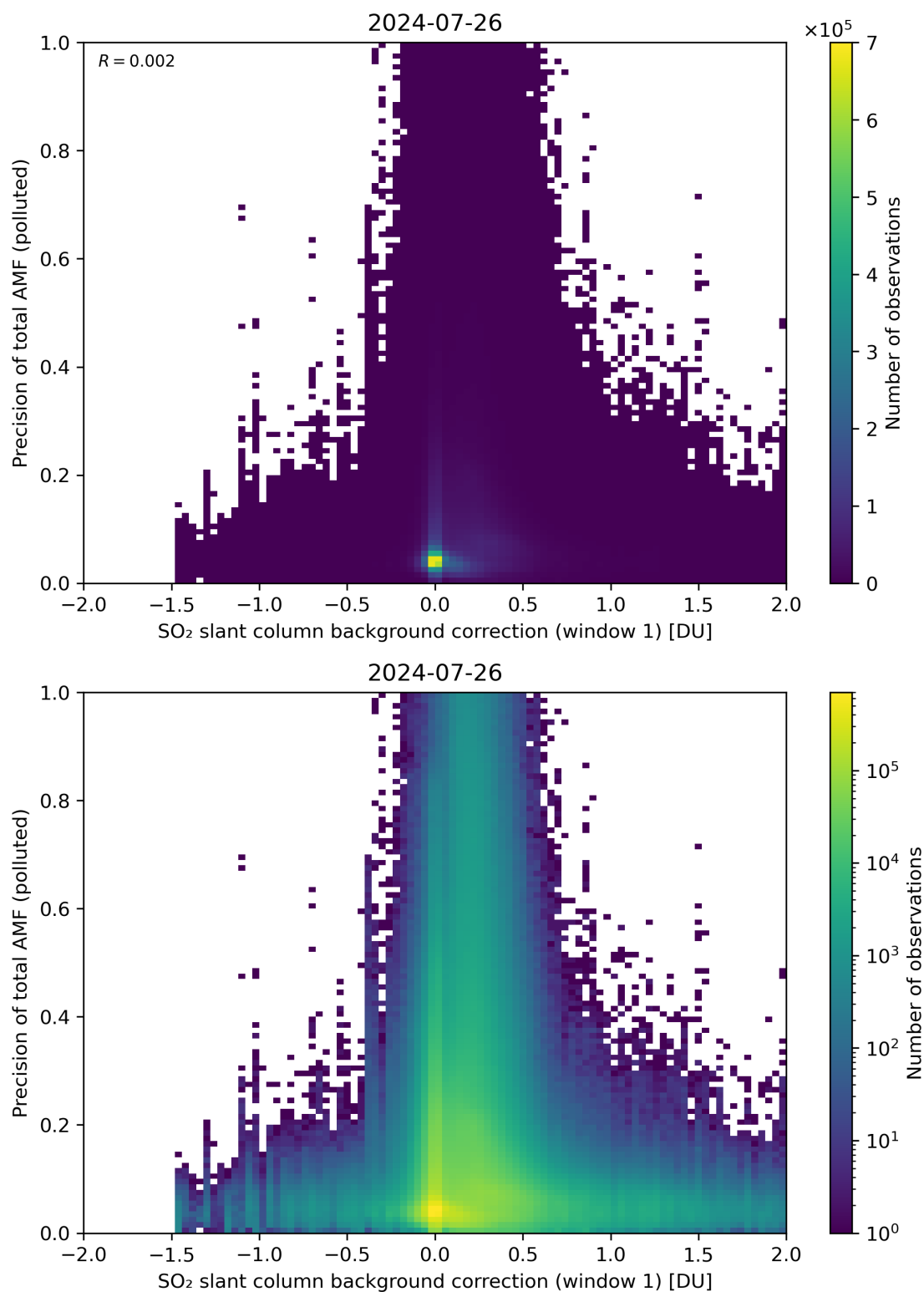
Figure 110: Scatter density plot of “SO 2 slant column background correction (window 1)” against “Precision of total AMF (polluted)” for 2024-07-26 to 2024-07-27.
