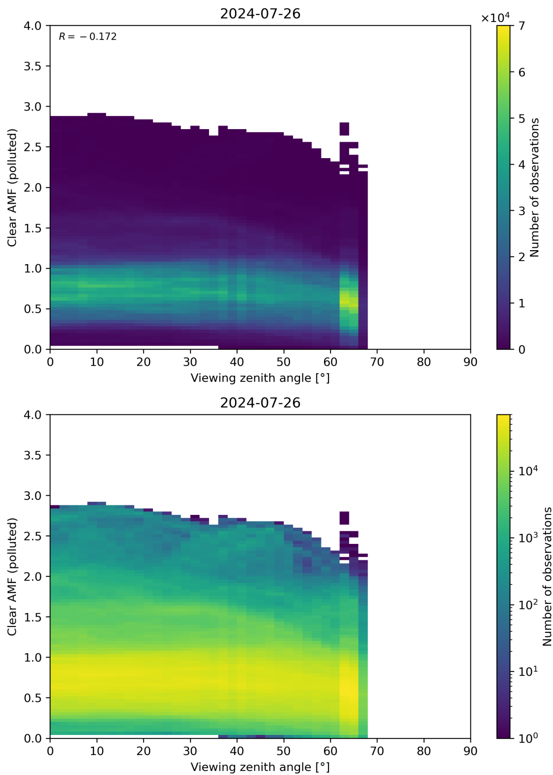
Figure 316: Scatter density plot of “Viewing zenith angle” against “Clear AMF (polluted)” for 2024-07-26 to 2024-07-27.
