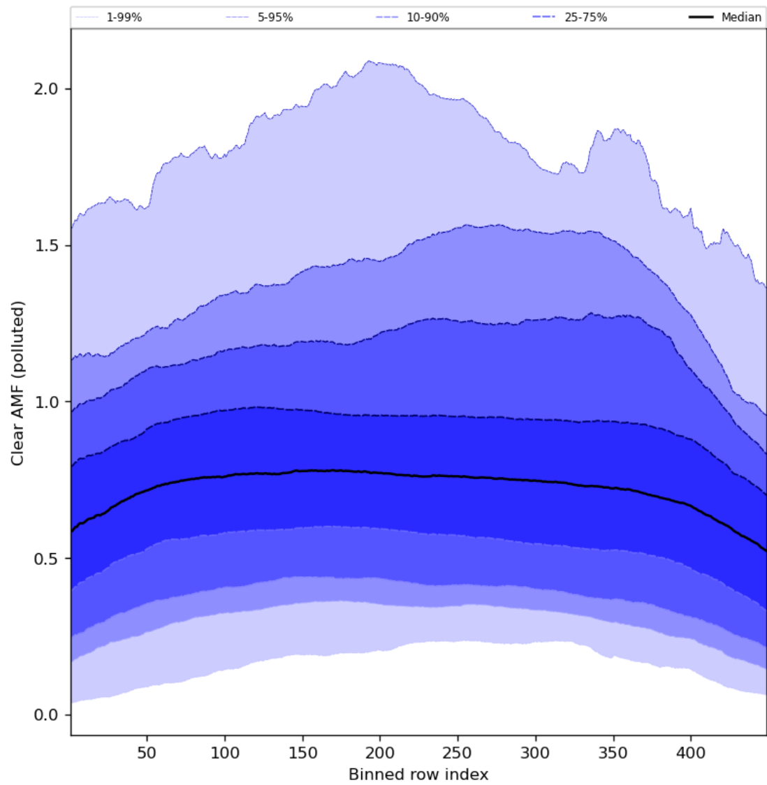
Figure 96: Along track statistics of “Clear AMF (polluted)” for 2024-07-26 to 2024-07-27
