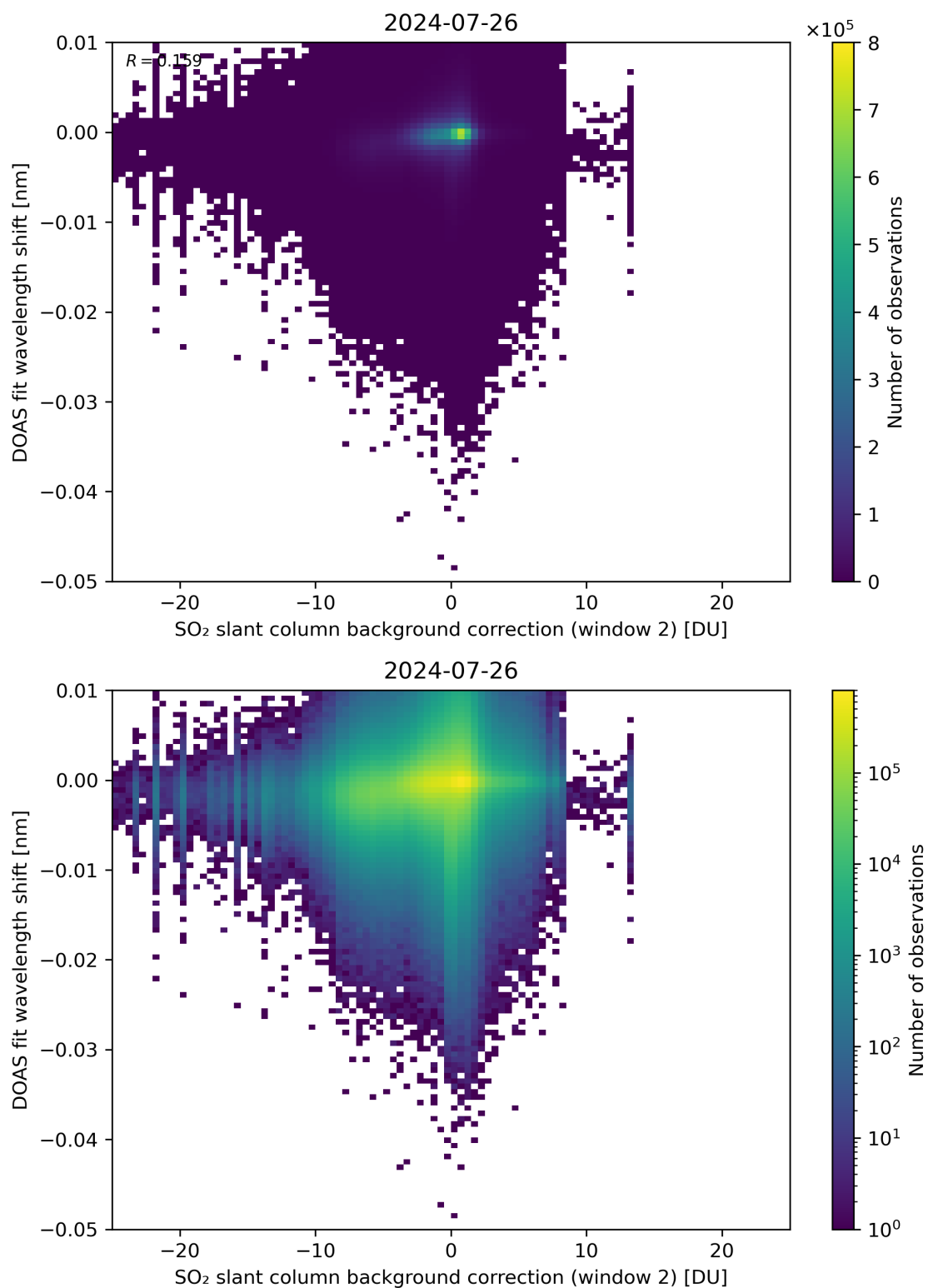
Figure 112: Scatter density plot of “SO 2 slant column background correction (window 2)” against “DOAS fit wavelength shift” for 2024-07-26 to 2024-07-27.
