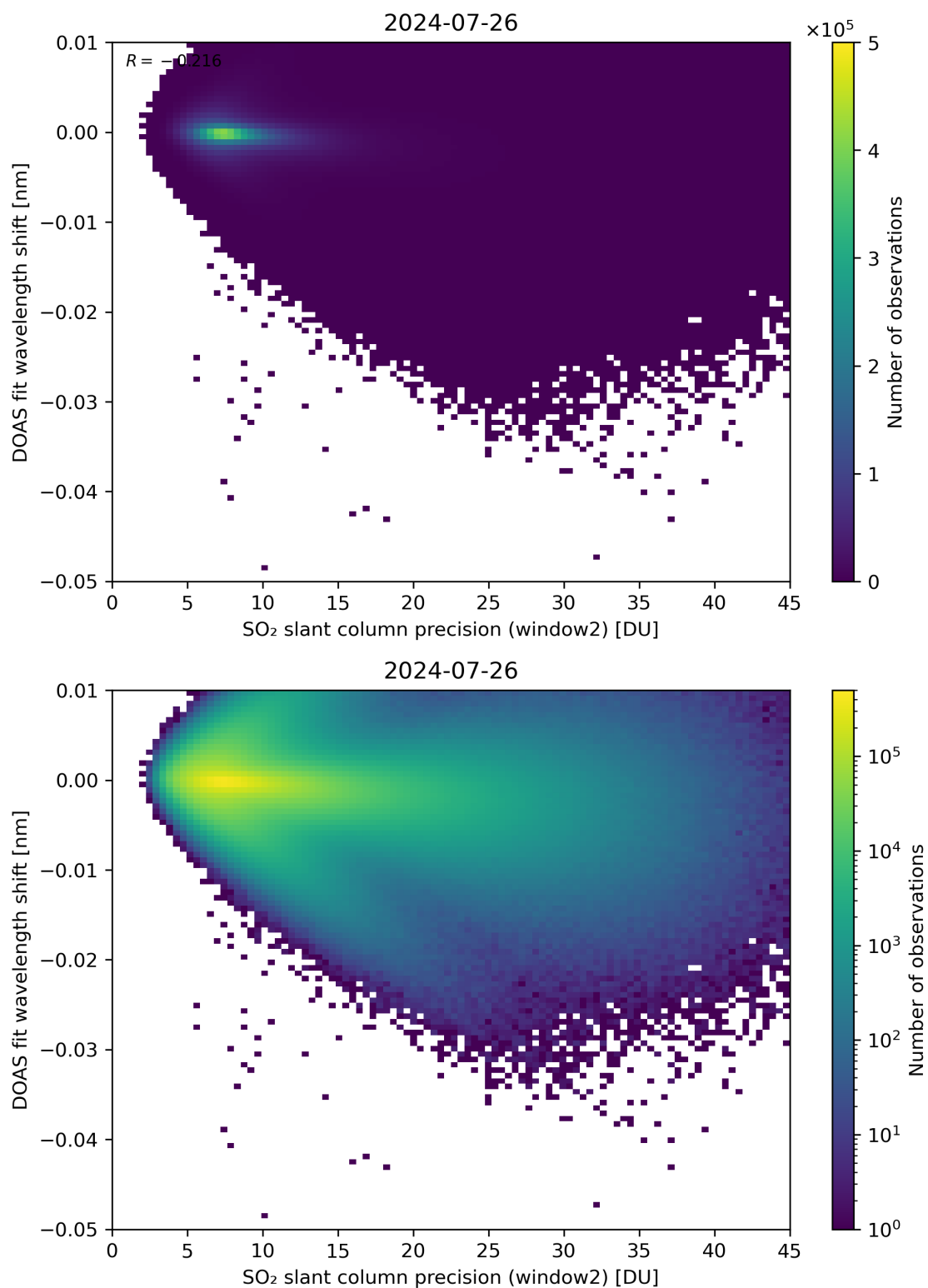
Figure 243: Scatter density plot of “SO 2 slant column precision (window2)” against “DOAS fit wavelength shift” for 2024-07-26 to 2024-07-27.
