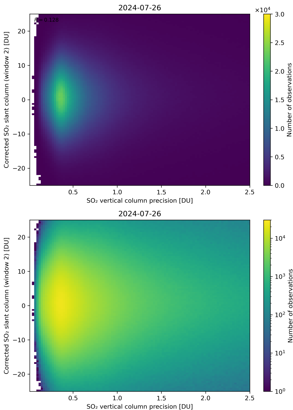
Figure 287: Scatter density plot of “SO 2 vertical column precision” against “Corrected SO 2 slant column (window 2)” for 2024-07-26 to 2024-07-27.
