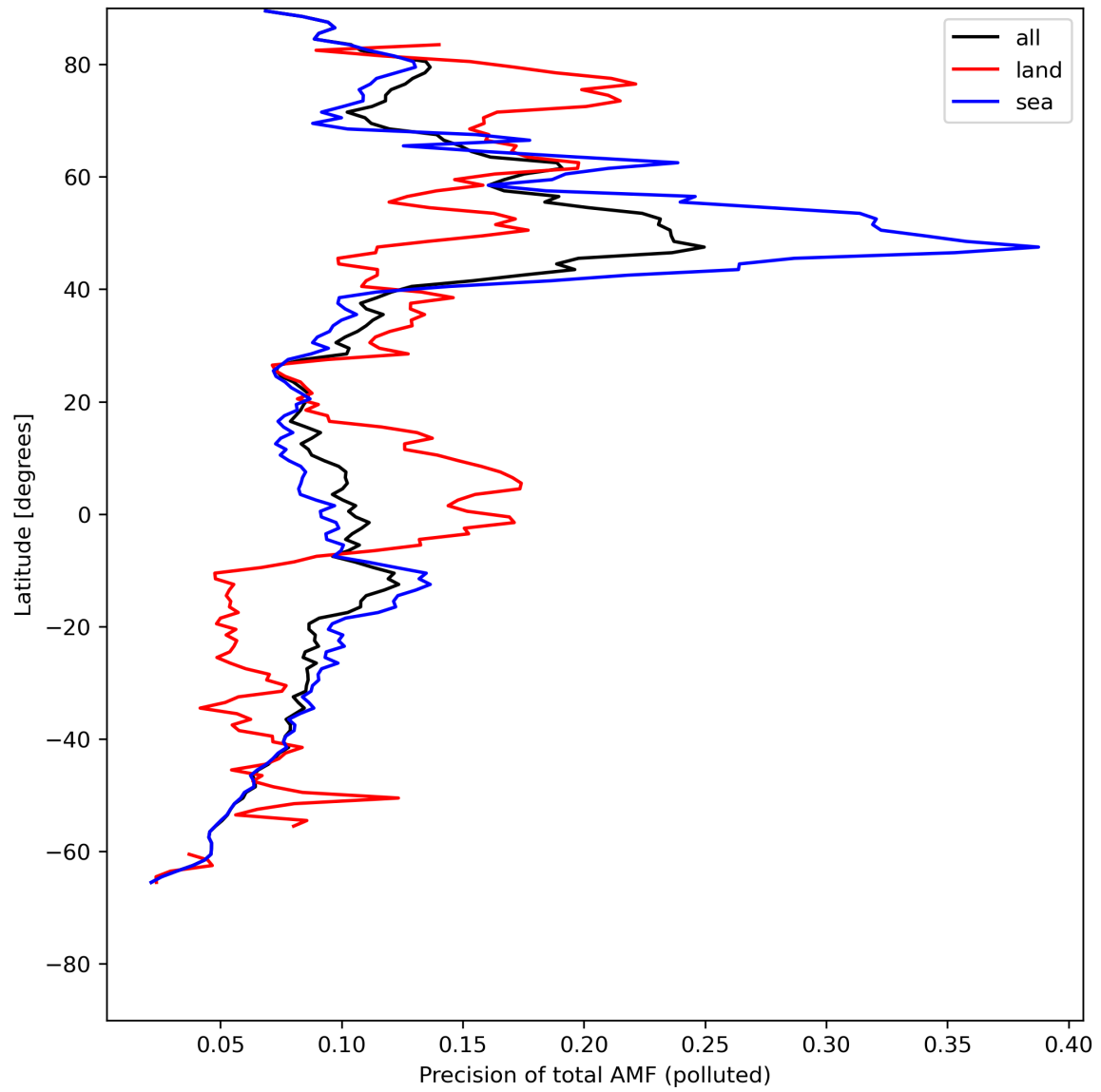
Figure 49: Zonal average of “Precision of total AMF (polluted)” for 2024-07-26 to 2024-07-27.
