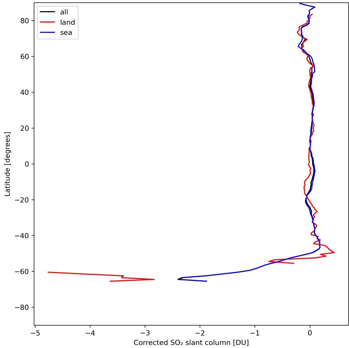
Figure 32: Zonal average of “Corrected SO 2 slant column” for 2024-07-26 to 2024-07-27.
