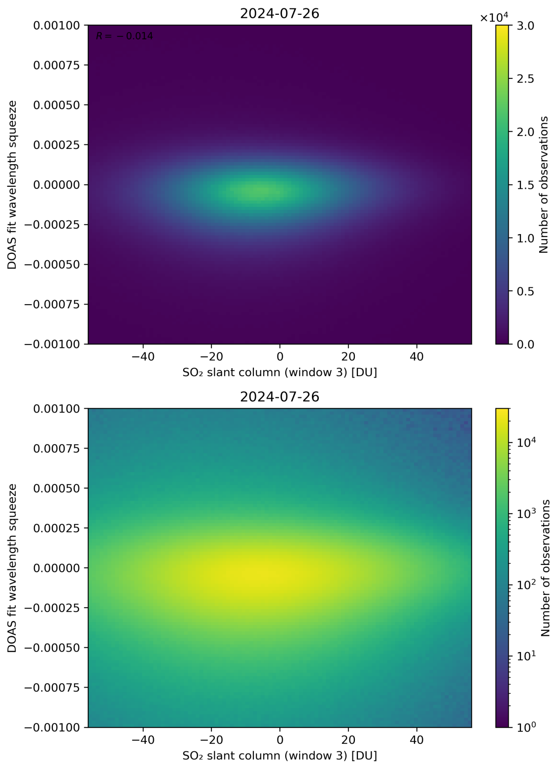
Figure 255: Scatter density plot of “SO 2 slant column (window 3)” against “DOAS fit wavelength squeeze” for 2024-07-26 to 2024-07-27.
