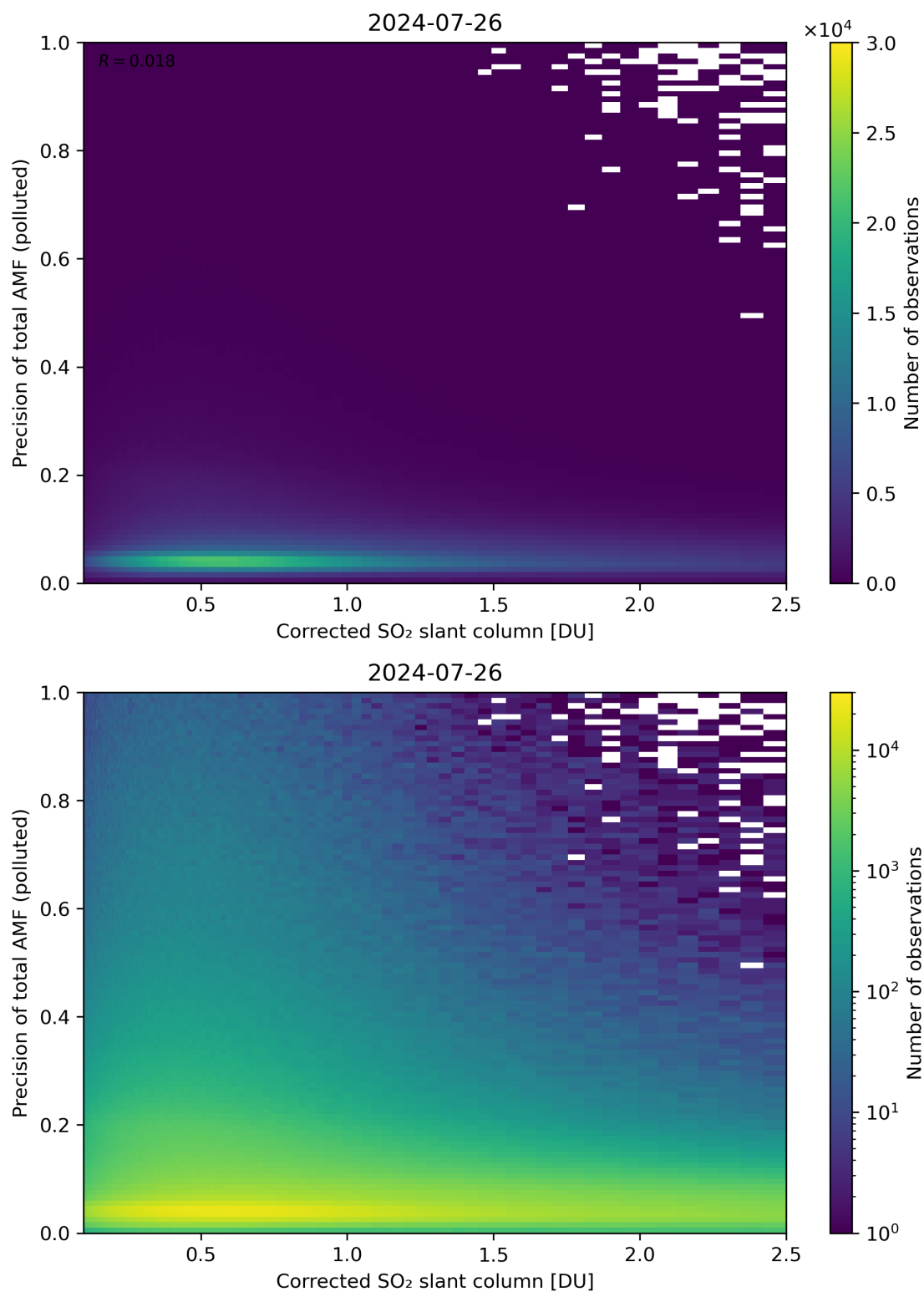
Figure 193: Scatter density plot of “Corrected SO 2 slant column” against “Precision of total AMF (polluted)” for 2024-07-26 to 2024-07-27.
