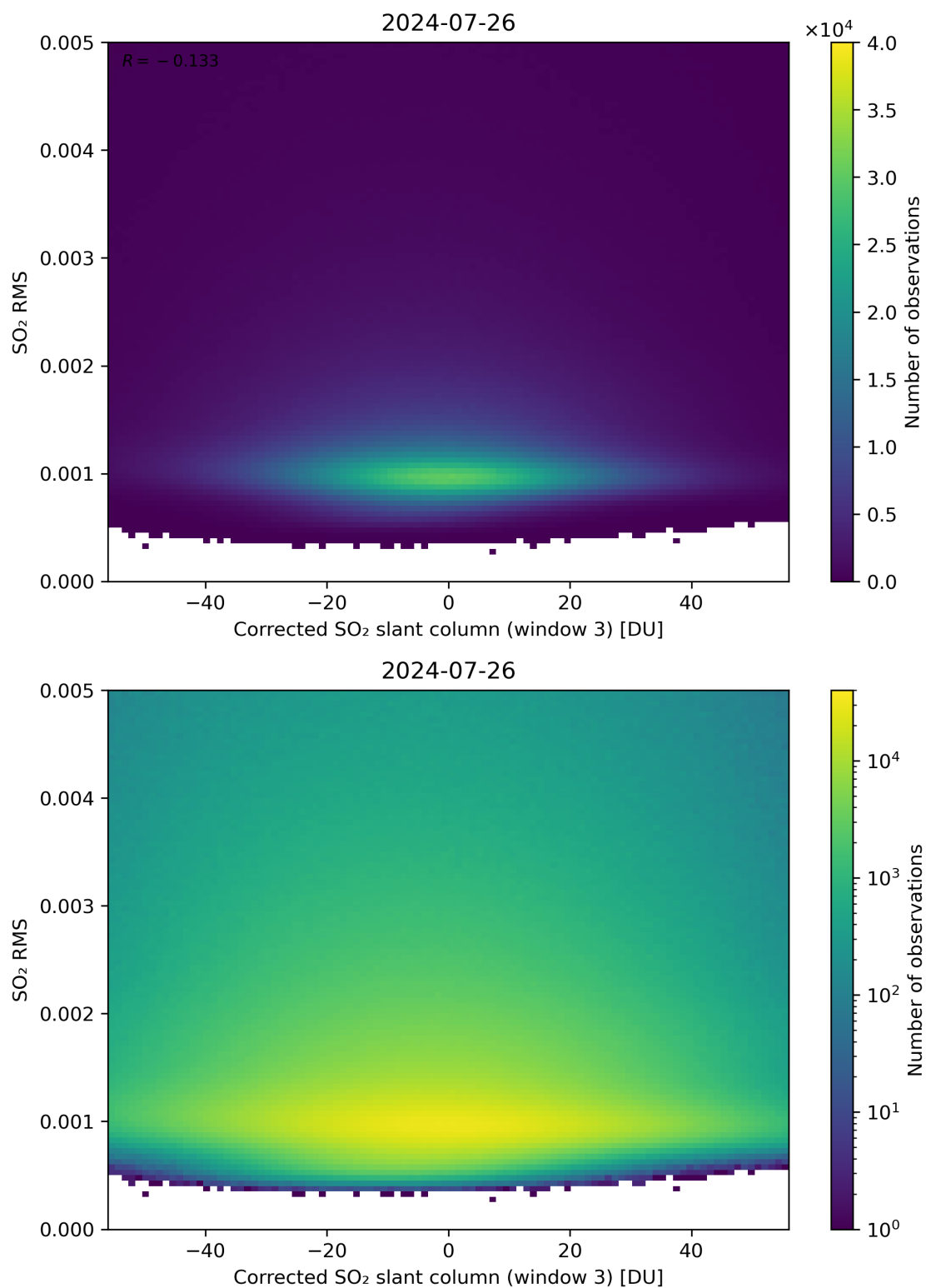
Figure 208: Scatter density plot of “Corrected SO 2 slant column (window 3)” against “SO 2 RMS” for 2024-07-26 to 2024-07-27.
