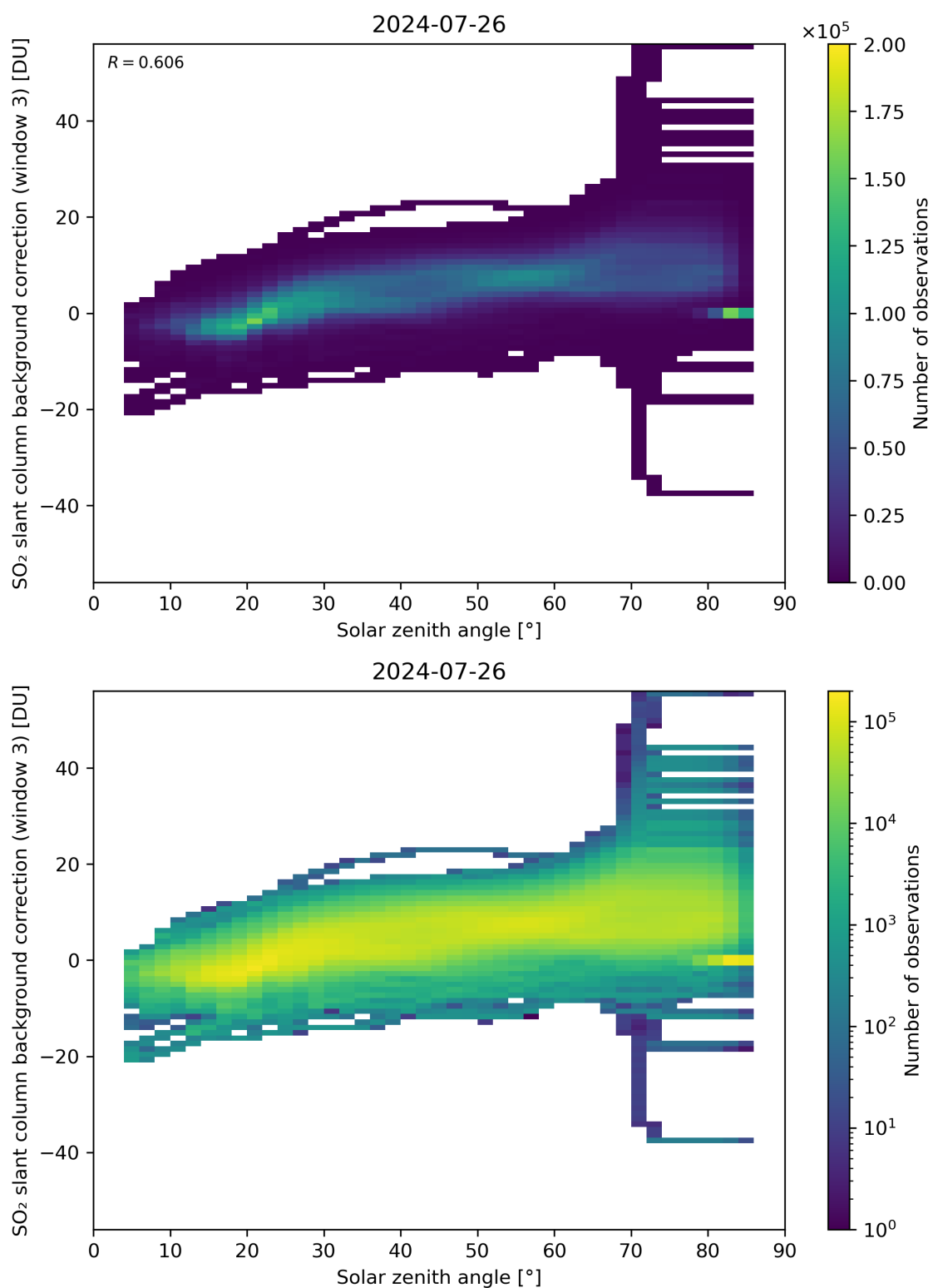
Figure 160: Scatter density plot of “Solar zenith angle” against “SO 2 slant column background correction (window 3)” for 2024-07-26 to 2024-07-27.
