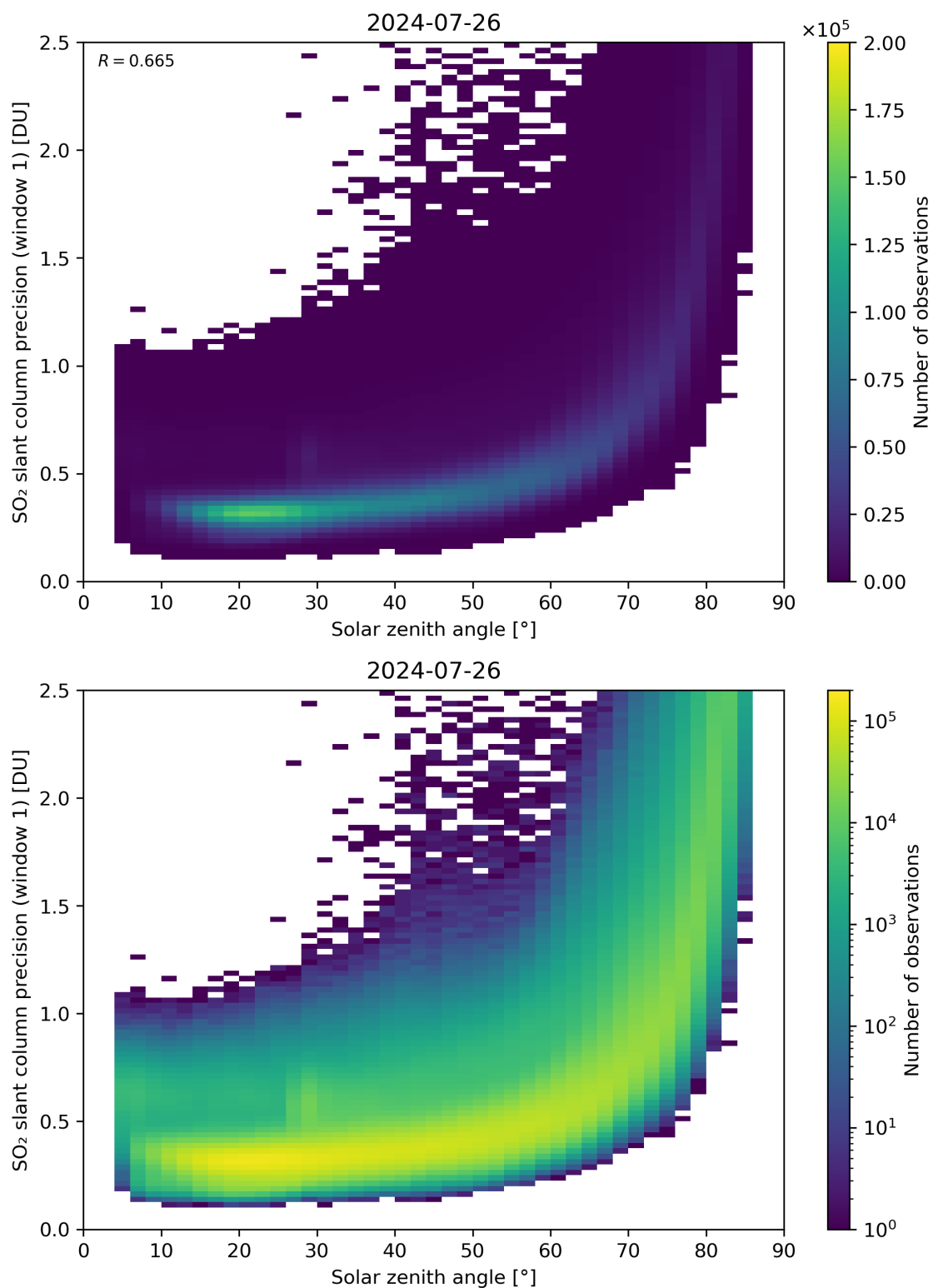
Figure 170: Scatter density plot of “Solar zenith angle” against “SO 2 slant column precision (window 1)” for 2024-07-26 to 2024-07-27.
