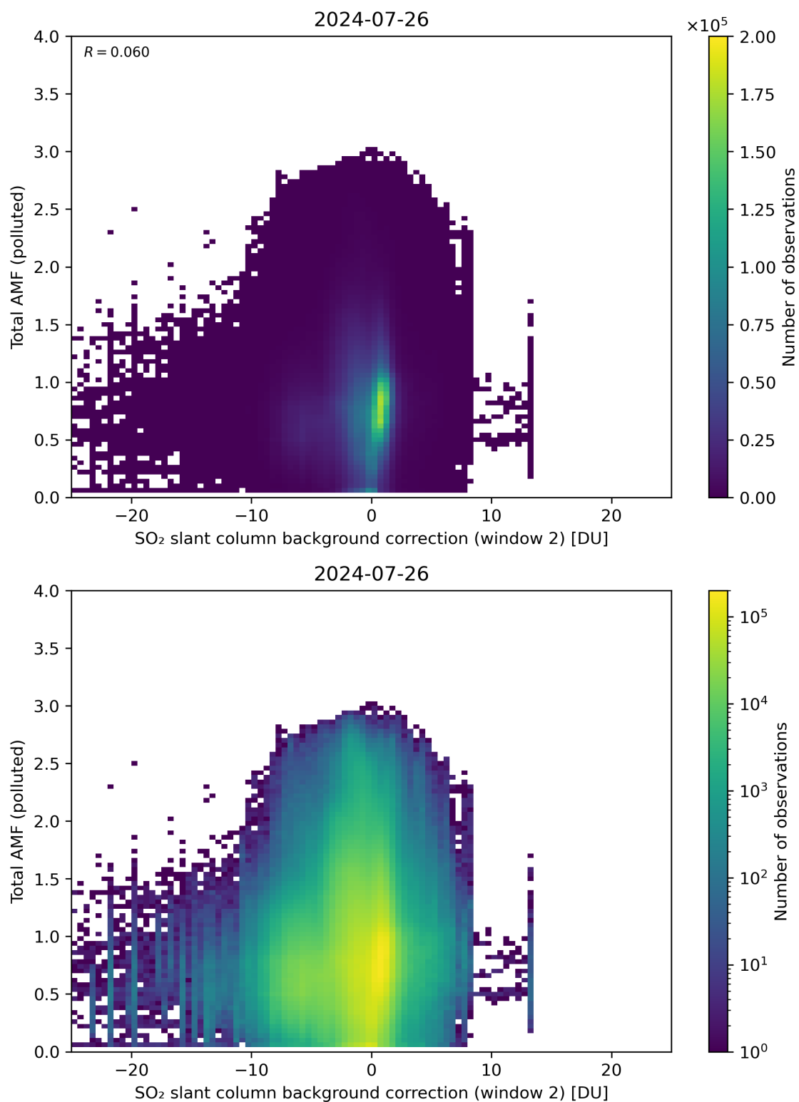
Figure 119: Scatter density plot of “SO 2 slant column background correction (window 2)” against “Total AMF (polluted)” for 2024-07-26 to 2024-07-27.
