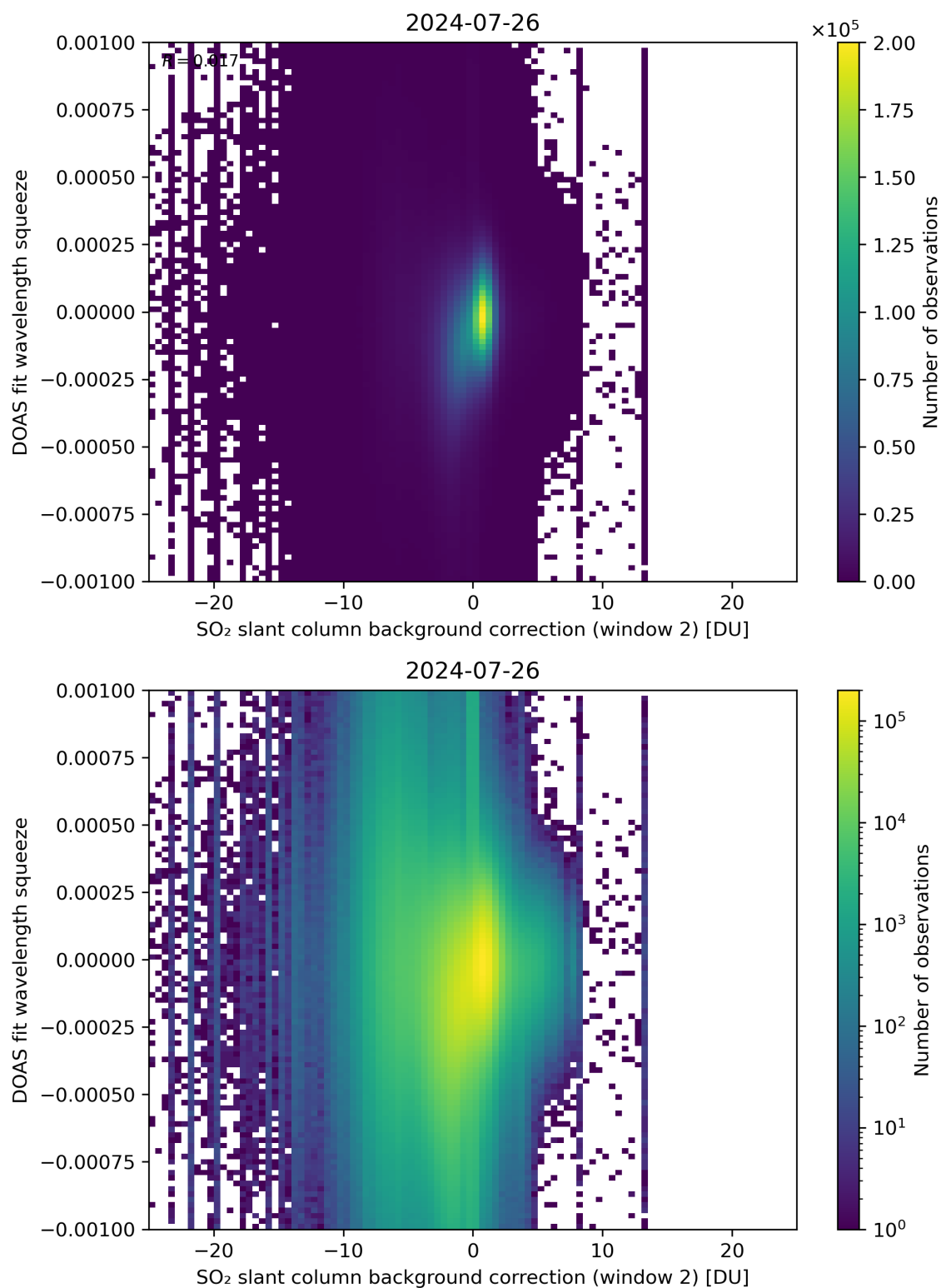
Figure 113: Scatter density plot of “SO 2 slant column background correction (window 2)” against “DOAS fit wavelength squeeze” for 2024-07-26 to 2024-07-27.
