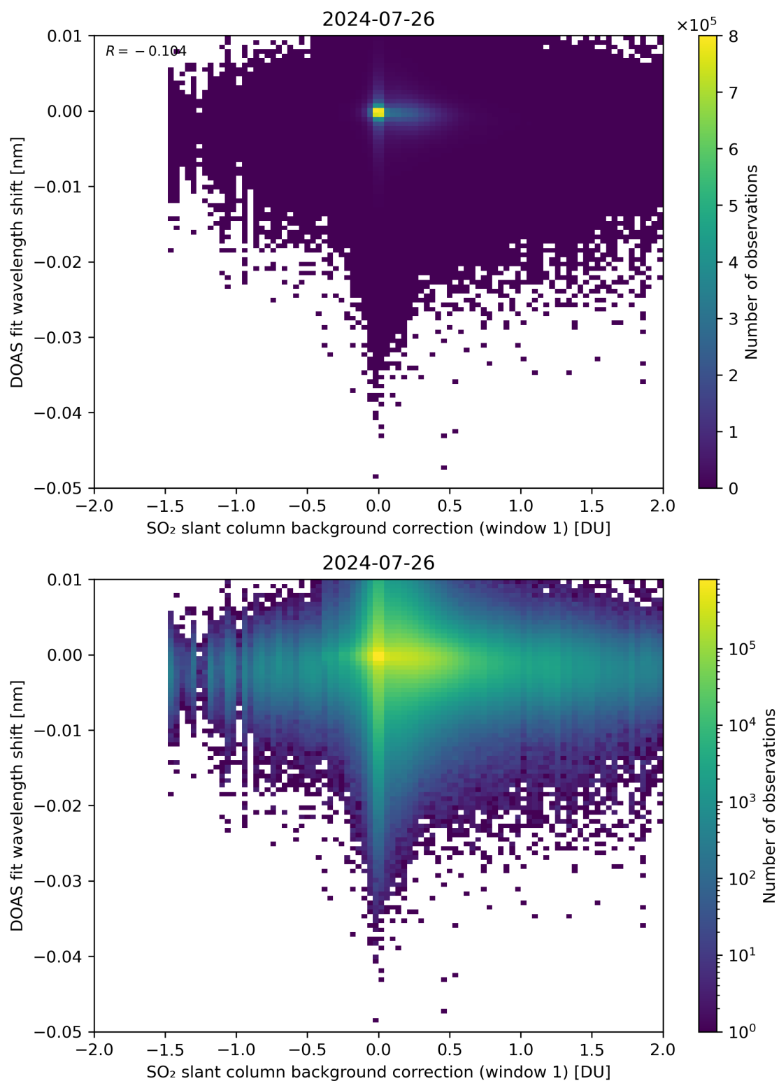
Figure 100: Scatter density plot of “SO 2 slant column background correction (window 1)” against “DOAS fit wavelength shift” for 2024-07-26 to 2024-07-27.
