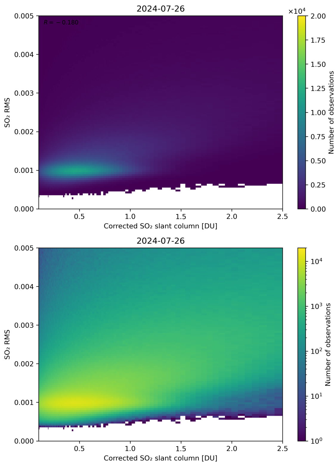
Figure 183: Scatter density plot of “Corrected SO 2 slant column” against “SO 2 RMS” for 2024-07-26 to 2024-07-27.
