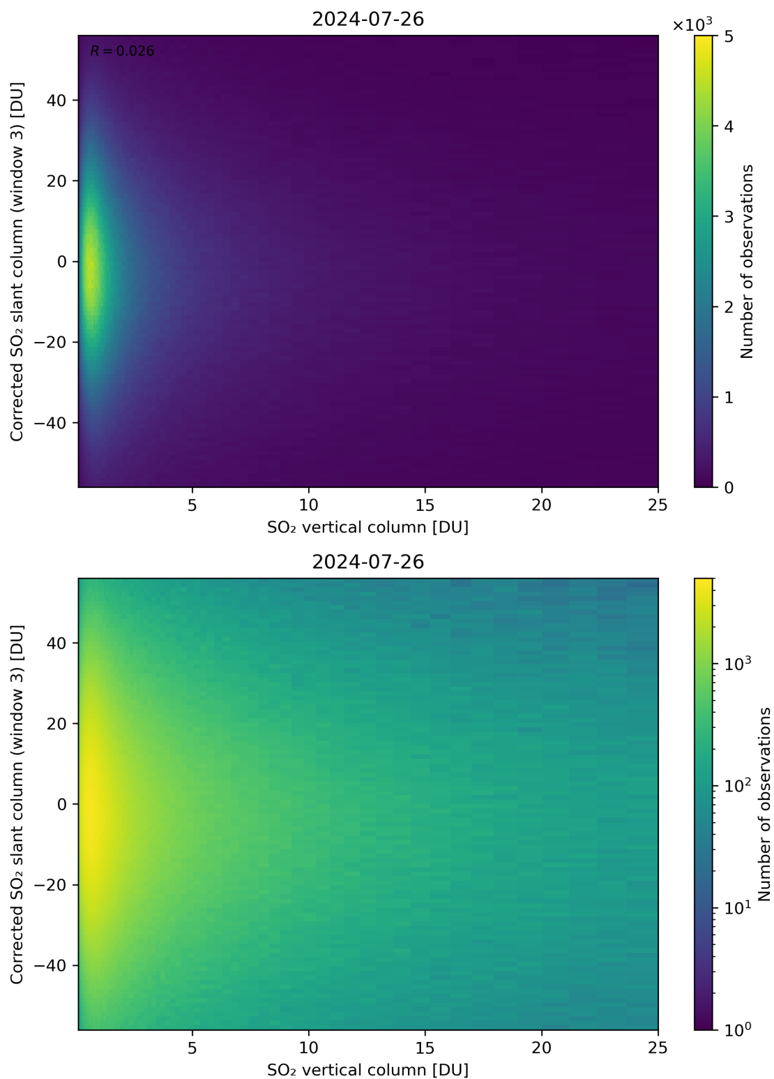
Figure 299: Scatter density plot of “SO 2 vertical column” against “Corrected SO 2 slant column (window 3)” for 2024-07-26 to 2024-07-27.
