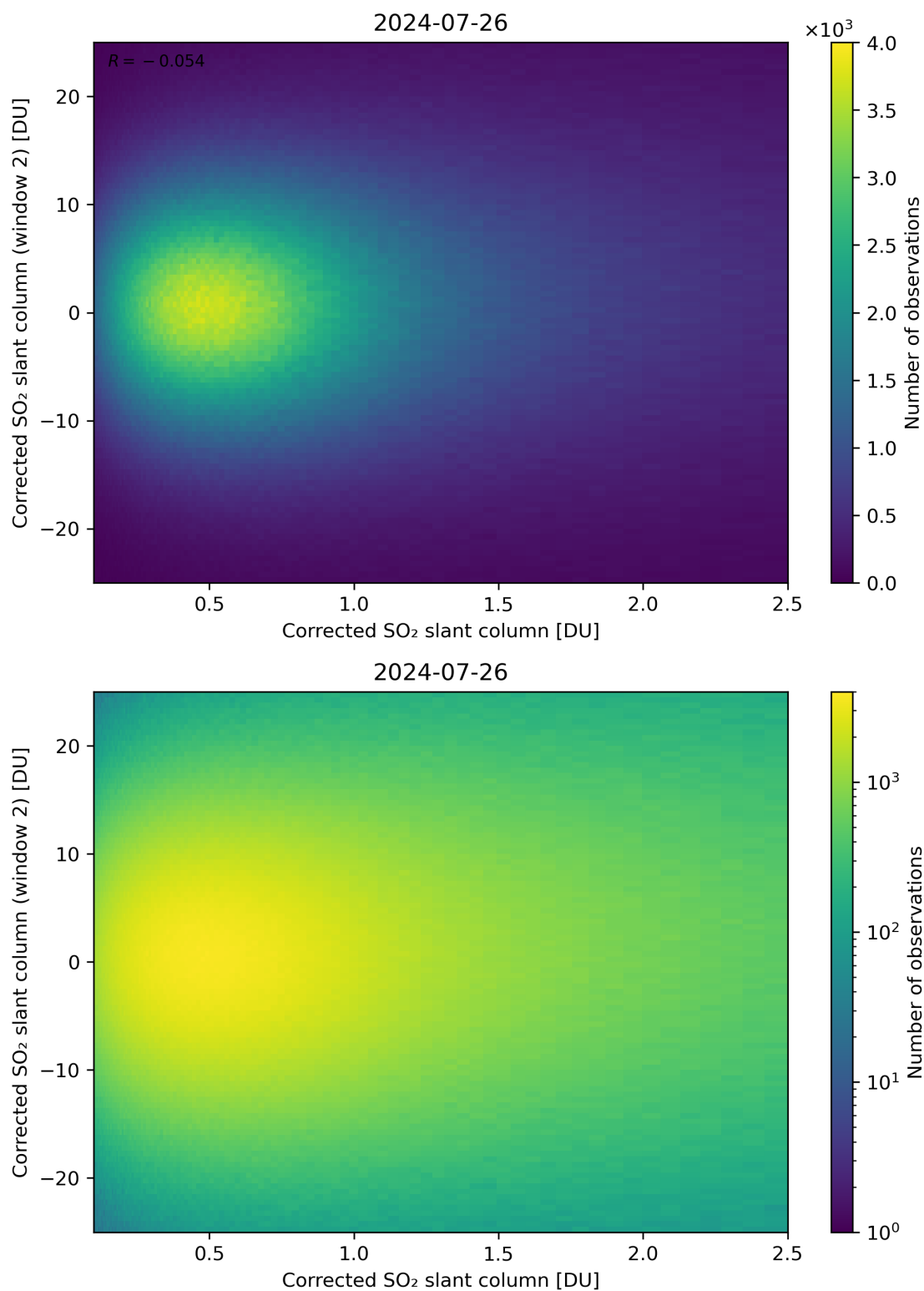
Figure 185: Scatter density plot of “Corrected SO 2 slant column” against “Corrected SO 2 slant column (window 2)” for 2024-07-26 to 2024-07-27.
