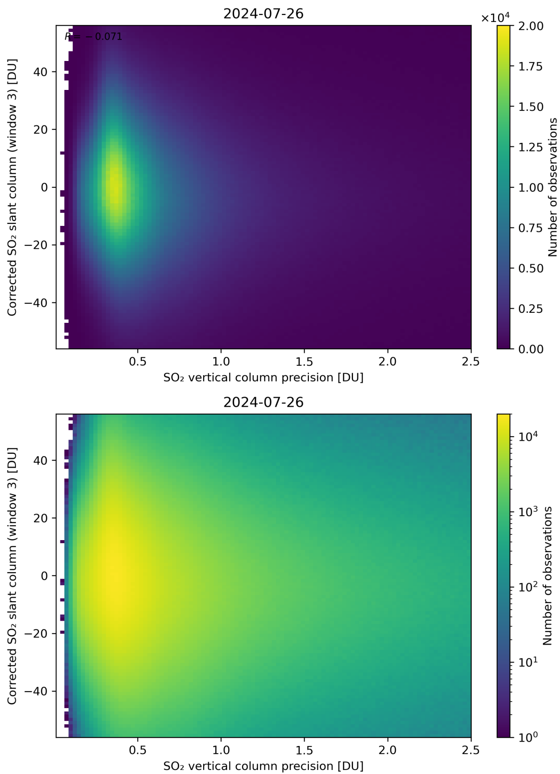
Figure 288: Scatter density plot of “SO 2 vertical column precision” against “Corrected SO 2 slant column (window 3)” for 2024-07-26 to 2024-07-27.
