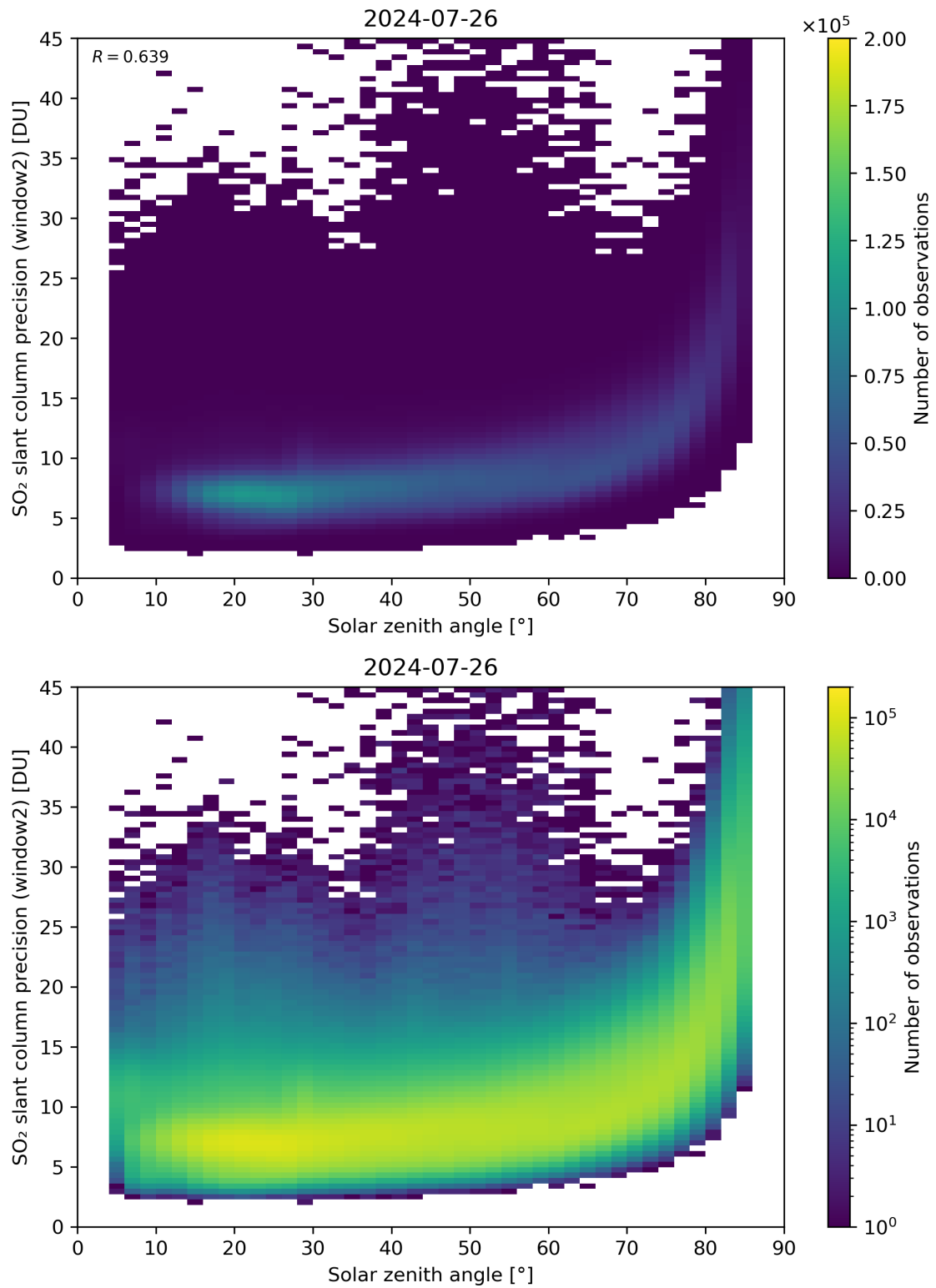
Figure 171: Scatter density plot of “Solar zenith angle” against “SO 2 slant column precision (window2)” for 2024-07-26 to 2024-07-27.
