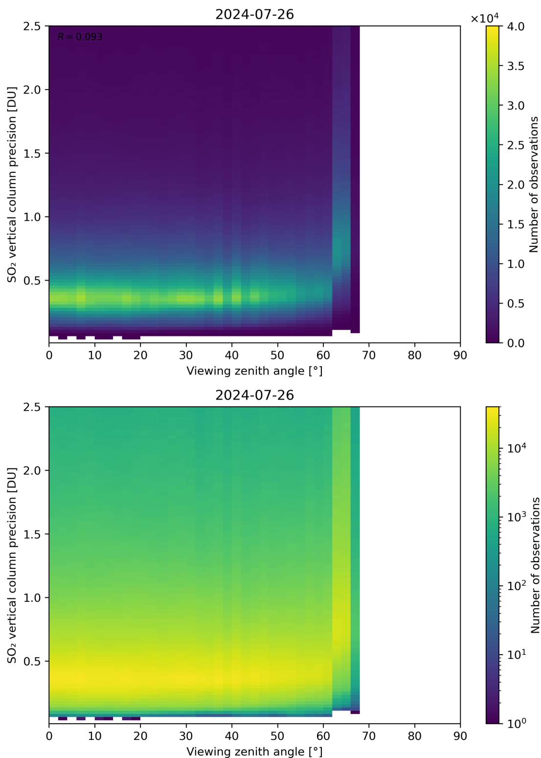
Figure 328: Scatter density plot of “Viewing zenith angle” against “SO 2 vertical column precision” for 2024-07-26 to 2024-07-27.
