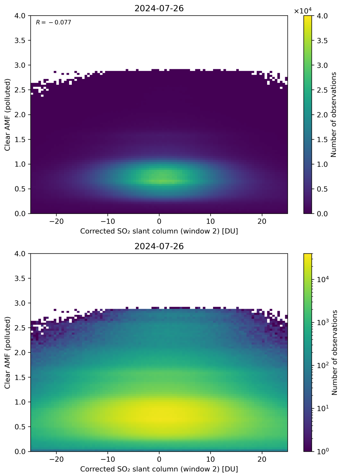
Figure 199: Scatter density plot of “Corrected SO 2 slant column (window 2)” against “Clear AMF (polluted)” for 2024-07-26 to 2024-07-27.
