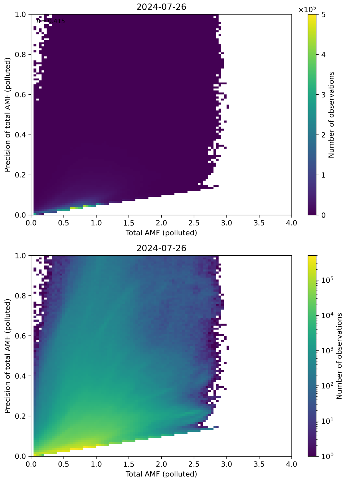
Figure 272: Scatter density plot of “Total AMF (polluted)” against “Precision of total AMF (polluted)” for 2024-07-26 to 2024-07-27.
