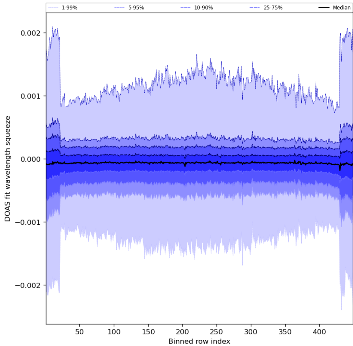
Figure 92: Along track statistics of “DOAS fit wavelength squeeze” for 2024-07-26 to 2024-07-27
