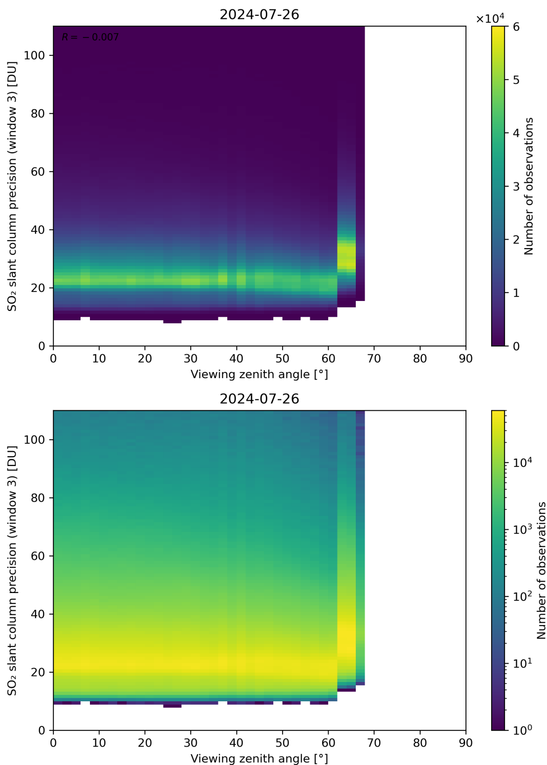
Figure 324: Scatter density plot of “Viewing zenith angle” against “SO 2 slant column precision (window 3)” for 2024-07-26 to 2024-07-27.
