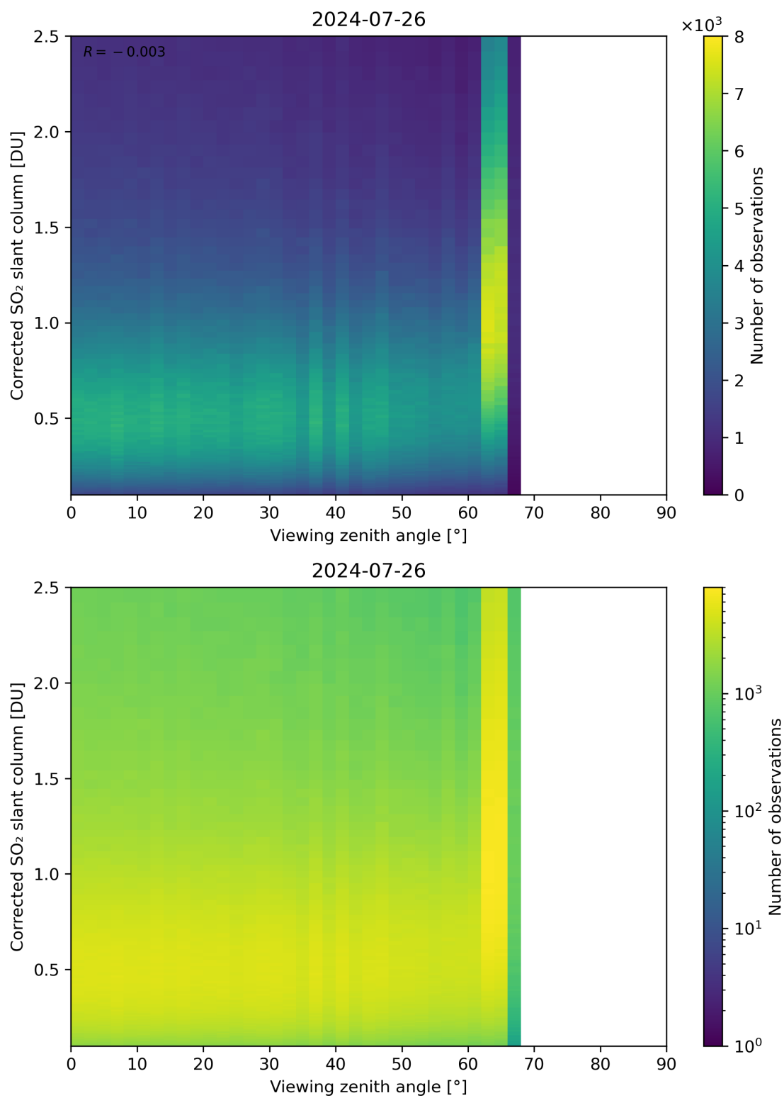
Figure 317: Scatter density plot of “Viewing zenith angle” against “Corrected SO 2 slant column” for 2024-07-26 to 2024-07-27.
