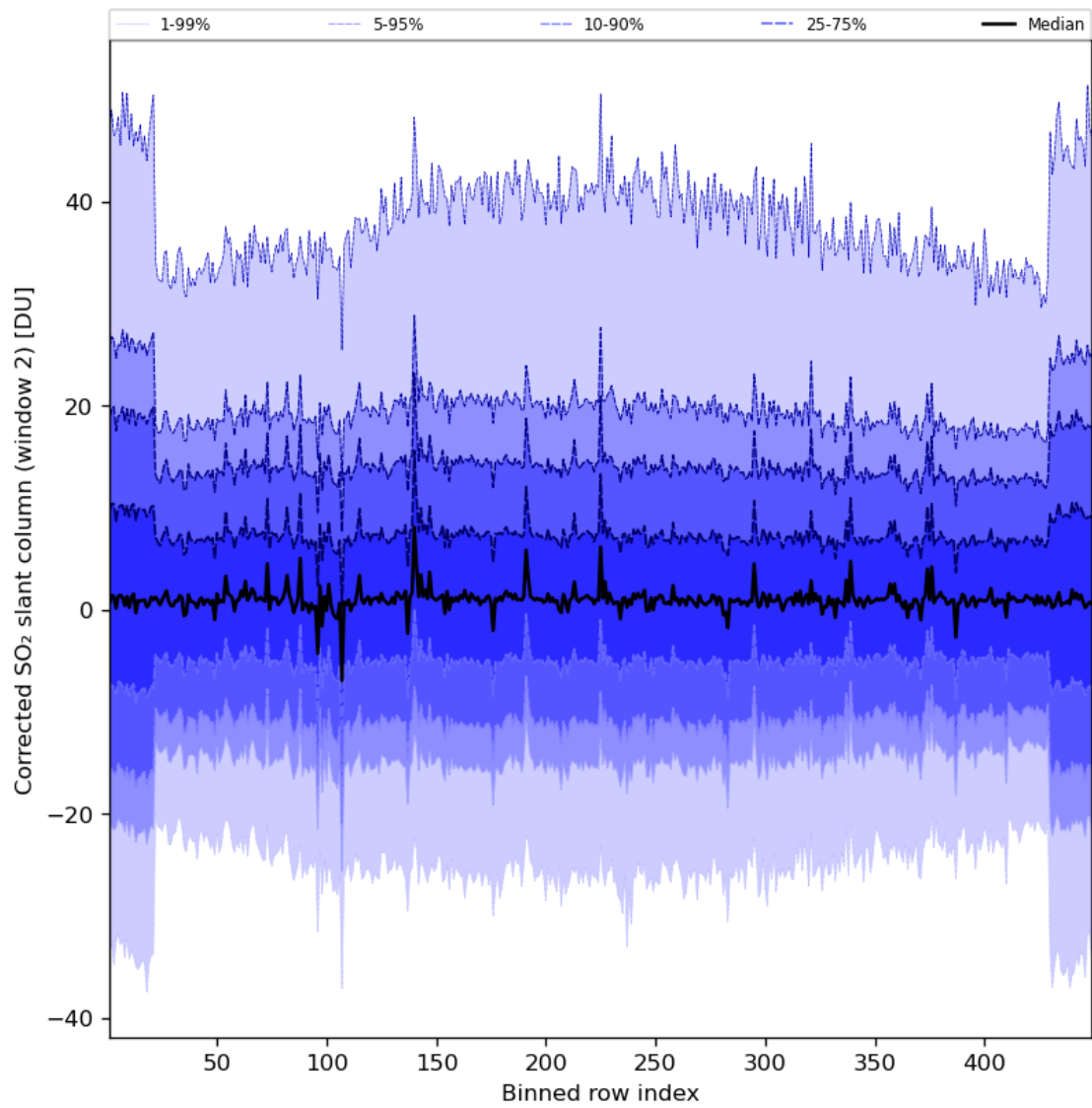
Figure 85: Along track statistics of “Corrected SO 2 slant column (window 2)” for 2024-07-26 to 2024-07-27
