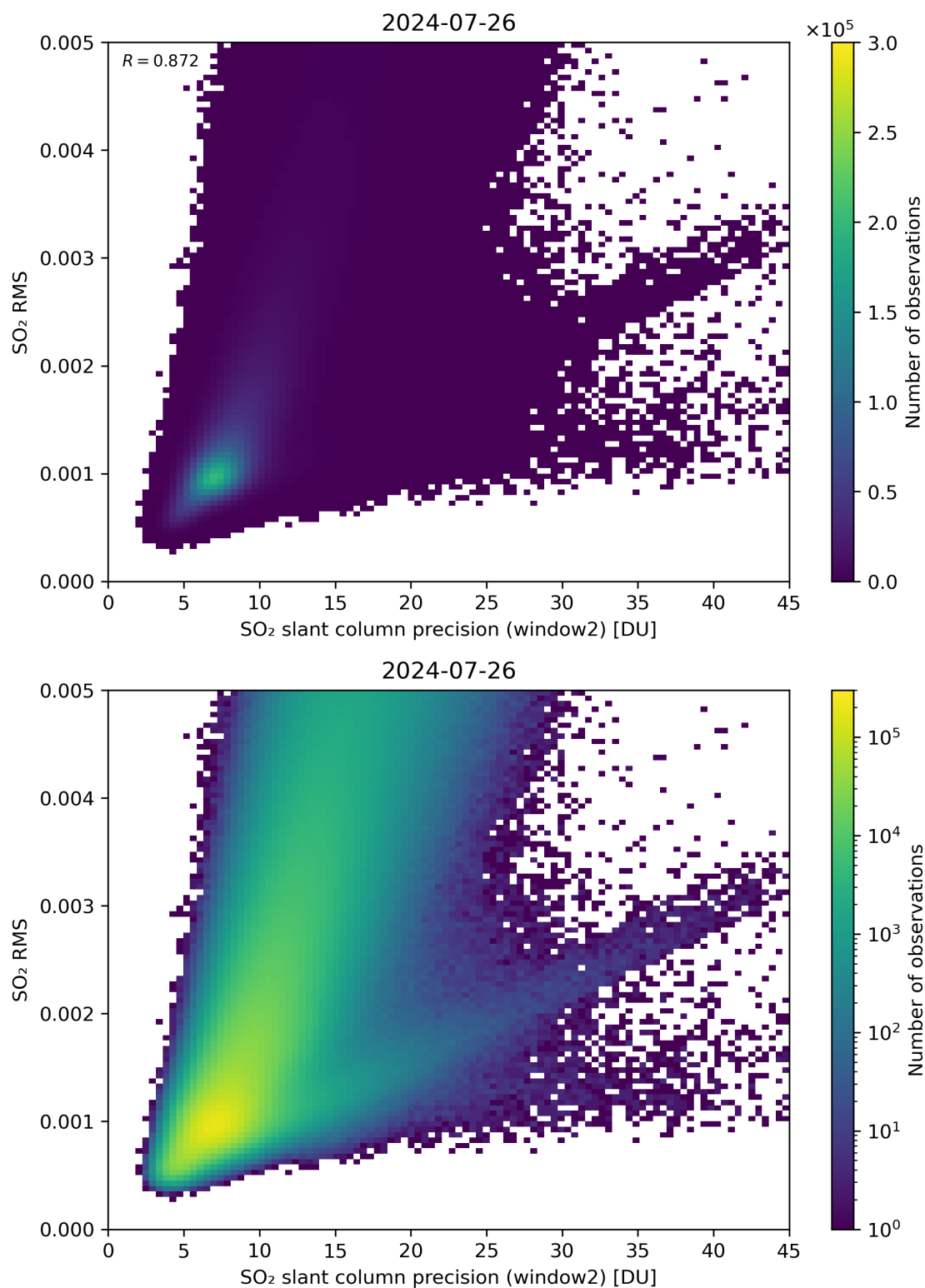
Figure 245: Scatter density plot of “SO 2 slant column precision (window2)” against “SO 2 RMS” for 2024-07-26 to 2024-07-27.
