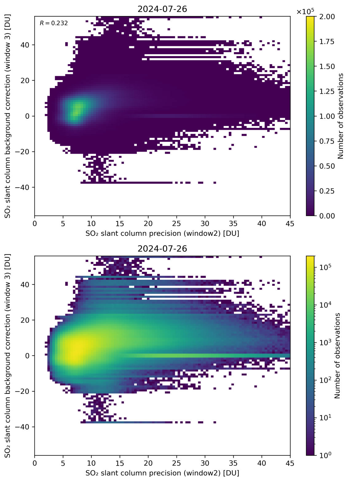
Figure 242: Scatter density plot of “SO 2 slant column precision (window2)” against “SO 2 slant column background correction (window 3)” for 2024-07-26 to 2024-07-27.
