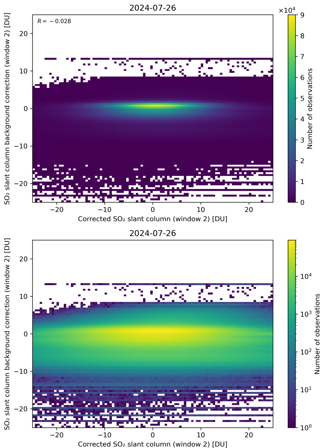
Figure 194: Scatter density plot of “Corrected SO 2 slant column (window 2)” against “SO 2 slant column background correction (window 2)” for 2024-07-26 to 2024-07-27.
