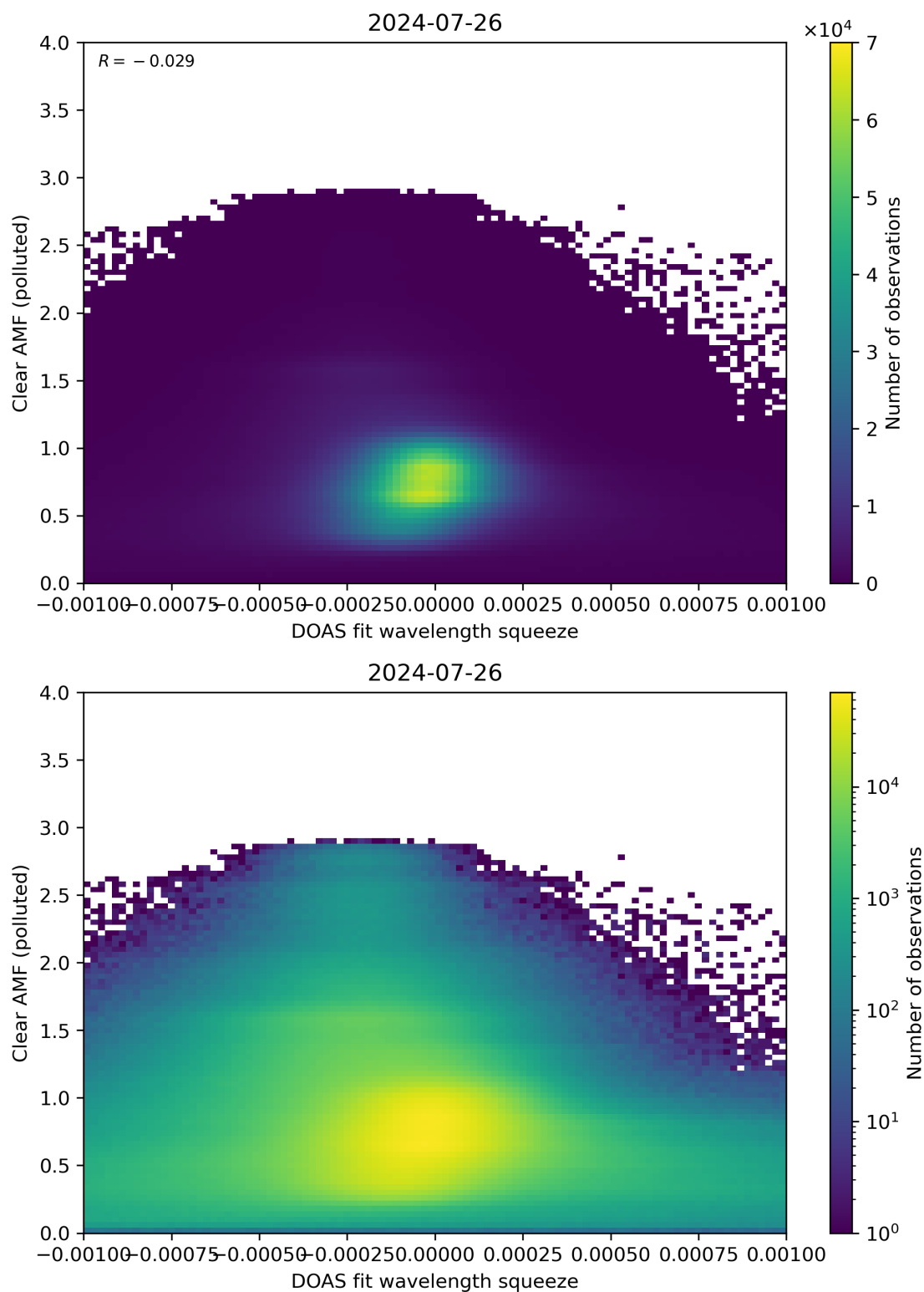
Figure 133: Scatter density plot of “DOAS fit wavelength squeeze” against “Clear AMF (polluted)” for 2024-07-26 to 2024-07-27.
