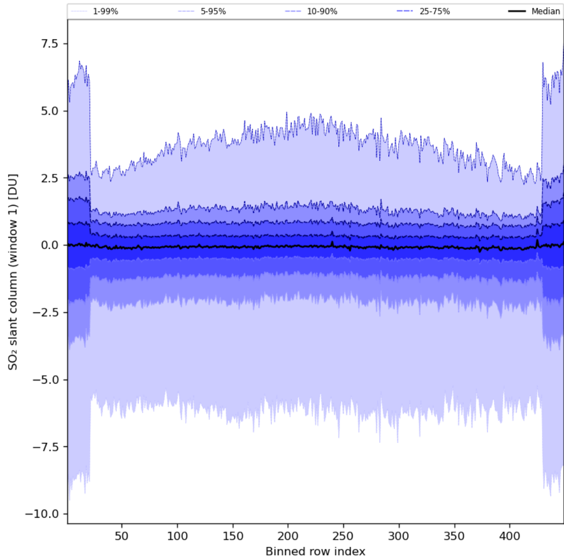
Figure 79: Along track statistics of “SO 2 slant column (window 1)” for 2024-07-26 to 2024-07-27
