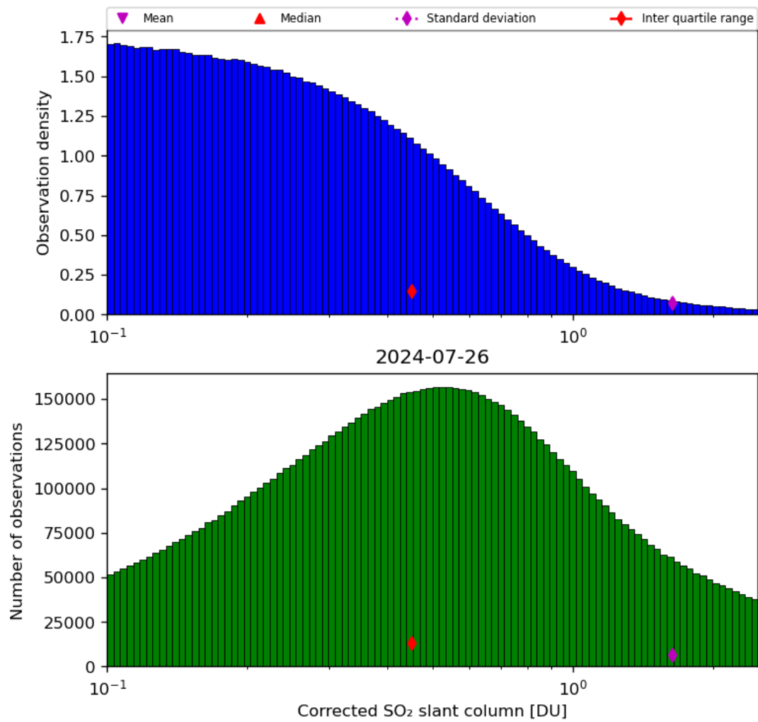
Figure 55: Histogram of “Corrected SO 2 slant column” for 2024-07-26 to 2024-07-27
