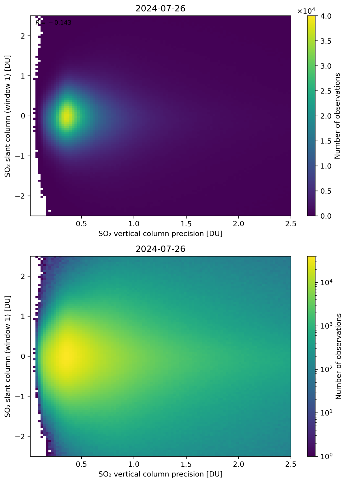
Figure 289: Scatter density plot of “SO 2 vertical column precision” against “SO 2 slant column (window 1)” for 2024-07-26 to 2024-07-27.
