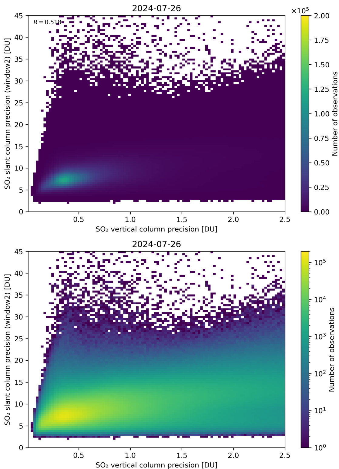
Figure 291: Scatter density plot of “SO 2 vertical column precision” against “SO 2 slant column precision (window2)” for 2024-07-26 to 2024-07-27.
