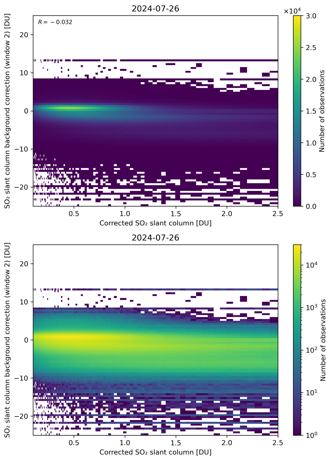
Figure 179: Scatter density plot of “Corrected SO 2 slant column” against “SO 2 slant column background correction (window 2)” for 2024-07-26 to 2024-07-27.
