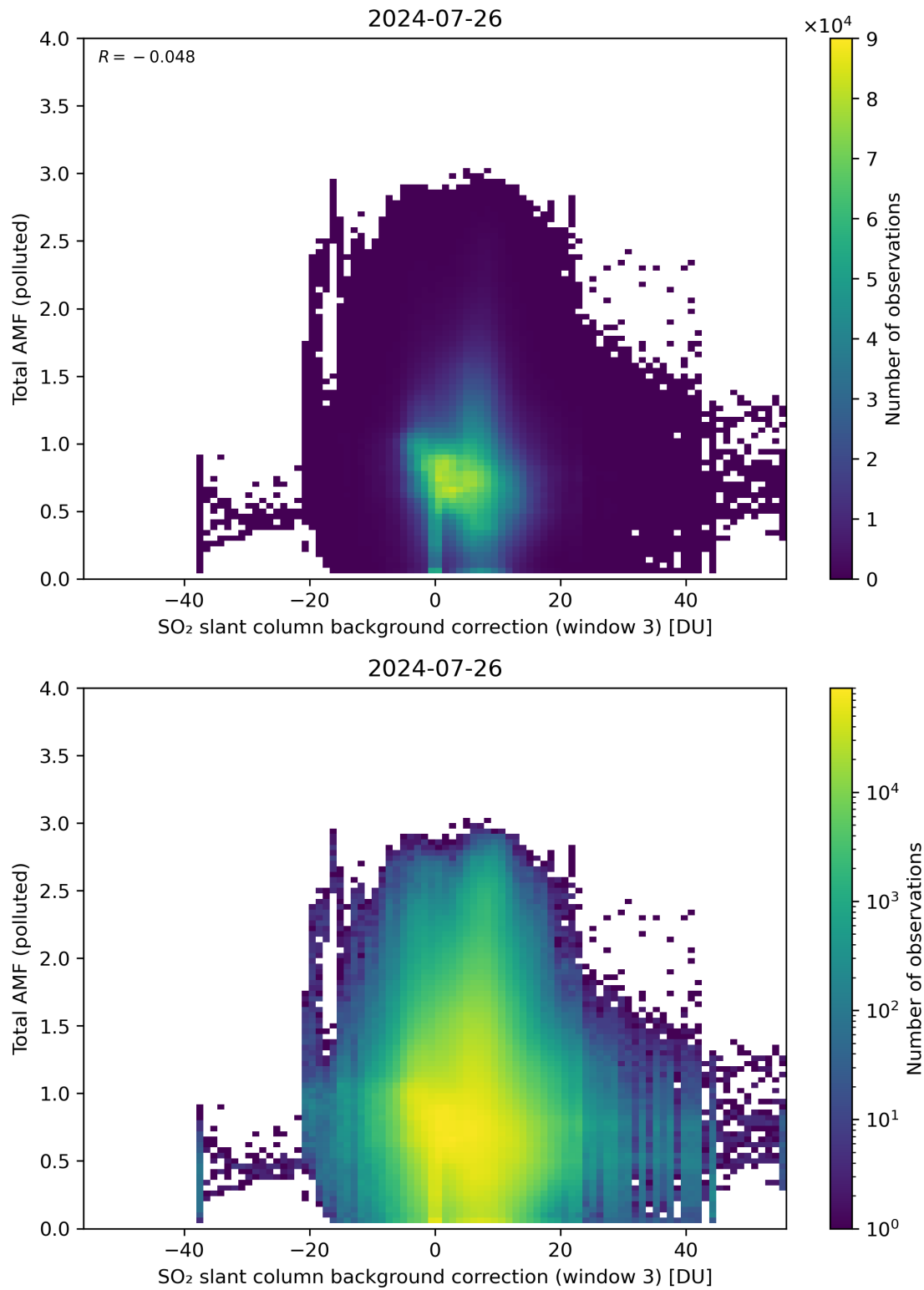
Figure 125: Scatter density plot of “SO 2 slant column background correction (window 3)” against “Total AMF (polluted)” for 2024-07-26 to 2024-07-27.
