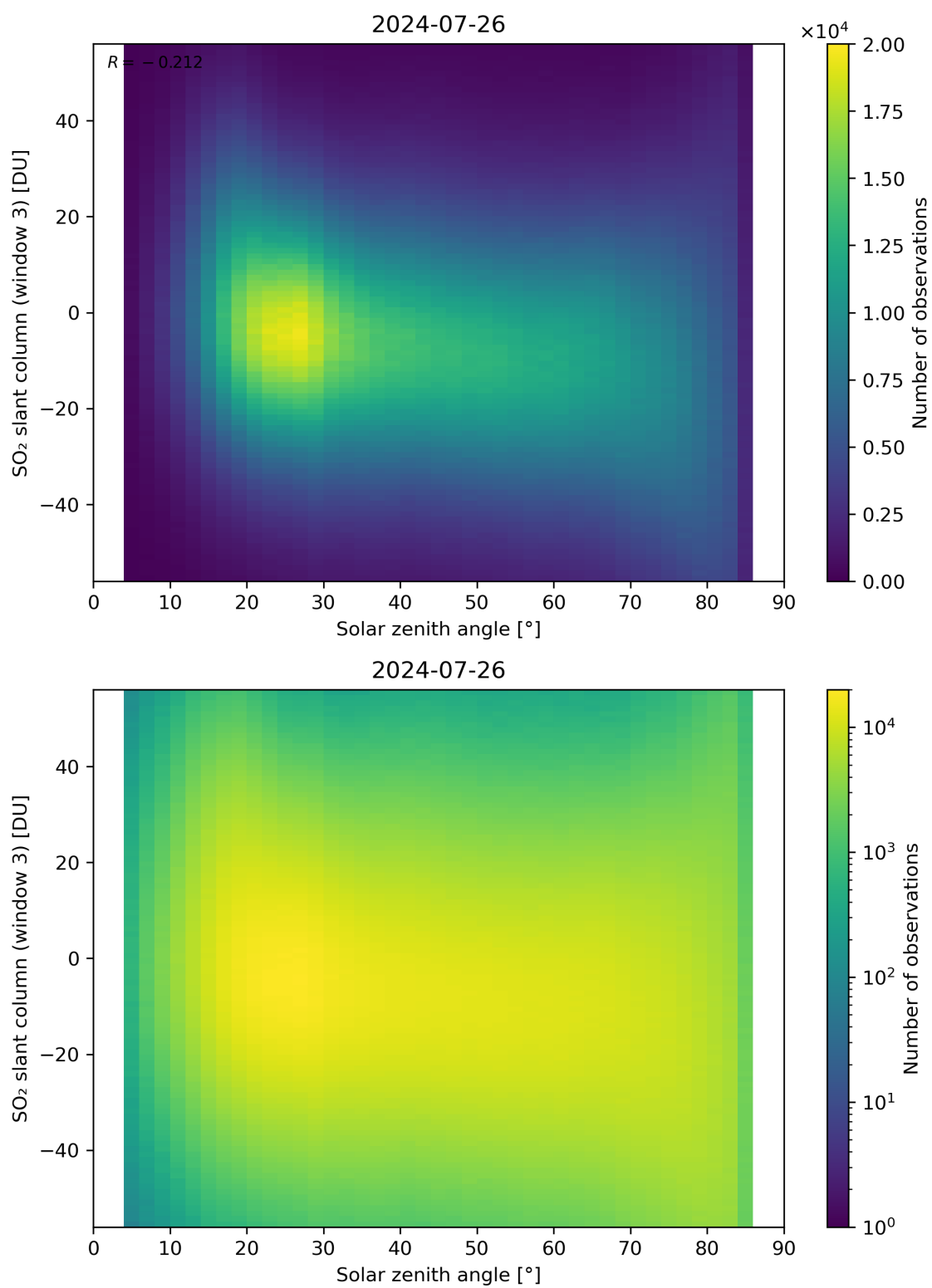
Figure 172: Scatter density plot of “Solar zenith angle” against “SO 2 slant column (window 3)” for 2024-07-26 to 2024-07-27.
