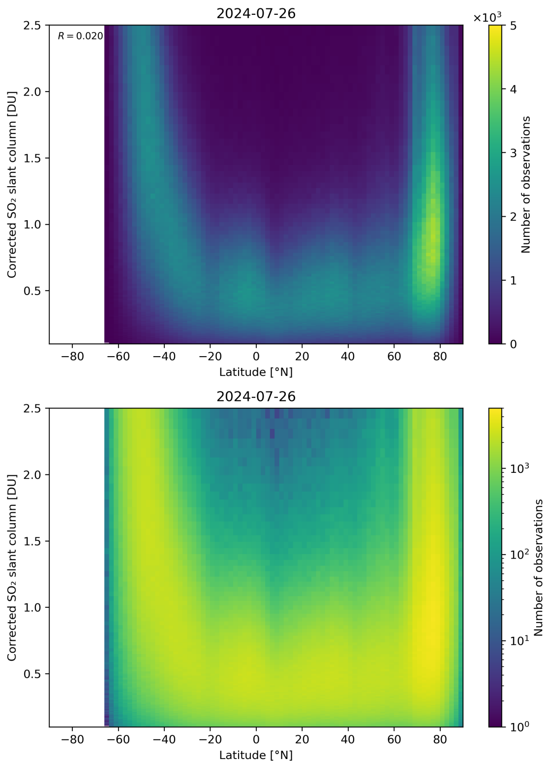
Figure 146: Scatter density plot of “Latitude” against “Corrected SO 2 slant column” for 2024-07-26 to 2024-07-27.
