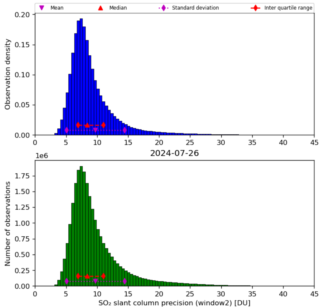
Figure 61: Histogram of “SO 2 slant column precision (window2)” for 2024-07-26 to 2024-07-27
