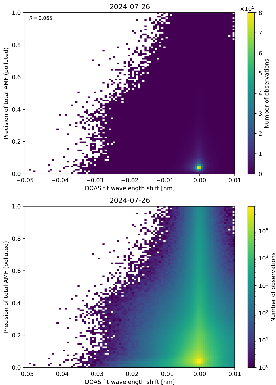
Figure 131: Scatter density plot of “DOAS fit wavelength shift” against “Precision of total AMF (polluted)” for 2024-07-26 to 2024-07-27.
