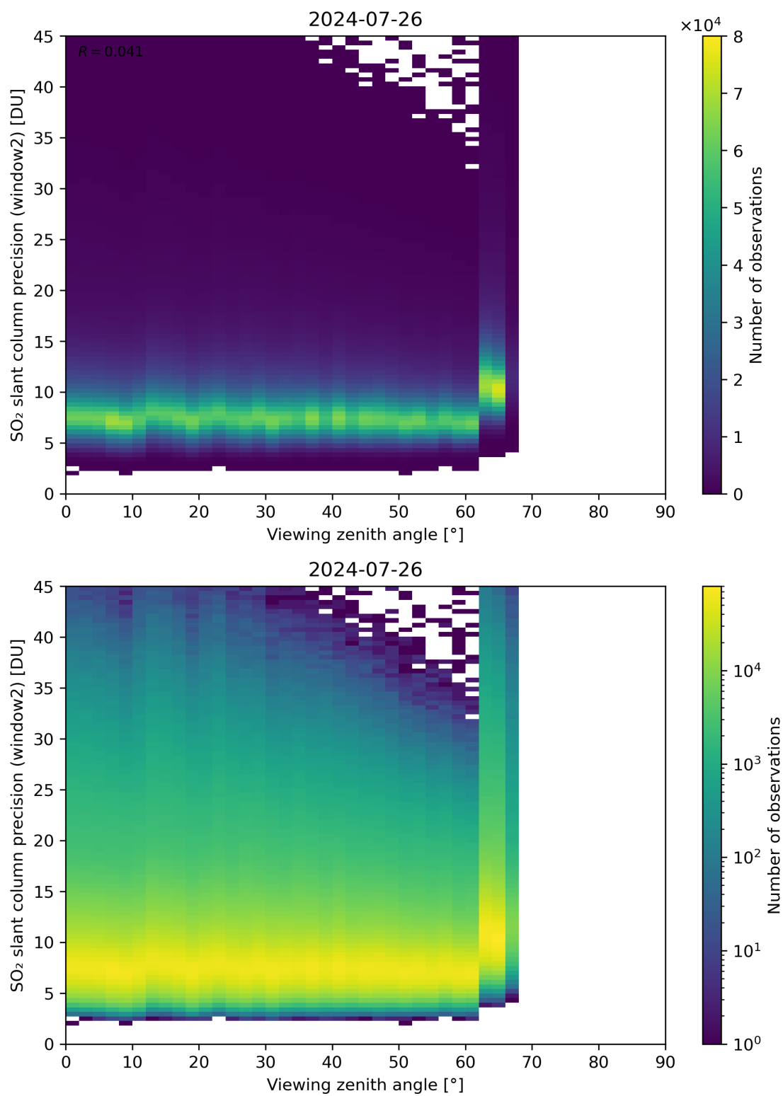
Figure 322: Scatter density plot of “Viewing zenith angle” against “SO 2 slant column precision (window2)” for 2024-07-26 to 2024-07-27.
