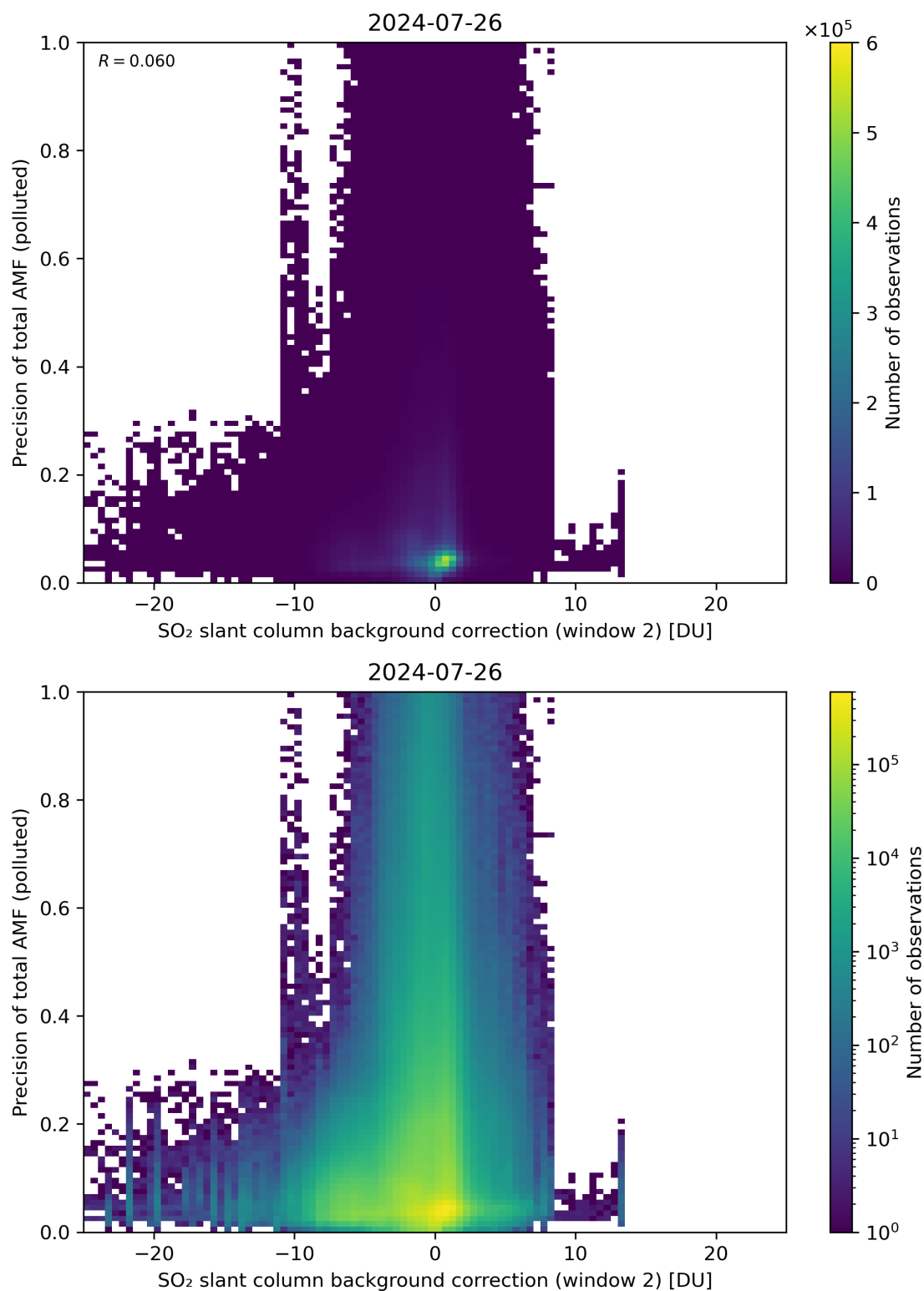
Figure 120: Scatter density plot of “SO 2 slant column background correction (window 2)” against “Precision of total AMF (polluted)” for 2024-07-26 to 2024-07-27.
