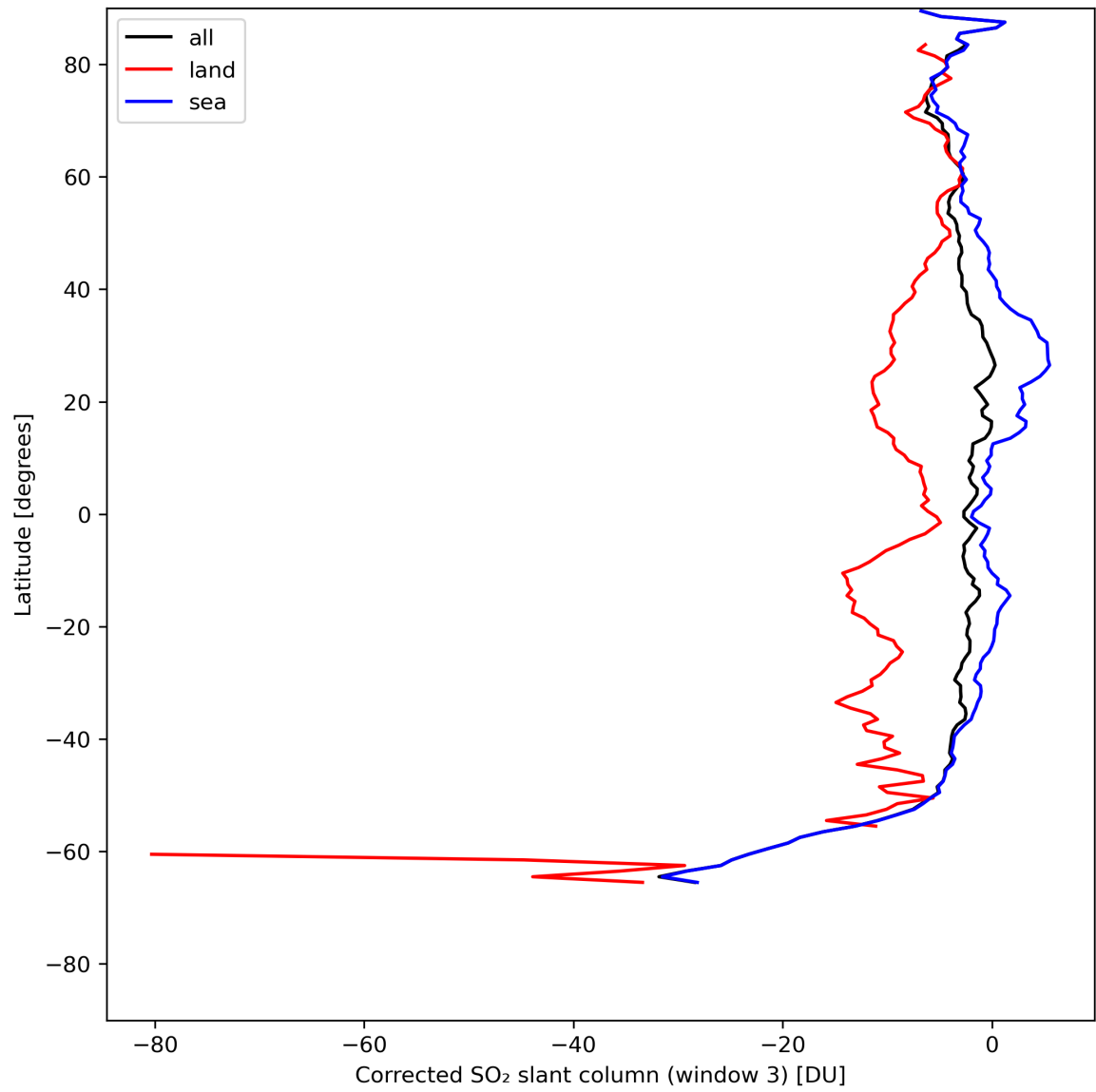
Figure 43: Zonal average of “Corrected SO 2 slant column (window 3)” for 2024-07-26 to 2024-07-27.
