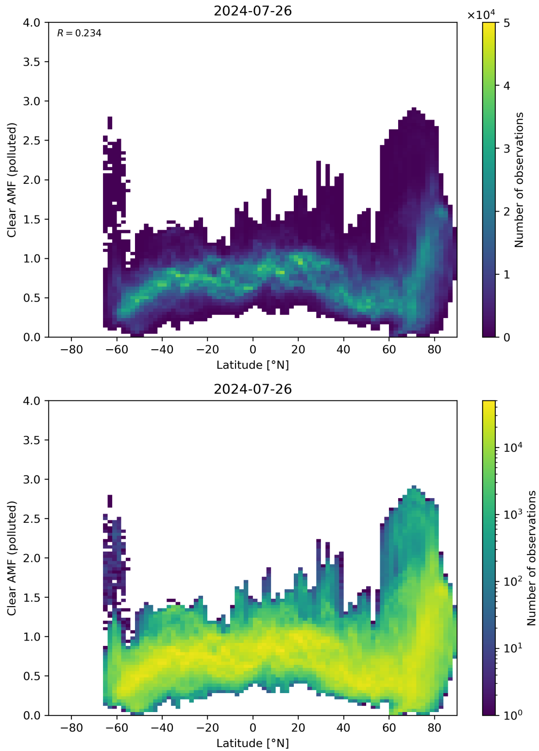
Figure 145: Scatter density plot of “Latitude” against “Clear AMF (polluted)” for 2024-07-26 to 2024-07-27.
