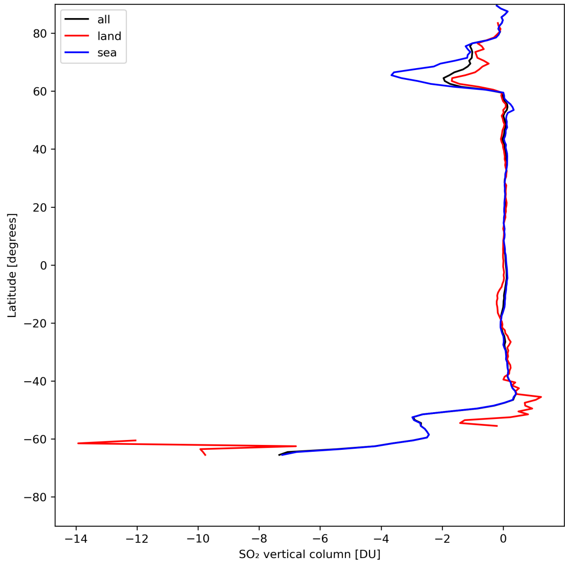
Figure 30: Zonal average of “SO 2 vertical column” for 2024-07-26 to 2024-07-27.
