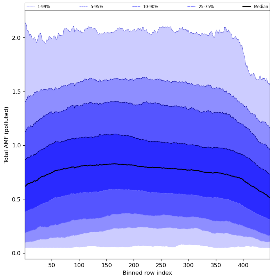
Figure 94: Along track statistics of “Total AMF (polluted)” for 2024-07-26 to 2024-07-27
