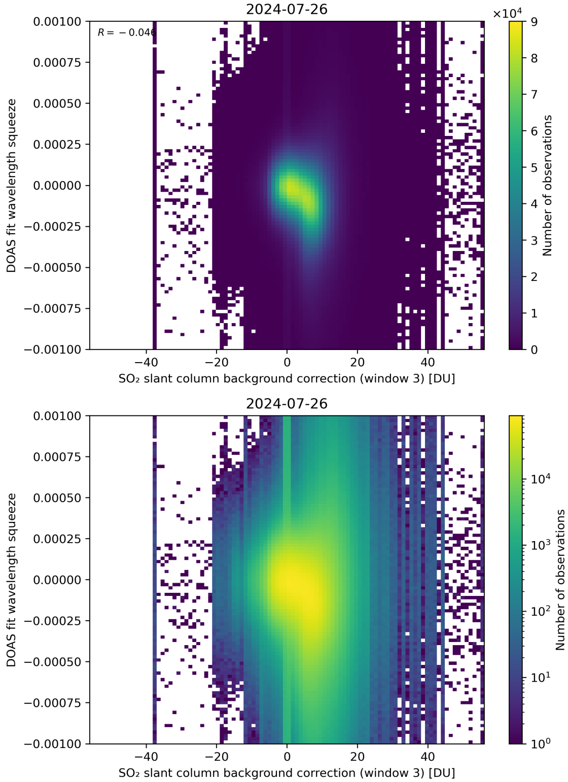
Figure 122: Scatter density plot of “SO 2 slant column background correction (window 3)” against “DOAS fit wavelength squeeze” for 2024-07-26 to 2024-07-27.
