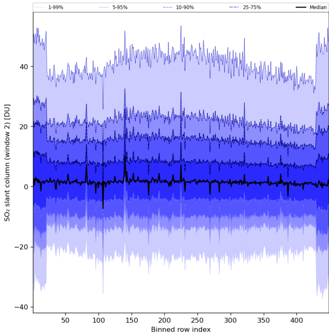
Figure 83: Along track statistics of “SO 2 slant column (window 2)” for 2024-07-26 to 2024-07-27
