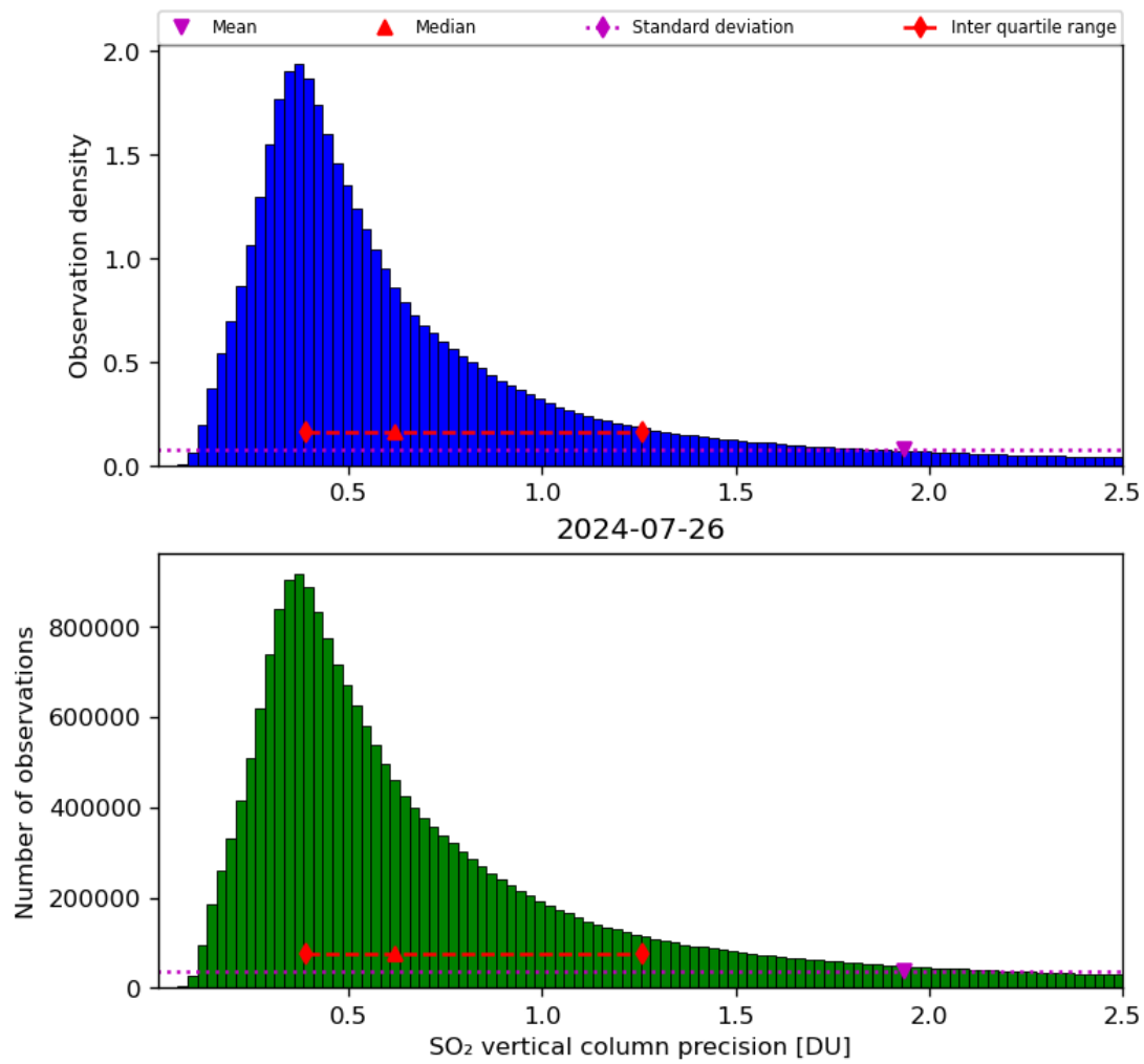
Figure 54: Histogram of “SO 2 vertical column precision” for 2024-07-26 to 2024-07-27
