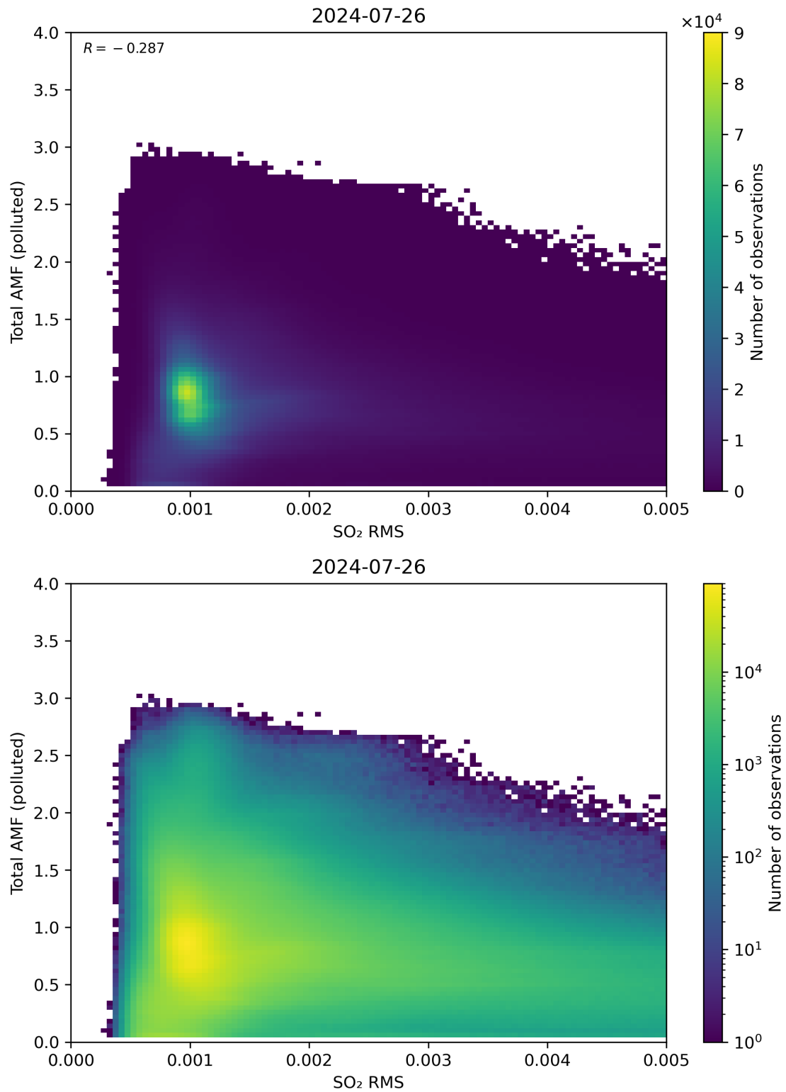
Figure 137: Scatter density plot of “SO 2 RMS” against “Total AMF (polluted)” for 2024-07-26 to 2024-07-27.
