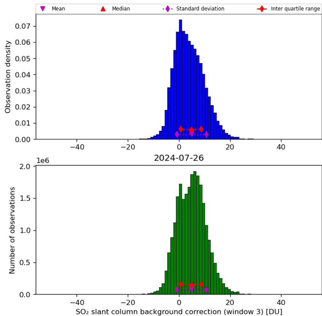
Figure 67: Histogram of “SO 2 slant column background correction (window 3)” for 2024-07-26 to 2024-07-27
