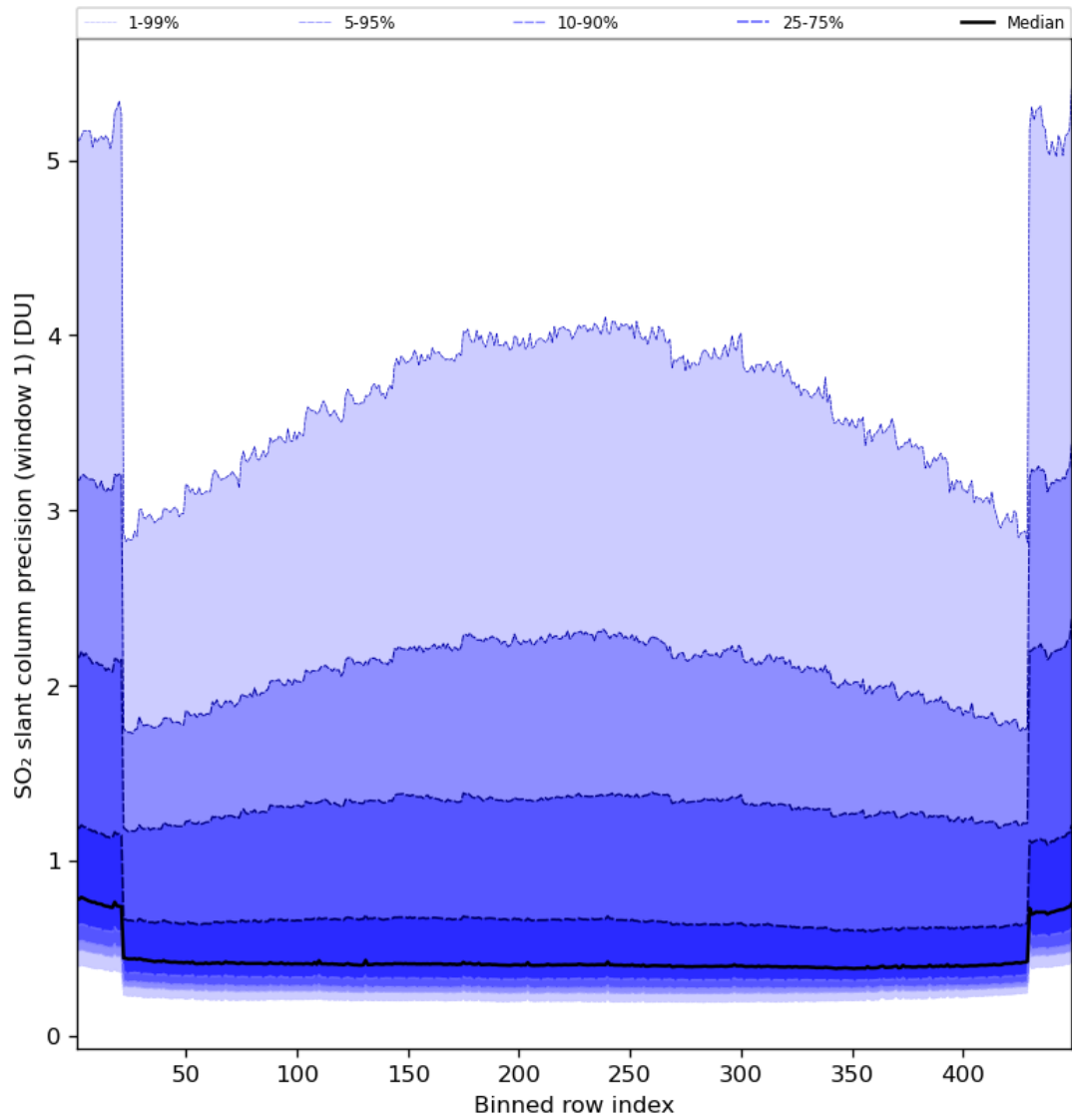
Figure 80: Along track statistics of “SO 2 slant column precision (window 1)” for 2024-07-26 to 2024-07-27
