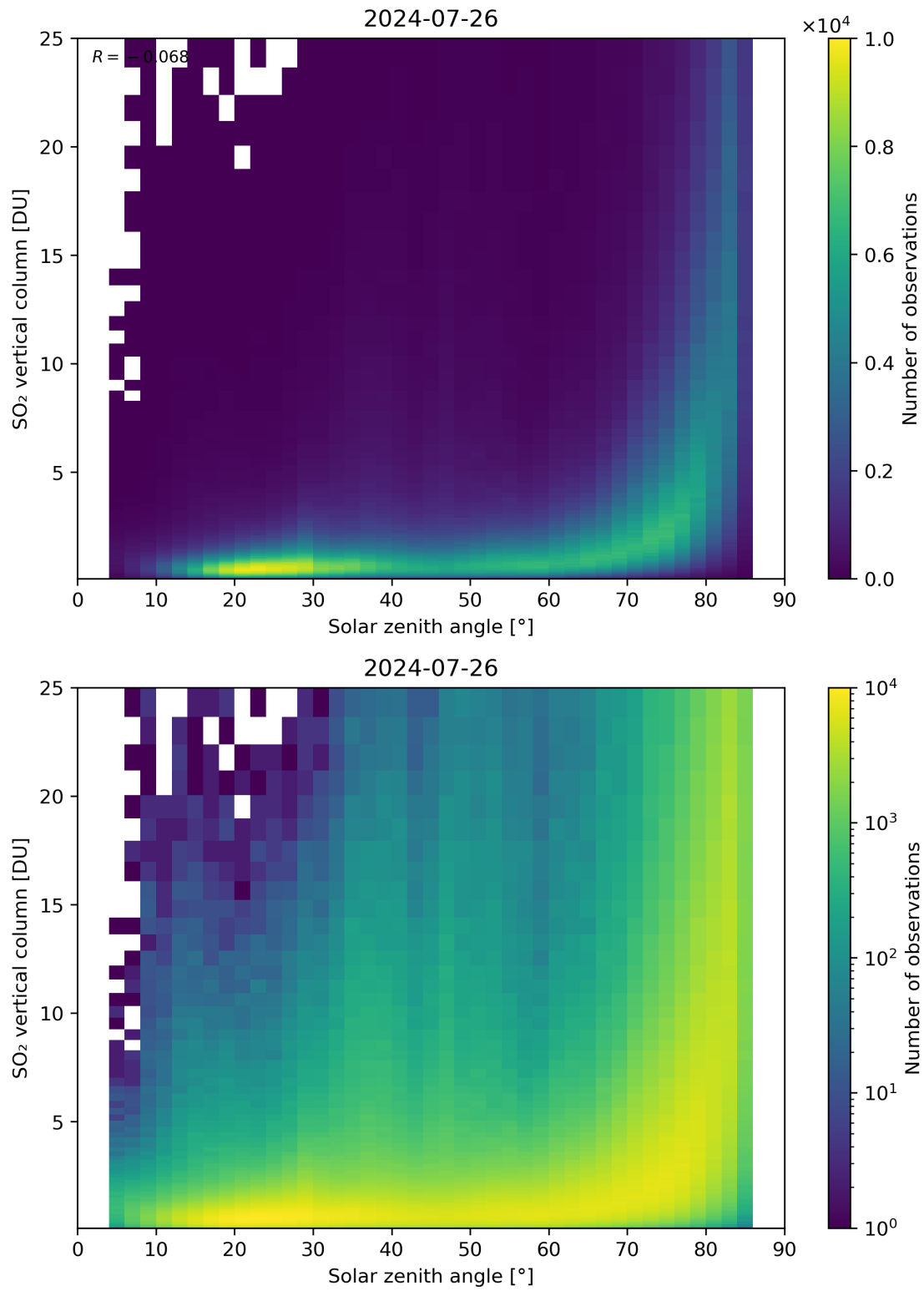
Figure 176: Scatter density plot of “Solar zenith angle” against “SO 2 vertical column” for 2024-07-26 to 2024-07-27.
