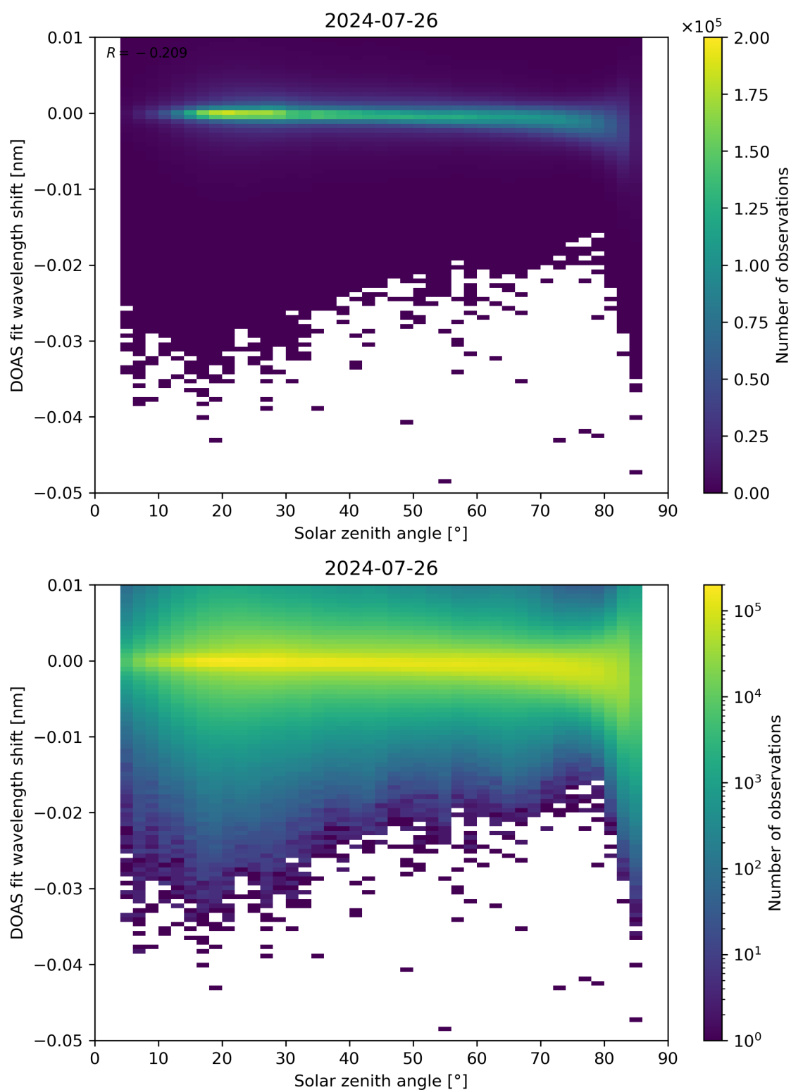
Figure 161: Scatter density plot of “Solar zenith angle” against “DOAS fit wavelength shift” for 2024-07-26 to 2024-07-27.
