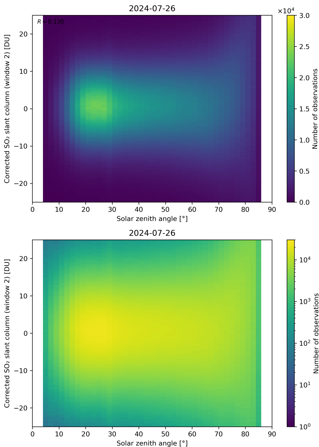
Figure 167: Scatter density plot of “Solar zenith angle” against “Corrected SO 2 slant column (window 2)” for 2024-07-26 to 2024-07-27.
