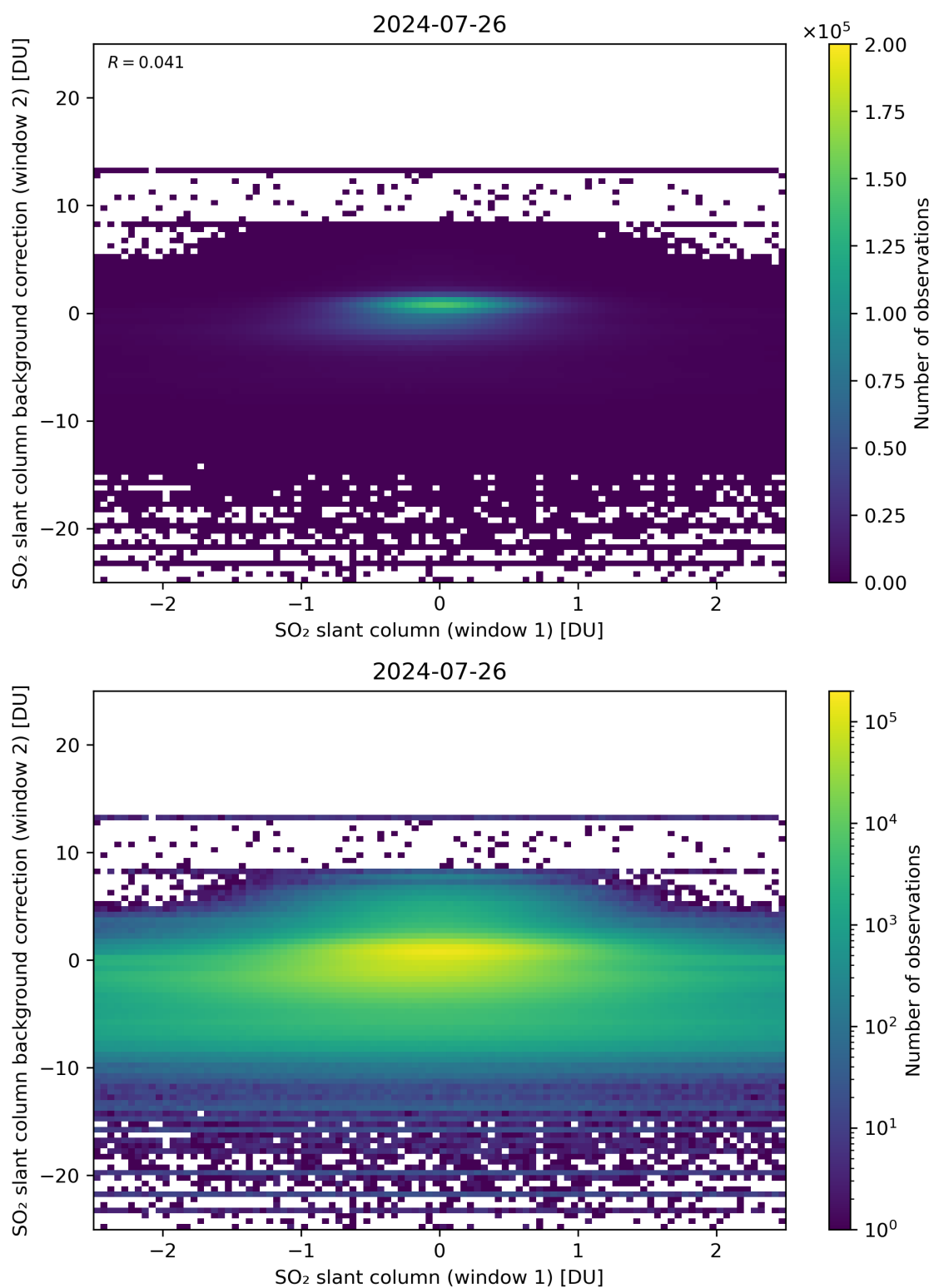
Figure 213: Scatter density plot of “SO 2 slant column (window 1)” against “SO 2 slant column background correction (window 2)” for 2024-07-26 to 2024-07-27.
