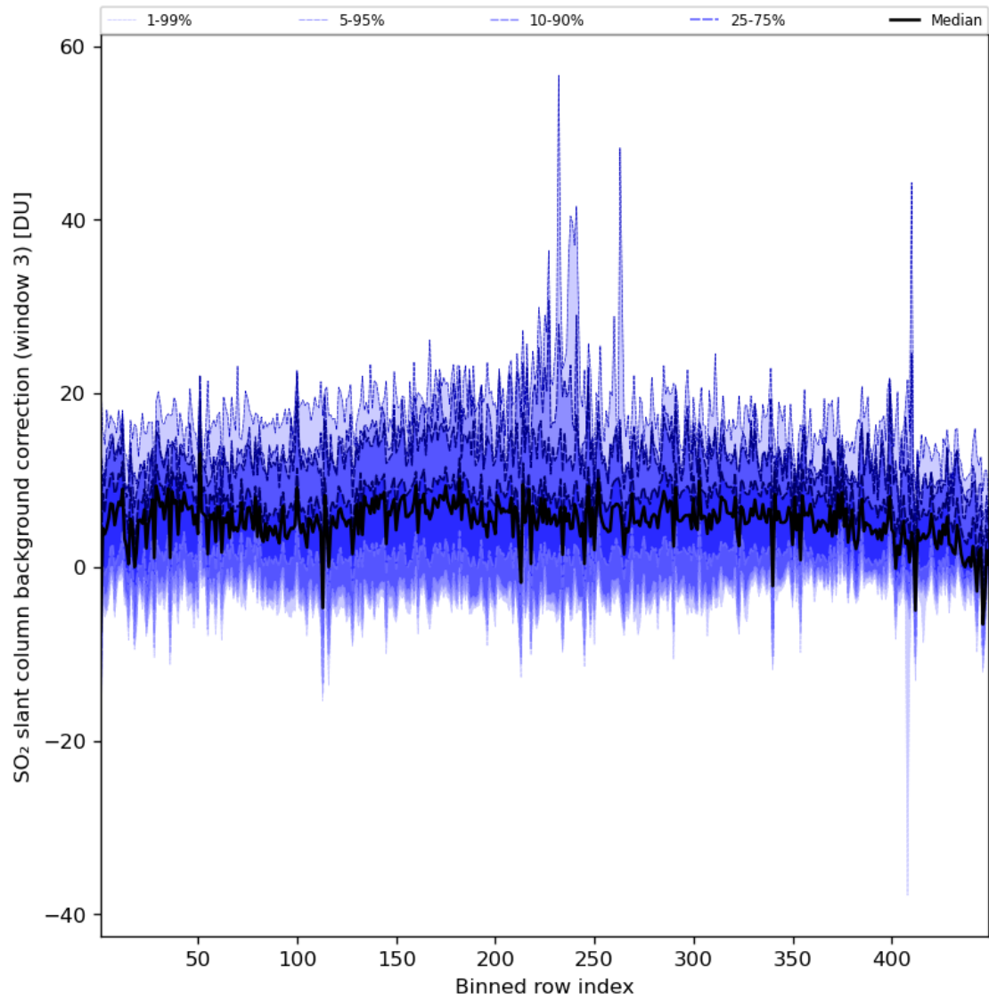
Figure 90: Along track statistics of “SO 2 slant column background correction (window 3)” for 2024-07-26 to 2024-07-27
