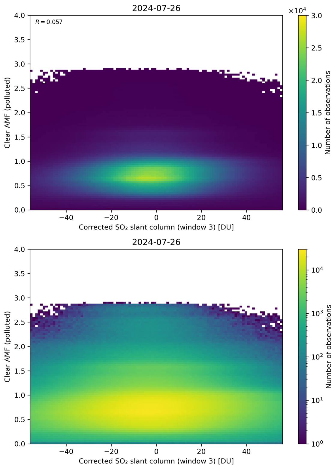
Figure 209: Scatter density plot of “Corrected SO 2 slant column (window 3)” against “Clear AMF (polluted)” for 2024-07-26 to 2024-07-27.
