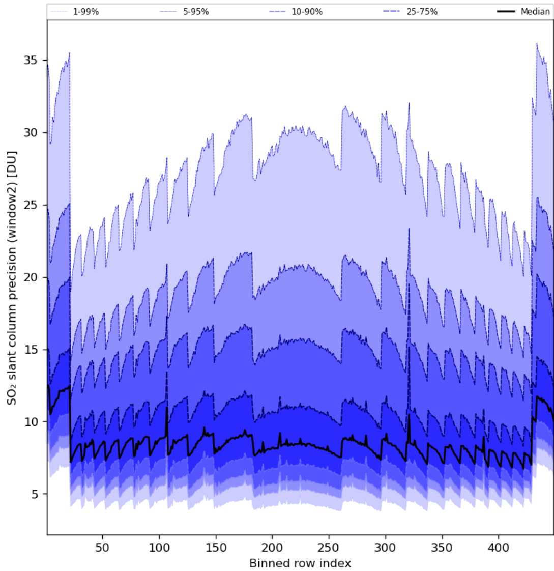
Figure 84: Along track statistics of “SO 2 slant column precision (window2)” for 2024-07-26 to 2024-07-27
