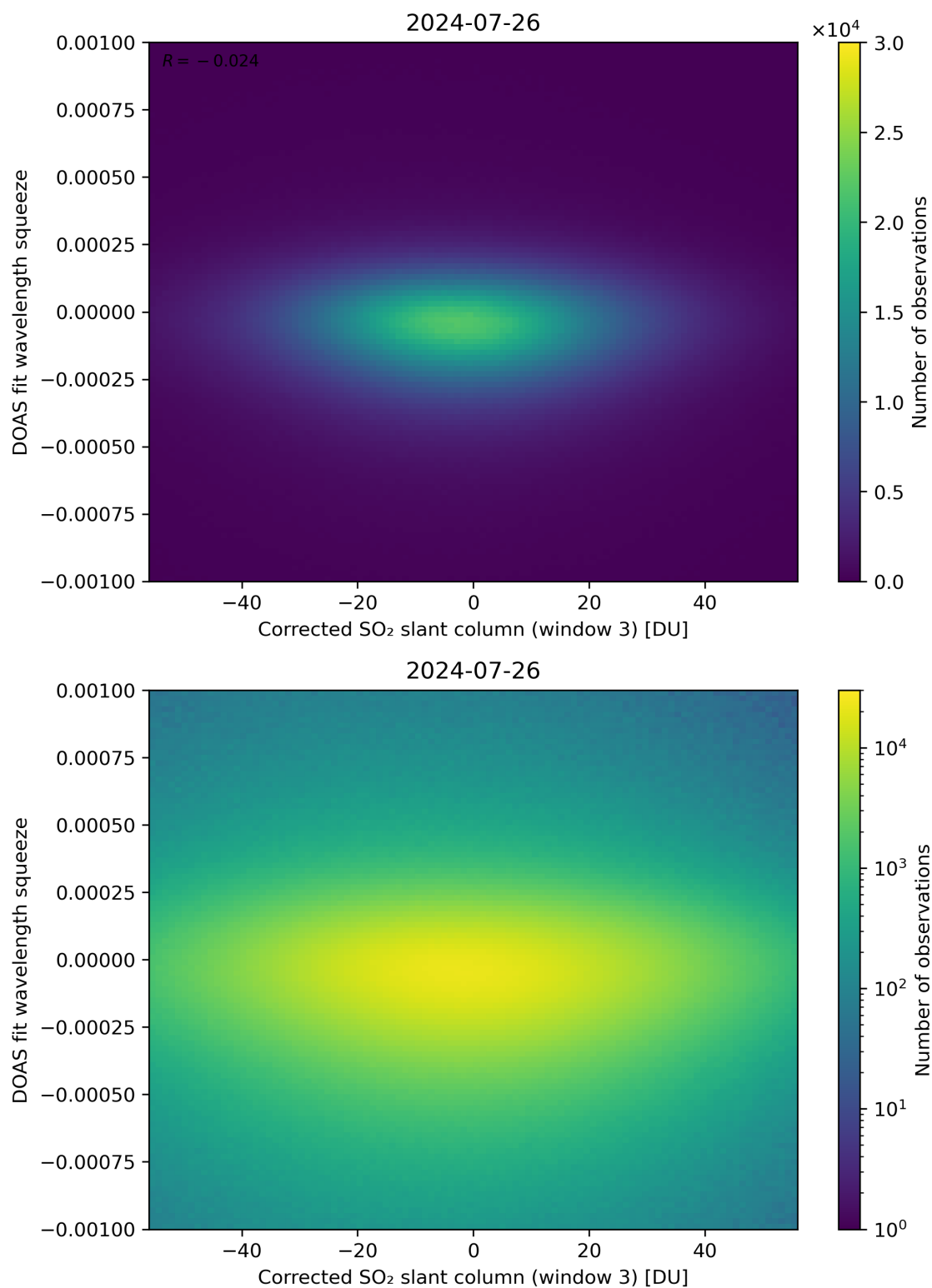
Figure 207: Scatter density plot of “Corrected SO 2 slant column (window 3)” against “DOAS fit wavelength squeeze” for 2024-07-26 to 2024-07-27.
