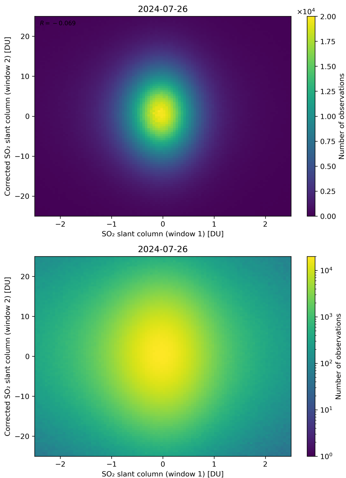
Figure 233: Scatter density plot of “SO 2 slant column (window 1)” against “Corrected SO 2 slant column (window 2)” for 2024-07-26 to 2024-07-27.
