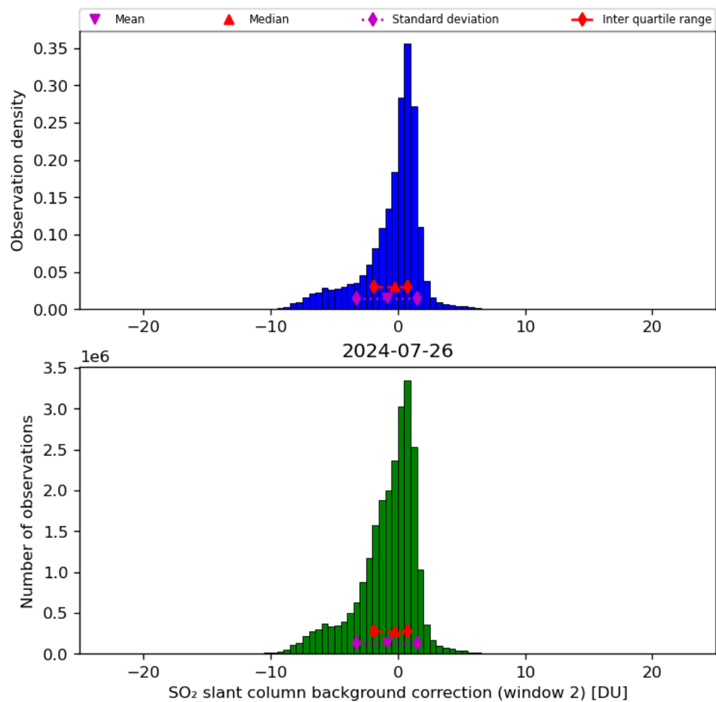
Figure 63: Histogram of “SO 2 slant column background correction (window 2)” for 2024-07-26 to 2024-07-27
