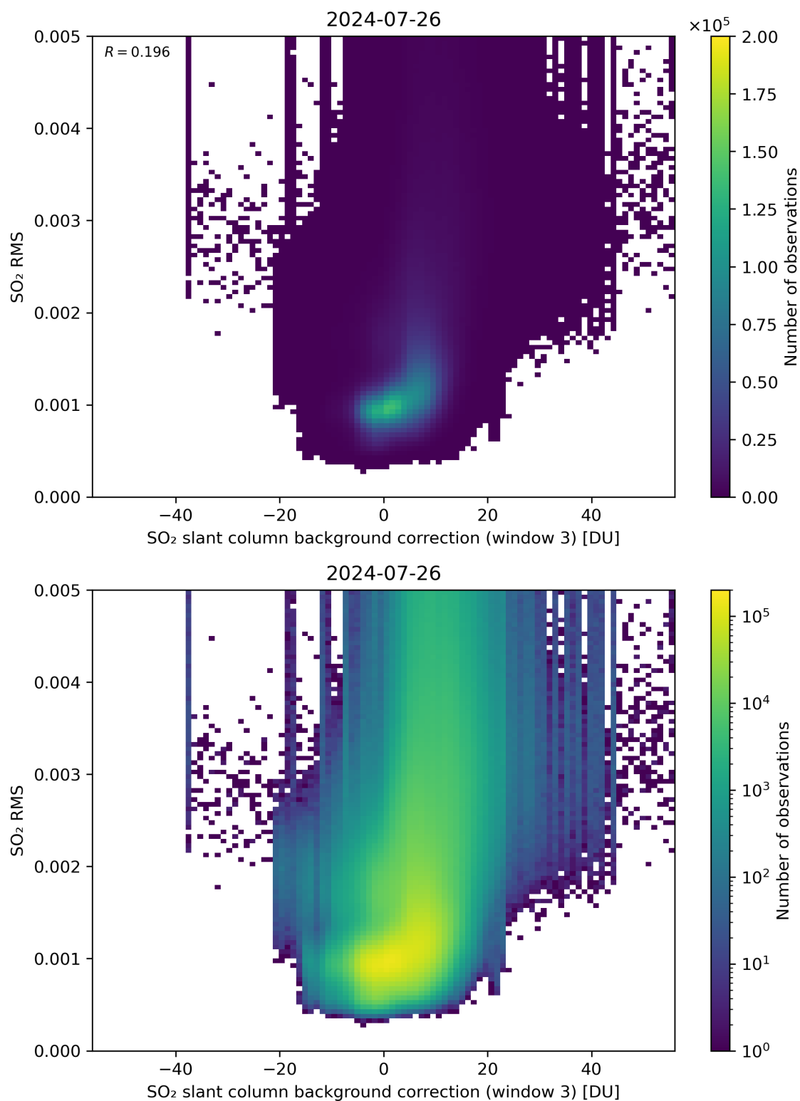
Figure 123: Scatter density plot of “SO 2 slant column background correction (window 3)” against “SO 2 RMS” for 2024-07-26 to 2024-07-27.
