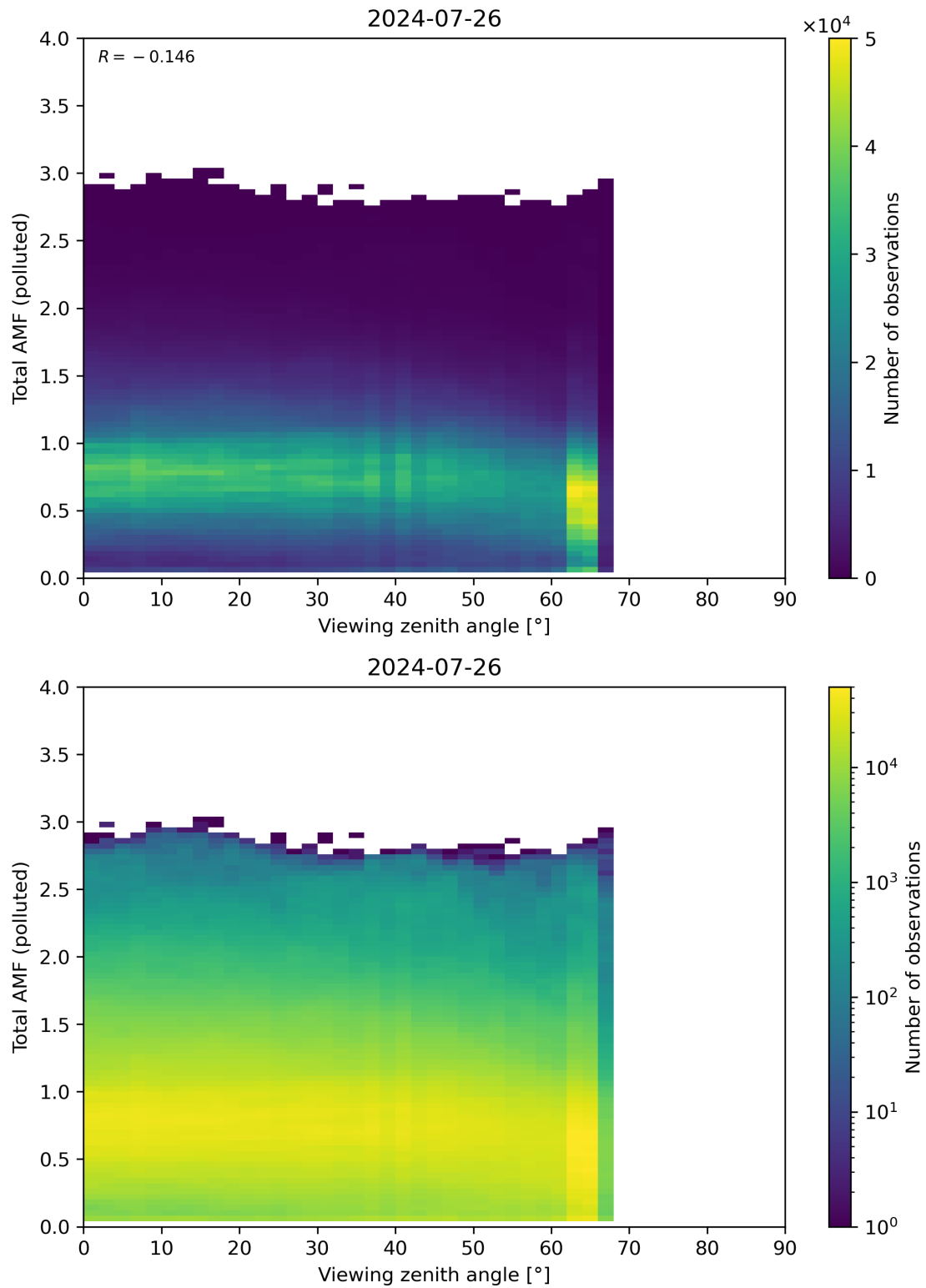
Figure 325: Scatter density plot of “Viewing zenith angle” against “Total AMF (polluted)” for 2024-07-26 to 2024-07-27.
