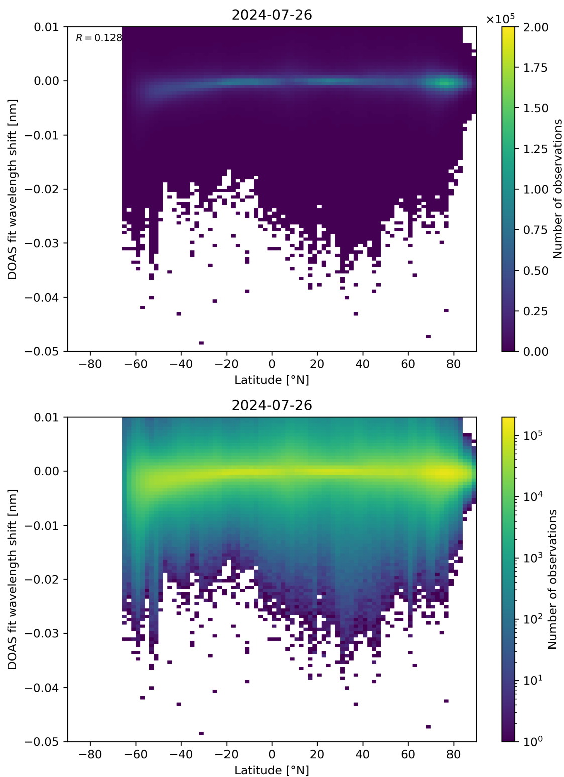
Figure 142: Scatter density plot of “Latitude” against “DOAS fit wavelength shift” for 2024-07-26 to 2024-07-27.
