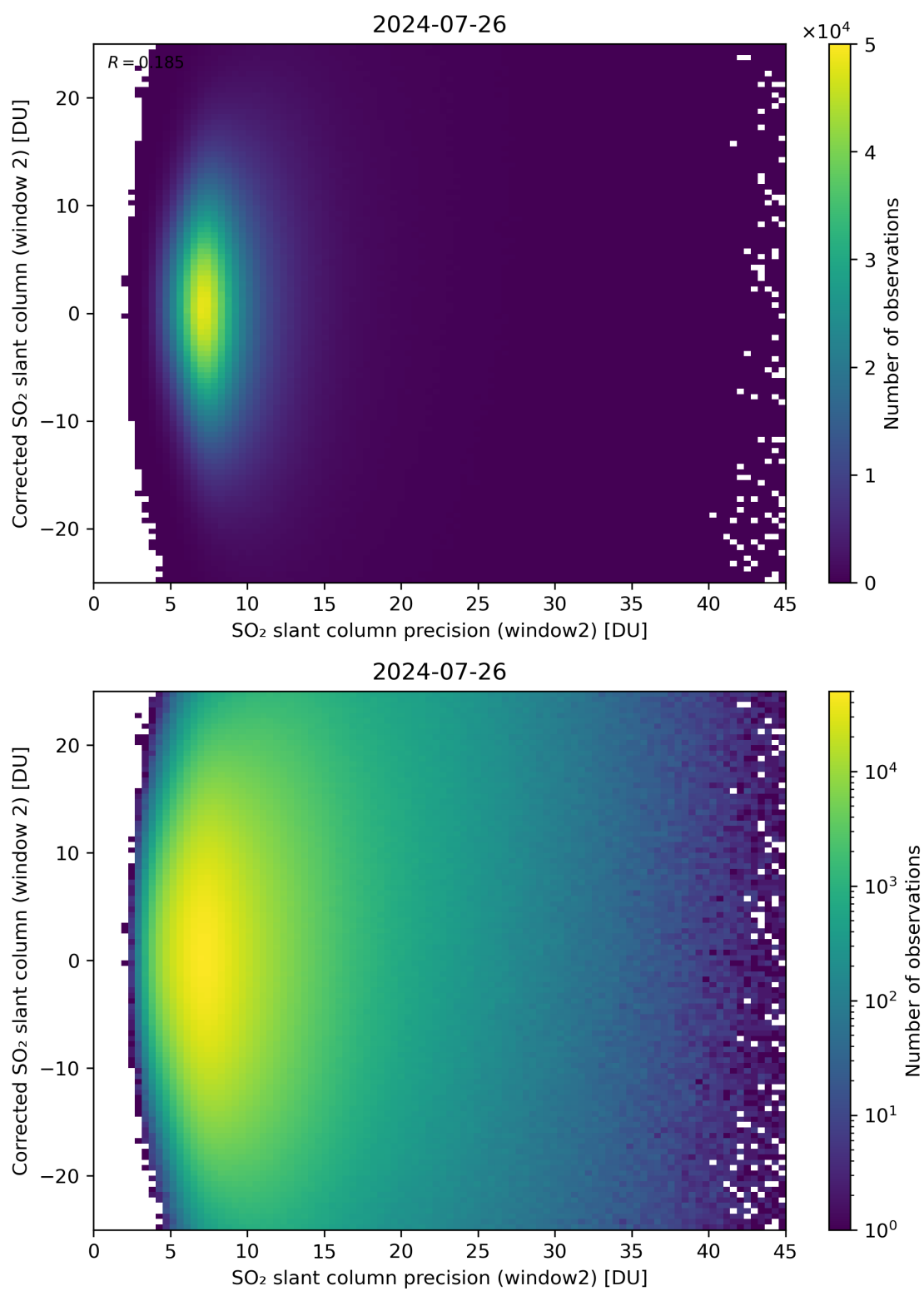
Figure 247: Scatter density plot of “SO 2 slant column precision (window2)” against “Corrected SO 2 slant column (window 2)” for 2024-07-26 to 2024-07-27.
