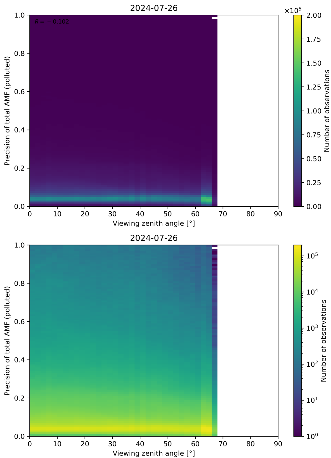
Figure 326: Scatter density plot of “Viewing zenith angle” against “Precision of total AMF (polluted)” for 2024-07-26 to 2024-07-27.
