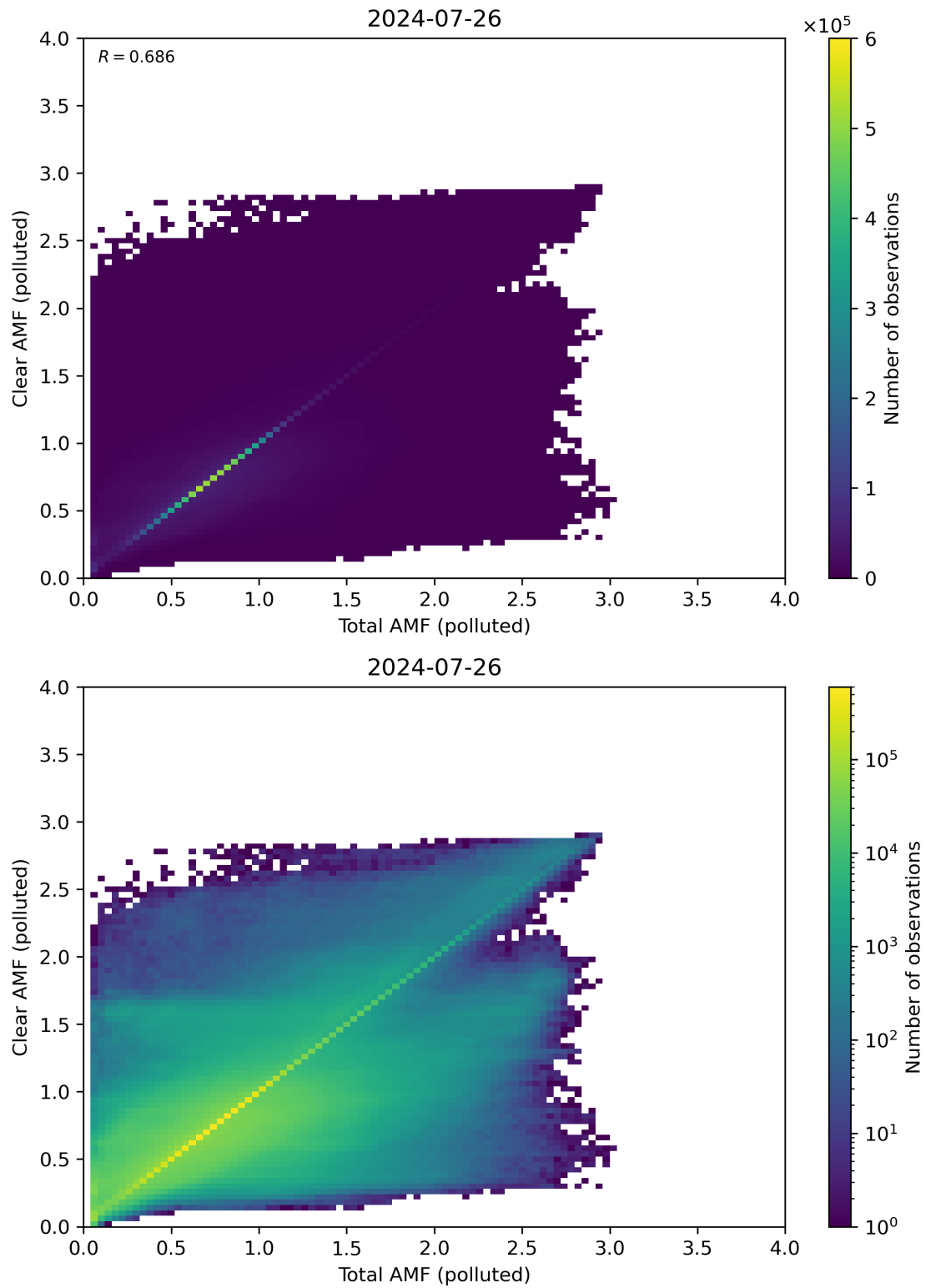
Figure 271: Scatter density plot of “Total AMF (polluted)” against “Clear AMF (polluted)” for 2024-07-26 to 2024-07-27.
