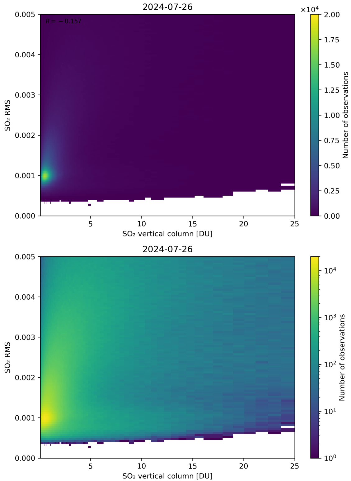
Figure 278: Scatter density plot of “SO 2 vertical column” against “SO 2 RMS” for 2024-07-26 to 2024-07-27.
