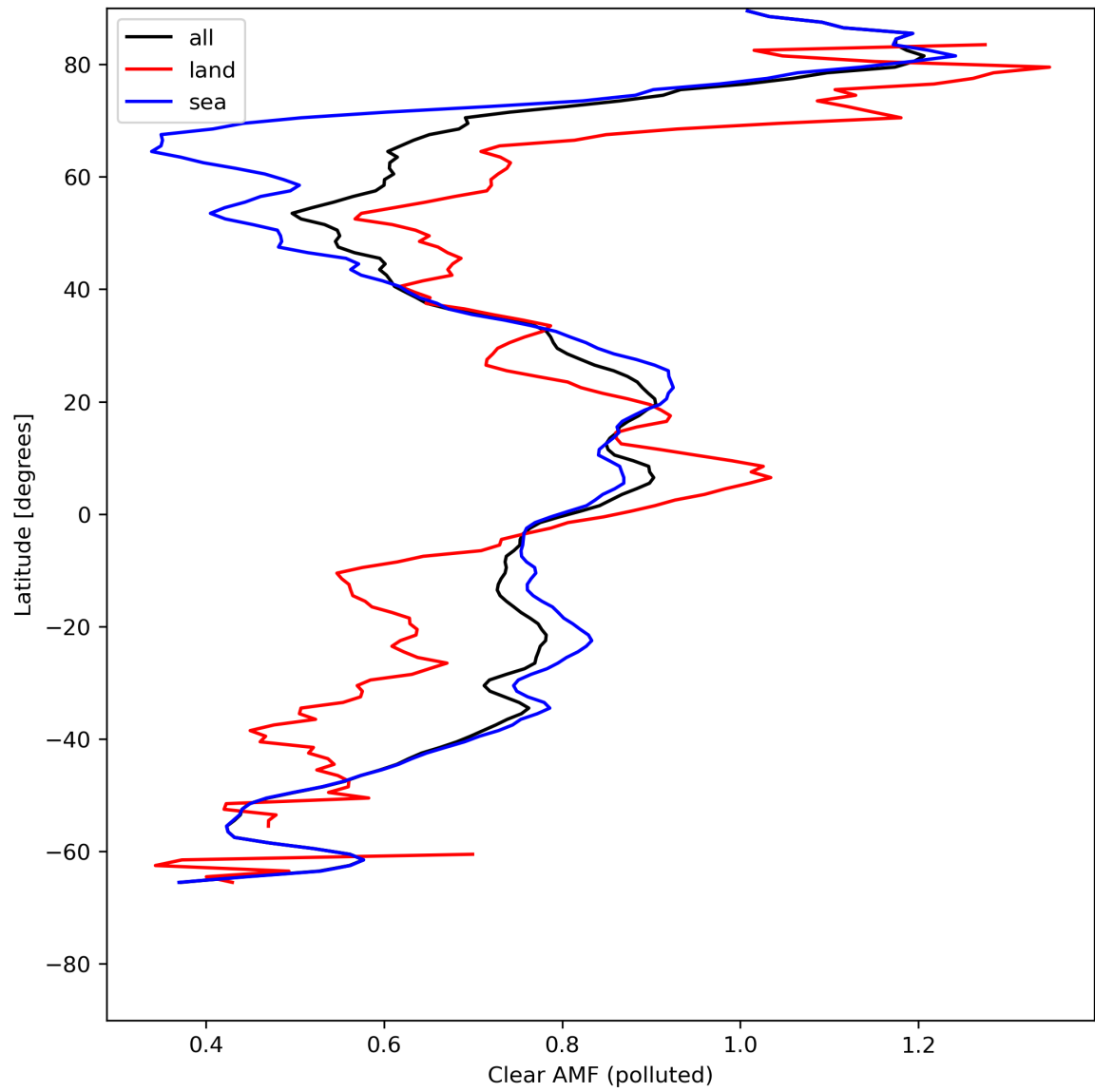
Figure 50: Zonal average of “Clear AMF (polluted)” for 2024-07-26 to 2024-07-27.
