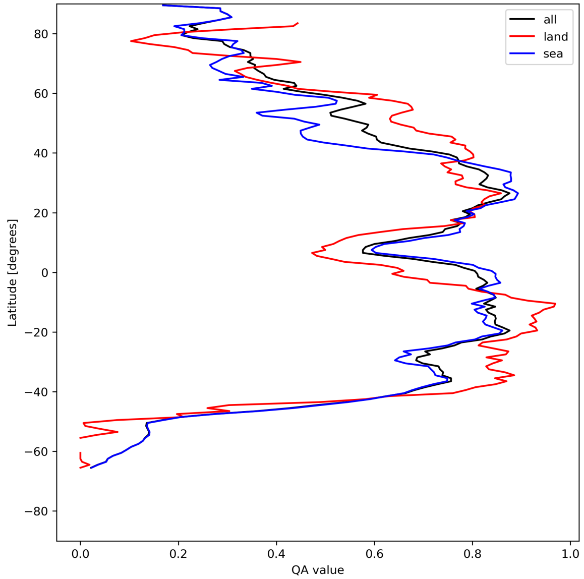
Figure 29: Zonal average of “QA value” for 2024-07-26 to 2024-07-27.
