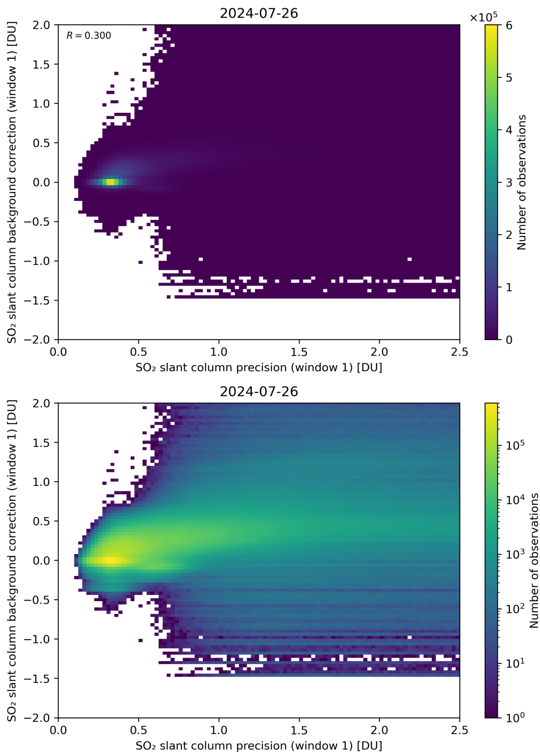
Figure 218: Scatter density plot of “SO 2 slant column precision (window 1)” against “SO 2 slant column background correction (window 1)” for 2024-07-26 to 2024-07-27.
