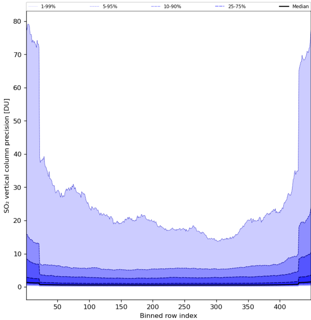
Figure 77: Along track statistics of “SO 2 vertical column precision” for 2024-07-26 to 2024-07-27
