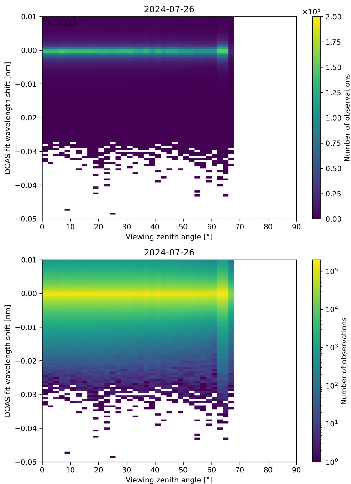
Figure 311: Scatter density plot of “Viewing zenith angle” against “DOAS fit wavelength shift” for 2024-07-26 to 2024-07-27.
