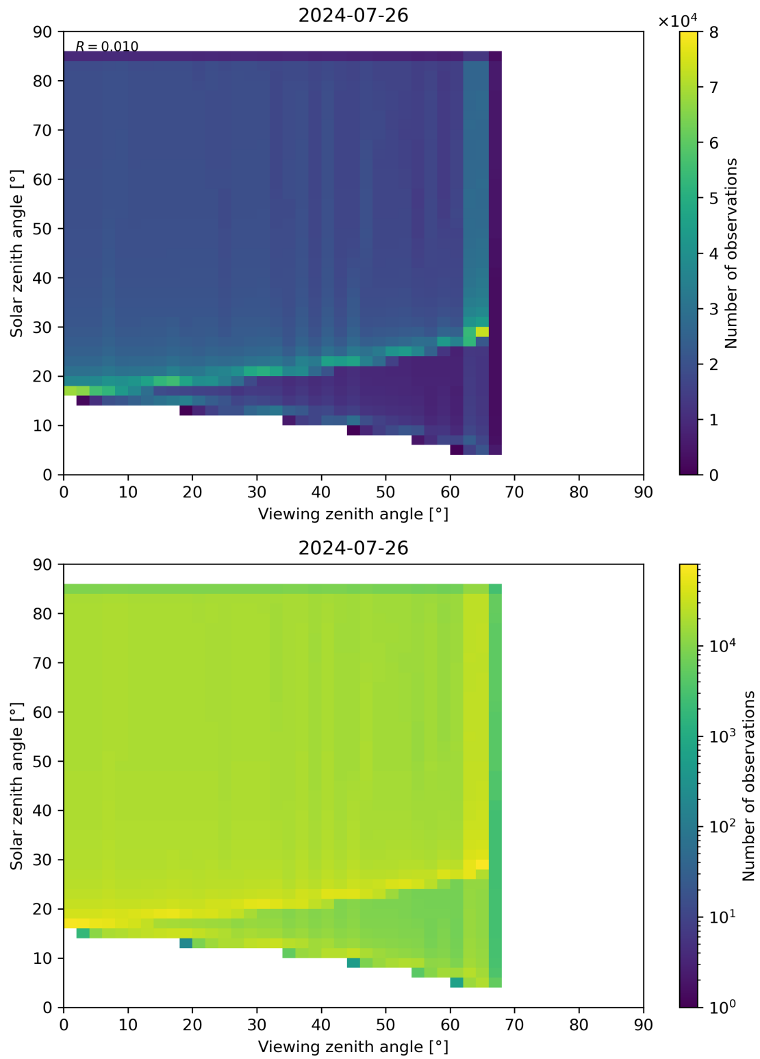
Figure 315: Scatter density plot of “Viewing zenith angle” against “Solar zenith angle” for 2024-07-26 to 2024-07-27.
