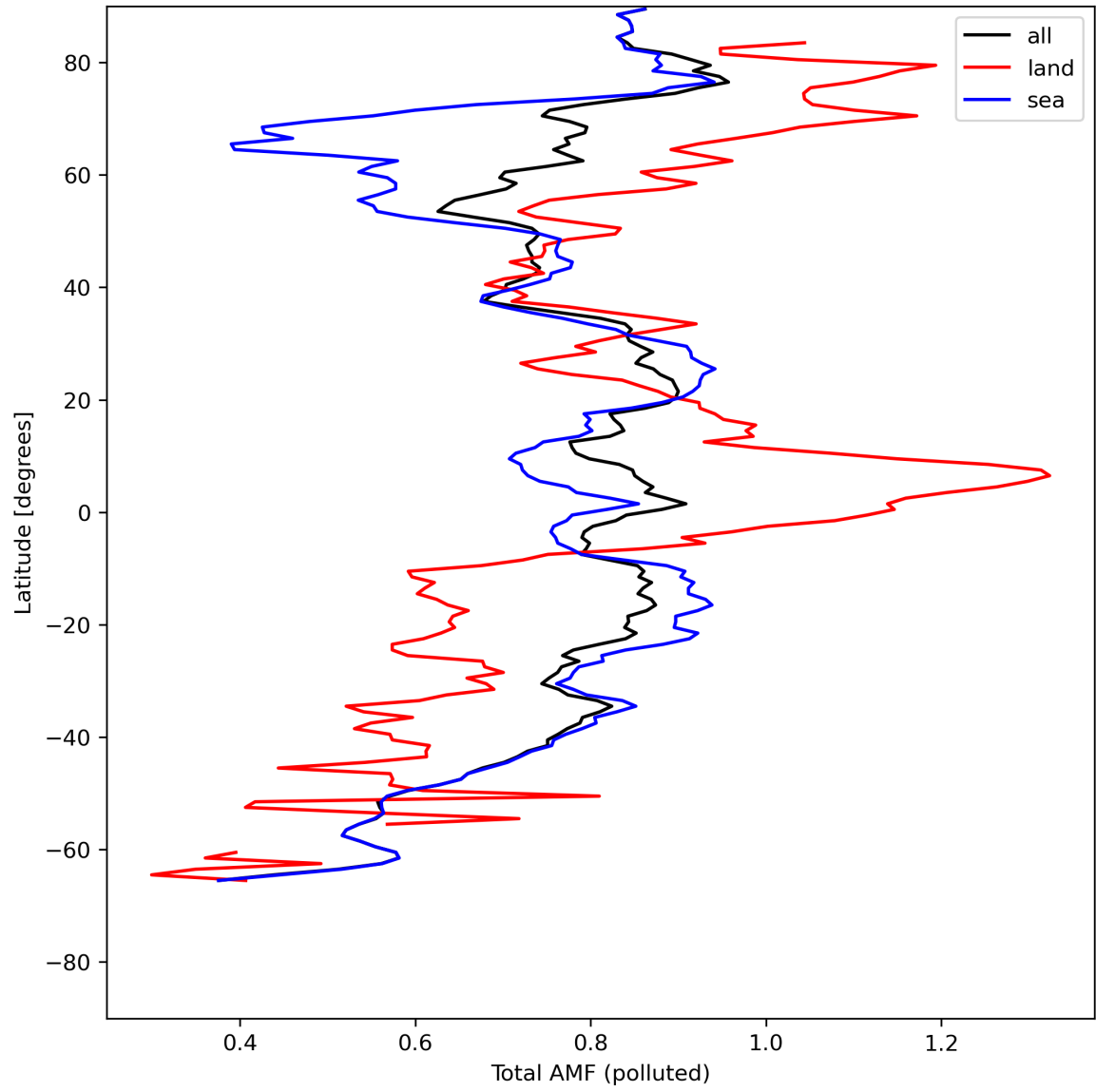
Figure 48: Zonal average of “Total AMF (polluted)” for 2024-07-26 to 2024-07-27.
