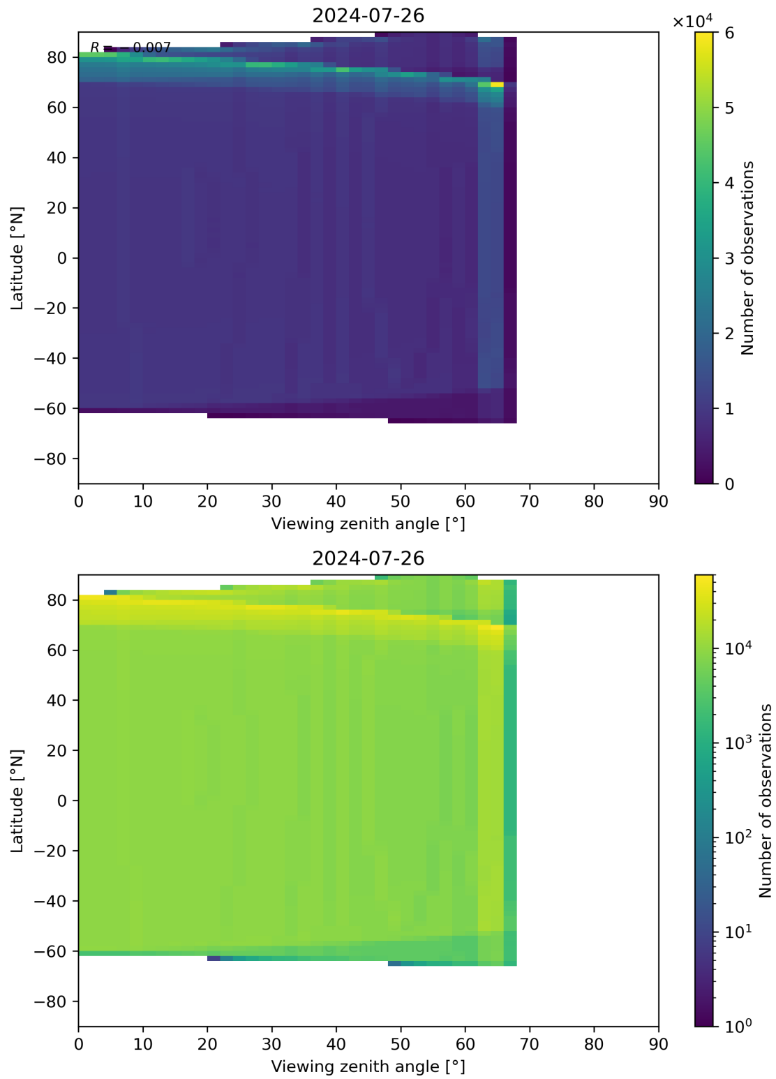
Figure 314: Scatter density plot of “Viewing zenith angle” against “Latitude” for 2024-07-26 to 2024-07-27.
