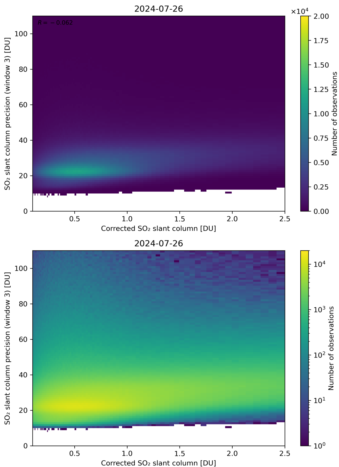
Figure 191: Scatter density plot of “Corrected SO 2 slant column” against “SO 2 slant column precision (window 3)” for 2024-07-26 to 2024-07-27.
