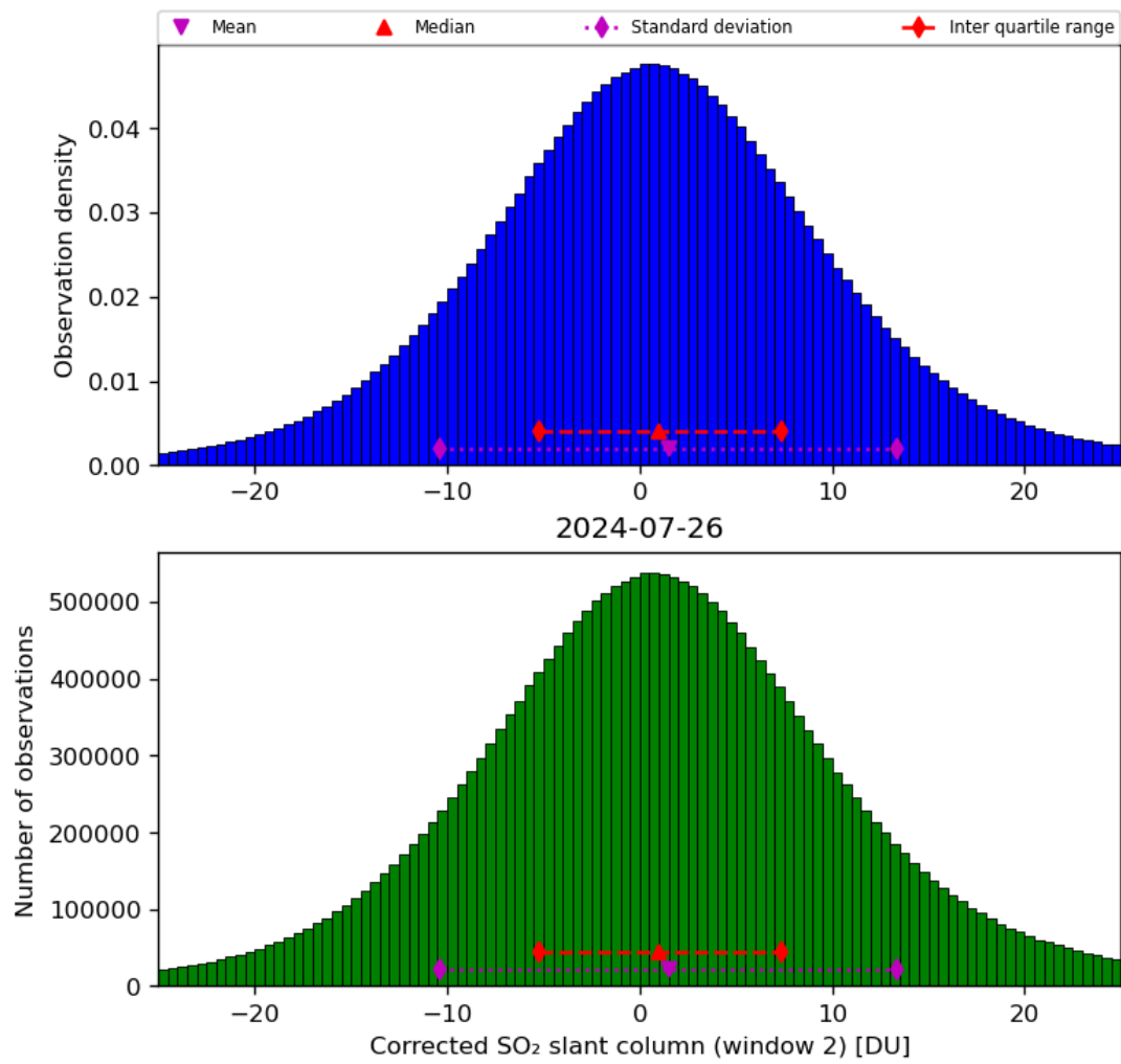
Figure 62: Histogram of “Corrected SO 2 slant column (window 2)” for 2024-07-26 to 2024-07-27
