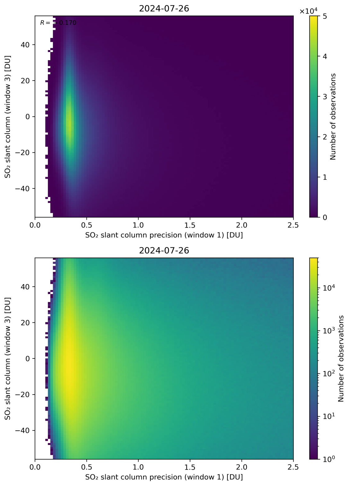
Figure 228: Scatter density plot of “SO 2 slant column precision (window 1)” against “SO 2 slant column (window 3)” for 2024-07-26 to 2024-07-27.
