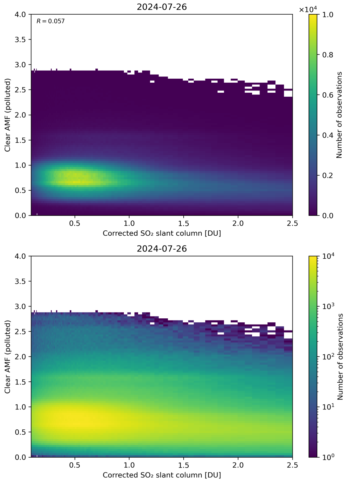
Figure 184: Scatter density plot of “Corrected SO 2 slant column” against “Clear AMF (polluted)” for 2024-07-26 to 2024-07-27.
