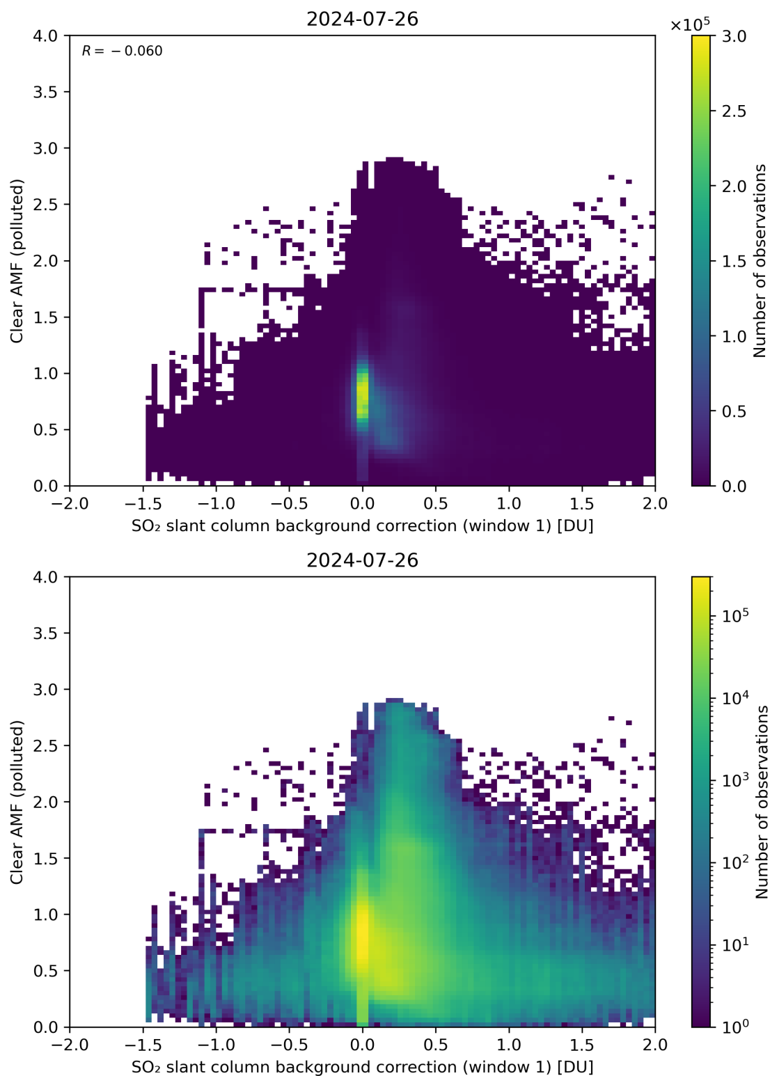
Figure 103: Scatter density plot of “SO 2 slant column background correction (window 1)” against “Clear AMF (polluted)” for 2024-07-26 to 2024-07-27.
