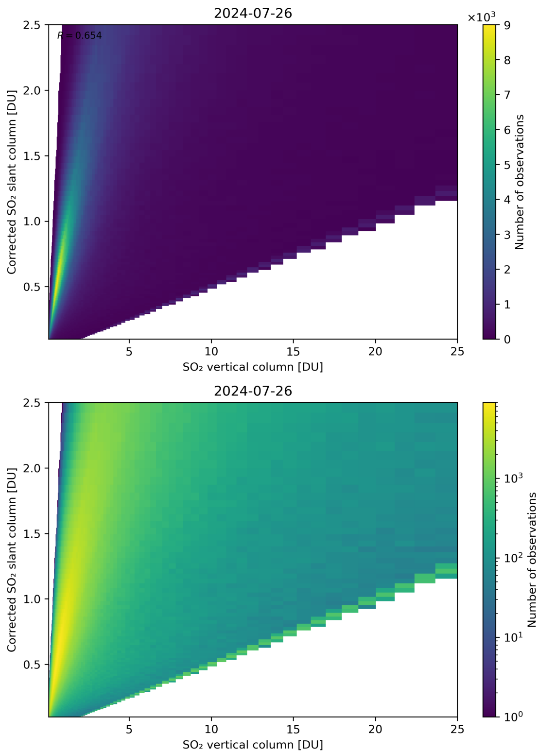
Figure 297: Scatter density plot of “SO 2 vertical column” against “Corrected SO 2 slant column” for 2024-07-26 to 2024-07-27.
