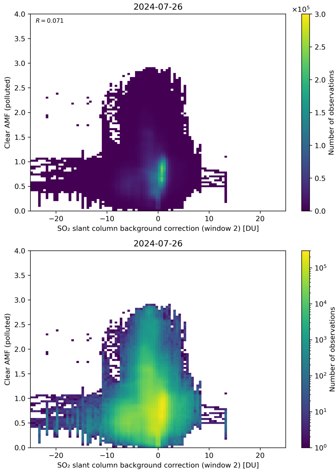
Figure 115: Scatter density plot of “SO 2 slant column background correction (window 2)” against “Clear AMF (polluted)” for 2024-07-26 to 2024-07-27.
