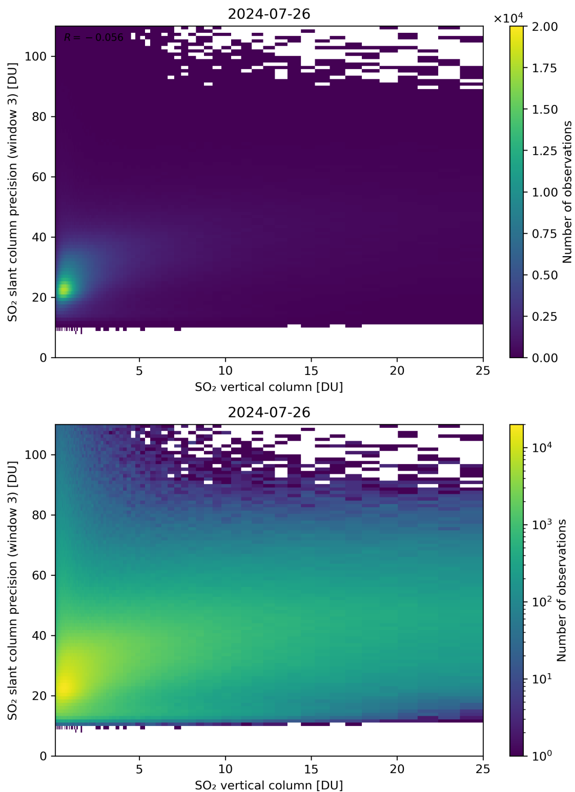
Figure 304: Scatter density plot of “SO 2 vertical column” against “SO 2 slant column precision (window 3)” for 2024-07-26 to 2024-07-27.
