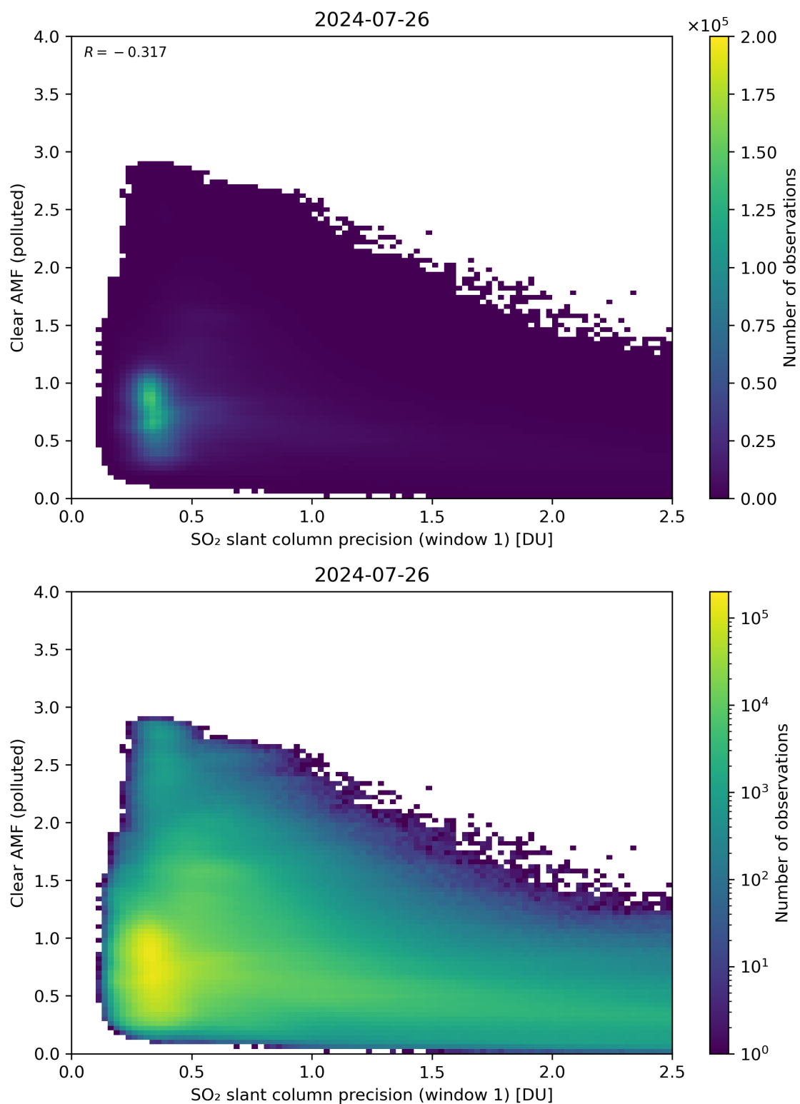
Figure 224: Scatter density plot of “SO 2 slant column precision (window 1)” against “Clear AMF (polluted)” for 2024-07-26 to 2024-07-27.
