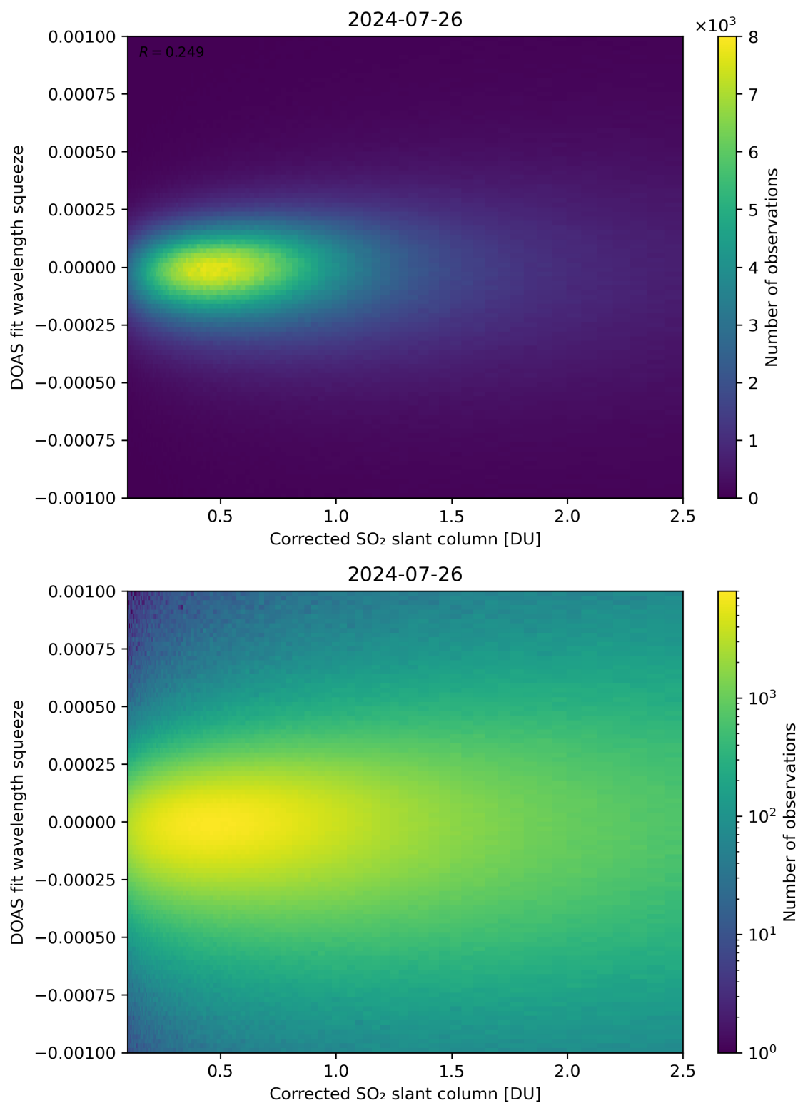
Figure 182: Scatter density plot of “Corrected SO 2 slant column” against “DOAS fit wavelength squeeze” for 2024-07-26 to 2024-07-27.
