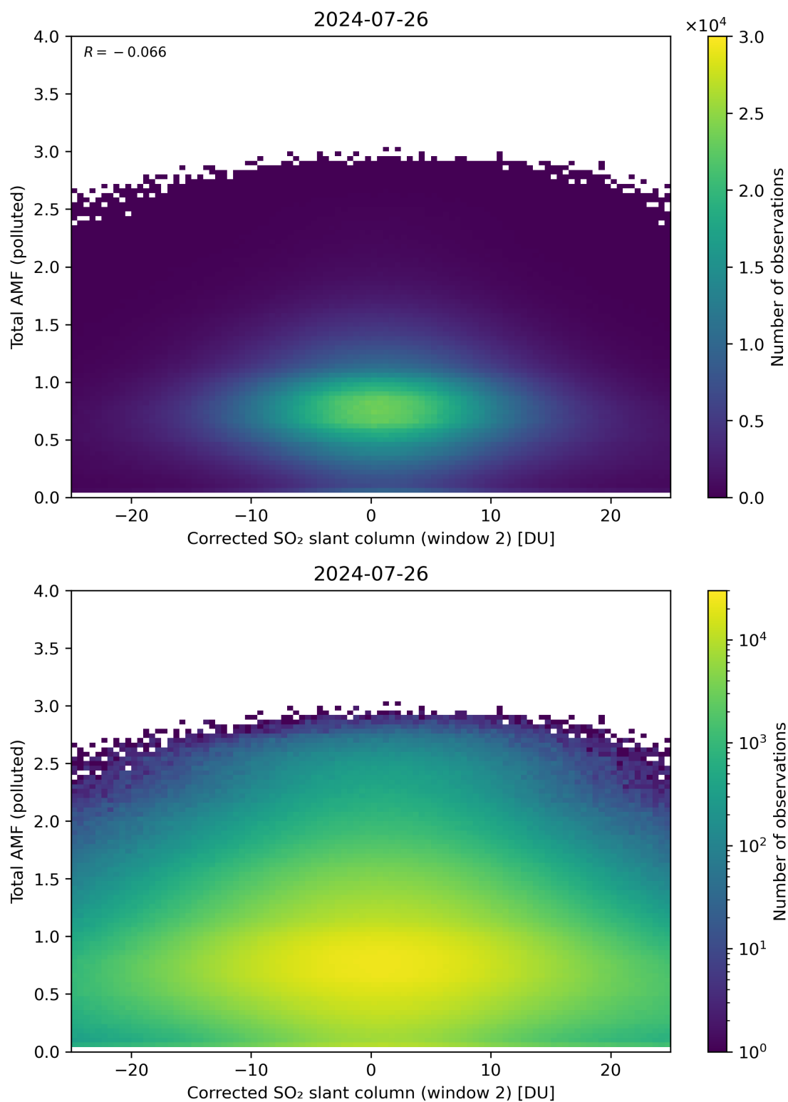
Figure 203: Scatter density plot of “Corrected SO 2 slant column (window 2)” against “Total AMF (polluted)” for 2024-07-26 to 2024-07-27.
