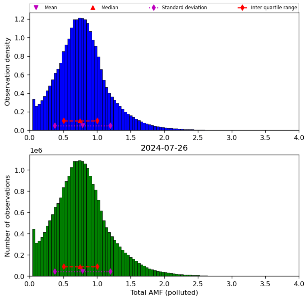
Figure 71: Histogram of “Total AMF (polluted)” for 2024-07-26 to 2024-07-27
