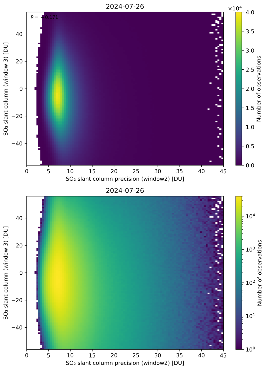
Figure 249: Scatter density plot of “SO 2 slant column precision (window2)” against “SO 2 slant column (window 3)” for 2024-07-26 to 2024-07-27.
