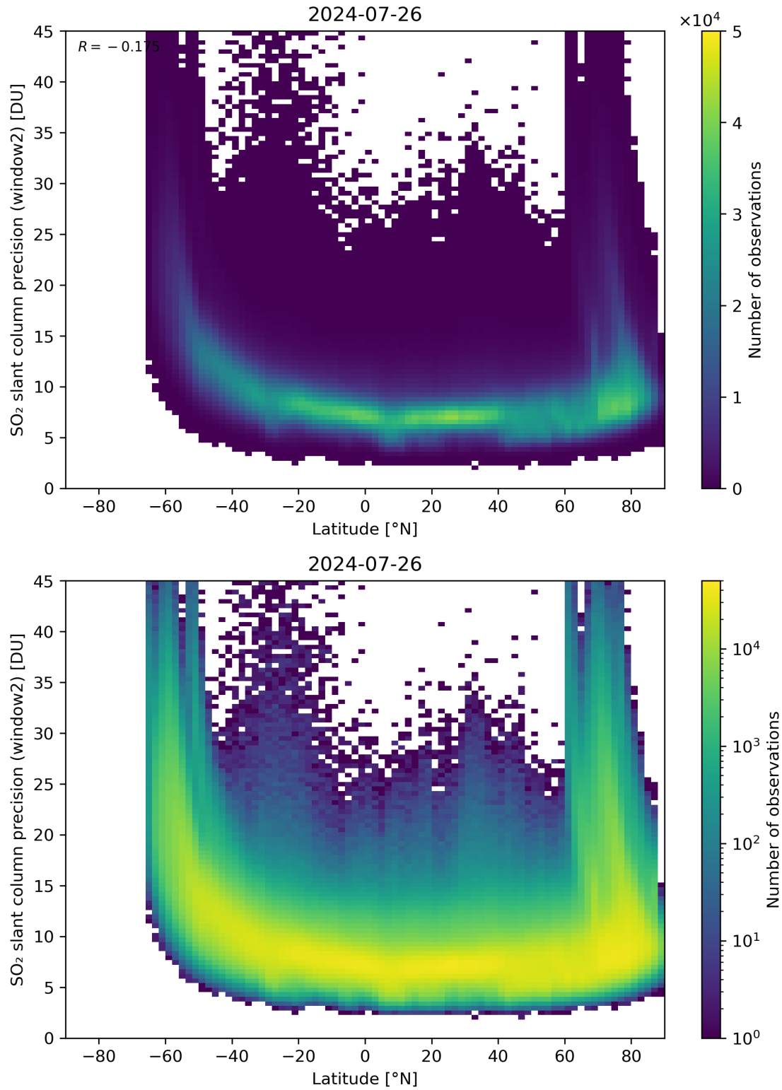
Figure 151: Scatter density plot of “Latitude” against “SO 2 slant column precision (window2)” for 2024-07-26 to 2024-07-27.
