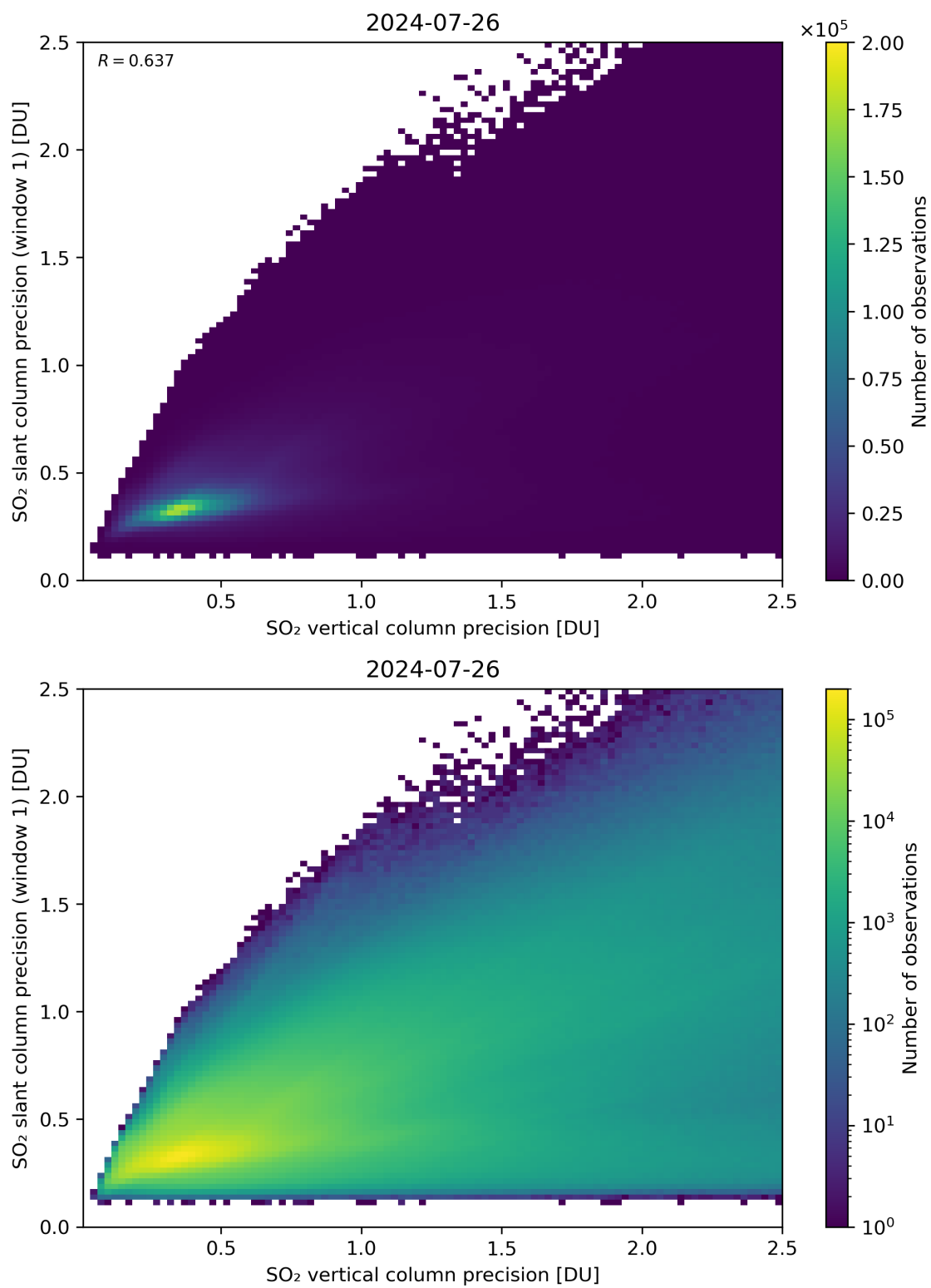
Figure 290: Scatter density plot of “SO 2 vertical column precision” against “SO 2 slant column precision (window 1)” for 2024-07-26 to 2024-07-27.
