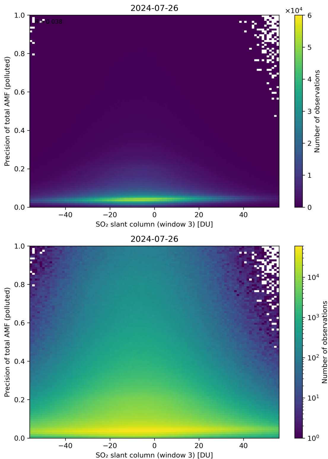
Figure 269: Scatter density plot of “SO 2 slant column (window 3)” against “Precision of total AMF (polluted)” for 2024-07-26 to 2024-07-27.
