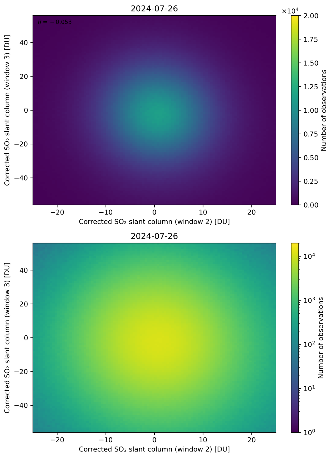
Figure 200: Scatter density plot of “Corrected SO 2 slant column (window 2)” against “Corrected SO 2 slant column (window 3)” for 2024-07-26 to 2024-07-27.
