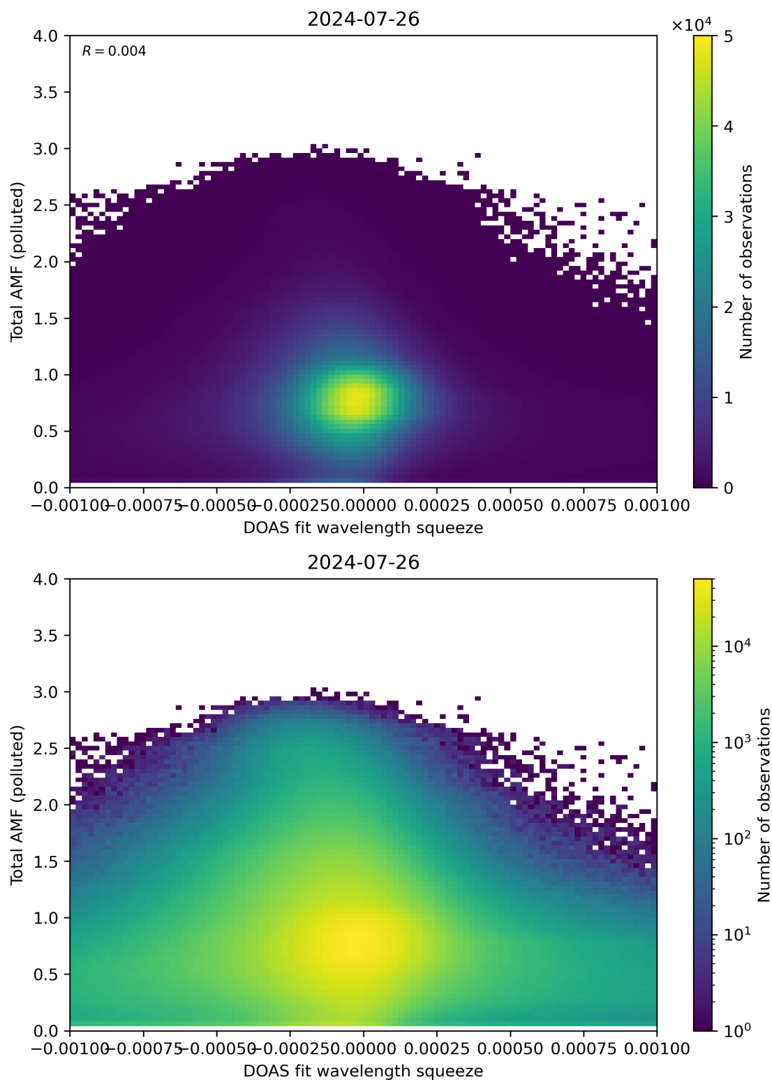
Figure 134: Scatter density plot of “DOAS fit wavelength squeeze” against “Total AMF (polluted)” for 2024-07-26 to 2024-07-27.
