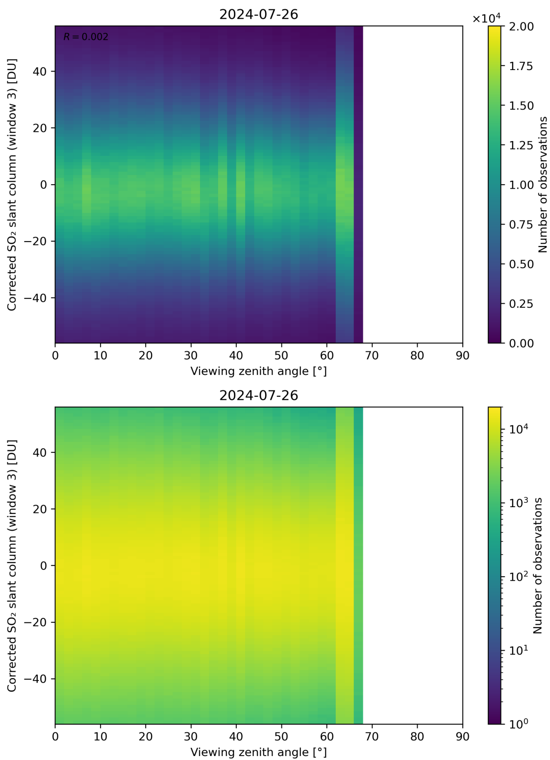
Figure 319: Scatter density plot of “Viewing zenith angle” against “Corrected SO 2 slant column (window 3)” for 2024-07-26 to 2024-07-27.
