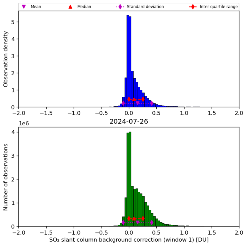
Figure 59: Histogram of “SO 2 slant column background correction (window 1)” for 2024-07-26 to 2024-07-27
