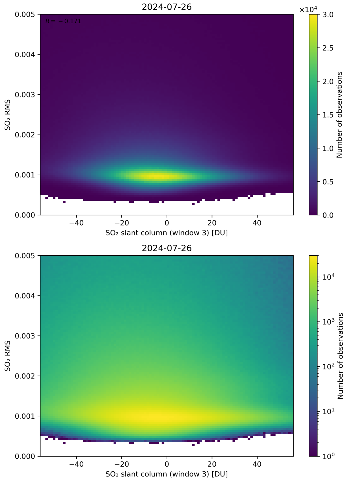
Figure 256: Scatter density plot of “SO 2 slant column (window 3)” against “SO 2 RMS” for 2024-07-26 to 2024-07-27.
