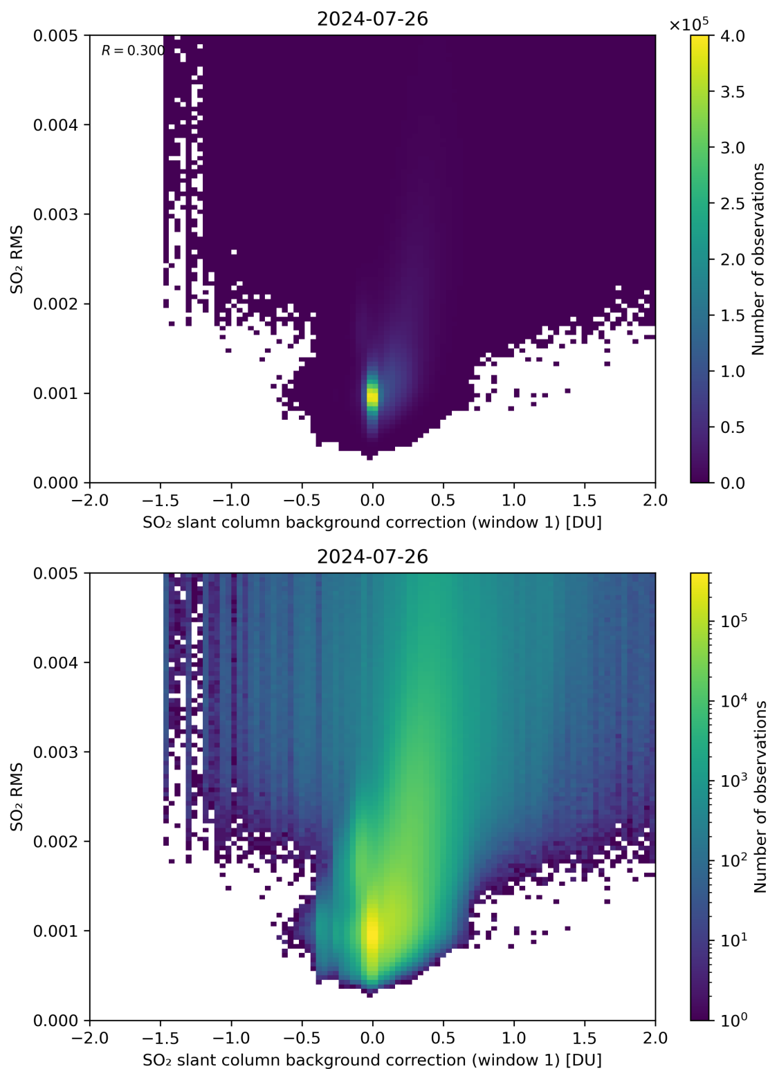
Figure 102: Scatter density plot of “SO 2 slant column background correction (window 1)” against “SO 2 RMS” for 2024-07-26 to 2024-07-27.
