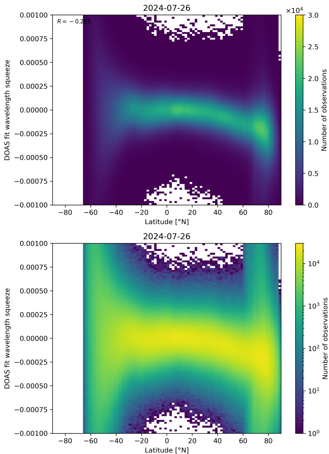
Figure 143: Scatter density plot of “Latitude” against “DOAS fit wavelength squeeze” for 2024-07-26 to 2024-07-27.
