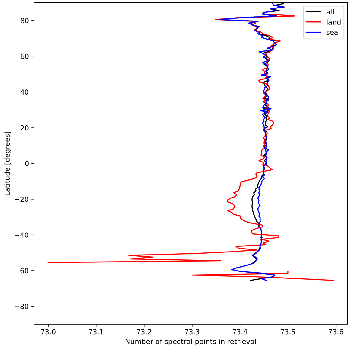
Figure 51: Zonal average of “Number of spectral points in retrieval” for 2024-07-26 to 2024-07-27.
