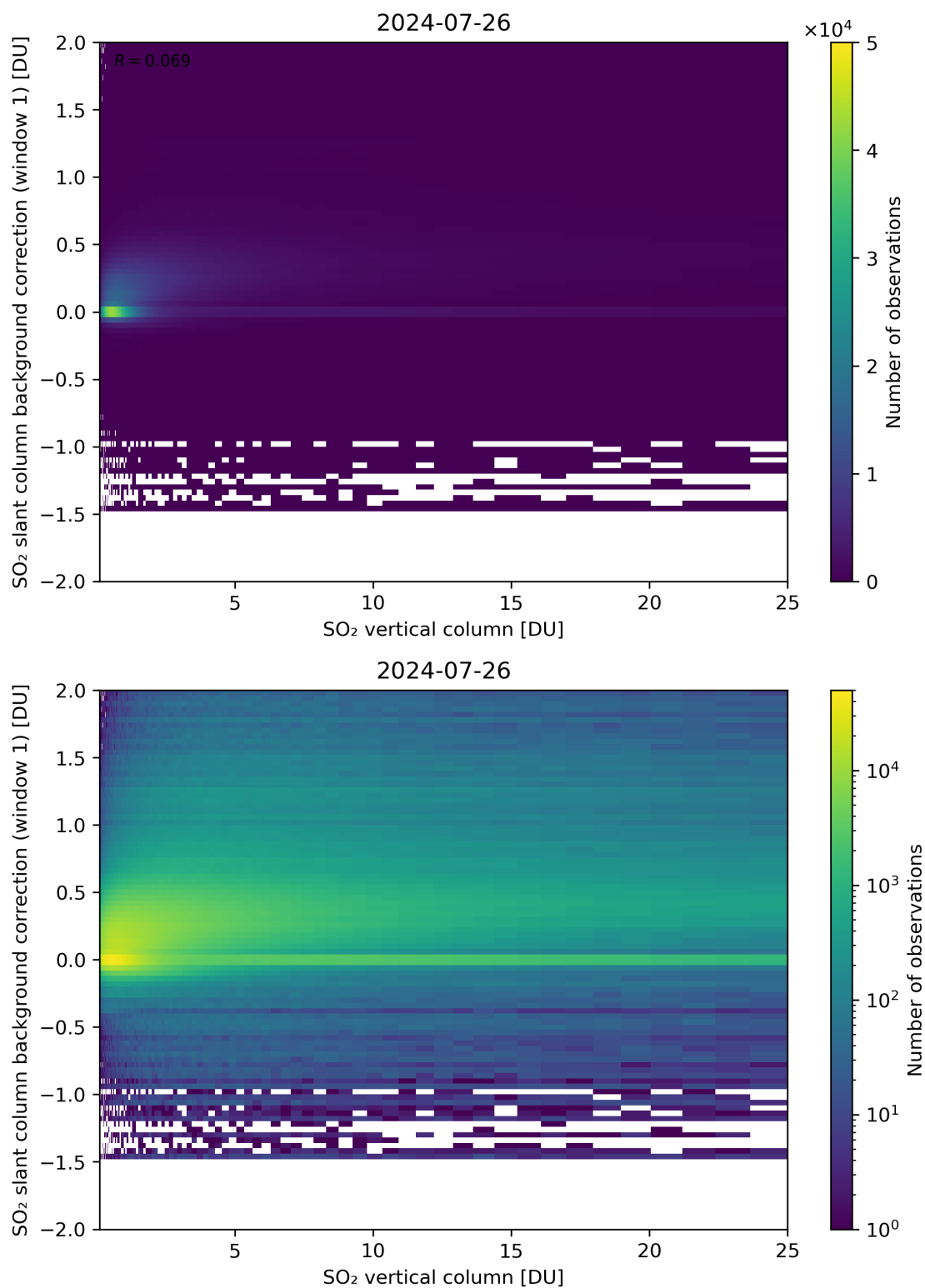
Figure 273: Scatter density plot of “SO 2 vertical column” against “SO 2 slant column background correction (window 1)” for 2024-07-26 to 2024-07-27.
