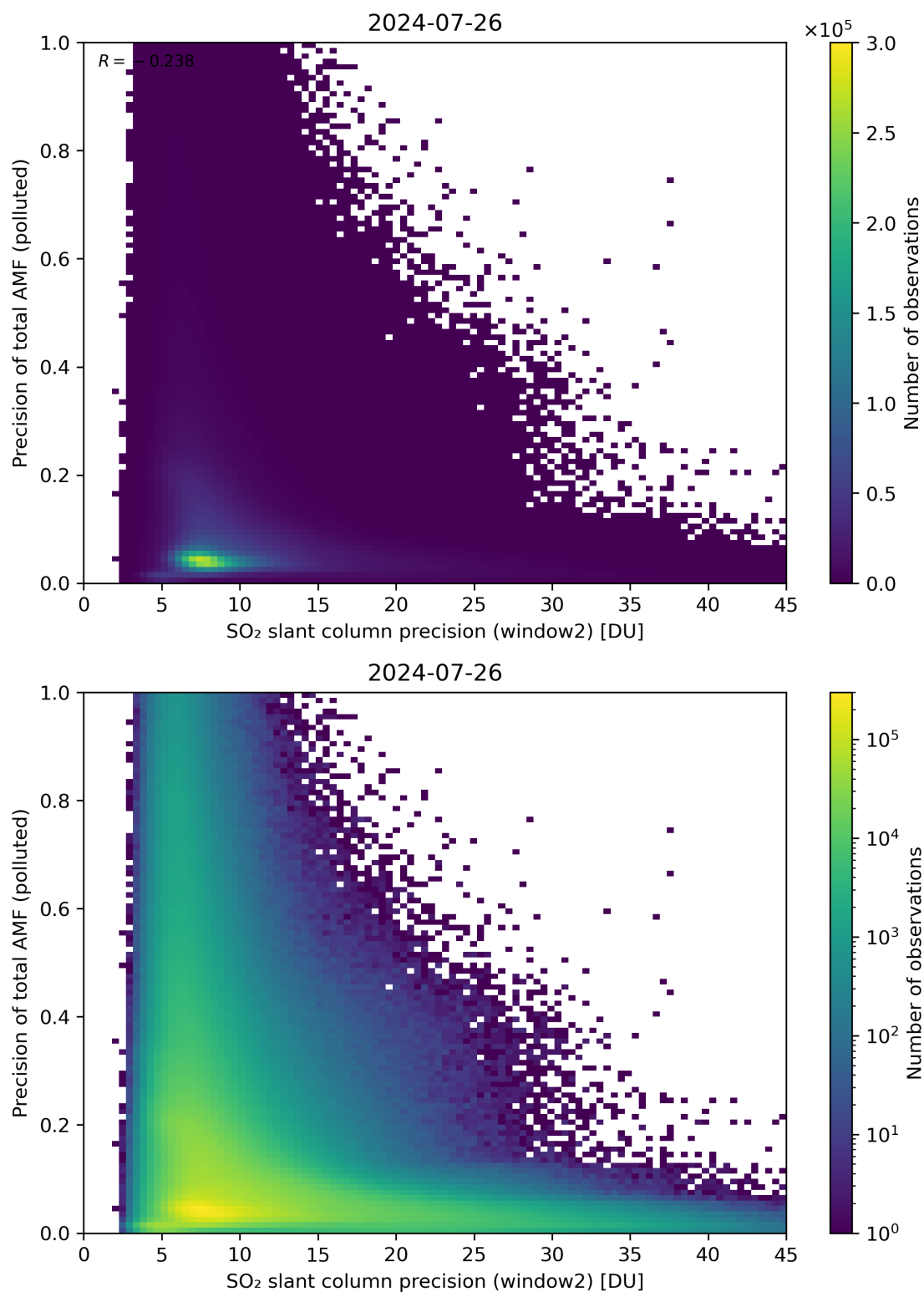
Figure 252: Scatter density plot of “SO 2 slant column precision (window2)” against “Precision of total AMF (polluted)” for 2024-07-26 to 2024-07-27.
