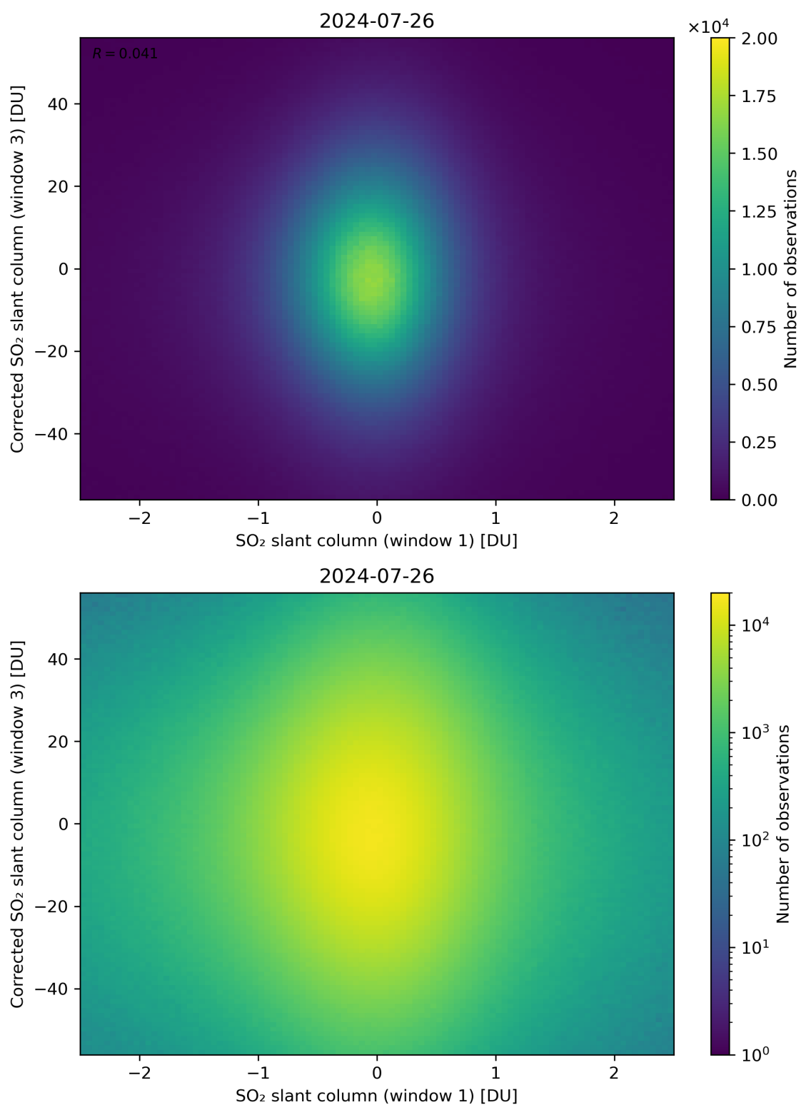
Figure 234: Scatter density plot of “SO 2 slant column (window 1)” against “Corrected SO 2 slant column (window 3)” for 2024-07-26 to 2024-07-27.
