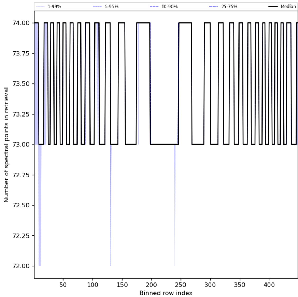
Figure 97: Along track statistics of “Number of spectral points in retrieval” for 2024-07-26 to 2024-07-27
