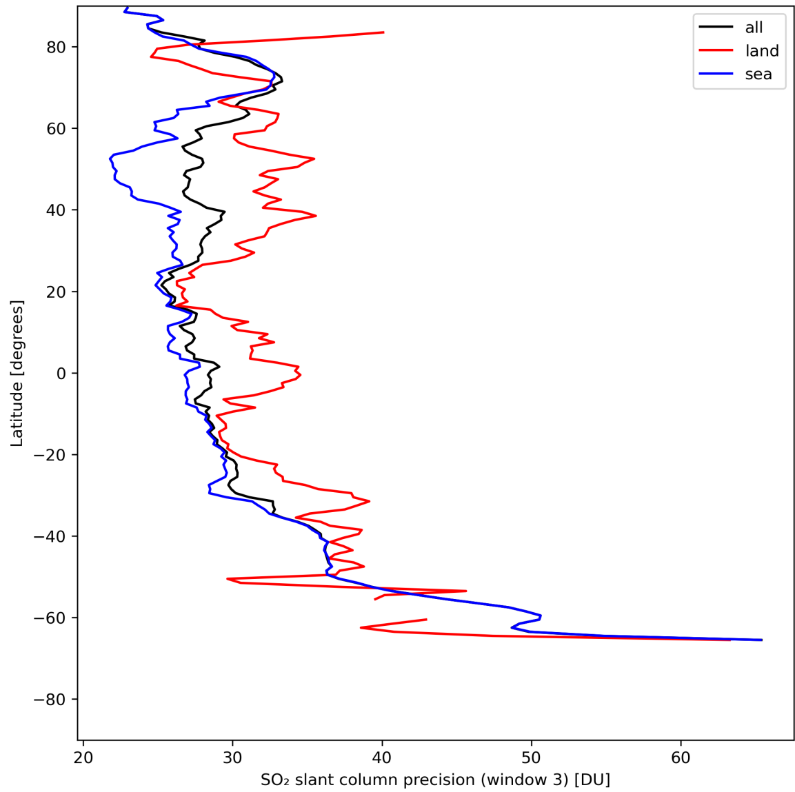
Figure 42: Zonal average of “SO 2 slant column precision (window 3)” for 2024-07-26 to 2024-07-27.
