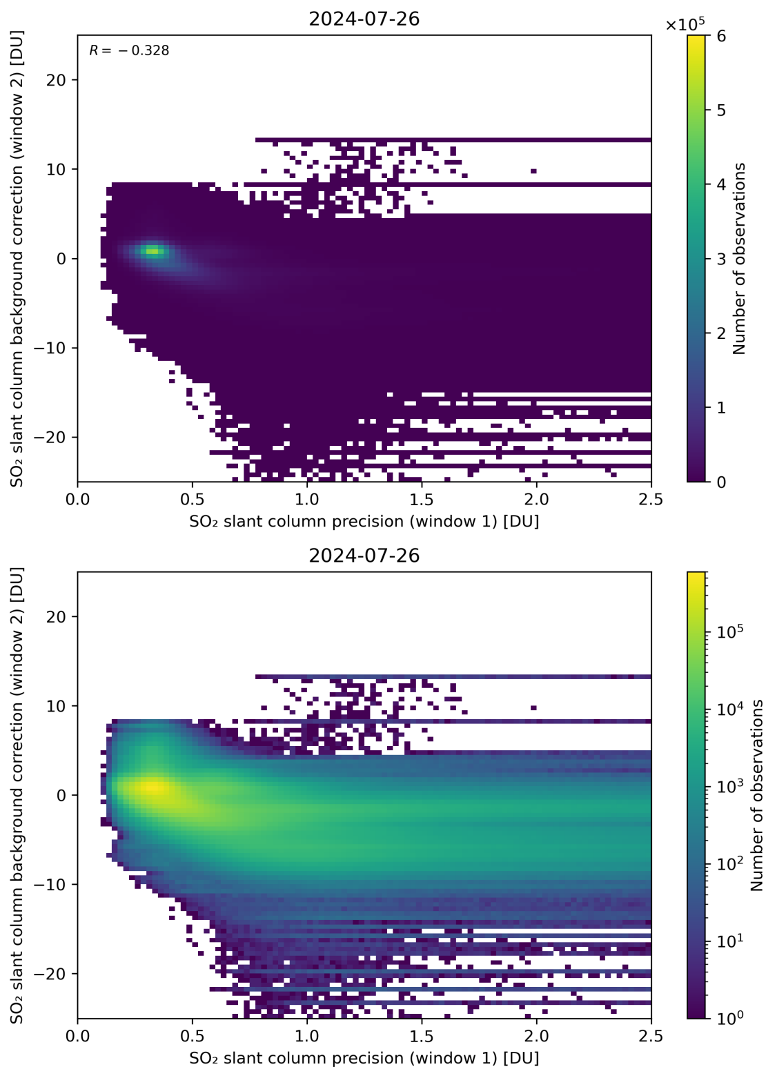
Figure 219: Scatter density plot of “SO 2 slant column precision (window 1)” against “SO 2 slant column background correction (window 2)” for 2024-07-26 to 2024-07-27.
