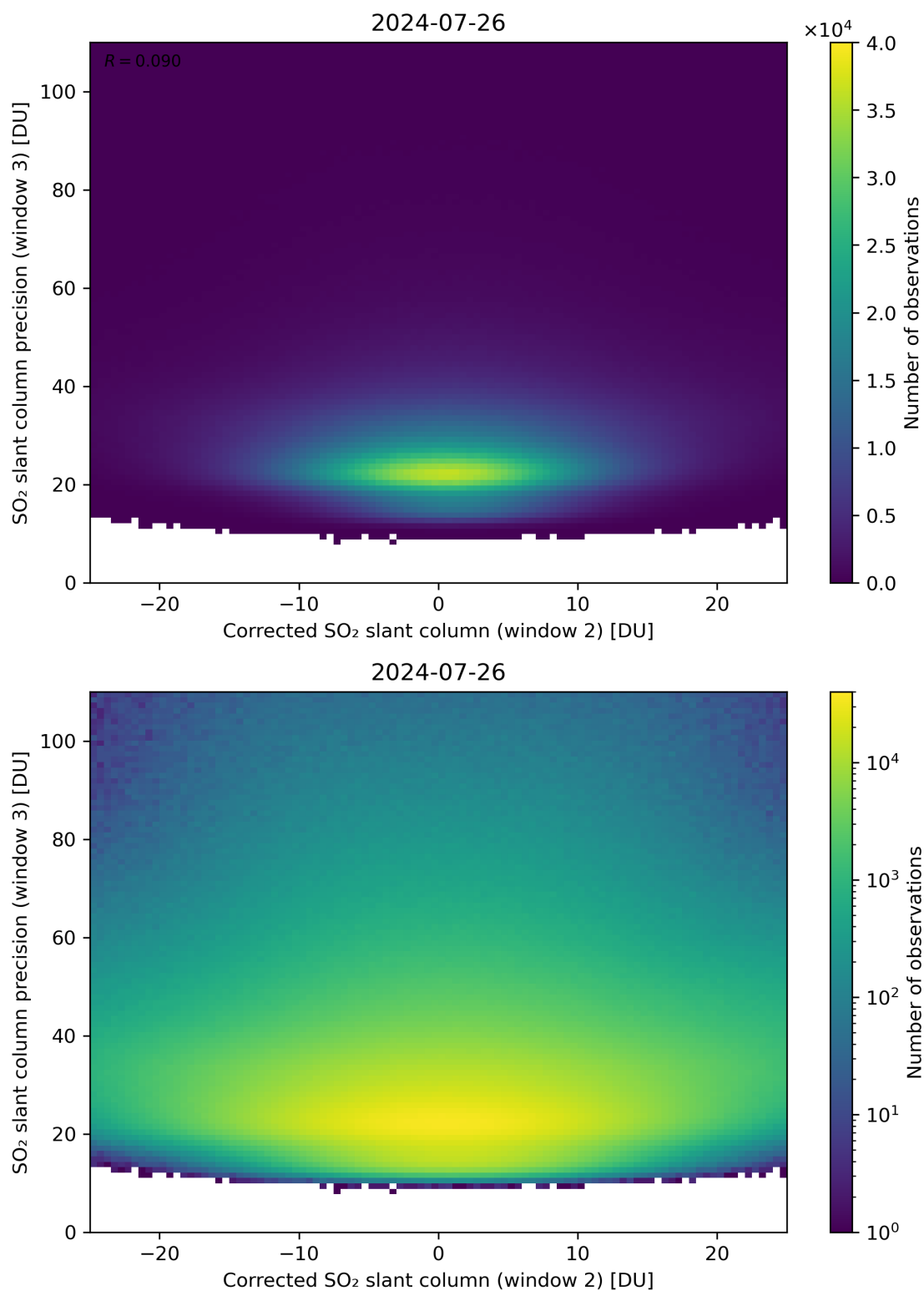
Figure 202: Scatter density plot of “Corrected SO 2 slant column (window 2)” against “SO 2 slant column precision (window 3)” for 2024-07-26 to 2024-07-27.
