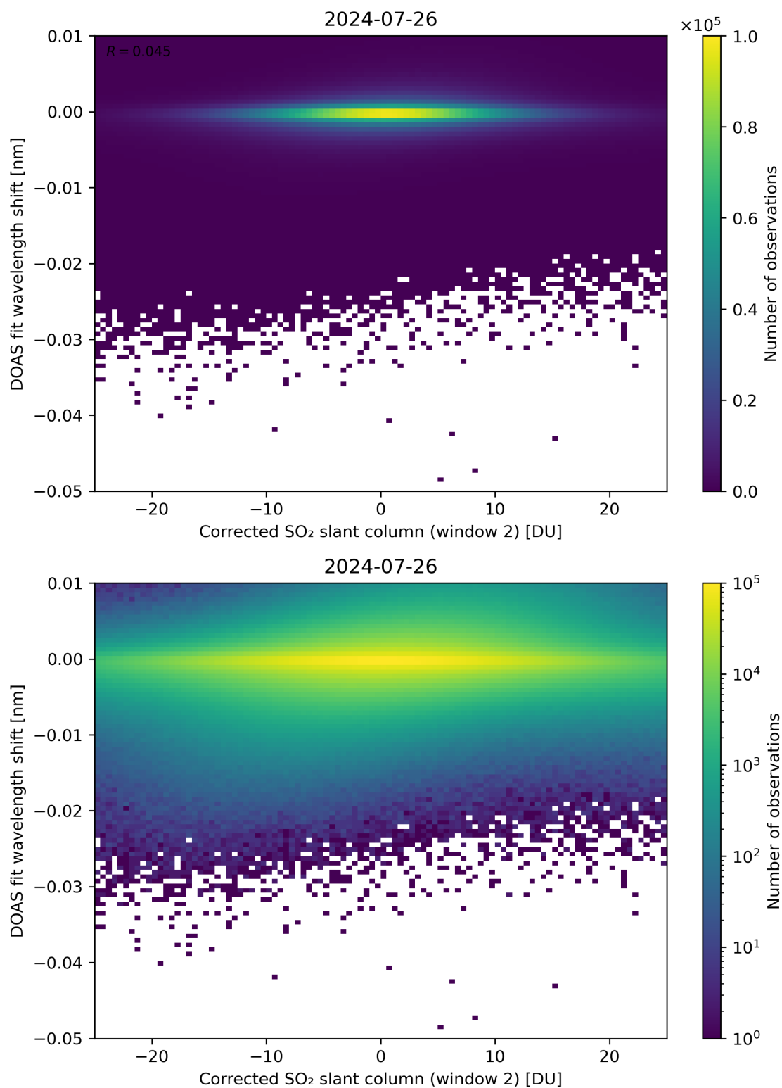
Figure 196: Scatter density plot of “Corrected SO 2 slant column (window 2)” against “DOAS fit wavelength shift” for 2024-07-26 to 2024-07-27.
