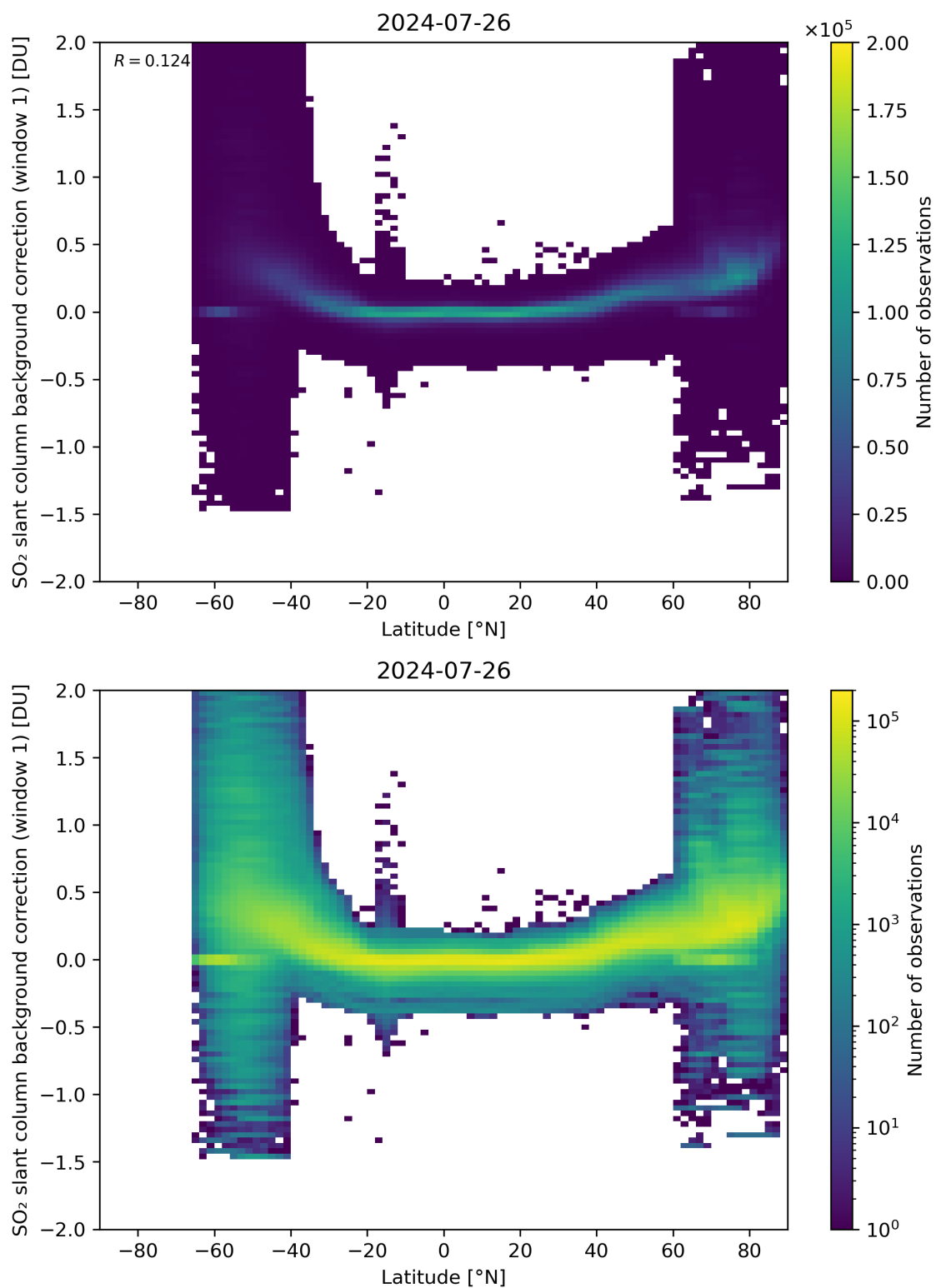
Figure 139: Scatter density plot of “Latitude” against “SO 2 slant column background correction (window 1)” for 2024-07-26 to 2024-07-27.
