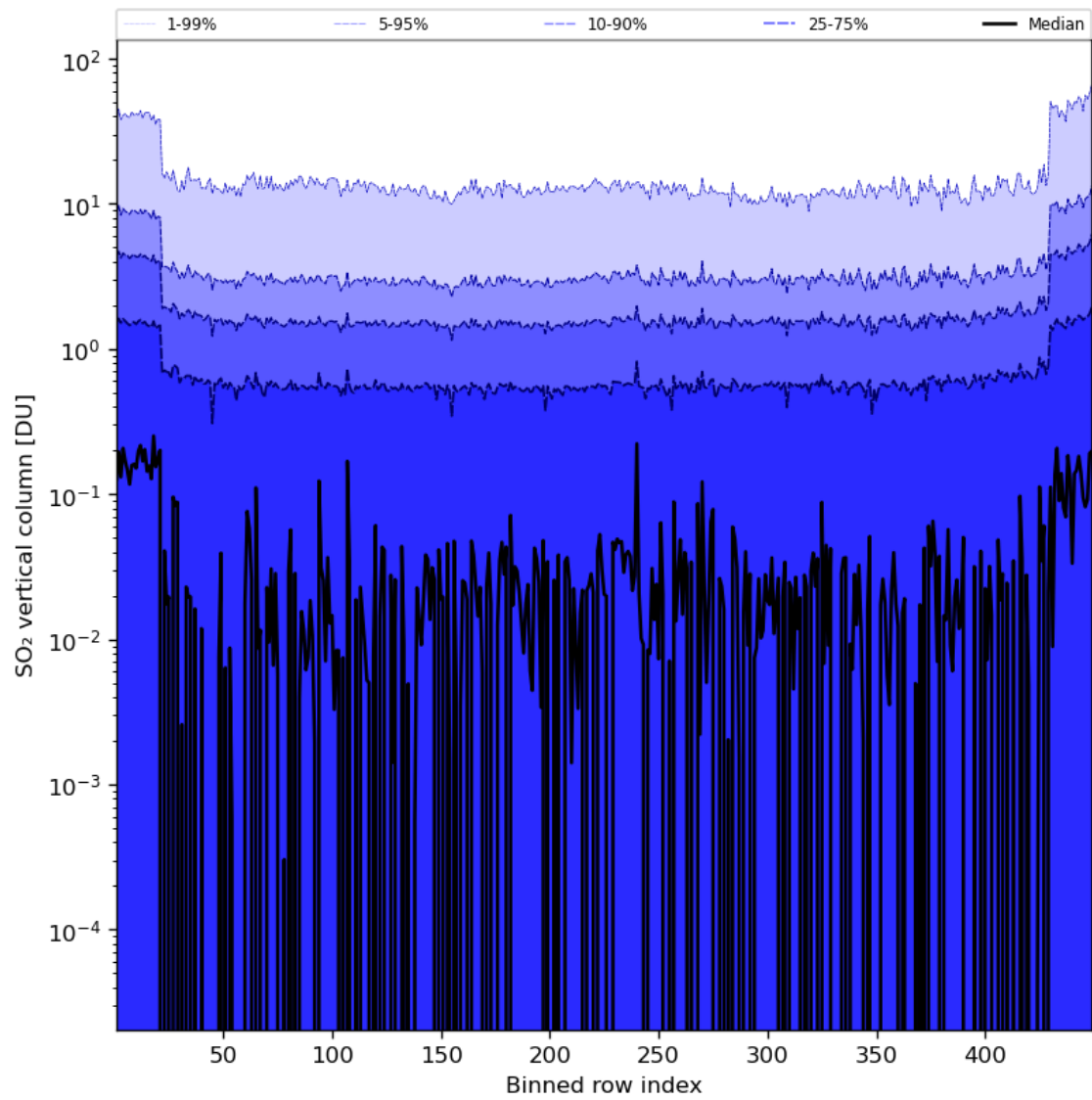
Figure 76: Along track statistics of “SO 2 vertical column” for 2024-07-26 to 2024-07-27
