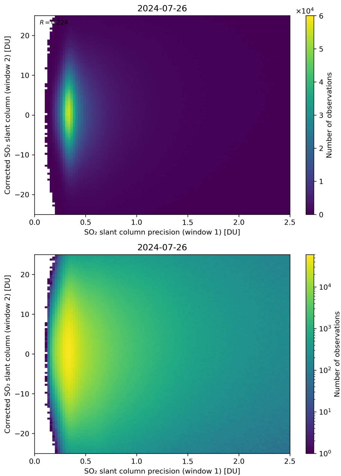
Figure 225: Scatter density plot of “SO 2 slant column precision (window 1)” against “Corrected SO 2 slant column (window 2)” for 2024-07-26 to 2024-07-27.
