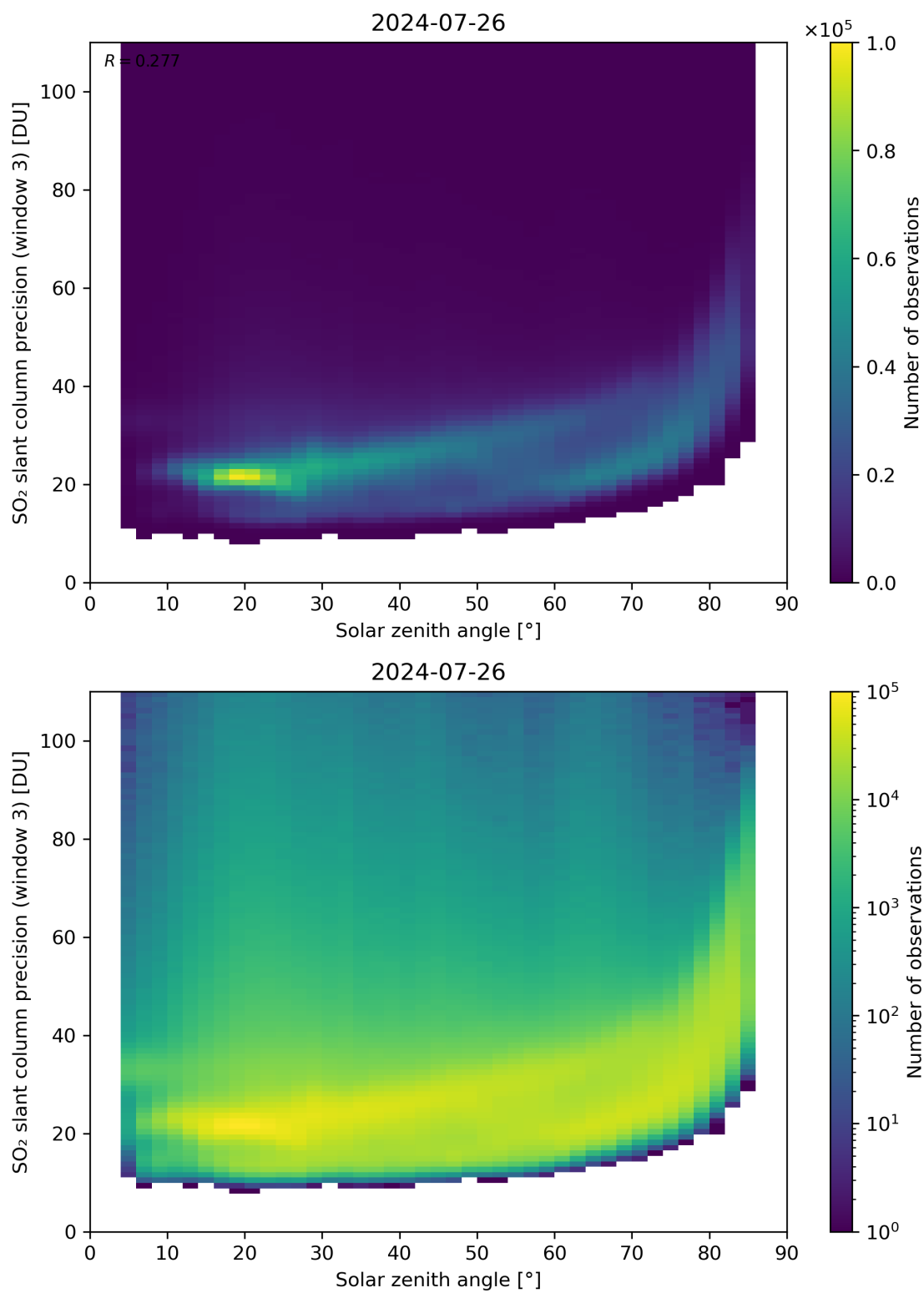
Figure 173: Scatter density plot of “Solar zenith angle” against “SO 2 slant column precision (window 3)” for 2024-07-26 to 2024-07-27.
