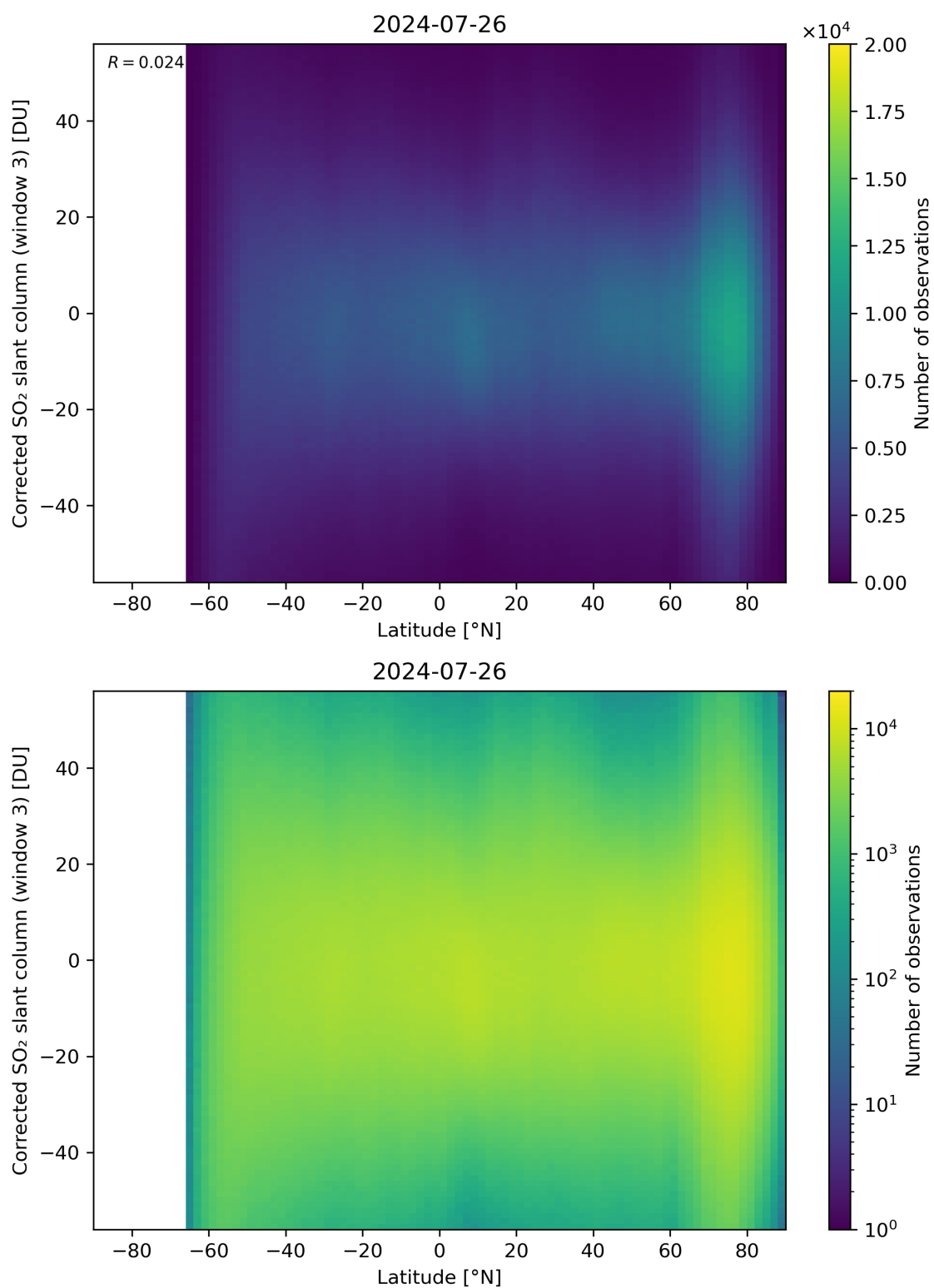
Figure 148: Scatter density plot of “Latitude” against “Corrected SO 2 slant column (window 3)” for 2024-07-26 to 2024-07-27.
