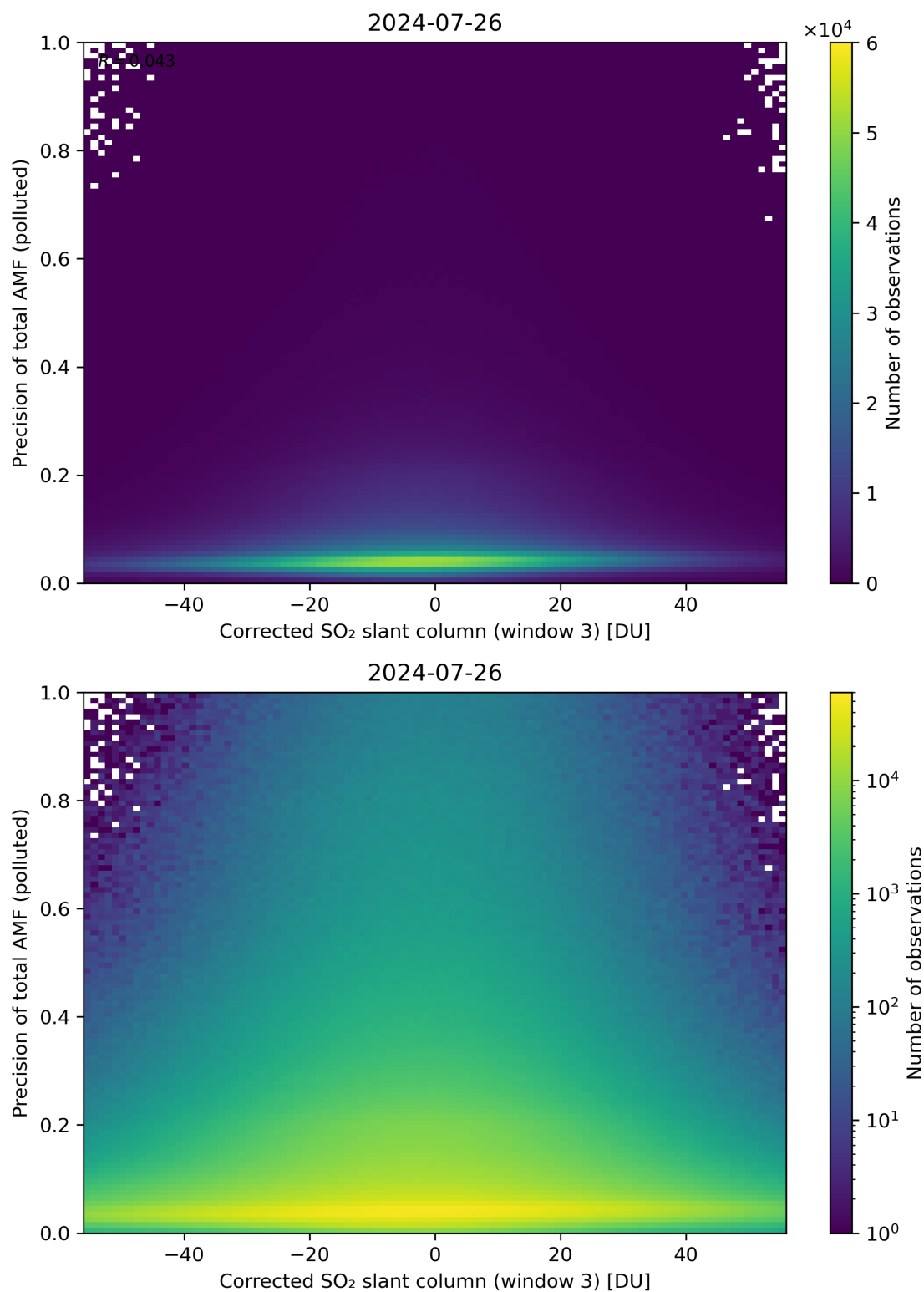
Figure 211: Scatter density plot of “Corrected SO 2 slant column (window 3)” against “Precision of total AMF (polluted)” for 2024-07-26 to 2024-07-27.
