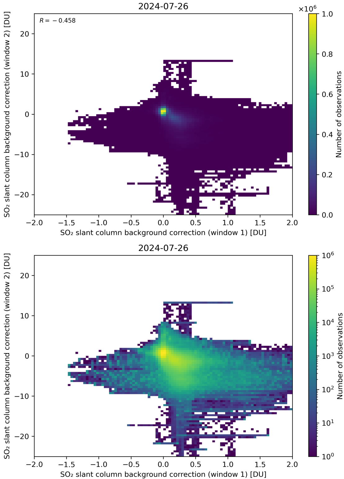
Figure 98: Scatter density plot of “SO 2 slant column background correction (window 1)” against “SO 2 slant column background correction (window 2)” for 2024-07-26 to 2024-07-27.
