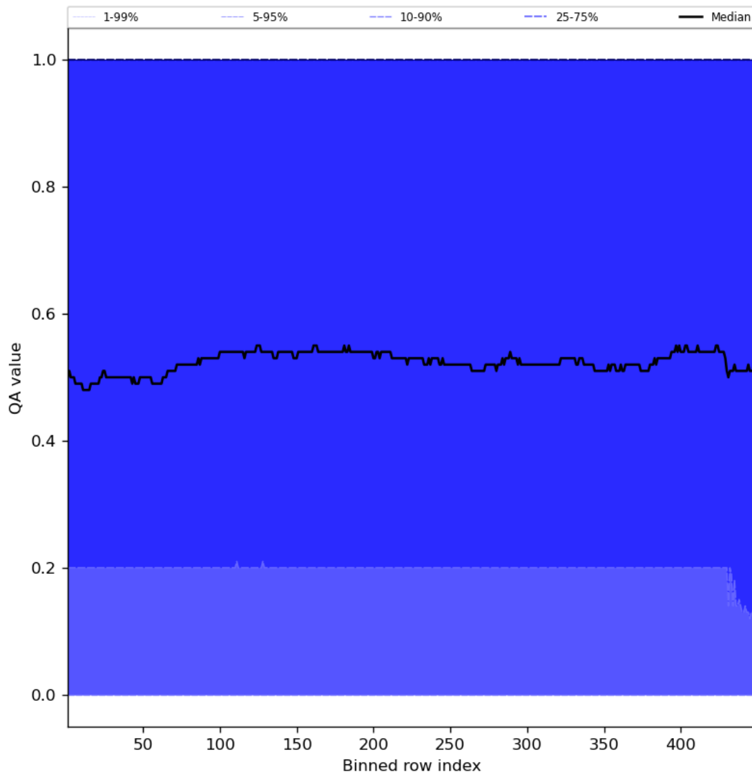
Figure 75: Along track statistics of “QA value” for 2024-07-26 to 2024-07-27
