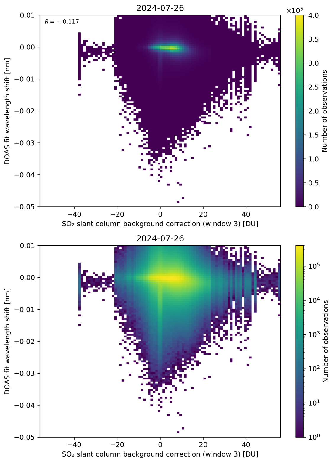
Figure 121: Scatter density plot of “SO 2 slant column background correction (window 3)” against “DOAS fit wavelength shift” for 2024-07-26 to 2024-07-27.
