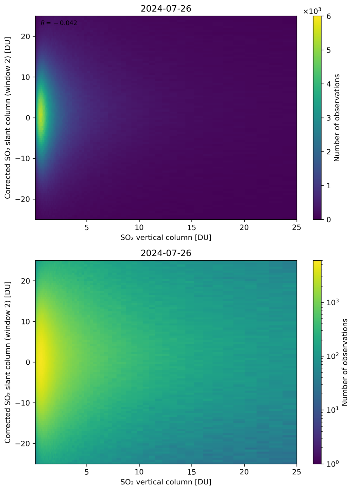
Figure 298: Scatter density plot of “SO 2 vertical column” against “Corrected SO 2 slant column (window 2)” for 2024-07-26 to 2024-07-27.
