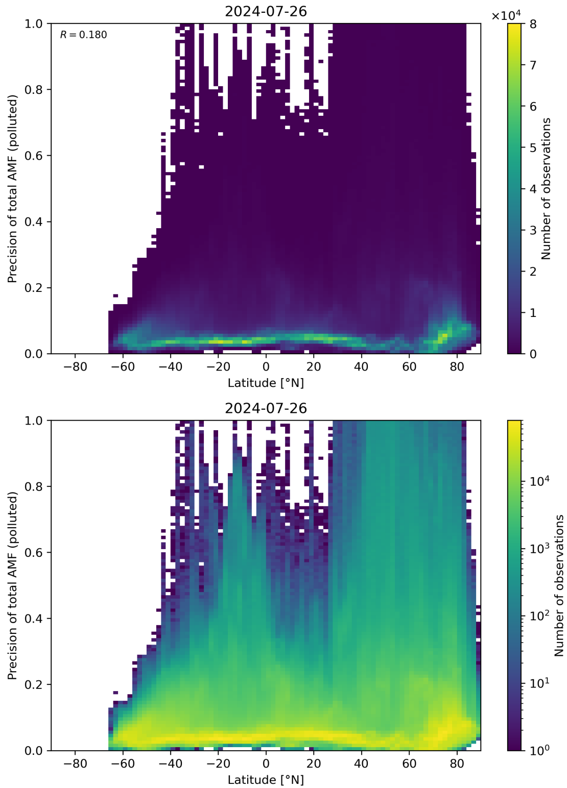
Figure 155: Scatter density plot of “Latitude” against “Precision of total AMF (polluted)” for 2024-07-26 to 2024-07-27.
