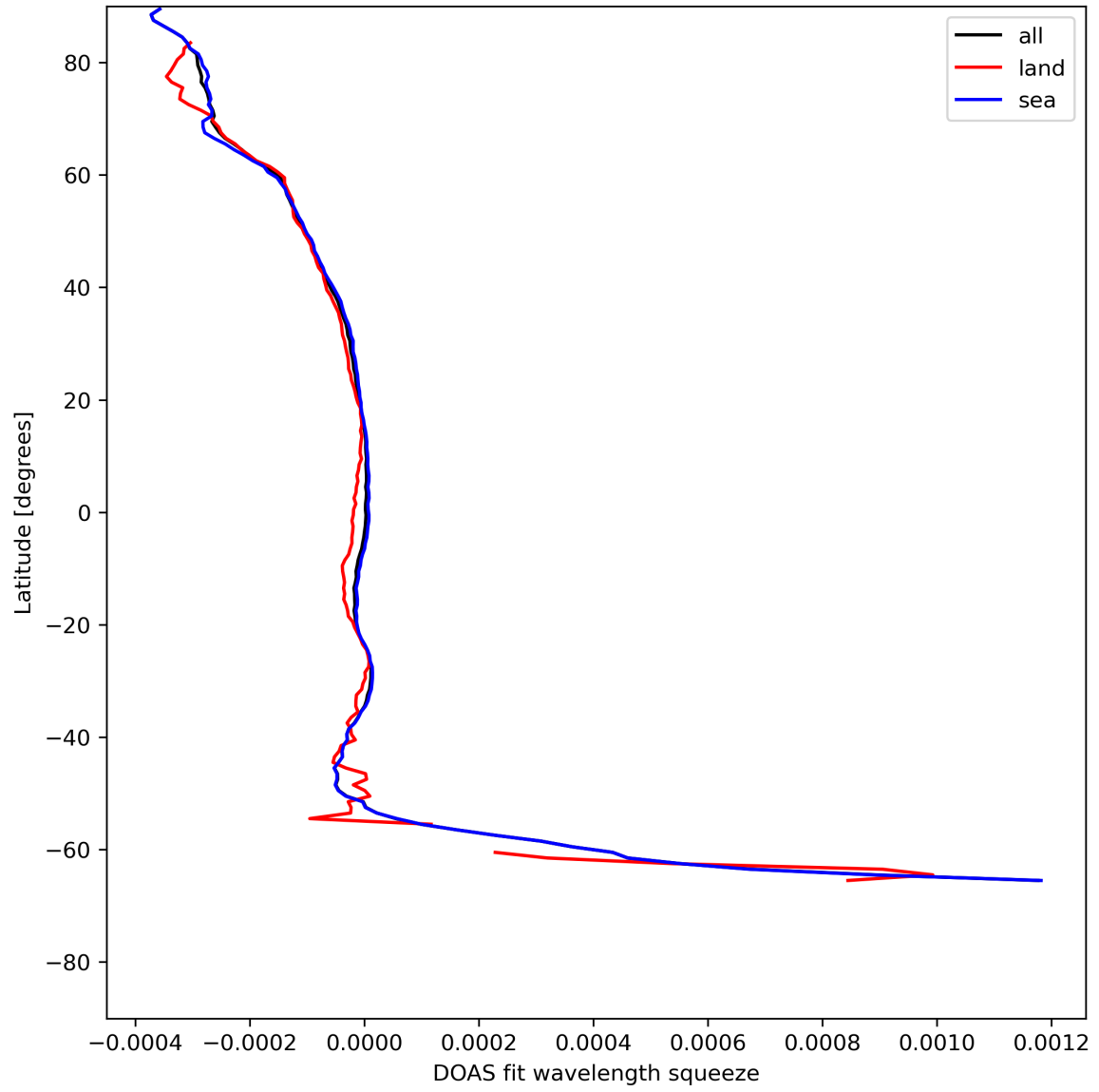
Figure 46: Zonal average of “DOAS fit wavelength squeeze” for 2024-07-26 to 2024-07-27.
