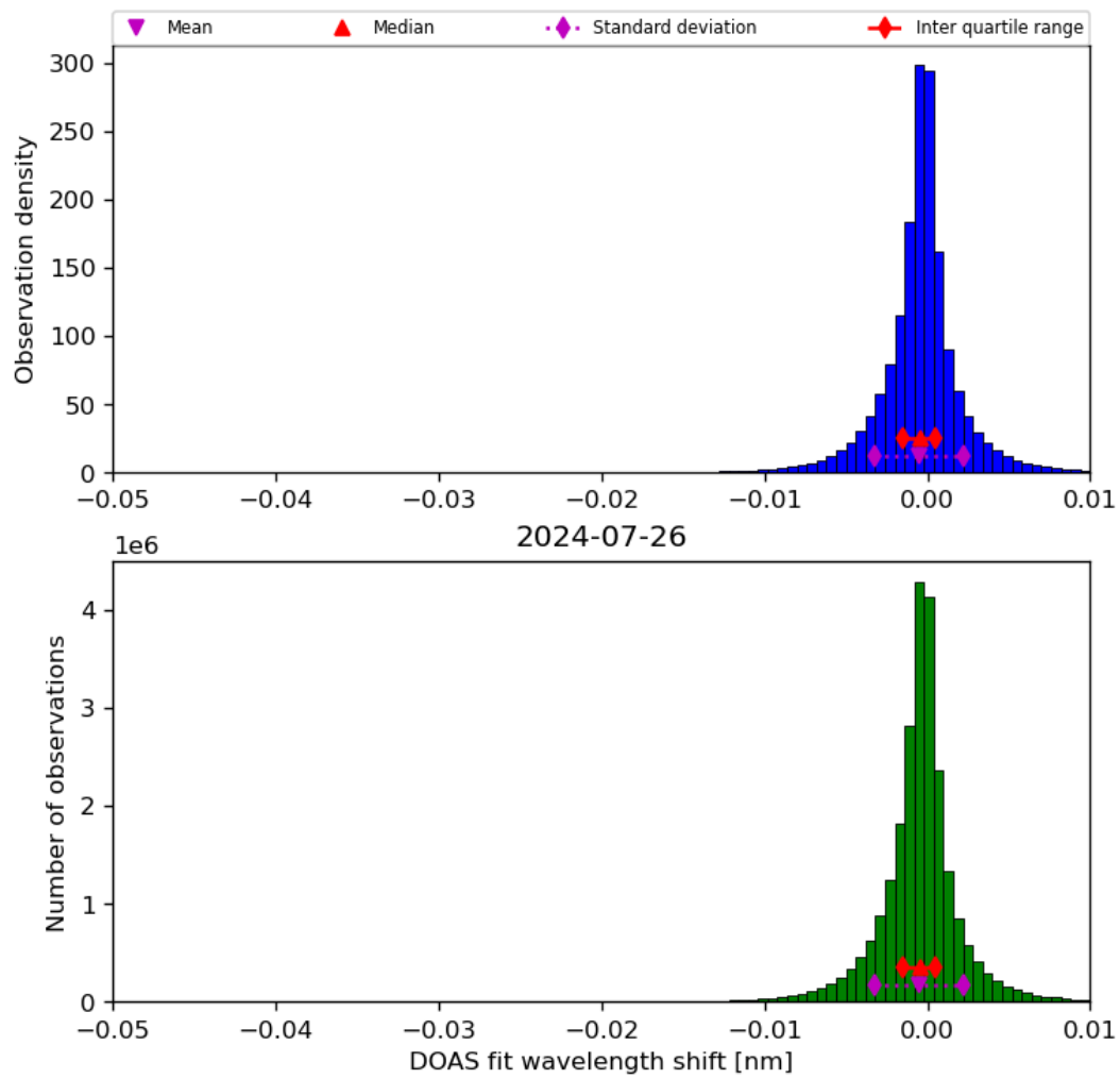
Figure 68: Histogram of “DOAS fit wavelength shift” for 2024-07-26 to 2024-07-27
