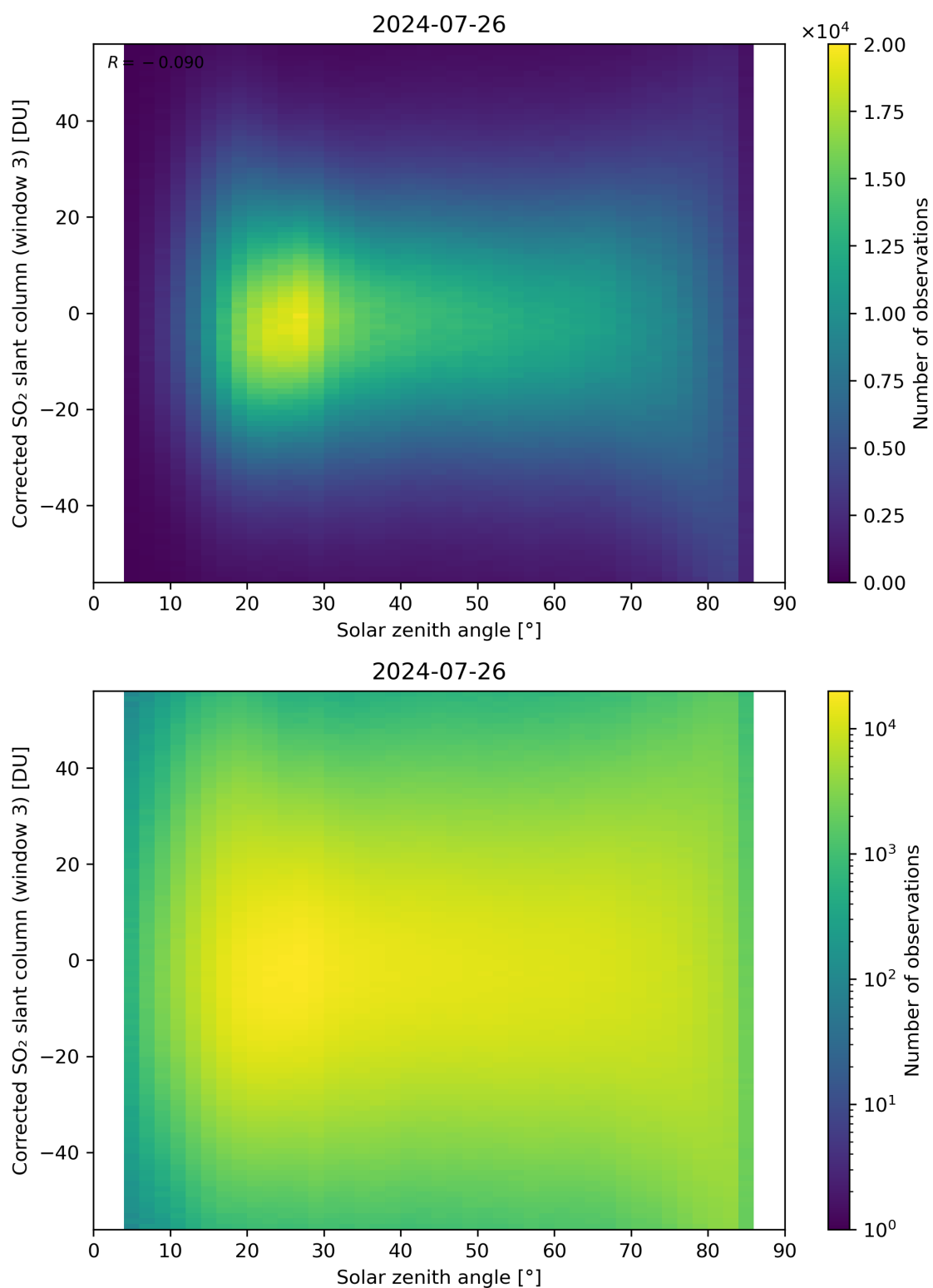
Figure 168: Scatter density plot of “Solar zenith angle” against “Corrected SO 2 slant column (window 3)” for 2024-07-26 to 2024-07-27.
