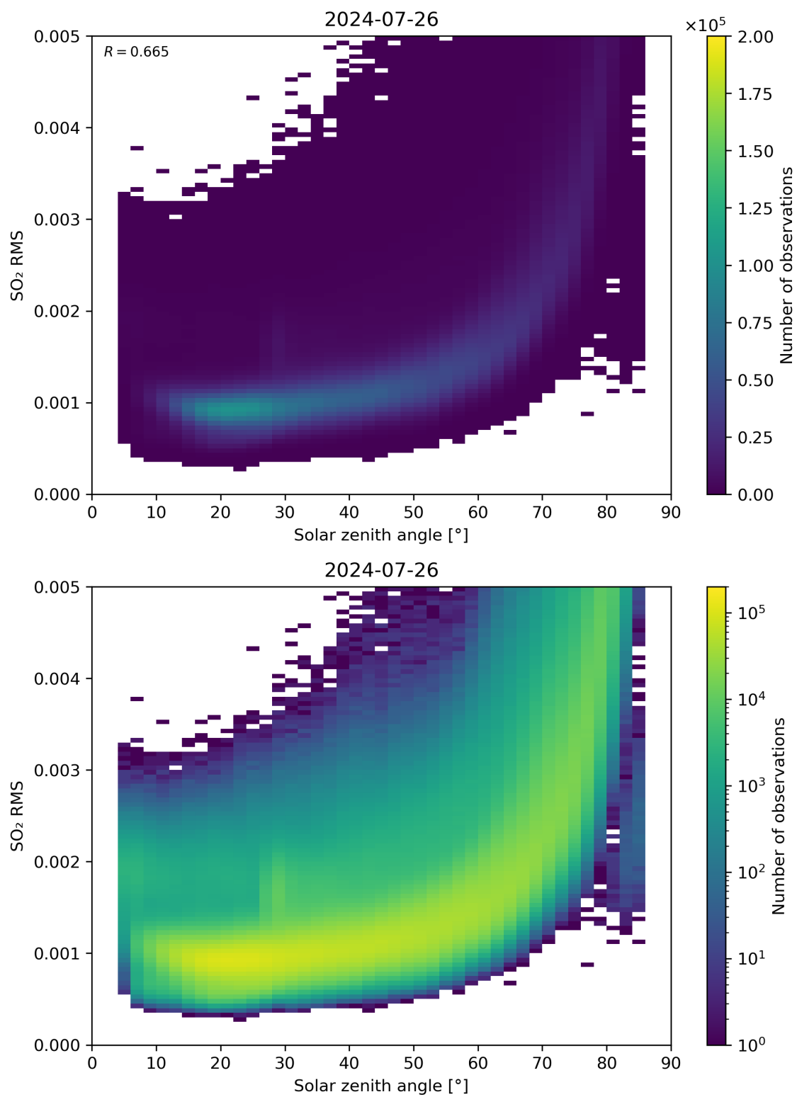
Figure 163: Scatter density plot of “Solar zenith angle” against “SO 2 RMS” for 2024-07-26 to 2024-07-27.
