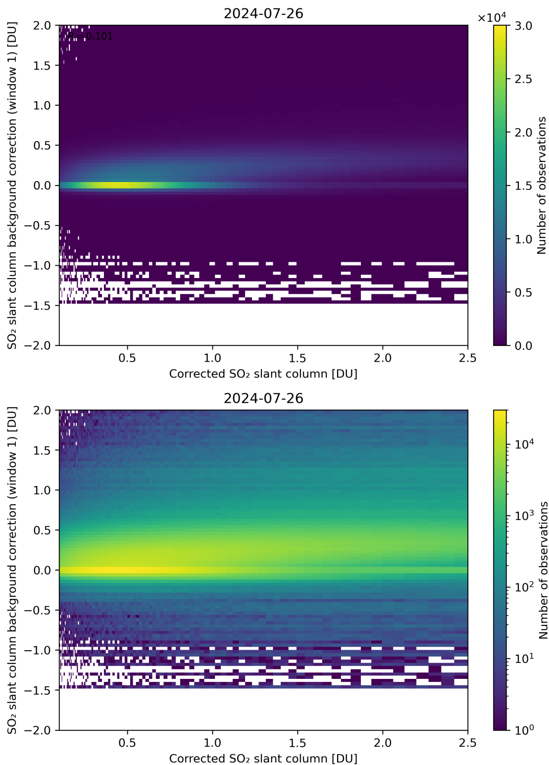
Figure 178: Scatter density plot of “Corrected SO 2 slant column” against “SO 2 slant column background correction (window 1)” for 2024-07-26 to 2024-07-27.
