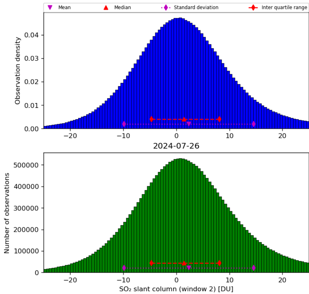
Figure 60: Histogram of “SO 2 slant column (window 2)” for 2024-07-26 to 2024-07-27
