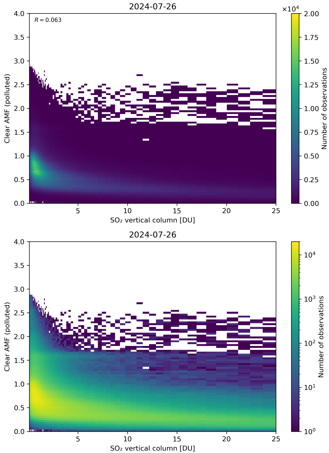
Figure 296: Scatter density plot of “SO 2 vertical column” against “Clear AMF (polluted)” for 2024-07-26 to 2024-07-27.
