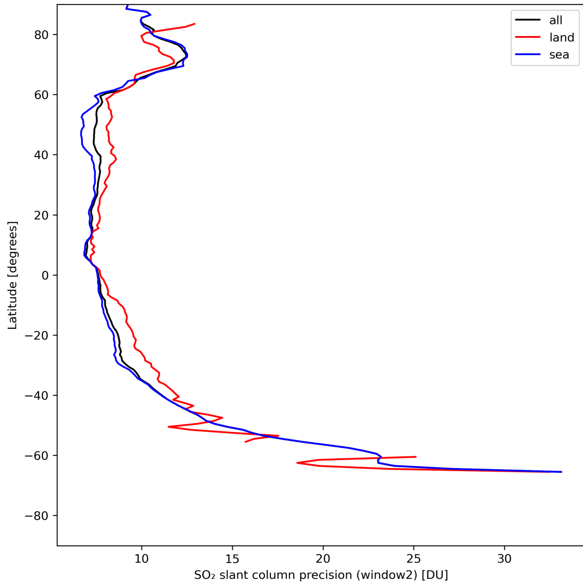
Figure 38: Zonal average of “SO 2 slant column precision (window2)” for 2024-07-26 to 2024-07-27.
