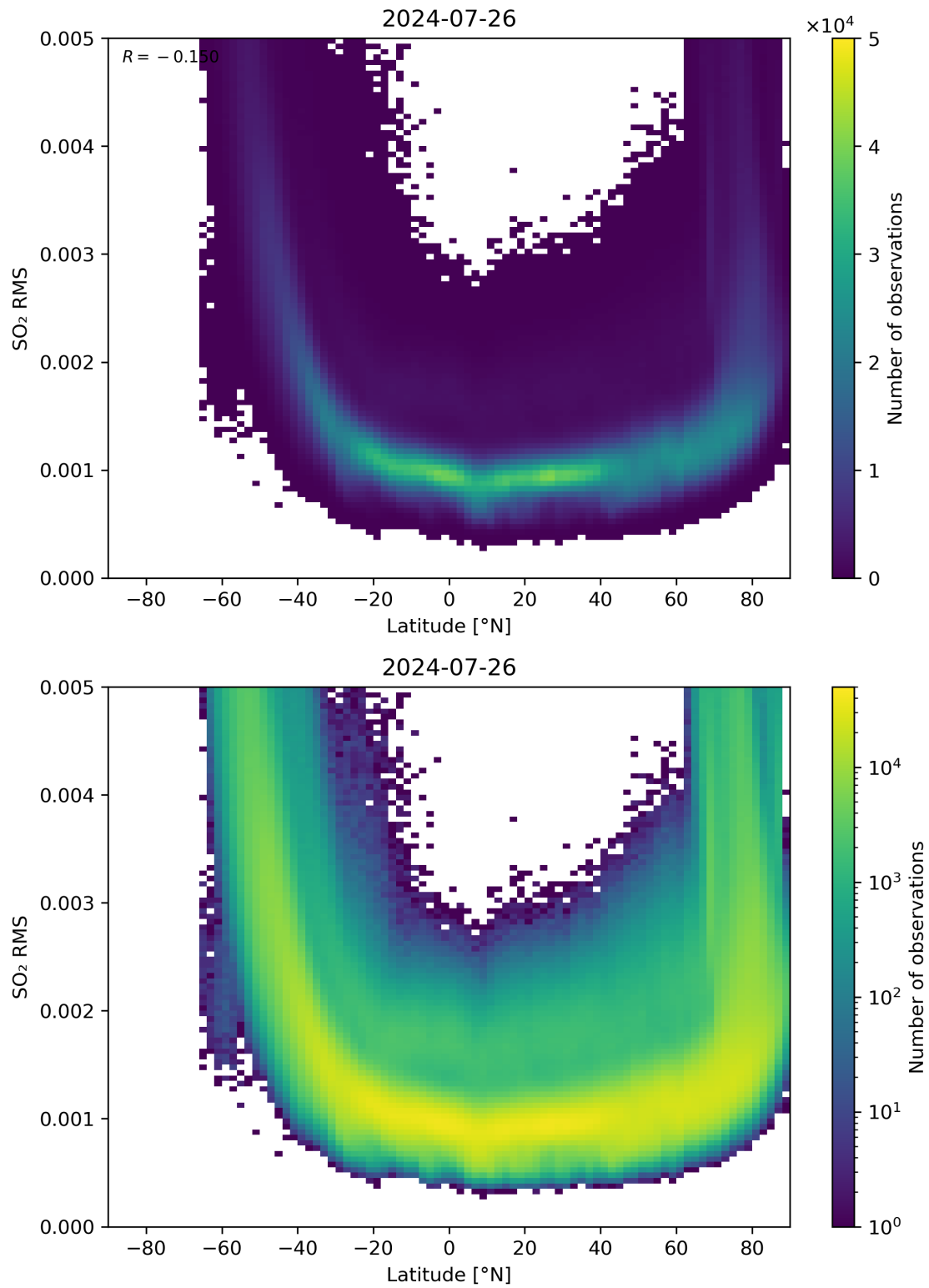
Figure 144: Scatter density plot of “Latitude” against “SO 2 RMS” for 2024-07-26 to 2024-07-27.
