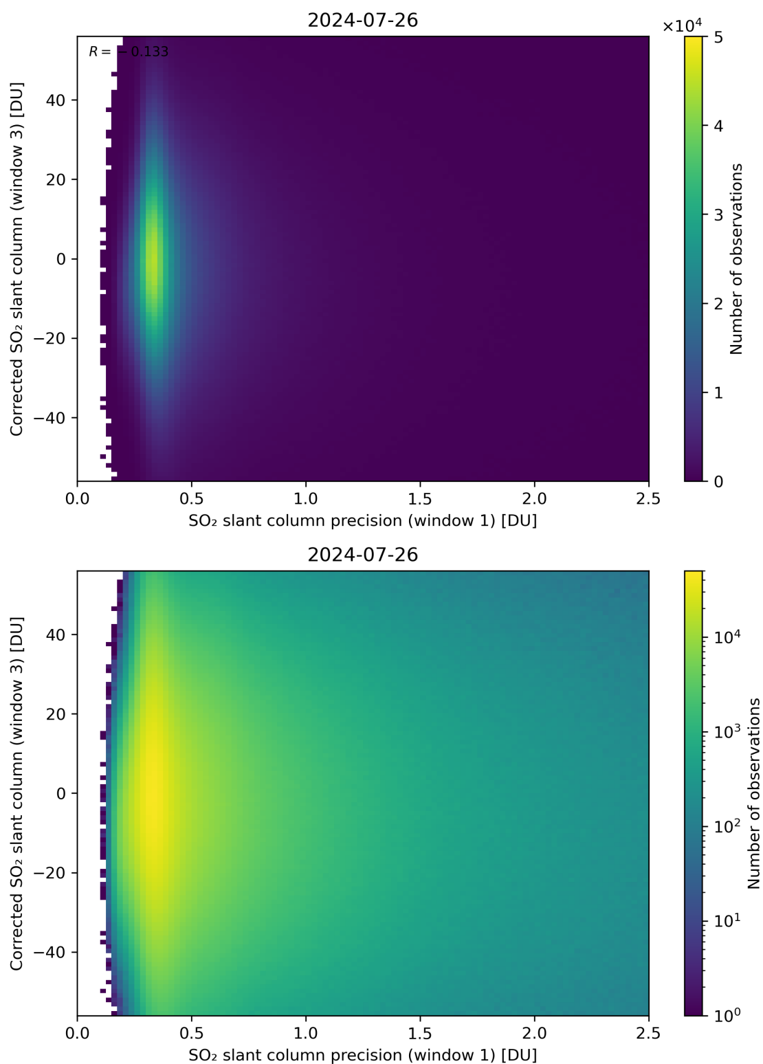
Figure 226: Scatter density plot of “SO 2 slant column precision (window 1)” against “Corrected SO 2 slant column (window 3)” for 2024-07-26 to 2024-07-27.
