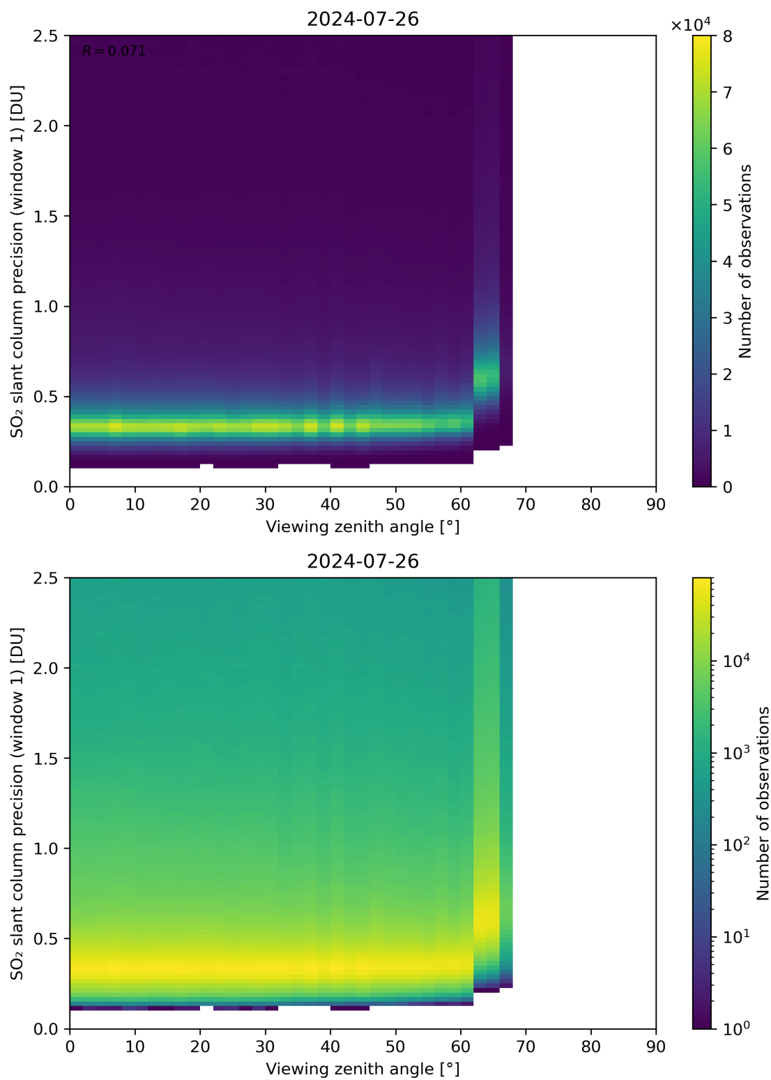
Figure 321: Scatter density plot of “Viewing zenith angle” against “SO 2 slant column precision (window 1)” for 2024-07-26 to 2024-07-27.
