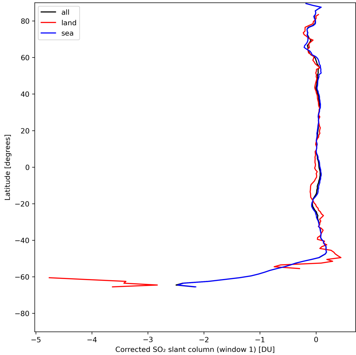
Figure 35: Zonal average of “Corrected SO 2 slant column (window 1)” for 2024-07-26 to 2024-07-27.
