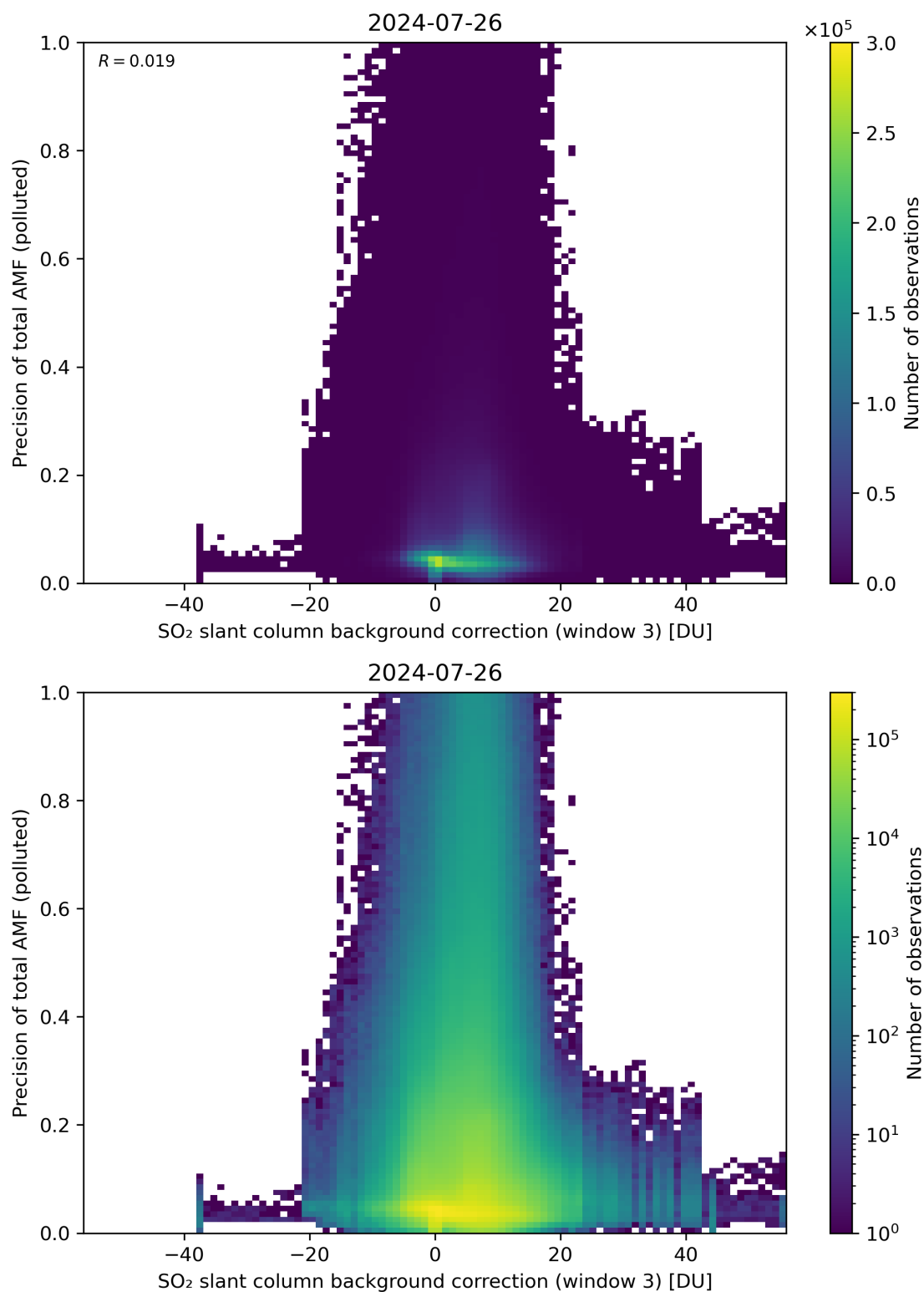
Figure 126: Scatter density plot of “SO 2 slant column background correction (window 3)” against “Precision of total AMF (polluted)” for 2024-07-26 to 2024-07-27.
