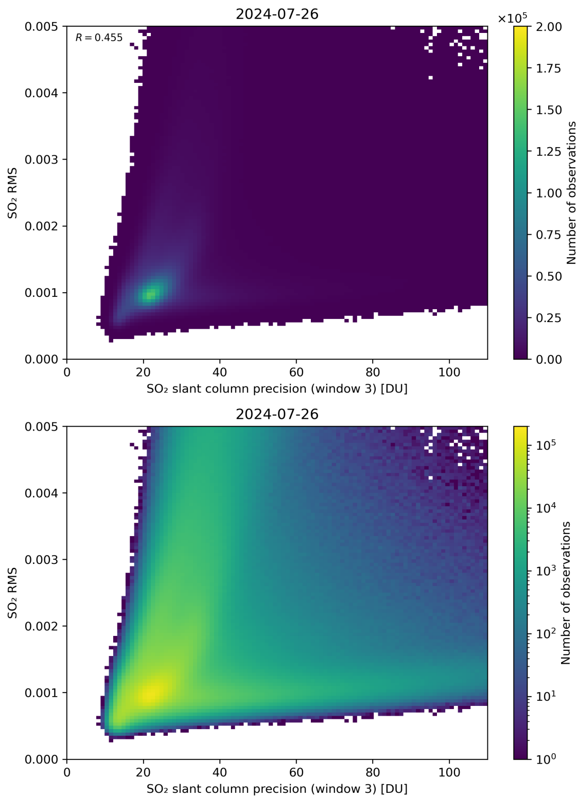
Figure 260: Scatter density plot of “SO 2 slant column precision (window 3)” against “SO 2 RMS” for 2024-07-26 to 2024-07-27.
