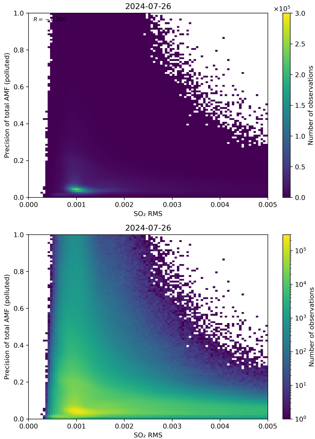
Figure 138: Scatter density plot of “SO 2 RMS” against “Precision of total AMF (polluted)” for 2024-07-26 to 2024-07-27.
