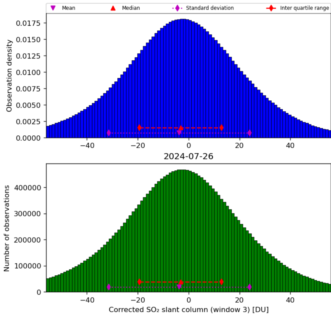
Figure 66: Histogram of “Corrected SO 2 slant column (window 3)” for 2024-07-26 to 2024-07-27
