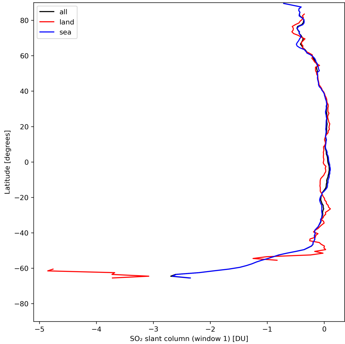
Figure 33: Zonal average of “SO 2 slant column (window 1)” for 2024-07-26 to 2024-07-27.
