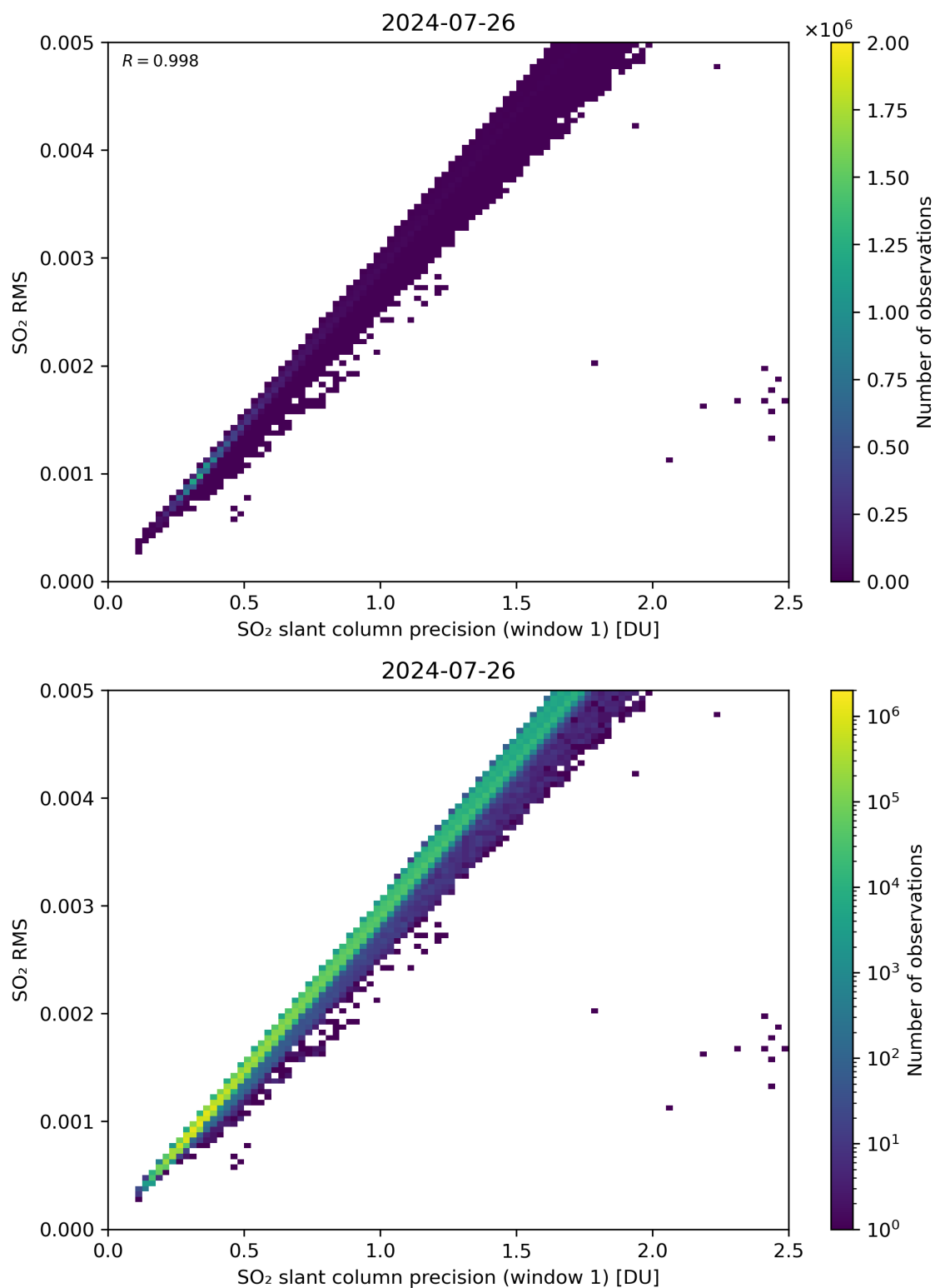
Figure 223: Scatter density plot of “SO 2 slant column precision (window 1)” against “SO 2 RMS” for 2024-07-26 to 2024-07-27.
