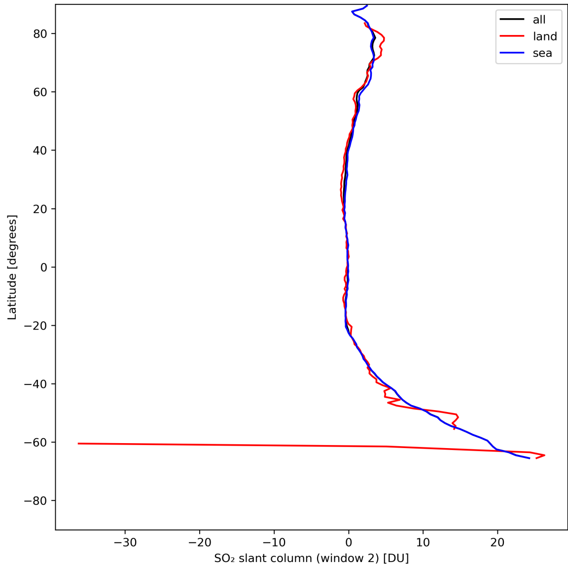
Figure 37: Zonal average of “SO 2 slant column (window 2)” for 2024-07-26 to 2024-07-27.
