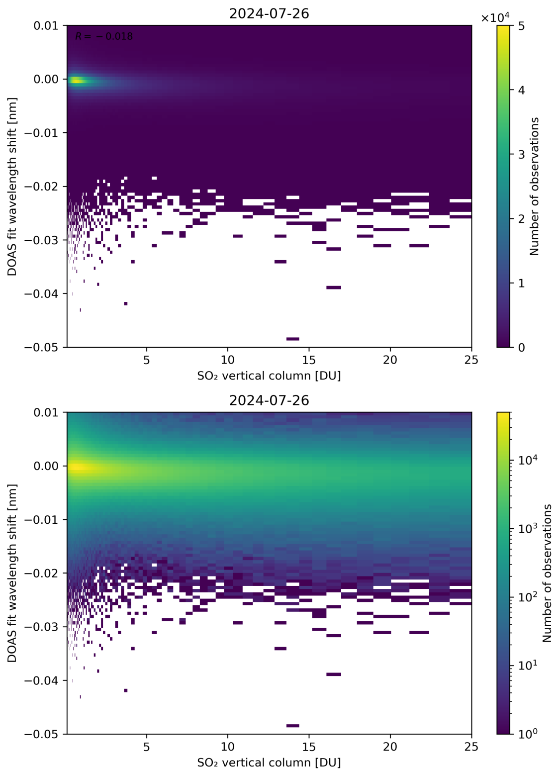
Figure 276: Scatter density plot of “SO 2 vertical column” against “DOAS fit wavelength shift” for 2024-07-26 to 2024-07-27.
