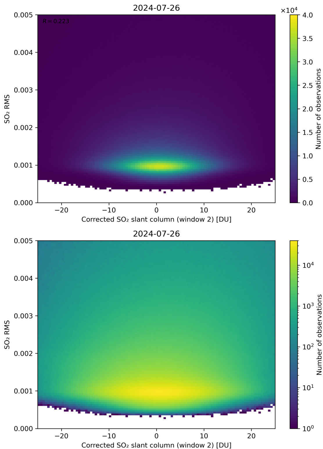
Figure 198: Scatter density plot of “Corrected SO 2 slant column (window 2)” against “SO 2 RMS” for 2024-07-26 to 2024-07-27.
