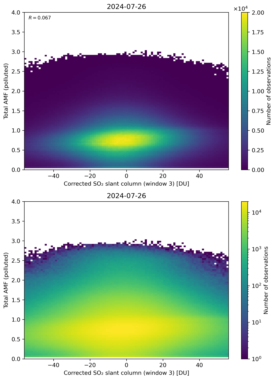
Figure 210: Scatter density plot of “Corrected SO 2 slant column (window 3)” against “Total AMF (polluted)” for 2024-07-26 to 2024-07-27.
