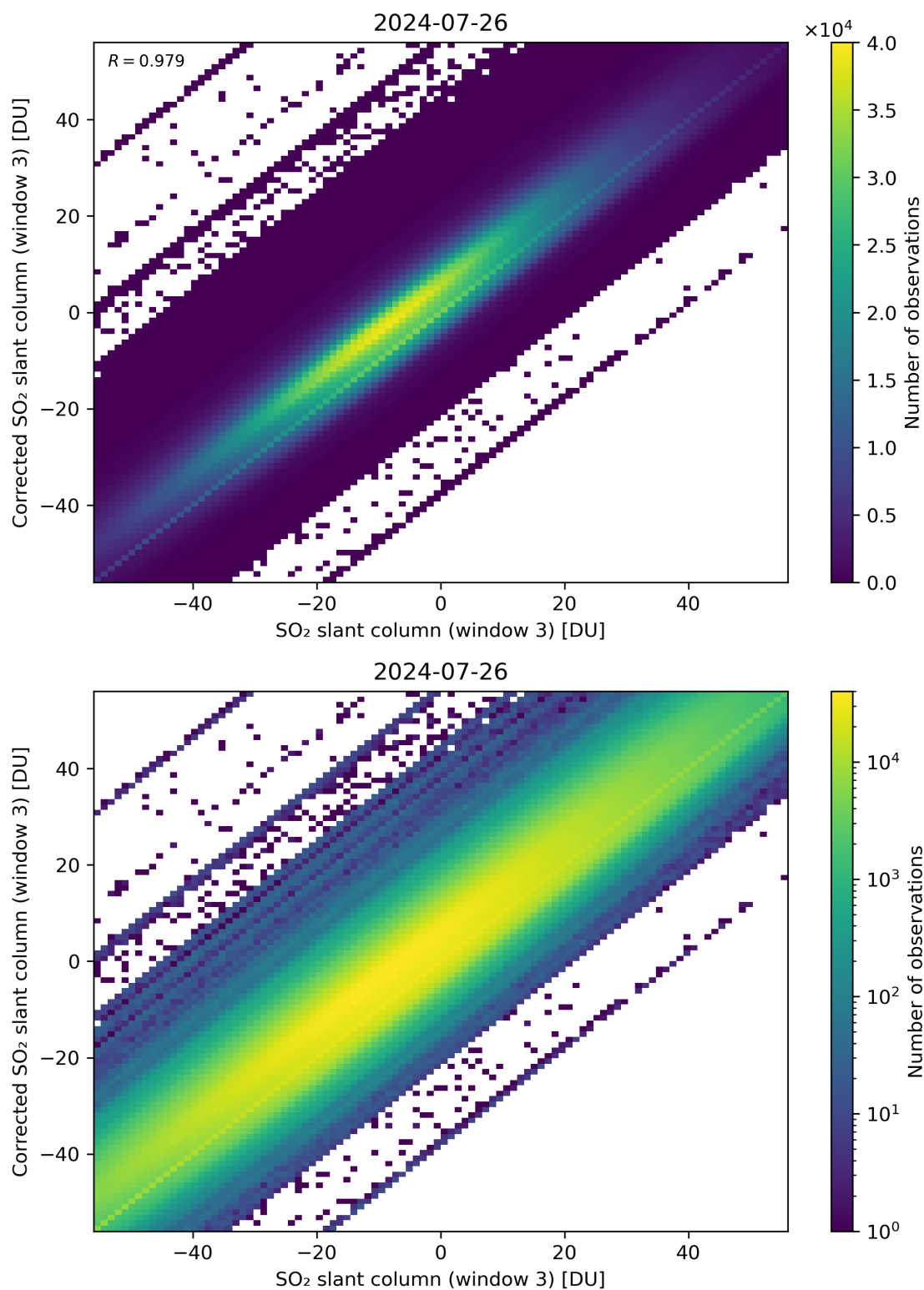
Figure 266: Scatter density plot of “SO 2 slant column (window 3)” against “Corrected SO 2 slant column (window 3)” for 2024-07-26 to 2024-07-27.
