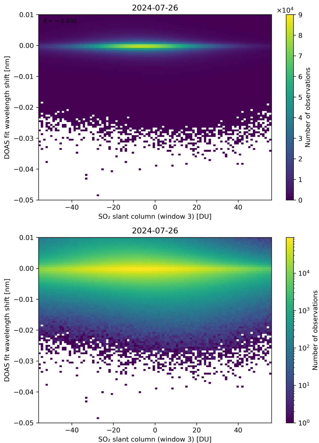
Figure 254: Scatter density plot of “SO 2 slant column (window 3)” against “DOAS fit wavelength shift” for 2024-07-26 to 2024-07-27.
