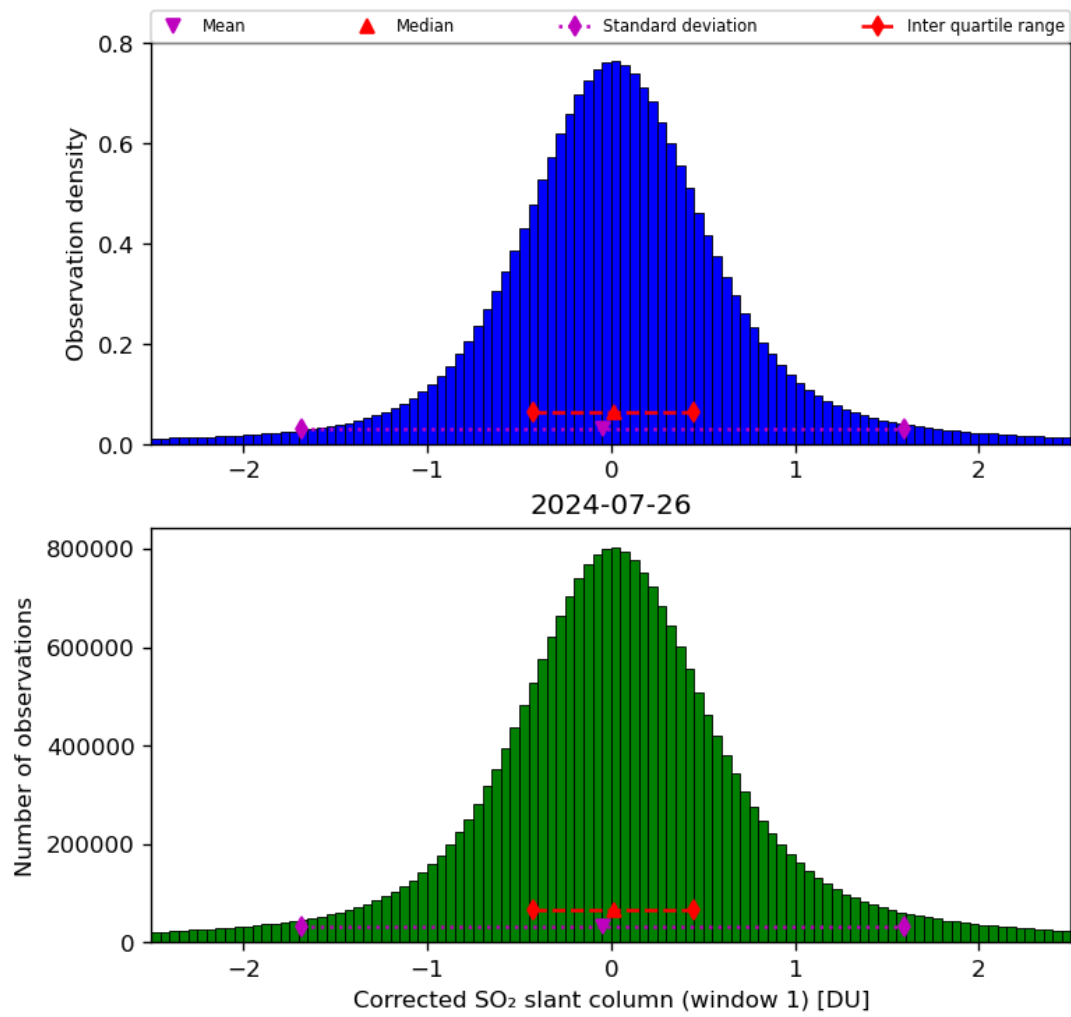
Figure 58: Histogram of “Corrected SO 2 slant column (window 1)” for 2024-07-26 to 2024-07-27
