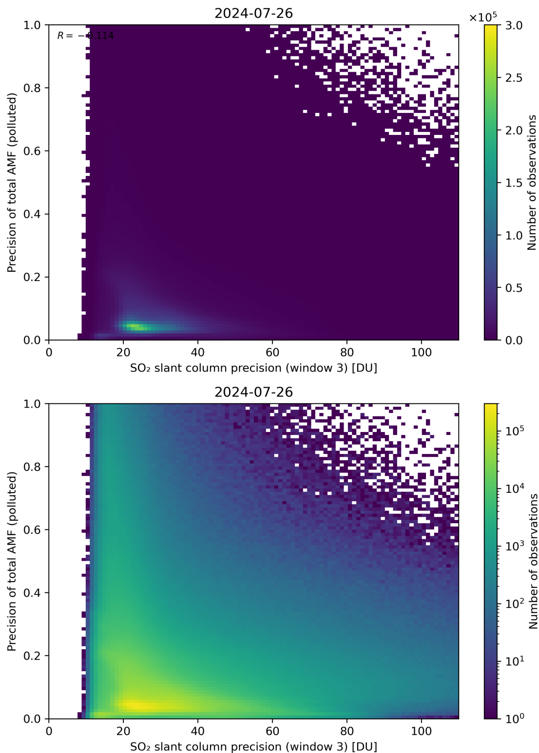
Figure 264: Scatter density plot of “SO 2 slant column precision (window 3)” against “Precision of total AMF (polluted)” for 2024-07-26 to 2024-07-27.
