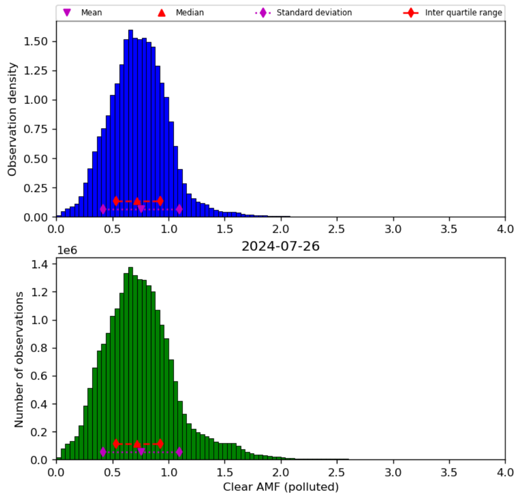
Figure 73: Histogram of “Clear AMF (polluted)” for 2024-07-26 to 2024-07-27
