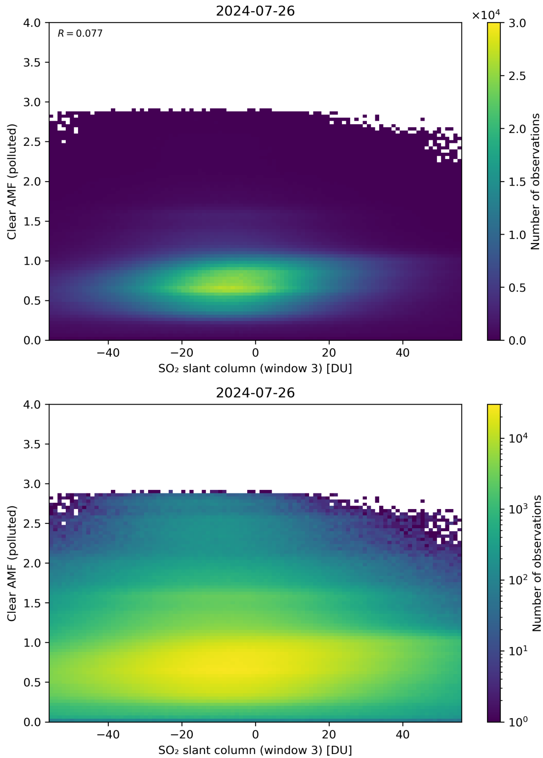
Figure 265: Scatter density plot of “SO 2 slant column (window 3)” against “Clear AMF (polluted)” for 2024-07-26 to 2024-07-27.
