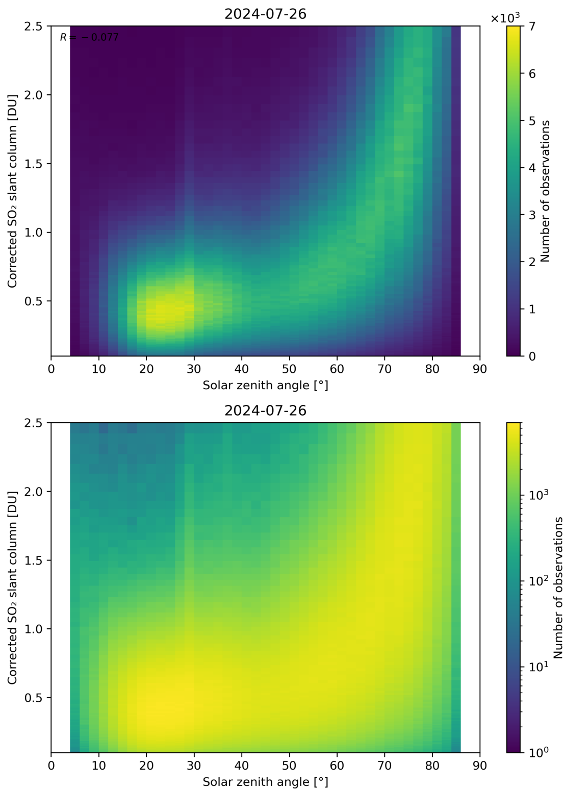
Figure 166: Scatter density plot of “Solar zenith angle” against “Corrected SO 2 slant column” for 2024-07-26 to 2024-07-27.
