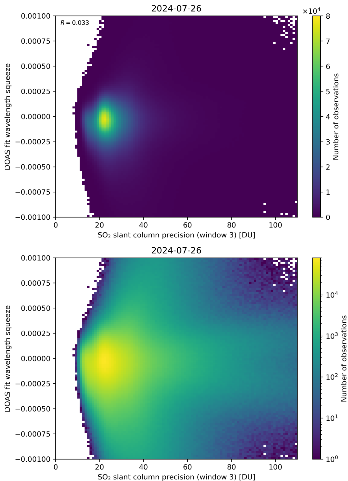
Figure 259: Scatter density plot of “SO 2 slant column precision (window 3)” against “DOAS fit wavelength squeeze” for 2024-07-26 to 2024-07-27.
