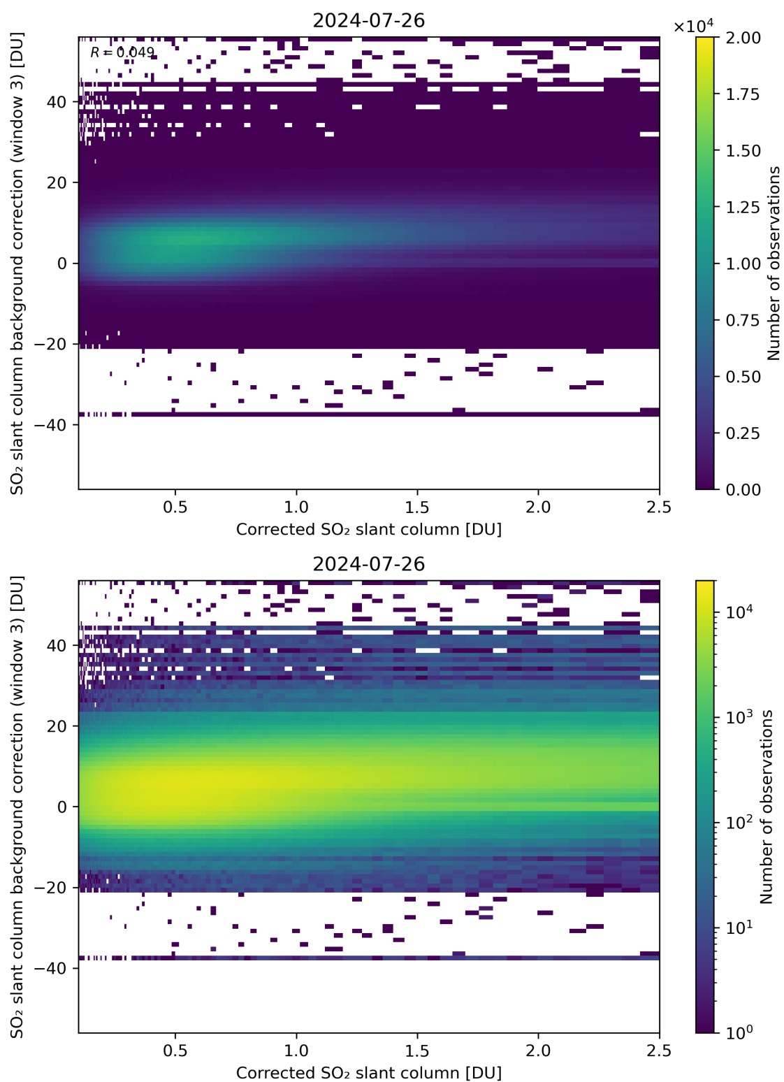
Figure 180: Scatter density plot of “Corrected SO 2 slant column” against “SO 2 slant column background correction (window 3)” for 2024-07-26 to 2024-07-27.
