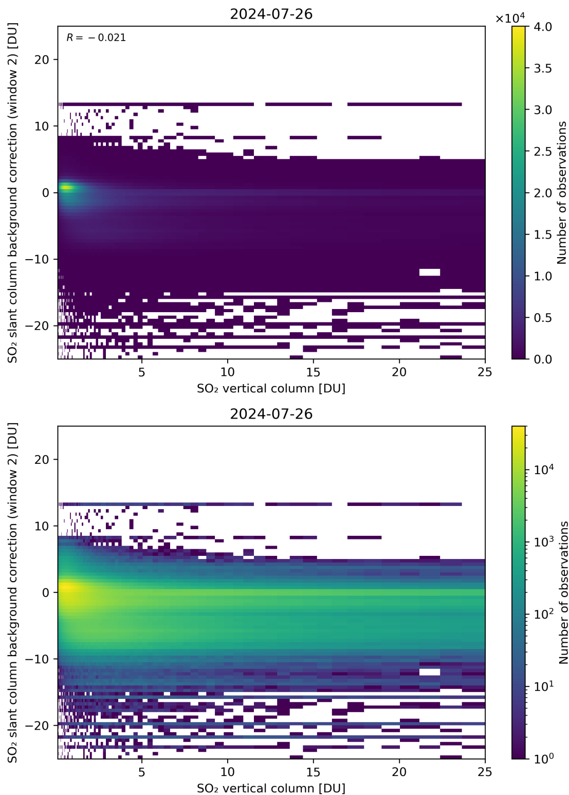
Figure 274: Scatter density plot of “SO 2 vertical column” against “SO 2 slant column background correction (window 2)” for 2024-07-26 to 2024-07-27.
