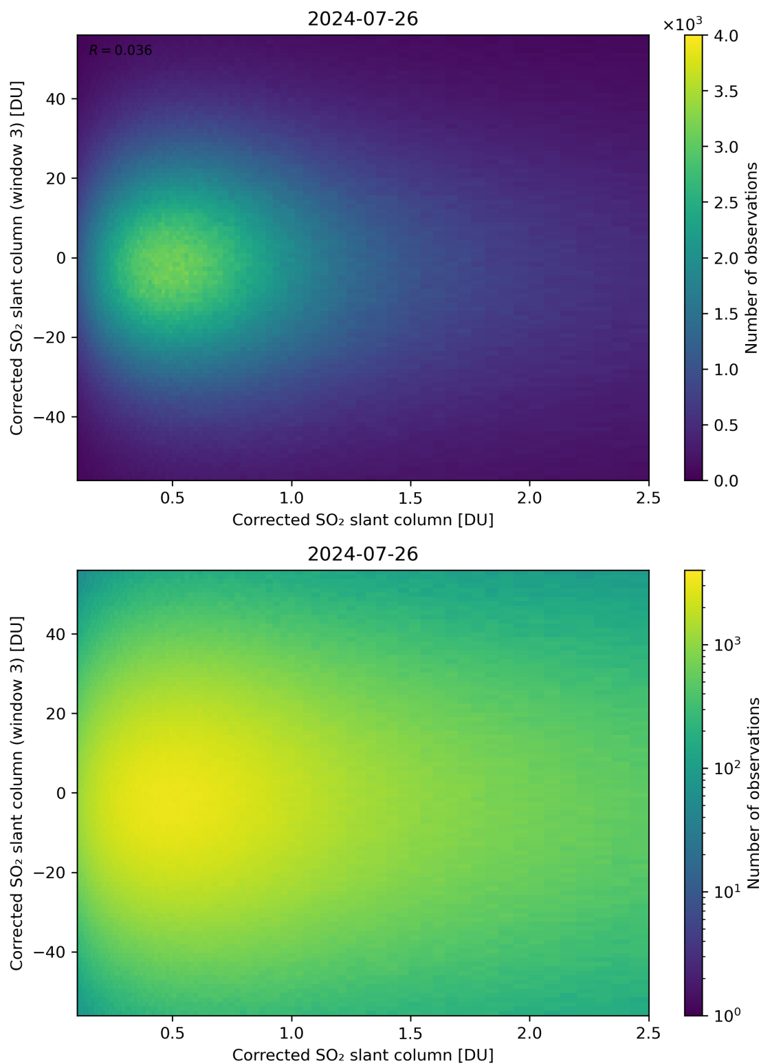
Figure 186: Scatter density plot of “Corrected SO 2 slant column” against “Corrected SO 2 slant column (window 3)” for 2024-07-26 to 2024-07-27.
