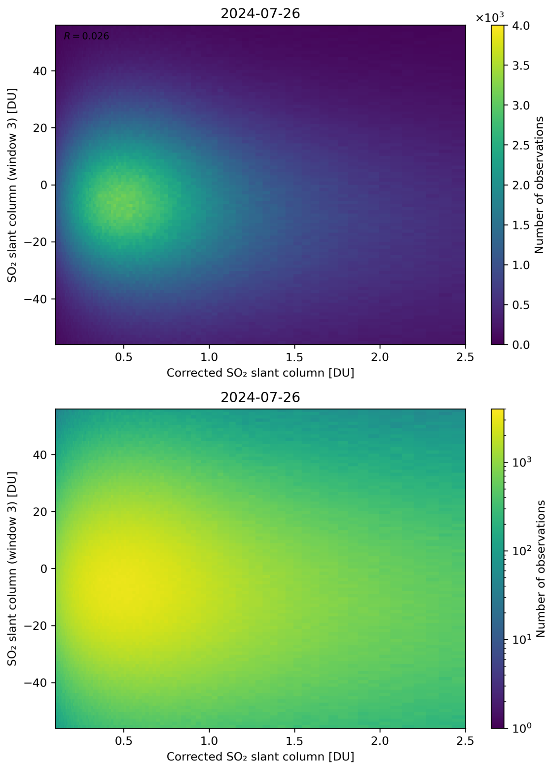
Figure 190: Scatter density plot of “Corrected SO 2 slant column” against “SO 2 slant column (window 3)” for 2024-07-26 to 2024-07-27.
