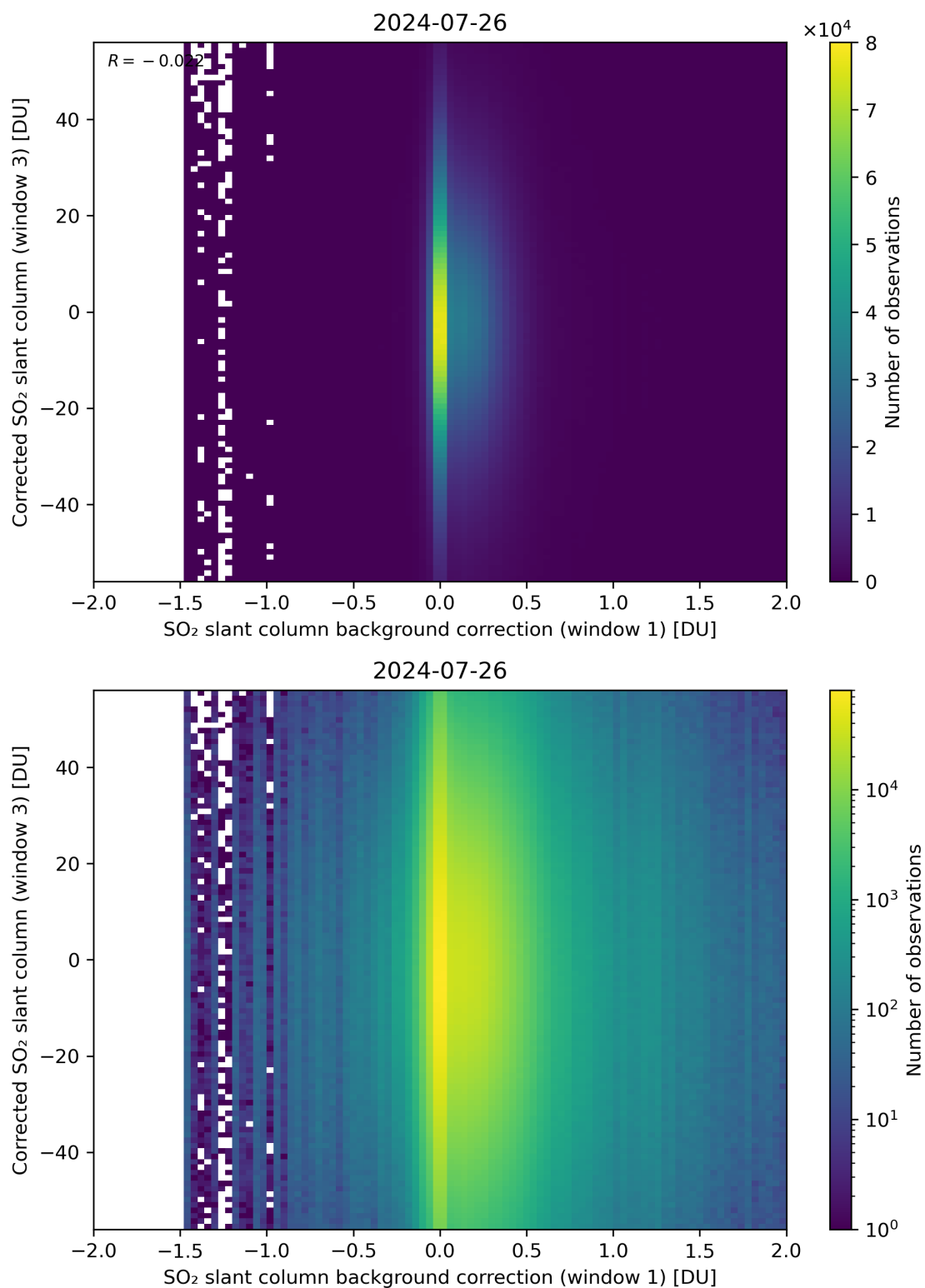
Figure 105: Scatter density plot of “SO 2 slant column background correction (window 1)” against “Corrected SO 2 slant column (window 3)” for 2024-07-26 to 2024-07-27.
