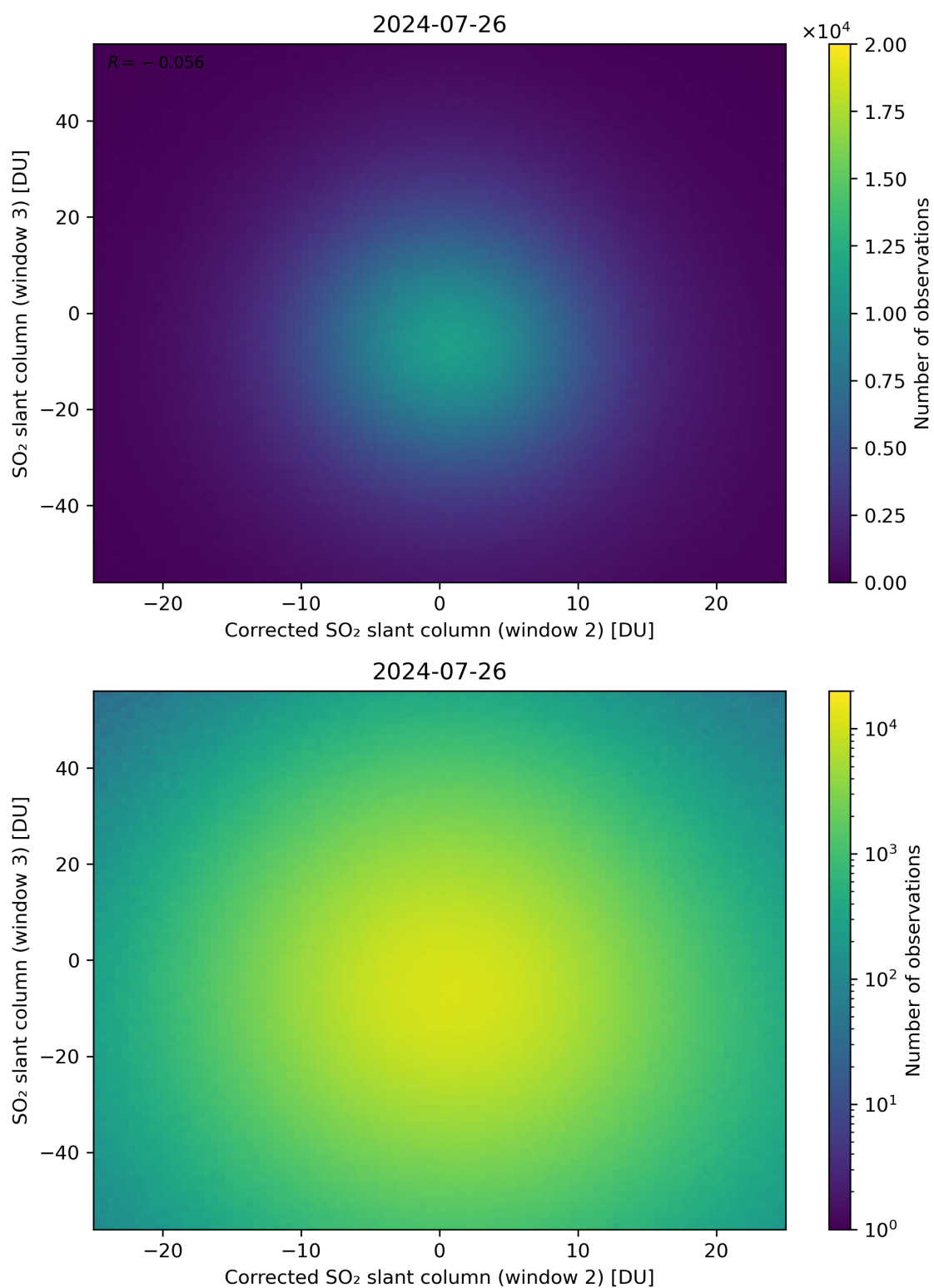
Figure 201: Scatter density plot of “Corrected SO 2 slant column (window 2)” against “SO 2 slant column (window 3)” for 2024-07-26 to 2024-07-27.
