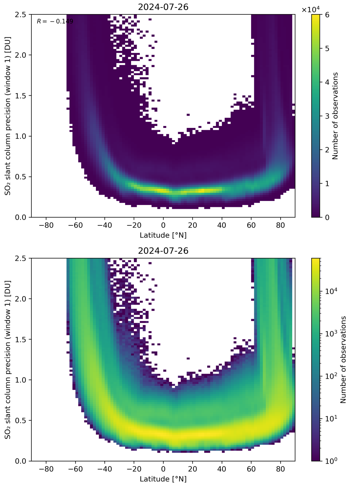
Figure 150: Scatter density plot of “Latitude” against “SO 2 slant column precision (window 1)” for 2024-07-26 to 2024-07-27.
