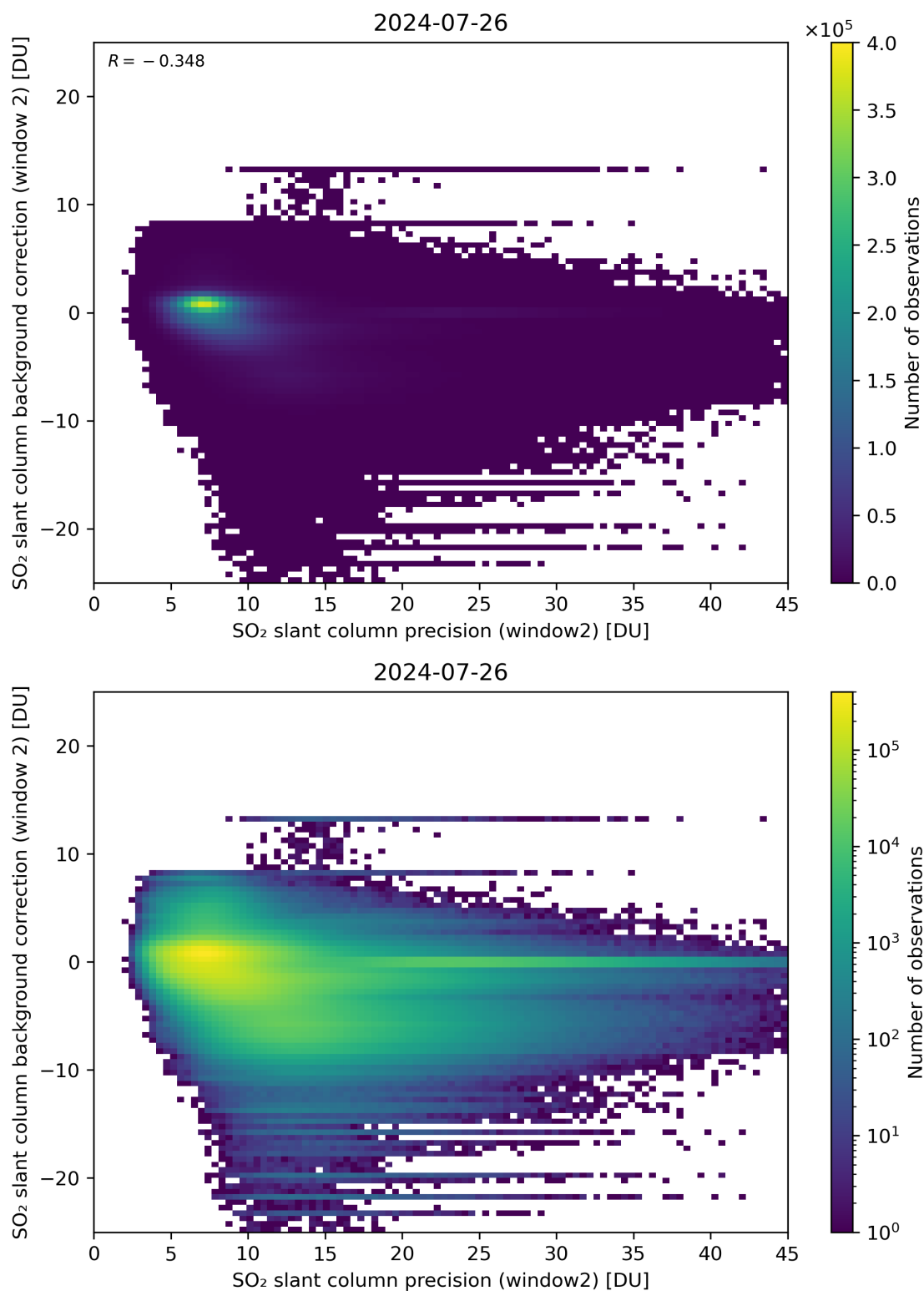
Figure 241: Scatter density plot of “SO 2 slant column precision (window2)” against “SO 2 slant column background correction (window 2)” for 2024-07-26 to 2024-07-27.
