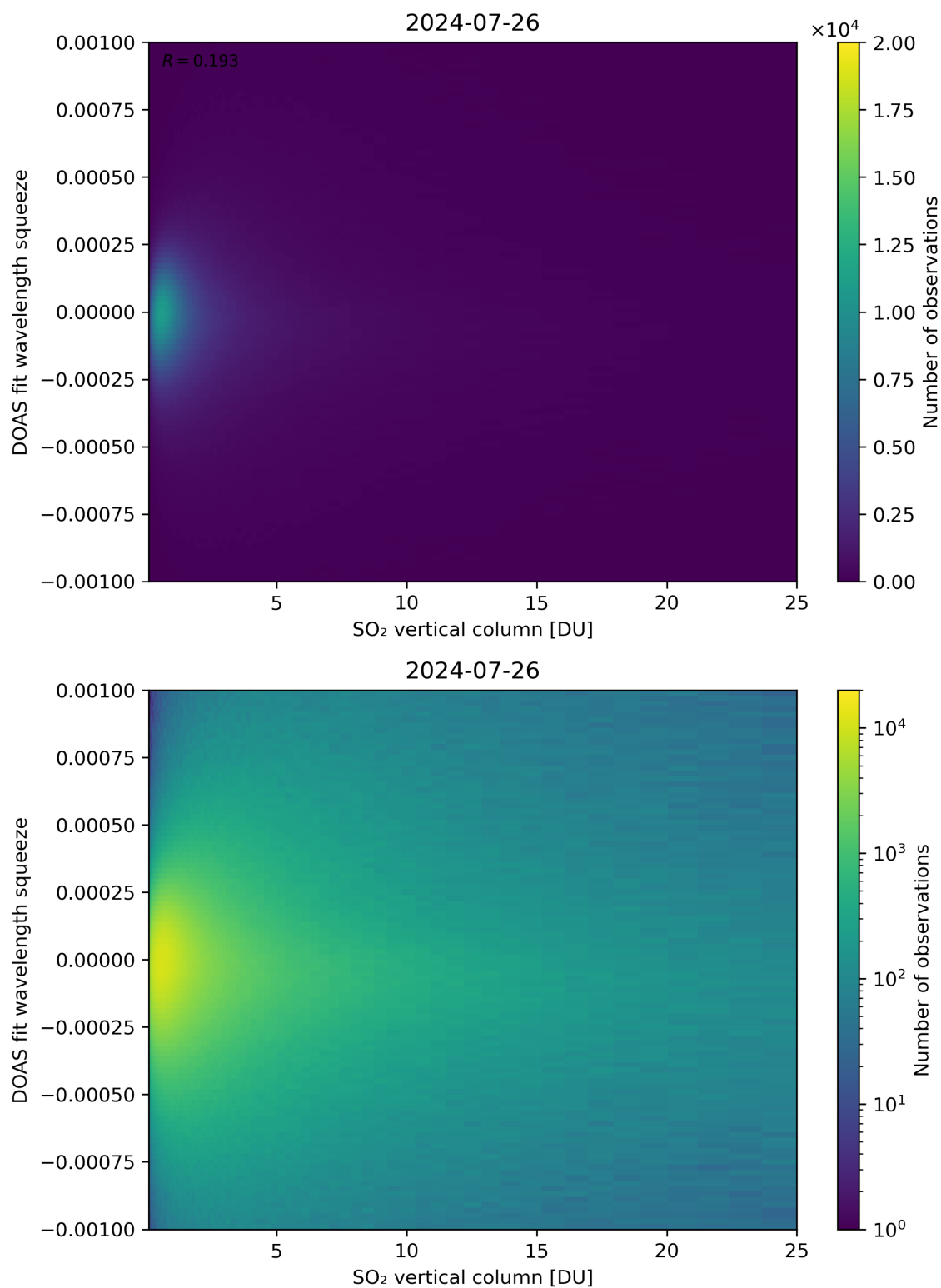
Figure 277: Scatter density plot of “SO 2 vertical column” against “DOAS fit wavelength squeeze” for 2024-07-26 to 2024-07-27.
