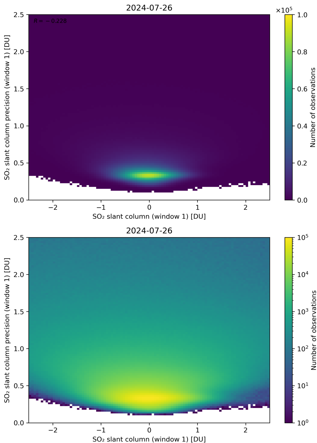
Figure 235: Scatter density plot of “SO 2 slant column (window 1)” against “SO 2 slant column precision (window 1)” for 2024-07-26 to 2024-07-27.
