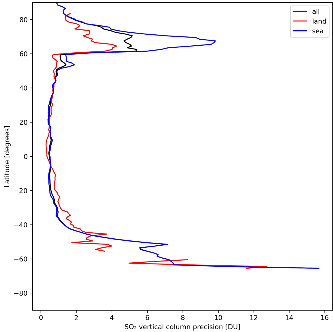
Figure 31: Zonal average of “SO 2 vertical column precision” for 2024-07-26 to 2024-07-27.
