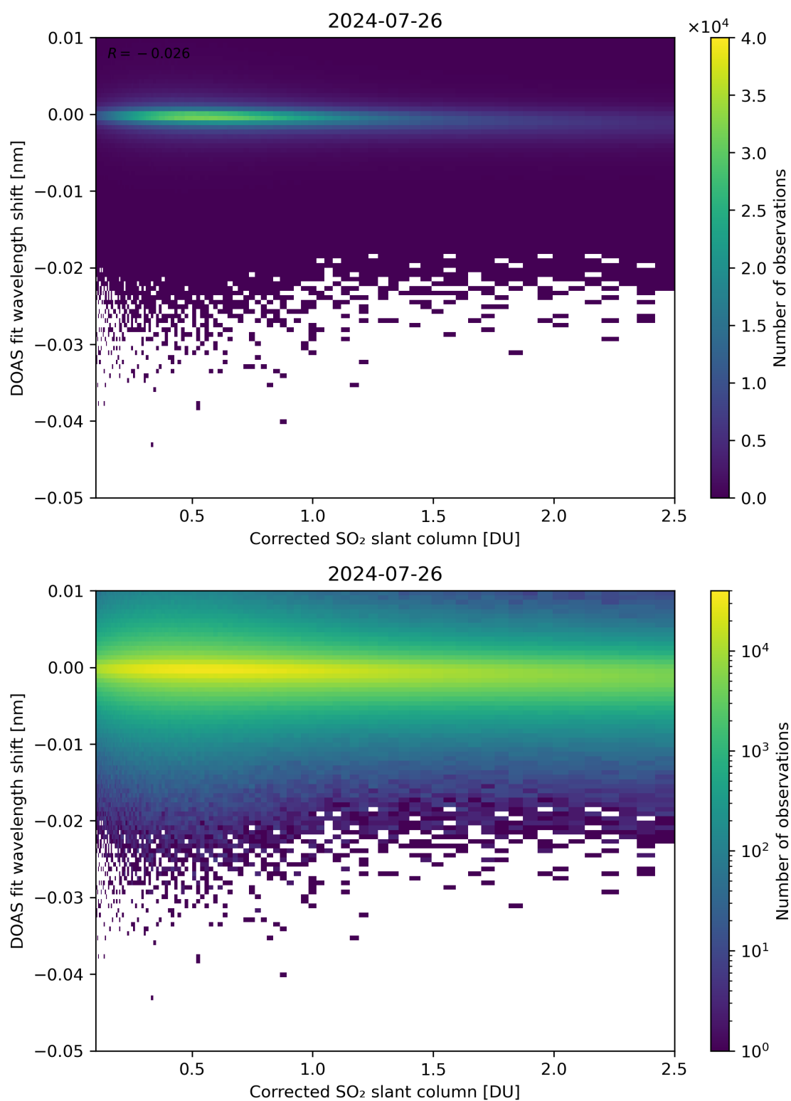
Figure 181: Scatter density plot of “Corrected SO 2 slant column” against “DOAS fit wavelength shift” for 2024-07-26 to 2024-07-27.
