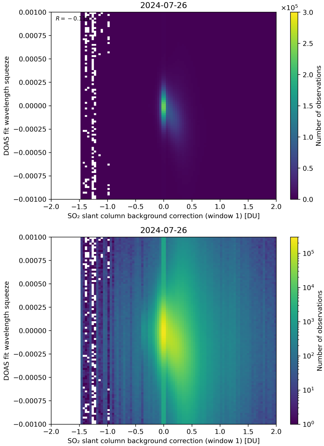
Figure 101: Scatter density plot of “SO 2 slant column background correction (window 1)” against “DOAS fit wavelength squeeze” for 2024-07-26 to 2024-07-27.
