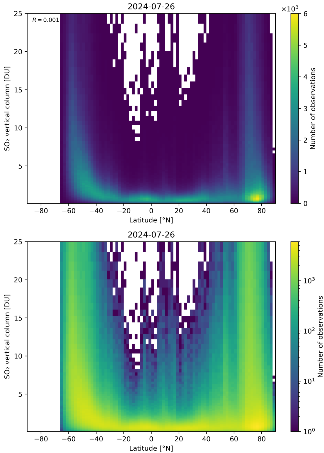
Figure 156: Scatter density plot of “Latitude” against “SO 2 vertical column” for 2024-07-26 to 2024-07-27.
