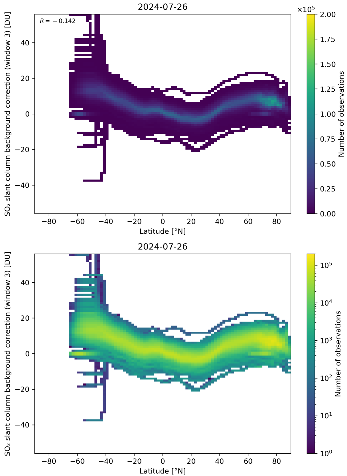
Figure 141: Scatter density plot of “Latitude” against “SO 2 slant column background correction (window 3)” for 2024-07-26 to 2024-07-27.
