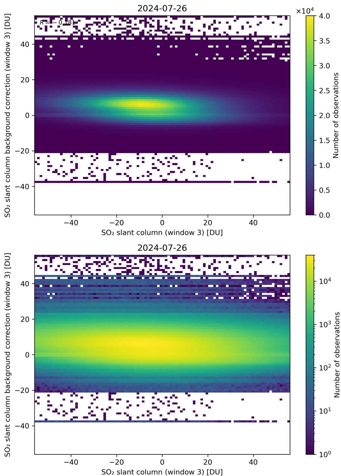
Figure 253: Scatter density plot of “SO 2 slant column (window 3)” against “SO 2 slant column background correction (window 3)” for 2024-07-26 to 2024-07-27.
