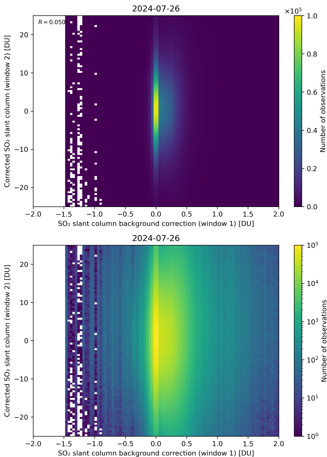
Figure 104: Scatter density plot of “SO 2 slant column background correction (window 1)” against “Corrected SO 2 slant column (window 2)” for 2024-07-26 to 2024-07-27.
