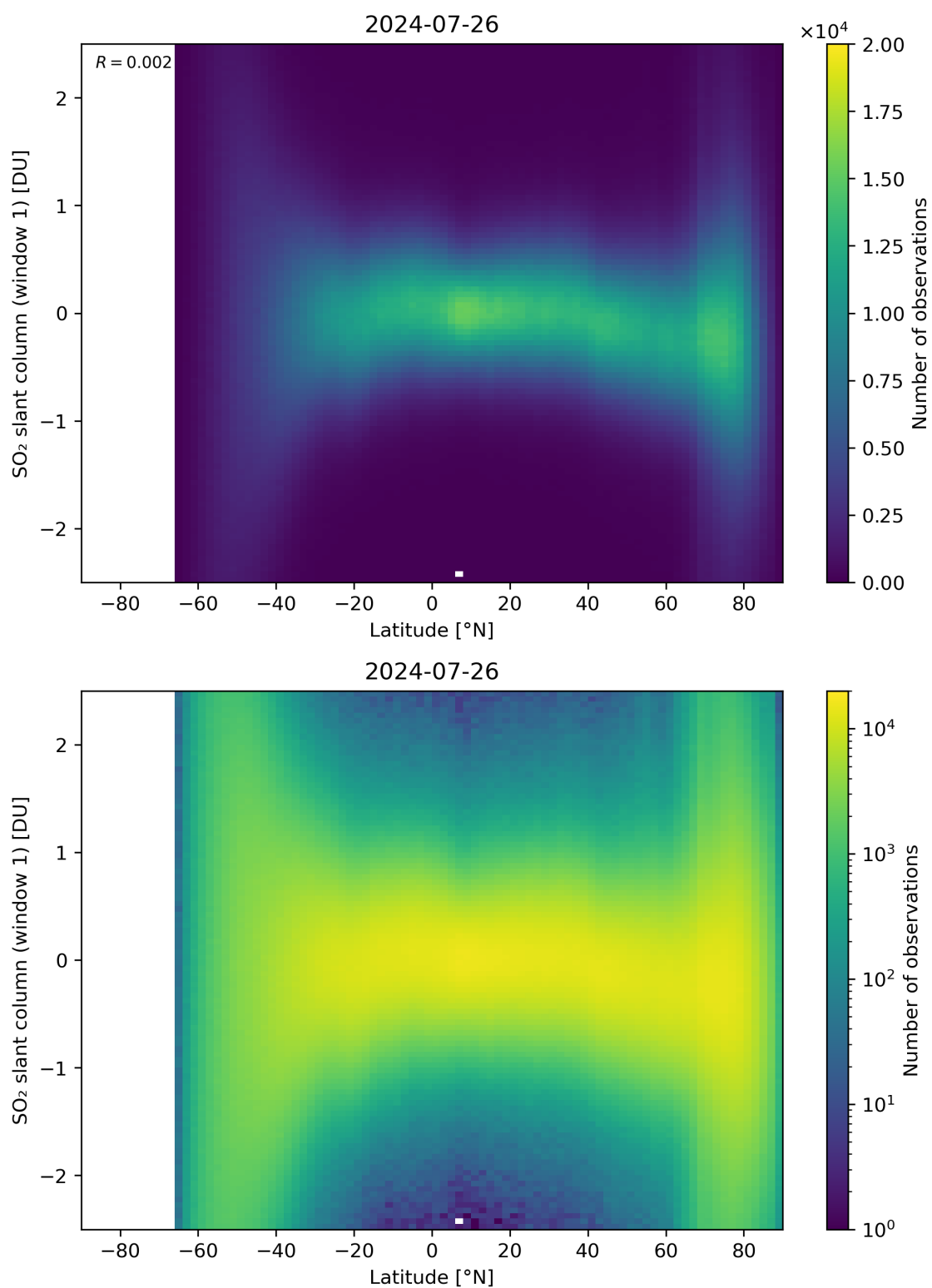
Figure 149: Scatter density plot of “Latitude” against “SO 2 slant column (window 1)” for 2024-07-26 to 2024-07-27.
