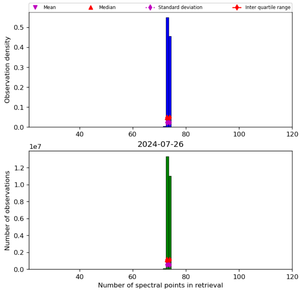
Figure 74: Histogram of “Number of spectral points in retrieval” for 2024-07-26 to 2024-07-27
