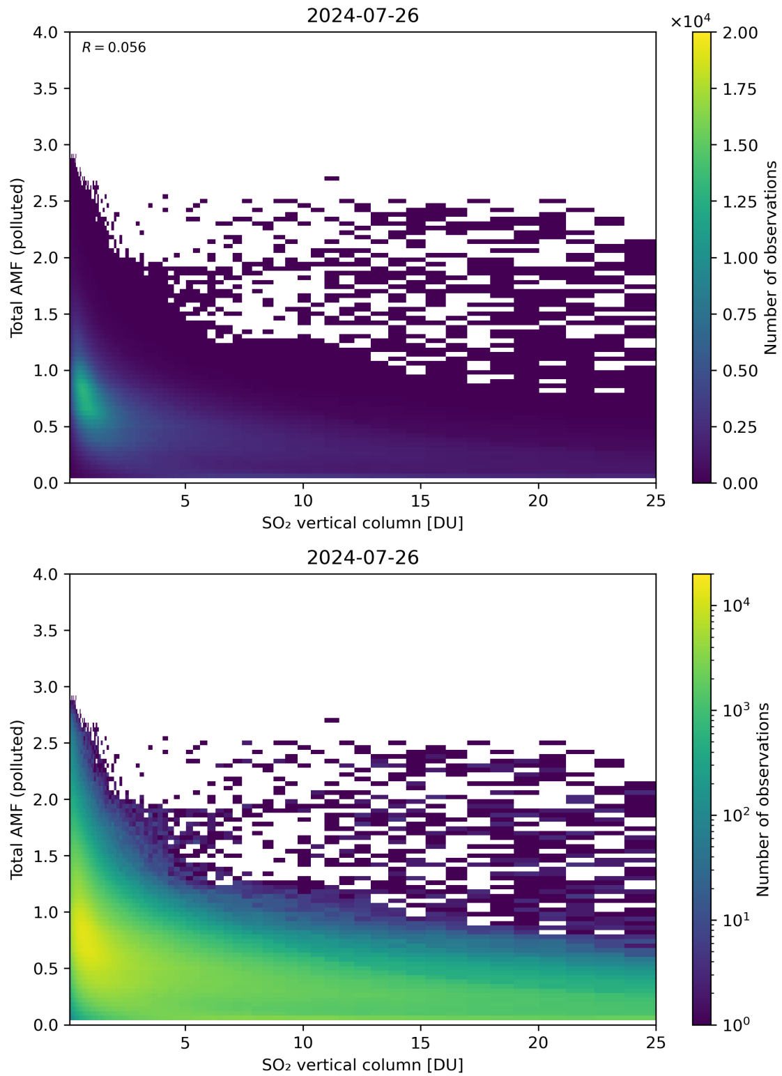
Figure 305: Scatter density plot of “SO 2 vertical column” against “Total AMF (polluted)” for 2024-07-26 to 2024-07-27.
