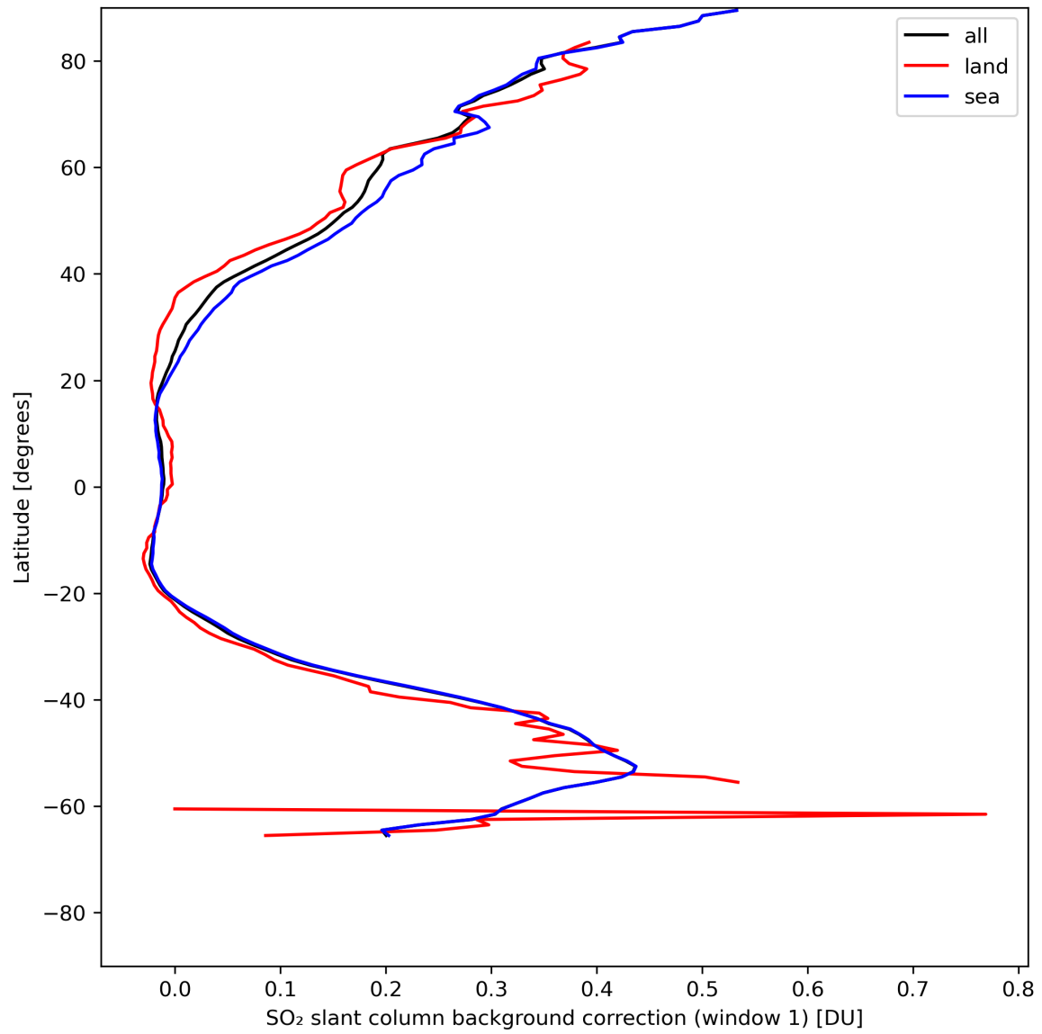
Figure 36: Zonal average of “SO 2 slant column background correction (window 1)” for 2024-07-26 to 2024-07-27.
