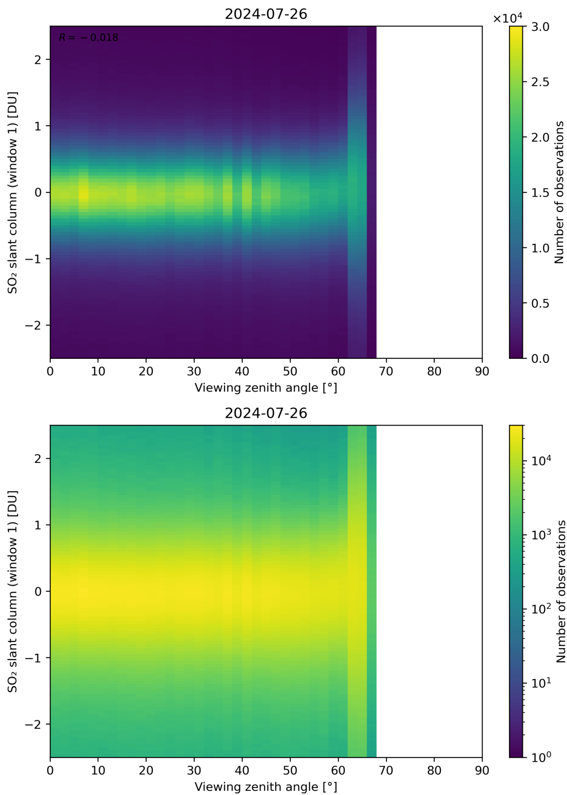
Figure 320: Scatter density plot of “Viewing zenith angle” against “SO 2 slant column (window 1)” for 2024-07-26 to 2024-07-27.
