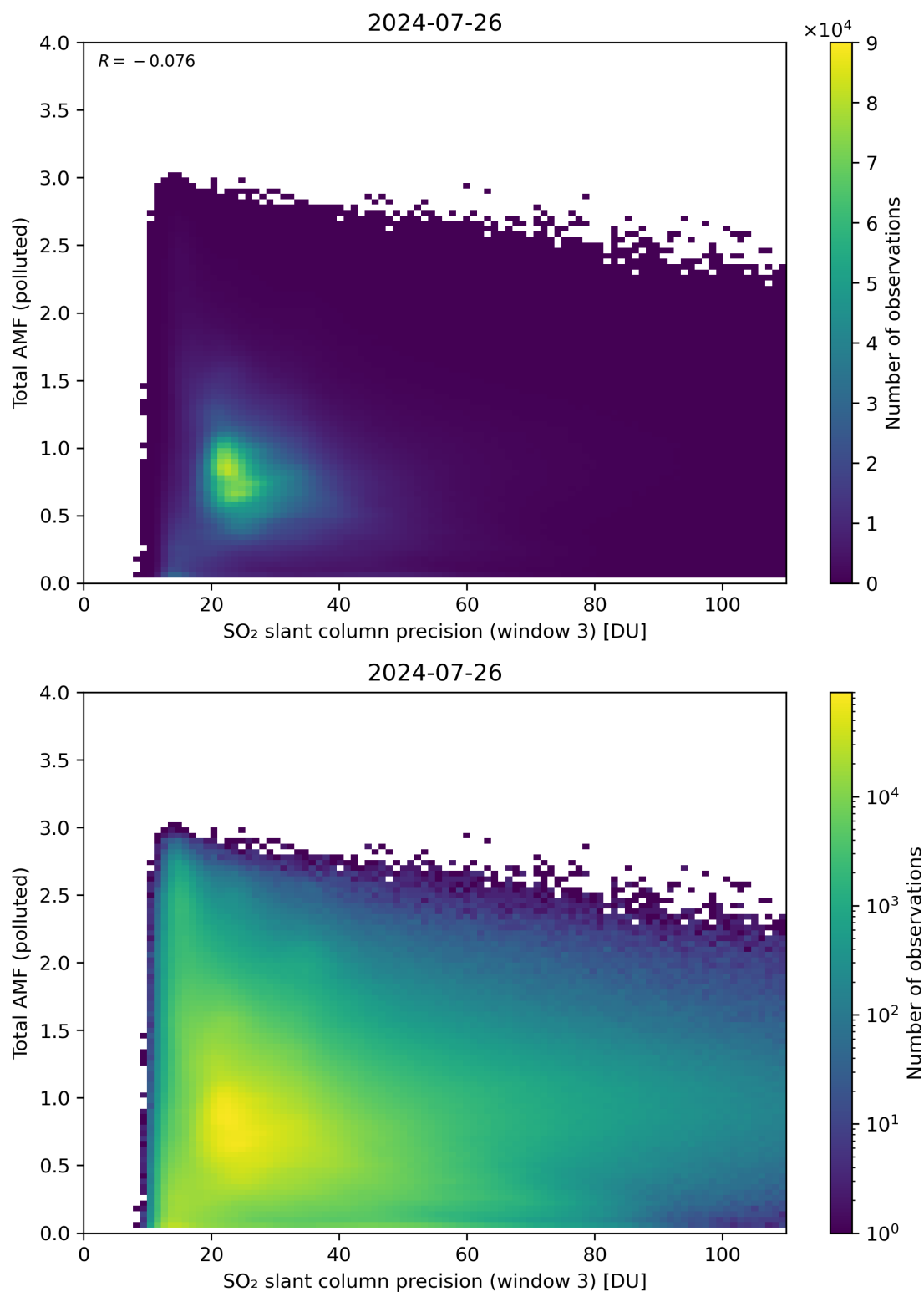
Figure 263: Scatter density plot of “SO 2 slant column precision (window 3)” against “Total AMF (polluted)” for 2024-07-26 to 2024-07-27.
