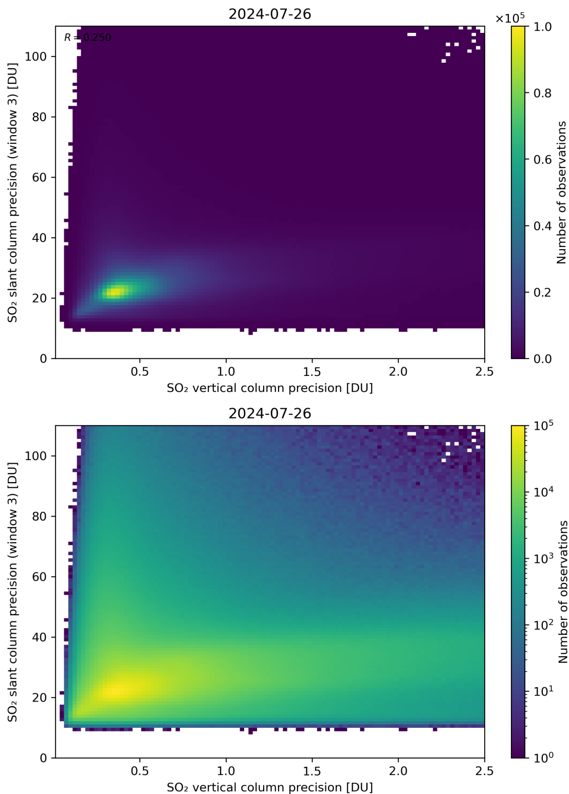
Figure 293: Scatter density plot of “SO 2 vertical column precision” against “SO 2 slant column precision (window 3)” for 2024-07-26 to 2024-07-27.
