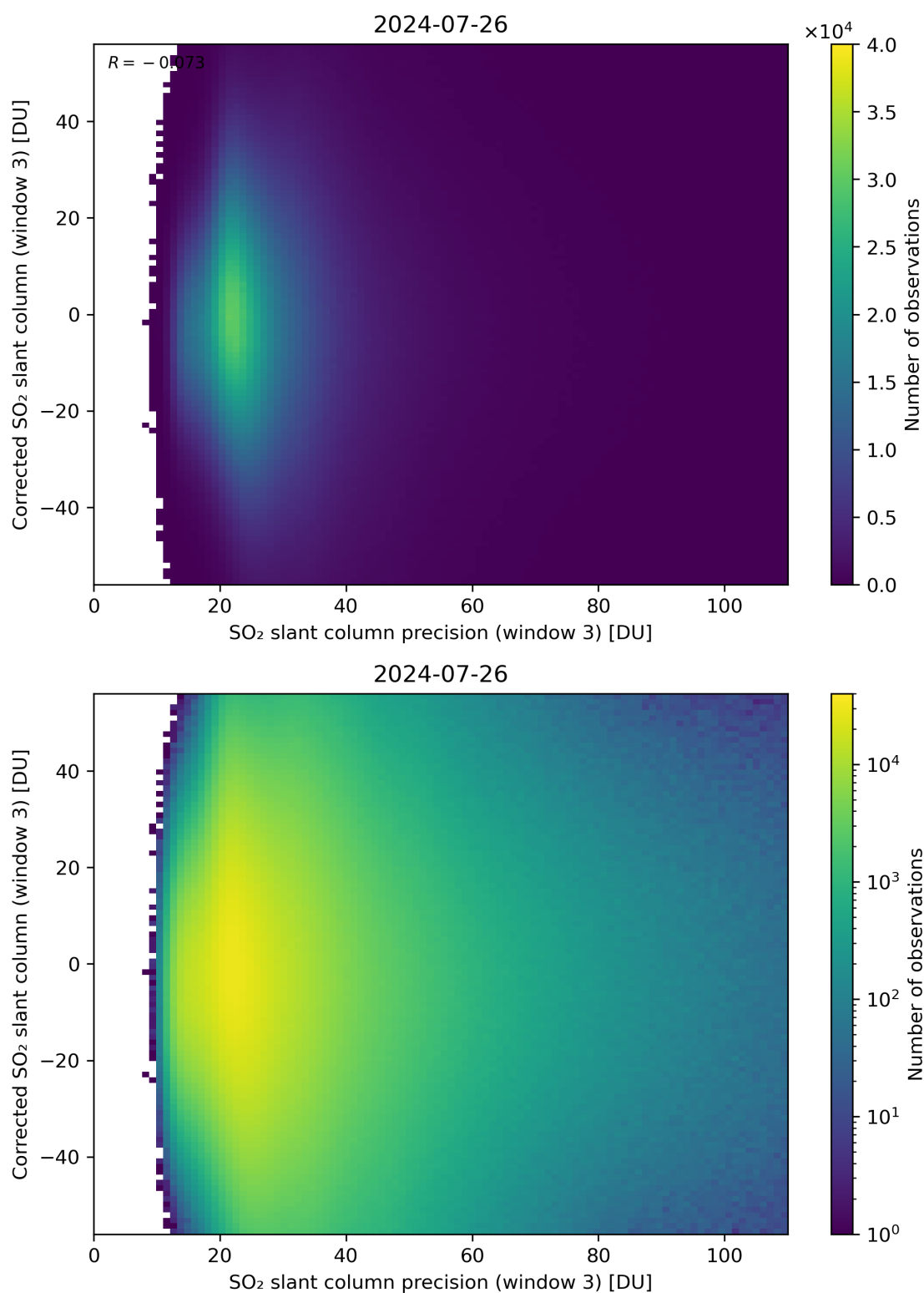
Figure 262: Scatter density plot of “SO 2 slant column precision (window 3)” against “Corrected SO 2 slant column (window 3)” for 2024-07-26 to 2024-07-27.
