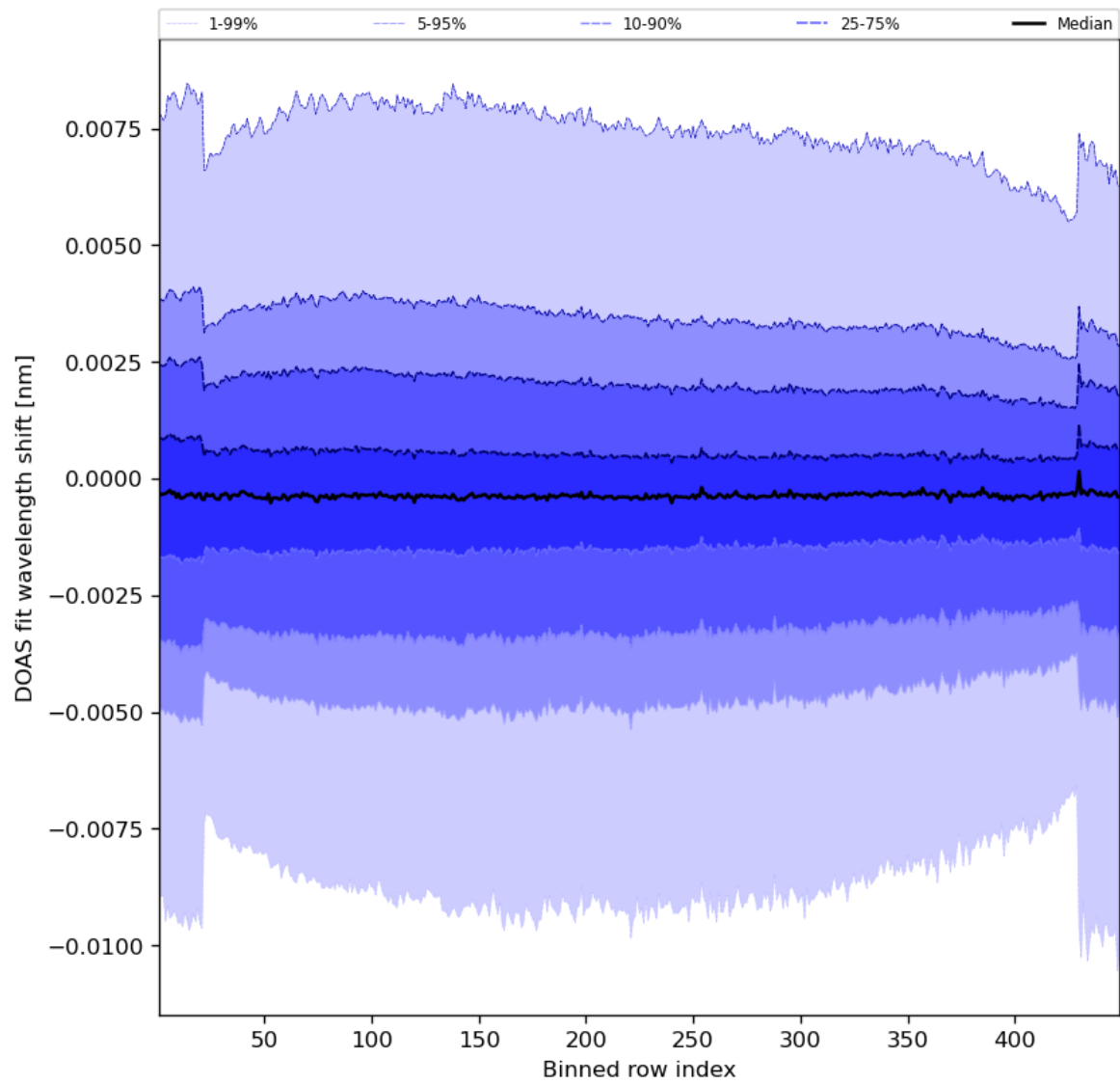
Figure 91: Along track statistics of “DOAS fit wavelength shift” for 2024-07-26 to 2024-07-27
