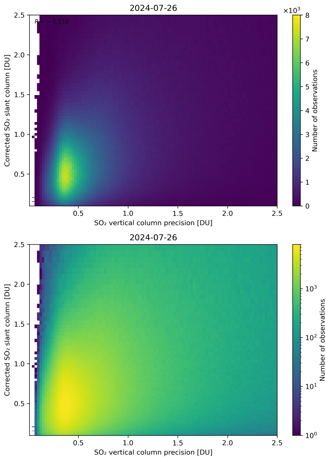
Figure 286: Scatter density plot of “SO 2 vertical column precision” against “Corrected SO 2 slant column” for 2024-07-26 to 2024-07-27.
