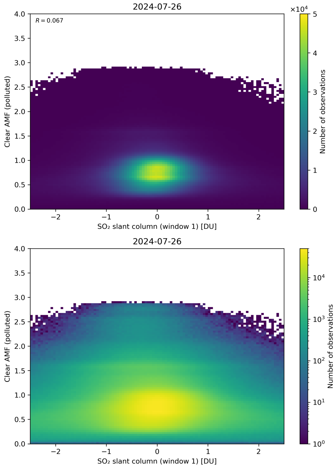
Figure 232: Scatter density plot of “SO 2 slant column (window 1)” against “Clear AMF (polluted)” for 2024-07-26 to 2024-07-27.
