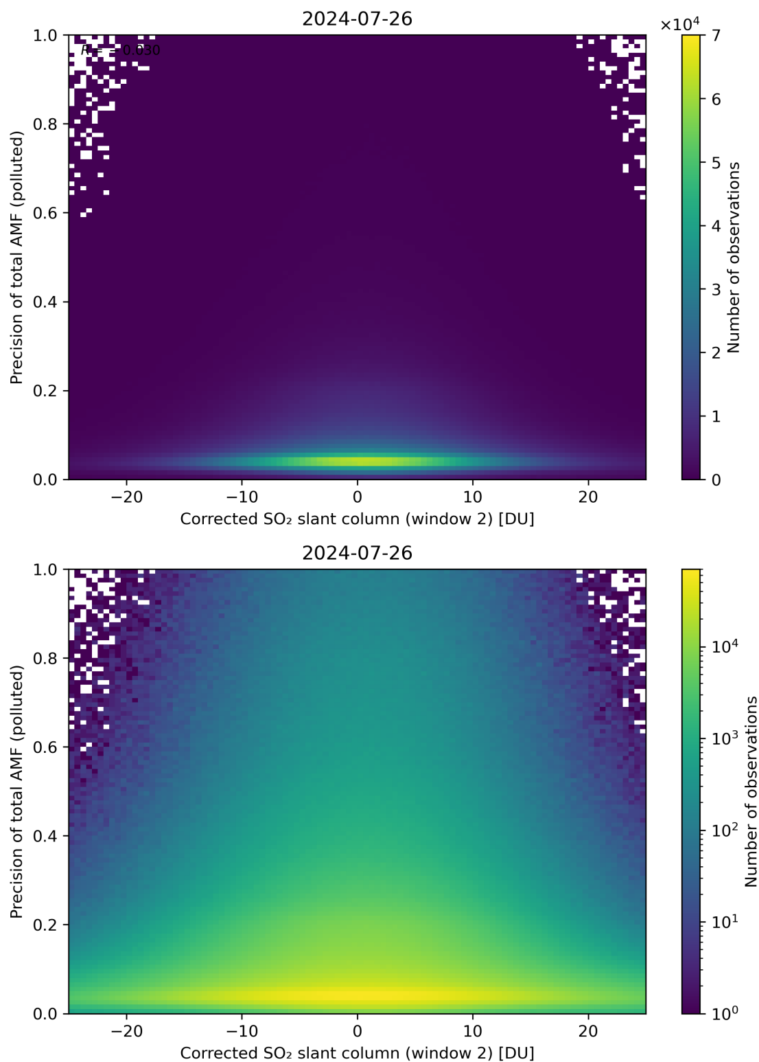
Figure 204: Scatter density plot of “Corrected SO 2 slant column (window 2)” against “Precision of total AMF (polluted)” for 2024-07-26 to 2024-07-27.
