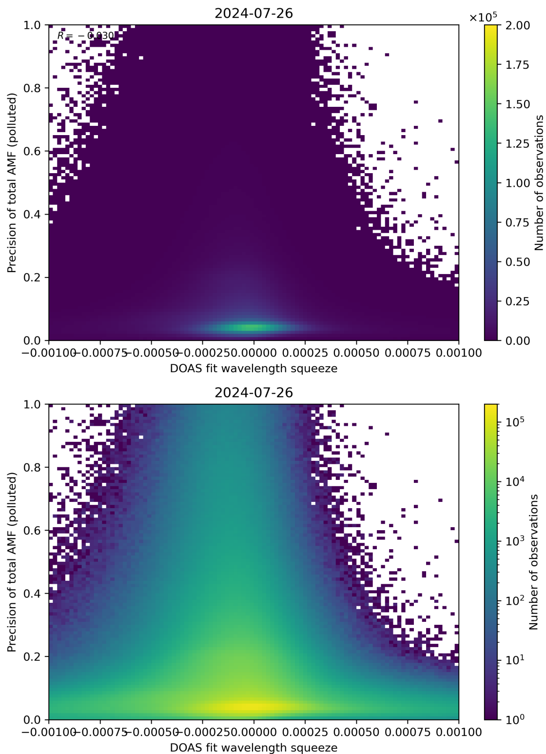
Figure 135: Scatter density plot of “DOAS fit wavelength squeeze” against “Precision of total AMF (polluted)” for 2024-07-26 to 2024-07-27.
