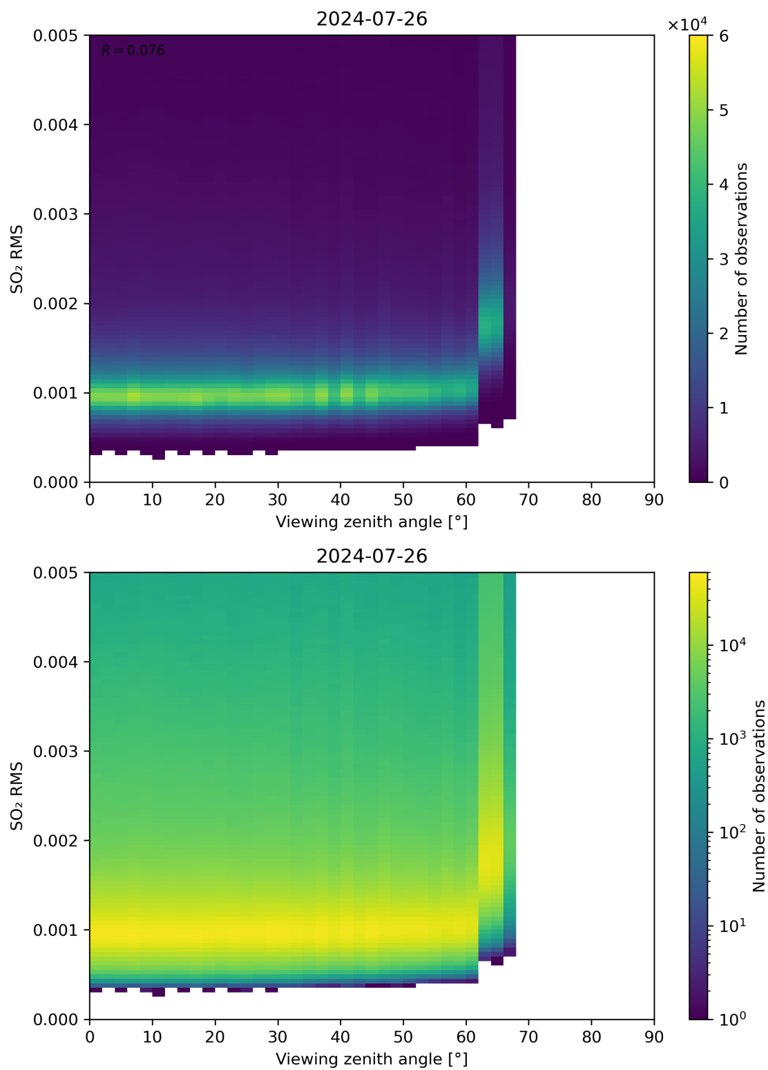
Figure 313: Scatter density plot of “Viewing zenith angle” against “SO 2 RMS” for 2024-07-26 to 2024-07-27.
