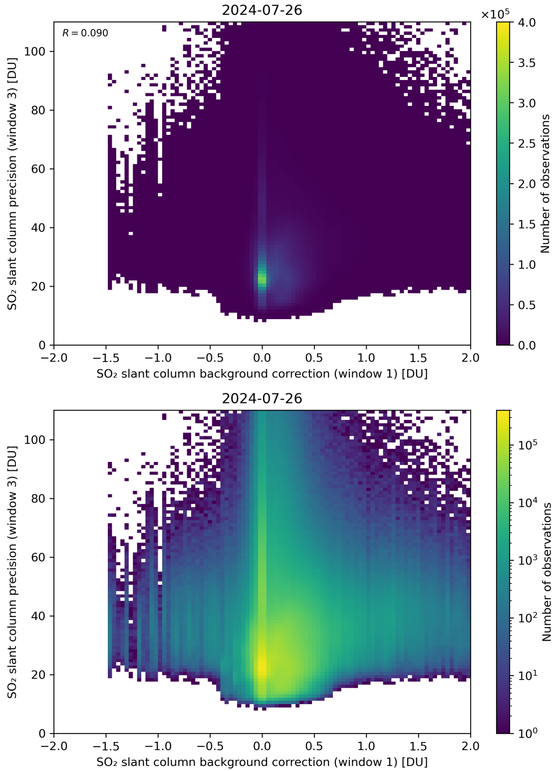
Figure 108: Scatter density plot of “SO 2 slant column background correction (window 1)” against “SO 2 slant column precision (window 3)” for 2024-07-26 to 2024-07-27.
