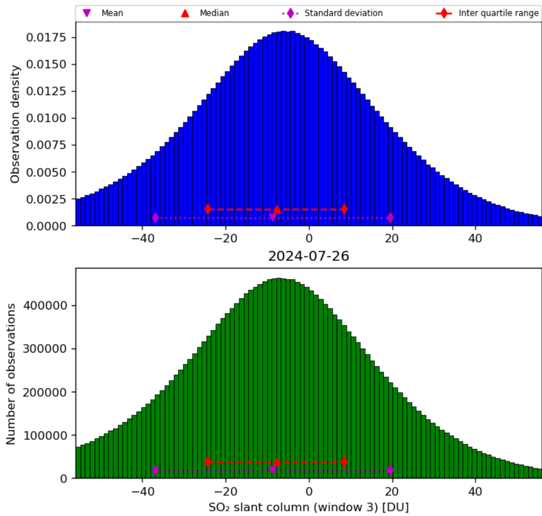
Figure 64: Histogram of “SO 2 slant column (window 3)” for 2024-07-26 to 2024-07-27
