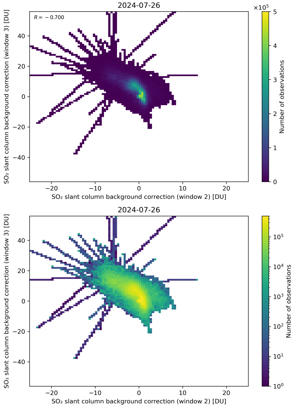
Figure 111: Scatter density plot of “SO 2 slant column background correction (window 2)” against “SO 2 slant column background correction (window 3)” for 2024-07-26 to 2024-07-27.
