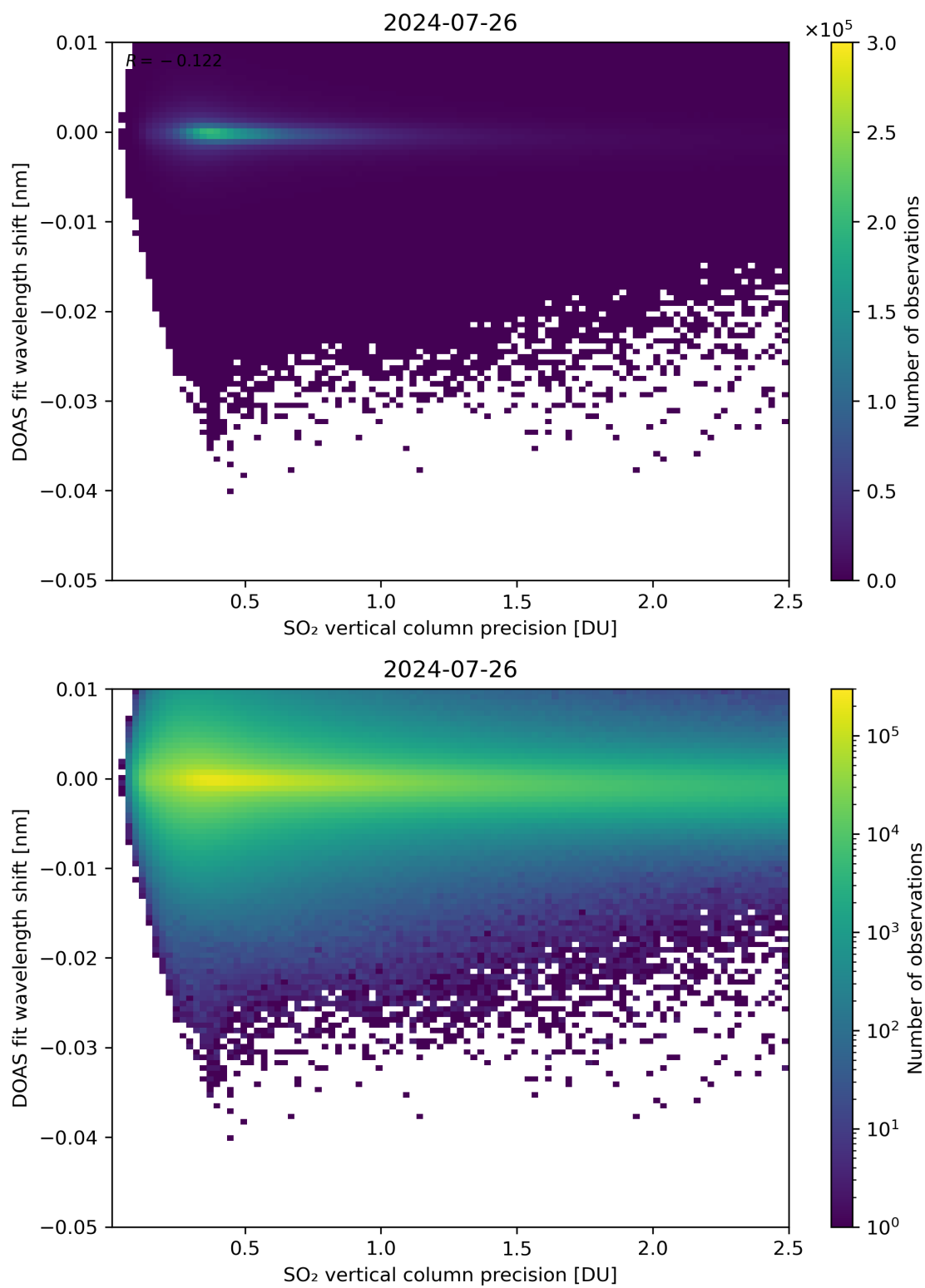
Figure 282: Scatter density plot of “SO 2 vertical column precision” against “DOAS fit wavelength shift” for 2024-07-26 to 2024-07-27.
