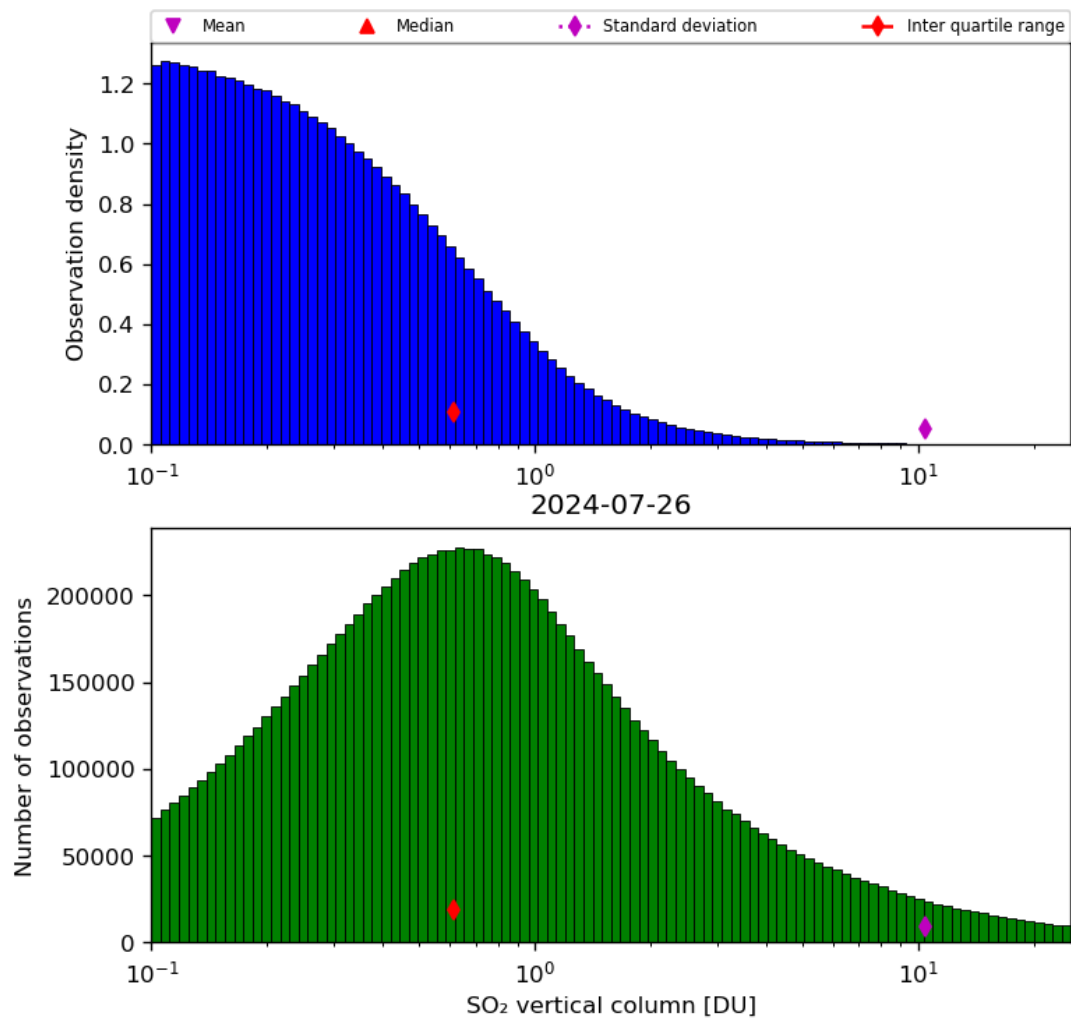
Figure 53: Histogram of “SO 2 vertical column” for 2024-07-26 to 2024-07-27
