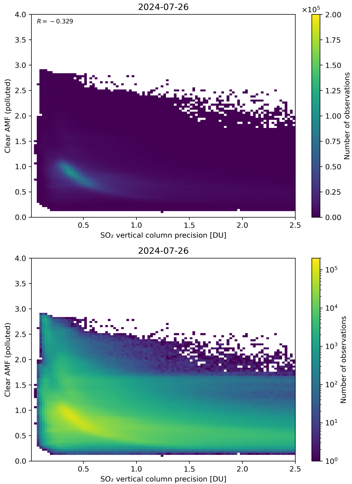
Figure 285: Scatter density plot of “SO 2 vertical column precision” against “Clear AMF (polluted)” for 2024-07-26 to 2024-07-27.
