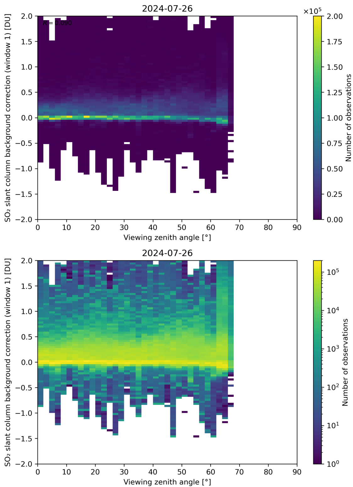
Figure 308: Scatter density plot of “Viewing zenith angle” against “SO 2 slant column background correction (window 1)” for 2024-07-26 to 2024-07-27.
