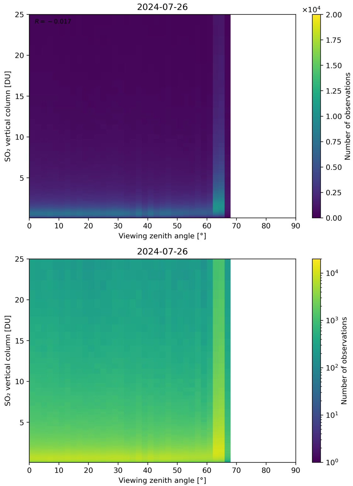
Figure 327: Scatter density plot of “Viewing zenith angle” against “SO 2 vertical column” for 2024-07-26 to 2024-07-27.
