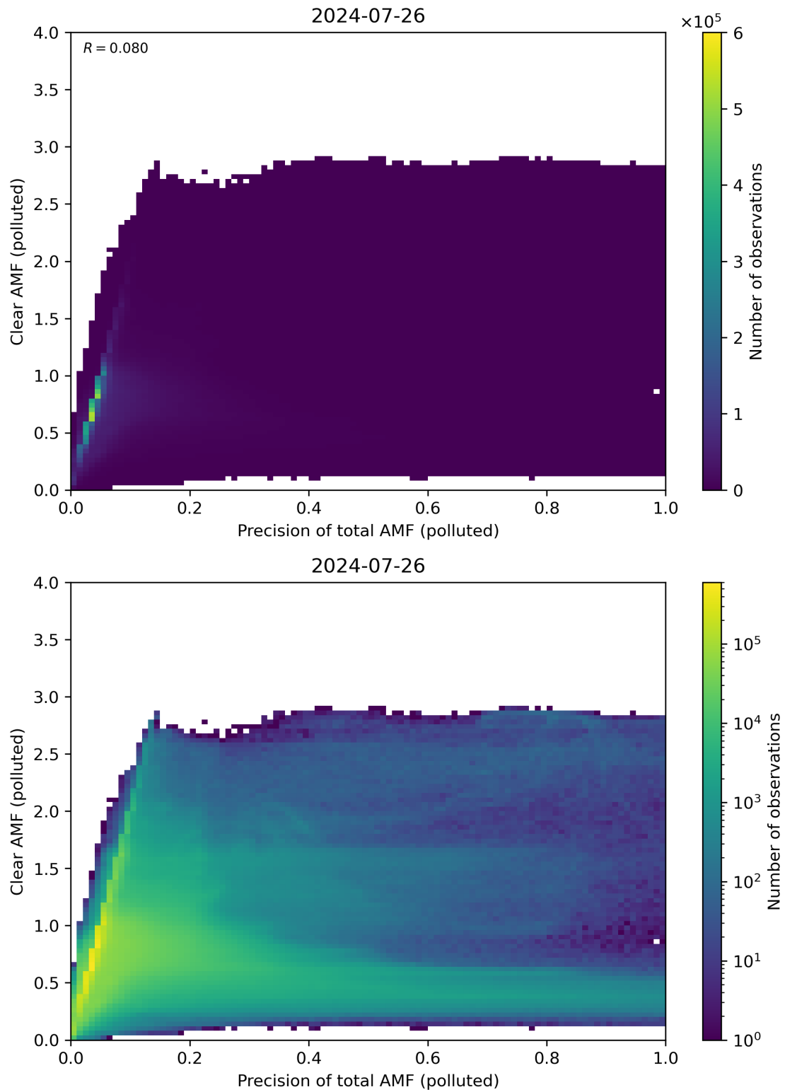
Figure 270: Scatter density plot of “Precision of total AMF (polluted)” against “Clear AMF (polluted)” for 2024-07-26 to 2024-07-27.
