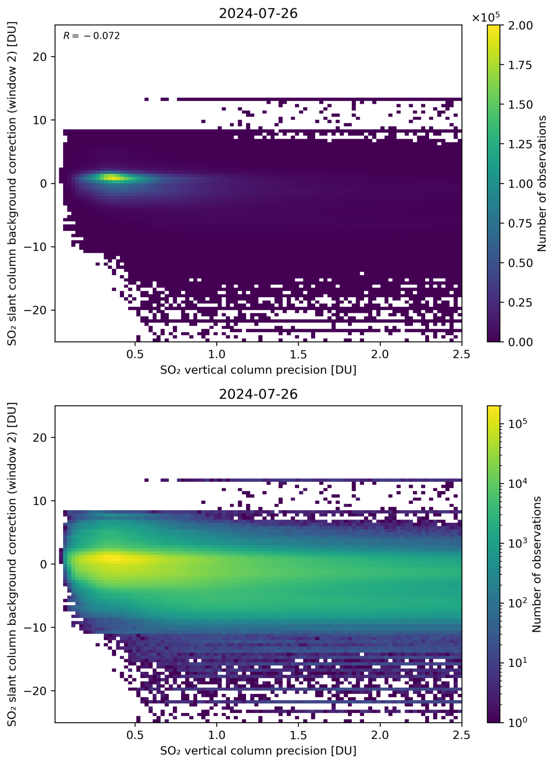
Figure 280: Scatter density plot of “SO 2 vertical column precision” against “SO 2 slant column background correction (window 2)” for 2024-07-26 to 2024-07-27.
