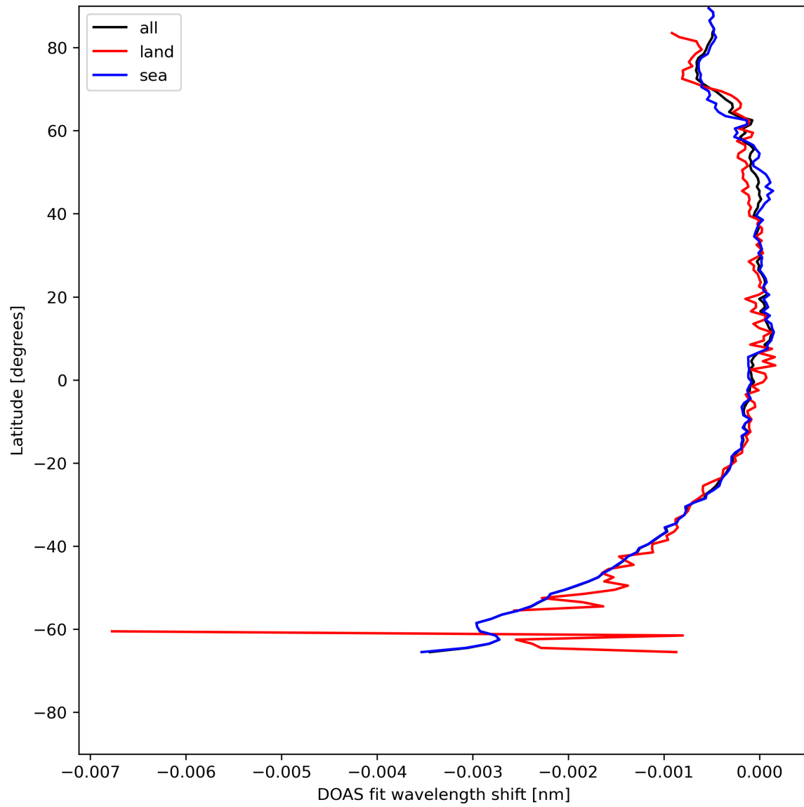
Figure 45: Zonal average of “DOAS fit wavelength shift” for 2024-07-26 to 2024-07-27.
