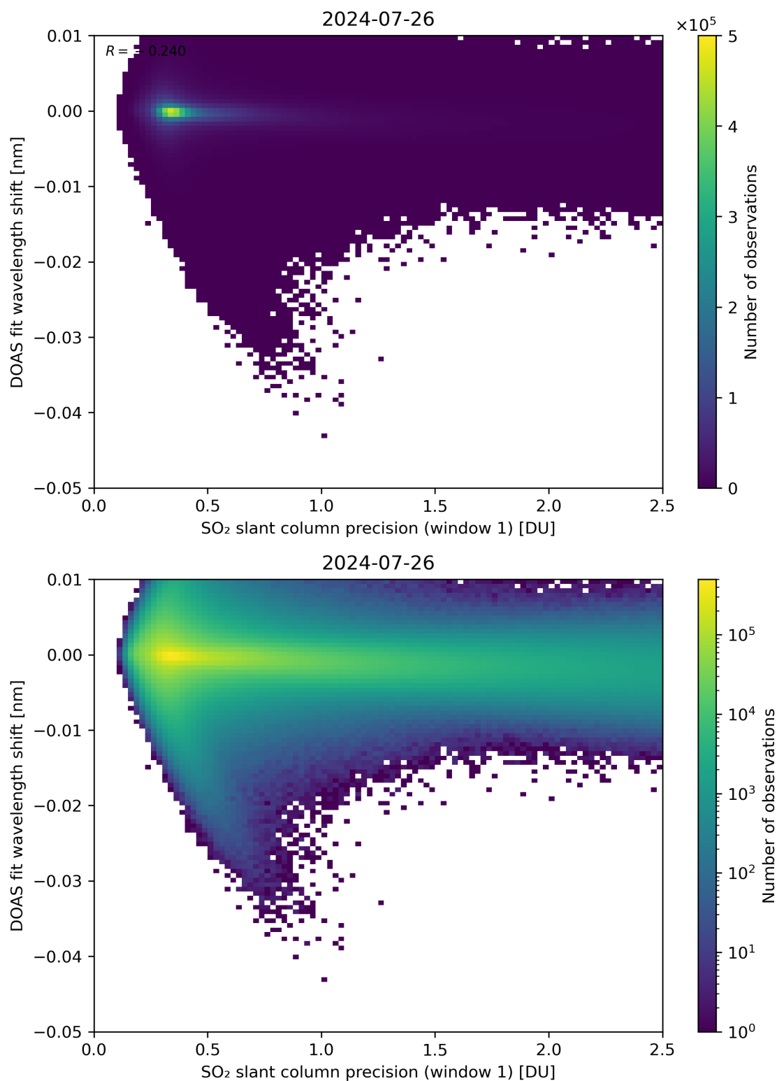
Figure 221: Scatter density plot of “SO 2 slant column precision (window 1)” against “DOAS fit wavelength shift” for 2024-07-26 to 2024-07-27.
