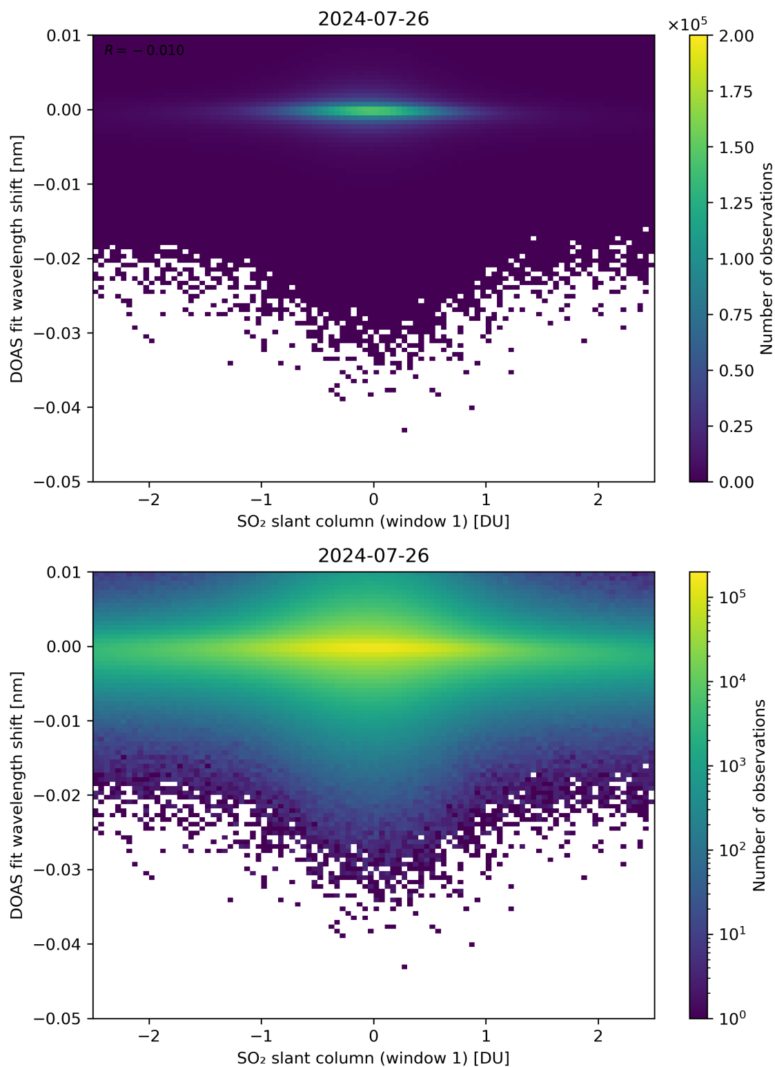
Figure 215: Scatter density plot of “SO 2 slant column (window 1)” against “DOAS fit wavelength shift” for 2024-07-26 to 2024-07-27.
