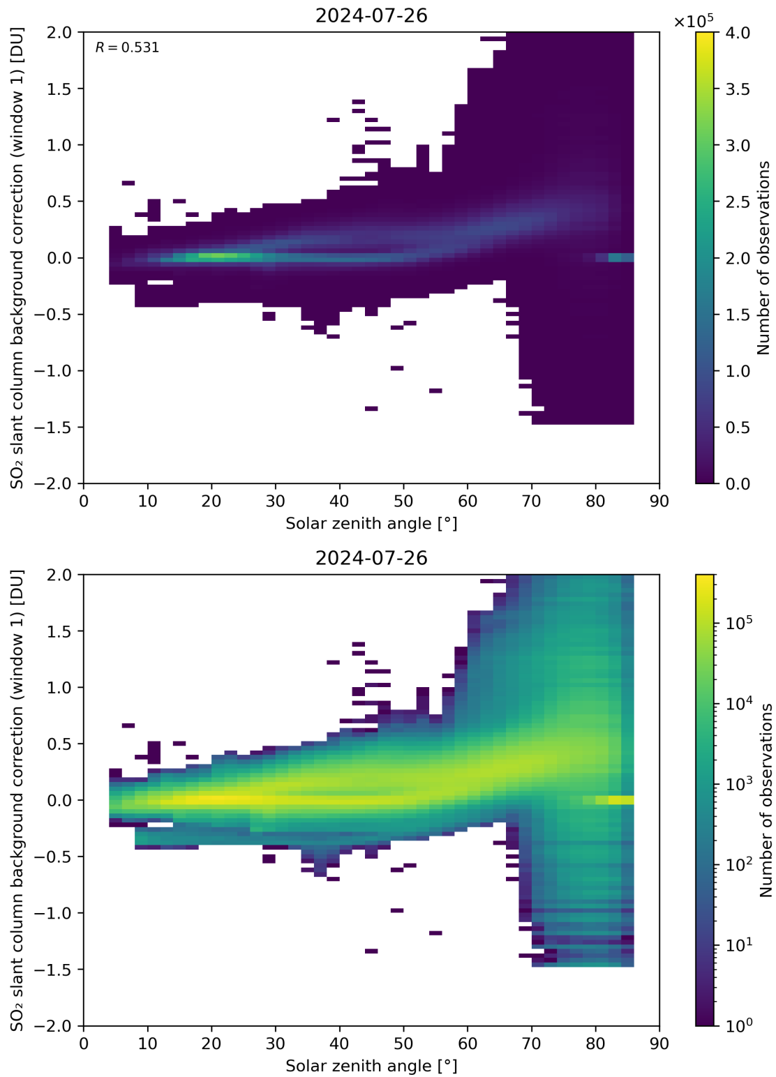
Figure 158: Scatter density plot of “Solar zenith angle” against “SO 2 slant column background correction (window 1)” for 2024-07-26 to 2024-07-27.
