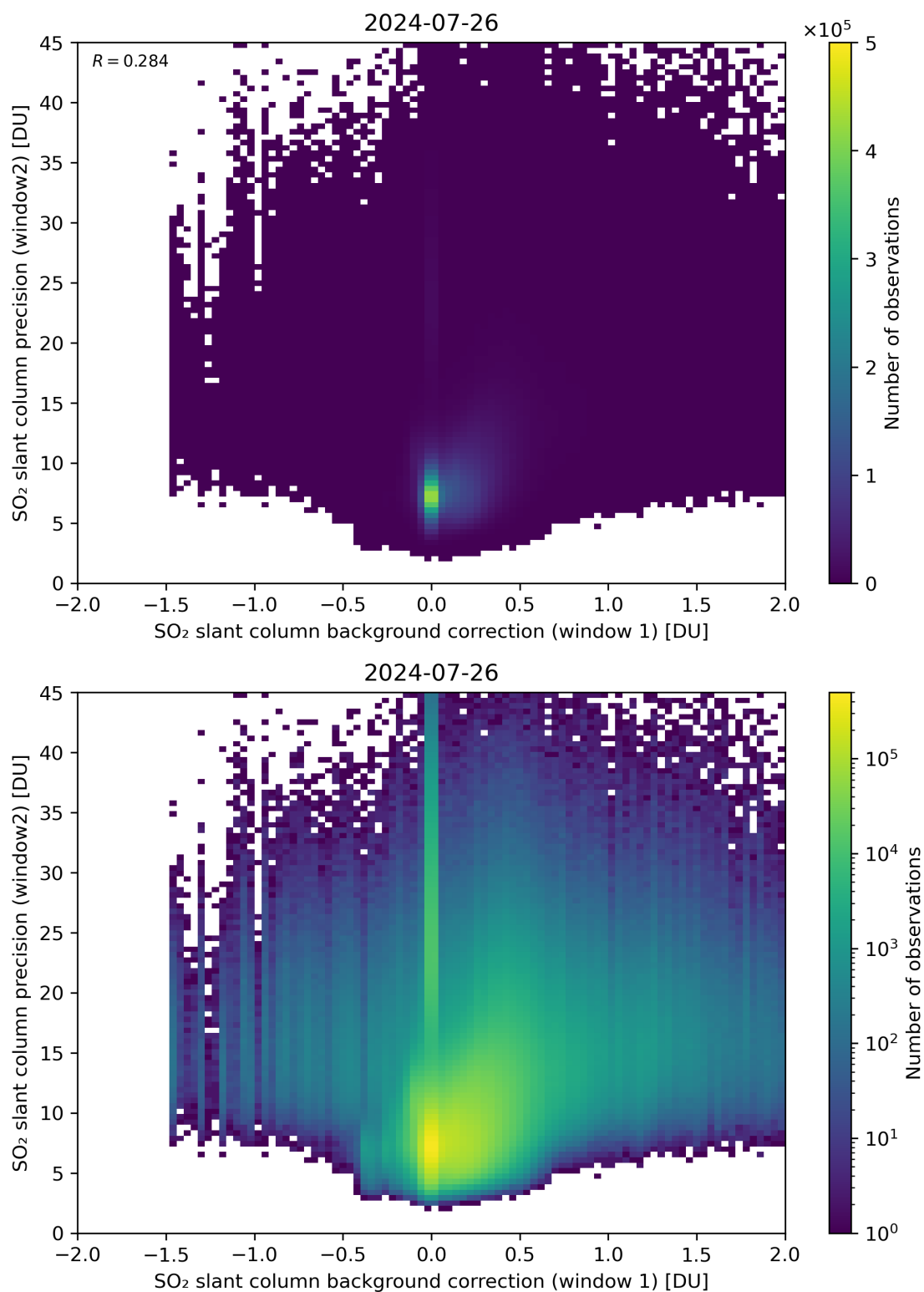
Figure 106: Scatter density plot of “SO 2 slant column background correction (window 1)” against “SO 2 slant column precision (window2)” for 2024-07-26 to 2024-07-27.
