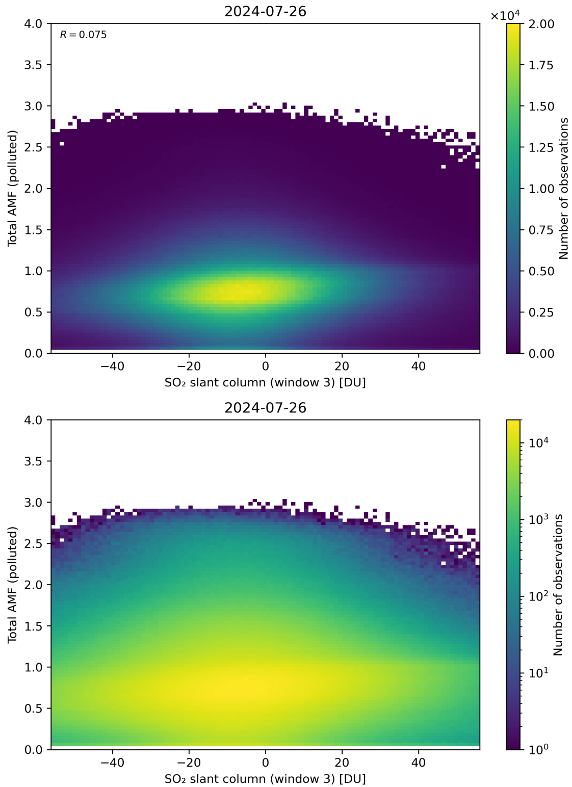
Figure 268: Scatter density plot of “SO 2 slant column (window 3)” against “Total AMF (polluted)” for 2024-07-26 to 2024-07-27.
