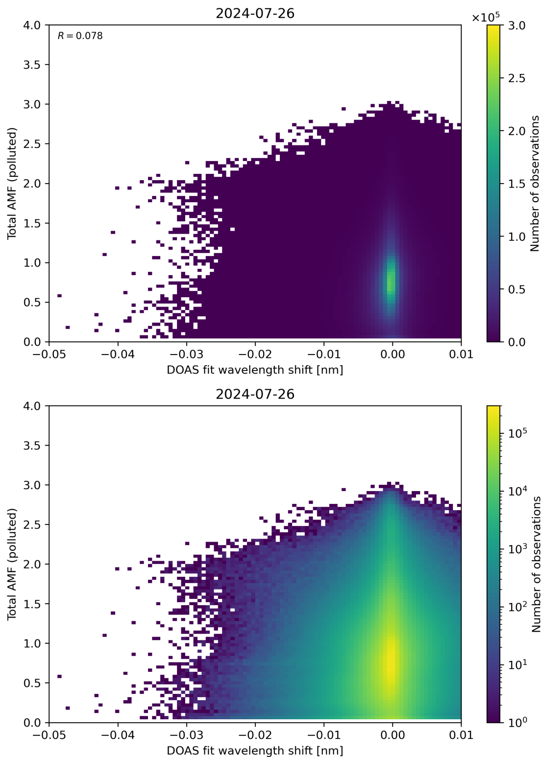
Figure 130: Scatter density plot of “DOAS fit wavelength shift” against “Total AMF (polluted)” for 2024-07-26 to 2024-07-27.
