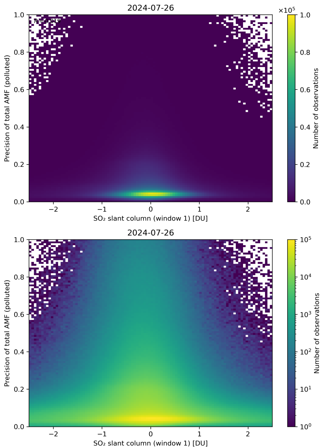
Figure 240: Scatter density plot of “SO 2 slant column (window 1)” against “Precision of total AMF (polluted)” for 2024-07-26 to 2024-07-27.
