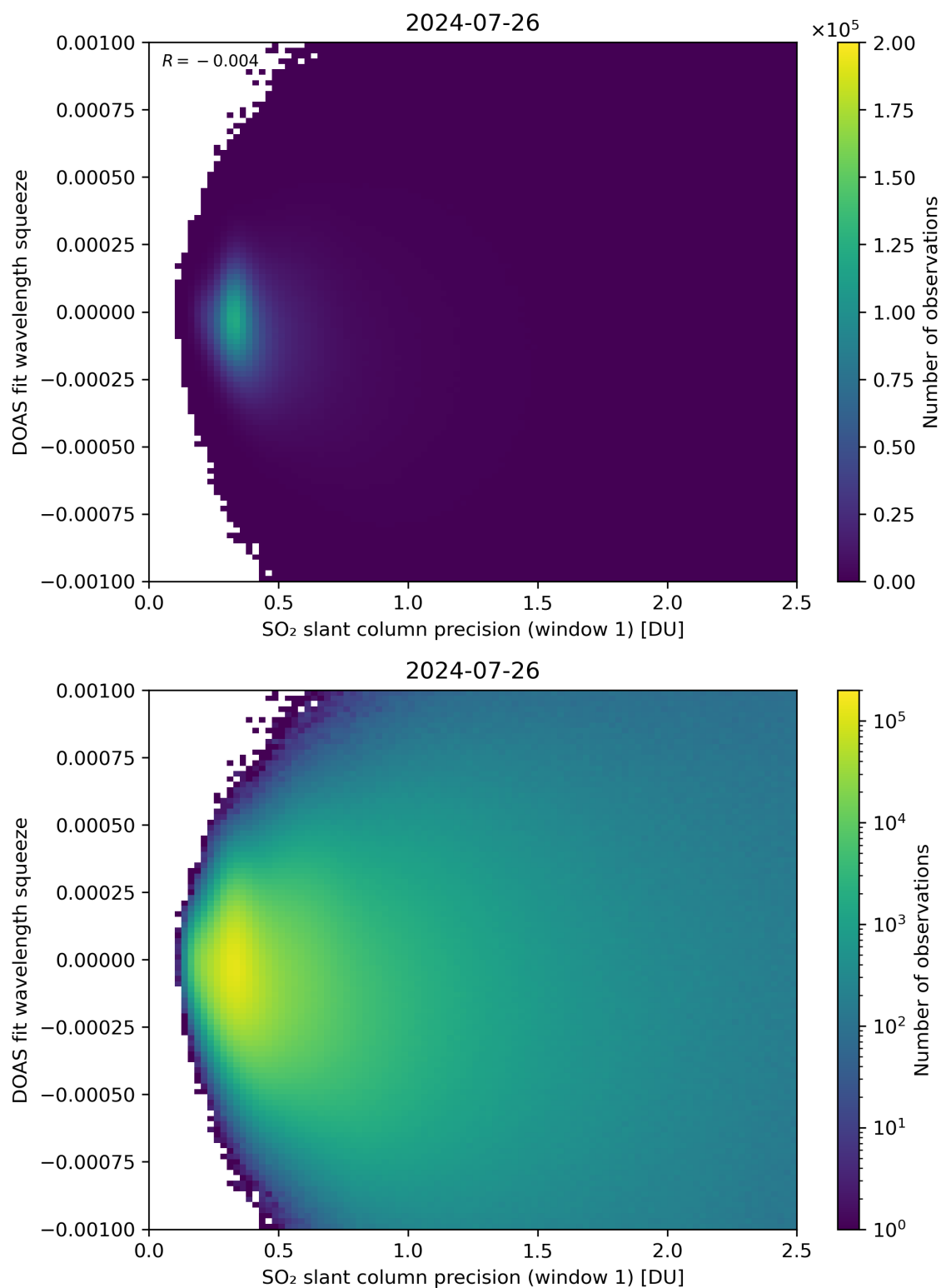
Figure 222: Scatter density plot of “SO 2 slant column precision (window 1)” against “DOAS fit wavelength squeeze” for 2024-07-26 to 2024-07-27.
