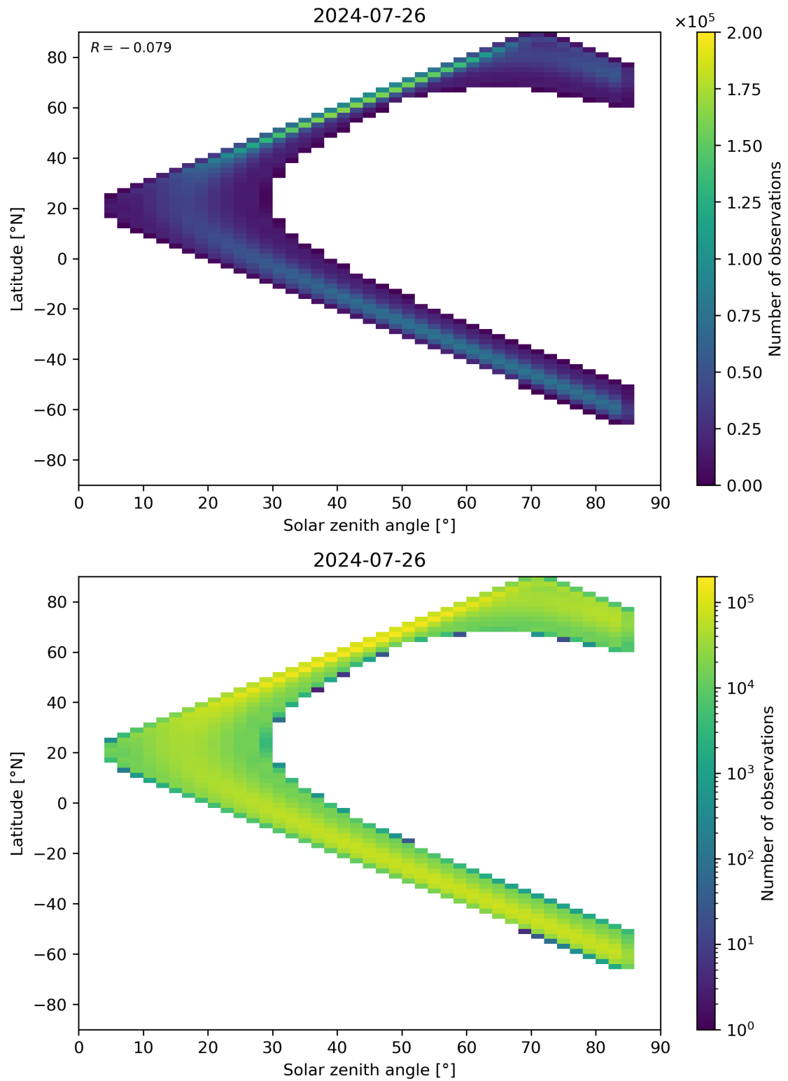
Figure 164: Scatter density plot of “Solar zenith angle” against “Latitude” for 2024-07-26 to 2024-07-27.
