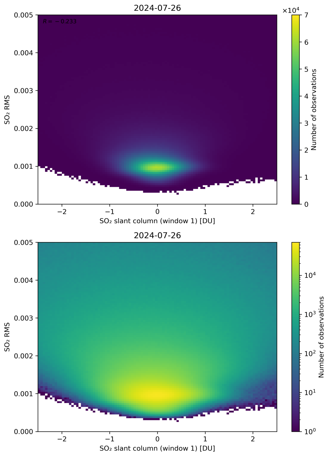
Figure 217: Scatter density plot of “SO 2 slant column (window 1)” against “SO 2 RMS” for 2024-07-26 to 2024-07-27.
