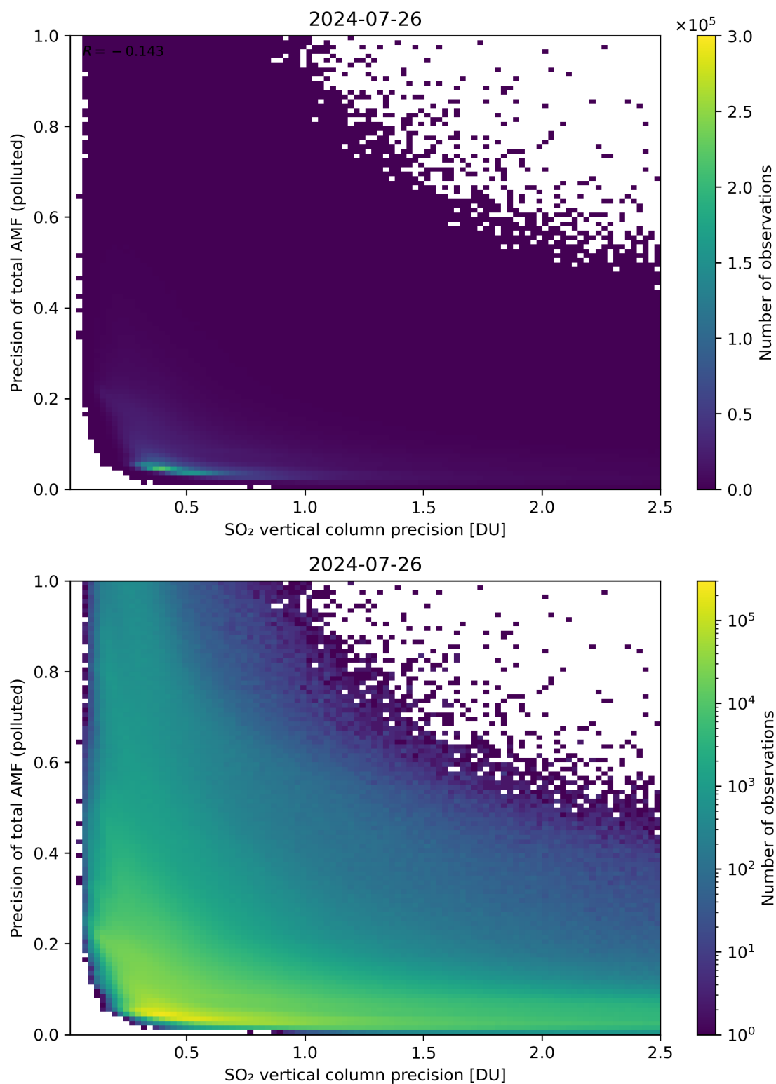
Figure 295: Scatter density plot of “SO 2 vertical column precision” against “Precision of total AMF (polluted)” for 2024-07-26 to 2024-07-27.
