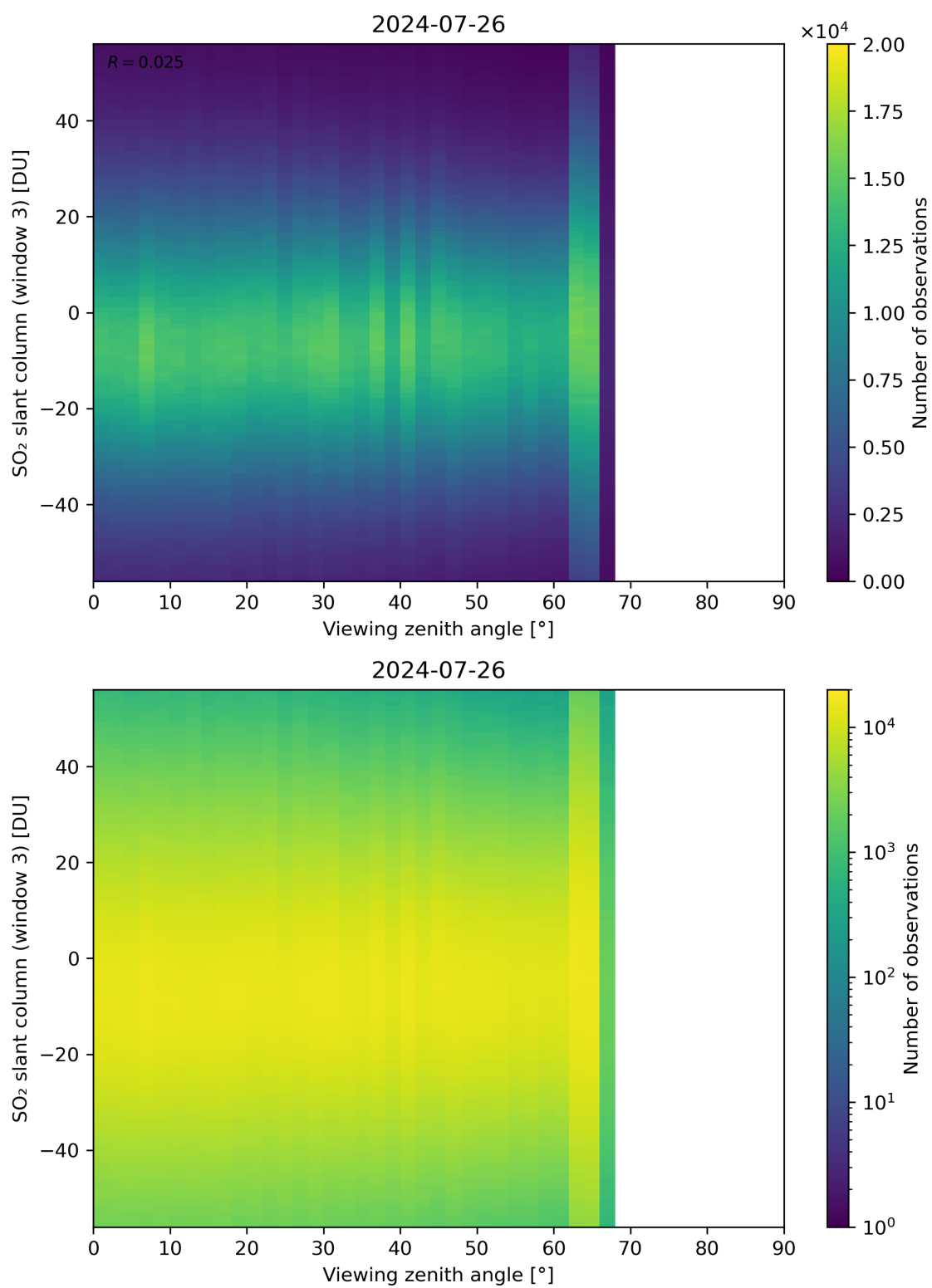
Figure 323: Scatter density plot of “Viewing zenith angle” against “SO 2 slant column (window 3)” for 2024-07-26 to 2024-07-27.
