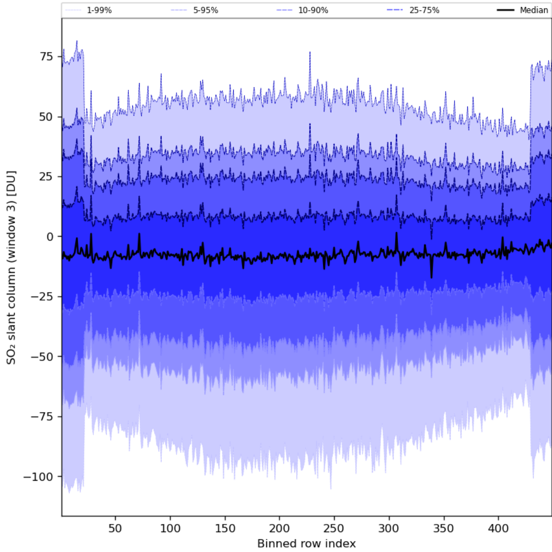
Figure 87: Along track statistics of “SO 2 slant column (window 3)” for 2024-07-26 to 2024-07-27
