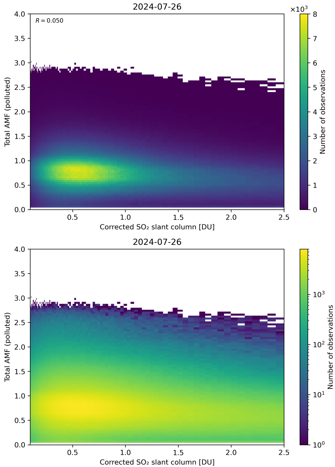
Figure 192: Scatter density plot of “Corrected SO 2 slant column” against “Total AMF (polluted)” for 2024-07-26 to 2024-07-27.
