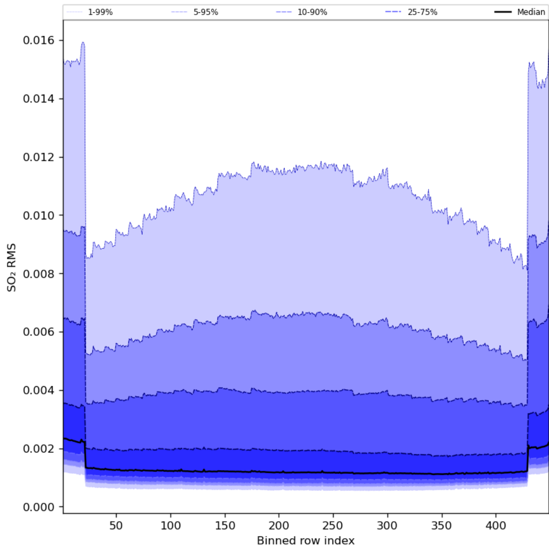
Figure 93: Along track statistics of “SO 2 RMS” for 2024-07-26 to 2024-07-27
