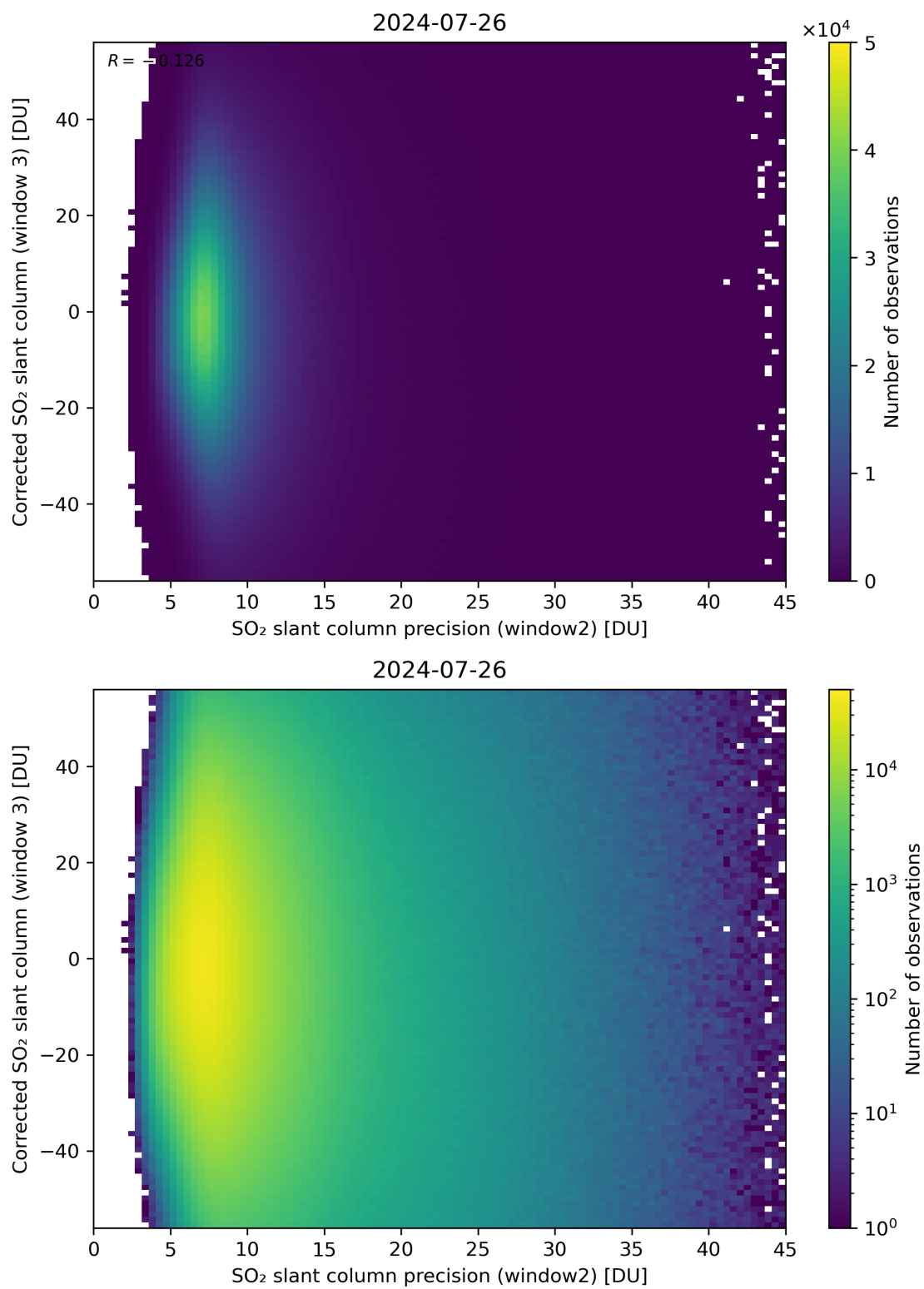
Figure 248: Scatter density plot of “SO 2 slant column precision (window2)” against “Corrected SO 2 slant column (window 3)” for 2024-07-26 to 2024-07-27.
