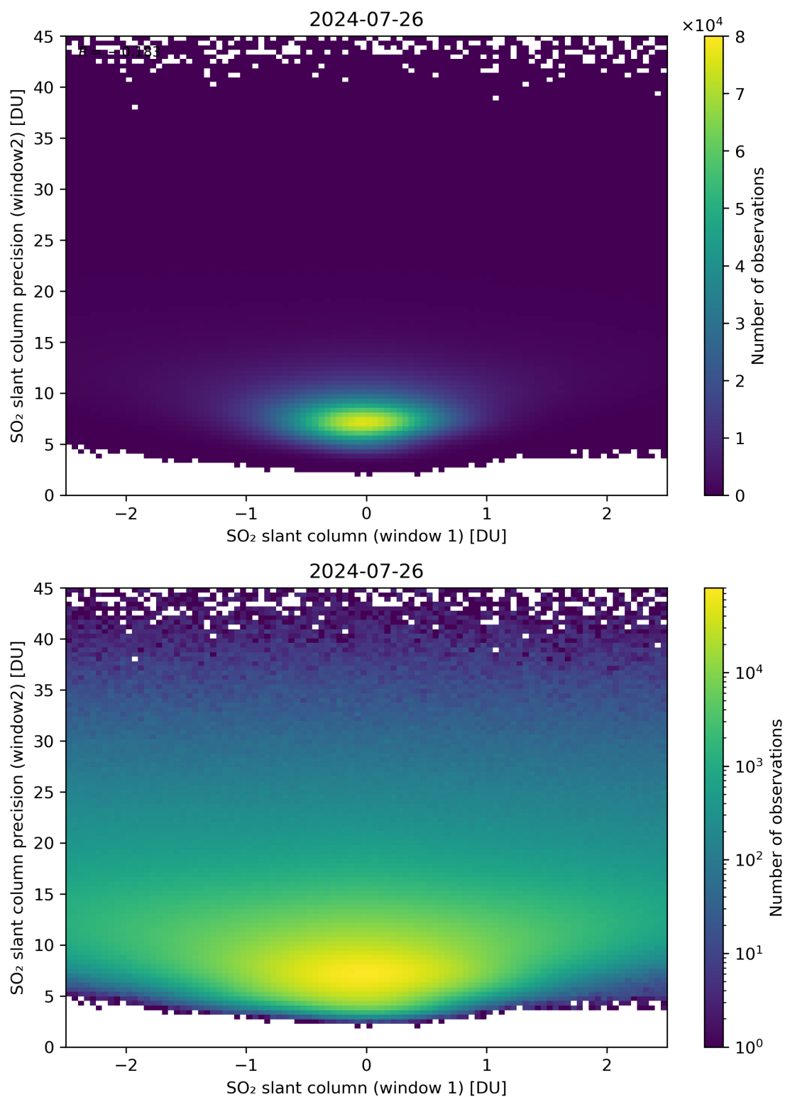
Figure 236: Scatter density plot of “SO 2 slant column (window 1)” against “SO 2 slant column precision (window2)” for 2024-07-26 to 2024-07-27.
