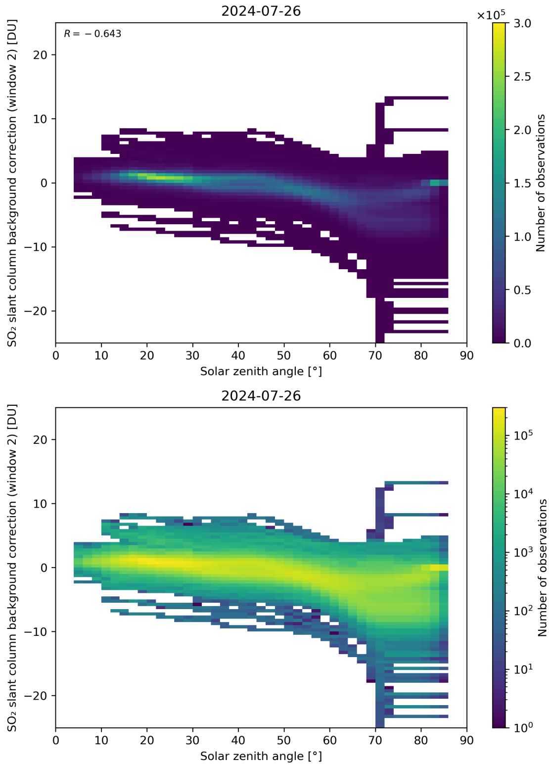
Figure 159: Scatter density plot of “Solar zenith angle” against “SO 2 slant column background correction (window 2)” for 2024-07-26 to 2024-07-27.
