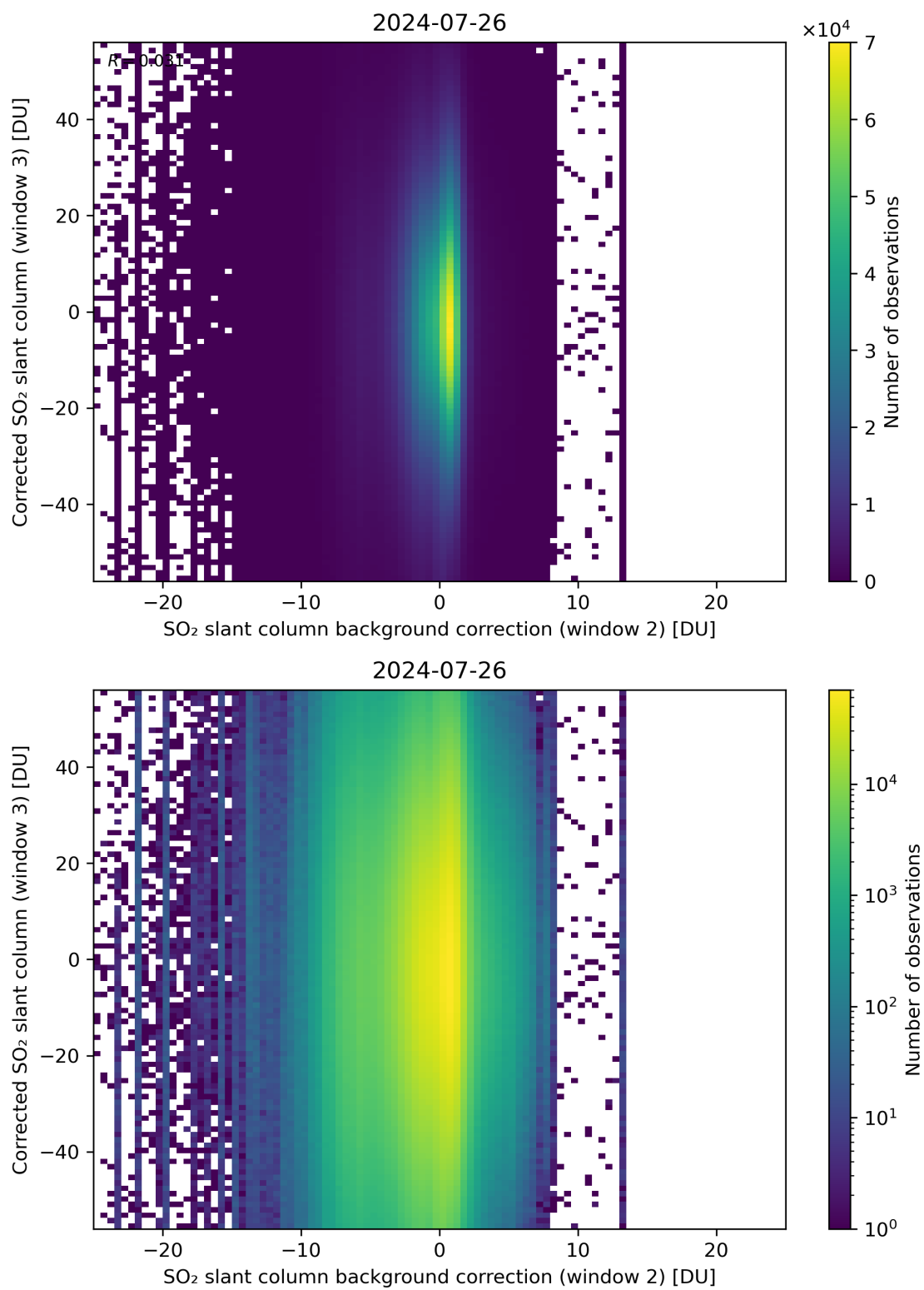
Figure 116: Scatter density plot of “SO 2 slant column background correction (window 2)” against “Corrected SO 2 slant column (window 3)” for 2024-07-26 to 2024-07-27.
