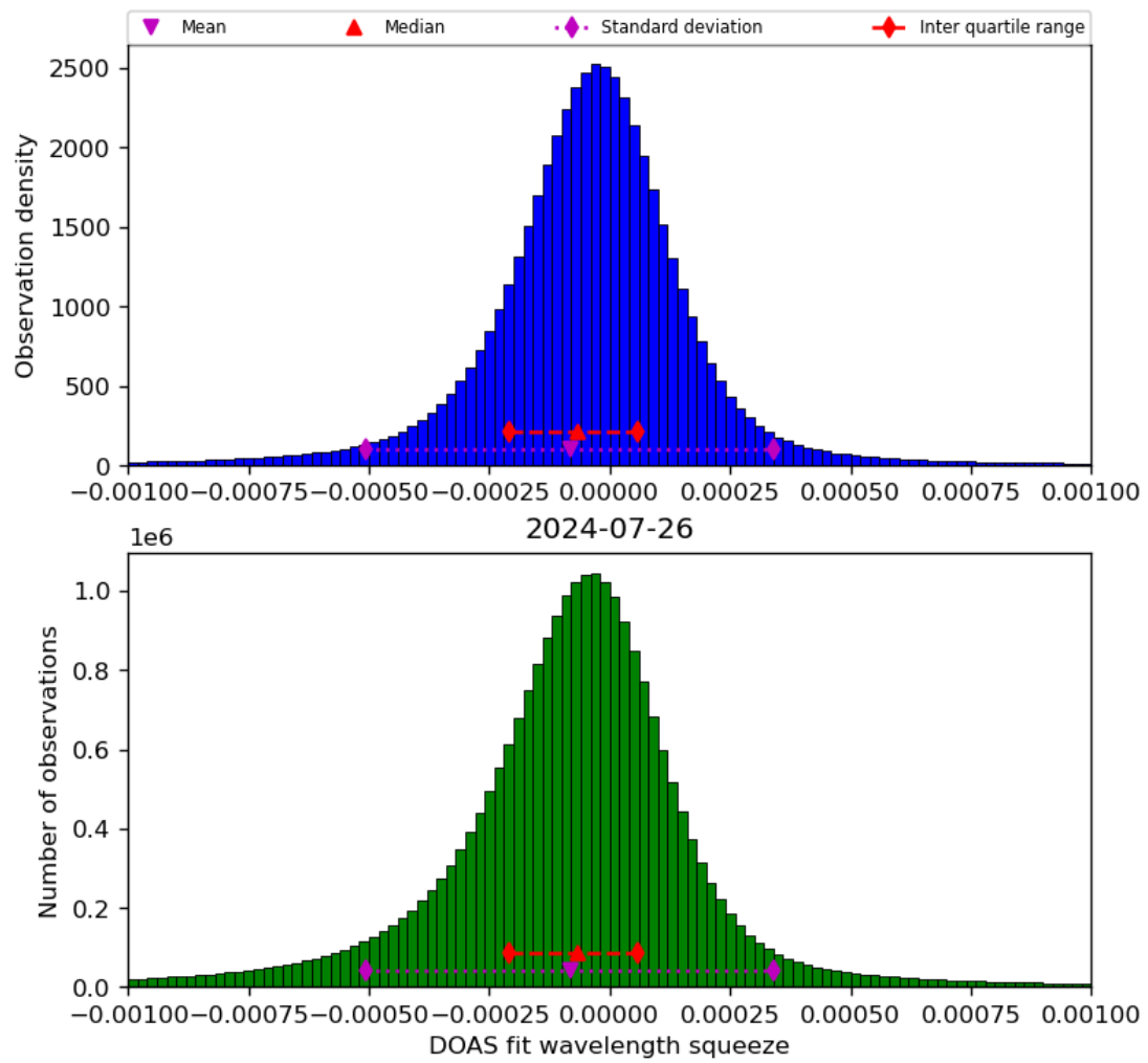
Figure 69: Histogram of “DOAS fit wavelength squeeze” for 2024-07-26 to 2024-07-27
