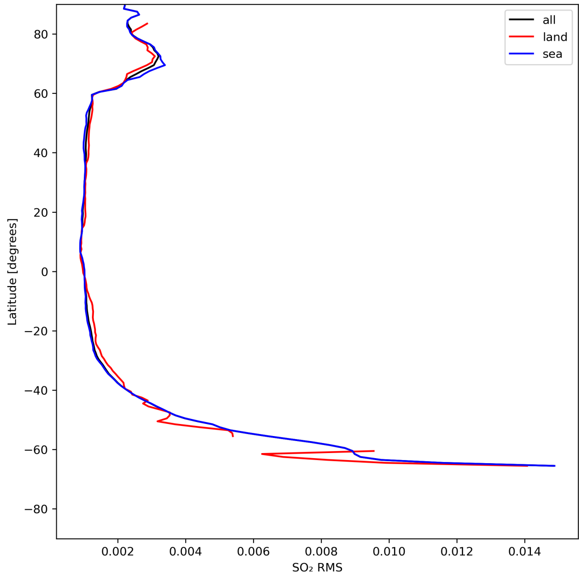
Figure 47: Zonal average of “SO 2 RMS” for 2024-07-26 to 2024-07-27.
