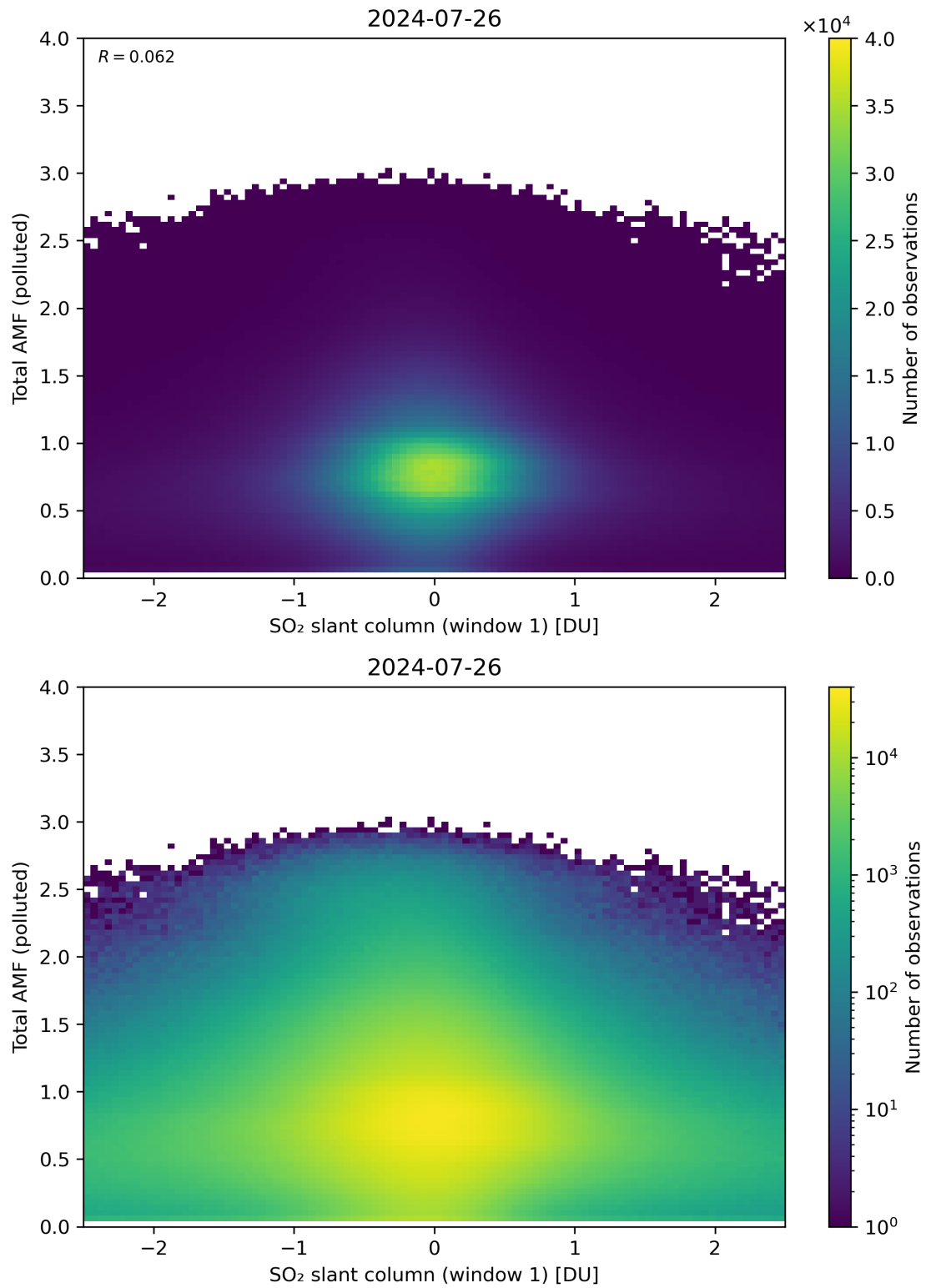
Figure 239: Scatter density plot of “SO 2 slant column (window 1)” against “Total AMF (polluted)” for 2024-07-26 to 2024-07-27.
