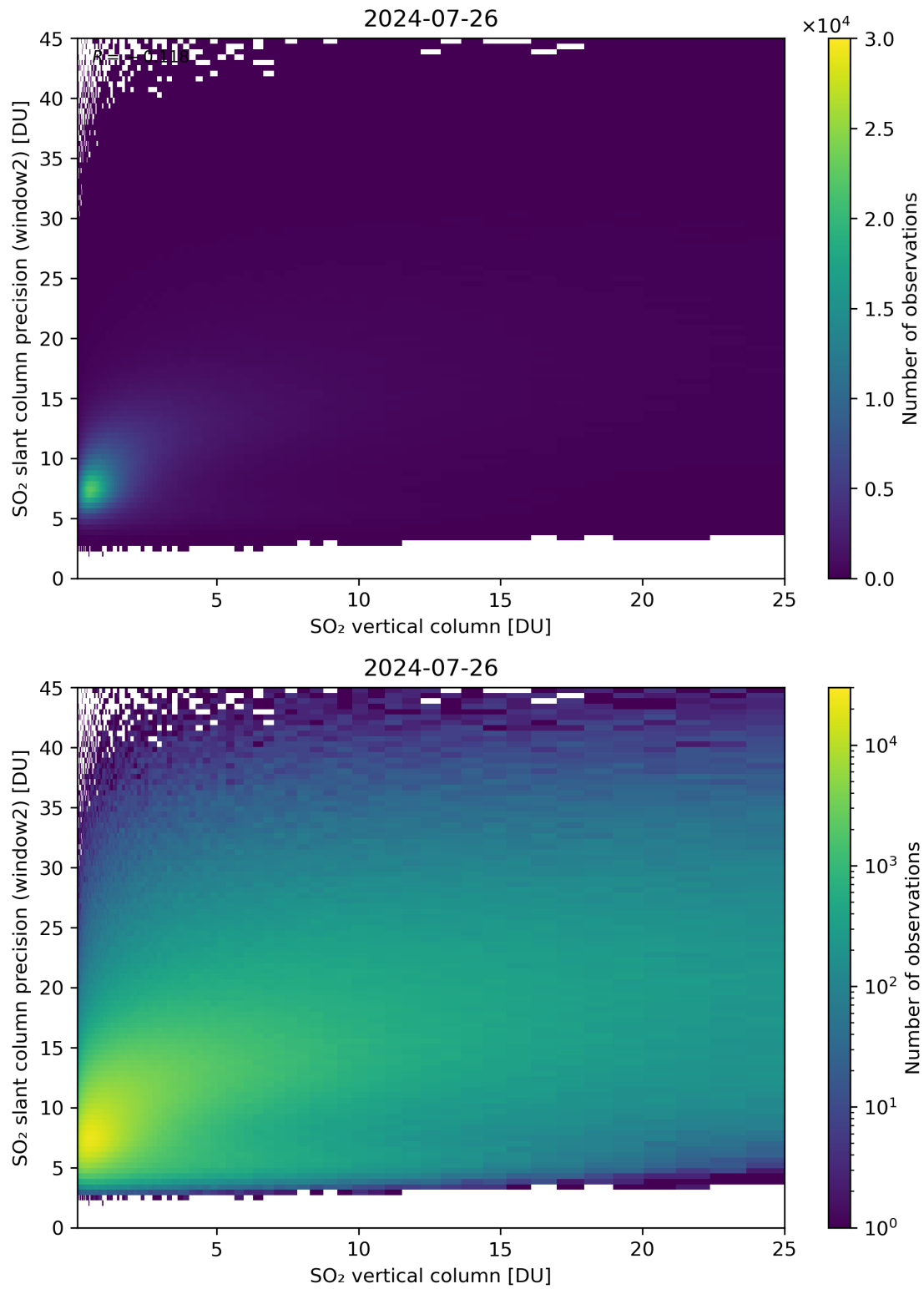
Figure 302: Scatter density plot of “SO 2 vertical column” against “SO 2 slant column precision (window2)” for 2024-07-26 to 2024-07-27.
