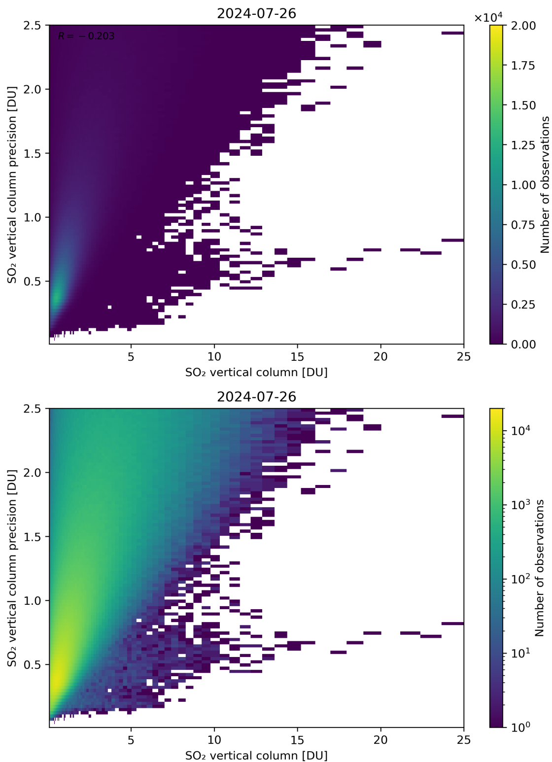
Figure 307: Scatter density plot of “SO 2 vertical column” against “SO 2 vertical column precision” for 2024-07-26 to 2024-07-27.
