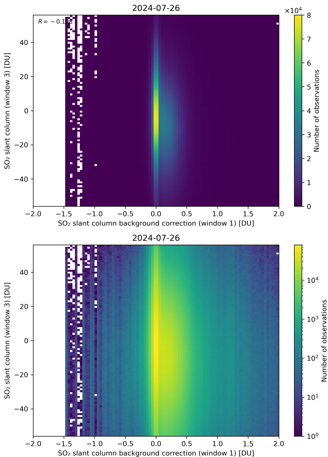
Figure 107: Scatter density plot of “SO 2 slant column background correction (window 1)” against “SO 2 slant column (window 3)” for 2024-07-26 to 2024-07-27.
