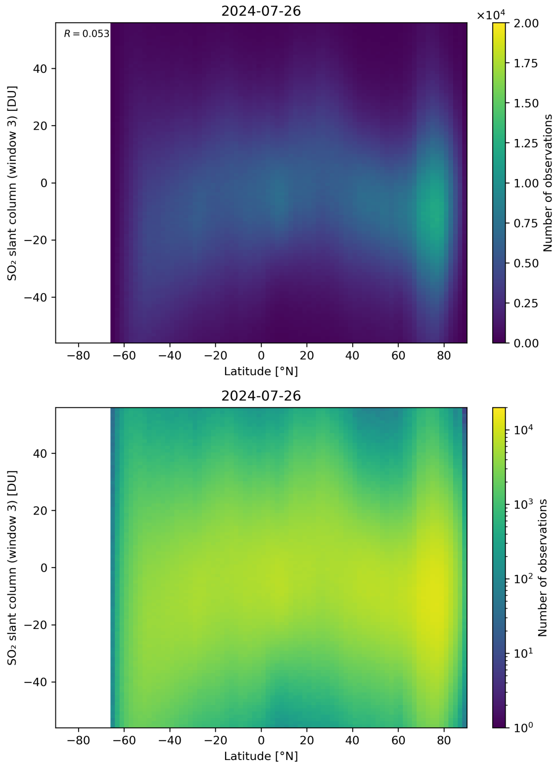
Figure 152: Scatter density plot of “Latitude” against “SO 2 slant column (window 3)” for 2024-07-26 to 2024-07-27.
