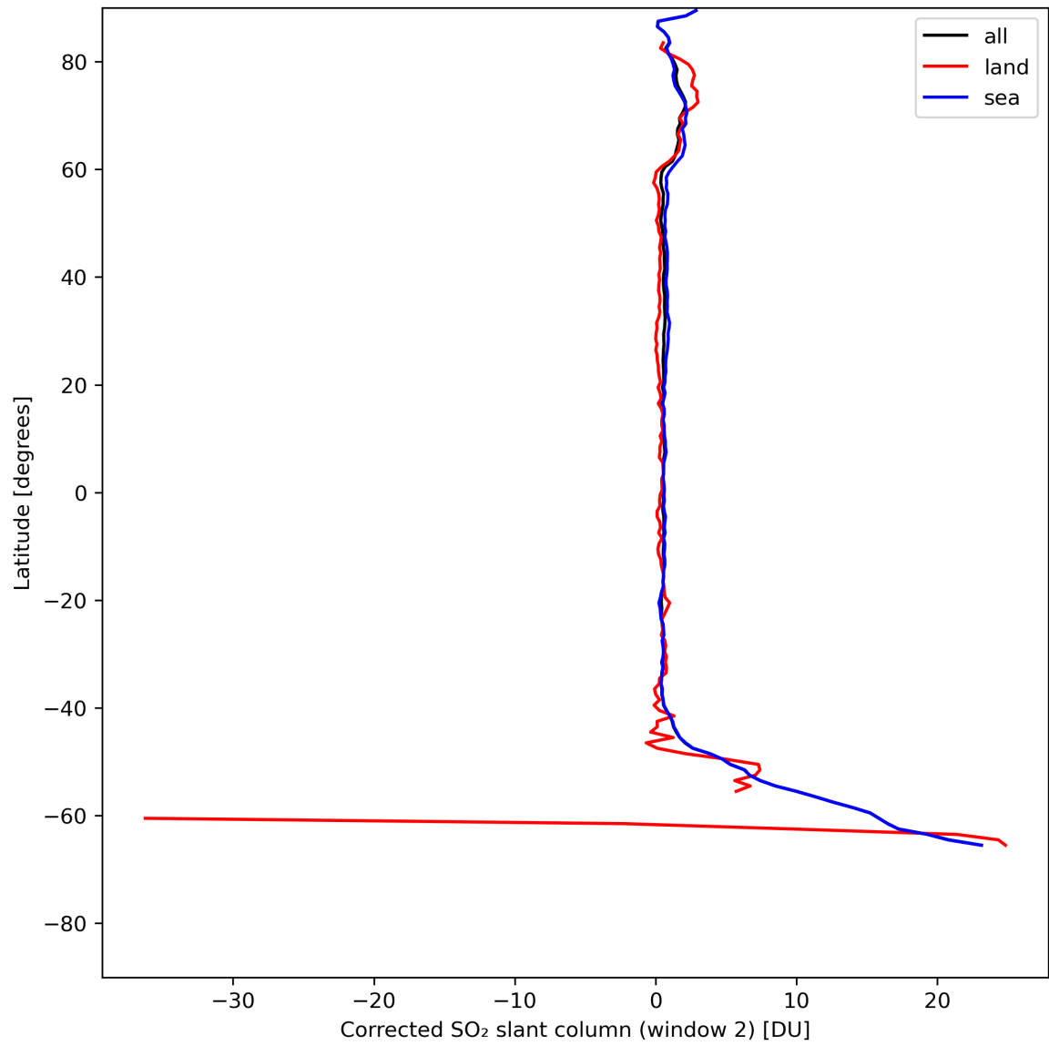
Figure 39: Zonal average of “Corrected SO 2 slant column (window 2)” for 2024-07-26 to 2024-07-27.
