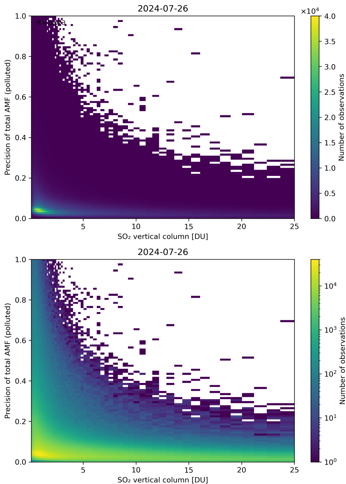
Figure 306: Scatter density plot of “SO 2 vertical column” against “Precision of total AMF (polluted)” for 2024-07-26 to 2024-07-27.
