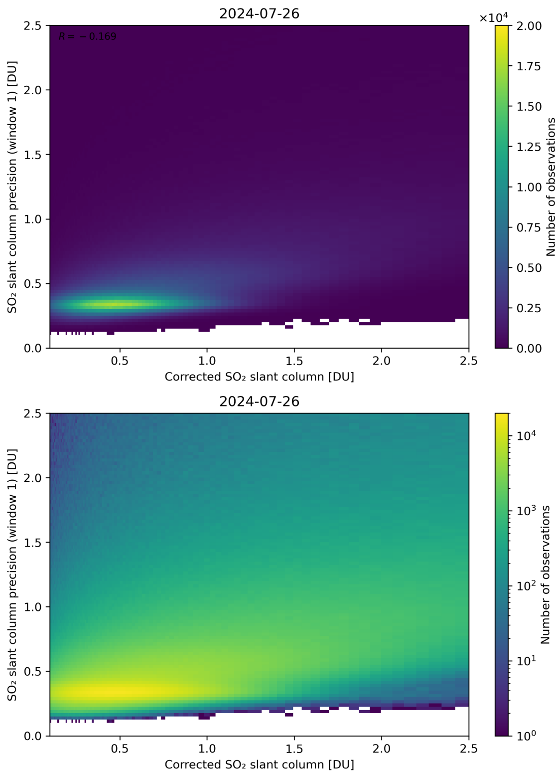
Figure 188: Scatter density plot of “Corrected SO 2 slant column” against “SO 2 slant column precision (window 1)” for 2024-07-26 to 2024-07-27.
