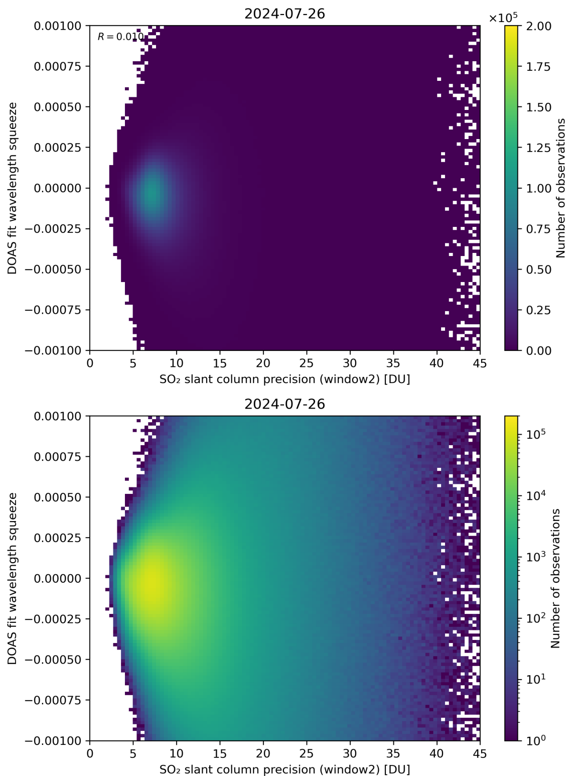
Figure 244: Scatter density plot of “SO 2 slant column precision (window2)” against “DOAS fit wavelength squeeze” for 2024-07-26 to 2024-07-27.
