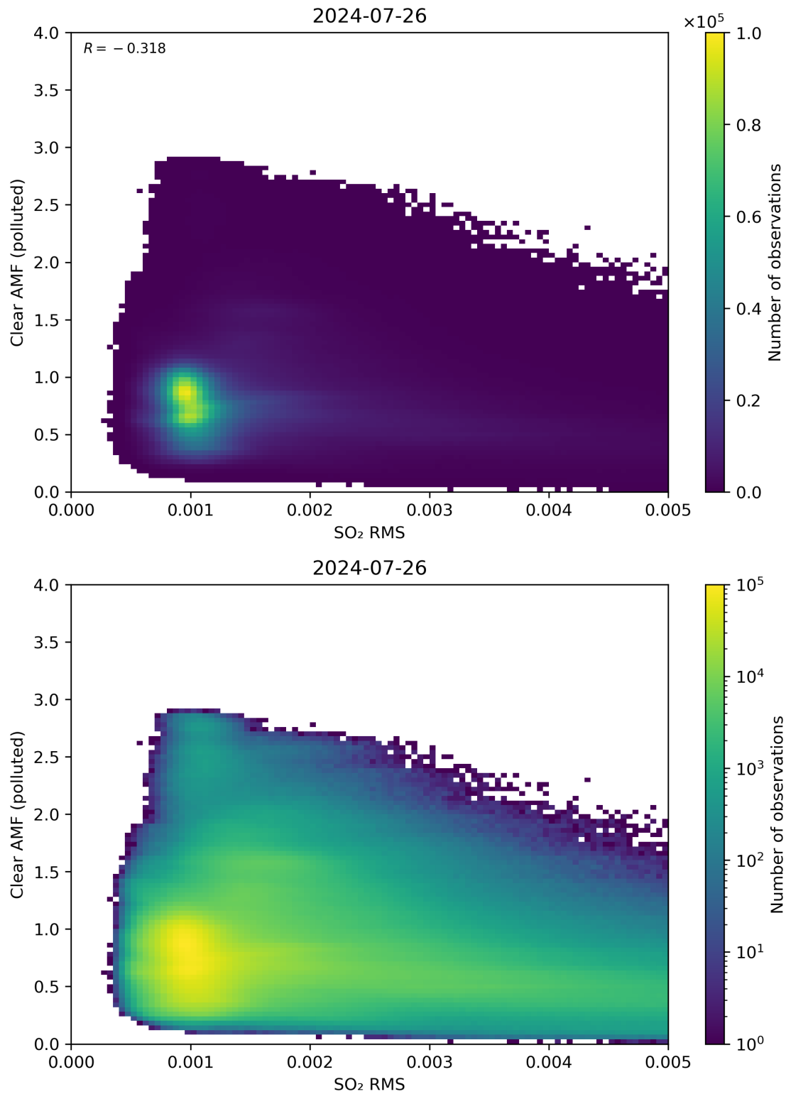
Figure 136: Scatter density plot of “SO 2 RMS” against “Clear AMF (polluted)” for 2024-07-26 to 2024-07-27.
