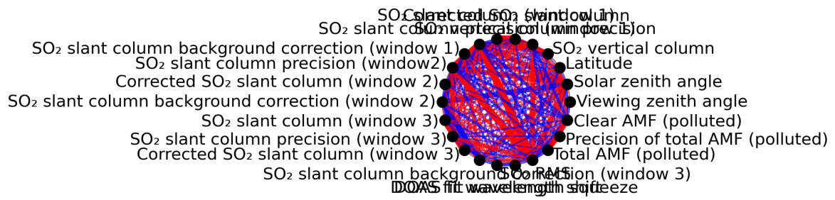
Figure 1: Map of correlation graph for 2024-07-26 to 2024-07-27.
