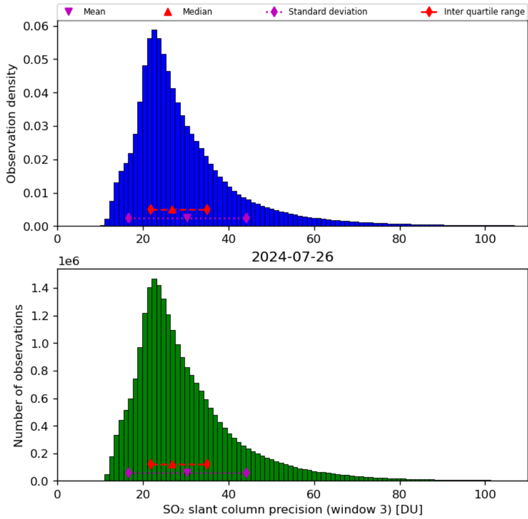
Figure 65: Histogram of “SO 2 slant column precision (window 3)” for 2024-07-26 to 2024-07-27
