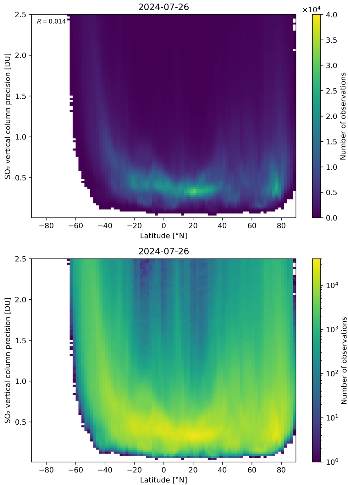
Figure 157: Scatter density plot of “Latitude” against “SO 2 vertical column precision” for 2024-07-26 to 2024-07-27.
