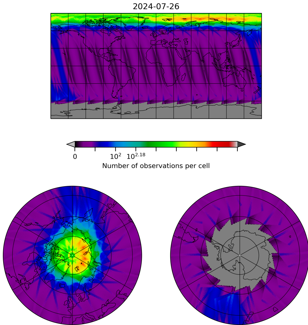
Figure 28: Map of the number of observations for 2024-07-26 to 2024-07-27
