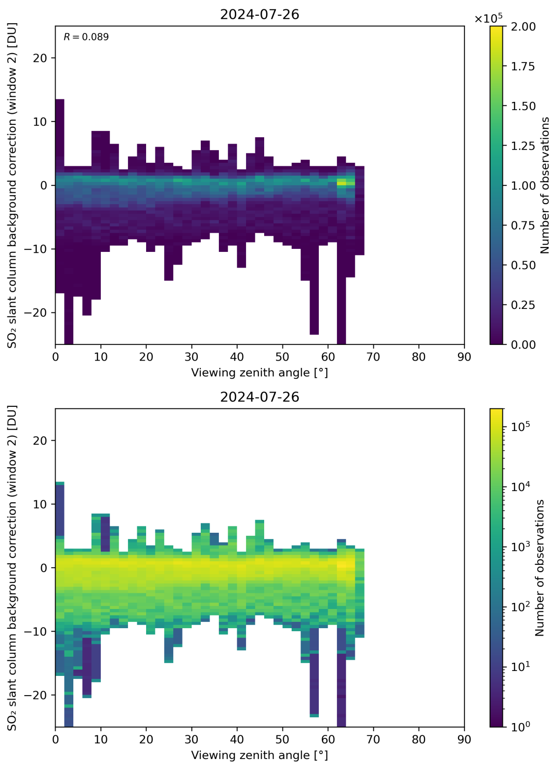
Figure 309: Scatter density plot of “Viewing zenith angle” against “SO 2 slant column background correction (window 2)” for 2024-07-26 to 2024-07-27.
