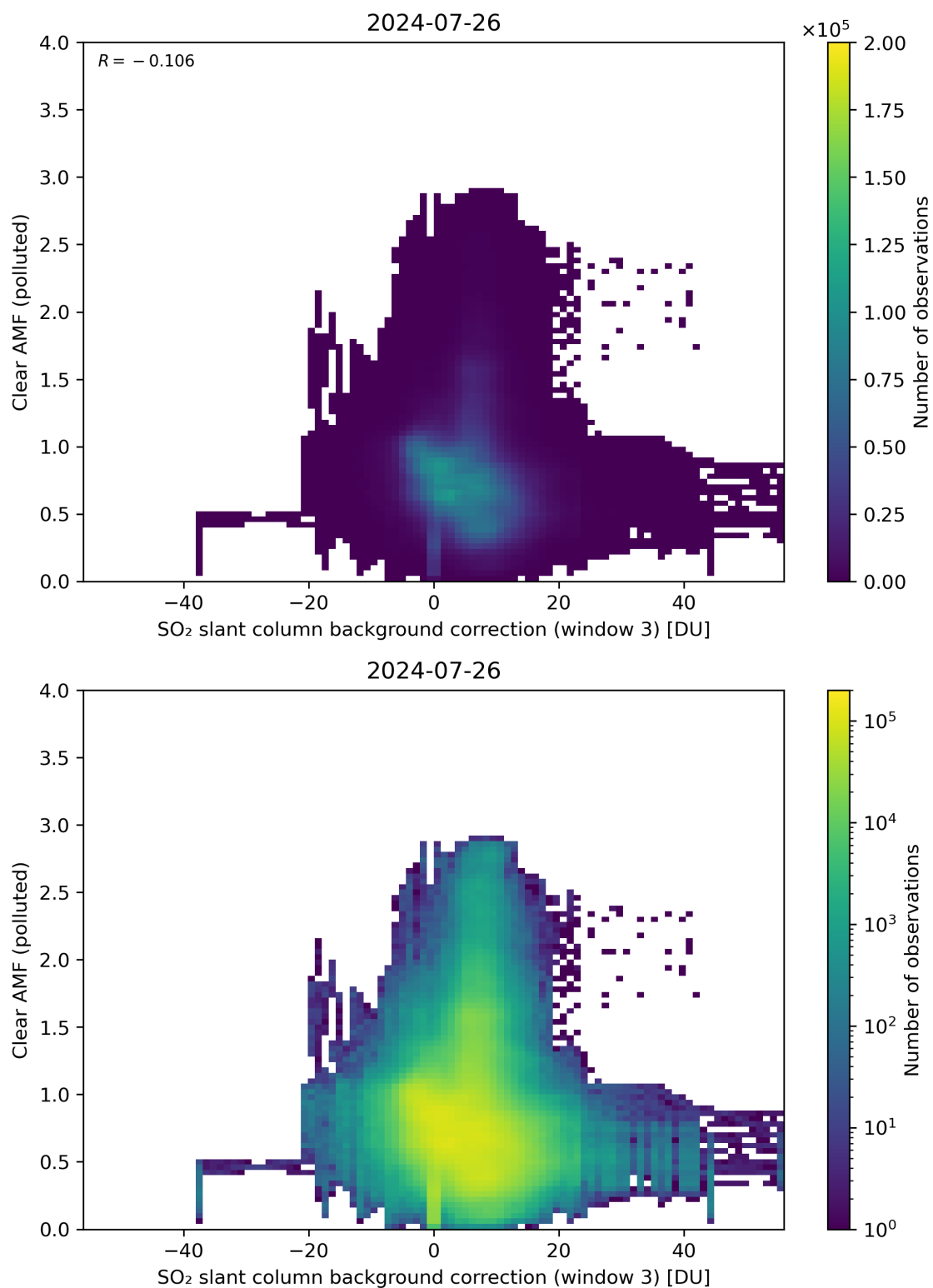
Figure 124: Scatter density plot of “SO 2 slant column background correction (window 3)” against “Clear AMF (polluted)” for 2024-07-26 to 2024-07-27.
