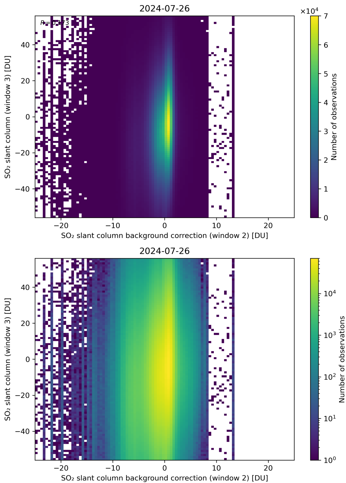
Figure 117: Scatter density plot of “SO 2 slant column background correction (window 2)” against “SO 2 slant column (window 3)” for 2024-07-26 to 2024-07-27.
