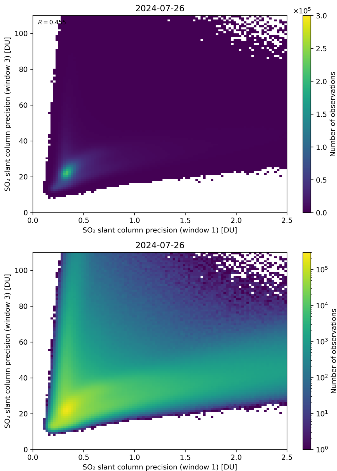
Figure 229: Scatter density plot of “SO 2 slant column precision (window 1)” against “SO 2 slant column precision (window 3)” for 2024-07-26 to 2024-07-27.
