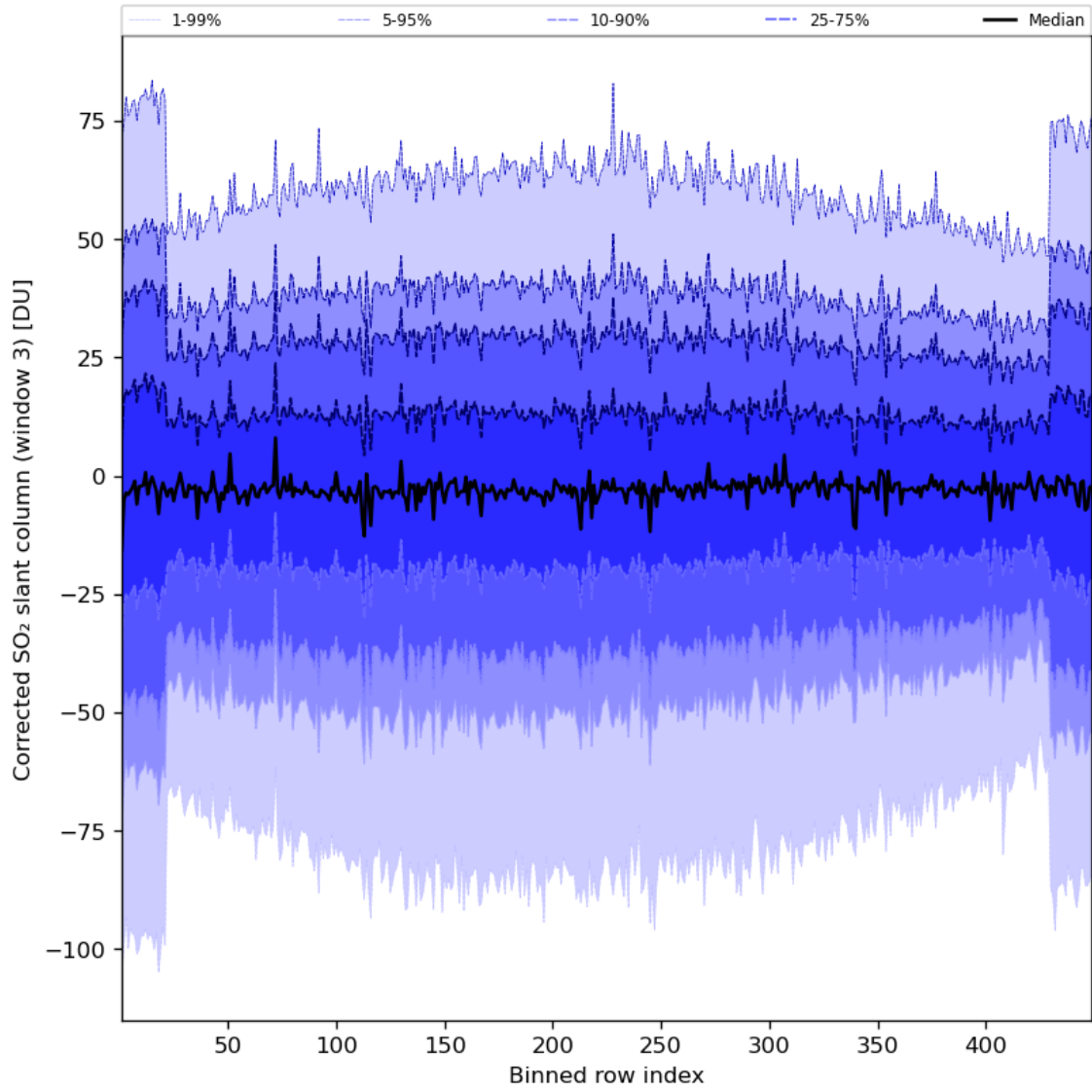
Figure 89: Along track statistics of “Corrected SO 2 slant column (window 3)” for 2024-07-26 to 2024-07-27
