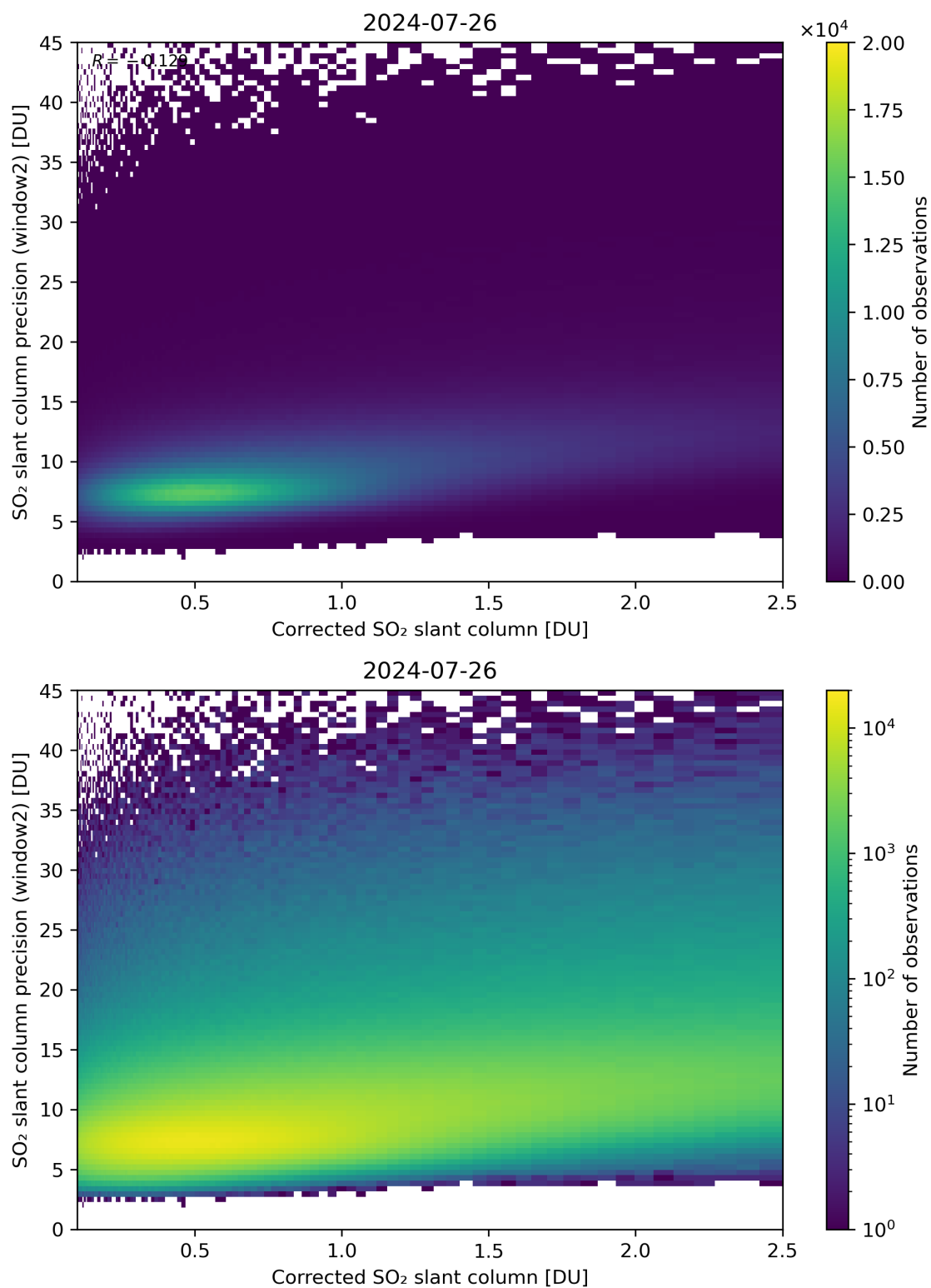
Figure 189: Scatter density plot of “Corrected SO 2 slant column” against “SO 2 slant column precision (window2)” for 2024-07-26 to 2024-07-27.
