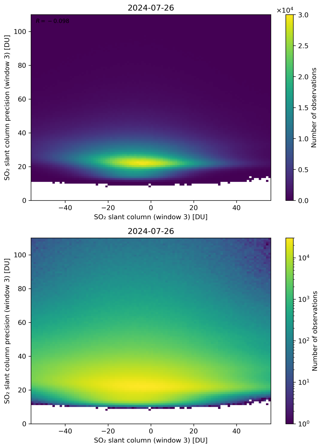
Figure 267: Scatter density plot of “SO 2 slant column (window 3)” against “SO 2 slant column precision (window 3)” for 2024-07-26 to 2024-07-27.
