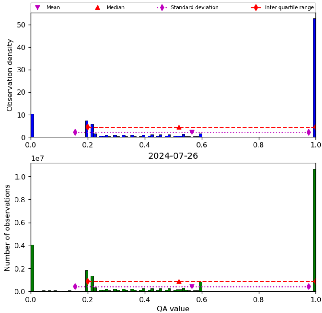
Figure 52: Histogram of “QA value” for 2024-07-26 to 2024-07-27
