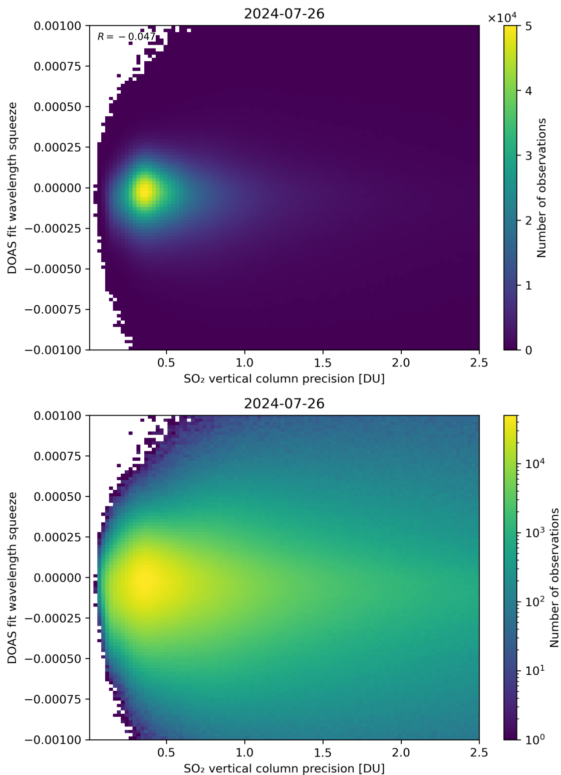
Figure 283: Scatter density plot of “SO 2 vertical column precision” against “DOAS fit wavelength squeeze” for 2024-07-26 to 2024-07-27.
