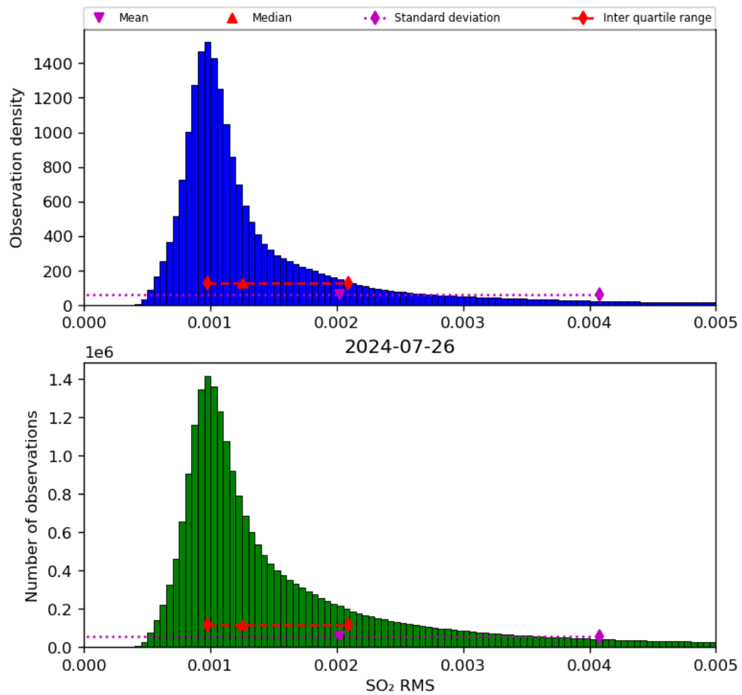
Figure 70: Histogram of “SO 2 RMS” for 2024-07-26 to 2024-07-27
