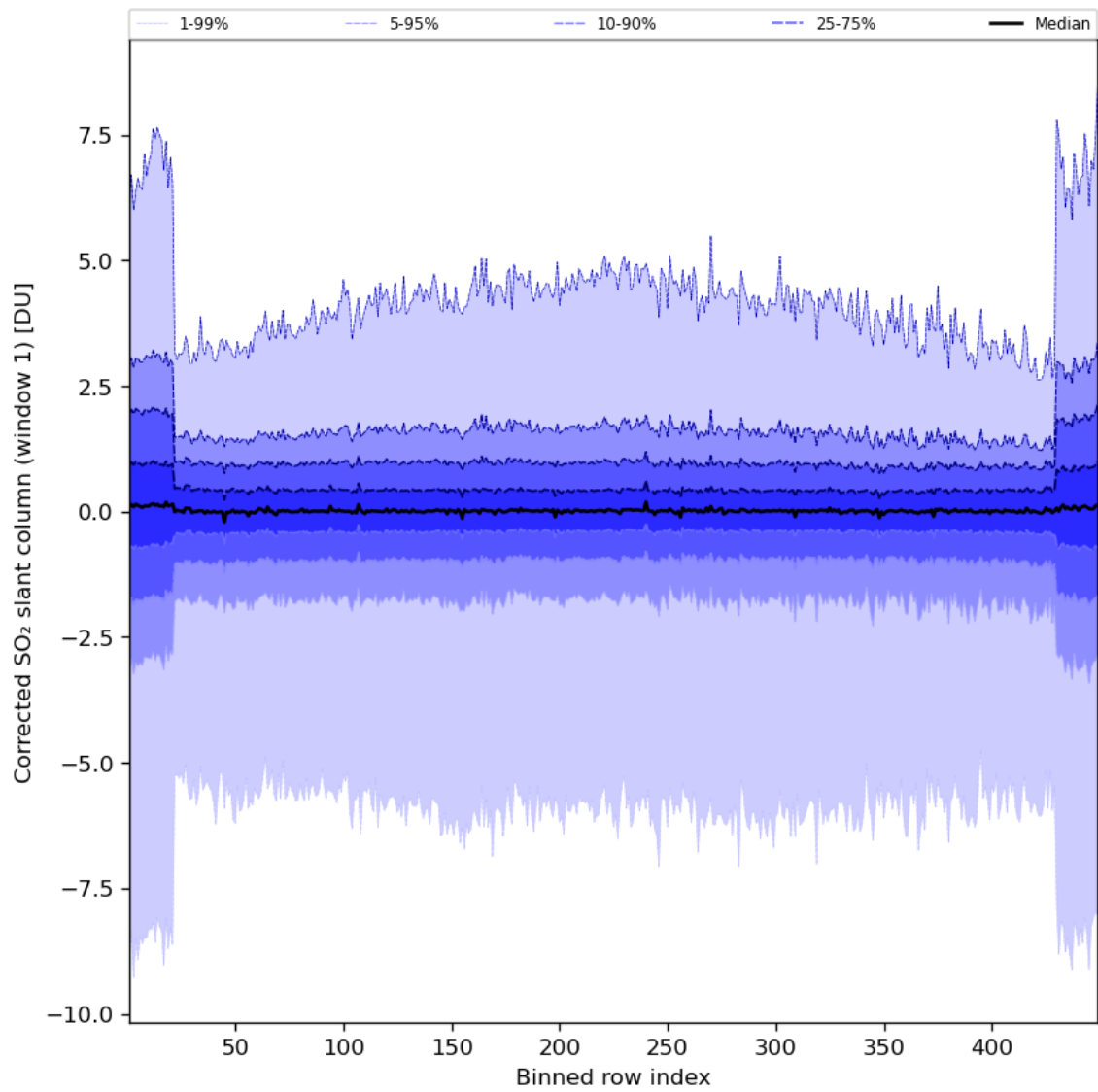
Figure 81: Along track statistics of “Corrected SO 2 slant column (window 1)” for 2024-07-26 to 2024-07-27
