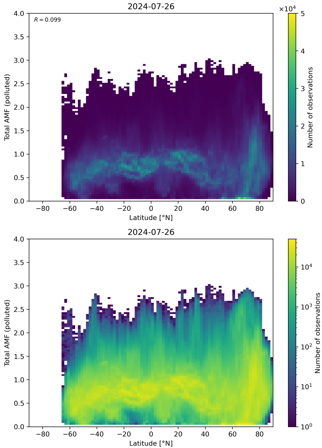
Figure 154: Scatter density plot of “Latitude” against “Total AMF (polluted)” for 2024-07-26 to 2024-07-27.
