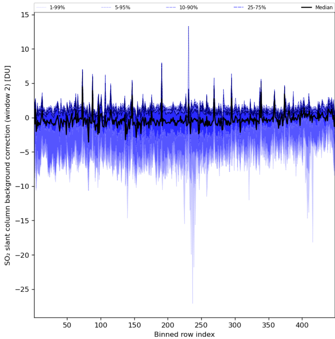
Figure 86: Along track statistics of “SO 2 slant column background correction (window 2)” for 2024-07-26 to 2024-07-27
