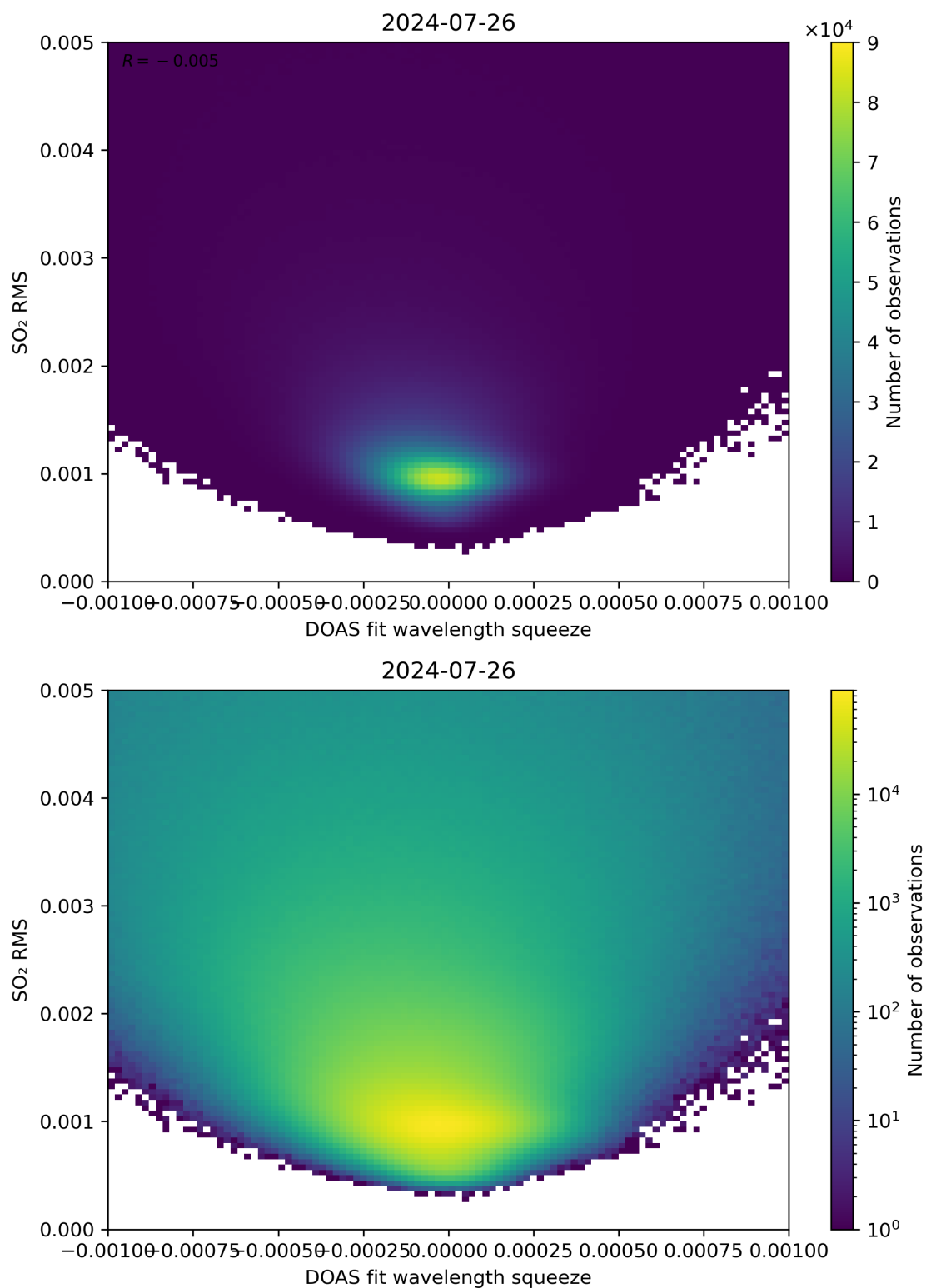
Figure 132: Scatter density plot of “DOAS fit wavelength squeeze” against “SO 2 RMS” for 2024-07-26 to 2024-07-27.
