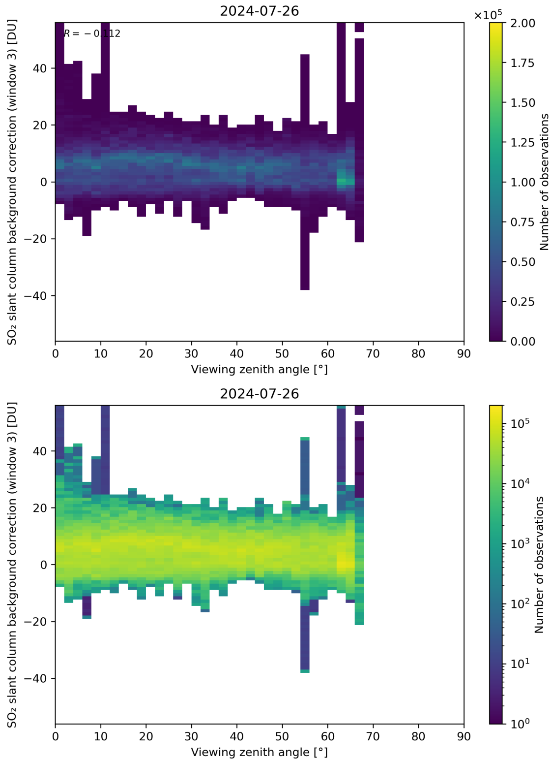
Figure 310: Scatter density plot of “Viewing zenith angle” against “SO 2 slant column background correction (window 3)” for 2024-07-26 to 2024-07-27.
