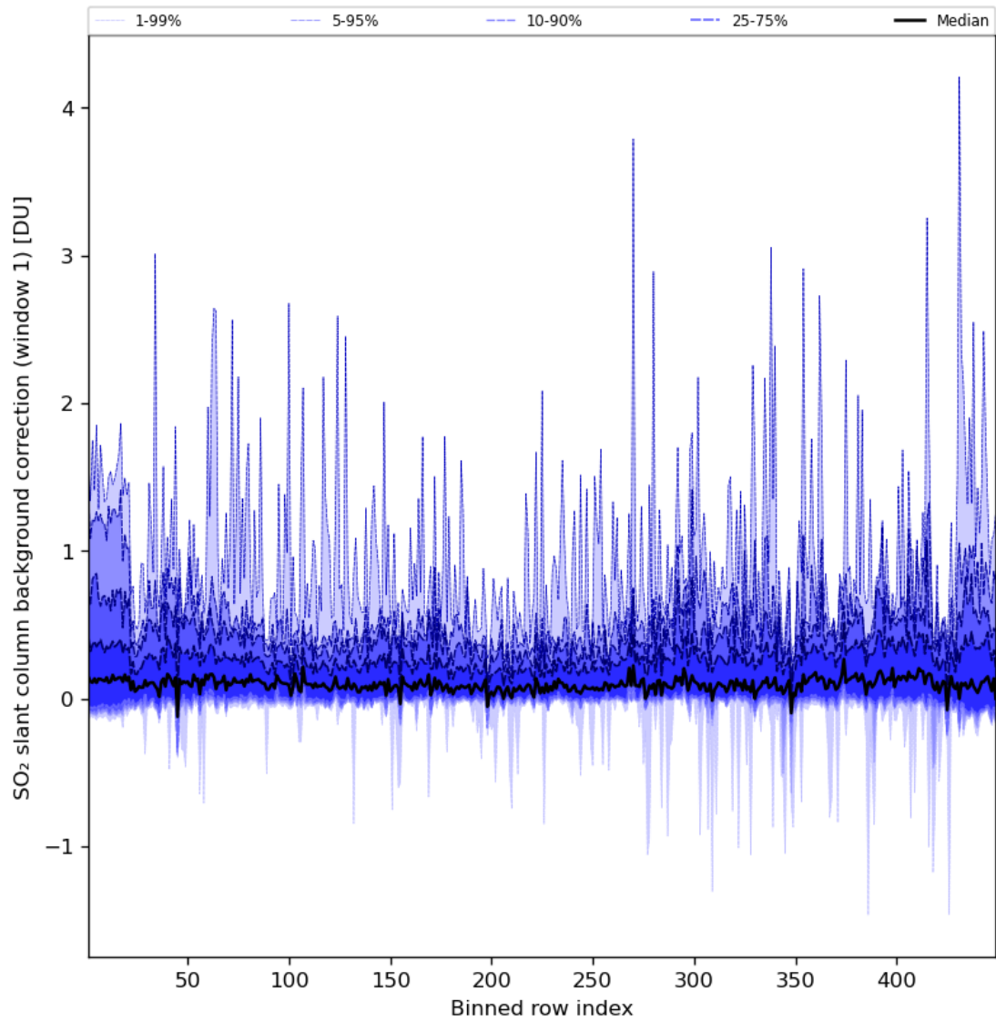
Figure 82: Along track statistics of “SO 2 slant column background correction (window 1)” for 2024-07-26 to 2024-07-27
