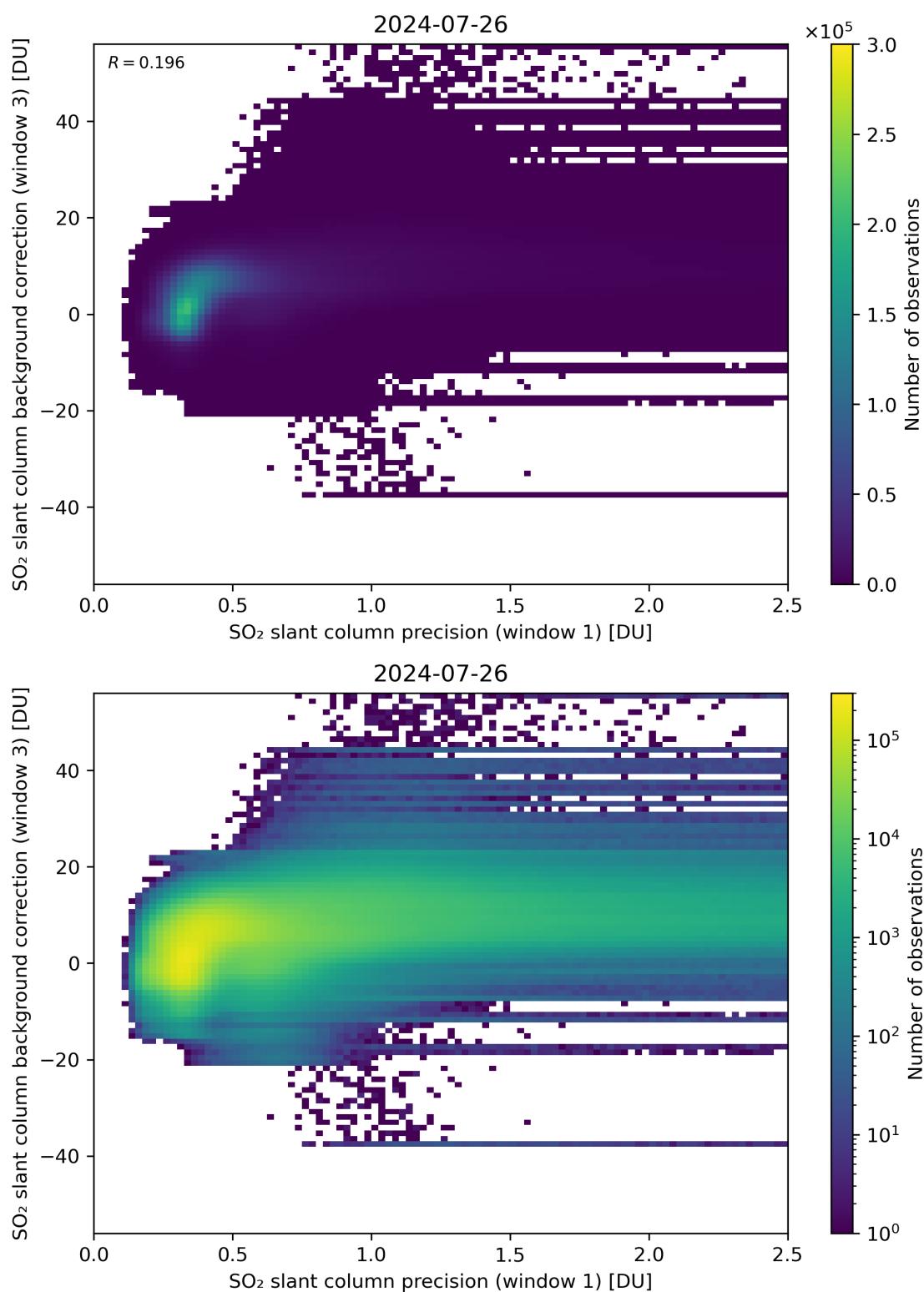
Figure 220: Scatter density plot of “SO 2 slant column precision (window 1)” against “SO 2 slant column background correction (window 3)” for 2024-07-26 to 2024-07-27.
