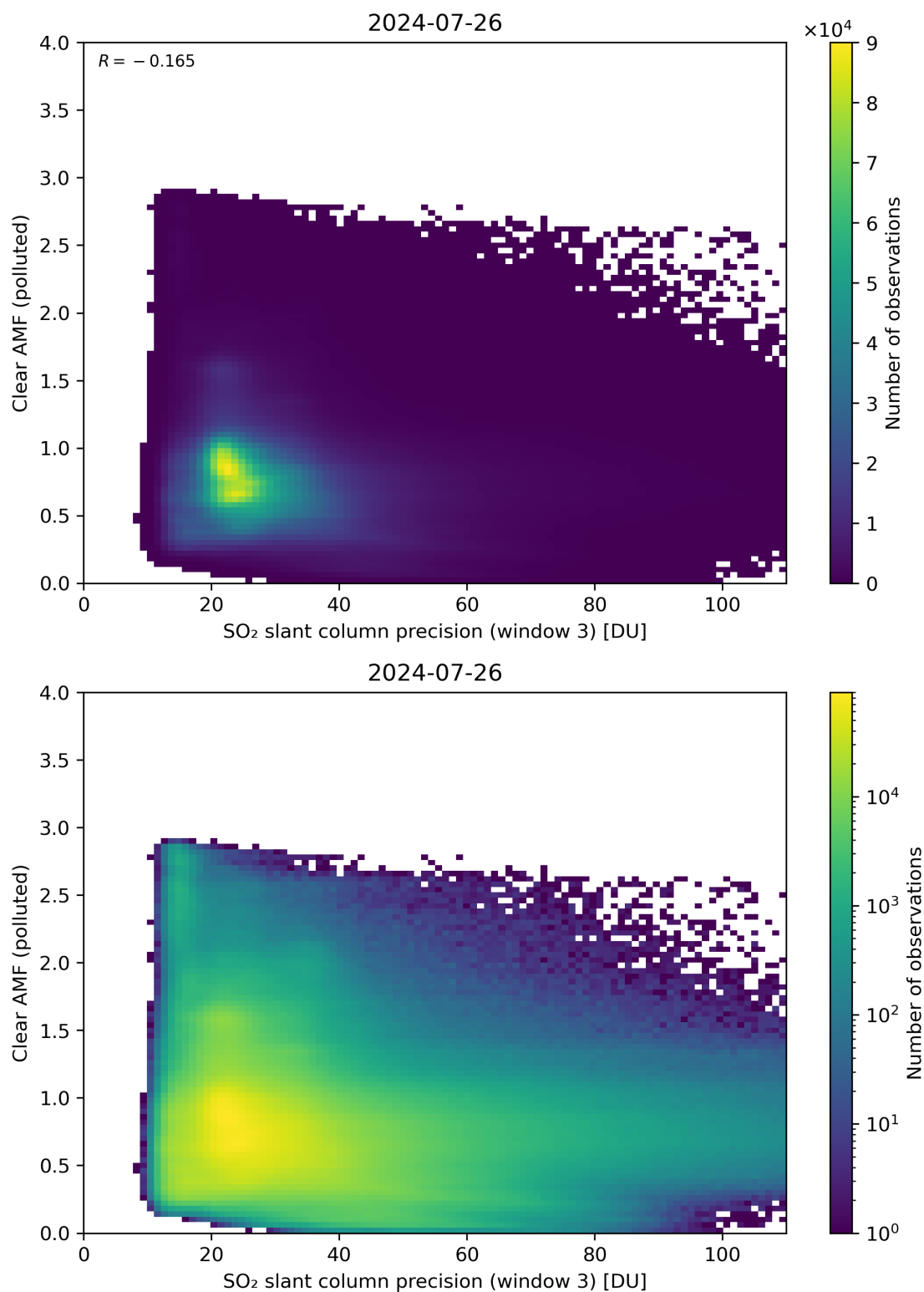
Figure 261: Scatter density plot of “SO 2 slant column precision (window 3)” against “Clear AMF (polluted)” for 2024-07-26 to 2024-07-27.
