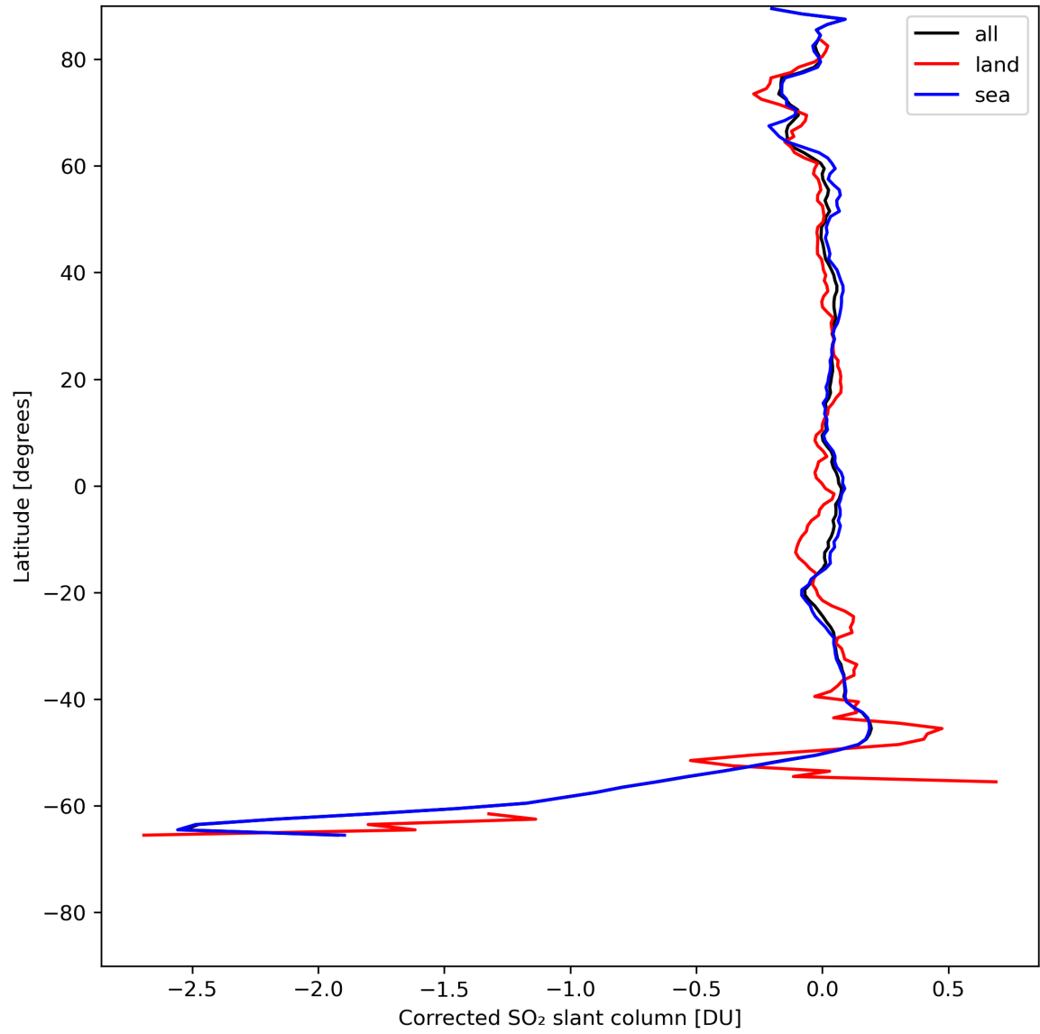
Figure 32: Zonal average of “Corrected SO 2 slant column” for 2024-07-26 to 2024-07-28.
