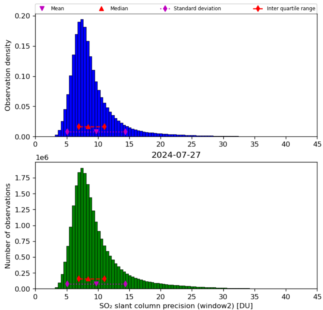
Figure 61: Histogram of “SO 2 slant column precision (window2)” for 2024-07-26 to 2024-07-28
