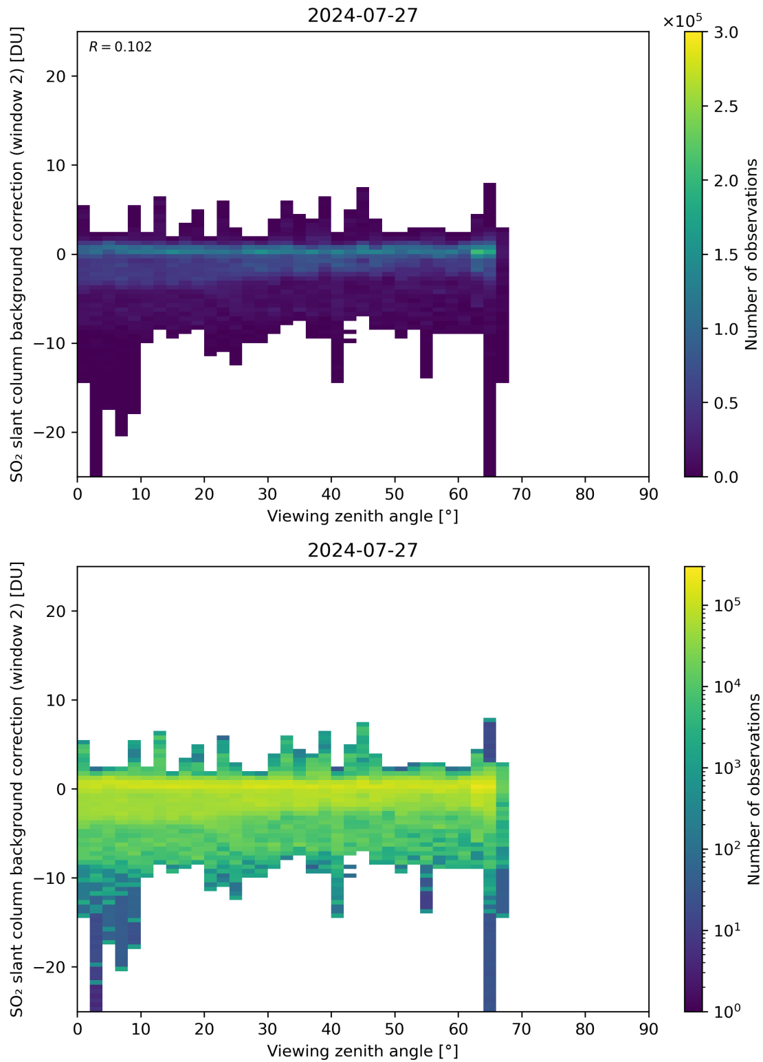
Figure 309: Scatter density plot of “Viewing zenith angle” against “SO 2 slant column background correction (window 2)” for 2024-07-26 to 2024-07-28.
