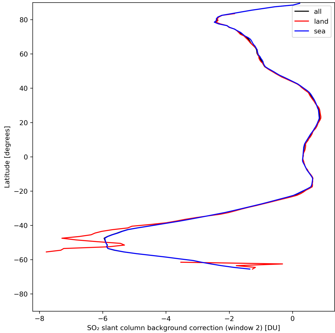
Figure 40: Zonal average of “SO 2 slant column background correction (window 2)” for 2024-07-26 to 2024-07-28.
