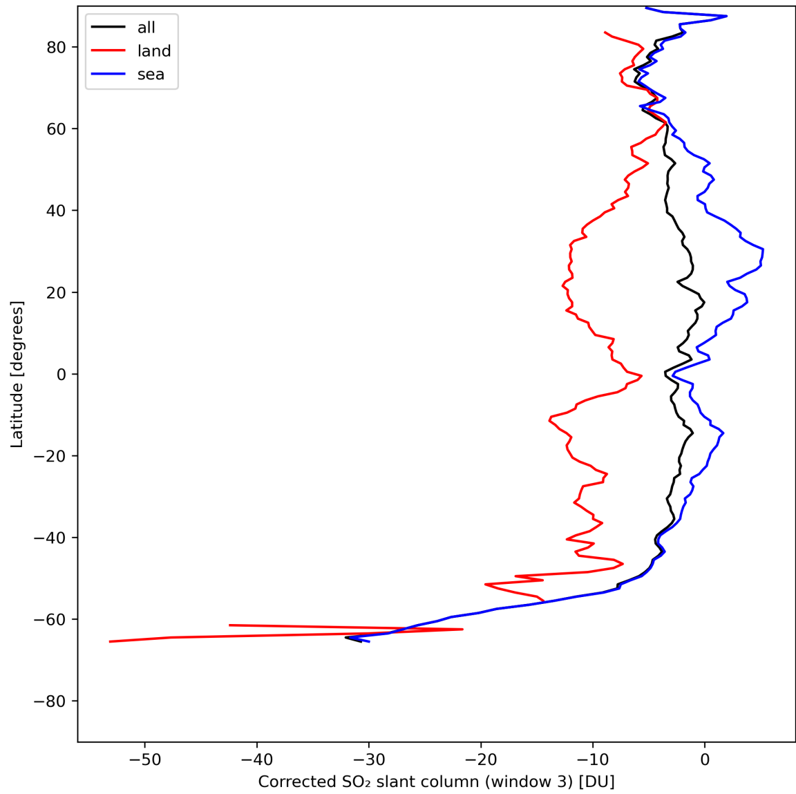
Figure 43: Zonal average of “Corrected SO 2 slant column (window 3)” for 2024-07-26 to 2024-07-28.
