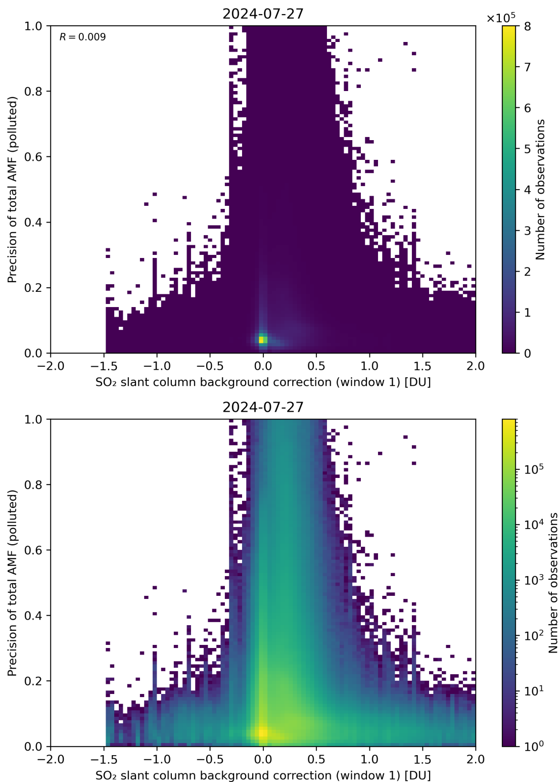
Figure 110: Scatter density plot of “SO 2 slant column background correction (window 1)” against “Precision of total AMF (polluted)” for 2024-07-26 to 2024-07-28.
