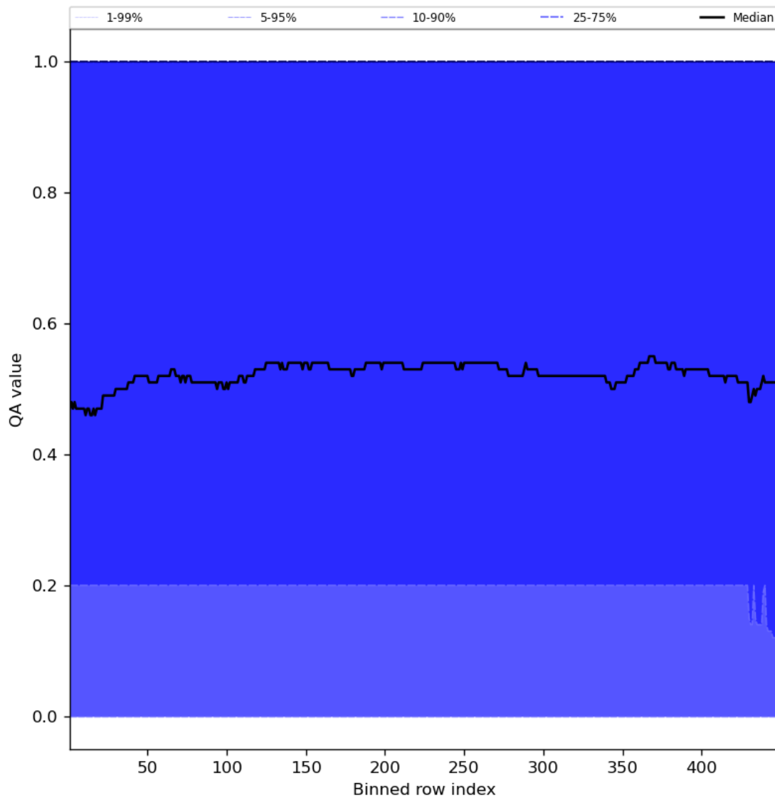
Figure 75: Along track statistics of “QA value” for 2024-07-26 to 2024-07-28
