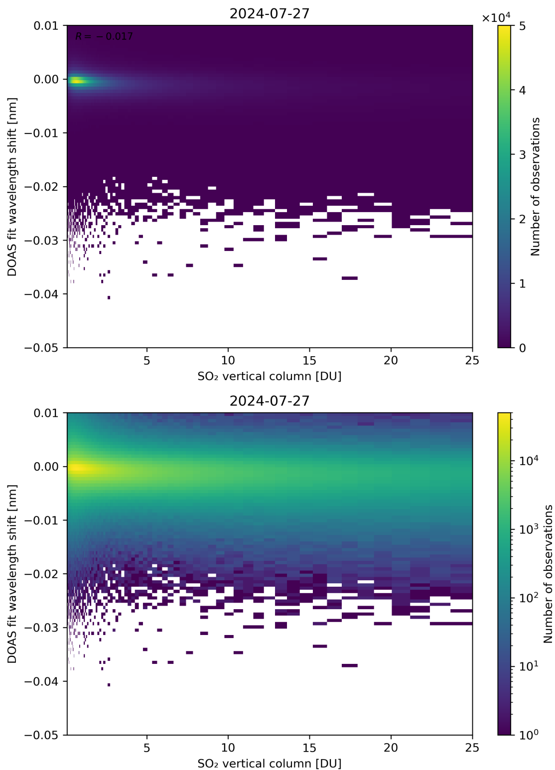
Figure 276: Scatter density plot of “SO 2 vertical column” against “DOAS fit wavelength shift” for 2024-07-26 to 2024-07-28.
