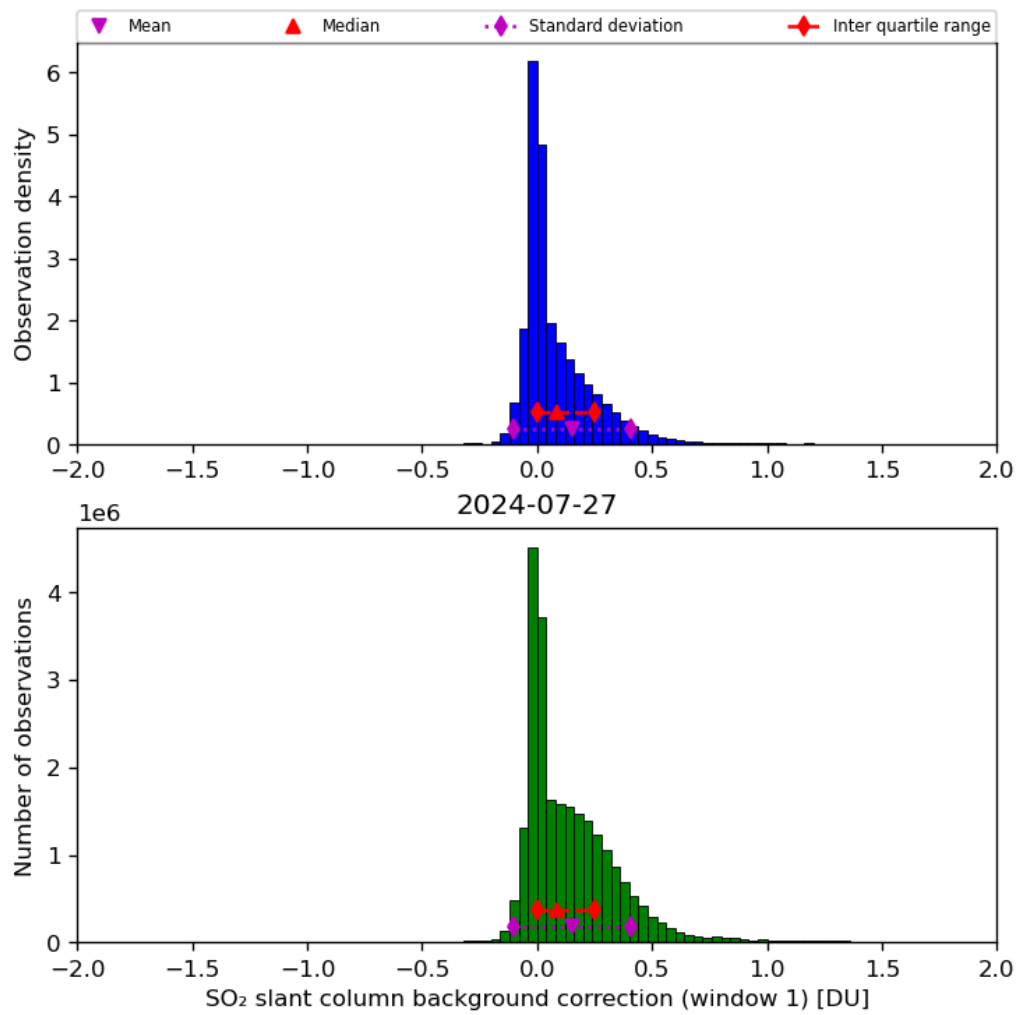
Figure 59: Histogram of “SO 2 slant column background correction (window 1)” for 2024-07-26 to 2024-07-28
