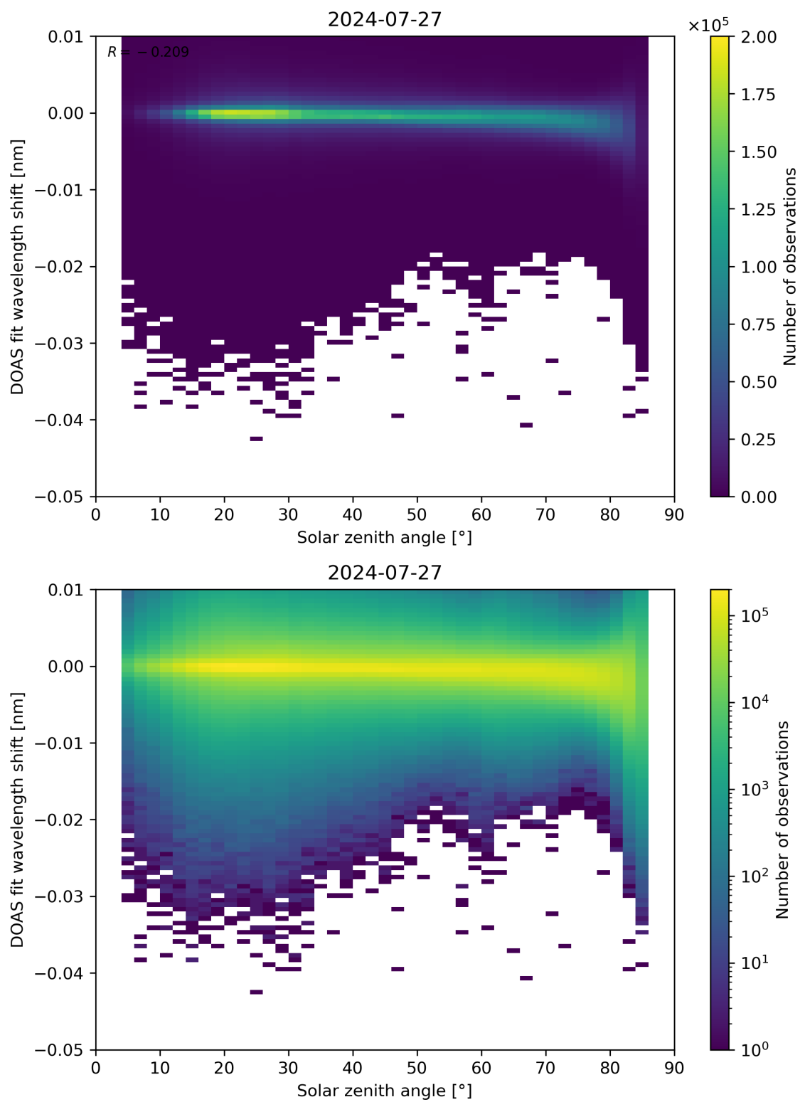
Figure 161: Scatter density plot of “Solar zenith angle” against “DOAS fit wavelength shift” for 2024-07-26 to 2024-07-28.
