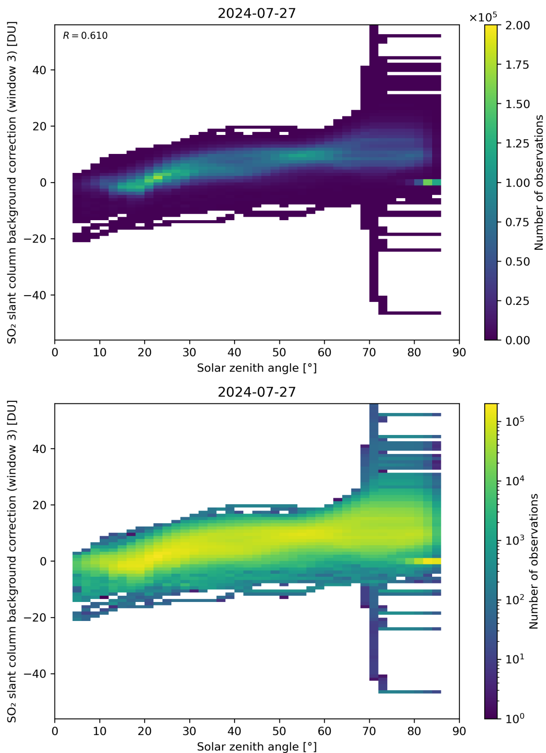
Figure 160: Scatter density plot of “Solar zenith angle” against “SO 2 slant column background correction (window 3)” for 2024-07-26 to 2024-07-28.
