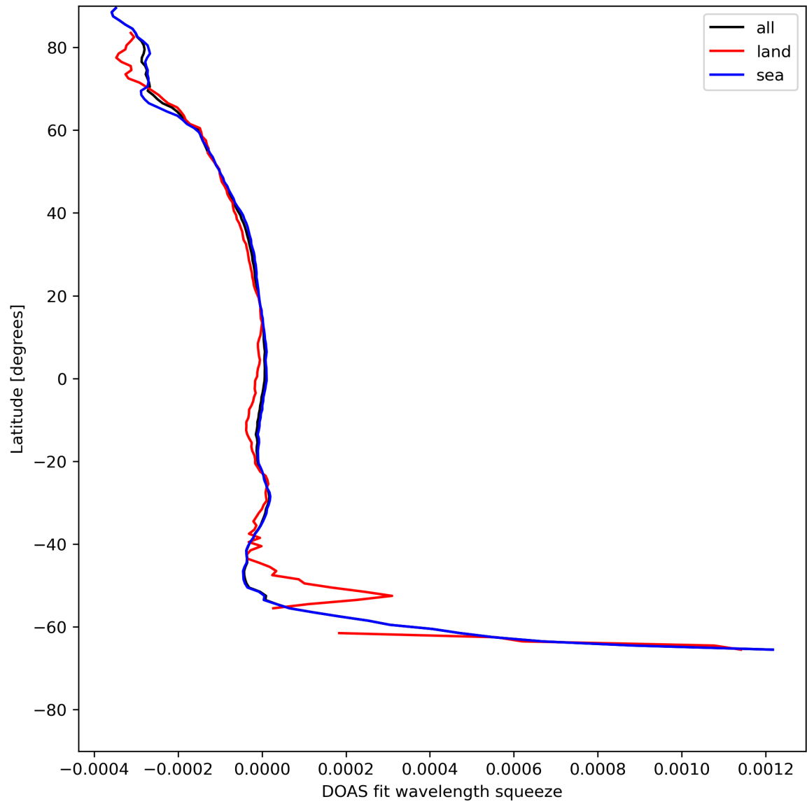
Figure 46: Zonal average of “DOAS fit wavelength squeeze” for 2024-07-26 to 2024-07-28.
