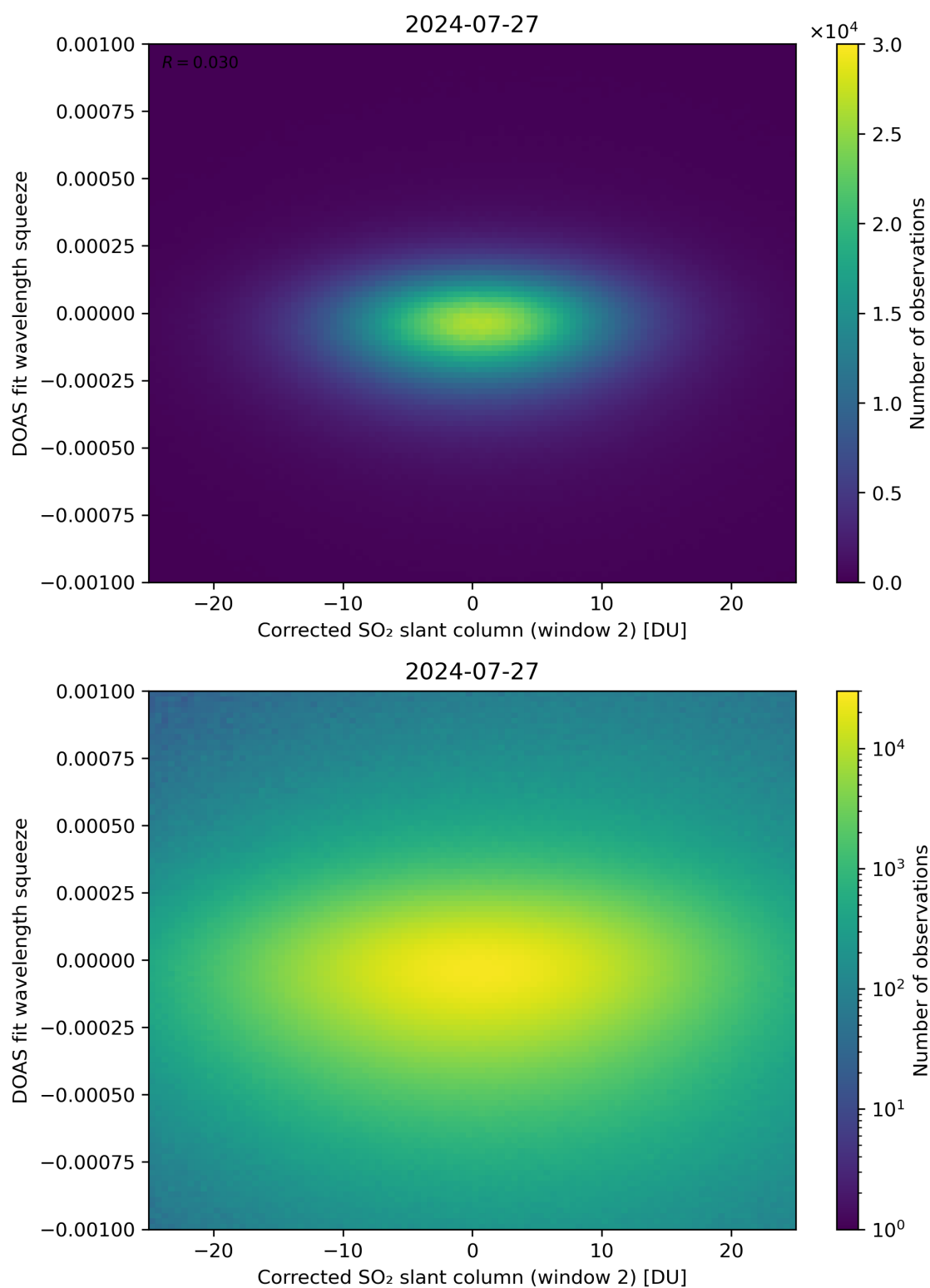
Figure 197: Scatter density plot of “Corrected SO 2 slant column (window 2)” against “DOAS fit wavelength squeeze” for 2024-07-26 to 2024-07-28.
