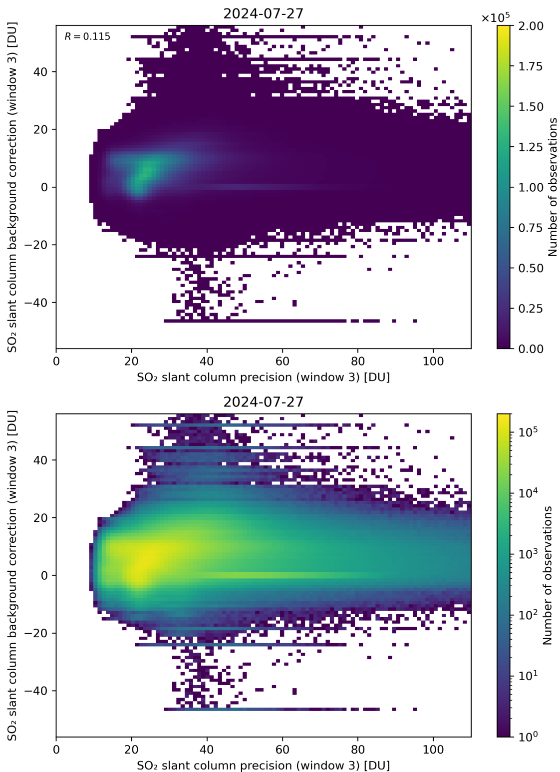
Figure 257: Scatter density plot of “SO 2 slant column precision (window 3)” against “SO 2 slant column background correction (window 3)” for 2024-07-26 to 2024-07-28.
