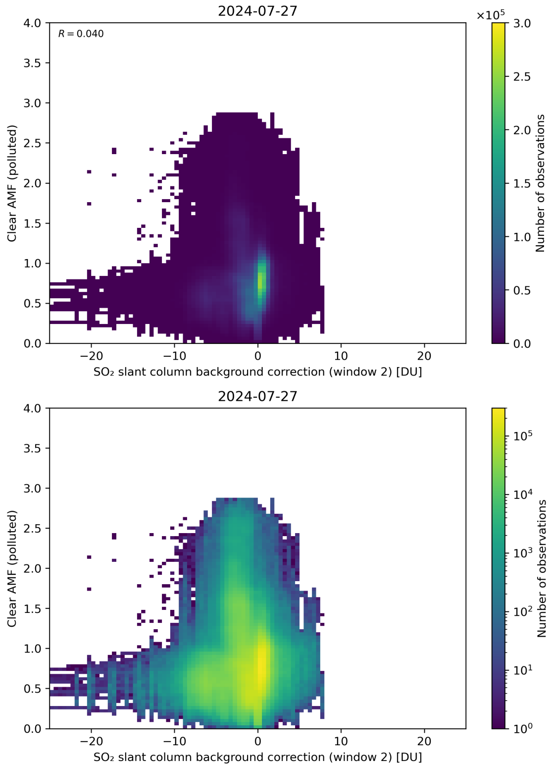
Figure 115: Scatter density plot of “SO 2 slant column background correction (window 2)” against “Clear AMF (polluted)” for 2024-07-26 to 2024-07-28.
