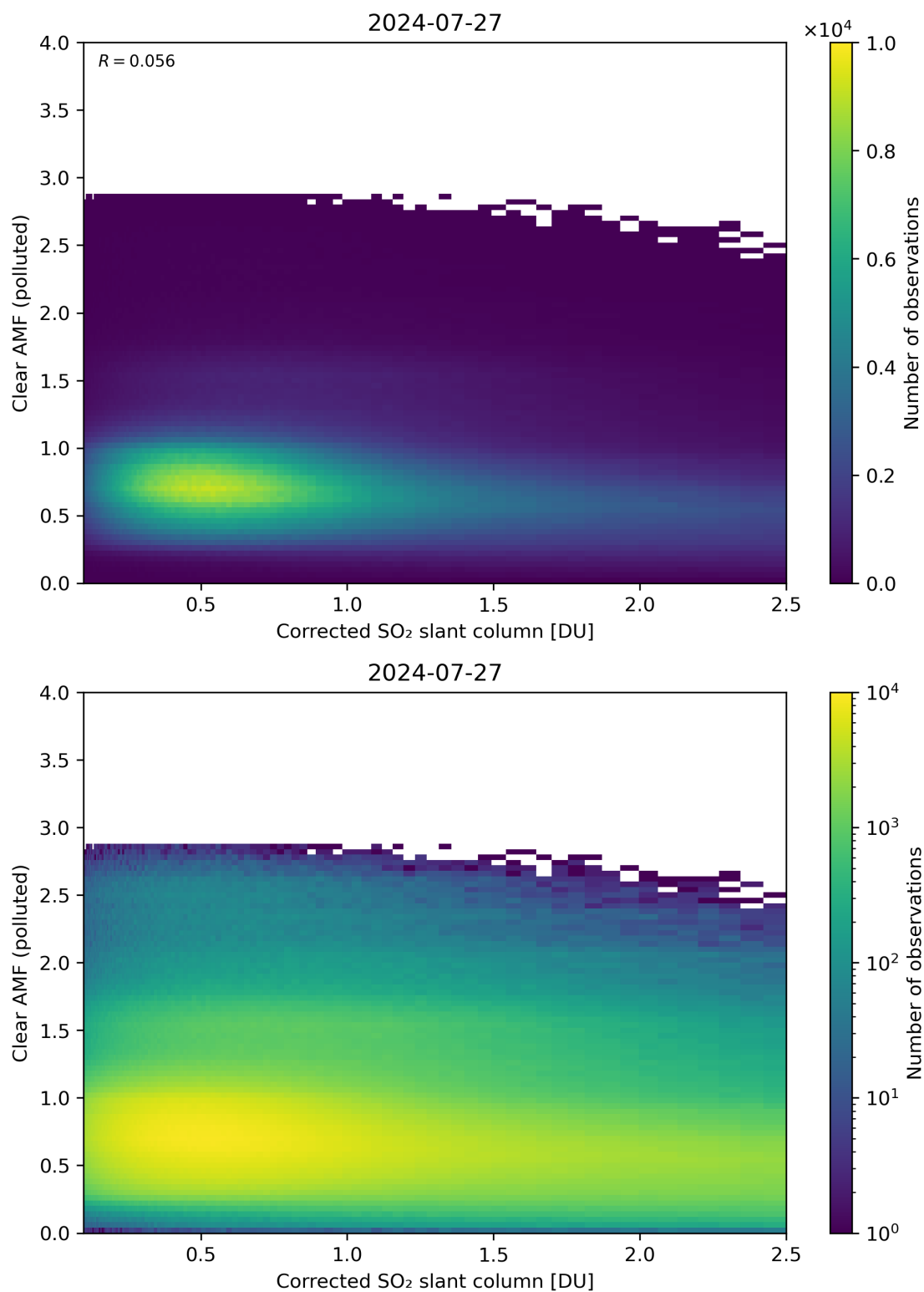
Figure 184: Scatter density plot of “Corrected SO 2 slant column” against “Clear AMF (polluted)” for 2024-07-26 to 2024-07-28.
