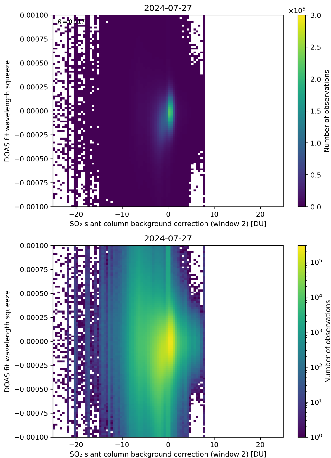
Figure 113: Scatter density plot of “SO 2 slant column background correction (window 2)” against “DOAS fit wavelength squeeze” for 2024-07-26 to 2024-07-28.
