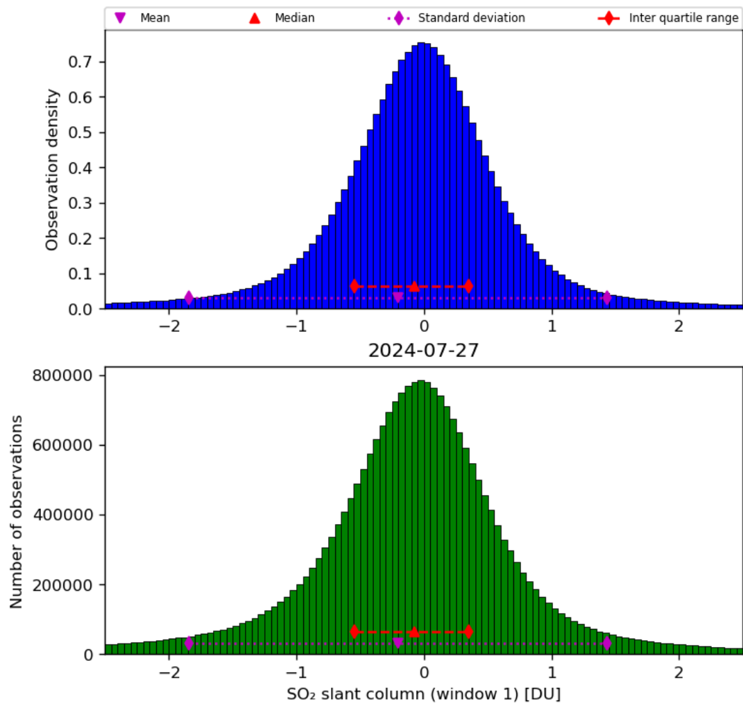
Figure 56: Histogram of “SO 2 slant column (window 1)” for 2024-07-26 to 2024-07-28
