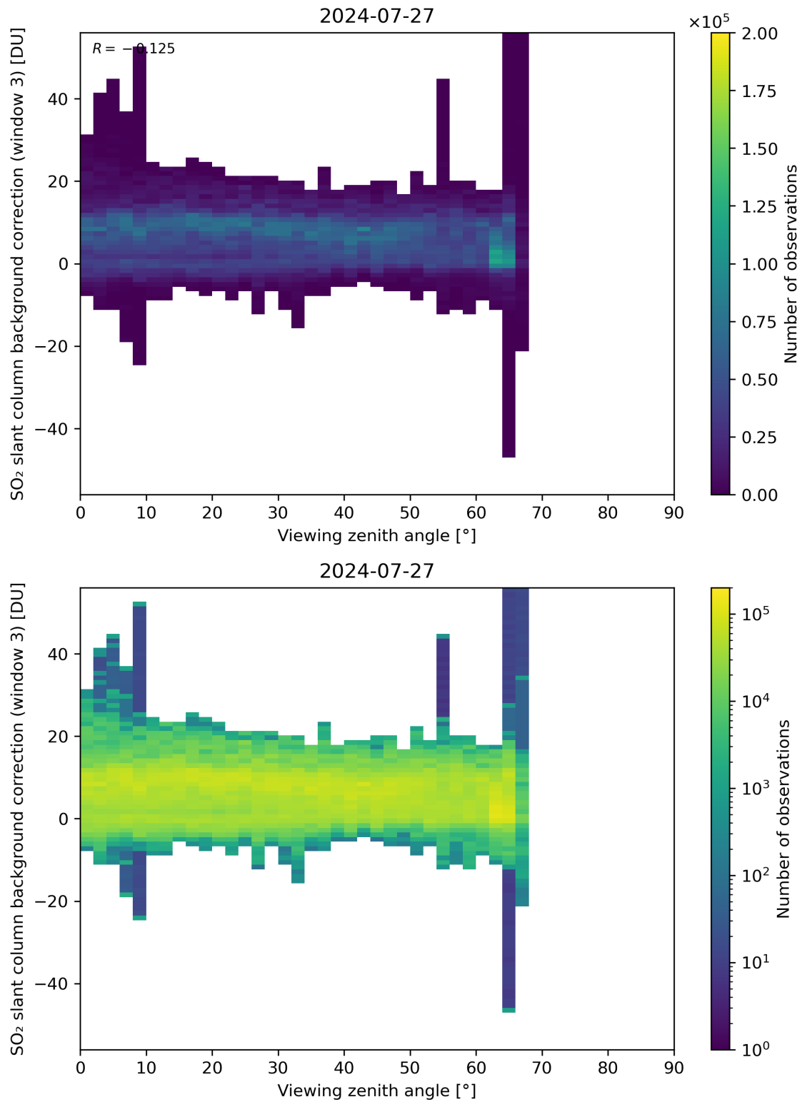
Figure 310: Scatter density plot of “Viewing zenith angle” against “SO 2 slant column background correction (window 3)” for 2024-07-26 to 2024-07-28.
