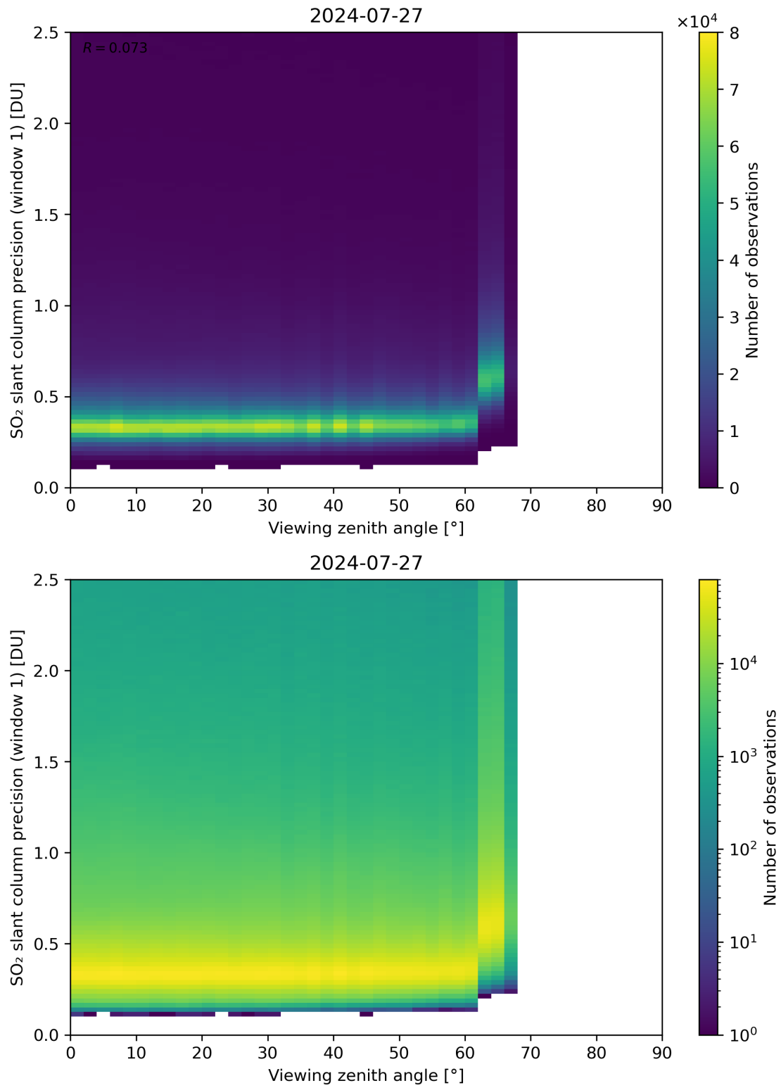
Figure 321: Scatter density plot of “Viewing zenith angle” against “SO 2 slant column precision (window 1)” for 2024-07-26 to 2024-07-28.
