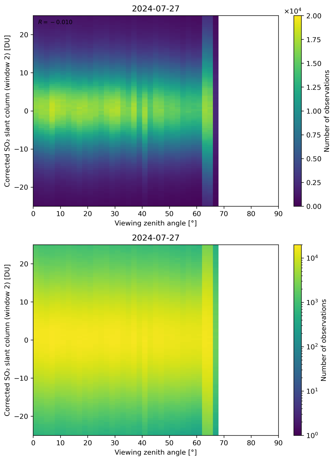
Figure 318: Scatter density plot of “Viewing zenith angle” against “Corrected SO 2 slant column (window 2)” for 2024-07-26 to 2024-07-28.
