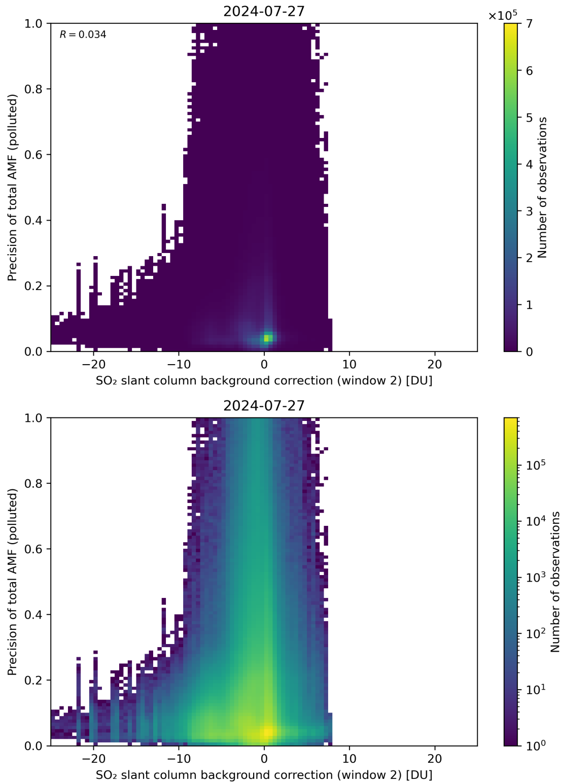
Figure 120: Scatter density plot of “SO 2 slant column background correction (window 2)” against “Precision of total AMF (polluted)” for 2024-07-26 to 2024-07-28.
