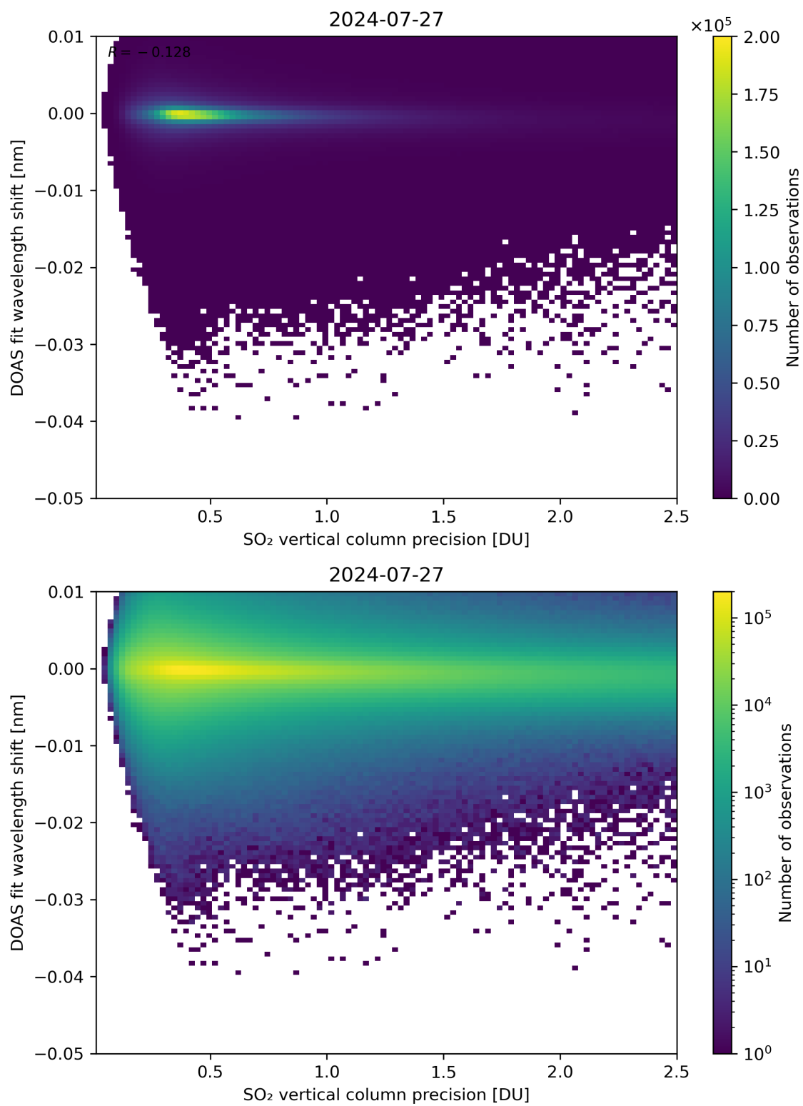
Figure 282: Scatter density plot of “SO 2 vertical column precision” against “DOAS fit wavelength shift” for 2024-07-26 to 2024-07-28.
