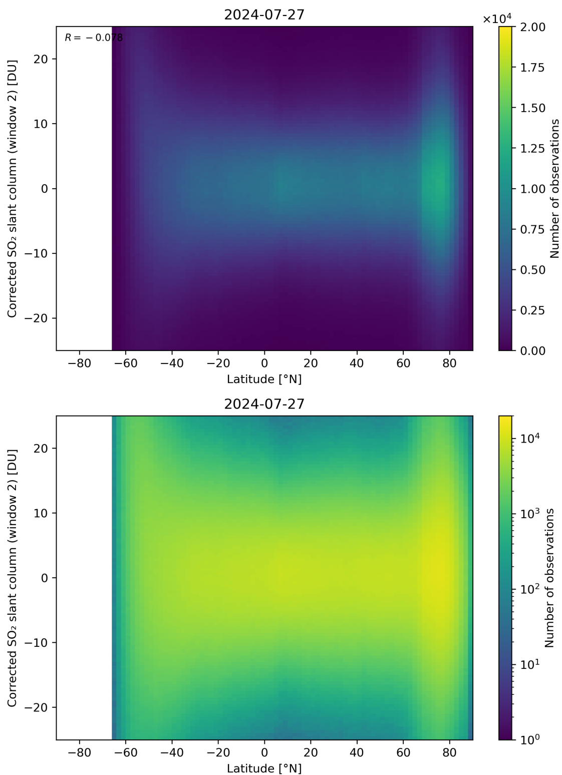
Figure 147: Scatter density plot of “Latitude” against “Corrected SO 2 slant column (window 2)” for 2024-07-26 to 2024-07-28.
