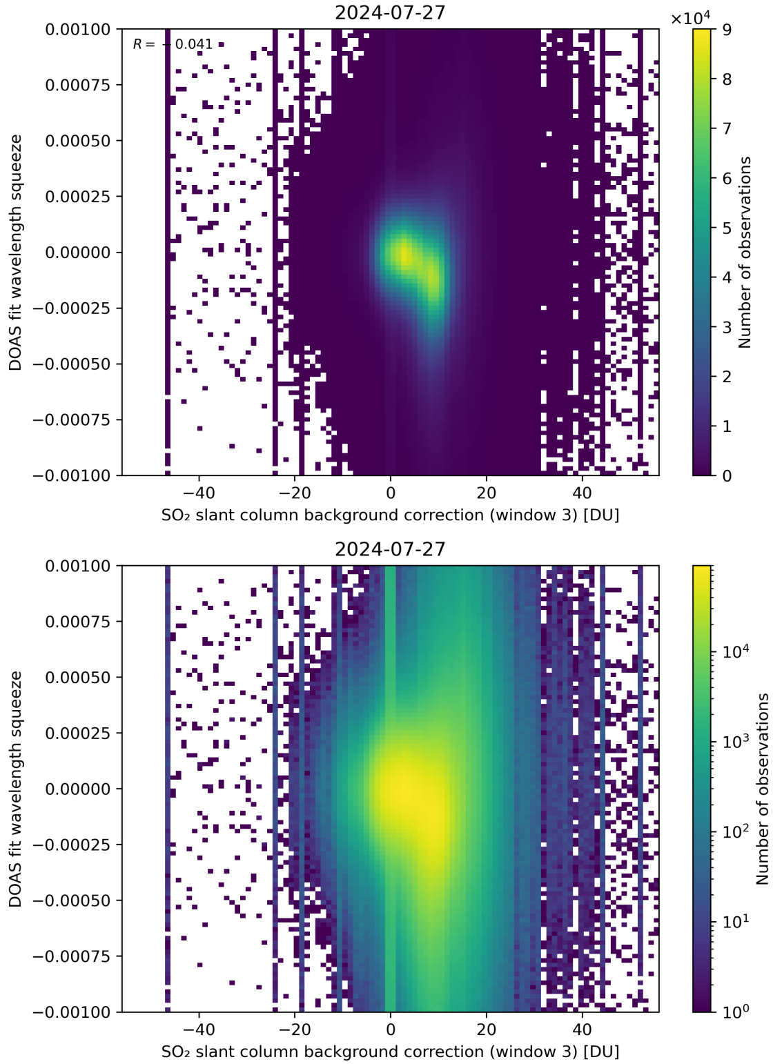
Figure 122: Scatter density plot of “SO 2 slant column background correction (window 3)” against “DOAS fit wavelength squeeze” for 2024-07-26 to 2024-07-28.
