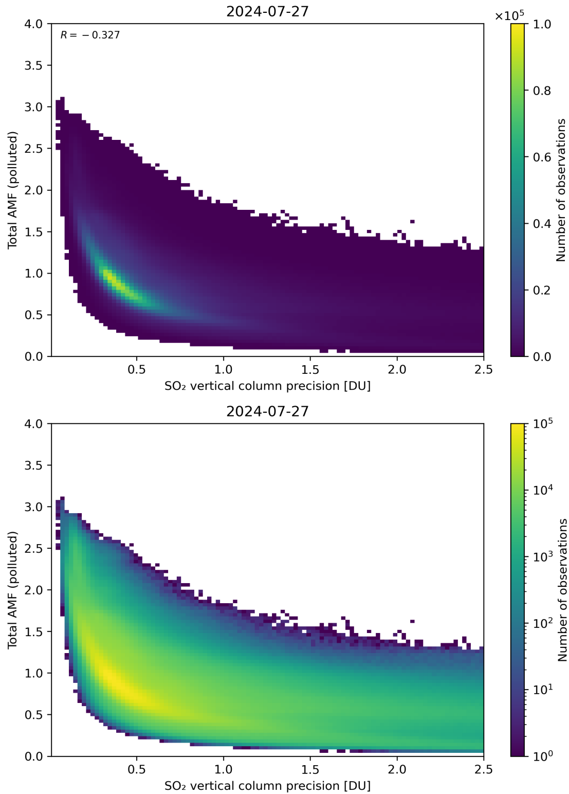
Figure 294: Scatter density plot of “SO 2 vertical column precision” against “Total AMF (polluted)” for 2024-07-26 to 2024-07-28.
