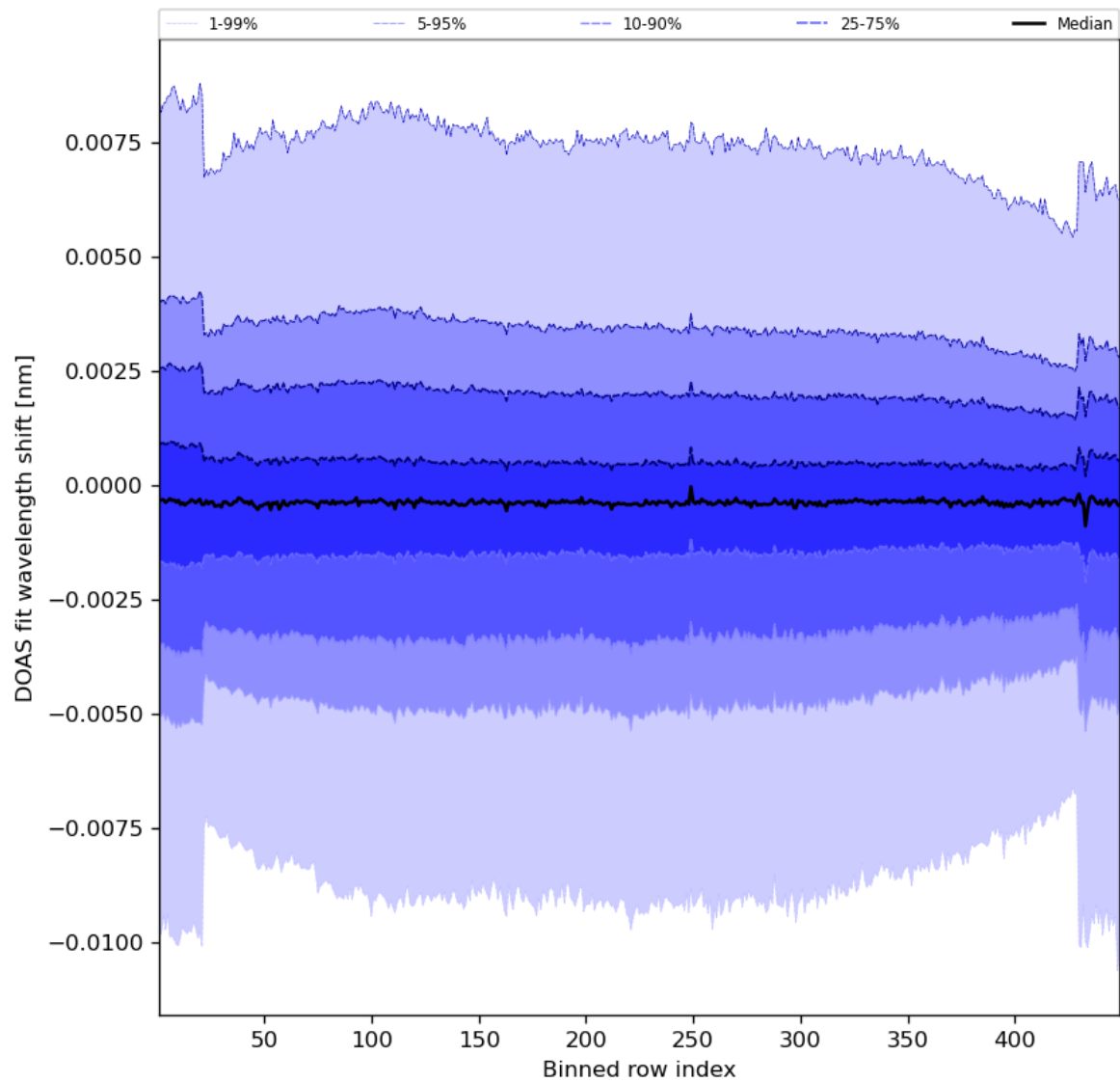
Figure 91: Along track statistics of “DOAS fit wavelength shift” for 2024-07-26 to 2024-07-28
