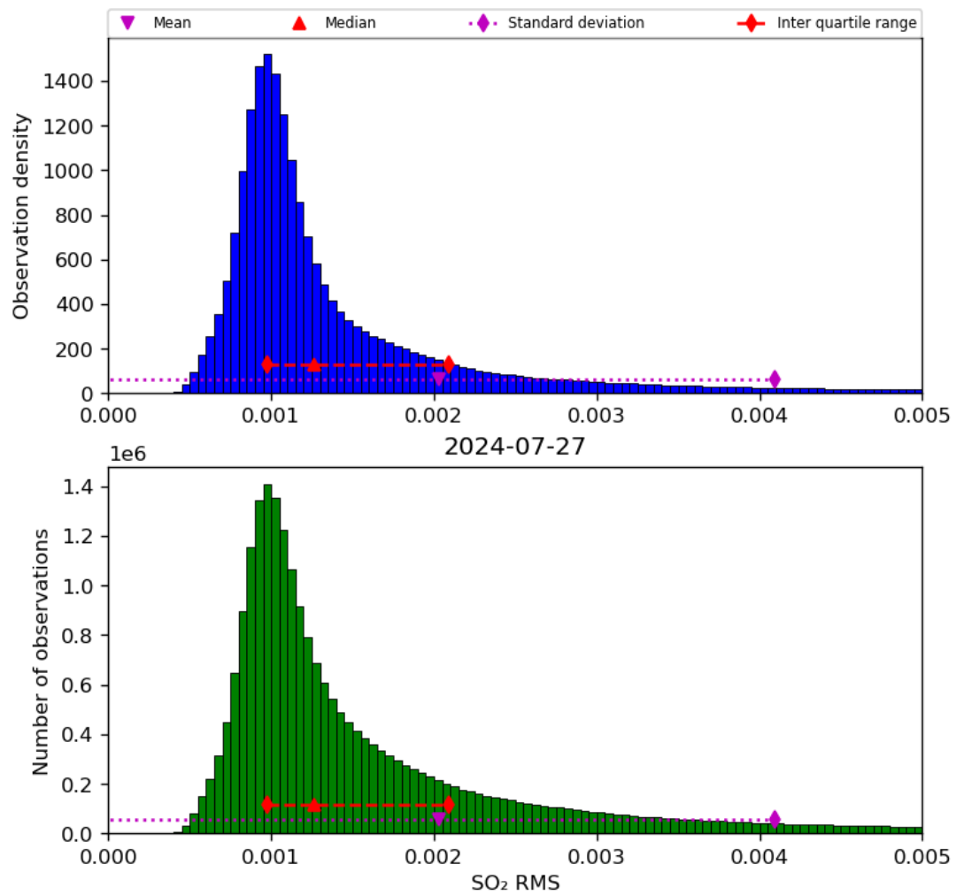
Figure 70: Histogram of “SO 2 RMS” for 2024-07-26 to 2024-07-28
