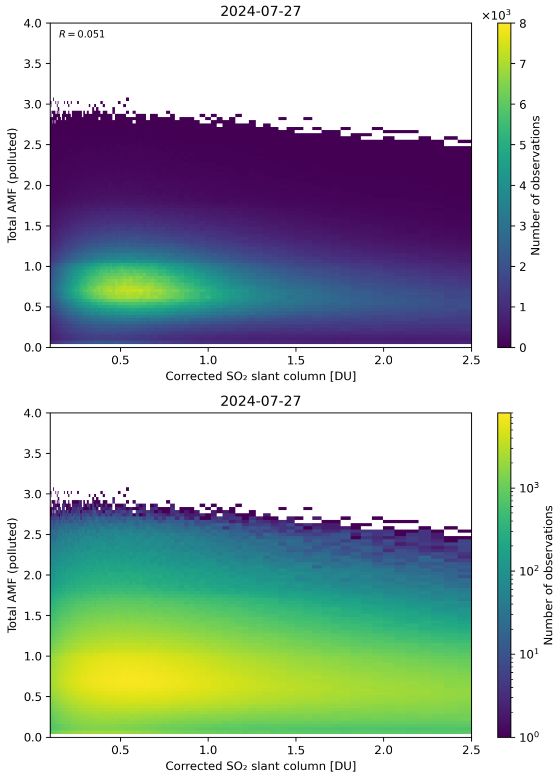
Figure 192: Scatter density plot of “Corrected SO 2 slant column” against “Total AMF (polluted)” for 2024-07-26 to 2024-07-28.
