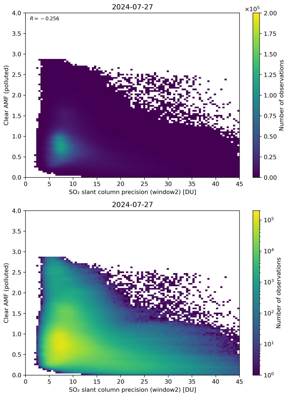
Figure 246: Scatter density plot of “SO 2 slant column precision (window2)” against “Clear AMF (polluted)” for 2024-07-26 to 2024-07-28.
