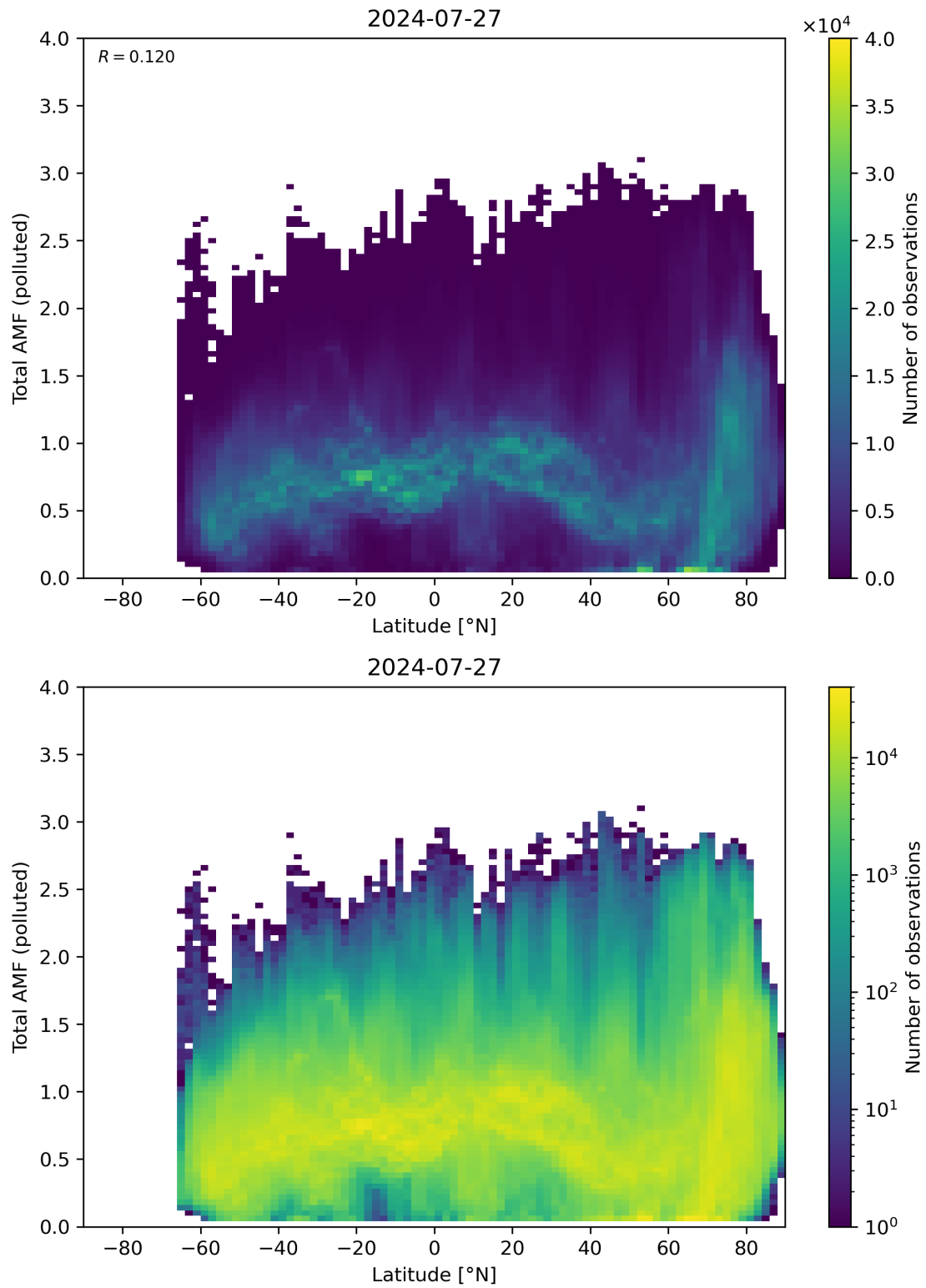
Figure 154: Scatter density plot of “Latitude” against “Total AMF (polluted)” for 2024-07-26 to 2024-07-28.
