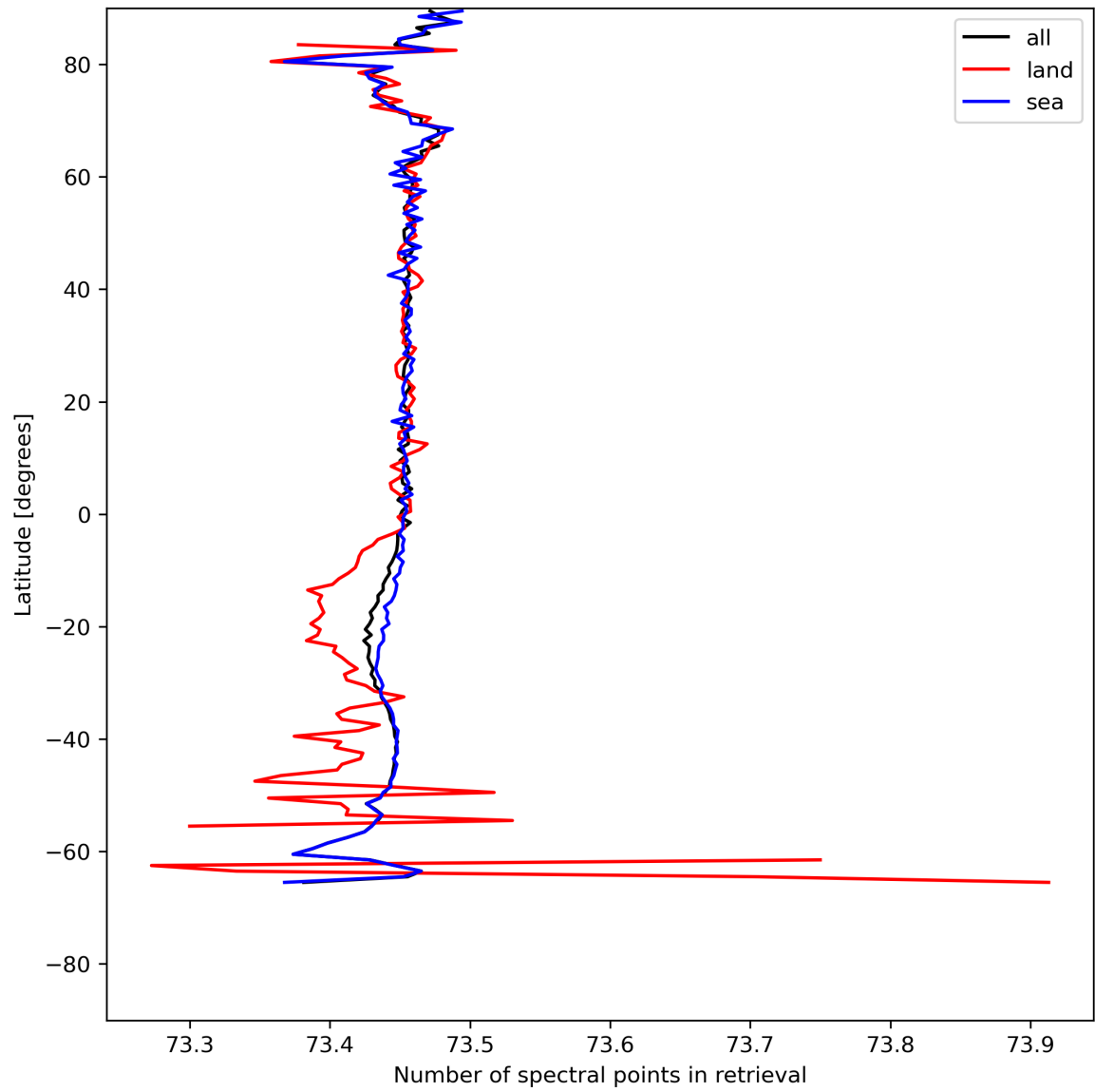
Figure 51: Zonal average of “Number of spectral points in retrieval” for 2024-07-26 to 2024-07-28.
