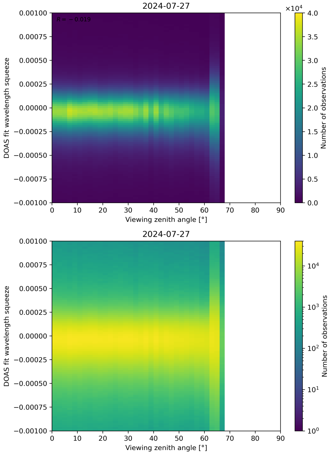
Figure 312: Scatter density plot of “Viewing zenith angle” against “DOAS fit wavelength squeeze” for 2024-07-26 to 2024-07-28.
