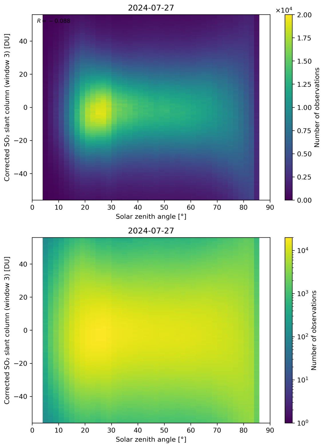
Figure 168: Scatter density plot of “Solar zenith angle” against “Corrected SO 2 slant column (window 3)” for 2024-07-26 to 2024-07-28.
