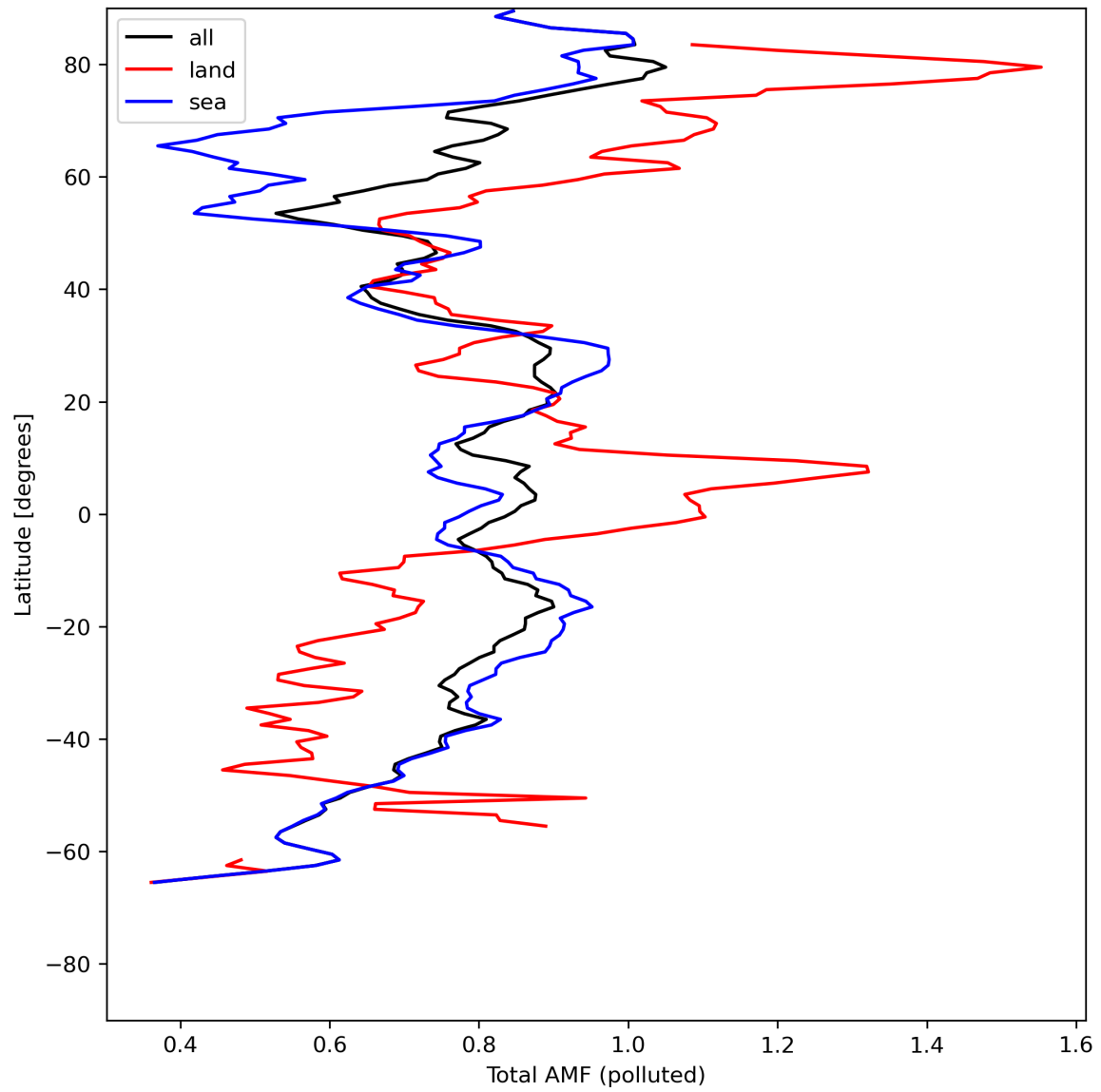
Figure 48: Zonal average of “Total AMF (polluted)” for 2024-07-26 to 2024-07-28.
