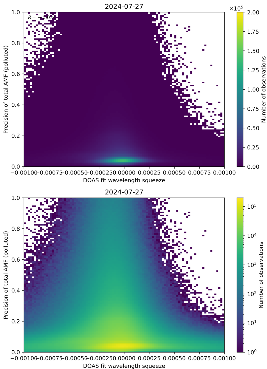
Figure 135: Scatter density plot of “DOAS fit wavelength squeeze” against “Precision of total AMF (polluted)” for 2024-07-26 to 2024-07-28.
