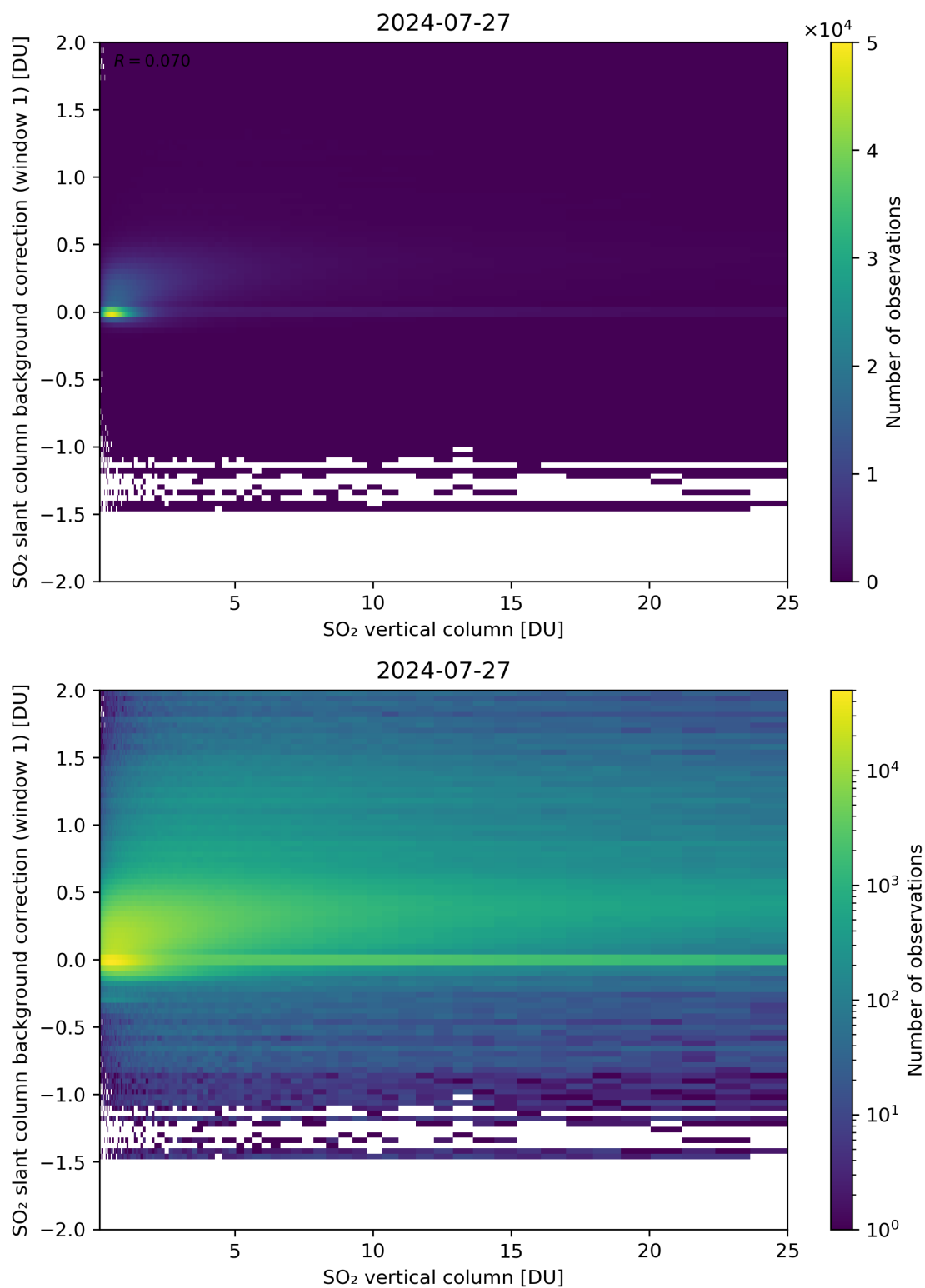
Figure 273: Scatter density plot of “SO 2 vertical column” against “SO 2 slant column background correction (window 1)” for 2024-07-26 to 2024-07-28.
