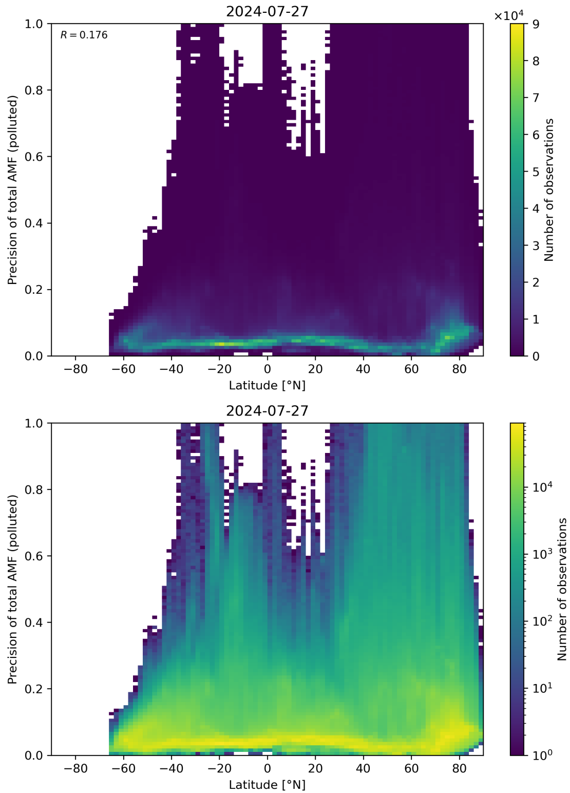
Figure 155: Scatter density plot of “Latitude” against “Precision of total AMF (polluted)” for 2024-07-26 to 2024-07-28.
