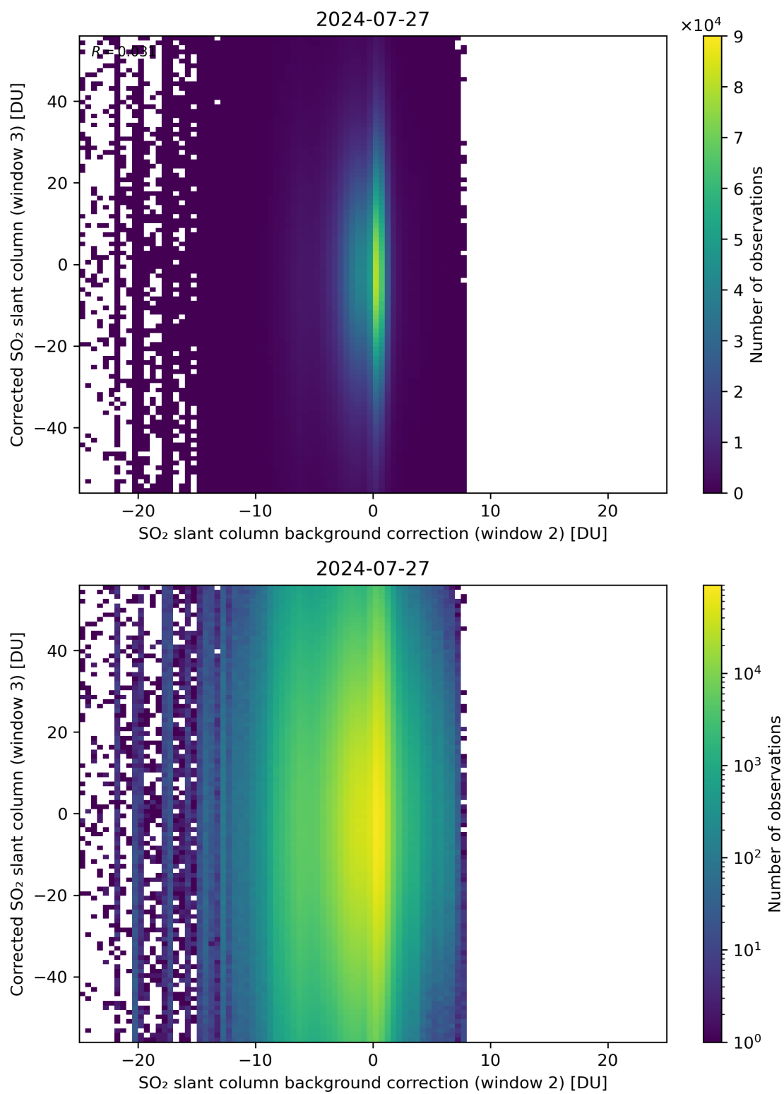
Figure 116: Scatter density plot of “SO 2 slant column background correction (window 2)” against “Corrected SO 2 slant column (window 3)” for 2024-07-26 to 2024-07-28.
