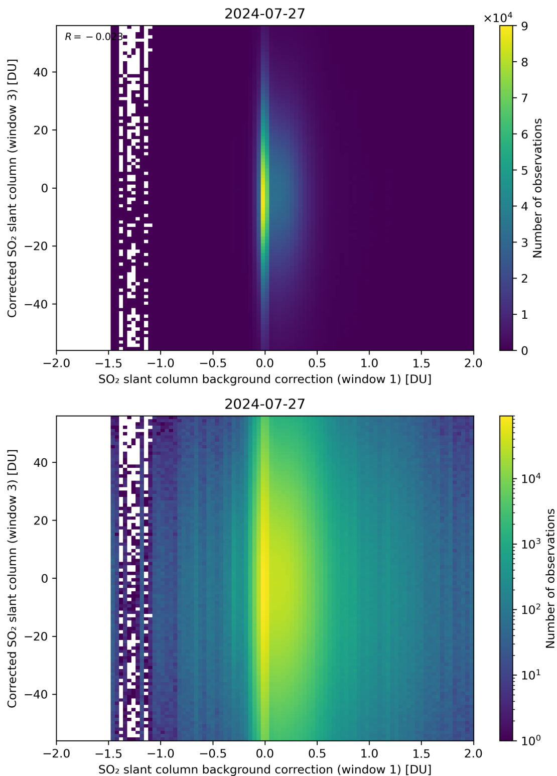
Figure 105: Scatter density plot of “SO 2 slant column background correction (window 1)” against “Corrected SO 2 slant column (window 3)” for 2024-07-26 to 2024-07-28.
