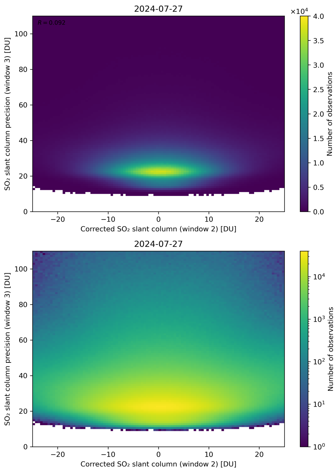
Figure 202: Scatter density plot of “Corrected SO 2 slant column (window 2)” against “SO 2 slant column precision (window 3)” for 2024-07-26 to 2024-07-28.
