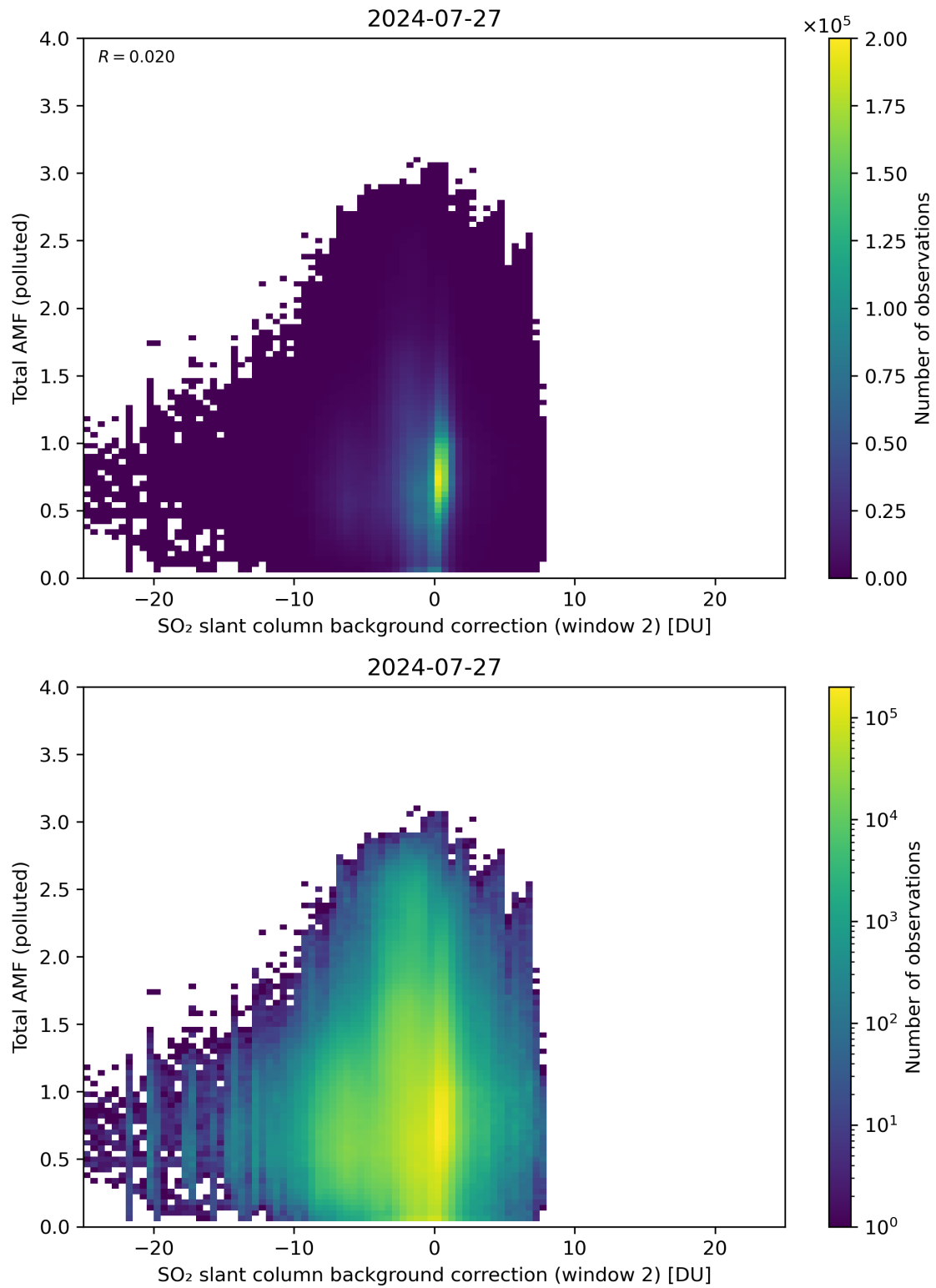
Figure 119: Scatter density plot of “SO 2 slant column background correction (window 2)” against “Total AMF (polluted)” for 2024-07-26 to 2024-07-28.
