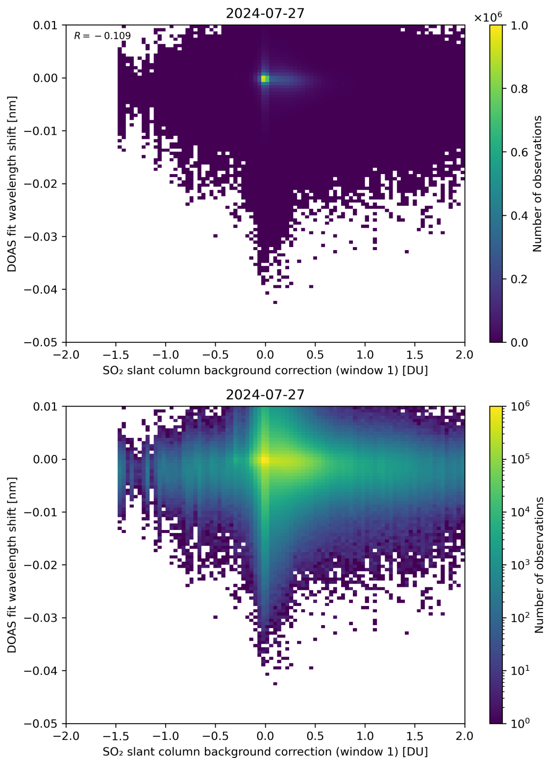
Figure 100: Scatter density plot of “SO 2 slant column background correction (window 1)” against “DOAS fit wavelength shift” for 2024-07-26 to 2024-07-28.
