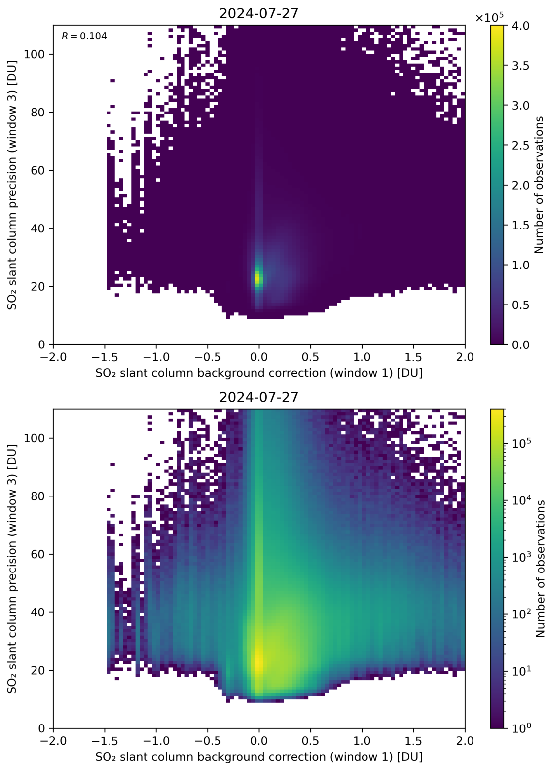
Figure 108: Scatter density plot of “SO 2 slant column background correction (window 1)” against “SO 2 slant column precision (window 3)” for 2024-07-26 to 2024-07-28.
