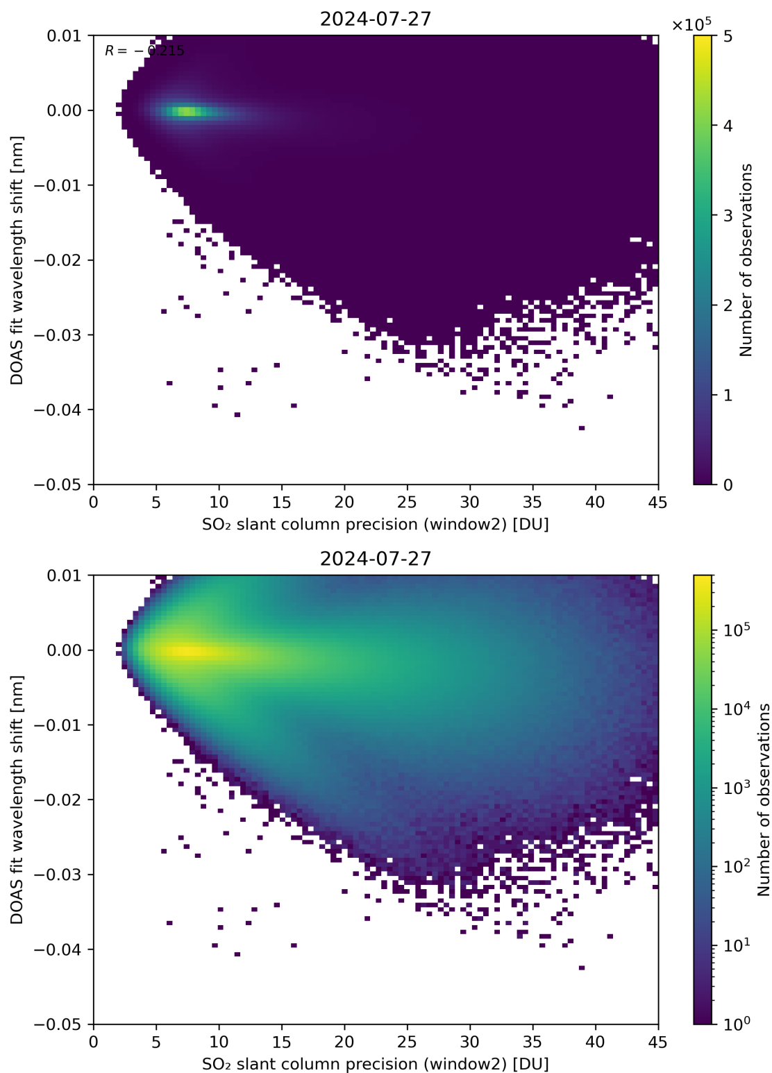
Figure 243: Scatter density plot of “SO 2 slant column precision (window2)” against “DOAS fit wavelength shift” for 2024-07-26 to 2024-07-28.
