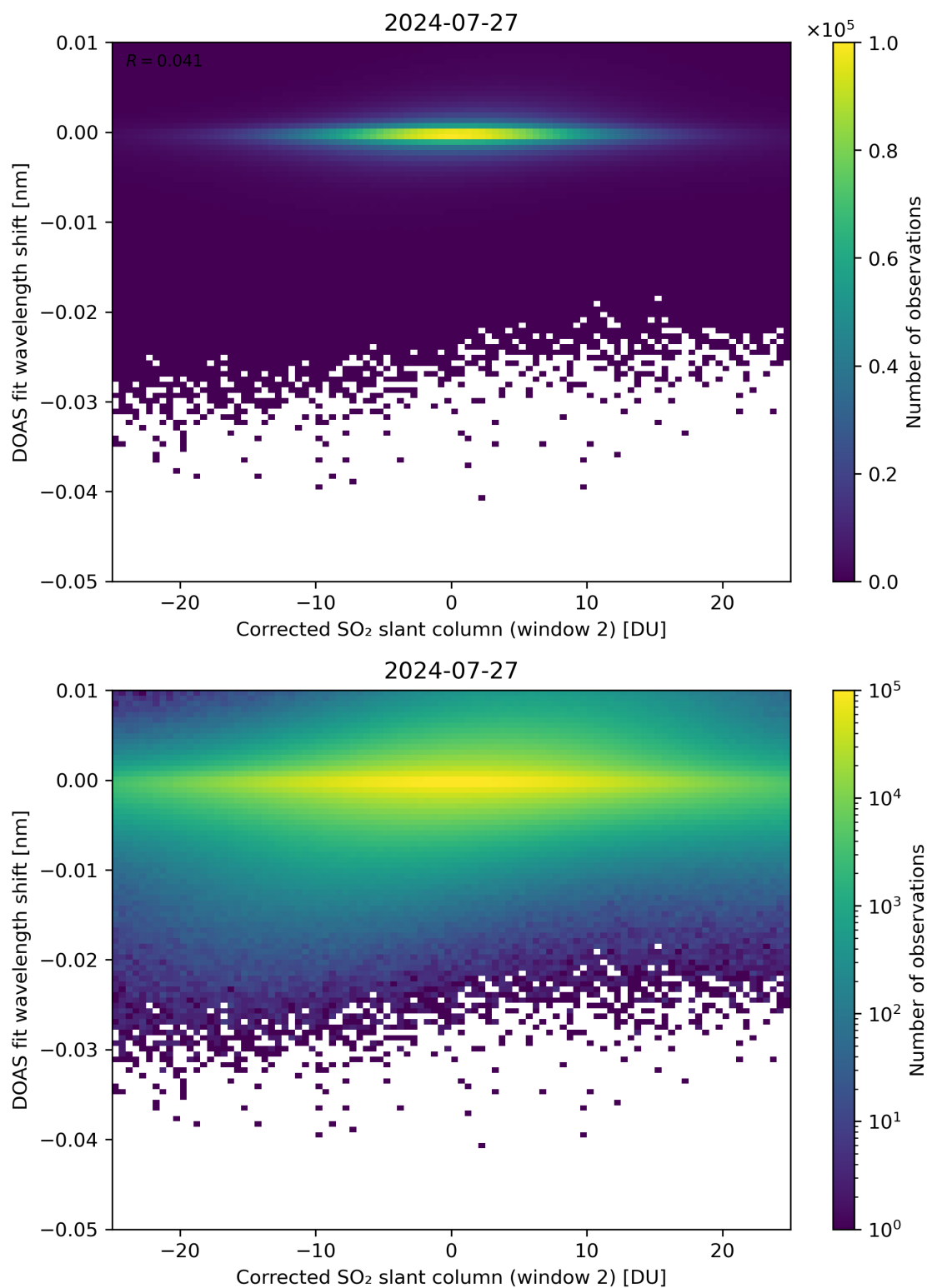
Figure 196: Scatter density plot of “Corrected SO 2 slant column (window 2)” against “DOAS fit wavelength shift” for 2024-07-26 to 2024-07-28.
