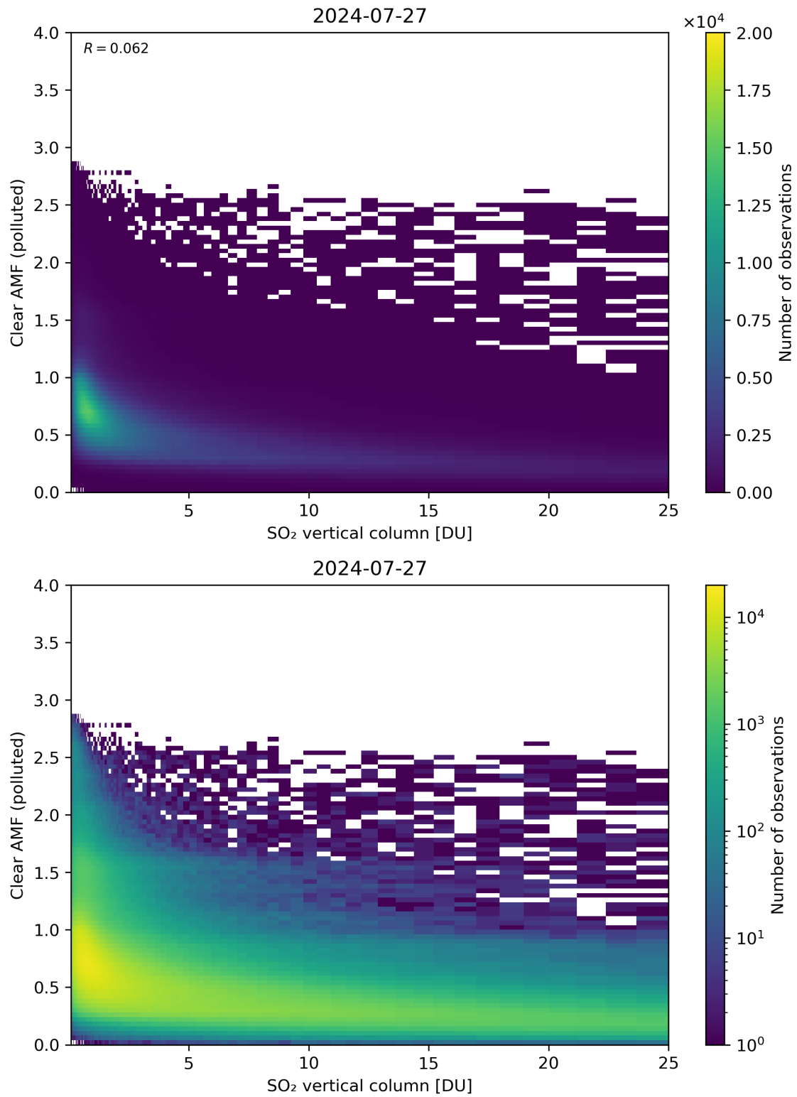
Figure 296: Scatter density plot of “SO 2 vertical column” against “Clear AMF (polluted)” for 2024-07-26 to 2024-07-28.
