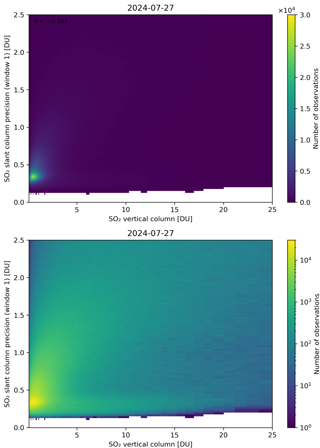
Figure 301: Scatter density plot of “SO 2 vertical column” against “SO 2 slant column precision (window 1)” for 2024-07-26 to 2024-07-28.
