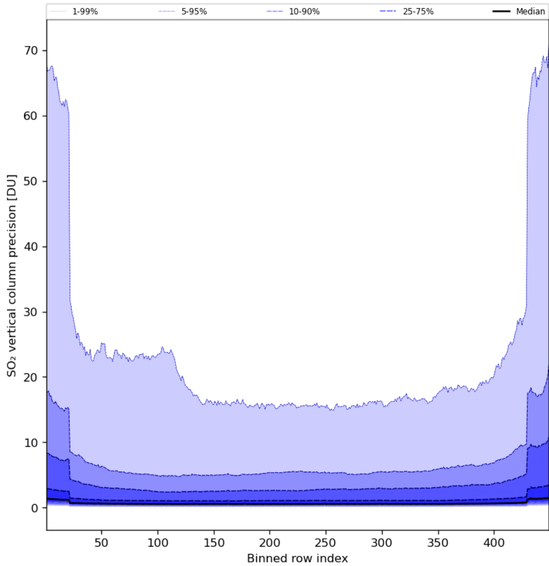
Figure 77: Along track statistics of “SO 2 vertical column precision” for 2024-07-26 to 2024-07-28
