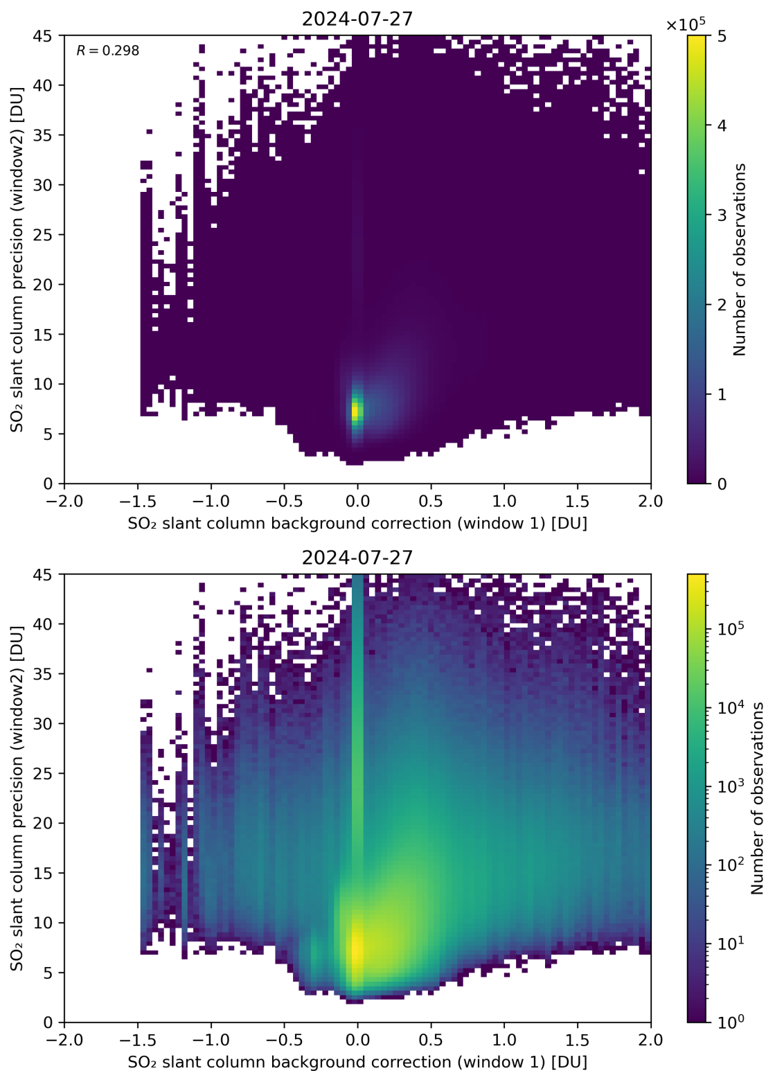
Figure 106: Scatter density plot of “SO 2 slant column background correction (window 1)” against “SO 2 slant column precision (window2)” for 2024-07-26 to 2024-07-28.
