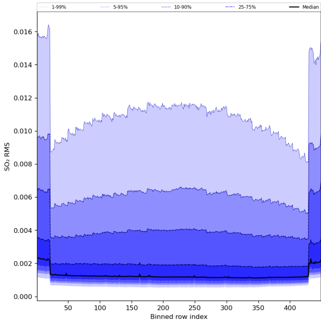
Figure 93: Along track statistics of “SO 2 RMS” for 2024-07-26 to 2024-07-28
