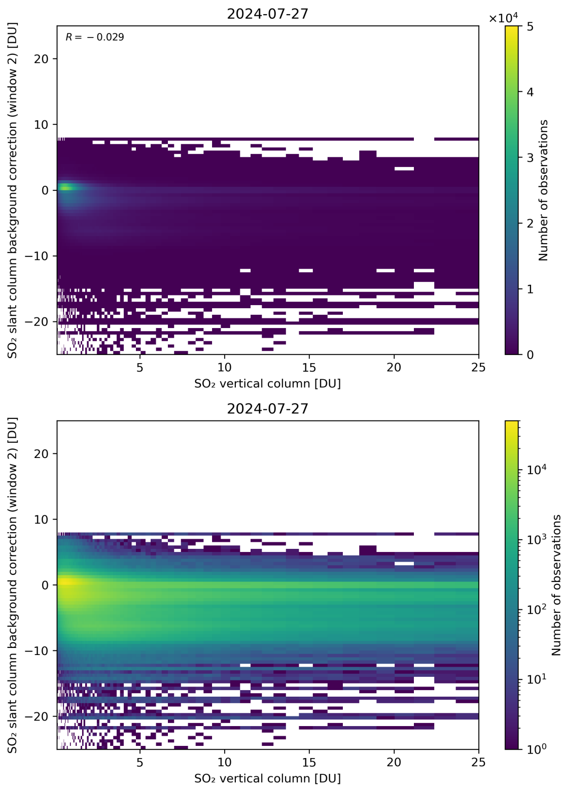
Figure 274: Scatter density plot of “SO 2 vertical column” against “SO 2 slant column background correction (window 2)” for 2024-07-26 to 2024-07-28.
