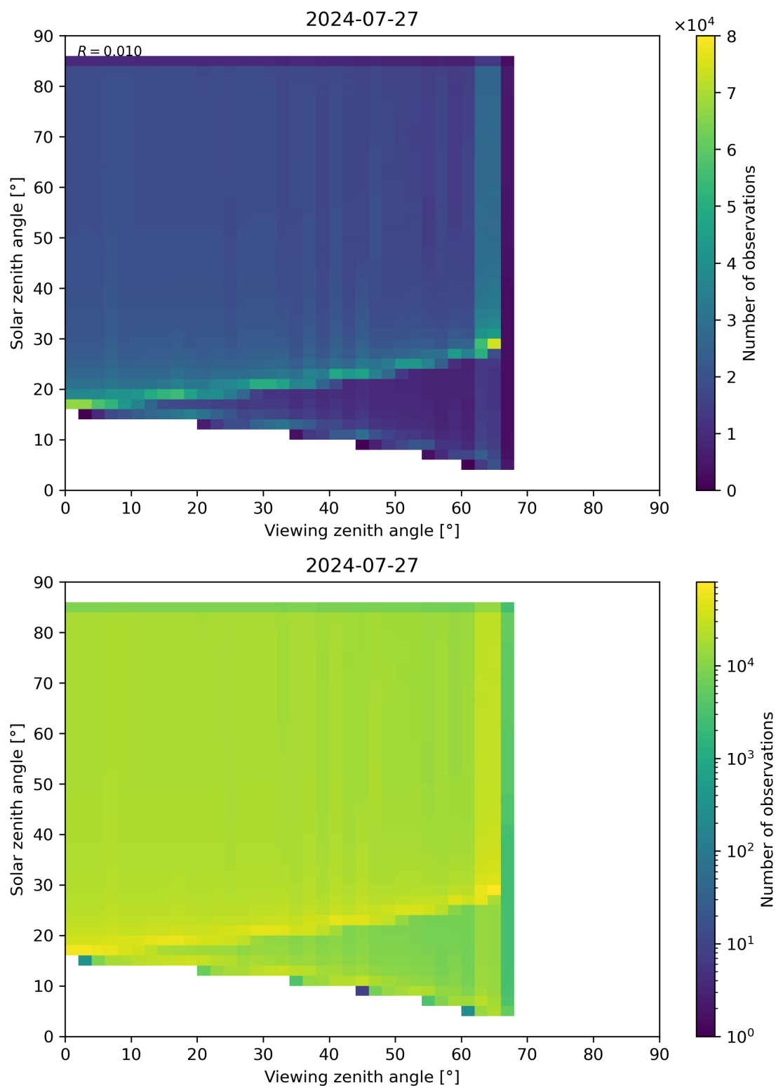
Figure 315: Scatter density plot of “Viewing zenith angle” against “Solar zenith angle” for 2024-07-26 to 2024-07-28.
