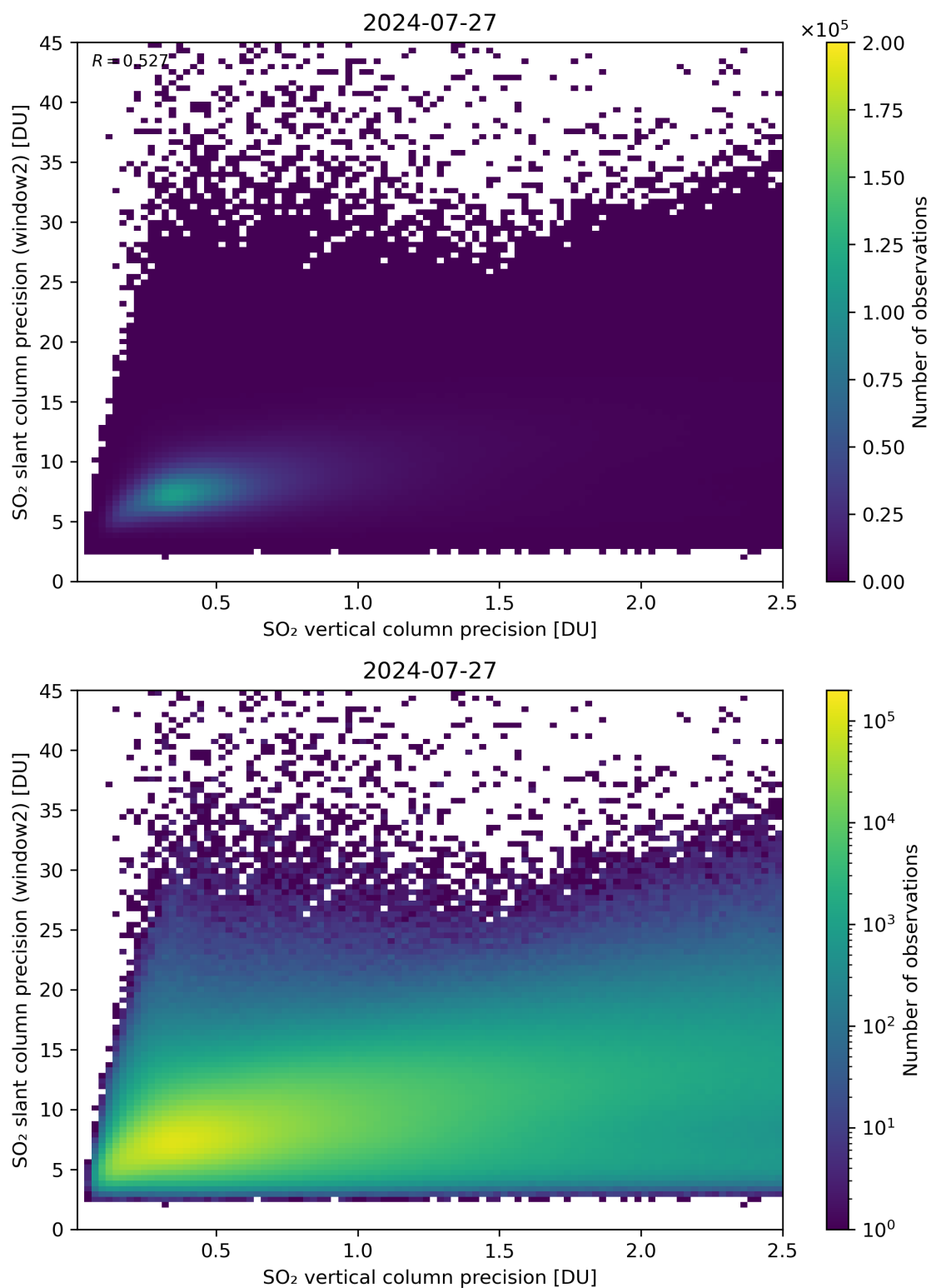
Figure 291: Scatter density plot of “SO 2 vertical column precision” against “SO 2 slant column precision (window2)” for 2024-07-26 to 2024-07-28.
