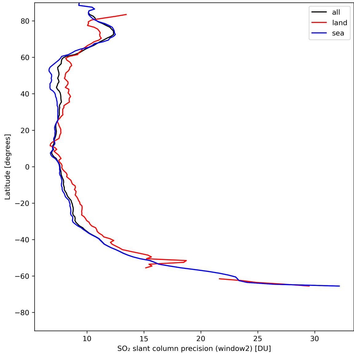
Figure 38: Zonal average of “SO 2 slant column precision (window2)” for 2024-07-26 to 2024-07-28.
