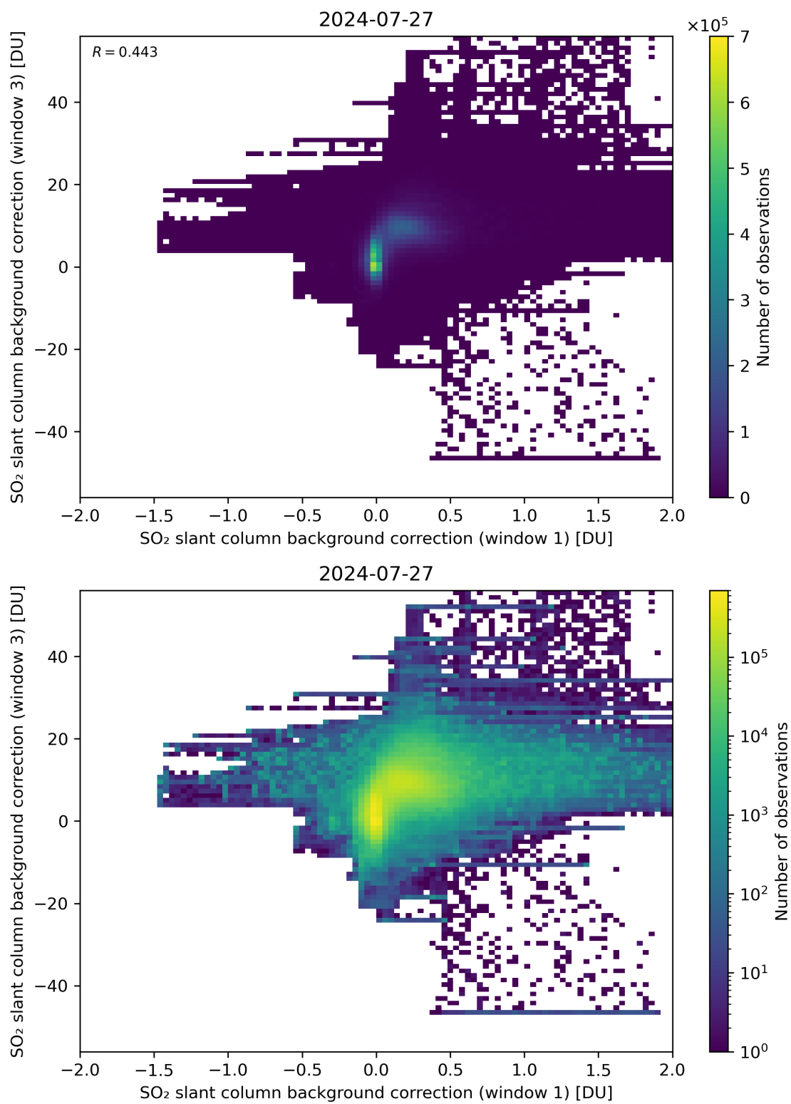
Figure 99: Scatter density plot of “SO 2 slant column background correction (window 1)” against “SO 2 slant column background correction (window 3)” for 2024-07-26 to 2024-07-28.
