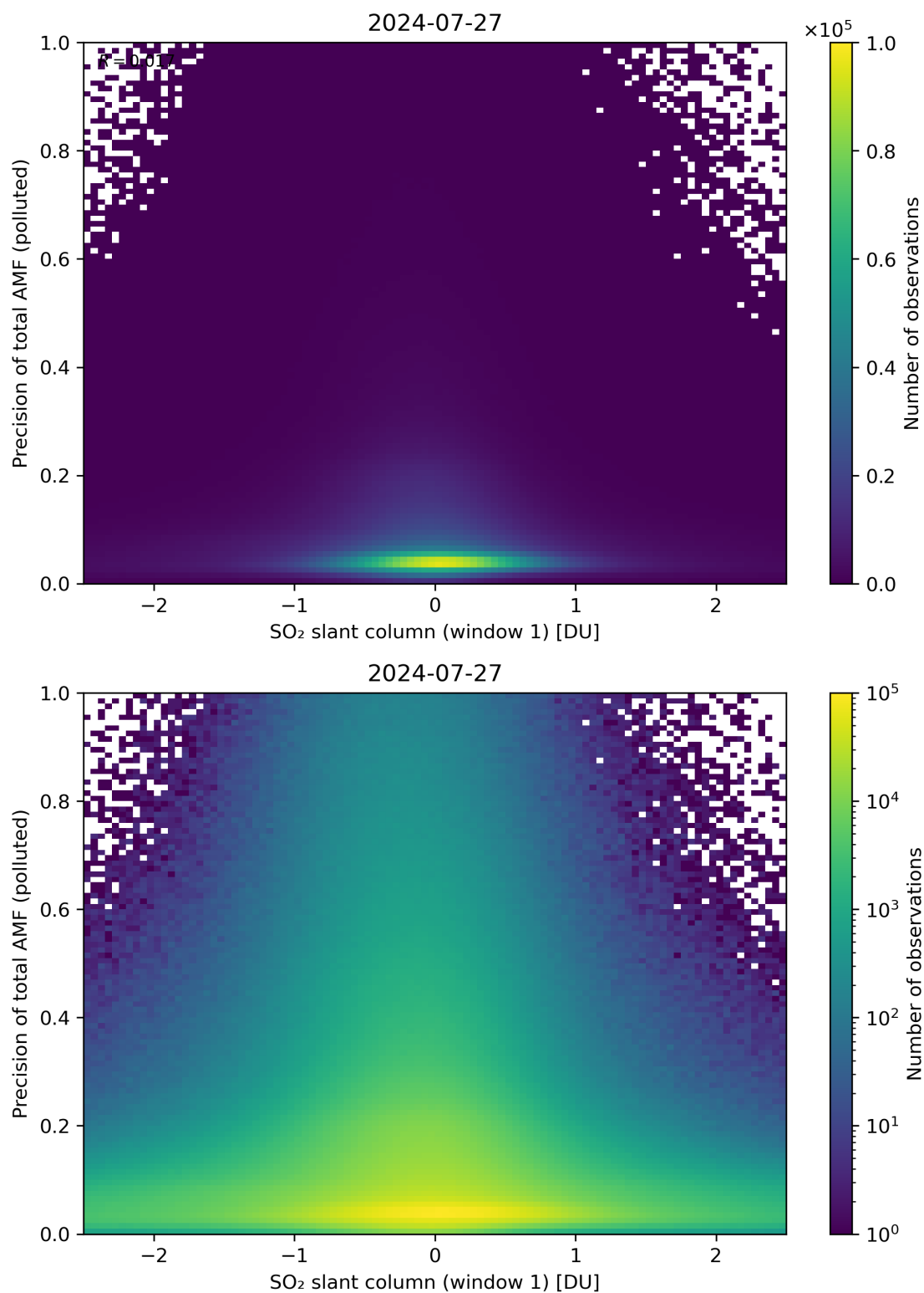
Figure 240: Scatter density plot of “SO 2 slant column (window 1)” against “Precision of total AMF (polluted)” for 2024-07-26 to 2024-07-28.
