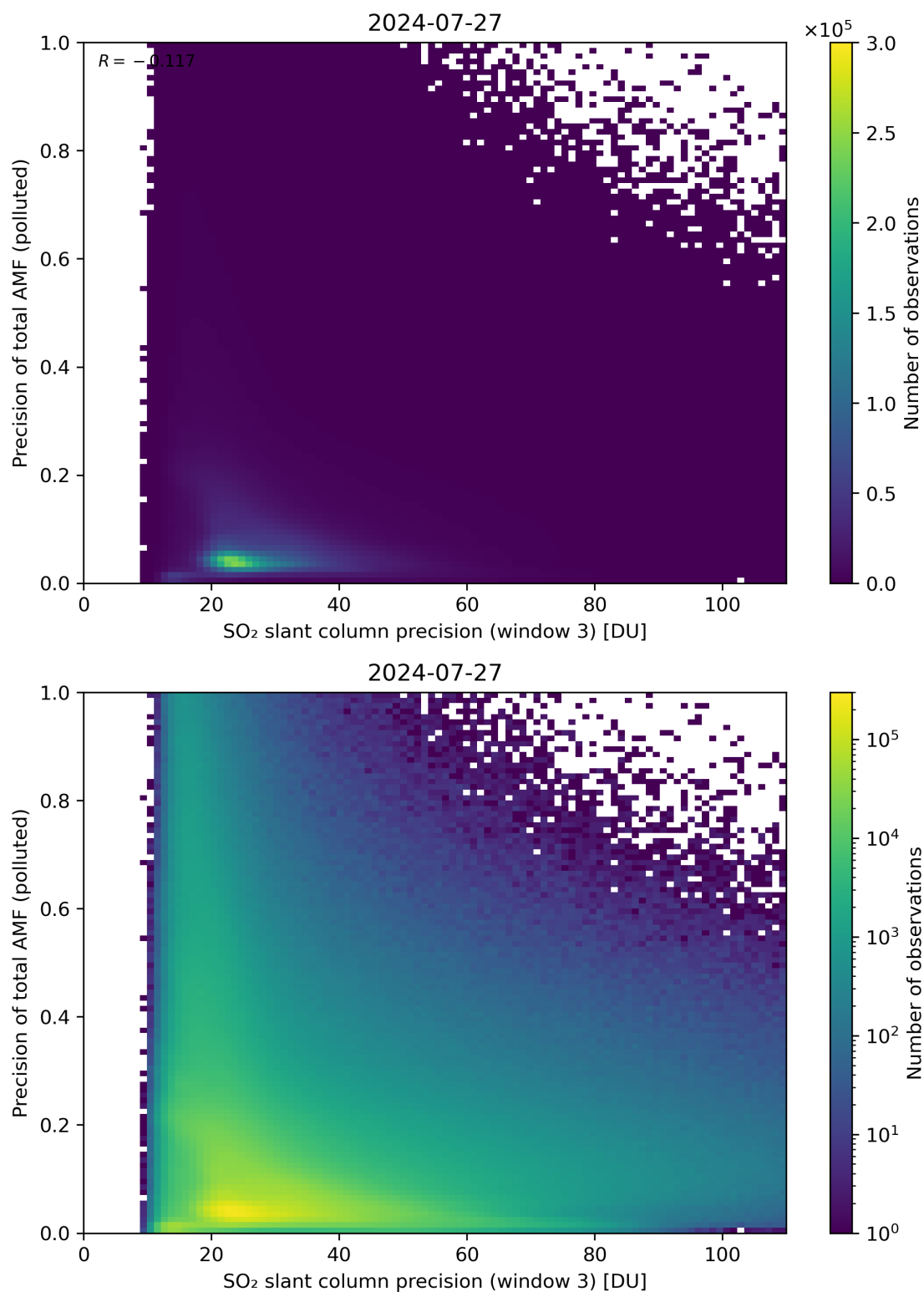
Figure 264: Scatter density plot of “SO 2 slant column precision (window 3)” against “Precision of total AMF (polluted)” for 2024-07-26 to 2024-07-28.
