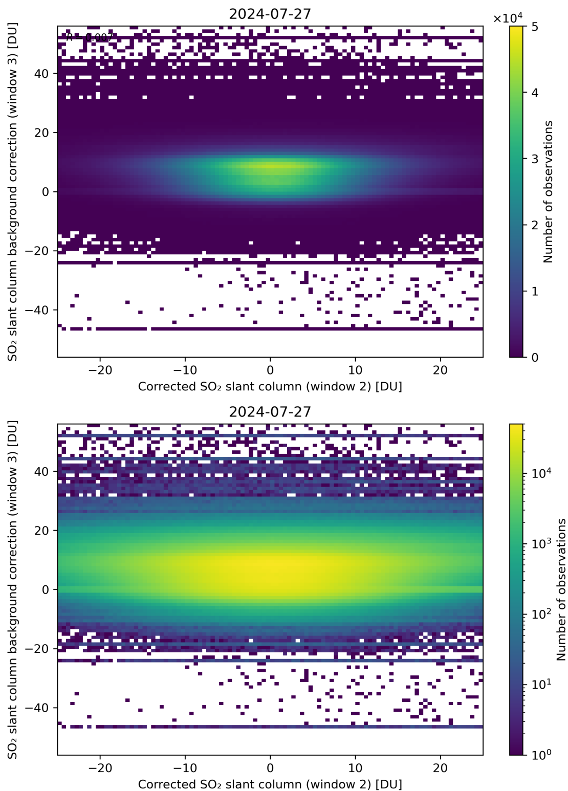
Figure 195: Scatter density plot of “Corrected SO 2 slant column (window 2)” against “SO 2 slant column background correction (window 3)” for 2024-07-26 to 2024-07-28.
