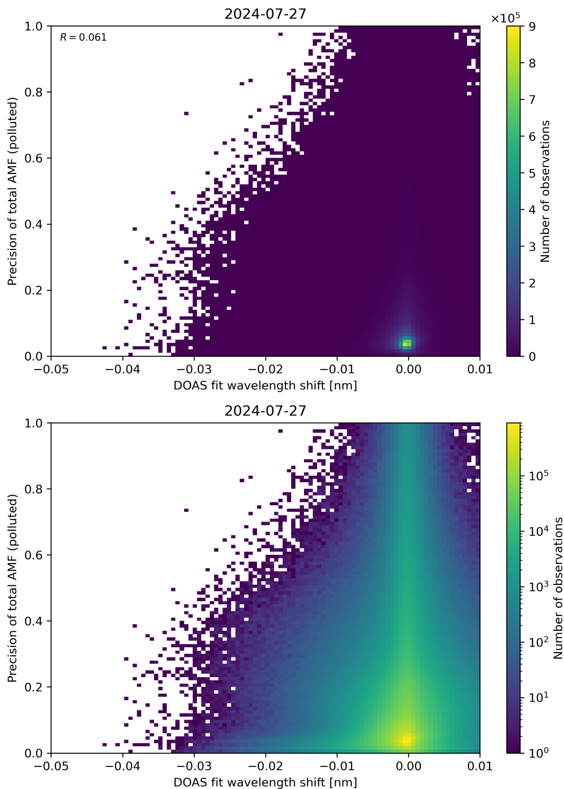
Figure 131: Scatter density plot of “DOAS fit wavelength shift” against “Precision of total AMF (polluted)” for 2024-07-26 to 2024-07-28.
