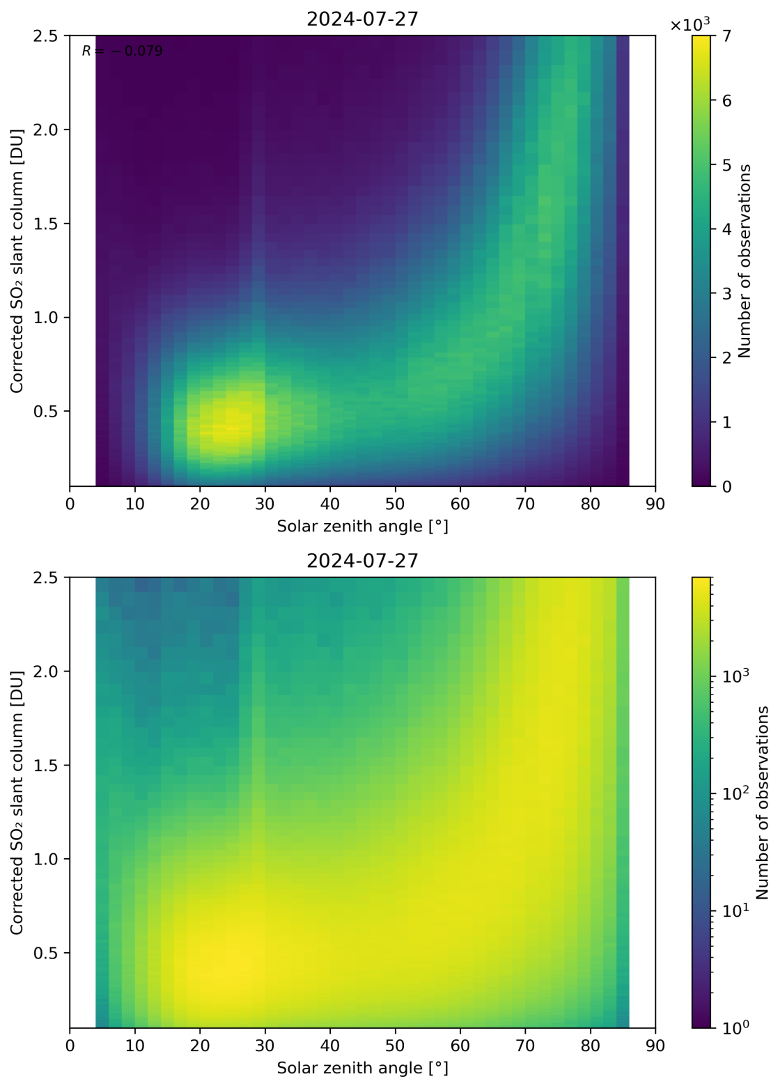
Figure 166: Scatter density plot of “Solar zenith angle” against “Corrected SO 2 slant column” for 2024-07-26 to 2024-07-28.
