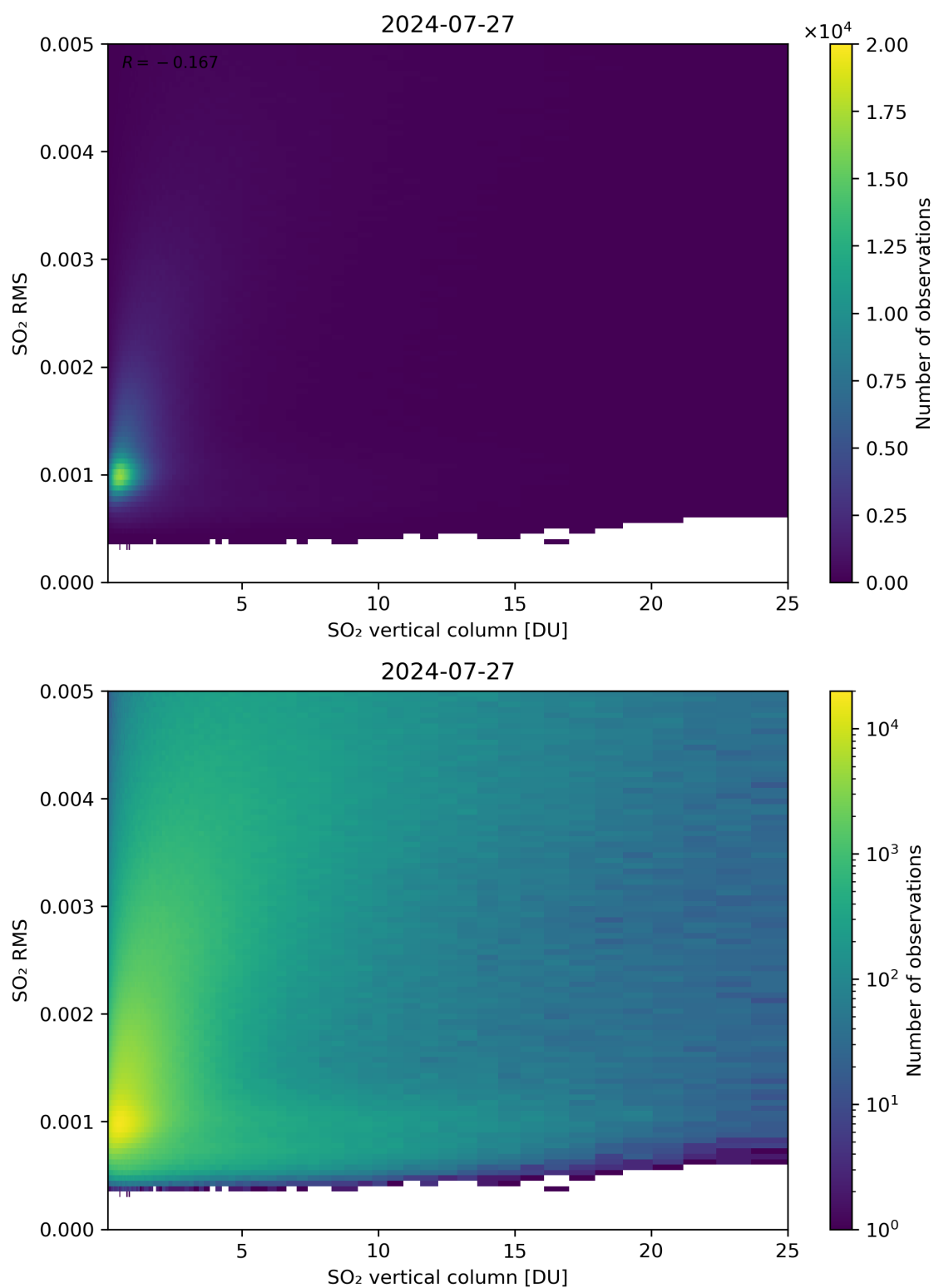
Figure 278: Scatter density plot of “SO 2 vertical column” against “SO 2 RMS” for 2024-07-26 to 2024-07-28.
