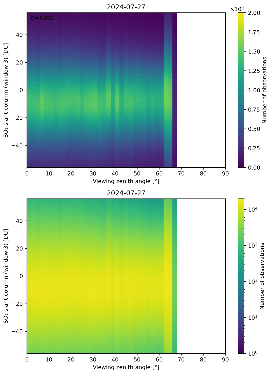
Figure 323: Scatter density plot of “Viewing zenith angle” against “SO 2 slant column (window 3)” for 2024-07-26 to 2024-07-28.
