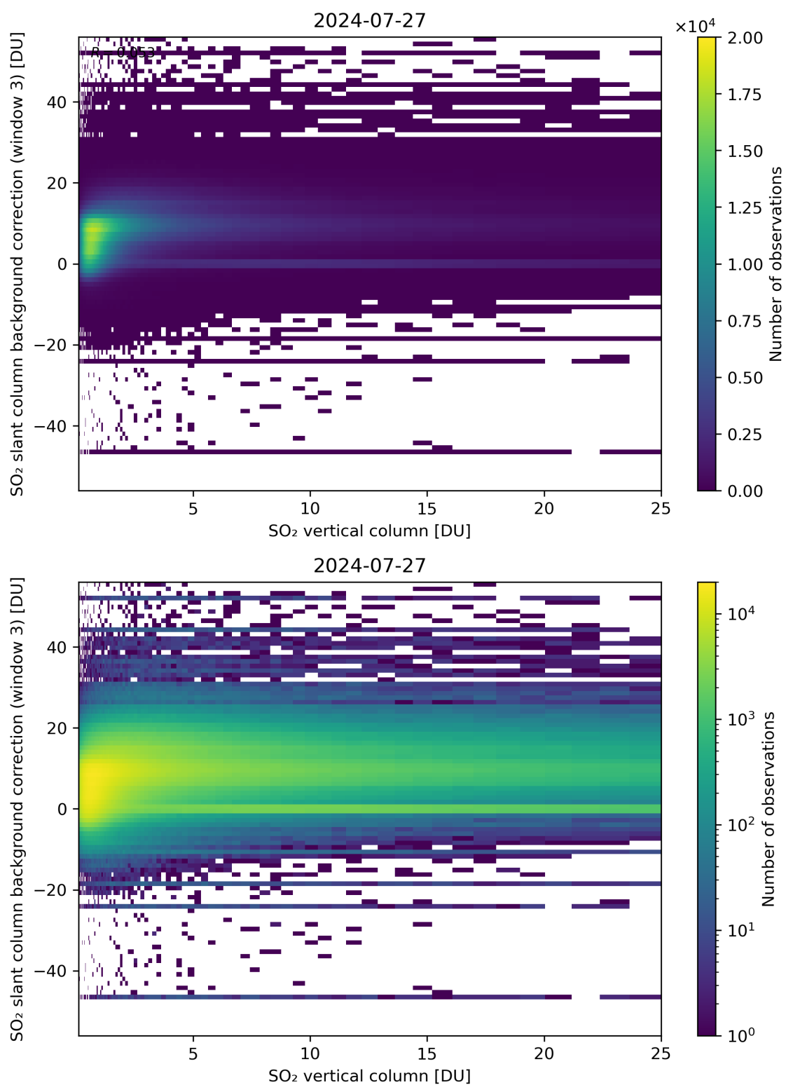
Figure 275: Scatter density plot of “SO 2 vertical column” against “SO 2 slant column background correction (window 3)” for 2024-07-26 to 2024-07-28.
