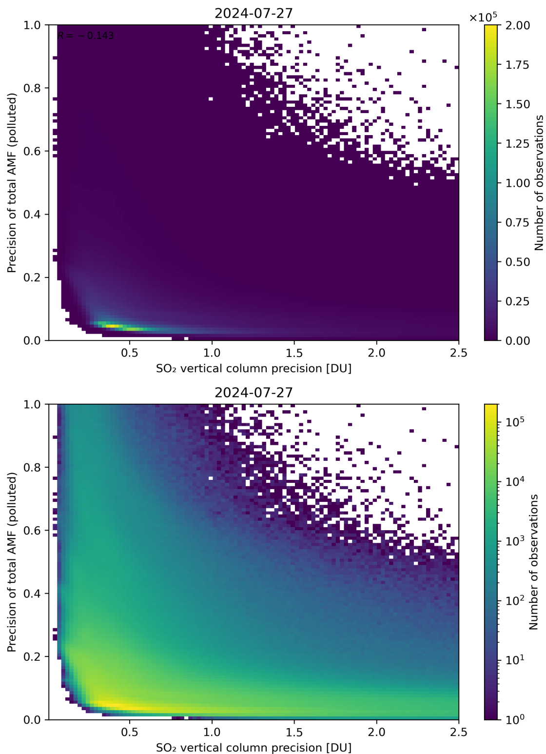
Figure 295: Scatter density plot of “SO 2 vertical column precision” against “Precision of total AMF (polluted)” for 2024-07-26 to 2024-07-28.
