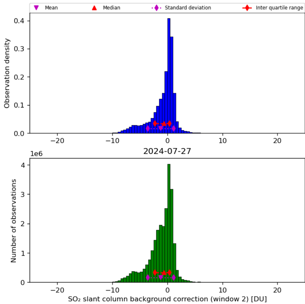
Figure 63: Histogram of “SO 2 slant column background correction (window 2)” for 2024-07-26 to 2024-07-28
