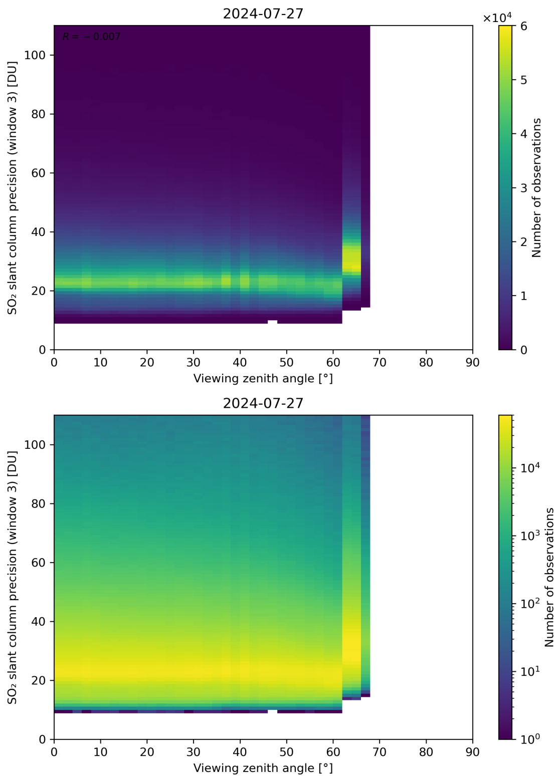
Figure 324: Scatter density plot of “Viewing zenith angle” against “SO 2 slant column precision (window 3)” for 2024-07-26 to 2024-07-28.
