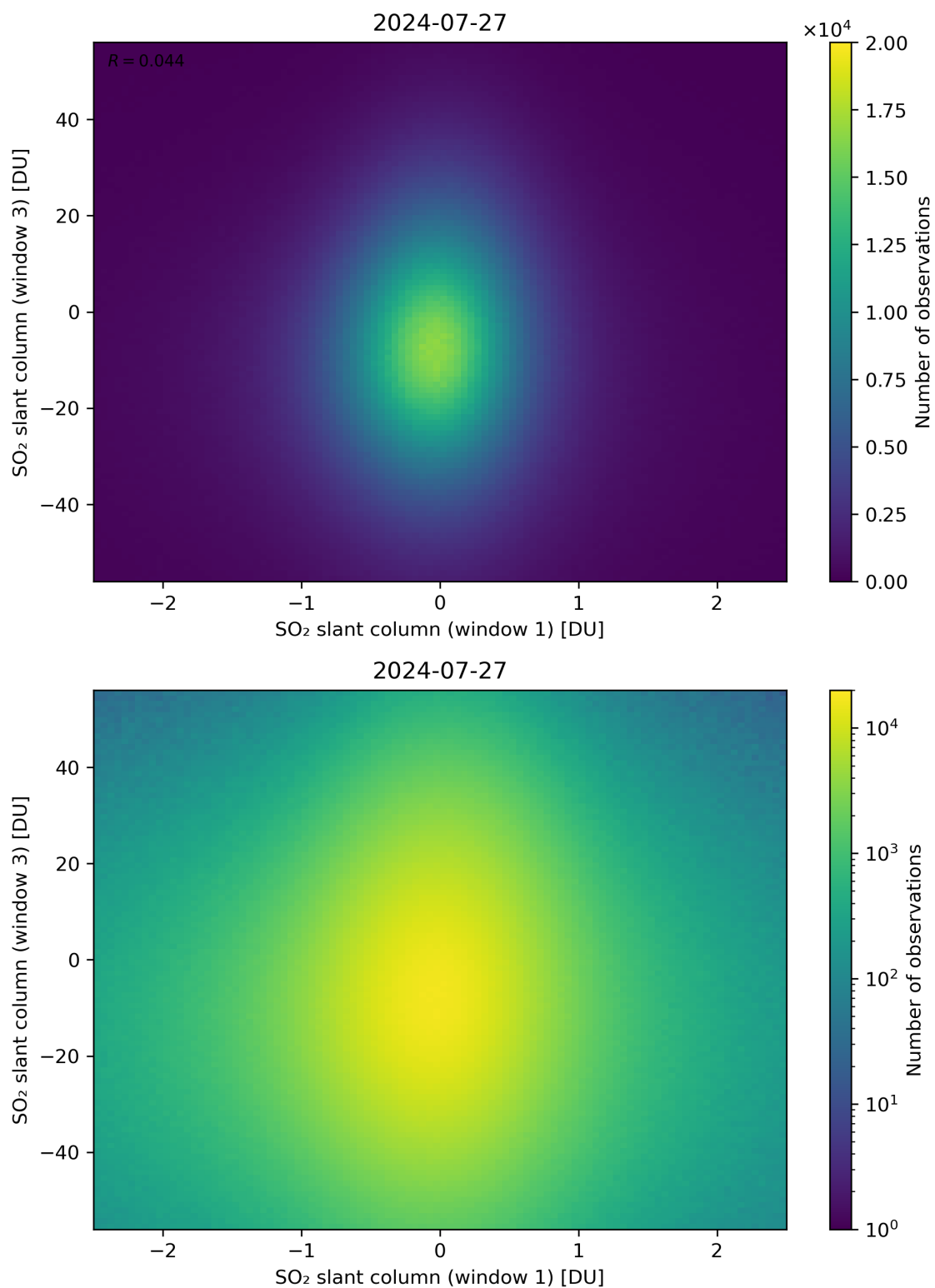
Figure 237: Scatter density plot of “SO 2 slant column (window 1)” against “SO 2 slant column (window 3)” for 2024-07-26 to 2024-07-28.
