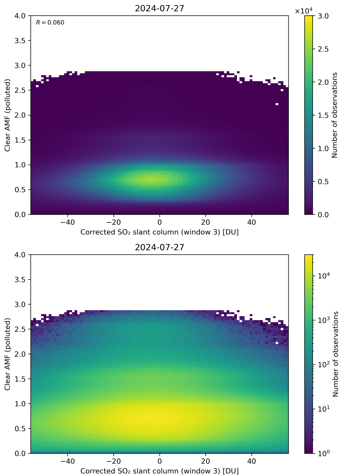
Figure 209: Scatter density plot of “Corrected SO 2 slant column (window 3)” against “Clear AMF (polluted)” for 2024-07-26 to 2024-07-28.
