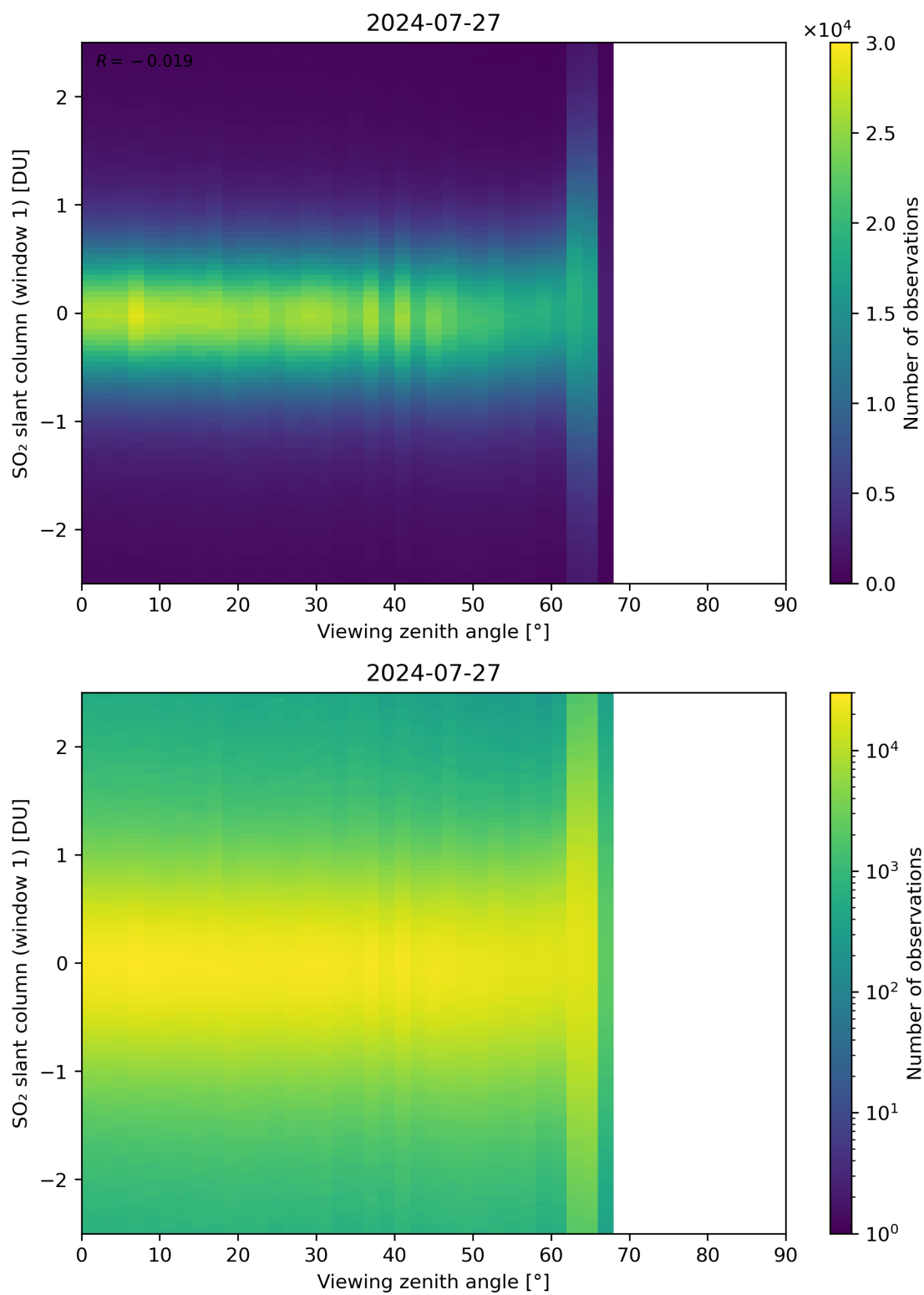
Figure 320: Scatter density plot of “Viewing zenith angle” against “SO 2 slant column (window 1)” for 2024-07-26 to 2024-07-28.
