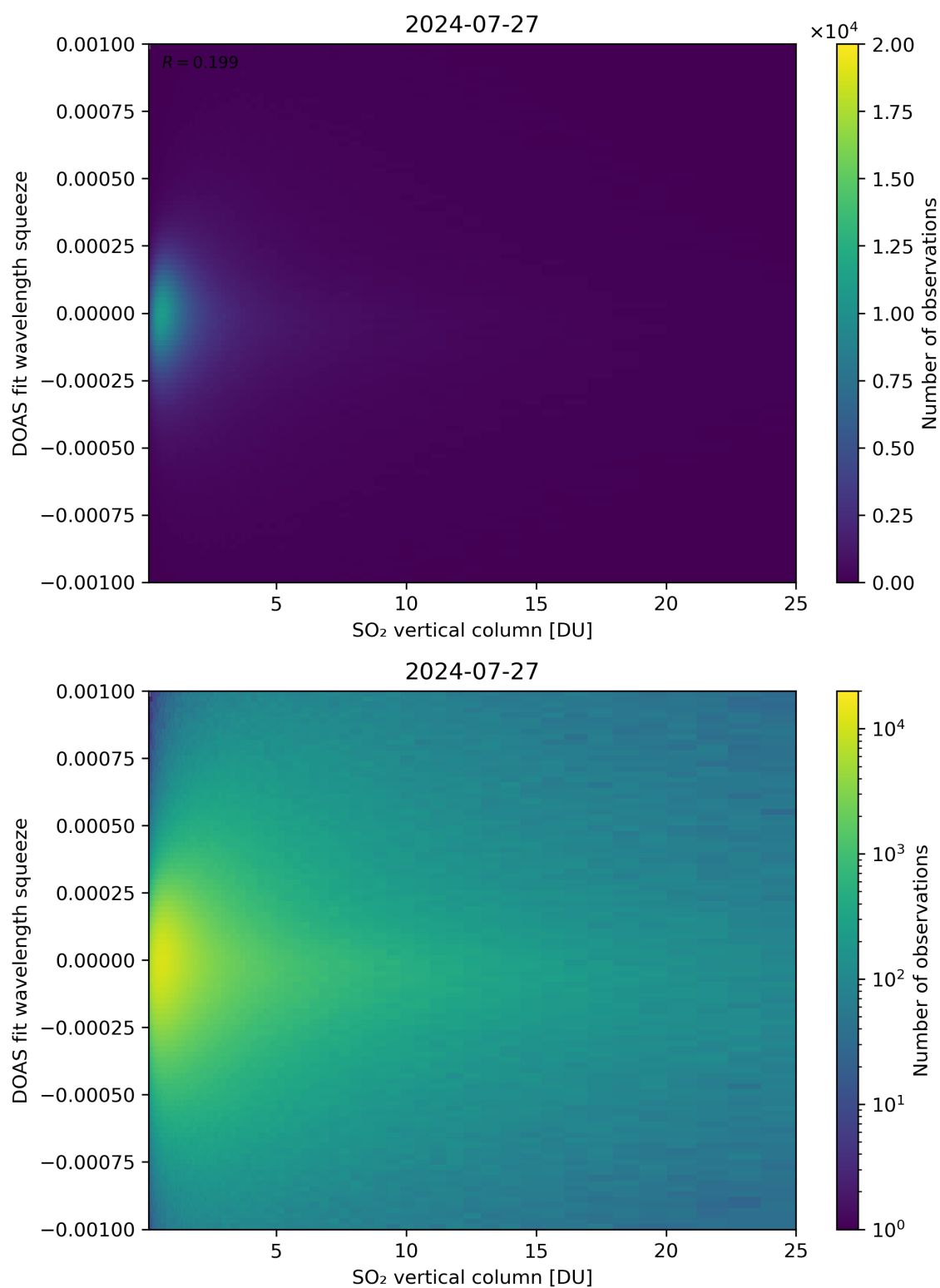
Figure 277: Scatter density plot of “SO 2 vertical column” against “DOAS fit wavelength squeeze” for 2024-07-26 to 2024-07-28.
