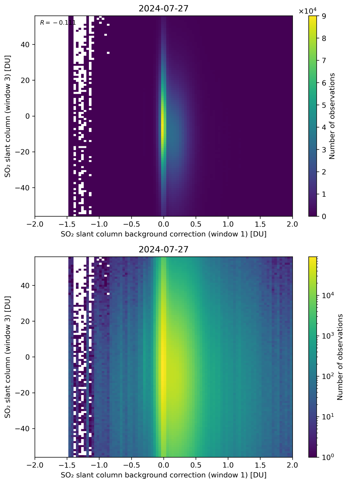
Figure 107: Scatter density plot of “SO 2 slant column background correction (window 1)” against “SO 2 slant column (window 3)” for 2024-07-26 to 2024-07-28.
