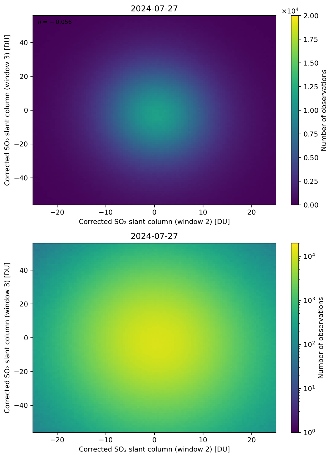
Figure 200: Scatter density plot of “Corrected SO 2 slant column (window 2)” against “Corrected SO 2 slant column (window 3)” for 2024-07-26 to 2024-07-28.
