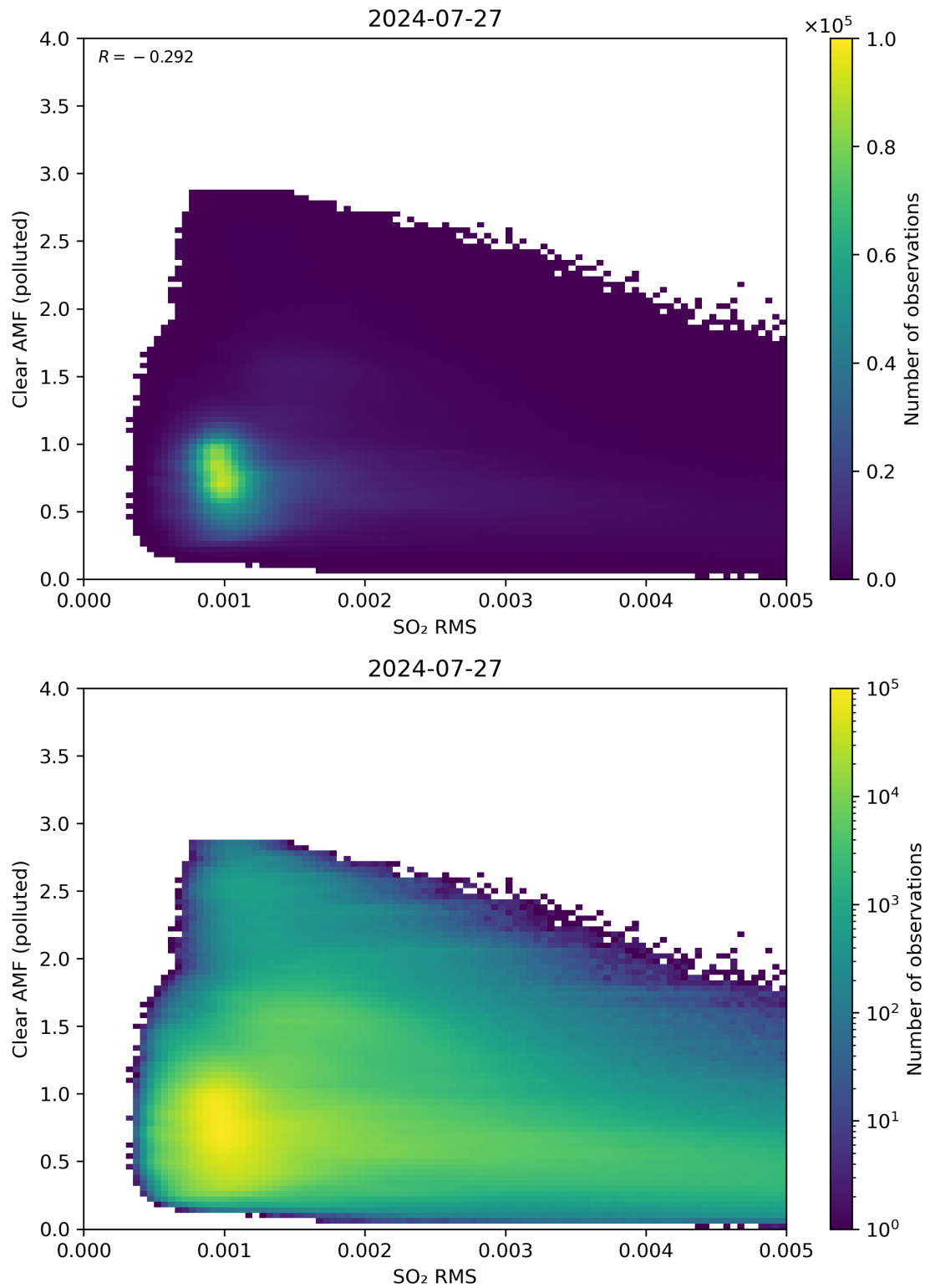
Figure 136: Scatter density plot of “SO 2 RMS” against “Clear AMF (polluted)” for 2024-07-26 to 2024-07-28.
