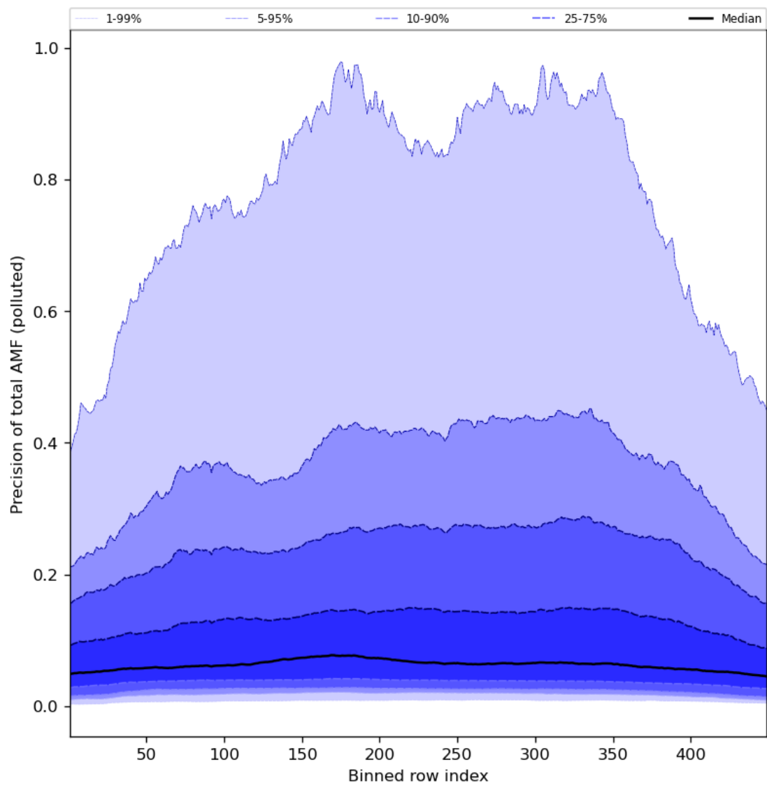
Figure 95: Along track statistics of “Precision of total AMF (polluted)” for 2024-07-26 to 2024-07-28
