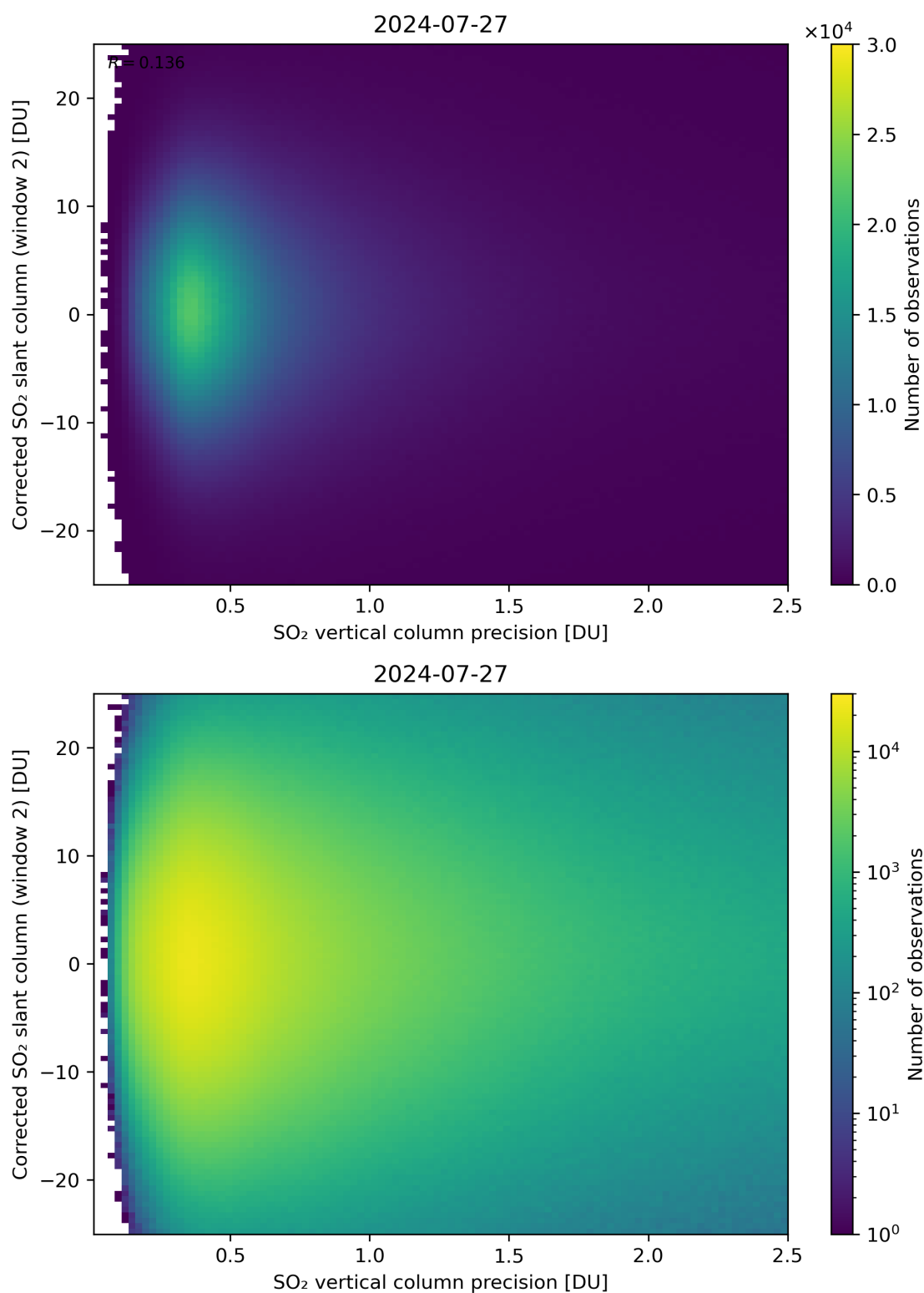
Figure 287: Scatter density plot of “SO 2 vertical column precision” against “Corrected SO 2 slant column (window 2)” for 2024-07-26 to 2024-07-28.
