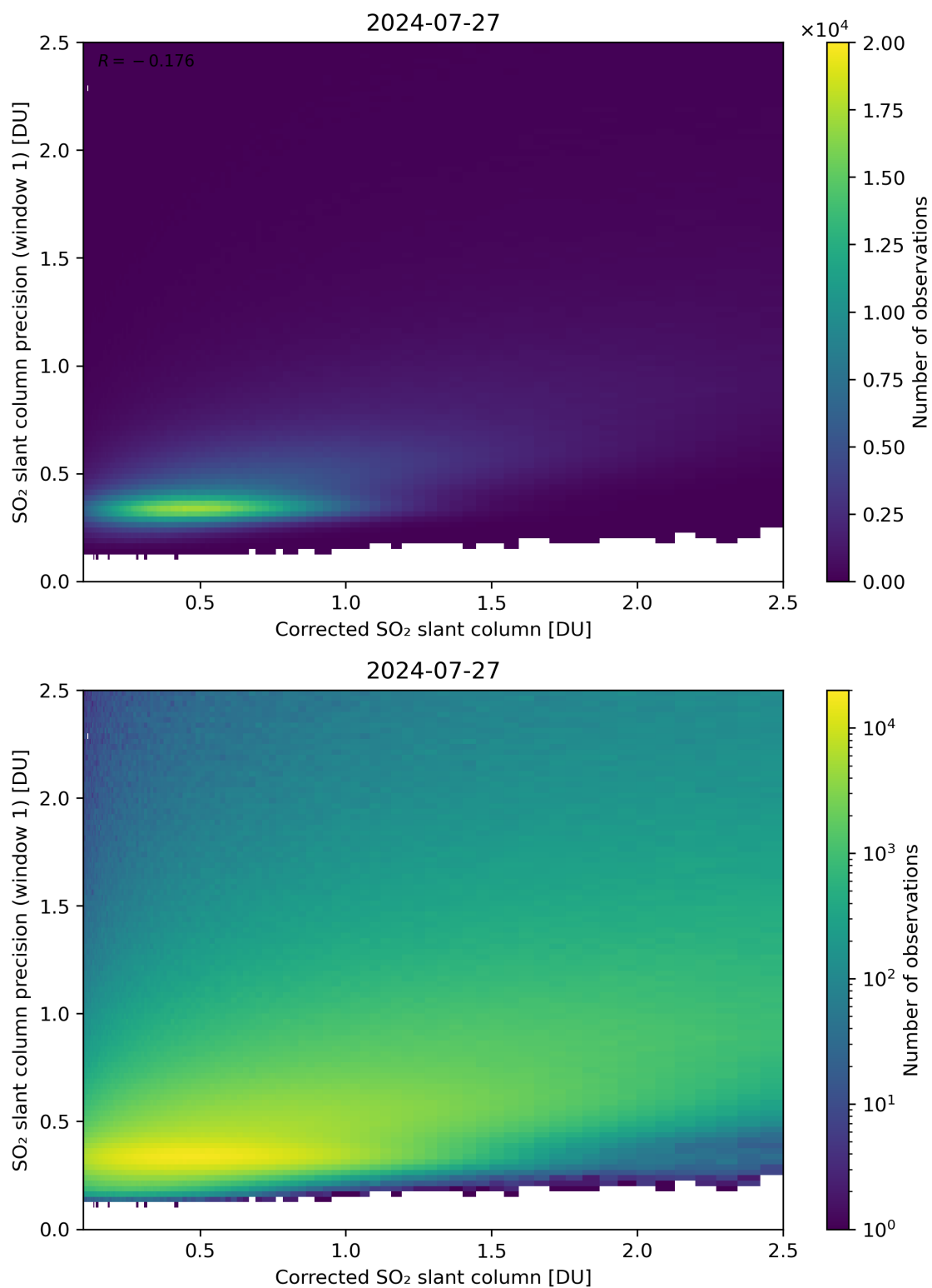
Figure 188: Scatter density plot of “Corrected SO 2 slant column” against “SO 2 slant column precision (window 1)” for 2024-07-26 to 2024-07-28.
