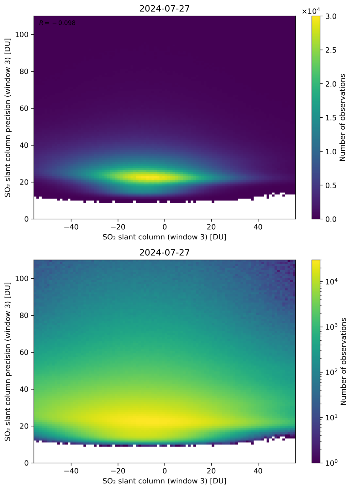
Figure 267: Scatter density plot of “SO 2 slant column (window 3)” against “SO 2 slant column precision (window 3)” for 2024-07-26 to 2024-07-28.
