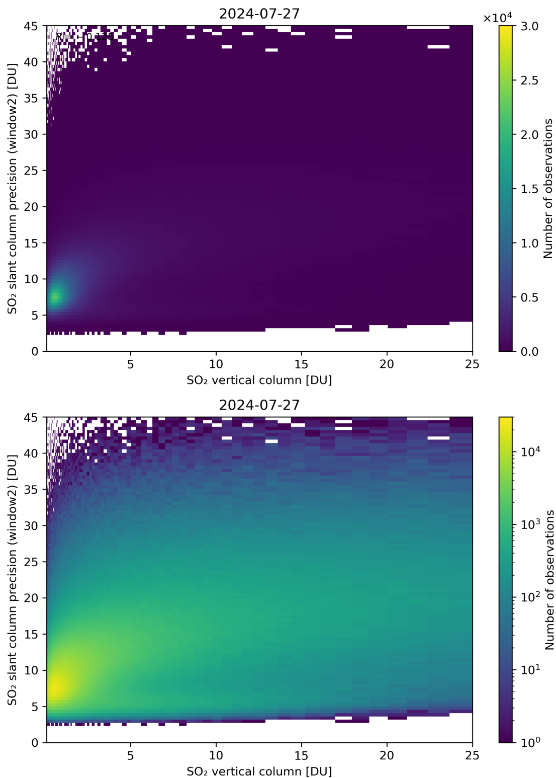
Figure 302: Scatter density plot of “SO 2 vertical column” against “SO 2 slant column precision (window2)” for 2024-07-26 to 2024-07-28.
