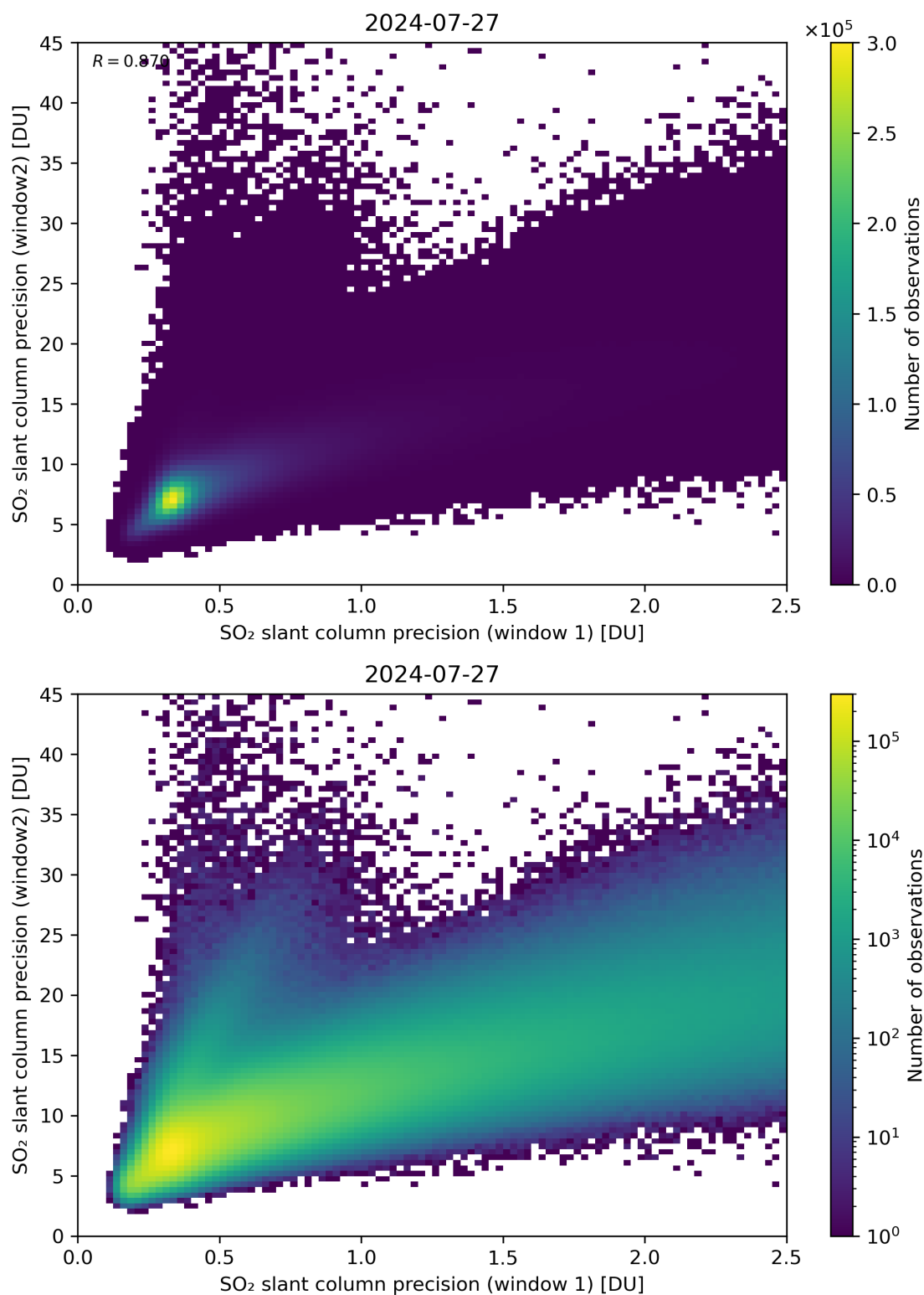
Figure 227: Scatter density plot of “SO 2 slant column precision (window 1)” against “SO 2 slant column precision (window2)” for 2024-07-26 to 2024-07-28.
