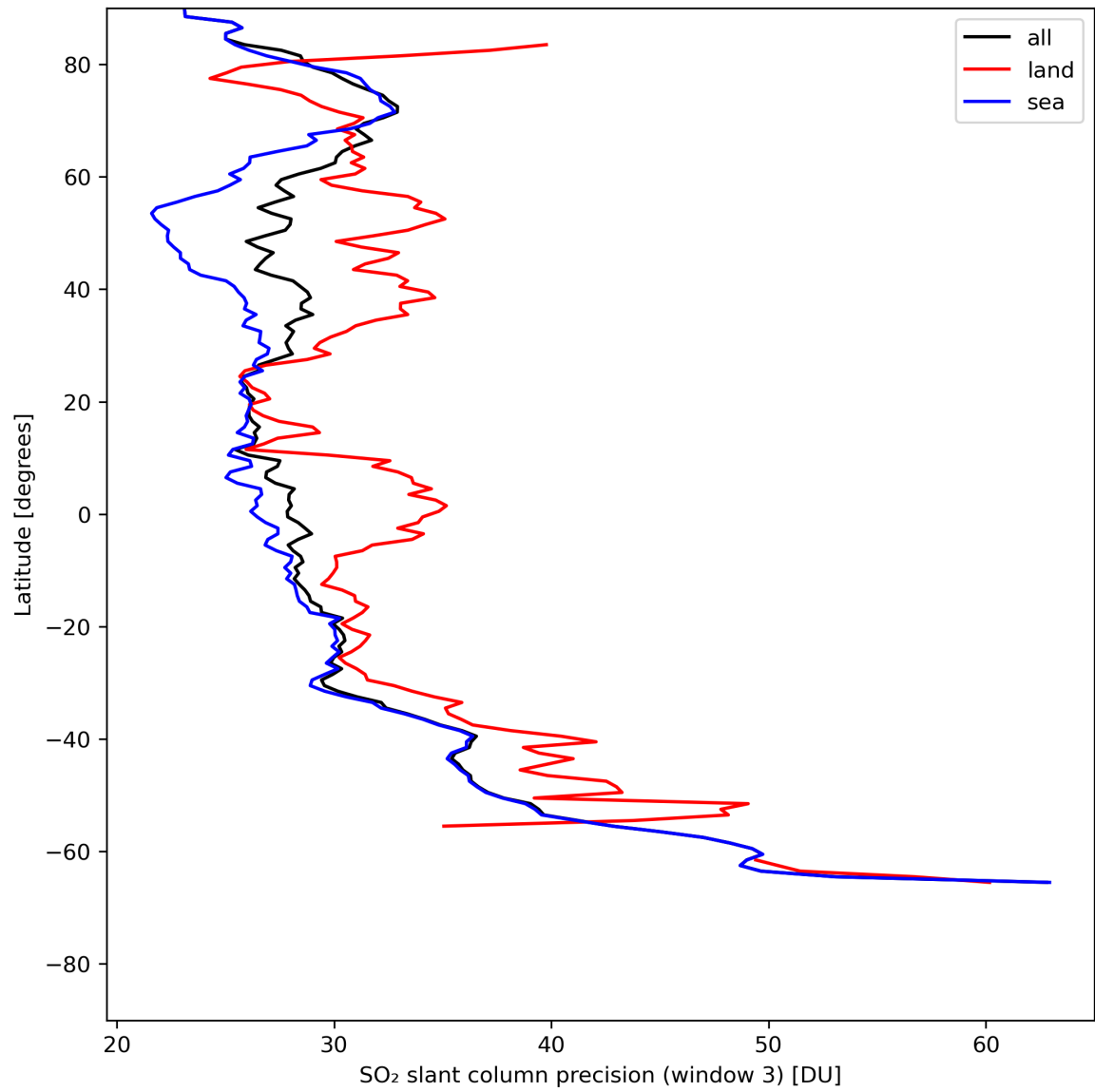
Figure 42: Zonal average of “SO 2 slant column precision (window 3)” for 2024-07-26 to 2024-07-28.
