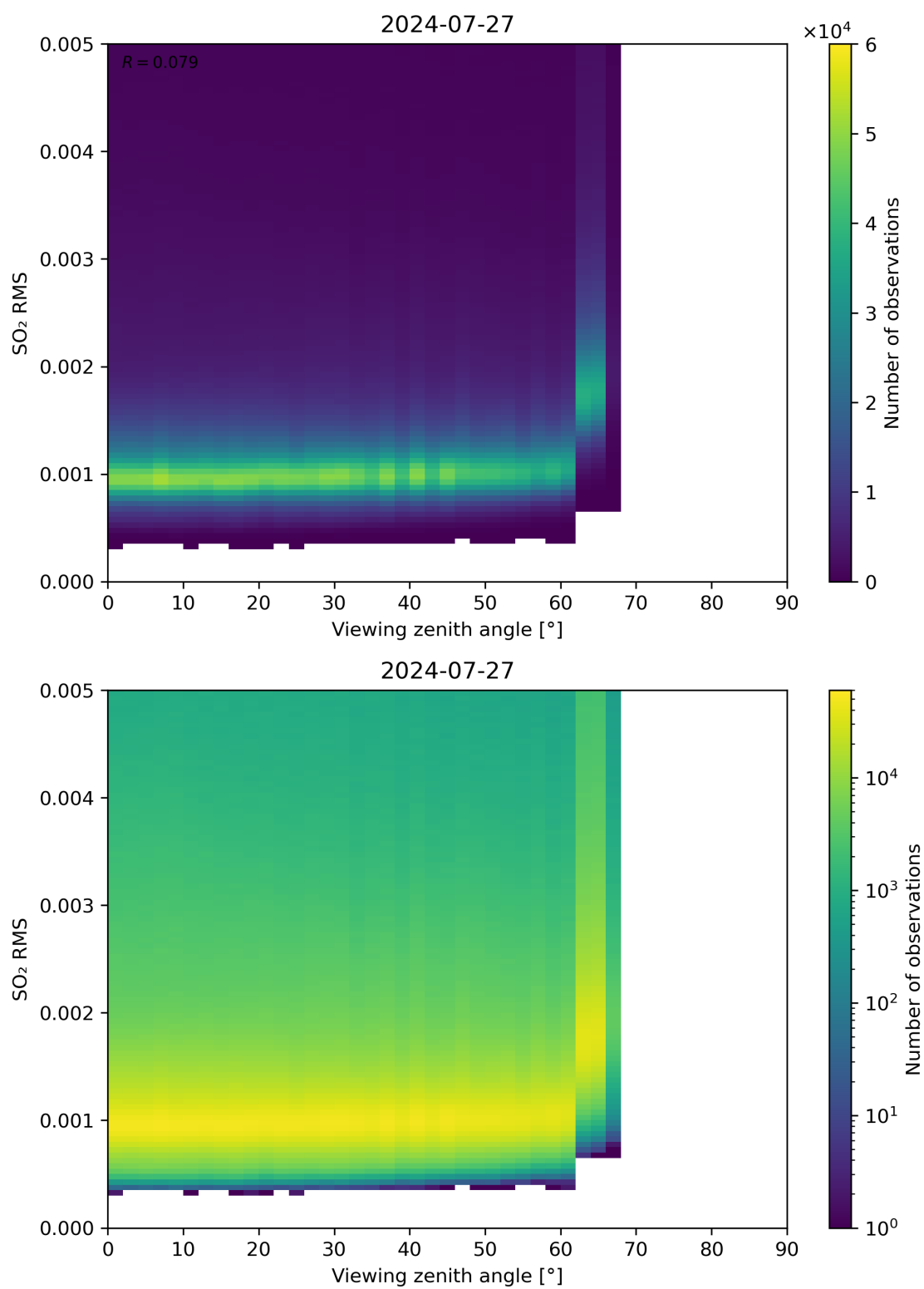
Figure 313: Scatter density plot of “Viewing zenith angle” against “SO 2 RMS” for 2024-07-26 to 2024-07-28.
