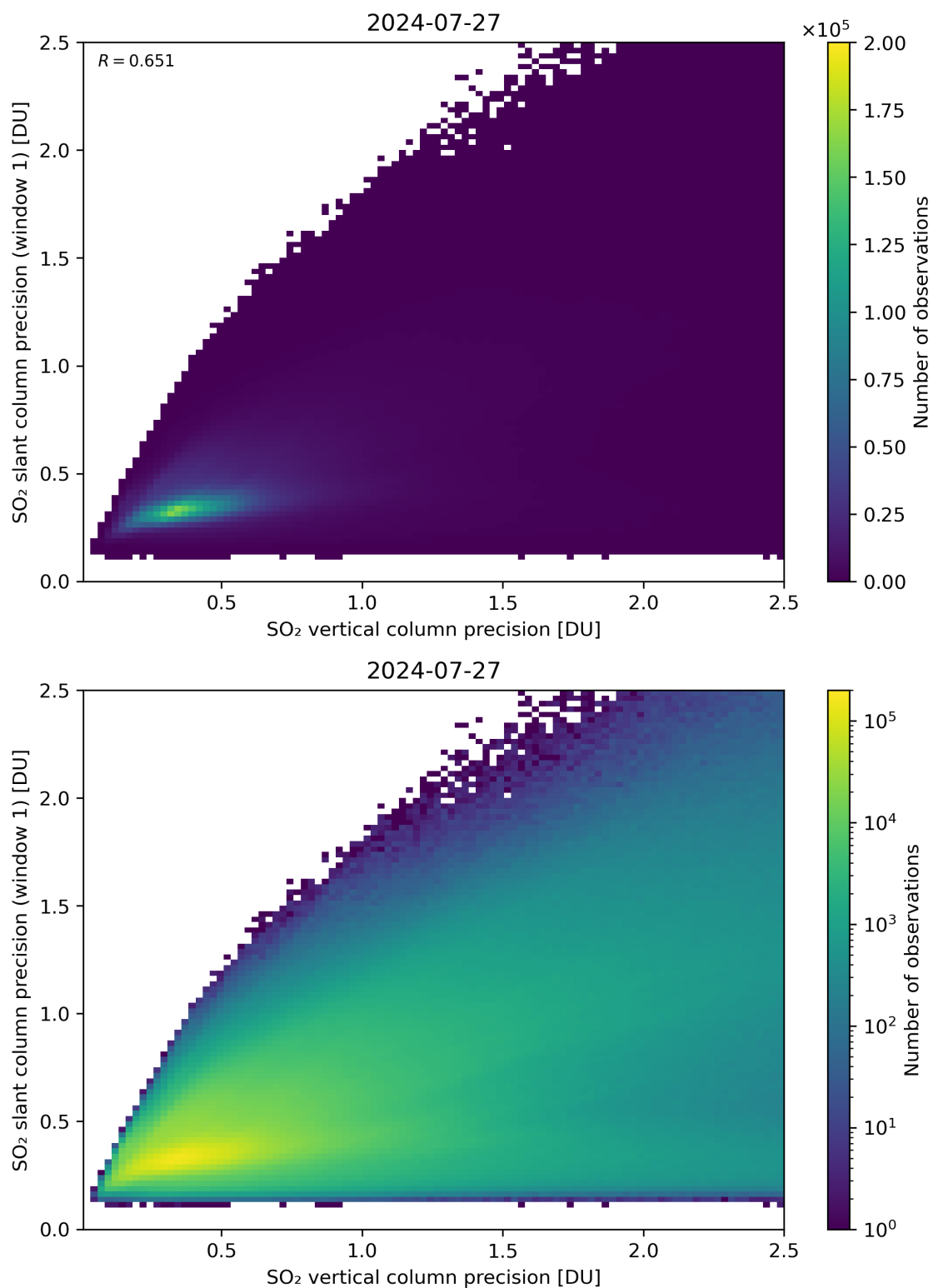
Figure 290: Scatter density plot of “SO 2 vertical column precision” against “SO 2 slant column precision (window 1)” for 2024-07-26 to 2024-07-28.
