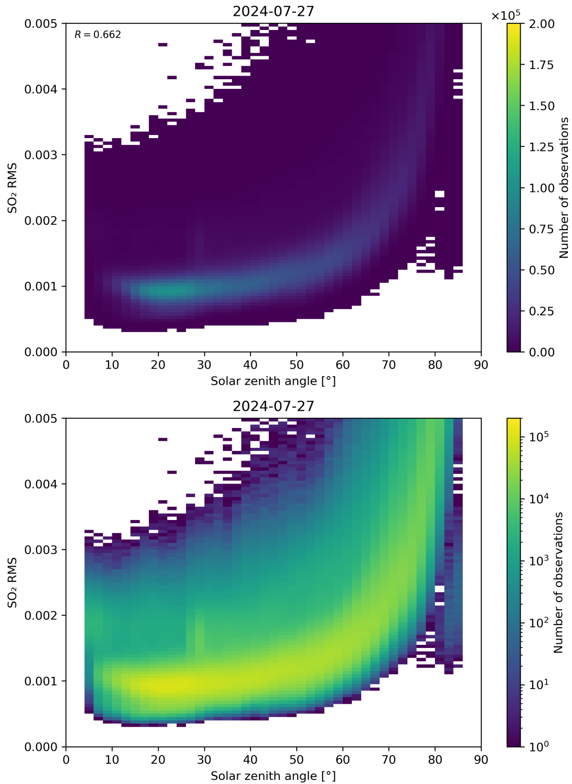
Figure 163: Scatter density plot of “Solar zenith angle” against “SO 2 RMS” for 2024-07-26 to 2024-07-28.
