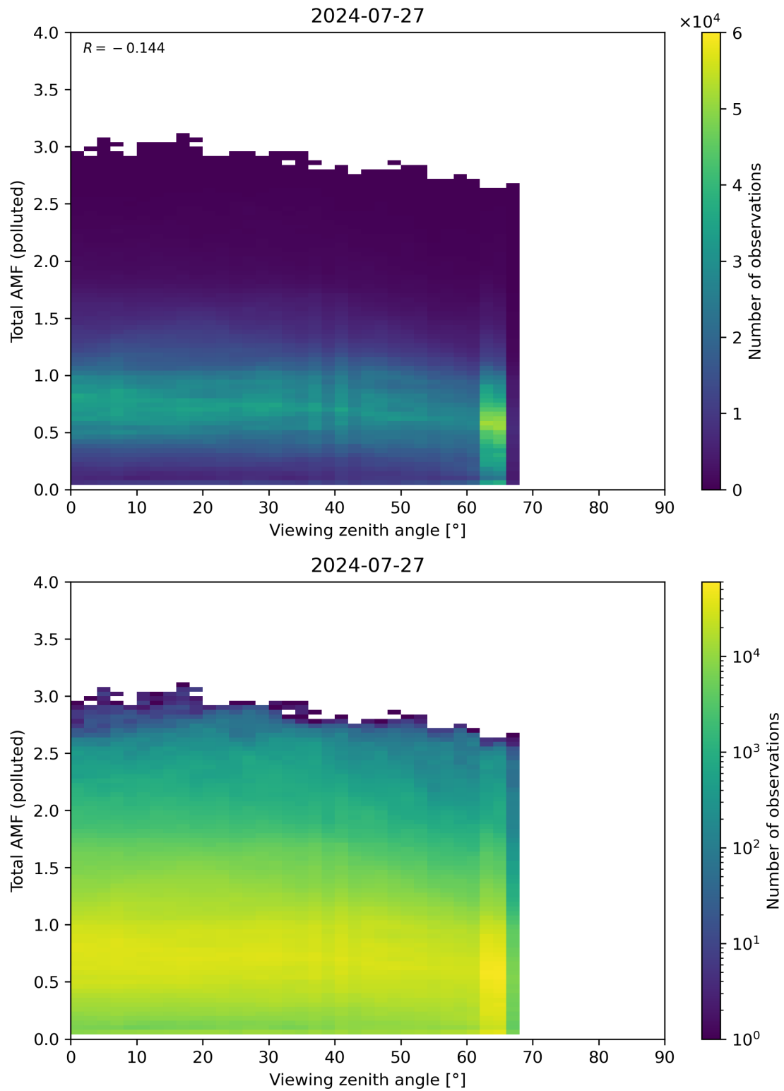
Figure 325: Scatter density plot of “Viewing zenith angle” against “Total AMF (polluted)” for 2024-07-26 to 2024-07-28.
