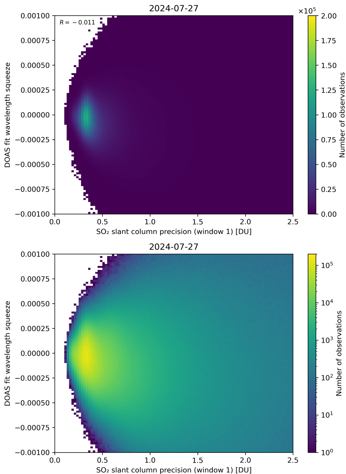
Figure 222: Scatter density plot of “SO 2 slant column precision (window 1)” against “DOAS fit wavelength squeeze” for 2024-07-26 to 2024-07-28.
