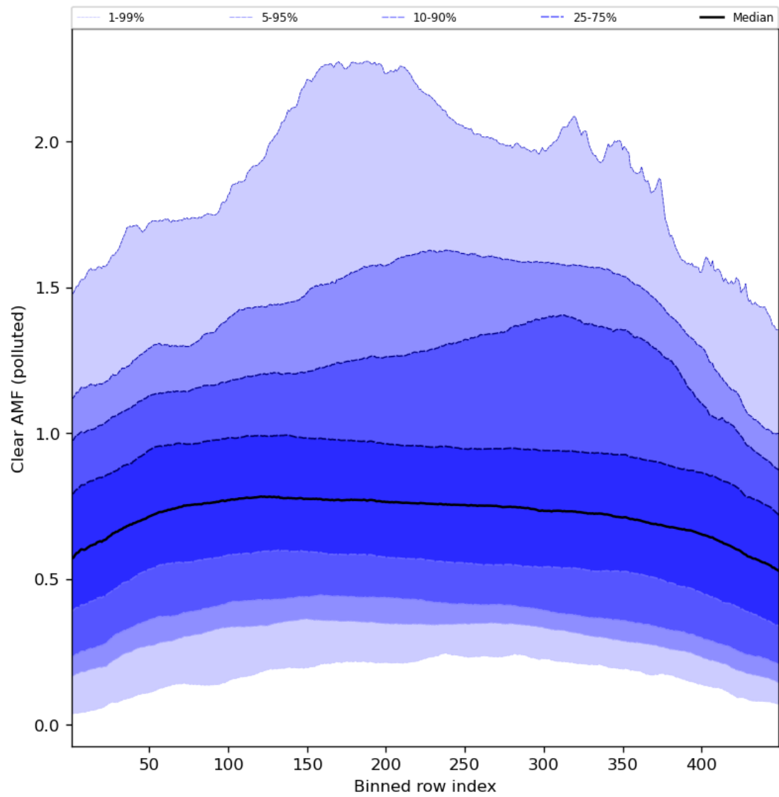
Figure 96: Along track statistics of “Clear AMF (polluted)” for 2024-07-26 to 2024-07-28
