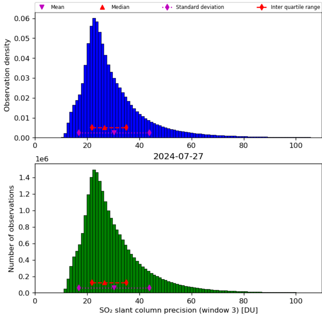
Figure 65: Histogram of “SO 2 slant column precision (window 3)” for 2024-07-26 to 2024-07-28
