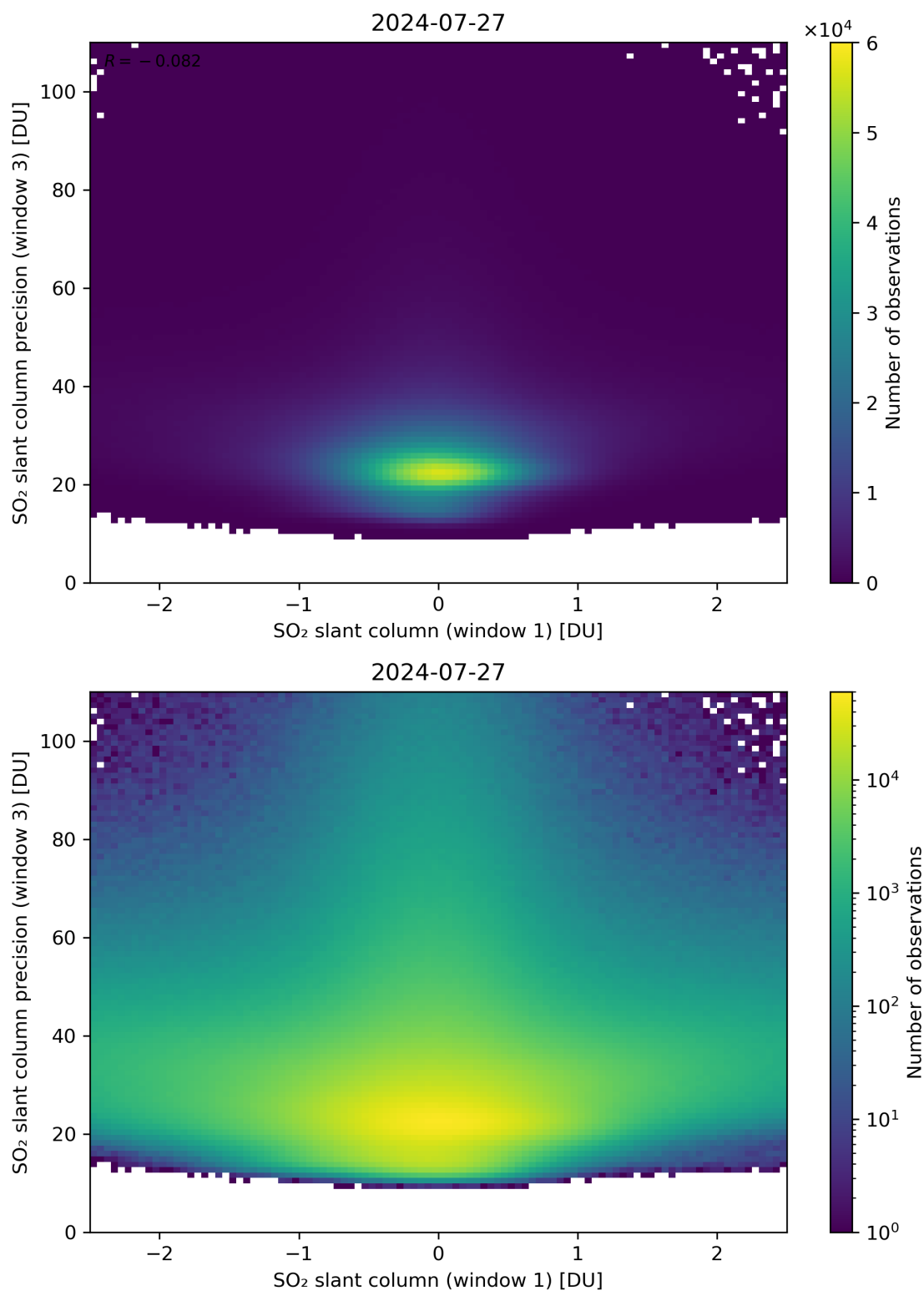
Figure 238: Scatter density plot of “SO 2 slant column (window 1)” against “SO 2 slant column precision (window 3)” for 2024-07-26 to 2024-07-28.
