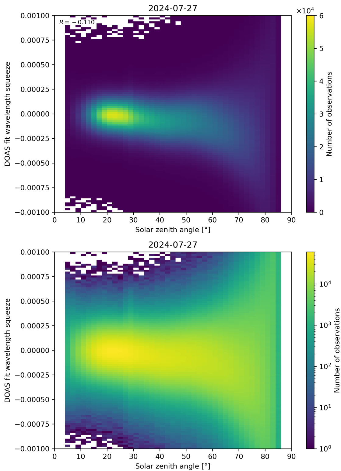
Figure 162: Scatter density plot of “Solar zenith angle” against “DOAS fit wavelength squeeze” for 2024-07-26 to 2024-07-28.
