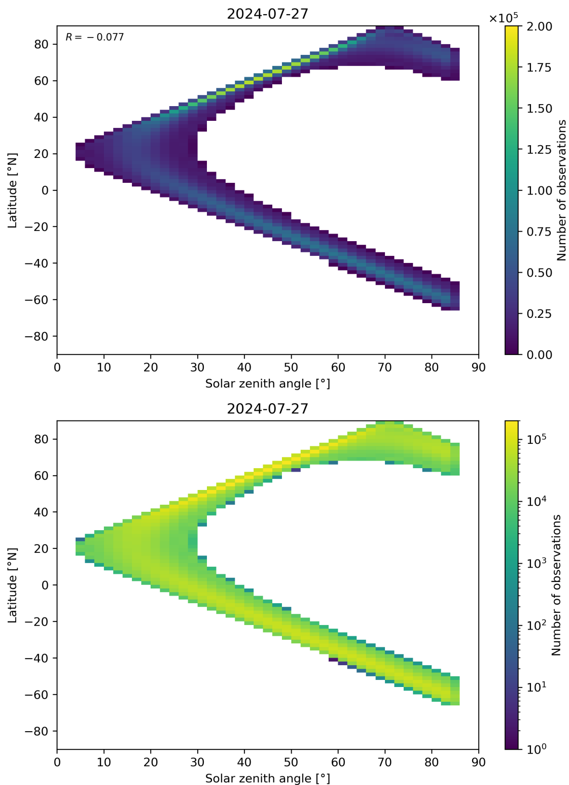
Figure 164: Scatter density plot of “Solar zenith angle” against “Latitude” for 2024-07-26 to 2024-07-28.
