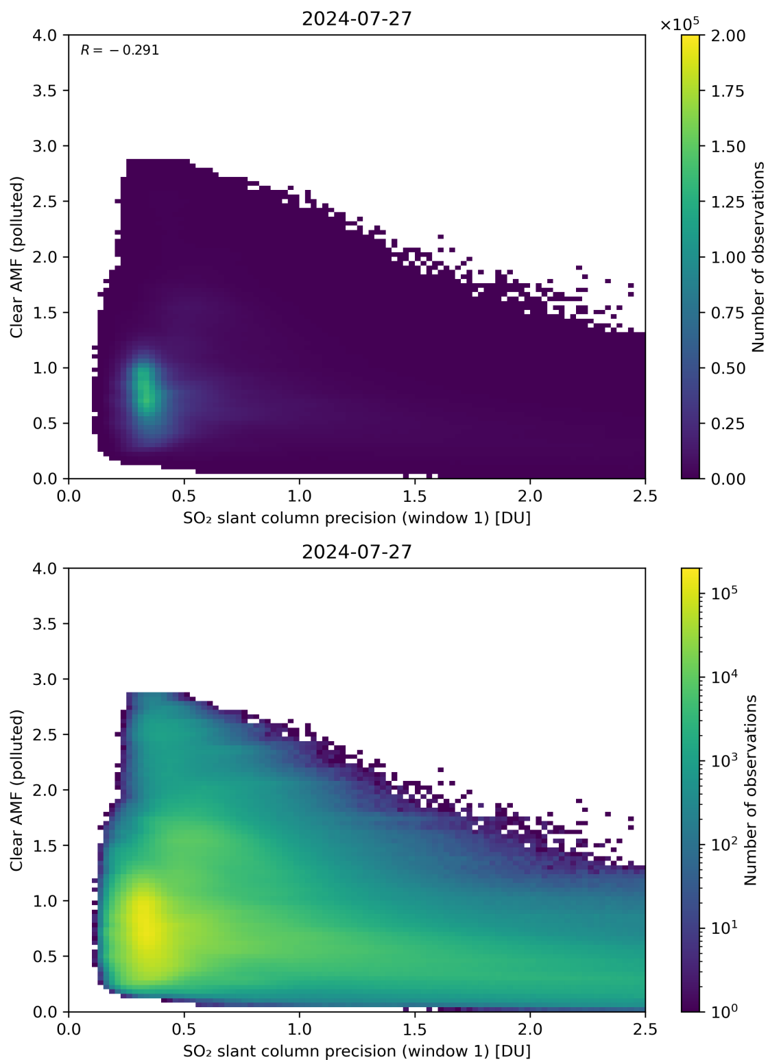
Figure 224: Scatter density plot of “SO 2 slant column precision (window 1)” against “Clear AMF (polluted)” for 2024-07-26 to 2024-07-28.
