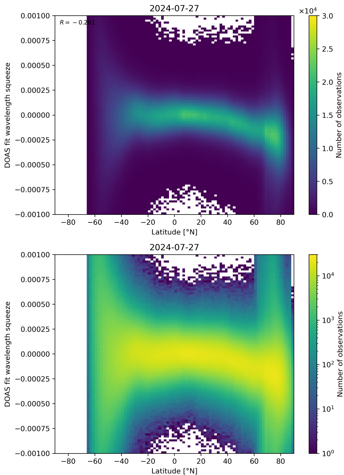
Figure 143: Scatter density plot of “Latitude” against “DOAS fit wavelength squeeze” for 2024-07-26 to 2024-07-28.
