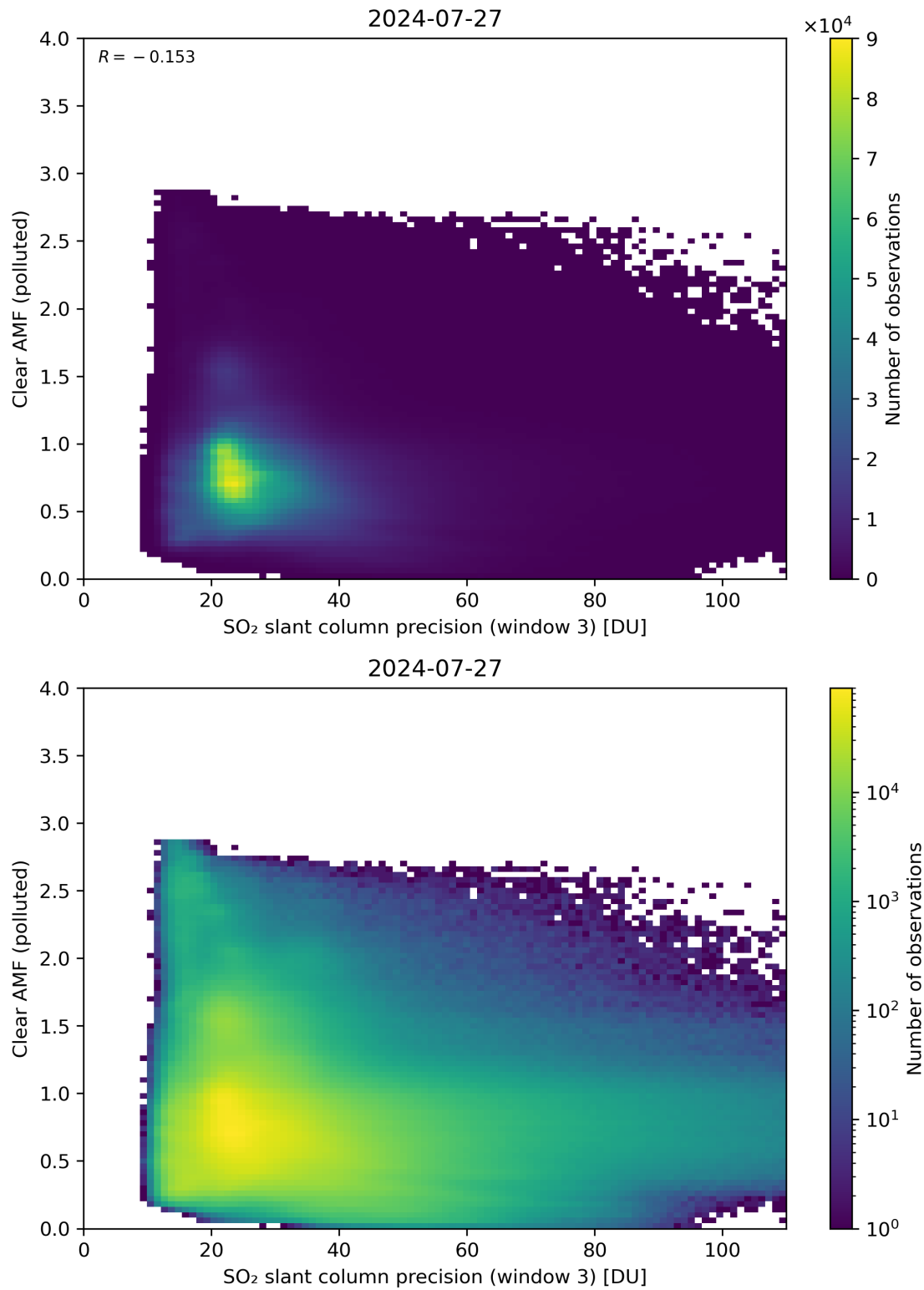
Figure 261: Scatter density plot of “SO 2 slant column precision (window 3)” against “Clear AMF (polluted)” for 2024-07-26 to 2024-07-28.
