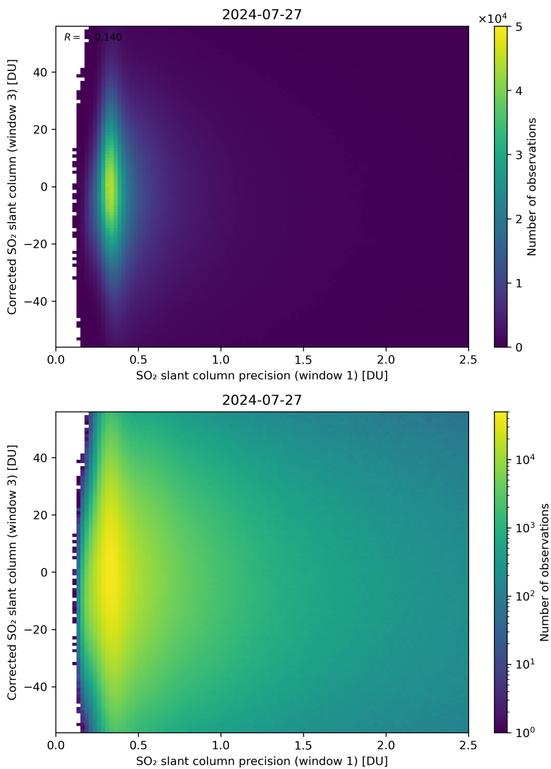
Figure 226: Scatter density plot of “SO 2 slant column precision (window 1)” against “Corrected SO 2 slant column (window 3)” for 2024-07-26 to 2024-07-28.
