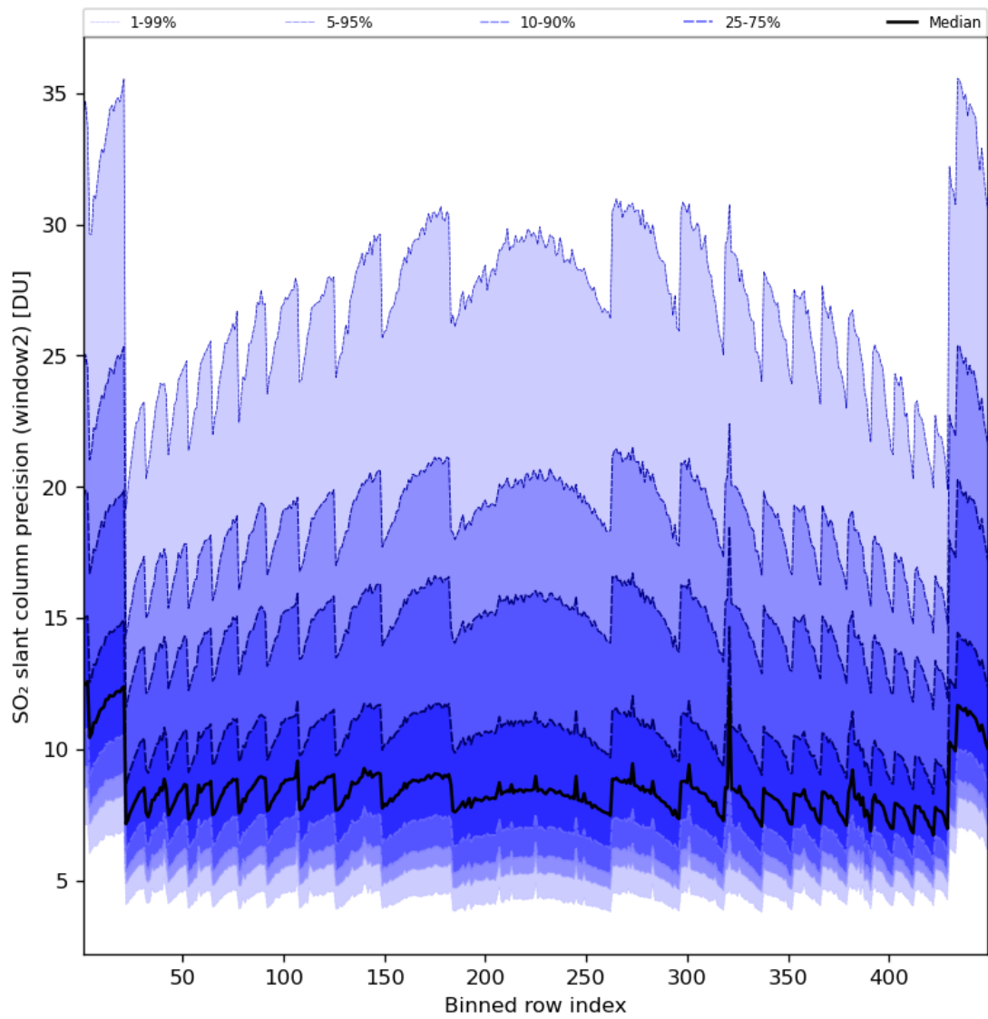
Figure 84: Along track statistics of “SO 2 slant column precision (window2)” for 2024-07-26 to 2024-07-28
