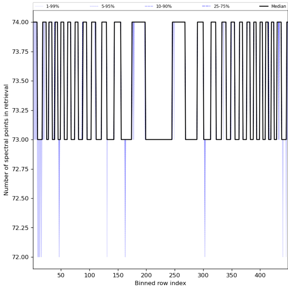
Figure 97: Along track statistics of “Number of spectral points in retrieval” for 2024-07-26 to 2024-07-28
