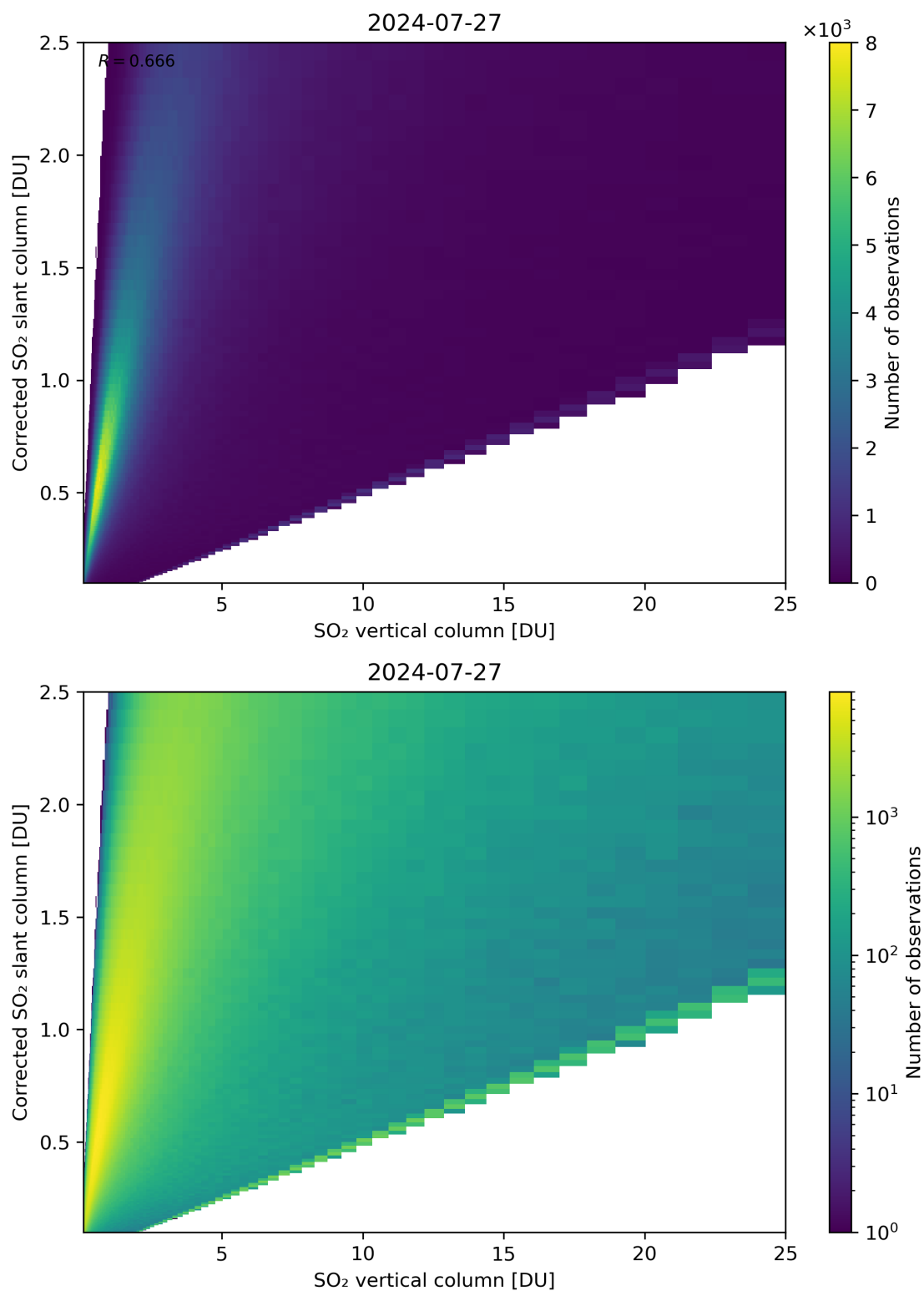
Figure 297: Scatter density plot of “SO 2 vertical column” against “Corrected SO 2 slant column” for 2024-07-26 to 2024-07-28.
