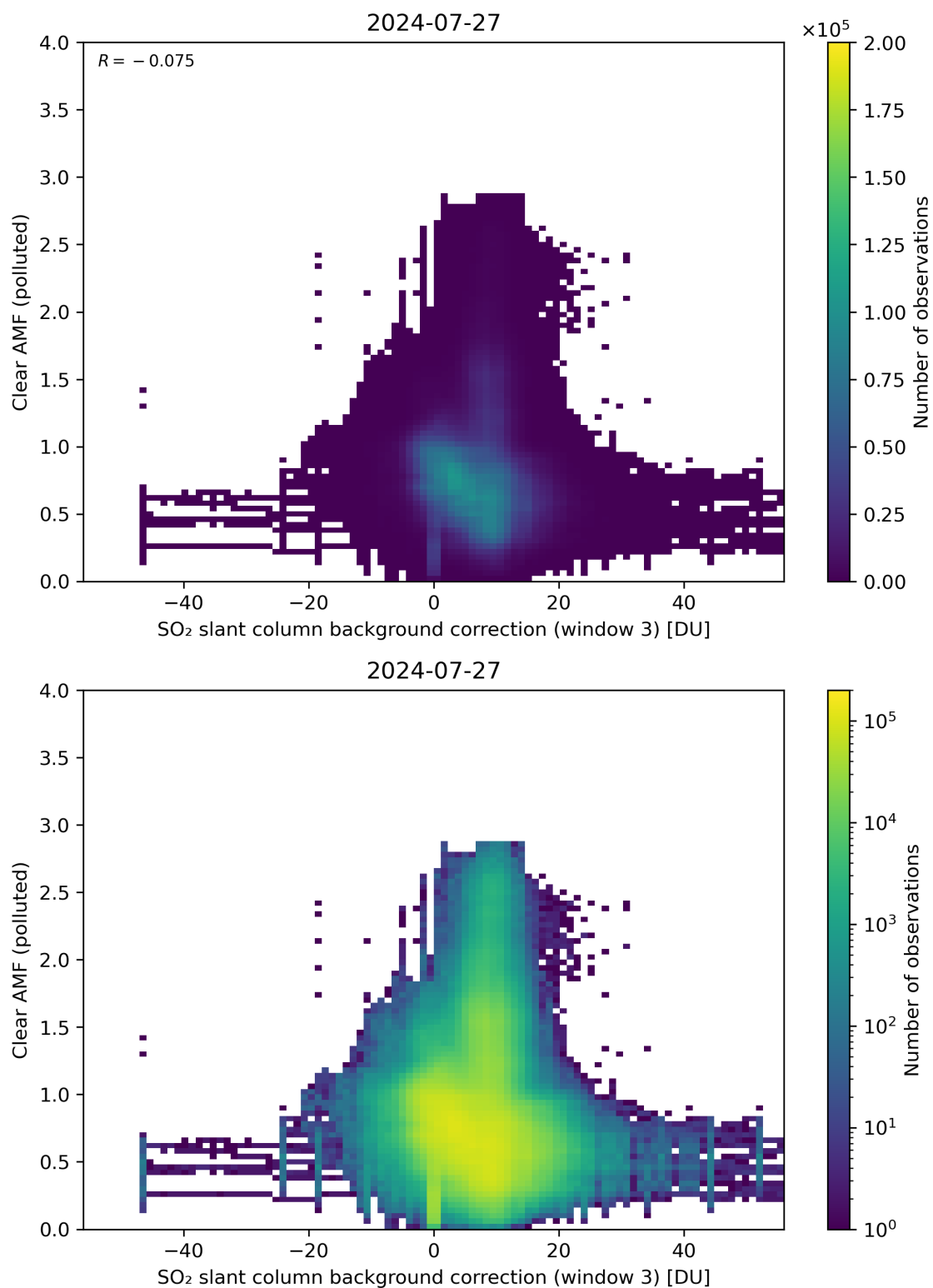
Figure 124: Scatter density plot of “SO 2 slant column background correction (window 3)” against “Clear AMF (polluted)” for 2024-07-26 to 2024-07-28.
