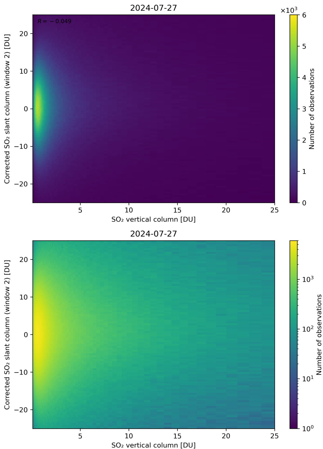
Figure 298: Scatter density plot of “SO 2 vertical column” against “Corrected SO 2 slant column (window 2)” for 2024-07-26 to 2024-07-28.
