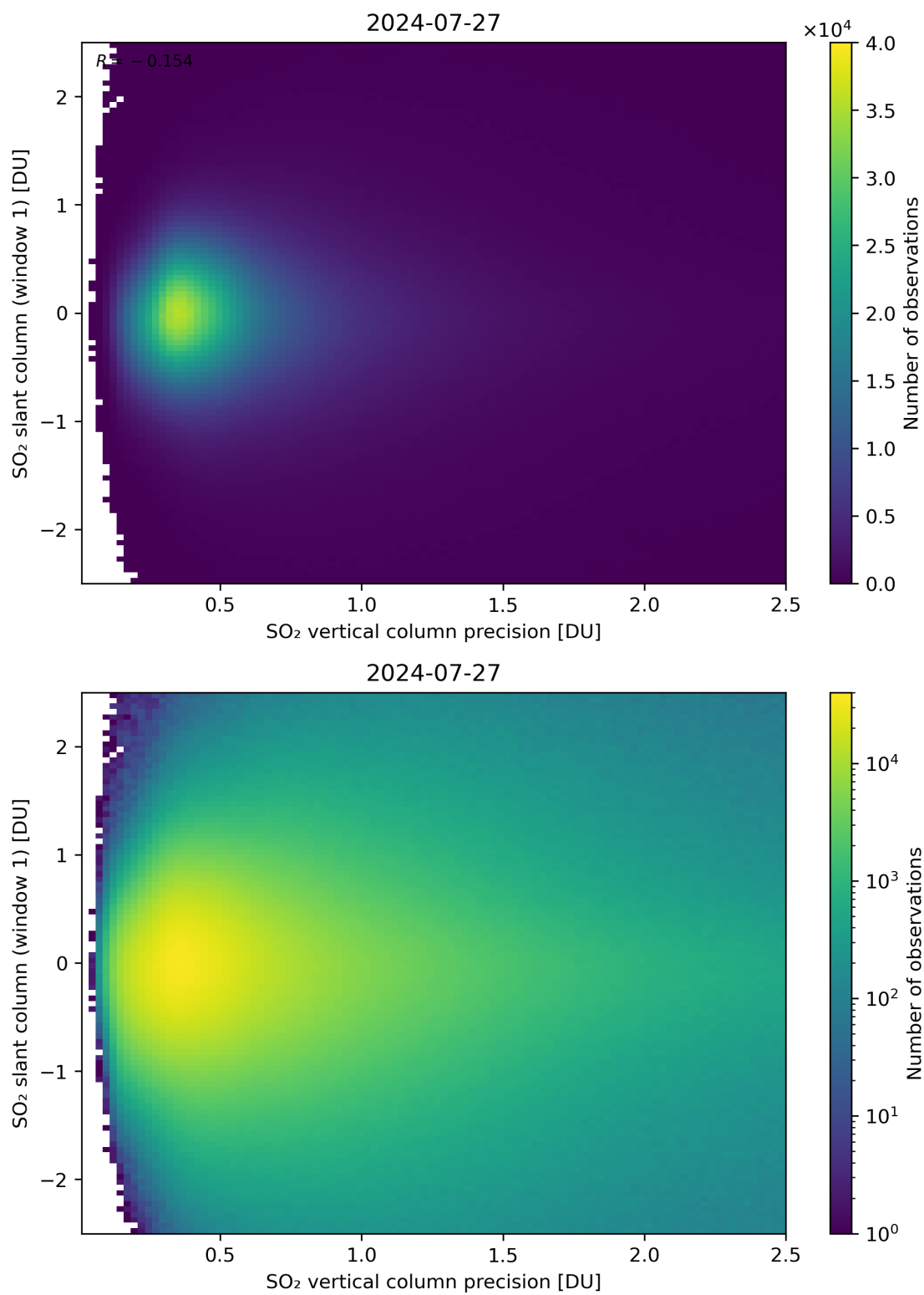
Figure 289: Scatter density plot of “SO 2 vertical column precision” against “SO 2 slant column (window 1)” for 2024-07-26 to 2024-07-28.
