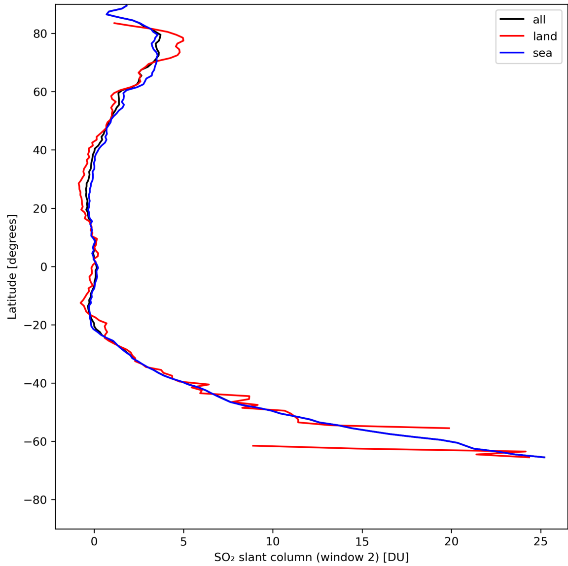
Figure 37: Zonal average of “SO 2 slant column (window 2)” for 2024-07-26 to 2024-07-28.
