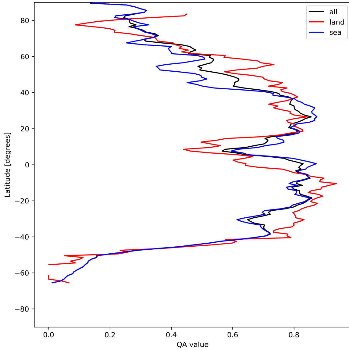
Figure 29: Zonal average of “QA value” for 2024-07-26 to 2024-07-28.
