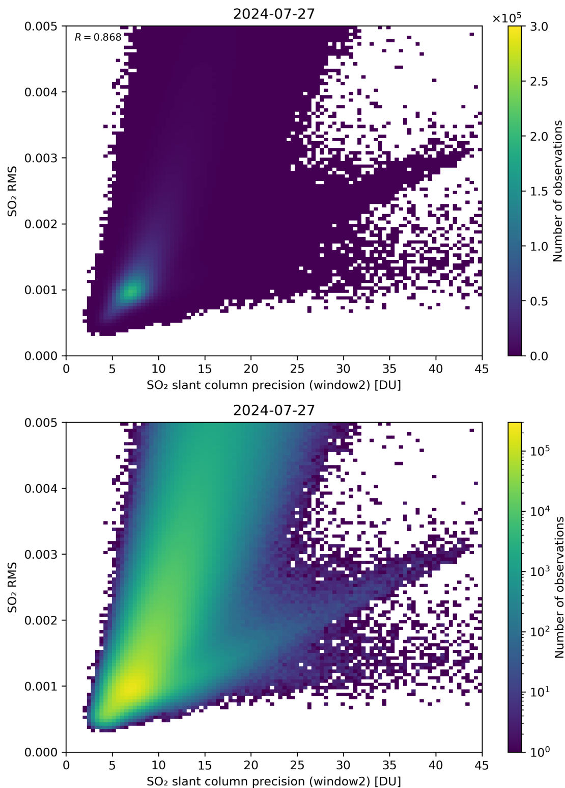
Figure 245: Scatter density plot of “SO 2 slant column precision (window2)” against “SO 2 RMS” for 2024-07-26 to 2024-07-28.
