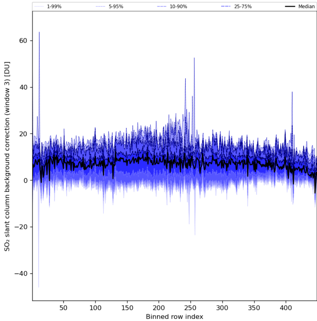
Figure 90: Along track statistics of “SO 2 slant column background correction (window 3)” for 2024-07-26 to 2024-07-28
