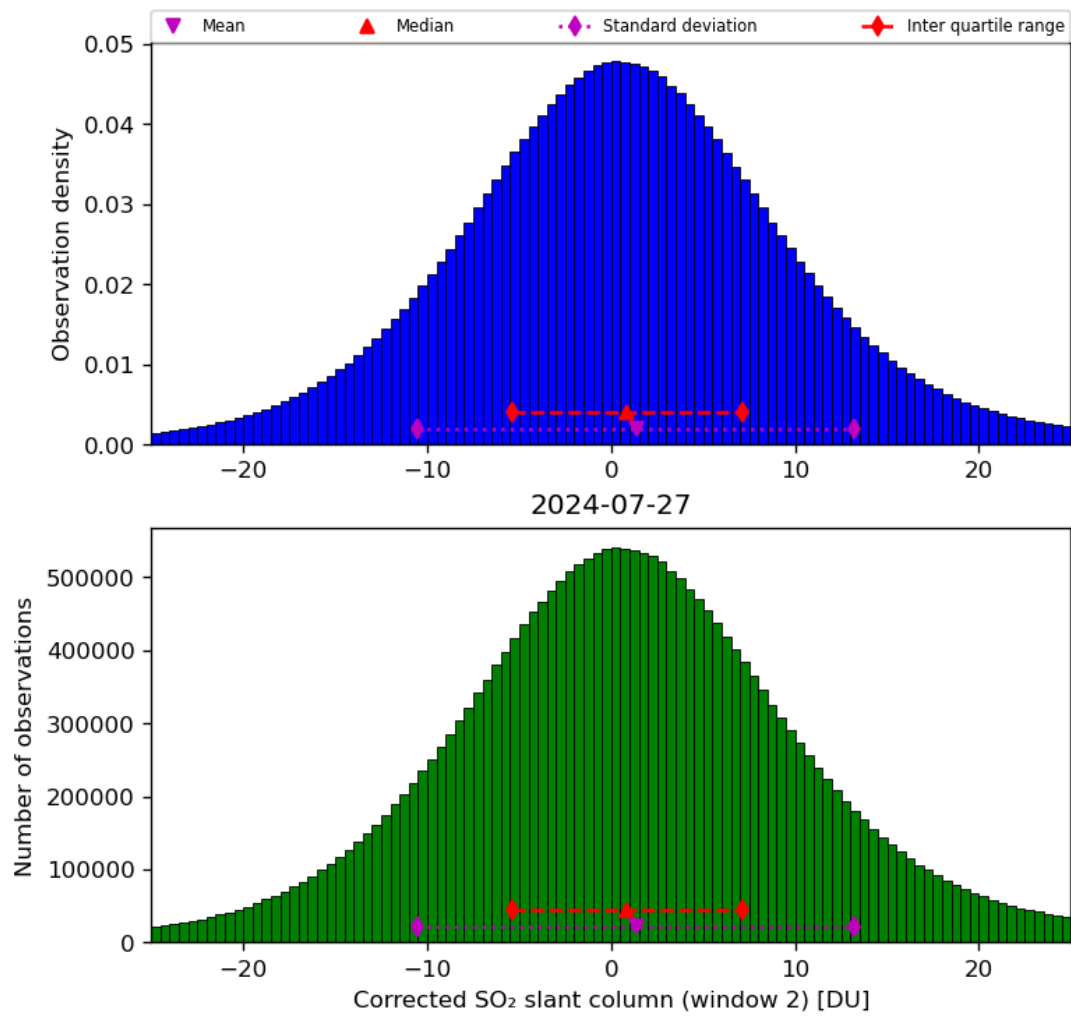
Figure 62: Histogram of “Corrected SO 2 slant column (window 2)” for 2024-07-26 to 2024-07-28
