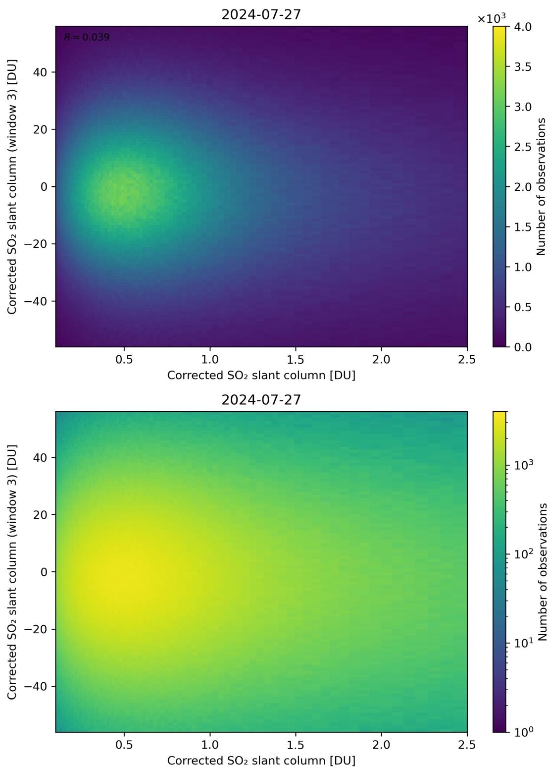
Figure 186: Scatter density plot of “Corrected SO 2 slant column” against “Corrected SO 2 slant column (window 3)” for 2024-07-26 to 2024-07-28.
