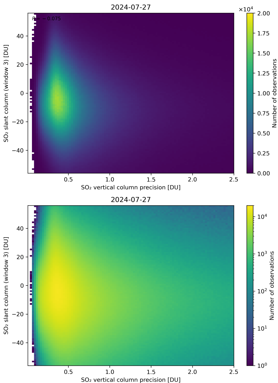
Figure 292: Scatter density plot of “SO 2 vertical column precision” against “SO 2 slant column (window 3)” for 2024-07-26 to 2024-07-28.
