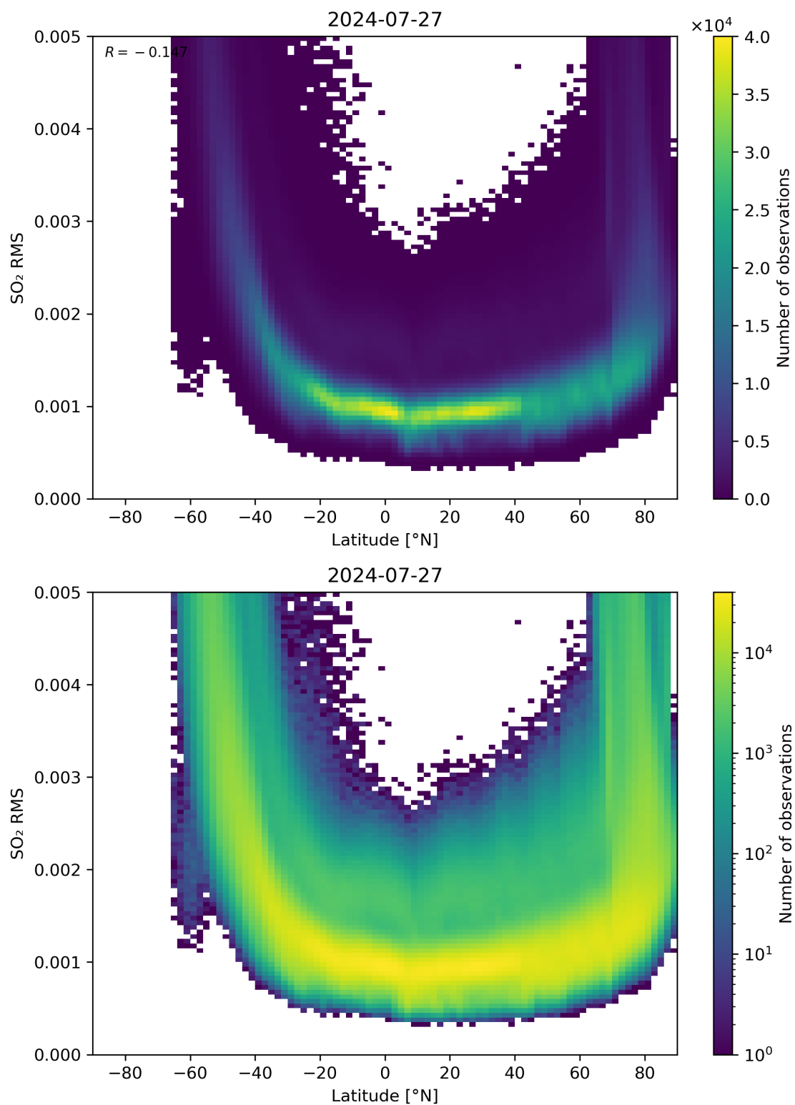
Figure 144: Scatter density plot of “Latitude” against “SO 2 RMS” for 2024-07-26 to 2024-07-28.
