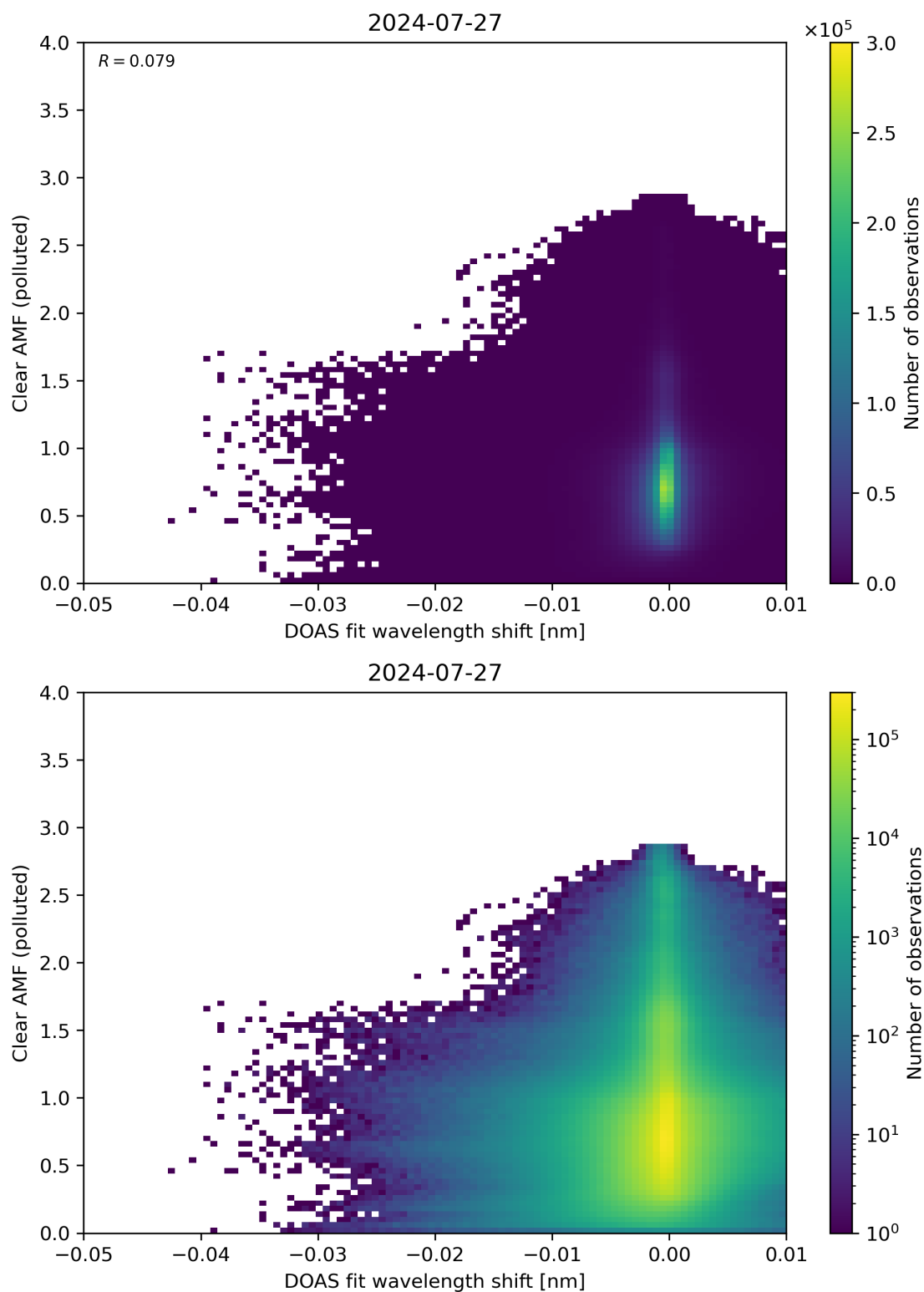
Figure 129: Scatter density plot of “DOAS fit wavelength shift” against “Clear AMF (polluted)” for 2024-07-26 to 2024-07-28.
