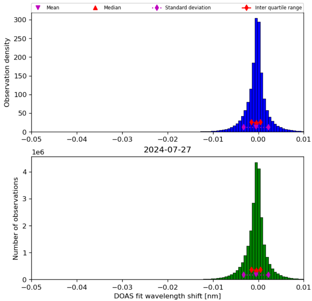
Figure 68: Histogram of “DOAS fit wavelength shift” for 2024-07-26 to 2024-07-28
