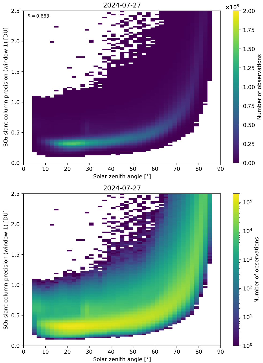
Figure 170: Scatter density plot of “Solar zenith angle” against “SO 2 slant column precision (window 1)” for 2024-07-26 to 2024-07-28.
