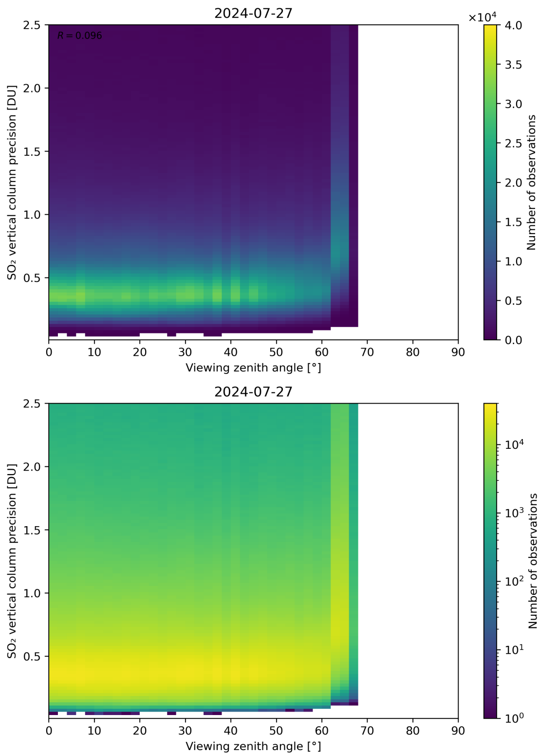
Figure 328: Scatter density plot of “Viewing zenith angle” against “SO 2 vertical column precision” for 2024-07-26 to 2024-07-28.
