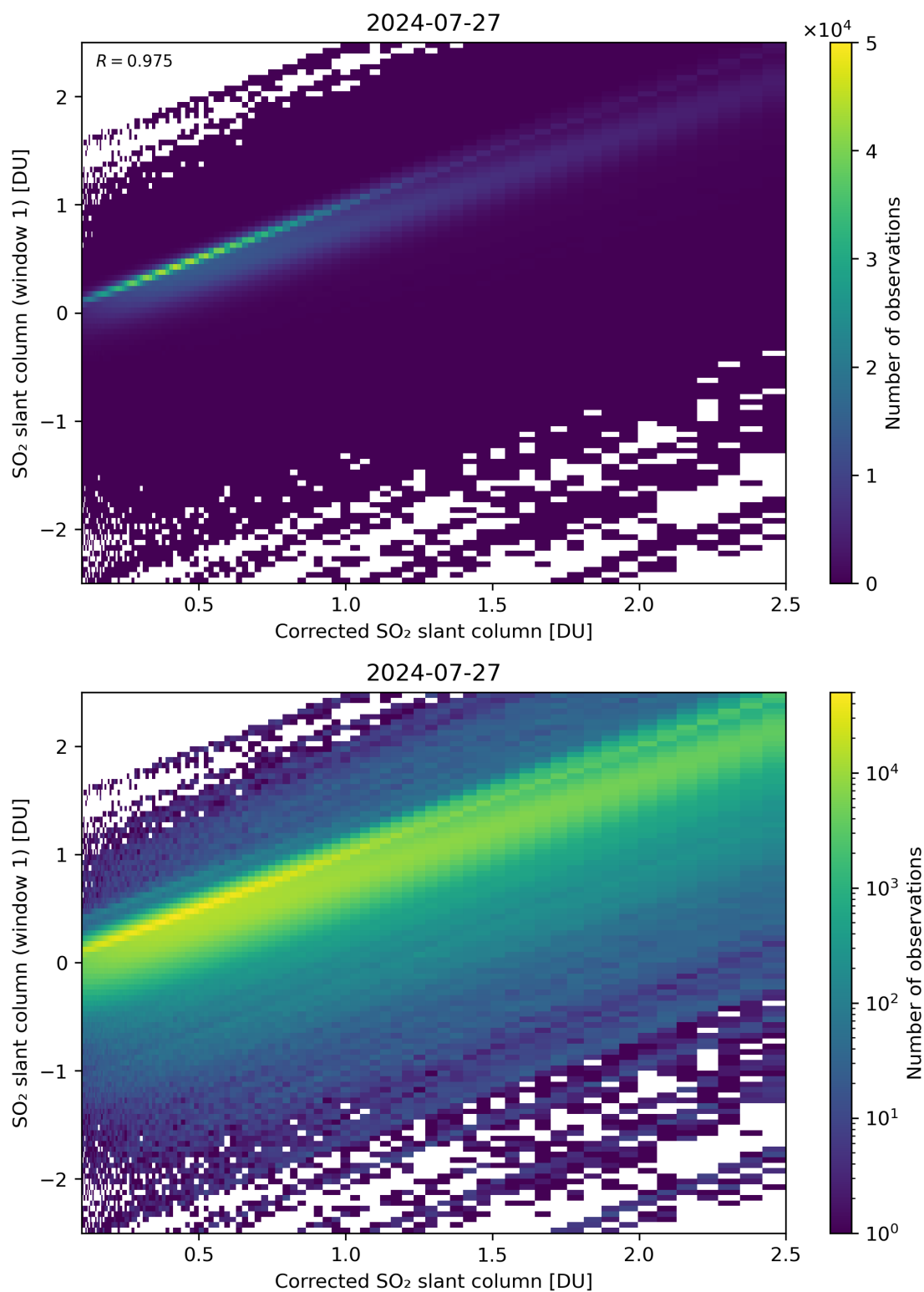
Figure 187: Scatter density plot of “Corrected SO 2 slant column” against “SO 2 slant column (window 1)” for 2024-07-26 to 2024-07-28.
