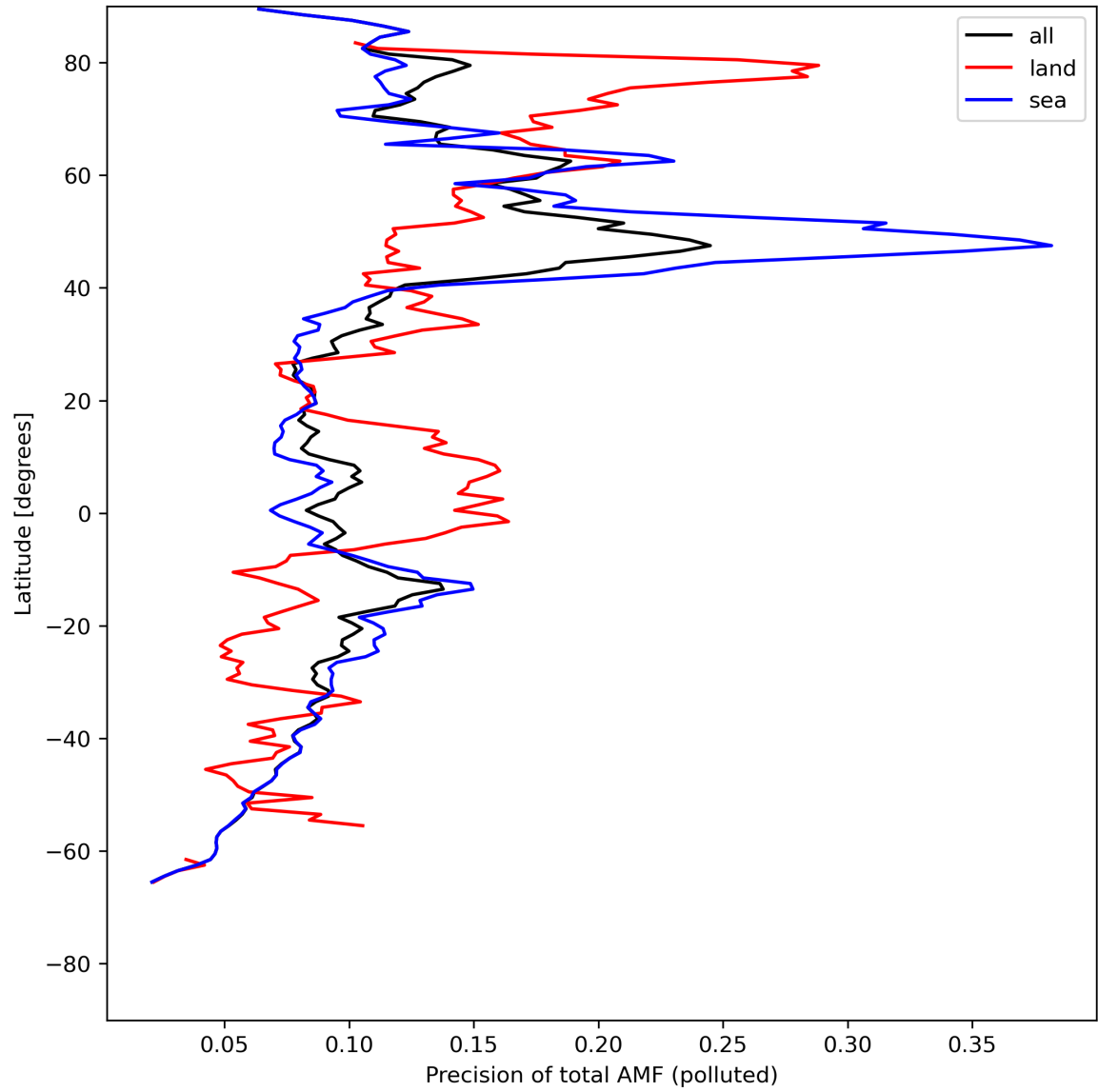
Figure 49: Zonal average of “Precision of total AMF (polluted)” for 2024-07-26 to 2024-07-28.
