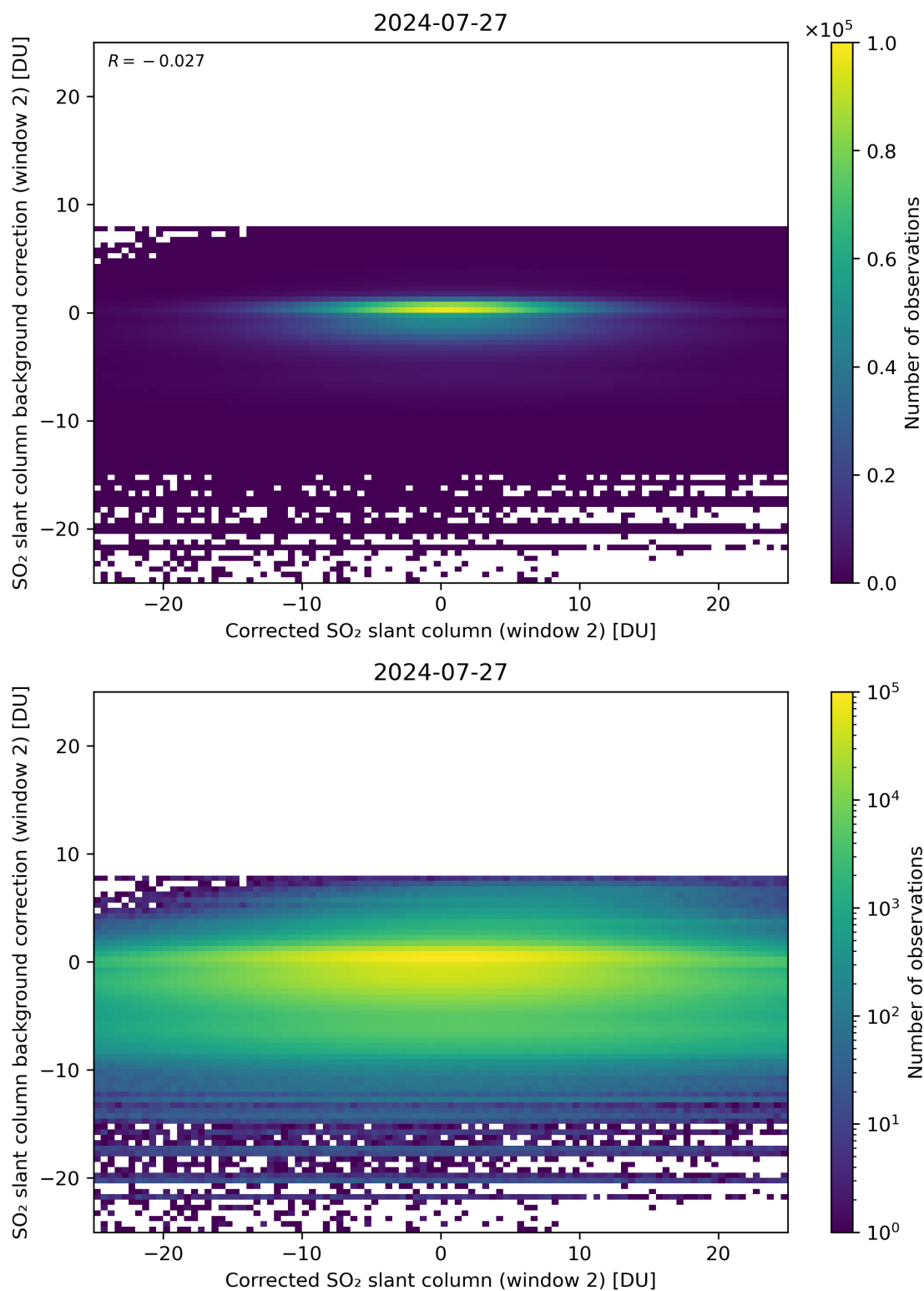
Figure 194: Scatter density plot of “Corrected SO 2 slant column (window 2)” against “SO 2 slant column background correction (window 2)” for 2024-07-26 to 2024-07-28.
