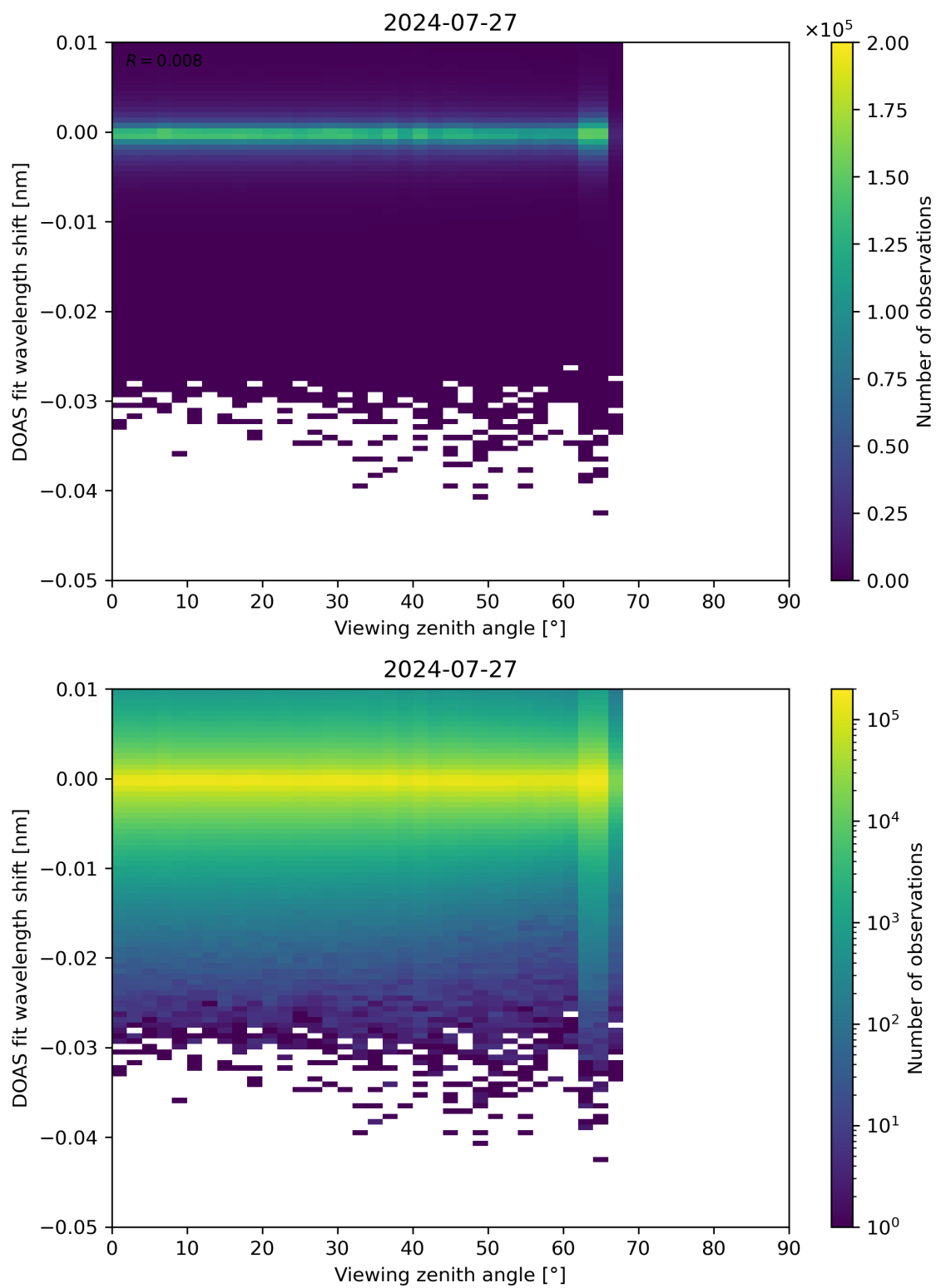
Figure 311: Scatter density plot of “Viewing zenith angle” against “DOAS fit wavelength shift” for 2024-07-26 to 2024-07-28.
