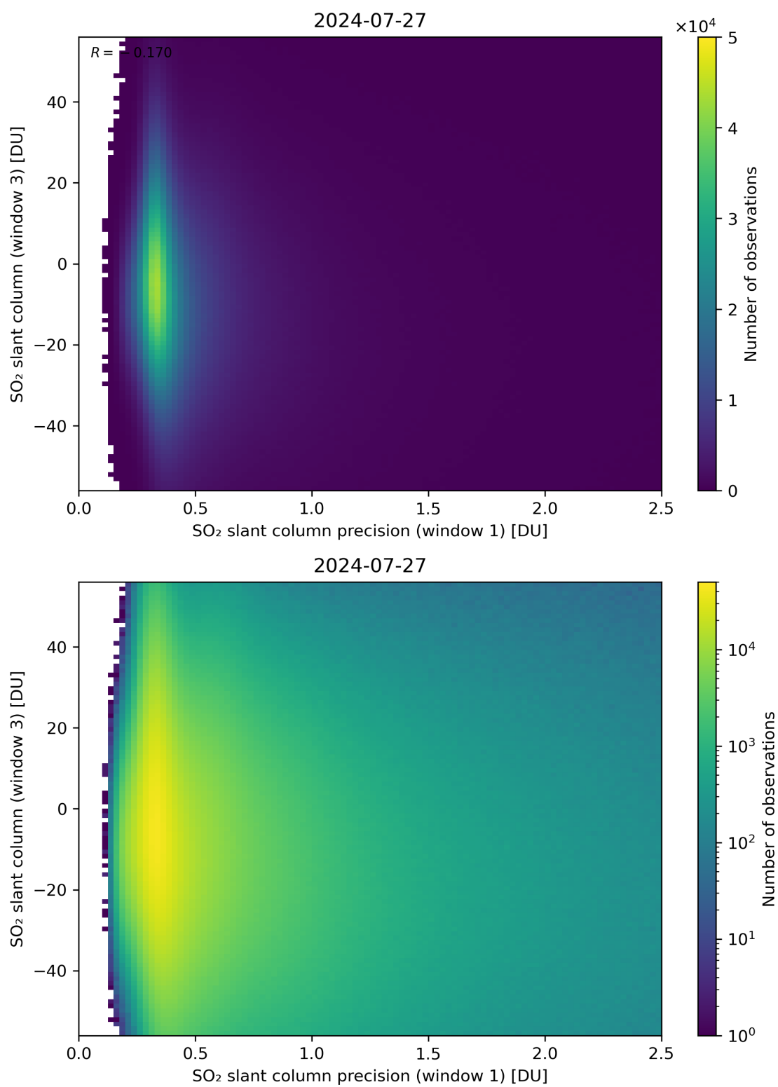
Figure 228: Scatter density plot of “SO 2 slant column precision (window 1)” against “SO 2 slant column (window 3)” for 2024-07-26 to 2024-07-28.
