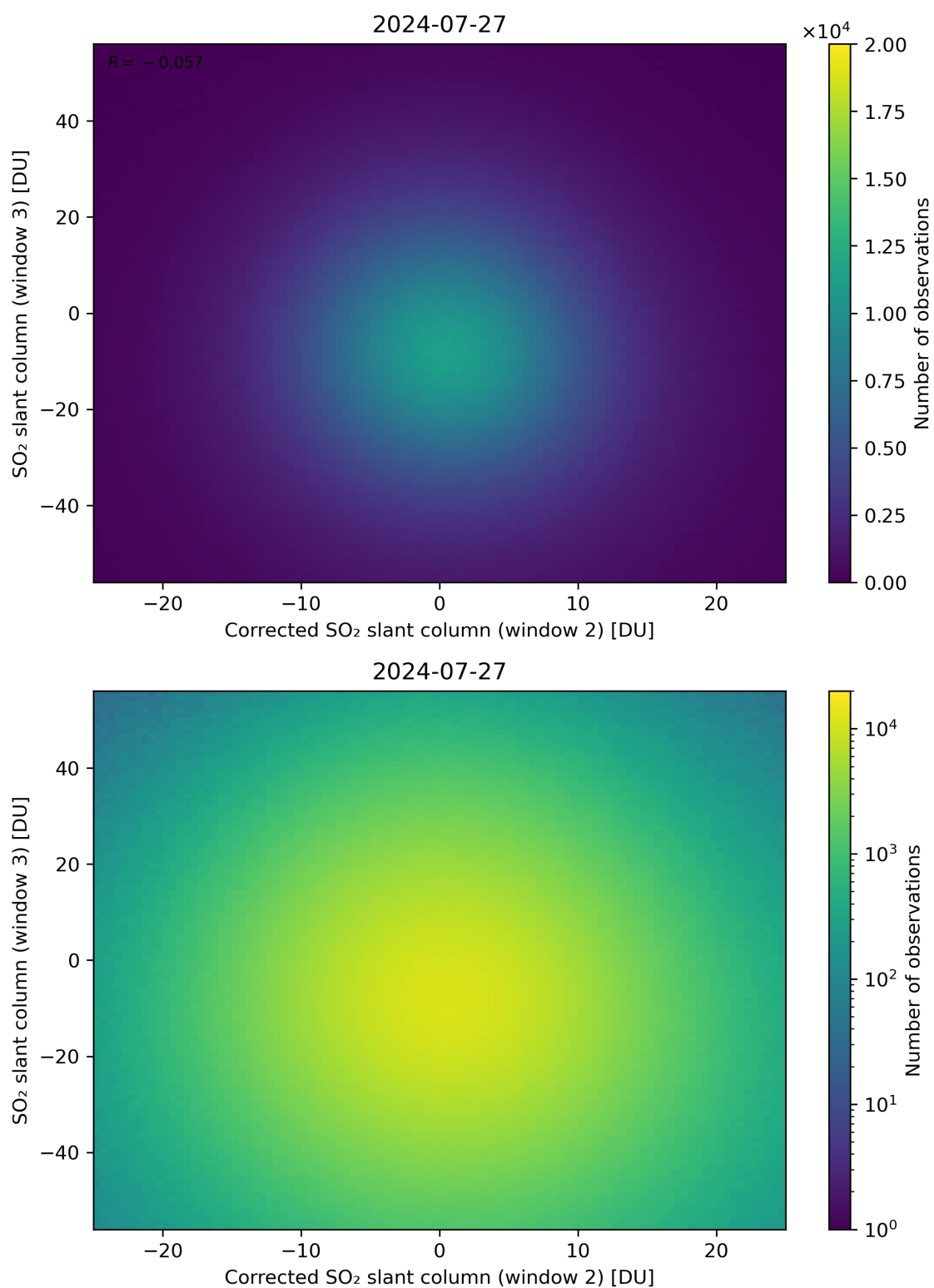
Figure 201: Scatter density plot of “Corrected SO 2 slant column (window 2)” against “SO 2 slant column (window 3)” for 2024-07-26 to 2024-07-28.
