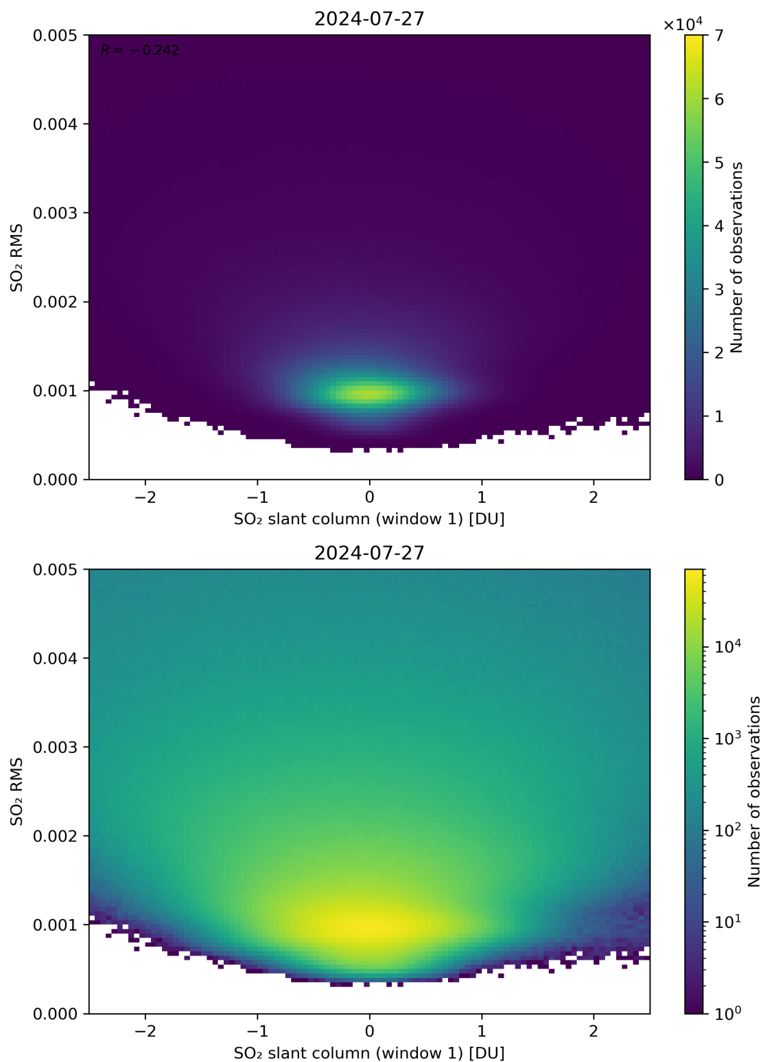
Figure 217: Scatter density plot of “SO 2 slant column (window 1)” against “SO 2 RMS” for 2024-07-26 to 2024-07-28.
