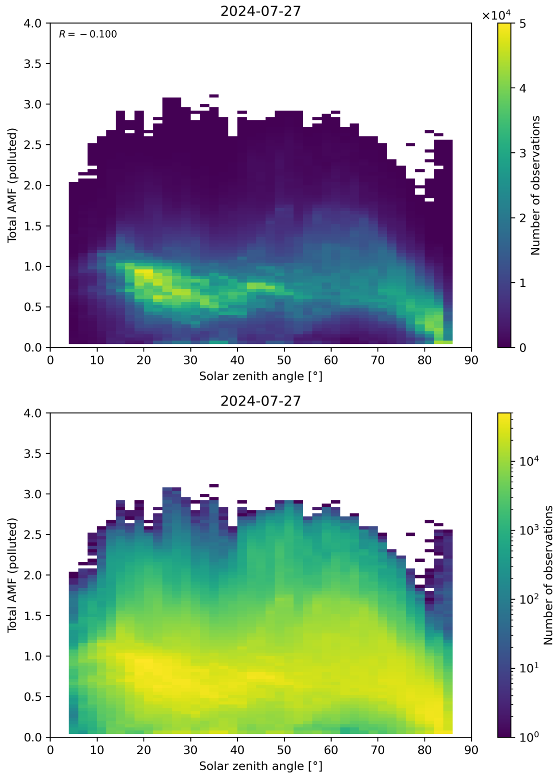
Figure 174: Scatter density plot of “Solar zenith angle” against “Total AMF (polluted)” for 2024-07-26 to 2024-07-28.
