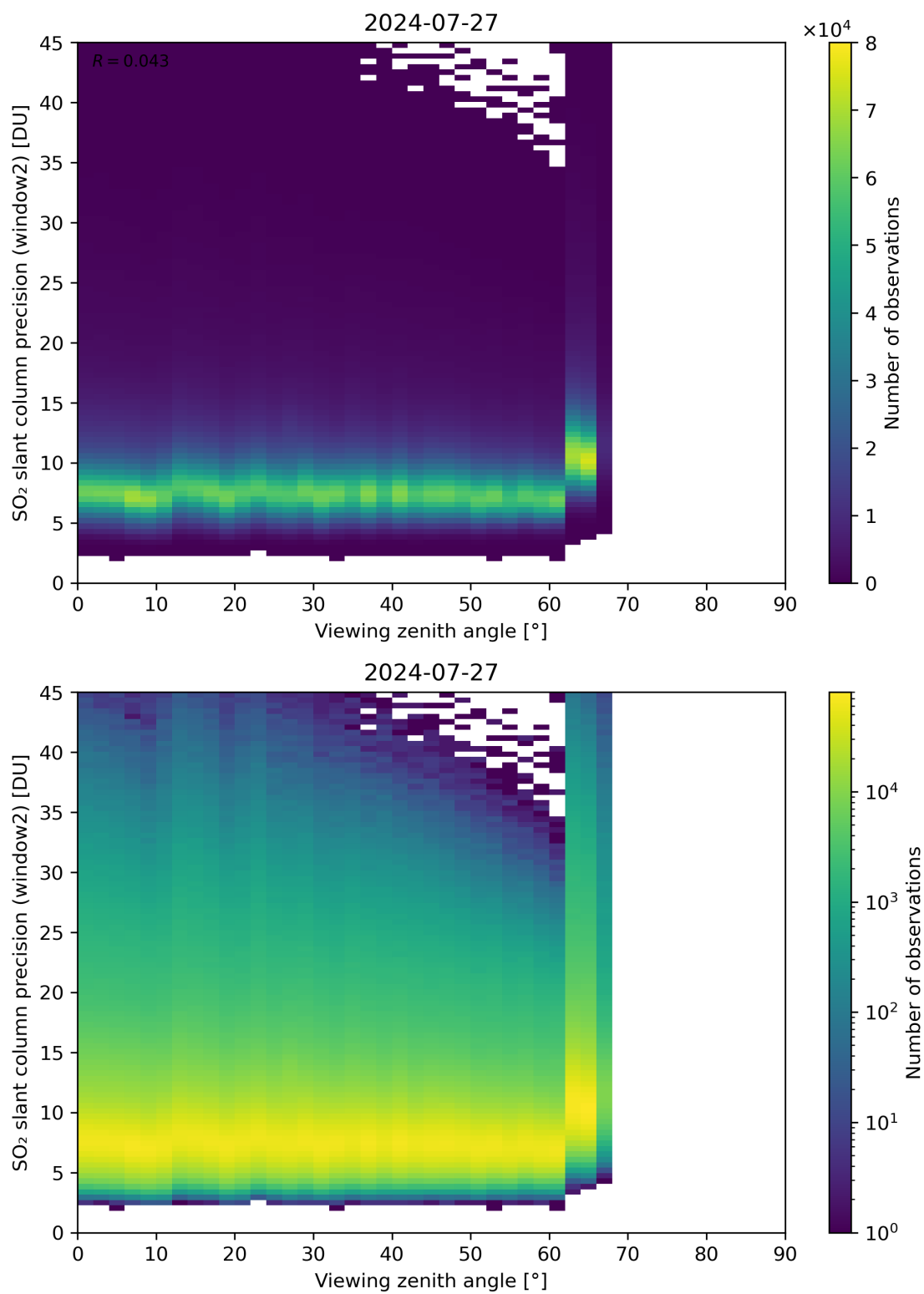
Figure 322: Scatter density plot of “Viewing zenith angle” against “SO 2 slant column precision (window2)” for 2024-07-26 to 2024-07-28.
