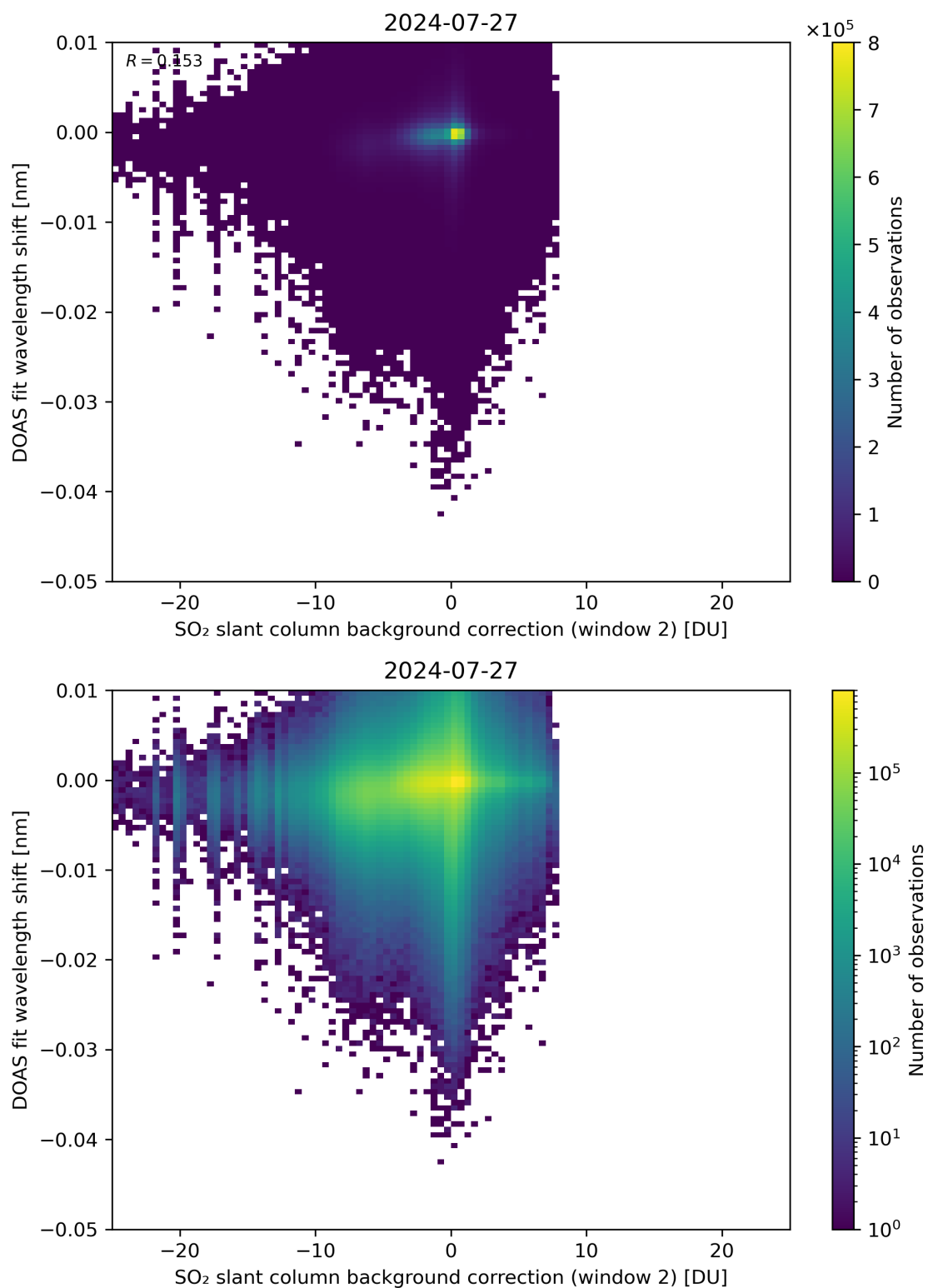
Figure 112: Scatter density plot of “SO 2 slant column background correction (window 2)” against “DOAS fit wavelength shift” for 2024-07-26 to 2024-07-28.
