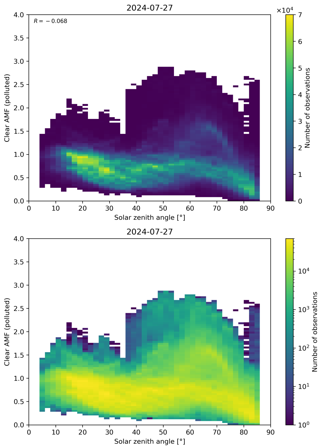
Figure 165: Scatter density plot of “Solar zenith angle” against “Clear AMF (polluted)” for 2024-07-26 to 2024-07-28.
