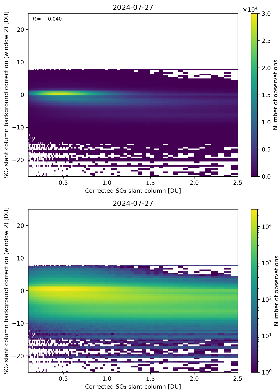
Figure 179: Scatter density plot of “Corrected SO 2 slant column” against “SO 2 slant column background correction (window 2)” for 2024-07-26 to 2024-07-28.
