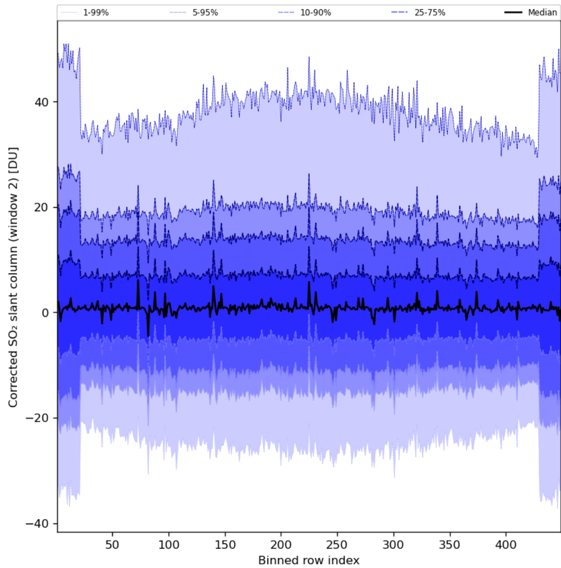
Figure 85: Along track statistics of “Corrected SO 2 slant column (window 2)” for 2024-07-26 to 2024-07-28
