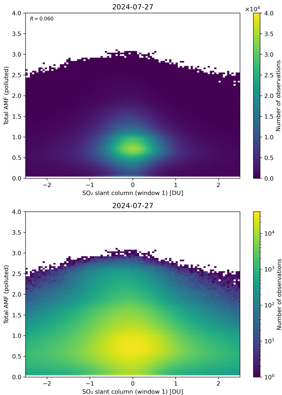
Figure 239: Scatter density plot of “SO 2 slant column (window 1)” against “Total AMF (polluted)” for 2024-07-26 to 2024-07-28.
