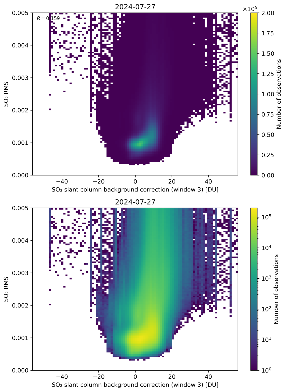
Figure 123: Scatter density plot of “SO 2 slant column background correction (window 3)” against “SO 2 RMS” for 2024-07-26 to 2024-07-28.
