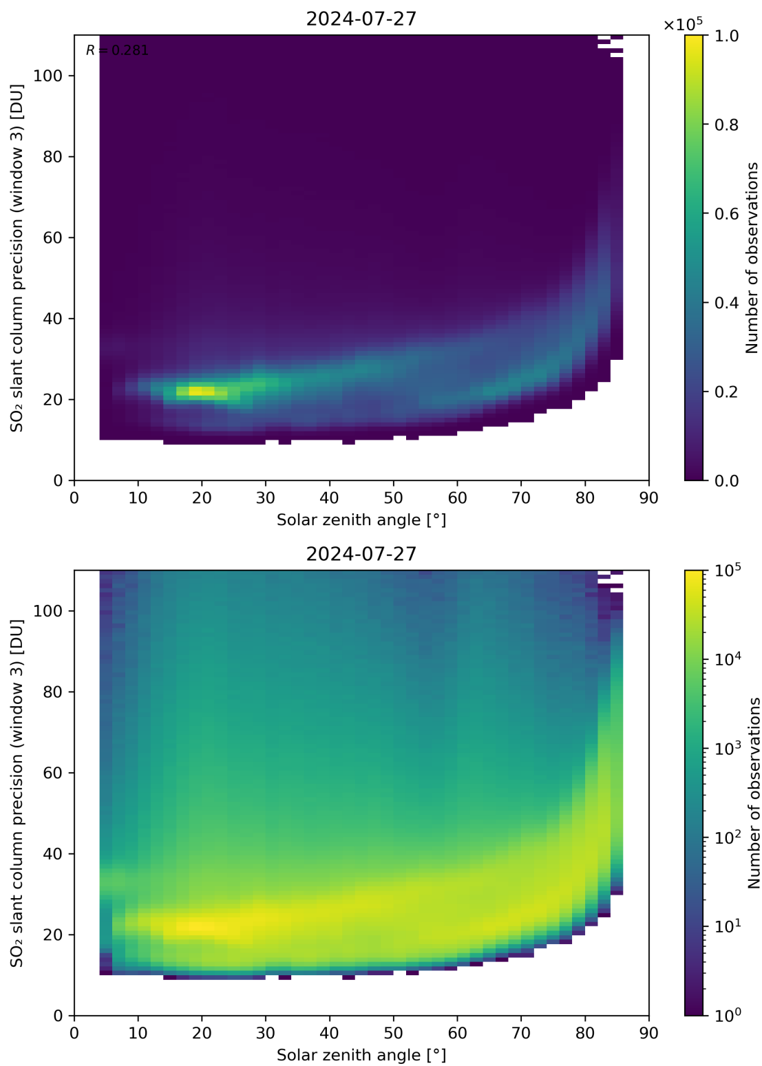
Figure 173: Scatter density plot of “Solar zenith angle” against “SO 2 slant column precision (window 3)” for 2024-07-26 to 2024-07-28.
