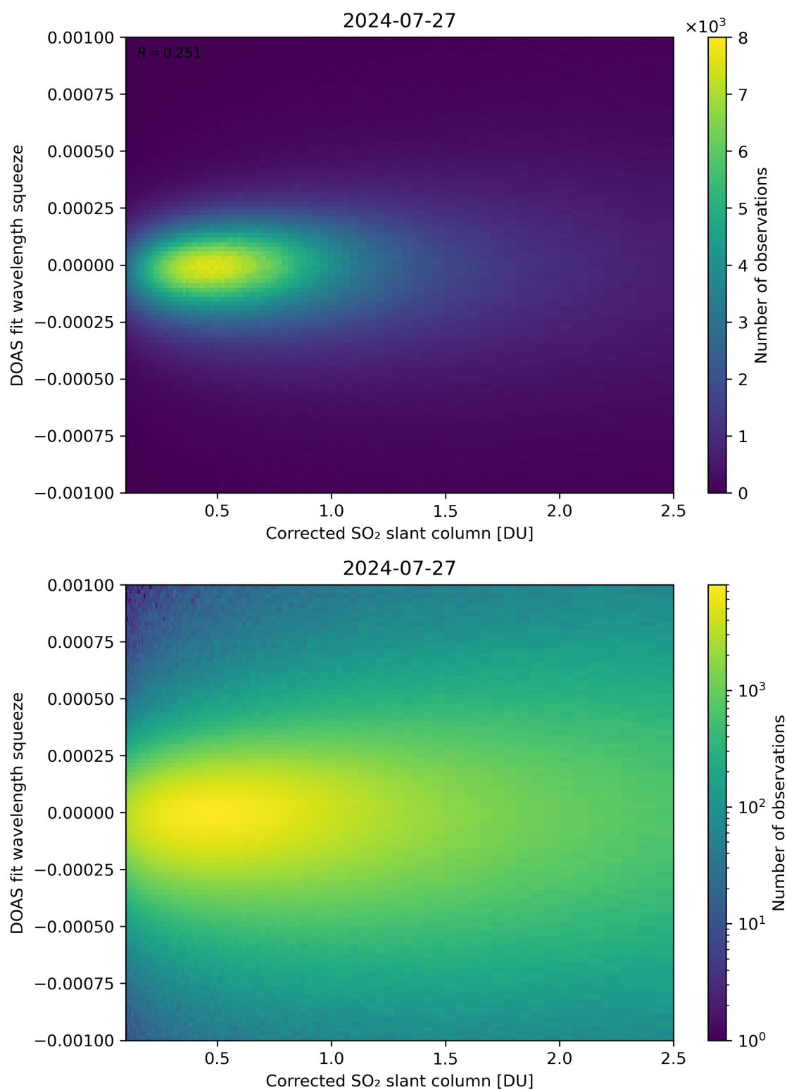
Figure 182: Scatter density plot of “Corrected SO 2 slant column” against “DOAS fit wavelength squeeze” for 2024-07-26 to 2024-07-28.
