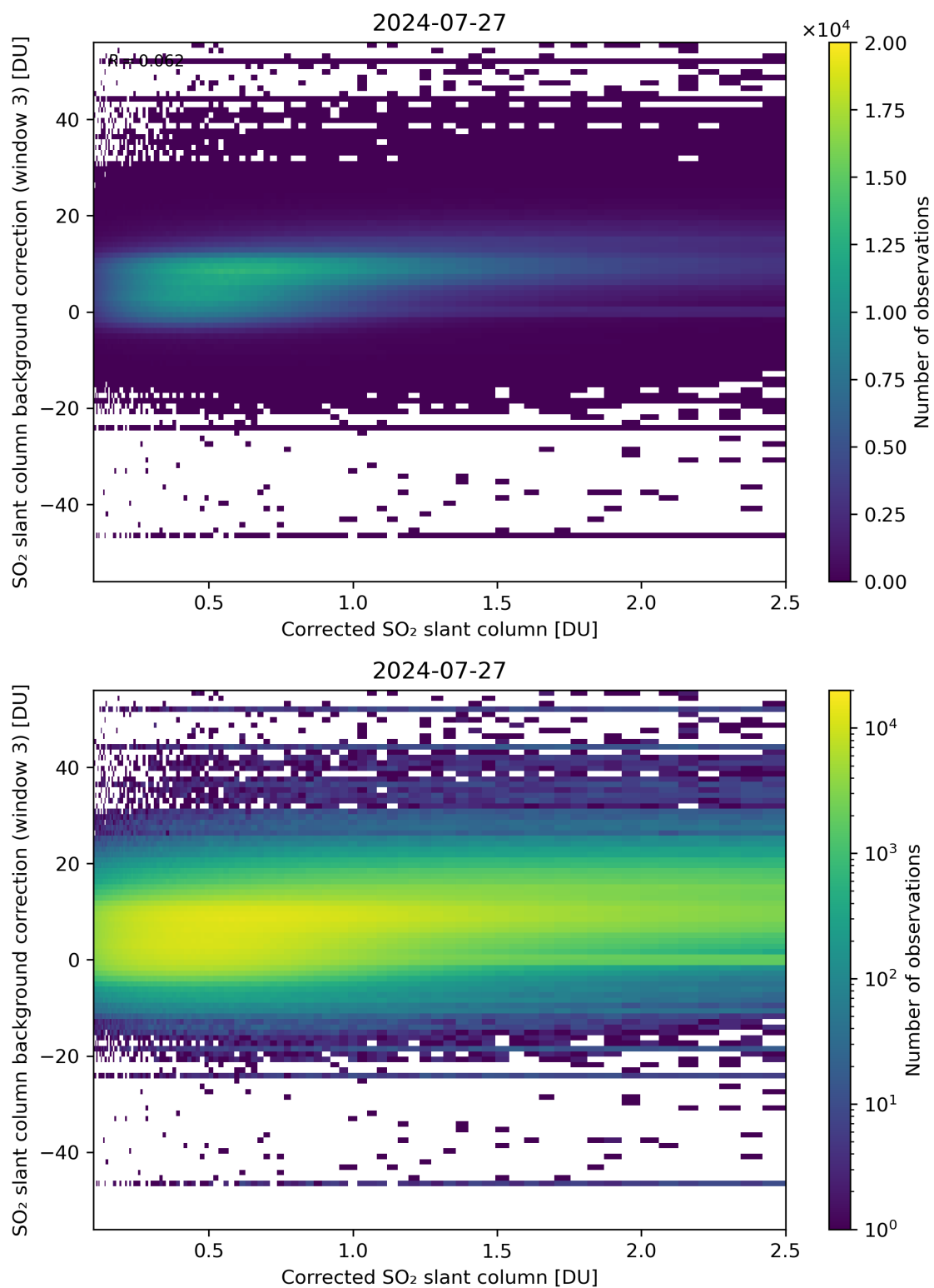
Figure 180: Scatter density plot of “Corrected SO 2 slant column” against “SO 2 slant column background correction (window 3)” for 2024-07-26 to 2024-07-28.
