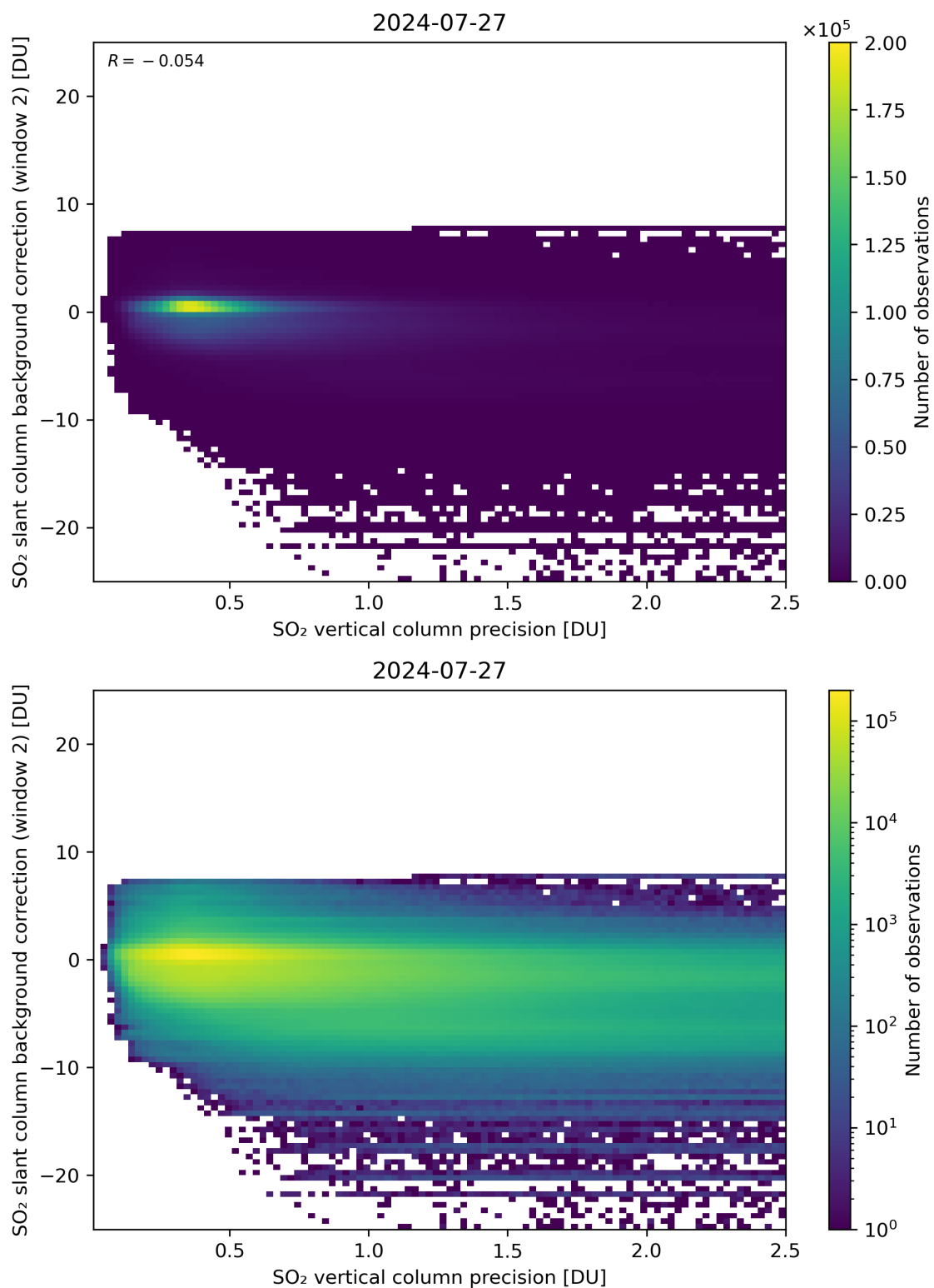
Figure 280: Scatter density plot of “SO 2 vertical column precision” against “SO 2 slant column background correction (window 2)” for 2024-07-26 to 2024-07-28.
