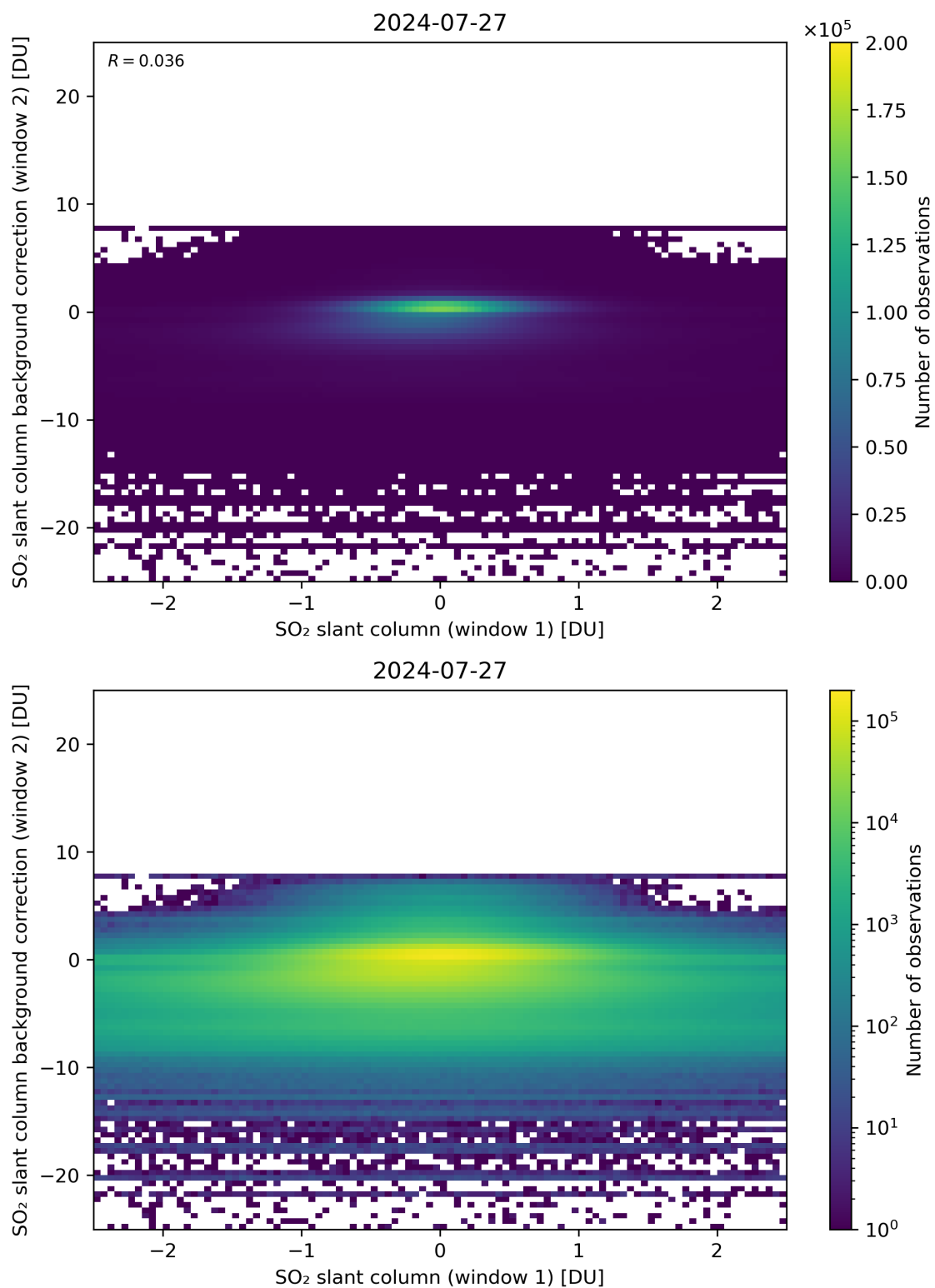
Figure 213: Scatter density plot of “SO 2 slant column (window 1)” against “SO 2 slant column background correction (window 2)” for 2024-07-26 to 2024-07-28.
