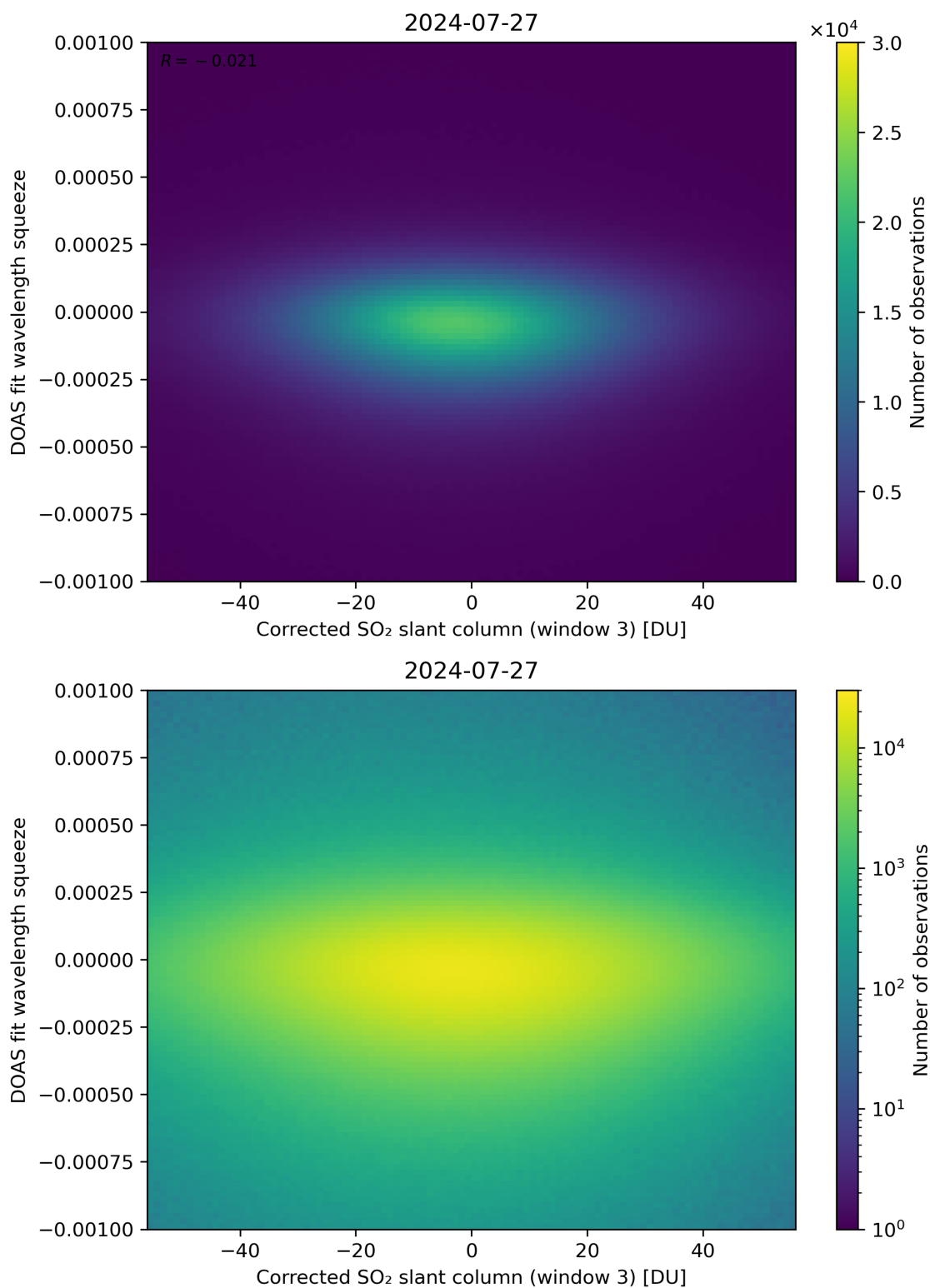
Figure 207: Scatter density plot of “Corrected SO 2 slant column (window 3)” against “DOAS fit wavelength squeeze” for 2024-07-26 to 2024-07-28.
