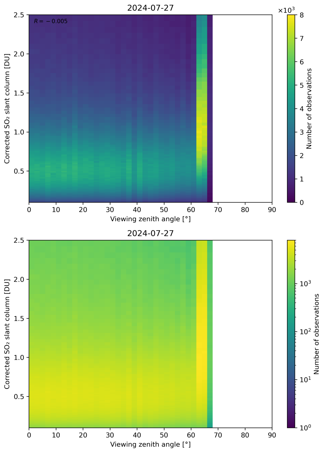
Figure 317: Scatter density plot of “Viewing zenith angle” against “Corrected SO 2 slant column” for 2024-07-26 to 2024-07-28.
