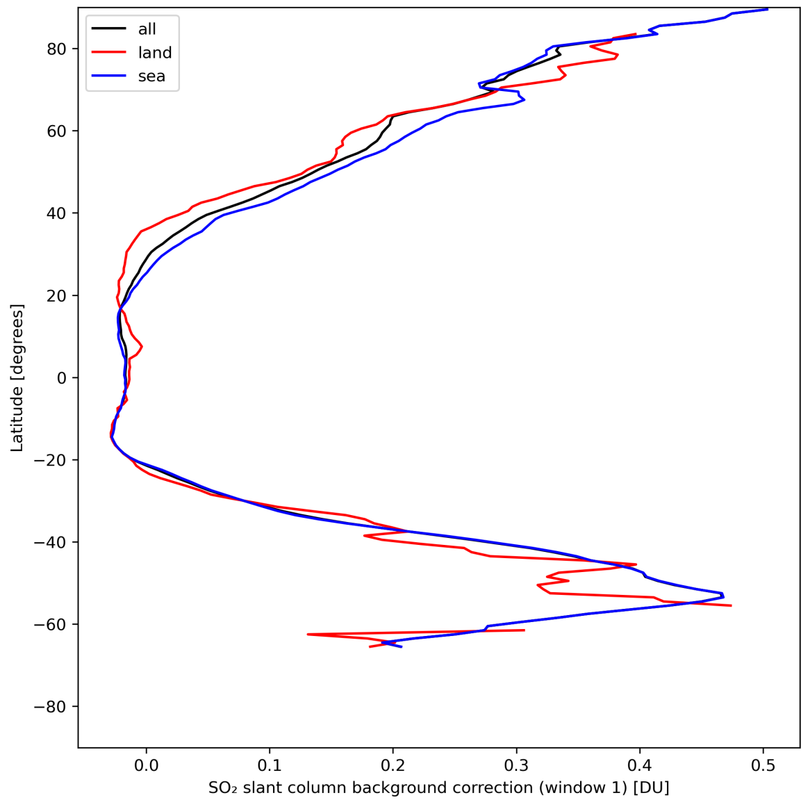
Figure 36: Zonal average of “SO 2 slant column background correction (window 1)” for 2024-07-26 to 2024-07-28.
