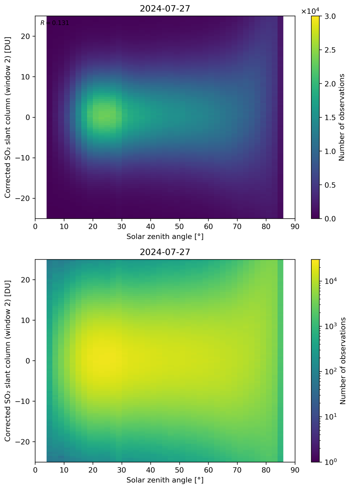
Figure 167: Scatter density plot of “Solar zenith angle” against “Corrected SO 2 slant column (window 2)” for 2024-07-26 to 2024-07-28.
