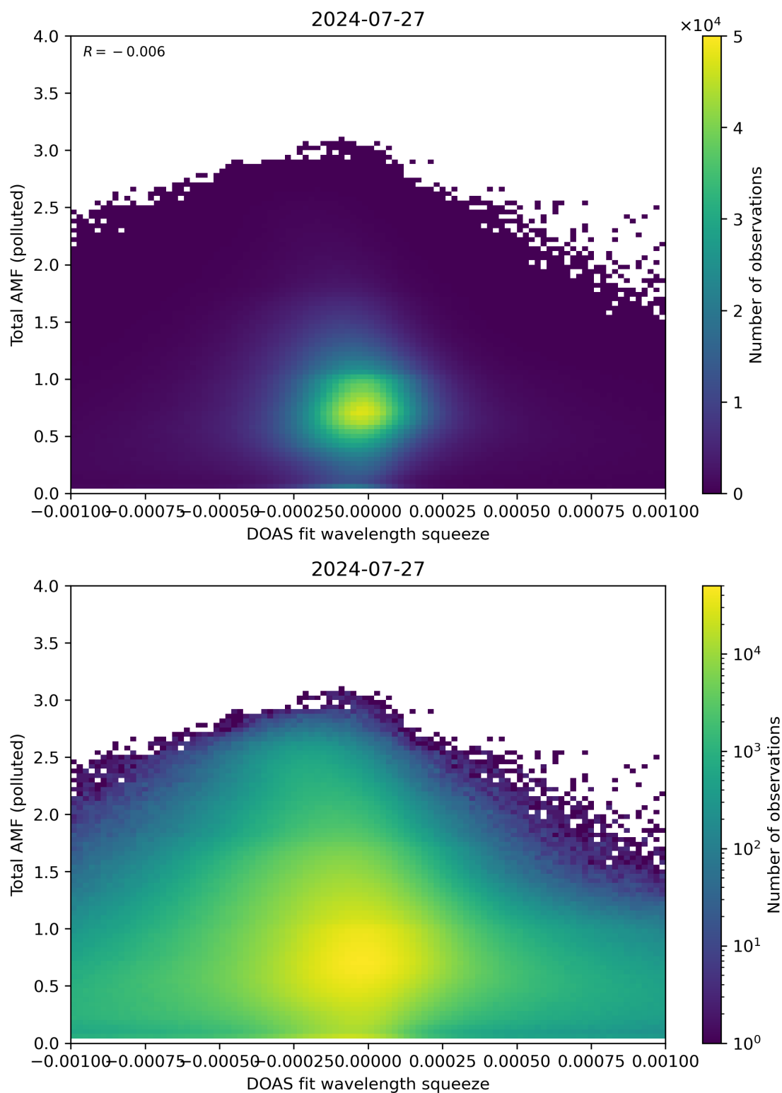
Figure 134: Scatter density plot of “DOAS fit wavelength squeeze” against “Total AMF (polluted)” for 2024-07-26 to 2024-07-28.
