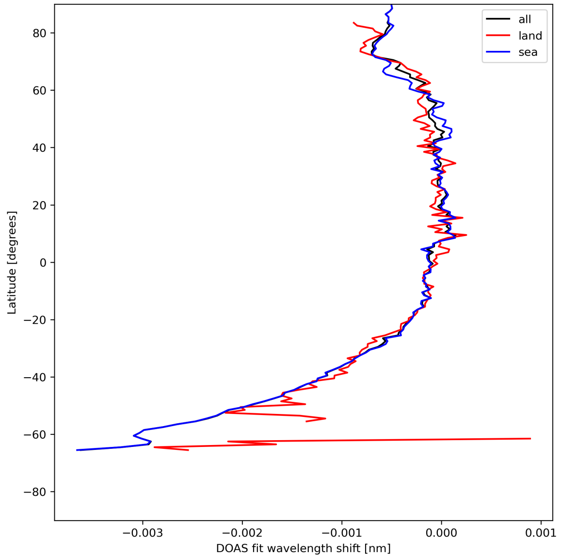
Figure 45: Zonal average of “DOAS fit wavelength shift” for 2024-07-26 to 2024-07-28.
