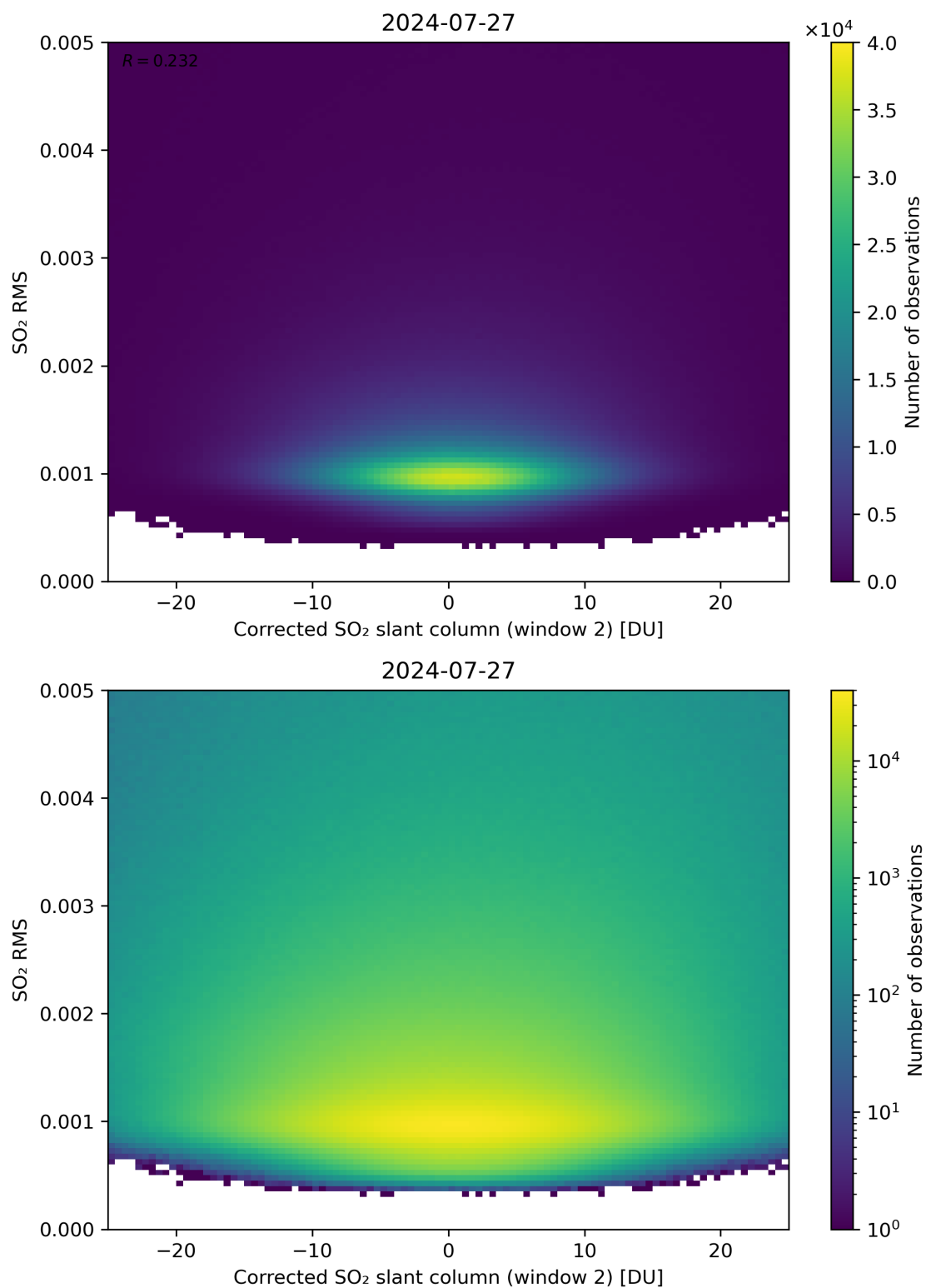
Figure 198: Scatter density plot of “Corrected SO 2 slant column (window 2)” against “SO 2 RMS” for 2024-07-26 to 2024-07-28.
