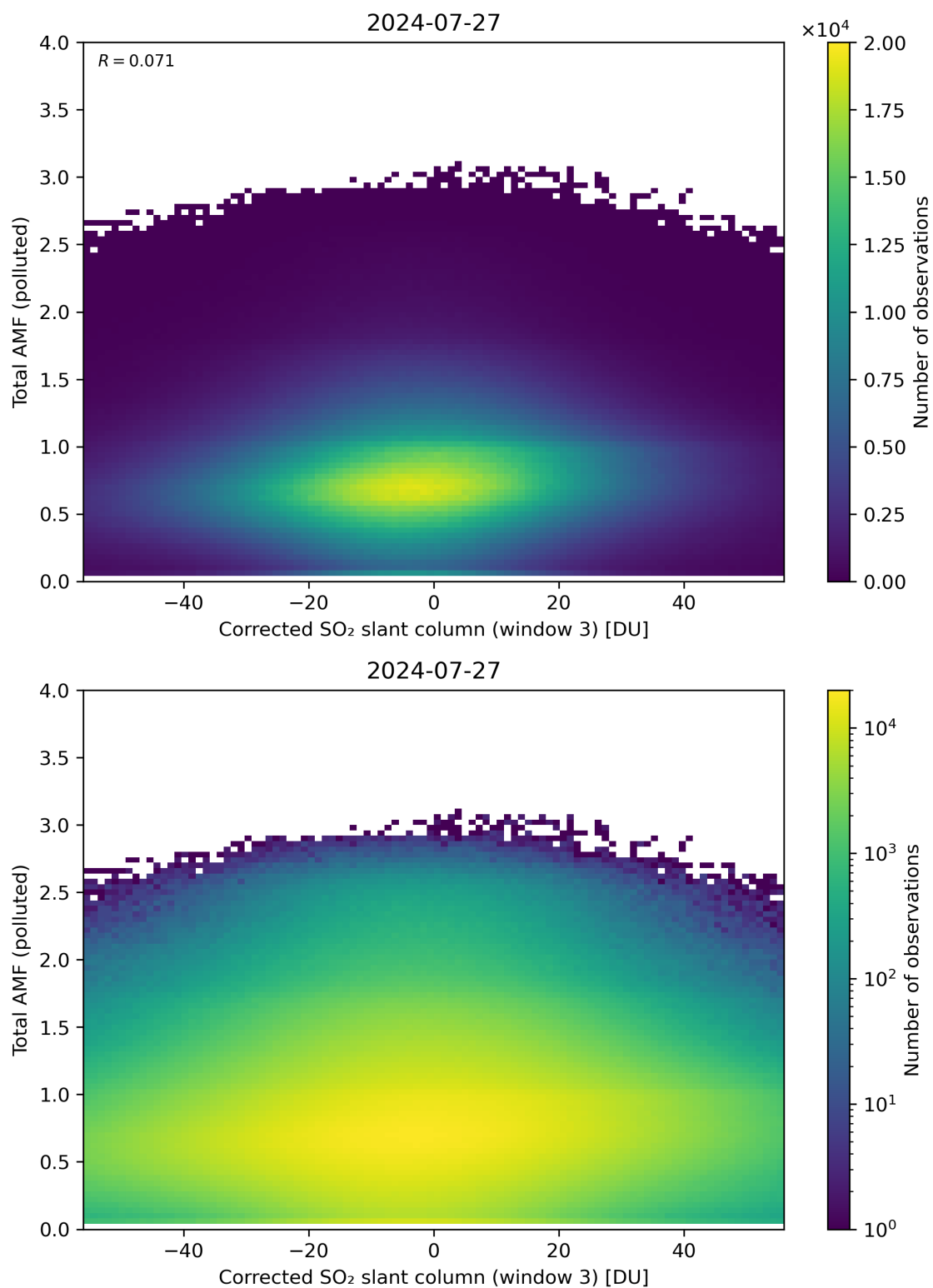
Figure 210: Scatter density plot of “Corrected SO 2 slant column (window 3)” against “Total AMF (polluted)” for 2024-07-26 to 2024-07-28.
