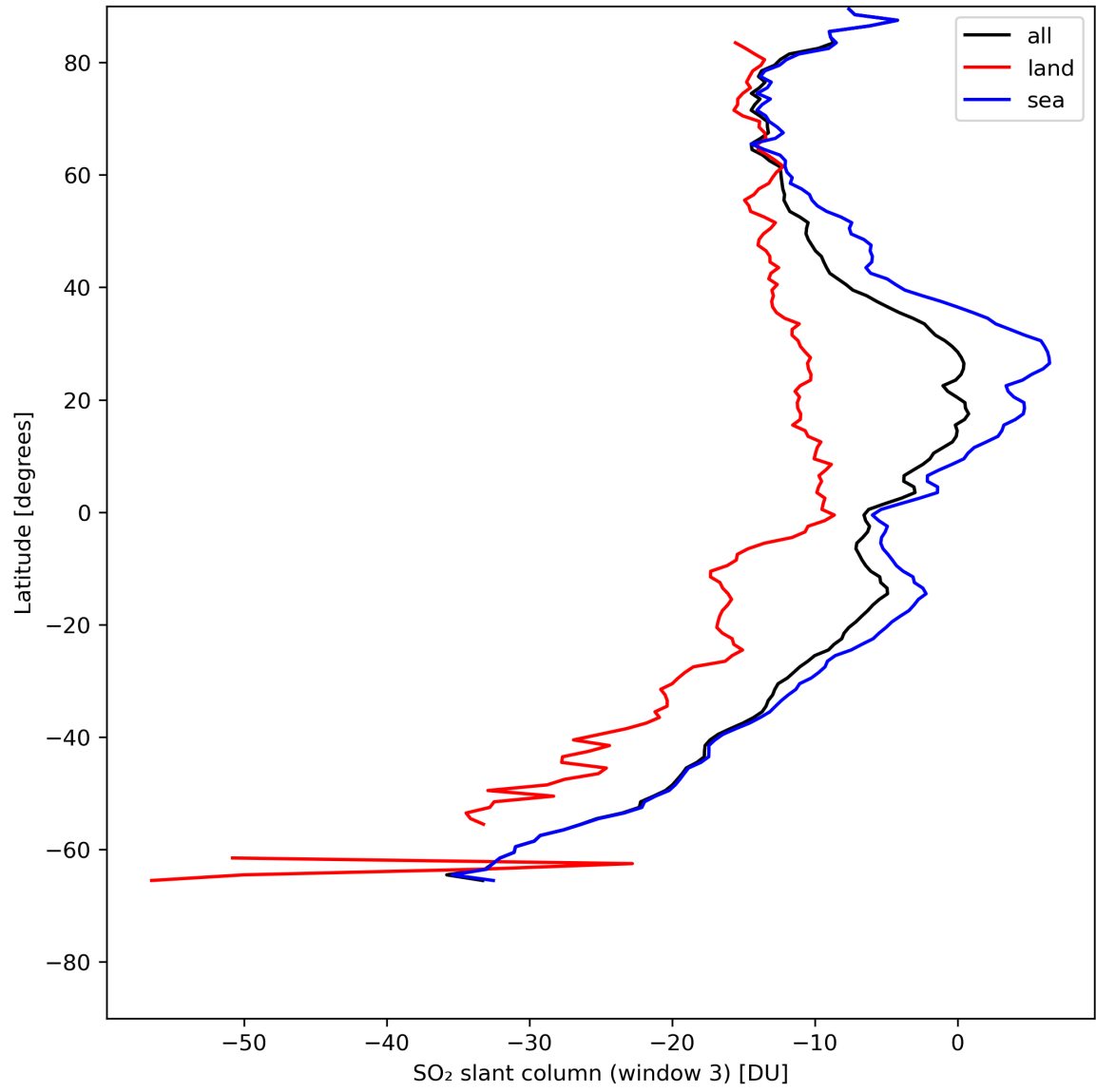
Figure 41: Zonal average of “SO 2 slant column (window 3)” for 2024-07-26 to 2024-07-28.
