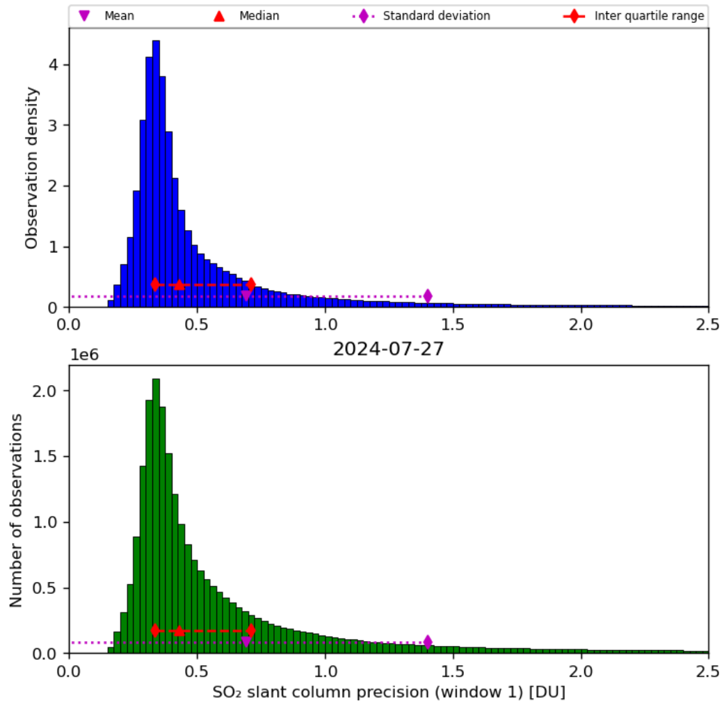
Figure 57: Histogram of “SO 2 slant column precision (window 1)” for 2024-07-26 to 2024-07-28
