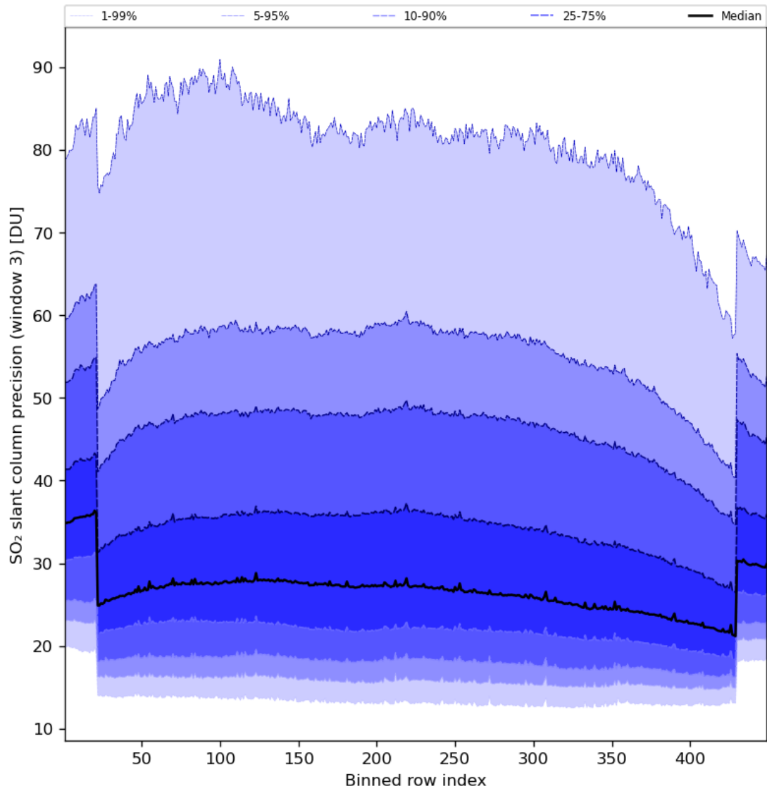
Figure 88: Along track statistics of “SO 2 slant column precision (window 3)” for 2024-07-26 to 2024-07-28
