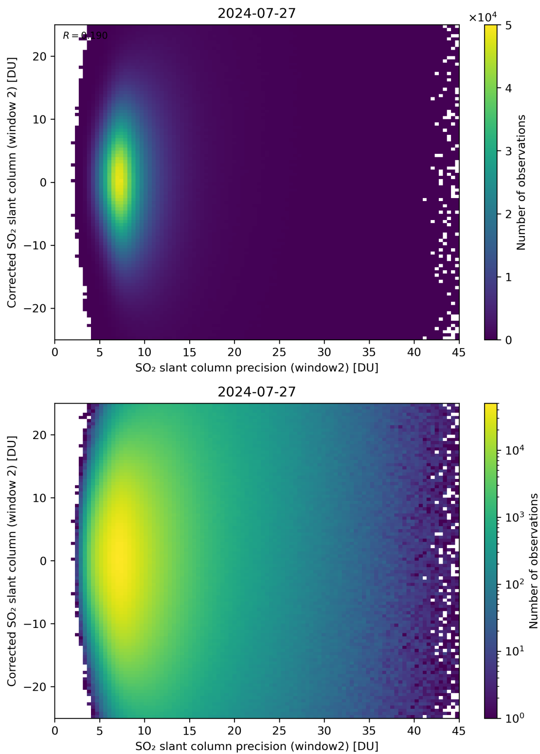
Figure 247: Scatter density plot of “SO 2 slant column precision (window2)” against “Corrected SO 2 slant column (window 2)” for 2024-07-26 to 2024-07-28.
