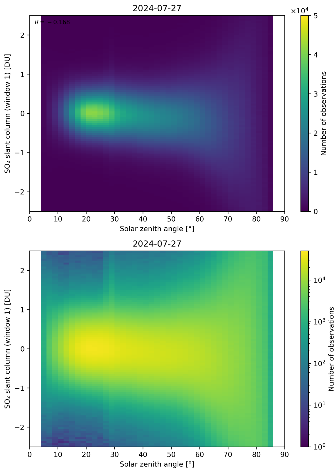
Figure 169: Scatter density plot of “Solar zenith angle” against “SO 2 slant column (window 1)” for 2024-07-26 to 2024-07-28.
