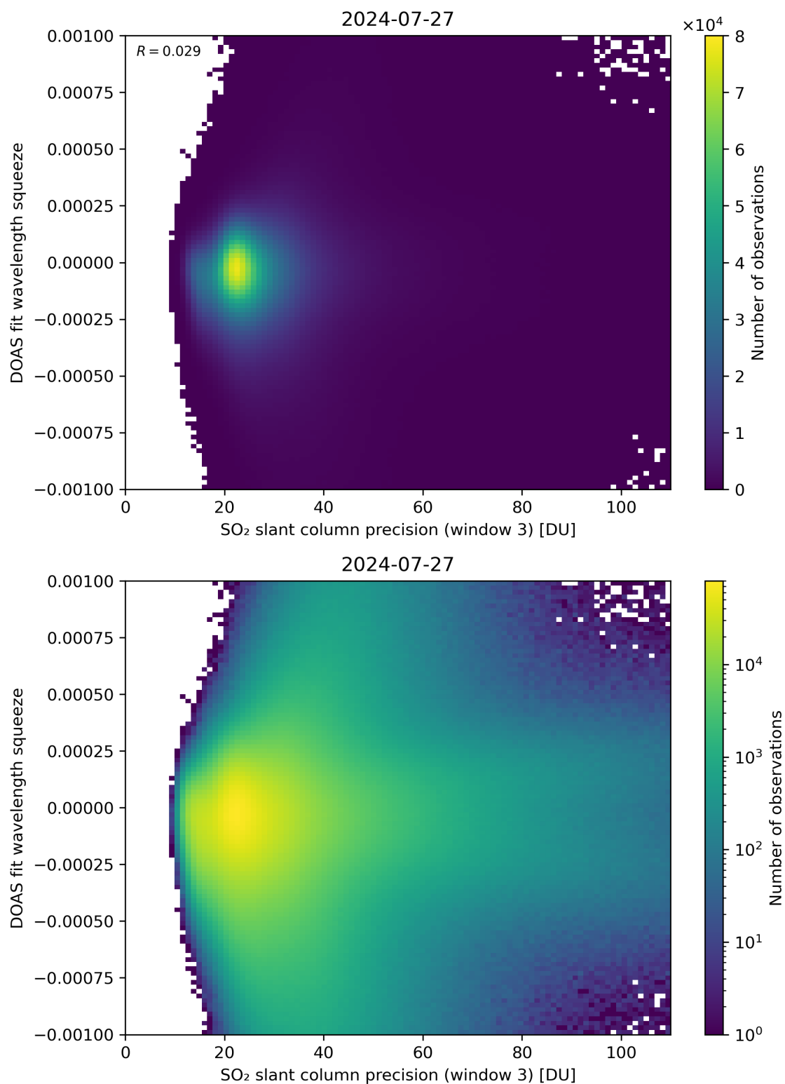
Figure 259: Scatter density plot of “SO 2 slant column precision (window 3)” against “DOAS fit wavelength squeeze” for 2024-07-26 to 2024-07-28.
