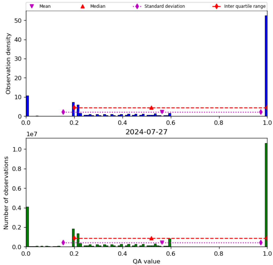
Figure 52: Histogram of “QA value” for 2024-07-26 to 2024-07-28
