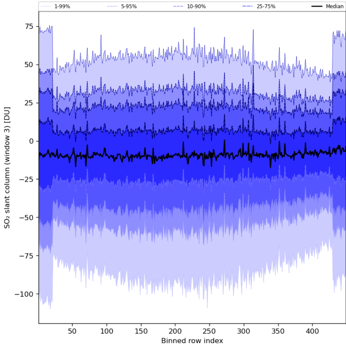
Figure 87: Along track statistics of “SO 2 slant column (window 3)” for 2024-07-26 to 2024-07-28
