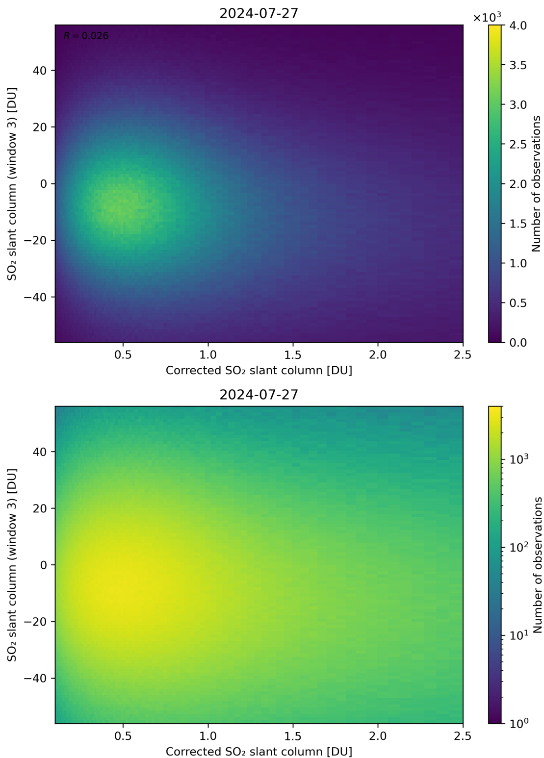
Figure 190: Scatter density plot of “Corrected SO 2 slant column” against “SO 2 slant column (window 3)” for 2024-07-26 to 2024-07-28.
