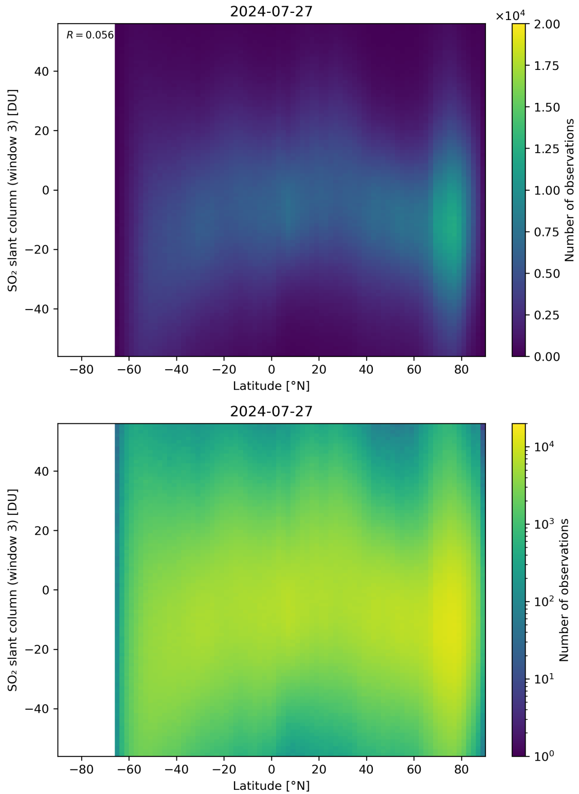
Figure 152: Scatter density plot of “Latitude” against “SO 2 slant column (window 3)” for 2024-07-26 to 2024-07-28.
