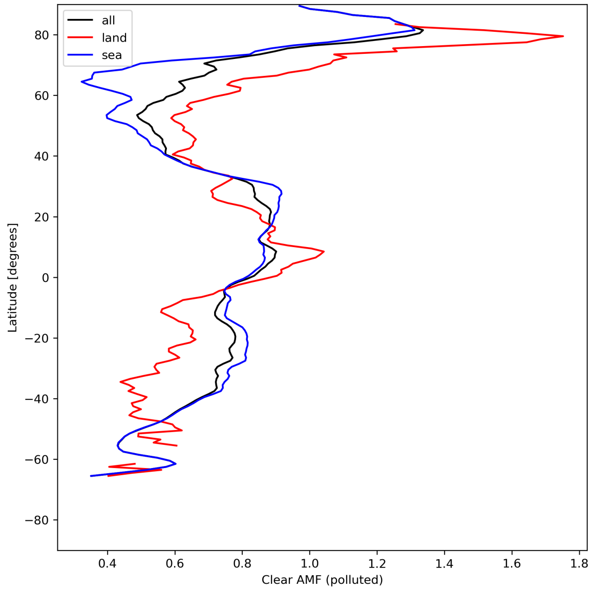
Figure 50: Zonal average of “Clear AMF (polluted)” for 2024-07-26 to 2024-07-28.
