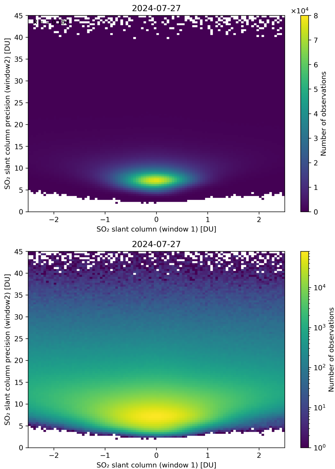
Figure 236: Scatter density plot of “SO 2 slant column (window 1)” against “SO 2 slant column precision (window2)” for 2024-07-26 to 2024-07-28.
