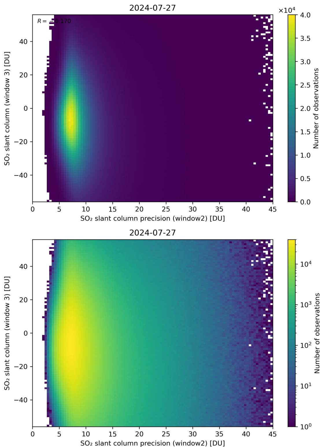
Figure 249: Scatter density plot of “SO 2 slant column precision (window2)” against “SO 2 slant column (window 3)” for 2024-07-26 to 2024-07-28.
