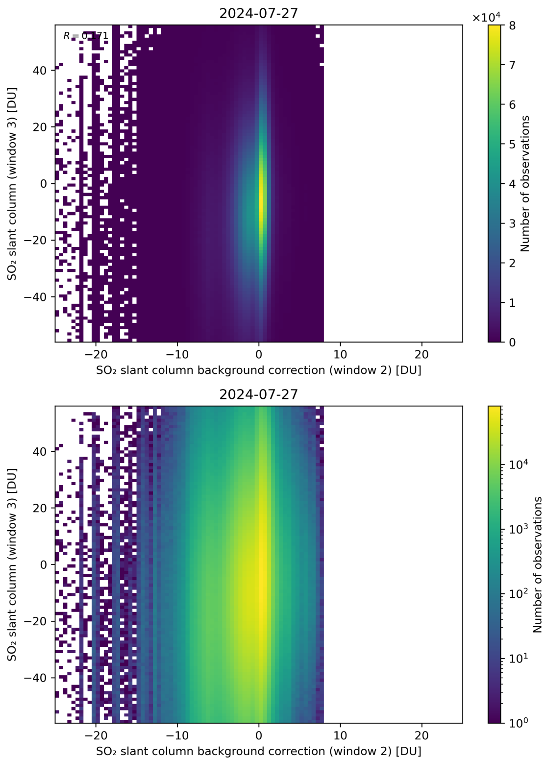
Figure 117: Scatter density plot of “SO 2 slant column background correction (window 2)” against “SO 2 slant column (window 3)” for 2024-07-26 to 2024-07-28.
