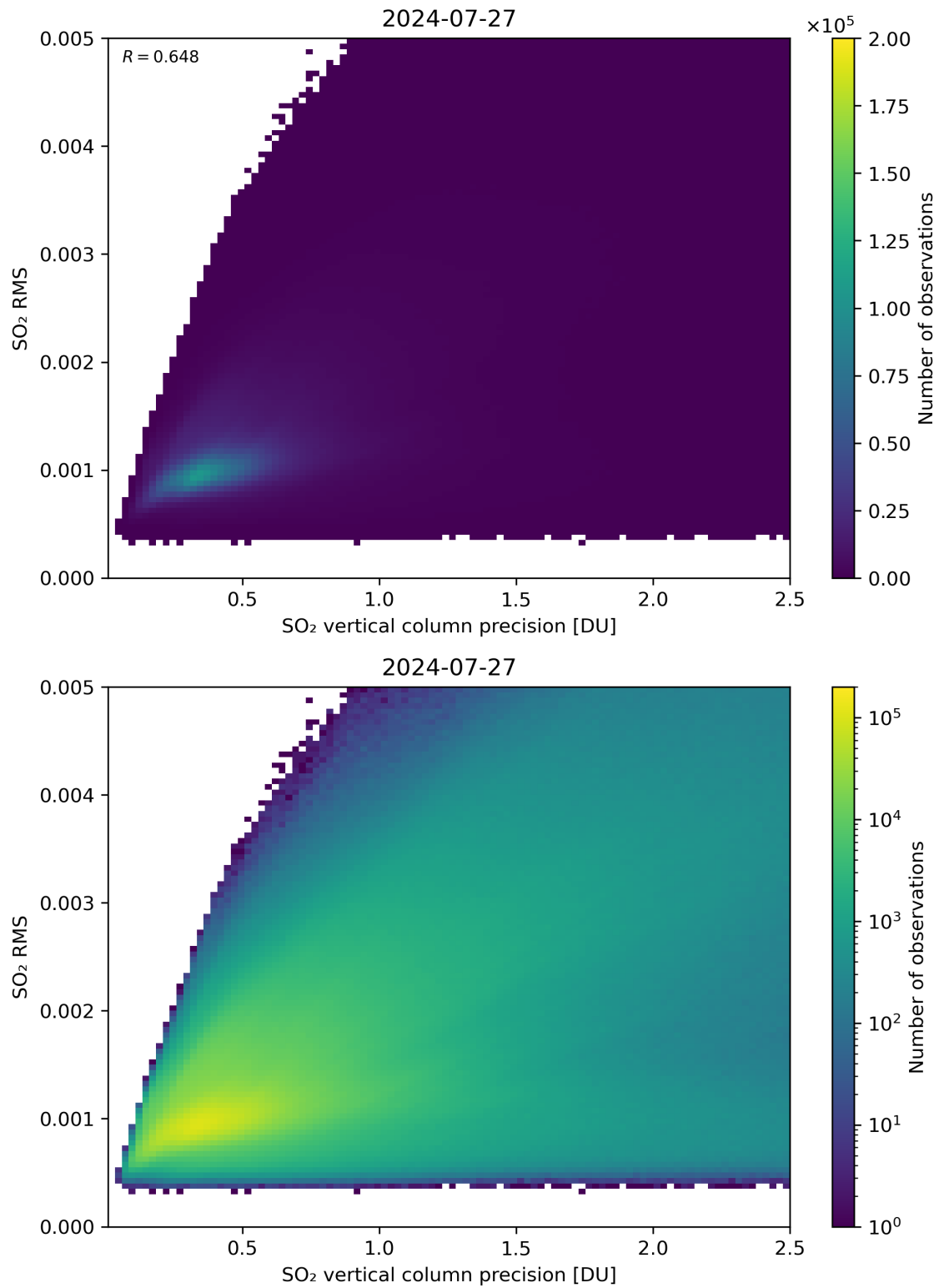
Figure 284: Scatter density plot of “SO 2 vertical column precision” against “SO 2 RMS” for 2024-07-26 to 2024-07-28.
