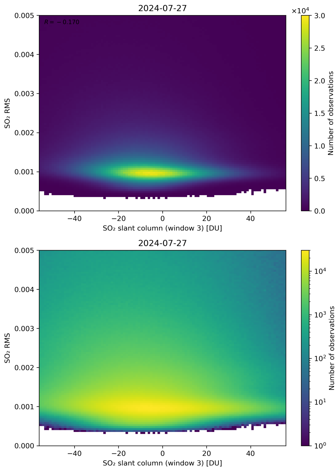
Figure 256: Scatter density plot of “SO 2 slant column (window 3)” against “SO 2 RMS” for 2024-07-26 to 2024-07-28.
