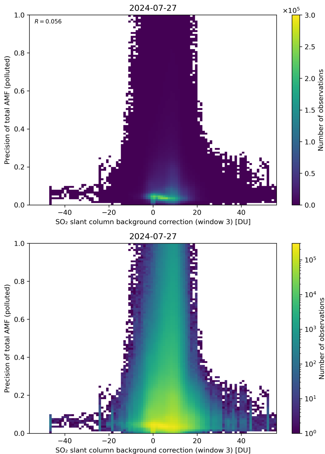
Figure 126: Scatter density plot of “SO 2 slant column background correction (window 3)” against “Precision of total AMF (polluted)” for 2024-07-26 to 2024-07-28.
