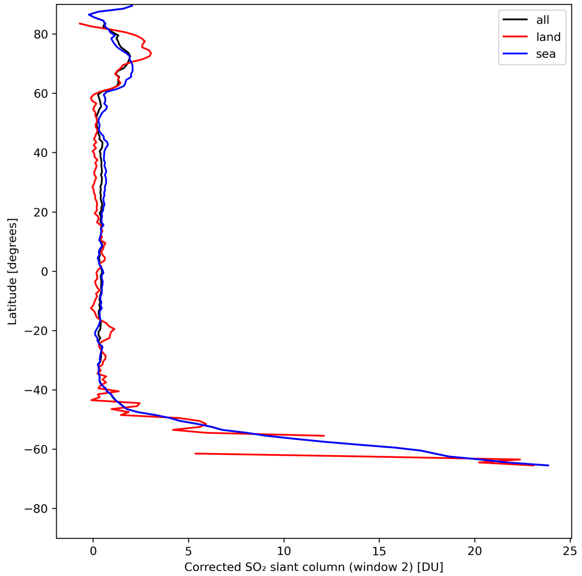
Figure 39: Zonal average of “Corrected SO 2 slant column (window 2)” for 2024-07-26 to 2024-07-28.
