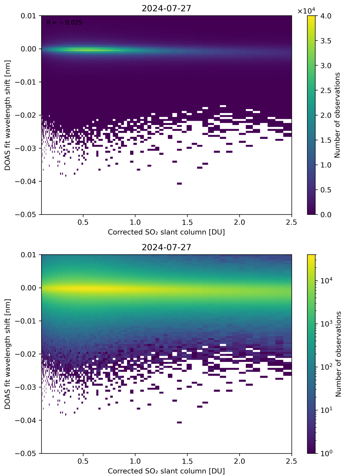
Figure 181: Scatter density plot of “Corrected SO 2 slant column” against “DOAS fit wavelength shift” for 2024-07-26 to 2024-07-28.
