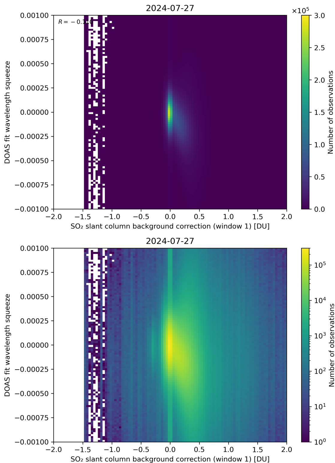
Figure 101: Scatter density plot of “SO 2 slant column background correction (window 1)” against “DOAS fit wavelength squeeze” for 2024-07-26 to 2024-07-28.
