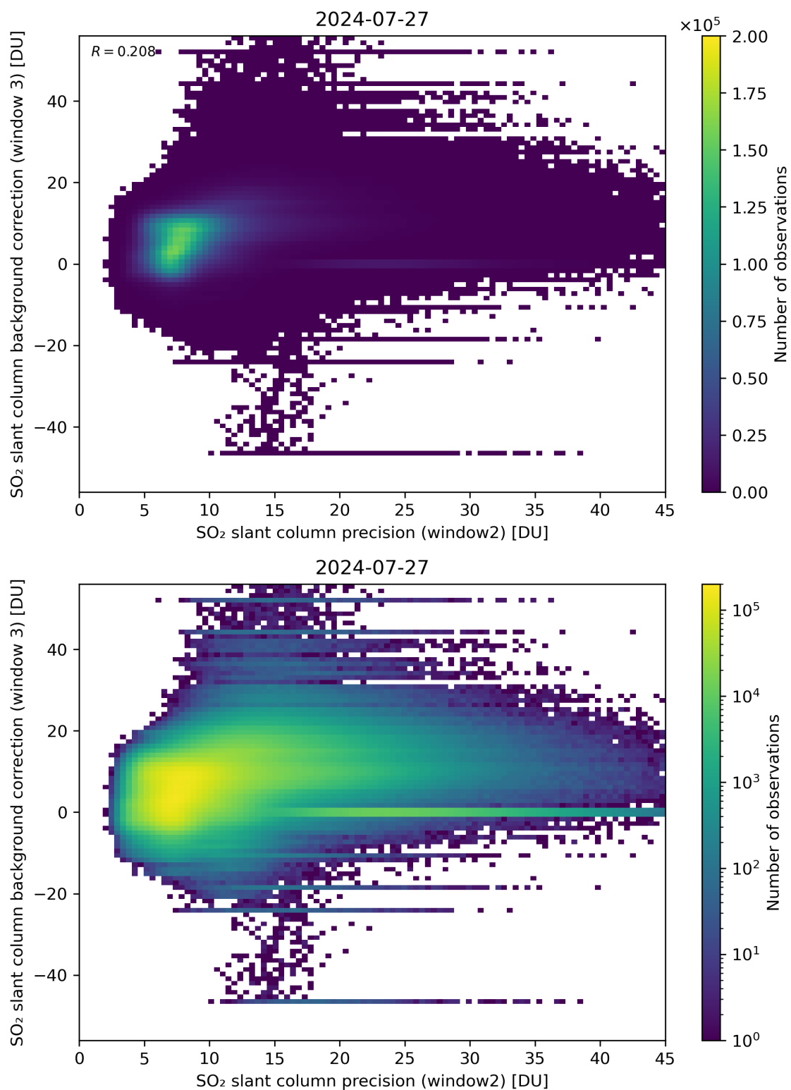
Figure 242: Scatter density plot of “SO 2 slant column precision (window2)” against “SO 2 slant column background correction (window 3)” for 2024-07-26 to 2024-07-28.
