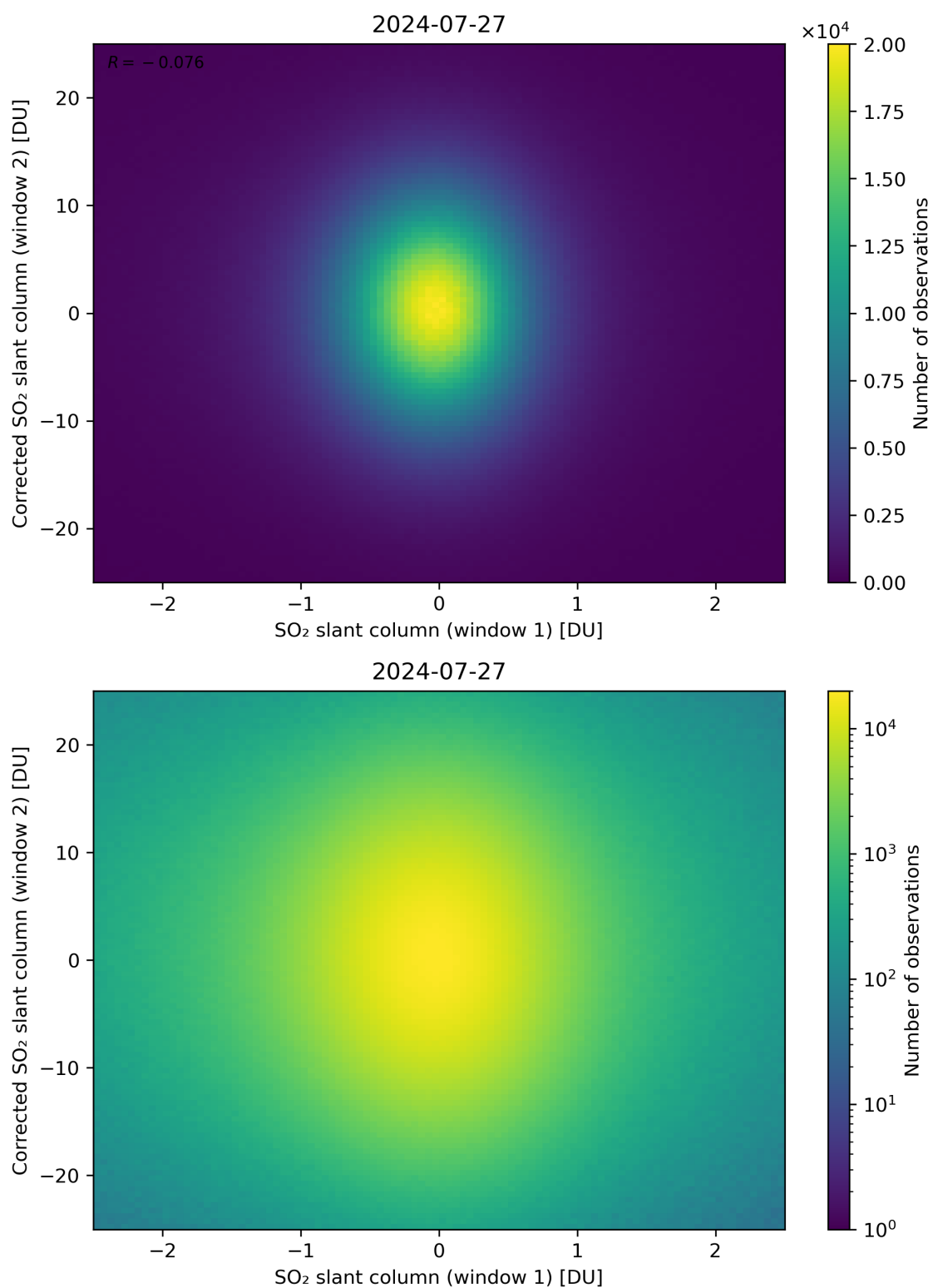
Figure 233: Scatter density plot of “SO 2 slant column (window 1)” against “Corrected SO 2 slant column (window 2)” for 2024-07-26 to 2024-07-28.
