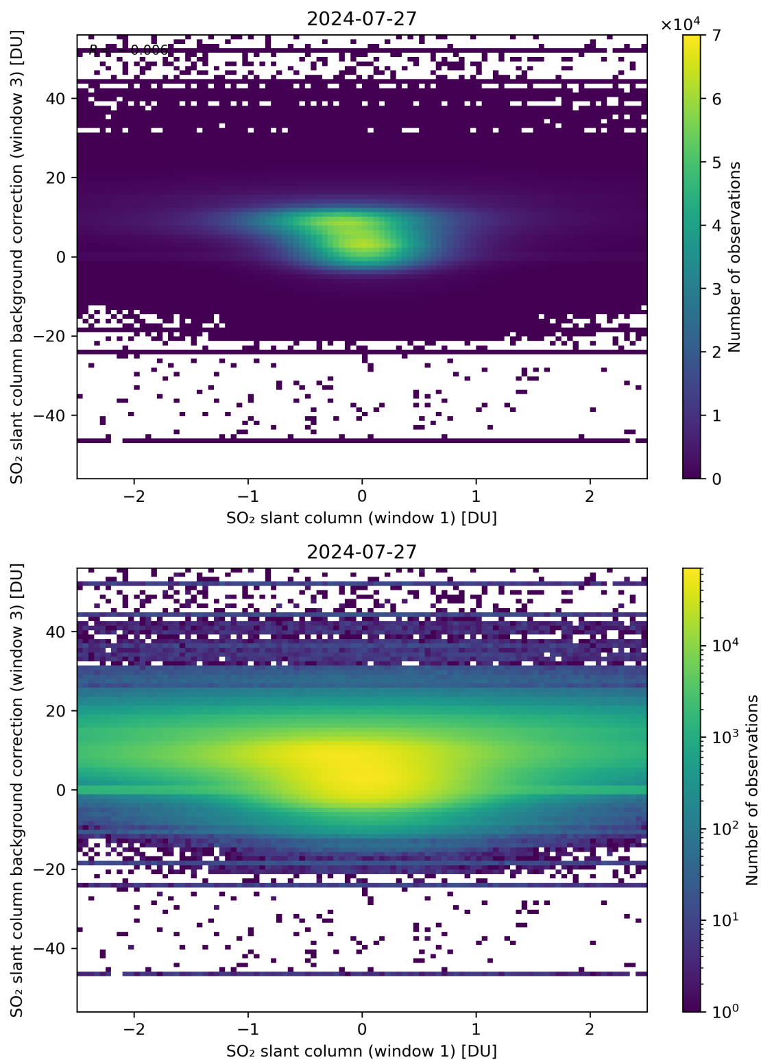
Figure 214: Scatter density plot of “SO 2 slant column (window 1)” against “SO 2 slant column background correction (window 3)” for 2024-07-26 to 2024-07-28.
