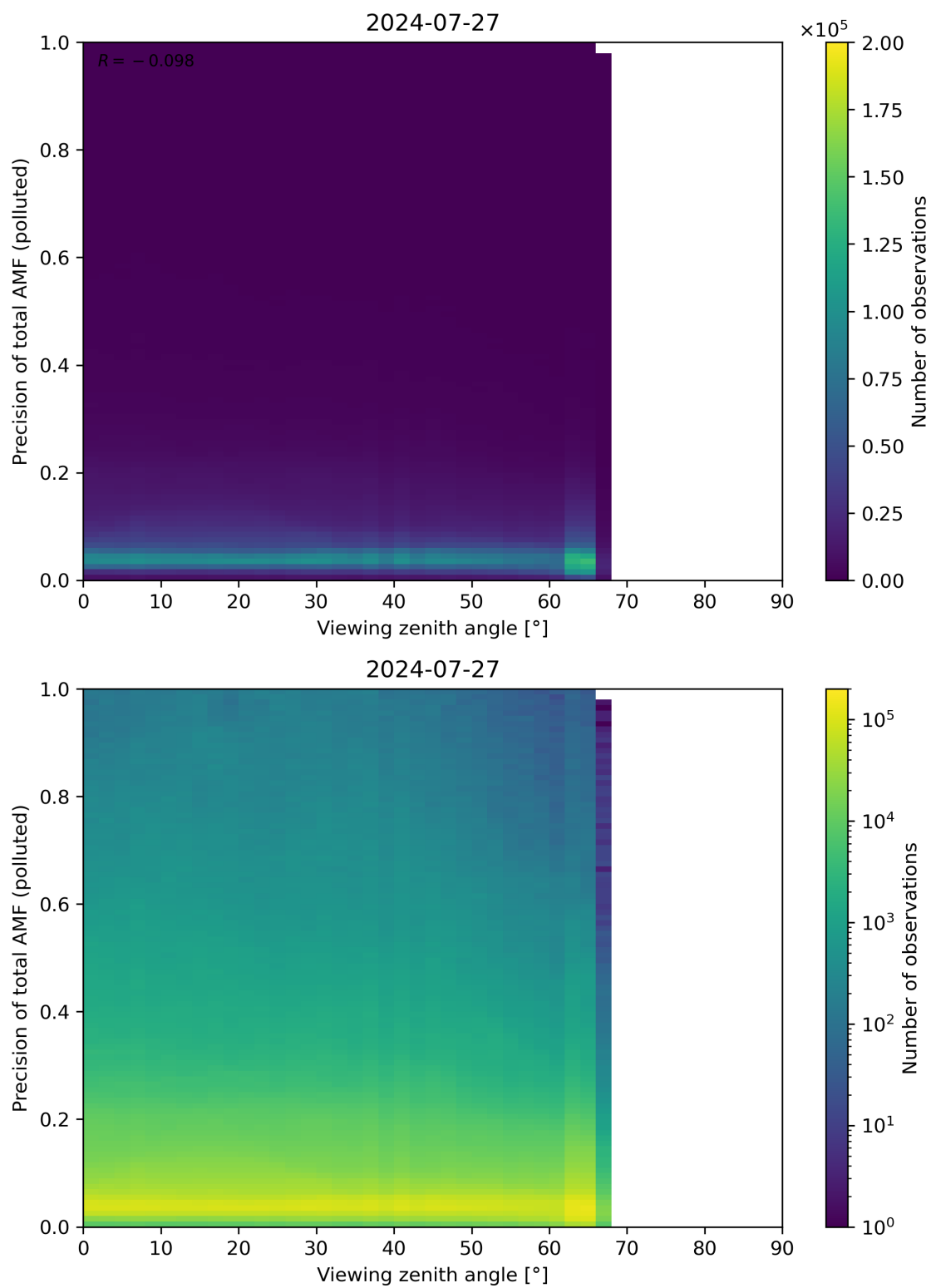
Figure 326: Scatter density plot of “Viewing zenith angle” against “Precision of total AMF (polluted)” for 2024-07-26 to 2024-07-28.
