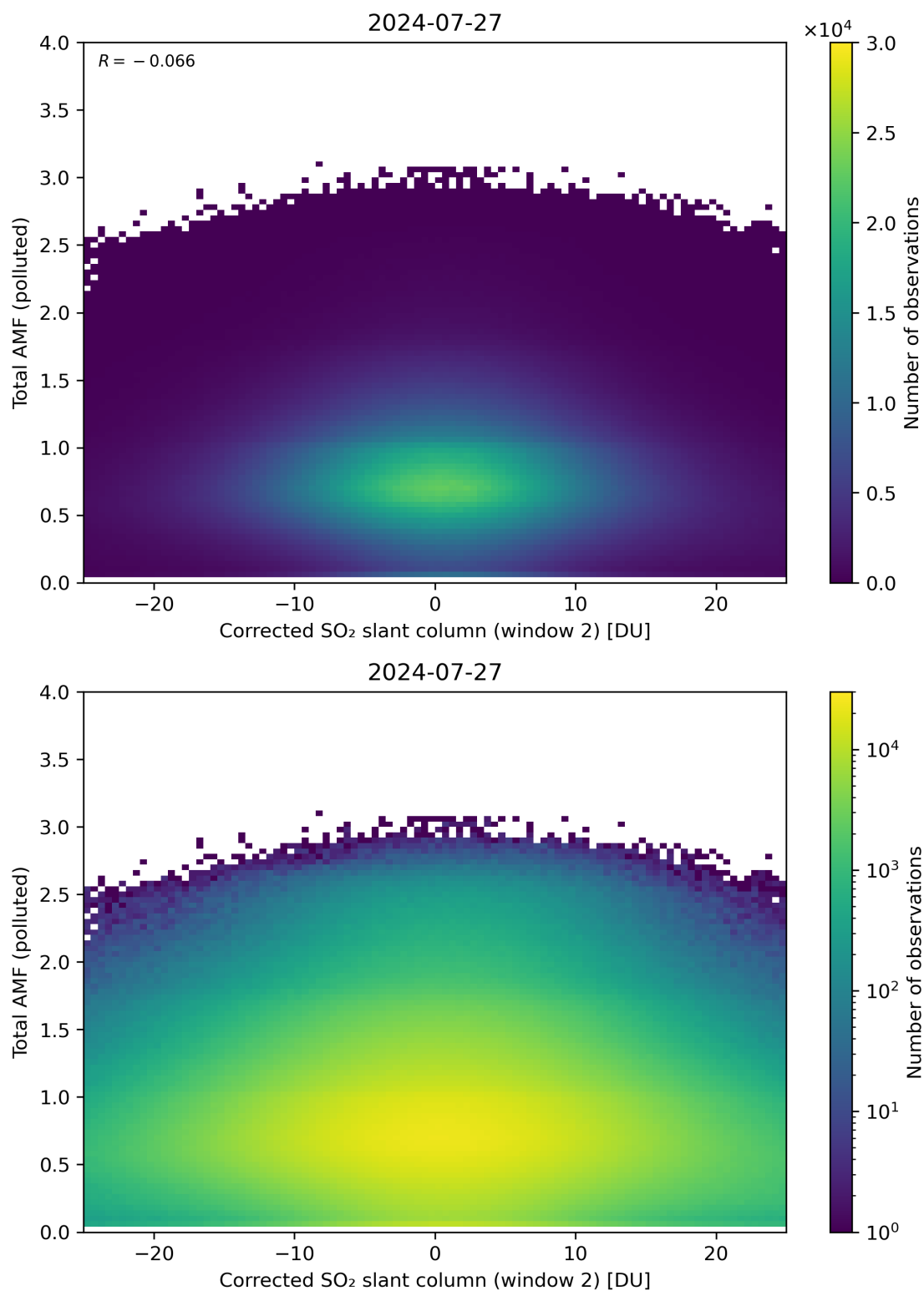
Figure 203: Scatter density plot of “Corrected SO 2 slant column (window 2)” against “Total AMF (polluted)” for 2024-07-26 to 2024-07-28.
