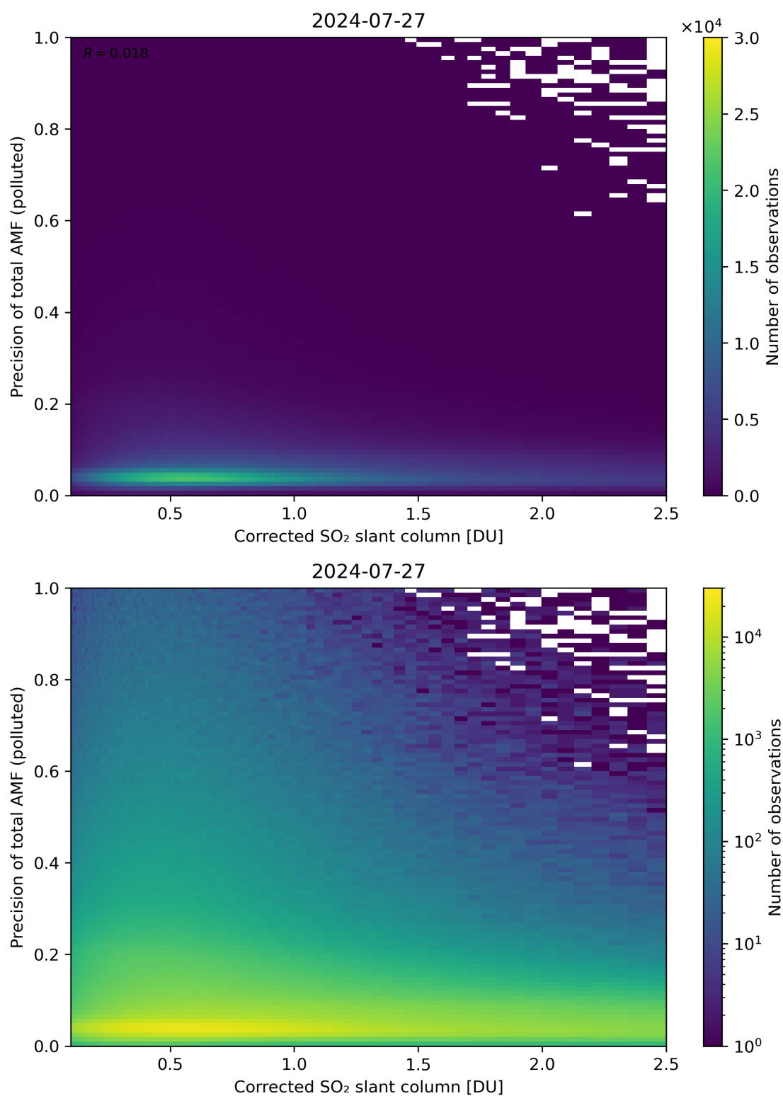
Figure 193: Scatter density plot of “Corrected SO 2 slant column” against “Precision of total AMF (polluted)” for 2024-07-26 to 2024-07-28.
