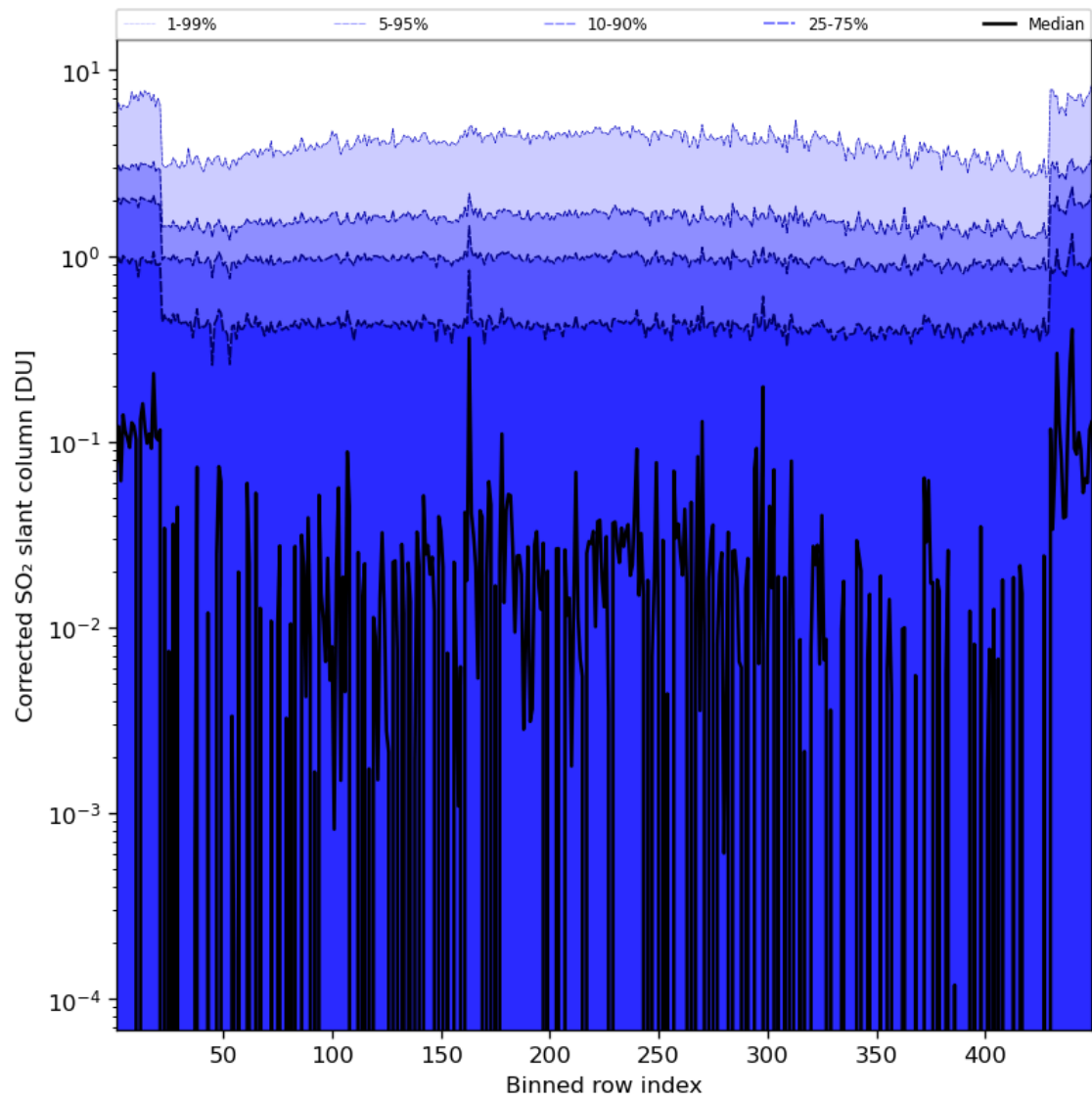
Figure 78: Along track statistics of "Corrected SO 2 slant column" for 2024-07-26 to 2024-07-28
