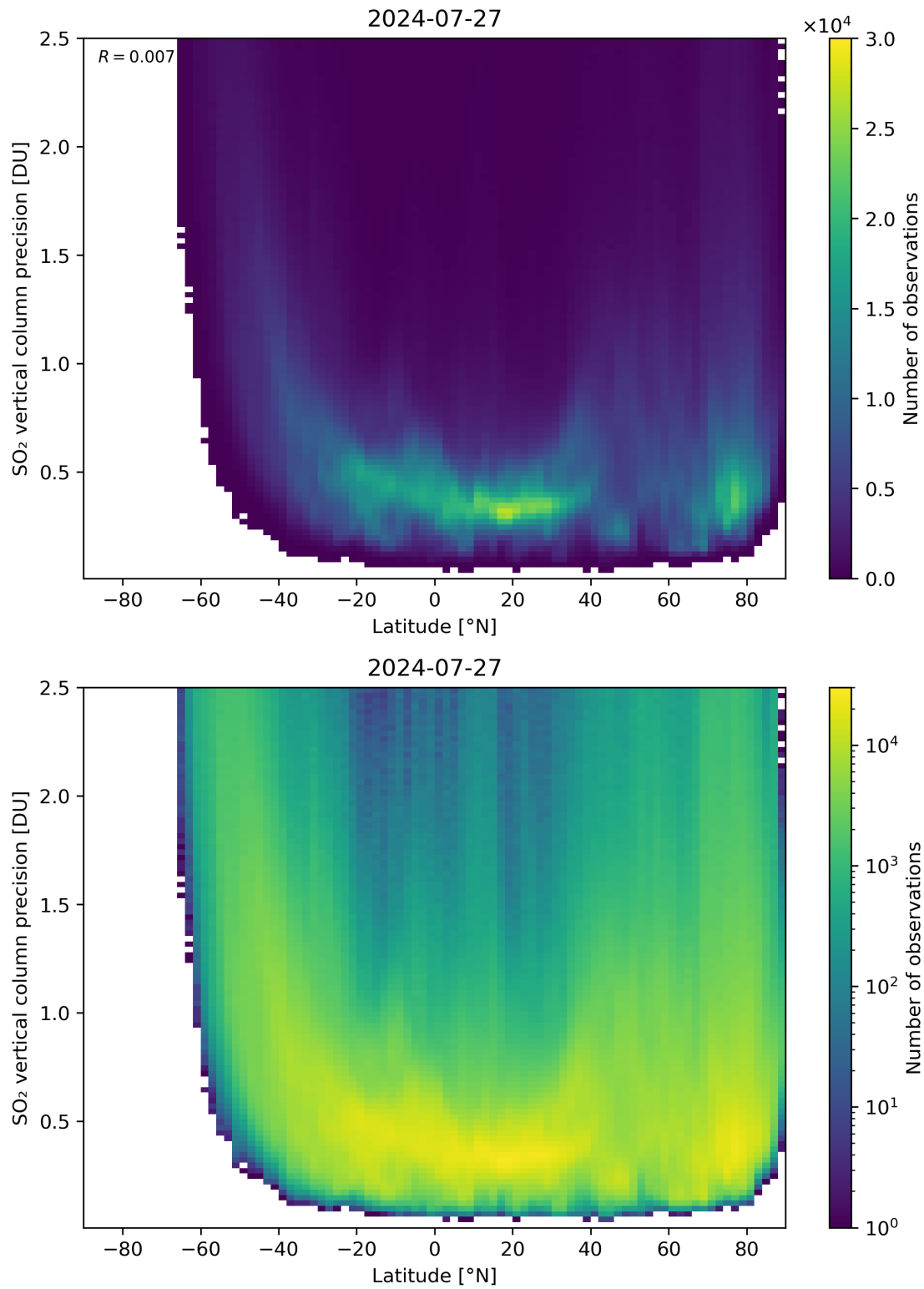
Figure 157: Scatter density plot of “Latitude” against “SO 2 vertical column precision” for 2024-07-26 to 2024-07-28.
