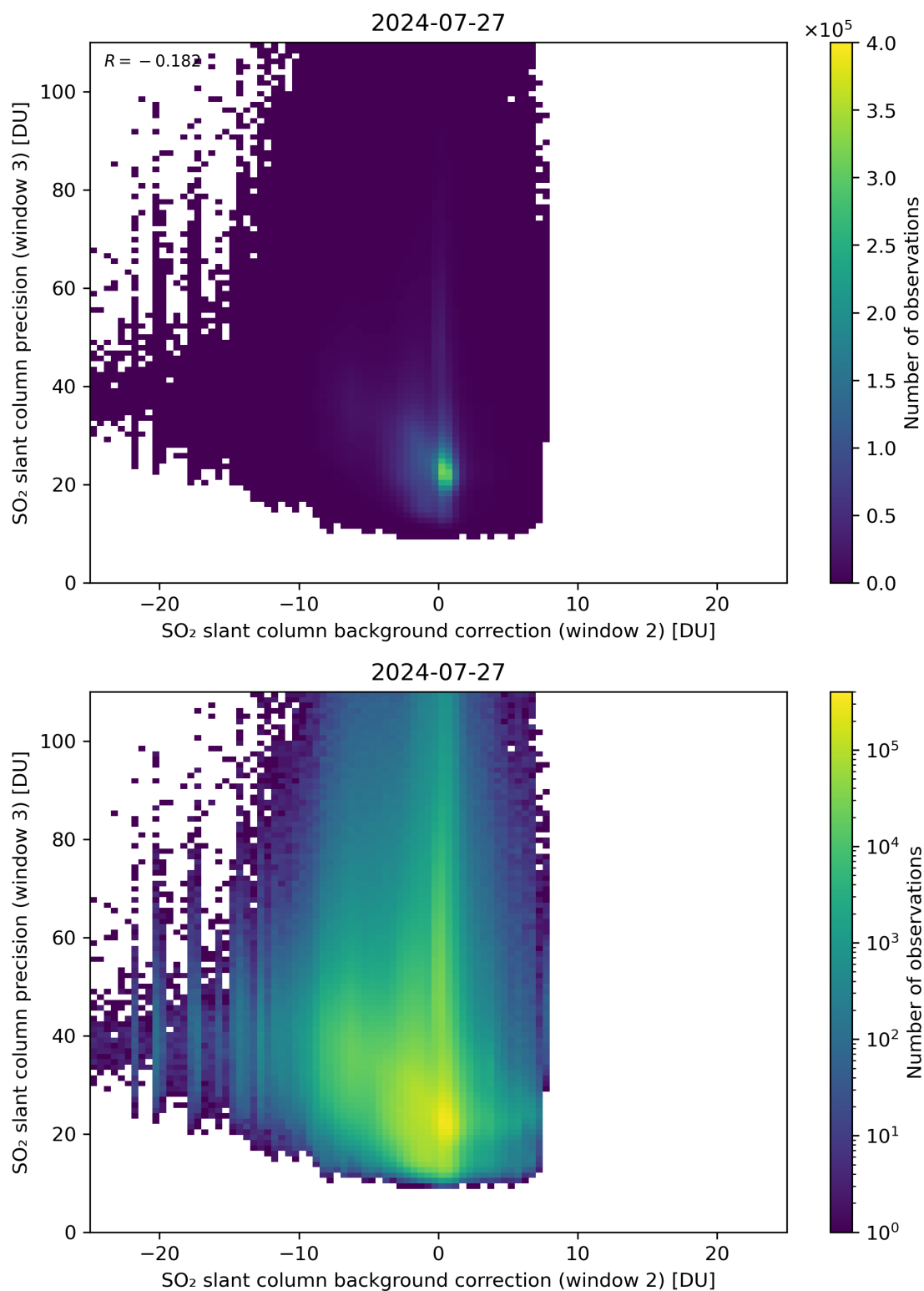
Figure 118: Scatter density plot of “SO 2 slant column background correction (window 2)” against “SO 2 slant column precision (window 3)” for 2024-07-26 to 2024-07-28.
