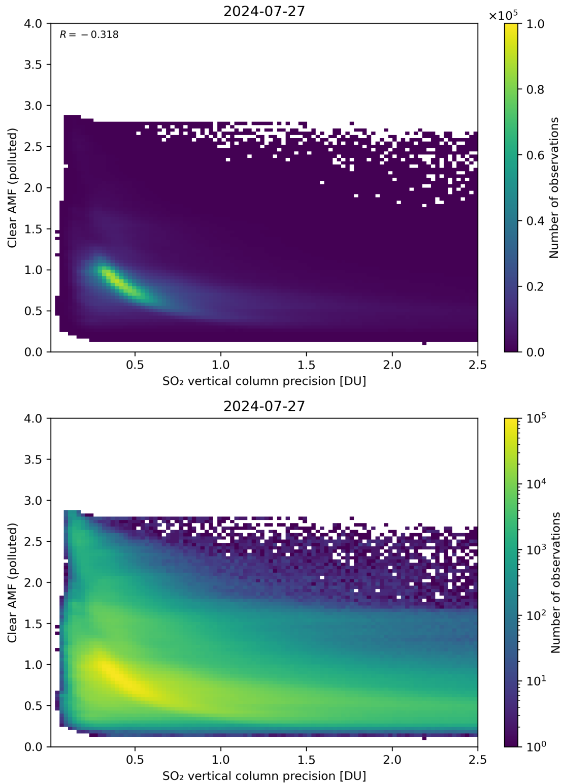
Figure 285: Scatter density plot of “SO 2 vertical column precision” against “Clear AMF (polluted)” for 2024-07-26 to 2024-07-28.
