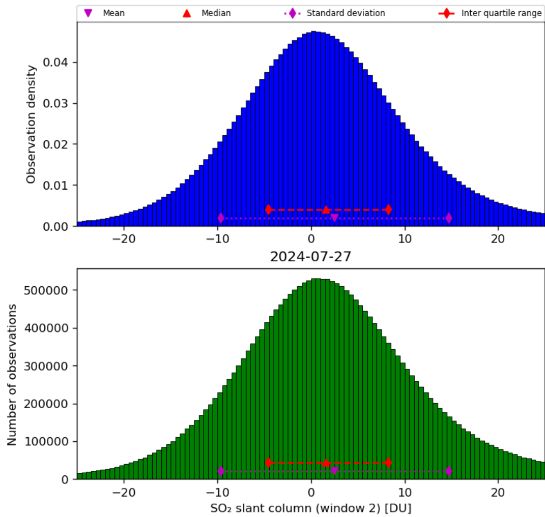
Figure 60: Histogram of “SO 2 slant column (window 2)” for 2024-07-26 to 2024-07-28
