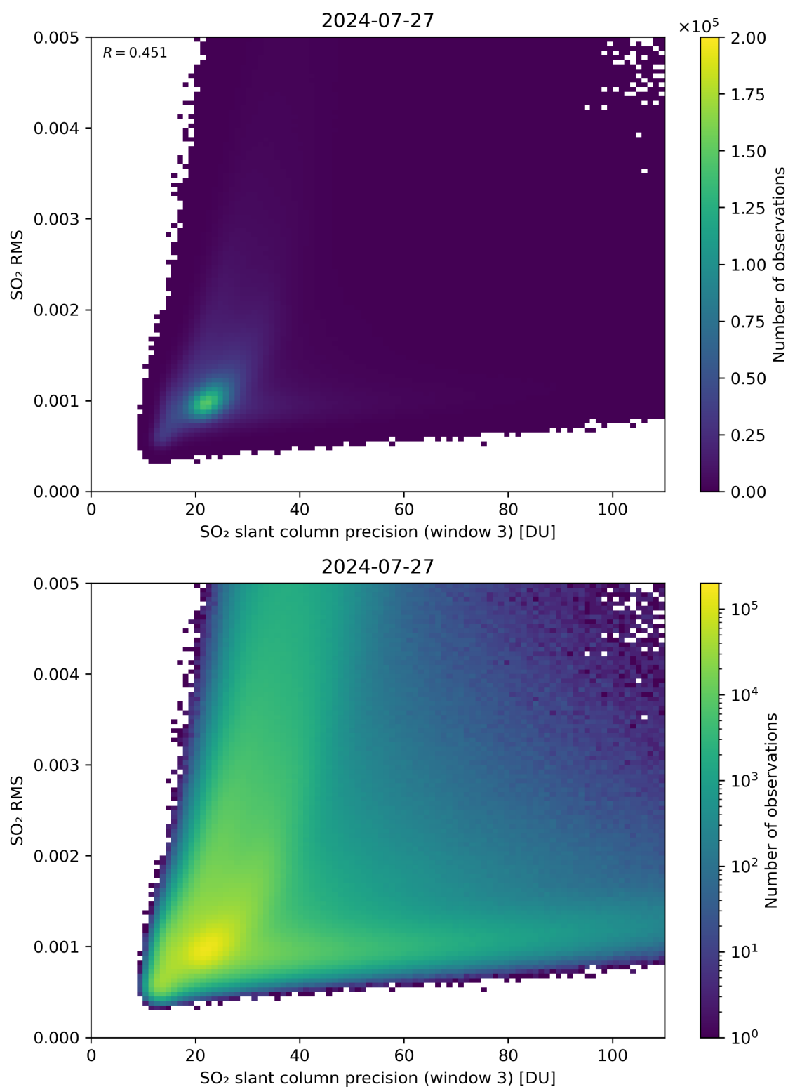
Figure 260: Scatter density plot of “SO 2 slant column precision (window 3)” against “SO 2 RMS” for 2024-07-26 to 2024-07-28.
