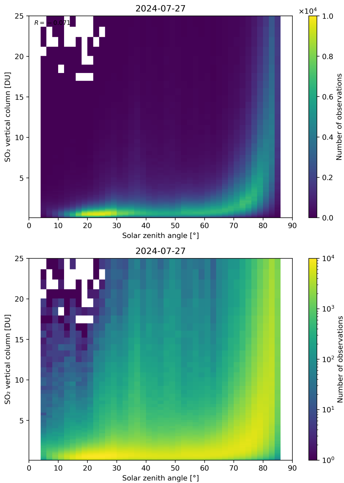
Figure 176: Scatter density plot of “Solar zenith angle” against “SO 2 vertical column” for 2024-07-26 to 2024-07-28.
