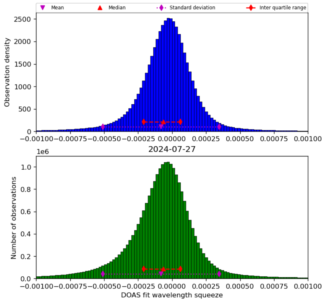
Figure 69: Histogram of “DOAS fit wavelength squeeze” for 2024-07-26 to 2024-07-28
