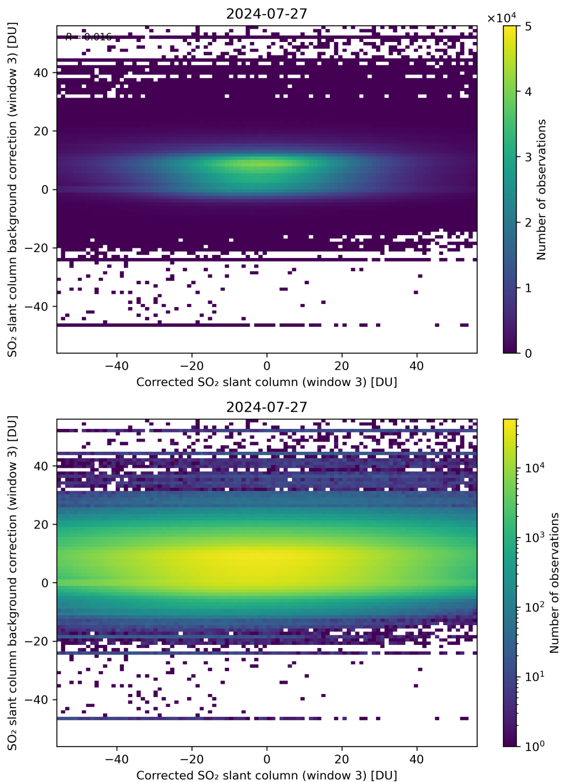
Figure 205: Scatter density plot of “Corrected SO 2 slant column (window 3)” against “SO 2 slant column background correction (window 3)” for 2024-07-26 to 2024-07-28.
