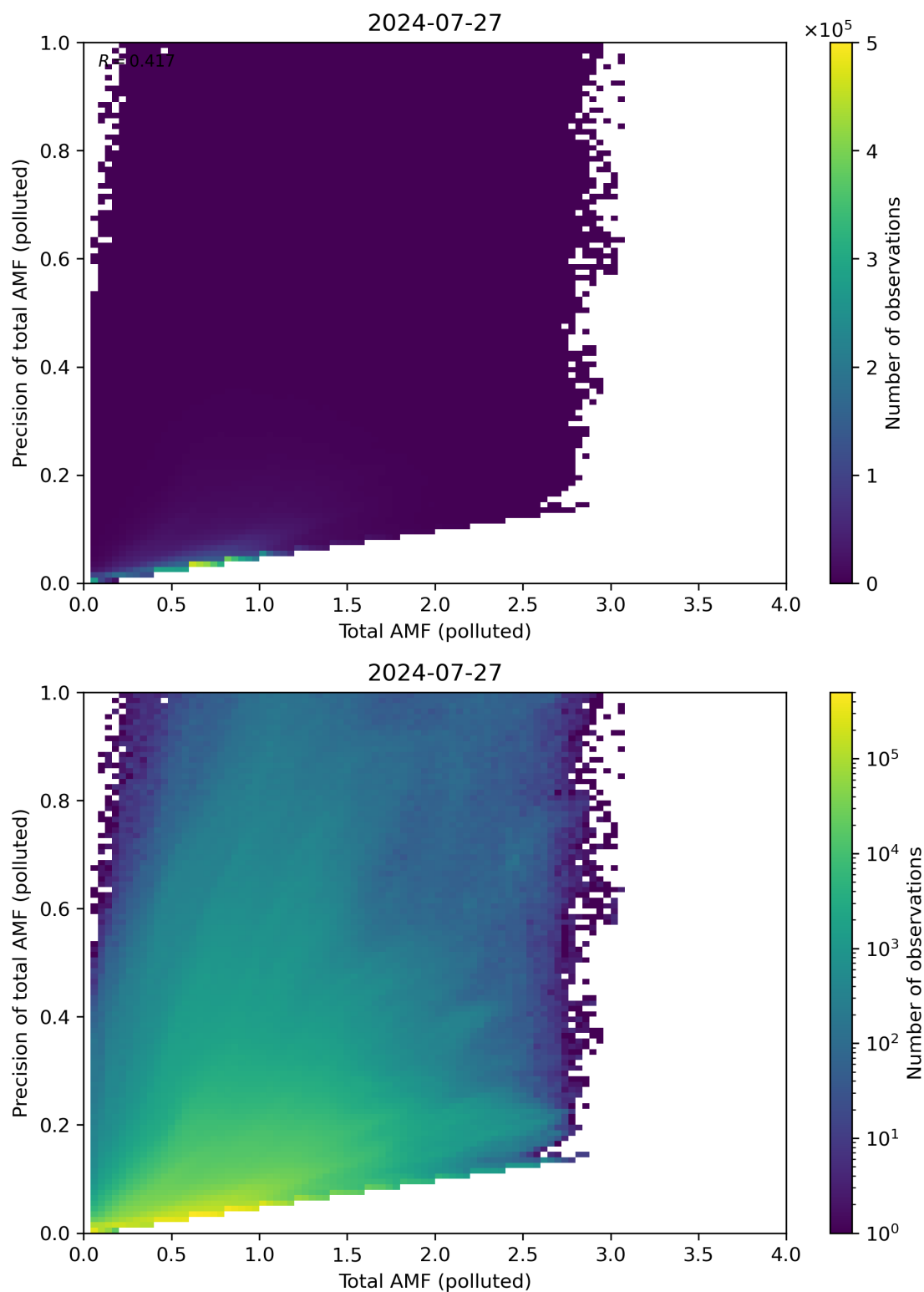
Figure 272: Scatter density plot of “Total AMF (polluted)” against “Precision of total AMF (polluted)” for 2024-07-26 to 2024-07-28.
