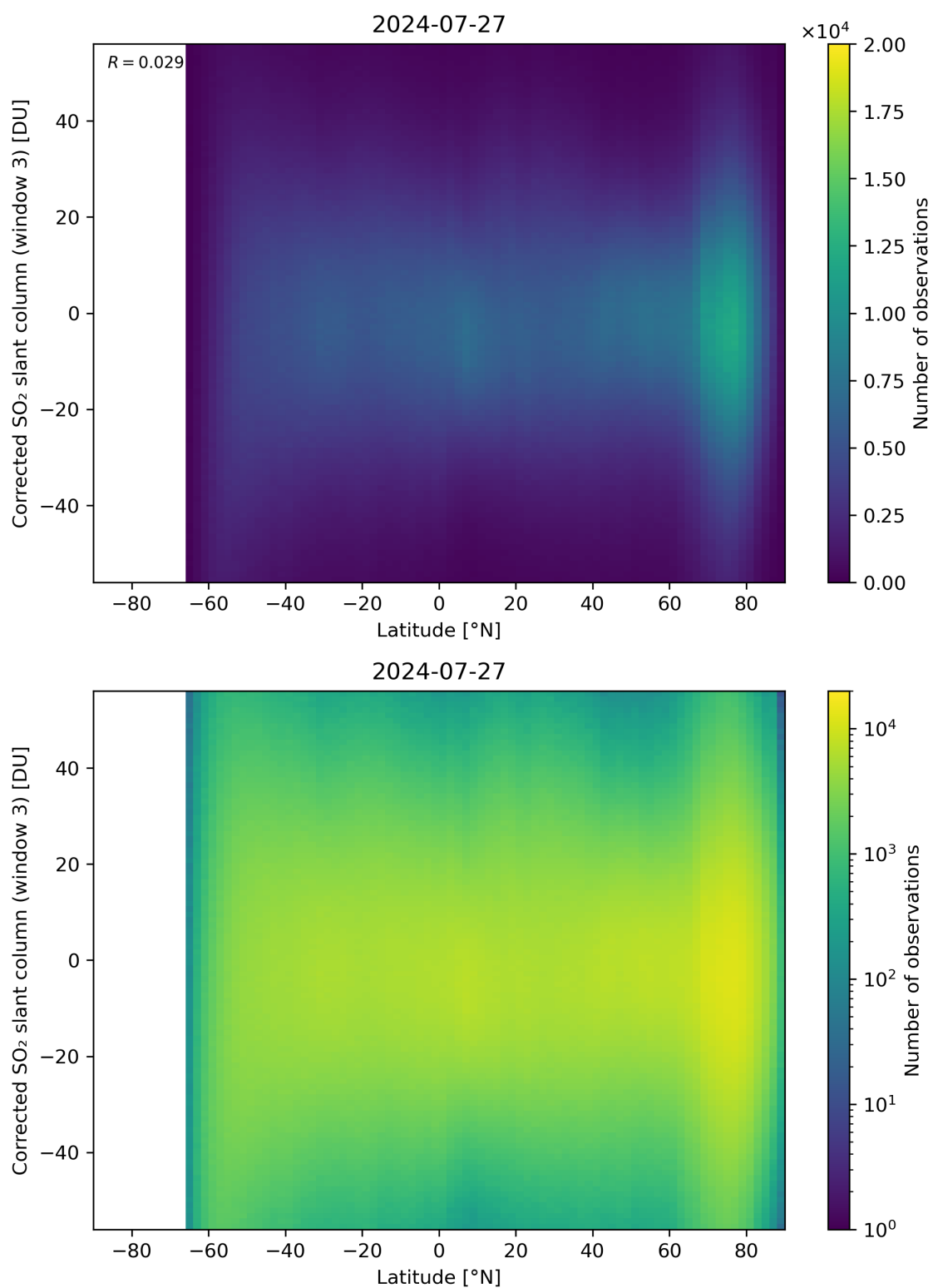
Figure 148: Scatter density plot of “Latitude” against “Corrected SO 2 slant column (window 3)” for 2024-07-26 to 2024-07-28.
