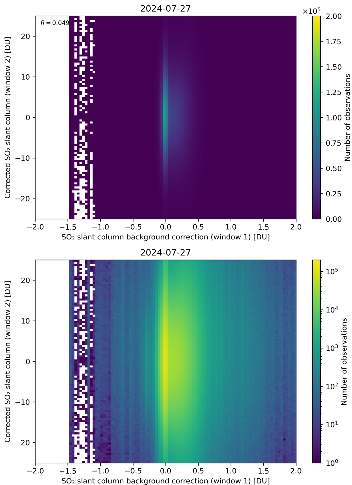
Figure 104: Scatter density plot of “SO 2 slant column background correction (window 1)” against “Corrected SO 2 slant column (window 2)” for 2024-07-26 to 2024-07-28.
