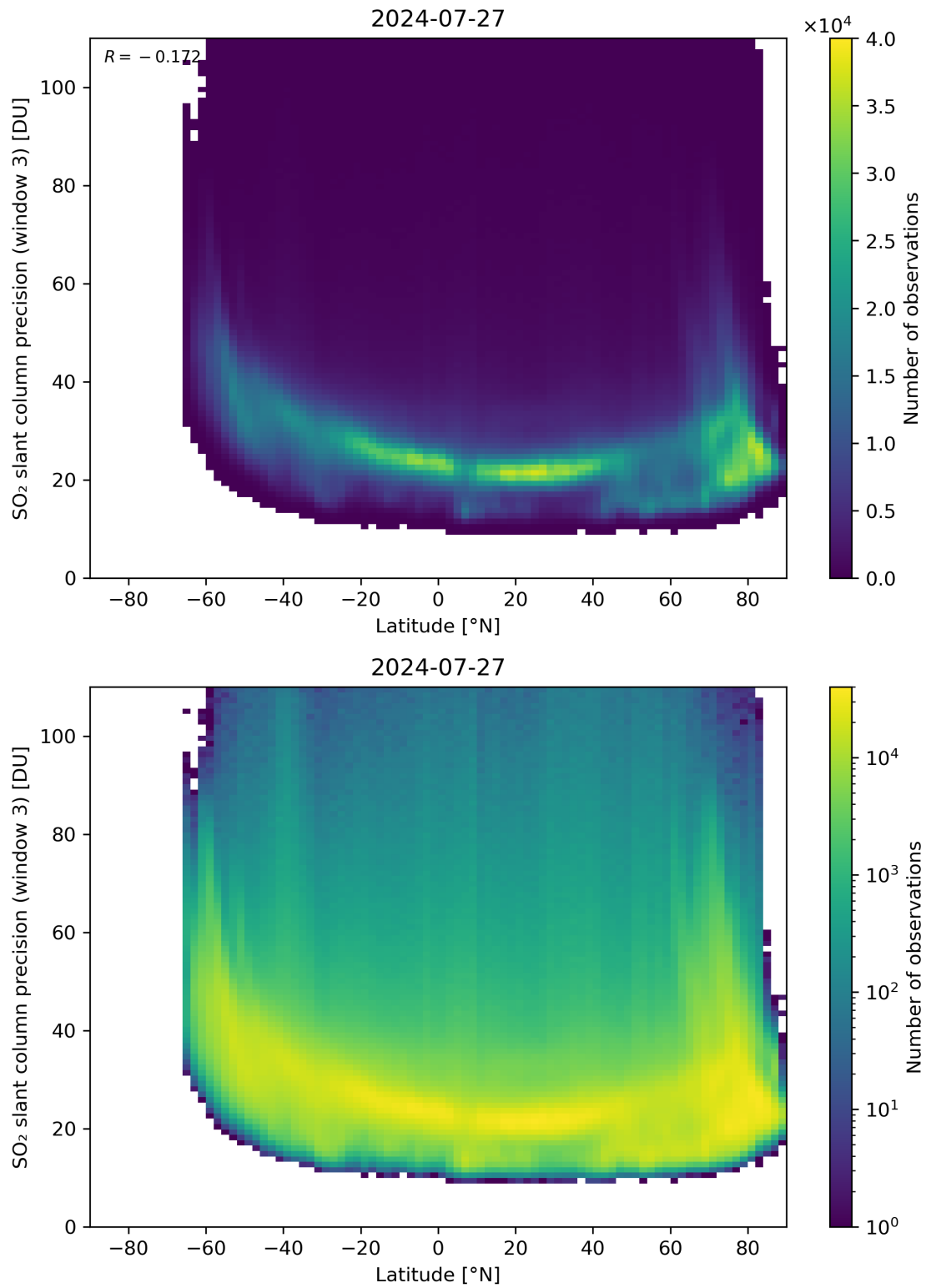
Figure 153: Scatter density plot of “Latitude” against “SO 2 slant column precision (window 3)” for 2024-07-26 to 2024-07-28.
