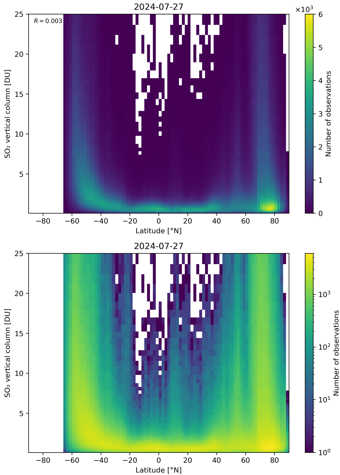
Figure 156: Scatter density plot of “Latitude” against “SO 2 vertical column” for 2024-07-26 to 2024-07-28.
