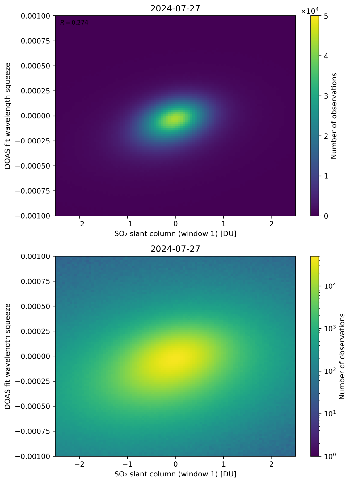
Figure 216: Scatter density plot of “SO 2 slant column (window 1)” against “DOAS fit wavelength squeeze” for 2024-07-26 to 2024-07-28.
