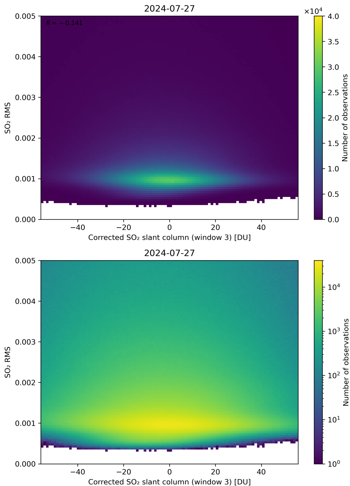
Figure 208: Scatter density plot of “Corrected SO 2 slant column (window 3)” against “SO 2 RMS” for 2024-07-26 to 2024-07-28.
