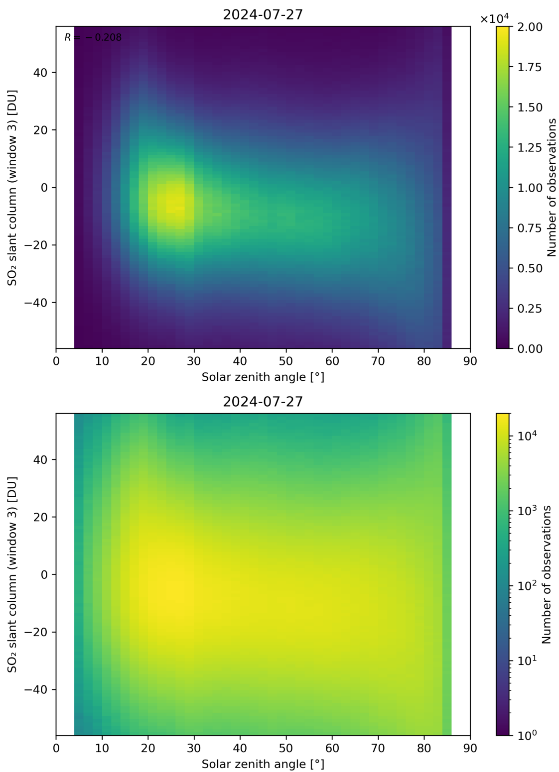
Figure 172: Scatter density plot of “Solar zenith angle” against “SO 2 slant column (window 3)” for 2024-07-26 to 2024-07-28.
