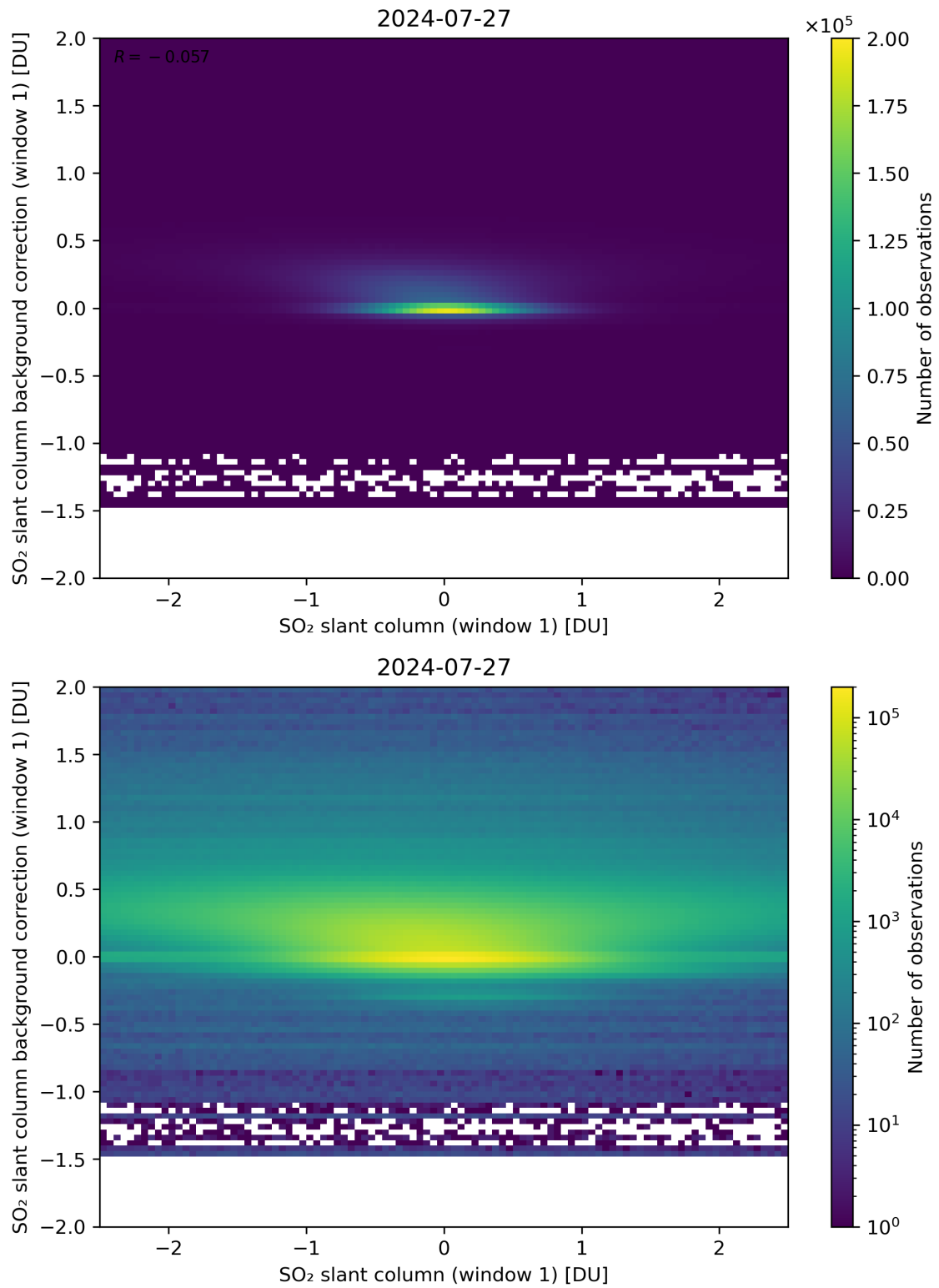
Figure 212: Scatter density plot of “SO 2 slant column (window 1)” against “SO 2 slant column background correction (window 1)” for 2024-07-26 to 2024-07-28.
