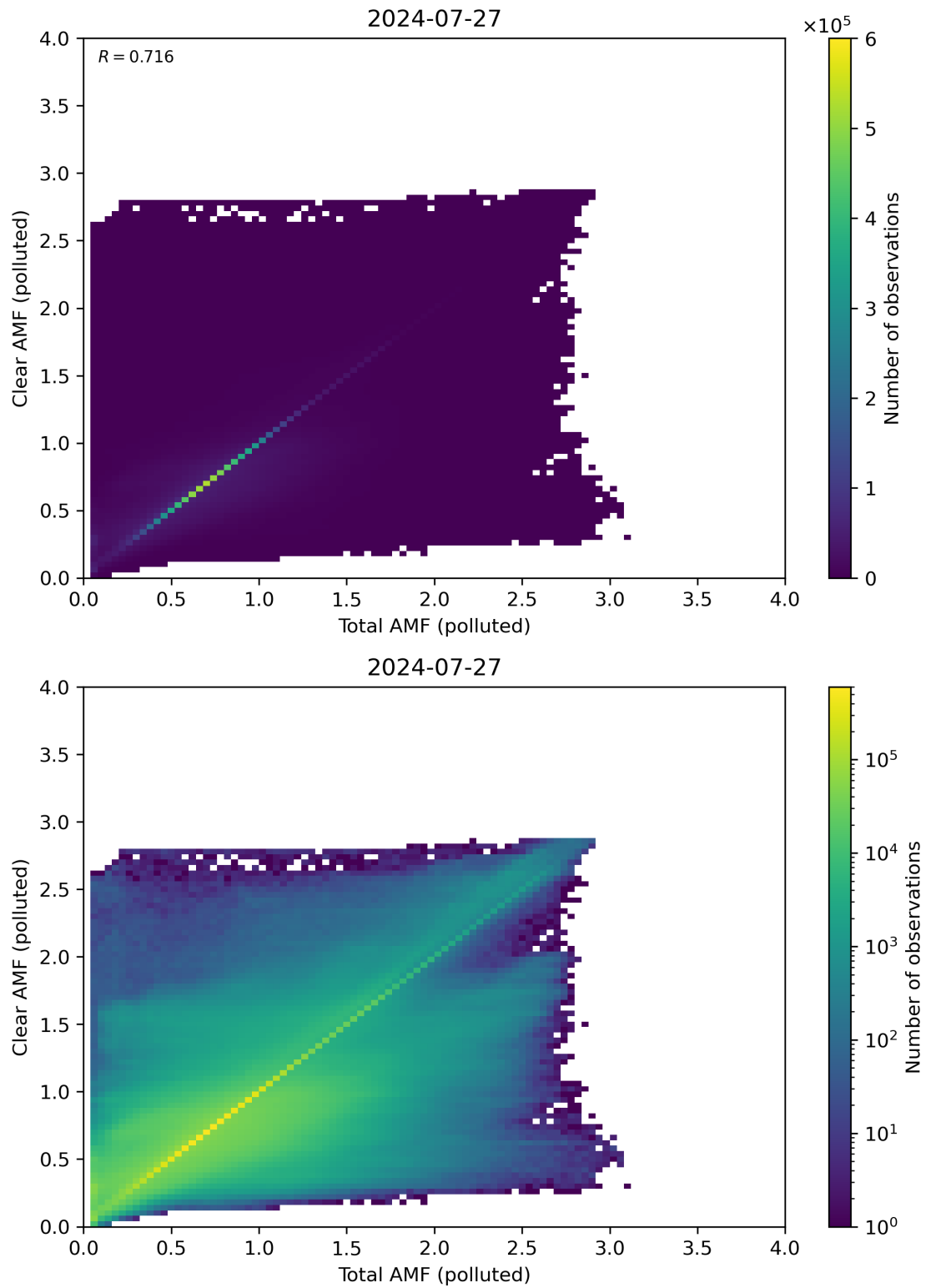
Figure 271: Scatter density plot of “Total AMF (polluted)” against “Clear AMF (polluted)” for 2024-07-26 to 2024-07-28.
