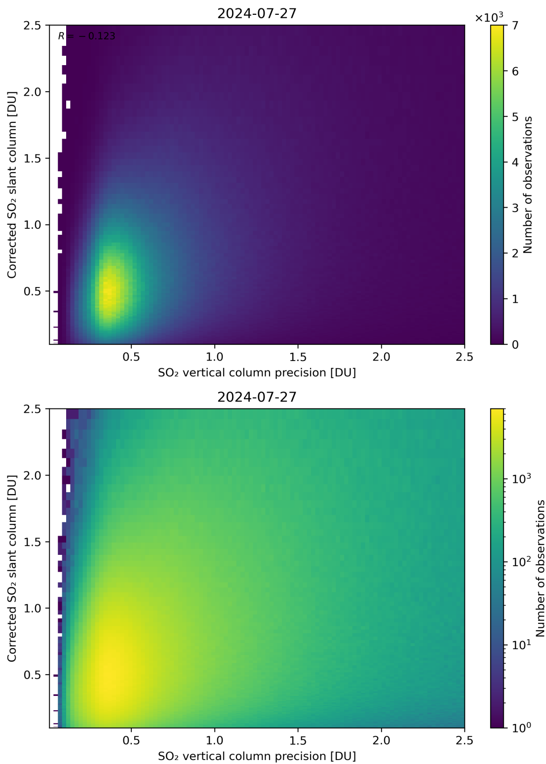
Figure 286: Scatter density plot of “SO 2 vertical column precision” against “Corrected SO 2 slant column” for 2024-07-26 to 2024-07-28.
