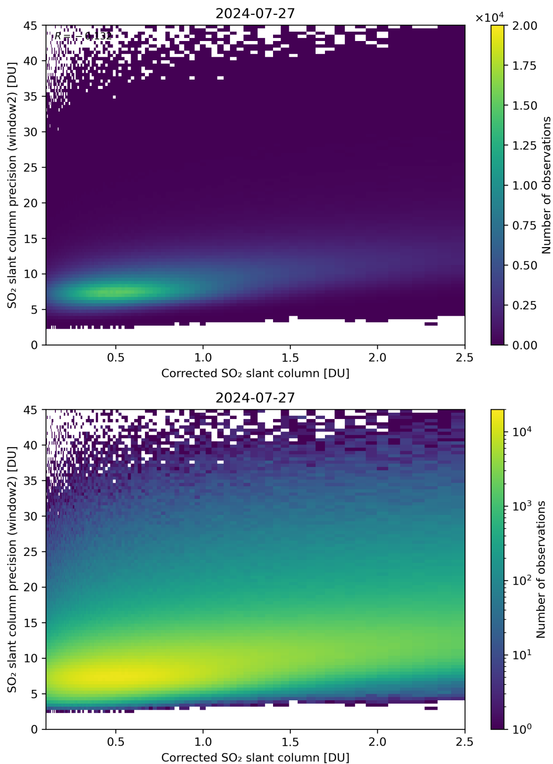
Figure 189: Scatter density plot of “Corrected SO 2 slant column” against “SO 2 slant column precision (window2)” for 2024-07-26 to 2024-07-28.
