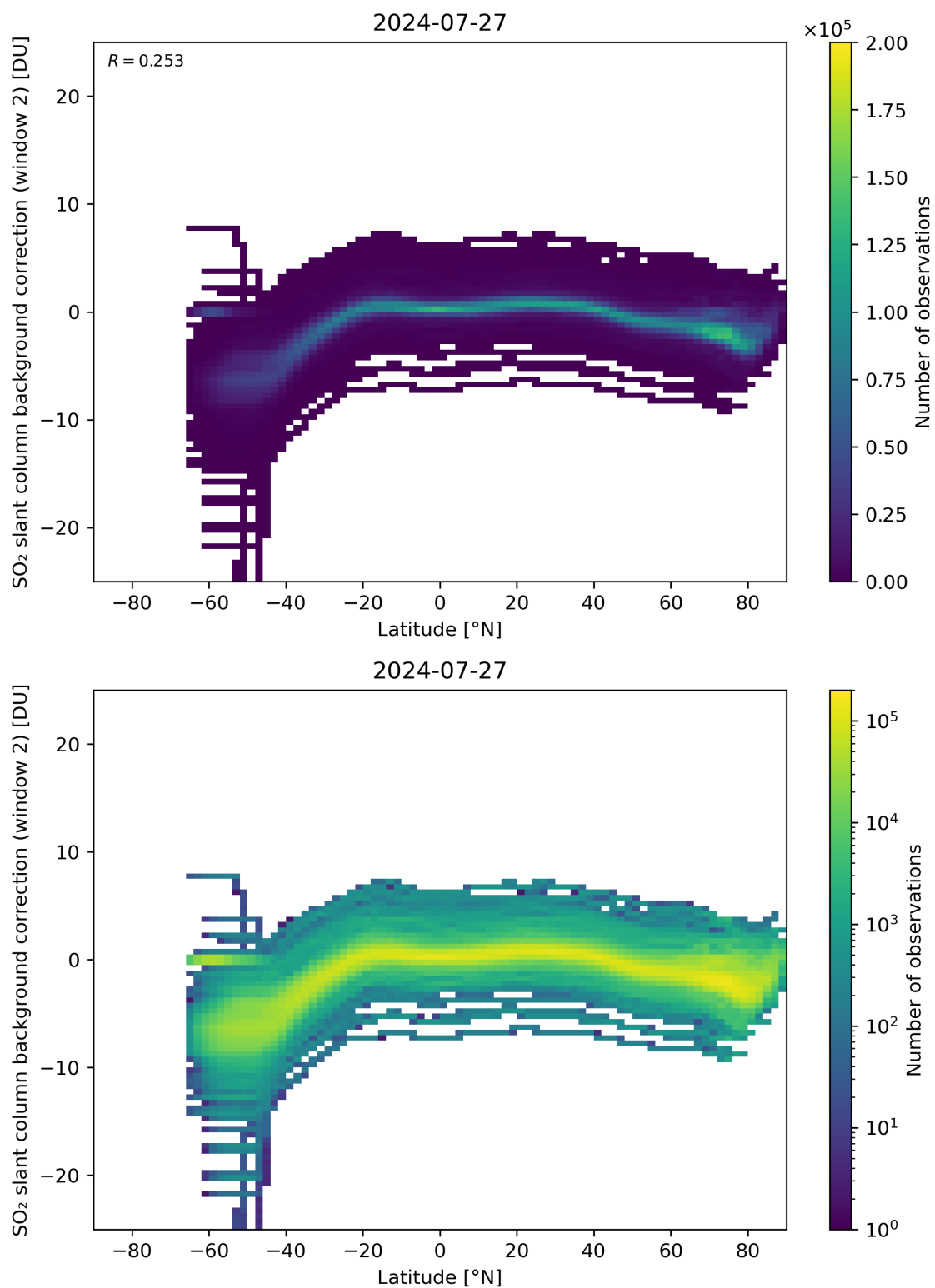
Figure 140: Scatter density plot of “Latitude” against “SO 2 slant column background correction (window 2)” for 2024-07-26 to 2024-07-28.
