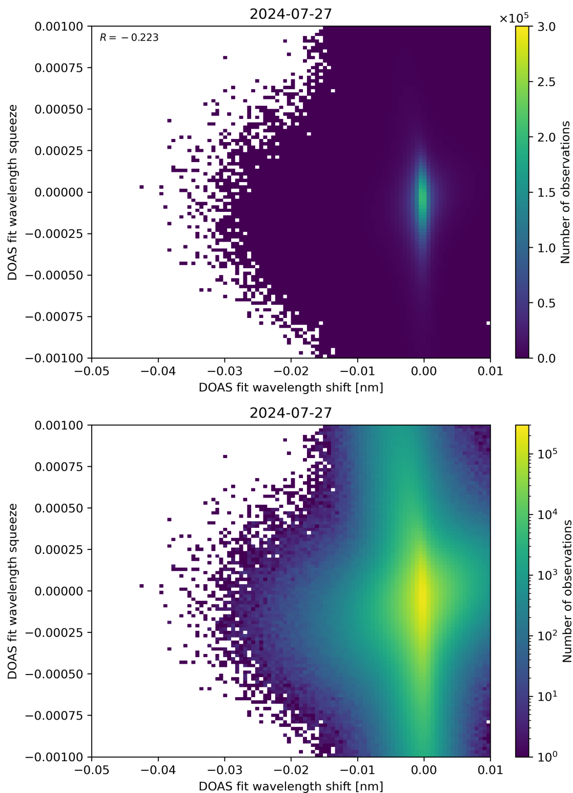
Figure 127: Scatter density plot of “DOAS fit wavelength shift” against “DOAS fit wavelength squeeze” for 2024-07-26 to 2024-07-28.
