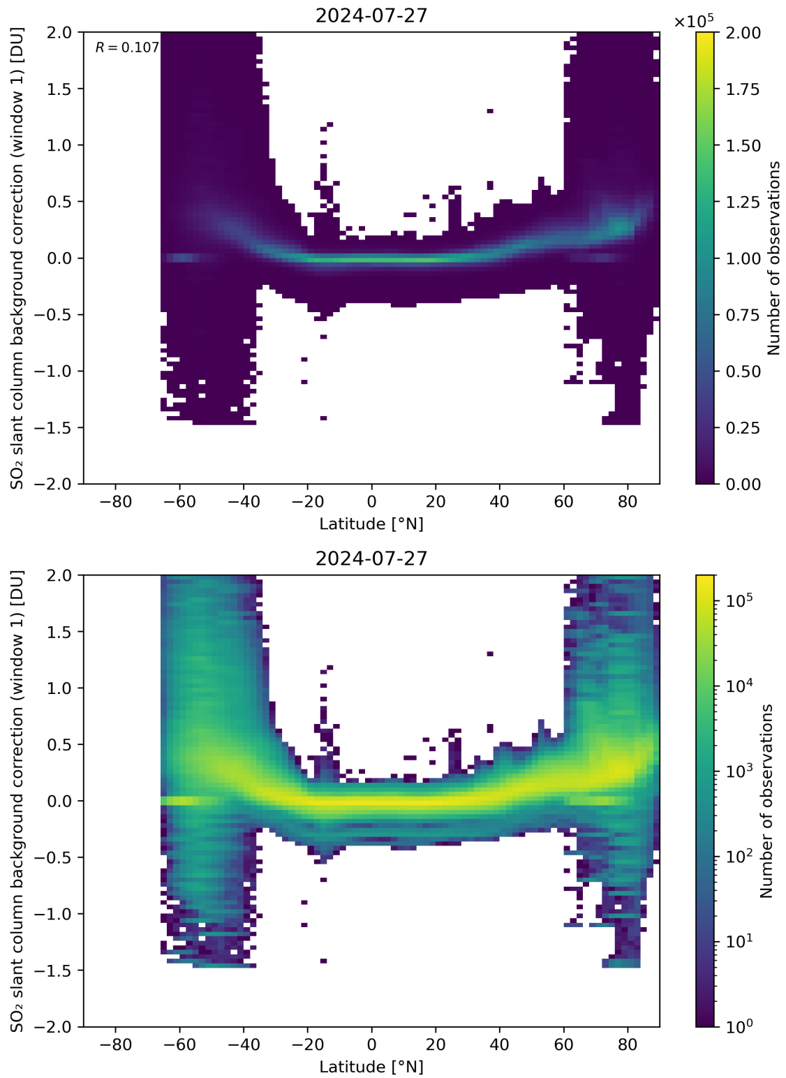
Figure 139: Scatter density plot of “Latitude” against “SO 2 slant column background correction (window 1)” for 2024-07-26 to 2024-07-28.
