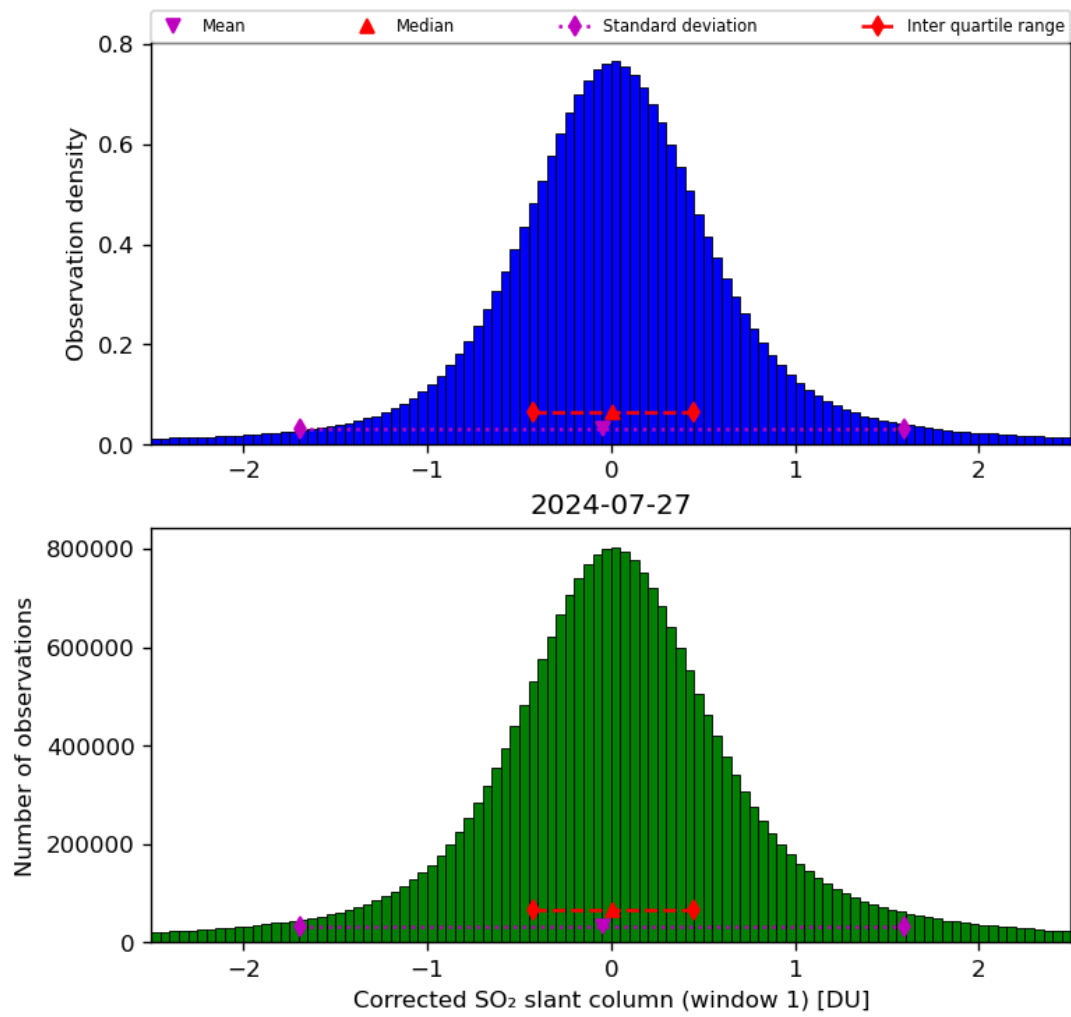
Figure 58: Histogram of “Corrected SO 2 slant column (window 1)” for 2024-07-26 to 2024-07-28
