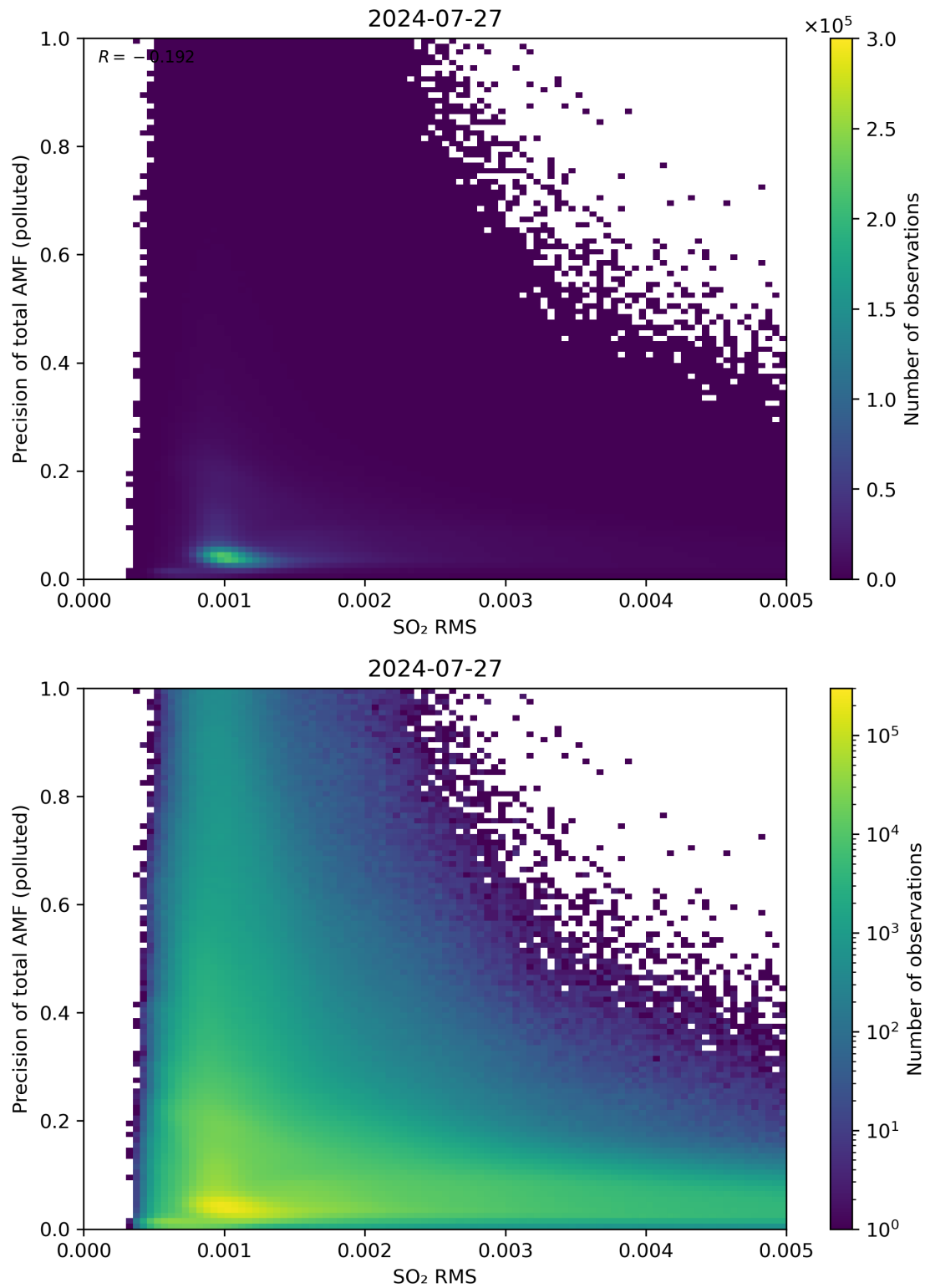
Figure 138: Scatter density plot of “SO 2 RMS” against “Precision of total AMF (polluted)” for 2024-07-26 to 2024-07-28.
