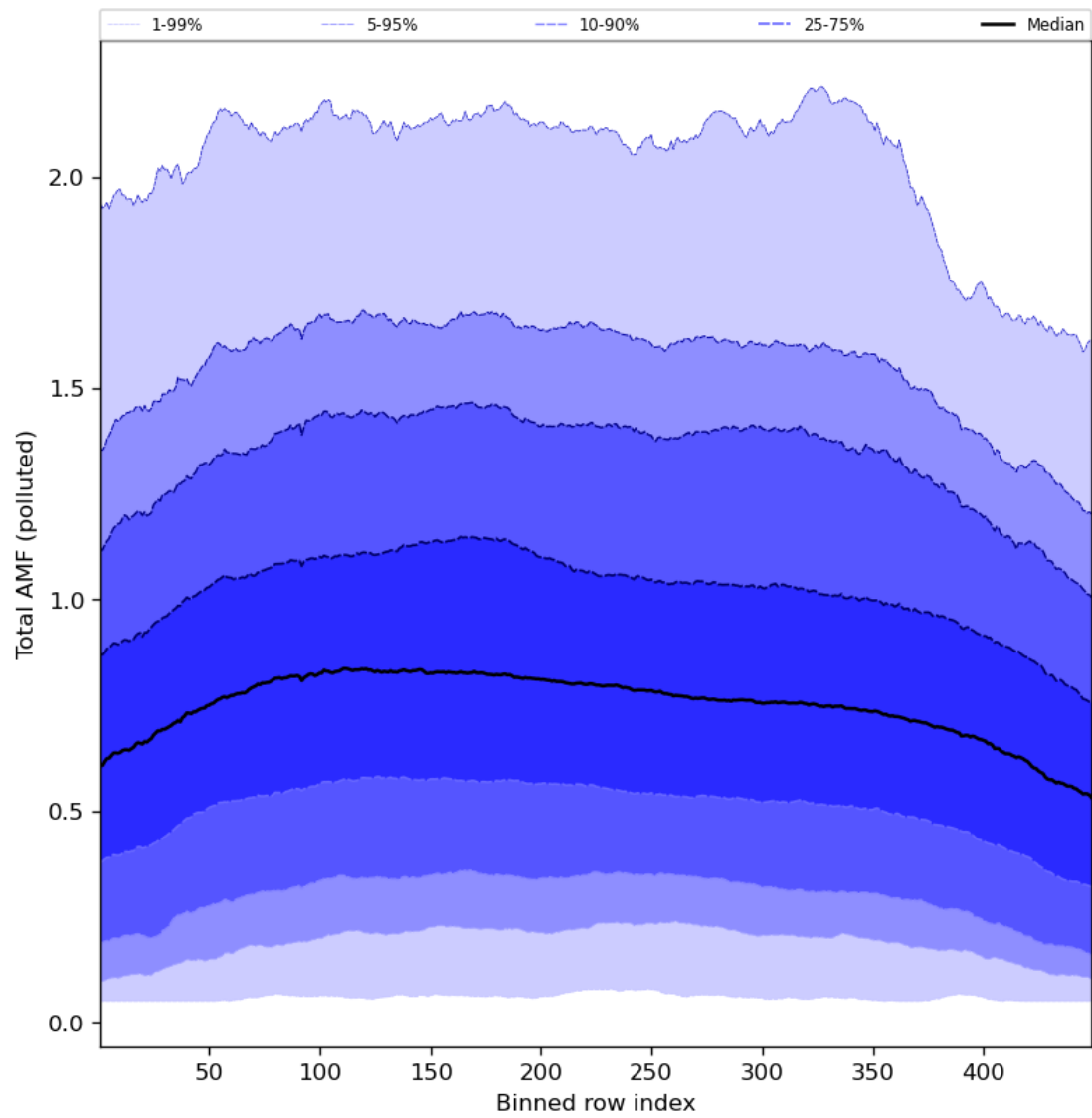
Figure 94: Along track statistics of “Total AMF (polluted)” for 2024-07-26 to 2024-07-28
