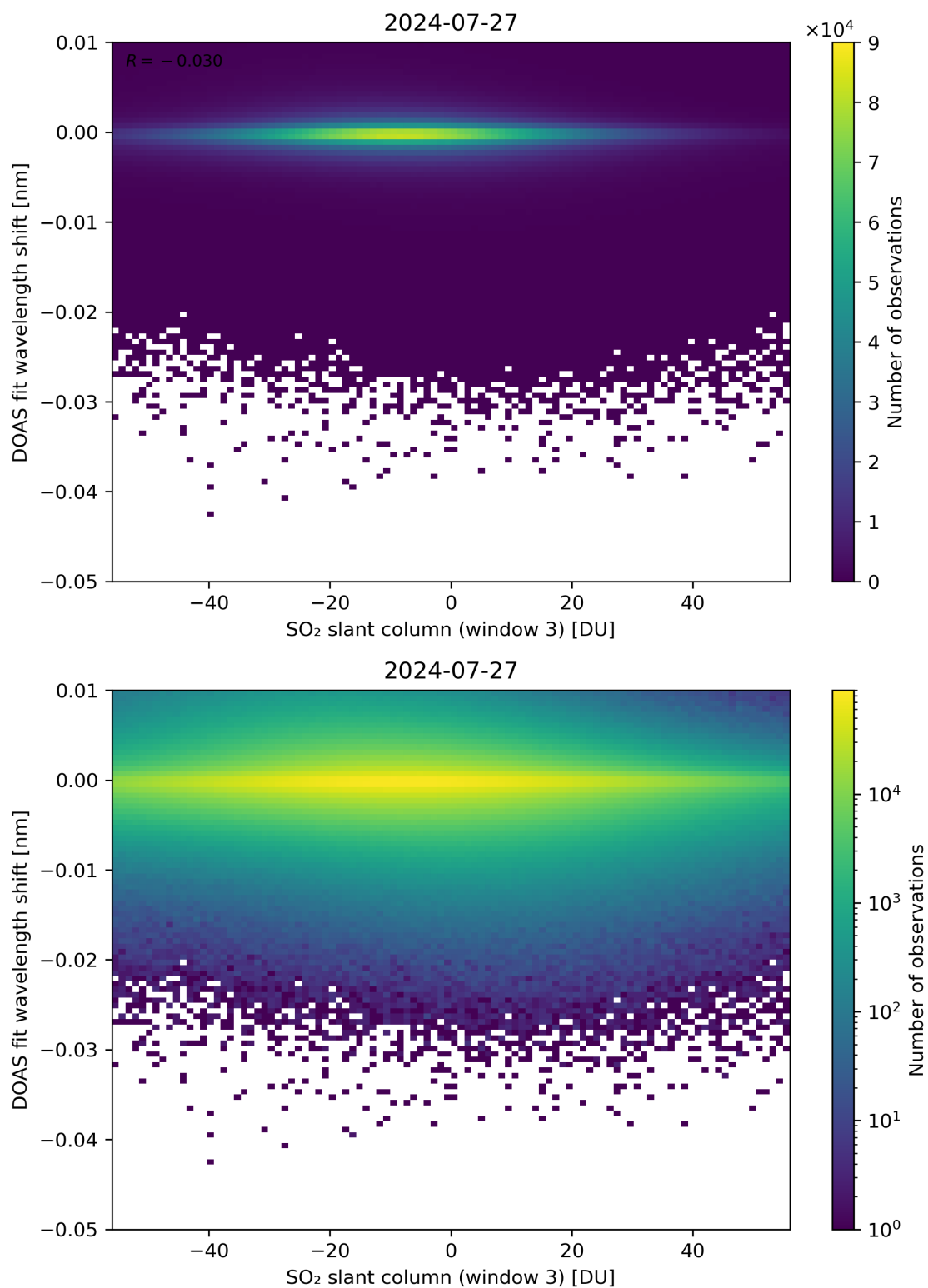
Figure 254: Scatter density plot of “SO 2 slant column (window 3)” against “DOAS fit wavelength shift” for 2024-07-26 to 2024-07-28.
