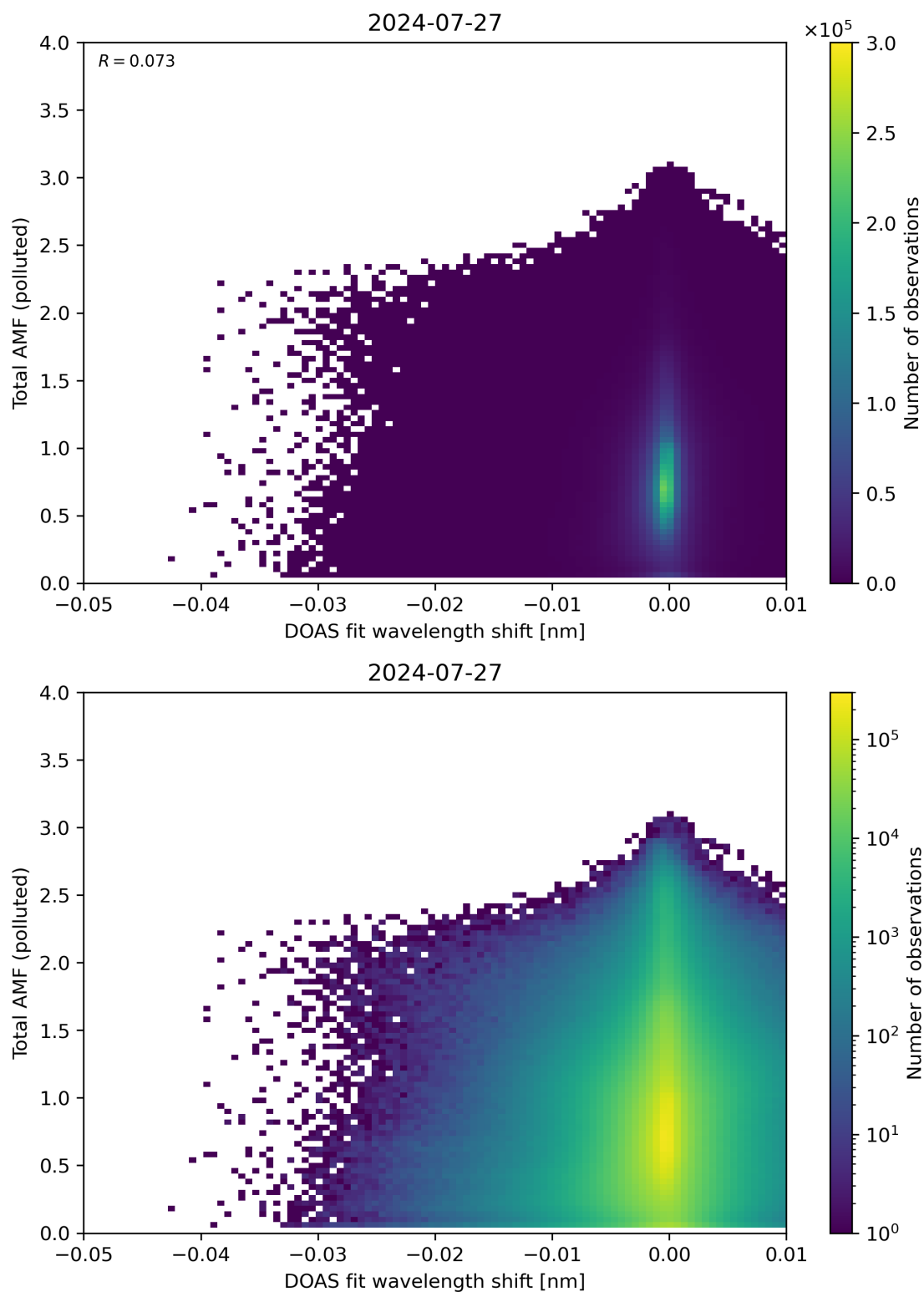
Figure 130: Scatter density plot of “DOAS fit wavelength shift” against “Total AMF (polluted)” for 2024-07-26 to 2024-07-28.
