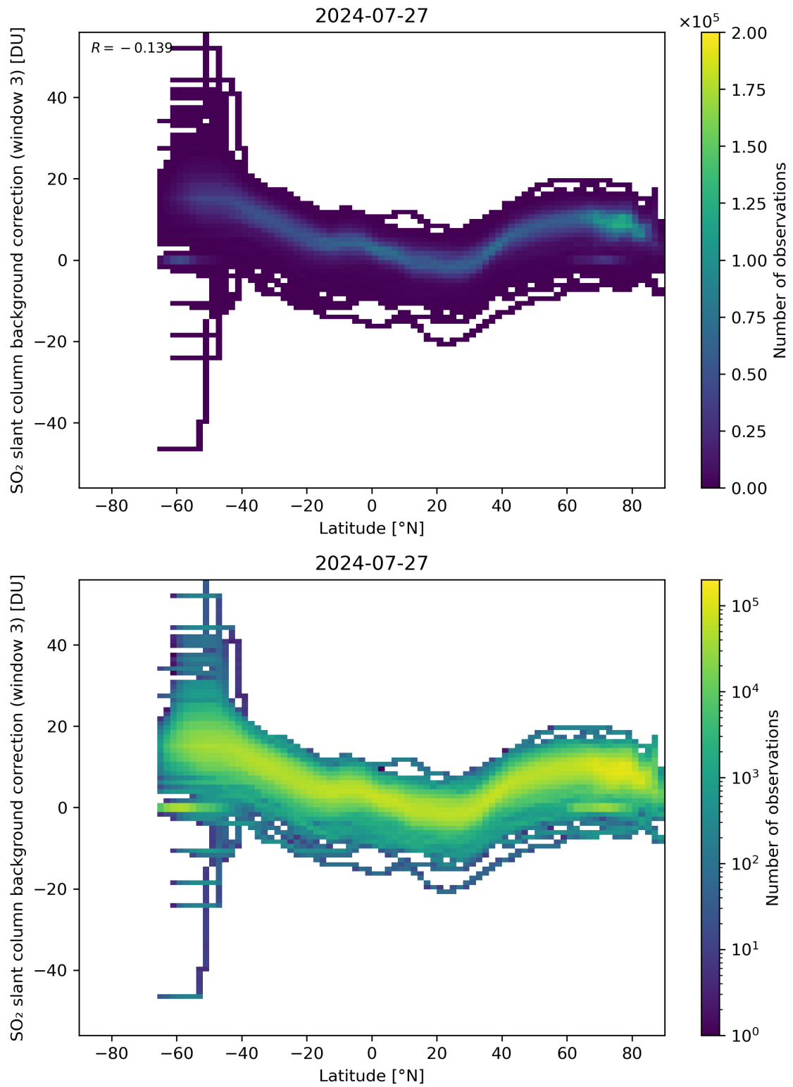
Figure 141: Scatter density plot of “Latitude” against “SO 2 slant column background correction (window 3)” for 2024-07-26 to 2024-07-28.
