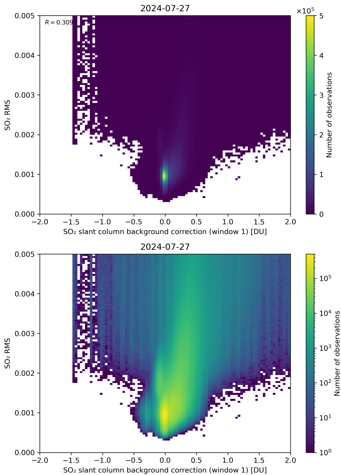
Figure 102: Scatter density plot of “SO 2 slant column background correction (window 1)” against “SO 2 RMS” for 2024-07-26 to 2024-07-28.
