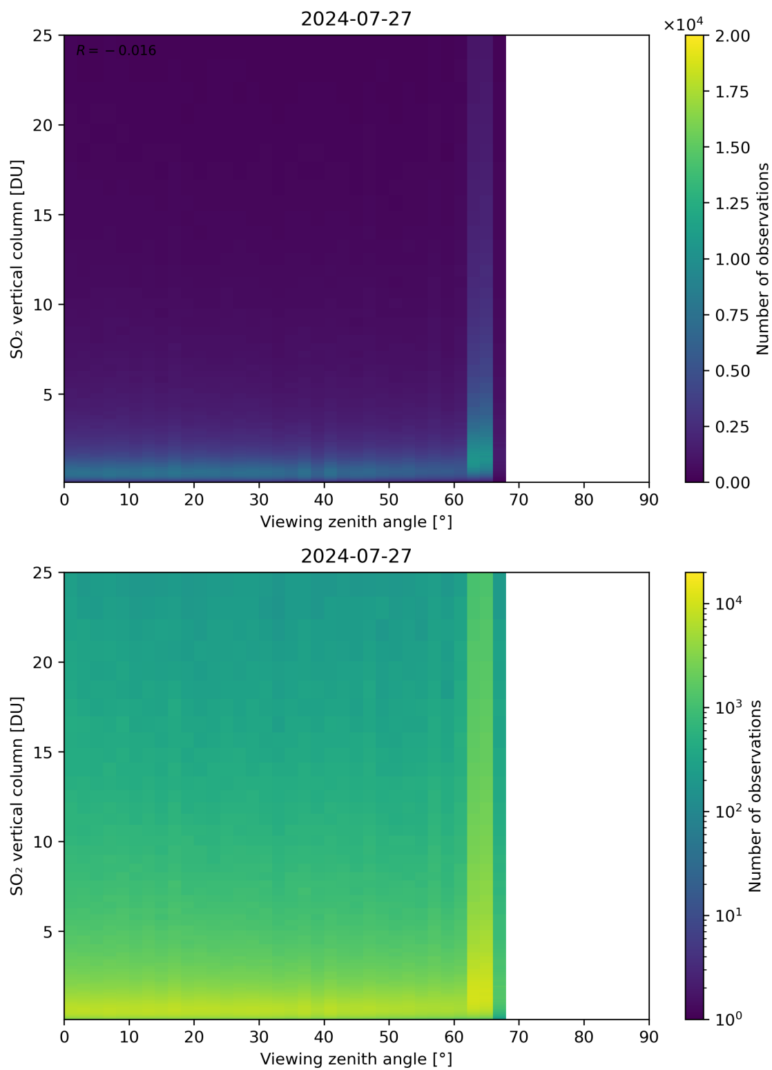
Figure 327: Scatter density plot of “Viewing zenith angle” against “SO 2 vertical column” for 2024-07-26 to 2024-07-28.
