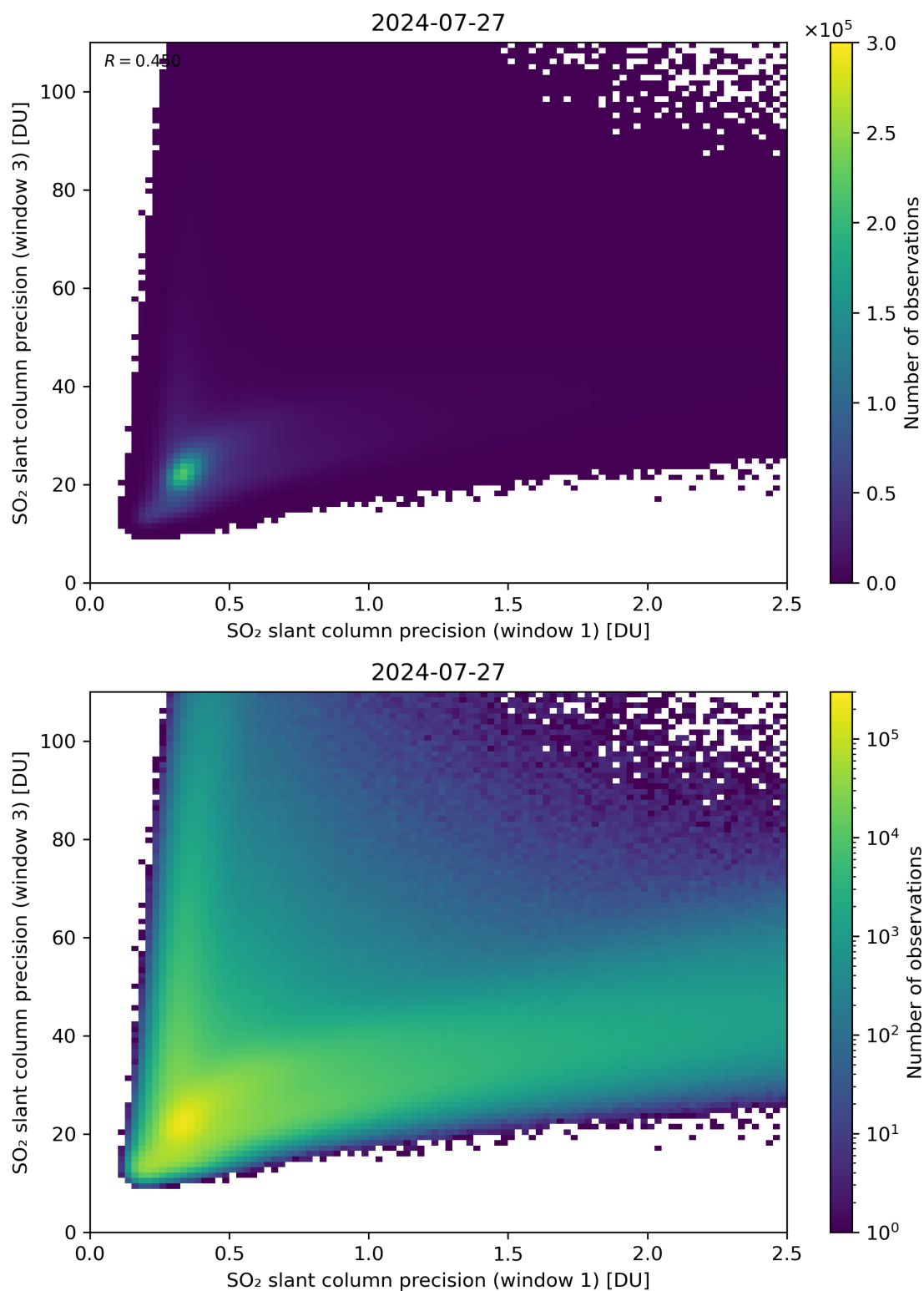
Figure 229: Scatter density plot of “SO 2 slant column precision (window 1)” against “SO 2 slant column precision (window 3)” for 2024-07-26 to 2024-07-28.
