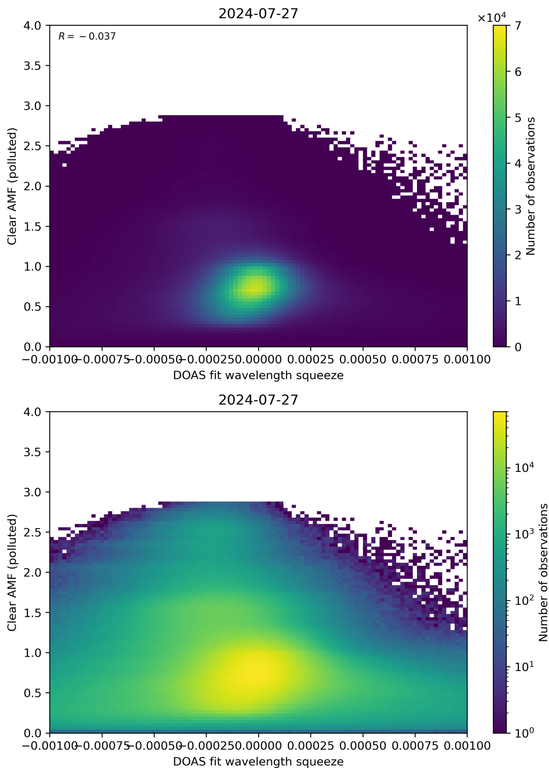
Figure 133: Scatter density plot of “DOAS fit wavelength squeeze” against “Clear AMF (polluted)” for 2024-07-26 to 2024-07-28.
