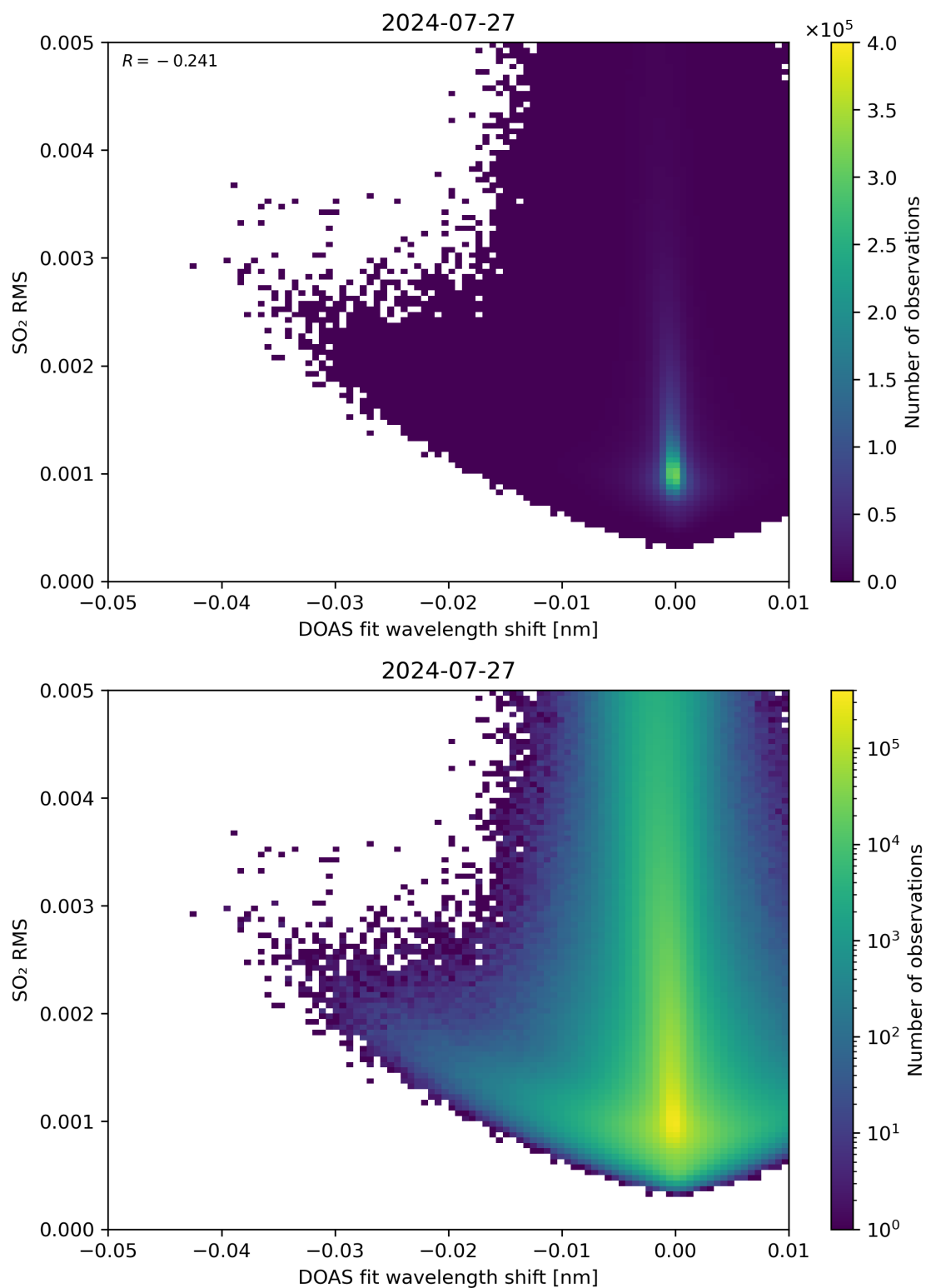
Figure 128: Scatter density plot of “DOAS fit wavelength shift” against “SO 2 RMS” for 2024-07-26 to 2024-07-28.
