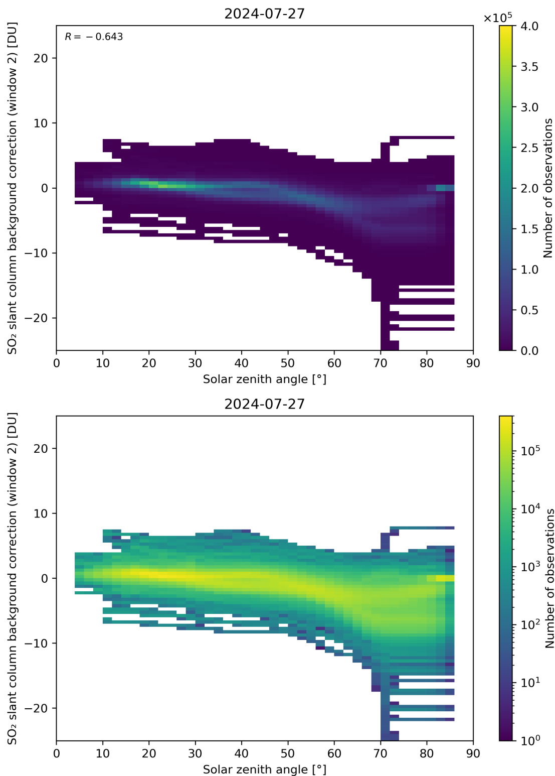
Figure 159: Scatter density plot of “Solar zenith angle” against “SO 2 slant column background correction (window 2)” for 2024-07-26 to 2024-07-28.
