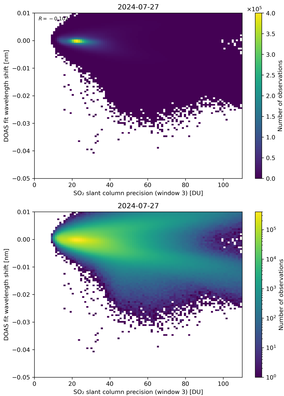
Figure 258: Scatter density plot of “SO 2 slant column precision (window 3)” against “DOAS fit wavelength shift” for 2024-07-26 to 2024-07-28.
