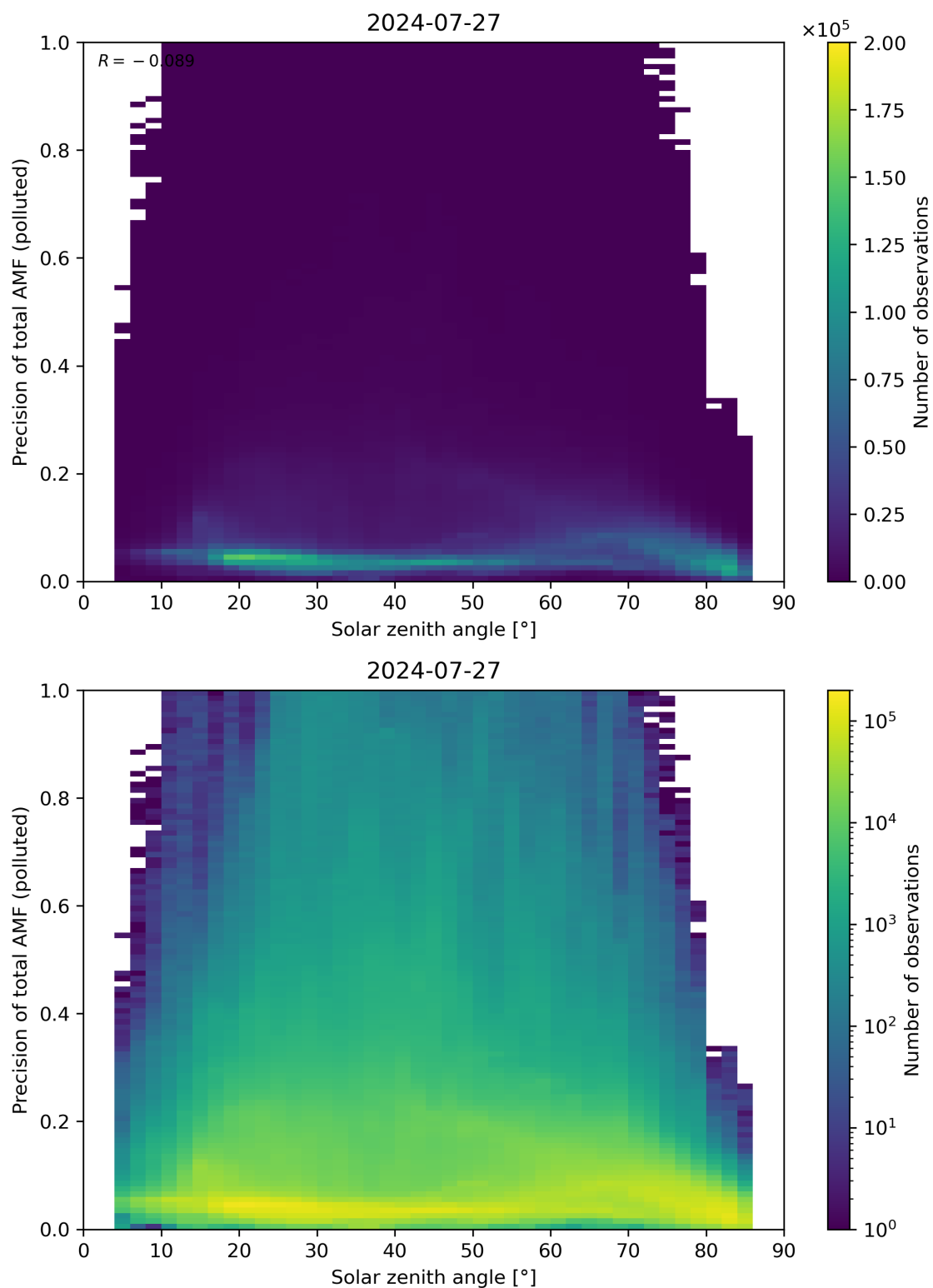
Figure 175: Scatter density plot of “Solar zenith angle” against “Precision of total AMF (polluted)” for 2024-07-26 to 2024-07-28.
