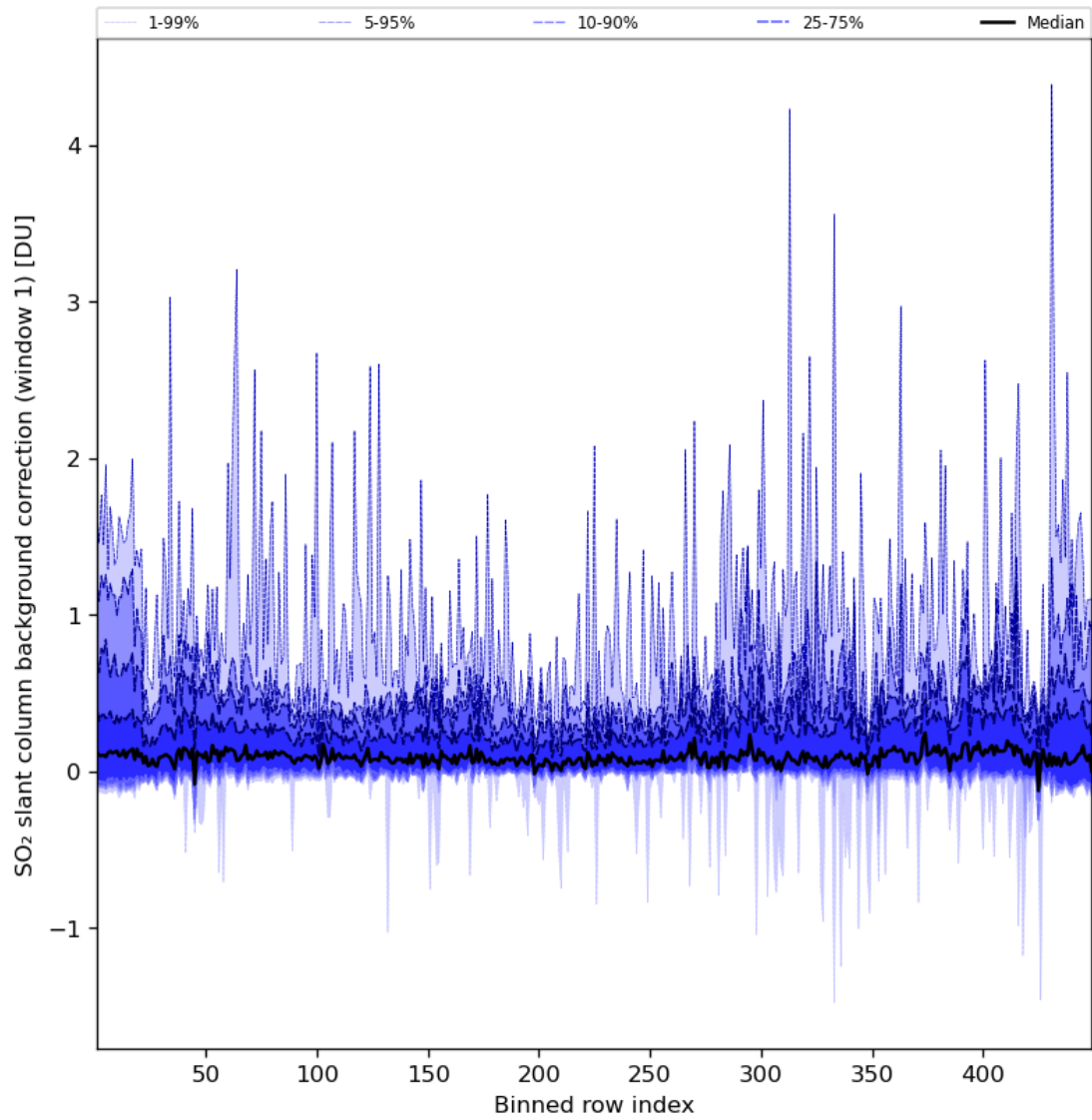
Figure 82: Along track statistics of "SO 2 slant column background correction (window 1)" for 2024-07-26 to 2024-07-28
