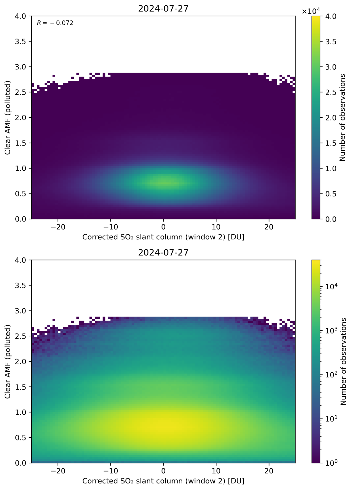
Figure 199: Scatter density plot of “Corrected SO 2 slant column (window 2)” against “Clear AMF (polluted)” for 2024-07-26 to 2024-07-28.
