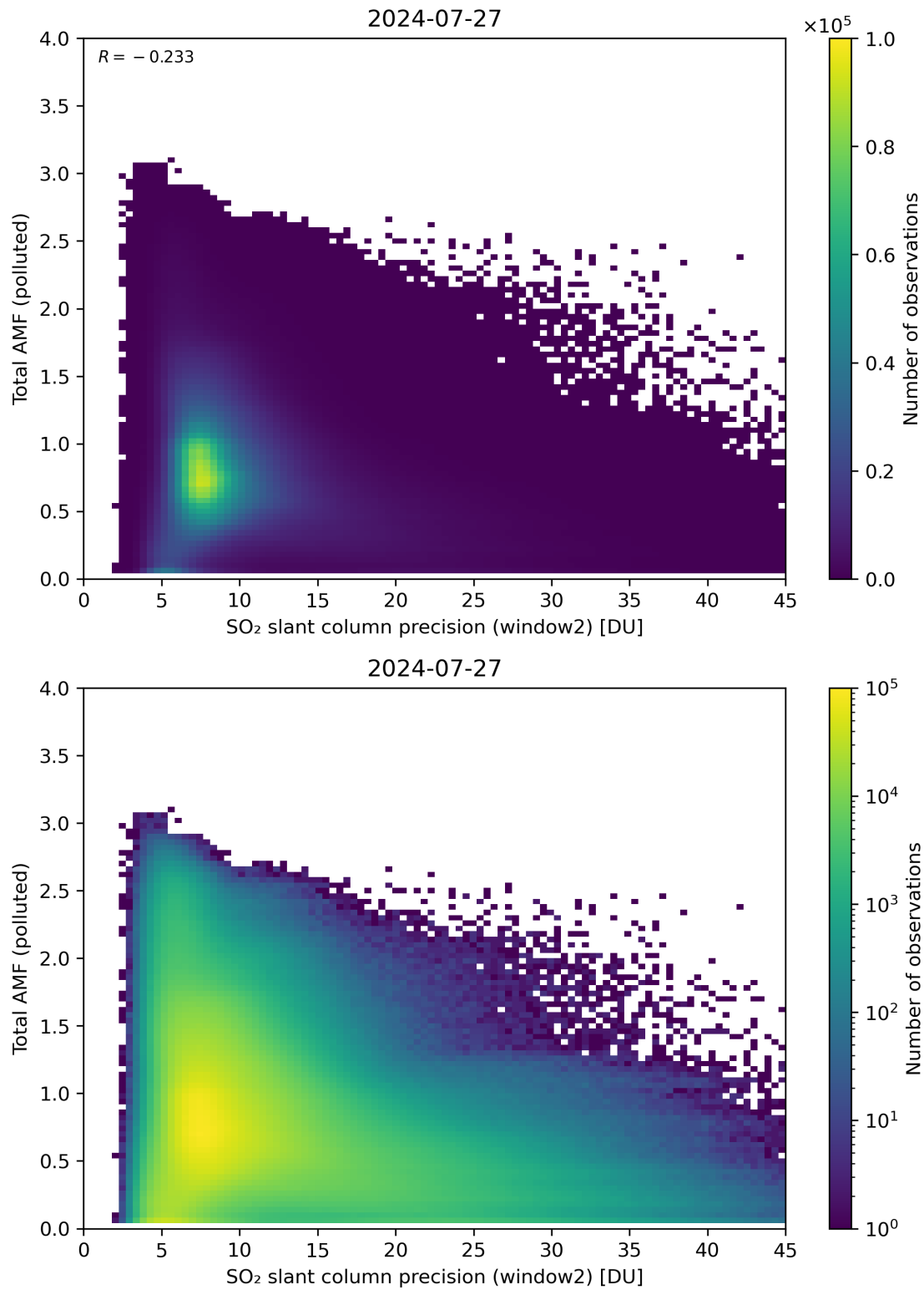
Figure 251: Scatter density plot of “SO 2 slant column precision (window2)” against “Total AMF (polluted)” for 2024-07-26 to 2024-07-28.
