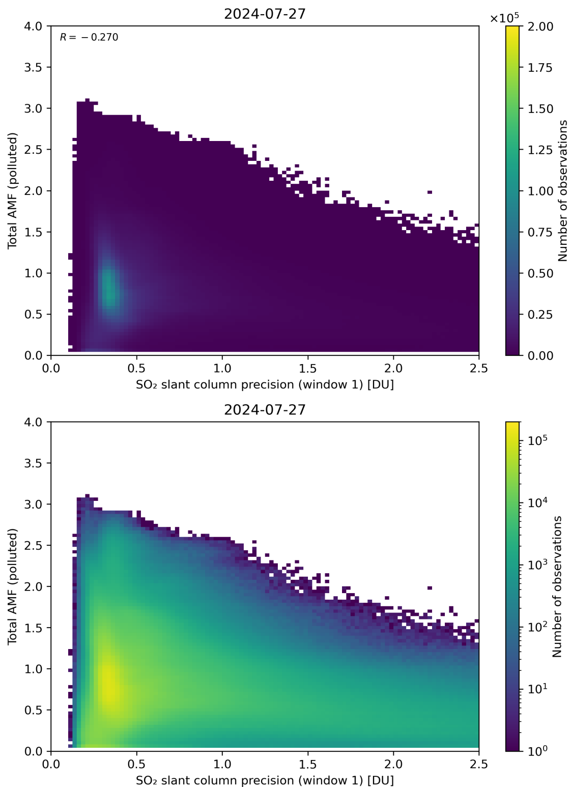
Figure 230: Scatter density plot of “SO 2 slant column precision (window 1)” against “Total AMF (polluted)” for 2024-07-26 to 2024-07-28.
