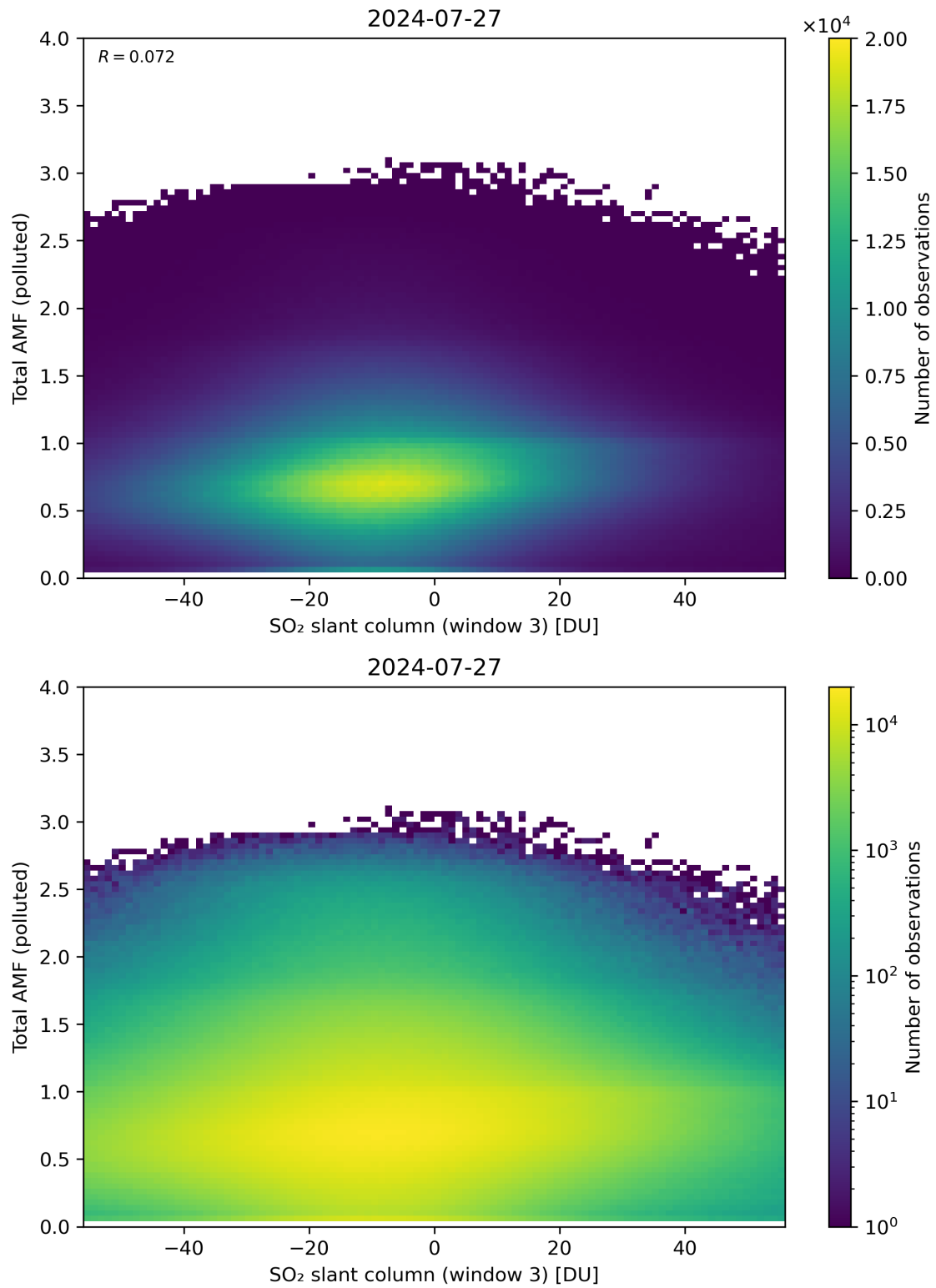
Figure 268: Scatter density plot of “SO 2 slant column (window 3)” against “Total AMF (polluted)” for 2024-07-26 to 2024-07-28.
