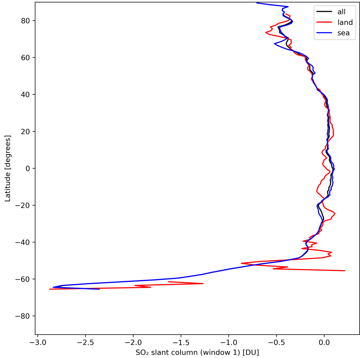
Figure 33: Zonal average of “SO 2 slant column (window 1)” for 2024-07-26 to 2024-07-28.
