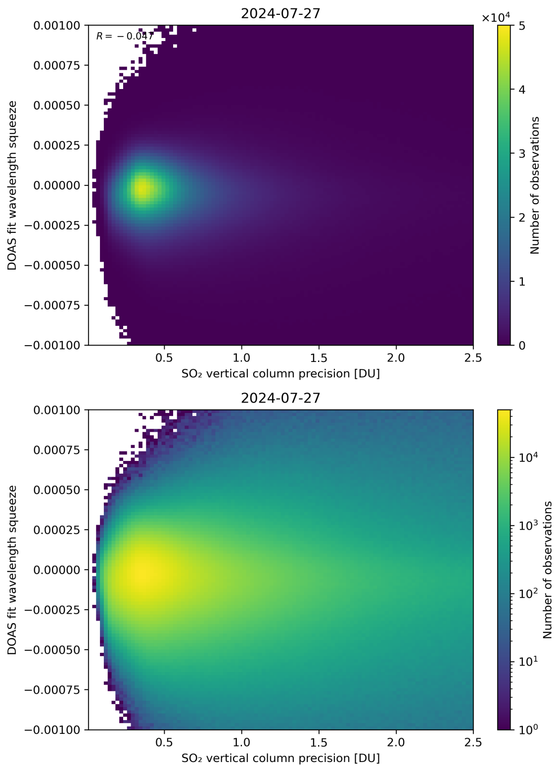
Figure 283: Scatter density plot of “SO 2 vertical column precision” against “DOAS fit wavelength squeeze” for 2024-07-26 to 2024-07-28.
