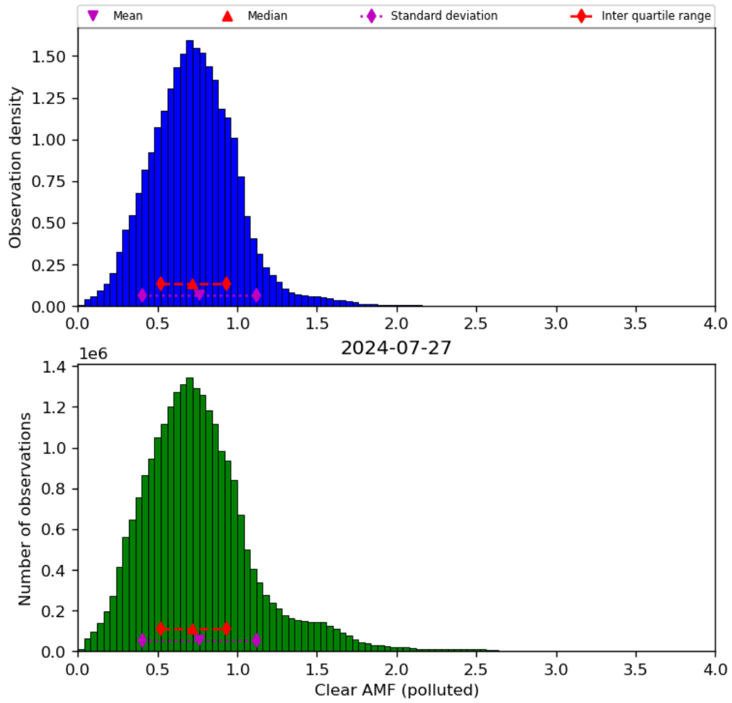
Figure 73: Histogram of “Clear AMF (polluted)” for 2024-07-26 to 2024-07-28
