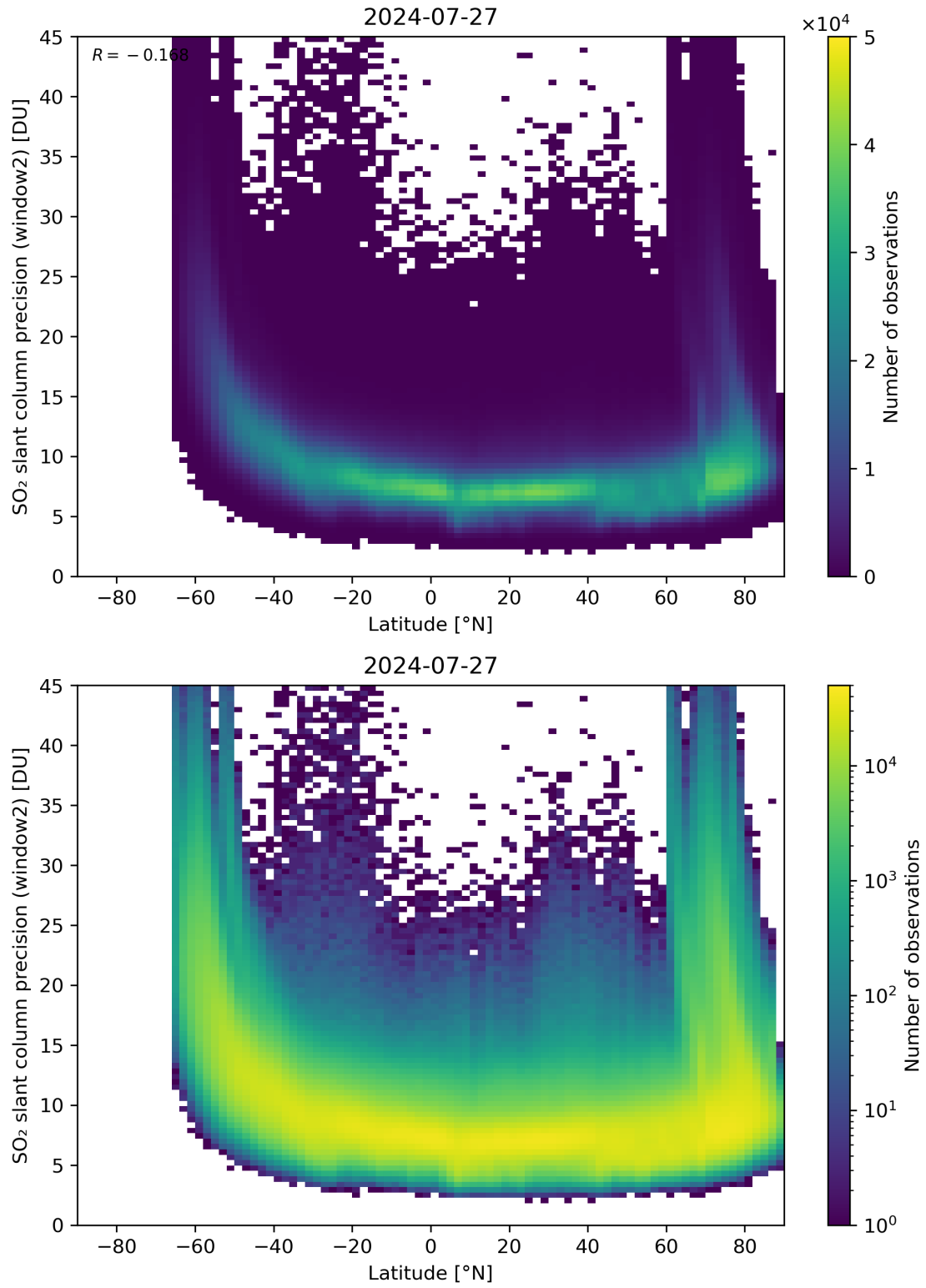
Figure 151: Scatter density plot of “Latitude” against “SO 2 slant column precision (window2)” for 2024-07-26 to 2024-07-28.
