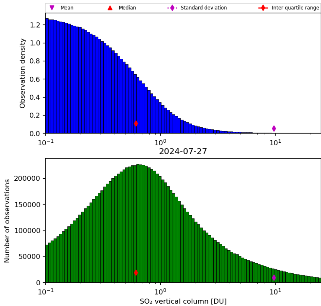
Figure 53: Histogram of “SO 2 vertical column” for 2024-07-26 to 2024-07-28
