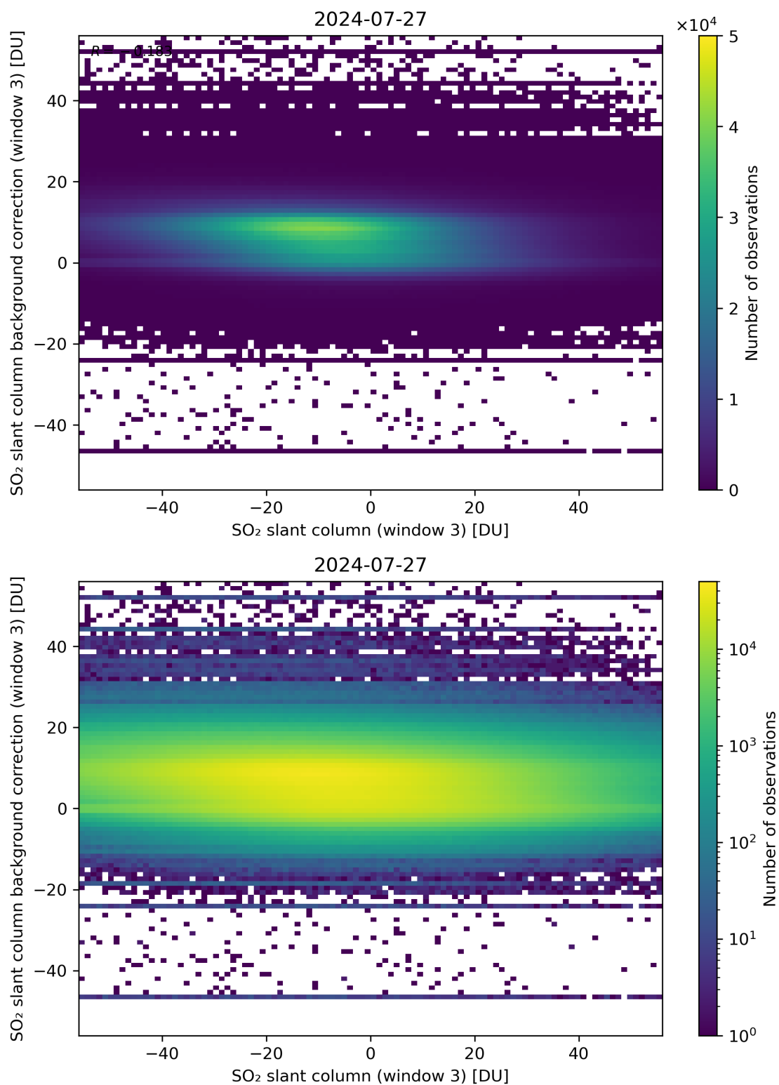
Figure 253: Scatter density plot of “SO 2 slant column (window 3)” against “SO 2 slant column background correction (window 3)” for 2024-07-26 to 2024-07-28.
