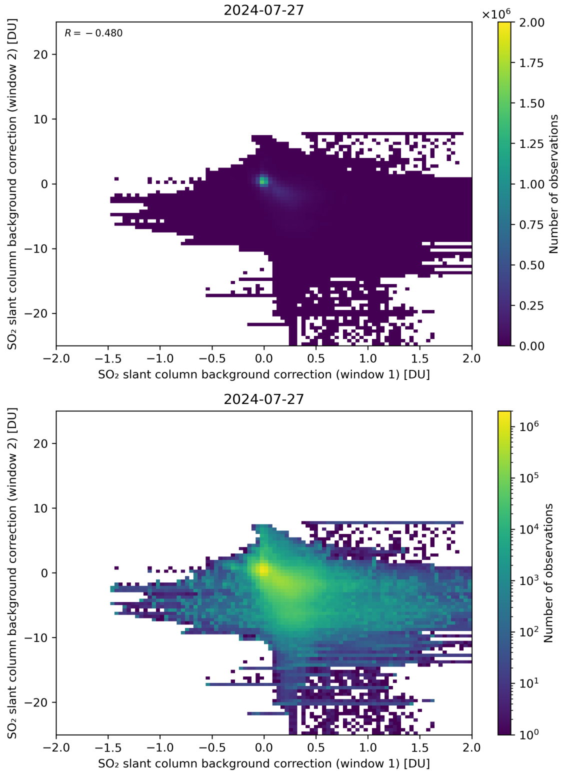
Figure 98: Scatter density plot of “SO 2 slant column background correction (window 1)” against “SO 2 slant column background correction (window 2)” for 2024-07-26 to 2024-07-28.
