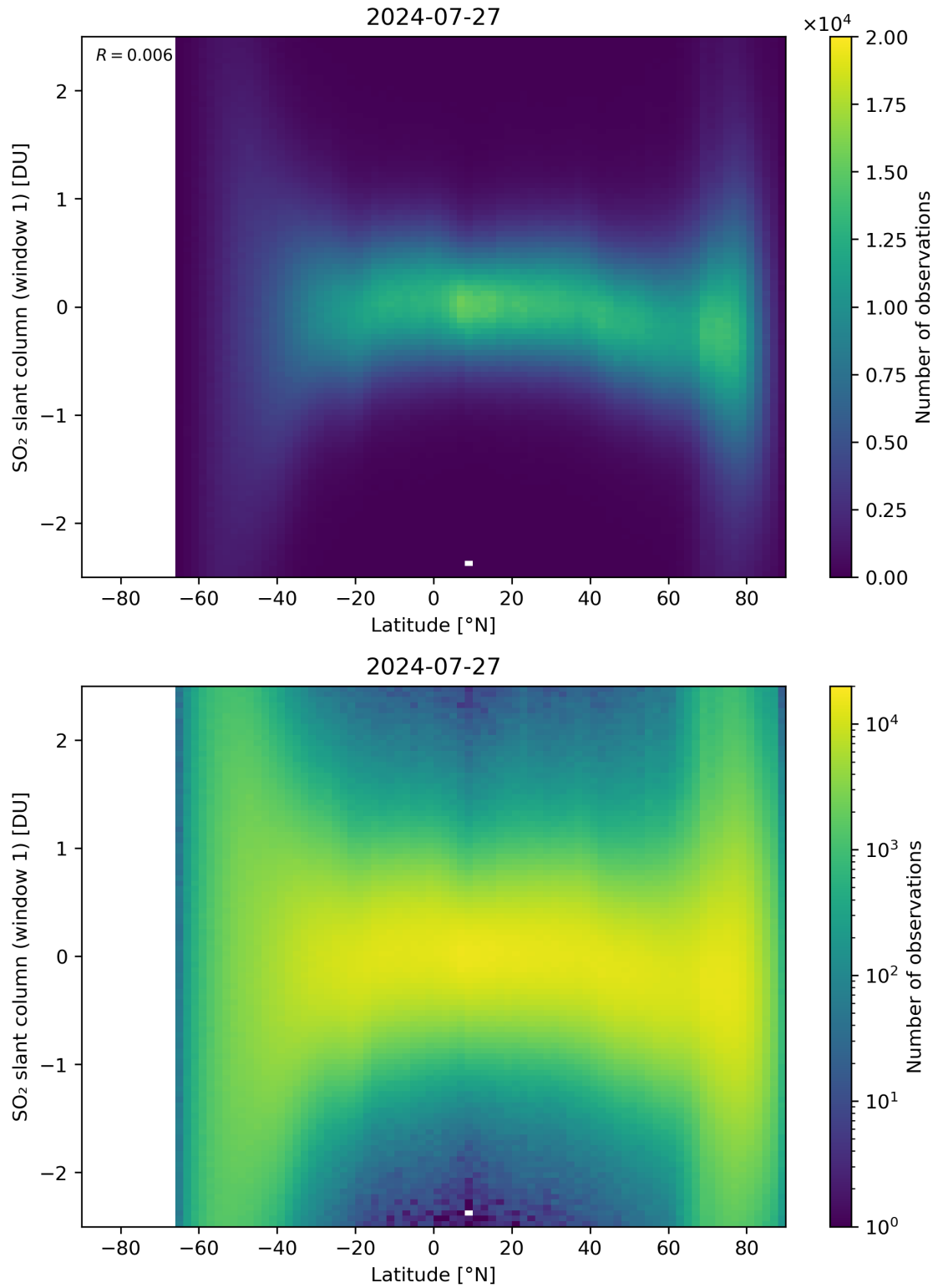
Figure 149: Scatter density plot of “Latitude” against “SO 2 slant column (window 1)” for 2024-07-26 to 2024-07-28.
