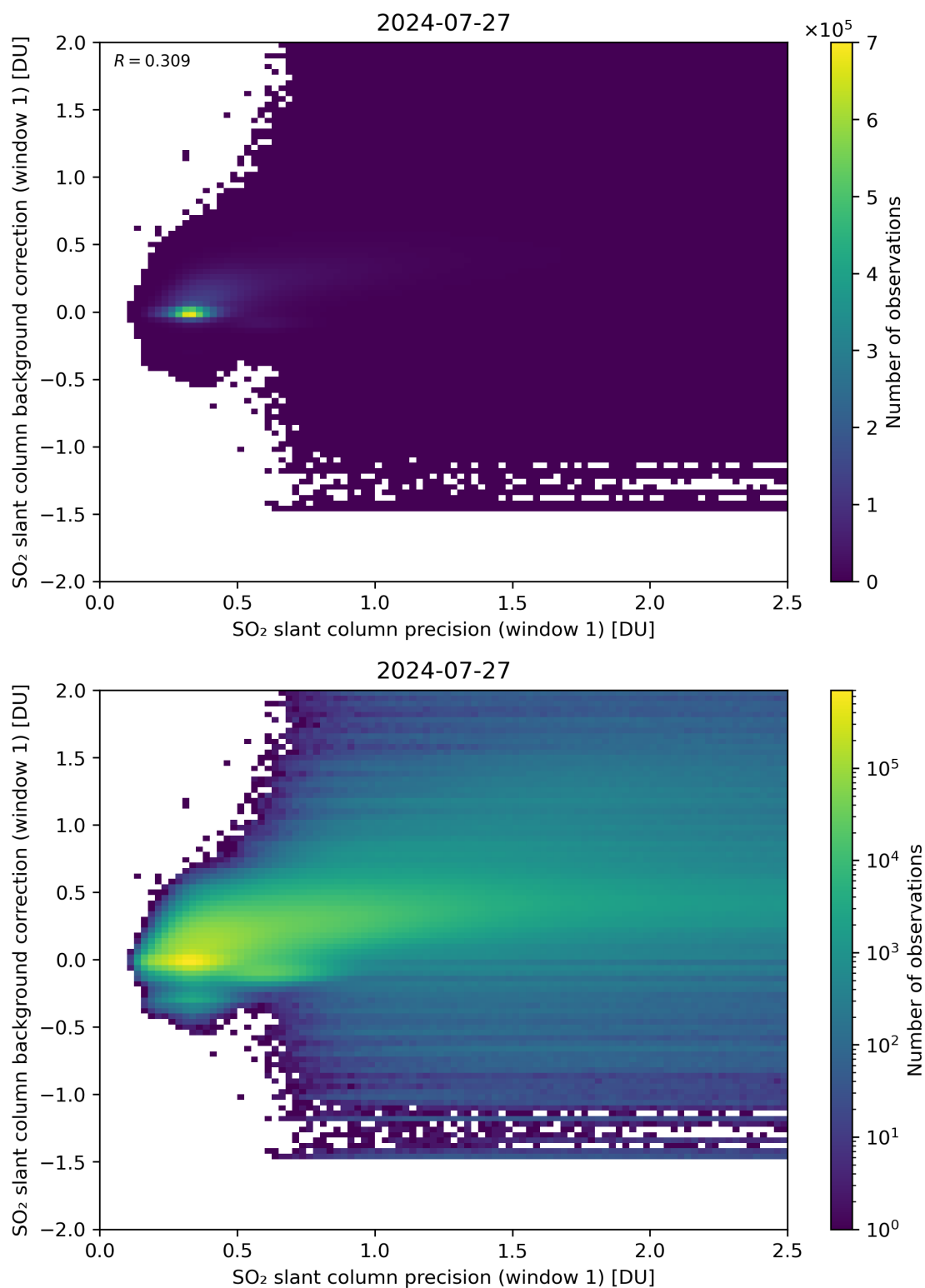
Figure 218: Scatter density plot of “SO 2 slant column precision (window 1)” against “SO 2 slant column background correction (window 1)” for 2024-07-26 to 2024-07-28.
