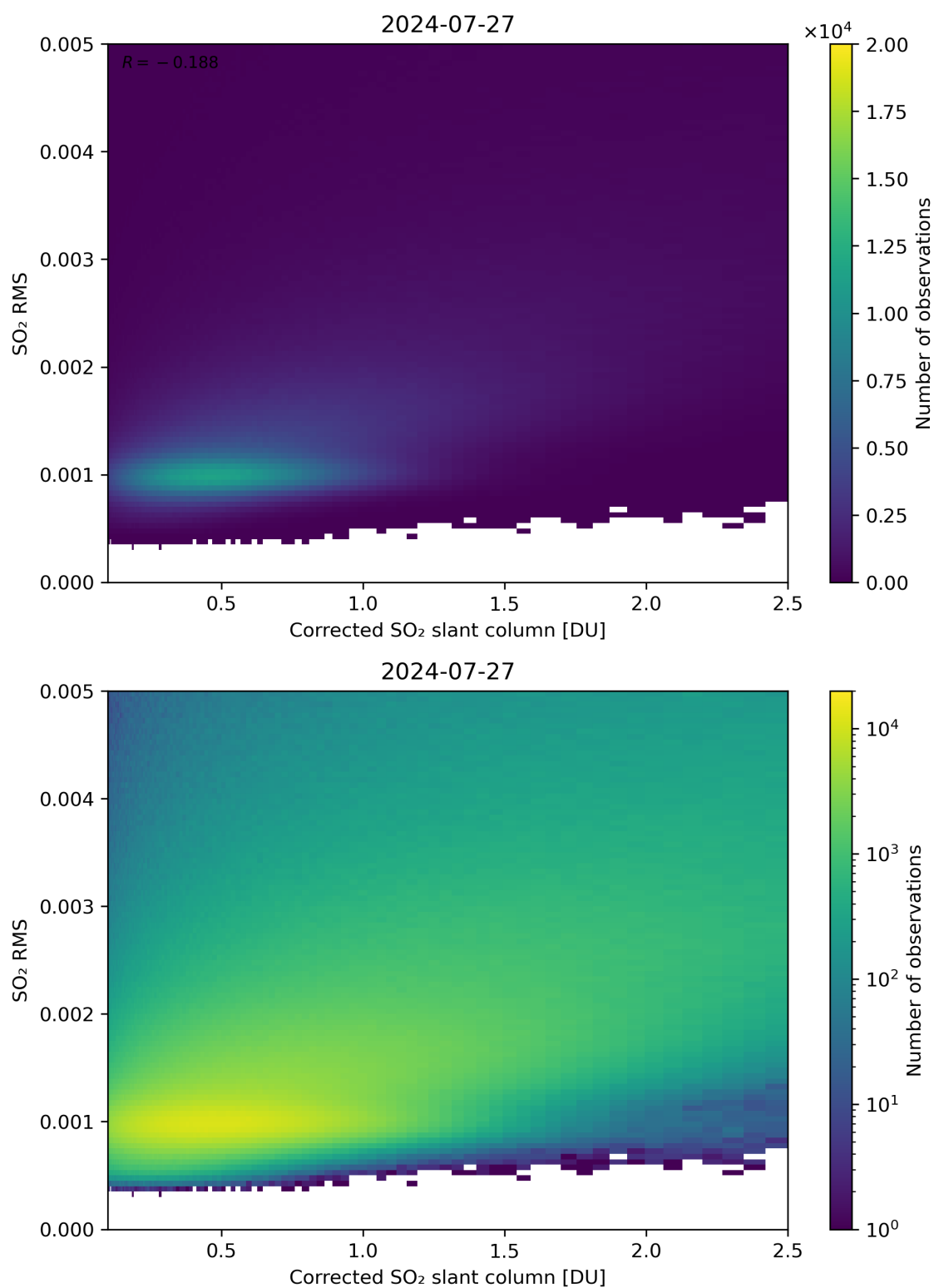
Figure 183: Scatter density plot of “Corrected SO 2 slant column” against “SO 2 RMS” for 2024-07-26 to 2024-07-28.
