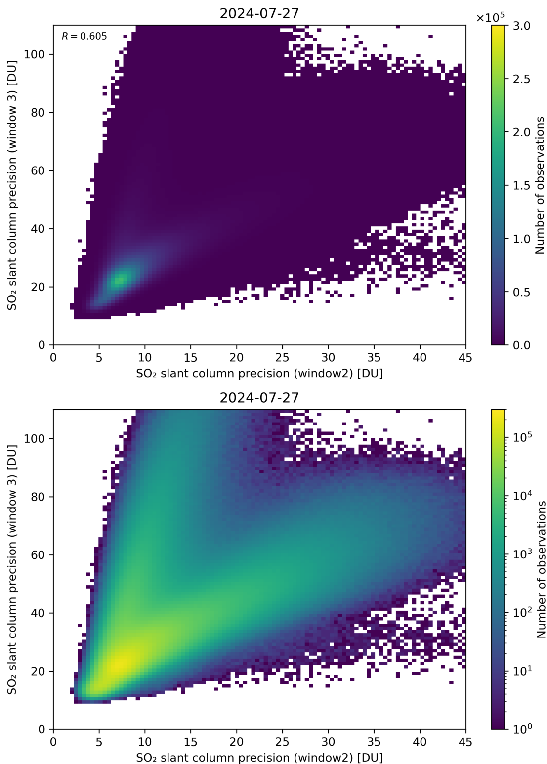
Figure 250: Scatter density plot of “SO 2 slant column precision (window2)” against “SO 2 slant column precision (window 3)” for 2024-07-26 to 2024-07-28.
