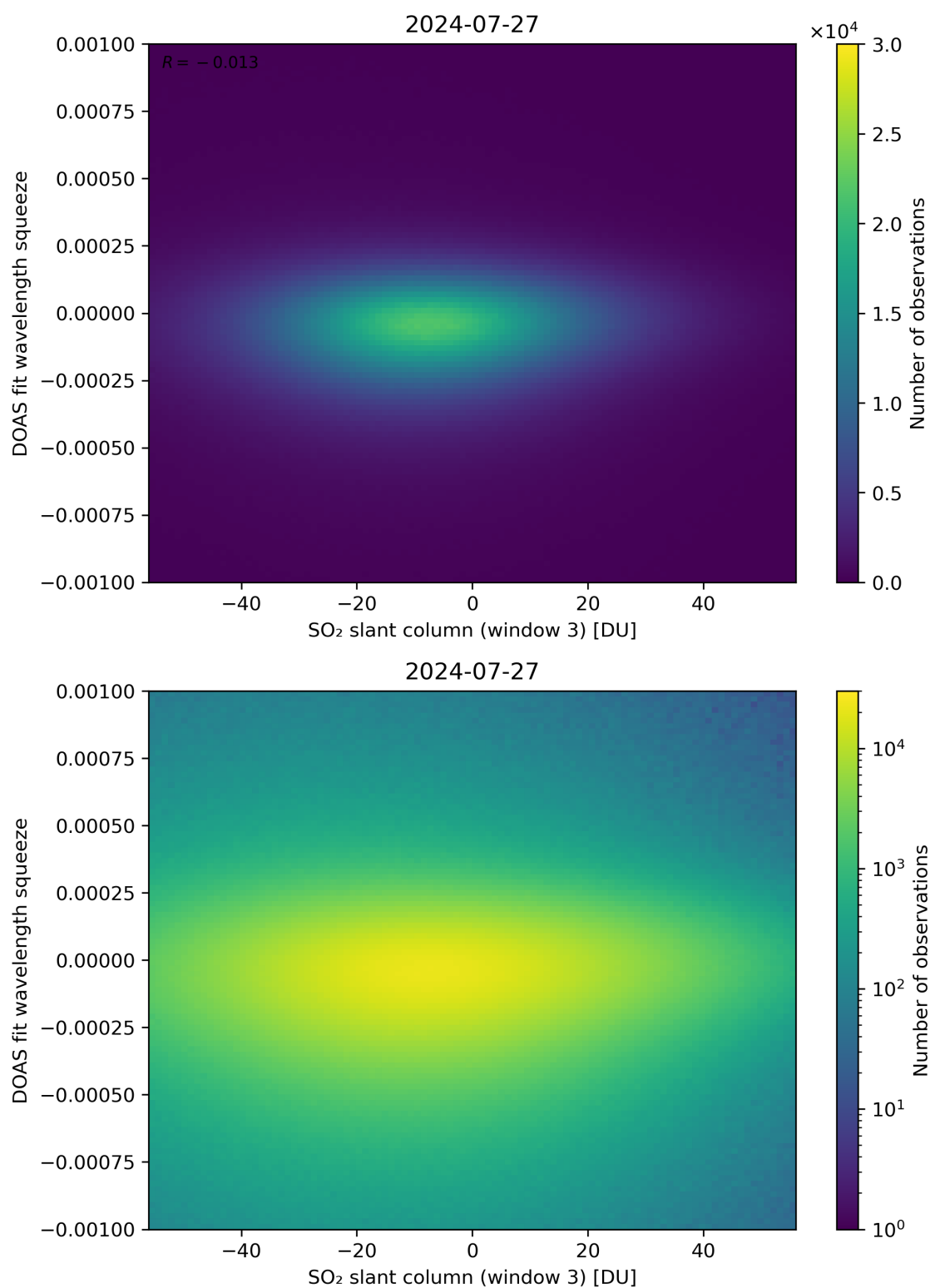
Figure 255: Scatter density plot of “SO 2 slant column (window 3)” against “DOAS fit wavelength squeeze” for 2024-07-26 to 2024-07-28.
