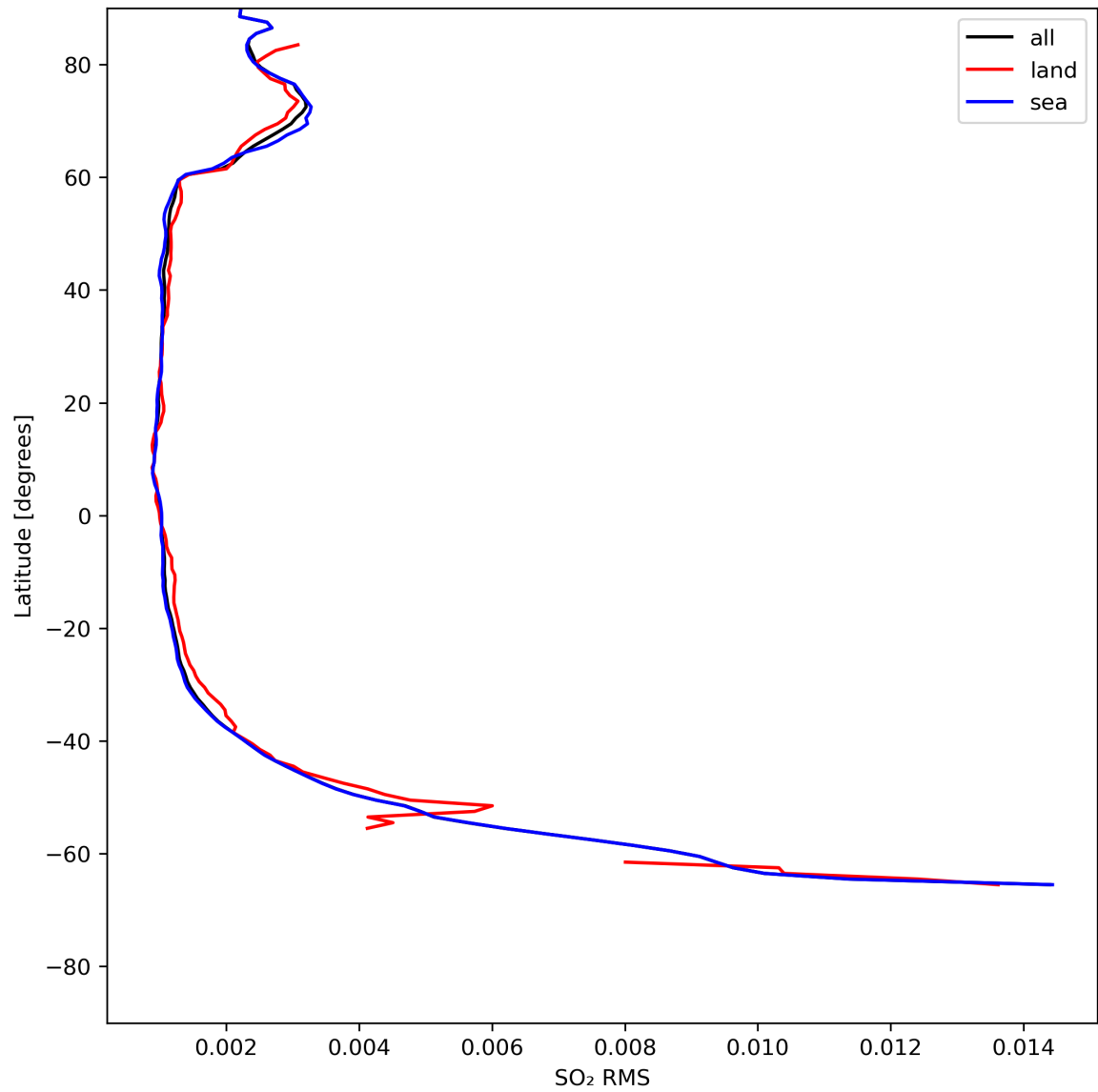
Figure 47: Zonal average of “SO 2 RMS” for 2024-07-26 to 2024-07-28.
