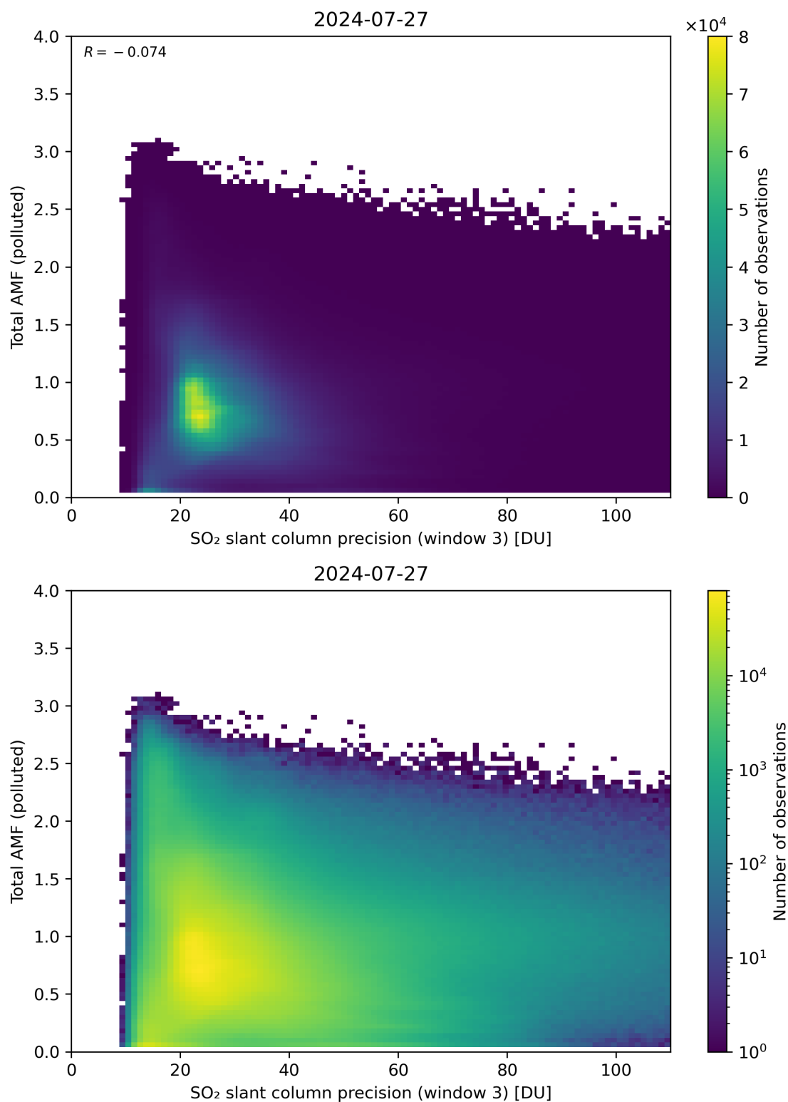
Figure 263: Scatter density plot of “SO 2 slant column precision (window 3)” against “Total AMF (polluted)” for 2024-07-26 to 2024-07-28.
