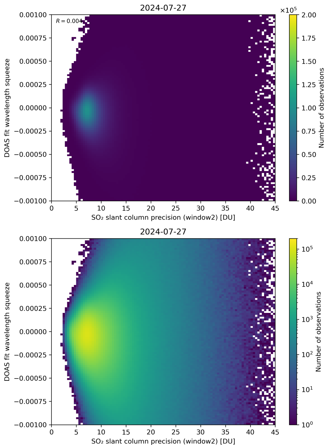
Figure 244: Scatter density plot of “SO 2 slant column precision (window2)” against “DOAS fit wavelength squeeze” for 2024-07-26 to 2024-07-28.
