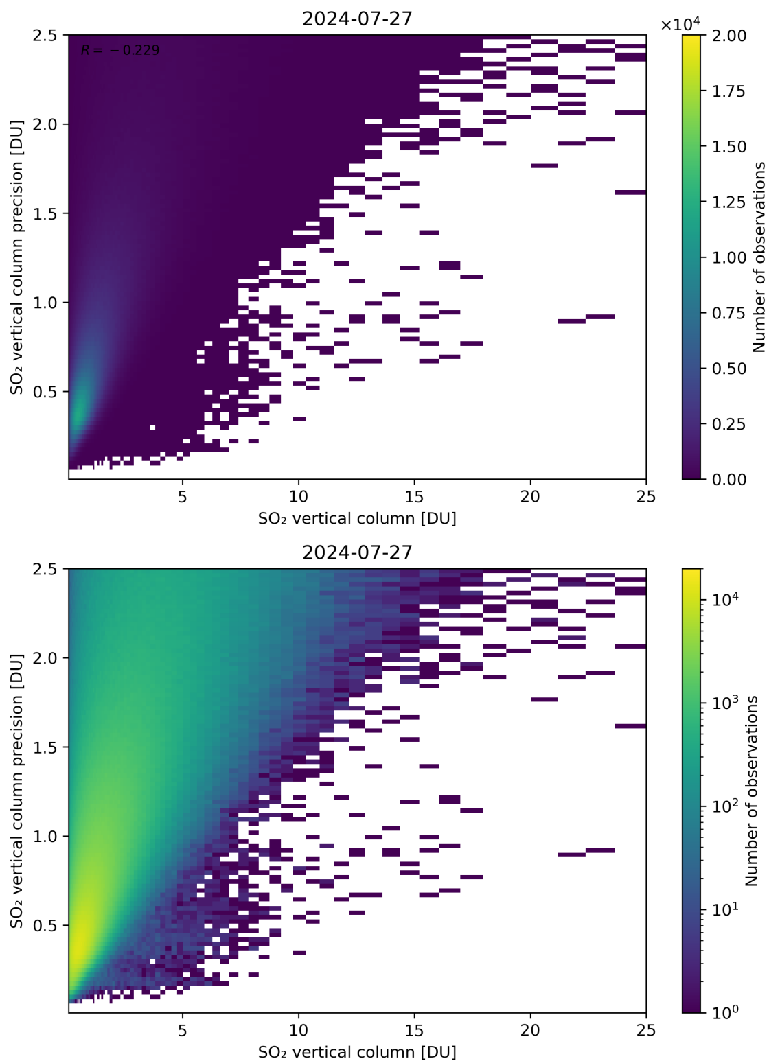
Figure 307: Scatter density plot of “SO 2 vertical column” against “SO 2 vertical column precision” for 2024-07-26 to 2024-07-28.
