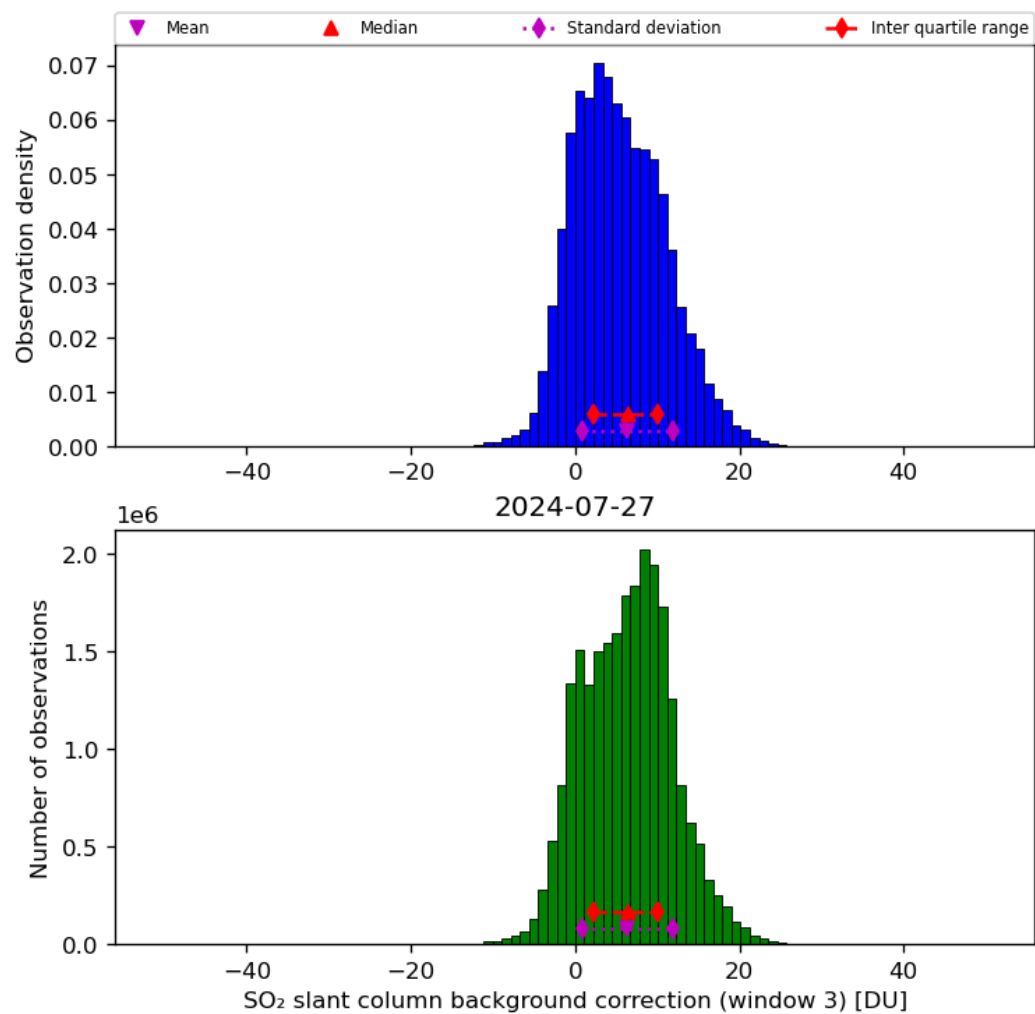
Figure 67: Histogram of “SO 2 slant column background correction (window 3)” for 2024-07-26 to 2024-07-28
