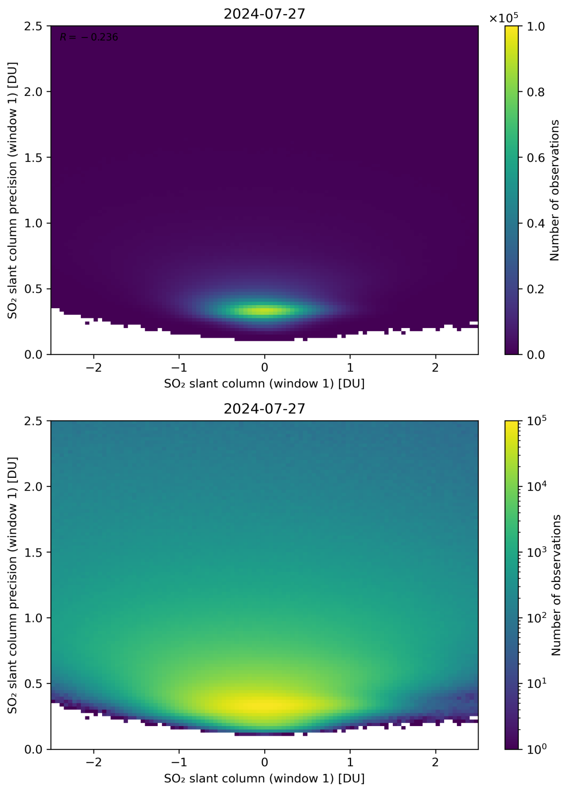
Figure 235: Scatter density plot of “SO 2 slant column (window 1)” against “SO 2 slant column precision (window 1)” for 2024-07-26 to 2024-07-28.
