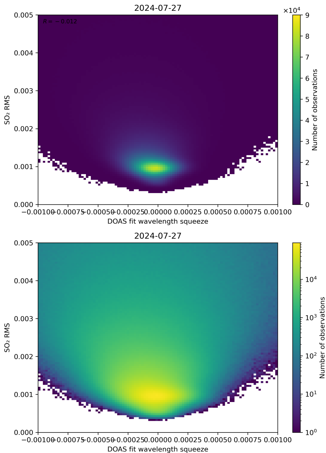
Figure 132: Scatter density plot of “DOAS fit wavelength squeeze” against “SO 2 RMS” for 2024-07-26 to 2024-07-28.
