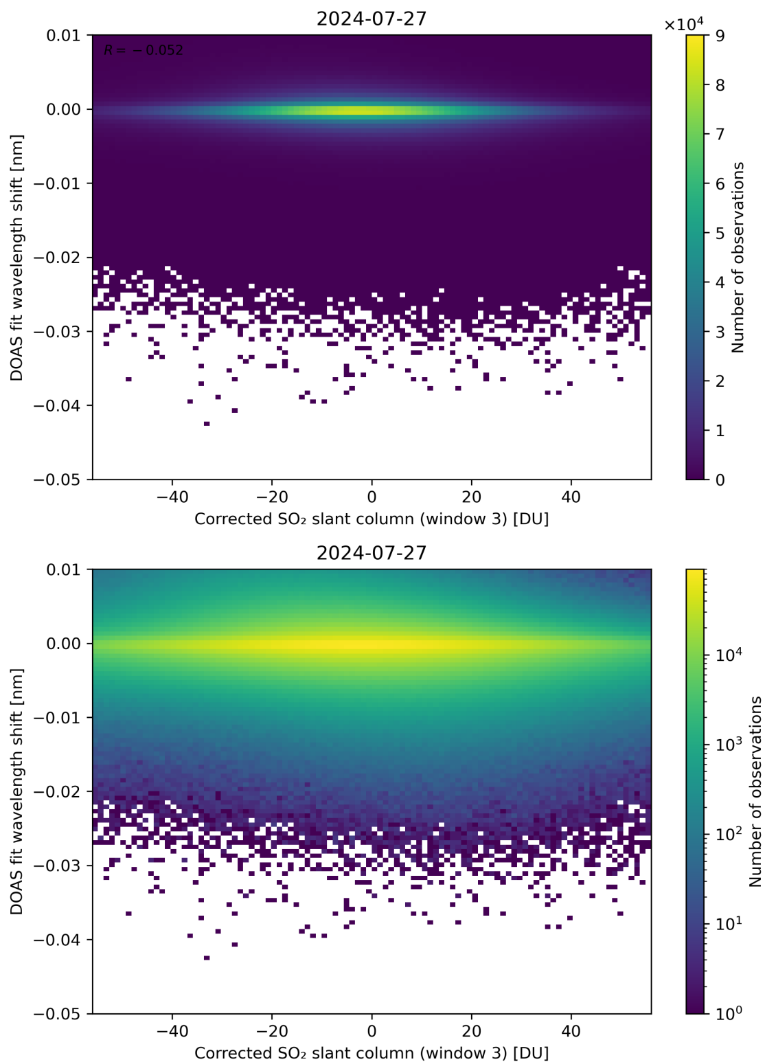
Figure 206: Scatter density plot of “Corrected SO 2 slant column (window 3)” against “DOAS fit wavelength shift” for 2024-07-26 to 2024-07-28.
