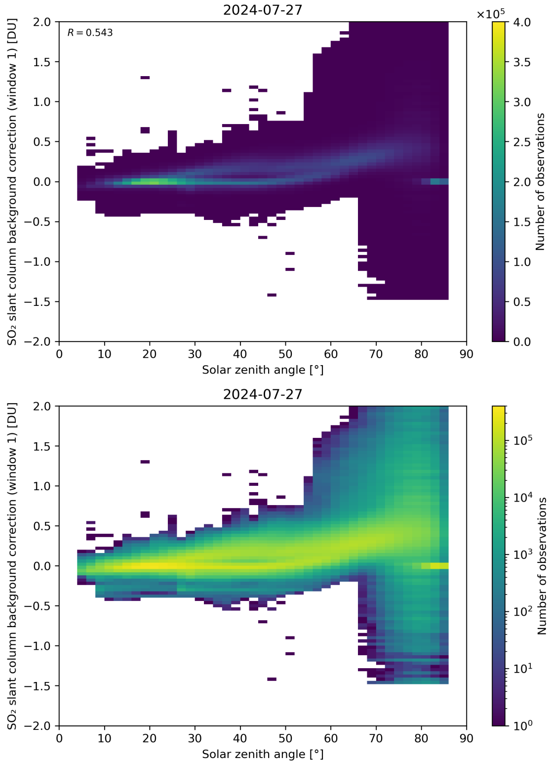
Figure 158: Scatter density plot of “Solar zenith angle” against “SO 2 slant column background correction (window 1)” for 2024-07-26 to 2024-07-28.
