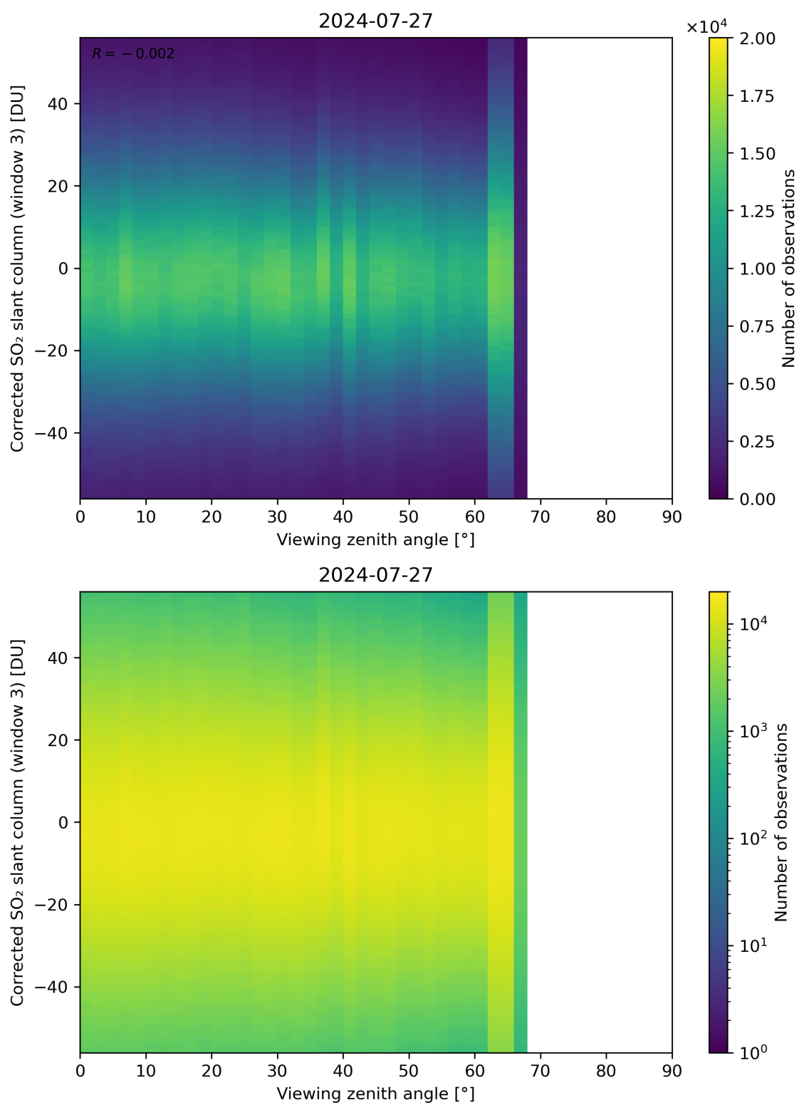
Figure 319: Scatter density plot of “Viewing zenith angle” against “Corrected SO 2 slant column (window 3)” for 2024-07-26 to 2024-07-28.
