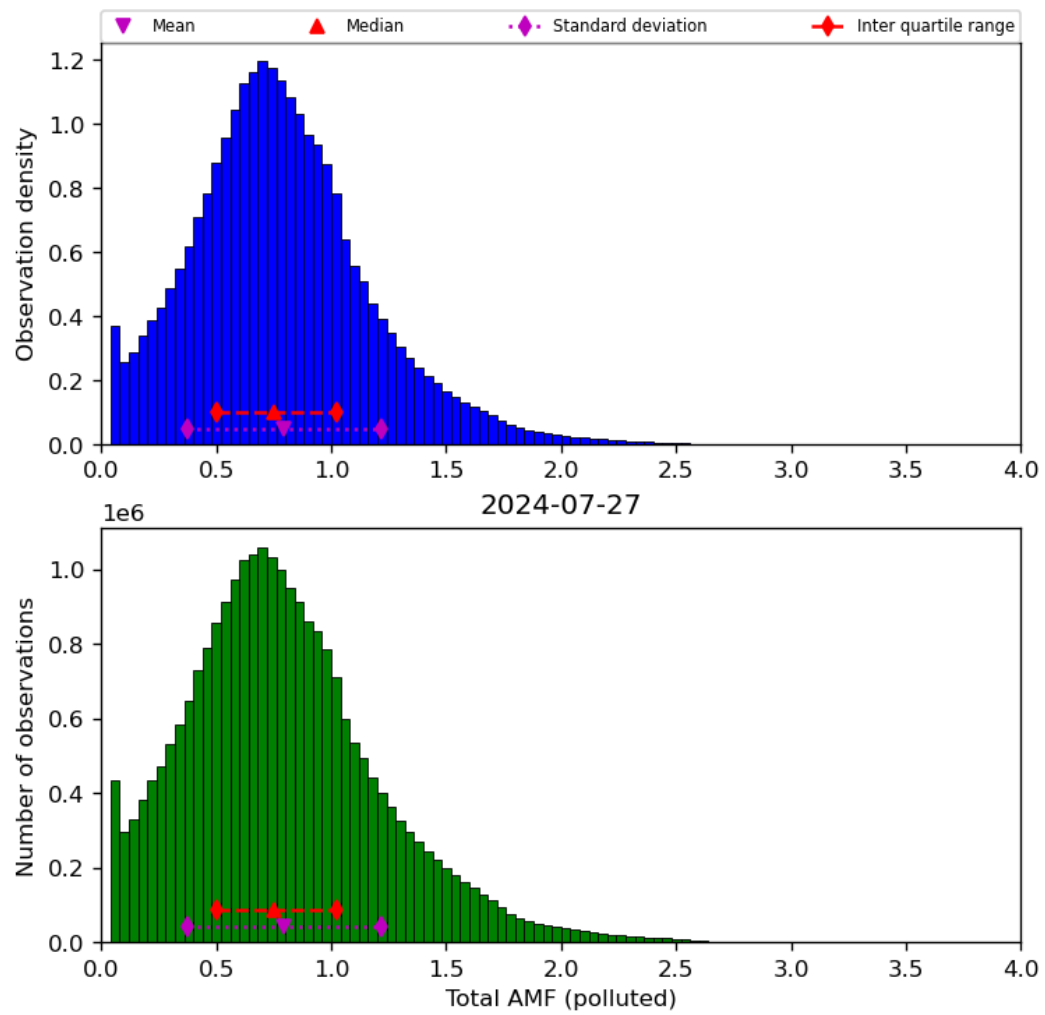
Figure 71: Histogram of “Total AMF (polluted)” for 2024-07-26 to 2024-07-28
