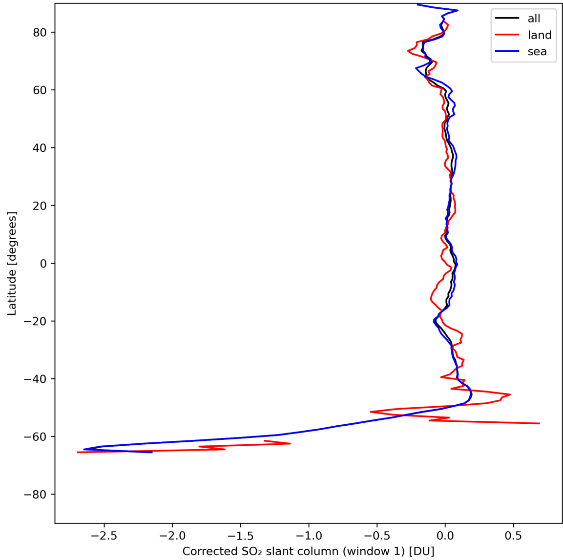
Figure 35: Zonal average of “Corrected SO 2 slant column (window 1)” for 2024-07-26 to 2024-07-28.
