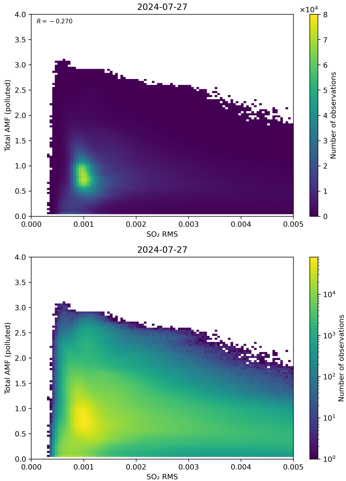
Figure 137: Scatter density plot of “SO 2 RMS” against “Total AMF (polluted)” for 2024-07-26 to 2024-07-28.
