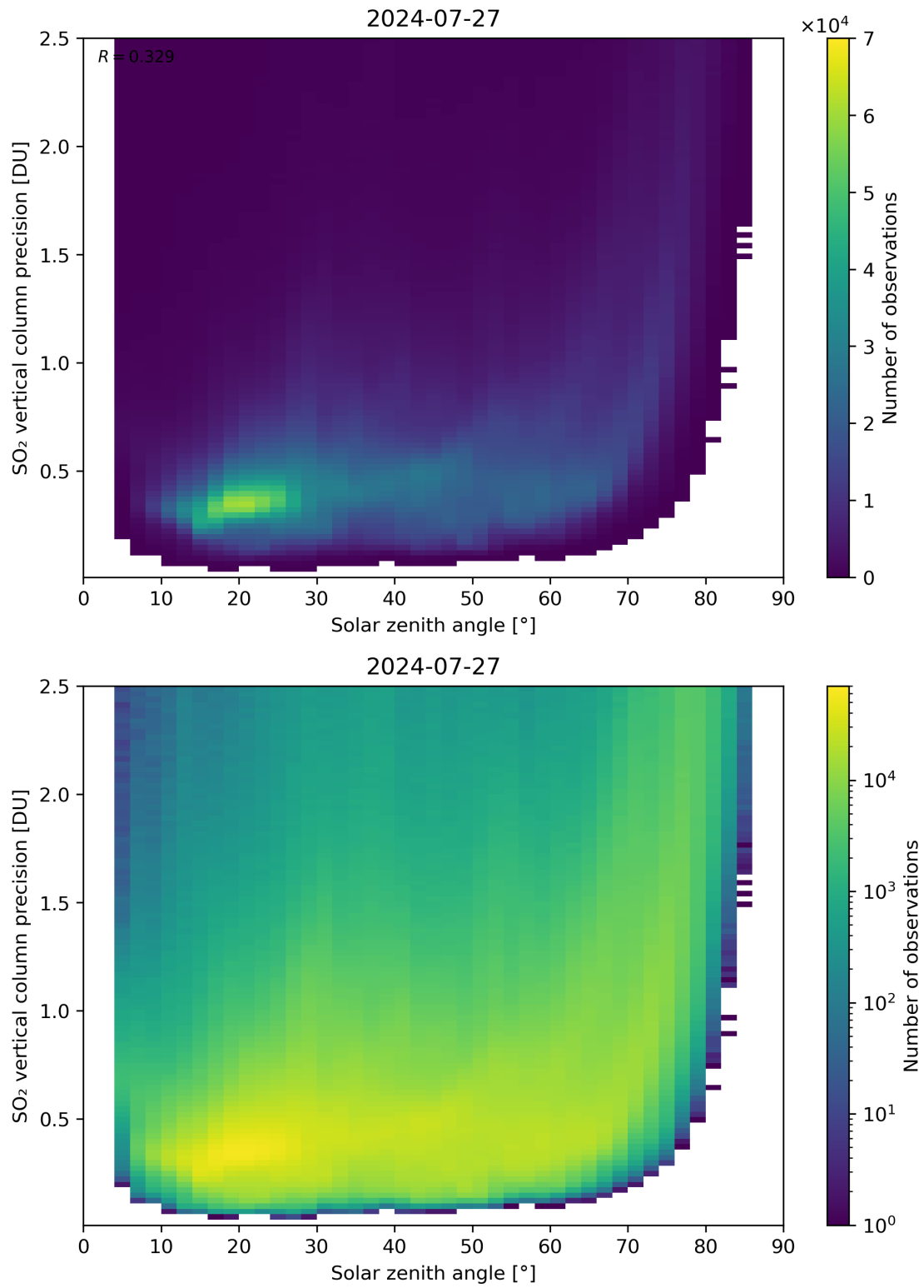
Figure 177: Scatter density plot of “Solar zenith angle” against “SO 2 vertical column precision” for 2024-07-26 to 2024-07-28.
