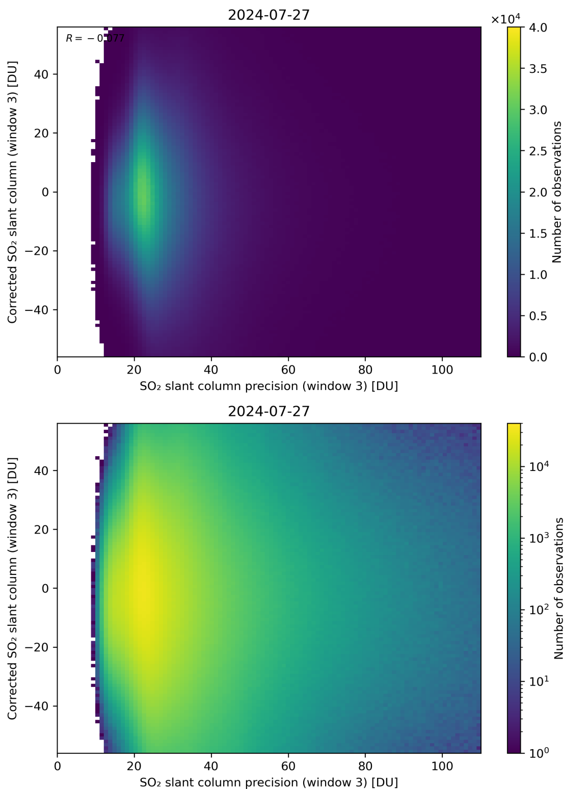
Figure 262: Scatter density plot of “SO 2 slant column precision (window 3)” against “Corrected SO 2 slant column (window 3)” for 2024-07-26 to 2024-07-28.
