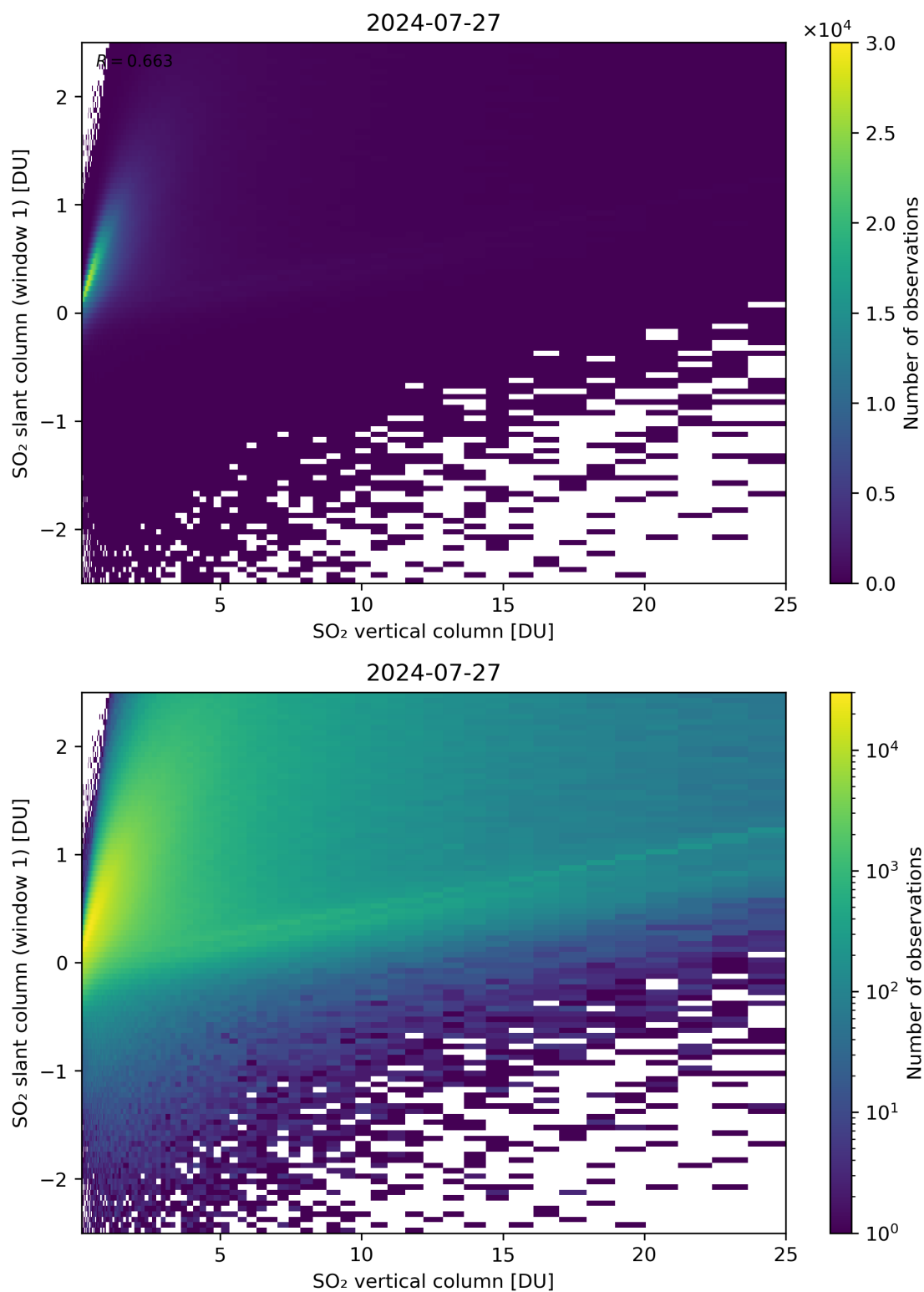
Figure 300: Scatter density plot of “SO 2 vertical column” against “SO 2 slant column (window 1)” for 2024-07-26 to 2024-07-28.
