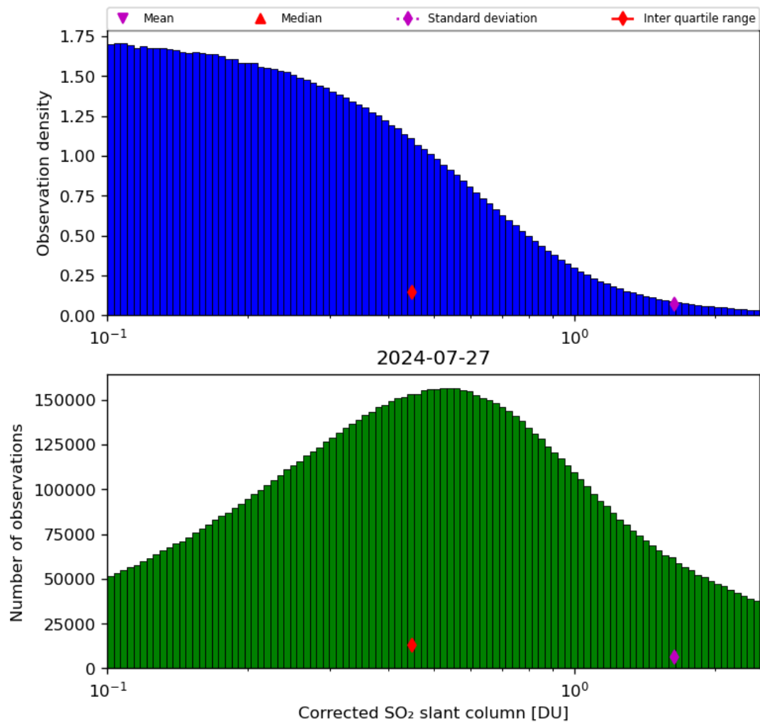
Figure 55: Histogram of “Corrected SO 2 slant column” for 2024-07-26 to 2024-07-28
