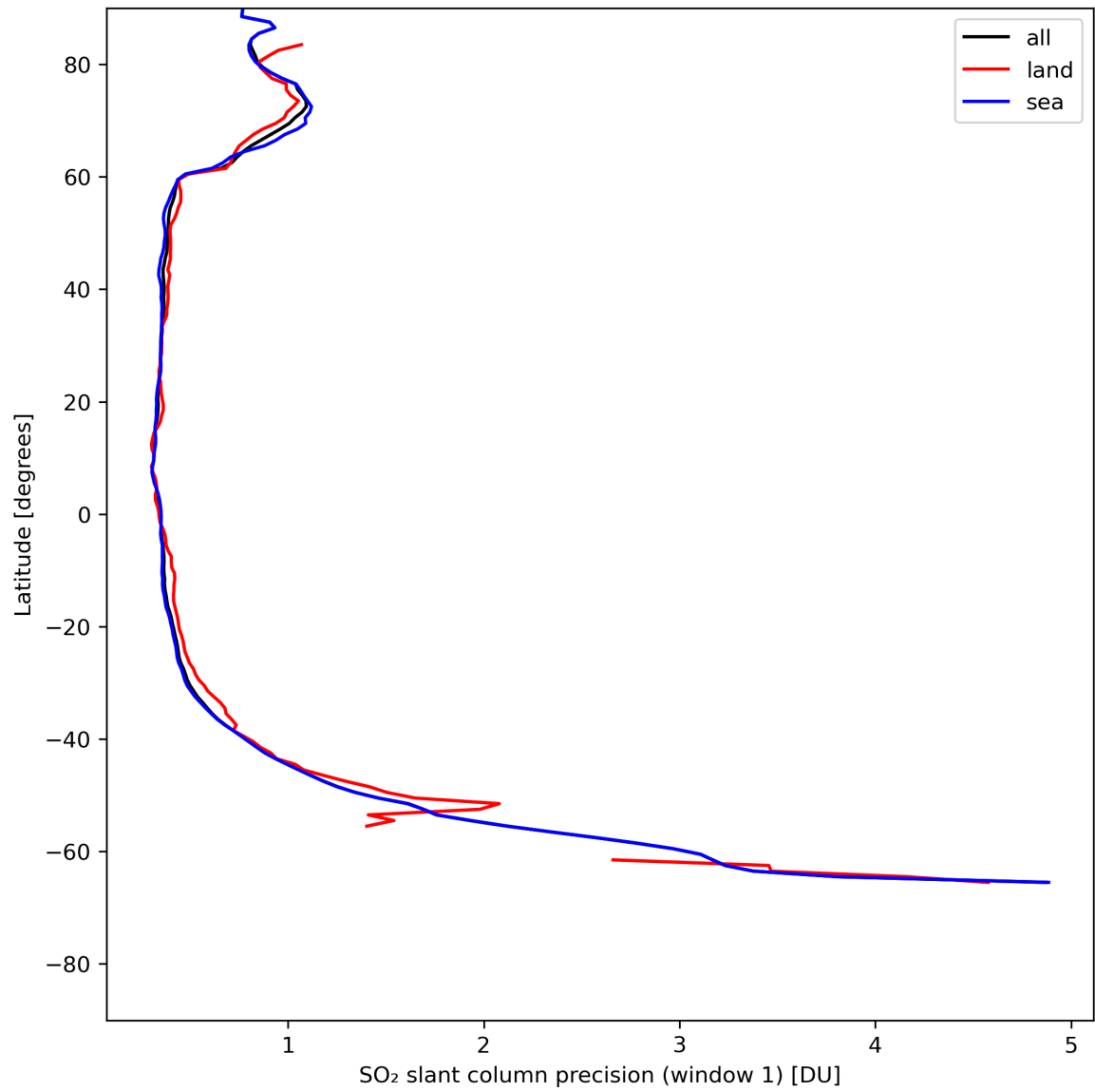
Figure 34: Zonal average of “SO 2 slant column precision (window 1)” for 2024-07-26 to 2024-07-28.
