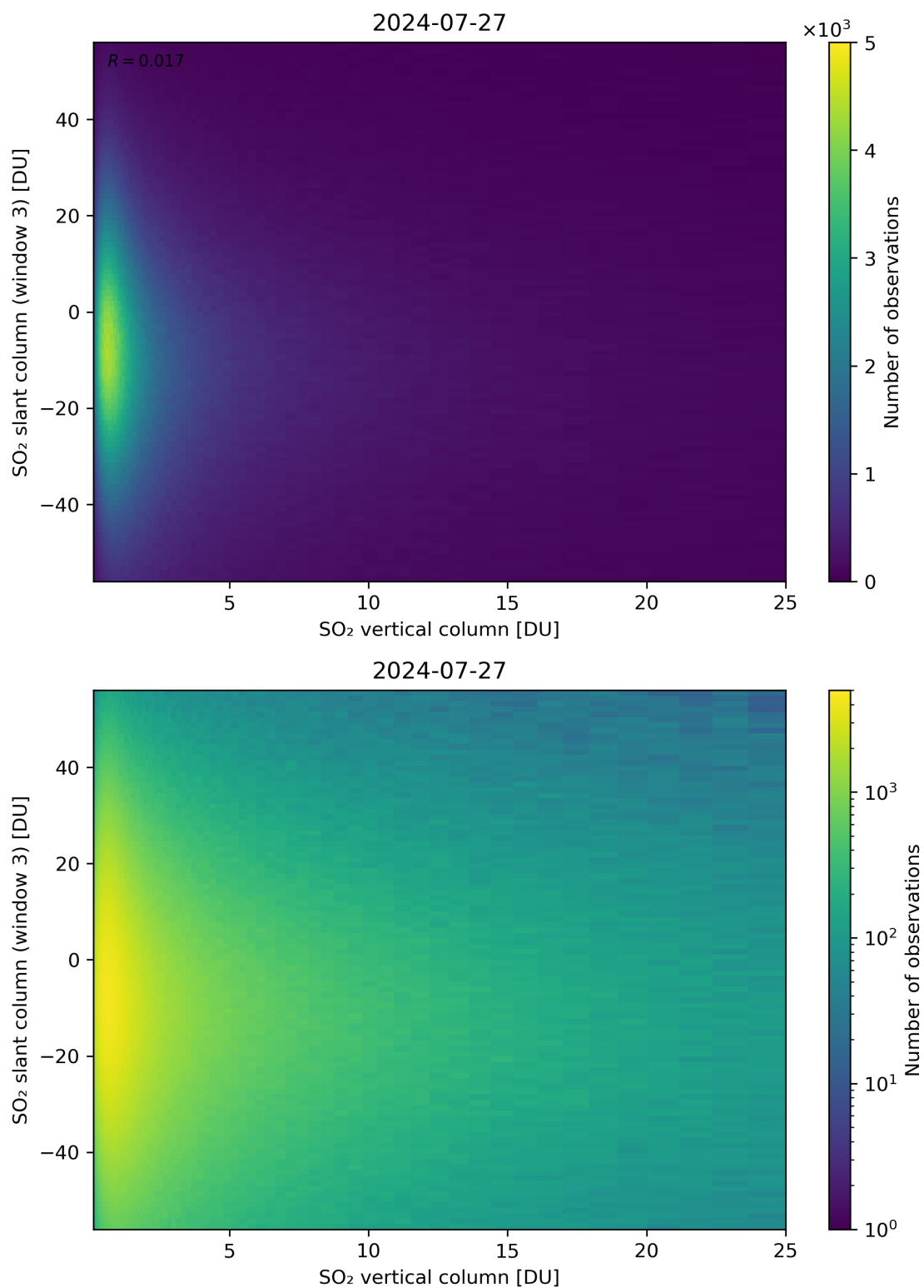
Figure 303: Scatter density plot of “SO 2 vertical column” against “SO 2 slant column (window 3)” for 2024-07-26 to 2024-07-28.
