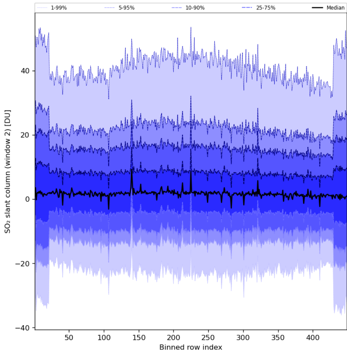
Figure 83: Along track statistics of “SO 2 slant column (window 2)” for 2024-07-26 to 2024-07-28
