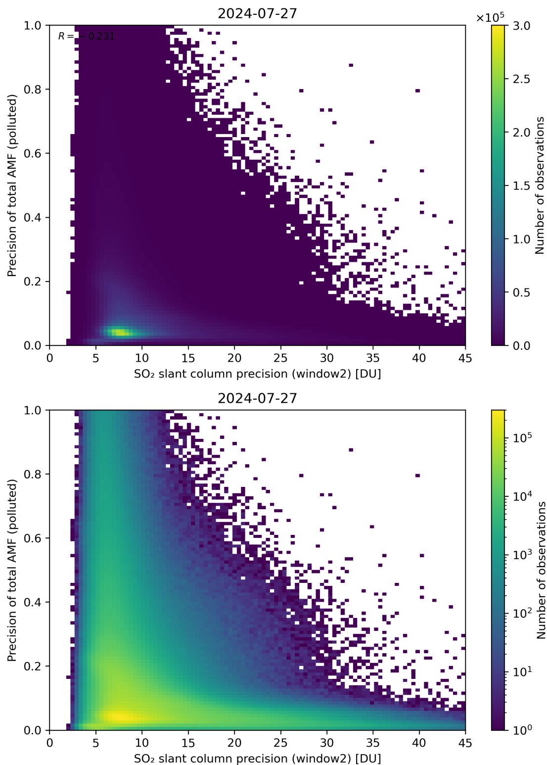
Figure 252: Scatter density plot of “SO 2 slant column precision (window2)” against “Precision of total AMF (polluted)” for 2024-07-26 to 2024-07-28.
