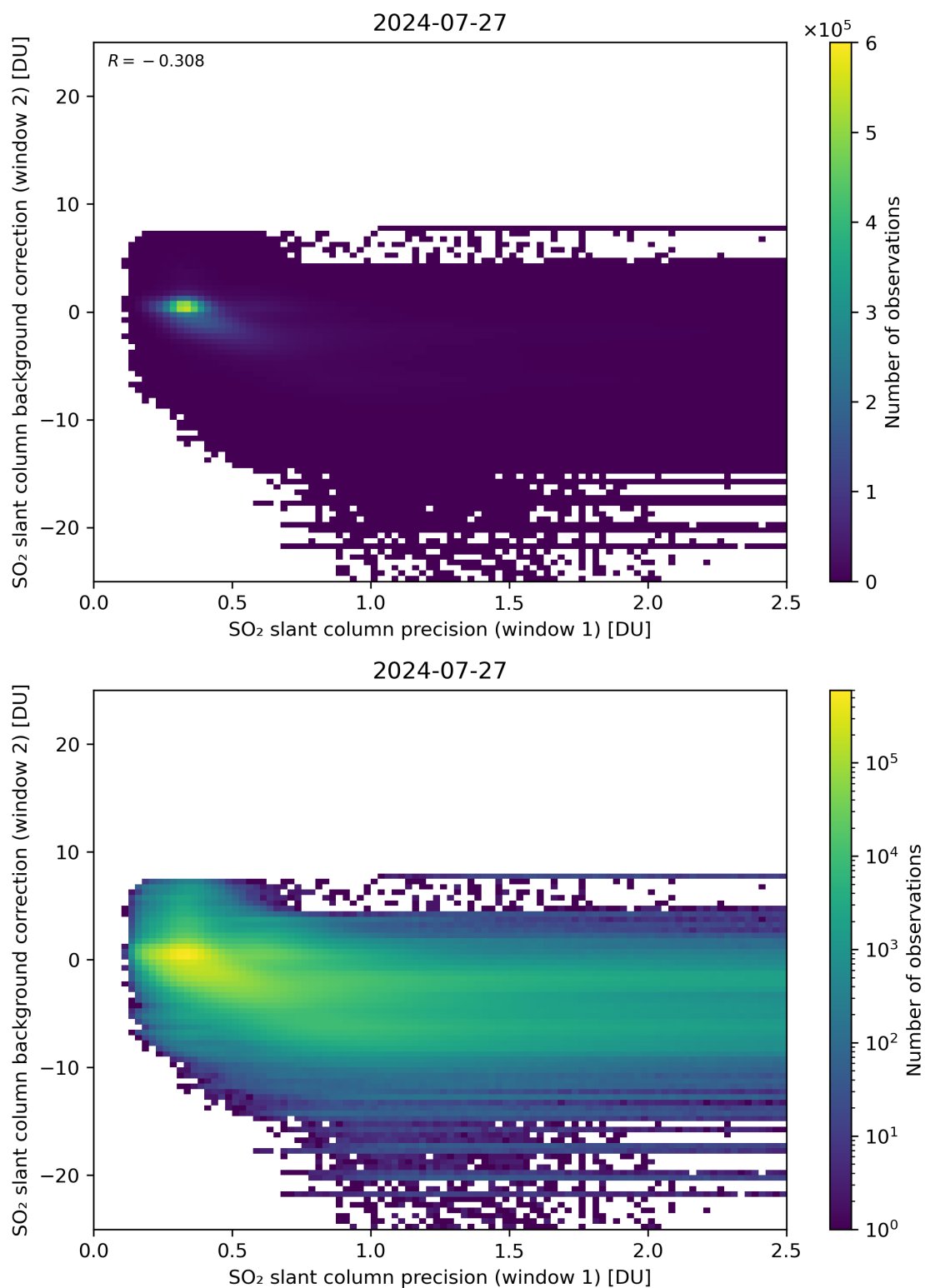
Figure 219: Scatter density plot of “SO 2 slant column precision (window 1)” against “SO 2 slant column background correction (window 2)” for 2024-07-26 to 2024-07-28.
