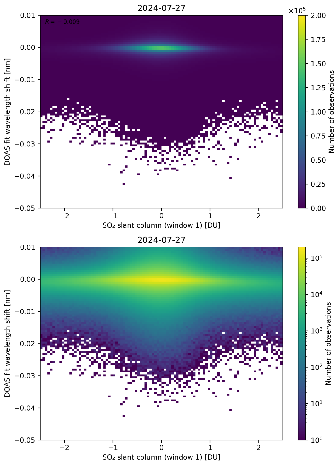
Figure 215: Scatter density plot of “SO 2 slant column (window 1)” against “DOAS fit wavelength shift” for 2024-07-26 to 2024-07-28.
