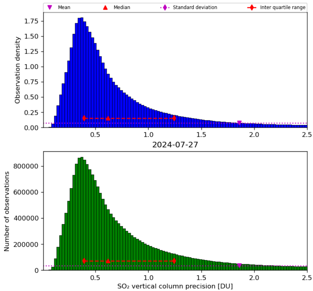
Figure 54: Histogram of “SO 2 vertical column precision” for 2024-07-26 to 2024-07-28
