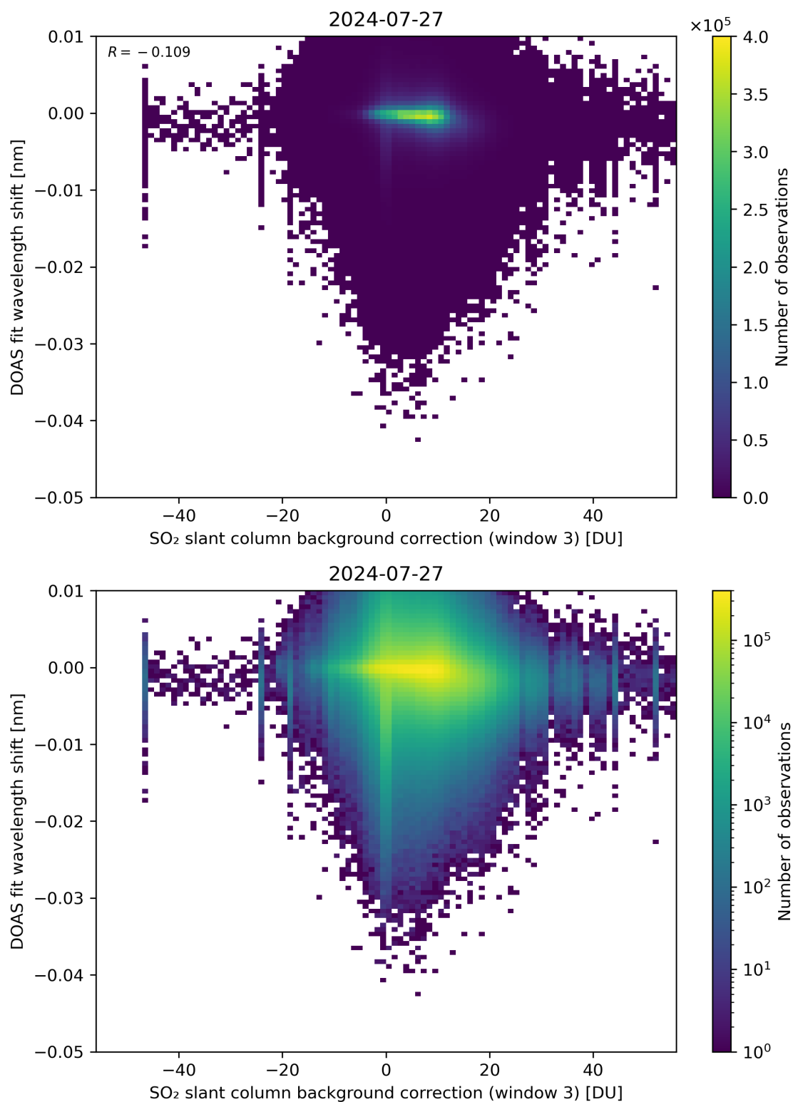
Figure 121: Scatter density plot of “SO 2 slant column background correction (window 3)” against “DOAS fit wavelength shift” for 2024-07-26 to 2024-07-28.
