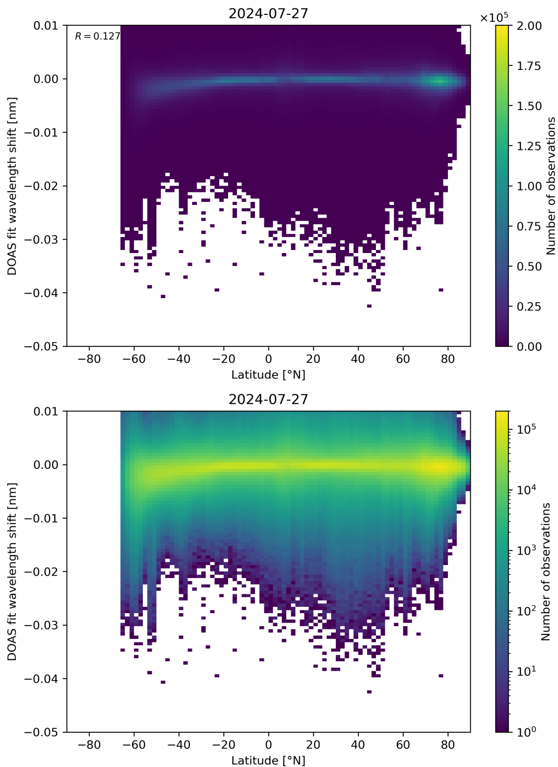
Figure 142: Scatter density plot of “Latitude” against “DOAS fit wavelength shift” for 2024-07-26 to 2024-07-28.
