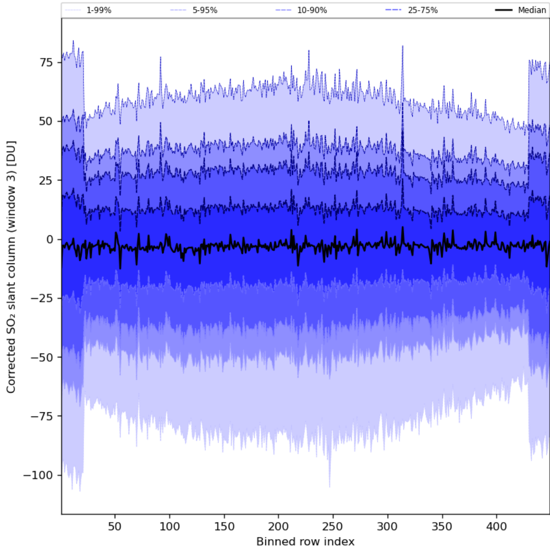
Figure 89: Along track statistics of “Corrected SO 2 slant column (window 3)” for 2024-07-26 to 2024-07-28
