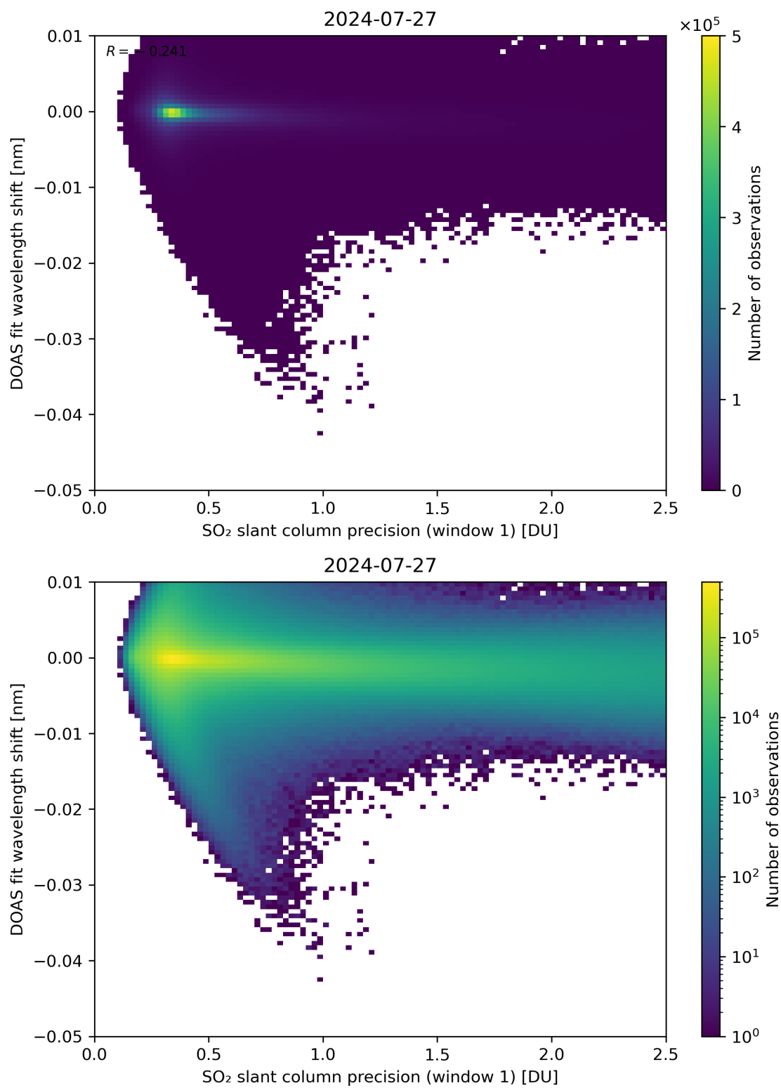
Figure 221: Scatter density plot of “SO 2 slant column precision (window 1)” against “DOAS fit wavelength shift” for 2024-07-26 to 2024-07-28.
