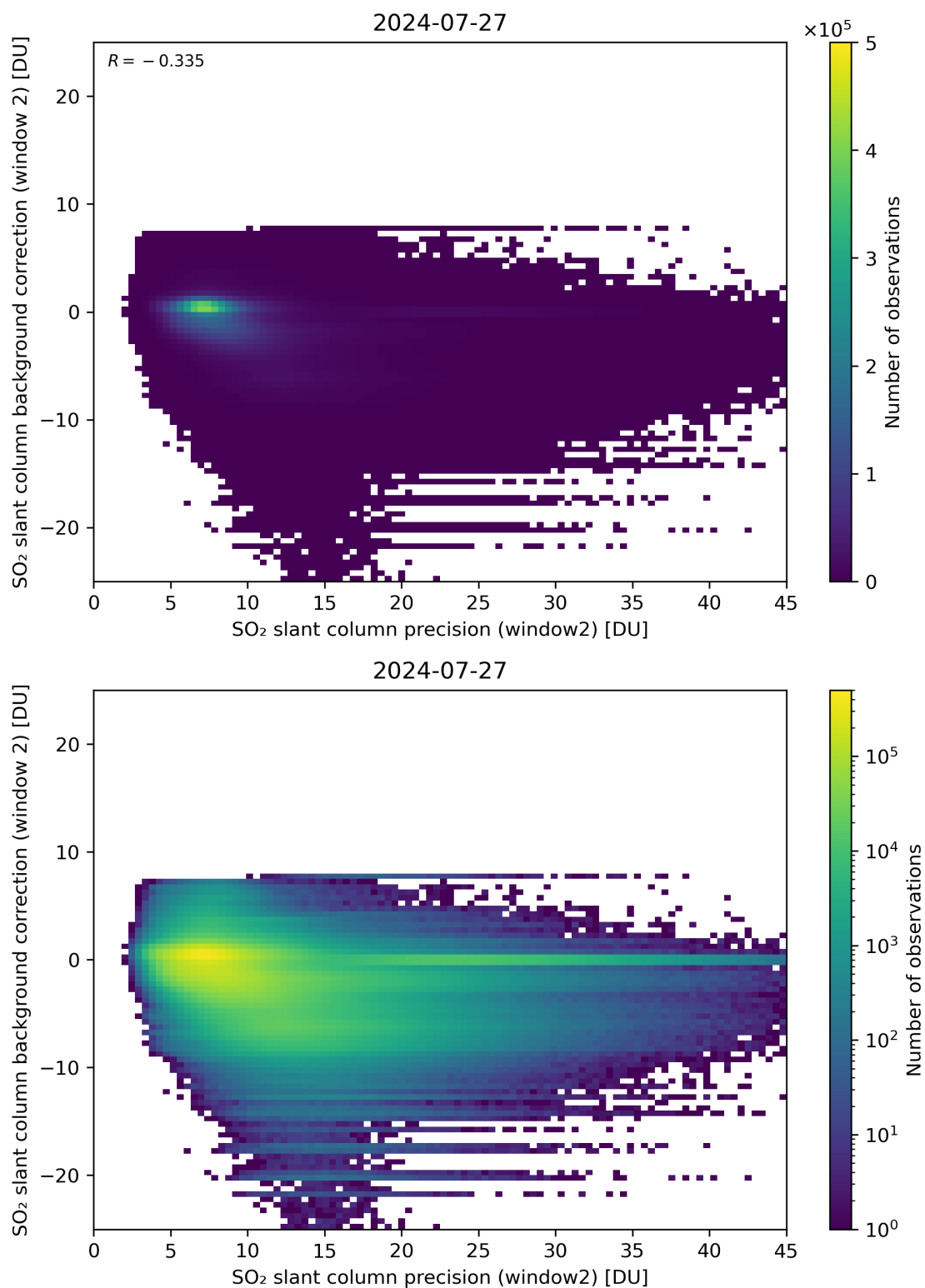
Figure 241: Scatter density plot of “SO 2 slant column precision (window2)” against “SO 2 slant column background correction (window 2)” for 2024-07-26 to 2024-07-28.
