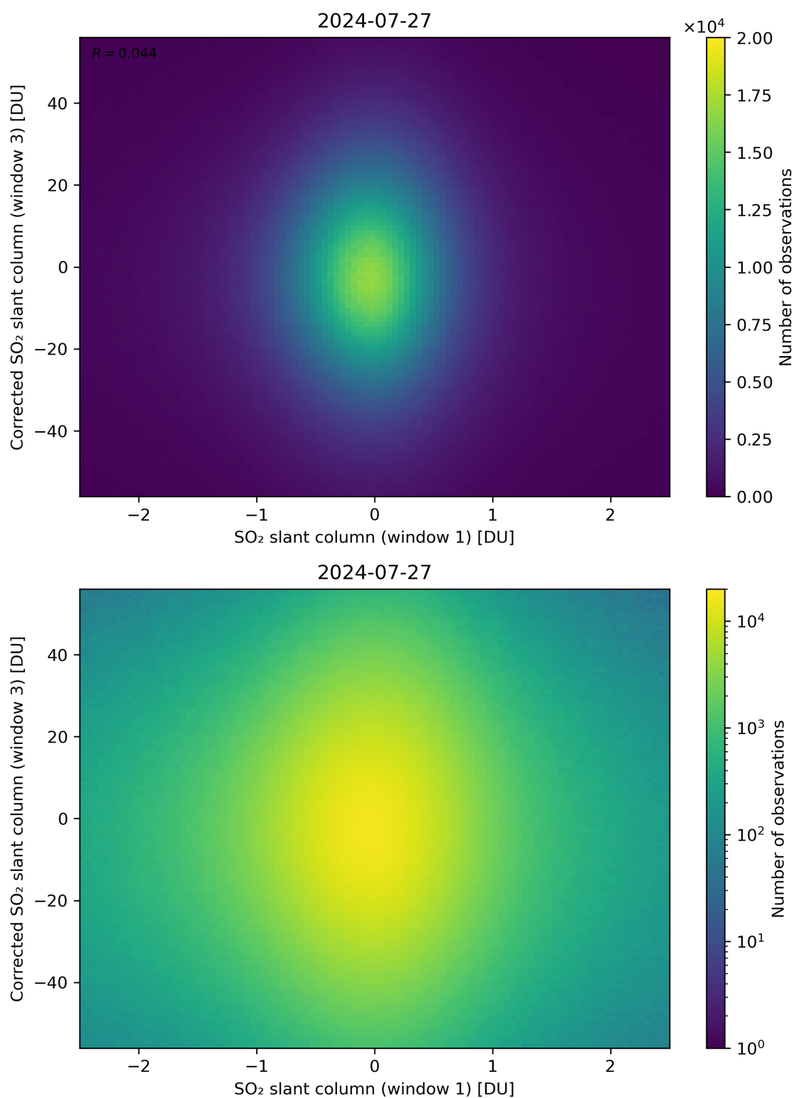
Figure 234: Scatter density plot of “SO 2 slant column (window 1)” against “Corrected SO 2 slant column (window 3)” for 2024-07-26 to 2024-07-28.
