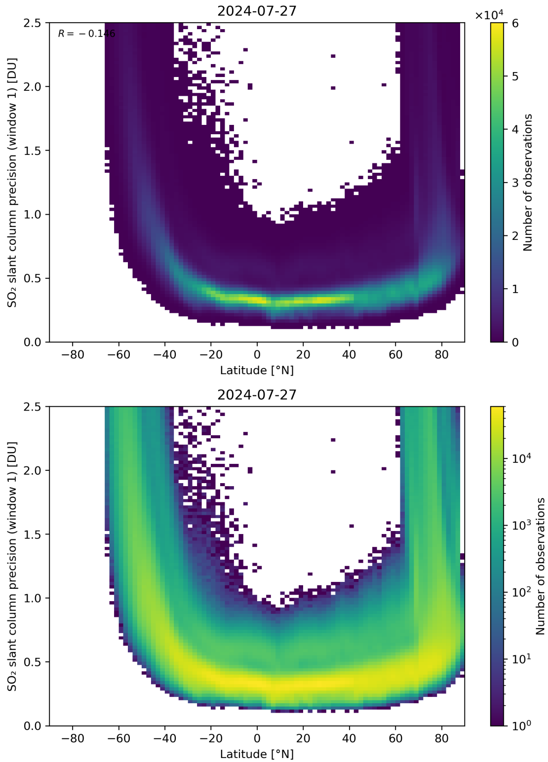
Figure 150: Scatter density plot of “Latitude” against “SO 2 slant column precision (window 1)” for 2024-07-26 to 2024-07-28.
