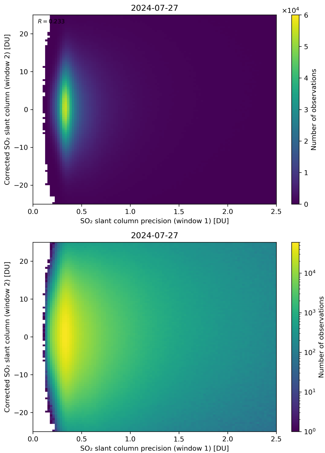
Figure 225: Scatter density plot of “SO 2 slant column precision (window 1)” against “Corrected SO 2 slant column (window 2)” for 2024-07-26 to 2024-07-28.
