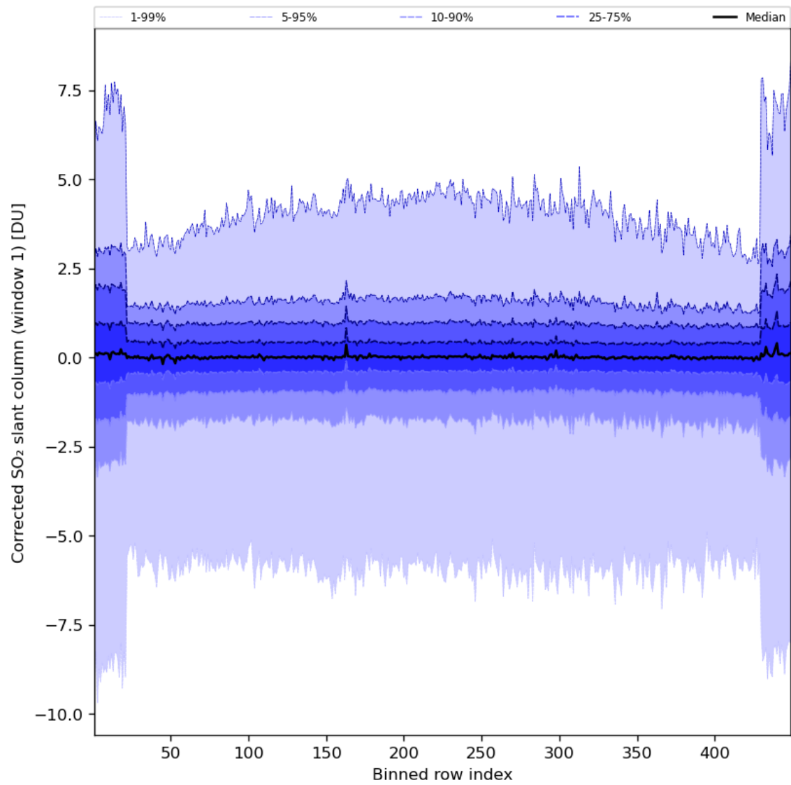
Figure 81: Along track statistics of “Corrected SO 2 slant column (window 1)” for 2024-07-26 to 2024-07-28
