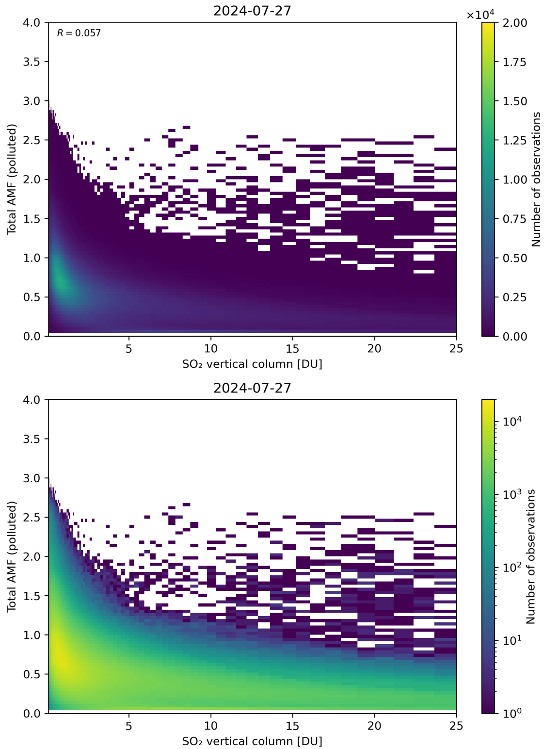
Figure 305: Scatter density plot of “SO 2 vertical column” against “Total AMF (polluted)” for 2024-07-26 to 2024-07-28.
