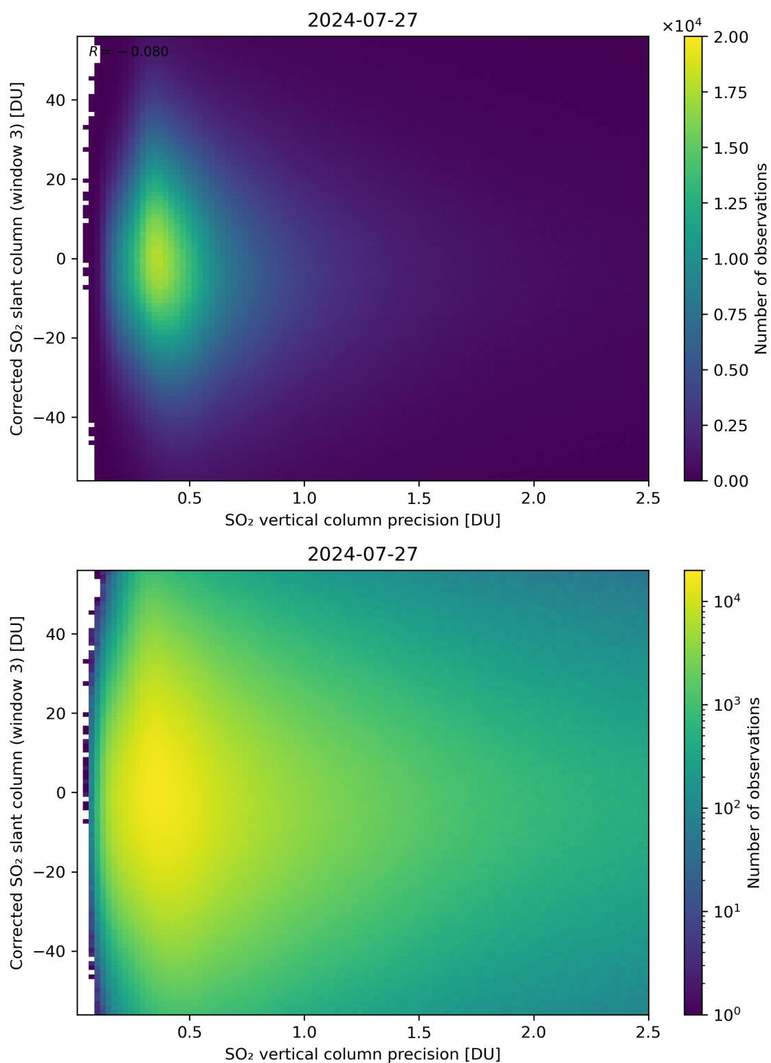
Figure 288: Scatter density plot of “SO 2 vertical column precision” against “Corrected SO 2 slant column (window 3)” for 2024-07-26 to 2024-07-28.
