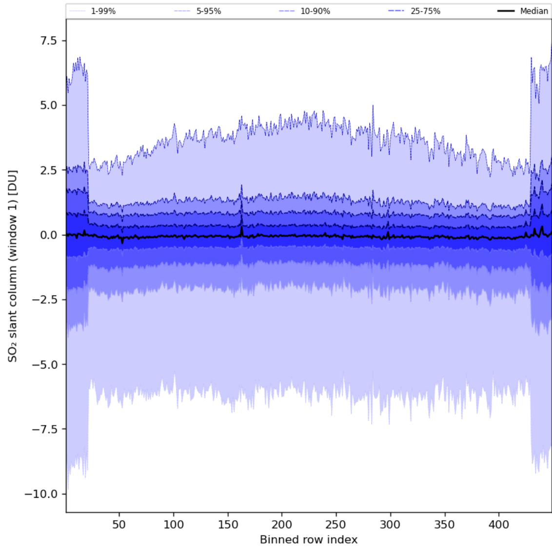
Figure 79: Along track statistics of “SO 2 slant column (window 1)” for 2024-07-26 to 2024-07-28
