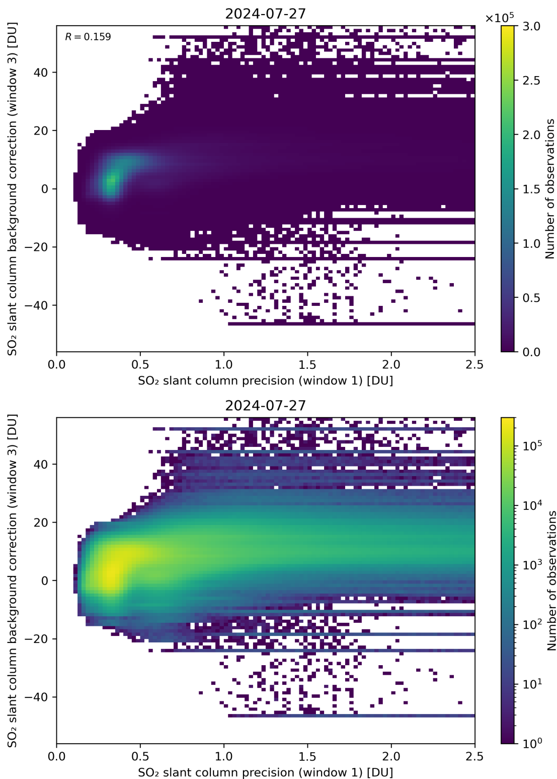
Figure 220: Scatter density plot of “SO 2 slant column precision (window 1)” against “SO 2 slant column background correction (window 3)” for 2024-07-26 to 2024-07-28.
