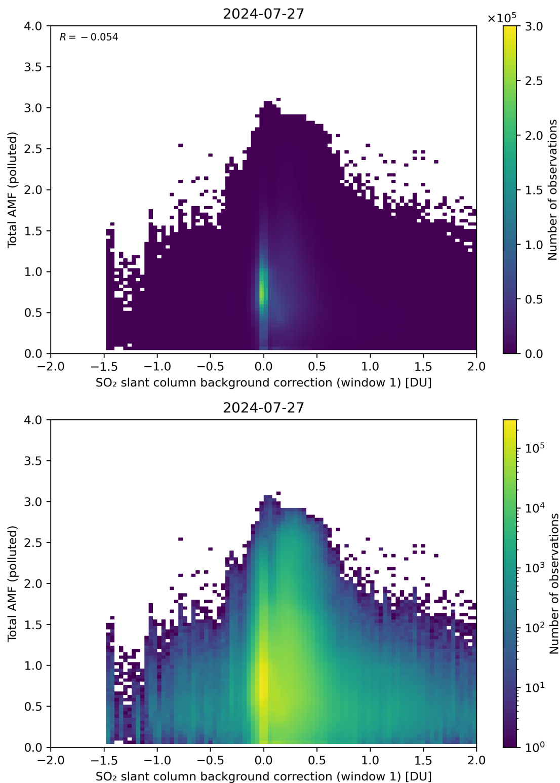
Figure 109: Scatter density plot of “SO 2 slant column background correction (window 1)” against “Total AMF (polluted)” for 2024-07-26 to 2024-07-28.
