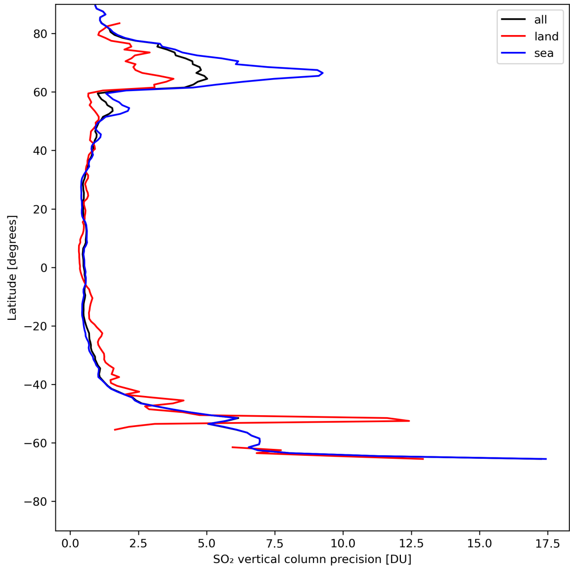
Figure 31: Zonal average of “SO 2 vertical column precision” for 2024-07-26 to 2024-07-28.
