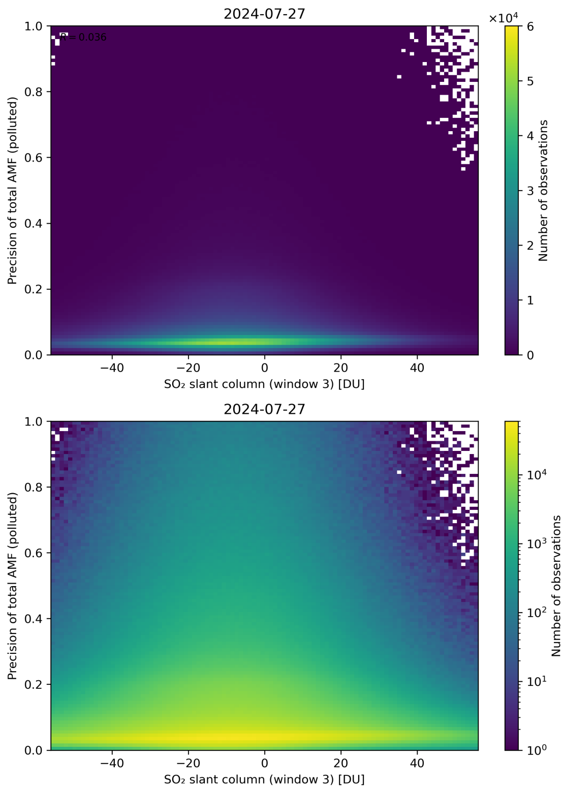
Figure 269: Scatter density plot of “SO 2 slant column (window 3)” against “Precision of total AMF (polluted)” for 2024-07-26 to 2024-07-28.
