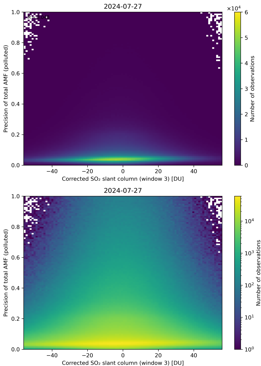
Figure 211: Scatter density plot of “Corrected SO 2 slant column (window 3)” against “Precision of total AMF (polluted)” for 2024-07-26 to 2024-07-28.
