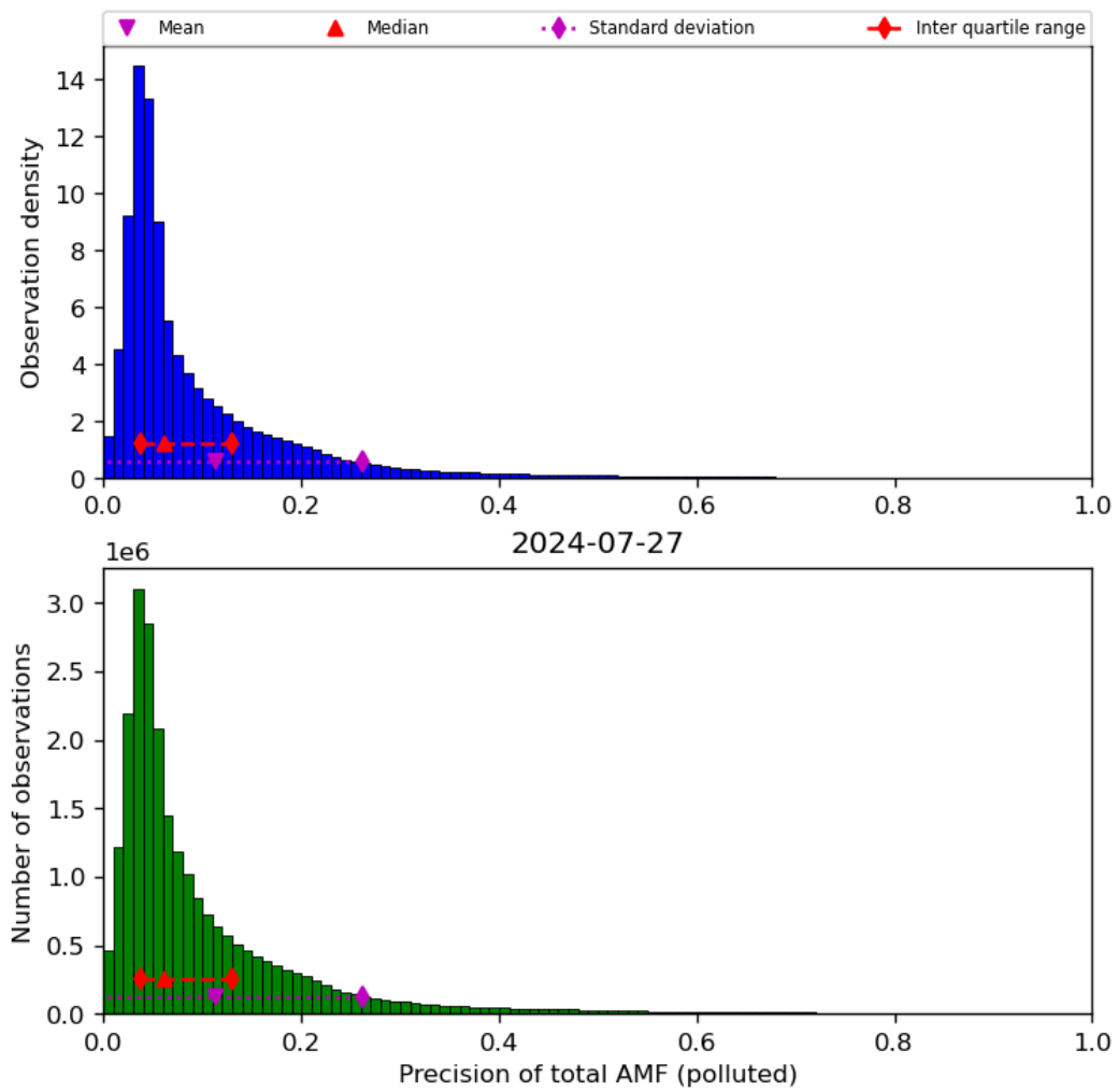
Figure 72: Histogram of “Precision of total AMF (polluted)” for 2024-07-26 to 2024-07-28
