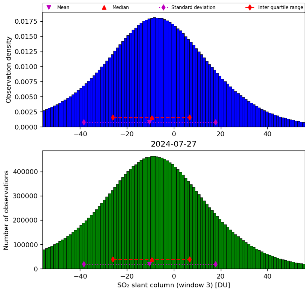
Figure 64: Histogram of “SO 2 slant column (window 3)” for 2024-07-26 to 2024-07-28
