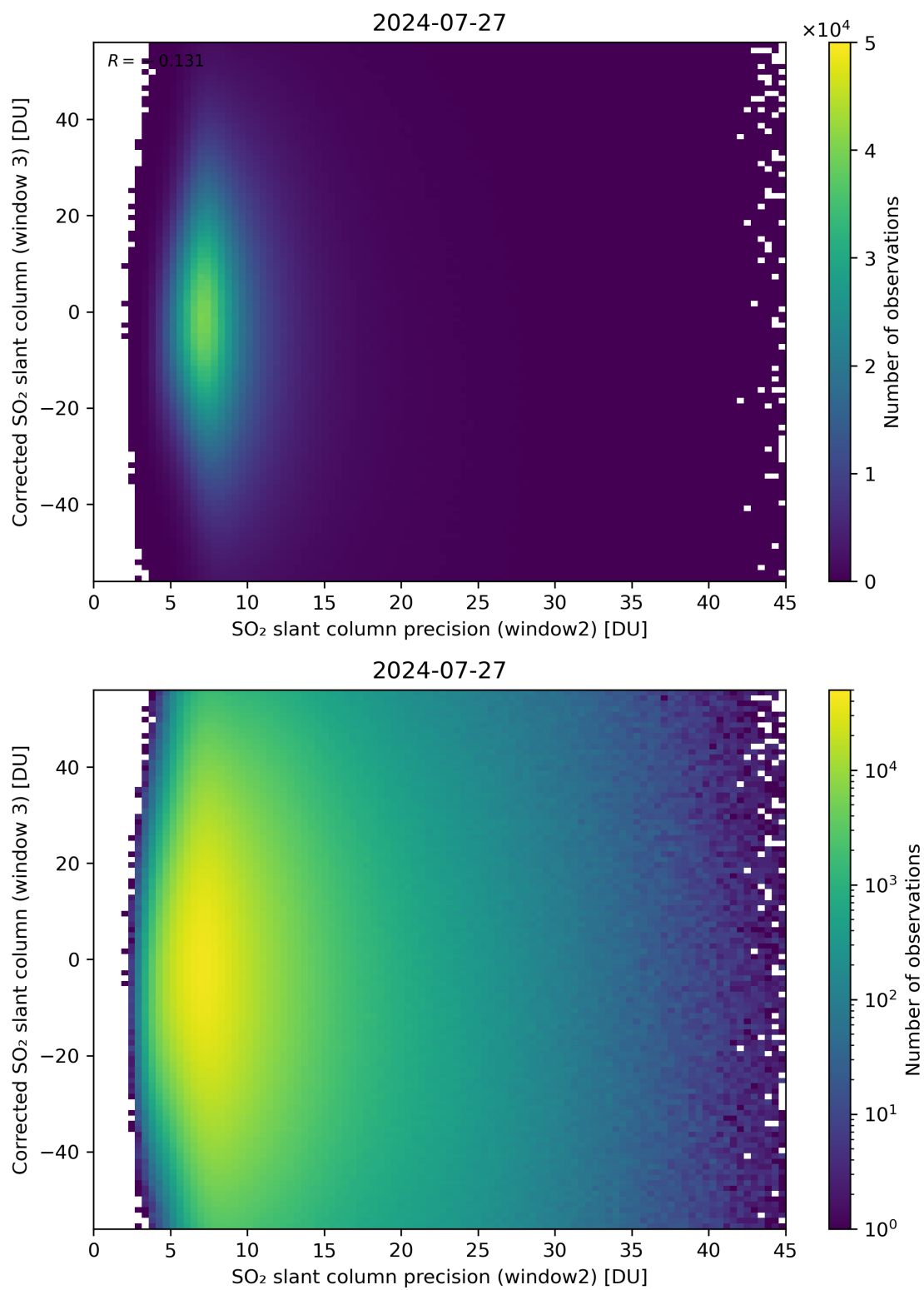
Figure 248: Scatter density plot of “SO 2 slant column precision (window2)” against “Corrected SO 2 slant column (window 3)” for 2024-07-26 to 2024-07-28.
