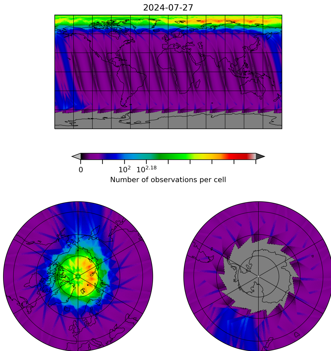
Figure 28: Map of the number of observations for 2024-07-26 to 2024-07-28
