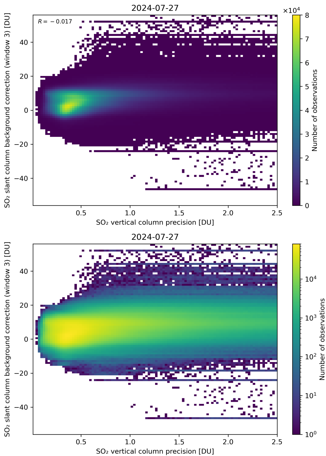
Figure 281: Scatter density plot of “SO 2 vertical column precision” against “SO 2 slant column background correction (window 3)” for 2024-07-26 to 2024-07-28.
