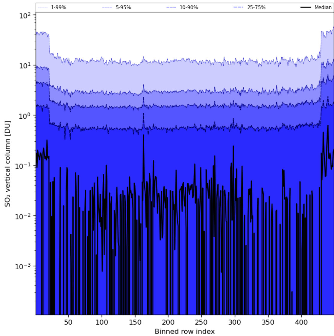
Figure 76: Along track statistics of “SO 2 vertical column” for 2024-07-26 to 2024-07-28
