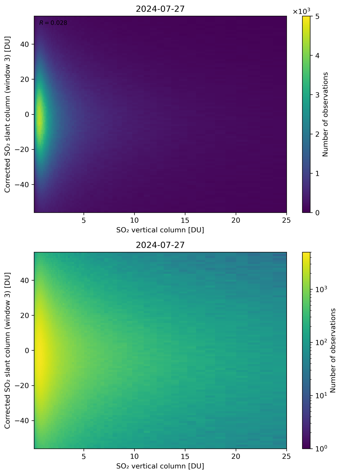
Figure 299: Scatter density plot of “SO 2 vertical column” against “Corrected SO 2 slant column (window 3)” for 2024-07-26 to 2024-07-28.
