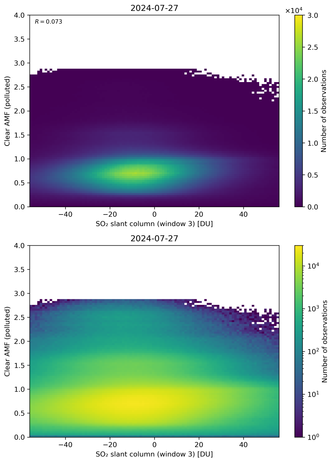
Figure 265: Scatter density plot of “SO 2 slant column (window 3)” against “Clear AMF (polluted)” for 2024-07-26 to 2024-07-28.
