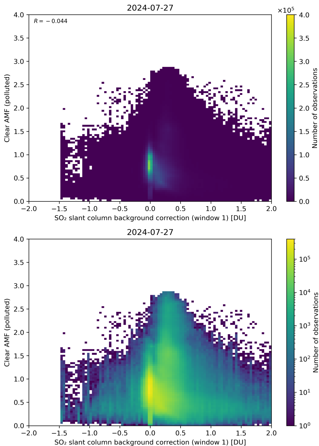
Figure 103: Scatter density plot of “SO 2 slant column background correction (window 1)” against “Clear AMF (polluted)” for 2024-07-26 to 2024-07-28.
