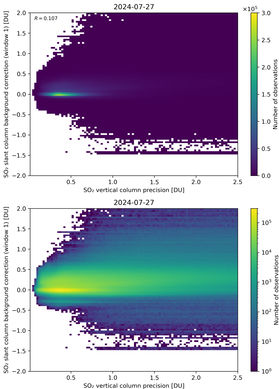
Figure 279: Scatter density plot of “SO 2 vertical column precision” against “SO 2 slant column background correction (window 1)” for 2024-07-26 to 2024-07-28.
