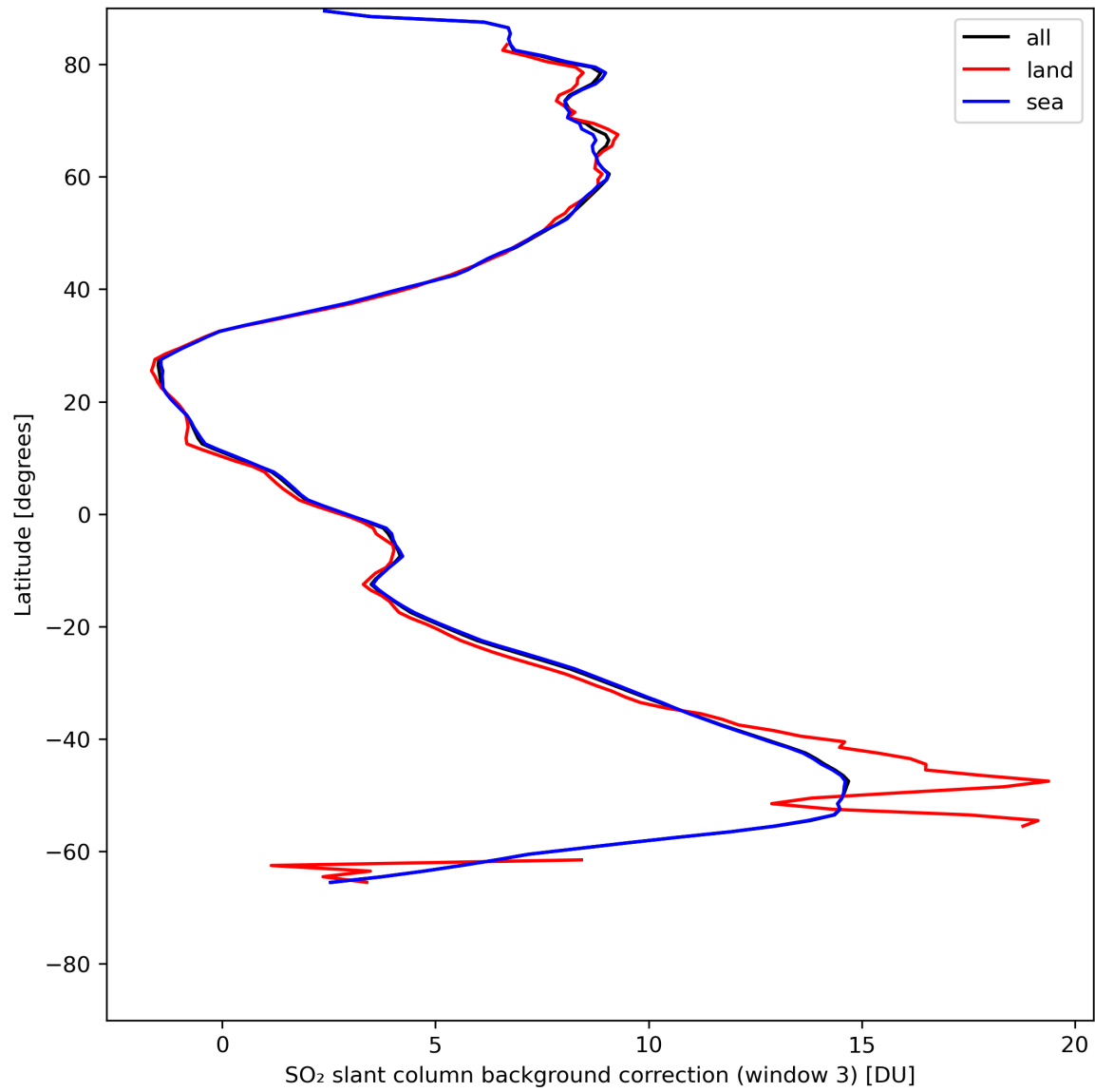
Figure 44: Zonal average of “SO 2 slant column background correction (window 3)” for 2024-07-26 to 2024-07-28.
