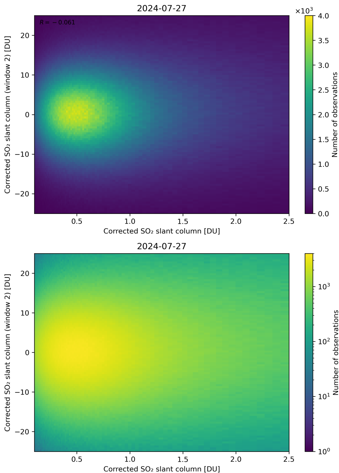
Figure 185: Scatter density plot of “Corrected SO 2 slant column” against “Corrected SO 2 slant column (window 2)” for 2024-07-26 to 2024-07-28.
