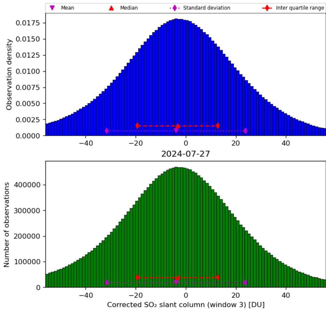
Figure 66: Histogram of “Corrected SO 2 slant column (window 3)” for 2024-07-26 to 2024-07-28
