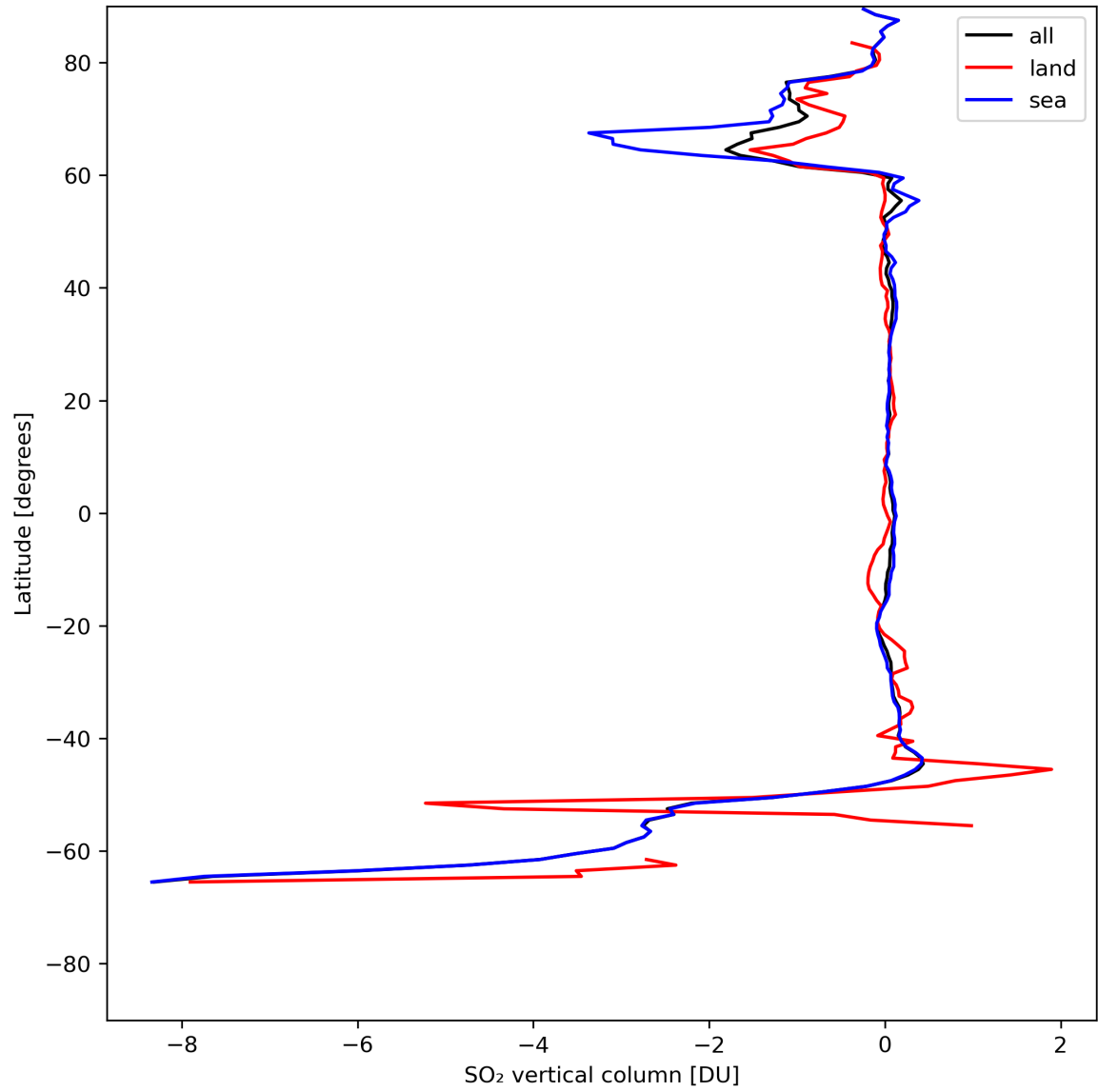
Figure 30: Zonal average of “SO 2 vertical column” for 2024-07-26 to 2024-07-28.
