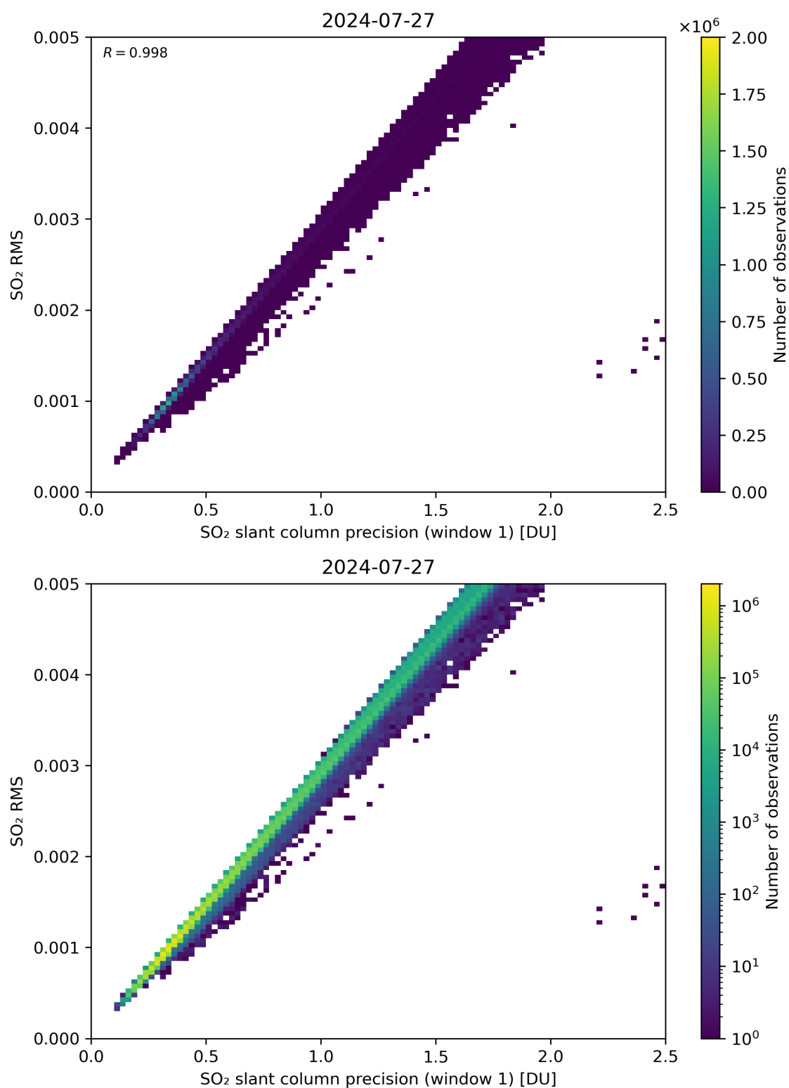
Figure 223: Scatter density plot of “SO 2 slant column precision (window 1)” against “SO 2 RMS” for 2024-07-26 to 2024-07-28.
