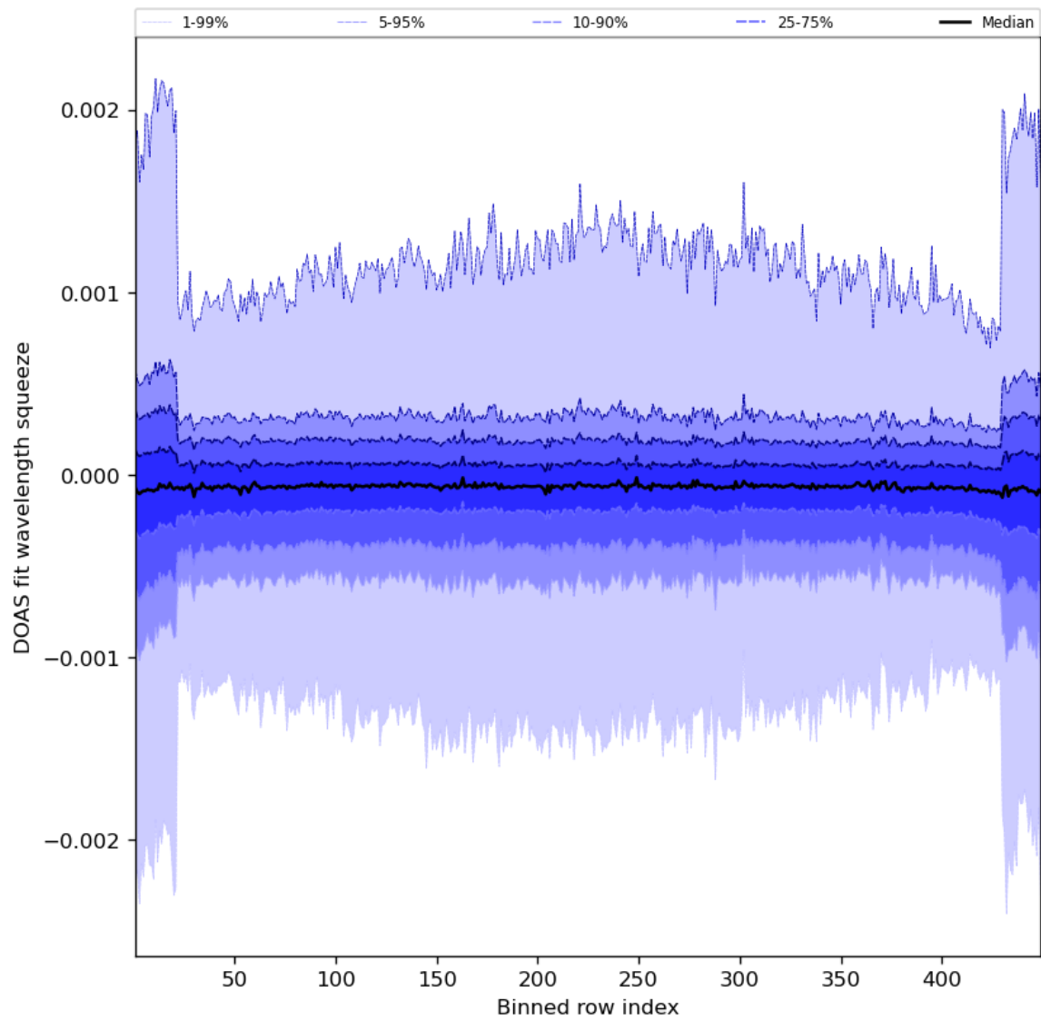
Figure 92: Along track statistics of “DOAS fit wavelength squeeze” for 2024-07-26 to 2024-07-28
