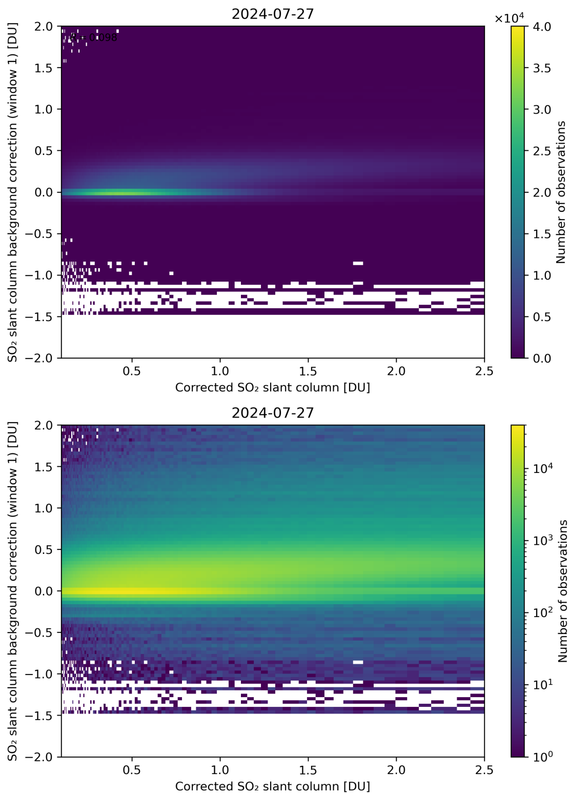
Figure 178: Scatter density plot of “Corrected SO 2 slant column” against “SO 2 slant column background correction (window 1)” for 2024-07-26 to 2024-07-28.
