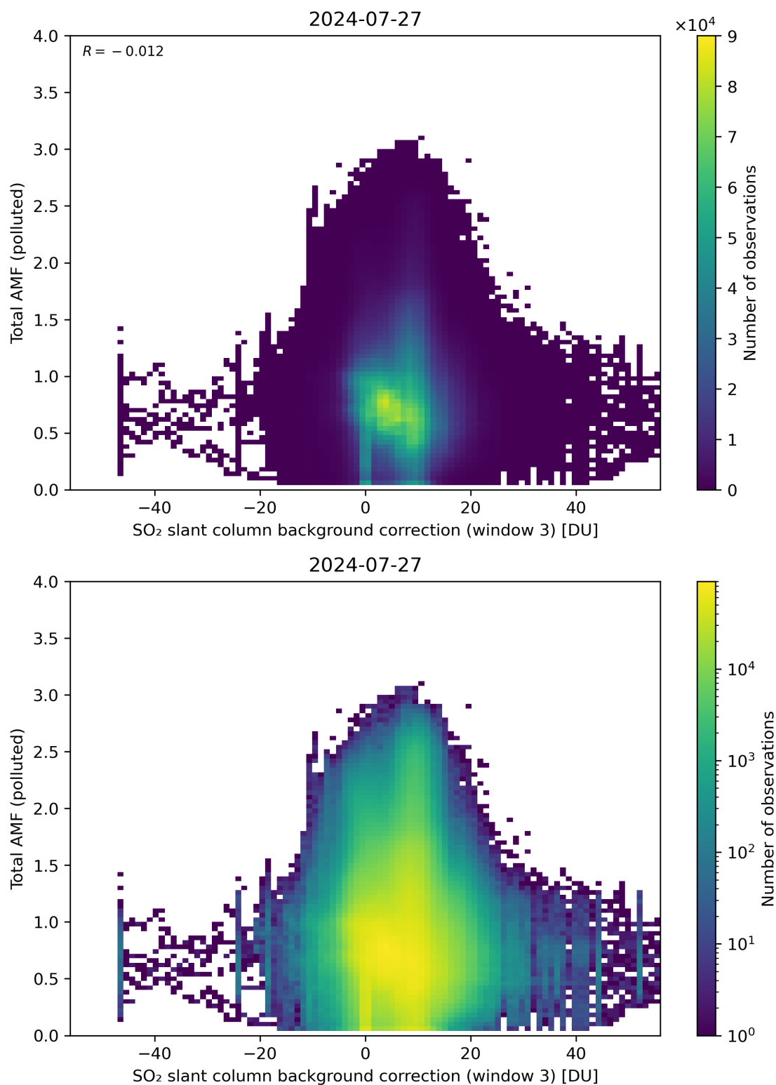
Figure 125: Scatter density plot of “SO 2 slant column background correction (window 3)” against “Total AMF (polluted)” for 2024-07-26 to 2024-07-28.
