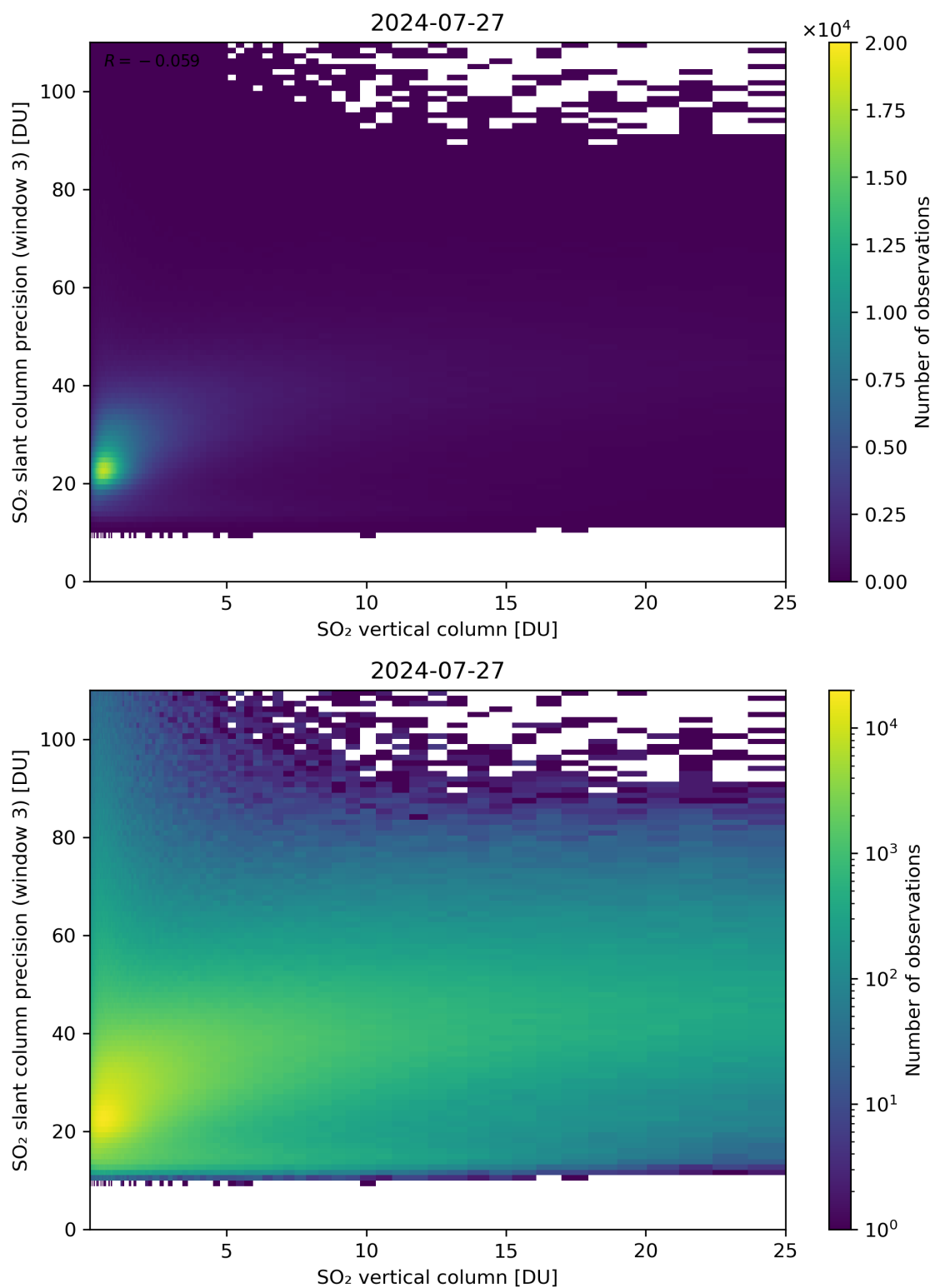
Figure 304: Scatter density plot of “SO 2 vertical column” against “SO 2 slant column precision (window 3)” for 2024-07-26 to 2024-07-28.
