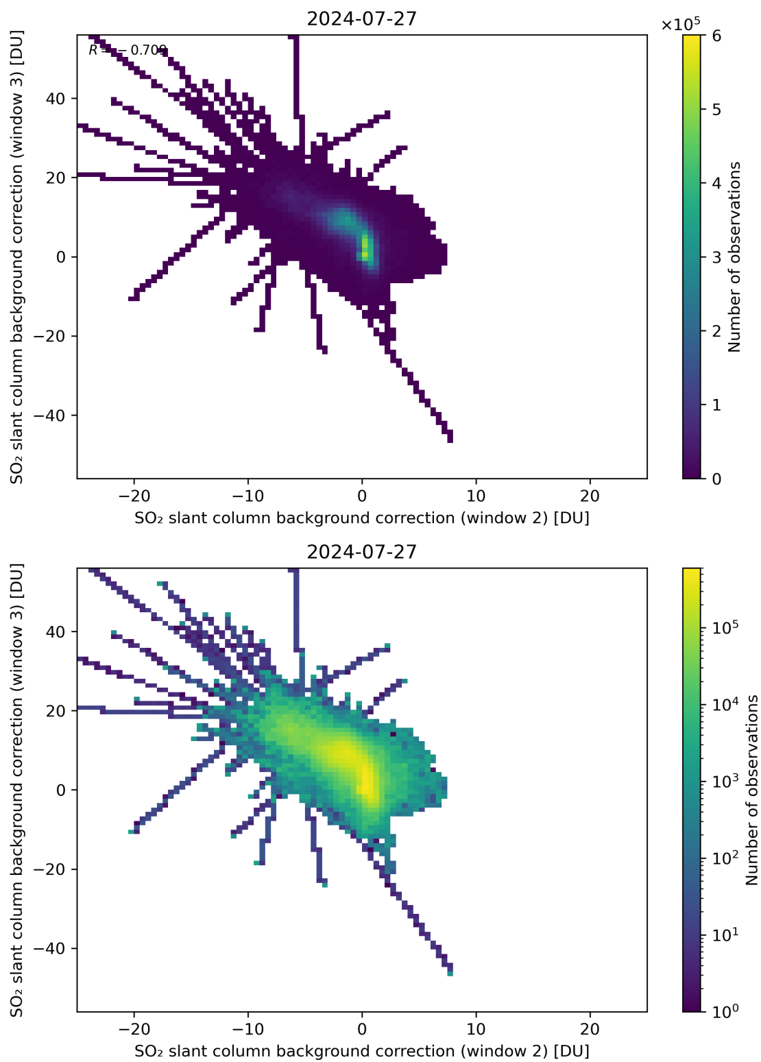
Figure 111: Scatter density plot of “SO 2 slant column background correction (window 2)” against “SO 2 slant column background correction (window 3)” for 2024-07-26 to 2024-07-28.
