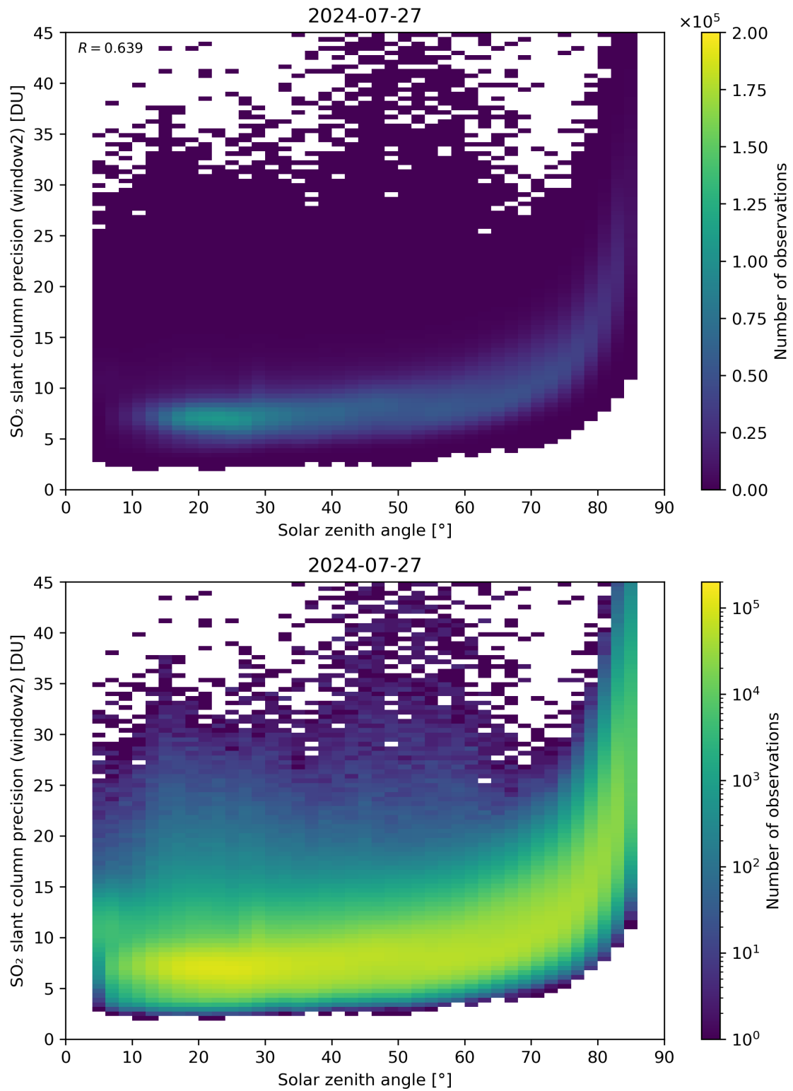
Figure 171: Scatter density plot of “Solar zenith angle” against “SO 2 slant column precision (window2)” for 2024-07-26 to 2024-07-28.
