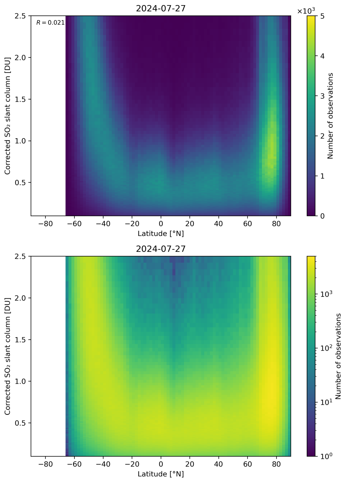
Figure 146: Scatter density plot of “Latitude” against “Corrected SO 2 slant column” for 2024-07-26 to 2024-07-28.
