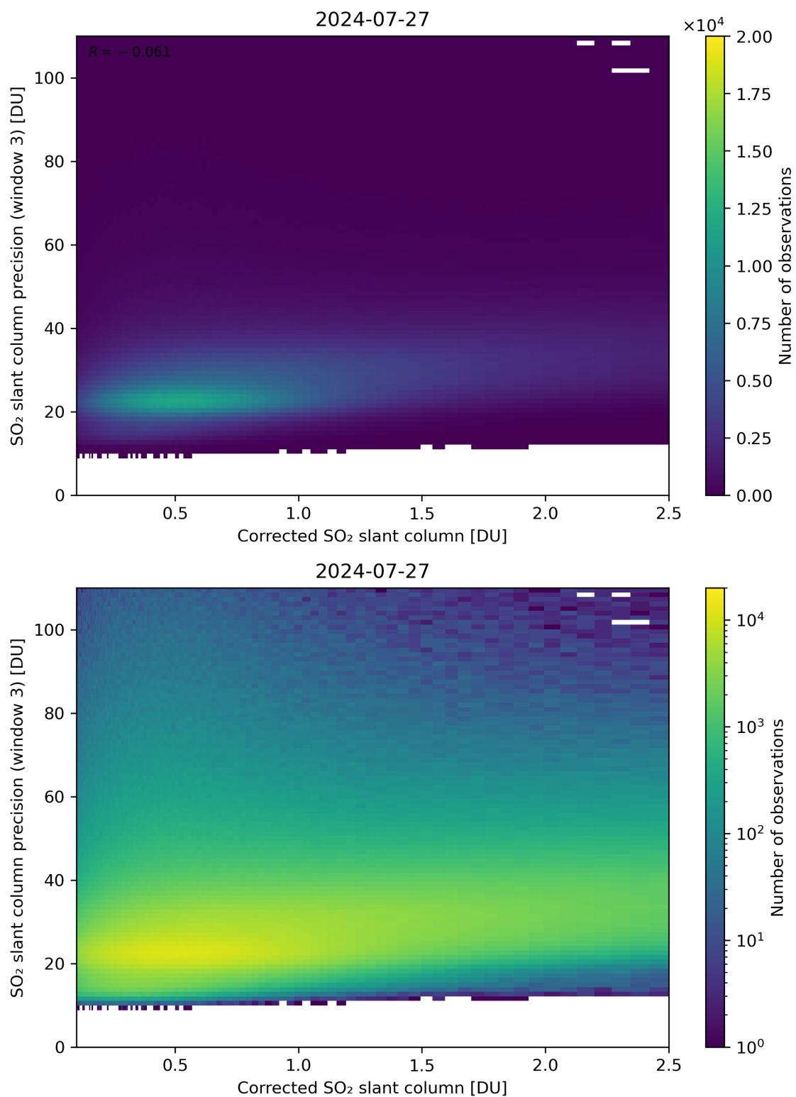
Figure 191: Scatter density plot of “Corrected SO 2 slant column” against “SO 2 slant column precision (window 3)” for 2024-07-26 to 2024-07-28.
