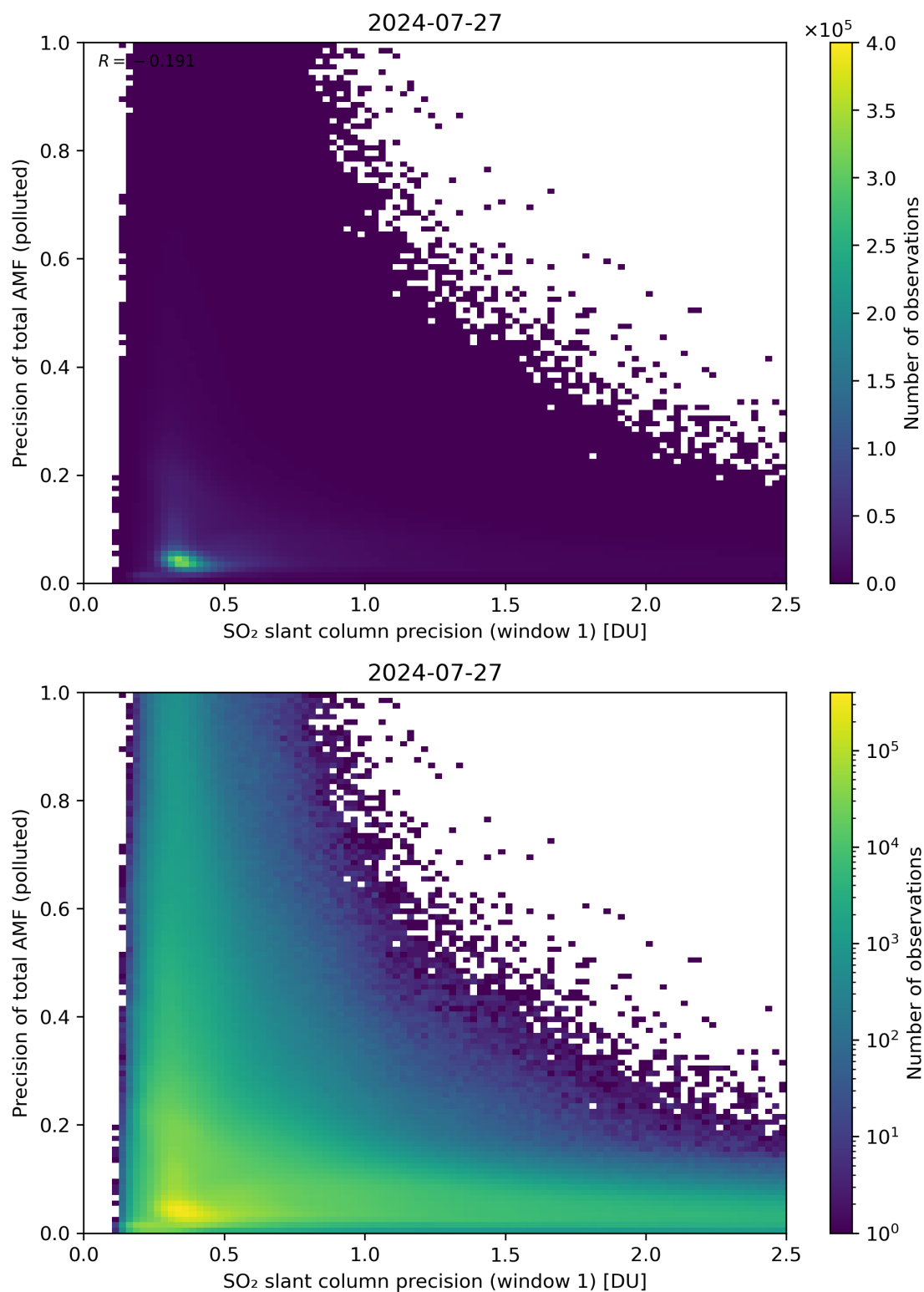
Figure 231: Scatter density plot of “SO 2 slant column precision (window 1)” against “Precision of total AMF (polluted)” for 2024-07-26 to 2024-07-28.
