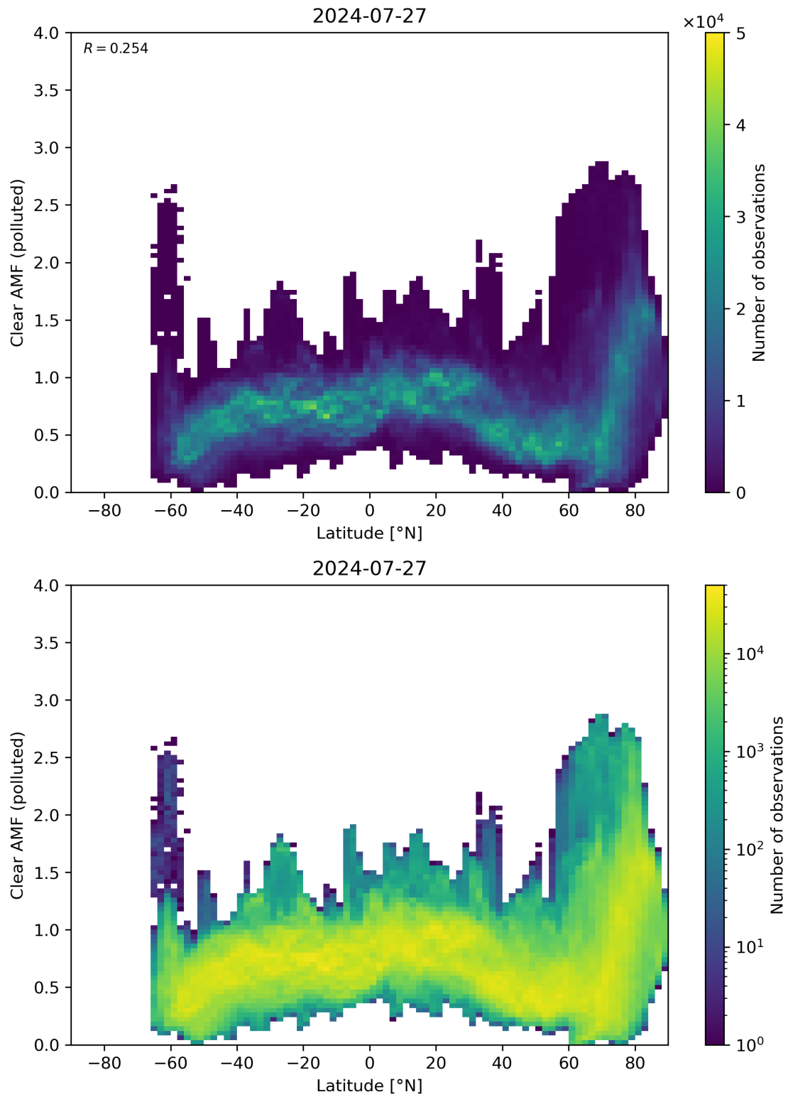
Figure 145: Scatter density plot of “Latitude” against “Clear AMF (polluted)” for 2024-07-26 to 2024-07-28.
