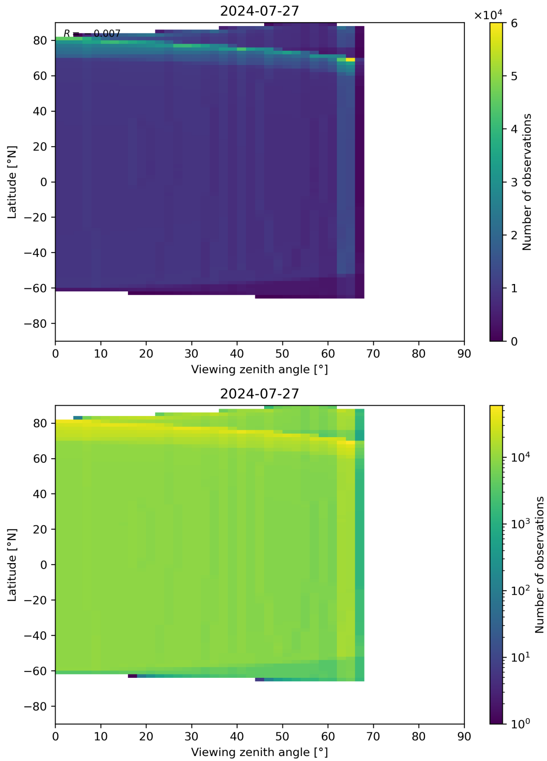
Figure 314: Scatter density plot of “Viewing zenith angle” against “Latitude” for 2024-07-26 to 2024-07-28.
