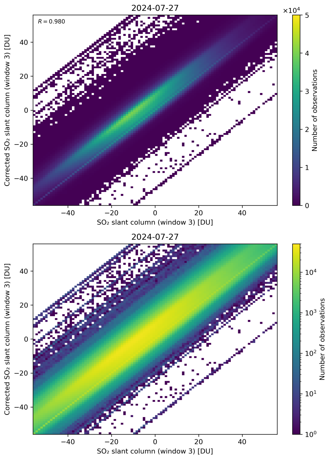
Figure 266: Scatter density plot of “SO 2 slant column (window 3)” against “Corrected SO 2 slant column (window 3)” for 2024-07-26 to 2024-07-28.
