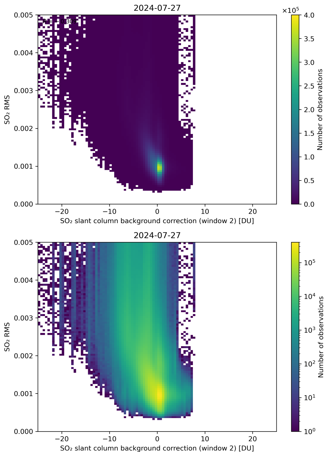
Figure 114: Scatter density plot of “SO 2 slant column background correction (window 2)” against “SO 2 RMS” for 2024-07-26 to 2024-07-28.
