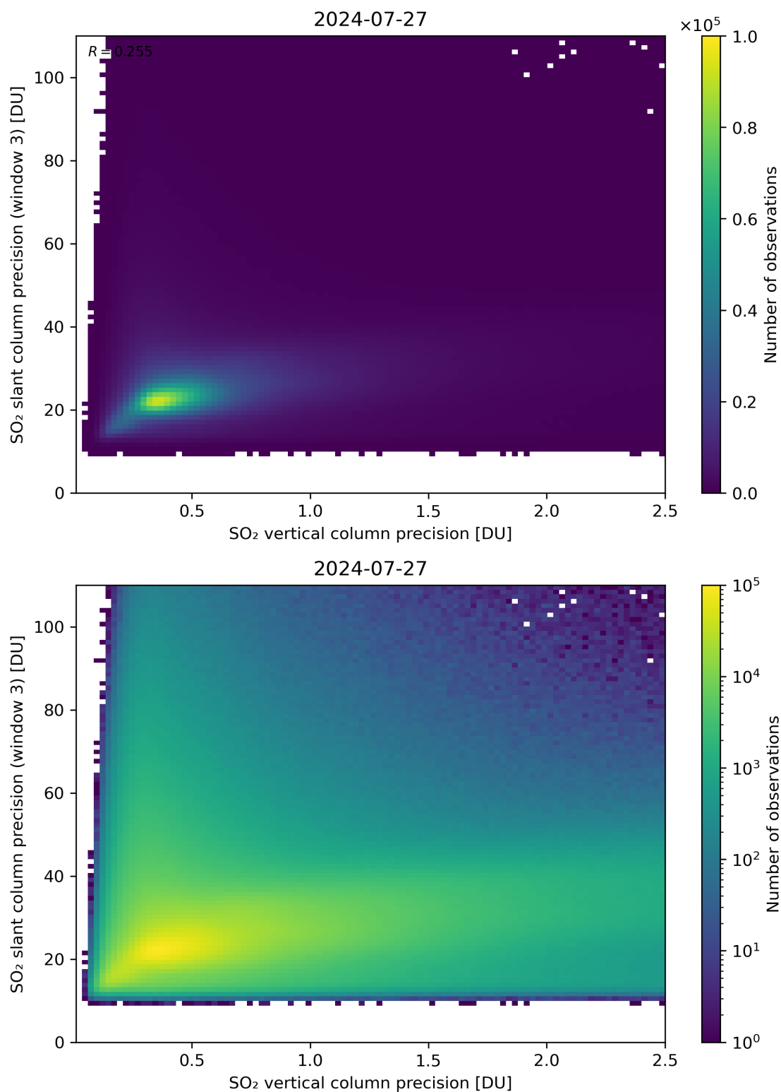
Figure 293: Scatter density plot of “SO 2 vertical column precision” against “SO 2 slant column precision (window 3)” for 2024-07-26 to 2024-07-28.
