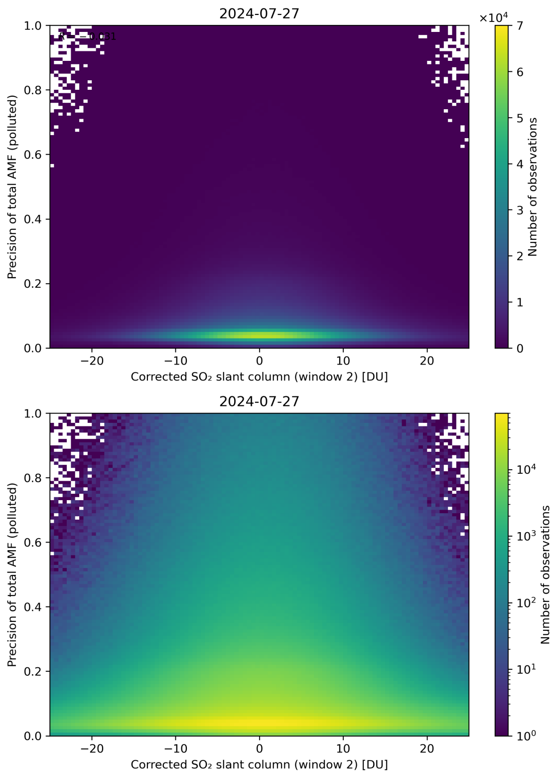
Figure 204: Scatter density plot of “Corrected SO 2 slant column (window 2)” against “Precision of total AMF (polluted)” for 2024-07-26 to 2024-07-28.
