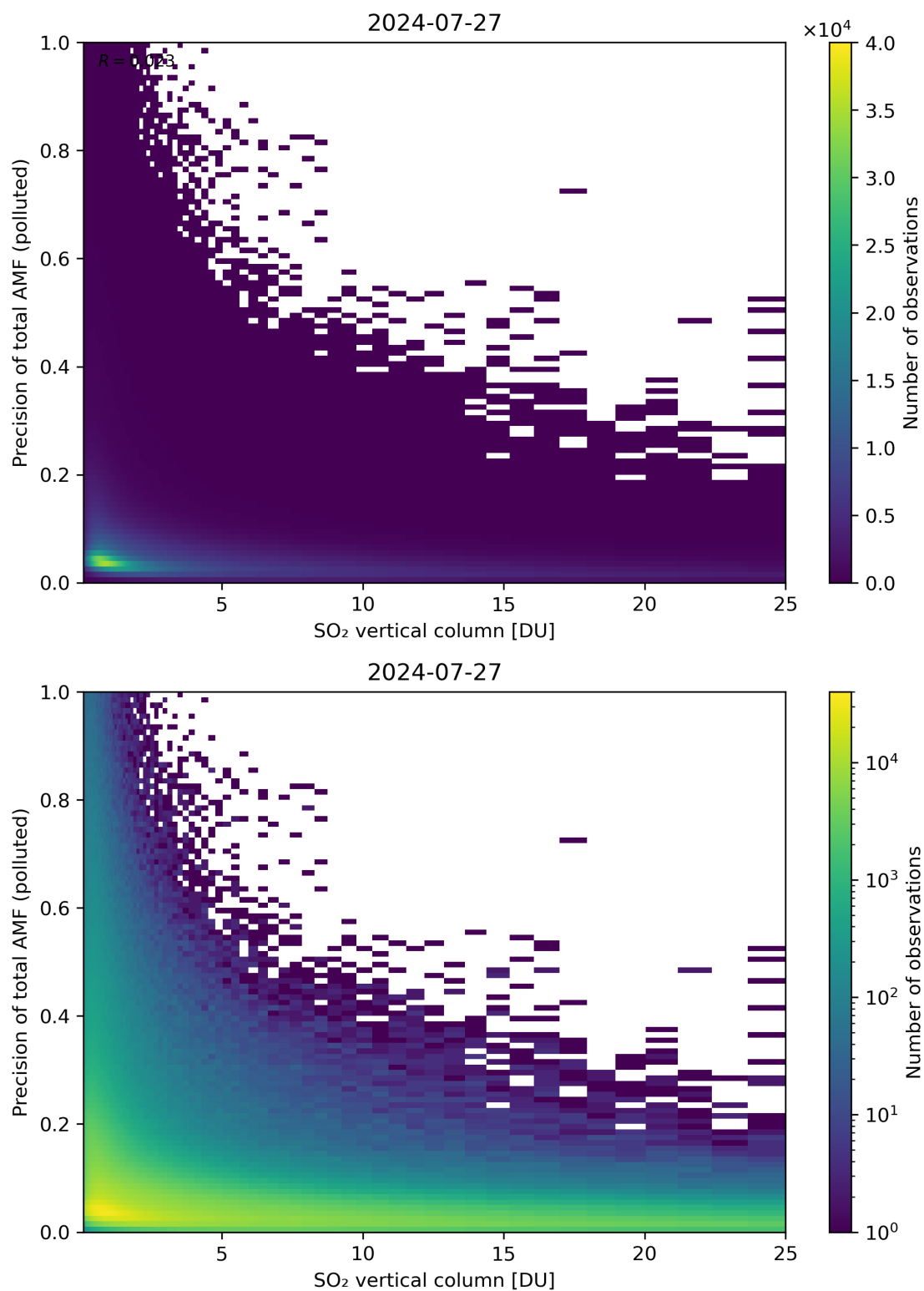
Figure 306: Scatter density plot of “SO 2 vertical column” against “Precision of total AMF (polluted)” for 2024-07-26 to 2024-07-28.
