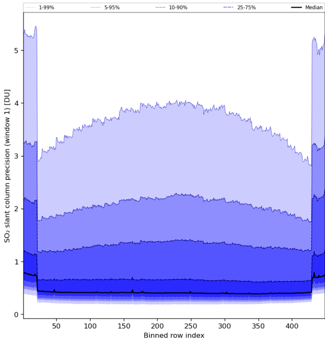
Figure 80: Along track statistics of “SO 2 slant column precision (window 1)” for 2024-07-26 to 2024-07-28
