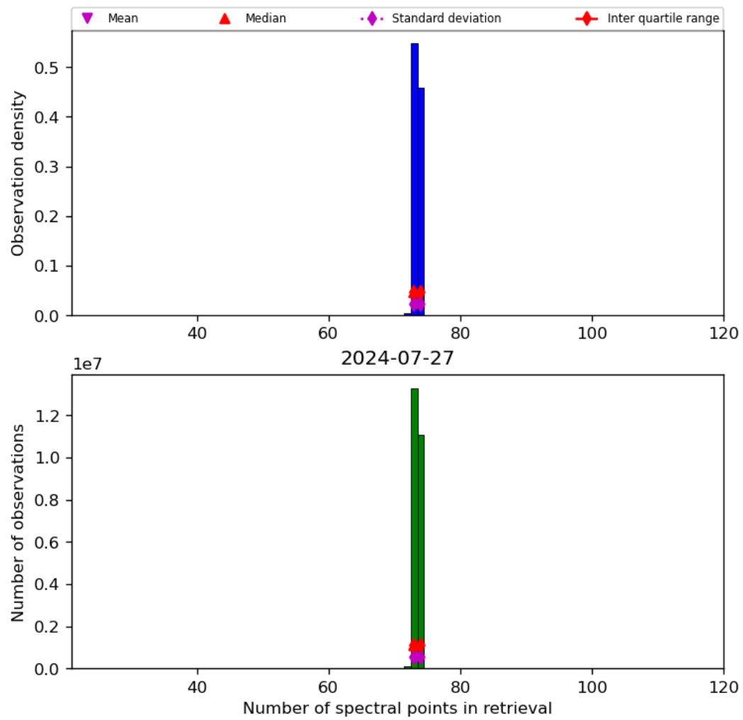
Figure 74: Histogram of “Number of spectral points in retrieval” for 2024-07-26 to 2024-07-28
