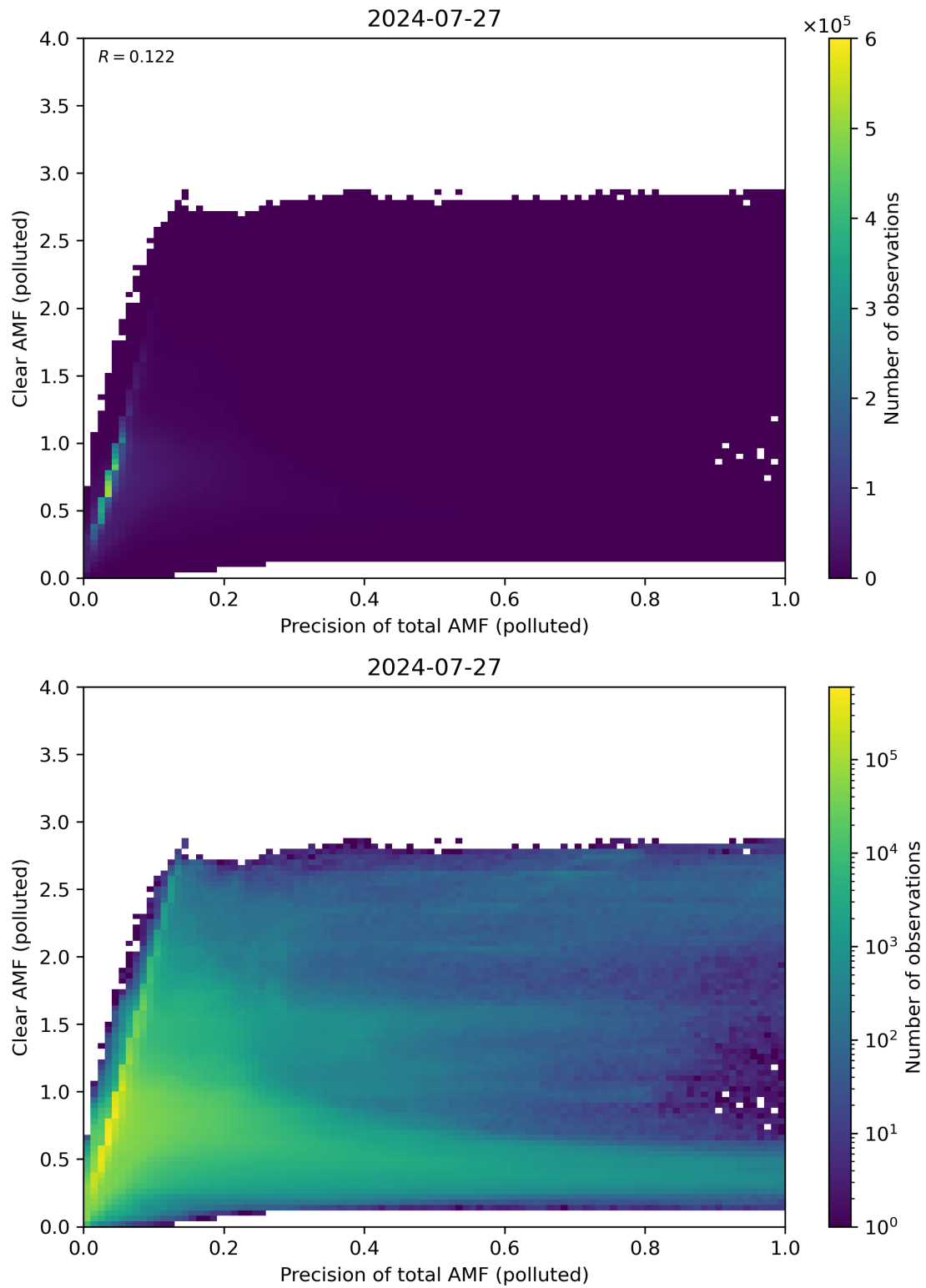
Figure 270: Scatter density plot of “Precision of total AMF (polluted)” against “Clear AMF (polluted)” for 2024-07-26 to 2024-07-28.
