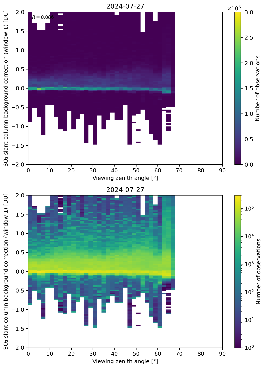
Figure 308: Scatter density plot of “Viewing zenith angle” against “SO 2 slant column background correction (window 1)” for 2024-07-26 to 2024-07-28.
