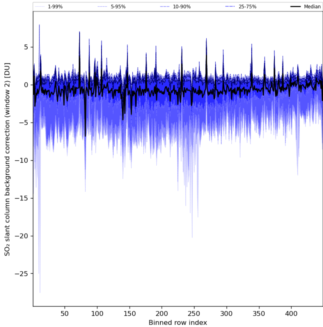
Figure 86: Along track statistics of “SO 2 slant column background correction (window 2)” for 2024-07-26 to 2024-07-28
