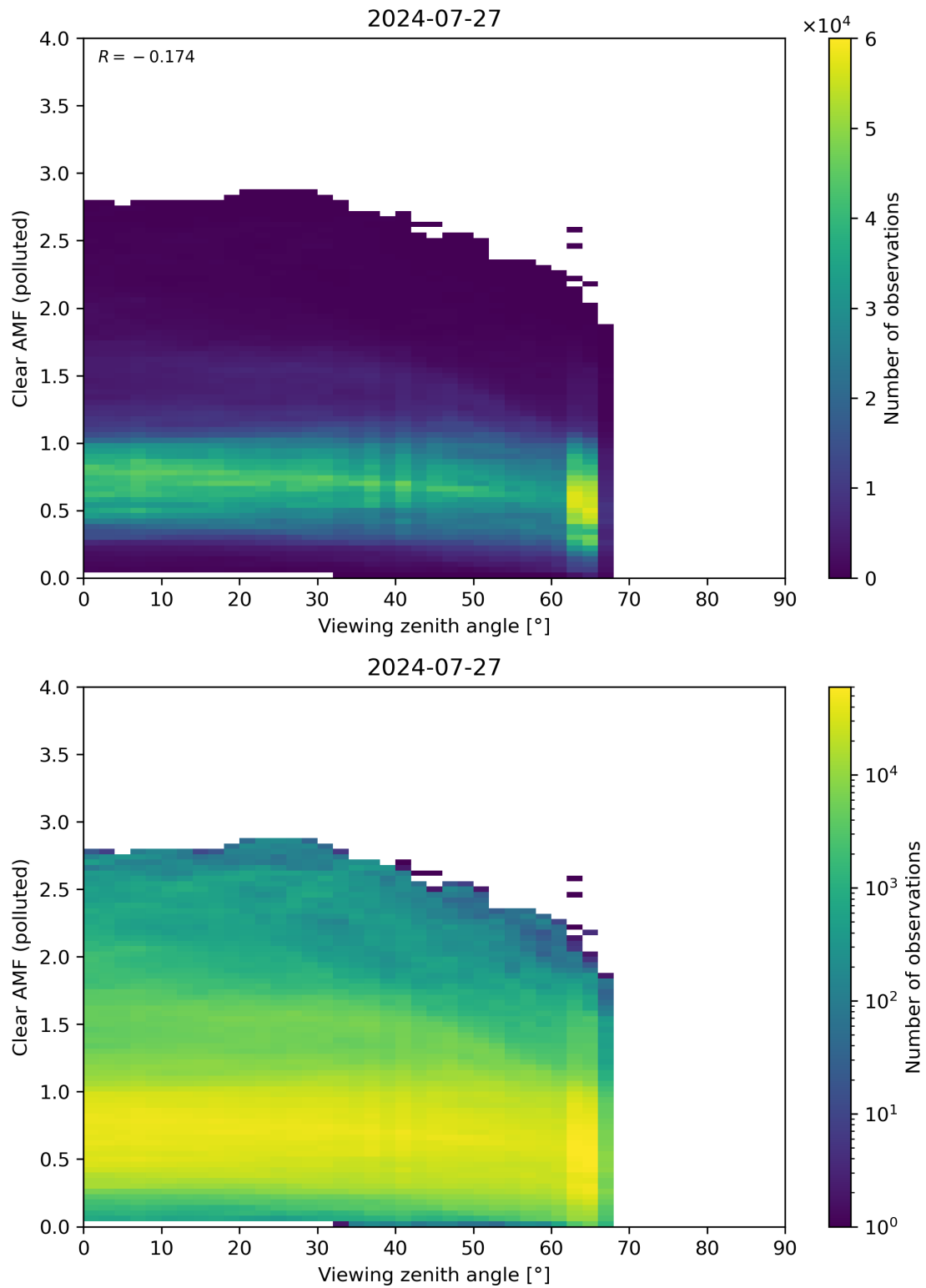
Figure 316: Scatter density plot of “Viewing zenith angle” against “Clear AMF (polluted)” for 2024-07-26 to 2024-07-28.
