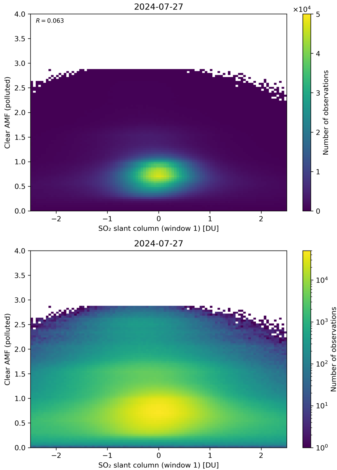
Figure 232: Scatter density plot of “SO 2 slant column (window 1)” against “Clear AMF (polluted)” for 2024-07-26 to 2024-07-28.
