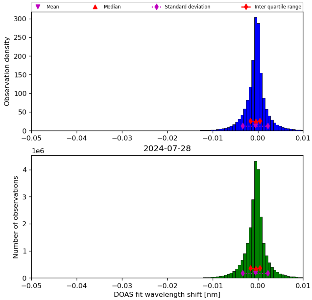
Figure 68: Histogram of “DOAS fit wavelength shift” for 2024-07-27 to 2024-07-29
