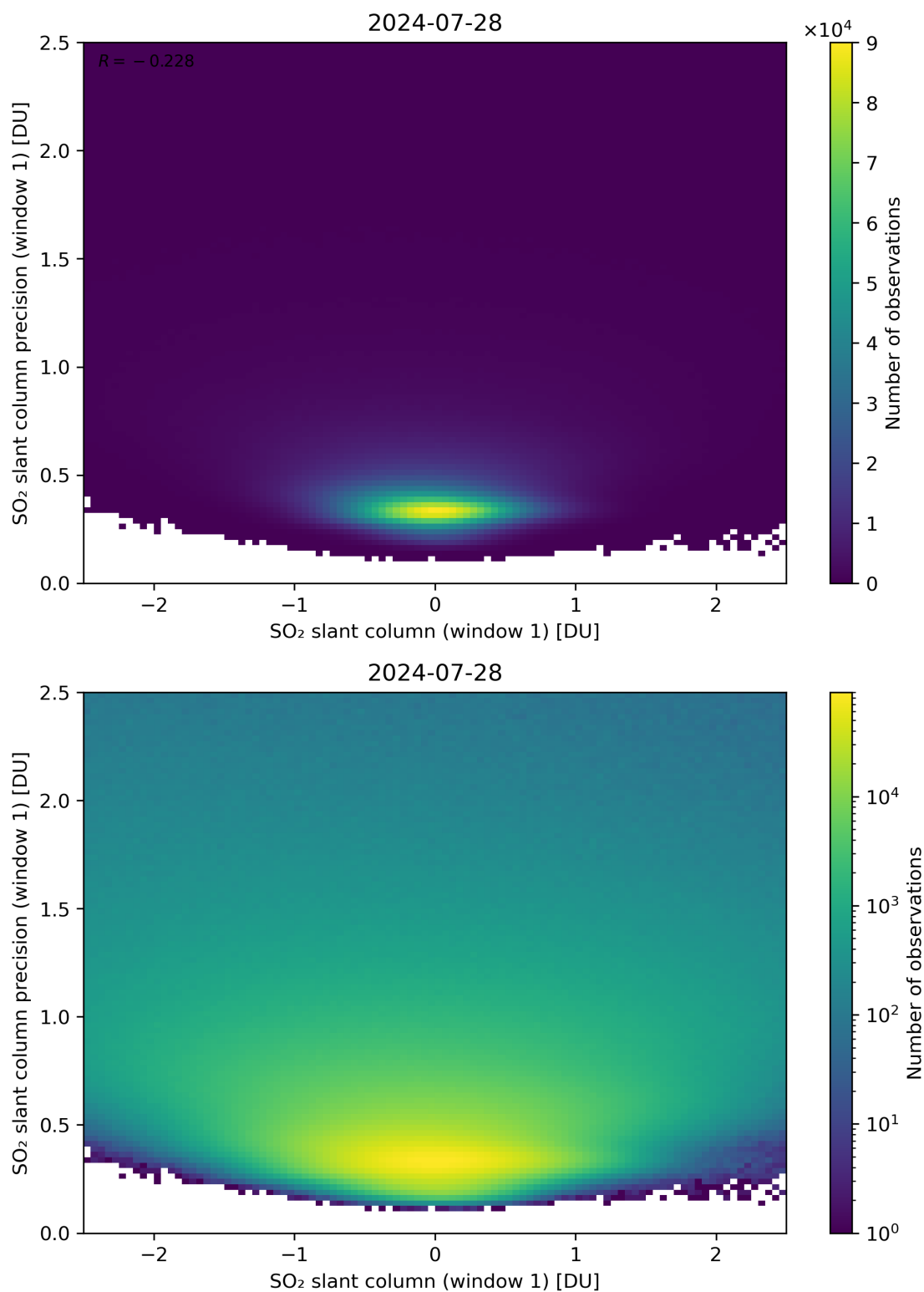
Figure 235: Scatter density plot of “SO 2 slant column (window 1)” against “SO 2 slant column precision (window 1)” for 2024-07-27 to 2024-07-29.
