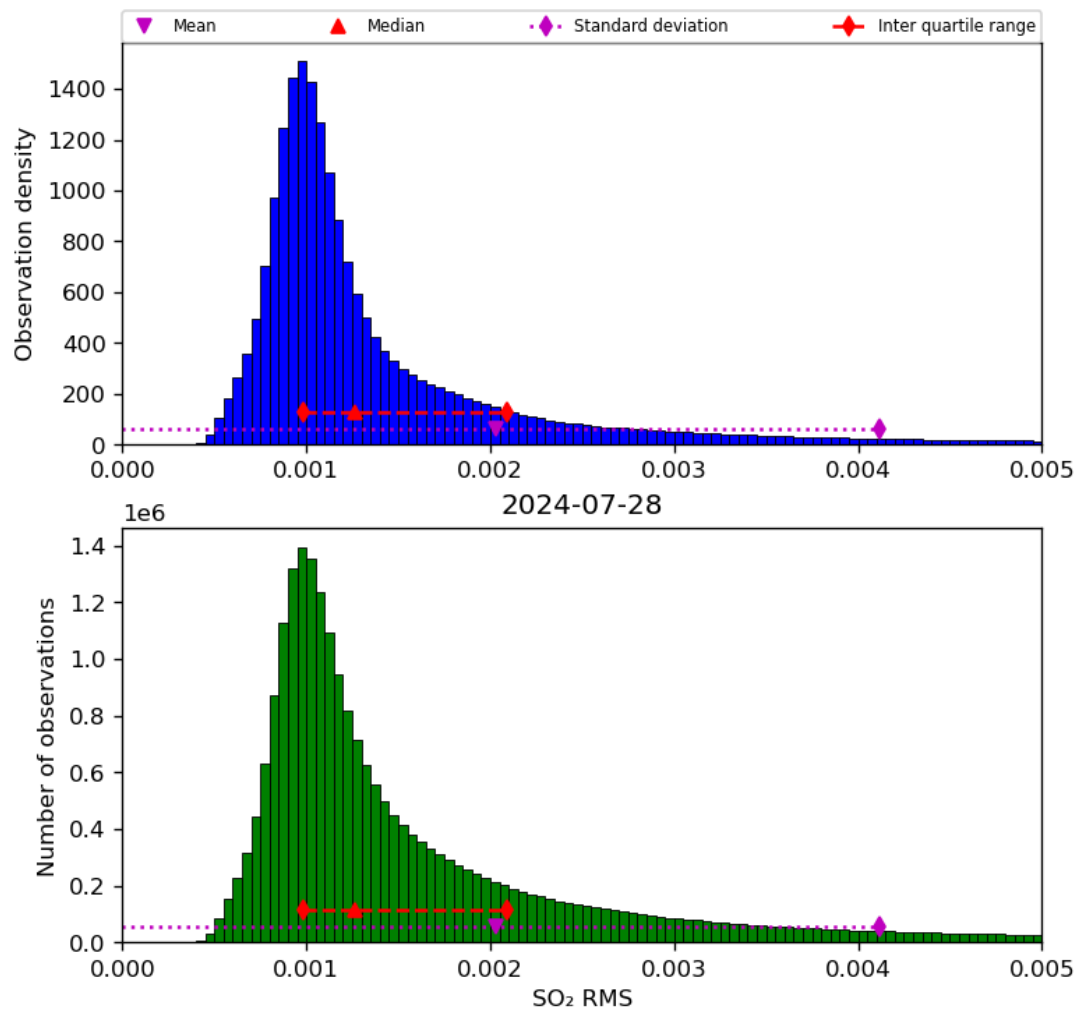
Figure 70: Histogram of “SO 2 RMS” for 2024-07-27 to 2024-07-29
