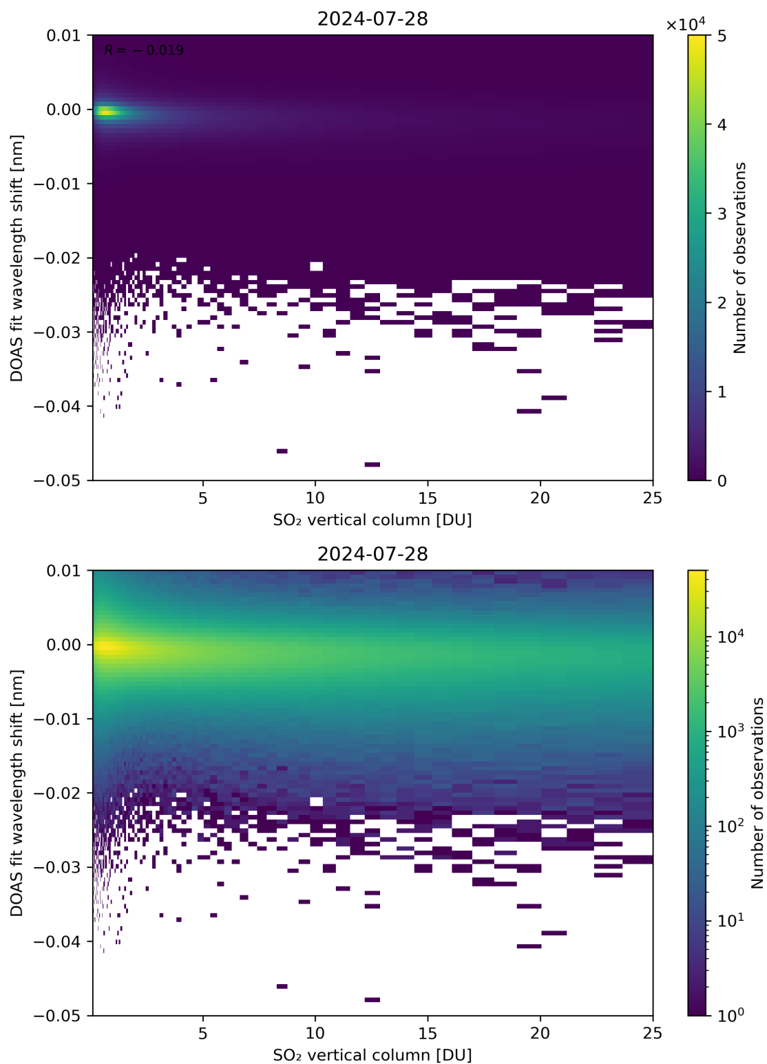
Figure 276: Scatter density plot of “SO 2 vertical column” against “DOAS fit wavelength shift” for 2024-07-27 to 2024-07-29.
