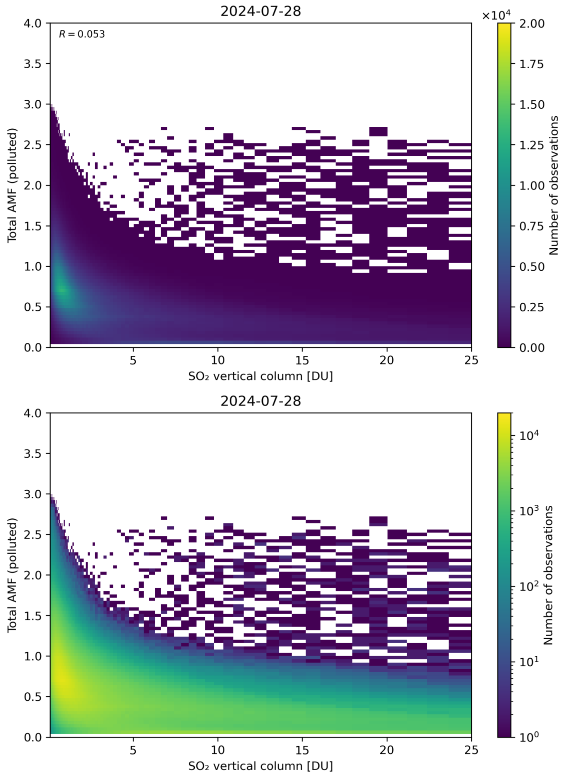
Figure 305: Scatter density plot of “SO 2 vertical column” against “Total AMF (polluted)” for 2024-07-27 to 2024-07-29.
