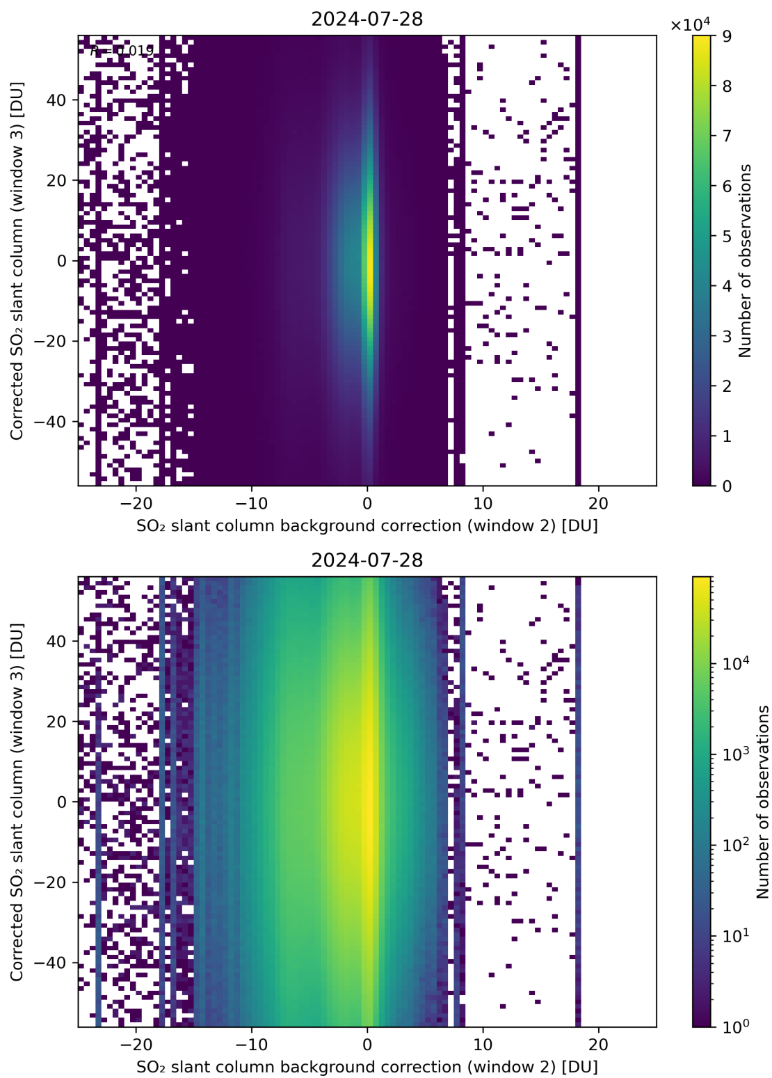
Figure 116: Scatter density plot of “SO 2 slant column background correction (window 2)” against “Corrected SO 2 slant column (window 3)” for 2024-07-27 to 2024-07-29.
