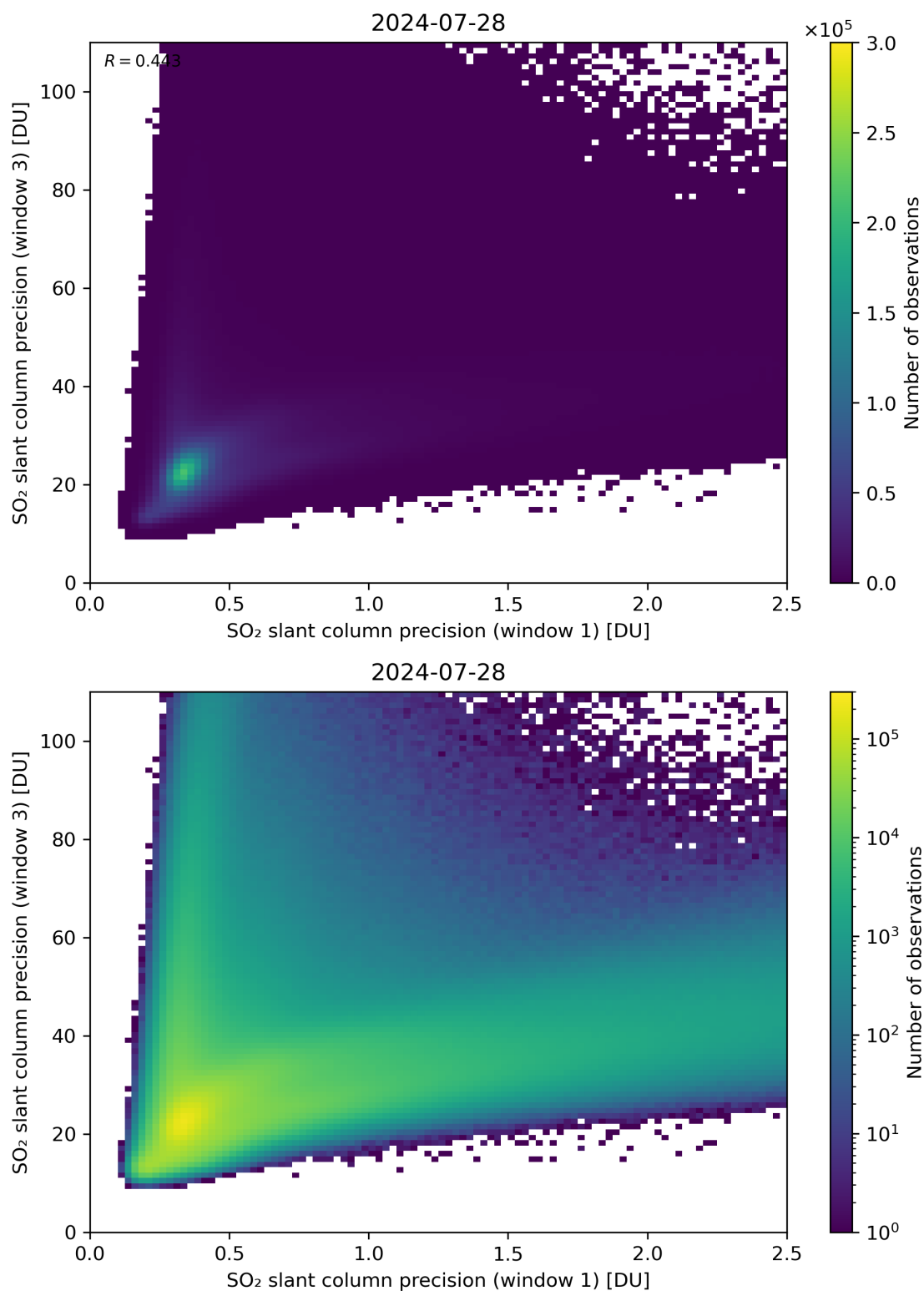
Figure 229: Scatter density plot of “SO 2 slant column precision (window 1)” against “SO 2 slant column precision (window 3)” for 2024-07-27 to 2024-07-29.
