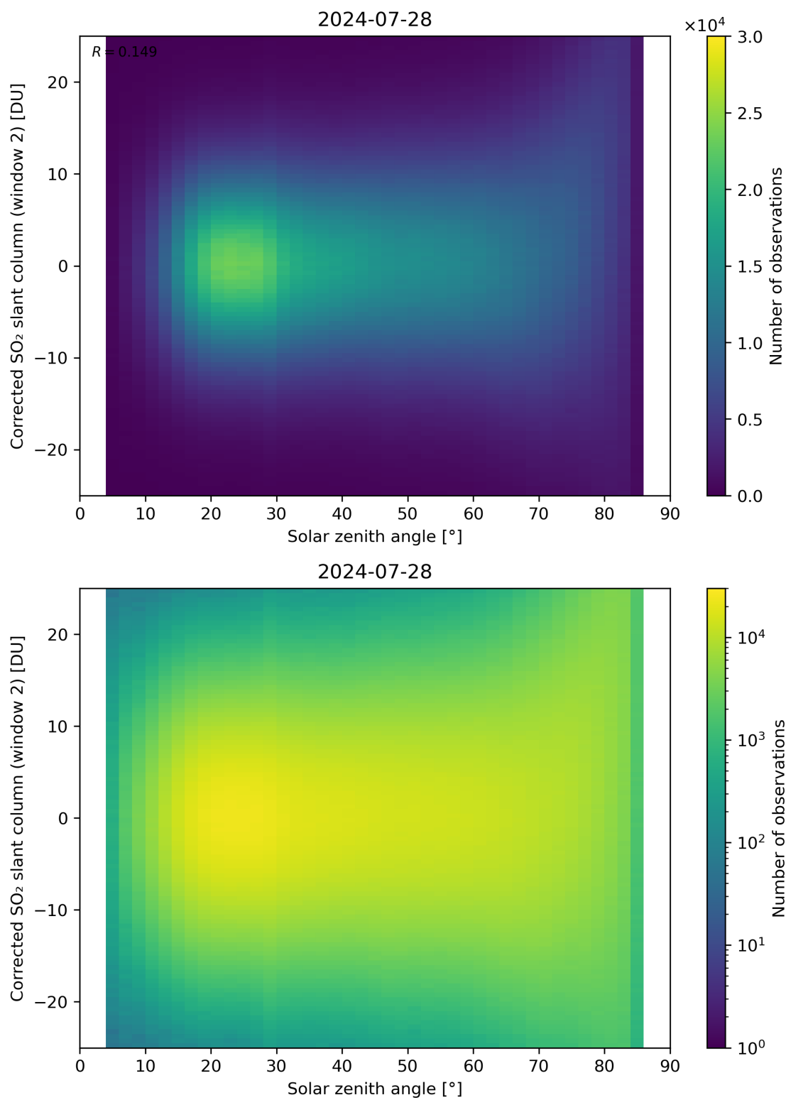
Figure 167: Scatter density plot of “Solar zenith angle” against “Corrected SO 2 slant column (window 2)” for 2024-07-27 to 2024-07-29.
