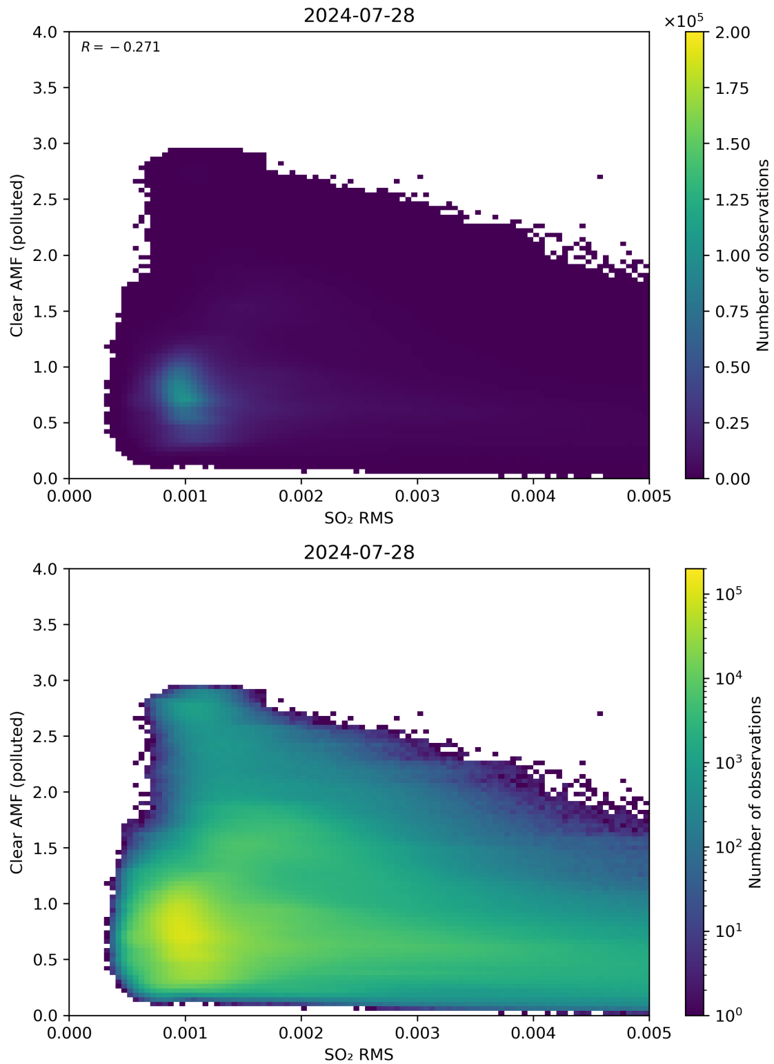
Figure 136: Scatter density plot of “SO 2 RMS” against “Clear AMF (polluted)” for 2024-07-27 to 2024-07-29.
