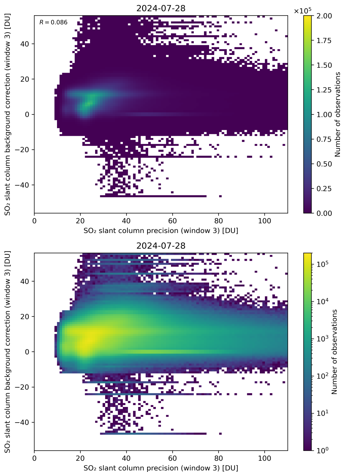
Figure 257: Scatter density plot of “SO 2 slant column precision (window 3)” against “SO 2 slant column background correction (window 3)” for 2024-07-27 to 2024-07-29.
