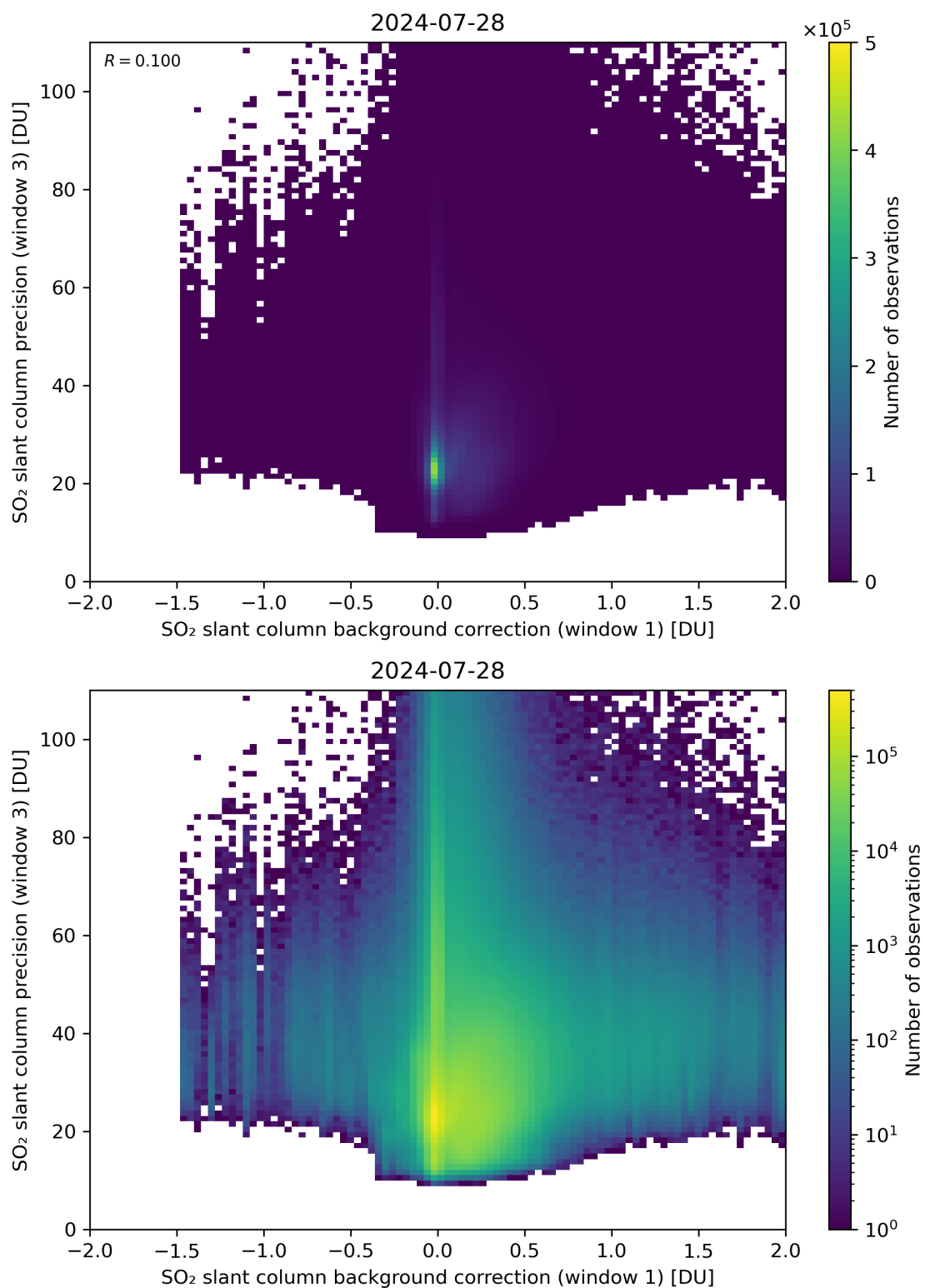
Figure 108: Scatter density plot of “SO 2 slant column background correction (window 1)” against “SO 2 slant column precision (window 3)” for 2024-07-27 to 2024-07-29.
