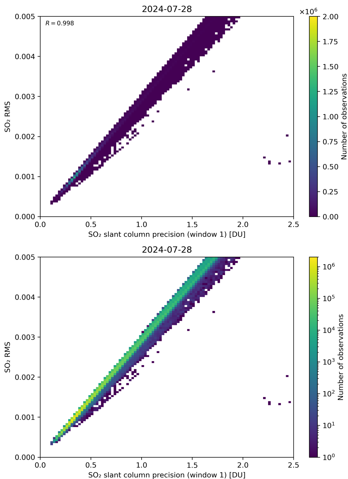
Figure 223: Scatter density plot of “SO 2 slant column precision (window 1)” against “SO 2 RMS” for 2024-07-27 to 2024-07-29.
