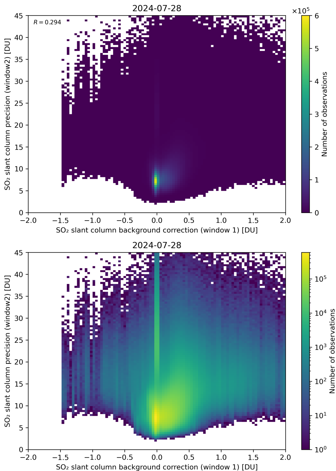
Figure 106: Scatter density plot of “SO 2 slant column background correction (window 1)” against “SO 2 slant column precision (window2)” for 2024-07-27 to 2024-07-29.
