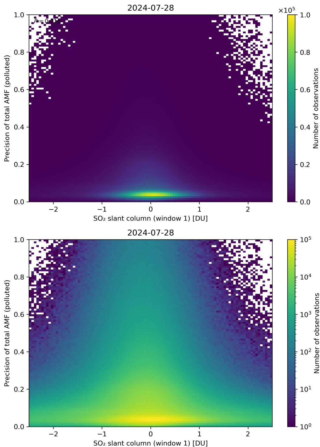
Figure 240: Scatter density plot of “SO 2 slant column (window 1)” against “Precision of total AMF (polluted)” for 2024-07-27 to 2024-07-29.
