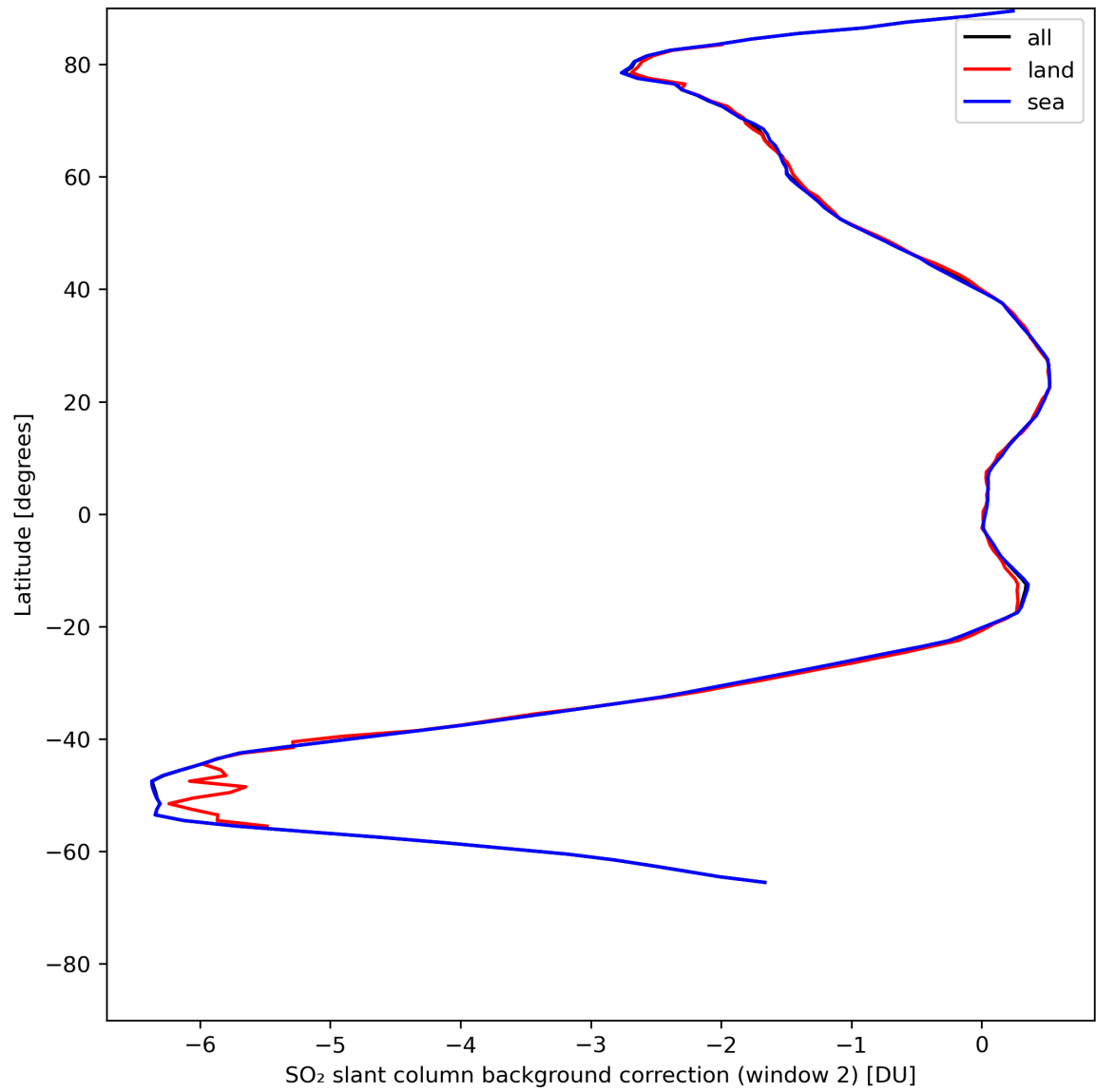
Figure 40: Zonal average of “SO 2 slant column background correction (window 2)” for 2024-07-27 to 2024-07-29.
