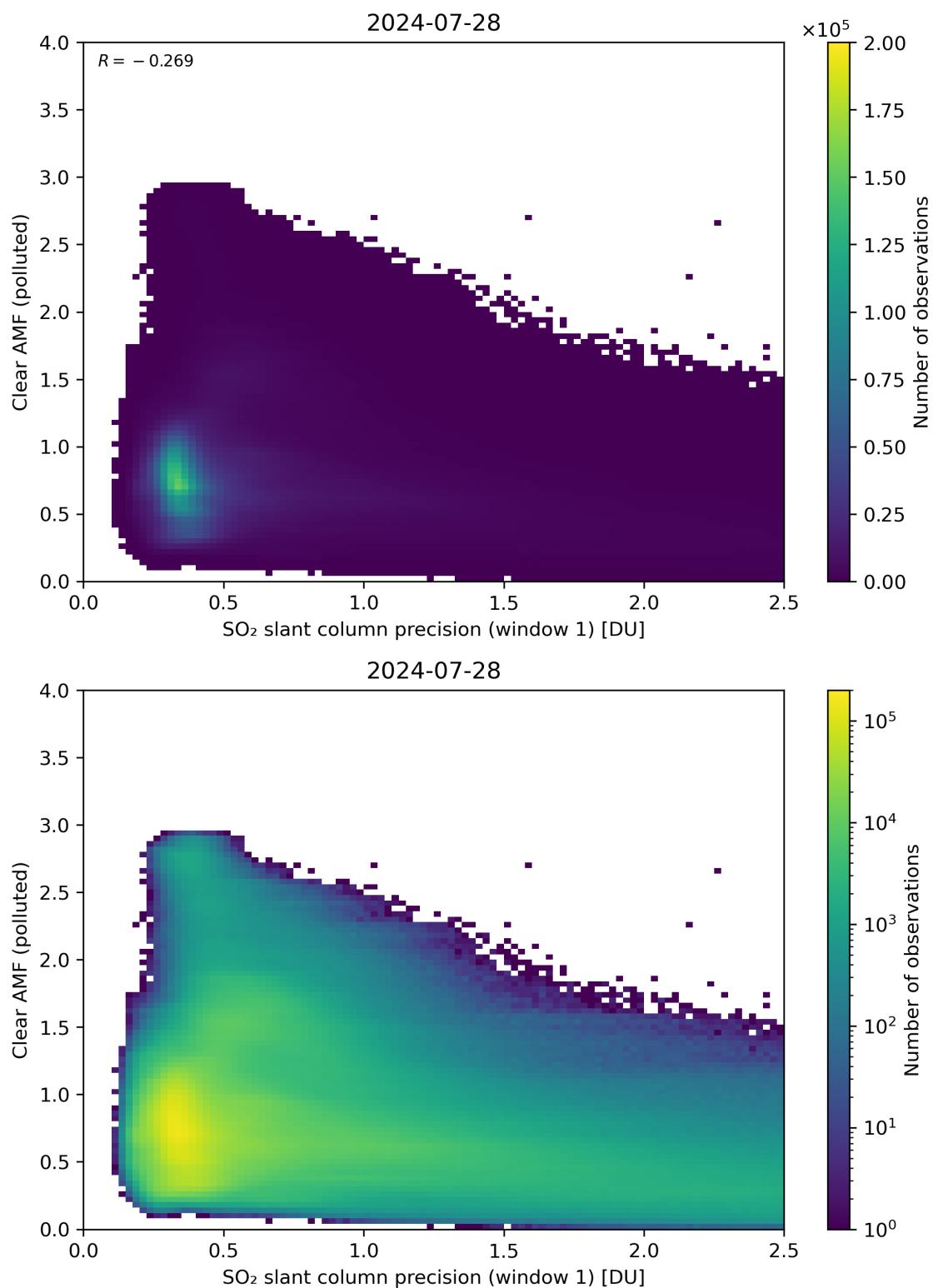
Figure 224: Scatter density plot of “SO 2 slant column precision (window 1)” against “Clear AMF (polluted)” for 2024-07-27 to 2024-07-29.
