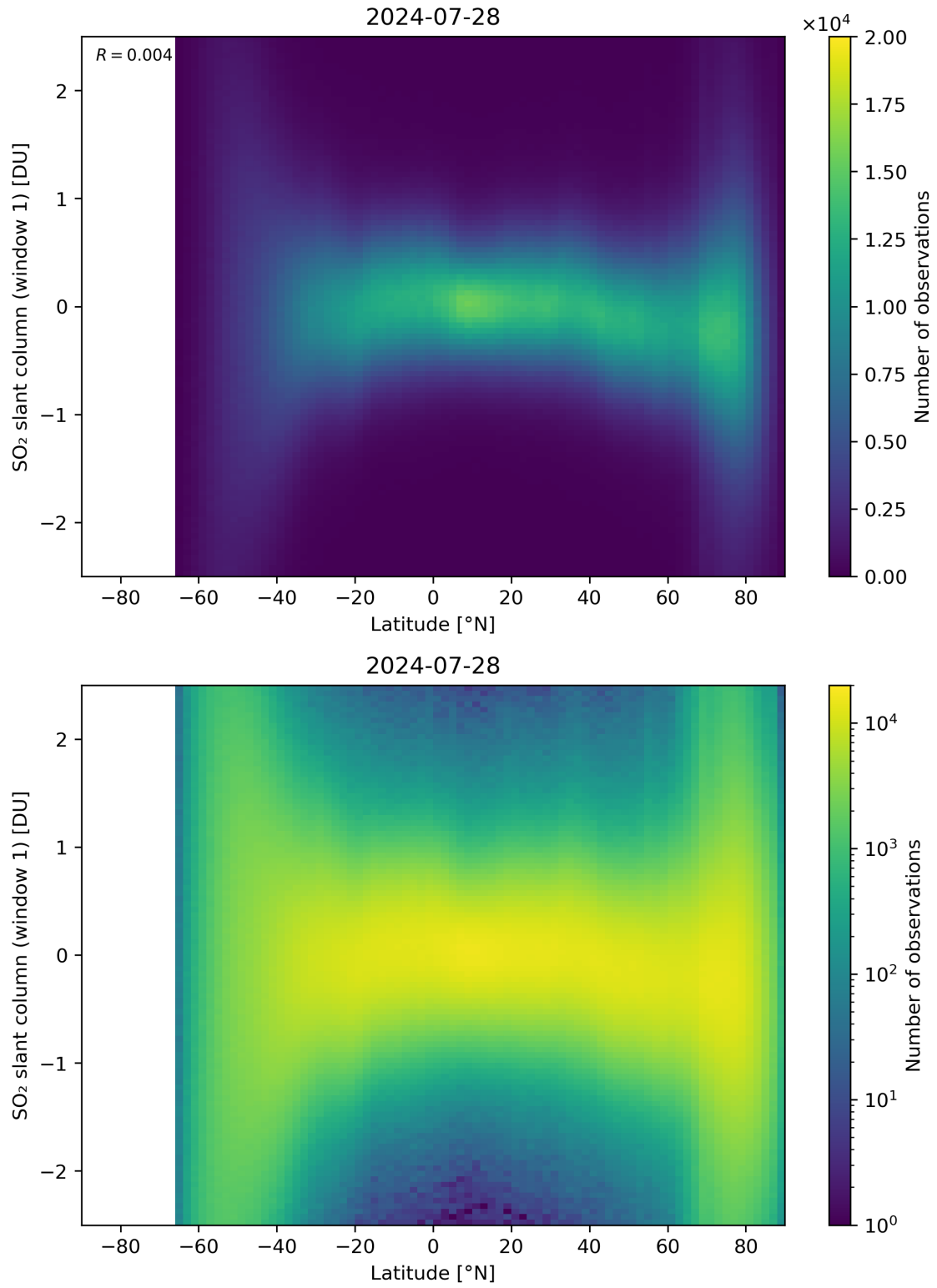
Figure 149: Scatter density plot of “Latitude” against “SO 2 slant column (window 1)” for 2024-07-27 to 2024-07-29.
