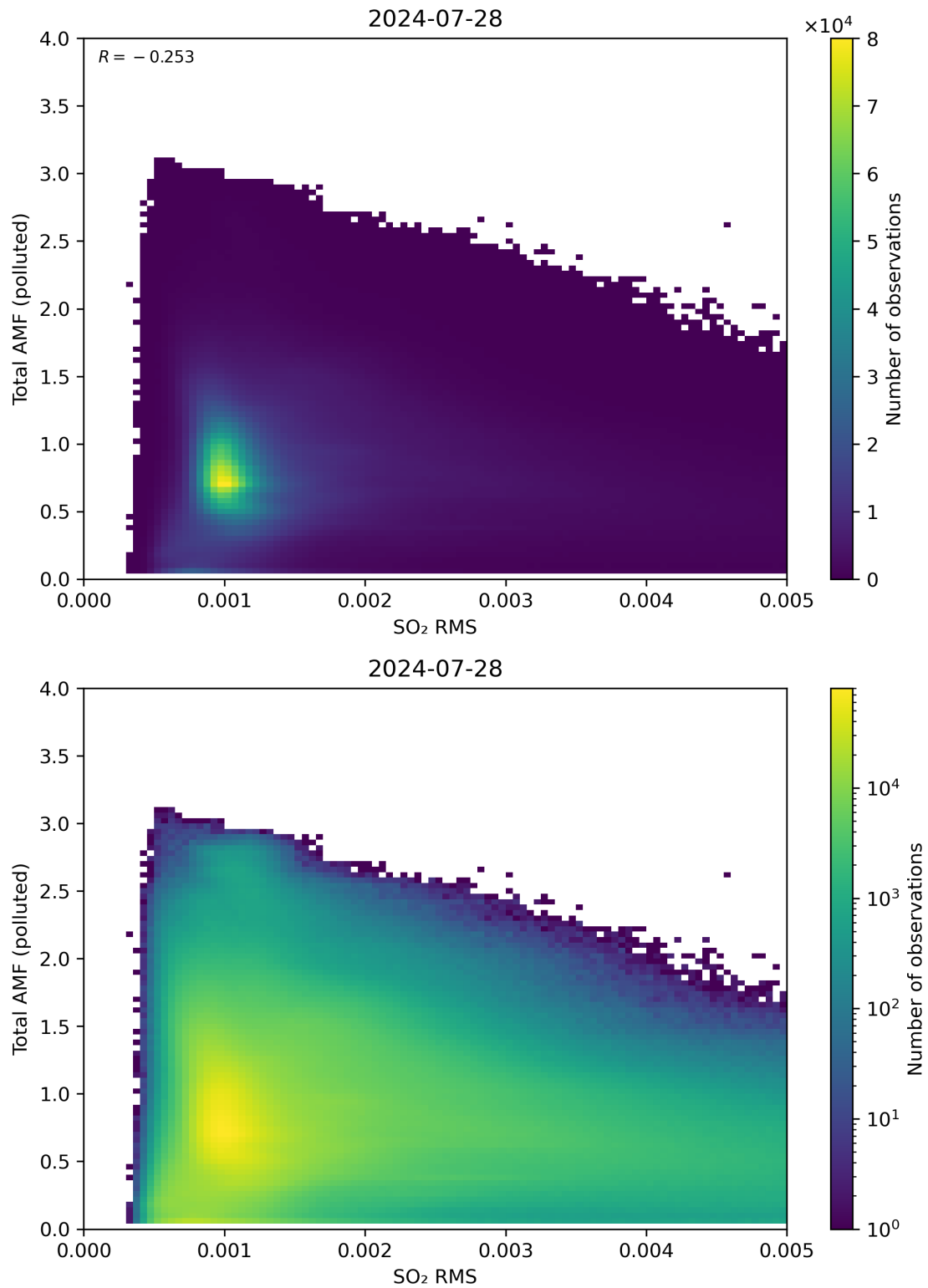
Figure 137: Scatter density plot of “SO 2 RMS” against “Total AMF (polluted)” for 2024-07-27 to 2024-07-29.
