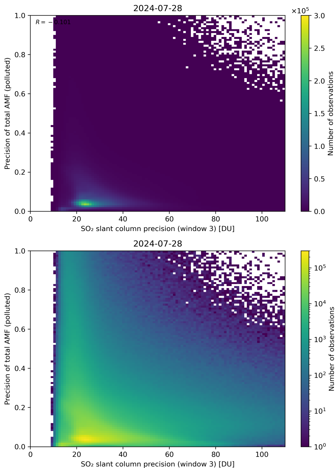
Figure 264: Scatter density plot of “SO 2 slant column precision (window 3)” against “Precision of total AMF (polluted)” for 2024-07-27 to 2024-07-29.
