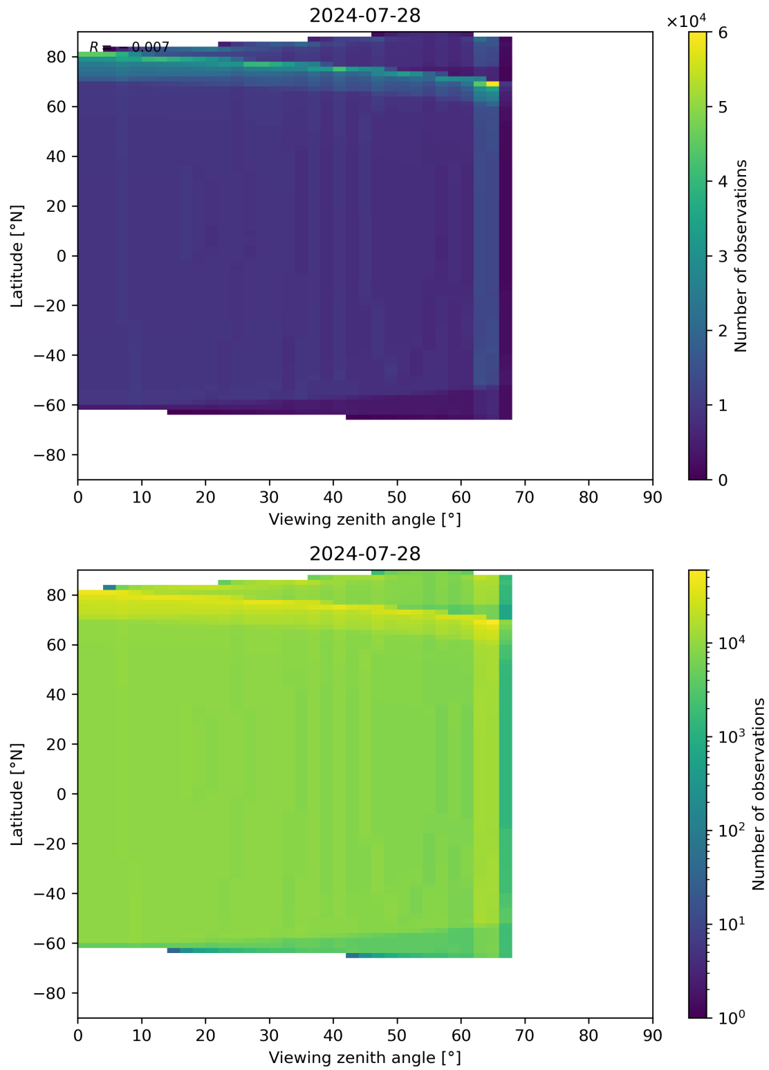
Figure 314: Scatter density plot of “Viewing zenith angle” against “Latitude” for 2024-07-27 to 2024-07-29.
