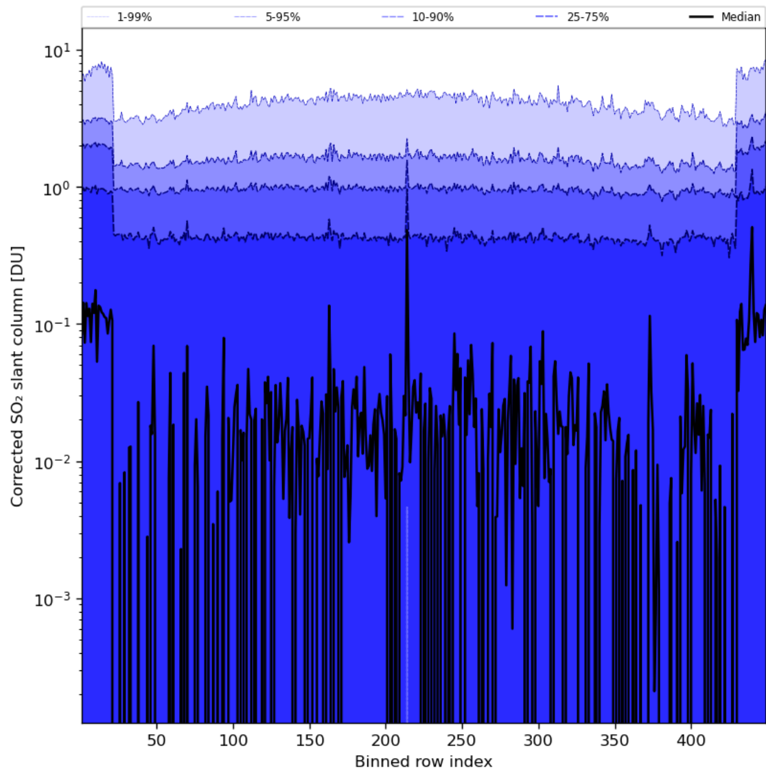
Figure 78: Along track statistics of “Corrected SO 2 slant column” for 2024-07-27 to 2024-07-29
