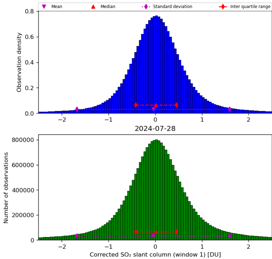
Figure 58: Histogram of “Corrected SO 2 slant column (window 1)” for 2024-07-27 to 2024-07-29
