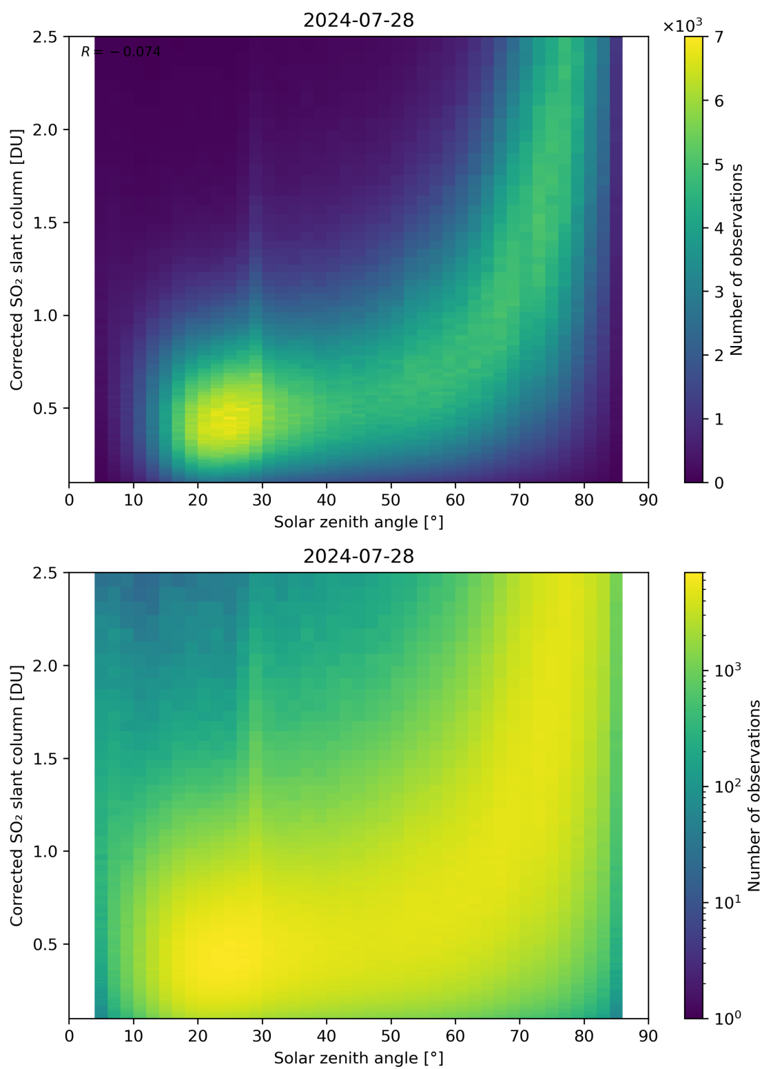
Figure 166: Scatter density plot of “Solar zenith angle” against “Corrected SO 2 slant column” for 2024-07-27 to 2024-07-29.
