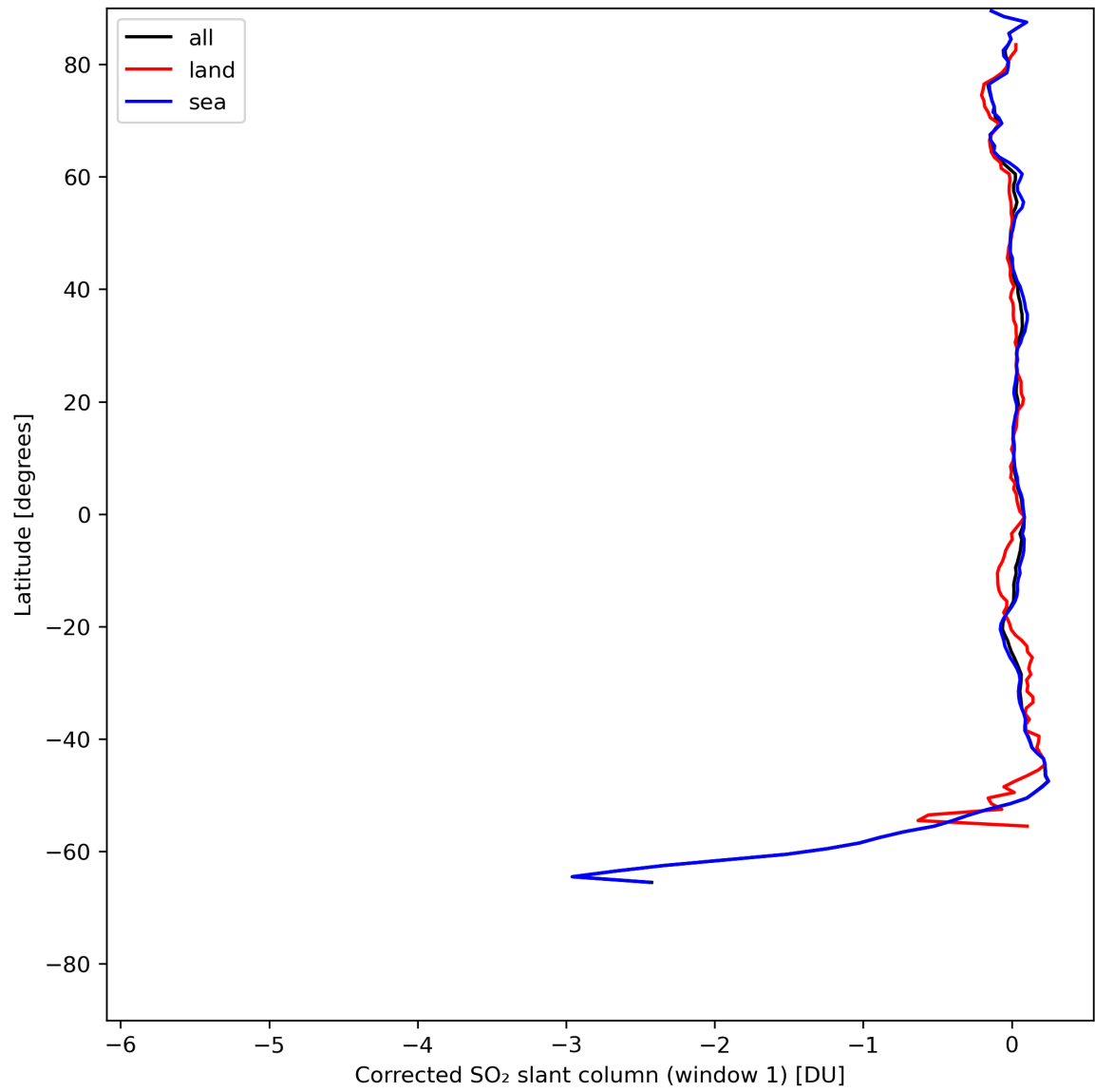
Figure 35: Zonal average of “Corrected SO 2 slant column (window 1)” for 2024-07-27 to 2024-07-29.
