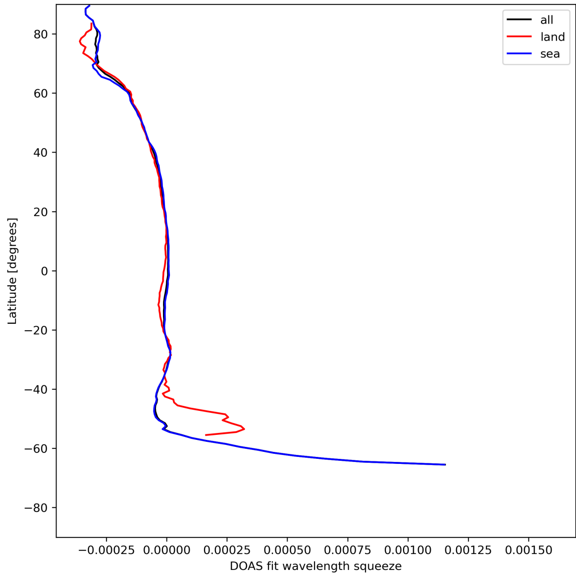
Figure 46: Zonal average of “DOAS fit wavelength squeeze” for 2024-07-27 to 2024-07-29.
