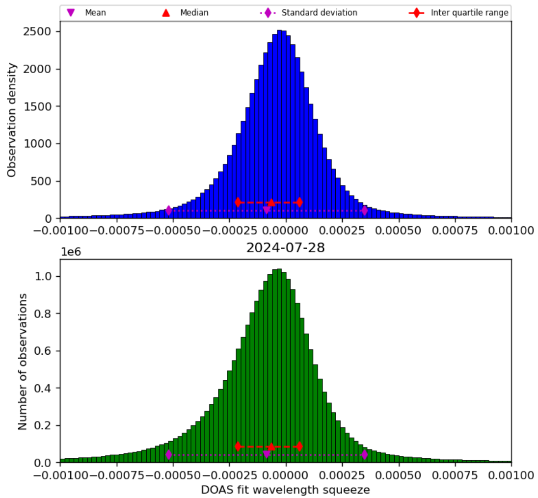
Figure 69: Histogram of “DOAS fit wavelength squeeze” for 2024-07-27 to 2024-07-29
