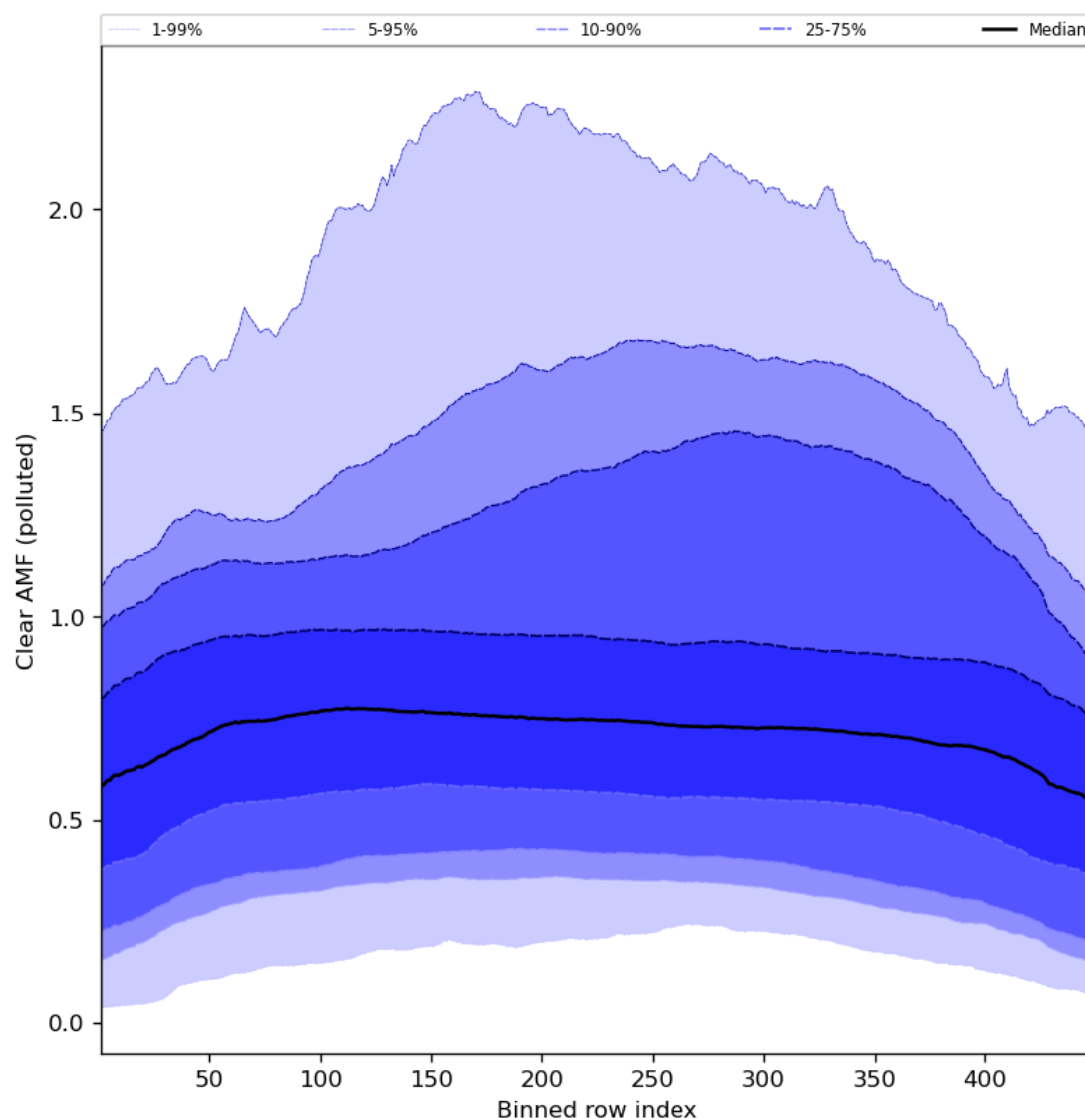
Figure 96: Along track statistics of “Clear AMF (polluted)” for 2024-07-27 to 2024-07-29
