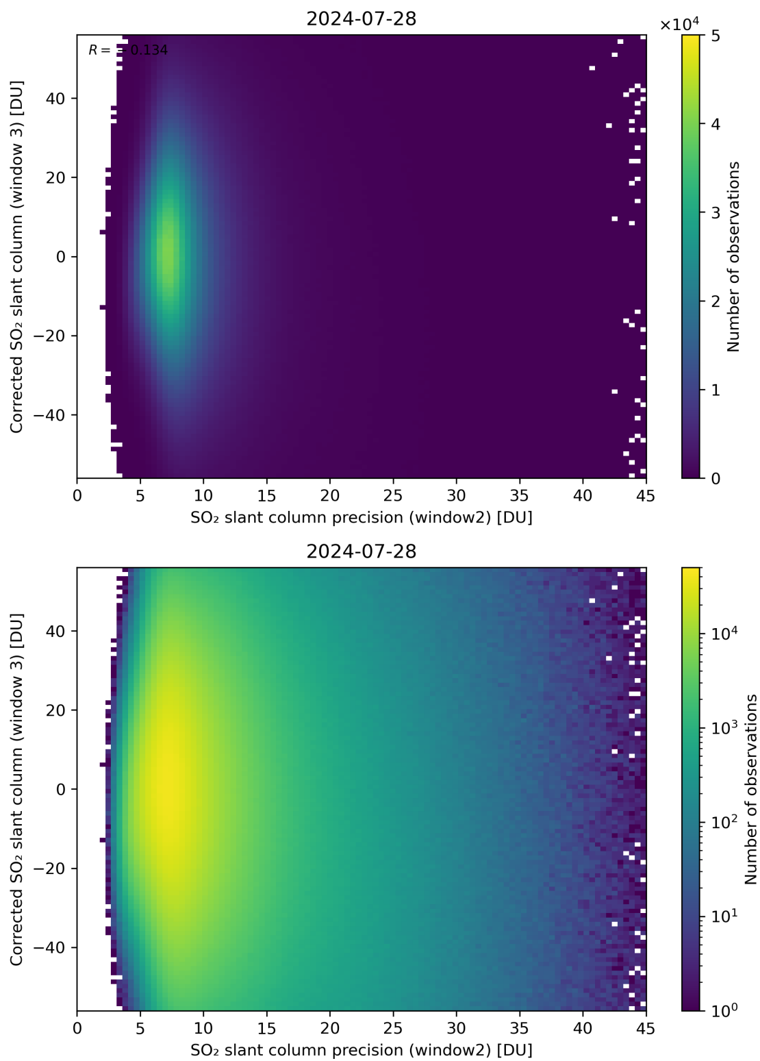
Figure 248: Scatter density plot of “SO 2 slant column precision (window2)” against “Corrected SO 2 slant column (window 3)” for 2024-07-27 to 2024-07-29.
