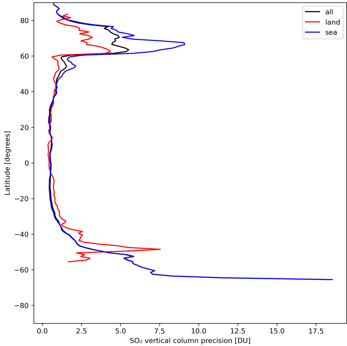
Figure 31: Zonal average of “SO 2 vertical column precision” for 2024-07-27 to 2024-07-29.
