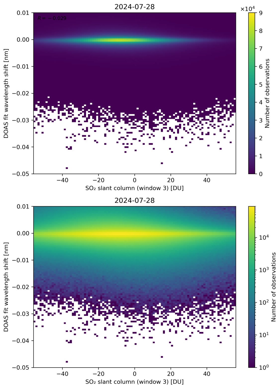
Figure 254: Scatter density plot of “SO 2 slant column (window 3)” against “DOAS fit wavelength shift” for 2024-07-27 to 2024-07-29.
