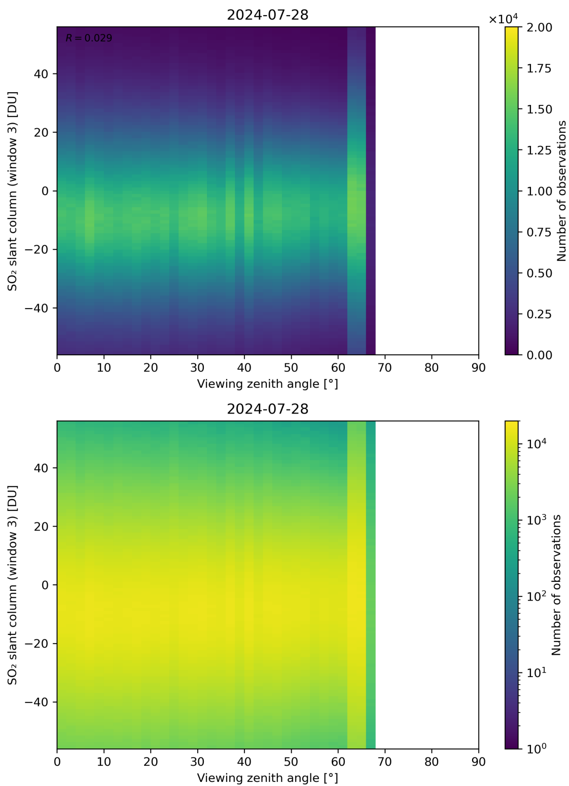
Figure 323: Scatter density plot of “Viewing zenith angle” against “SO 2 slant column (window 3)” for 2024-07-27 to 2024-07-29.
