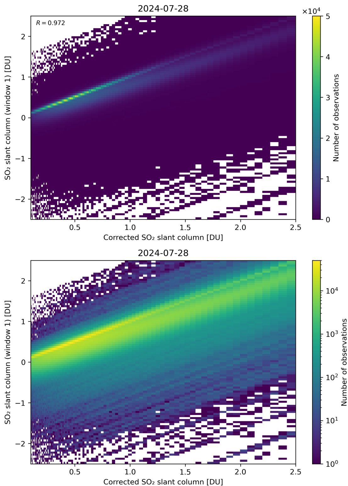
Figure 187: Scatter density plot of “Corrected SO 2 slant column” against “SO 2 slant column (window 1)” for 2024-07-27 to 2024-07-29.
