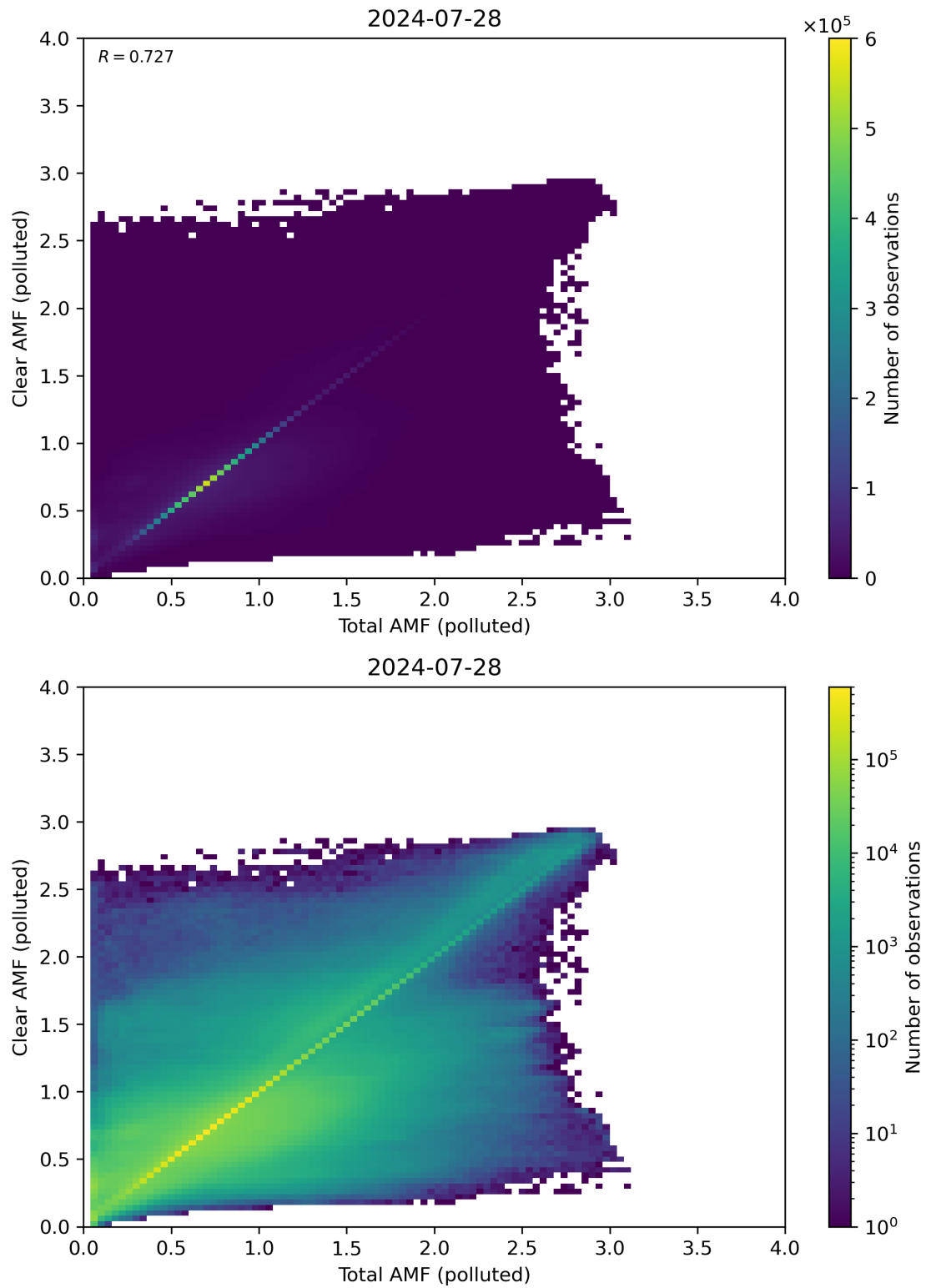
Figure 271: Scatter density plot of “Total AMF (polluted)” against “Clear AMF (polluted)” for 2024-07-27 to 2024-07-29.
