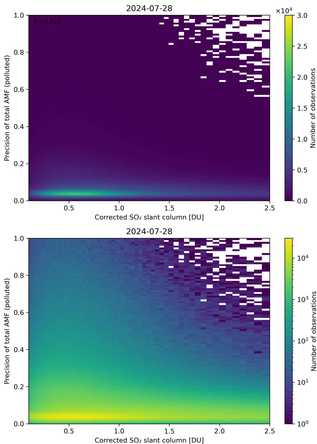
Figure 193: Scatter density plot of “Corrected SO 2 slant column” against “Precision of total AMF (polluted)” for 2024-07-27 to 2024-07-29.
