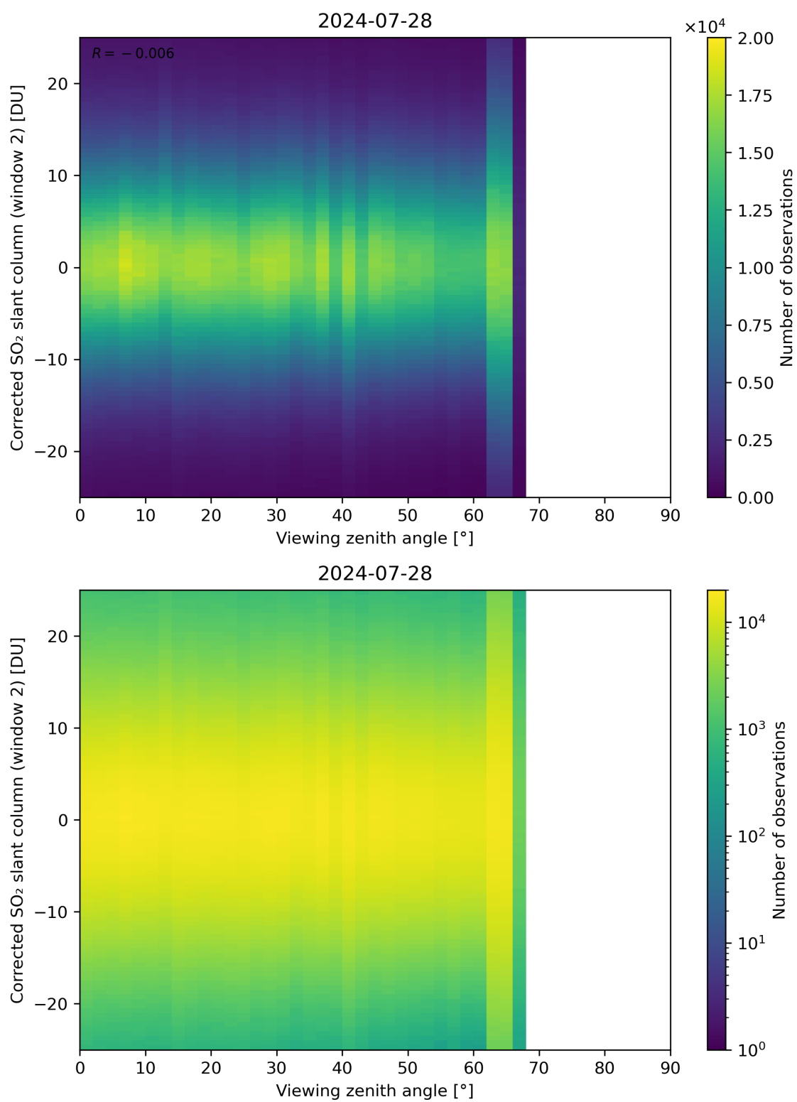
Figure 318: Scatter density plot of “Viewing zenith angle” against “Corrected SO 2 slant column (window 2)” for 2024-07-27 to 2024-07-29.
