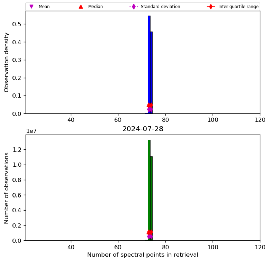
Figure 74: Histogram of “Number of spectral points in retrieval” for 2024-07-27 to 2024-07-29
