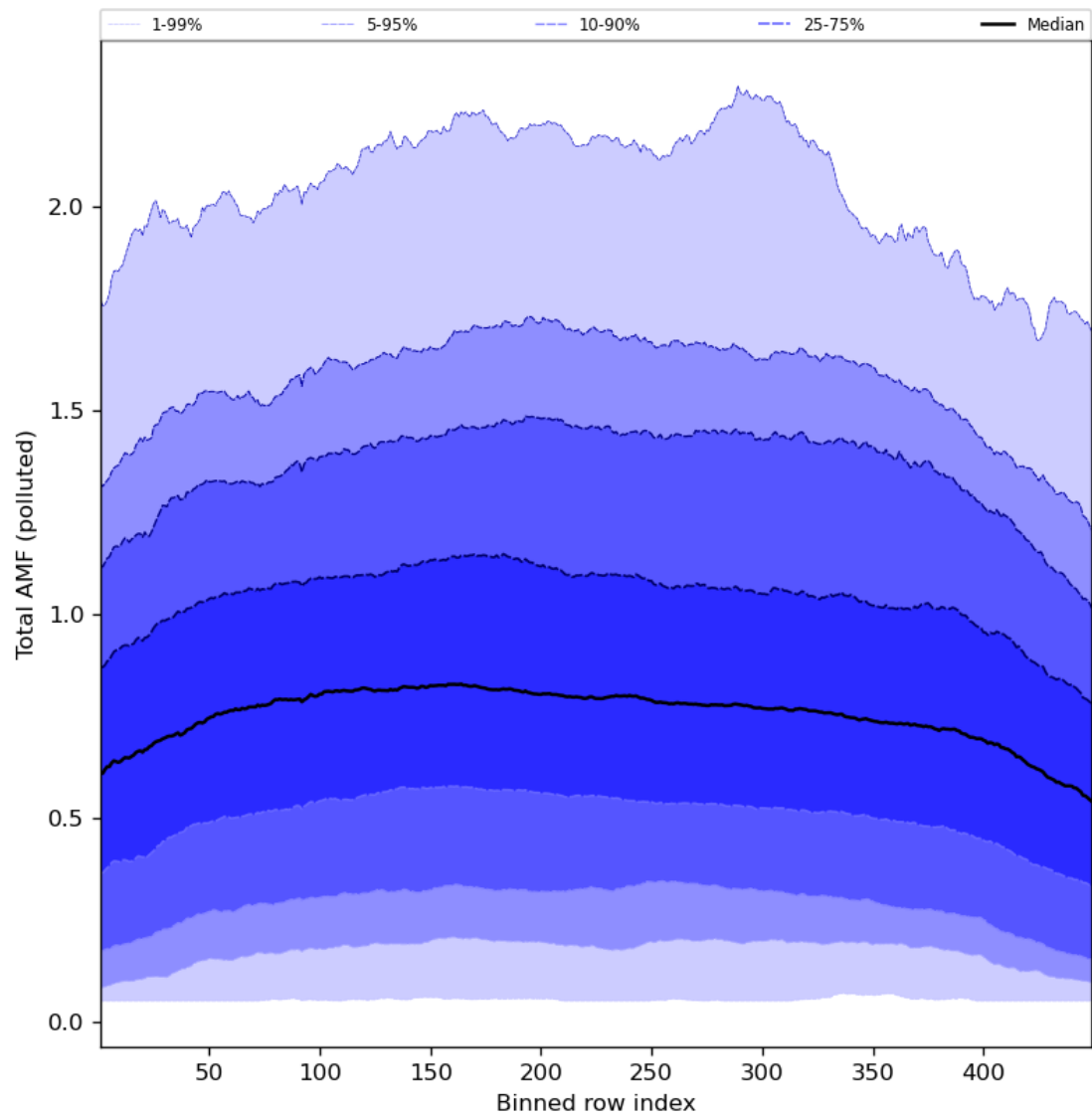
Figure 94: Along track statistics of “Total AMF (polluted)” for 2024-07-27 to 2024-07-29
