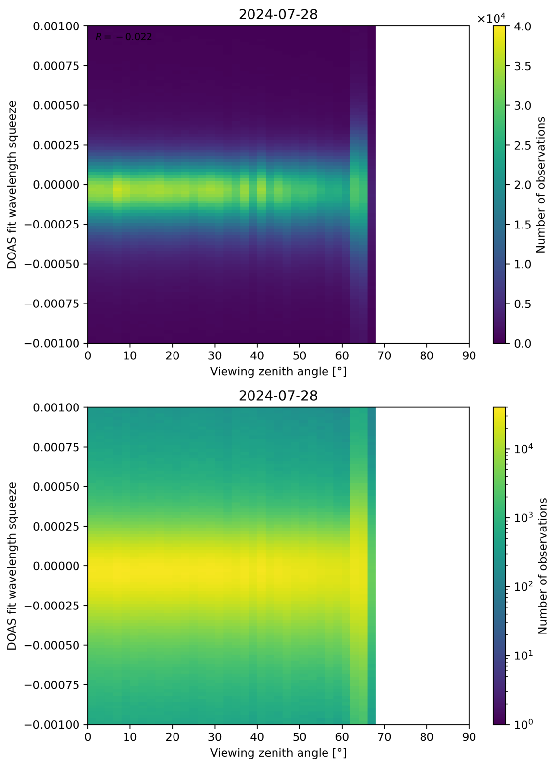
Figure 312: Scatter density plot of “Viewing zenith angle” against “DOAS fit wavelength squeeze” for 2024-07-27 to 2024-07-29.
