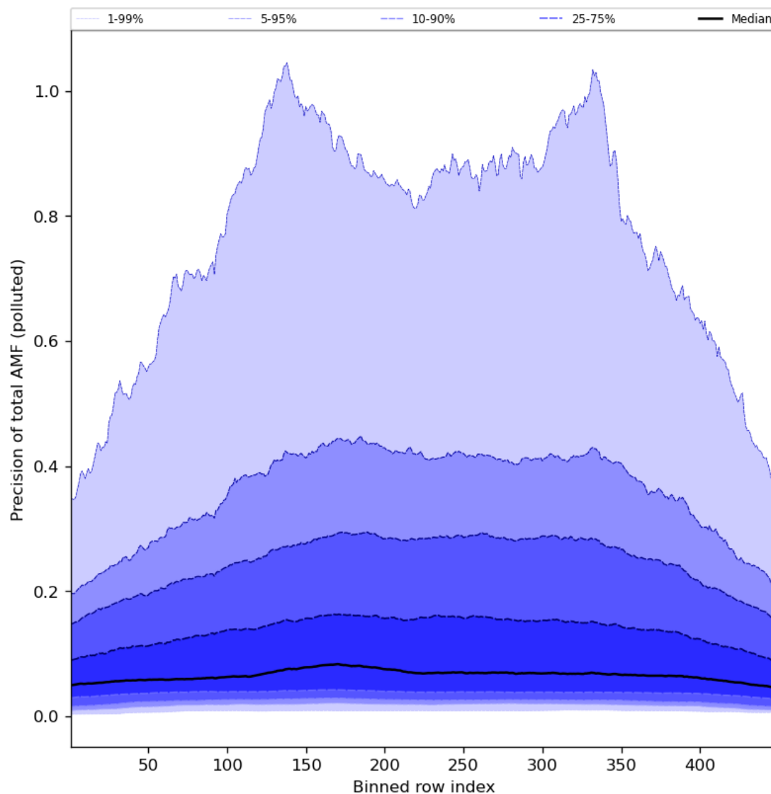
Figure 95: Along track statistics of “Precision of total AMF (polluted)” for 2024-07-27 to 2024-07-29
