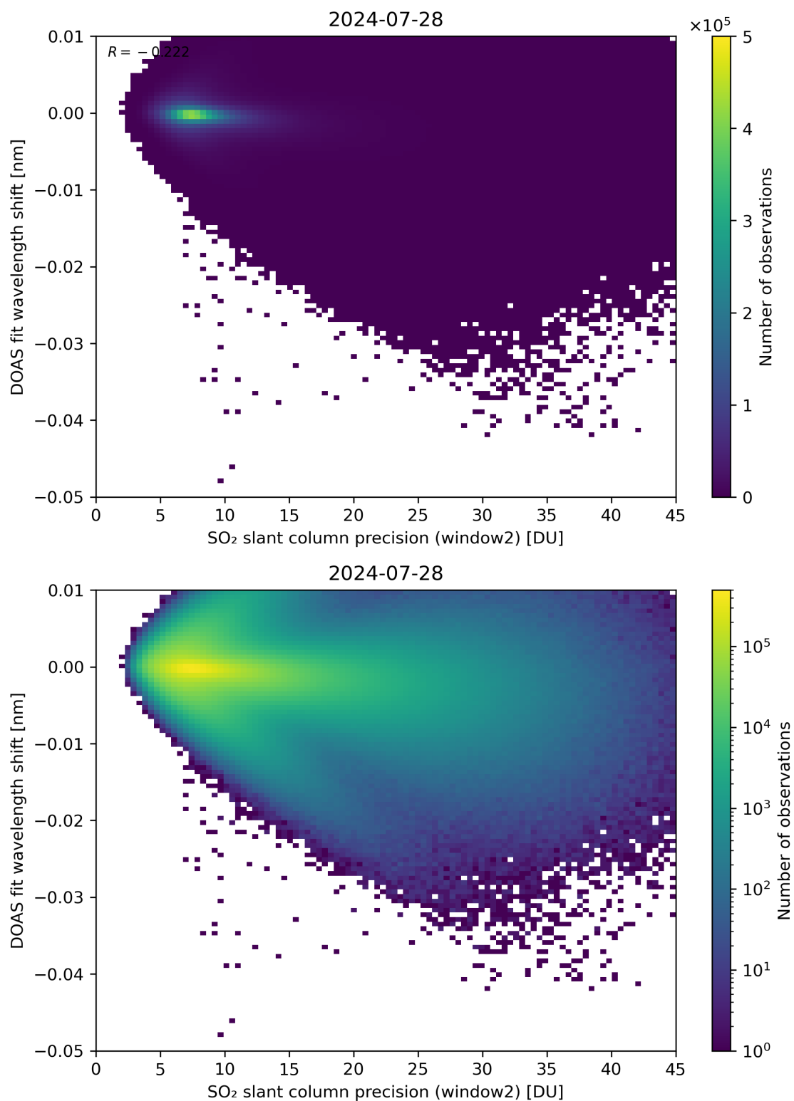
Figure 243: Scatter density plot of “SO 2 slant column precision (window2)” against “DOAS fit wavelength shift” for 2024-07-27 to 2024-07-29.
