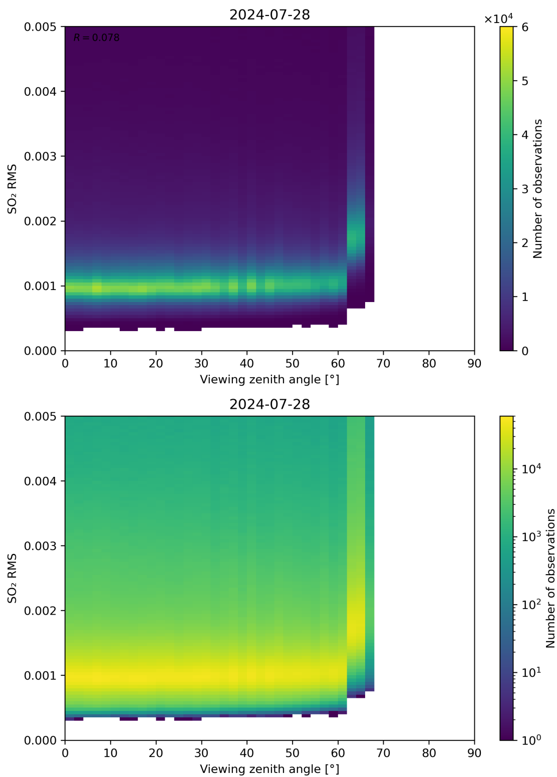
Figure 313: Scatter density plot of “Viewing zenith angle” against “SO 2 RMS” for 2024-07-27 to 2024-07-29.
