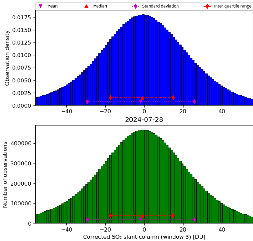
Figure 66: Histogram of “Corrected SO 2 slant column (window 3)” for 2024-07-27 to 2024-07-29
