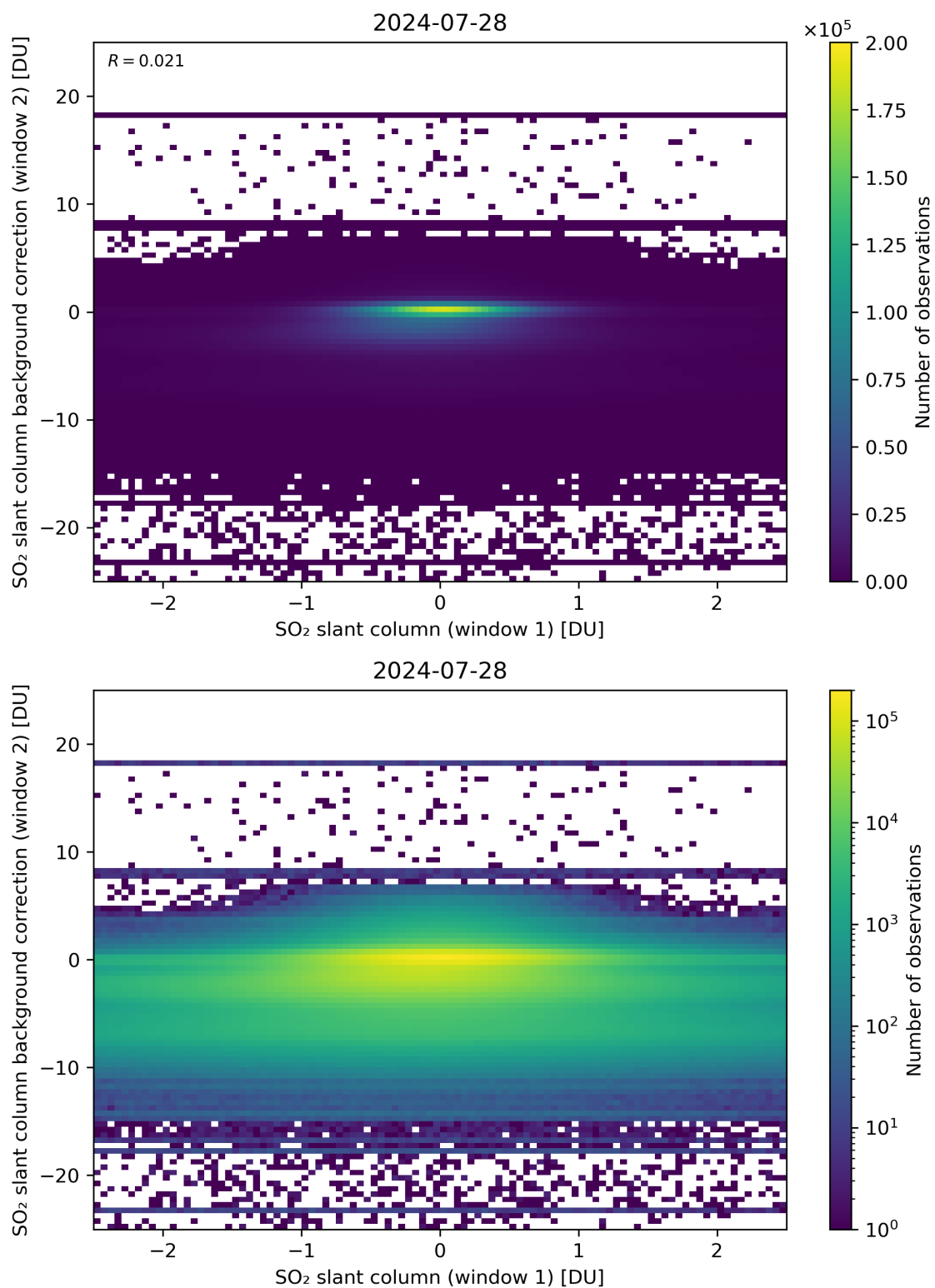
Figure 213: Scatter density plot of “SO 2 slant column (window 1)” against “SO 2 slant column background correction (window 2)” for 2024-07-27 to 2024-07-29.
