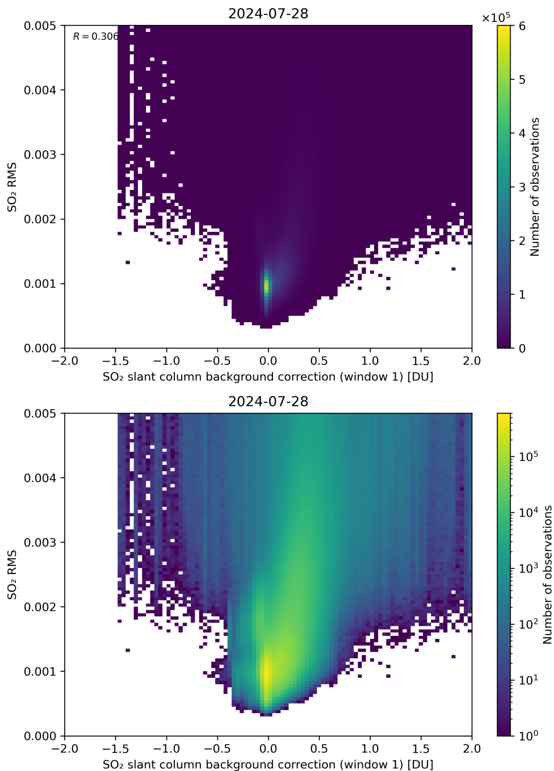
Figure 102: Scatter density plot of “SO 2 slant column background correction (window 1)” against “SO 2 RMS” for 2024-07-27 to 2024-07-29.
