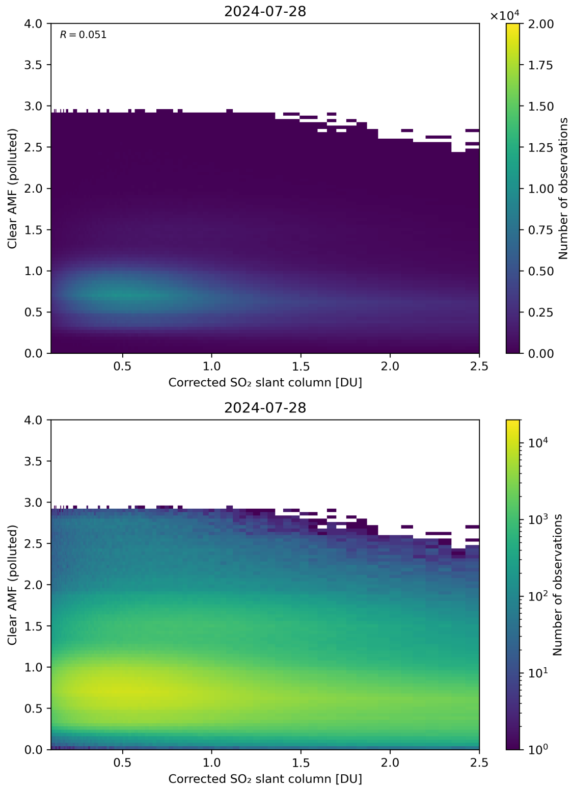
Figure 184: Scatter density plot of “Corrected SO 2 slant column” against “Clear AMF (polluted)” for 2024-07-27 to 2024-07-29.
