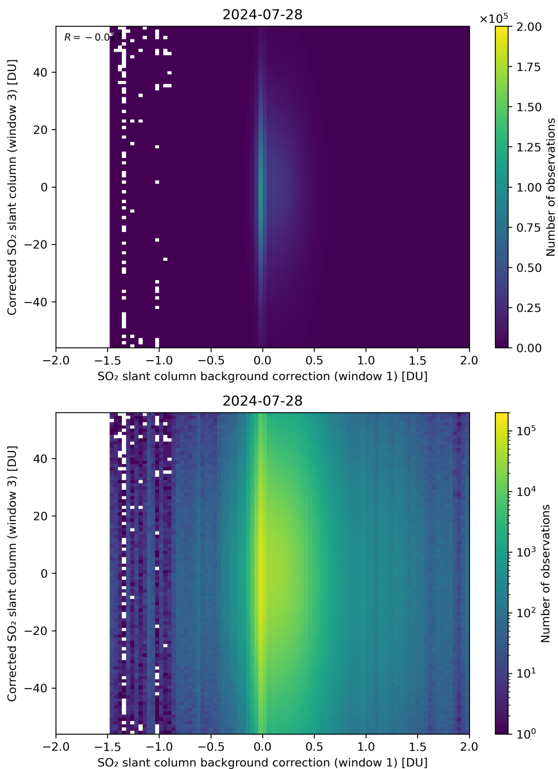
Figure 105: Scatter density plot of “SO 2 slant column background correction (window 1)” against “Corrected SO 2 slant column (window 3)” for 2024-07-27 to 2024-07-29.
