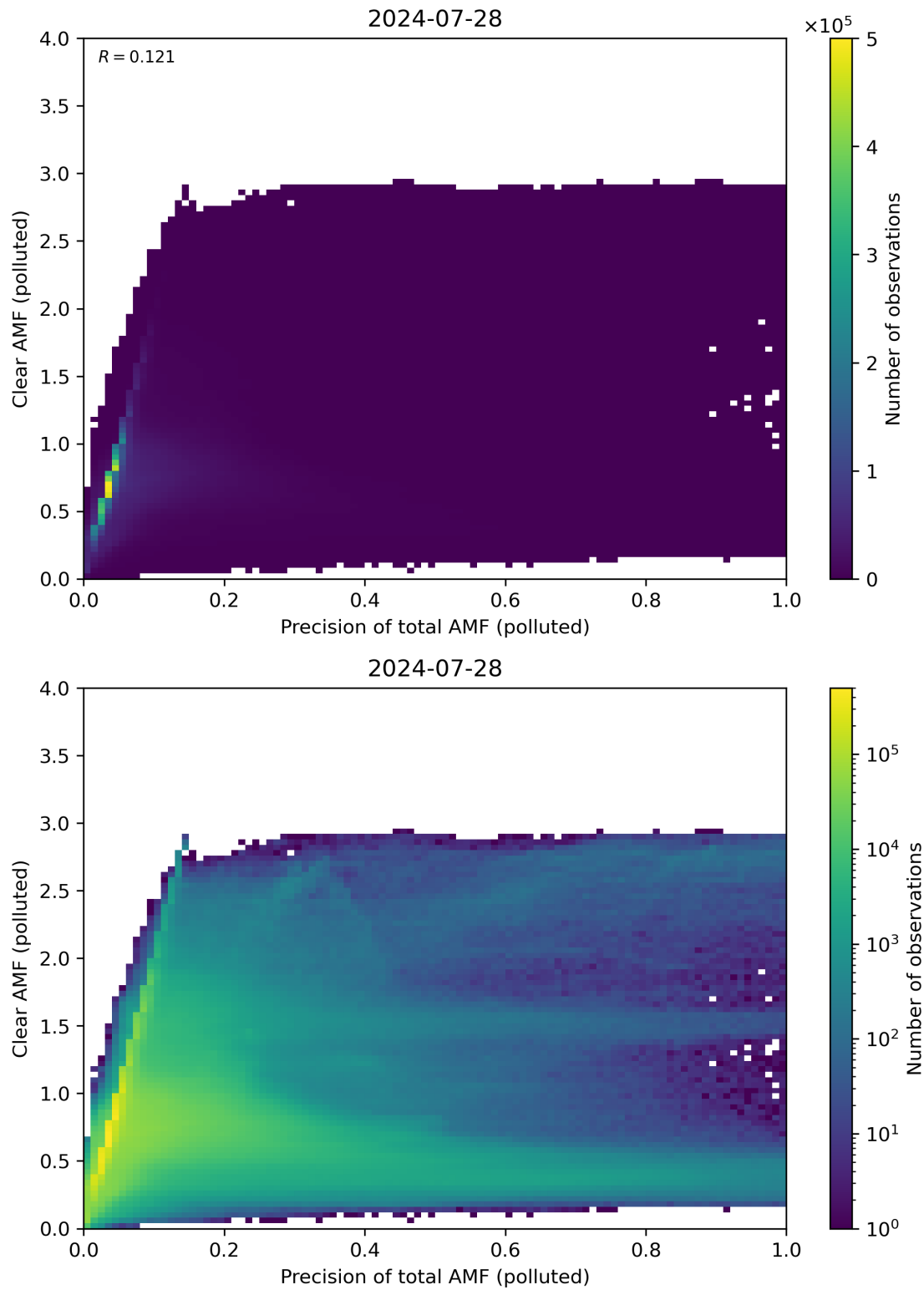
Figure 270: Scatter density plot of “Precision of total AMF (polluted)” against “Clear AMF (polluted)” for 2024-07-27 to 2024-07-29.
