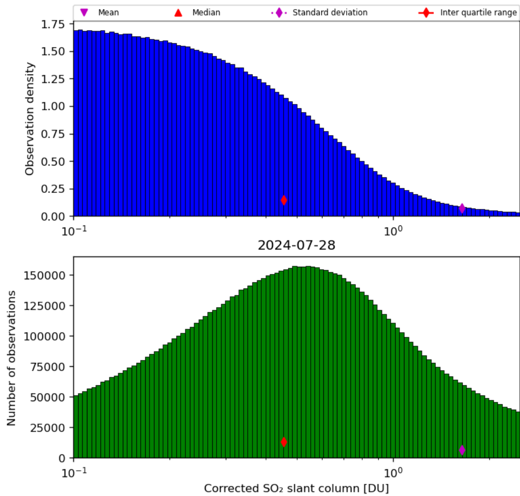
Figure 55: Histogram of “Corrected SO 2 slant column” for 2024-07-27 to 2024-07-29
