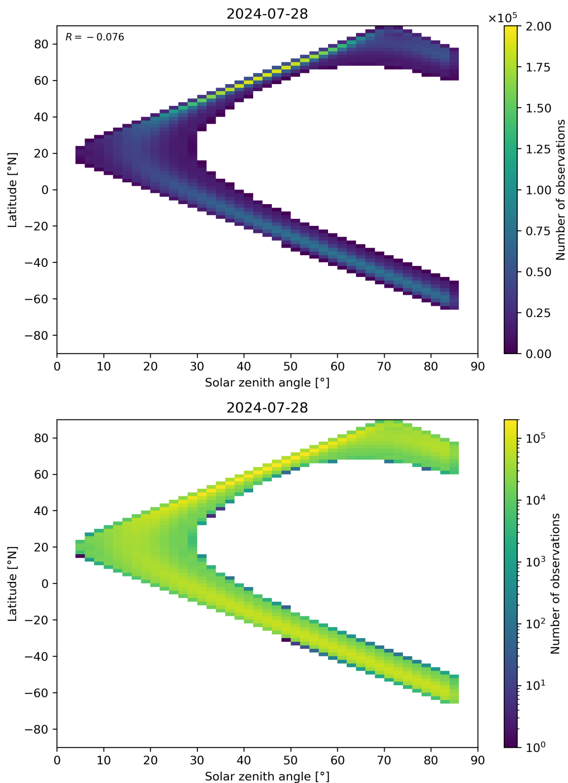
Figure 164: Scatter density plot of “Solar zenith angle” against “Latitude” for 2024-07-27 to 2024-07-29.
