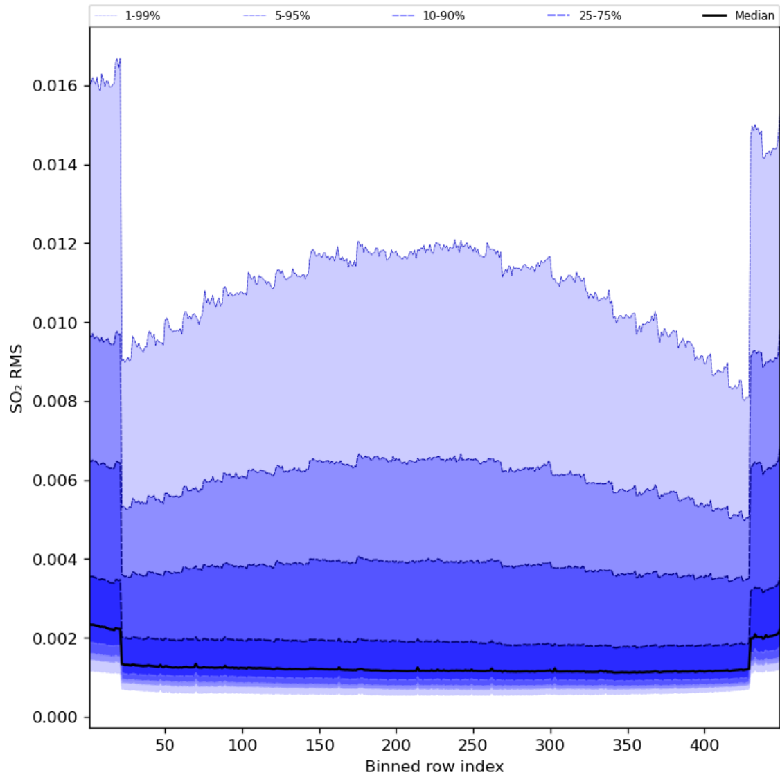
Figure 93: Along track statistics of “SO 2 RMS” for 2024-07-27 to 2024-07-29
