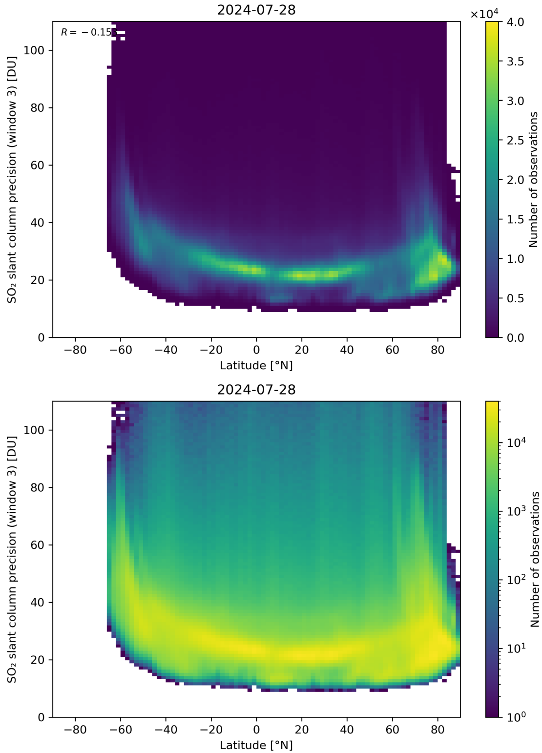
Figure 153: Scatter density plot of “Latitude” against “SO 2 slant column precision (window 3)” for 2024-07-27 to 2024-07-29.
