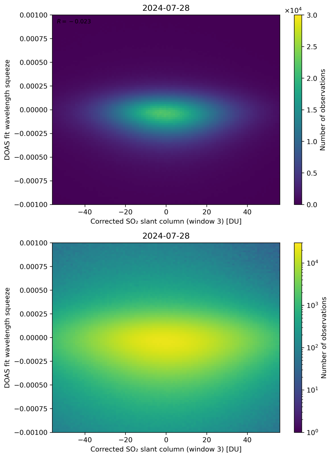
Figure 207: Scatter density plot of “Corrected SO 2 slant column (window 3)” against “DOAS fit wavelength squeeze” for 2024-07-27 to 2024-07-29.
