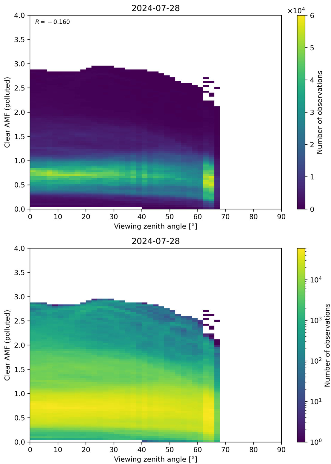
Figure 316: Scatter density plot of “Viewing zenith angle” against “Clear AMF (polluted)” for 2024-07-27 to 2024-07-29.
