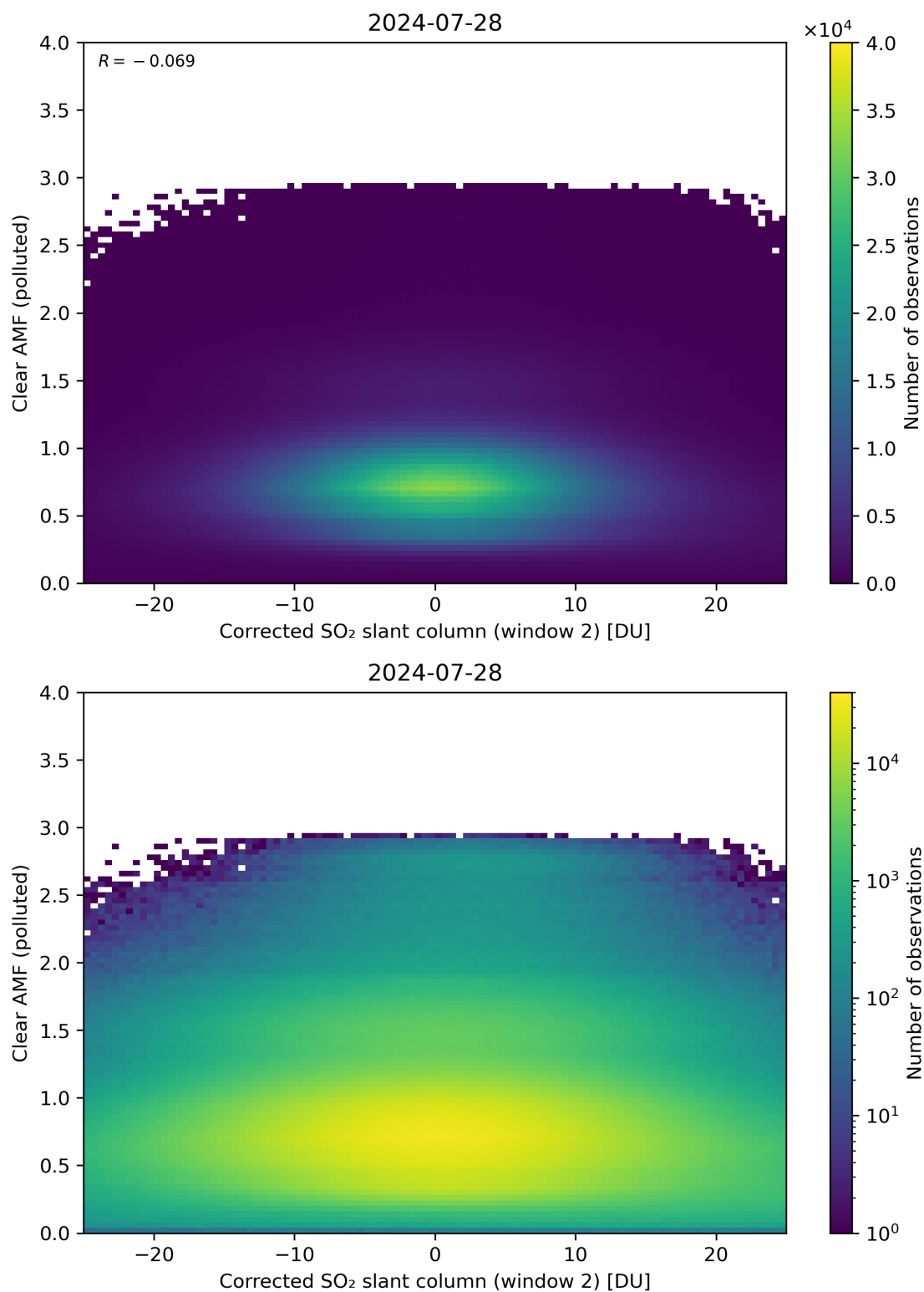
Figure 199: Scatter density plot of “Corrected SO 2 slant column (window 2)” against “Clear AMF (polluted)” for 2024-07-27 to 2024-07-29.
