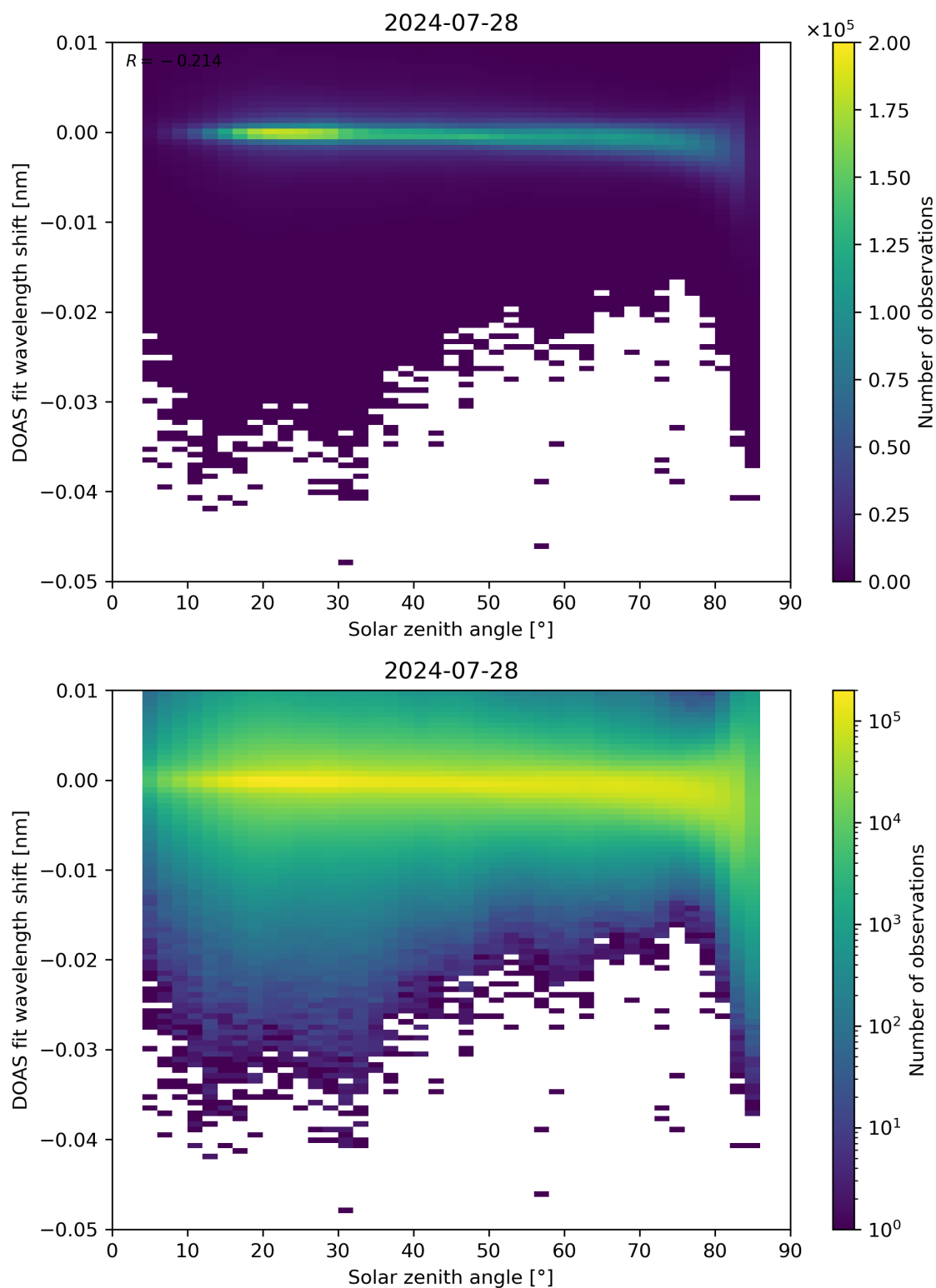
Figure 161: Scatter density plot of “Solar zenith angle” against “DOAS fit wavelength shift” for 2024-07-27 to 2024-07-29.
