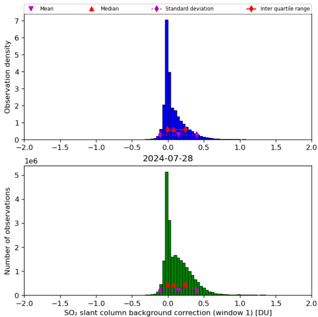
Figure 59: Histogram of “SO 2 slant column background correction (window 1)” for 2024-07-27 to 2024-07-29
