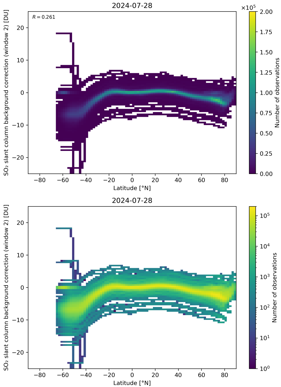
Figure 140: Scatter density plot of “Latitude” against “SO 2 slant column background correction (window 2)” for 2024-07-27 to 2024-07-29.
