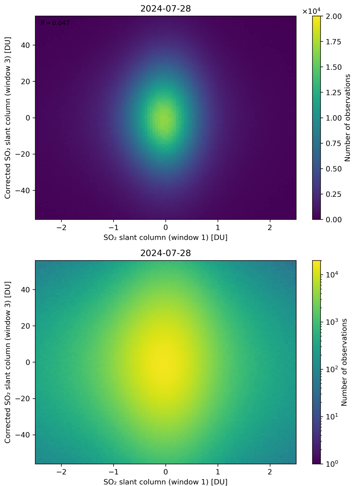
Figure 234: Scatter density plot of “SO 2 slant column (window 1)” against “Corrected SO 2 slant column (window 3)” for 2024-07-27 to 2024-07-29.
