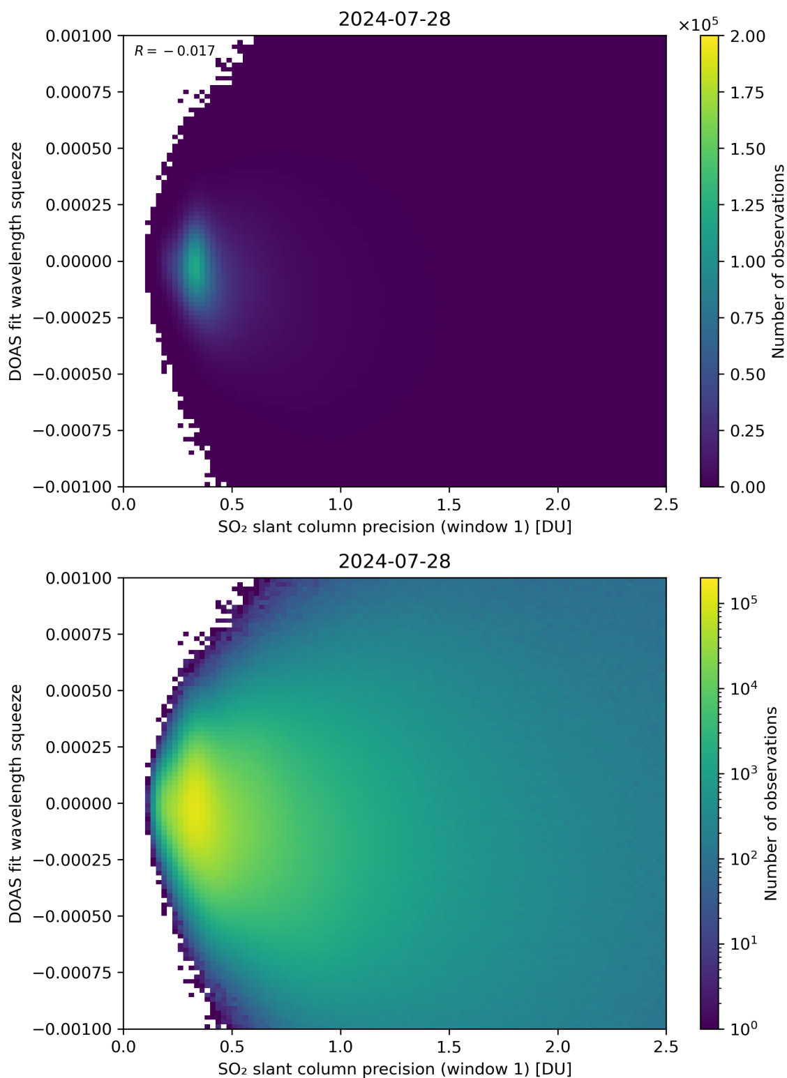
Figure 222: Scatter density plot of “SO 2 slant column precision (window 1)” against “DOAS fit wavelength squeeze” for 2024-07-27 to 2024-07-29.
