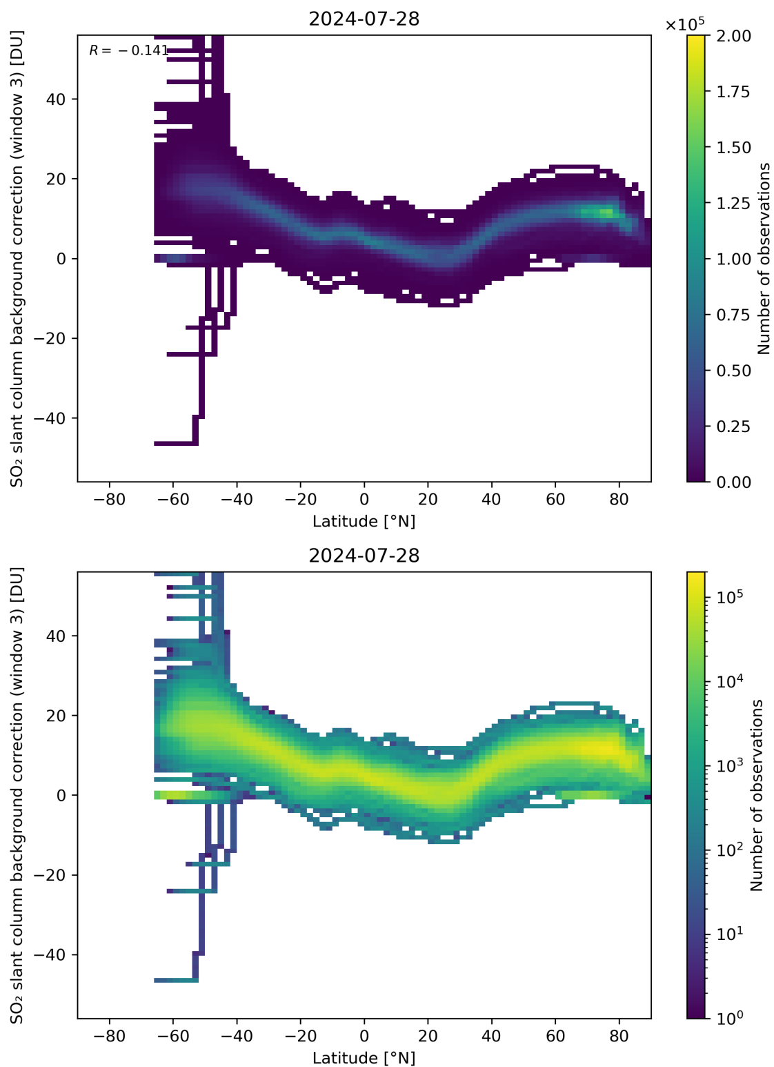
Figure 141: Scatter density plot of “Latitude” against “SO 2 slant column background correction (window 3)” for 2024-07-27 to 2024-07-29.
