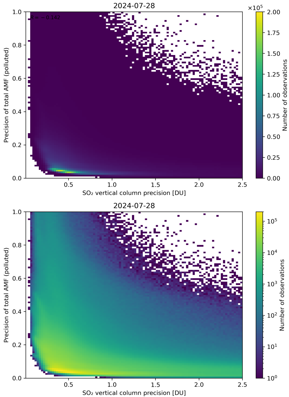
Figure 295: Scatter density plot of “SO 2 vertical column precision” against “Precision of total AMF (polluted)” for 2024-07-27 to 2024-07-29.
