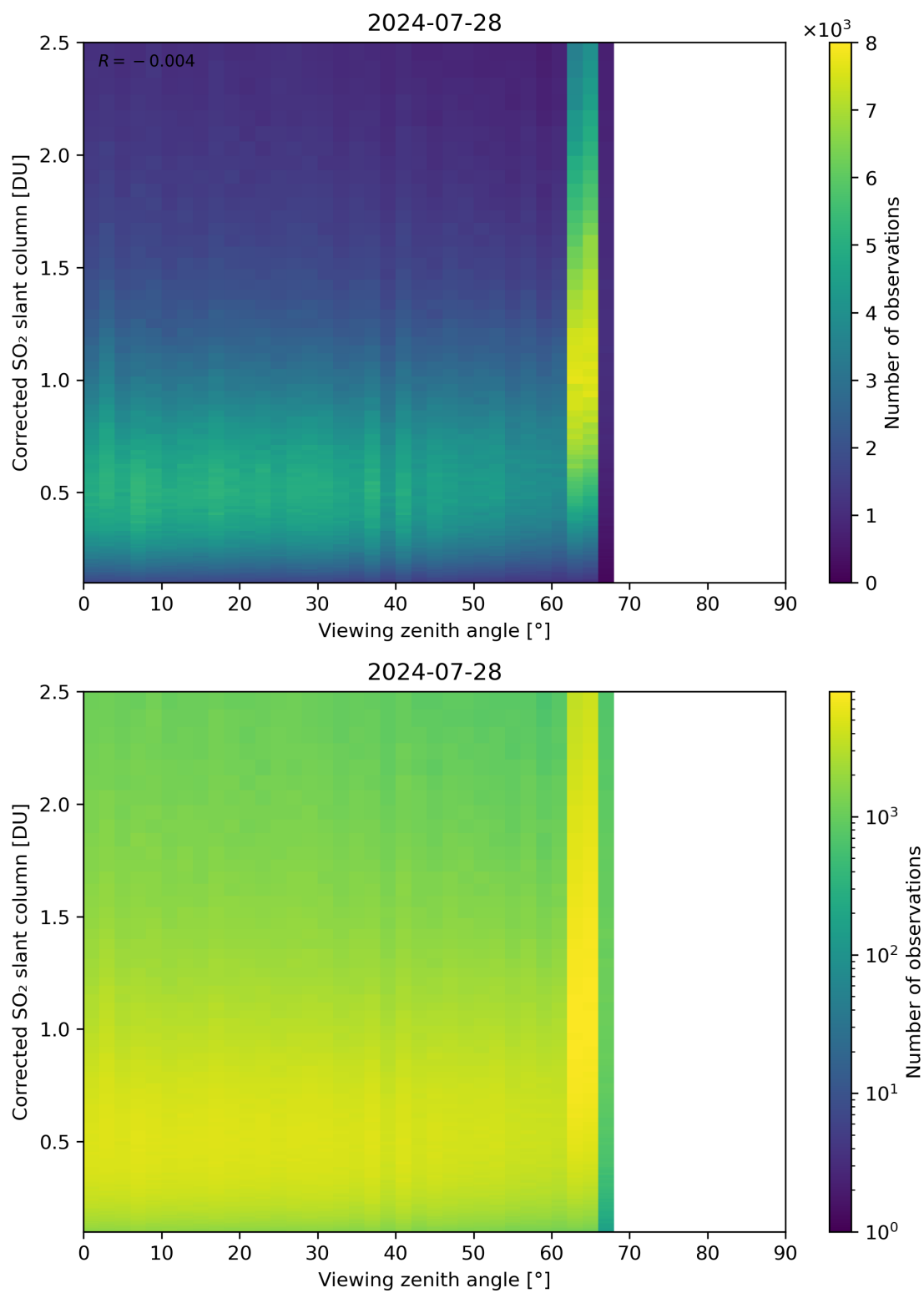
Figure 317: Scatter density plot of “Viewing zenith angle” against “Corrected SO 2 slant column” for 2024-07-27 to 2024-07-29.
