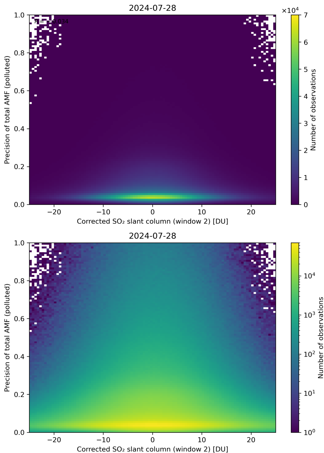
Figure 204: Scatter density plot of “Corrected SO 2 slant column (window 2)” against “Precision of total AMF (polluted)” for 2024-07-27 to 2024-07-29.
