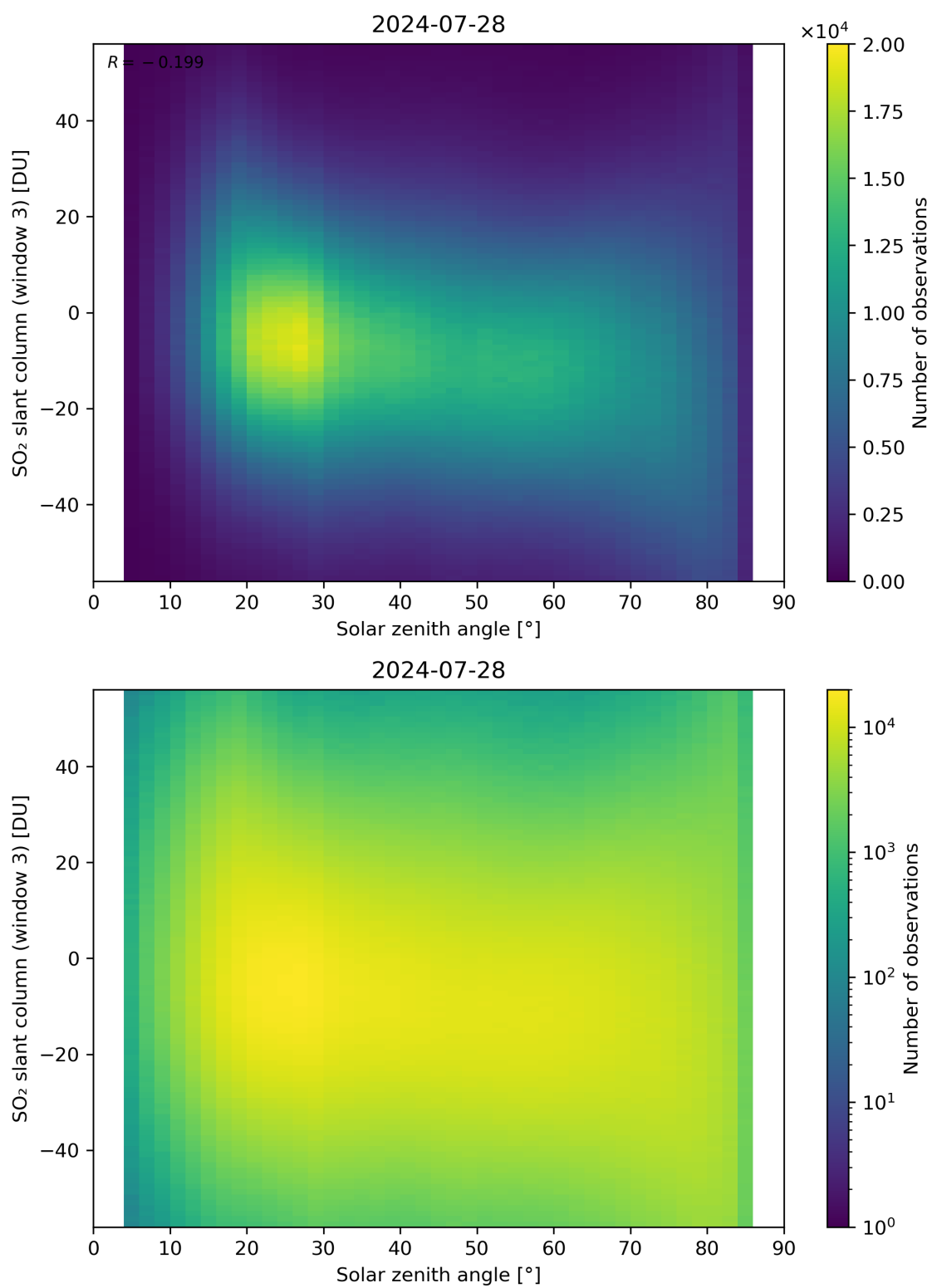
Figure 172: Scatter density plot of “Solar zenith angle” against “SO 2 slant column (window 3)” for 2024-07-27 to 2024-07-29.
