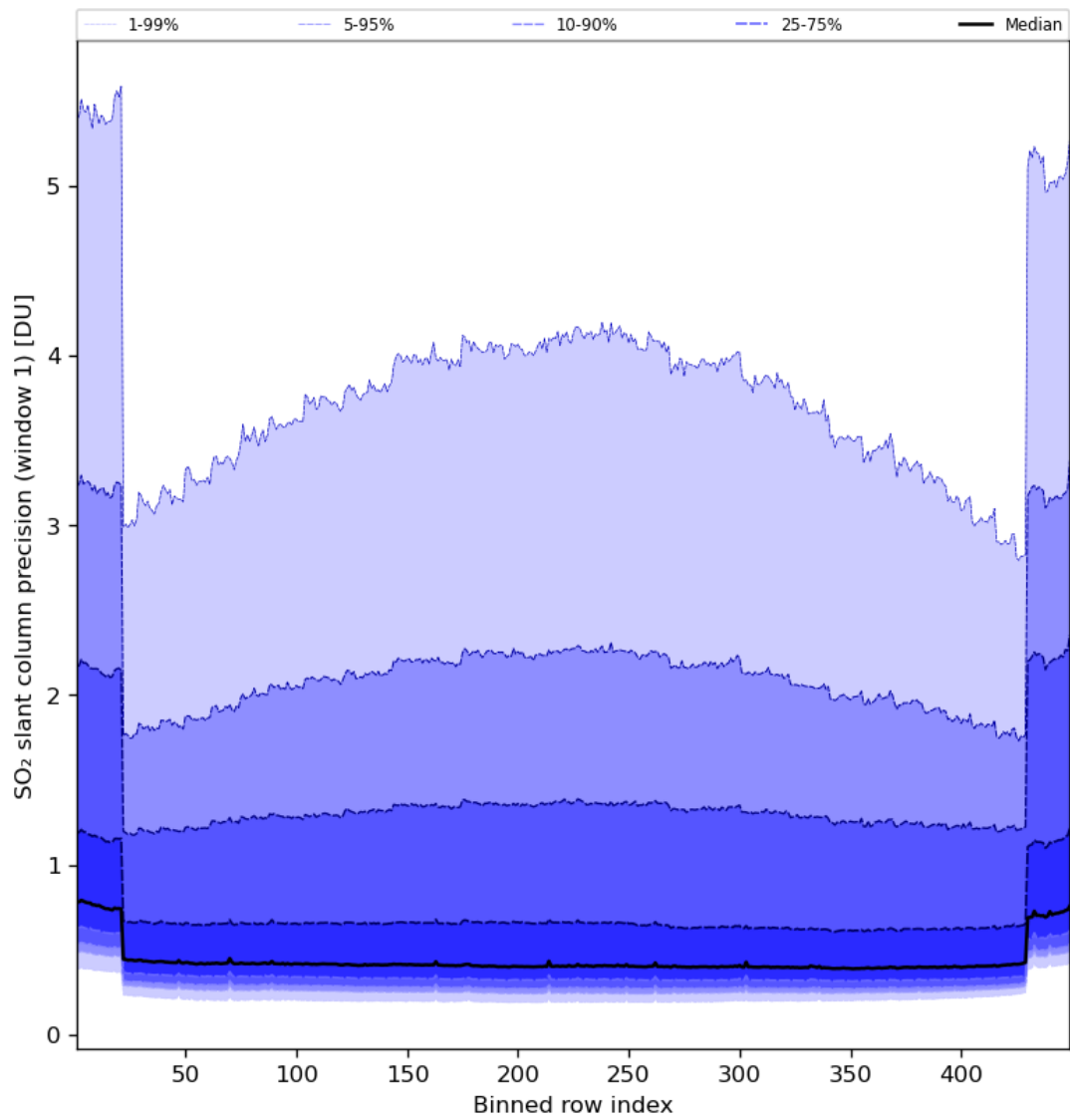
Figure 80: Along track statistics of “SO 2 slant column precision (window 1)” for 2024-07-27 to 2024-07-29
