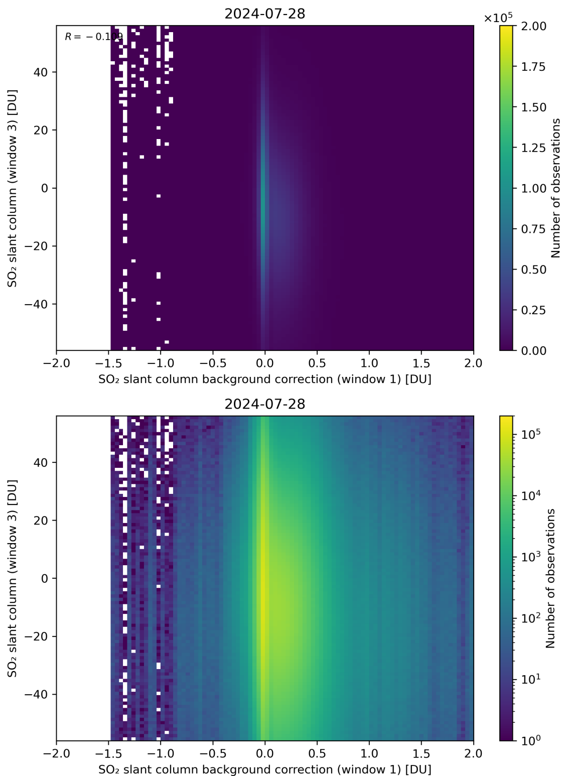
Figure 107: Scatter density plot of “SO 2 slant column background correction (window 1)” against “SO 2 slant column (window 3)” for 2024-07-27 to 2024-07-29.
