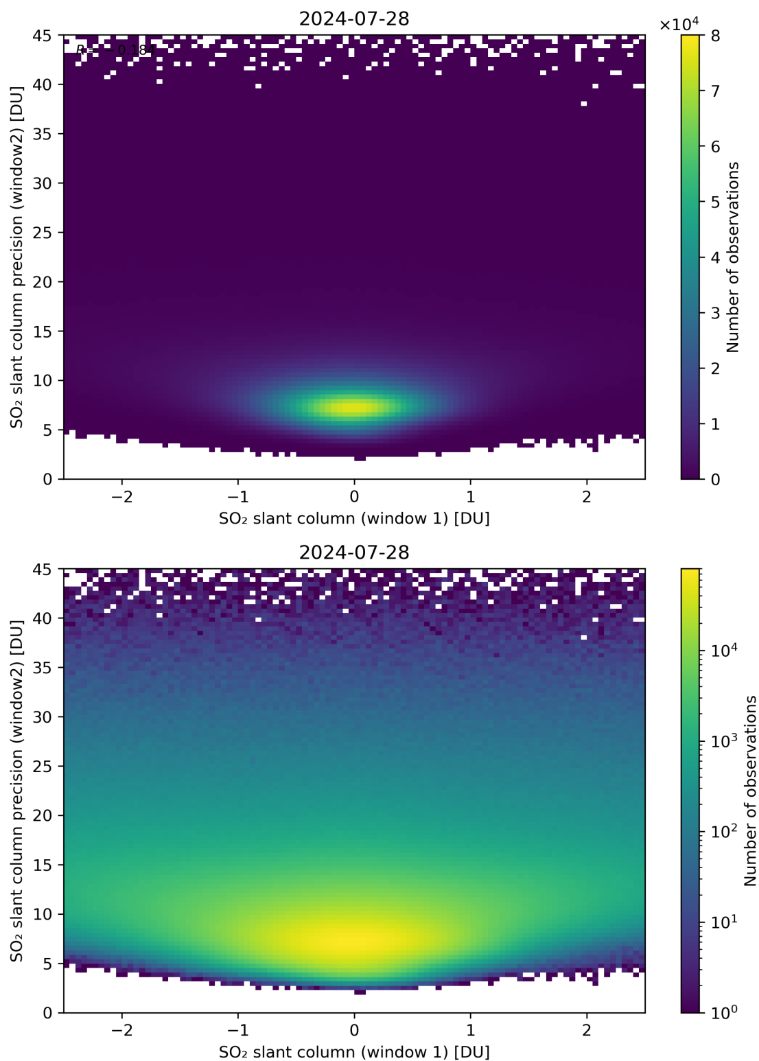
Figure 236: Scatter density plot of “SO 2 slant column (window 1)” against “SO 2 slant column precision (window2)” for 2024-07-27 to 2024-07-29.
