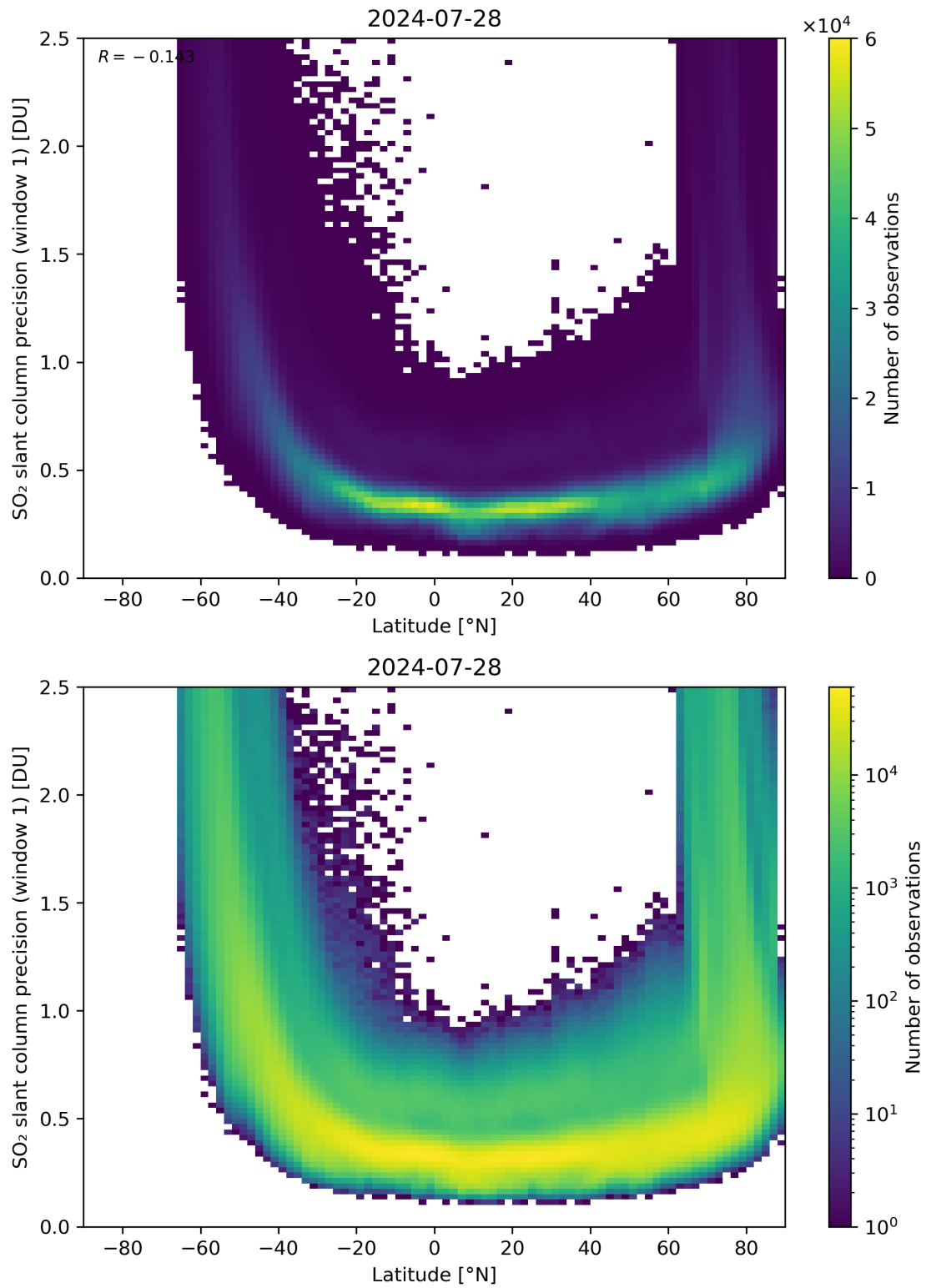
Figure 150: Scatter density plot of “Latitude” against “SO 2 slant column precision (window 1)” for 2024-07-27 to 2024-07-29.
