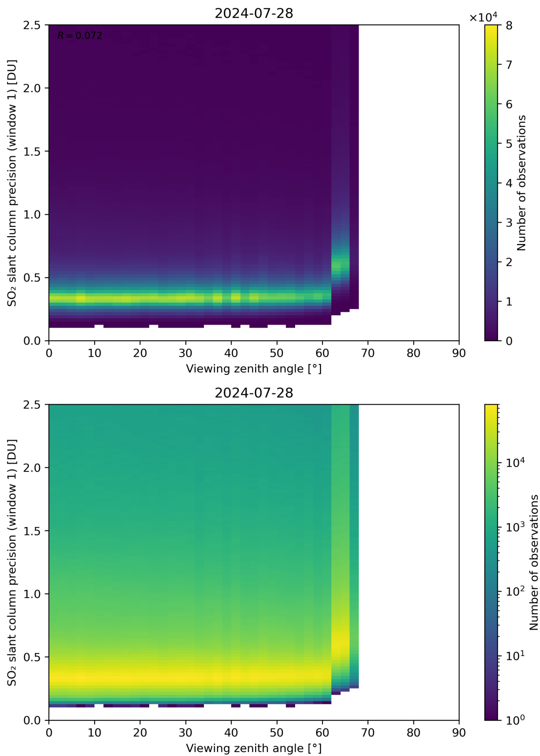
Figure 321: Scatter density plot of “Viewing zenith angle” against “SO 2 slant column precision (window 1)” for 2024-07-27 to 2024-07-29.
