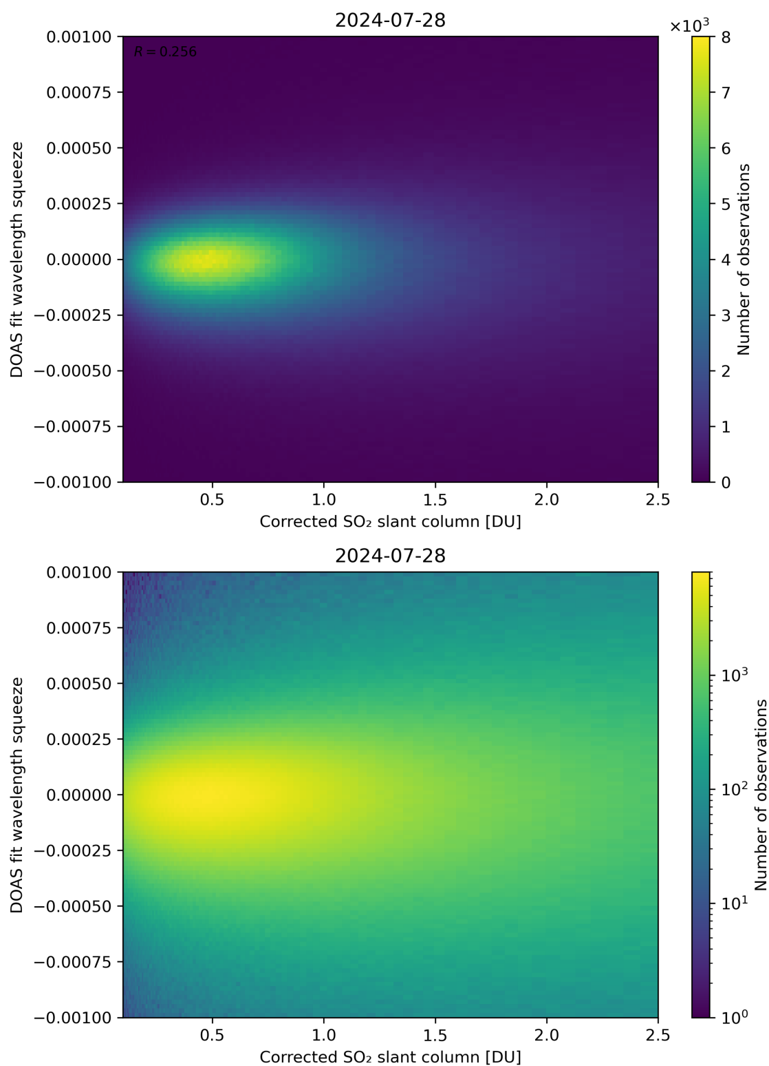
Figure 182: Scatter density plot of “Corrected SO 2 slant column” against “DOAS fit wavelength squeeze” for 2024-07-27 to 2024-07-29.
