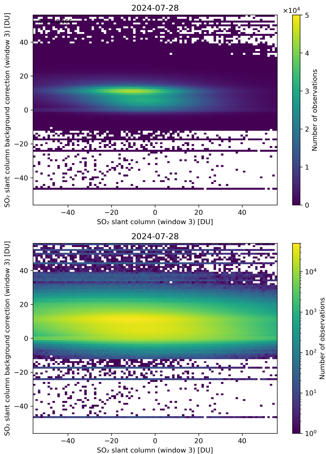
Figure 253: Scatter density plot of “SO 2 slant column (window 3)” against “SO 2 slant column background correction (window 3)” for 2024-07-27 to 2024-07-29.
