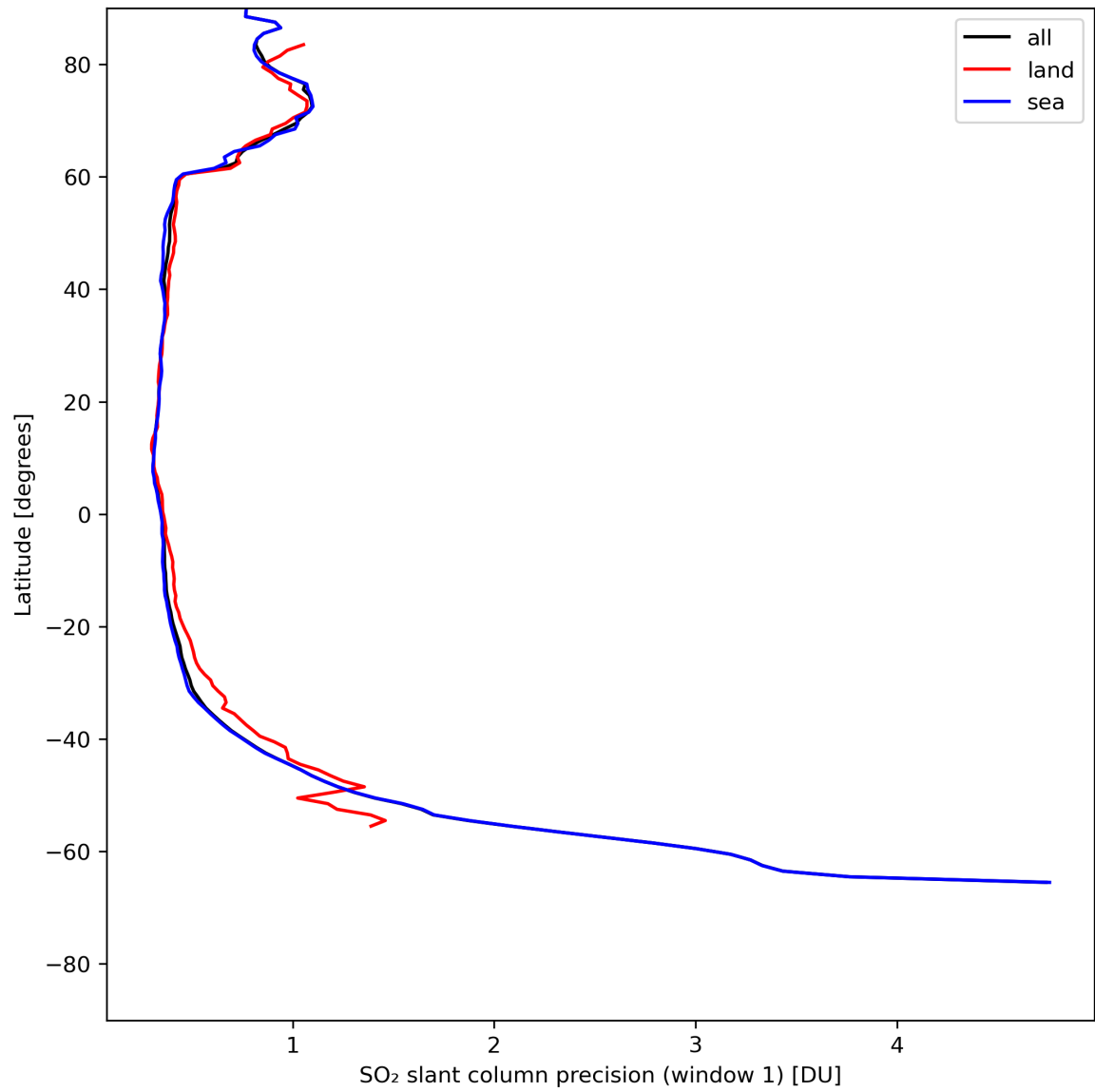
Figure 34: Zonal average of “SO 2 slant column precision (window 1)” for 2024-07-27 to 2024-07-29.
