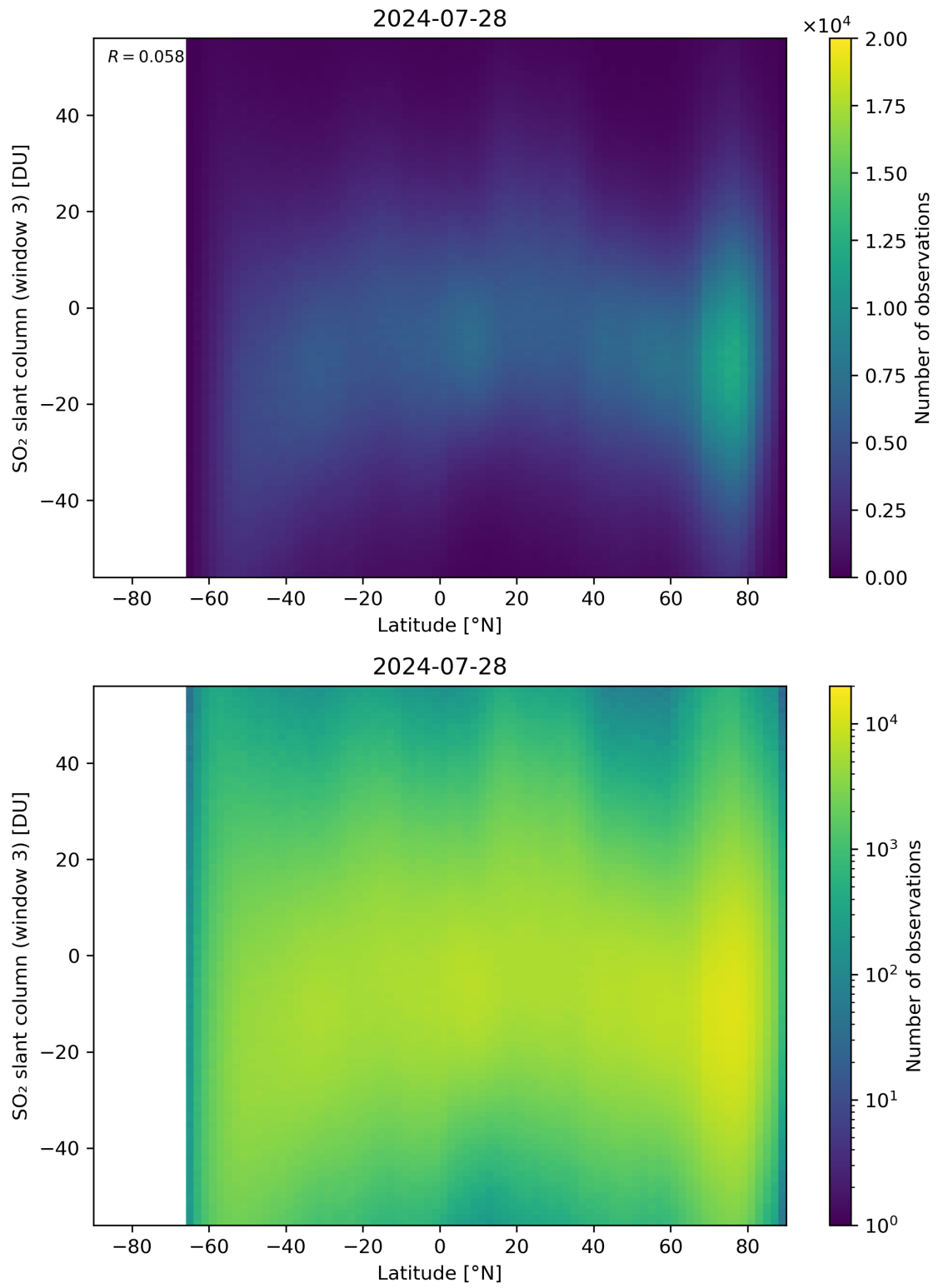
Figure 152: Scatter density plot of “Latitude” against “SO 2 slant column (window 3)” for 2024-07-27 to 2024-07-29.
