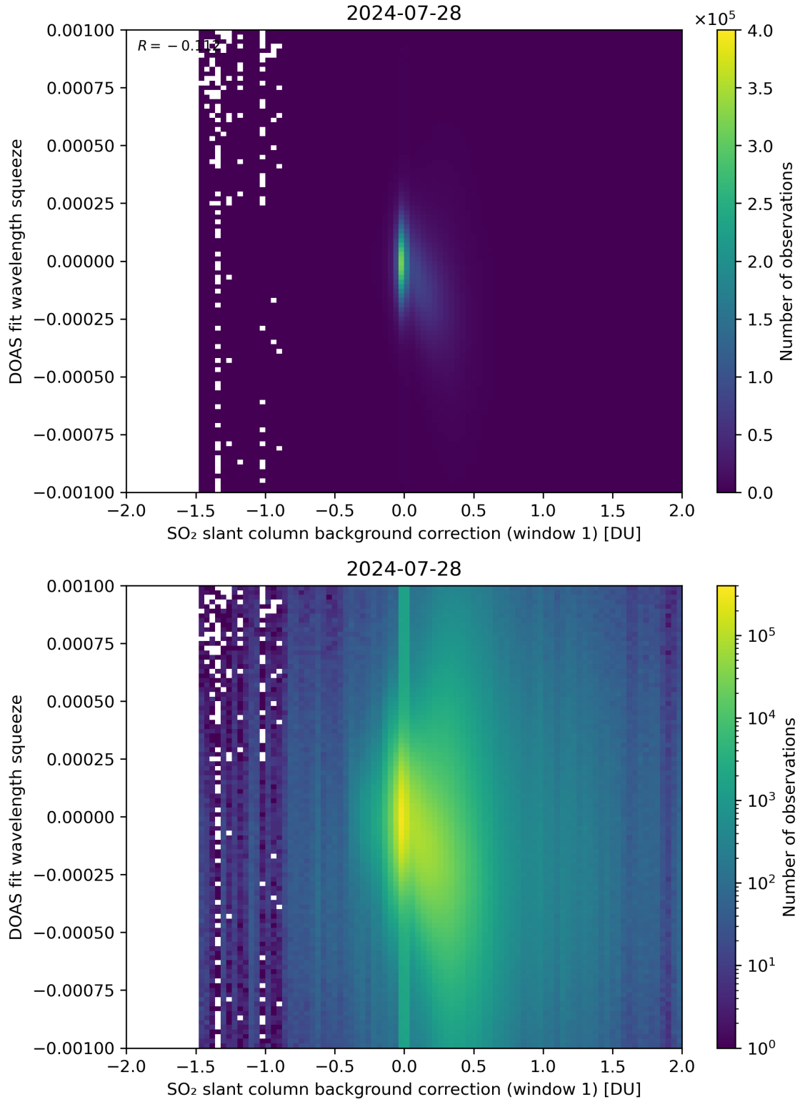
Figure 101: Scatter density plot of “SO 2 slant column background correction (window 1)” against “DOAS fit wavelength squeeze” for 2024-07-27 to 2024-07-29.
