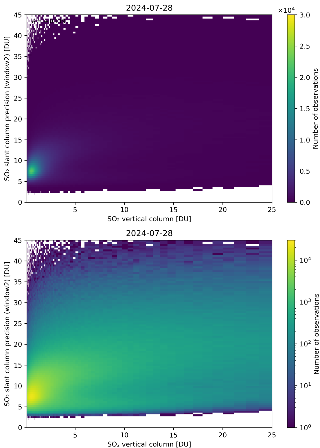
Figure 302: Scatter density plot of “SO 2 vertical column” against “SO 2 slant column precision (window2)” for 2024-07-27 to 2024-07-29.
