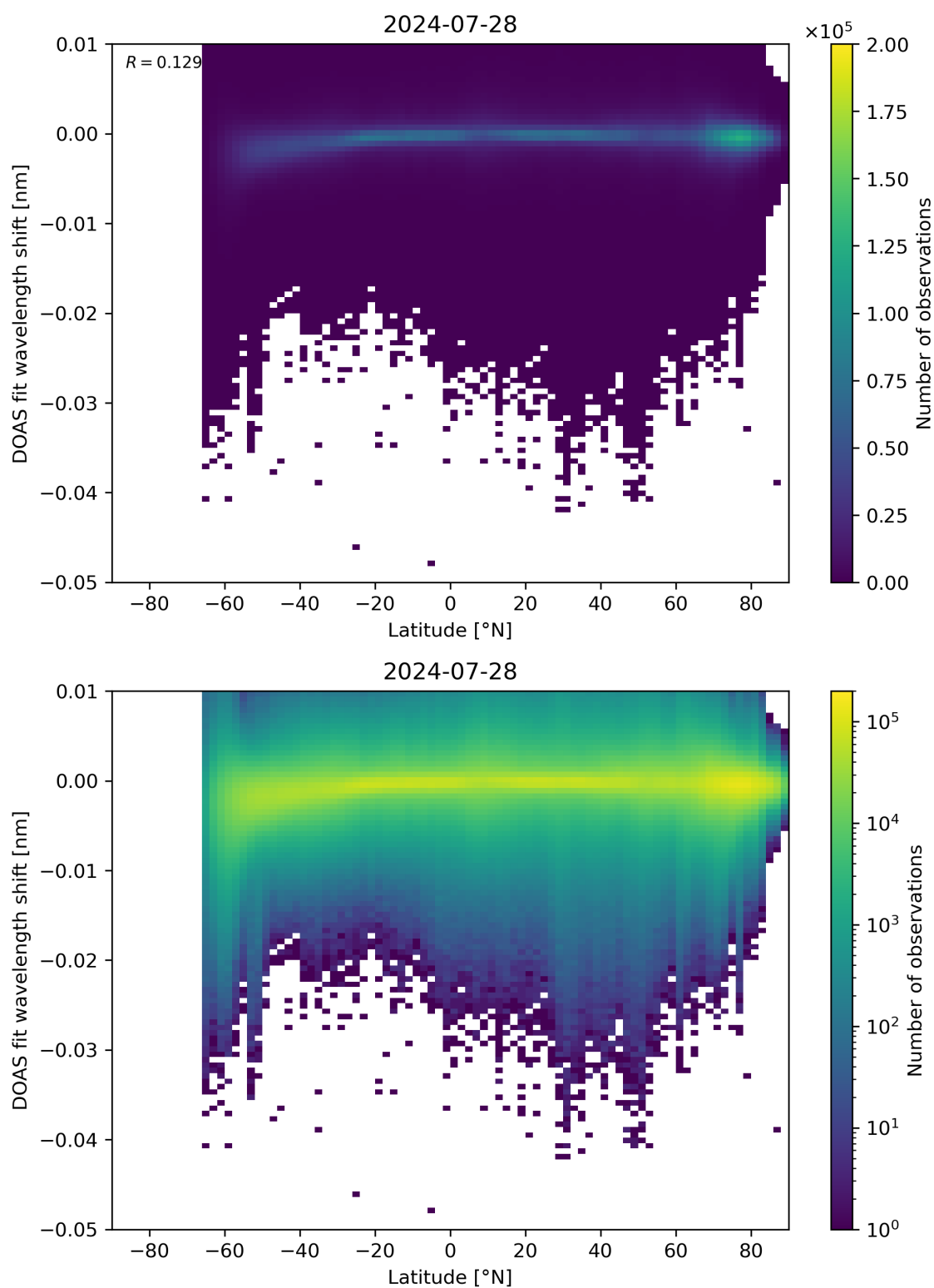
Figure 142: Scatter density plot of “Latitude” against “DOAS fit wavelength shift” for 2024-07-27 to 2024-07-29.
