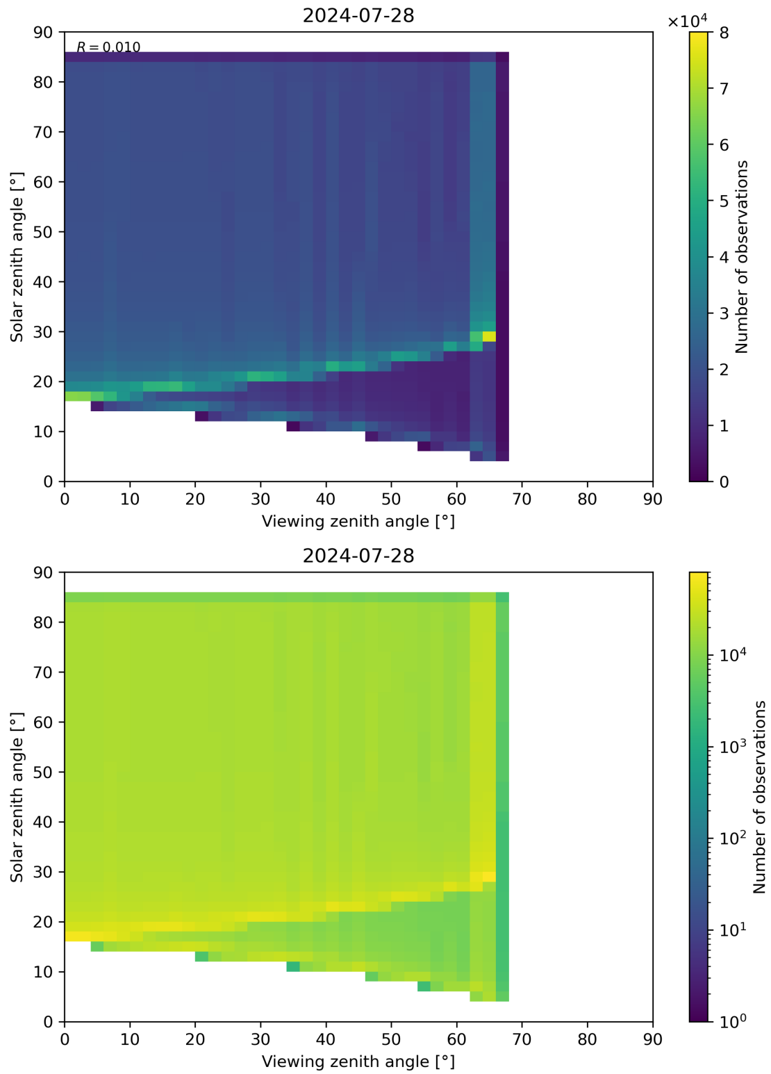
Figure 315: Scatter density plot of “Viewing zenith angle” against “Solar zenith angle” for 2024-07-27 to 2024-07-29.
