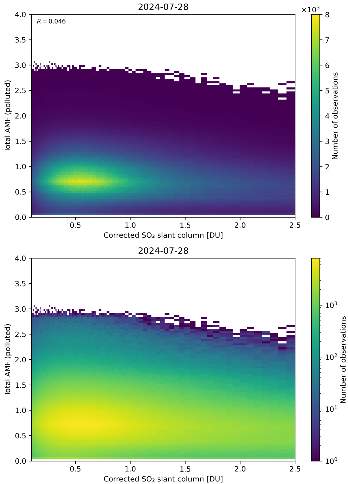
Figure 192: Scatter density plot of “Corrected SO 2 slant column” against “Total AMF (polluted)” for 2024-07-27 to 2024-07-29.
