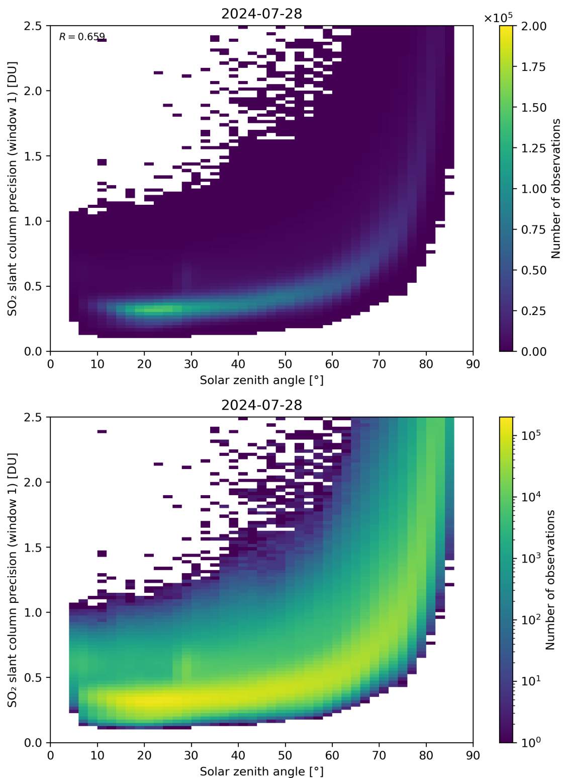
Figure 170: Scatter density plot of “Solar zenith angle” against “SO 2 slant column precision (window 1)” for 2024-07-27 to 2024-07-29.
