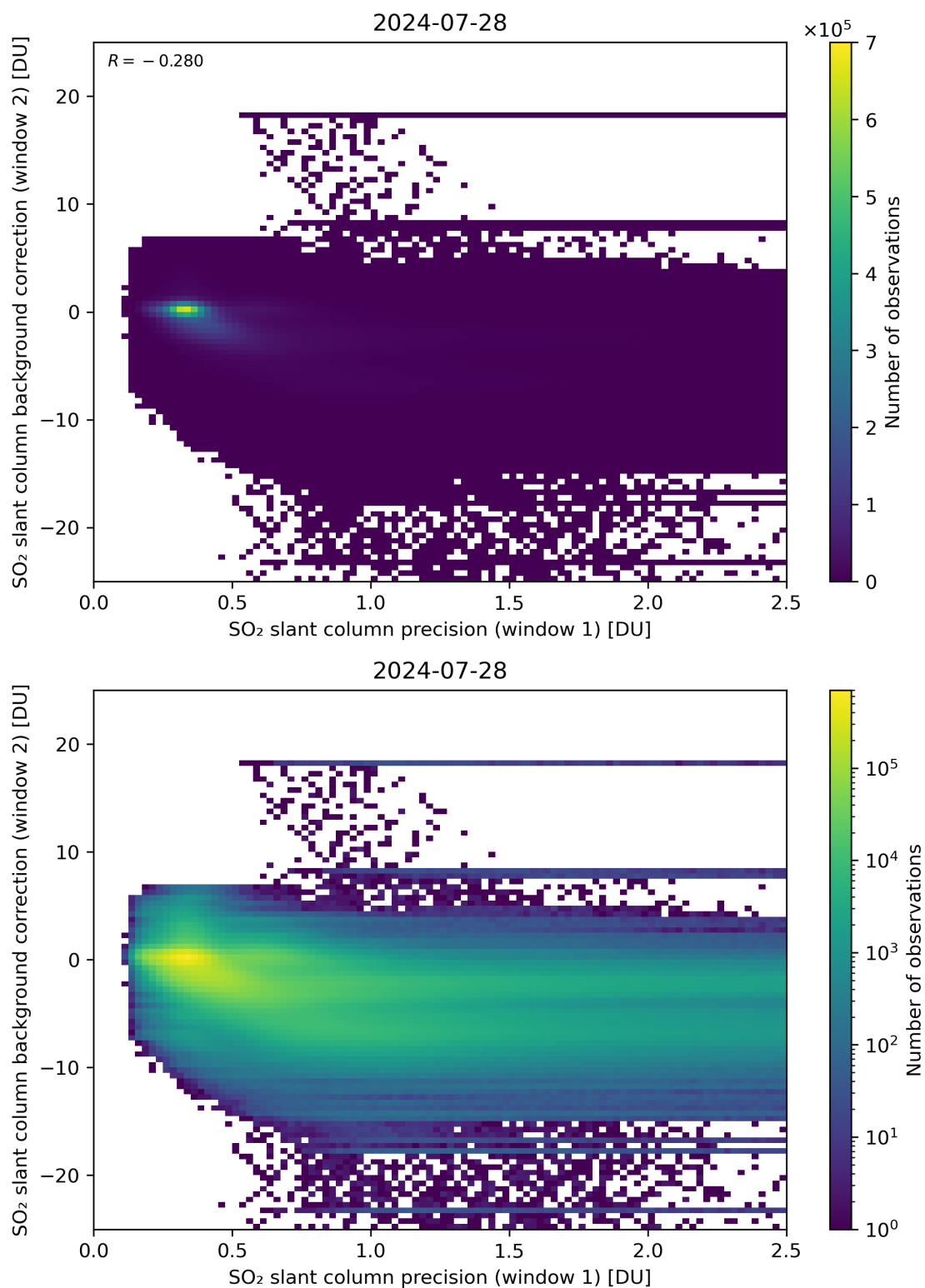
Figure 219: Scatter density plot of “SO 2 slant column precision (window 1)” against “SO 2 slant column background correction (window 2)” for 2024-07-27 to 2024-07-29.
