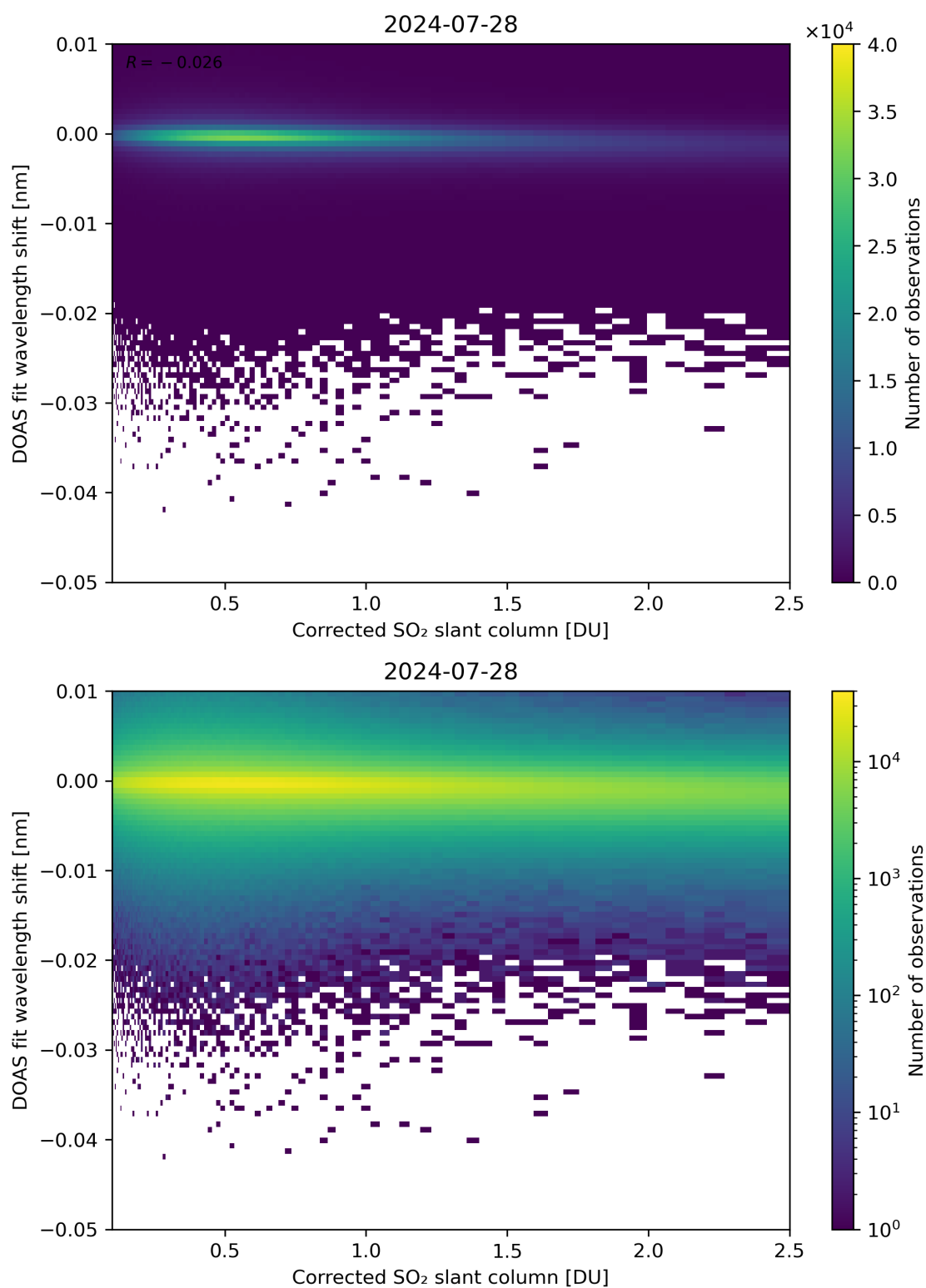
Figure 181: Scatter density plot of “Corrected SO 2 slant column” against “DOAS fit wavelength shift” for 2024-07-27 to 2024-07-29.
