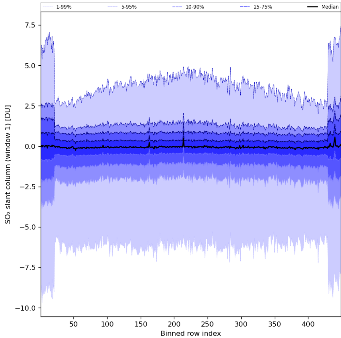
Figure 79: Along track statistics of “SO 2 slant column (window 1)” for 2024-07-27 to 2024-07-29
