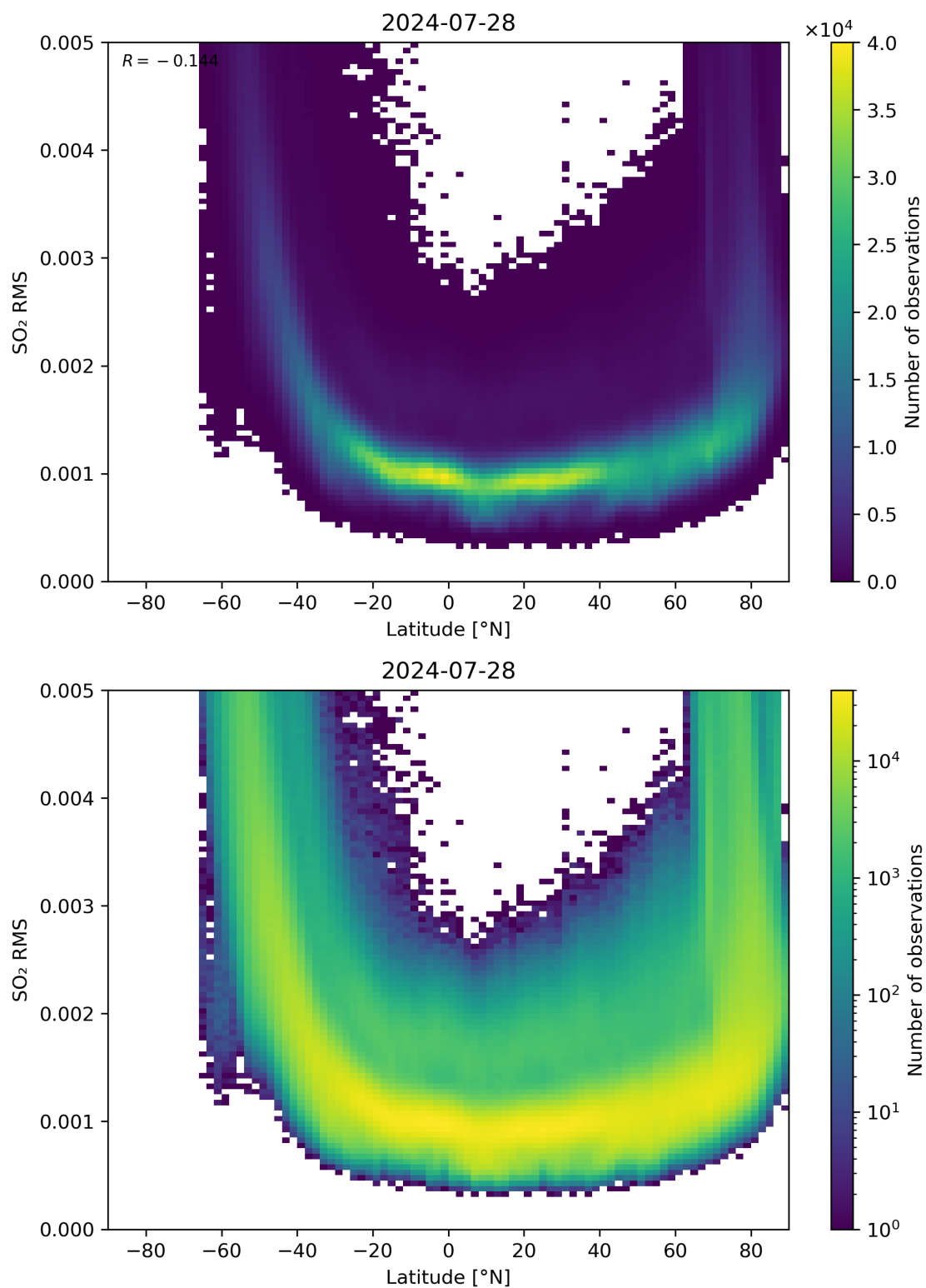
Figure 144: Scatter density plot of “Latitude” against “SO 2 RMS” for 2024-07-27 to 2024-07-29.
