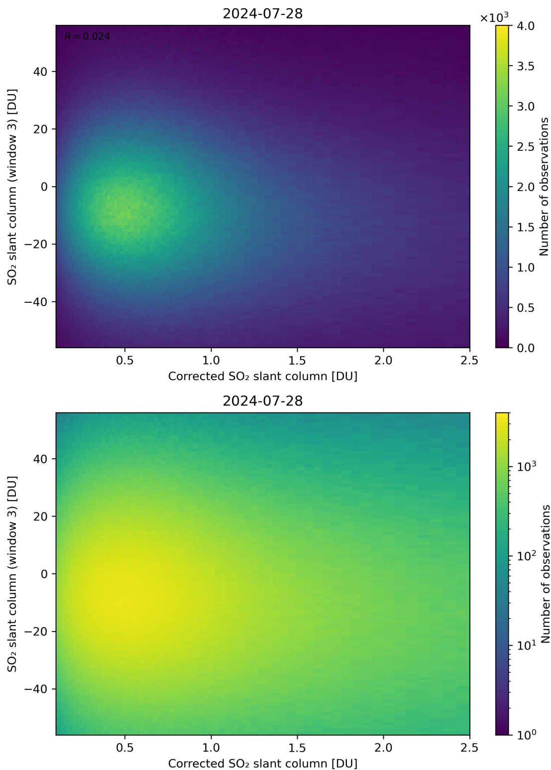
Figure 190: Scatter density plot of “Corrected SO 2 slant column” against “SO 2 slant column (window 3)” for 2024-07-27 to 2024-07-29.
