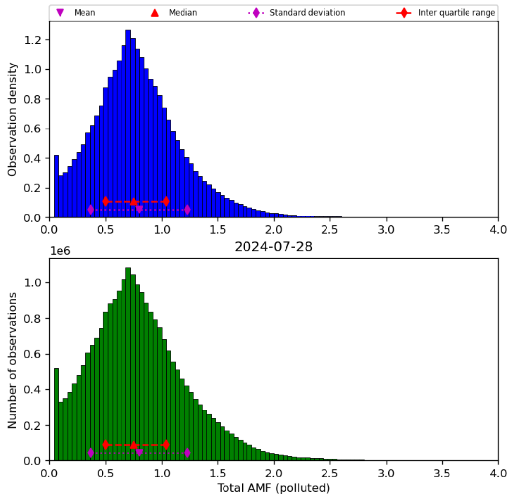
Figure 71: Histogram of “Total AMF (polluted)” for 2024-07-27 to 2024-07-29
