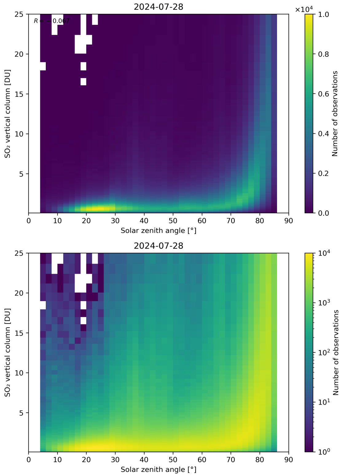
Figure 176: Scatter density plot of “Solar zenith angle” against “SO 2 vertical column” for 2024-07-27 to 2024-07-29.
