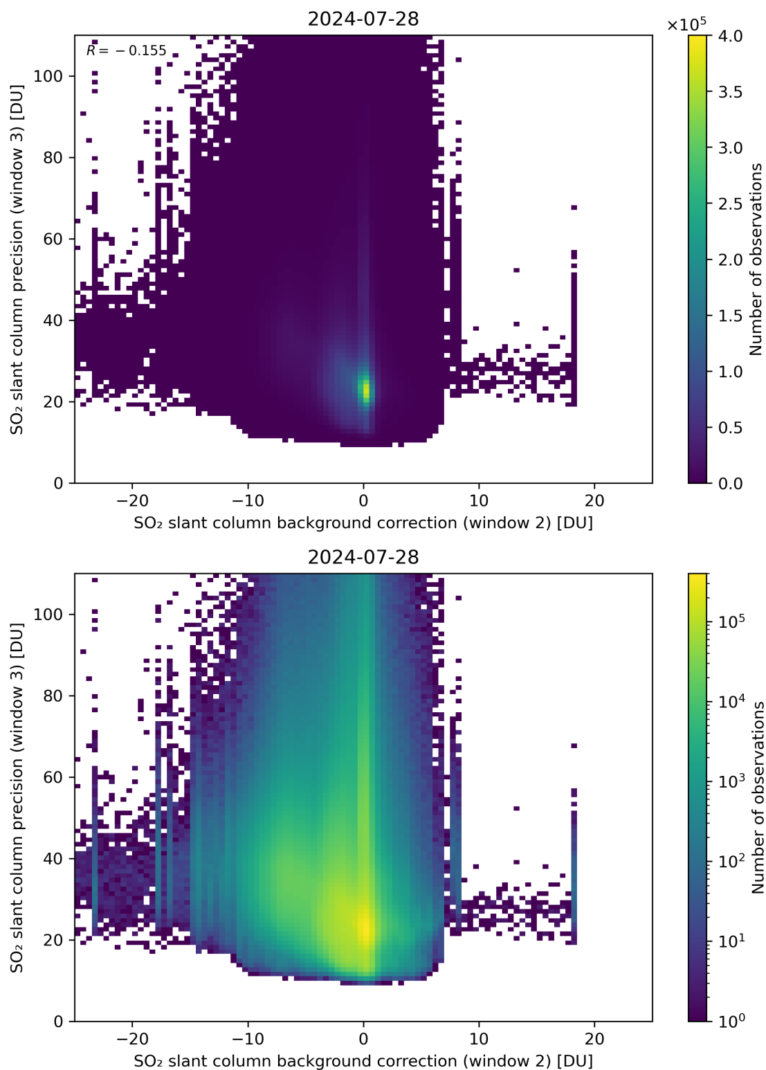
Figure 118: Scatter density plot of “SO 2 slant column background correction (window 2)” against “SO 2 slant column precision (window 3)” for 2024-07-27 to 2024-07-29.
