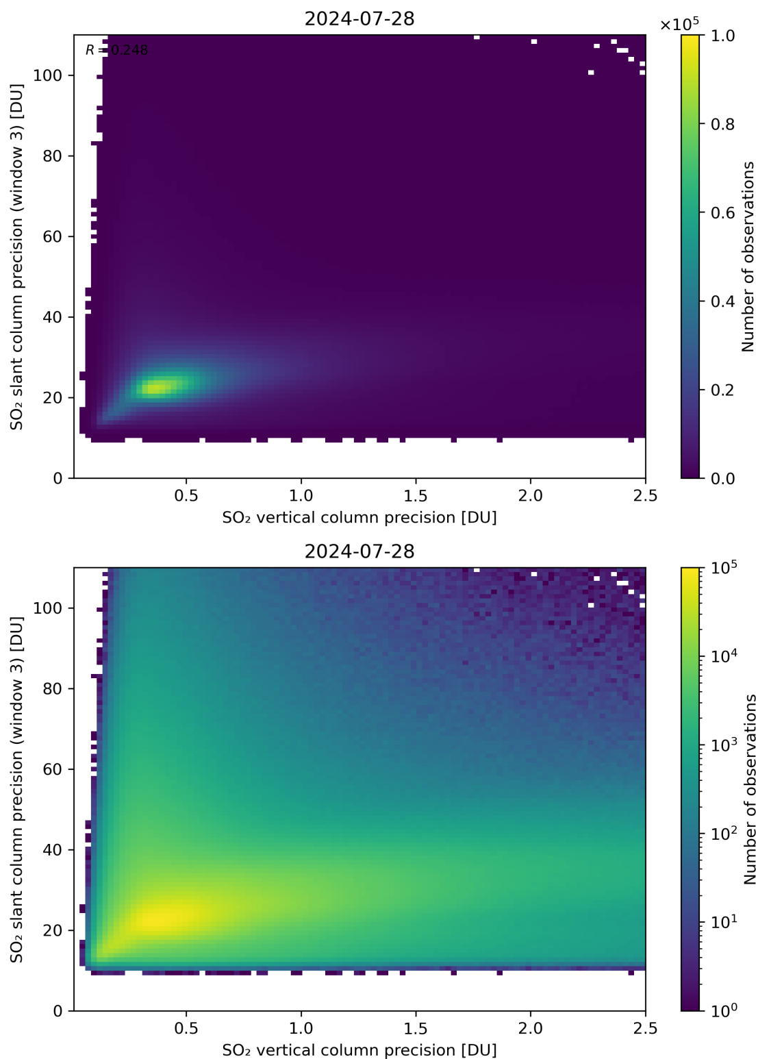
Figure 293: Scatter density plot of “SO 2 vertical column precision” against “SO 2 slant column precision (window 3)” for 2024-07-27 to 2024-07-29.
