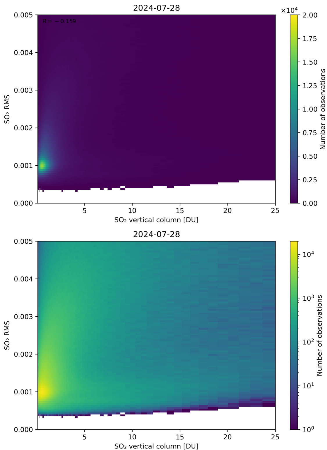
Figure 278: Scatter density plot of “SO 2 vertical column” against “SO 2 RMS” for 2024-07-27 to 2024-07-29.
