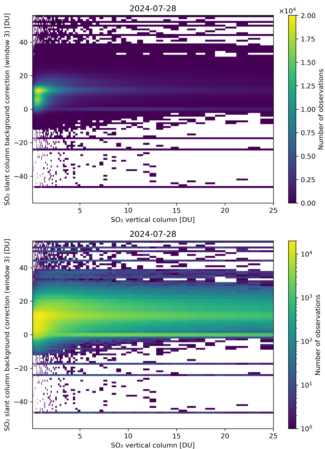
Figure 275: Scatter density plot of “SO 2 vertical column” against “SO 2 slant column background correction (window 3)” for 2024-07-27 to 2024-07-29.
