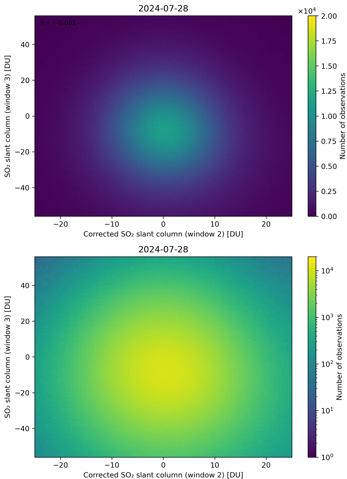
Figure 201: Scatter density plot of “Corrected SO 2 slant column (window 2)” against “SO 2 slant column (window 3)” for 2024-07-27 to 2024-07-29.
