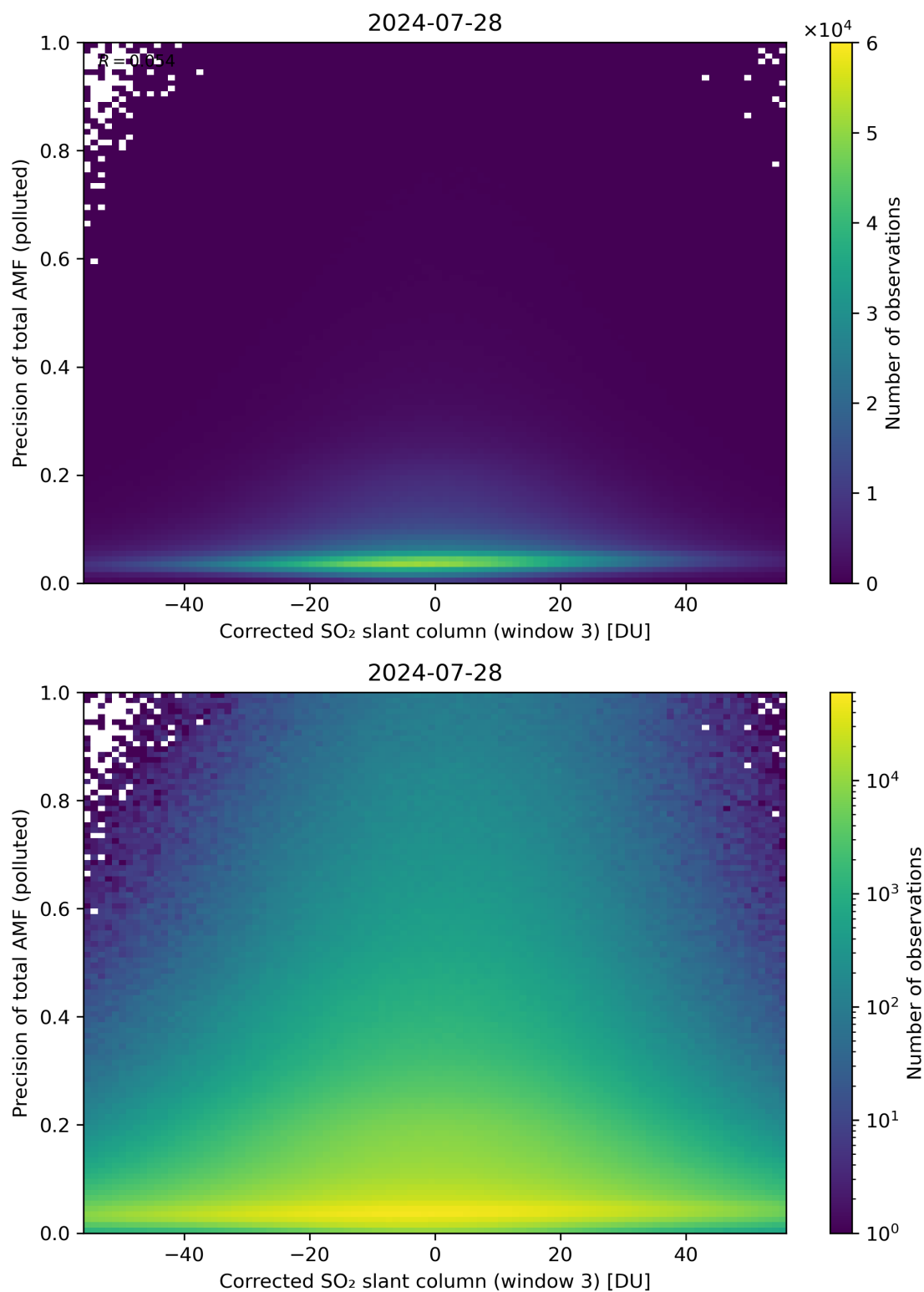
Figure 211: Scatter density plot of “Corrected SO 2 slant column (window 3)” against “Precision of total AMF (polluted)” for 2024-07-27 to 2024-07-29.
