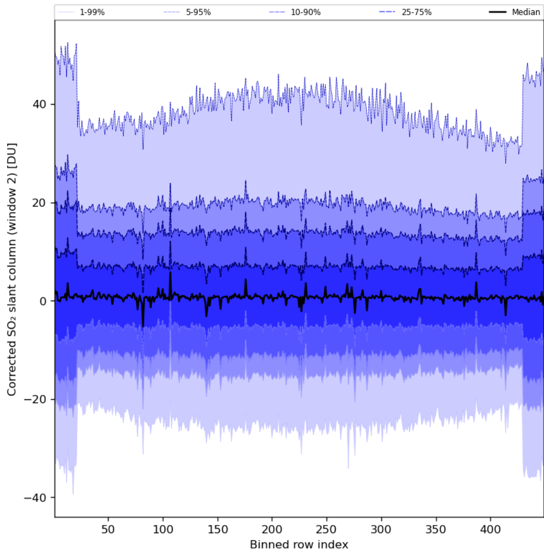
Figure 85: Along track statistics of “Corrected SO 2 slant column (window 2)” for 2024-07-27 to 2024-07-29
