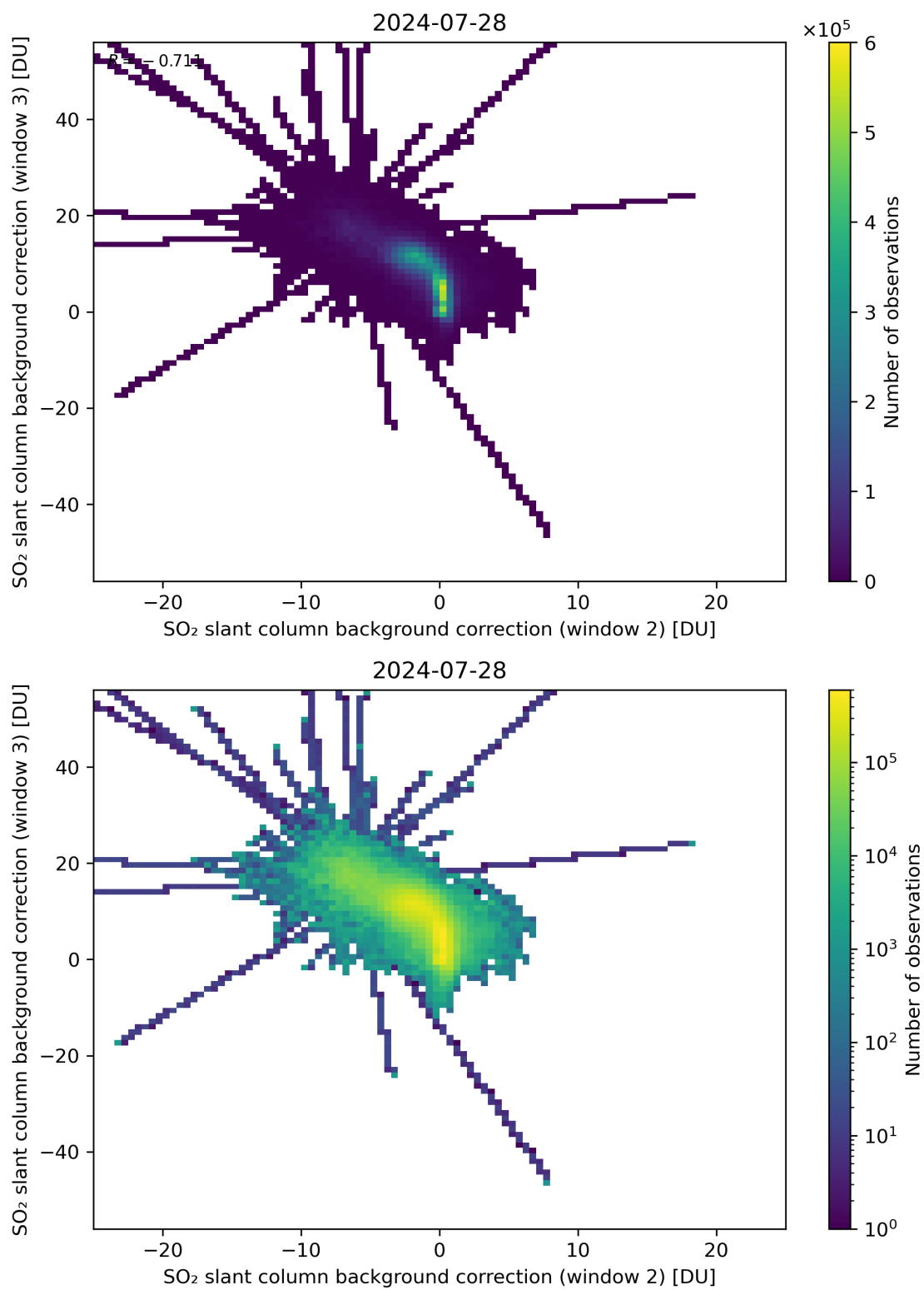
Figure 111: Scatter density plot of “SO 2 slant column background correction (window 2)” against “SO 2 slant column background correction (window 3)” for 2024-07-27 to 2024-07-29.
