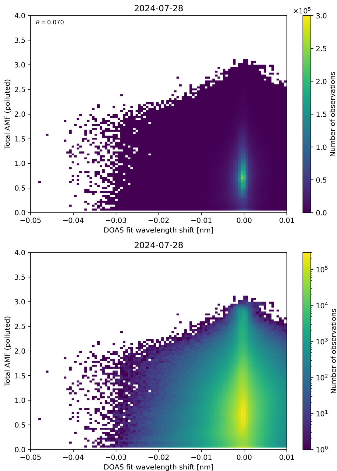
Figure 130: Scatter density plot of “DOAS fit wavelength shift” against “Total AMF (polluted)” for 2024-07-27 to 2024-07-29.
