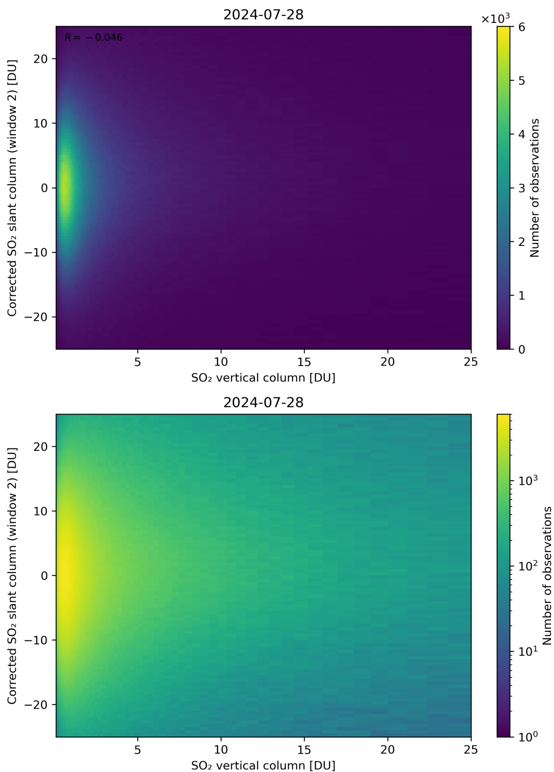
Figure 298: Scatter density plot of “SO 2 vertical column” against “Corrected SO 2 slant column (window 2)” for 2024-07-27 to 2024-07-29.
