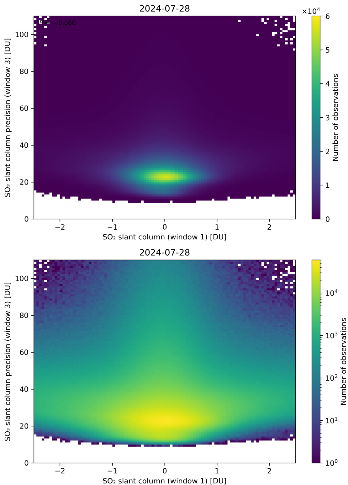
Figure 238: Scatter density plot of “SO 2 slant column (window 1)” against “SO 2 slant column precision (window 3)” for 2024-07-27 to 2024-07-29.
