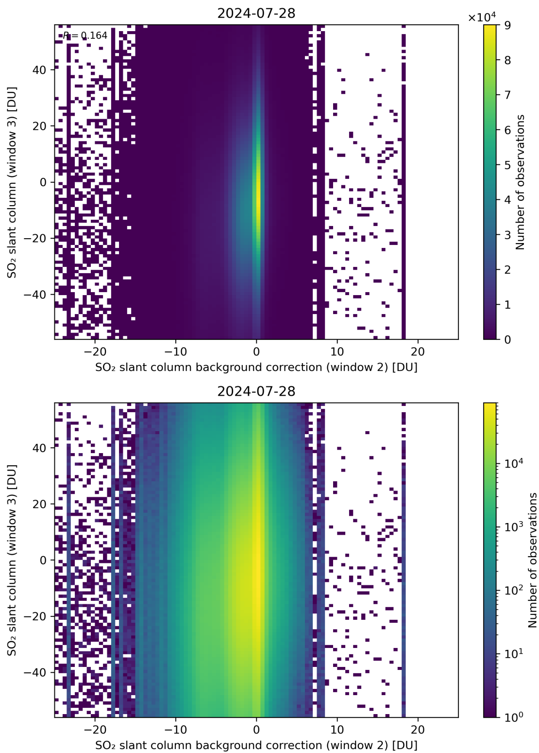
Figure 117: Scatter density plot of “SO 2 slant column background correction (window 2)” against “SO 2 slant column (window 3)” for 2024-07-27 to 2024-07-29.
