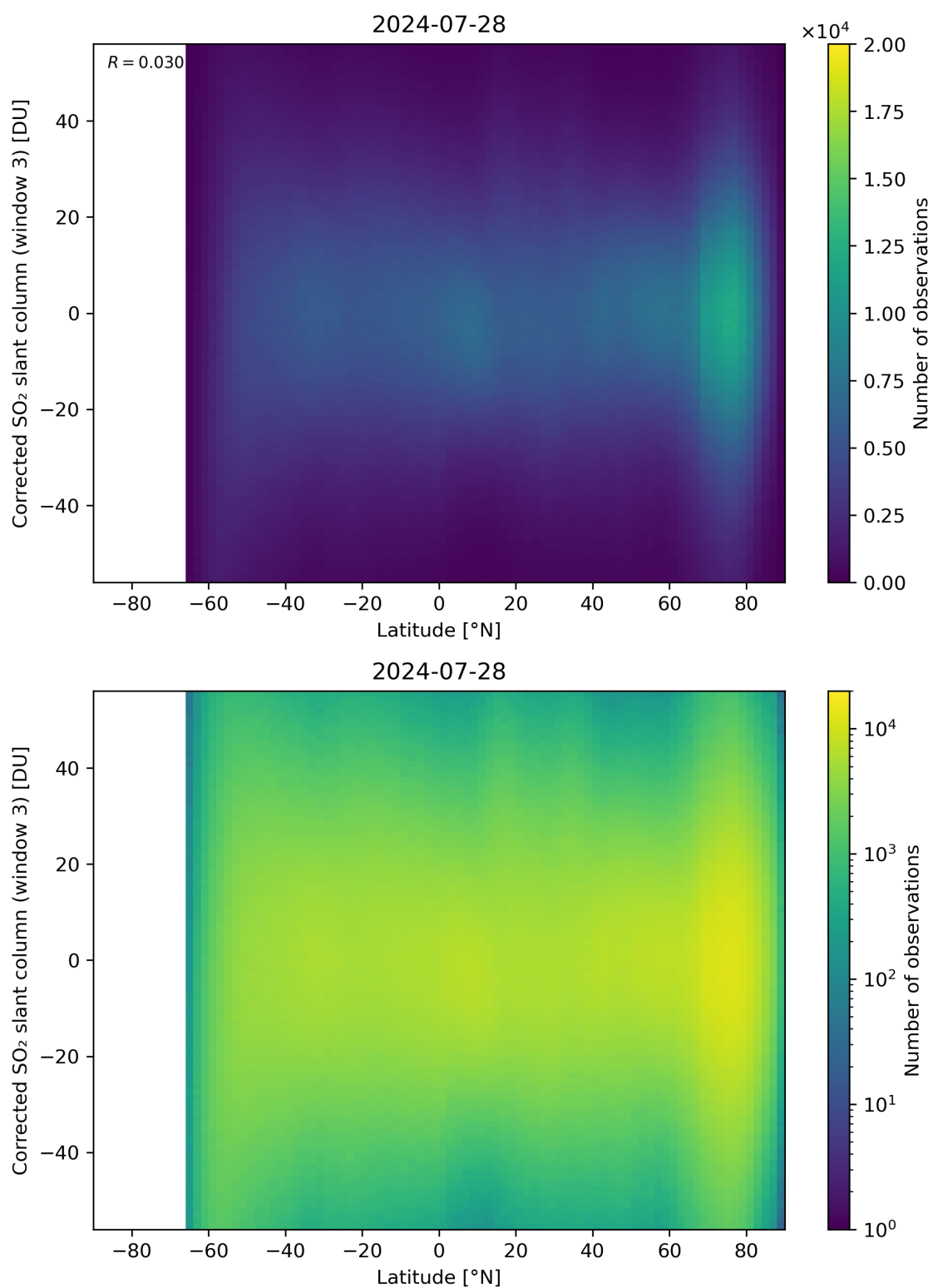
Figure 148: Scatter density plot of “Latitude” against “Corrected SO 2 slant column (window 3)” for 2024-07-27 to 2024-07-29.
