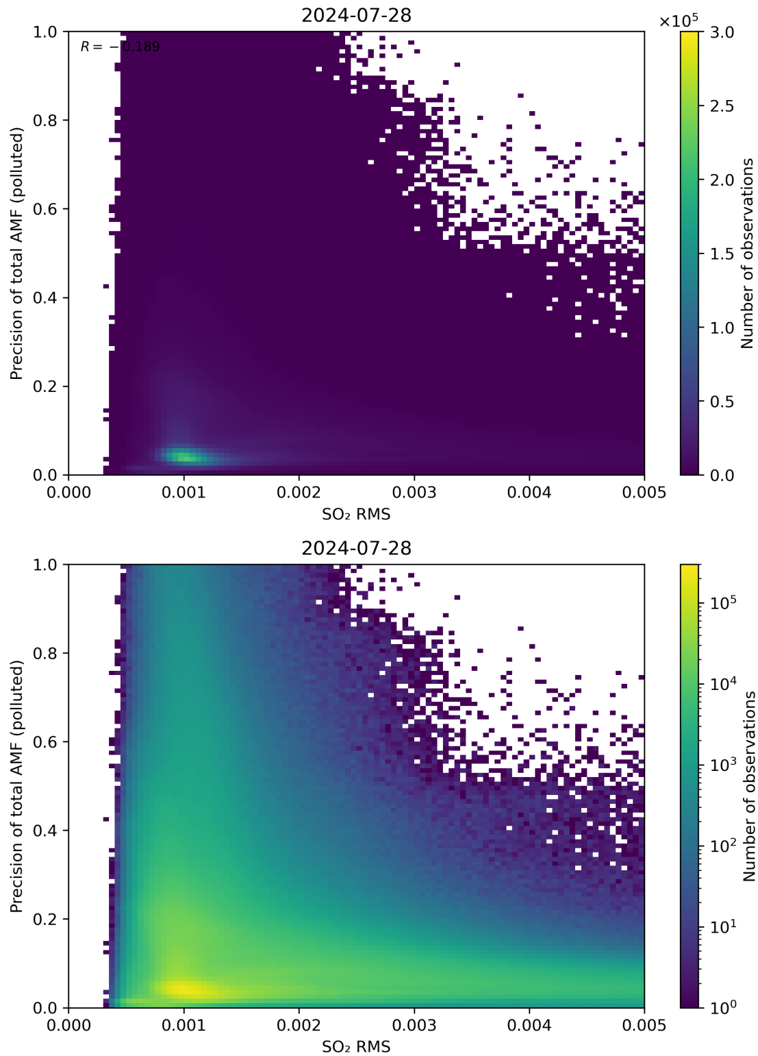
Figure 138: Scatter density plot of “SO 2 RMS” against “Precision of total AMF (polluted)” for 2024-07-27 to 2024-07-29.
