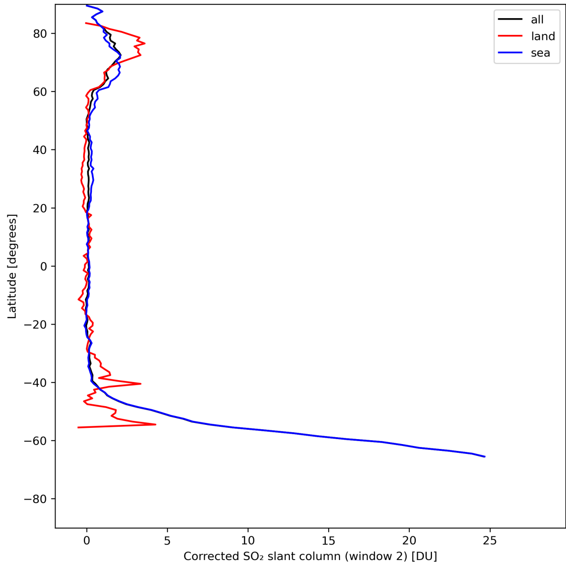
Figure 39: Zonal average of “Corrected SO 2 slant column (window 2)” for 2024-07-27 to 2024-07-29.
