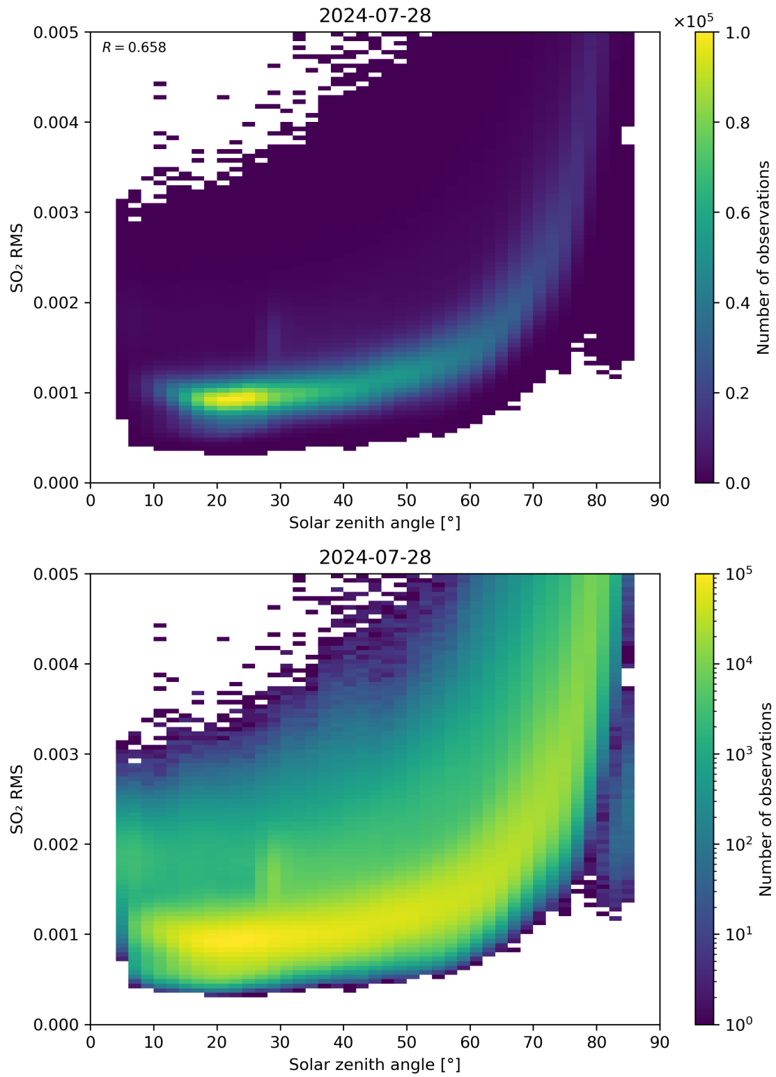
Figure 163: Scatter density plot of “Solar zenith angle” against “SO 2 RMS” for 2024-07-27 to 2024-07-29.
