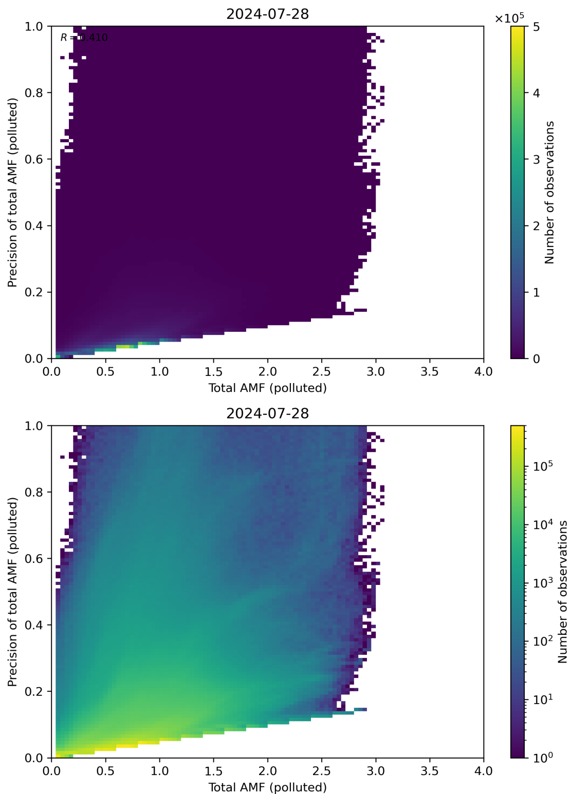
Figure 272: Scatter density plot of “Total AMF (polluted)” against “Precision of total AMF (polluted)” for 2024-07-27 to 2024-07-29.
