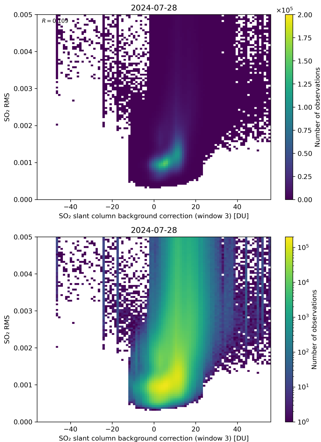
Figure 123: Scatter density plot of “SO 2 slant column background correction (window 3)” against “SO 2 RMS” for 2024-07-27 to 2024-07-29.
