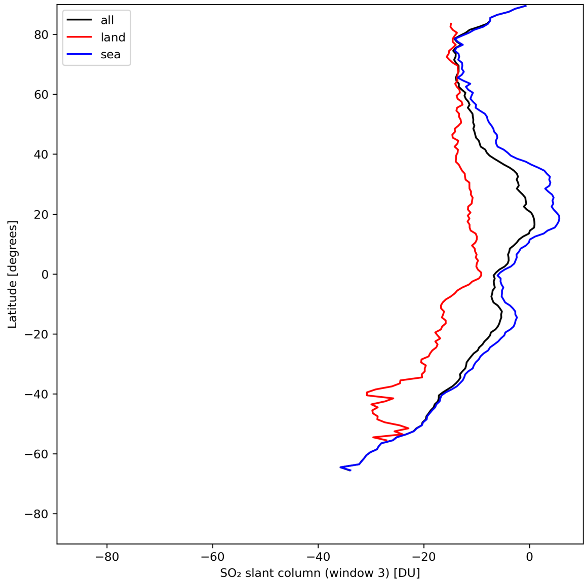
Figure 41: Zonal average of “SO 2 slant column (window 3)” for 2024-07-27 to 2024-07-29.
