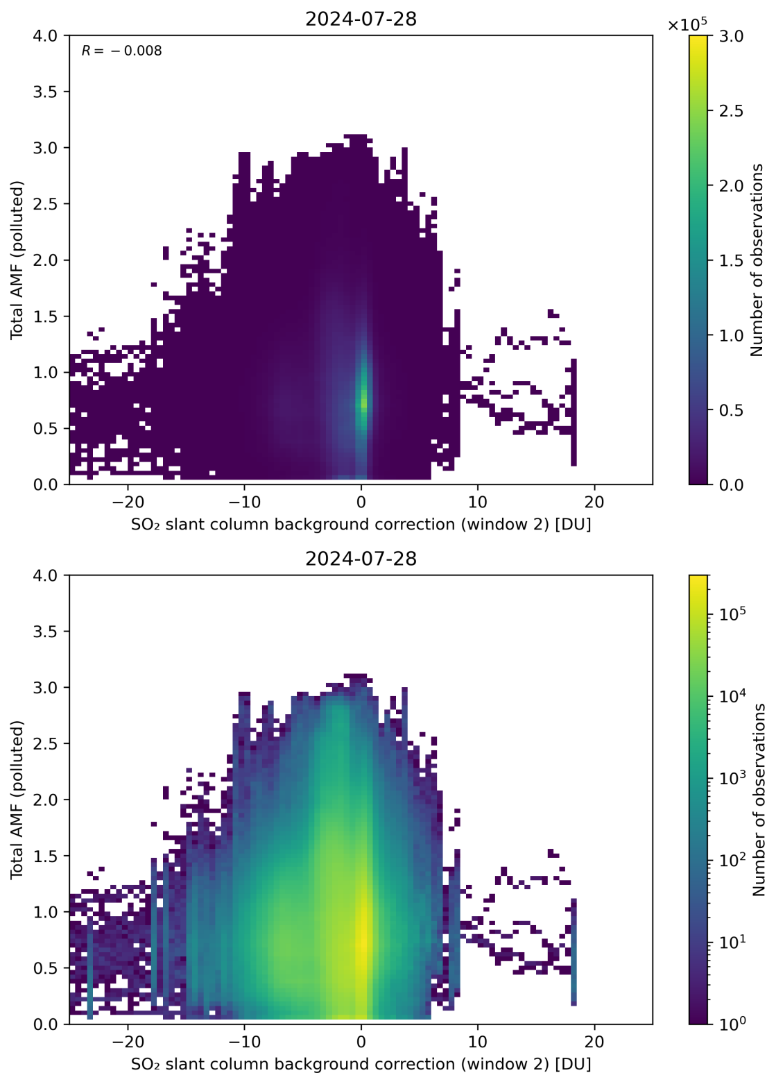
Figure 119: Scatter density plot of “SO 2 slant column background correction (window 2)” against “Total AMF (polluted)” for 2024-07-27 to 2024-07-29.
