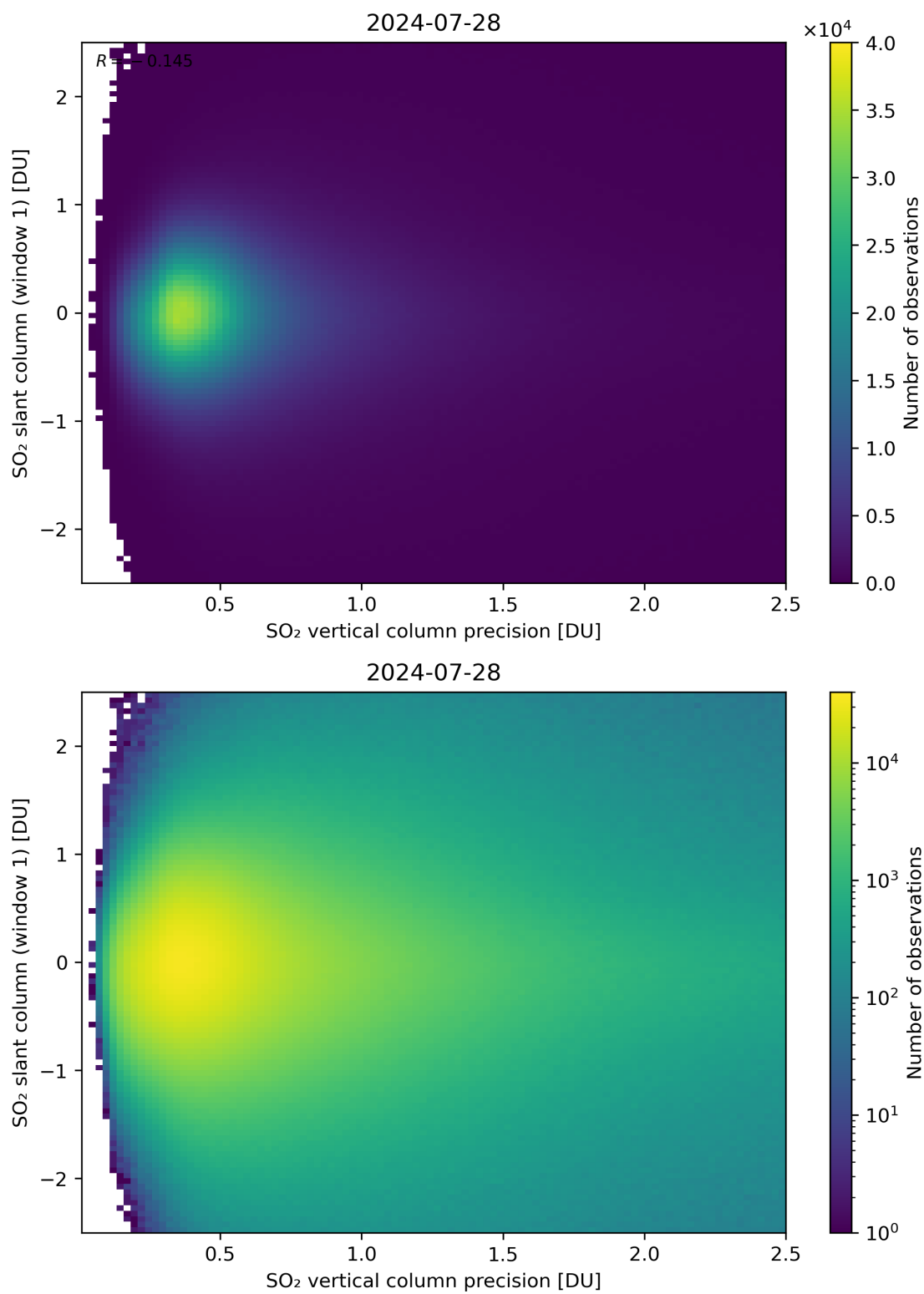
Figure 289: Scatter density plot of “SO 2 vertical column precision” against “SO 2 slant column (window 1)” for 2024-07-27 to 2024-07-29.
