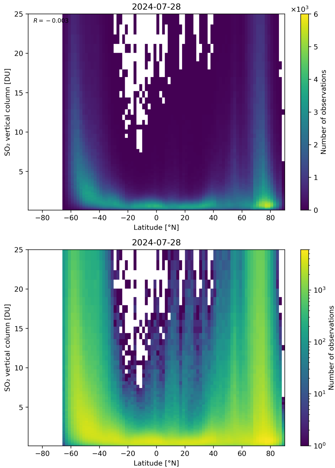
Figure 156: Scatter density plot of “Latitude” against “SO 2 vertical column” for 2024-07-27 to 2024-07-29.
