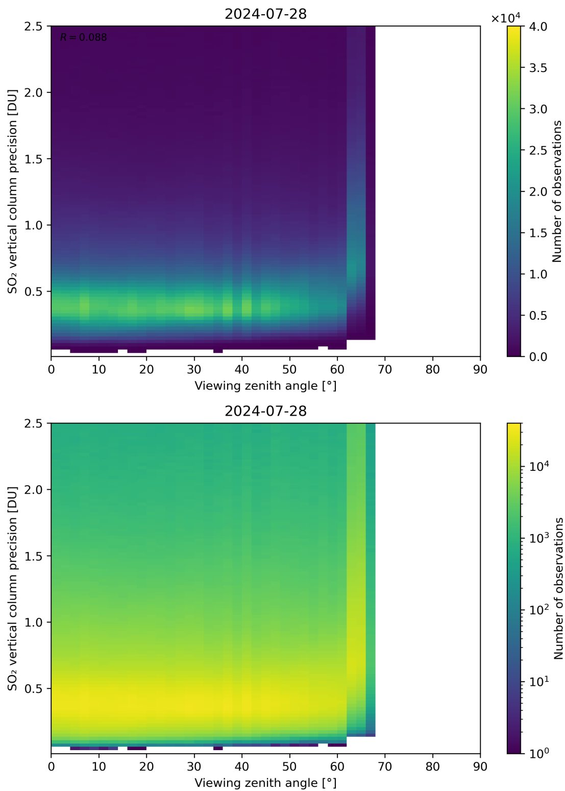
Figure 328: Scatter density plot of “Viewing zenith angle” against “SO 2 vertical column precision” for 2024-07-27 to 2024-07-29.
