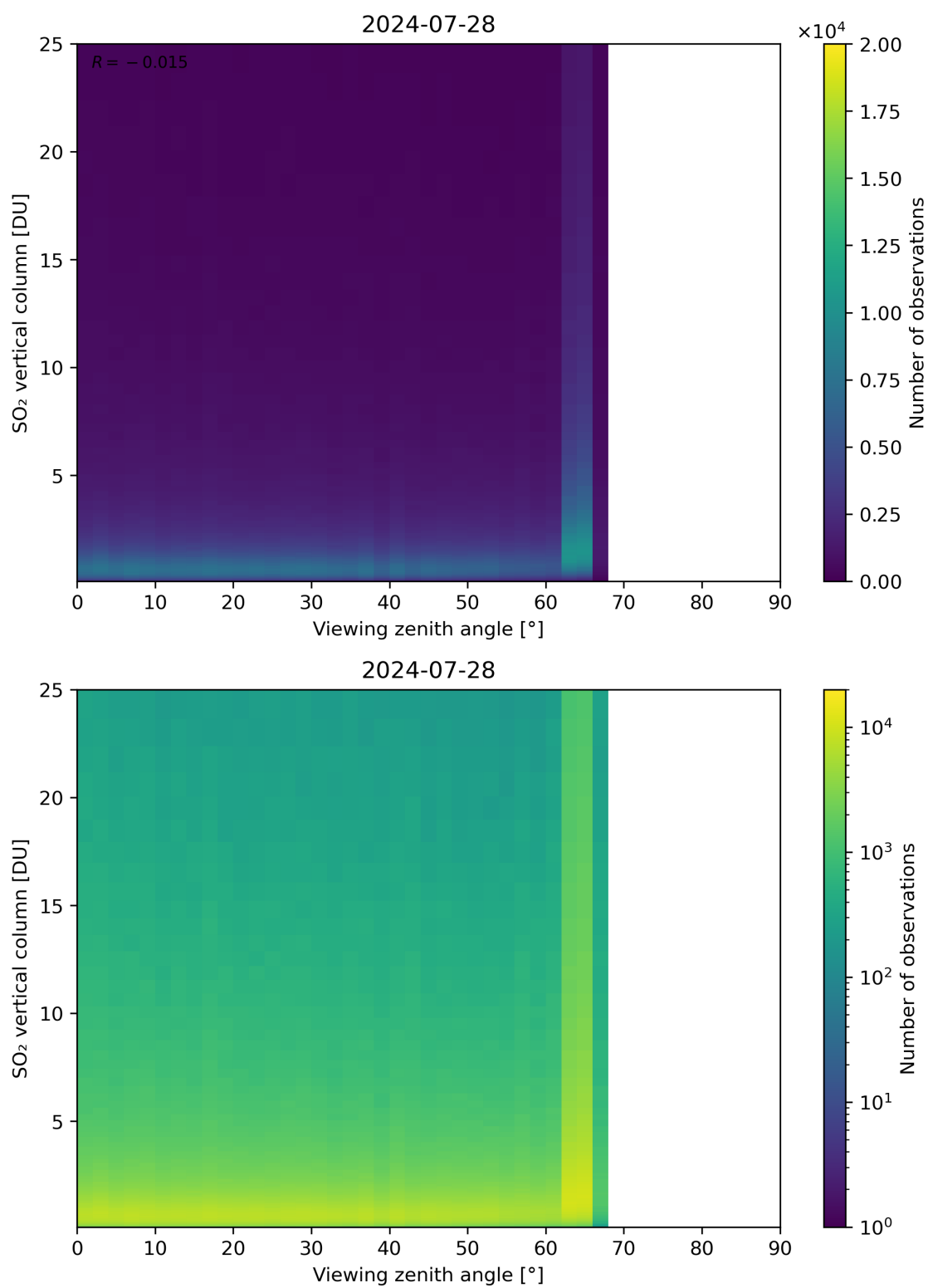
Figure 327: Scatter density plot of “Viewing zenith angle” against “SO 2 vertical column” for 2024-07-27 to 2024-07-29.
