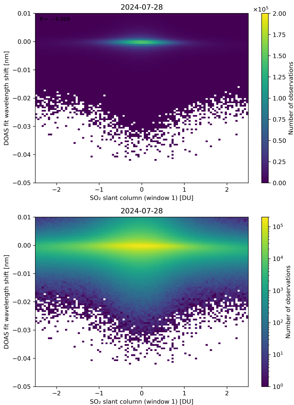
Figure 215: Scatter density plot of “SO 2 slant column (window 1)” against “DOAS fit wavelength shift” for 2024-07-27 to 2024-07-29.
