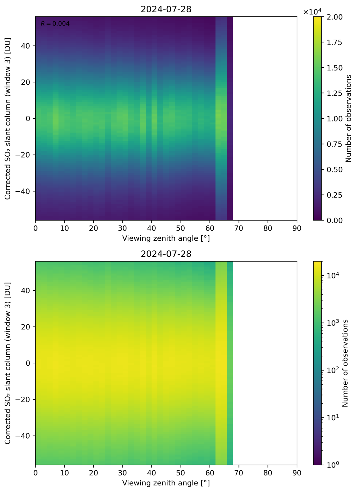
Figure 319: Scatter density plot of “Viewing zenith angle” against “Corrected SO 2 slant column (window 3)” for 2024-07-27 to 2024-07-29.
