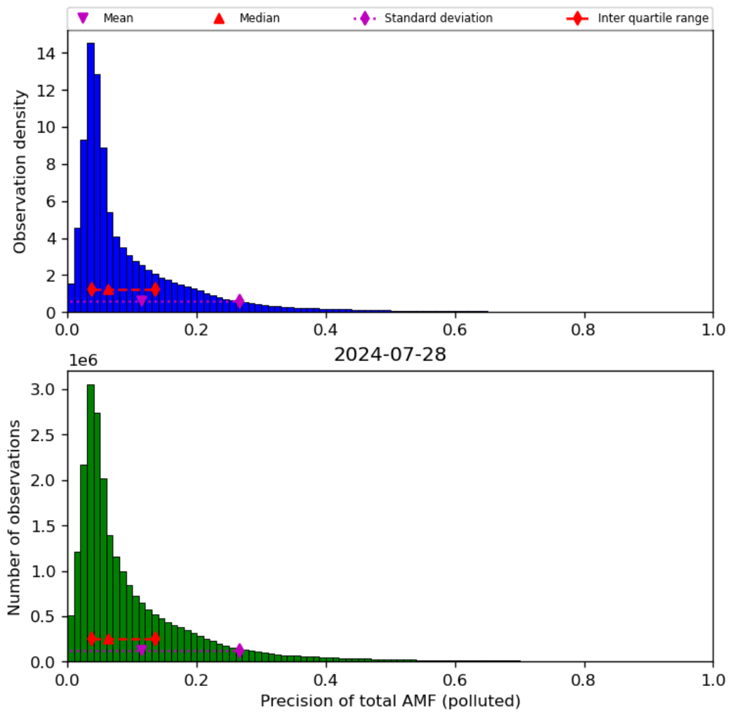
Figure 72: Histogram of “Precision of total AMF (polluted)” for 2024-07-27 to 2024-07-29
