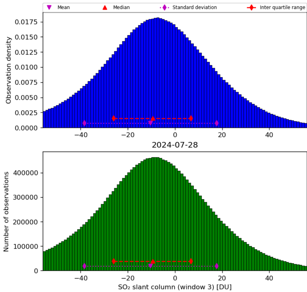
Figure 64: Histogram of “SO 2 slant column (window 3)” for 2024-07-27 to 2024-07-29
