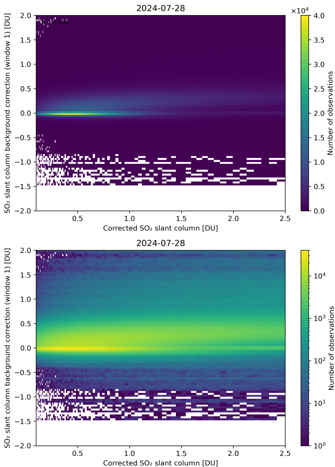
Figure 178: Scatter density plot of “Corrected SO 2 slant column” against “SO 2 slant column background correction (window 1)” for 2024-07-27 to 2024-07-29.
