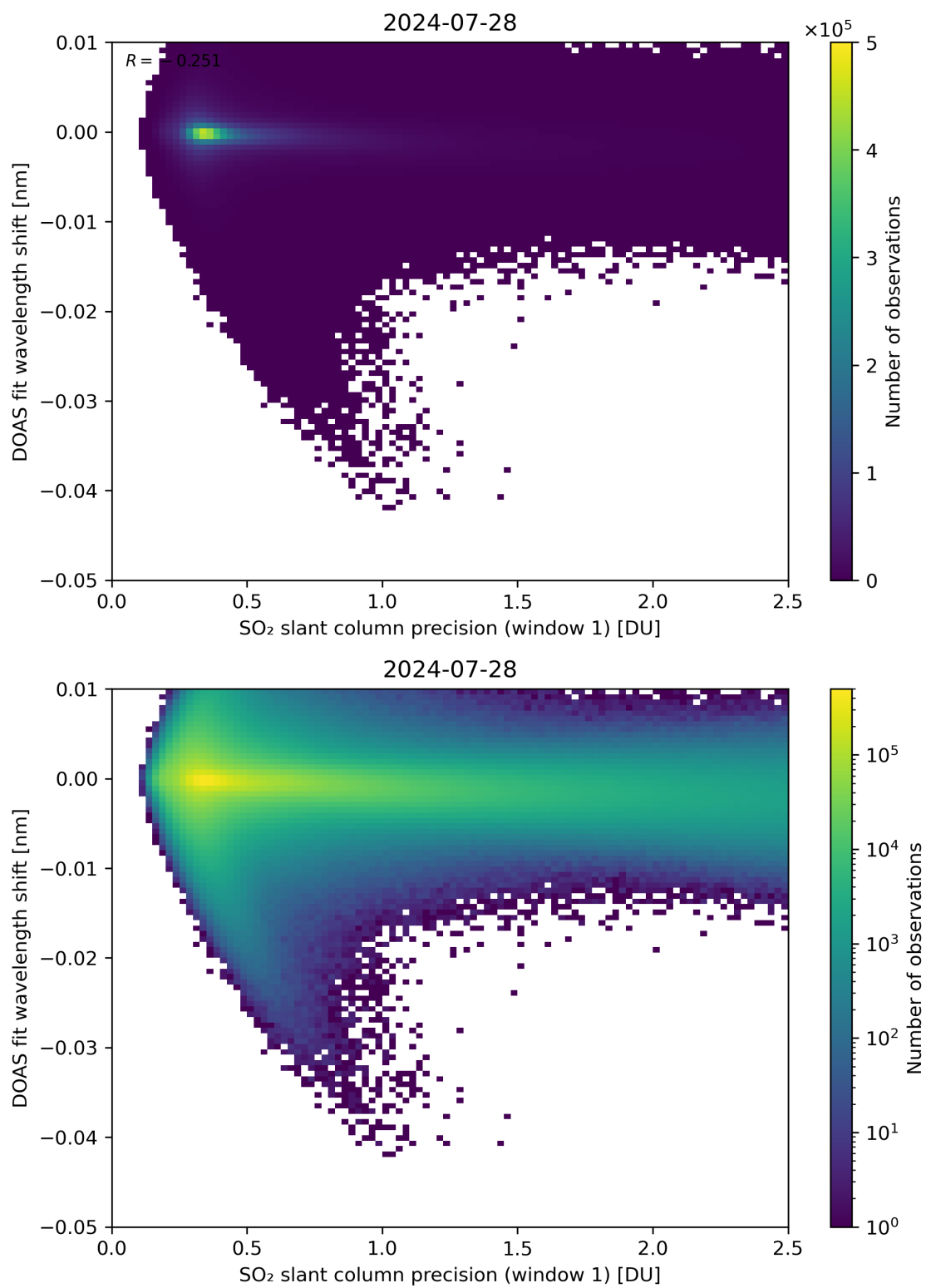
Figure 221: Scatter density plot of “SO 2 slant column precision (window 1)” against “DOAS fit wavelength shift” for 2024-07-27 to 2024-07-29.
