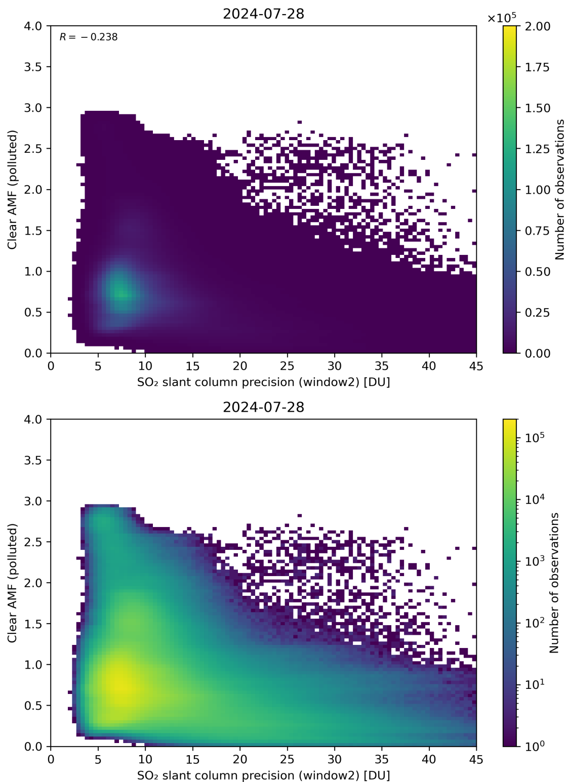
Figure 246: Scatter density plot of “SO 2 slant column precision (window2)” against “Clear AMF (polluted)” for 2024-07-27 to 2024-07-29.
