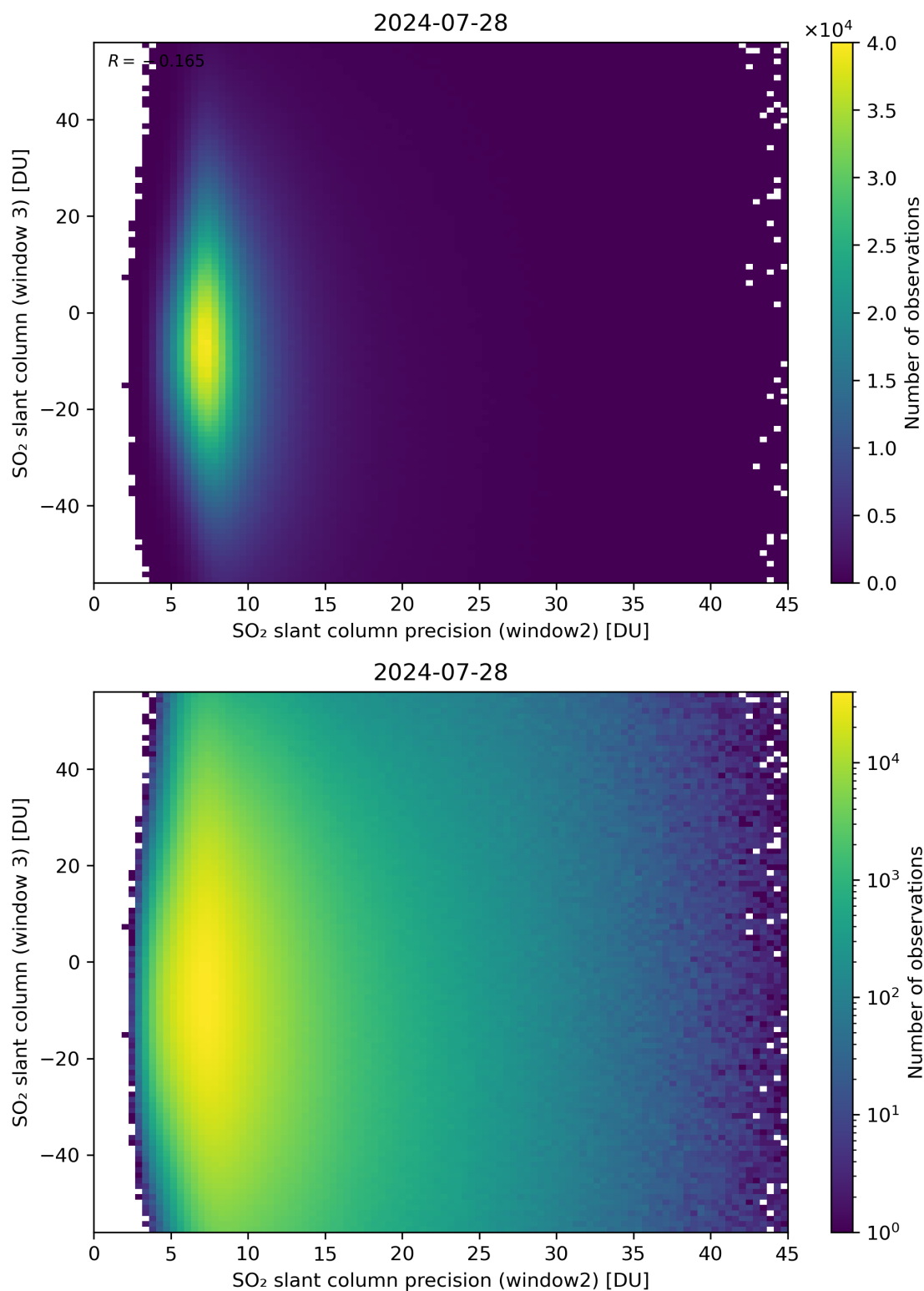
Figure 249: Scatter density plot of “SO 2 slant column precision (window2)” against “SO 2 slant column (window 3)” for 2024-07-27 to 2024-07-29.
