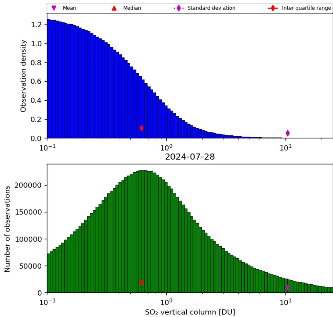
Figure 53: Histogram of “SO 2 vertical column” for 2024-07-27 to 2024-07-29
