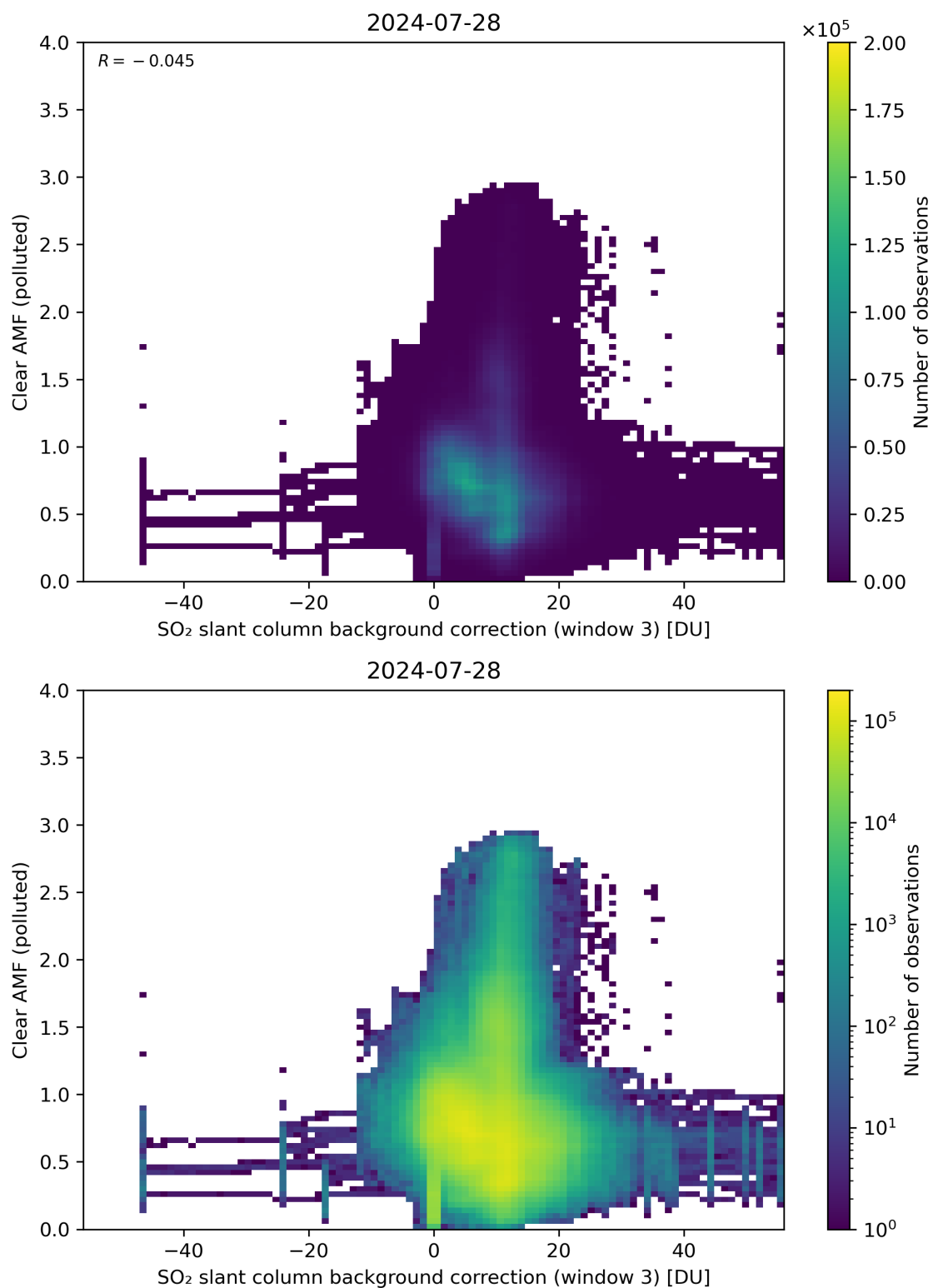
Figure 124: Scatter density plot of “SO 2 slant column background correction (window 3)” against “Clear AMF (polluted)” for 2024-07-27 to 2024-07-29.
