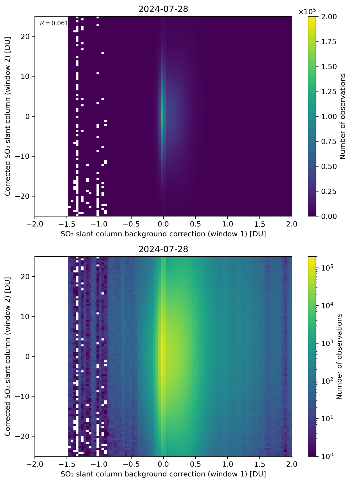
Figure 104: Scatter density plot of “SO 2 slant column background correction (window 1)” against “Corrected SO 2 slant column (window 2)” for 2024-07-27 to 2024-07-29.
