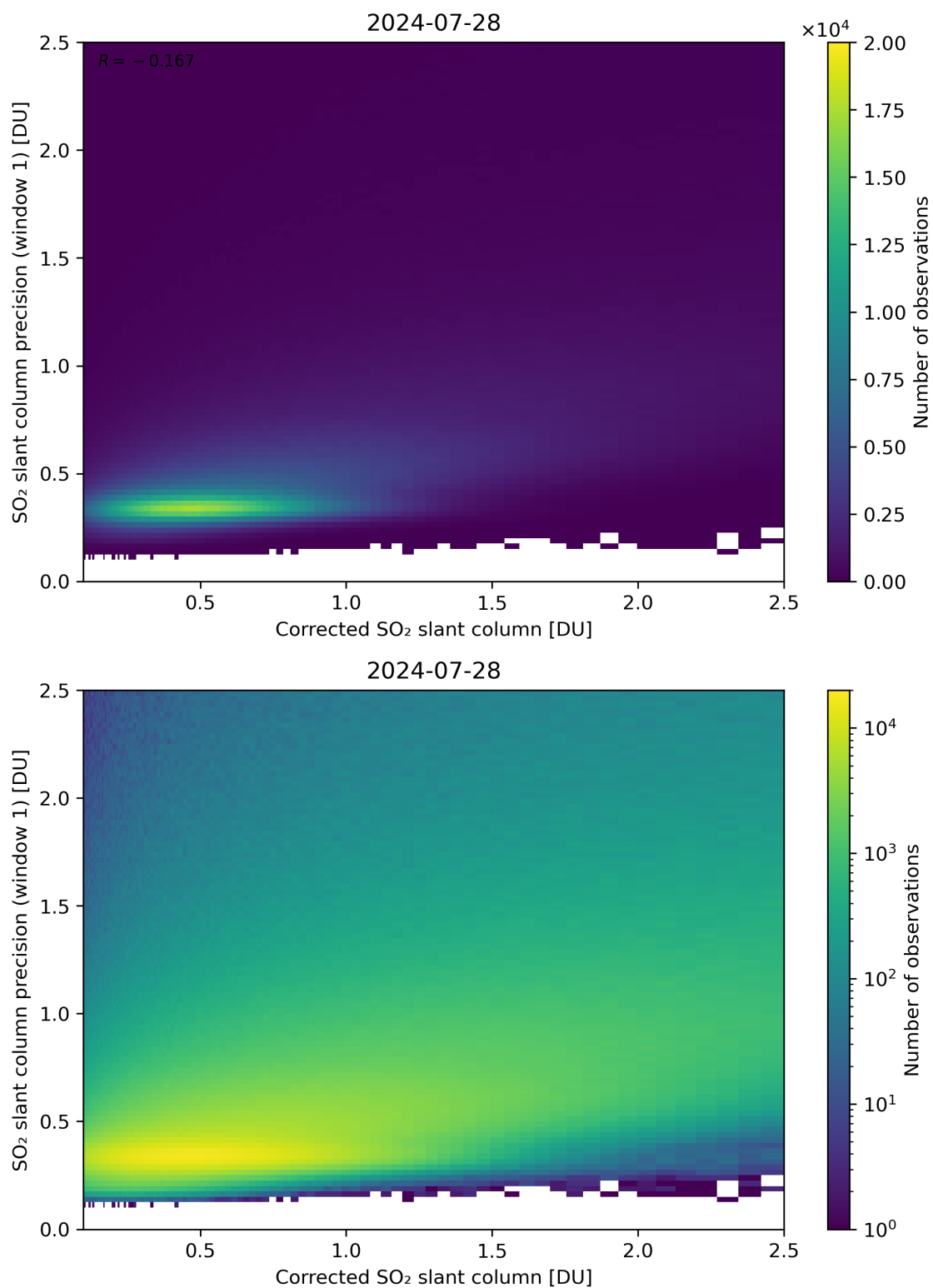
Figure 188: Scatter density plot of “Corrected SO 2 slant column” against “SO 2 slant column precision (window 1)” for 2024-07-27 to 2024-07-29.
