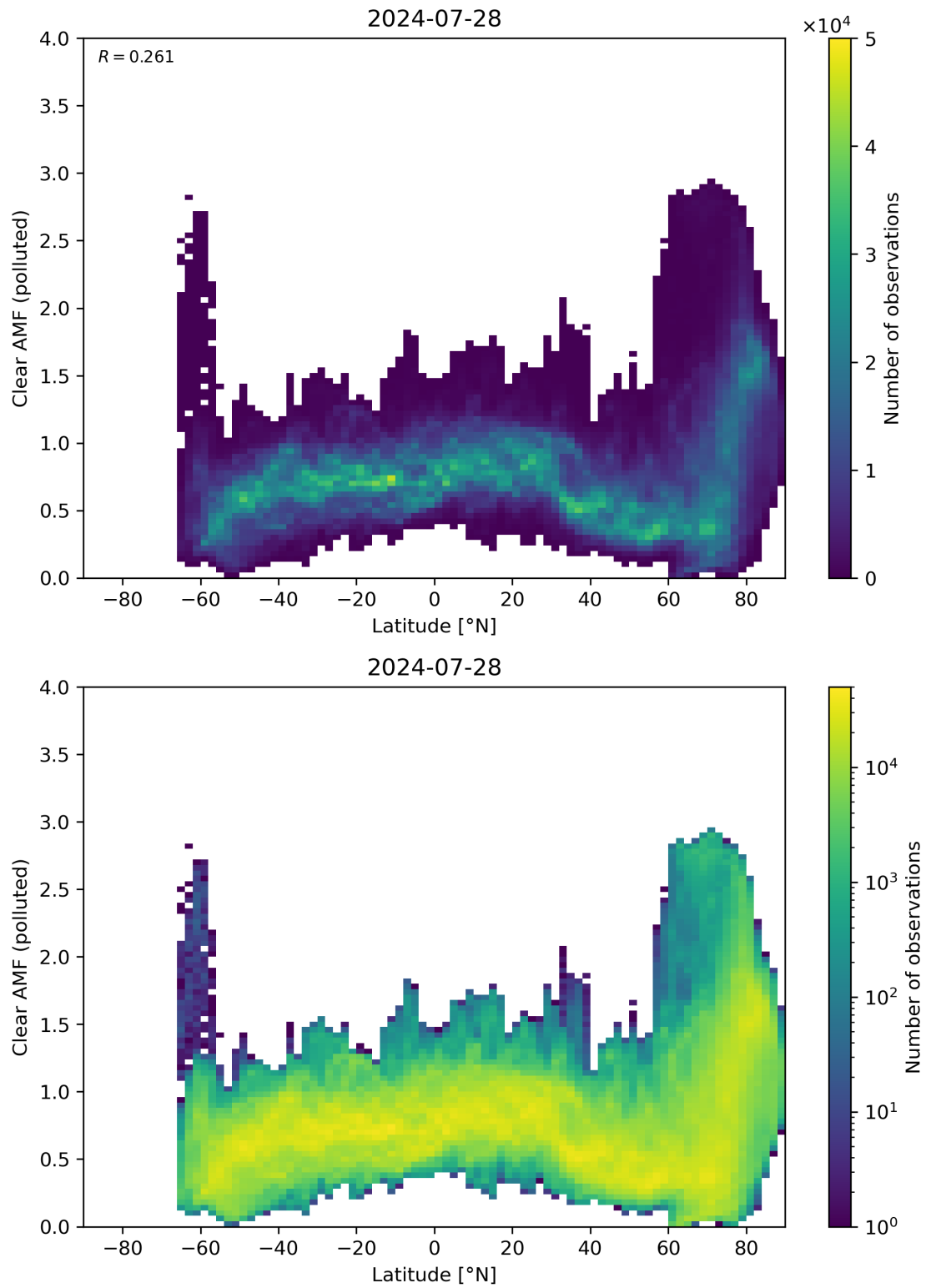
Figure 145: Scatter density plot of “Latitude” against “Clear AMF (polluted)” for 2024-07-27 to 2024-07-29.
