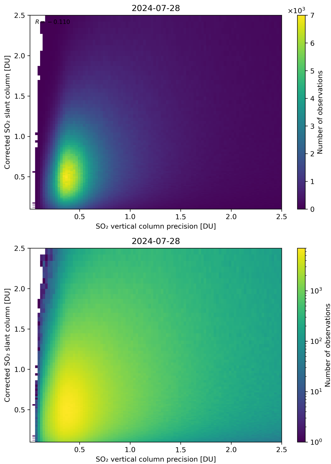
Figure 286: Scatter density plot of “SO 2 vertical column precision” against “Corrected SO 2 slant column” for 2024-07-27 to 2024-07-29.
