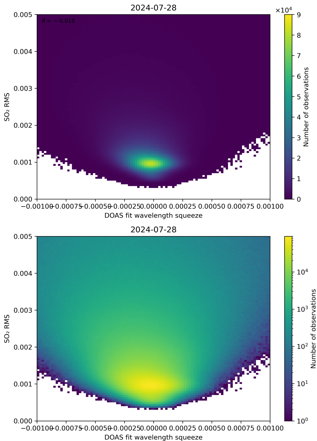
Figure 132: Scatter density plot of “DOAS fit wavelength squeeze” against “SO 2 RMS” for 2024-07-27 to 2024-07-29.
