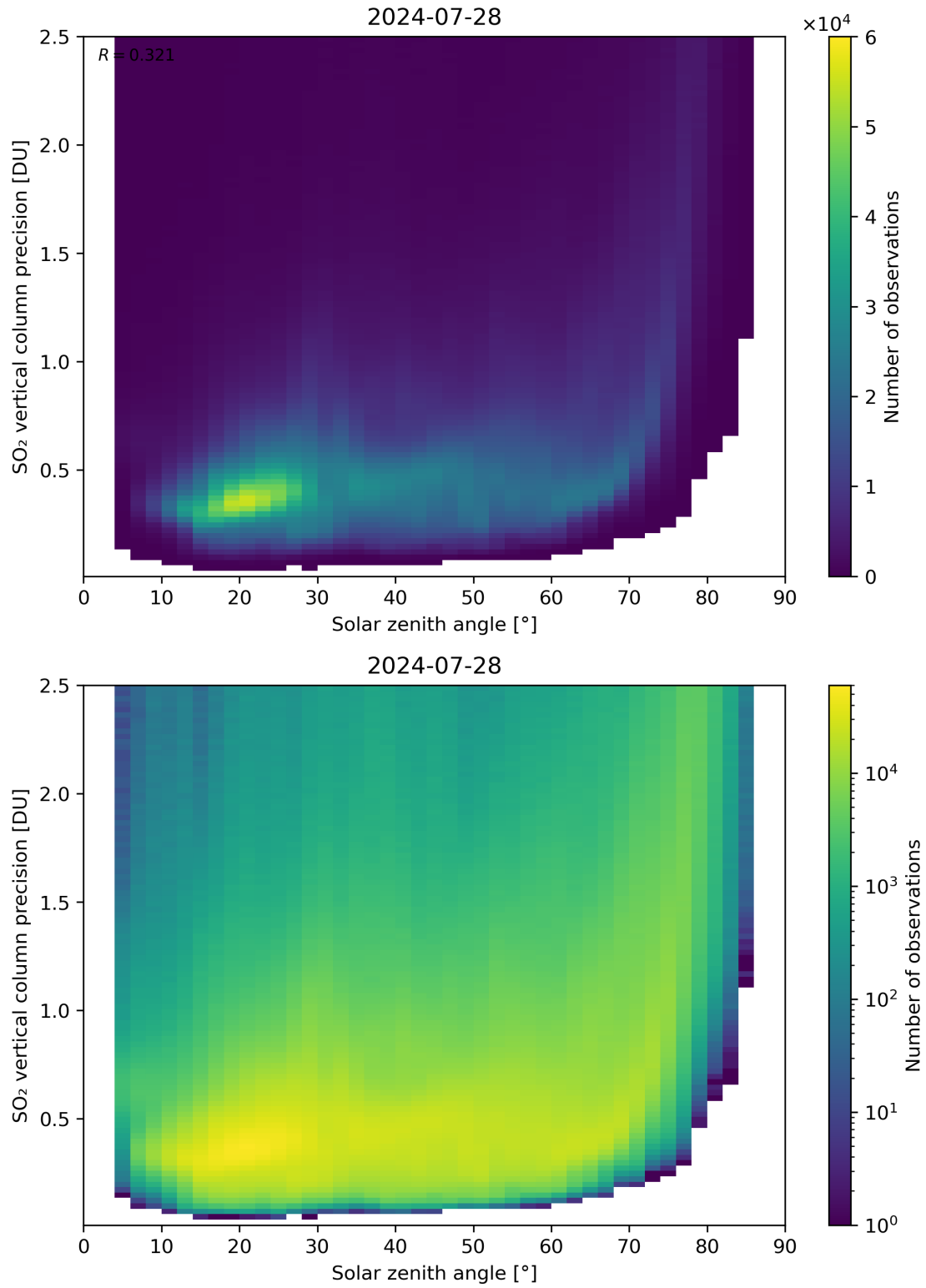
Figure 177: Scatter density plot of “Solar zenith angle” against “SO 2 vertical column precision” for 2024-07-27 to 2024-07-29.
