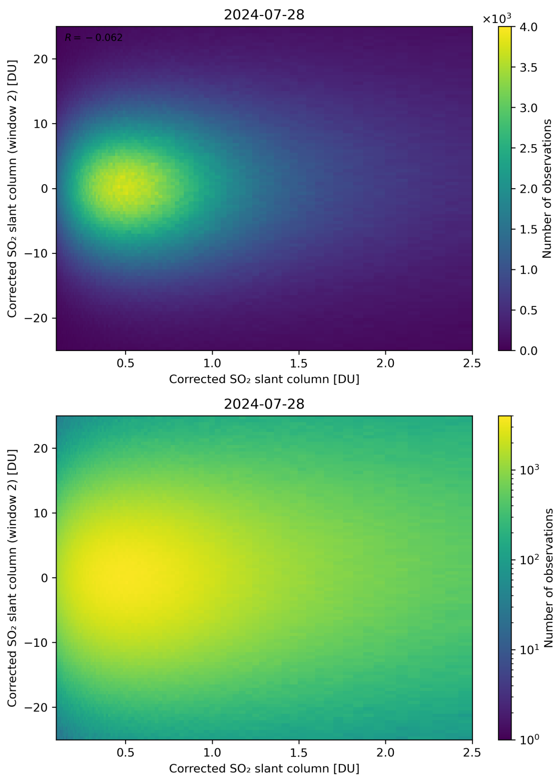
Figure 185: Scatter density plot of “Corrected SO 2 slant column” against “Corrected SO 2 slant column (window 2)” for 2024-07-27 to 2024-07-29.
