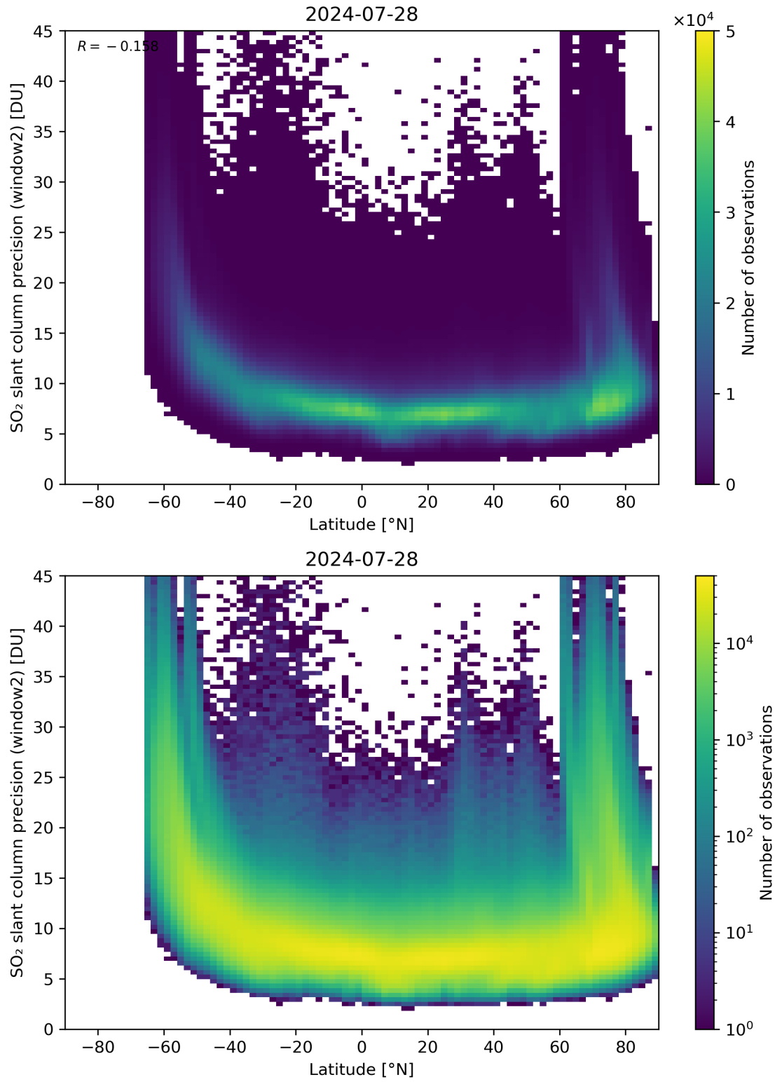
Figure 151: Scatter density plot of “Latitude” against “SO 2 slant column precision (window2)” for 2024-07-27 to 2024-07-29.
