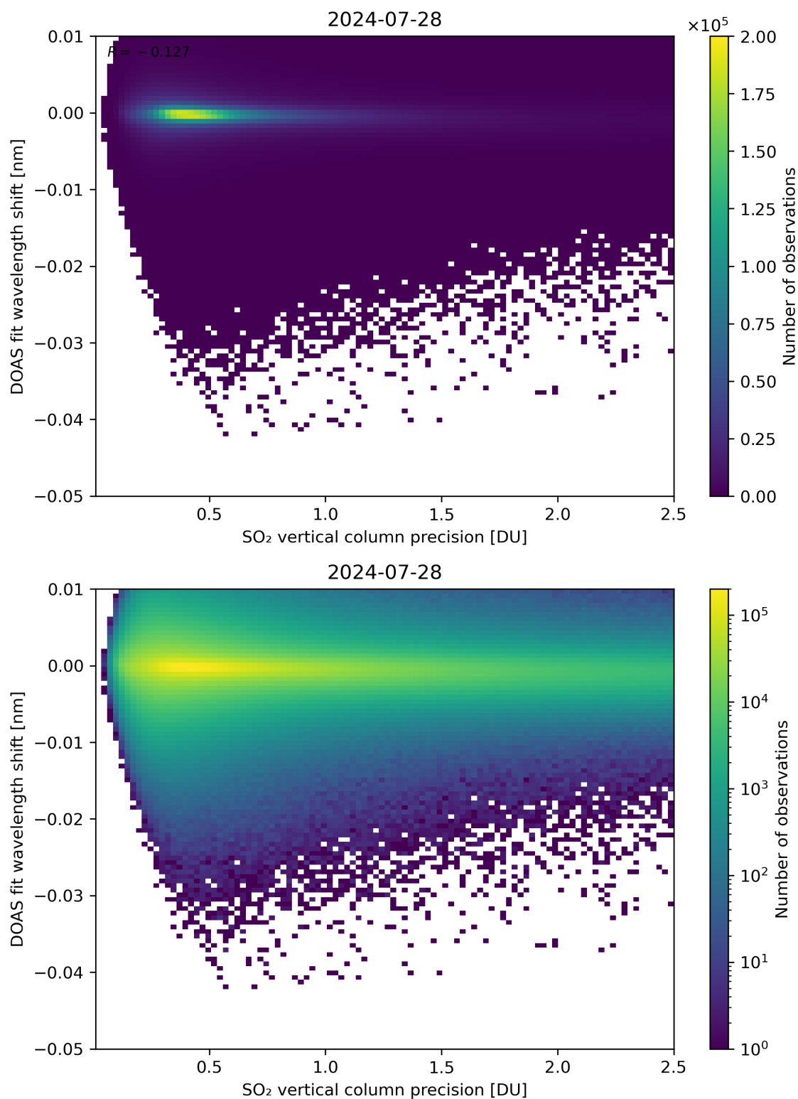
Figure 282: Scatter density plot of “SO 2 vertical column precision” against “DOAS fit wavelength shift” for 2024-07-27 to 2024-07-29.
