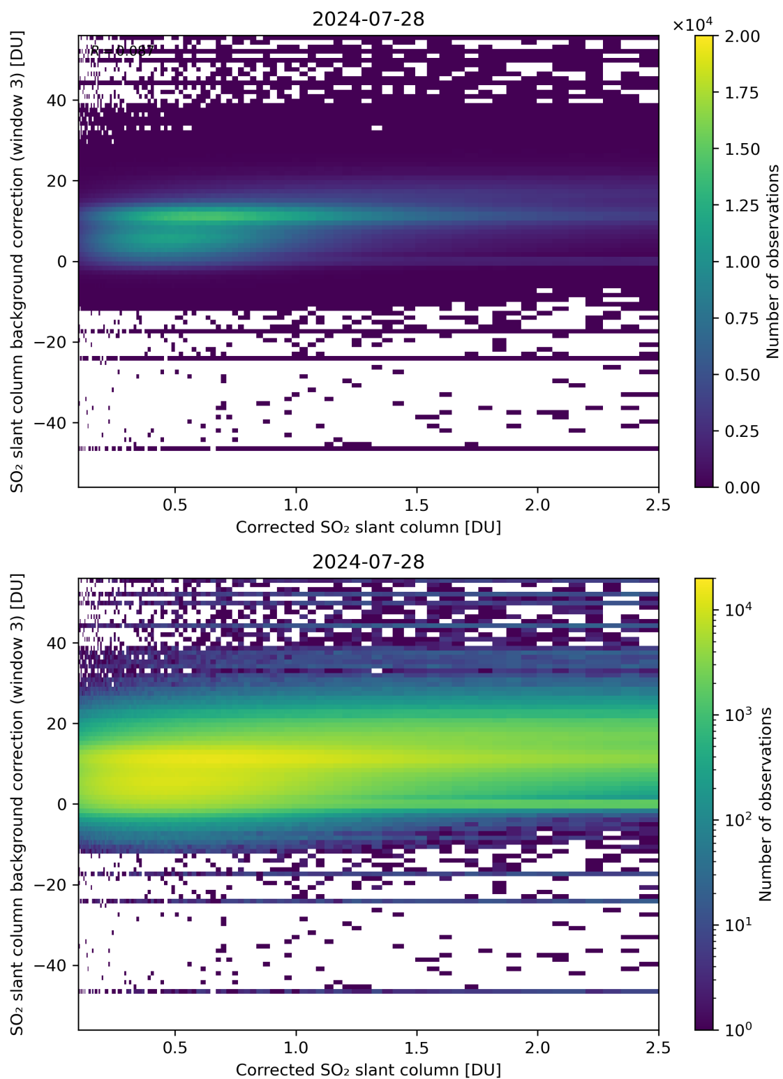
Figure 180: Scatter density plot of “Corrected SO 2 slant column” against “SO 2 slant column background correction (window 3)” for 2024-07-27 to 2024-07-29.
