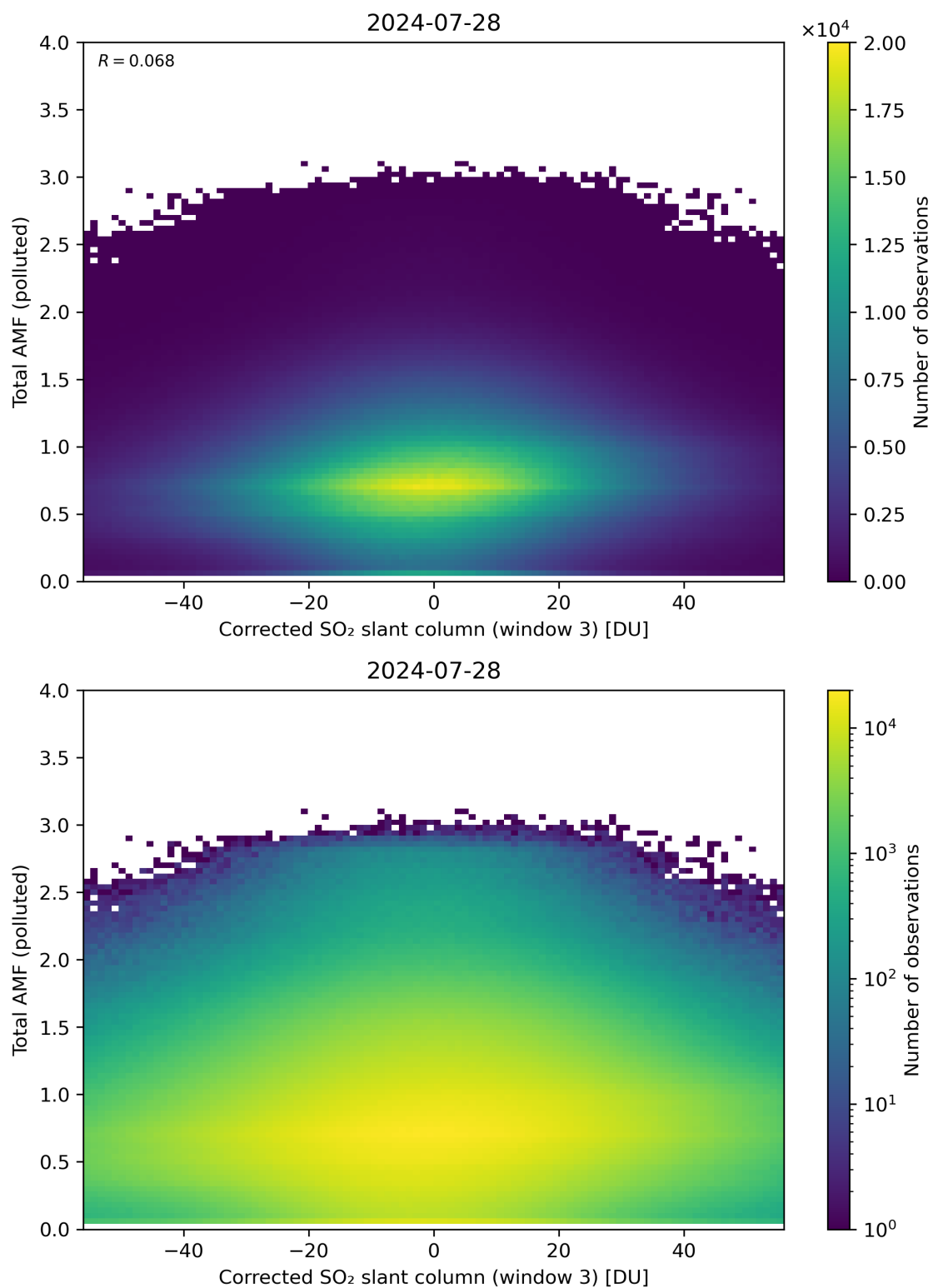
Figure 210: Scatter density plot of “Corrected SO 2 slant column (window 3)” against “Total AMF (polluted)” for 2024-07-27 to 2024-07-29.
