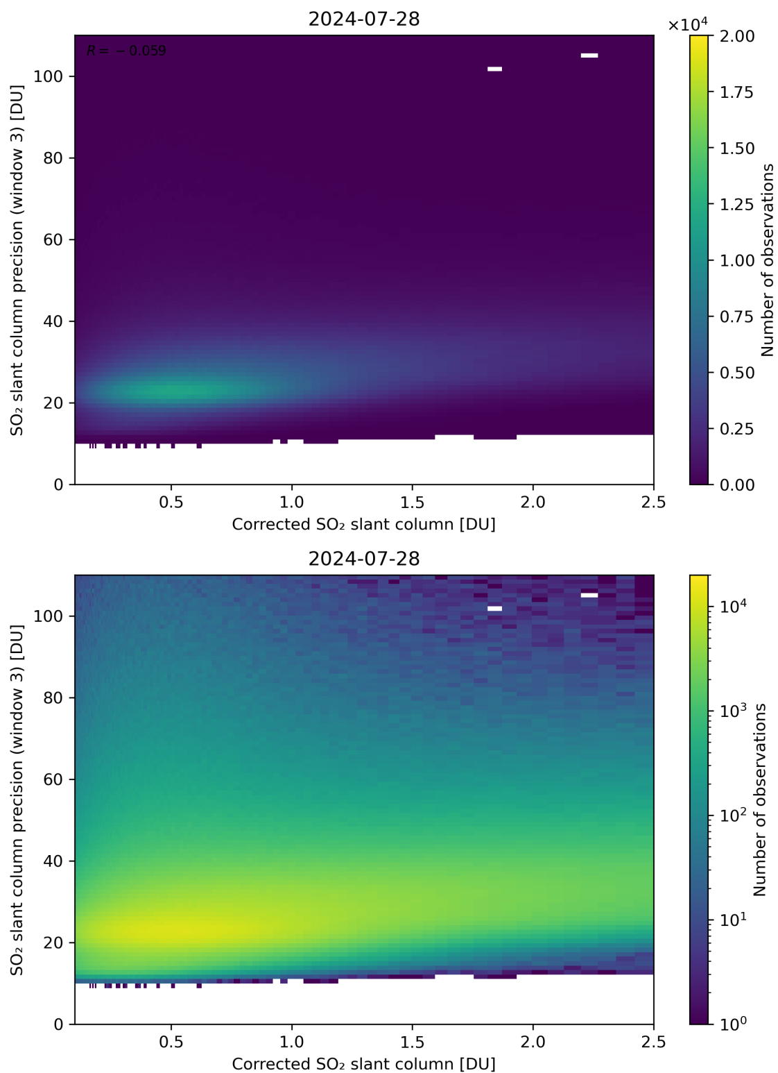
Figure 191: Scatter density plot of “Corrected SO 2 slant column” against “SO 2 slant column precision (window 3)” for 2024-07-27 to 2024-07-29.
