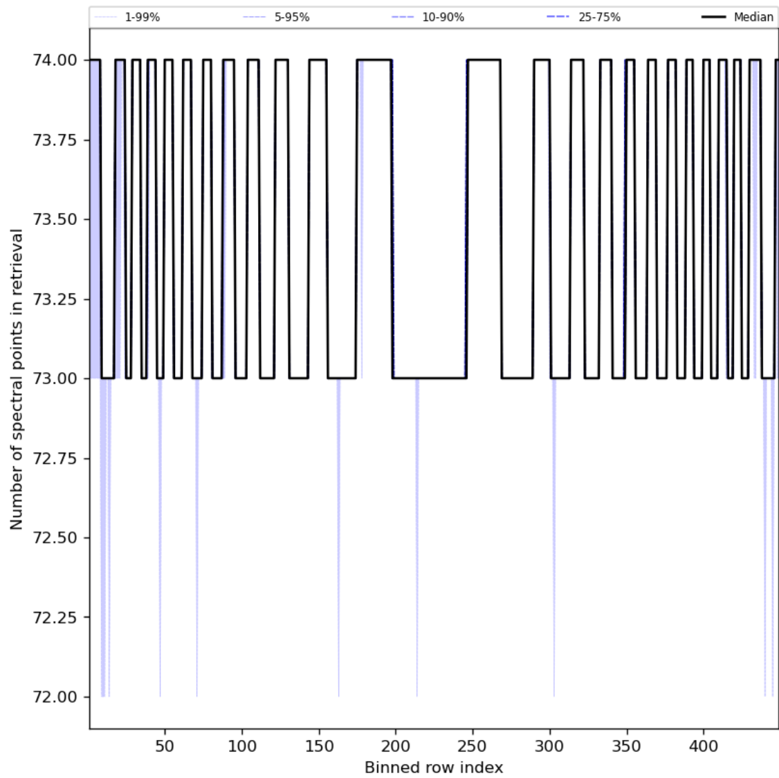
Figure 97: Along track statistics of “Number of spectral points in retrieval” for 2024-07-27 to 2024-07-29
