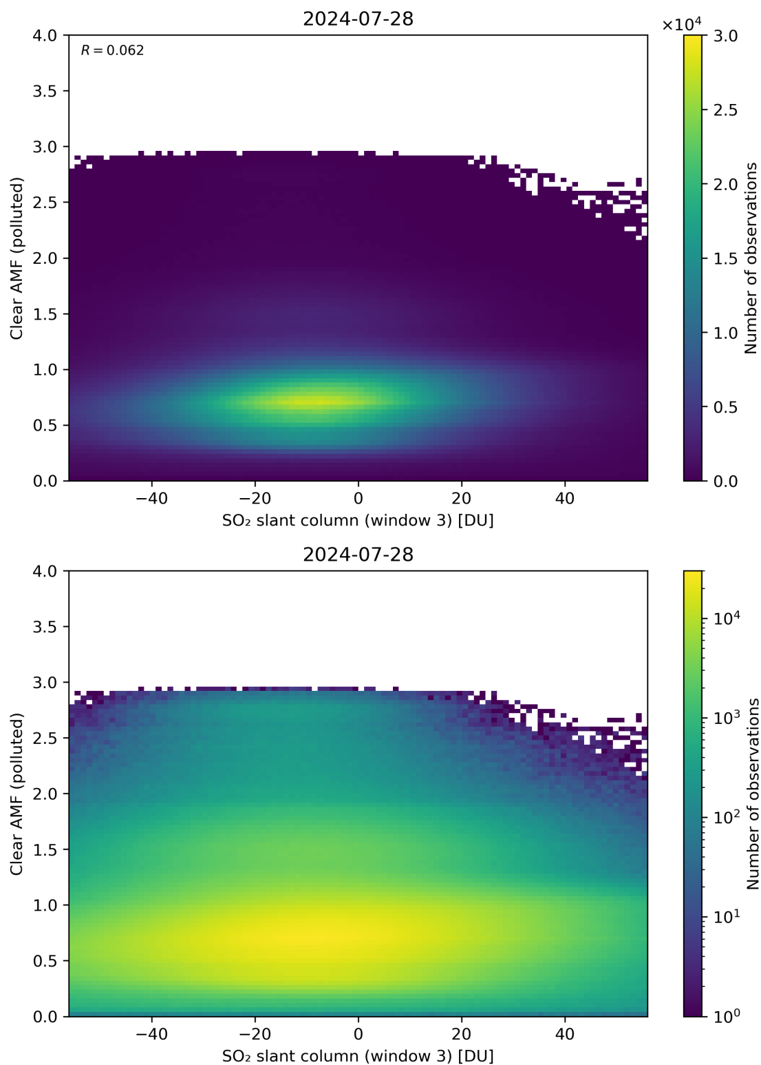
Figure 265: Scatter density plot of “SO 2 slant column (window 3)” against “Clear AMF (polluted)” for 2024-07-27 to 2024-07-29.
