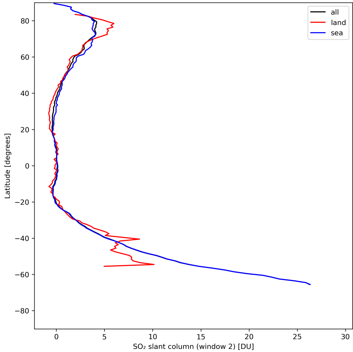
Figure 37: Zonal average of “SO 2 slant column (window 2)” for 2024-07-27 to 2024-07-29.
