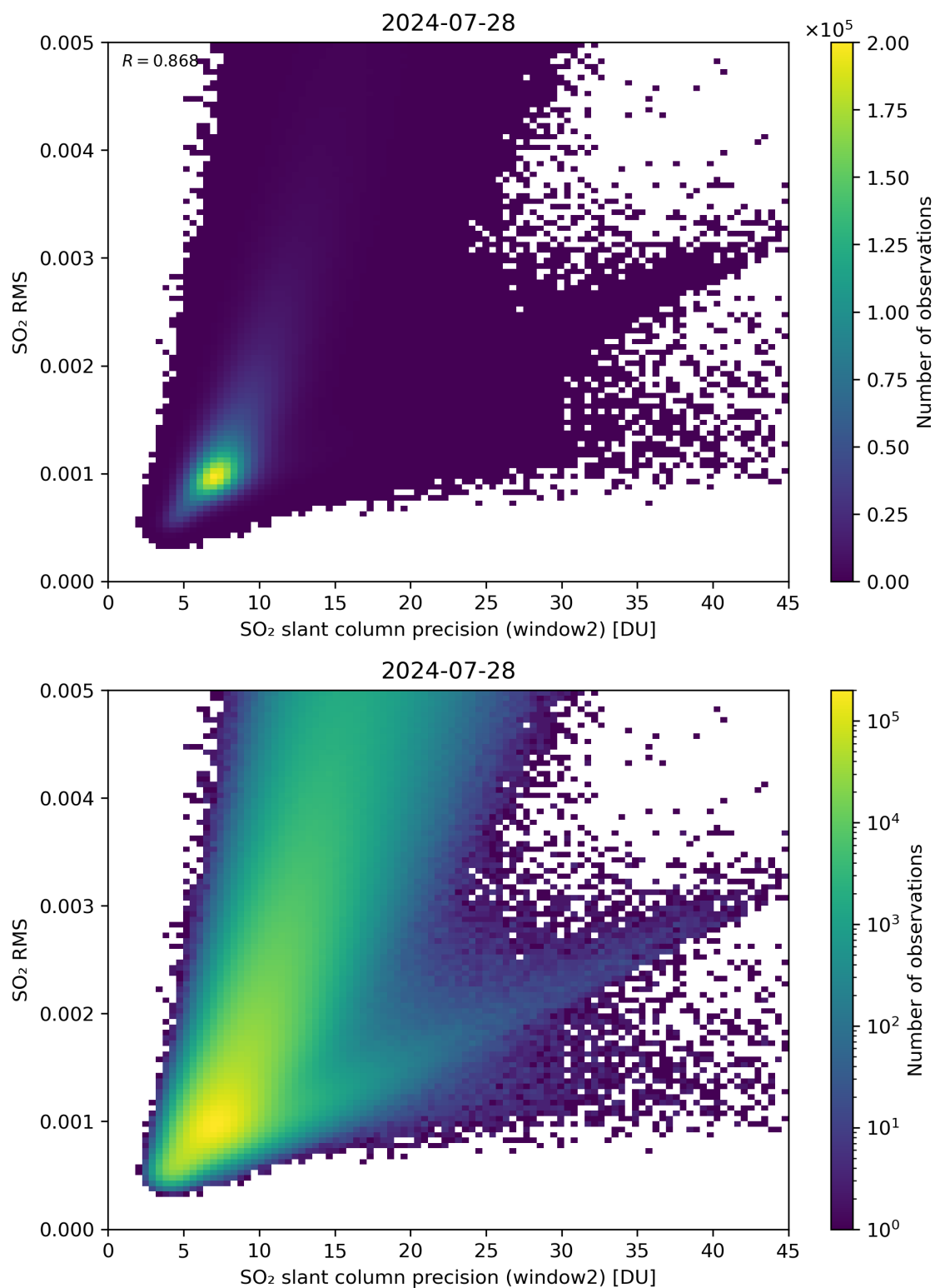
Figure 245: Scatter density plot of “SO 2 slant column precision (window2)” against “SO 2 RMS” for 2024-07-27 to 2024-07-29.
