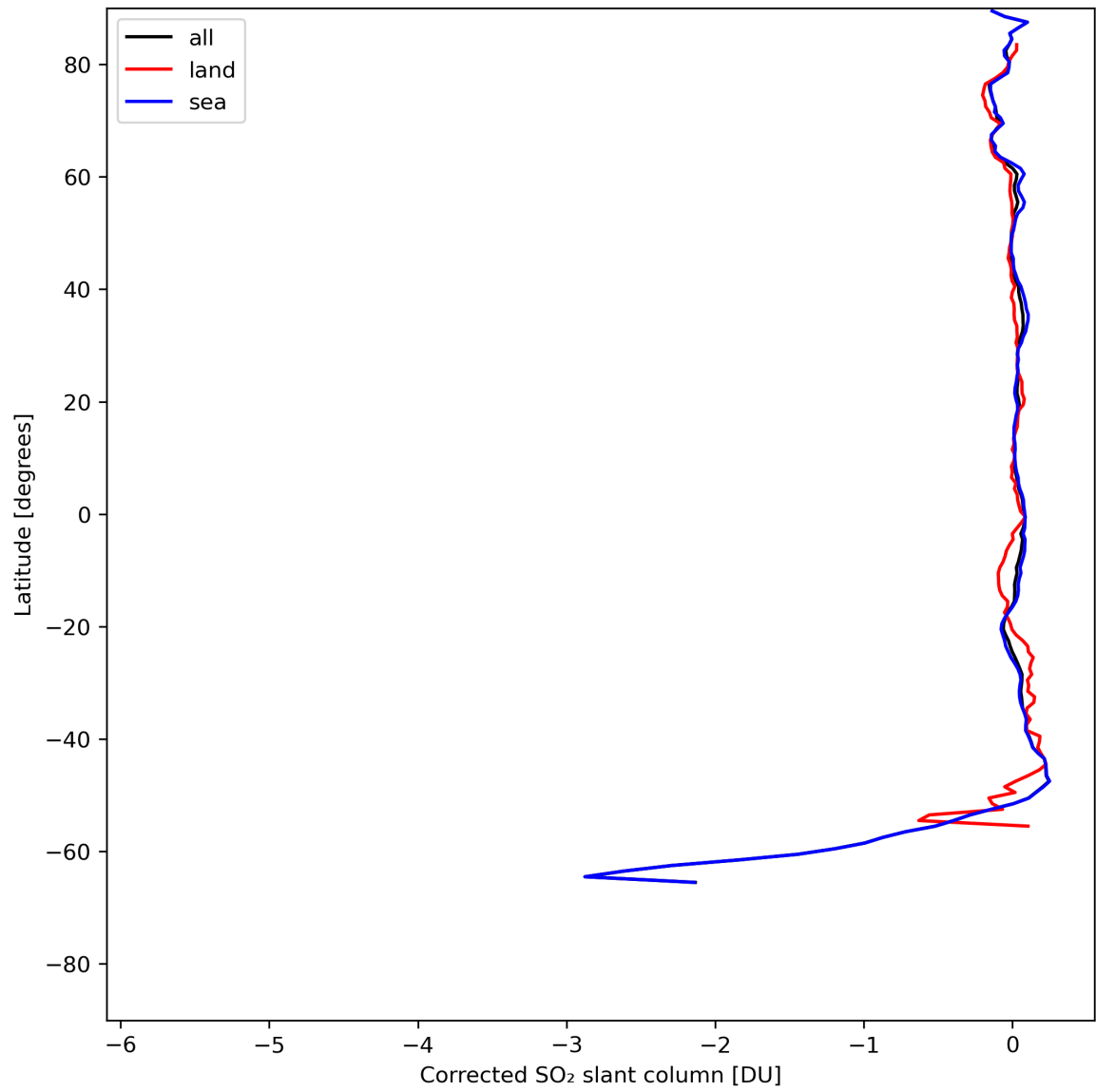
Figure 32: Zonal average of “Corrected SO 2 slant column” for 2024-07-27 to 2024-07-29.
