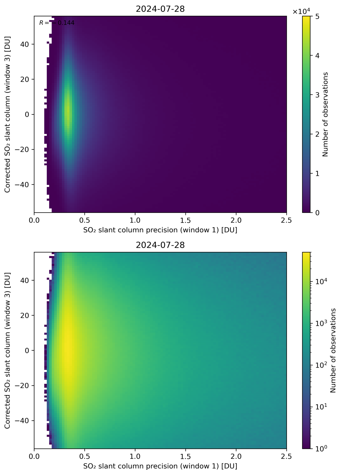
Figure 226: Scatter density plot of “SO 2 slant column precision (window 1)” against “Corrected SO 2 slant column (window 3)” for 2024-07-27 to 2024-07-29.
