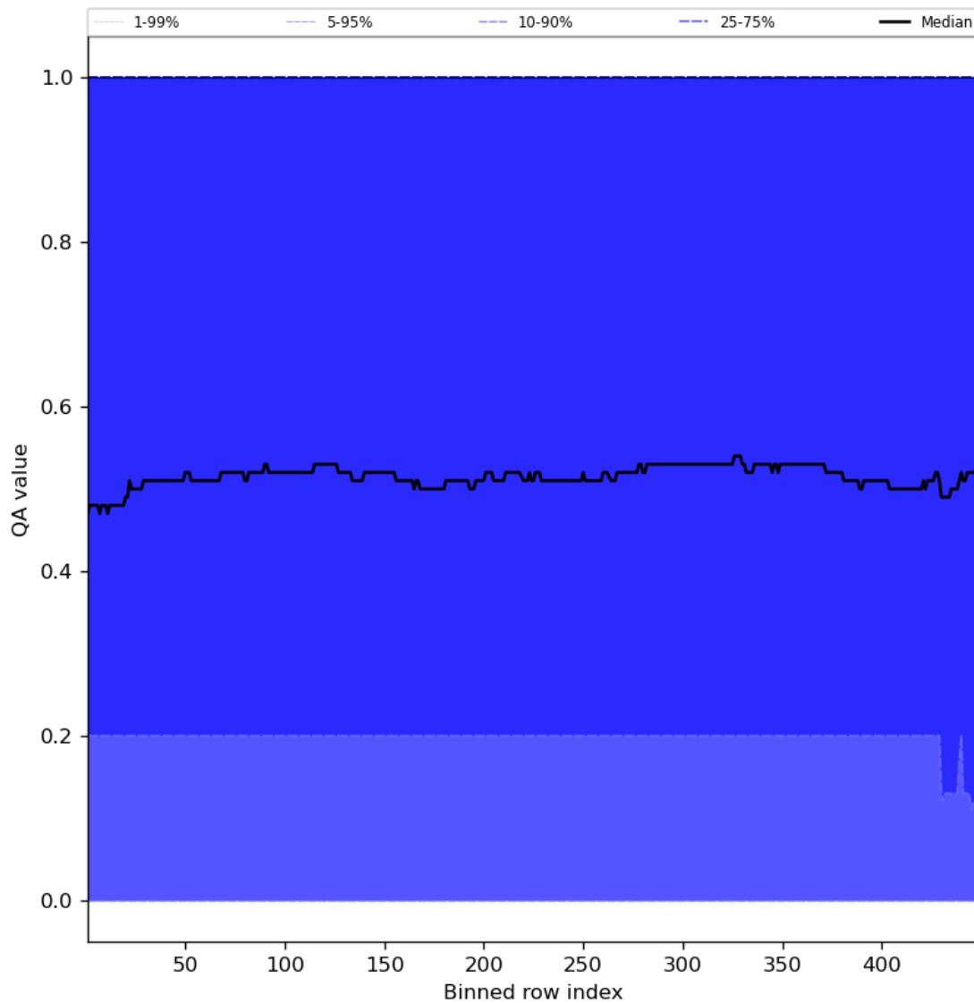
Figure 75: Along track statistics of “QA value” for 2024-07-27 to 2024-07-29
