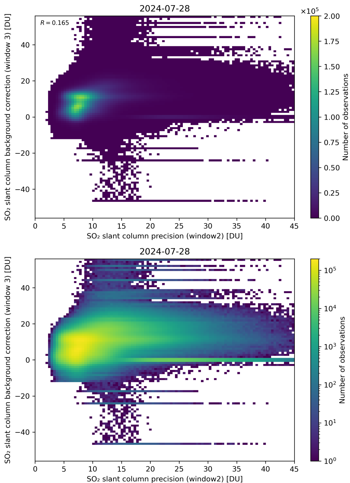
Figure 242: Scatter density plot of “SO 2 slant column precision (window2)” against “SO 2 slant column background correction (window 3)” for 2024-07-27 to 2024-07-29.
