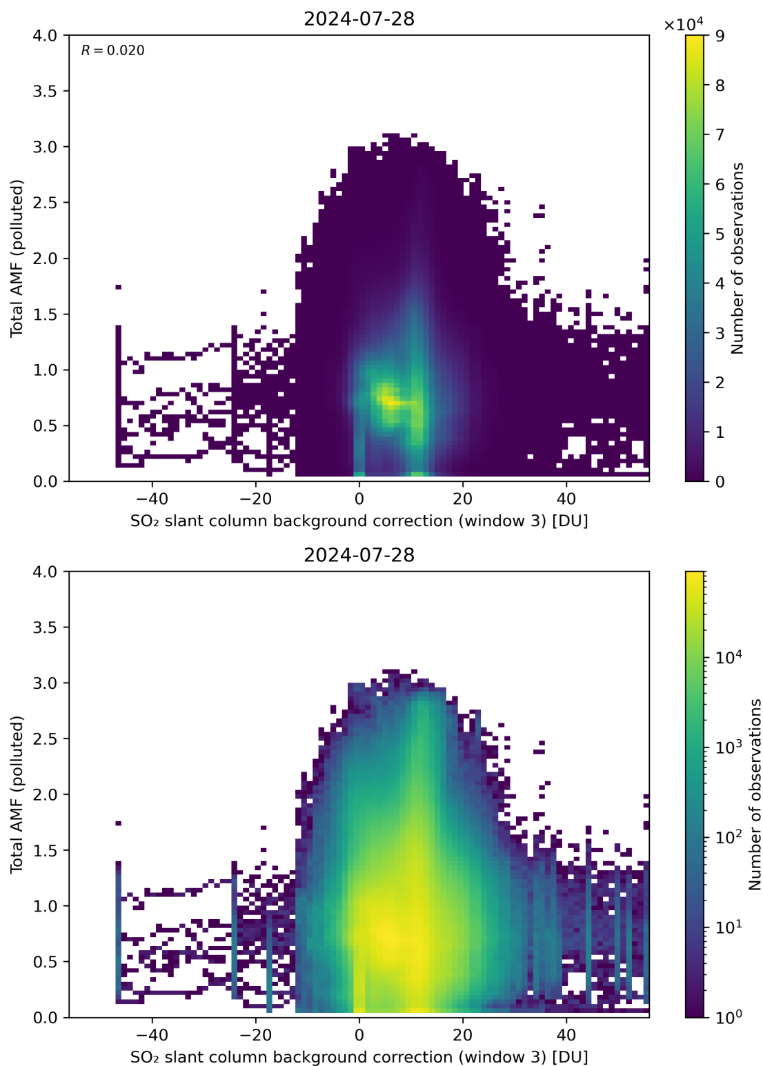
Figure 125: Scatter density plot of “SO 2 slant column background correction (window 3)” against “Total AMF (polluted)” for 2024-07-27 to 2024-07-29.
