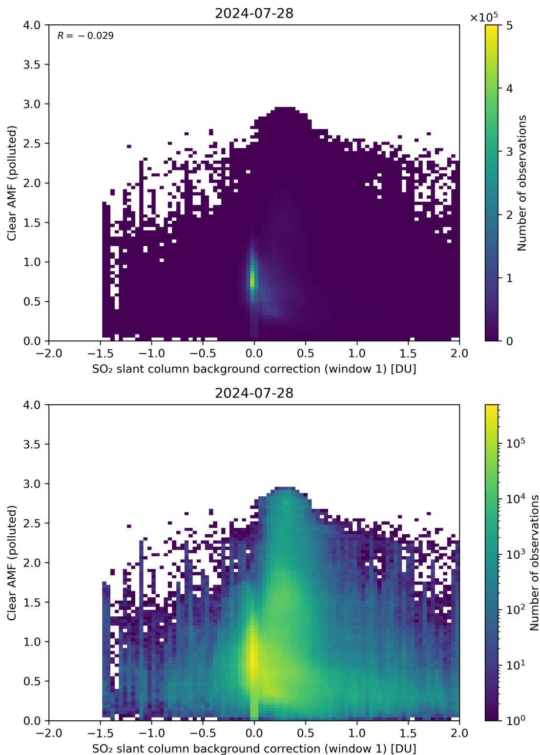
Figure 103: Scatter density plot of “SO 2 slant column background correction (window 1)” against “Clear AMF (polluted)” for 2024-07-27 to 2024-07-29.
