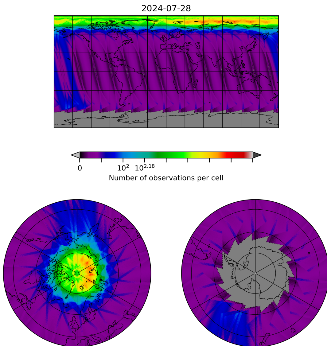
Figure 28: Map of the number of observations for 2024-07-27 to 2024-07-29
