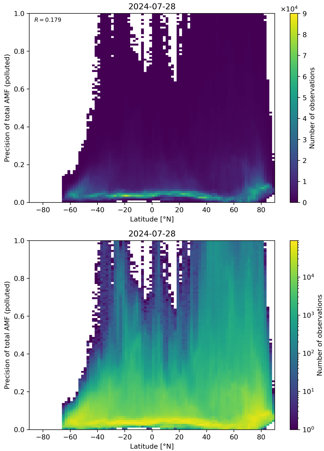
Figure 155: Scatter density plot of “Latitude” against “Precision of total AMF (polluted)” for 2024-07-27 to 2024-07-29.
