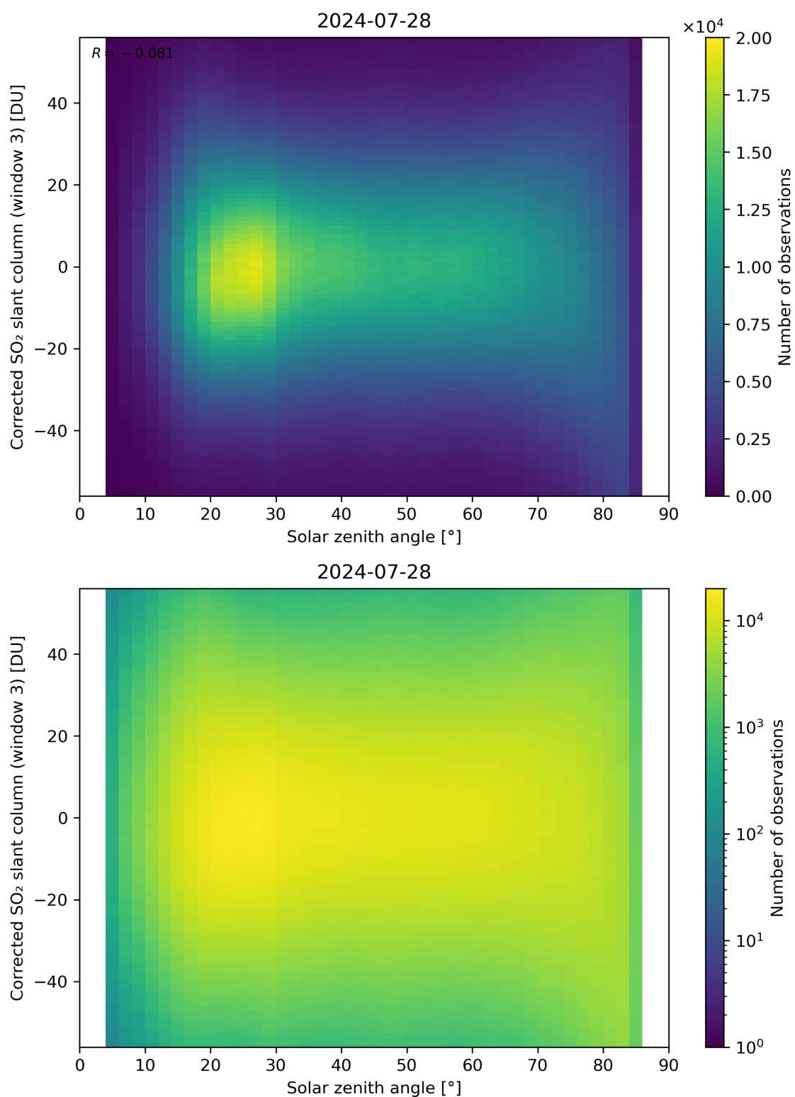
Figure 168: Scatter density plot of “Solar zenith angle” against “Corrected SO 2 slant column (window 3)” for 2024-07-27 to 2024-07-29.
