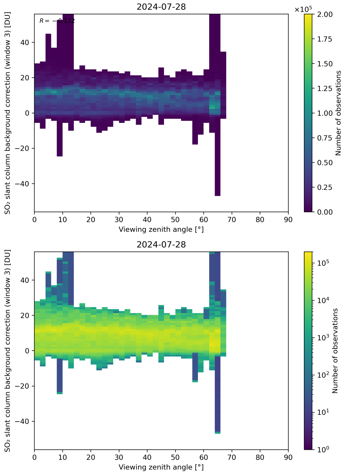
Figure 310: Scatter density plot of “Viewing zenith angle” against “SO 2 slant column background correction (window 3)” for 2024-07-27 to 2024-07-29.
