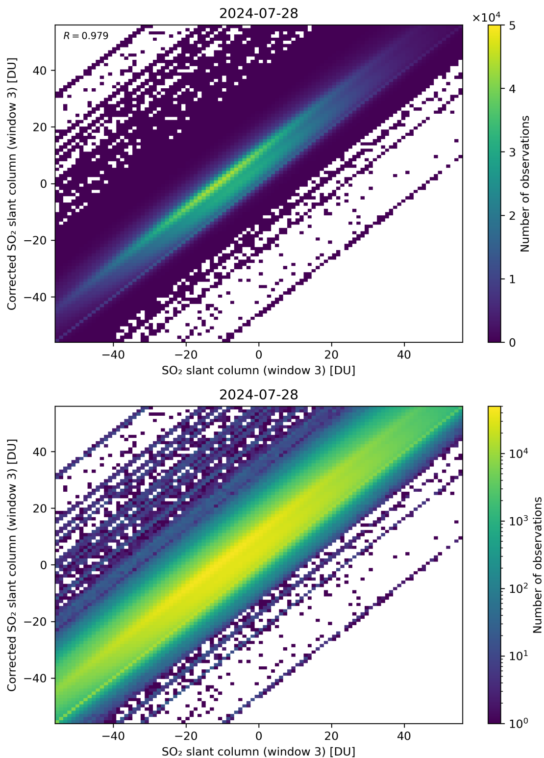
Figure 266: Scatter density plot of “SO 2 slant column (window 3)” against “Corrected SO 2 slant column (window 3)” for 2024-07-27 to 2024-07-29.
