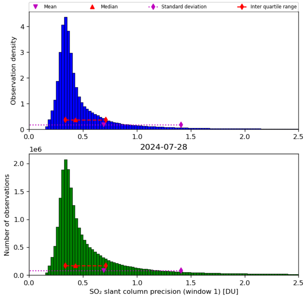
Figure 57: Histogram of “SO 2 slant column precision (window 1)” for 2024-07-27 to 2024-07-29
