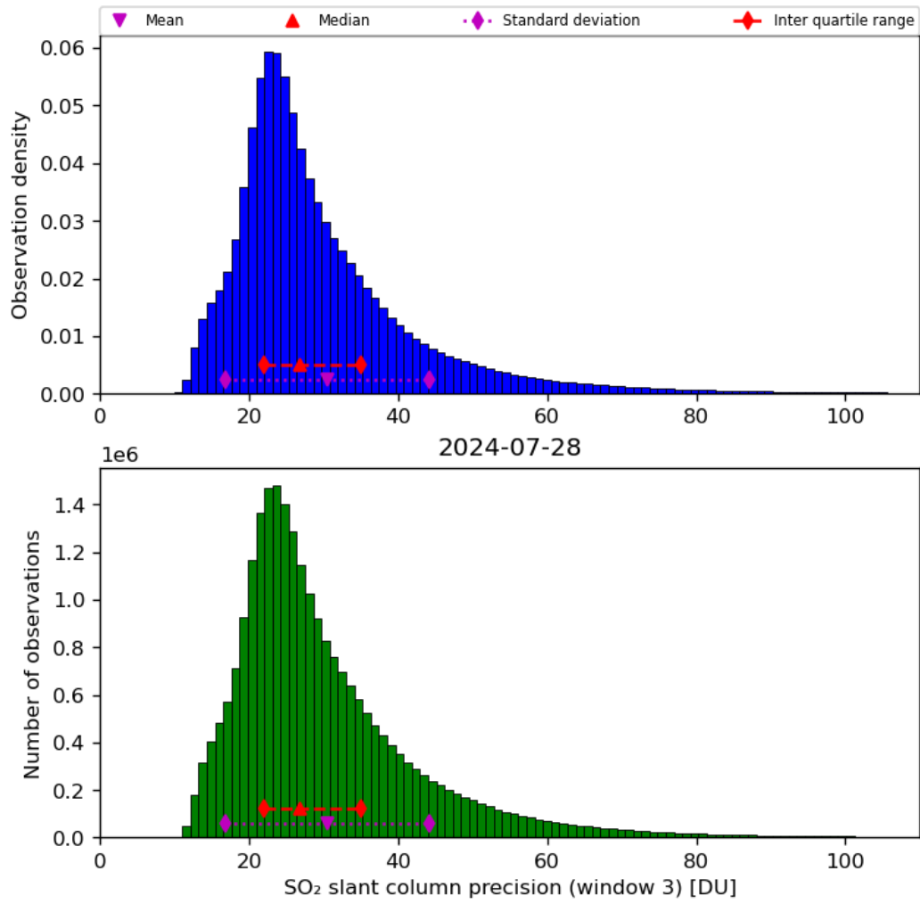
Figure 65: Histogram of “SO 2 slant column precision (window 3)” for 2024-07-27 to 2024-07-29
