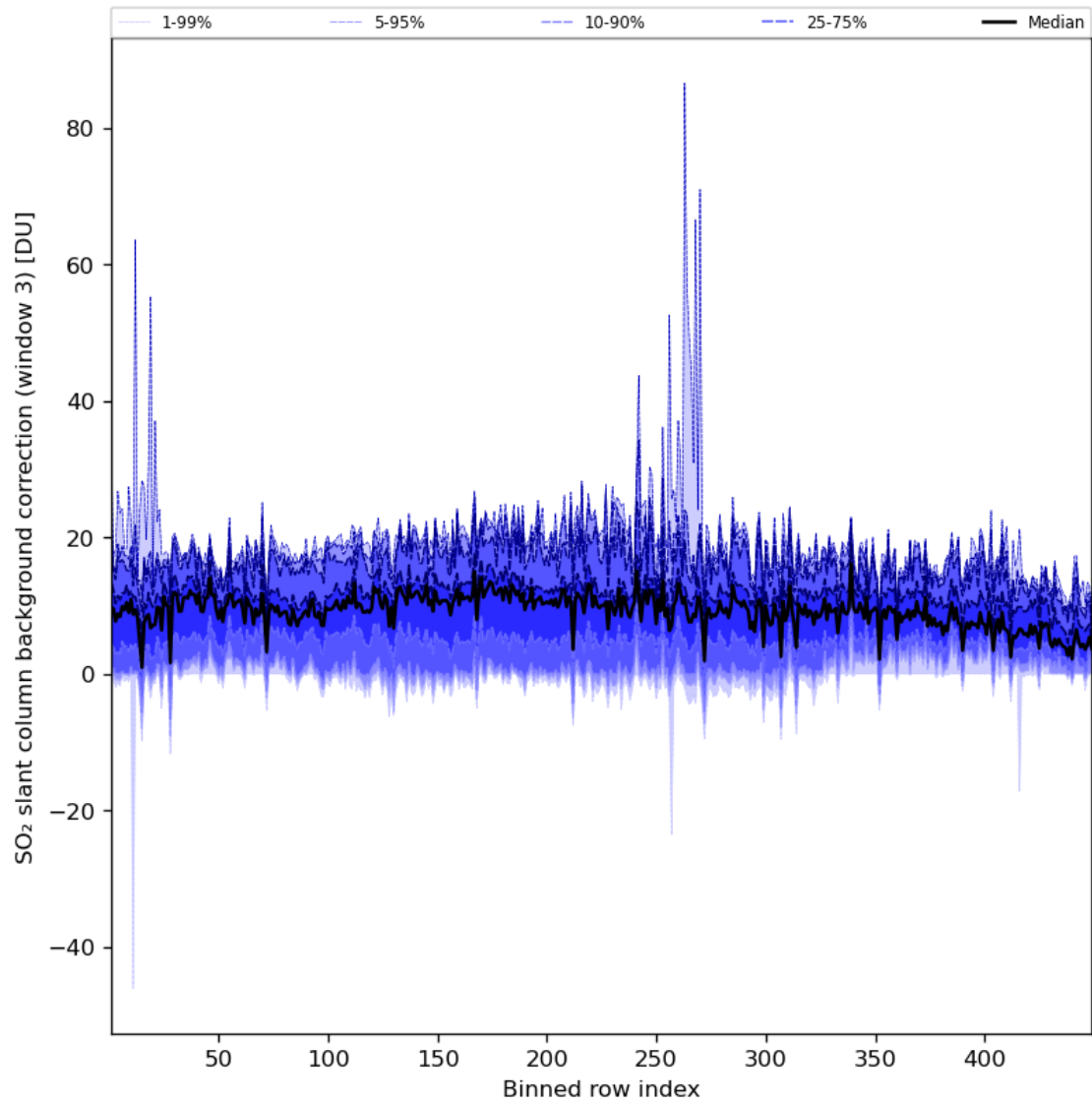
Figure 90: Along track statistics of “SO 2 slant column background correction (window 3)” for 2024-07-27 to 2024-07-29
