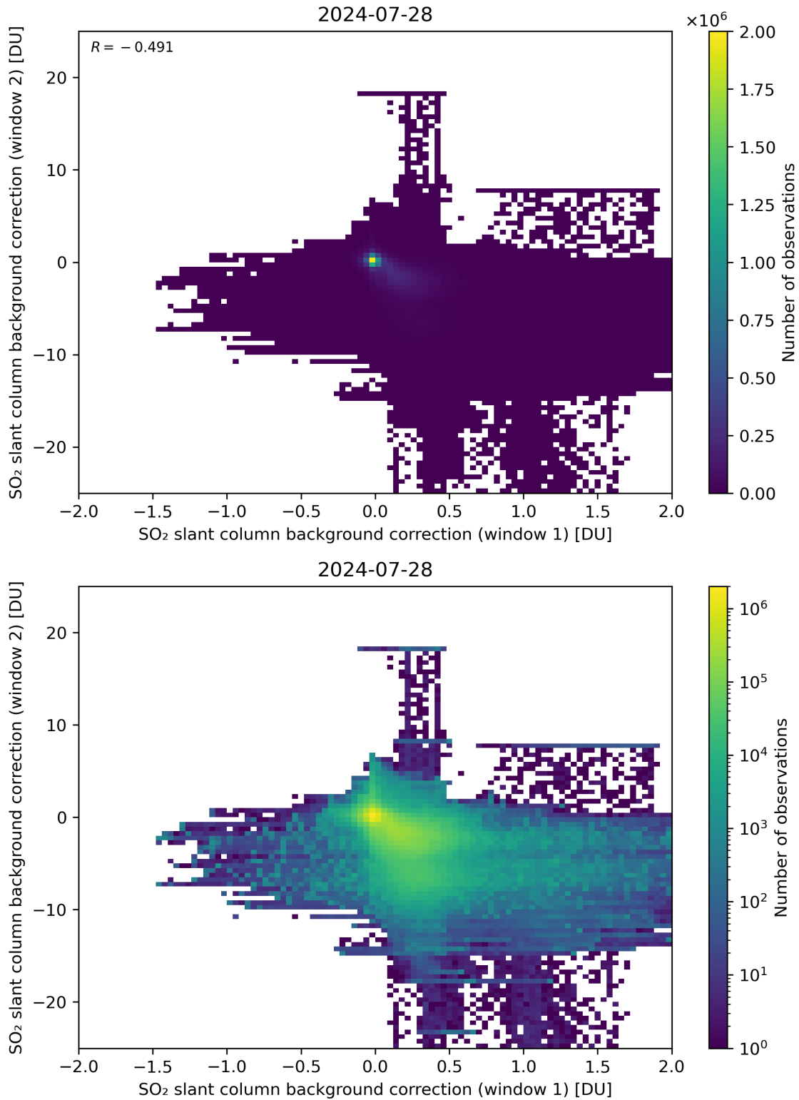
Figure 98: Scatter density plot of “SO 2 slant column background correction (window 1)” against “SO 2 slant column background correction (window 2)” for 2024-07-27 to 2024-07-29.
