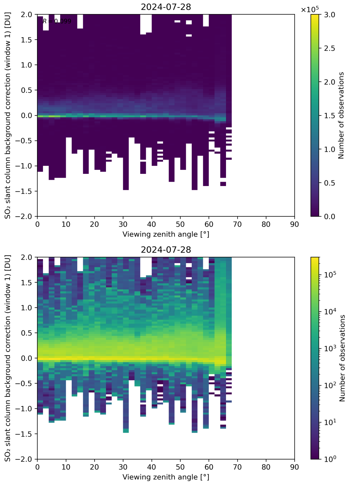
Figure 308: Scatter density plot of “Viewing zenith angle” against “SO 2 slant column background correction (window 1)” for 2024-07-27 to 2024-07-29.
