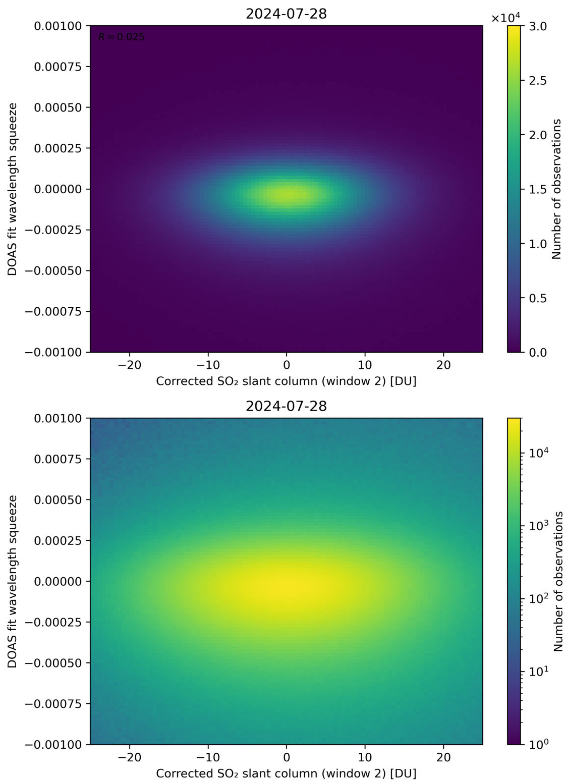
Figure 197: Scatter density plot of “Corrected SO 2 slant column (window 2)” against “DOAS fit wavelength squeeze” for 2024-07-27 to 2024-07-29.
