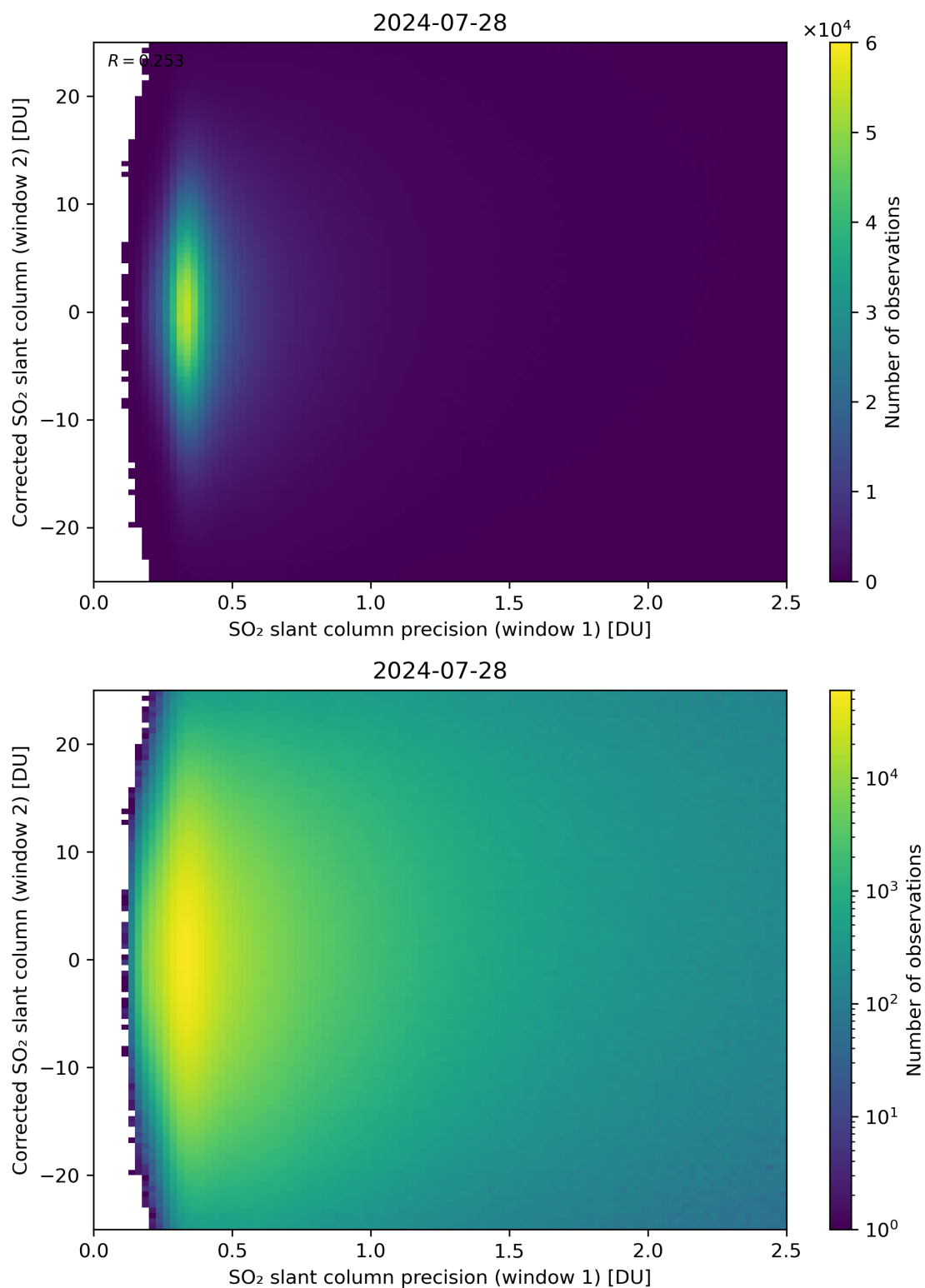
Figure 225: Scatter density plot of “SO 2 slant column precision (window 1)” against “Corrected SO 2 slant column (window 2)” for 2024-07-27 to 2024-07-29.
