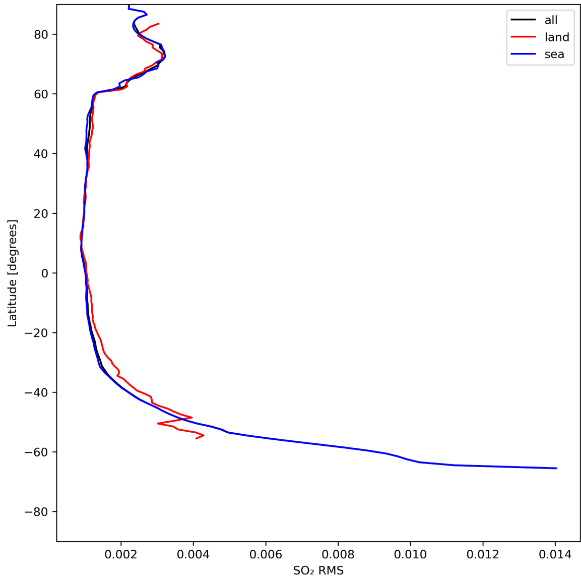
Figure 47: Zonal average of “SO 2 RMS” for 2024-07-27 to 2024-07-29.
