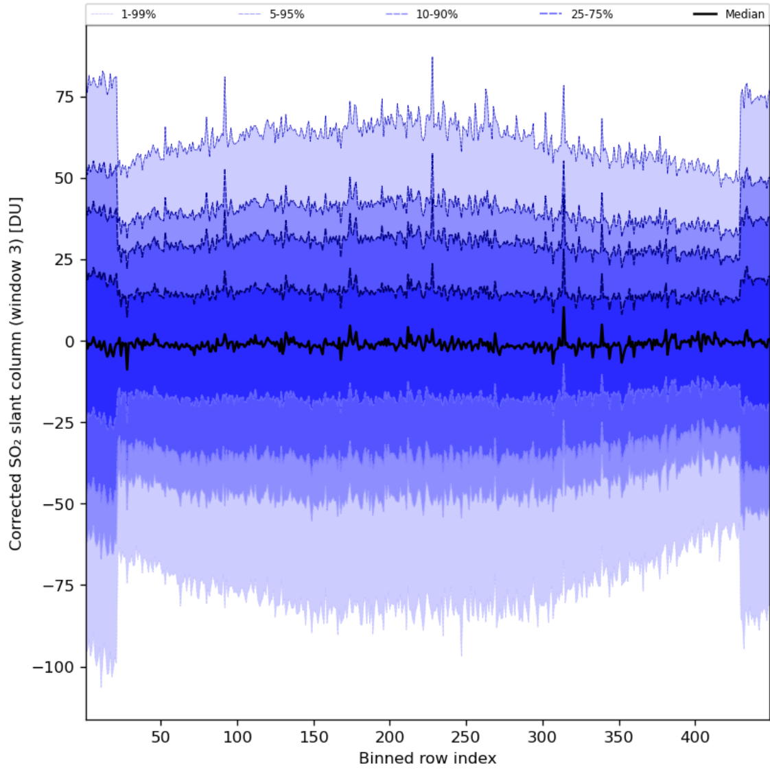
Figure 89: Along track statistics of “Corrected SO 2 slant column (window 3)” for 2024-07-27 to 2024-07-29
