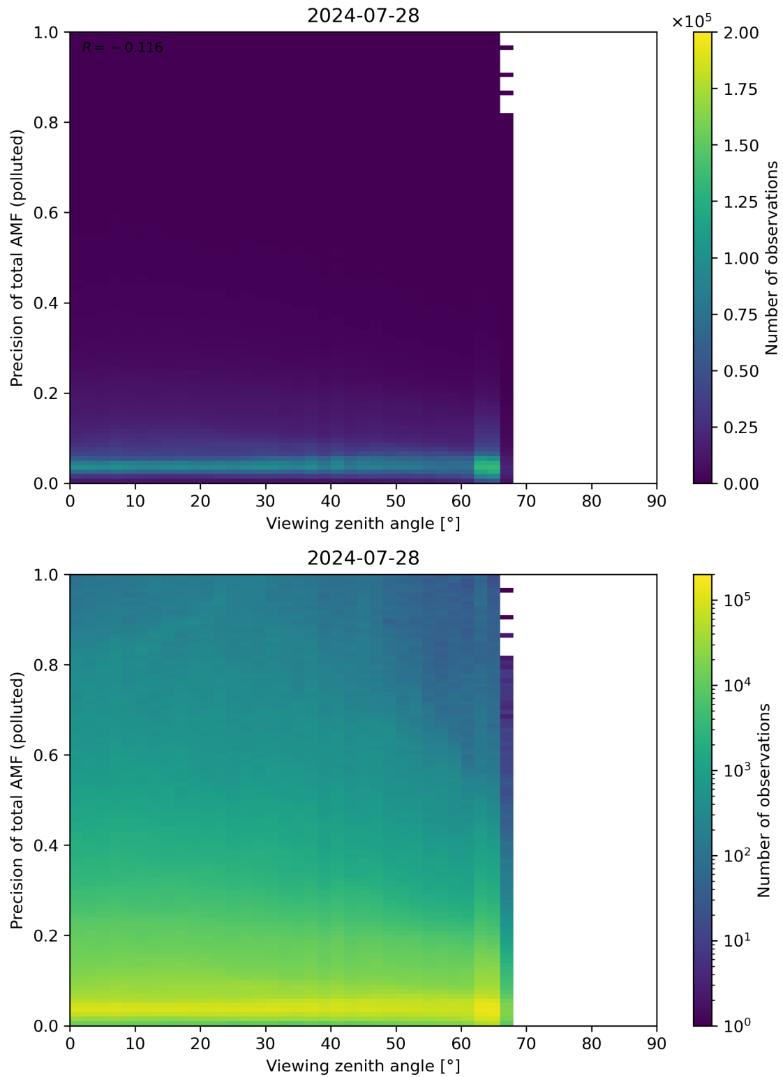
Figure 326: Scatter density plot of “Viewing zenith angle” against “Precision of total AMF (polluted)” for 2024-07-27 to 2024-07-29.
