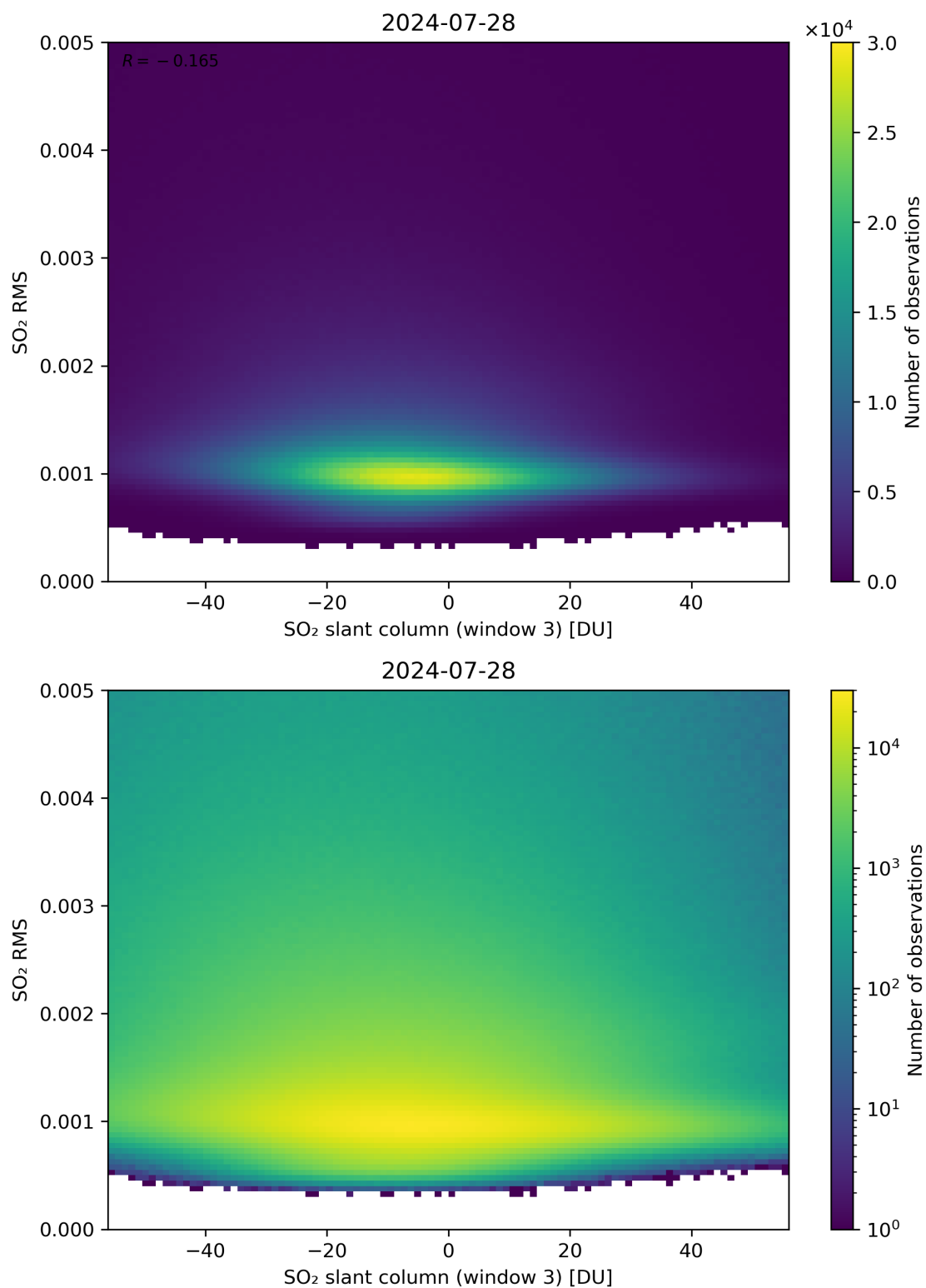
Figure 256: Scatter density plot of “SO 2 slant column (window 3)” against “SO 2 RMS” for 2024-07-27 to 2024-07-29.
