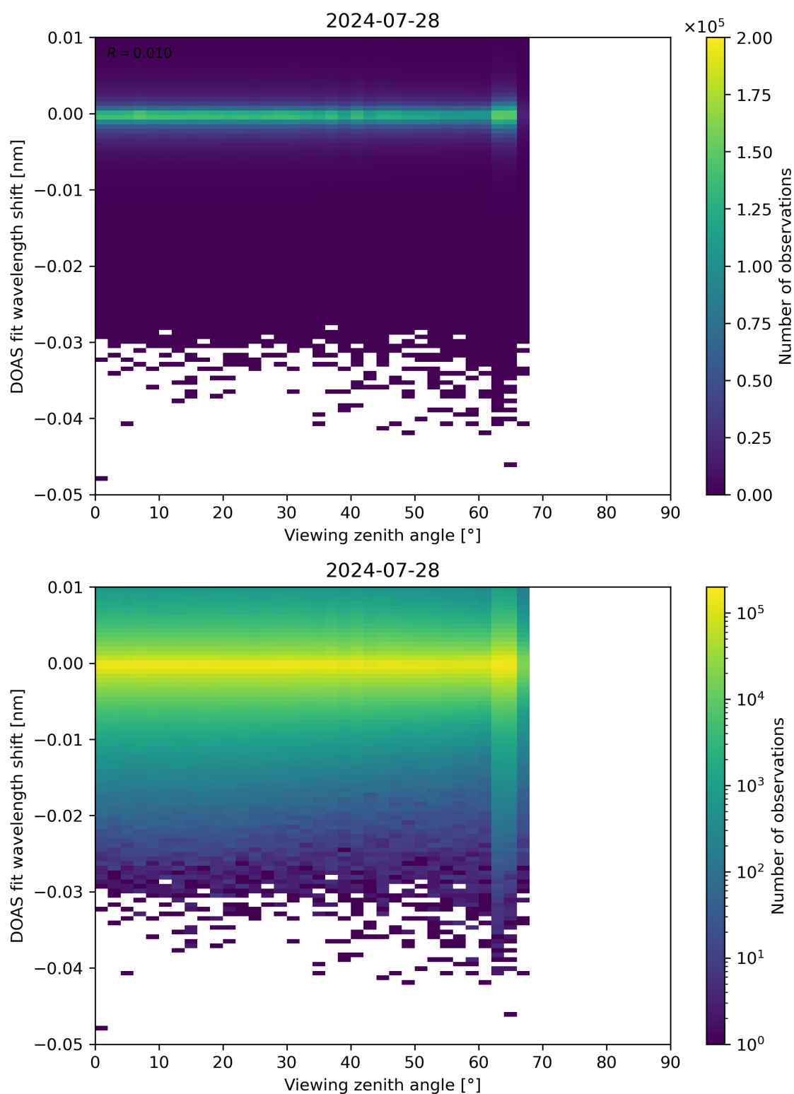
Figure 311: Scatter density plot of “Viewing zenith angle” against “DOAS fit wavelength shift” for 2024-07-27 to 2024-07-29.
