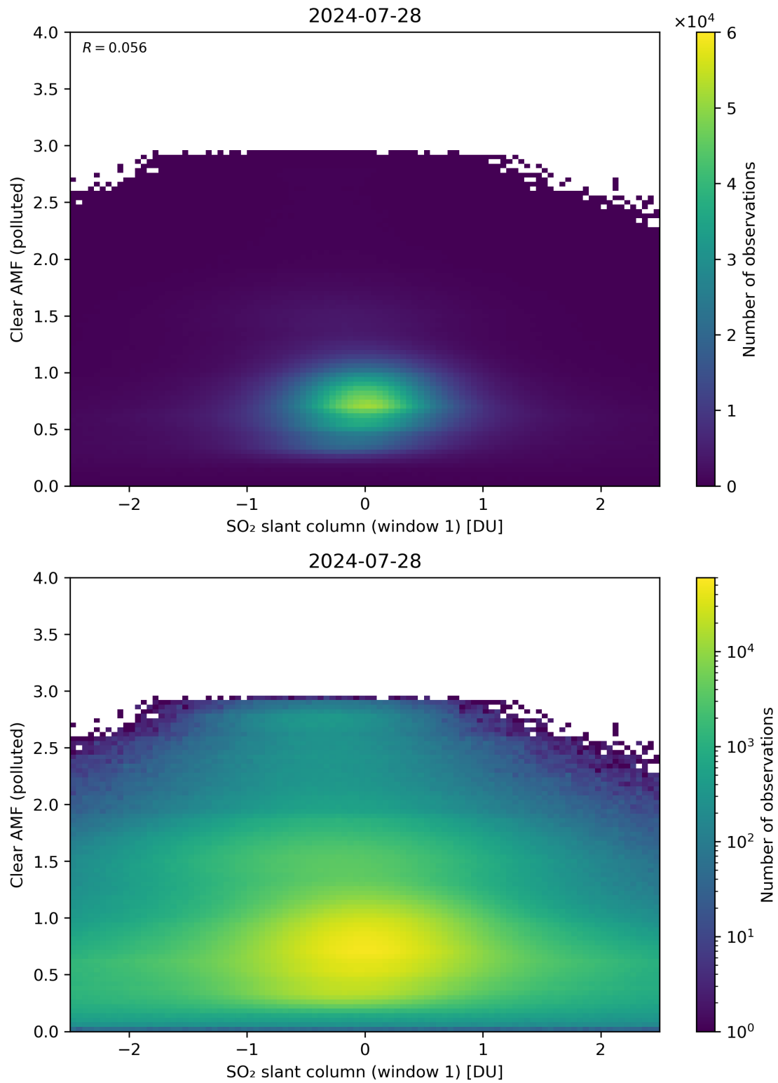
Figure 232: Scatter density plot of “SO 2 slant column (window 1)” against “Clear AMF (polluted)” for 2024-07-27 to 2024-07-29.
