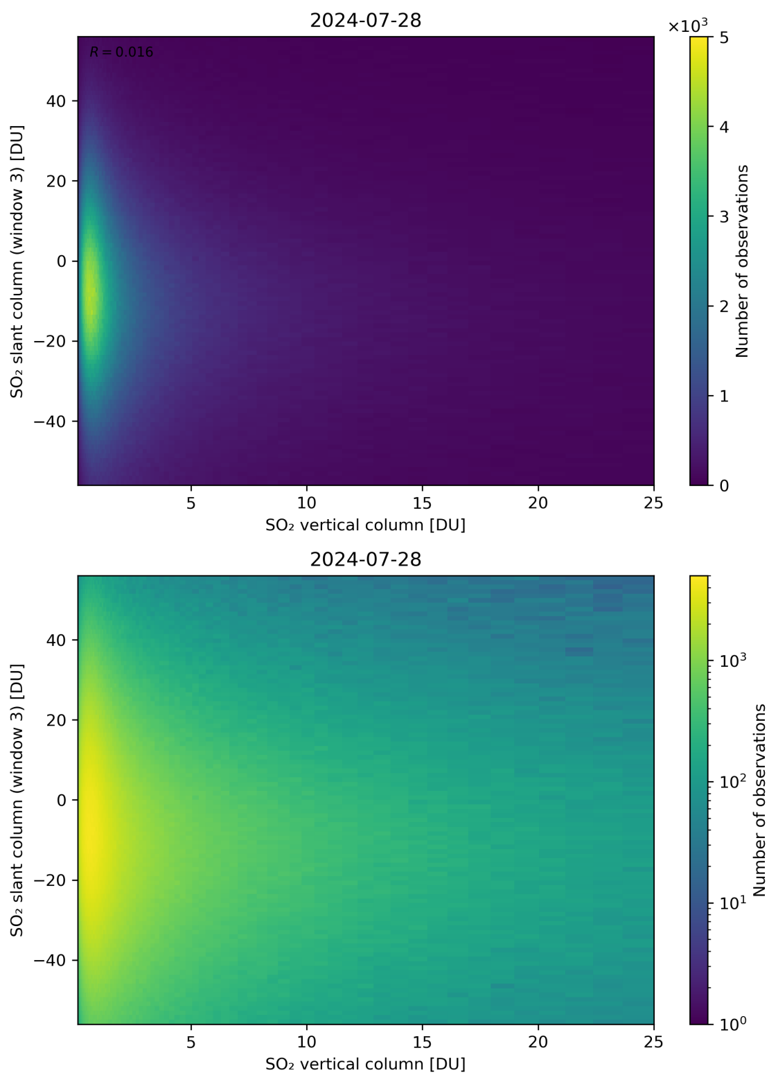
Figure 303: Scatter density plot of “SO 2 vertical column” against “SO 2 slant column (window 3)” for 2024-07-27 to 2024-07-29.
