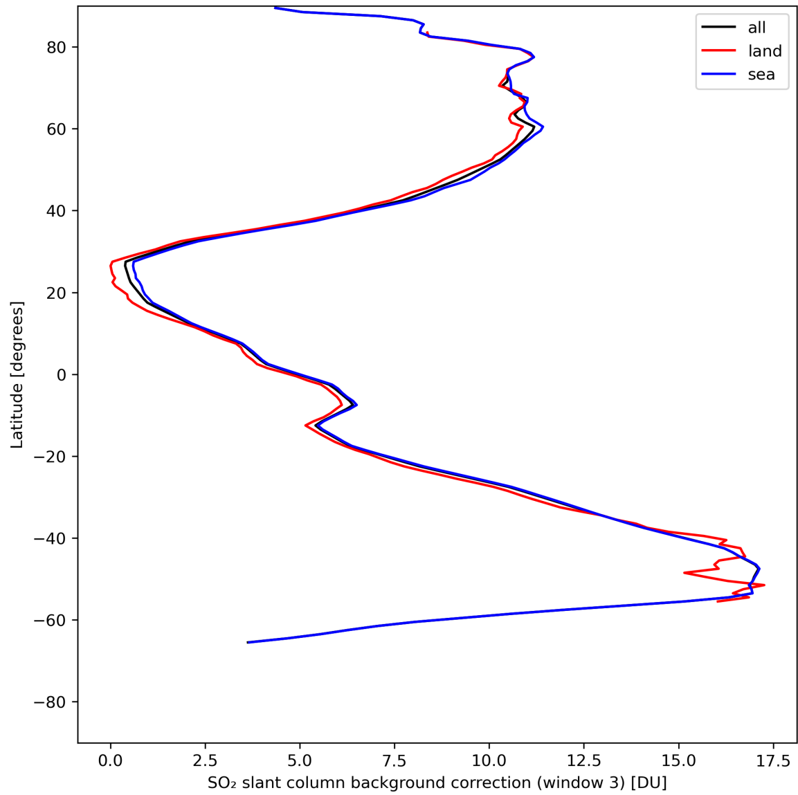
Figure 44: Zonal average of “SO 2 slant column background correction (window 3)” for 2024-07-27 to 2024-07-29.
