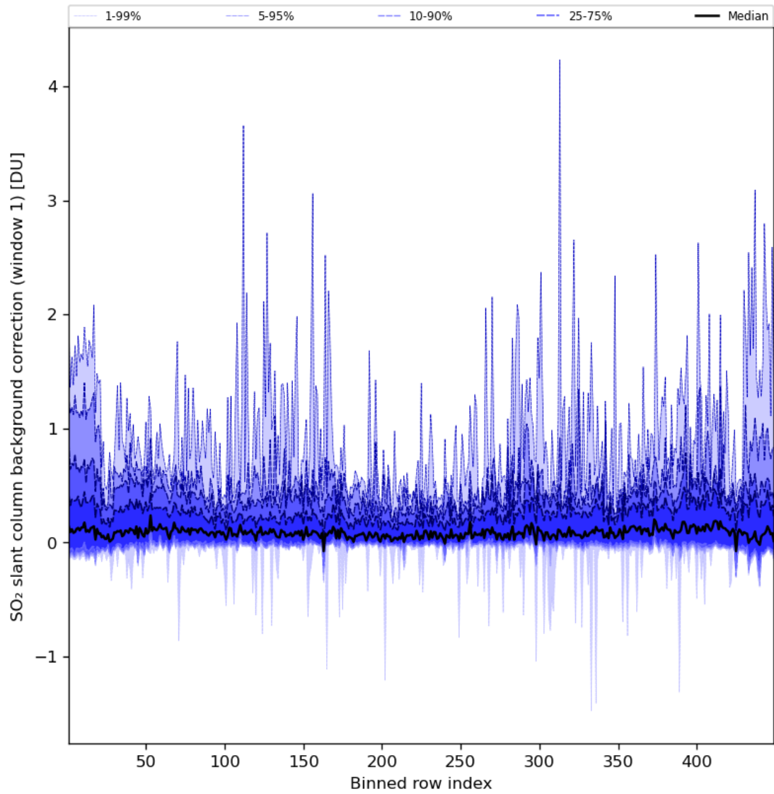
Figure 82: Along track statistics of “SO 2 slant column background correction (window 1)” for 2024-07-27 to 2024-07-29
