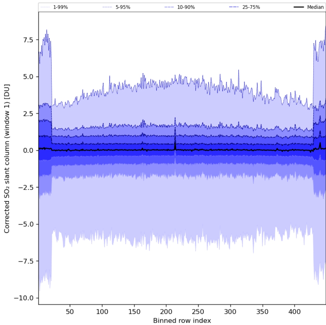
Figure 81: Along track statistics of “Corrected SO 2 slant column (window 1)” for 2024-07-27 to 2024-07-29
