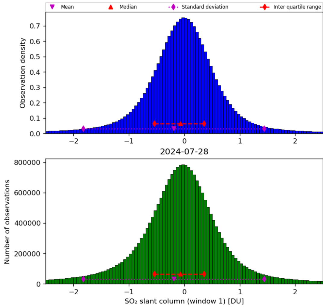
Figure 56: Histogram of “SO 2 slant column (window 1)” for 2024-07-27 to 2024-07-29
