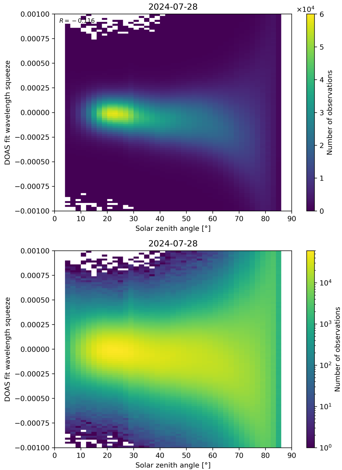
Figure 162: Scatter density plot of “Solar zenith angle” against “DOAS fit wavelength squeeze” for 2024-07-27 to 2024-07-29.
