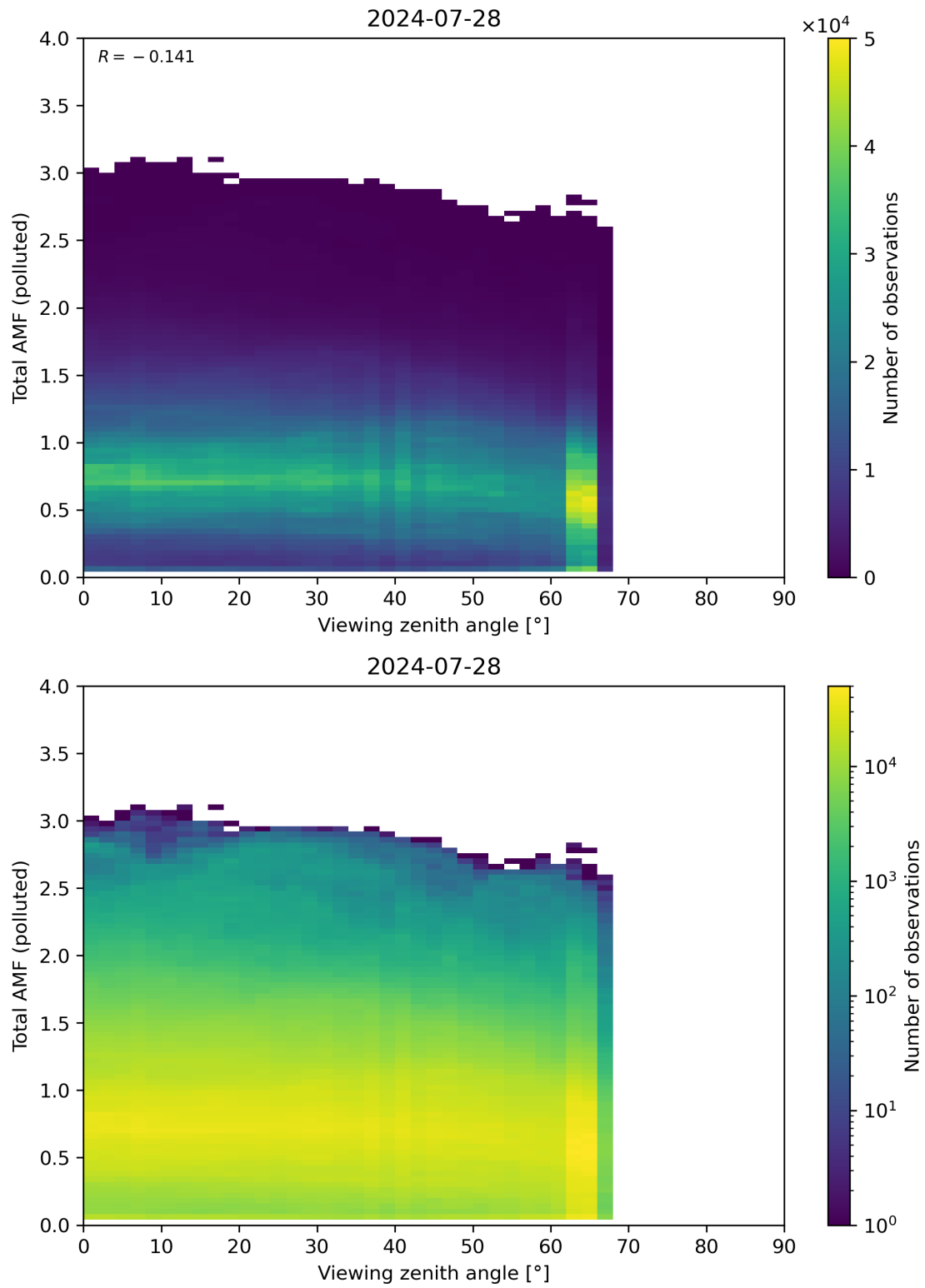
Figure 325: Scatter density plot of “Viewing zenith angle” against “Total AMF (polluted)” for 2024-07-27 to 2024-07-29.
