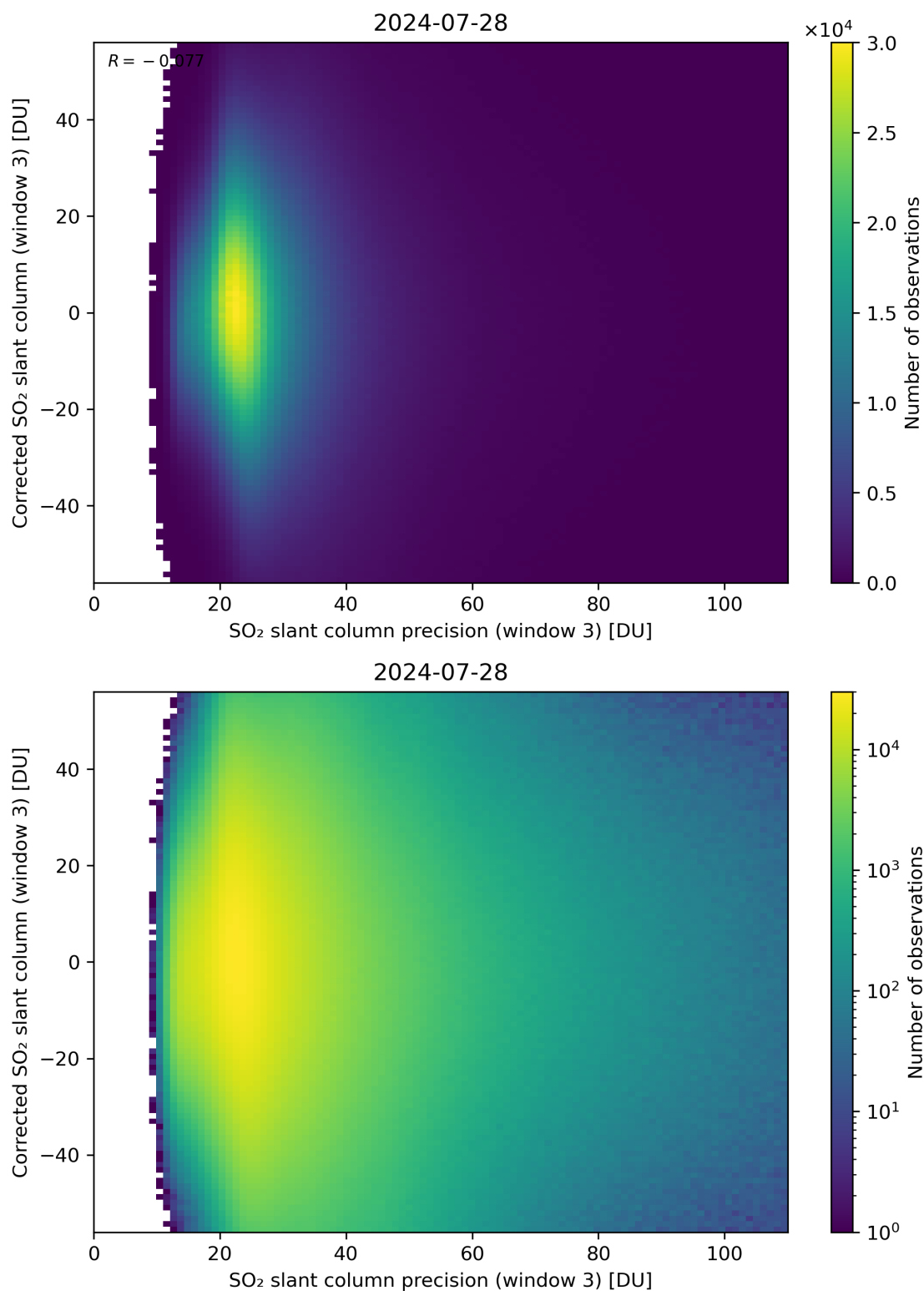
Figure 262: Scatter density plot of “SO 2 slant column precision (window 3)” against “Corrected SO 2 slant column (window 3)” for 2024-07-27 to 2024-07-29.
