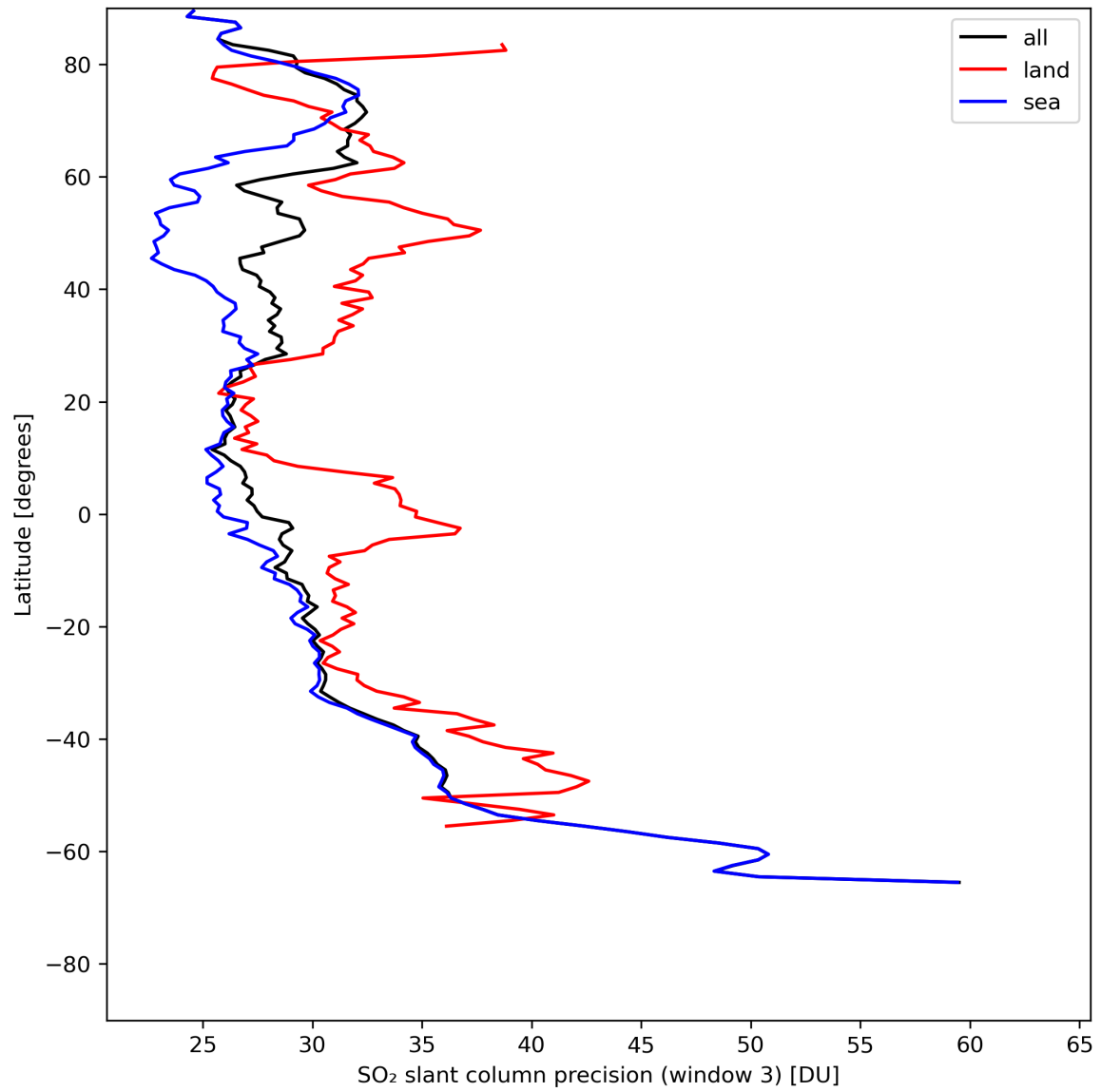
Figure 42: Zonal average of “SO 2 slant column precision (window 3)” for 2024-07-27 to 2024-07-29.
