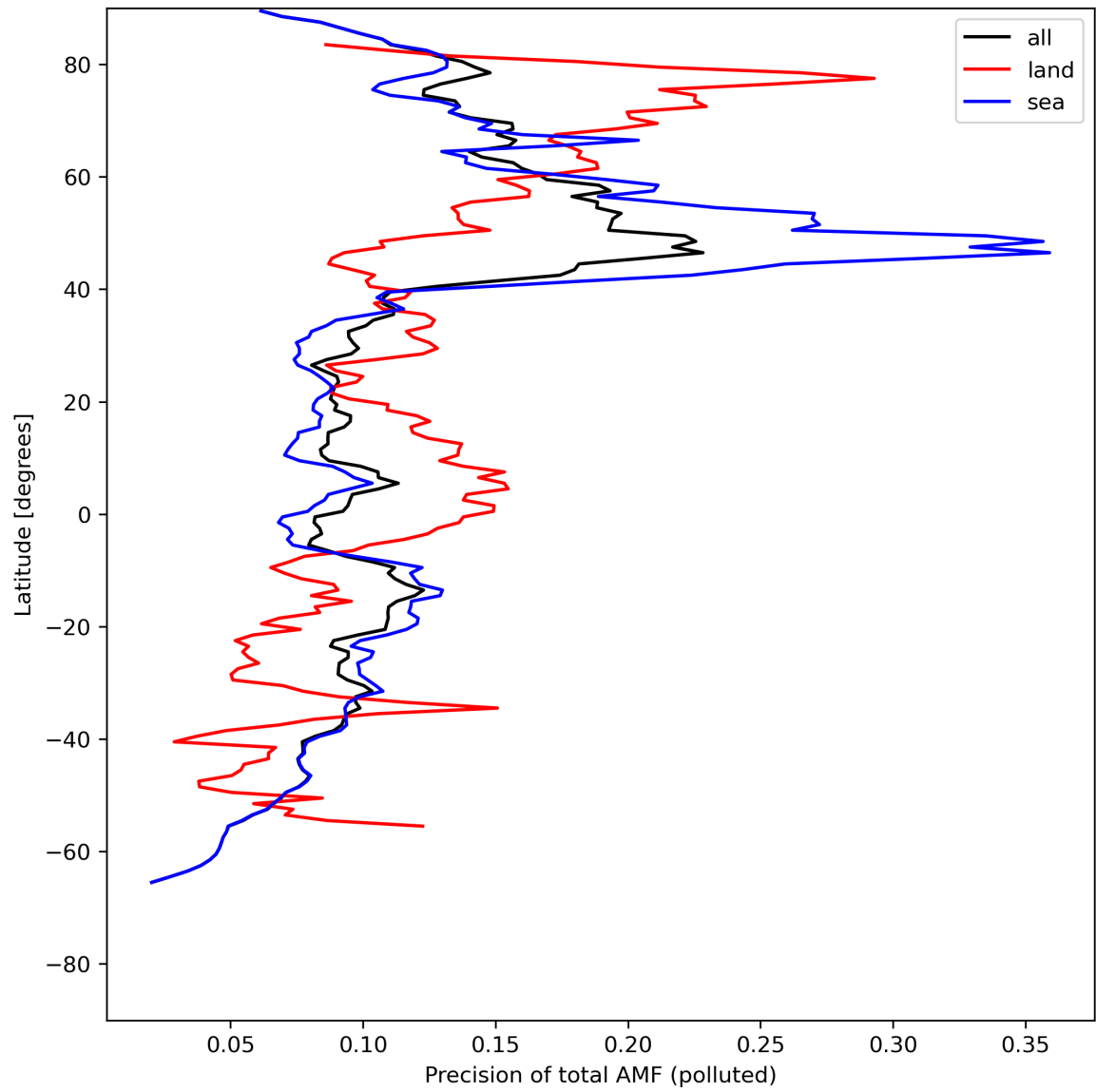
Figure 49: Zonal average of “Precision of total AMF (polluted)” for 2024-07-27 to 2024-07-29.
