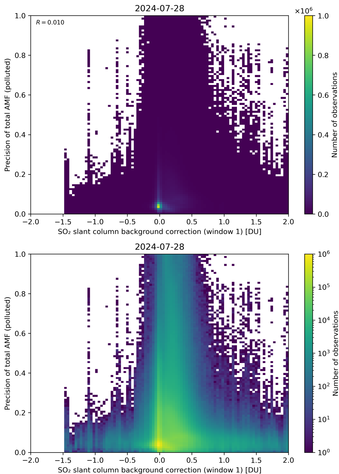
Figure 110: Scatter density plot of “SO 2 slant column background correction (window 1)” against “Precision of total AMF (polluted)” for 2024-07-27 to 2024-07-29.
