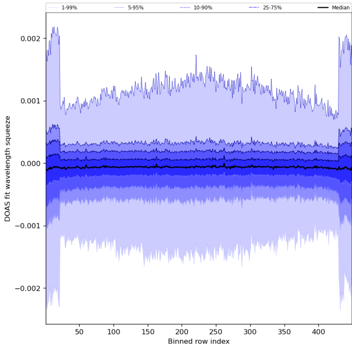
Figure 92: Along track statistics of “DOAS fit wavelength squeeze” for 2024-07-27 to 2024-07-29
