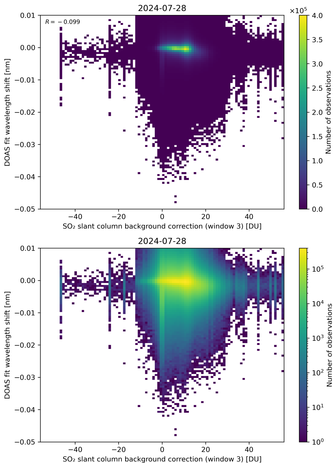
Figure 121: Scatter density plot of “SO 2 slant column background correction (window 3)” against “DOAS fit wavelength shift” for 2024-07-27 to 2024-07-29.
