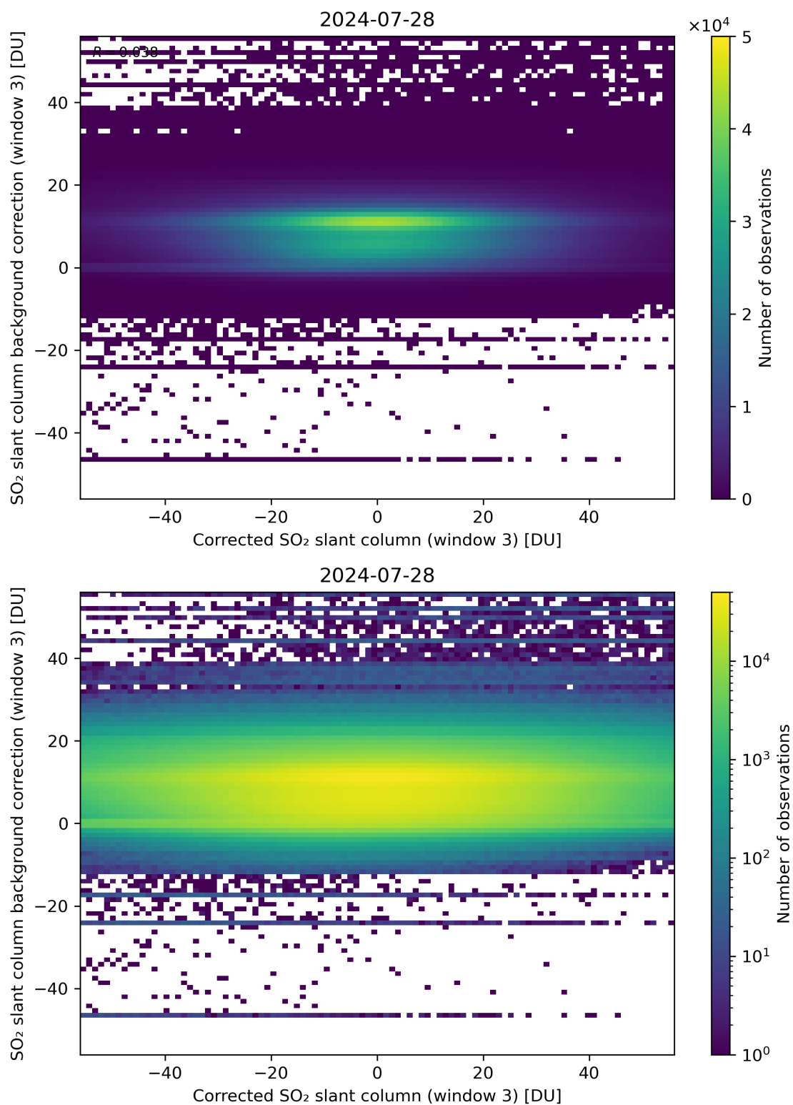
Figure 205: Scatter density plot of “Corrected SO 2 slant column (window 3)” against “SO 2 slant column background correction (window 3)” for 2024-07-27 to 2024-07-29.
