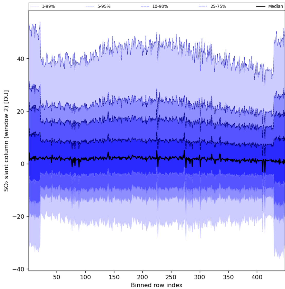
Figure 83: Along track statistics of “SO 2 slant column (window 2)” for 2024-07-27 to 2024-07-29
