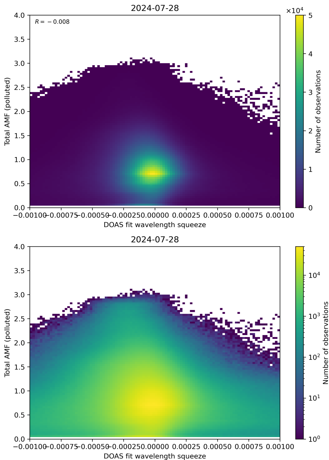
Figure 134: Scatter density plot of “DOAS fit wavelength squeeze” against “Total AMF (polluted)” for 2024-07-27 to 2024-07-29.
