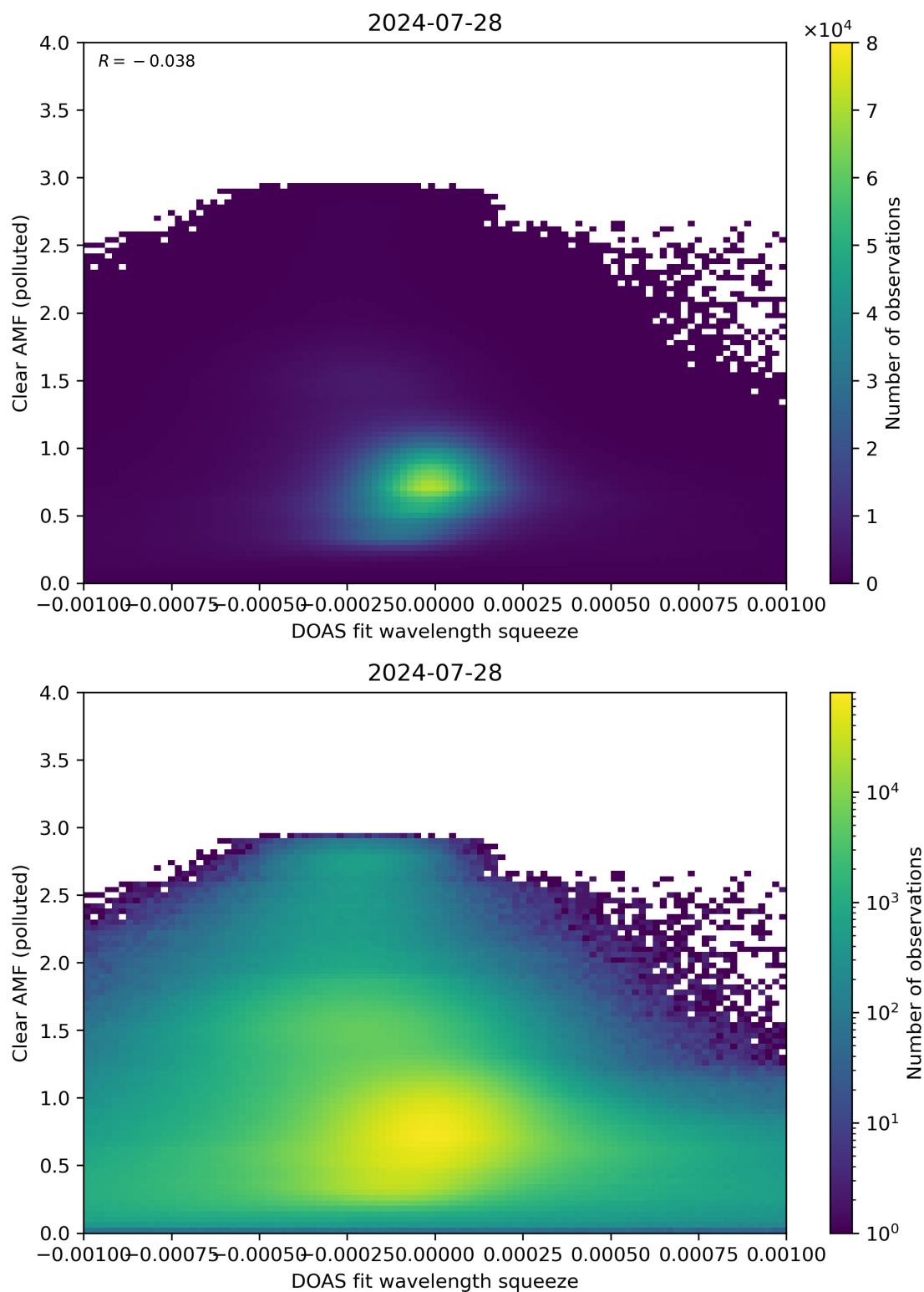
Figure 133: Scatter density plot of “DOAS fit wavelength squeeze” against “Clear AMF (polluted)” for 2024-07-27 to 2024-07-29.
