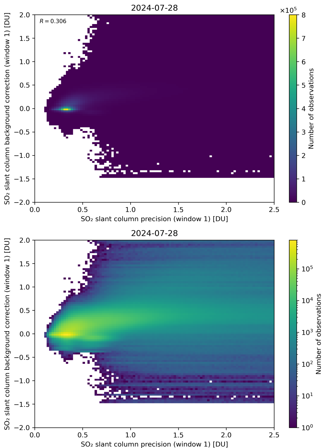
Figure 218: Scatter density plot of “SO 2 slant column precision (window 1)” against “SO 2 slant column background correction (window 1)” for 2024-07-27 to 2024-07-29.
