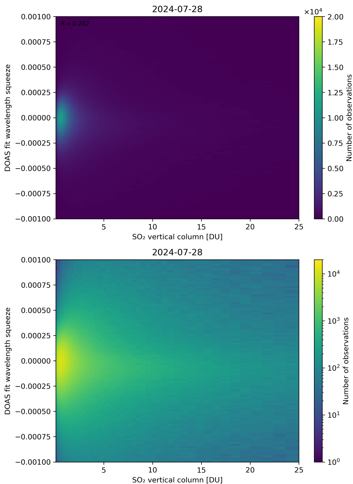
Figure 277: Scatter density plot of “SO 2 vertical column” against “DOAS fit wavelength squeeze” for 2024-07-27 to 2024-07-29.
