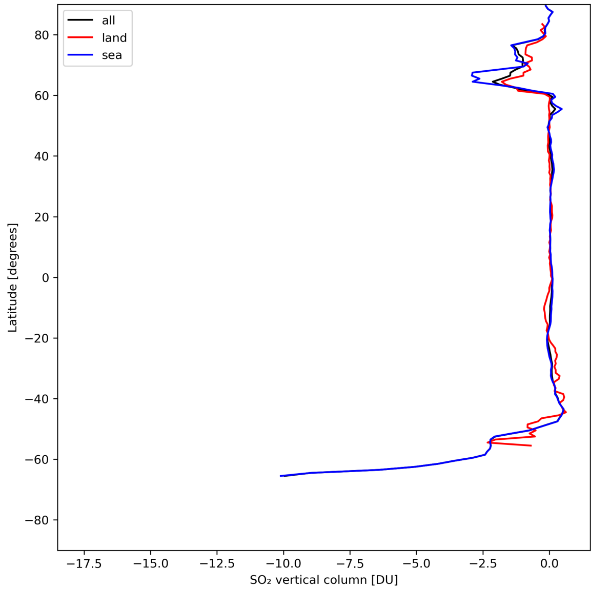
Figure 30: Zonal average of “SO 2 vertical column” for 2024-07-27 to 2024-07-29.
