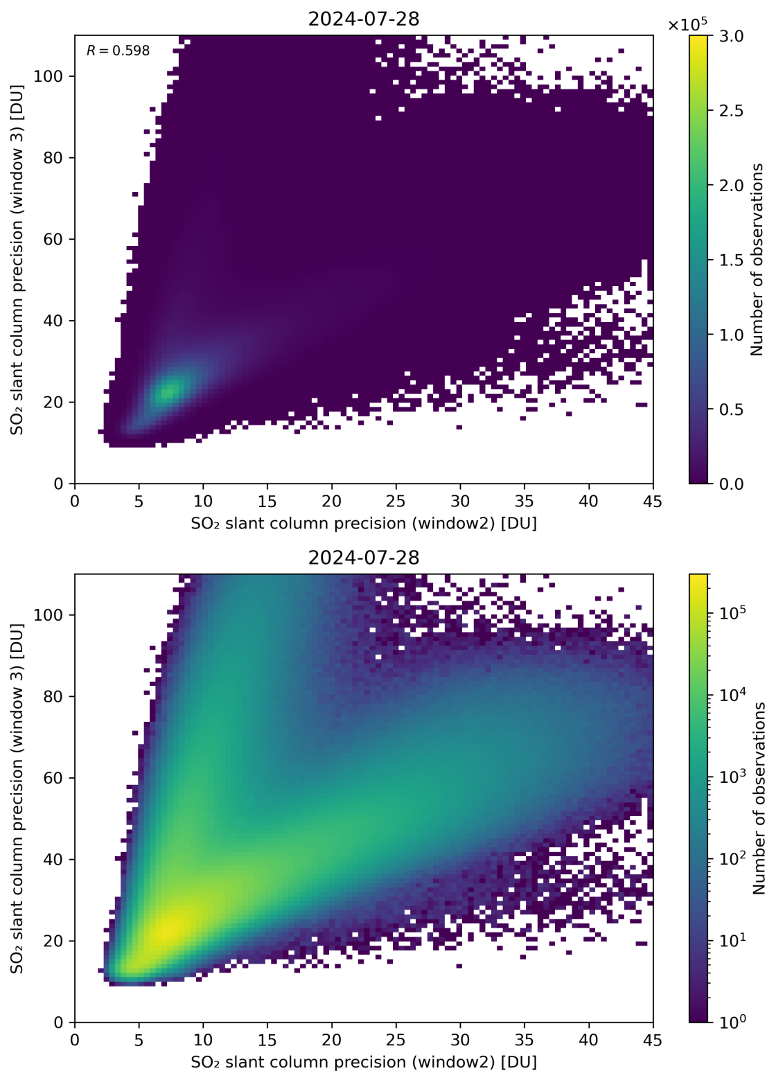
Figure 250: Scatter density plot of “SO 2 slant column precision (window2)” against “SO 2 slant column precision (window 3)” for 2024-07-27 to 2024-07-29.
