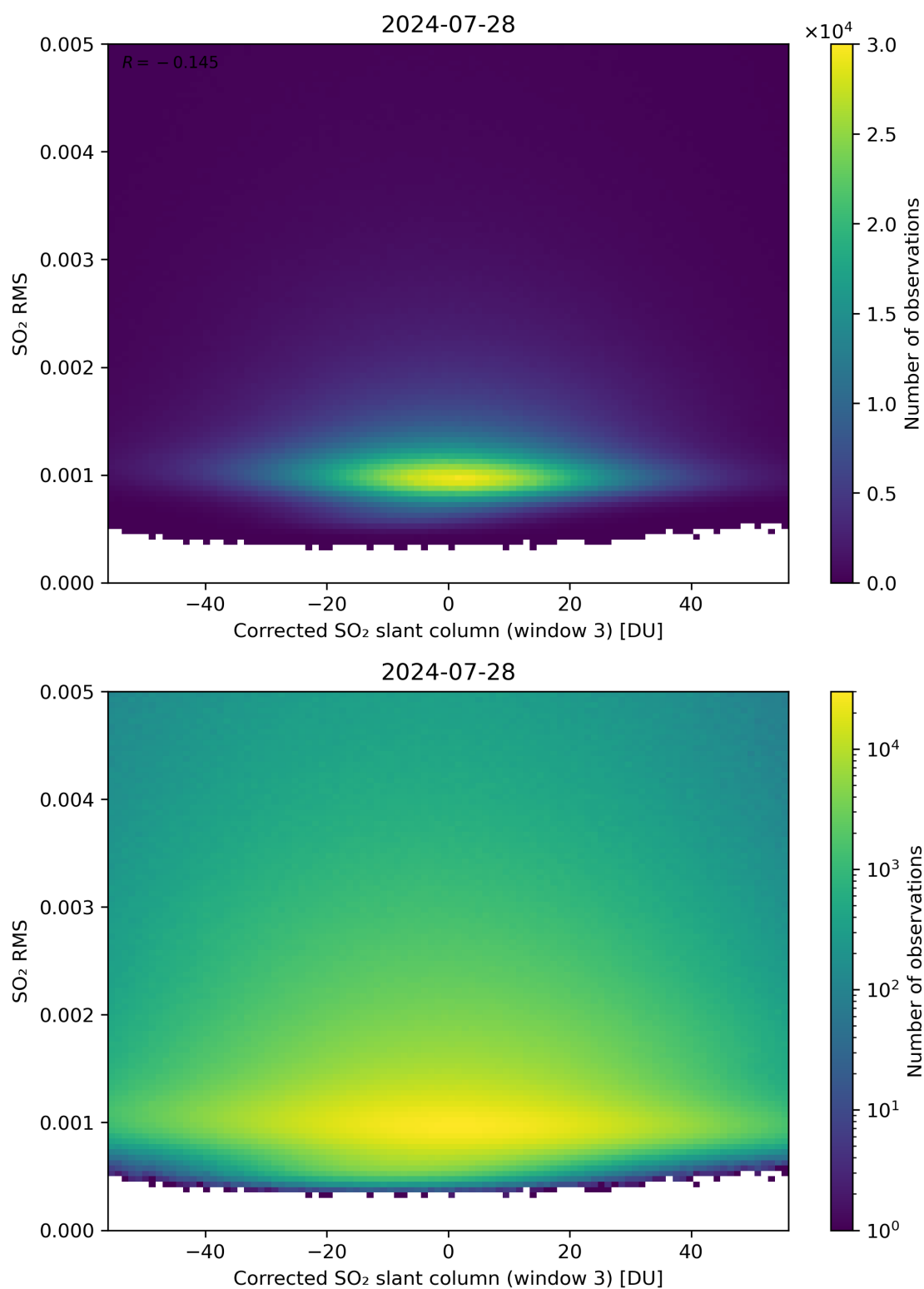
Figure 208: Scatter density plot of “Corrected SO 2 slant column (window 3)” against “SO 2 RMS” for 2024-07-27 to 2024-07-29.
