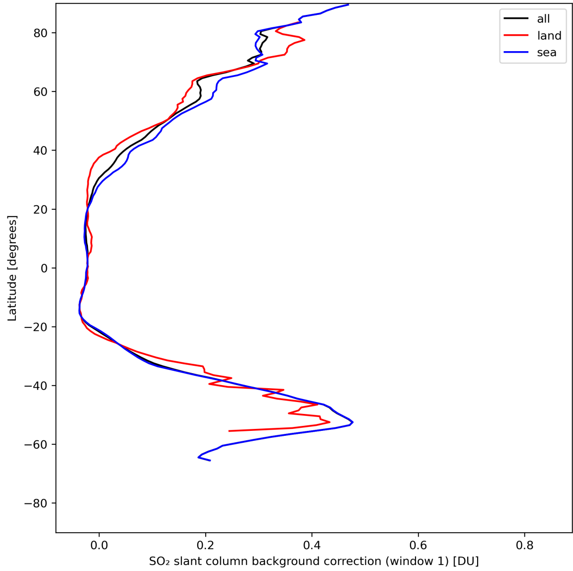
Figure 36: Zonal average of “SO 2 slant column background correction (window 1)” for 2024-07-27 to 2024-07-29.
