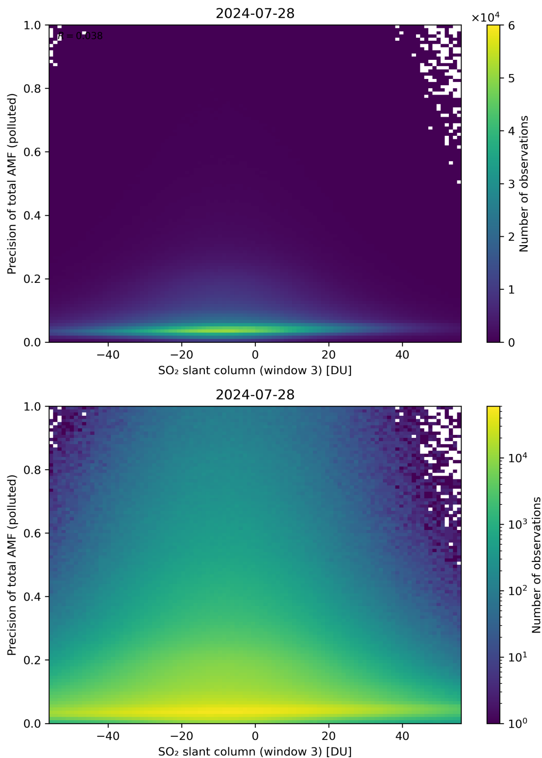
Figure 269: Scatter density plot of “SO 2 slant column (window 3)” against “Precision of total AMF (polluted)” for 2024-07-27 to 2024-07-29.
