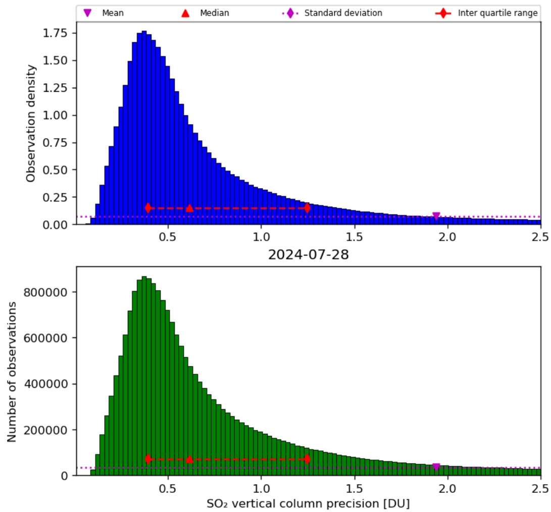
Figure 54: Histogram of “SO 2 vertical column precision” for 2024-07-27 to 2024-07-29
