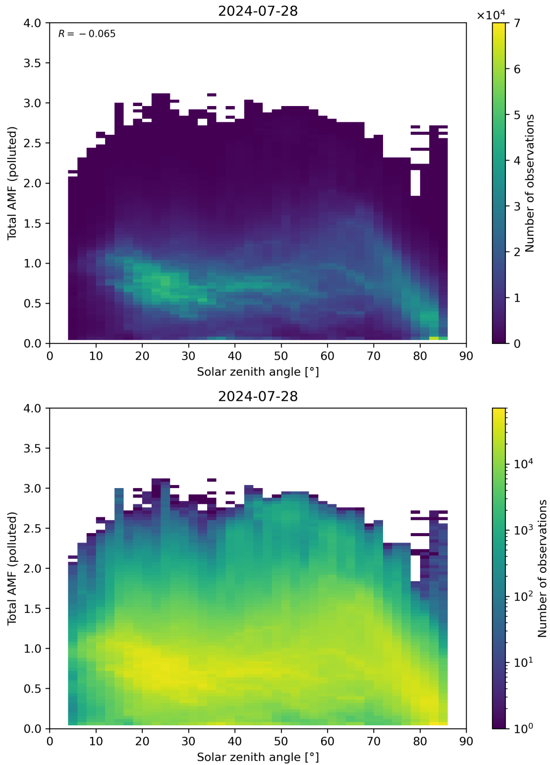
Figure 174: Scatter density plot of “Solar zenith angle” against “Total AMF (polluted)” for 2024-07-27 to 2024-07-29.
