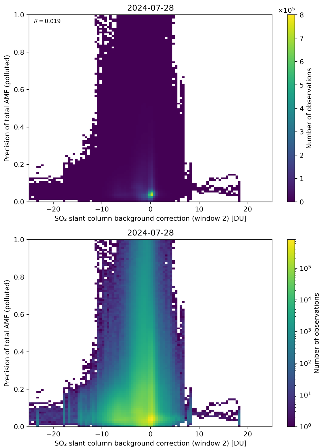
Figure 120: Scatter density plot of “SO 2 slant column background correction (window 2)” against “Precision of total AMF (polluted)” for 2024-07-27 to 2024-07-29.
