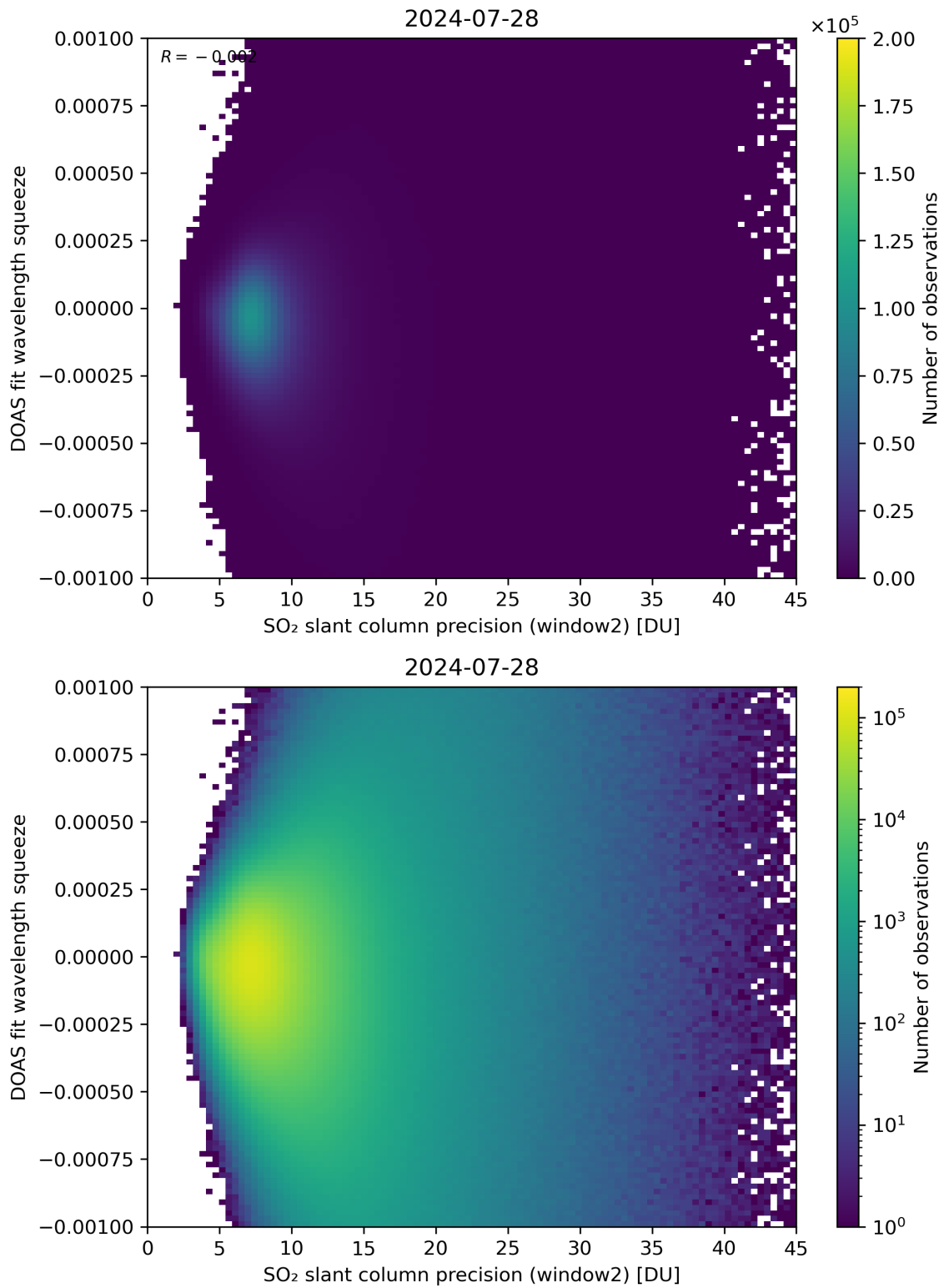
Figure 244: Scatter density plot of “SO 2 slant column precision (window2)” against “DOAS fit wavelength squeeze” for 2024-07-27 to 2024-07-29.
