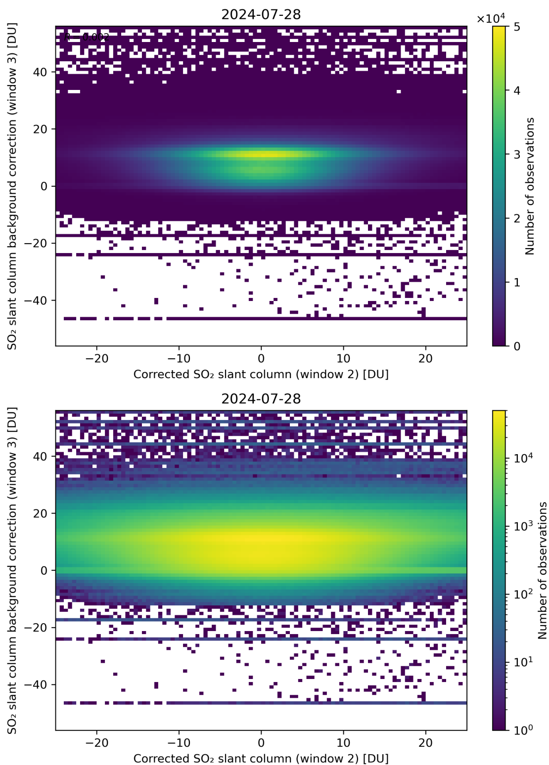
Figure 195: Scatter density plot of “Corrected SO 2 slant column (window 2)” against “SO 2 slant column background correction (window 3)” for 2024-07-27 to 2024-07-29.
