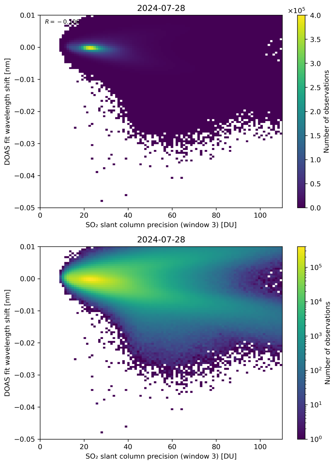
Figure 258: Scatter density plot of “SO 2 slant column precision (window 3)” against “DOAS fit wavelength shift” for 2024-07-27 to 2024-07-29.
