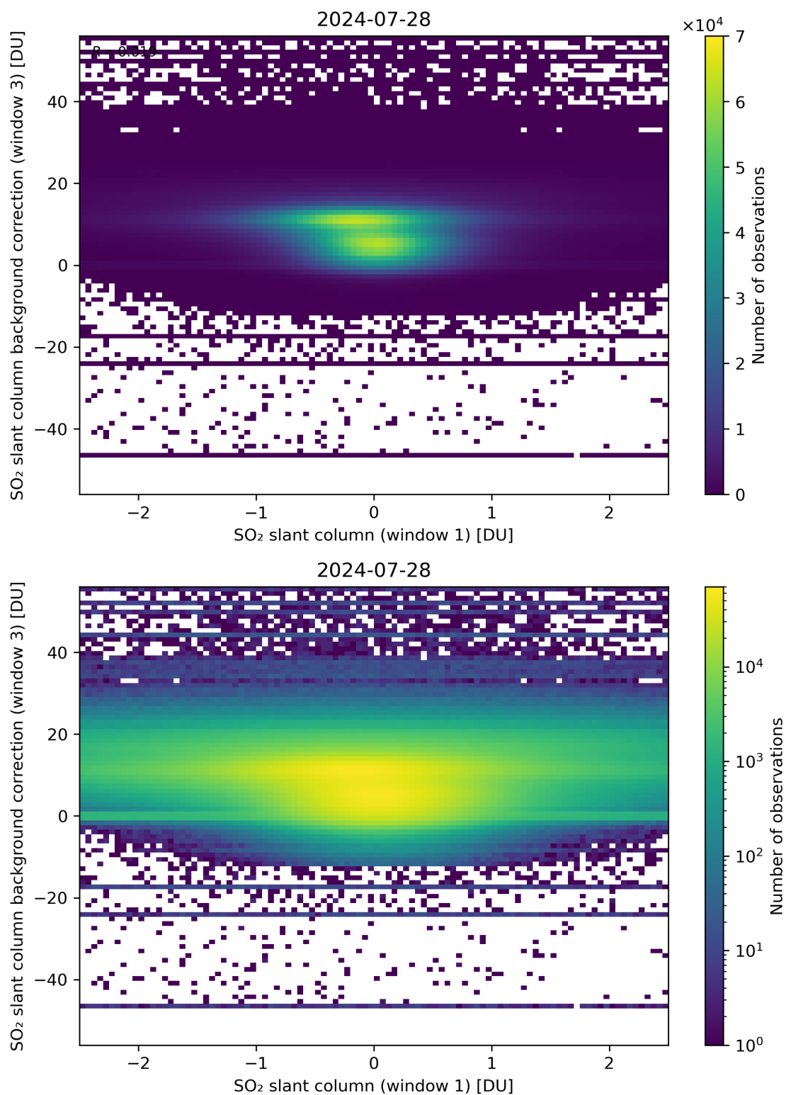
Figure 214: Scatter density plot of “SO 2 slant column (window 1)” against “SO 2 slant column background correction (window 3)” for 2024-07-27 to 2024-07-29.
