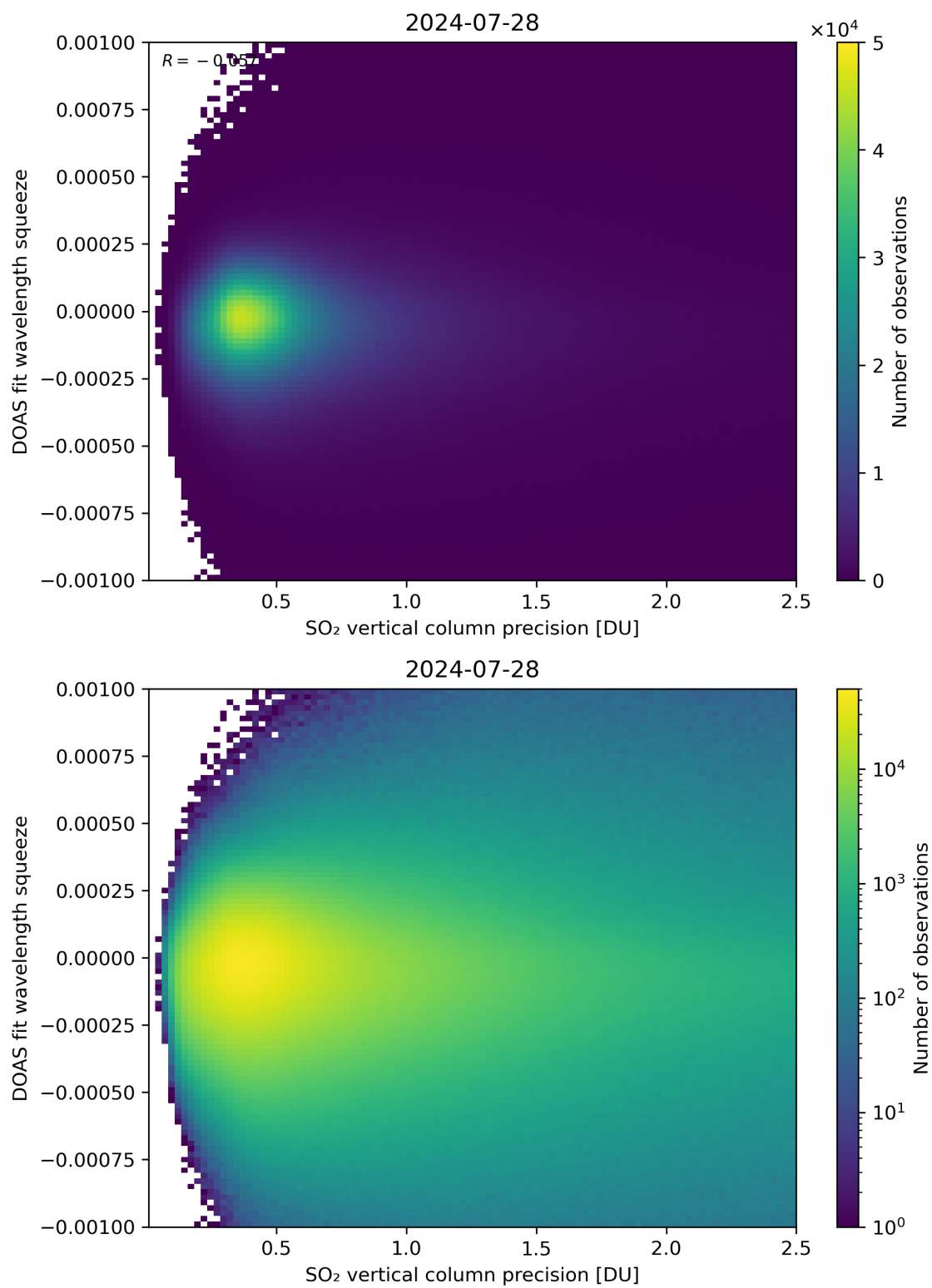
Figure 283: Scatter density plot of “SO 2 vertical column precision” against “DOAS fit wavelength squeeze” for 2024-07-27 to 2024-07-29.
