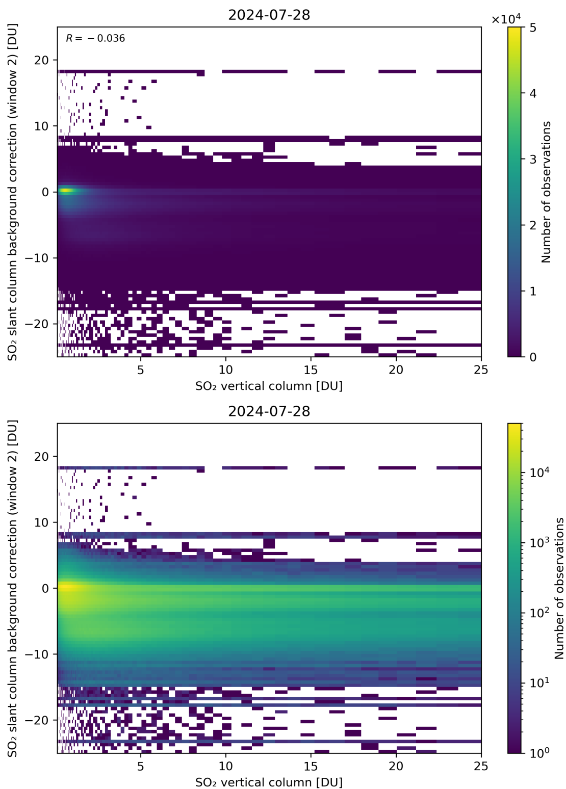
Figure 274: Scatter density plot of “SO 2 vertical column” against “SO 2 slant column background correction (window 2)” for 2024-07-27 to 2024-07-29.
