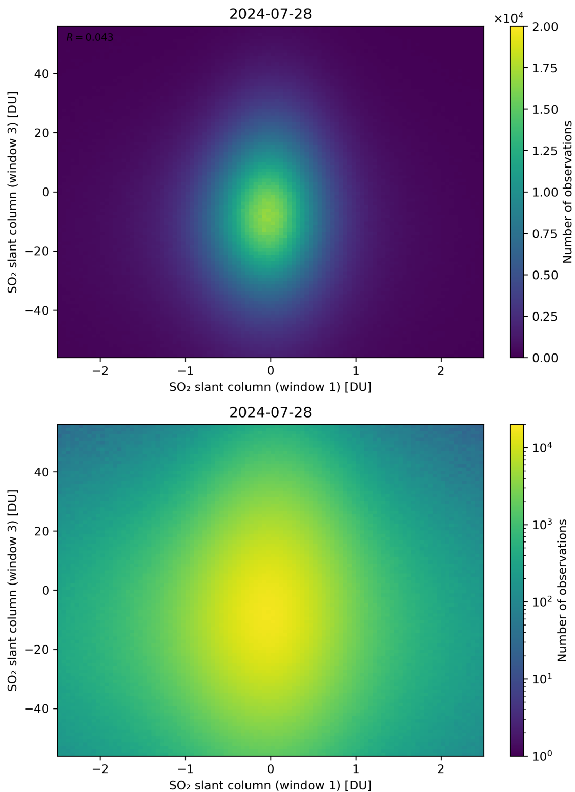
Figure 237: Scatter density plot of “SO 2 slant column (window 1)” against “SO 2 slant column (window 3)” for 2024-07-27 to 2024-07-29.
