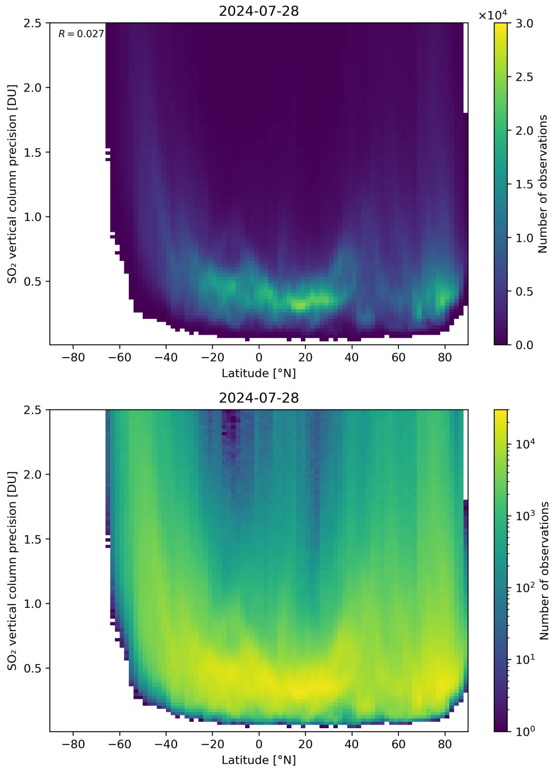
Figure 157: Scatter density plot of “Latitude” against “SO 2 vertical column precision” for 2024-07-27 to 2024-07-29.
