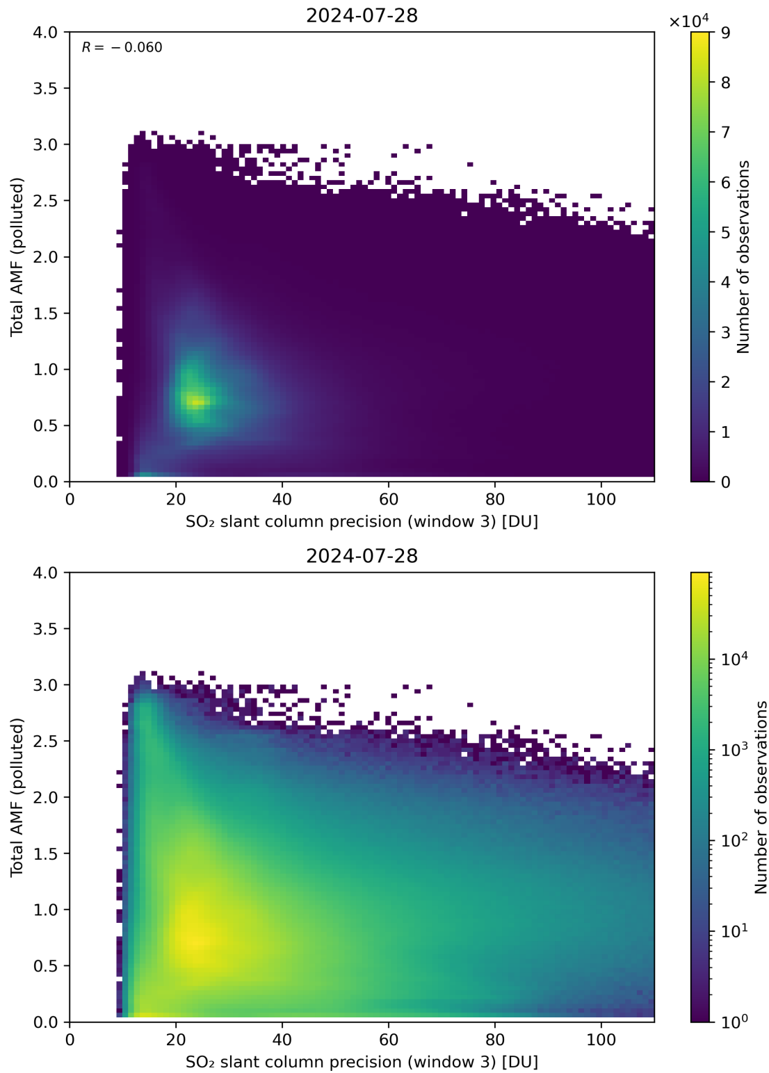
Figure 263: Scatter density plot of “SO 2 slant column precision (window 3)” against “Total AMF (polluted)” for 2024-07-27 to 2024-07-29.
