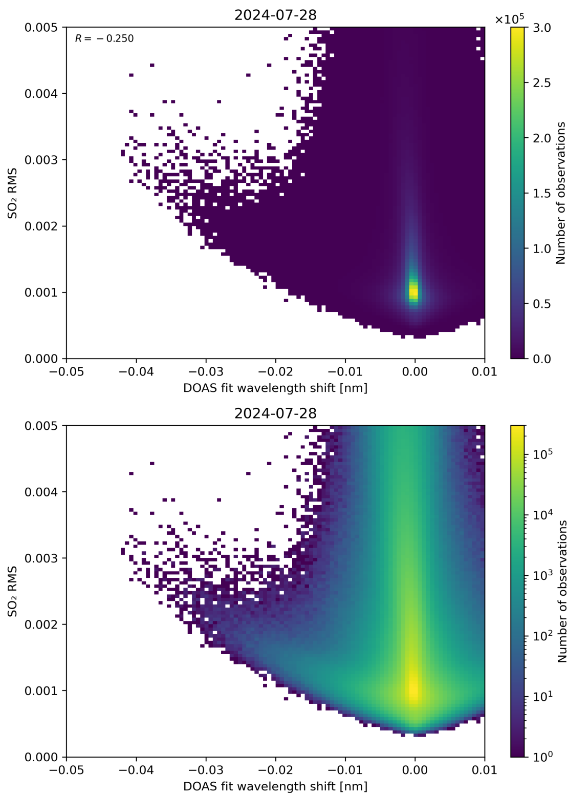
Figure 128: Scatter density plot of “DOAS fit wavelength shift” against “SO 2 RMS” for 2024-07-27 to 2024-07-29.
