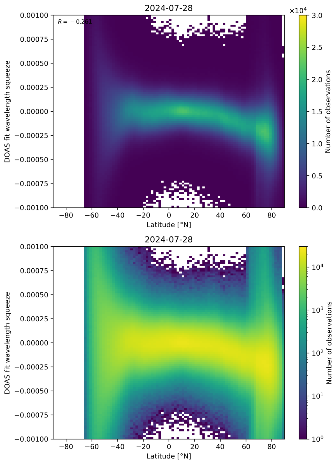
Figure 143: Scatter density plot of “Latitude” against “DOAS fit wavelength squeeze” for 2024-07-27 to 2024-07-29.
