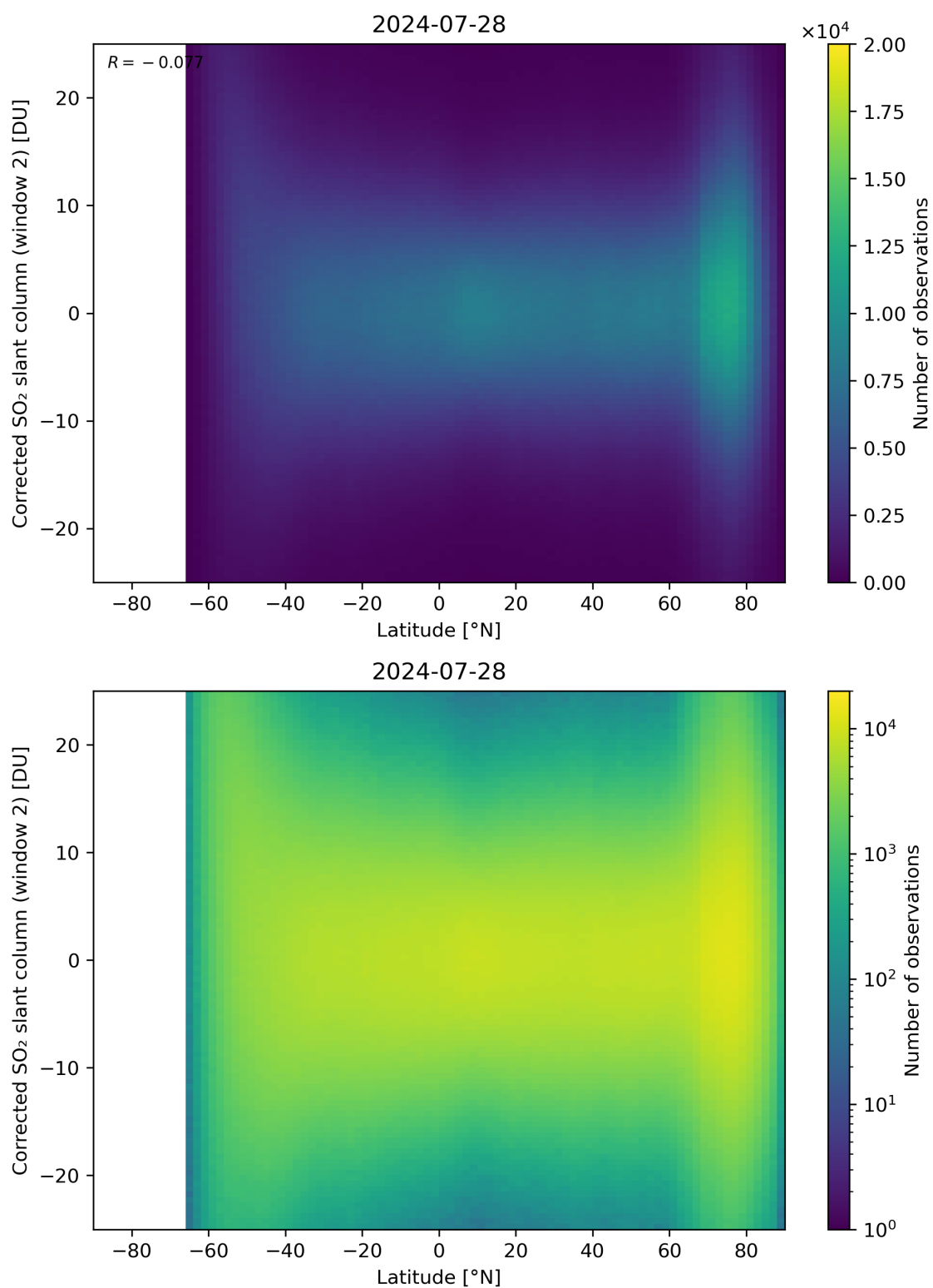
Figure 147: Scatter density plot of “Latitude” against “Corrected SO 2 slant column (window 2)” for 2024-07-27 to 2024-07-29.
