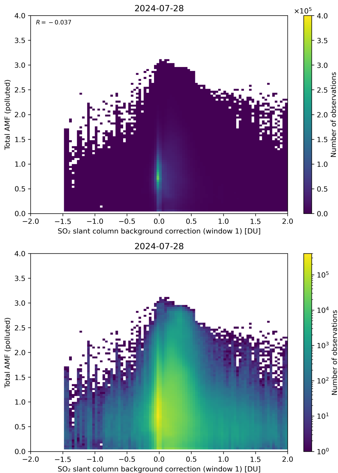
Figure 109: Scatter density plot of “SO 2 slant column background correction (window 1)” against “Total AMF (polluted)” for 2024-07-27 to 2024-07-29.
