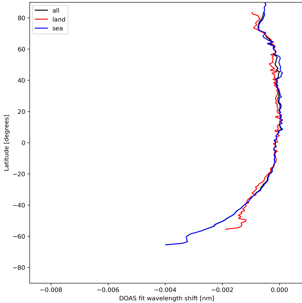
Figure 45: Zonal average of “DOAS fit wavelength shift” for 2024-07-27 to 2024-07-29.
