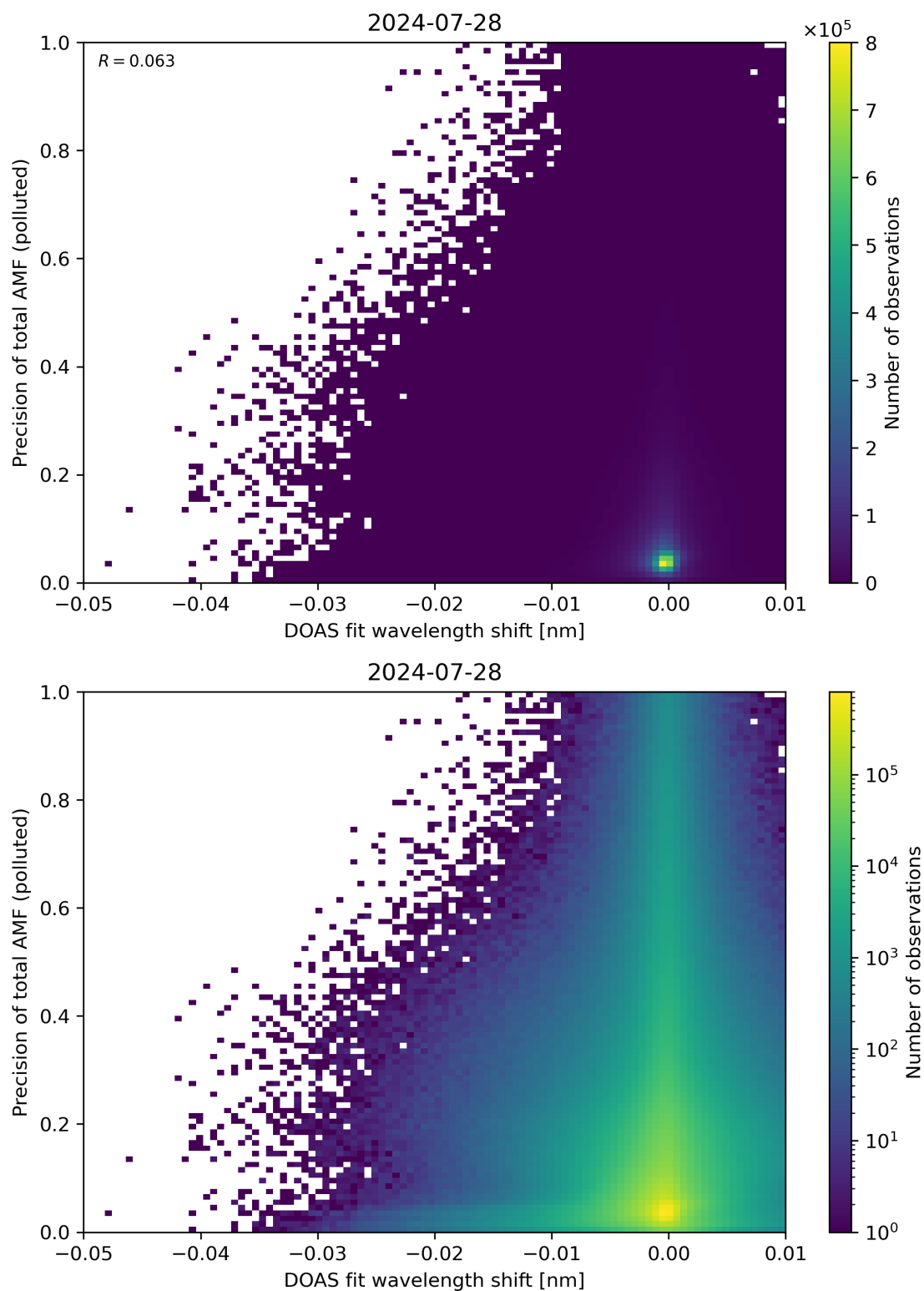
Figure 131: Scatter density plot of “DOAS fit wavelength shift” against “Precision of total AMF (polluted)” for 2024-07-27 to 2024-07-29.
