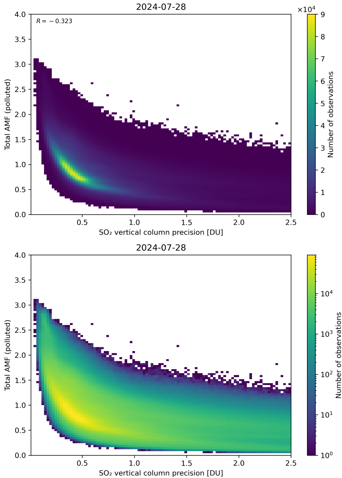
Figure 294: Scatter density plot of “SO 2 vertical column precision” against “Total AMF (polluted)” for 2024-07-27 to 2024-07-29.
