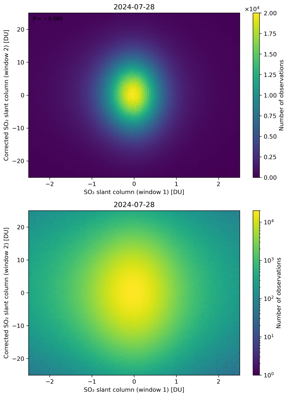
Figure 233: Scatter density plot of “SO 2 slant column (window 1)” against “Corrected SO 2 slant column (window 2)” for 2024-07-27 to 2024-07-29.
