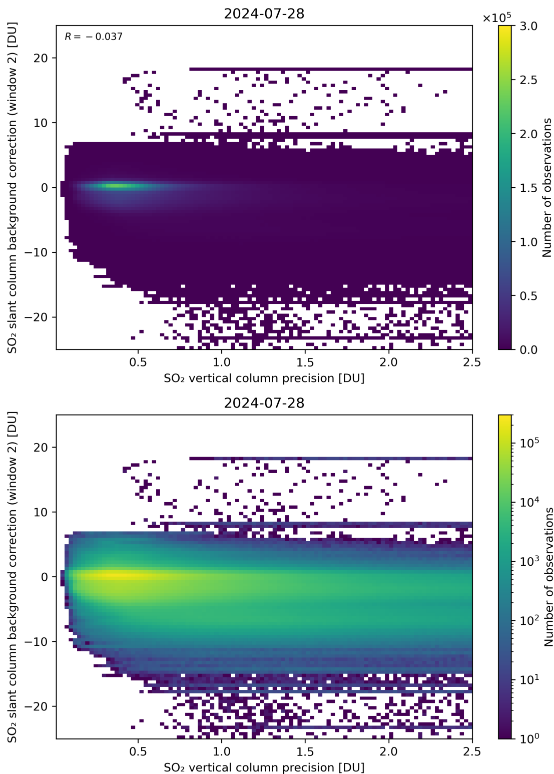
Figure 280: Scatter density plot of “SO 2 vertical column precision” against “SO 2 slant column background correction (window 2)” for 2024-07-27 to 2024-07-29.
