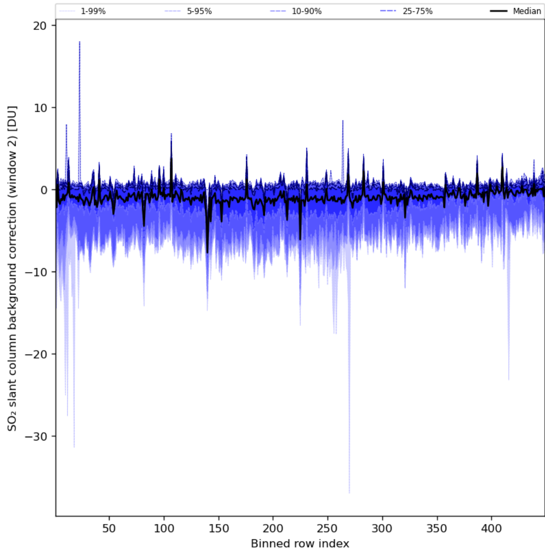
Figure 86: Along track statistics of “SO 2 slant column background correction (window 2)” for 2024-07-27 to 2024-07-29
