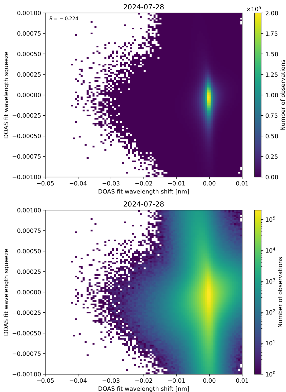
Figure 127: Scatter density plot of “DOAS fit wavelength shift” against “DOAS fit wavelength squeeze” for 2024-07-27 to 2024-07-29.
