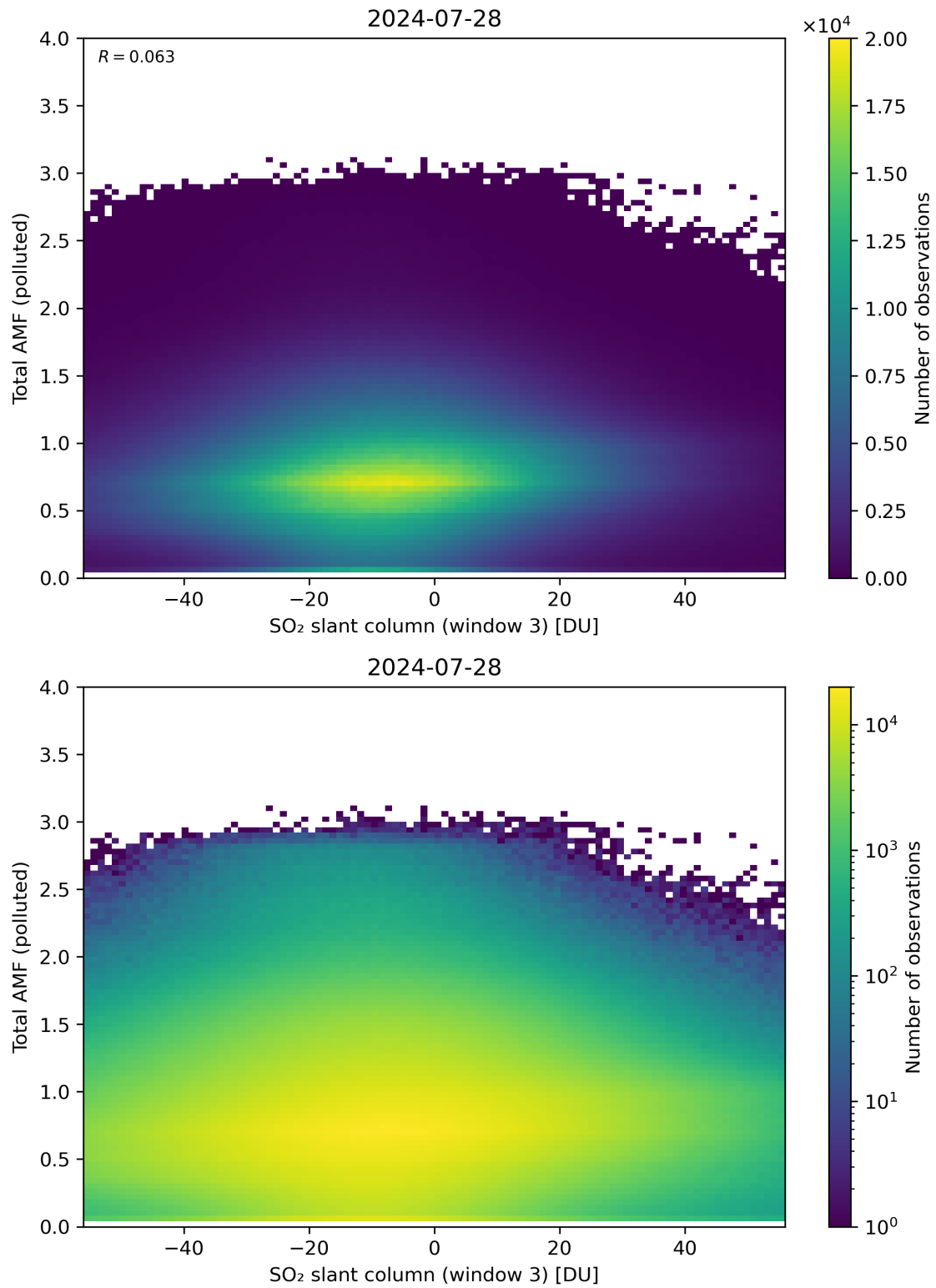
Figure 268: Scatter density plot of “SO 2 slant column (window 3)” against “Total AMF (polluted)” for 2024-07-27 to 2024-07-29.
