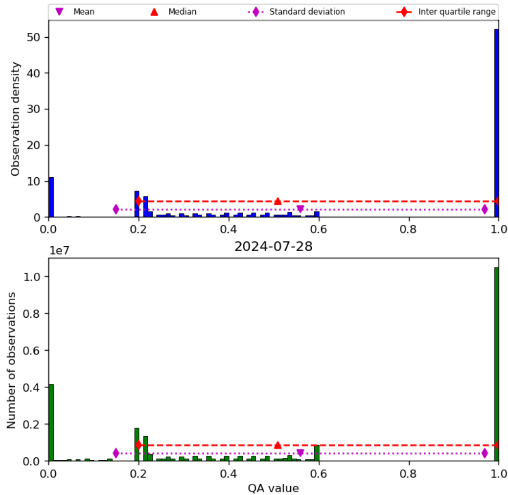
Figure 52: Histogram of “QA value” for 2024-07-27 to 2024-07-29
