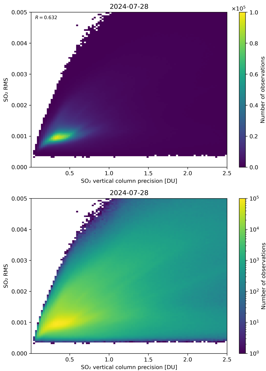
Figure 284: Scatter density plot of “SO 2 vertical column precision” against “SO 2 RMS” for 2024-07-27 to 2024-07-29.
