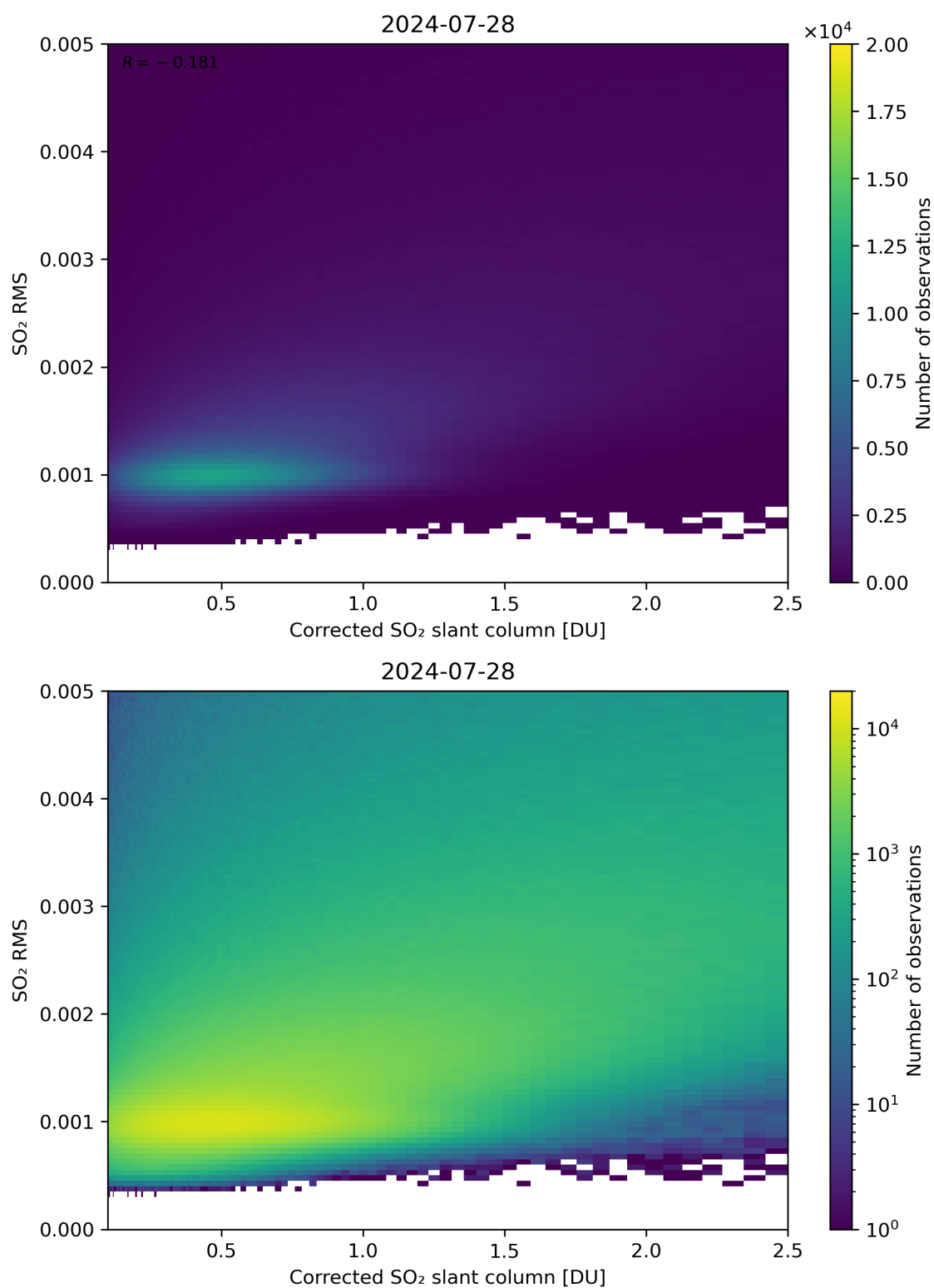
Figure 183: Scatter density plot of “Corrected SO 2 slant column” against “SO 2 RMS” for 2024-07-27 to 2024-07-29.
