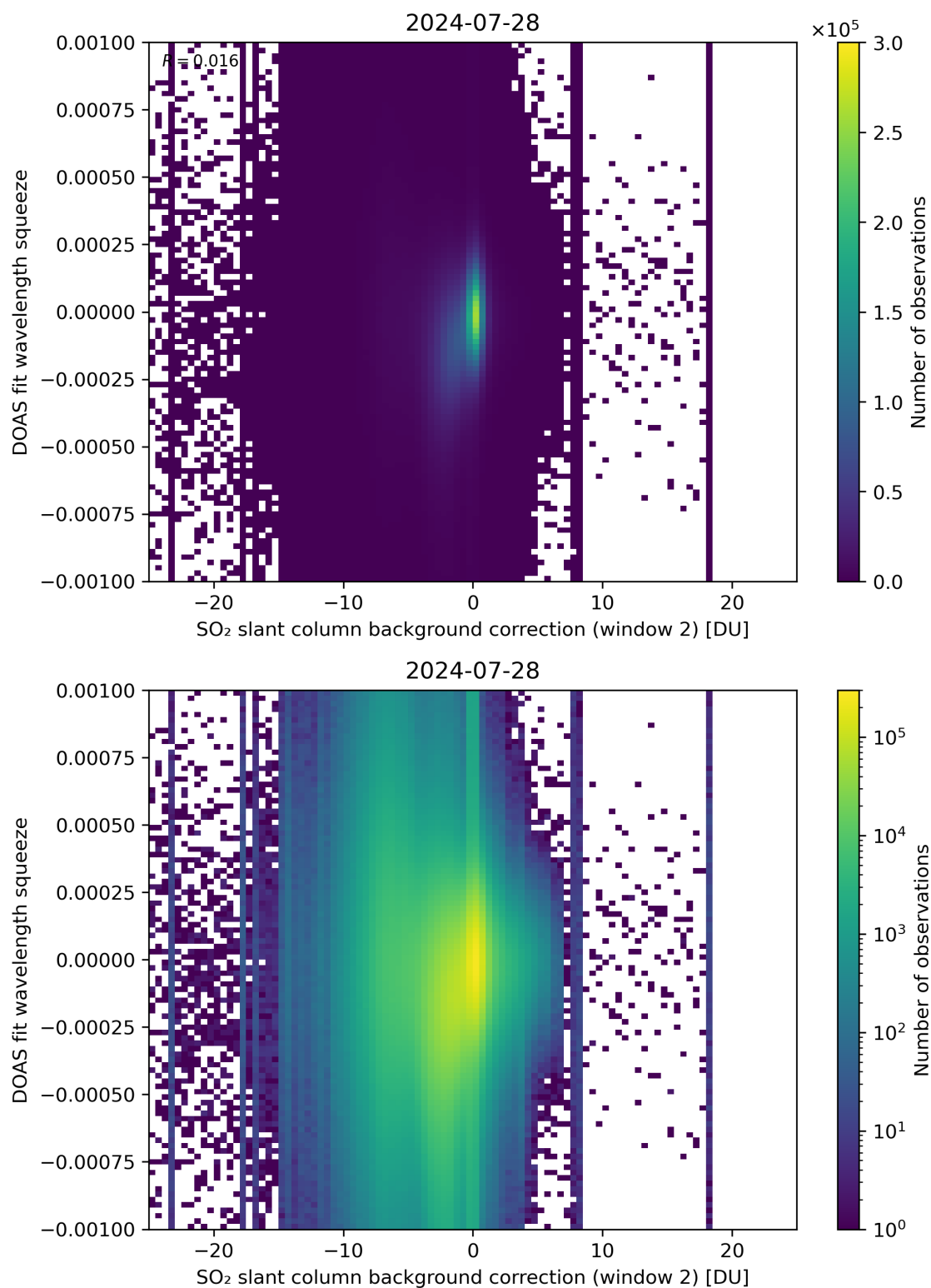
Figure 113: Scatter density plot of “SO 2 slant column background correction (window 2)” against “DOAS fit wavelength squeeze” for 2024-07-27 to 2024-07-29.
