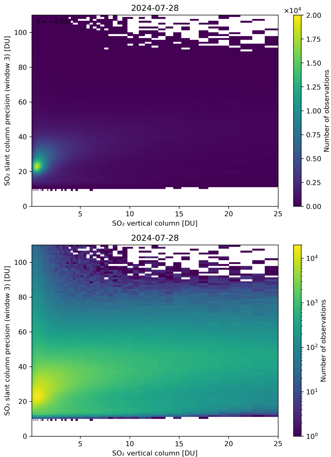
Figure 304: Scatter density plot of “SO 2 vertical column” against “SO 2 slant column precision (window 3)” for 2024-07-27 to 2024-07-29.
