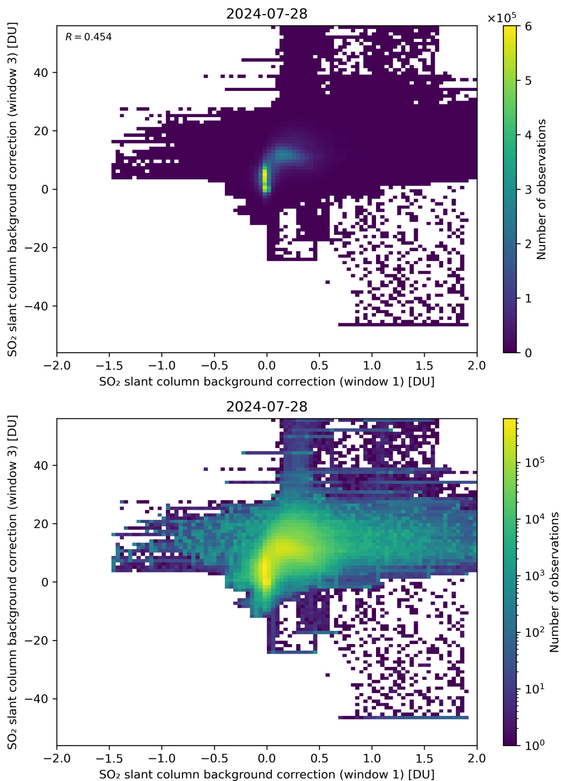
Figure 99: Scatter density plot of “SO 2 slant column background correction (window 1)” against “SO 2 slant column background correction (window 3)” for 2024-07-27 to 2024-07-29.
