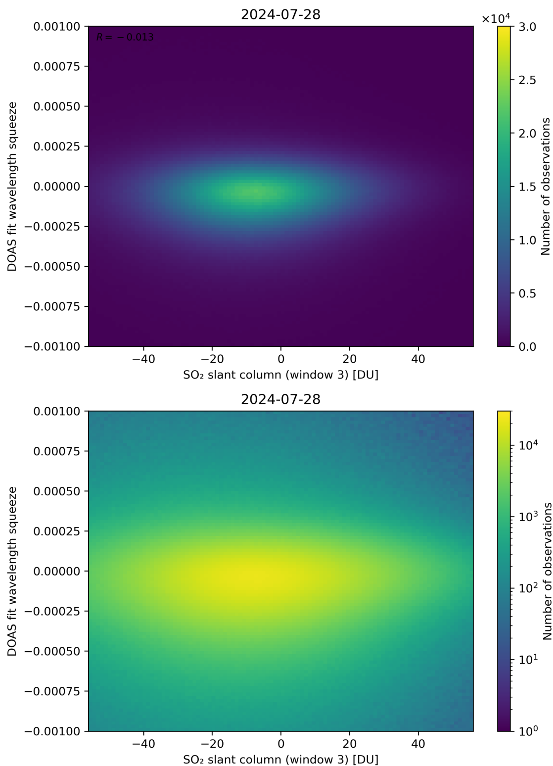
Figure 255: Scatter density plot of “SO 2 slant column (window 3)” against “DOAS fit wavelength squeeze” for 2024-07-27 to 2024-07-29.
