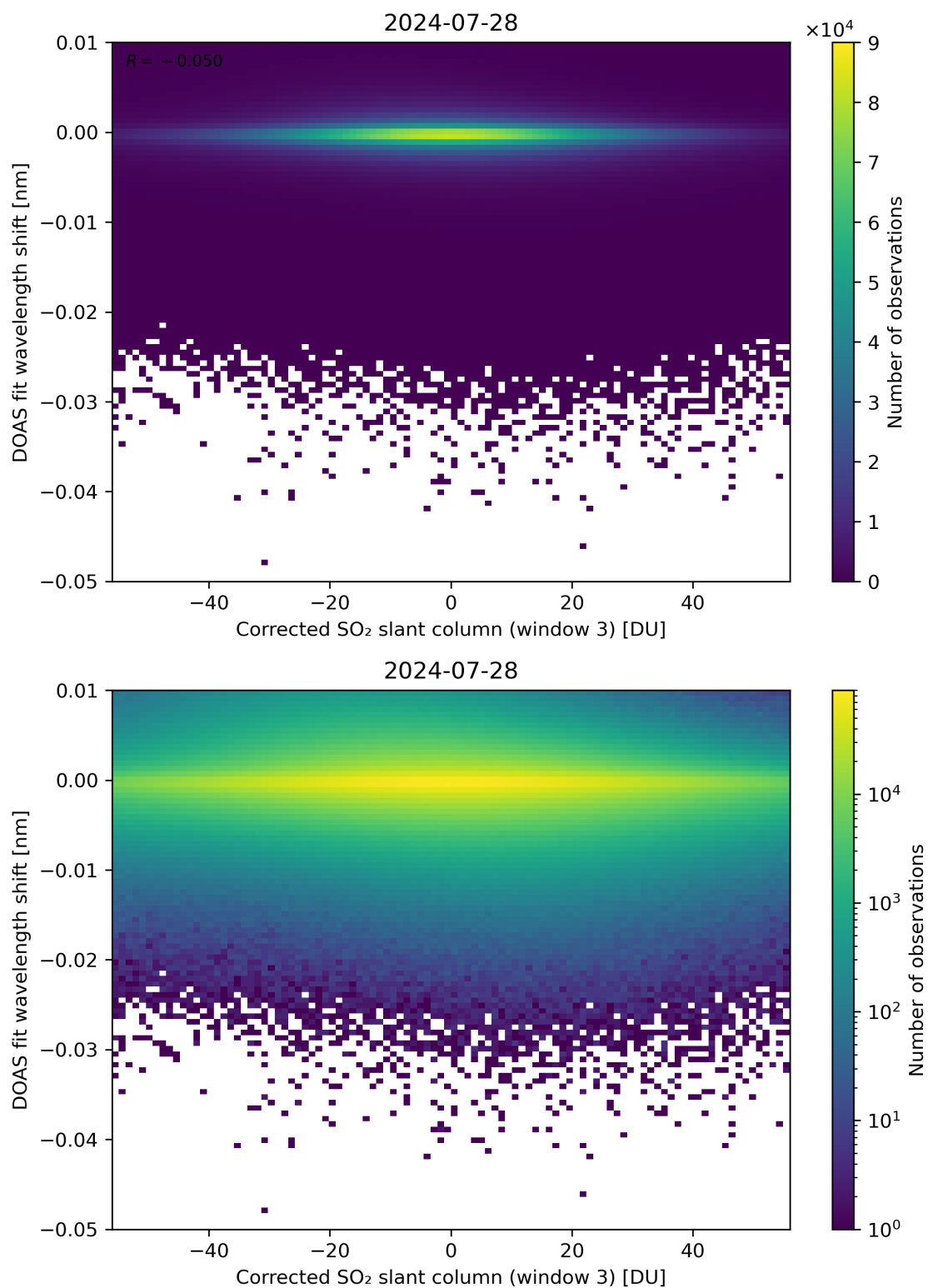
Figure 206: Scatter density plot of “Corrected SO 2 slant column (window 3)” against “DOAS fit wavelength shift” for 2024-07-27 to 2024-07-29.
