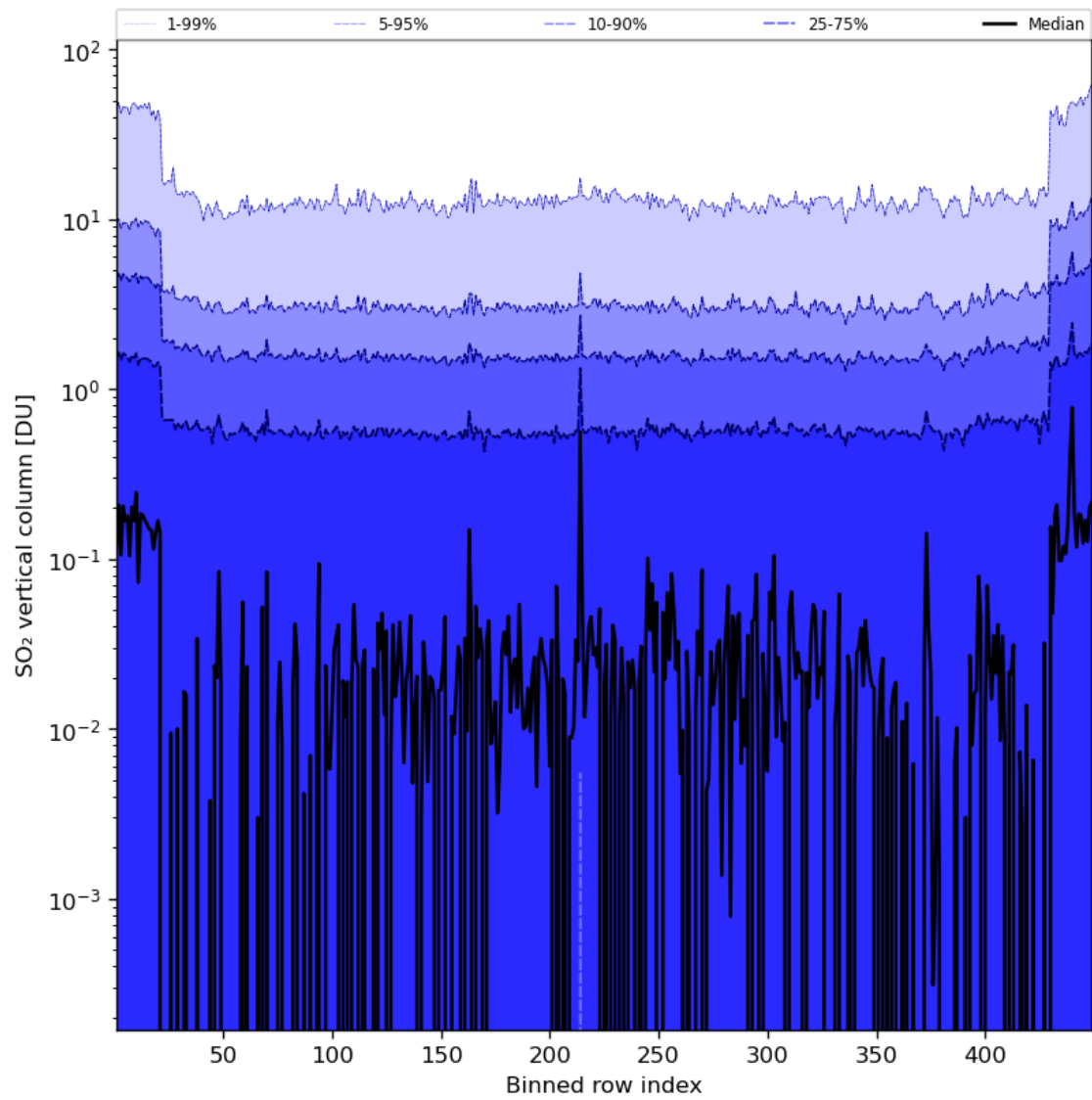
Figure 76: Along track statistics of “SO 2 vertical column” for 2024-07-27 to 2024-07-29
