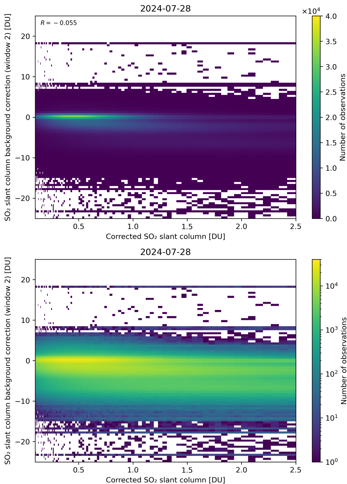
Figure 179: Scatter density plot of “Corrected SO 2 slant column” against “SO 2 slant column background correction (window 2)” for 2024-07-27 to 2024-07-29.
