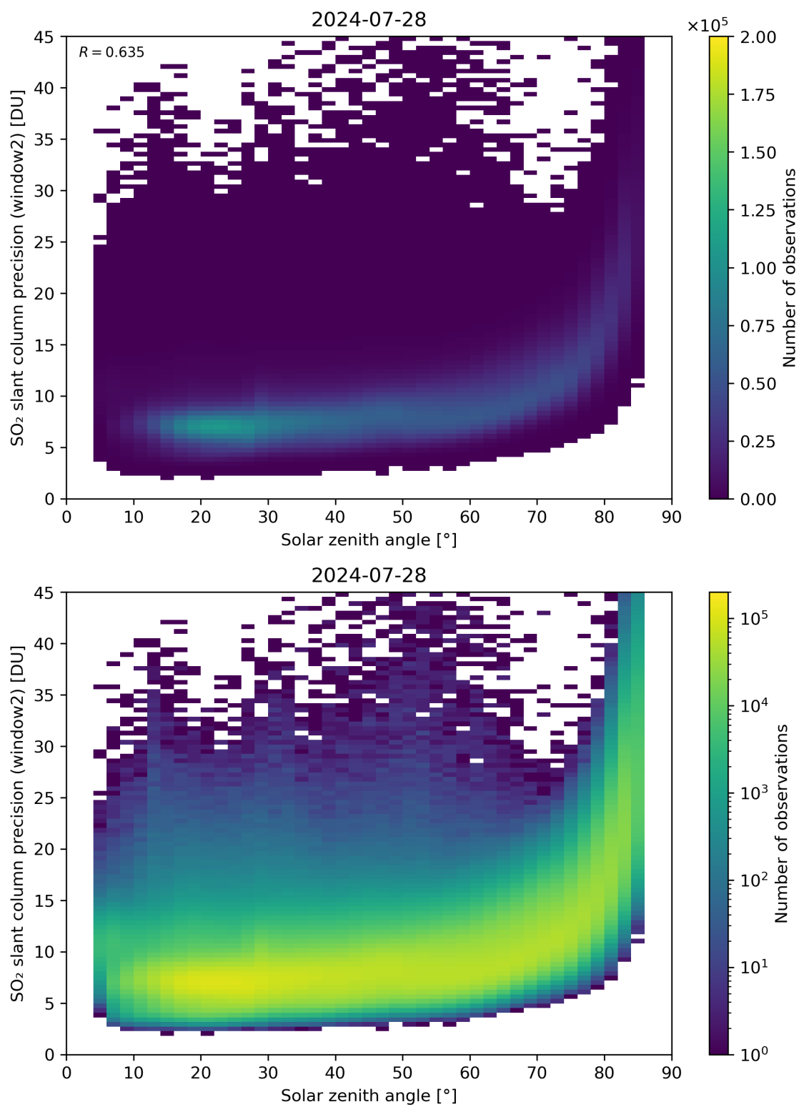
Figure 171: Scatter density plot of “Solar zenith angle” against “SO 2 slant column precision (window2)” for 2024-07-27 to 2024-07-29.
