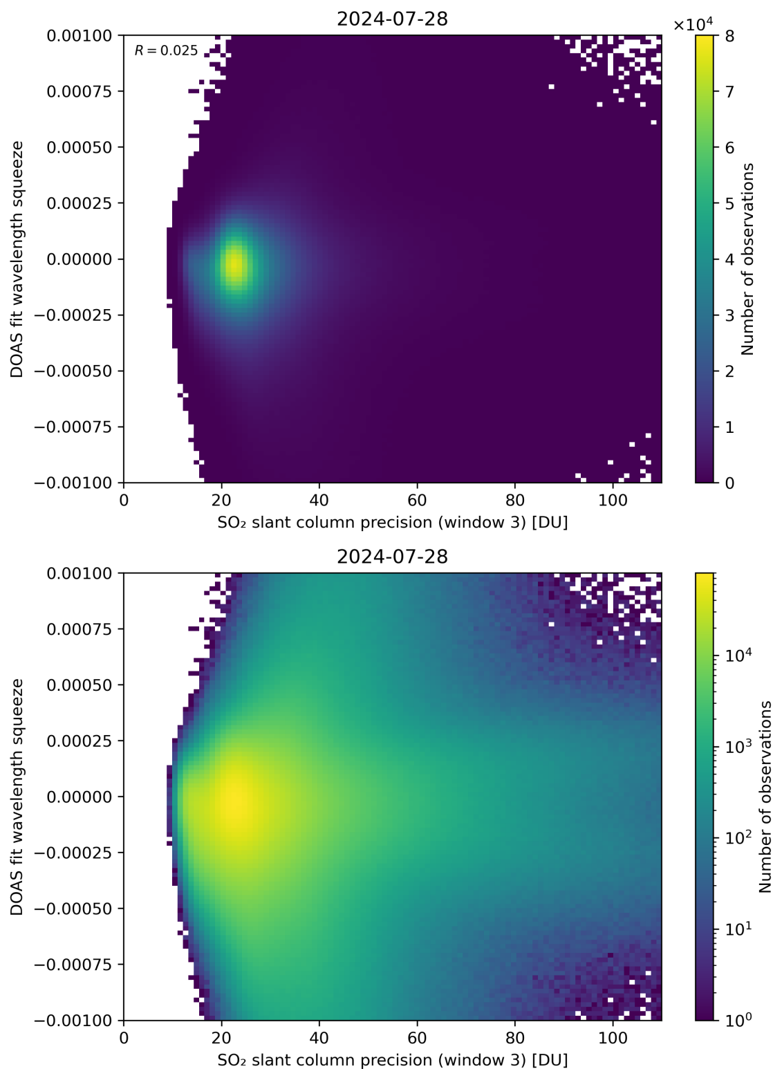
Figure 259: Scatter density plot of “SO 2 slant column precision (window 3)” against “DOAS fit wavelength squeeze” for 2024-07-27 to 2024-07-29.
