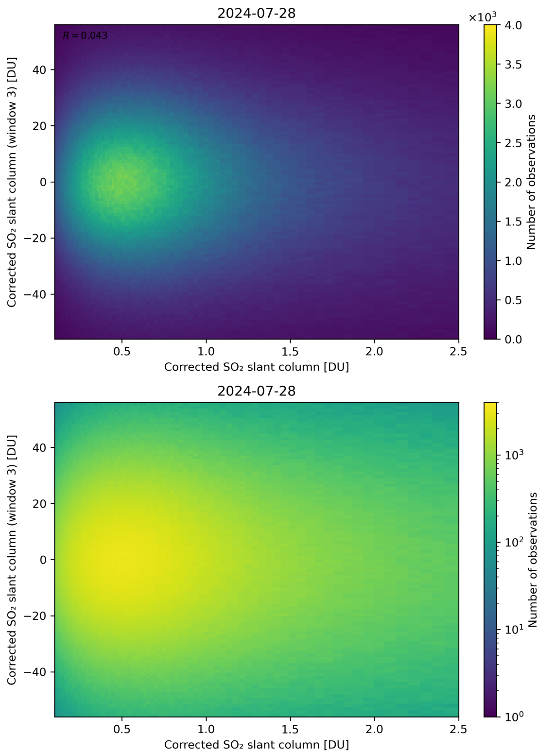
Figure 186: Scatter density plot of “Corrected SO 2 slant column” against “Corrected SO 2 slant column (window 3)” for 2024-07-27 to 2024-07-29.
