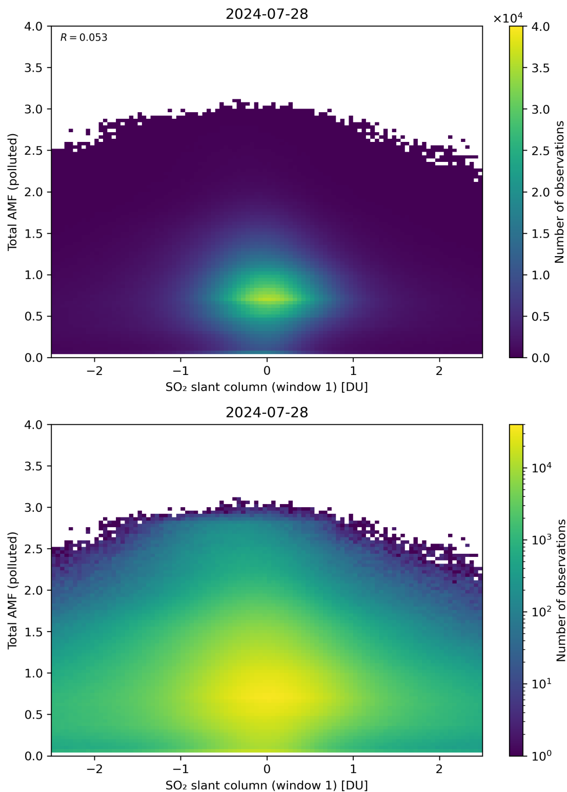
Figure 239: Scatter density plot of “SO 2 slant column (window 1)” against “Total AMF (polluted)” for 2024-07-27 to 2024-07-29.
