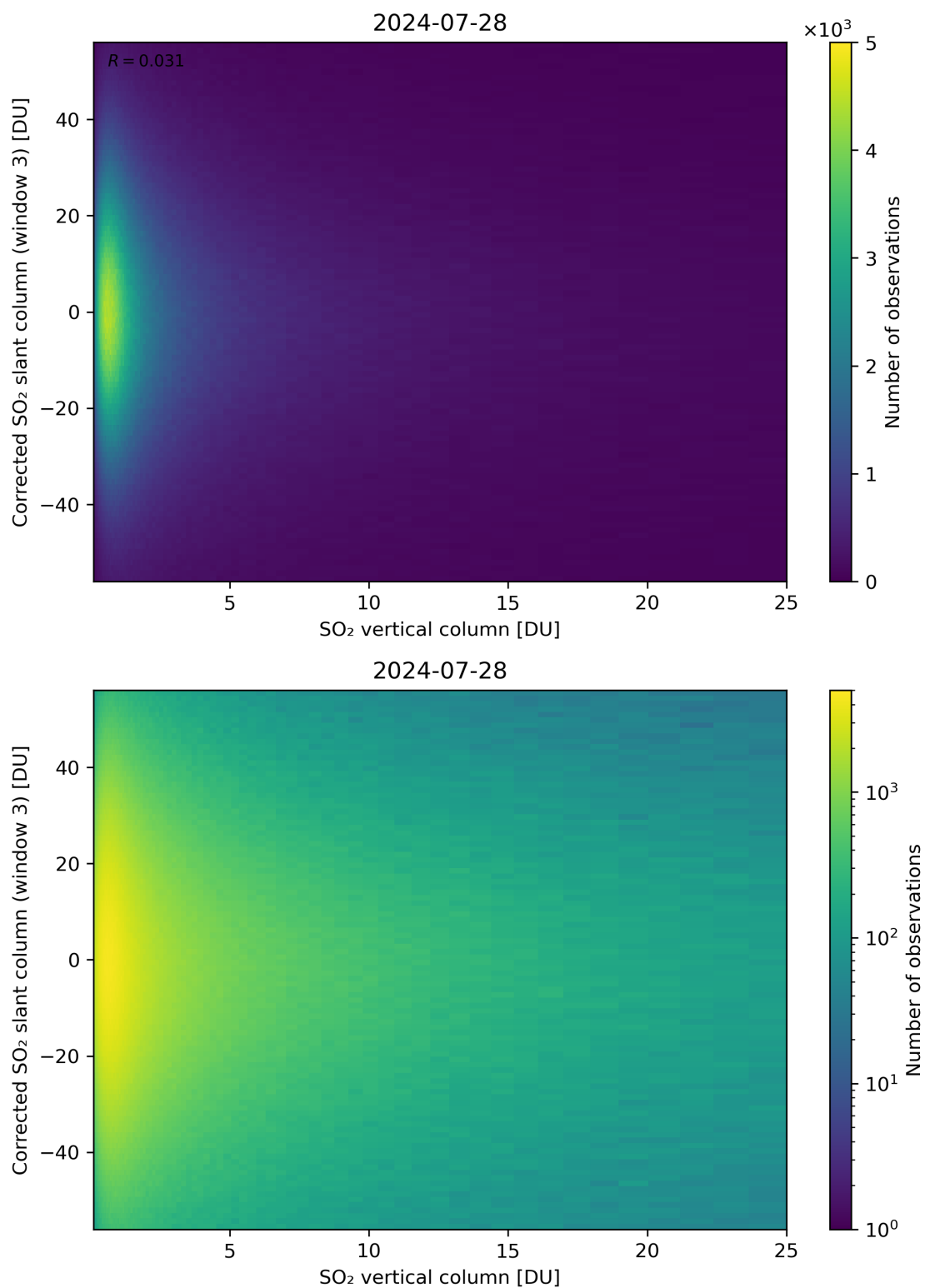
Figure 299: Scatter density plot of “SO 2 vertical column” against “Corrected SO 2 slant column (window 3)” for 2024-07-27 to 2024-07-29.
