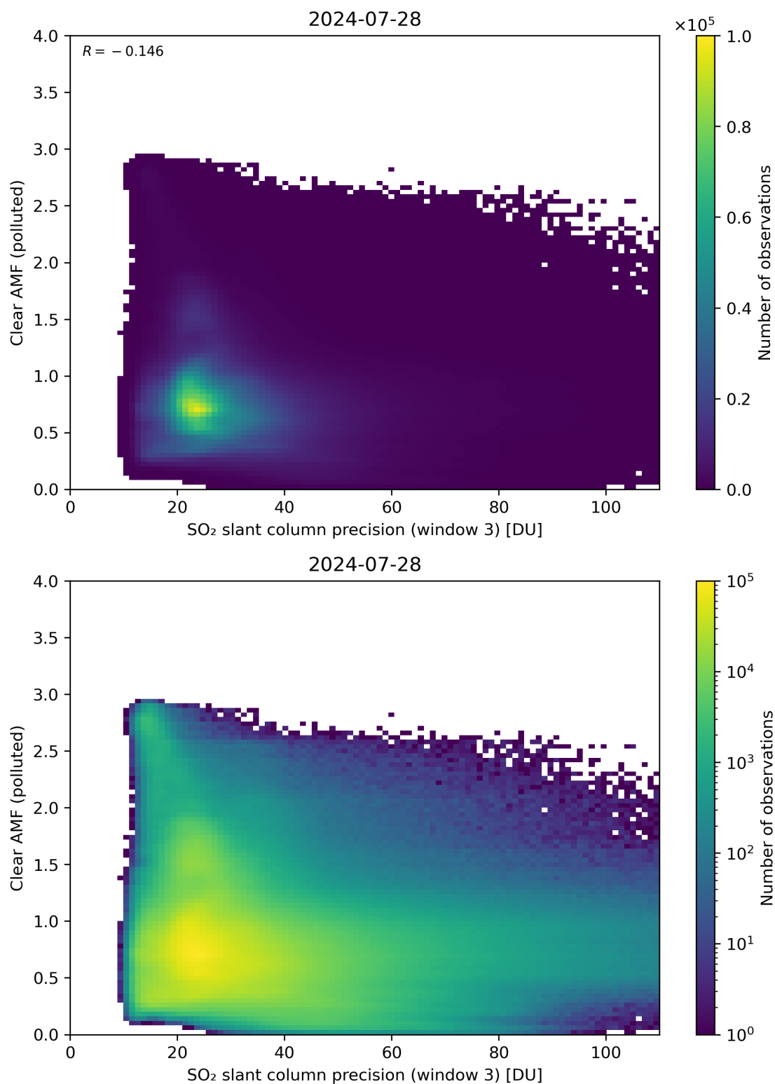
Figure 261: Scatter density plot of “SO 2 slant column precision (window 3)” against “Clear AMF (polluted)” for 2024-07-27 to 2024-07-29.
