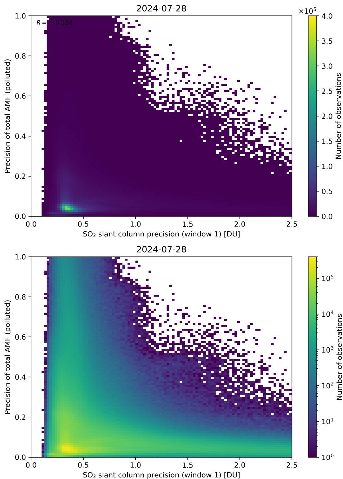
Figure 231: Scatter density plot of “SO 2 slant column precision (window 1)” against “Precision of total AMF (polluted)” for 2024-07-27 to 2024-07-29.
