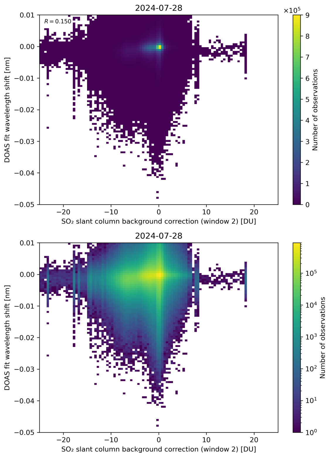
Figure 112: Scatter density plot of “SO 2 slant column background correction (window 2)” against “DOAS fit wavelength shift” for 2024-07-27 to 2024-07-29.
