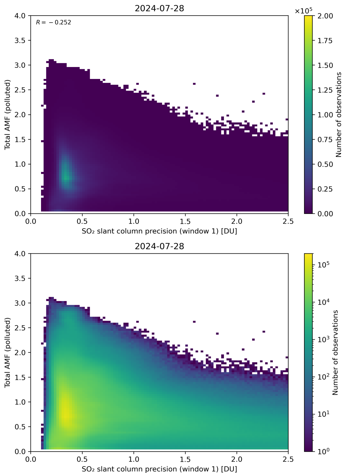
Figure 230: Scatter density plot of “SO 2 slant column precision (window 1)” against “Total AMF (polluted)” for 2024-07-27 to 2024-07-29.
