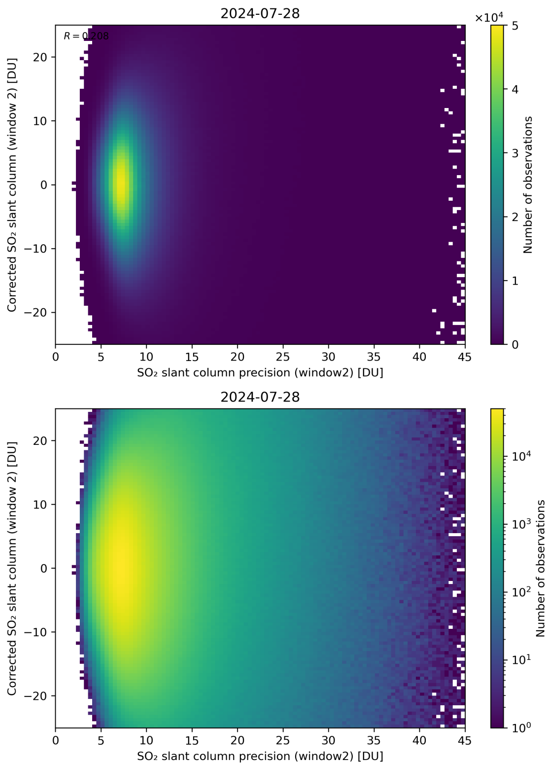
Figure 247: Scatter density plot of “SO 2 slant column precision (window2)” against “Corrected SO 2 slant column (window 2)” for 2024-07-27 to 2024-07-29.
