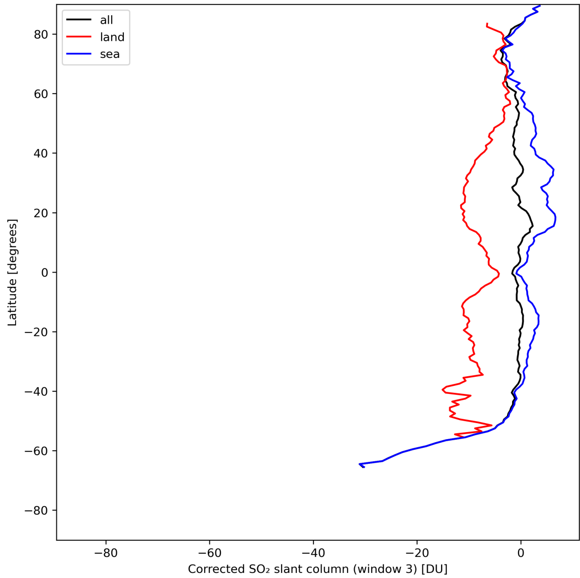
Figure 43: Zonal average of “Corrected SO 2 slant column (window 3)” for 2024-07-27 to 2024-07-29.
