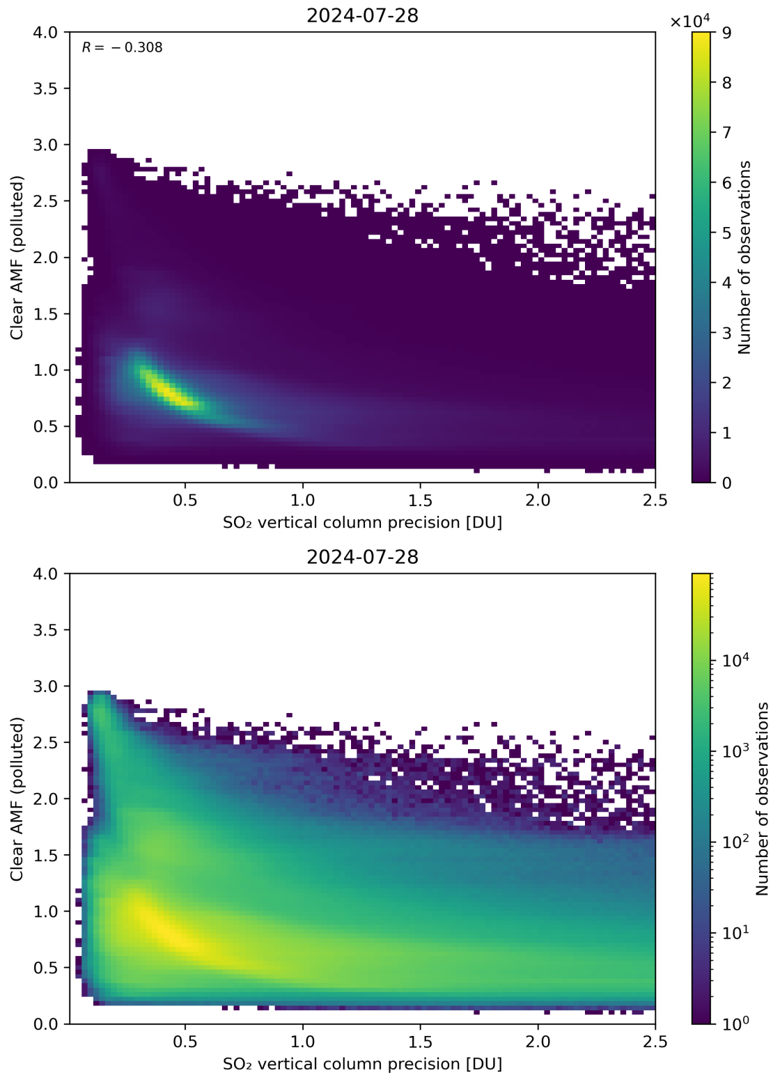
Figure 285: Scatter density plot of “SO 2 vertical column precision” against “Clear AMF (polluted)” for 2024-07-27 to 2024-07-29.
