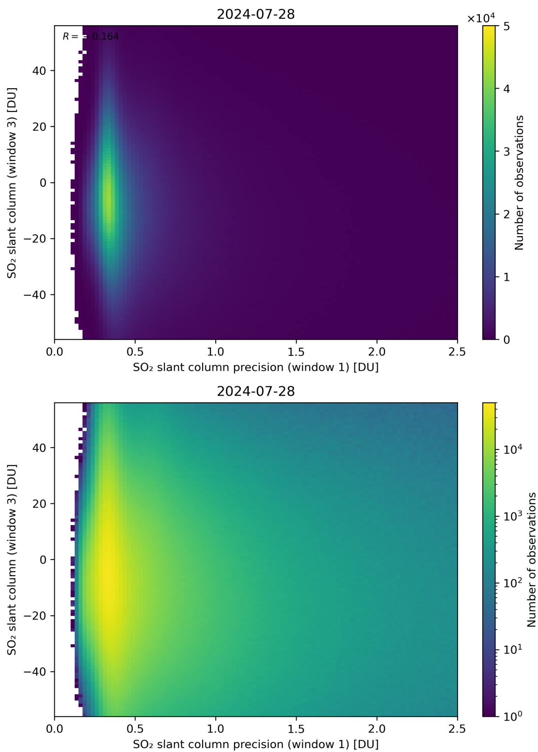
Figure 228: Scatter density plot of “SO 2 slant column precision (window 1)” against “SO 2 slant column (window 3)” for 2024-07-27 to 2024-07-29.
