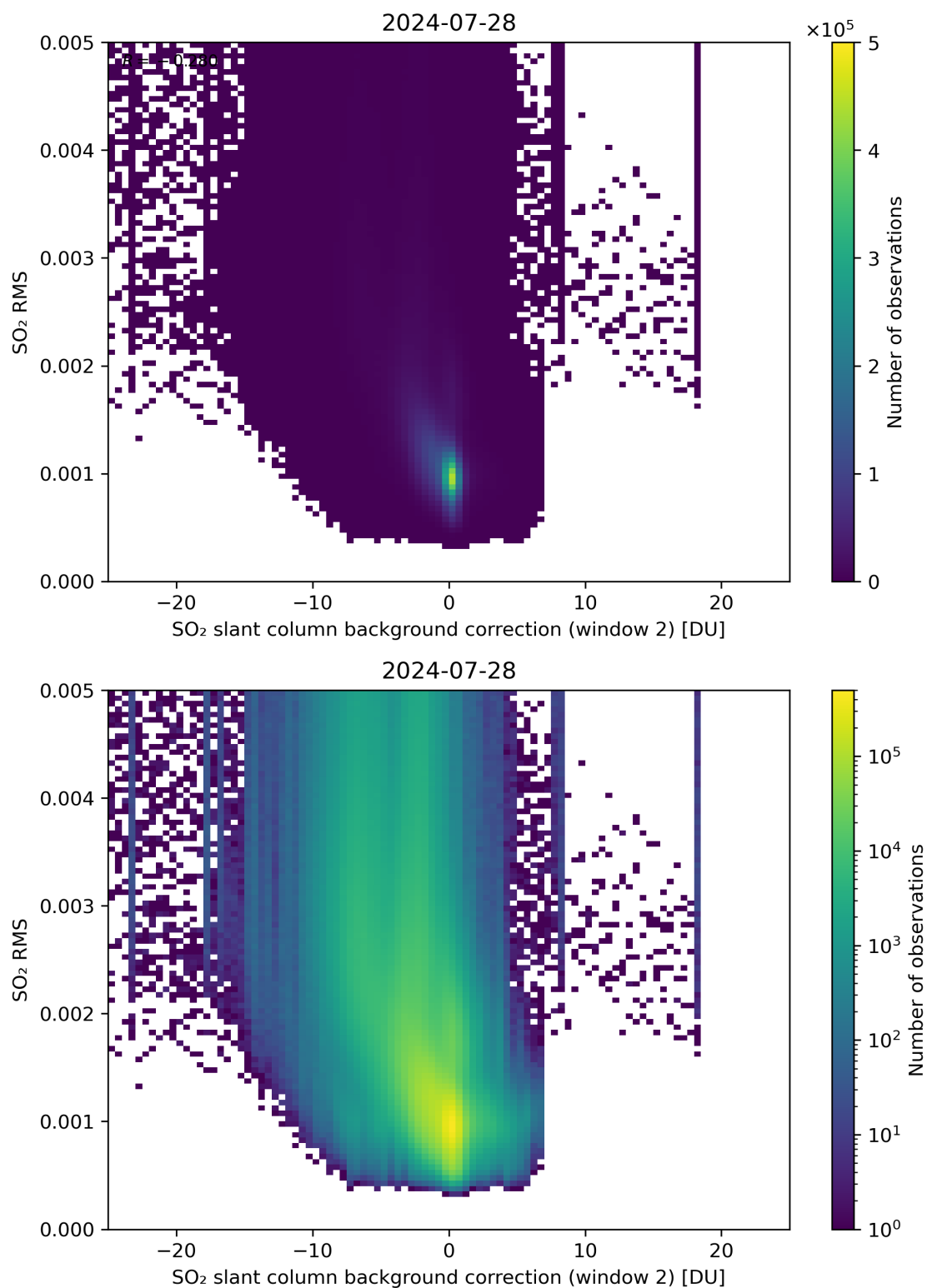
Figure 114: Scatter density plot of “SO 2 slant column background correction (window 2)” against “SO 2 RMS” for 2024-07-27 to 2024-07-29.
