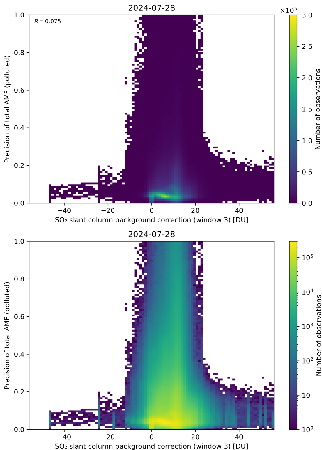
Figure 126: Scatter density plot of “SO 2 slant column background correction (window 3)” against “Precision of total AMF (polluted)” for 2024-07-27 to 2024-07-29.
