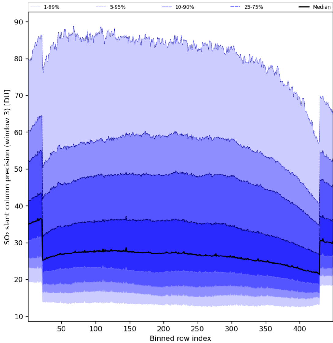
Figure 88: Along track statistics of “SO 2 slant column precision (window 3)” for 2024-07-27 to 2024-07-29
