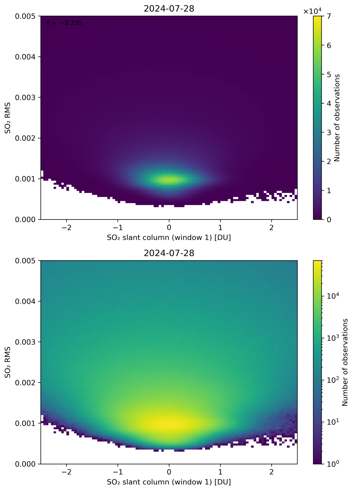
Figure 217: Scatter density plot of “SO 2 slant column (window 1)” against “SO 2 RMS” for 2024-07-27 to 2024-07-29.
