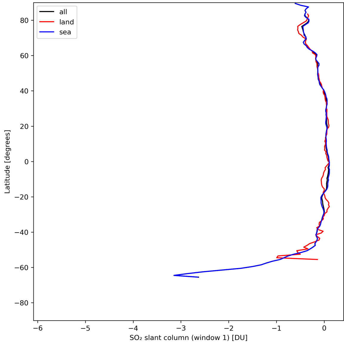
Figure 33: Zonal average of “SO 2 slant column (window 1)” for 2024-07-27 to 2024-07-29.
