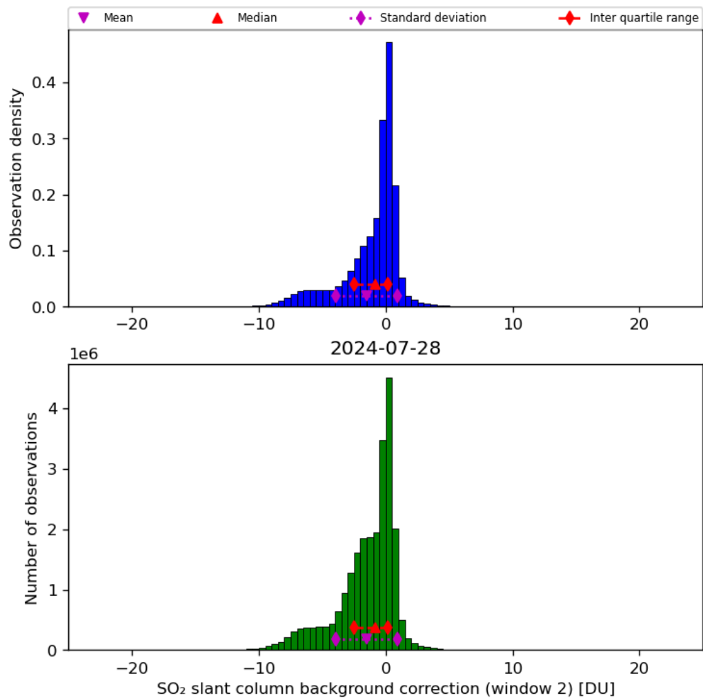
Figure 63: Histogram of “SO 2 slant column background correction (window 2)” for 2024-07-27 to 2024-07-29
