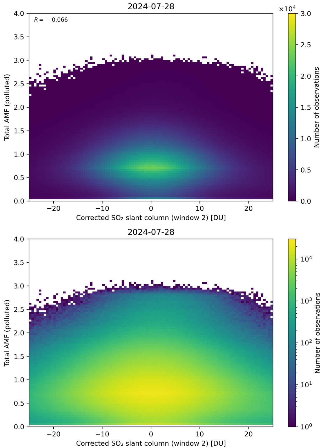
Figure 203: Scatter density plot of “Corrected SO 2 slant column (window 2)” against “Total AMF (polluted)” for 2024-07-27 to 2024-07-29.
