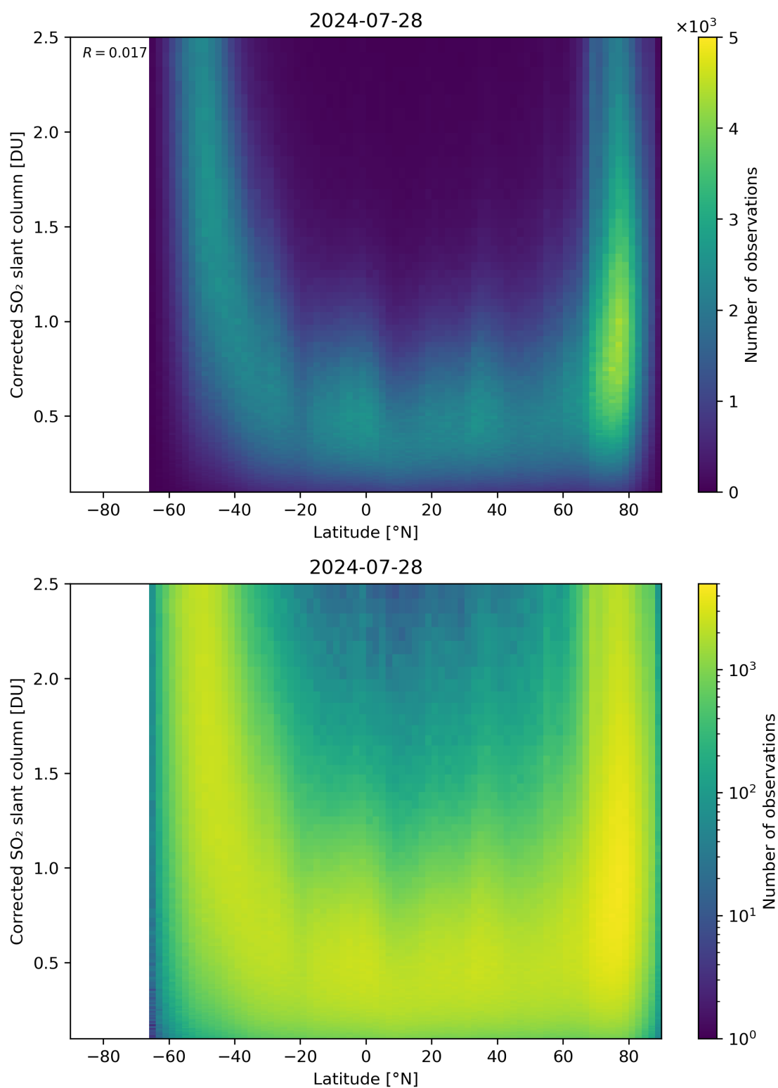
Figure 146: Scatter density plot of “Latitude” against “Corrected SO 2 slant column” for 2024-07-27 to 2024-07-29.
