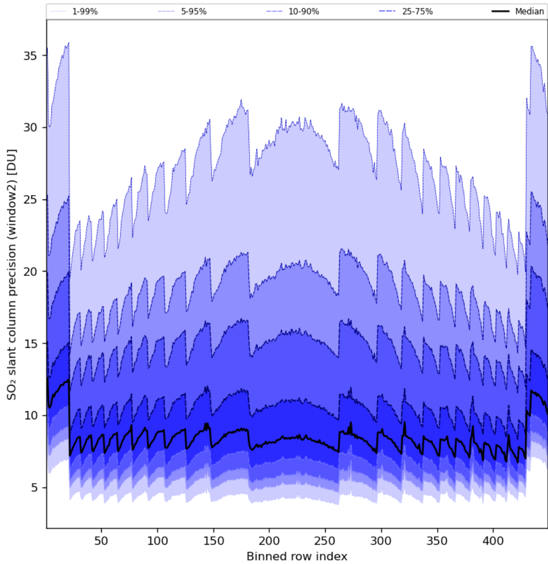
Figure 84: Along track statistics of “SO 2 slant column precision (window2)” for 2024-07-27 to 2024-07-29
