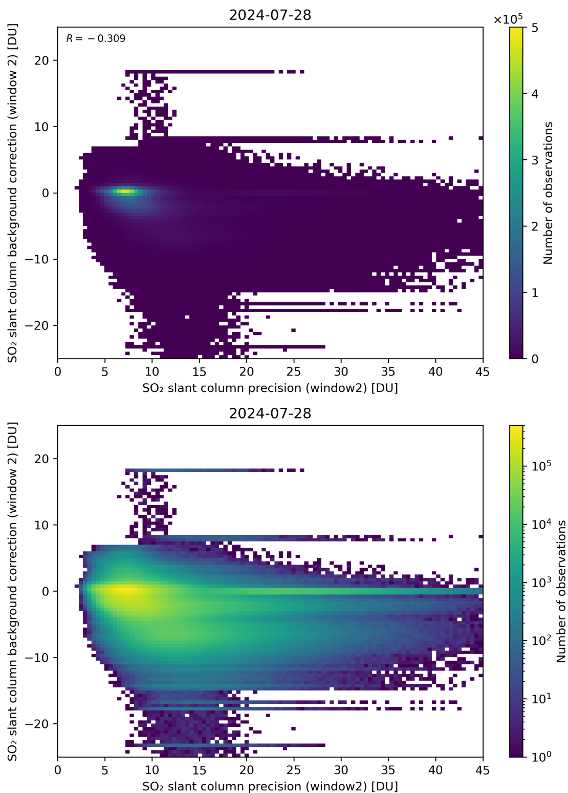
Figure 241: Scatter density plot of “SO 2 slant column precision (window2)” against “SO 2 slant column background correction (window 2)” for 2024-07-27 to 2024-07-29.
