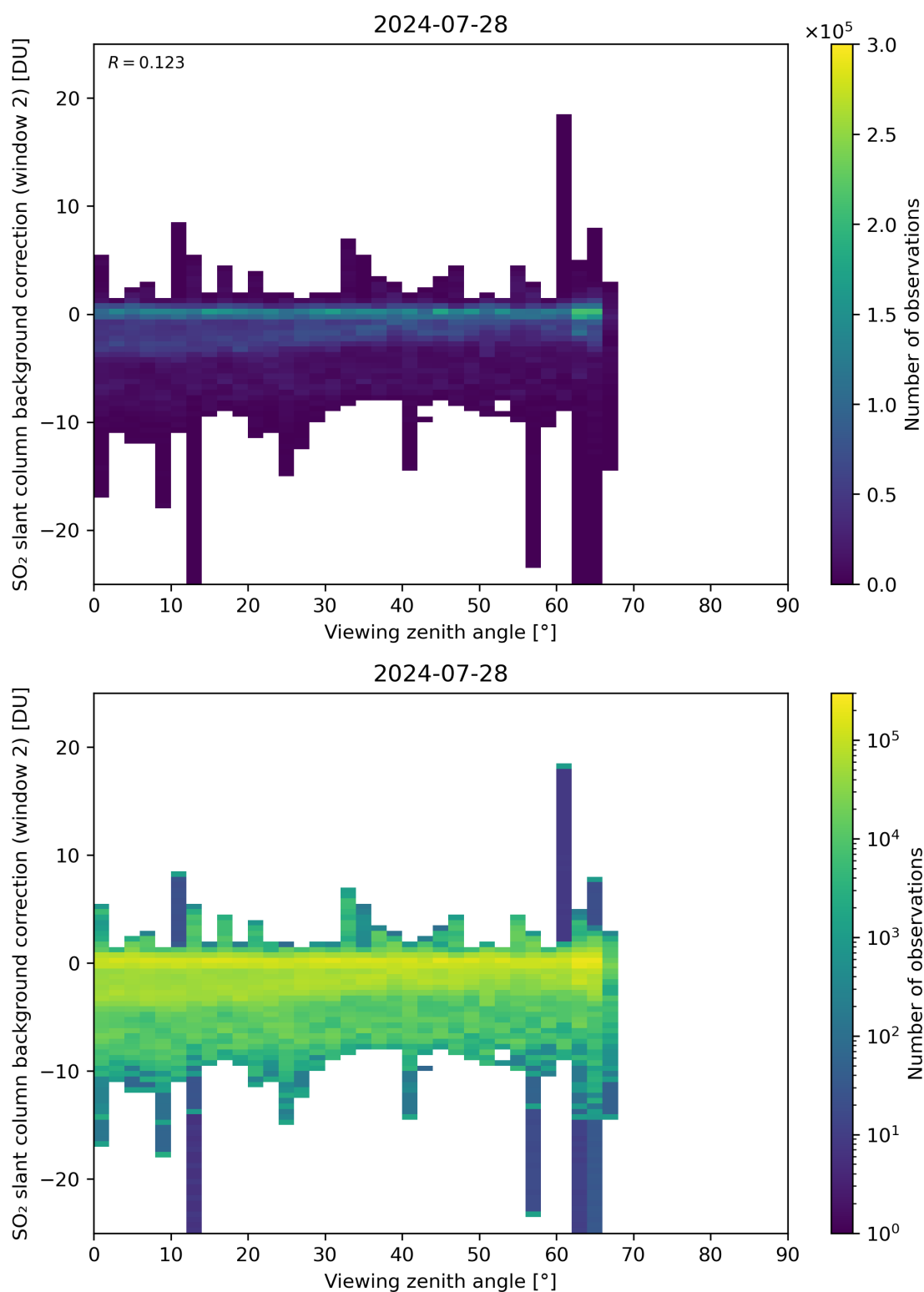
Figure 309: Scatter density plot of “Viewing zenith angle” against “SO 2 slant column background correction (window 2)” for 2024-07-27 to 2024-07-29.
