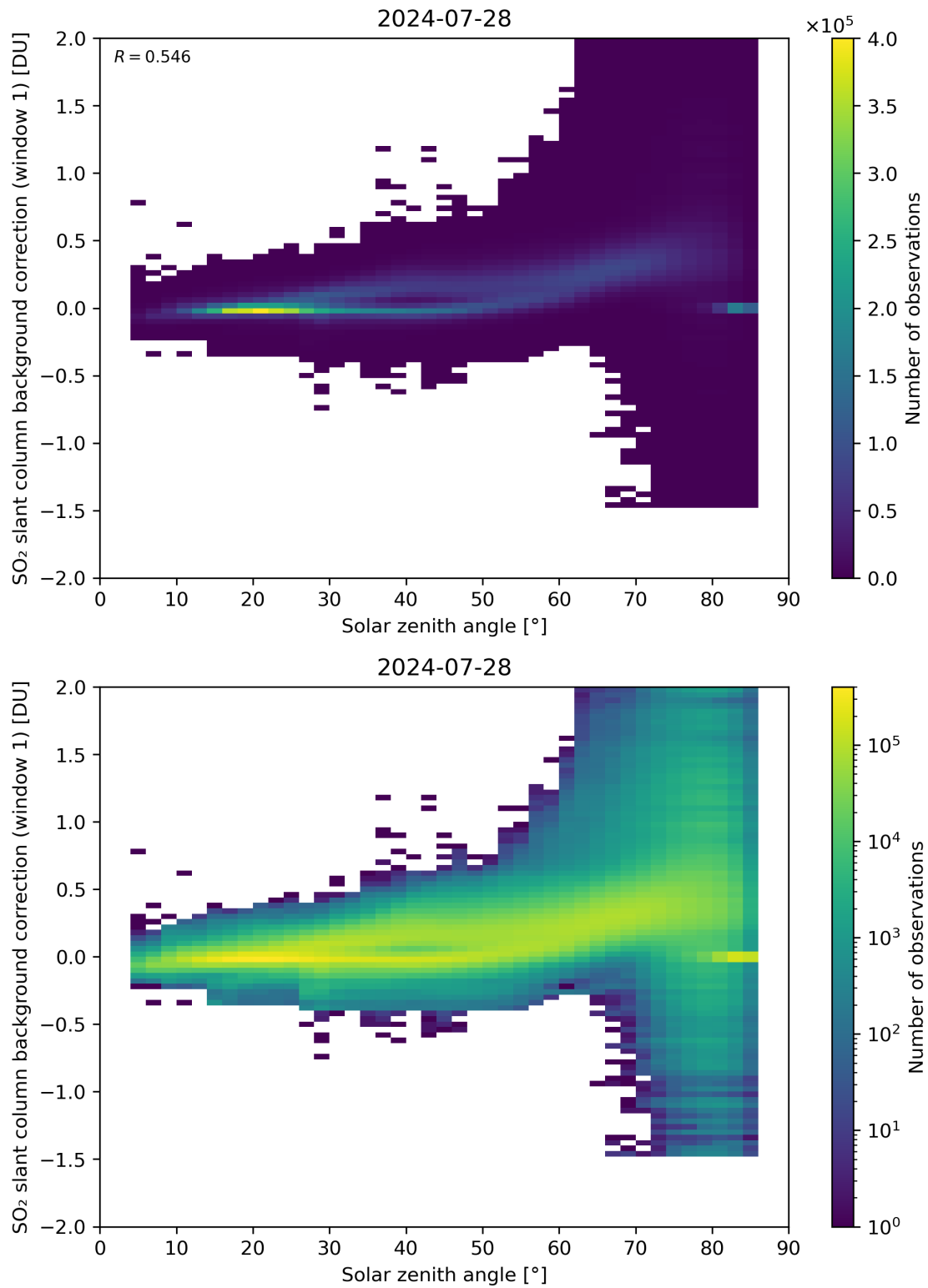
Figure 158: Scatter density plot of “Solar zenith angle” against “SO 2 slant column background correction (window 1)” for 2024-07-27 to 2024-07-29.
