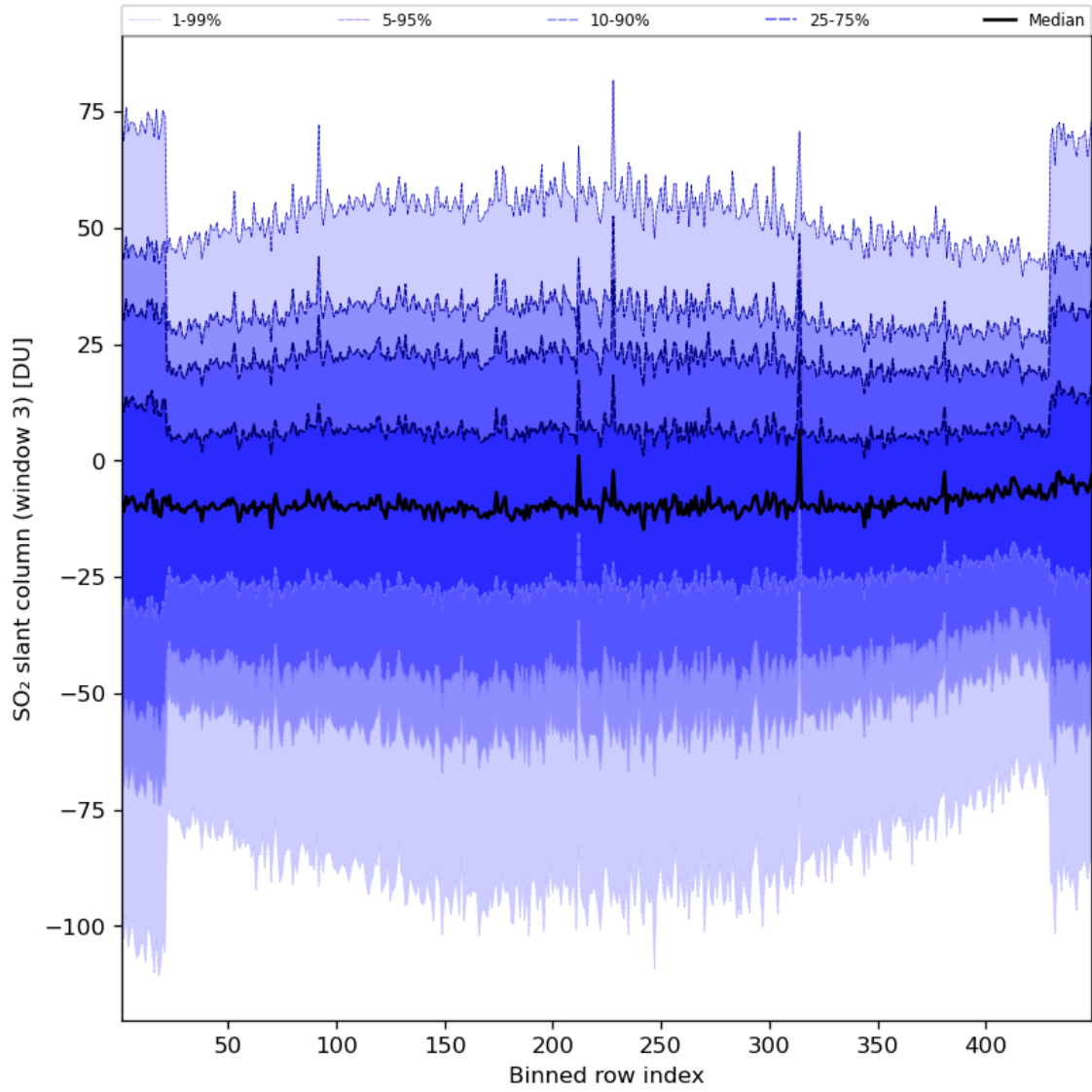
Figure 87: Along track statistics of “SO 2 slant column (window 3)” for 2024-07-27 to 2024-07-29
