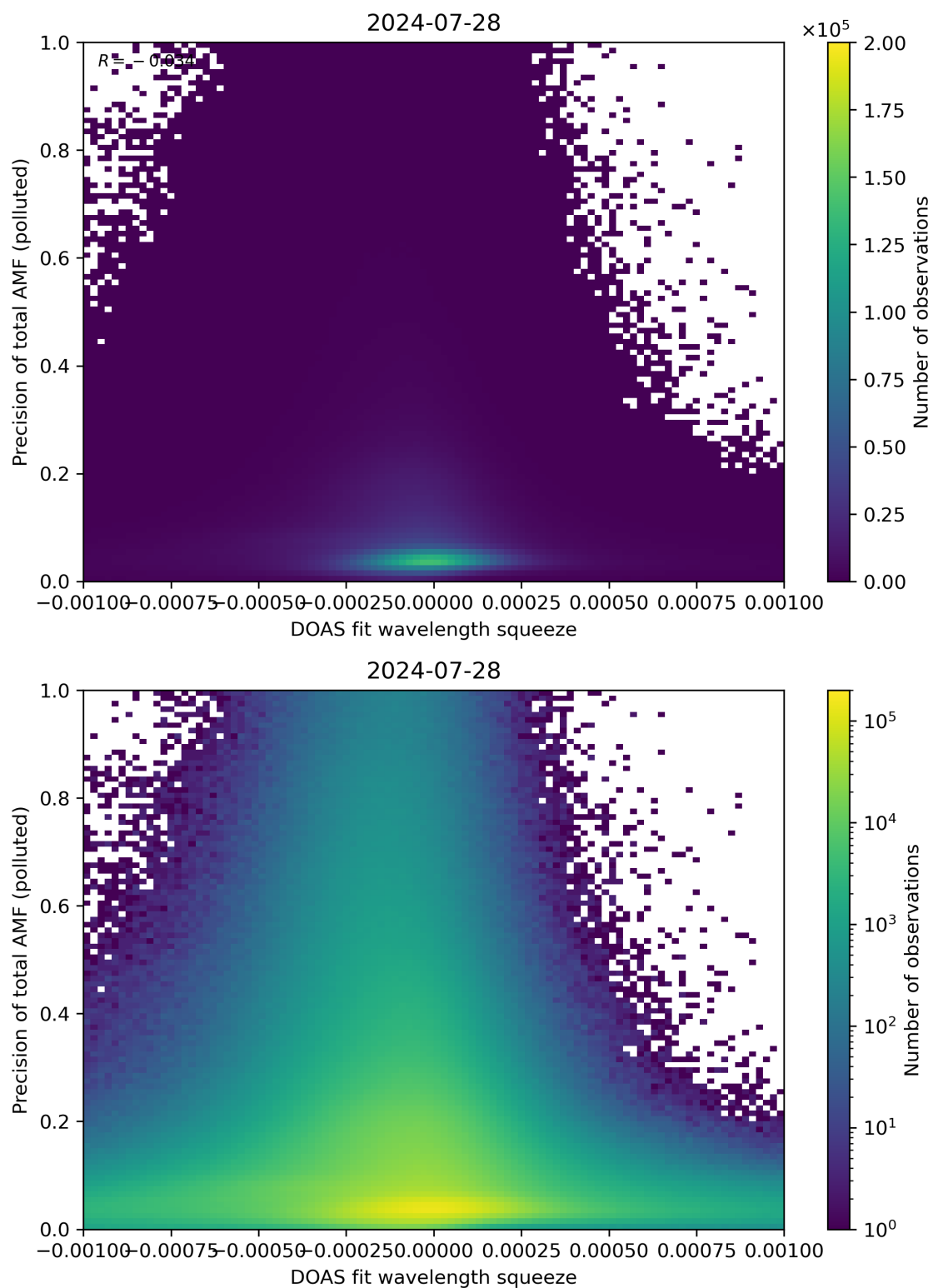
Figure 135: Scatter density plot of “DOAS fit wavelength squeeze” against “Precision of total AMF (polluted)” for 2024-07-27 to 2024-07-29.
