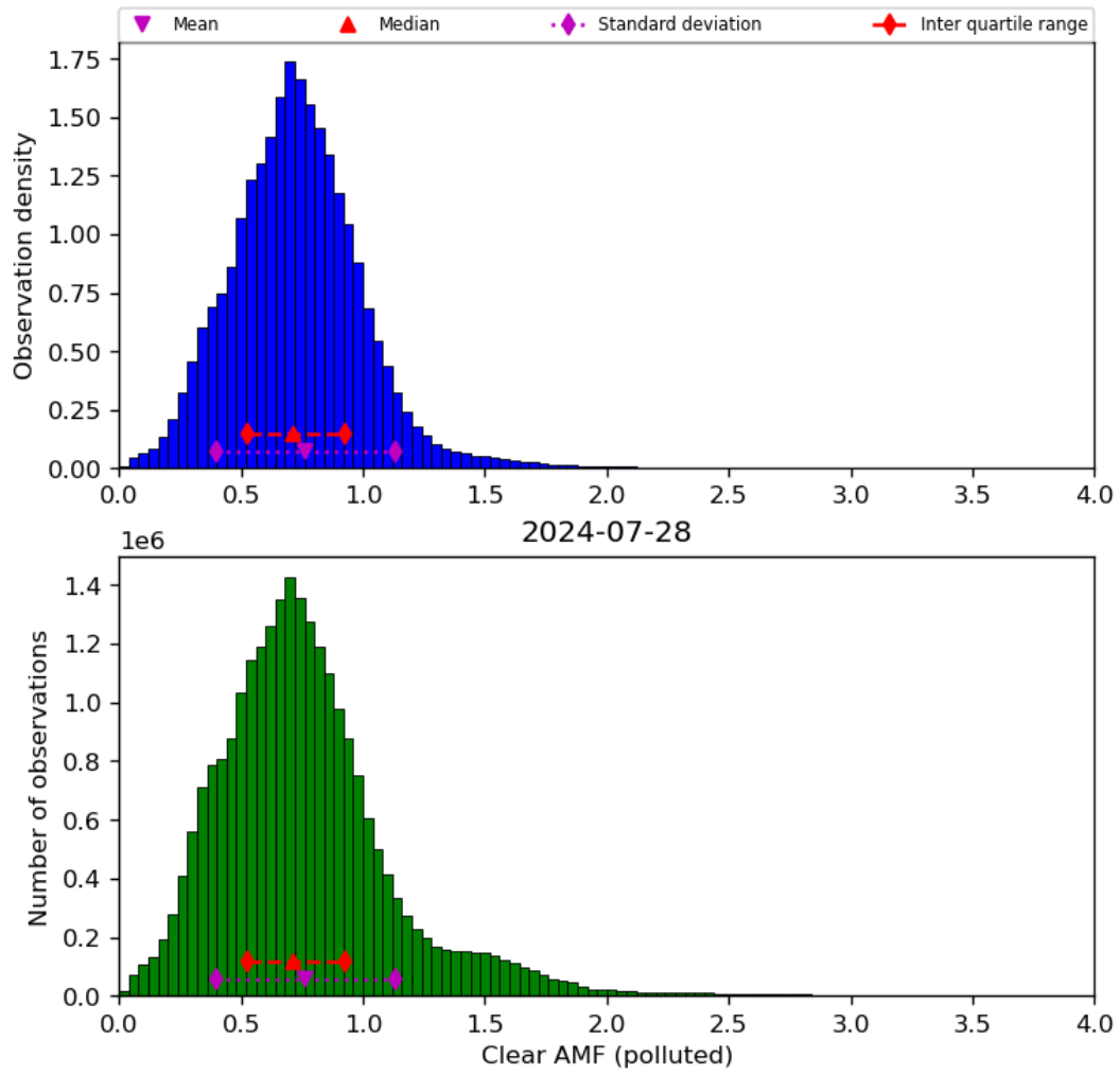
Figure 73: Histogram of "Clear AMF (polluted)" for 2024-07-27 to 2024-07-29
