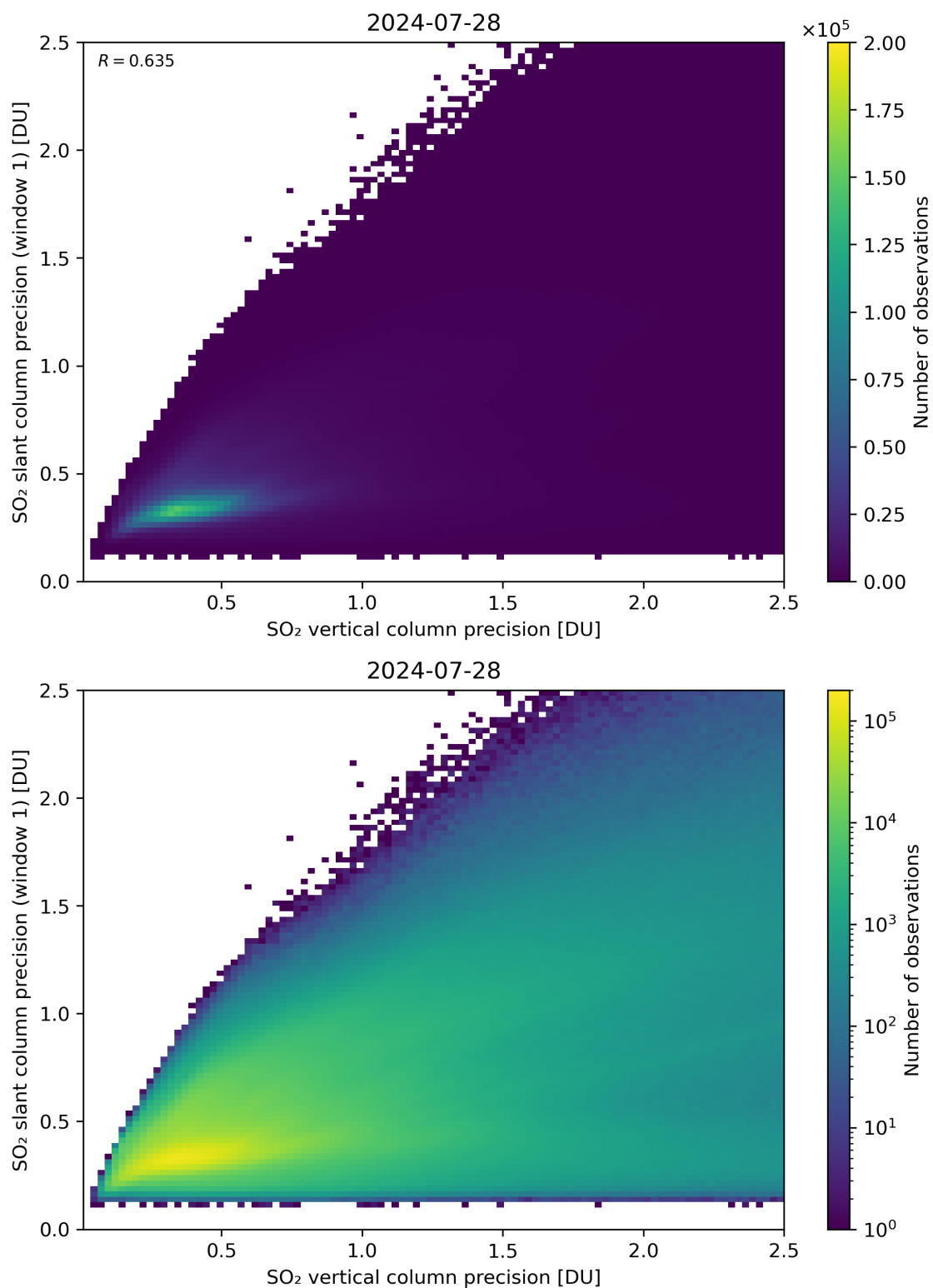
Figure 290: Scatter density plot of “SO 2 vertical column precision” against “SO 2 slant column precision (window 1)” for 2024-07-27 to 2024-07-29.
