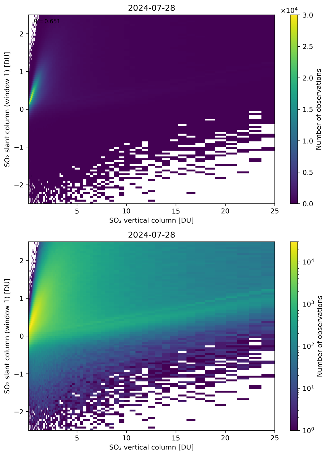
Figure 300: Scatter density plot of “SO 2 vertical column” against “SO 2 slant column (window 1)” for 2024-07-27 to 2024-07-29.
