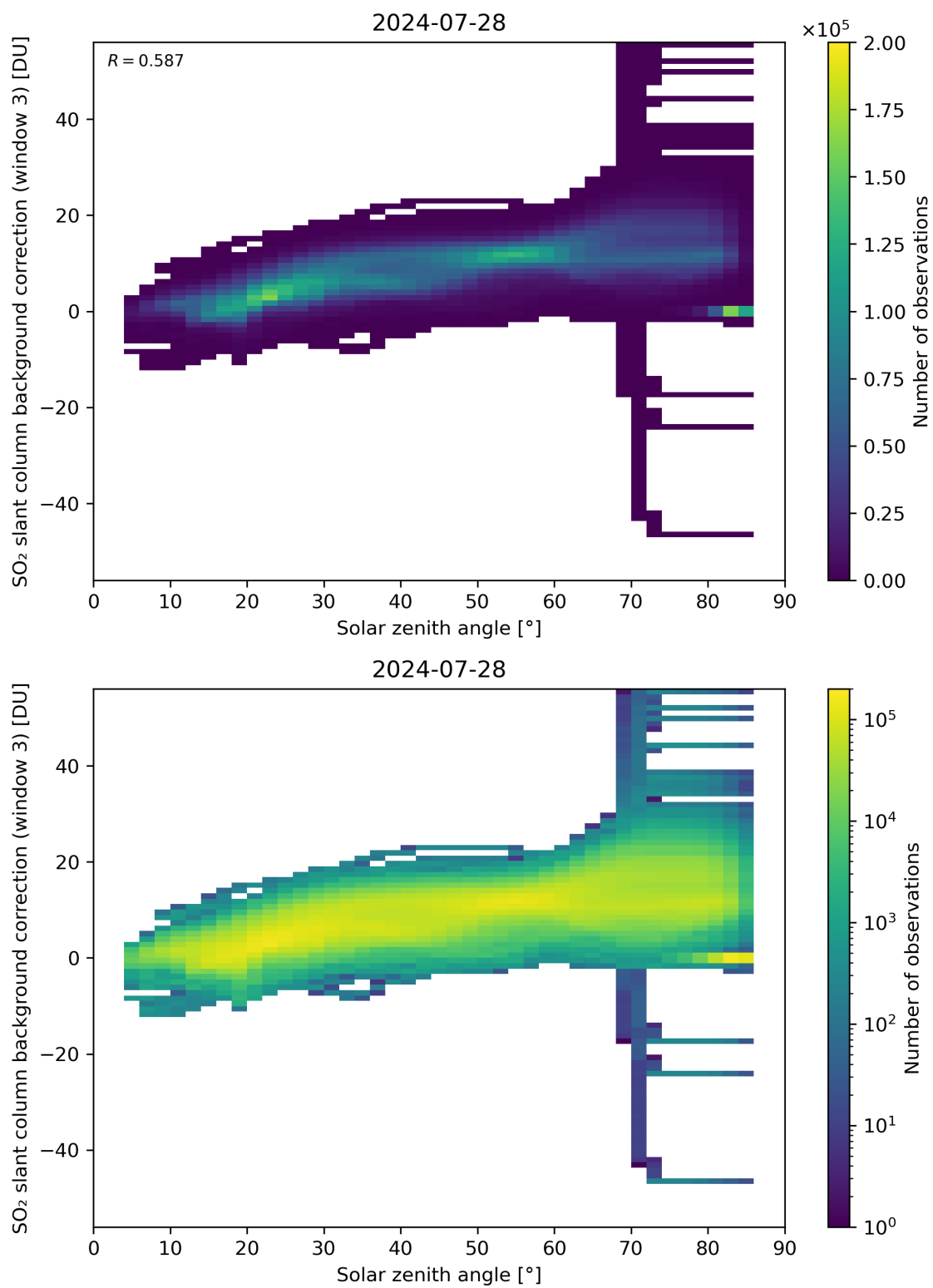
Figure 160: Scatter density plot of “Solar zenith angle” against “SO 2 slant column background correction (window 3)” for 2024-07-27 to 2024-07-29.
