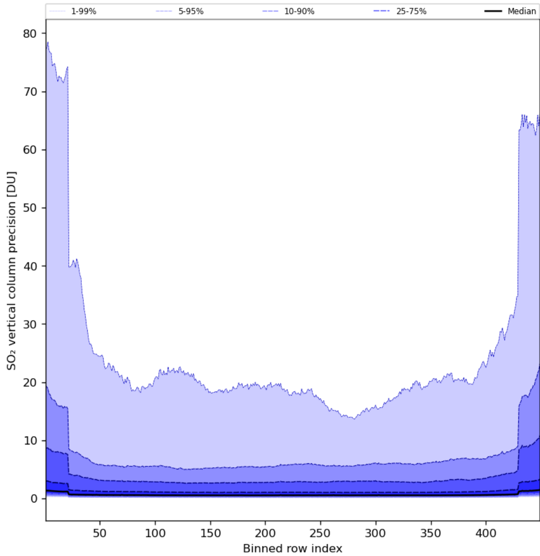
Figure 77: Along track statistics of “SO 2 vertical column precision” for 2024-07-27 to 2024-07-29
