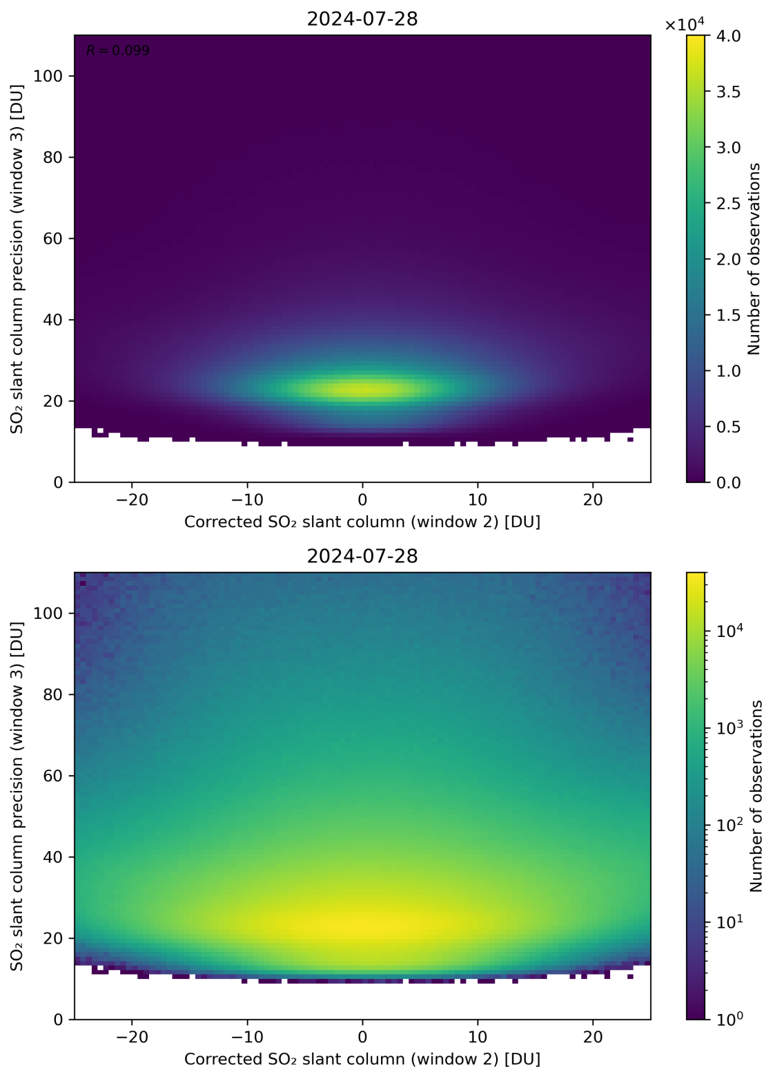
Figure 202: Scatter density plot of “Corrected SO 2 slant column (window 2)” against “SO 2 slant column precision (window 3)” for 2024-07-27 to 2024-07-29.
