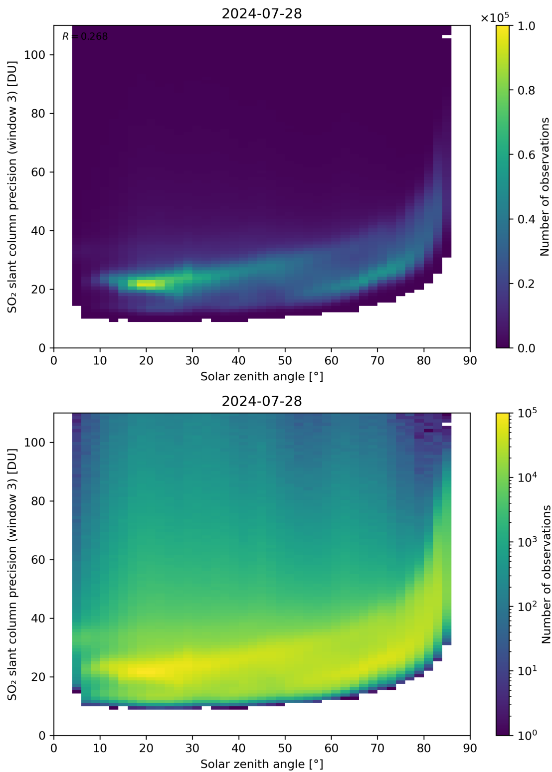
Figure 173: Scatter density plot of “Solar zenith angle” against “SO 2 slant column precision (window 3)” for 2024-07-27 to 2024-07-29.
