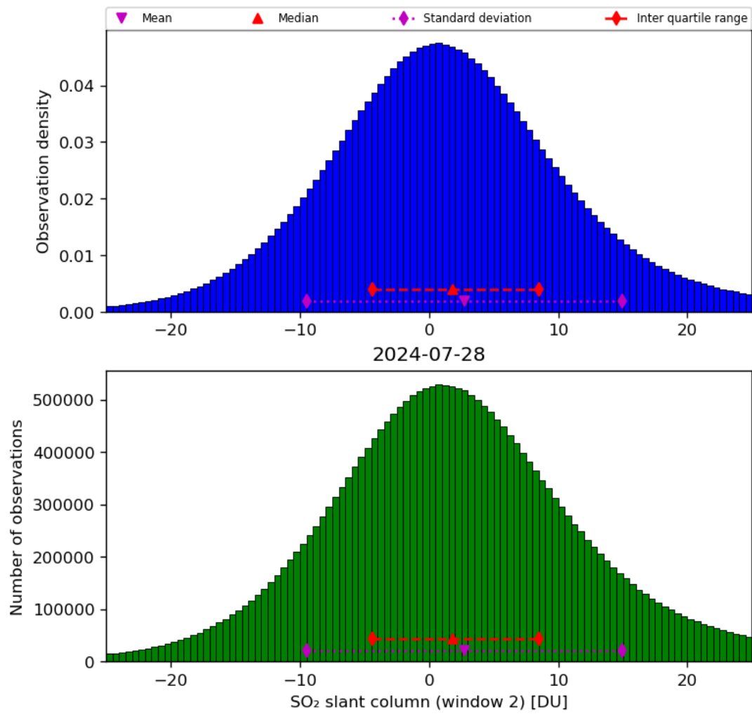
Figure 60: Histogram of “SO 2 slant column (window 2)” for 2024-07-27 to 2024-07-29
