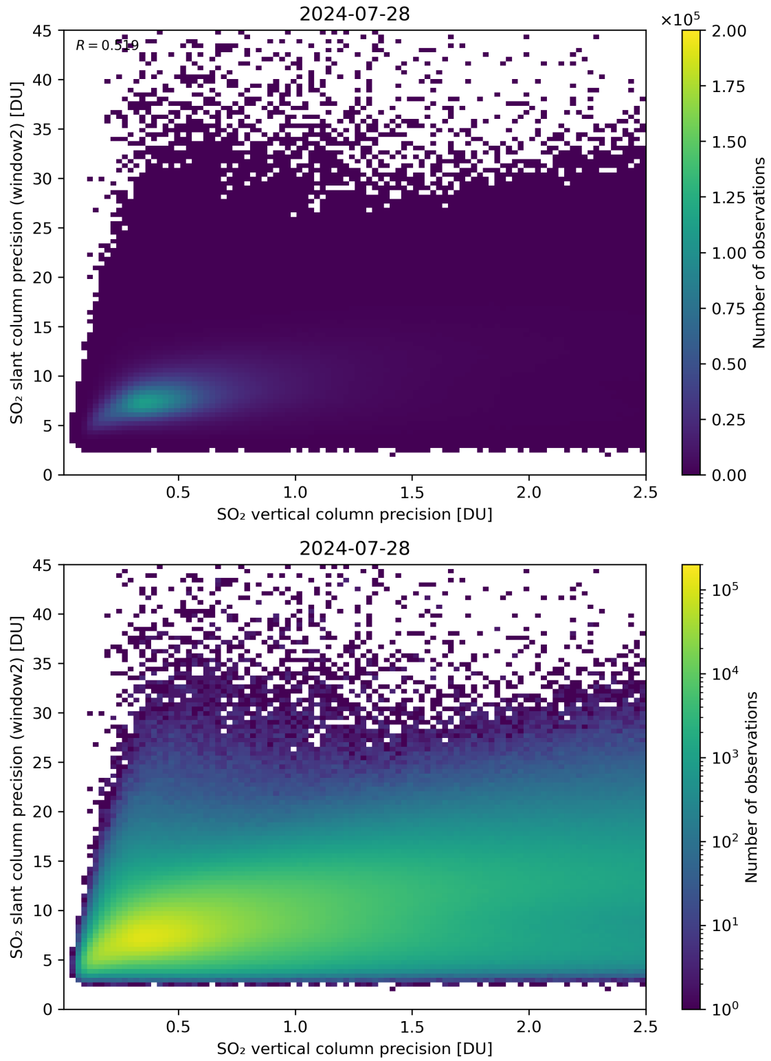
Figure 291: Scatter density plot of “SO 2 vertical column precision” against “SO 2 slant column precision (window2)” for 2024-07-27 to 2024-07-29.
