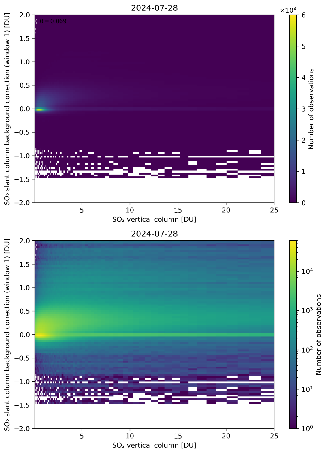
Figure 273: Scatter density plot of “SO 2 vertical column” against “SO 2 slant column background correction (window 1)” for 2024-07-27 to 2024-07-29.
