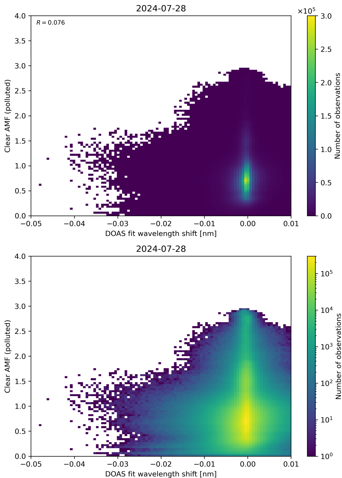
Figure 129: Scatter density plot of “DOAS fit wavelength shift” against “Clear AMF (polluted)” for 2024-07-27 to 2024-07-29.
