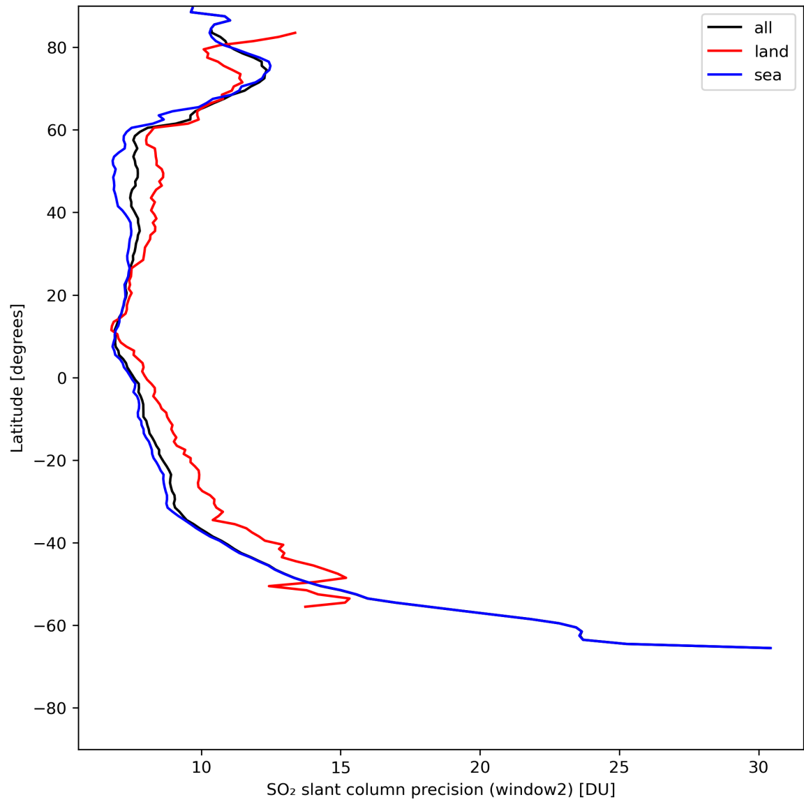
Figure 38: Zonal average of “SO 2 slant column precision (window2)” for 2024-07-27 to 2024-07-29.
