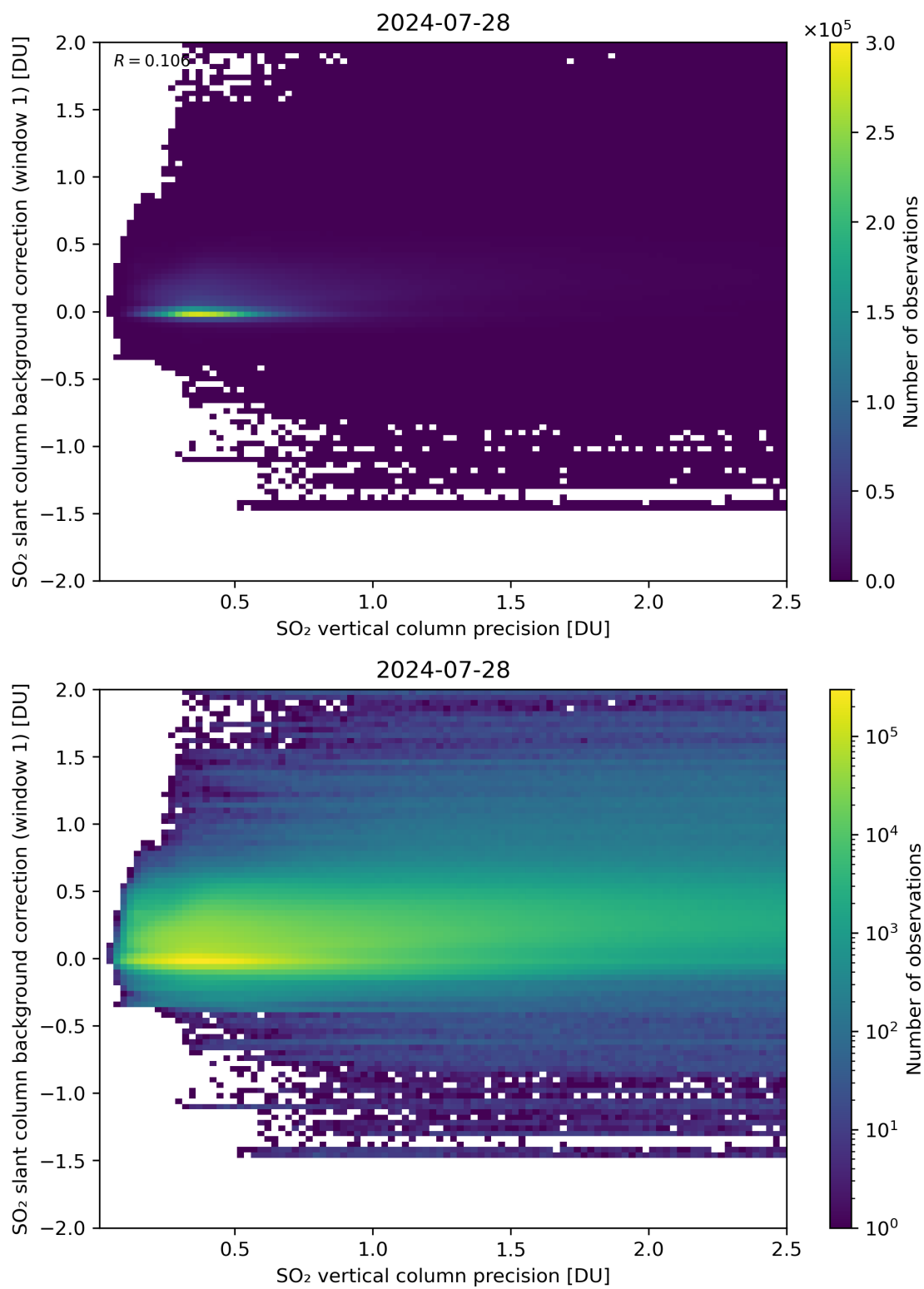
Figure 279: Scatter density plot of “SO 2 vertical column precision” against “SO 2 slant column background correction (window 1)” for 2024-07-27 to 2024-07-29.
