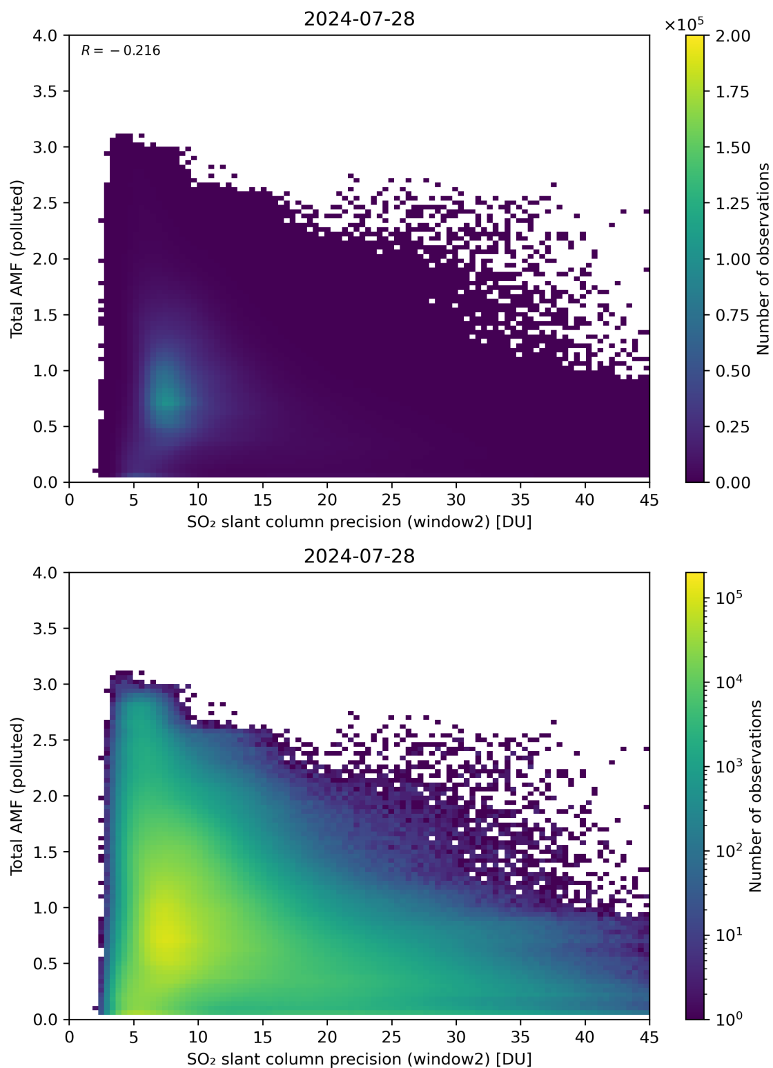
Figure 251: Scatter density plot of “SO 2 slant column precision (window2)” against “Total AMF (polluted)” for 2024-07-27 to 2024-07-29.
