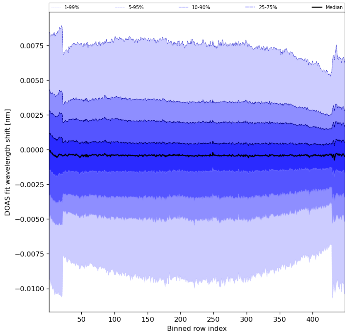
Figure 91: Along track statistics of “DOAS fit wavelength shift” for 2024-07-27 to 2024-07-29
