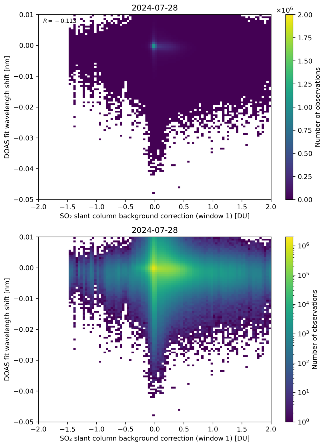
Figure 100: Scatter density plot of “SO 2 slant column background correction (window 1)” against “DOAS fit wavelength shift” for 2024-07-27 to 2024-07-29.
