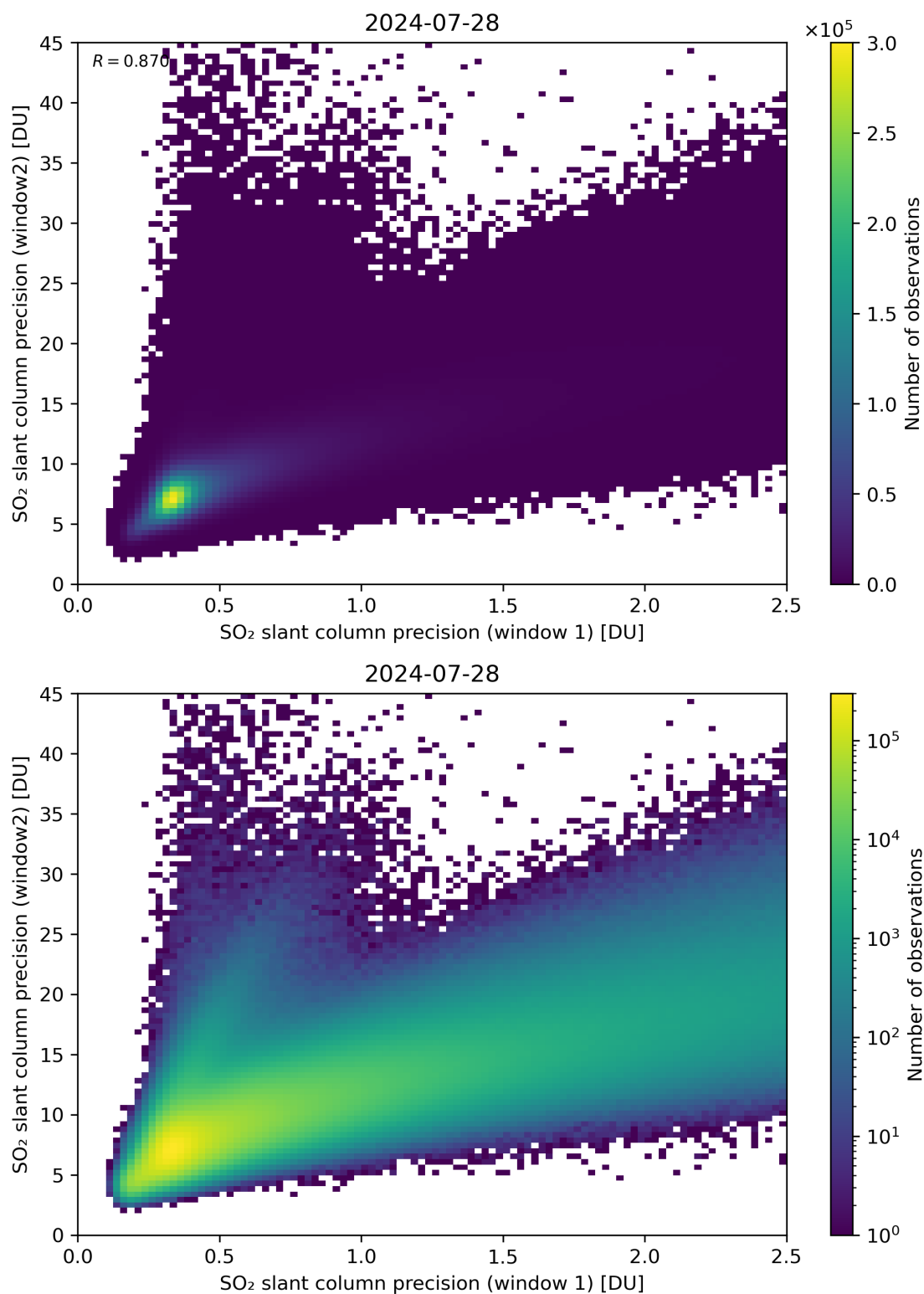
Figure 227: Scatter density plot of “SO 2 slant column precision (window 1)” against “SO 2 slant column precision (window2)” for 2024-07-27 to 2024-07-29.
