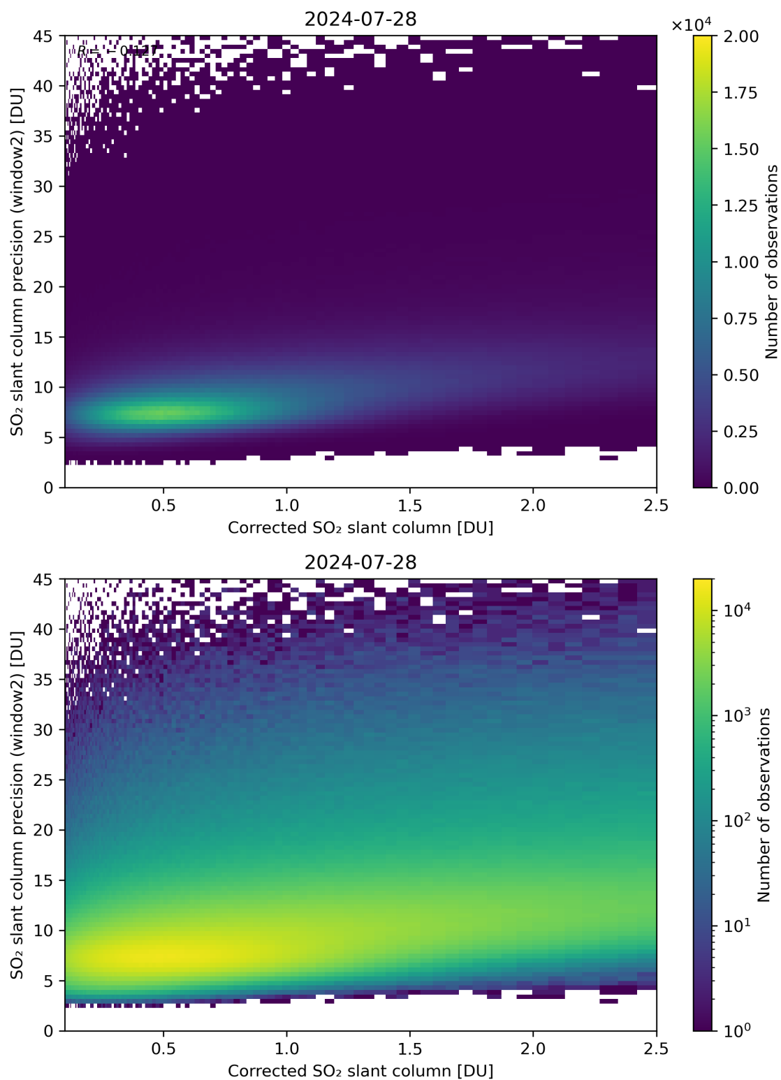
Figure 189: Scatter density plot of “Corrected SO 2 slant column” against “SO 2 slant column precision (window2)” for 2024-07-27 to 2024-07-29.
