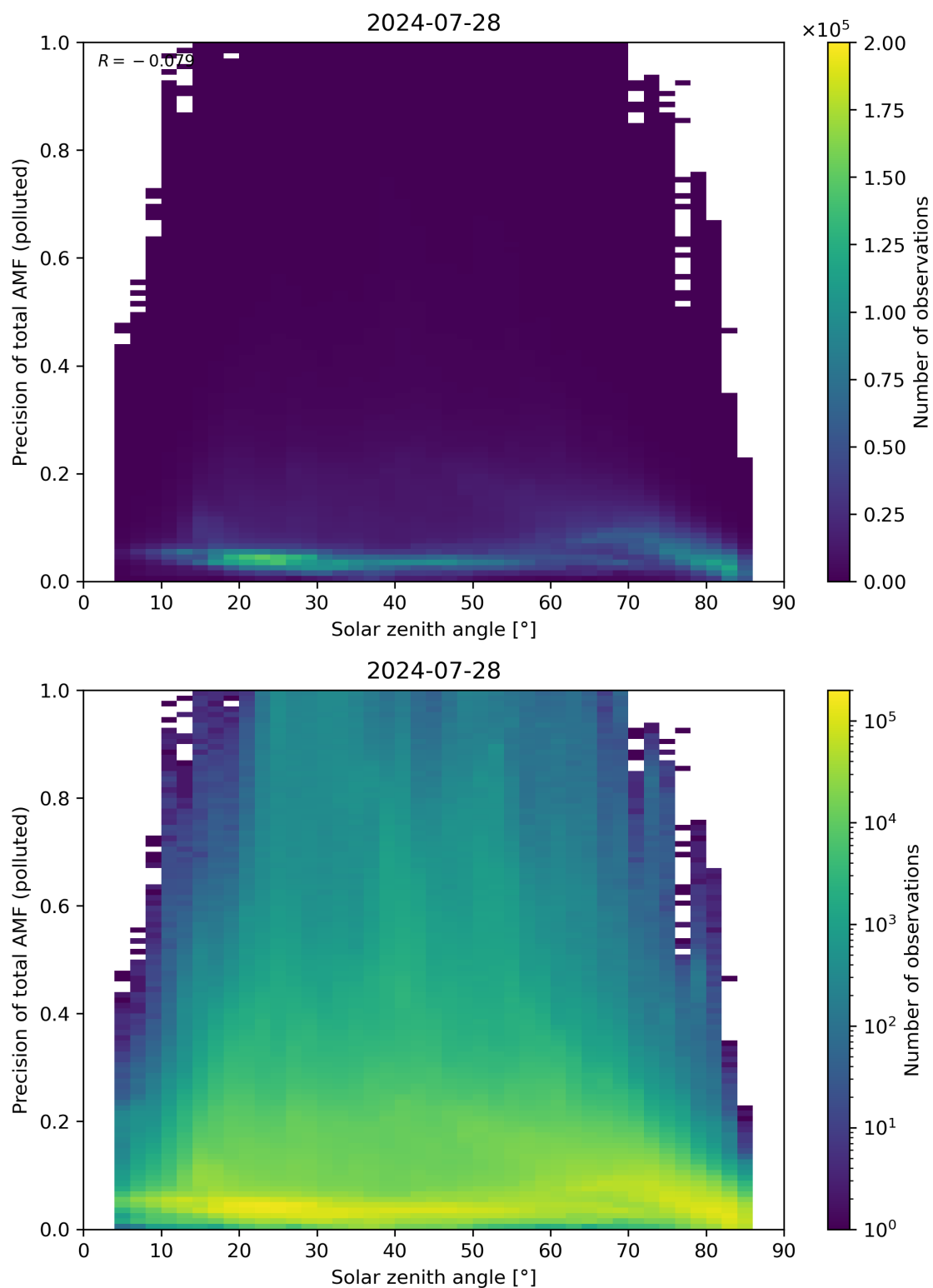
Figure 175: Scatter density plot of “Solar zenith angle” against “Precision of total AMF (polluted)” for 2024-07-27 to 2024-07-29.
