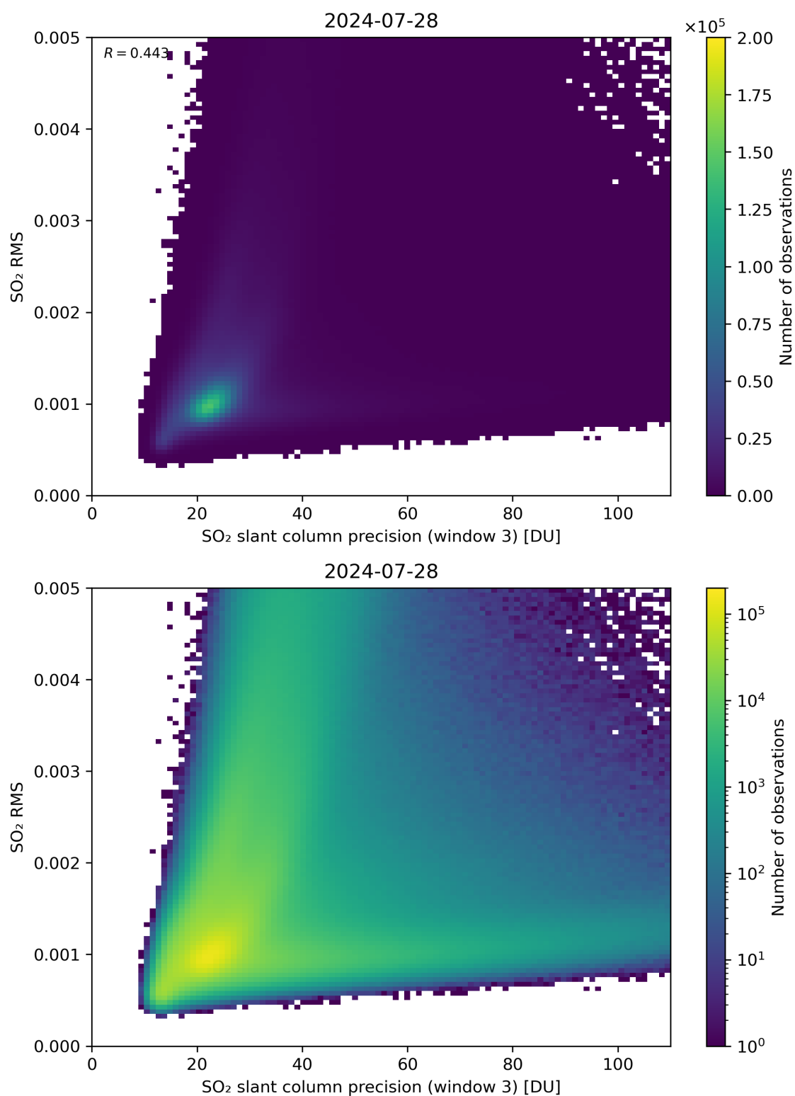
Figure 260: Scatter density plot of “SO 2 slant column precision (window 3)” against “SO 2 RMS” for 2024-07-27 to 2024-07-29.
