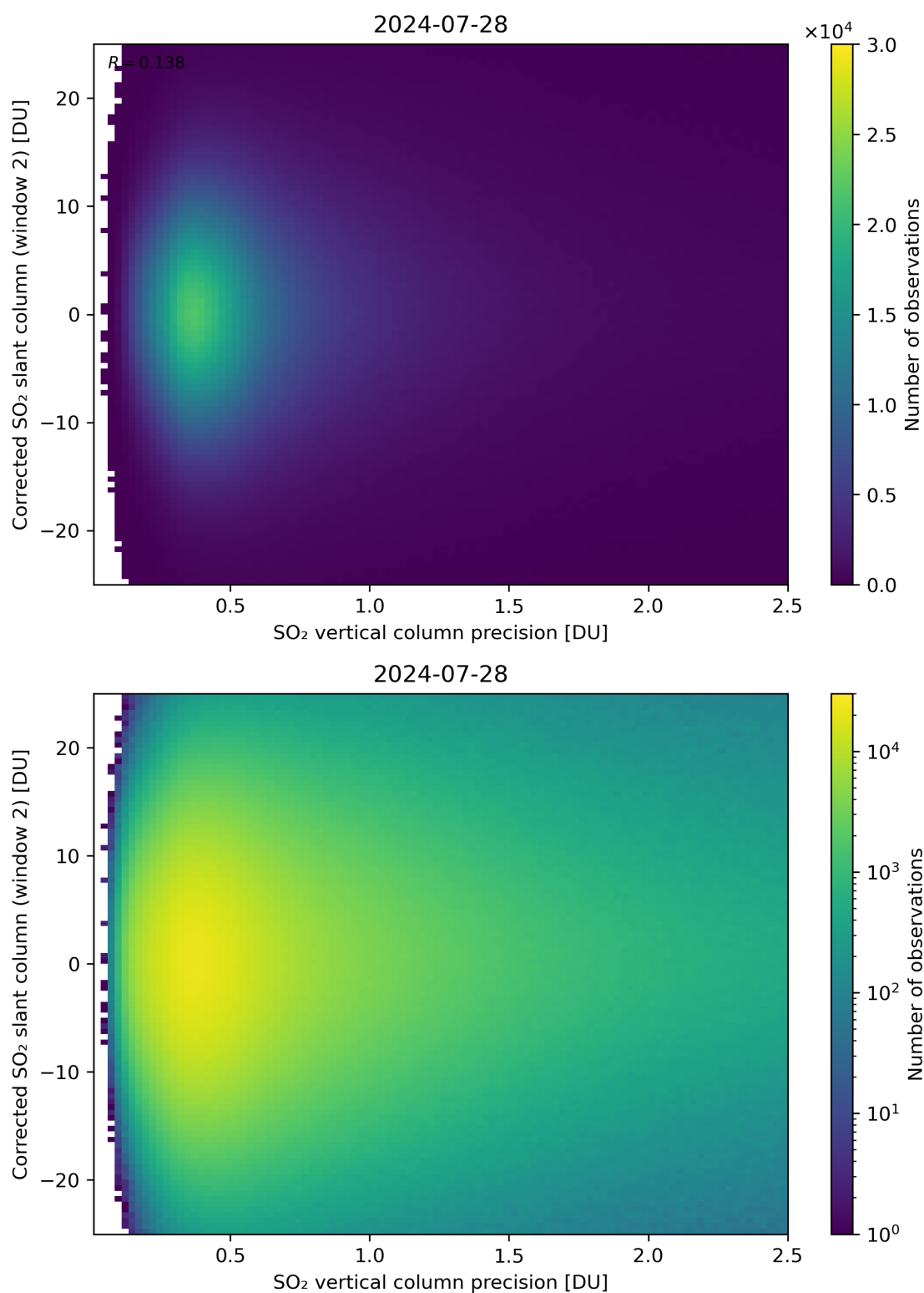
Figure 287: Scatter density plot of “SO 2 vertical column precision” against “Corrected SO 2 slant column (window 2)” for 2024-07-27 to 2024-07-29.
