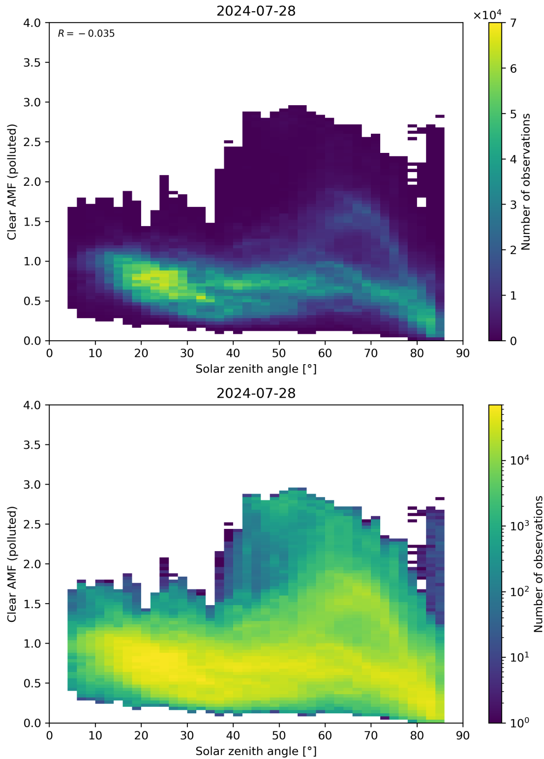
Figure 165: Scatter density plot of “Solar zenith angle” against “Clear AMF (polluted)” for 2024-07-27 to 2024-07-29.
