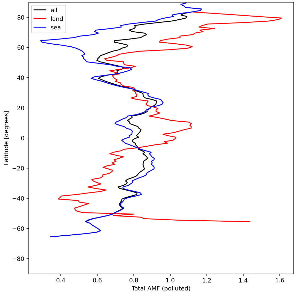
Figure 48: Zonal average of “Total AMF (polluted)” for 2024-07-27 to 2024-07-29.
