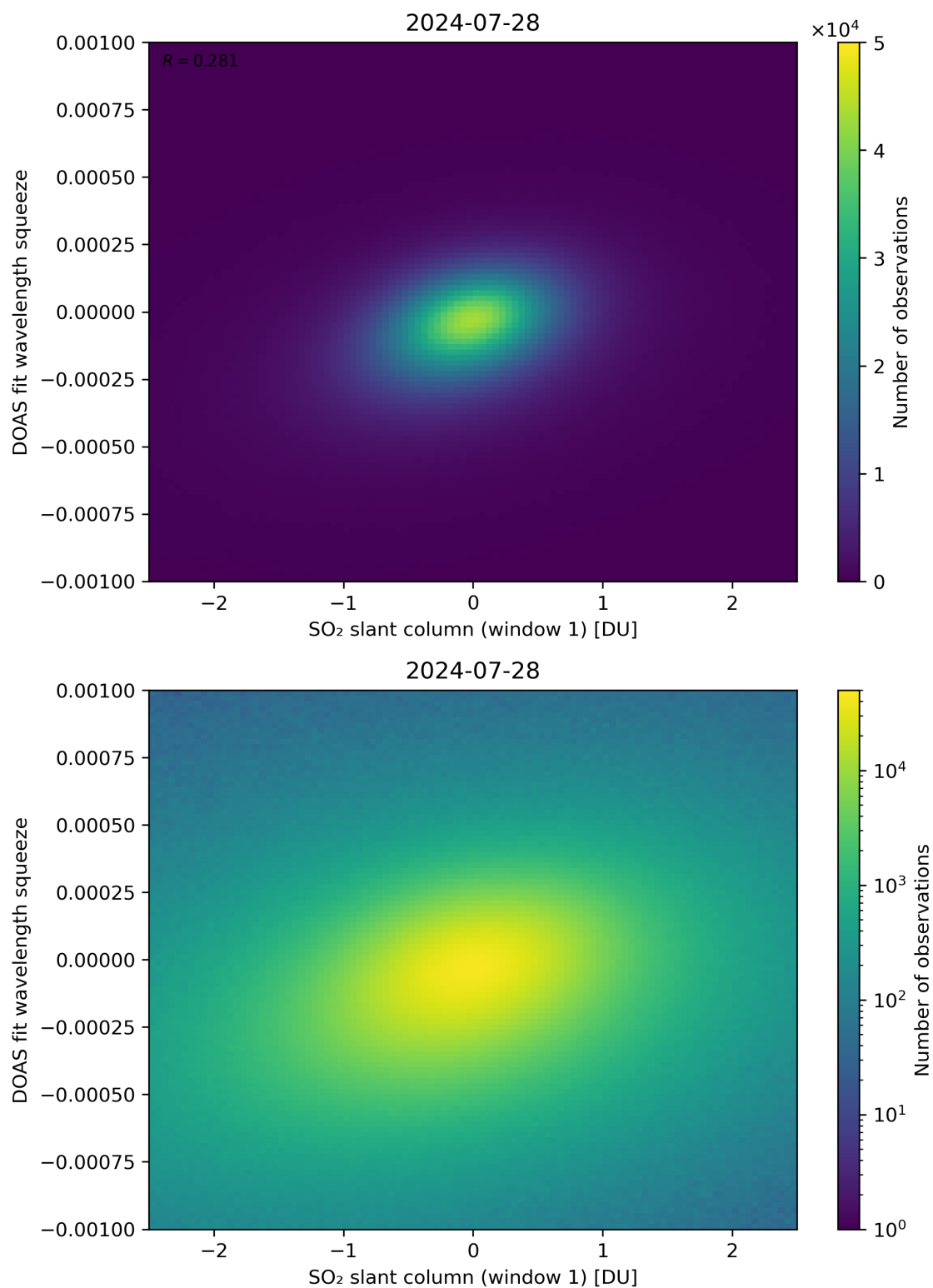
Figure 216: Scatter density plot of “SO 2 slant column (window 1)” against “DOAS fit wavelength squeeze” for 2024-07-27 to 2024-07-29.
