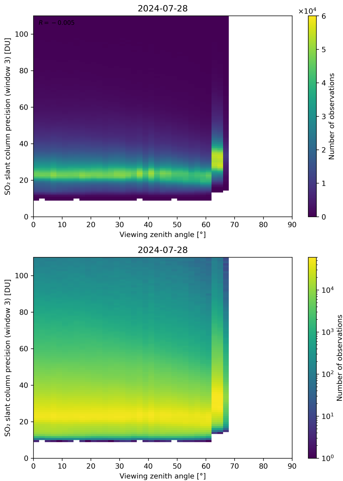
Figure 324: Scatter density plot of “Viewing zenith angle” against “SO 2 slant column precision (window 3)” for 2024-07-27 to 2024-07-29.
