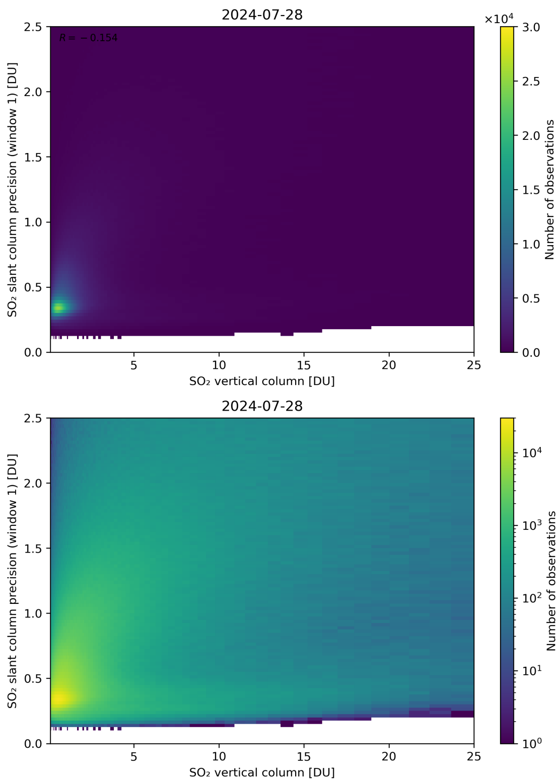
Figure 301: Scatter density plot of “SO 2 vertical column” against “SO 2 slant column precision (window 1)” for 2024-07-27 to 2024-07-29.
