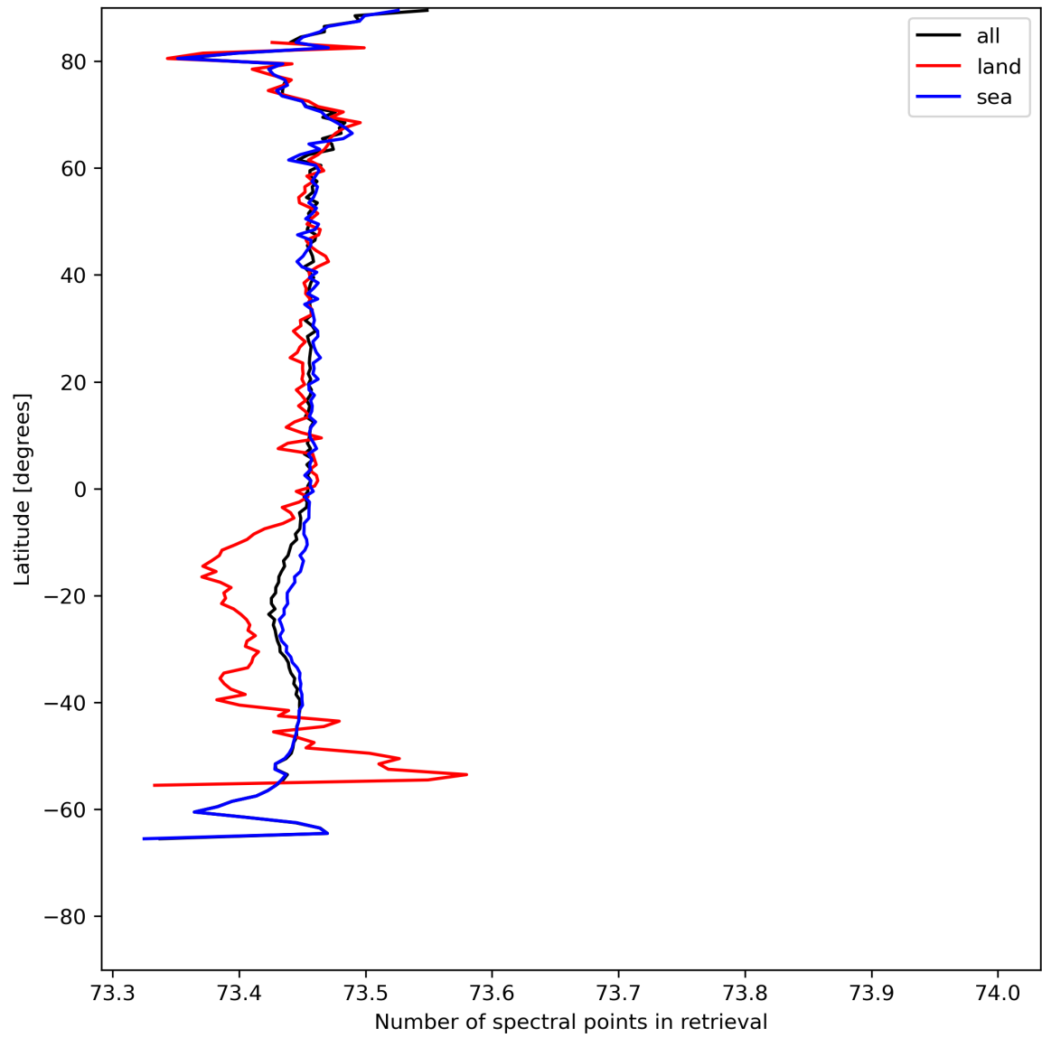
Figure 51: Zonal average of “Number of spectral points in retrieval” for 2024-07-27 to 2024-07-29.
