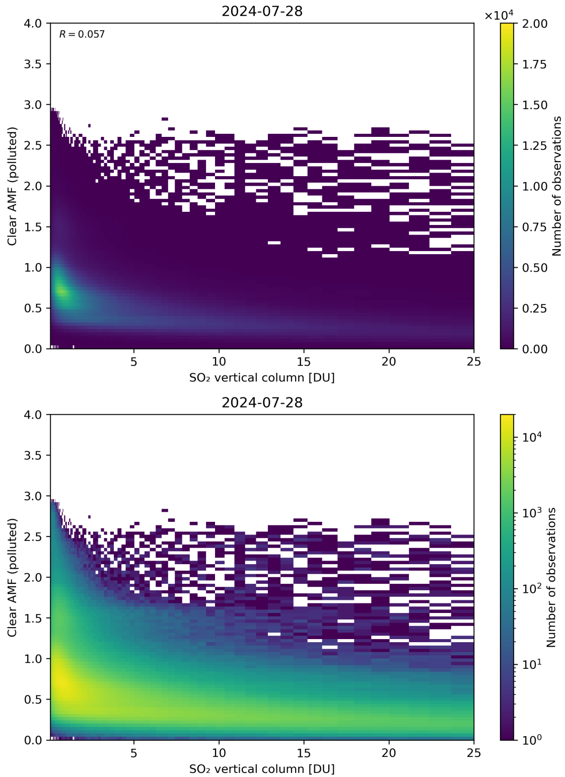
Figure 296: Scatter density plot of “SO 2 vertical column” against “Clear AMF (polluted)” for 2024-07-27 to 2024-07-29.
