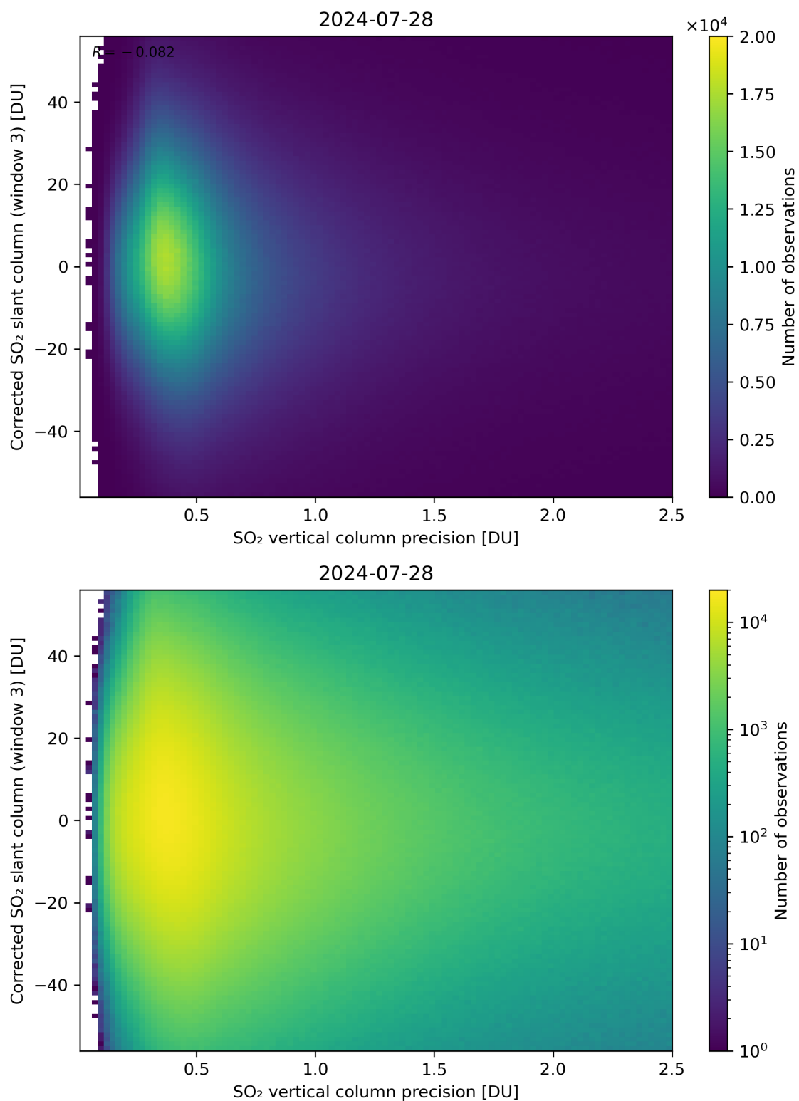
Figure 288: Scatter density plot of “SO 2 vertical column precision” against “Corrected SO 2 slant column (window 3)” for 2024-07-27 to 2024-07-29.
