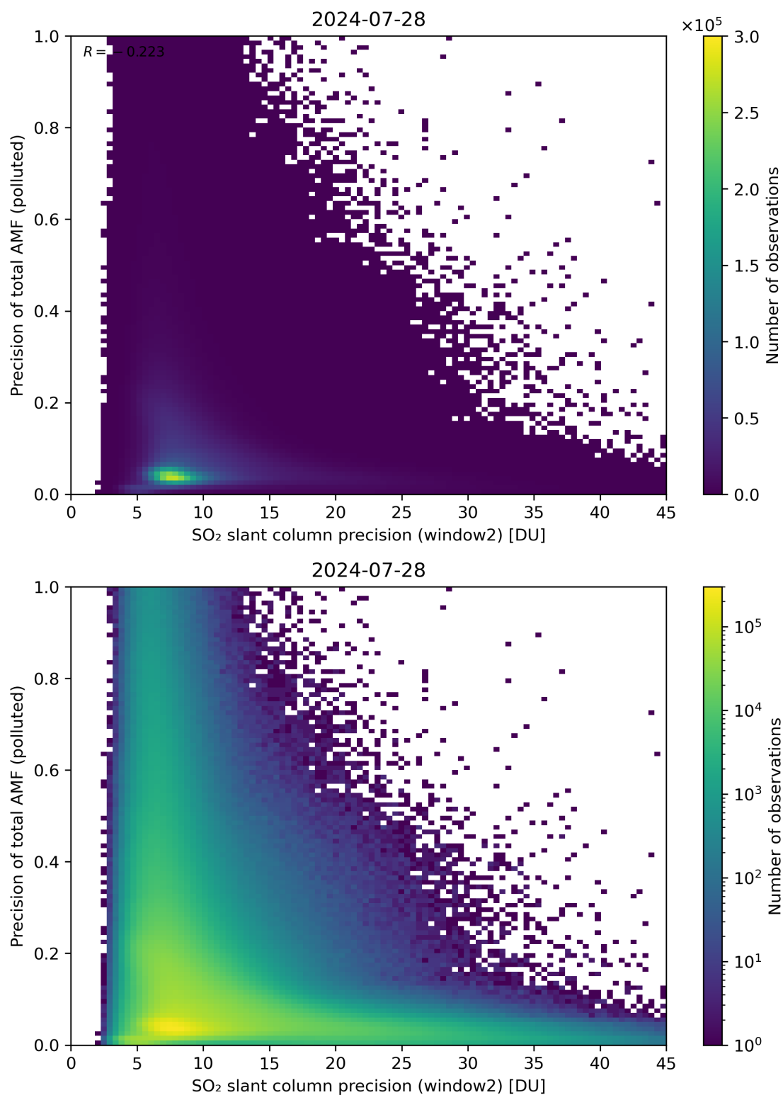
Figure 252: Scatter density plot of “SO 2 slant column precision (window2)” against “Precision of total AMF (polluted)” for 2024-07-27 to 2024-07-29.
