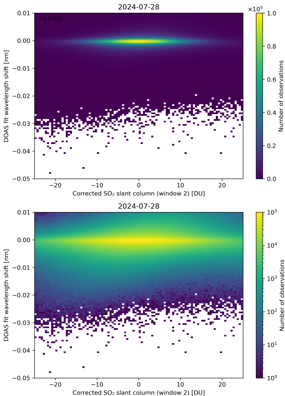
Figure 196: Scatter density plot of “Corrected SO 2 slant column (window 2)” against “DOAS fit wavelength shift” for 2024-07-27 to 2024-07-29.
