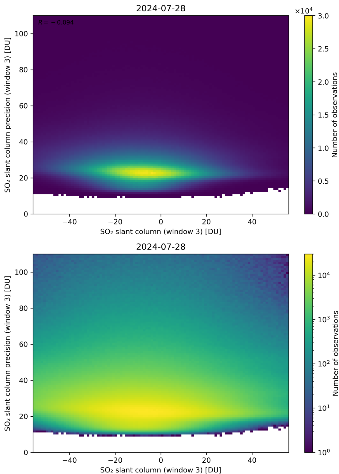
Figure 267: Scatter density plot of “SO 2 slant column (window 3)” against “SO 2 slant column precision (window 3)” for 2024-07-27 to 2024-07-29.
