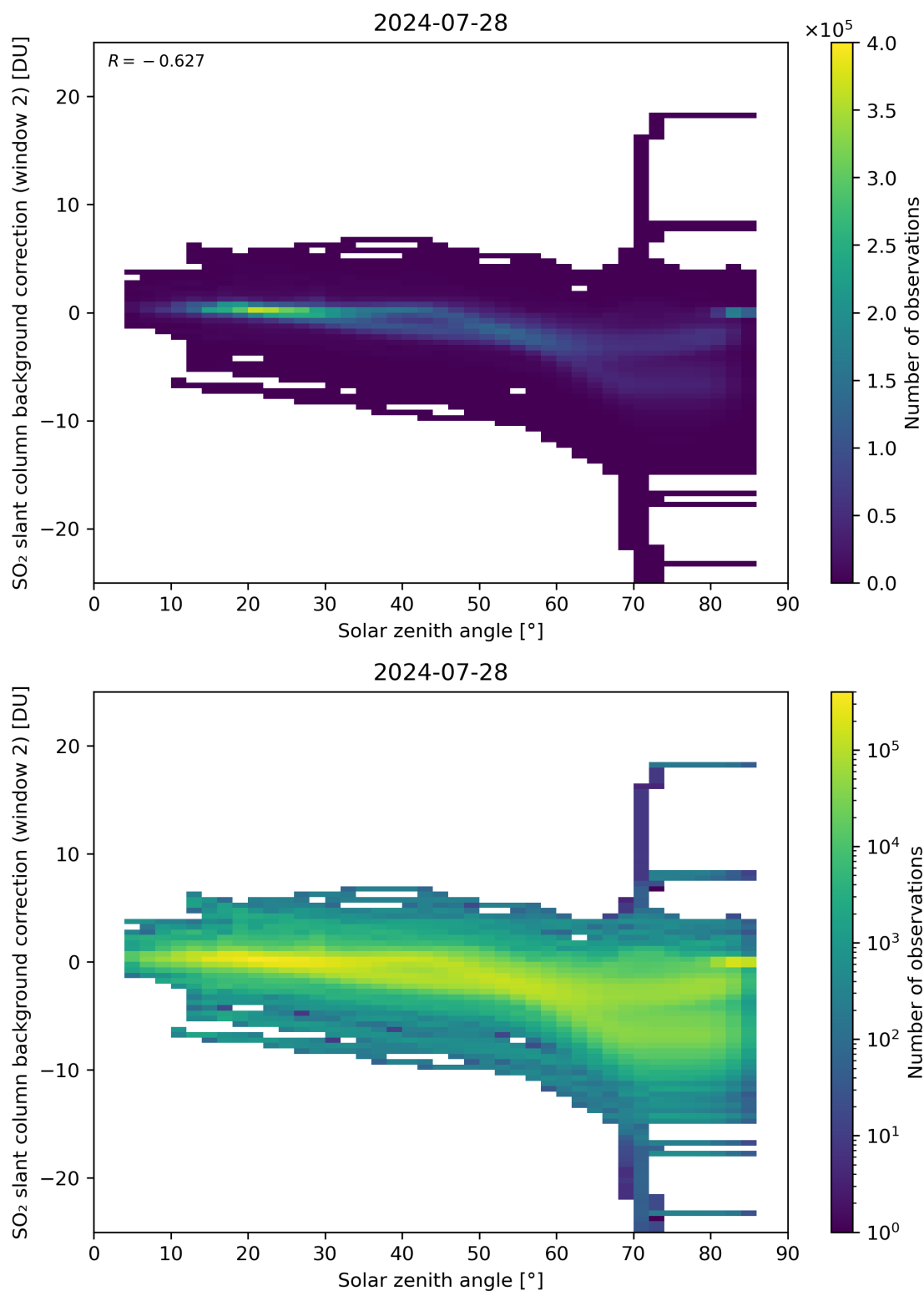
Figure 159: Scatter density plot of “Solar zenith angle” against “SO 2 slant column background correction (window 2)” for 2024-07-27 to 2024-07-29.
