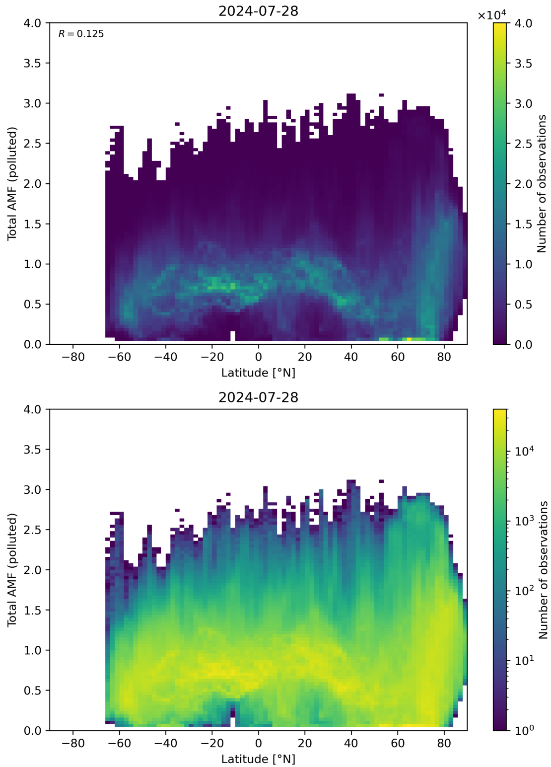
Figure 154: Scatter density plot of “Latitude” against “Total AMF (polluted)” for 2024-07-27 to 2024-07-29.
