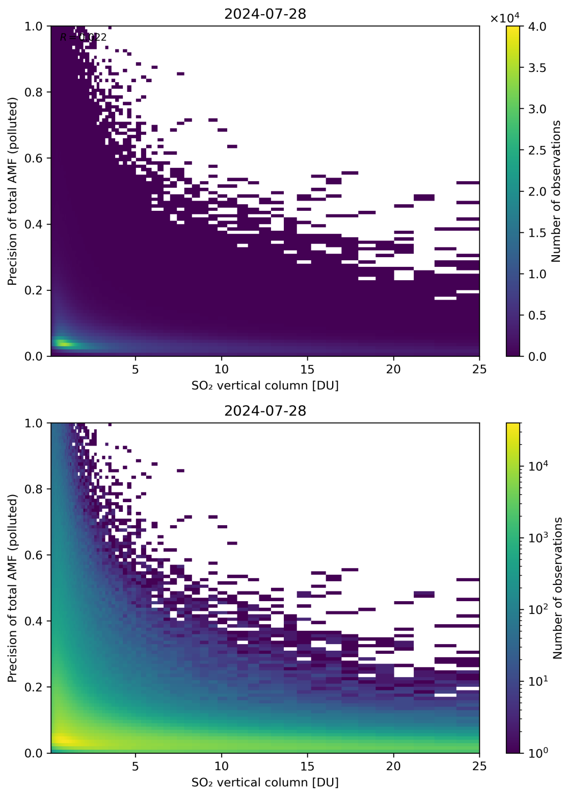
Figure 306: Scatter density plot of “SO 2 vertical column” against “Precision of total AMF (polluted)” for 2024-07-27 to 2024-07-29.
