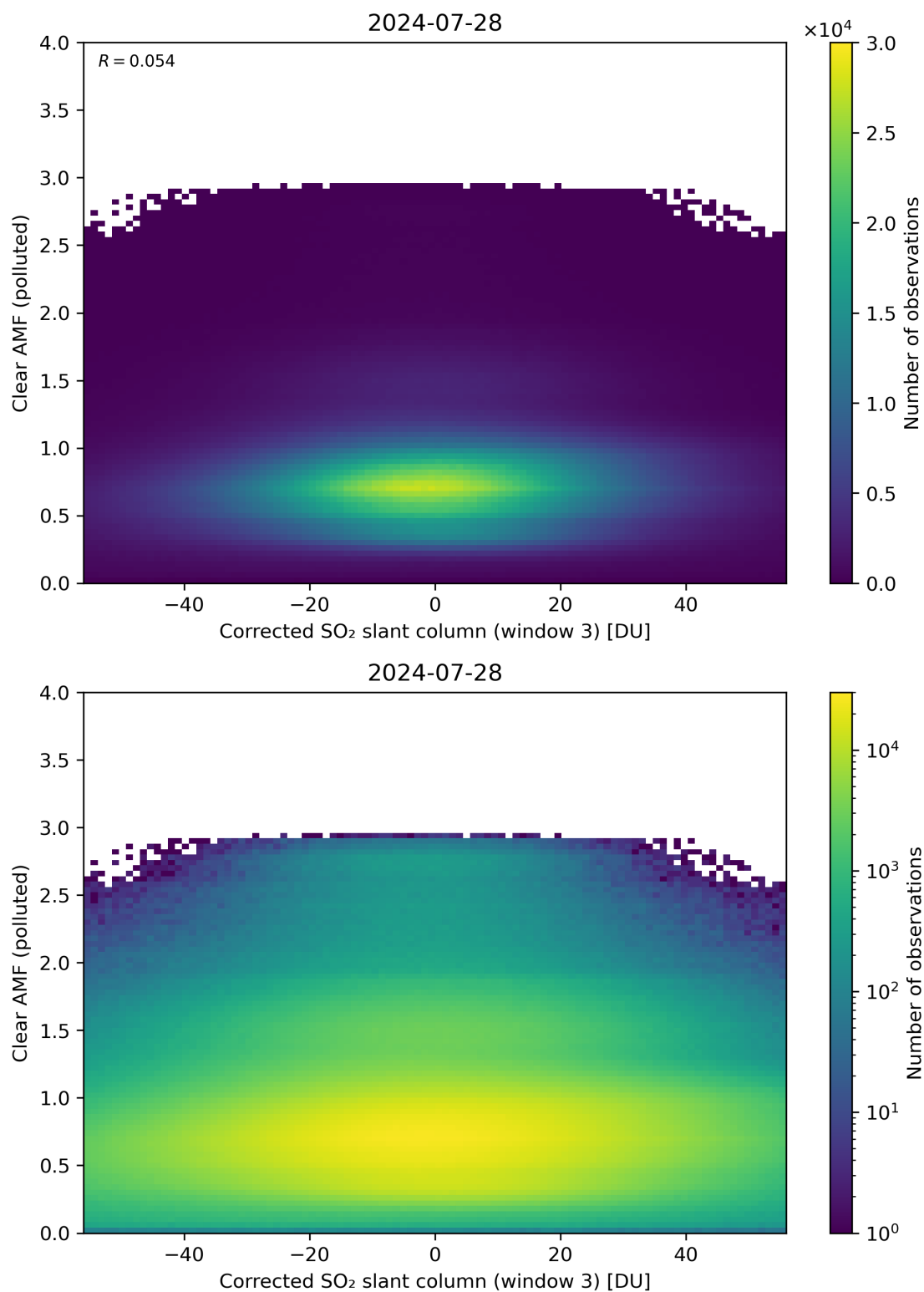
Figure 209: Scatter density plot of “Corrected SO 2 slant column (window 3)” against “Clear AMF (polluted)” for 2024-07-27 to 2024-07-29.
