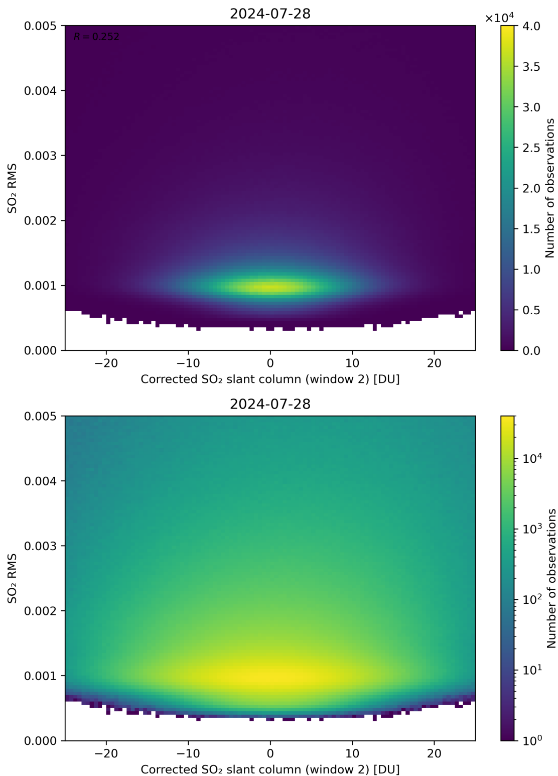
Figure 198: Scatter density plot of “Corrected SO 2 slant column (window 2)” against “SO 2 RMS” for 2024-07-27 to 2024-07-29.
