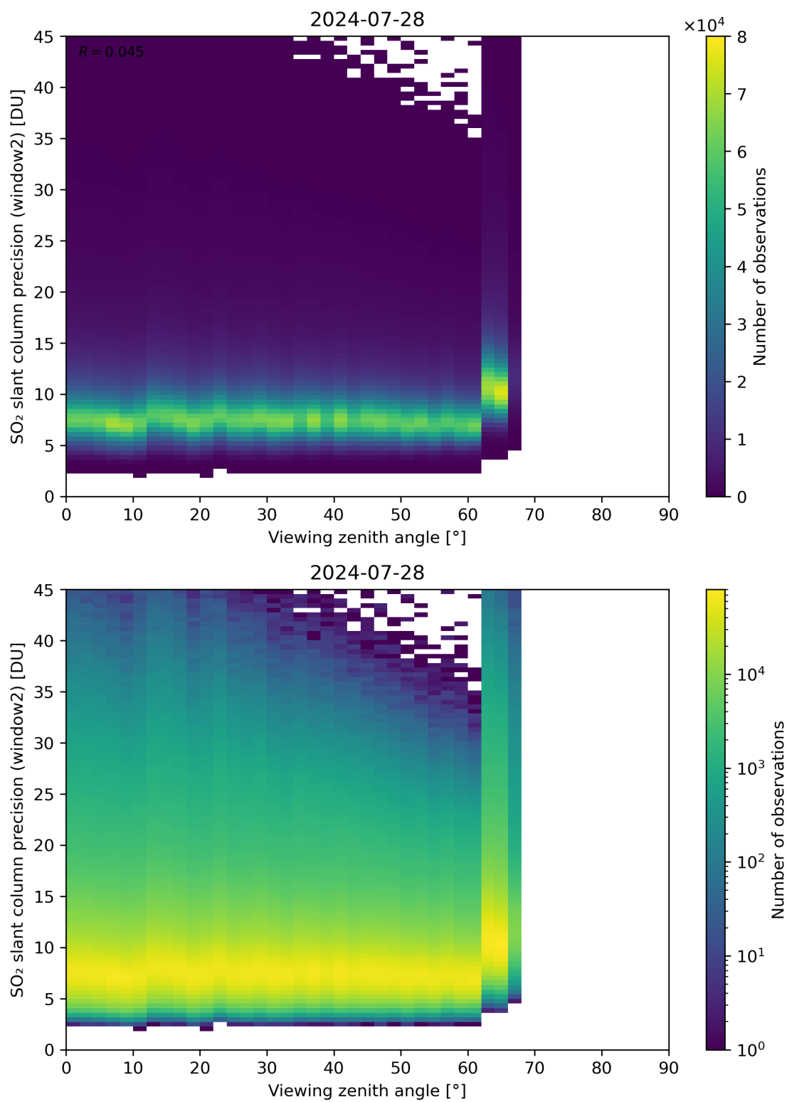
Figure 322: Scatter density plot of “Viewing zenith angle” against “SO 2 slant column precision (window2)” for 2024-07-27 to 2024-07-29.
