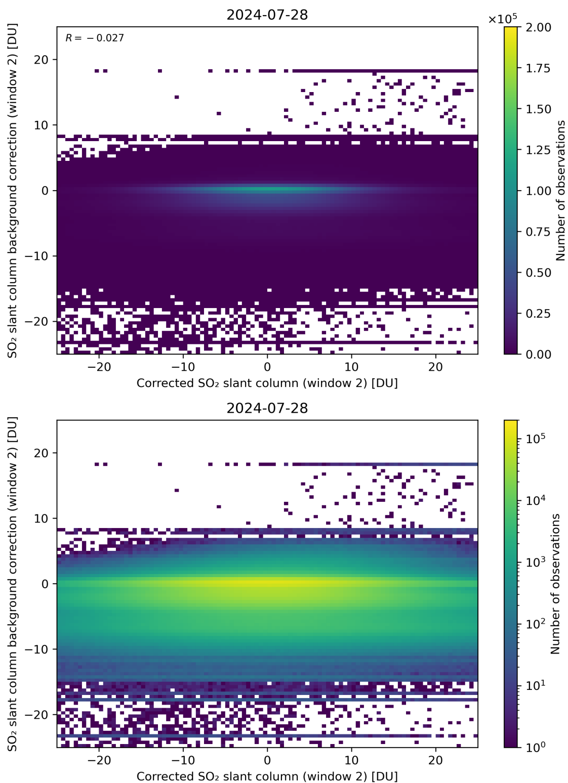
Figure 194: Scatter density plot of “Corrected SO 2 slant column (window 2)” against “SO 2 slant column background correction (window 2)” for 2024-07-27 to 2024-07-29.
