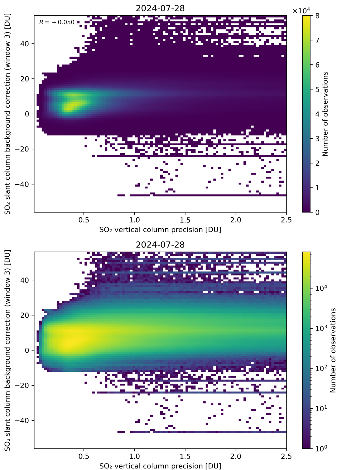
Figure 281: Scatter density plot of “SO 2 vertical column precision” against “SO 2 slant column background correction (window 3)” for 2024-07-27 to 2024-07-29.
