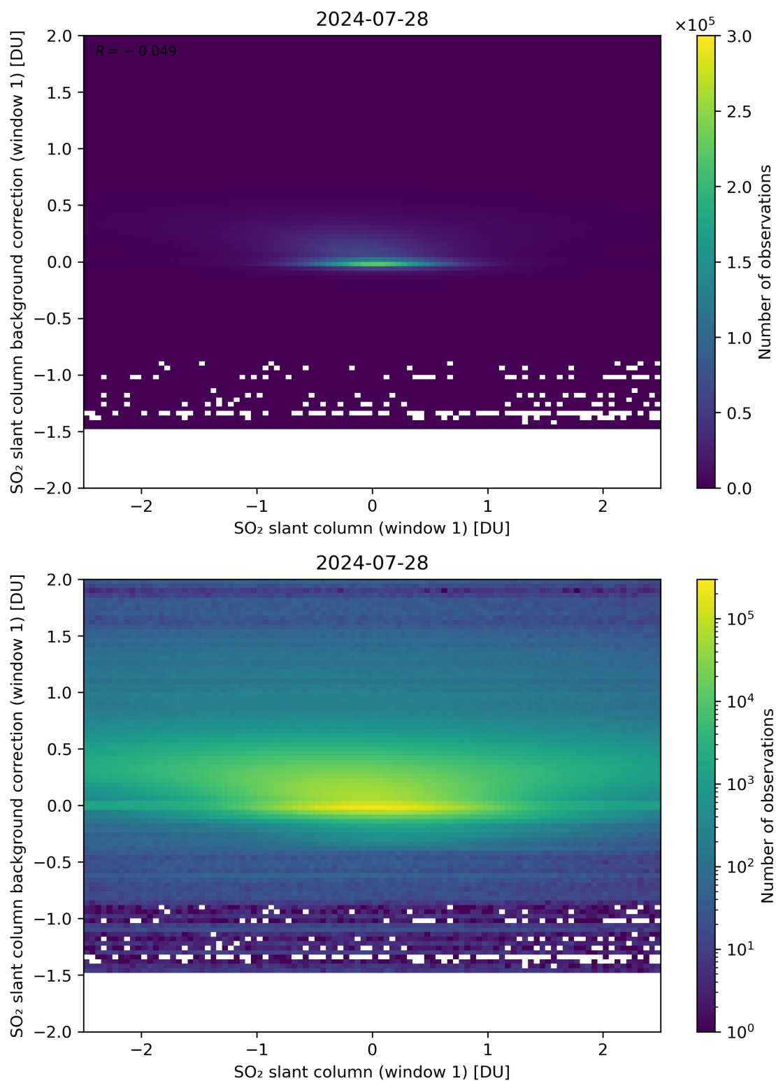
Figure 212: Scatter density plot of “SO 2 slant column (window 1)” against “SO 2 slant column background correction (window 1)” for 2024-07-27 to 2024-07-29.
