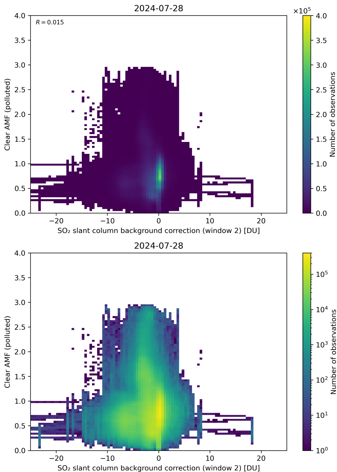
Figure 115: Scatter density plot of “SO 2 slant column background correction (window 2)” against “Clear AMF (polluted)” for 2024-07-27 to 2024-07-29.
