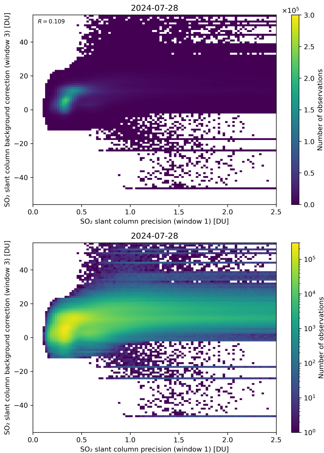
Figure 220: Scatter density plot of “SO 2 slant column precision (window 1)” against “SO 2 slant column background correction (window 3)” for 2024-07-27 to 2024-07-29.
