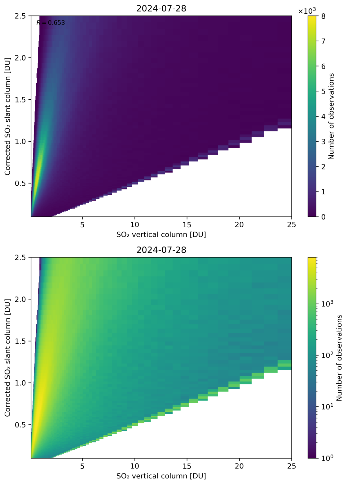
Figure 297: Scatter density plot of “SO 2 vertical column” against “Corrected SO 2 slant column” for 2024-07-27 to 2024-07-29.
