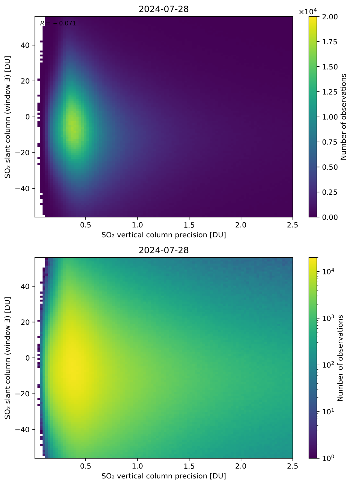
Figure 292: Scatter density plot of “SO 2 vertical column precision” against “SO 2 slant column (window 3)” for 2024-07-27 to 2024-07-29.
