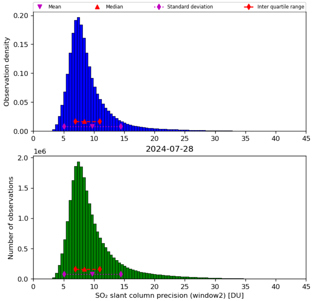
Figure 61: Histogram of “SO 2 slant column precision (window2)” for 2024-07-27 to 2024-07-29
