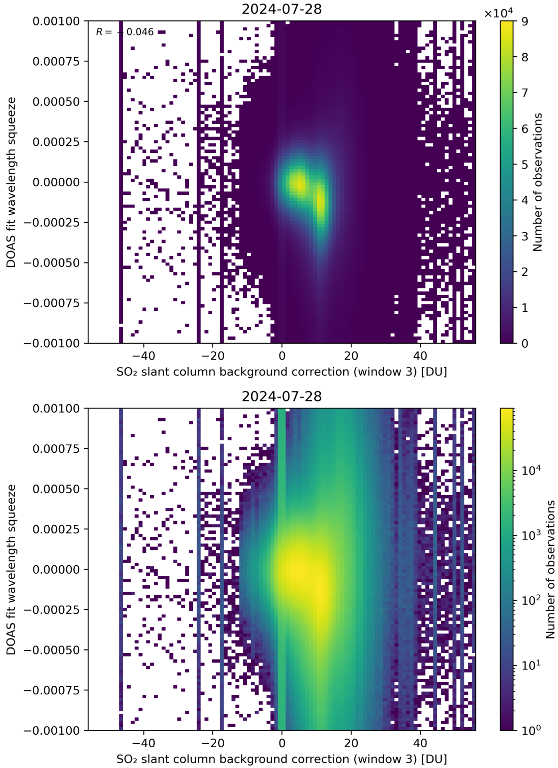
Figure 122: Scatter density plot of “SO 2 slant column background correction (window 3)” against “DOAS fit wavelength squeeze” for 2024-07-27 to 2024-07-29.
