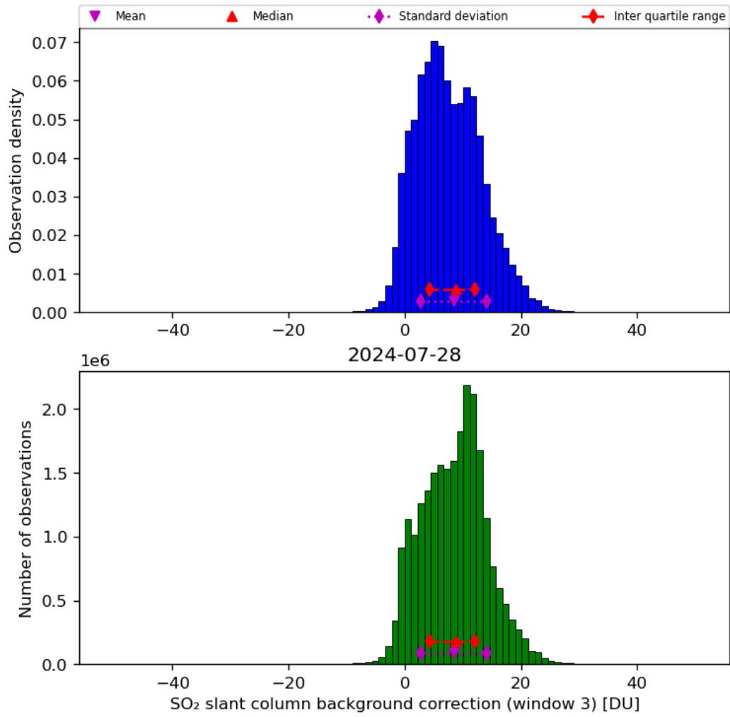
Figure 67: Histogram of “SO 2 slant column background correction (window 3)” for 2024-07-27 to 2024-07-29
