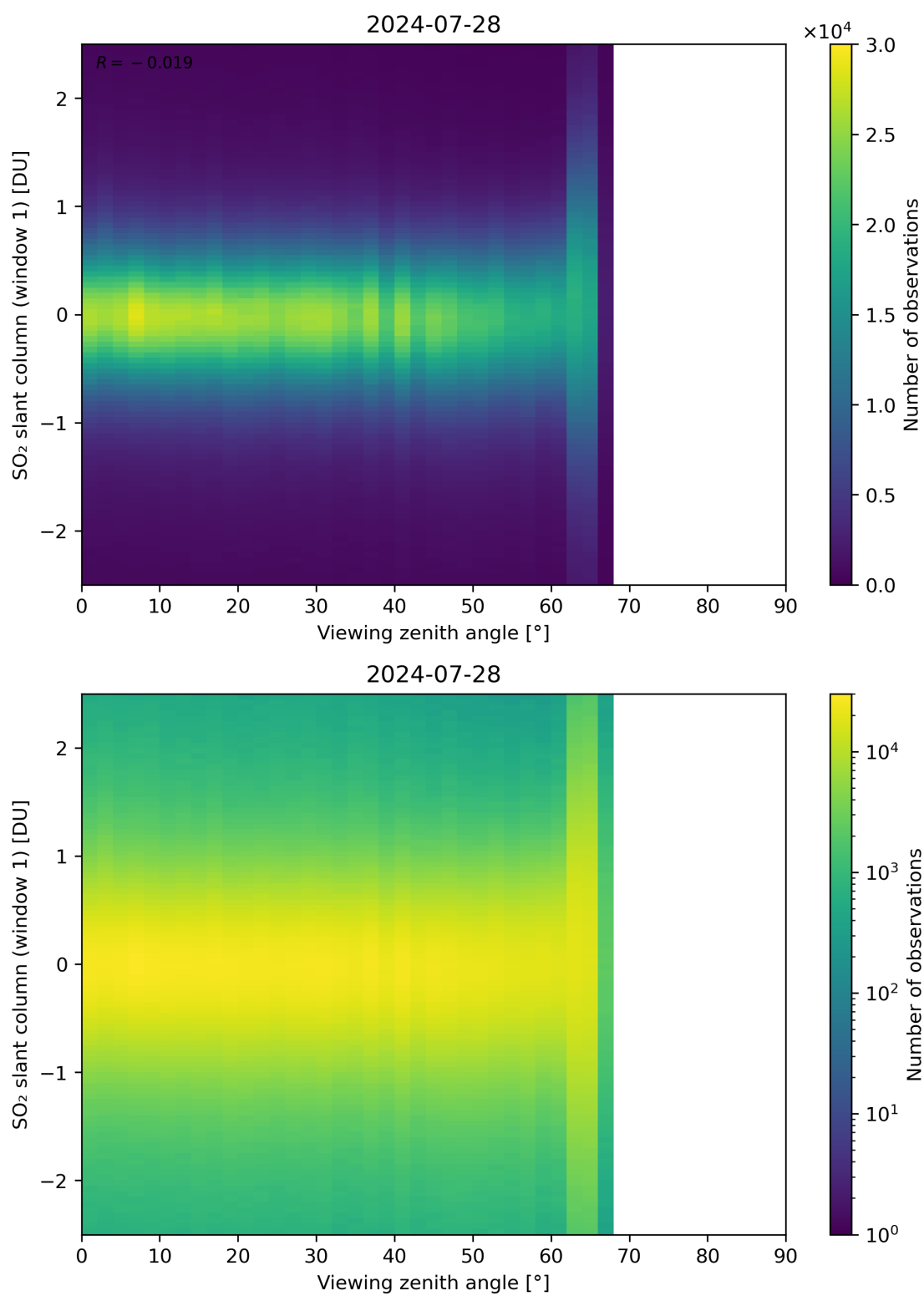
Figure 320: Scatter density plot of “Viewing zenith angle” against “SO 2 slant column (window 1)” for 2024-07-27 to 2024-07-29.
