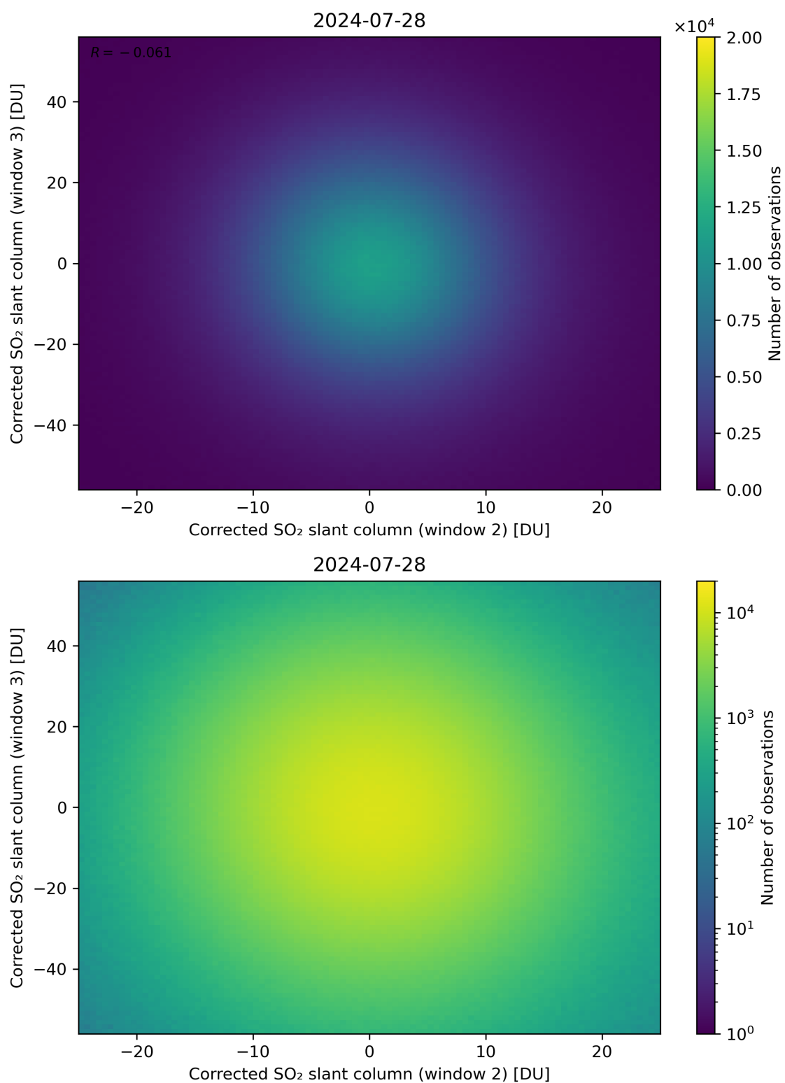
Figure 200: Scatter density plot of “Corrected SO 2 slant column (window 2)” against “Corrected SO 2 slant column (window 3)” for 2024-07-27 to 2024-07-29.
