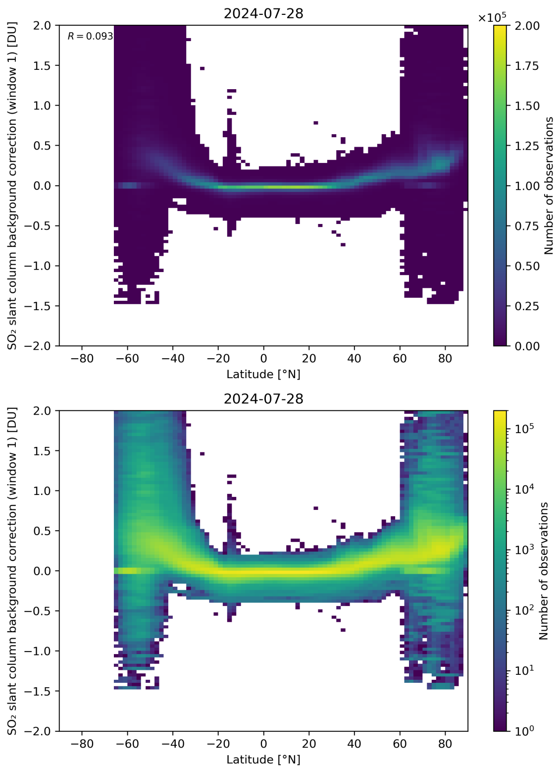
Figure 139: Scatter density plot of “Latitude” against “SO 2 slant column background correction (window 1)” for 2024-07-27 to 2024-07-29.
