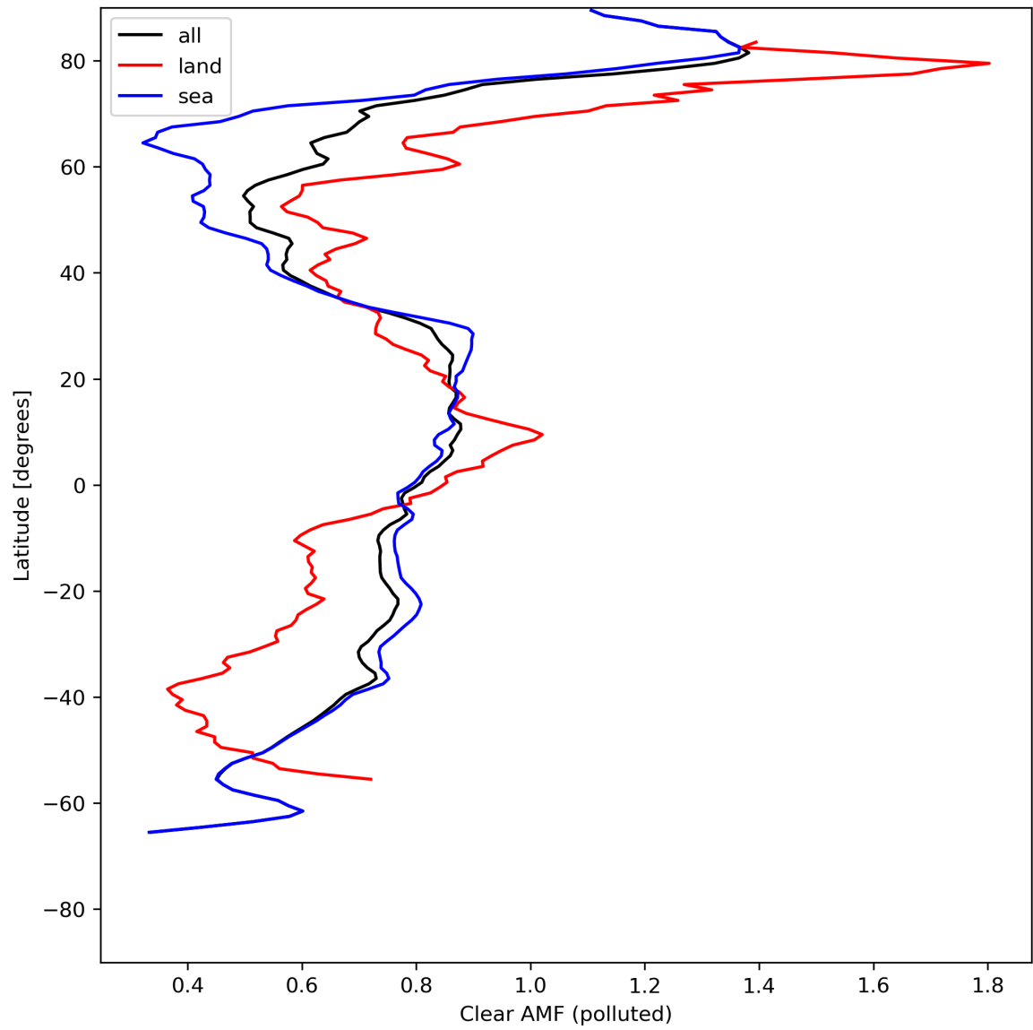
Figure 50: Zonal average of “Clear AMF (polluted)” for 2024-07-27 to 2024-07-29.
