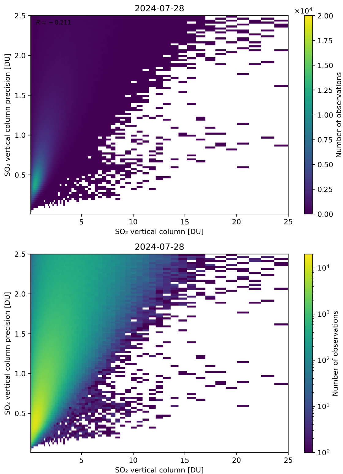
Figure 307: Scatter density plot of “SO 2 vertical column” against “SO 2 vertical column precision” for 2024-07-27 to 2024-07-29.
