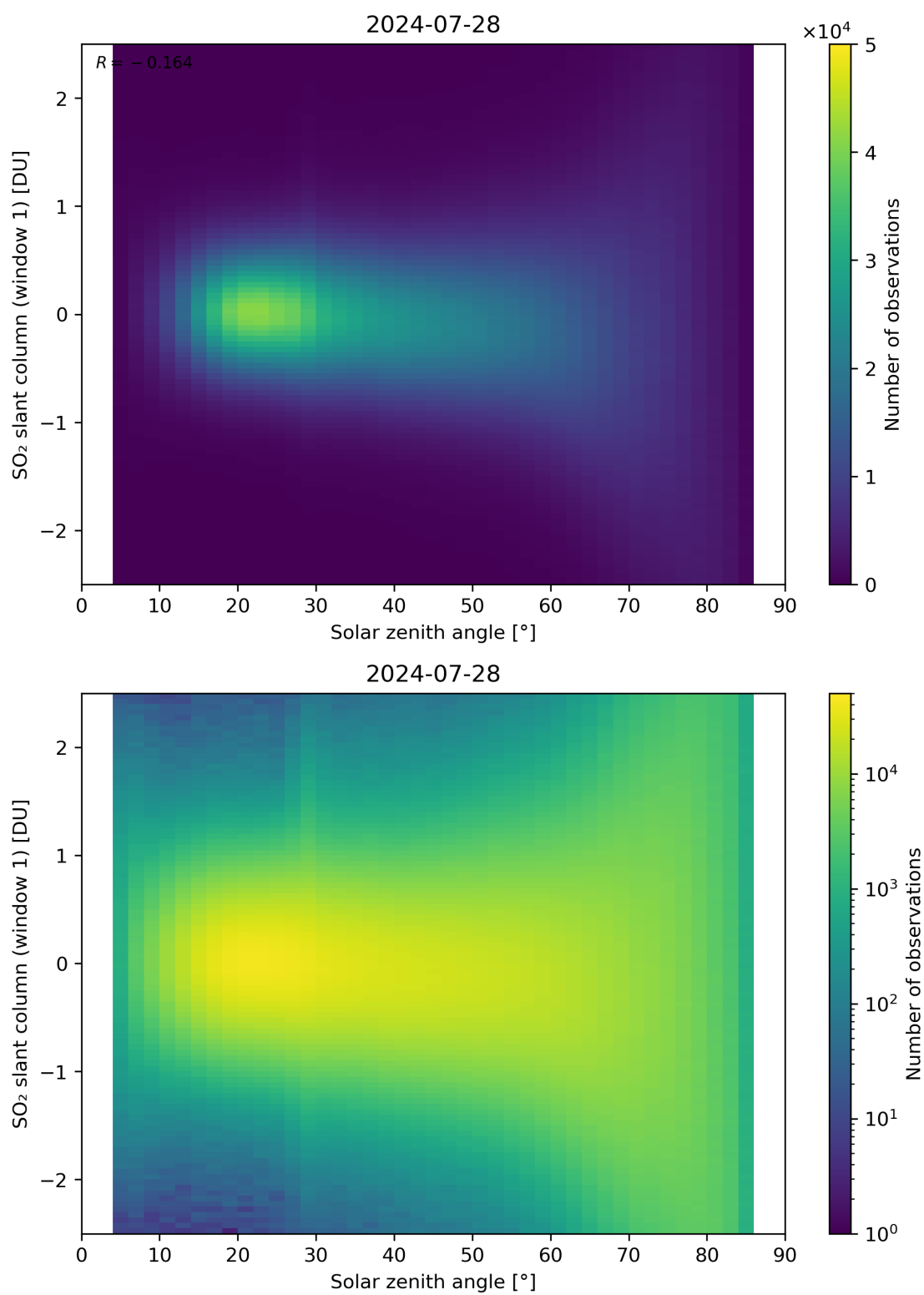
Figure 169: Scatter density plot of “Solar zenith angle” against “SO 2 slant column (window 1)” for 2024-07-27 to 2024-07-29.
