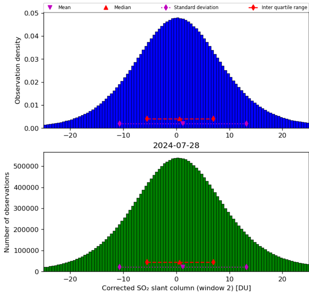
Figure 62: Histogram of “Corrected SO 2 slant column (window 2)” for 2024-07-27 to 2024-07-29
