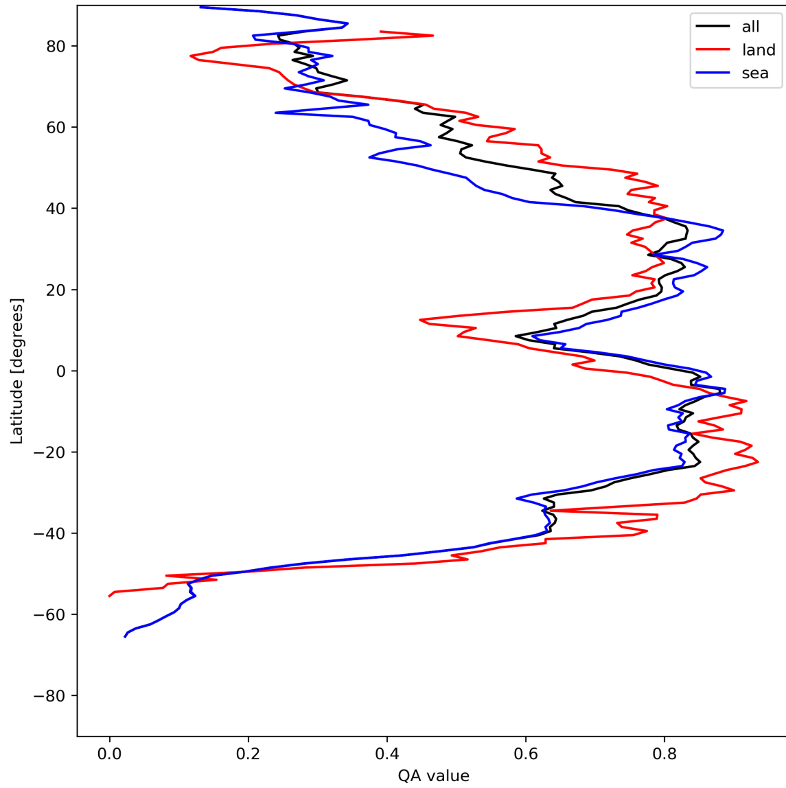
Figure 29: Zonal average of “QA value” for 2024-07-27 to 2024-07-29.
