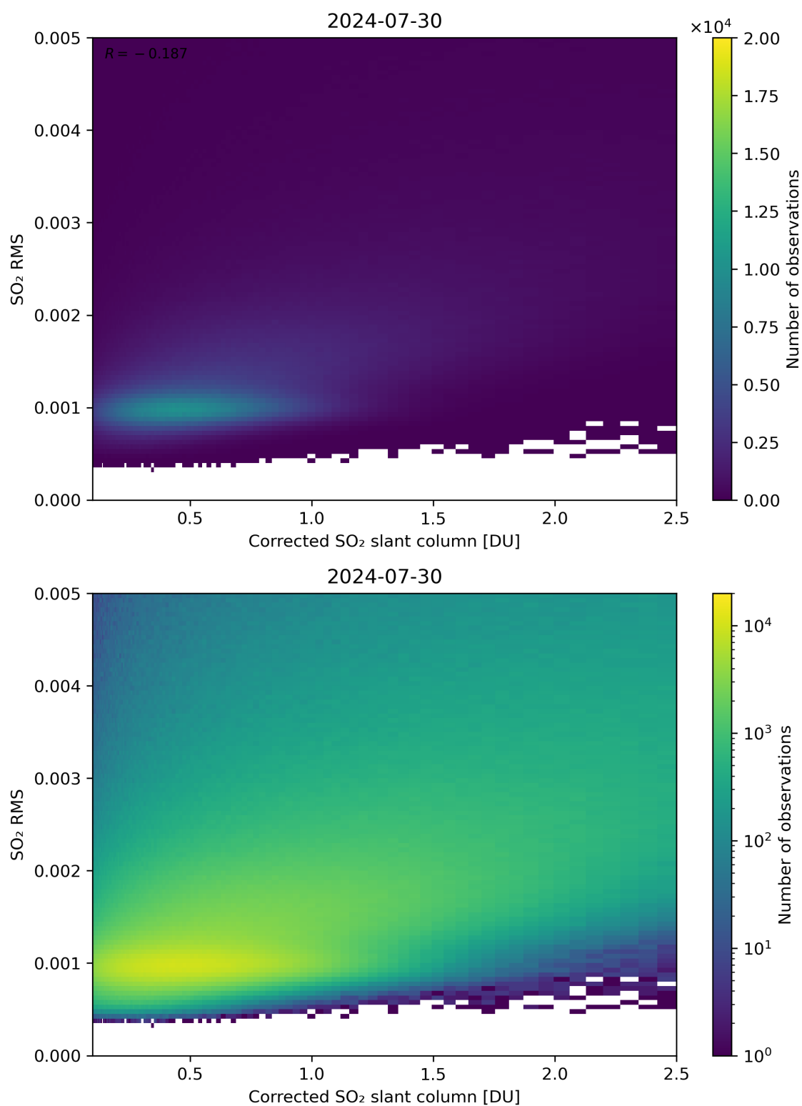
Figure 183: Scatter density plot of “Corrected SO 2 slant column” against “SO 2 RMS” for 2024-07-29 to 2024-07-31.
