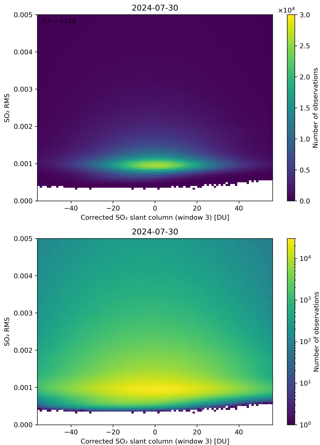
Figure 208: Scatter density plot of “Corrected SO 2 slant column (window 3)” against “SO 2 RMS” for 2024-07-29 to 2024-07-31.
