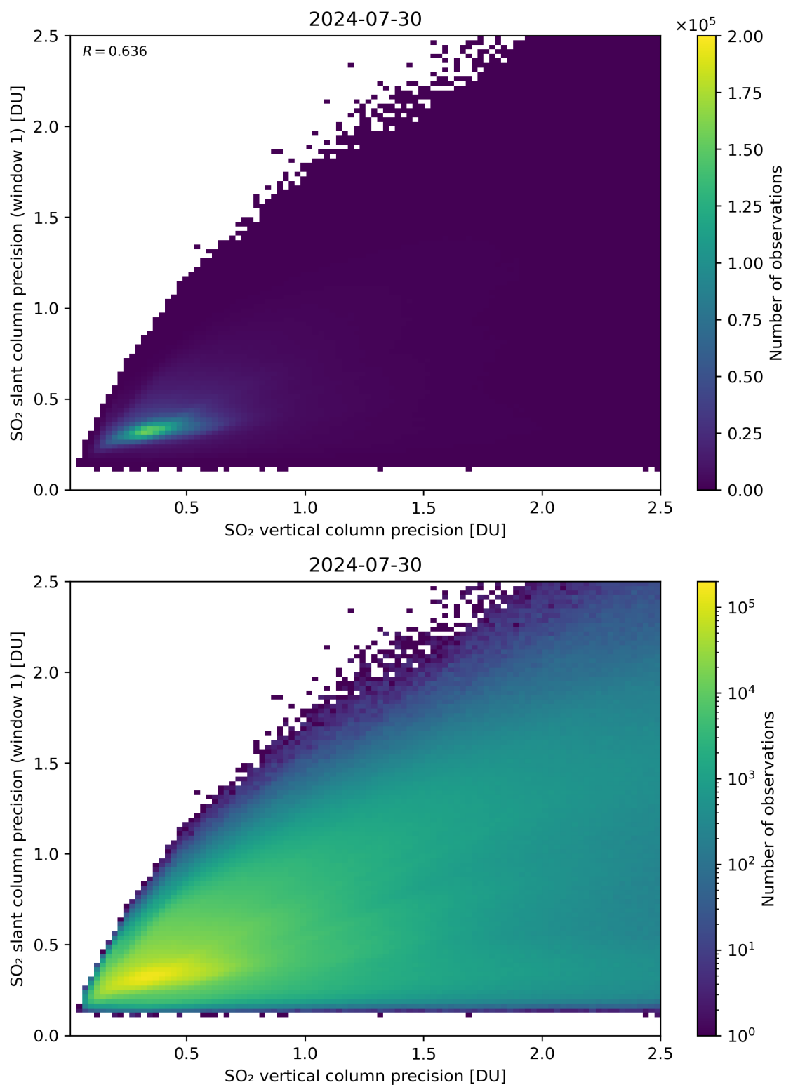
Figure 290: Scatter density plot of “SO 2 vertical column precision” against “SO 2 slant column precision (window 1)” for 2024-07-29 to 2024-07-31.
