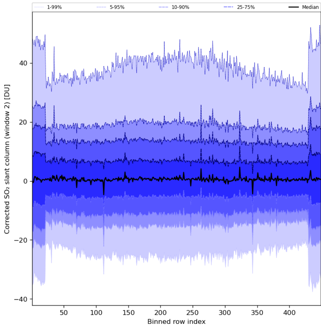
Figure 85: Along track statistics of “Corrected SO 2 slant column (window 2)” for 2024-07-29 to 2024-07-31
