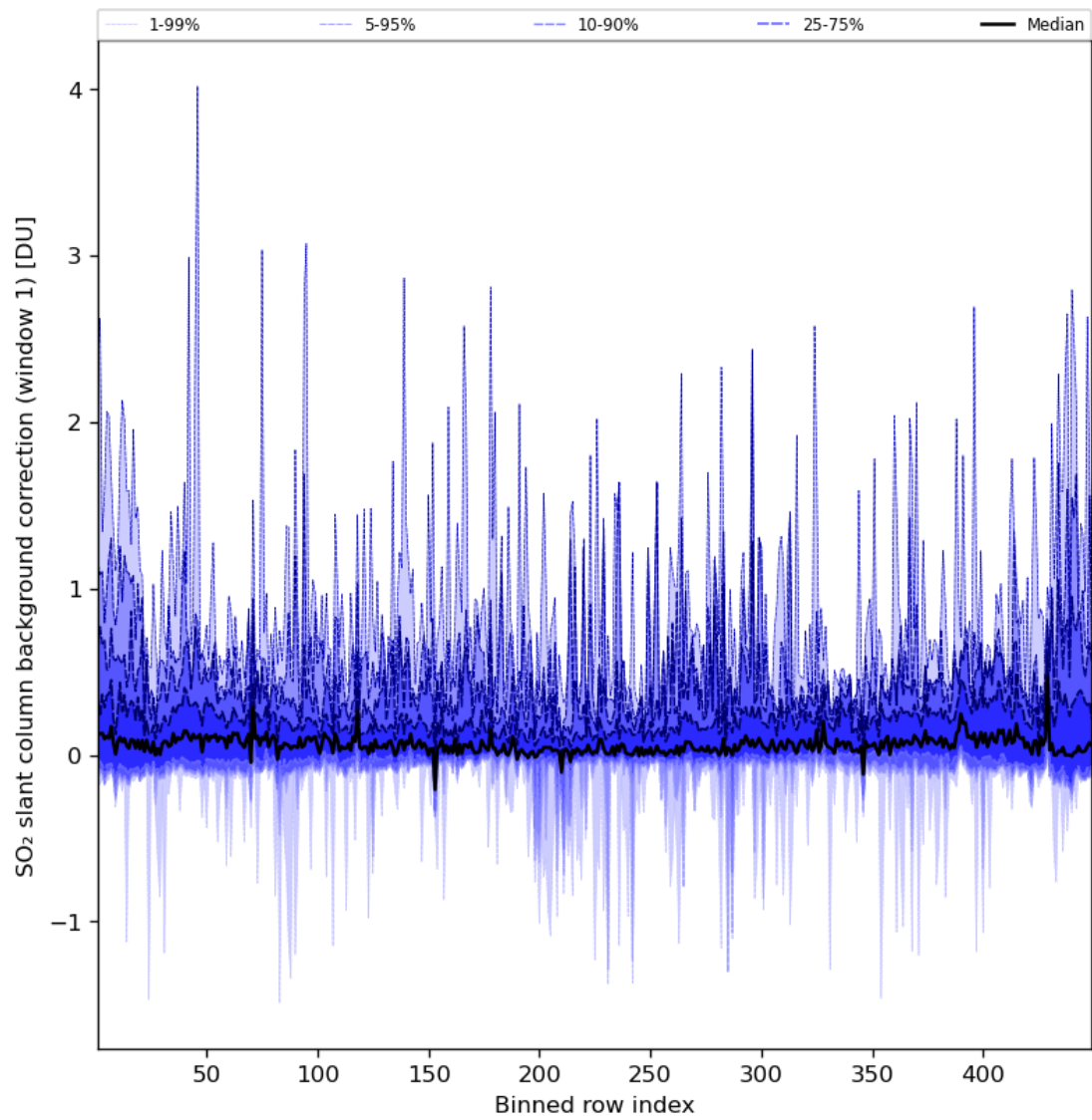
Figure 82: Along track statistics of “SO 2 slant column background correction (window 1)” for 2024-07-29 to 2024-07-31
