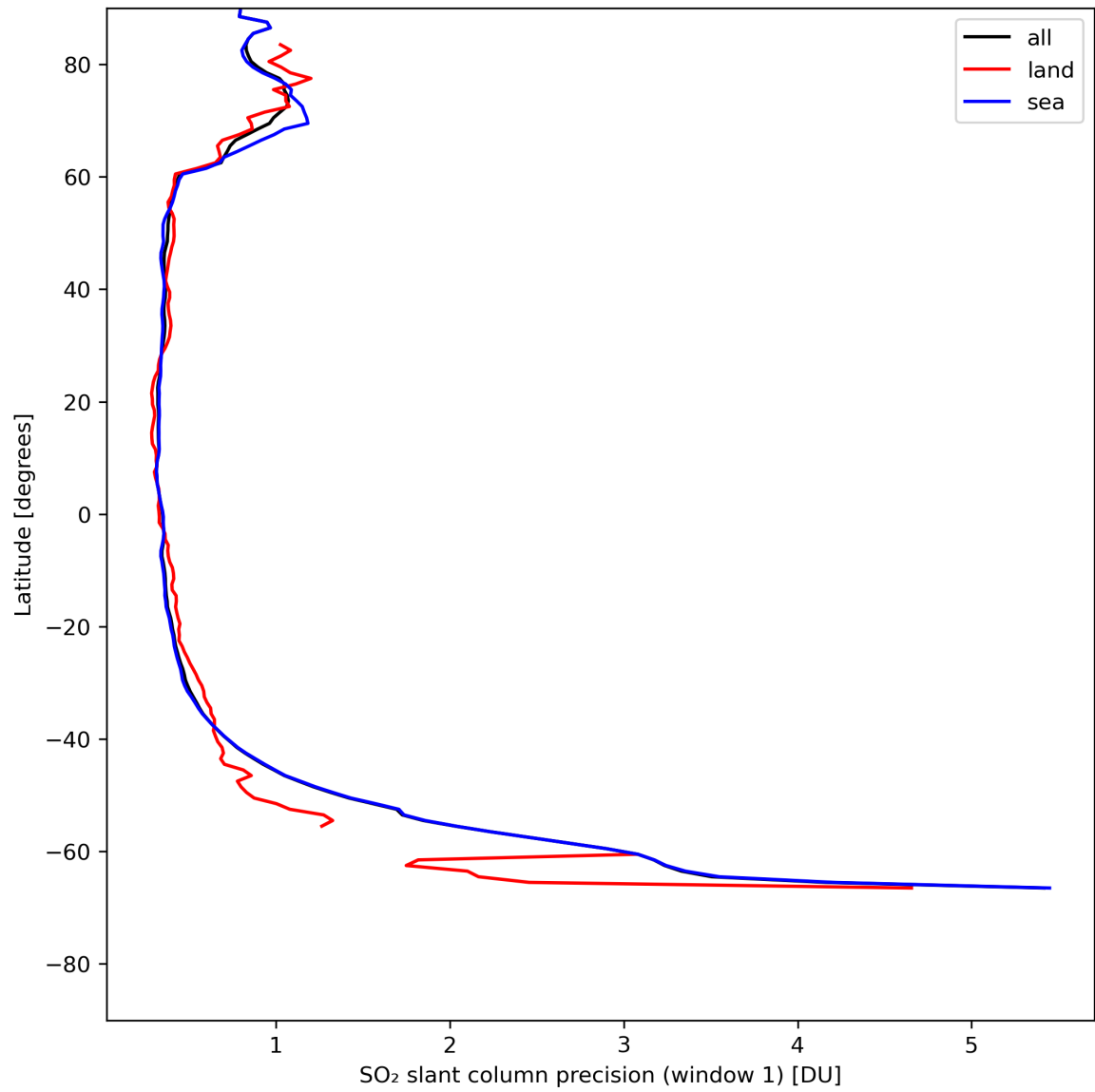
Figure 34: Zonal average of “SO 2 slant column precision (window 1)” for 2024-07-29 to 2024-07-31.
