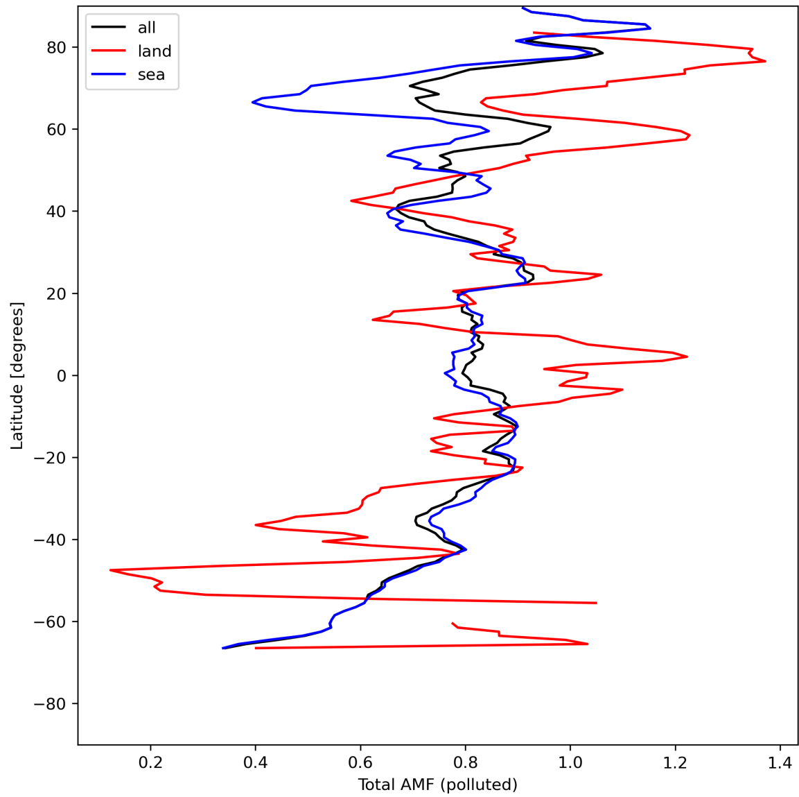
Figure 48: Zonal average of “Total AMF (polluted)” for 2024-07-29 to 2024-07-31.
