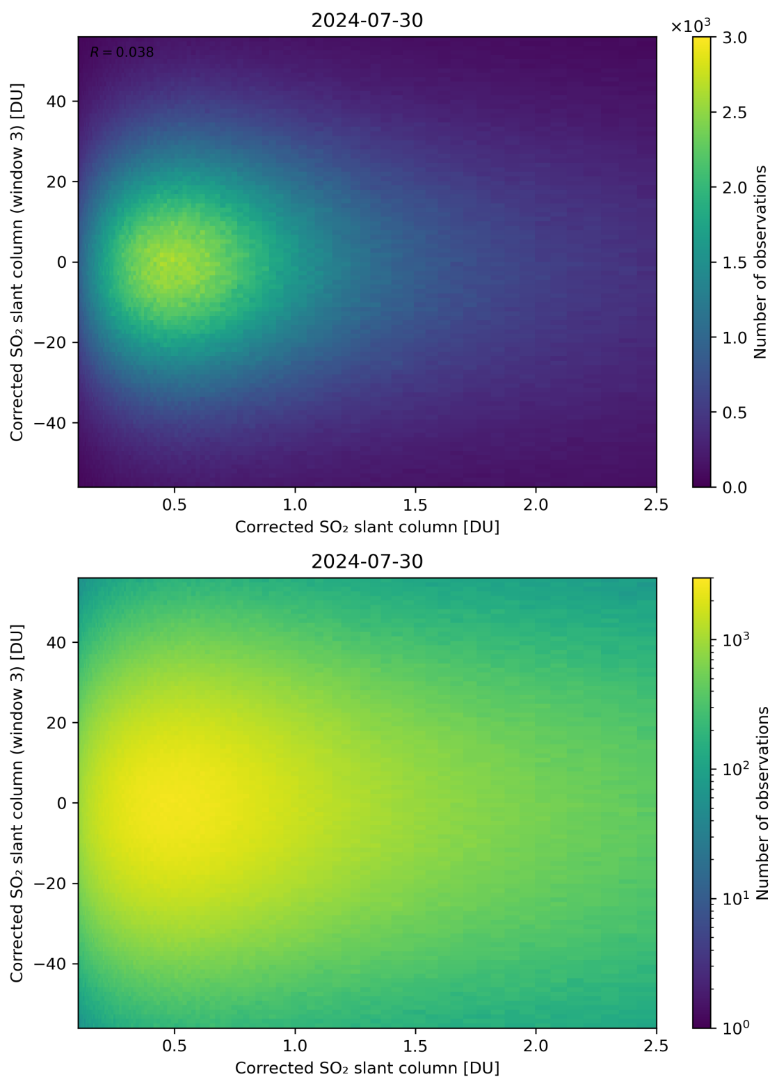
Figure 186: Scatter density plot of “Corrected SO 2 slant column” against “Corrected SO 2 slant column (window 3)” for 2024-07-29 to 2024-07-31.
