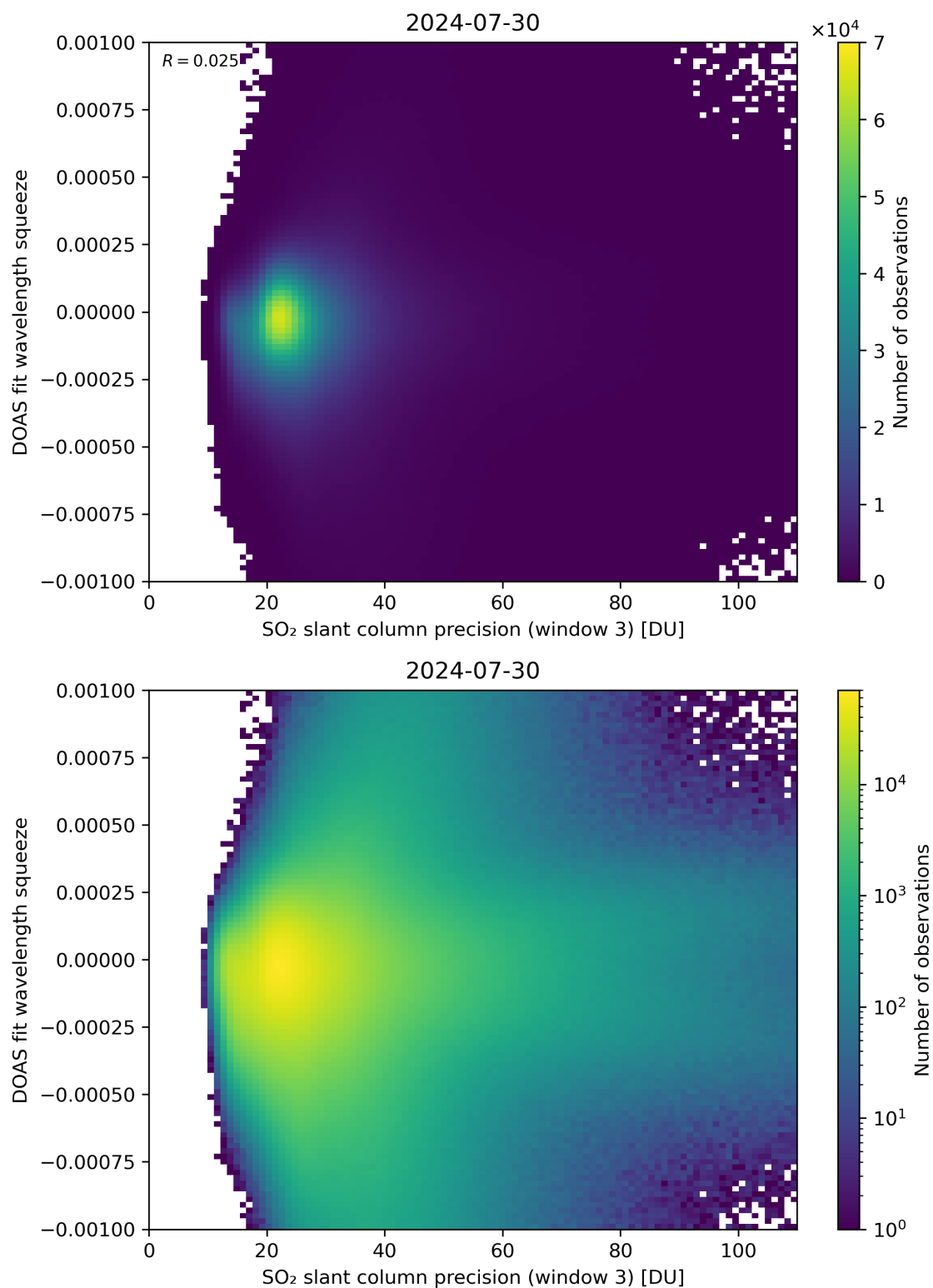
Figure 259: Scatter density plot of “SO 2 slant column precision (window 3)” against “DOAS fit wavelength squeeze” for 2024-07-29 to 2024-07-31.
