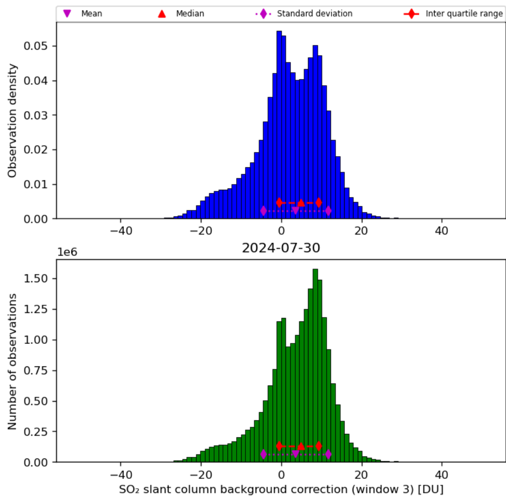
Figure 67: Histogram of “SO 2 slant column background correction (window 3)” for 2024-07-29 to 2024-07-31
