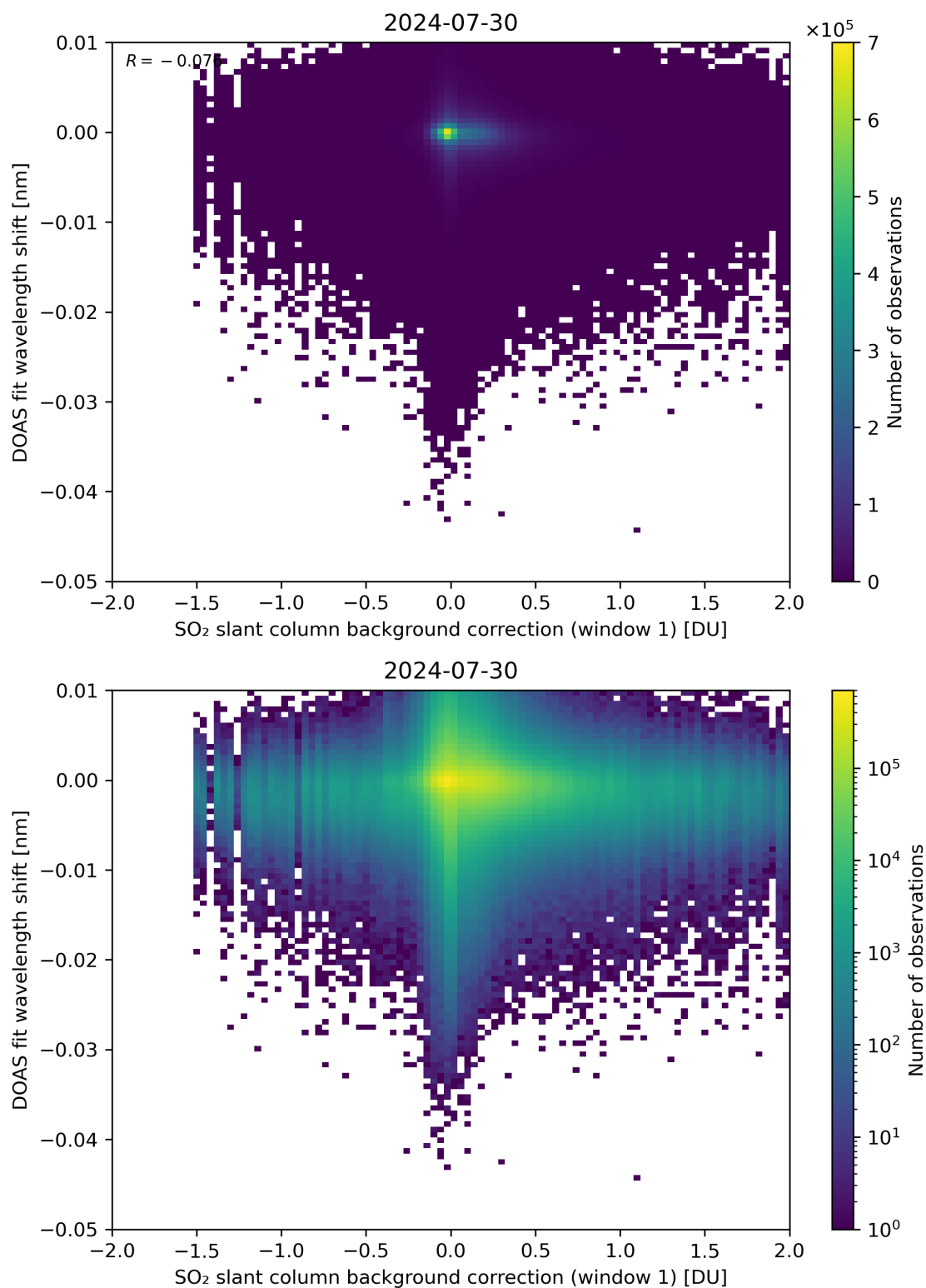
Figure 100: Scatter density plot of “SO 2 slant column background correction (window 1)” against “DOAS fit wavelength shift” for 2024-07-29 to 2024-07-31.
