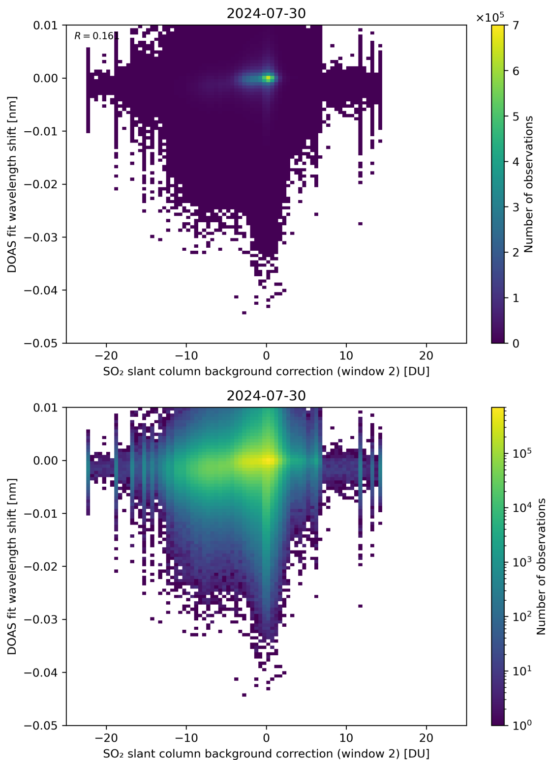
Figure 112: Scatter density plot of “SO 2 slant column background correction (window 2)” against “DOAS fit wavelength shift” for 2024-07-29 to 2024-07-31.
