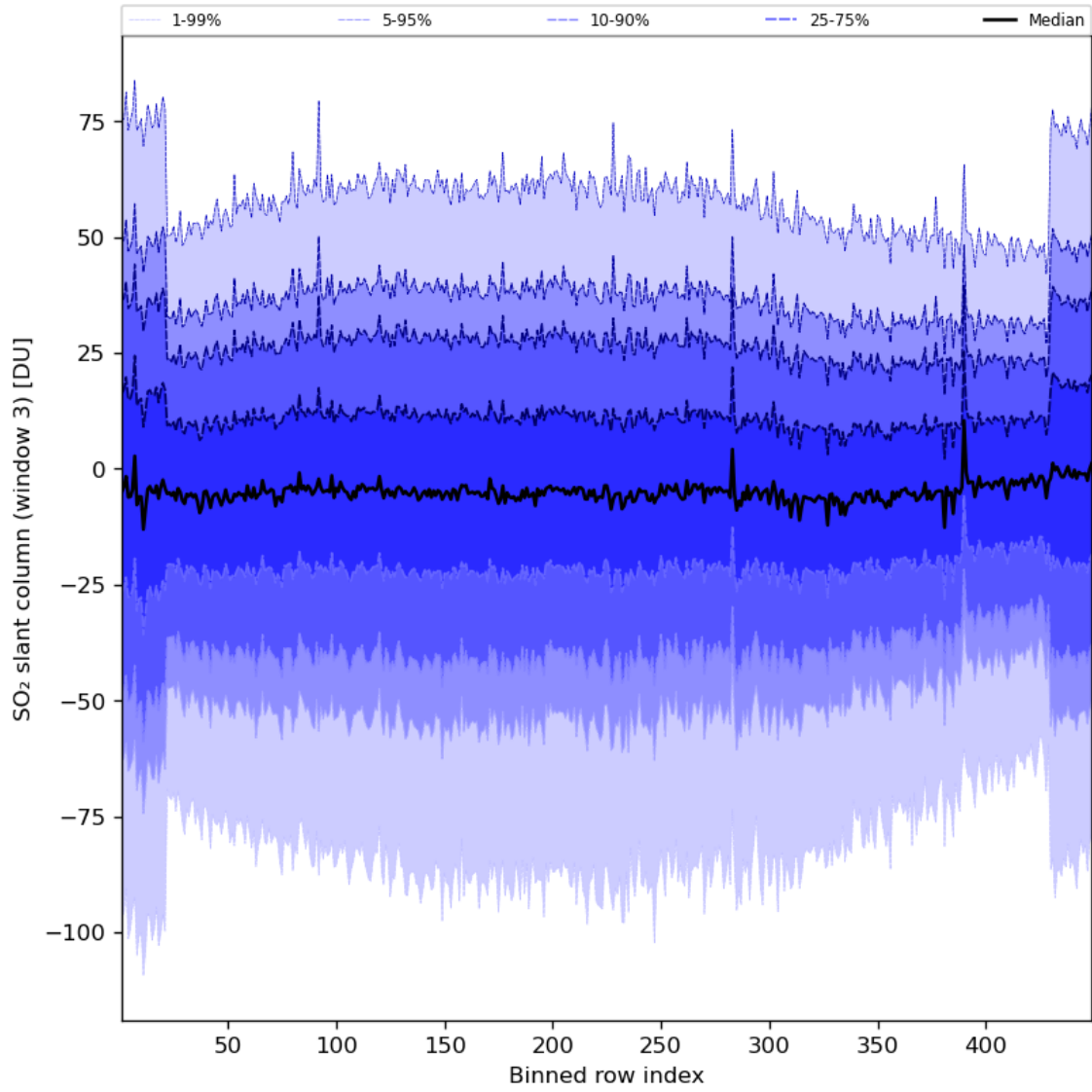
Figure 87: Along track statistics of "SO 2 slant column (window 3)" for 2024-07-29 to 2024-07-31
