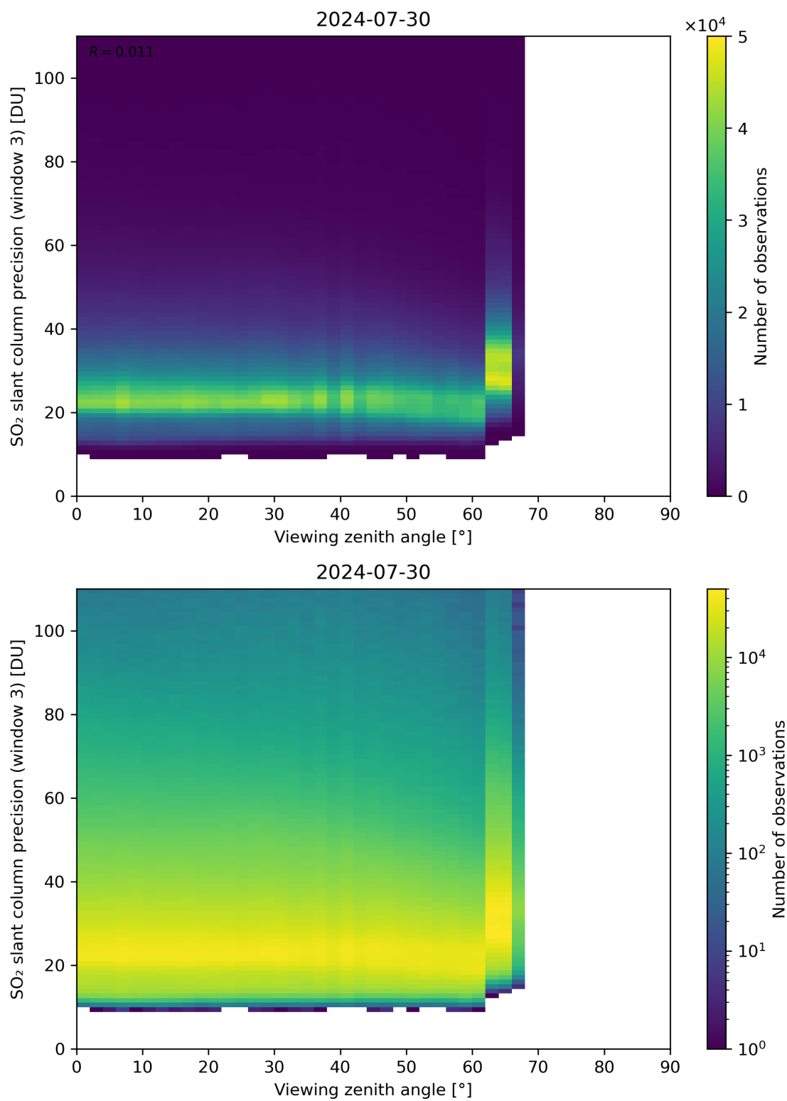
Figure 324: Scatter density plot of “Viewing zenith angle” against “SO 2 slant column precision (window 3)” for 2024-07-29 to 2024-07-31.
