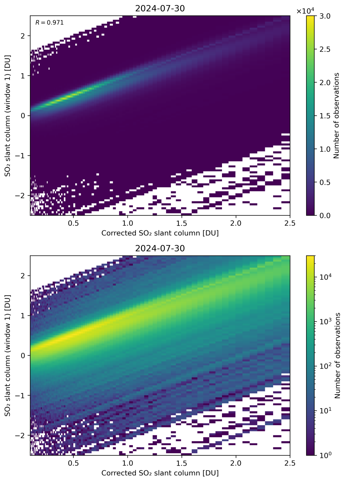
Figure 187: Scatter density plot of “Corrected SO 2 slant column” against “SO 2 slant column (window 1)” for 2024-07-29 to 2024-07-31.
