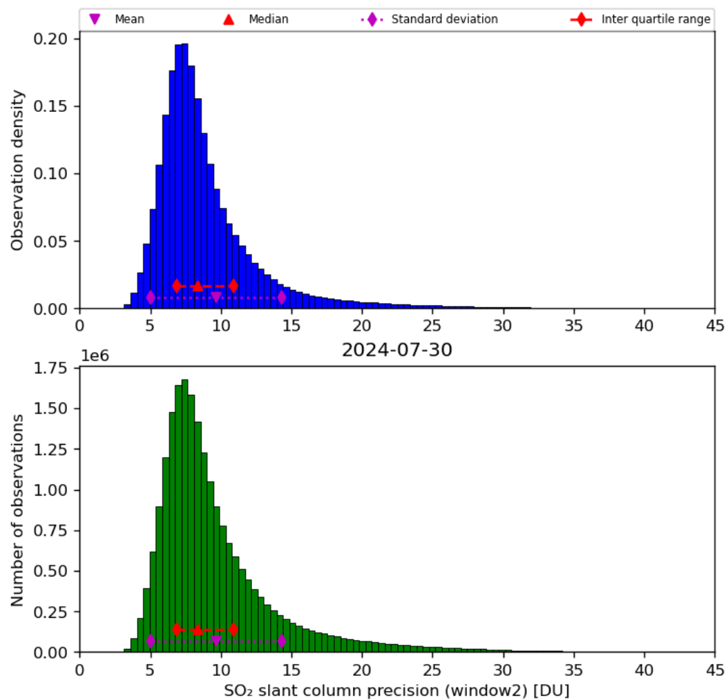
Figure 61: Histogram of “SO 2 slant column precision (window2)” for 2024-07-29 to 2024-07-31
