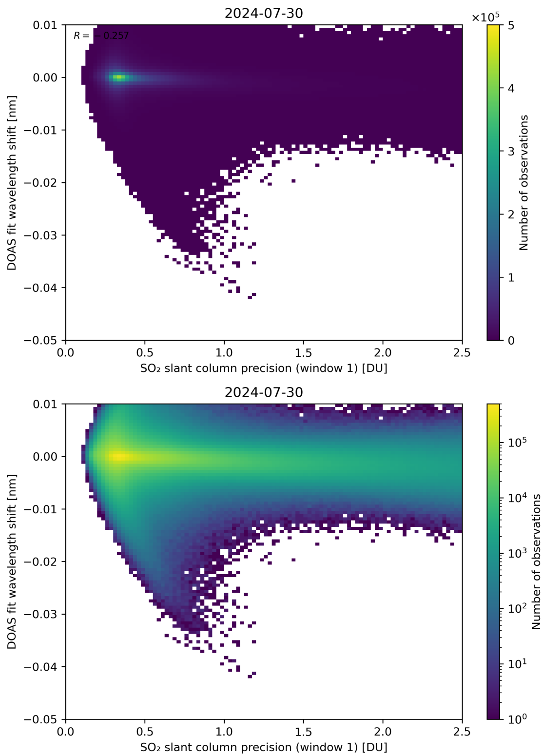
Figure 221: Scatter density plot of “SO 2 slant column precision (window 1)” against “DOAS fit wavelength shift” for 2024-07-29 to 2024-07-31.
