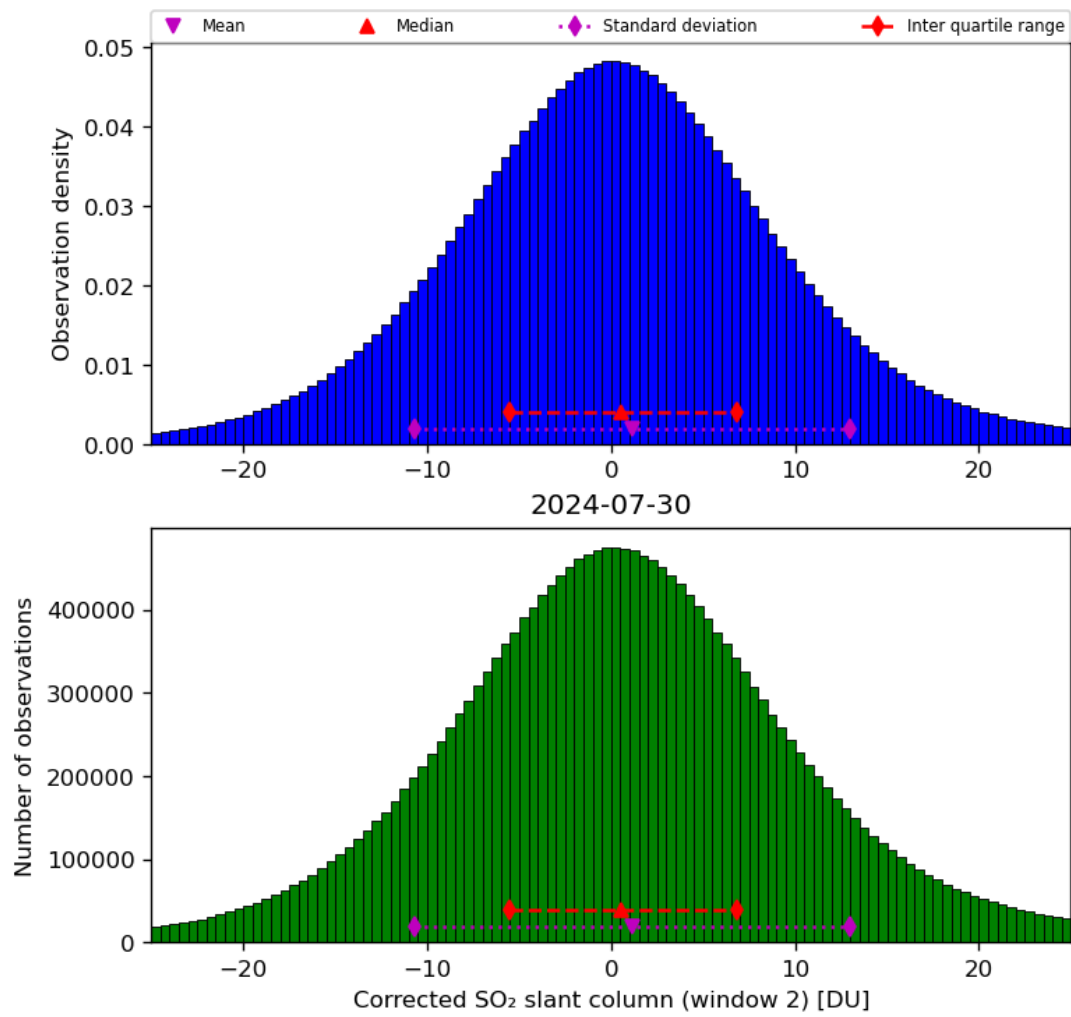
Figure 62: Histogram of “Corrected SO 2 slant column (window 2)” for 2024-07-29 to 2024-07-31
