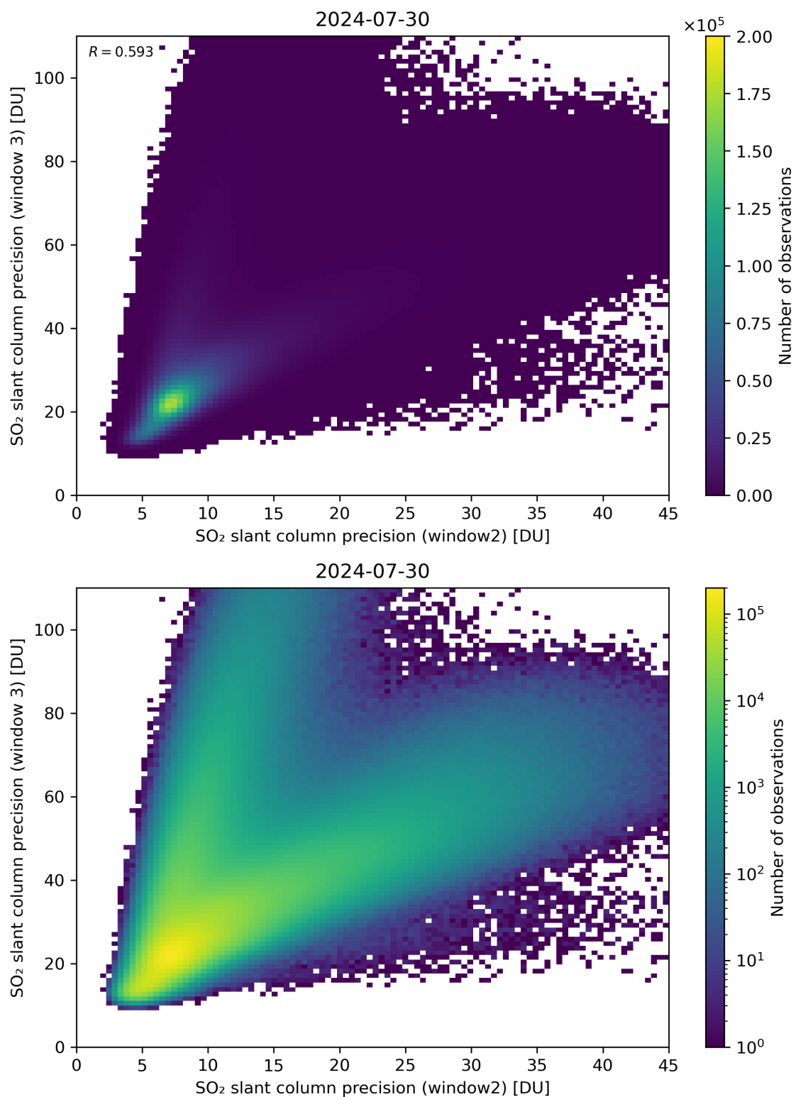
Figure 250: Scatter density plot of “SO 2 slant column precision (window2)” against “SO 2 slant column precision (window 3)” for 2024-07-29 to 2024-07-31.
