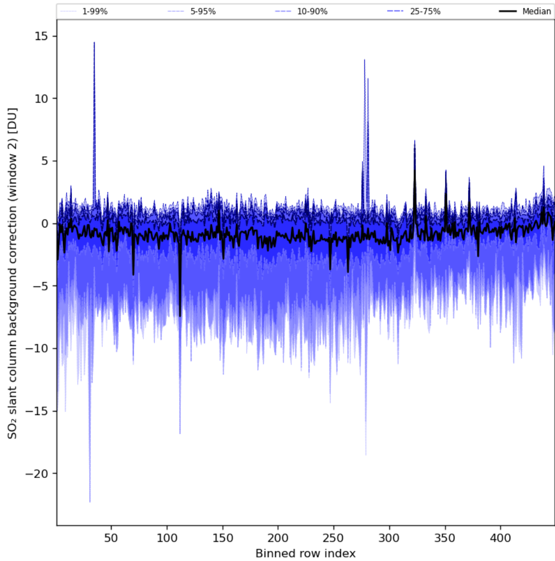
Figure 86: Along track statistics of “SO 2 slant column background correction (window 2)” for 2024-07-29 to 2024-07-31
