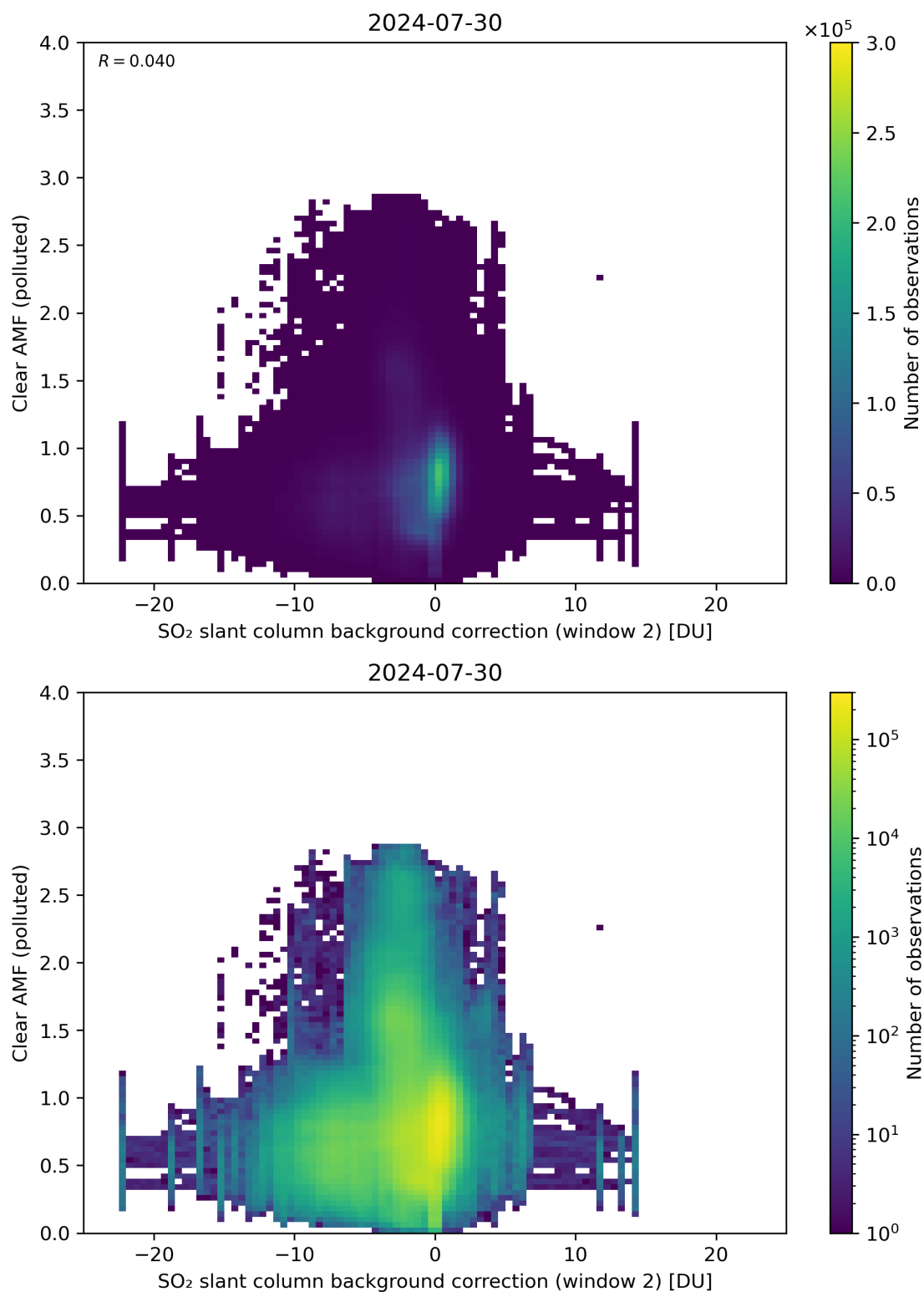
Figure 115: Scatter density plot of “SO 2 slant column background correction (window 2)” against “Clear AMF (polluted)” for 2024-07-29 to 2024-07-31.
