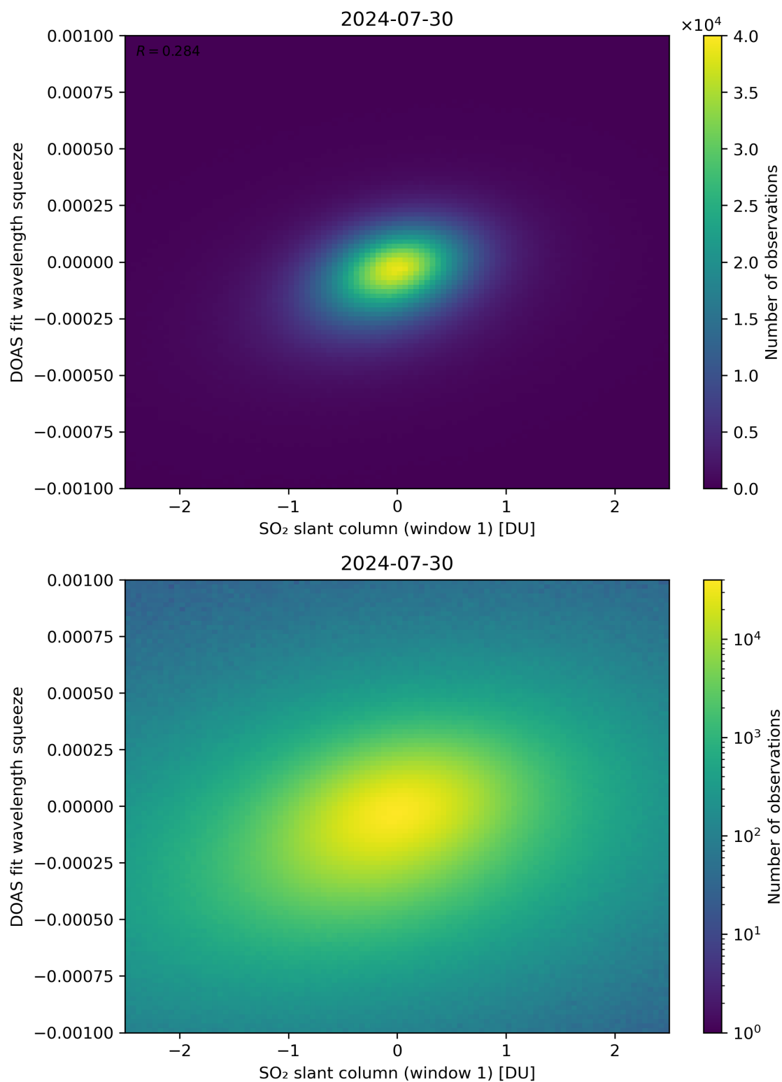
Figure 216: Scatter density plot of “SO 2 slant column (window 1)” against “DOAS fit wavelength squeeze” for 2024-07-29 to 2024-07-31.
