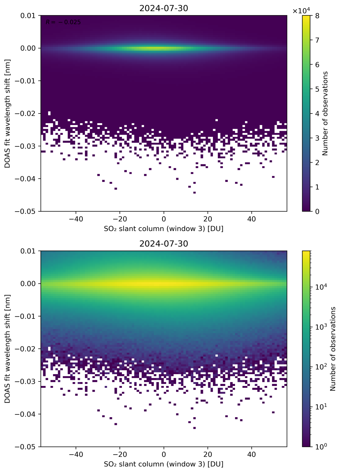
Figure 254: Scatter density plot of “SO 2 slant column (window 3)” against “DOAS fit wavelength shift” for 2024-07-29 to 2024-07-31.
