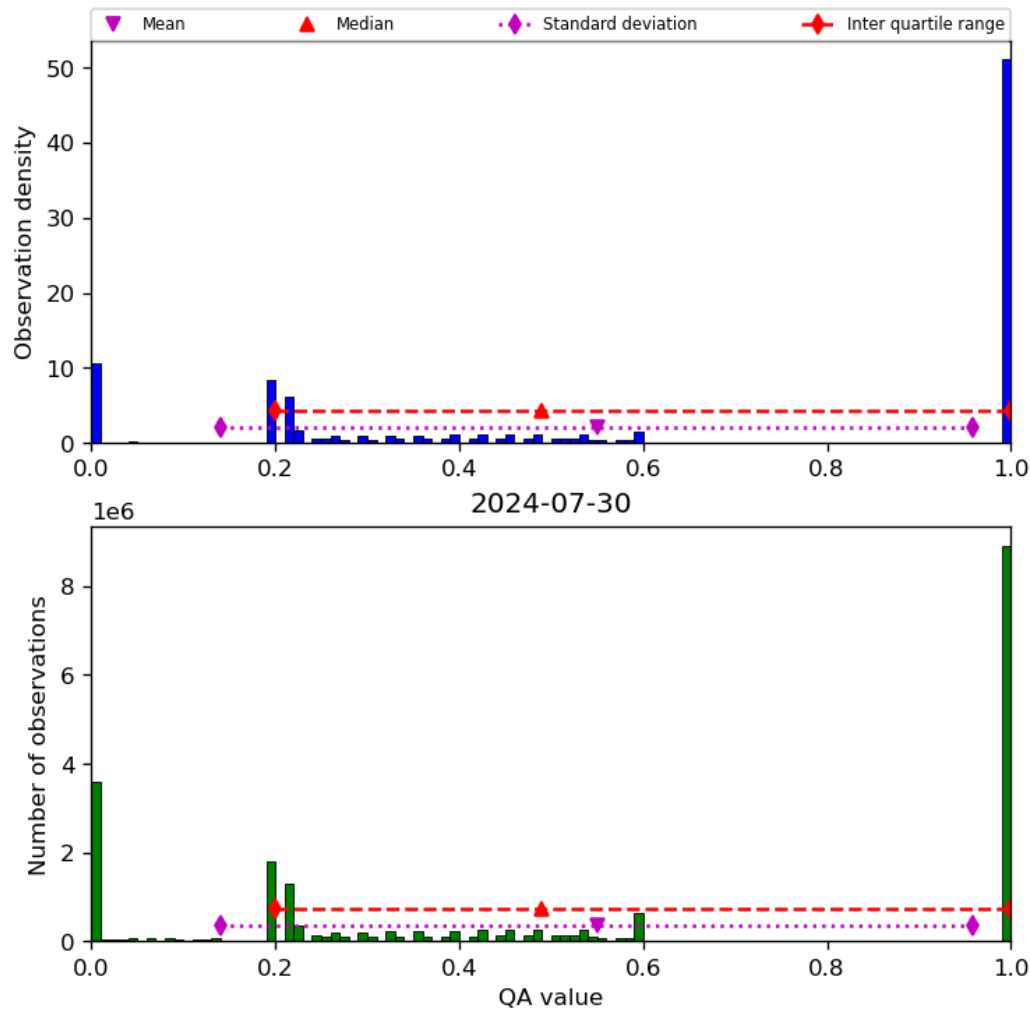
Figure 52: Histogram of “QA value” for 2024-07-29 to 2024-07-31
