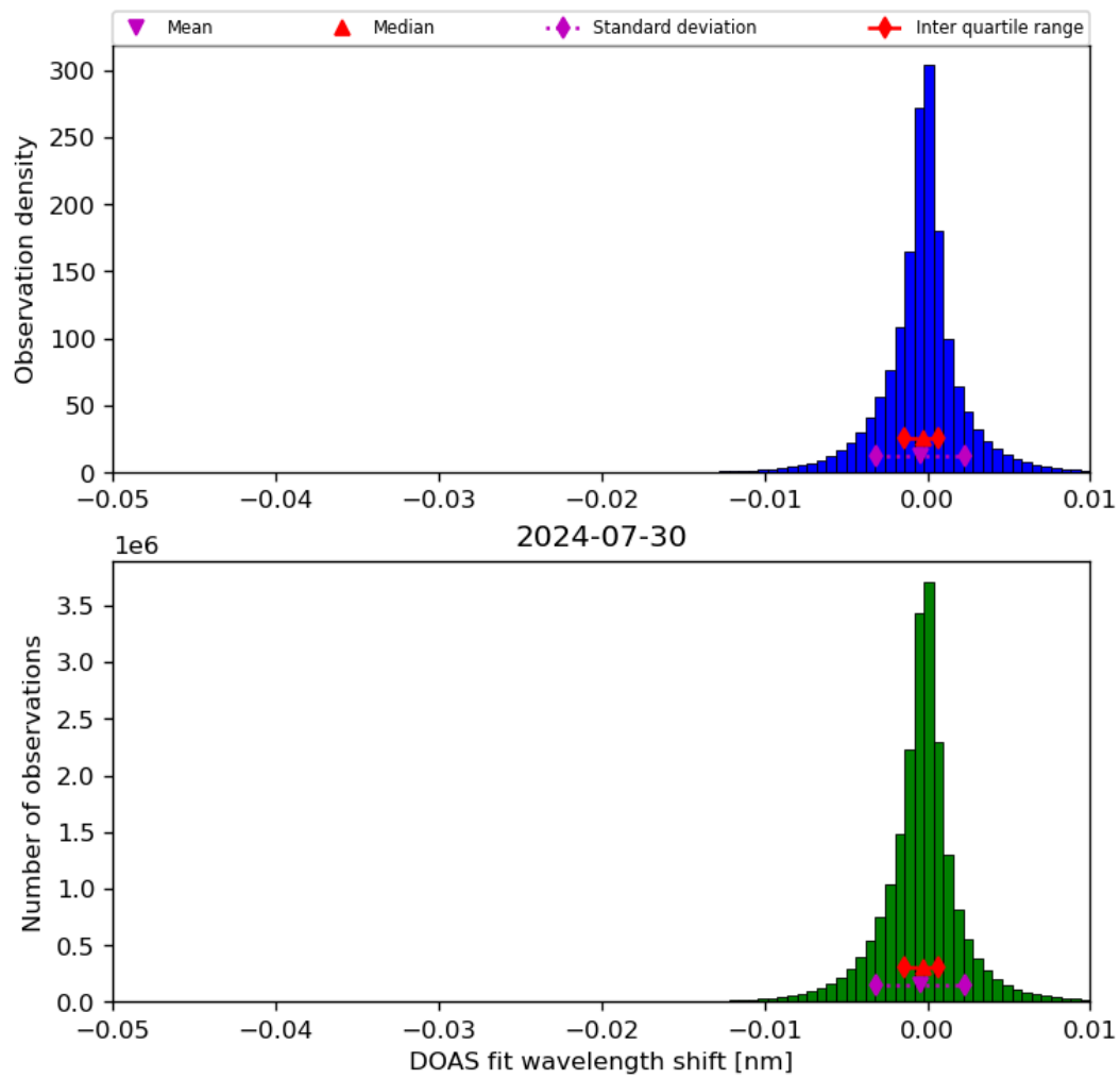
Figure 68: Histogram of “DOAS fit wavelength shift” for 2024-07-29 to 2024-07-31
