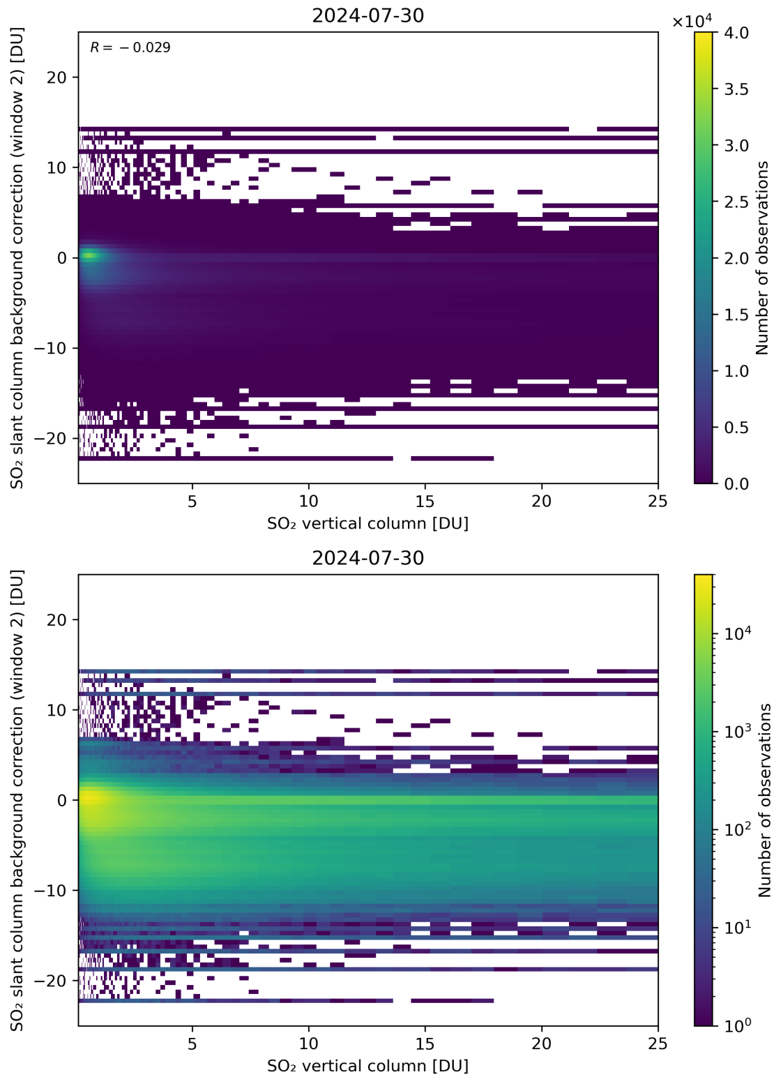
Figure 274: Scatter density plot of “SO 2 vertical column” against “SO 2 slant column background correction (window 2)” for 2024-07-29 to 2024-07-31.
