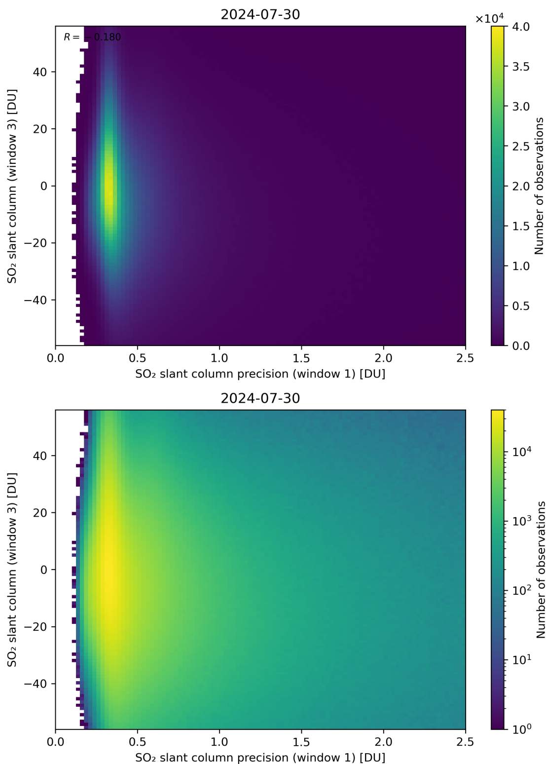
Figure 228: Scatter density plot of “SO 2 slant column precision (window 1)” against “SO 2 slant column (window 3)” for 2024-07-29 to 2024-07-31.
