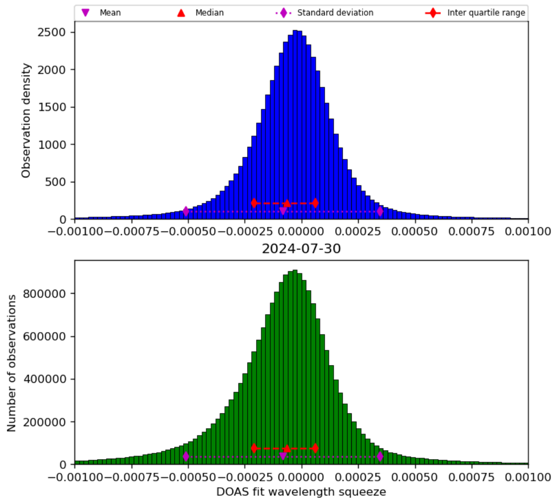
Figure 69: Histogram of “DOAS fit wavelength squeeze” for 2024-07-29 to 2024-07-31
