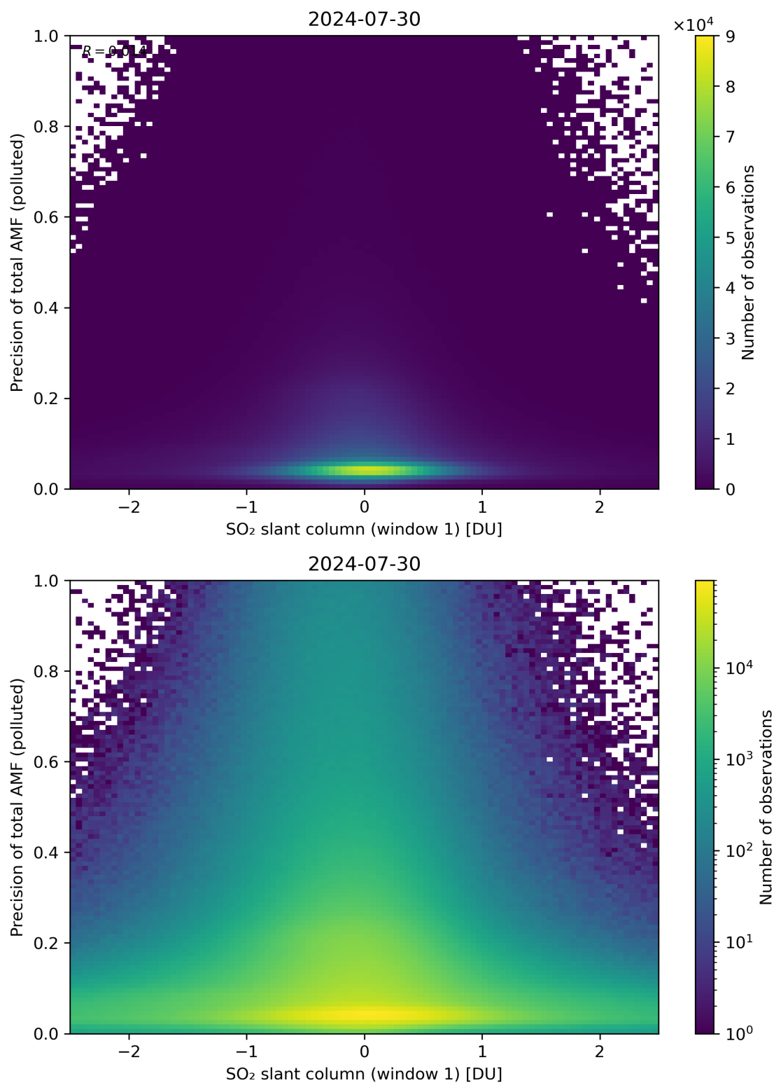
Figure 240: Scatter density plot of “SO 2 slant column (window 1)” against “Precision of total AMF (polluted)” for 2024-07-29 to 2024-07-31.
