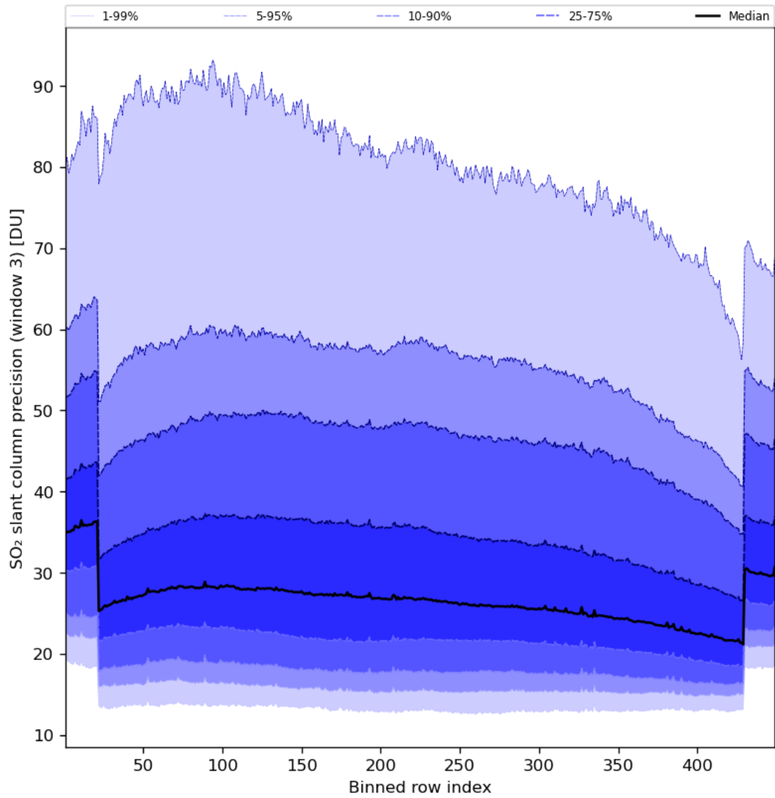
Figure 88: Along track statistics of “SO 2 slant column precision (window 3)” for 2024-07-29 to 2024-07-31
