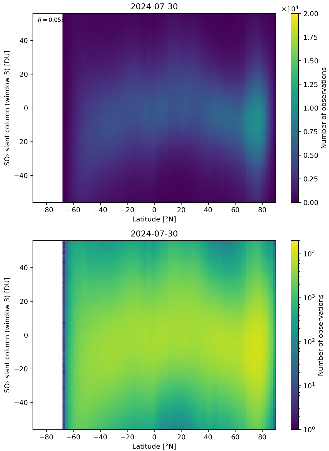
Figure 152: Scatter density plot of “Latitude” against “SO 2 slant column (window 3)” for 2024-07-29 to 2024-07-31.
