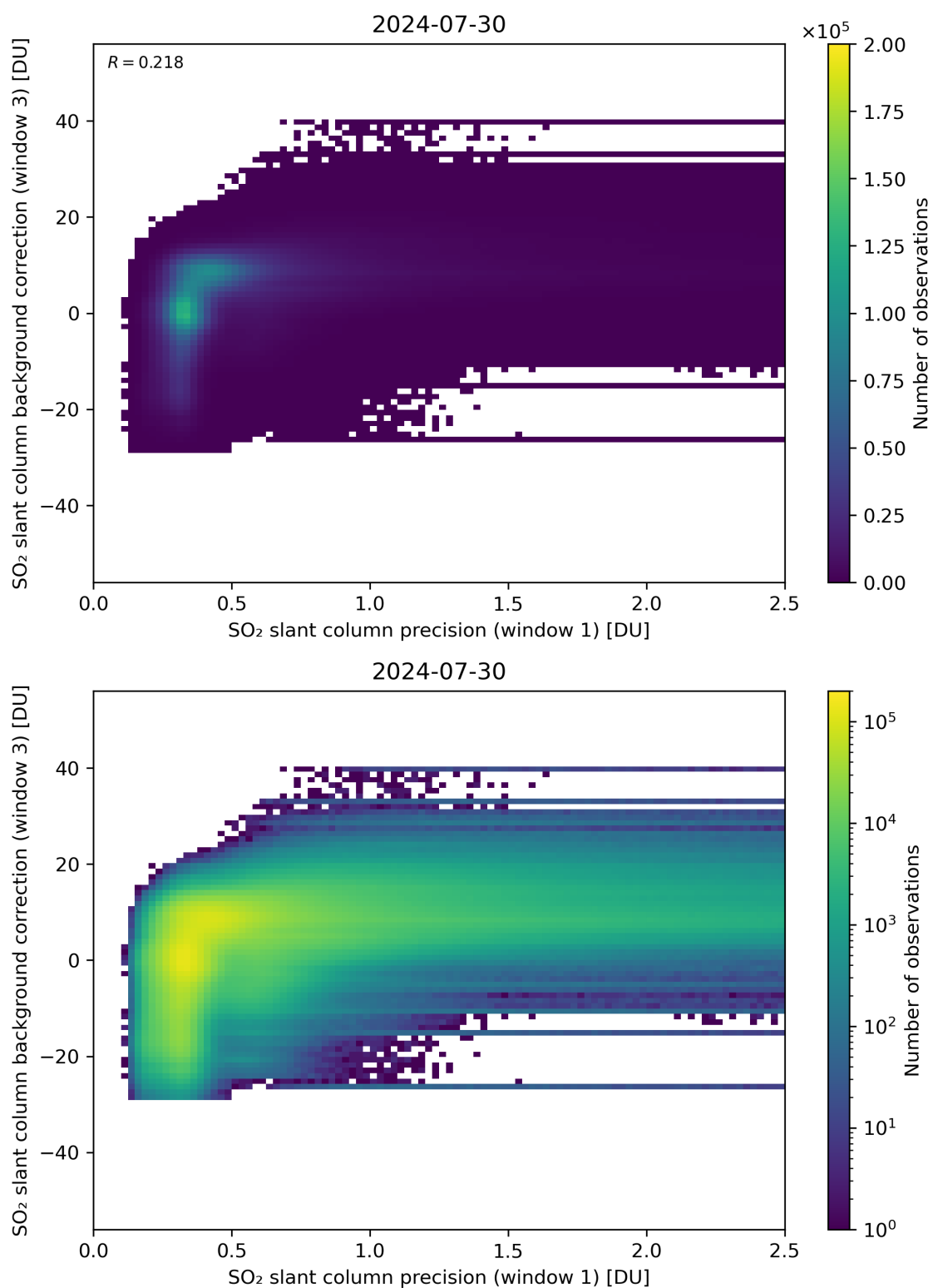
Figure 220: Scatter density plot of “SO 2 slant column precision (window 1)” against “SO 2 slant column background correction (window 3)” for 2024-07-29 to 2024-07-31.
