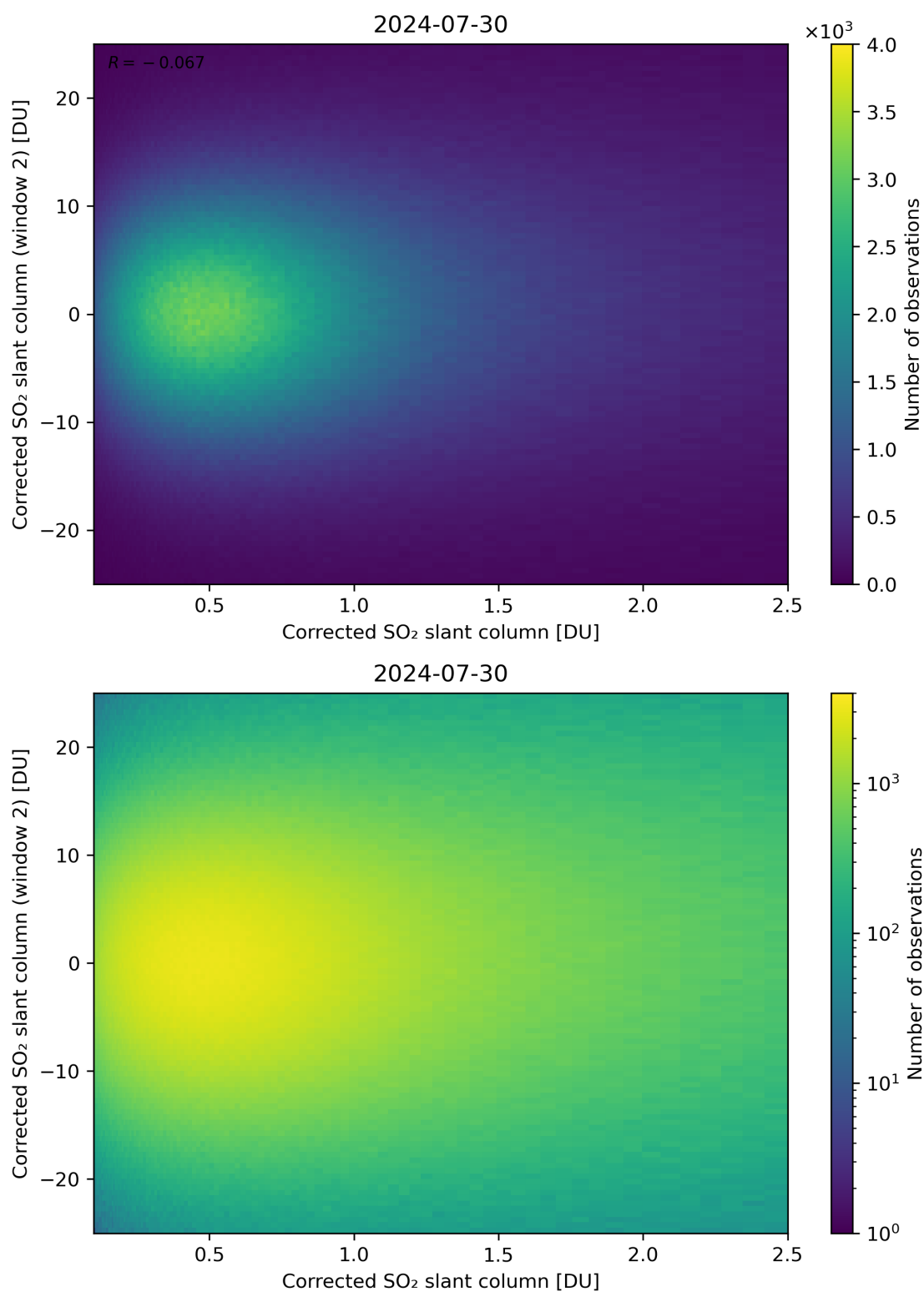
Figure 185: Scatter density plot of “Corrected SO 2 slant column” against “Corrected SO 2 slant column (window 2)” for 2024-07-29 to 2024-07-31.
