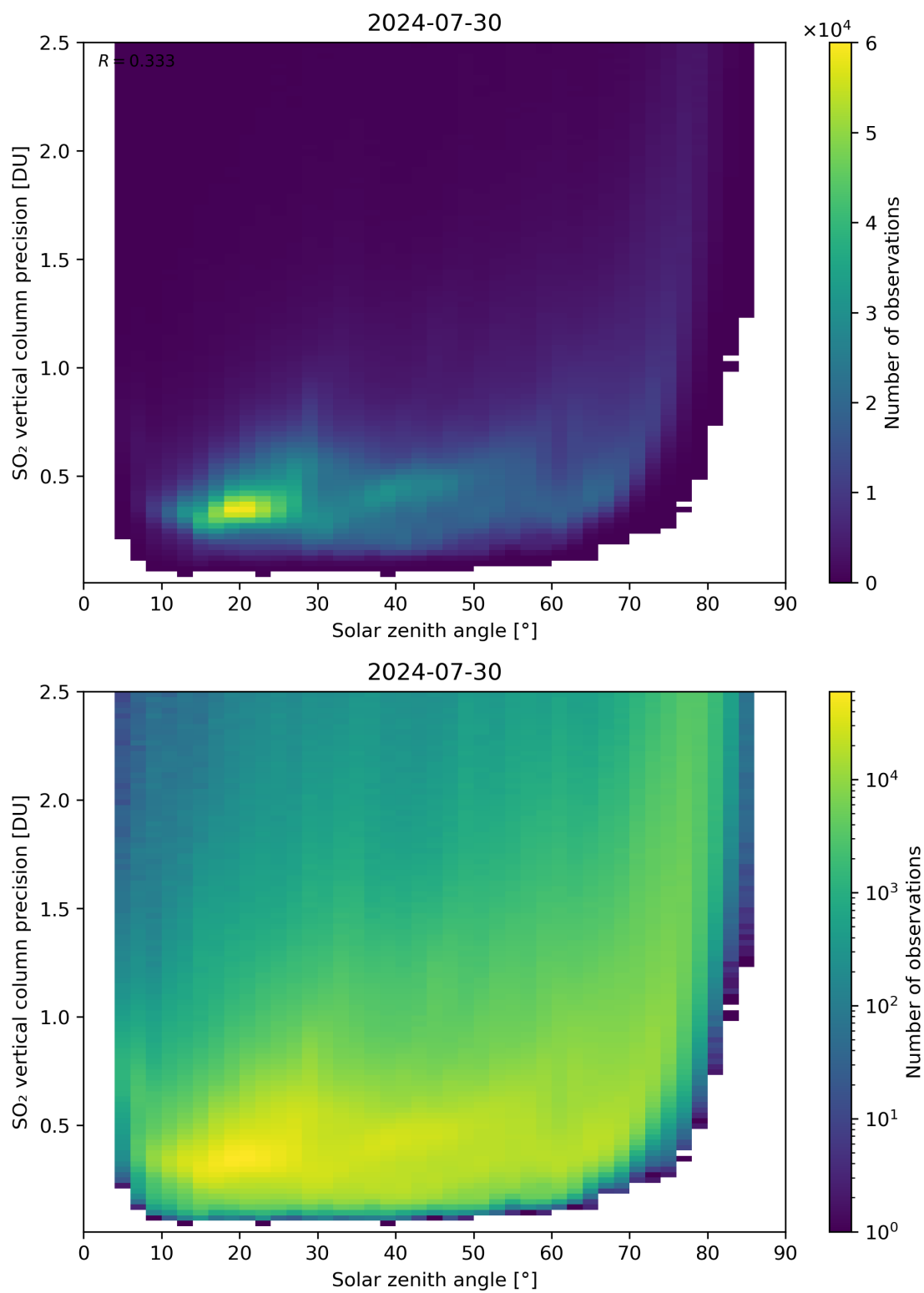
Figure 177: Scatter density plot of “Solar zenith angle” against “SO 2 vertical column precision” for 2024-07-29 to 2024-07-31.
