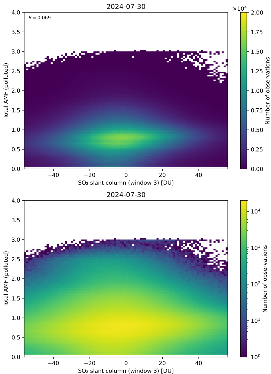
Figure 268: Scatter density plot of “SO 2 slant column (window 3)” against “Total AMF (polluted)” for 2024-07-29 to 2024-07-31.
