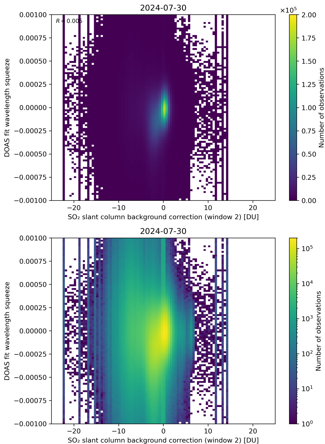
Figure 113: Scatter density plot of “SO 2 slant column background correction (window 2)” against “DOAS fit wavelength squeeze” for 2024-07-29 to 2024-07-31.
