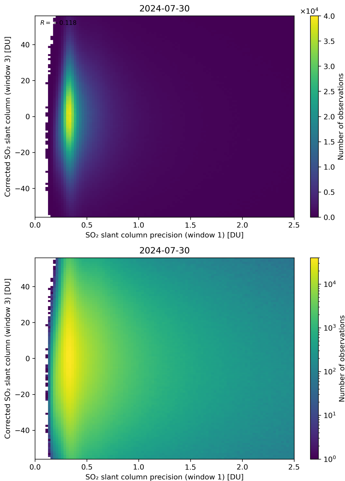
Figure 226: Scatter density plot of “SO 2 slant column precision (window 1)” against “Corrected SO 2 slant column (window 3)” for 2024-07-29 to 2024-07-31.
