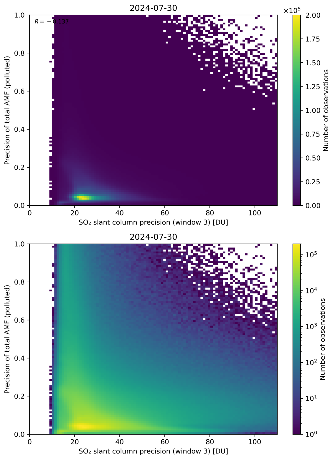
Figure 264: Scatter density plot of “SO 2 slant column precision (window 3)” against “Precision of total AMF (polluted)” for 2024-07-29 to 2024-07-31.
