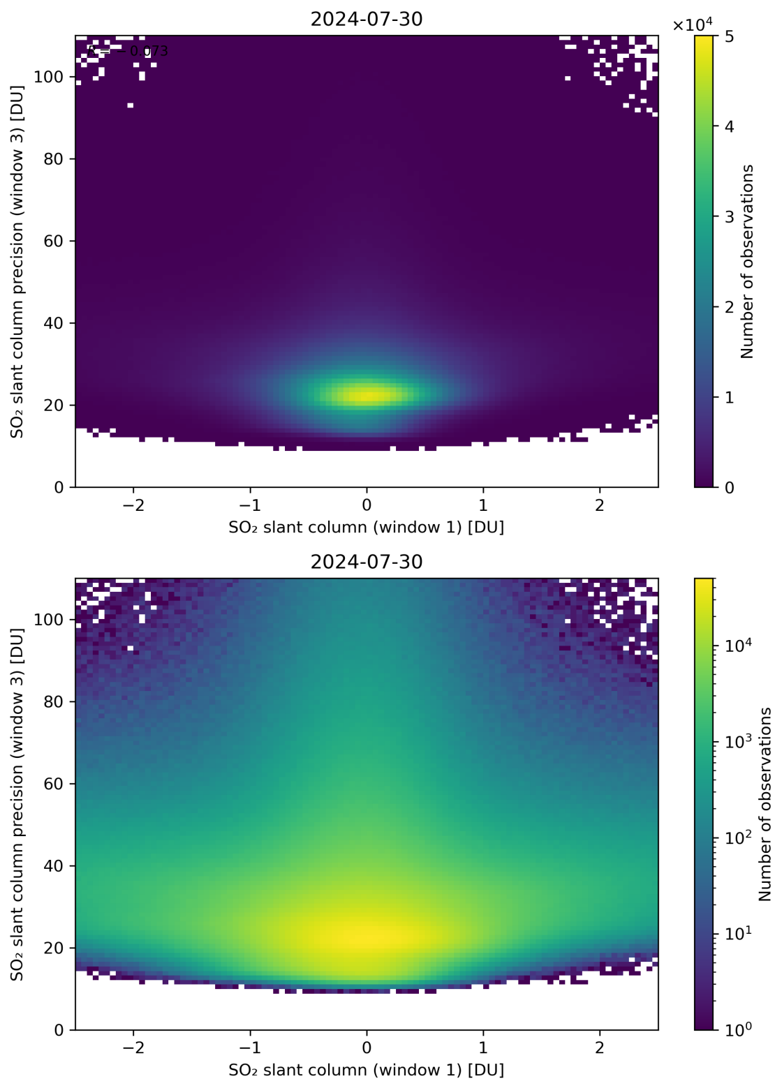
Figure 238: Scatter density plot of “SO 2 slant column (window 1)” against “SO 2 slant column precision (window 3)” for 2024-07-29 to 2024-07-31.
