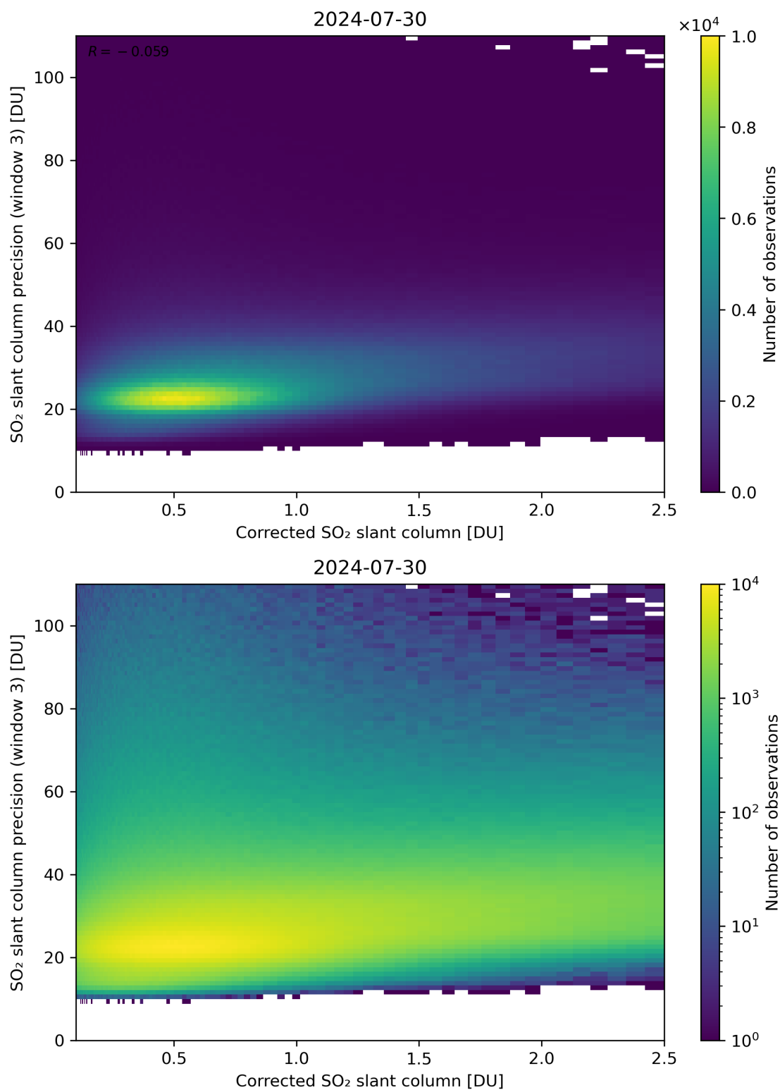
Figure 191: Scatter density plot of “Corrected SO 2 slant column” against “SO 2 slant column precision (window 3)” for 2024-07-29 to 2024-07-31.
