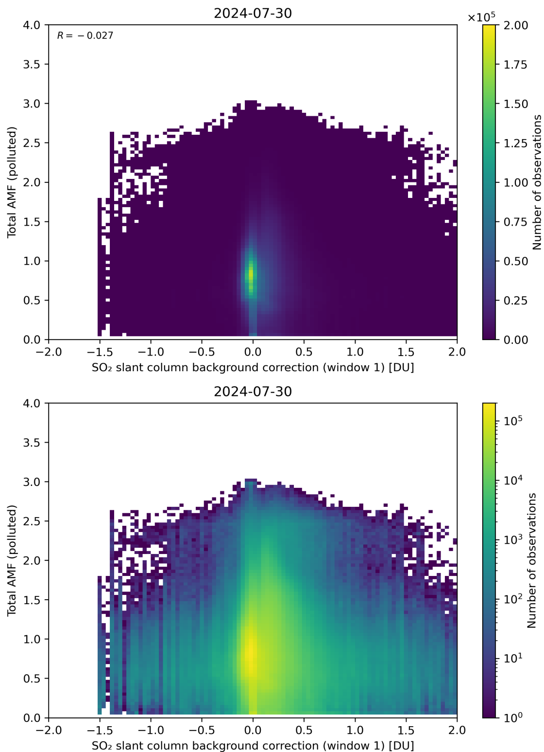
Figure 109: Scatter density plot of “SO 2 slant column background correction (window 1)” against “Total AMF (polluted)” for 2024-07-29 to 2024-07-31.
