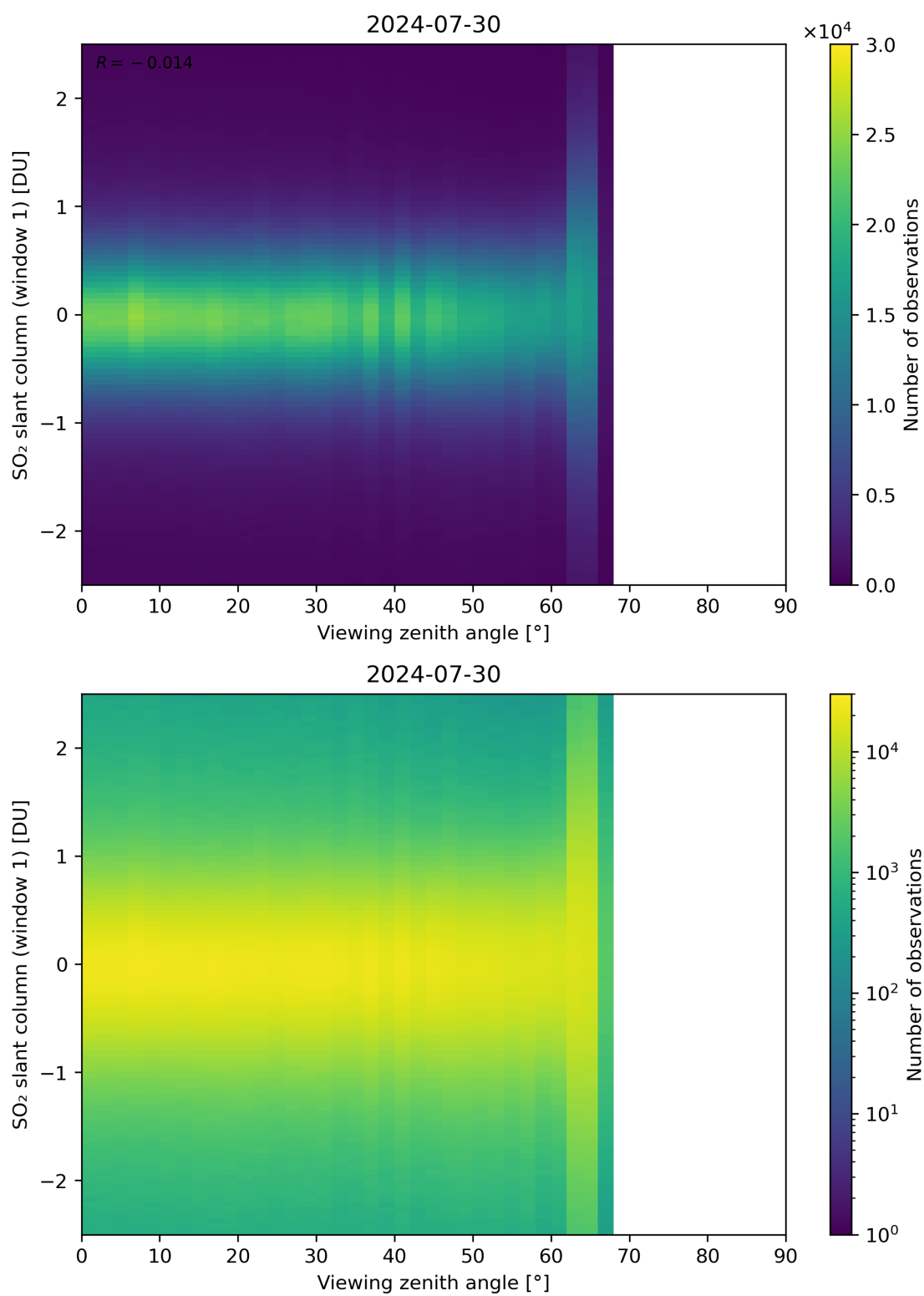
Figure 320: Scatter density plot of “Viewing zenith angle” against “SO 2 slant column (window 1)” for 2024-07-29 to 2024-07-31.
