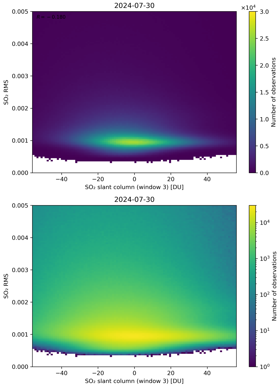
Figure 256: Scatter density plot of “SO 2 slant column (window 3)” against “SO 2 RMS” for 2024-07-29 to 2024-07-31.
