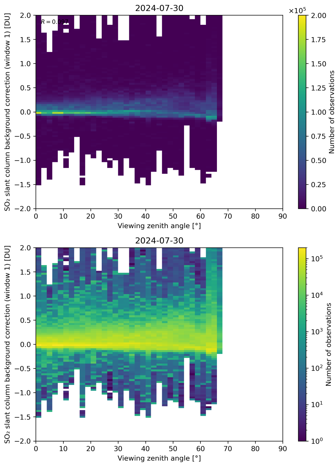
Figure 308: Scatter density plot of “Viewing zenith angle” against “SO 2 slant column background correction (window 1)” for 2024-07-29 to 2024-07-31.
