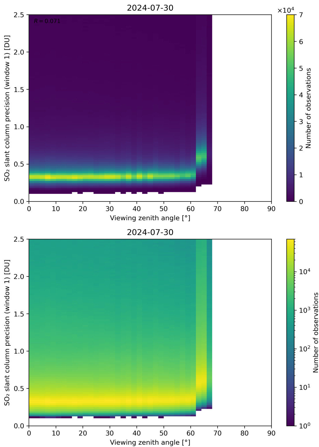
Figure 321: Scatter density plot of “Viewing zenith angle” against “SO 2 slant column precision (window 1)” for 2024-07-29 to 2024-07-31.
