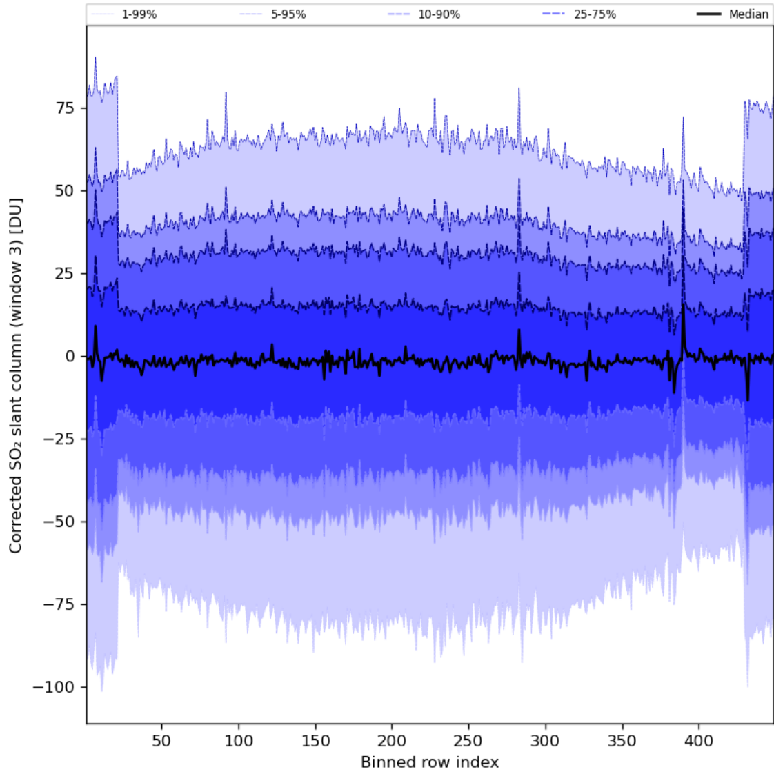
Figure 89: Along track statistics of “Corrected SO 2 slant column (window 3)” for 2024-07-29 to 2024-07-31
