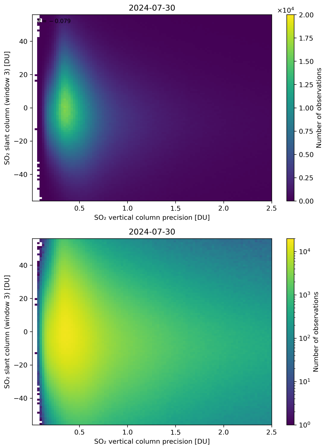
Figure 292: Scatter density plot of “SO 2 vertical column precision” against “SO 2 slant column (window 3)” for 2024-07-29 to 2024-07-31.
