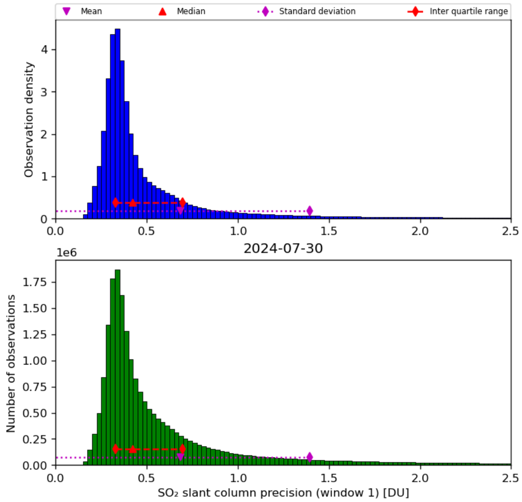
Figure 57: Histogram of “SO 2 slant column precision (window 1)” for 2024-07-29 to 2024-07-31
