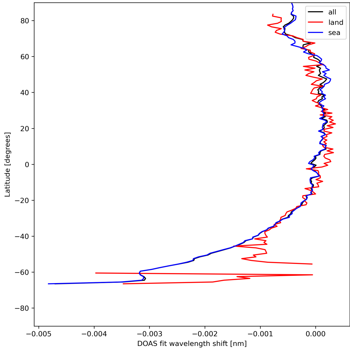
Figure 45: Zonal average of “DOAS fit wavelength shift” for 2024-07-29 to 2024-07-31.
