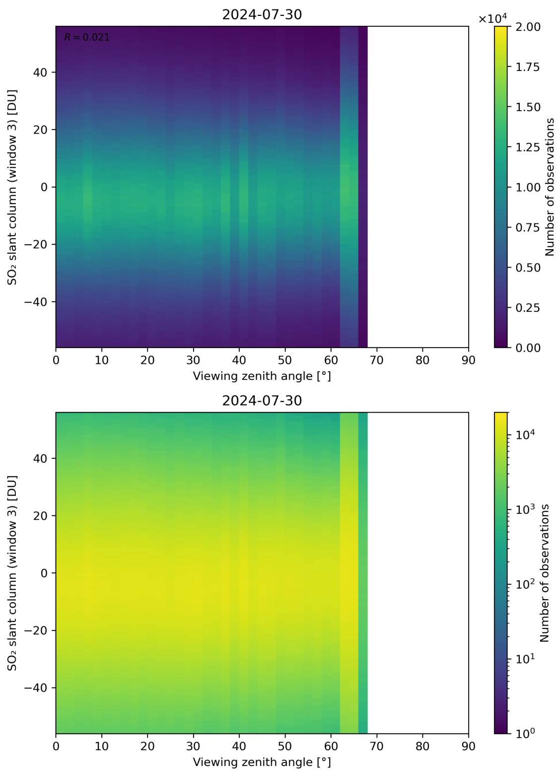
Figure 323: Scatter density plot of “Viewing zenith angle” against “SO 2 slant column (window 3)” for 2024-07-29 to 2024-07-31.
