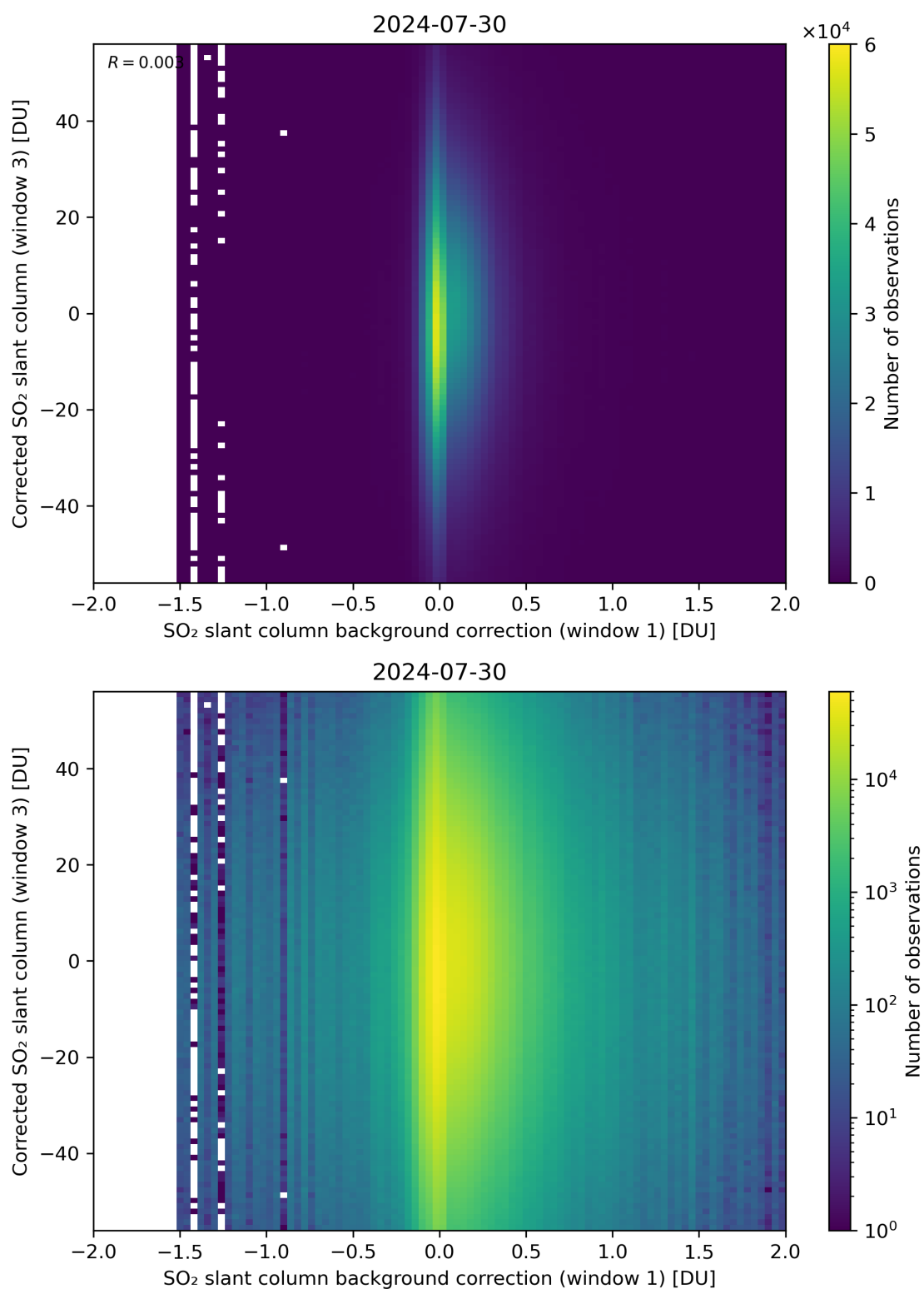
Figure 105: Scatter density plot of “SO 2 slant column background correction (window 1)” against “Corrected SO 2 slant column (window 3)” for 2024-07-29 to 2024-07-31.
