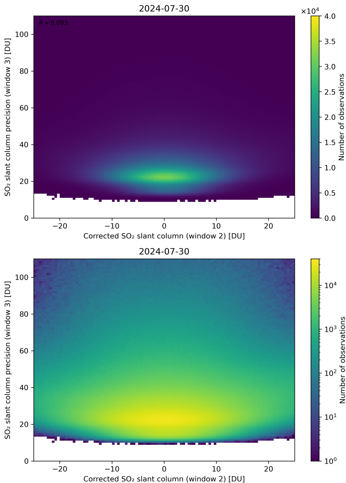
Figure 202: Scatter density plot of “Corrected SO 2 slant column (window 2)” against “SO 2 slant column precision (window 3)” for 2024-07-29 to 2024-07-31.
