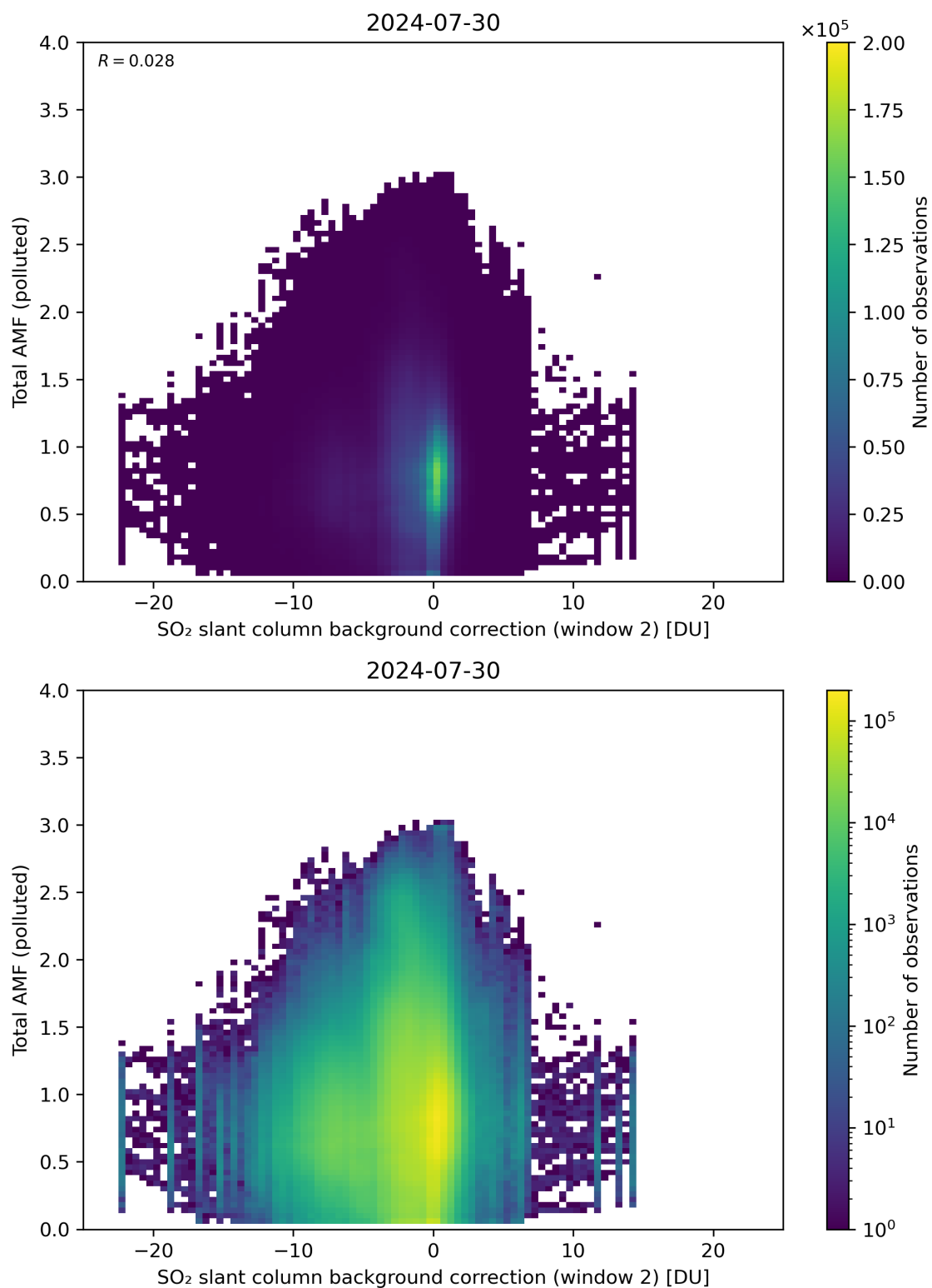
Figure 119: Scatter density plot of “SO 2 slant column background correction (window 2)” against “Total AMF (polluted)” for 2024-07-29 to 2024-07-31.
