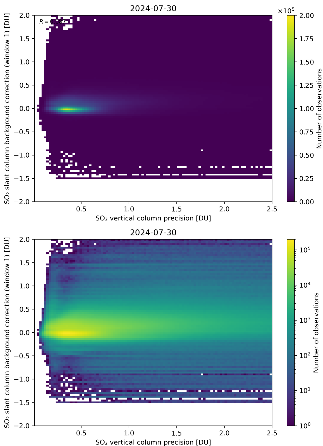
Figure 279: Scatter density plot of “SO 2 vertical column precision” against “SO 2 slant column background correction (window 1)” for 2024-07-29 to 2024-07-31.
