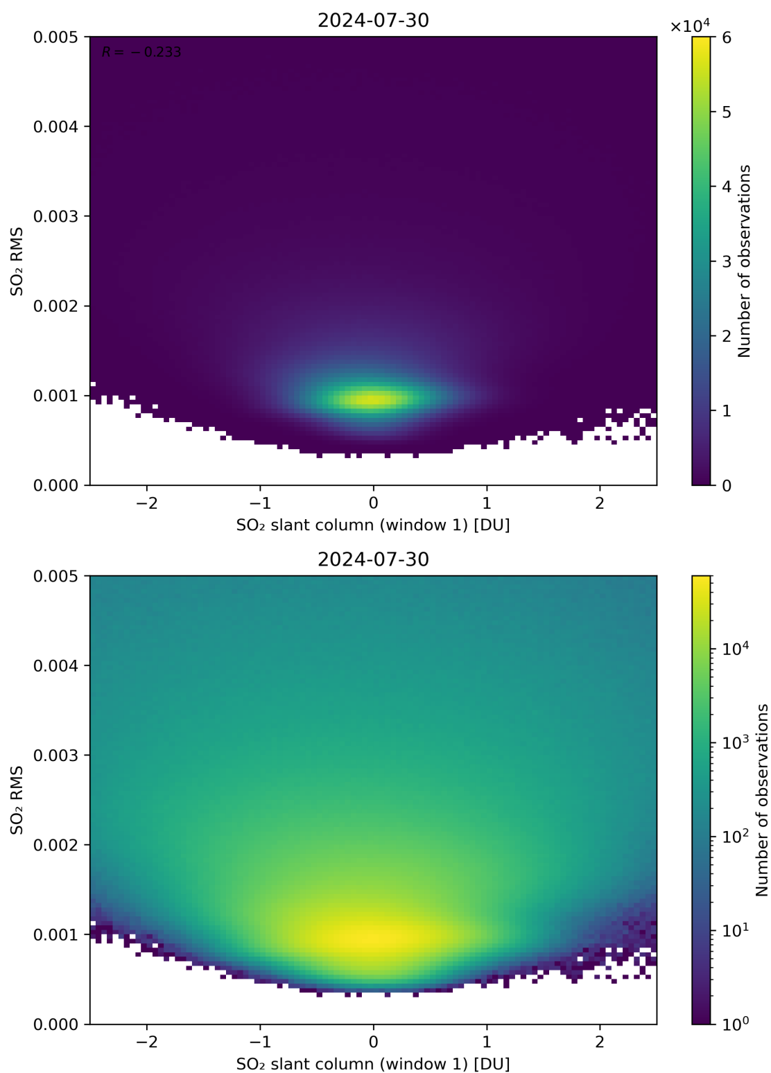
Figure 217: Scatter density plot of “SO 2 slant column (window 1)” against “SO 2 RMS” for 2024-07-29 to 2024-07-31.
