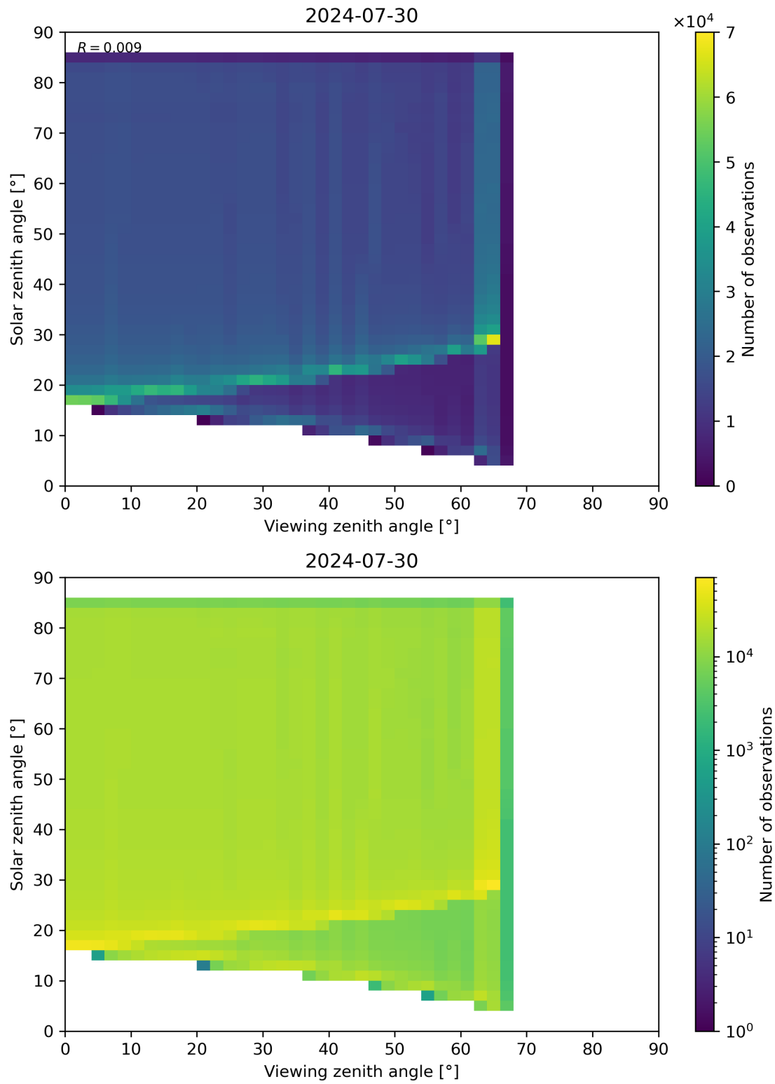
Figure 315: Scatter density plot of “Viewing zenith angle” against “Solar zenith angle” for 2024-07-29 to 2024-07-31.
