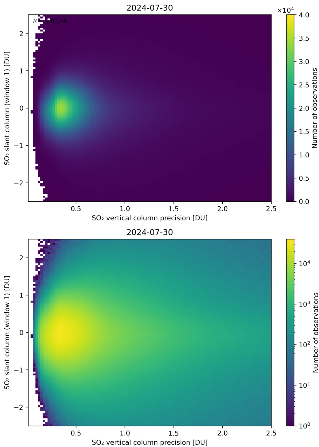
Figure 289: Scatter density plot of “SO 2 vertical column precision” against “SO 2 slant column (window 1)” for 2024-07-29 to 2024-07-31.
