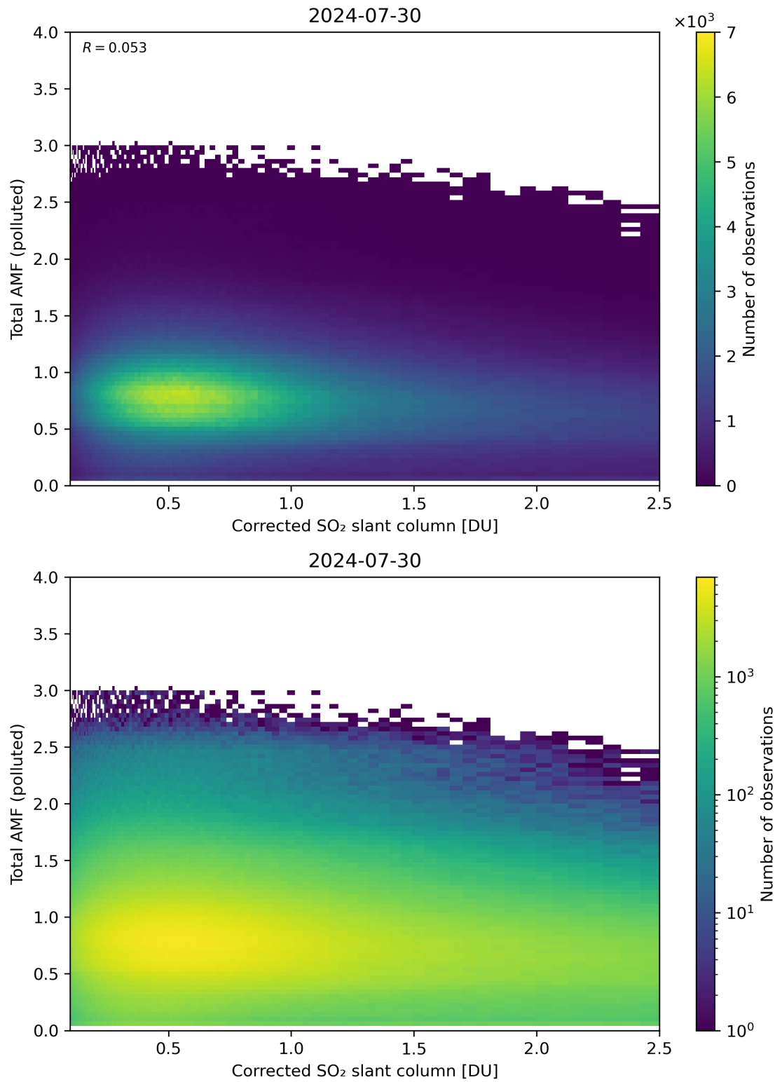
Figure 192: Scatter density plot of “Corrected SO 2 slant column” against “Total AMF (polluted)” for 2024-07-29 to 2024-07-31.
