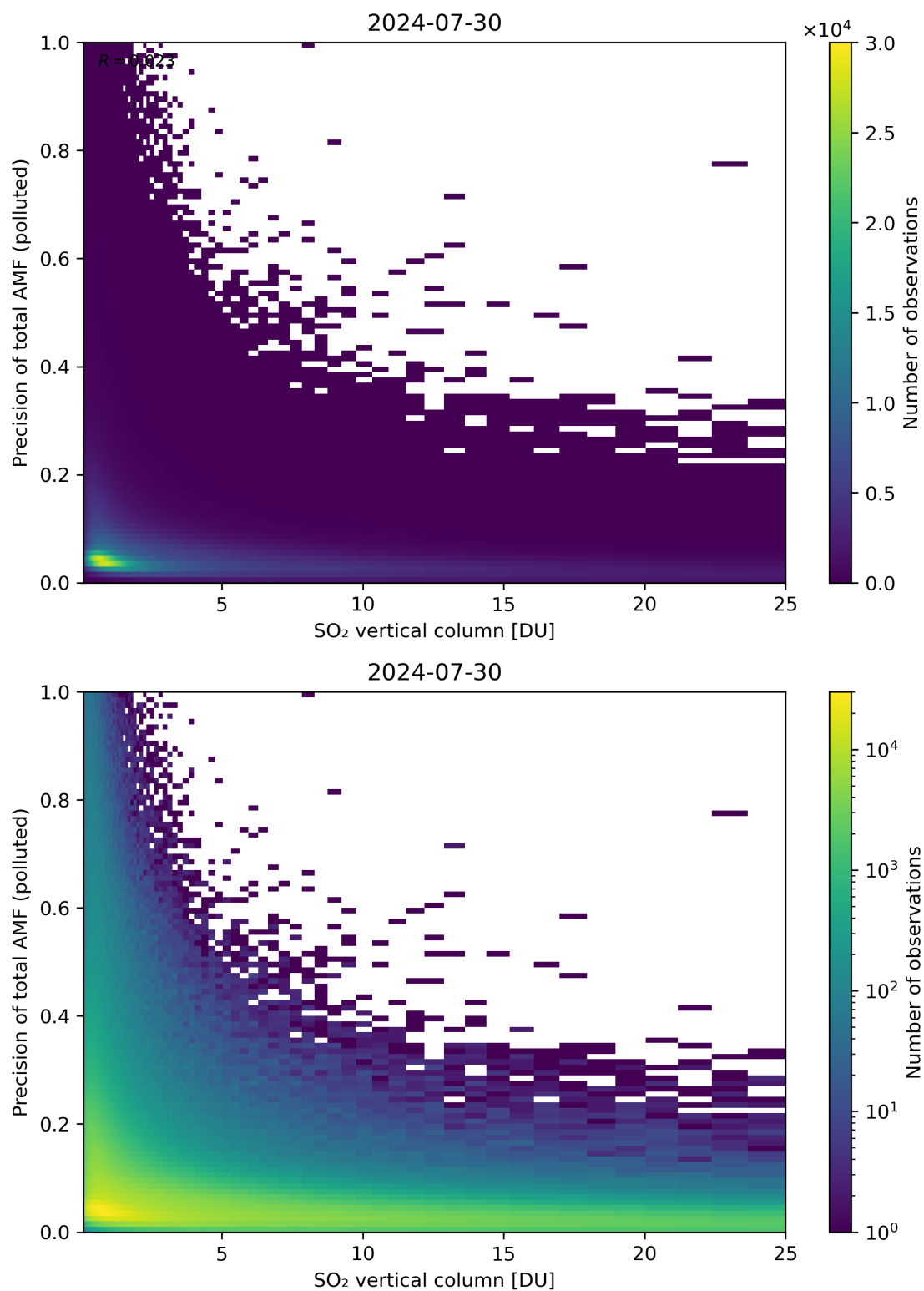
Figure 306: Scatter density plot of “SO 2 vertical column” against “Precision of total AMF (polluted)” for 2024-07-29 to 2024-07-31.
