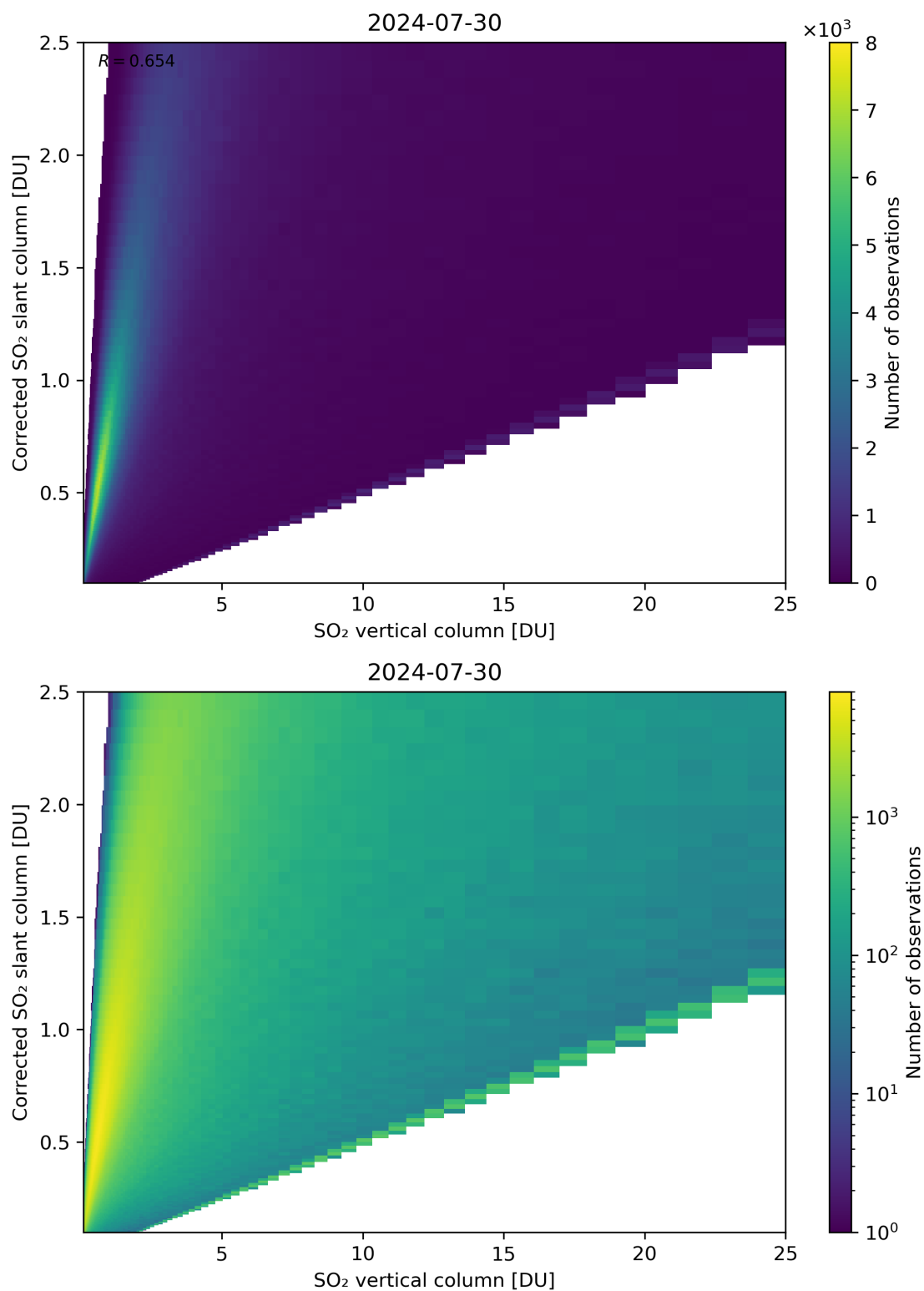
Figure 297: Scatter density plot of “SO 2 vertical column” against “Corrected SO 2 slant column” for 2024-07-29 to 2024-07-31.
