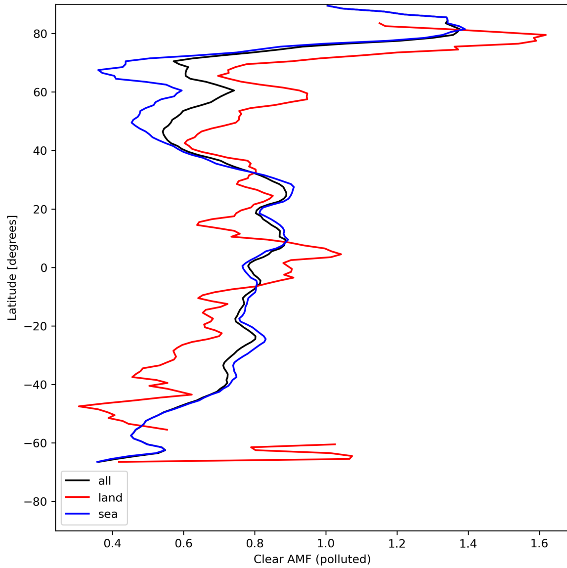
Figure 50: Zonal average of “Clear AMF (polluted)” for 2024-07-29 to 2024-07-31.
