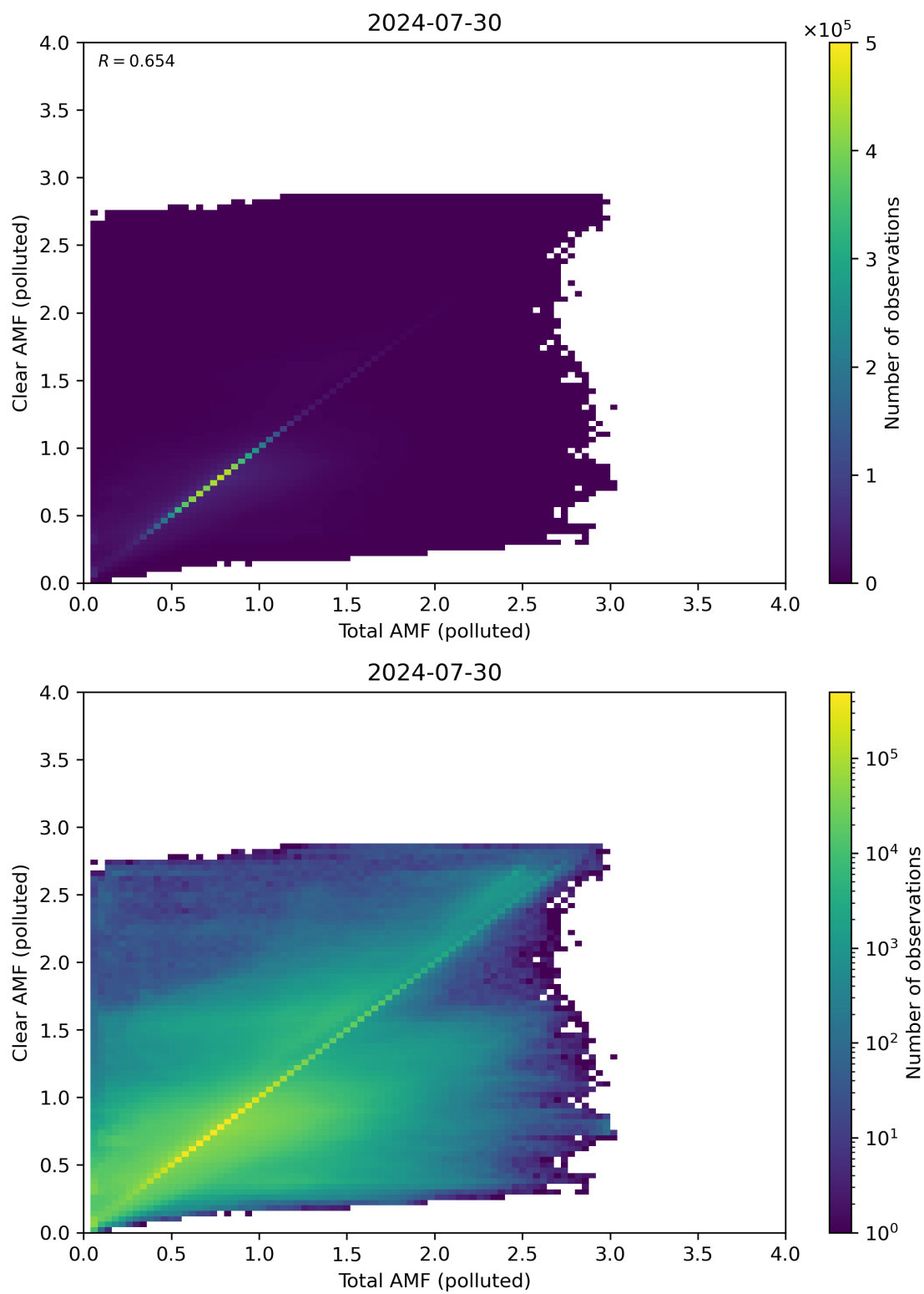
Figure 271: Scatter density plot of “Total AMF (polluted)” against “Clear AMF (polluted)” for 2024-07-29 to 2024-07-31.
