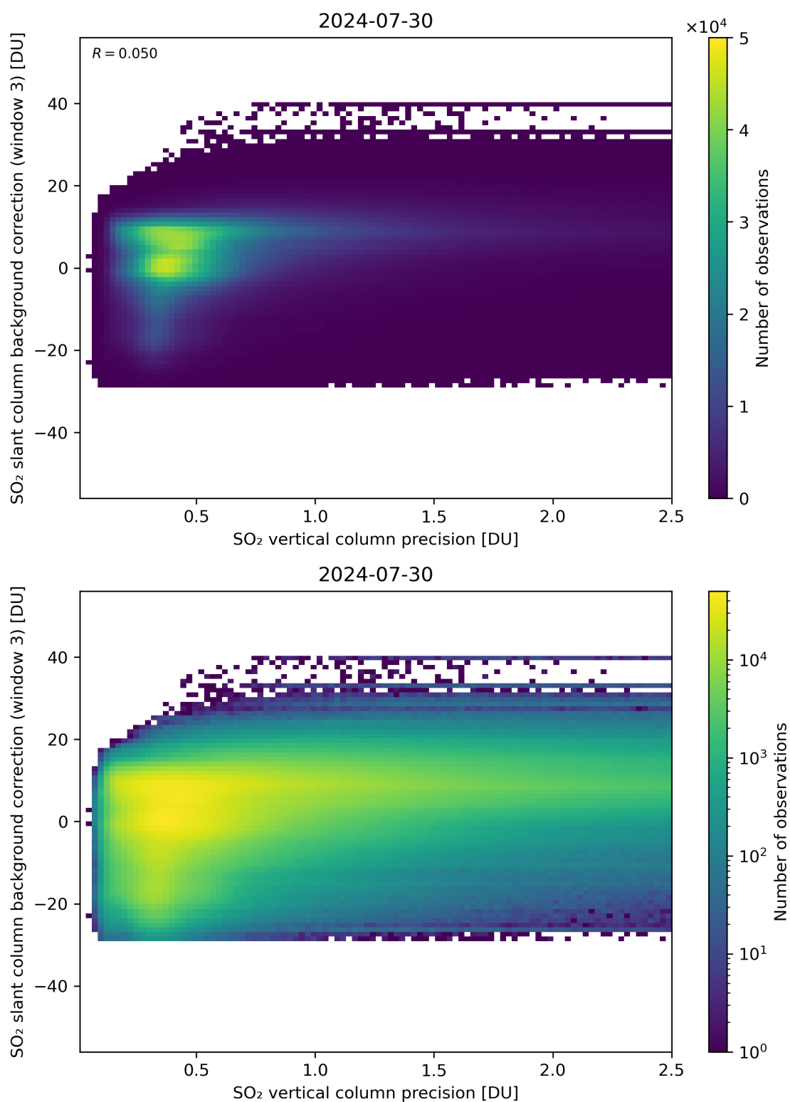
Figure 281: Scatter density plot of “SO 2 vertical column precision” against “SO 2 slant column background correction (window 3)” for 2024-07-29 to 2024-07-31.
