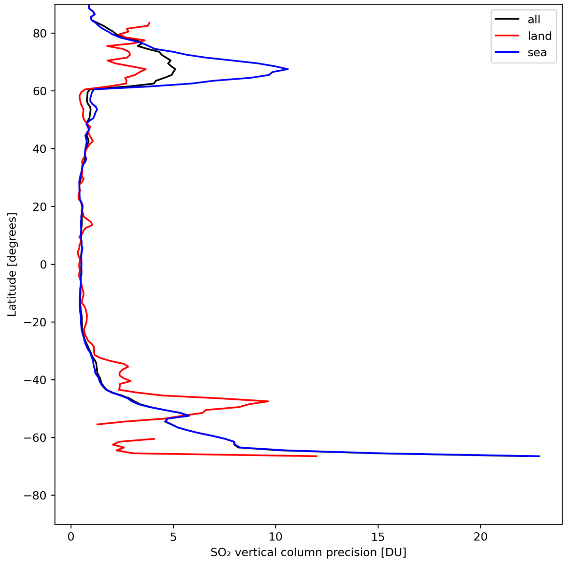
Figure 31: Zonal average of “SO 2 vertical column precision” for 2024-07-29 to 2024-07-31.
