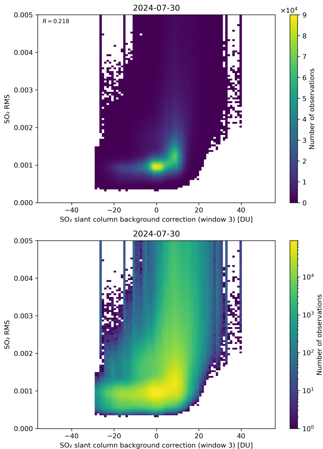
Figure 123: Scatter density plot of “SO 2 slant column background correction (window 3)” against “SO 2 RMS” for 2024-07-29 to 2024-07-31.
