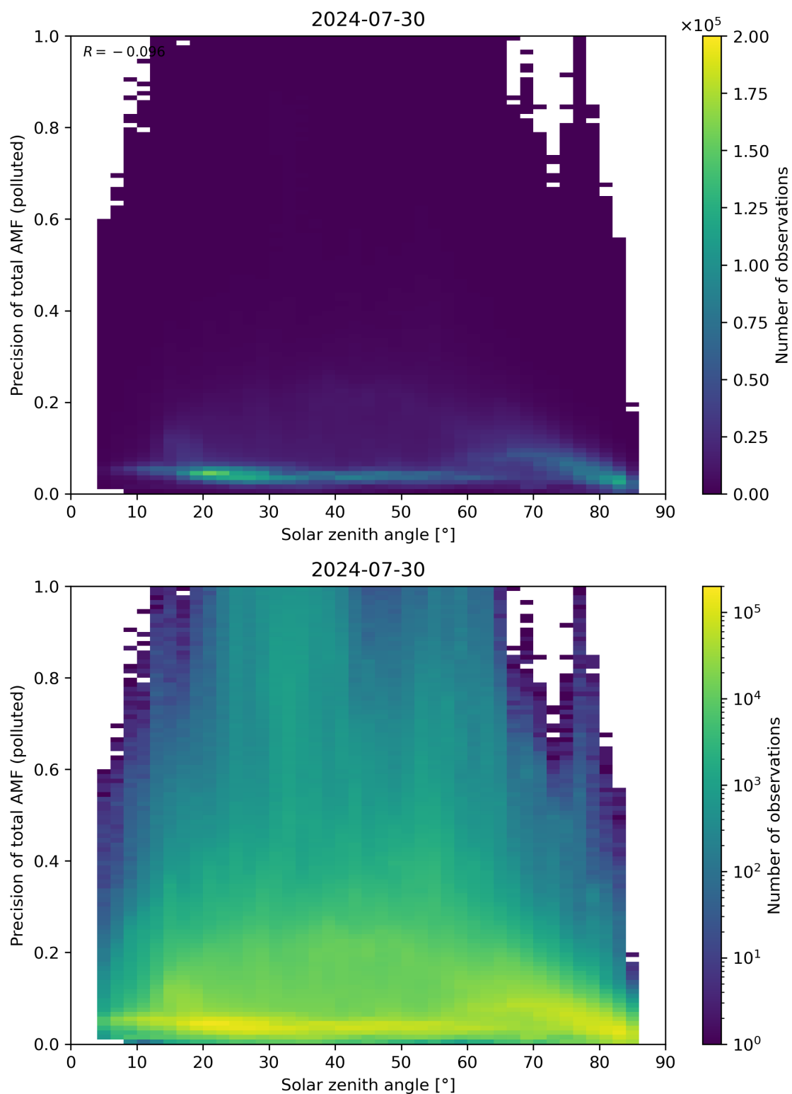
Figure 175: Scatter density plot of “Solar zenith angle” against “Precision of total AMF (polluted)” for 2024-07-29 to 2024-07-31.
