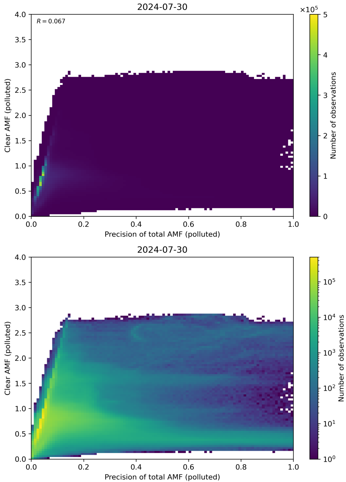
Figure 270: Scatter density plot of “Precision of total AMF (polluted)” against “Clear AMF (polluted)” for 2024-07-29 to 2024-07-31.
