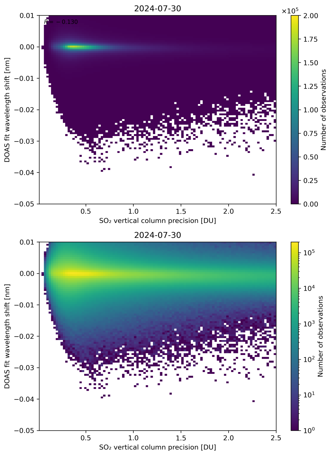
Figure 282: Scatter density plot of “SO 2 vertical column precision” against “DOAS fit wavelength shift” for 2024-07-29 to 2024-07-31.
