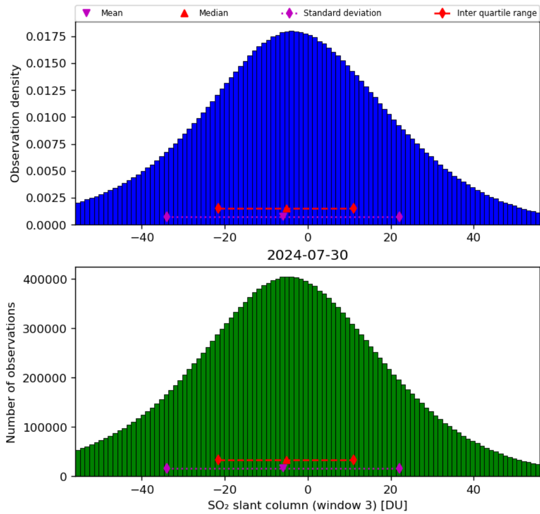
Figure 64: Histogram of “SO 2 slant column (window 3)” for 2024-07-29 to 2024-07-31
