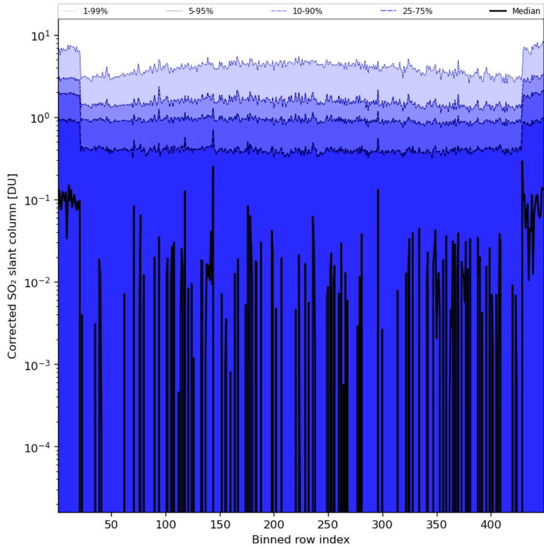
Figure 78: Along track statistics of “Corrected SO 2 slant column” for 2024-07-29 to 2024-07-31
