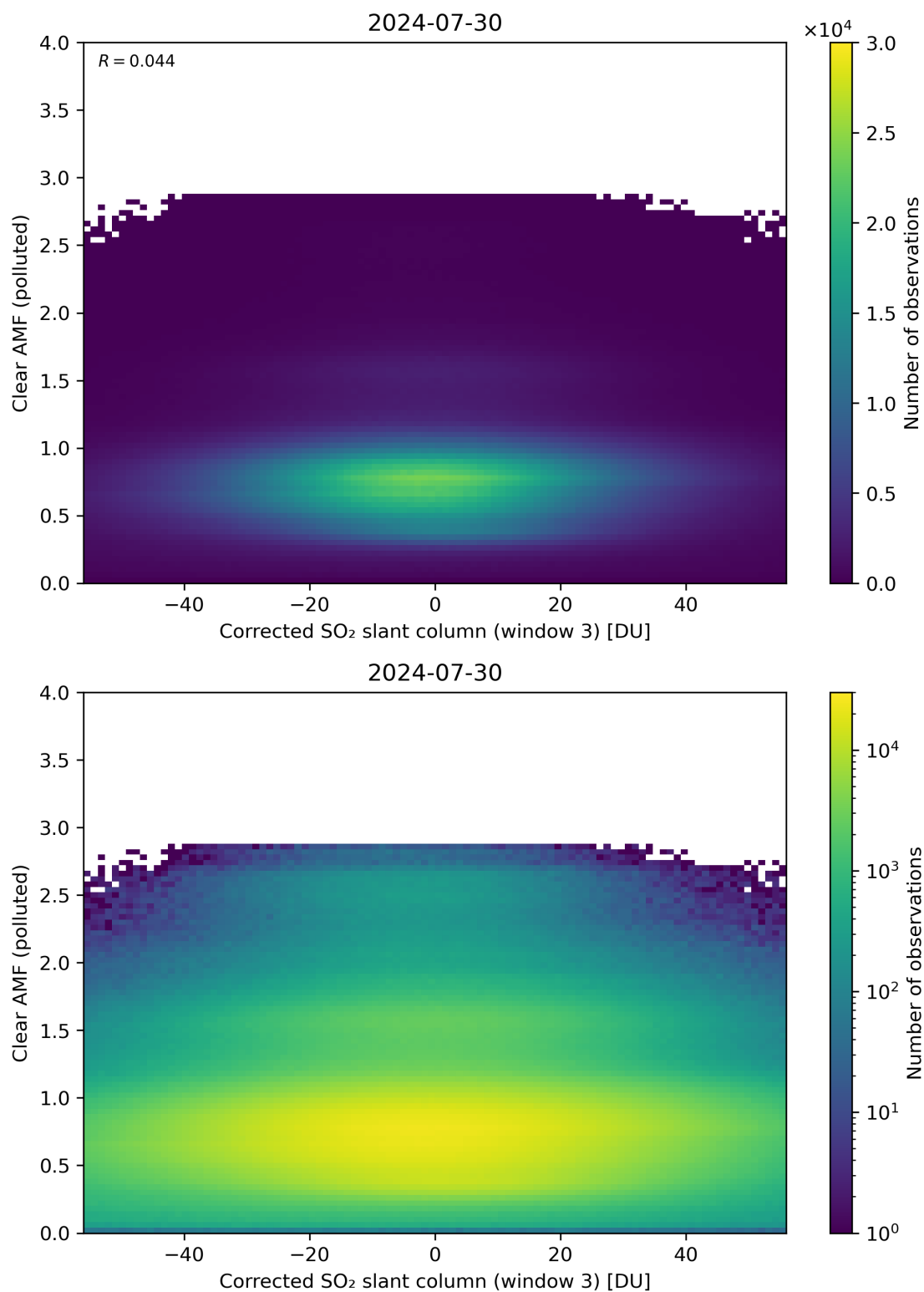
Figure 209: Scatter density plot of “Corrected SO 2 slant column (window 3)” against “Clear AMF (polluted)” for 2024-07-29 to 2024-07-31.
