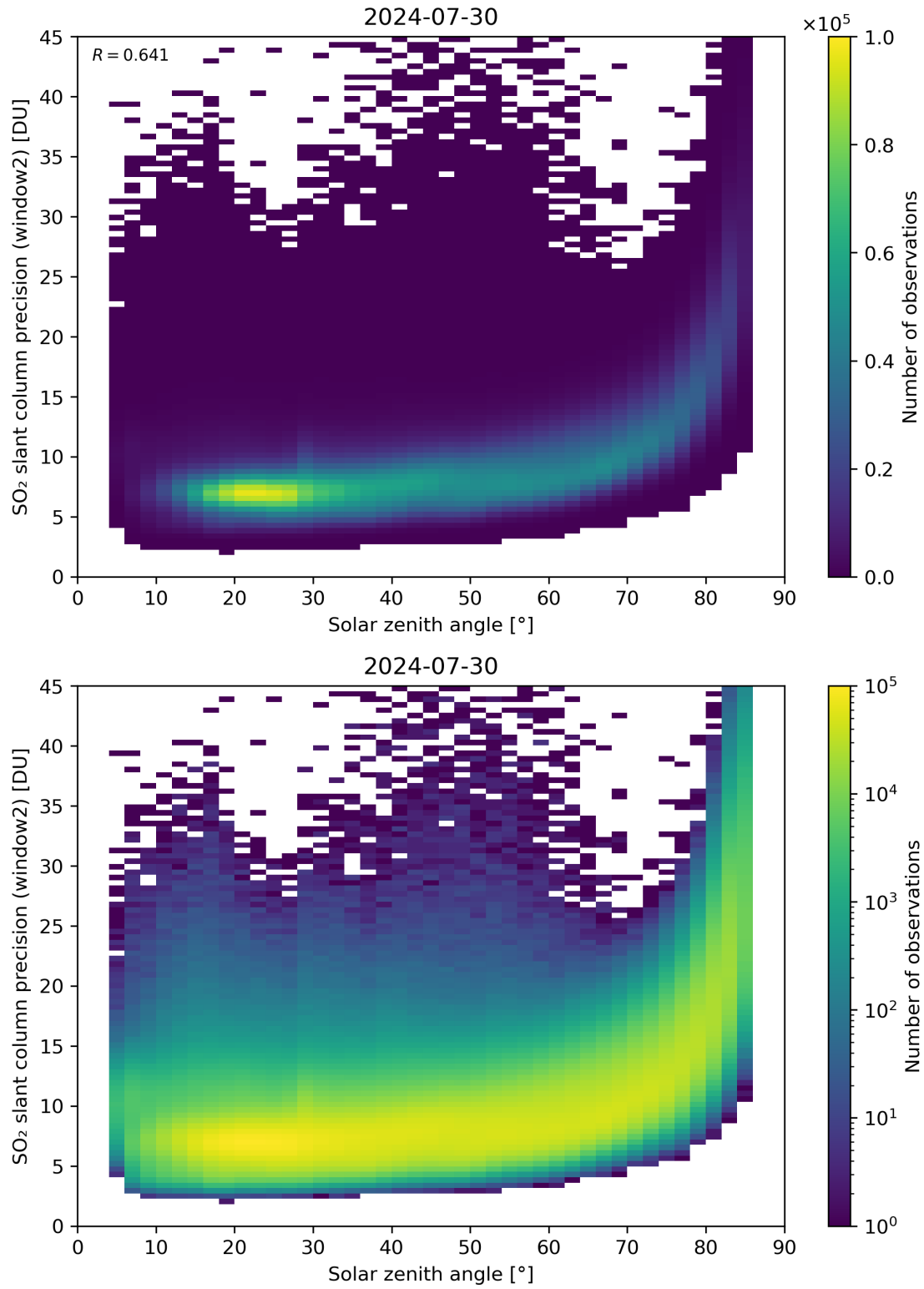
Figure 171: Scatter density plot of “Solar zenith angle” against “SO 2 slant column precision (window2)” for 2024-07-29 to 2024-07-31.
