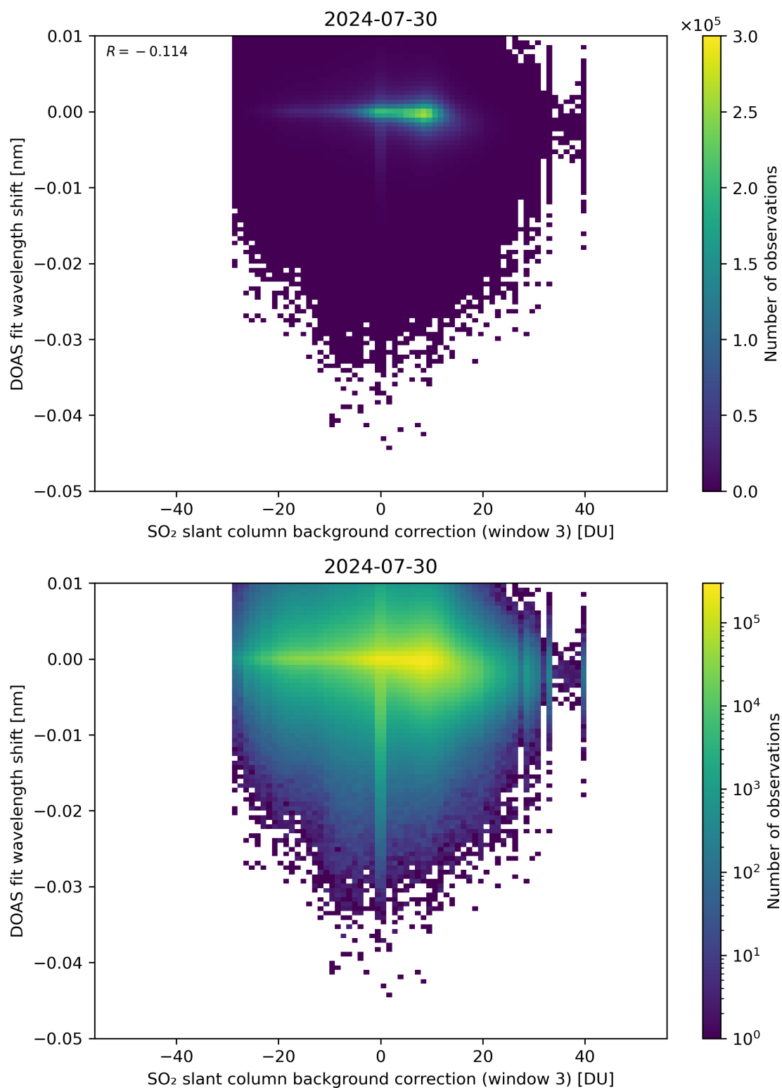
Figure 121: Scatter density plot of “SO 2 slant column background correction (window 3)” against “DOAS fit wavelength shift” for 2024-07-29 to 2024-07-31.
