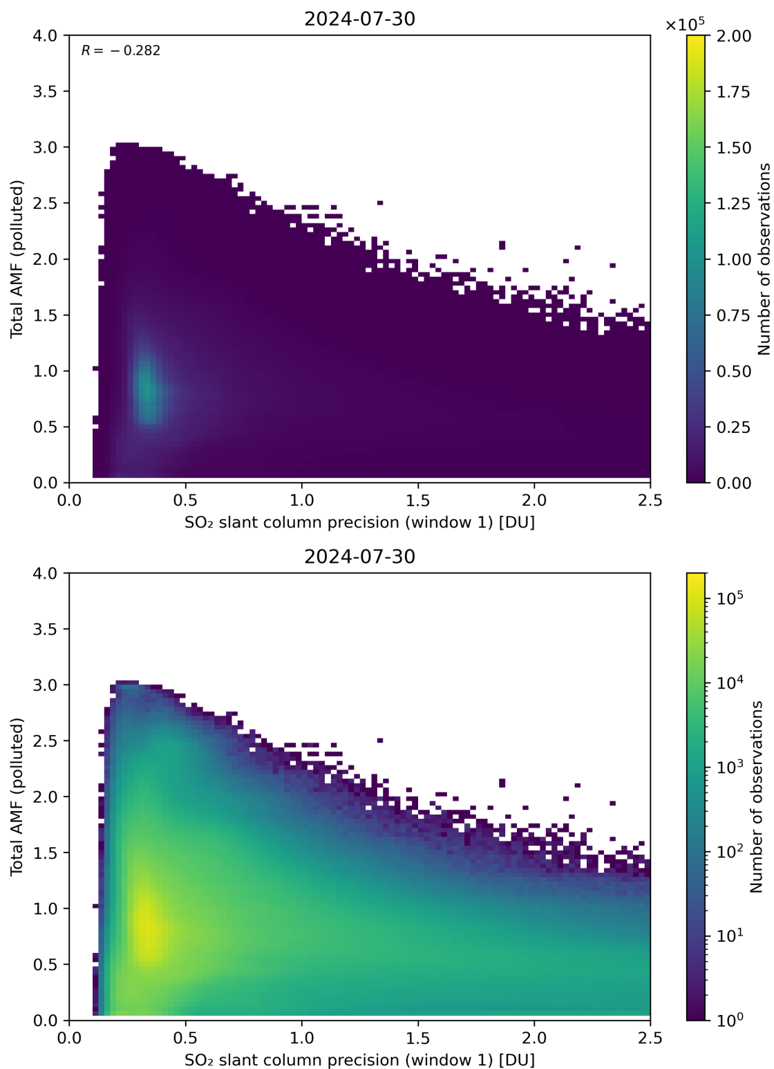
Figure 230: Scatter density plot of “SO 2 slant column precision (window 1)” against “Total AMF (polluted)” for 2024-07-29 to 2024-07-31.
