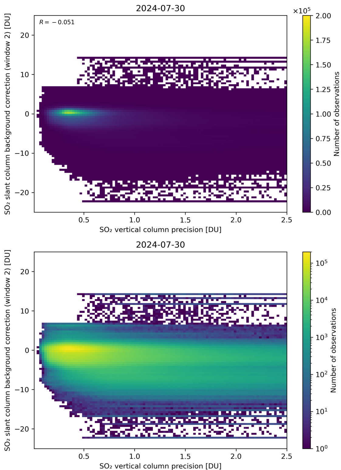
Figure 280: Scatter density plot of “SO 2 vertical column precision” against “SO 2 slant column background correction (window 2)” for 2024-07-29 to 2024-07-31.
