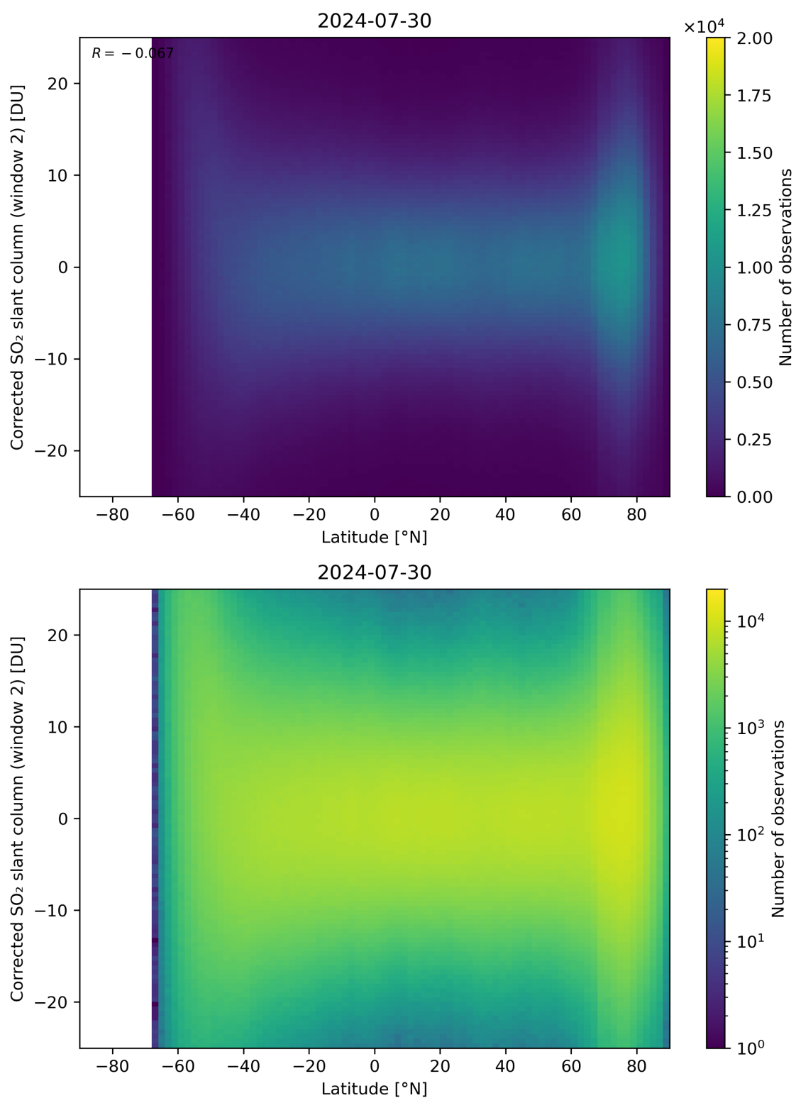
Figure 147: Scatter density plot of “Latitude” against “Corrected SO 2 slant column (window 2)” for 2024-07-29 to 2024-07-31.
