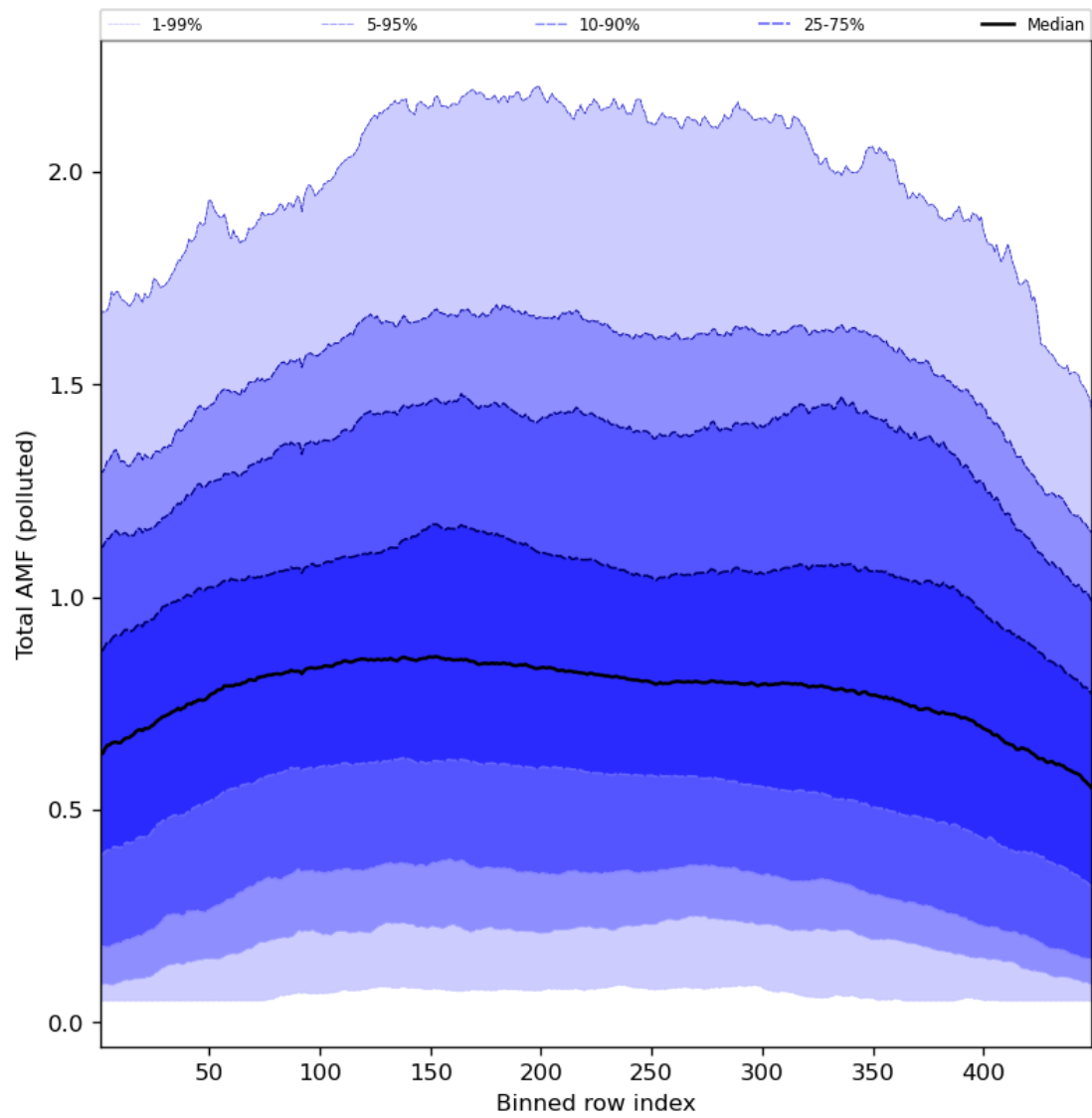
Figure 94: Along track statistics of “Total AMF (polluted)” for 2024-07-29 to 2024-07-31
