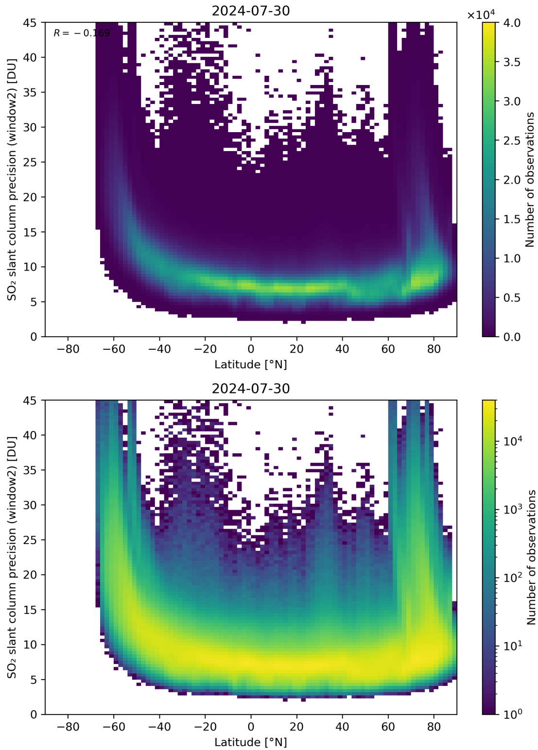
Figure 151: Scatter density plot of “Latitude” against “SO 2 slant column precision (window2)” for 2024-07-29 to 2024-07-31.
