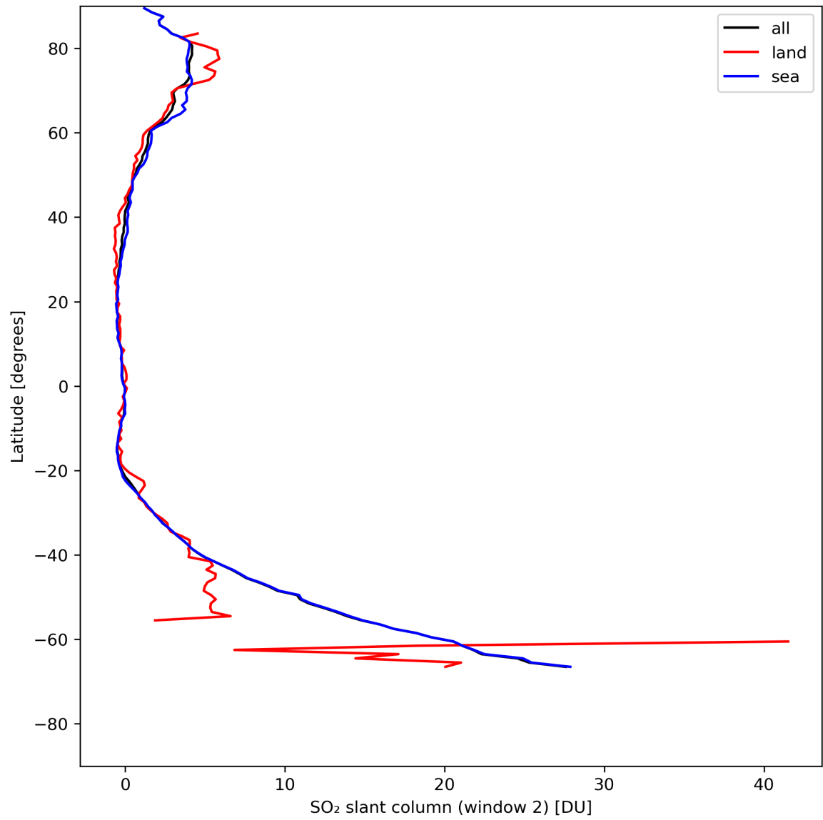
Figure 37: Zonal average of “SO 2 slant column (window 2)” for 2024-07-29 to 2024-07-31.
