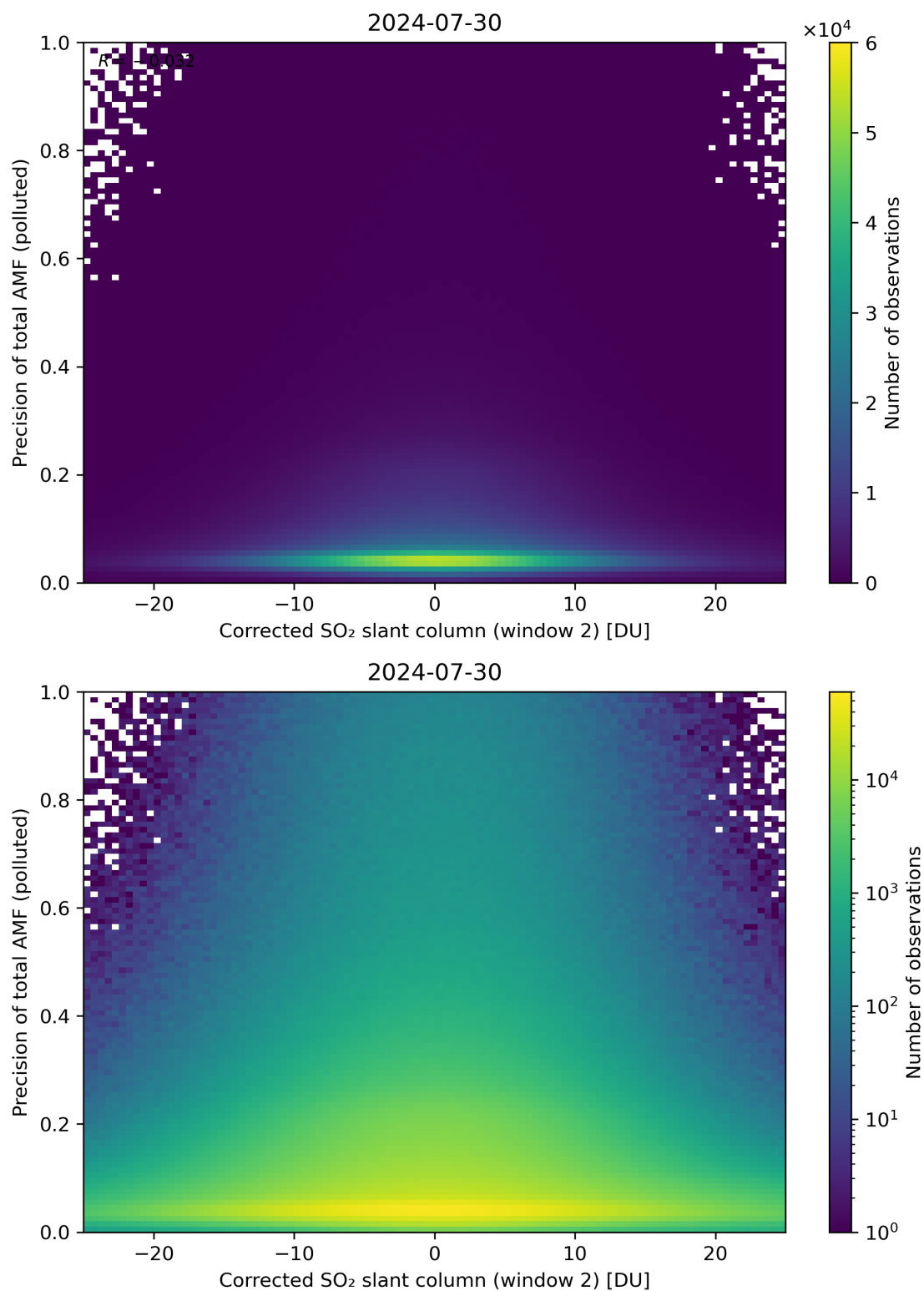
Figure 204: Scatter density plot of “Corrected SO 2 slant column (window 2)” against “Precision of total AMF (polluted)” for 2024-07-29 to 2024-07-31.
