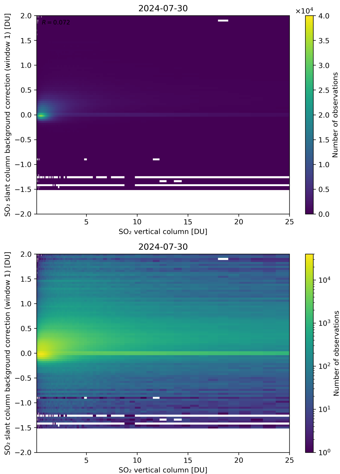
Figure 273: Scatter density plot of “SO 2 vertical column” against “SO 2 slant column background correction (window 1)” for 2024-07-29 to 2024-07-31.
