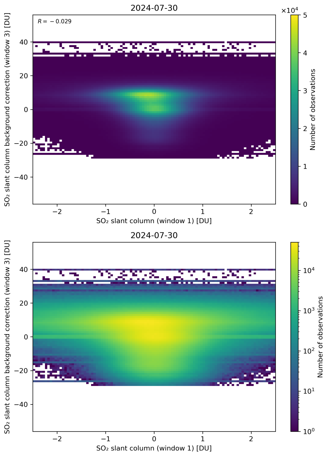
Figure 214: Scatter density plot of “SO 2 slant column (window 1)” against “SO 2 slant column background correction (window 3)” for 2024-07-29 to 2024-07-31.
