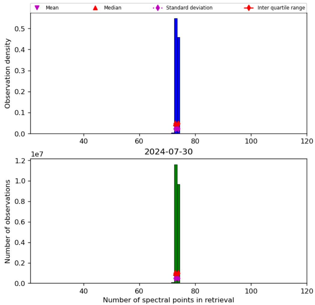
Figure 74: Histogram of “Number of spectral points in retrieval” for 2024-07-29 to 2024-07-31
