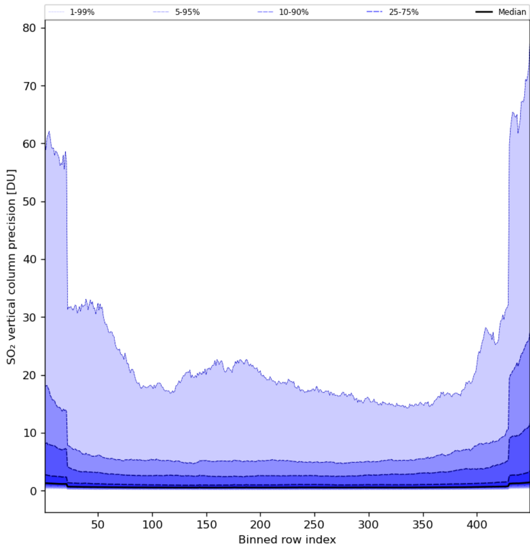
Figure 77: Along track statistics of “SO 2 vertical column precision” for 2024-07-29 to 2024-07-31
