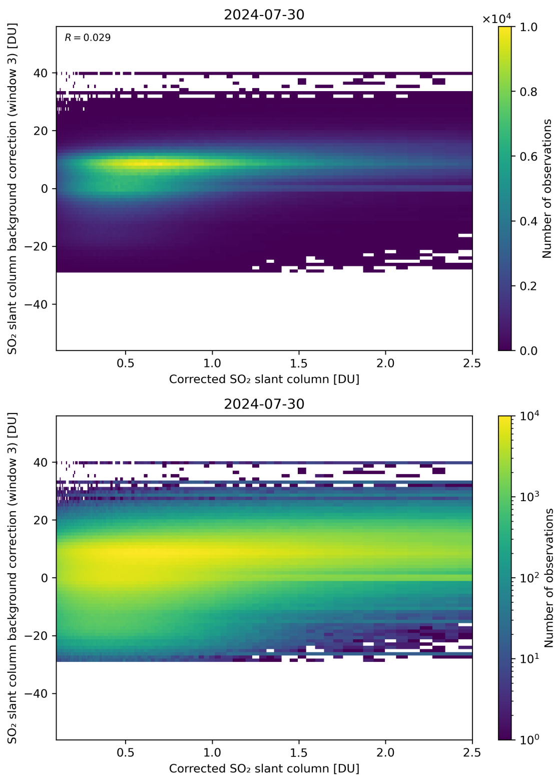
Figure 180: Scatter density plot of “Corrected SO 2 slant column” against “SO 2 slant column background correction (window 3)” for 2024-07-29 to 2024-07-31.
