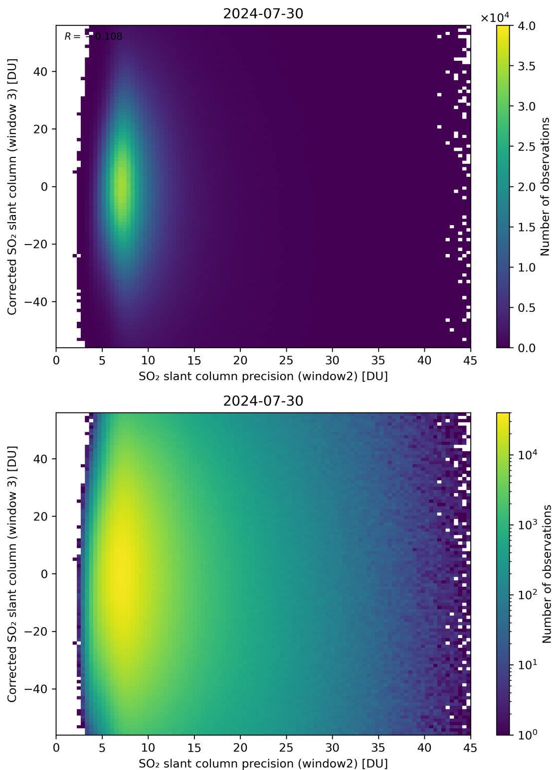
Figure 248: Scatter density plot of “SO 2 slant column precision (window2)” against “Corrected SO 2 slant column (window 3)” for 2024-07-29 to 2024-07-31.
