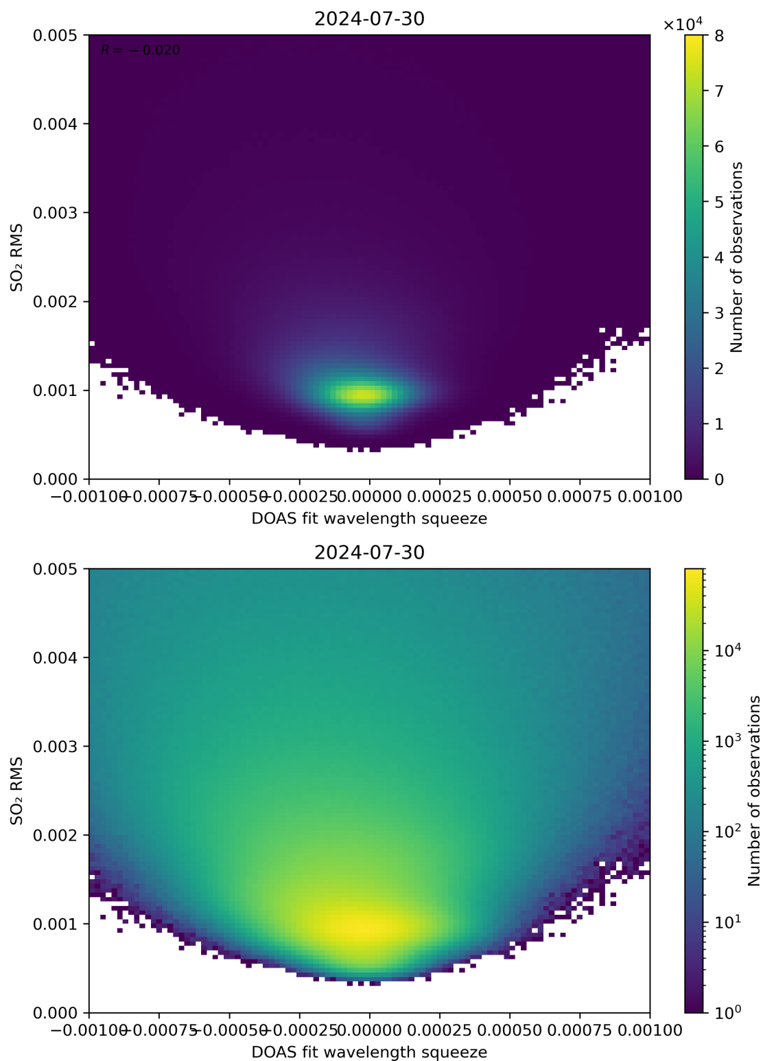
Figure 132: Scatter density plot of “DOAS fit wavelength squeeze” against “SO 2 RMS” for 2024-07-29 to 2024-07-31.
