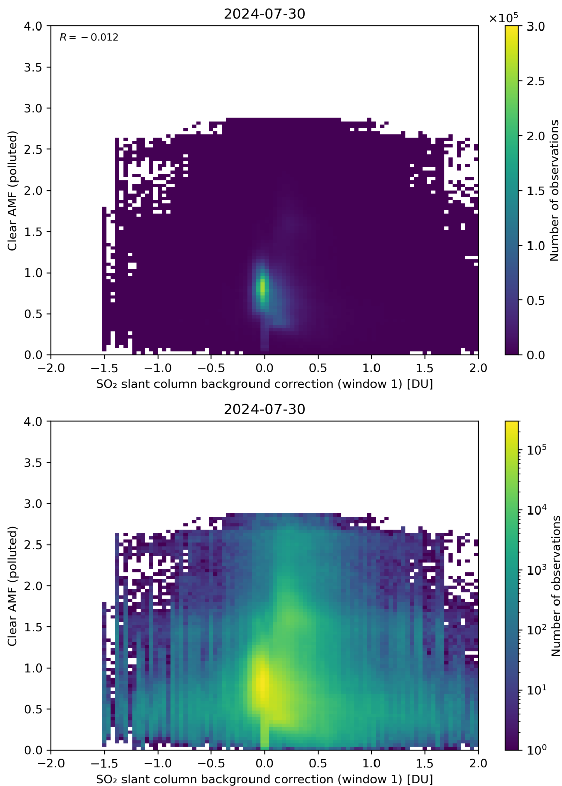
Figure 103: Scatter density plot of “SO 2 slant column background correction (window 1)” against “Clear AMF (polluted)” for 2024-07-29 to 2024-07-31.
