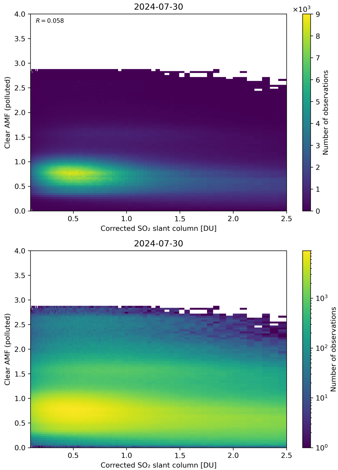
Figure 184: Scatter density plot of “Corrected SO 2 slant column” against “Clear AMF (polluted)” for 2024-07-29 to 2024-07-31.
