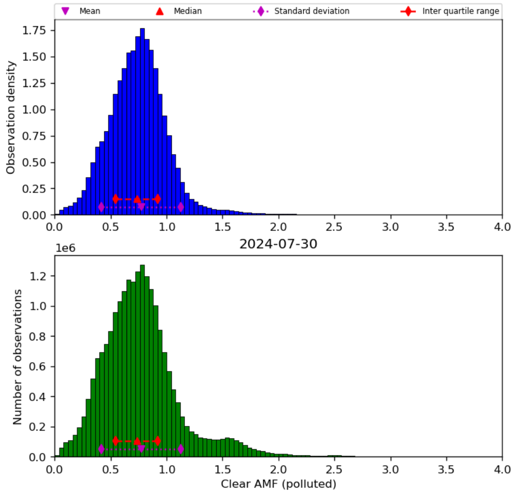
Figure 73: Histogram of “Clear AMF (polluted)” for 2024-07-29 to 2024-07-31
