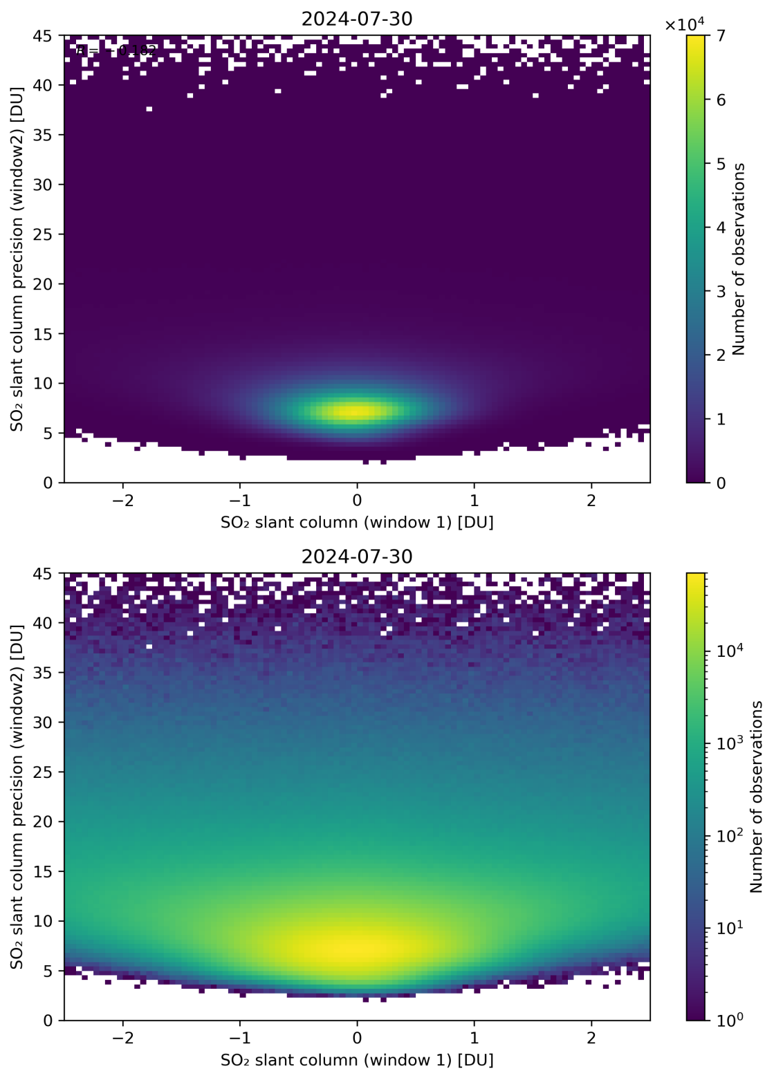
Figure 236: Scatter density plot of “SO 2 slant column (window 1)” against “SO 2 slant column precision (window2)” for 2024-07-29 to 2024-07-31.
