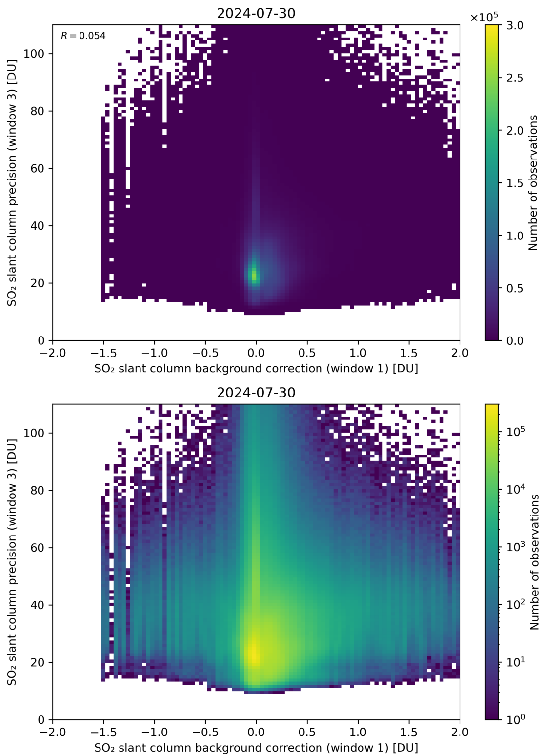
Figure 108: Scatter density plot of “SO 2 slant column background correction (window 1)” against “SO 2 slant column precision (window 3)” for 2024-07-29 to 2024-07-31.
