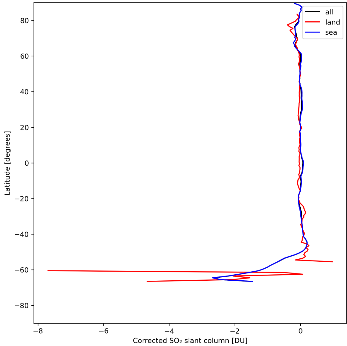
Figure 32: Zonal average of “Corrected SO 2 slant column” for 2024-07-29 to 2024-07-31.
