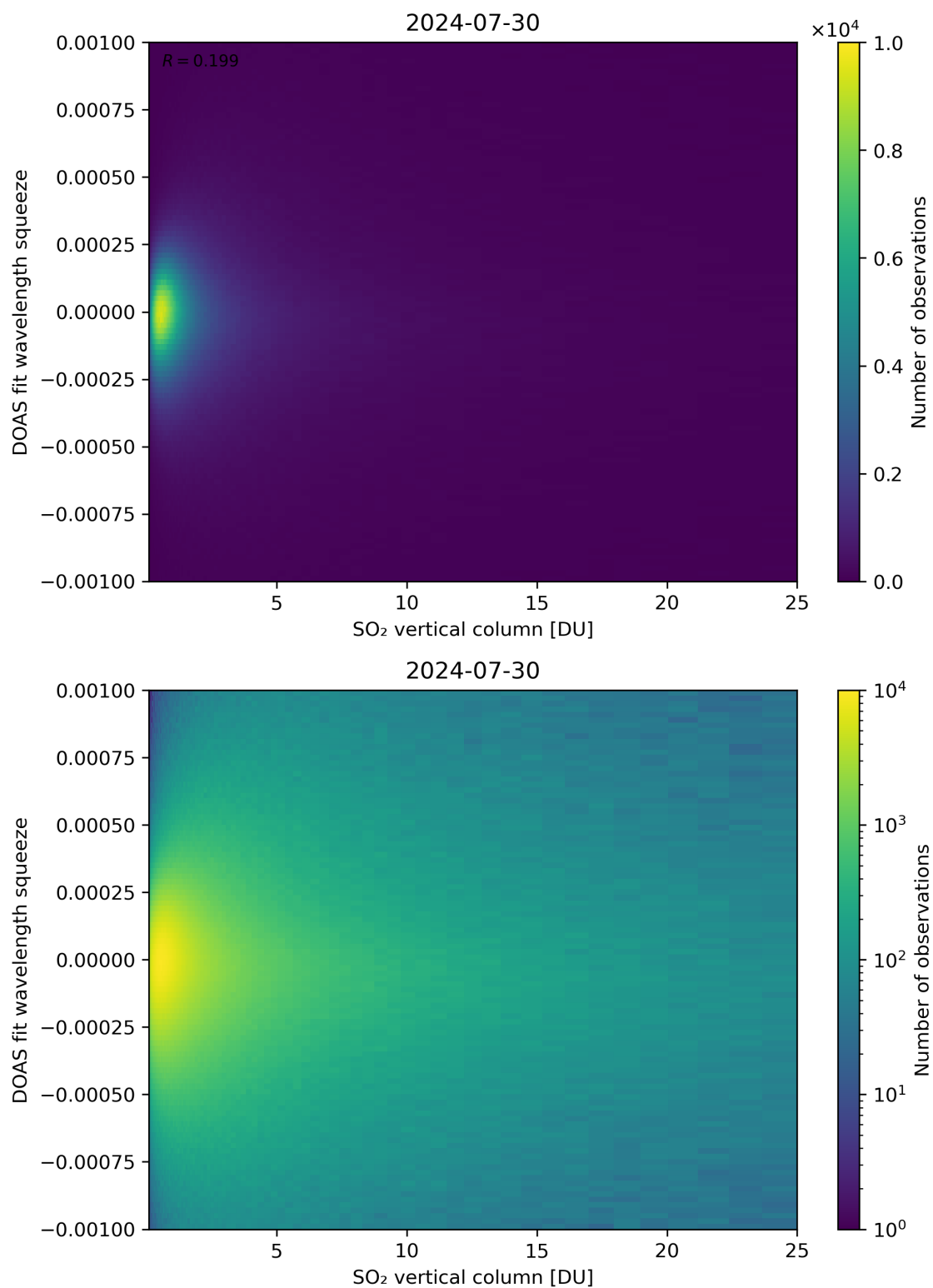
Figure 277: Scatter density plot of “SO 2 vertical column” against “DOAS fit wavelength squeeze” for 2024-07-29 to 2024-07-31.
