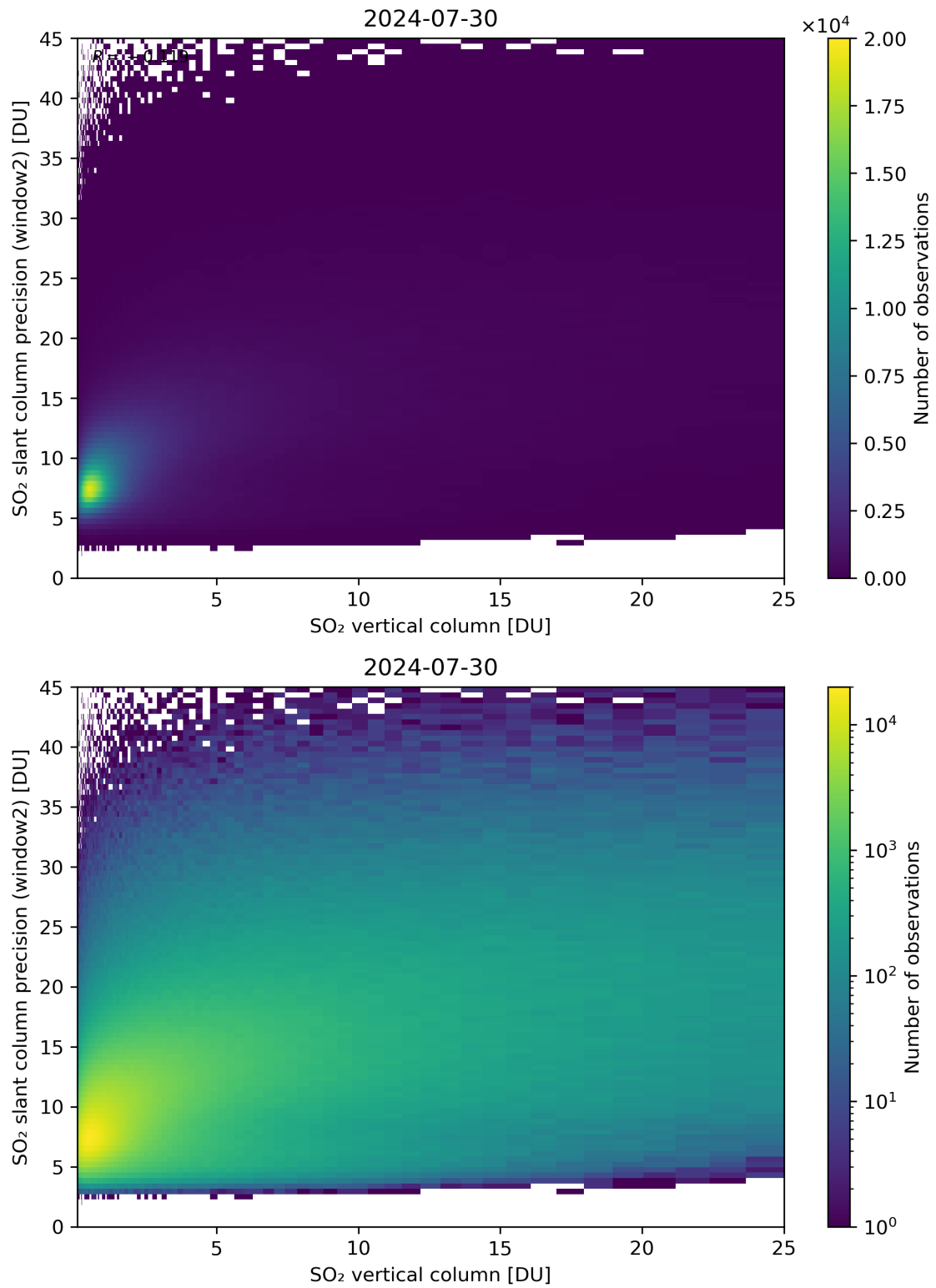
Figure 302: Scatter density plot of “SO 2 vertical column” against “SO 2 slant column precision (window2)” for 2024-07-29 to 2024-07-31.
