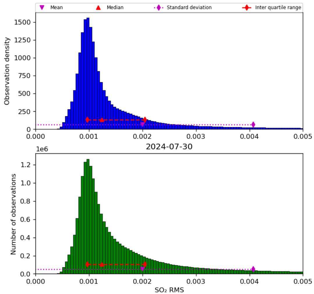
Figure 70: Histogram of “SO 2 RMS” for 2024-07-29 to 2024-07-31
