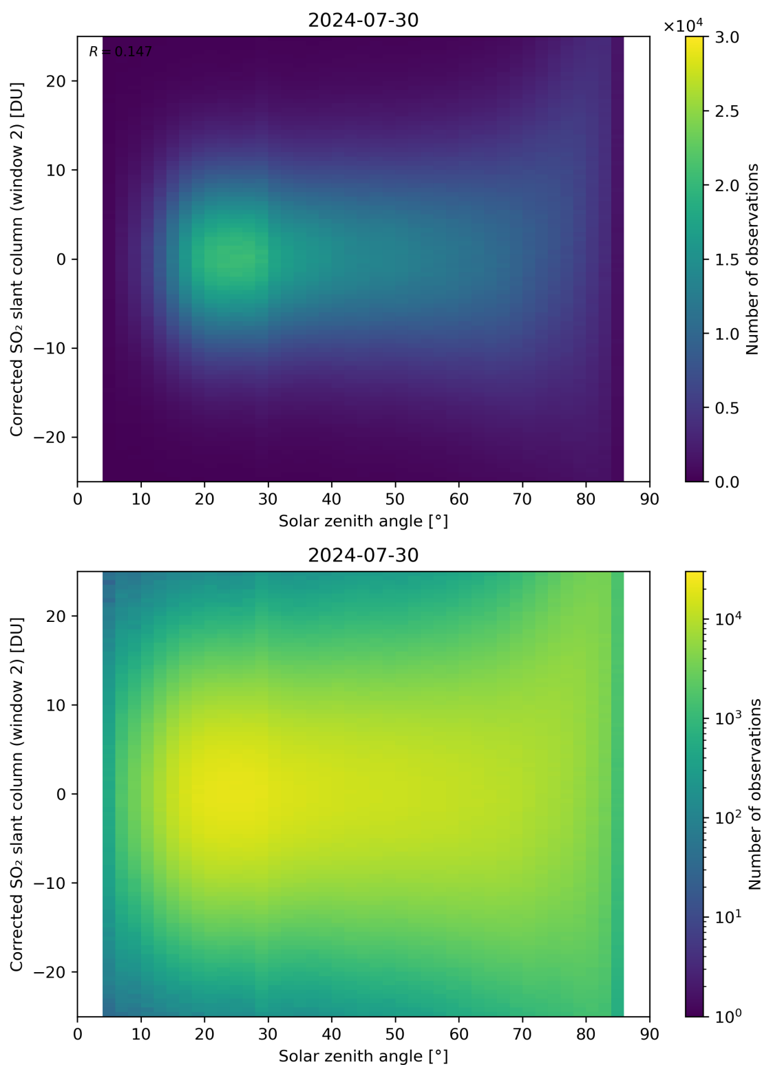
Figure 167: Scatter density plot of “Solar zenith angle” against “Corrected SO 2 slant column (window 2)” for 2024-07-29 to 2024-07-31.
