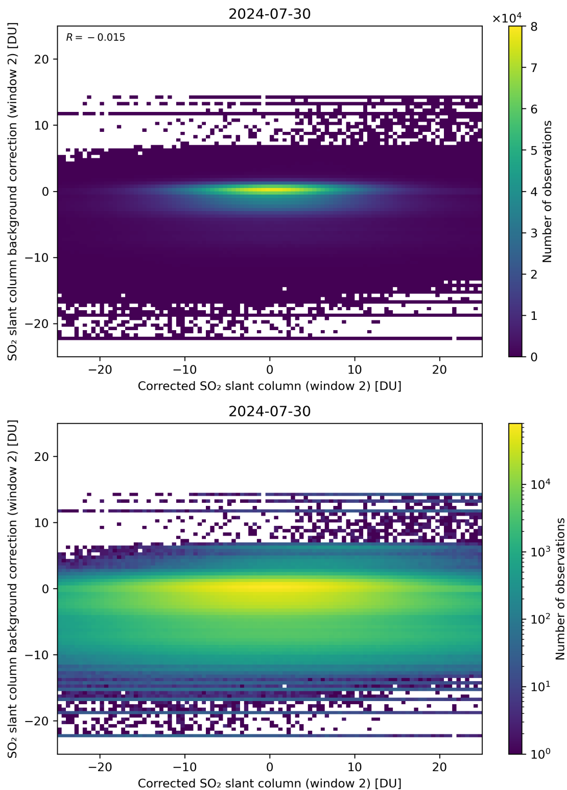
Figure 194: Scatter density plot of “Corrected SO 2 slant column (window 2)” against “SO 2 slant column background correction (window 2)” for 2024-07-29 to 2024-07-31.
