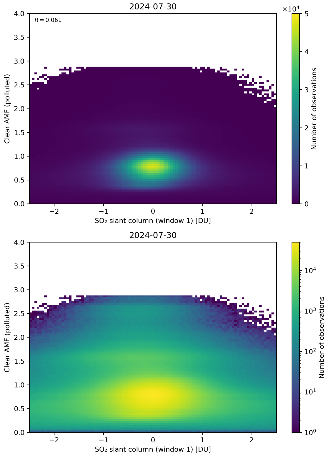
Figure 232: Scatter density plot of “SO 2 slant column (window 1)” against “Clear AMF (polluted)” for 2024-07-29 to 2024-07-31.
