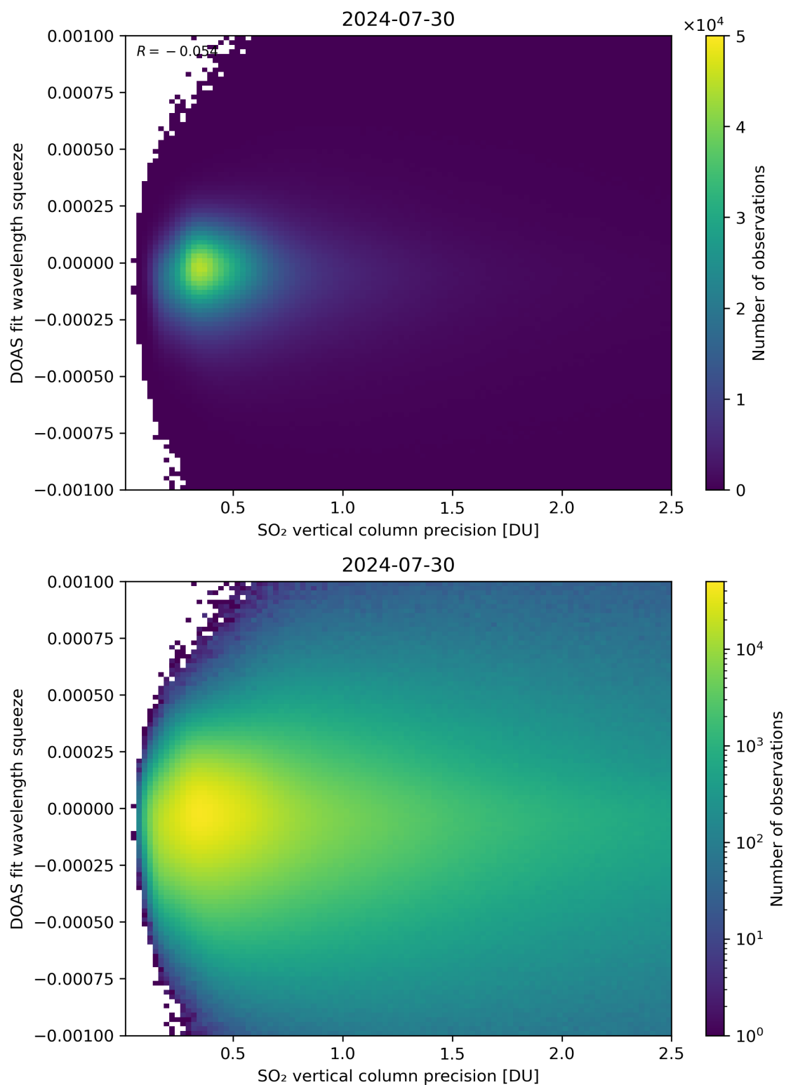
Figure 283: Scatter density plot of “SO 2 vertical column precision” against “DOAS fit wavelength squeeze” for 2024-07-29 to 2024-07-31.
