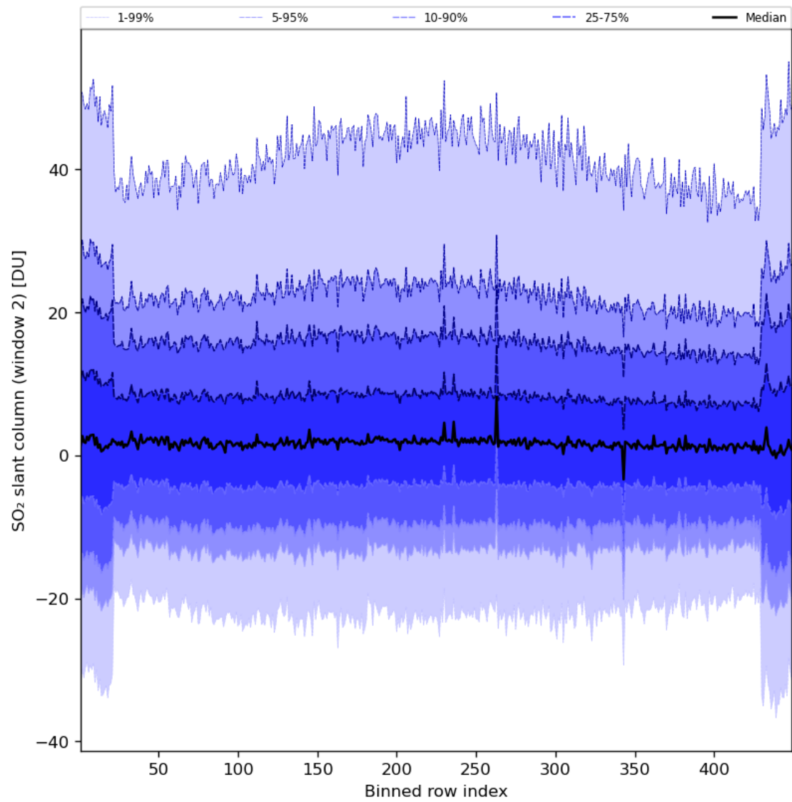
Figure 83: Along track statistics of “SO 2 slant column (window 2)” for 2024-07-29 to 2024-07-31
