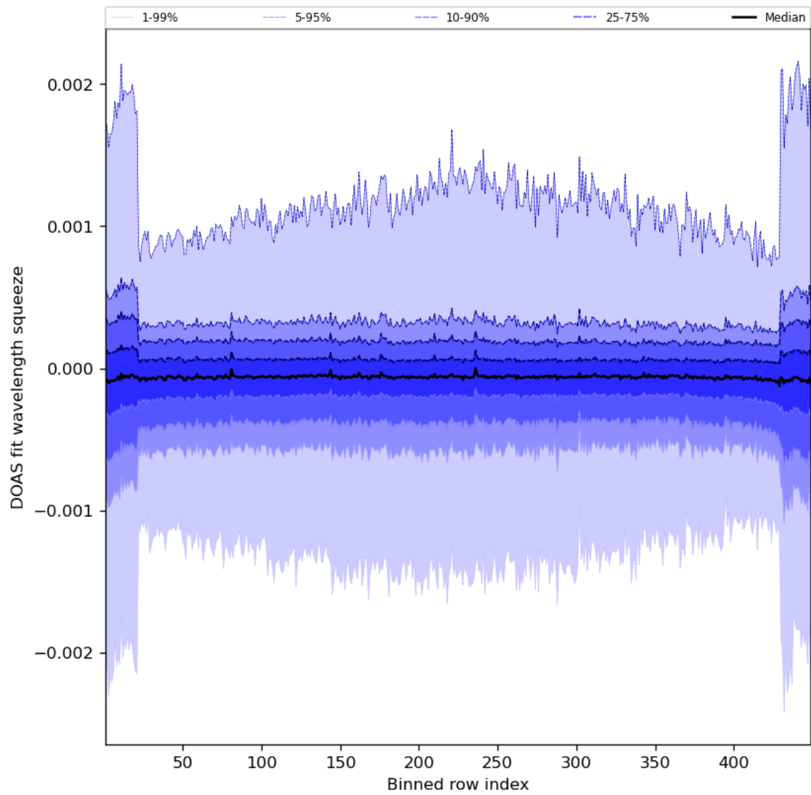
Figure 92: Along track statistics of “DOAS fit wavelength squeeze” for 2024-07-29 to 2024-07-31
