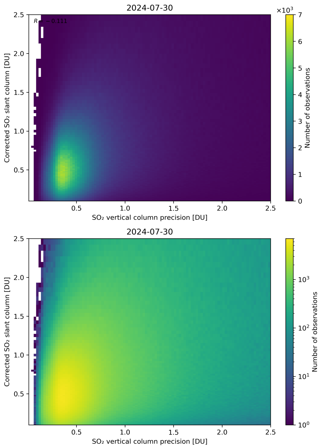
Figure 286: Scatter density plot of “SO 2 vertical column precision” against “Corrected SO 2 slant column” for 2024-07-29 to 2024-07-31.
