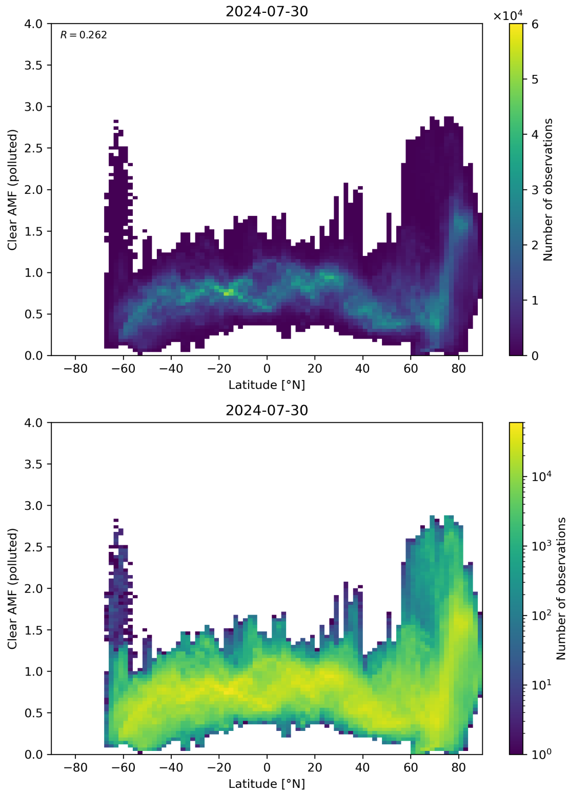
Figure 145: Scatter density plot of “Latitude” against “Clear AMF (polluted)” for 2024-07-29 to 2024-07-31.
