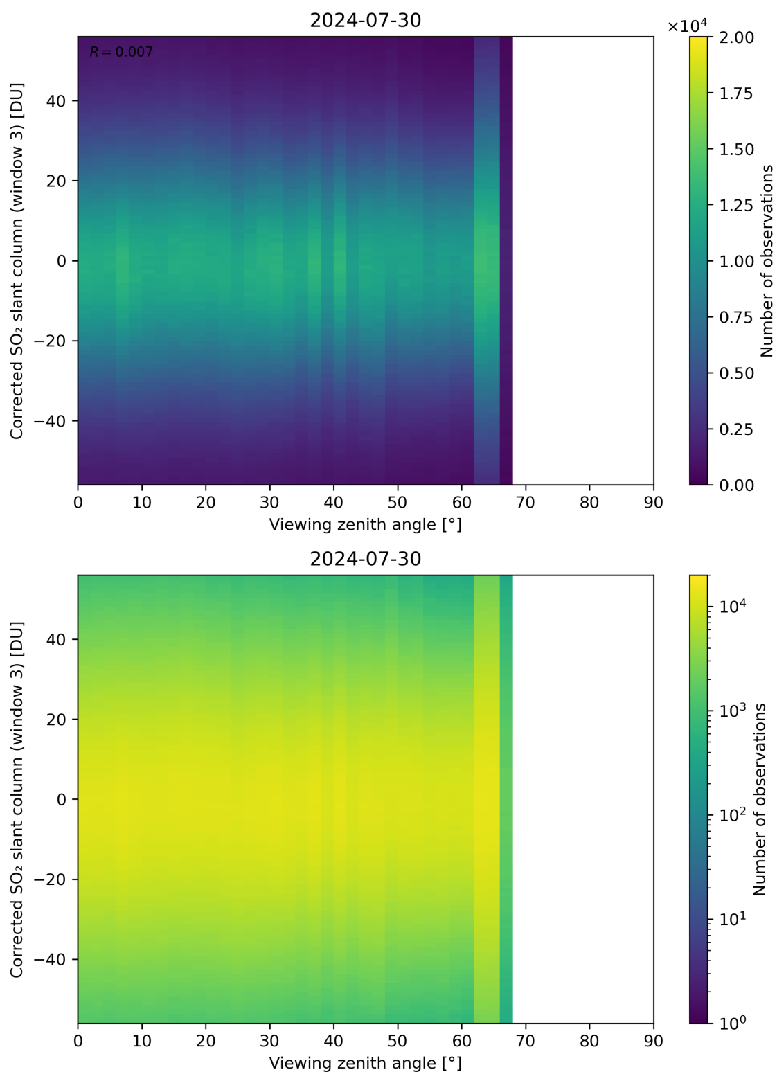
Figure 319: Scatter density plot of “Viewing zenith angle” against “Corrected SO 2 slant column (window 3)” for 2024-07-29 to 2024-07-31.
