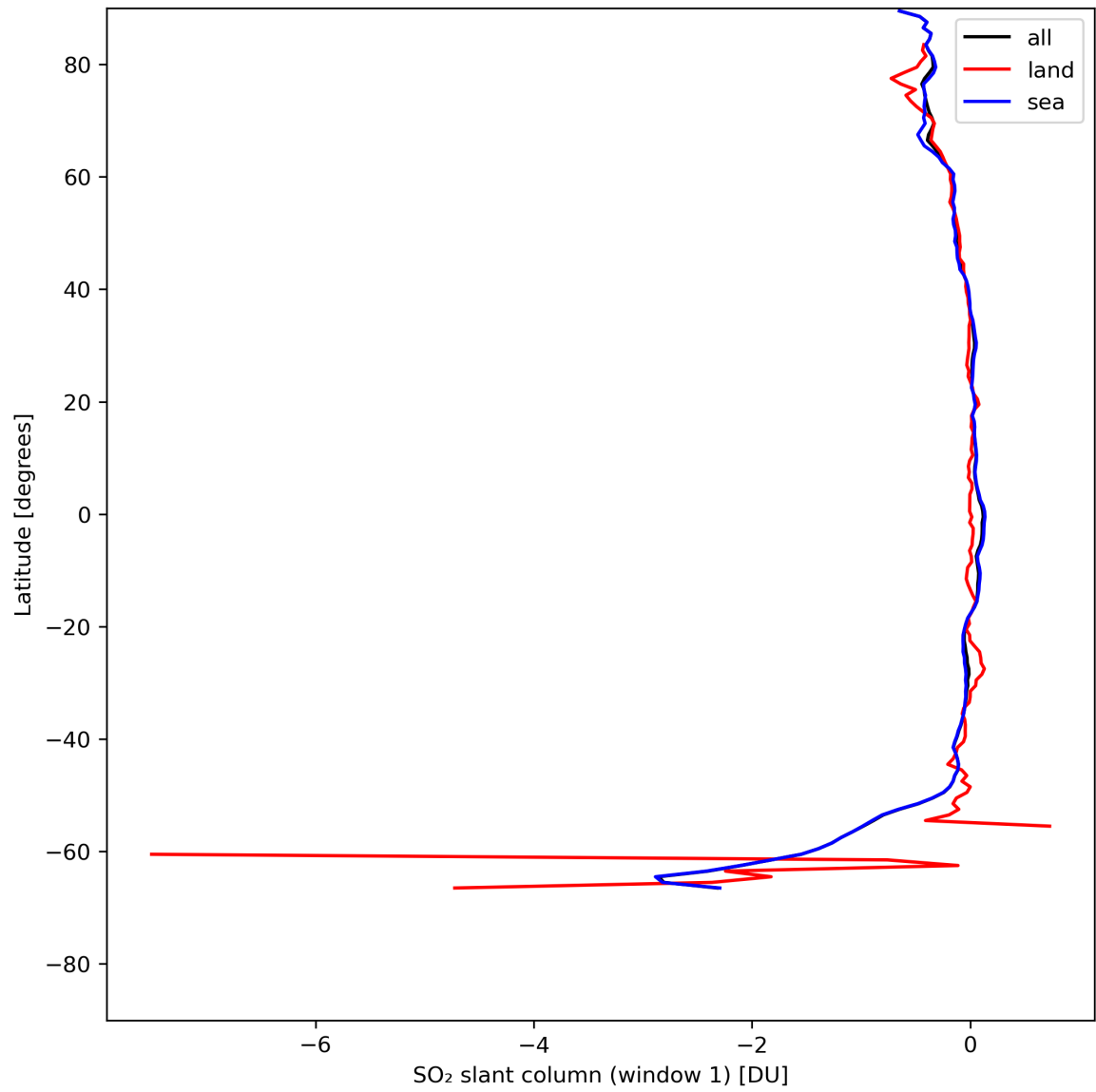
Figure 33: Zonal average of “SO 2 slant column (window 1)” for 2024-07-29 to 2024-07-31.
