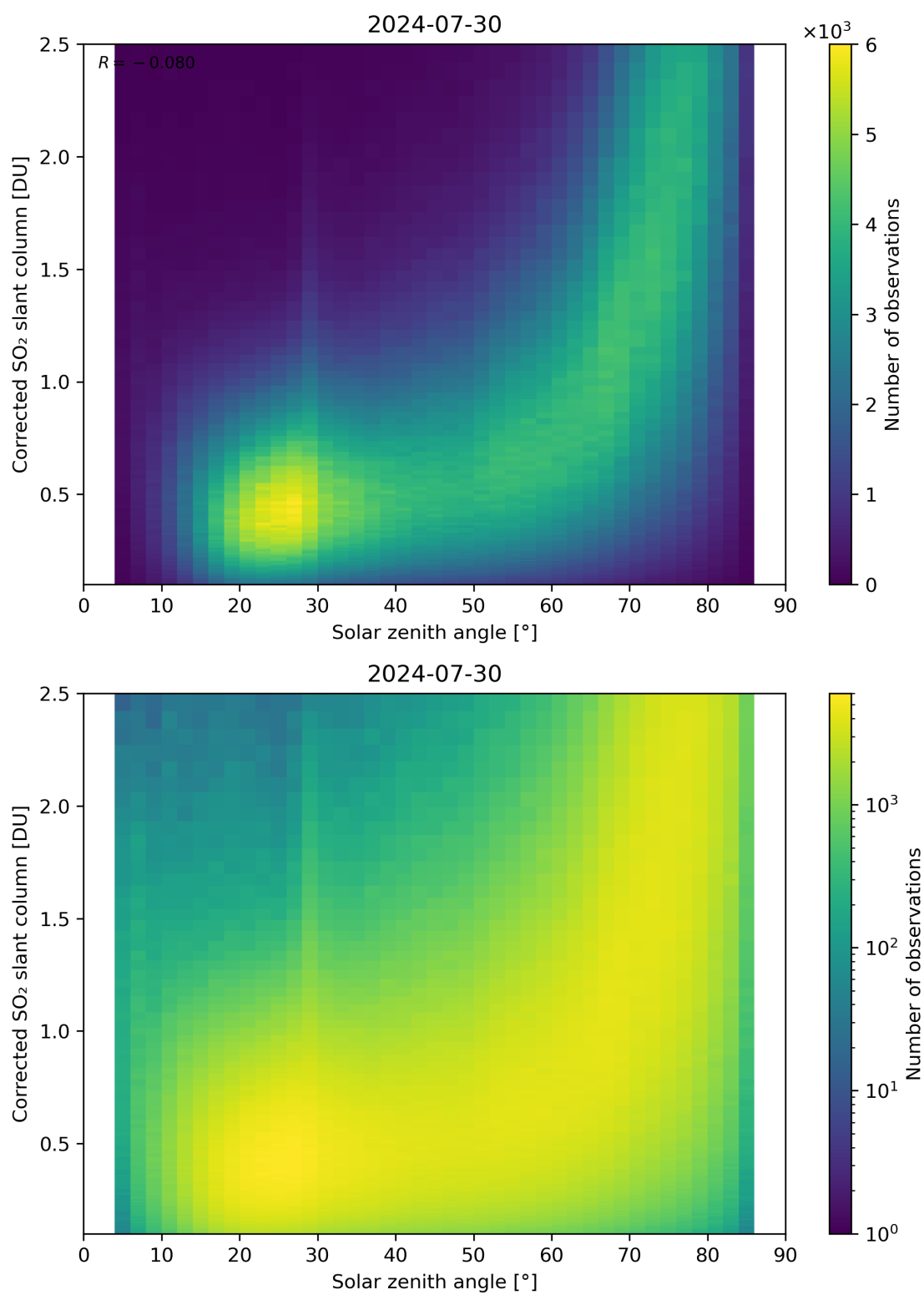
Figure 166: Scatter density plot of “Solar zenith angle” against “Corrected SO 2 slant column” for 2024-07-29 to 2024-07-31.
