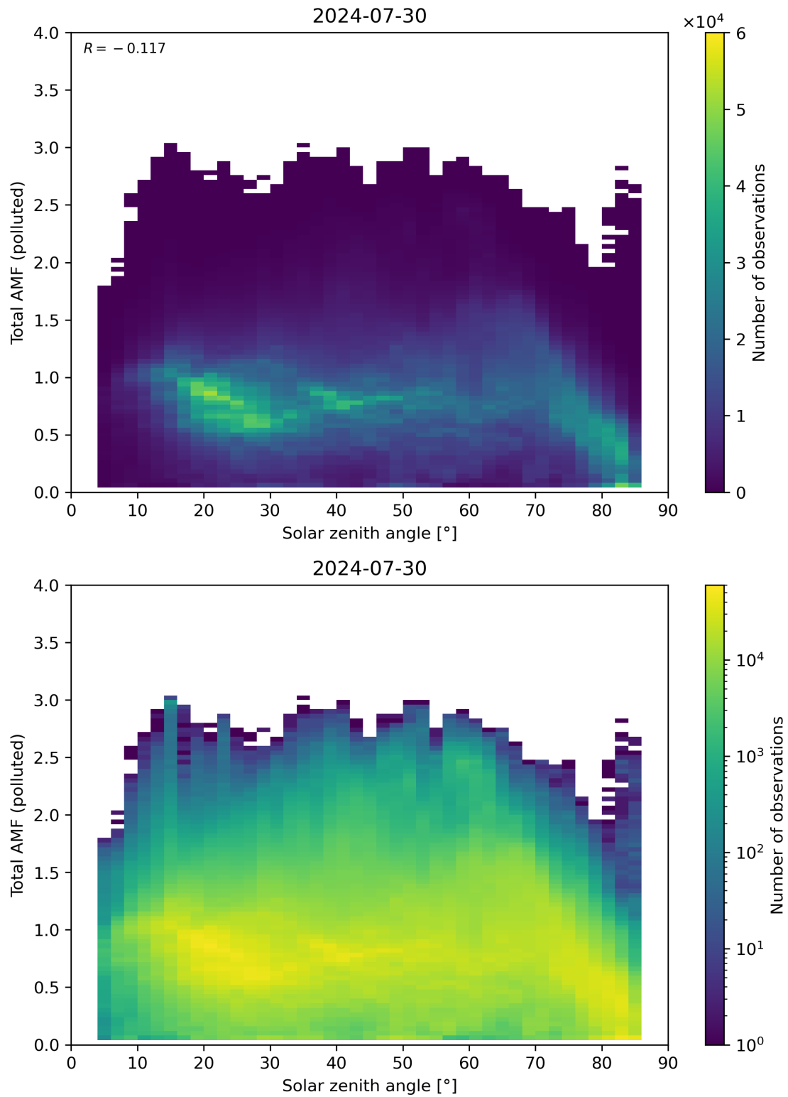
Figure 174: Scatter density plot of “Solar zenith angle” against “Total AMF (polluted)” for 2024-07-29 to 2024-07-31.
