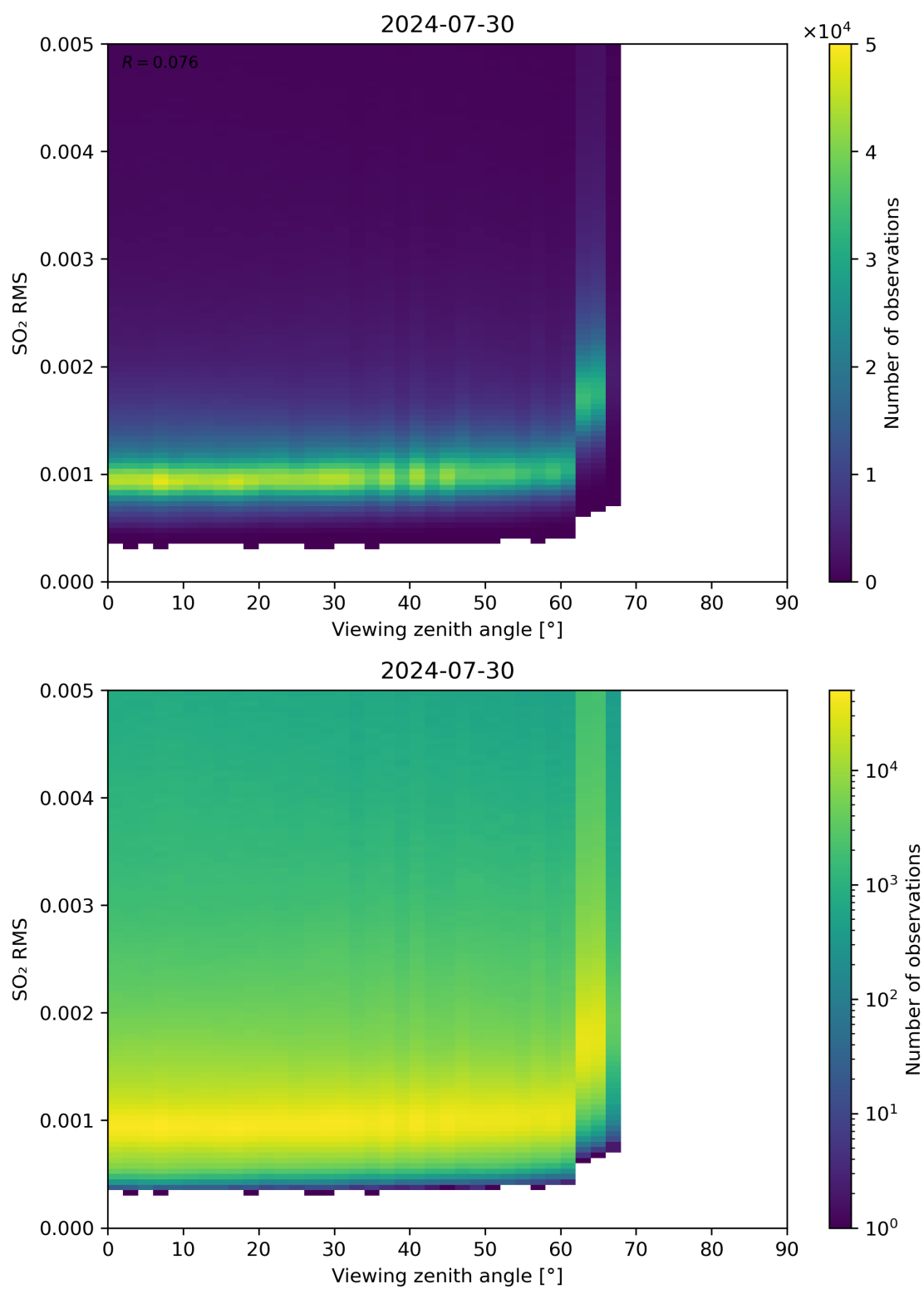
Figure 313: Scatter density plot of “Viewing zenith angle” against “SO 2 RMS” for 2024-07-29 to 2024-07-31.
