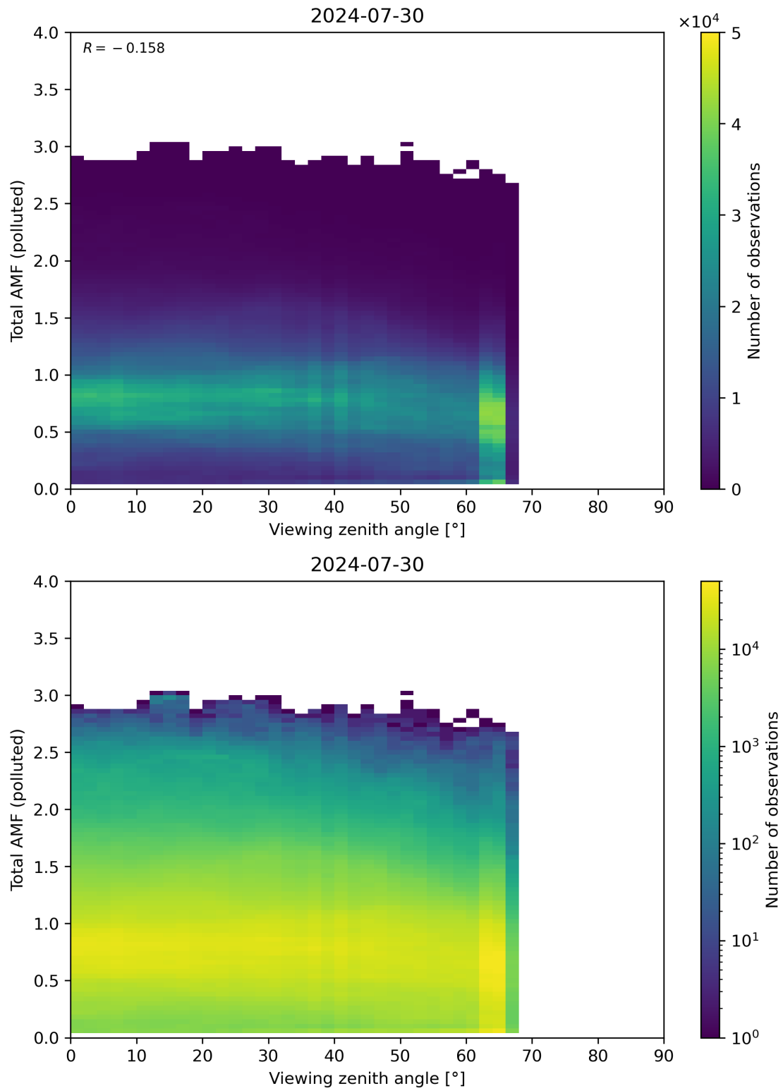
Figure 325: Scatter density plot of “Viewing zenith angle” against “Total AMF (polluted)” for 2024-07-29 to 2024-07-31.
