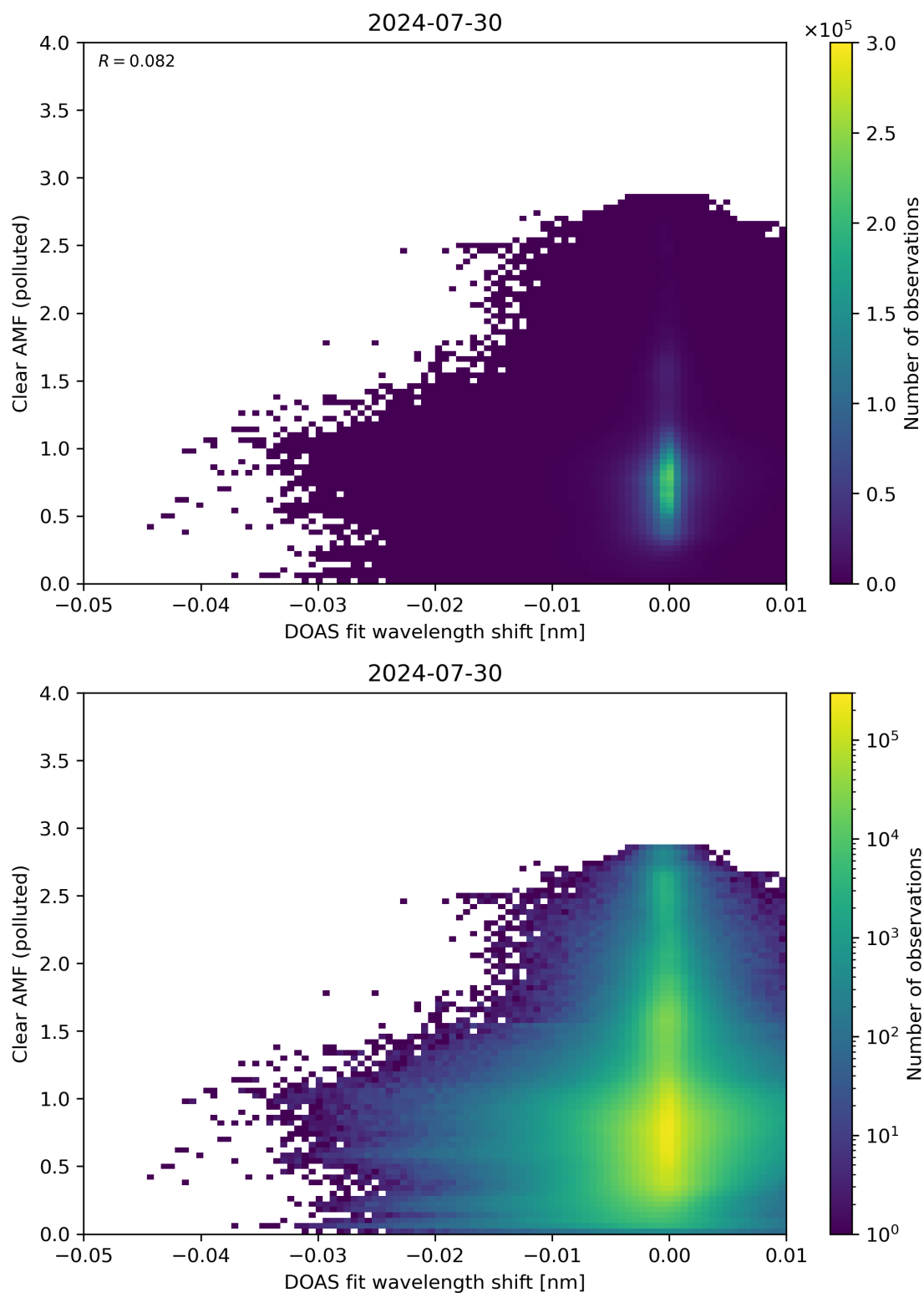
Figure 129: Scatter density plot of “DOAS fit wavelength shift” against “Clear AMF (polluted)” for 2024-07-29 to 2024-07-31.
