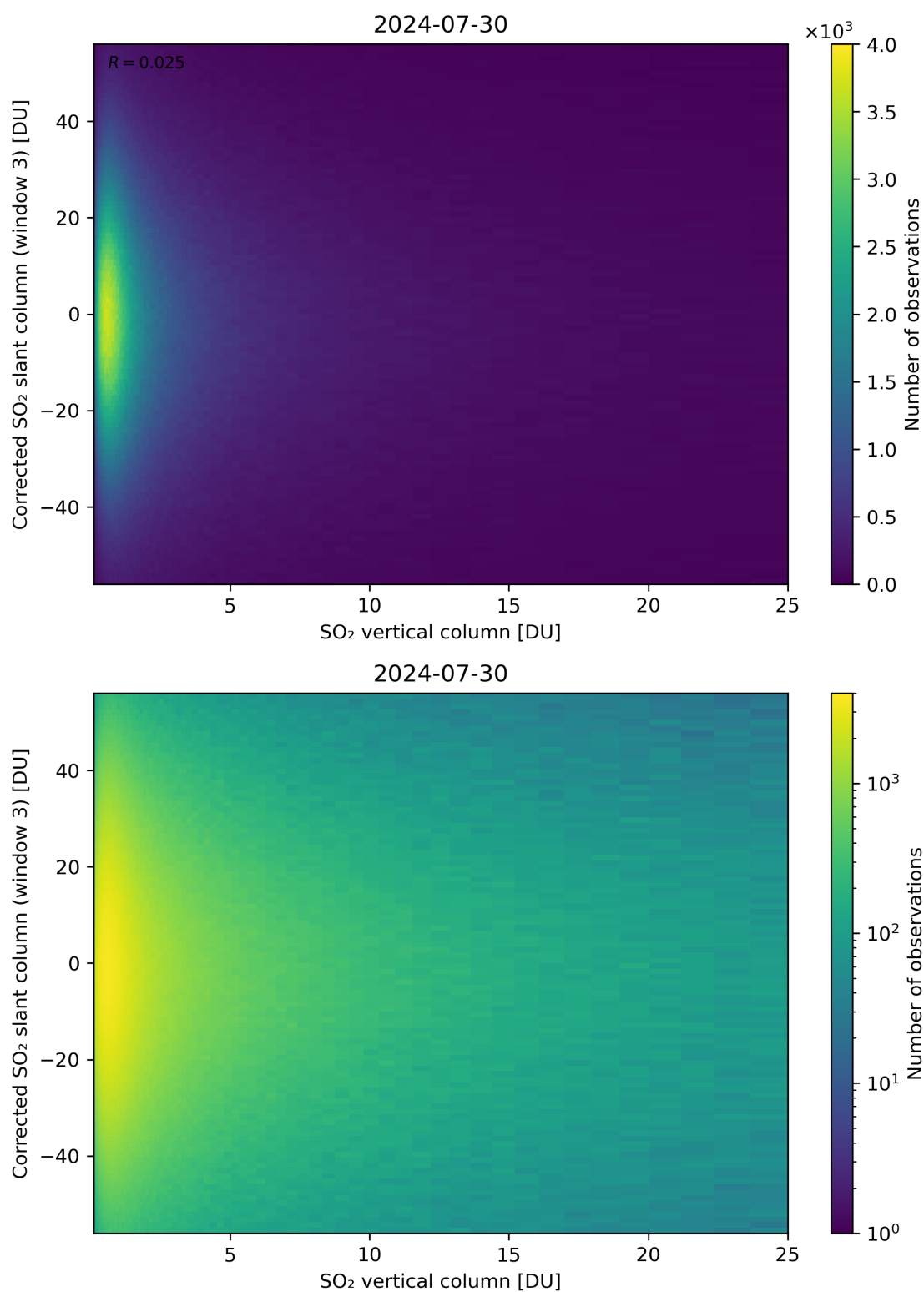
Figure 299: Scatter density plot of “SO 2 vertical column” against “Corrected SO 2 slant column (window 3)” for 2024-07-29 to 2024-07-31.
