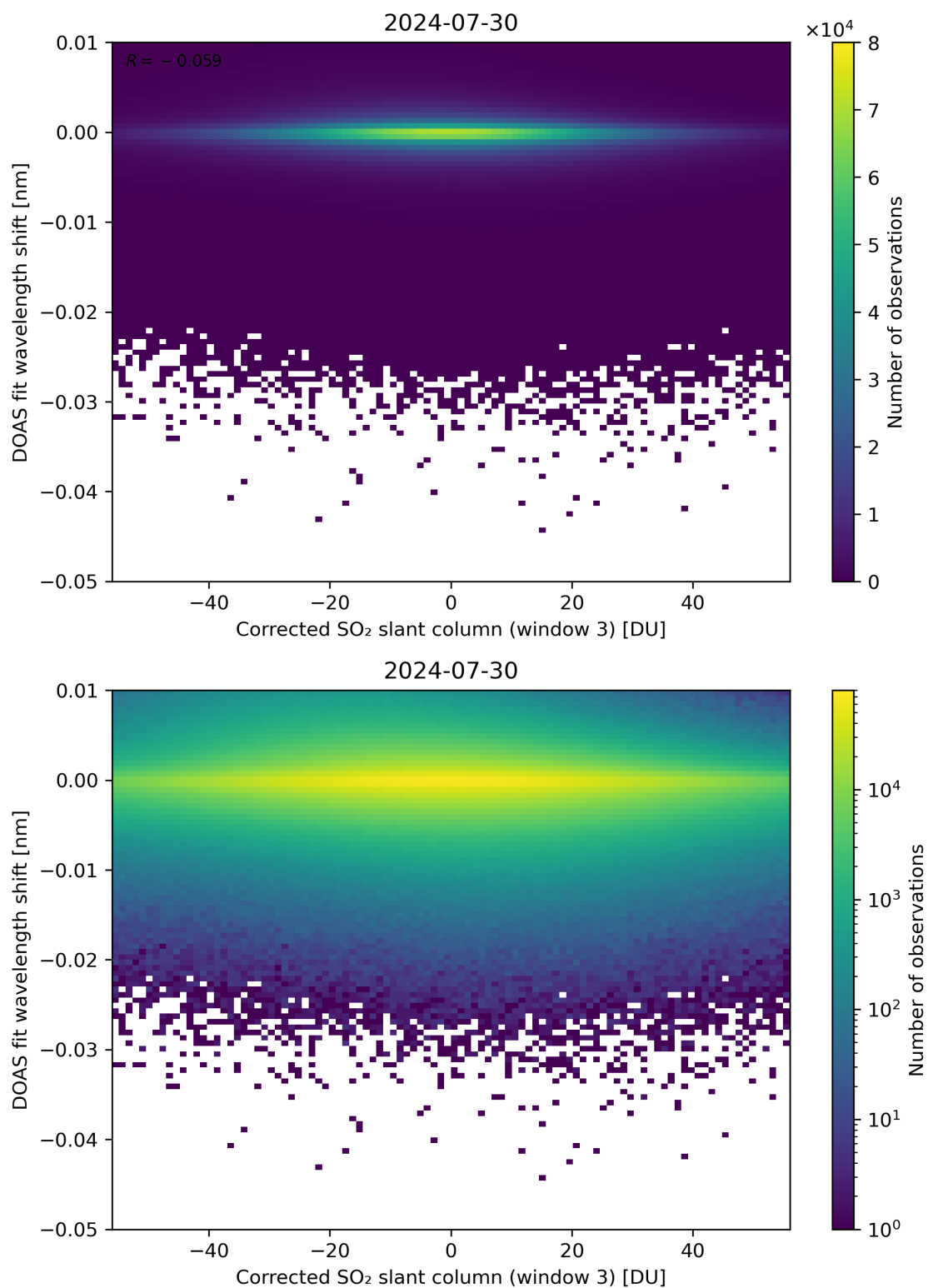
Figure 206: Scatter density plot of “Corrected SO 2 slant column (window 3)” against “DOAS fit wavelength shift” for 2024-07-29 to 2024-07-31.
