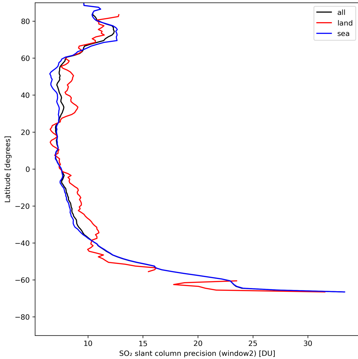
Figure 38: Zonal average of “SO 2 slant column precision (window2)” for 2024-07-29 to 2024-07-31.
