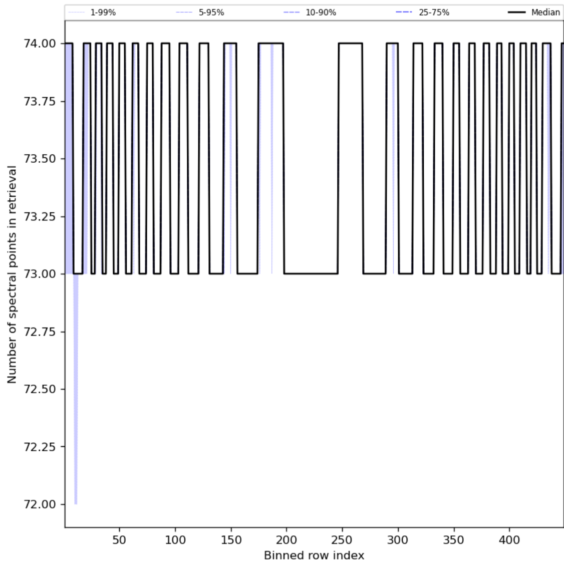
Figure 97: Along track statistics of “Number of spectral points in retrieval” for 2024-07-29 to 2024-07-31
