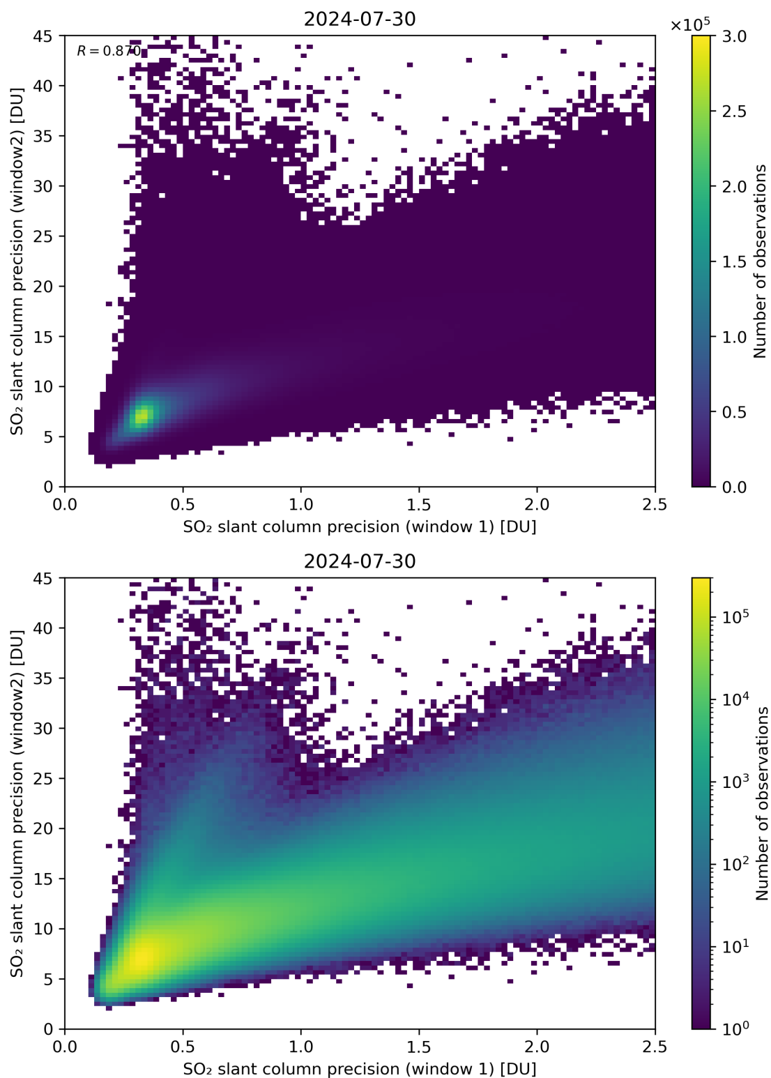
Figure 227: Scatter density plot of “SO 2 slant column precision (window 1)” against “SO 2 slant column precision (window 2)” for 2024-07-29 to 2024-07-31.
