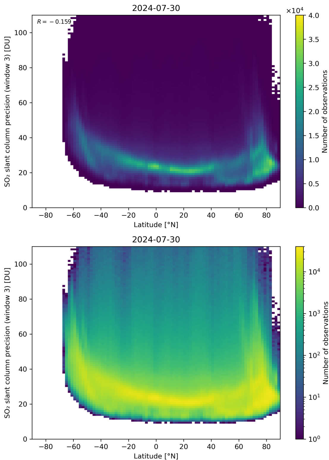
Figure 153: Scatter density plot of “Latitude” against “SO 2 slant column precision (window 3)” for 2024-07-29 to 2024-07-31.
