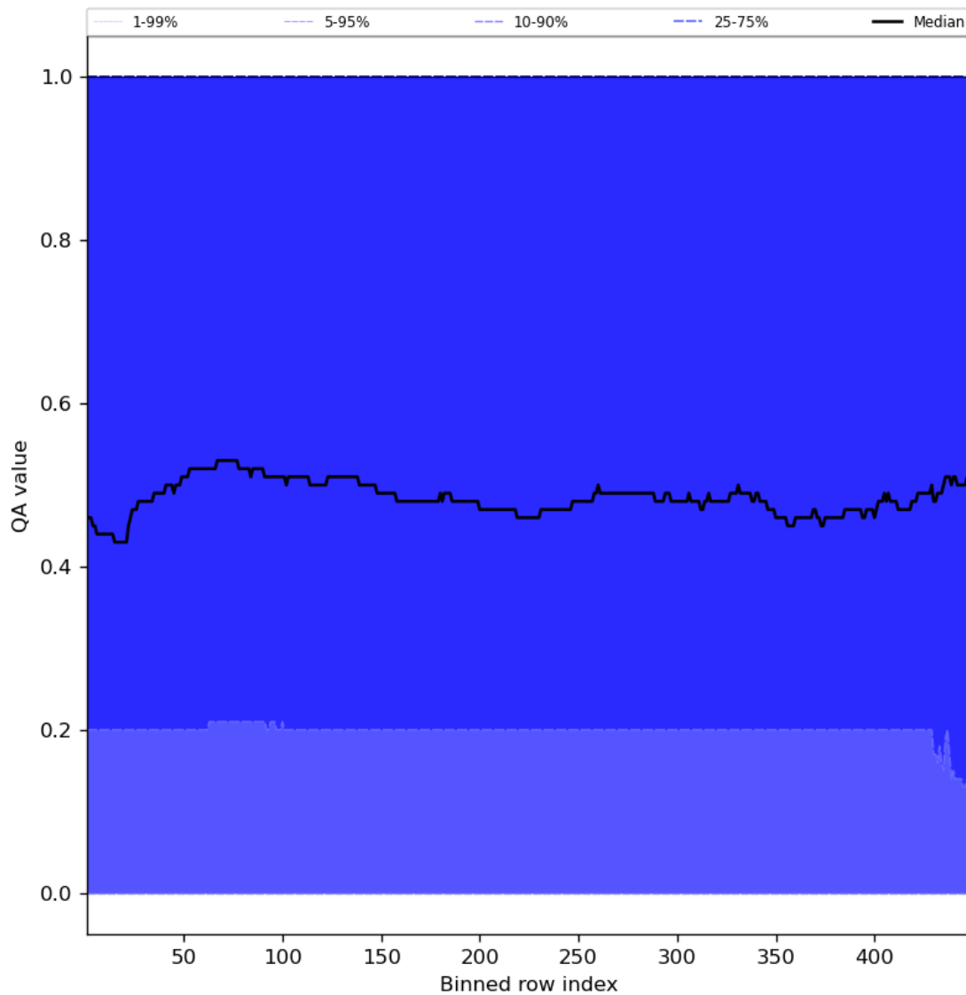
Figure 75: Along track statistics of “QA value” for 2024-07-29 to 2024-07-31
