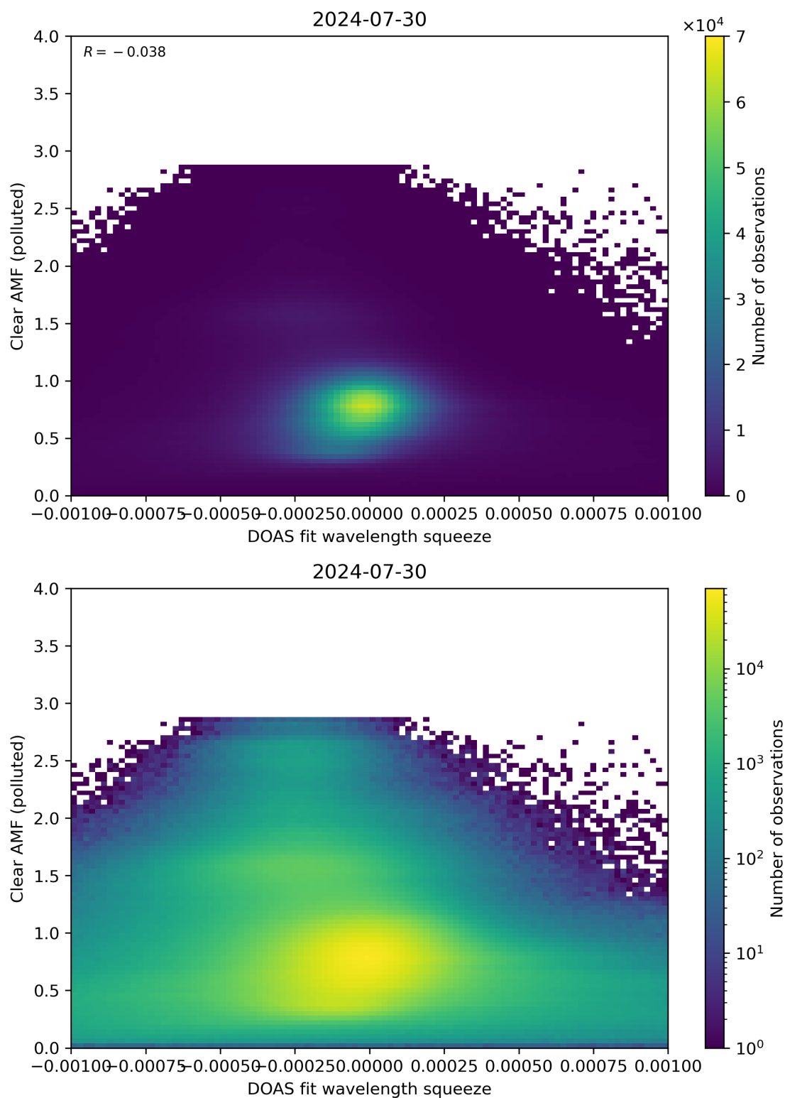
Figure 133: Scatter density plot of “DOAS fit wavelength squeeze” against “Clear AMF (polluted)” for 2024-07-29 to 2024-07-31.
