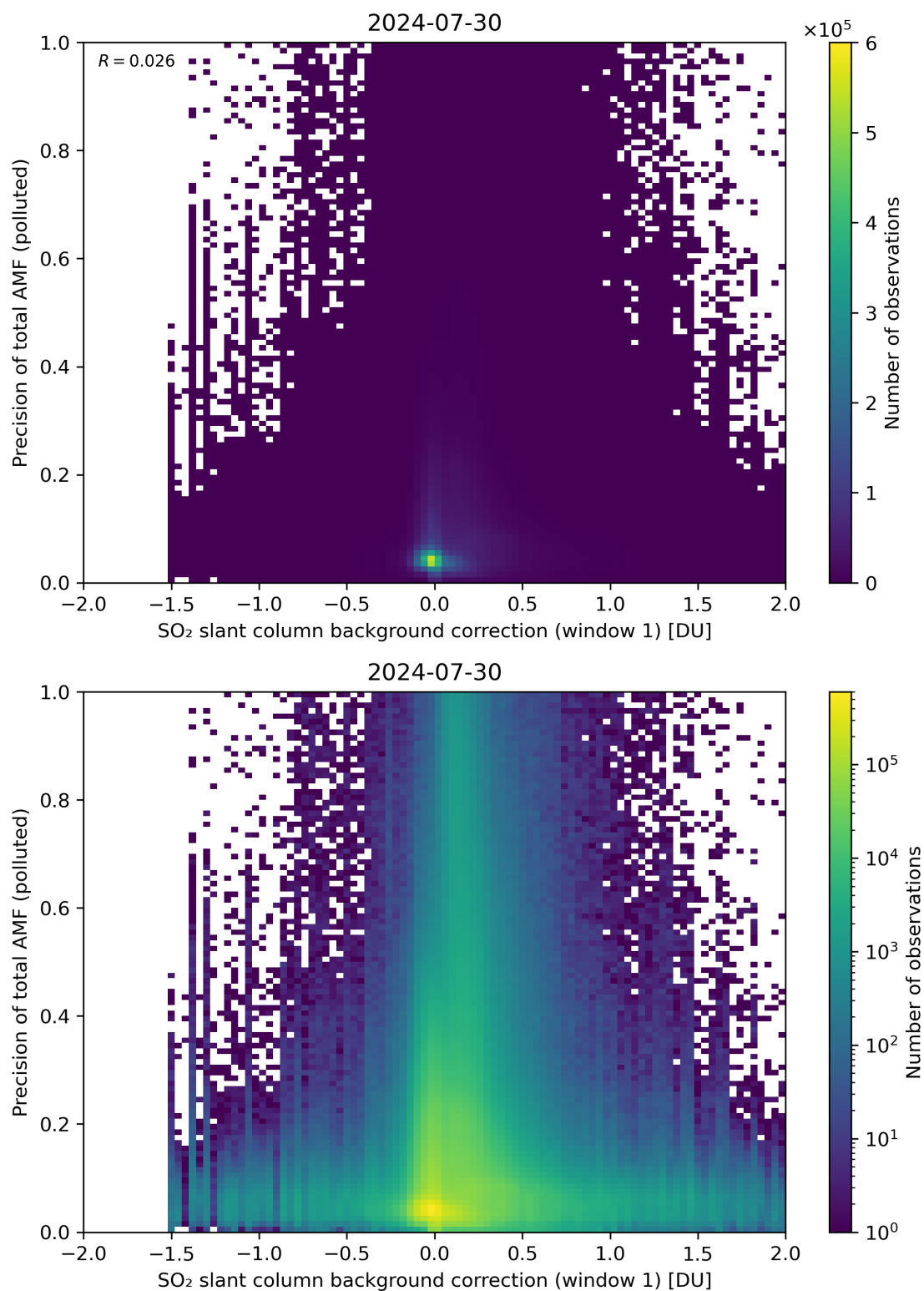
Figure 110: Scatter density plot of “SO 2 slant column background correction (window 1)” against “Precision of total AMF (polluted)” for 2024-07-29 to 2024-07-31.
