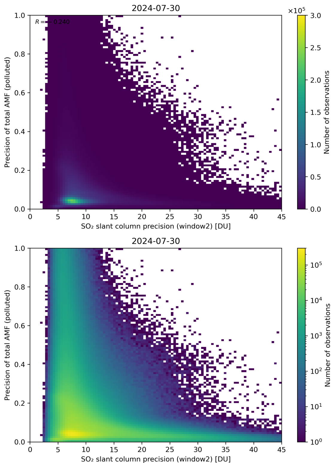
Figure 252: Scatter density plot of “SO 2 slant column precision (window2)” against “Precision of total AMF (polluted)” for 2024-07-29 to 2024-07-31.
