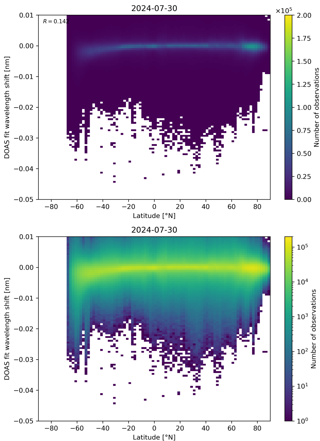
Figure 142: Scatter density plot of “Latitude” against “DOAS fit wavelength shift” for 2024-07-29 to 2024-07-31.
