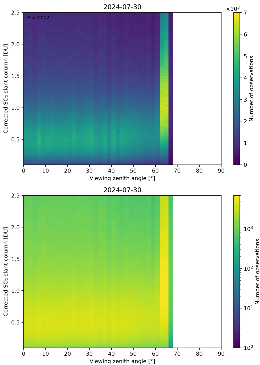
Figure 317: Scatter density plot of “Viewing zenith angle” against “Corrected SO 2 slant column” for 2024-07-29 to 2024-07-31.
