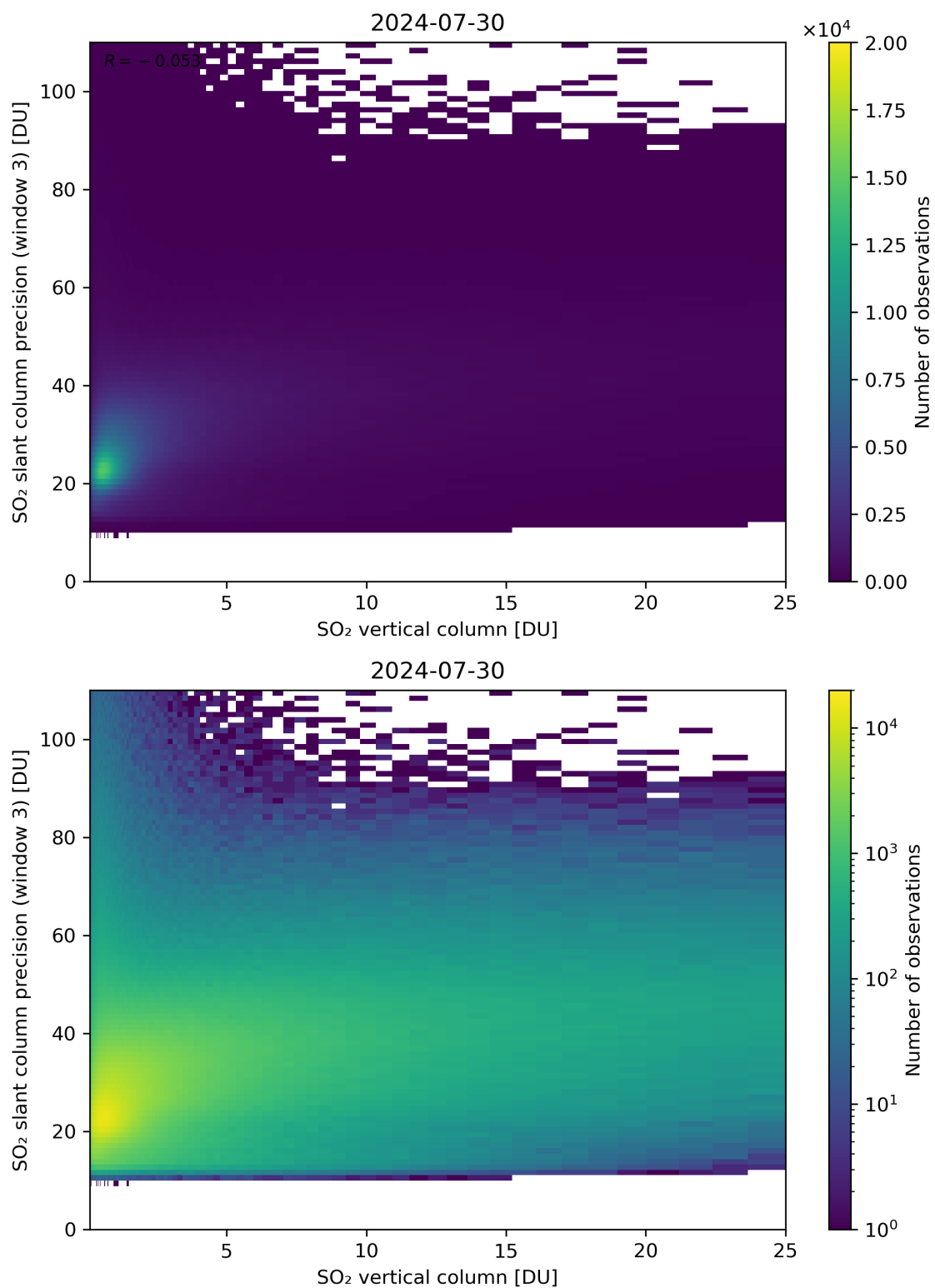
Figure 304: Scatter density plot of “SO 2 vertical column” against “SO 2 slant column precision (window 3)” for 2024-07-29 to 2024-07-31.
