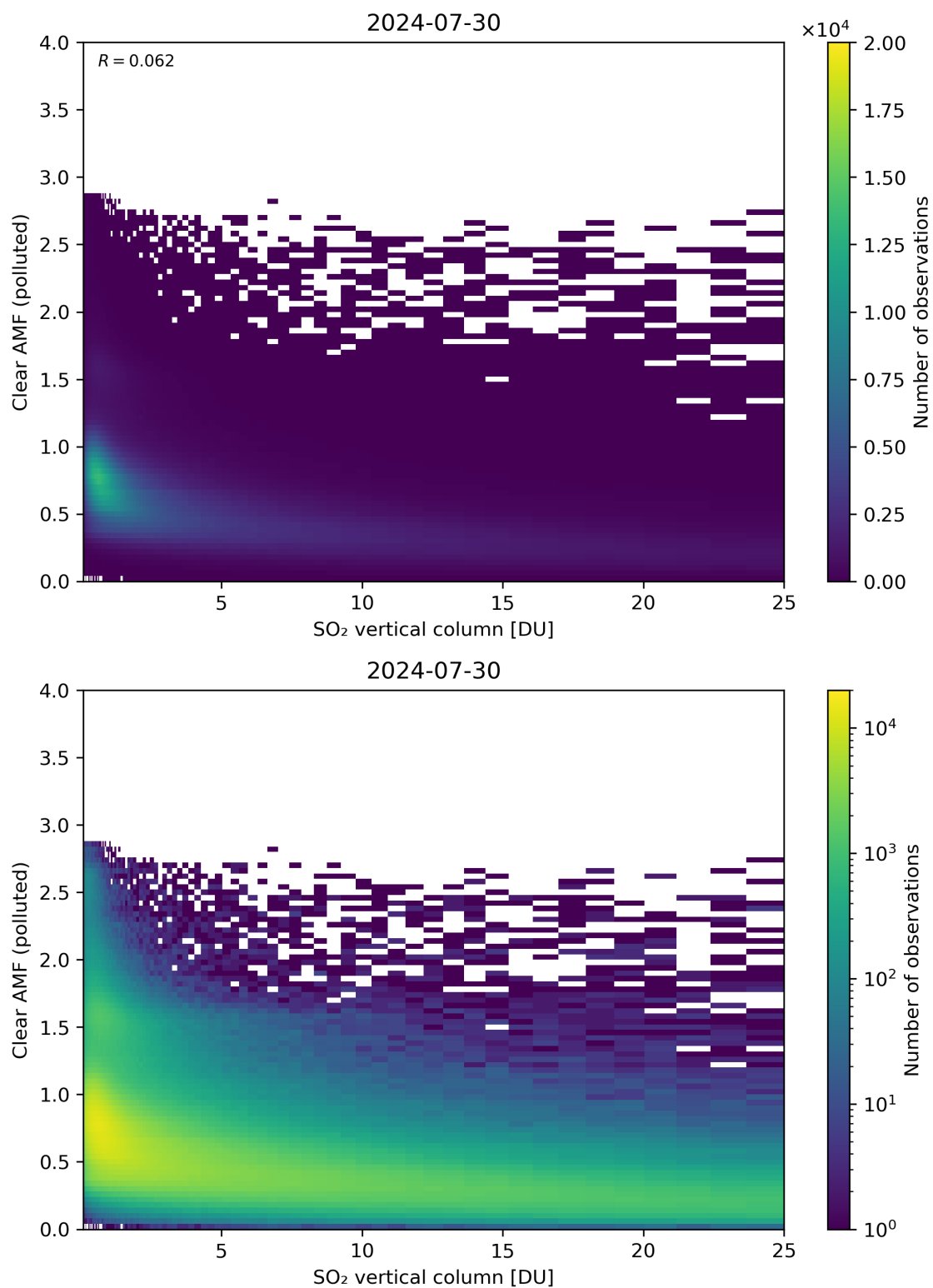
Figure 296: Scatter density plot of “SO 2 vertical column” against “Clear AMF (polluted)” for 2024-07-29 to 2024-07-31.
