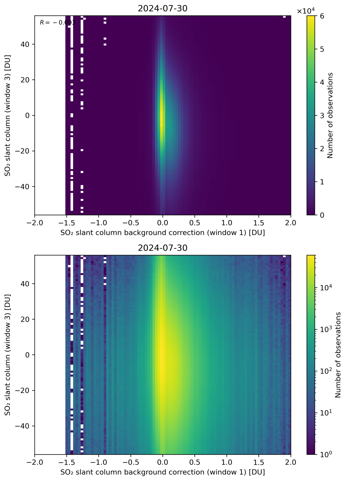
Figure 107: Scatter density plot of “SO 2 slant column background correction (window 1)” against “SO 2 slant column (window 3)” for 2024-07-29 to 2024-07-31.
