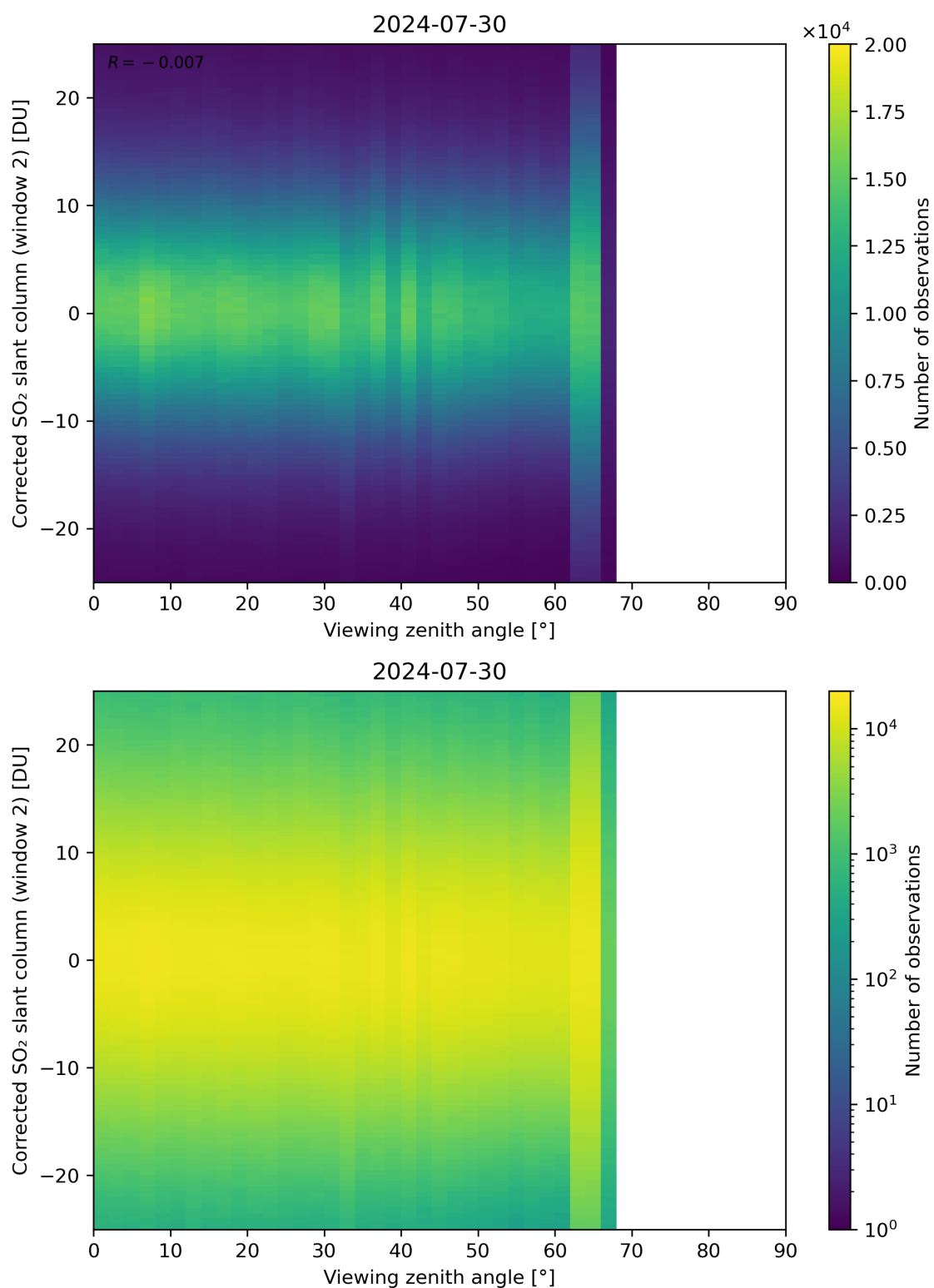
Figure 318: Scatter density plot of “Viewing zenith angle” against “Corrected SO 2 slant column (window 2)” for 2024-07-29 to 2024-07-31.
