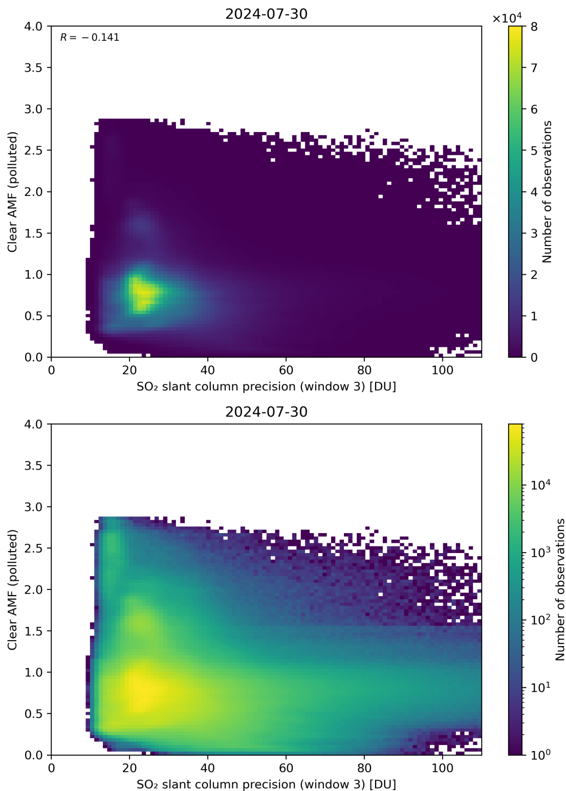
Figure 261: Scatter density plot of “SO 2 slant column precision (window 3)” against “Clear AMF (polluted)” for 2024-07-29 to 2024-07-31.
