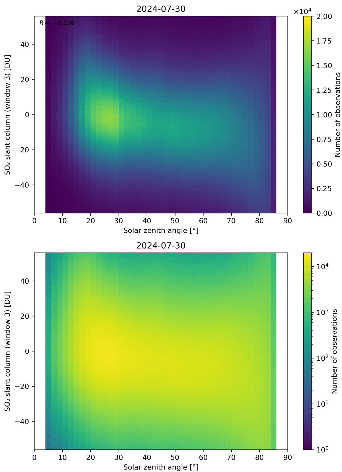
Figure 172: Scatter density plot of “Solar zenith angle” against “SO 2 slant column (window 3)” for 2024-07-29 to 2024-07-31.
