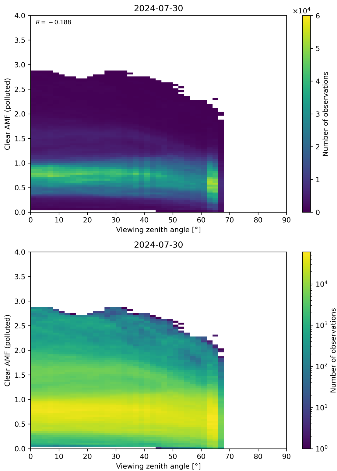
Figure 316: Scatter density plot of “Viewing zenith angle” against “Clear AMF (polluted)” for 2024-07-29 to 2024-07-31.
