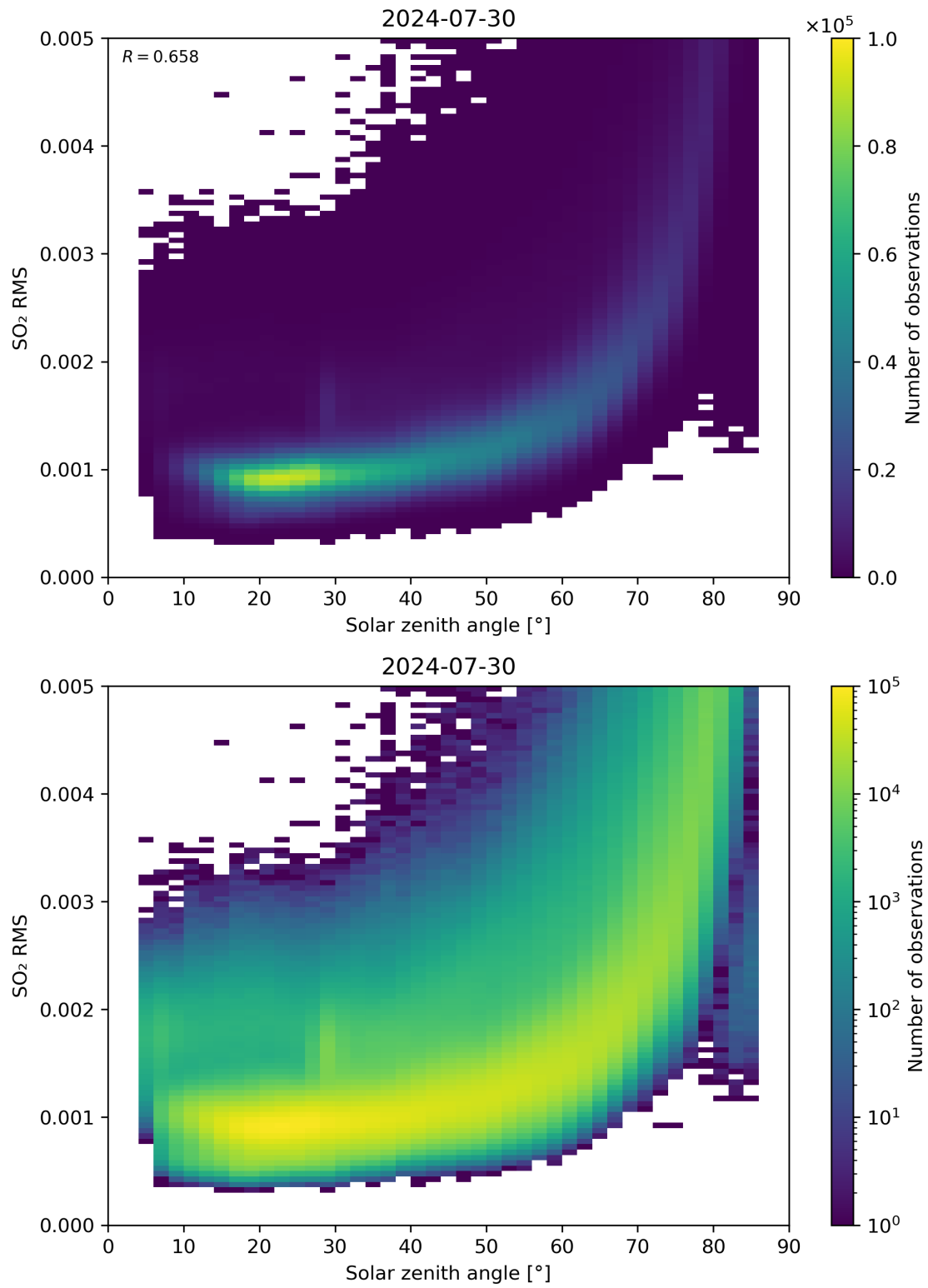
Figure 163: Scatter density plot of “Solar zenith angle” against “SO 2 RMS” for 2024-07-29 to 2024-07-31.
