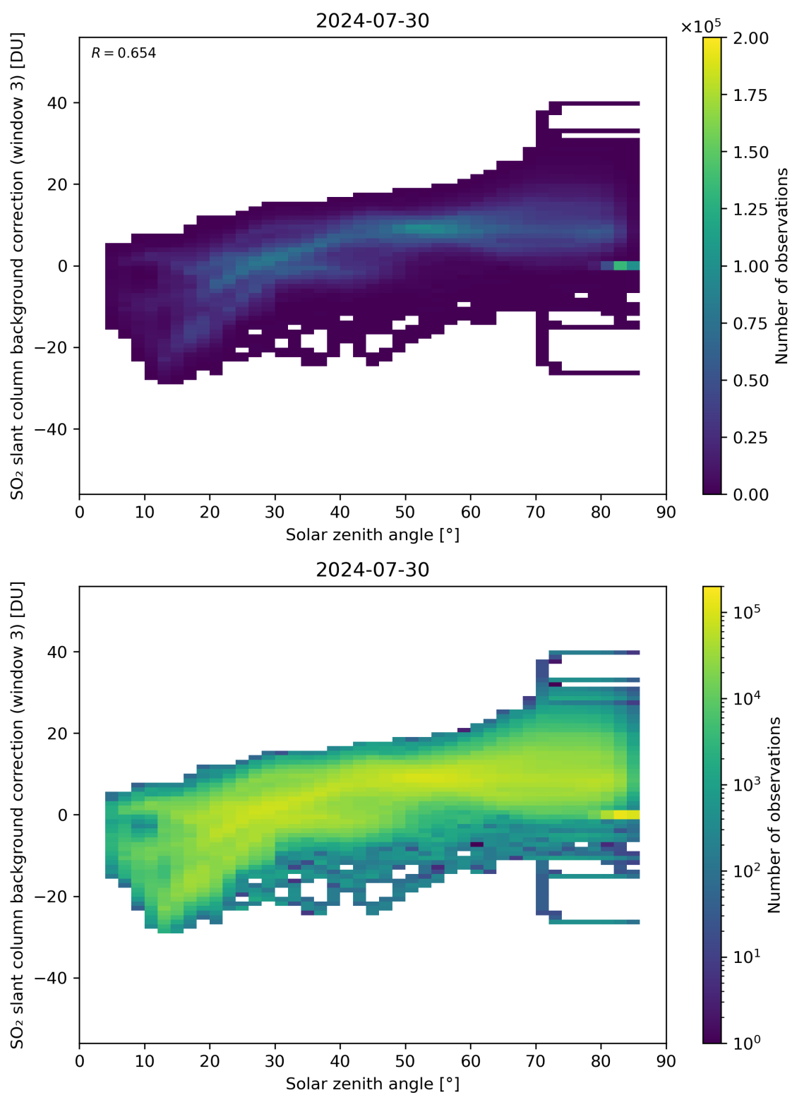
Figure 160: Scatter density plot of “Solar zenith angle” against “SO 2 slant column background correction (window 3)” for 2024-07-29 to 2024-07-31.
