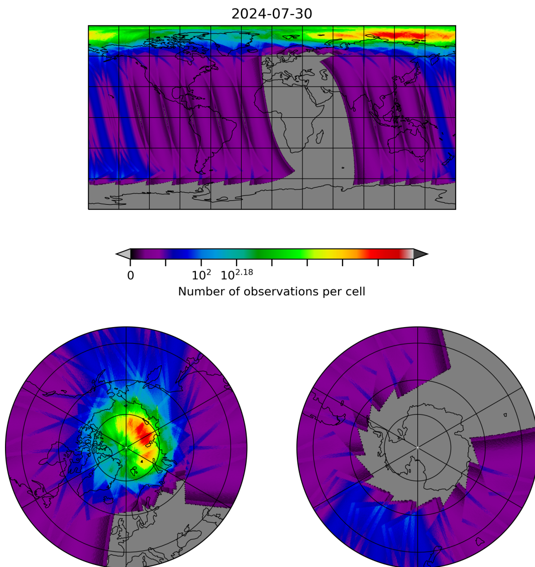
Figure 28: Map of the number of observations for 2024-07-29 to 2024-07-31
