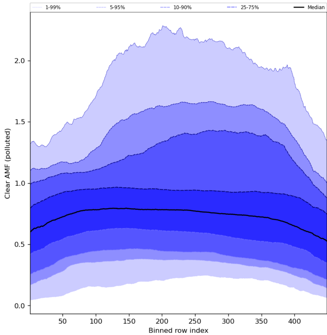
Figure 96: Along track statistics of “Clear AMF (polluted)” for 2024-07-29 to 2024-07-31
