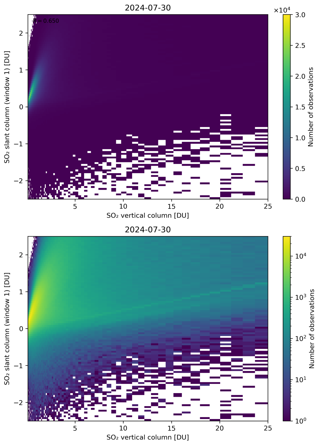
Figure 300: Scatter density plot of “SO 2 vertical column” against “SO 2 slant column (window 1)” for 2024-07-29 to 2024-07-31.
