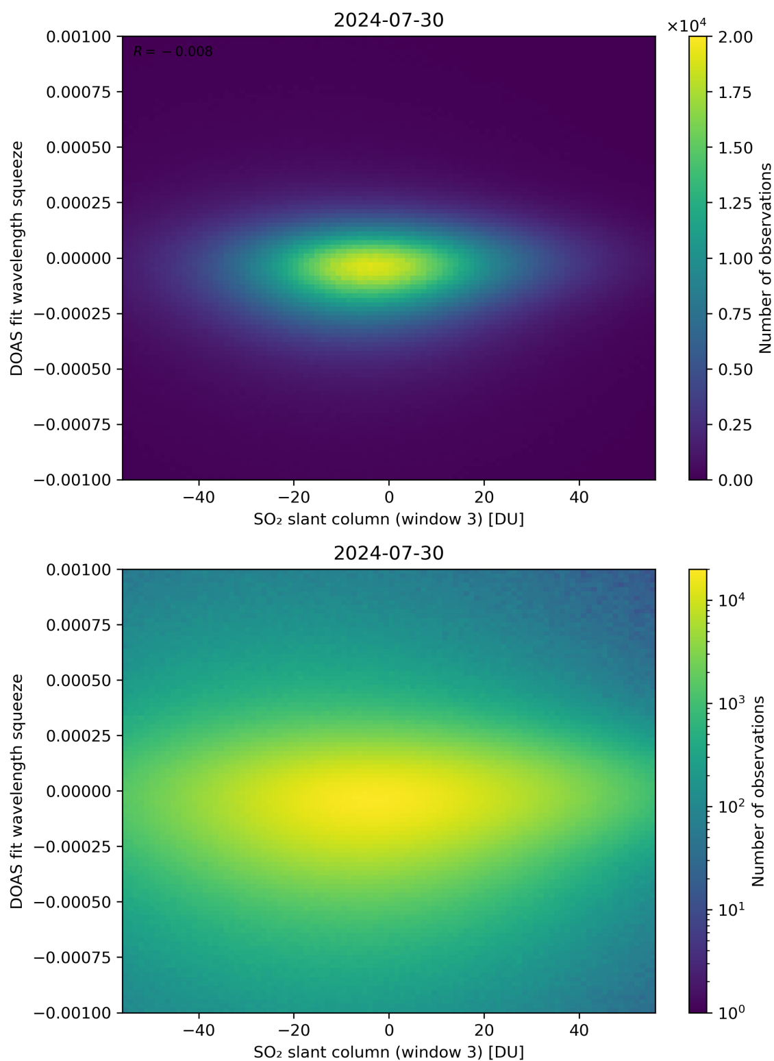
Figure 255: Scatter density plot of “SO 2 slant column (window 3)” against “DOAS fit wavelength squeeze” for 2024-07-29 to 2024-07-31.
