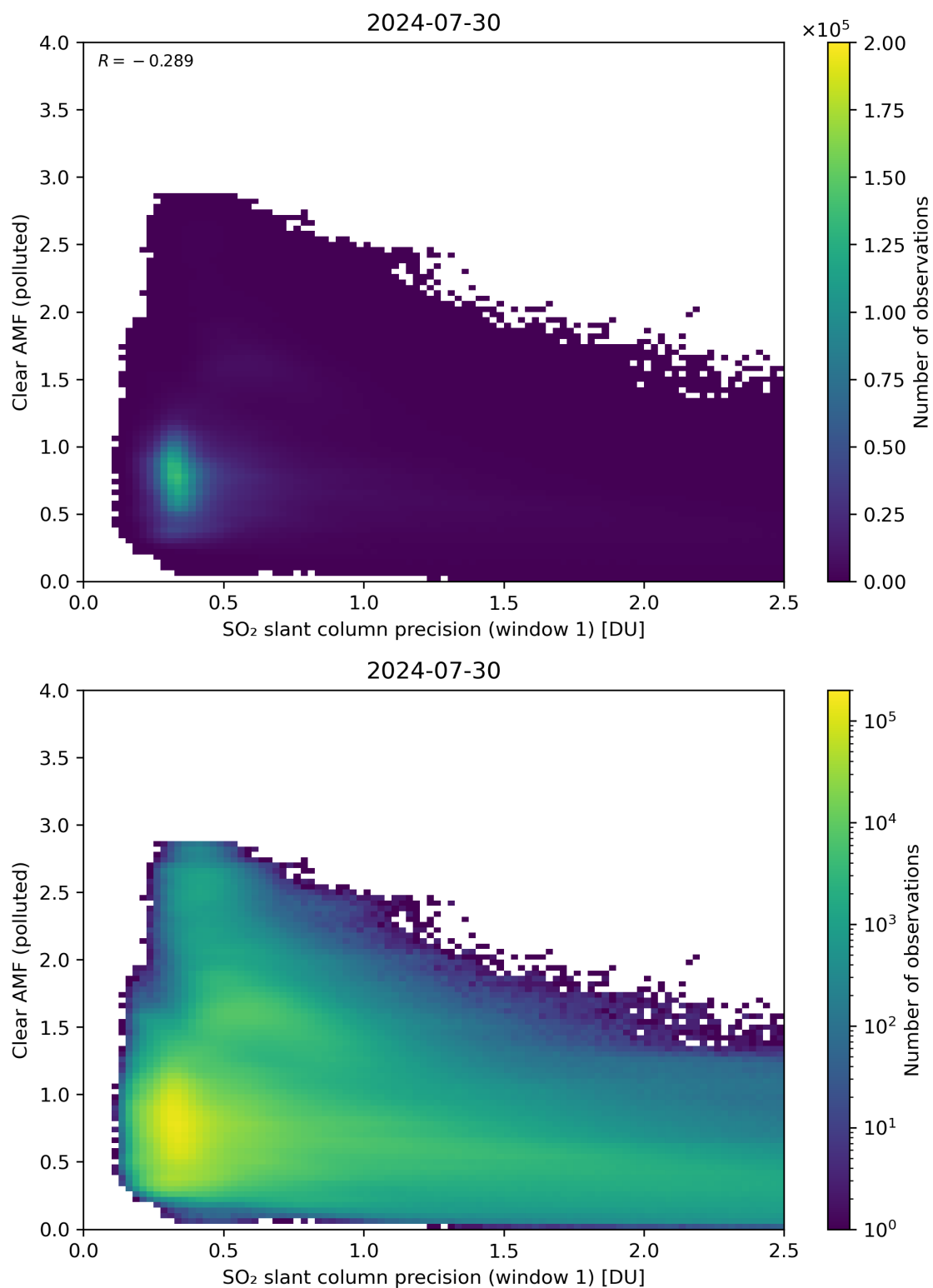
Figure 224: Scatter density plot of “SO 2 slant column precision (window 1)” against “Clear AMF (polluted)” for 2024-07-29 to 2024-07-31.
