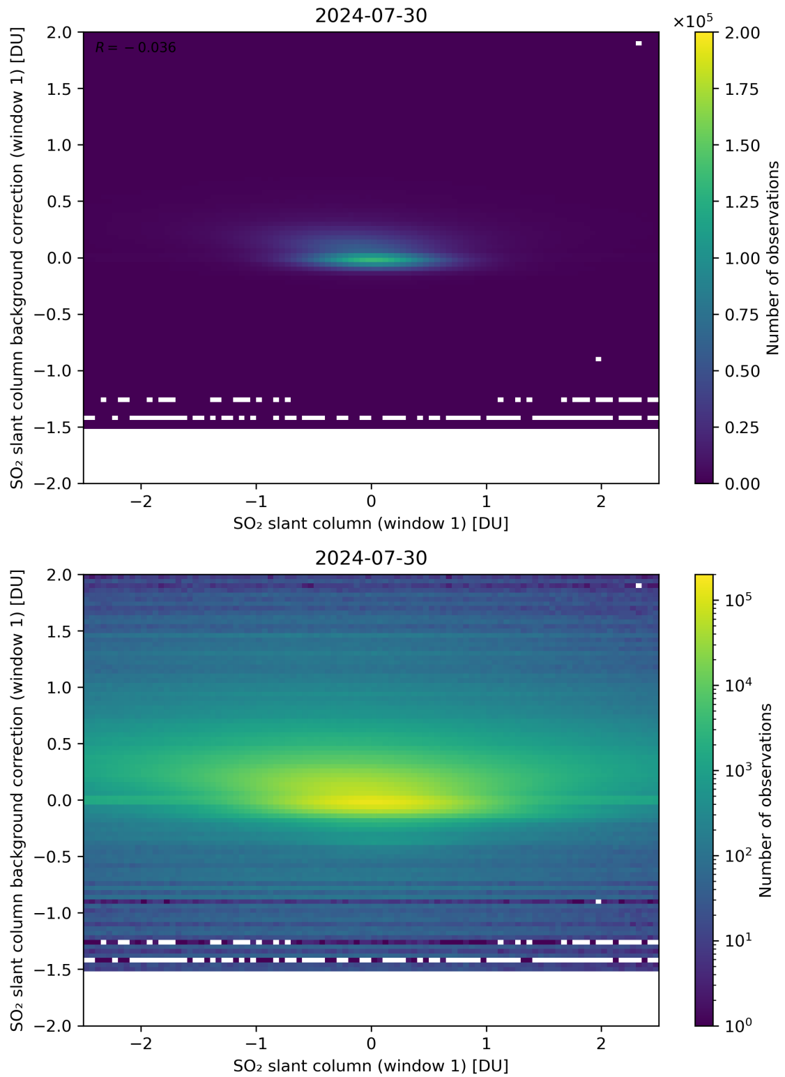
Figure 212: Scatter density plot of “SO 2 slant column (window 1)” against “SO 2 slant column background correction (window 1)” for 2024-07-29 to 2024-07-31.
