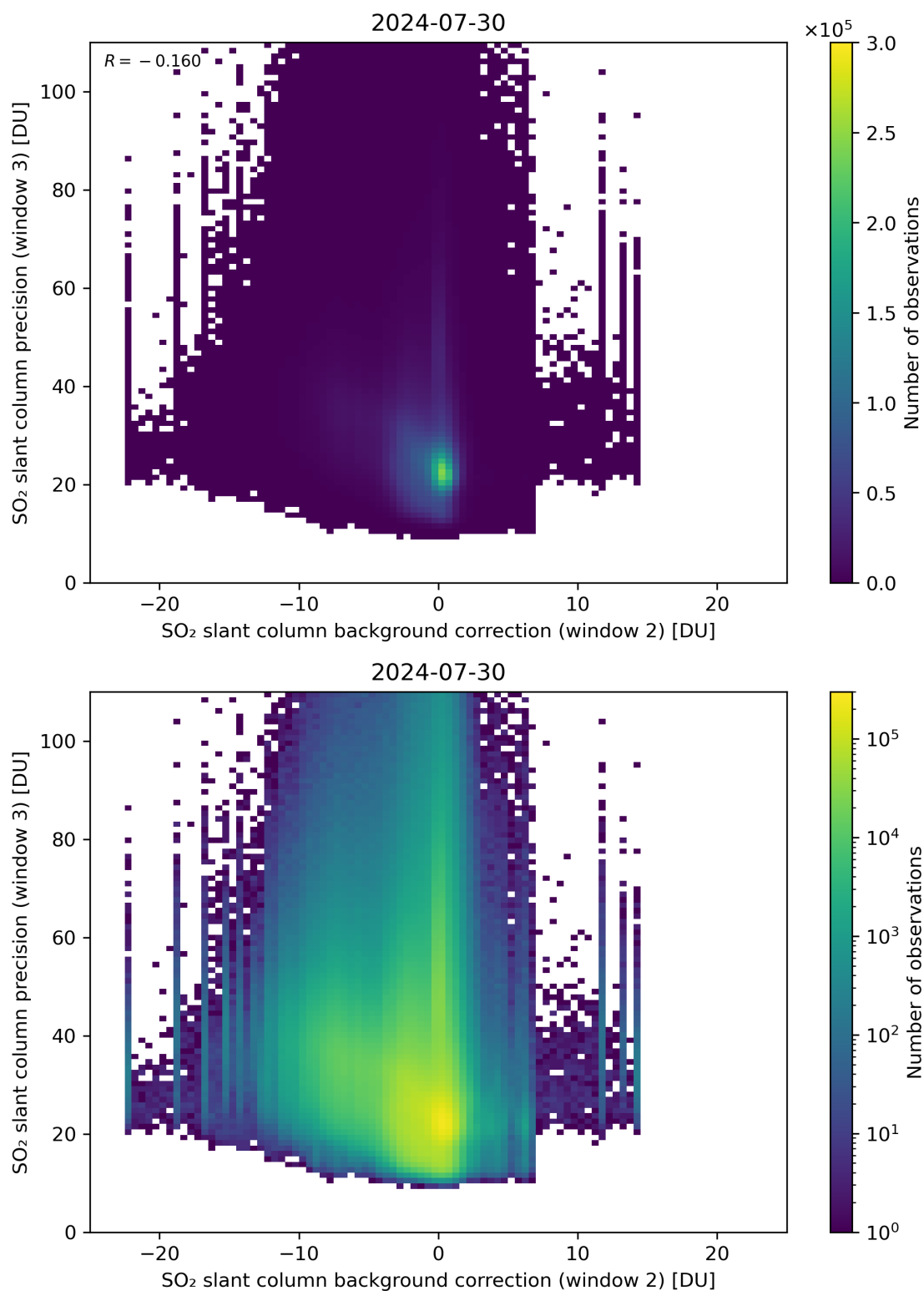
Figure 118: Scatter density plot of “SO 2 slant column background correction (window 2)” against “SO 2 slant column precision (window 3)” for 2024-07-29 to 2024-07-31.
