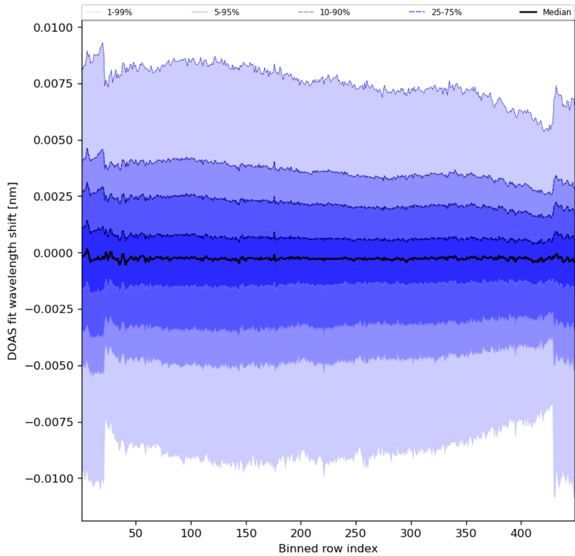
Figure 91: Along track statistics of “DOAS fit wavelength shift” for 2024-07-29 to 2024-07-31
