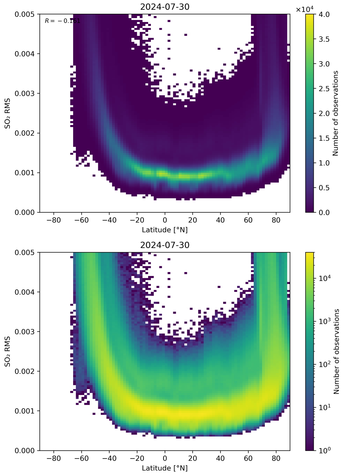
Figure 144: Scatter density plot of “Latitude” against “SO 2 RMS” for 2024-07-29 to 2024-07-31.
