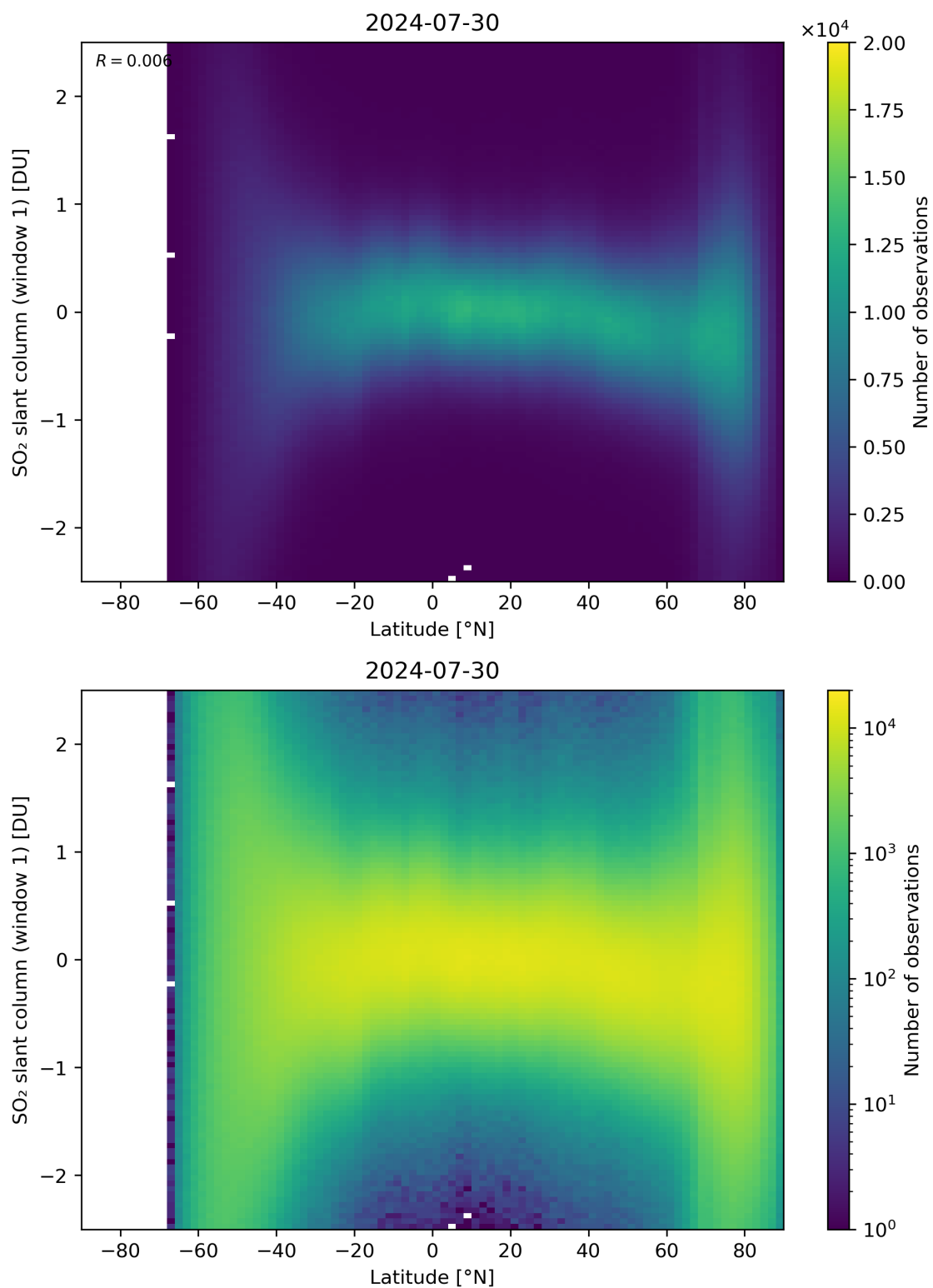
Figure 149: Scatter density plot of “Latitude” against “SO 2 slant column (window 1)” for 2024-07-29 to 2024-07-31.
