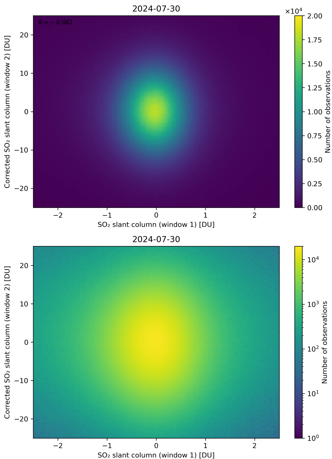
Figure 233: Scatter density plot of “SO 2 slant column (window 1)” against “Corrected SO 2 slant column (window 2)” for 2024-07-29 to 2024-07-31.
