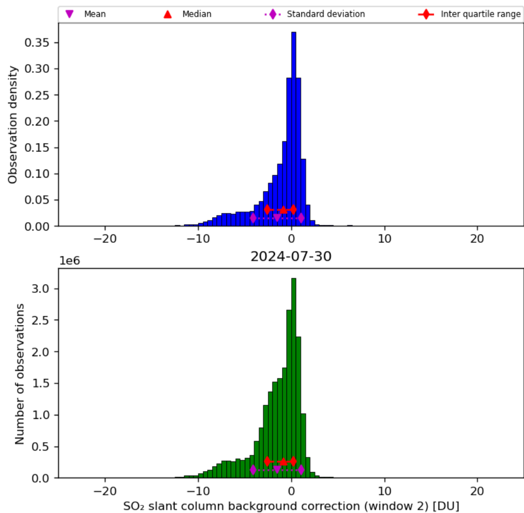
Figure 63: Histogram of “SO 2 slant column background correction (window 2)” for 2024-07-29 to 2024-07-31
