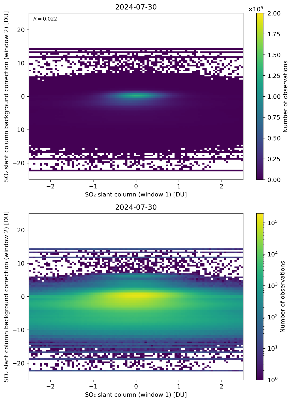
Figure 213: Scatter density plot of “SO 2 slant column (window 1)” against “SO 2 slant column background correction (window 2)” for 2024-07-29 to 2024-07-31.
