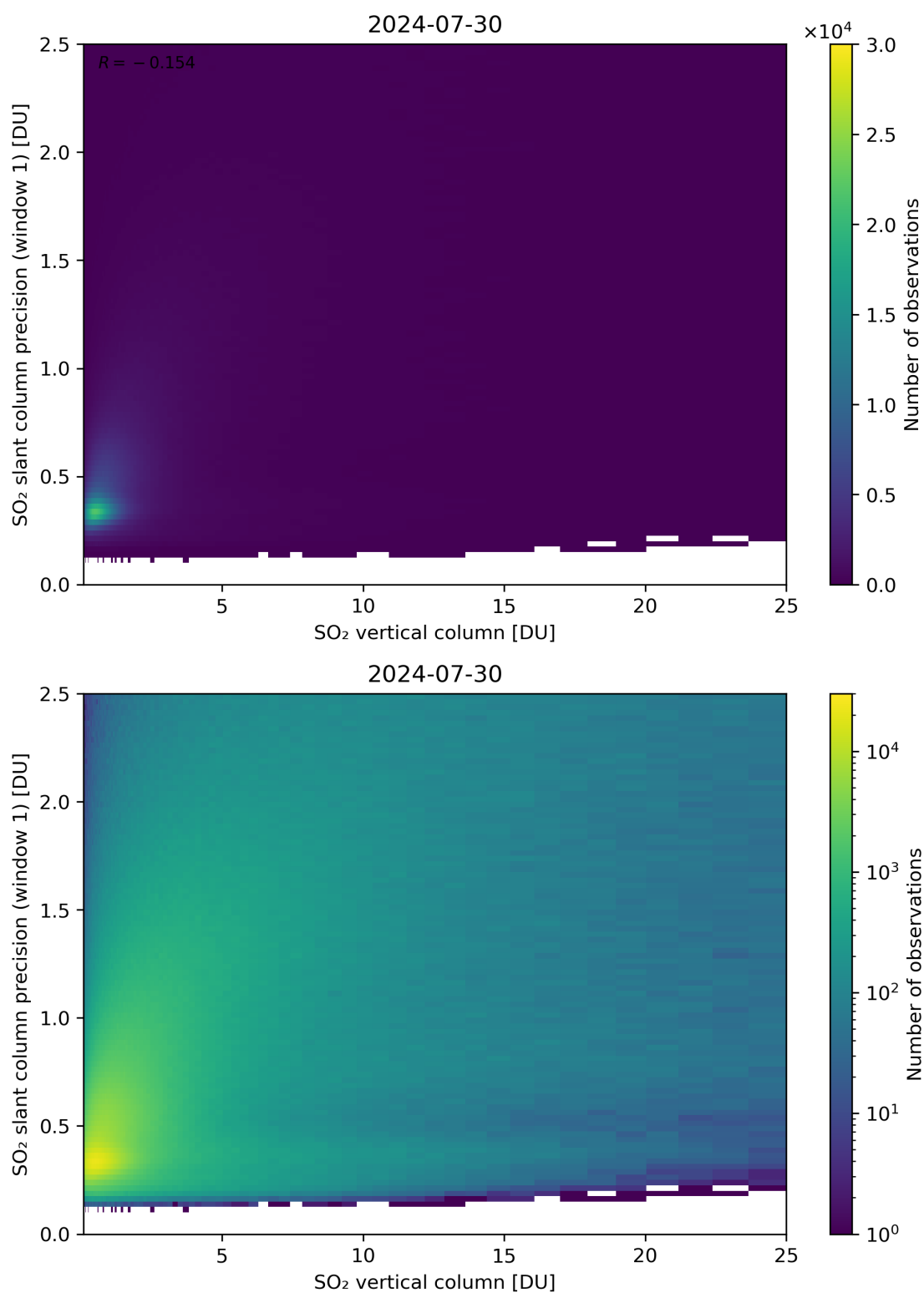
Figure 301: Scatter density plot of “SO 2 vertical column” against “SO 2 slant column precision (window 1)” for 2024-07-29 to 2024-07-31.
