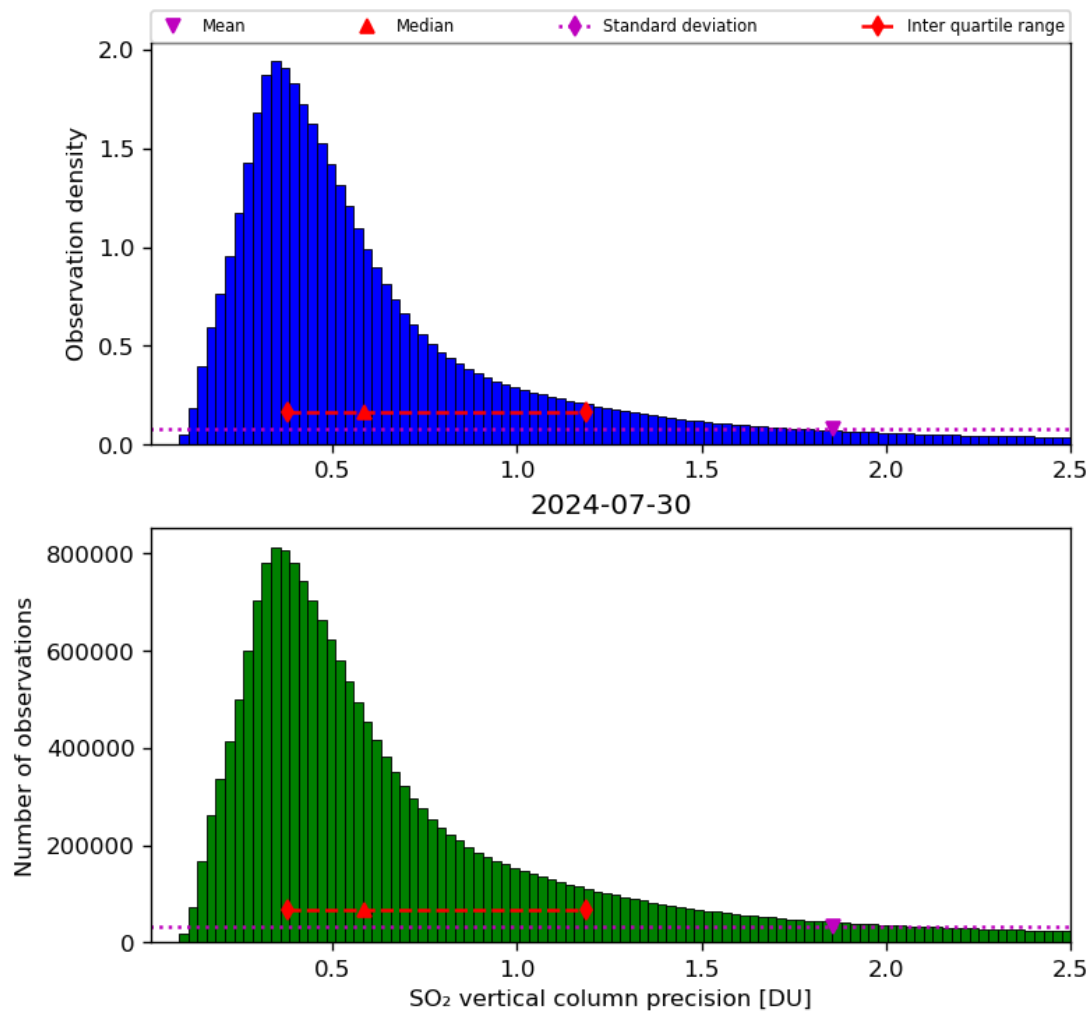
Figure 54: Histogram of “SO 2 vertical column precision” for 2024-07-29 to 2024-07-31
