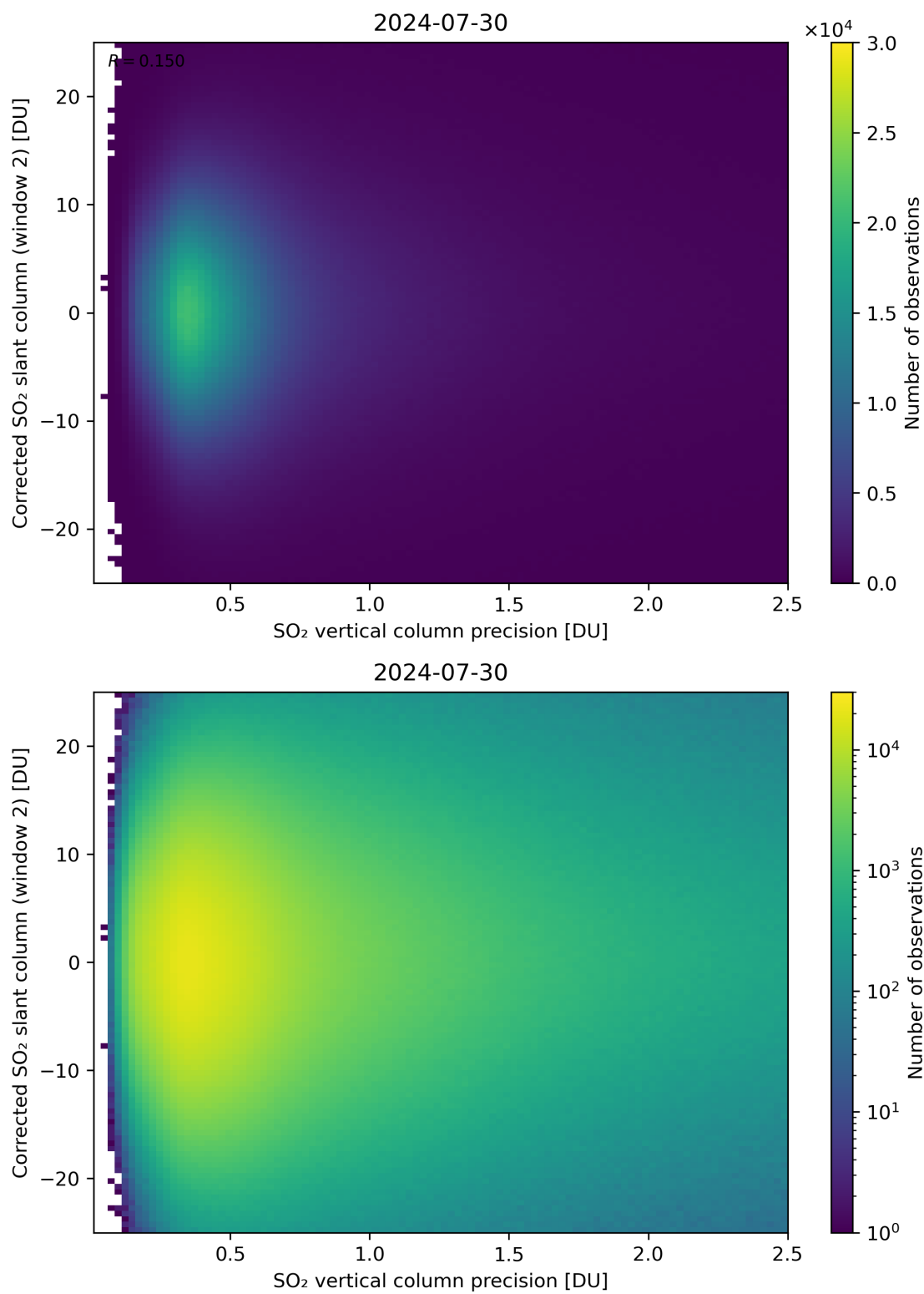
Figure 287: Scatter density plot of “SO 2 vertical column precision” against “Corrected SO 2 slant column (window 2)” for 2024-07-29 to 2024-07-31.
