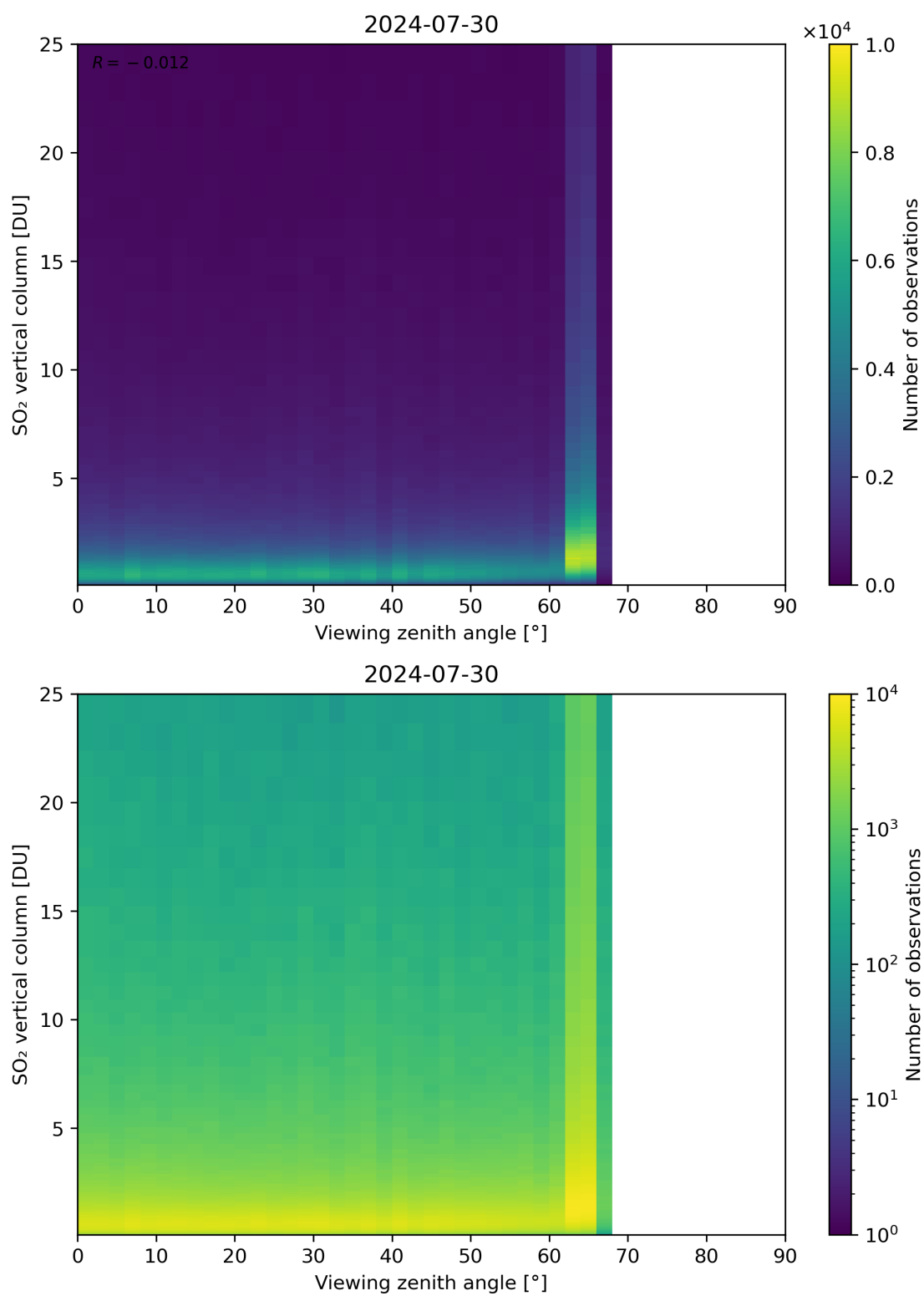
Figure 327: Scatter density plot of “Viewing zenith angle” against “SO 2 vertical column” for 2024-07-29 to 2024-07-31.
