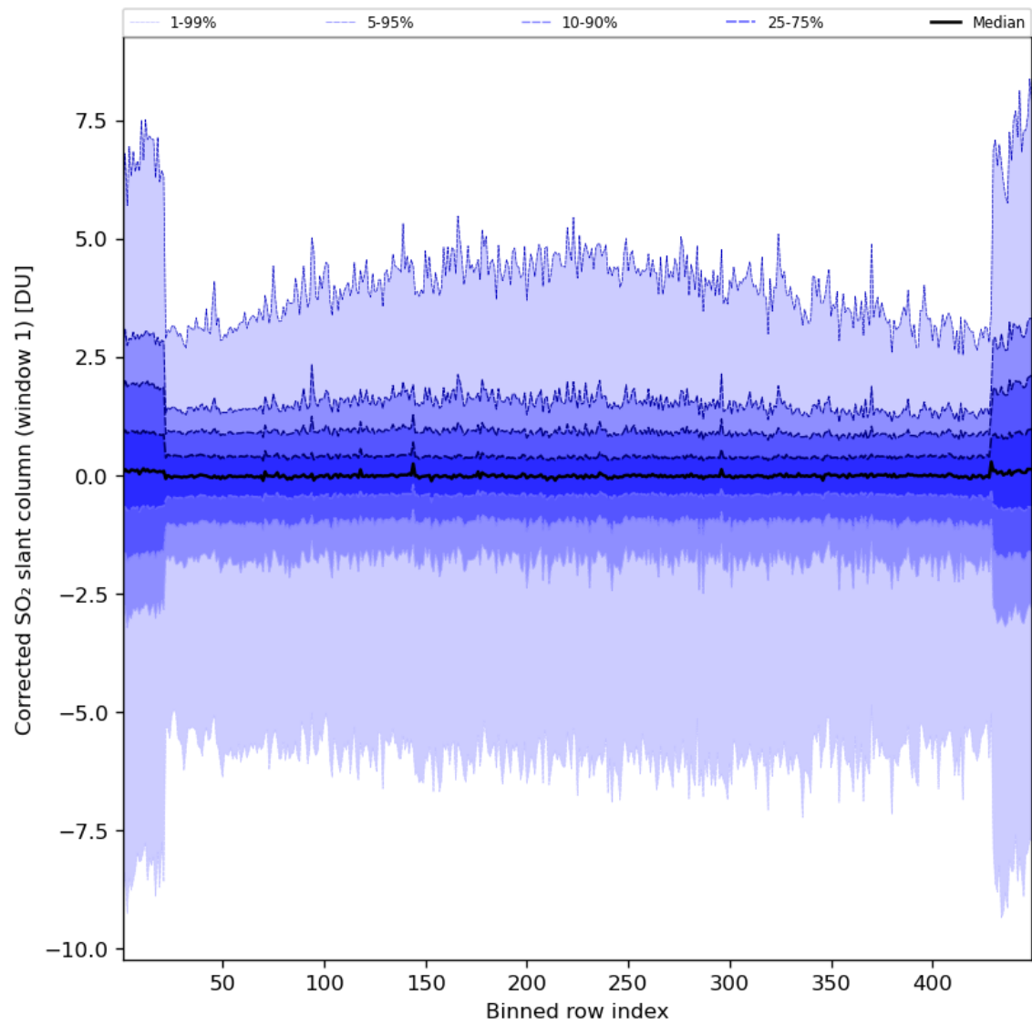
Figure 81: Along track statistics of "Corrected SO 2 slant column (window 1)" for 2024-07-29 to 2024-07-31
