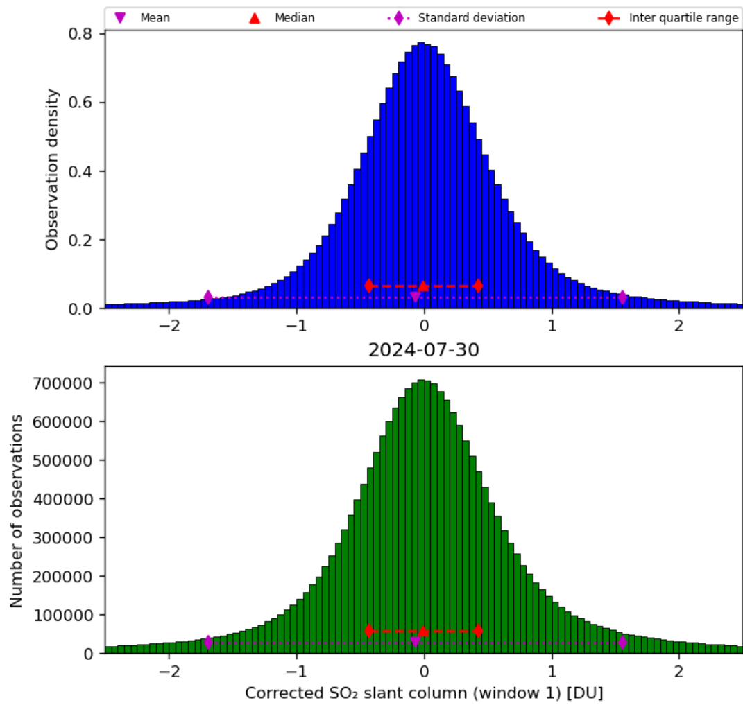
Figure 58: Histogram of “Corrected SO 2 slant column (window 1)” for 2024-07-29 to 2024-07-31
