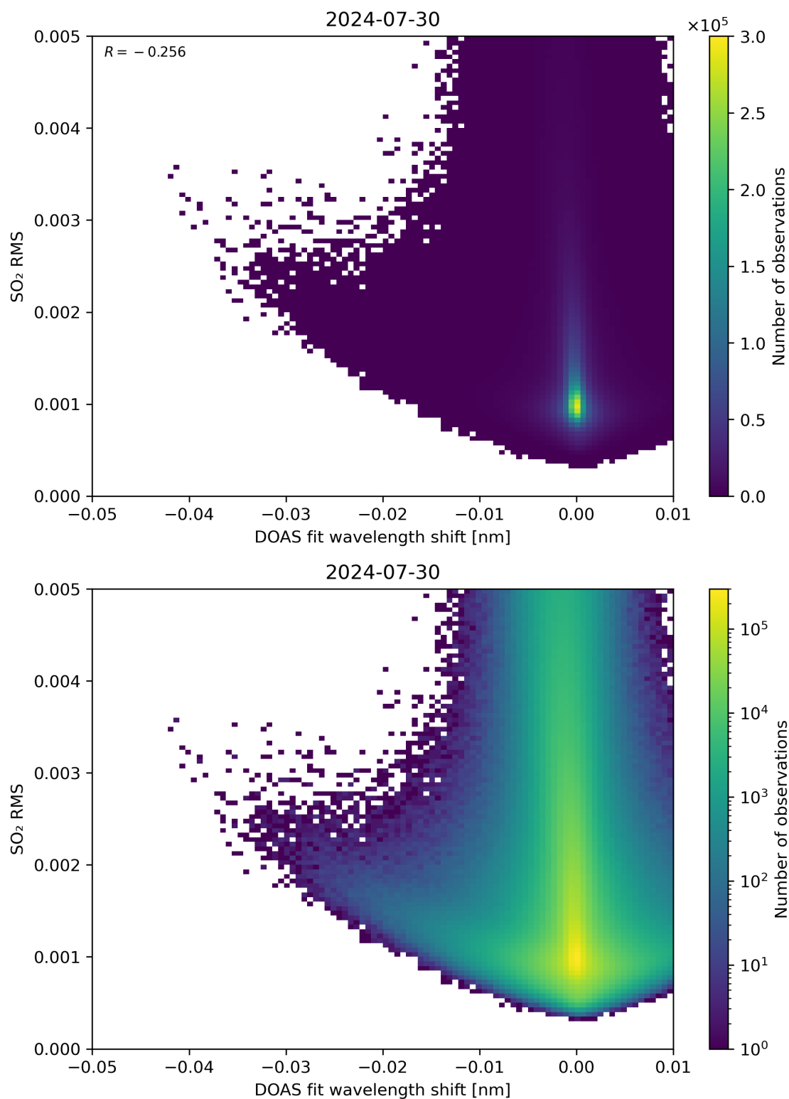
Figure 128: Scatter density plot of “DOAS fit wavelength shift” against “SO 2 RMS” for 2024-07-29 to 2024-07-31.
