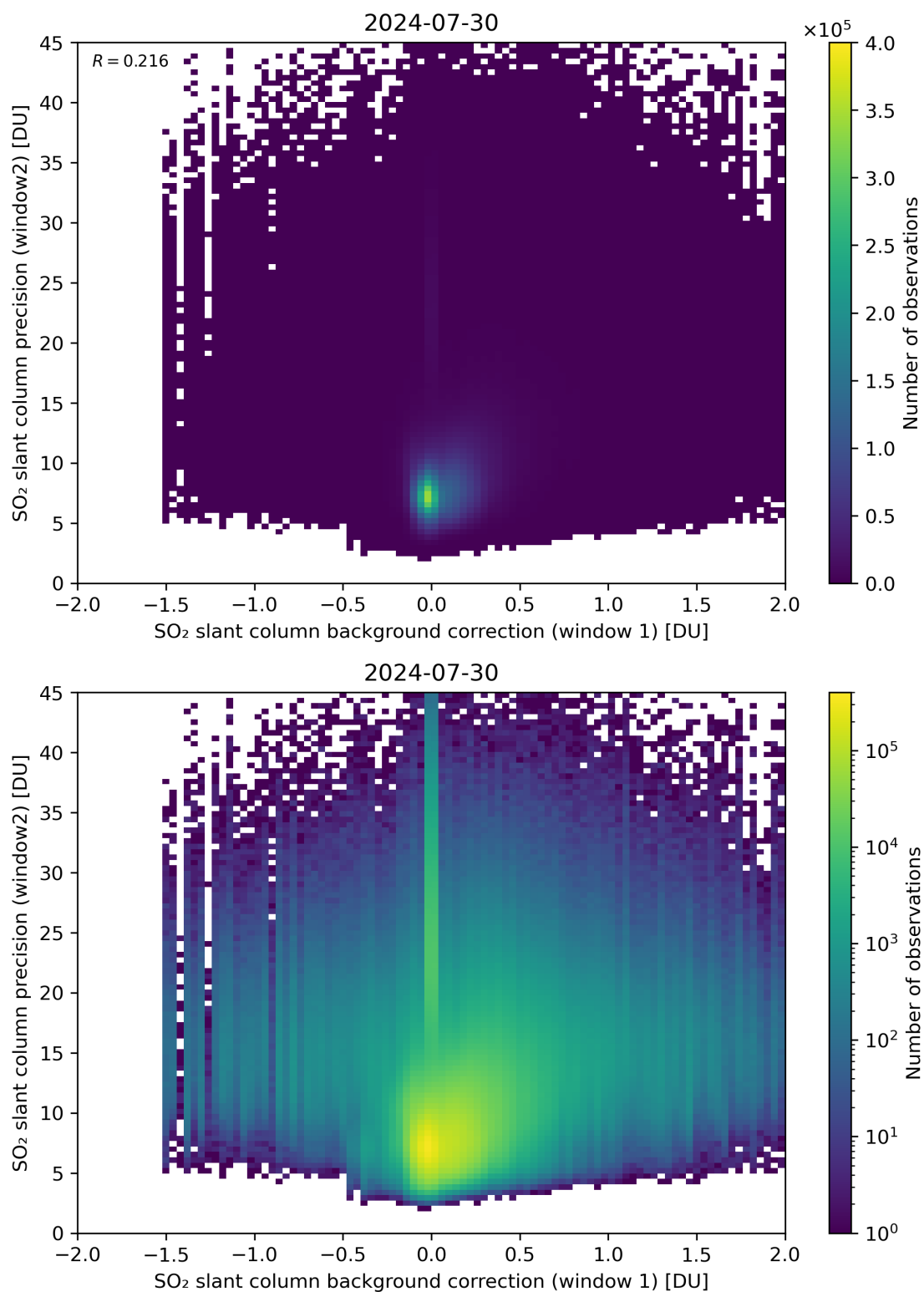
Figure 106: Scatter density plot of “SO 2 slant column background correction (window 1)” against “SO 2 slant column precision (window2)” for 2024-07-29 to 2024-07-31.
