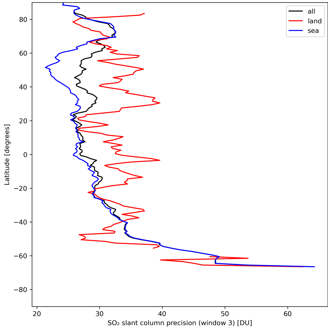
Figure 42: Zonal average of “SO 2 slant column precision (window 3)” for 2024-07-29 to 2024-07-31.
