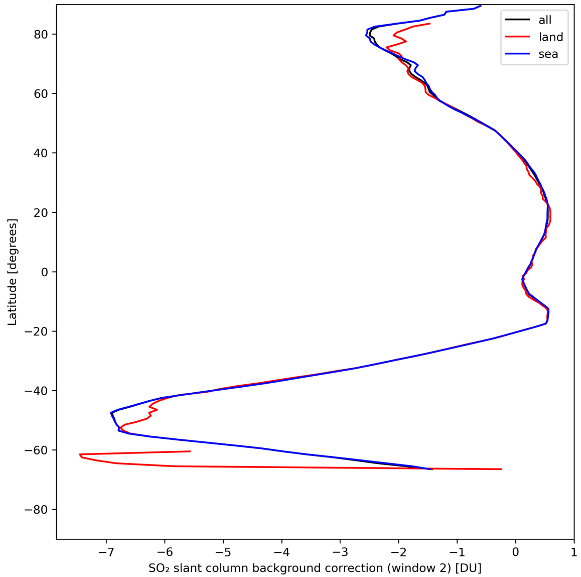
Figure 40: Zonal average of “SO 2 slant column background correction (window 2)” for 2024-07-29 to 2024-07-31.
