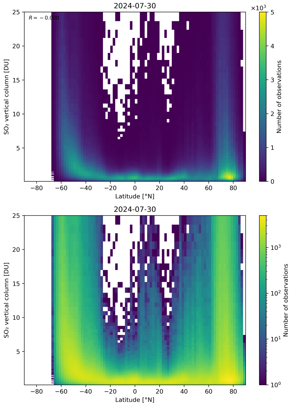
Figure 156: Scatter density plot of “Latitude” against “SO 2 vertical column” for 2024-07-29 to 2024-07-31.
