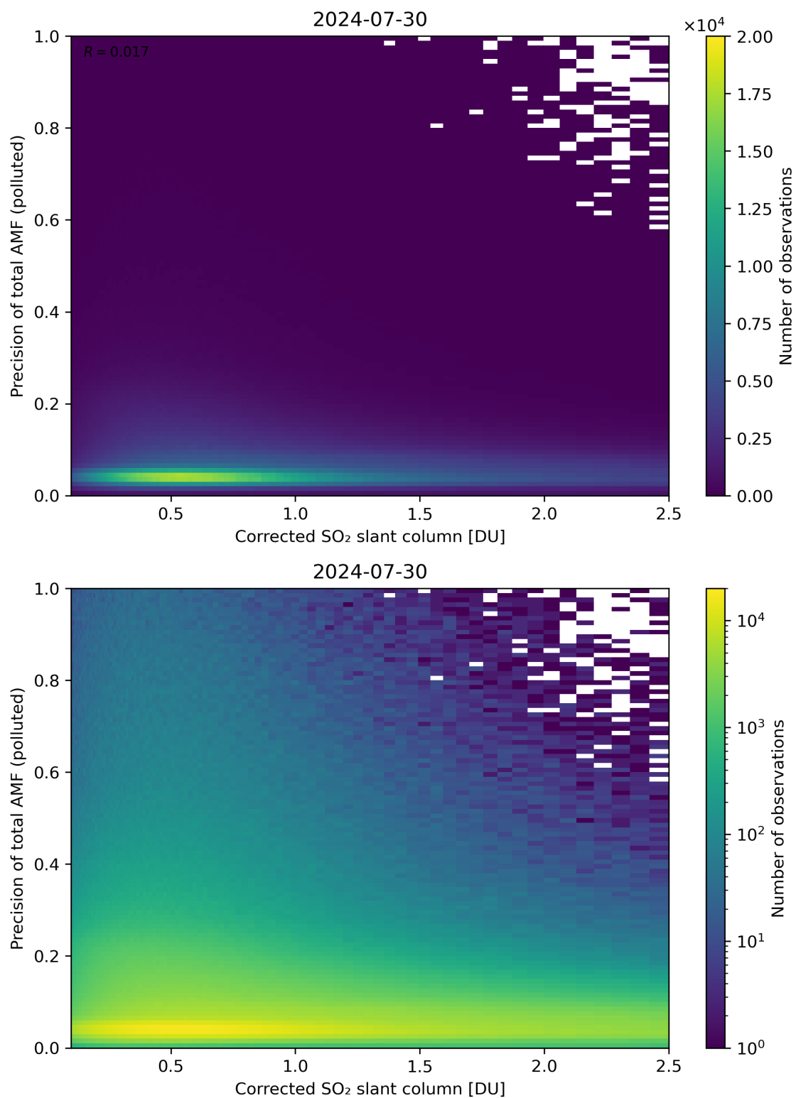
Figure 193: Scatter density plot of “Corrected SO 2 slant column” against “Precision of total AMF (polluted)” for 2024-07-29 to 2024-07-31.
