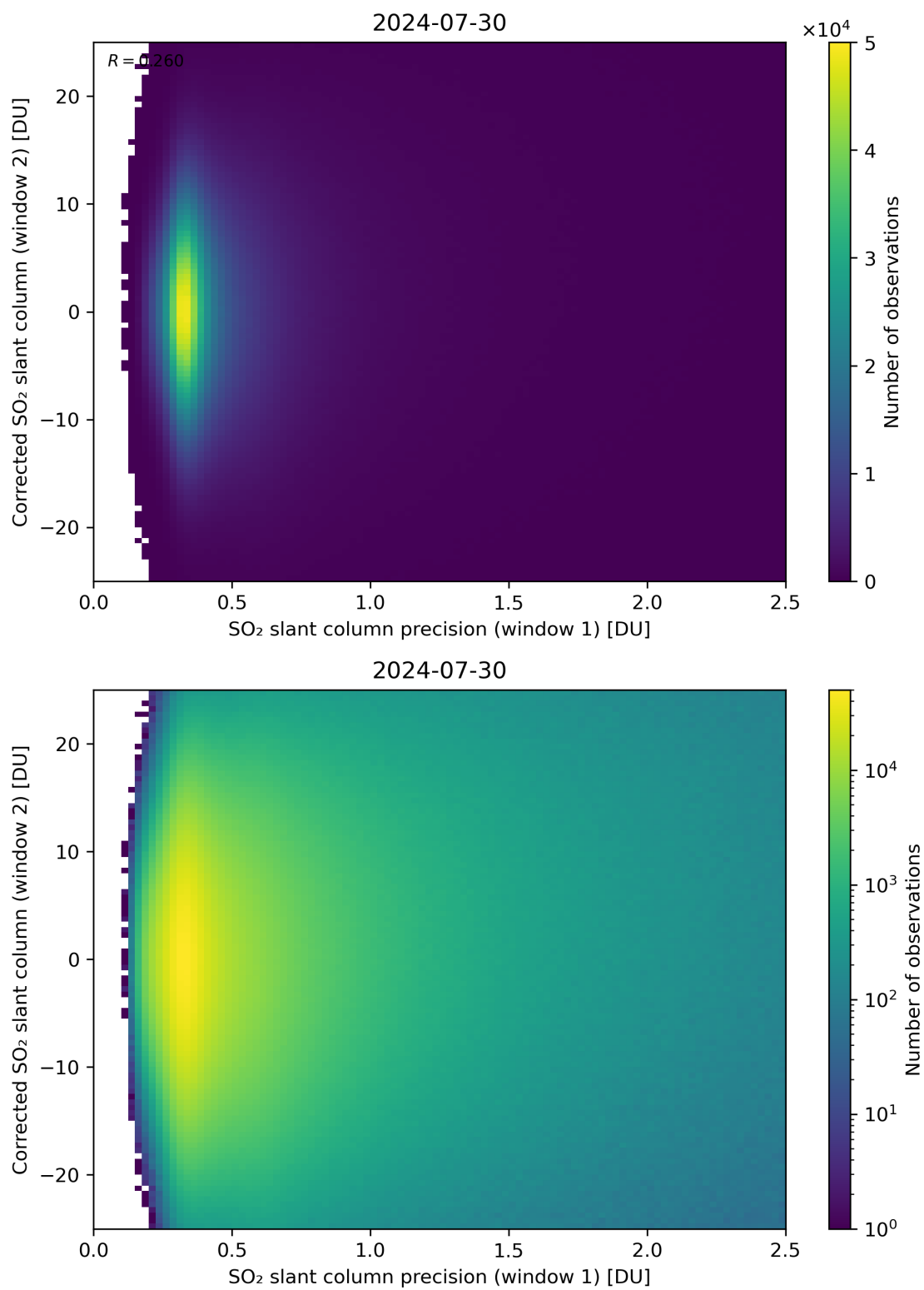
Figure 225: Scatter density plot of “SO 2 slant column precision (window 1)” against “Corrected SO 2 slant column (window 2)” for 2024-07-29 to 2024-07-31.
