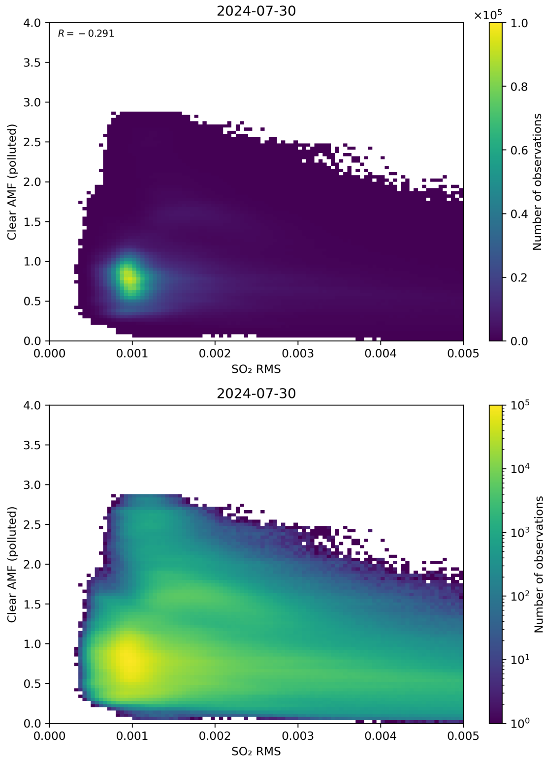
Figure 136: Scatter density plot of “SO 2 RMS” against “Clear AMF (polluted)” for 2024-07-29 to 2024-07-31.
