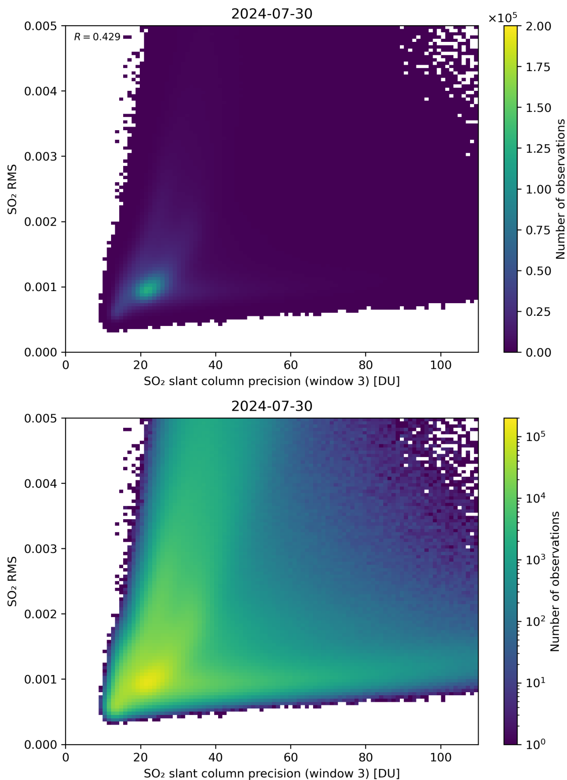
Figure 260: Scatter density plot of “SO 2 slant column precision (window 3)” against “SO 2 RMS” for 2024-07-29 to 2024-07-31.
