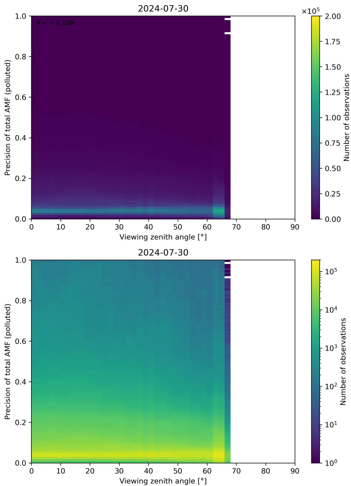
Figure 326: Scatter density plot of “Viewing zenith angle” against “Precision of total AMF (polluted)” for 2024-07-29 to 2024-07-31.
