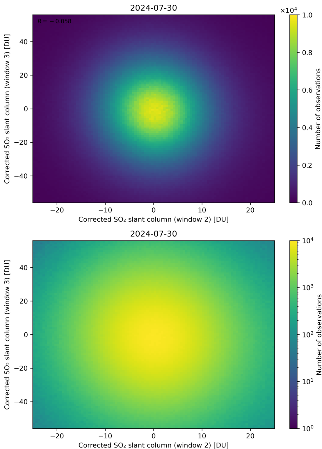
Figure 200: Scatter density plot of “Corrected SO 2 slant column (window 2)” against “Corrected SO 2 slant column (window 3)” for 2024-07-29 to 2024-07-31.
