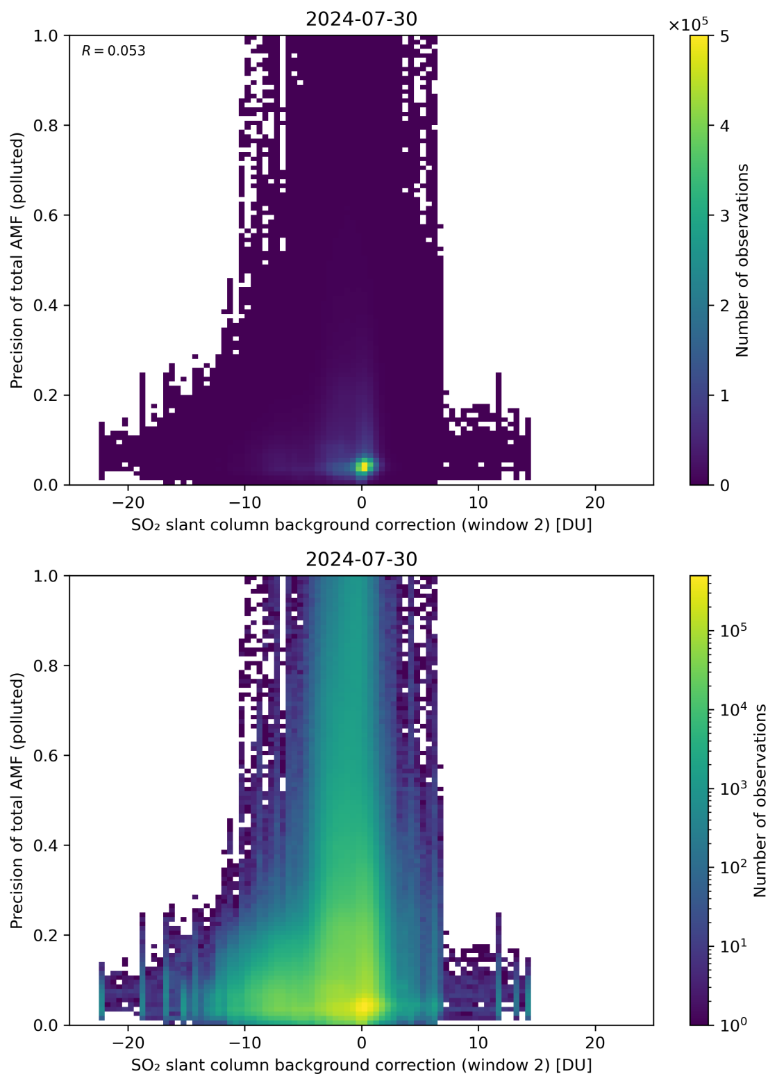
Figure 120: Scatter density plot of “SO 2 slant column background correction (window 2)” against “Precision of total AMF (polluted)” for 2024-07-29 to 2024-07-31.
