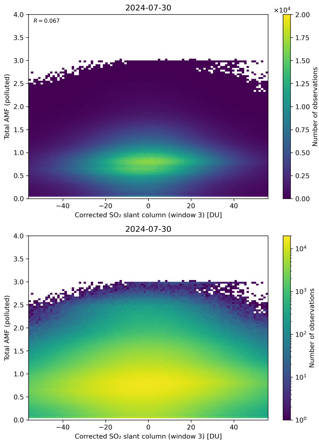
Figure 210: Scatter density plot of “Corrected SO 2 slant column (window 3)” against “Total AMF (polluted)” for 2024-07-29 to 2024-07-31.
