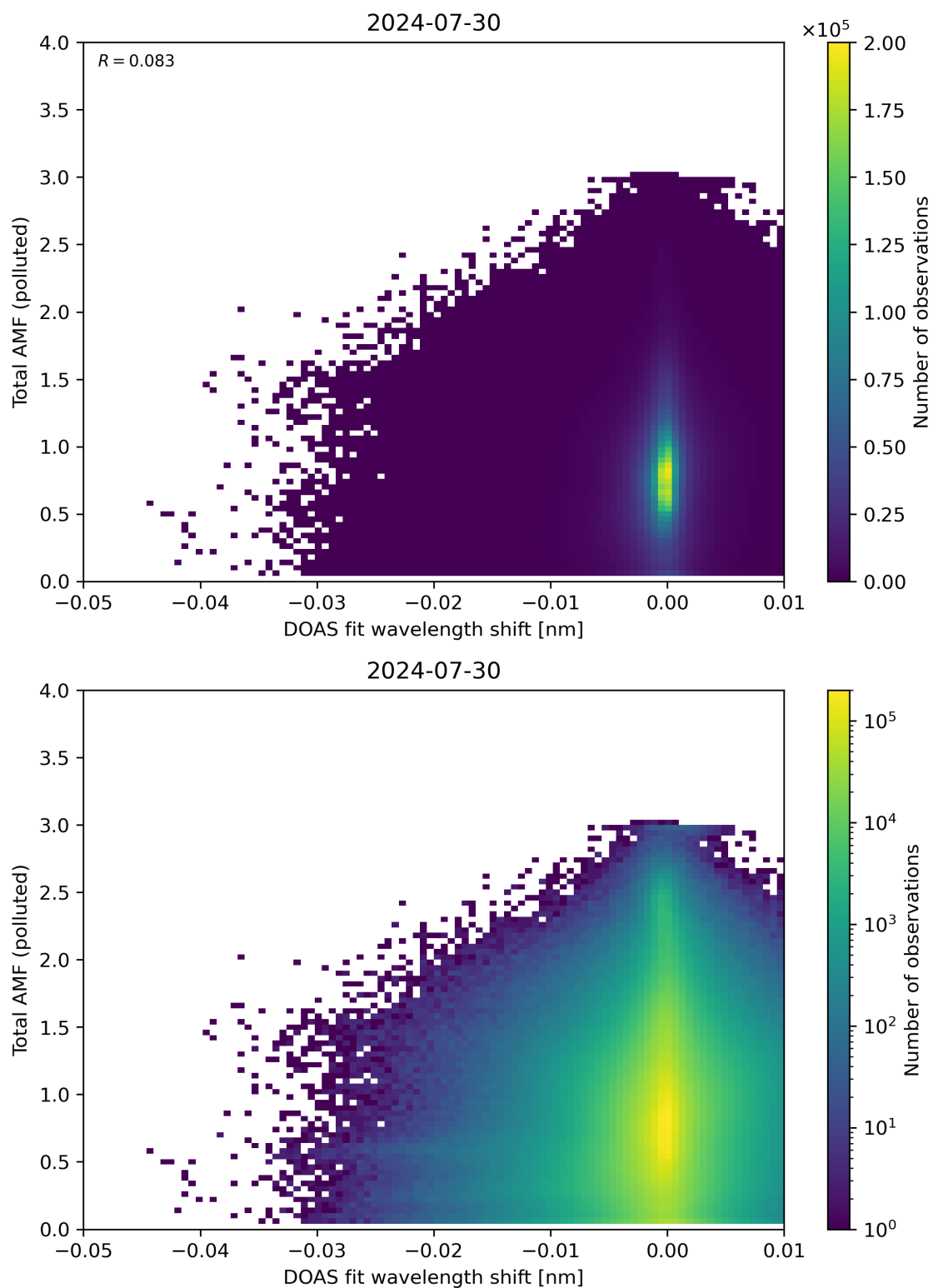
Figure 130: Scatter density plot of “DOAS fit wavelength shift” against “Total AMF (polluted)” for 2024-07-29 to 2024-07-31.
