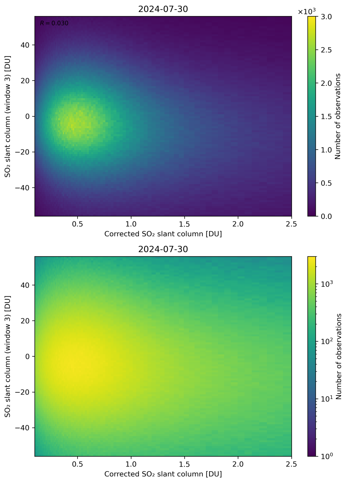
Figure 190: Scatter density plot of “Corrected SO 2 slant column” against “SO 2 slant column (window 3)” for 2024-07-29 to 2024-07-31.
