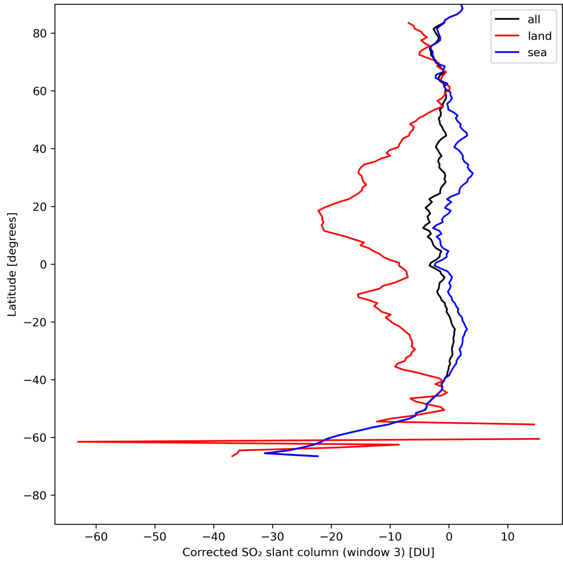
Figure 43: Zonal average of “Corrected SO 2 slant column (window 3)” for 2024-07-29 to 2024-07-31.
