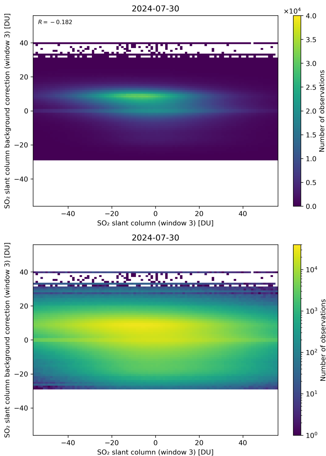
Figure 253: Scatter density plot of “SO 2 slant column (window 3)” against “SO 2 slant column background correction (window 3)” for 2024-07-29 to 2024-07-31.
