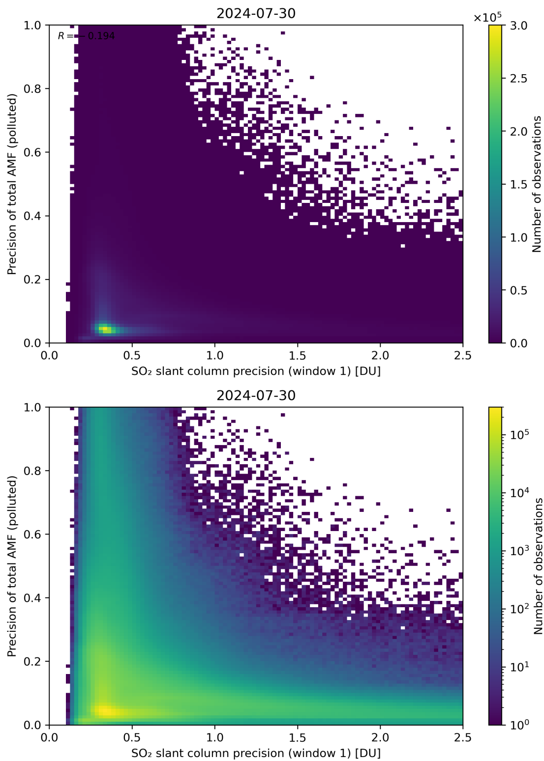
Figure 231: Scatter density plot of “SO 2 slant column precision (window 1)” against “Precision of total AMF (polluted)” for 2024-07-29 to 2024-07-31.
