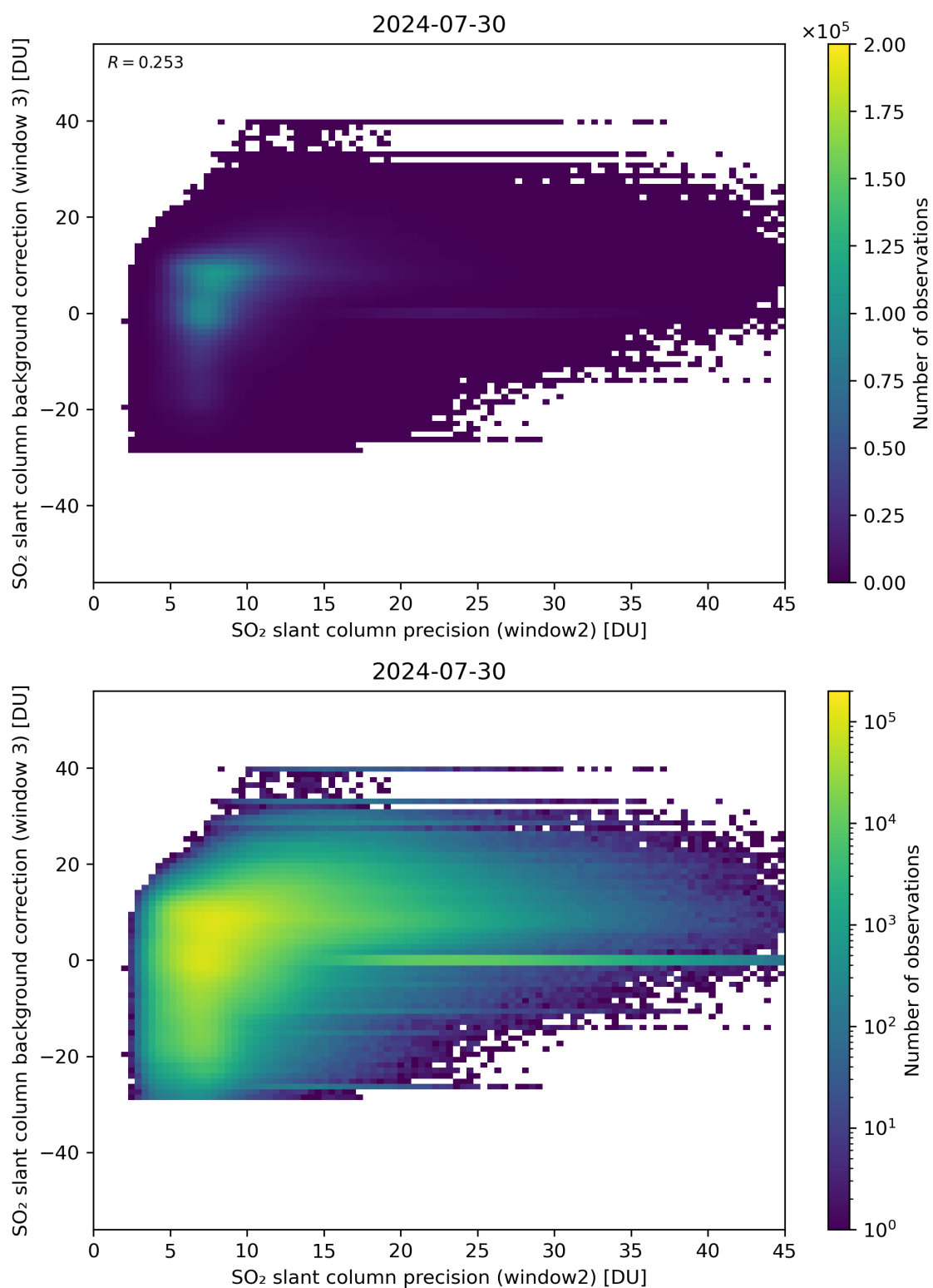
Figure 242: Scatter density plot of “SO 2 slant column precision (window2)” against “SO 2 slant column background correction (window 3)” for 2024-07-29 to 2024-07-31.
