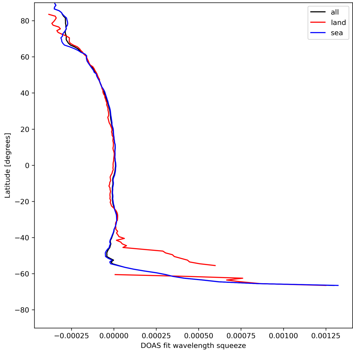
Figure 46: Zonal average of “DOAS fit wavelength squeeze” for 2024-07-29 to 2024-07-31.
