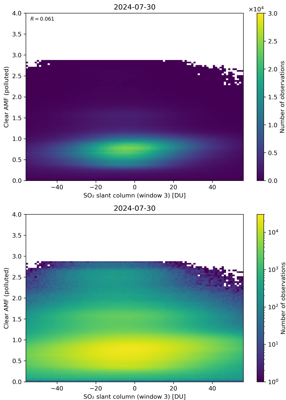
Figure 265: Scatter density plot of “SO 2 slant column (window 3)” against “Clear AMF (polluted)” for 2024-07-29 to 2024-07-31.
