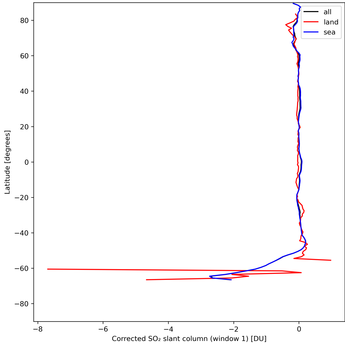
Figure 35: Zonal average of “Corrected SO 2 slant column (window 1)” for 2024-07-29 to 2024-07-31.
