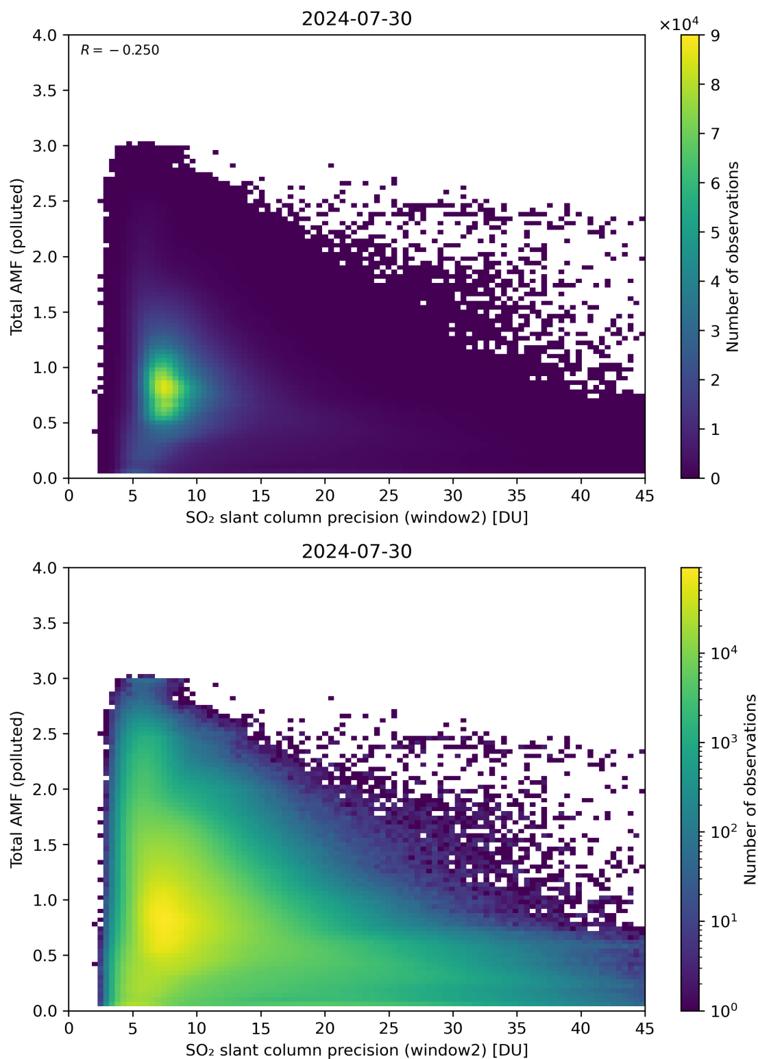
Figure 251: Scatter density plot of “SO 2 slant column precision (window2)” against “Total AMF (polluted)” for 2024-07-29 to 2024-07-31.
