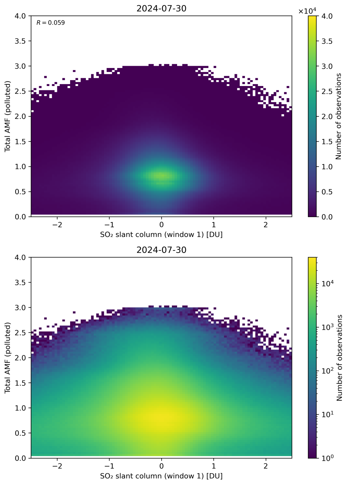
Figure 239: Scatter density plot of “SO 2 slant column (window 1)” against “Total AMF (polluted)” for 2024-07-29 to 2024-07-31.
