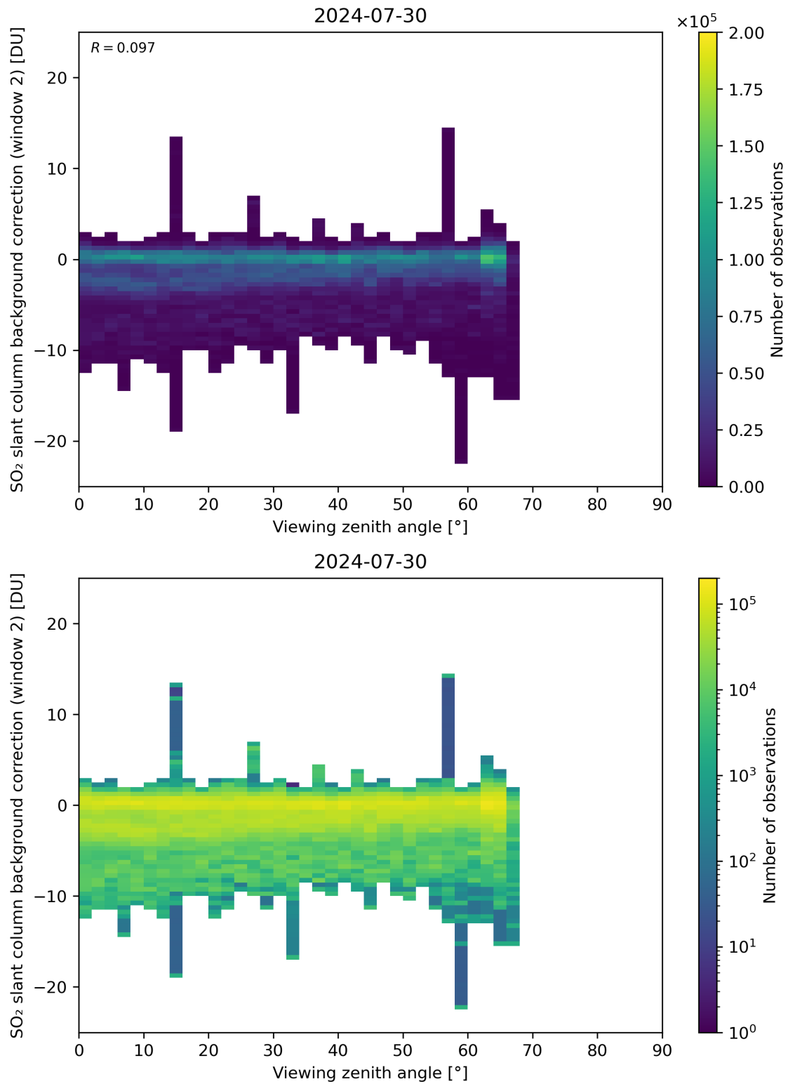
Figure 309: Scatter density plot of “Viewing zenith angle” against “SO 2 slant column background correction (window 2)” for 2024-07-29 to 2024-07-31.
