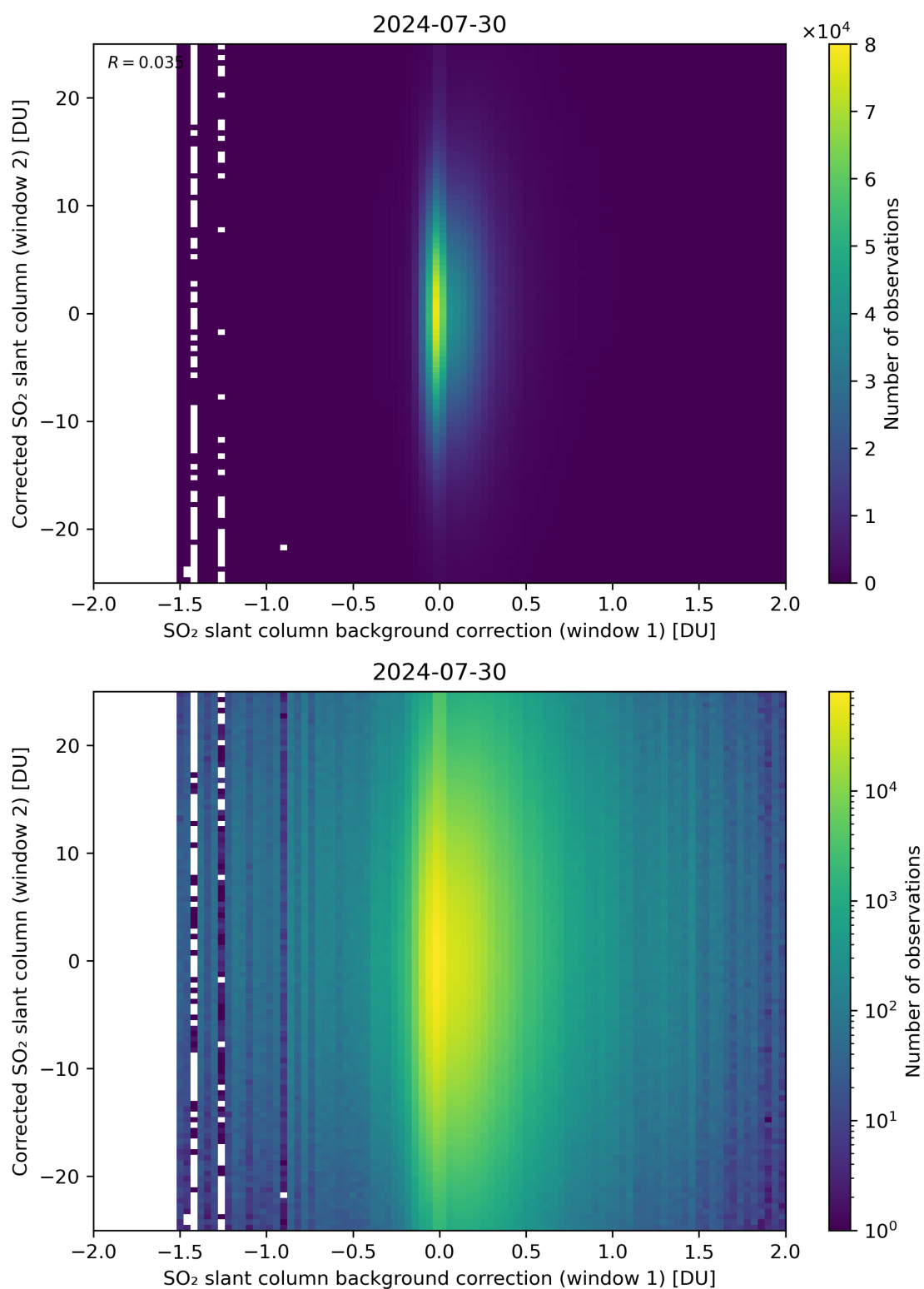
Figure 104: Scatter density plot of “SO 2 slant column background correction (window 1)” against “Corrected SO 2 slant column (window 2)” for 2024-07-29 to 2024-07-31.
