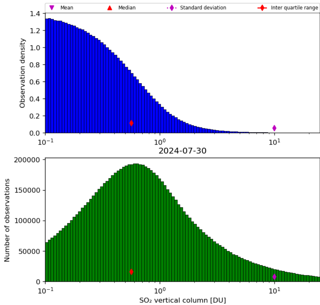
Figure 53: Histogram of "SO 2 vertical column" for 2024-07-29 to 2024-07-31
