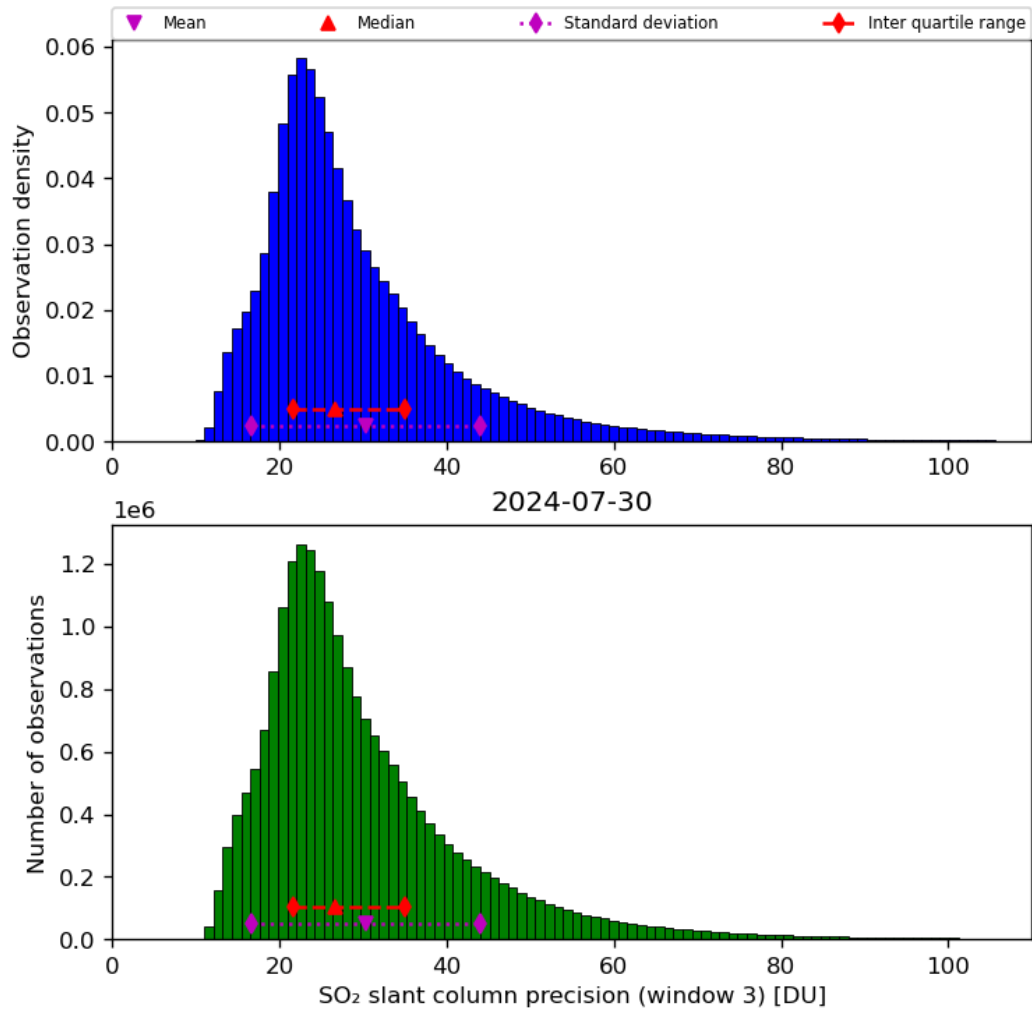
Figure 65: Histogram of “SO 2 slant column precision (window 3)” for 2024-07-29 to 2024-07-31
