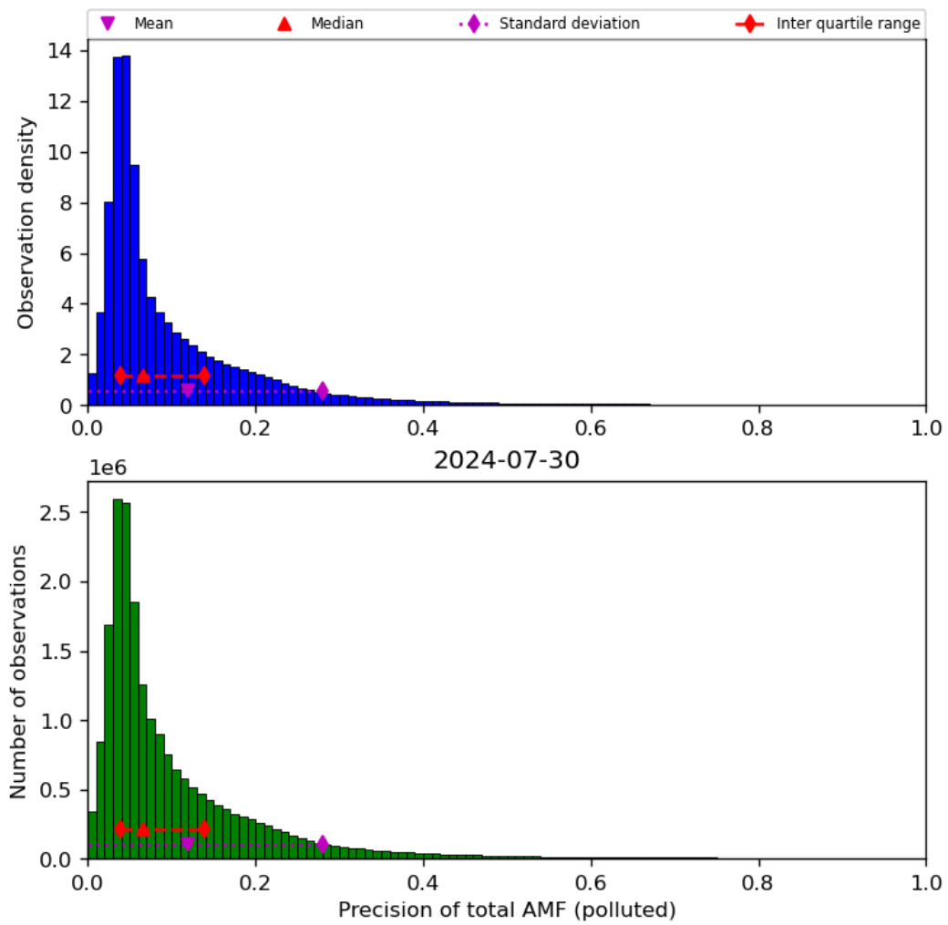
Figure 72: Histogram of “Precision of total AMF (polluted)” for 2024-07-29 to 2024-07-31
