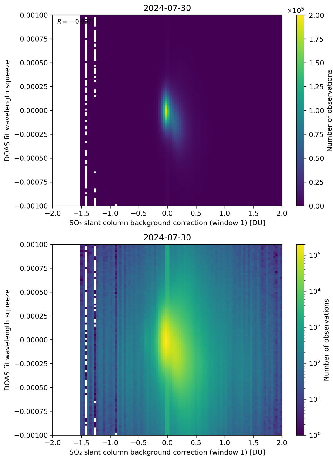
Figure 101: Scatter density plot of “SO 2 slant column background correction (window 1)” against “DOAS fit wavelength squeeze” for 2024-07-29 to 2024-07-31.
