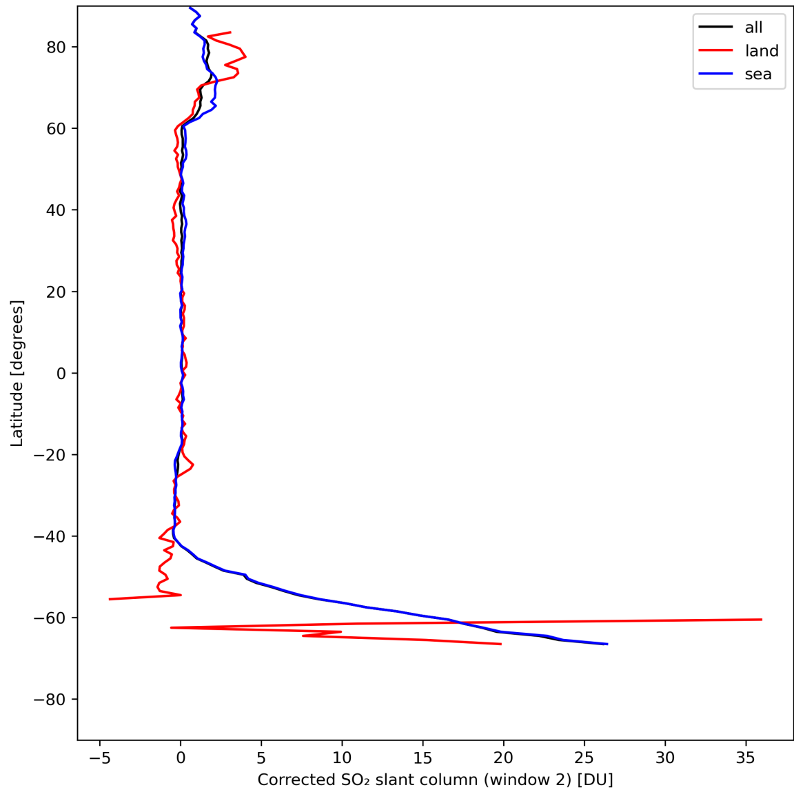
Figure 39: Zonal average of “Corrected SO 2 slant column (window 2)” for 2024-07-29 to 2024-07-31.
