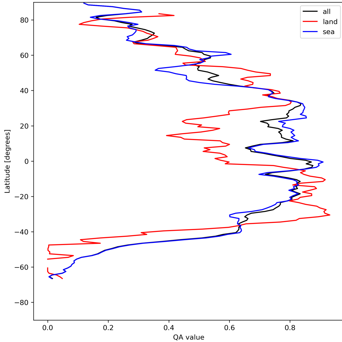
Figure 29: Zonal average of “QA value” for 2024-07-29 to 2024-07-31.
