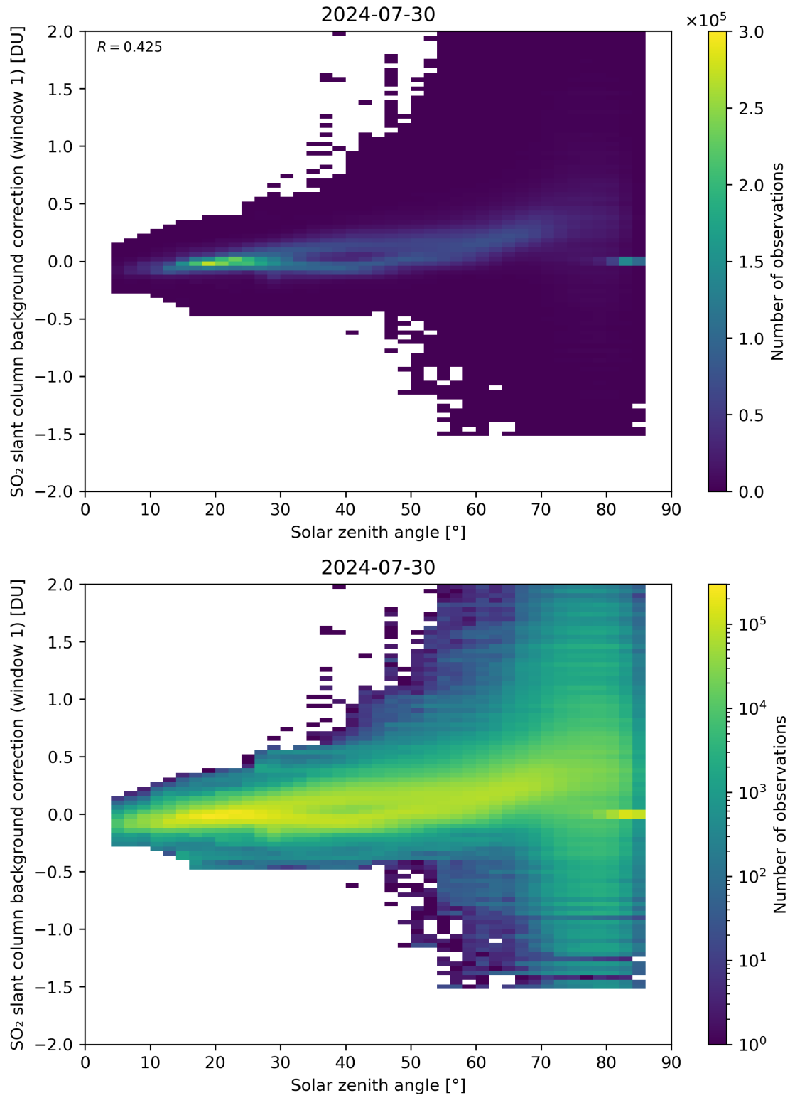
Figure 158: Scatter density plot of “Solar zenith angle” against “SO 2 slant column background correction (window 1)” for 2024-07-29 to 2024-07-31.
