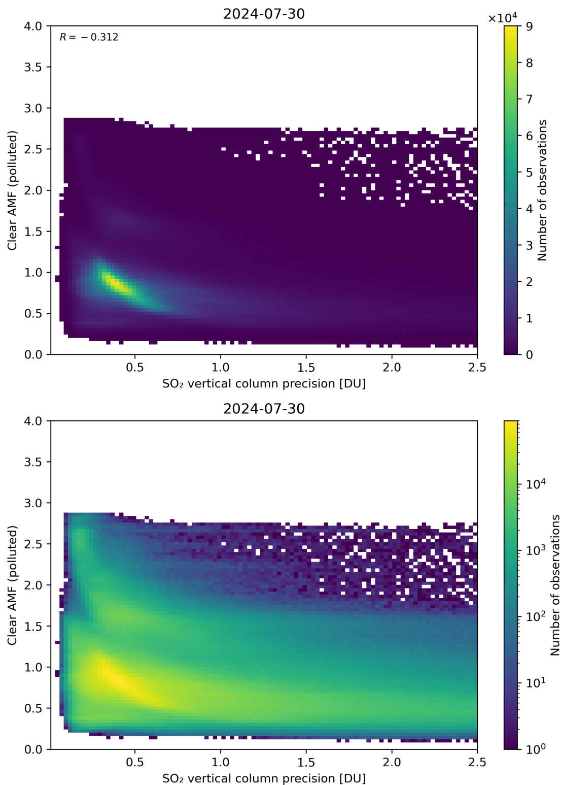
Figure 285: Scatter density plot of “SO 2 vertical column precision” against “Clear AMF (polluted)” for 2024-07-29 to 2024-07-31.
