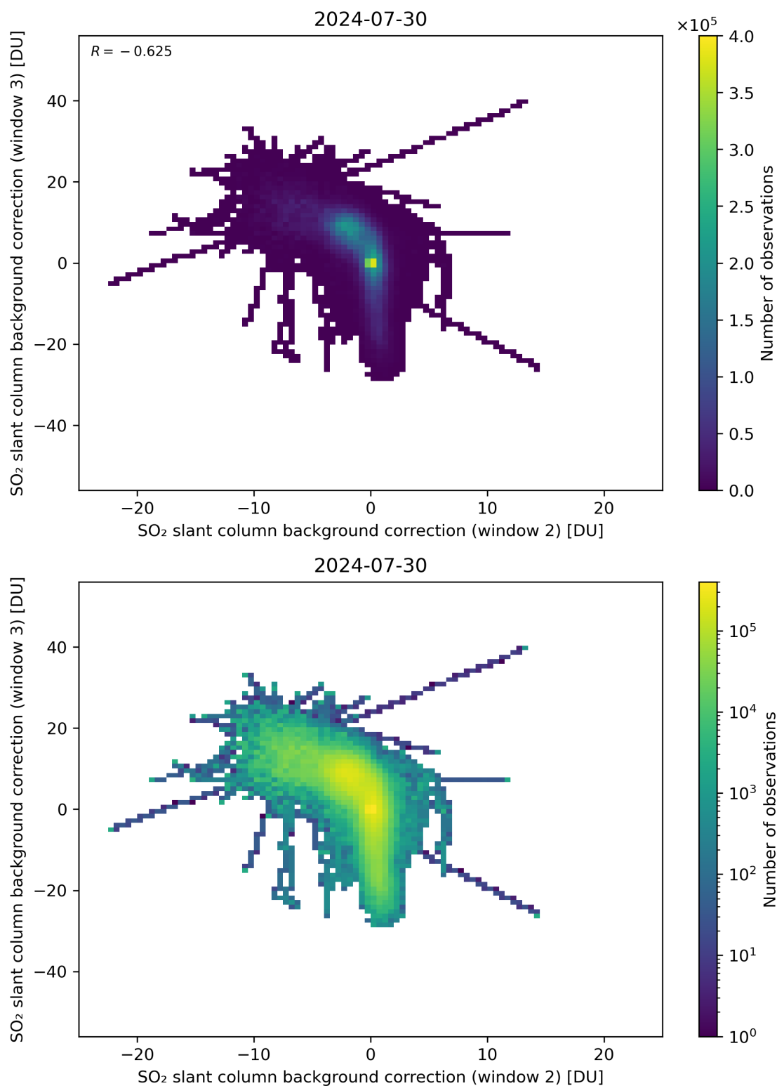
Figure 111: Scatter density plot of “SO 2 slant column background correction (window 2)” against “SO 2 slant column background correction (window 3)” for 2024-07-29 to 2024-07-31.
