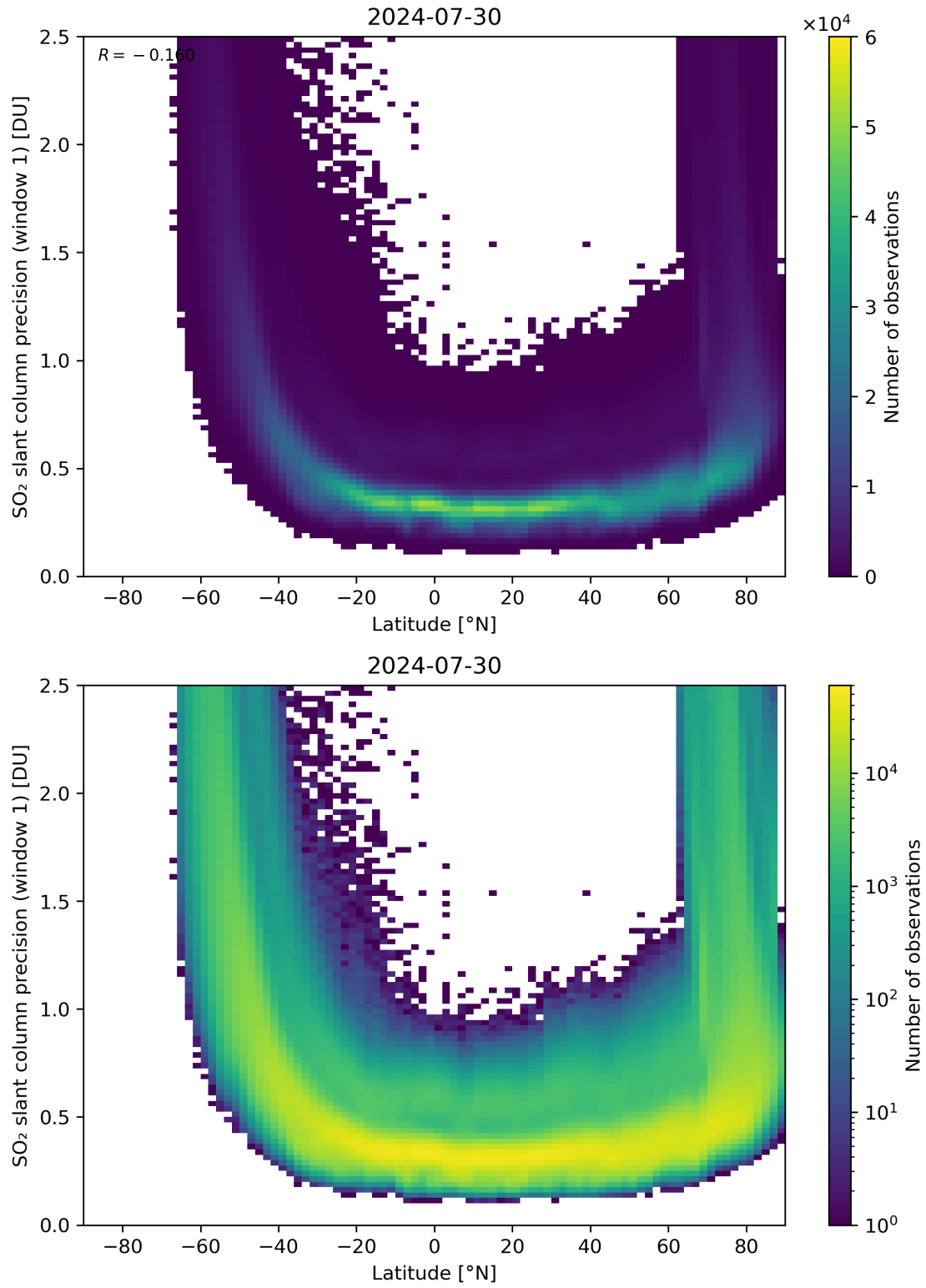
Figure 150: Scatter density plot of “Latitude” against “SO 2 slant column precision (window 1)” for 2024-07-29 to 2024-07-31.
