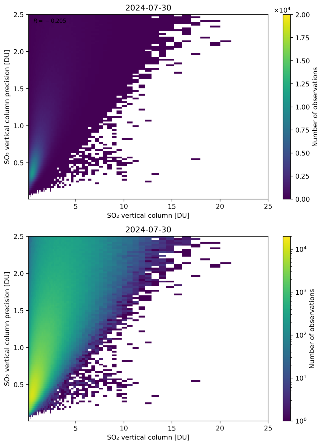
Figure 307: Scatter density plot of “SO 2 vertical column” against “SO 2 vertical column precision” for 2024-07-29 to 2024-07-31.
