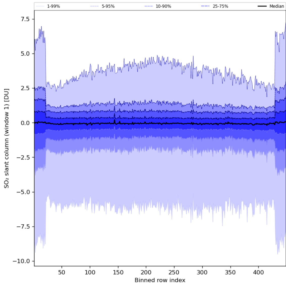
Figure 79: Along track statistics of “SO 2 slant column (window 1)” for 2024-07-29 to 2024-07-31
