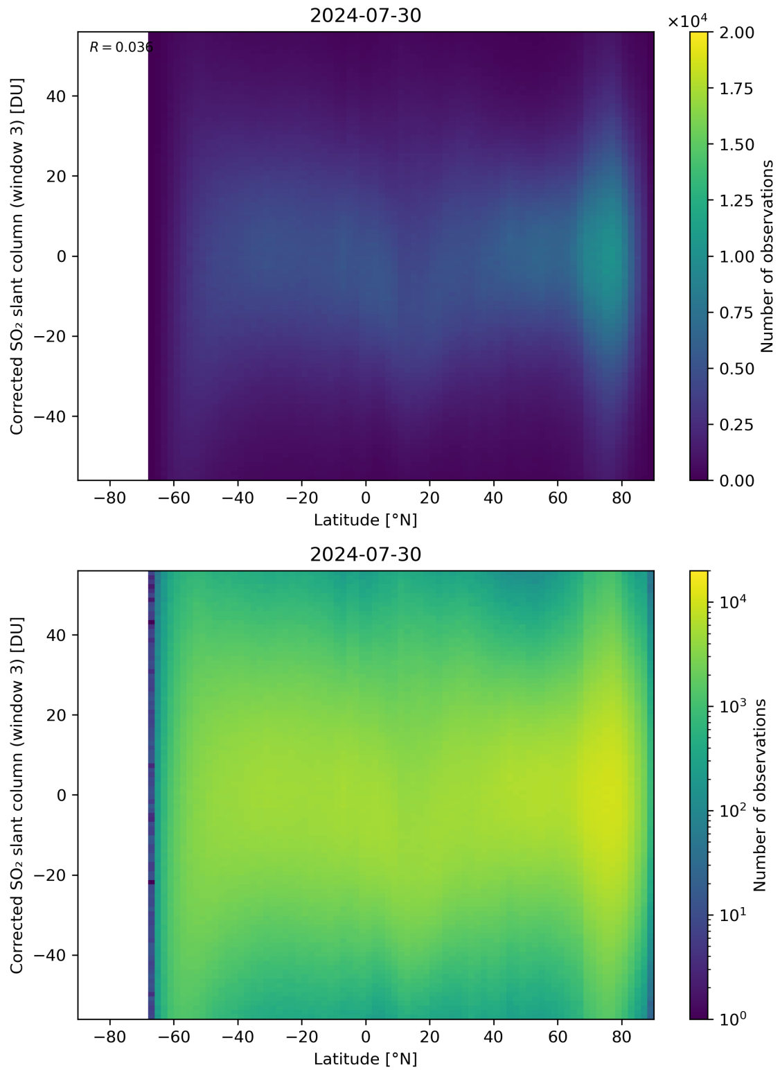
Figure 148: Scatter density plot of “Latitude” against “Corrected SO 2 slant column (window 3)” for 2024-07-29 to 2024-07-31.
