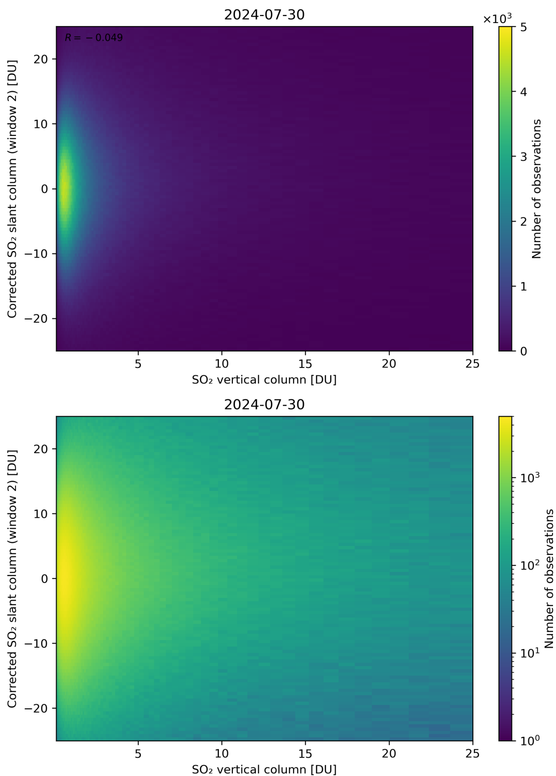
Figure 298: Scatter density plot of “SO 2 vertical column” against “Corrected SO 2 slant column (window 2)” for 2024-07-29 to 2024-07-31.
