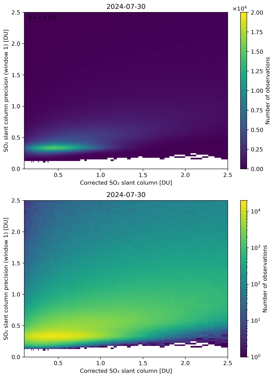
Figure 188: Scatter density plot of “Corrected SO 2 slant column” against “SO 2 slant column precision (window 1)” for 2024-07-29 to 2024-07-31.
