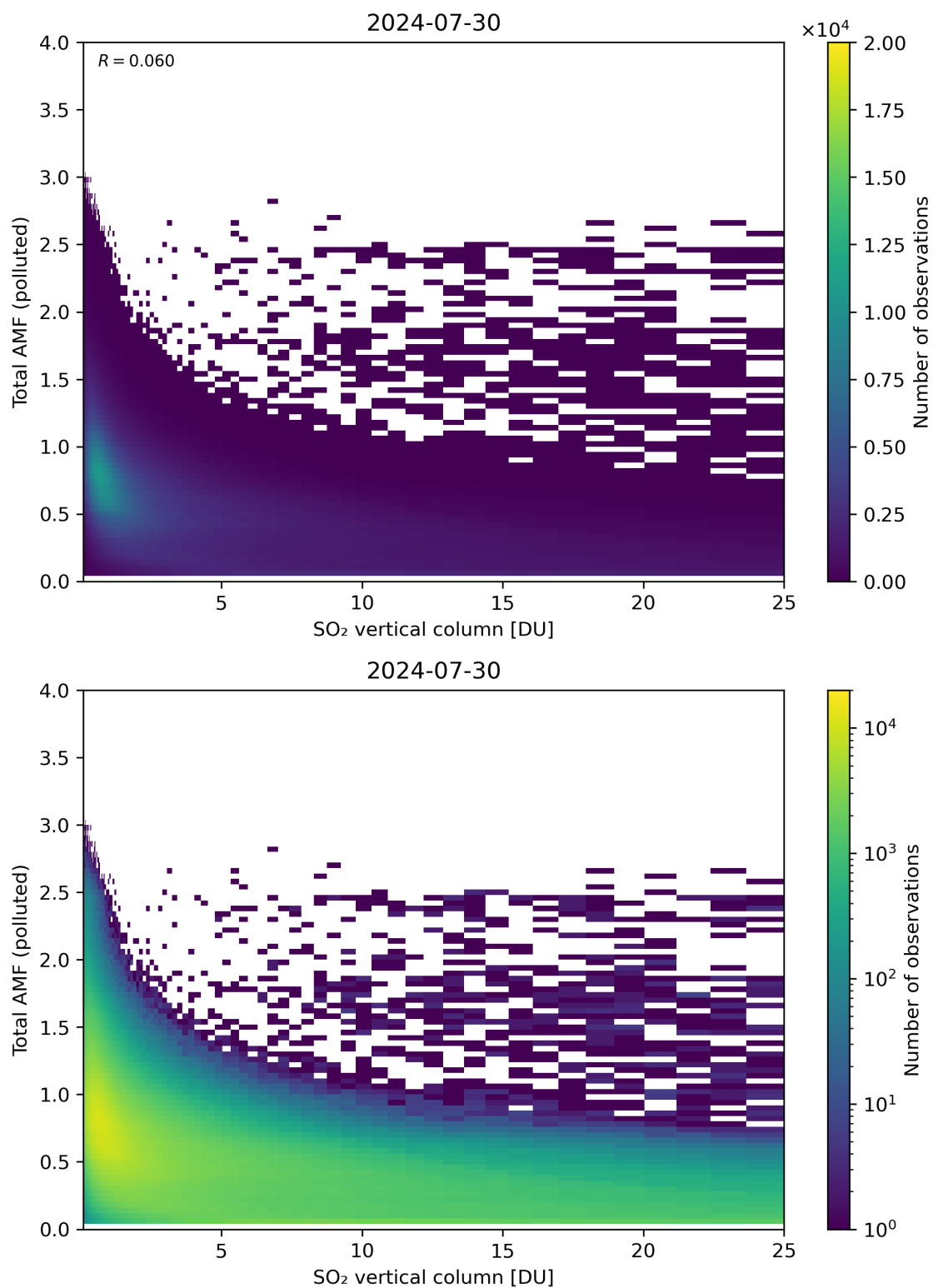
Figure 305: Scatter density plot of “SO 2 vertical column” against “Total AMF (polluted)” for 2024-07-29 to 2024-07-31.
