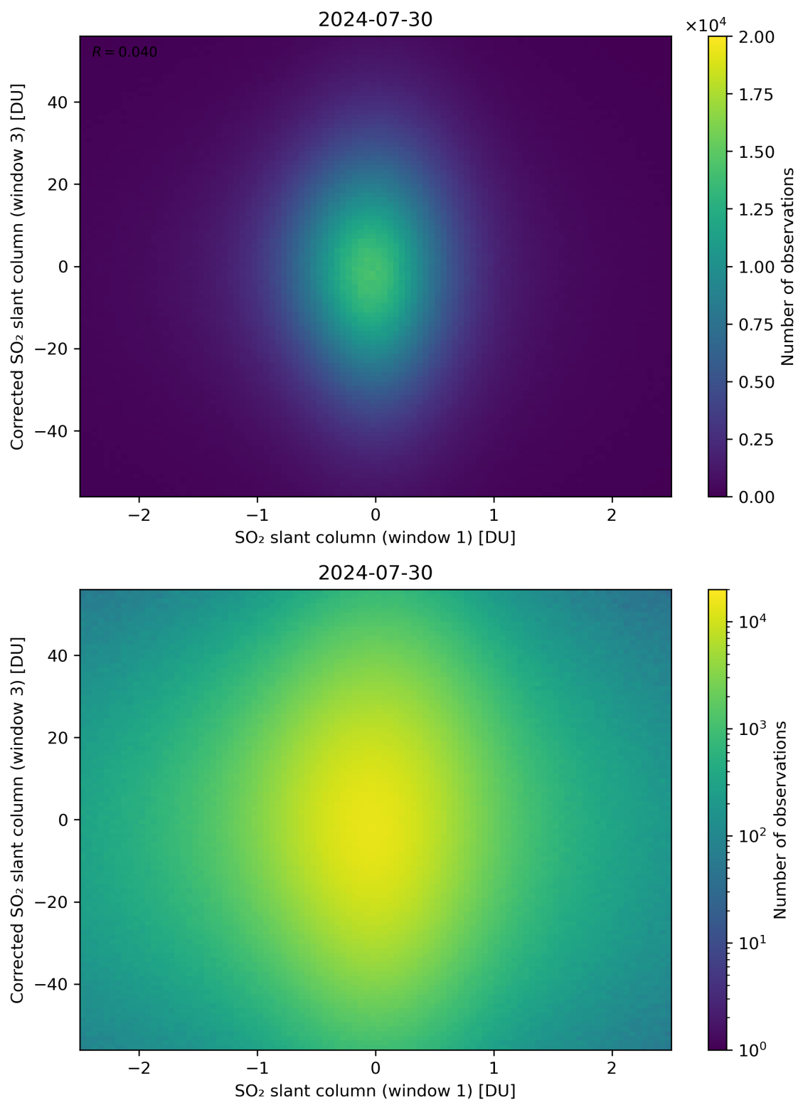
Figure 234: Scatter density plot of “SO 2 slant column (window 1)” against “Corrected SO 2 slant column (window 3)” for 2024-07-29 to 2024-07-31.
