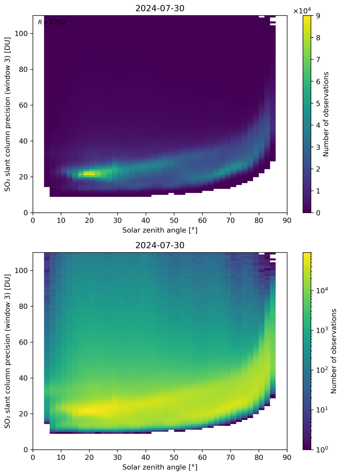
Figure 173: Scatter density plot of “Solar zenith angle” against “SO 2 slant column precision (window 3)” for 2024-07-29 to 2024-07-31.
