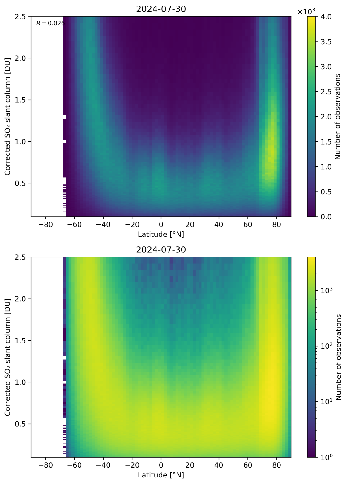
Figure 146: Scatter density plot of “Latitude” against “Corrected SO 2 slant column” for 2024-07-29 to 2024-07-31.
