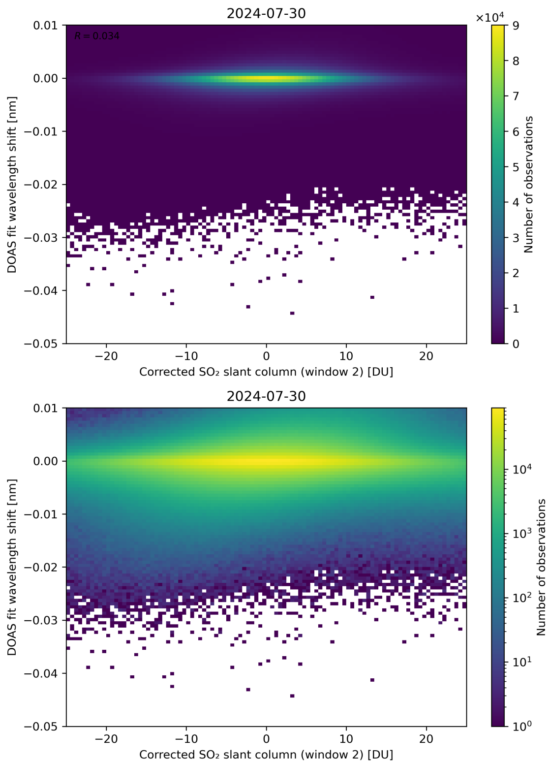
Figure 196: Scatter density plot of “Corrected SO 2 slant column (window 2)” against “DOAS fit wavelength shift” for 2024-07-29 to 2024-07-31.
