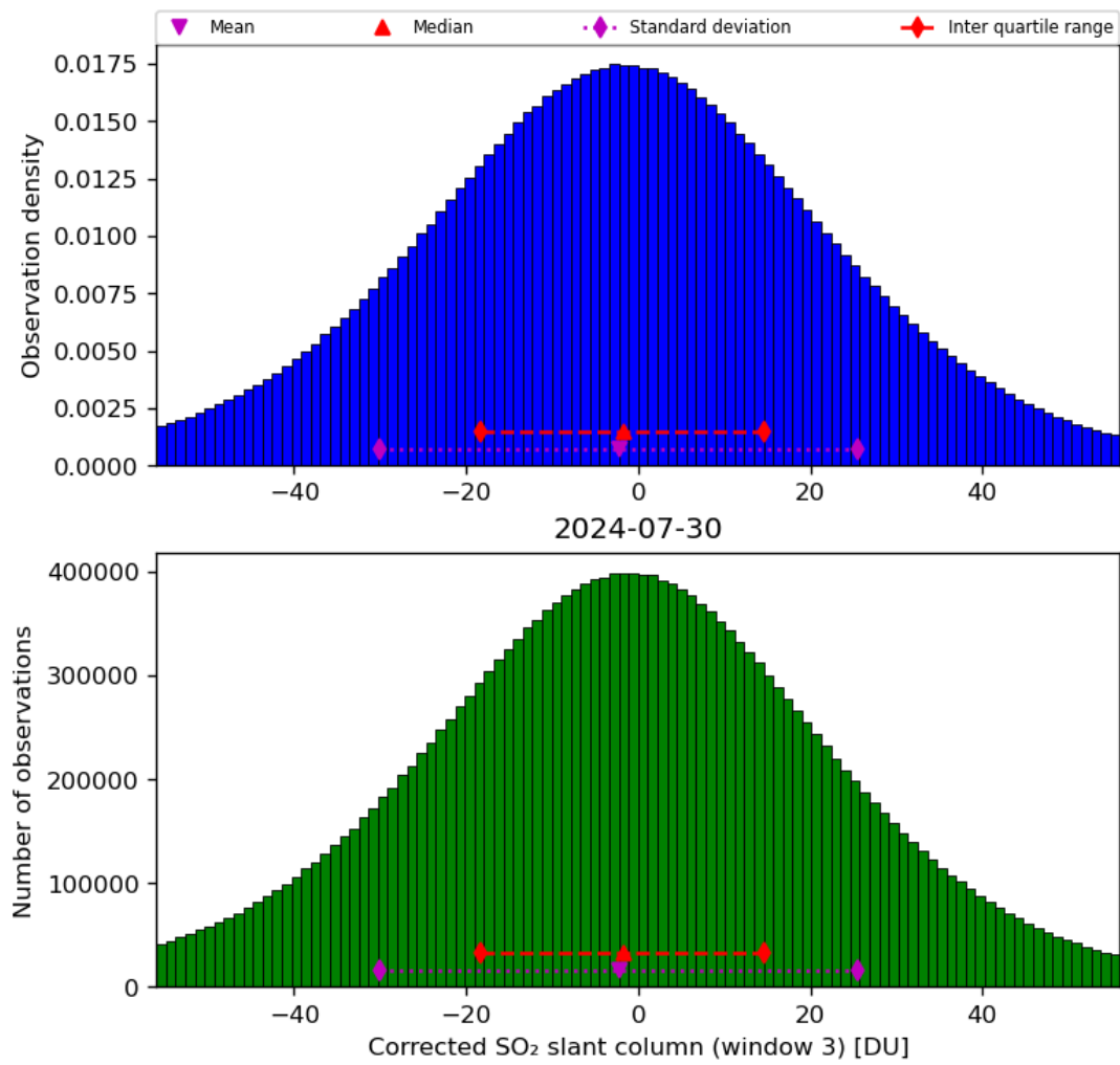
Figure 66: Histogram of “Corrected SO 2 slant column (window 3)” for 2024-07-29 to 2024-07-31
