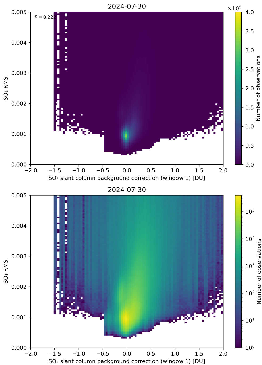
Figure 102: Scatter density plot of “SO 2 slant column background correction (window 1)” against “SO 2 RMS” for 2024-07-29 to 2024-07-31.
