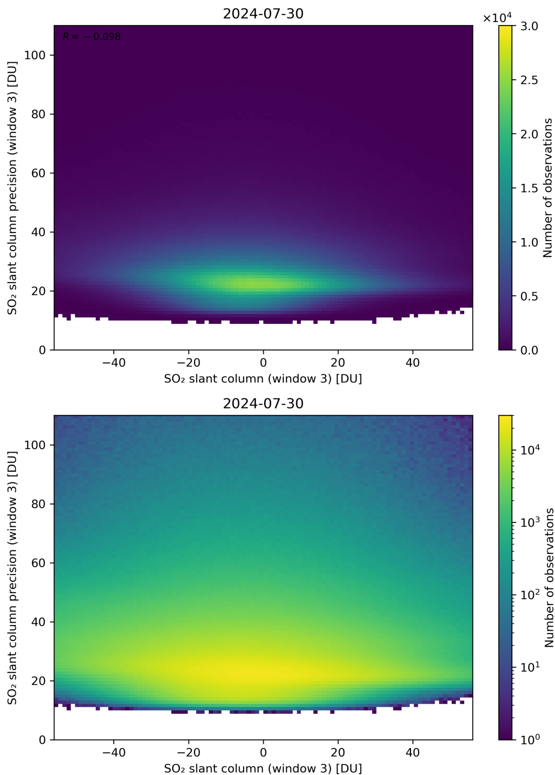
Figure 267: Scatter density plot of “SO 2 slant column (window 3)” against “SO 2 slant column precision (window 3)” for 2024-07-29 to 2024-07-31.
