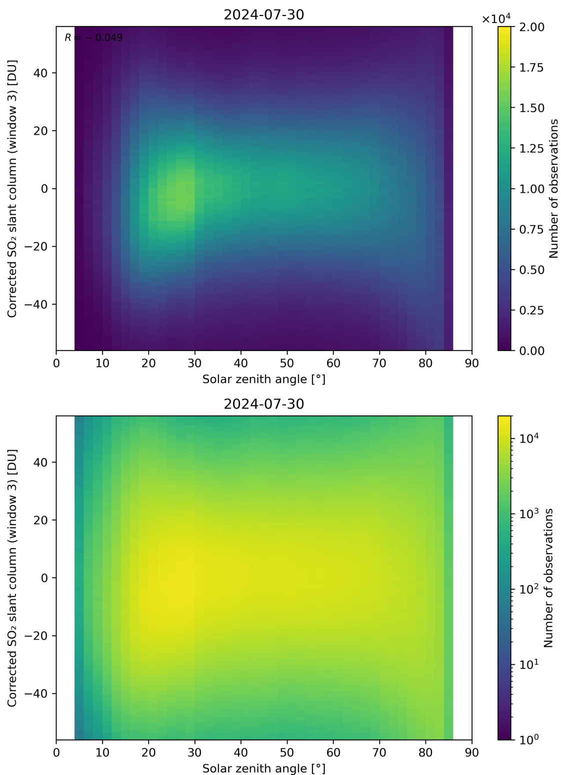
Figure 168: Scatter density plot of “Solar zenith angle” against “Corrected SO 2 slant column (window 3)” for 2024-07-29 to 2024-07-31.
