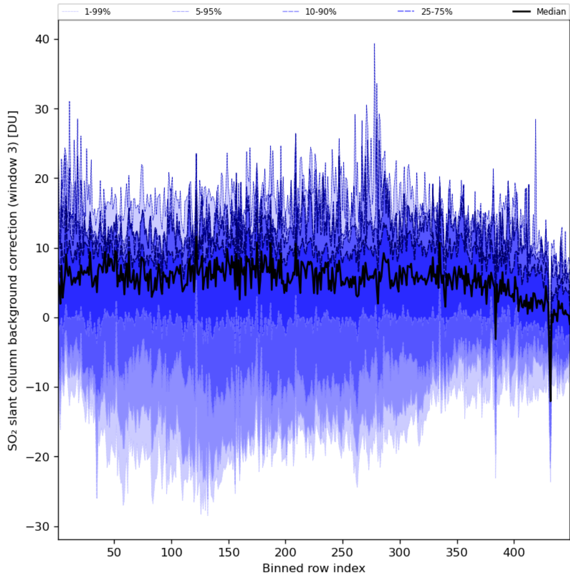
Figure 90: Along track statistics of “SO 2 slant column background correction (window 3)” for 2024-07-29 to 2024-07-31
