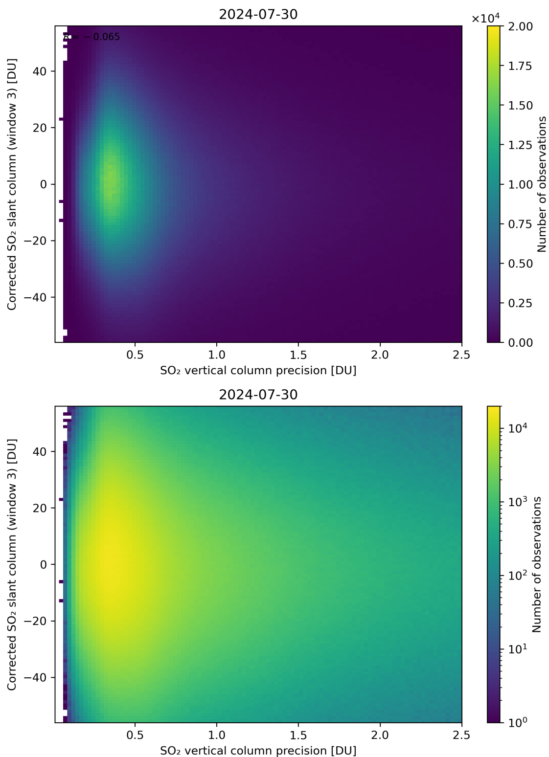
Figure 288: Scatter density plot of “SO 2 vertical column precision” against “Corrected SO 2 slant column (window 3)” for 2024-07-29 to 2024-07-31.
