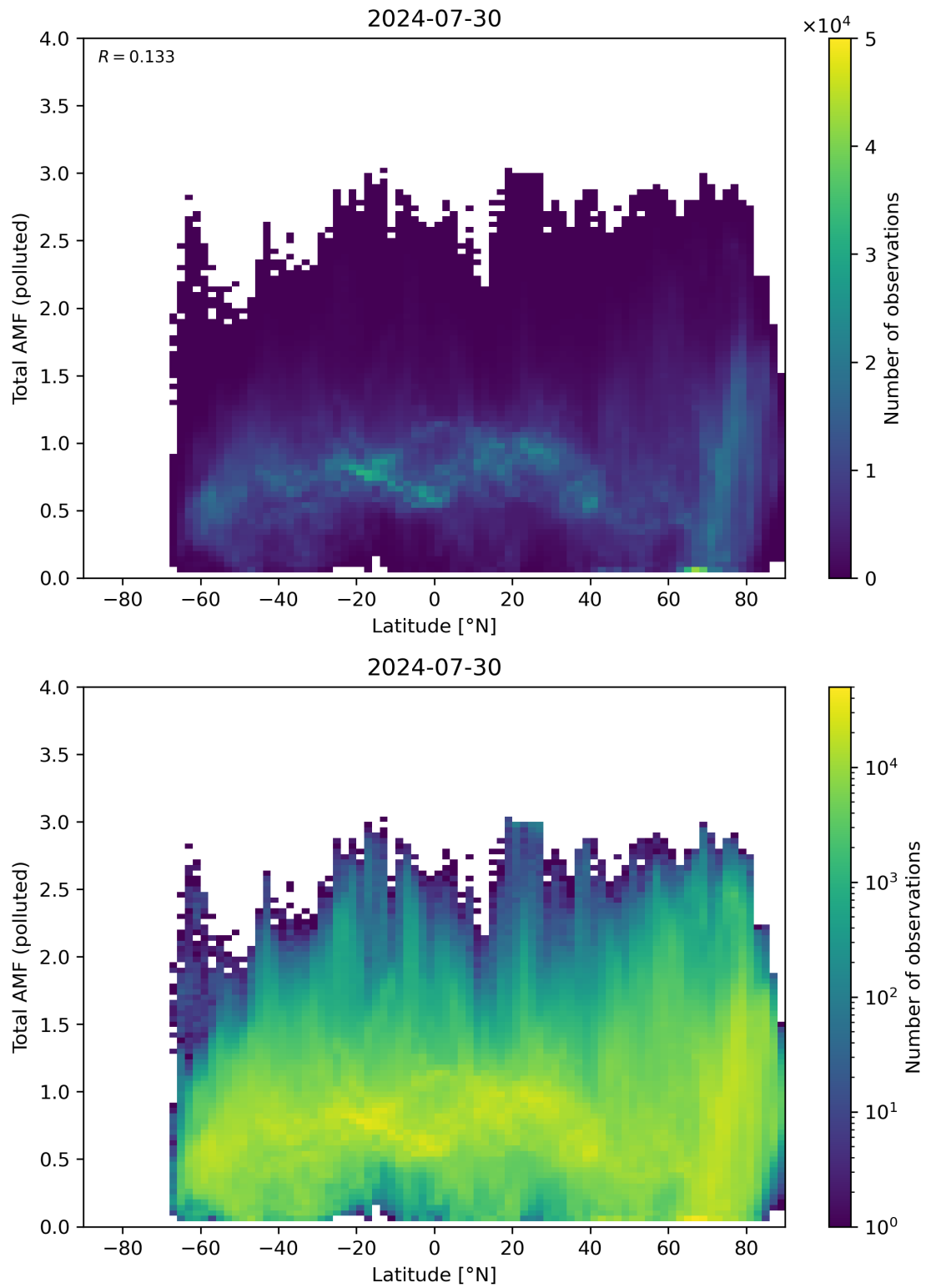
Figure 154: Scatter density plot of “Latitude” against “Total AMF (polluted)” for 2024-07-29 to 2024-07-31.
