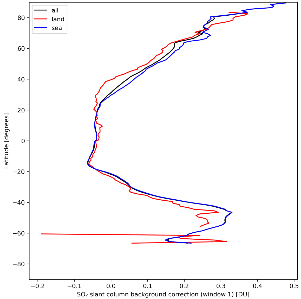
Figure 36: Zonal average of “SO 2 slant column background correction (window 1)” for 2024-07-29 to 2024-07-31.
