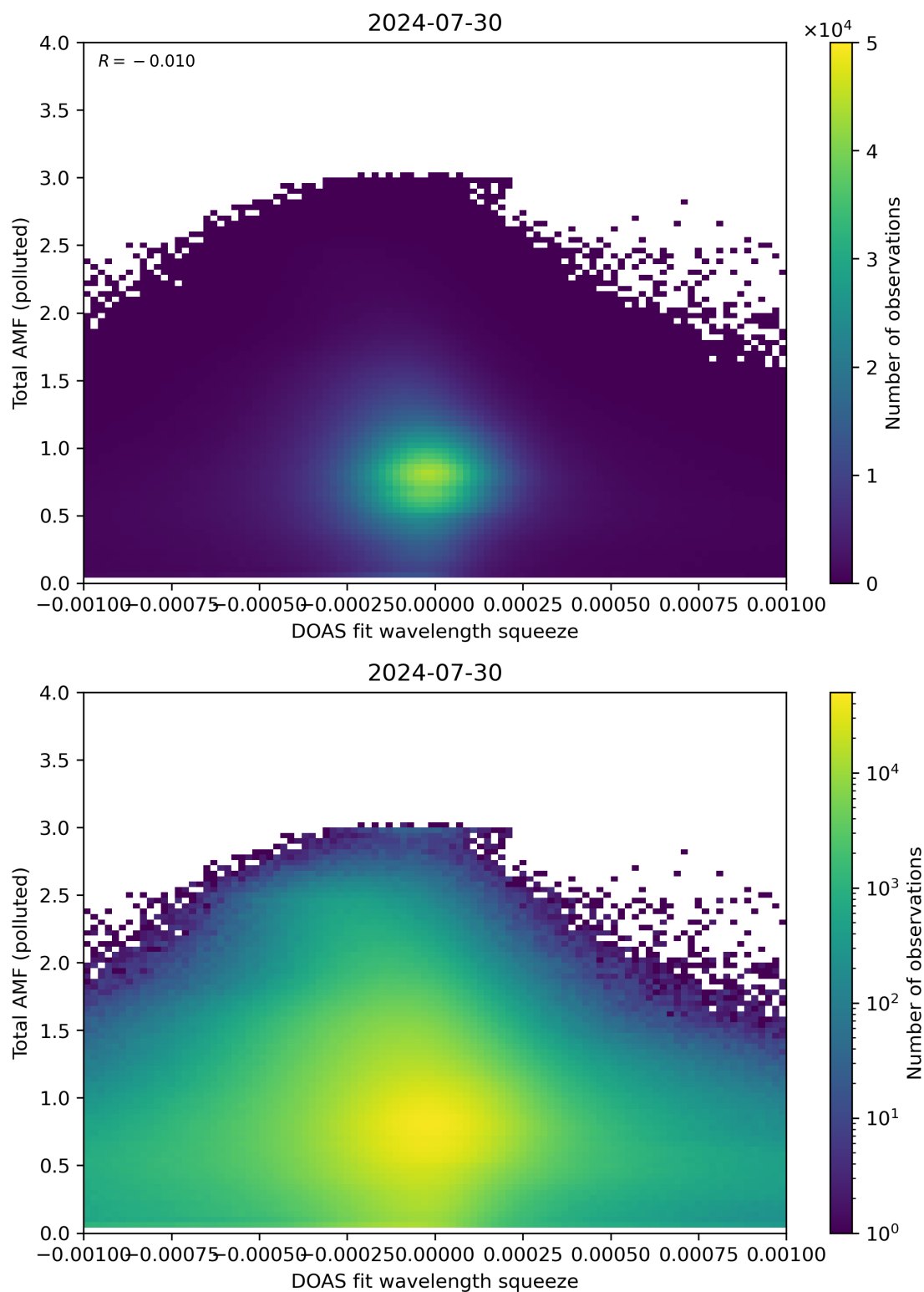
Figure 134: Scatter density plot of “DOAS fit wavelength squeeze” against “Total AMF (polluted)” for 2024-07-29 to 2024-07-31.
