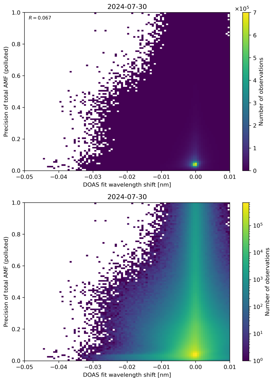
Figure 131: Scatter density plot of “DOAS fit wavelength shift” against “Precision of total AMF (polluted)” for 2024-07-29 to 2024-07-31.
