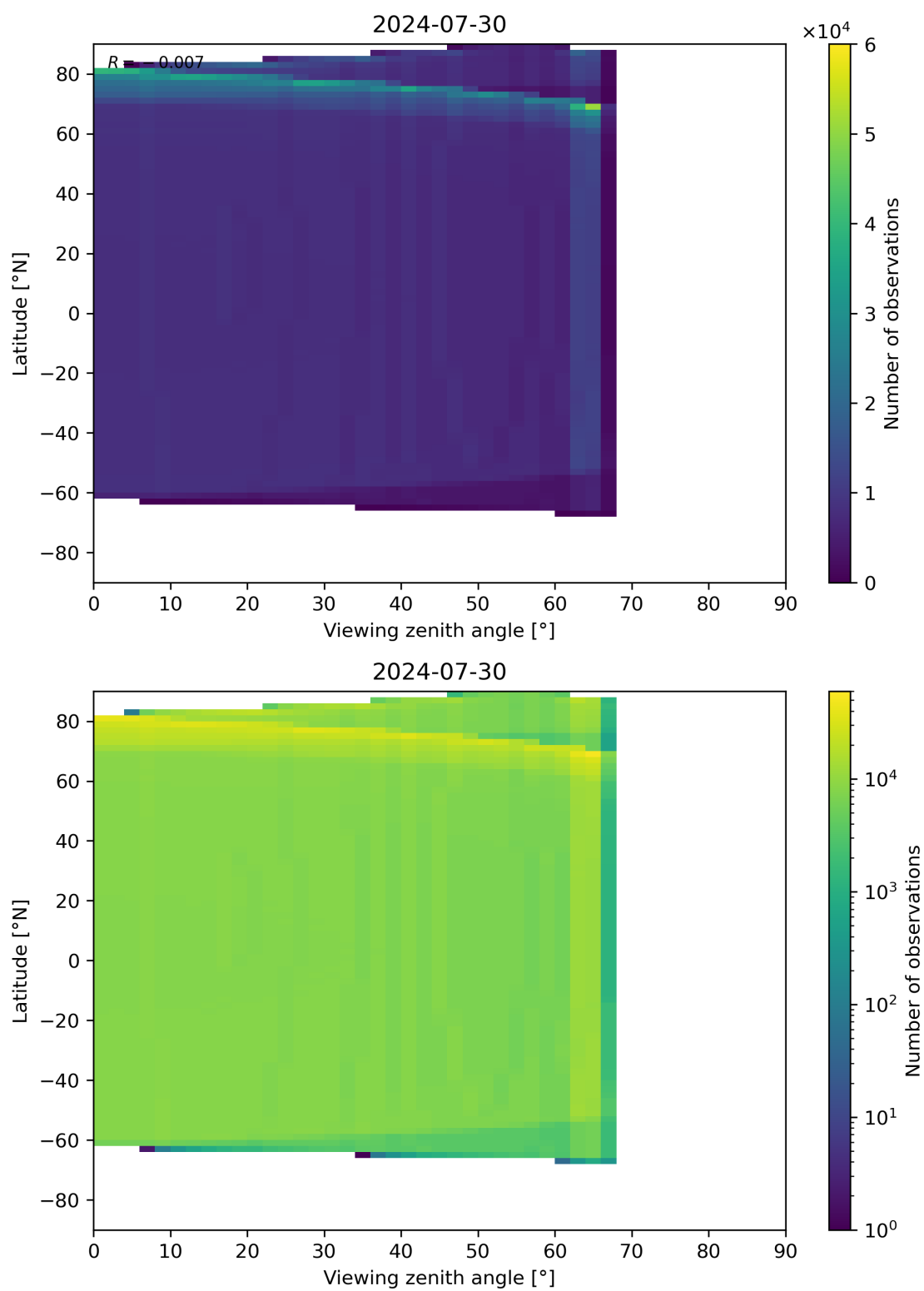
Figure 314: Scatter density plot of “Viewing zenith angle” against “Latitude” for 2024-07-29 to 2024-07-31.
