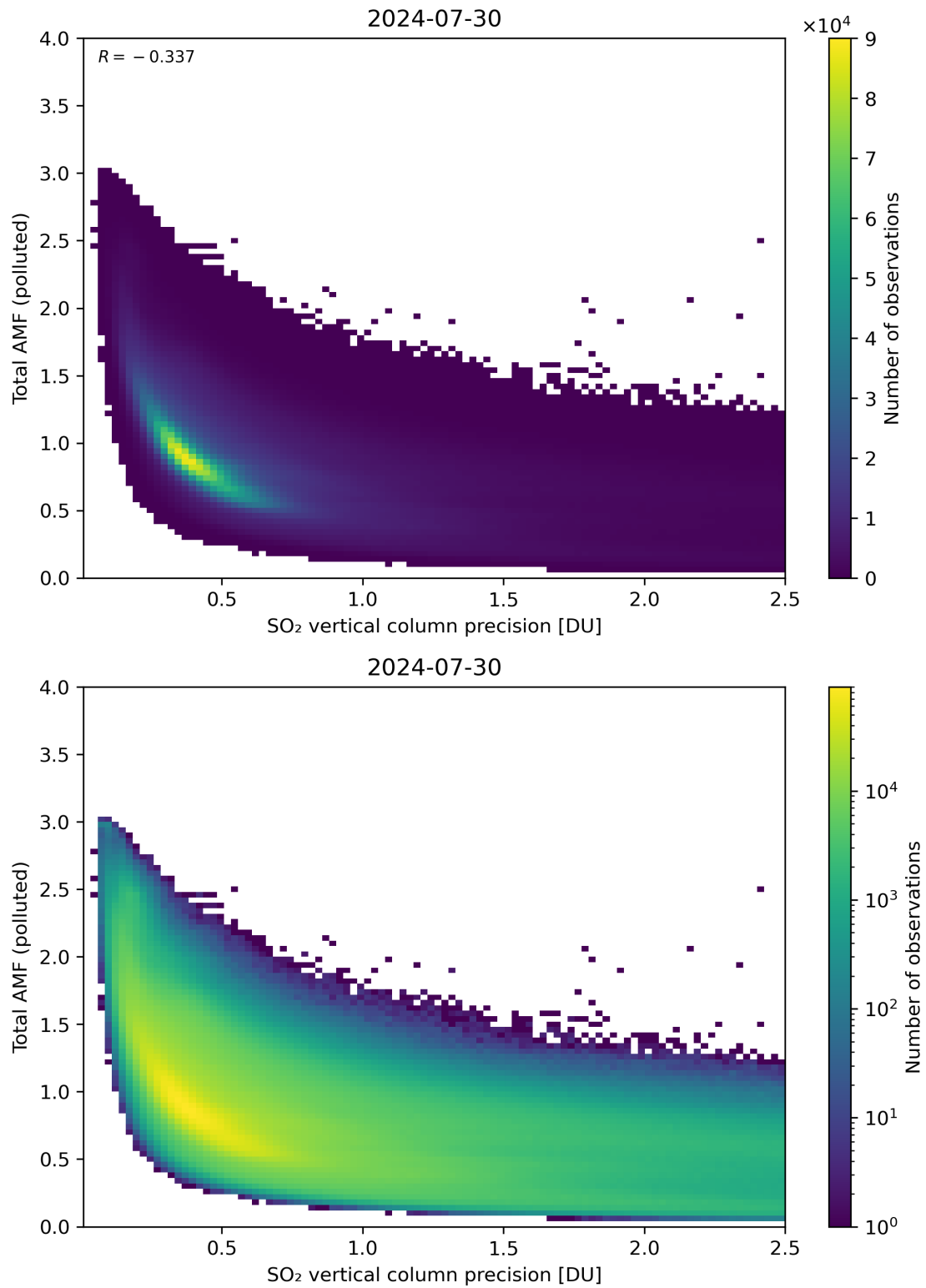
Figure 294: Scatter density plot of “SO 2 vertical column precision” against “Total AMF (polluted)” for 2024-07-29 to 2024-07-31.
