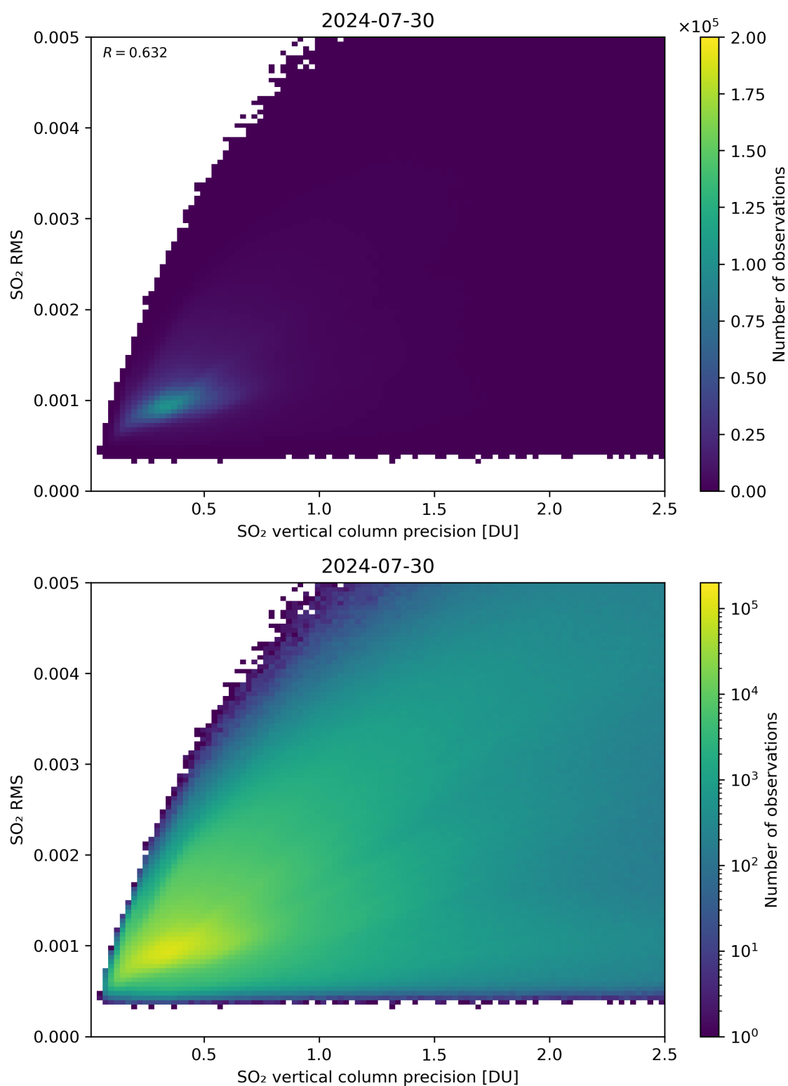
Figure 284: Scatter density plot of “SO 2 vertical column precision” against “SO 2 RMS” for 2024-07-29 to 2024-07-31.
