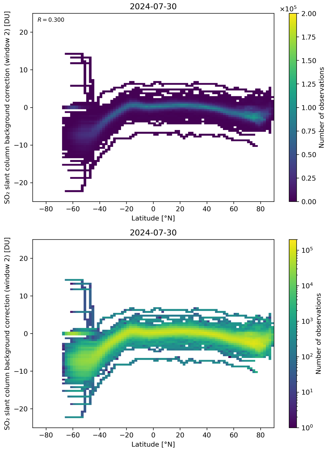
Figure 140: Scatter density plot of “Latitude” against “SO 2 slant column background correction (window 2)” for 2024-07-29 to 2024-07-31.
