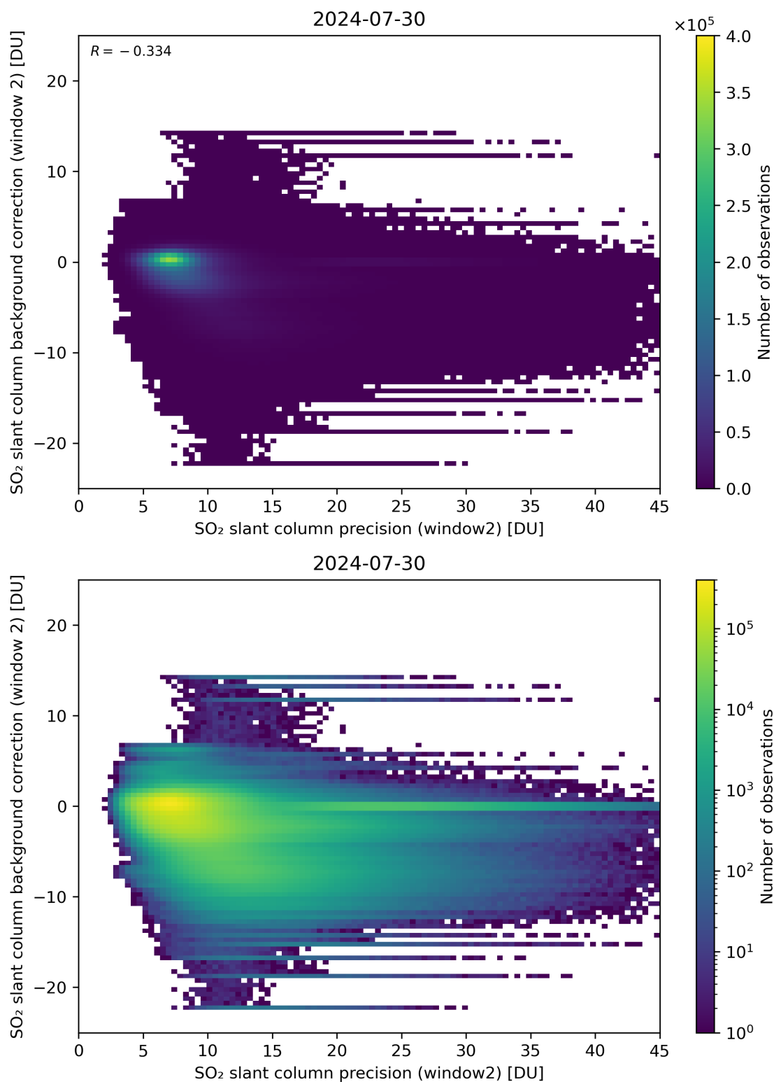
Figure 241: Scatter density plot of “SO 2 slant column precision (window2)” against “SO 2 slant column background correction (window 2)” for 2024-07-29 to 2024-07-31.
