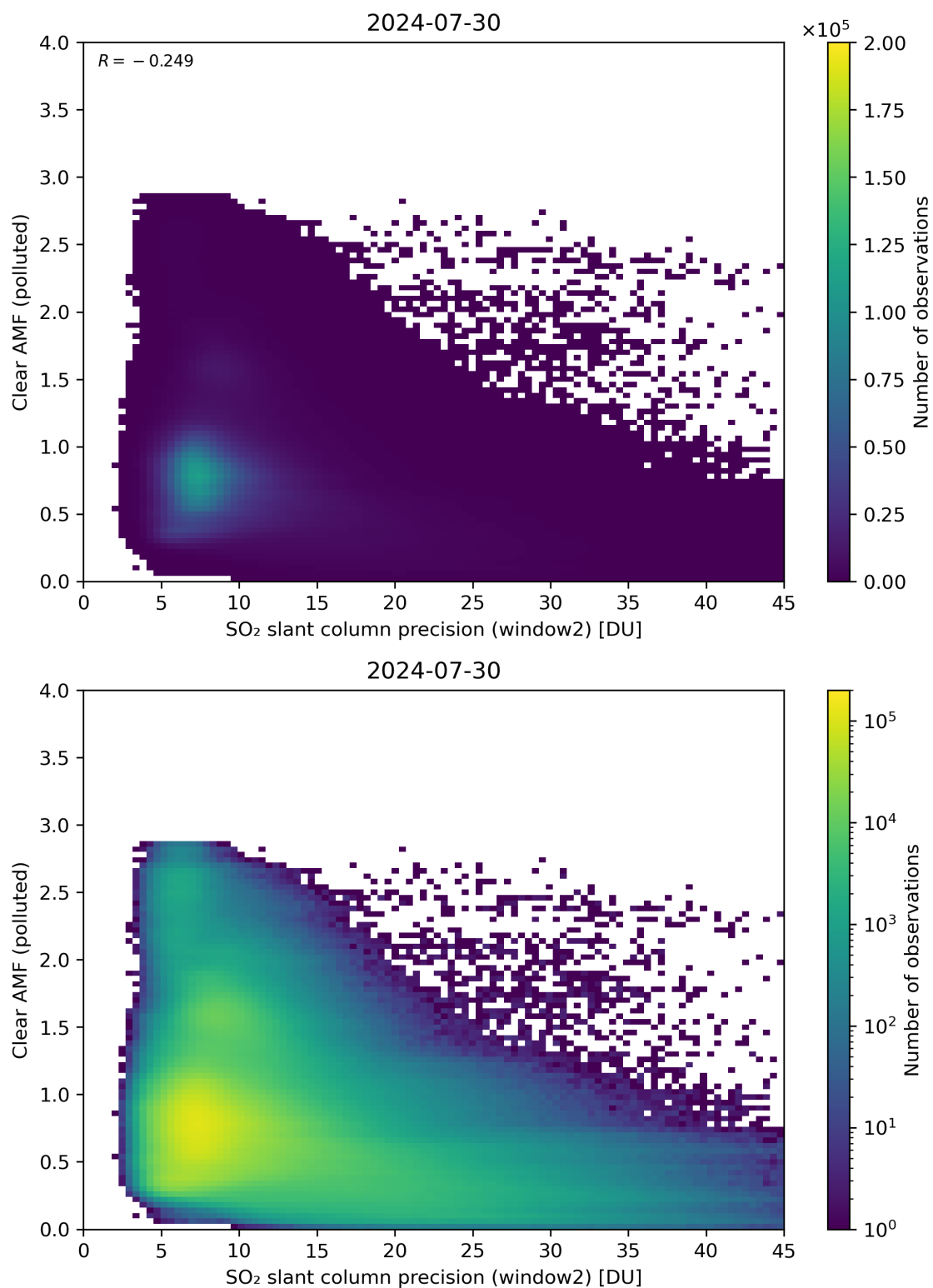
Figure 246: Scatter density plot of “SO 2 slant column precision (window2)” against “Clear AMF (polluted)” for 2024-07-29 to 2024-07-31.
