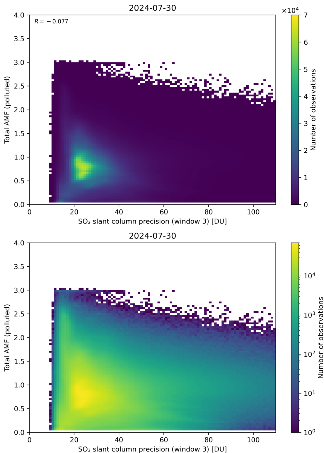
Figure 263: Scatter density plot of “SO 2 slant column precision (window 3)” against “Total AMF (polluted)” for 2024-07-29 to 2024-07-31.
