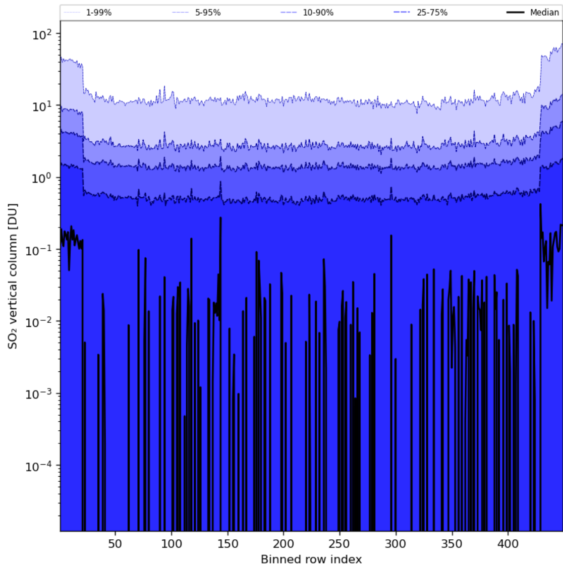
Figure 76: Along track statistics of “SO 2 vertical column” for 2024-07-29 to 2024-07-31
