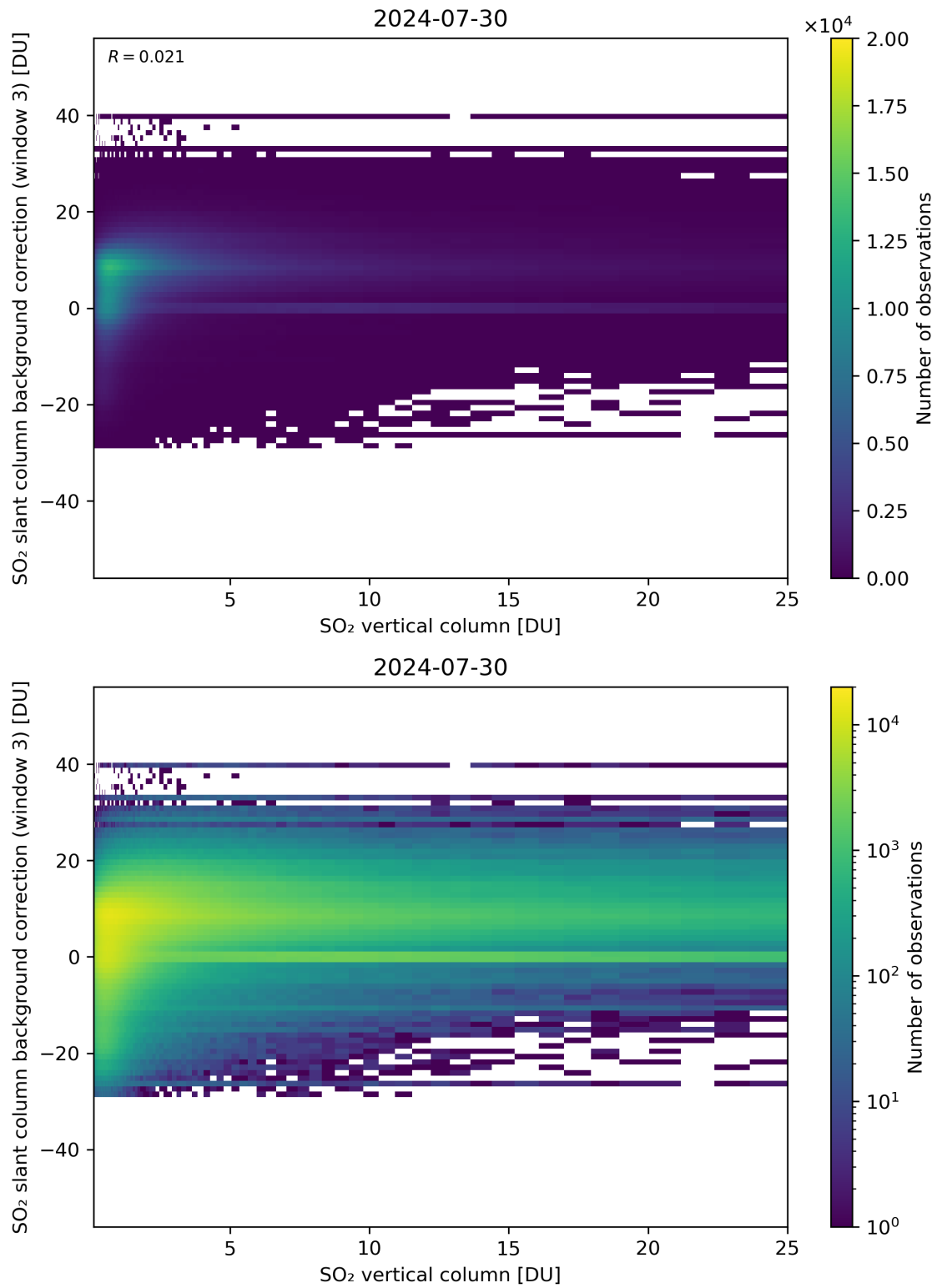
Figure 275: Scatter density plot of “SO 2 vertical column” against “SO 2 slant column background correction (window 3)” for 2024-07-29 to 2024-07-31.
