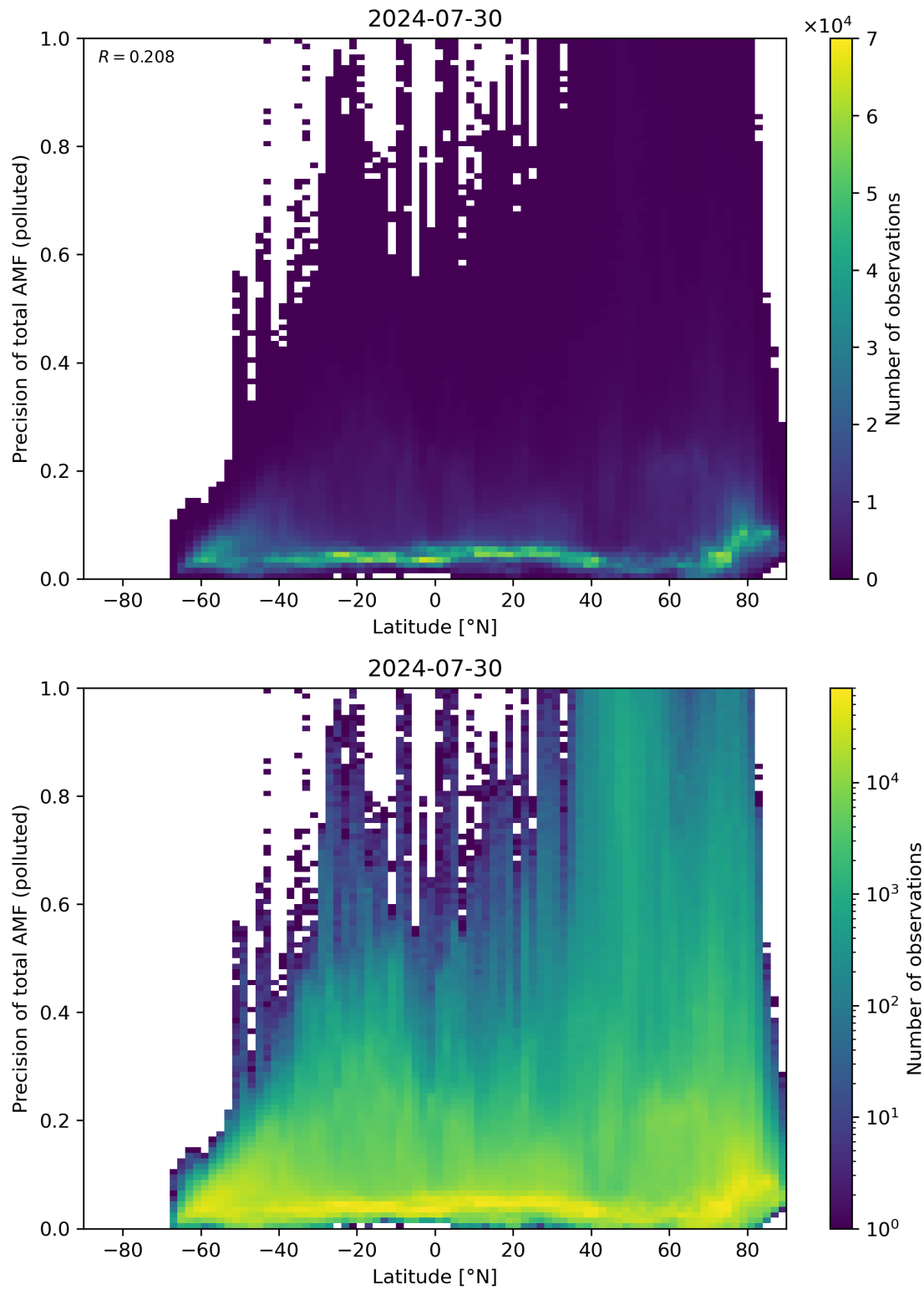
Figure 155: Scatter density plot of “Latitude” against “Precision of total AMF (polluted)” for 2024-07-29 to 2024-07-31.
