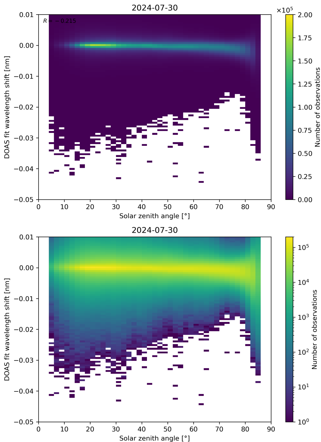
Figure 161: Scatter density plot of “Solar zenith angle” against “DOAS fit wavelength shift” for 2024-07-29 to 2024-07-31.
