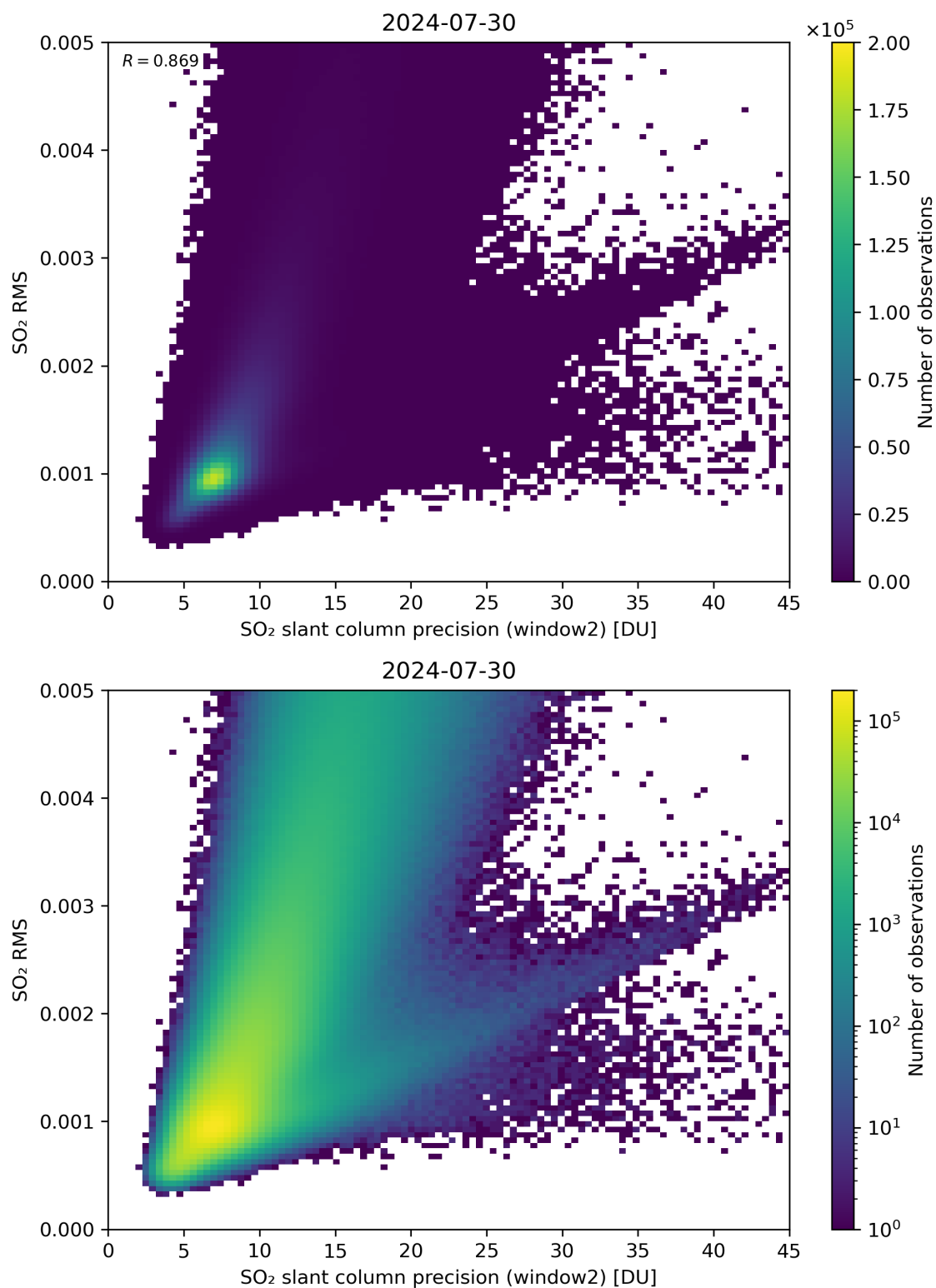
Figure 245: Scatter density plot of “SO 2 slant column precision (window2)” against “SO 2 RMS” for 2024-07-29 to 2024-07-31.
