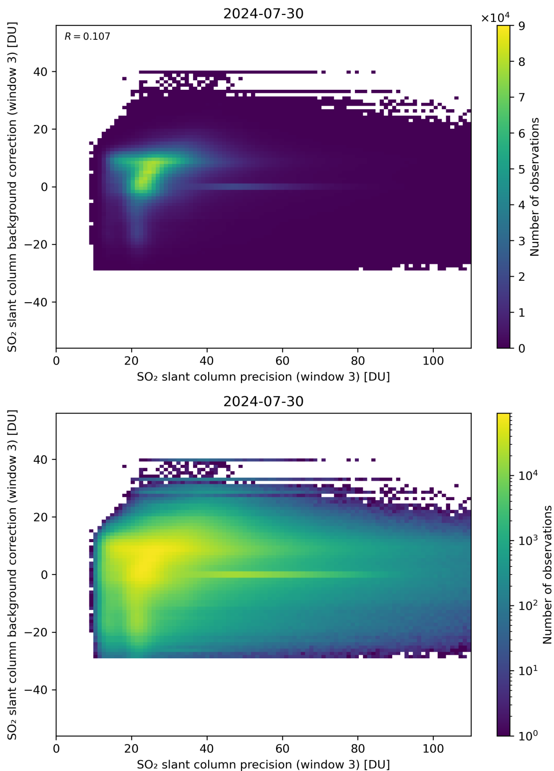
Figure 257: Scatter density plot of “SO 2 slant column precision (window 3)” against “SO 2 slant column background correction (window 3)” for 2024-07-29 to 2024-07-31.
