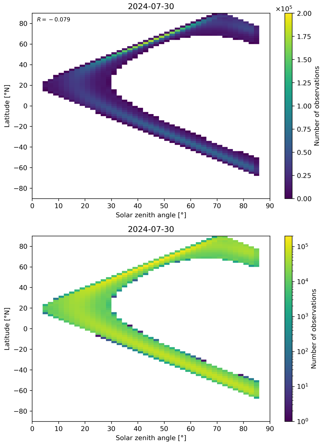
Figure 164: Scatter density plot of “Solar zenith angle” against “Latitude” for 2024-07-29 to 2024-07-31.
