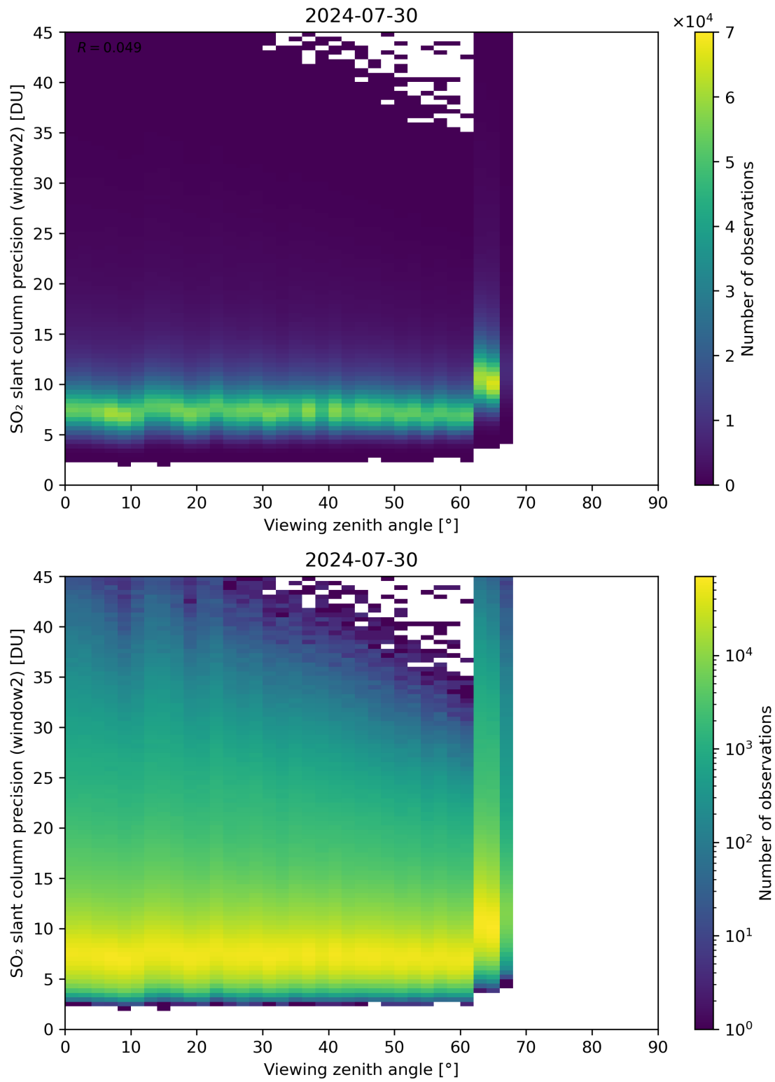
Figure 322: Scatter density plot of “Viewing zenith angle” against “SO 2 slant column precision (window2)” for 2024-07-29 to 2024-07-31.
