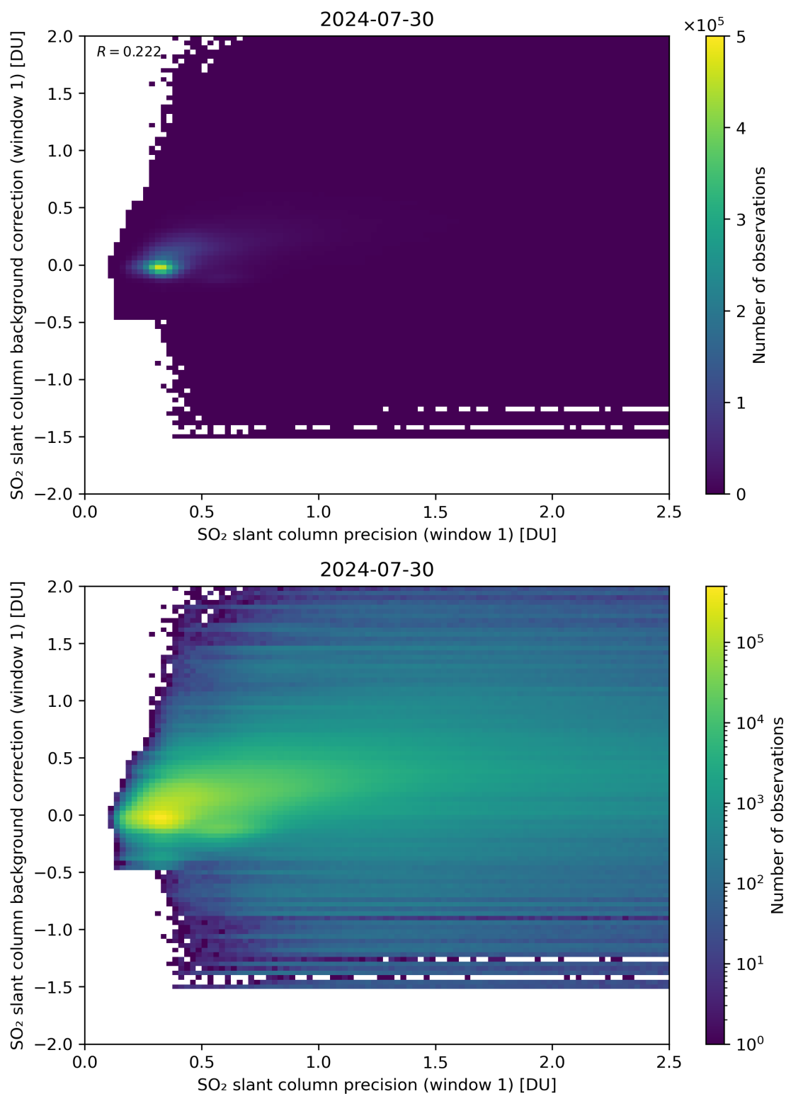
Figure 218: Scatter density plot of “SO 2 slant column precision (window 1)” against “SO 2 slant column background correction (window 1)” for 2024-07-29 to 2024-07-31.
