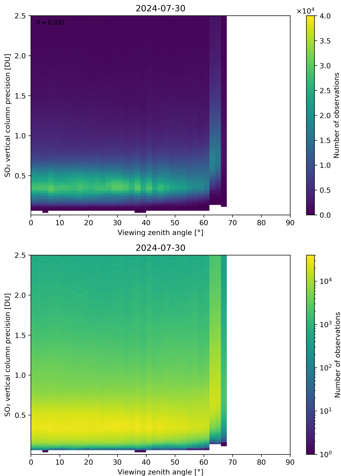
Figure 328: Scatter density plot of “Viewing zenith angle” against “SO 2 vertical column precision” for 2024-07-29 to 2024-07-31.
