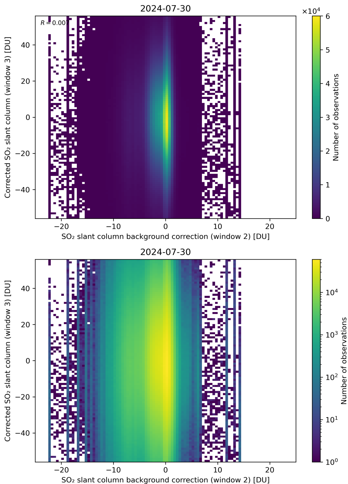
Figure 116: Scatter density plot of “SO 2 slant column background correction (window 2)” against “Corrected SO 2 slant column (window 3)” for 2024-07-29 to 2024-07-31.
