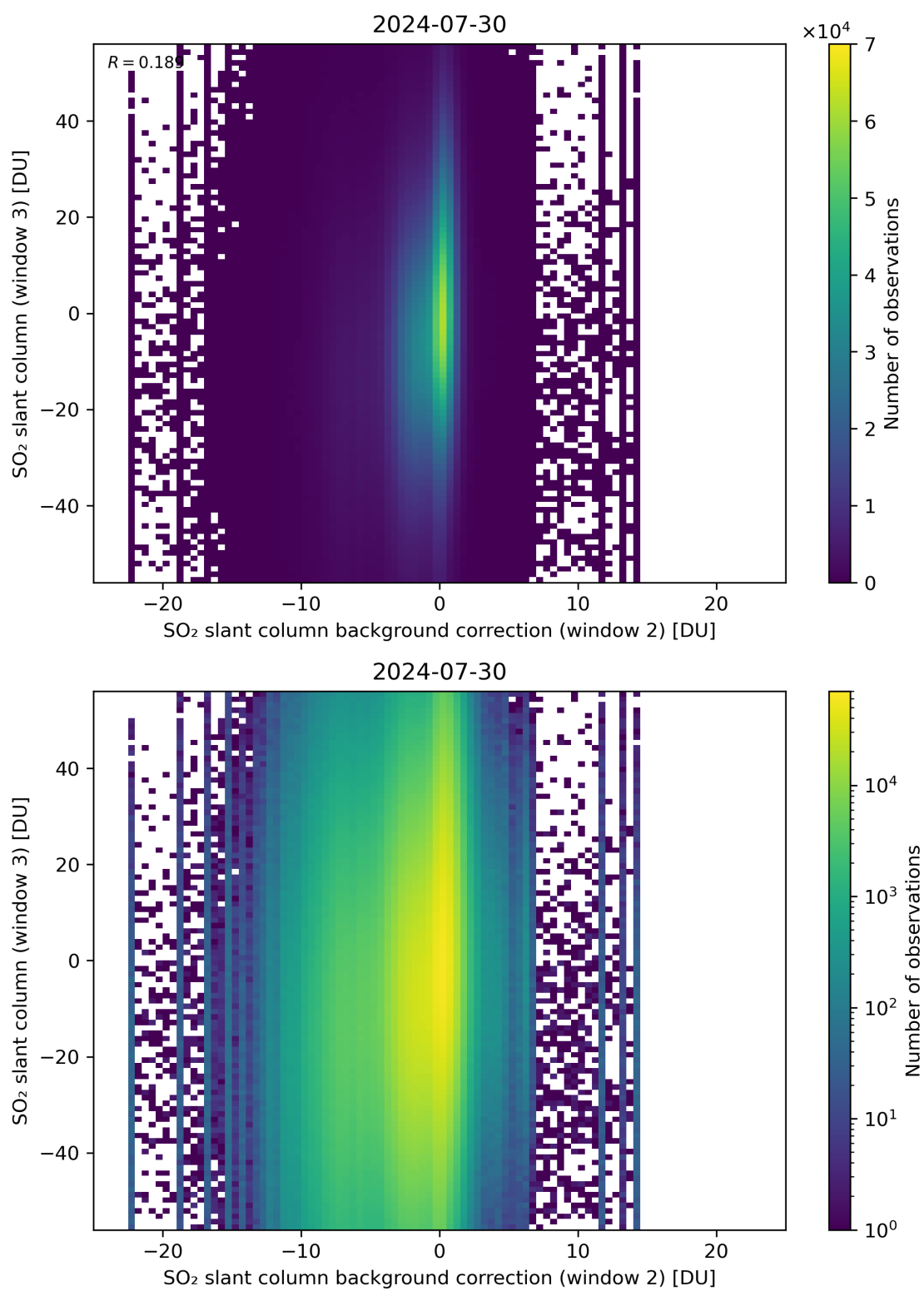
Figure 117: Scatter density plot of “SO 2 slant column background correction (window 2)” against “SO 2 slant column (window 3)” for 2024-07-29 to 2024-07-31.
