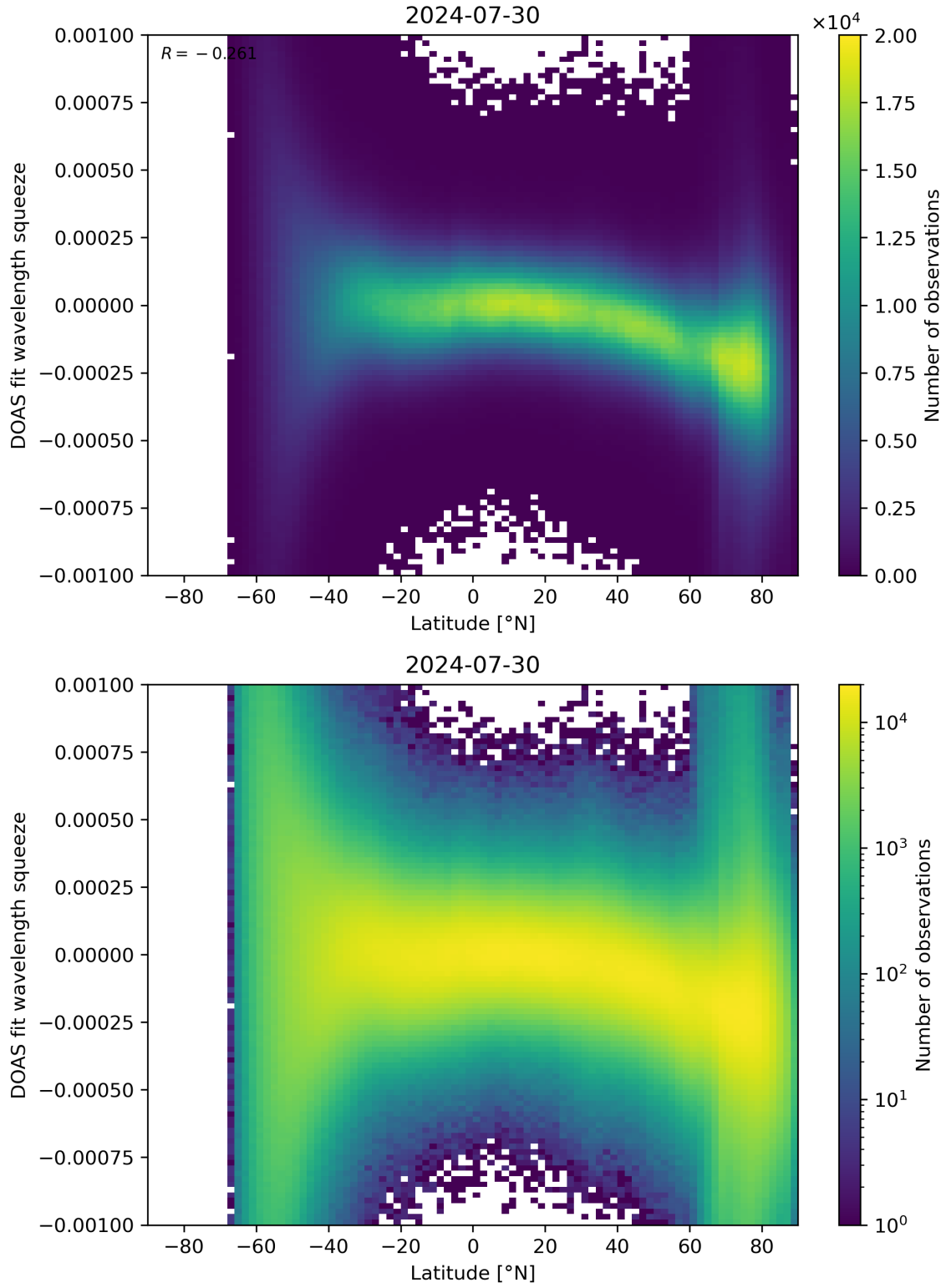
Figure 143: Scatter density plot of “Latitude” against “DOAS fit wavelength squeeze” for 2024-07-29 to 2024-07-31.
