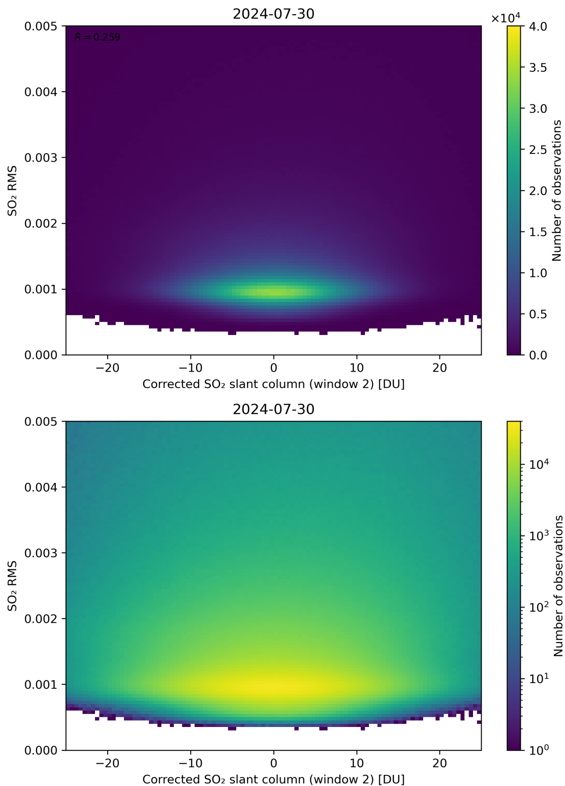
Figure 198: Scatter density plot of “Corrected SO 2 slant column (window 2)” against “SO 2 RMS” for 2024-07-29 to 2024-07-31.
