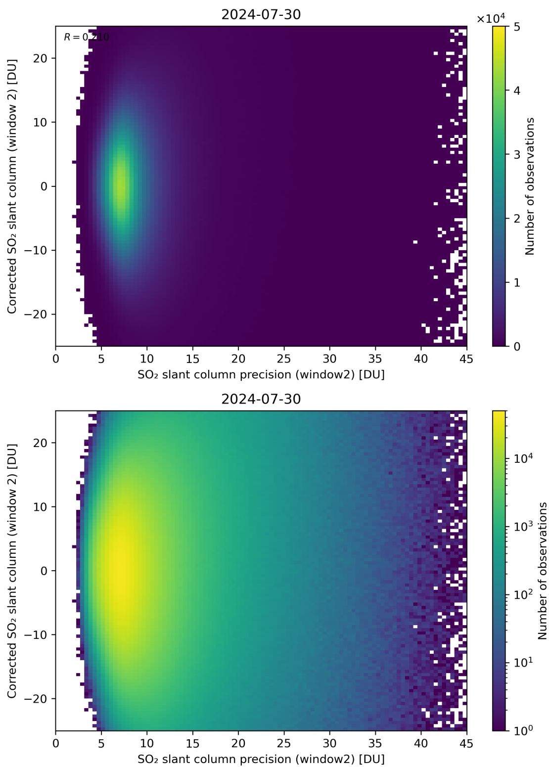
Figure 247: Scatter density plot of “SO 2 slant column precision (window2)” against “Corrected SO 2 slant column (window 2)” for 2024-07-29 to 2024-07-31.
