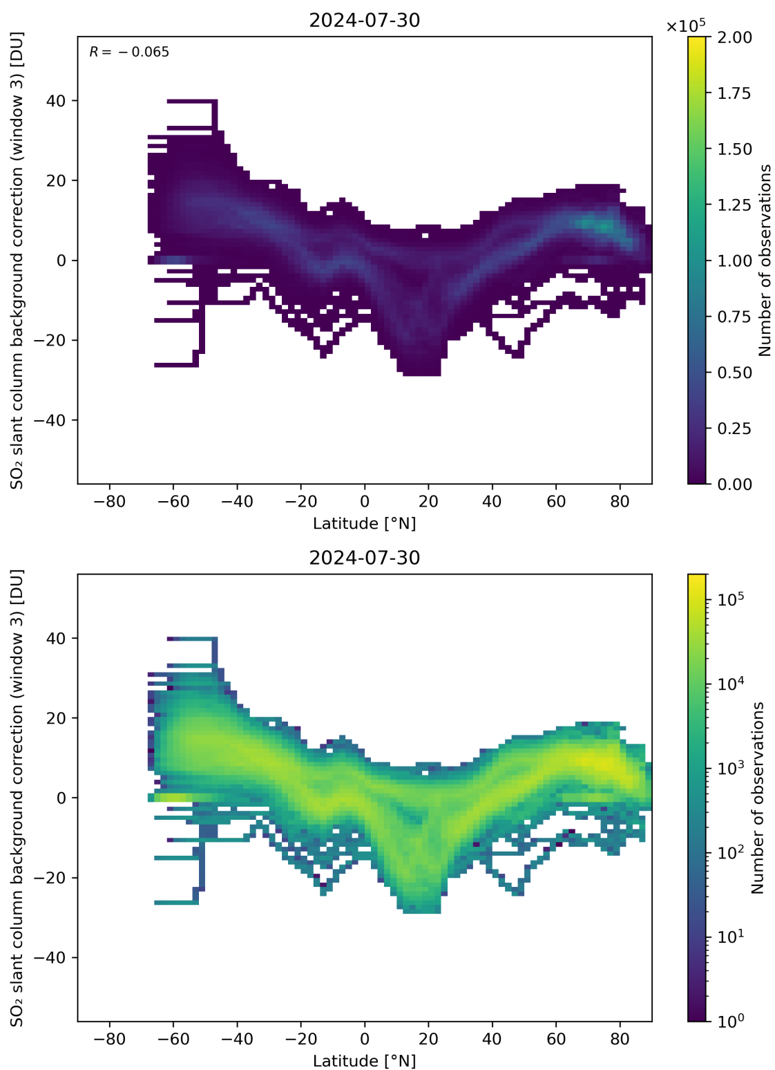
Figure 141: Scatter density plot of “Latitude” against “SO 2 slant column background correction (window 3)” for 2024-07-29 to 2024-07-31.
