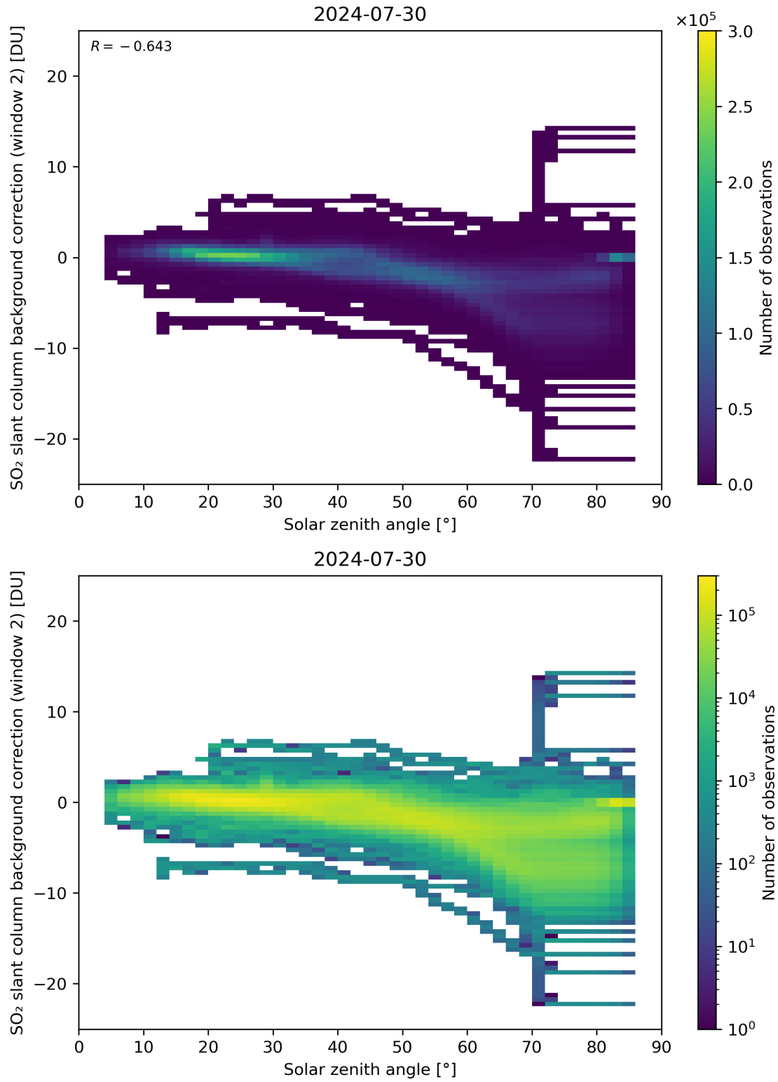
Figure 159: Scatter density plot of “Solar zenith angle” against “SO 2 slant column background correction (window 2)” for 2024-07-29 to 2024-07-31.
