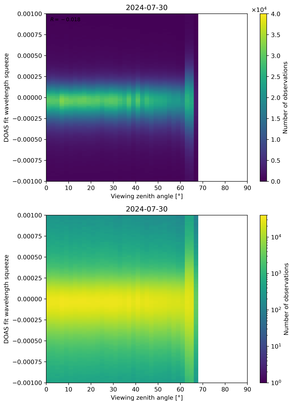
Figure 312: Scatter density plot of “Viewing zenith angle” against “DOAS fit wavelength squeeze” for 2024-07-29 to 2024-07-31.
