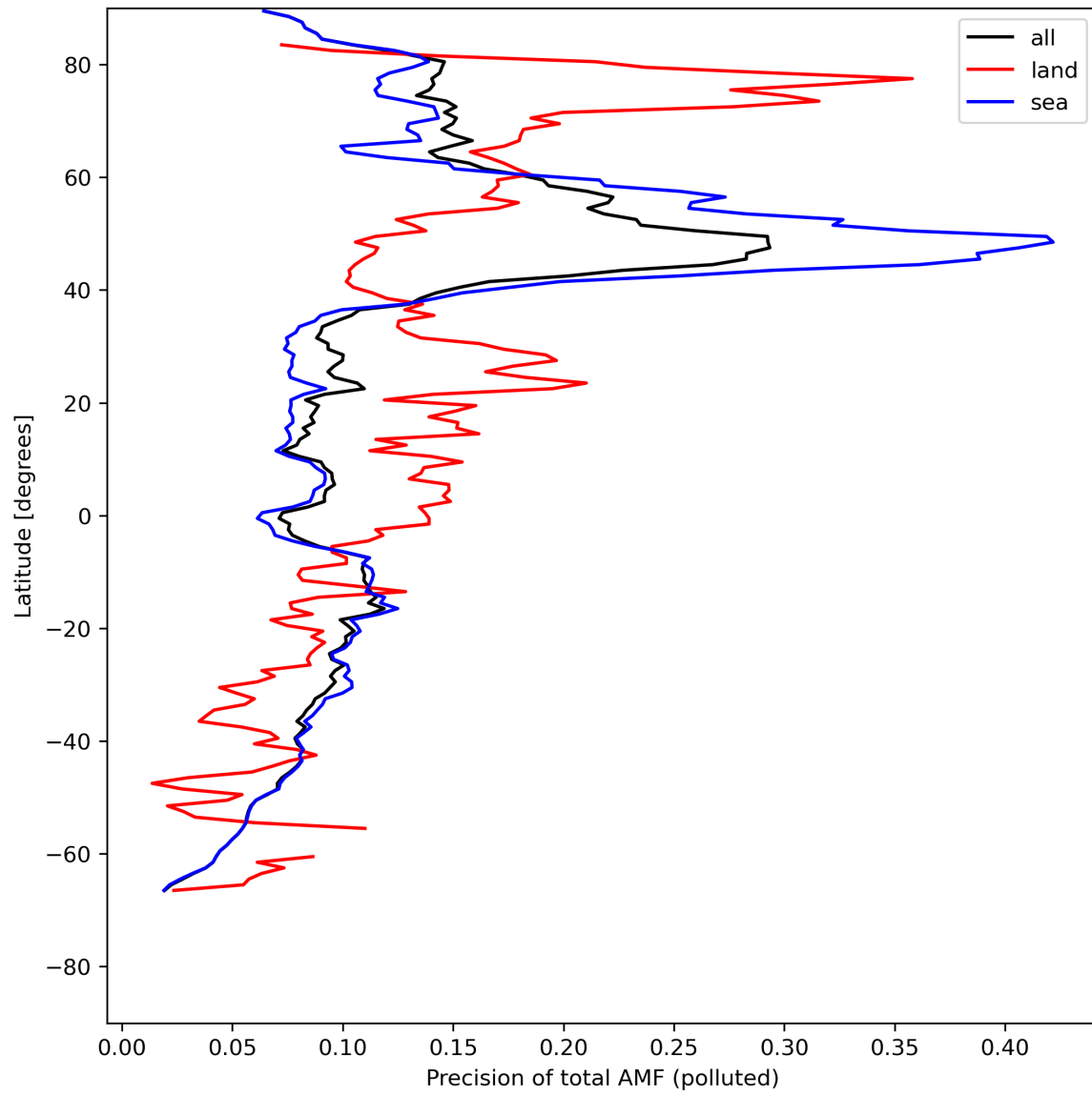
Figure 49: Zonal average of “Precision of total AMF (polluted)” for 2024-07-29 to 2024-07-31.
