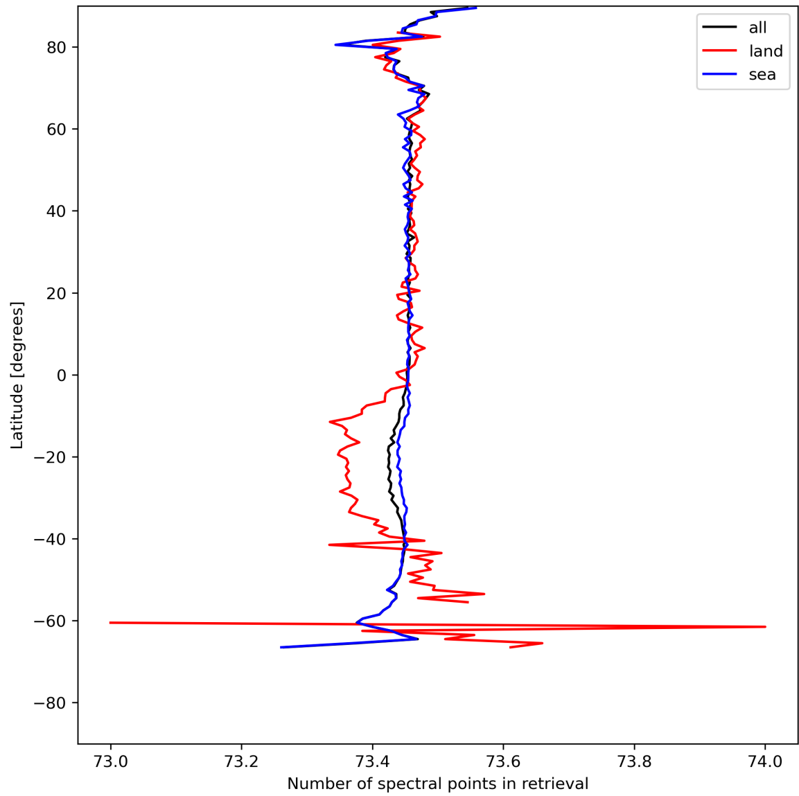
Figure 51: Zonal average of “Number of spectral points in retrieval” for 2024-07-29 to 2024-07-31.
