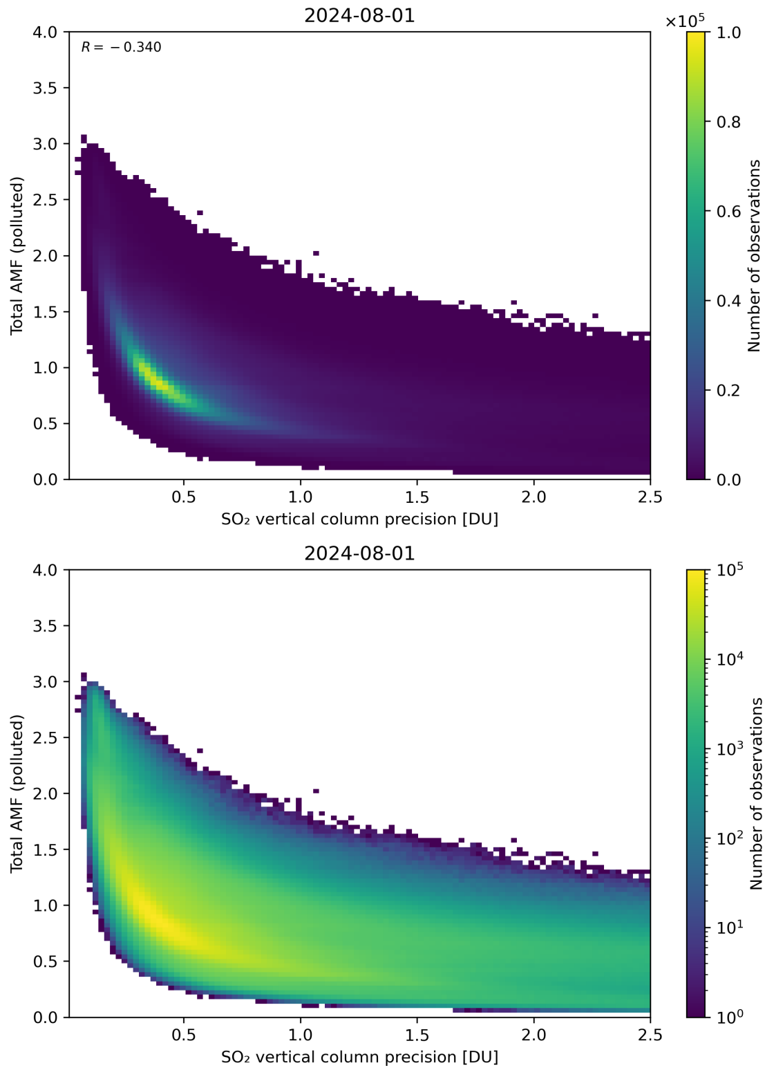
Figure 294: Scatter density plot of “SO 2 vertical column precision” against “Total AMF (polluted)” for 2024-07-31 to 2024-08-02.
