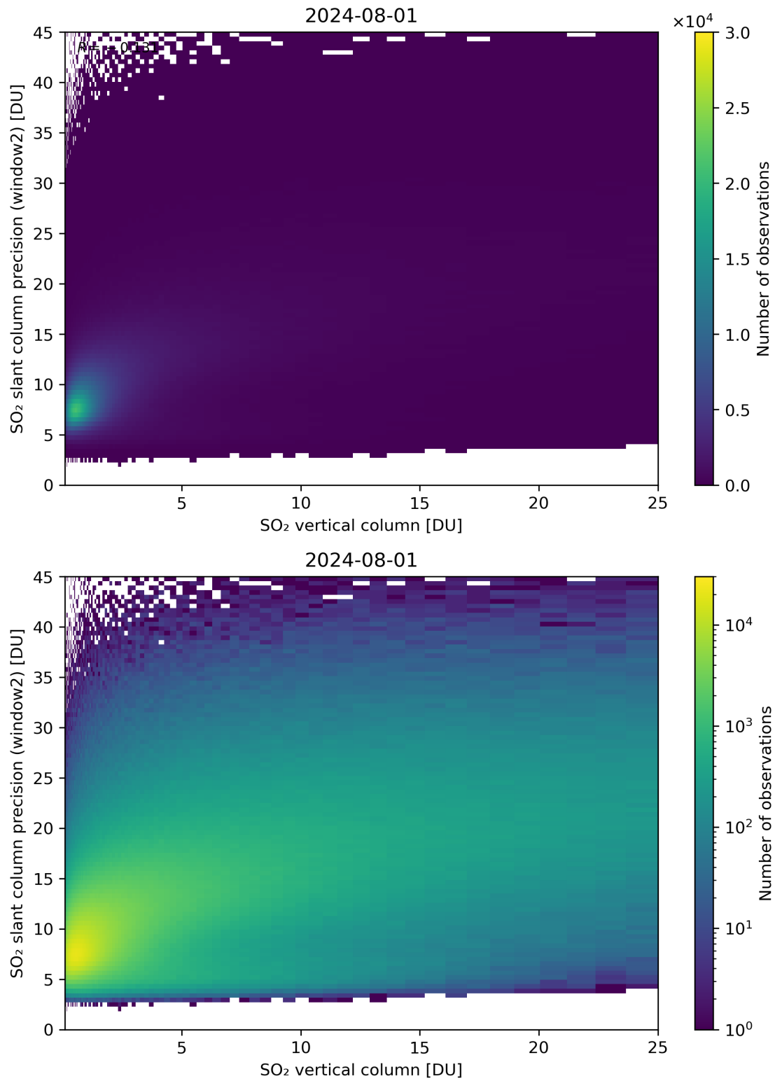
Figure 302: Scatter density plot of “SO 2 vertical column” against “SO 2 slant column precision (window2)” for 2024-07-31 to 2024-08-02.
