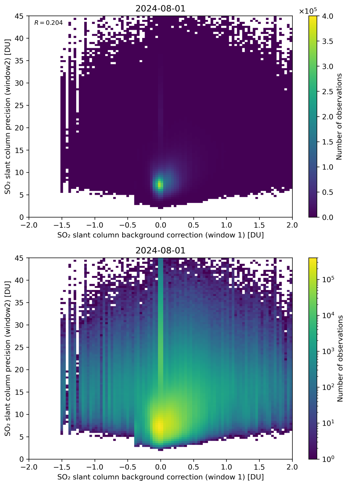
Figure 106: Scatter density plot of “SO 2 slant column background correction (window 1)” against “SO 2 slant column precision (window2)” for 2024-07-31 to 2024-08-02.
