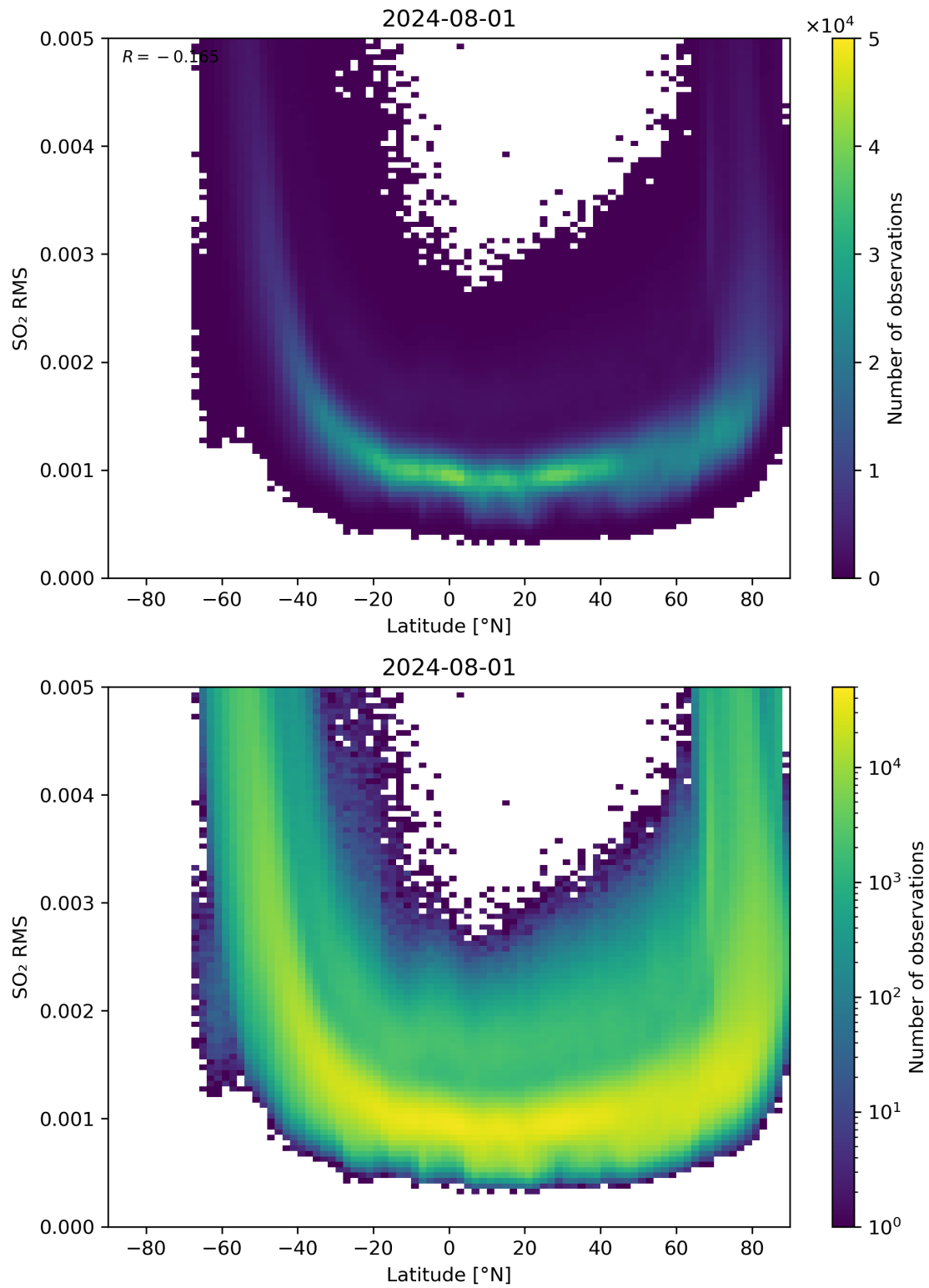
Figure 144: Scatter density plot of “Latitude” against “SO 2 RMS” for 2024-07-31 to 2024-08-02.
