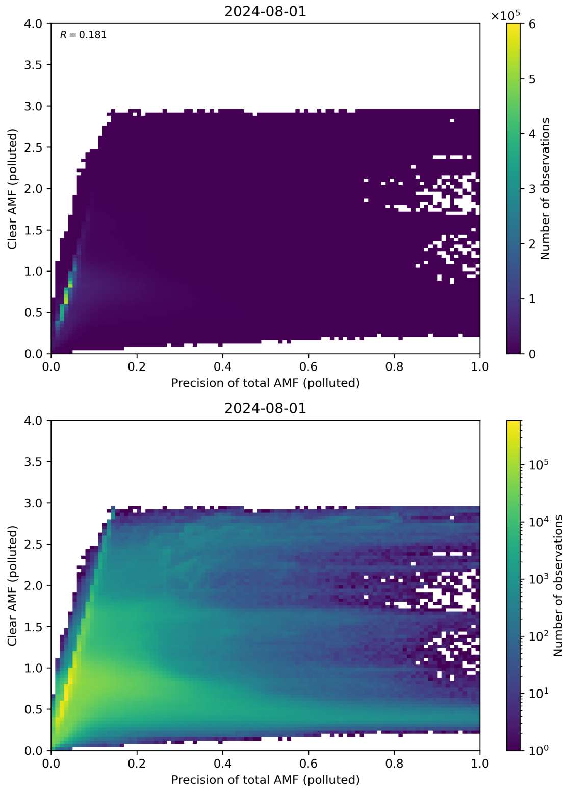
Figure 270: Scatter density plot of “Precision of total AMF (polluted)” against “Clear AMF (polluted)” for 2024-07-31 to 2024-08-02.
