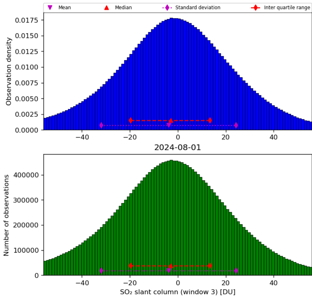
Figure 64: Histogram of “SO 2 slant column (window 3)” for 2024-07-31 to 2024-08-02
