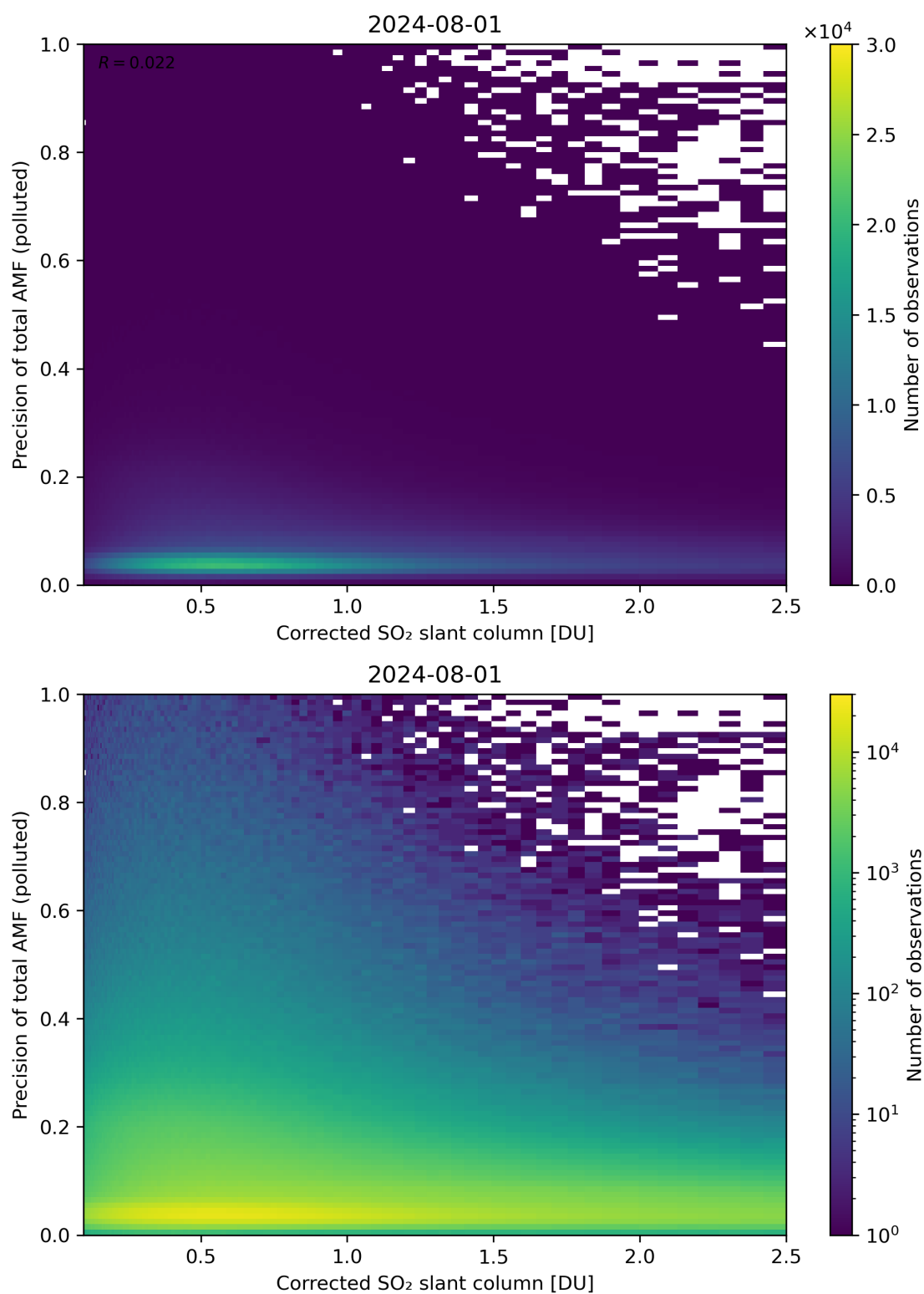
Figure 193: Scatter density plot of “Corrected SO 2 slant column” against “Precision of total AMF (polluted)” for 2024-07-31 to 2024-08-02.
