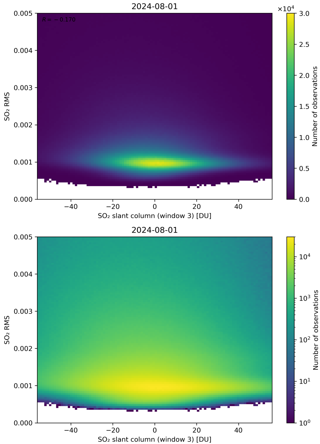
Figure 256: Scatter density plot of “SO 2 slant column (window 3)” against “SO 2 RMS” for 2024-07-31 to 2024-08-02.
