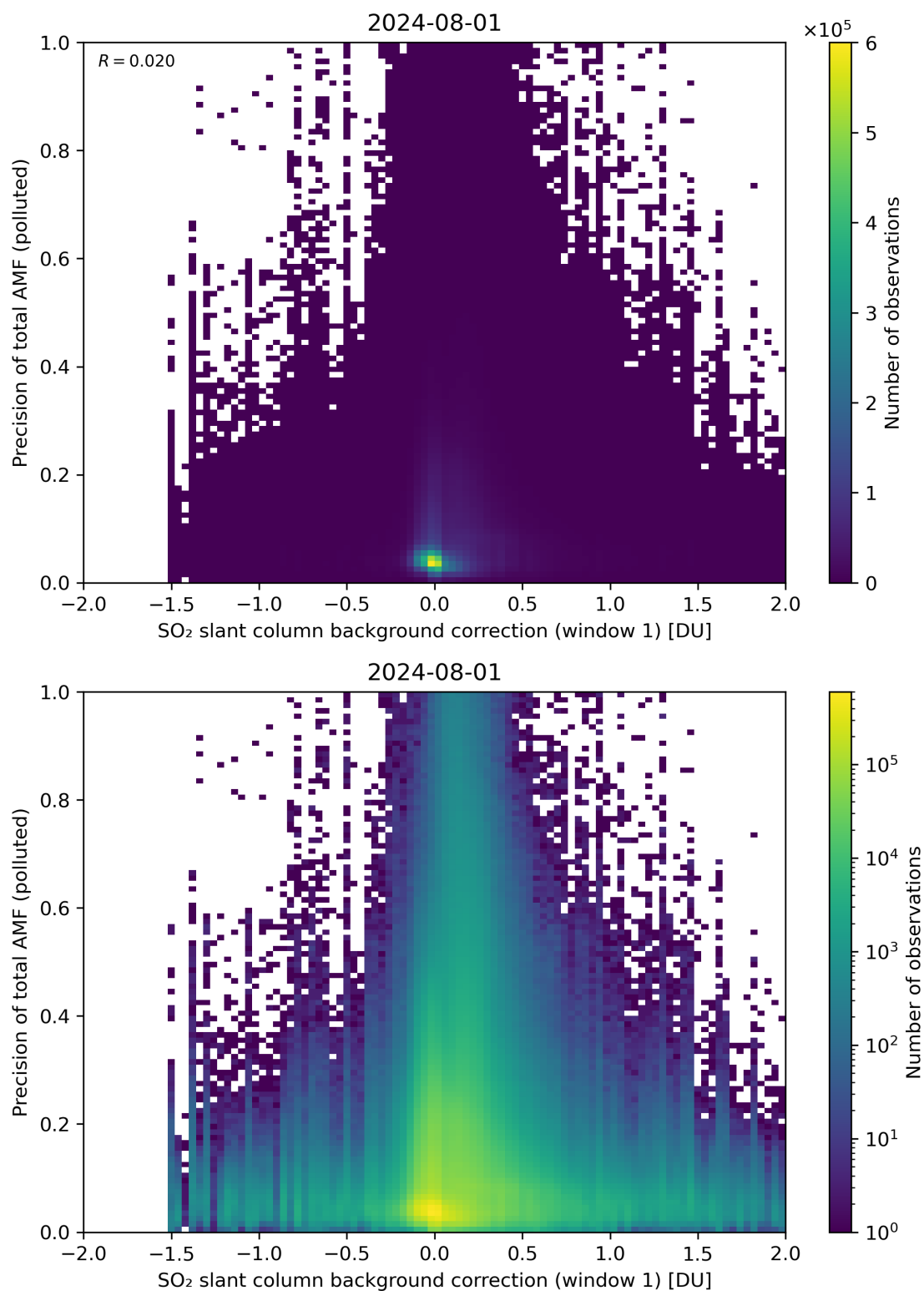
Figure 110: Scatter density plot of “SO 2 slant column background correction (window 1)” against “Precision of total AMF (polluted)” for 2024-07-31 to 2024-08-02.
