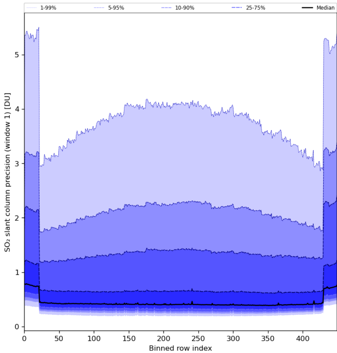
Figure 80: Along track statistics of “SO 2 slant column precision (window 1)” for 2024-07-31 to 2024-08-02
