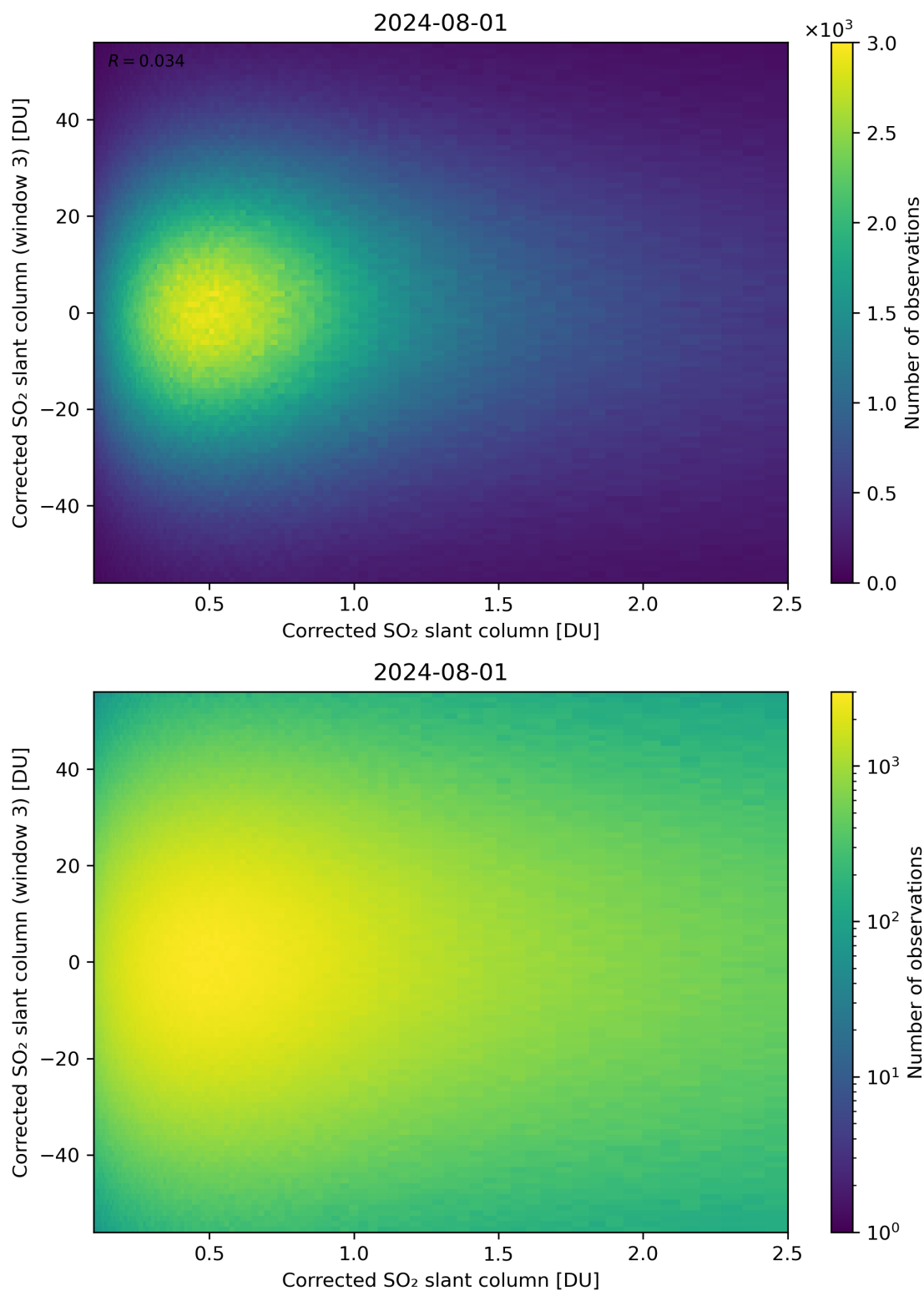
Figure 186: Scatter density plot of “Corrected SO 2 slant column” against “Corrected SO 2 slant column (window 3)” for 2024-07-31 to 2024-08-02.
