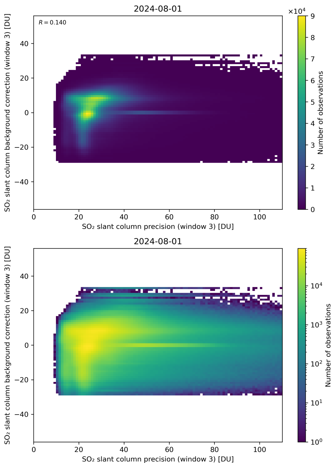
Figure 257: Scatter density plot of “SO 2 slant column precision (window 3)” against “SO 2 slant column background correction (window 3)” for 2024-07-31 to 2024-08-02.
