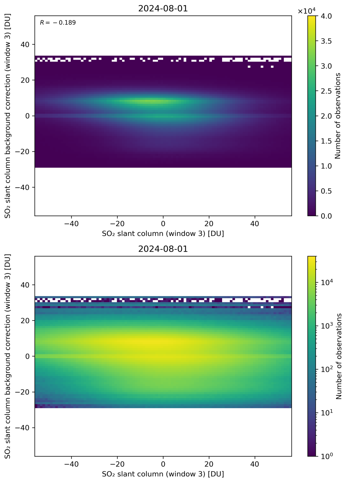
Figure 253: Scatter density plot of “SO 2 slant column (window 3)” against “SO 2 slant column background correction (window 3)” for 2024-07-31 to 2024-08-02.
