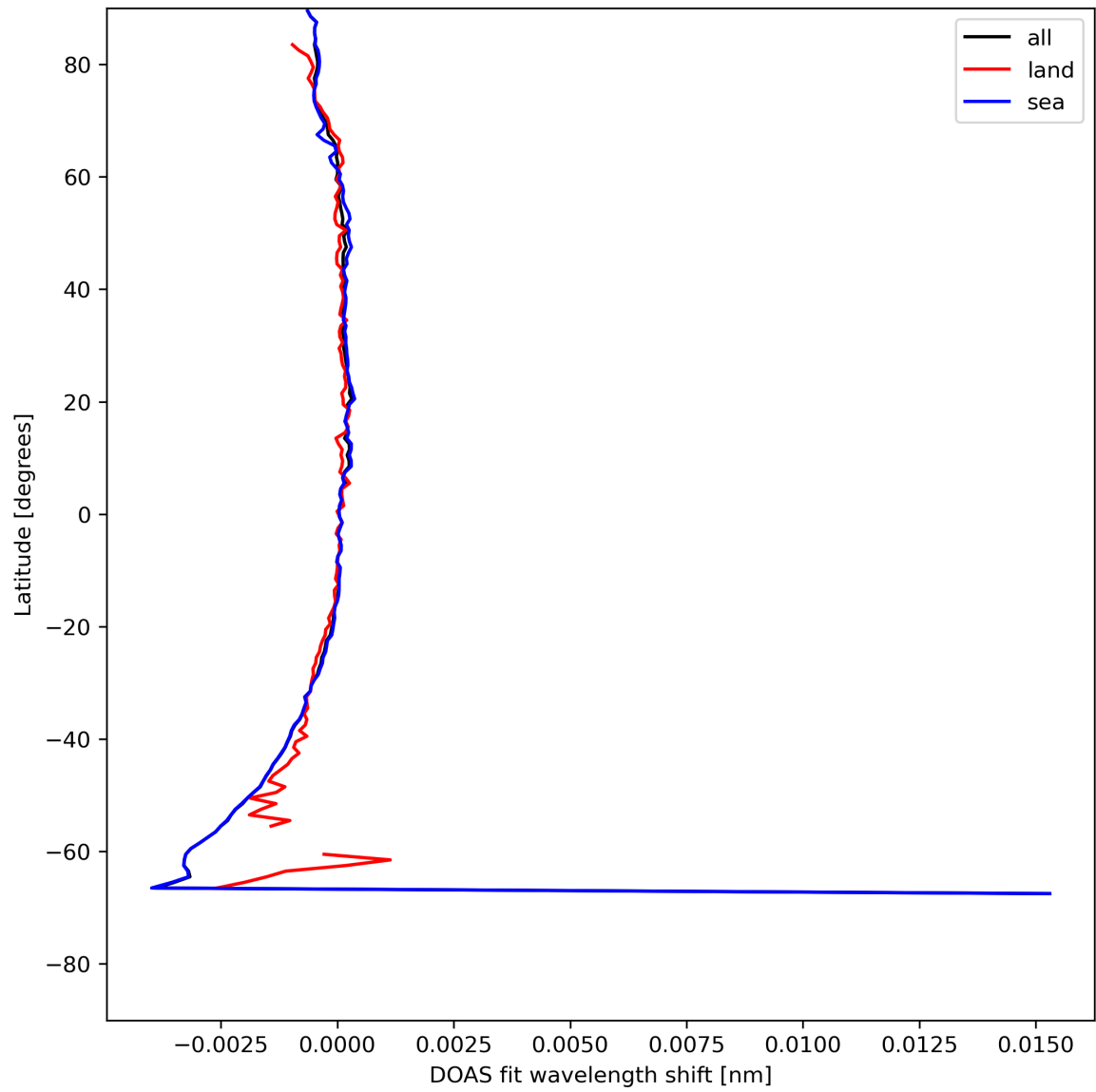
Figure 45: Zonal average of "DOAS fit wavelength shift" for 2024-07-31 to 2024-08-02.
