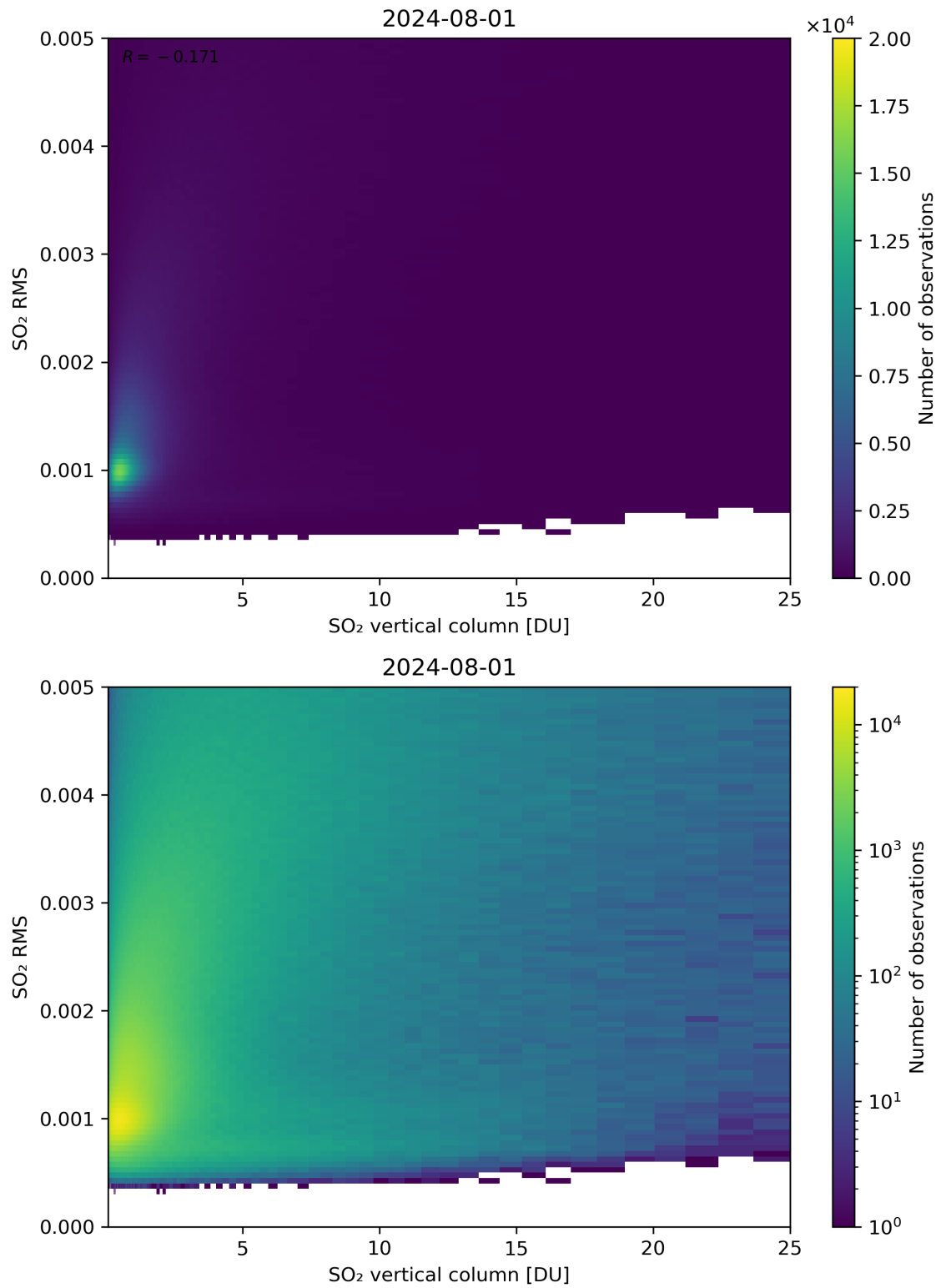
Figure 278: Scatter density plot of “SO 2 vertical column” against “SO 2 RMS” for 2024-07-31 to 2024-08-02.
