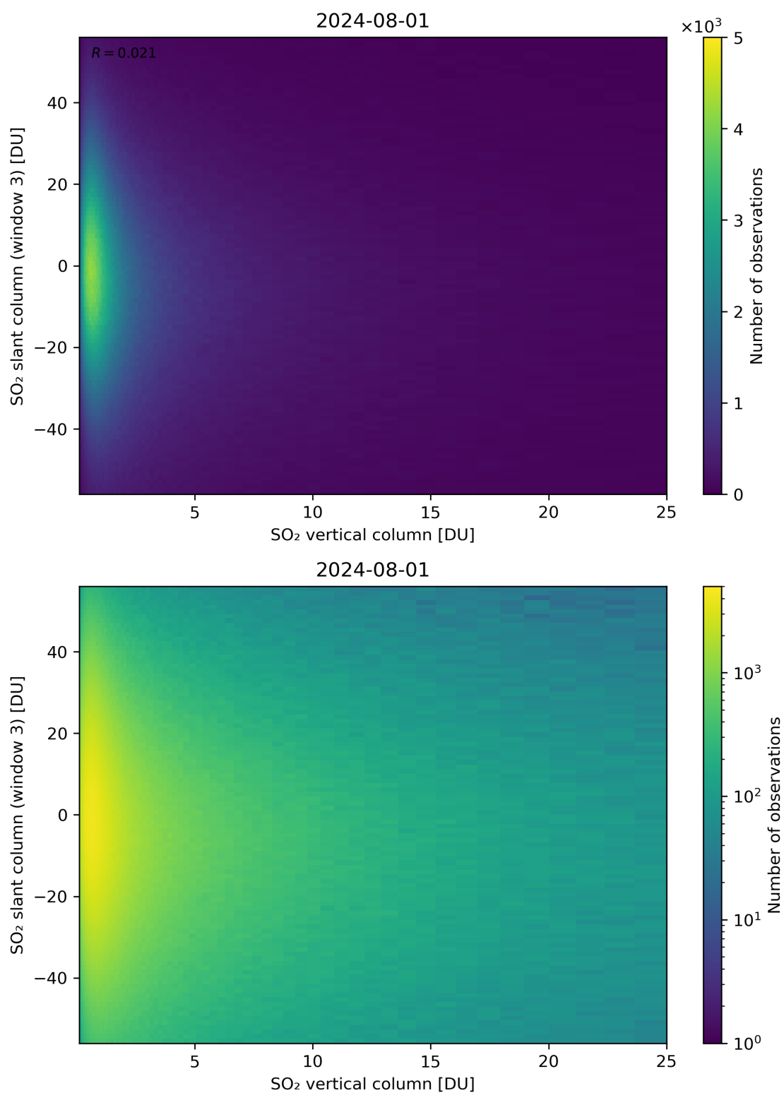
Figure 303: Scatter density plot of “SO 2 vertical column” against “SO 2 slant column (window 3)” for 2024-07-31 to 2024-08-02.
