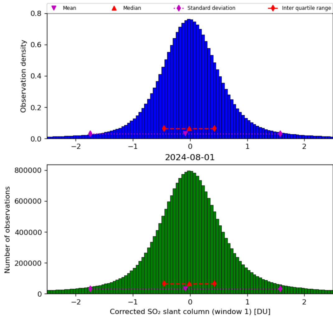
Figure 58: Histogram of “Corrected SO 2 slant column (window 1)” for 2024-07-31 to 2024-08-02
