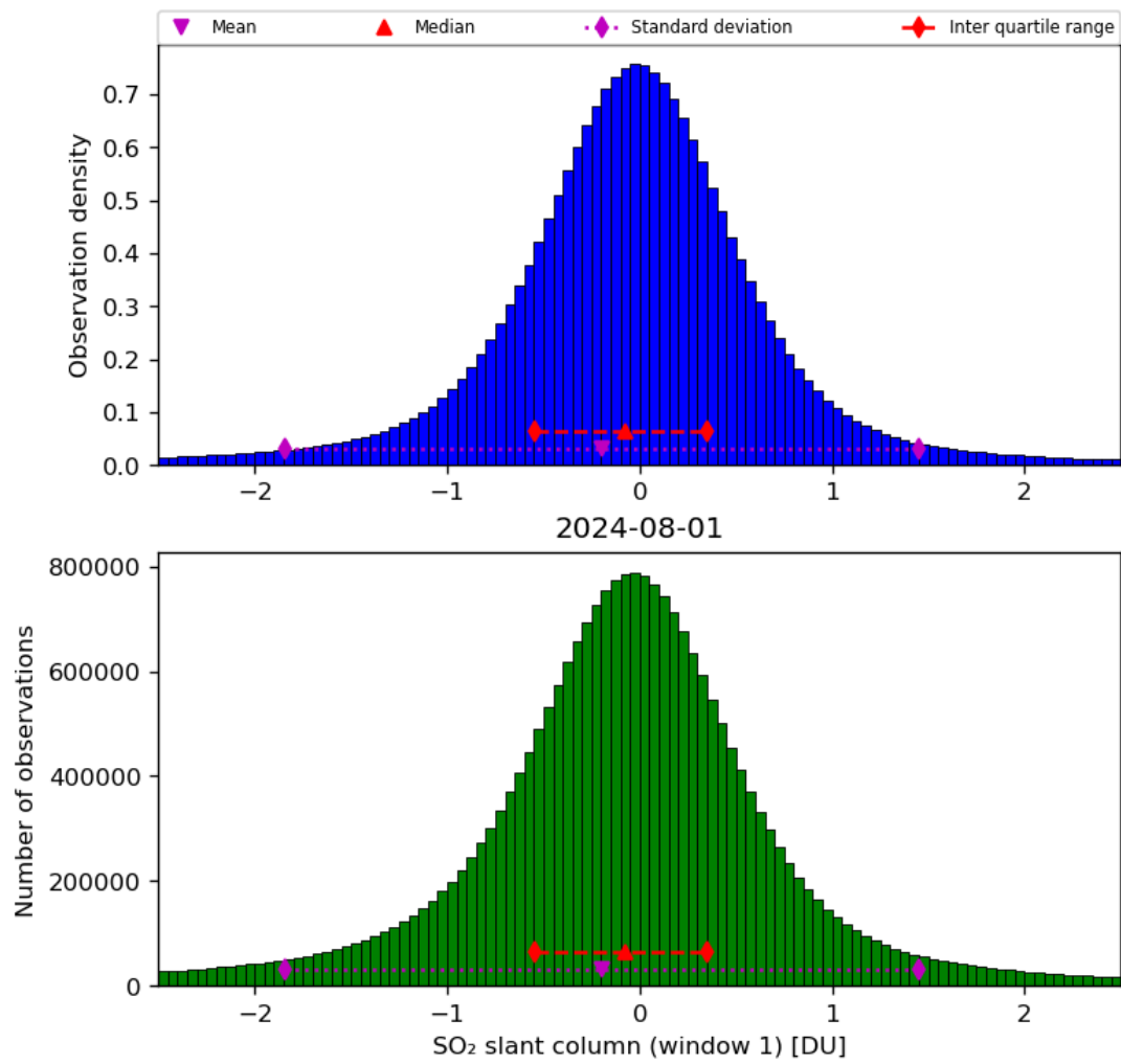
Figure 56: Histogram of “SO 2 slant column (window 1)” for 2024-07-31 to 2024-08-02
