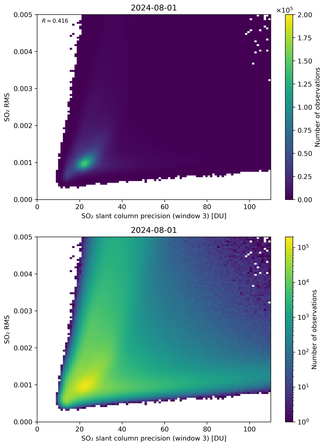
Figure 260: Scatter density plot of “SO 2 slant column precision (window 3)” against “SO 2 RMS” for 2024-07-31 to 2024-08-02.
