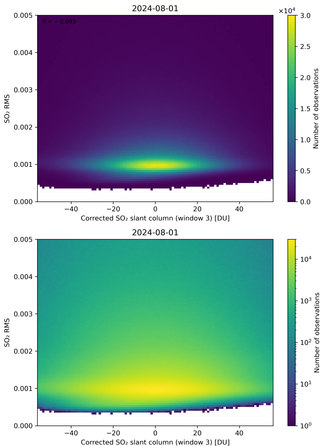
Figure 208: Scatter density plot of “Corrected SO 2 slant column (window 3)” against “SO 2 RMS” for 2024-07-31 to 2024-08-02.
