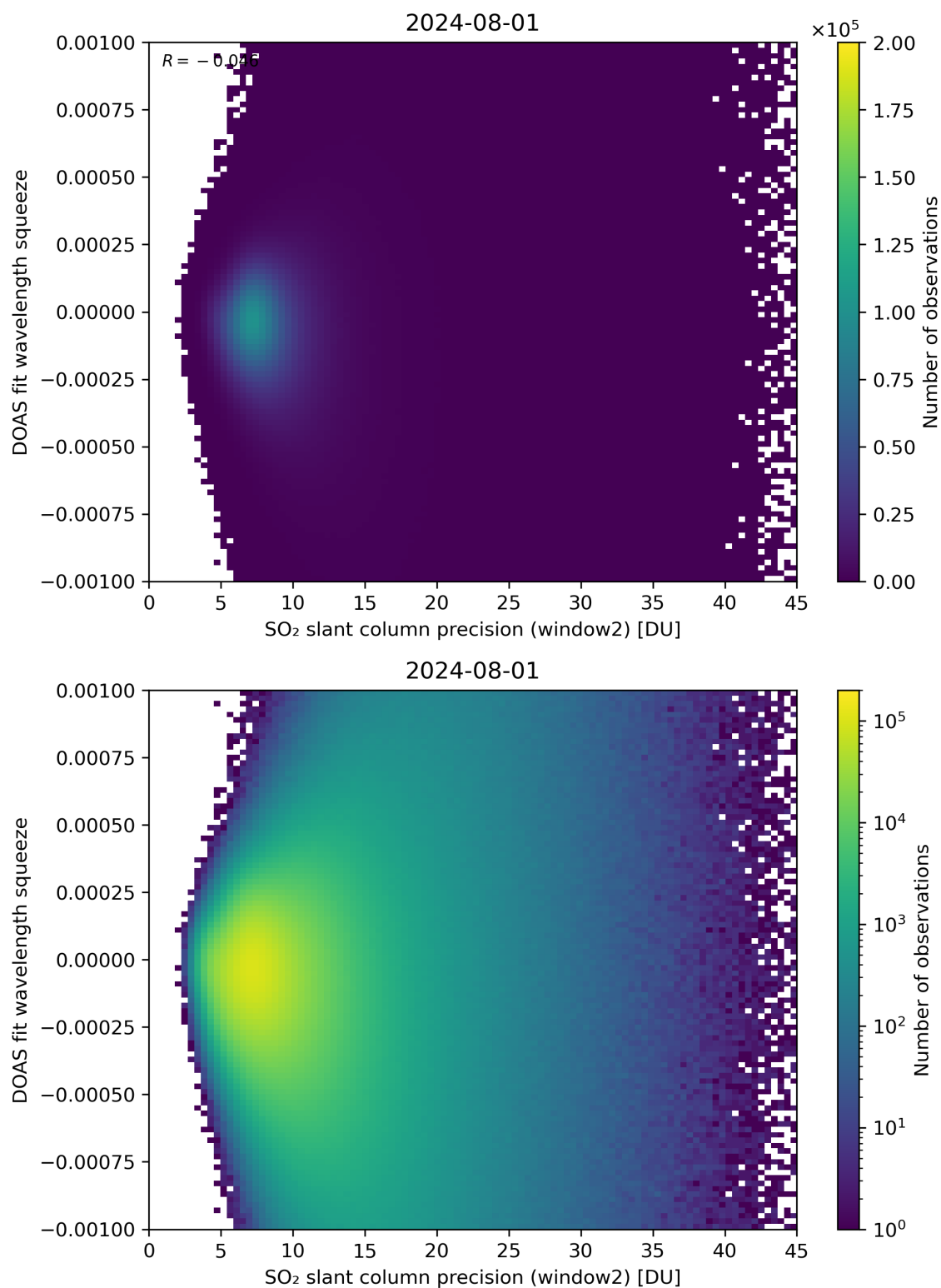
Figure 244: Scatter density plot of “SO 2 slant column precision (window2)” against “DOAS fit wavelength squeeze” for 2024-07-31 to 2024-08-02.
