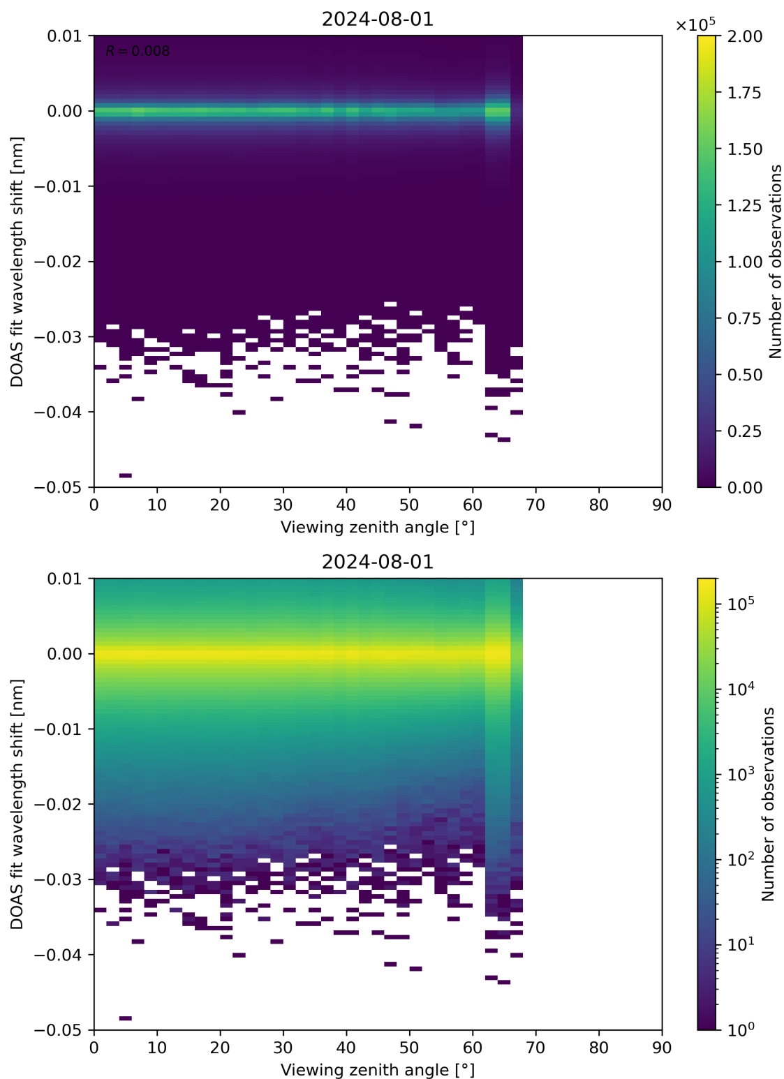
Figure 311: Scatter density plot of “Viewing zenith angle” against “DOAS fit wavelength shift” for 2024-07-31 to 2024-08-02.
