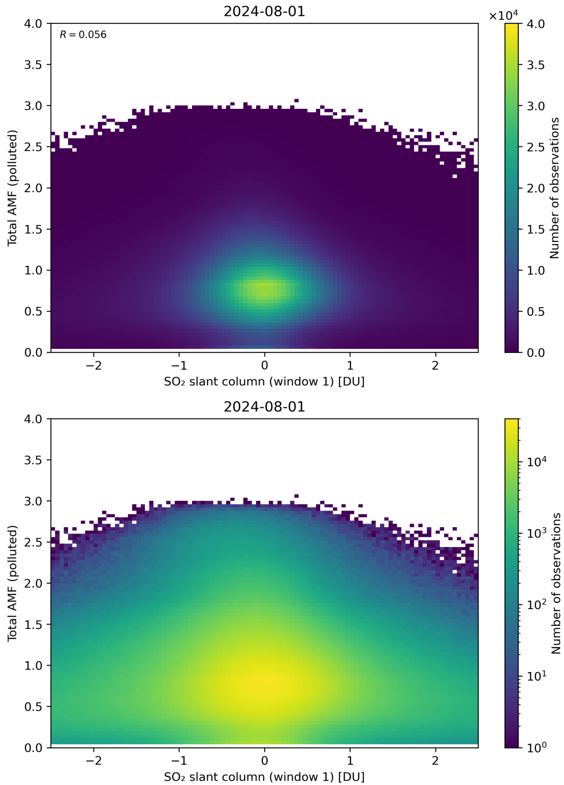
Figure 239: Scatter density plot of “SO 2 slant column (window 1)” against “Total AMF (polluted)” for 2024-07-31 to 2024-08-02.
