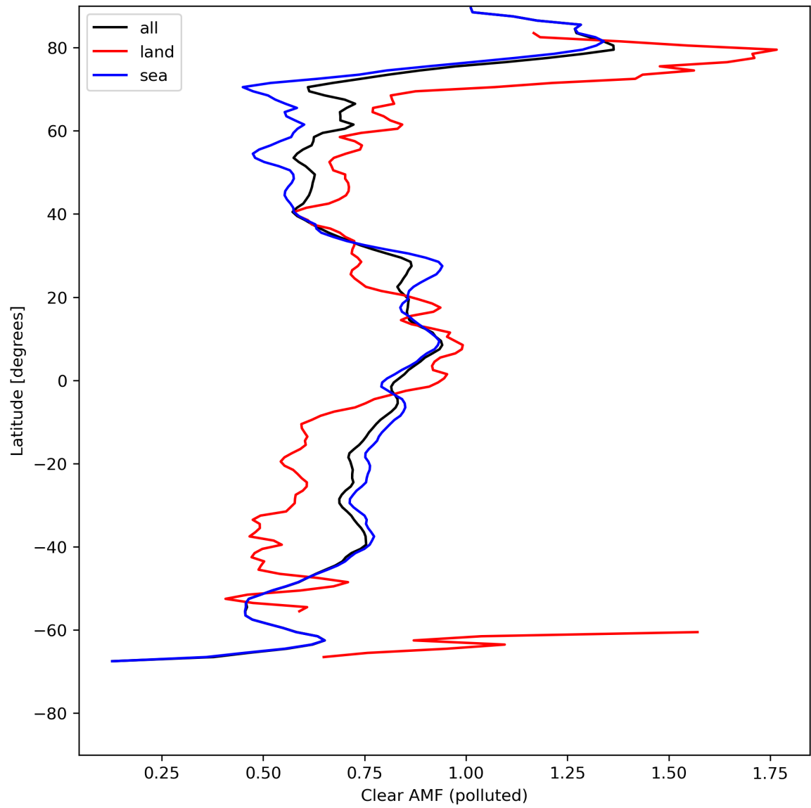
Figure 50: Zonal average of “Clear AMF (polluted)” for 2024-07-31 to 2024-08-02.
