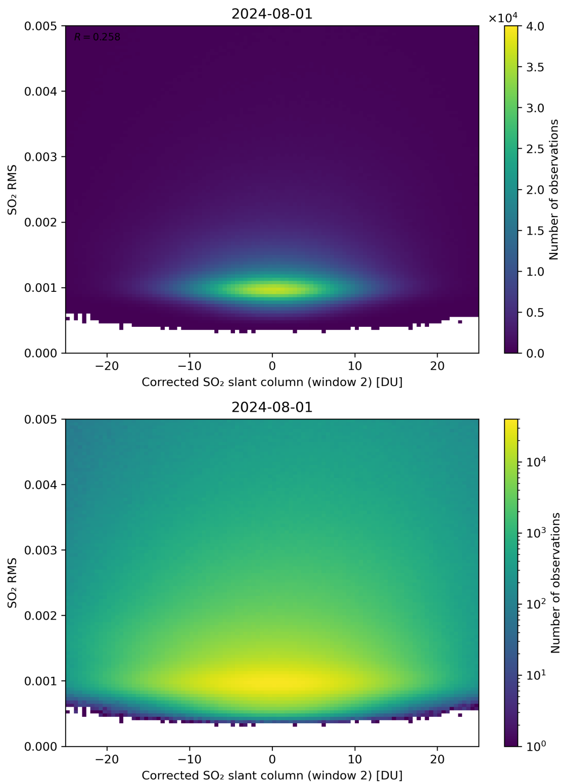
Figure 198: Scatter density plot of “Corrected SO 2 slant column (window 2)” against “SO 2 RMS” for 2024-07-31 to 2024-08-02.
