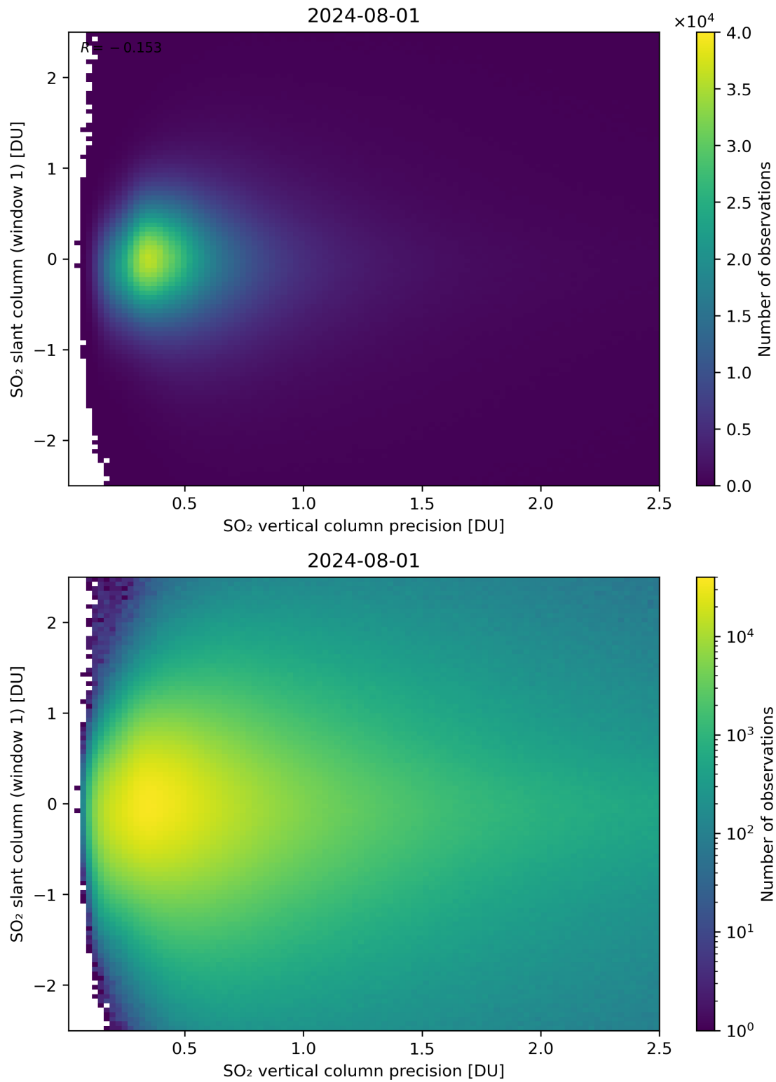
Figure 289: Scatter density plot of “SO 2 vertical column precision” against “SO 2 slant column (window 1)” for 2024-07-31 to 2024-08-02.
