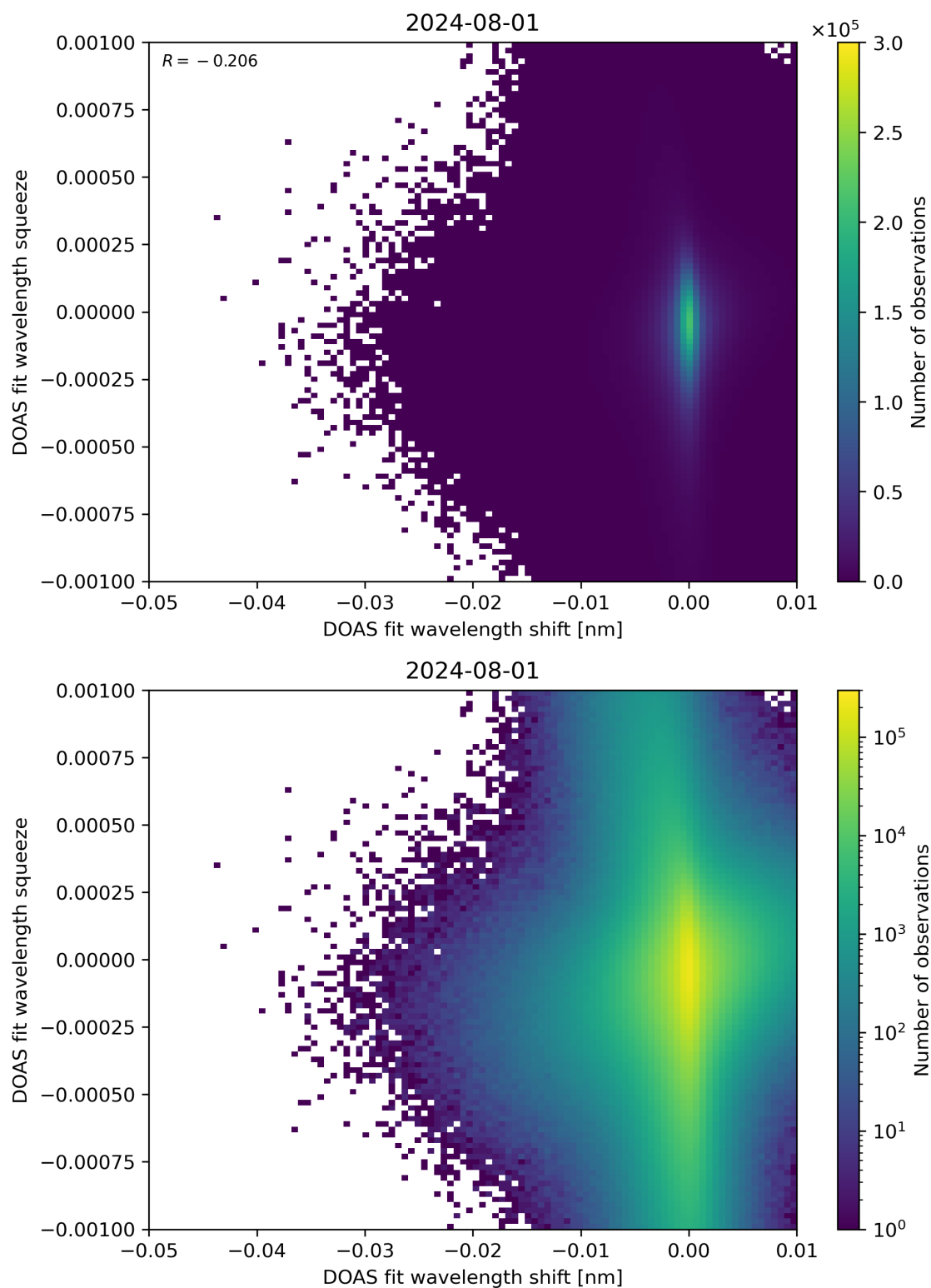
Figure 127: Scatter density plot of “DOAS fit wavelength shift” against “DOAS fit wavelength squeeze” for 2024-07-31 to 2024-08-02.
