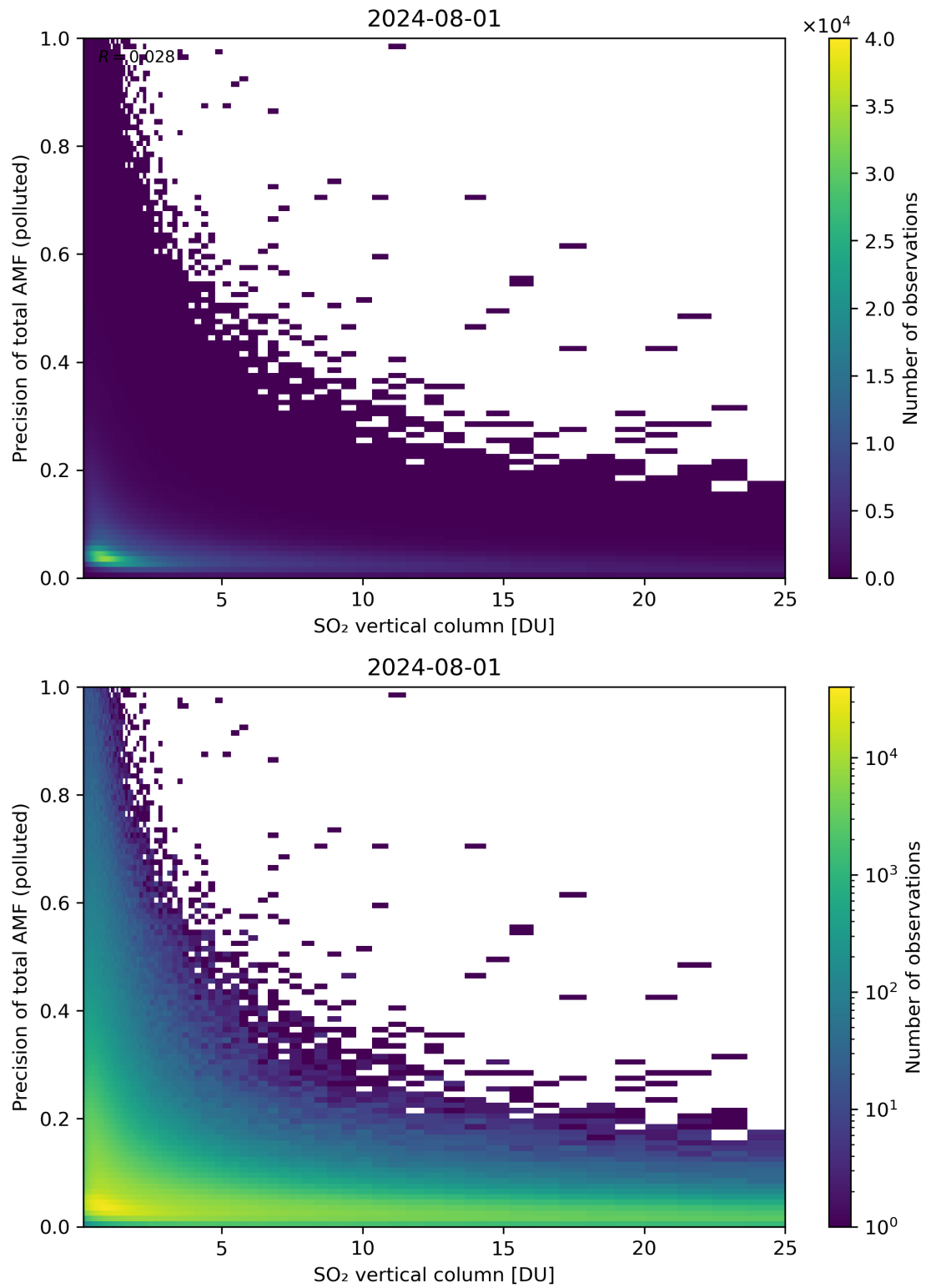
Figure 306: Scatter density plot of “SO 2 vertical column” against “Precision of total AMF (polluted)” for 2024-07-31 to 2024-08-02.
