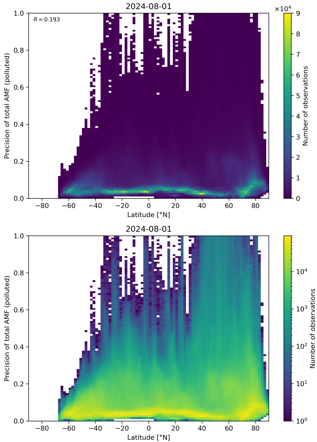
Figure 155: Scatter density plot of “Latitude” against “Precision of total AMF (polluted)” for 2024-07-31 to 2024-08-02.
