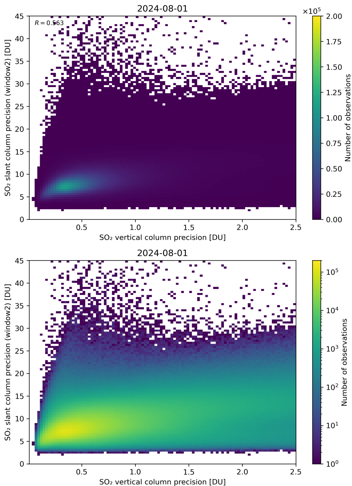
Figure 291: Scatter density plot of “SO 2 vertical column precision” against “SO 2 slant column precision (window2)” for 2024-07-31 to 2024-08-02.
