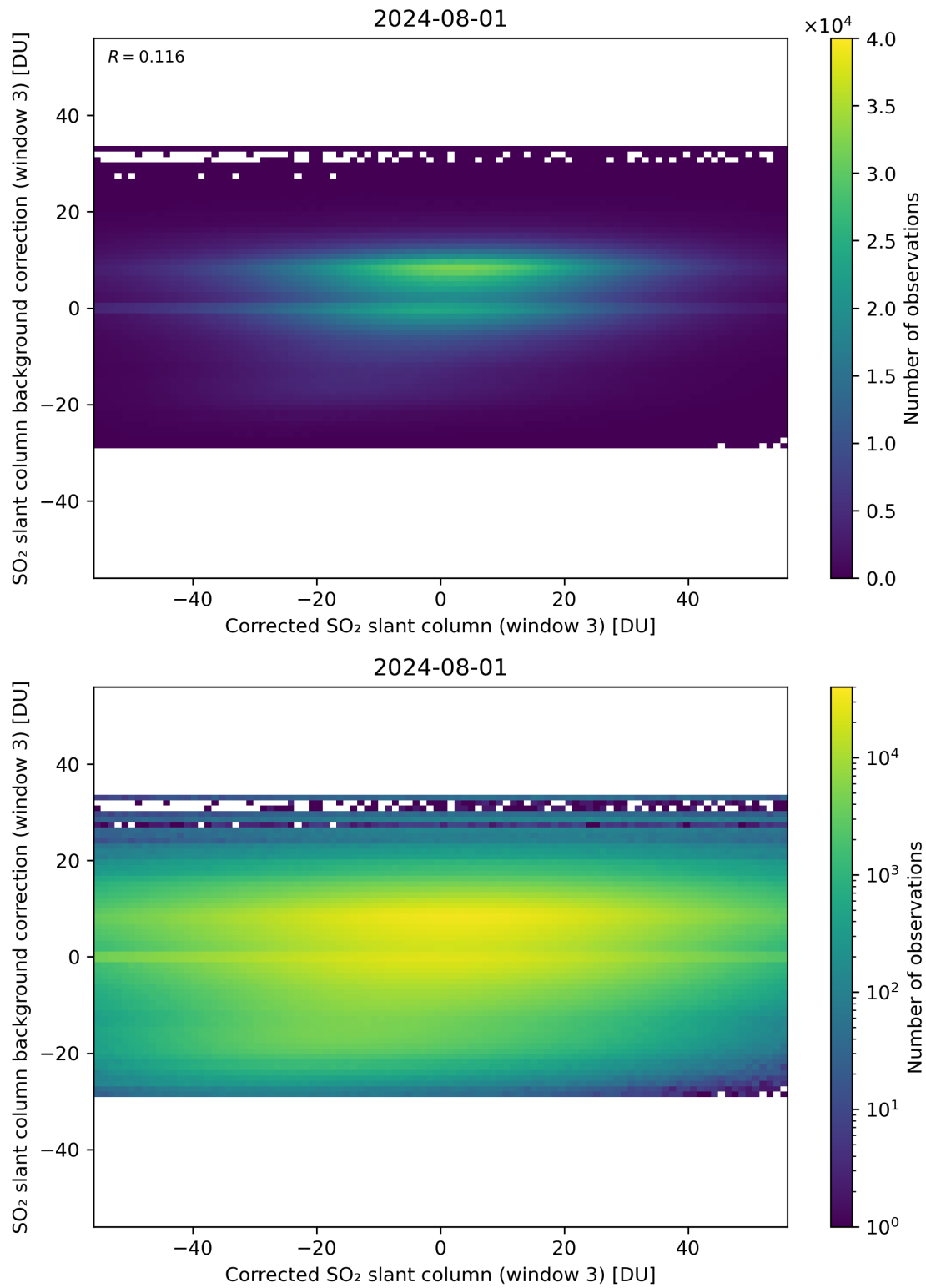
Figure 205: Scatter density plot of “Corrected SO 2 slant column (window 3)” against “SO 2 slant column background correction (window 3)” for 2024-07-31 to 2024-08-02.
