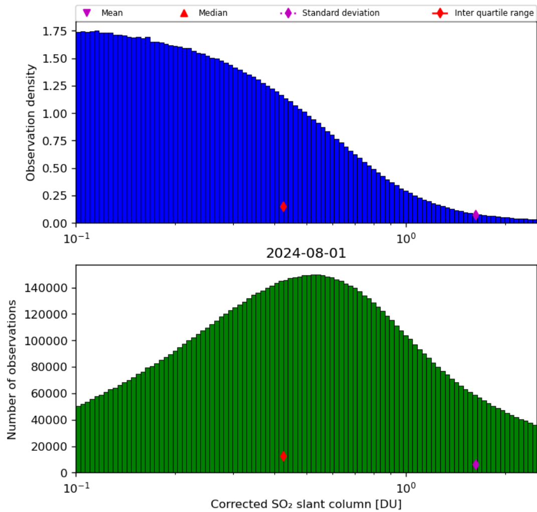
Figure 55: Histogram of “Corrected SO 2 slant column” for 2024-07-31 to 2024-08-02
