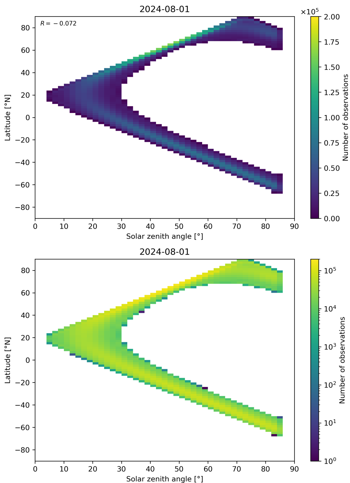
Figure 164: Scatter density plot of “Solar zenith angle” against “Latitude” for 2024-07-31 to 2024-08-02.
