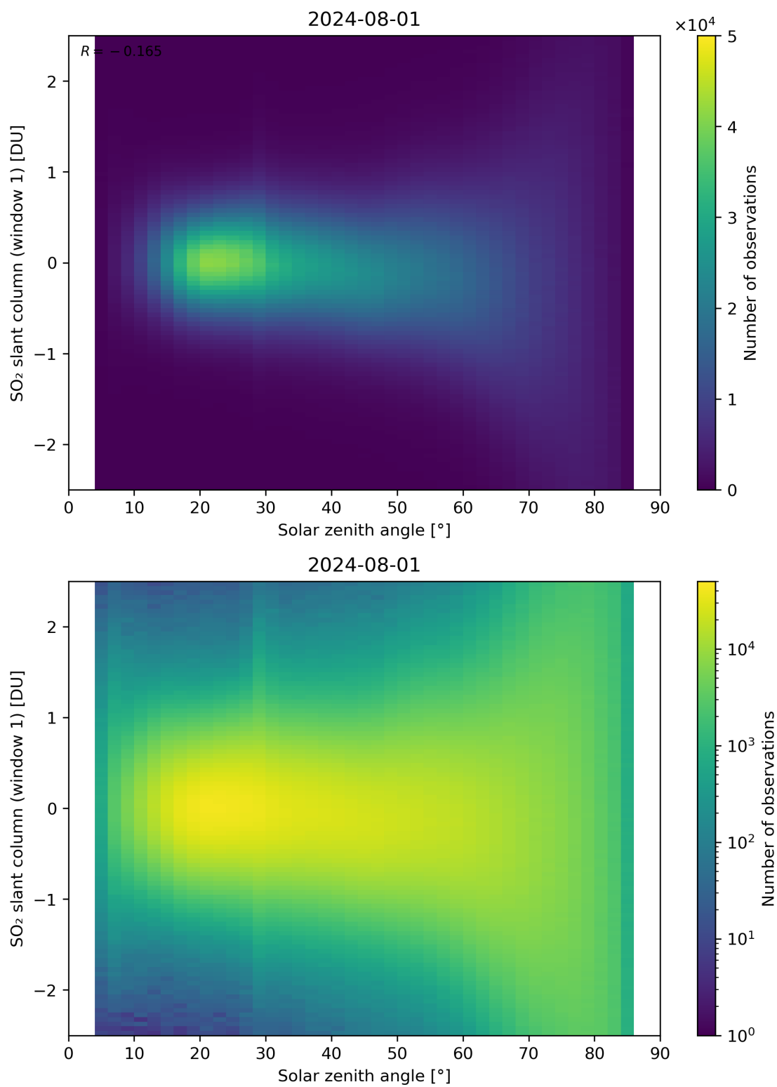
Figure 169: Scatter density plot of “Solar zenith angle” against “SO 2 slant column (window 1)” for 2024-07-31 to 2024-08-02.
