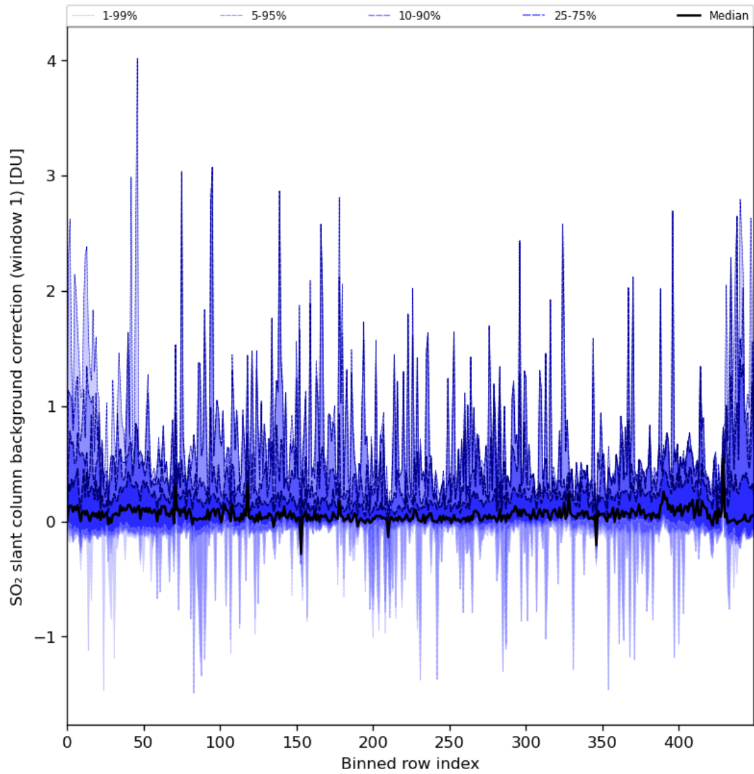
Figure 82: Along track statistics of “SO 2 slant column background correction (window 1)” for 2024-07-31 to 2024-08-02
