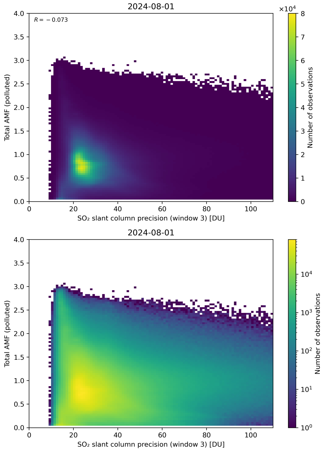
Figure 263: Scatter density plot of “SO 2 slant column precision (window 3)” against “Total AMF (polluted)” for 2024-07-31 to 2024-08-02.
