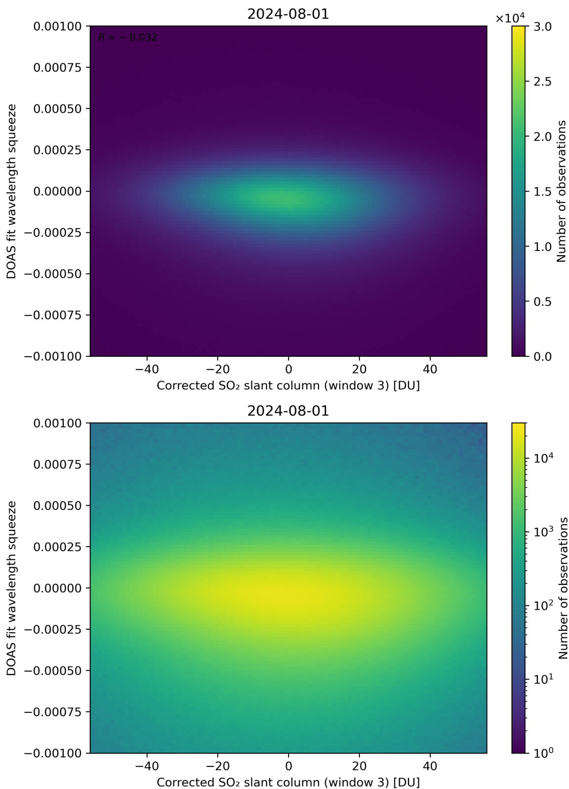
Figure 207: Scatter density plot of “Corrected SO 2 slant column (window 3)” against “DOAS fit wavelength squeeze” for 2024-07-31 to 2024-08-02.
