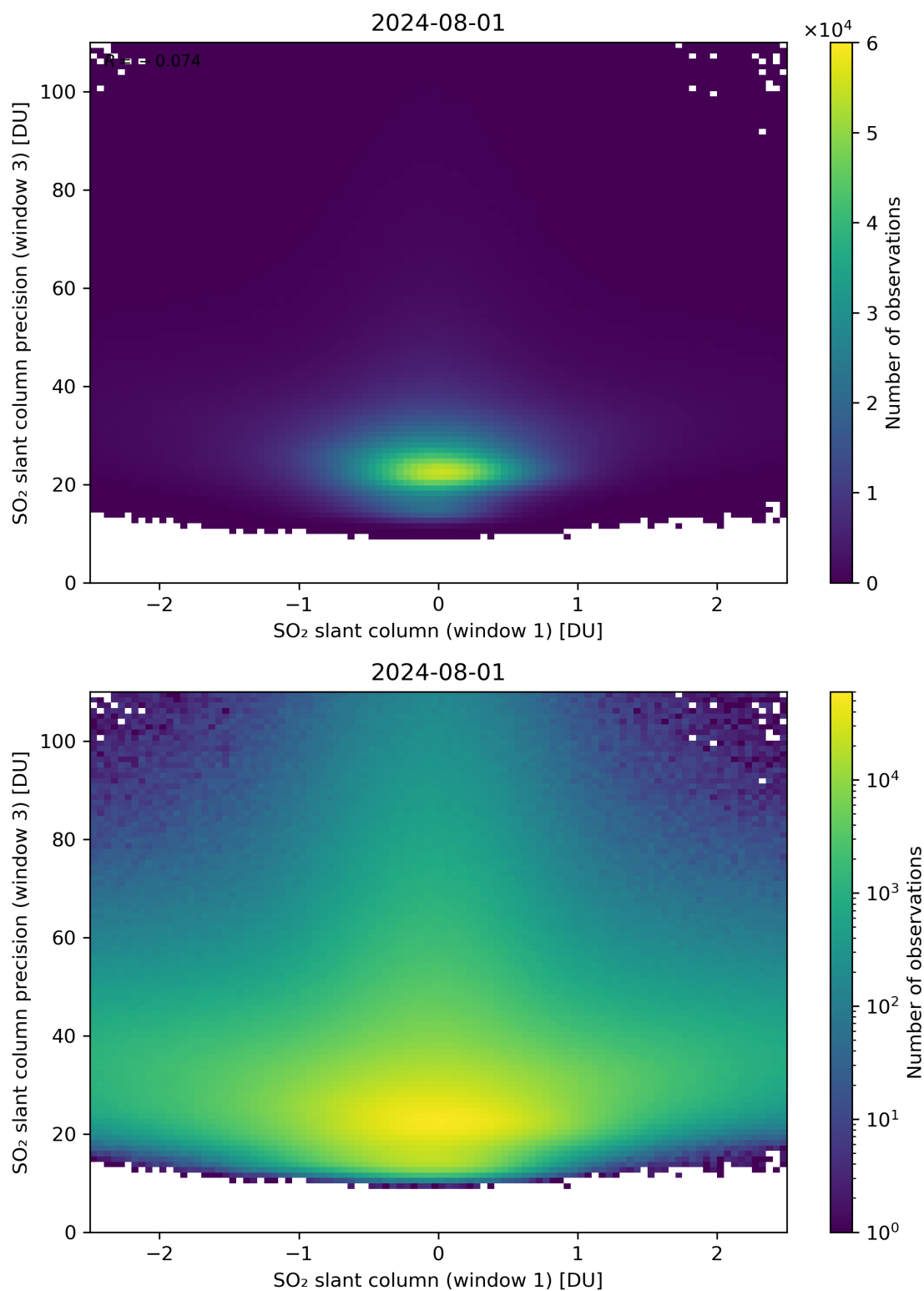
Figure 238: Scatter density plot of “SO 2 slant column (window 1)” against “SO 2 slant column precision (window 3)” for 2024-07-31 to 2024-08-02.
