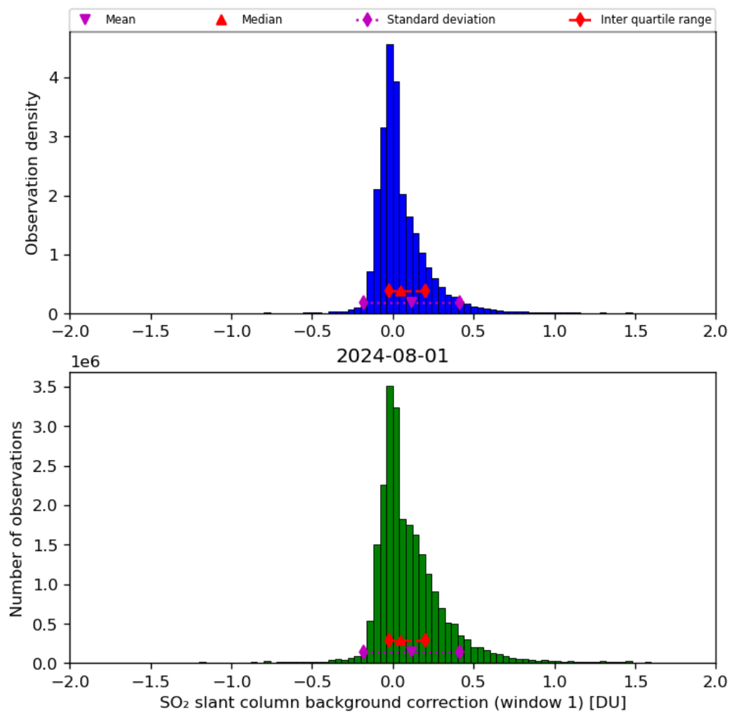
Figure 59: Histogram of “SO 2 slant column background correction (window 1)” for 2024-07-31 to 2024-08-02
