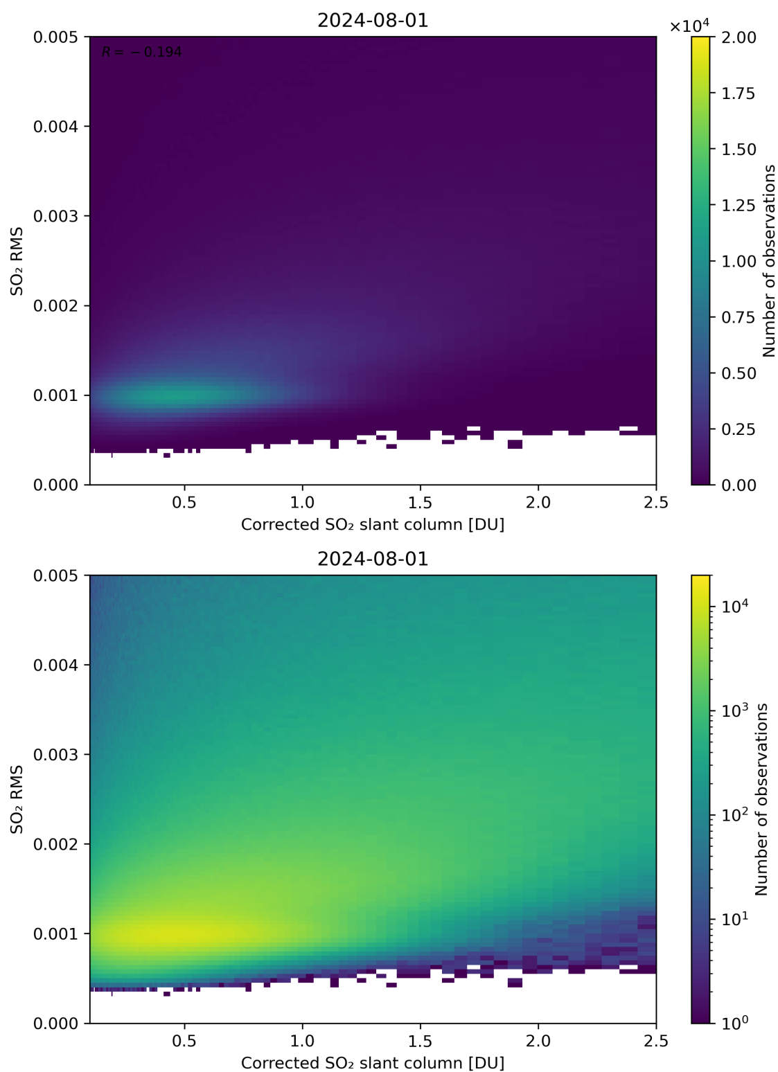
Figure 183: Scatter density plot of “Corrected SO 2 slant column” against “SO 2 RMS” for 2024-07-31 to 2024-08-02.
