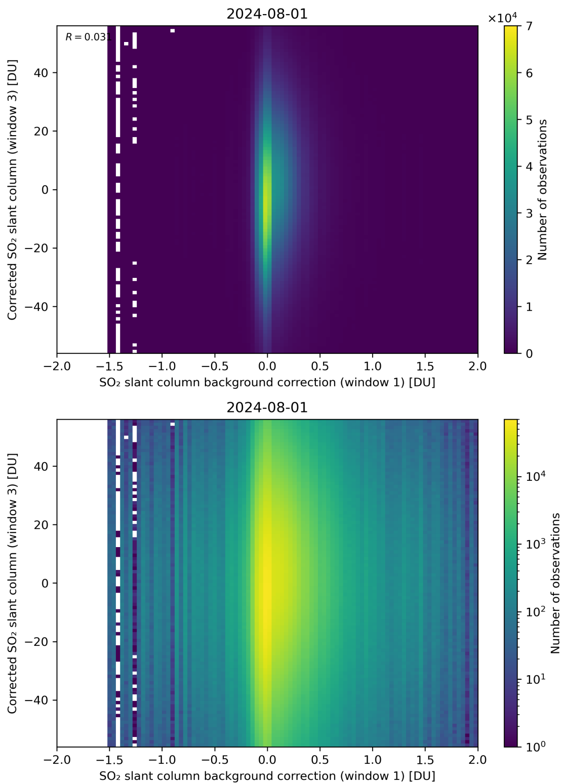
Figure 105: Scatter density plot of “SO 2 slant column background correction (window 1)” against “Corrected SO 2 slant column (window 3)” for 2024-07-31 to 2024-08-02.
