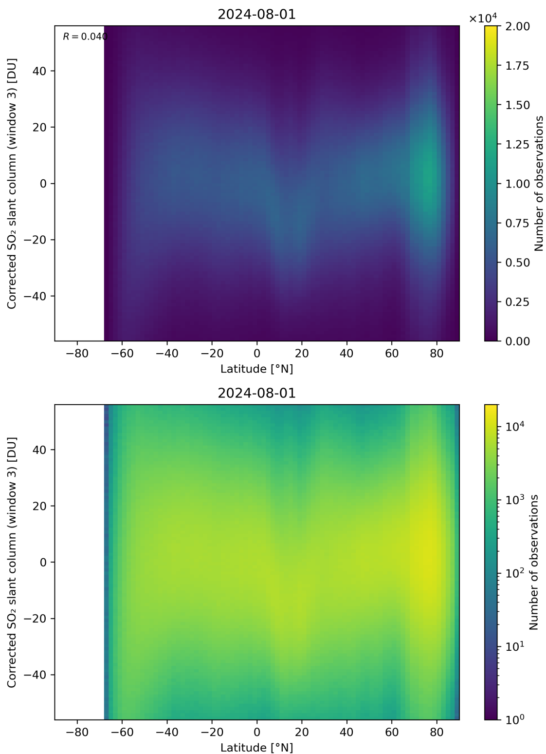
Figure 148: Scatter density plot of “Latitude” against “Corrected SO 2 slant column (window 3)” for 2024-07-31 to 2024-08-02.
