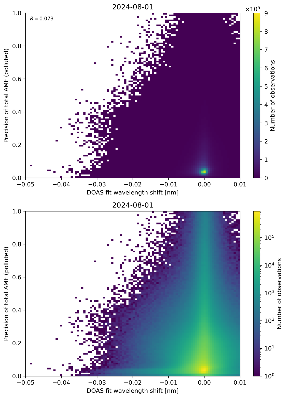
Figure 131: Scatter density plot of “DOAS fit wavelength shift” against “Precision of total AMF (polluted)” for 2024-07-31 to 2024-08-02.
