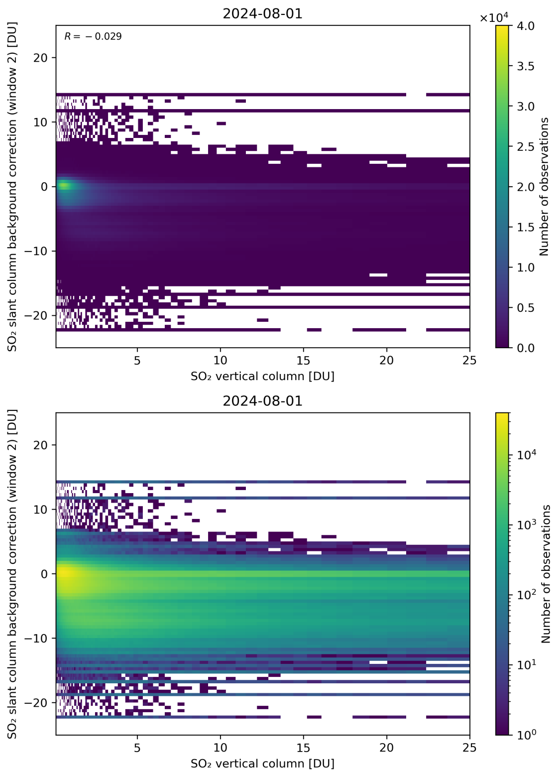
Figure 274: Scatter density plot of “SO 2 vertical column” against “SO 2 slant column background correction (window 2)” for 2024-07-31 to 2024-08-02.
