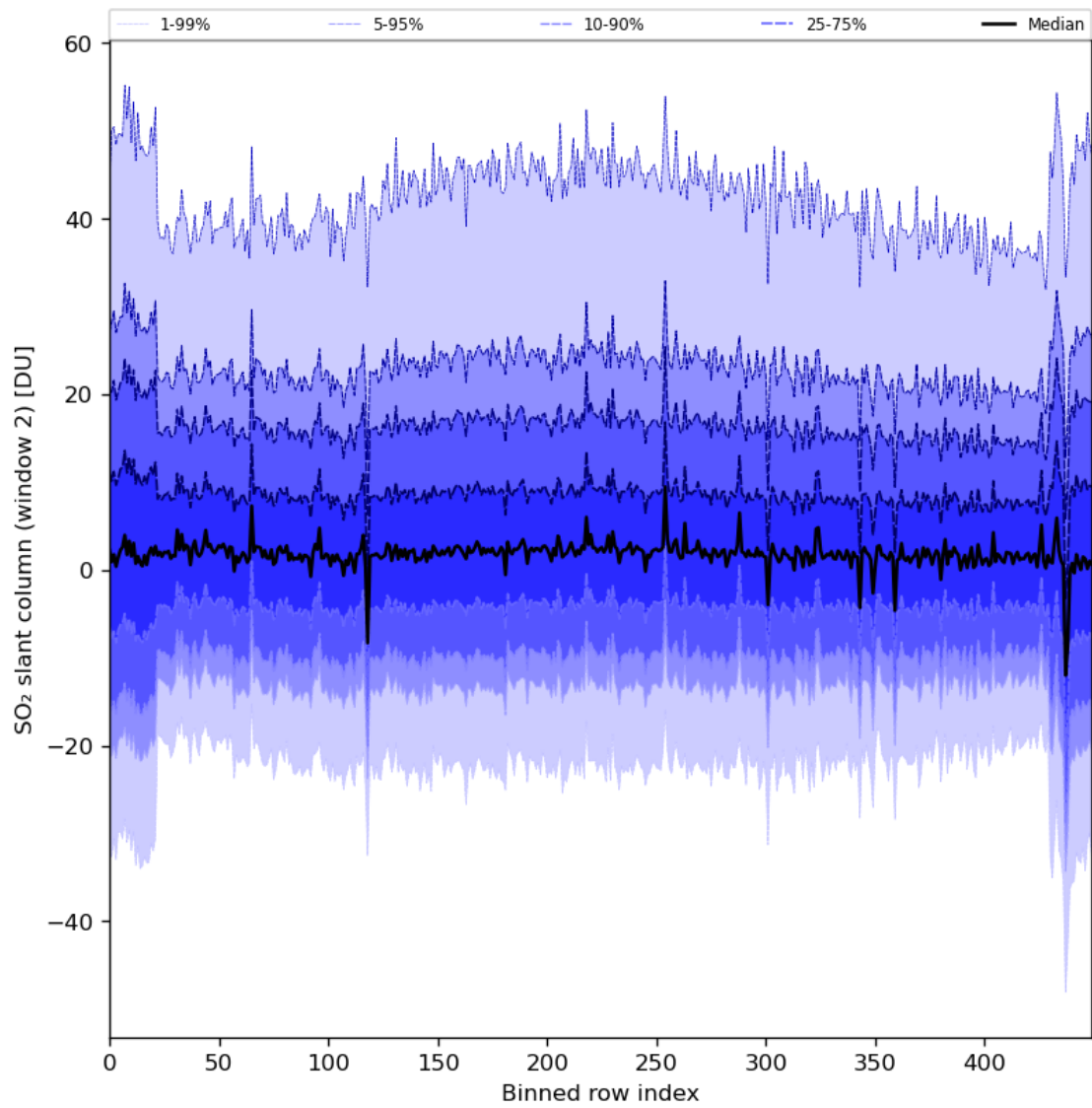
Figure 83: Along track statistics of “SO 2 slant column (window 2)” for 2024-07-31 to 2024-08-02
