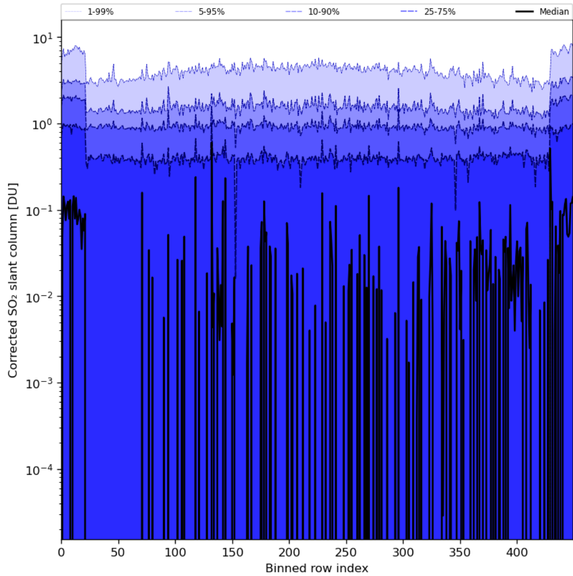
Figure 78: Along track statistics of “Corrected SO 2 slant column” for 2024-07-31 to 2024-08-02
