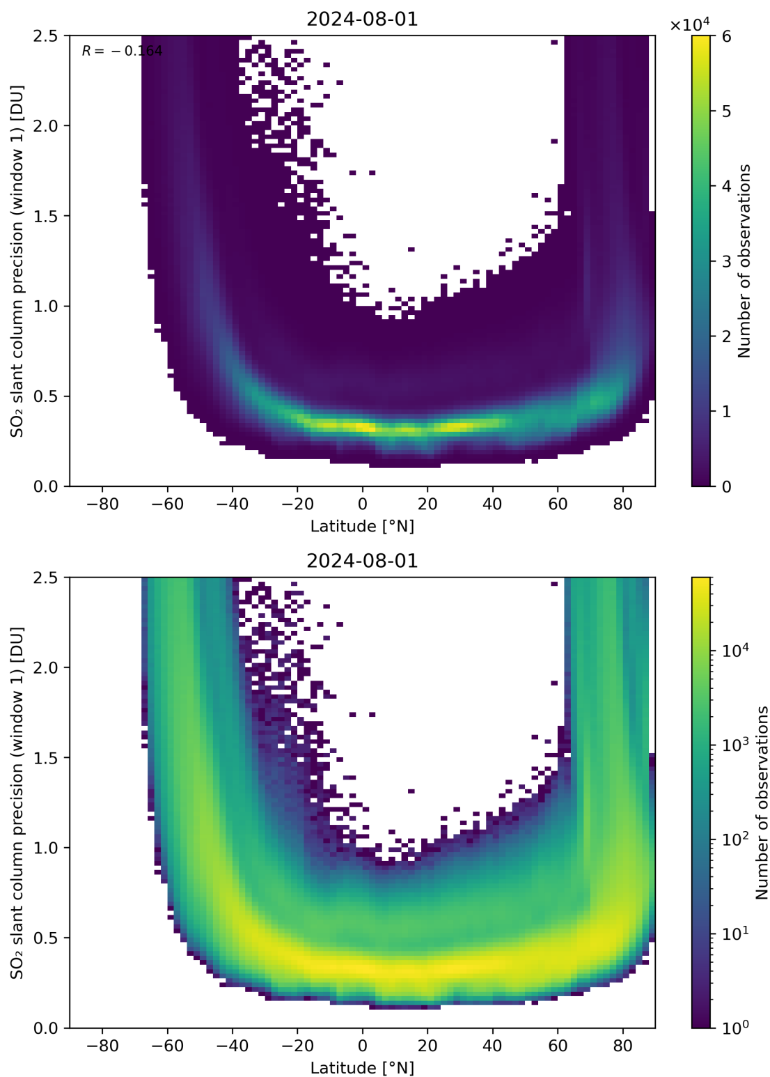
Figure 150: Scatter density plot of “Latitude” against “SO 2 slant column precision (window 1)” for 2024-07-31 to 2024-08-02.
