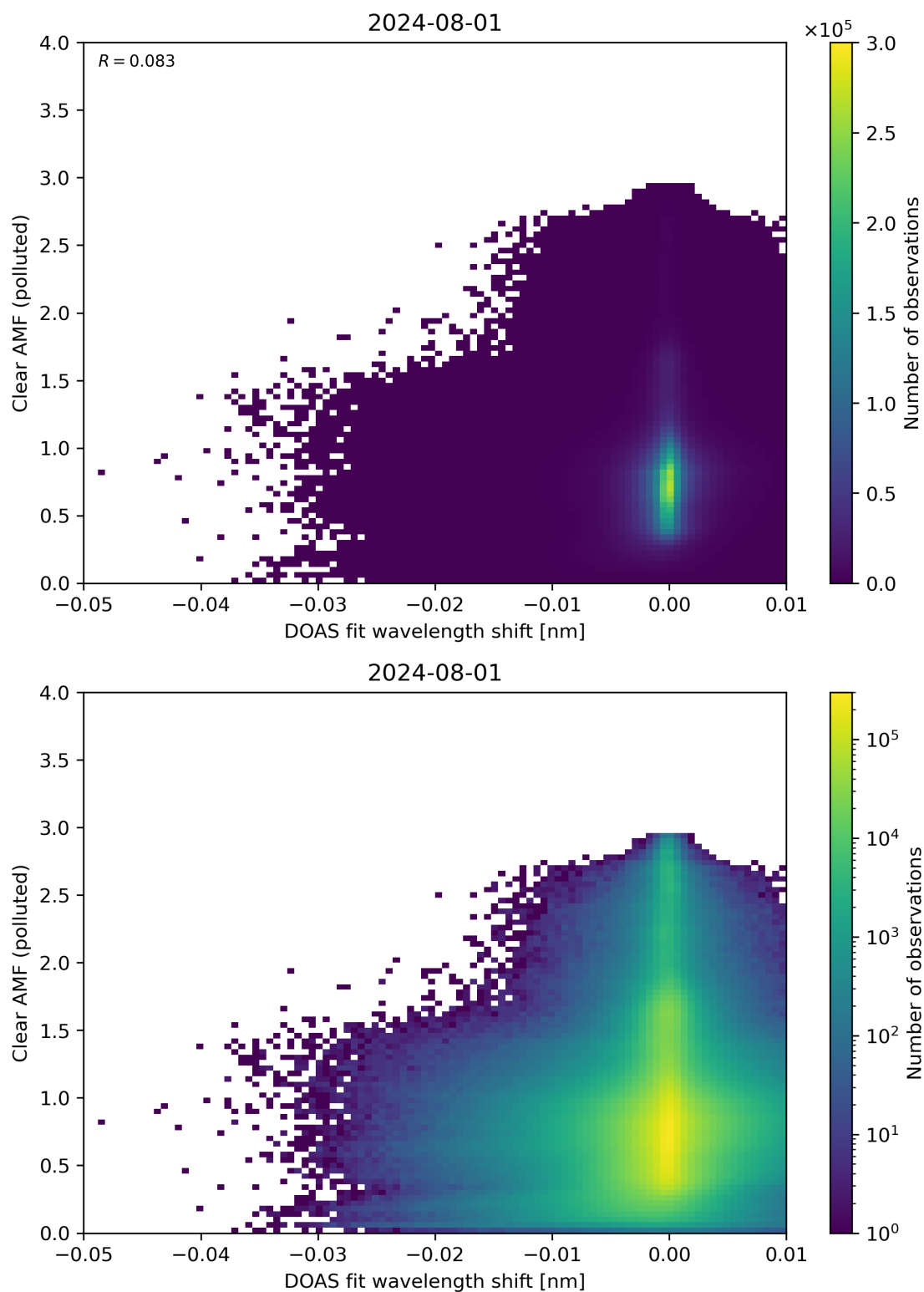
Figure 129: Scatter density plot of “DOAS fit wavelength shift” against “Clear AMF (polluted)” for 2024-07-31 to 2024-08-02.
