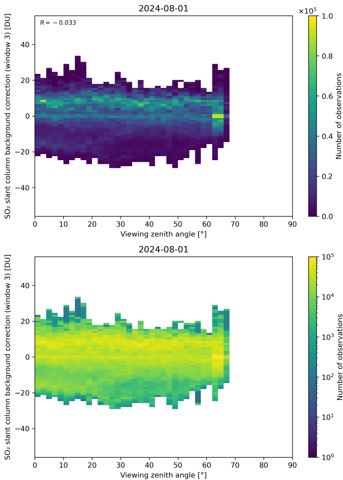
Figure 310: Scatter density plot of “Viewing zenith angle” against “SO 2 slant column background correction (window 3)” for 2024-07-31 to 2024-08-02.
