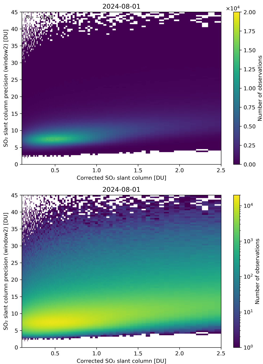
Figure 189: Scatter density plot of “Corrected SO 2 slant column” against “SO 2 slant column precision (window2)” for 2024-07-31 to 2024-08-02.
