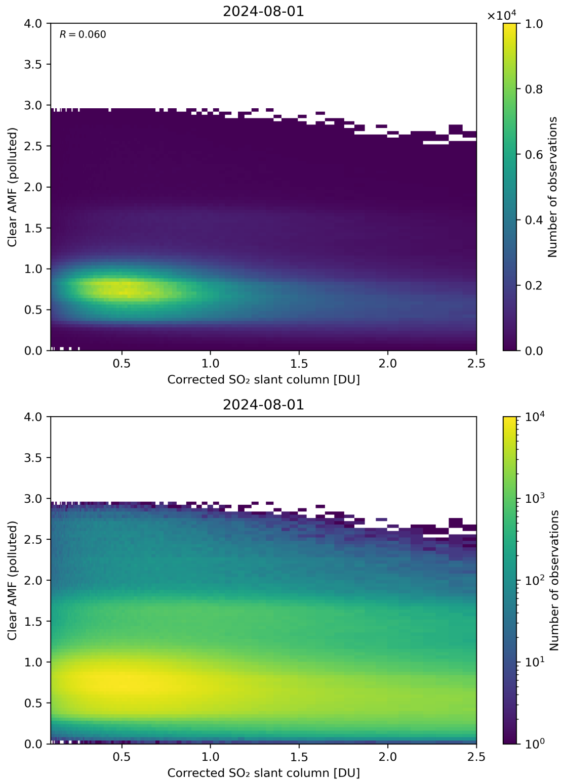
Figure 184: Scatter density plot of “Corrected SO 2 slant column” against “Clear AMF (polluted)” for 2024-07-31 to 2024-08-02.
