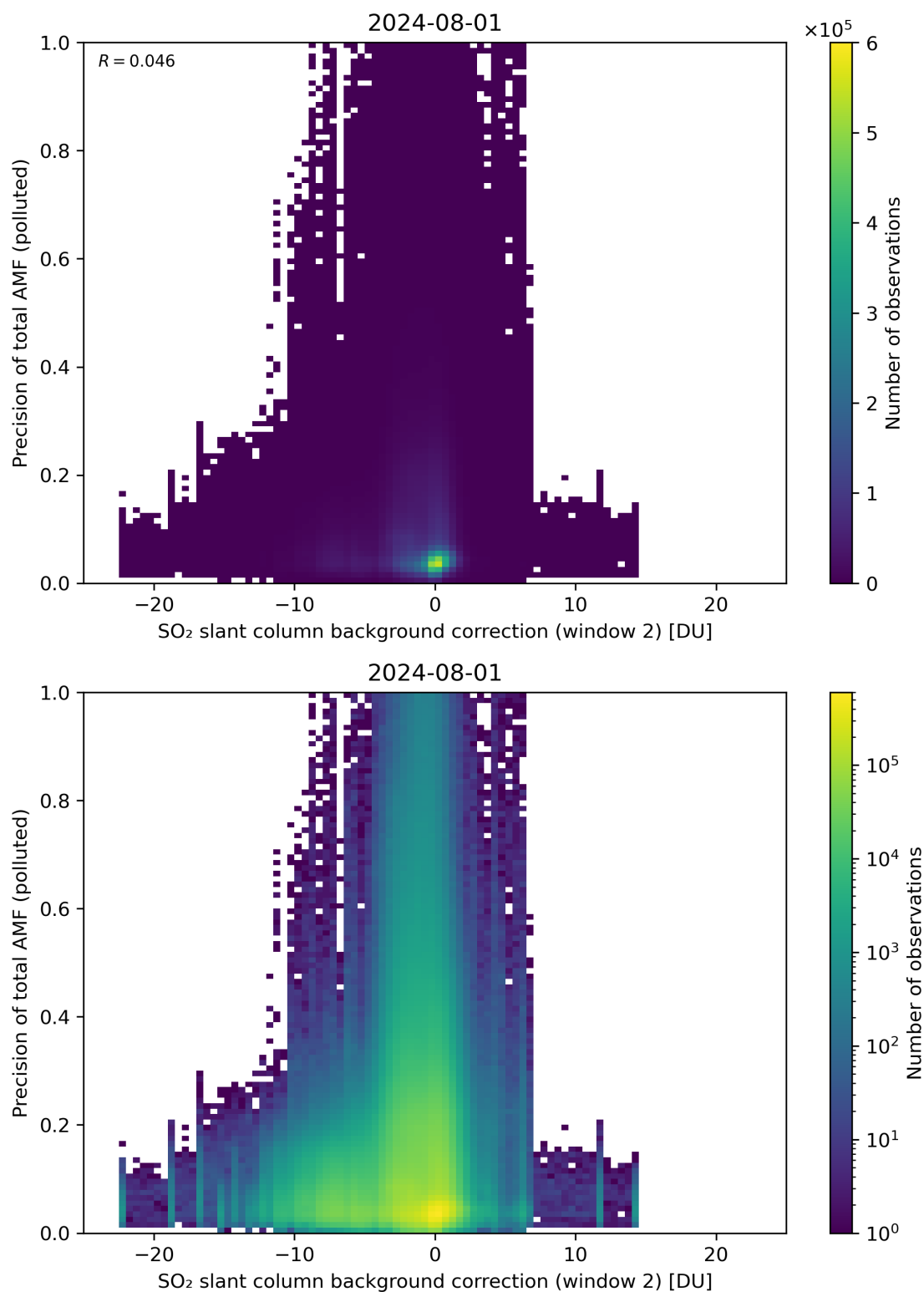
Figure 120: Scatter density plot of “SO 2 slant column background correction (window 2)” against “Precision of total AMF (polluted)” for 2024-07-31 to 2024-08-02.
