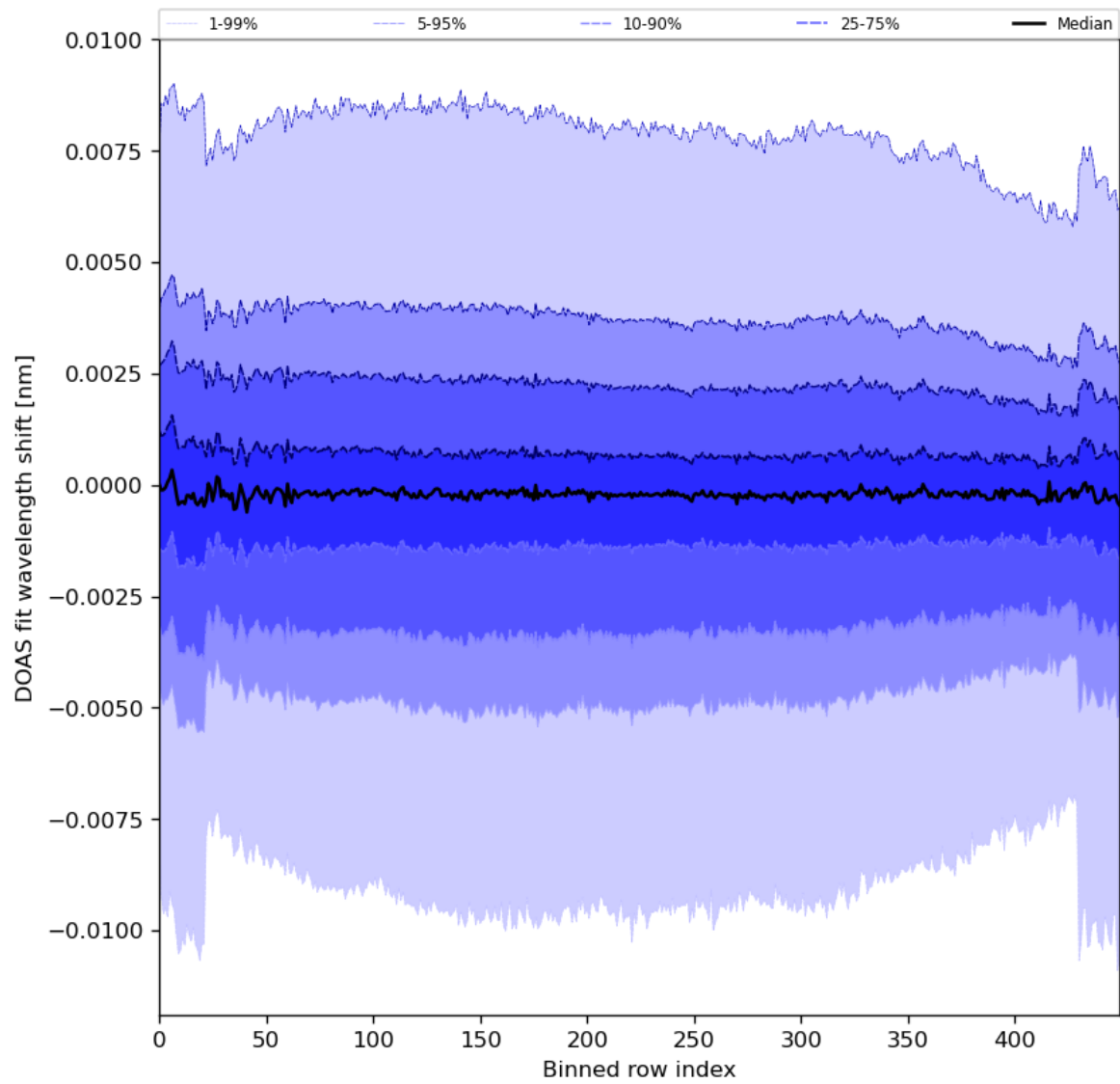
Figure 91: Along track statistics of “DOAS fit wavelength shift” for 2024-07-31 to 2024-08-02
