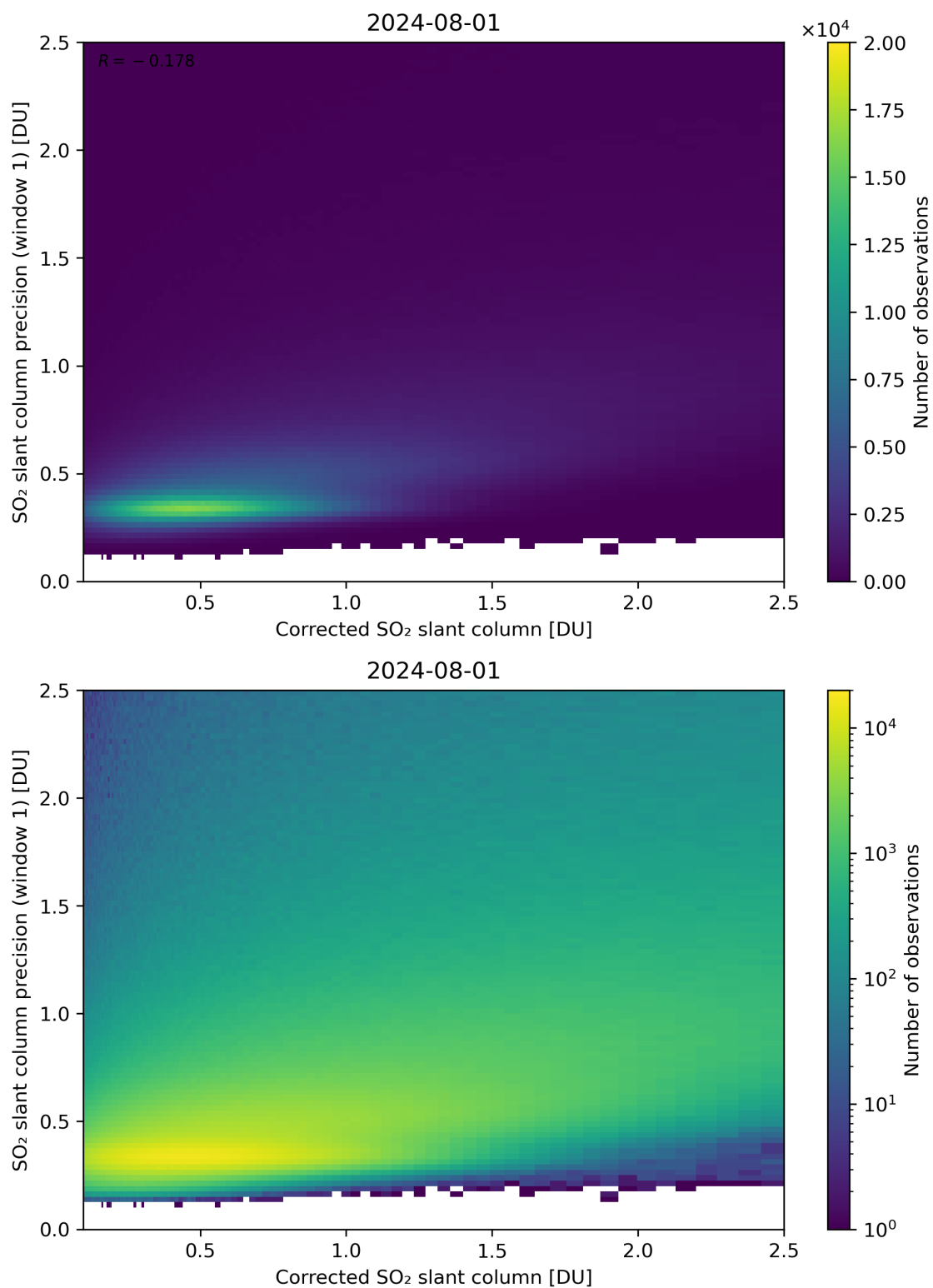
Figure 188: Scatter density plot of “Corrected SO 2 slant column” against “SO 2 slant column precision (window 1)” for 2024-07-31 to 2024-08-02.
