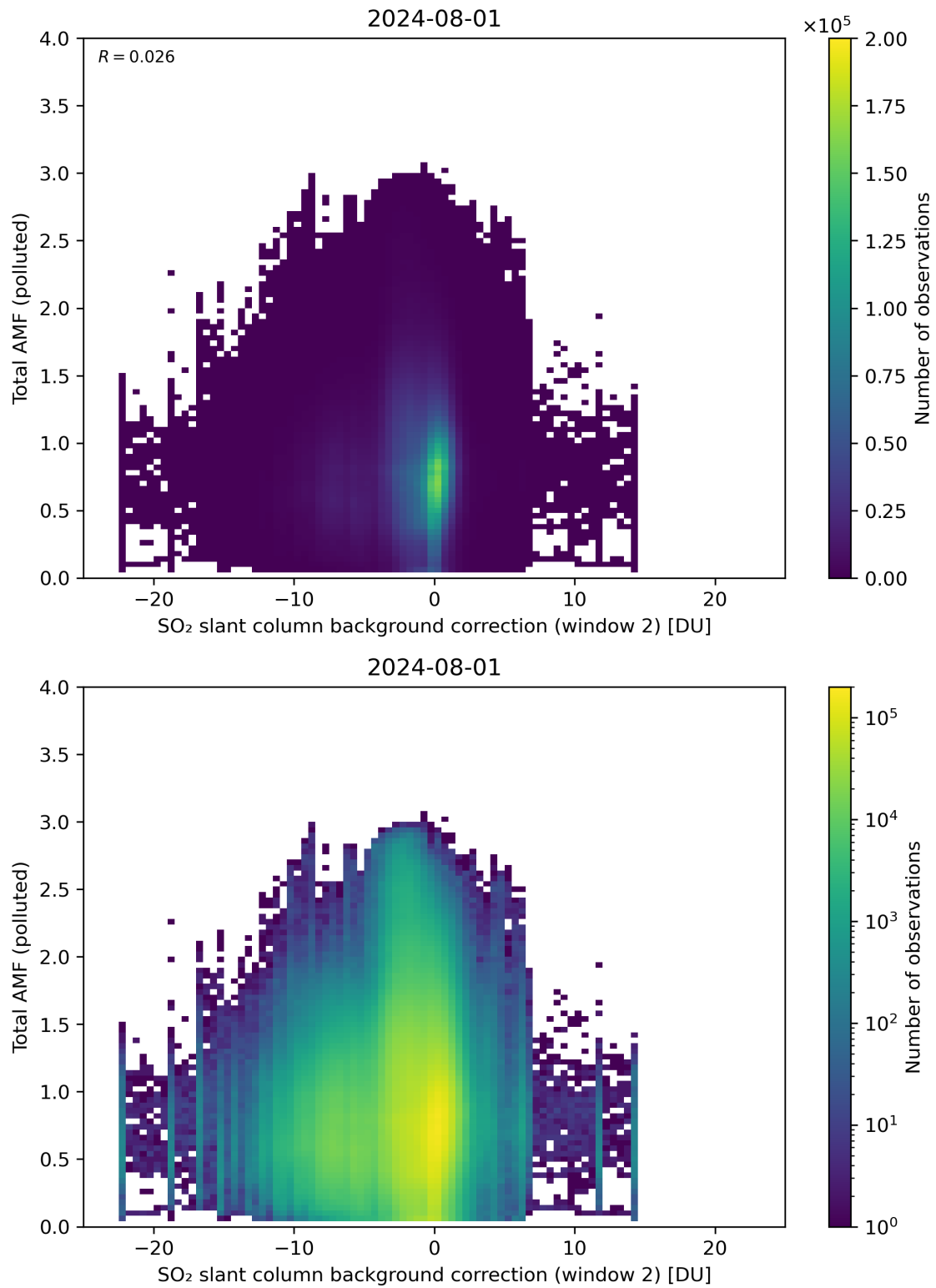
Figure 119: Scatter density plot of “SO 2 slant column background correction (window 2)” against “Total AMF (polluted)” for 2024-07-31 to 2024-08-02.
