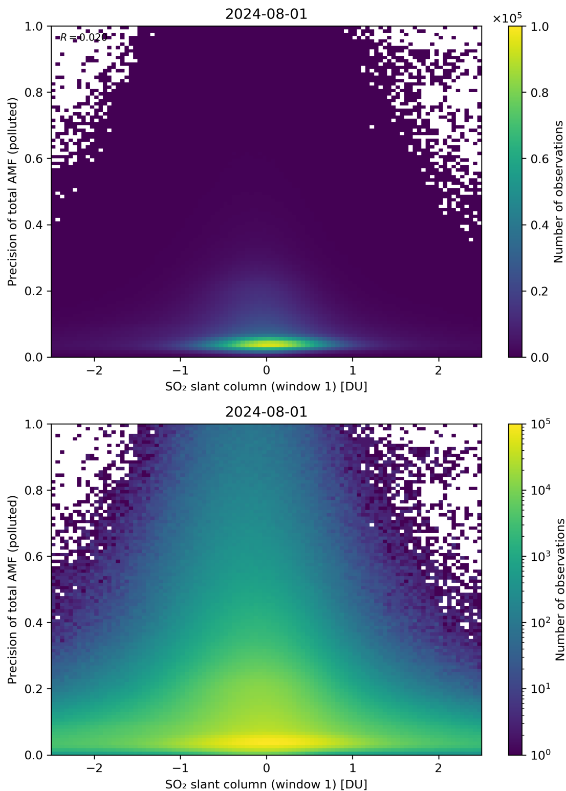
Figure 240: Scatter density plot of “SO 2 slant column (window 1)” against “Precision of total AMF (polluted)” for 2024-07-31 to 2024-08-02.
