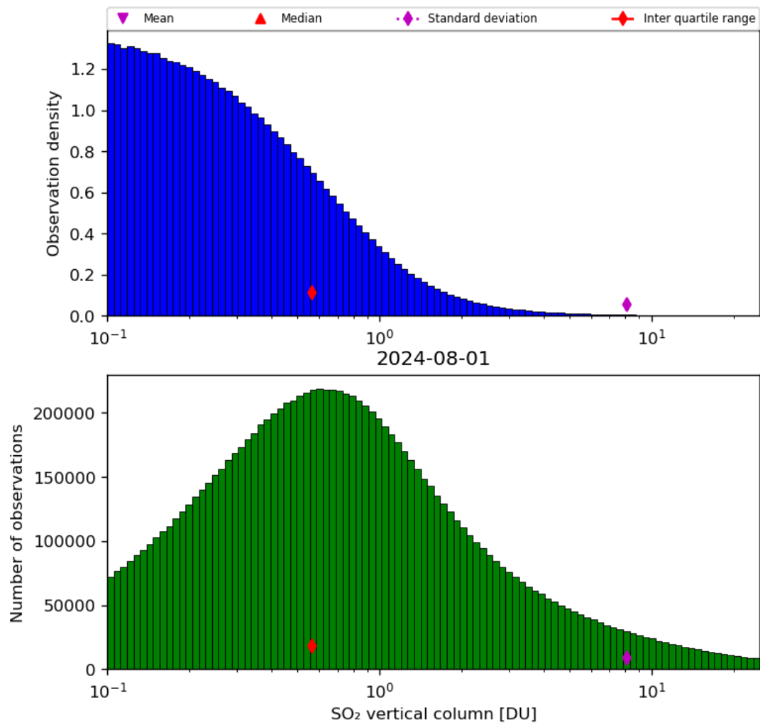
Figure 53: Histogram of “SO 2 vertical column” for 2024-07-31 to 2024-08-02
