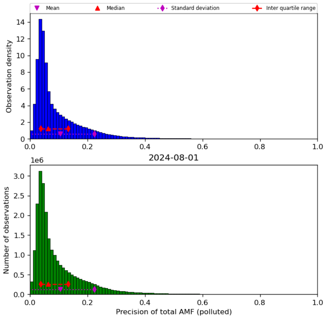
Figure 72: Histogram of “Precision of total AMF (polluted)” for 2024-07-31 to 2024-08-02
