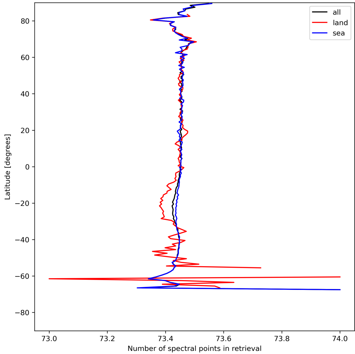
Figure 51: Zonal average of “Number of spectral points in retrieval” for 2024-07-31 to 2024-08-02.
