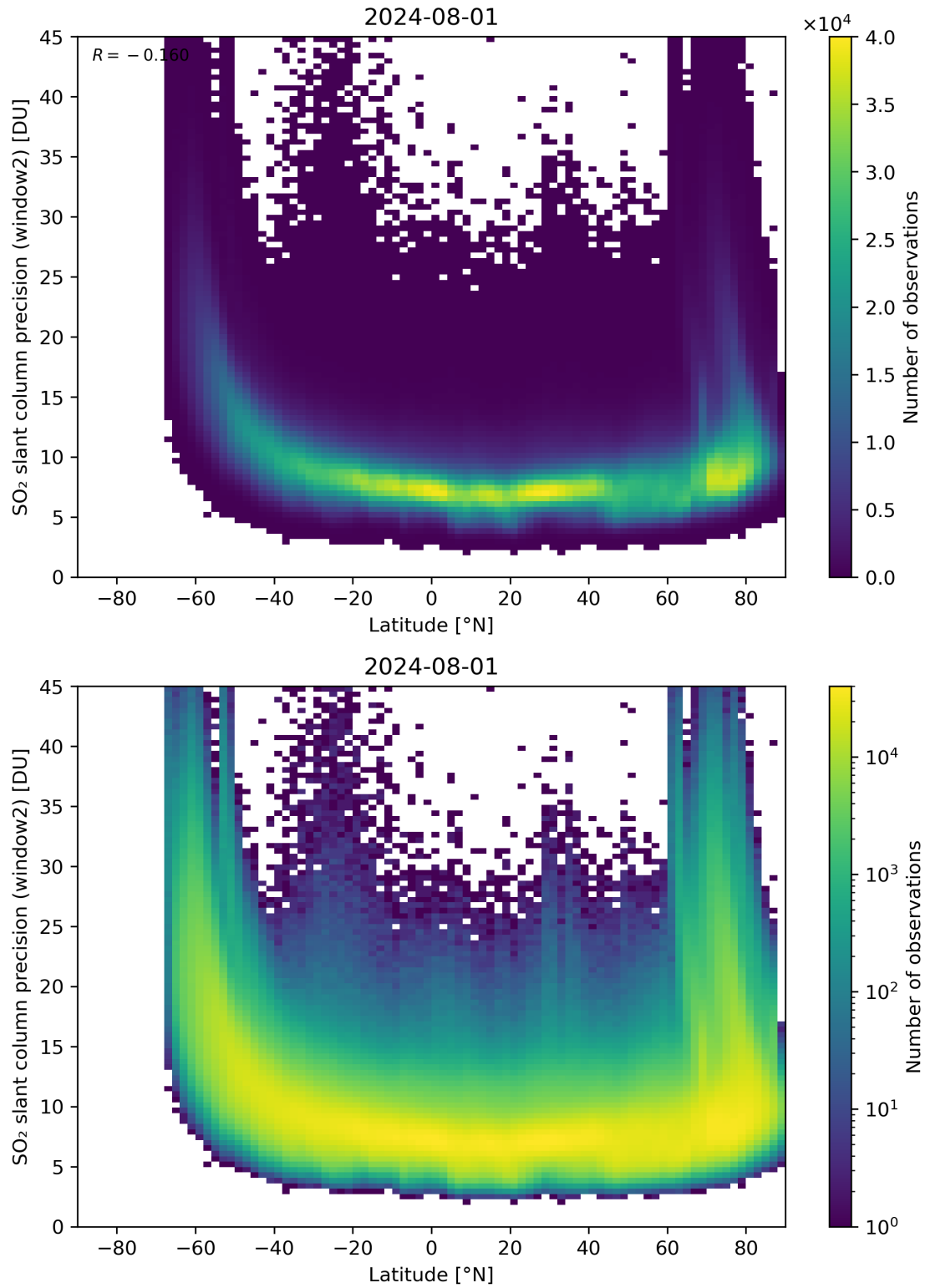
Figure 151: Scatter density plot of “Latitude” against “SO 2 slant column precision (window2)” for 2024-07-31 to 2024-08-02.
