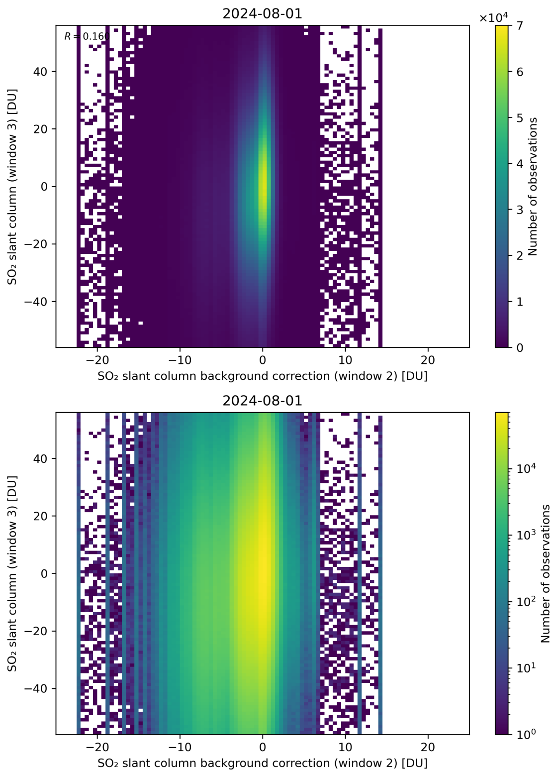
Figure 117: Scatter density plot of “SO 2 slant column background correction (window 2)” against “SO 2 slant column (window 3)” for 2024-07-31 to 2024-08-02.
