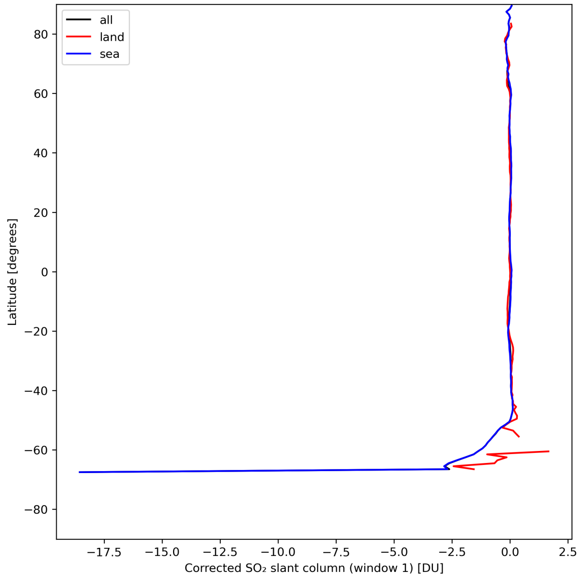
Figure 35: Zonal average of “Corrected SO 2 slant column (window 1)” for 2024-07-31 to 2024-08-02.
