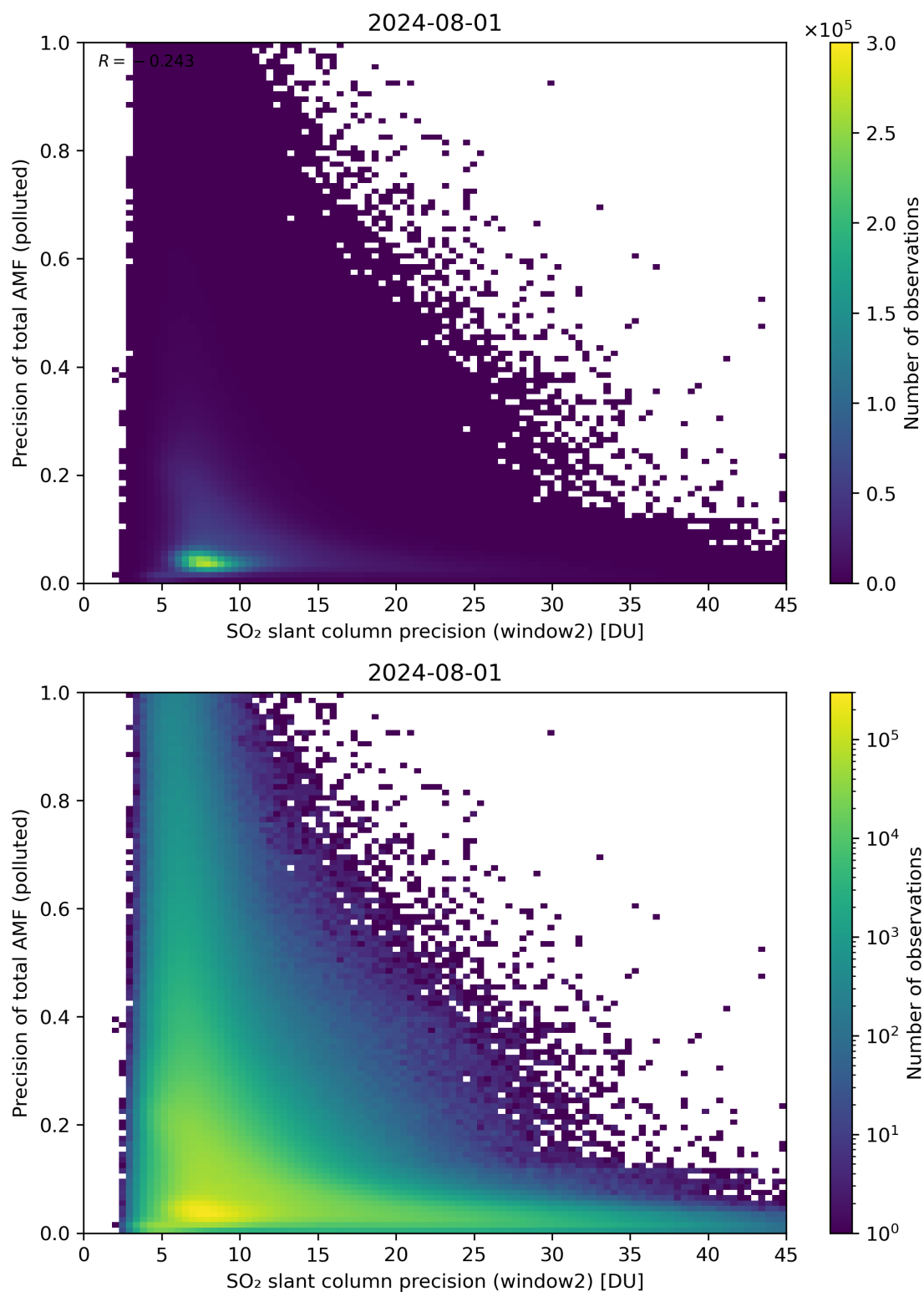
Figure 252: Scatter density plot of “SO 2 slant column precision (window2)” against “Precision of total AMF (polluted)” for 2024-07-31 to 2024-08-02.
