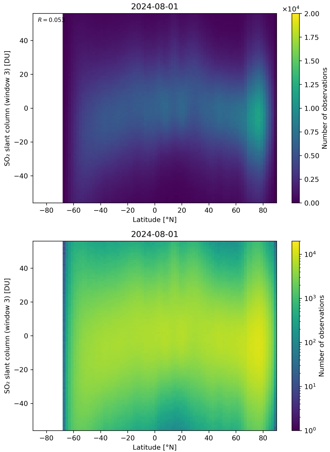
Figure 152: Scatter density plot of “Latitude” against “SO 2 slant column (window 3)” for 2024-07-31 to 2024-08-02.
