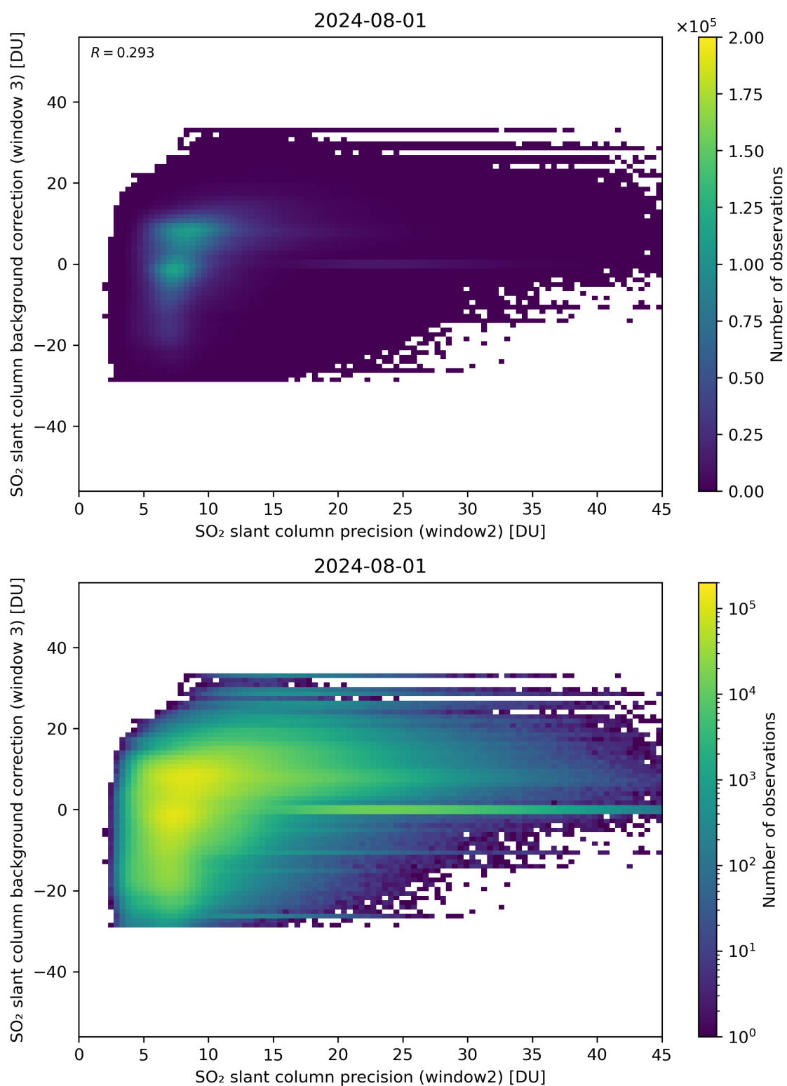
Figure 242: Scatter density plot of “SO 2 slant column precision (window2)” against “SO 2 slant column background correction (window 3)” for 2024-07-31 to 2024-08-02.
