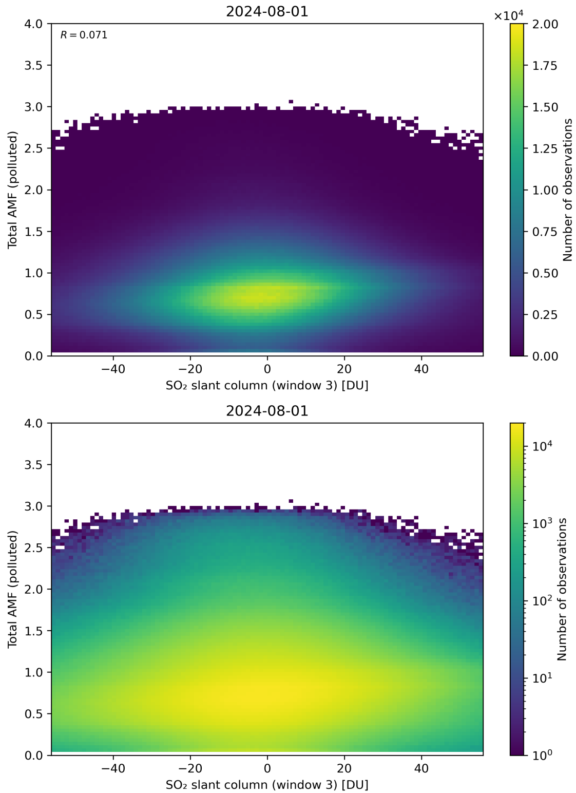
Figure 268: Scatter density plot of “SO 2 slant column (window 3)” against “Total AMF (polluted)” for 2024-07-31 to 2024-08-02.
