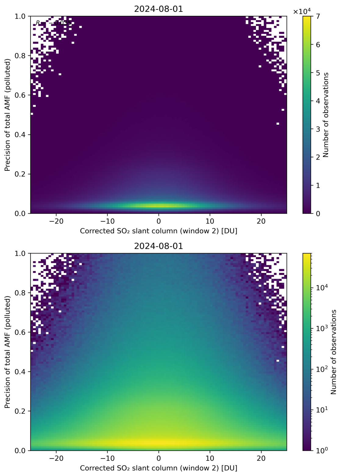
Figure 204: Scatter density plot of “Corrected SO 2 slant column (window 2)” against “Precision of total AMF (polluted)” for 2024-07-31 to 2024-08-02.
