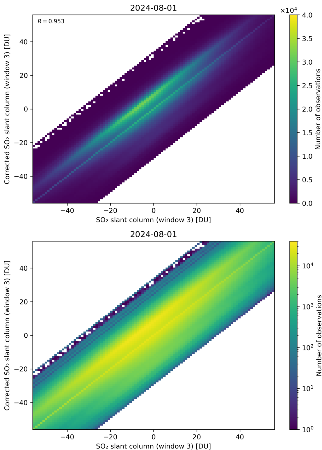
Figure 266: Scatter density plot of “SO 2 slant column (window 3)” against “Corrected SO 2 slant column (window 3)” for 2024-07-31 to 2024-08-02.
