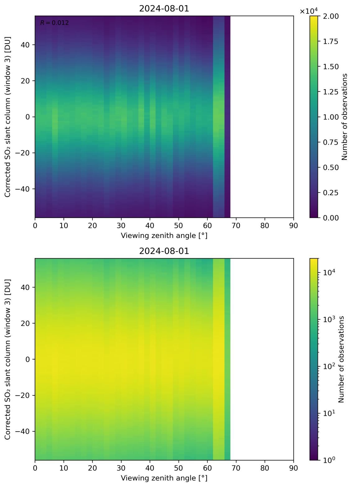
Figure 319: Scatter density plot of “Viewing zenith angle” against “Corrected SO 2 slant column (window 3)” for 2024-07-31 to 2024-08-02.
