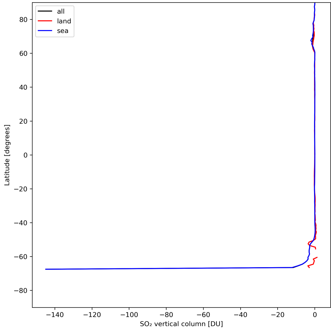
Figure 30: Zonal average of “SO 2 vertical column” for 2024-07-31 to 2024-08-02.
