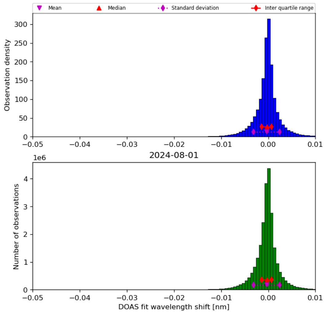
Figure 68: Histogram of “DOAS fit wavelength shift” for 2024-07-31 to 2024-08-02
