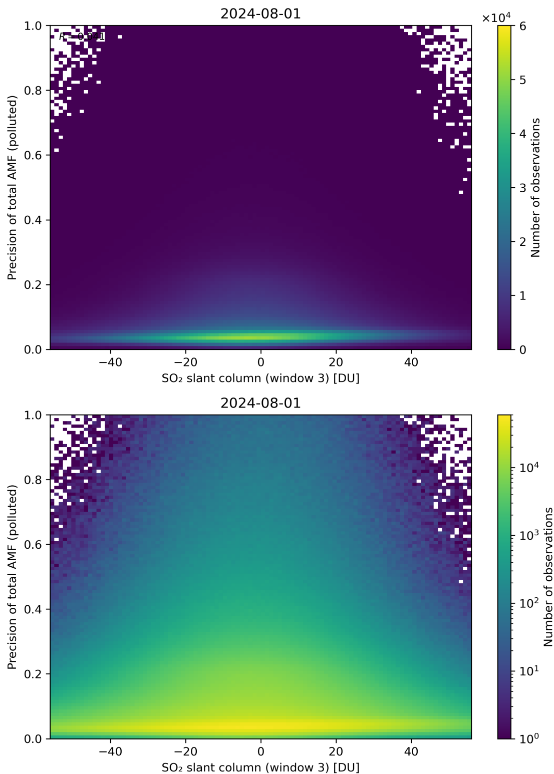
Figure 269: Scatter density plot of “SO 2 slant column (window 3)” against “Precision of total AMF (polluted)” for 2024-07-31 to 2024-08-02.
