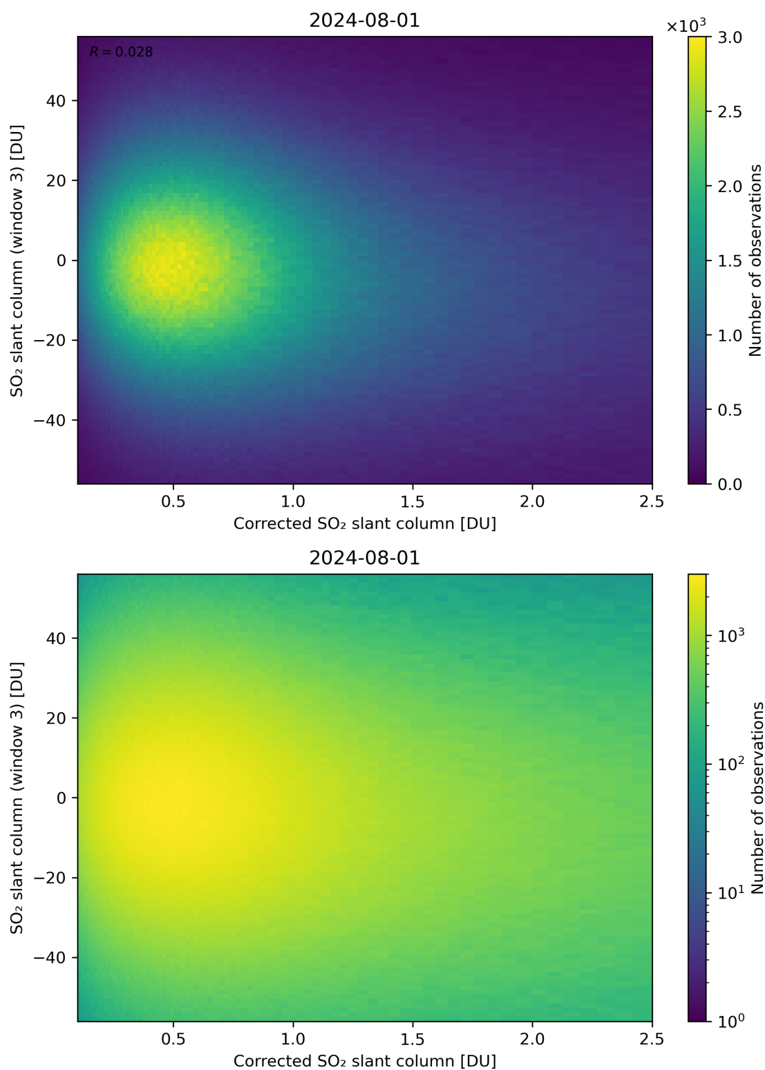
Figure 190: Scatter density plot of “Corrected SO 2 slant column” against “SO 2 slant column (window 3)” for 2024-07-31 to 2024-08-02.
