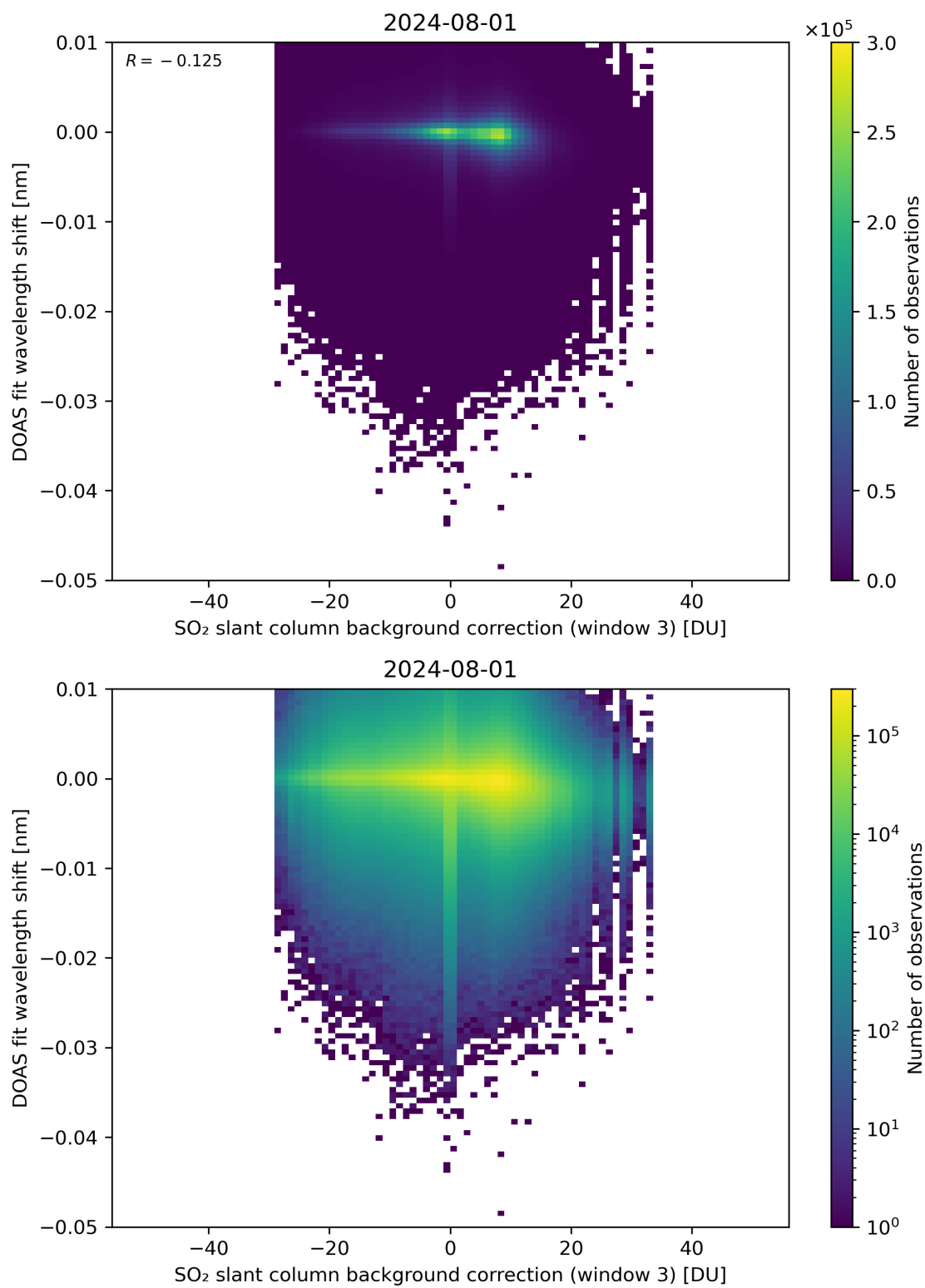
Figure 121: Scatter density plot of “SO 2 slant column background correction (window 3)” against “DOAS fit wavelength shift” for 2024-07-31 to 2024-08-02.
