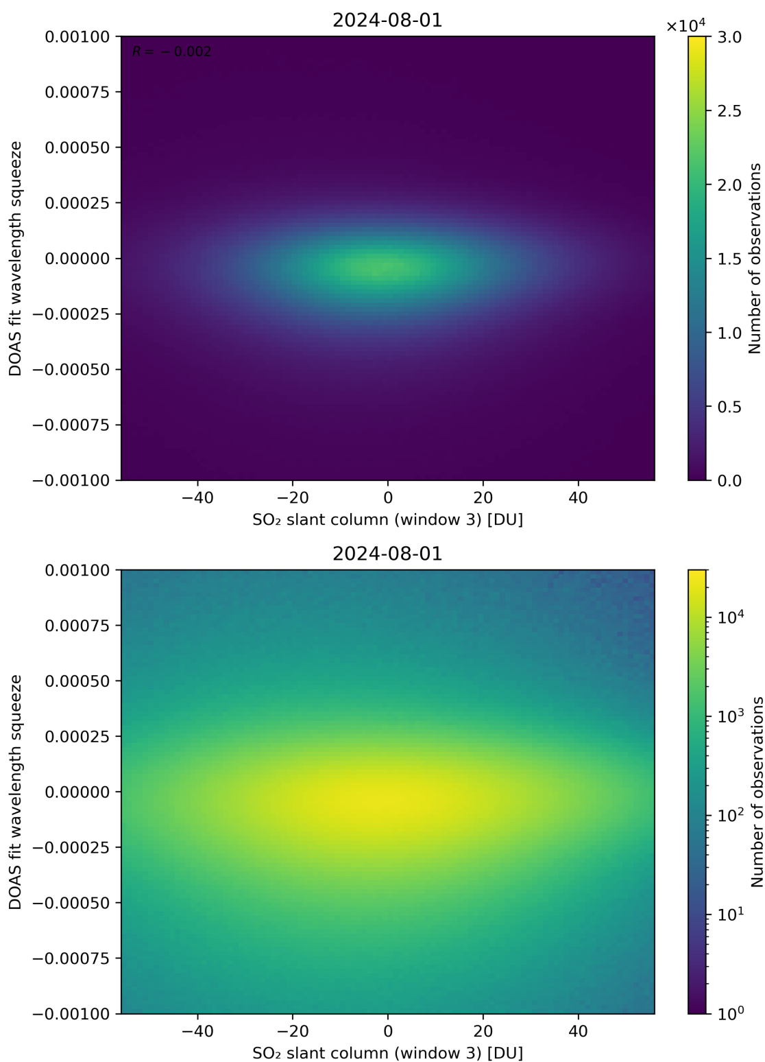
Figure 255: Scatter density plot of “SO 2 slant column (window 3)” against “DOAS fit wavelength squeeze” for 2024-07-31 to 2024-08-02.
