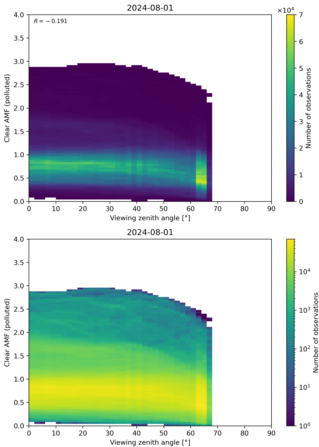
Figure 316: Scatter density plot of “Viewing zenith angle” against “Clear AMF (polluted)” for 2024-07-31 to 2024-08-02.
