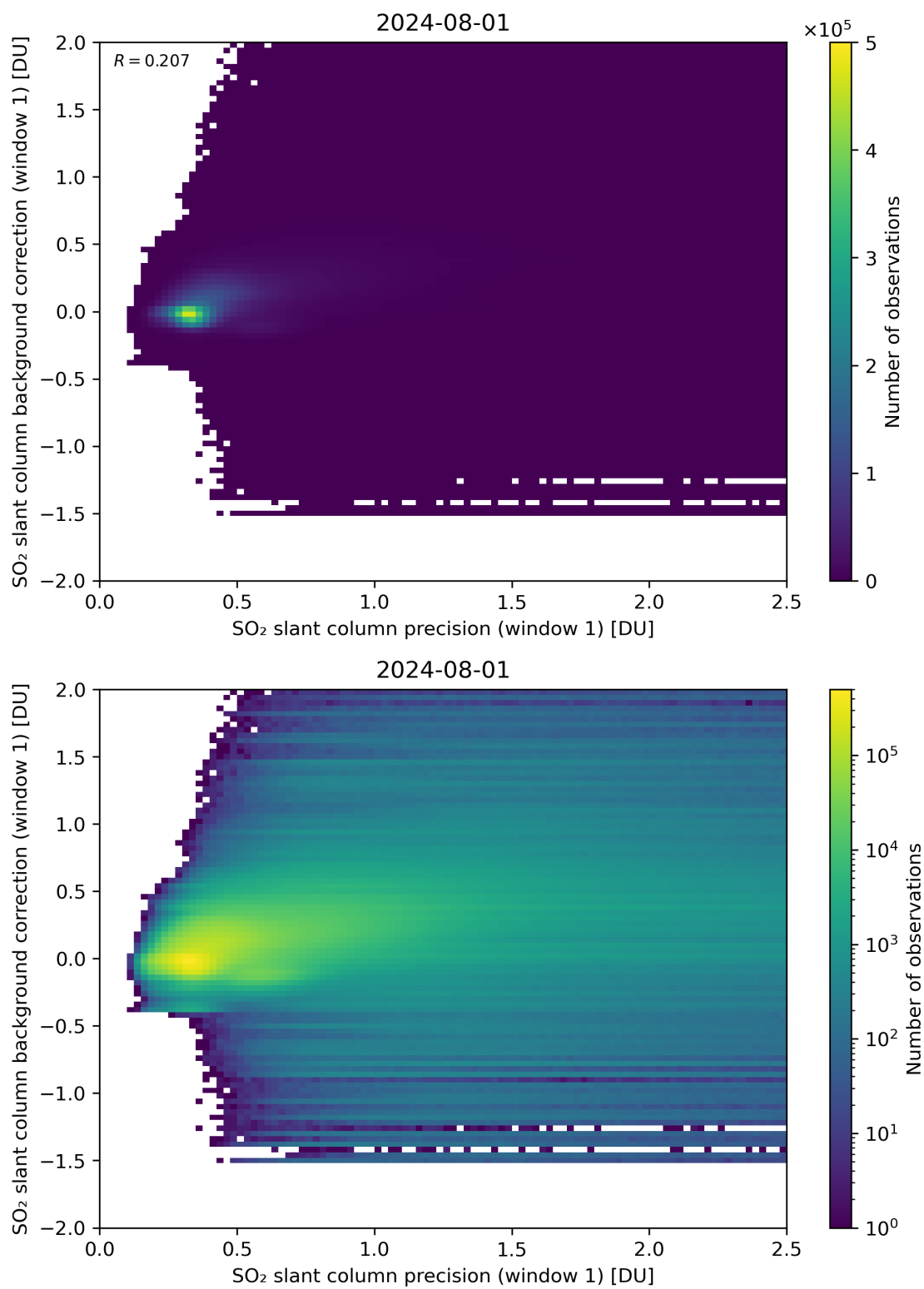
Figure 218: Scatter density plot of “SO 2 slant column precision (window 1)” against “SO 2 slant column background correction (window 1)” for 2024-07-31 to 2024-08-02.
