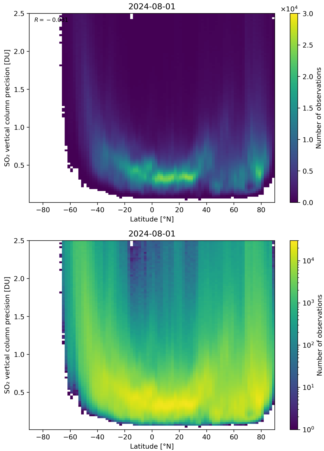
Figure 157: Scatter density plot of “Latitude” against “SO 2 vertical column precision” for 2024-07-31 to 2024-08-02.
