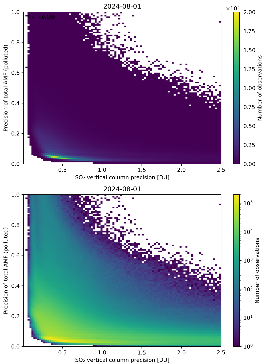
Figure 295: Scatter density plot of “SO 2 vertical column precision” against “Precision of total AMF (polluted)” for 2024-07-31 to 2024-08-02.
