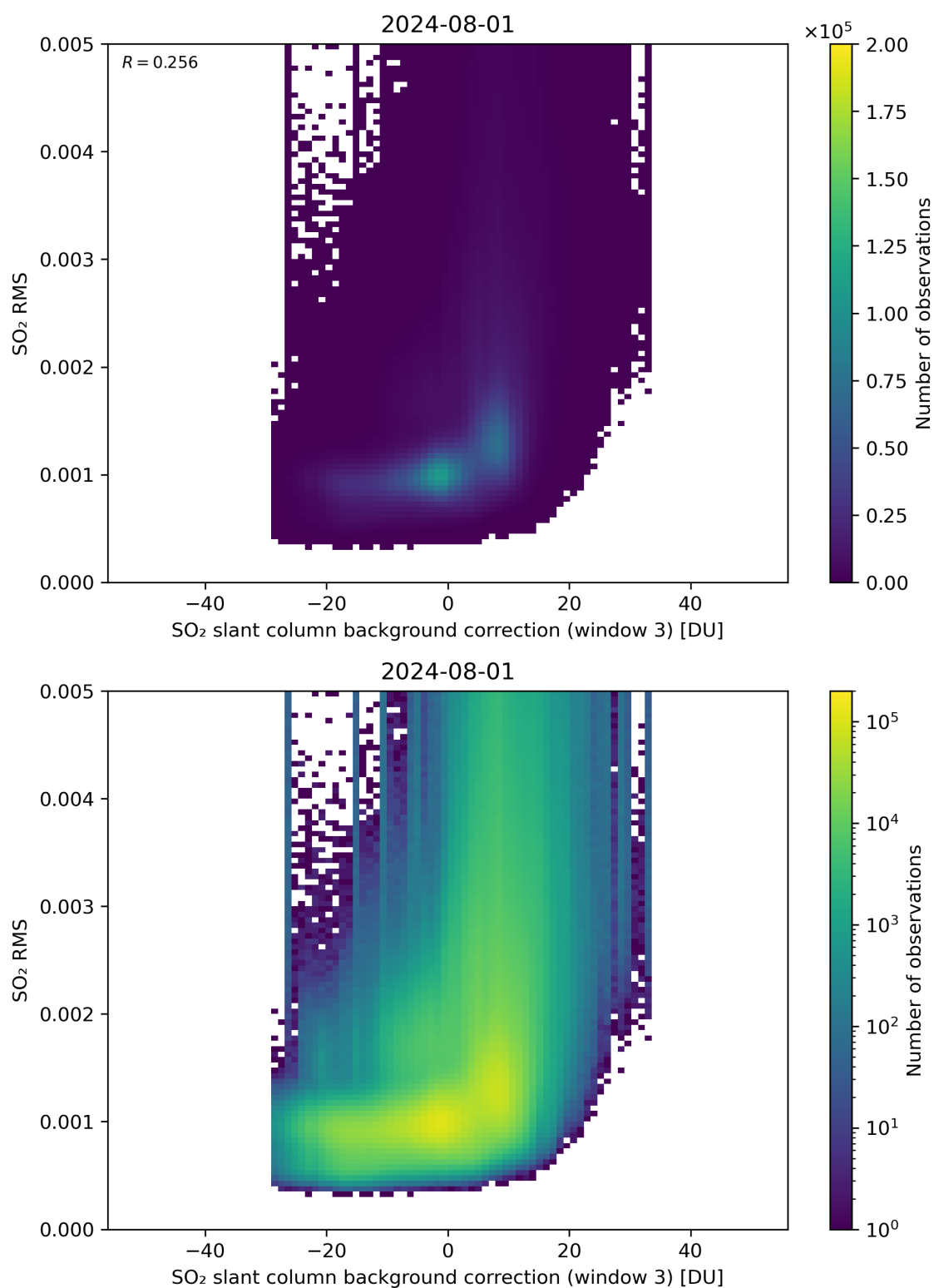
Figure 123: Scatter density plot of “SO 2 slant column background correction (window 3)” against “SO 2 RMS” for 2024-07-31 to 2024-08-02.
