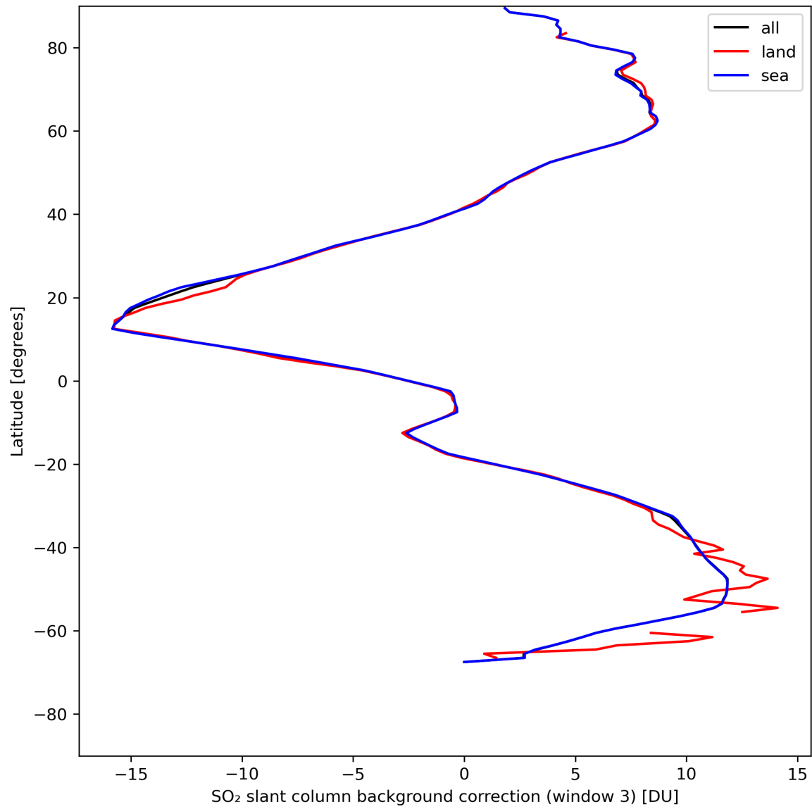
Figure 44: Zonal average of “SO 2 slant column background correction (window 3)” for 2024-07-31 to 2024-08-02.
