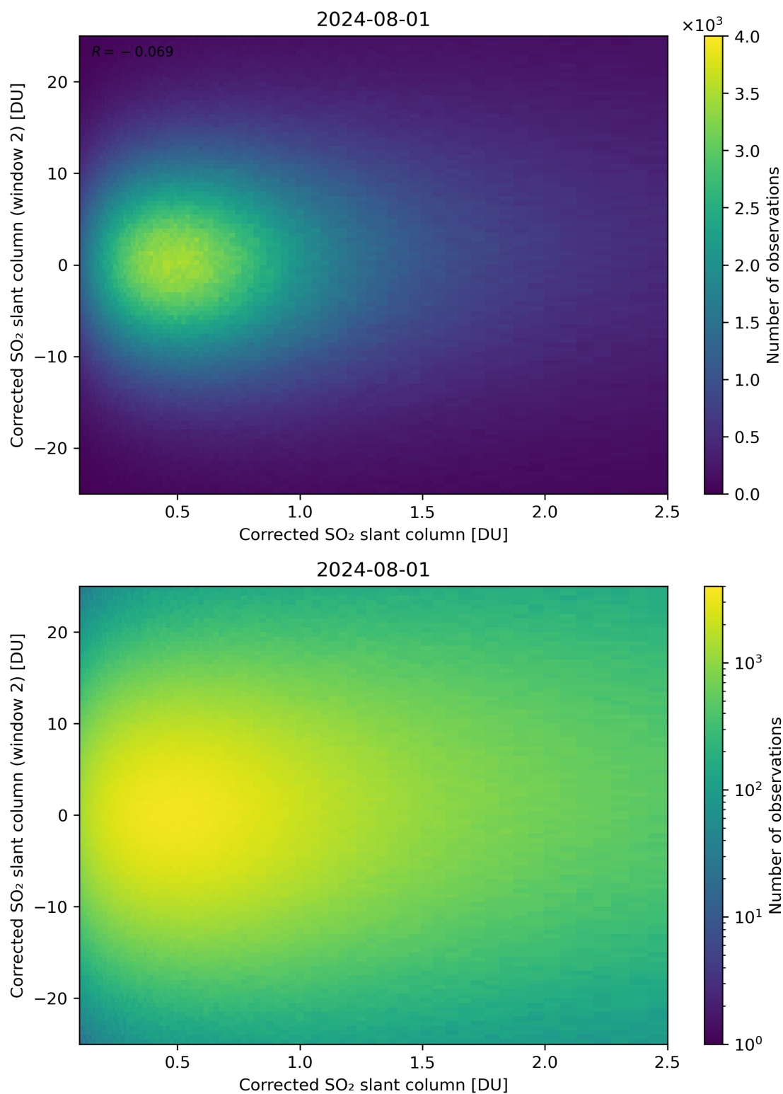
Figure 185: Scatter density plot of “Corrected SO 2 slant column” against “Corrected SO 2 slant column (window 2)” for 2024-07-31 to 2024-08-02.
