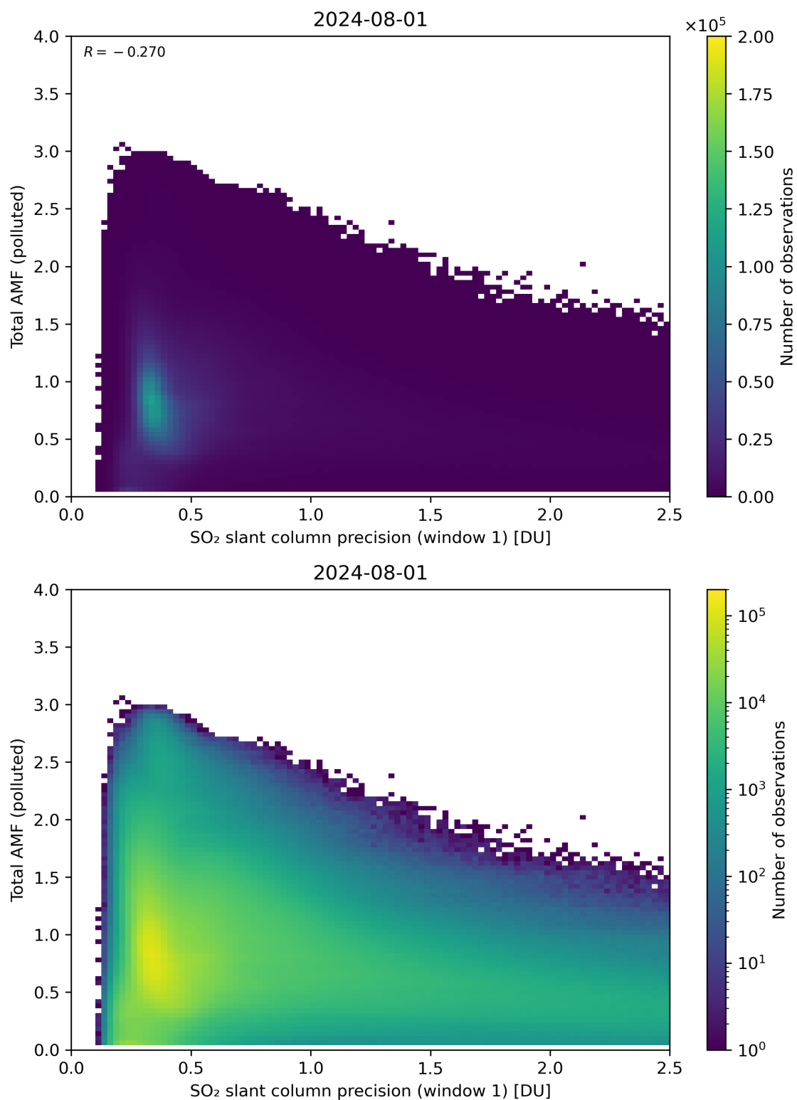
Figure 230: Scatter density plot of “SO 2 slant column precision (window 1)” against “Total AMF (polluted)” for 2024-07-31 to 2024-08-02.
