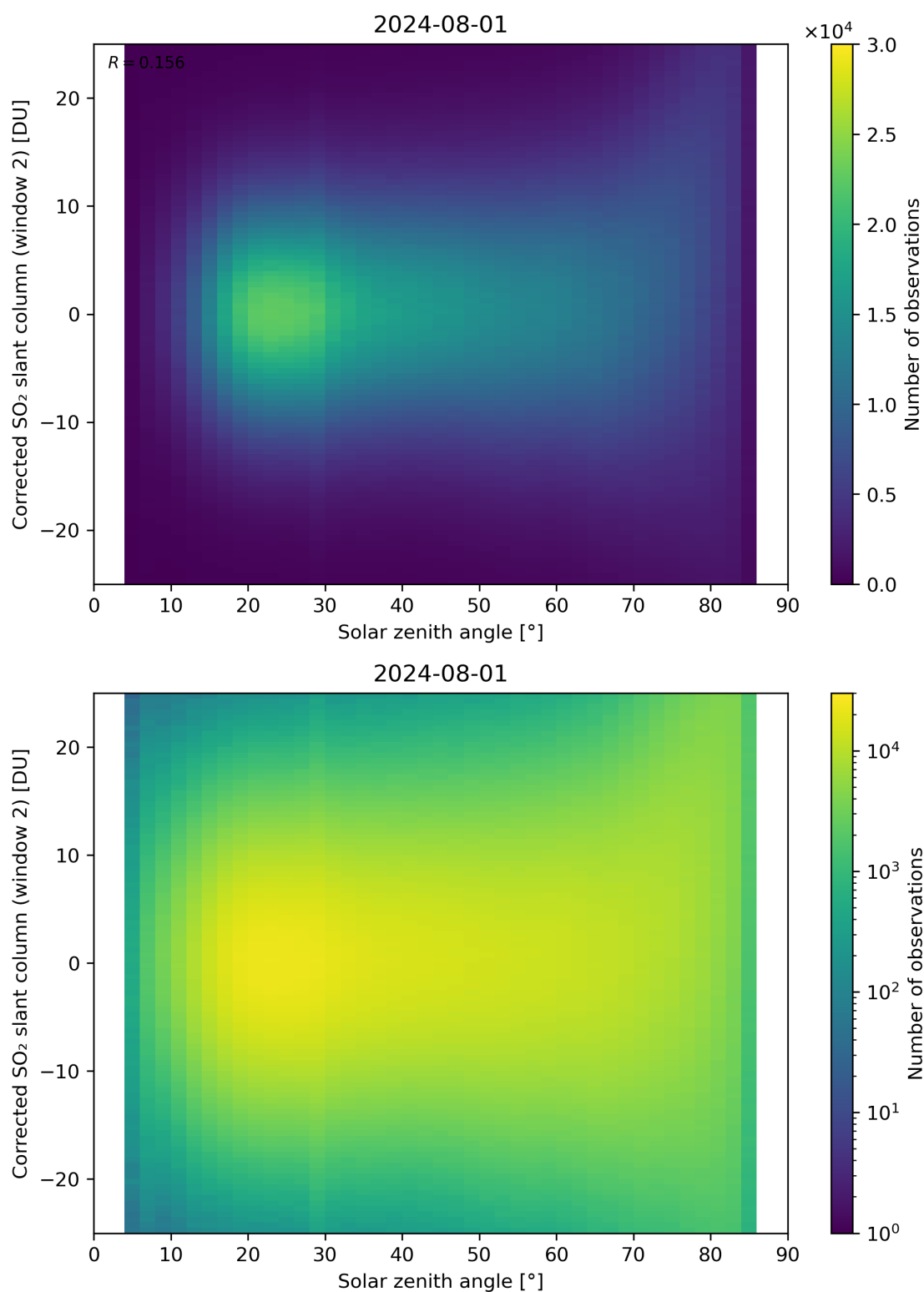
Figure 167: Scatter density plot of “Solar zenith angle” against “Corrected SO 2 slant column (window 2)” for 2024-07-31 to 2024-08-02.
