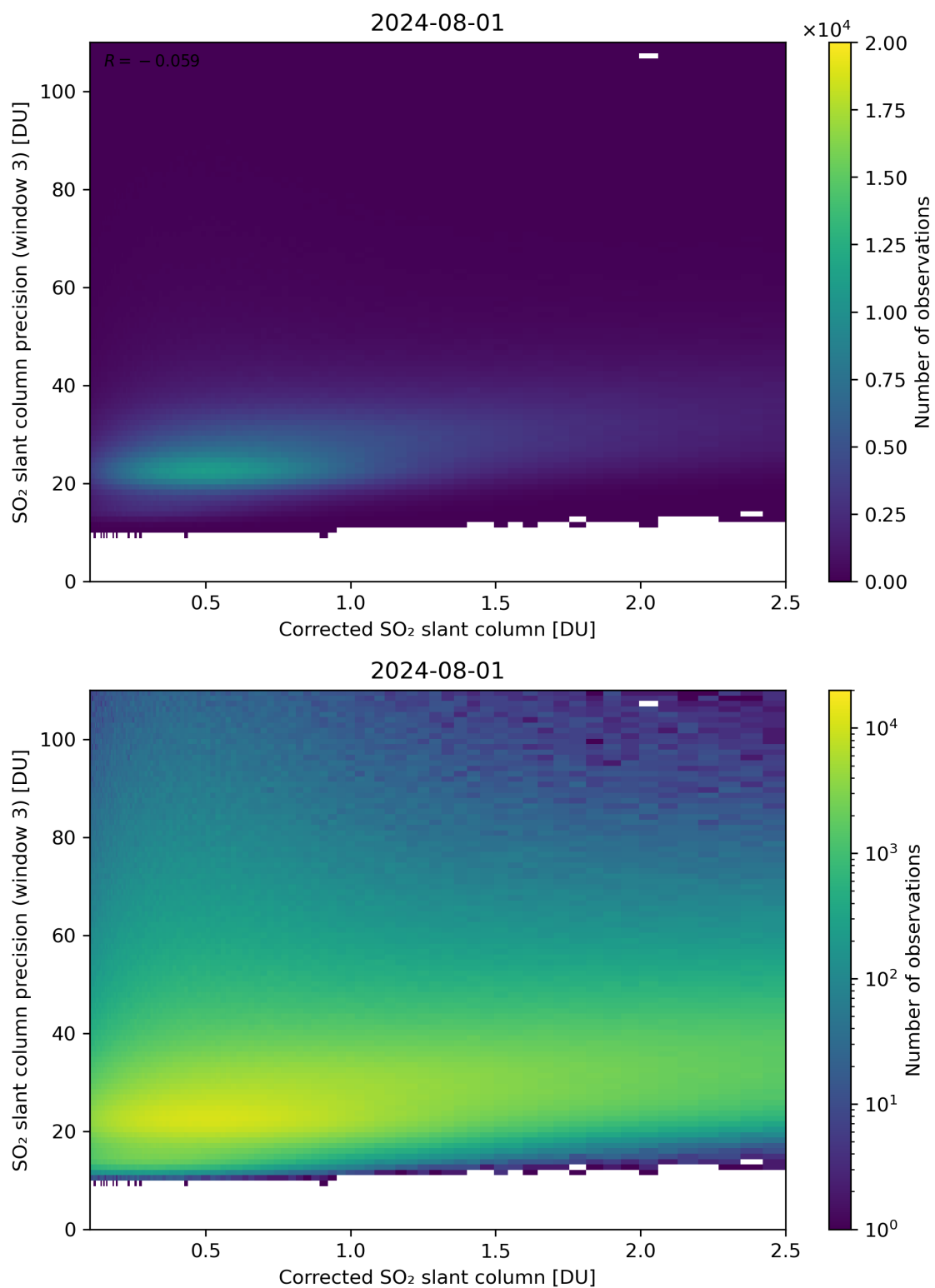
Figure 191: Scatter density plot of “Corrected SO 2 slant column” against “SO 2 slant column precision (window 3)” for 2024-07-31 to 2024-08-02.
