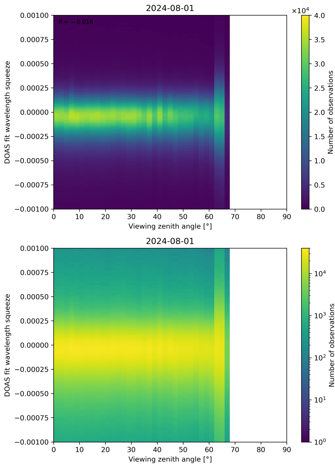
Figure 312: Scatter density plot of “Viewing zenith angle” against “DOAS fit wavelength squeeze” for 2024-07-31 to 2024-08-02.
