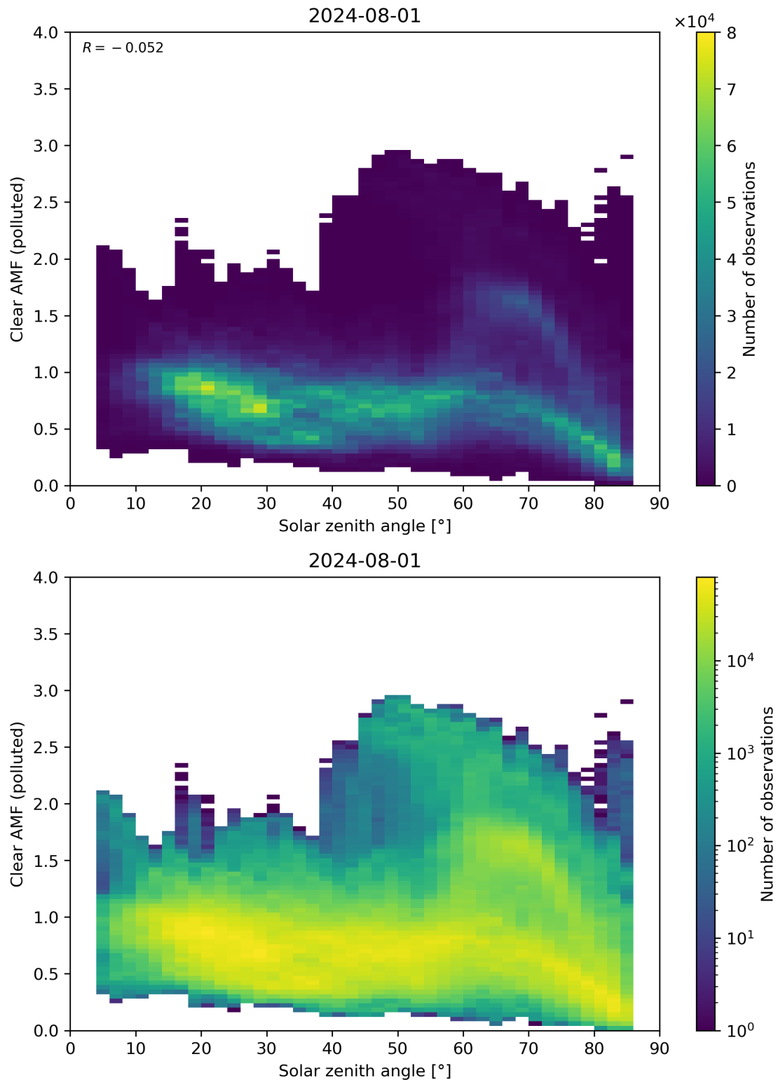
Figure 165: Scatter density plot of “Solar zenith angle” against “Clear AMF (polluted)” for 2024-07-31 to 2024-08-02.
