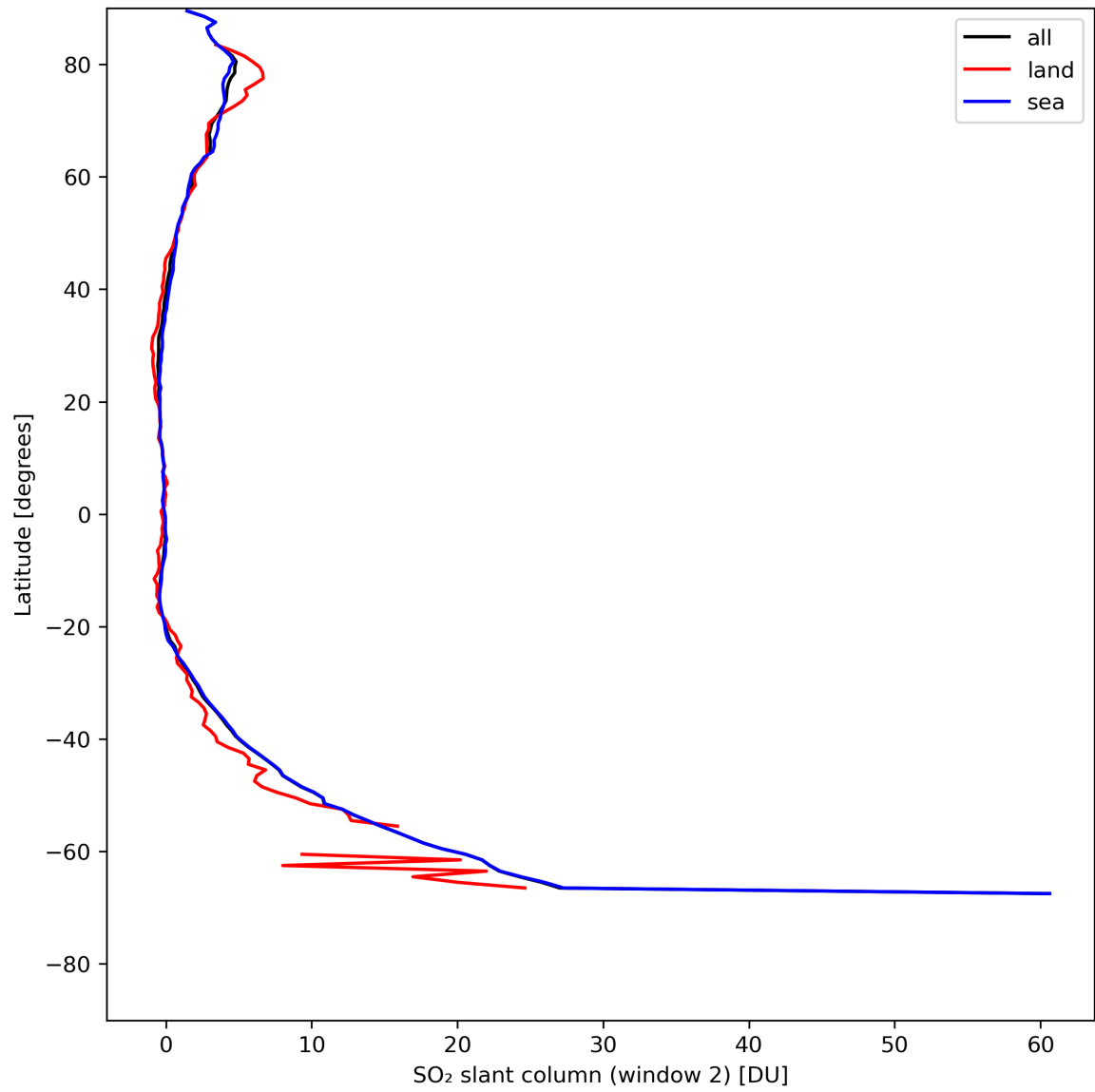
Figure 37: Zonal average of “SO 2 slant column (window 2)” for 2024-07-31 to 2024-08-02.
