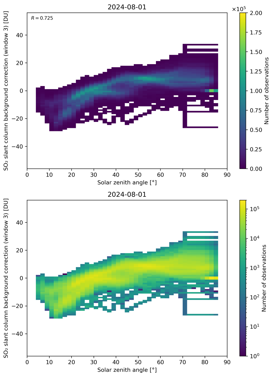
Figure 160: Scatter density plot of “Solar zenith angle” against “SO 2 slant column background correction (window 3)” for 2024-07-31 to 2024-08-02.
