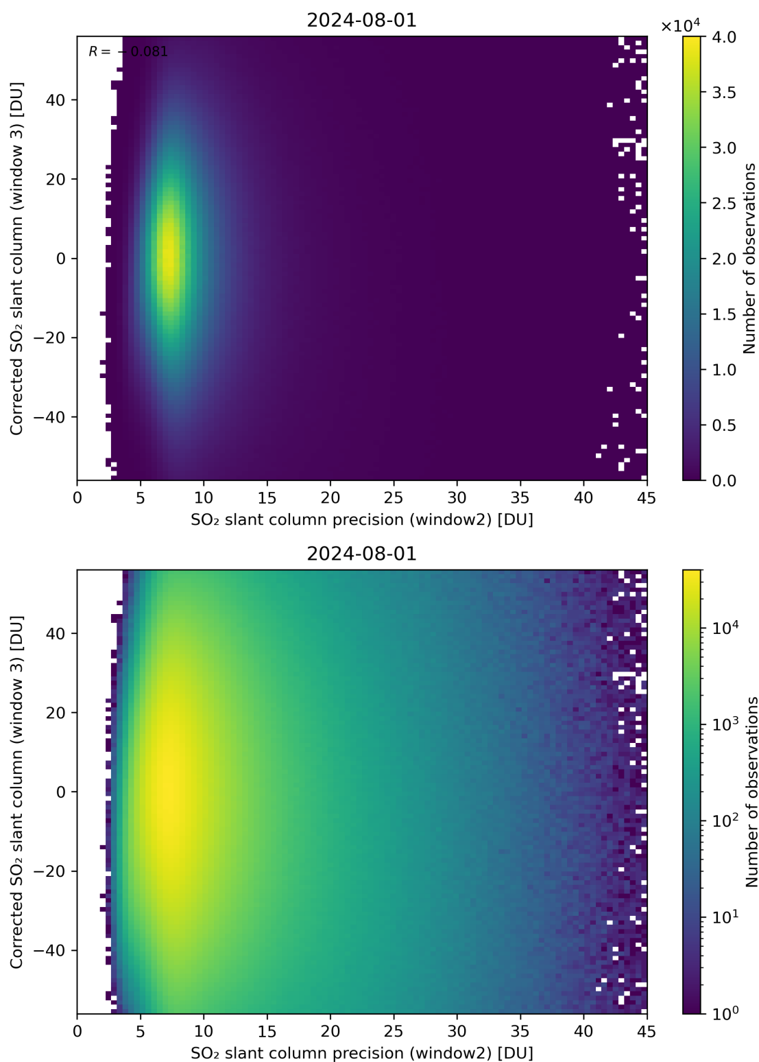
Figure 248: Scatter density plot of “SO 2 slant column precision (window2)” against “Corrected SO 2 slant column (window 3)” for 2024-07-31 to 2024-08-02.
