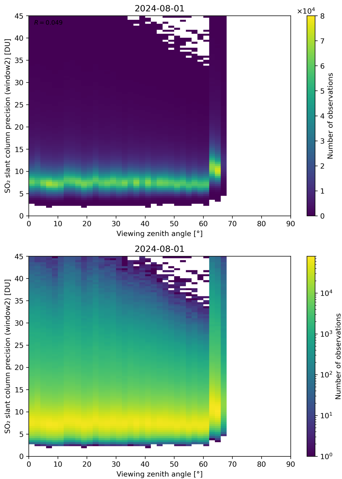
Figure 322: Scatter density plot of “Viewing zenith angle” against “SO 2 slant column precision (window2)” for 2024-07-31 to 2024-08-02.
