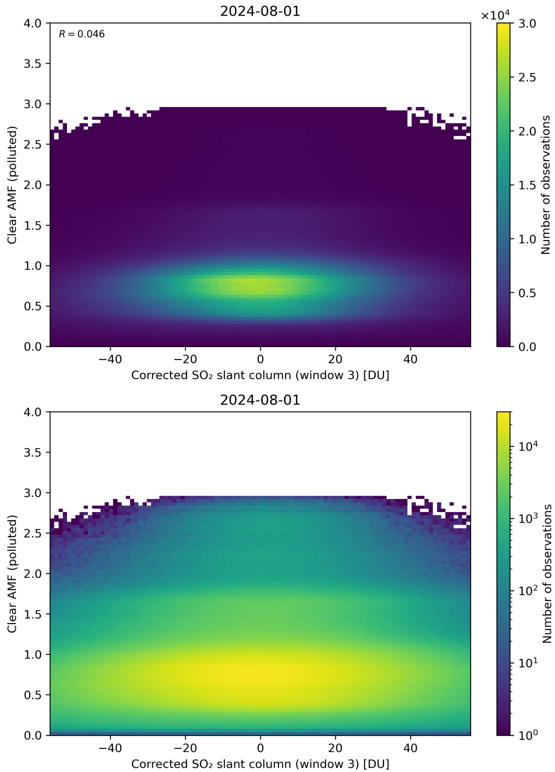
Figure 209: Scatter density plot of “Corrected SO 2 slant column (window 3)” against “Clear AMF (polluted)” for 2024-07-31 to 2024-08-02.
