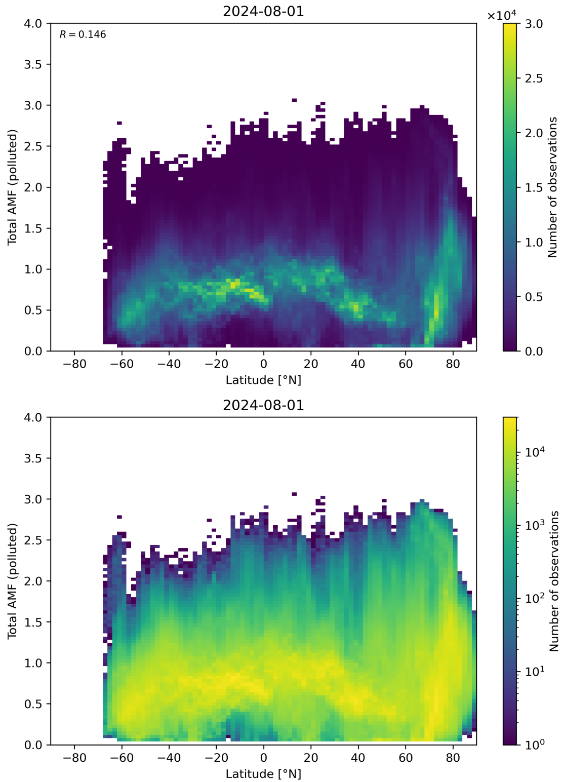
Figure 154: Scatter density plot of “Latitude” against “Total AMF (polluted)” for 2024-07-31 to 2024-08-02.
