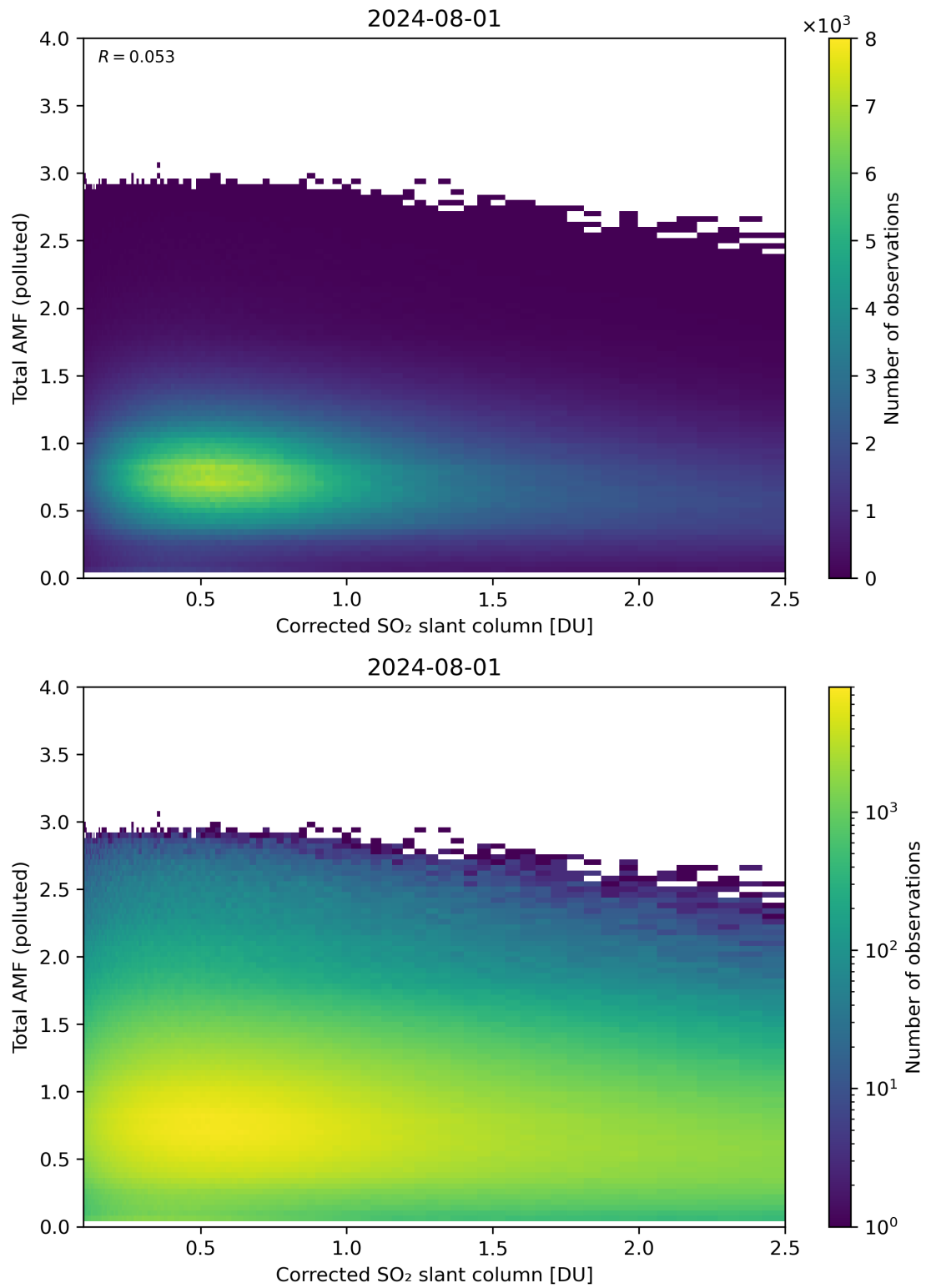
Figure 192: Scatter density plot of “Corrected SO 2 slant column” against “Total AMF (polluted)” for 2024-07-31 to 2024-08-02.
