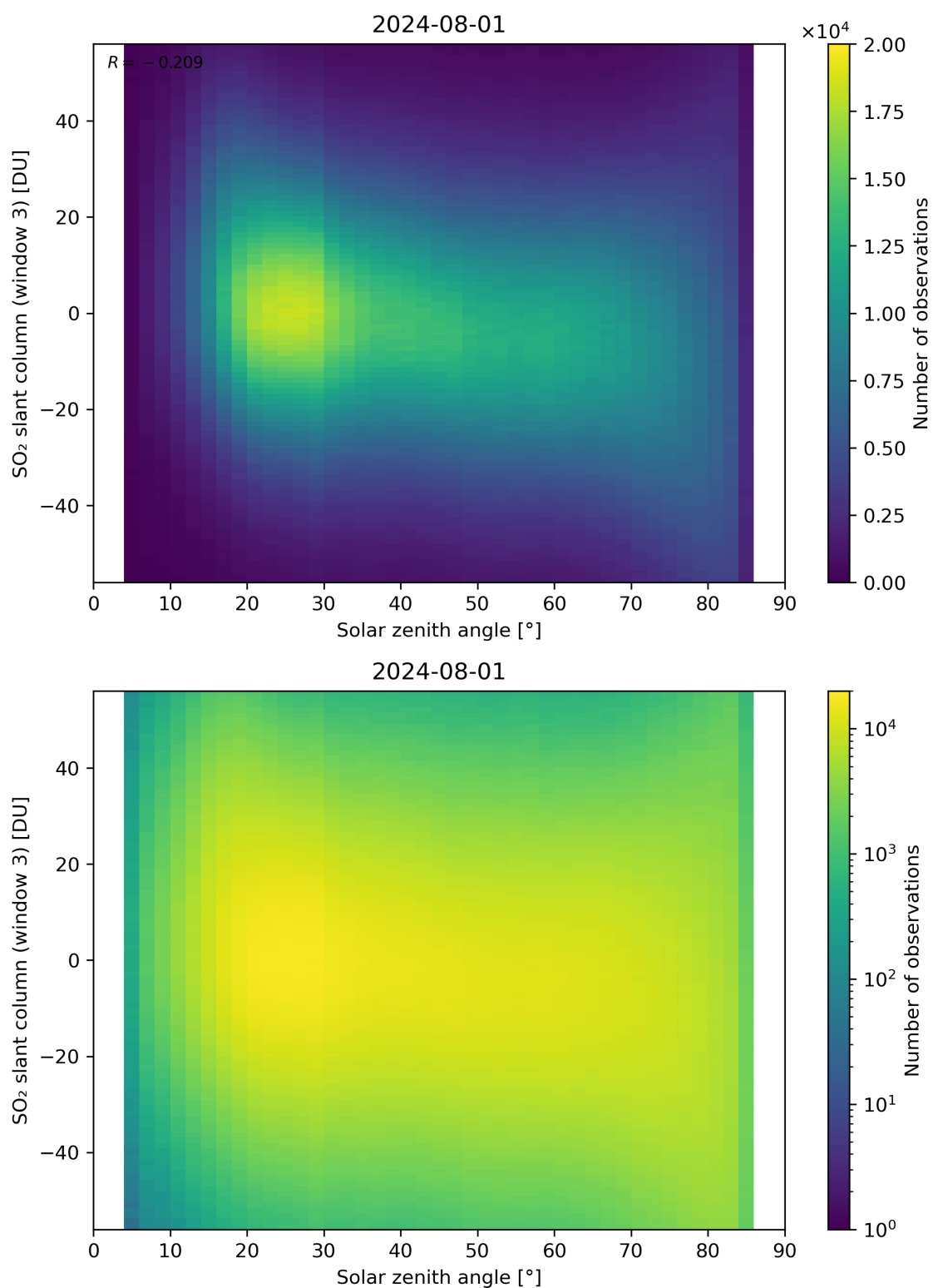
Figure 172: Scatter density plot of “Solar zenith angle” against “SO 2 slant column (window 3)” for 2024-07-31 to 2024-08-02.
