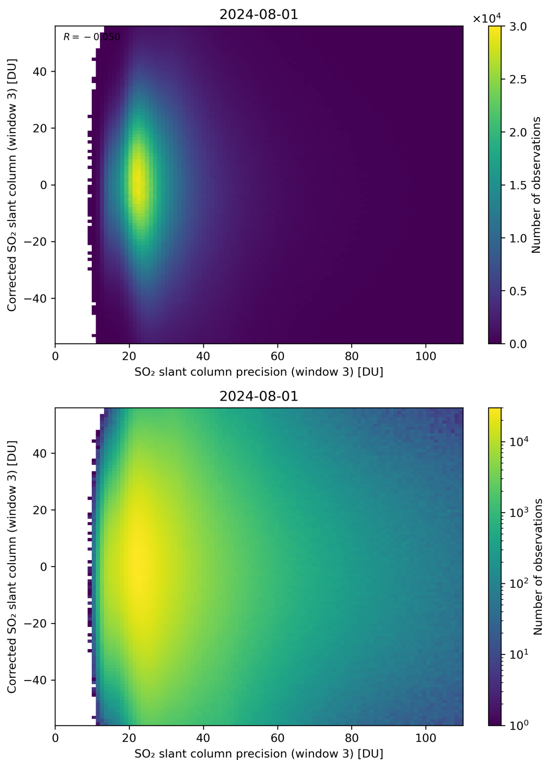
Figure 262: Scatter density plot of “SO 2 slant column precision (window 3)” against “Corrected SO 2 slant column (window 3)” for 2024-07-31 to 2024-08-02.
