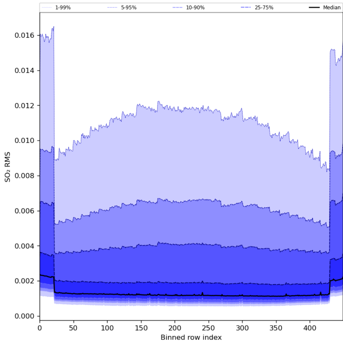
Figure 93: Along track statistics of “SO 2 RMS” for 2024-07-31 to 2024-08-02
