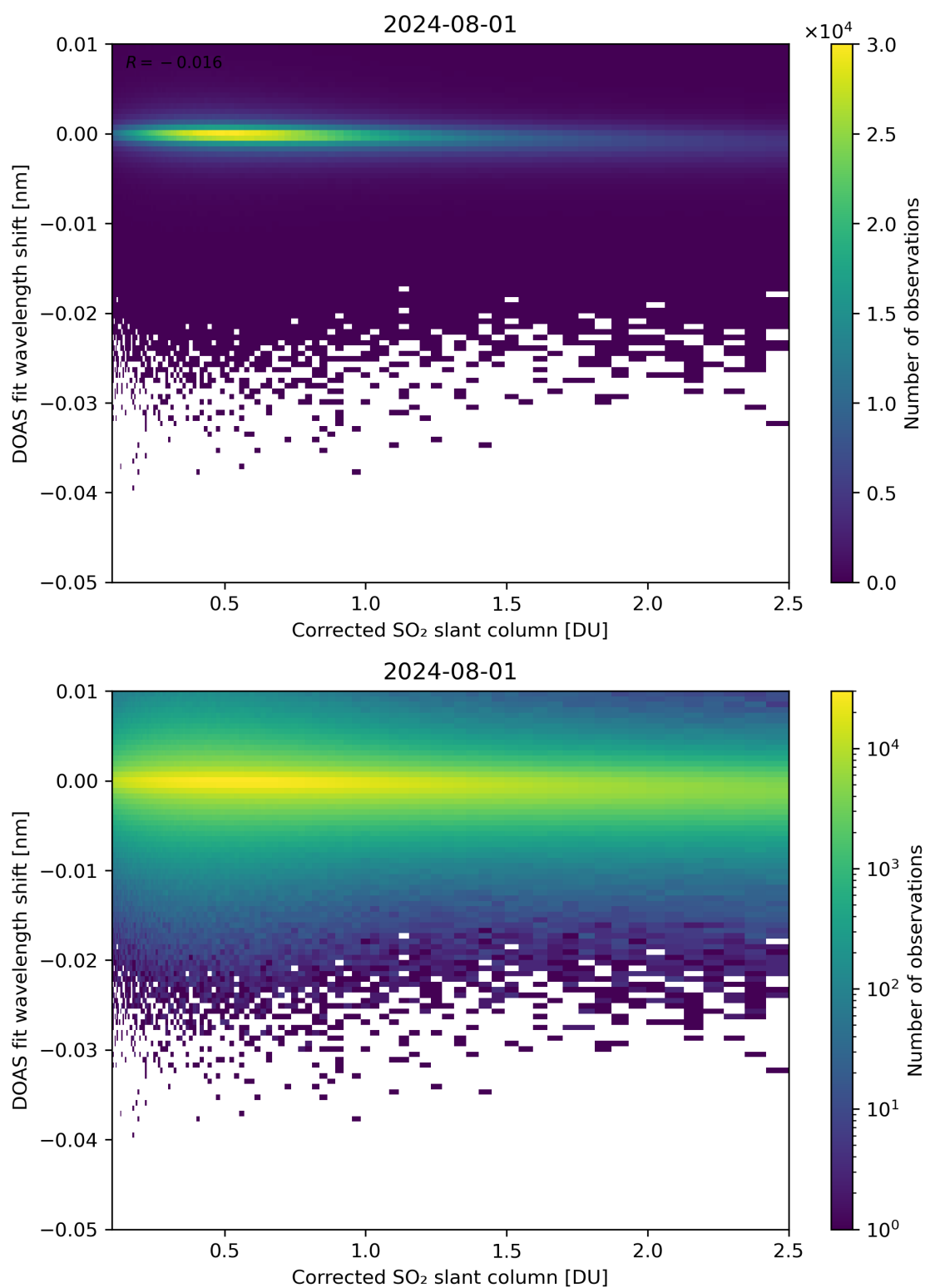
Figure 181: Scatter density plot of “Corrected SO 2 slant column” against “DOAS fit wavelength shift” for 2024-07-31 to 2024-08-02.
