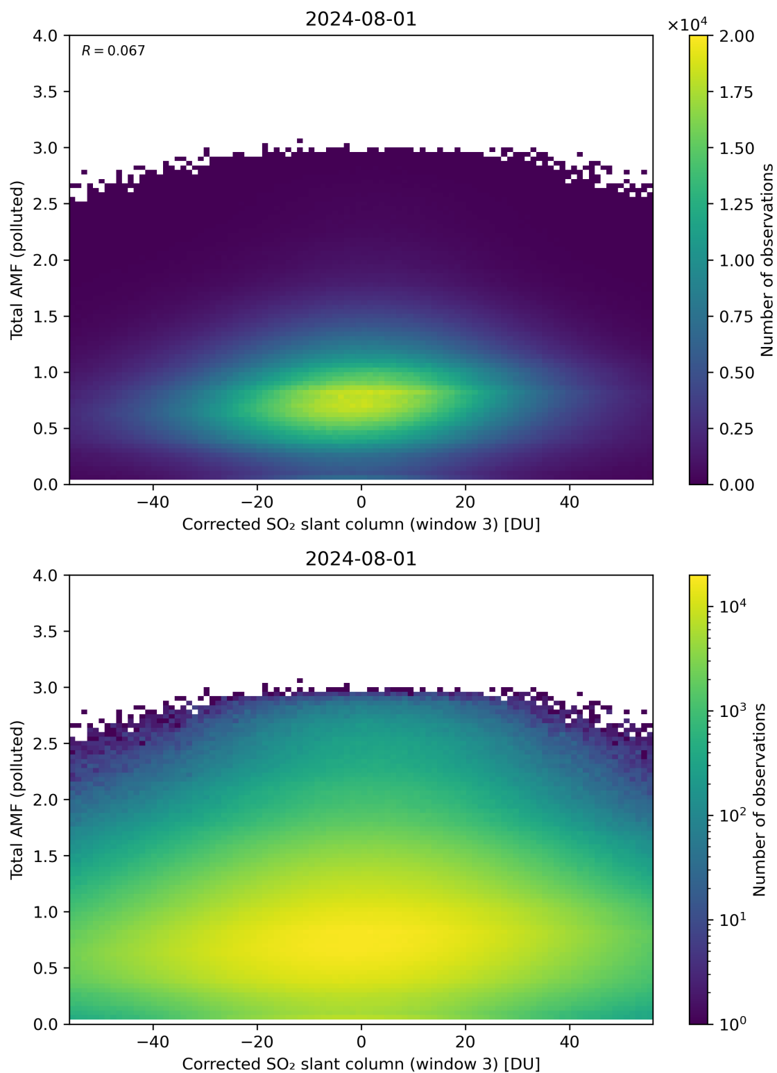
Figure 210: Scatter density plot of “Corrected SO 2 slant column (window 3)” against “Total AMF (polluted)” for 2024-07-31 to 2024-08-02.
