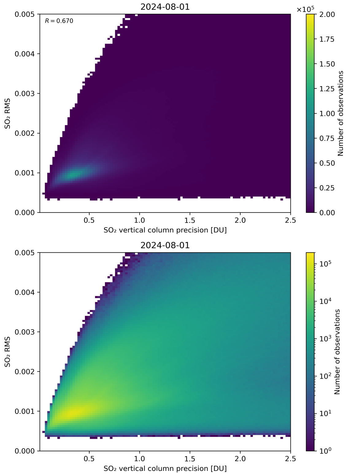
Figure 284: Scatter density plot of “SO 2 vertical column precision” against “SO 2 RMS” for 2024-07-31 to 2024-08-02.
