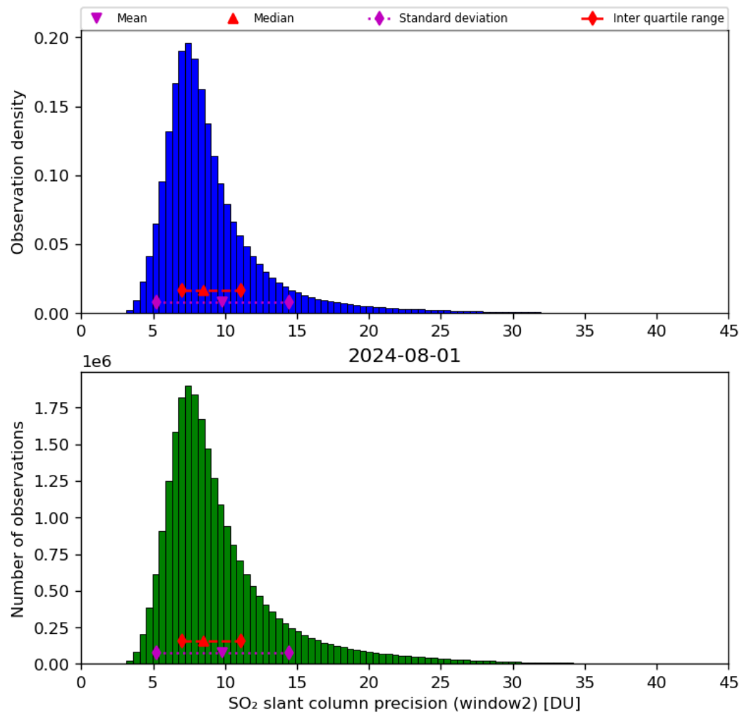
Figure 61: Histogram of “SO 2 slant column precision (window2)” for 2024-07-31 to 2024-08-02
