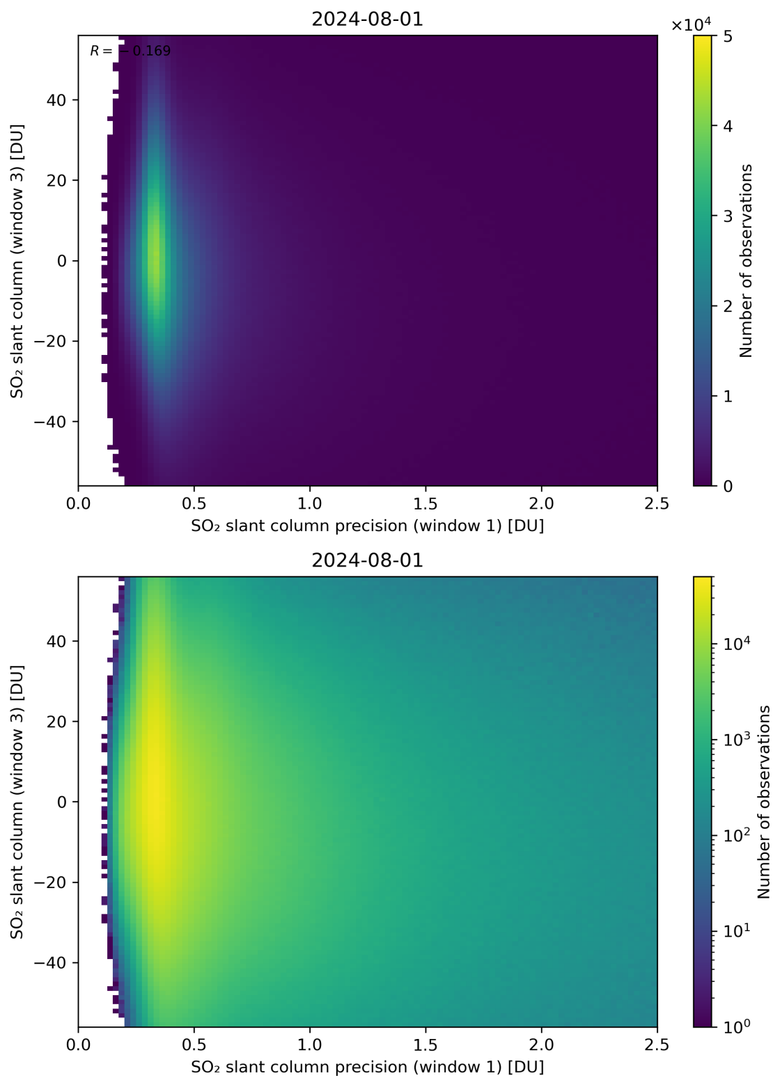
Figure 228: Scatter density plot of “SO 2 slant column precision (window 1)” against “SO 2 slant column (window 3)” for 2024-07-31 to 2024-08-02.
