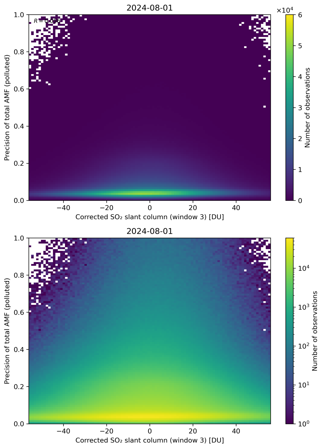
Figure 211: Scatter density plot of “Corrected SO 2 slant column (window 3)” against “Precision of total AMF (polluted)” for 2024-07-31 to 2024-08-02.
