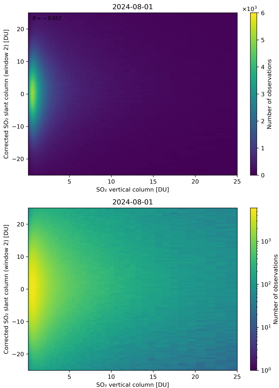
Figure 298: Scatter density plot of “SO 2 vertical column” against “Corrected SO 2 slant column (window 2)” for 2024-07-31 to 2024-08-02.
