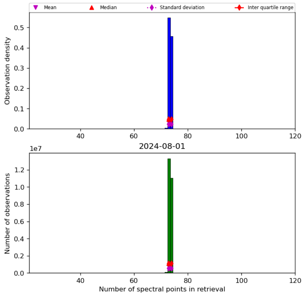
Figure 74: Histogram of “Number of spectral points in retrieval” for 2024-07-31 to 2024-08-02
