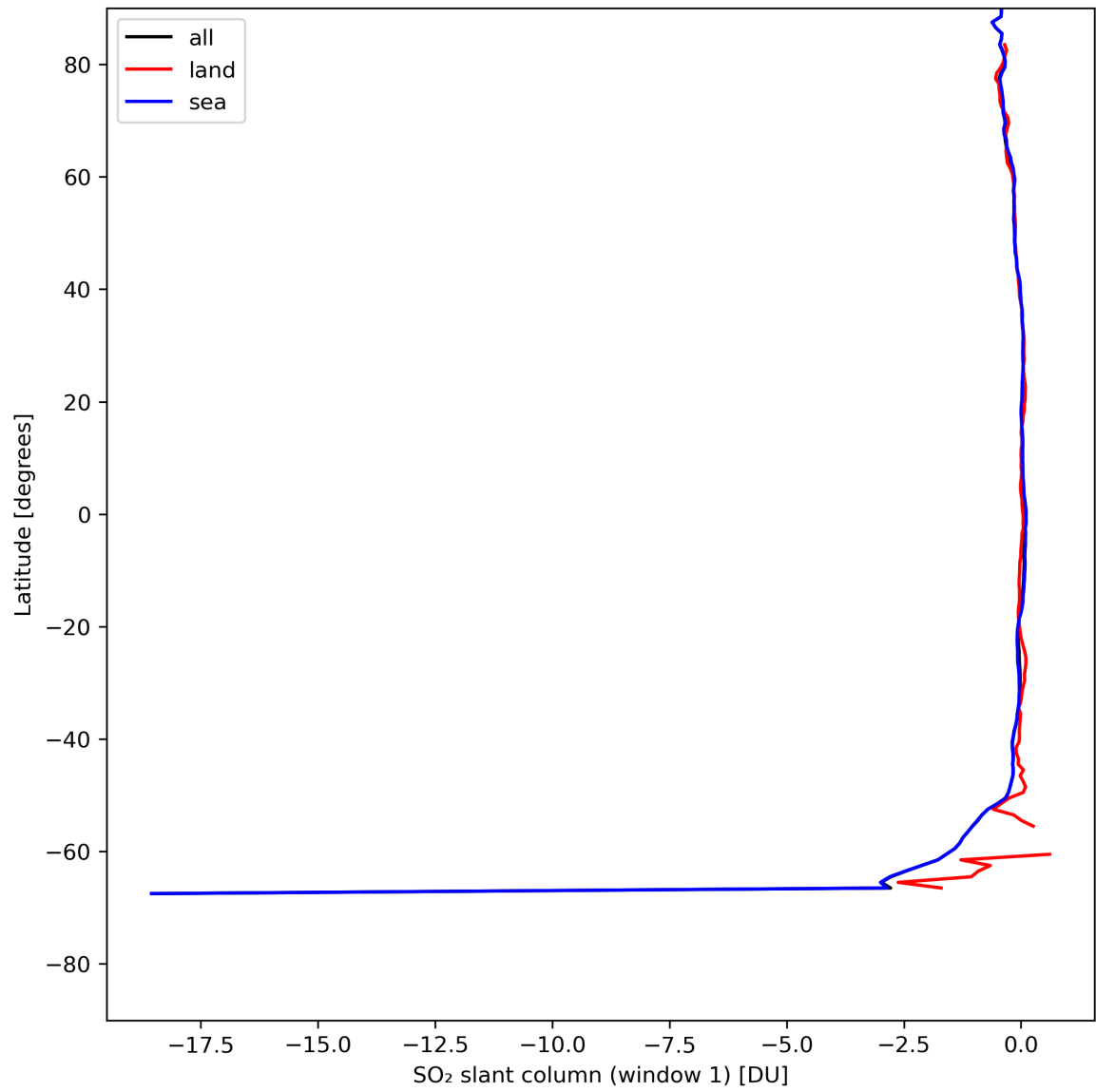
Figure 33: Zonal average of “SO 2 slant column (window 1)” for 2024-07-31 to 2024-08-02.
