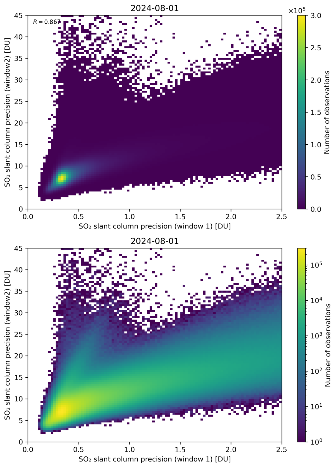
Figure 227: Scatter density plot of “SO 2 slant column precision (window 1)” against “SO 2 slant column precision (window2)” for 2024-07-31 to 2024-08-02.
