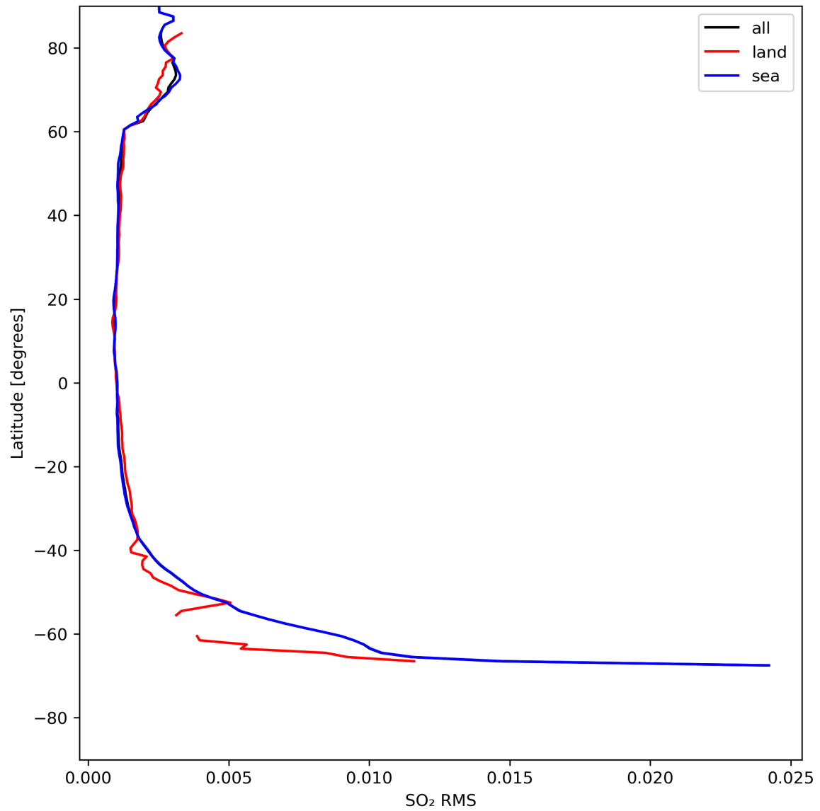
Figure 47: Zonal average of “SO 2 RMS” for 2024-07-31 to 2024-08-02.
