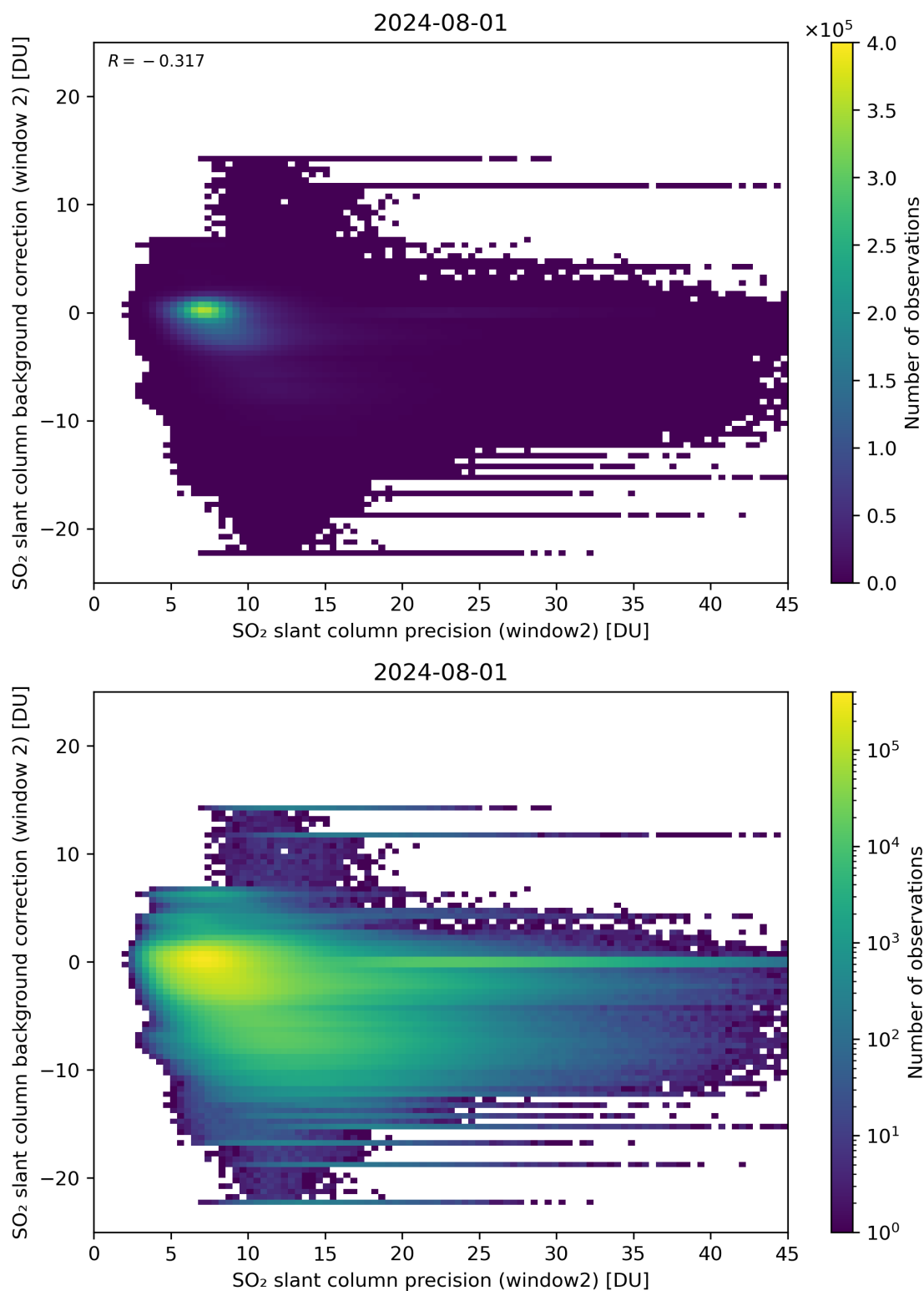
Figure 241: Scatter density plot of “SO 2 slant column precision (window2)” against “SO 2 slant column background correction (window 2)” for 2024-07-31 to 2024-08-02.
