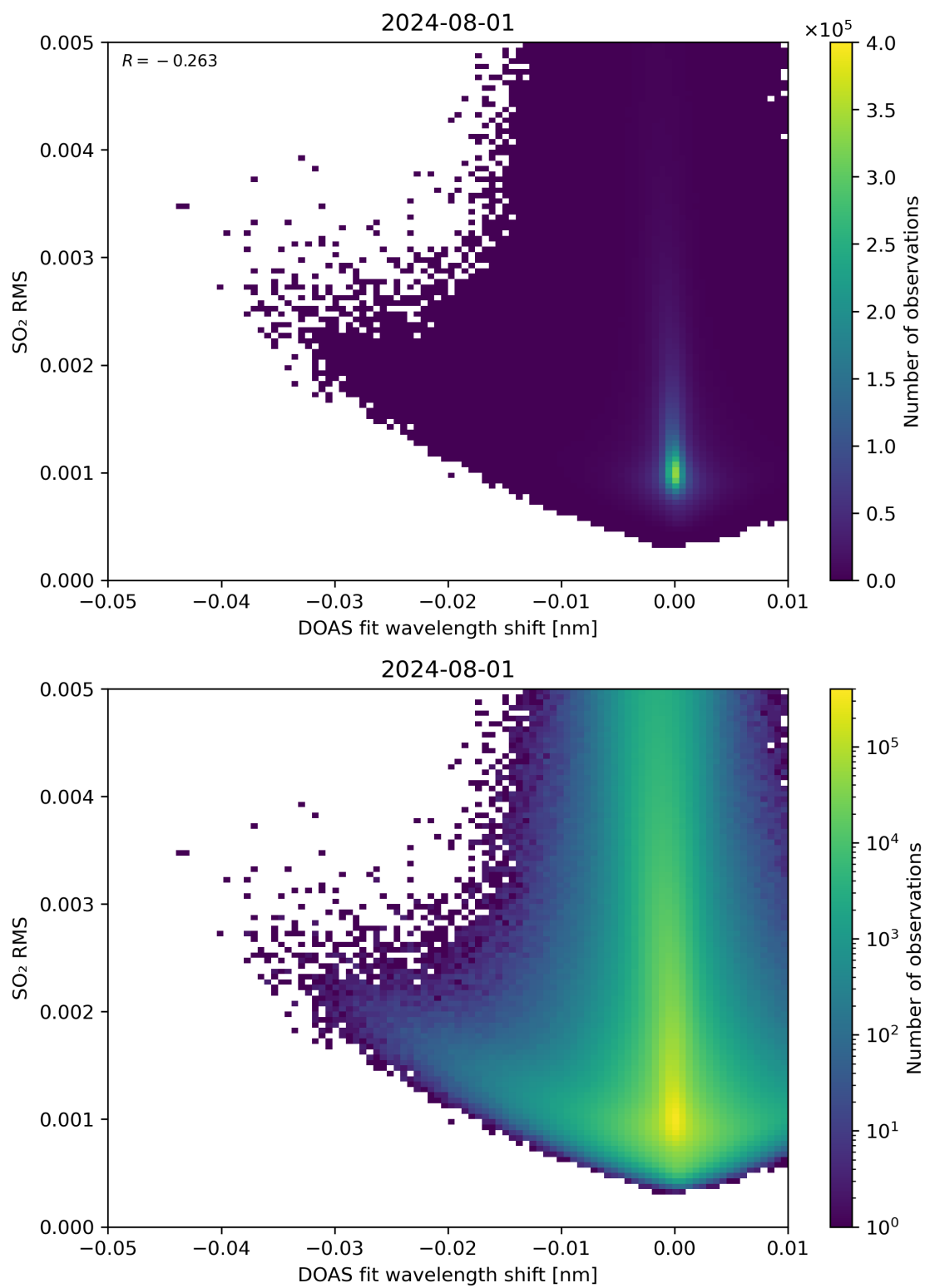
Figure 128: Scatter density plot of “DOAS fit wavelength shift” against “SO 2 RMS” for 2024-07-31 to 2024-08-02.
