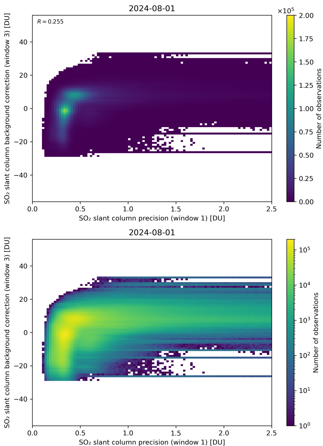
Figure 220: Scatter density plot of “SO 2 slant column precision (window 1)” against “SO 2 slant column background correction (window 3)” for 2024-07-31 to 2024-08-02.
