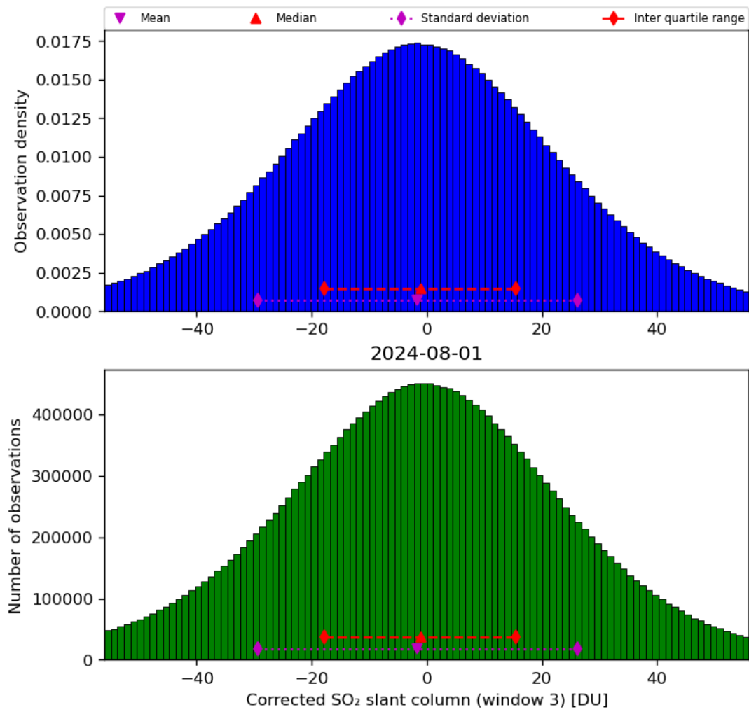
Figure 66: Histogram of “Corrected SO 2 slant column (window 3)” for 2024-07-31 to 2024-08-02
