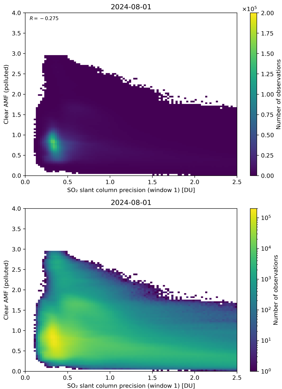
Figure 224: Scatter density plot of “SO 2 slant column precision (window 1)” against “Clear AMF (polluted)” for 2024-07-31 to 2024-08-02.
