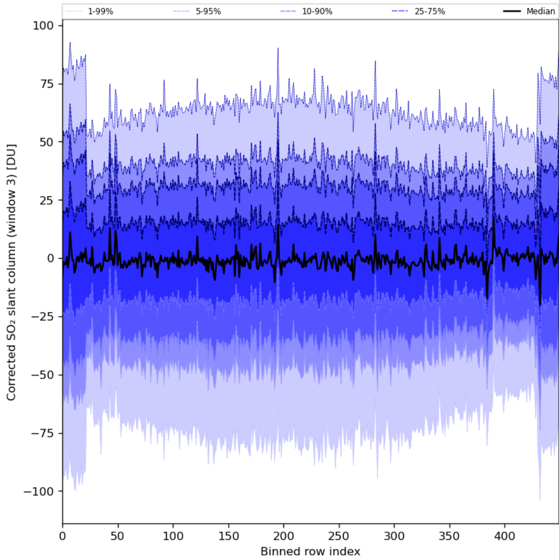
Figure 89: Along track statistics of “Corrected SO 2 slant column (window 3)” for 2024-07-31 to 2024-08-02
