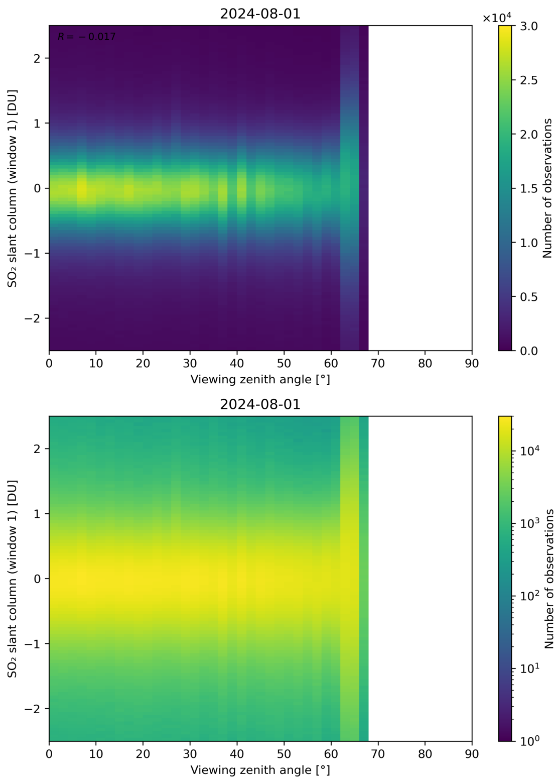
Figure 320: Scatter density plot of “Viewing zenith angle” against “SO 2 slant column (window 1)” for 2024-07-31 to 2024-08-02.
