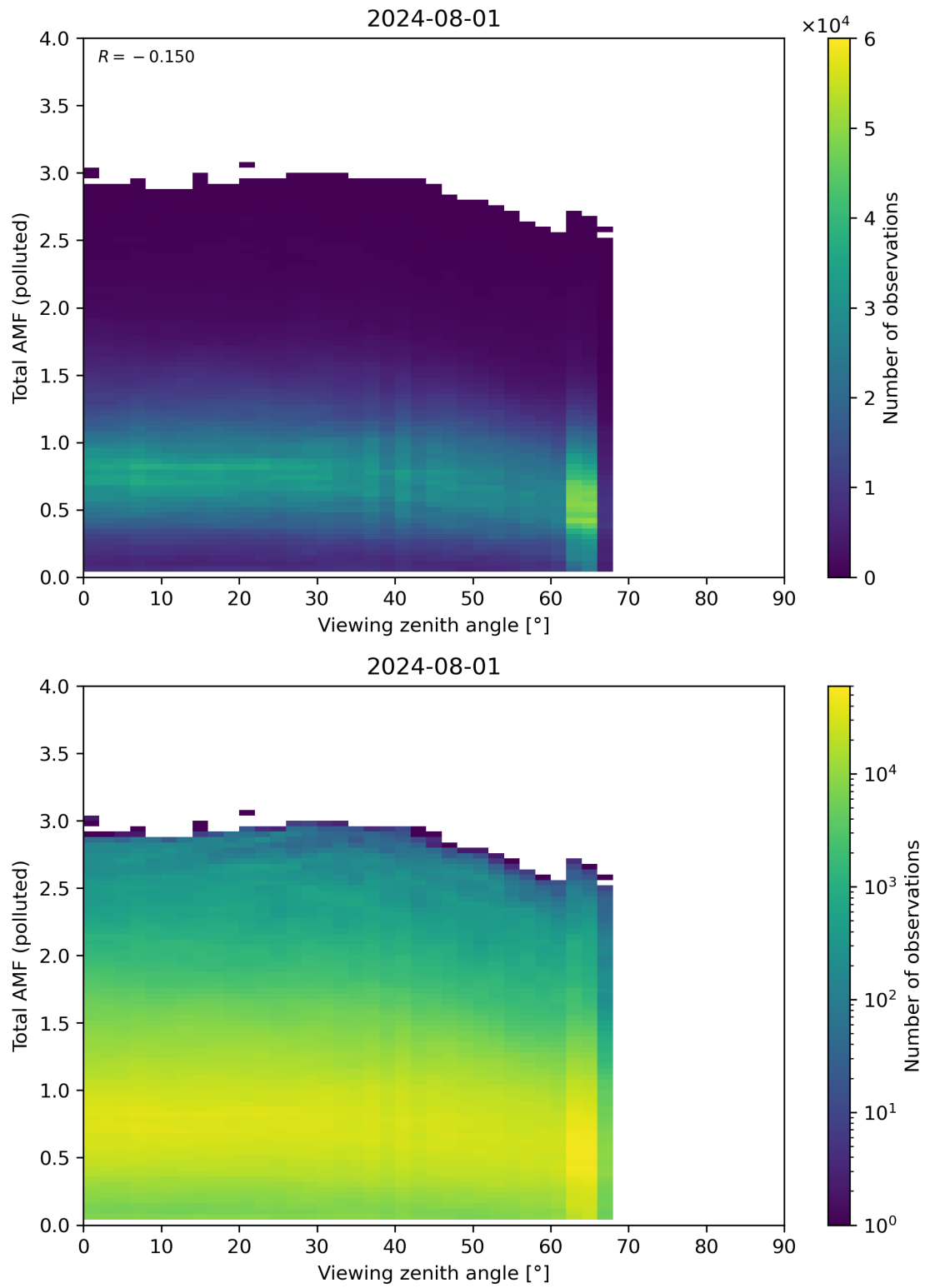
Figure 325: Scatter density plot of “Viewing zenith angle” against “Total AMF (polluted)” for 2024-07-31 to 2024-08-02.
