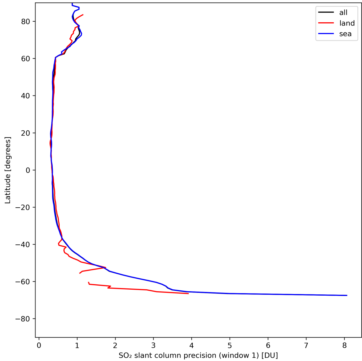
Figure 34: Zonal average of “SO 2 slant column precision (window 1)” for 2024-07-31 to 2024-08-02.
