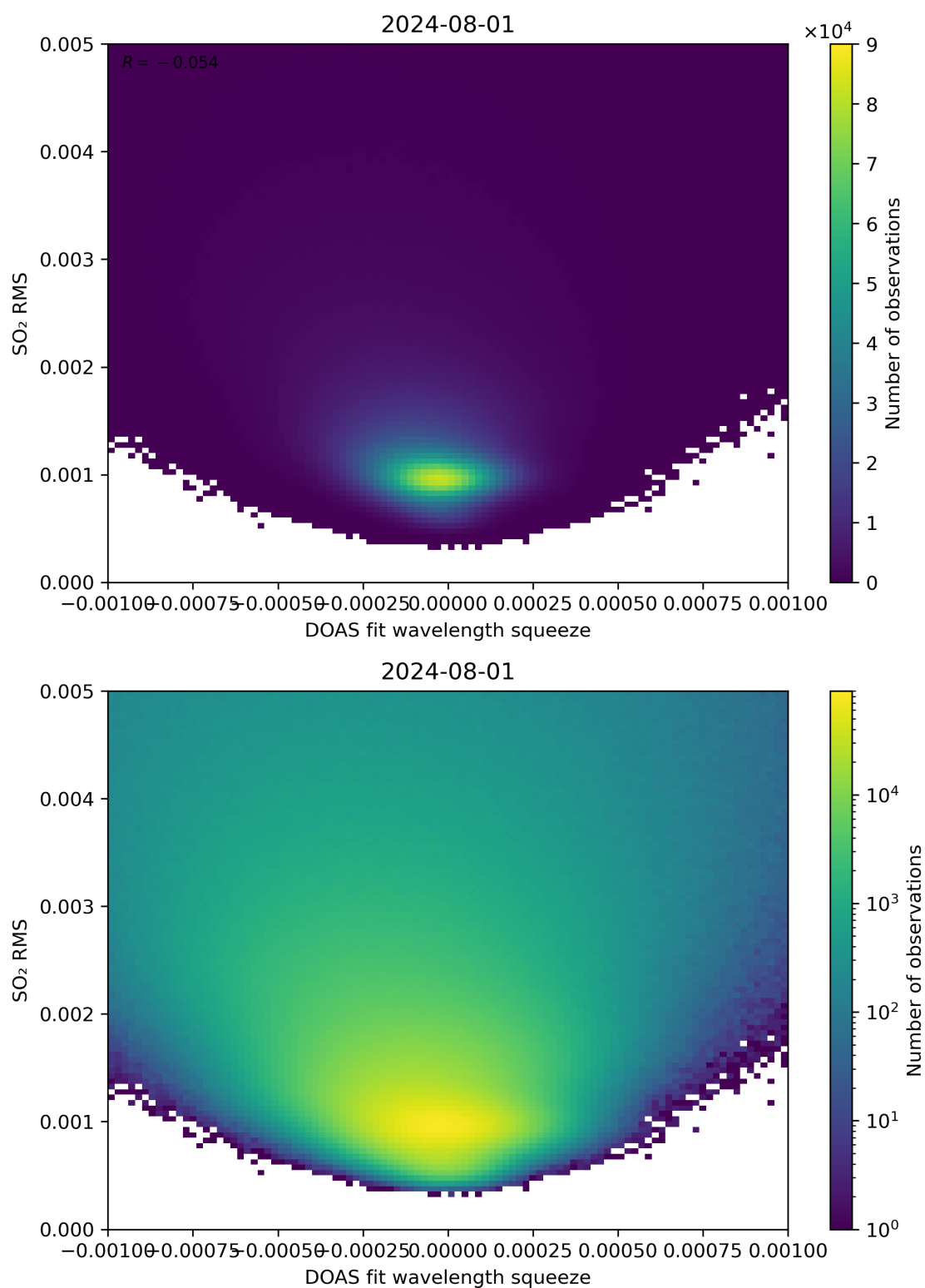
Figure 132: Scatter density plot of “DOAS fit wavelength squeeze” against “SO 2 RMS” for 2024-07-31 to 2024-08-02.
