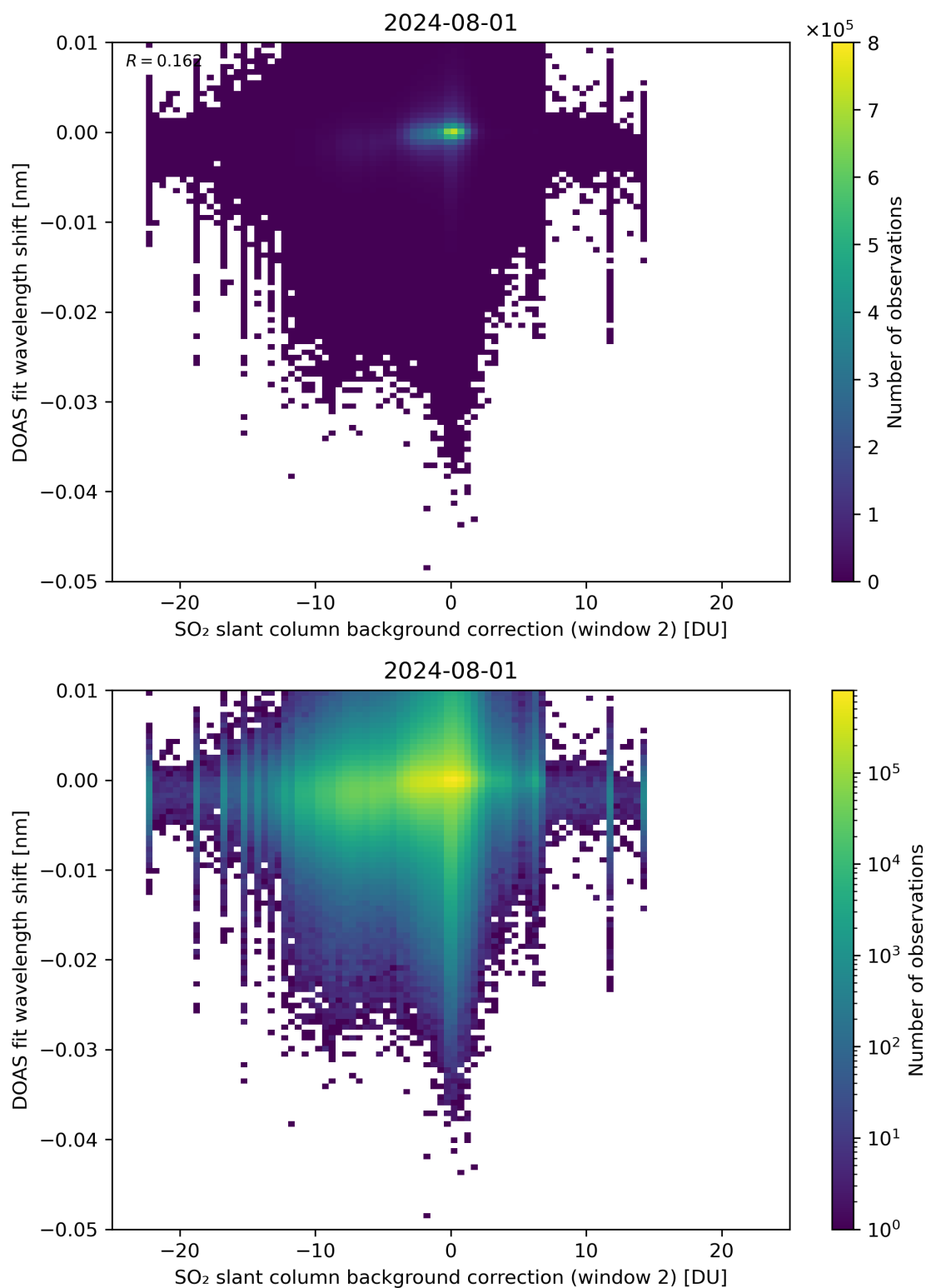
Figure 112: Scatter density plot of “SO 2 slant column background correction (window 2)” against “DOAS fit wavelength shift” for 2024-07-31 to 2024-08-02.
