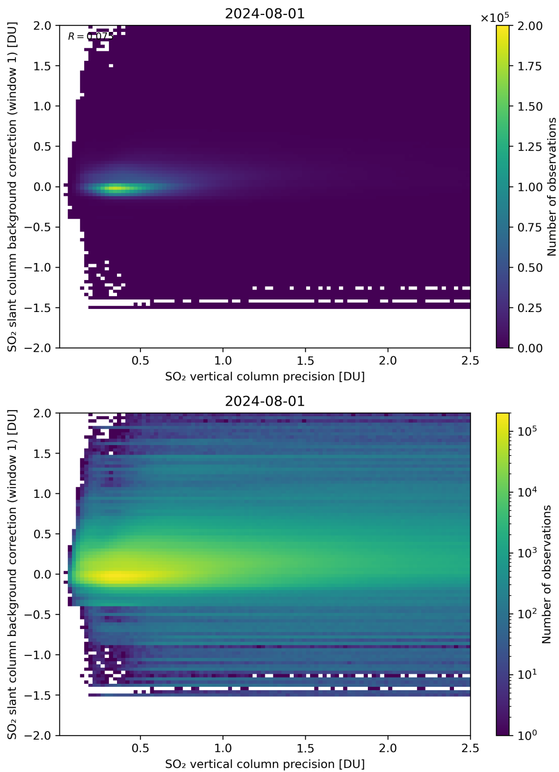
Figure 279: Scatter density plot of “SO 2 vertical column precision” against “SO 2 slant column background correction (window 1)” for 2024-07-31 to 2024-08-02.
