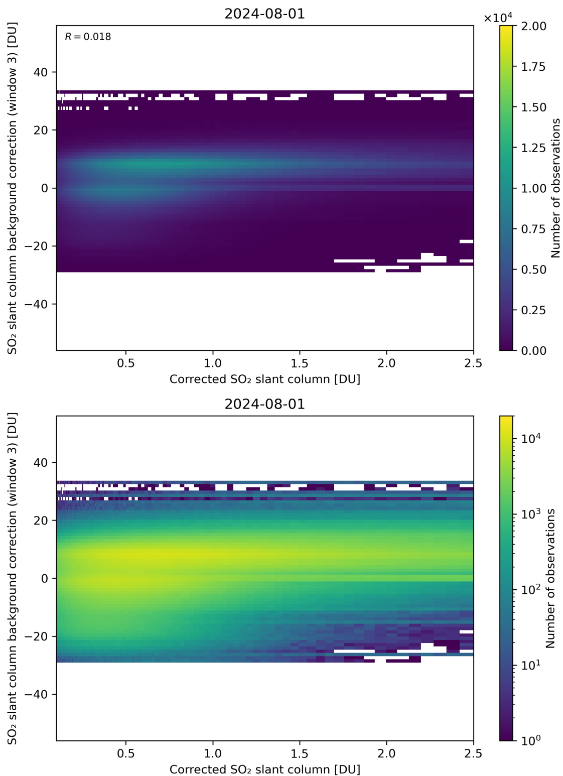
Figure 180: Scatter density plot of “Corrected SO 2 slant column” against “SO 2 slant column background correction (window 3)” for 2024-07-31 to 2024-08-02.
