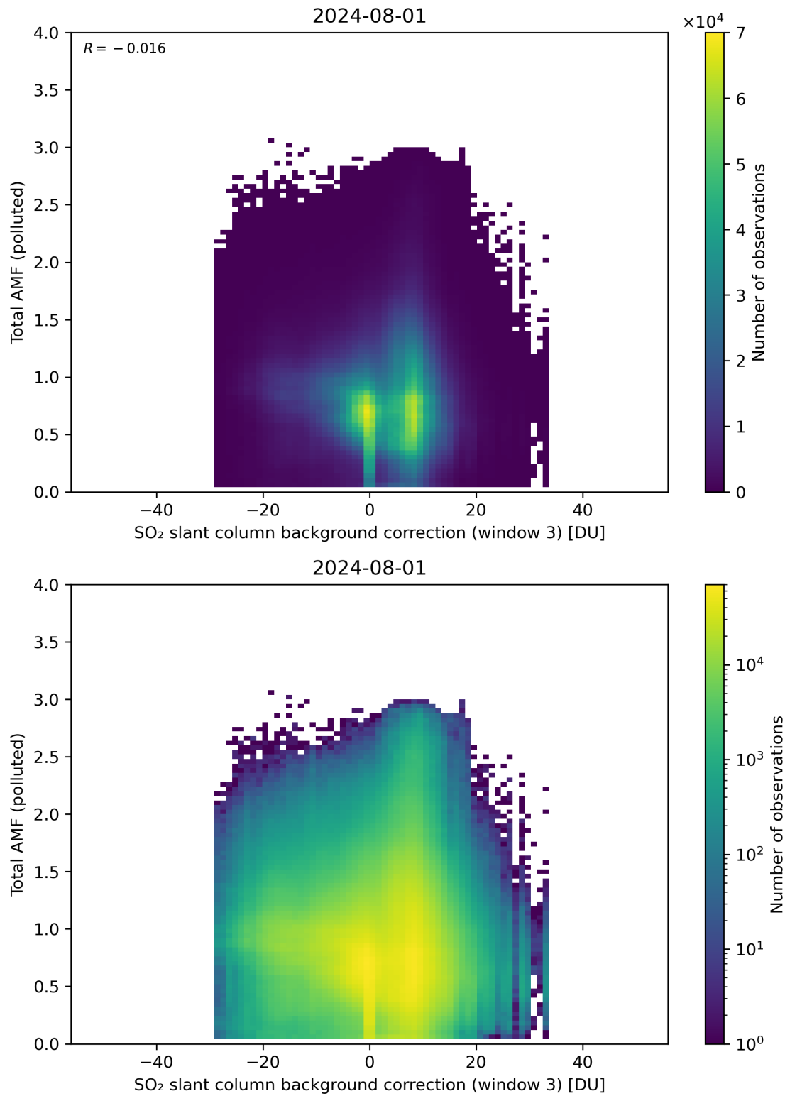
Figure 125: Scatter density plot of “SO 2 slant column background correction (window 3)” against “Total AMF (polluted)” for 2024-07-31 to 2024-08-02.
