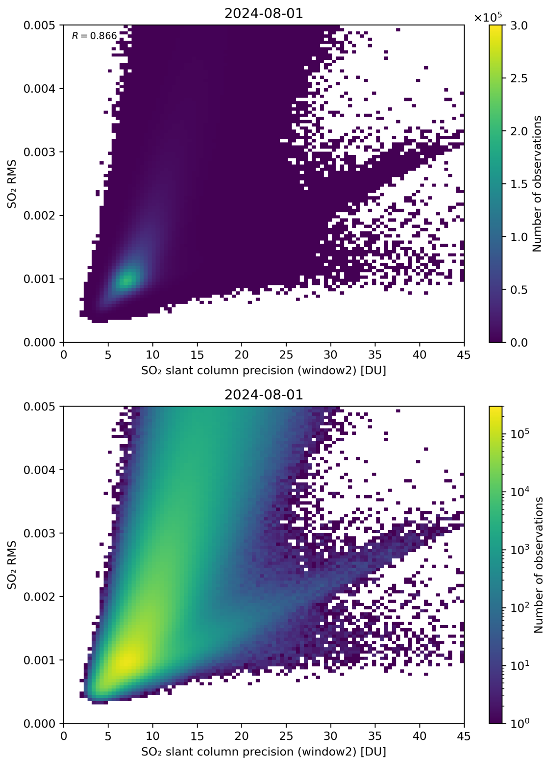
Figure 245: Scatter density plot of “SO 2 slant column precision (window2)” against “SO 2 RMS” for 2024-07-31 to 2024-08-02.
