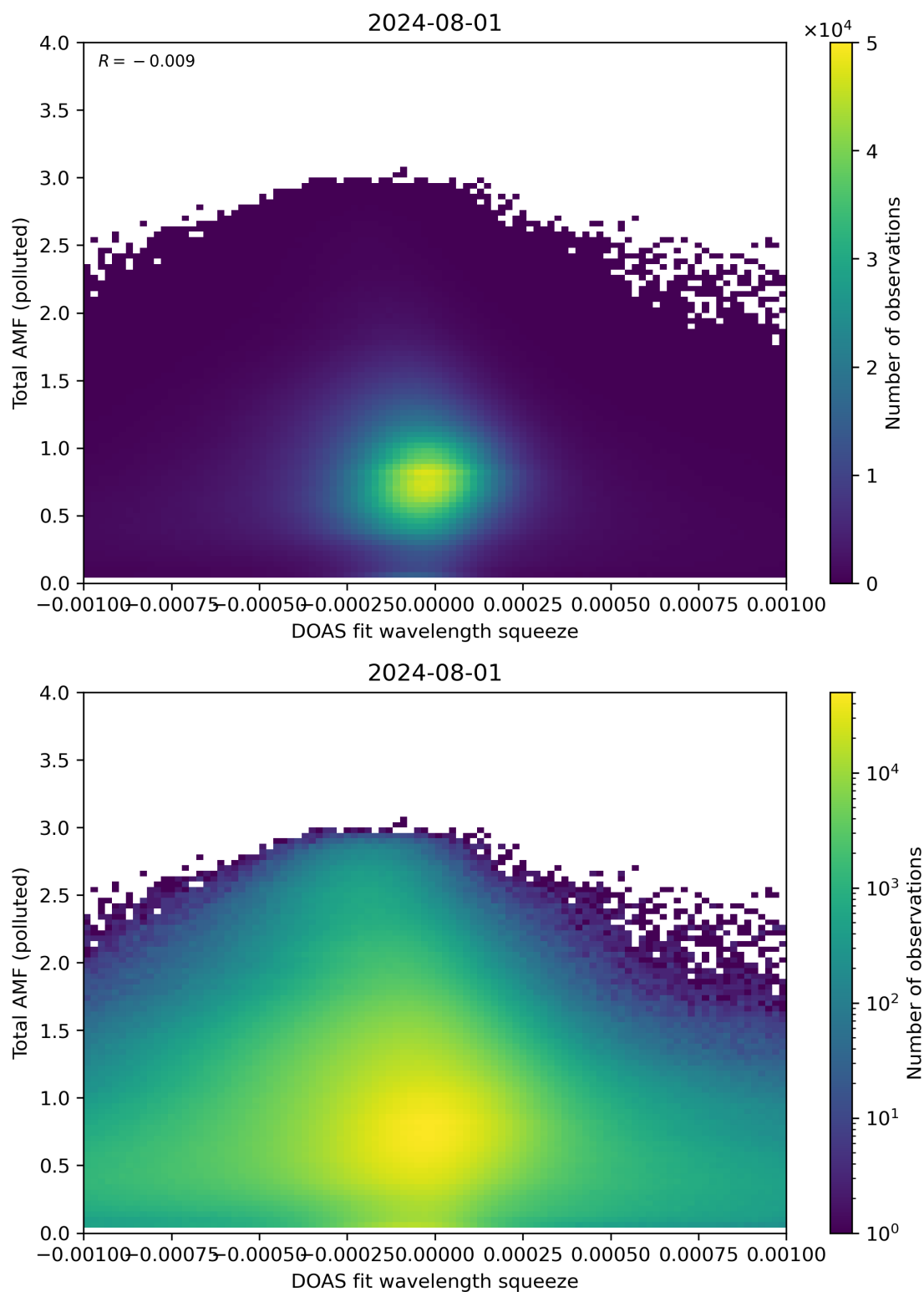
Figure 134: Scatter density plot of “DOAS fit wavelength squeeze” against “Total AMF (polluted)” for 2024-07-31 to 2024-08-02.
