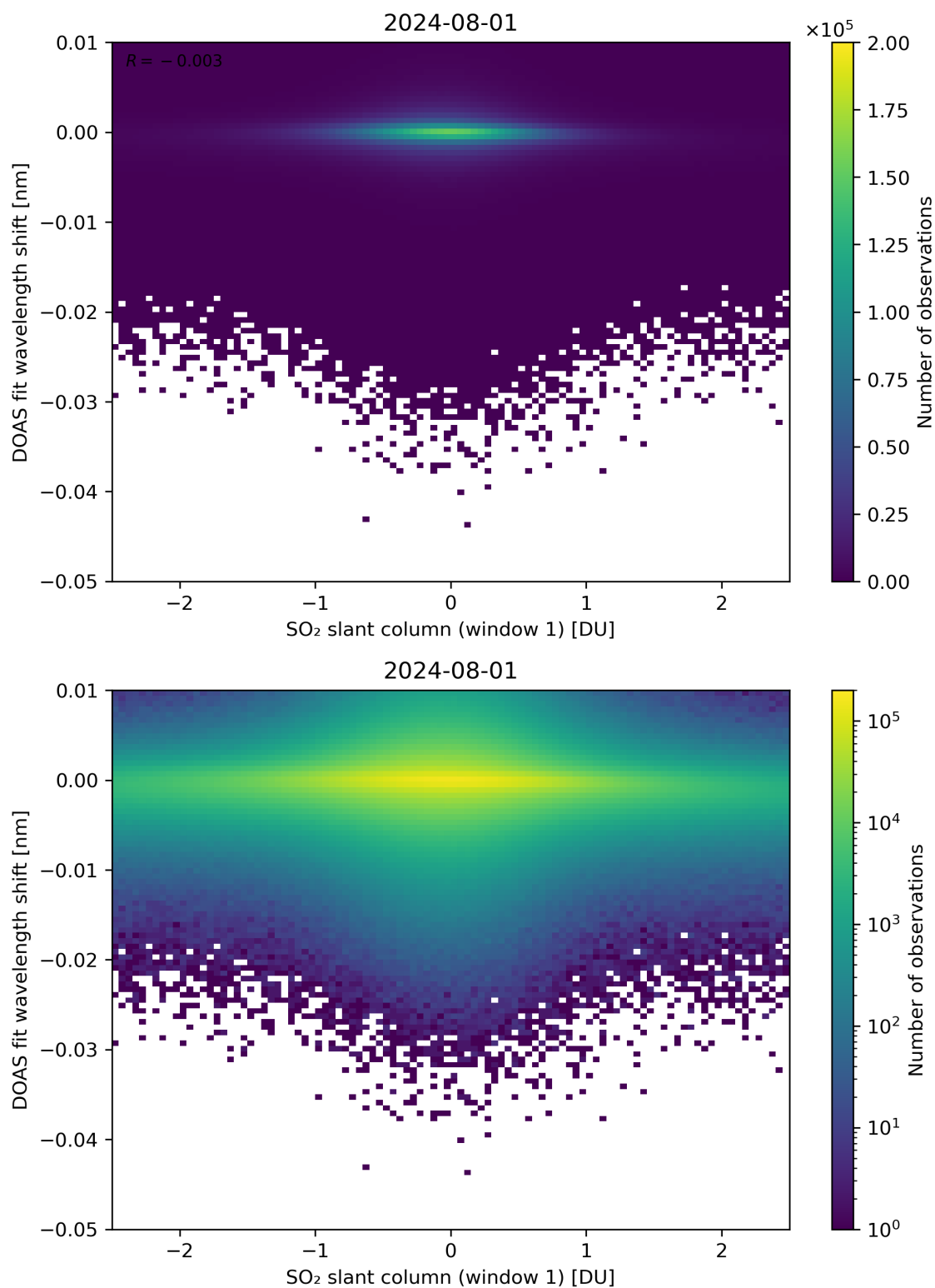
Figure 215: Scatter density plot of “SO 2 slant column (window 1)” against “DOAS fit wavelength shift” for 2024-07-31 to 2024-08-02.
