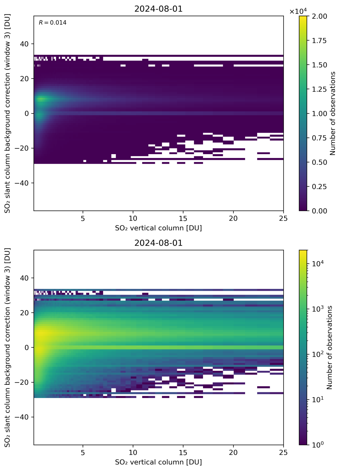
Figure 275: Scatter density plot of “SO 2 vertical column” against “SO 2 slant column background correction (window 3)” for 2024-07-31 to 2024-08-02.
