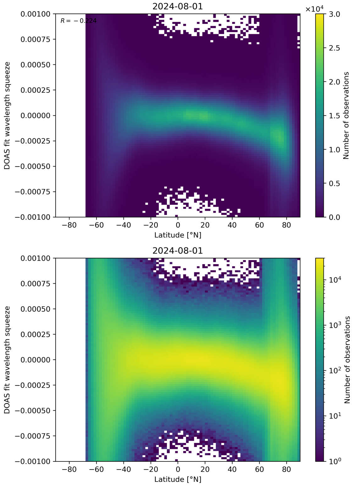
Figure 143: Scatter density plot of “Latitude” against “DOAS fit wavelength squeeze” for 2024-07-31 to 2024-08-02.
