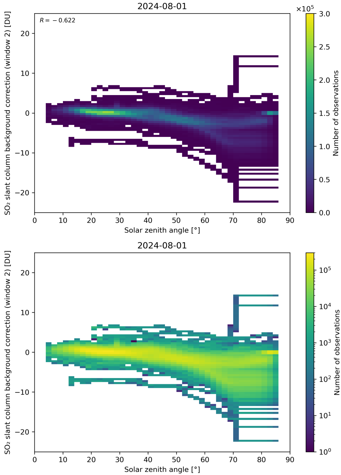
Figure 159: Scatter density plot of “Solar zenith angle” against “SO 2 slant column background correction (window 2)” for 2024-07-31 to 2024-08-02.
