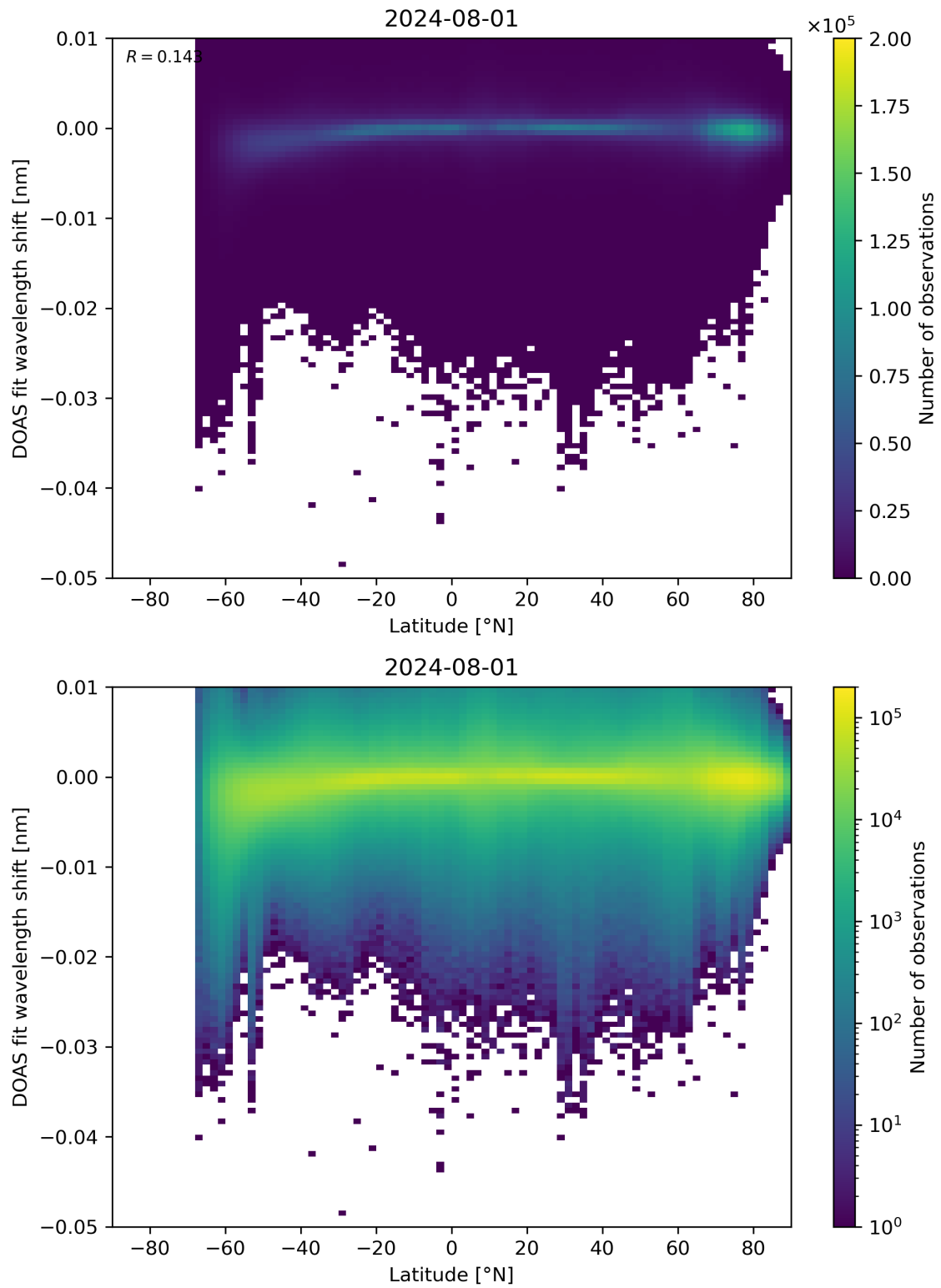
Figure 142: Scatter density plot of “Latitude” against “DOAS fit wavelength shift” for 2024-07-31 to 2024-08-02.
