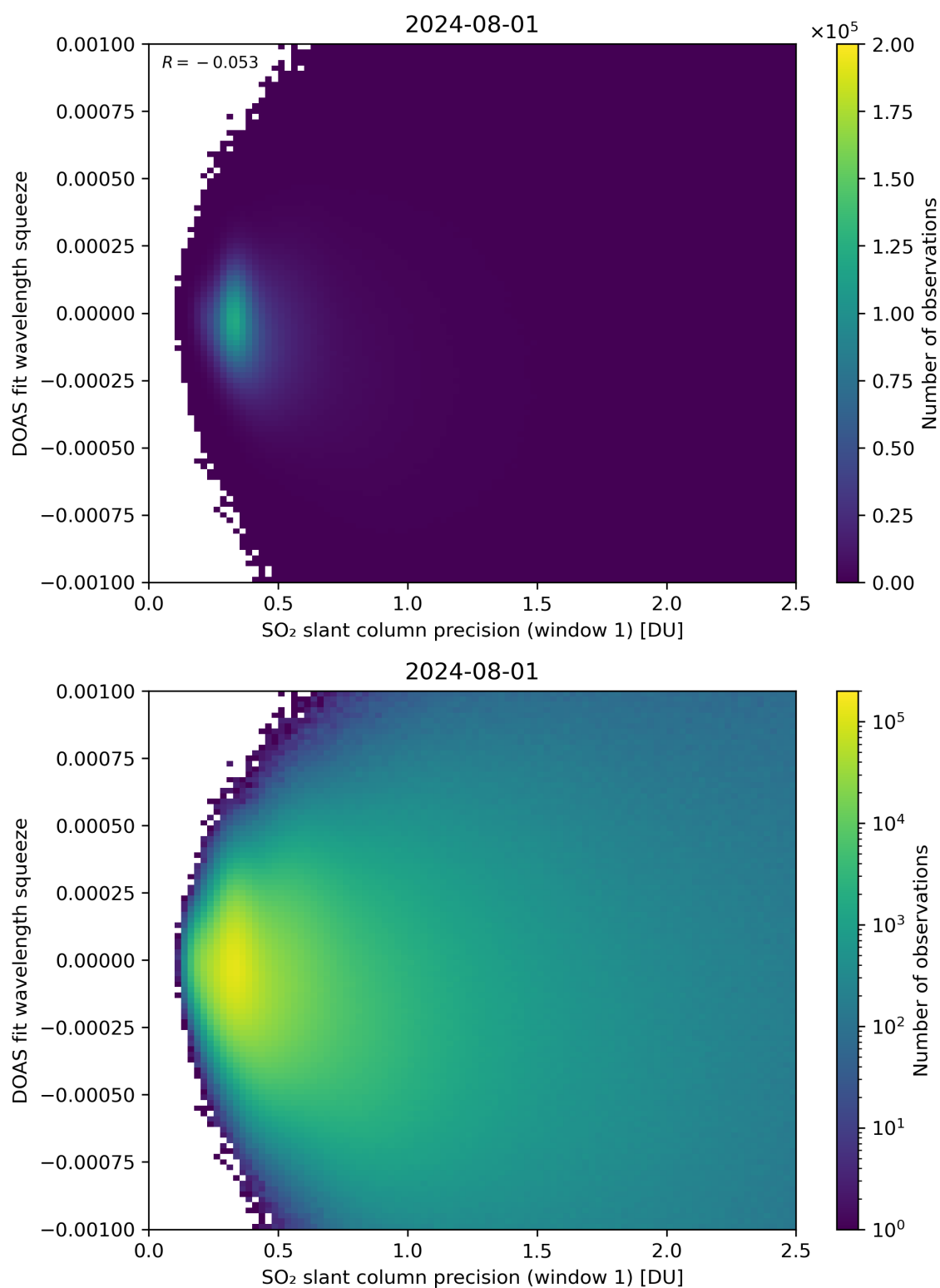
Figure 222: Scatter density plot of “SO 2 slant column precision (window 1)” against “DOAS fit wavelength squeeze” for 2024-07-31 to 2024-08-02.
