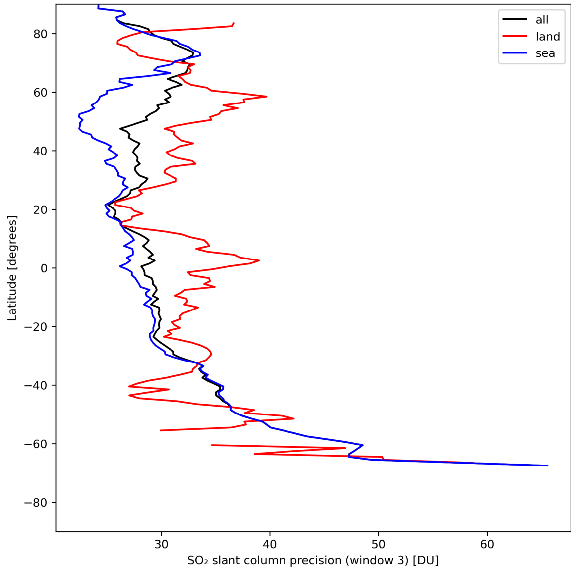
Figure 42: Zonal average of “SO 2 slant column precision (window 3)” for 2024-07-31 to 2024-08-02.
