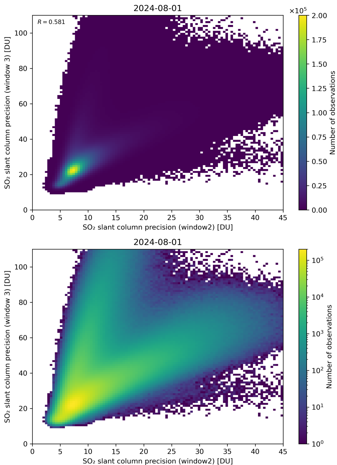
Figure 250: Scatter density plot of “SO 2 slant column precision (window2)” against “SO 2 slant column precision (window 3)” for 2024-07-31 to 2024-08-02.
