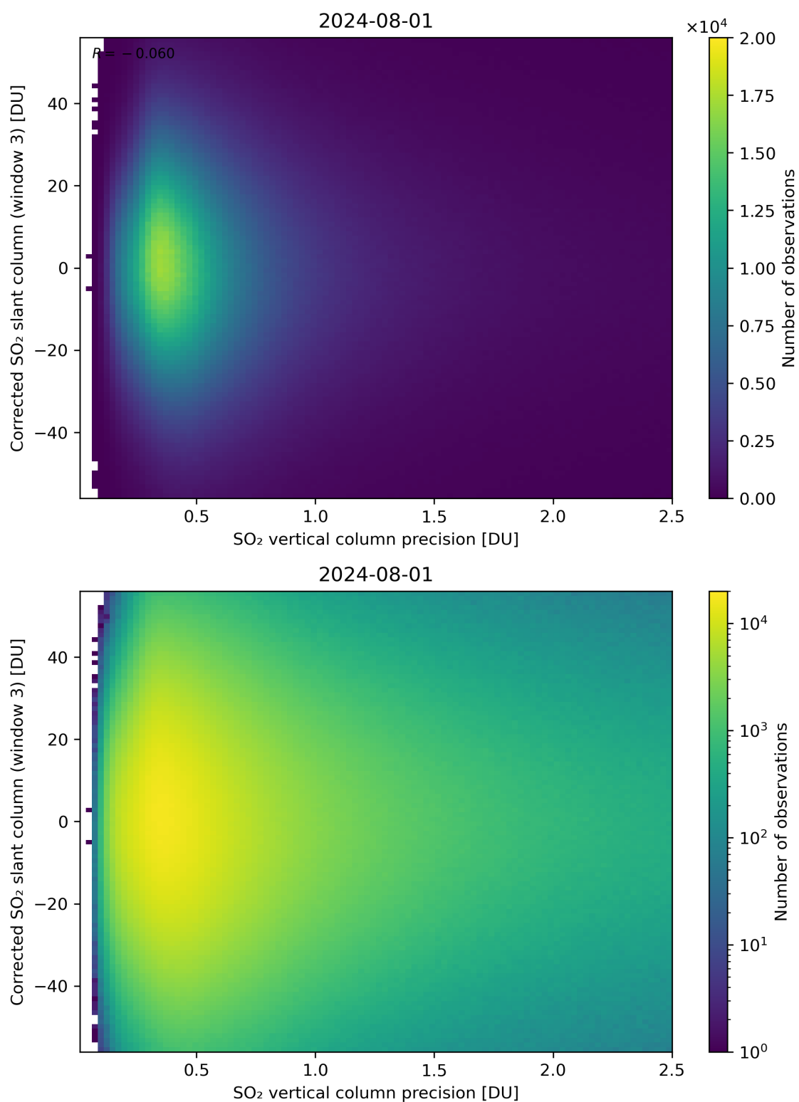
Figure 288: Scatter density plot of “SO 2 vertical column precision” against “Corrected SO 2 slant column (window 3)” for 2024-07-31 to 2024-08-02.
