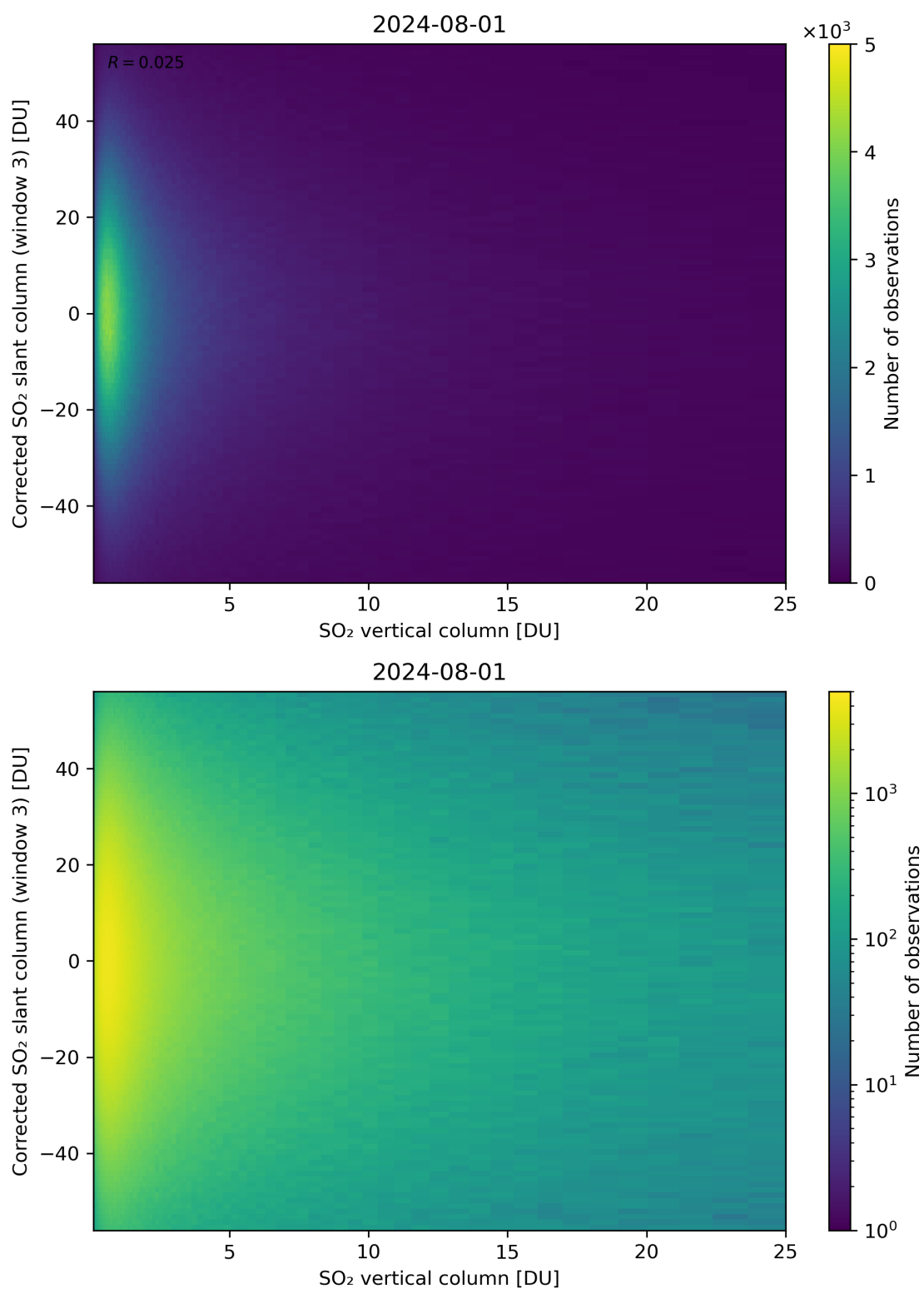
Figure 299: Scatter density plot of “SO 2 vertical column” against “Corrected SO 2 slant column (window 3)” for 2024-07-31 to 2024-08-02.
