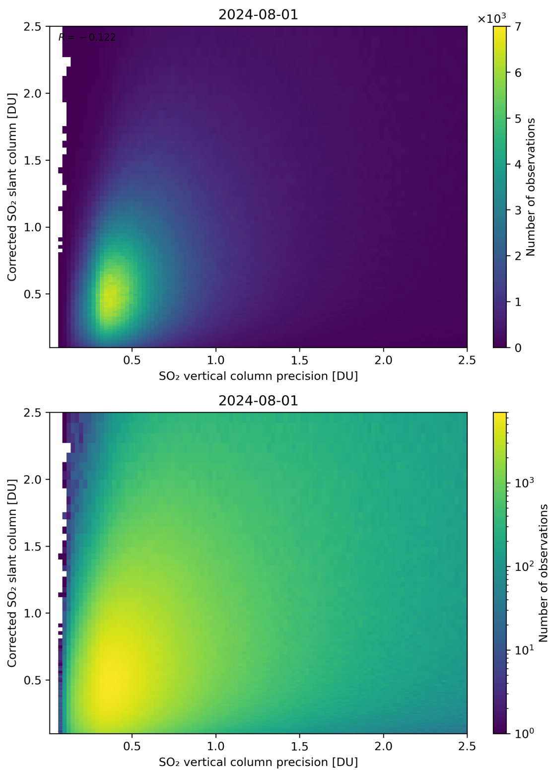
Figure 286: Scatter density plot of “SO 2 vertical column precision” against “Corrected SO 2 slant column” for 2024-07-31 to 2024-08-02.
