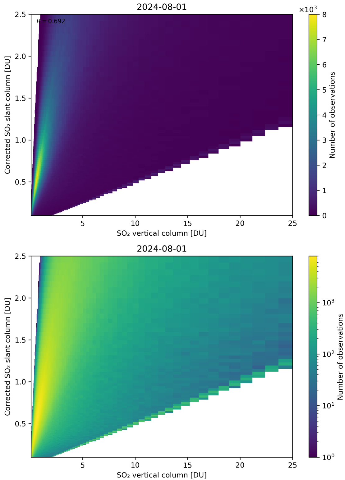
Figure 297: Scatter density plot of “SO 2 vertical column” against “Corrected SO 2 slant column” for 2024-07-31 to 2024-08-02.
