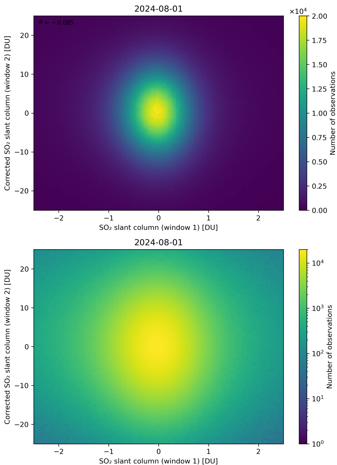
Figure 233: Scatter density plot of “SO 2 slant column (window 1)” against “Corrected SO 2 slant column (window 2)” for 2024-07-31 to 2024-08-02.
