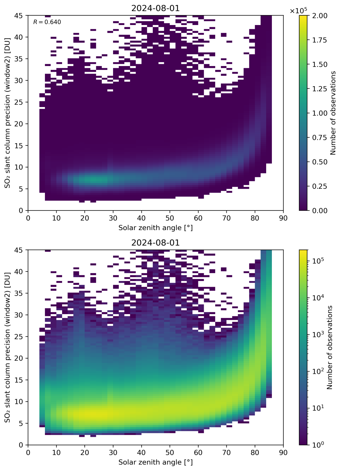
Figure 171: Scatter density plot of “Solar zenith angle” against “SO 2 slant column precision (window2)” for 2024-07-31 to 2024-08-02.
