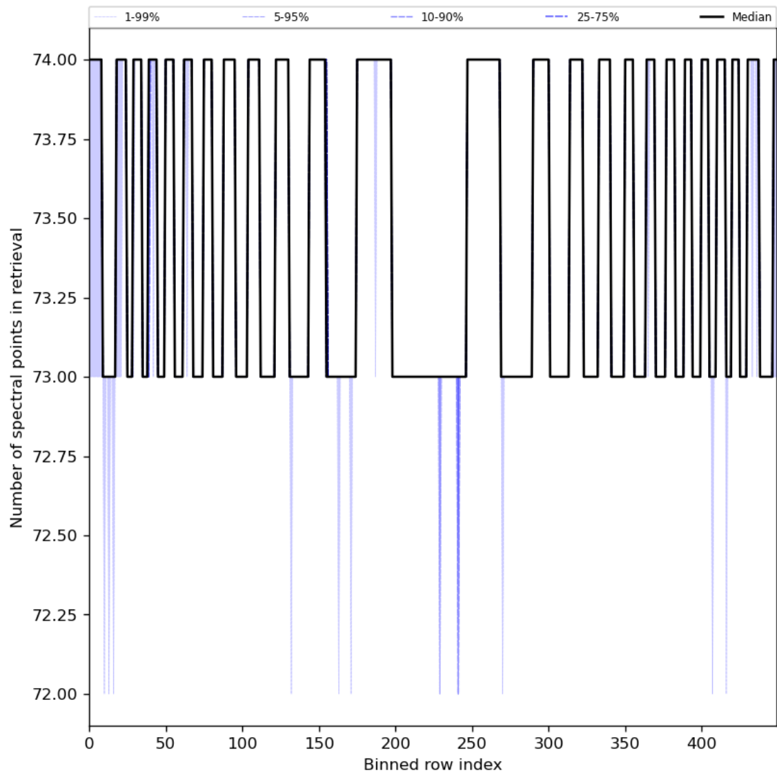
Figure 97: Along track statistics of “Number of spectral points in retrieval” for 2024-07-31 to 2024-08-02
