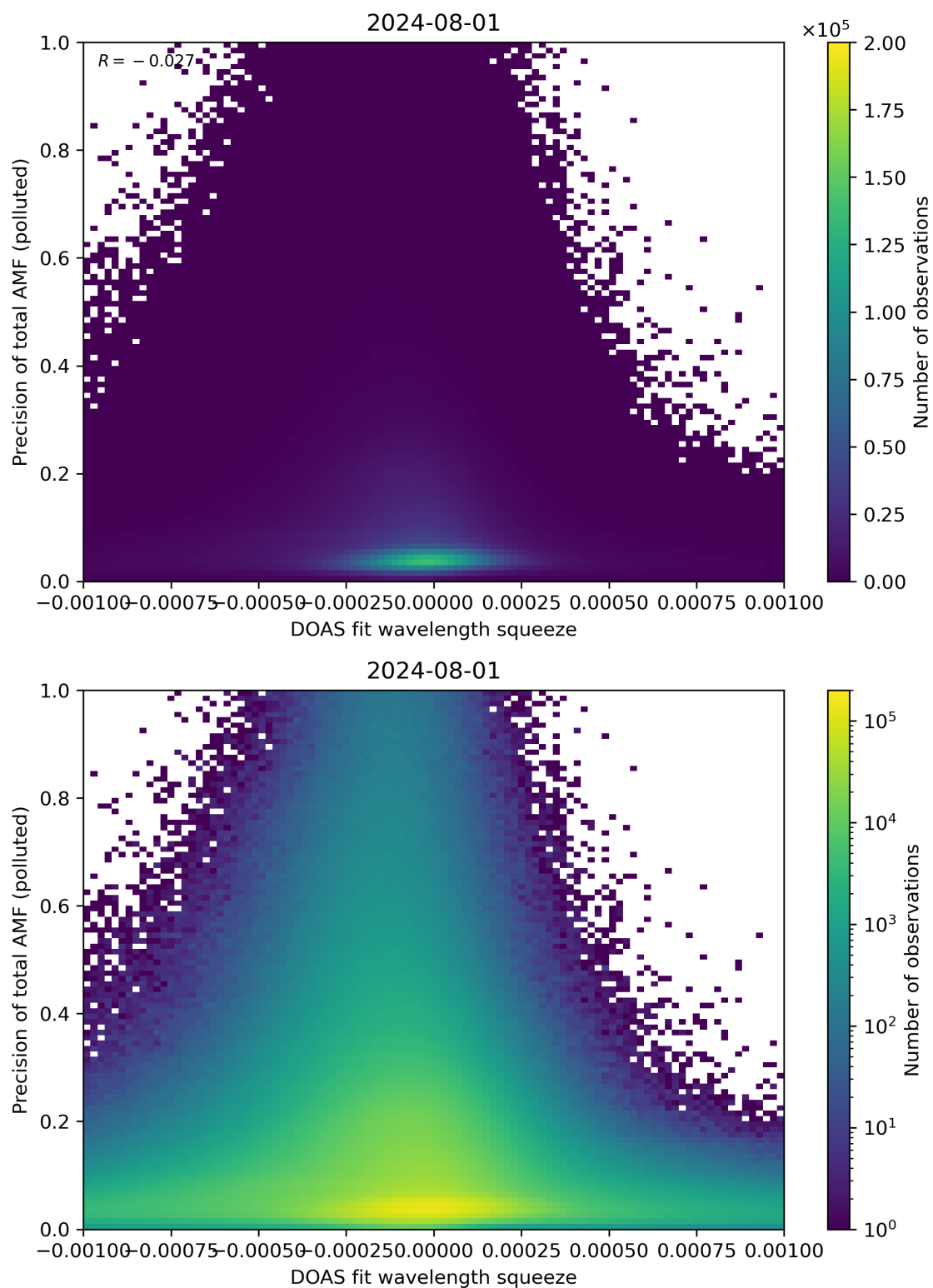
Figure 135: Scatter density plot of “DOAS fit wavelength squeeze” against “Precision of total AMF (polluted)” for 2024-07-31 to 2024-08-02.
