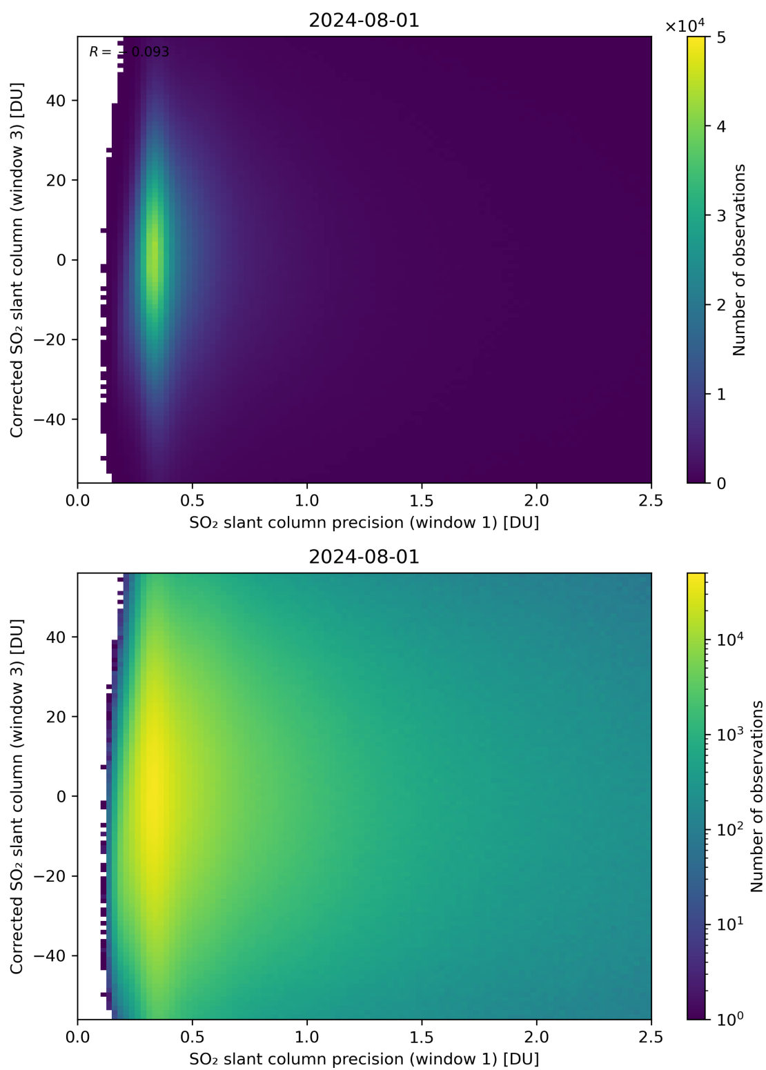
Figure 226: Scatter density plot of “SO 2 slant column precision (window 1)” against “Corrected SO 2 slant column (window 3)” for 2024-07-31 to 2024-08-02.
