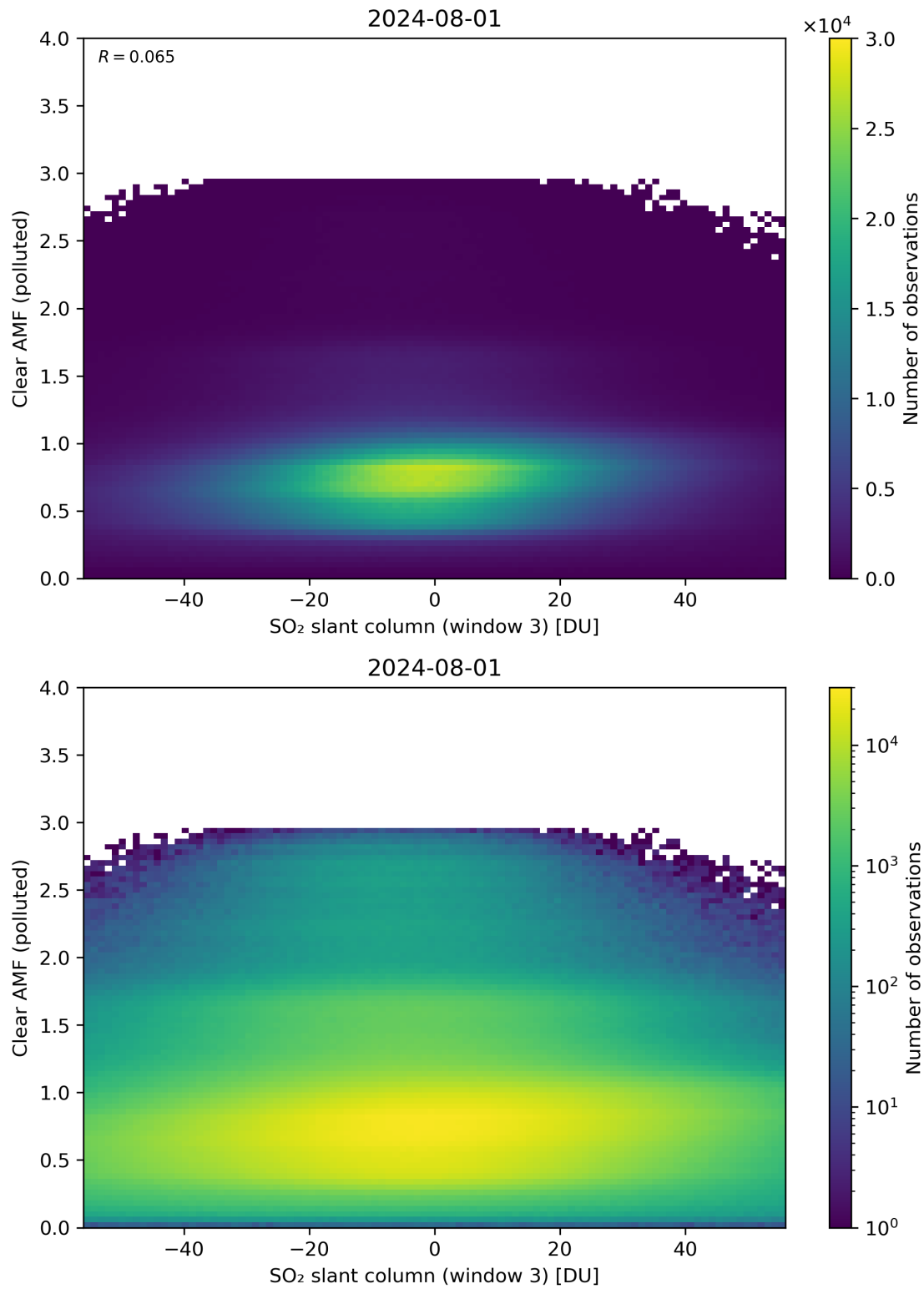
Figure 265: Scatter density plot of “SO 2 slant column (window 3)” against “Clear AMF (polluted)” for 2024-07-31 to 2024-08-02.
