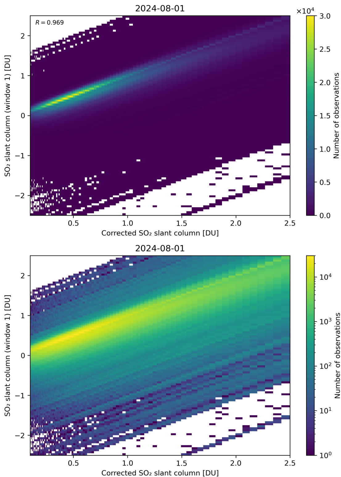
Figure 187: Scatter density plot of “Corrected SO 2 slant column” against “SO 2 slant column (window 1)” for 2024-07-31 to 2024-08-02.
