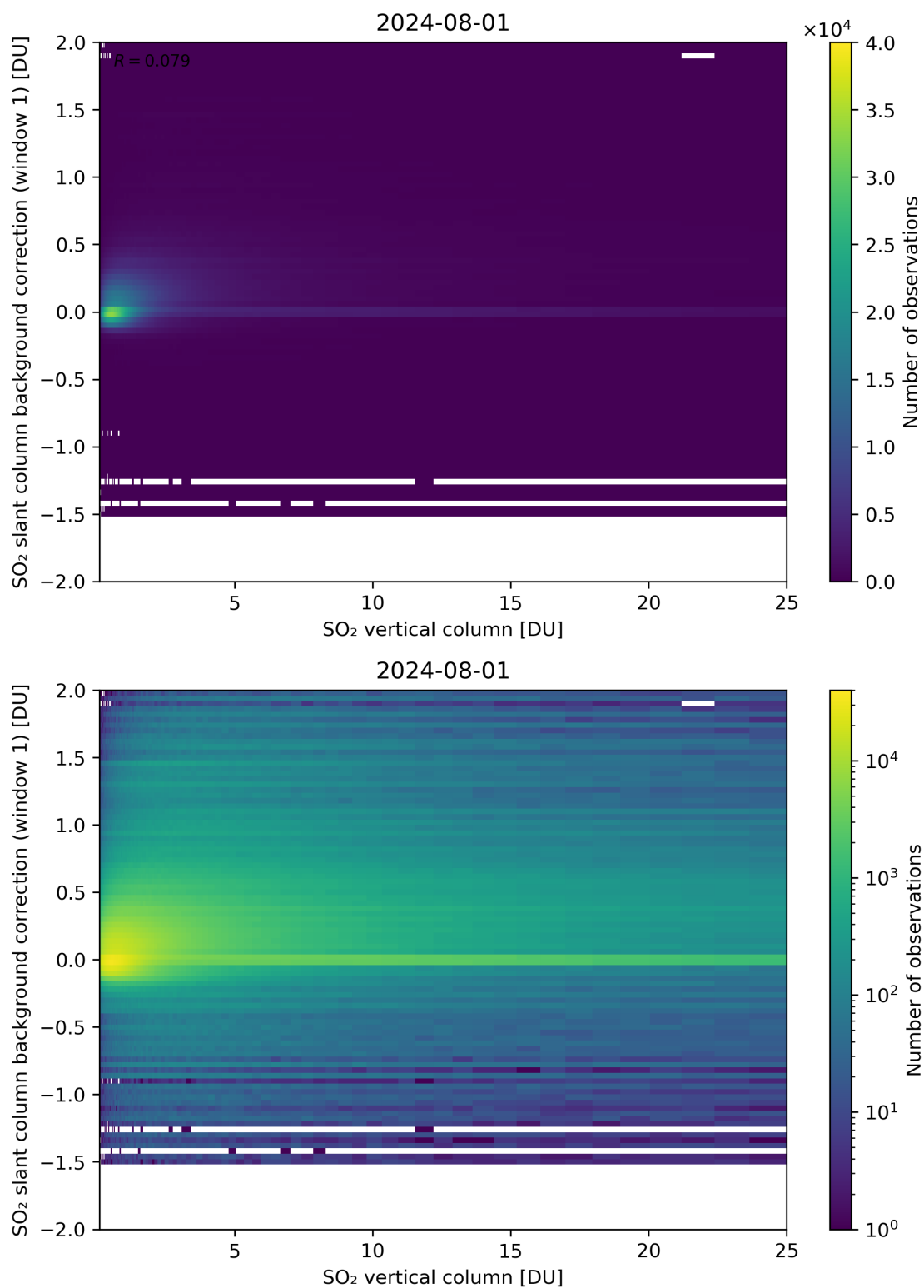
Figure 273: Scatter density plot of “SO 2 vertical column” against “SO 2 slant column background correction (window 1)” for 2024-07-31 to 2024-08-02.
