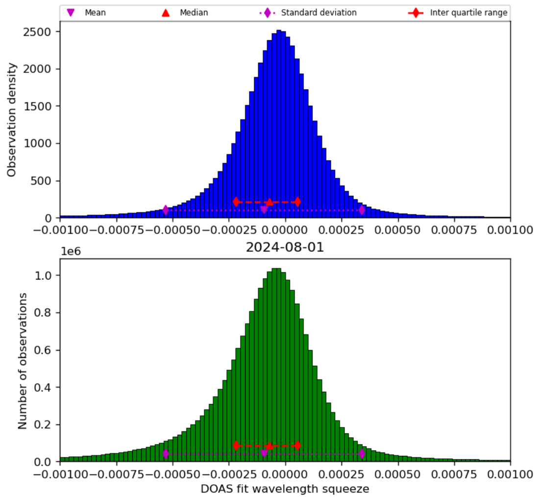
Figure 69: Histogram of “DOAS fit wavelength squeeze” for 2024-07-31 to 2024-08-02
