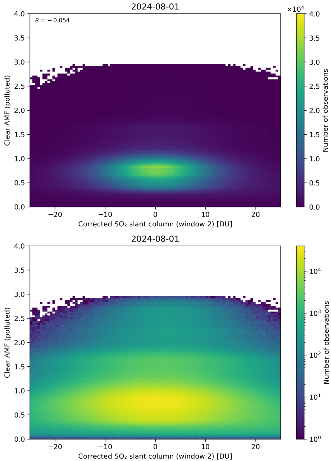
Figure 199: Scatter density plot of “Corrected SO 2 slant column (window 2)” against “Clear AMF (polluted)” for 2024-07-31 to 2024-08-02.
