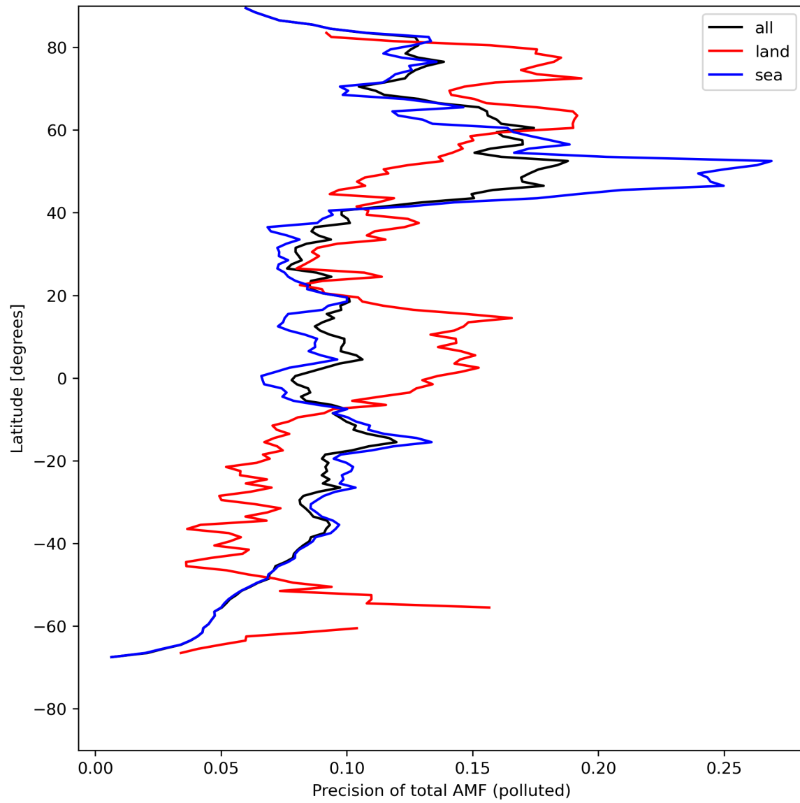
Figure 49: Zonal average of “Precision of total AMF (polluted)” for 2024-07-31 to 2024-08-02.
