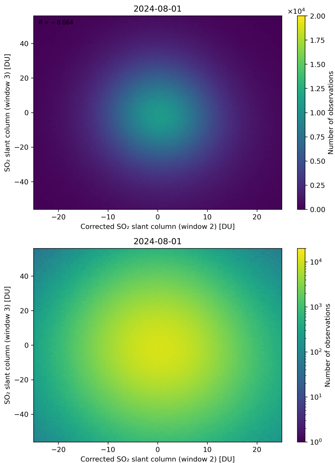
Figure 201: Scatter density plot of “Corrected SO 2 slant column (window 2)” against “SO 2 slant column (window 3)” for 2024-07-31 to 2024-08-02.
