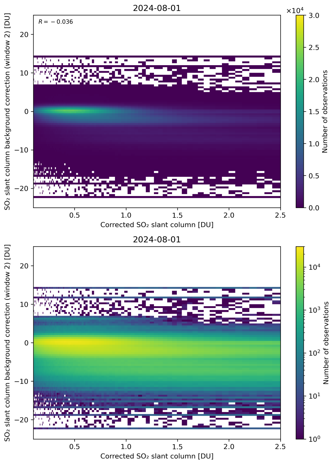
Figure 179: Scatter density plot of “Corrected SO 2 slant column” against “SO 2 slant column background correction (window 2)” for 2024-07-31 to 2024-08-02.
