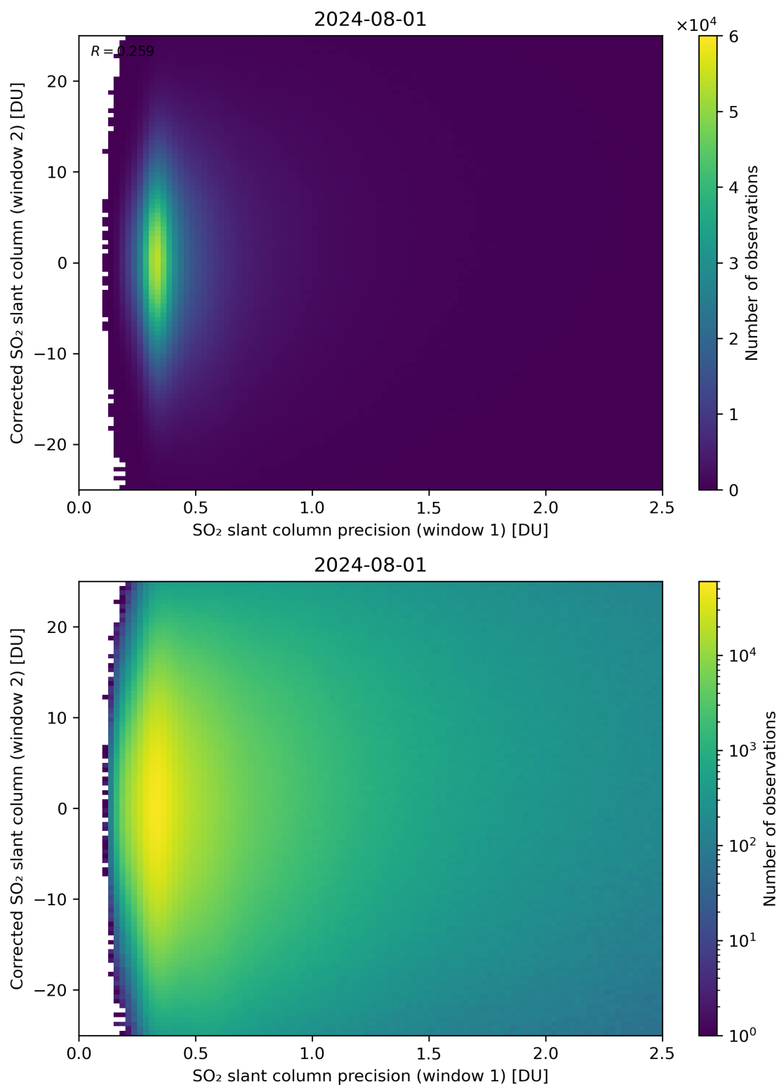
Figure 225: Scatter density plot of “SO 2 slant column precision (window 1)” against “Corrected SO 2 slant column (window 2)” for 2024-07-31 to 2024-08-02.
