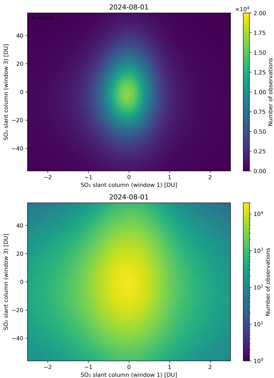
Figure 237: Scatter density plot of “SO 2 slant column (window 1)” against “SO 2 slant column (window 3)” for 2024-07-31 to 2024-08-02.
