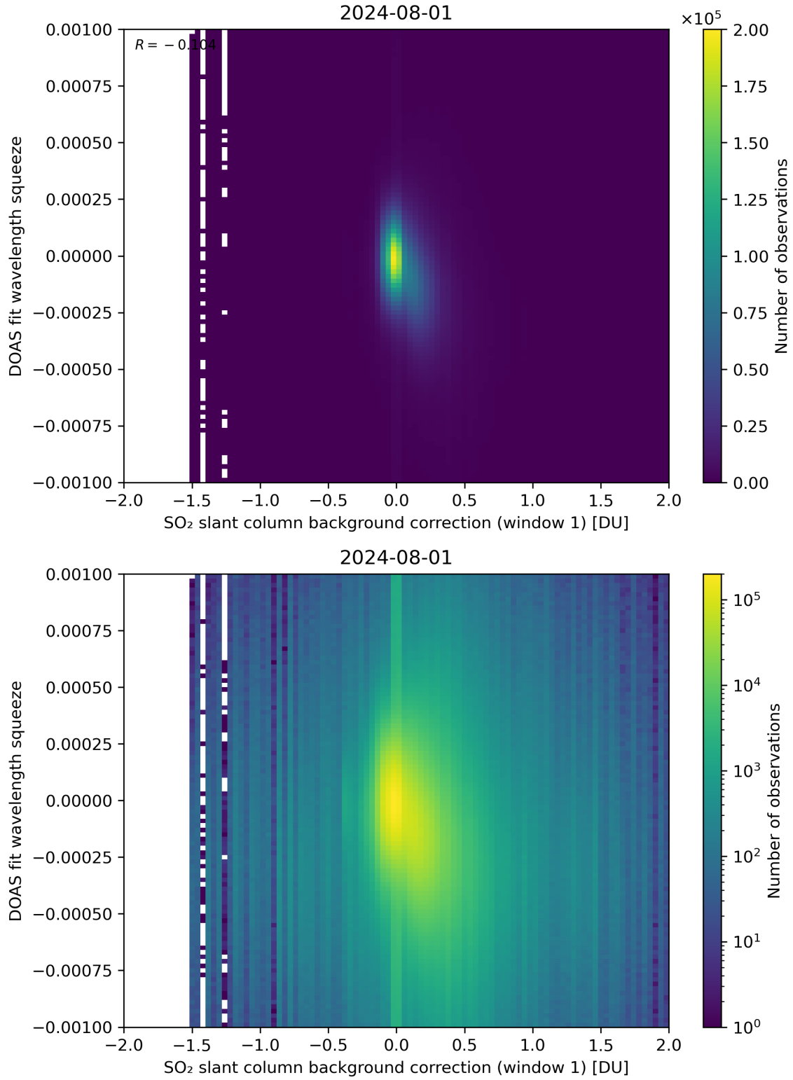
Figure 101: Scatter density plot of “SO 2 slant column background correction (window 1)” against “DOAS fit wavelength squeeze” for 2024-07-31 to 2024-08-02.
