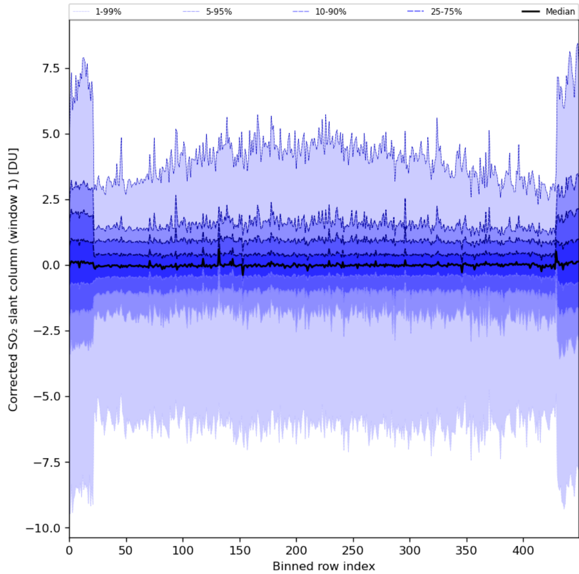
Figure 81: Along track statistics of “Corrected SO 2 slant column (window 1)” for 2024-07-31 to 2024-08-02
