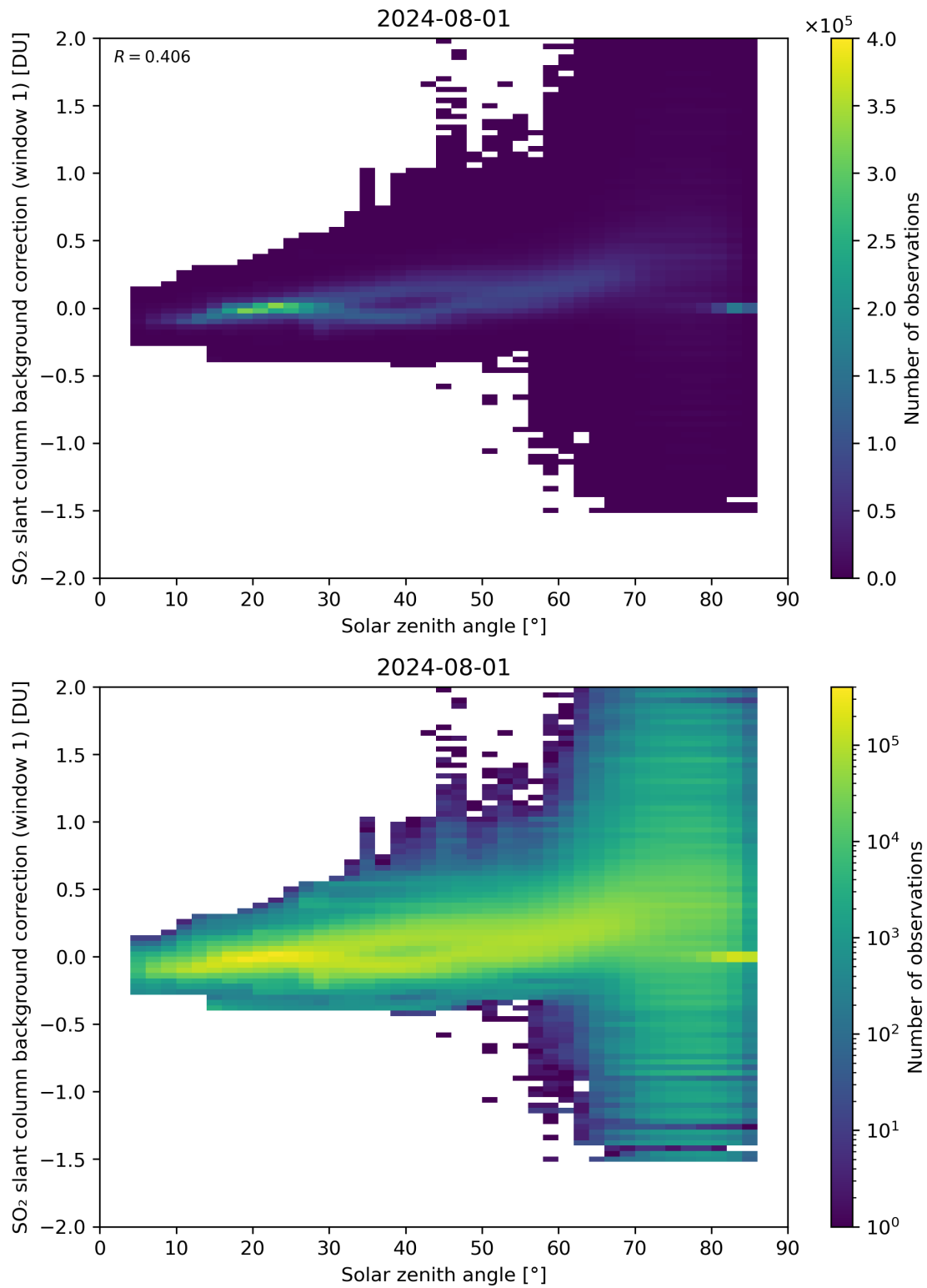
Figure 158: Scatter density plot of “Solar zenith angle” against “SO 2 slant column background correction (window 1)” for 2024-07-31 to 2024-08-02.
