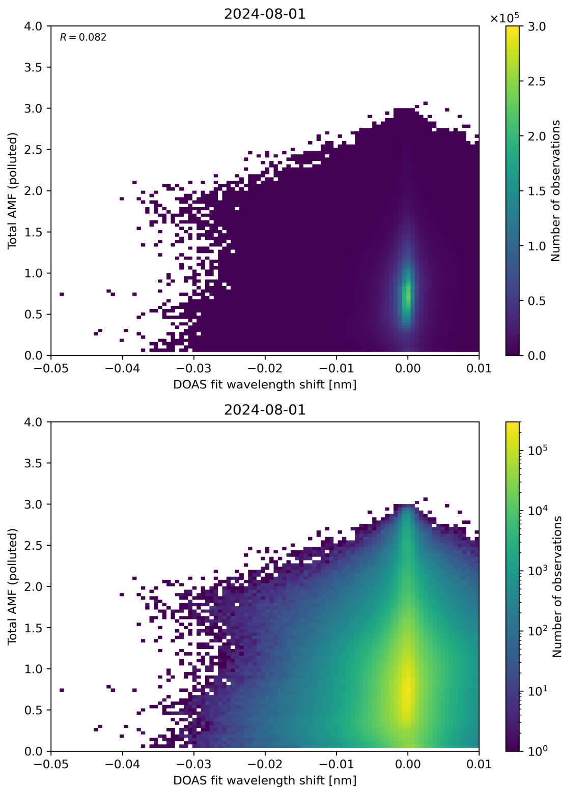
Figure 130: Scatter density plot of “DOAS fit wavelength shift” against “Total AMF (polluted)” for 2024-07-31 to 2024-08-02.
