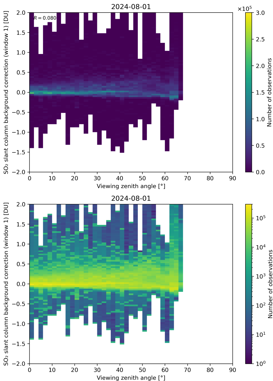
Figure 308: Scatter density plot of “Viewing zenith angle” against “SO 2 slant column background correction (window 1)” for 2024-07-31 to 2024-08-02.
