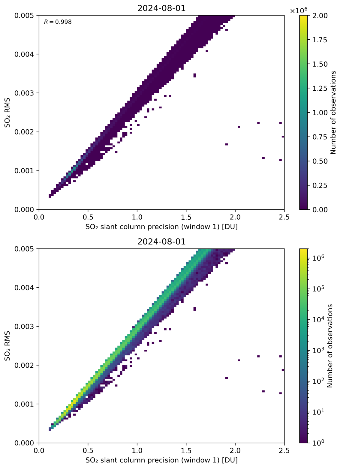
Figure 223: Scatter density plot of “SO 2 slant column precision (window 1)” against “SO 2 RMS” for 2024-07-31 to 2024-08-02.
