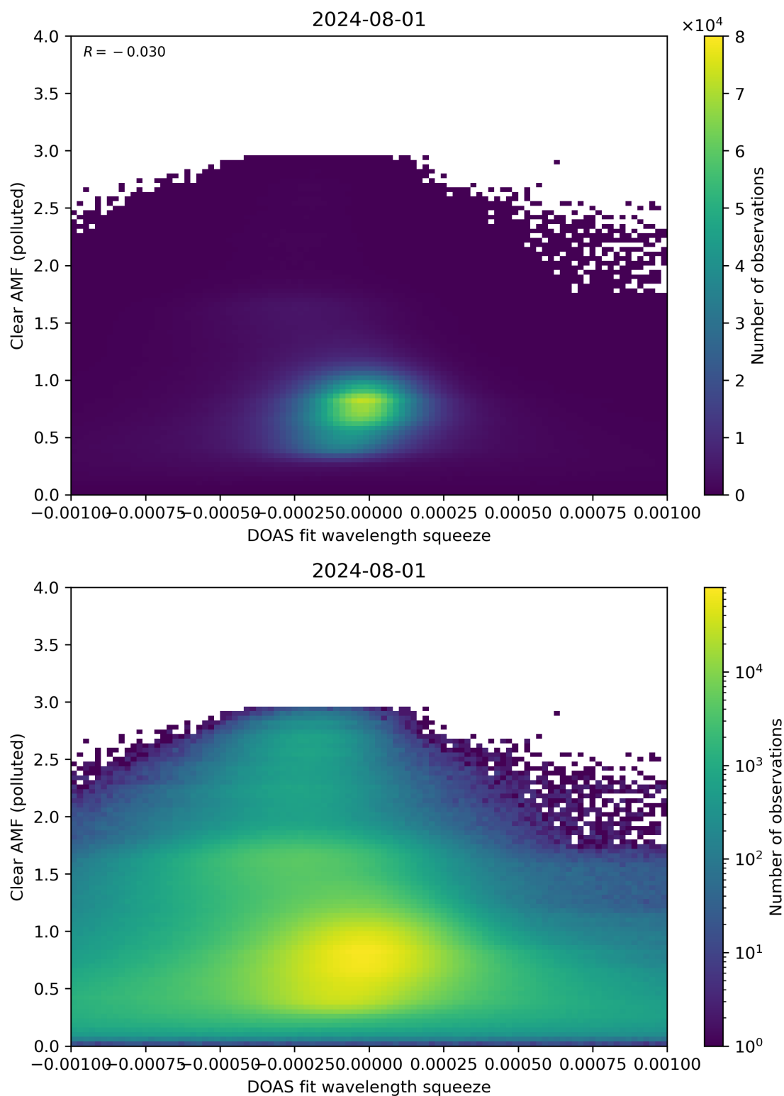
Figure 133: Scatter density plot of “DOAS fit wavelength squeeze” against “Clear AMF (polluted)” for 2024-07-31 to 2024-08-02.
