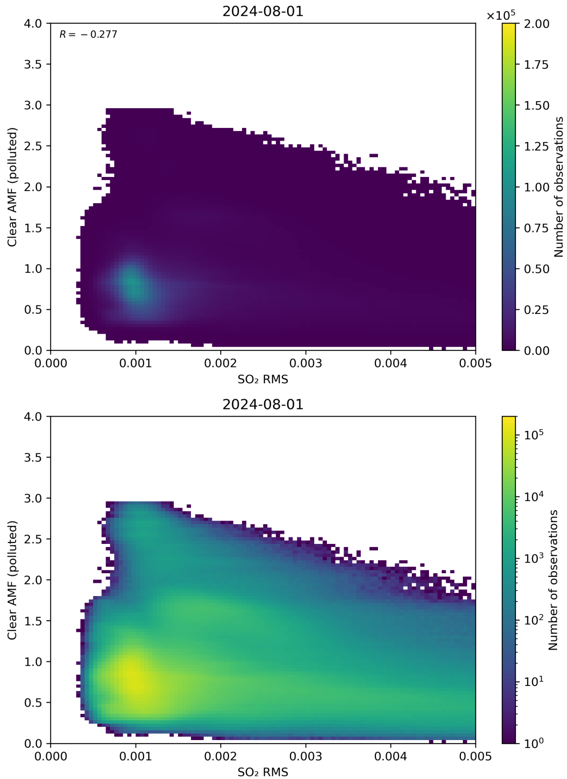
Figure 136: Scatter density plot of “SO 2 RMS” against “Clear AMF (polluted)” for 2024-07-31 to 2024-08-02.
