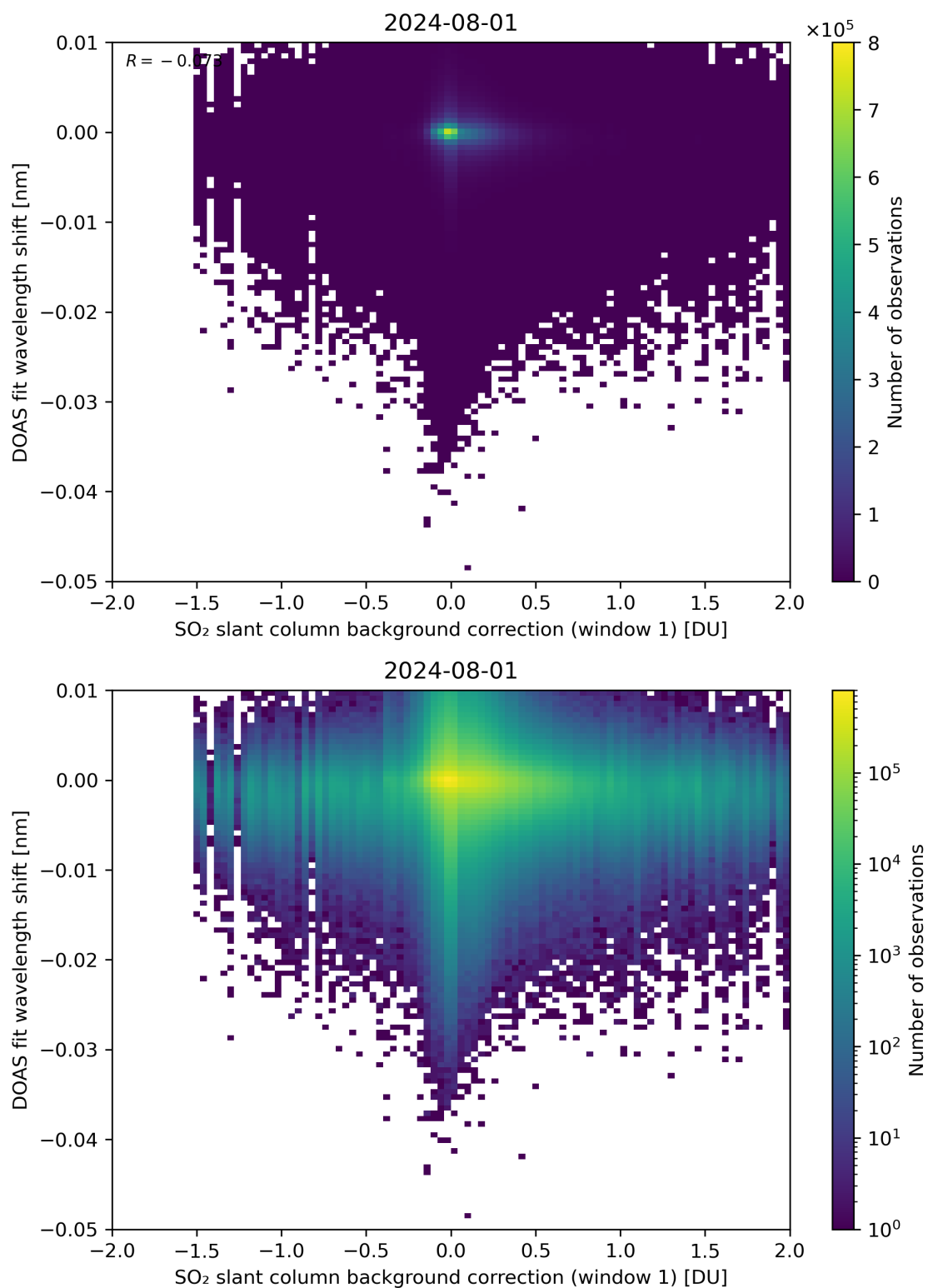
Figure 100: Scatter density plot of “SO 2 slant column background correction (window 1)” against “DOAS fit wavelength shift” for 2024-07-31 to 2024-08-02.
