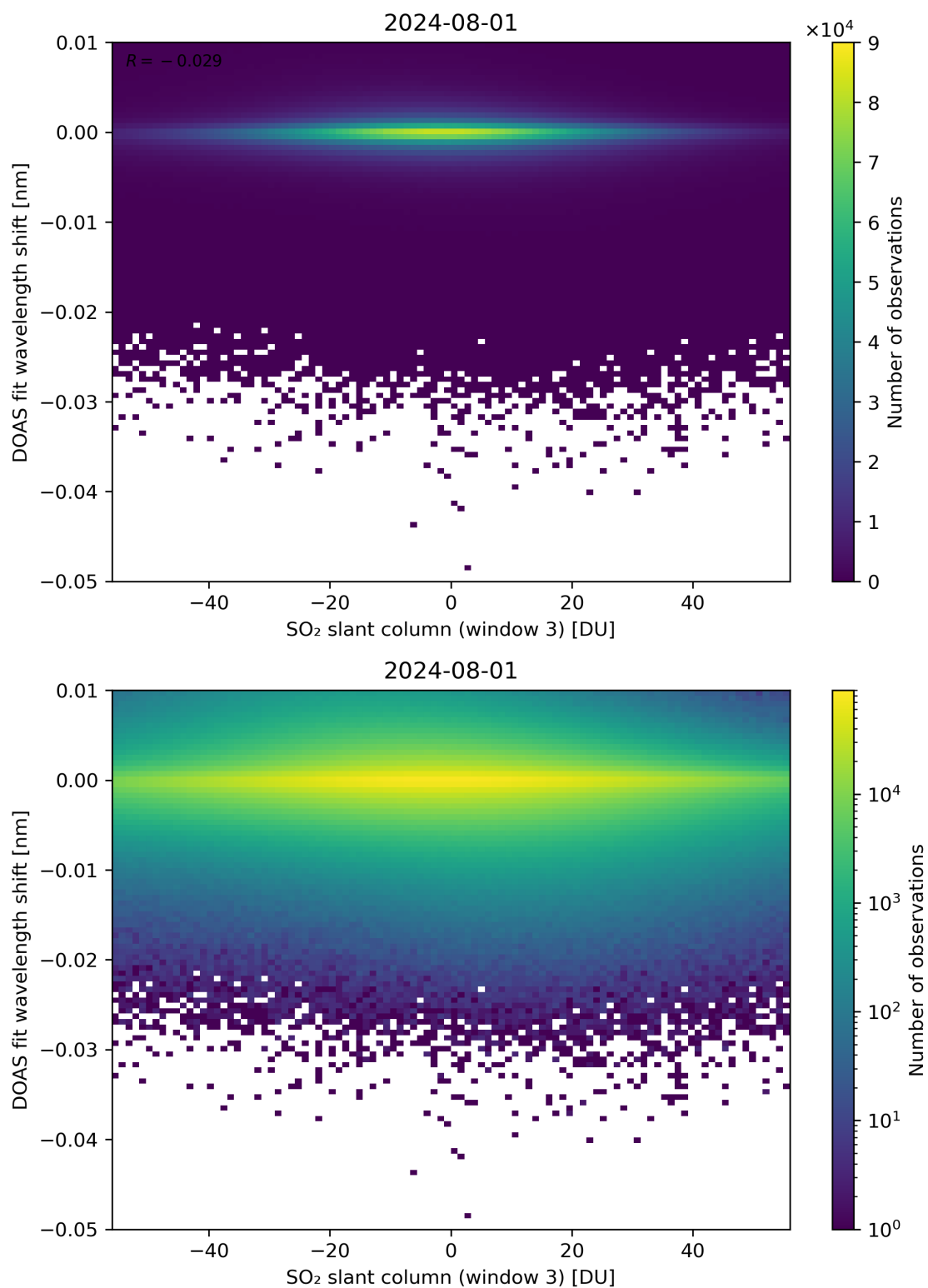
Figure 254: Scatter density plot of “SO 2 slant column (window 3)” against “DOAS fit wavelength shift” for 2024-07-31 to 2024-08-02.
