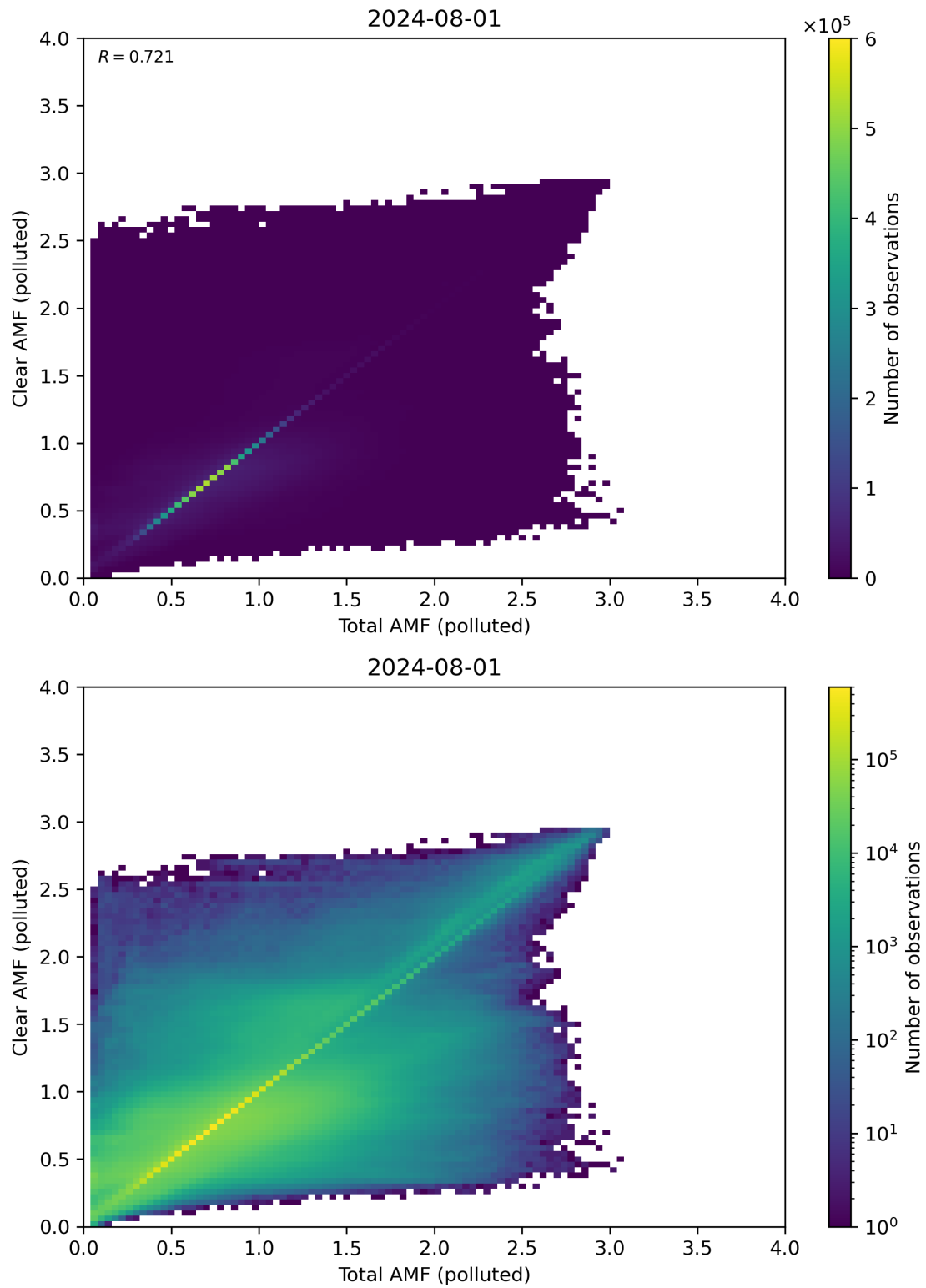
Figure 271: Scatter density plot of “Total AMF (polluted)” against “Clear AMF (polluted)” for 2024-07-31 to 2024-08-02.
