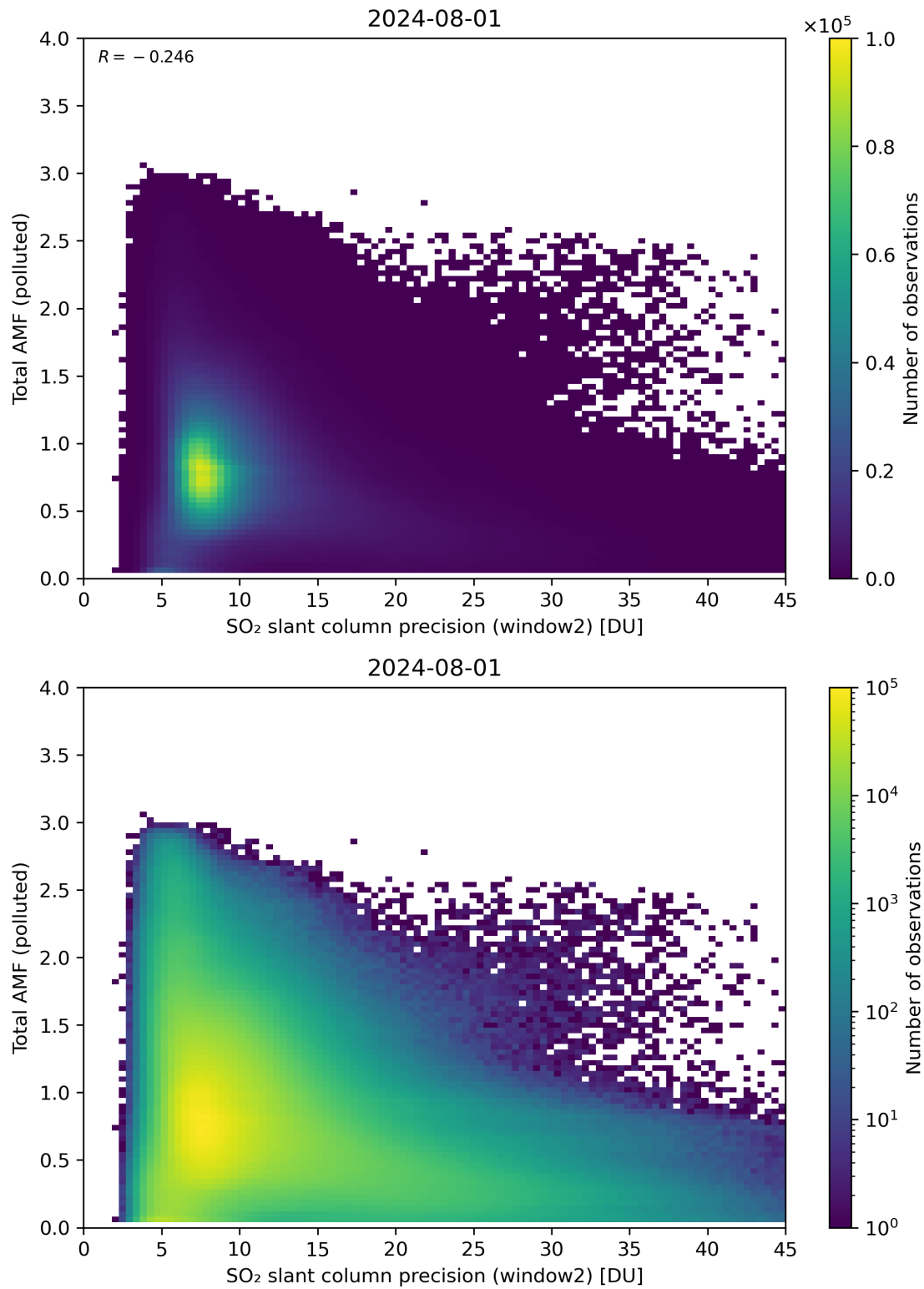
Figure 251: Scatter density plot of “SO 2 slant column precision (window2)” against “Total AMF (polluted)” for 2024-07-31 to 2024-08-02.
