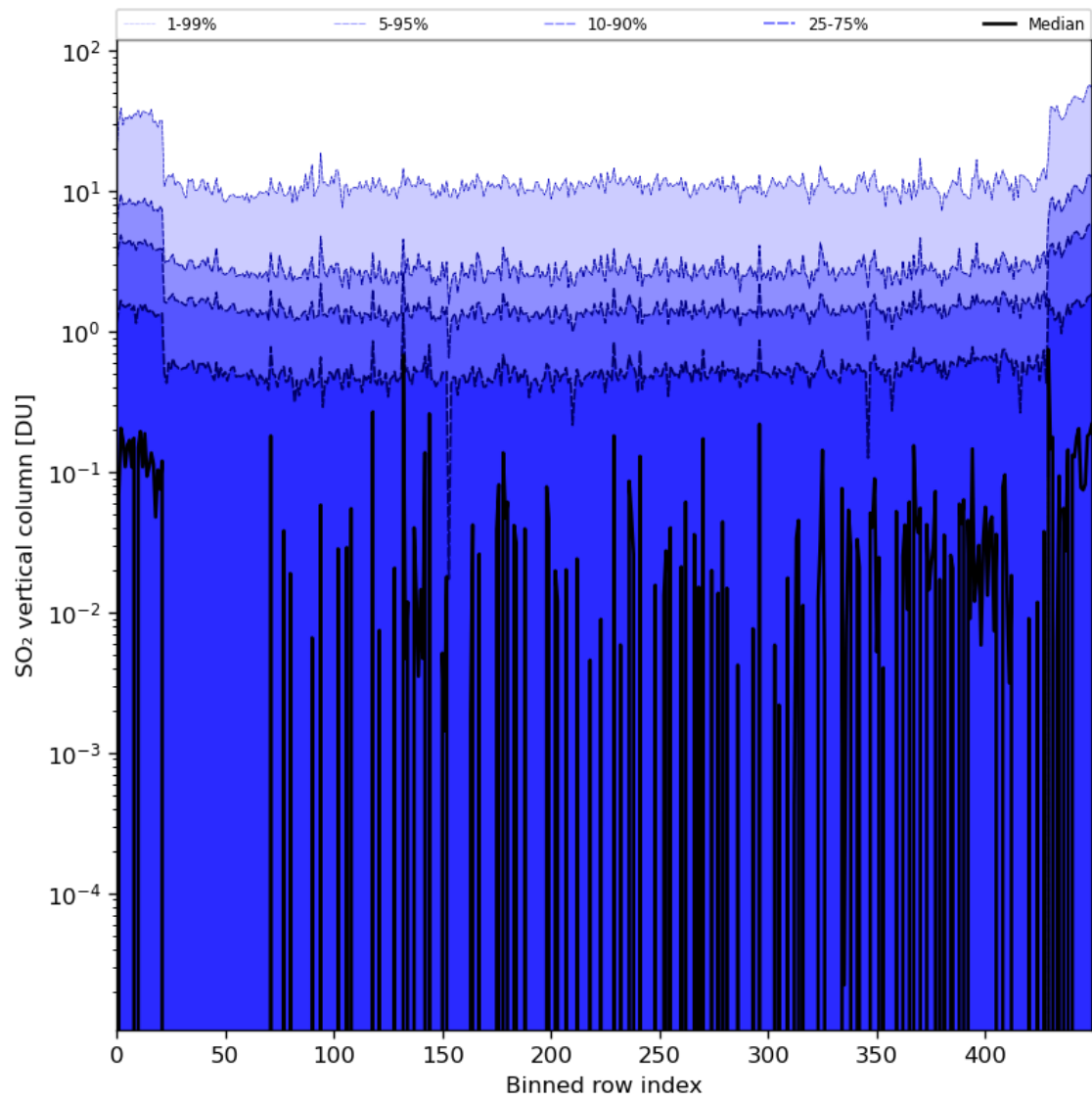
Figure 76: Along track statistics of “SO 2 vertical column” for 2024-07-31 to 2024-08-02
