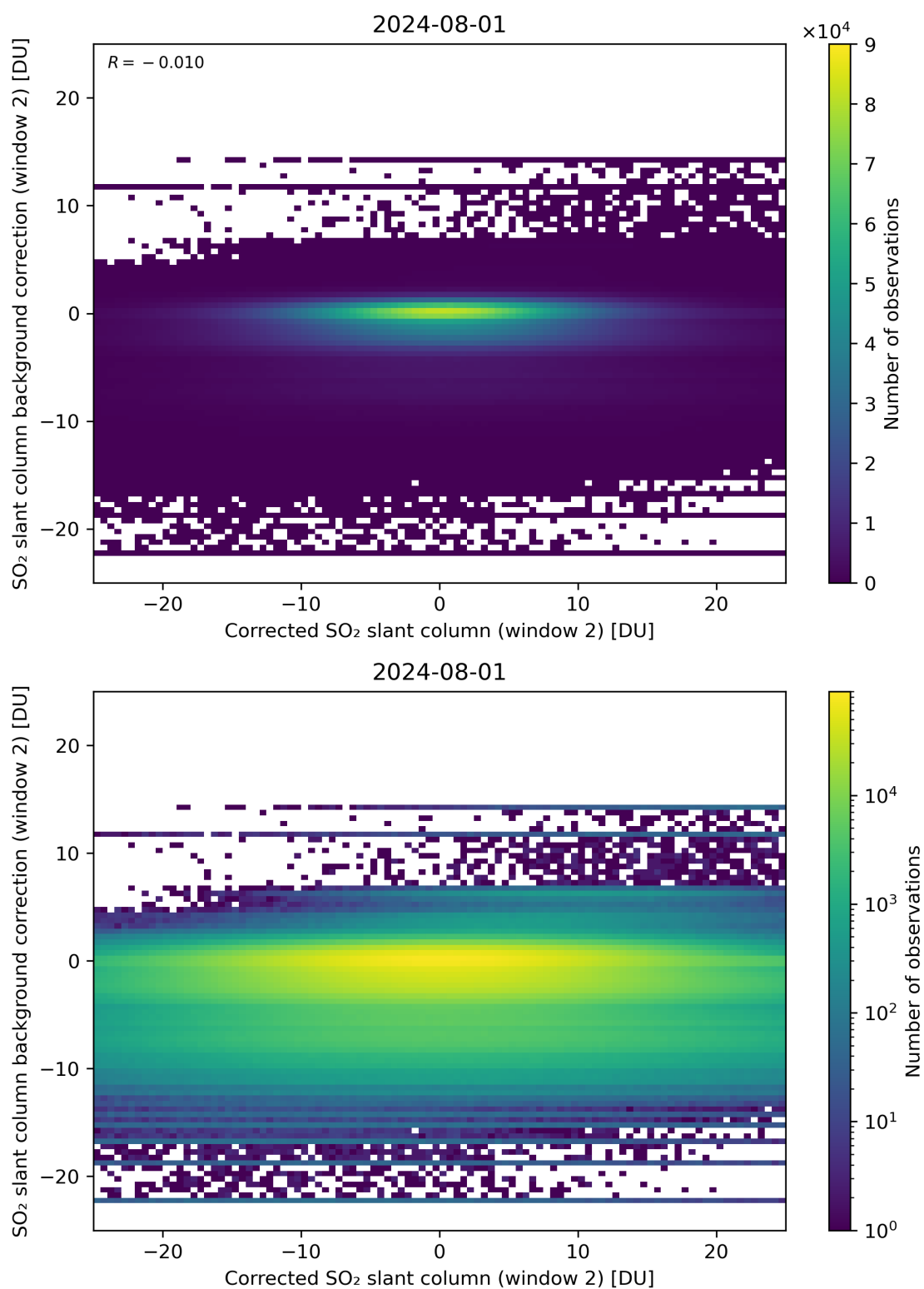
Figure 194: Scatter density plot of “Corrected SO 2 slant column (window 2)” against “SO 2 slant column background correction (window 2)” for 2024-07-31 to 2024-08-02.
