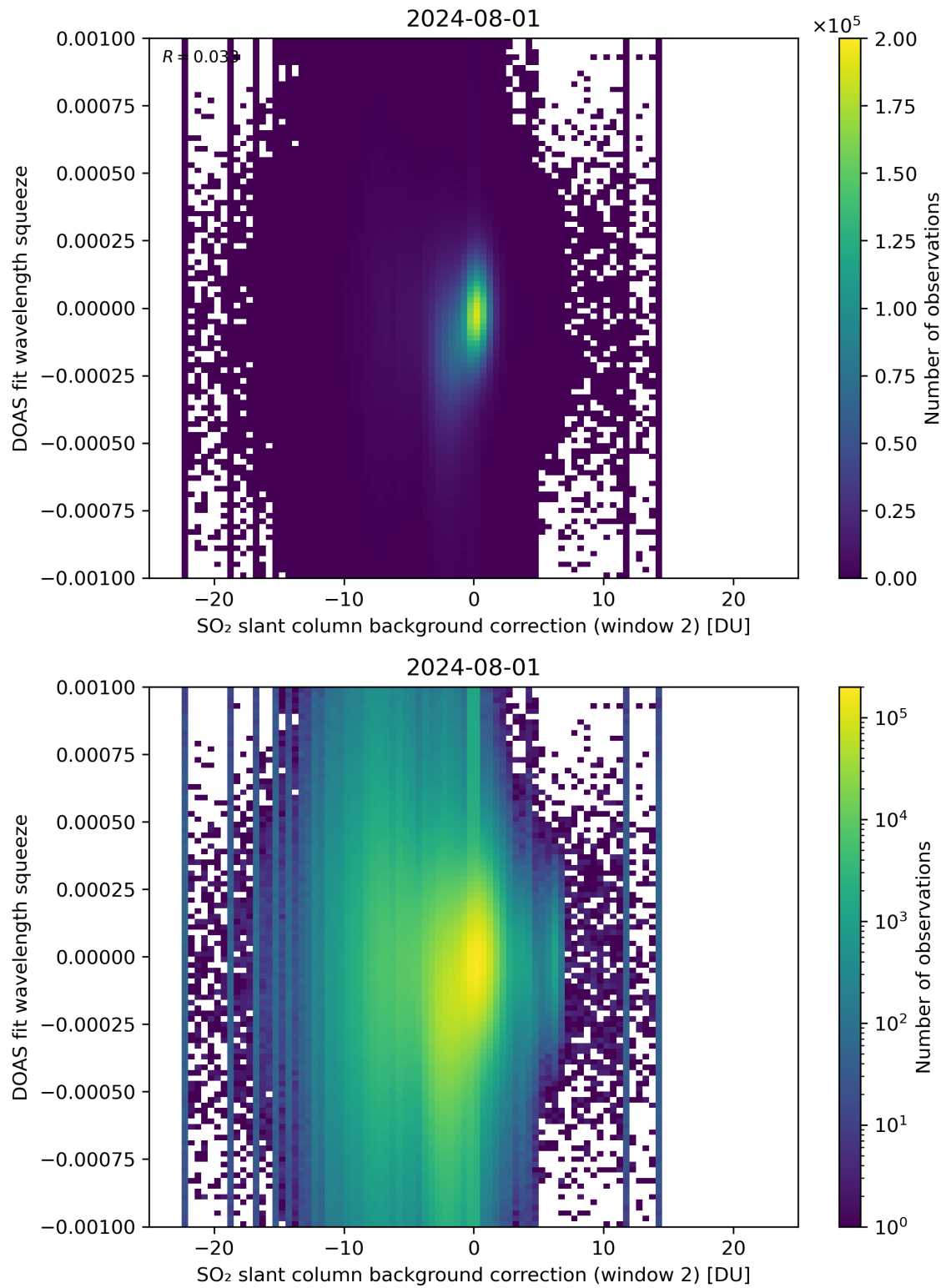
Figure 113: Scatter density plot of “SO 2 slant column background correction (window 2)” against “DOAS fit wavelength squeeze” for 2024-07-31 to 2024-08-02.
