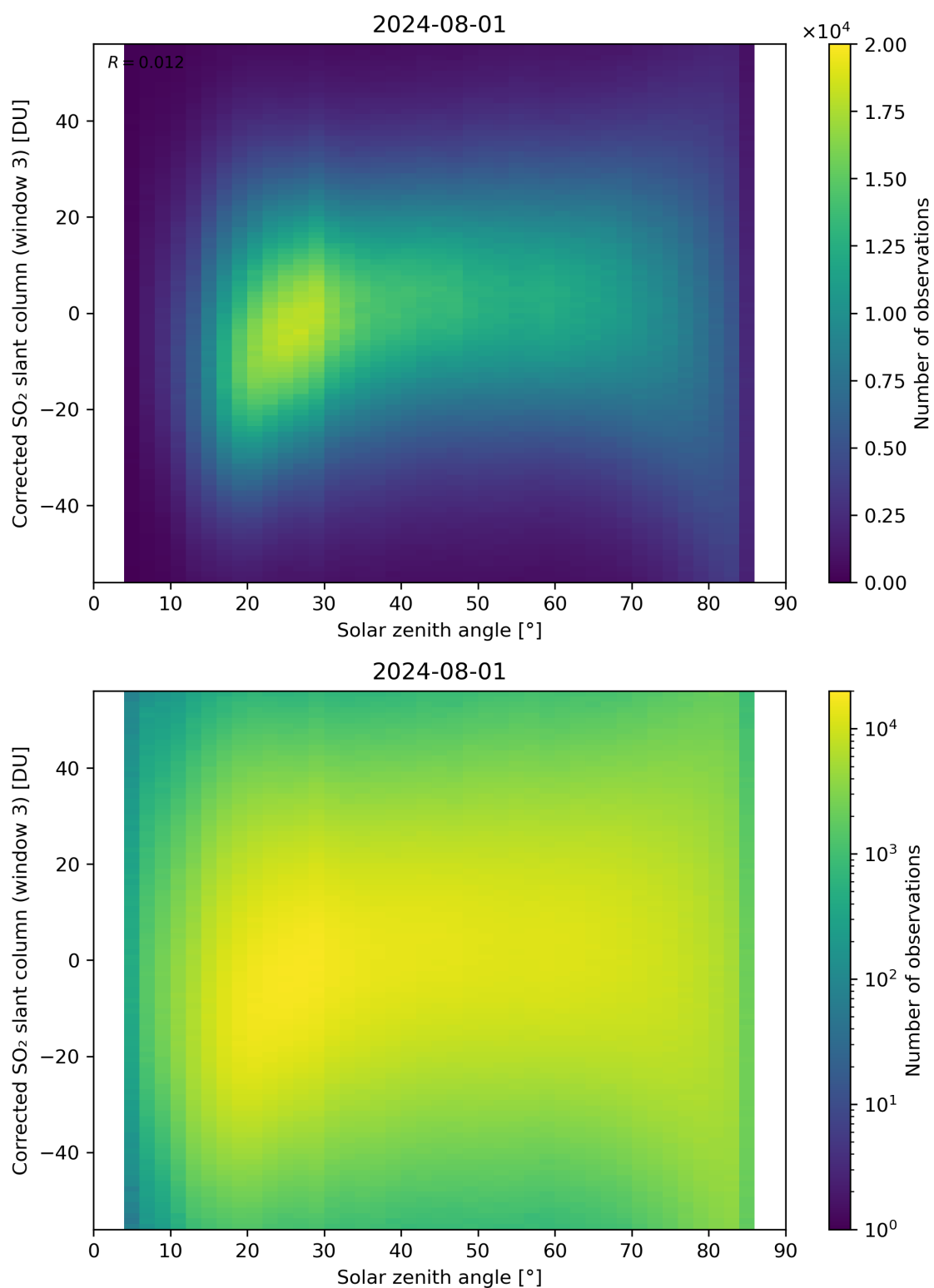
Figure 168: Scatter density plot of “Solar zenith angle” against “Corrected SO 2 slant column (window 3)” for 2024-07-31 to 2024-08-02.
