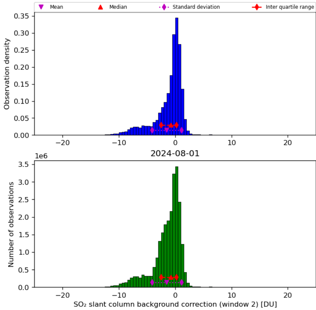
Figure 63: Histogram of “SO 2 slant column background correction (window 2)” for 2024-07-31 to 2024-08-02
