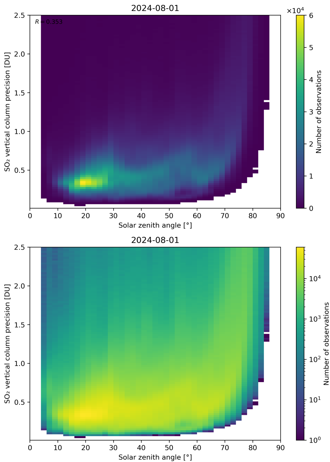
Figure 177: Scatter density plot of “Solar zenith angle” against “SO 2 vertical column precision” for 2024-07-31 to 2024-08-02.
