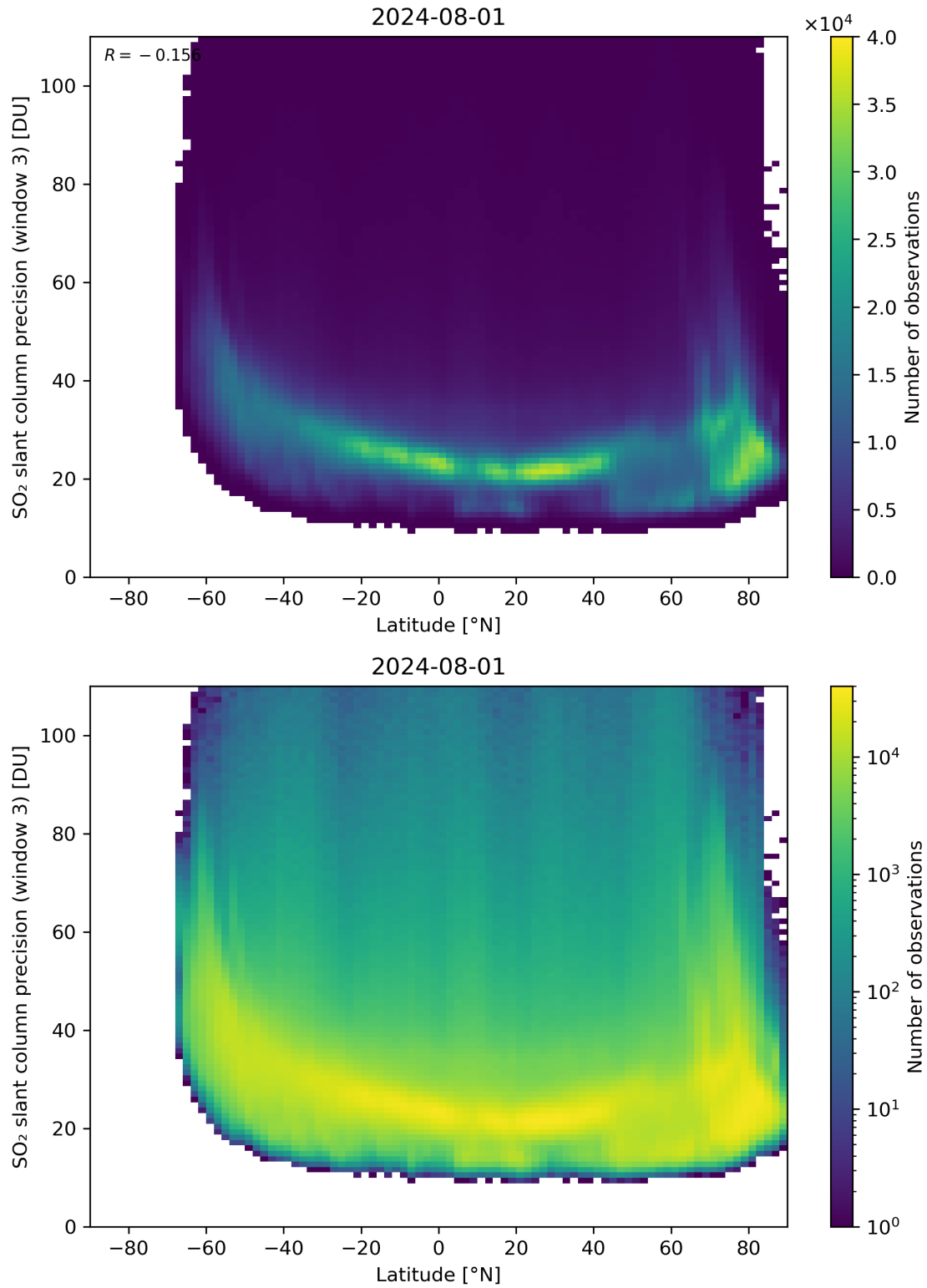
Figure 153: Scatter density plot of “Latitude” against “SO 2 slant column precision (window 3)” for 2024-07-31 to 2024-08-02.
