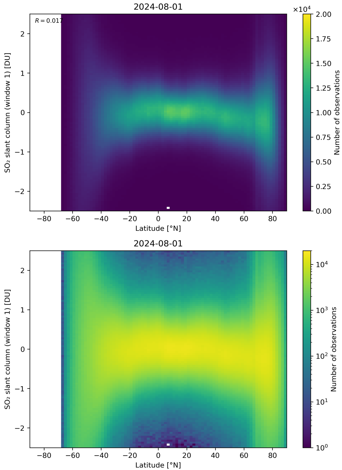
Figure 149: Scatter density plot of “Latitude” against “SO 2 slant column (window 1)” for 2024-07-31 to 2024-08-02.
