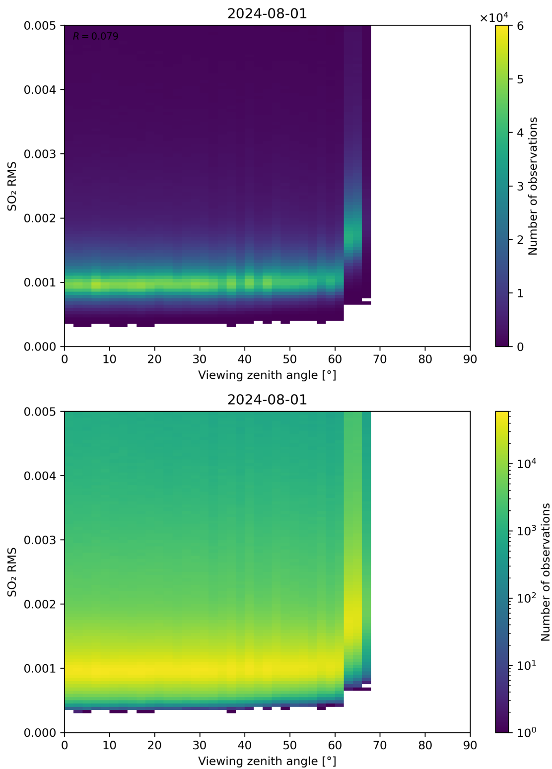
Figure 313: Scatter density plot of “Viewing zenith angle” against “SO 2 RMS” for 2024-07-31 to 2024-08-02.
