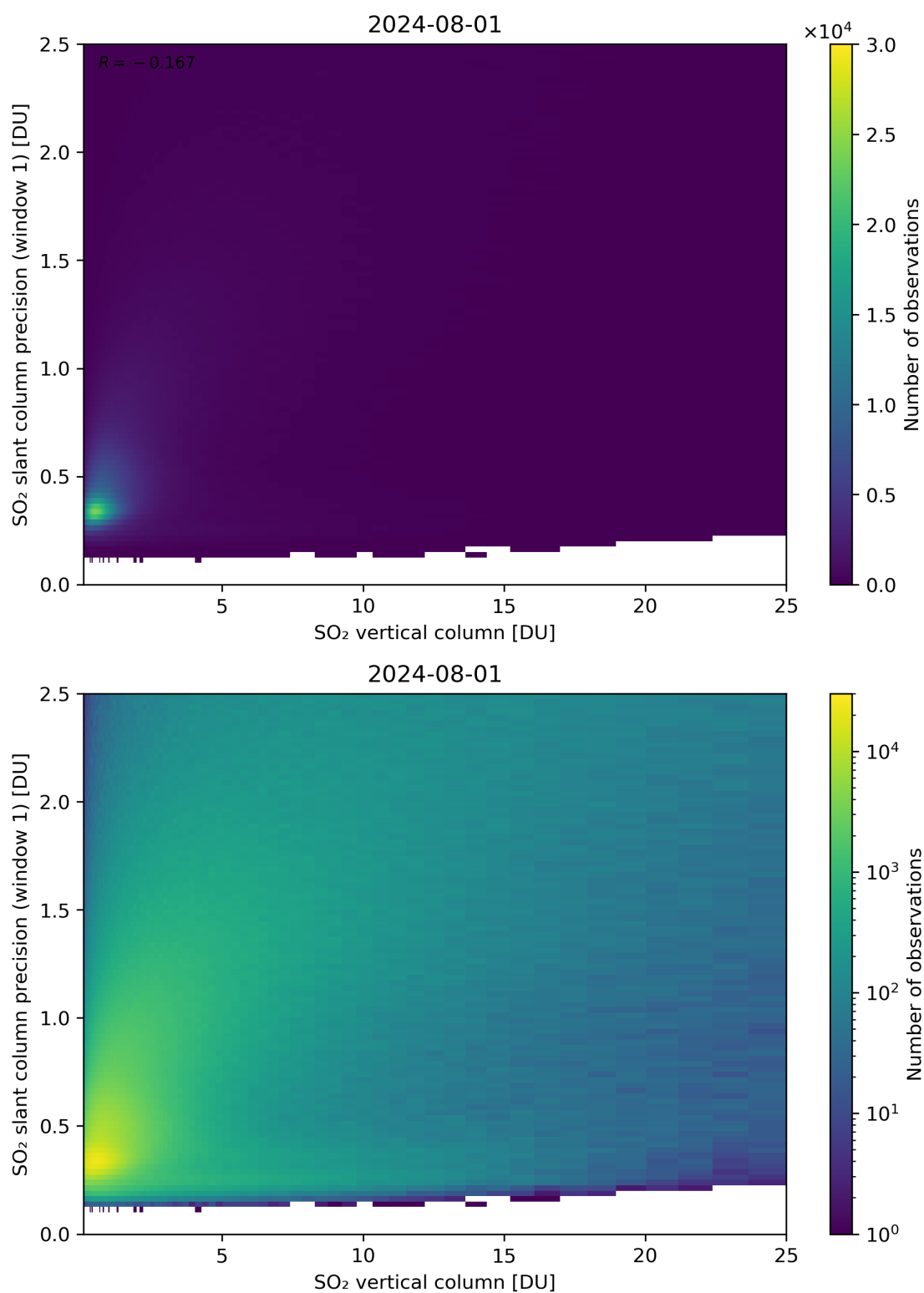
Figure 301: Scatter density plot of “SO 2 vertical column” against “SO 2 slant column precision (window 1)” for 2024-07-31 to 2024-08-02.
