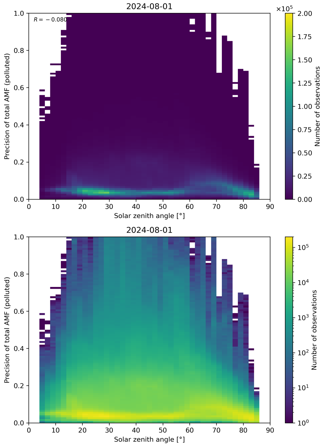
Figure 175: Scatter density plot of “Solar zenith angle” against “Precision of total AMF (polluted)” for 2024-07-31 to 2024-08-02.
