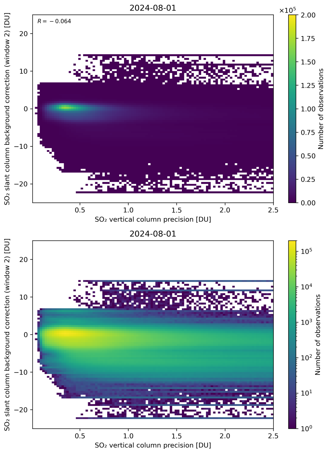
Figure 280: Scatter density plot of “SO 2 vertical column precision” against “SO 2 slant column background correction (window 2)” for 2024-07-31 to 2024-08-02.
