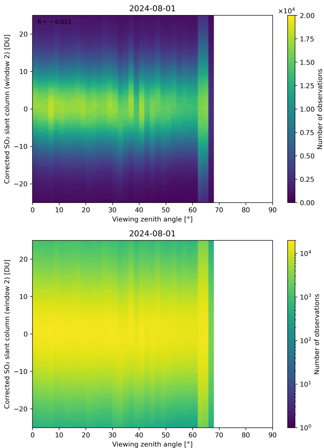
Figure 318: Scatter density plot of “Viewing zenith angle” against “Corrected SO 2 slant column (window 2)” for 2024-07-31 to 2024-08-02.
