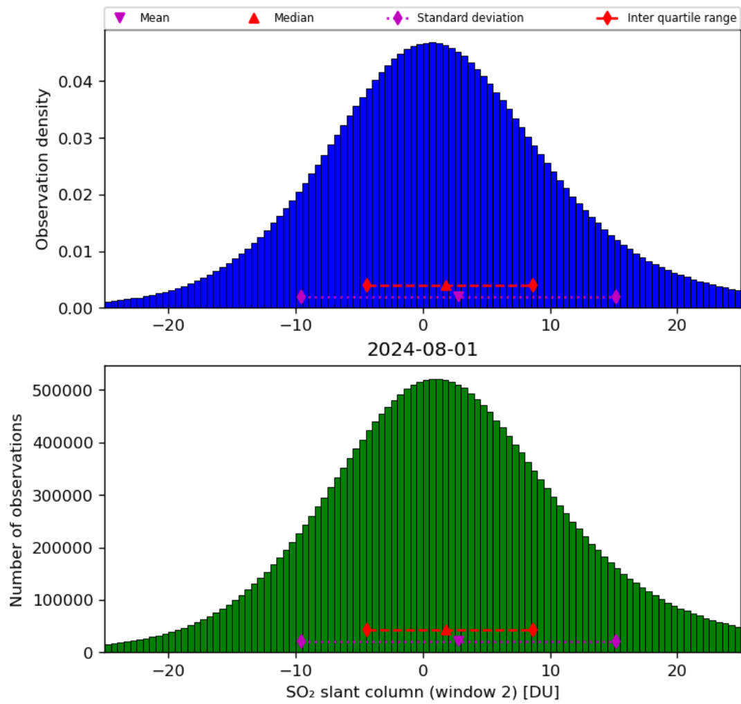
Figure 60: Histogram of “SO 2 slant column (window 2)” for 2024-07-31 to 2024-08-02
