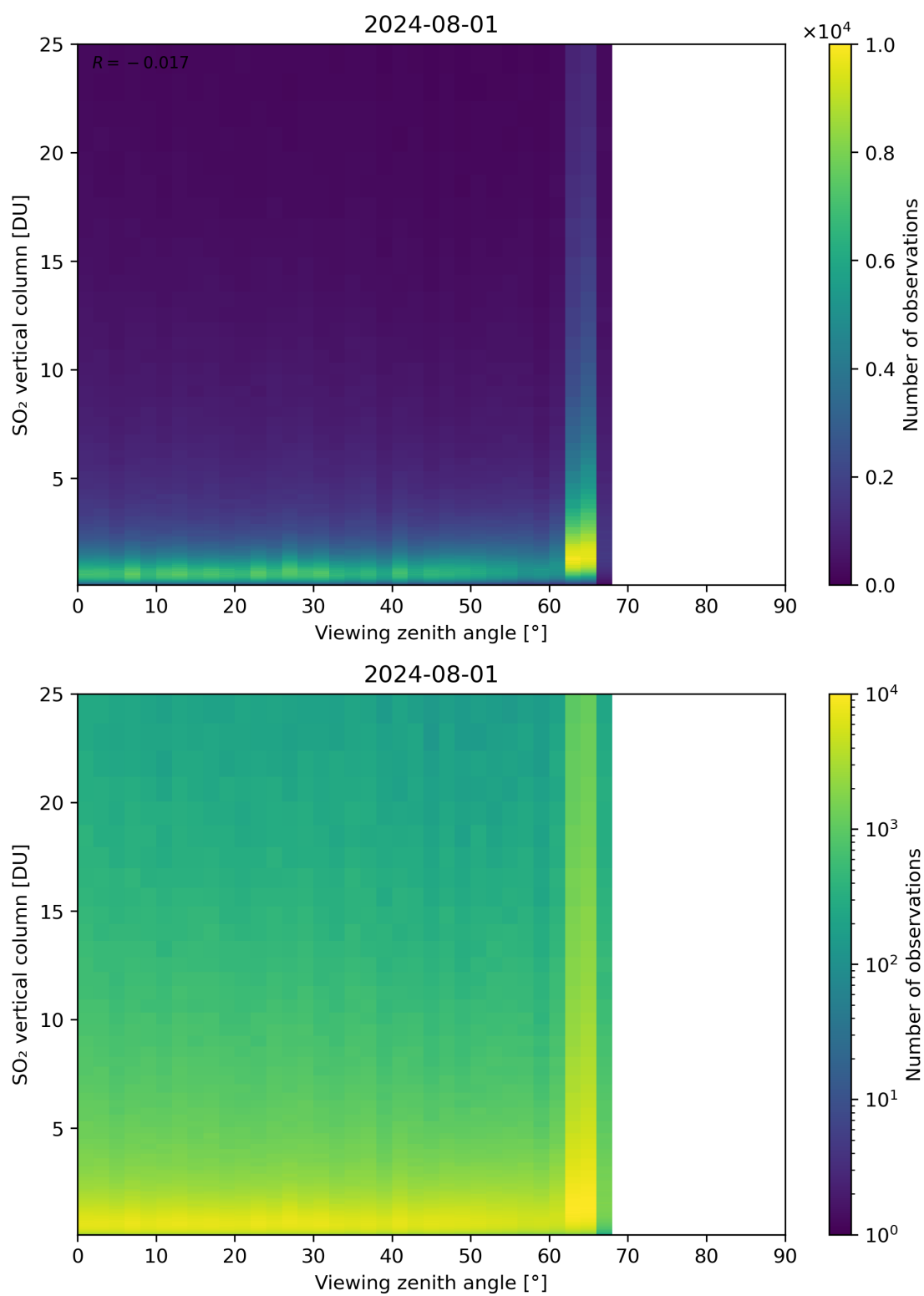
Figure 327: Scatter density plot of “Viewing zenith angle” against “SO 2 vertical column” for 2024-07-31 to 2024-08-02.
