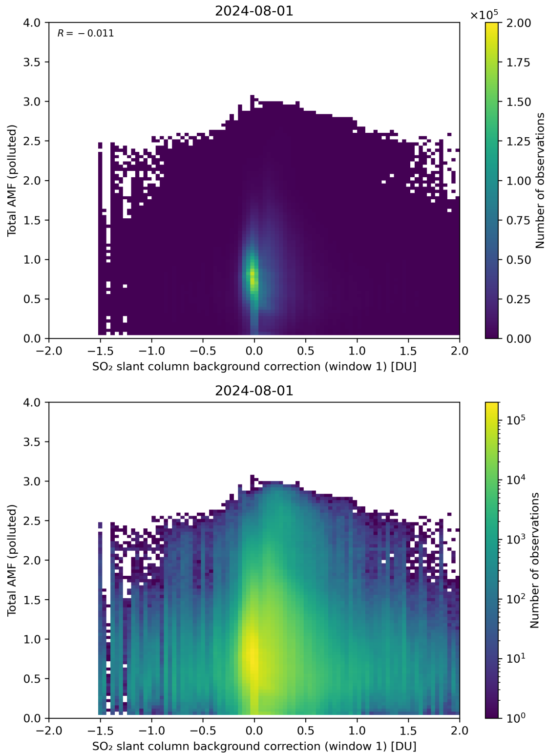
Figure 109: Scatter density plot of “SO 2 slant column background correction (window 1)” against “Total AMF (polluted)” for 2024-07-31 to 2024-08-02.
