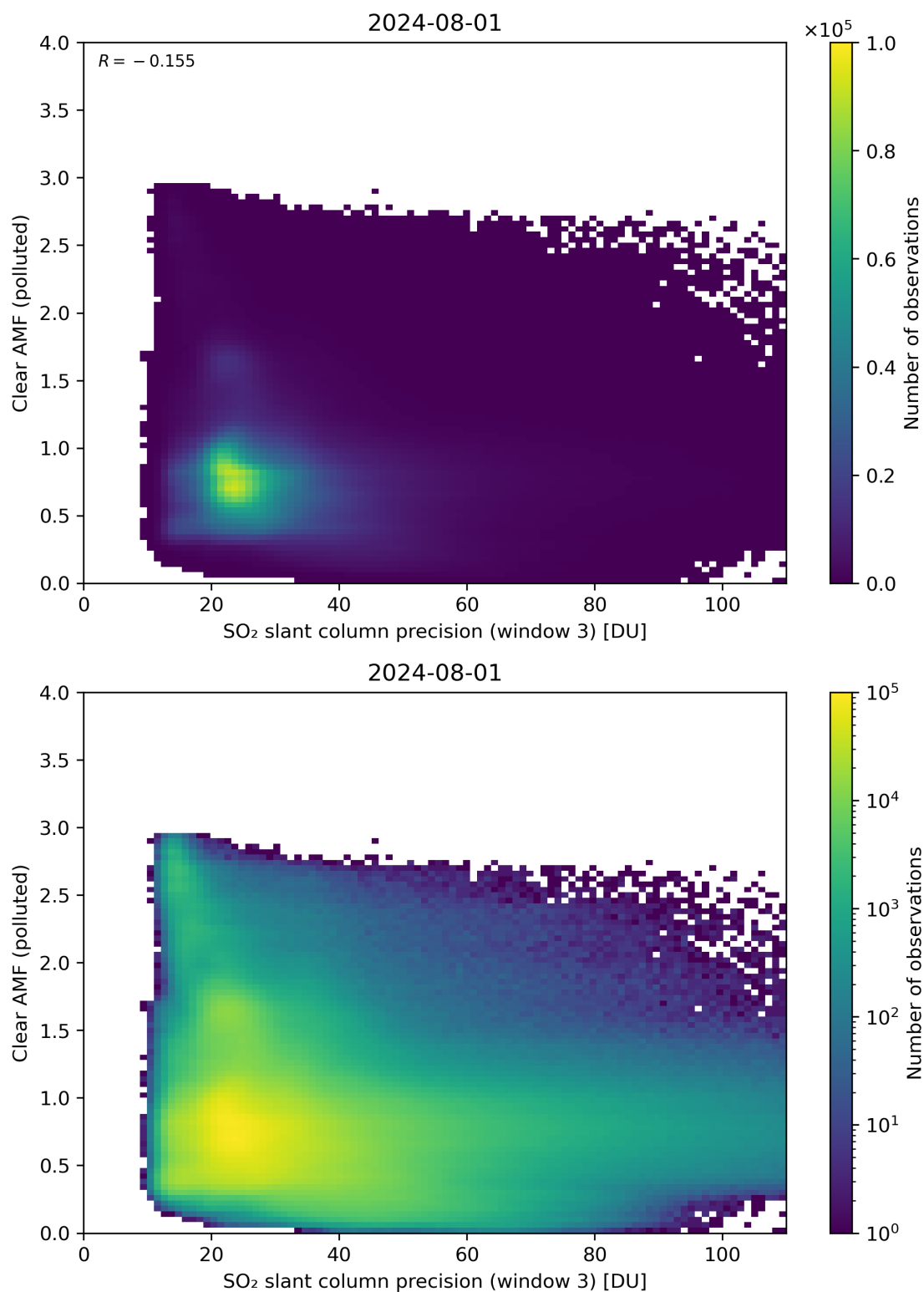
Figure 261: Scatter density plot of “SO 2 slant column precision (window 3)” against “Clear AMF (polluted)” for 2024-07-31 to 2024-08-02.
