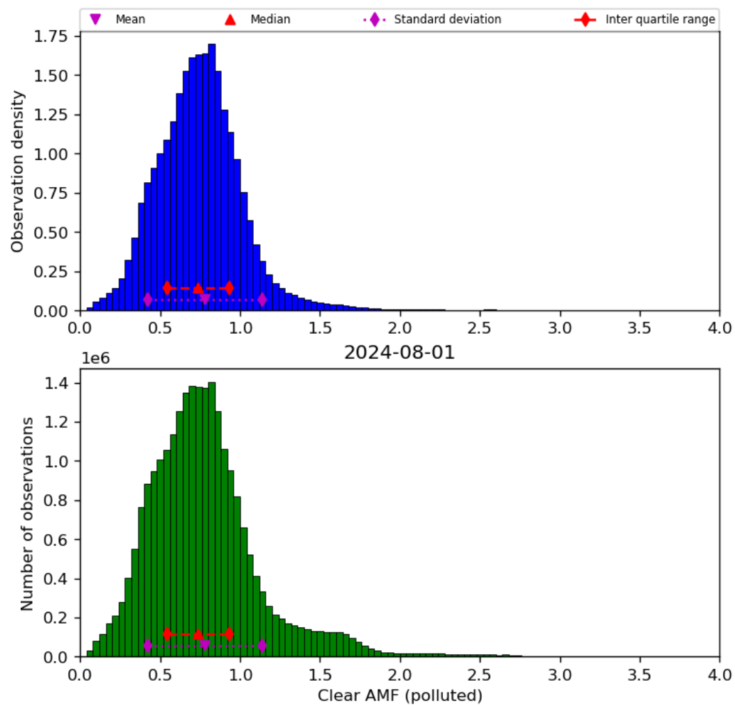
Figure 73: Histogram of “Clear AMF (polluted)” for 2024-07-31 to 2024-08-02
