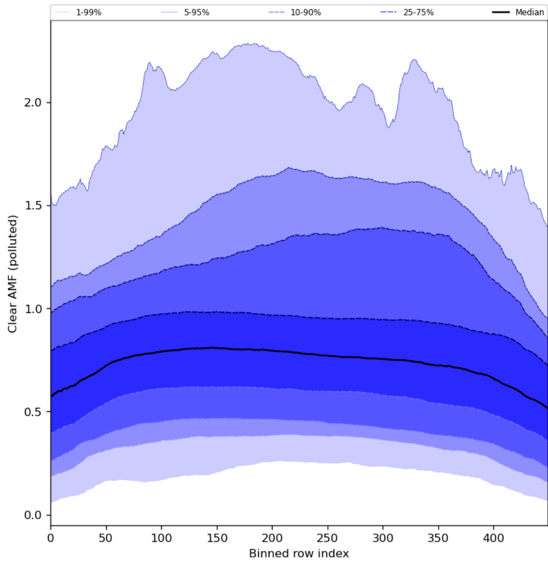
Figure 96: Along track statistics of “Clear AMF (polluted)” for 2024-07-31 to 2024-08-02
