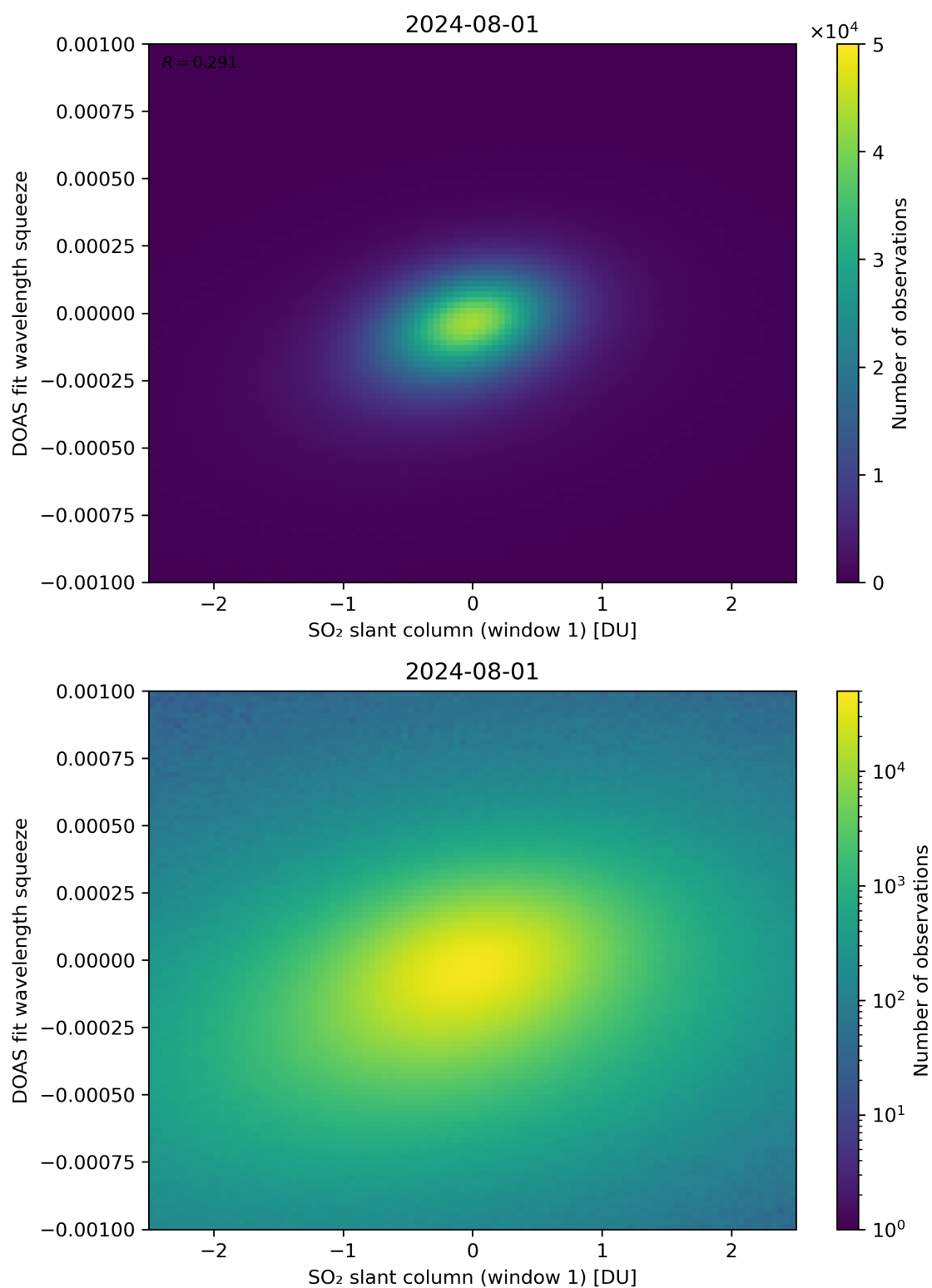
Figure 216: Scatter density plot of “SO 2 slant column (window 1)” against “DOAS fit wavelength squeeze” for 2024-07-31 to 2024-08-02.
