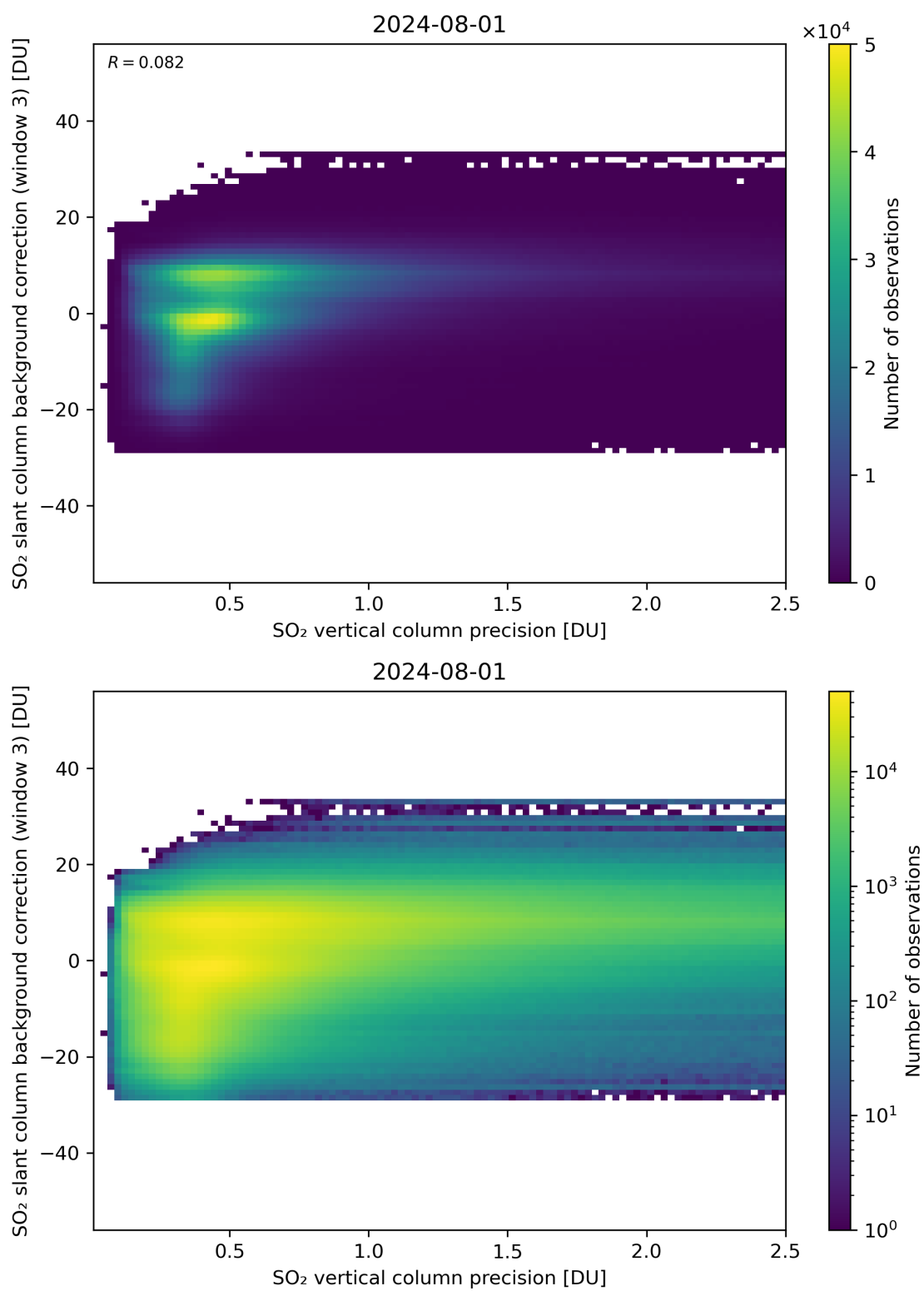
Figure 281: Scatter density plot of “SO 2 vertical column precision” against “SO 2 slant column background correction (window 3)” for 2024-07-31 to 2024-08-02.
