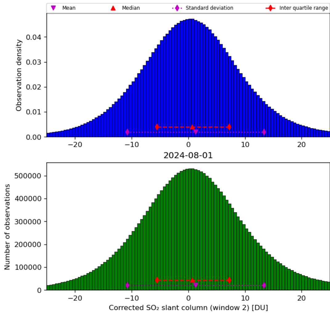
Figure 62: Histogram of “Corrected SO 2 slant column (window 2)” for 2024-07-31 to 2024-08-02
