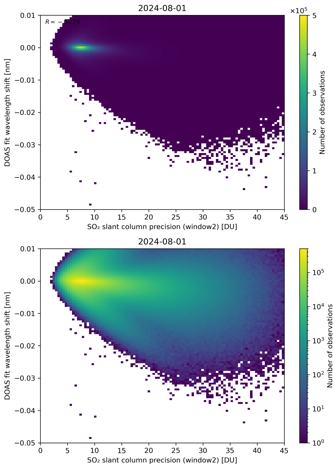
Figure 243: Scatter density plot of “SO 2 slant column precision (window2)” against “DOAS fit wavelength shift” for 2024-07-31 to 2024-08-02.
