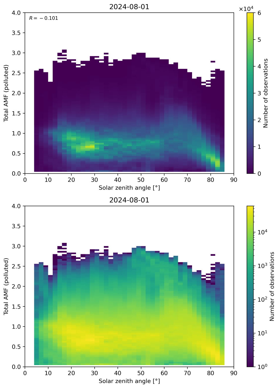
Figure 174: Scatter density plot of “Solar zenith angle” against “Total AMF (polluted)” for 2024-07-31 to 2024-08-02.
