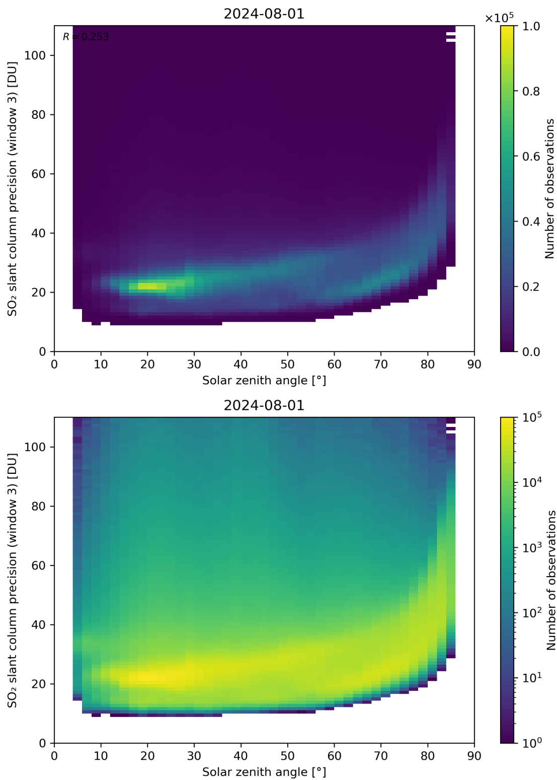
Figure 173: Scatter density plot of “Solar zenith angle” against “SO 2 slant column precision (window 3)” for 2024-07-31 to 2024-08-02.
