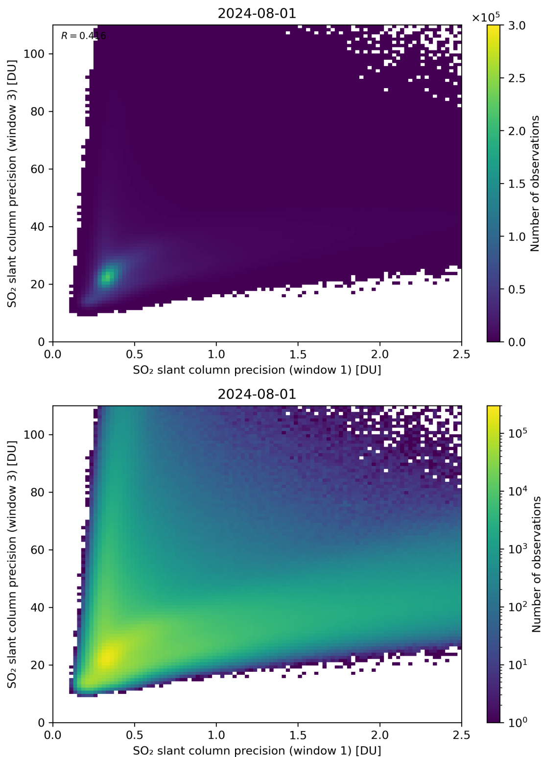
Figure 229: Scatter density plot of “SO 2 slant column precision (window 1)” against “SO 2 slant column precision (window 3)” for 2024-07-31 to 2024-08-02.
