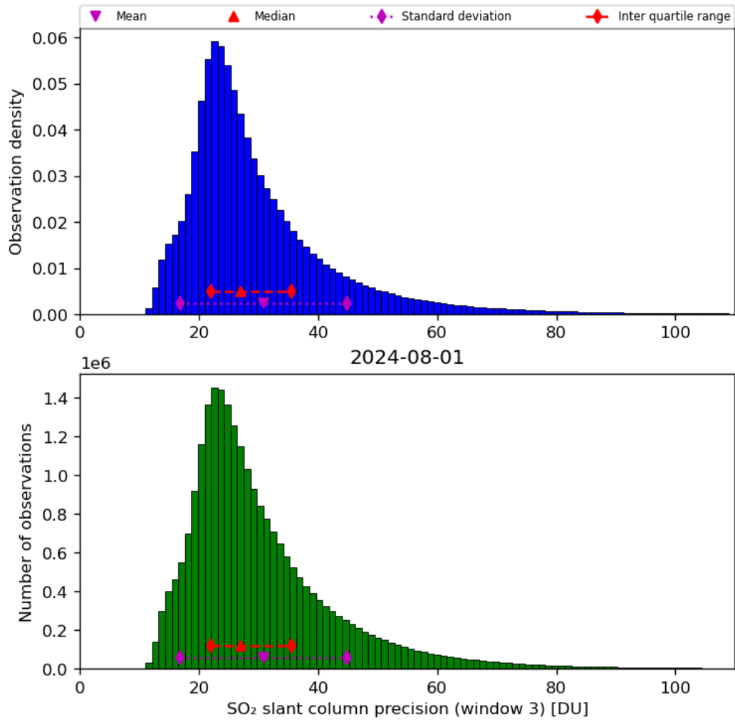
Figure 65: Histogram of “SO 2 slant column precision (window 3)” for 2024-07-31 to 2024-08-02
