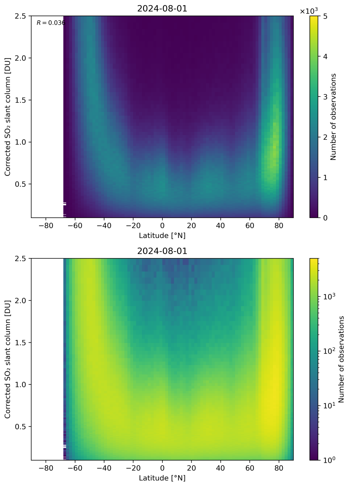
Figure 146: Scatter density plot of “Latitude” against “Corrected SO 2 slant column” for 2024-07-31 to 2024-08-02.
