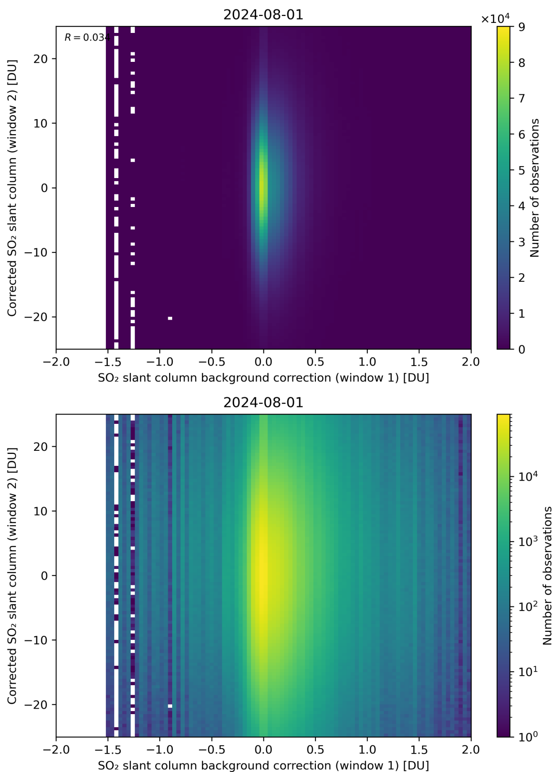
Figure 104: Scatter density plot of “SO 2 slant column background correction (window 1)” against “Corrected SO 2 slant column (window 2)” for 2024-07-31 to 2024-08-02.
