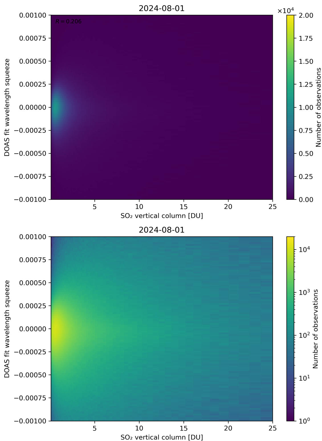
Figure 277: Scatter density plot of “SO 2 vertical column” against “DOAS fit wavelength squeeze” for 2024-07-31 to 2024-08-02.
