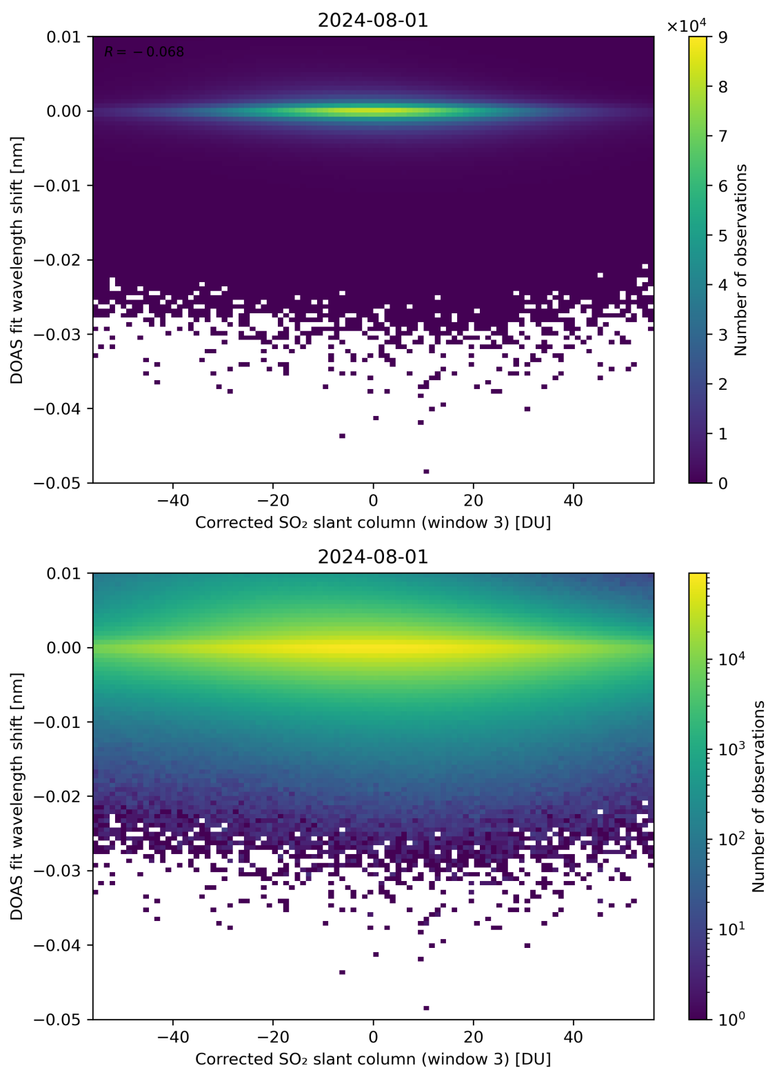
Figure 206: Scatter density plot of “Corrected SO 2 slant column (window 3)” against “DOAS fit wavelength shift” for 2024-07-31 to 2024-08-02.
