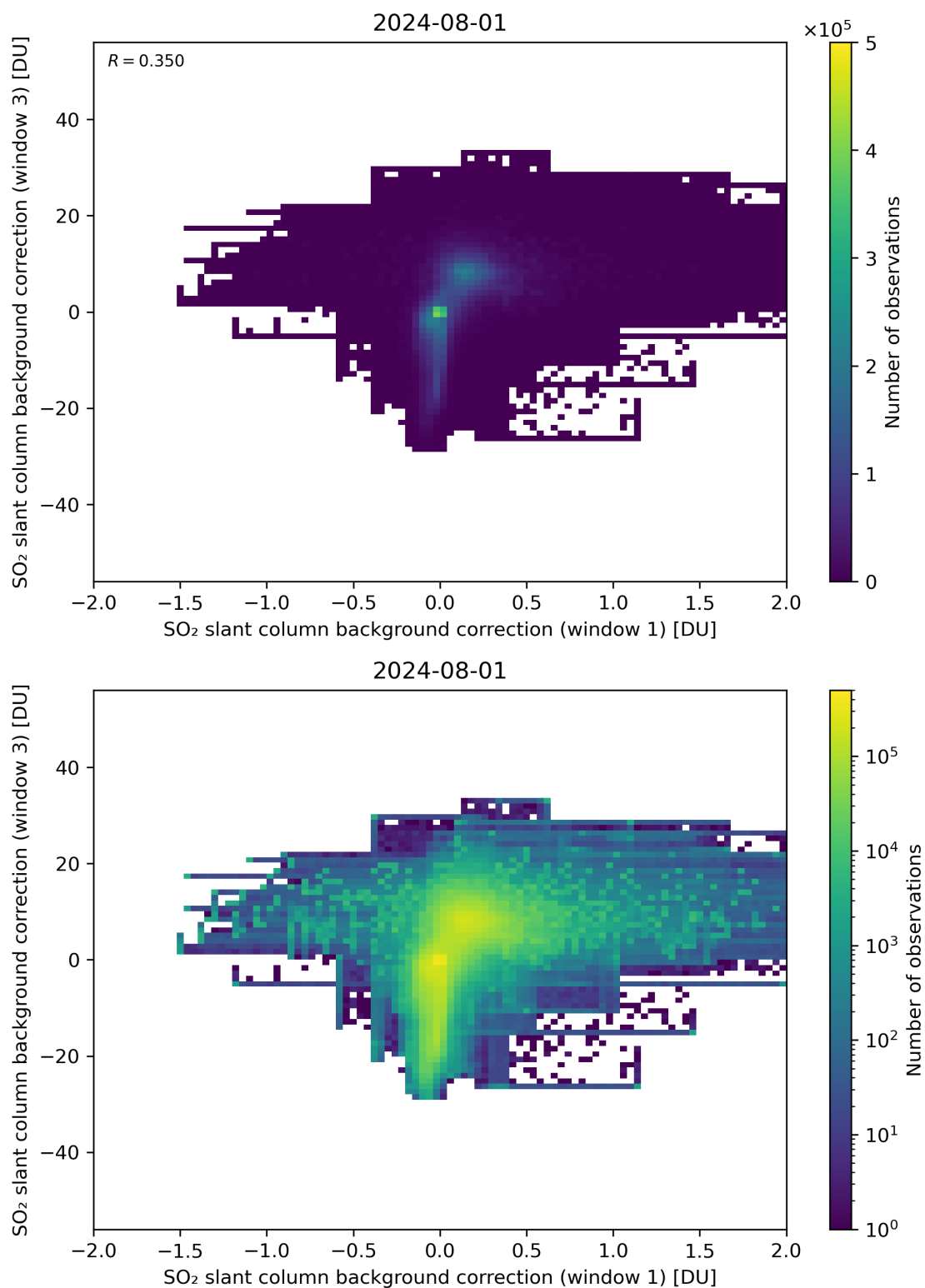
Figure 99: Scatter density plot of “SO 2 slant column background correction (window 1)” against “SO 2 slant column background correction (window 3)” for 2024-07-31 to 2024-08-02.
