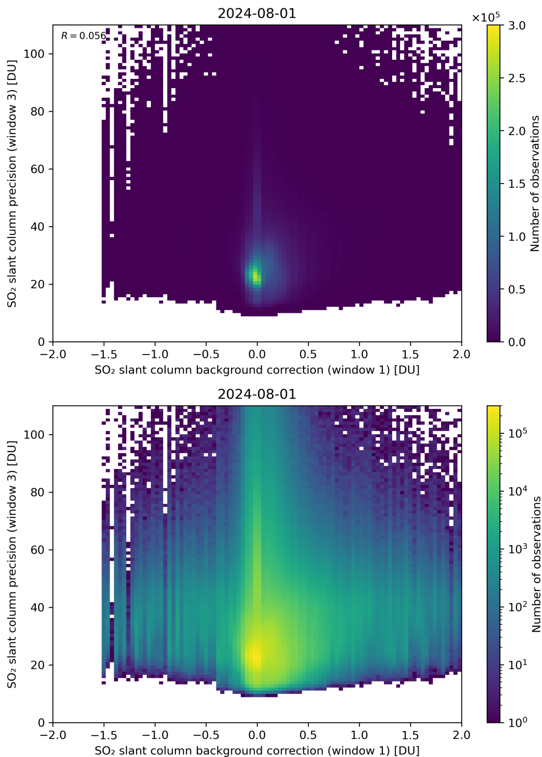
Figure 108: Scatter density plot of “SO 2 slant column background correction (window 1)” against “SO 2 slant column precision (window 3)” for 2024-07-31 to 2024-08-02.
