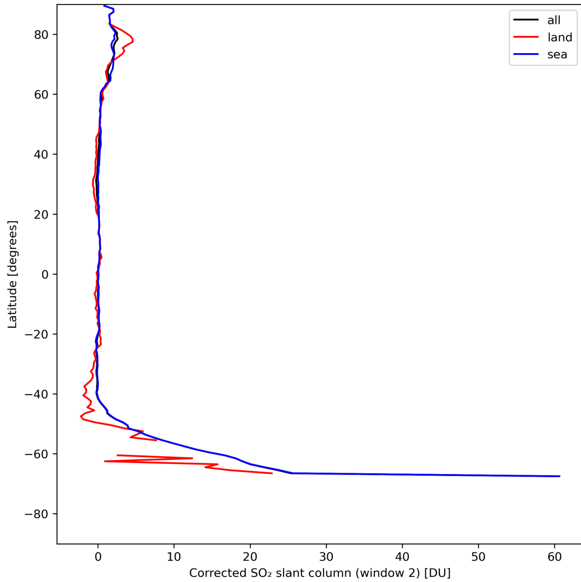
Figure 39: Zonal average of “Corrected SO 2 slant column (window 2)” for 2024-07-31 to 2024-08-02.
