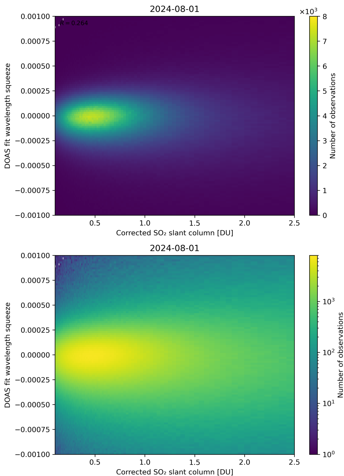
Figure 182: Scatter density plot of “Corrected SO 2 slant column” against “DOAS fit wavelength squeeze” for 2024-07-31 to 2024-08-02.
