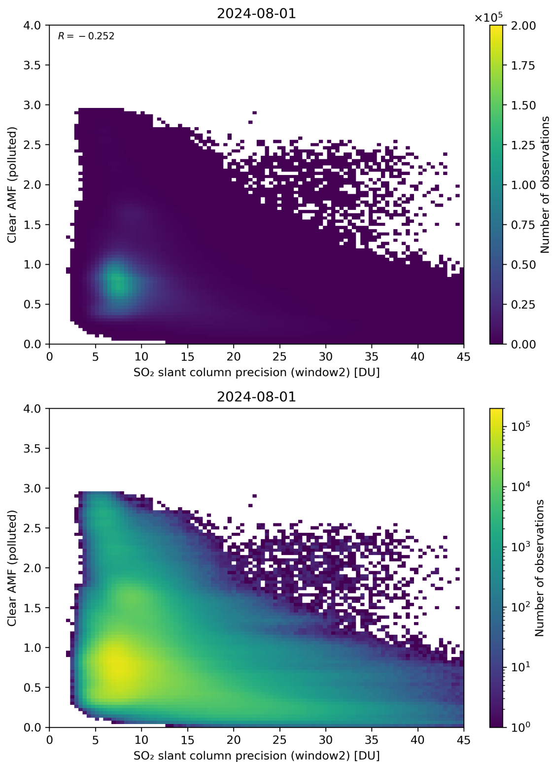
Figure 246: Scatter density plot of “SO 2 slant column precision (window2)” against “Clear AMF (polluted)” for 2024-07-31 to 2024-08-02.
