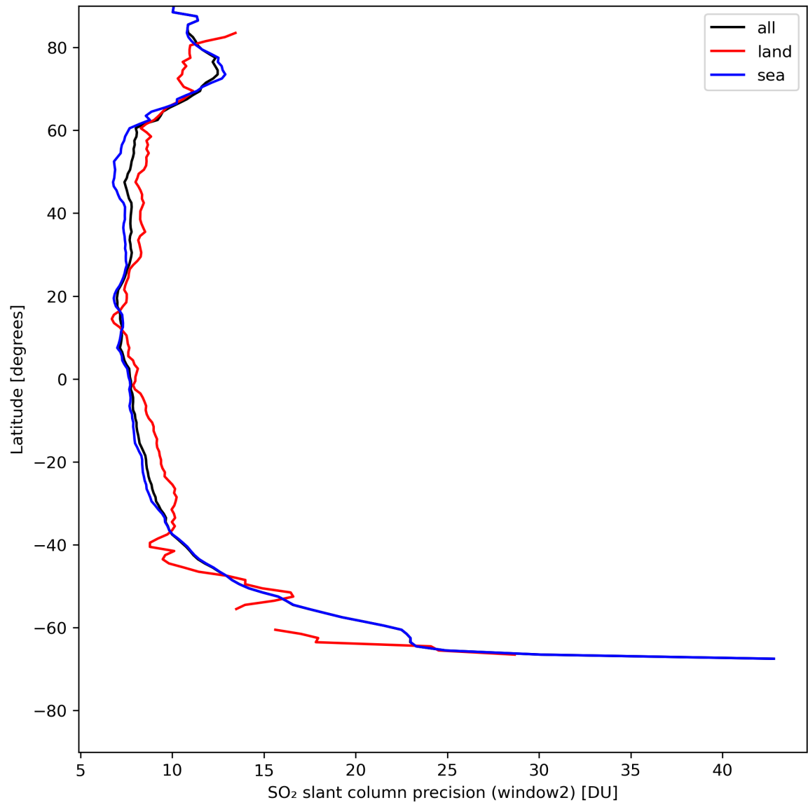
Figure 38: Zonal average of “SO 2 slant column precision (window2)” for 2024-07-31 to 2024-08-02.
