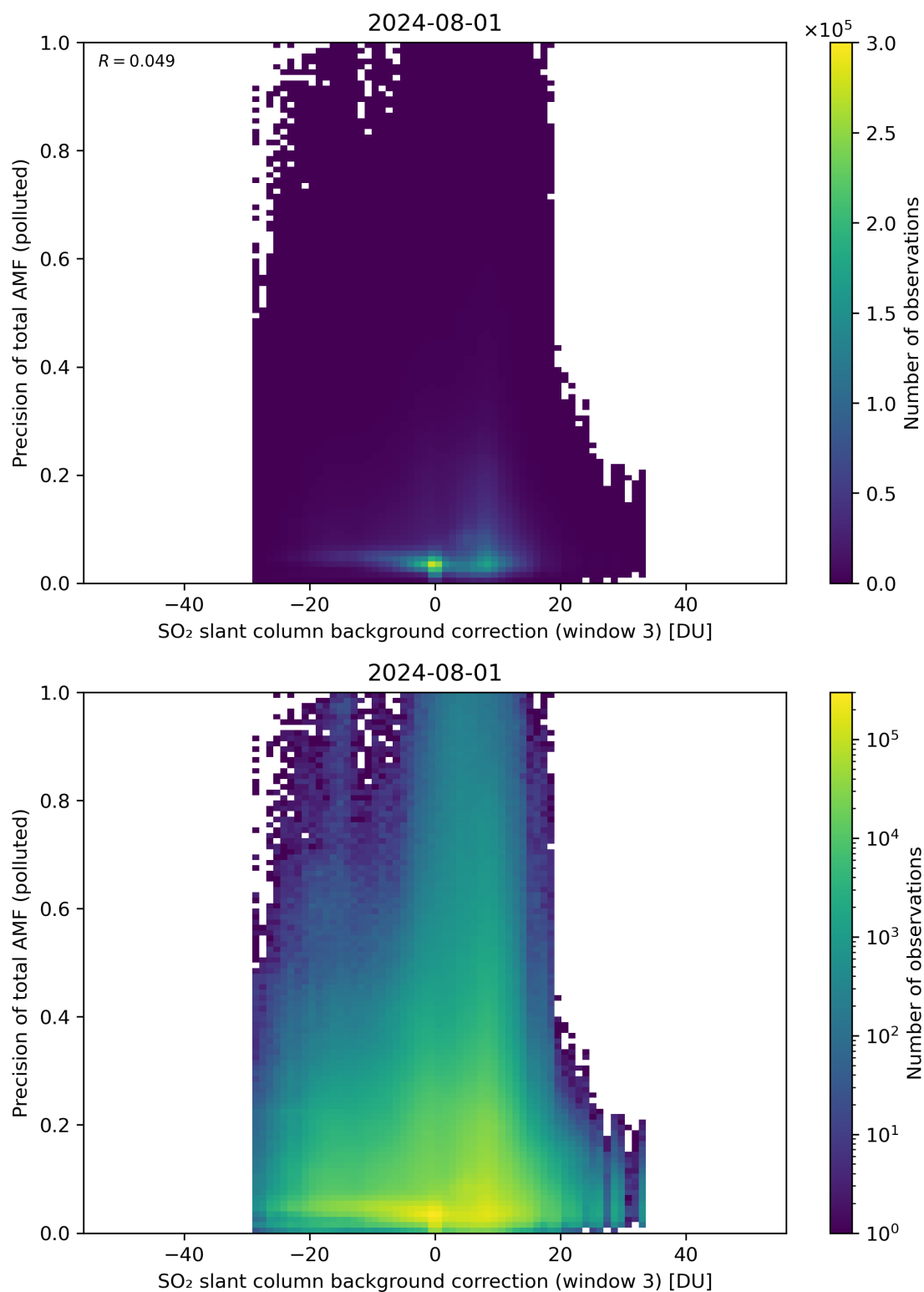
Figure 126: Scatter density plot of “SO 2 slant column background correction (window 3)” against “Precision of total AMF (polluted)” for 2024-07-31 to 2024-08-02.
