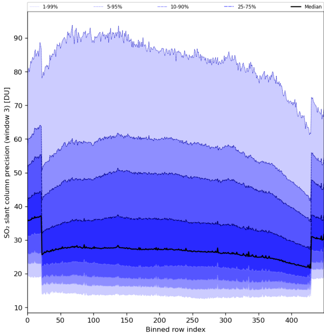
Figure 88: Along track statistics of “SO 2 slant column precision (window 3)” for 2024-07-31 to 2024-08-02
