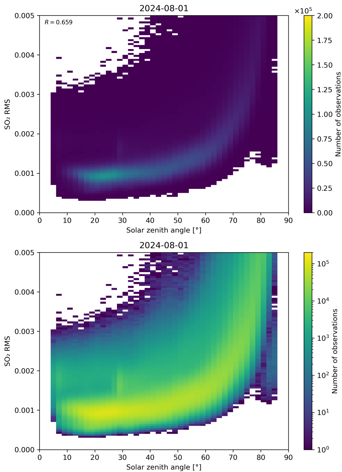
Figure 163: Scatter density plot of “Solar zenith angle” against “SO 2 RMS” for 2024-07-31 to 2024-08-02.
