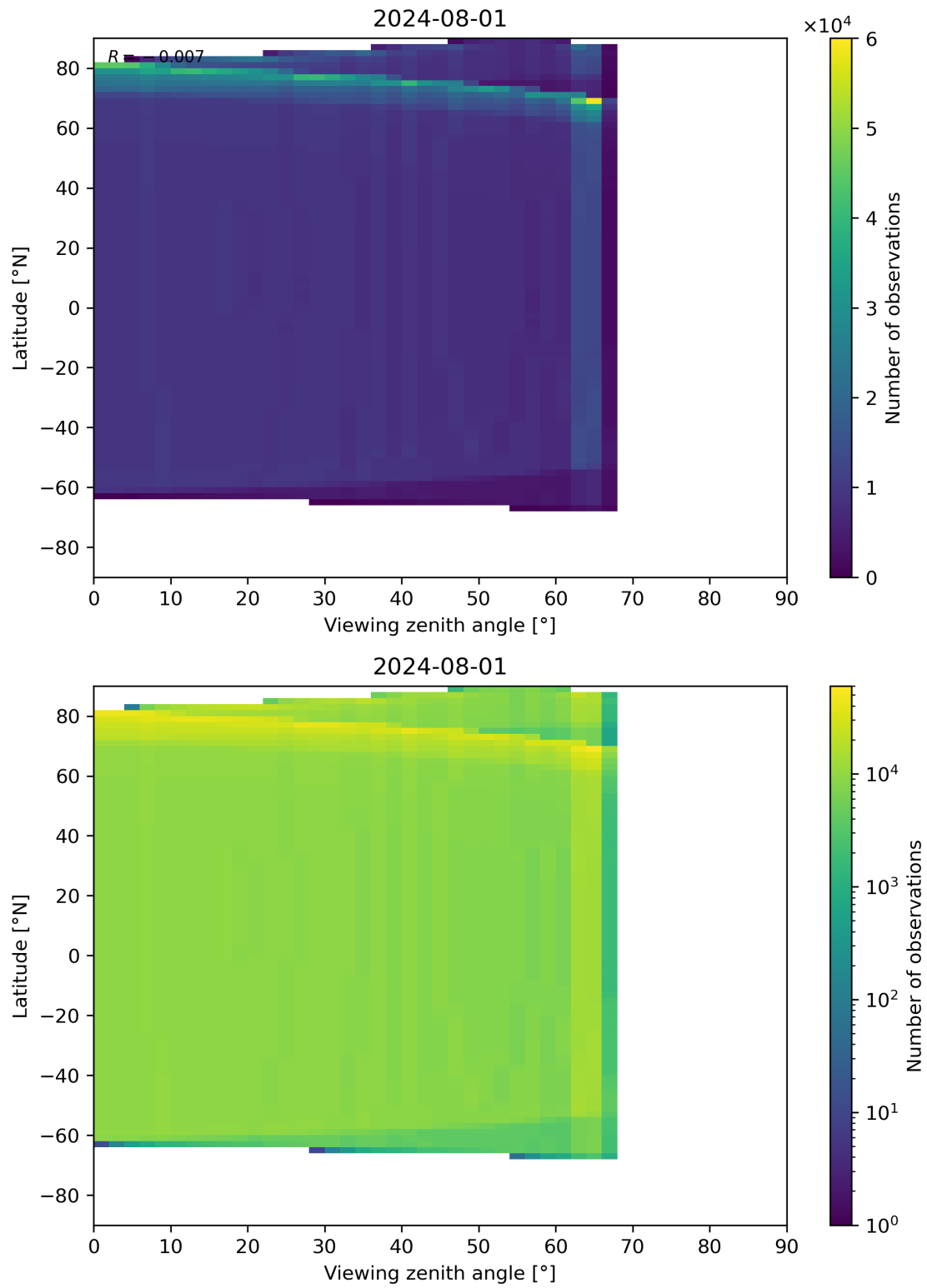
Figure 314: Scatter density plot of “Viewing zenith angle” against “Latitude” for 2024-07-31 to 2024-08-02.
