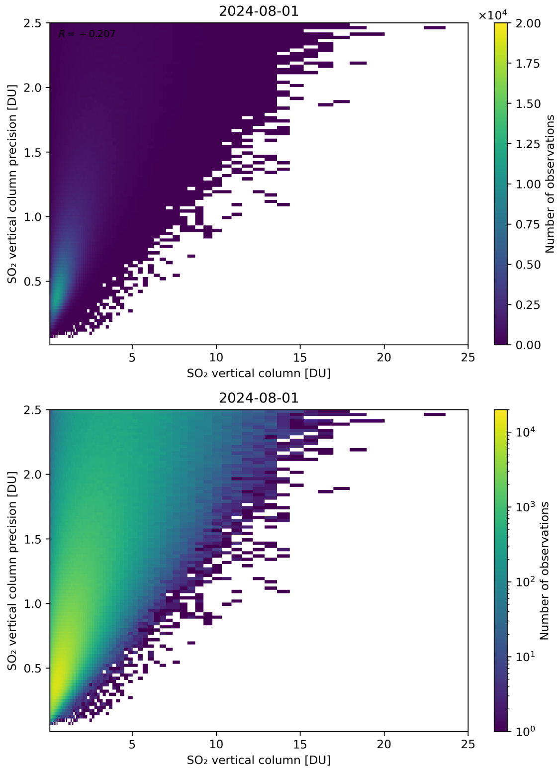
Figure 307: Scatter density plot of “SO 2 vertical column” against “SO 2 vertical column precision” for 2024-07-31 to 2024-08-02.
