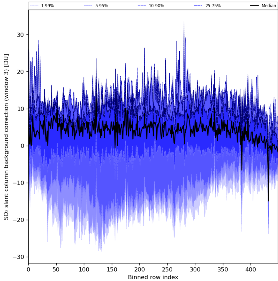
Figure 90: Along track statistics of “SO 2 slant column background correction (window 3)” for 2024-07-31 to 2024-08-02
