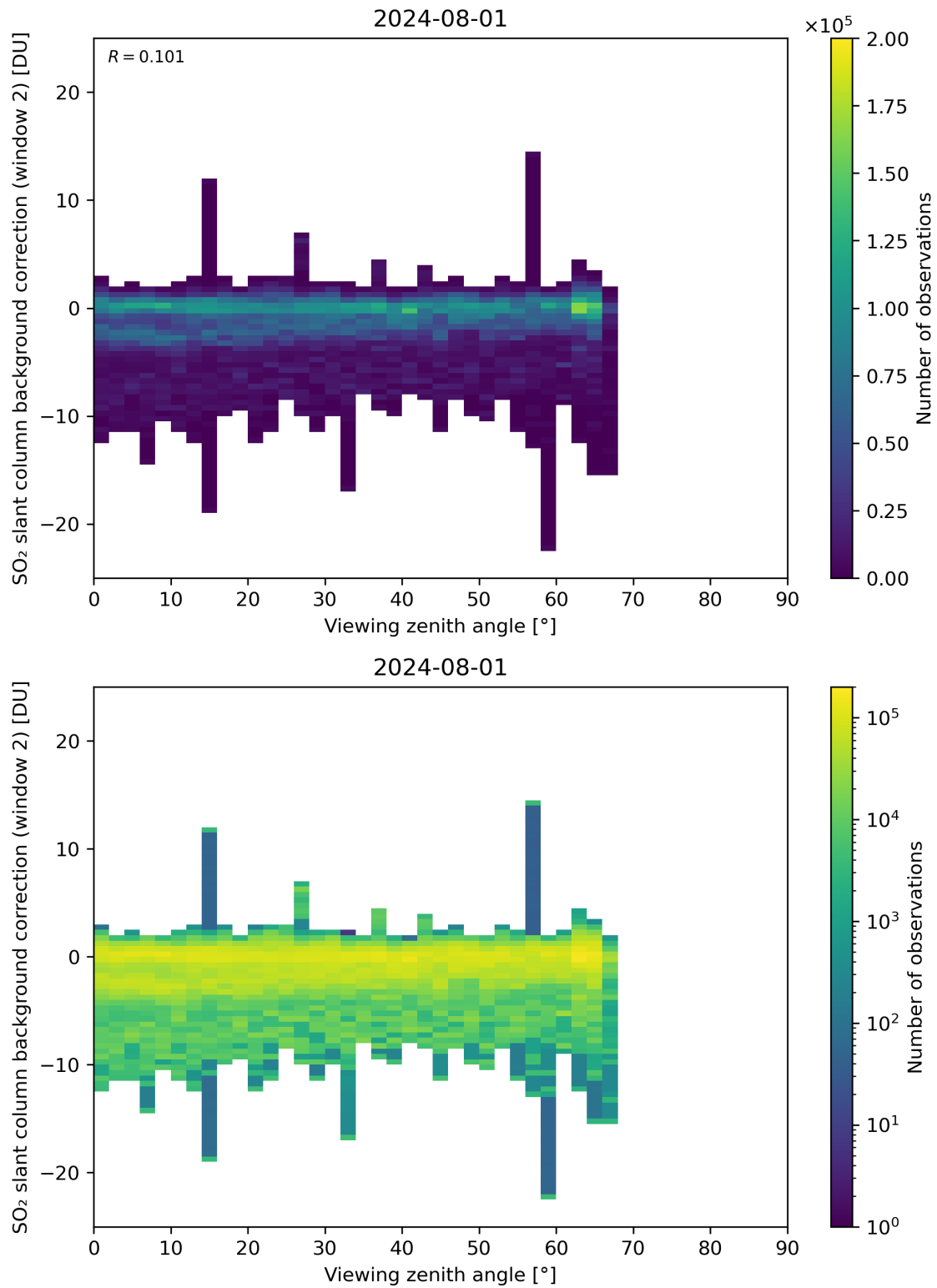
Figure 309: Scatter density plot of “Viewing zenith angle” against “SO 2 slant column background correction (window 2)” for 2024-07-31 to 2024-08-02.
