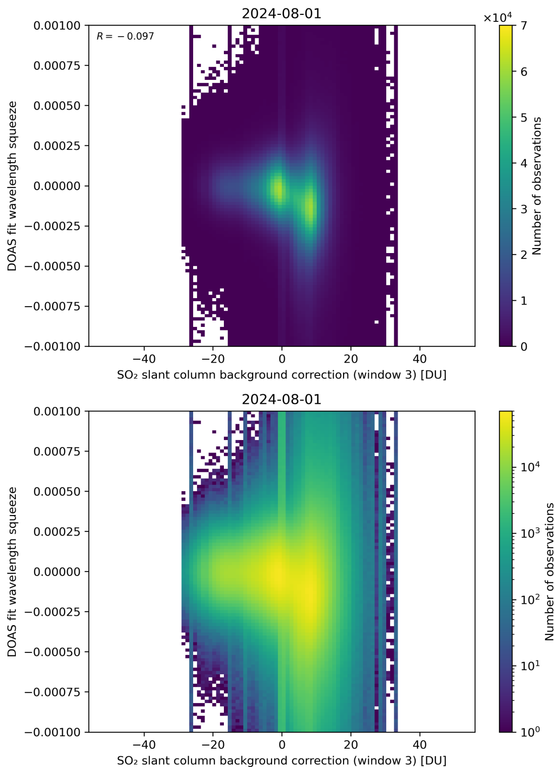
Figure 122: Scatter density plot of “SO 2 slant column background correction (window 3)” against “DOAS fit wavelength squeeze” for 2024-07-31 to 2024-08-02.
