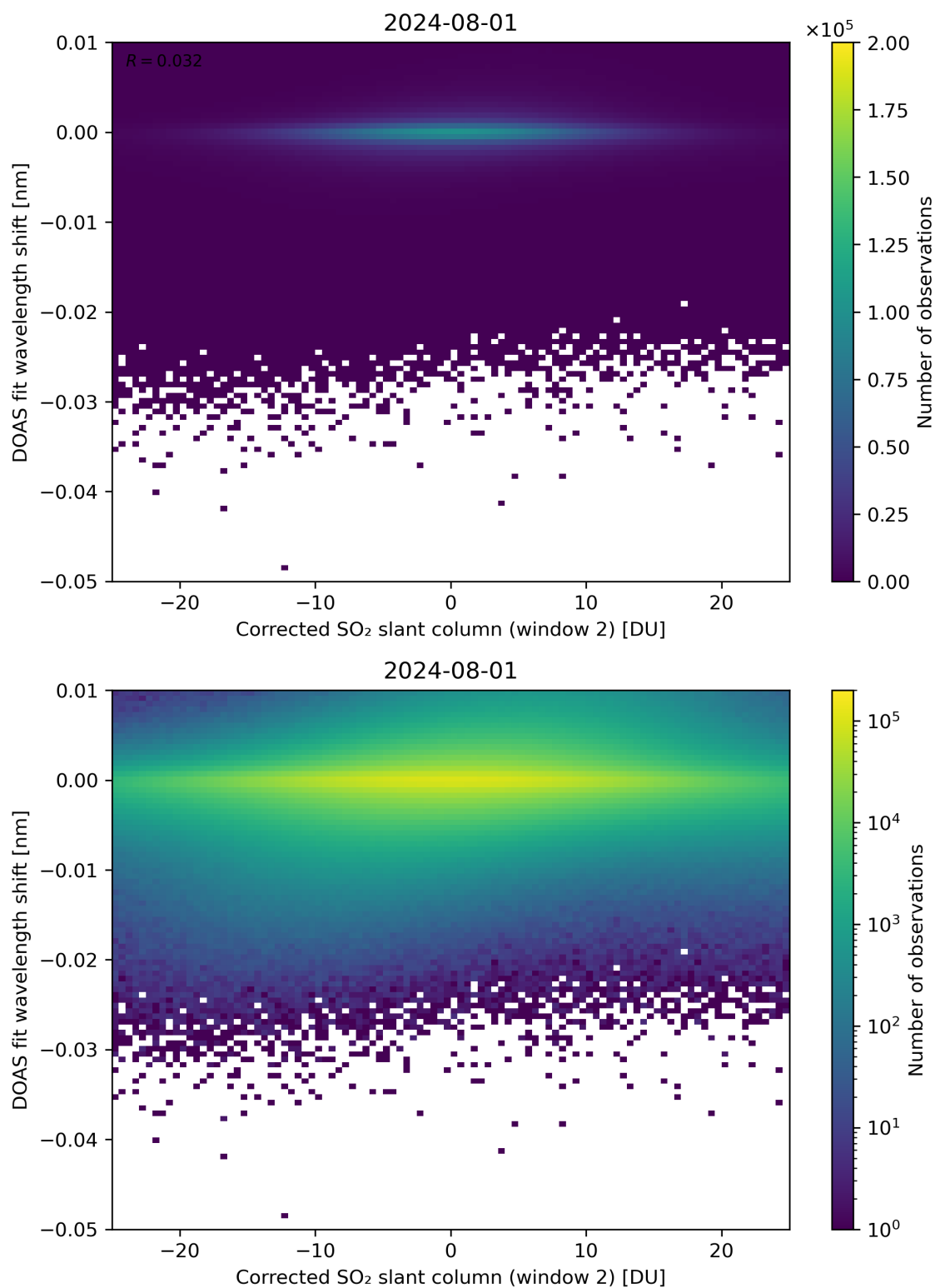
Figure 196: Scatter density plot of “Corrected SO 2 slant column (window 2)” against “DOAS fit wavelength shift” for 2024-07-31 to 2024-08-02.
