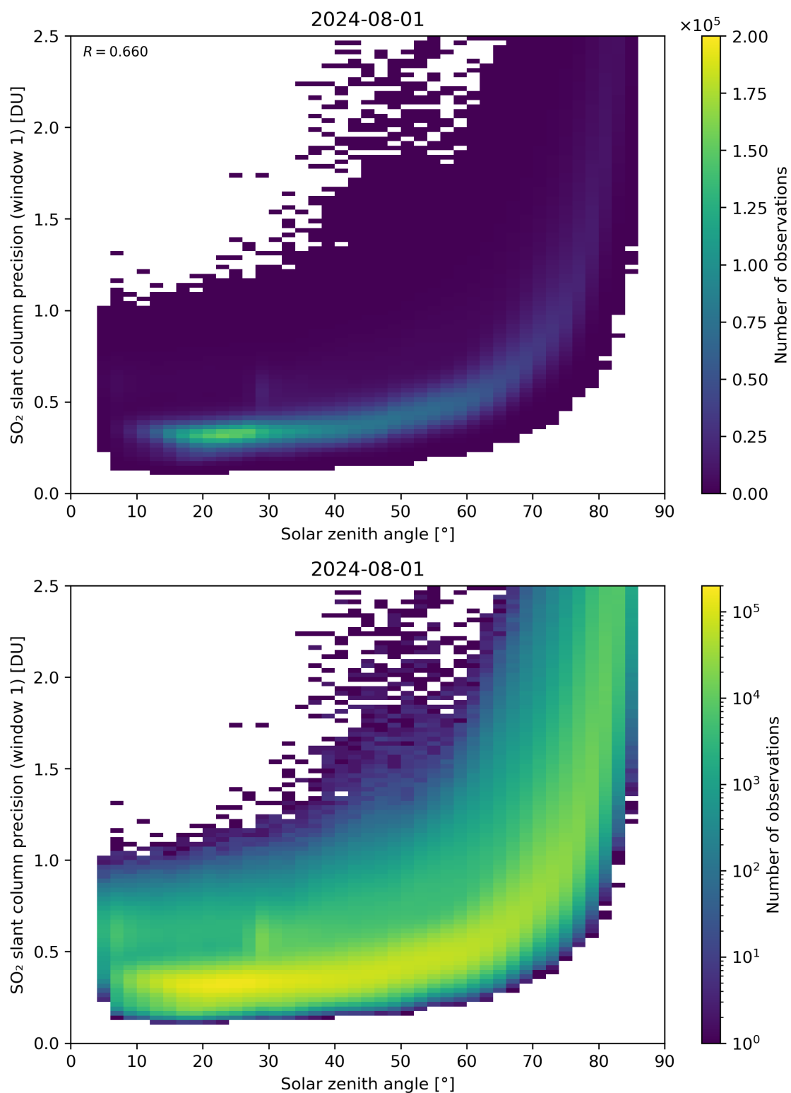
Figure 170: Scatter density plot of “Solar zenith angle” against “SO 2 slant column precision (window 1)” for 2024-07-31 to 2024-08-02.
