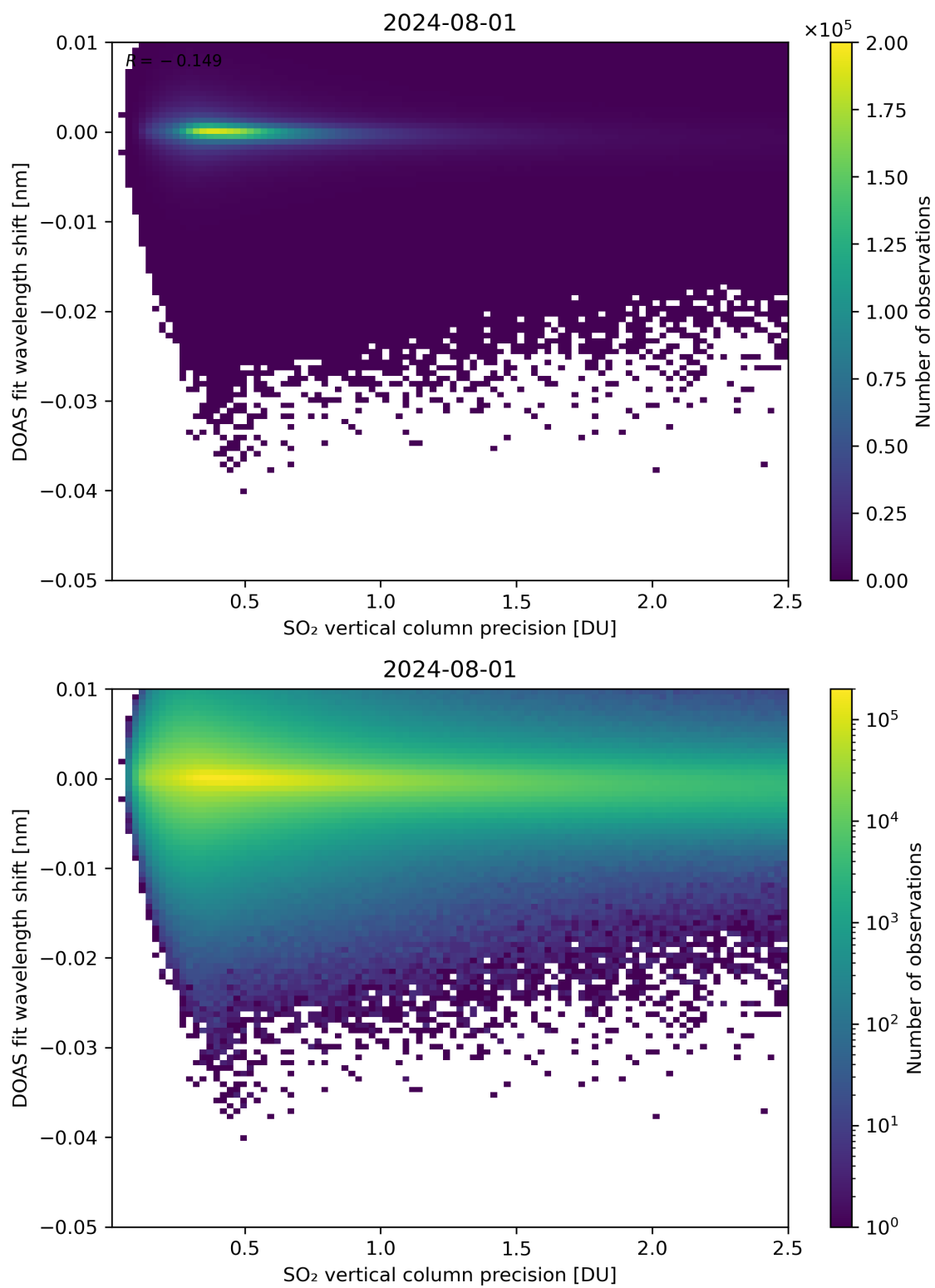
Figure 282: Scatter density plot of “SO 2 vertical column precision” against “DOAS fit wavelength shift” for 2024-07-31 to 2024-08-02.
