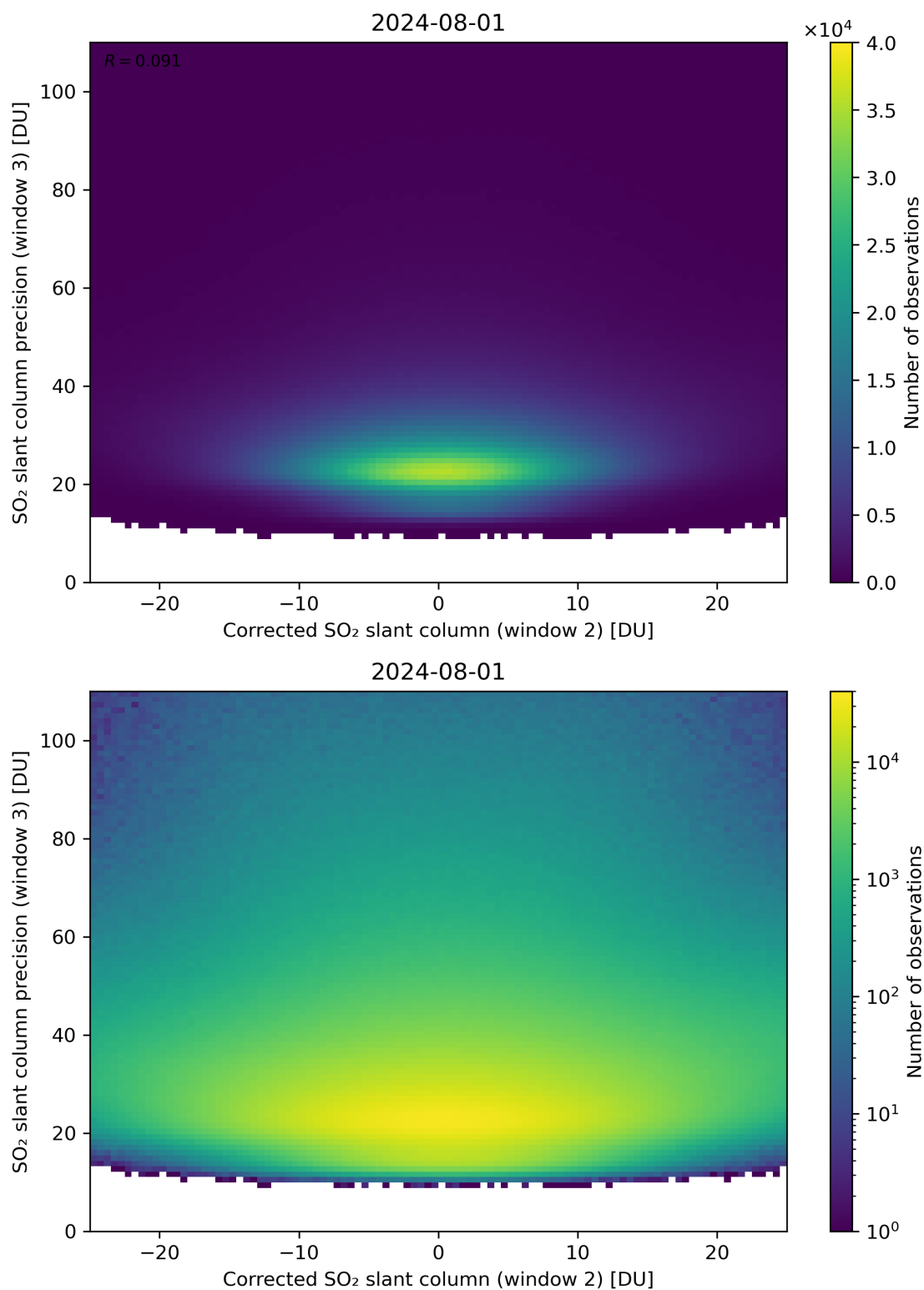
Figure 202: Scatter density plot of “Corrected SO 2 slant column (window 2)” against “SO 2 slant column precision (window 3)” for 2024-07-31 to 2024-08-02.
