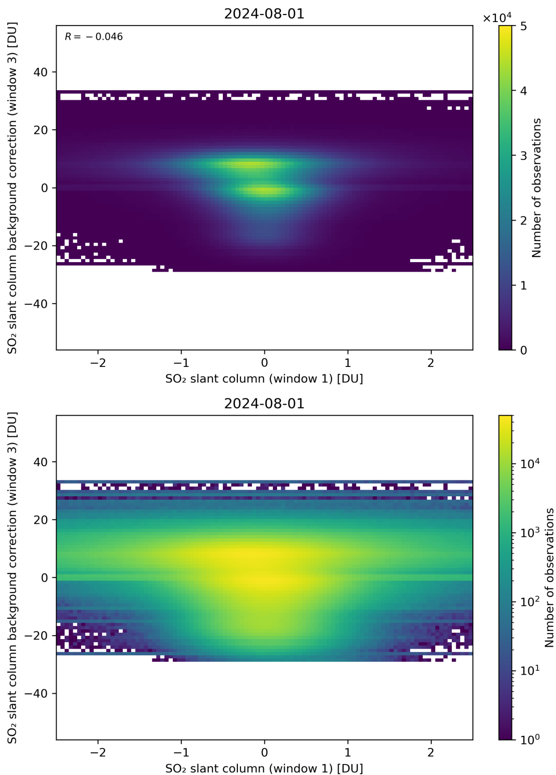
Figure 214: Scatter density plot of “SO 2 slant column (window 1)” against “SO 2 slant column background correction (window 3)” for 2024-07-31 to 2024-08-02.
