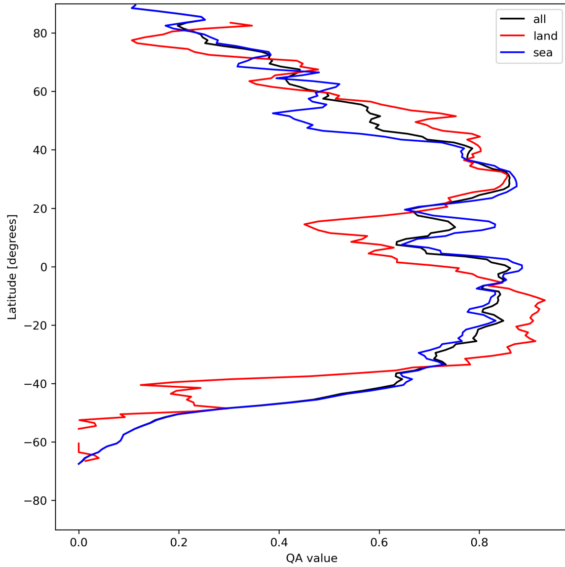
Figure 29: Zonal average of “QA value” for 2024-07-31 to 2024-08-02.
