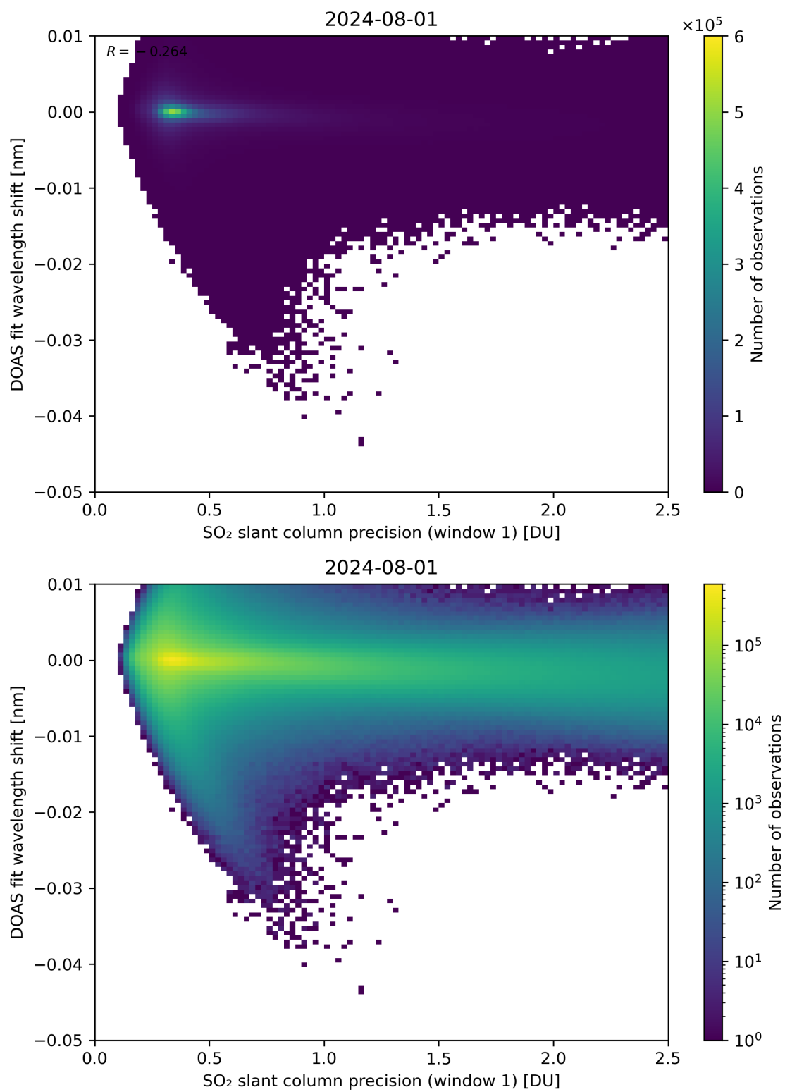
Figure 221: Scatter density plot of “SO 2 slant column precision (window 1)” against “DOAS fit wavelength shift” for 2024-07-31 to 2024-08-02.
