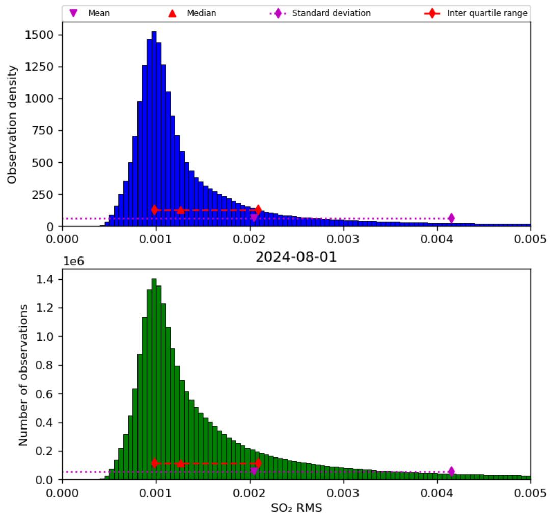
Figure 70: Histogram of “SO 2 RMS” for 2024-07-31 to 2024-08-02
