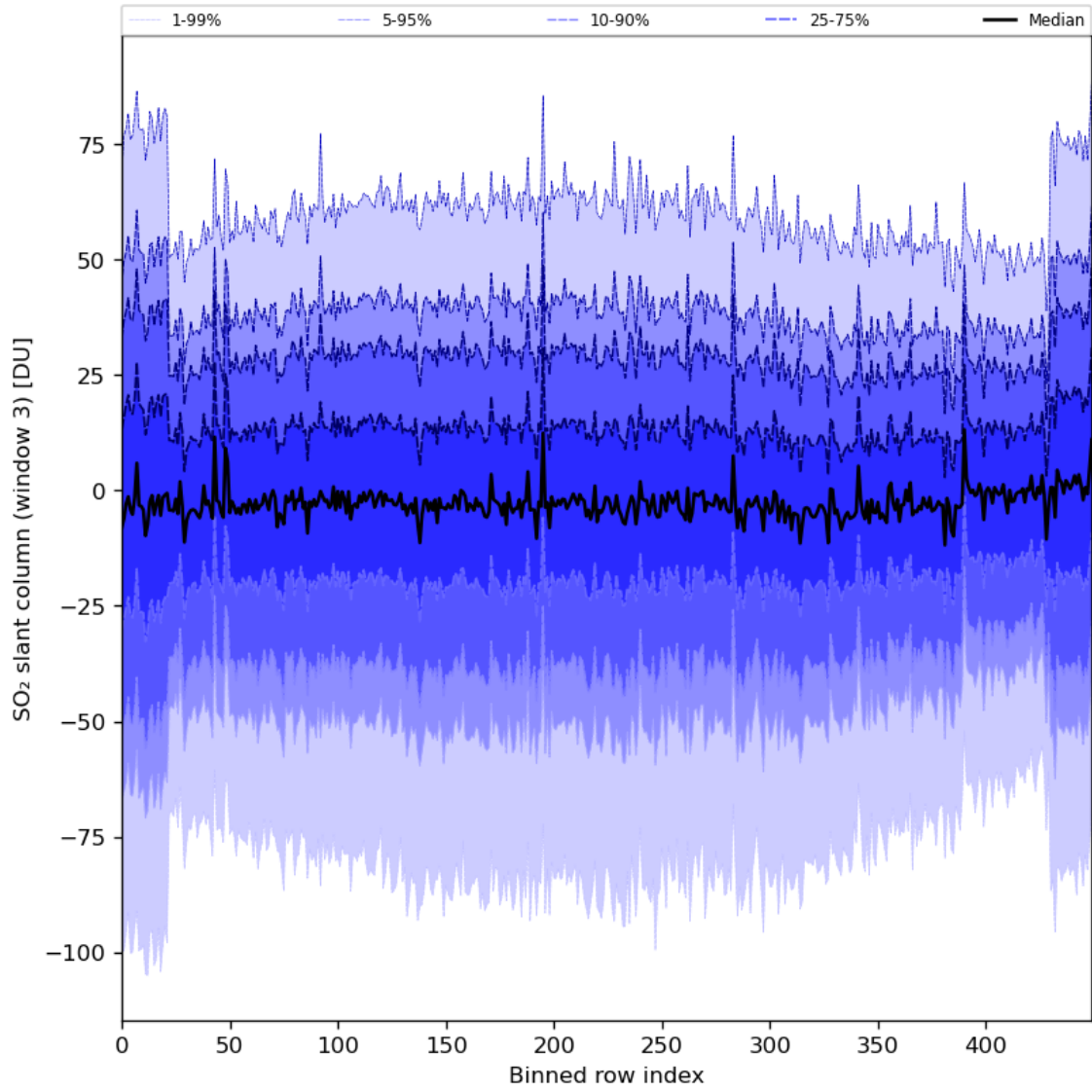
Figure 87: Along track statistics of “SO 2 slant column (window 3)” for 2024-07-31 to 2024-08-02
