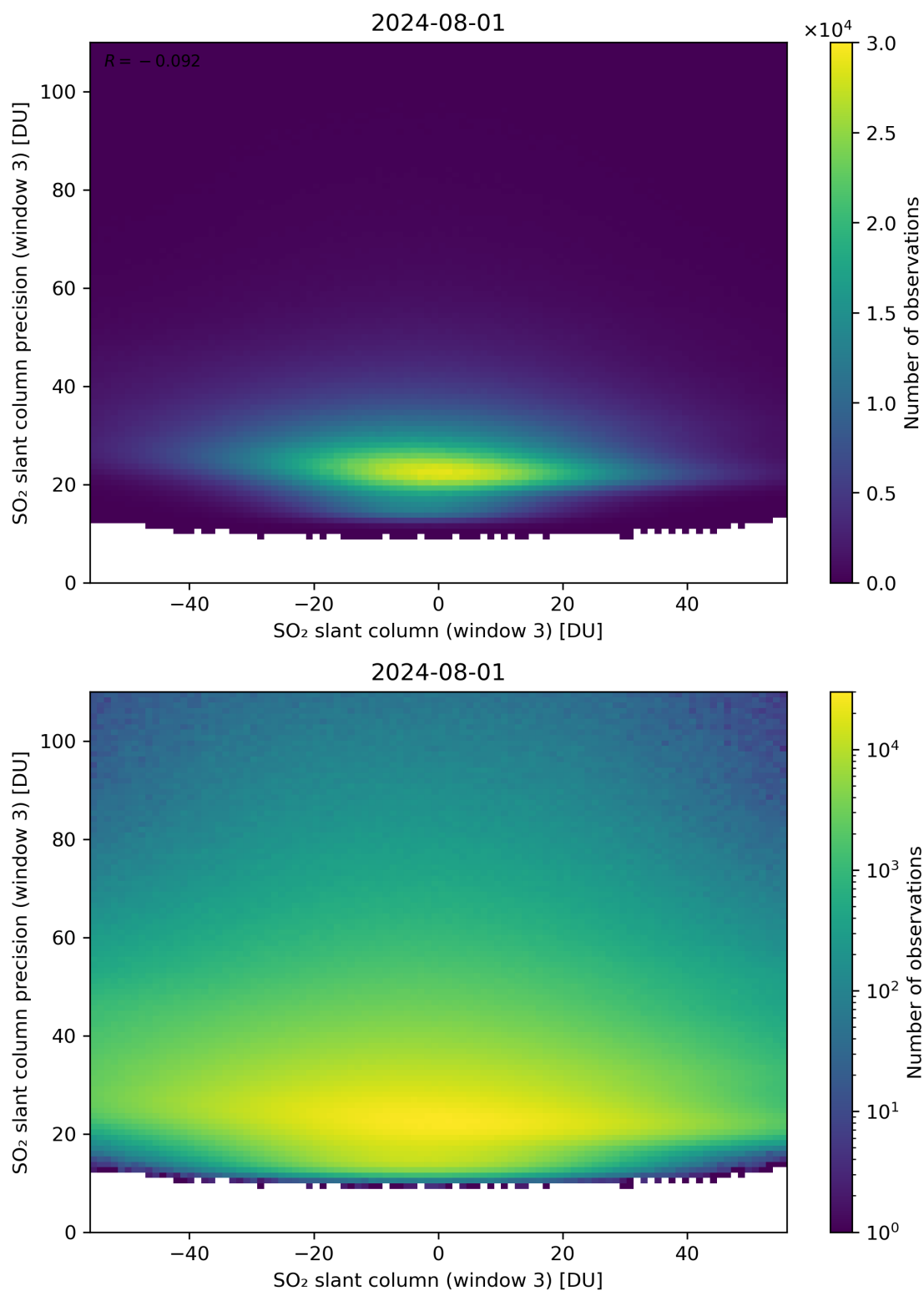
Figure 267: Scatter density plot of “SO 2 slant column (window 3)” against “SO 2 slant column precision (window 3)” for 2024-07-31 to 2024-08-02.
