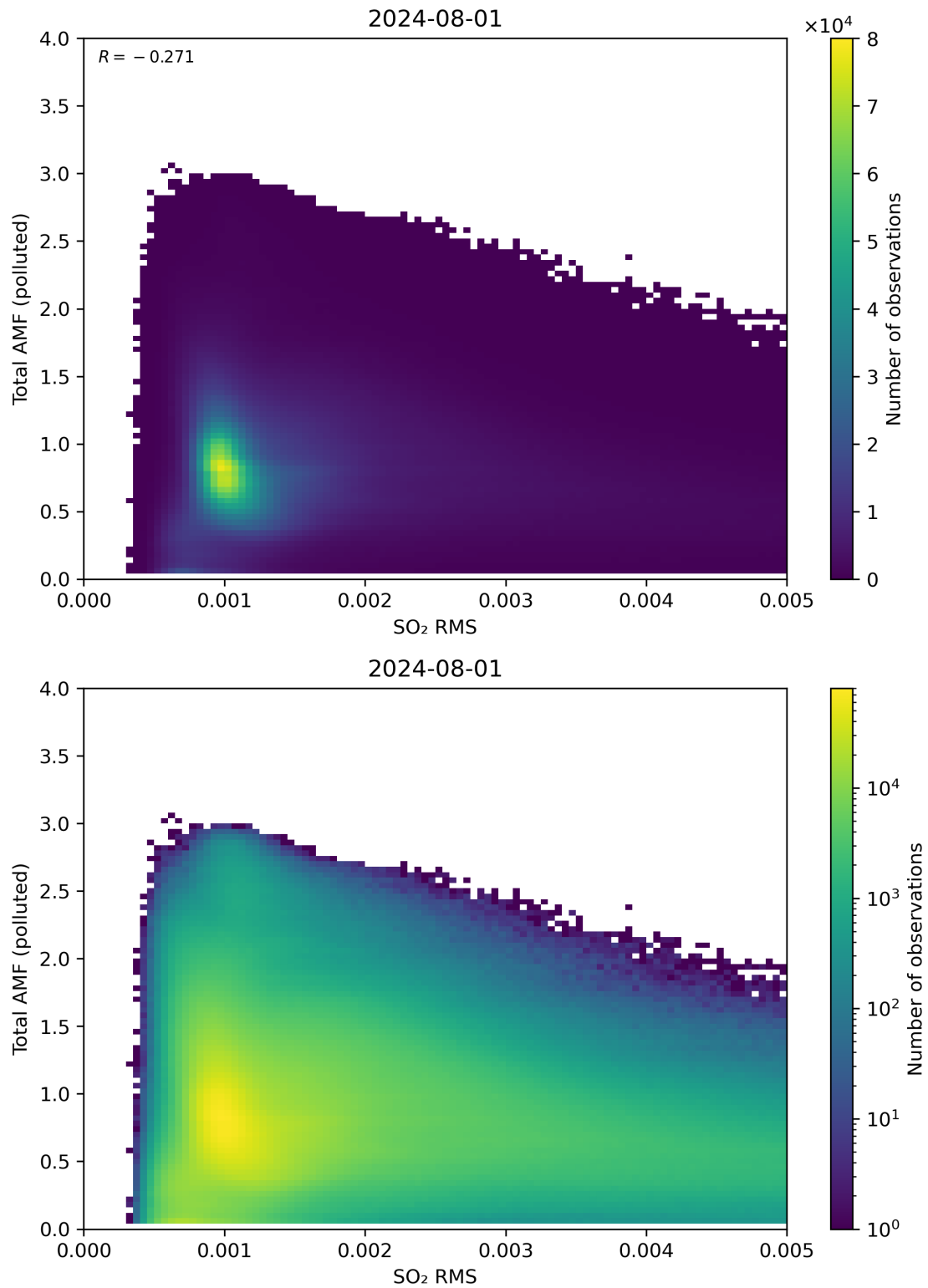
Figure 137: Scatter density plot of “SO 2 RMS” against “Total AMF (polluted)” for 2024-07-31 to 2024-08-02.
