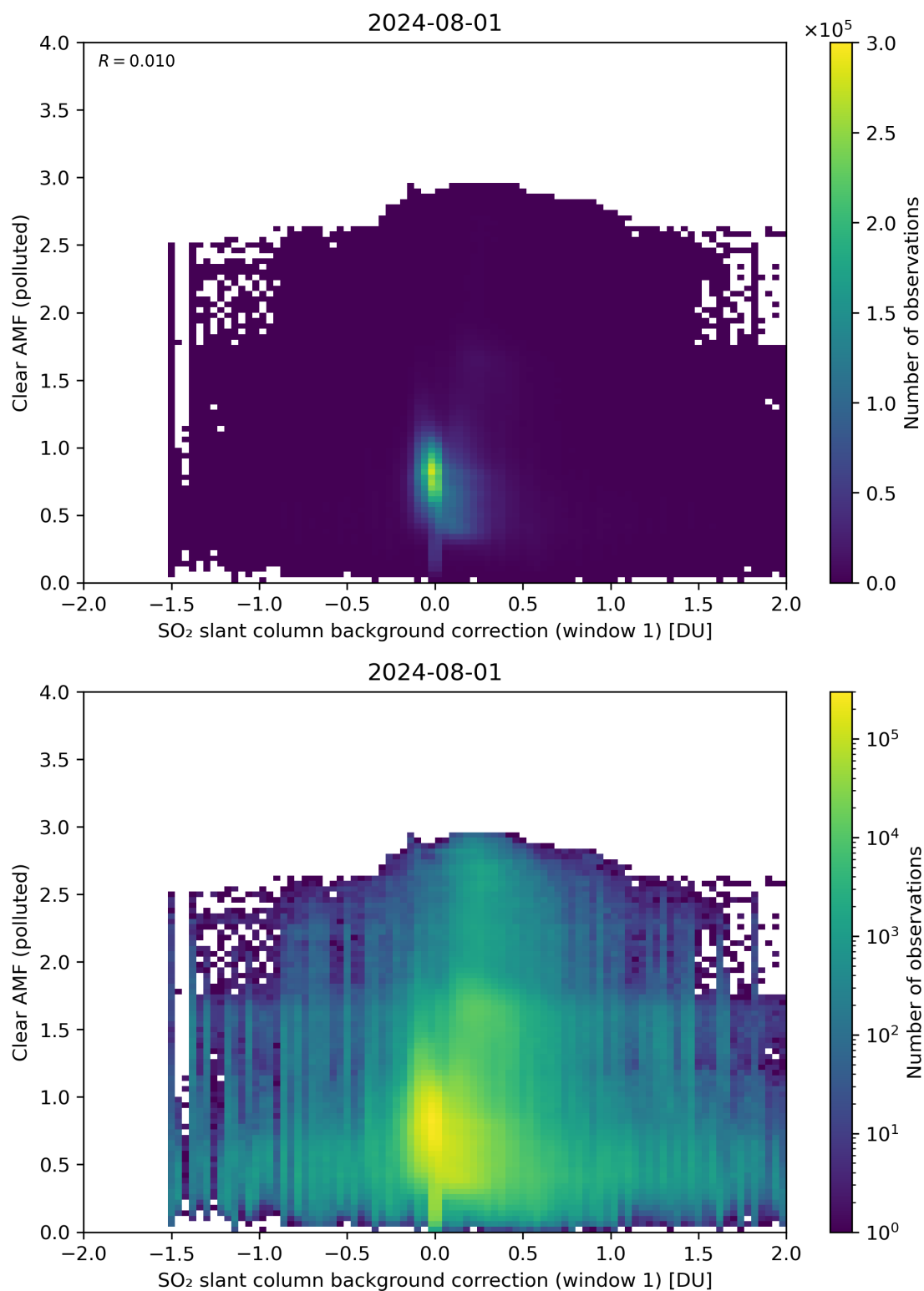
Figure 103: Scatter density plot of “SO 2 slant column background correction (window 1)” against “Clear AMF (polluted)” for 2024-07-31 to 2024-08-02.
