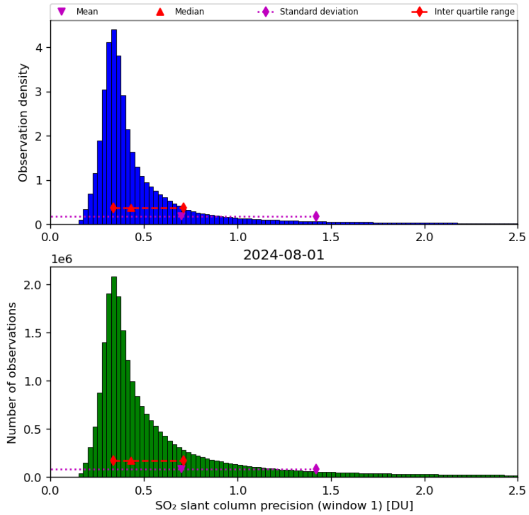
Figure 57: Histogram of “SO 2 slant column precision (window 1)” for 2024-07-31 to 2024-08-02
