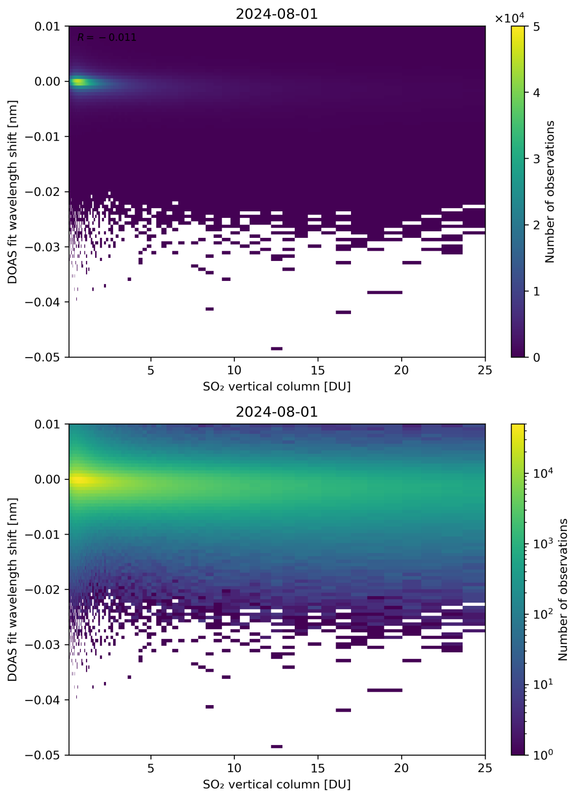
Figure 276: Scatter density plot of “SO 2 vertical column” against “DOAS fit wavelength shift” for 2024-07-31 to 2024-08-02.
