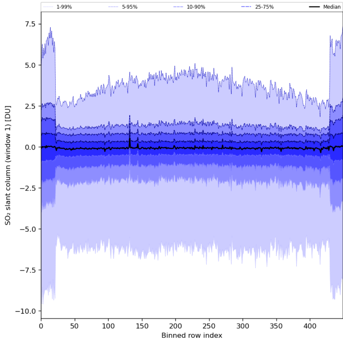
Figure 79: Along track statistics of “SO 2 slant column (window 1)” for 2024-07-31 to 2024-08-02
