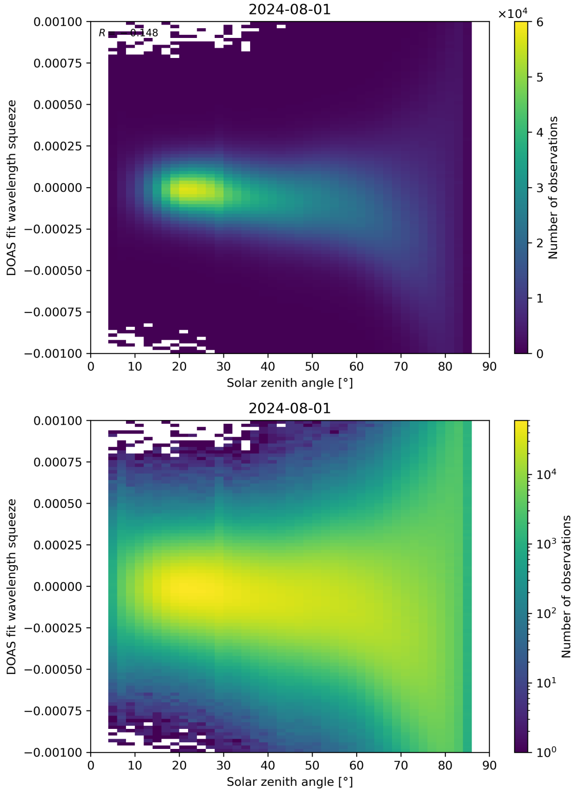
Figure 162: Scatter density plot of “Solar zenith angle” against “DOAS fit wavelength squeeze” for 2024-07-31 to 2024-08-02.
