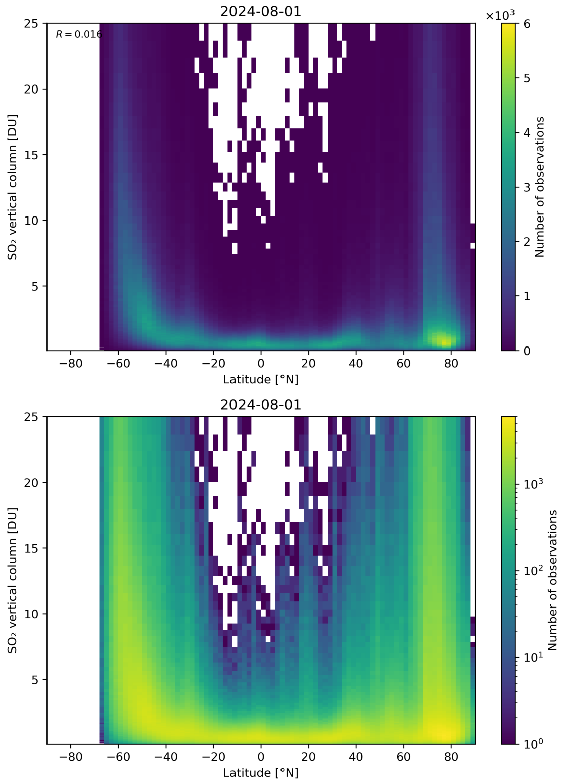
Figure 156: Scatter density plot of “Latitude” against “SO 2 vertical column” for 2024-07-31 to 2024-08-02.
