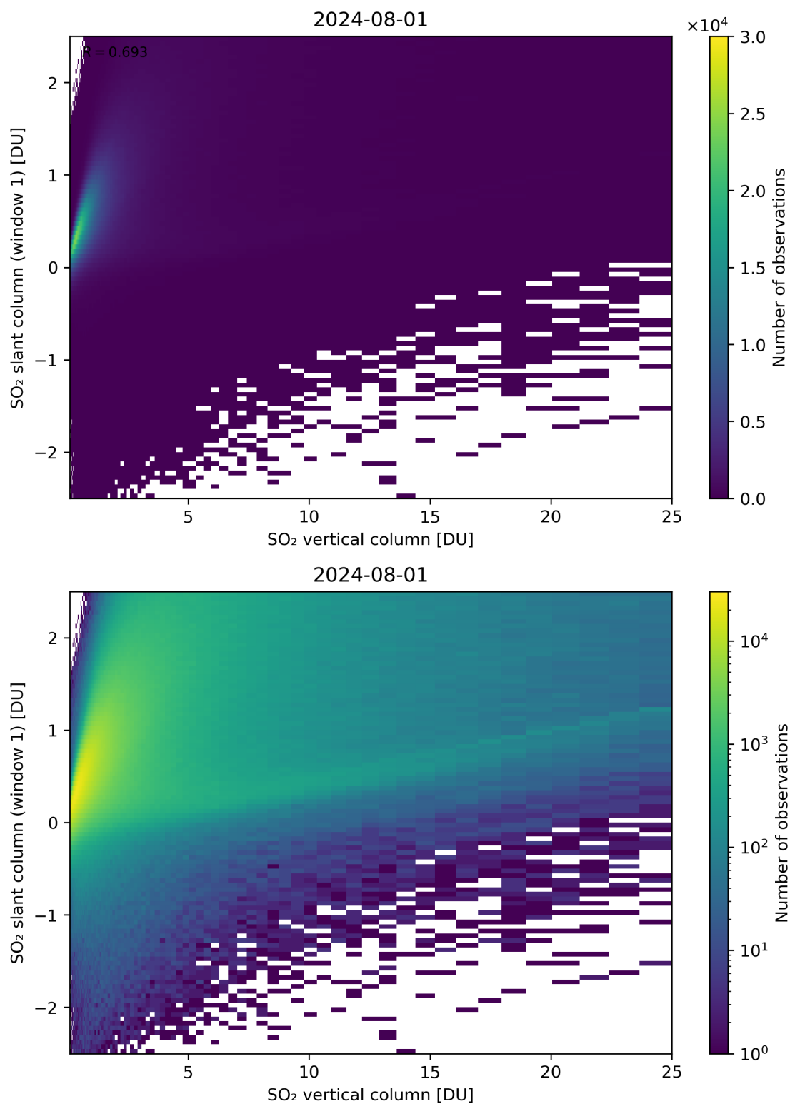
Figure 300: Scatter density plot of “SO 2 vertical column” against “SO 2 slant column (window 1)” for 2024-07-31 to 2024-08-02.
