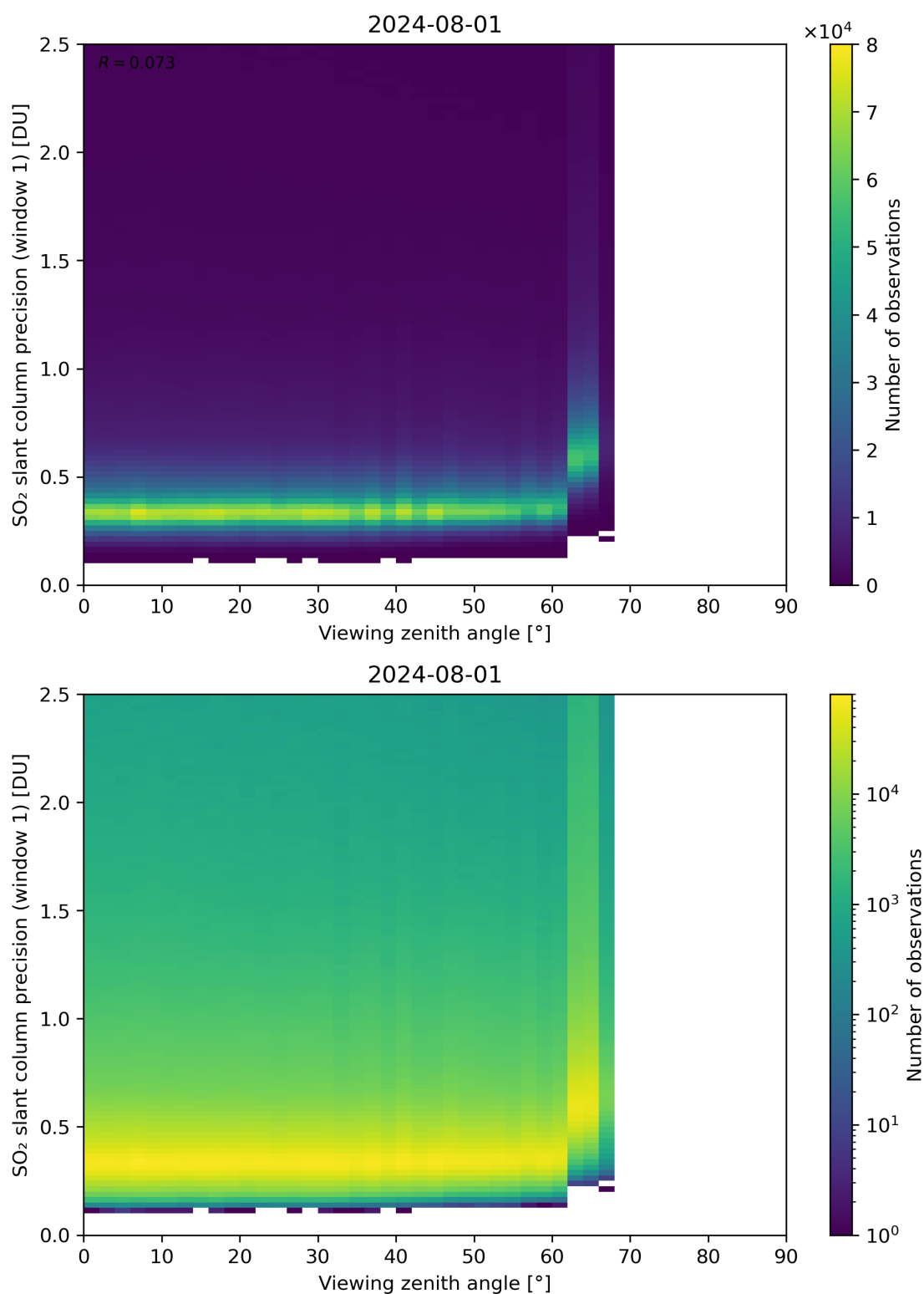
Figure 321: Scatter density plot of “Viewing zenith angle” against “SO 2 slant column precision (window 1)” for 2024-07-31 to 2024-08-02.
