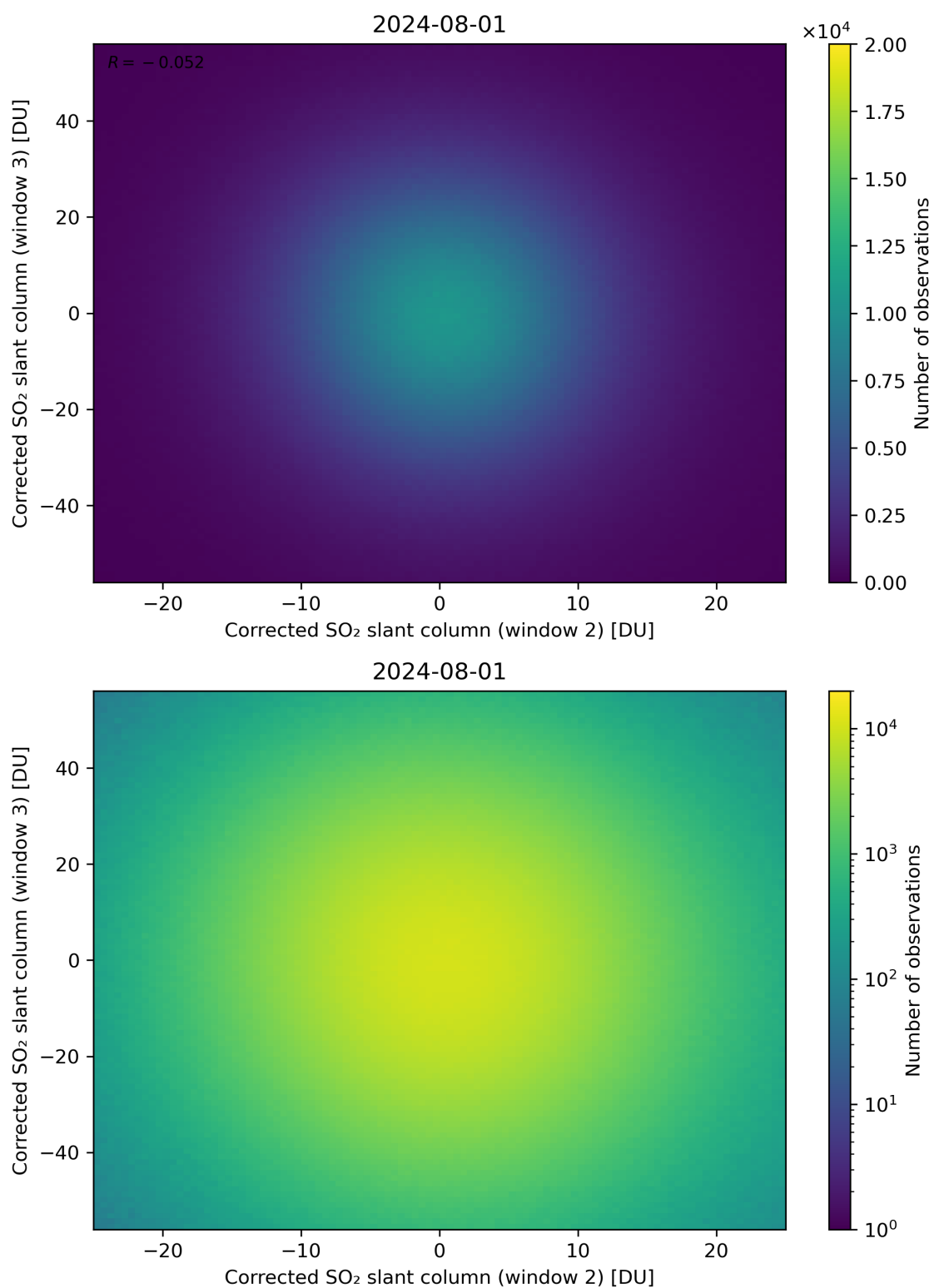
Figure 200: Scatter density plot of “Corrected SO 2 slant column (window 2)” against “Corrected SO 2 slant column (window 3)” for 2024-07-31 to 2024-08-02.
