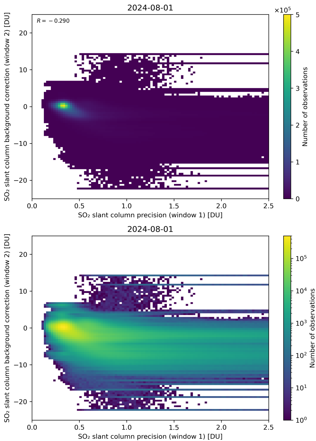
Figure 219: Scatter density plot of “SO 2 slant column precision (window 1)” against “SO 2 slant column background correction (window 2)” for 2024-07-31 to 2024-08-02.
