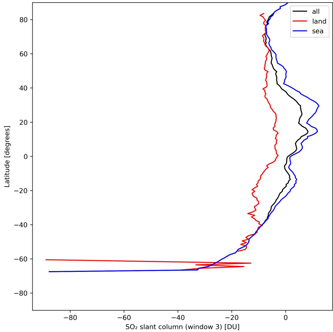
Figure 41: Zonal average of “SO 2 slant column (window 3)” for 2024-07-31 to 2024-08-02.
