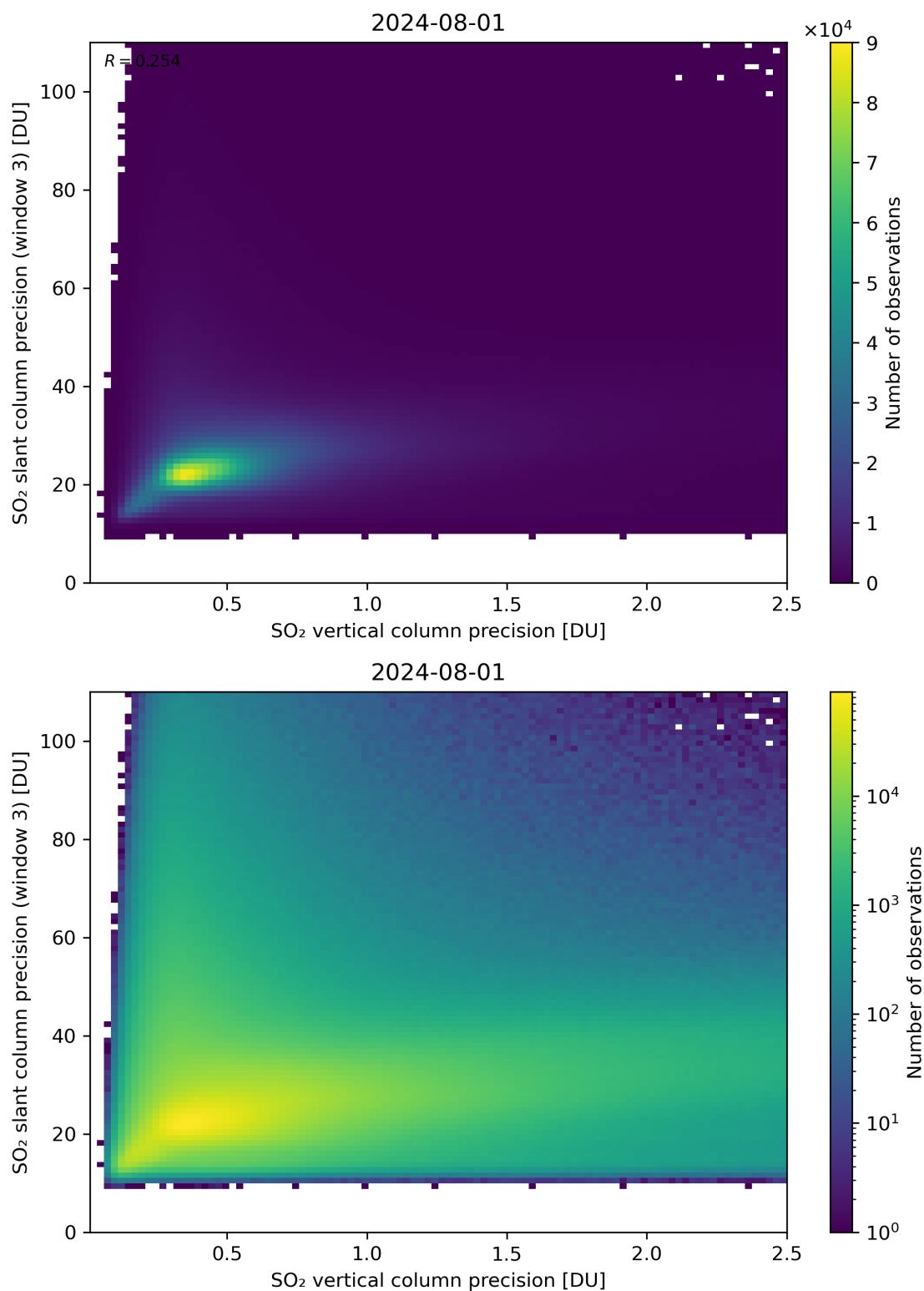
Figure 293: Scatter density plot of “SO 2 vertical column precision” against “SO 2 slant column precision (window 3)” for 2024-07-31 to 2024-08-02.
