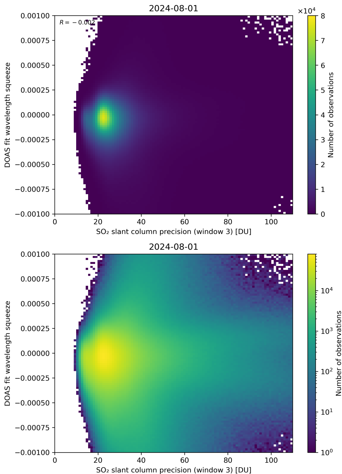
Figure 259: Scatter density plot of “SO 2 slant column precision (window 3)” against “DOAS fit wavelength squeeze” for 2024-07-31 to 2024-08-02.
