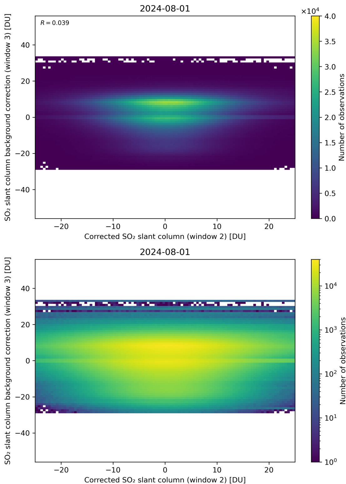
Figure 195: Scatter density plot of “Corrected SO 2 slant column (window 2)” against “SO 2 slant column background correction (window 3)” for 2024-07-31 to 2024-08-02.
