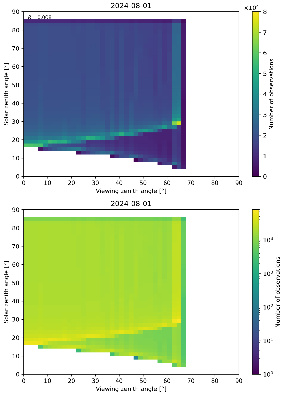
Figure 315: Scatter density plot of “Viewing zenith angle” against “Solar zenith angle” for 2024-07-31 to 2024-08-02.
