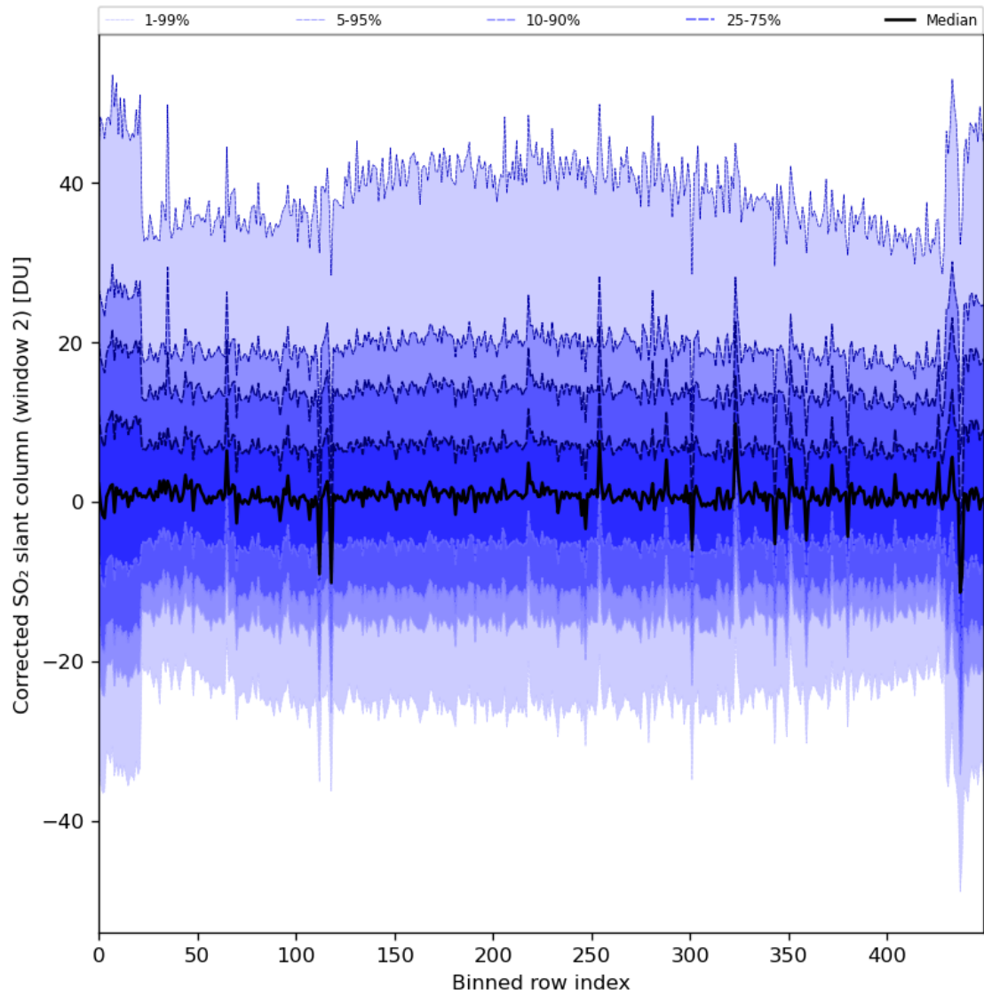
Figure 85: Along track statistics of "Corrected SO 2 slant column (window 2)" for 2024-07-31 to 2024-08-02
