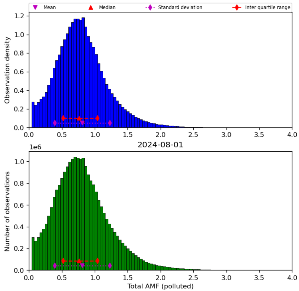
Figure 71: Histogram of “Total AMF (polluted)” for 2024-07-31 to 2024-08-02
