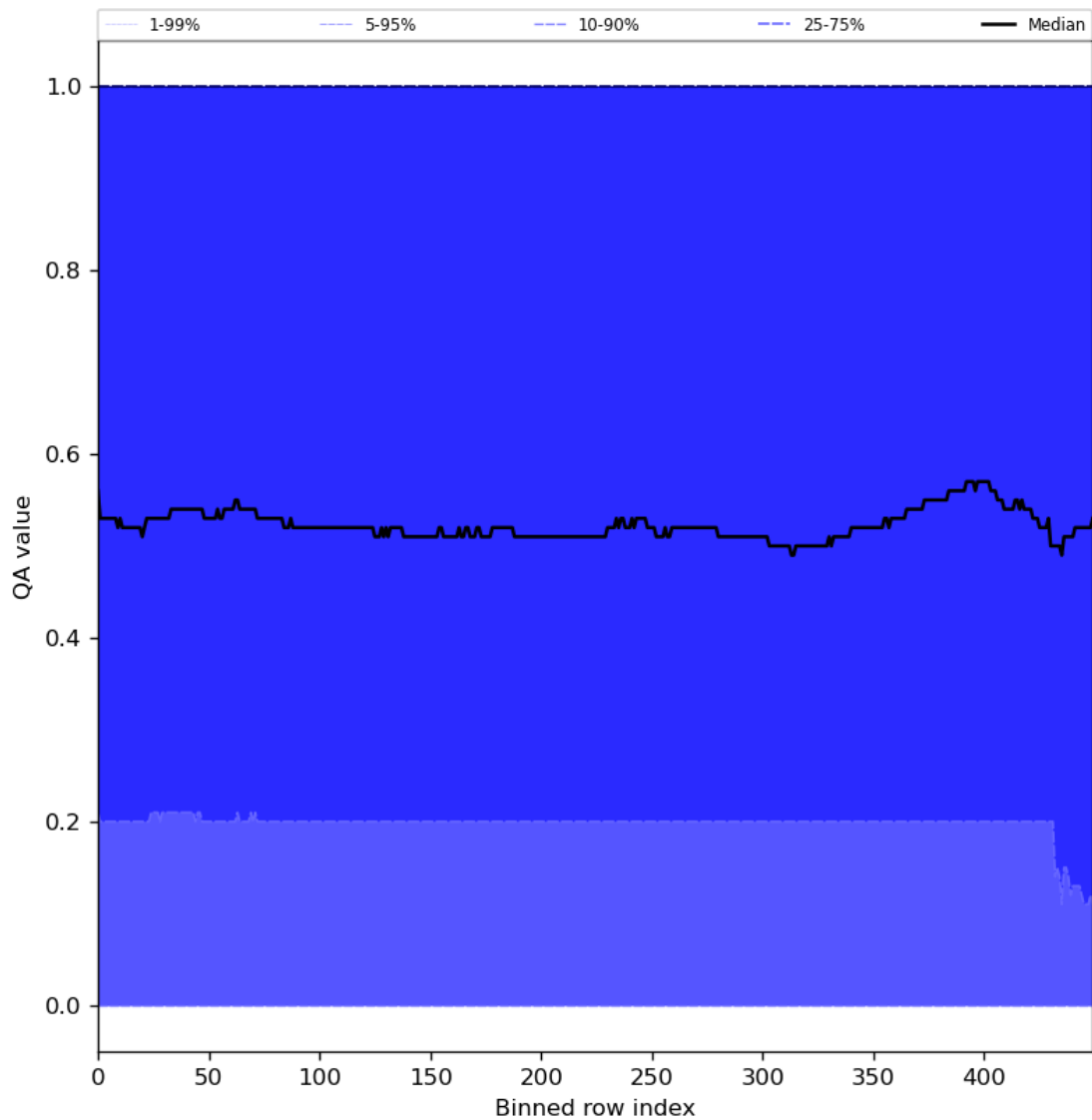
Figure 75: Along track statistics of “QA value” for 2024-07-31 to 2024-08-02
