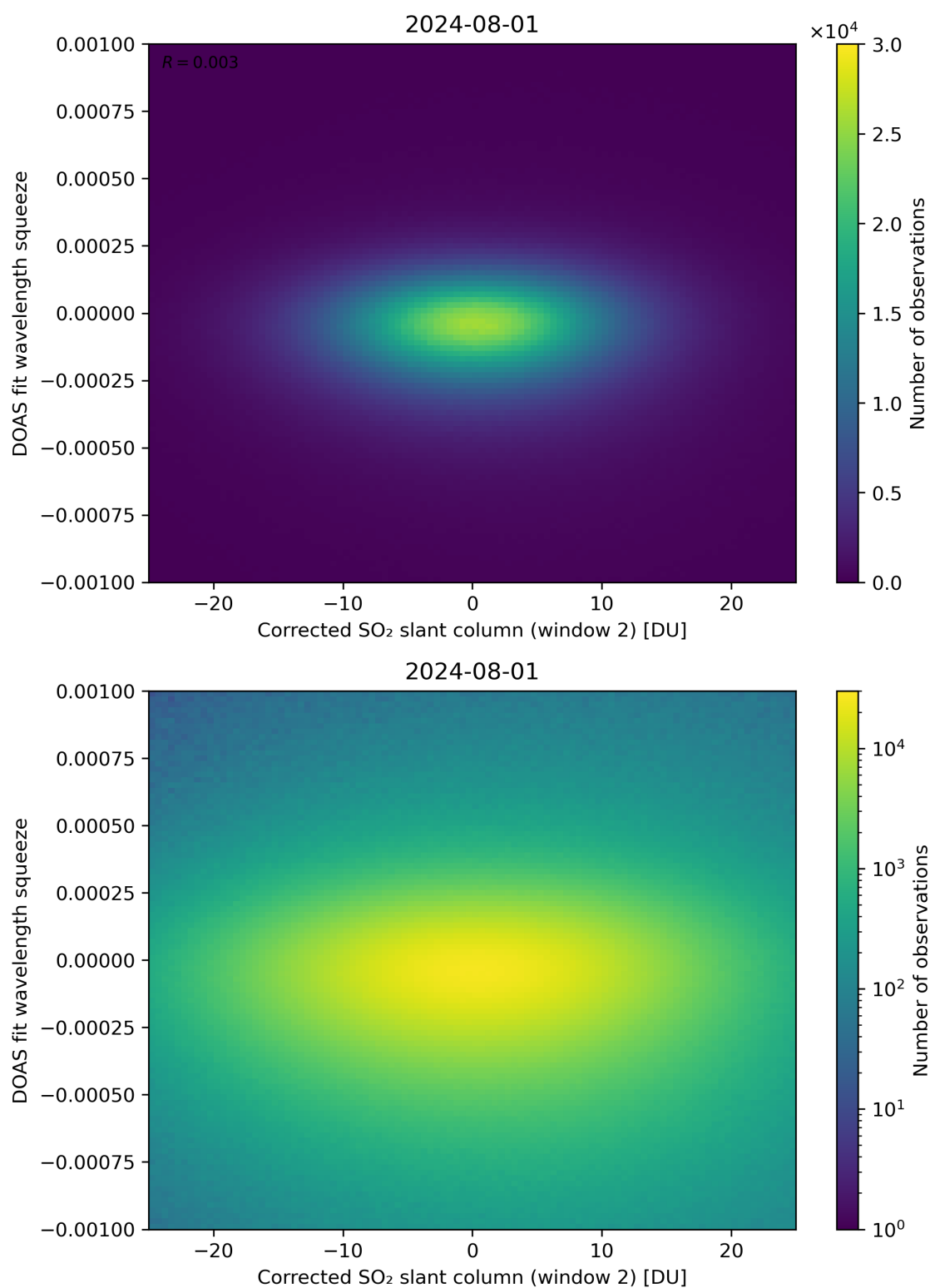
Figure 197: Scatter density plot of “Corrected SO 2 slant column (window 2)” against “DOAS fit wavelength squeeze” for 2024-07-31 to 2024-08-02.
