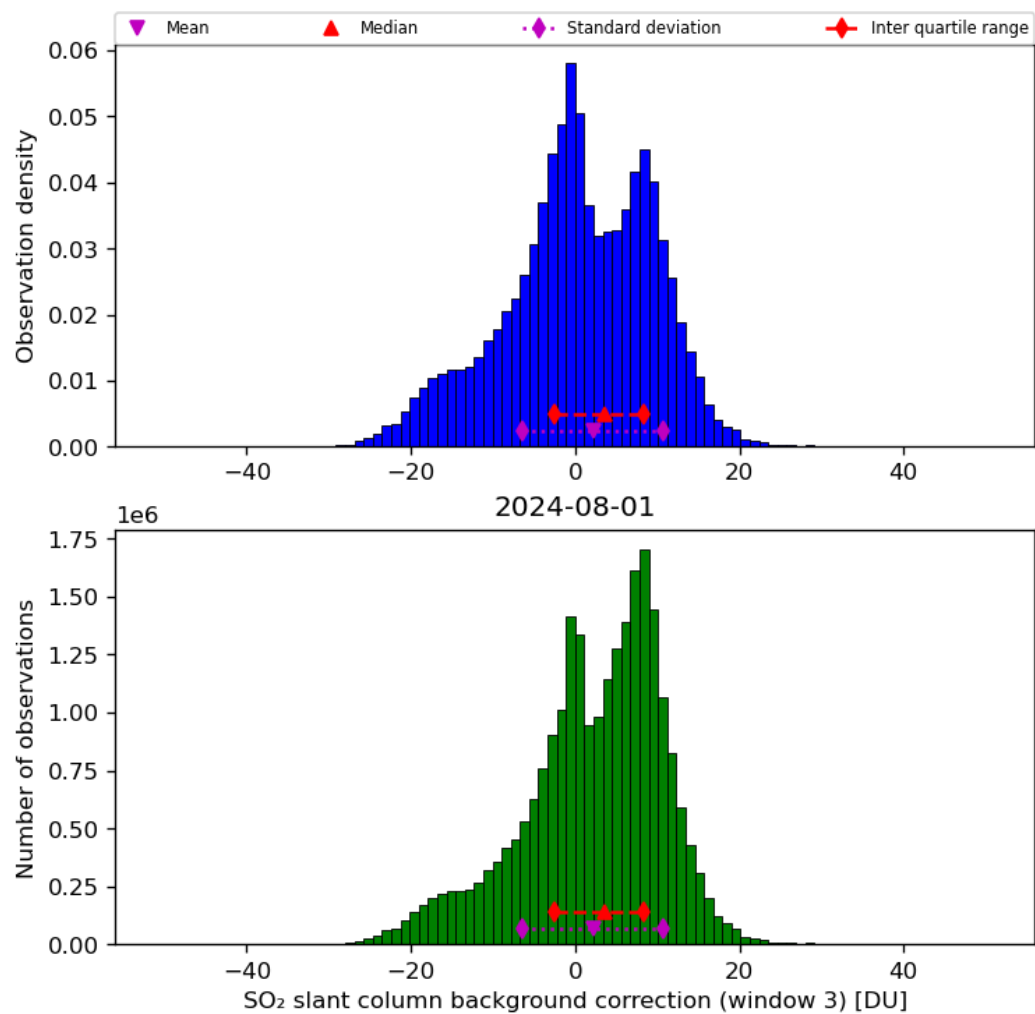
Figure 67: Histogram of “SO 2 slant column background correction (window 3)” for 2024-07-31 to 2024-08-02
