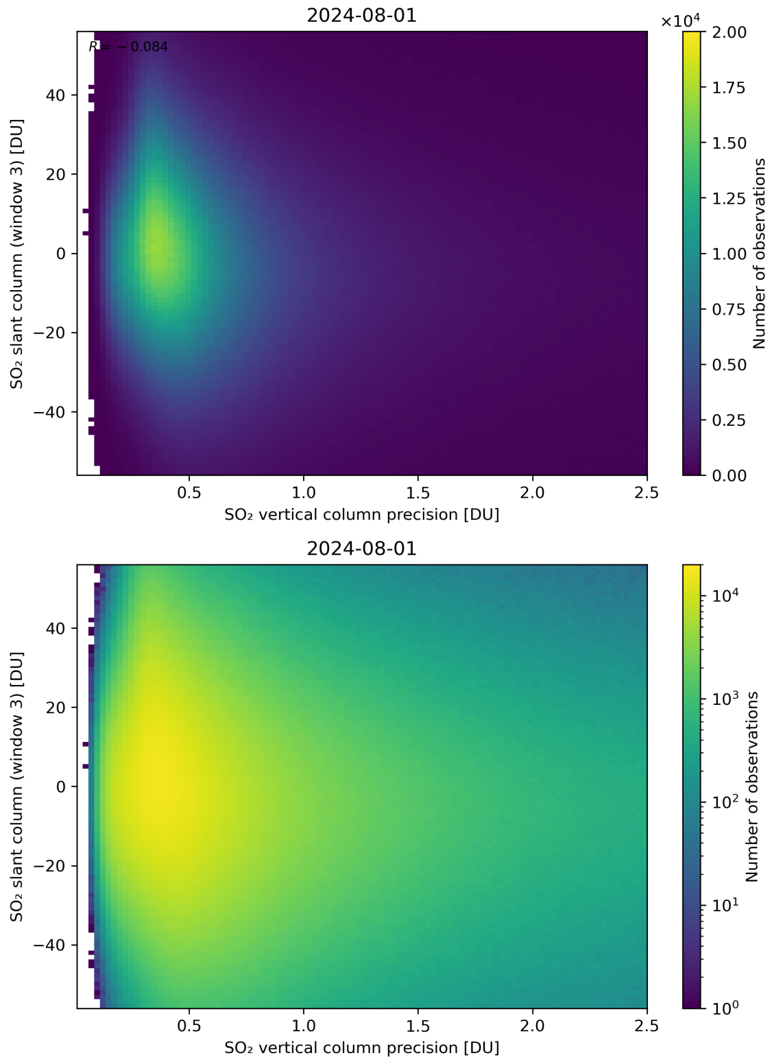
Figure 292: Scatter density plot of “SO 2 vertical column precision” against “SO 2 slant column (window 3)” for 2024-07-31 to 2024-08-02.
