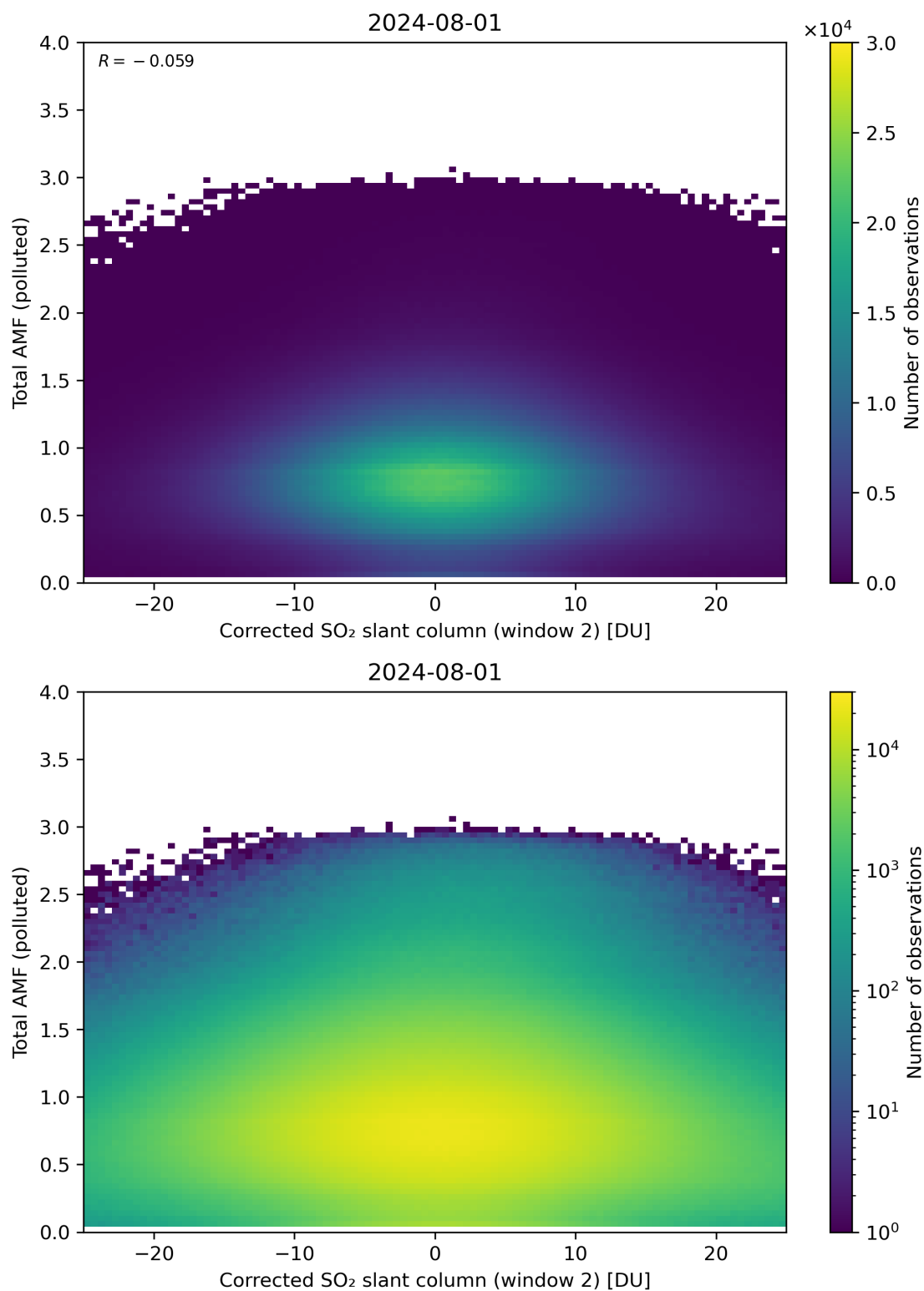
Figure 203: Scatter density plot of “Corrected SO 2 slant column (window 2)” against “Total AMF (polluted)” for 2024-07-31 to 2024-08-02.
