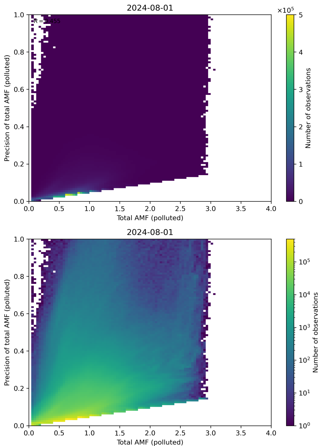
Figure 272: Scatter density plot of “Total AMF (polluted)” against “Precision of total AMF (polluted)” for 2024-07-31 to 2024-08-02.
