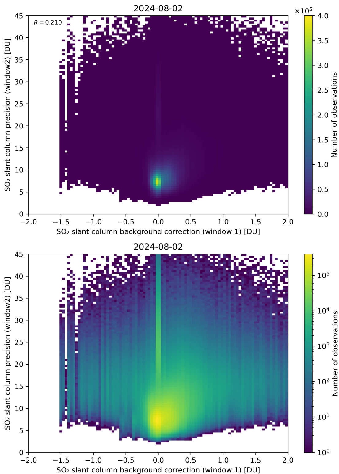
Figure 106: Scatter density plot of “SO 2 slant column background correction (window 1)” against “SO 2 slant column precision (window2)” for 2024-08-01 to 2024-08-03.
