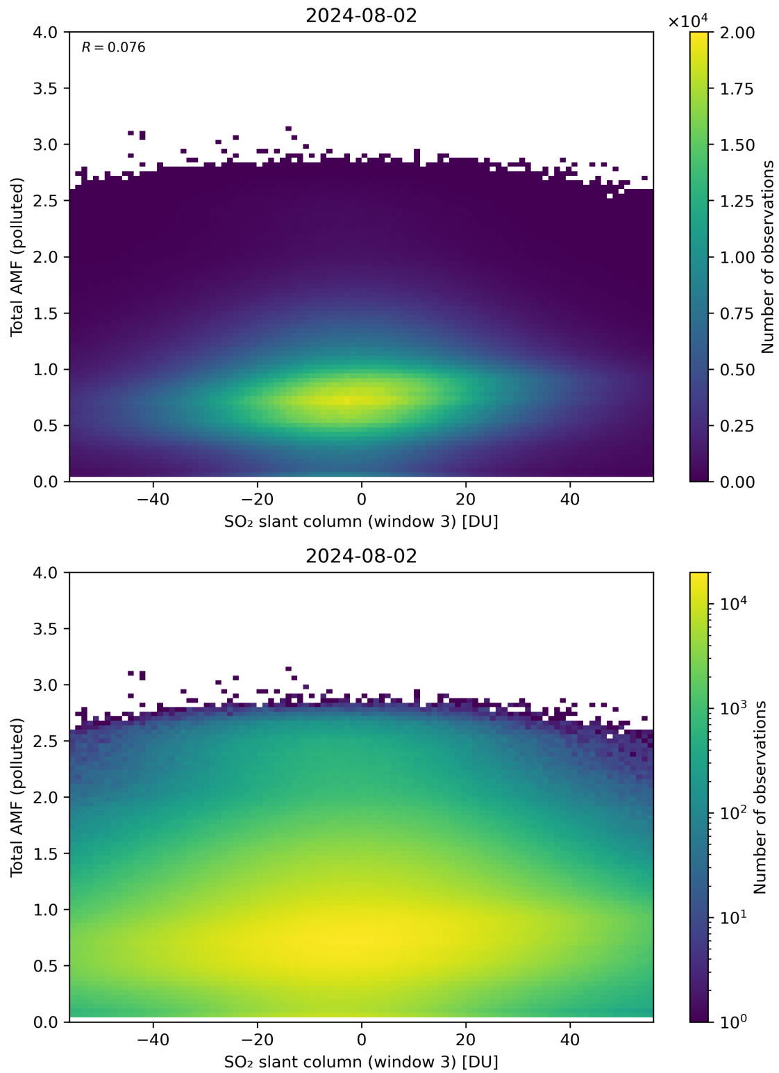
Figure 268: Scatter density plot of “SO 2 slant column (window 3)” against “Total AMF (polluted)” for 2024-08-01 to 2024-08-03.
