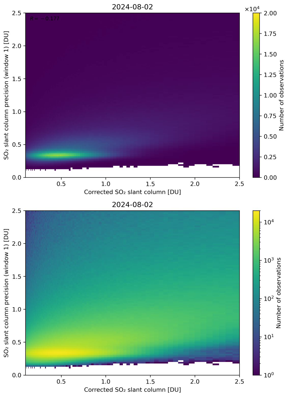
Figure 188: Scatter density plot of “Corrected SO 2 slant column” against “SO 2 slant column precision (window 1)” for 2024-08-01 to 2024-08-03.
