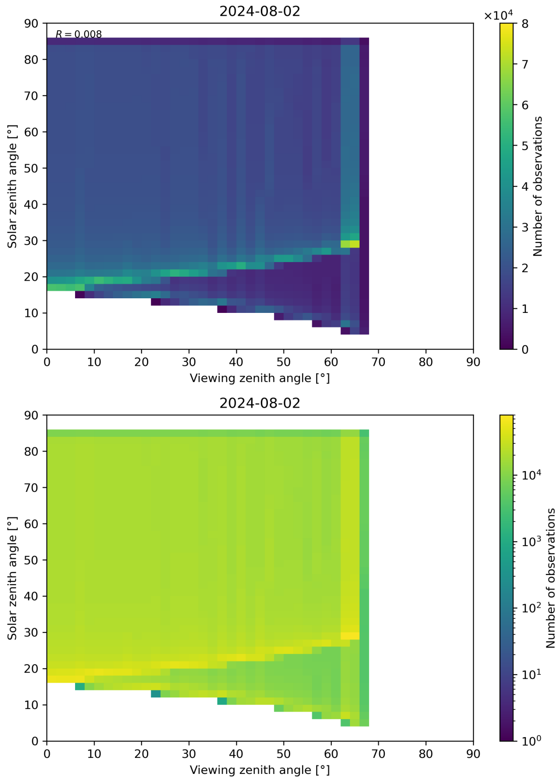
Figure 315: Scatter density plot of “Viewing zenith angle” against “Solar zenith angle” for 2024-08-01 to 2024-08-03.
