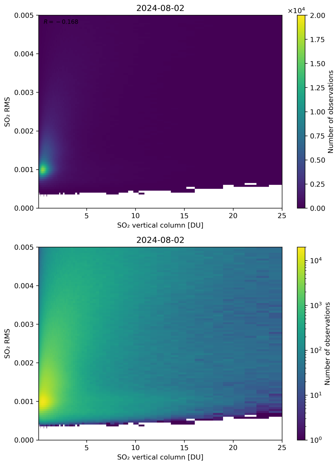
Figure 278: Scatter density plot of “SO 2 vertical column” against “SO 2 RMS” for 2024-08-01 to 2024-08-03.
