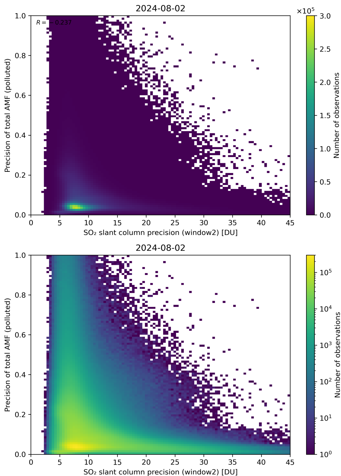
Figure 252: Scatter density plot of “SO 2 slant column precision (window2)” against “Precision of total AMF (polluted)” for 2024-08-01 to 2024-08-03.
