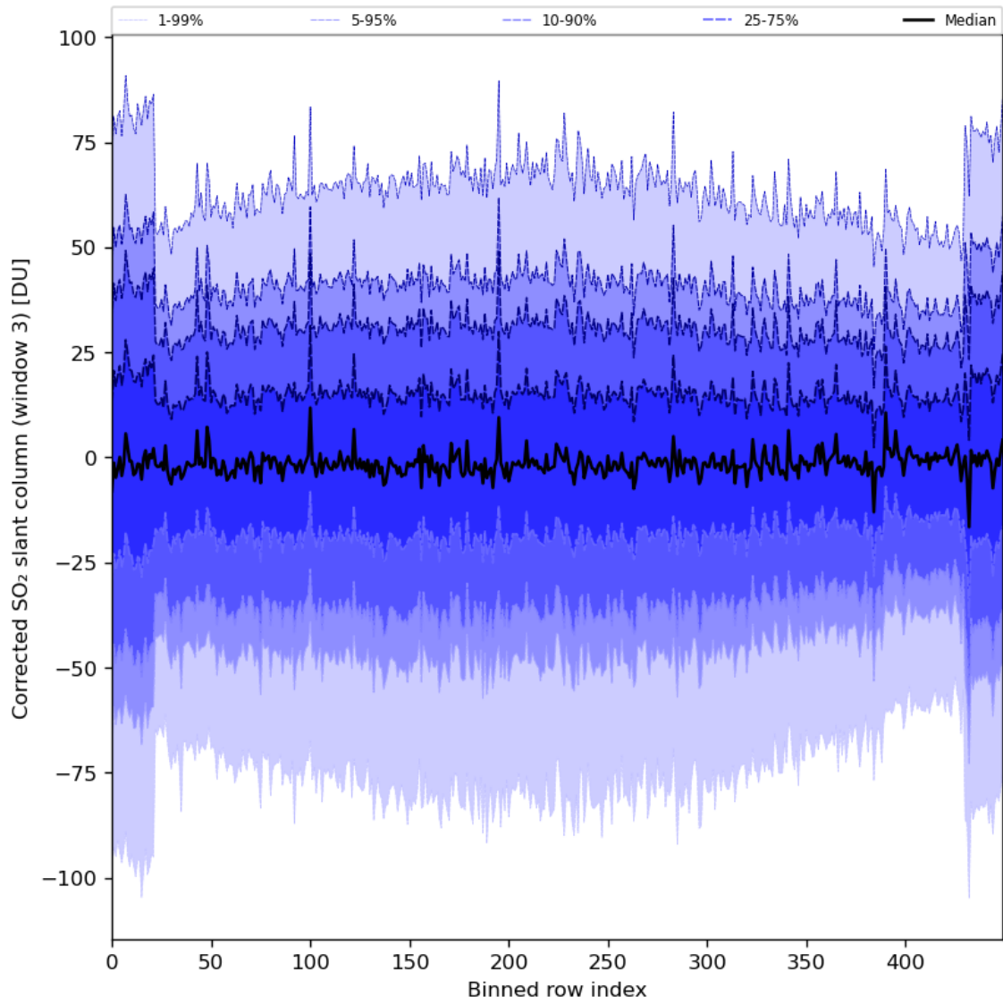
Figure 89: Along track statistics of “Corrected SO 2 slant column (window 3)” for 2024-08-01 to 2024-08-03
