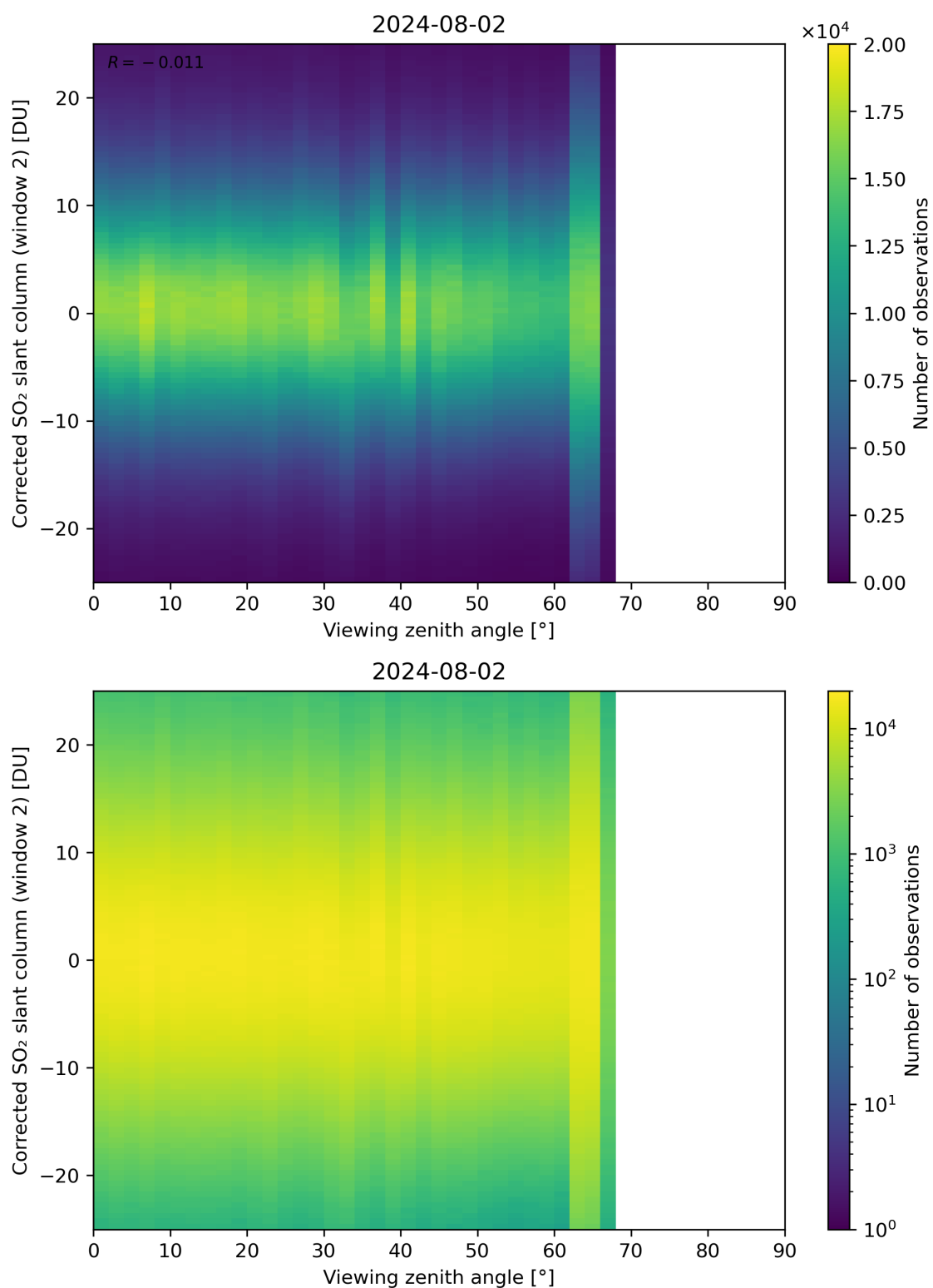
Figure 318: Scatter density plot of “Viewing zenith angle” against “Corrected SO 2 slant column (window 2)” for 2024-08-01 to 2024-08-03.
