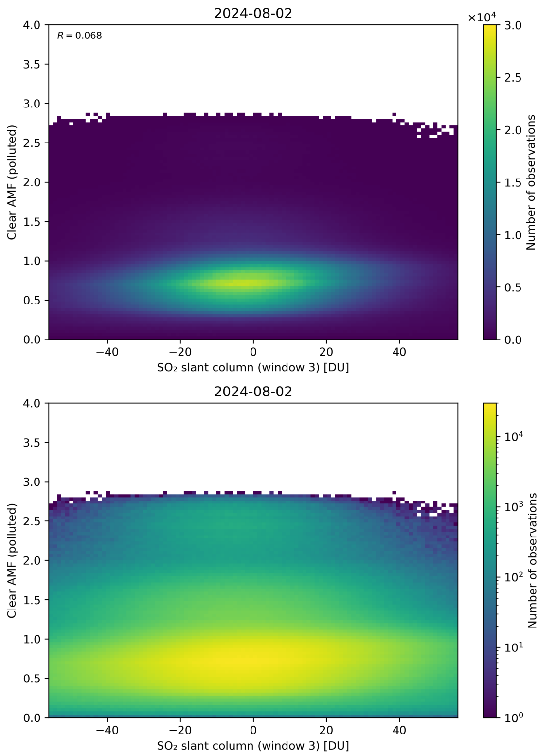
Figure 265: Scatter density plot of “SO 2 slant column (window 3)” against “Clear AMF (polluted)” for 2024-08-01 to 2024-08-03.
