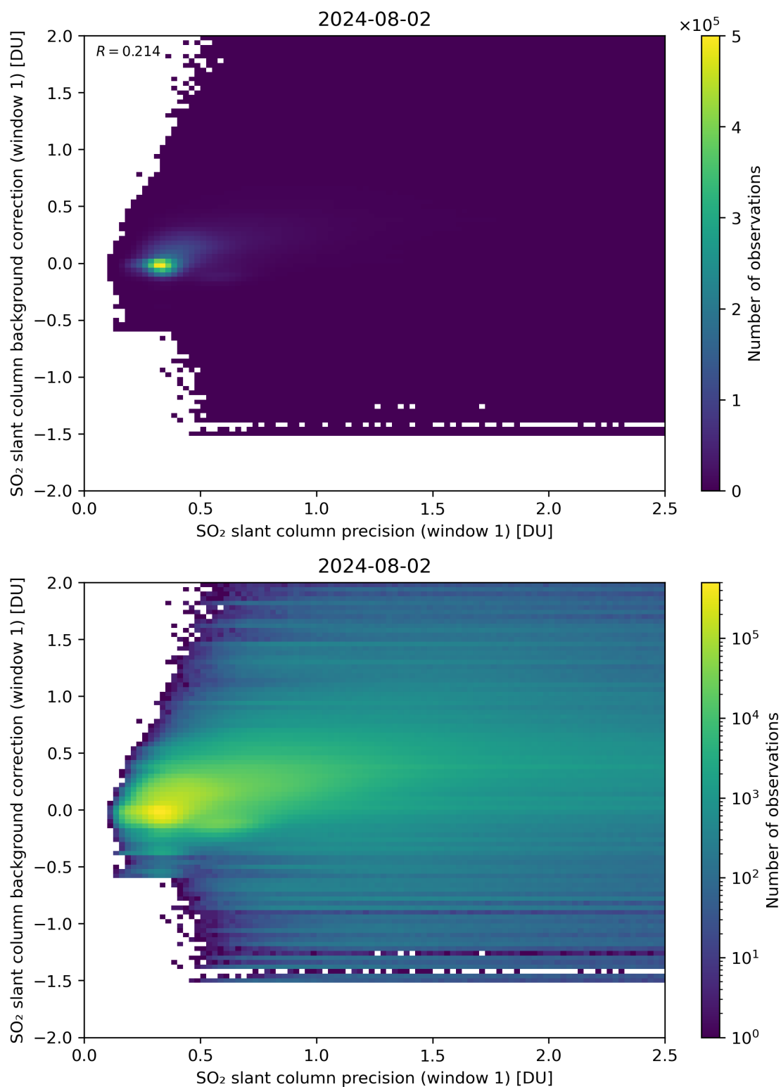
Figure 218: Scatter density plot of “SO 2 slant column precision (window 1)” against “SO 2 slant column background correction (window 1)” for 2024-08-01 to 2024-08-03.
