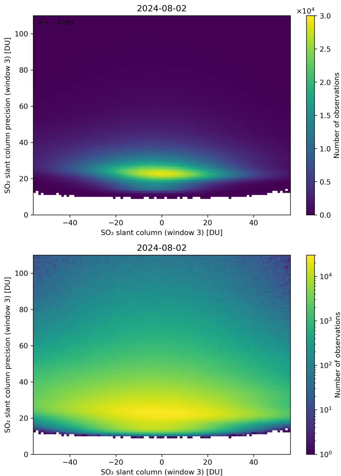
Figure 267: Scatter density plot of “SO 2 slant column (window 3)” against “SO 2 slant column precision (window 3)” for 2024-08-01 to 2024-08-03.
