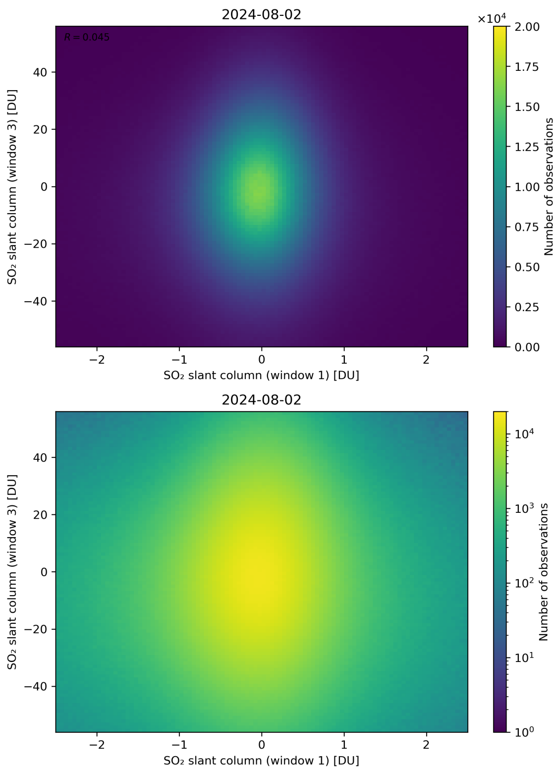
Figure 237: Scatter density plot of “SO 2 slant column (window 1)” against “SO 2 slant column (window 3)” for 2024-08-01 to 2024-08-03.
