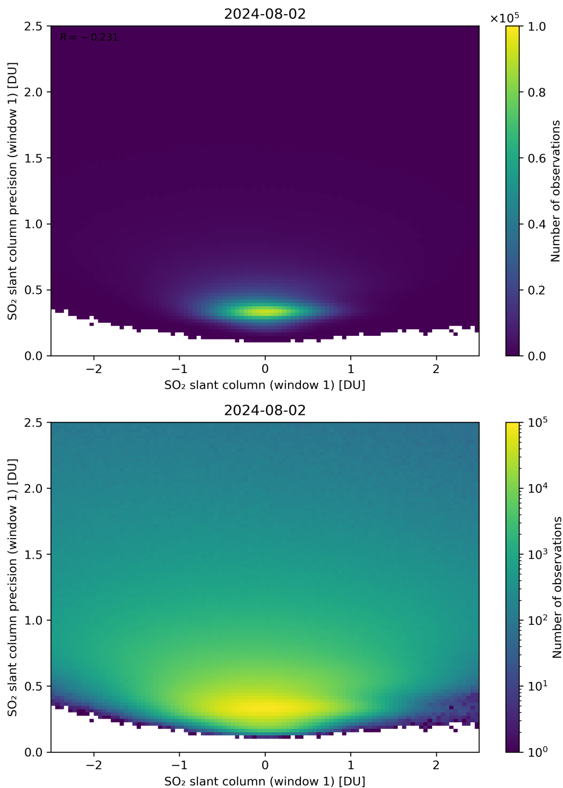
Figure 235: Scatter density plot of “SO 2 slant column (window 1)” against “SO 2 slant column precision (window 1)” for 2024-08-01 to 2024-08-03.
