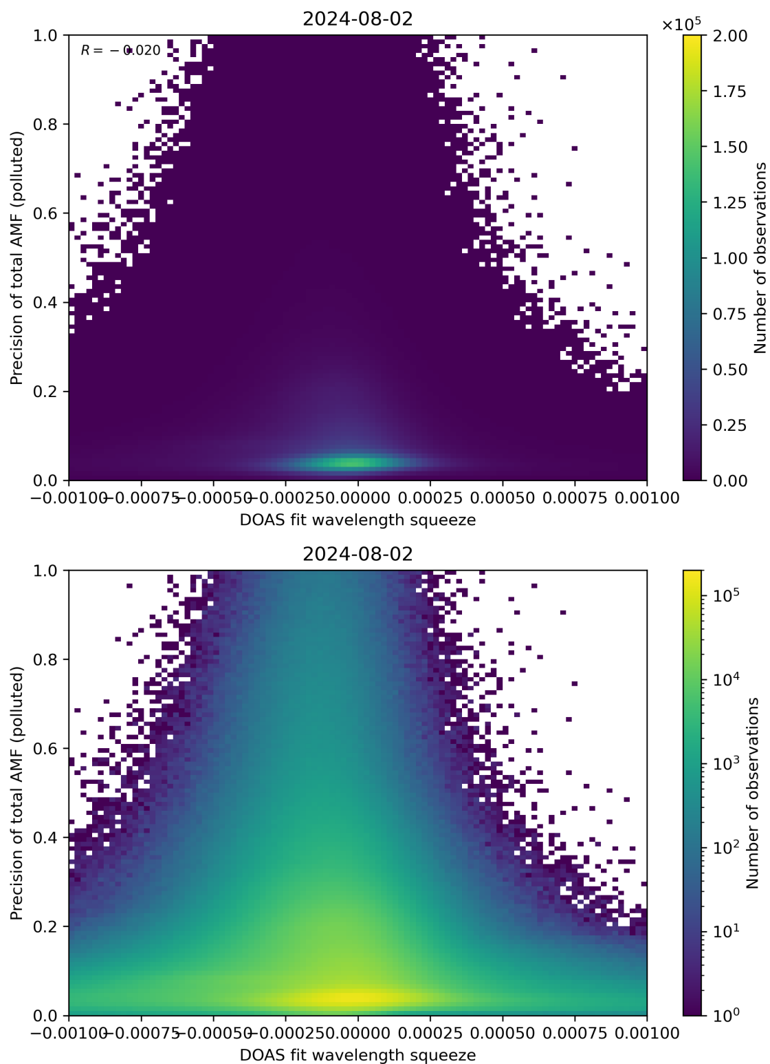
Figure 135: Scatter density plot of “DOAS fit wavelength squeeze” against “Precision of total AMF (polluted)” for 2024-08-01 to 2024-08-03.
