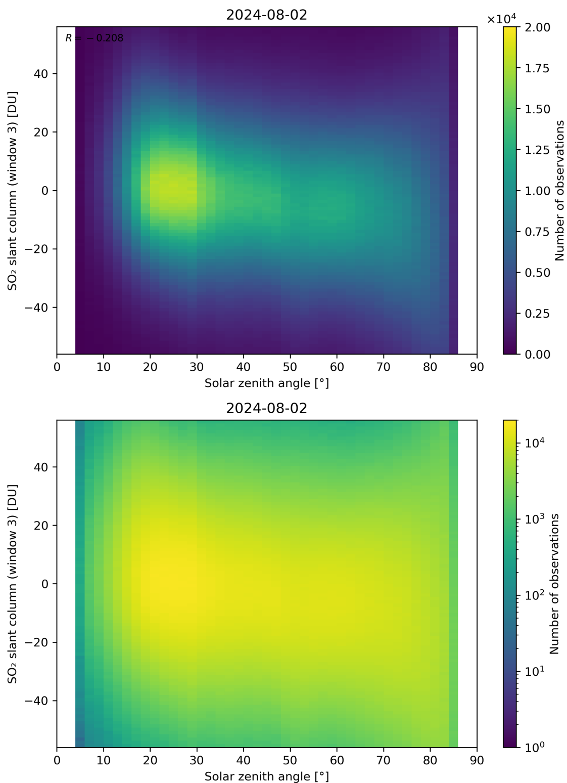
Figure 172: Scatter density plot of “Solar zenith angle” against “SO 2 slant column (window 3)” for 2024-08-01 to 2024-08-03.
