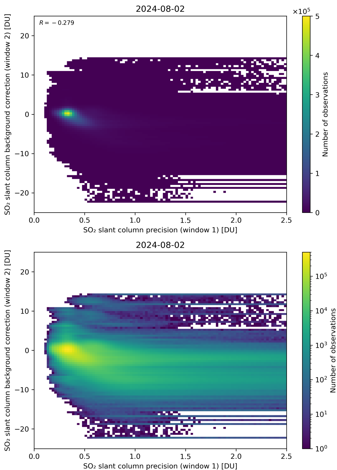
Figure 219: Scatter density plot of “SO 2 slant column precision (window 1)” against “SO 2 slant column background correction (window 2)” for 2024-08-01 to 2024-08-03.
