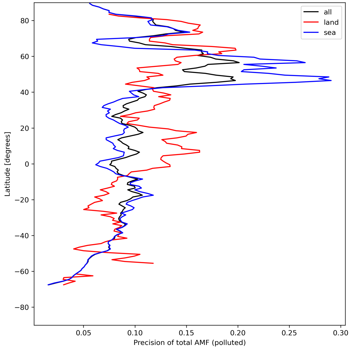
Figure 49: Zonal average of “Precision of total AMF (polluted)” for 2024-08-01 to 2024-08-03.
