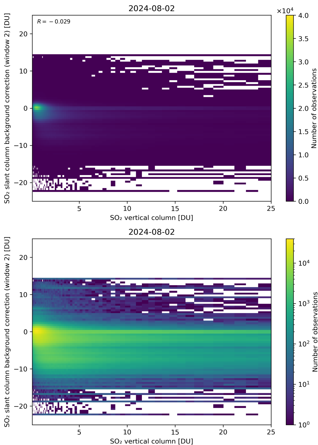
Figure 274: Scatter density plot of “SO 2 vertical column” against “SO 2 slant column background correction (window 2)” for 2024-08-01 to 2024-08-03.
