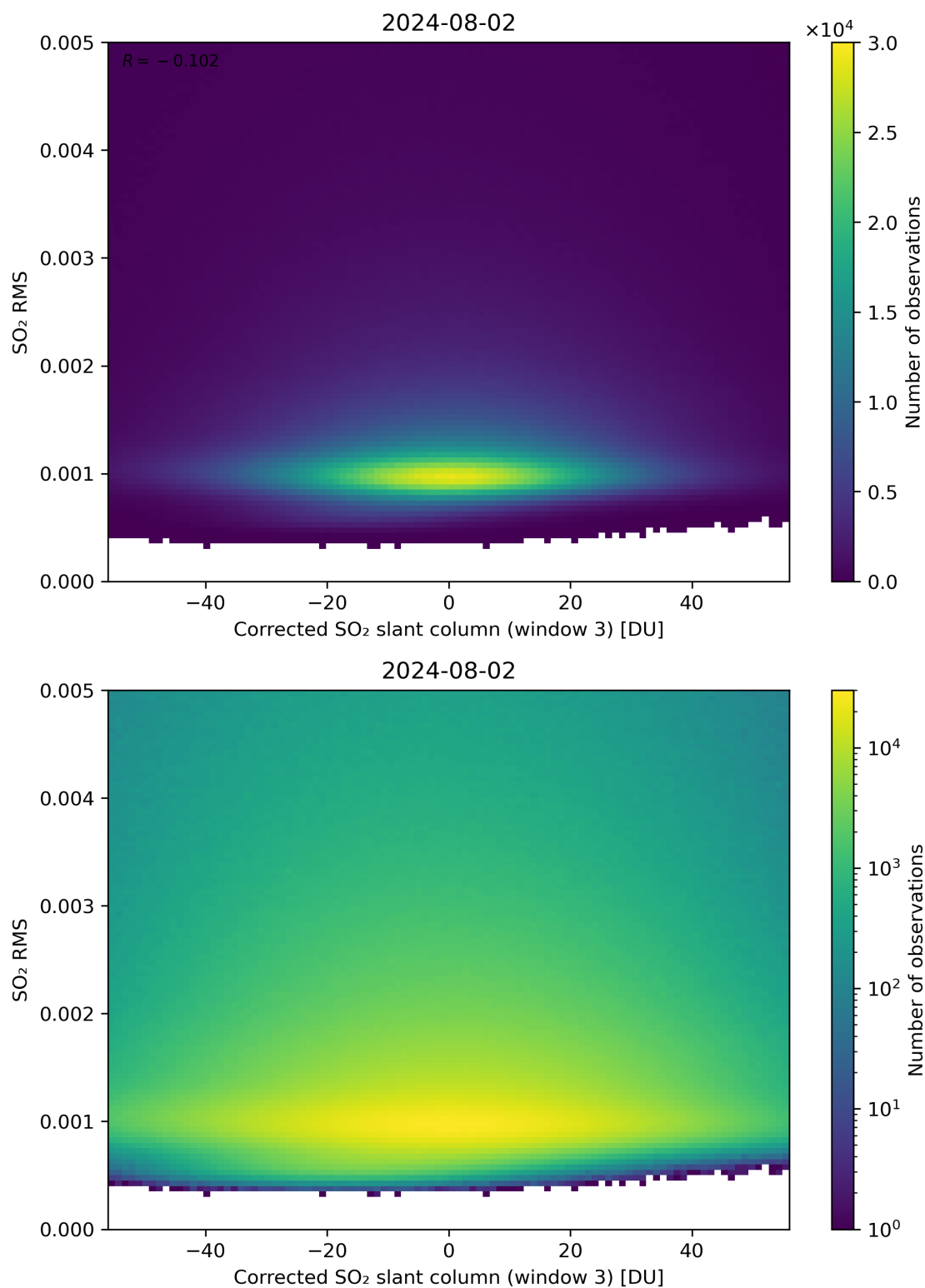
Figure 208: Scatter density plot of “Corrected SO 2 slant column (window 3)” against “SO 2 RMS” for 2024-08-01 to 2024-08-03.
