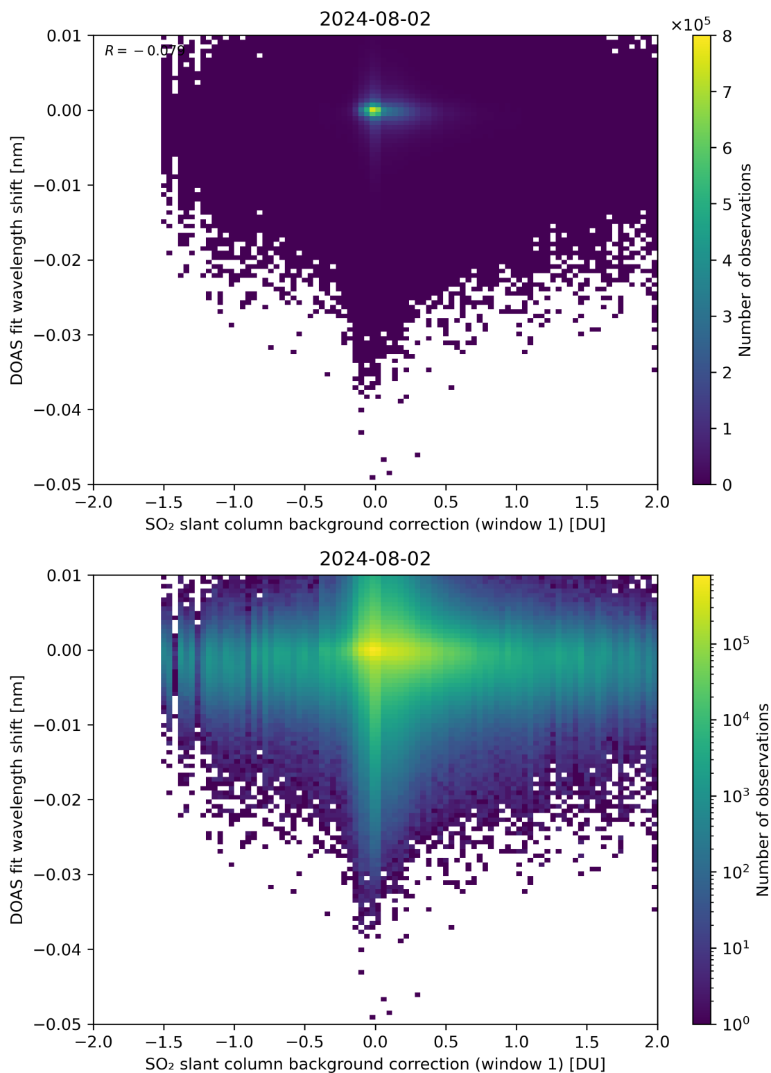
Figure 100: Scatter density plot of “SO 2 slant column background correction (window 1)” against “DOAS fit wavelength shift” for 2024-08-01 to 2024-08-03.
