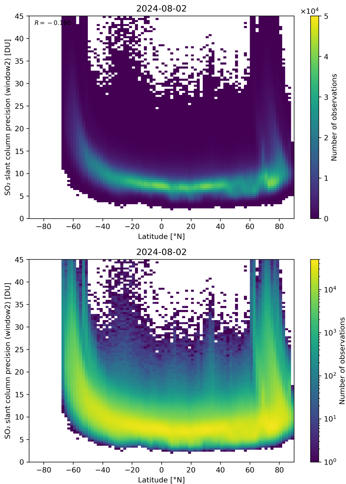
Figure 151: Scatter density plot of “Latitude” against “SO 2 slant column precision (window2)” for 2024-08-01 to 2024-08-03.
