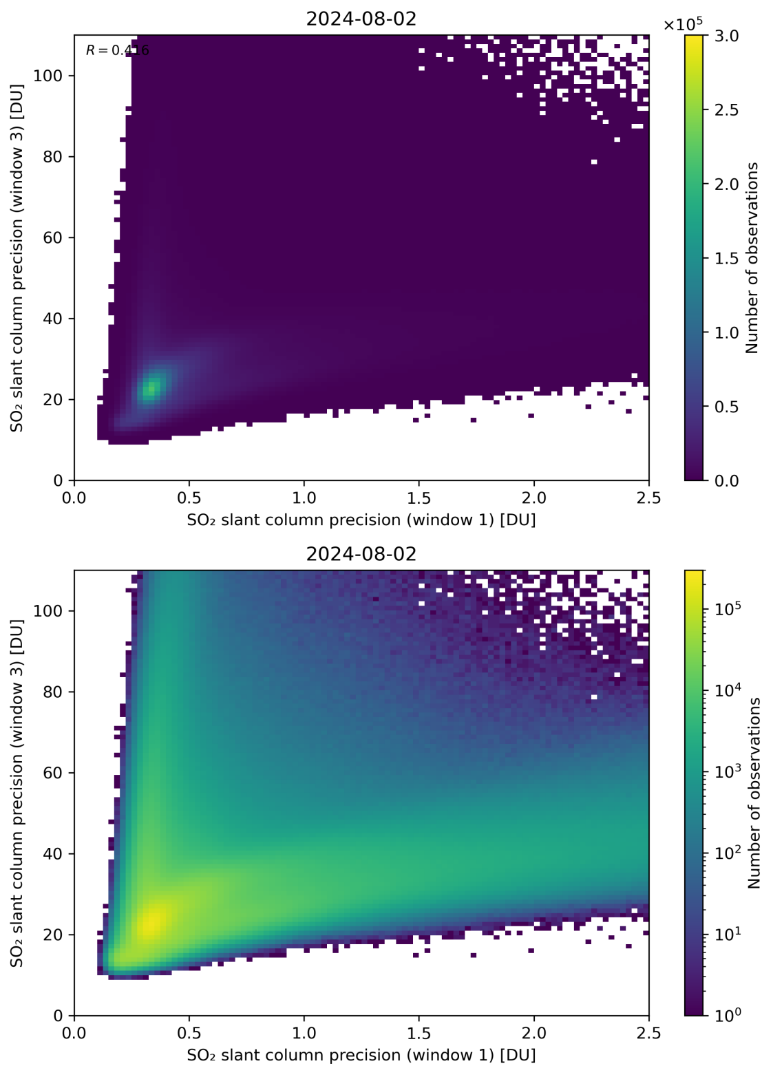
Figure 229: Scatter density plot of “SO 2 slant column precision (window 1)” against “SO 2 slant column precision (window 3)” for 2024-08-01 to 2024-08-03.
