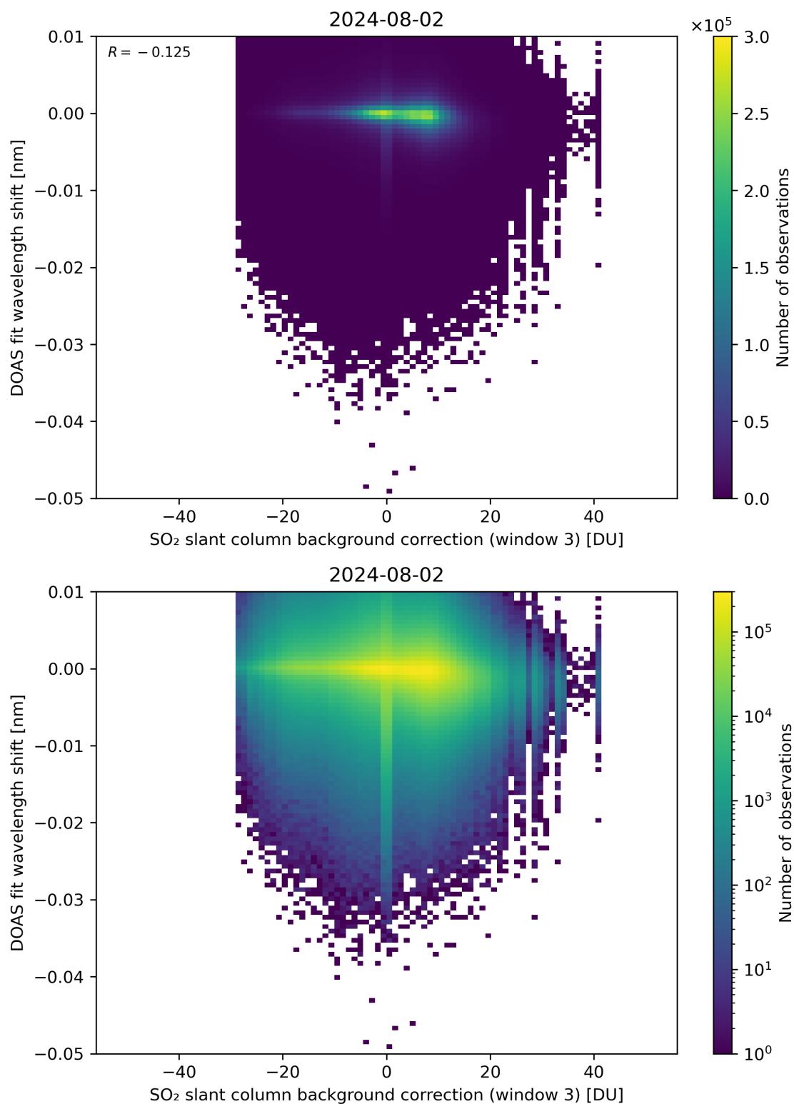
Figure 121: Scatter density plot of “SO 2 slant column background correction (window 3)” against “DOAS fit wavelength shift” for 2024-08-01 to 2024-08-03.
