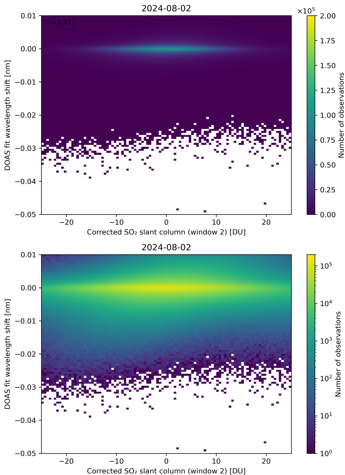
Figure 196: Scatter density plot of “Corrected SO 2 slant column (window 2)” against “DOAS fit wavelength shift” for 2024-08-01 to 2024-08-03.
