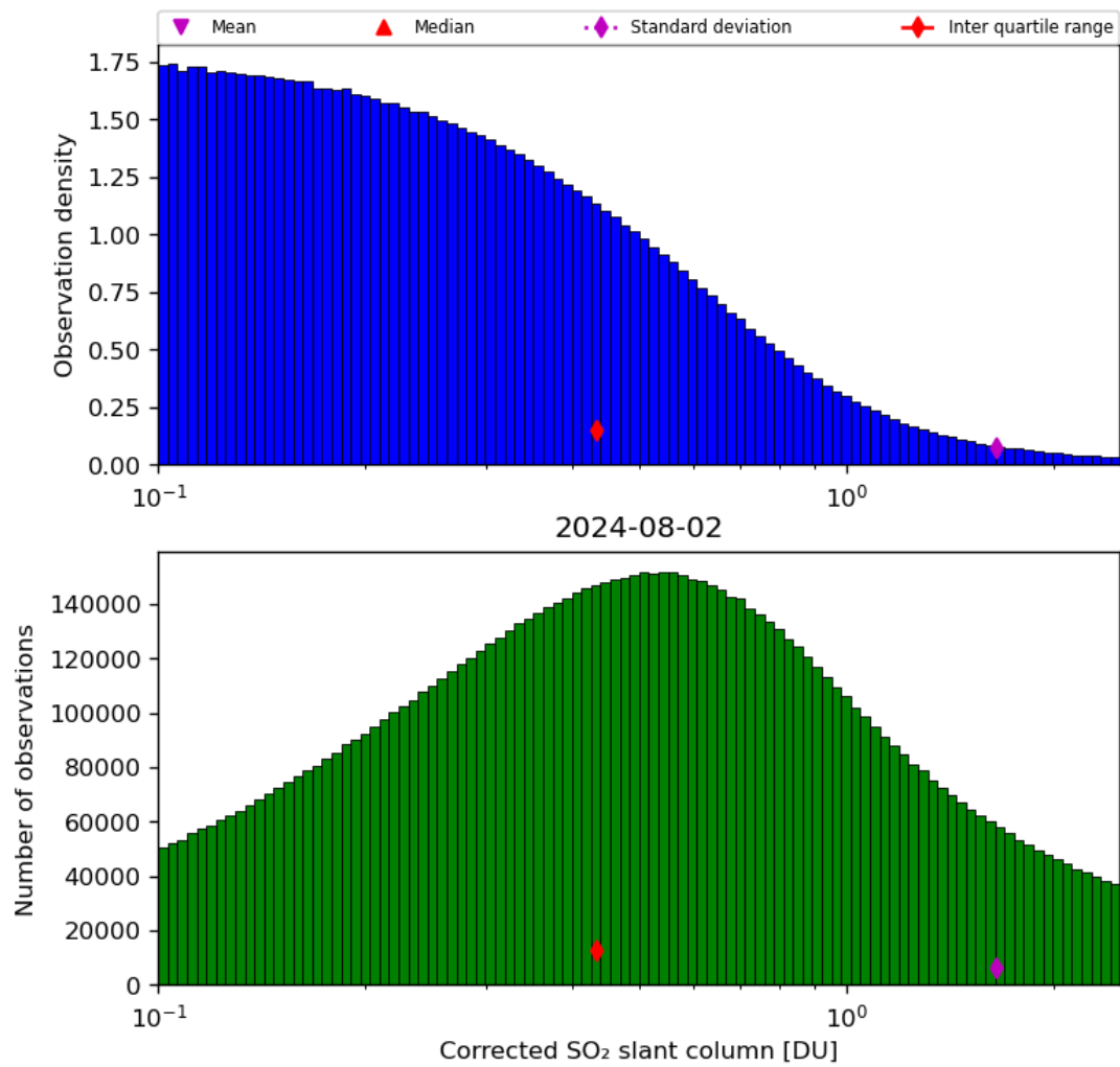
Figure 55: Histogram of "Corrected SO 2 slant column" for 2024-08-01 to 2024-08-03
