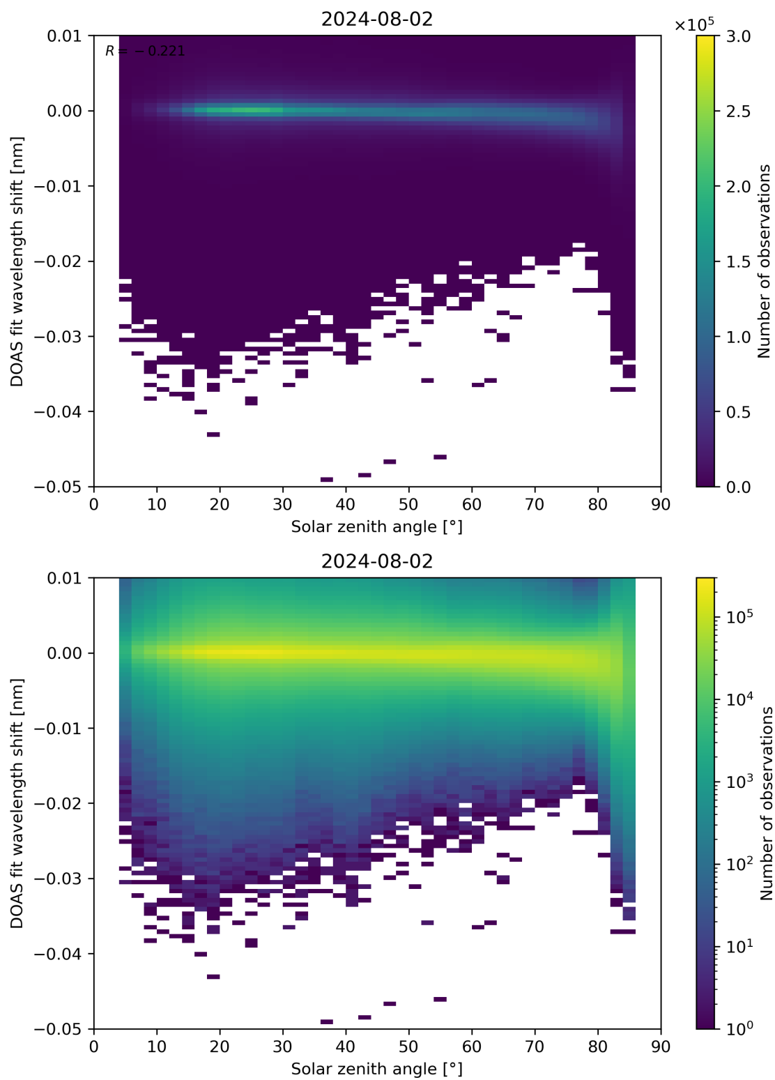
Figure 161: Scatter density plot of “Solar zenith angle” against “DOAS fit wavelength shift” for 2024-08-01 to 2024-08-03.
