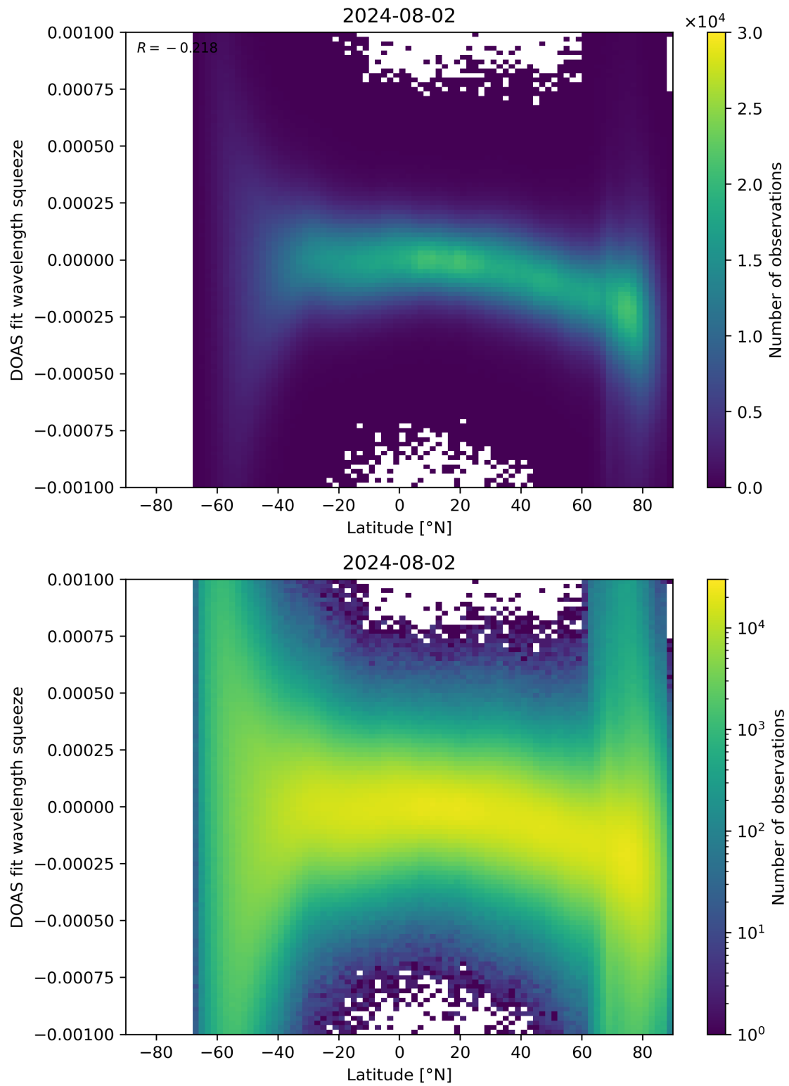
Figure 143: Scatter density plot of “Latitude” against “DOAS fit wavelength squeeze” for 2024-08-01 to 2024-08-03.
