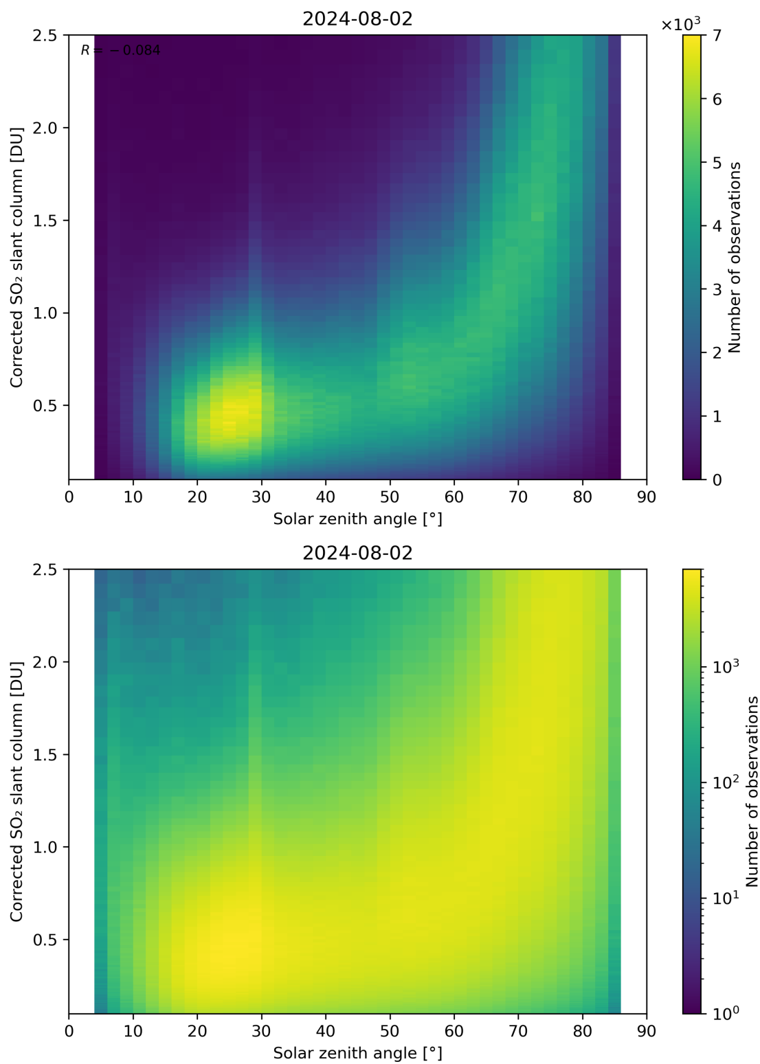
Figure 166: Scatter density plot of “Solar zenith angle” against “Corrected SO 2 slant column” for 2024-08-01 to 2024-08-03.
