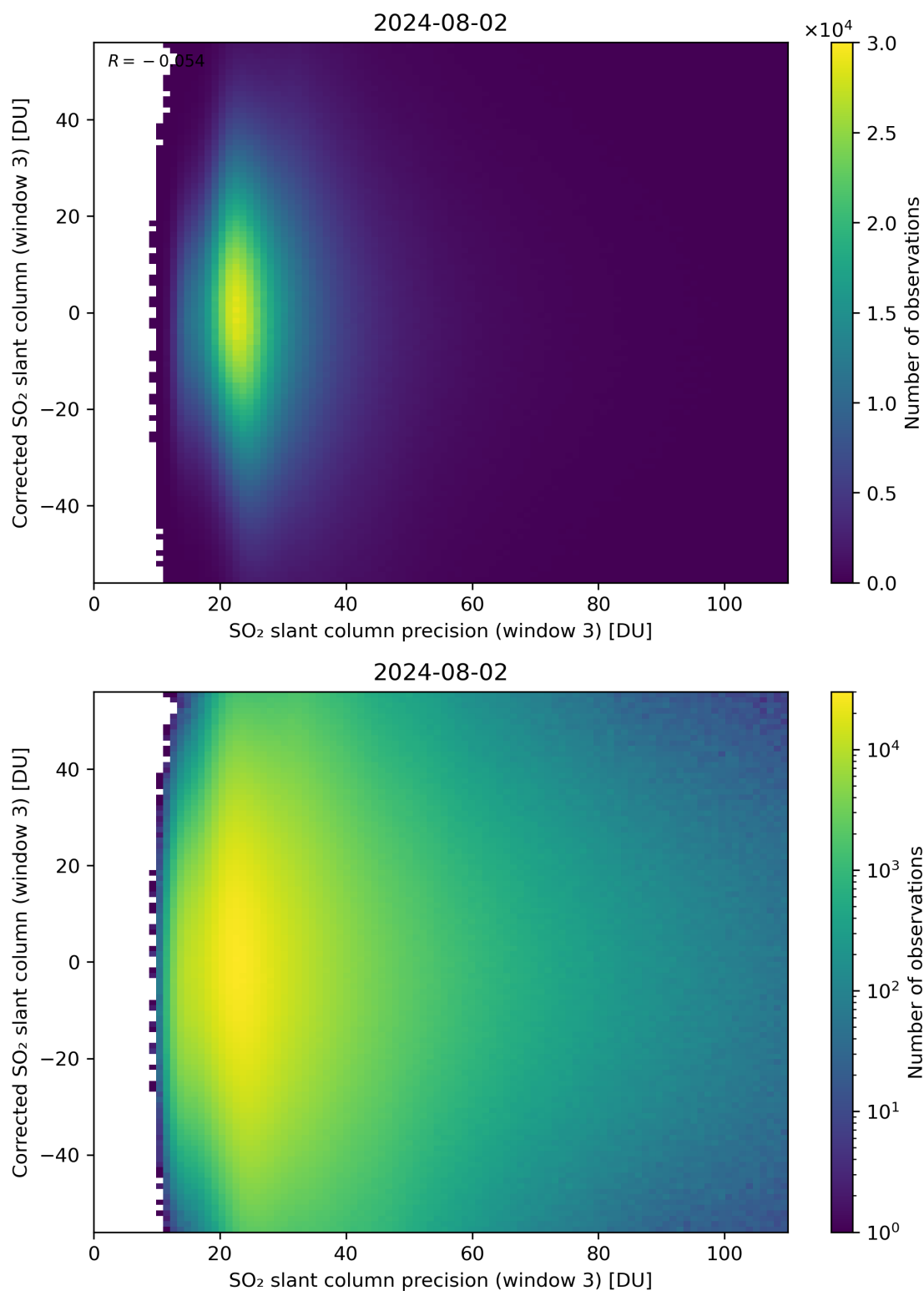
Figure 262: Scatter density plot of “SO 2 slant column precision (window 3)” against “Corrected SO 2 slant column (window 3)” for 2024-08-01 to 2024-08-03.
