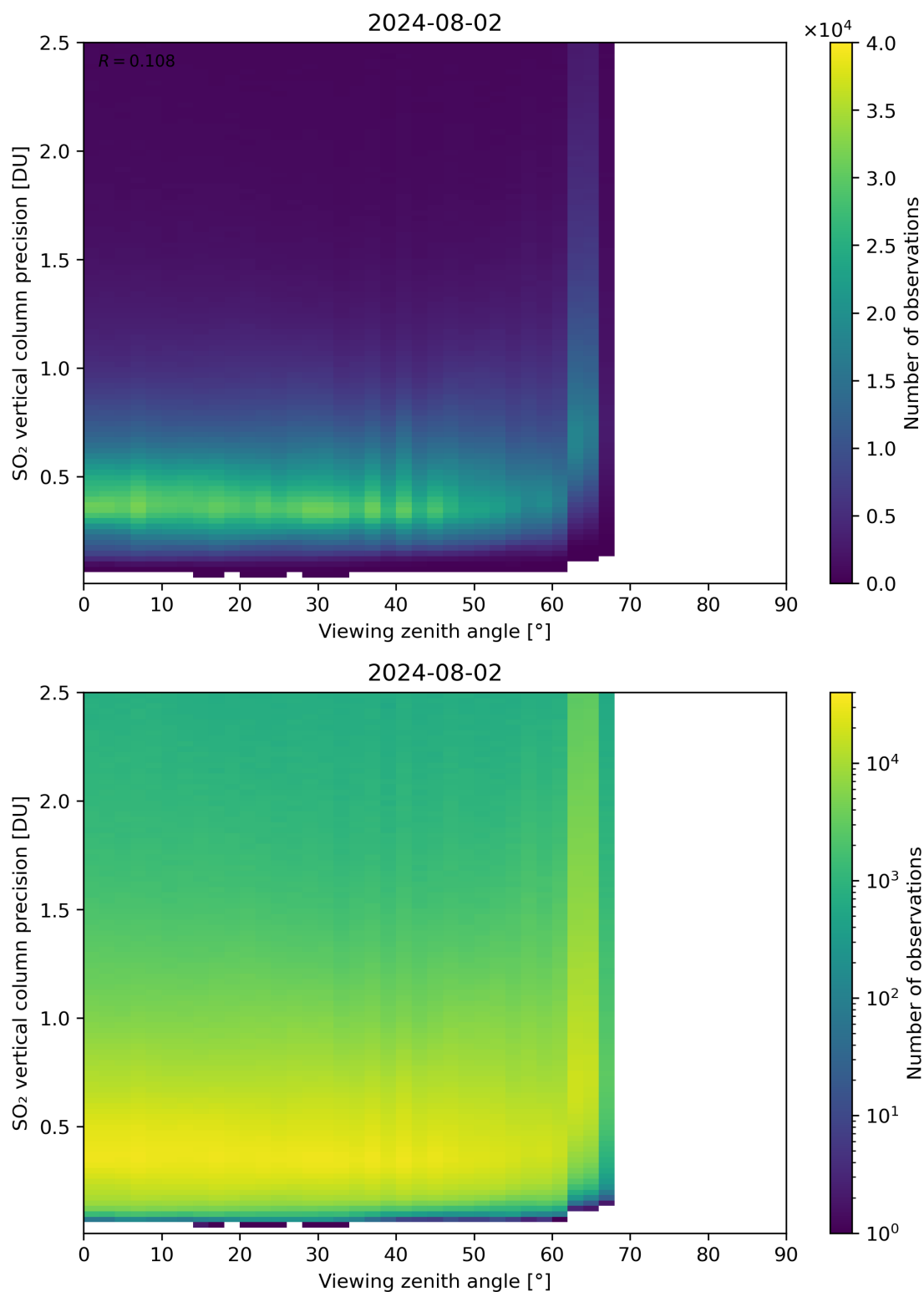
Figure 328: Scatter density plot of “Viewing zenith angle” against “SO 2 vertical column precision” for 2024-08-01 to 2024-08-03.
