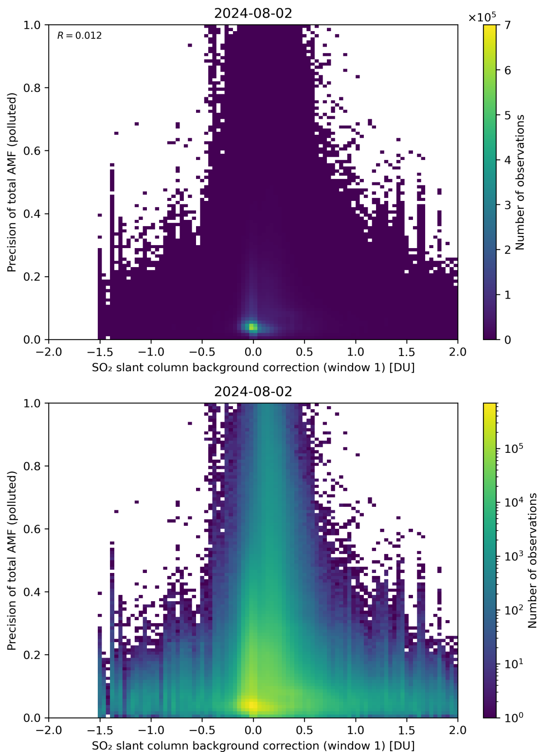
Figure 110: Scatter density plot of “SO 2 slant column background correction (window 1)” against “Precision of total AMF (polluted)” for 2024-08-01 to 2024-08-03.
