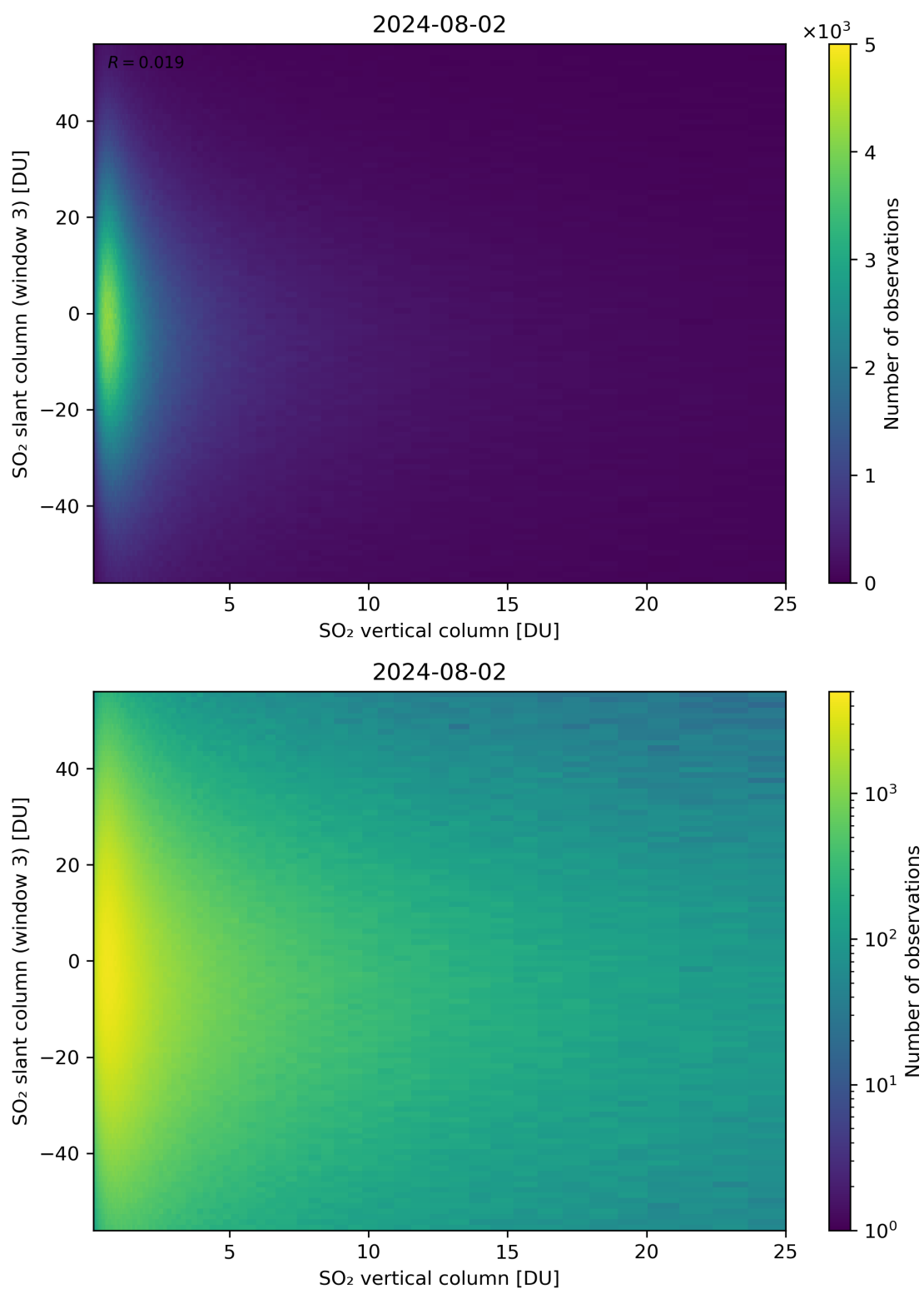
Figure 303: Scatter density plot of “SO 2 vertical column” against “SO 2 slant column (window 3)” for 2024-08-01 to 2024-08-03.
