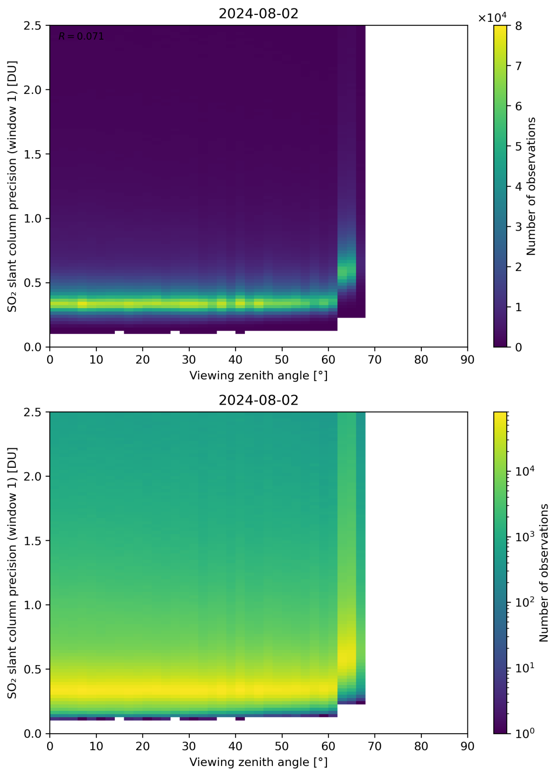
Figure 321: Scatter density plot of “Viewing zenith angle” against “SO 2 slant column precision (window 1)” for 2024-08-01 to 2024-08-03.
