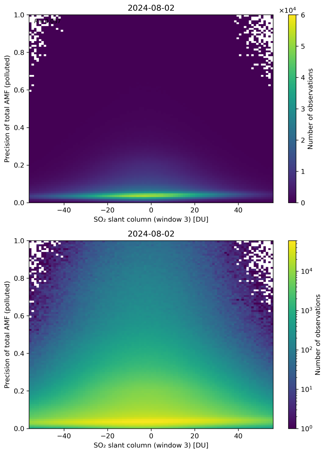
Figure 269: Scatter density plot of “SO 2 slant column (window 3)” against “Precision of total AMF (polluted)” for 2024-08-01 to 2024-08-03.
