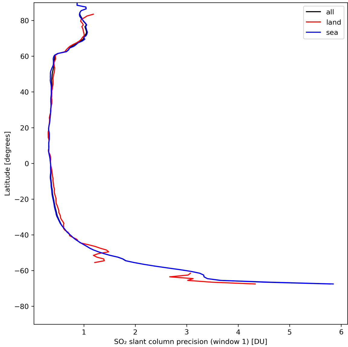
Figure 34: Zonal average of “SO 2 slant column precision (window 1)” for 2024-08-01 to 2024-08-03.
