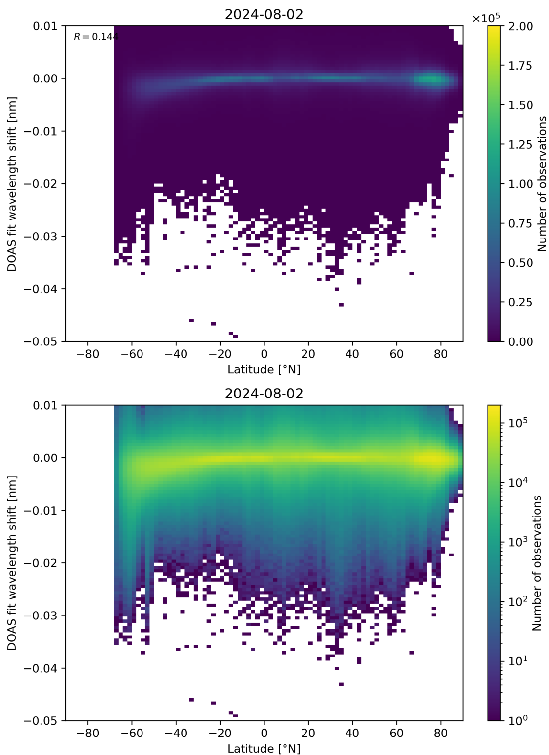
Figure 142: Scatter density plot of “Latitude” against “DOAS fit wavelength shift” for 2024-08-01 to 2024-08-03.
