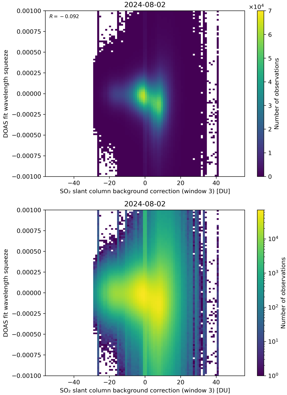
Figure 122: Scatter density plot of “SO 2 slant column background correction (window 3)” against “DOAS fit wavelength squeeze” for 2024-08-01 to 2024-08-03.
