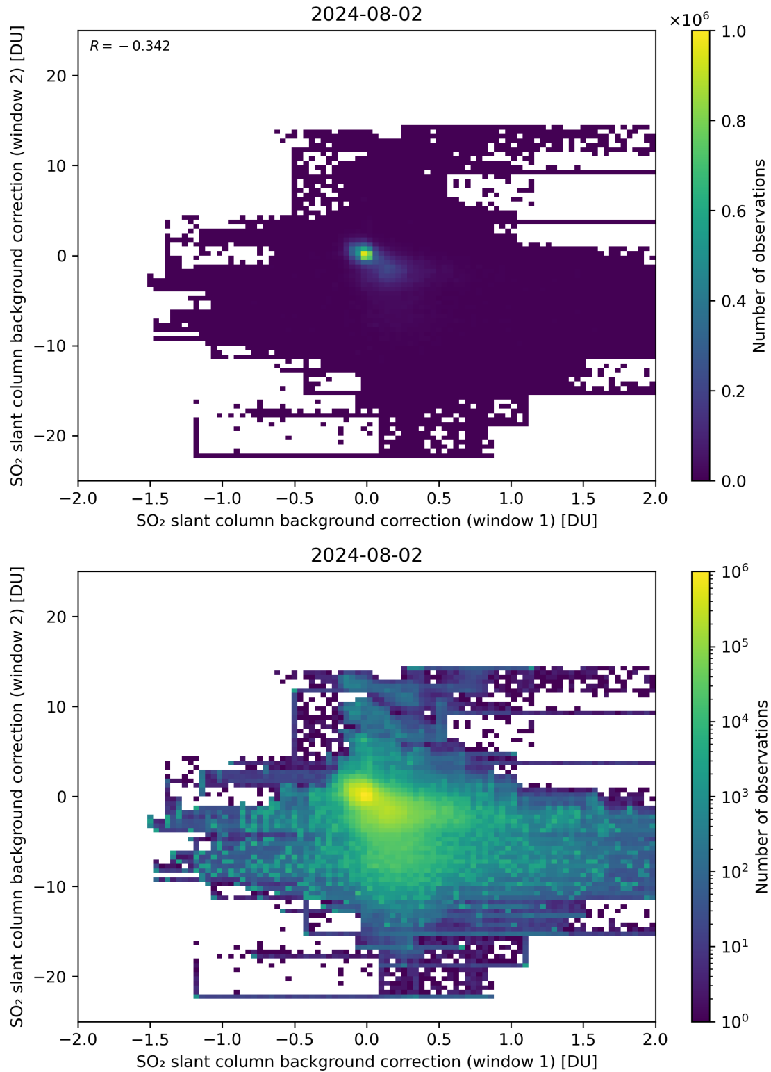
Figure 98: Scatter density plot of “SO 2 slant column background correction (window 1)” against “SO 2 slant column background correction (window 2)” for 2024-08-01 to 2024-08-03.
