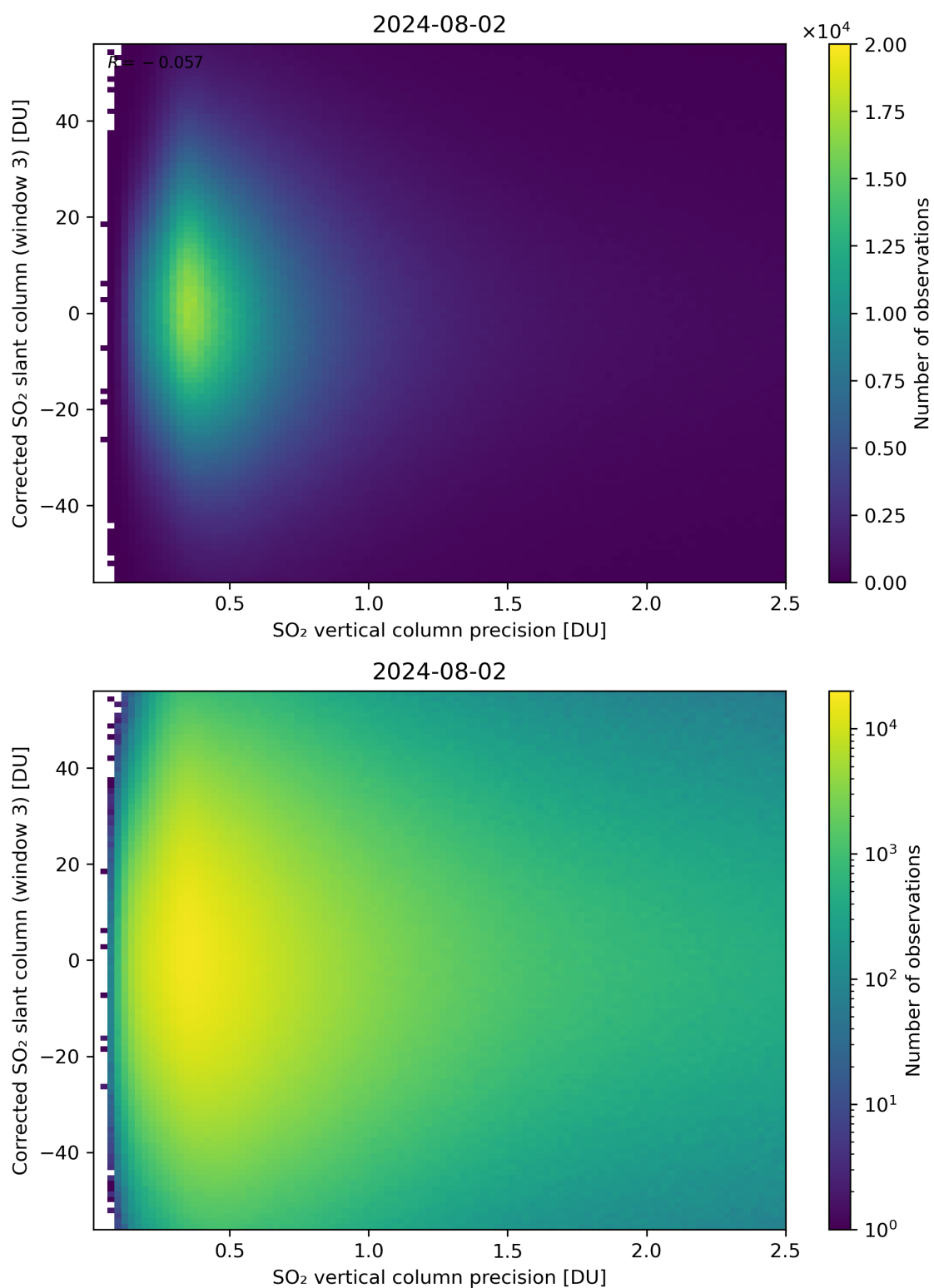
Figure 288: Scatter density plot of “SO 2 vertical column precision” against “Corrected SO 2 slant column (window 3)” for 2024-08-01 to 2024-08-03.
