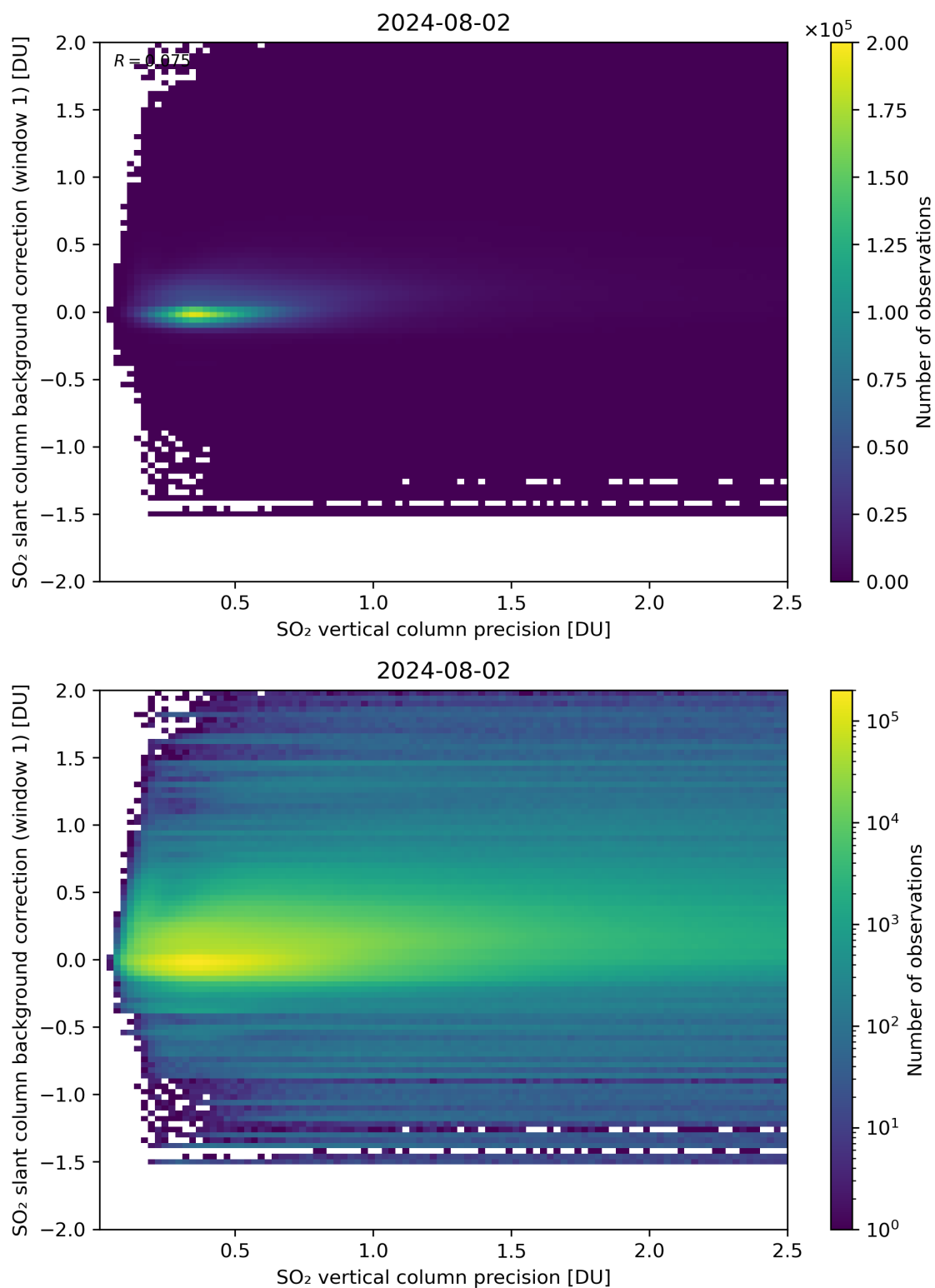
Figure 279: Scatter density plot of “SO 2 vertical column precision” against “SO 2 slant column background correction (window 1)” for 2024-08-01 to 2024-08-03.
