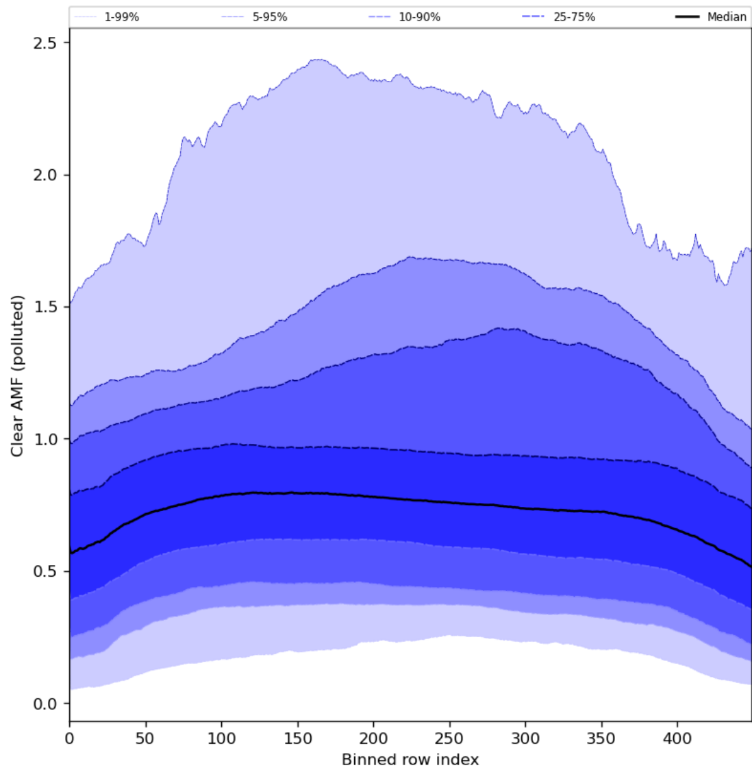
Figure 96: Along track statistics of “Clear AMF (polluted)” for 2024-08-01 to 2024-08-03
