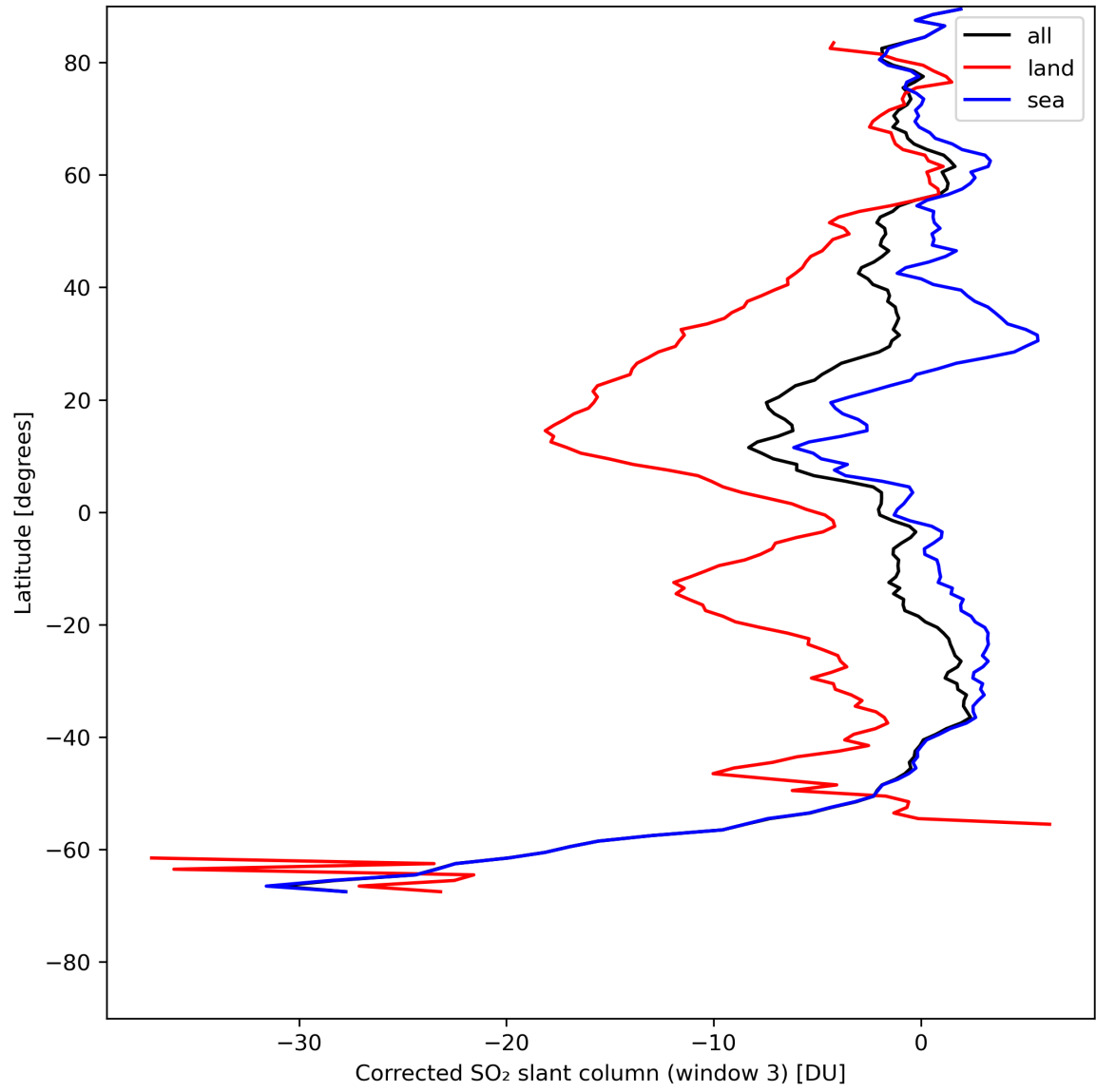
Figure 43: Zonal average of “Corrected SO 2 slant column (window 3)” for 2024-08-01 to 2024-08-03.
