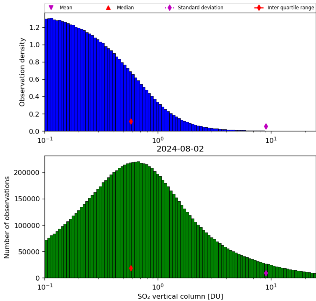
Figure 53: Histogram of “SO 2 vertical column” for 2024-08-01 to 2024-08-03
