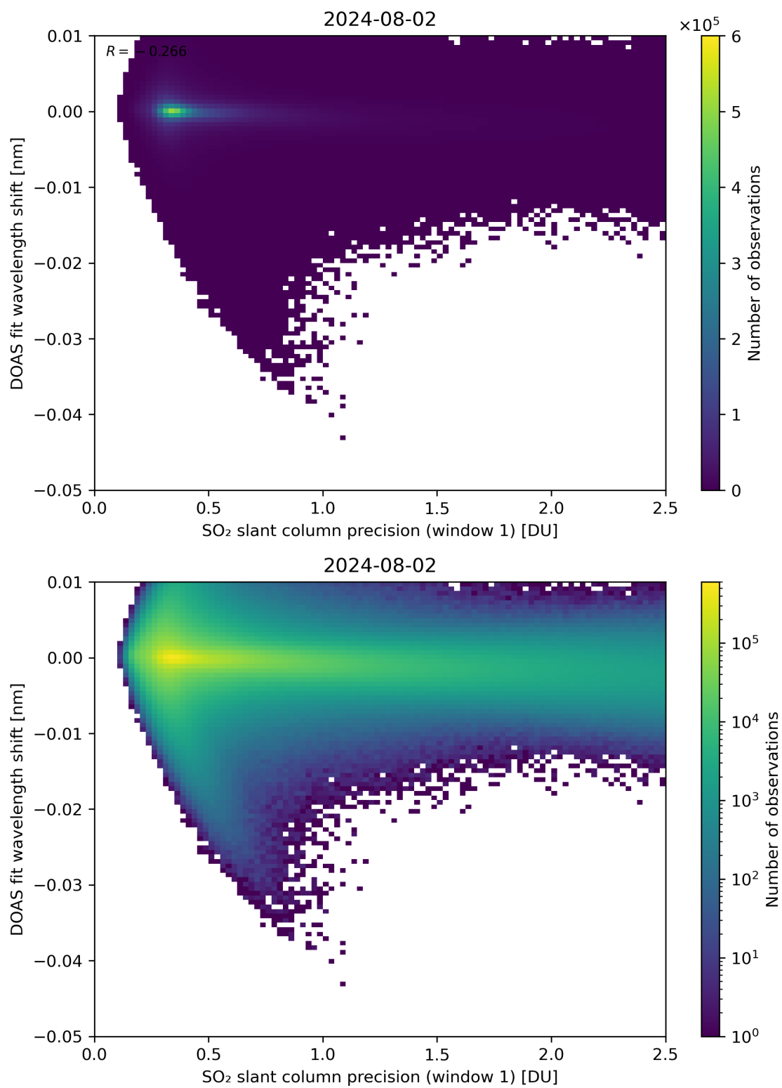
Figure 221: Scatter density plot of “SO 2 slant column precision (window 1)” against “DOAS fit wavelength shift” for 2024-08-01 to 2024-08-03.
