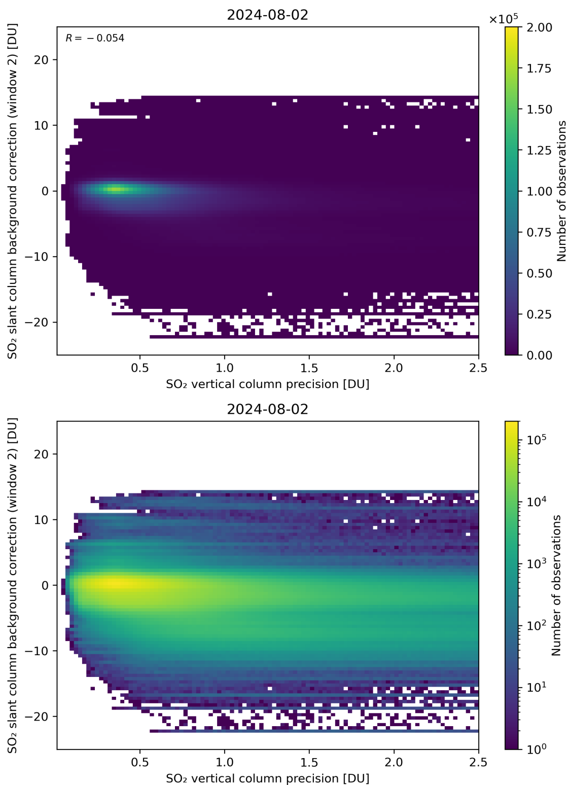
Figure 280: Scatter density plot of “SO 2 vertical column precision” against “SO 2 slant column background correction (window 2)” for 2024-08-01 to 2024-08-03.
