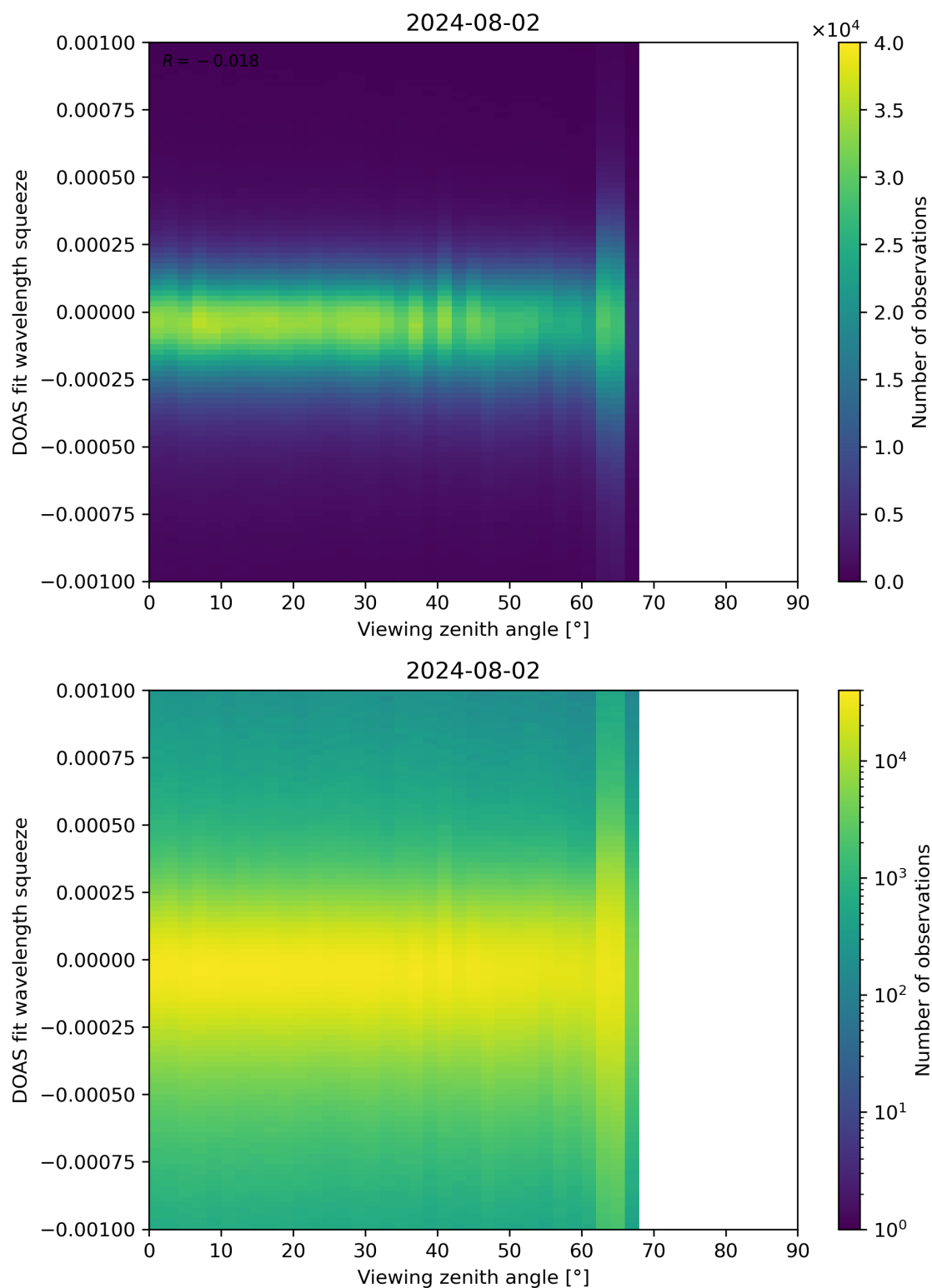
Figure 312: Scatter density plot of “Viewing zenith angle” against “DOAS fit wavelength squeeze” for 2024-08-01 to 2024-08-03.
