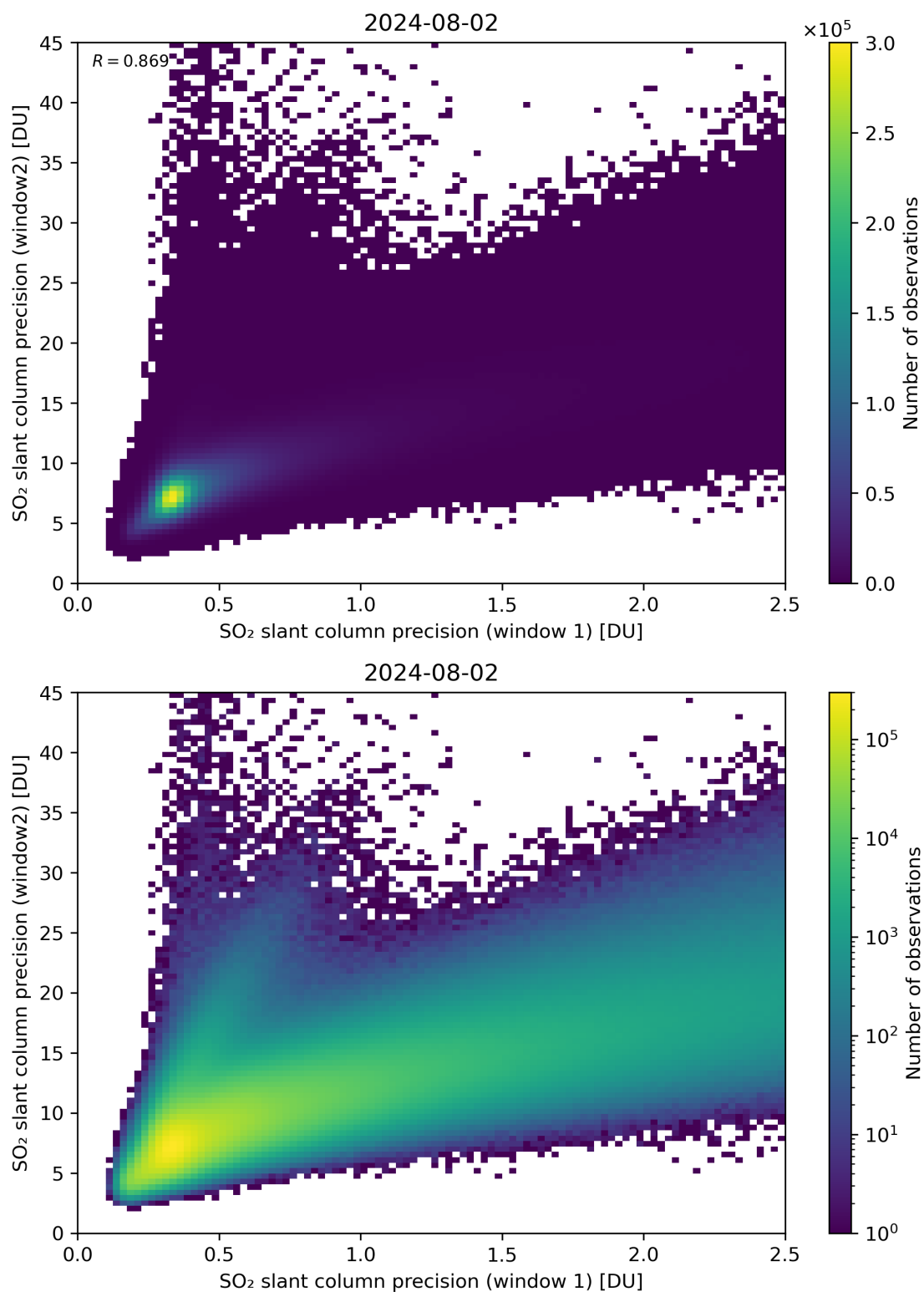
Figure 227: Scatter density plot of “SO 2 slant column precision (window 1)” against “SO 2 slant column precision (window2)” for 2024-08-01 to 2024-08-03.
