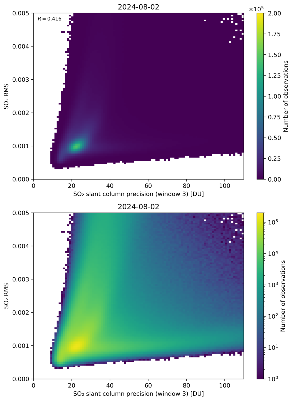
Figure 260: Scatter density plot of “SO 2 slant column precision (window 3)” against “SO 2 RMS” for 2024-08-01 to 2024-08-03.
