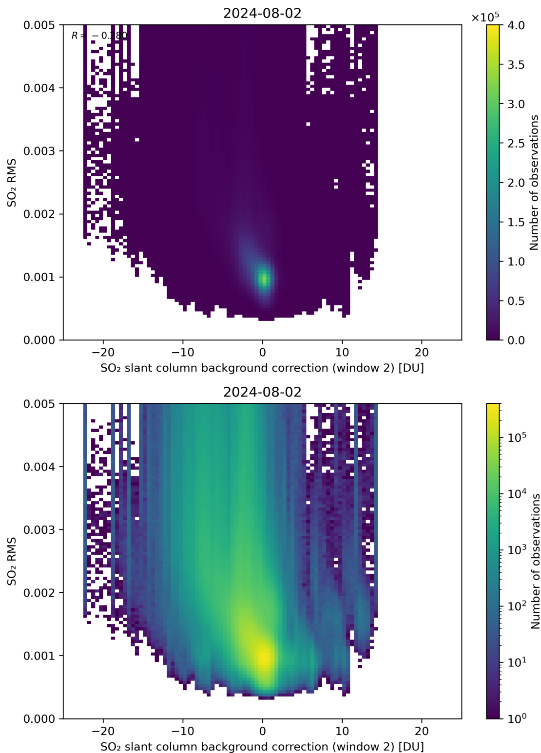
Figure 114: Scatter density plot of “SO 2 slant column background correction (window 2)” against “SO 2 RMS” for 2024-08-01 to 2024-08-03.
