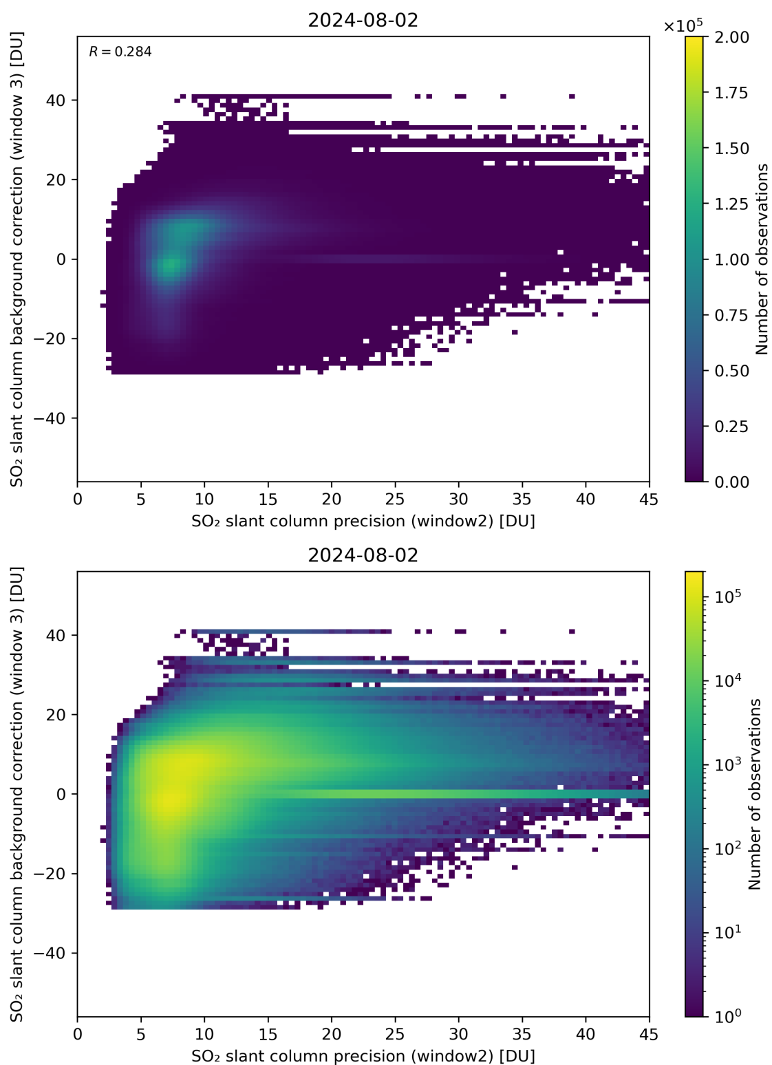
Figure 242: Scatter density plot of “SO 2 slant column precision (window2)” against “SO 2 slant column background correction (window 3)” for 2024-08-01 to 2024-08-03.
