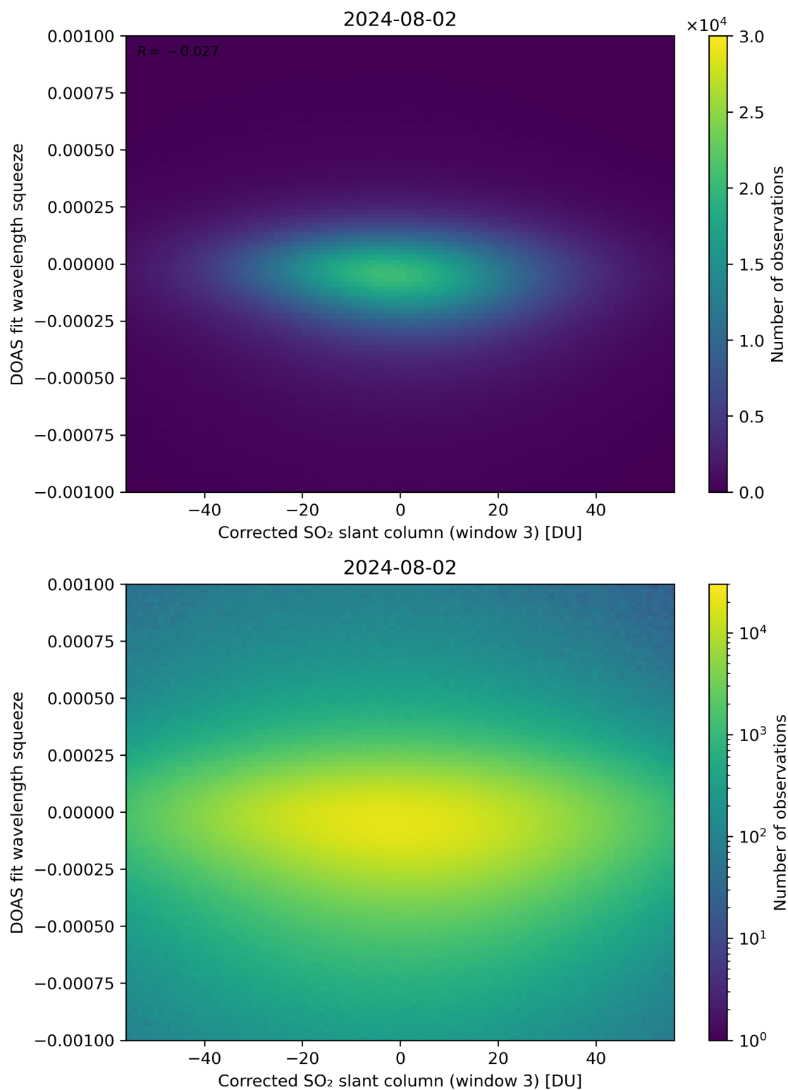
Figure 207: Scatter density plot of “Corrected SO 2 slant column (window 3)” against “DOAS fit wavelength squeeze” for 2024-08-01 to 2024-08-03.
