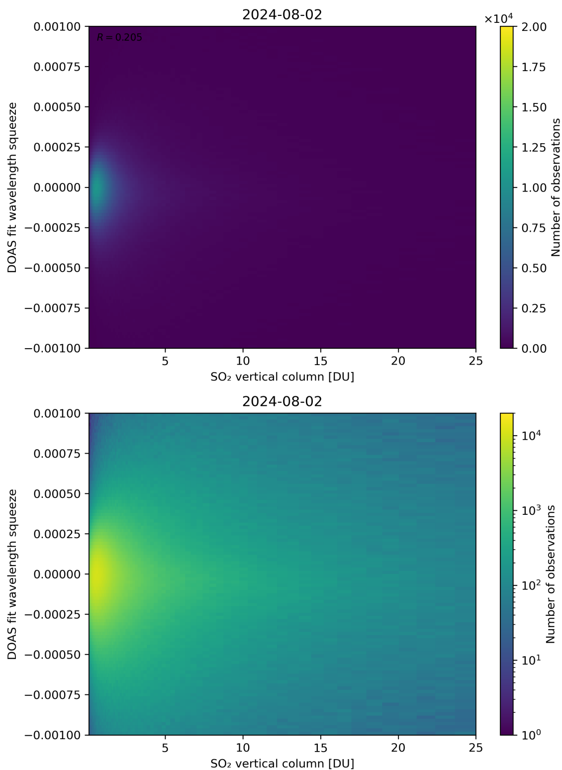
Figure 277: Scatter density plot of “SO 2 vertical column” against “DOAS fit wavelength squeeze” for 2024-08-01 to 2024-08-03.
