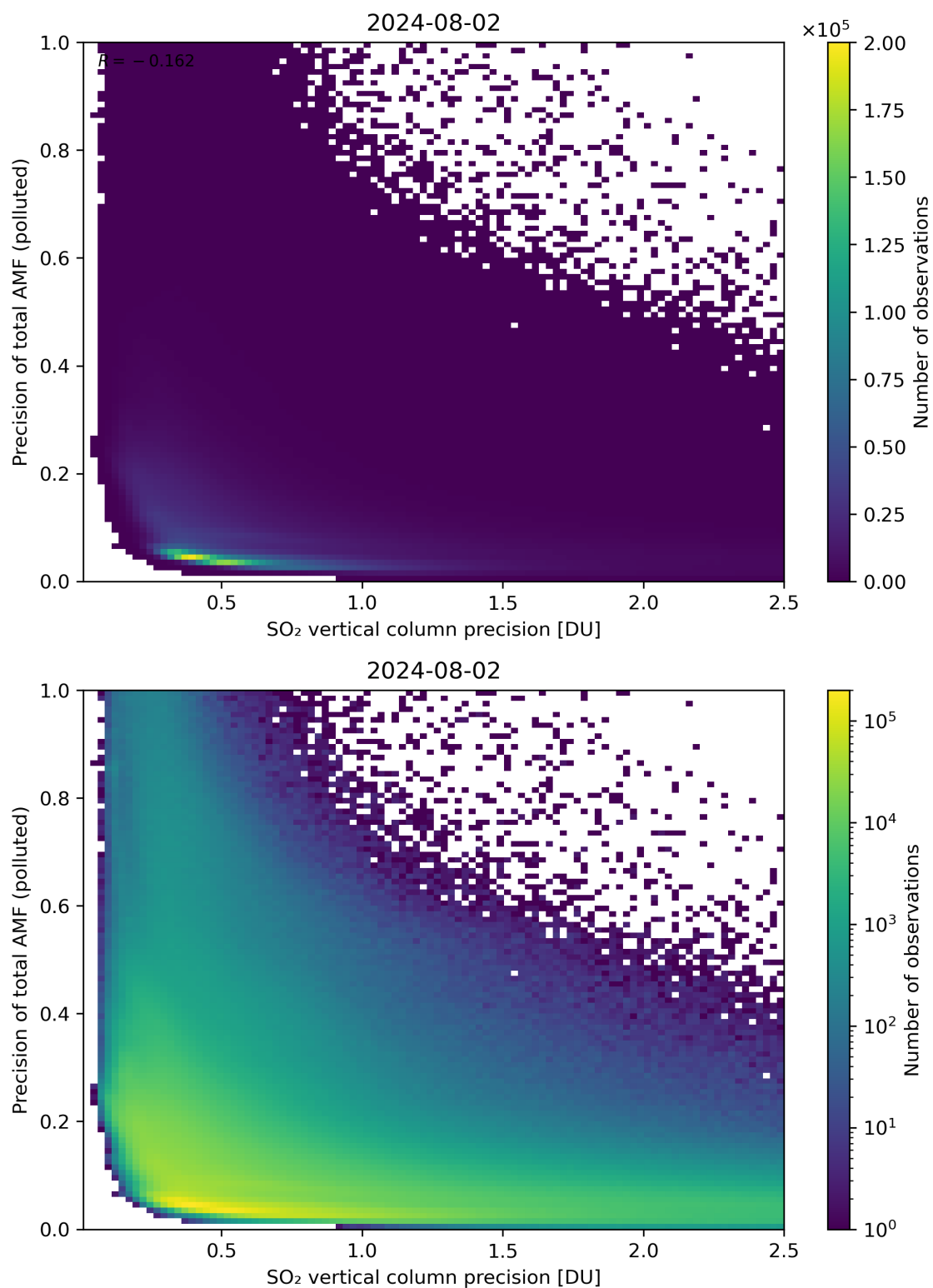
Figure 295: Scatter density plot of “SO 2 vertical column precision” against “Precision of total AMF (polluted)” for 2024-08-01 to 2024-08-03.
