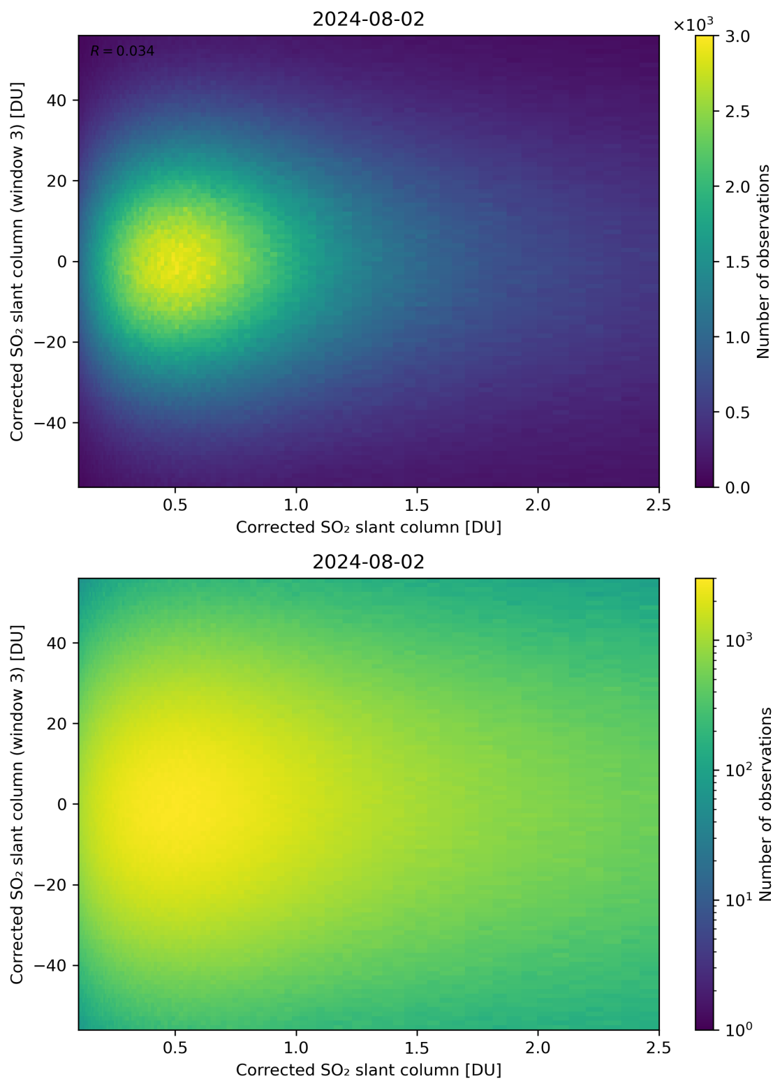
Figure 186: Scatter density plot of “Corrected SO 2 slant column” against “Corrected SO 2 slant column (window 3)” for 2024-08-01 to 2024-08-03.
