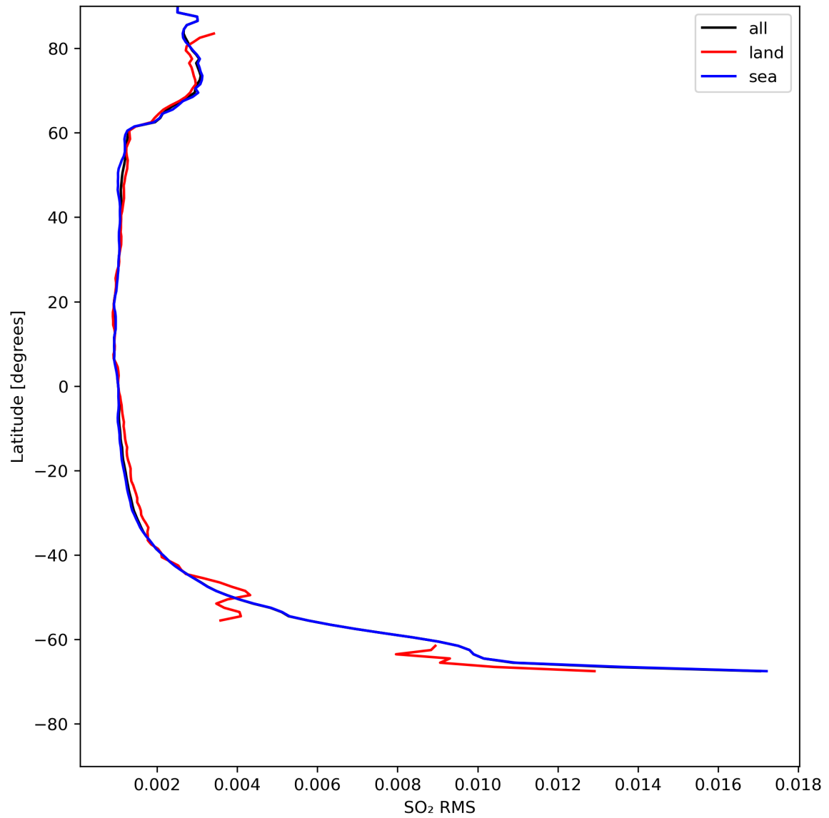
Figure 47: Zonal average of “SO 2 RMS” for 2024-08-01 to 2024-08-03.
