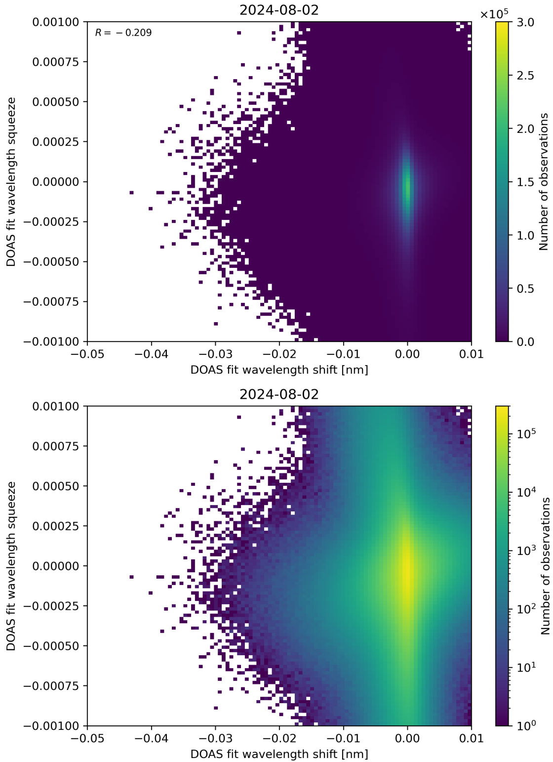
Figure 127: Scatter density plot of “DOAS fit wavelength shift” against “DOAS fit wavelength squeeze” for 2024-08-01 to 2024-08-03.
