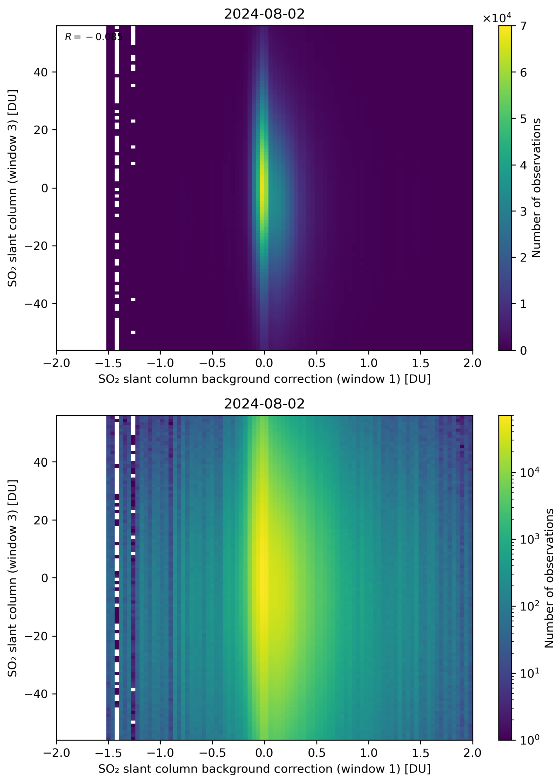
Figure 107: Scatter density plot of “SO 2 slant column background correction (window 1)” against “SO 2 slant column (window 3)” for 2024-08-01 to 2024-08-03.
