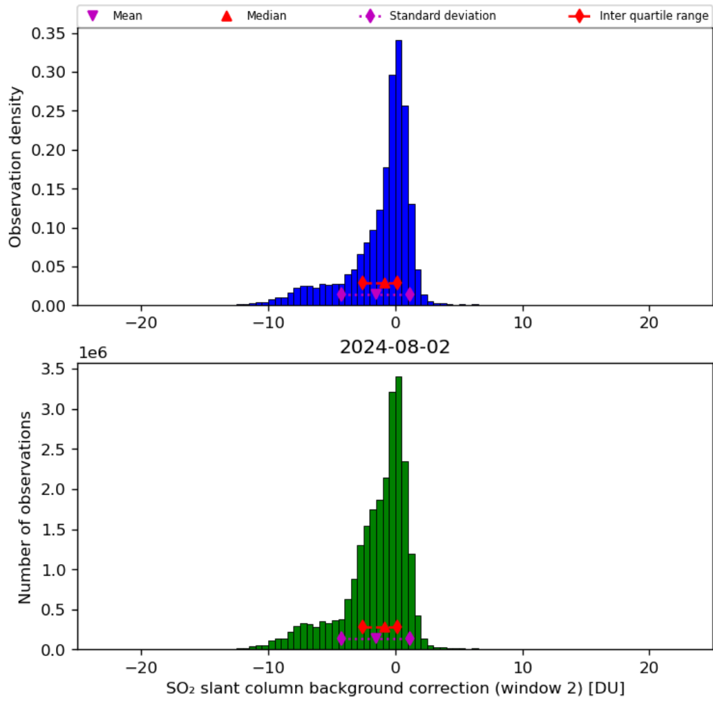
Figure 63: Histogram of “SO 2 slant column background correction (window 2)” for 2024-08-01 to 2024-08-03
