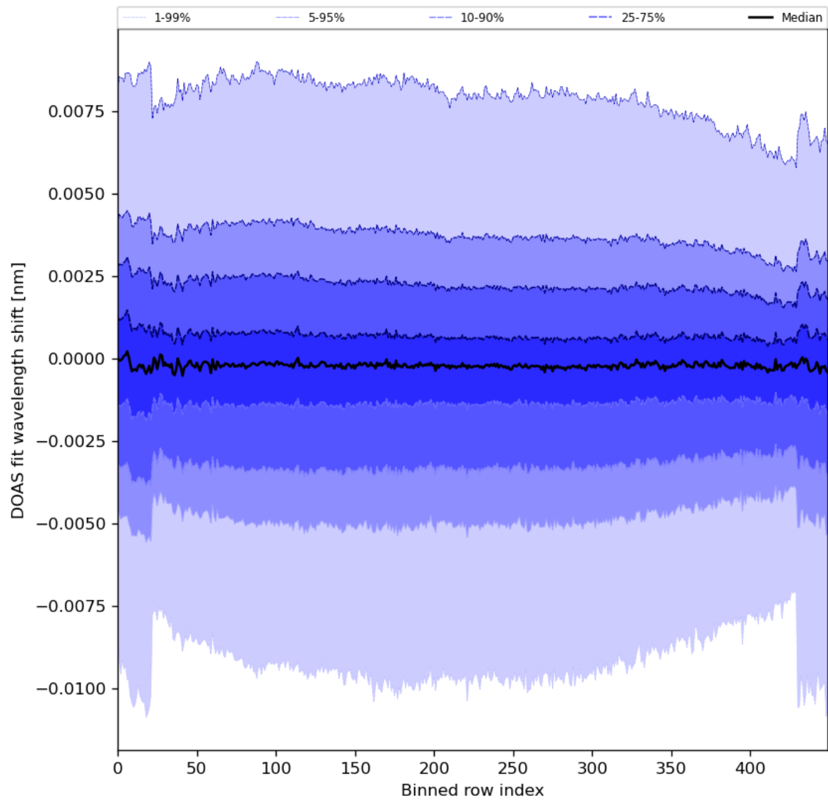
Figure 91: Along track statistics of “DOAS fit wavelength shift” for 2024-08-01 to 2024-08-03
