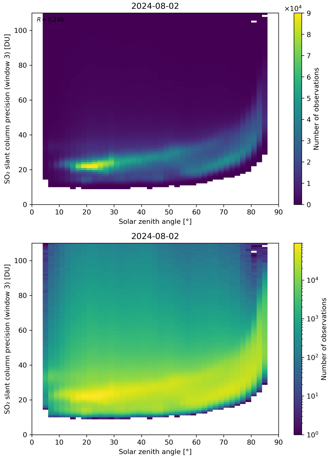
Figure 173: Scatter density plot of “Solar zenith angle” against “SO 2 slant column precision (window 3)” for 2024-08-01 to 2024-08-03.
