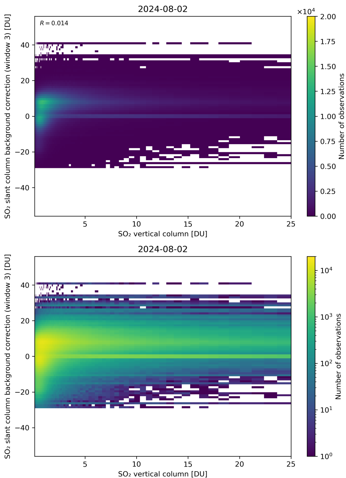
Figure 275: Scatter density plot of “SO 2 vertical column” against “SO 2 slant column background correction (window 3)” for 2024-08-01 to 2024-08-03.
