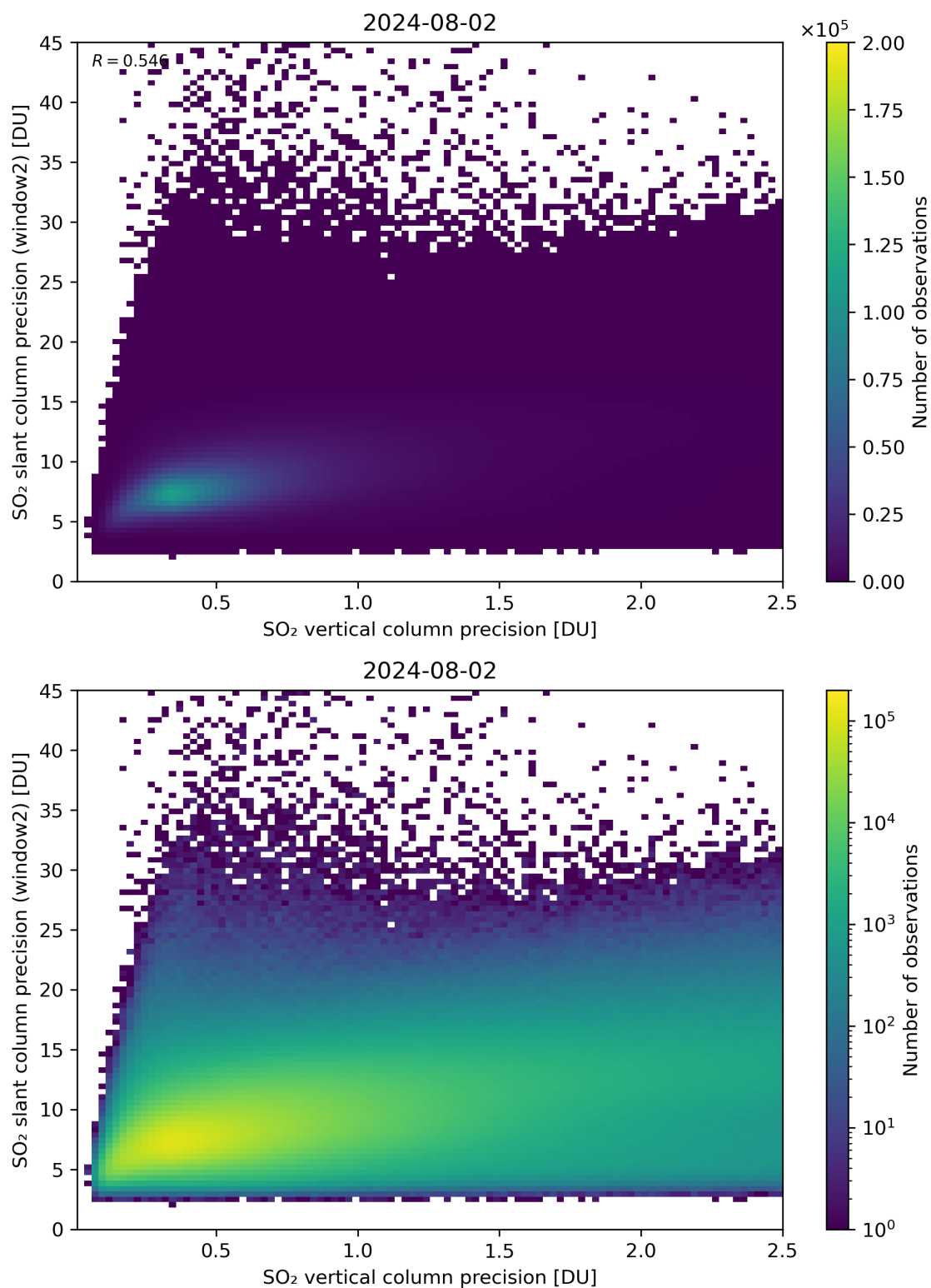
Figure 291: Scatter density plot of “SO 2 vertical column precision” against “SO 2 slant column precision (window2)” for 2024-08-01 to 2024-08-03.
