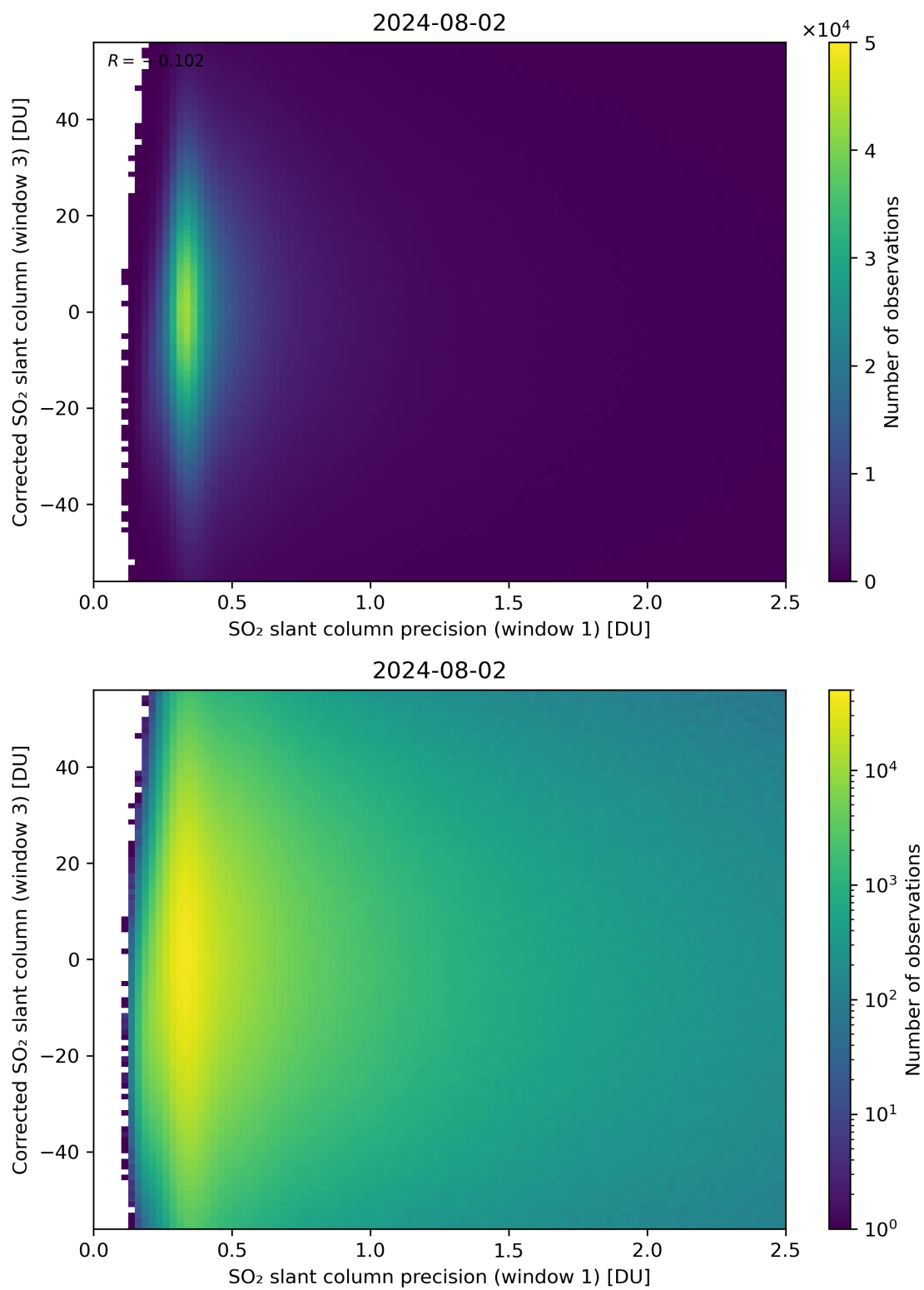
Figure 226: Scatter density plot of “SO 2 slant column precision (window 1)” against “Corrected SO 2 slant column (window 3)” for 2024-08-01 to 2024-08-03.
