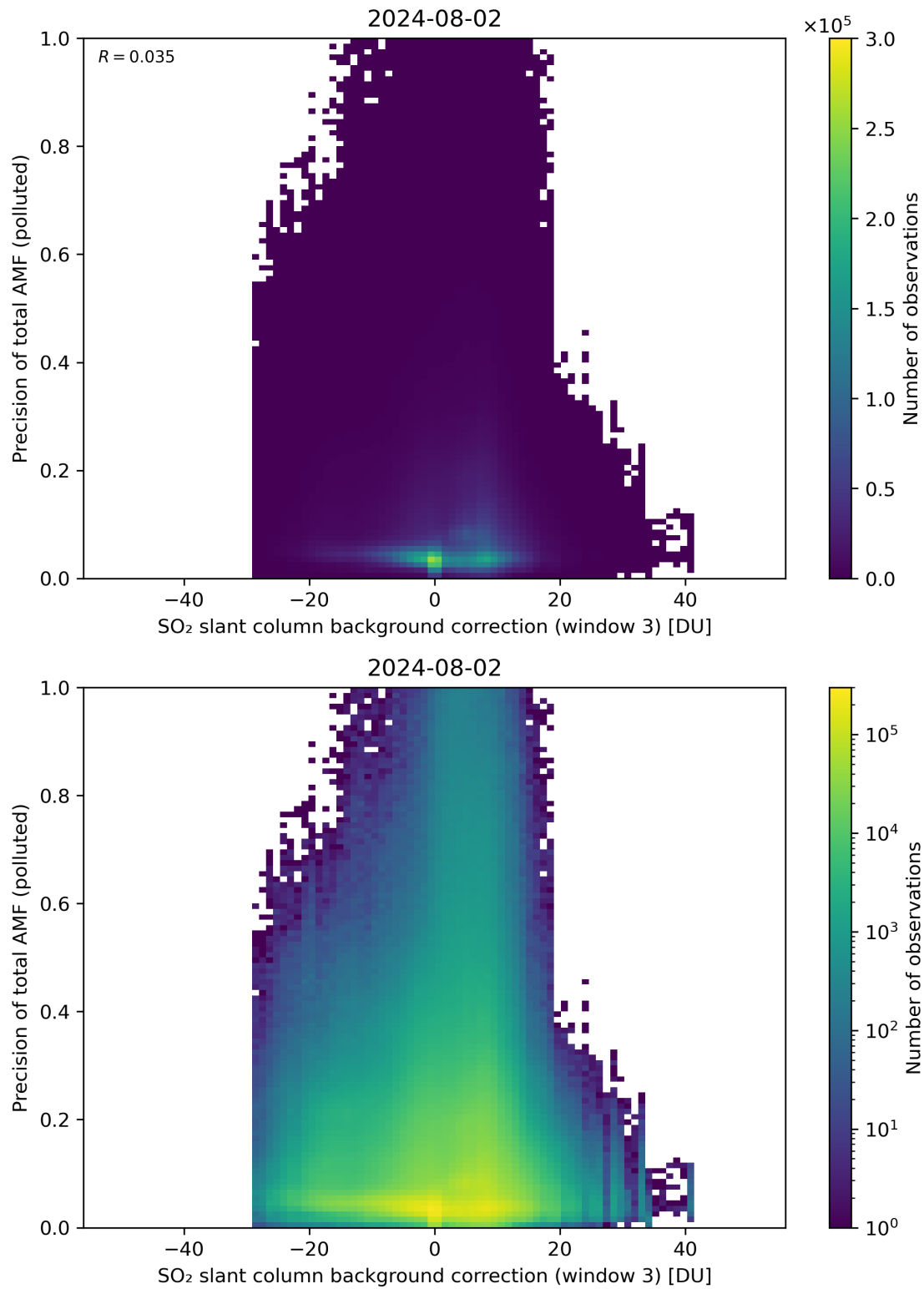
Figure 126: Scatter density plot of “SO 2 slant column background correction (window 3)” against “Precision of total AMF (polluted)” for 2024-08-01 to 2024-08-03.
