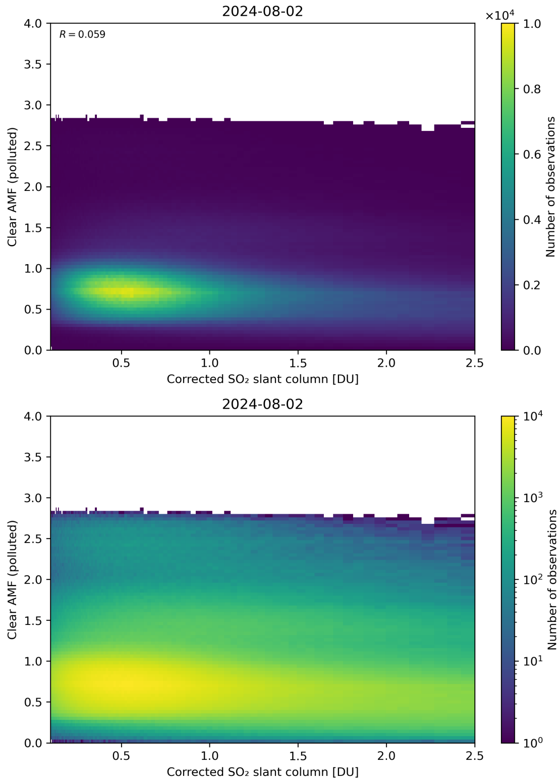
Figure 184: Scatter density plot of “Corrected SO 2 slant column” against “Clear AMF (polluted)” for 2024-08-01 to 2024-08-03.
