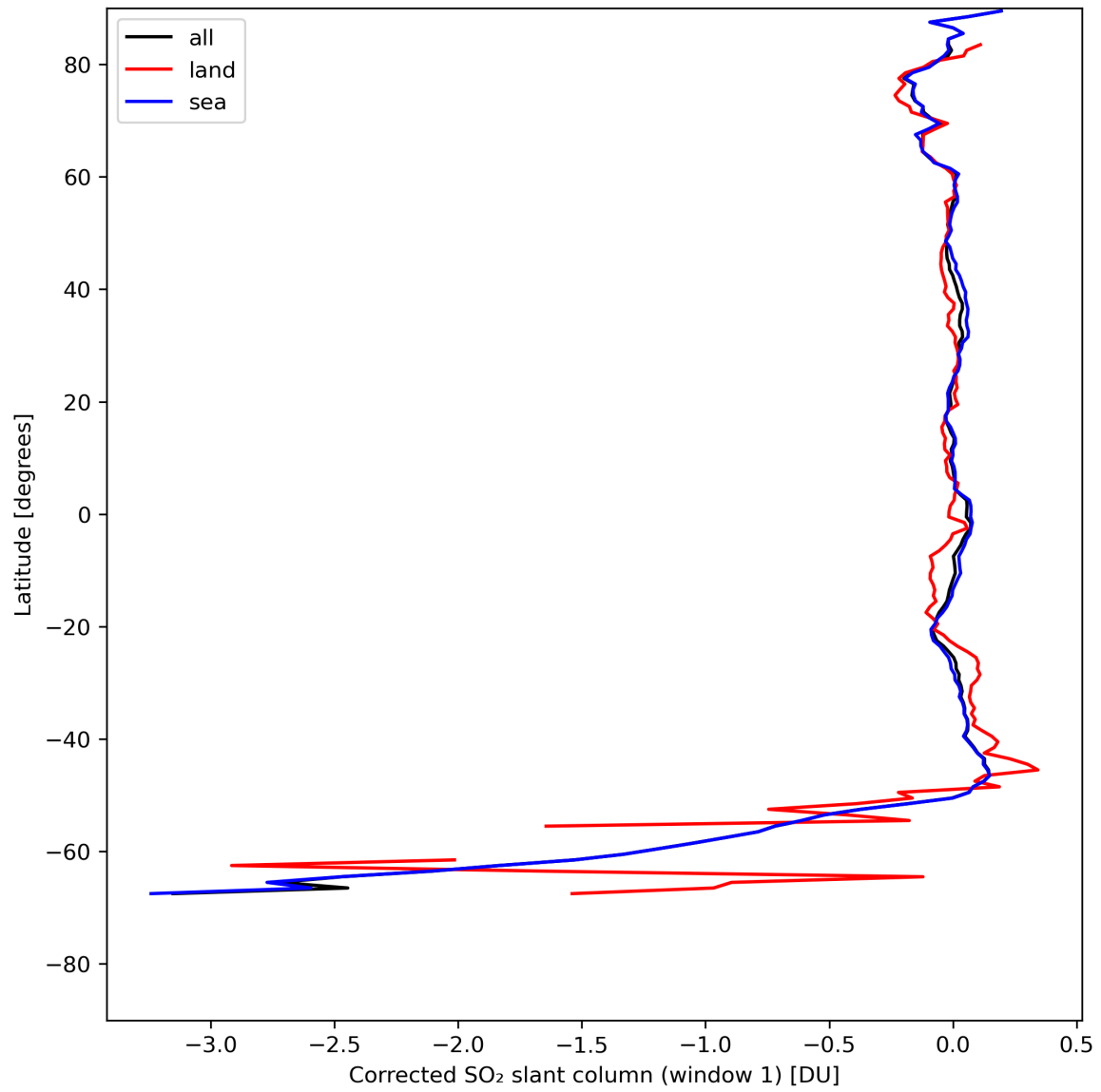
Figure 35: Zonal average of “Corrected SO 2 slant column (window 1)” for 2024-08-01 to 2024-08-03.
