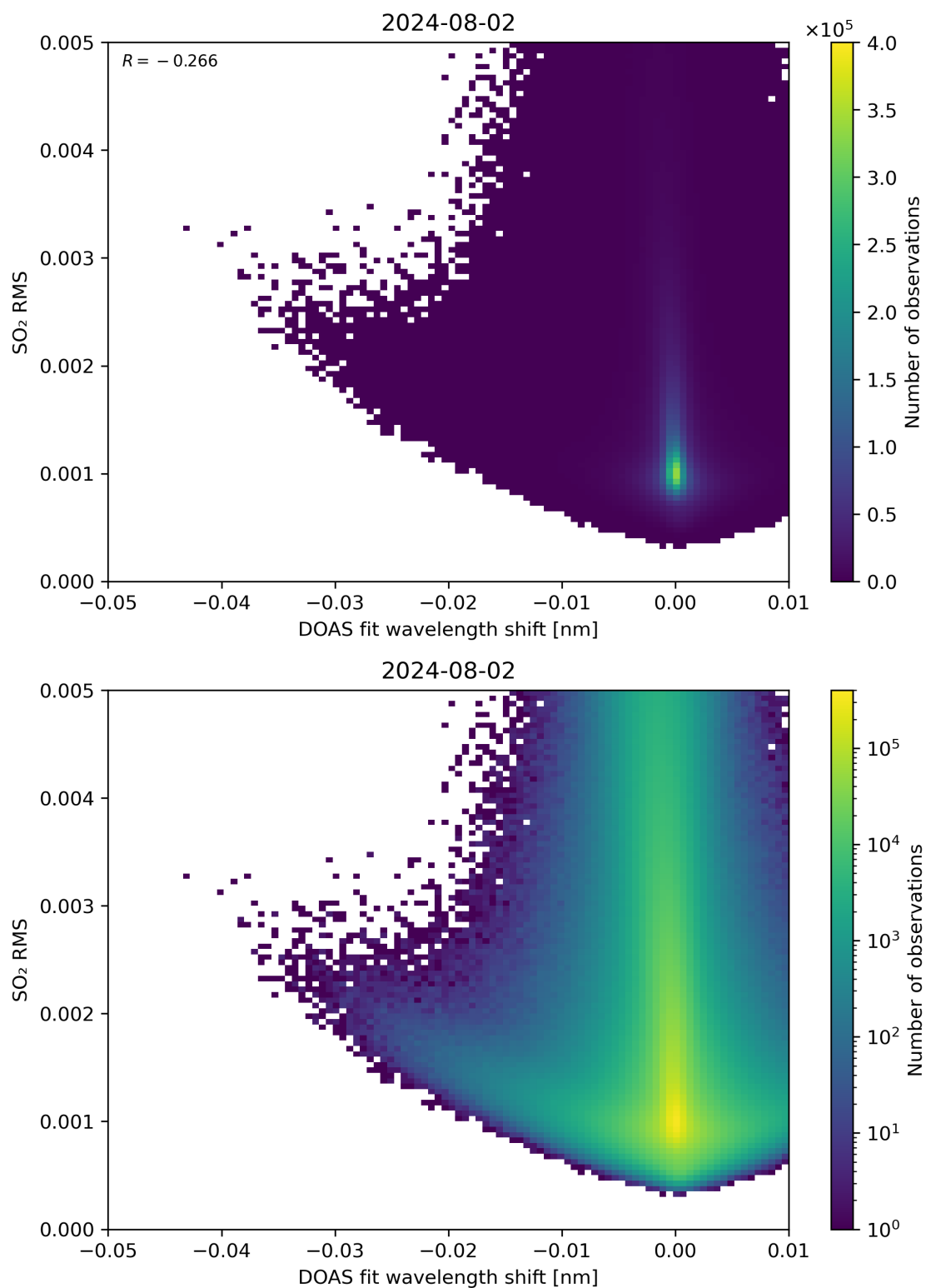
Figure 128: Scatter density plot of “DOAS fit wavelength shift” against “SO 2 RMS” for 2024-08-01 to 2024-08-03.
