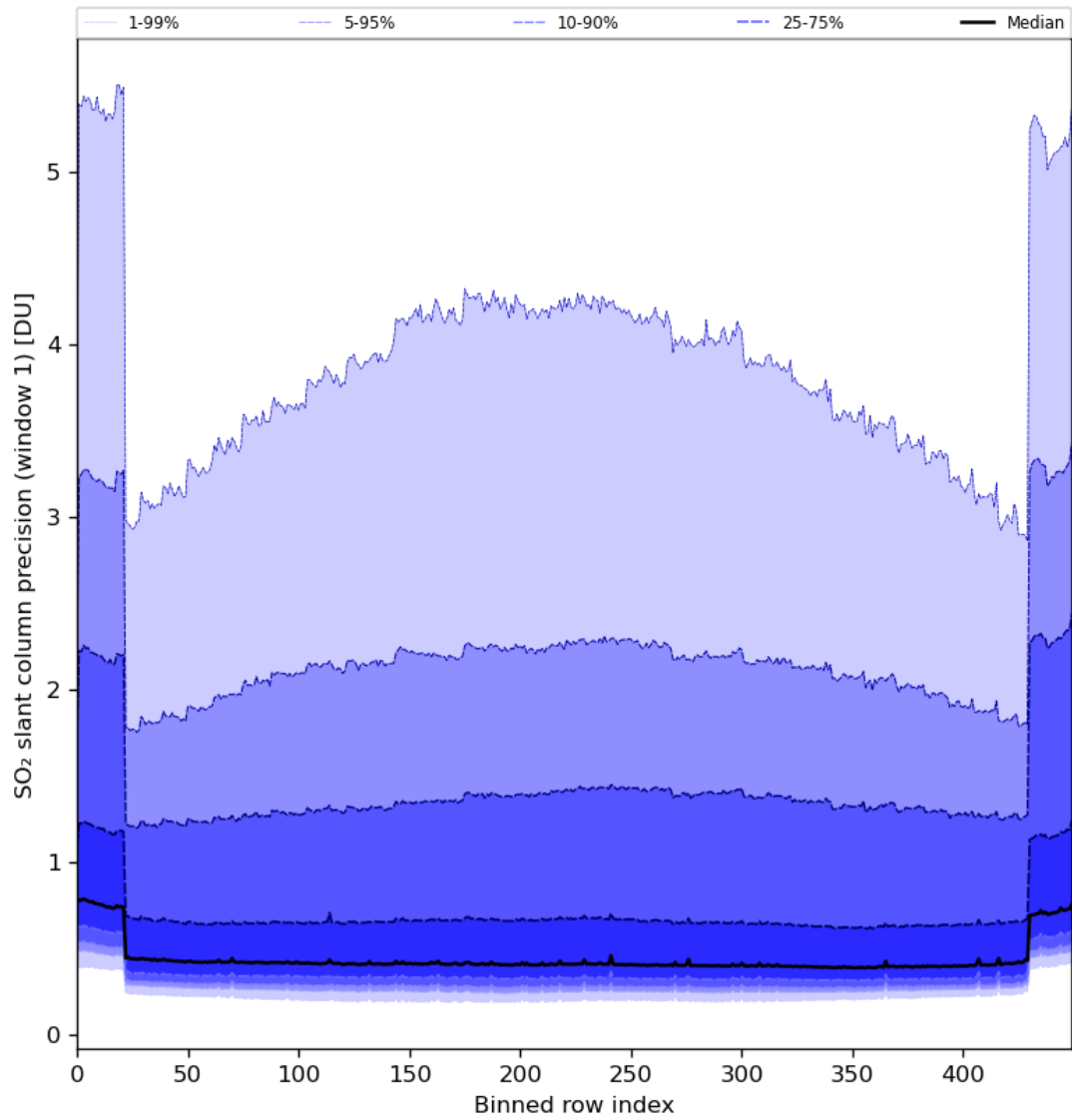
Figure 80: Along track statistics of “SO 2 slant column precision (window 1)” for 2024-08-01 to 2024-08-03
