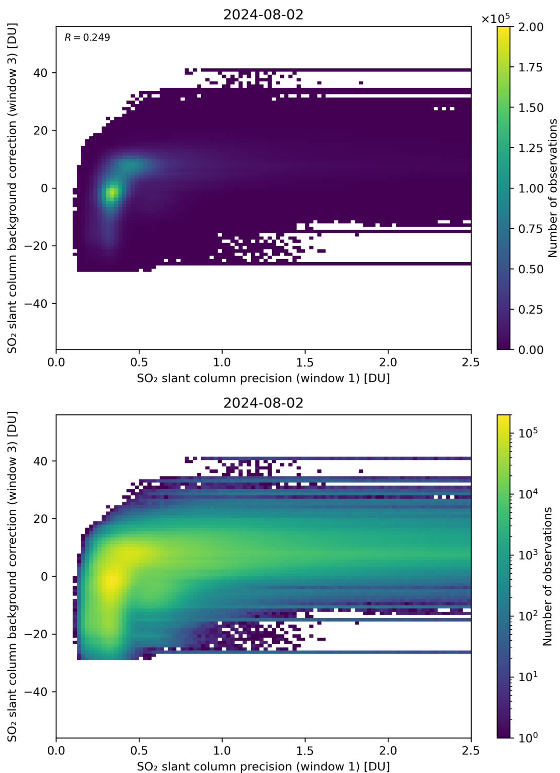
Figure 220: Scatter density plot of “SO 2 slant column precision (window 1)” against “SO 2 slant column background correction (window 3)” for 2024-08-01 to 2024-08-03.
