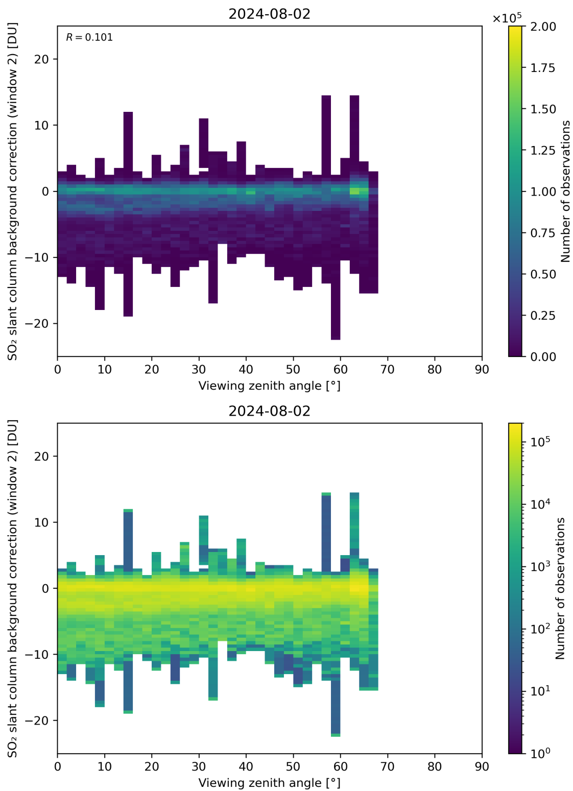
Figure 309: Scatter density plot of “Viewing zenith angle” against “SO 2 slant column background correction (window 2)” for 2024-08-01 to 2024-08-03.
