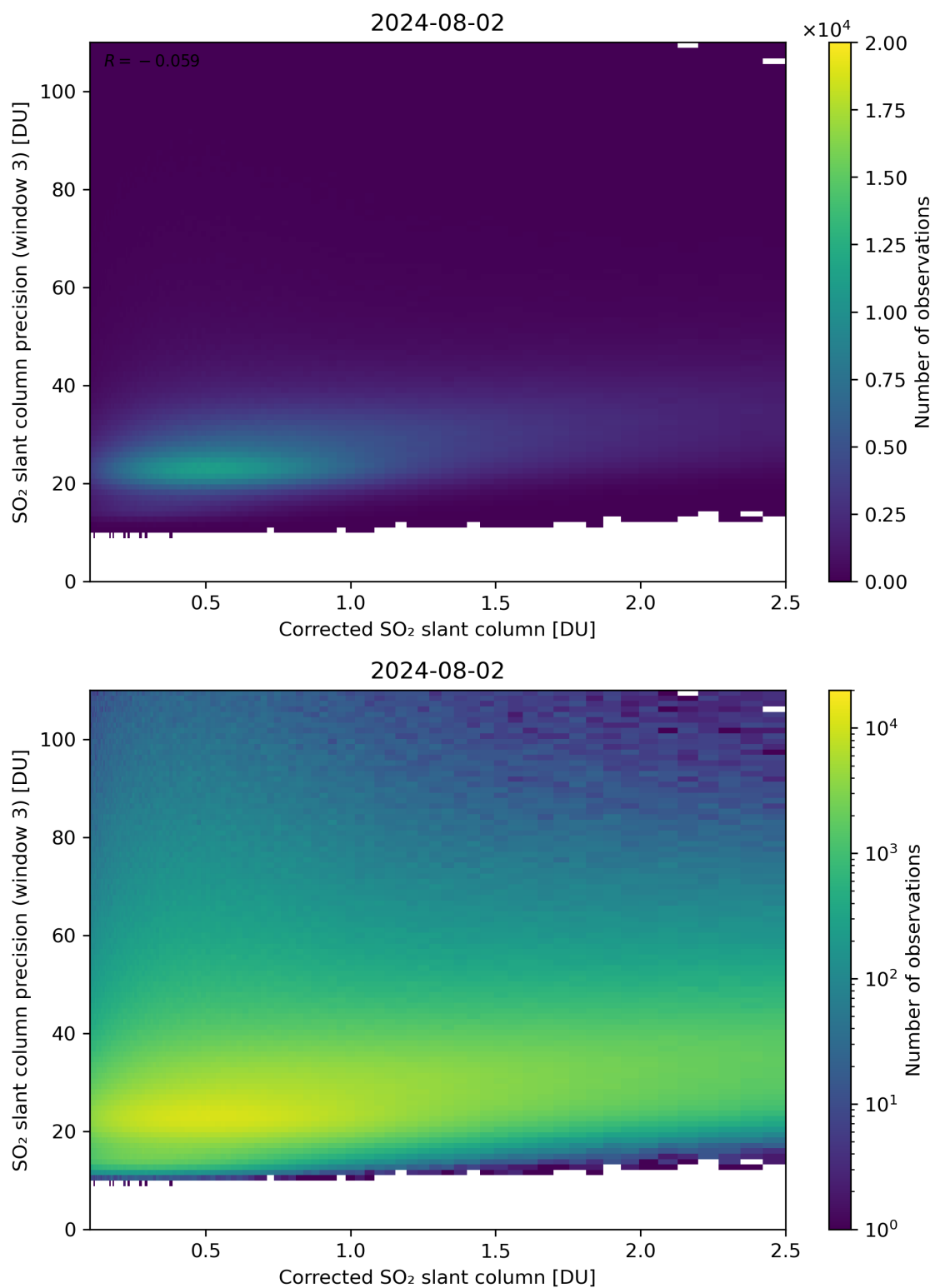
Figure 191: Scatter density plot of “Corrected SO 2 slant column” against “SO 2 slant column precision (window 3)” for 2024-08-01 to 2024-08-03.
