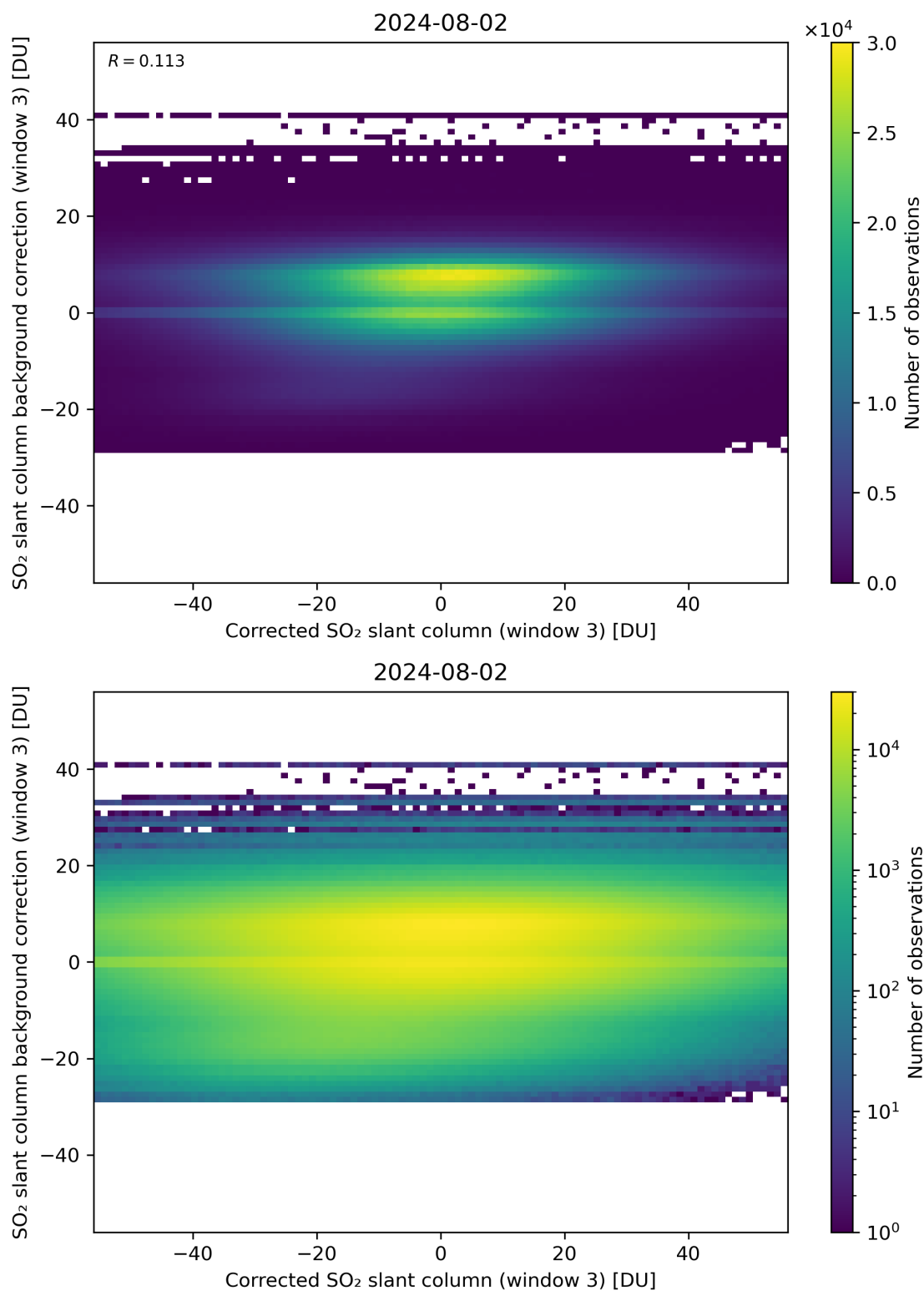
Figure 205: Scatter density plot of “Corrected SO 2 slant column (window 3)” against “SO 2 slant column background correction (window 3)” for 2024-08-01 to 2024-08-03.
