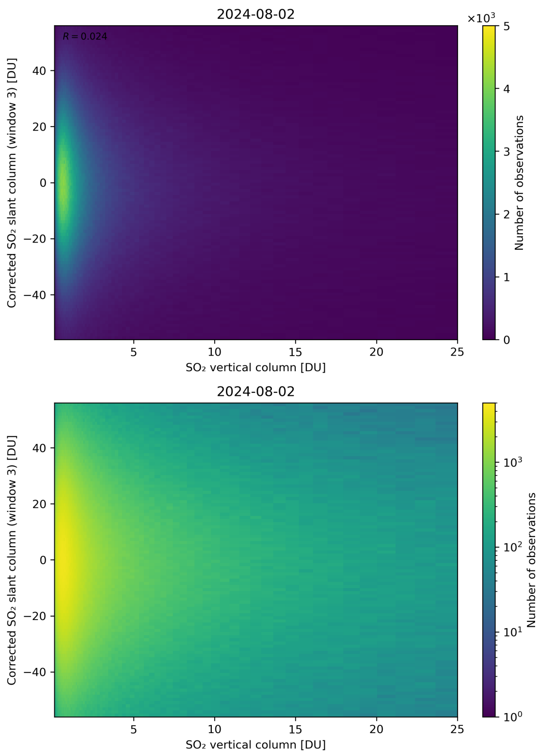
Figure 299: Scatter density plot of “SO 2 vertical column” against “Corrected SO 2 slant column (window 3)” for 2024-08-01 to 2024-08-03.
