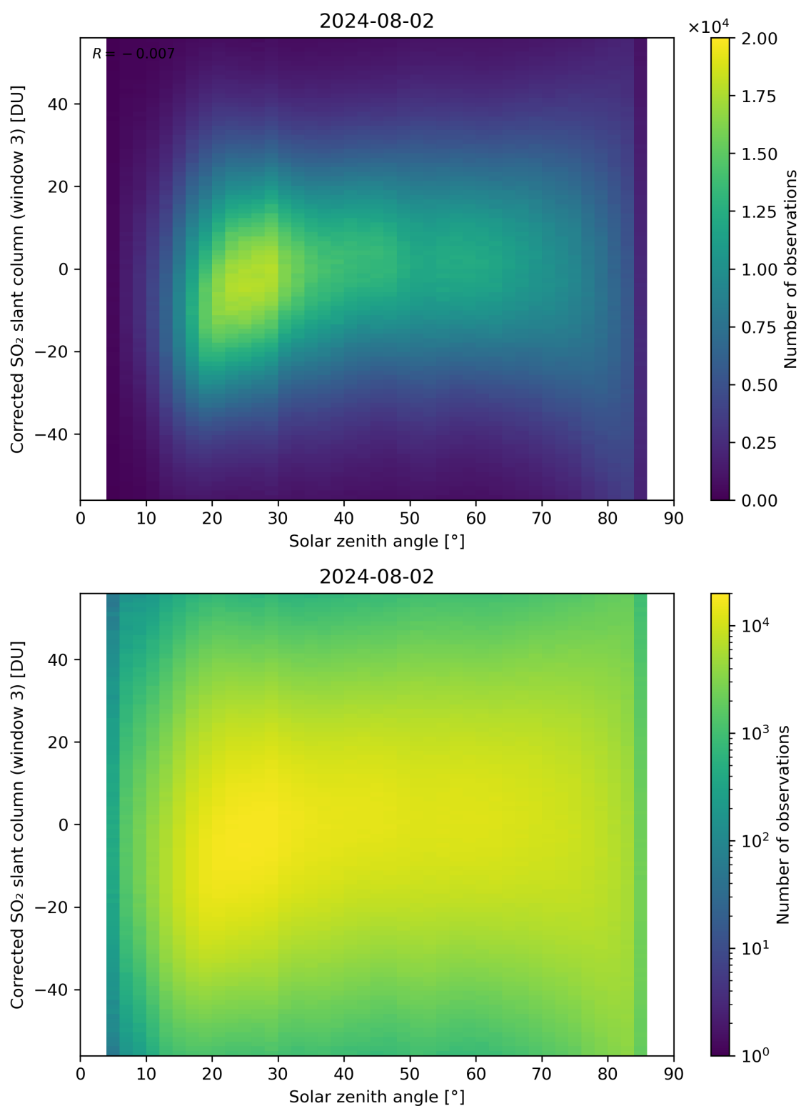
Figure 168: Scatter density plot of “Solar zenith angle” against “Corrected SO 2 slant column (window 3)” for 2024-08-01 to 2024-08-03.
