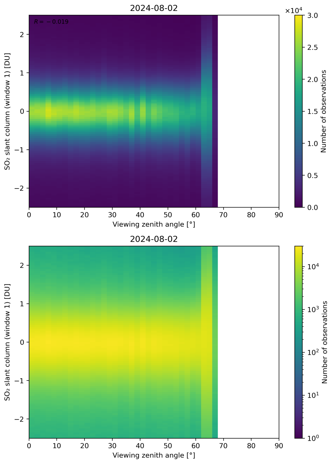
Figure 320: Scatter density plot of “Viewing zenith angle” against “SO 2 slant column (window 1)” for 2024-08-01 to 2024-08-03.
