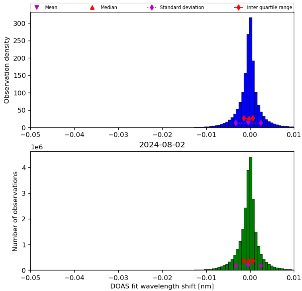
Figure 68: Histogram of “DOAS fit wavelength shift” for 2024-08-01 to 2024-08-03
