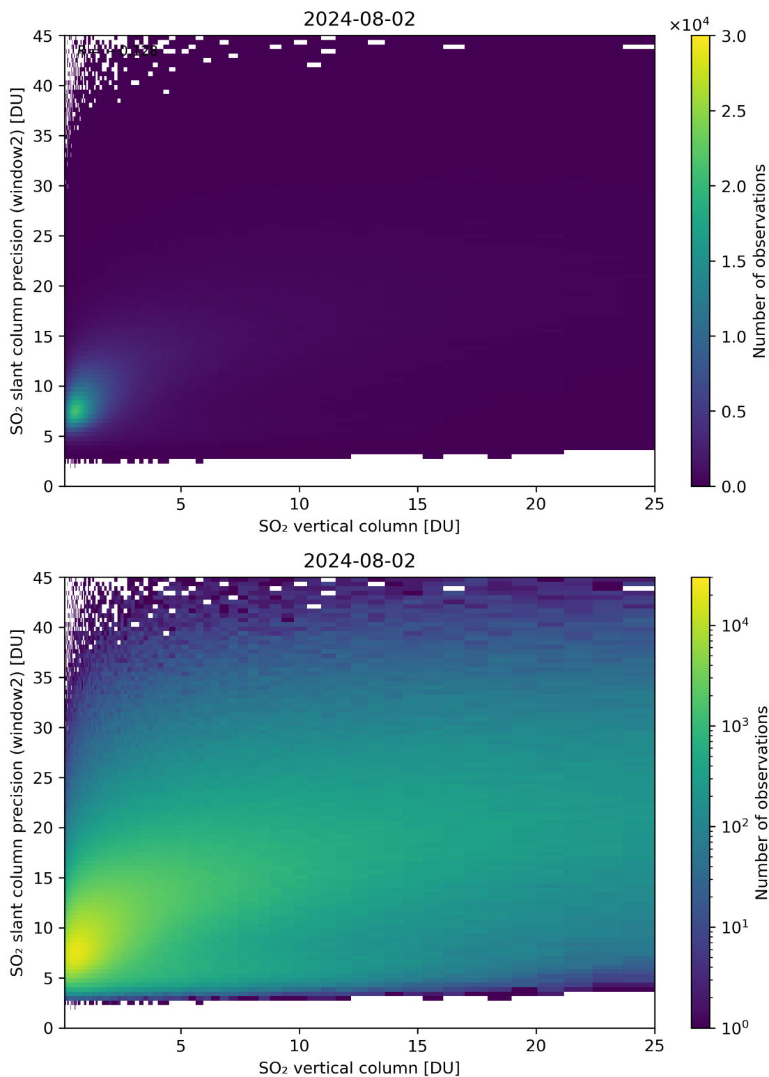
Figure 302: Scatter density plot of “SO 2 vertical column” against “SO 2 slant column precision (window2)” for 2024-08-01 to 2024-08-03.
