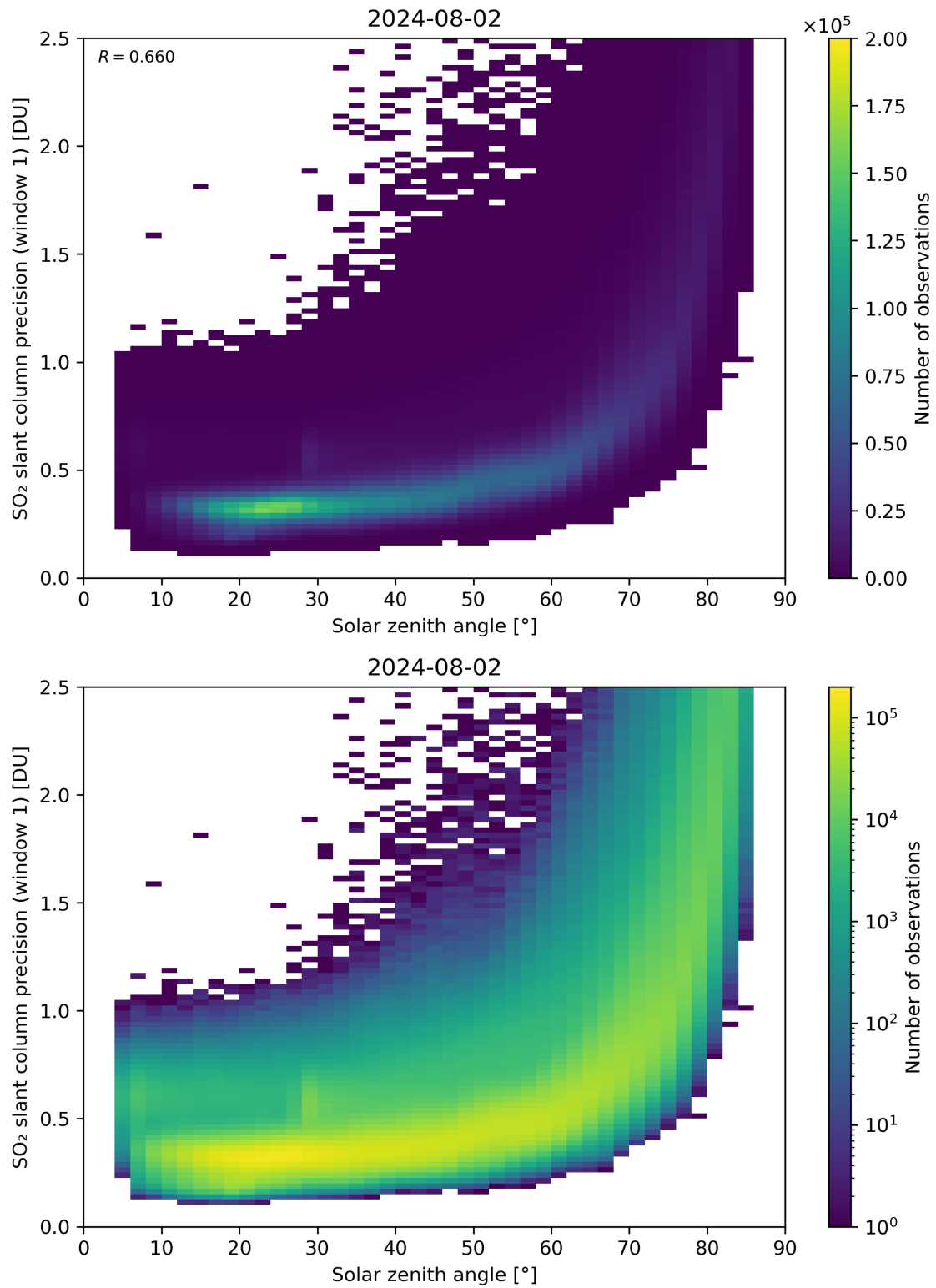
Figure 170: Scatter density plot of “Solar zenith angle” against “SO 2 slant column precision (window 1)” for 2024-08-01 to 2024-08-03.
