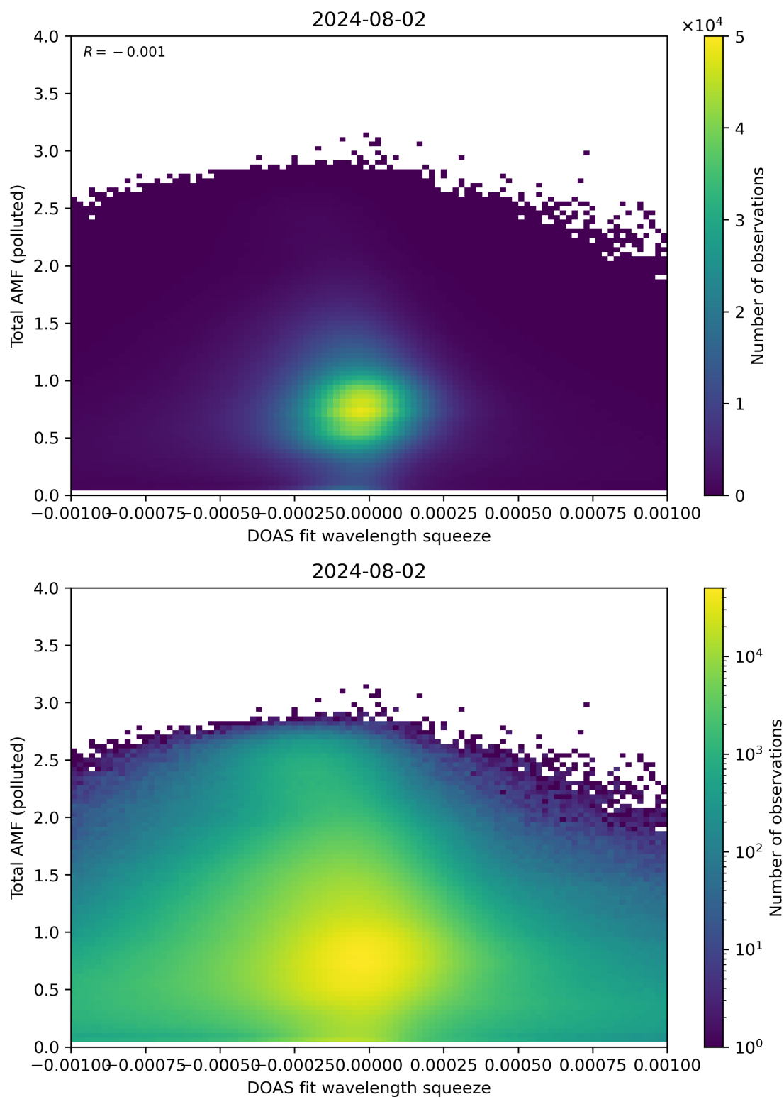
Figure 134: Scatter density plot of “DOAS fit wavelength squeeze” against “Total AMF (polluted)” for 2024-08-01 to 2024-08-03.
