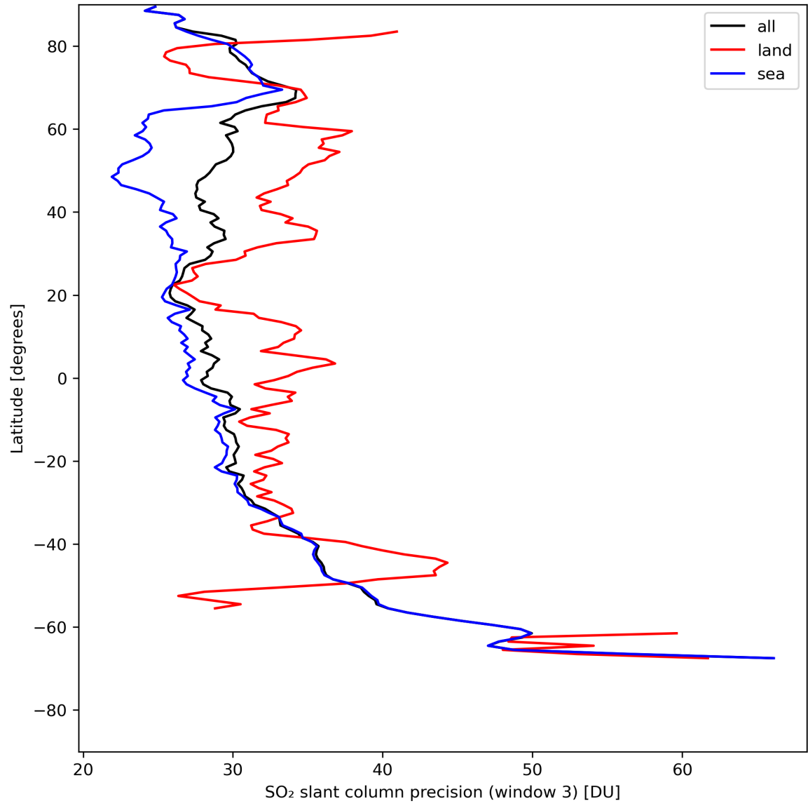
Figure 42: Zonal average of “SO 2 slant column precision (window 3)” for 2024-08-01 to 2024-08-03.
