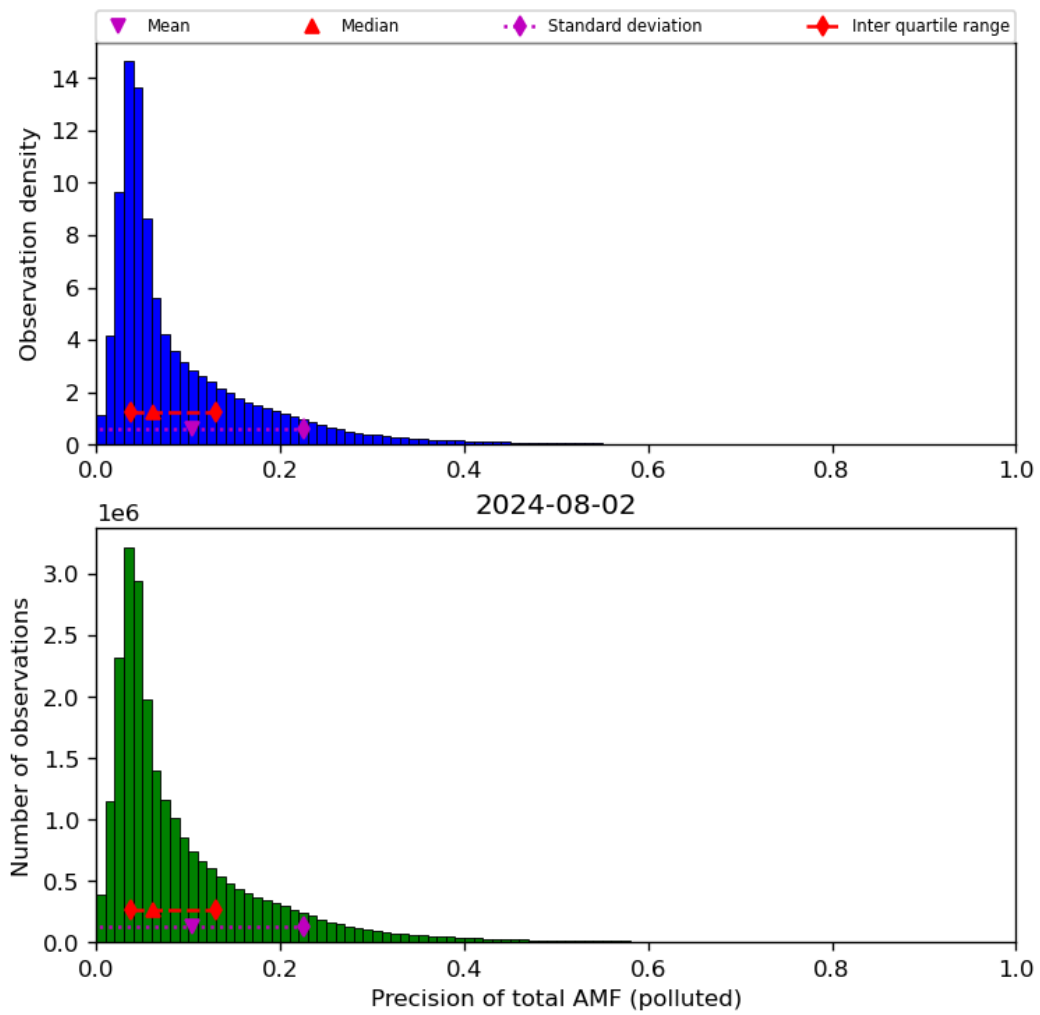
Figure 72: Histogram of “Precision of total AMF (polluted)” for 2024-08-01 to 2024-08-03
