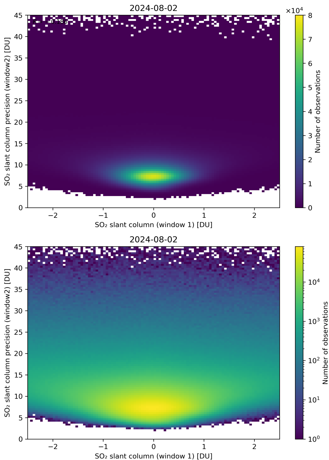
Figure 236: Scatter density plot of “SO 2 slant column (window 1)” against “SO 2 slant column precision (window2)” for 2024-08-01 to 2024-08-03.
