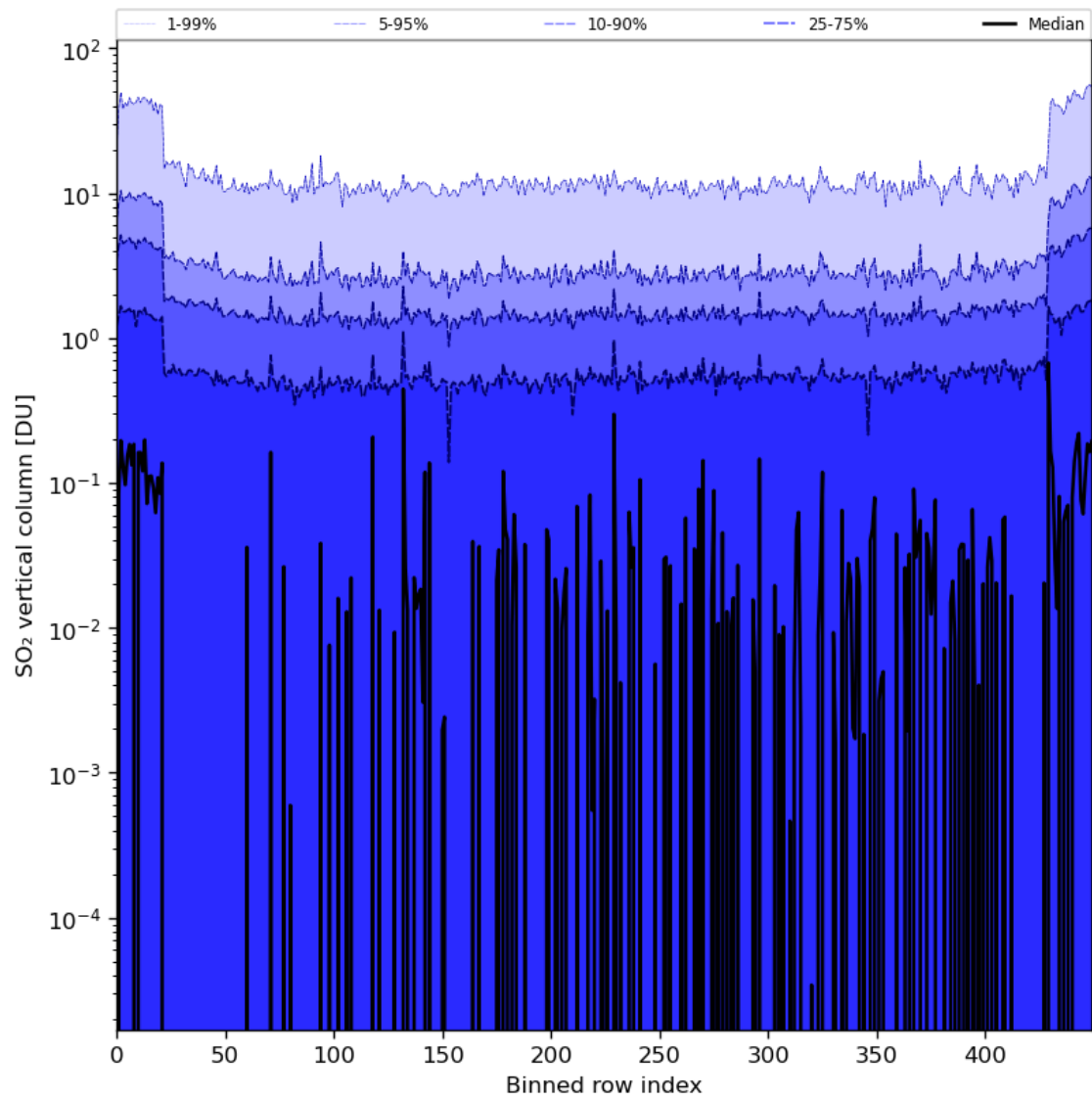
Figure 76: Along track statistics of “SO 2 vertical column” for 2024-08-01 to 2024-08-03
