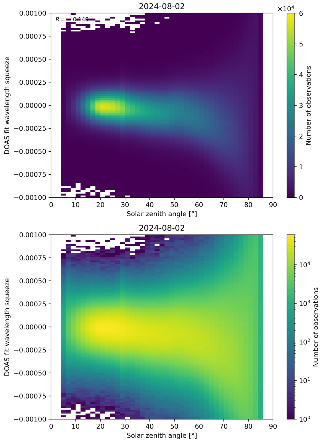
Figure 162: Scatter density plot of “Solar zenith angle” against “DOAS fit wavelength squeeze” for 2024-08-01 to 2024-08-03.
