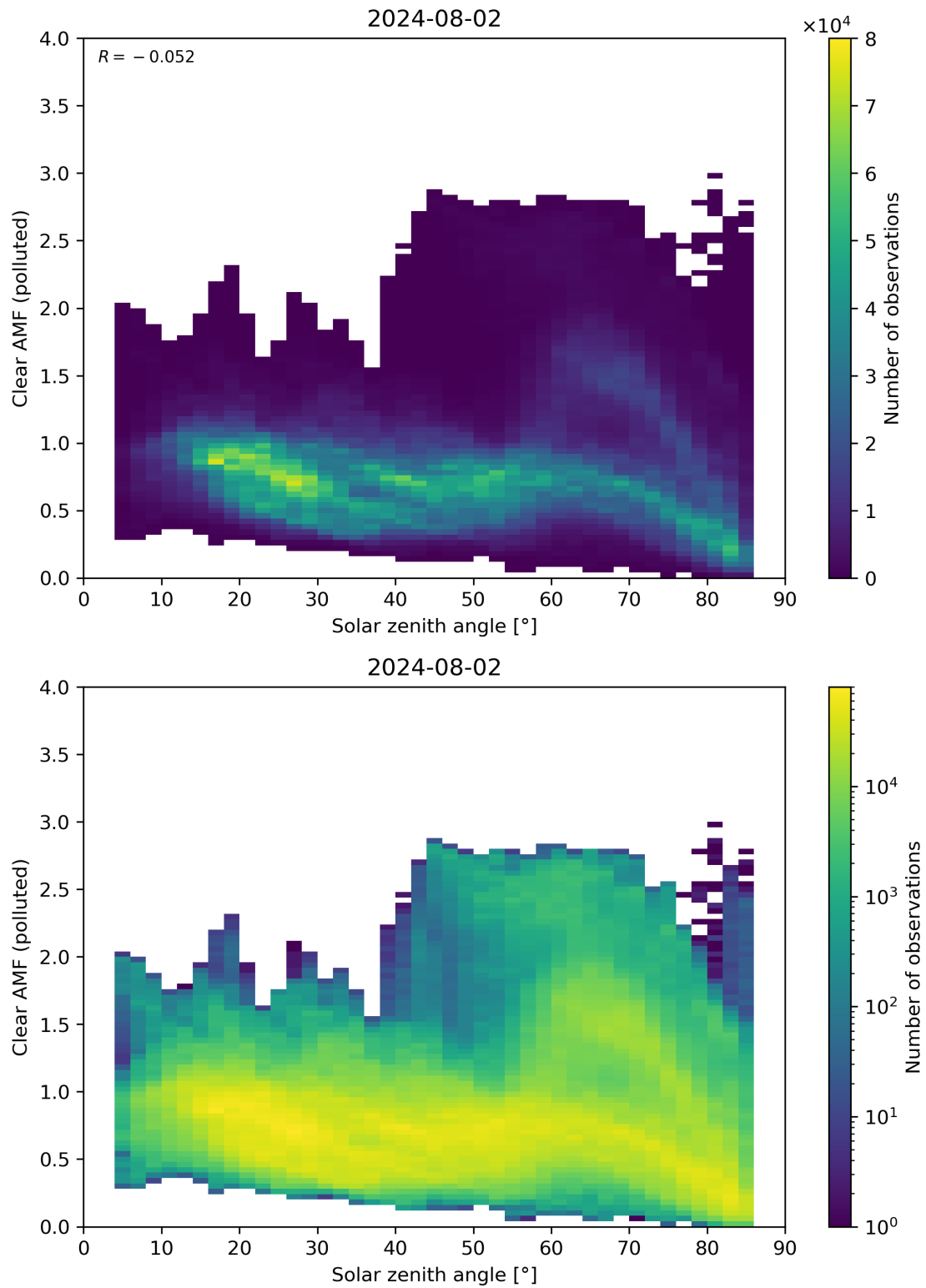
Figure 165: Scatter density plot of “Solar zenith angle” against “Clear AMF (polluted)” for 2024-08-01 to 2024-08-03.
