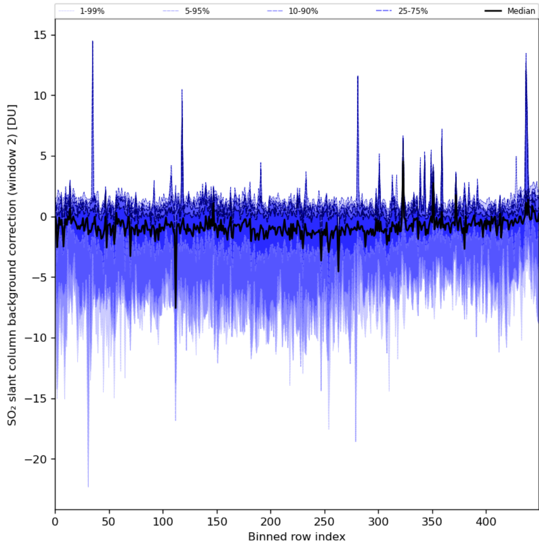
Figure 86: Along track statistics of “SO 2 slant column background correction (window 2)” for 2024-08-01 to 2024-08-03
