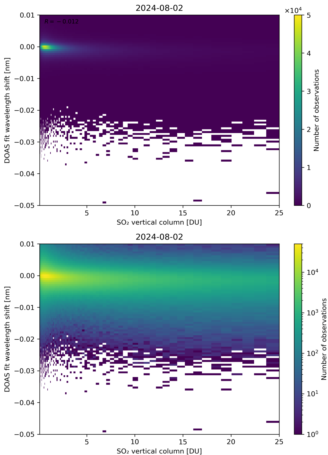
Figure 276: Scatter density plot of “SO 2 vertical column” against “DOAS fit wavelength shift” for 2024-08-01 to 2024-08-03.
