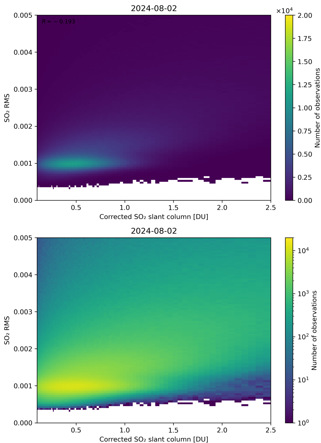
Figure 183: Scatter density plot of “Corrected SO 2 slant column” against “SO 2 RMS” for 2024-08-01 to 2024-08-03.
