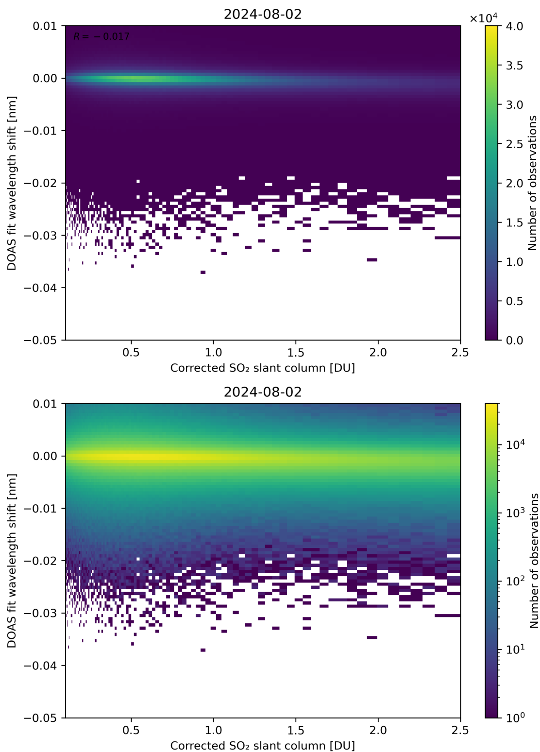
Figure 181: Scatter density plot of “Corrected SO 2 slant column” against “DOAS fit wavelength shift” for 2024-08-01 to 2024-08-03.
