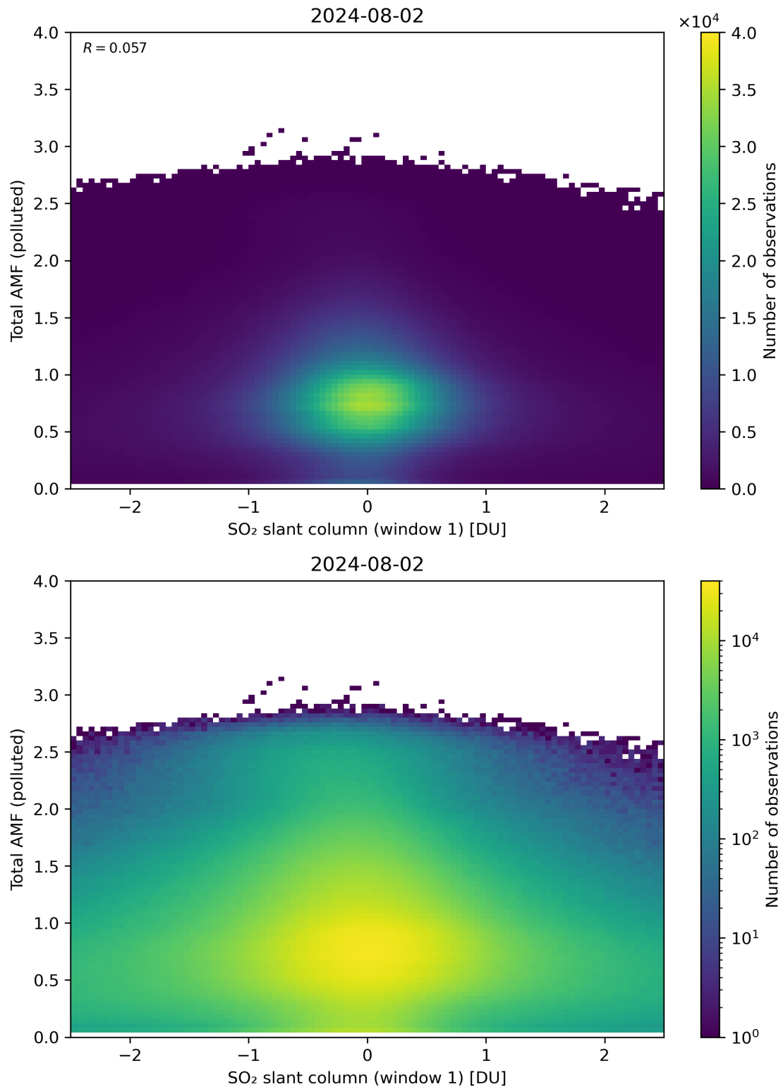
Figure 239: Scatter density plot of “SO 2 slant column (window 1)” against “Total AMF (polluted)” for 2024-08-01 to 2024-08-03.
