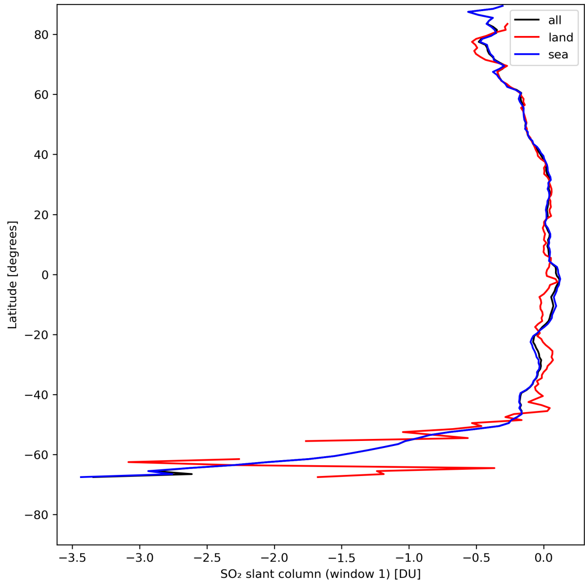
Figure 33: Zonal average of “SO 2 slant column (window 1)” for 2024-08-01 to 2024-08-03.
