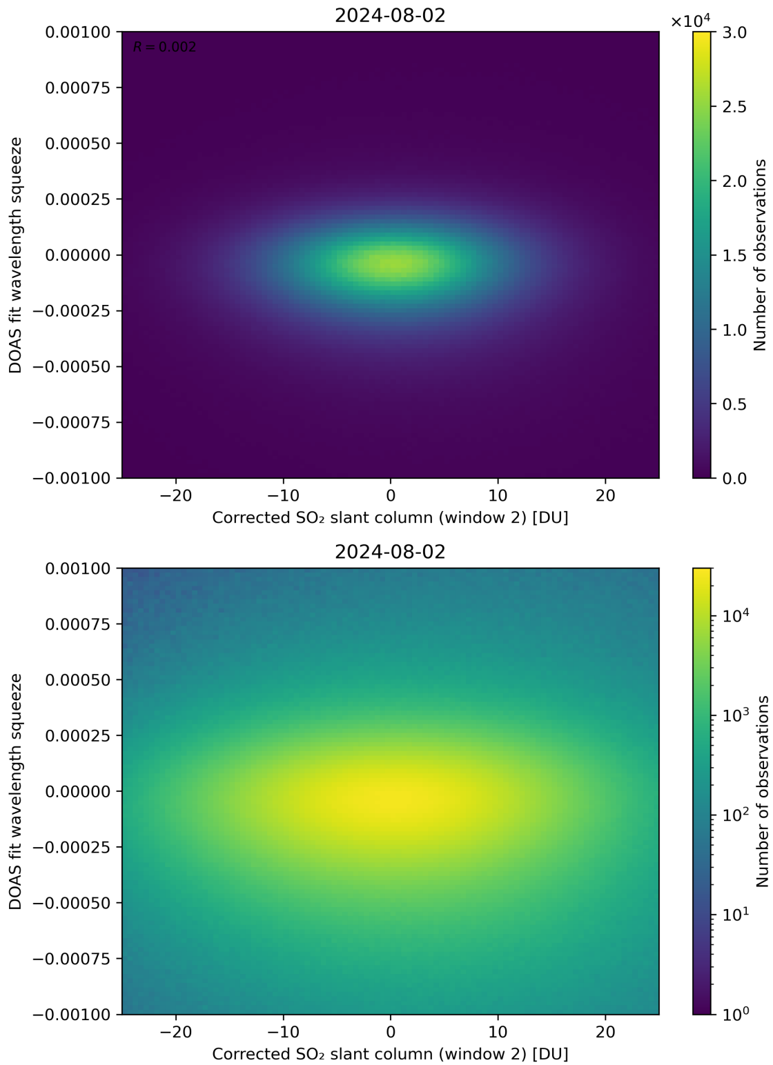
Figure 197: Scatter density plot of “Corrected SO 2 slant column (window 2)” against “DOAS fit wavelength squeeze” for 2024-08-01 to 2024-08-03.
