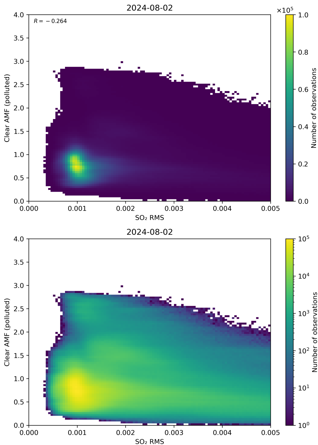
Figure 136: Scatter density plot of “SO 2 RMS” against “Clear AMF (polluted)” for 2024-08-01 to 2024-08-03.
