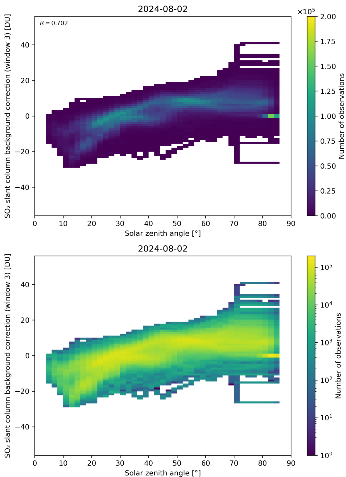
Figure 160: Scatter density plot of “Solar zenith angle” against “SO 2 slant column background correction (window 3)” for 2024-08-01 to 2024-08-03.
