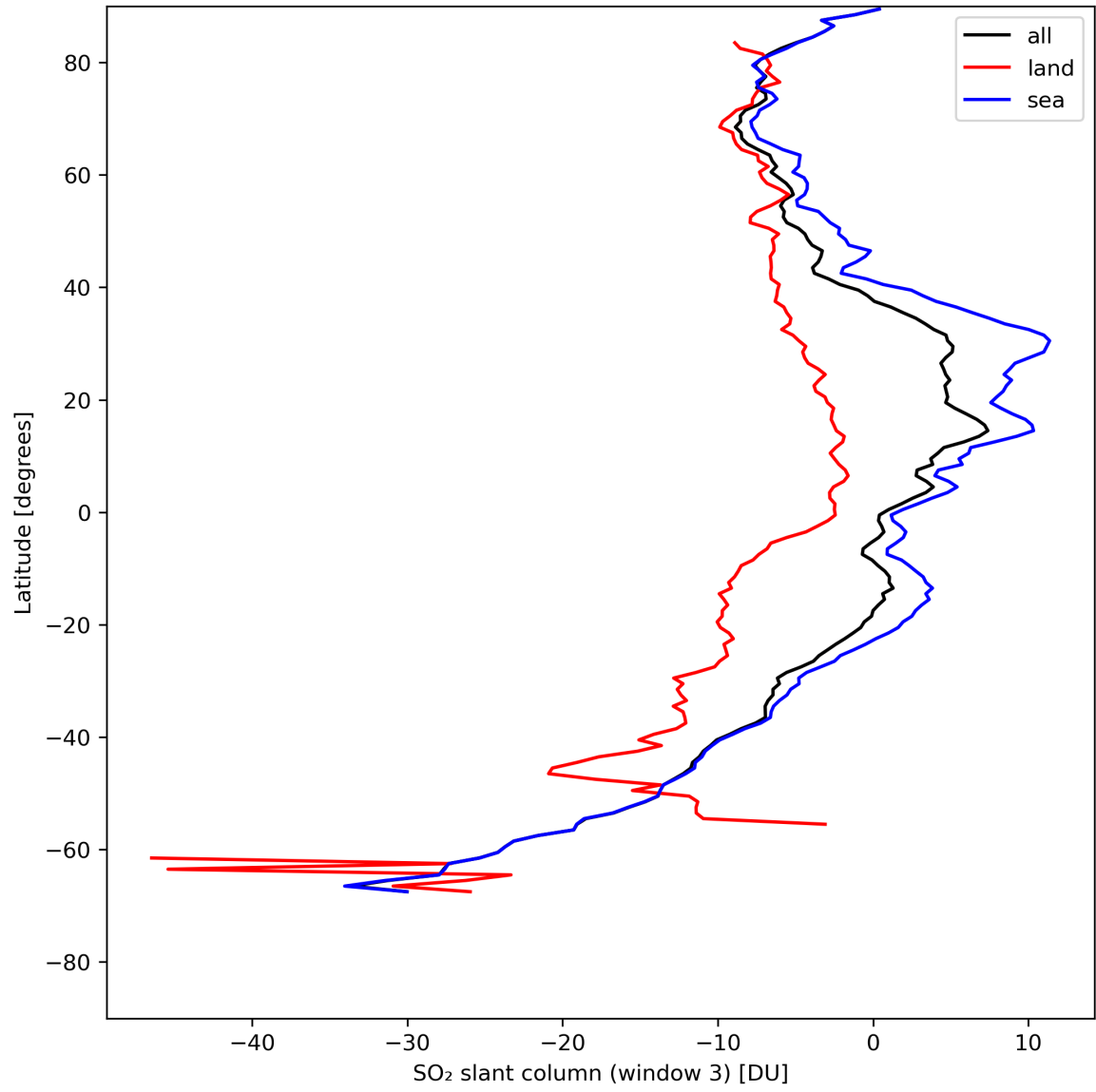
Figure 41: Zonal average of “SO 2 slant column (window 3)” for 2024-08-01 to 2024-08-03.
