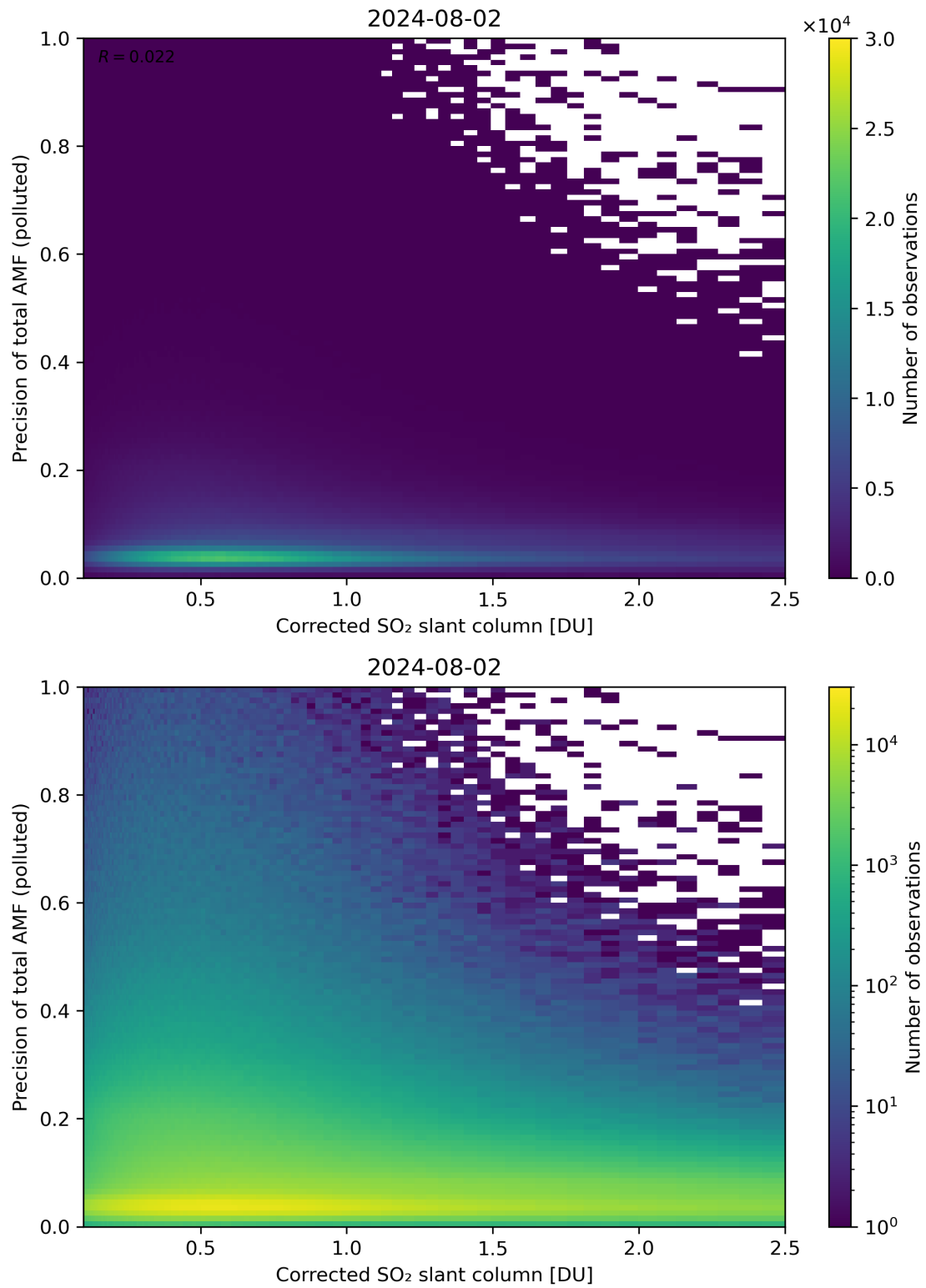
Figure 193: Scatter density plot of “Corrected SO 2 slant column” against “Precision of total AMF (polluted)” for 2024-08-01 to 2024-08-03.
