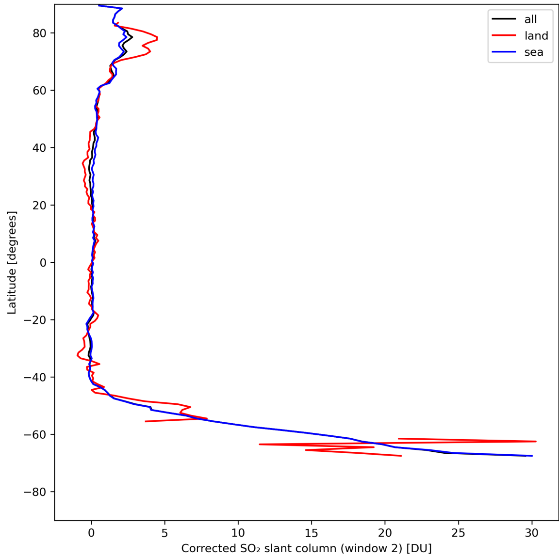
Figure 39: Zonal average of “Corrected SO 2 slant column (window 2)” for 2024-08-01 to 2024-08-03.
