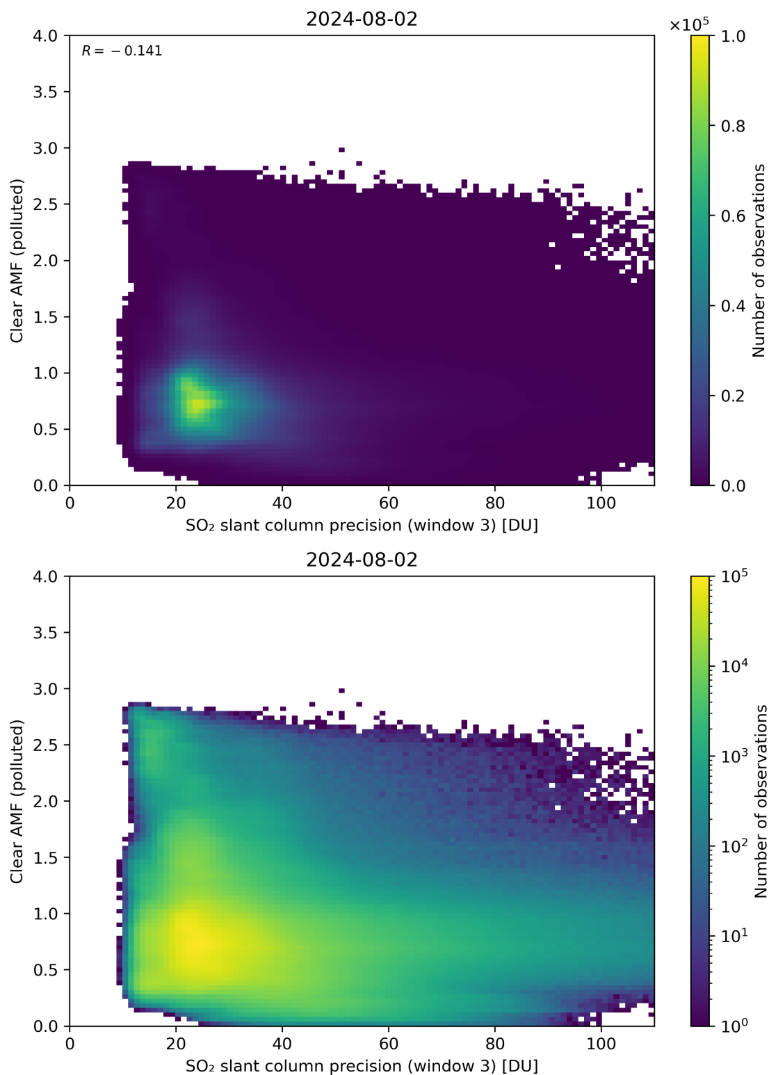
Figure 261: Scatter density plot of “SO 2 slant column precision (window 3)” against “Clear AMF (polluted)” for 2024-08-01 to 2024-08-03.
