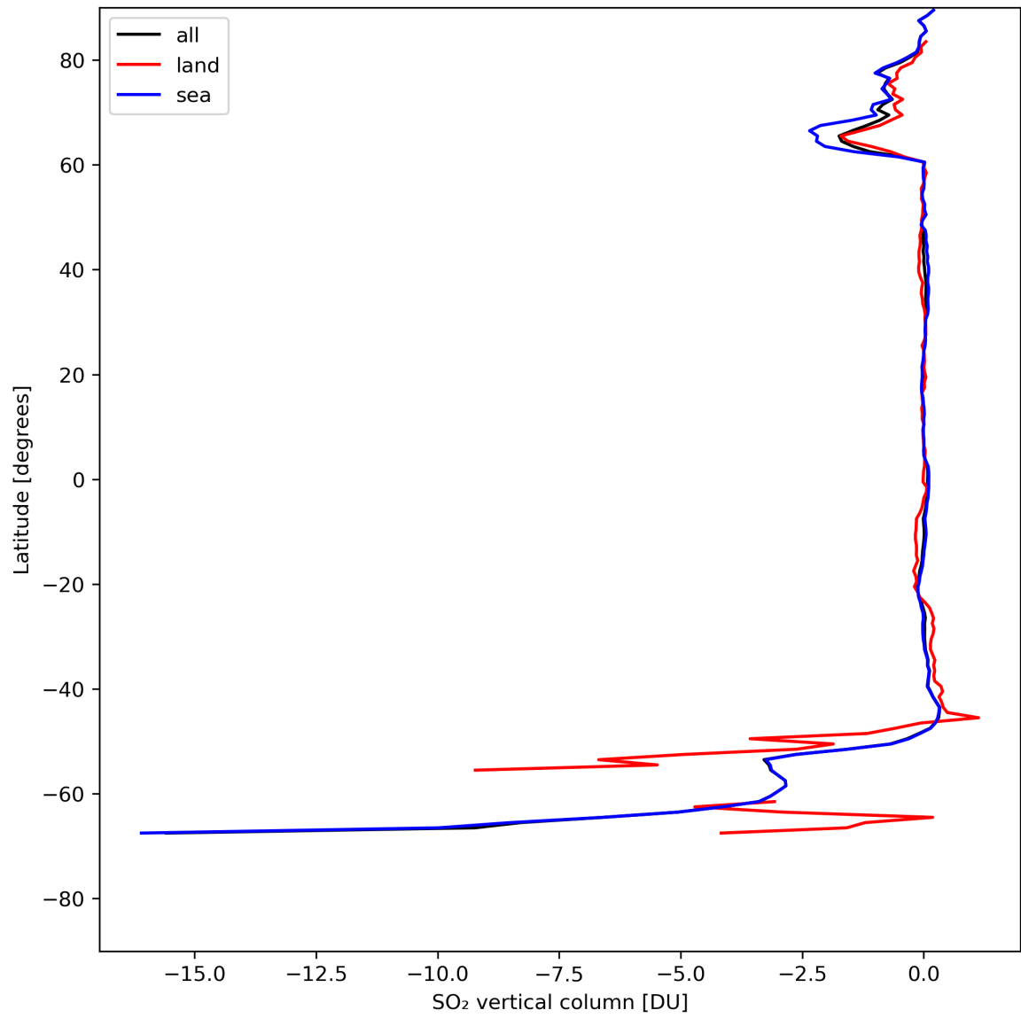
Figure 30: Zonal average of “SO 2 vertical column” for 2024-08-01 to 2024-08-03.
