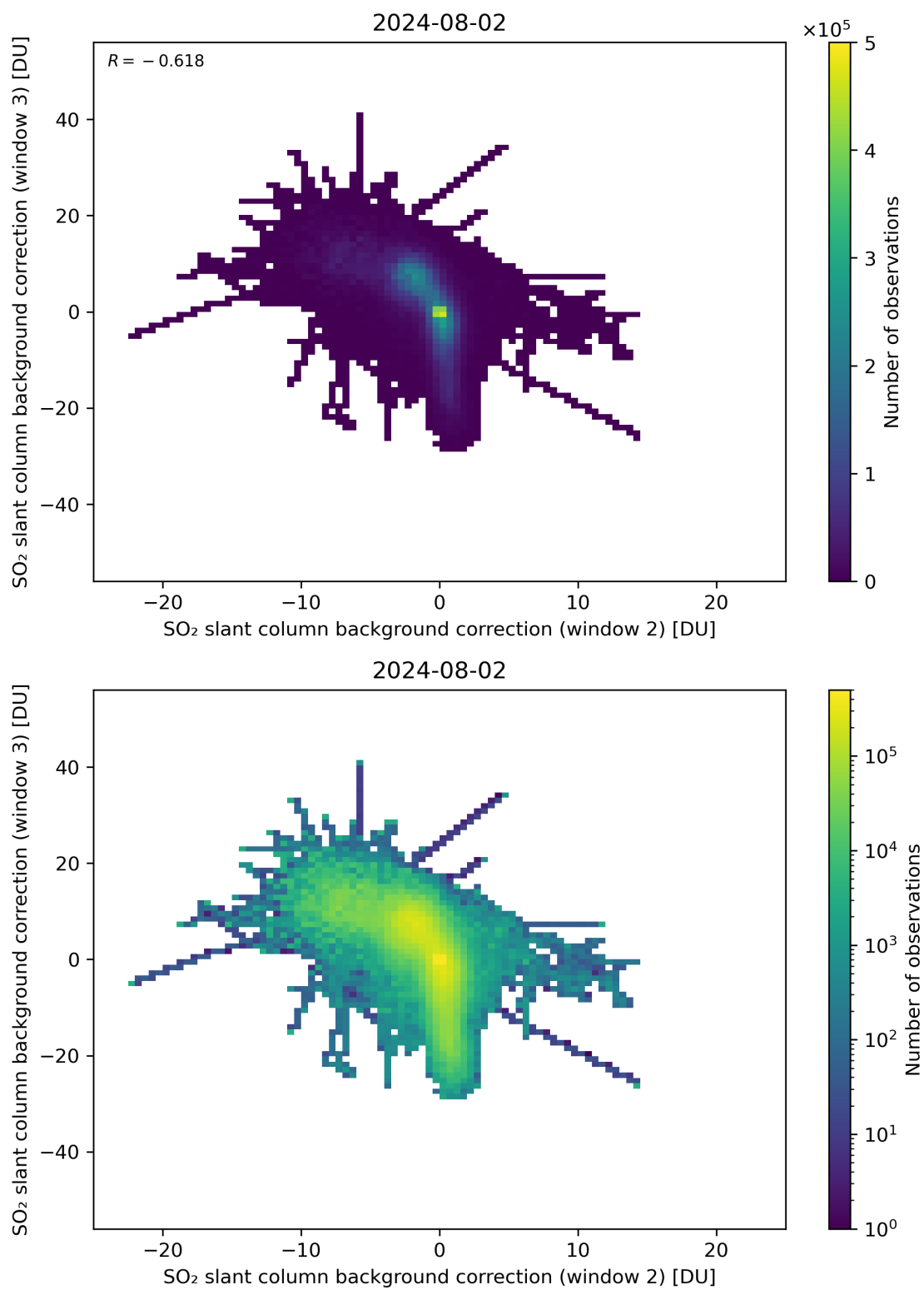
Figure 111: Scatter density plot of “SO 2 slant column background correction (window 2)” against “SO 2 slant column background correction (window 3)” for 2024-08-01 to 2024-08-03.
