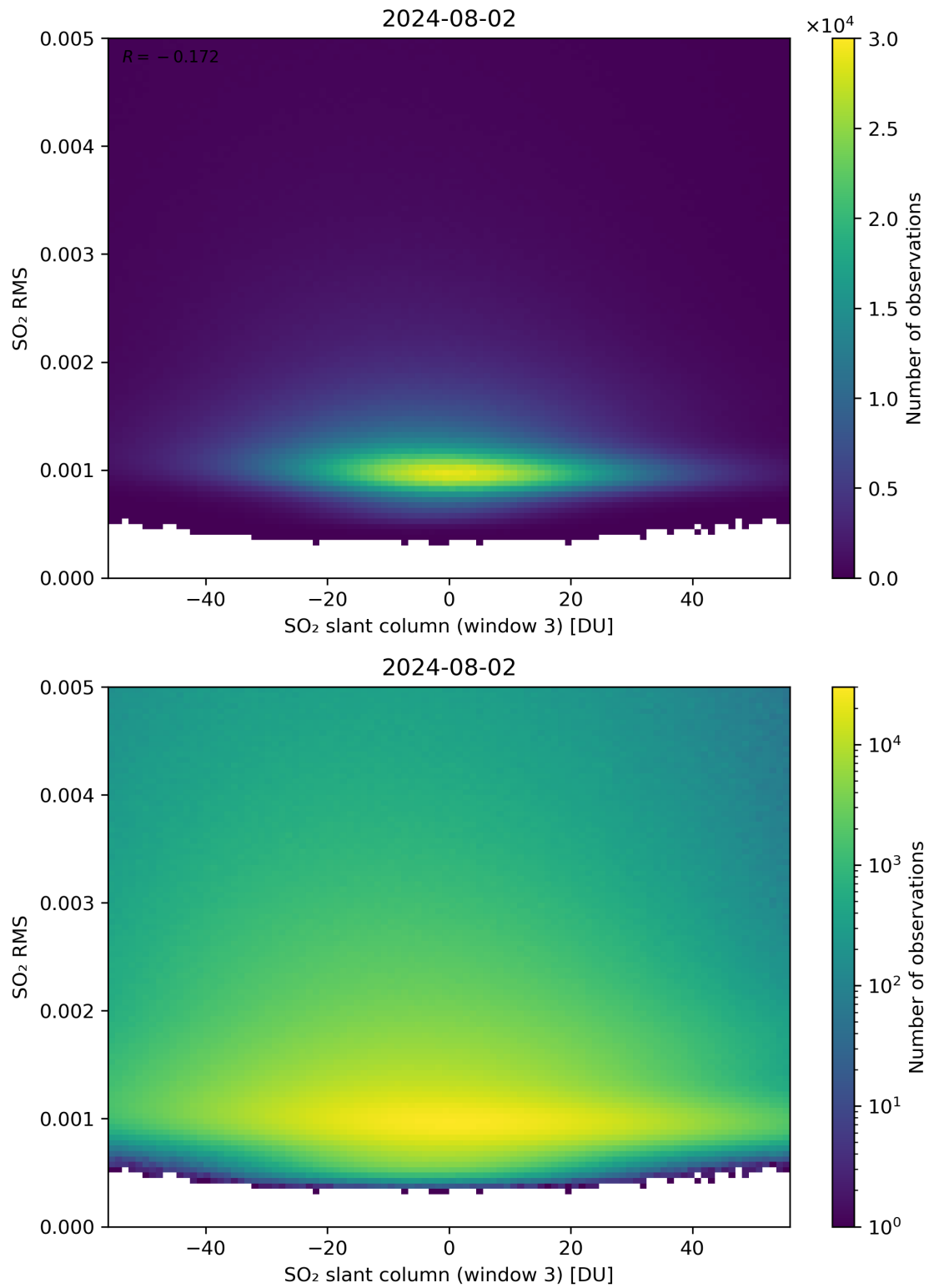
Figure 256: Scatter density plot of “SO 2 slant column (window 3)” against “SO 2 RMS” for 2024-08-01 to 2024-08-03.
