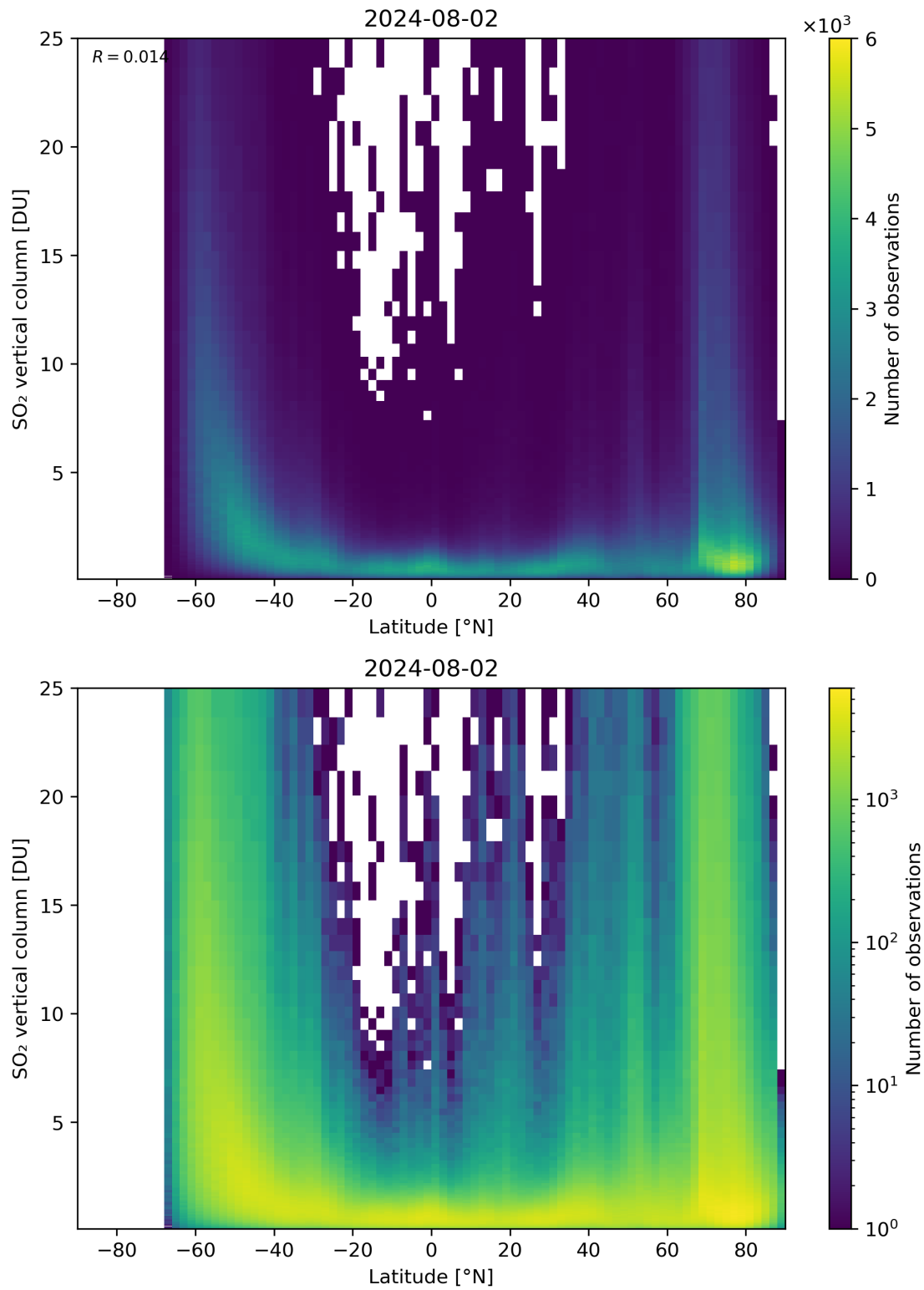
Figure 156: Scatter density plot of “Latitude” against “SO 2 vertical column” for 2024-08-01 to 2024-08-03.
