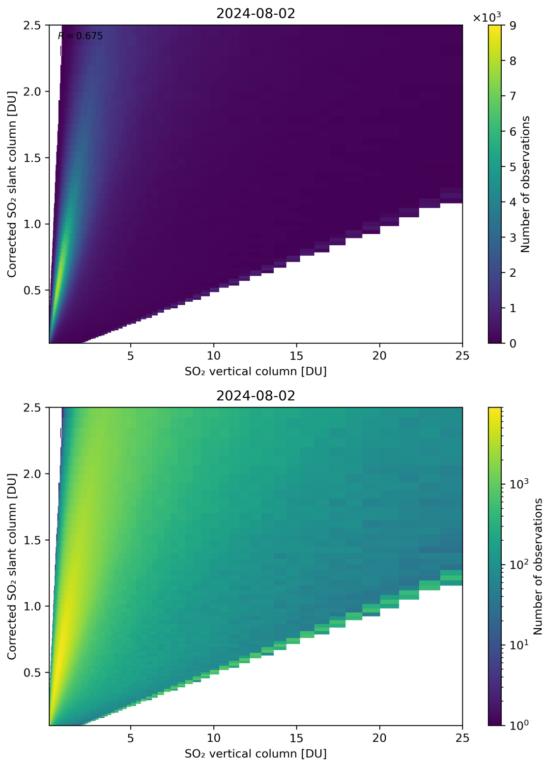
Figure 297: Scatter density plot of “SO 2 vertical column” against “Corrected SO 2 slant column” for 2024-08-01 to 2024-08-03.
