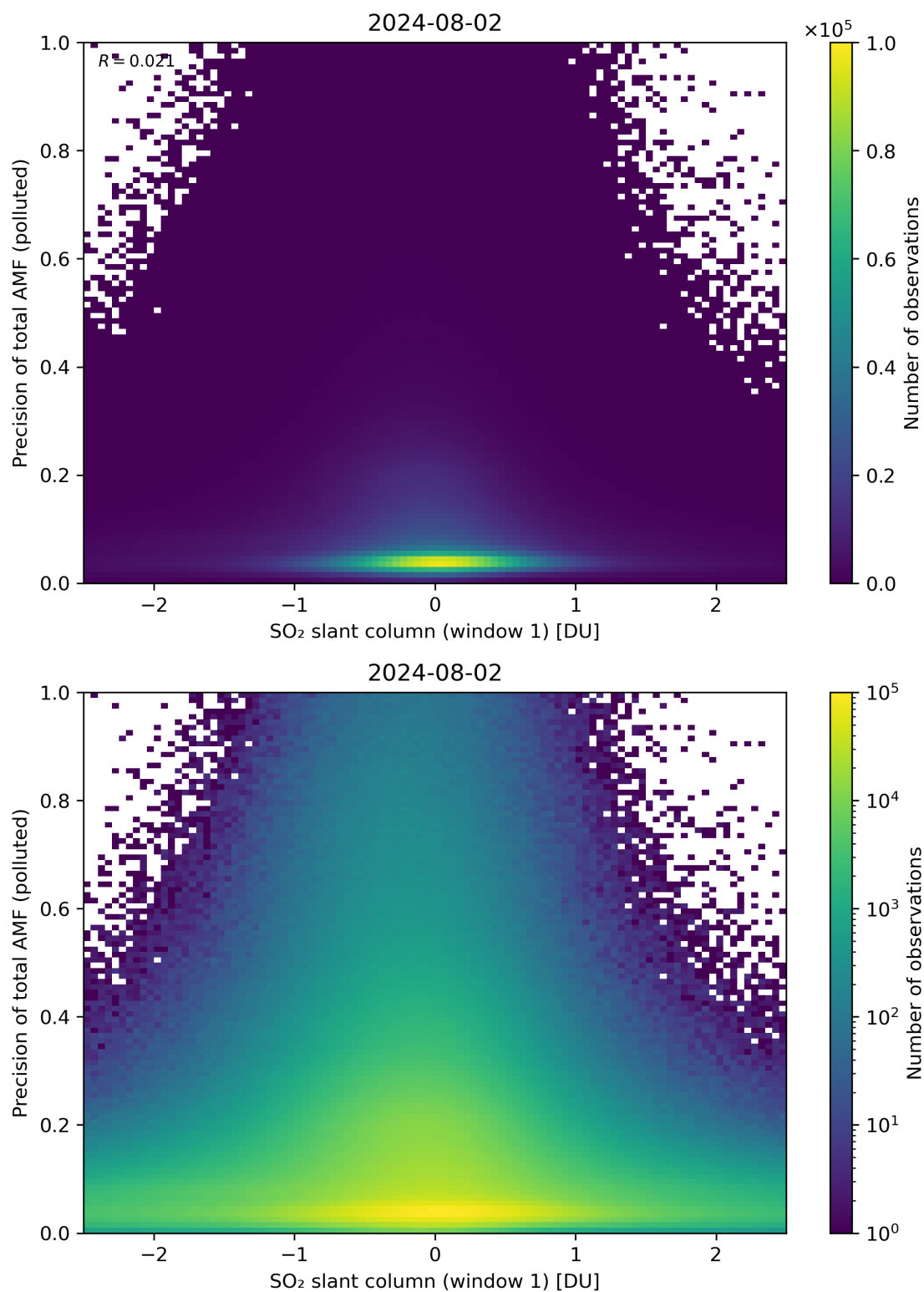
Figure 240: Scatter density plot of “SO 2 slant column (window 1)” against “Precision of total AMF (polluted)” for 2024-08-01 to 2024-08-03.
