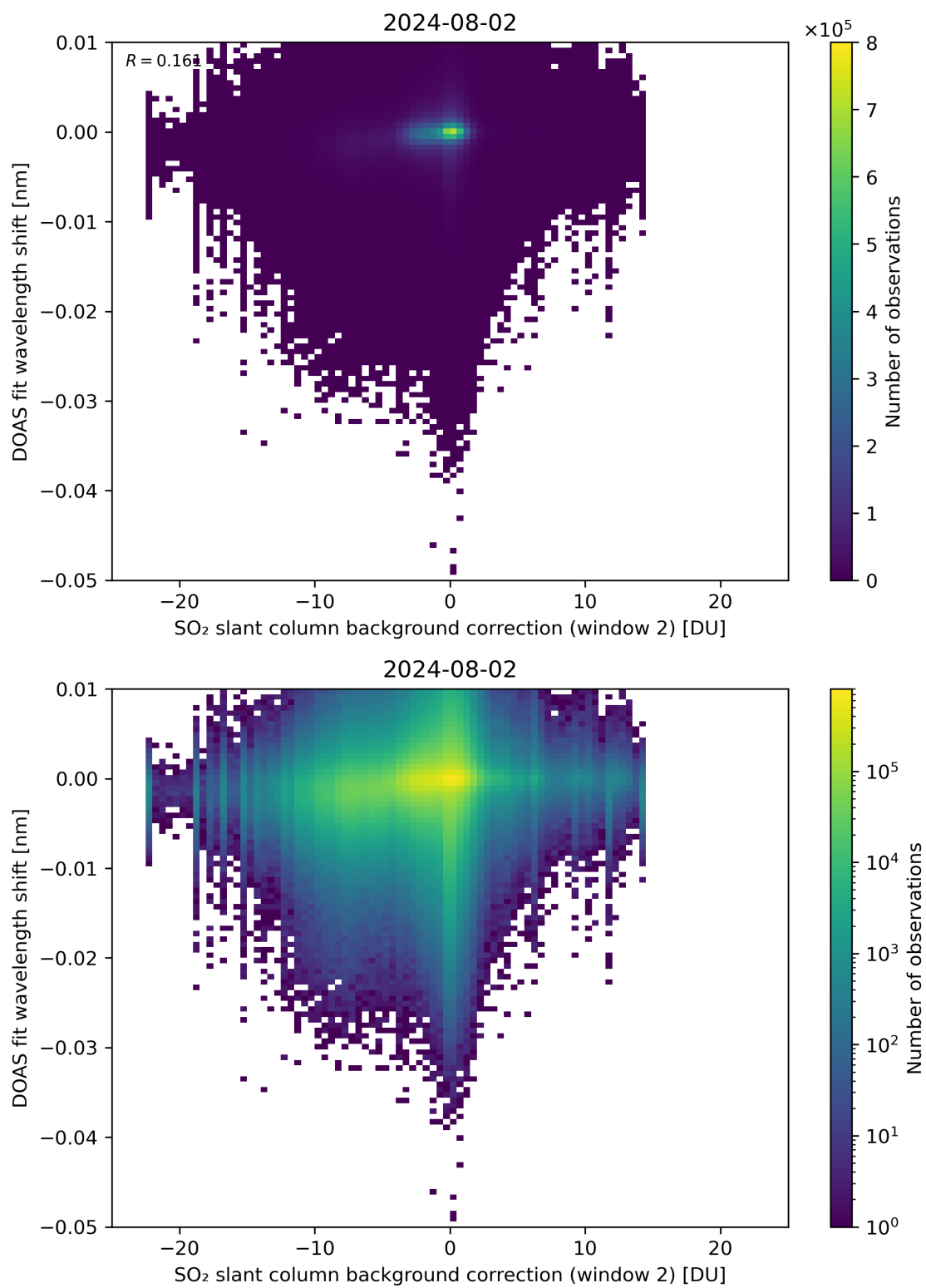
Figure 112: Scatter density plot of “SO 2 slant column background correction (window 2)” against “DOAS fit wavelength shift” for 2024-08-01 to 2024-08-03.
