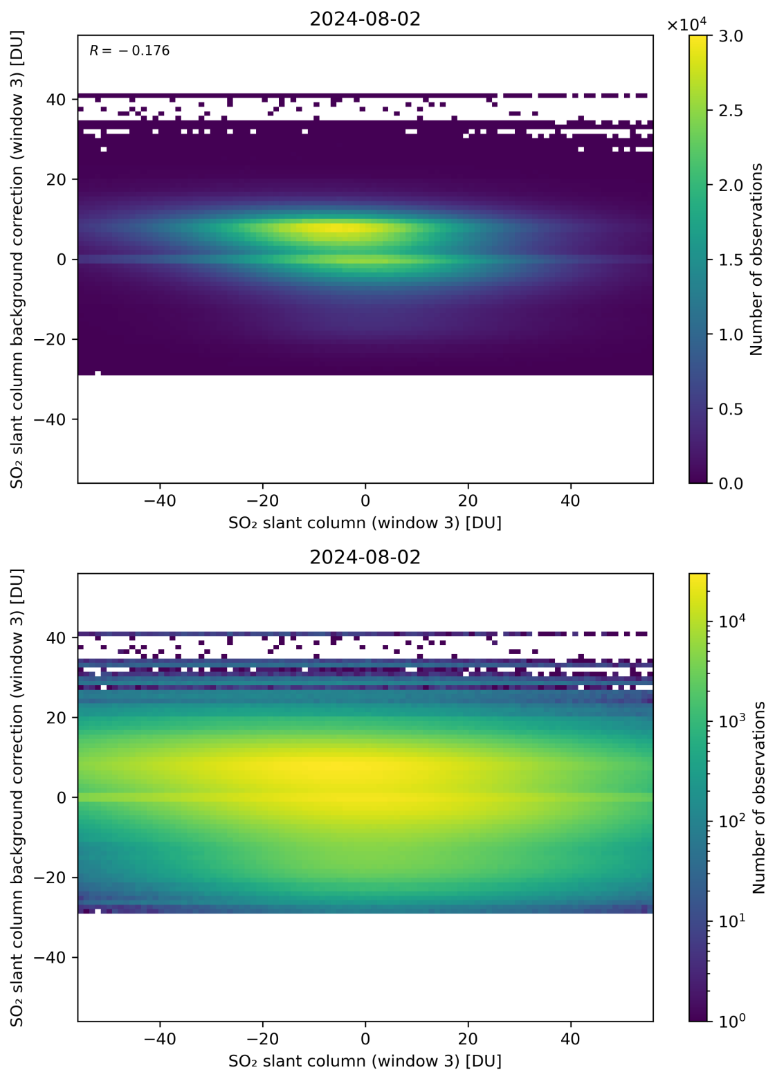
Figure 253: Scatter density plot of “SO 2 slant column (window 3)” against “SO 2 slant column background correction (window 3)” for 2024-08-01 to 2024-08-03.
