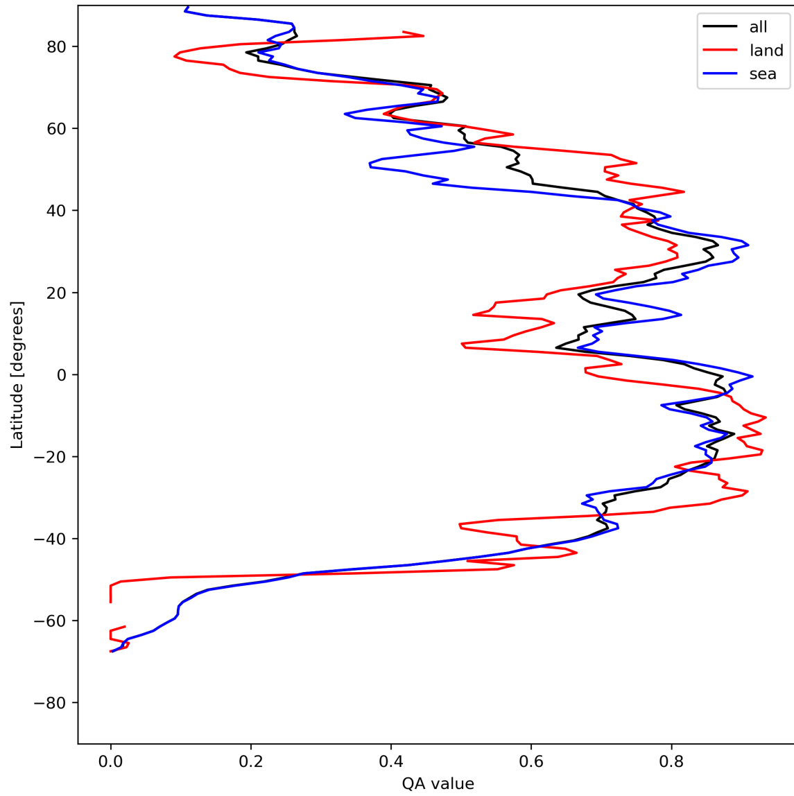
Figure 29: Zonal average of “QA value” for 2024-08-01 to 2024-08-03.
