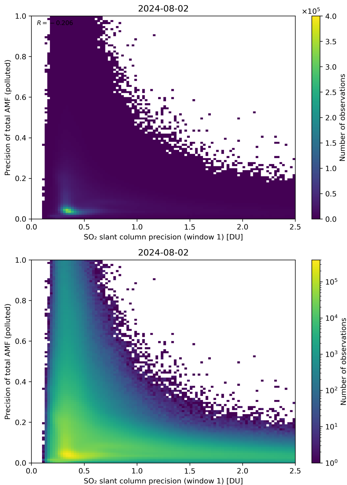
Figure 231: Scatter density plot of “SO 2 slant column precision (window 1)” against “Precision of total AMF (polluted)” for 2024-08-01 to 2024-08-03.
