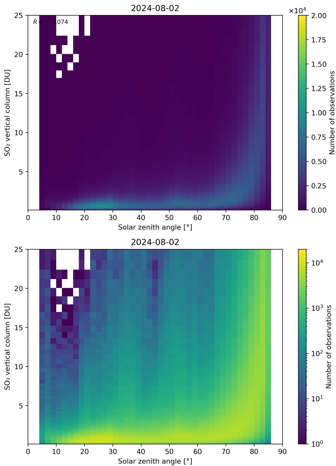
Figure 176: Scatter density plot of “Solar zenith angle” against “SO 2 vertical column” for 2024-08-01 to 2024-08-03.
