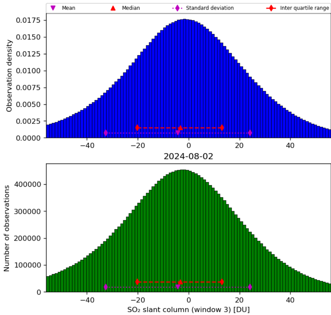
Figure 64: Histogram of “SO 2 slant column (window 3)” for 2024-08-01 to 2024-08-03
