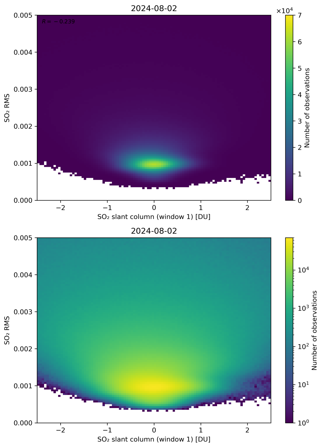
Figure 217: Scatter density plot of “SO 2 slant column (window 1)” against “SO 2 RMS” for 2024-08-01 to 2024-08-03.
