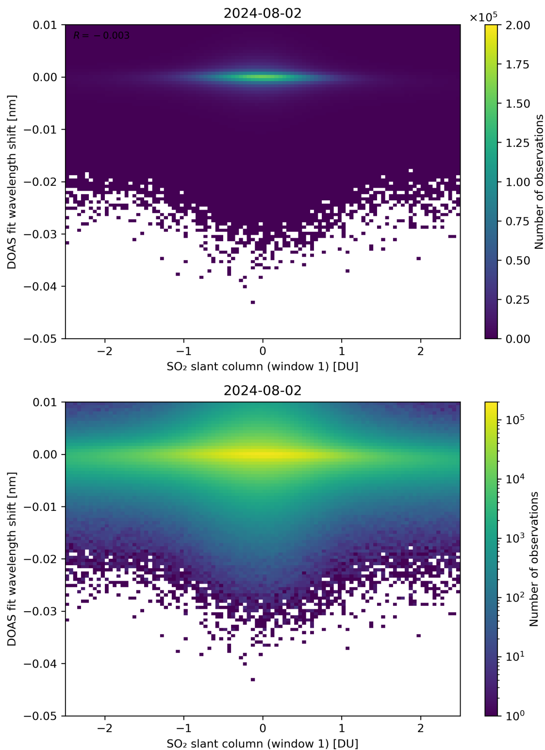
Figure 215: Scatter density plot of “SO 2 slant column (window 1)” against “DOAS fit wavelength shift” for 2024-08-01 to 2024-08-03.
