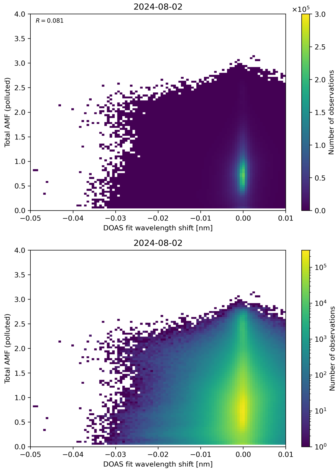
Figure 130: Scatter density plot of “DOAS fit wavelength shift” against “Total AMF (polluted)” for 2024-08-01 to 2024-08-03.
