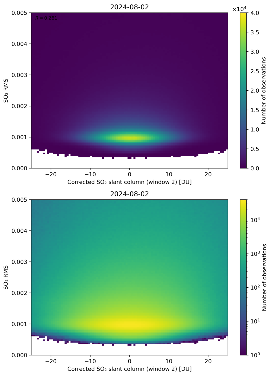
Figure 198: Scatter density plot of “Corrected SO 2 slant column (window 2)” against “SO 2 RMS” for 2024-08-01 to 2024-08-03.
