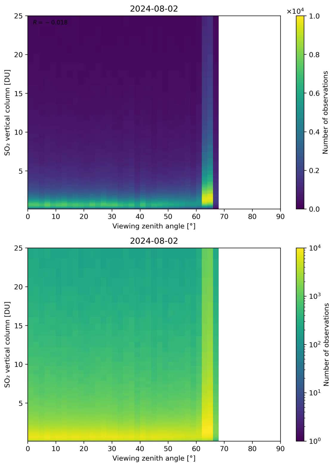
Figure 327: Scatter density plot of “Viewing zenith angle” against “SO 2 vertical column” for 2024-08-01 to 2024-08-03.
