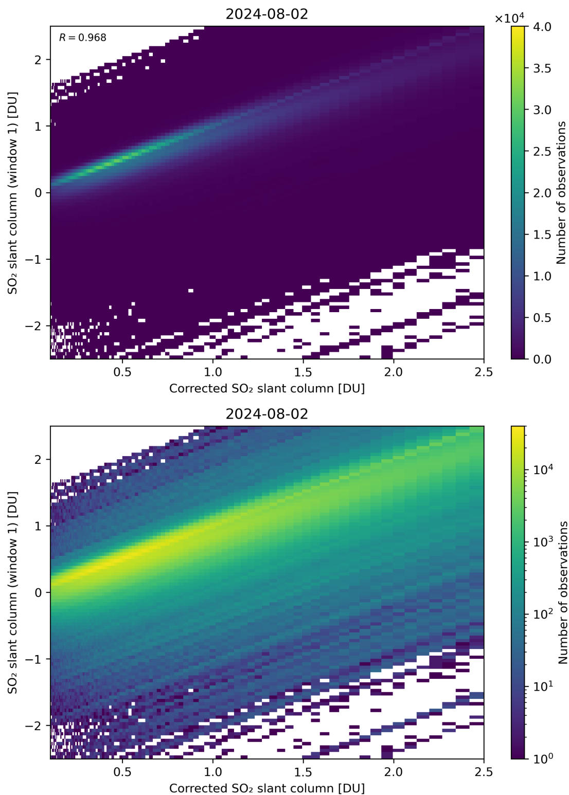
Figure 187: Scatter density plot of “Corrected SO 2 slant column” against “SO 2 slant column (window 1)” for 2024-08-01 to 2024-08-03.
