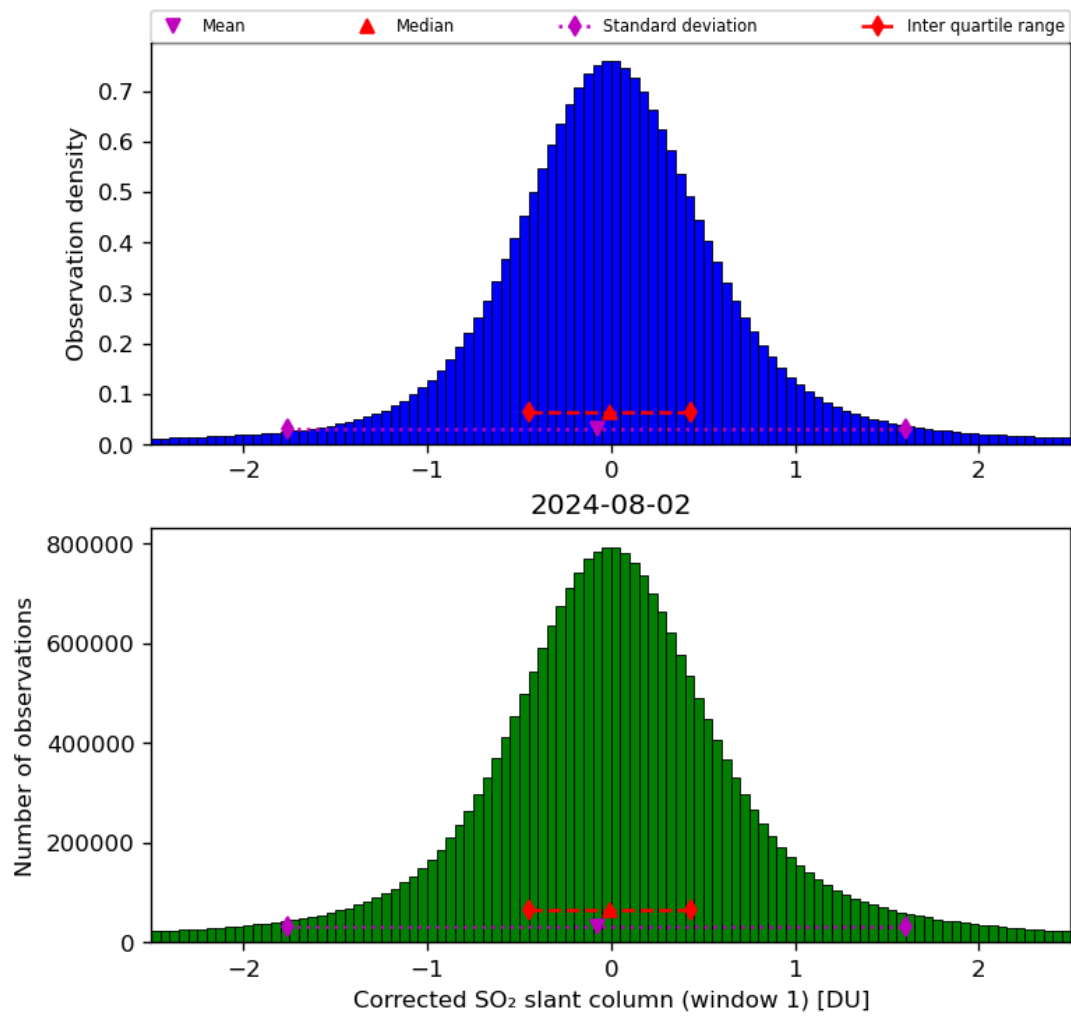
Figure 58: Histogram of “Corrected SO 2 slant column (window 1)” for 2024-08-01 to 2024-08-03
