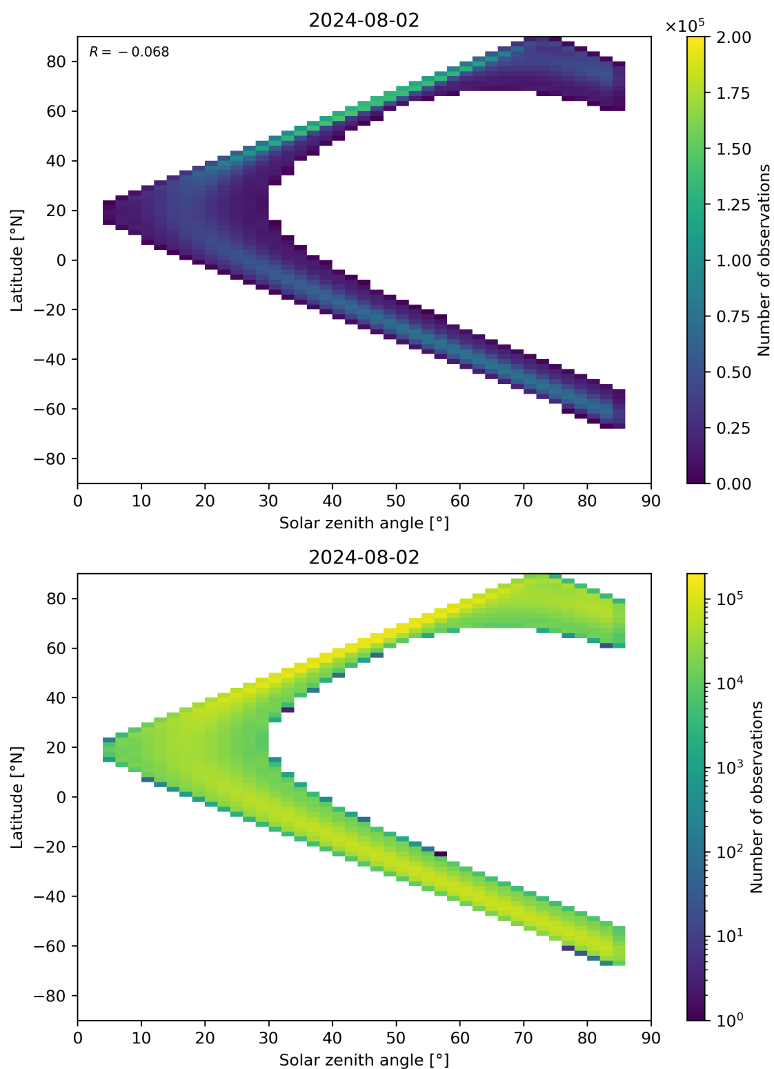
Figure 164: Scatter density plot of “Solar zenith angle” against “Latitude” for 2024-08-01 to 2024-08-03.
