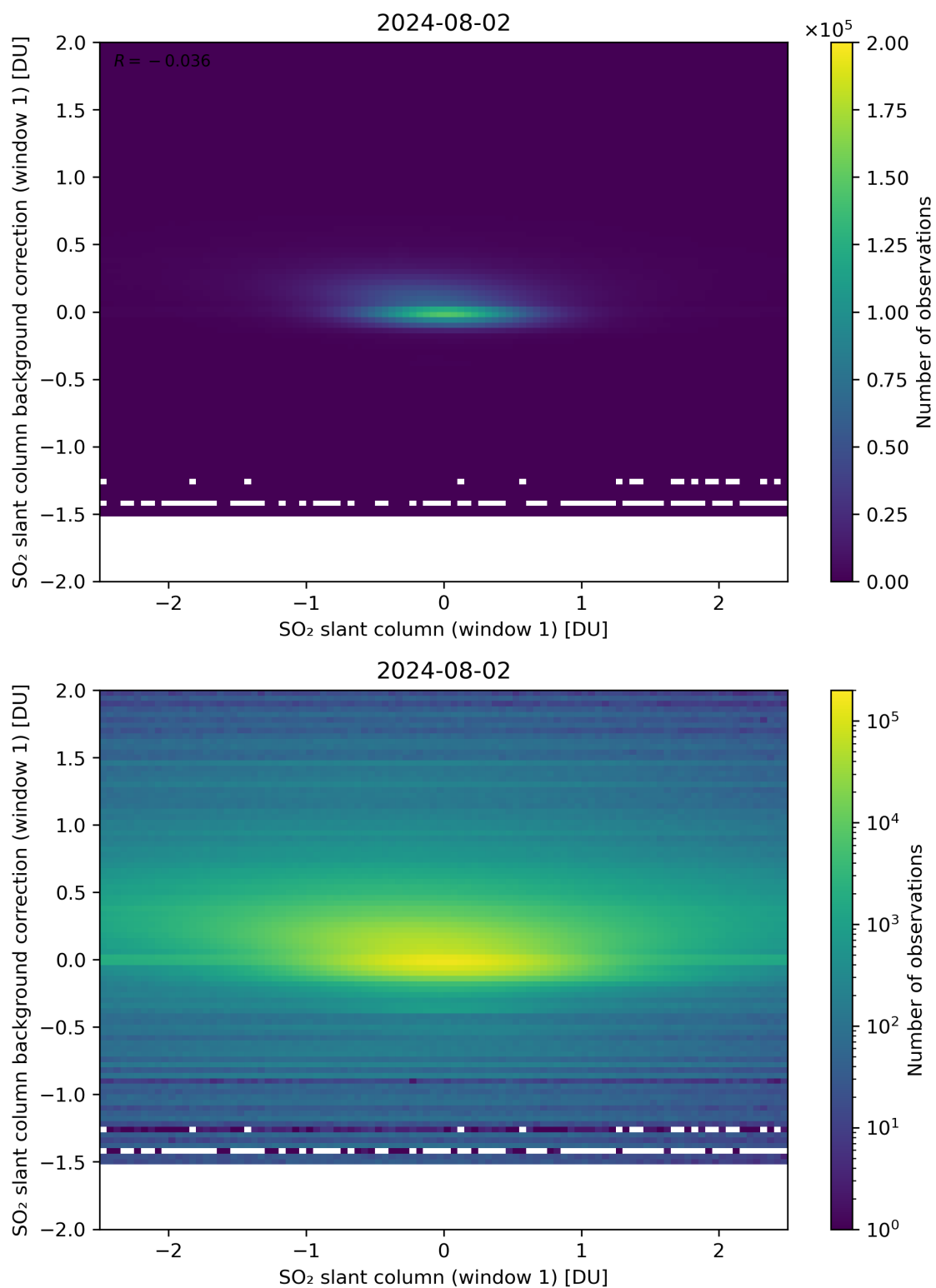
Figure 212: Scatter density plot of “SO 2 slant column (window 1)” against “SO 2 slant column background correction (window 1)” for 2024-08-01 to 2024-08-03.
