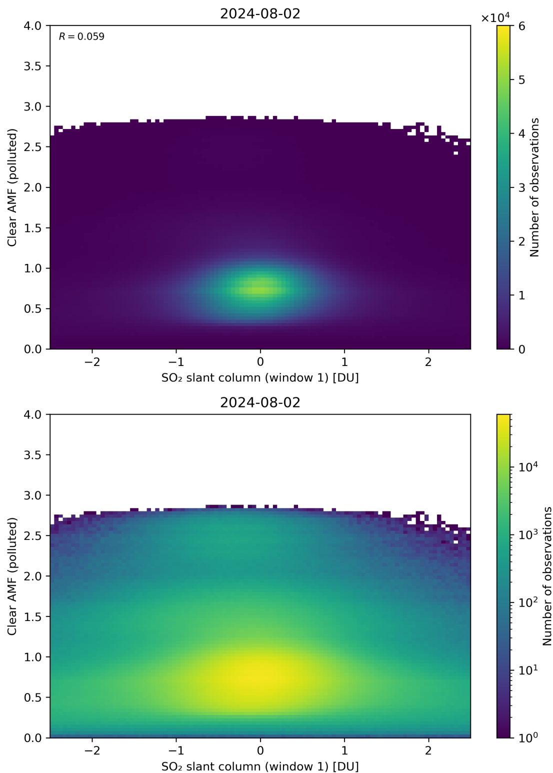
Figure 232: Scatter density plot of “SO 2 slant column (window 1)” against “Clear AMF (polluted)” for 2024-08-01 to 2024-08-03.
