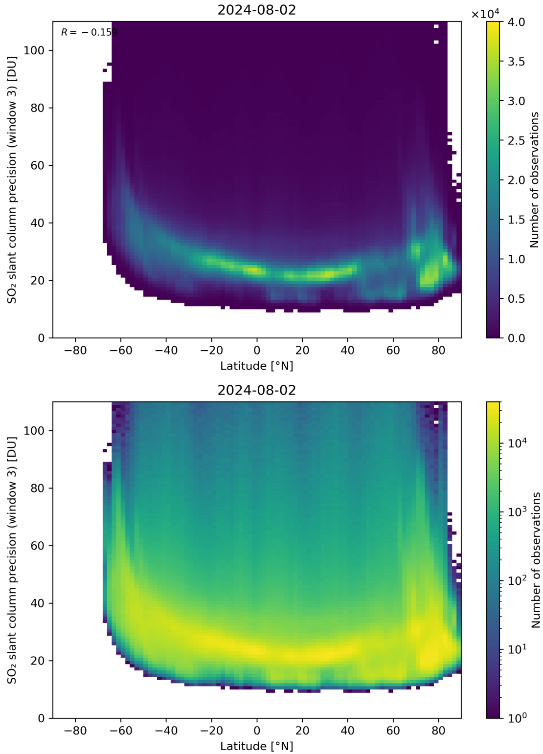
Figure 153: Scatter density plot of “Latitude” against “SO 2 slant column precision (window 3)” for 2024-08-01 to 2024-08-03.
