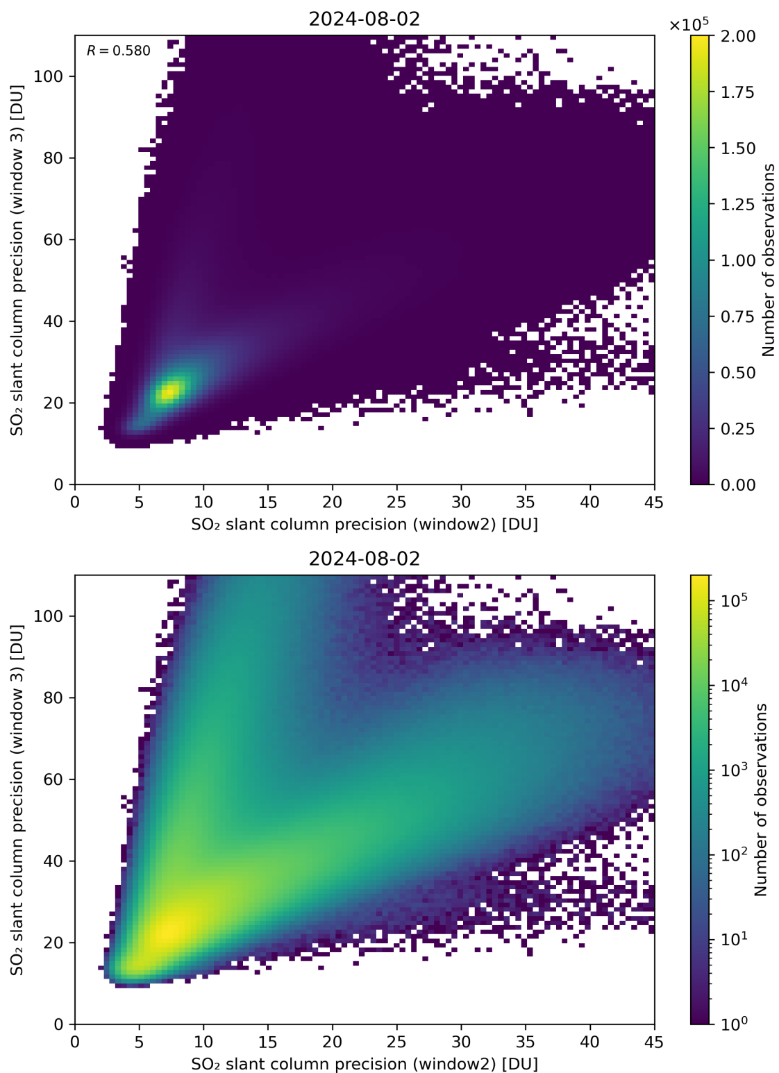
Figure 250: Scatter density plot of “SO 2 slant column precision (window2)” against “SO 2 slant column precision (window 3)” for 2024-08-01 to 2024-08-03.
