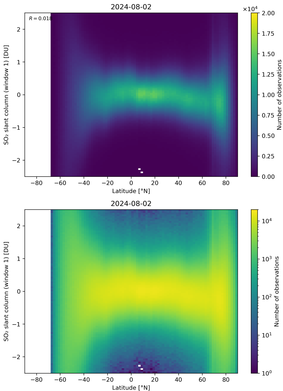
Figure 149: Scatter density plot of “Latitude” against “SO 2 slant column (window 1)” for 2024-08-01 to 2024-08-03.
