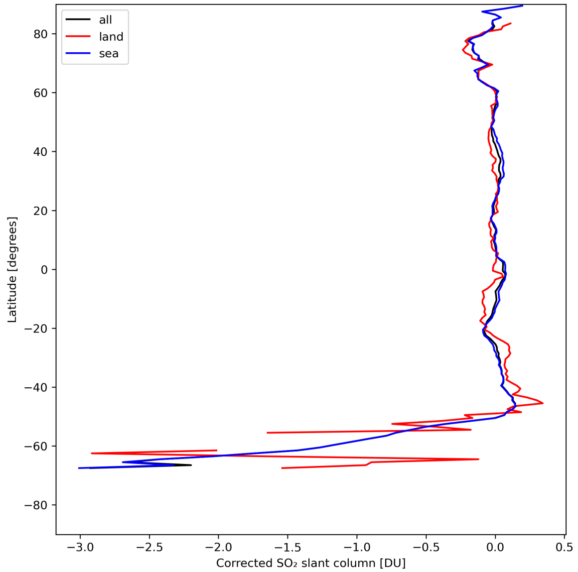
Figure 32: Zonal average of “Corrected SO 2 slant column” for 2024-08-01 to 2024-08-03.
