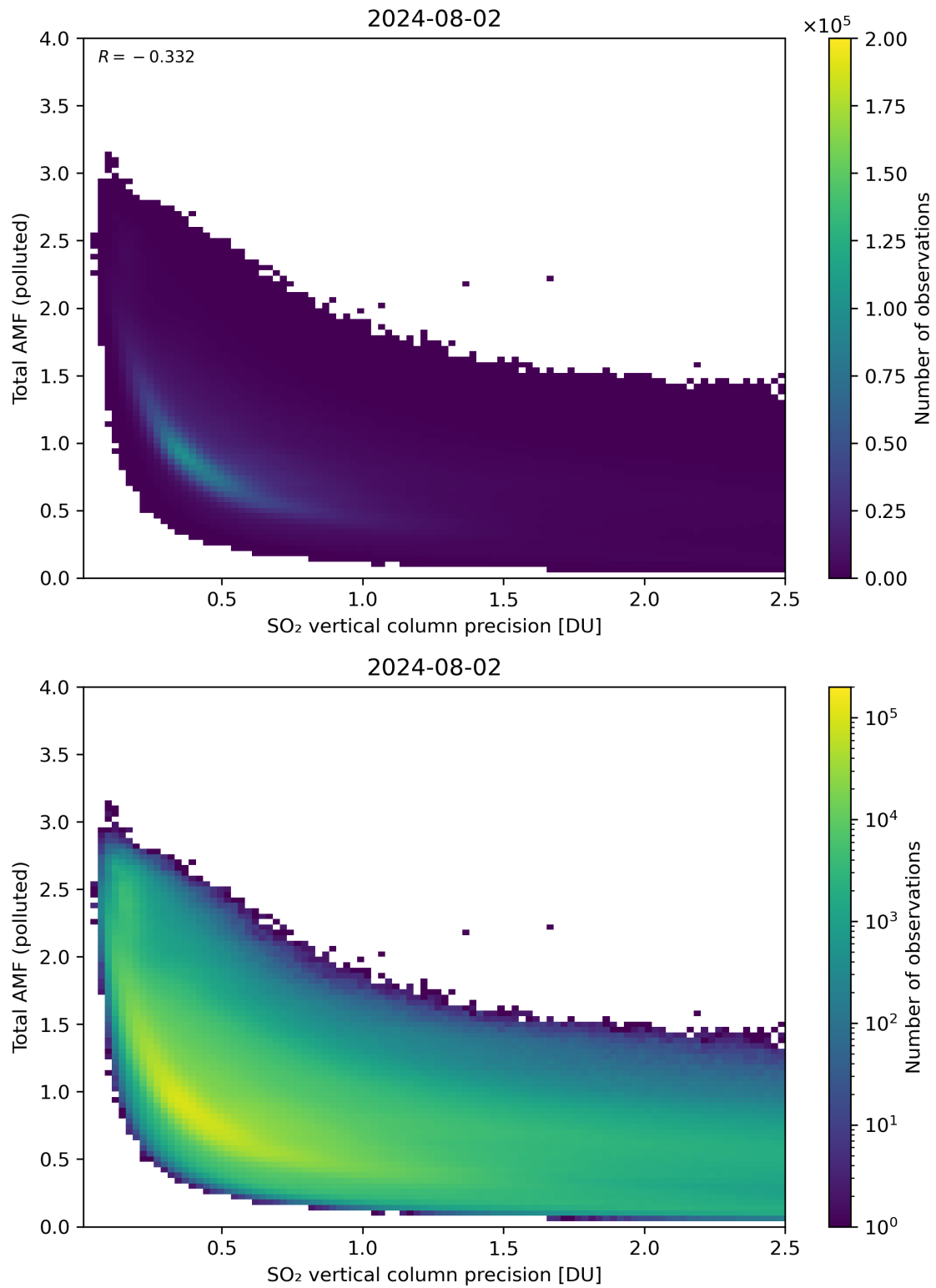
Figure 294: Scatter density plot of “SO 2 vertical column precision” against “Total AMF (polluted)” for 2024-08-01 to 2024-08-03.
