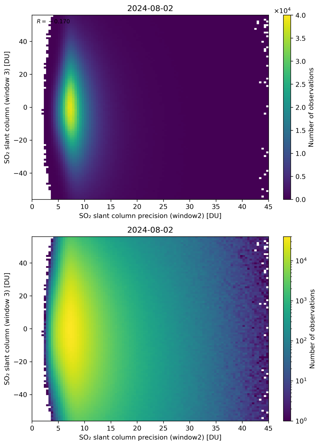
Figure 249: Scatter density plot of “SO 2 slant column precision (window2)” against “SO 2 slant column (window 3)” for 2024-08-01 to 2024-08-03.
