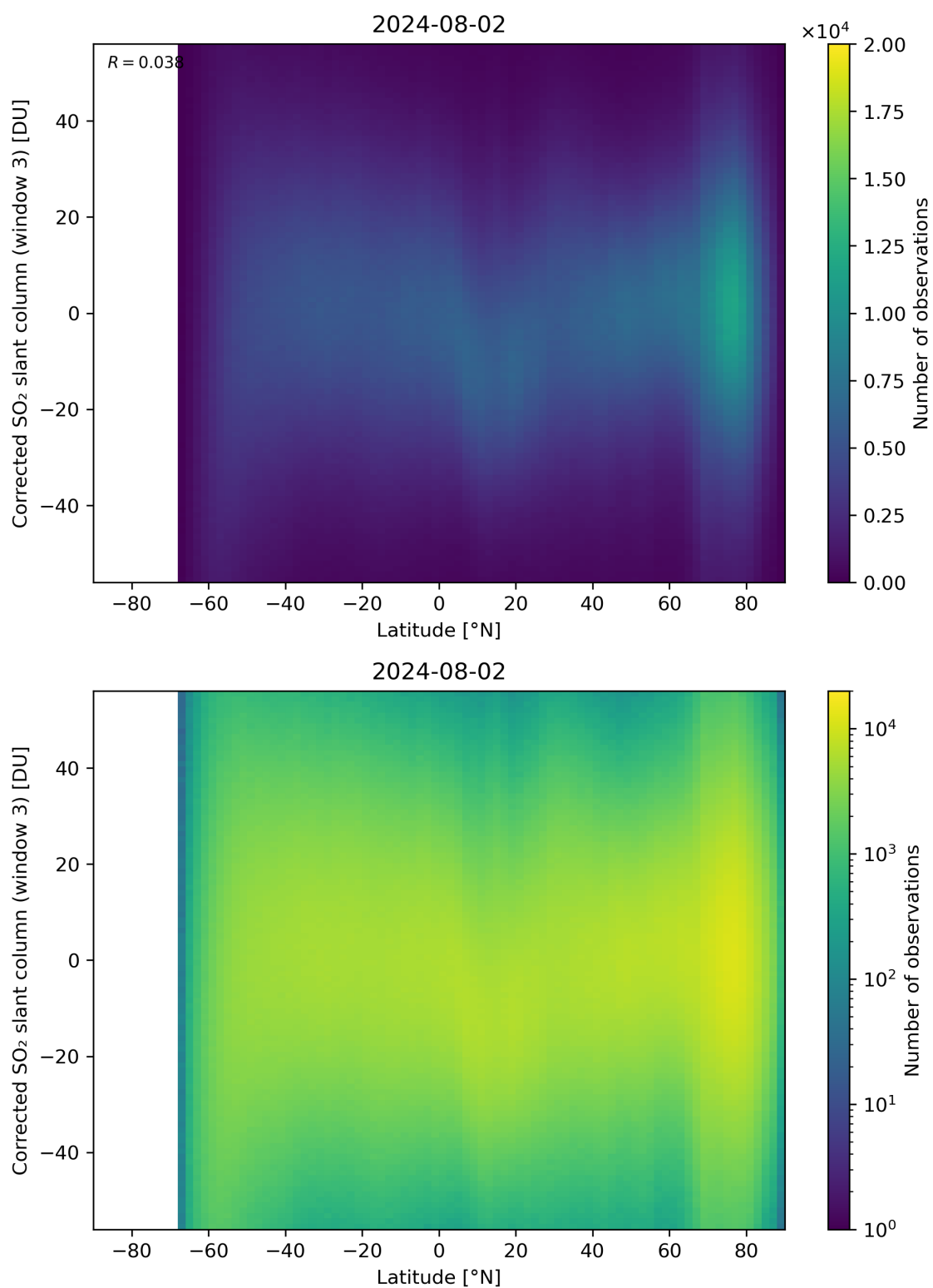
Figure 148: Scatter density plot of “Latitude” against “Corrected SO 2 slant column (window 3)” for 2024-08-01 to 2024-08-03.
