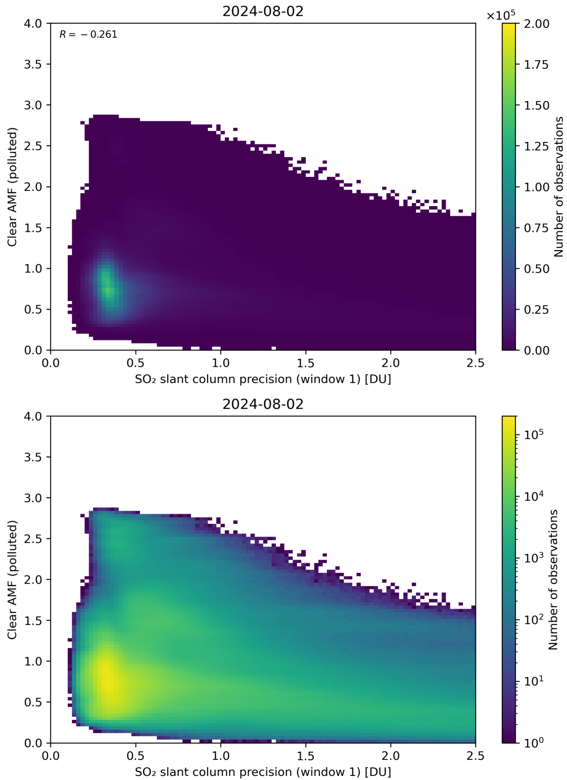
Figure 224: Scatter density plot of “SO 2 slant column precision (window 1)” against “Clear AMF (polluted)” for 2024-08-01 to 2024-08-03.
