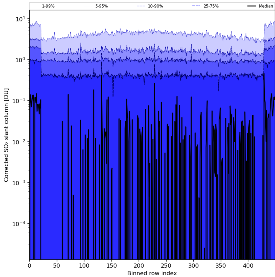
Figure 78: Along track statistics of “Corrected SO 2 slant column” for 2024-08-01 to 2024-08-03
