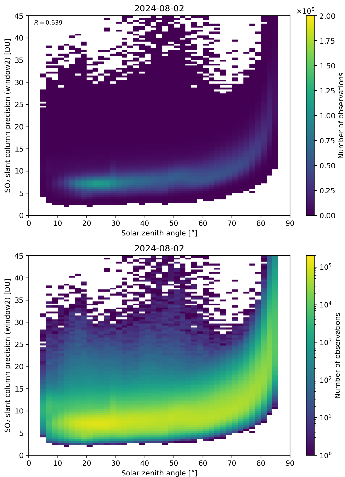
Figure 171: Scatter density plot of “Solar zenith angle” against “SO 2 slant column precision (window2)” for 2024-08-01 to 2024-08-03.
