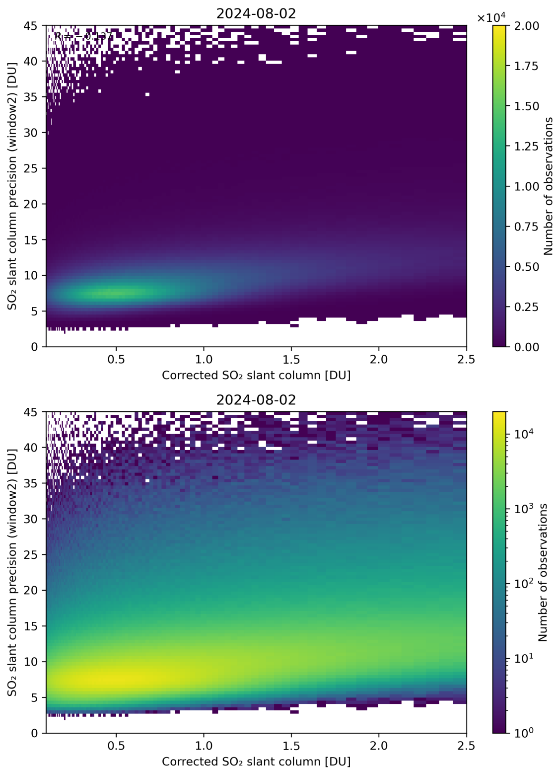
Figure 189: Scatter density plot of “Corrected SO 2 slant column” against “SO 2 slant column precision (window2)” for 2024-08-01 to 2024-08-03.
