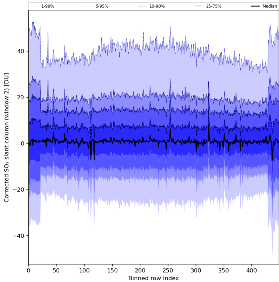
Figure 85: Along track statistics of “Corrected SO 2 slant column (window 2)” for 2024-08-01 to 2024-08-03
