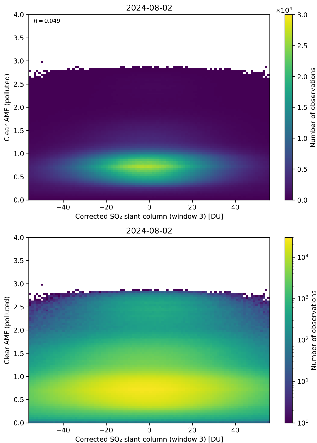
Figure 209: Scatter density plot of “Corrected SO 2 slant column (window 3)” against “Clear AMF (polluted)” for 2024-08-01 to 2024-08-03.
