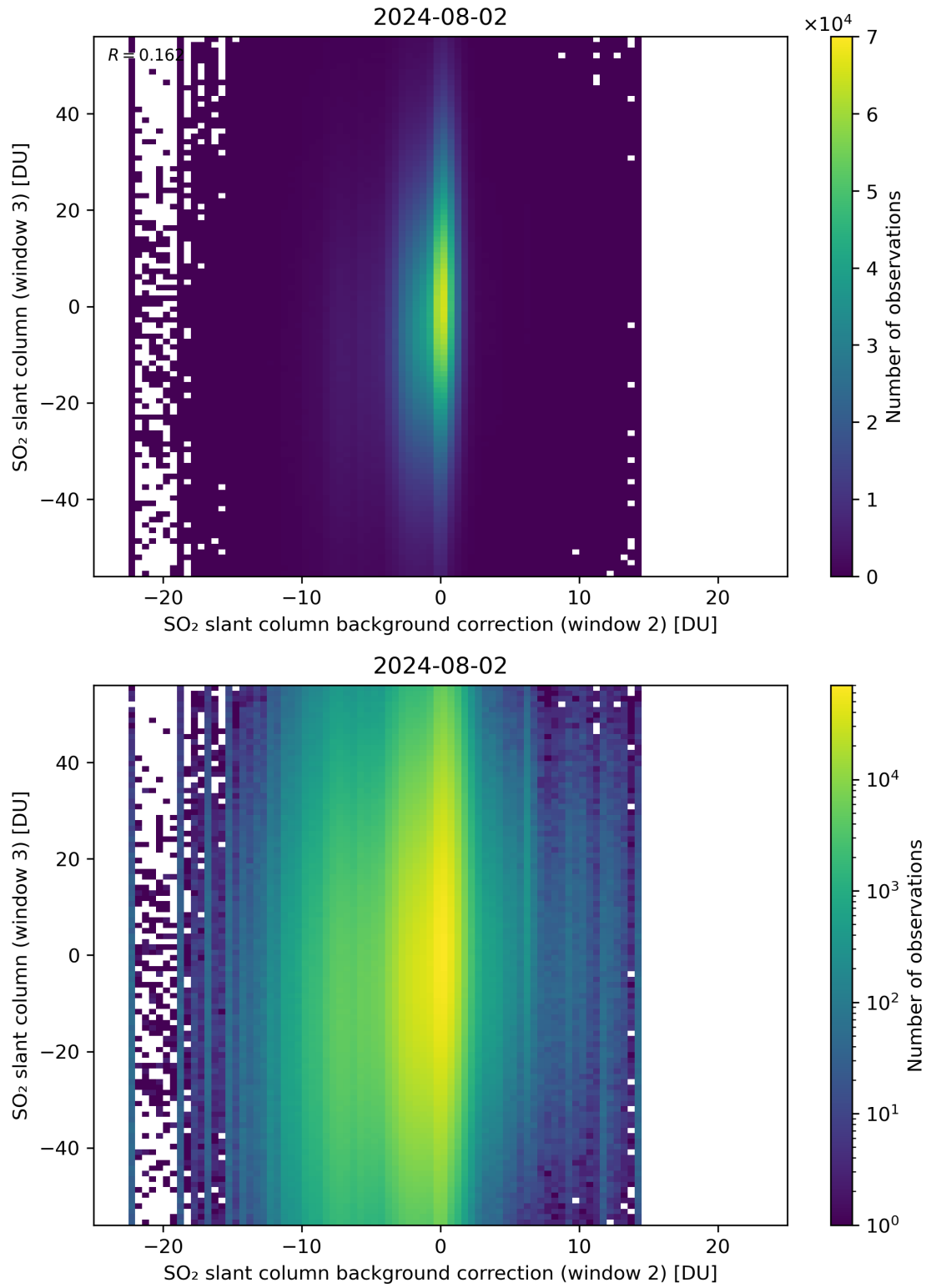
Figure 117: Scatter density plot of “SO 2 slant column background correction (window 2)” against “SO 2 slant column (window 3)” for 2024-08-01 to 2024-08-03.
