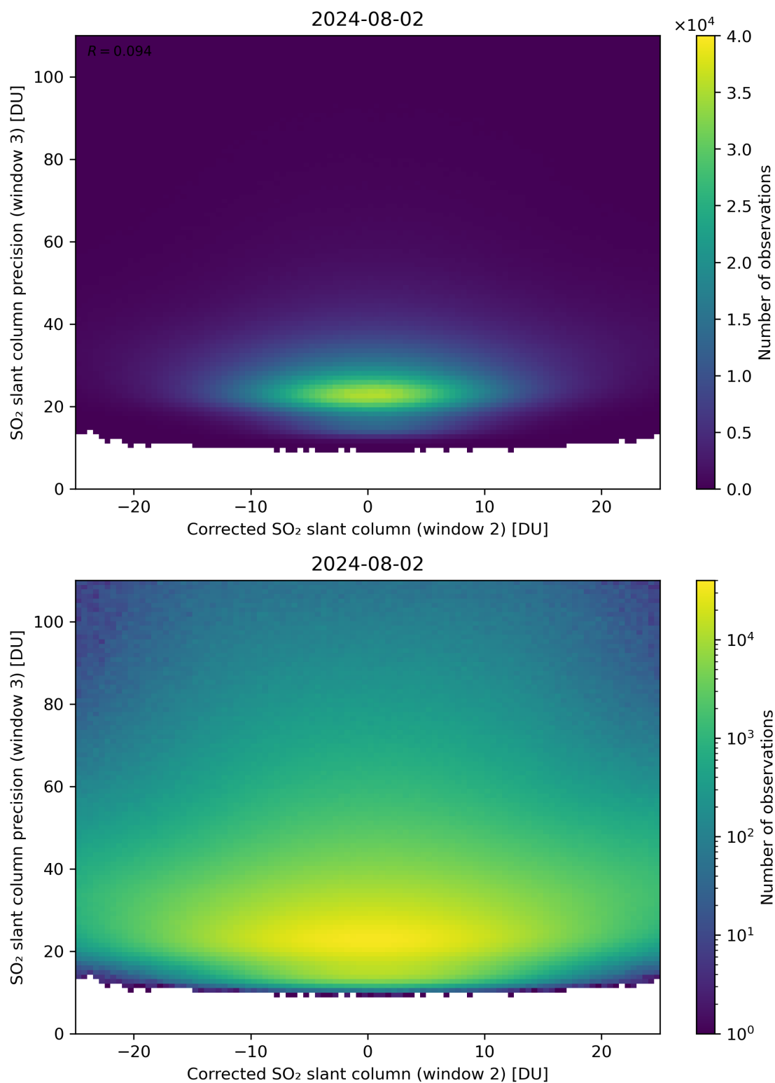
Figure 202: Scatter density plot of “Corrected SO 2 slant column (window 2)” against “SO 2 slant column precision (window 3)” for 2024-08-01 to 2024-08-03.
