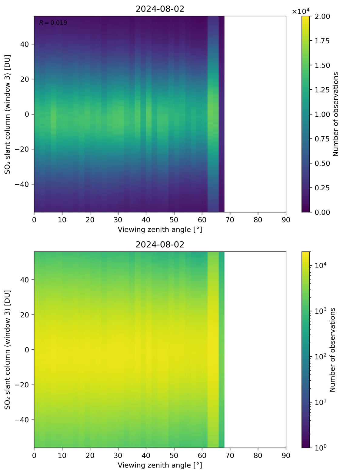
Figure 323: Scatter density plot of “Viewing zenith angle” against “SO 2 slant column (window 3)” for 2024-08-01 to 2024-08-03.
