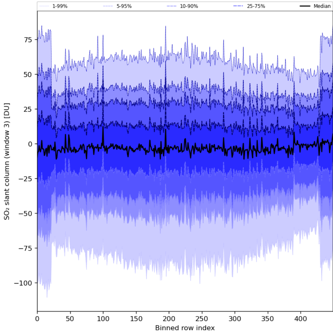
Figure 87: Along track statistics of “SO 2 slant column (window 3)” for 2024-08-01 to 2024-08-03
