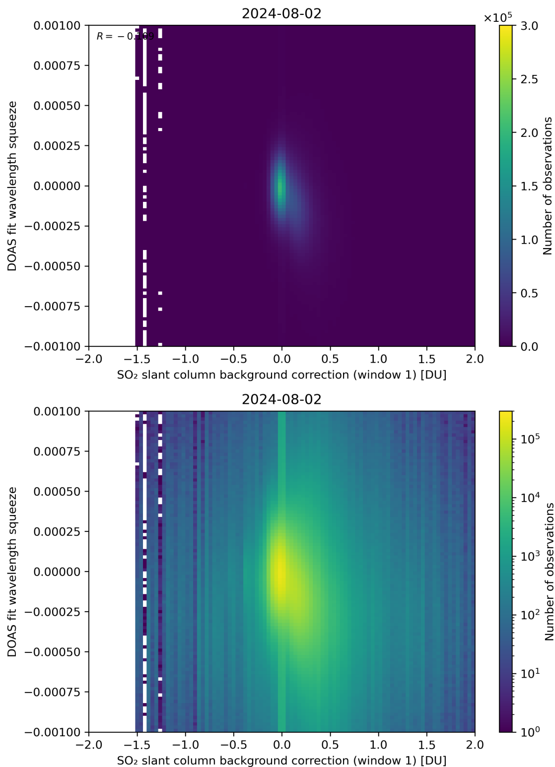
Figure 101: Scatter density plot of “SO 2 slant column background correction (window 1)” against “DOAS fit wavelength squeeze” for 2024-08-01 to 2024-08-03.
