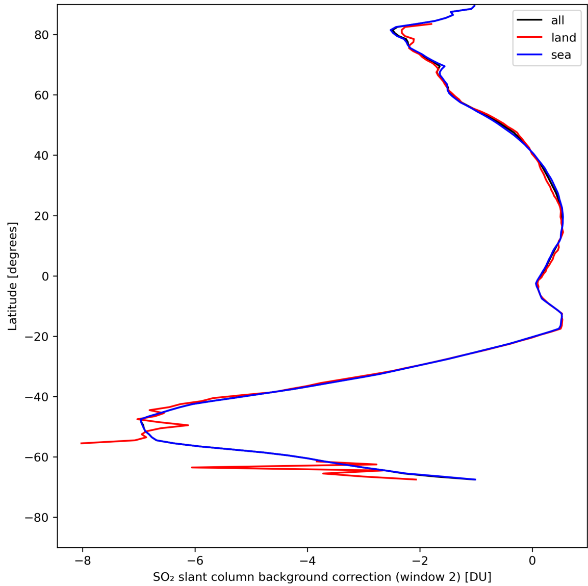
Figure 40: Zonal average of “SO 2 slant column background correction (window 2)” for 2024-08-01 to 2024-08-03.
