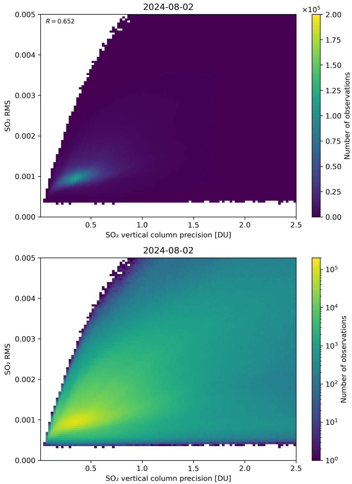
Figure 284: Scatter density plot of “SO 2 vertical column precision” against “SO 2 RMS” for 2024-08-01 to 2024-08-03.
