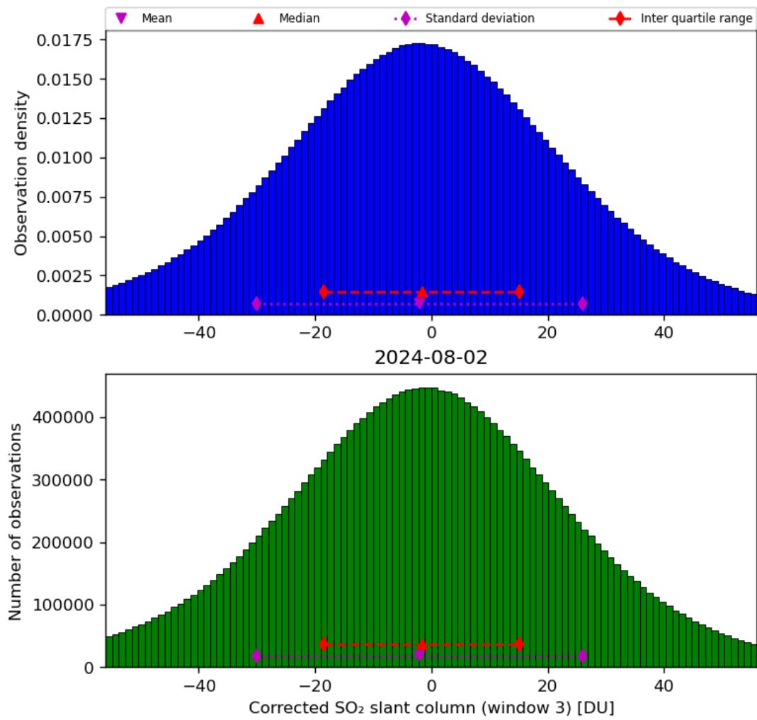
Figure 66: Histogram of “Corrected SO 2 slant column (window 3)” for 2024-08-01 to 2024-08-03
