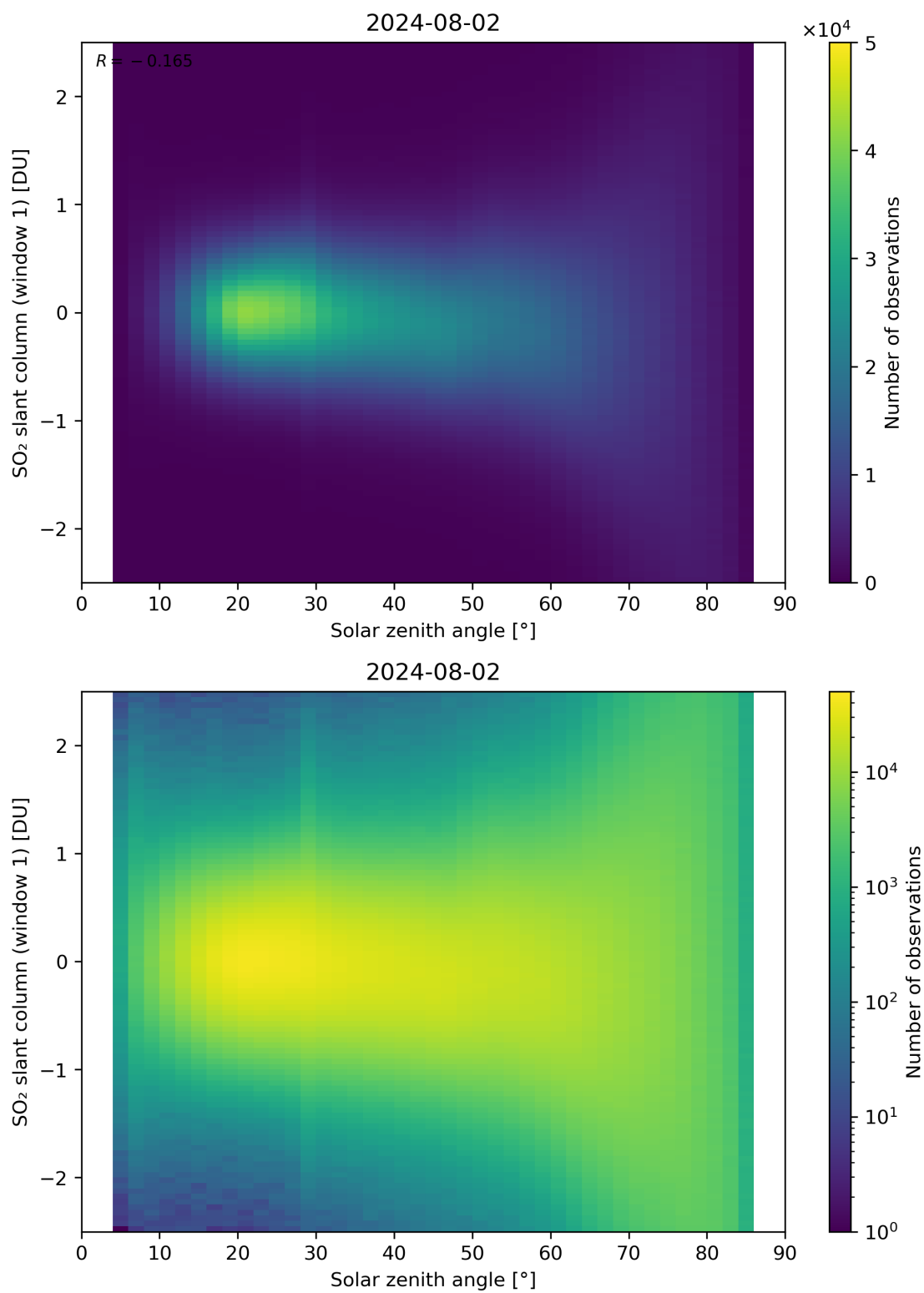
Figure 169: Scatter density plot of “Solar zenith angle” against “SO 2 slant column (window 1)” for 2024-08-01 to 2024-08-03.
