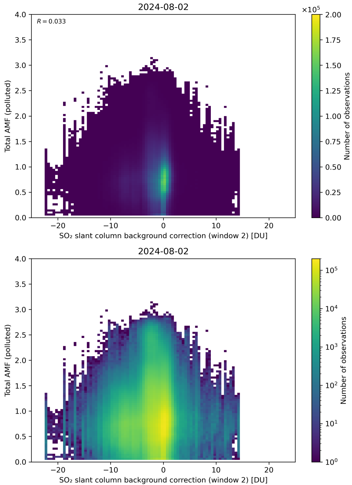
Figure 119: Scatter density plot of “SO 2 slant column background correction (window 2)” against “Total AMF (polluted)” for 2024-08-01 to 2024-08-03.
