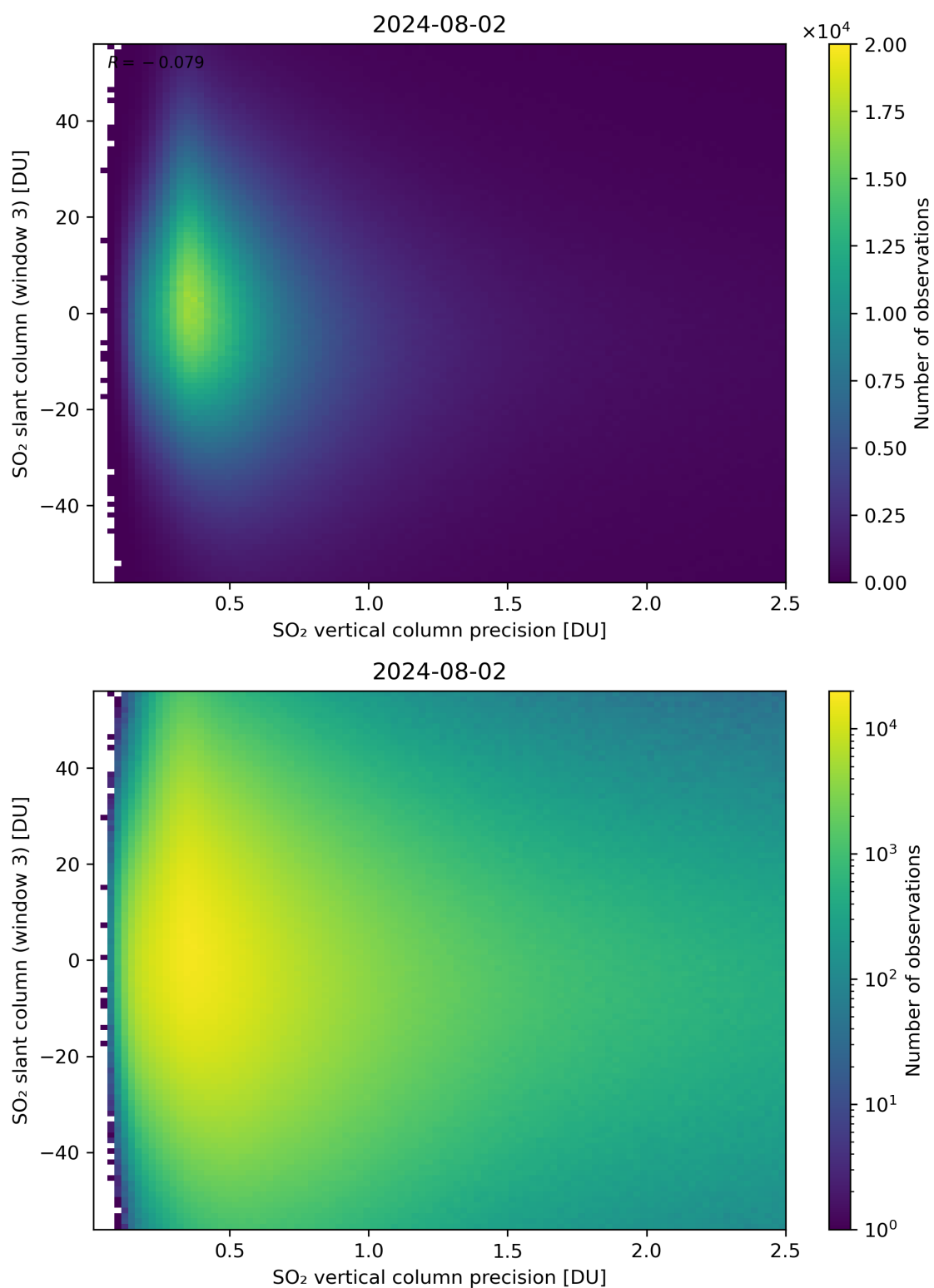
Figure 292: Scatter density plot of “SO 2 vertical column precision” against “SO 2 slant column (window 3)” for 2024-08-01 to 2024-08-03.
