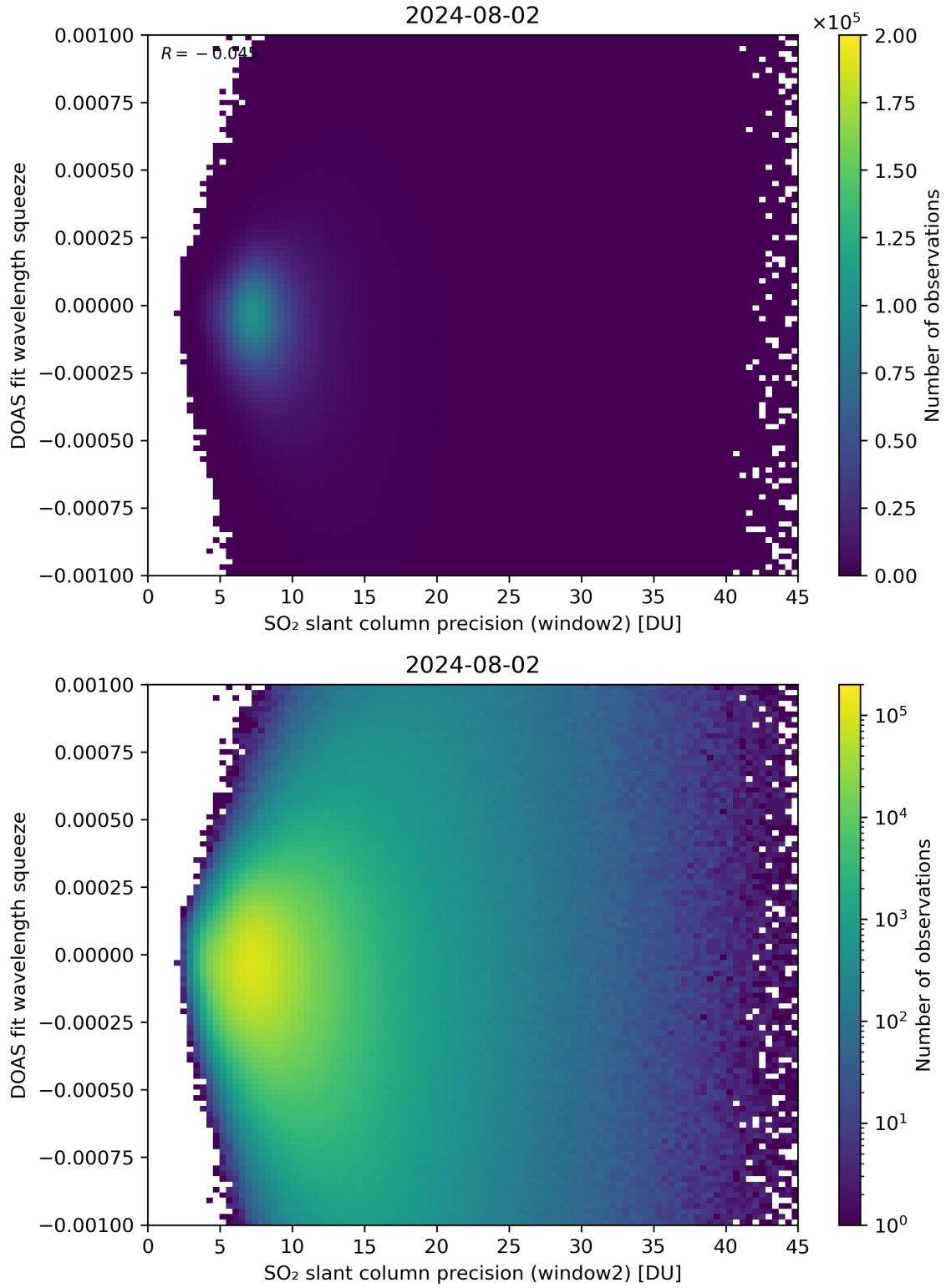
Figure 244: Scatter density plot of “SO 2 slant column precision (window2)” against “DOAS fit wavelength squeeze” for 2024-08-01 to 2024-08-03.
