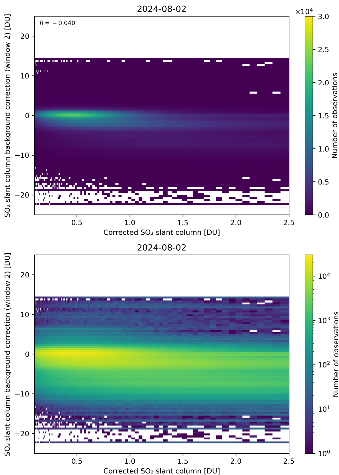
Figure 179: Scatter density plot of “Corrected SO 2 slant column” against “SO 2 slant column background correction (window 2)” for 2024-08-01 to 2024-08-03.
