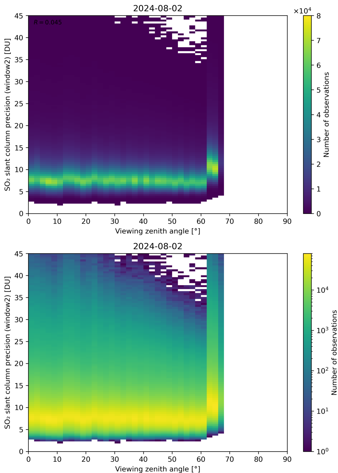
Figure 322: Scatter density plot of “Viewing zenith angle” against “SO 2 slant column precision (window2)” for 2024-08-01 to 2024-08-03.
