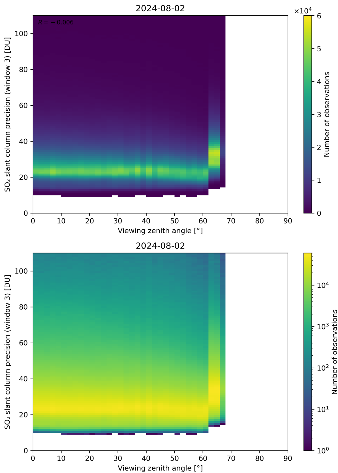
Figure 324: Scatter density plot of “Viewing zenith angle” against “SO 2 slant column precision (window 3)” for 2024-08-01 to 2024-08-03.
