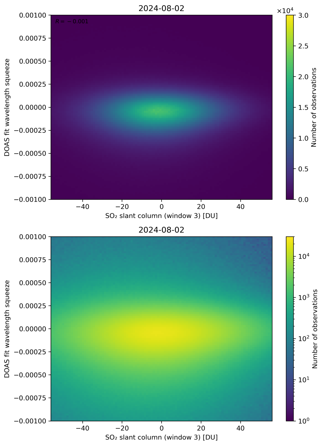
Figure 255: Scatter density plot of “SO 2 slant column (window 3)” against “DOAS fit wavelength squeeze” for 2024-08-01 to 2024-08-03.
