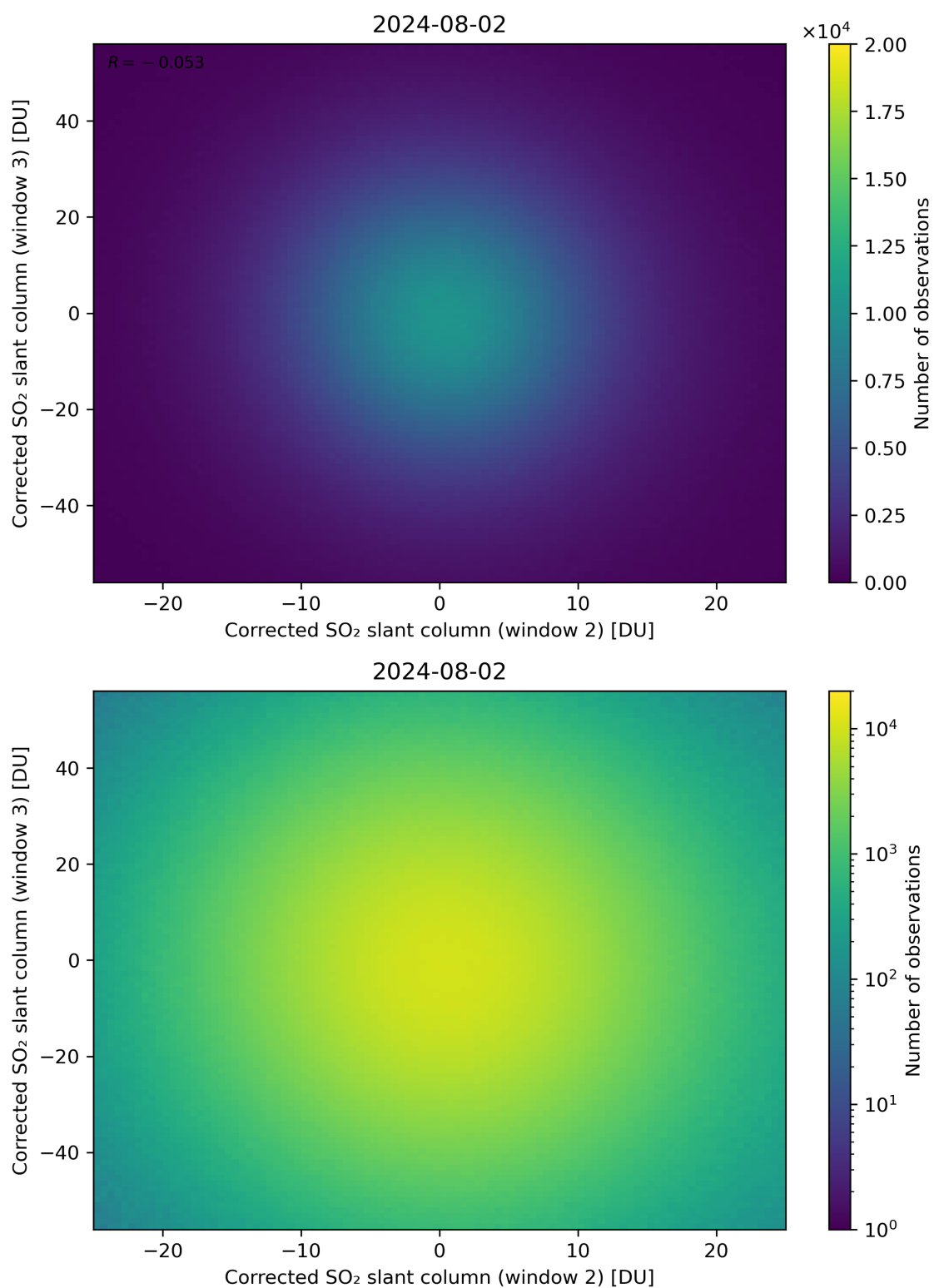
Figure 200: Scatter density plot of “Corrected SO 2 slant column (window 2)” against “Corrected SO 2 slant column (window 3)” for 2024-08-01 to 2024-08-03.
