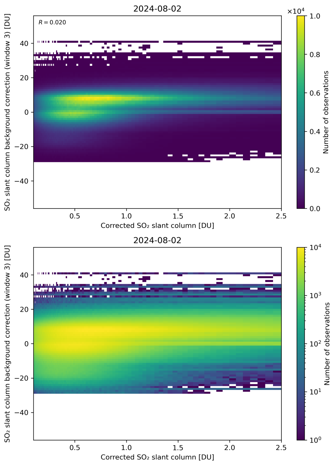
Figure 180: Scatter density plot of “Corrected SO 2 slant column” against “SO 2 slant column background correction (window 3)” for 2024-08-01 to 2024-08-03.
