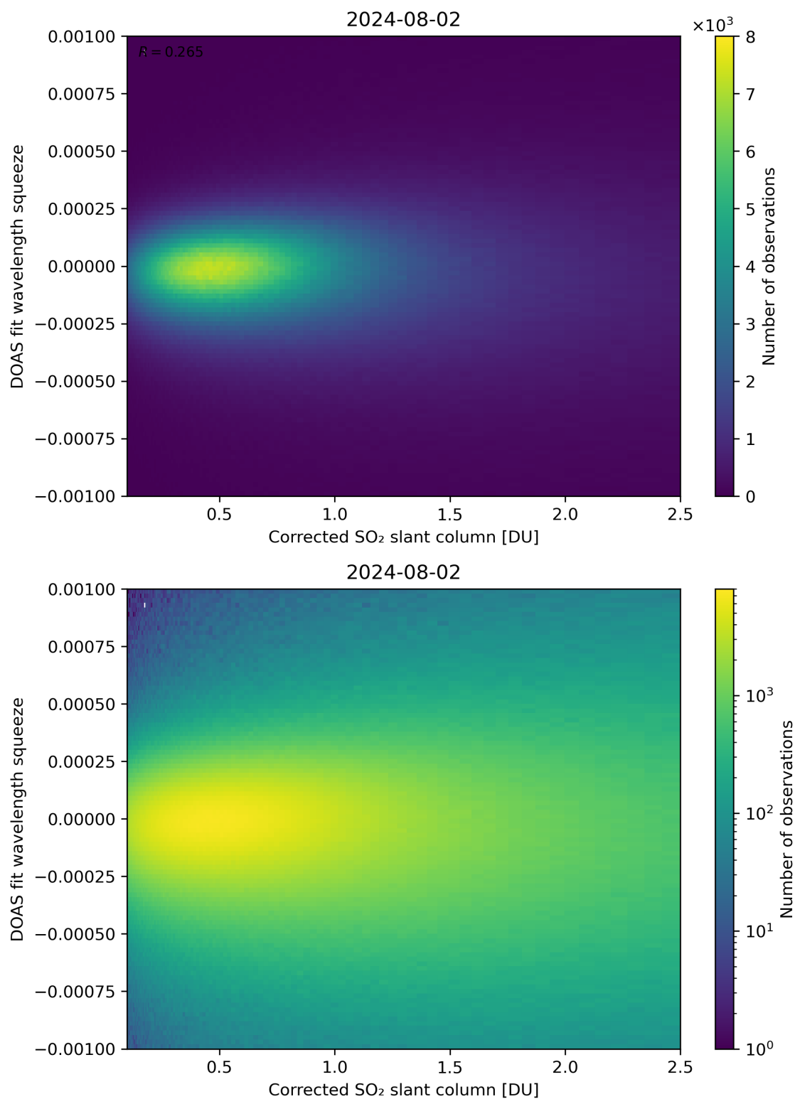
Figure 182: Scatter density plot of “Corrected SO 2 slant column” against “DOAS fit wavelength squeeze” for 2024-08-01 to 2024-08-03.
