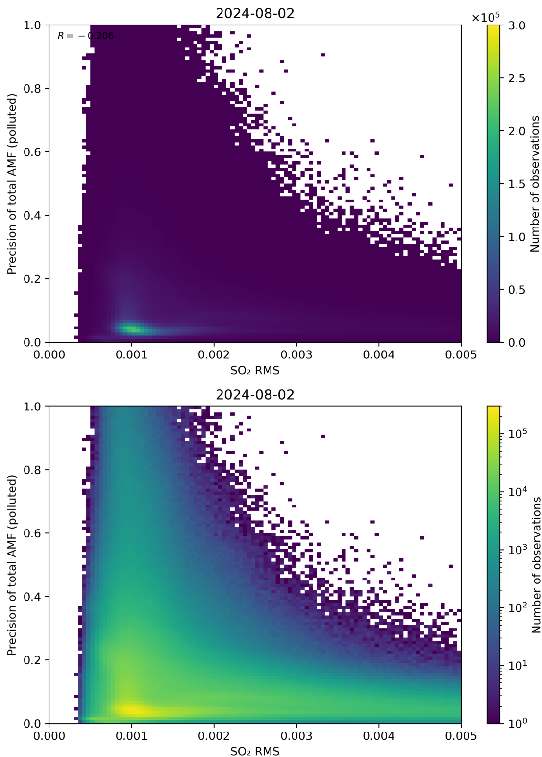
Figure 138: Scatter density plot of “SO 2 RMS” against “Precision of total AMF (polluted)” for 2024-08-01 to 2024-08-03.
