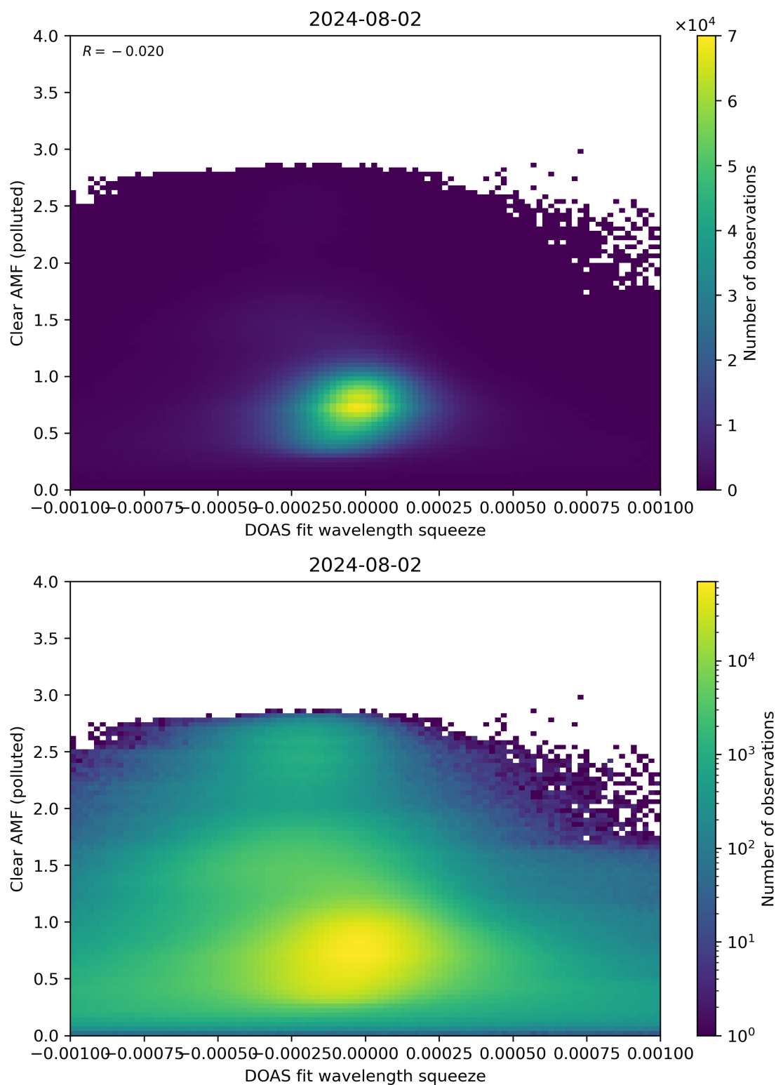
Figure 133: Scatter density plot of “DOAS fit wavelength squeeze” against “Clear AMF (polluted)” for 2024-08-01 to 2024-08-03.
