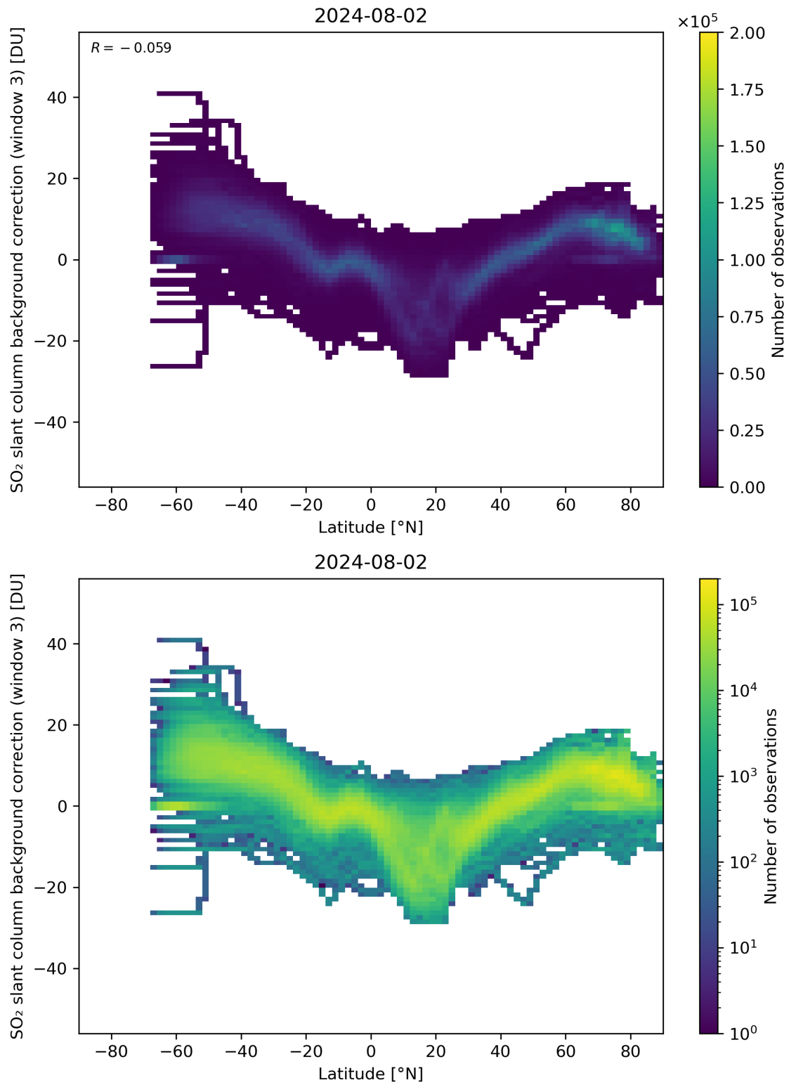
Figure 141: Scatter density plot of “Latitude” against “SO 2 slant column background correction (window 3)” for 2024-08-01 to 2024-08-03.
