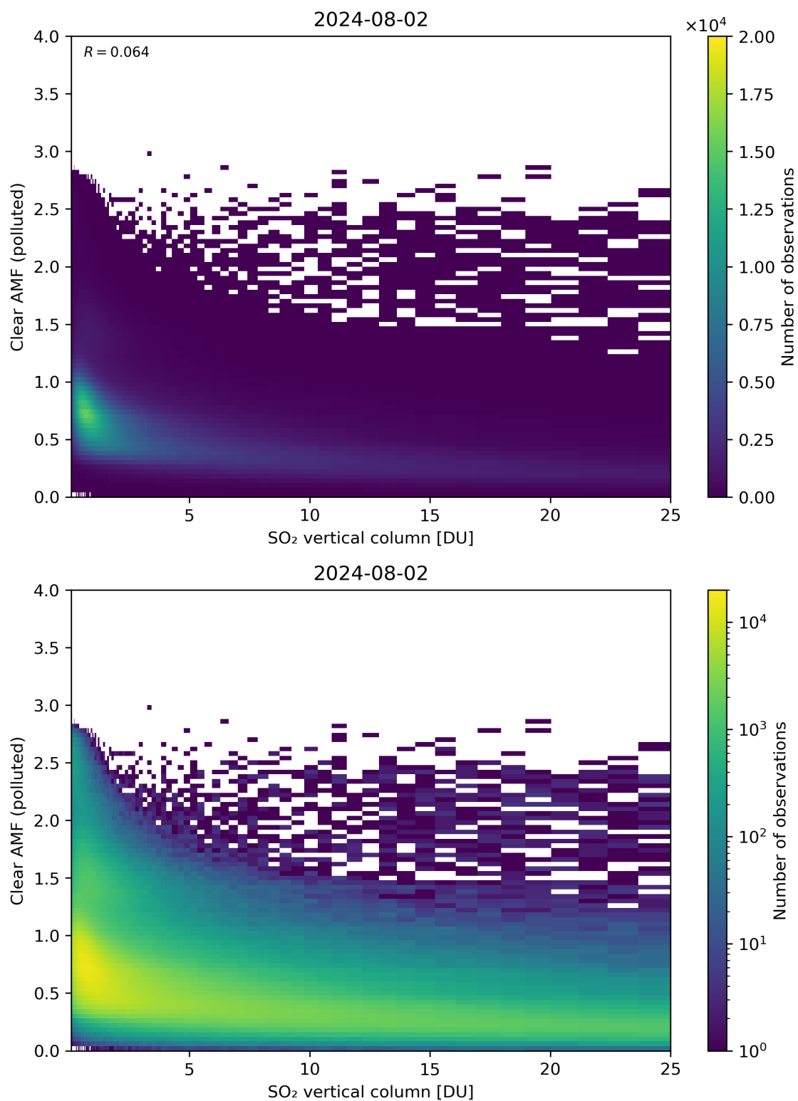
Figure 296: Scatter density plot of “SO 2 vertical column” against “Clear AMF (polluted)” for 2024-08-01 to 2024-08-03.
