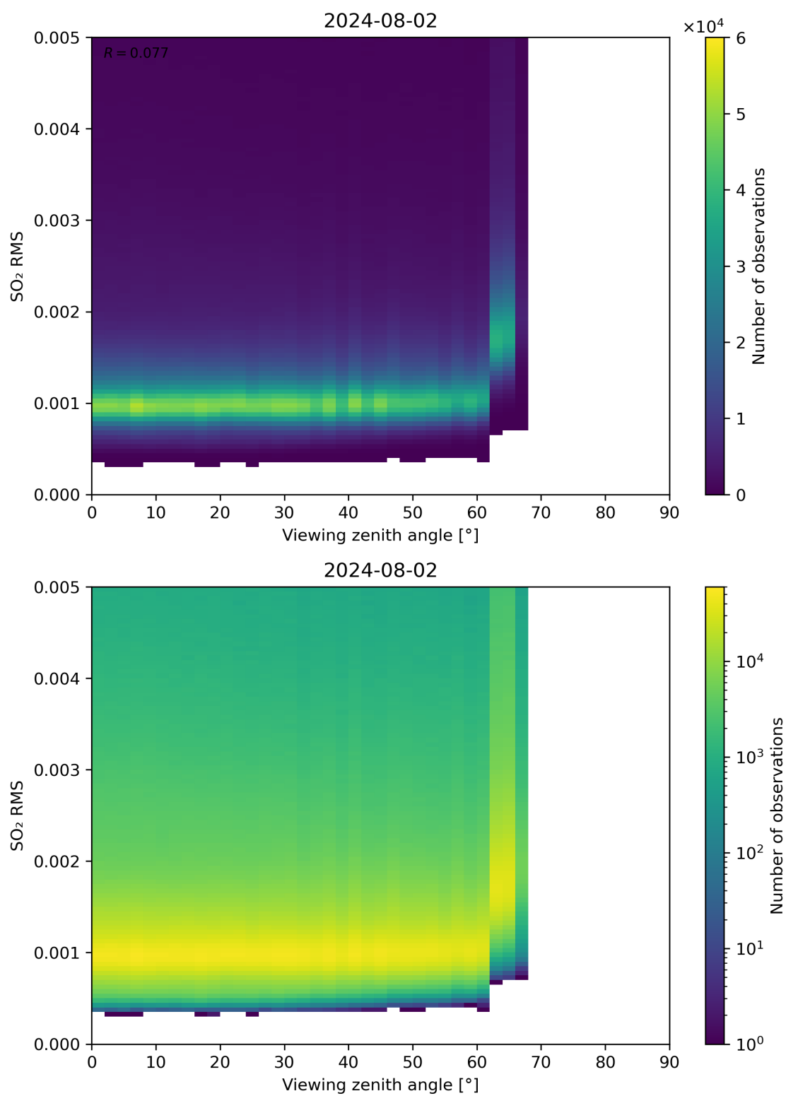
Figure 313: Scatter density plot of “Viewing zenith angle” against “SO 2 RMS” for 2024-08-01 to 2024-08-03.
