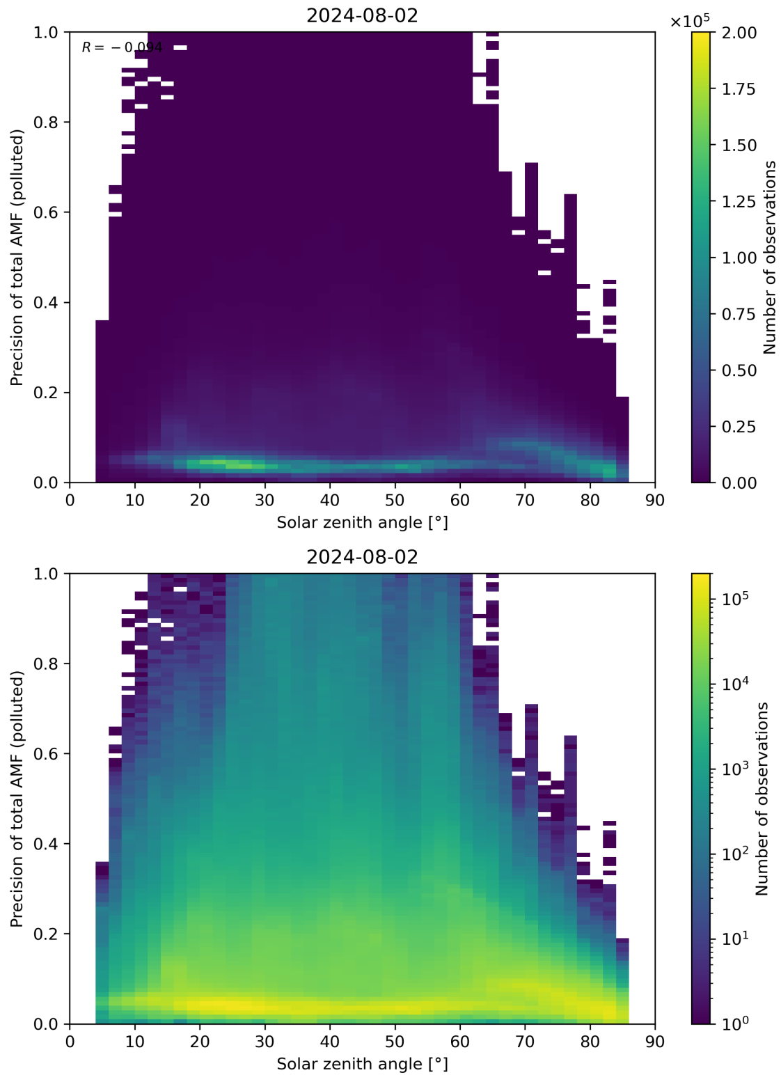
Figure 175: Scatter density plot of “Solar zenith angle” against “Precision of total AMF (polluted)” for 2024-08-01 to 2024-08-03.
