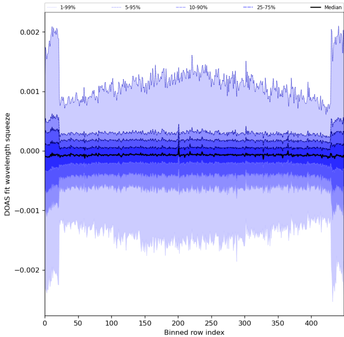
Figure 92: Along track statistics of “DOAS fit wavelength squeeze” for 2024-08-01 to 2024-08-03
