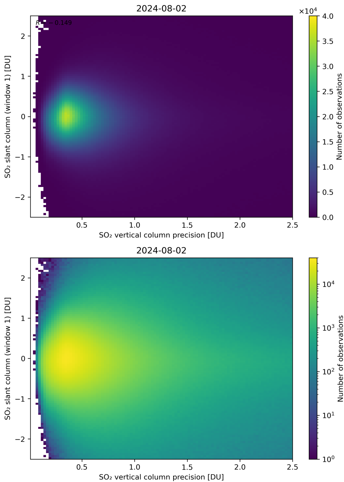
Figure 289: Scatter density plot of “SO 2 vertical column precision” against “SO 2 slant column (window 1)” for 2024-08-01 to 2024-08-03.
