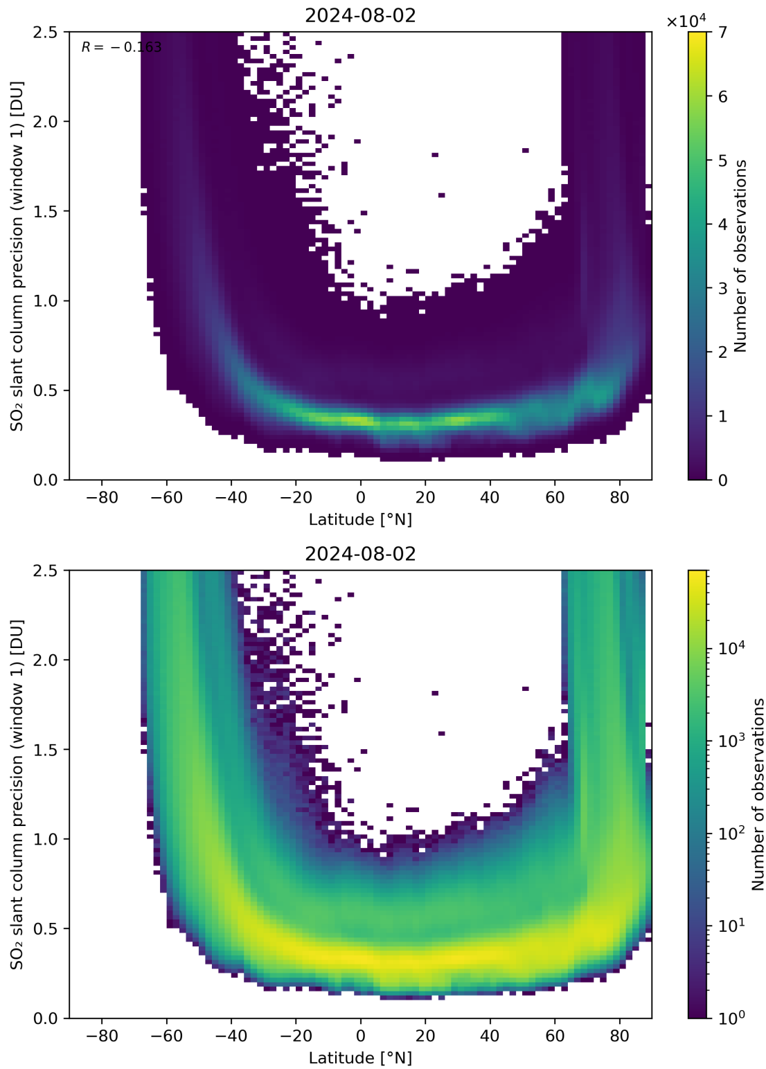
Figure 150: Scatter density plot of “Latitude” against “SO 2 slant column precision (window 1)” for 2024-08-01 to 2024-08-03.
