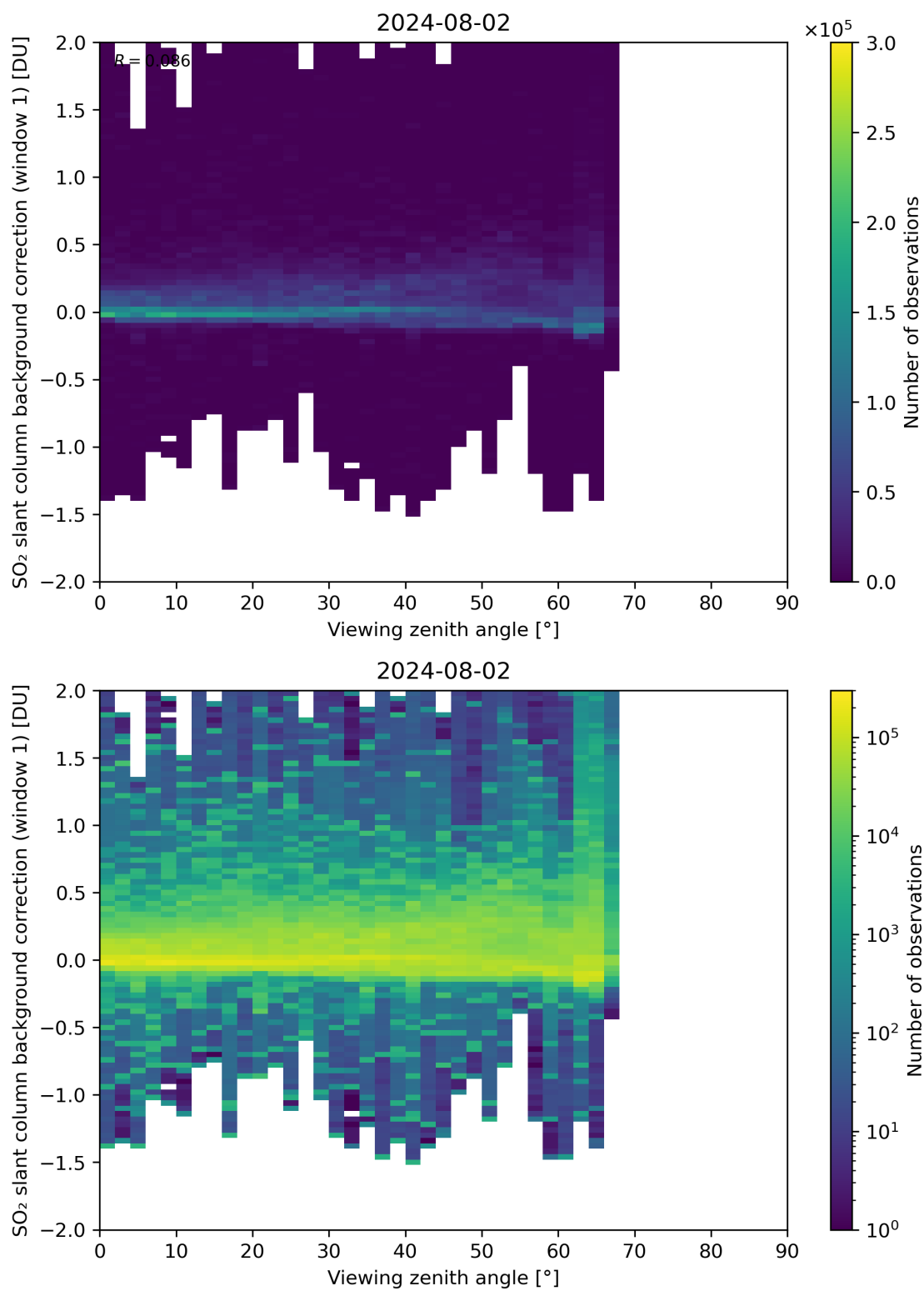
Figure 308: Scatter density plot of “Viewing zenith angle” against “SO 2 slant column background correction (window 1)” for 2024-08-01 to 2024-08-03.
