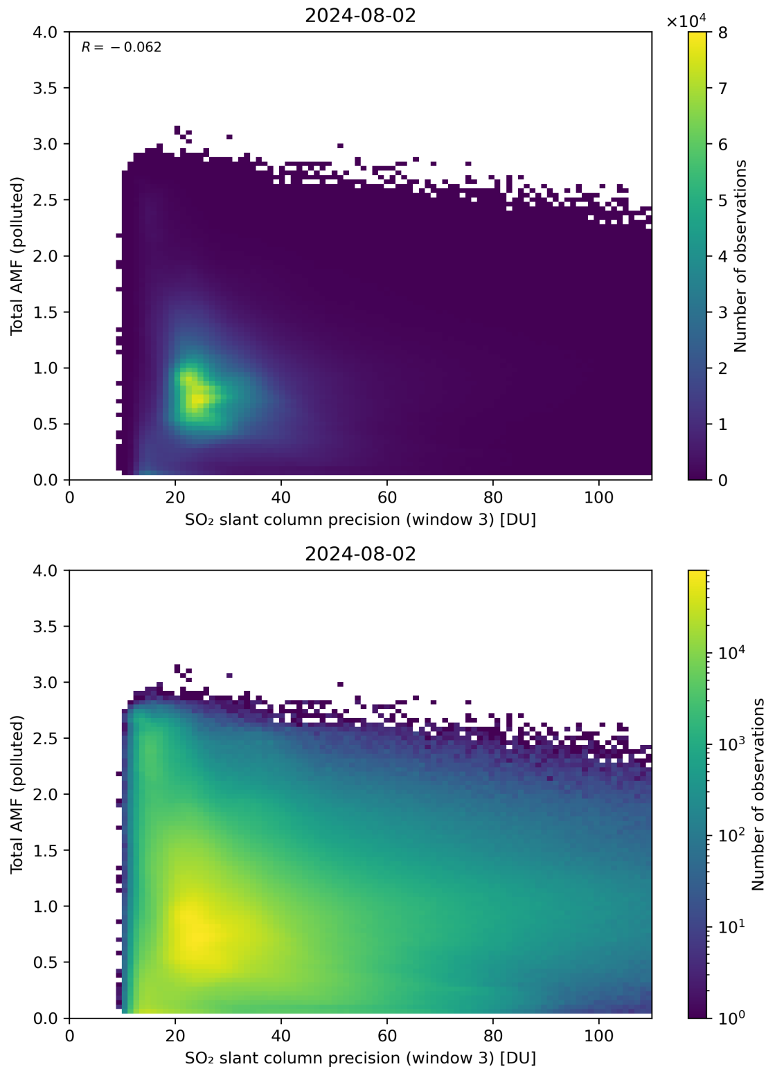
Figure 263: Scatter density plot of “SO 2 slant column precision (window 3)” against “Total AMF (polluted)” for 2024-08-01 to 2024-08-03.
