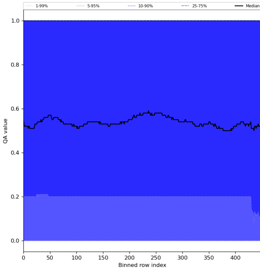
Figure 75: Along track statistics of “QA value” for 2024-08-01 to 2024-08-03
