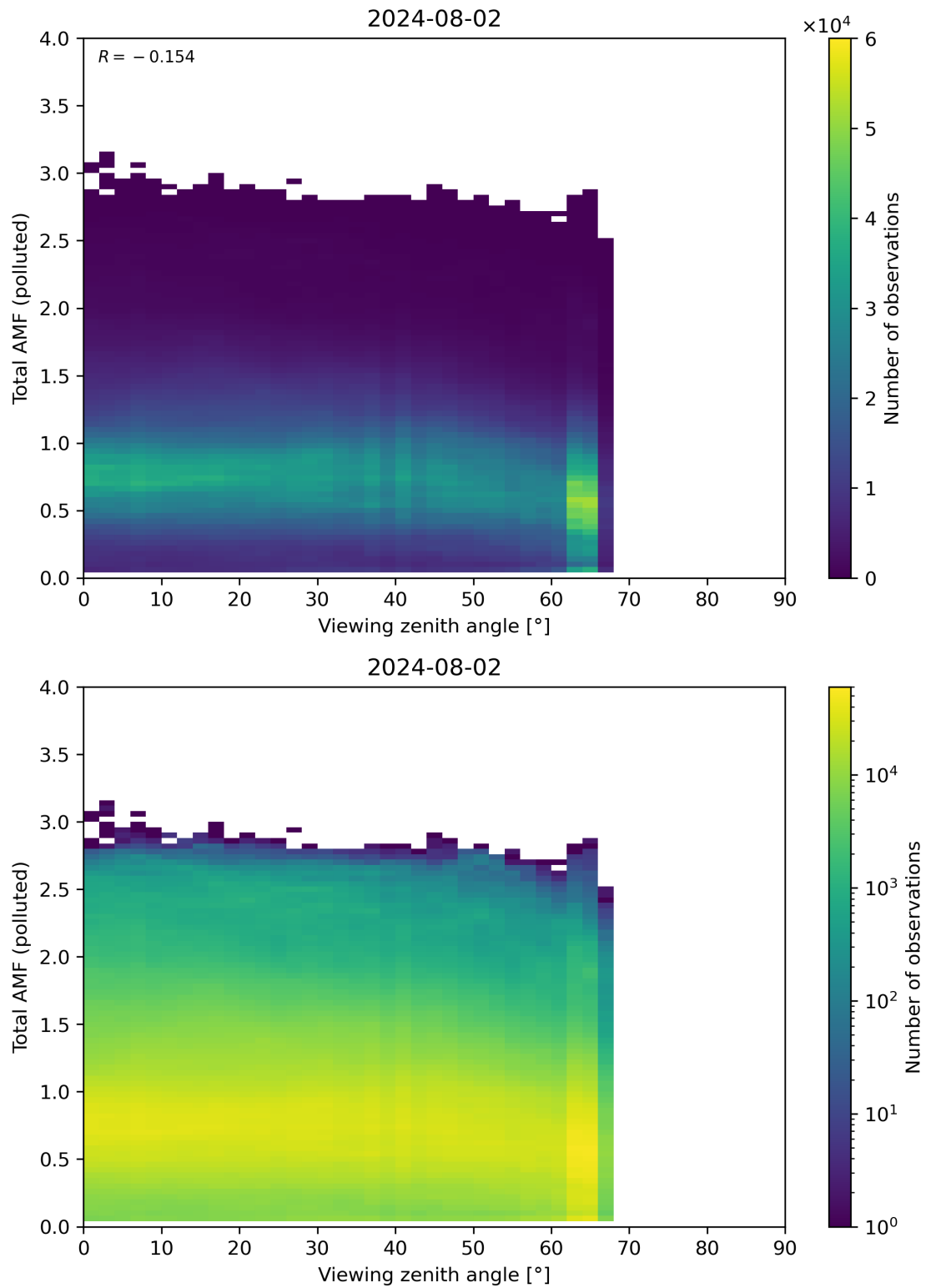
Figure 325: Scatter density plot of “Viewing zenith angle” against “Total AMF (polluted)” for 2024-08-01 to 2024-08-03.
