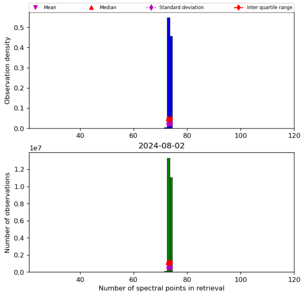
Figure 74: Histogram of “Number of spectral points in retrieval” for 2024-08-01 to 2024-08-03
