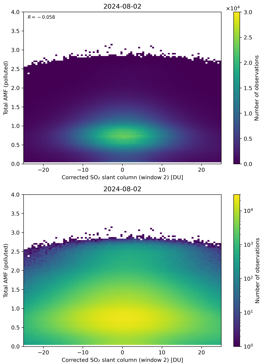
Figure 203: Scatter density plot of “Corrected SO 2 slant column (window 2)” against “Total AMF (polluted)” for 2024-08-01 to 2024-08-03.
