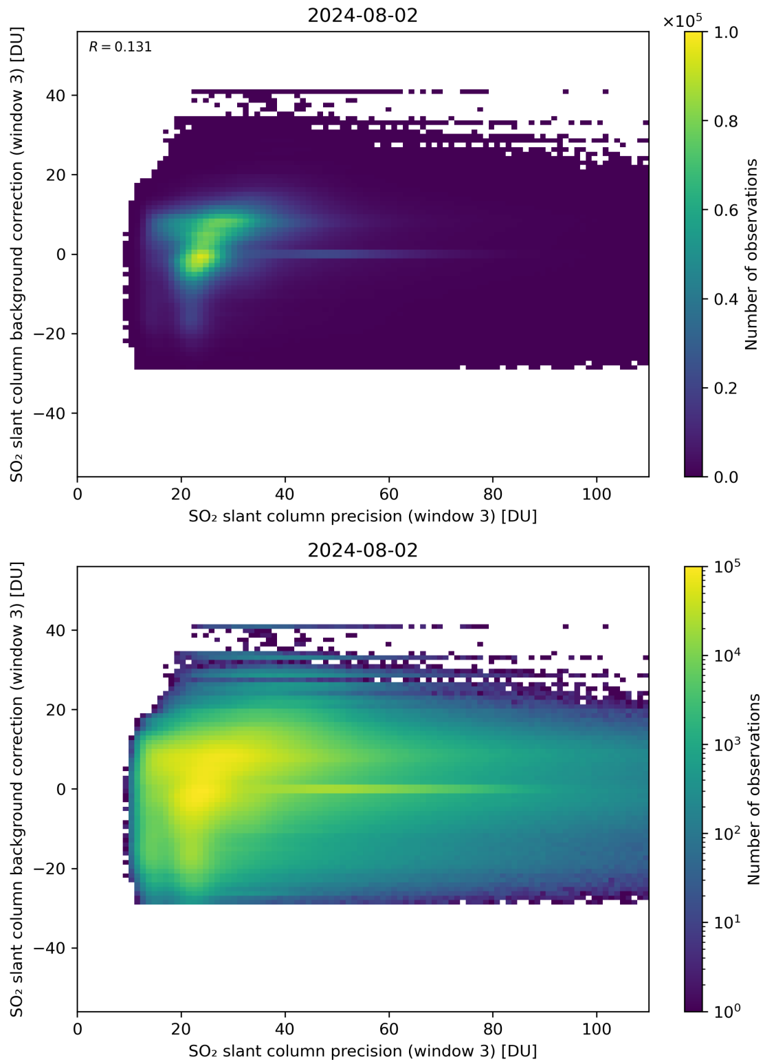
Figure 257: Scatter density plot of “SO 2 slant column precision (window 3)” against “SO 2 slant column background correction (window 3)” for 2024-08-01 to 2024-08-03.
