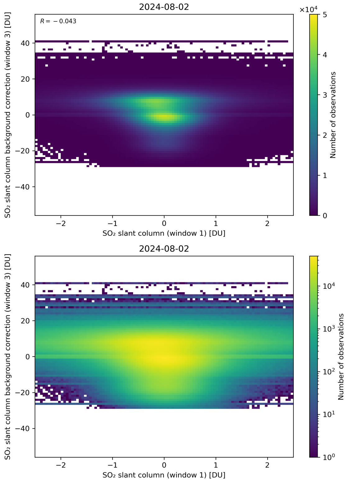
Figure 214: Scatter density plot of “SO 2 slant column (window 1)” against “SO 2 slant column background correction (window 3)” for 2024-08-01 to 2024-08-03.
