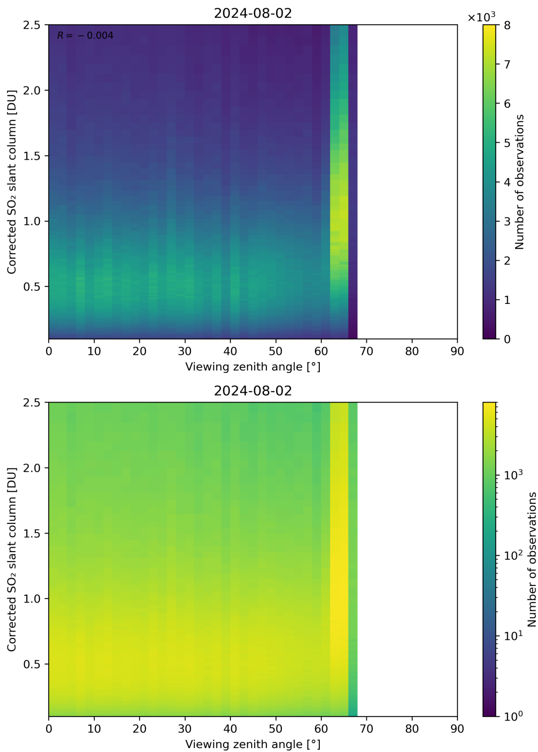
Figure 317: Scatter density plot of “Viewing zenith angle” against “Corrected SO 2 slant column” for 2024-08-01 to 2024-08-03.
