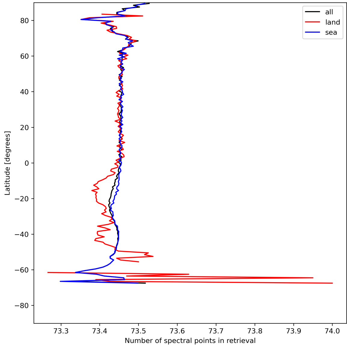
Figure 51: Zonal average of “Number of spectral points in retrieval” for 2024-08-01 to 2024-08-03.
