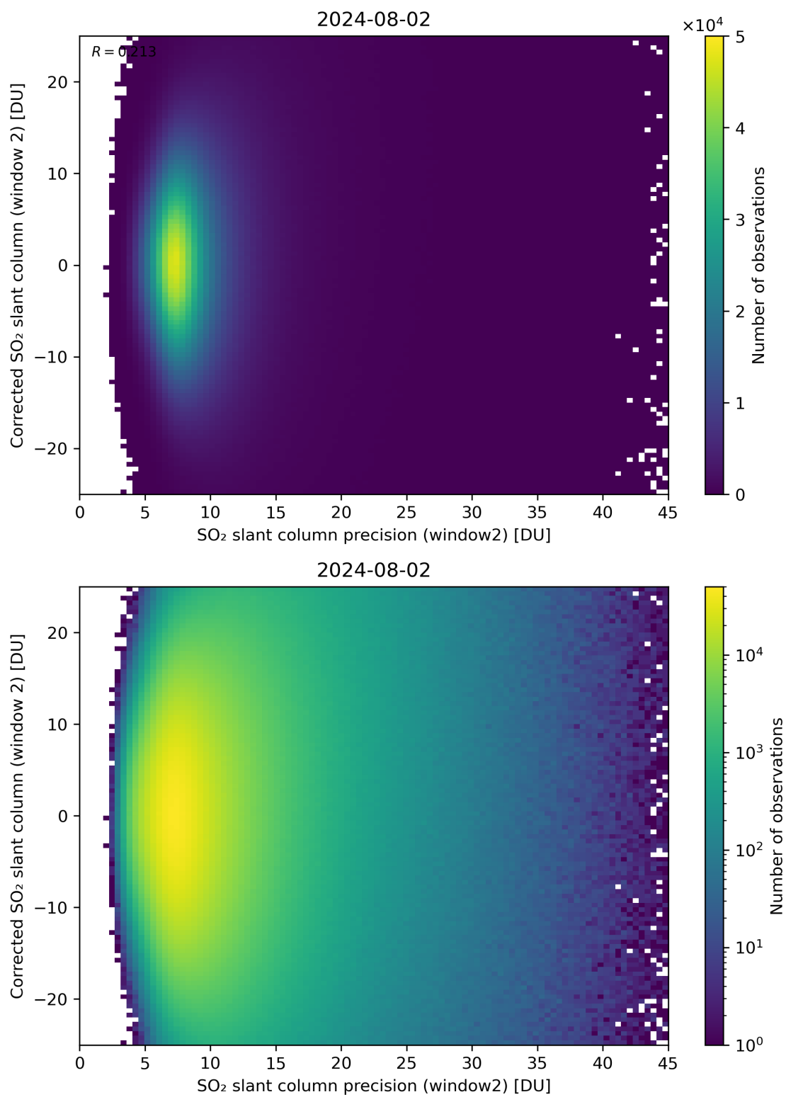
Figure 247: Scatter density plot of “SO 2 slant column precision (window2)” against “Corrected SO 2 slant column (window 2)” for 2024-08-01 to 2024-08-03.
