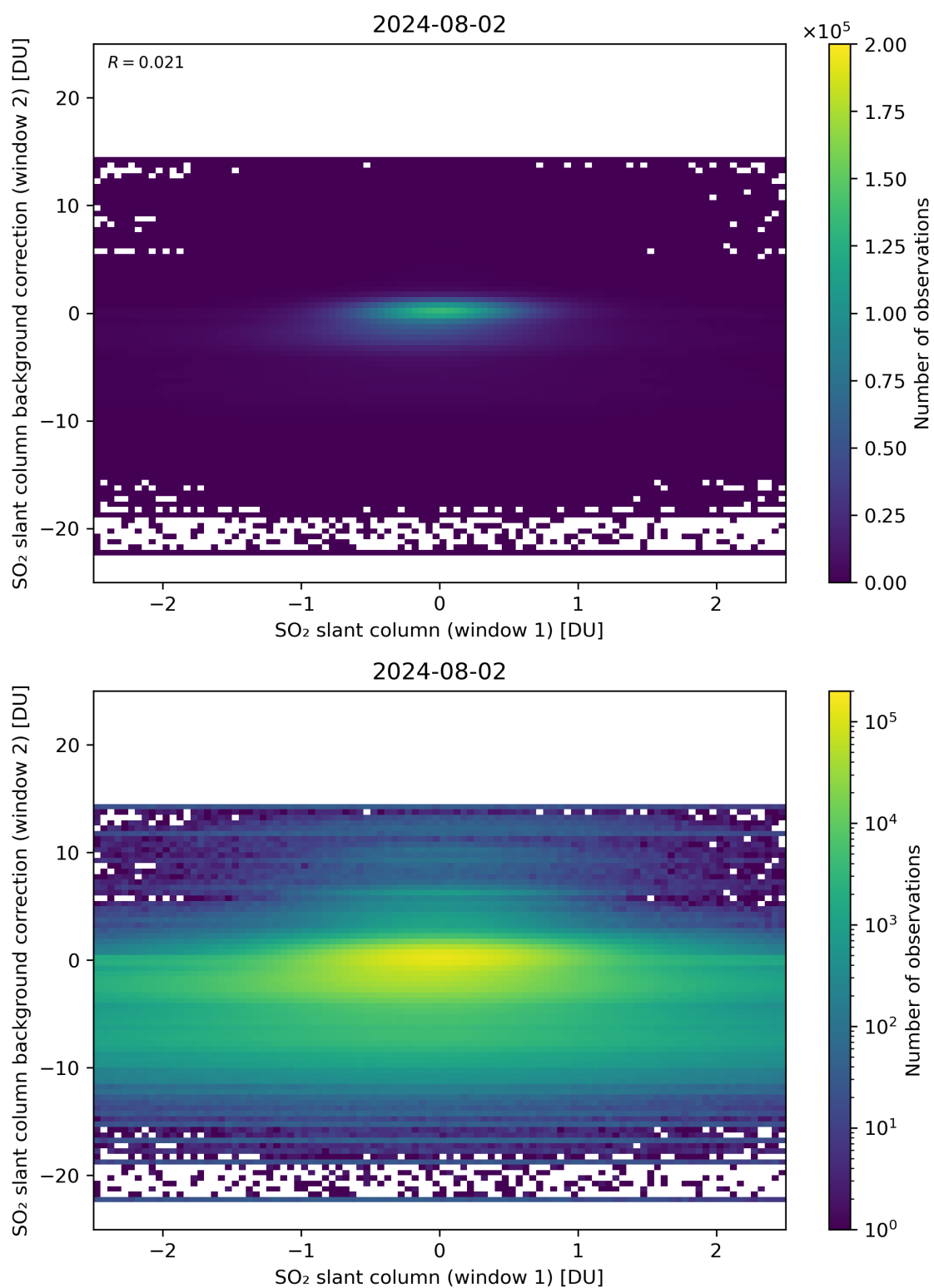
Figure 213: Scatter density plot of “SO 2 slant column (window 1)” against “SO 2 slant column background correction (window 2)” for 2024-08-01 to 2024-08-03.
