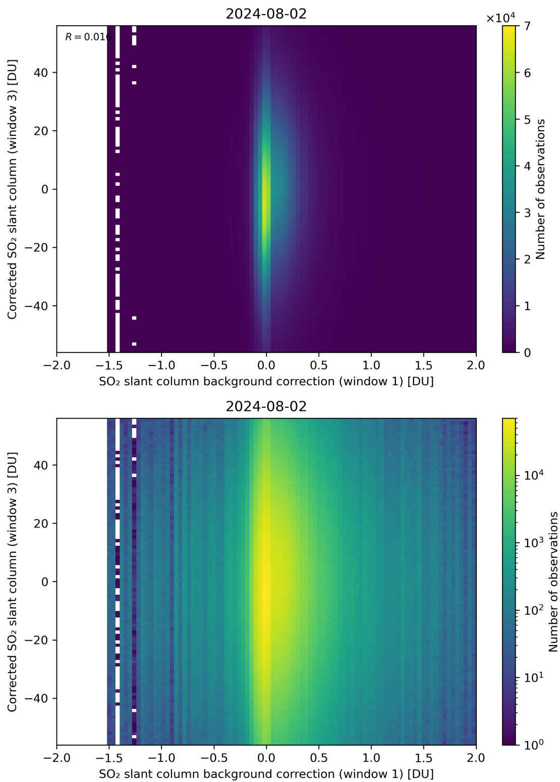
Figure 105: Scatter density plot of “SO 2 slant column background correction (window 1)” against “Corrected SO 2 slant column (window 3)” for 2024-08-01 to 2024-08-03.
