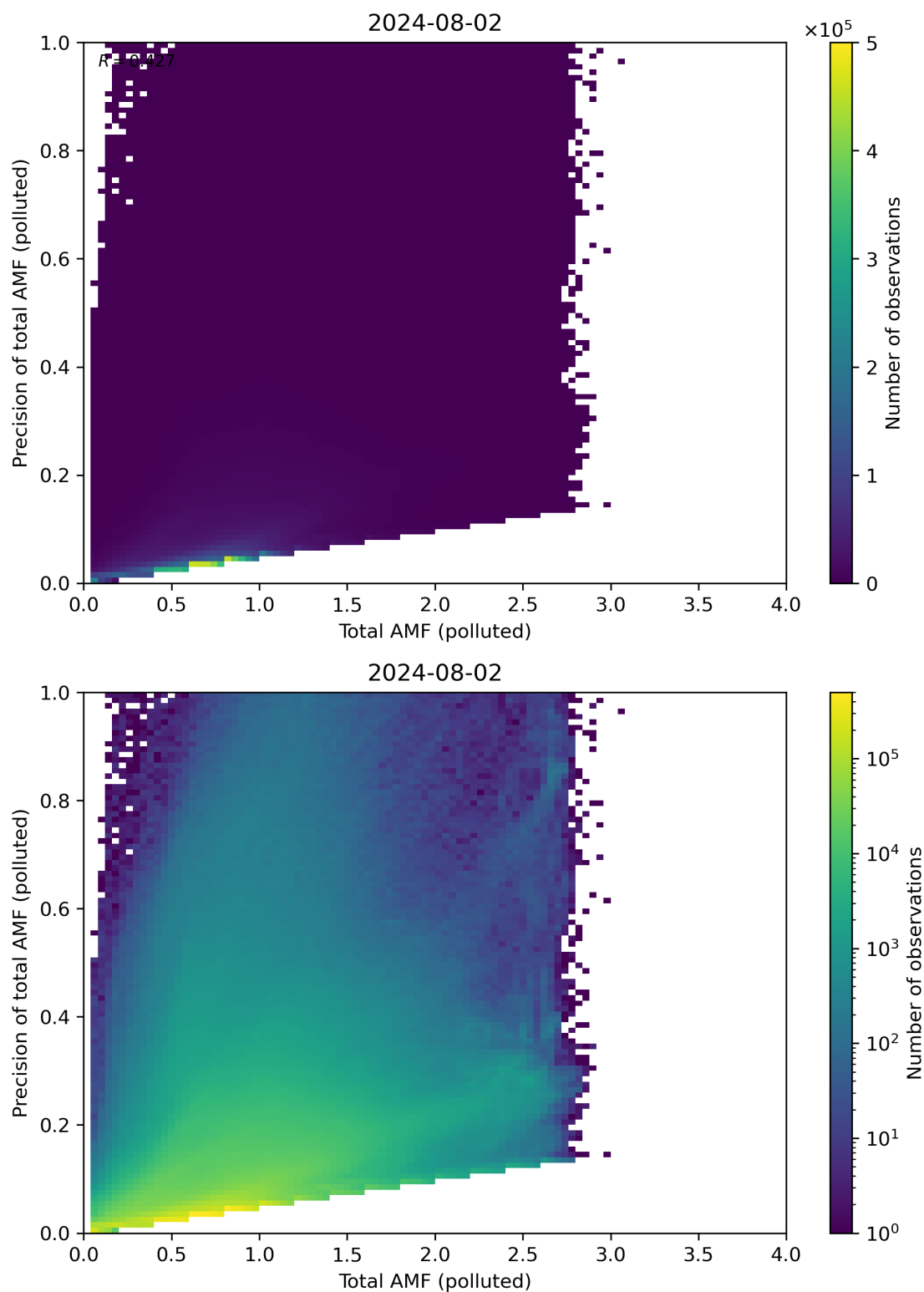
Figure 272: Scatter density plot of “Total AMF (polluted)” against “Precision of total AMF (polluted)” for 2024-08-01 to 2024-08-03.
