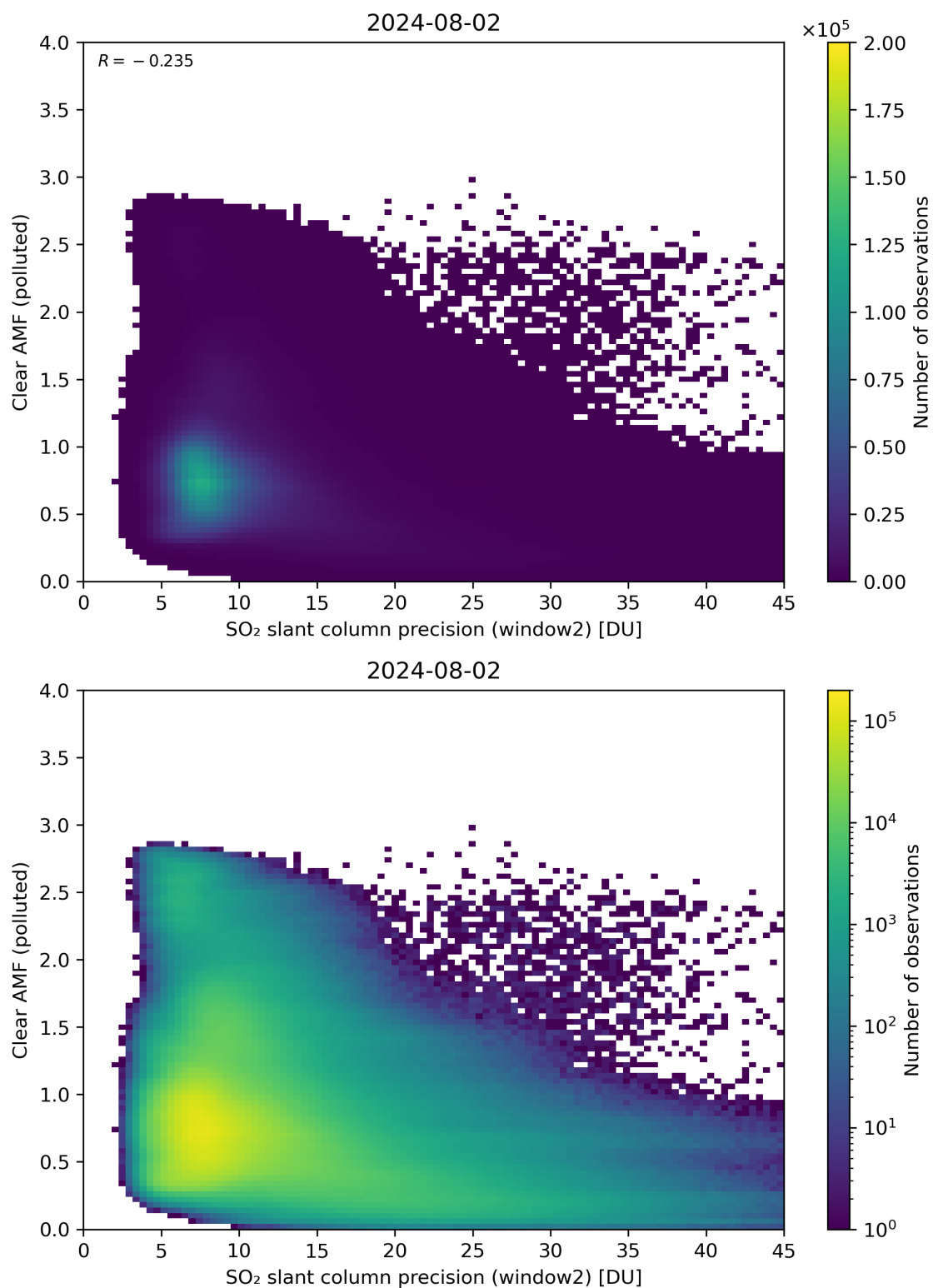
Figure 246: Scatter density plot of “SO 2 slant column precision (window2)” against “Clear AMF (polluted)” for 2024-08-01 to 2024-08-03.
