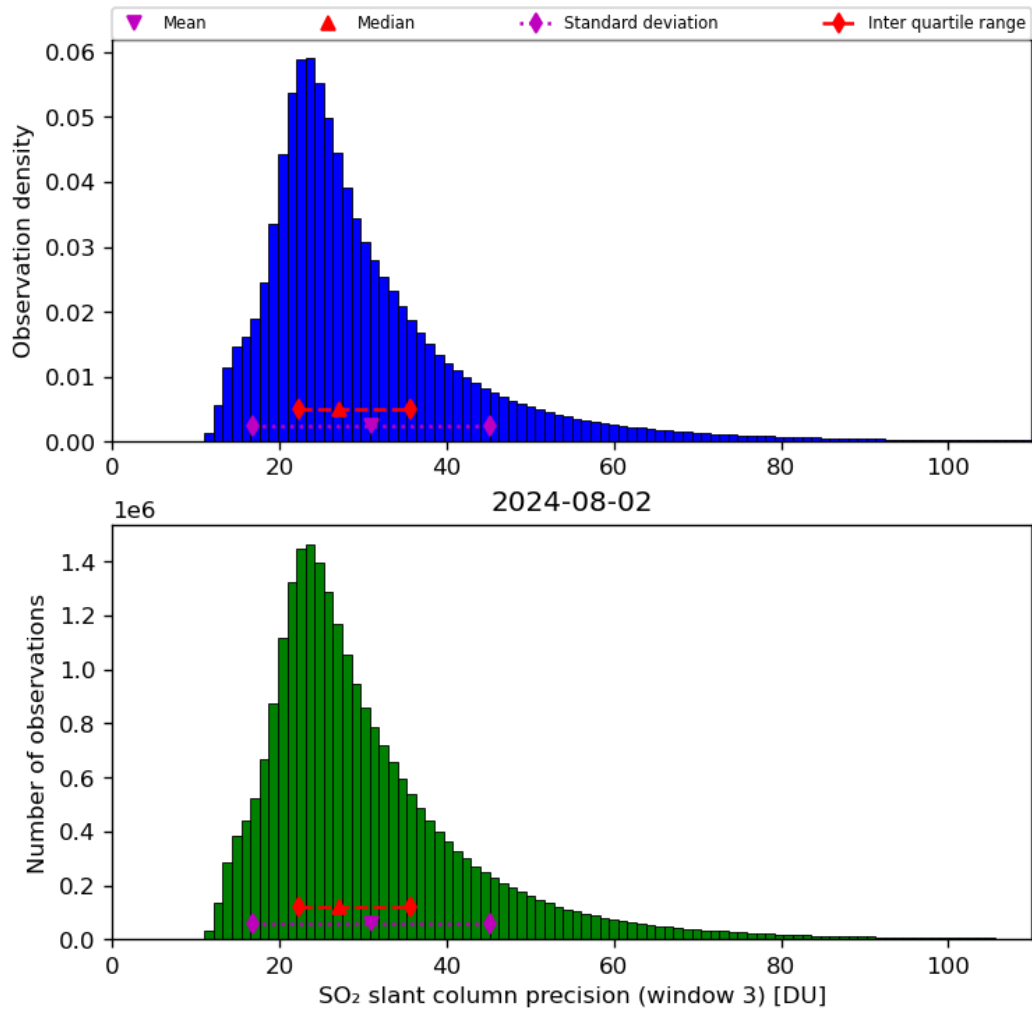
Figure 65: Histogram of “SO 2 slant column precision (window 3)” for 2024-08-01 to 2024-08-03
