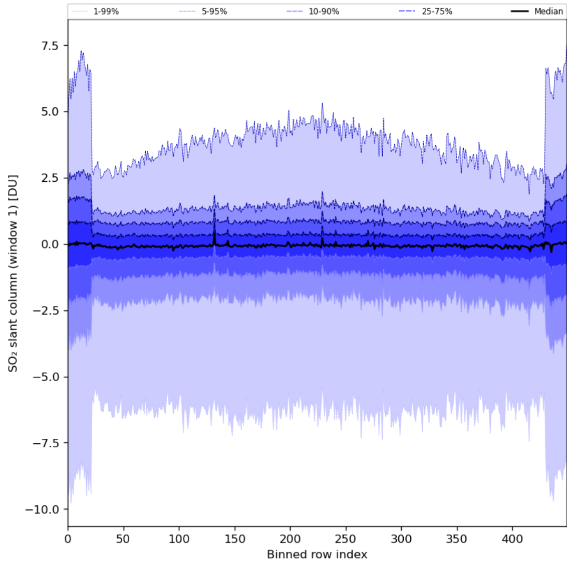
Figure 79: Along track statistics of “SO 2 slant column (window 1)” for 2024-08-01 to 2024-08-03
