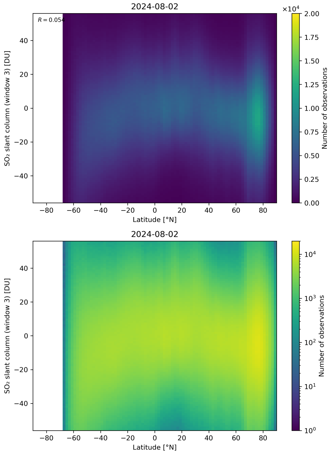
Figure 152: Scatter density plot of “Latitude” against “SO 2 slant column (window 3)” for 2024-08-01 to 2024-08-03.
