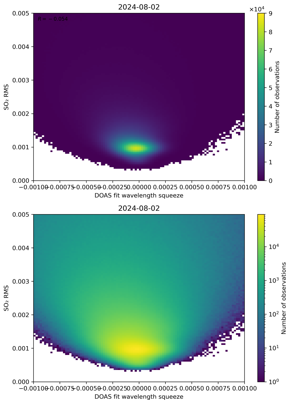
Figure 132: Scatter density plot of “DOAS fit wavelength squeeze” against “SO 2 RMS” for 2024-08-01 to 2024-08-03.
