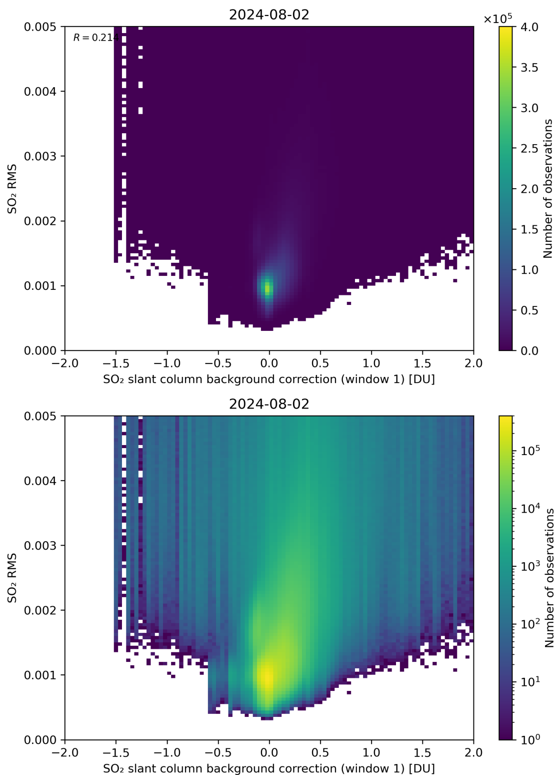
Figure 102: Scatter density plot of “SO 2 slant column background correction (window 1)” against “SO 2 RMS” for 2024-08-01 to 2024-08-03.
