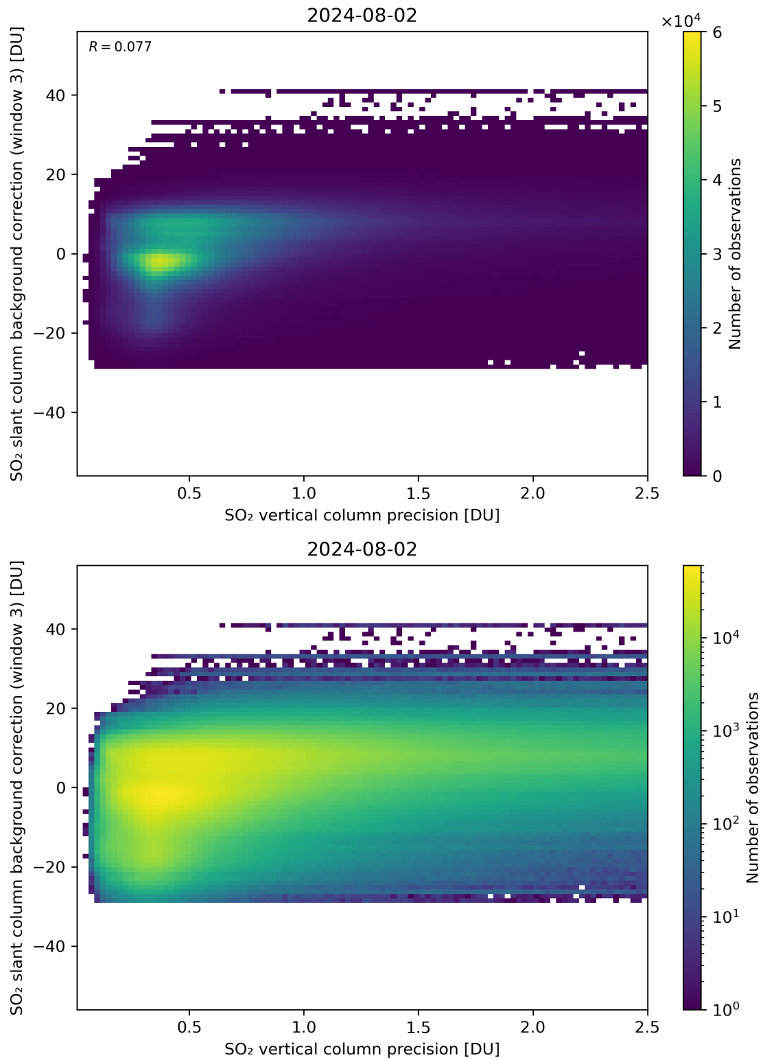
Figure 281: Scatter density plot of “SO 2 vertical column precision” against “SO 2 slant column background correction (window 3)” for 2024-08-01 to 2024-08-03.
