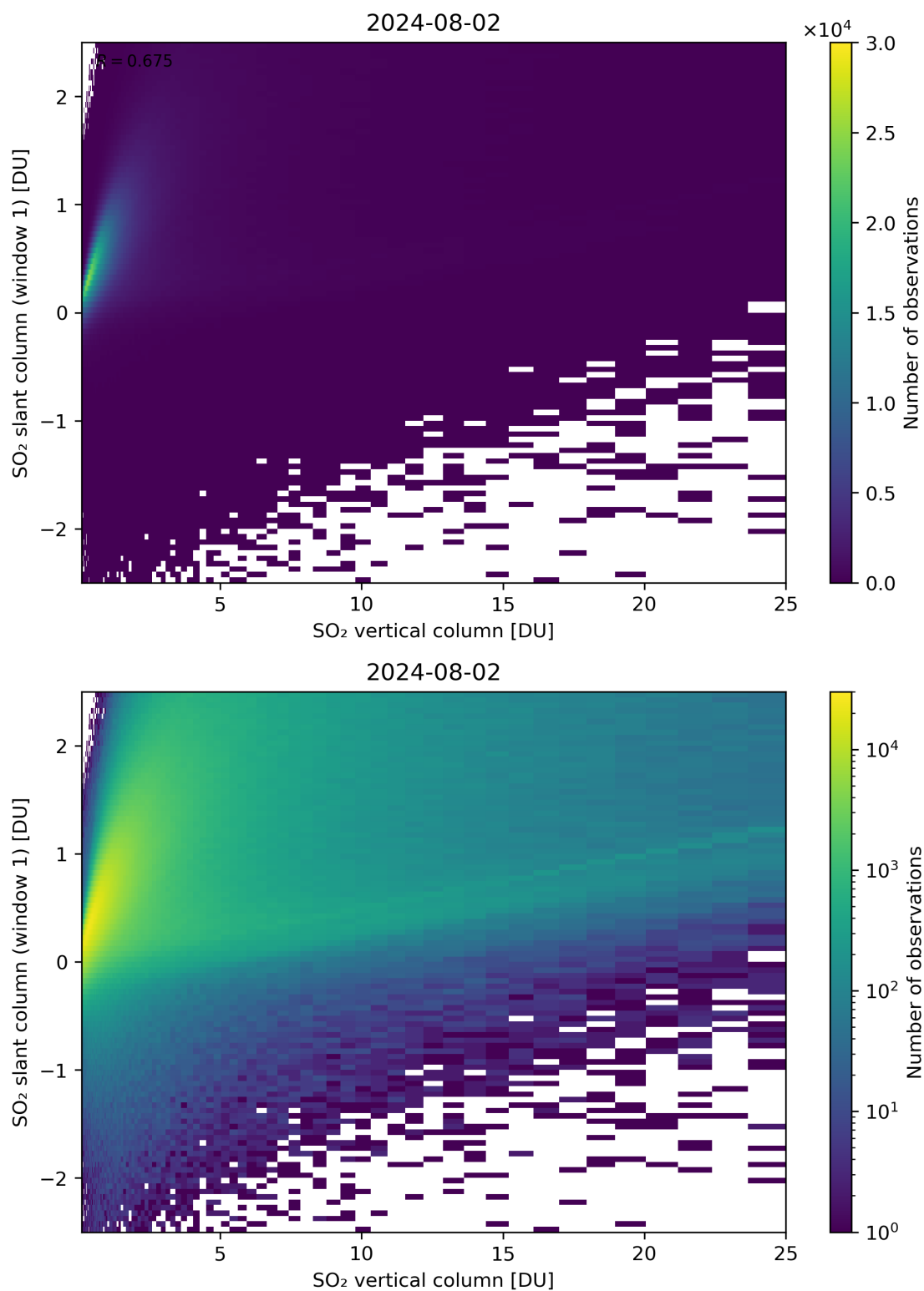
Figure 300: Scatter density plot of “SO 2 vertical column” against “SO 2 slant column (window 1)” for 2024-08-01 to 2024-08-03.
