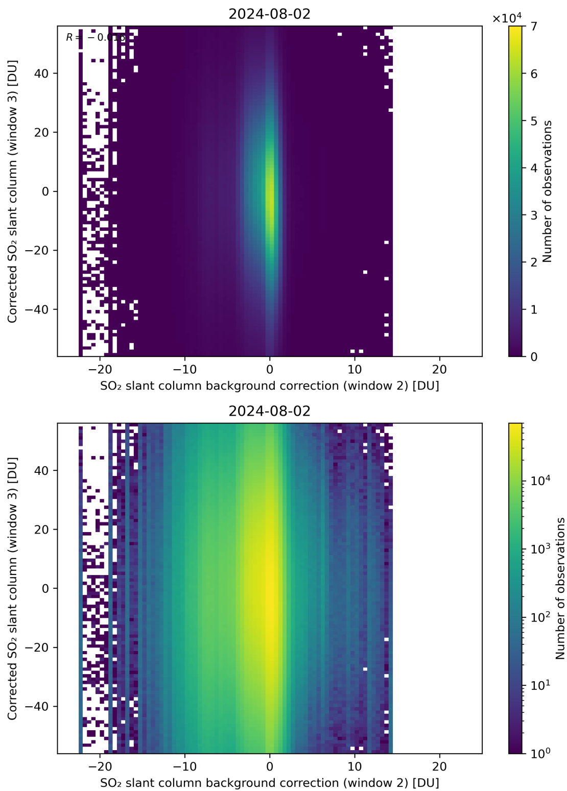
Figure 116: Scatter density plot of “SO 2 slant column background correction (window 2)” against “Corrected SO 2 slant column (window 3)” for 2024-08-01 to 2024-08-03.
