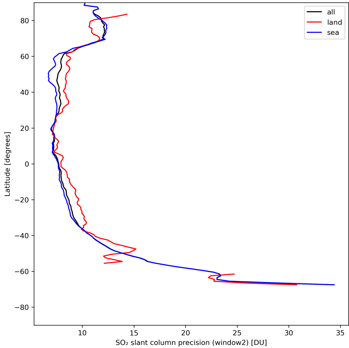
Figure 38: Zonal average of “SO 2 slant column precision (window2)” for 2024-08-01 to 2024-08-03.
