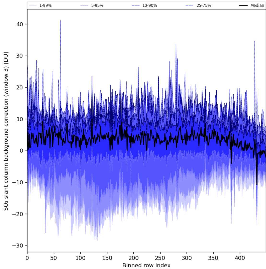
Figure 90: Along track statistics of “SO 2 slant column background correction (window 3)” for 2024-08-01 to 2024-08-03
