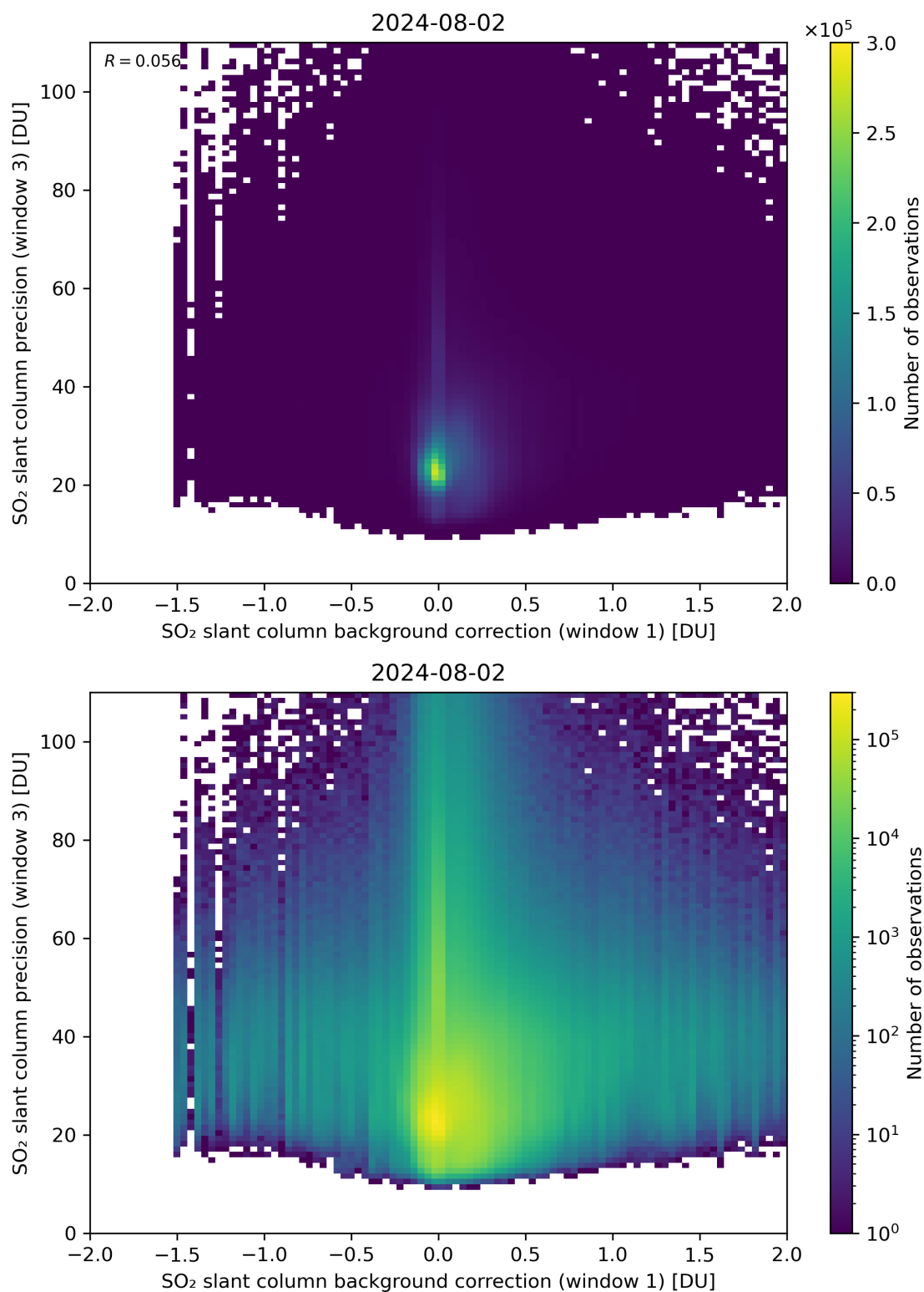
Figure 108: Scatter density plot of “SO 2 slant column background correction (window 1)” against “SO 2 slant column precision (window 3)” for 2024-08-01 to 2024-08-03.
