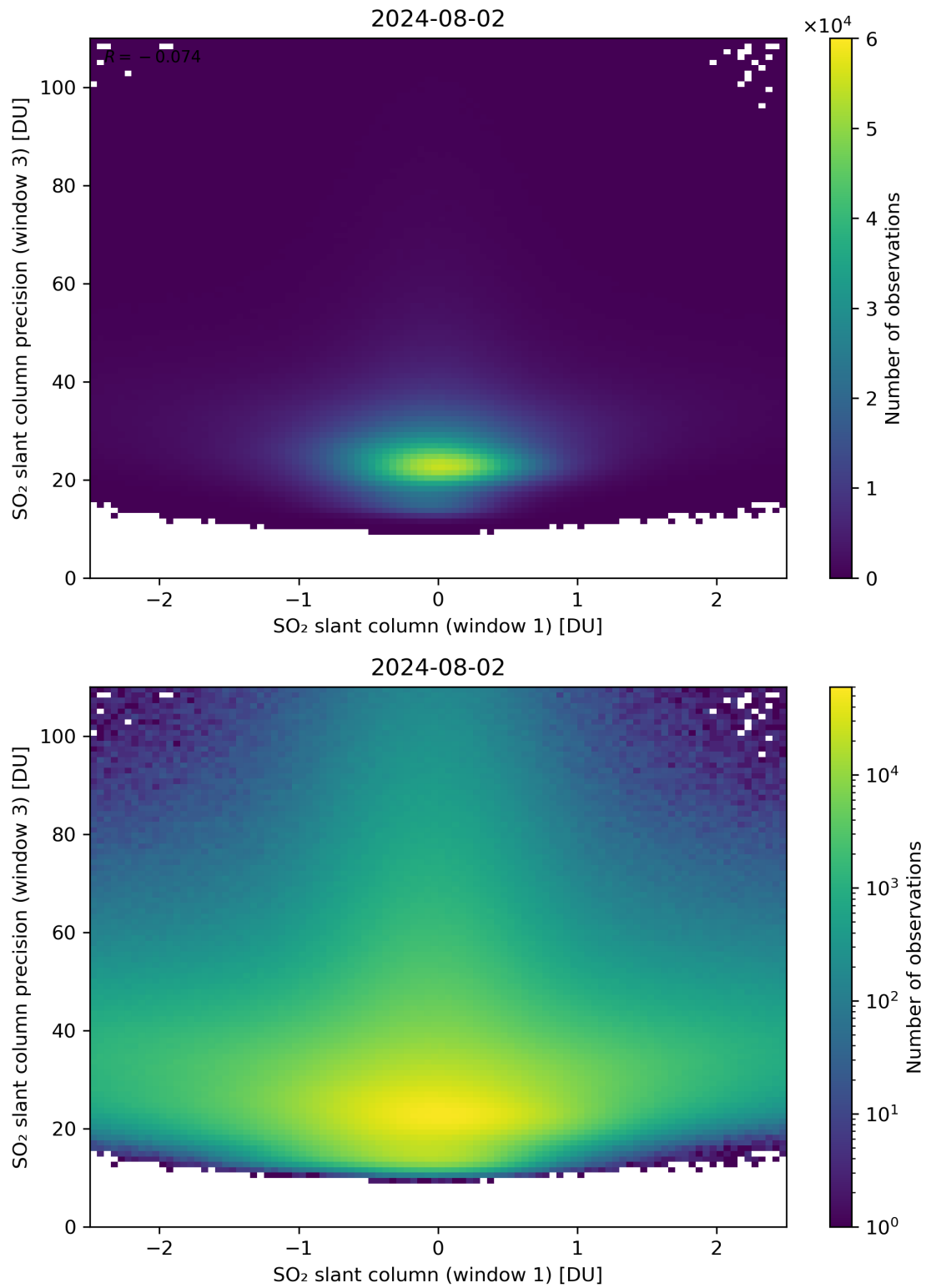
Figure 238: Scatter density plot of “SO 2 slant column (window 1)” against “SO 2 slant column precision (window 3)” for 2024-08-01 to 2024-08-03.
