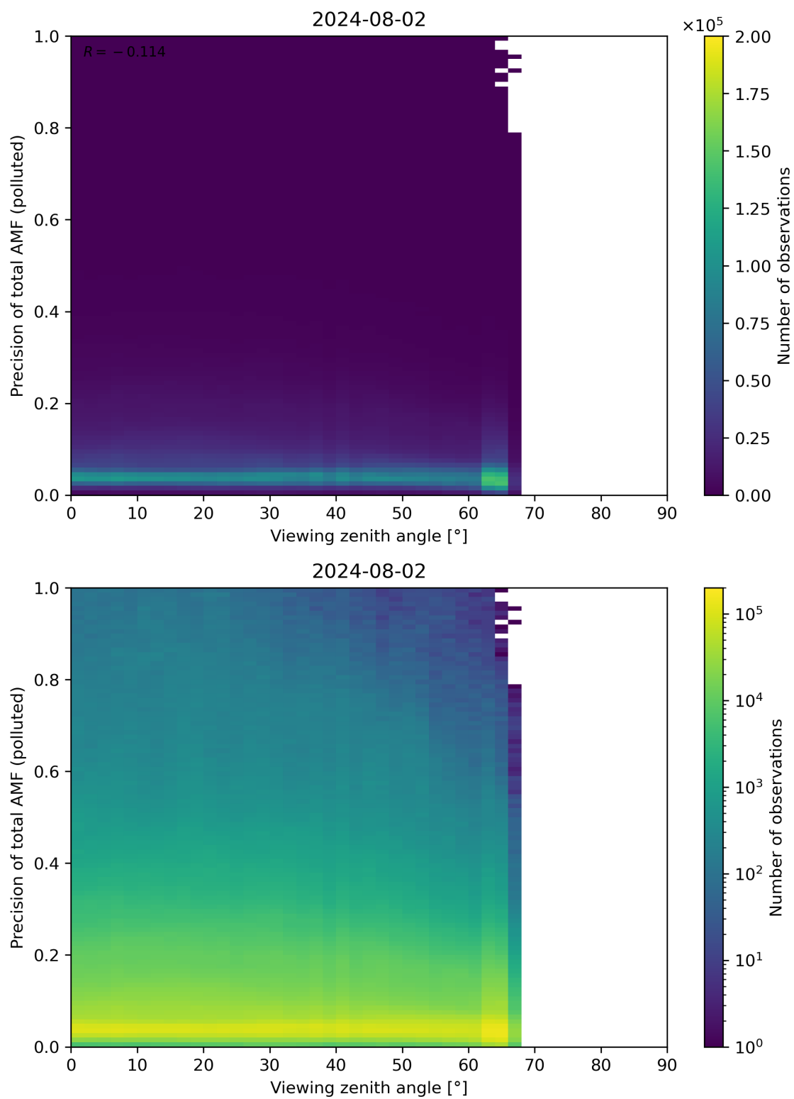
Figure 326: Scatter density plot of “Viewing zenith angle” against “Precision of total AMF (polluted)” for 2024-08-01 to 2024-08-03.
