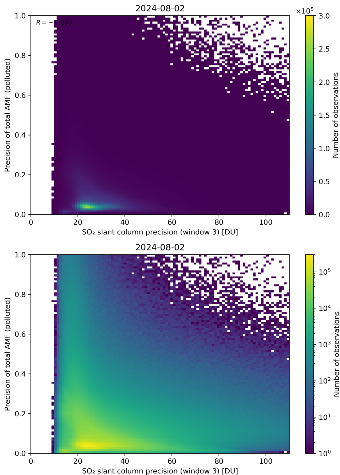
Figure 264: Scatter density plot of “SO 2 slant column precision (window 3)” against “Precision of total AMF (polluted)” for 2024-08-01 to 2024-08-03.
