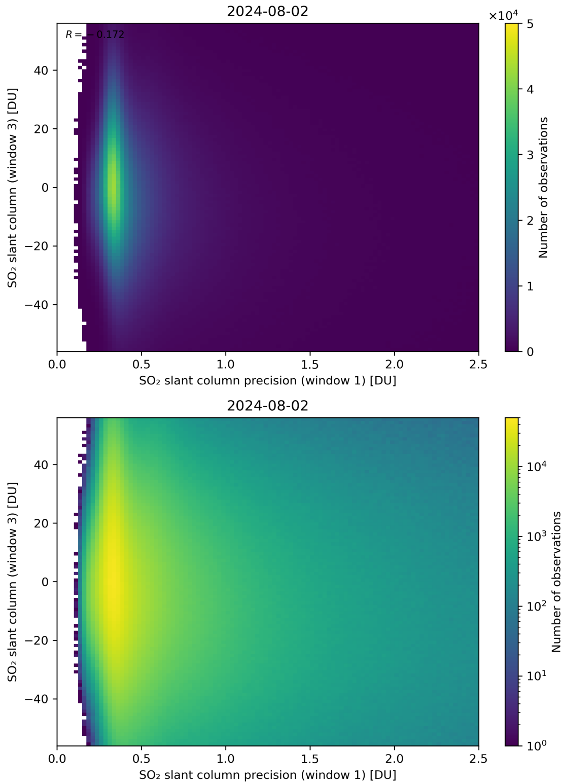
Figure 228: Scatter density plot of “SO 2 slant column precision (window 1)” against “SO 2 slant column (window 3)” for 2024-08-01 to 2024-08-03.
