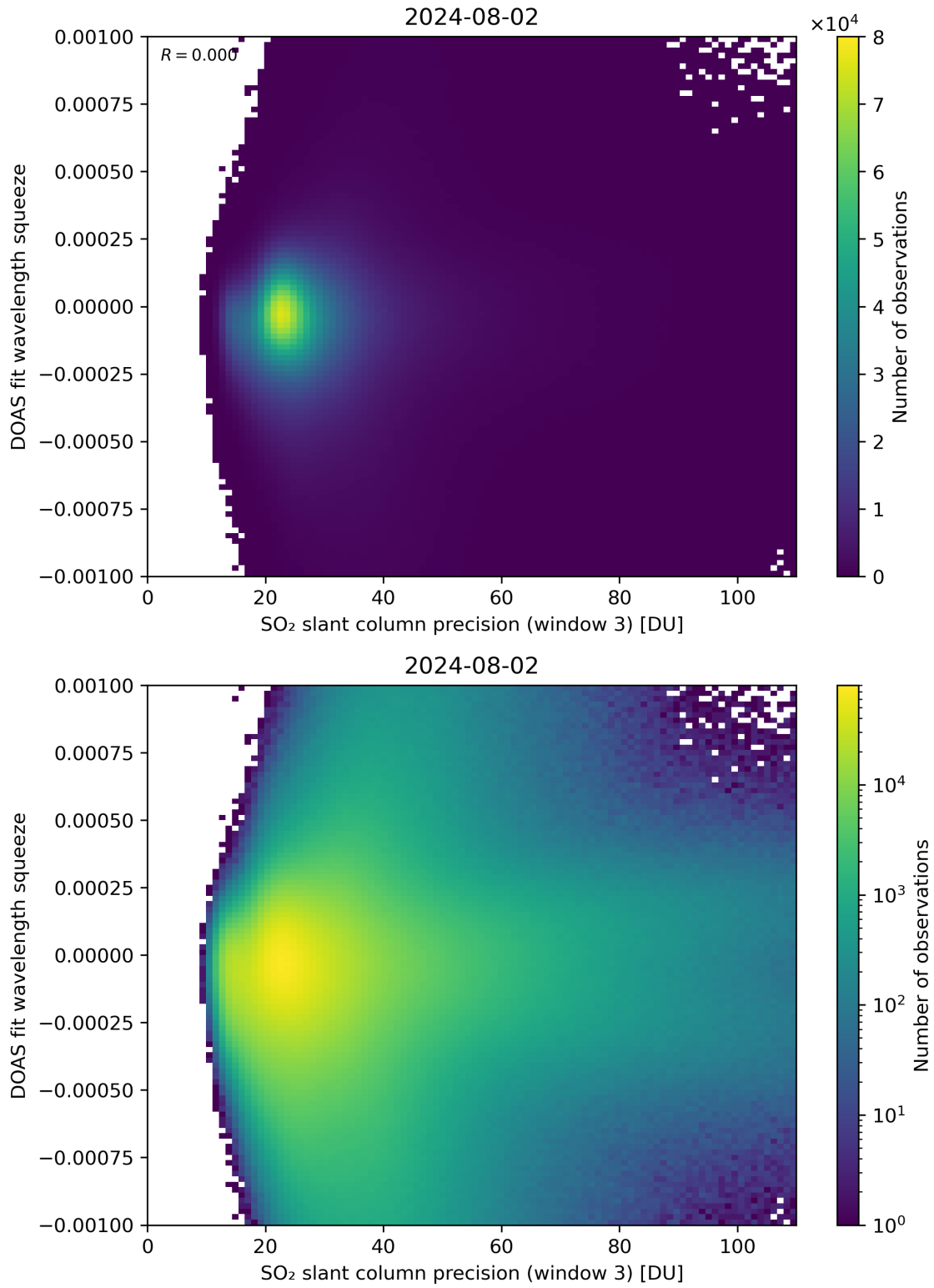
Figure 259: Scatter density plot of “SO 2 slant column precision (window 3)” against “DOAS fit wavelength squeeze” for 2024-08-01 to 2024-08-03.
