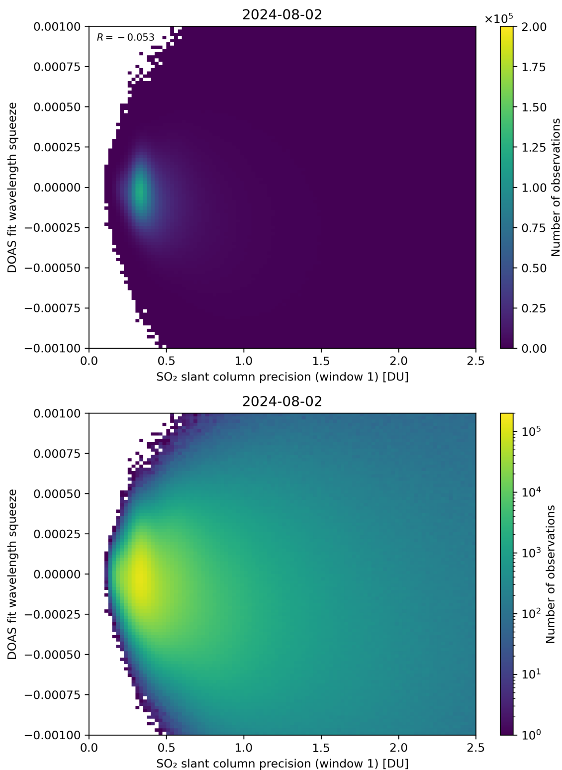
Figure 222: Scatter density plot of “SO 2 slant column precision (window 1)” against “DOAS fit wavelength squeeze” for 2024-08-01 to 2024-08-03.
