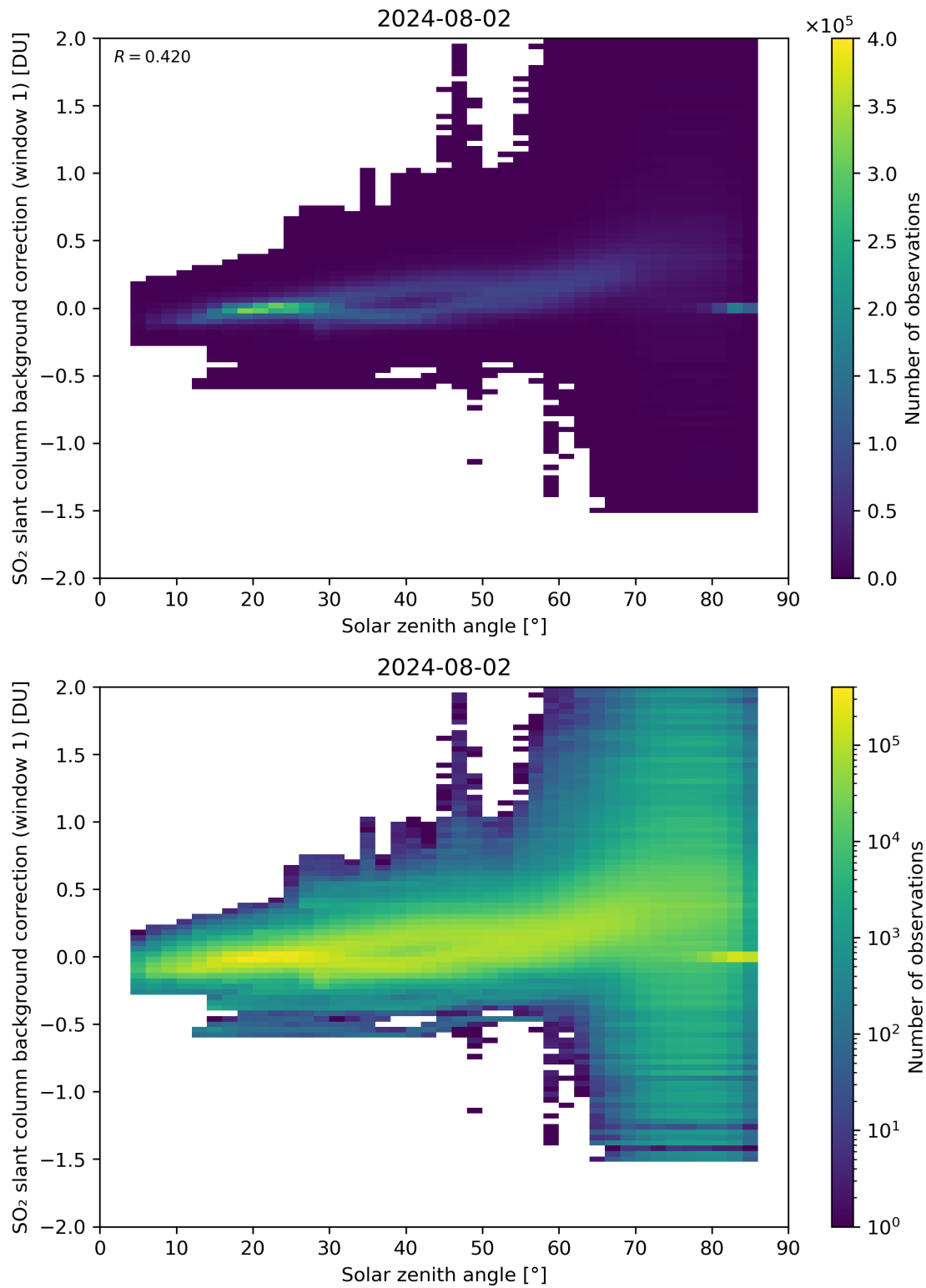
Figure 158: Scatter density plot of “Solar zenith angle” against “SO 2 slant column background correction (window 1)” for 2024-08-01 to 2024-08-03.
