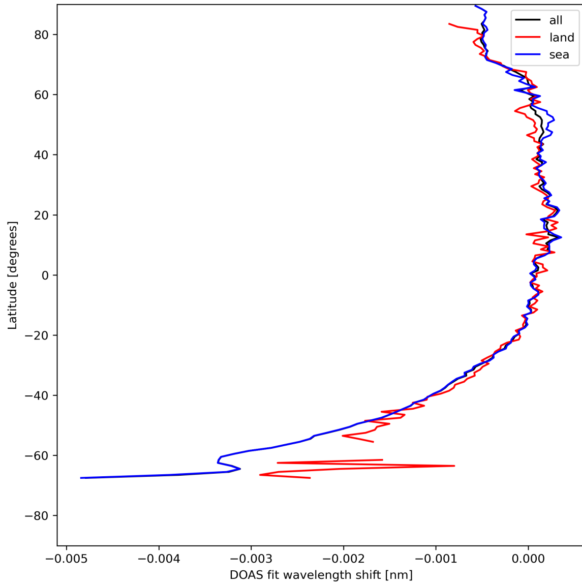
Figure 45: Zonal average of “DOAS fit wavelength shift” for 2024-08-01 to 2024-08-03.
