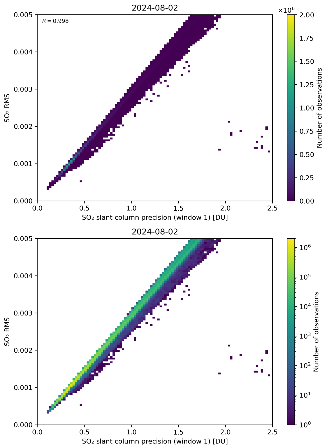
Figure 223: Scatter density plot of “SO 2 slant column precision (window 1)” against “SO 2 RMS” for 2024-08-01 to 2024-08-03.
