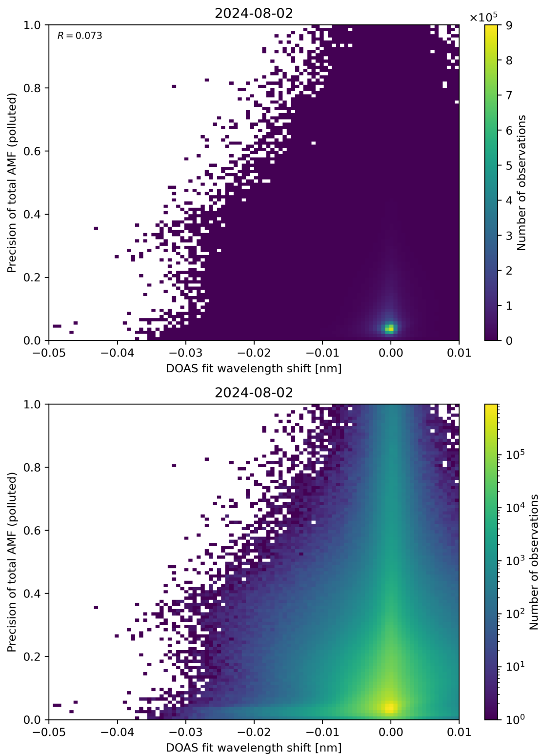
Figure 131: Scatter density plot of “DOAS fit wavelength shift” against “Precision of total AMF (polluted)” for 2024-08-01 to 2024-08-03.
