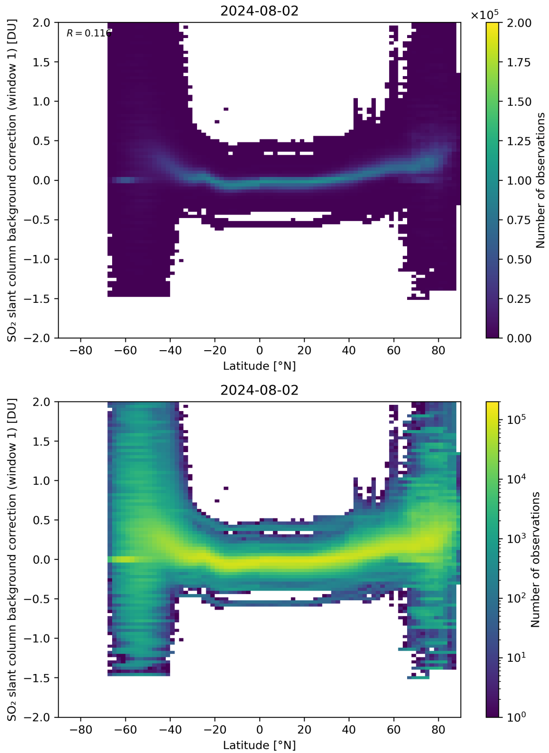
Figure 139: Scatter density plot of “Latitude” against “SO 2 slant column background correction (window 1)” for 2024-08-01 to 2024-08-03.
