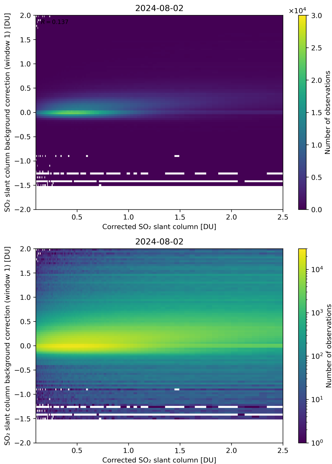
Figure 178: Scatter density plot of “Corrected SO 2 slant column” against “SO 2 slant column background correction (window 1)” for 2024-08-01 to 2024-08-03.
