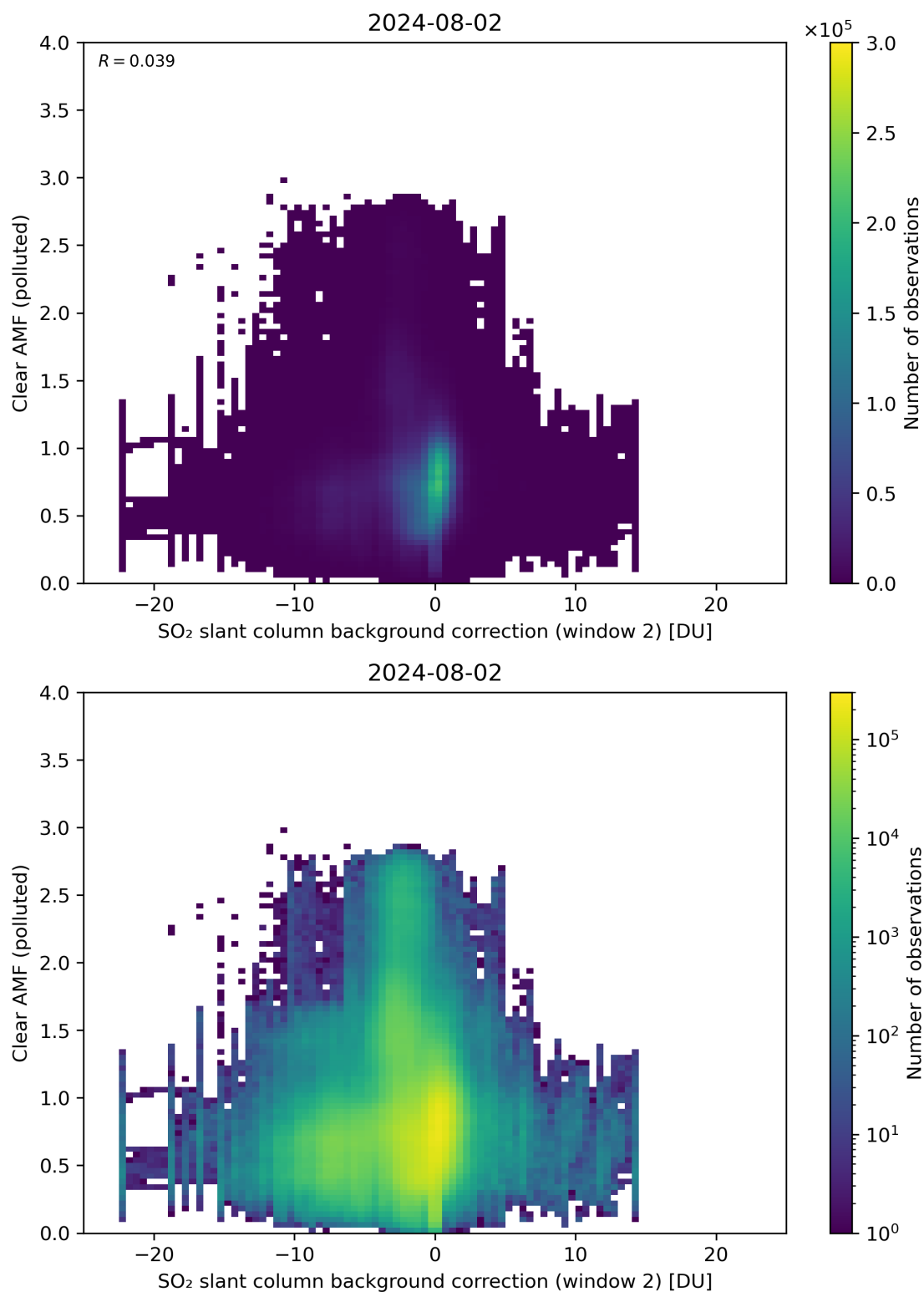
Figure 115: Scatter density plot of “SO 2 slant column background correction (window 2)” against “Clear AMF (polluted)” for 2024-08-01 to 2024-08-03.
