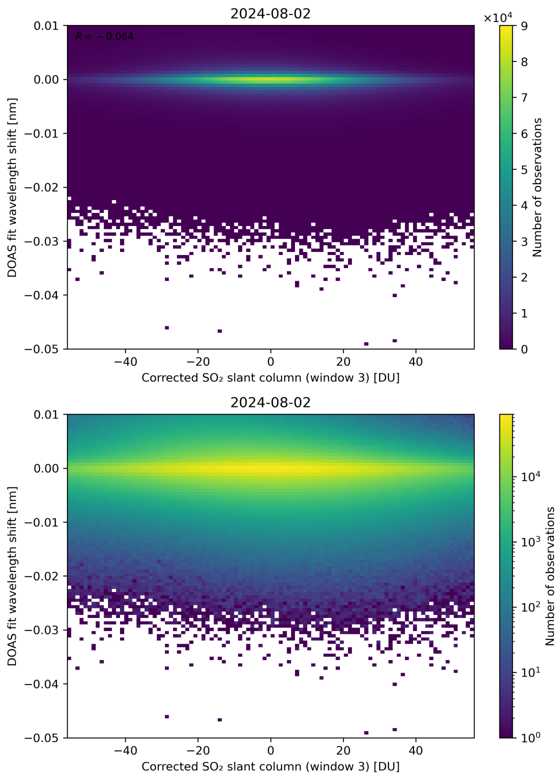
Figure 206: Scatter density plot of “Corrected SO 2 slant column (window 3)” against “DOAS fit wavelength shift” for 2024-08-01 to 2024-08-03.
