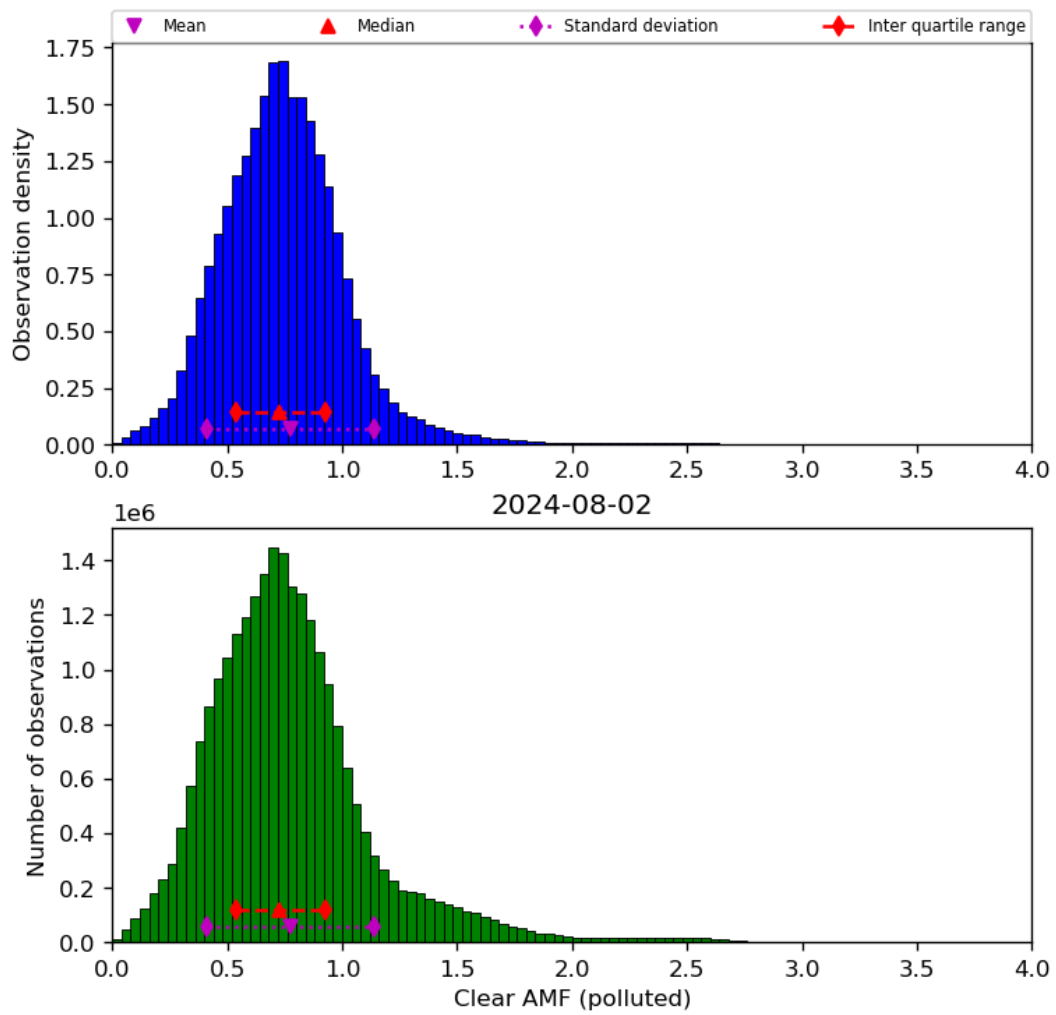
Figure 73: Histogram of “Clear AMF (polluted)” for 2024-08-01 to 2024-08-03
