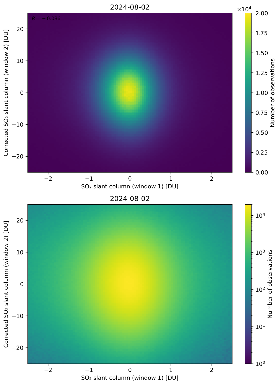
Figure 233: Scatter density plot of “SO 2 slant column (window 1)” against “Corrected SO 2 slant column (window 2)” for 2024-08-01 to 2024-08-03.
