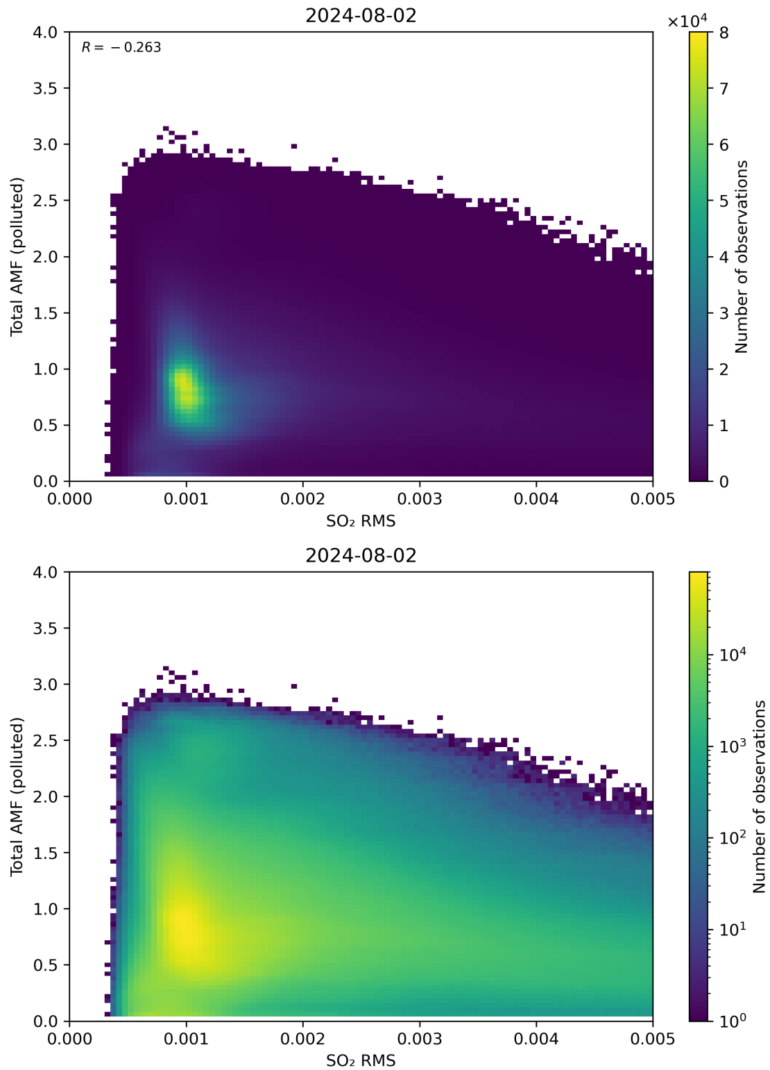
Figure 137: Scatter density plot of “SO 2 RMS” against “Total AMF (polluted)” for 2024-08-01 to 2024-08-03.
