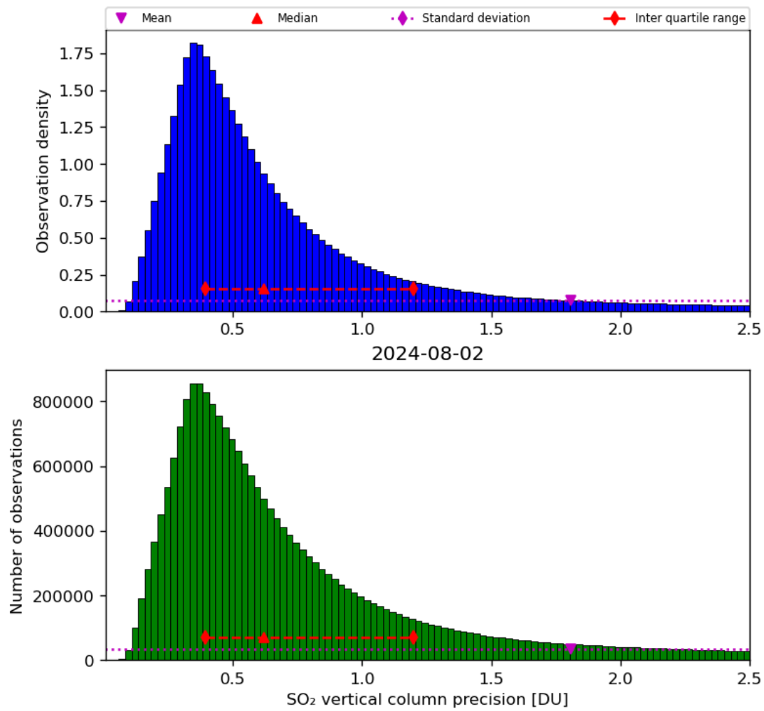
Figure 54: Histogram of “SO 2 vertical column precision” for 2024-08-01 to 2024-08-03
