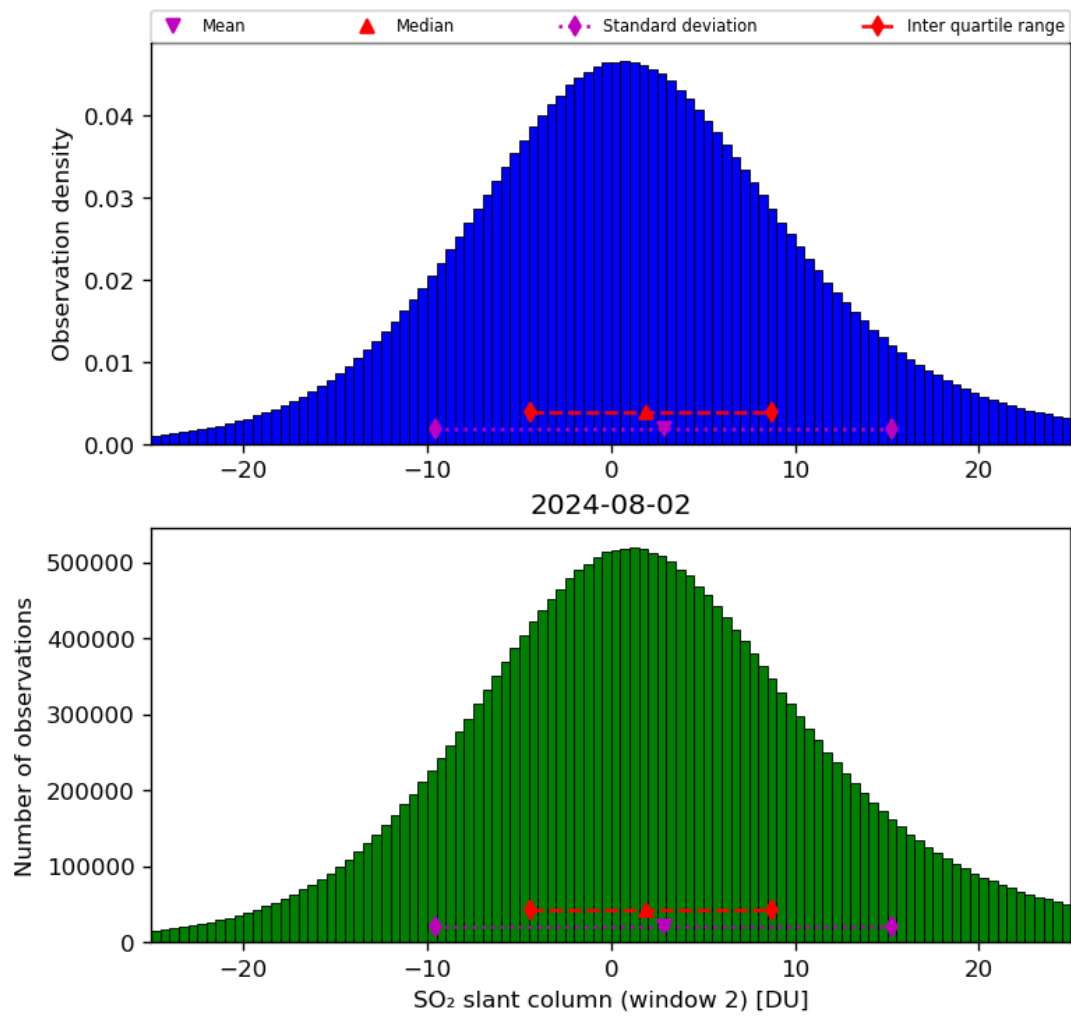
Figure 60: Histogram of “SO 2 slant column (window 2)” for 2024-08-01 to 2024-08-03
