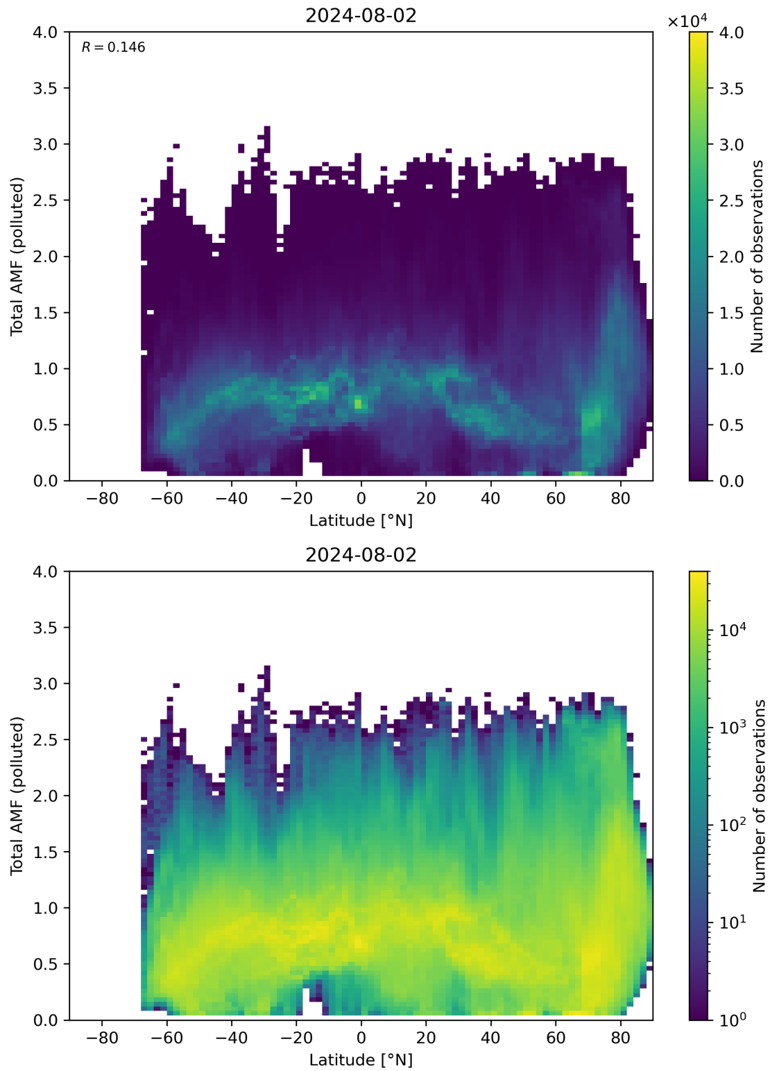
Figure 154: Scatter density plot of “Latitude” against “Total AMF (polluted)” for 2024-08-01 to 2024-08-03.
