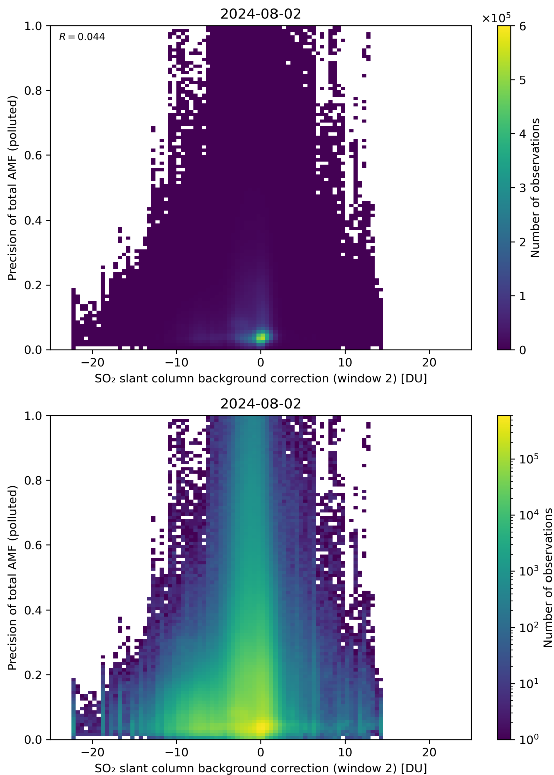
Figure 120: Scatter density plot of “SO 2 slant column background correction (window 2)” against “Precision of total AMF (polluted)” for 2024-08-01 to 2024-08-03.
