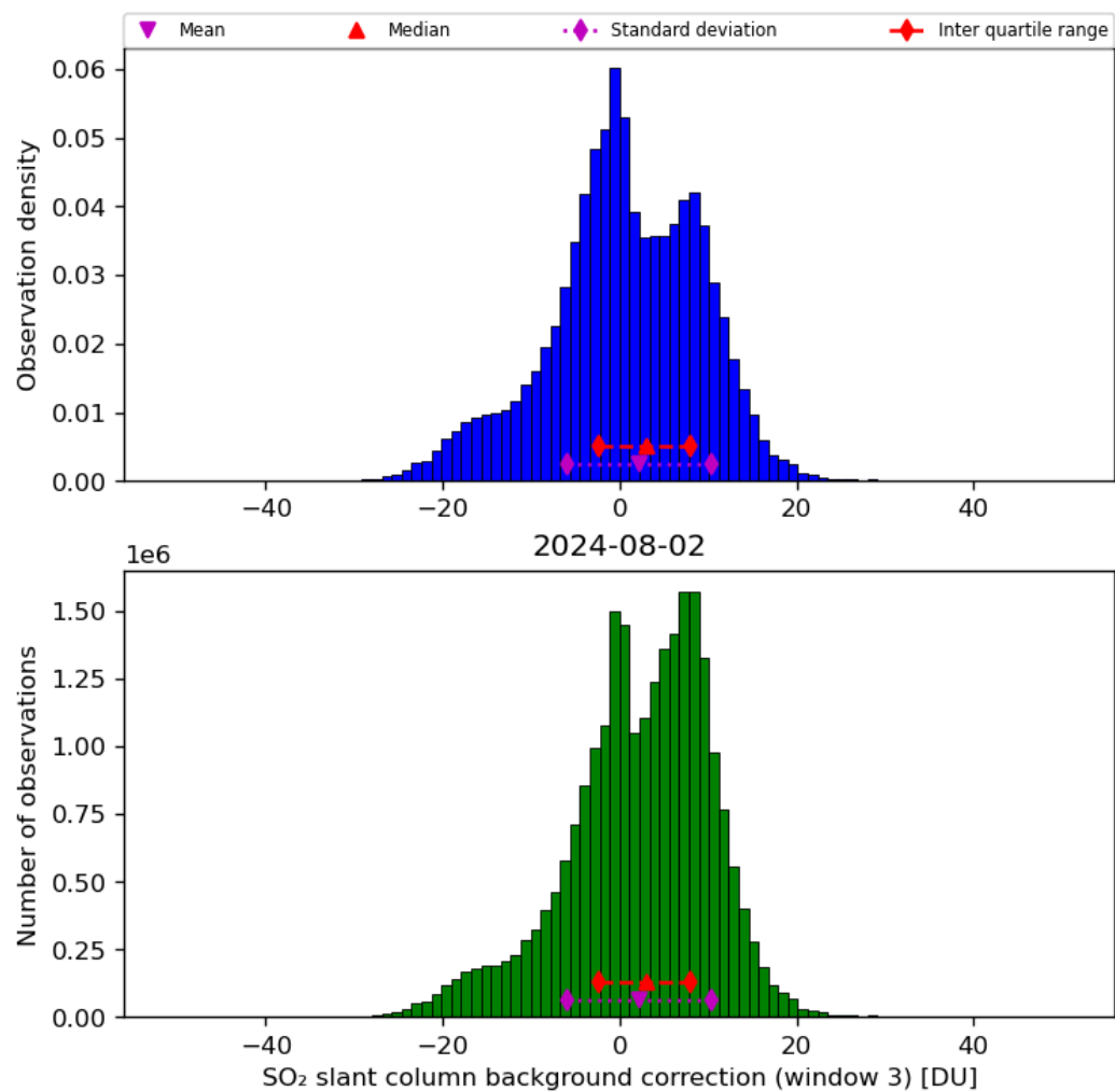
Figure 67: Histogram of “SO 2 slant column background correction (window 3)” for 2024-08-01 to 2024-08-03
