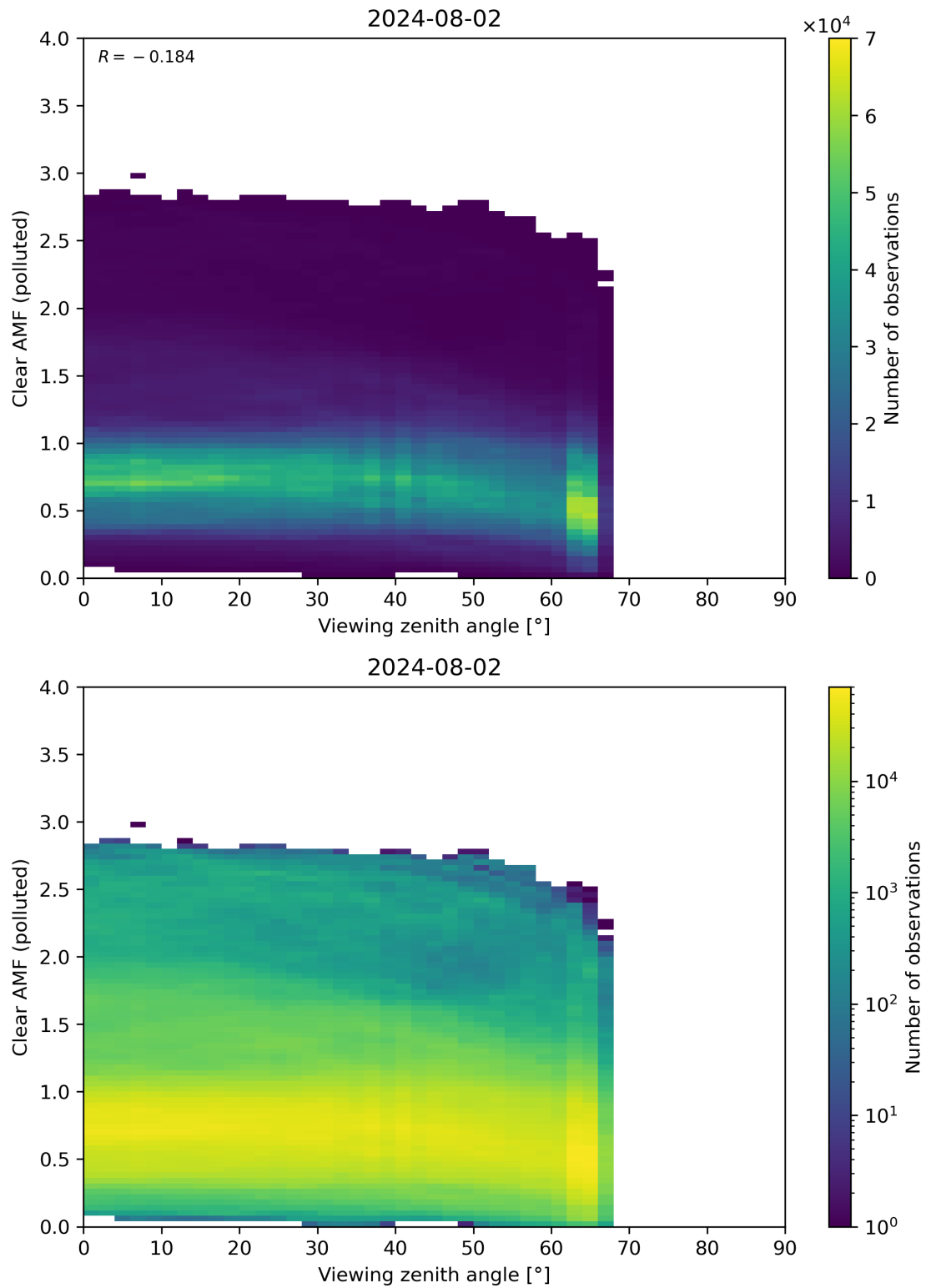
Figure 316: Scatter density plot of “Viewing zenith angle” against “Clear AMF (polluted)” for 2024-08-01 to 2024-08-03.
