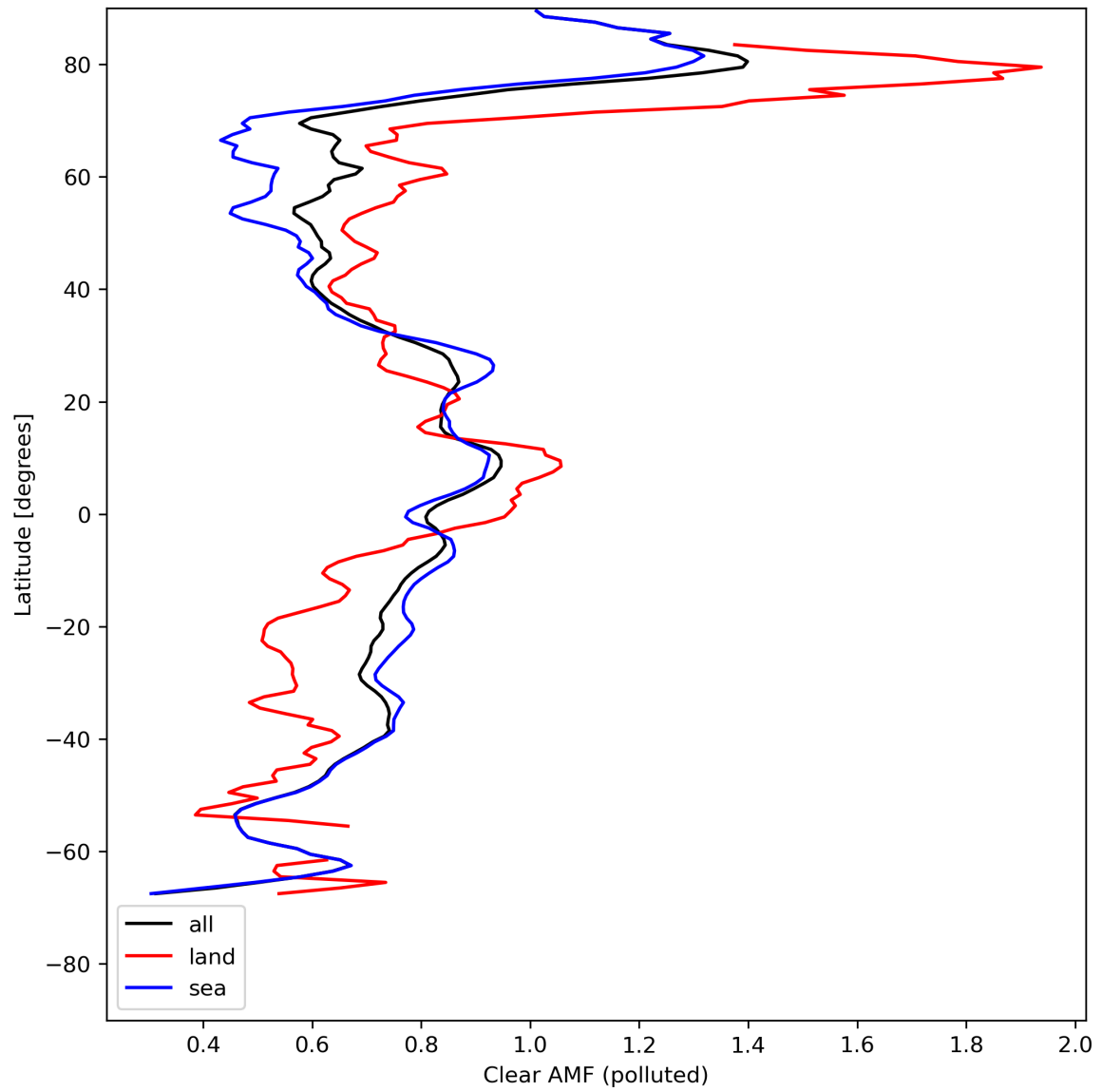
Figure 50: Zonal average of “Clear AMF (polluted)” for 2024-08-01 to 2024-08-03.
