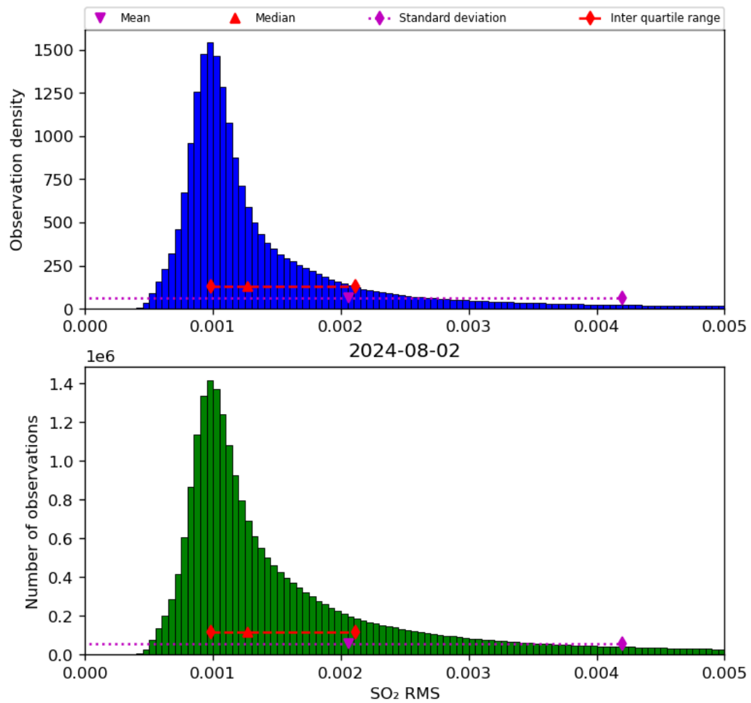
Figure 70: Histogram of “SO 2 RMS” for 2024-08-01 to 2024-08-03
