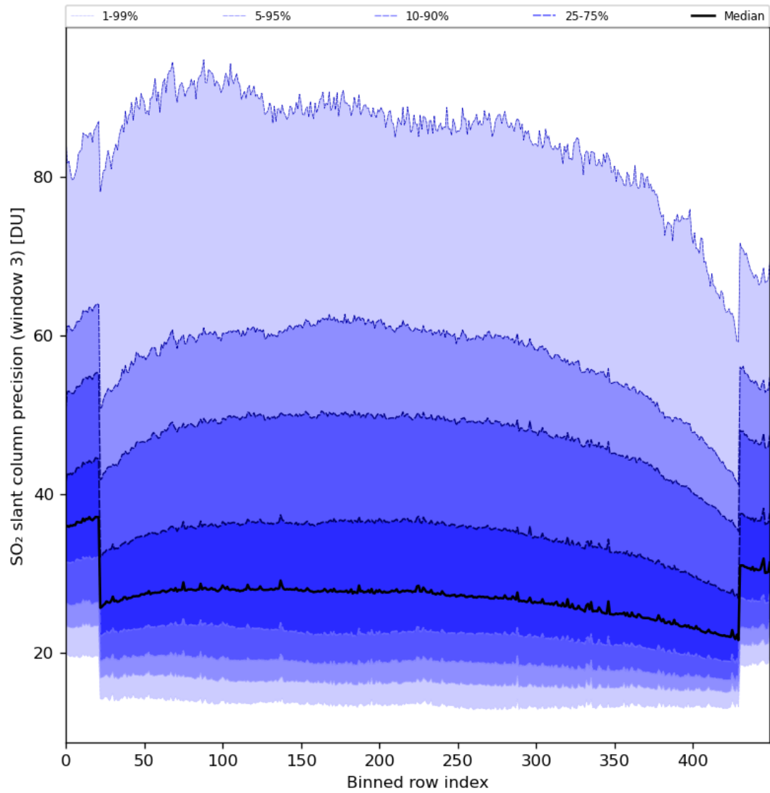
Figure 88: Along track statistics of “SO 2 slant column precision (window 3)” for 2024-08-01 to 2024-08-03
