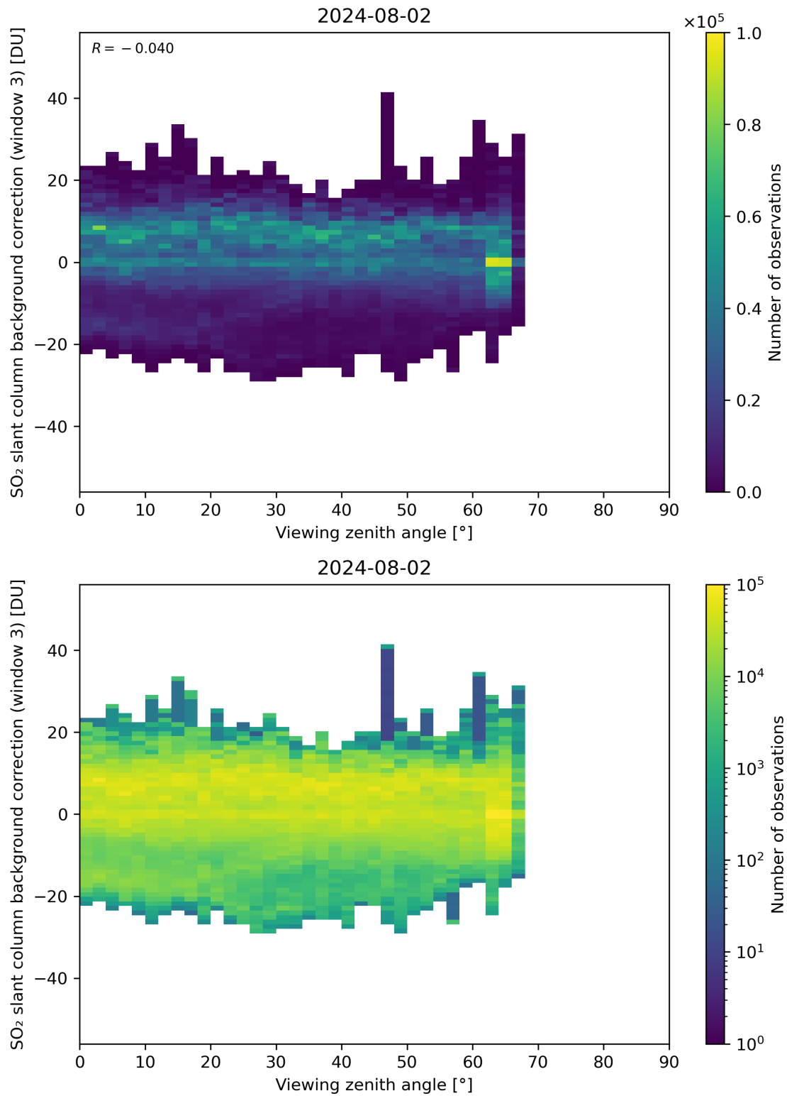
Figure 310: Scatter density plot of “Viewing zenith angle” against “SO 2 slant column background correction (window 3)” for 2024-08-01 to 2024-08-03.
