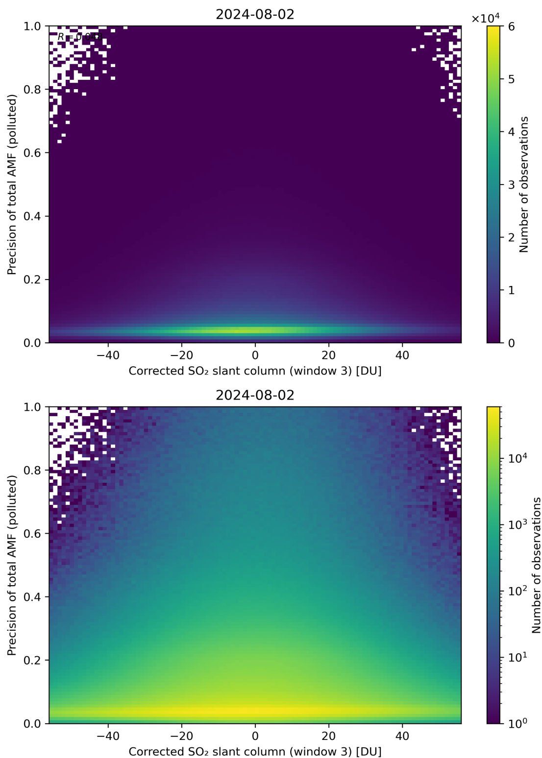
Figure 211: Scatter density plot of “Corrected SO 2 slant column (window 3)” against “Precision of total AMF (polluted)” for 2024-08-01 to 2024-08-03.
