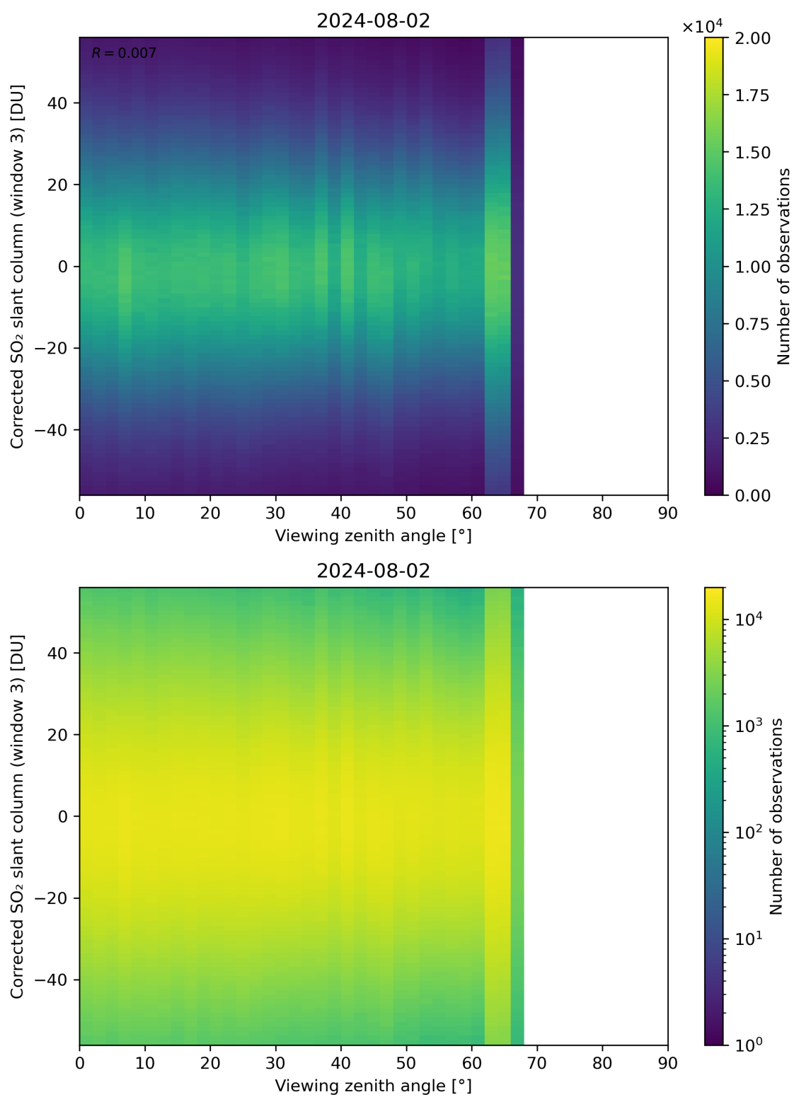
Figure 319: Scatter density plot of “Viewing zenith angle” against “Corrected SO 2 slant column (window 3)” for 2024-08-01 to 2024-08-03.
