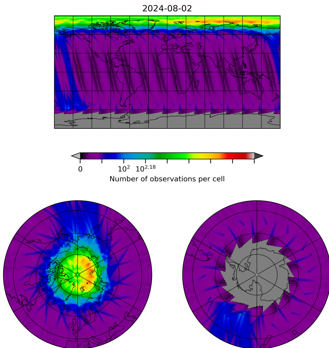
Figure 28: Map of the number of observations for 2024-08-01 to 2024-08-03
