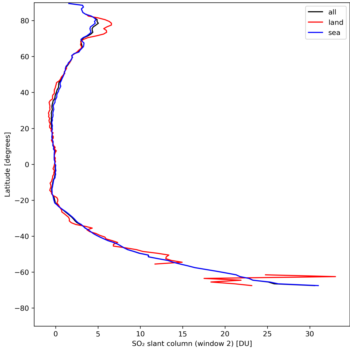
Figure 37: Zonal average of “SO 2 slant column (window 2)” for 2024-08-01 to 2024-08-03.
