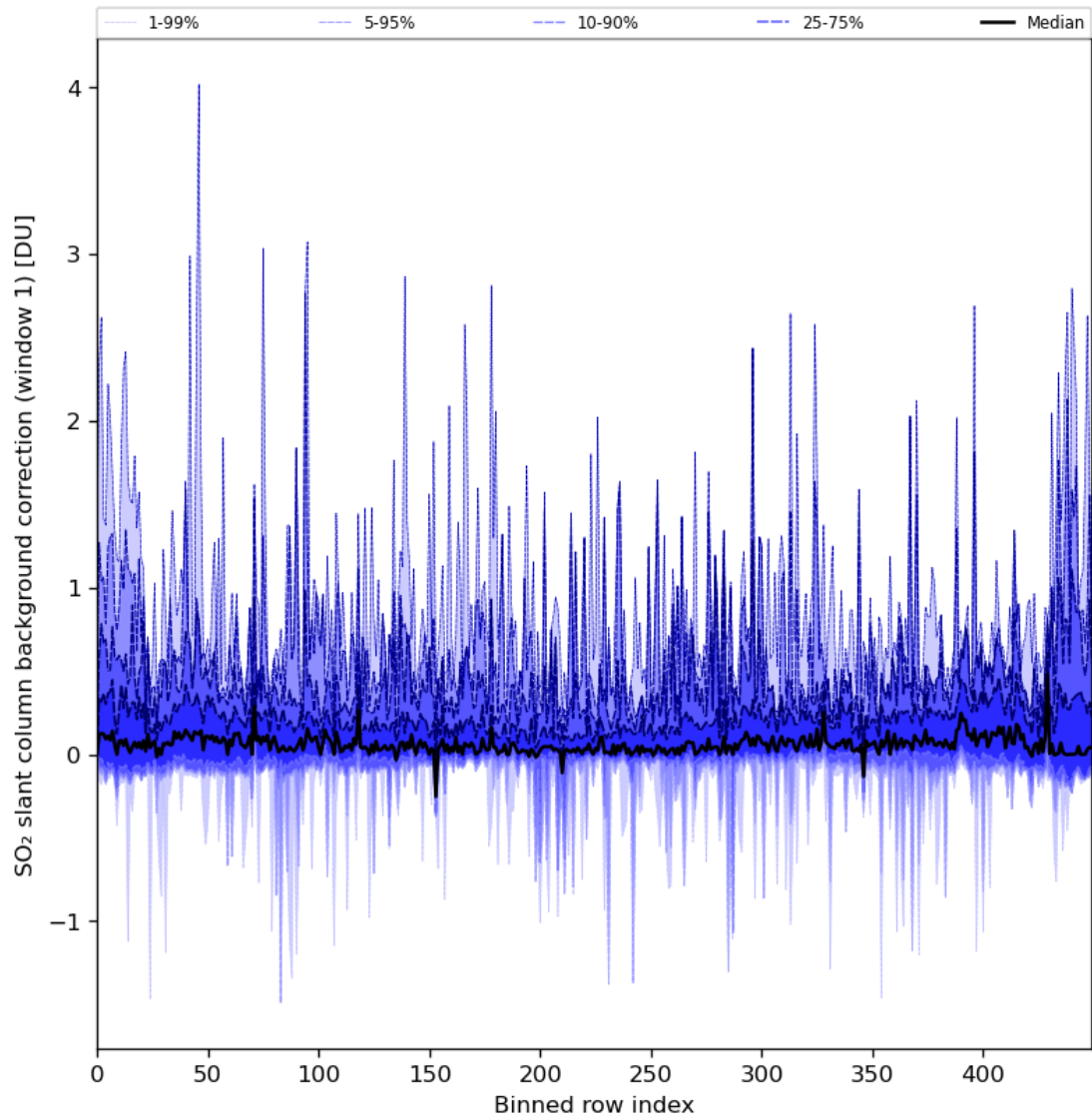
Figure 82: Along track statistics of “SO 2 slant column background correction (window 1)” for 2024-08-01 to 2024-08-03
