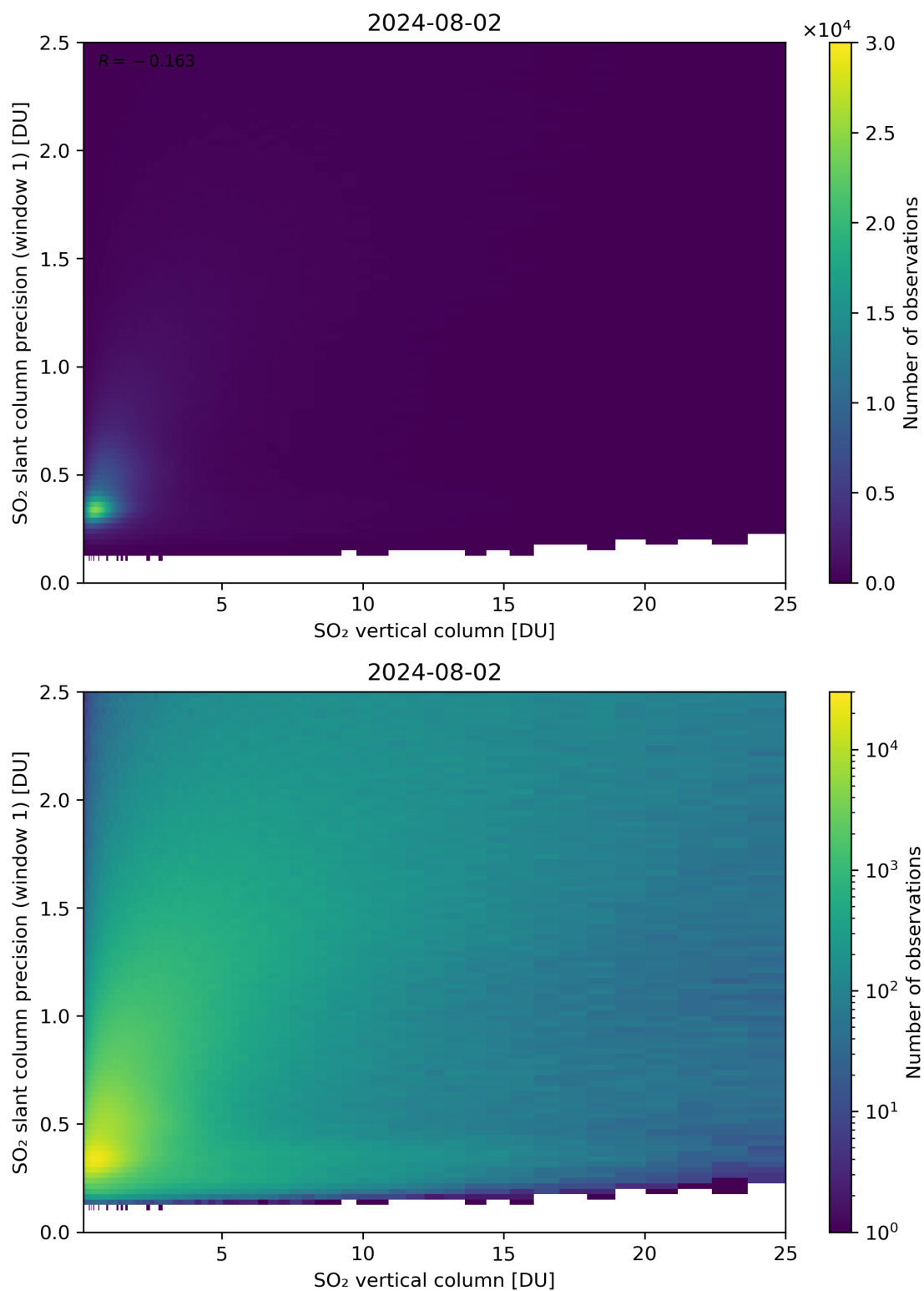
Figure 301: Scatter density plot of “SO 2 vertical column” against “SO 2 slant column precision (window 1)” for 2024-08-01 to 2024-08-03.
