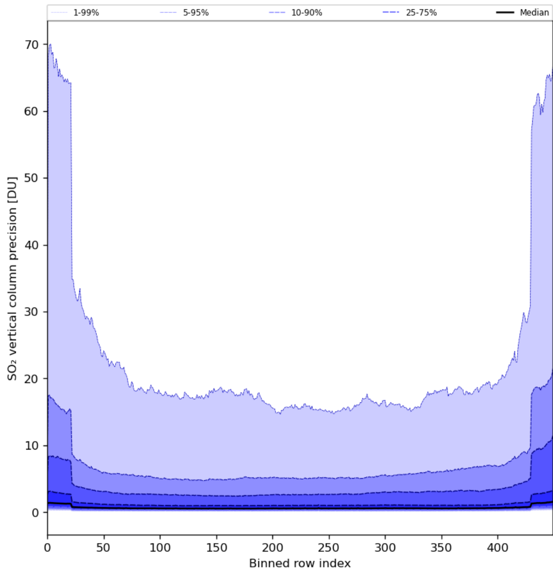
Figure 77: Along track statistics of “SO 2 vertical column precision” for 2024-08-01 to 2024-08-03
