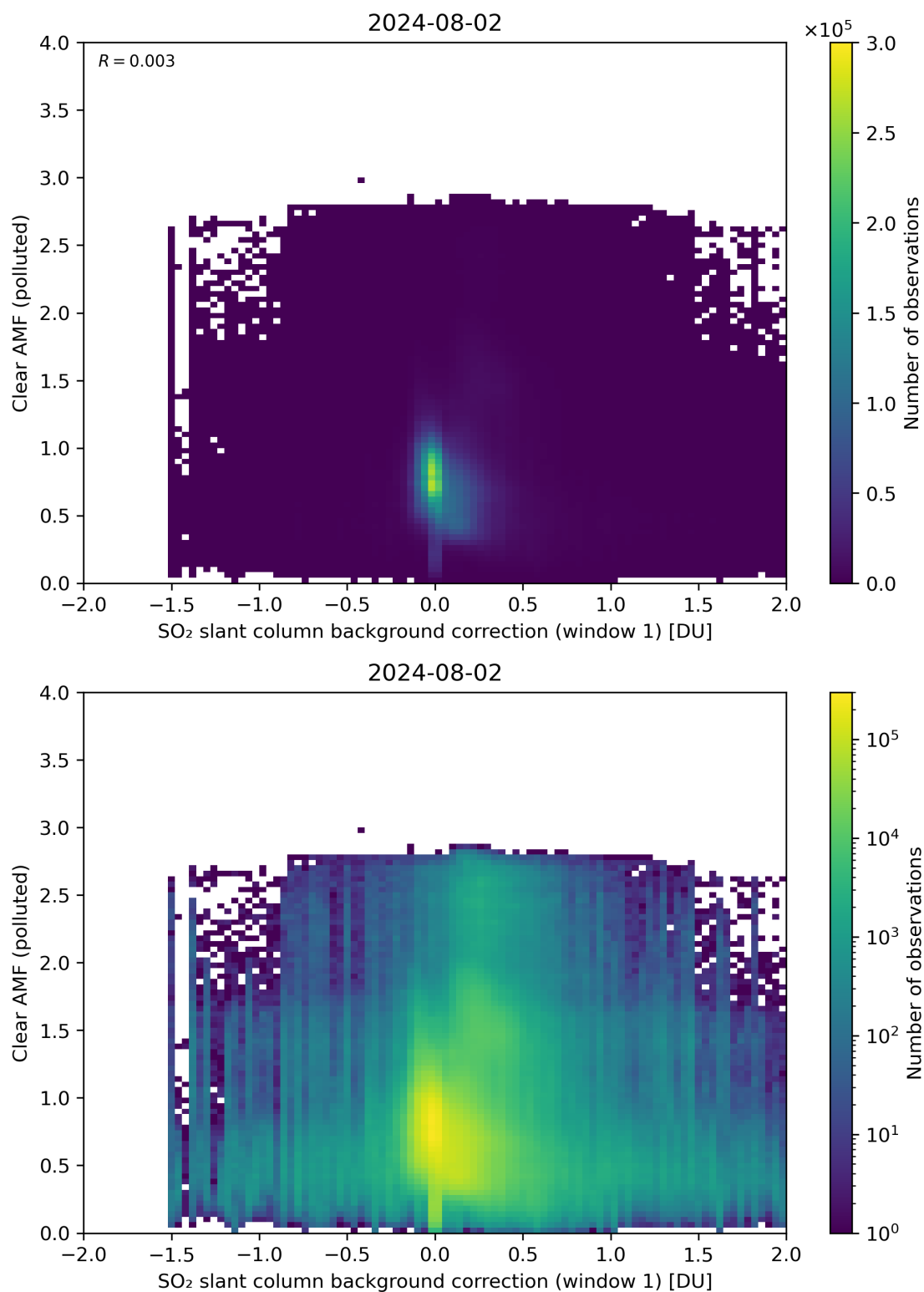
Figure 103: Scatter density plot of “SO 2 slant column background correction (window 1)” against “Clear AMF (polluted)” for 2024-08-01 to 2024-08-03.
