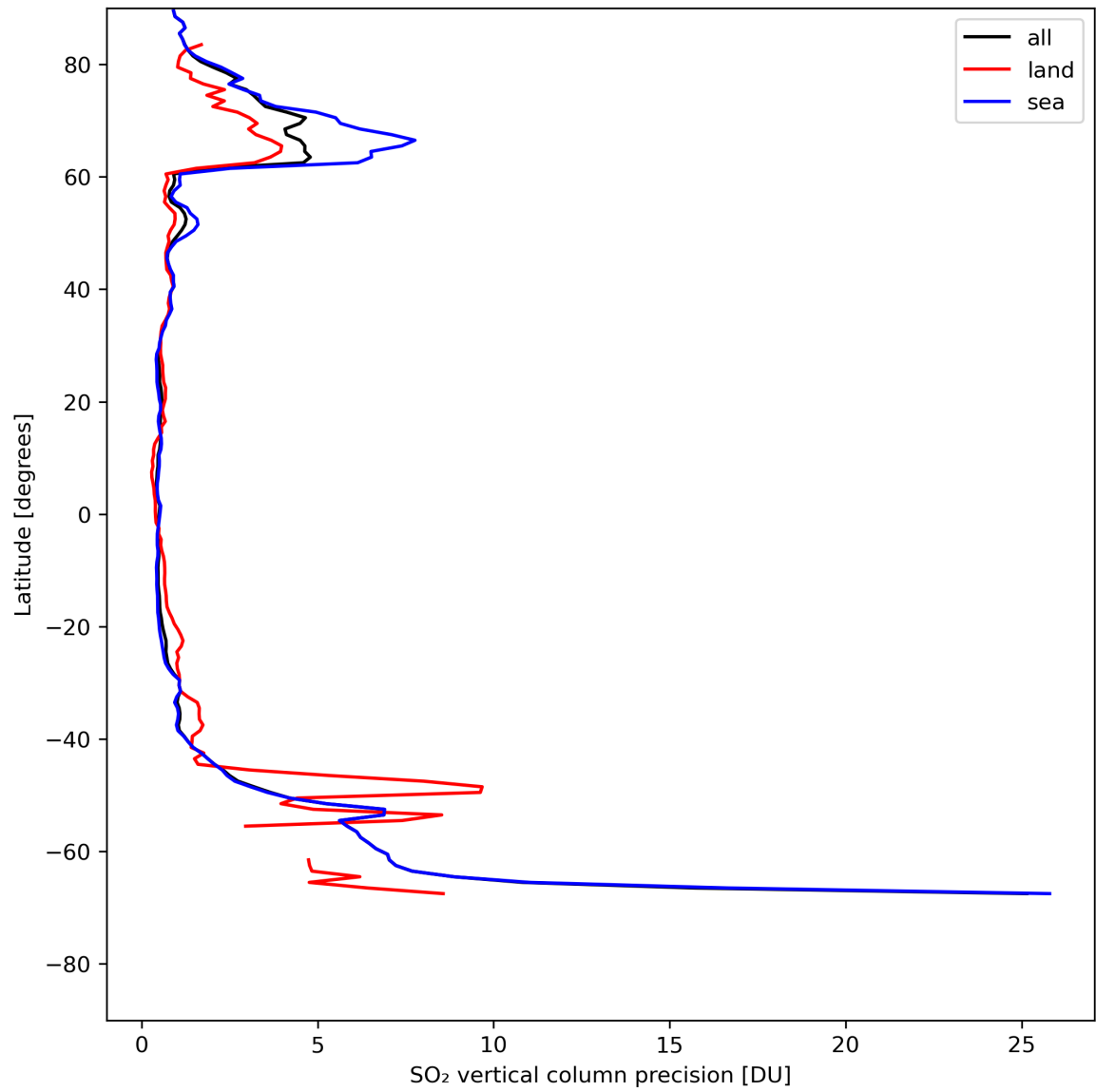
Figure 31: Zonal average of “SO 2 vertical column precision” for 2024-08-01 to 2024-08-03.
