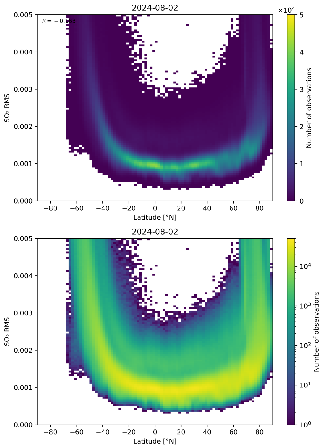
Figure 144: Scatter density plot of “Latitude” against “SO 2 RMS” for 2024-08-01 to 2024-08-03.
