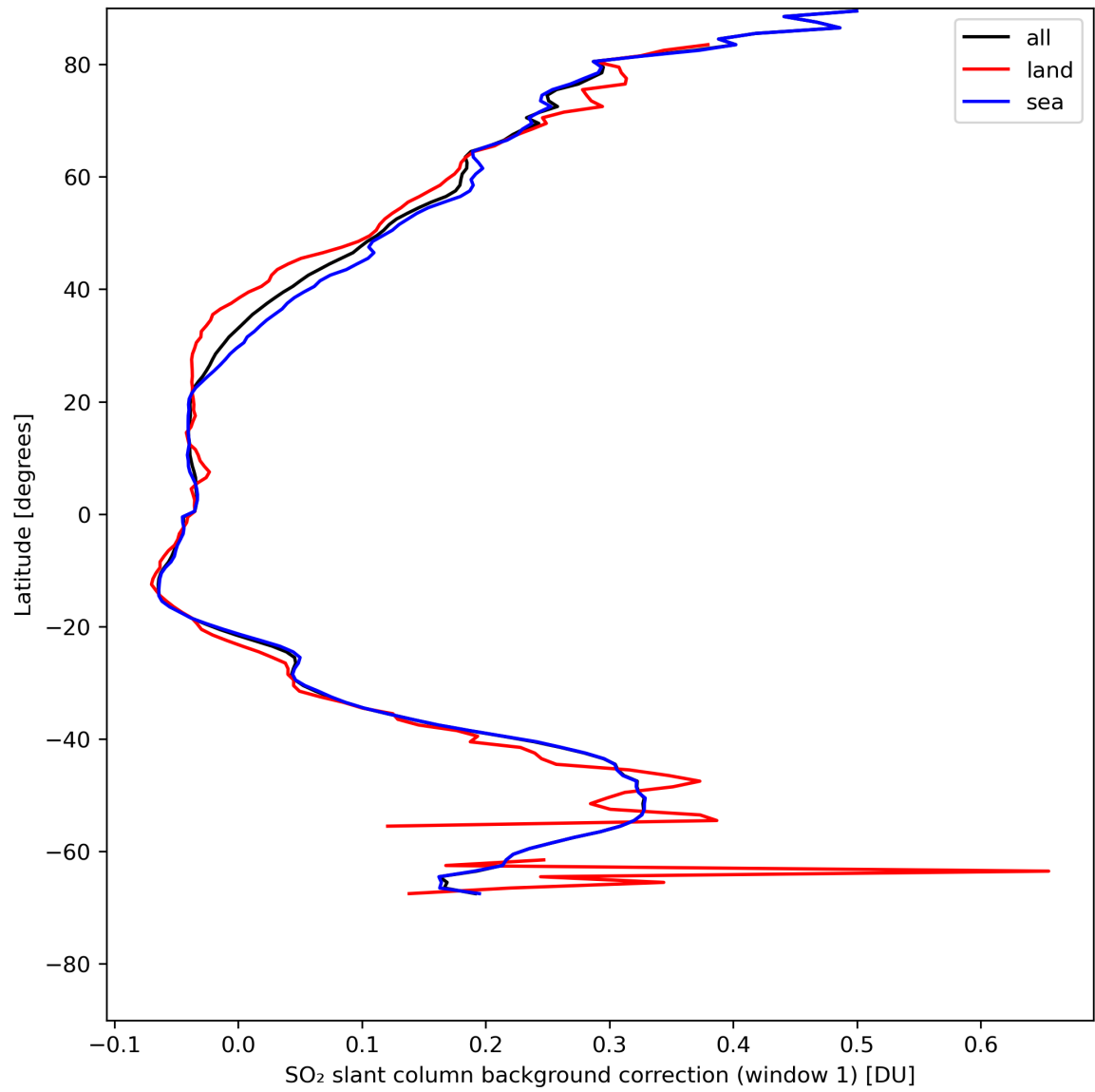
Figure 36: Zonal average of “SO 2 slant column background correction (window 1)” for 2024-08-01 to 2024-08-03.
