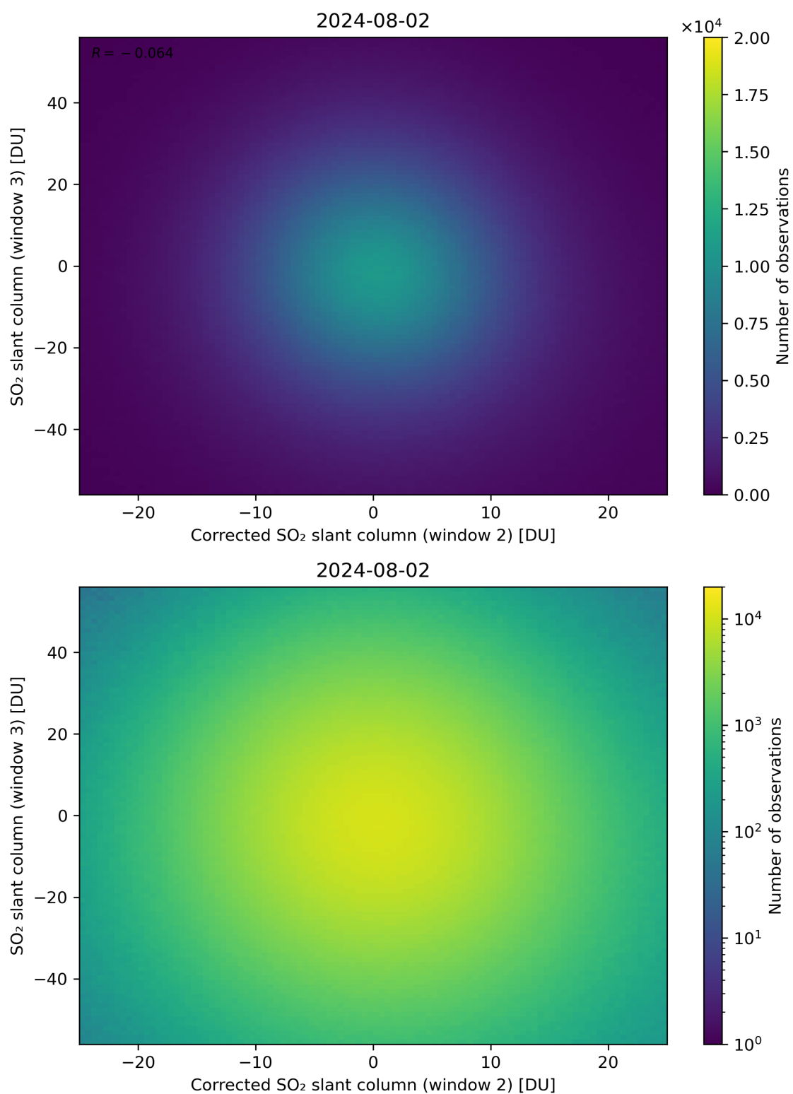
Figure 201: Scatter density plot of “Corrected SO 2 slant column (window 2)” against “SO 2 slant column (window 3)” for 2024-08-01 to 2024-08-03.
