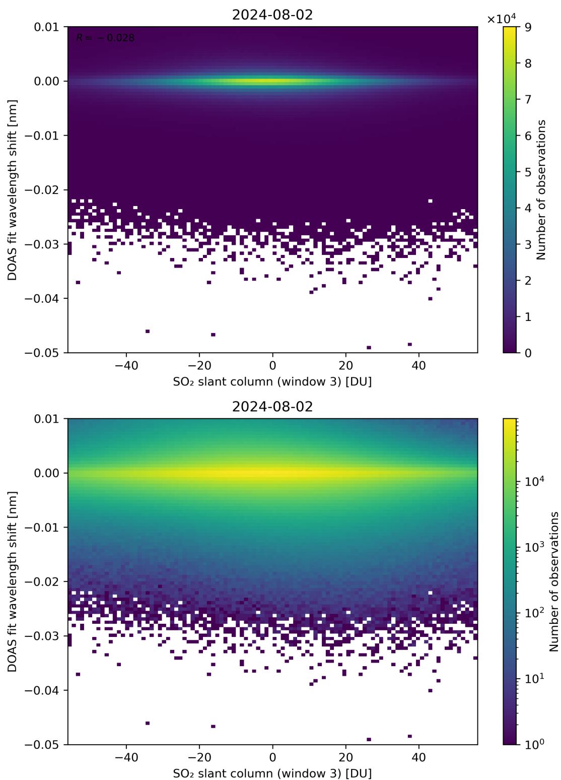
Figure 254: Scatter density plot of “SO 2 slant column (window 3)” against “DOAS fit wavelength shift” for 2024-08-01 to 2024-08-03.
