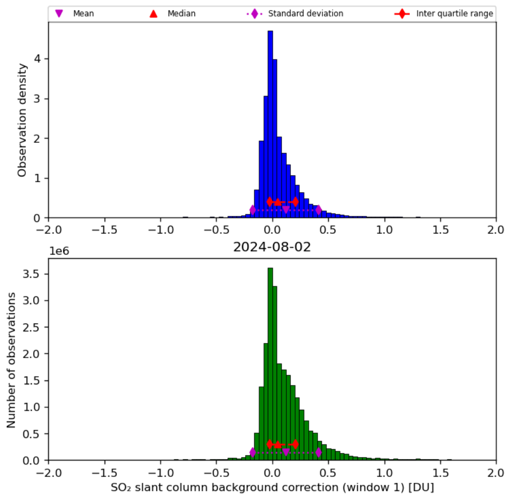
Figure 59: Histogram of “SO 2 slant column background correction (window 1)” for 2024-08-01 to 2024-08-03
