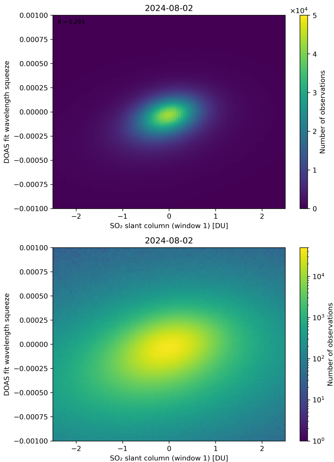
Figure 216: Scatter density plot of “SO 2 slant column (window 1)” against “DOAS fit wavelength squeeze” for 2024-08-01 to 2024-08-03.
