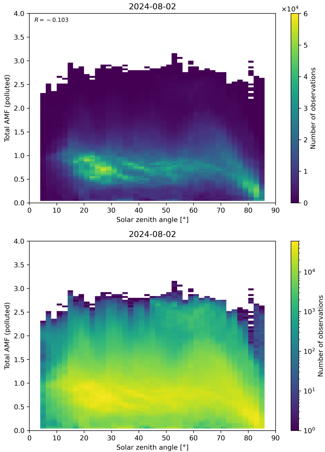
Figure 174: Scatter density plot of “Solar zenith angle” against “Total AMF (polluted)” for 2024-08-01 to 2024-08-03.
