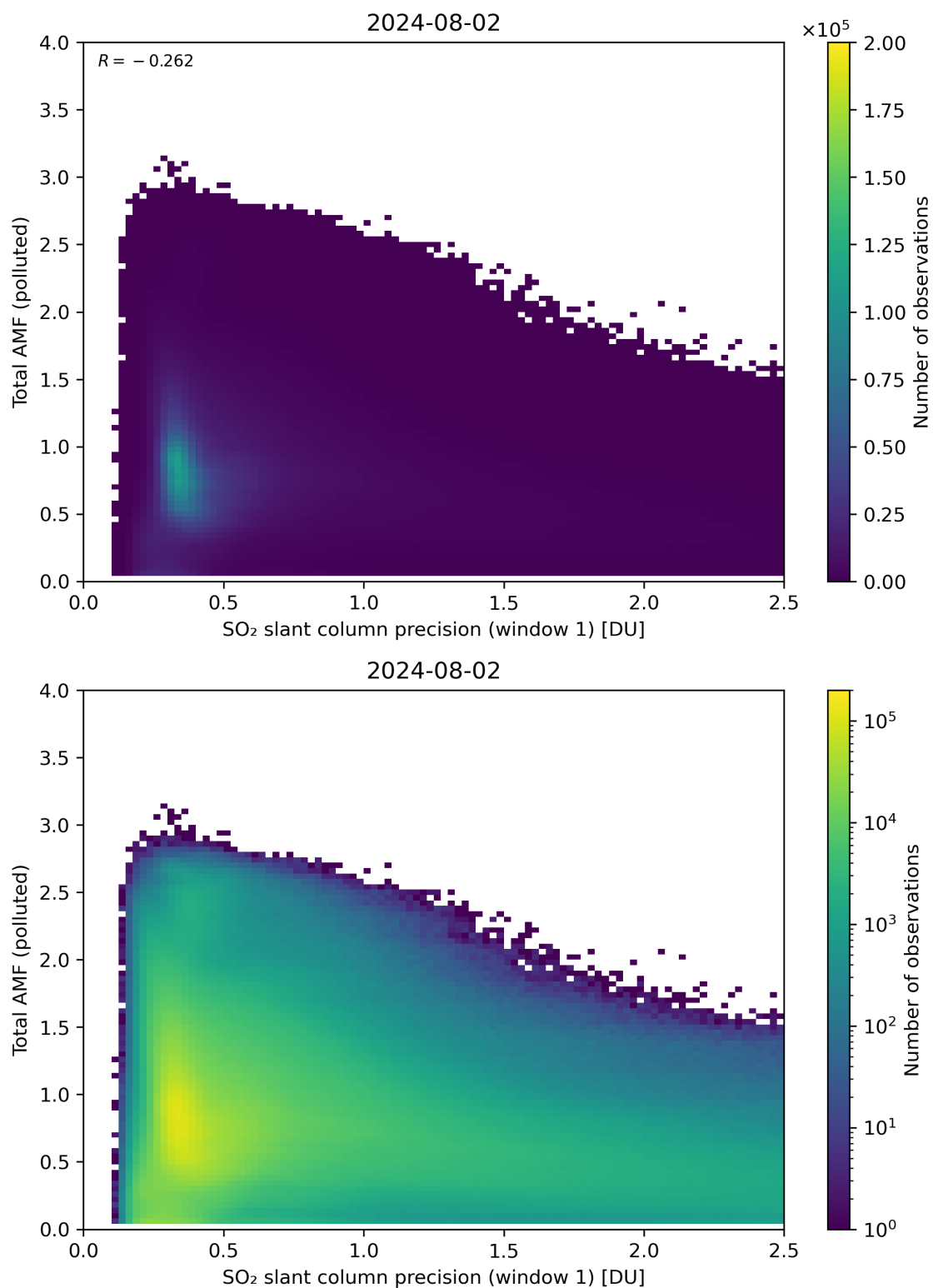
Figure 230: Scatter density plot of “SO 2 slant column precision (window 1)” against “Total AMF (polluted)” for 2024-08-01 to 2024-08-03.
