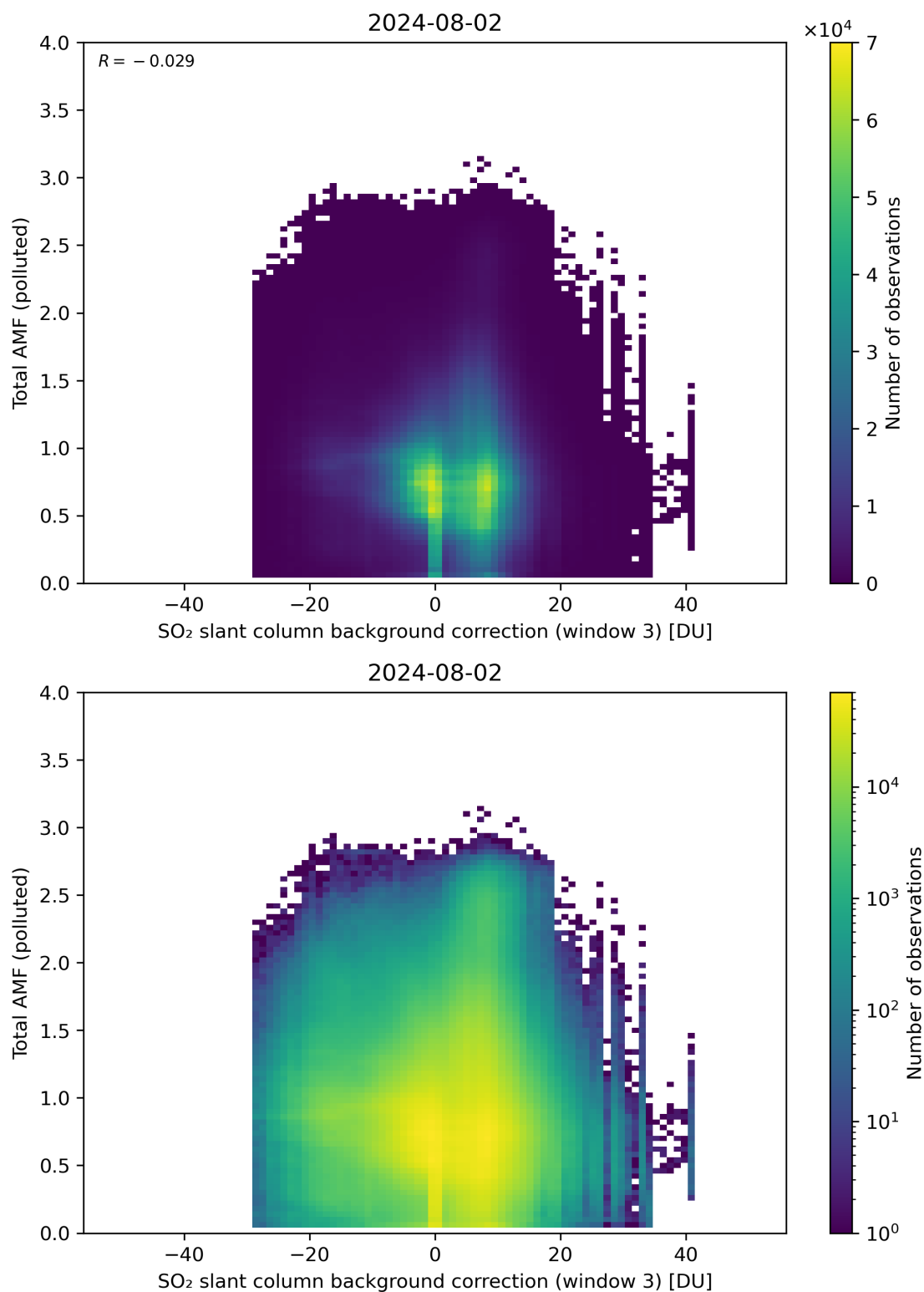
Figure 125: Scatter density plot of “SO 2 slant column background correction (window 3)” against “Total AMF (polluted)” for 2024-08-01 to 2024-08-03.
