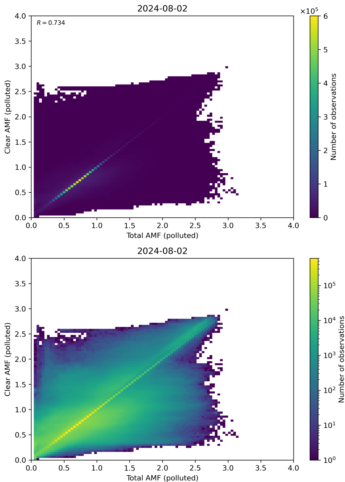
Figure 271: Scatter density plot of “Total AMF (polluted)” against “Clear AMF (polluted)” for 2024-08-01 to 2024-08-03.
