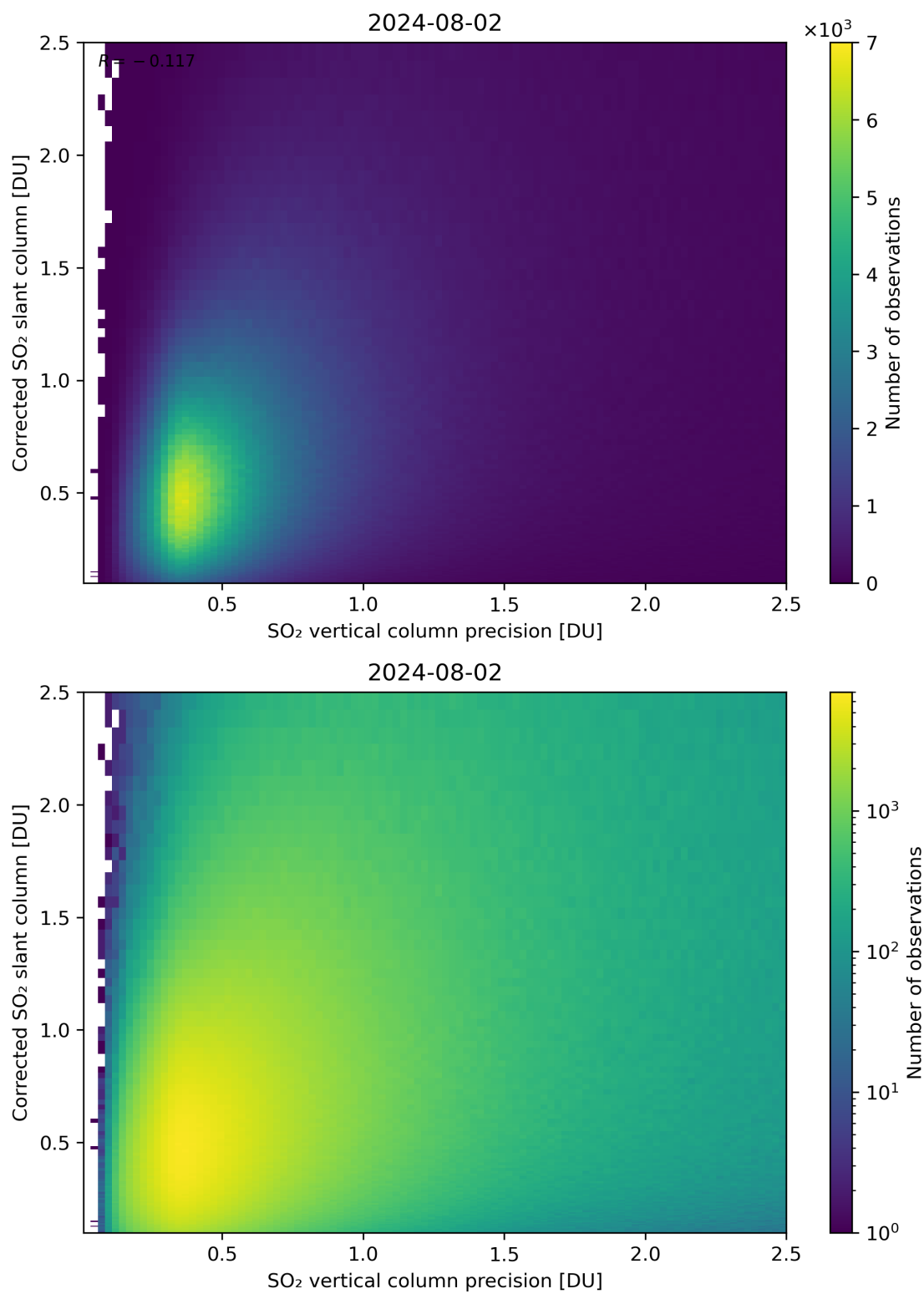
Figure 286: Scatter density plot of “SO 2 vertical column precision” against “Corrected SO 2 slant column” for 2024-08-01 to 2024-08-03.
