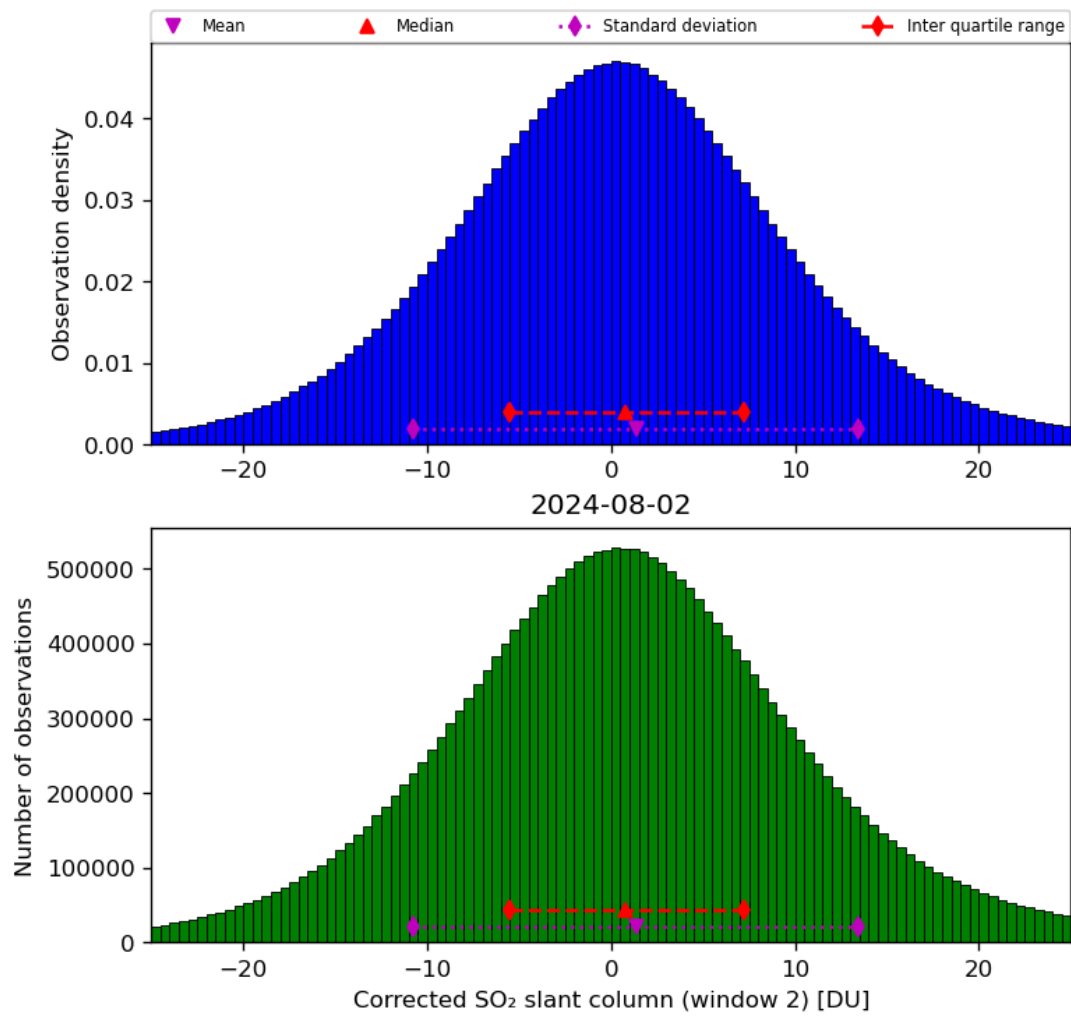
Figure 62: Histogram of “Corrected SO 2 slant column (window 2)” for 2024-08-01 to 2024-08-03
