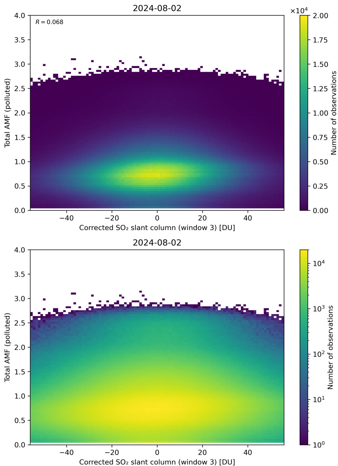
Figure 210: Scatter density plot of “Corrected SO 2 slant column (window 3)” against “Total AMF (polluted)” for 2024-08-01 to 2024-08-03.
