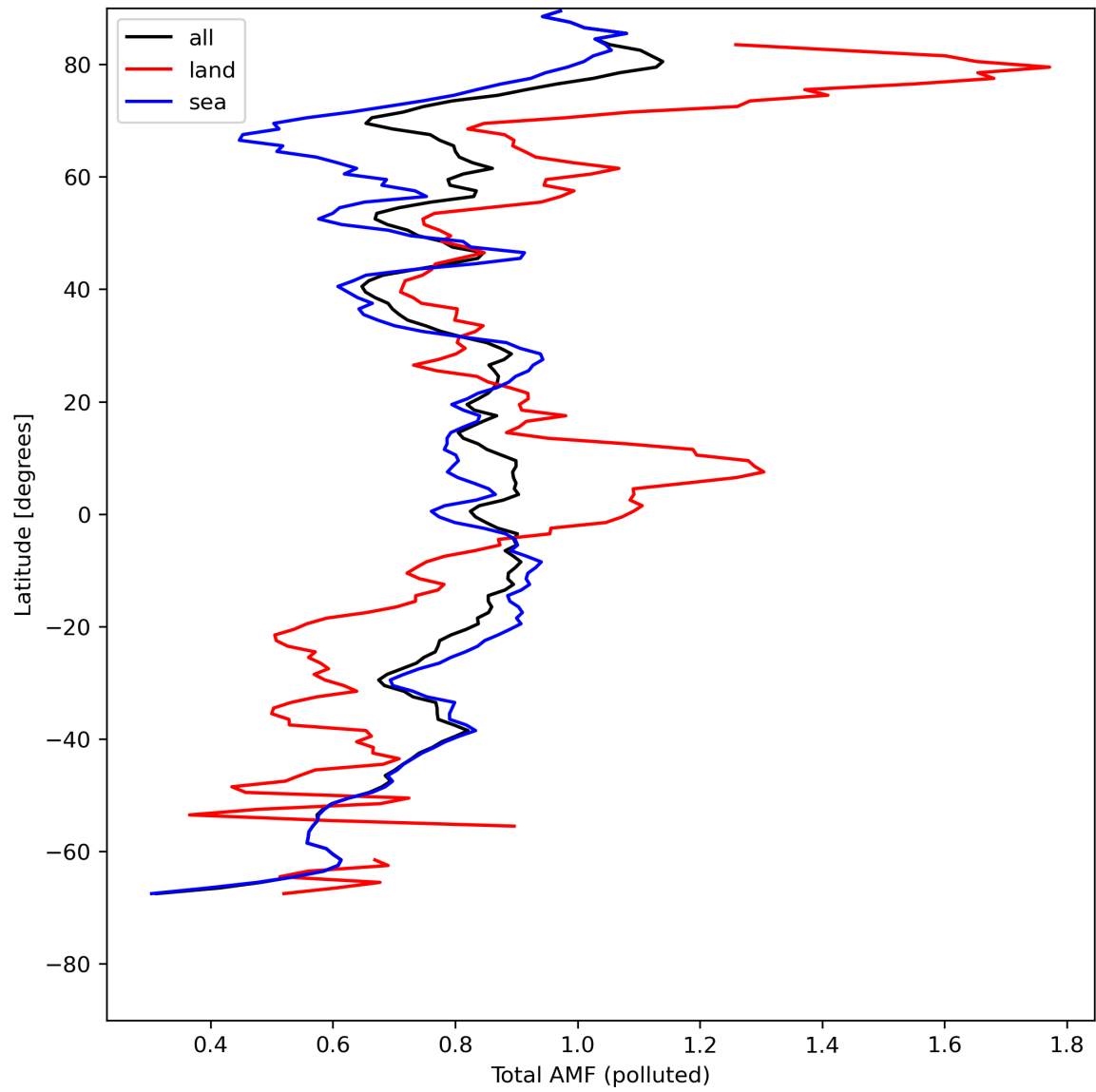
Figure 48: Zonal average of “Total AMF (polluted)” for 2024-08-01 to 2024-08-03.
