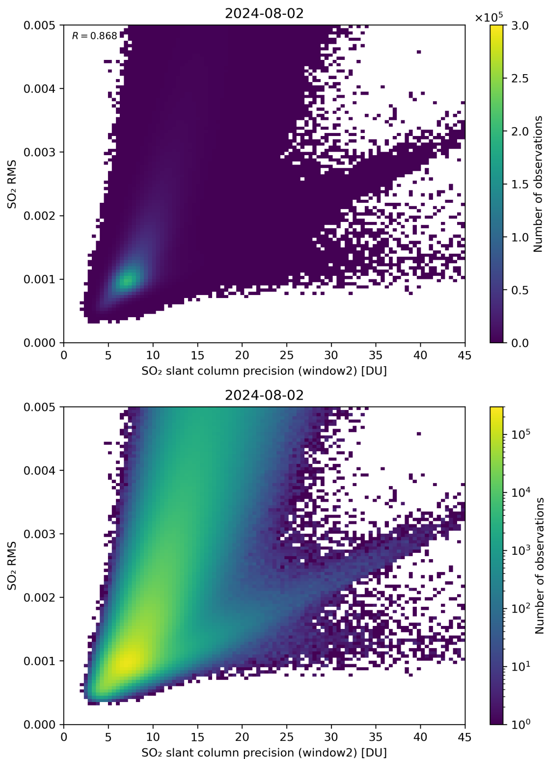
Figure 245: Scatter density plot of “SO 2 slant column precision (window2)” against “SO 2 RMS” for 2024-08-01 to 2024-08-03.
