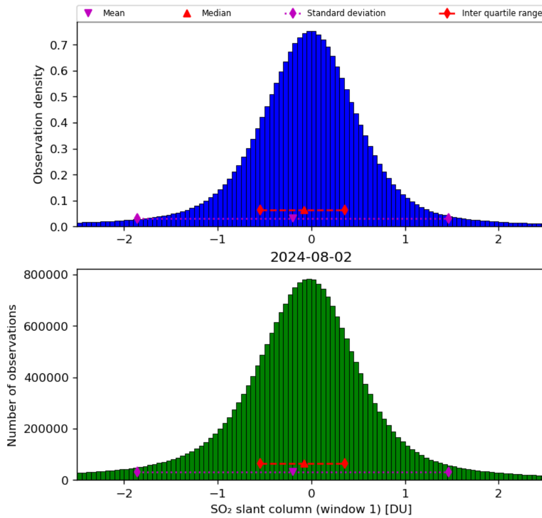
Figure 56: Histogram of “SO 2 slant column (window 1)” for 2024-08-01 to 2024-08-03
