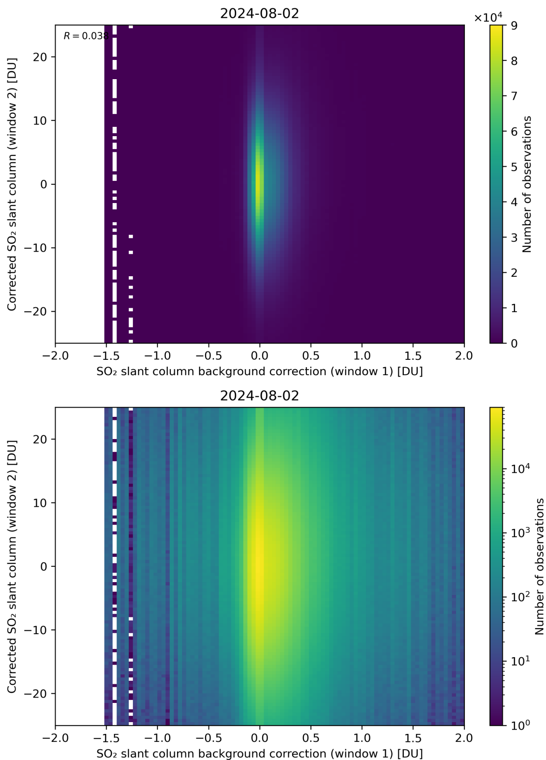
Figure 104: Scatter density plot of “SO 2 slant column background correction (window 1)” against “Corrected SO 2 slant column (window 2)” for 2024-08-01 to 2024-08-03.
