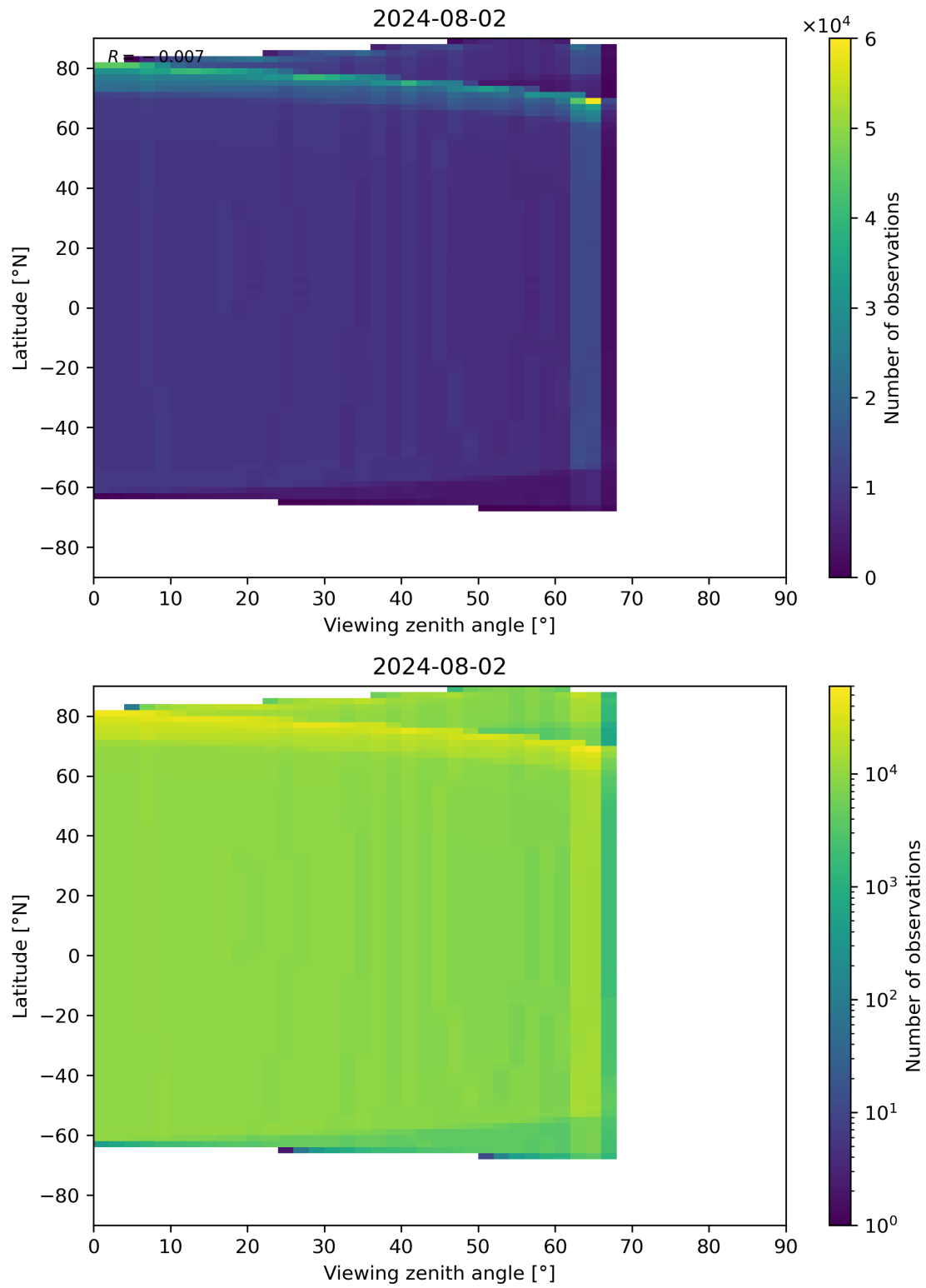
Figure 314: Scatter density plot of “Viewing zenith angle” against “Latitude” for 2024-08-01 to 2024-08-03.
