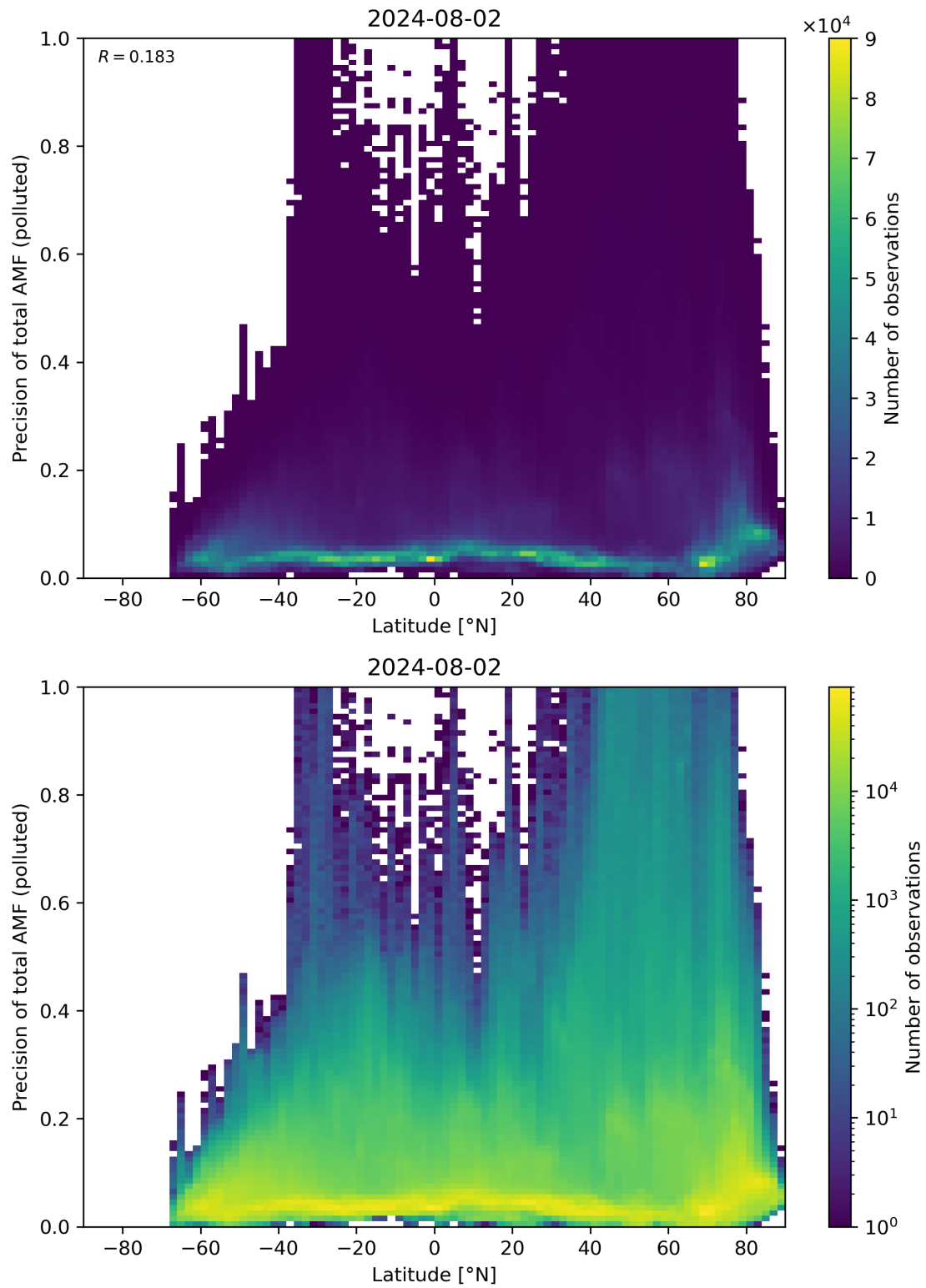
Figure 155: Scatter density plot of “Latitude” against “Precision of total AMF (polluted)” for 2024-08-01 to 2024-08-03.
