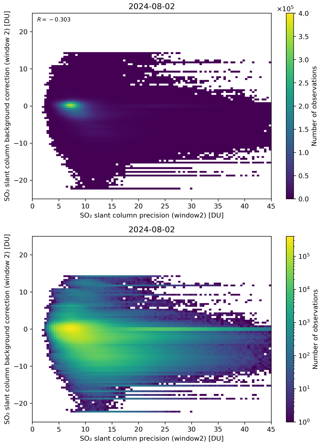
Figure 241: Scatter density plot of “SO 2 slant column precision (window2)” against “SO 2 slant column background correction (window 2)” for 2024-08-01 to 2024-08-03.
