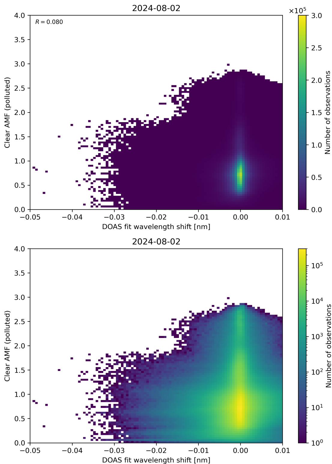
Figure 129: Scatter density plot of “DOAS fit wavelength shift” against “Clear AMF (polluted)” for 2024-08-01 to 2024-08-03.
