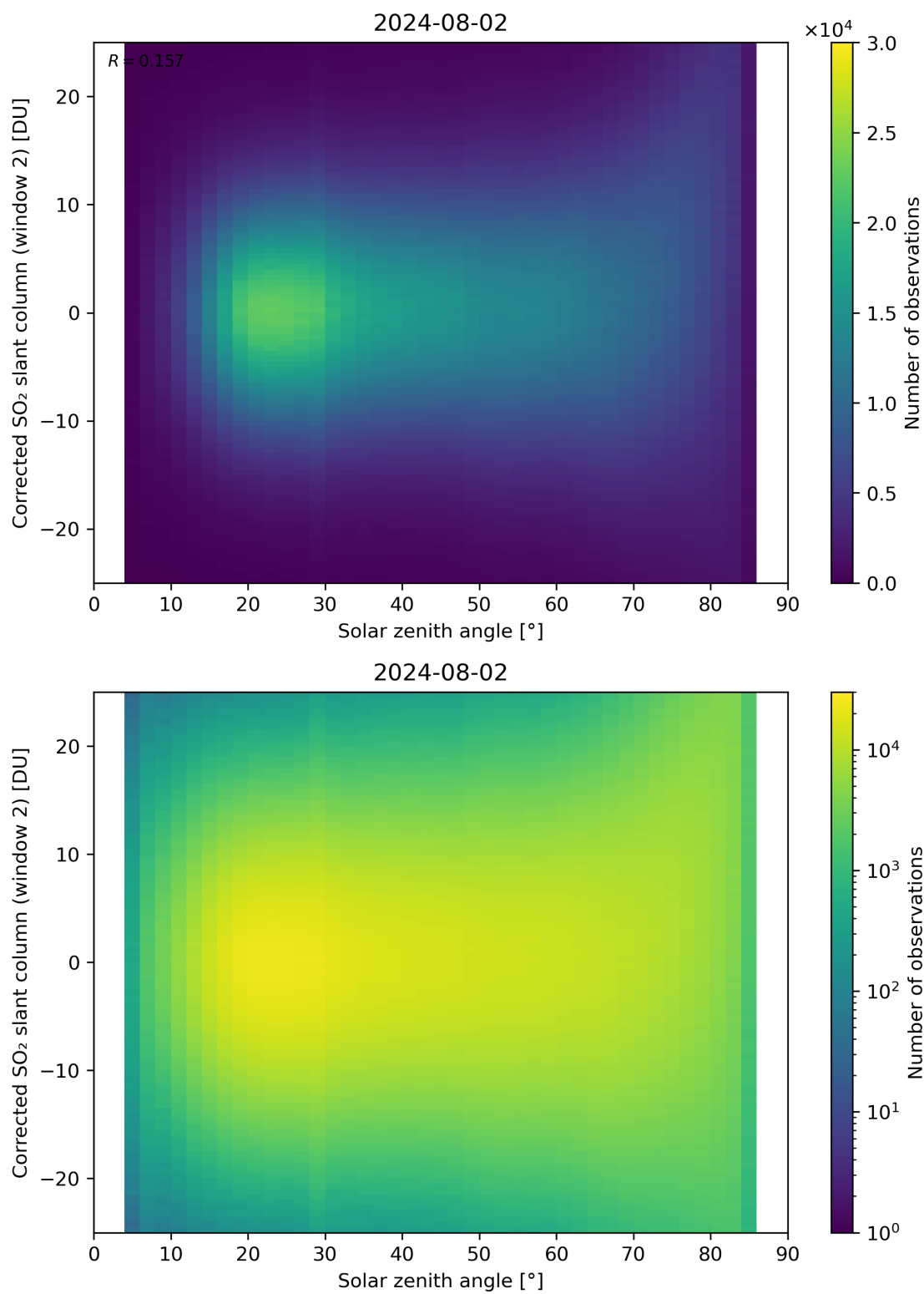
Figure 167: Scatter density plot of “Solar zenith angle” against “Corrected SO 2 slant column (window 2)” for 2024-08-01 to 2024-08-03.
