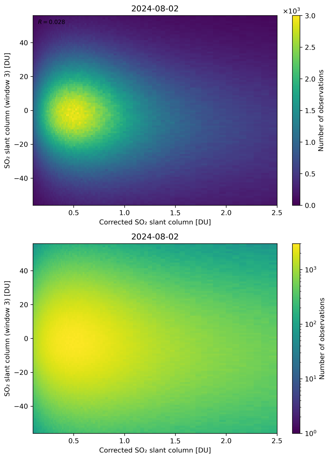
Figure 190: Scatter density plot of “Corrected SO 2 slant column” against “SO 2 slant column (window 3)” for 2024-08-01 to 2024-08-03.
