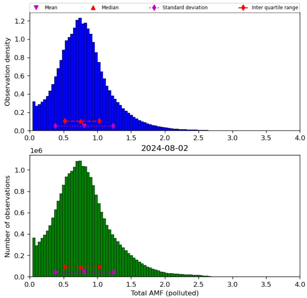
Figure 71: Histogram of “Total AMF (polluted)” for 2024-08-01 to 2024-08-03
