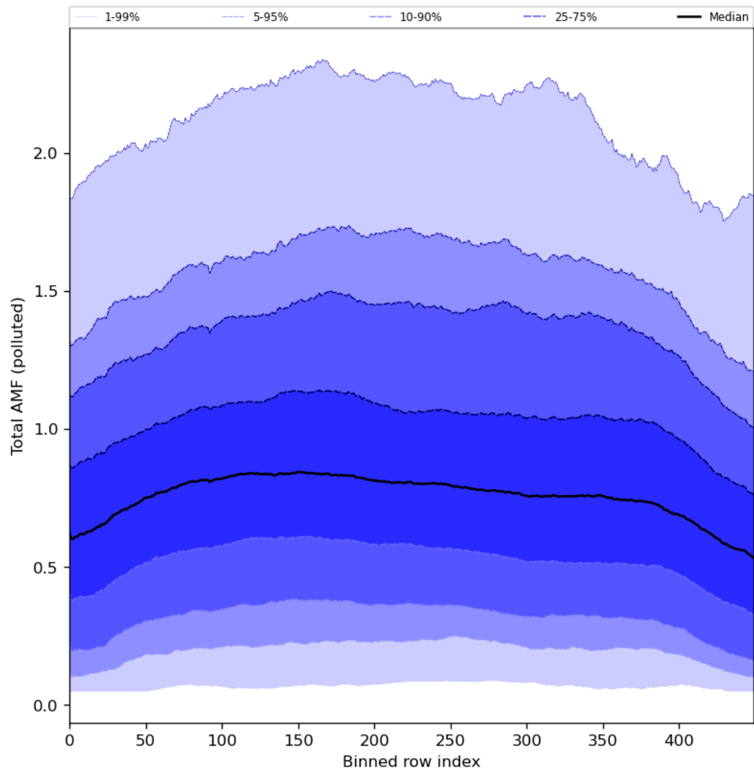
Figure 94: Along track statistics of “Total AMF (polluted)” for 2024-08-01 to 2024-08-03
