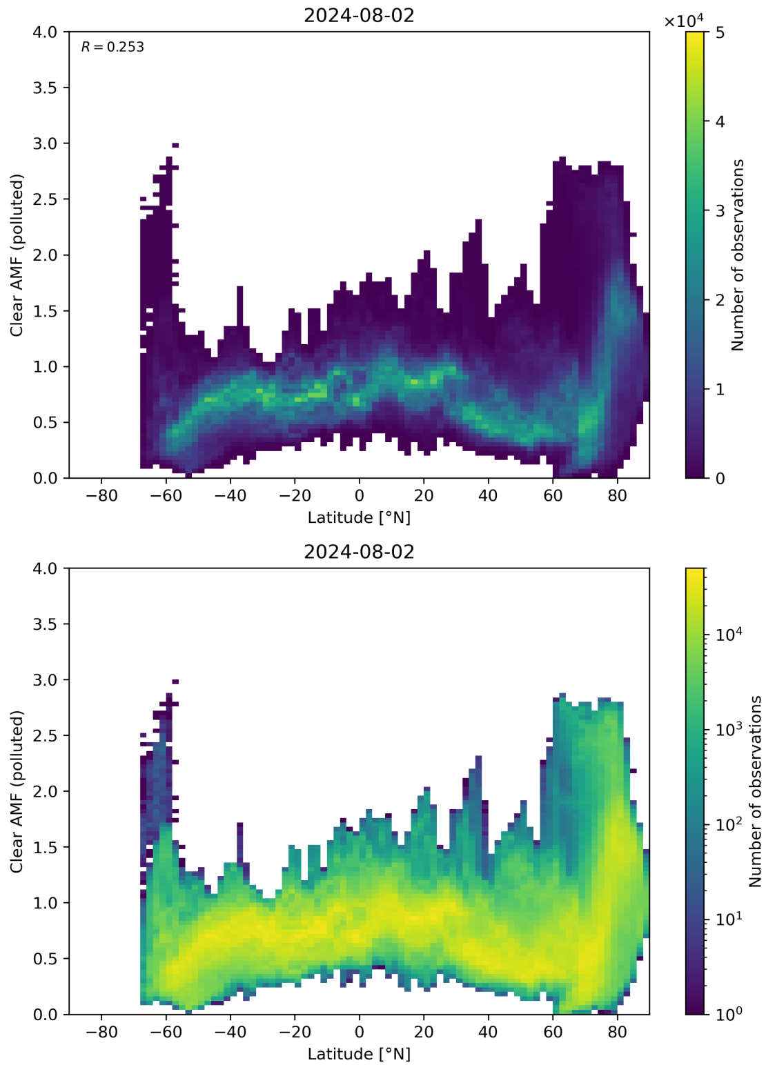
Figure 145: Scatter density plot of “Latitude” against “Clear AMF (polluted)” for 2024-08-01 to 2024-08-03.
