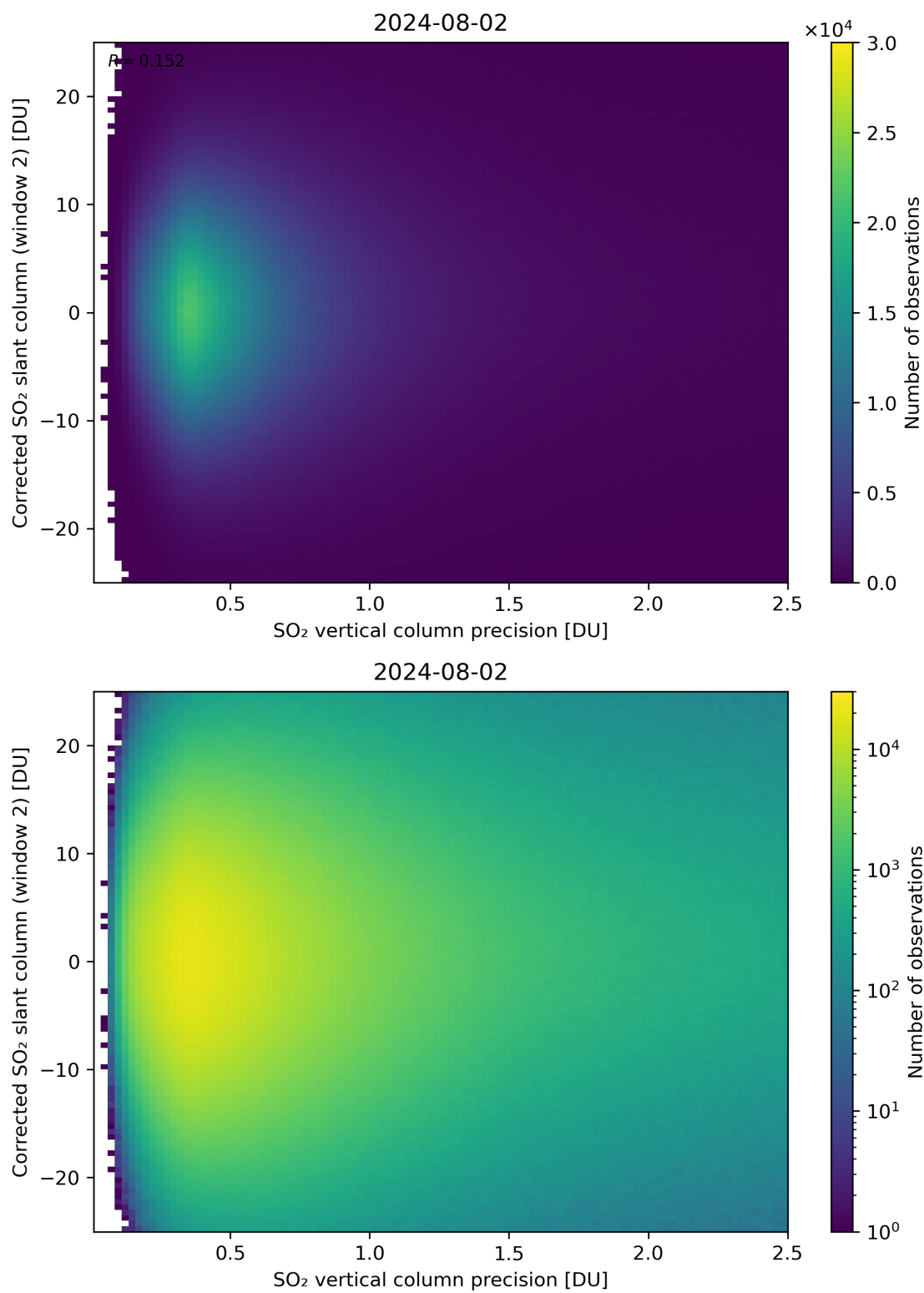
Figure 287: Scatter density plot of “SO 2 vertical column precision” against “Corrected SO 2 slant column (window 2)” for 2024-08-01 to 2024-08-03.
