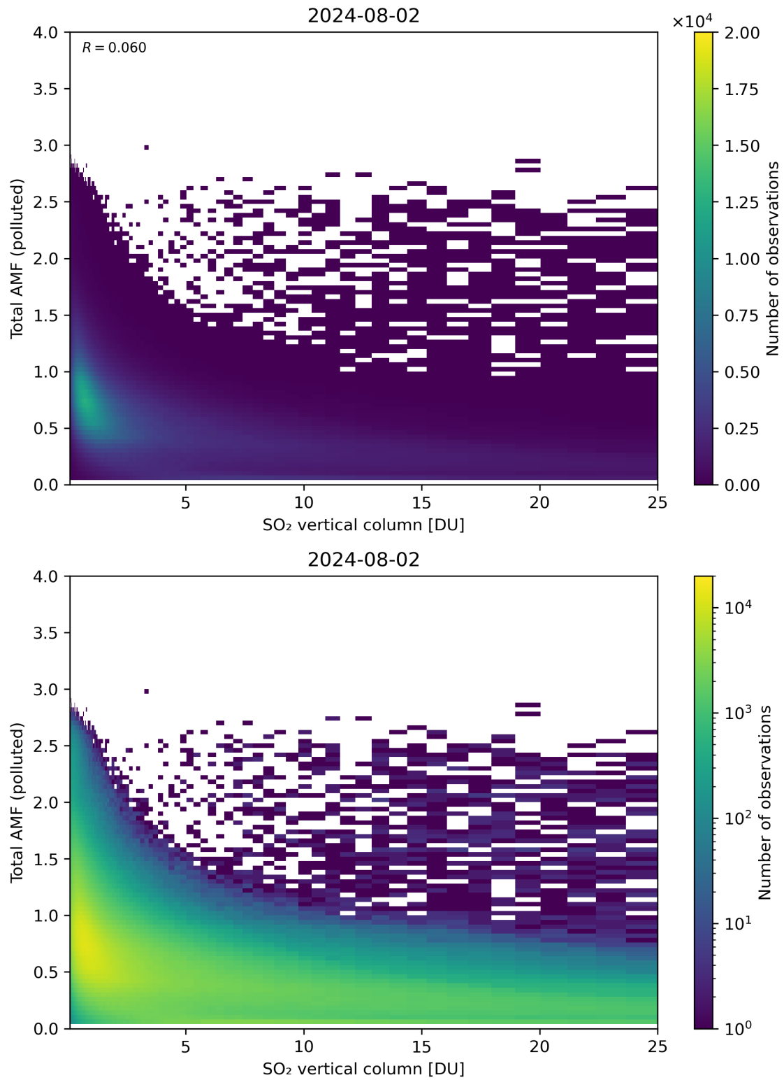
Figure 305: Scatter density plot of “SO 2 vertical column” against “Total AMF (polluted)” for 2024-08-01 to 2024-08-03.
