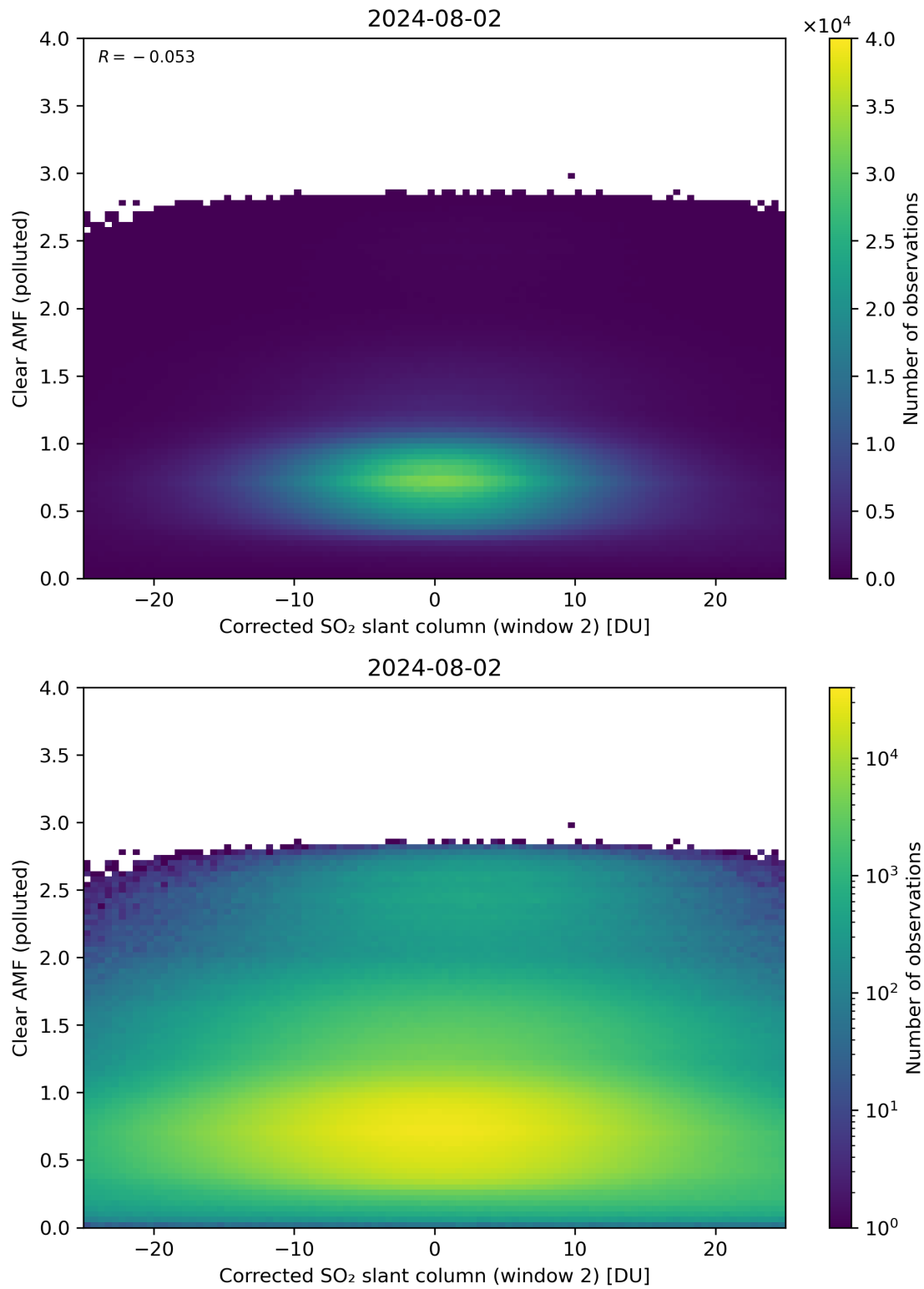
Figure 199: Scatter density plot of “Corrected SO 2 slant column (window 2)” against “Clear AMF (polluted)” for 2024-08-01 to 2024-08-03.
