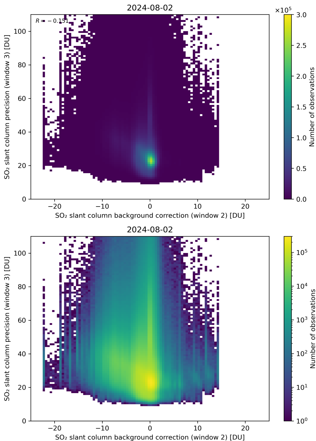
Figure 118: Scatter density plot of “SO 2 slant column background correction (window 2)” against “SO 2 slant column precision (window 3)” for 2024-08-01 to 2024-08-03.
