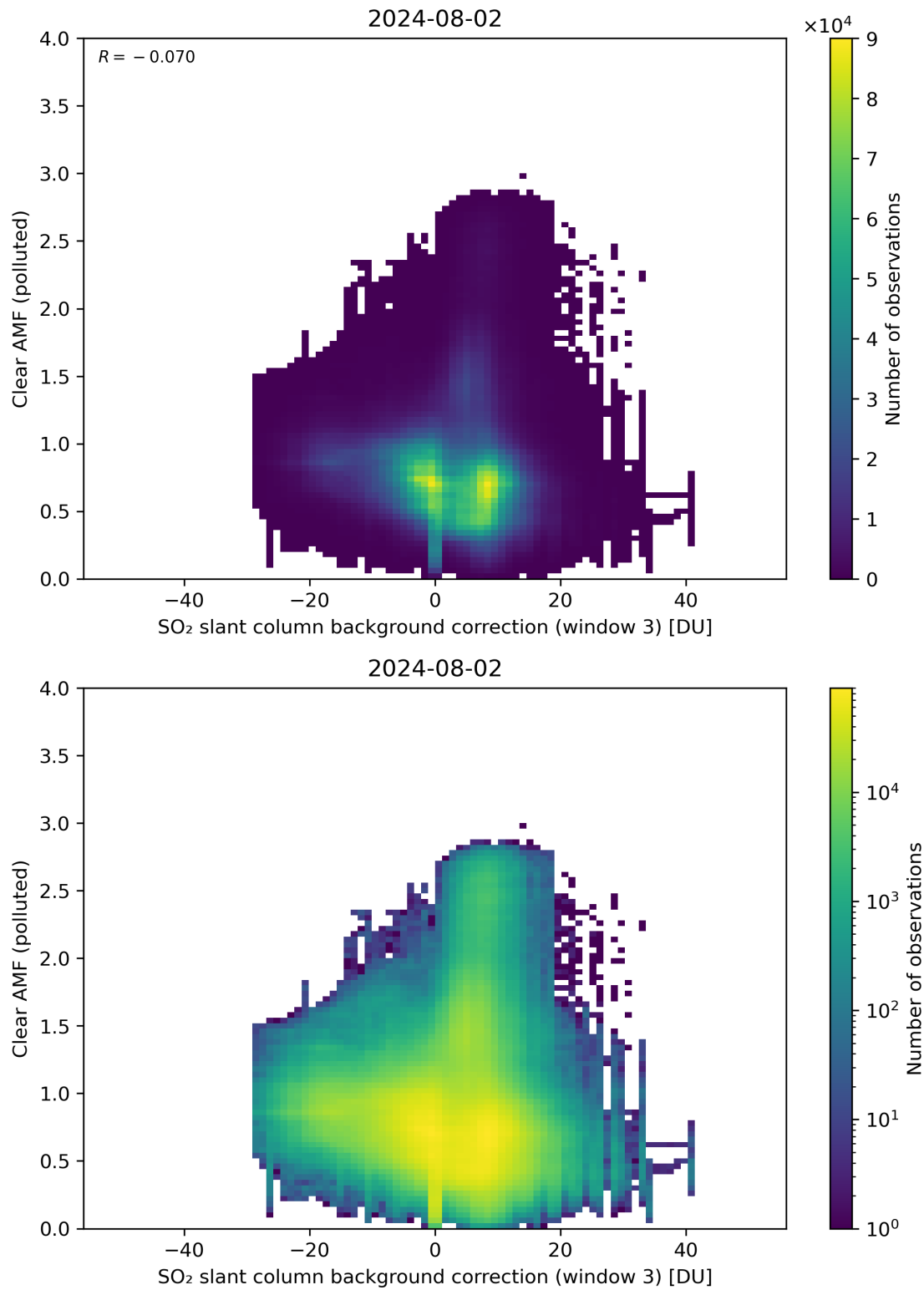
Figure 124: Scatter density plot of “SO 2 slant column background correction (window 3)” against “Clear AMF (polluted)” for 2024-08-01 to 2024-08-03.
