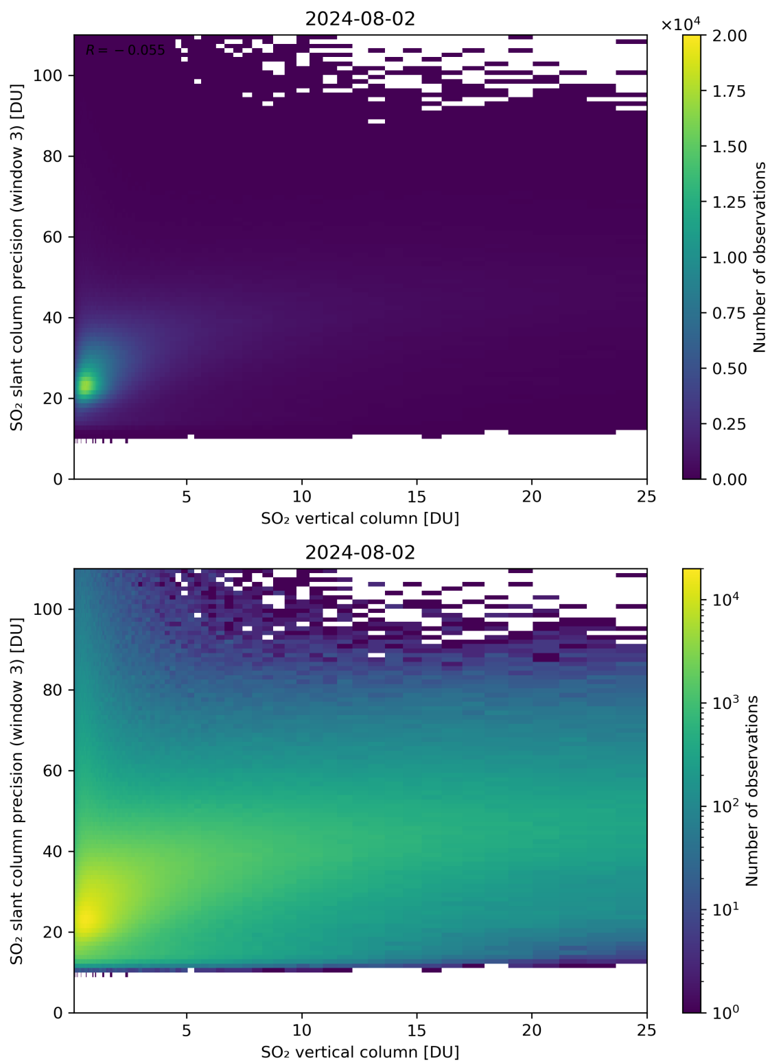
Figure 304: Scatter density plot of “SO 2 vertical column” against “SO 2 slant column precision (window 3)” for 2024-08-01 to 2024-08-03.
