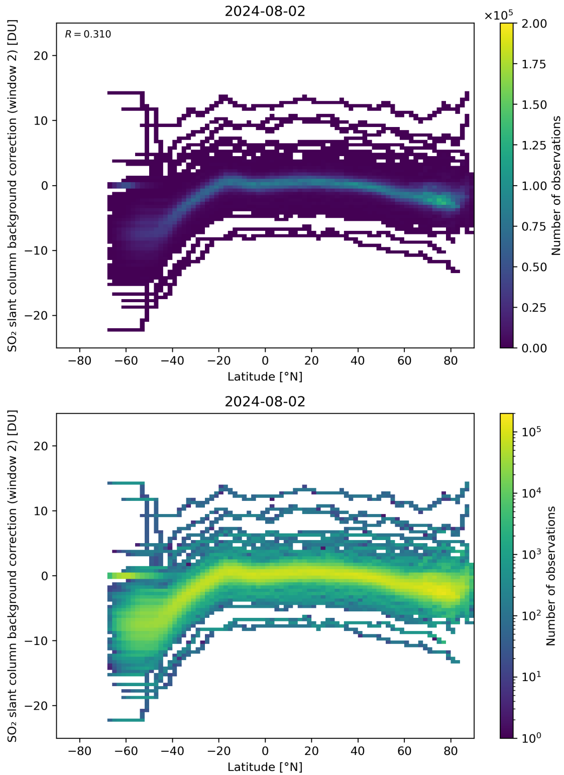
Figure 140: Scatter density plot of “Latitude” against “SO 2 slant column background correction (window 2)” for 2024-08-01 to 2024-08-03.
