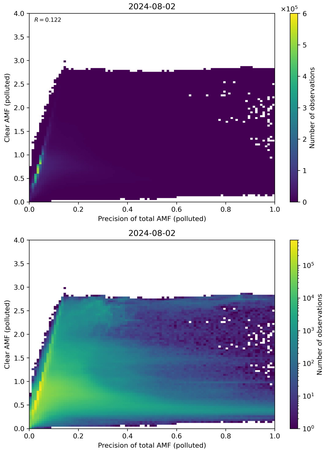
Figure 270: Scatter density plot of “Precision of total AMF (polluted)” against “Clear AMF (polluted)” for 2024-08-01 to 2024-08-03.
