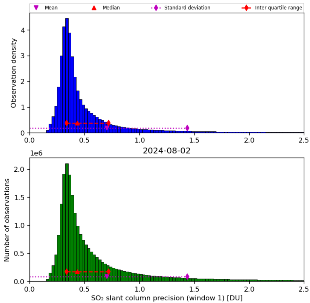
Figure 57: Histogram of “SO 2 slant column precision (window 1)” for 2024-08-01 to 2024-08-03
