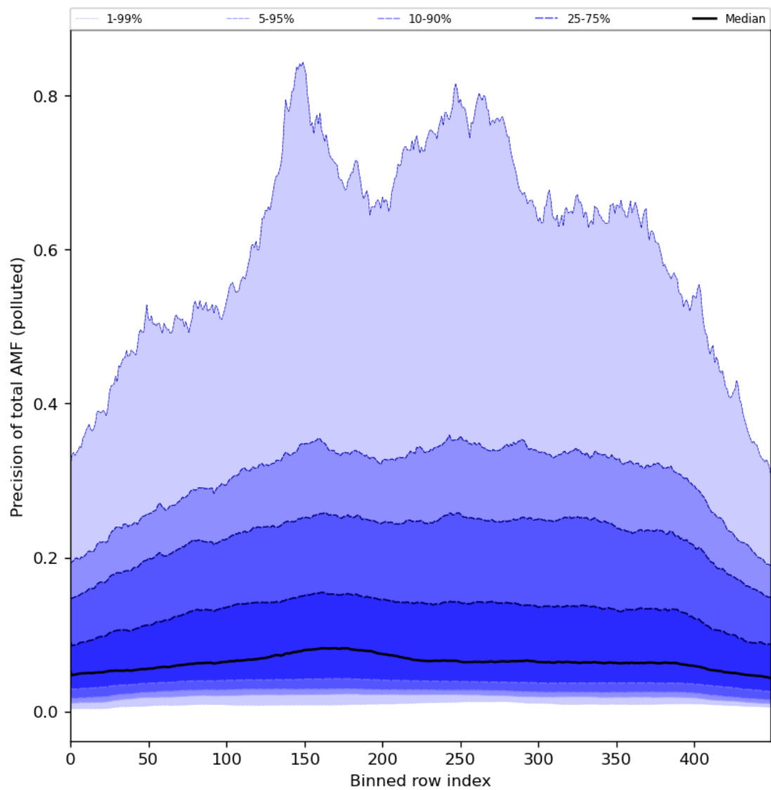
Figure 95: Along track statistics of “Precision of total AMF (polluted)” for 2024-08-01 to 2024-08-03
