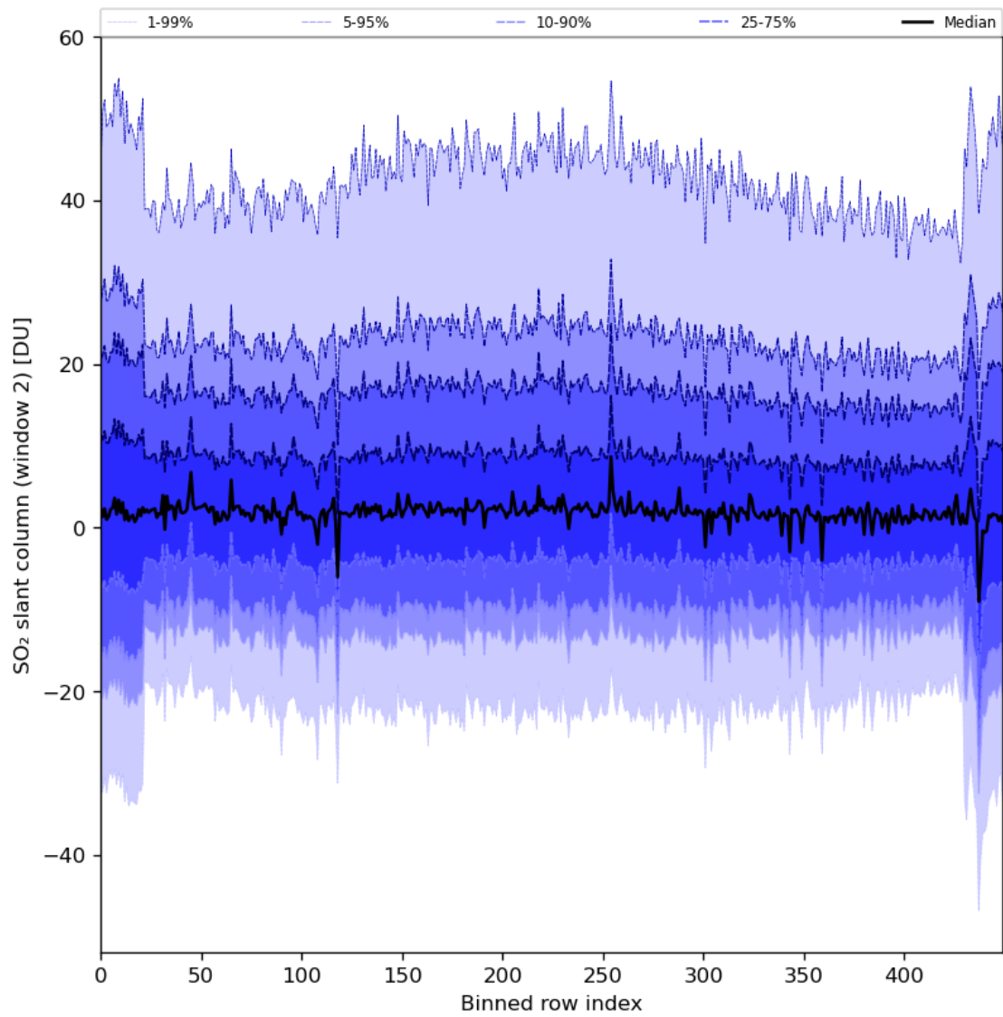
Figure 83: Along track statistics of “SO 2 slant column (window 2)” for 2024-08-01 to 2024-08-03
