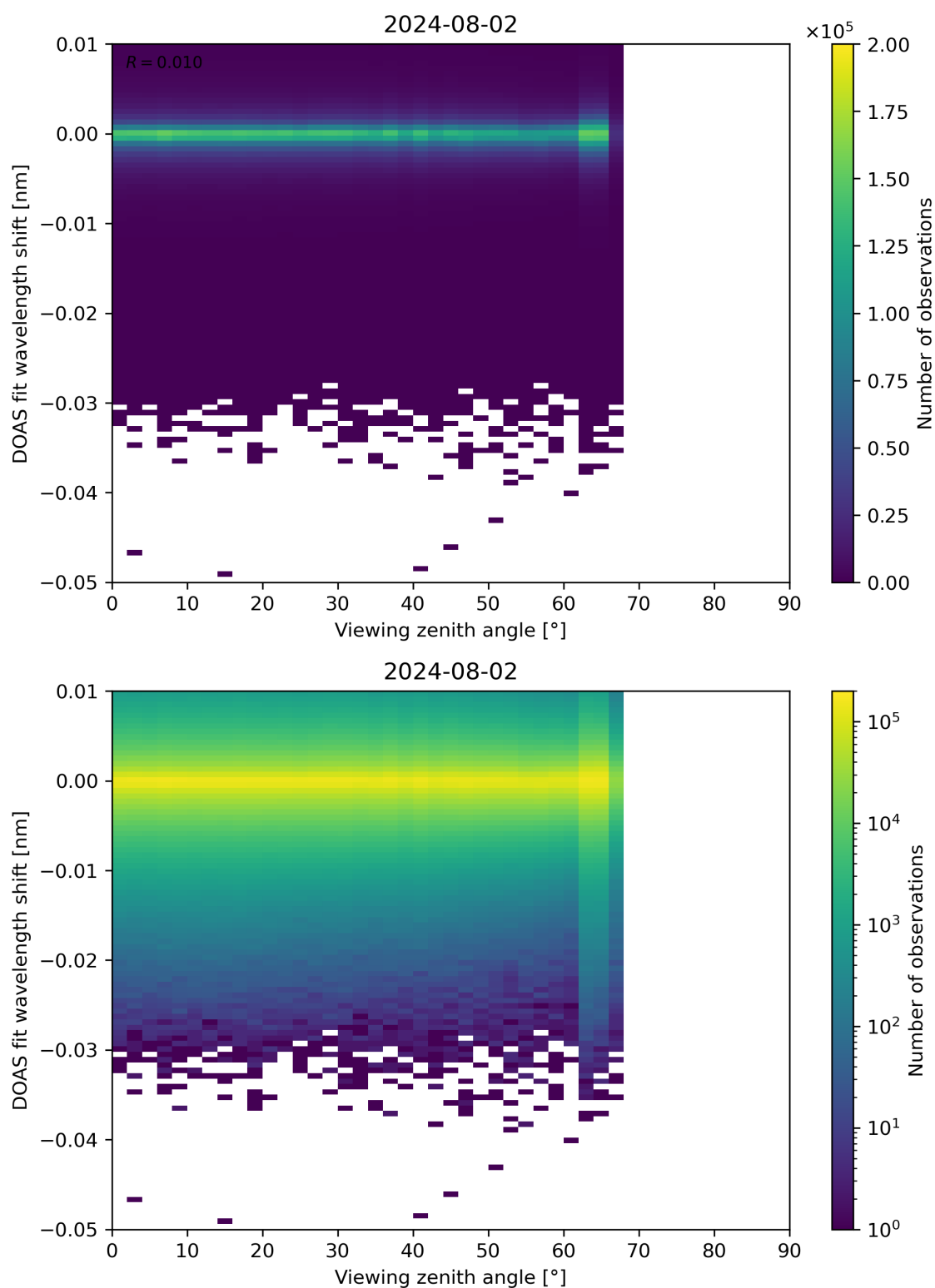
Figure 311: Scatter density plot of “Viewing zenith angle” against “DOAS fit wavelength shift” for 2024-08-01 to 2024-08-03.
