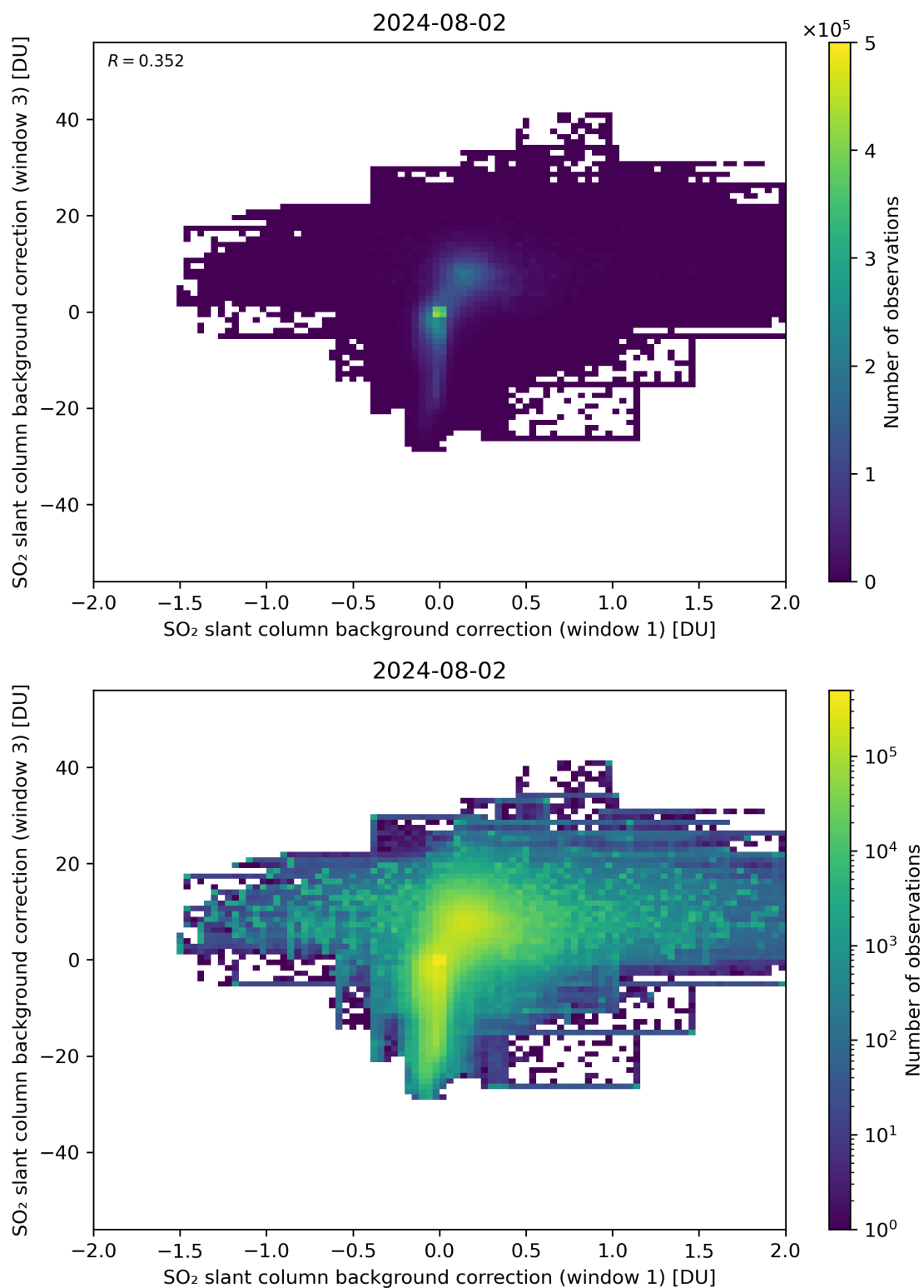
Figure 99: Scatter density plot of “SO 2 slant column background correction (window 1)” against “SO 2 slant column background correction (window 3)” for 2024-08-01 to 2024-08-03.
