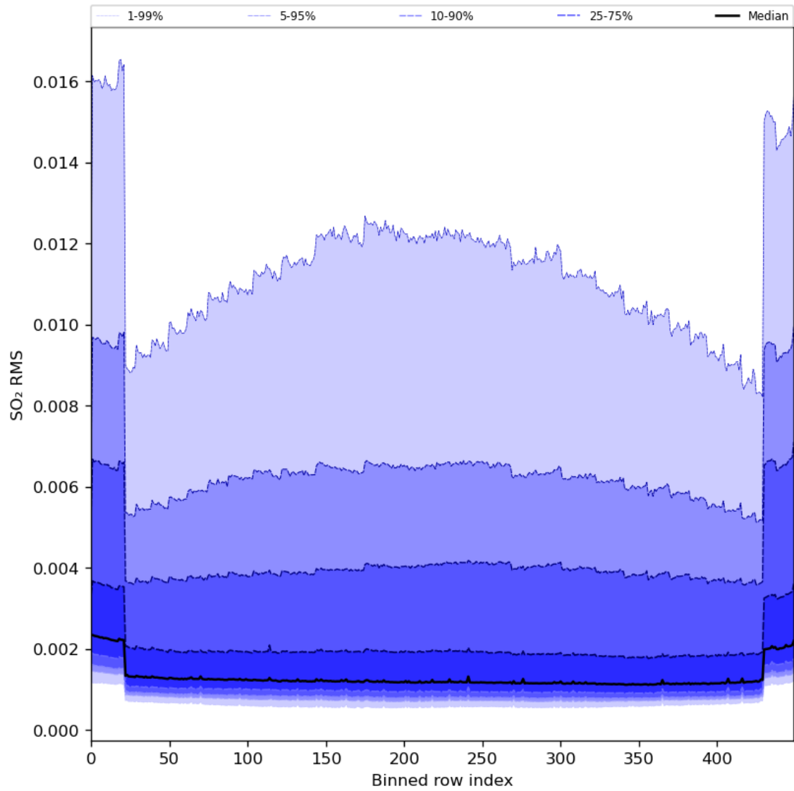
Figure 93: Along track statistics of “SO 2 RMS” for 2024-08-01 to 2024-08-03
