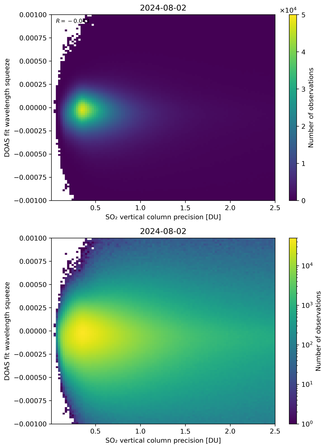
Figure 283: Scatter density plot of “SO 2 vertical column precision” against “DOAS fit wavelength squeeze” for 2024-08-01 to 2024-08-03.
