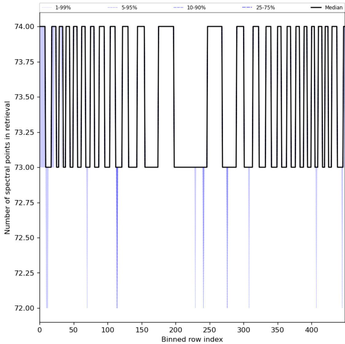
Figure 97: Along track statistics of “Number of spectral points in retrieval” for 2024-08-01 to 2024-08-03
