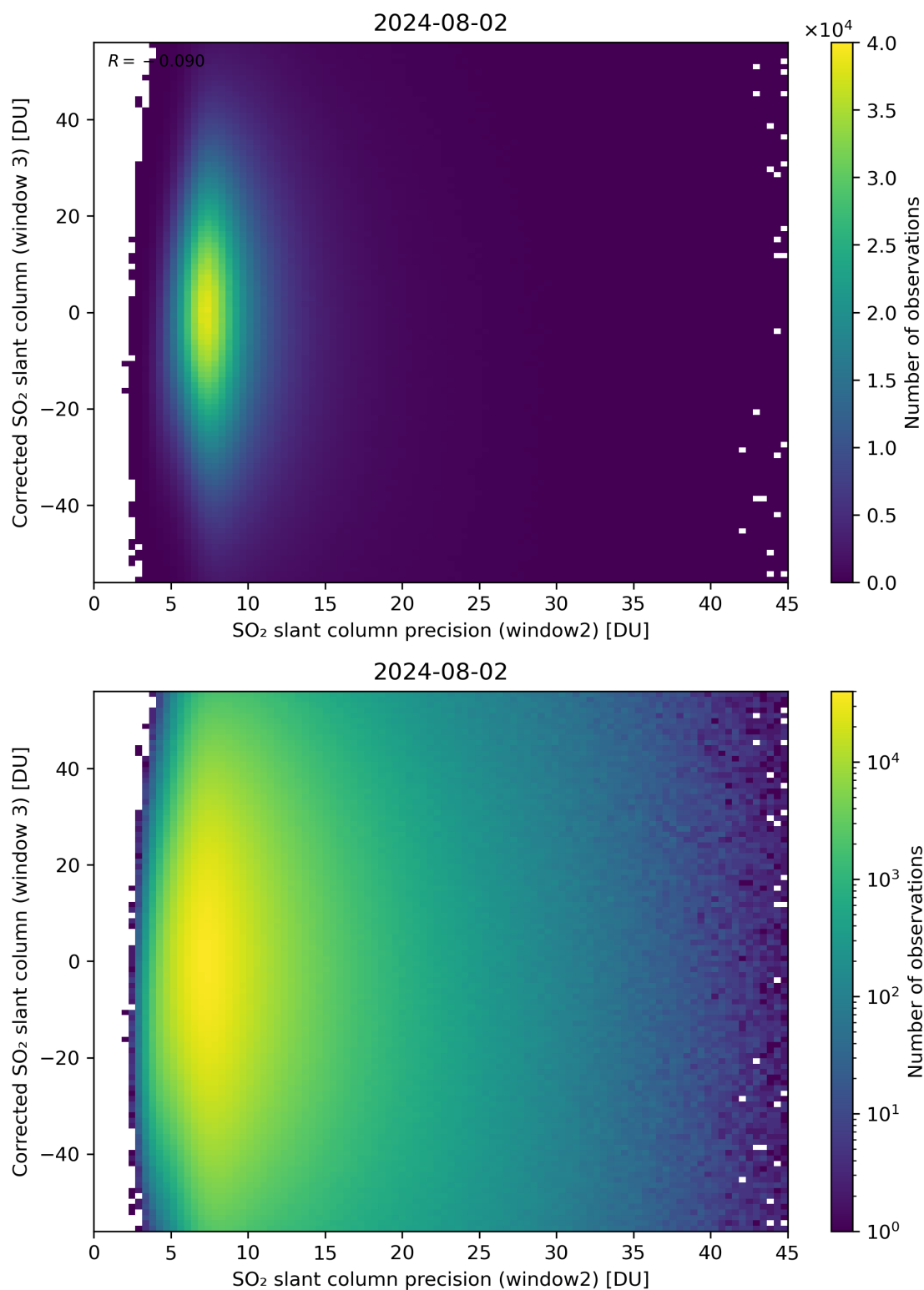
Figure 248: Scatter density plot of “SO 2 slant column precision (window2)” against “Corrected SO 2 slant column (window 3)” for 2024-08-01 to 2024-08-03.
