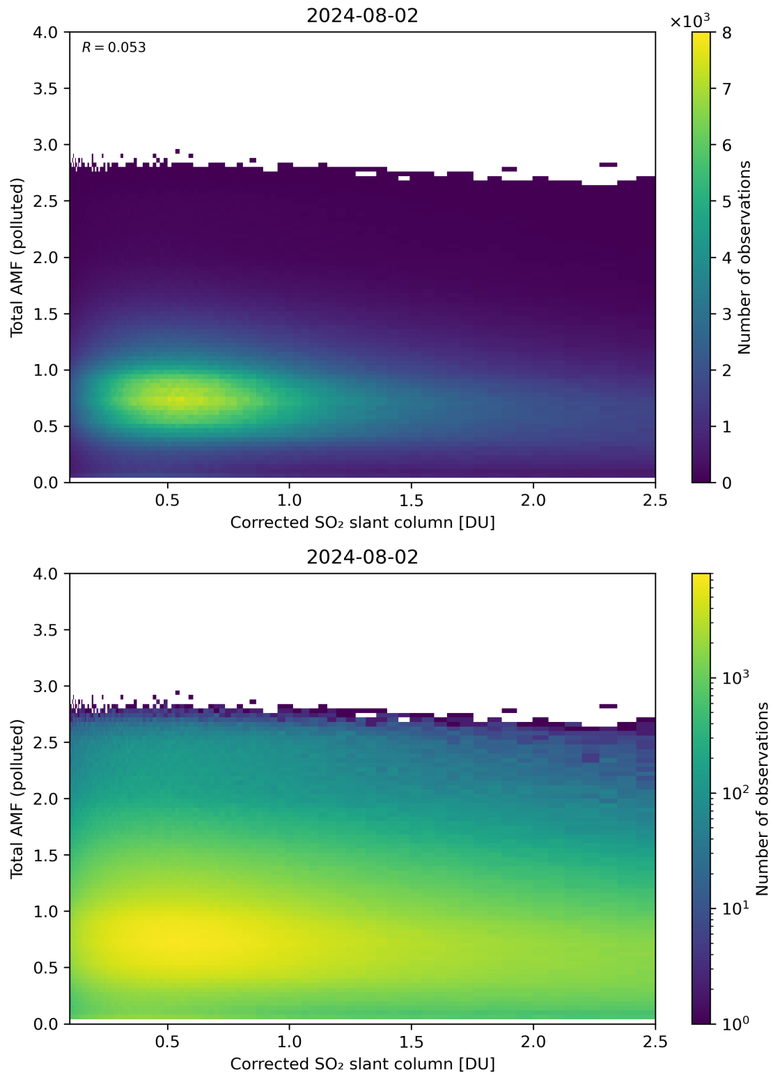
Figure 192: Scatter density plot of “Corrected SO 2 slant column” against “Total AMF (polluted)” for 2024-08-01 to 2024-08-03.
