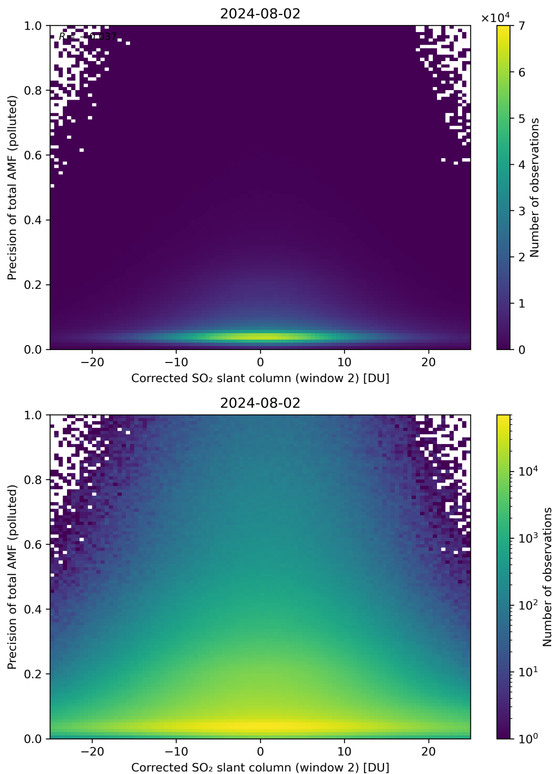
Figure 204: Scatter density plot of “Corrected SO 2 slant column (window 2)” against “Precision of total AMF (polluted)” for 2024-08-01 to 2024-08-03.
