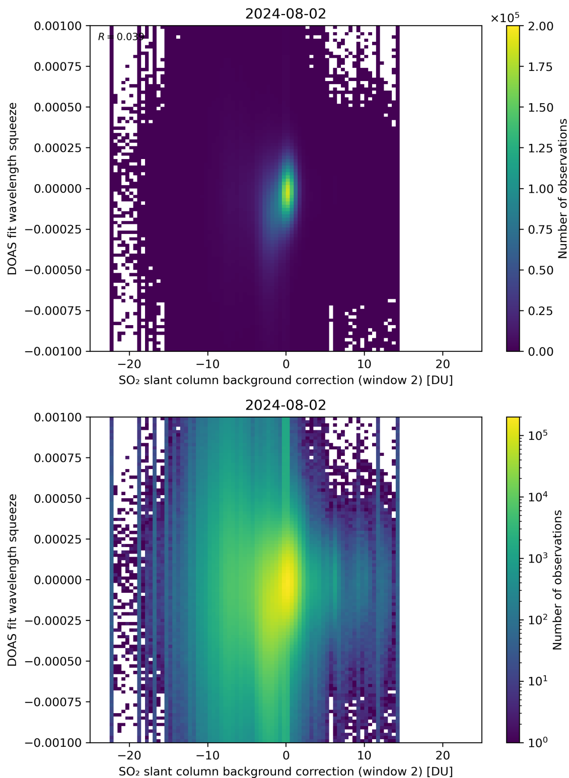
Figure 113: Scatter density plot of “SO 2 slant column background correction (window 2)” against “DOAS fit wavelength squeeze” for 2024-08-01 to 2024-08-03.
