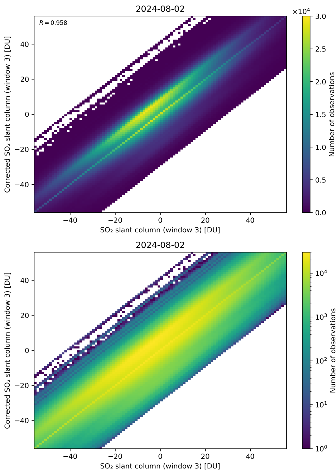
Figure 266: Scatter density plot of “SO 2 slant column (window 3)” against “Corrected SO 2 slant column (window 3)” for 2024-08-01 to 2024-08-03.
