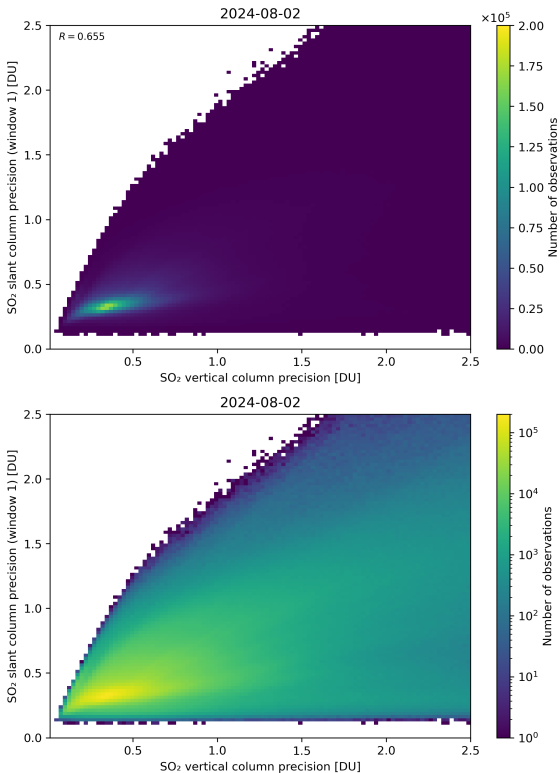
Figure 290: Scatter density plot of “SO 2 vertical column precision” against “SO 2 slant column precision (window 1)” for 2024-08-01 to 2024-08-03.
