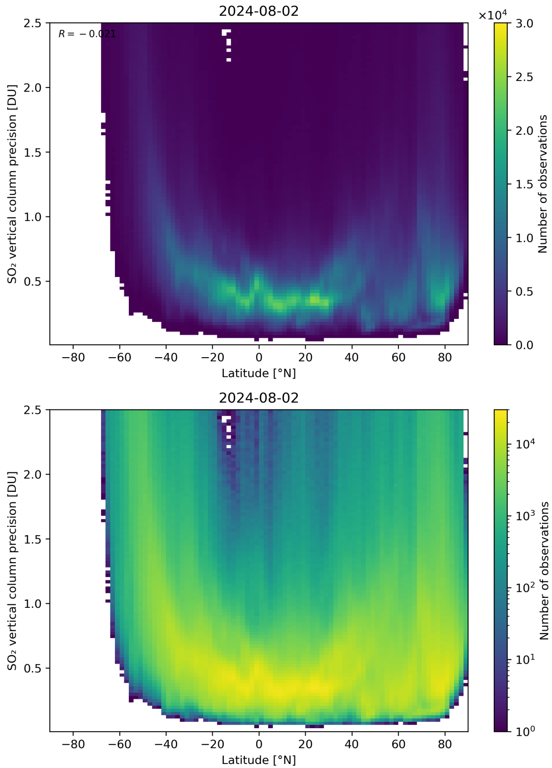
Figure 157: Scatter density plot of “Latitude” against “SO 2 vertical column precision” for 2024-08-01 to 2024-08-03.
