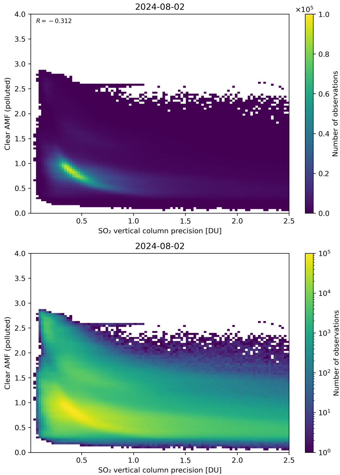
Figure 285: Scatter density plot of “SO 2 vertical column precision” against “Clear AMF (polluted)” for 2024-08-01 to 2024-08-03.
