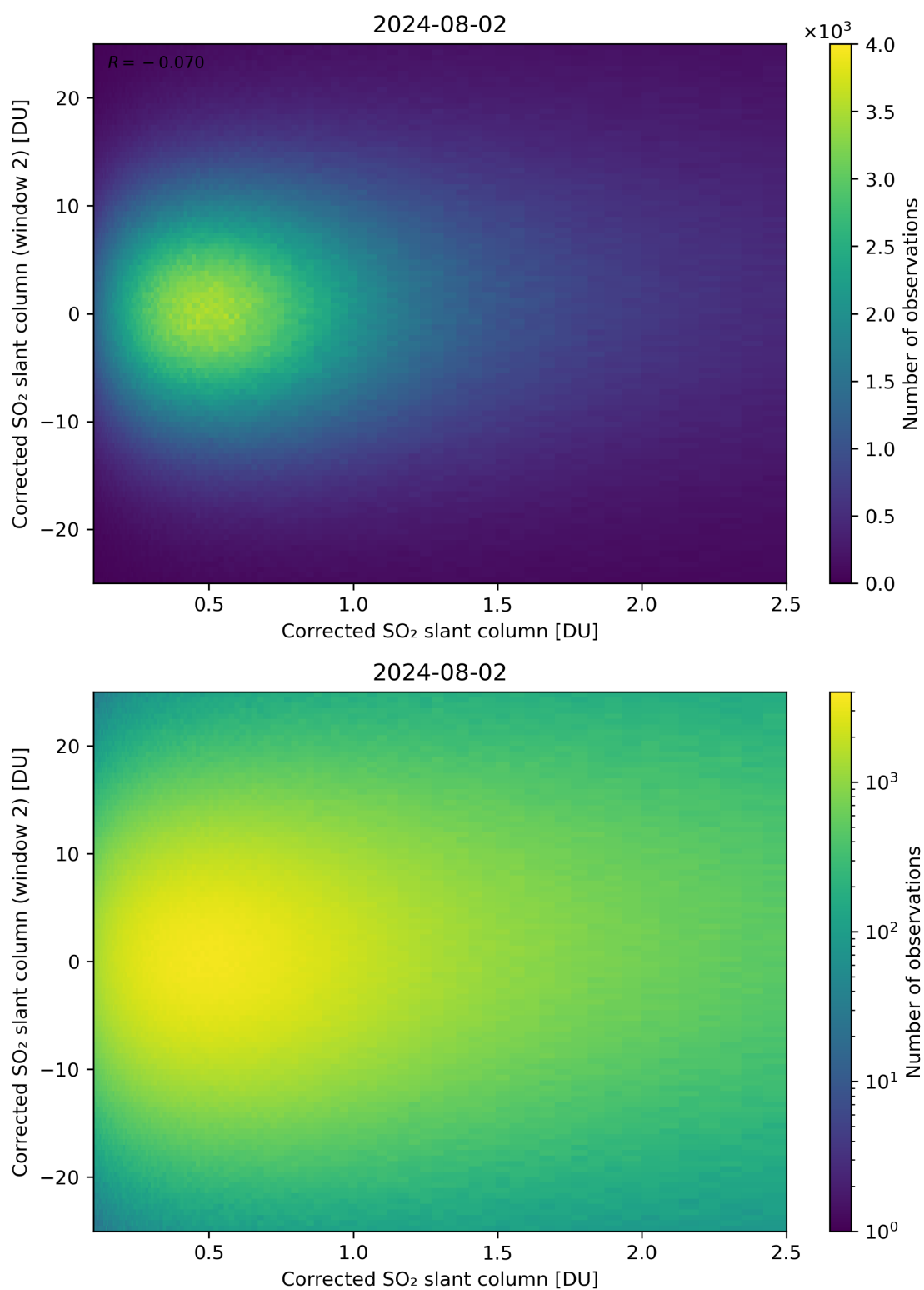
Figure 185: Scatter density plot of “Corrected SO 2 slant column” against “Corrected SO 2 slant column (window 2)” for 2024-08-01 to 2024-08-03.
