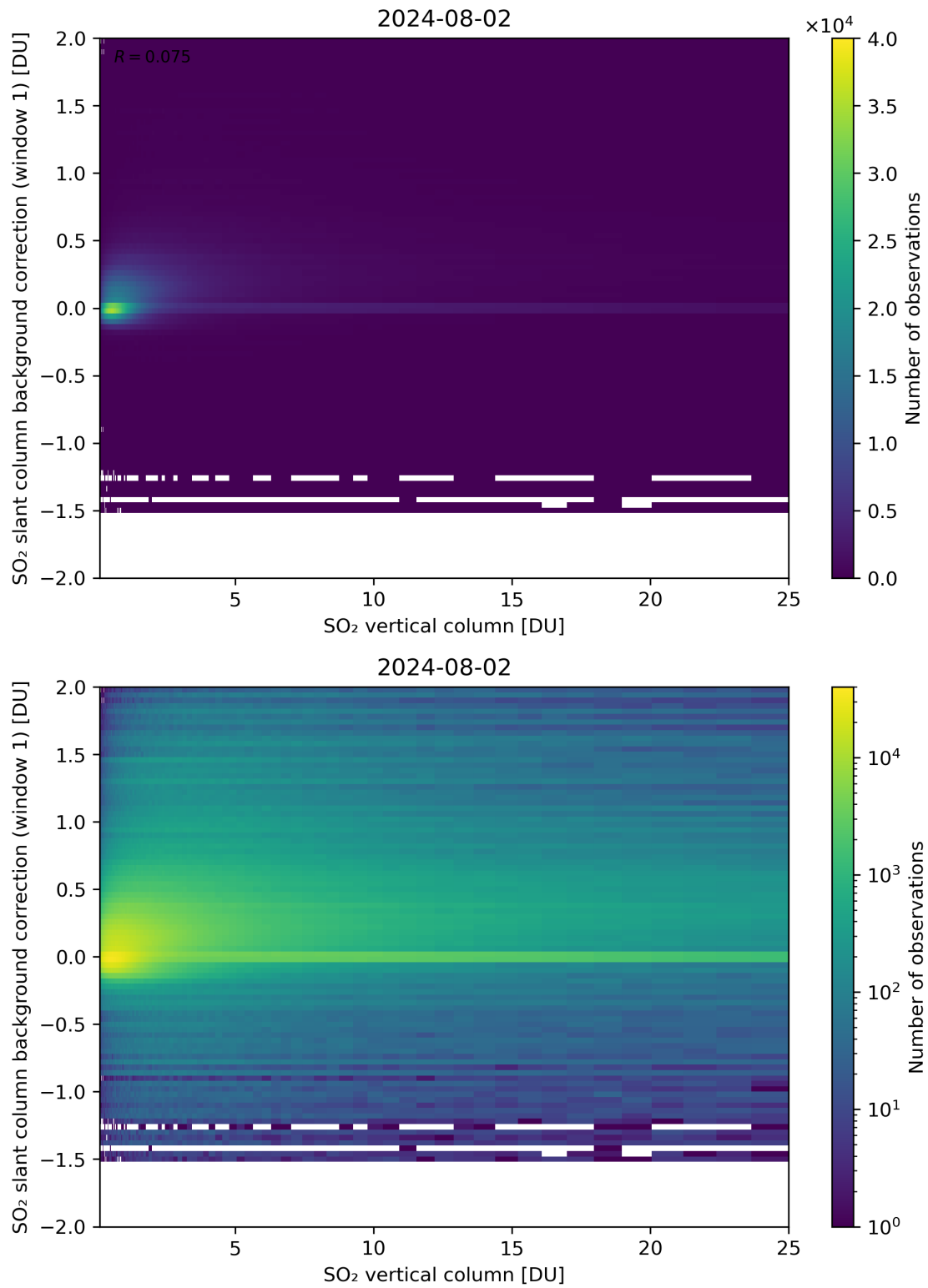
Figure 273: Scatter density plot of “SO 2 vertical column” against “SO 2 slant column background correction (window 1)” for 2024-08-01 to 2024-08-03.
