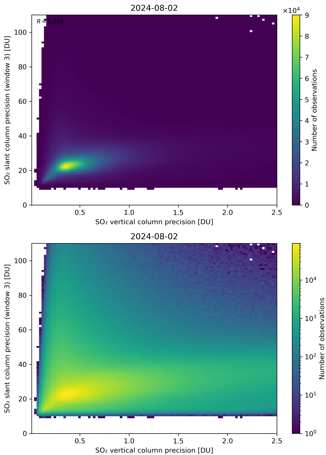
Figure 293: Scatter density plot of “SO 2 vertical column precision” against “SO 2 slant column precision (window 3)” for 2024-08-01 to 2024-08-03.
