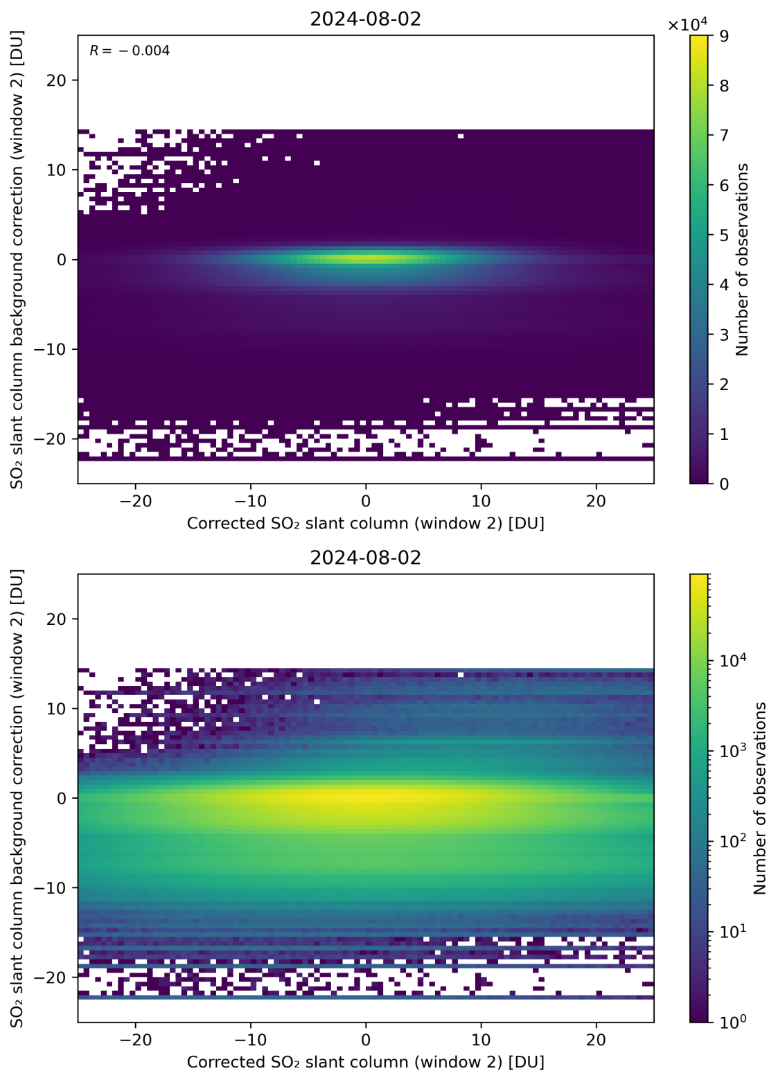
Figure 194: Scatter density plot of “Corrected SO 2 slant column (window 2)” against “SO 2 slant column background correction (window 2)” for 2024-08-01 to 2024-08-03.
