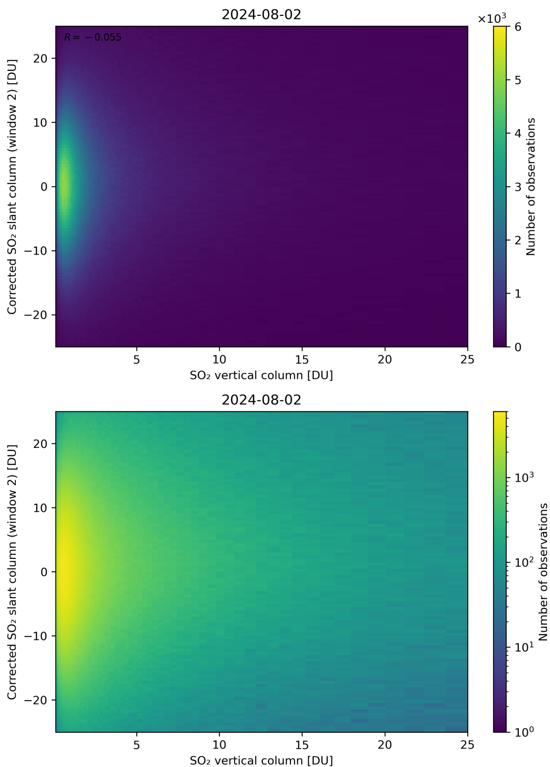
Figure 298: Scatter density plot of “SO 2 vertical column” against “Corrected SO 2 slant column (window 2)” for 2024-08-01 to 2024-08-03.
