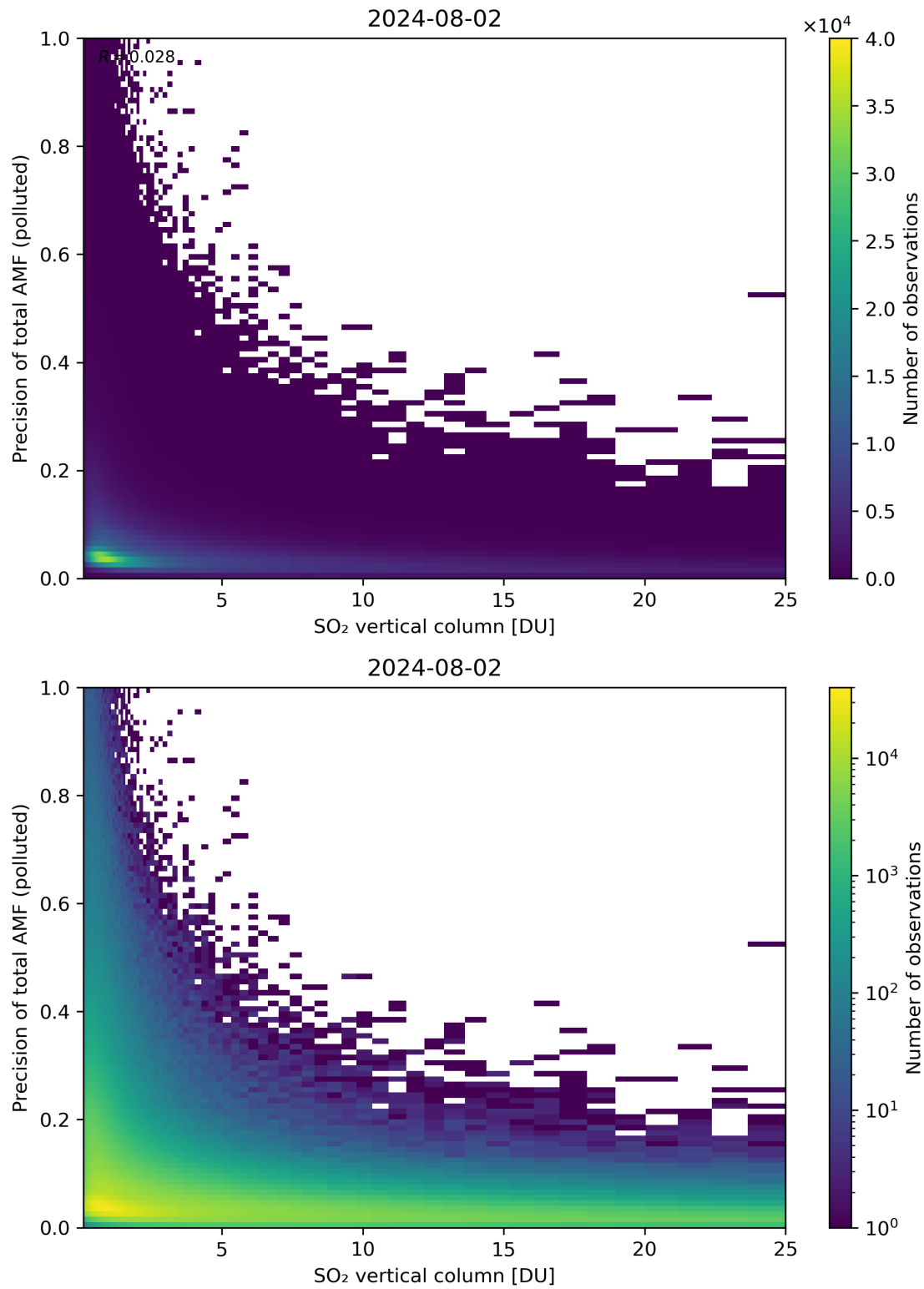
Figure 306: Scatter density plot of “SO 2 vertical column” against “Precision of total AMF (polluted)” for 2024-08-01 to 2024-08-03.
