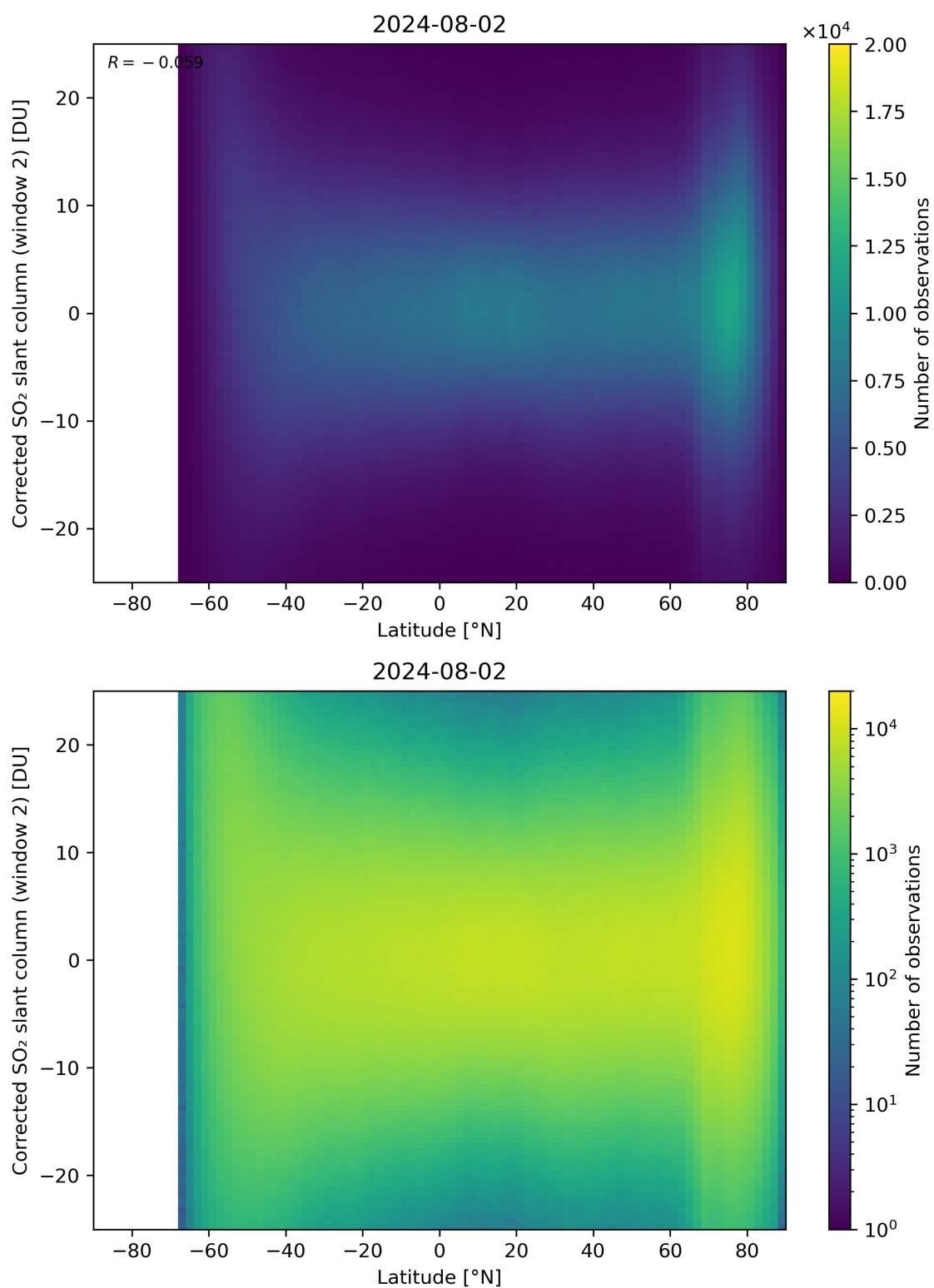
Figure 147: Scatter density plot of “Latitude” against “Corrected SO 2 slant column (window 2)” for 2024-08-01 to 2024-08-03.
