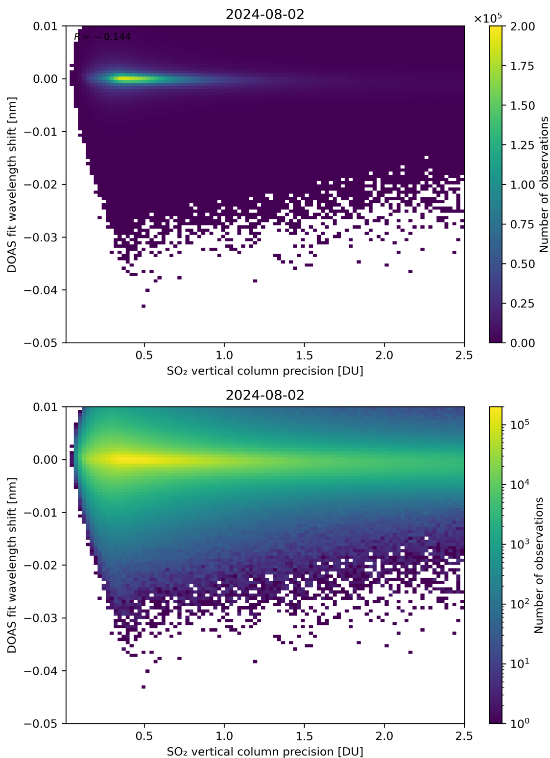
Figure 282: Scatter density plot of “SO 2 vertical column precision” against “DOAS fit wavelength shift” for 2024-08-01 to 2024-08-03.
