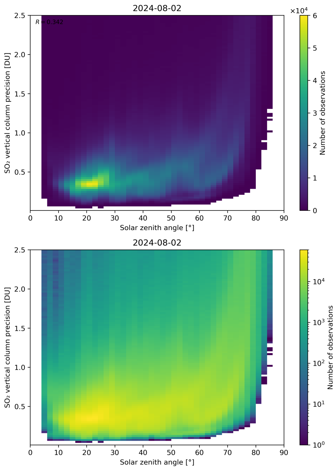
Figure 177: Scatter density plot of “Solar zenith angle” against “SO 2 vertical column precision” for 2024-08-01 to 2024-08-03.
