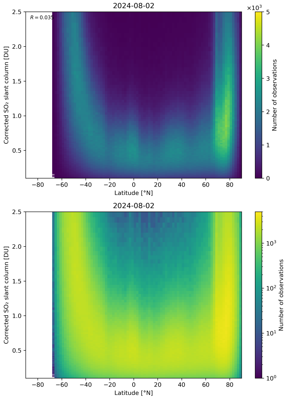
Figure 146: Scatter density plot of “Latitude” against “Corrected SO 2 slant column” for 2024-08-01 to 2024-08-03.
