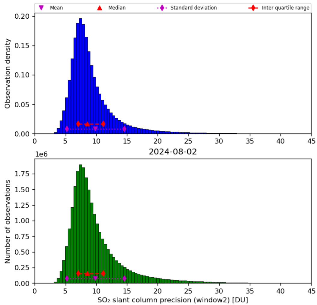
Figure 61: Histogram of “SO 2 slant column precision (window2)” for 2024-08-01 to 2024-08-03
