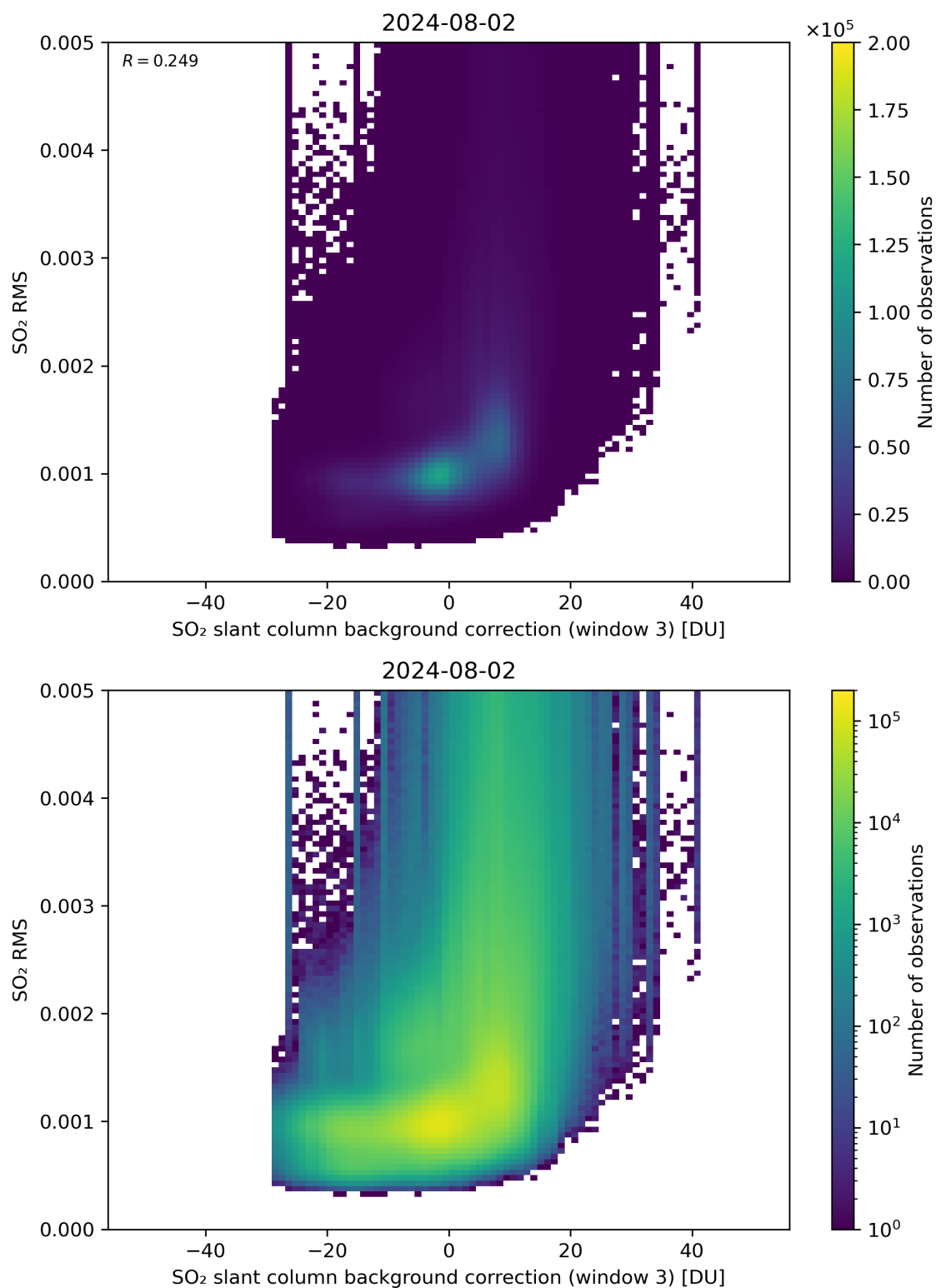
Figure 123: Scatter density plot of “SO 2 slant column background correction (window 3)” against “SO 2 RMS” for 2024-08-01 to 2024-08-03.
