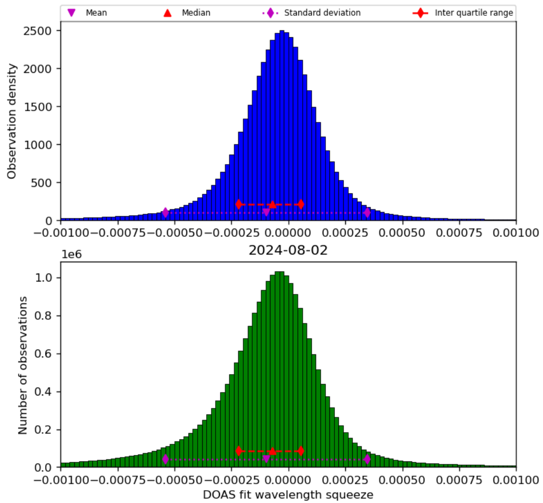
Figure 69: Histogram of “DOAS fit wavelength squeeze” for 2024-08-01 to 2024-08-03
