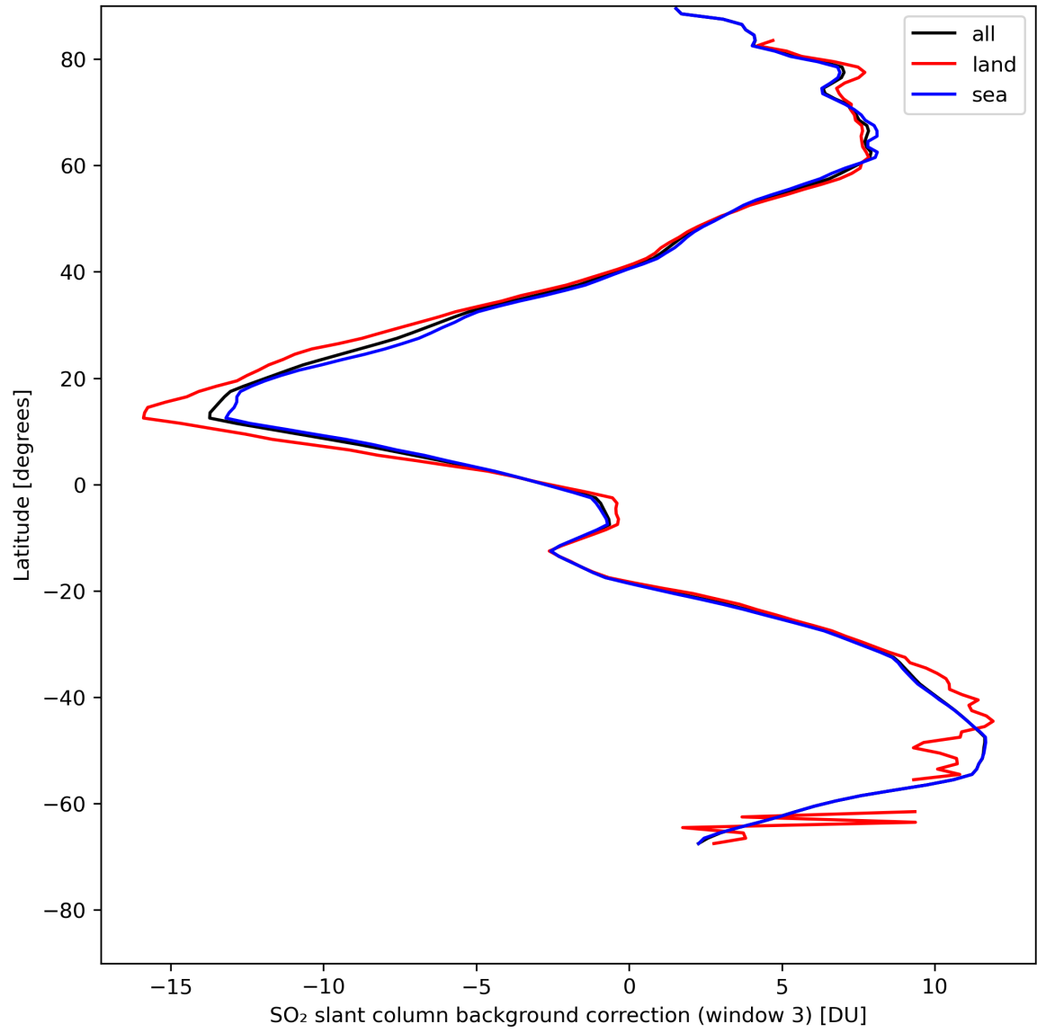
Figure 44: Zonal average of “SO 2 slant column background correction (window 3)” for 2024-08-01 to 2024-08-03.
