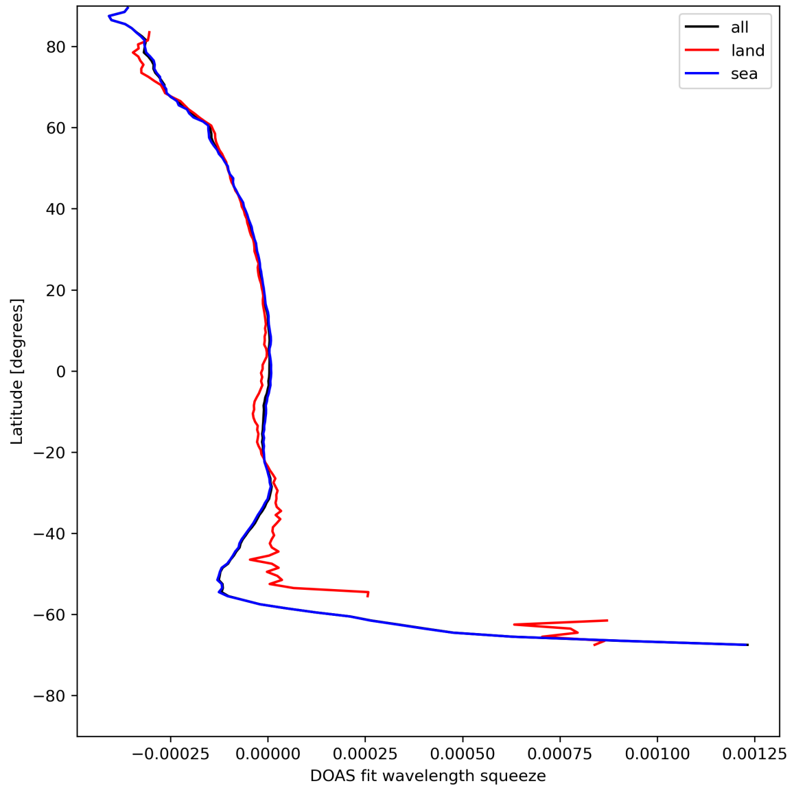
Figure 46: Zonal average of “DOAS fit wavelength squeeze” for 2024-08-01 to 2024-08-03.
