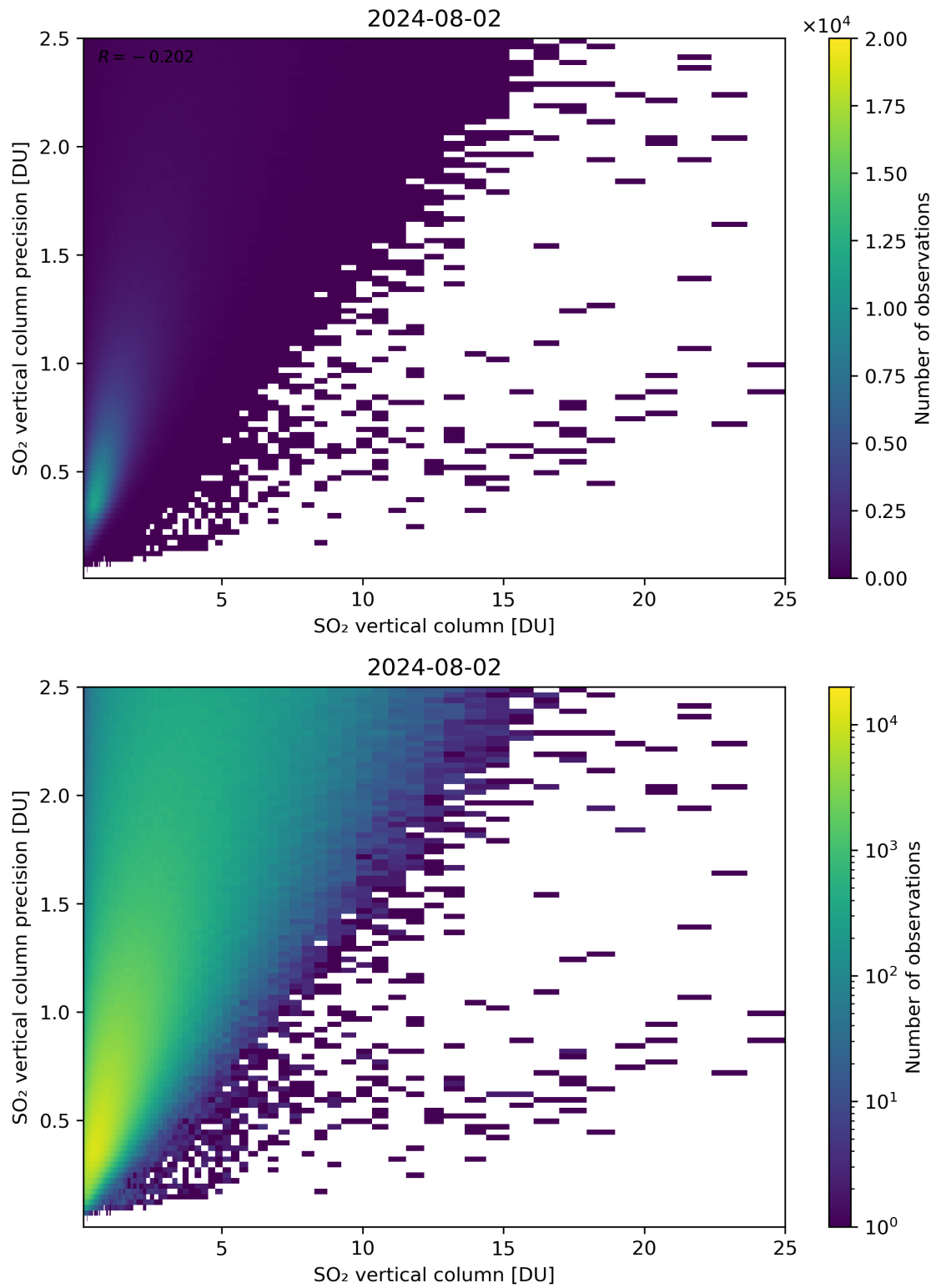
Figure 307: Scatter density plot of “SO 2 vertical column” against “SO 2 vertical column precision” for 2024-08-01 to 2024-08-03.
