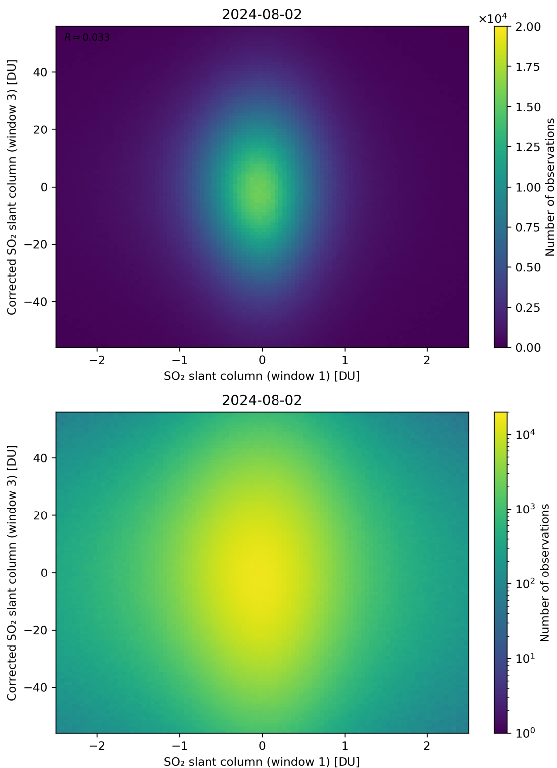
Figure 234: Scatter density plot of “SO 2 slant column (window 1)” against “Corrected SO 2 slant column (window 3)” for 2024-08-01 to 2024-08-03.
