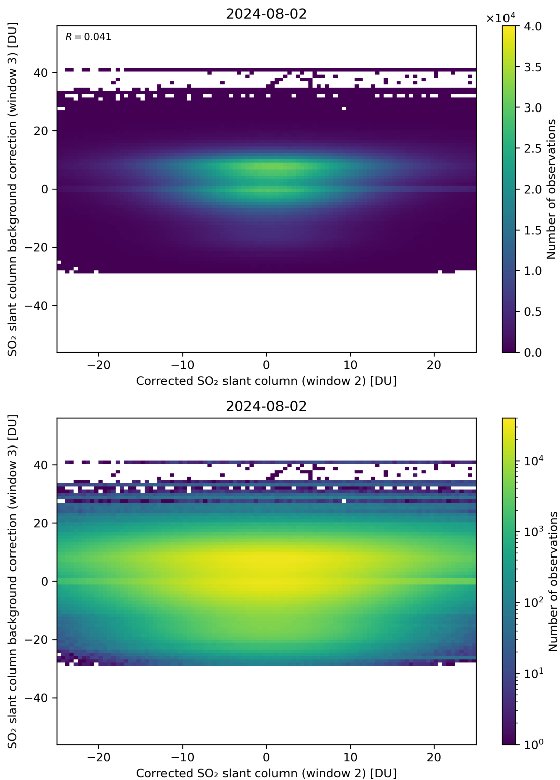
Figure 195: Scatter density plot of “Corrected SO 2 slant column (window 2)” against “SO 2 slant column background correction (window 3)” for 2024-08-01 to 2024-08-03.
