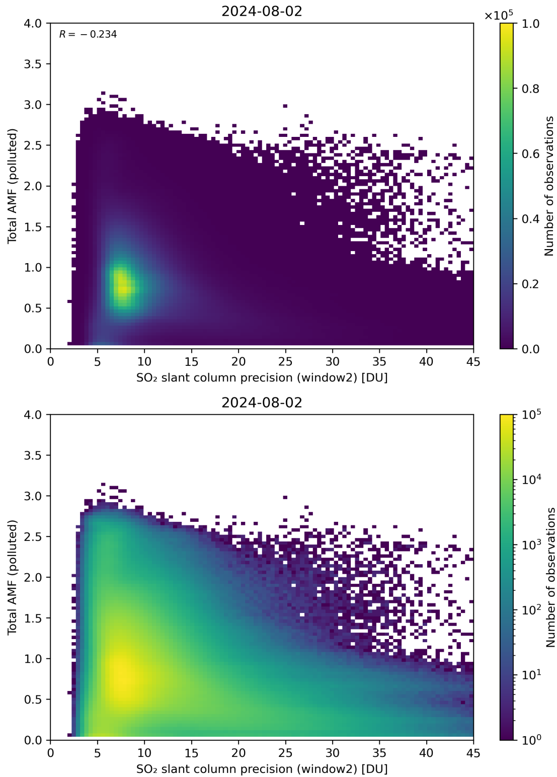
Figure 251: Scatter density plot of “SO 2 slant column precision (window2)” against “Total AMF (polluted)” for 2024-08-01 to 2024-08-03.
