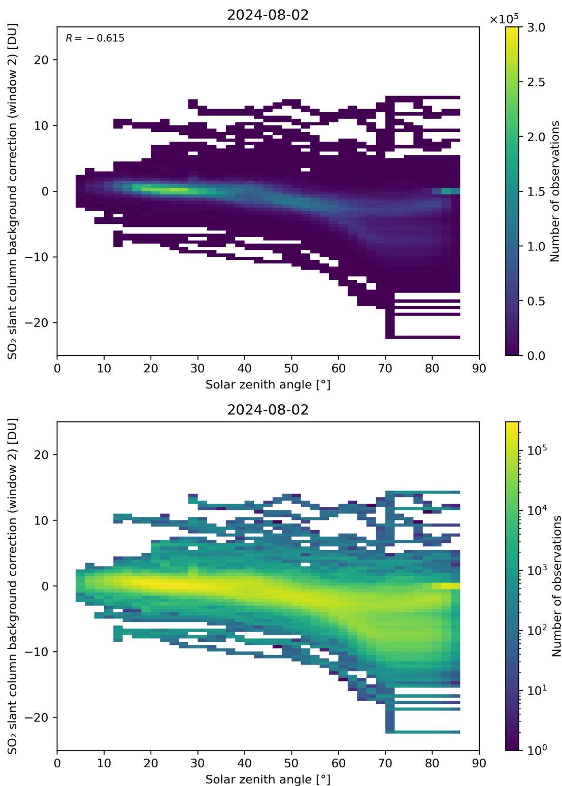
Figure 159: Scatter density plot of “Solar zenith angle” against “SO 2 slant column background correction (window 2)” for 2024-08-01 to 2024-08-03.
