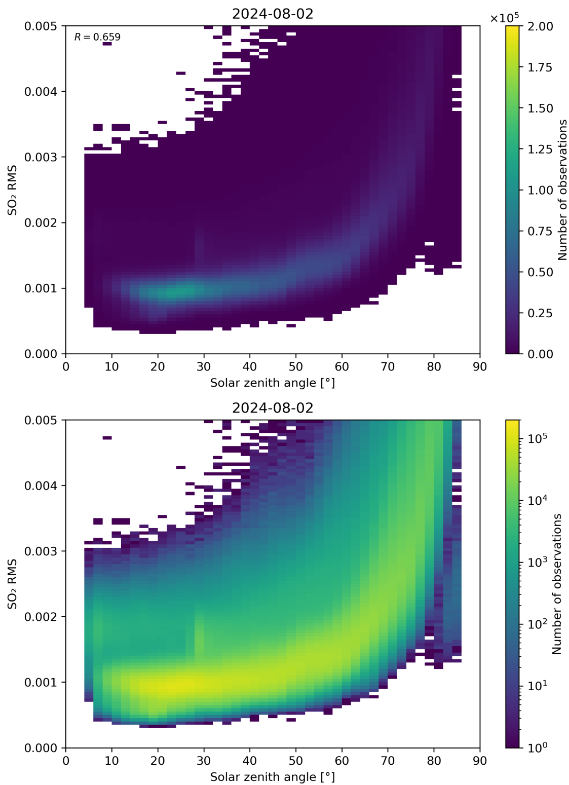
Figure 163: Scatter density plot of “Solar zenith angle” against “SO 2 RMS” for 2024-08-01 to 2024-08-03.
