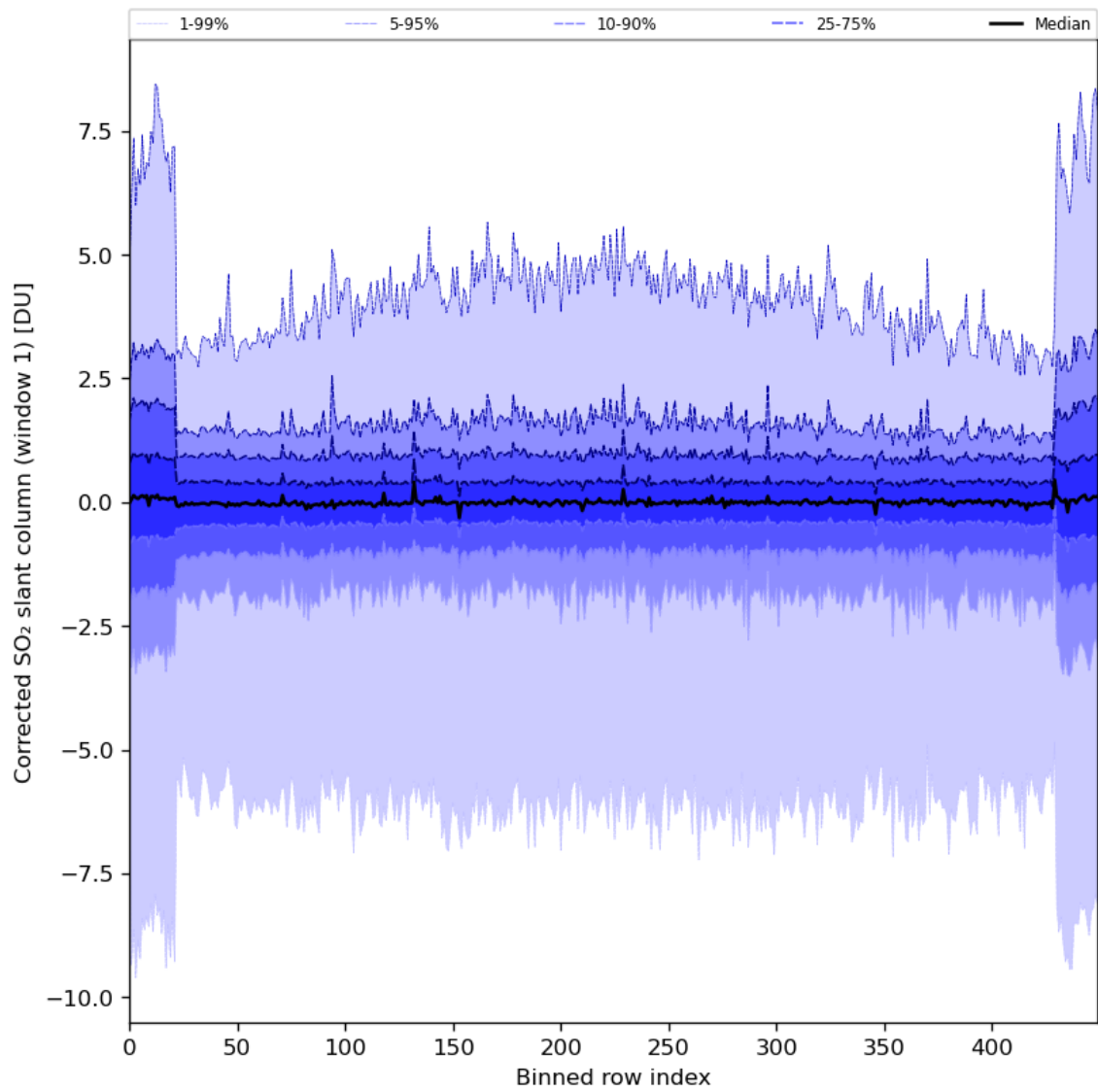
Figure 81: Along track statistics of “Corrected SO 2 slant column (window 1)” for 2024-08-01 to 2024-08-03
