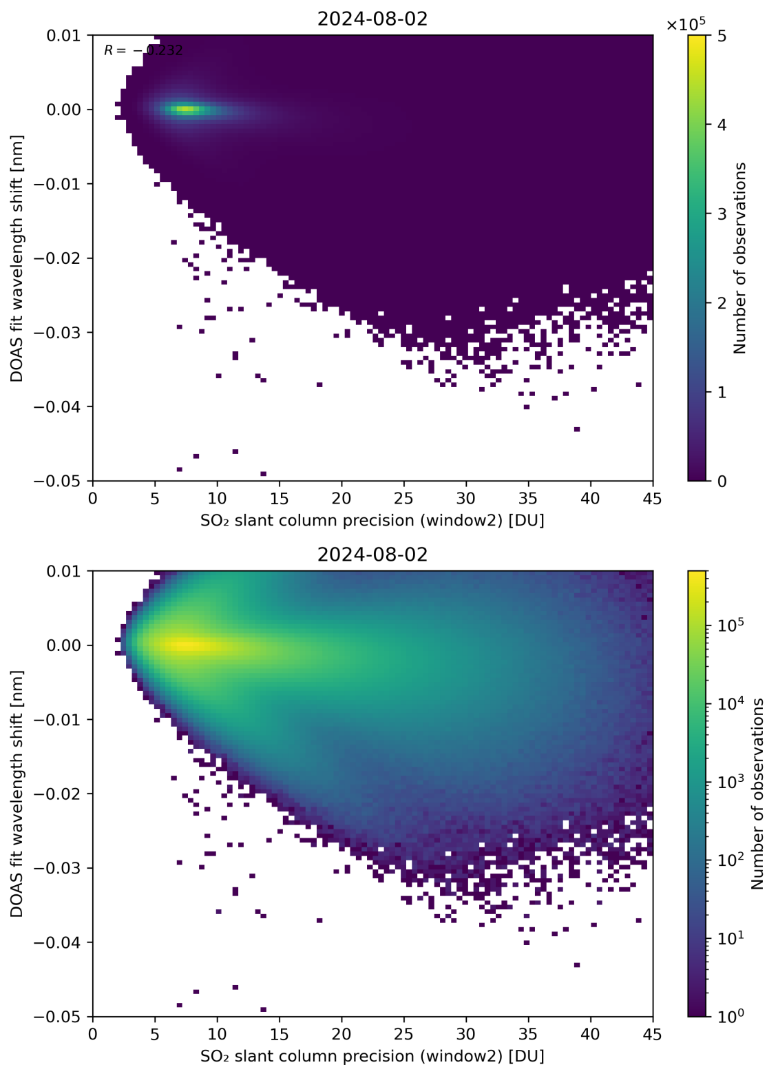
Figure 243: Scatter density plot of “SO 2 slant column precision (window2)” against “DOAS fit wavelength shift” for 2024-08-01 to 2024-08-03.
