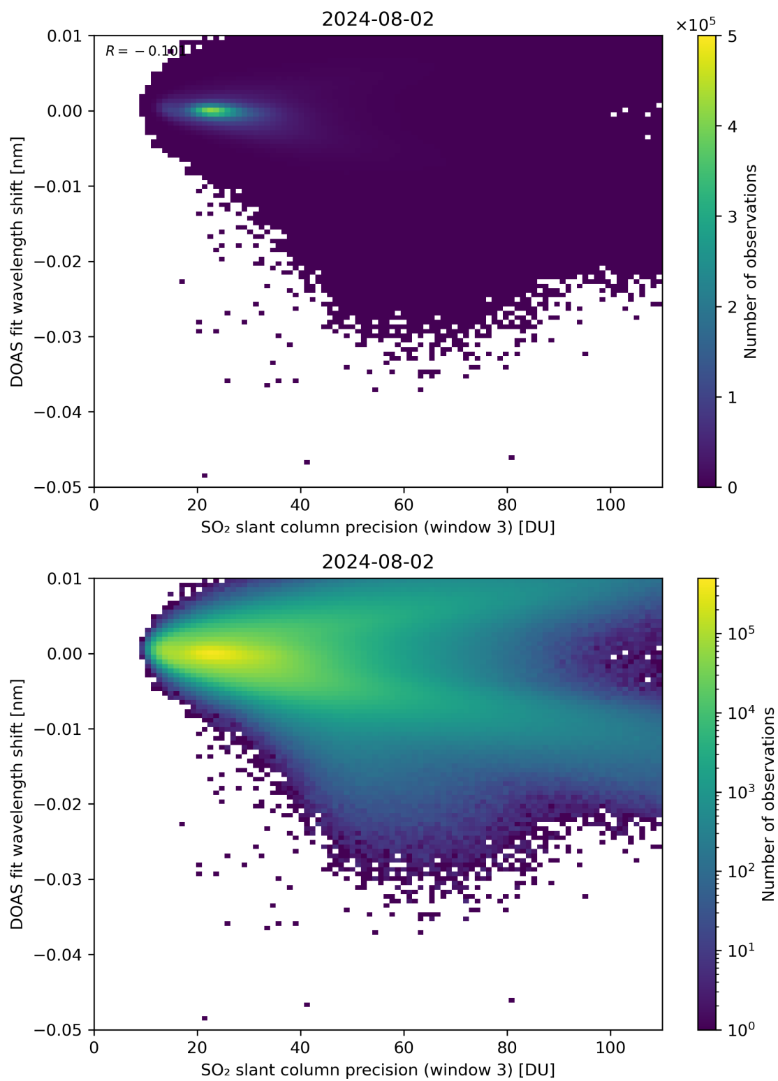
Figure 258: Scatter density plot of “SO 2 slant column precision (window 3)” against “DOAS fit wavelength shift” for 2024-08-01 to 2024-08-03.
