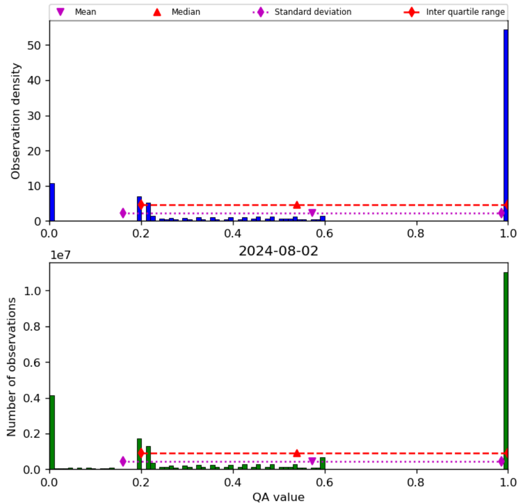
Figure 52: Histogram of “QA value” for 2024-08-01 to 2024-08-03
