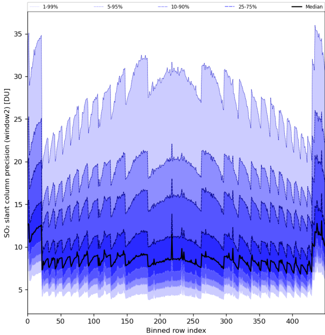
Figure 84: Along track statistics of “SO 2 slant column precision (window2)” for 2024-08-01 to 2024-08-03
