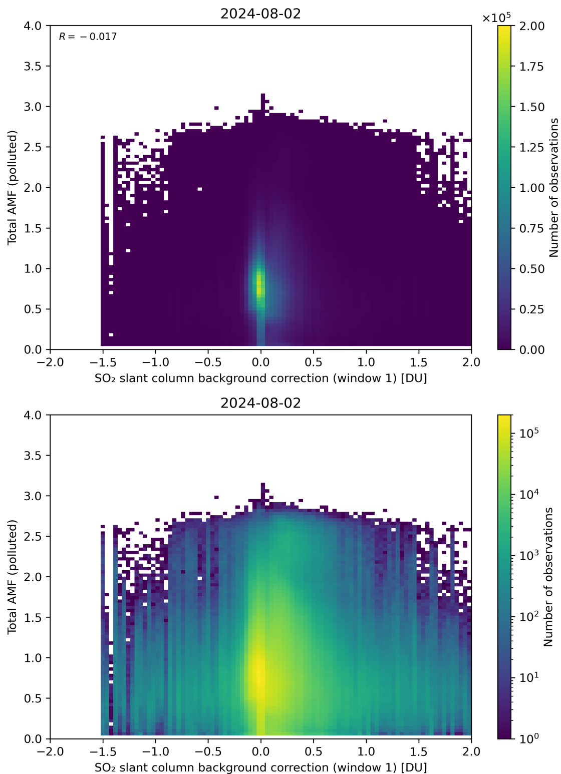
Figure 109: Scatter density plot of “SO 2 slant column background correction (window 1)” against “Total AMF (polluted)” for 2024-08-01 to 2024-08-03.
