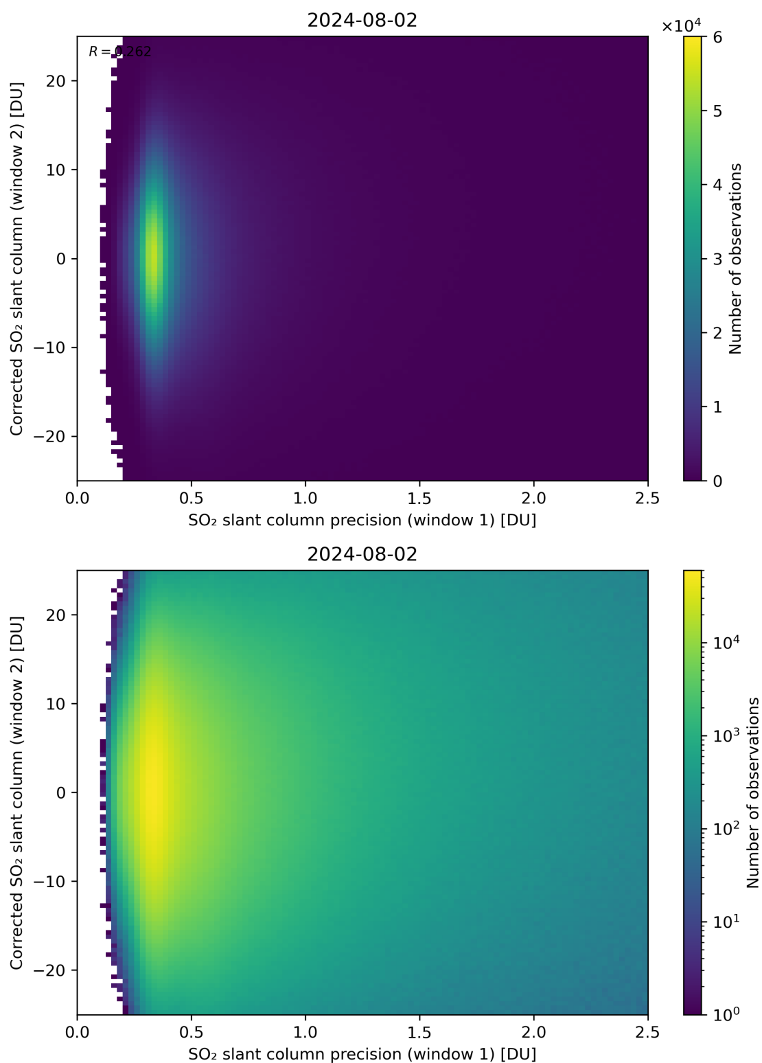
Figure 225: Scatter density plot of “SO 2 slant column precision (window 1)” against “Corrected SO 2 slant column (window 2)” for 2024-08-01 to 2024-08-03.
