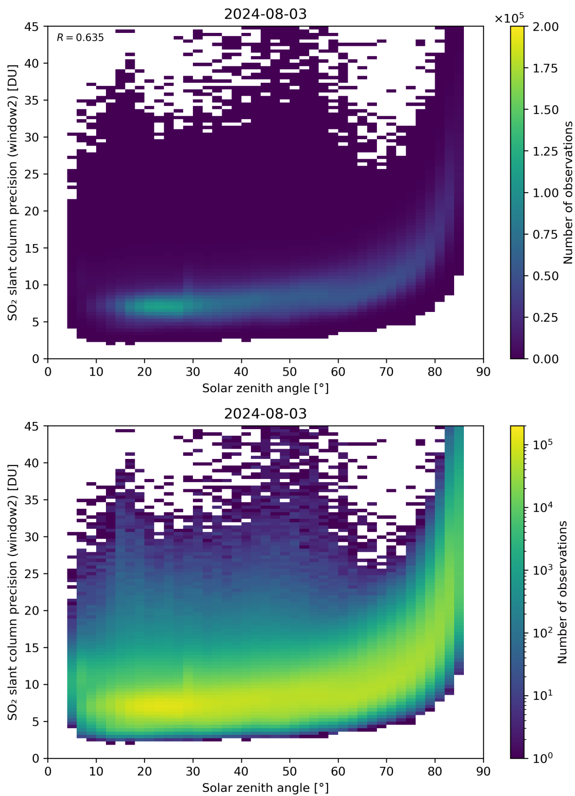
Figure 171: Scatter density plot of “Solar zenith angle” against “SO 2 slant column precision (window2)” for 2024-08-02 to 2024-08-04.
