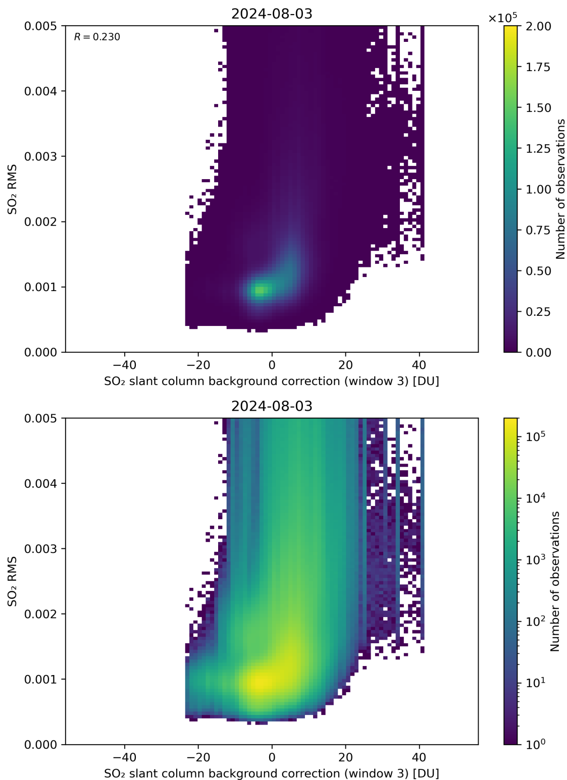
Figure 123: Scatter density plot of “SO 2 slant column background correction (window 3)” against “SO 2 RMS” for 2024-08-02 to 2024-08-04.
