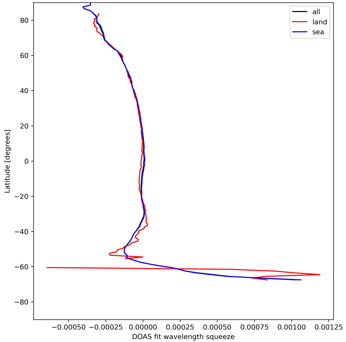
Figure 46: Zonal average of “DOAS fit wavelength squeeze” for 2024-08-02 to 2024-08-04.
