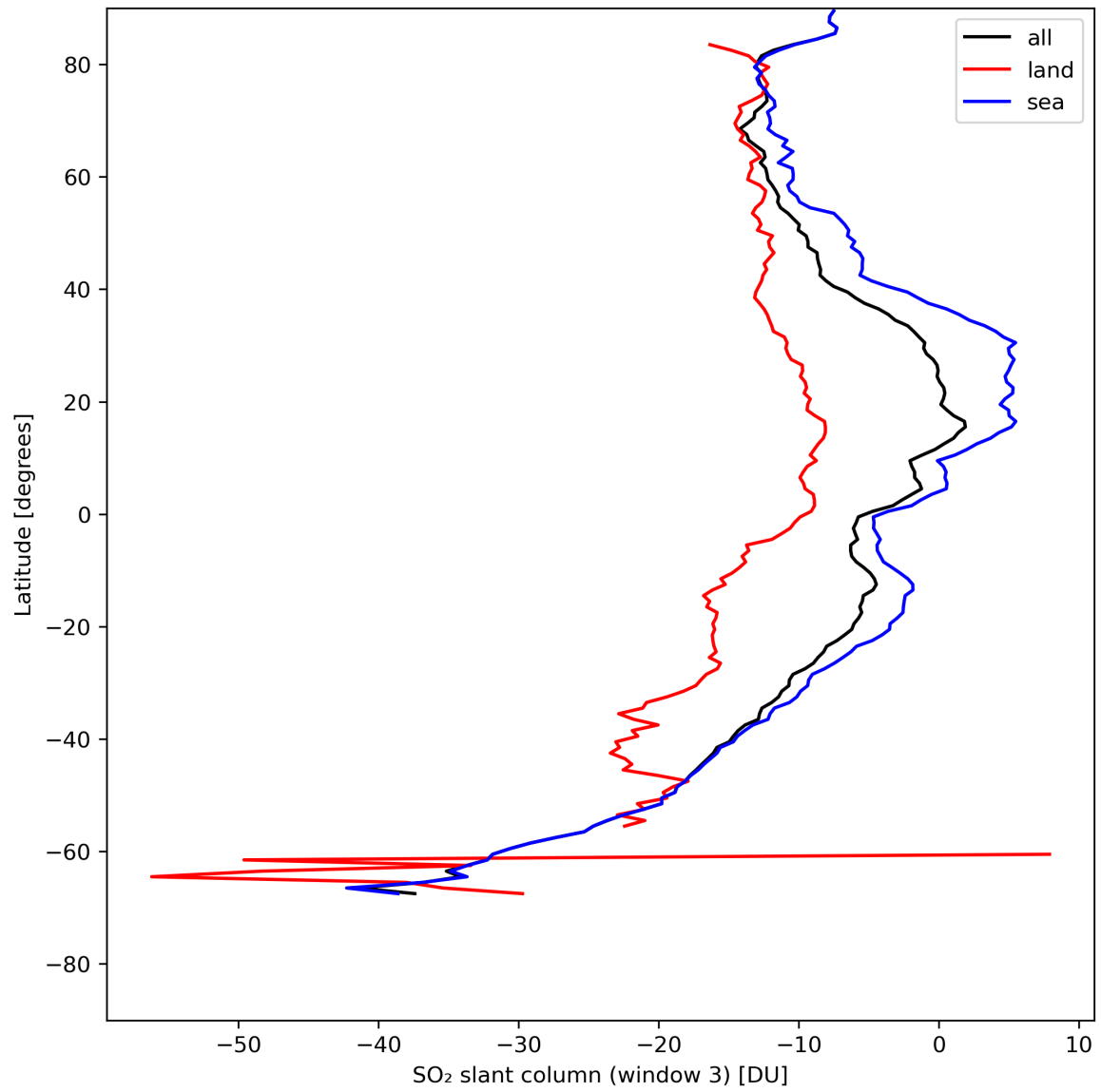
Figure 41: Zonal average of “SO 2 slant column (window 3)” for 2024-08-02 to 2024-08-04.
