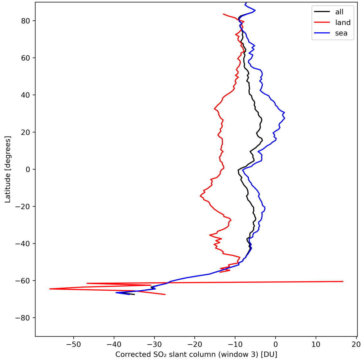
Figure 43: Zonal average of “Corrected SO 2 slant column (window 3)” for 2024-08-02 to 2024-08-04.
