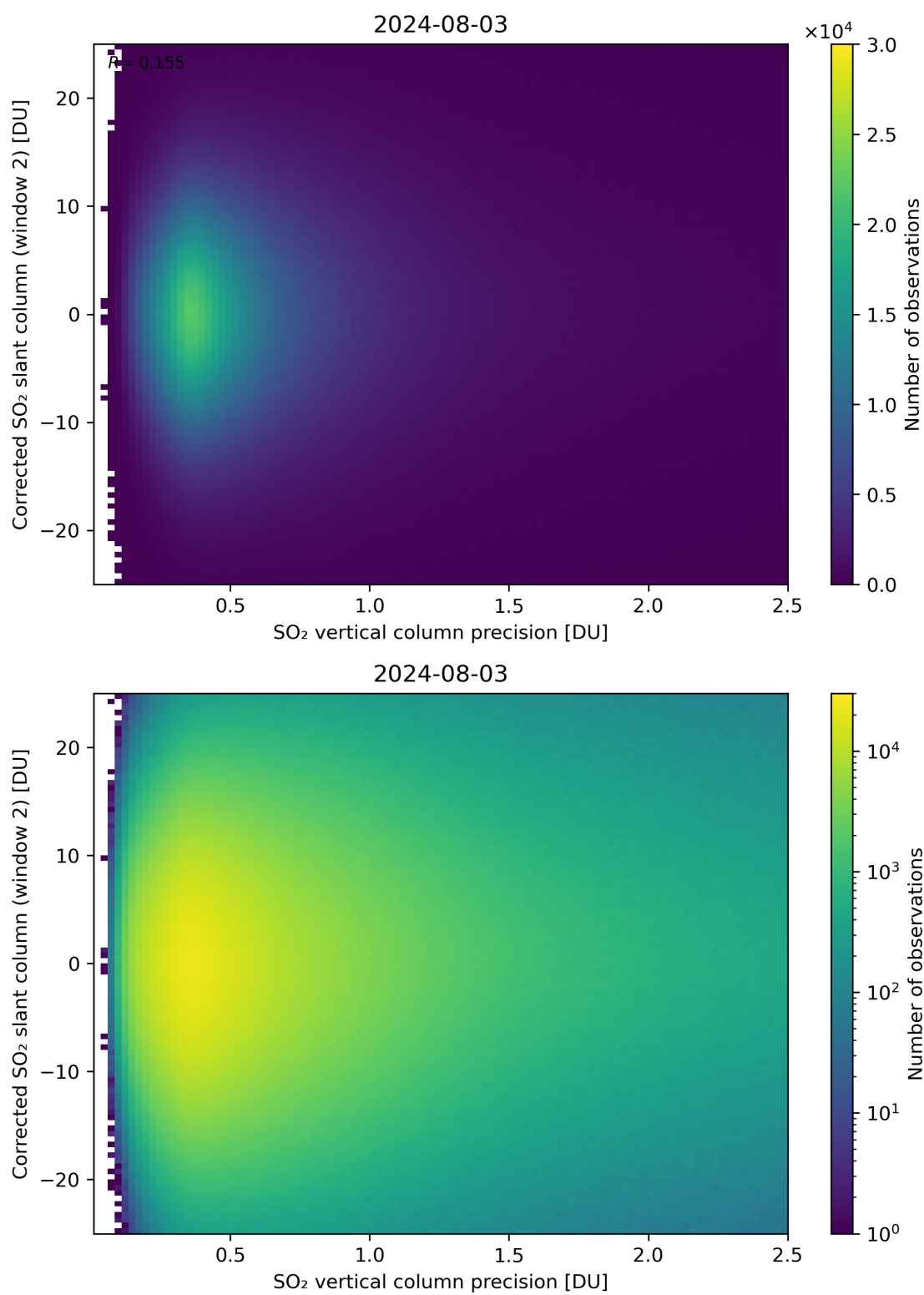
Figure 287: Scatter density plot of “SO 2 vertical column precision” against “Corrected SO 2 slant column (window 2)” for 2024-08-02 to 2024-08-04.
