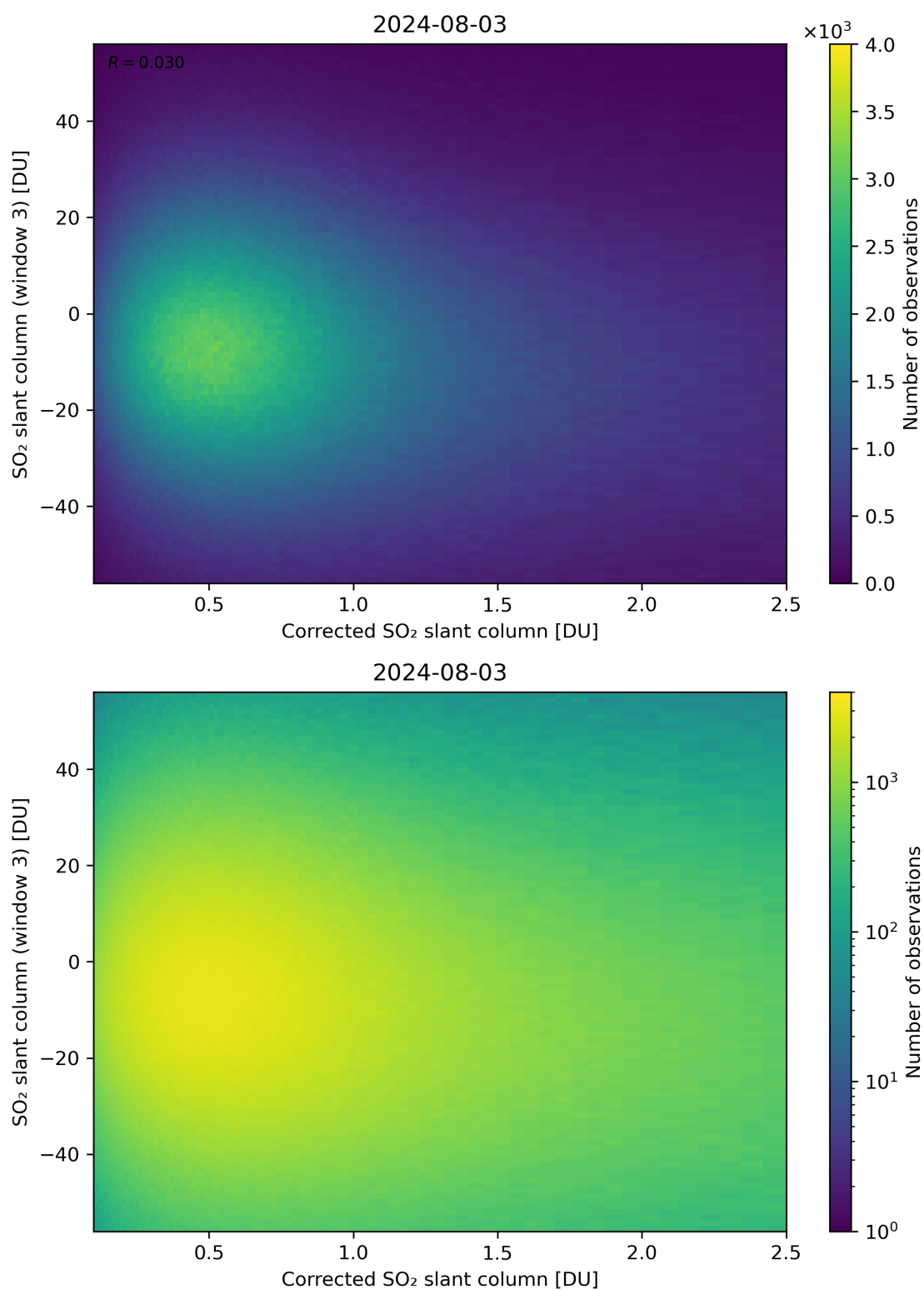
Figure 190: Scatter density plot of “Corrected SO 2 slant column” against “SO 2 slant column (window 3)” for 2024-08-02 to 2024-08-04.
