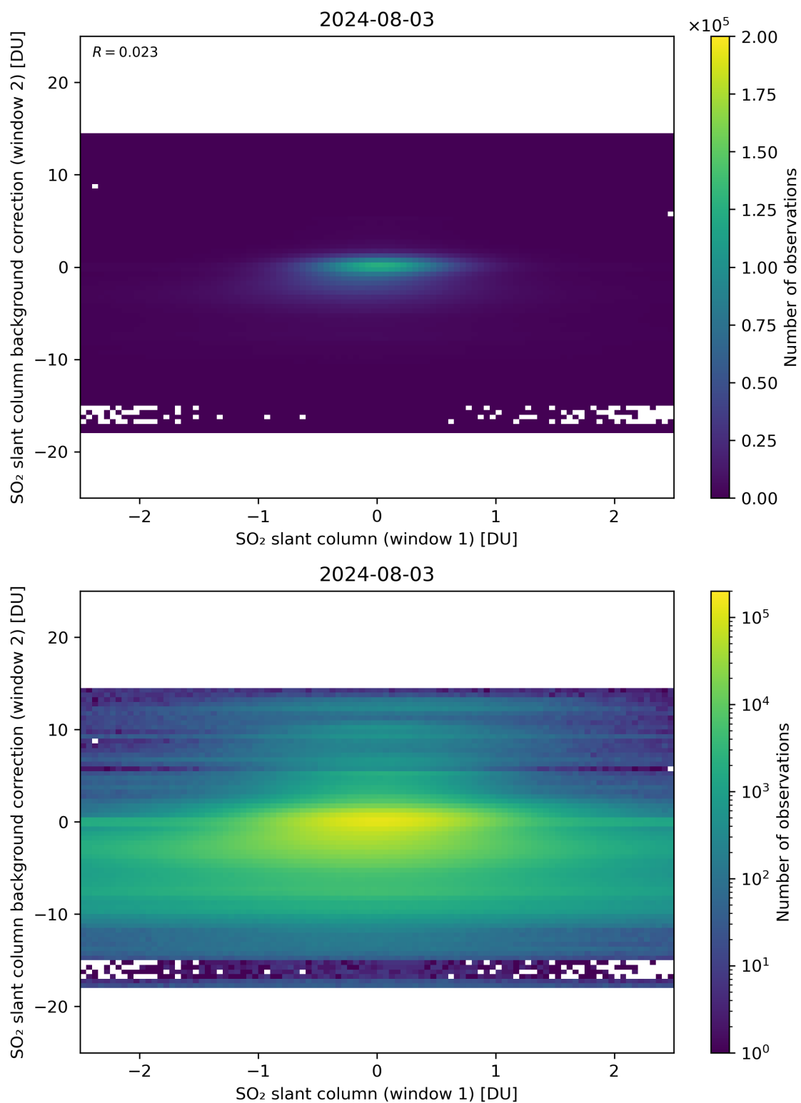
Figure 213: Scatter density plot of “SO 2 slant column (window 1)” against “SO 2 slant column background correction (window 2)” for 2024-08-02 to 2024-08-04.
