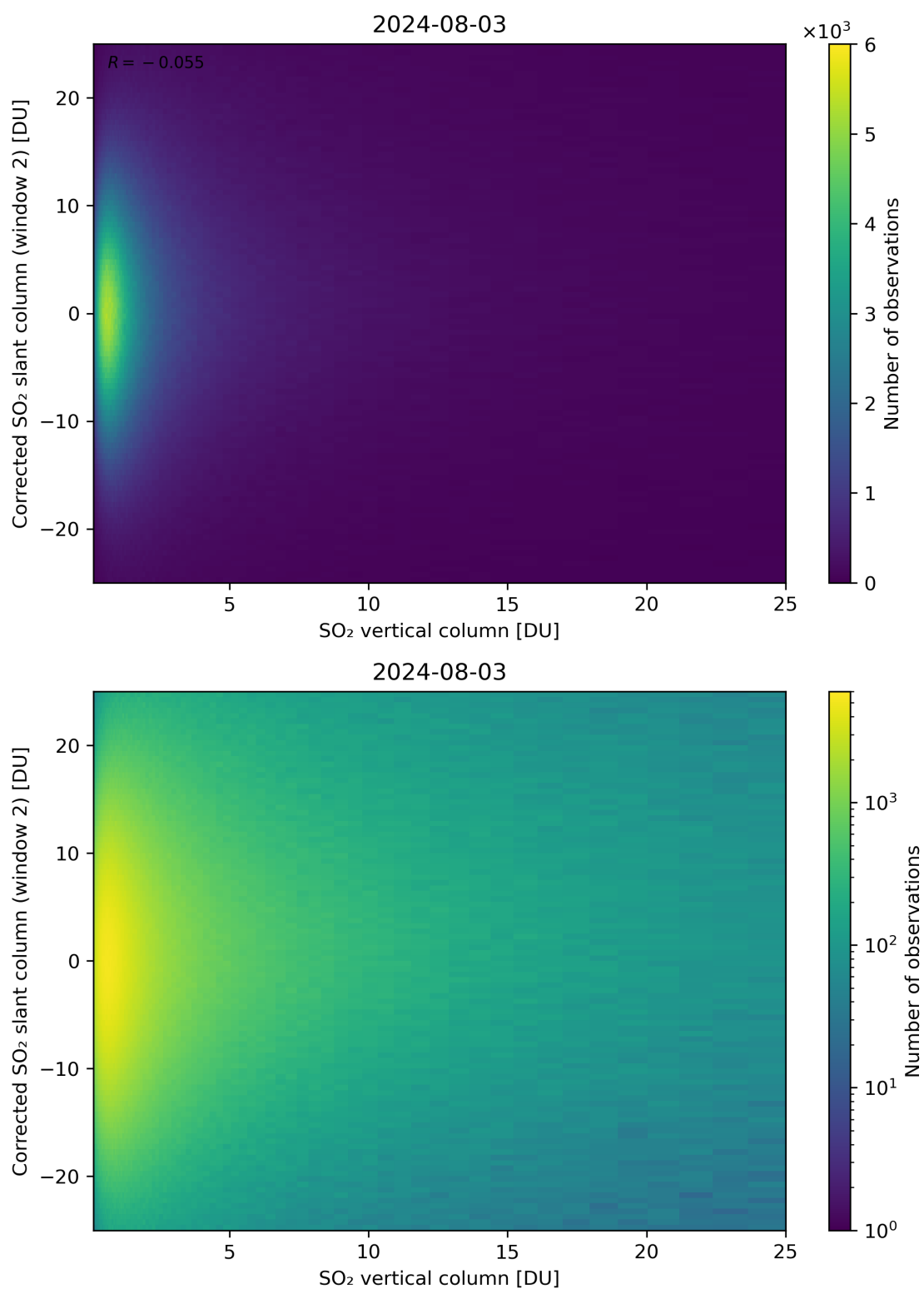
Figure 298: Scatter density plot of “SO 2 vertical column” against “Corrected SO 2 slant column (window 2)” for 2024-08-02 to 2024-08-04.
