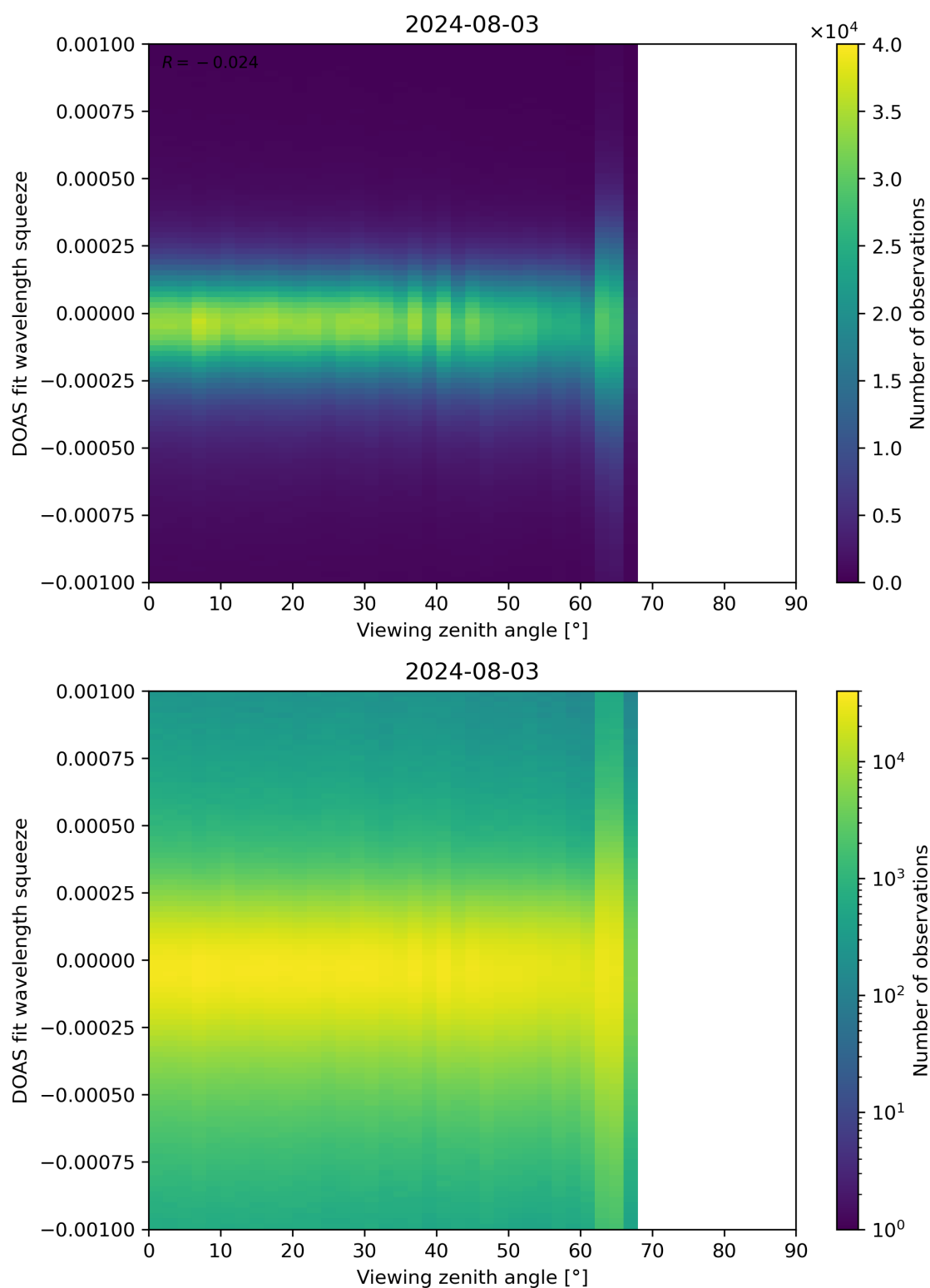
Figure 312: Scatter density plot of “Viewing zenith angle” against “DOAS fit wavelength squeeze” for 2024-08-02 to 2024-08-04.
