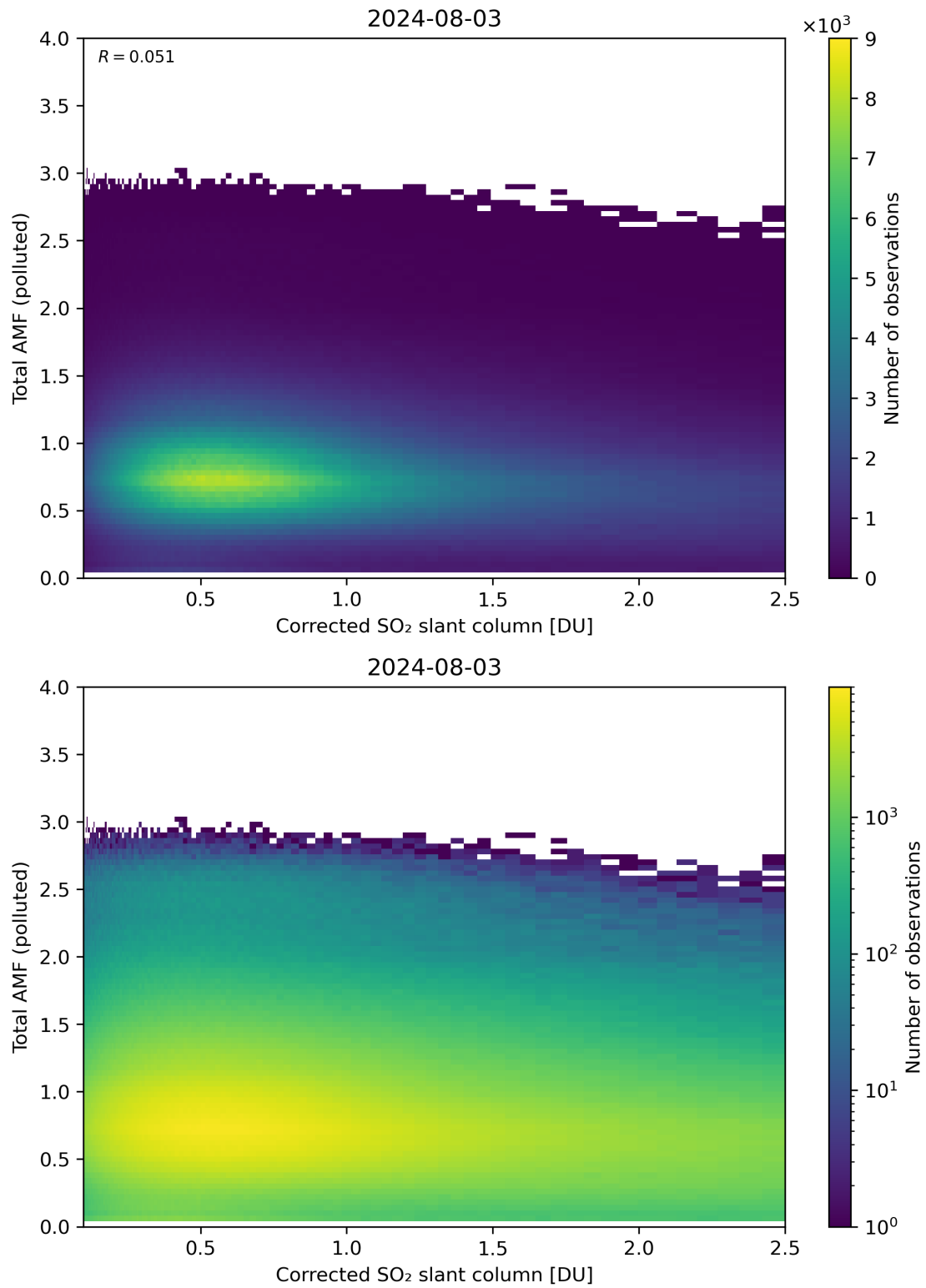
Figure 192: Scatter density plot of “Corrected SO 2 slant column” against “Total AMF (polluted)” for 2024-08-02 to 2024-08-04.
