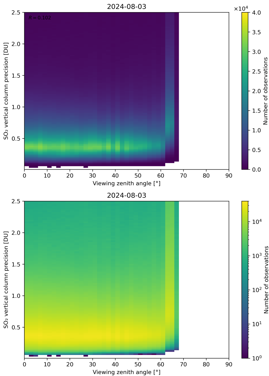
Figure 328: Scatter density plot of “Viewing zenith angle” against “SO 2 vertical column precision” for 2024-08-02 to 2024-08-04.
