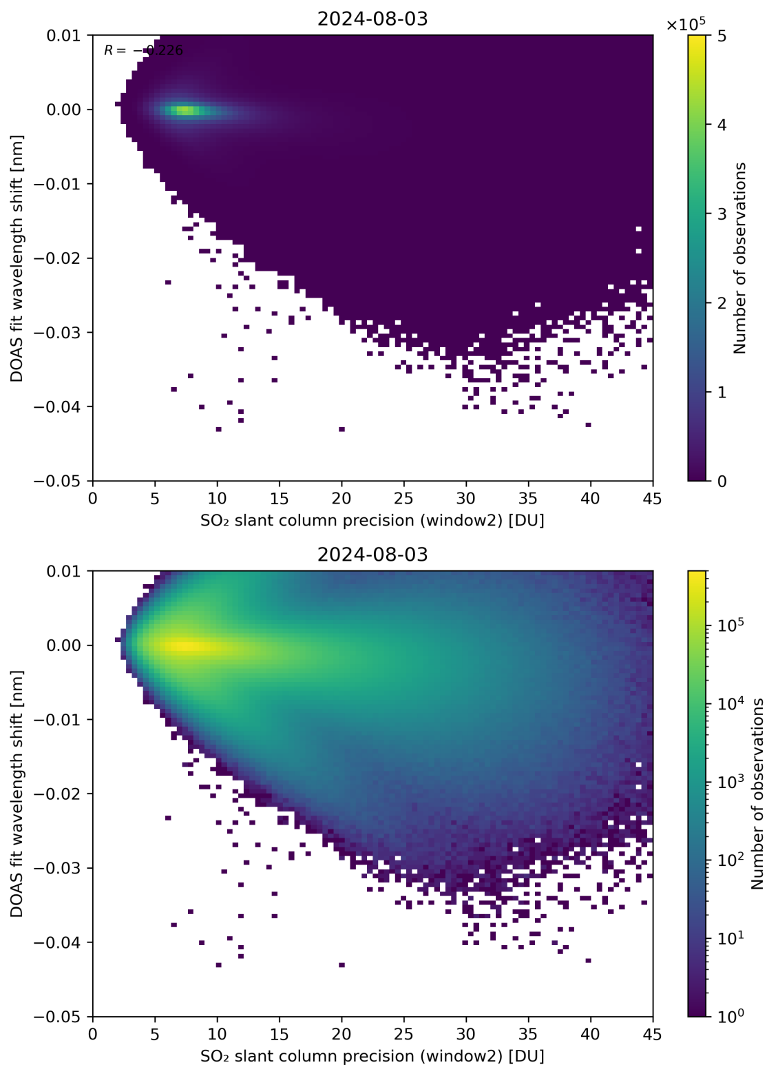
Figure 243: Scatter density plot of “SO 2 slant column precision (window2)” against “DOAS fit wavelength shift” for 2024-08-02 to 2024-08-04.
