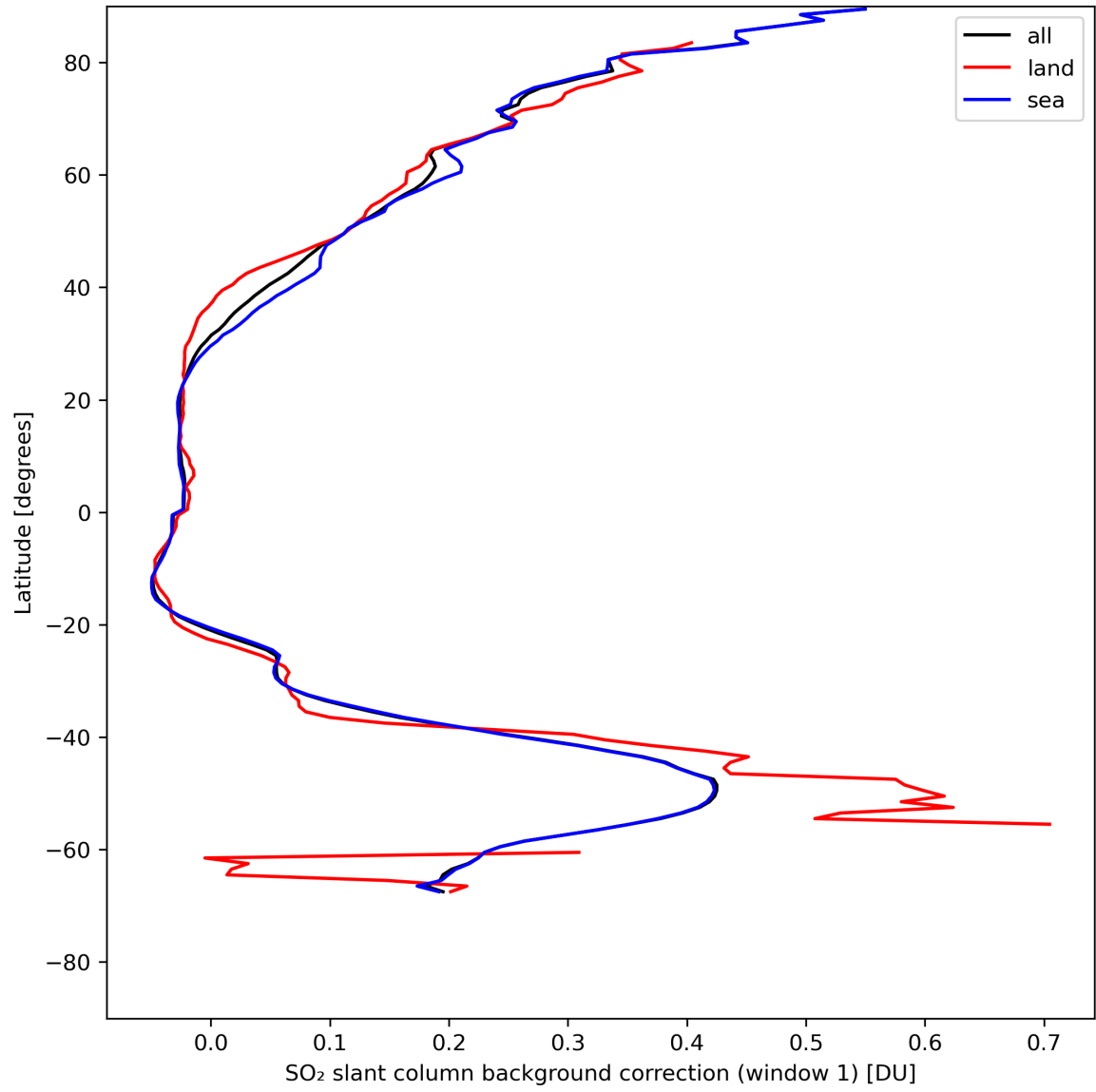
Figure 36: Zonal average of “SO 2 slant column background correction (window 1)” for 2024-08-02 to 2024-08-04.
