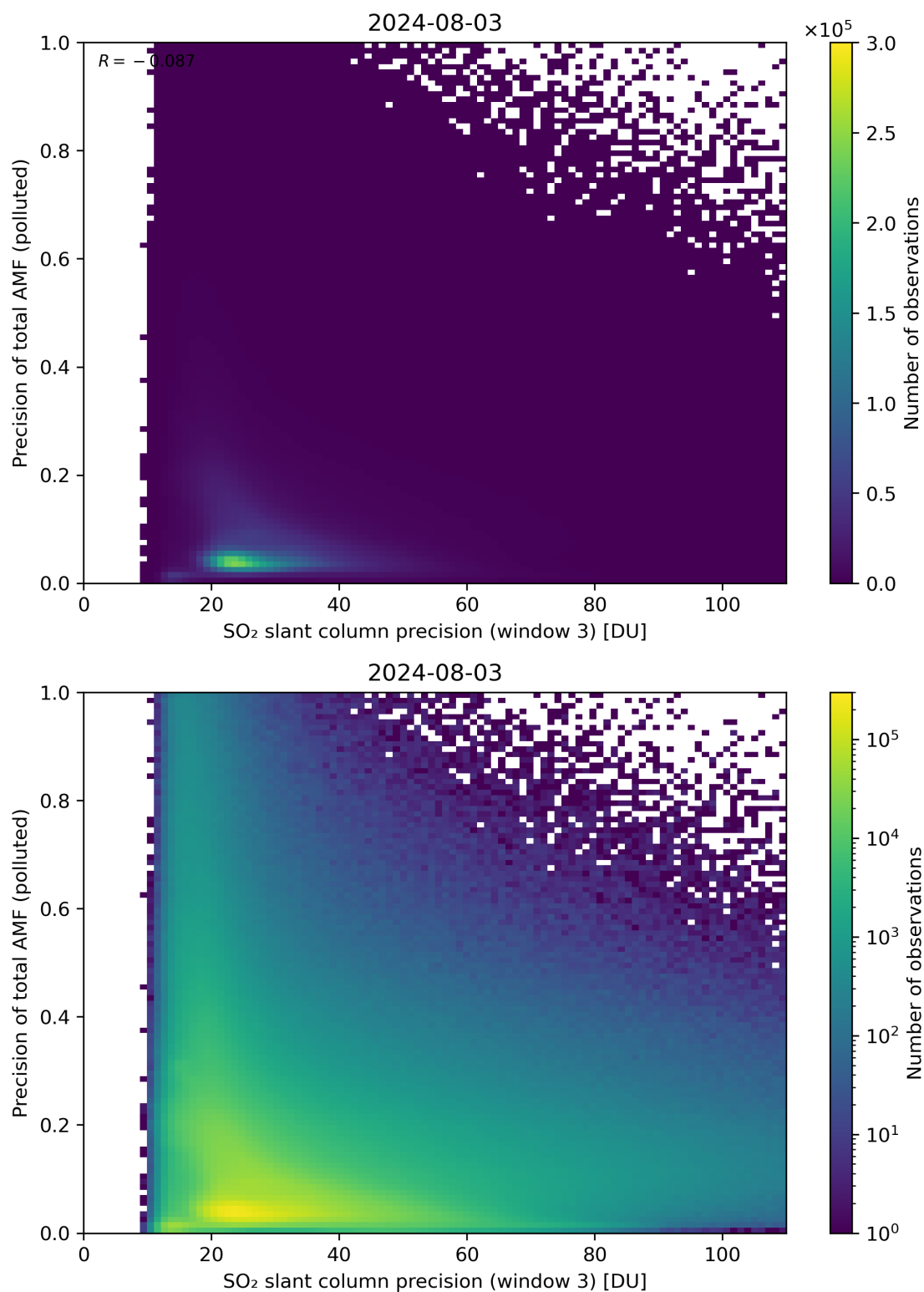
Figure 264: Scatter density plot of “SO 2 slant column precision (window 3)” against “Precision of total AMF (polluted)” for 2024-08-02 to 2024-08-04.
