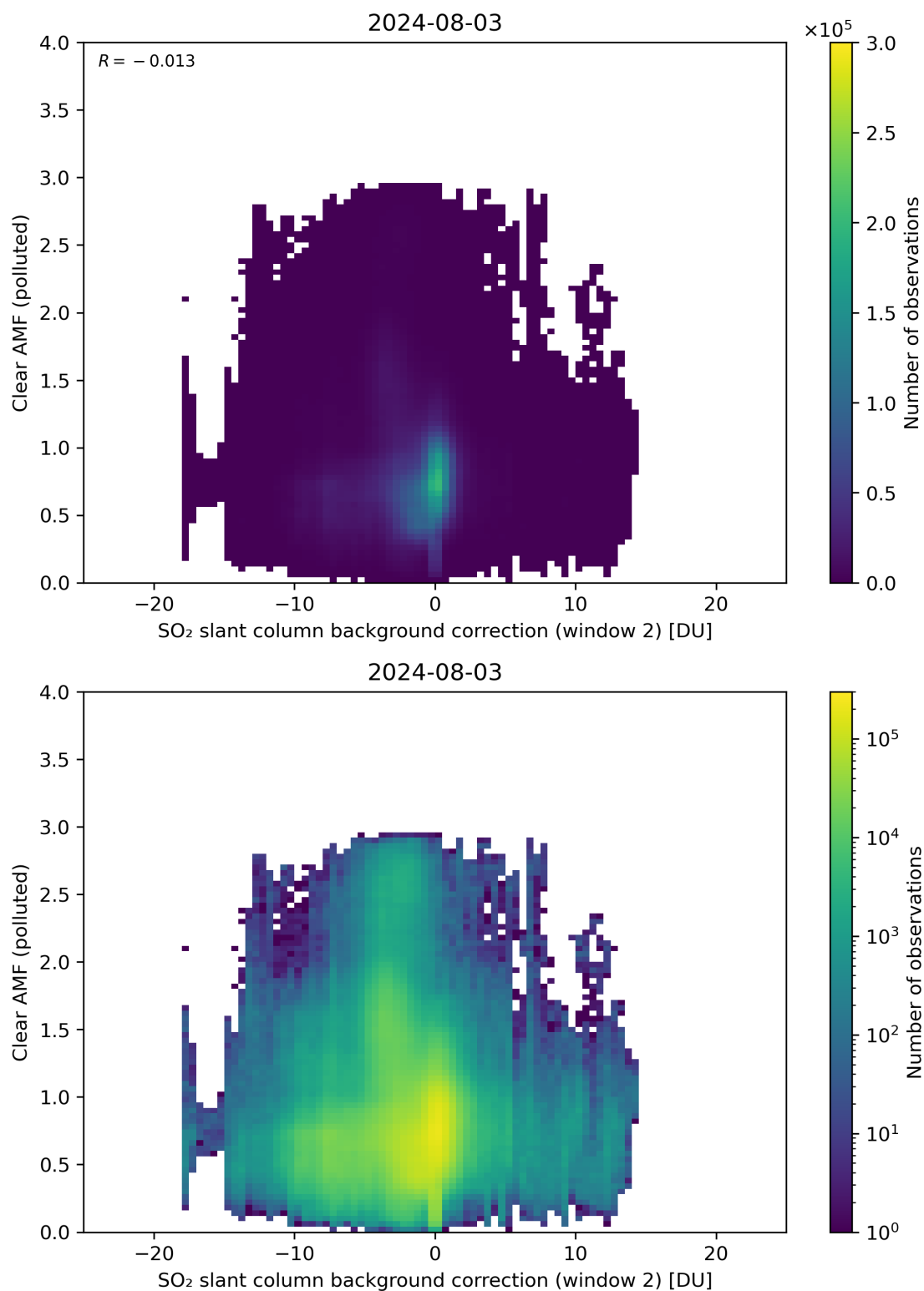
Figure 115: Scatter density plot of “SO 2 slant column background correction (window 2)” against “Clear AMF (polluted)” for 2024-08-02 to 2024-08-04.
