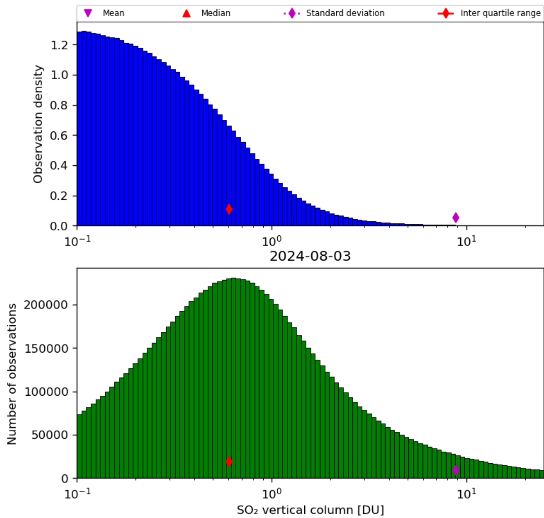
Figure 53: Histogram of “SO 2 vertical column” for 2024-08-02 to 2024-08-04
