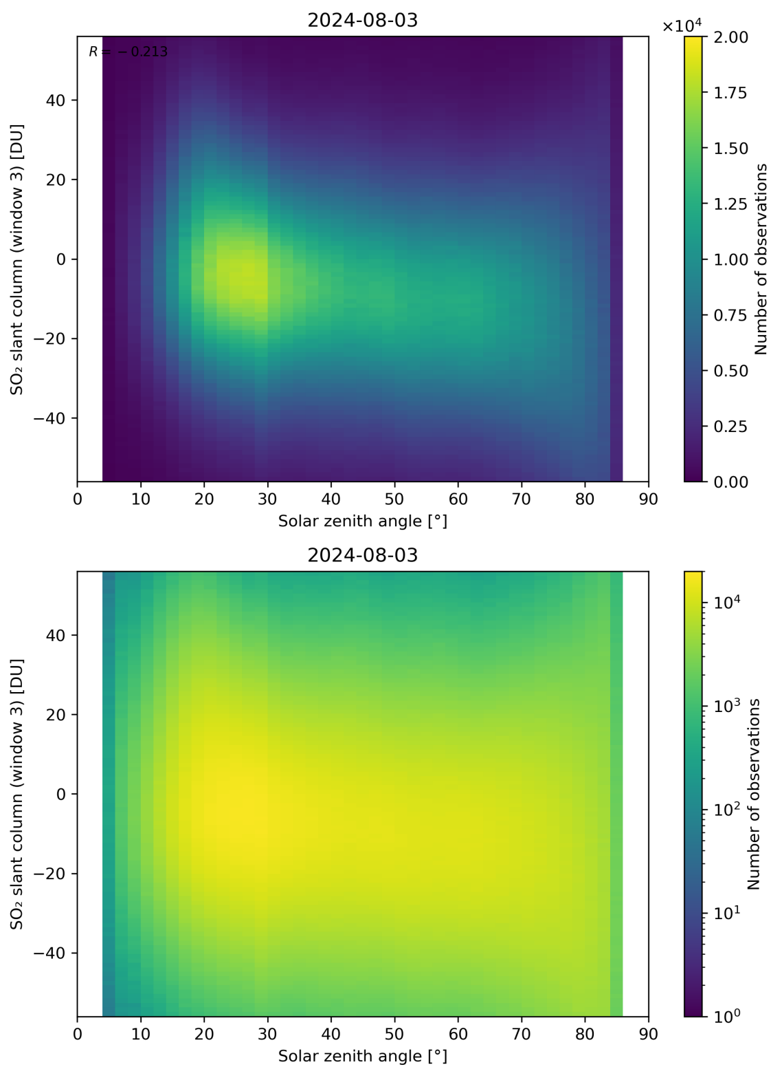
Figure 172: Scatter density plot of “Solar zenith angle” against “SO 2 slant column (window 3)” for 2024-08-02 to 2024-08-04.
