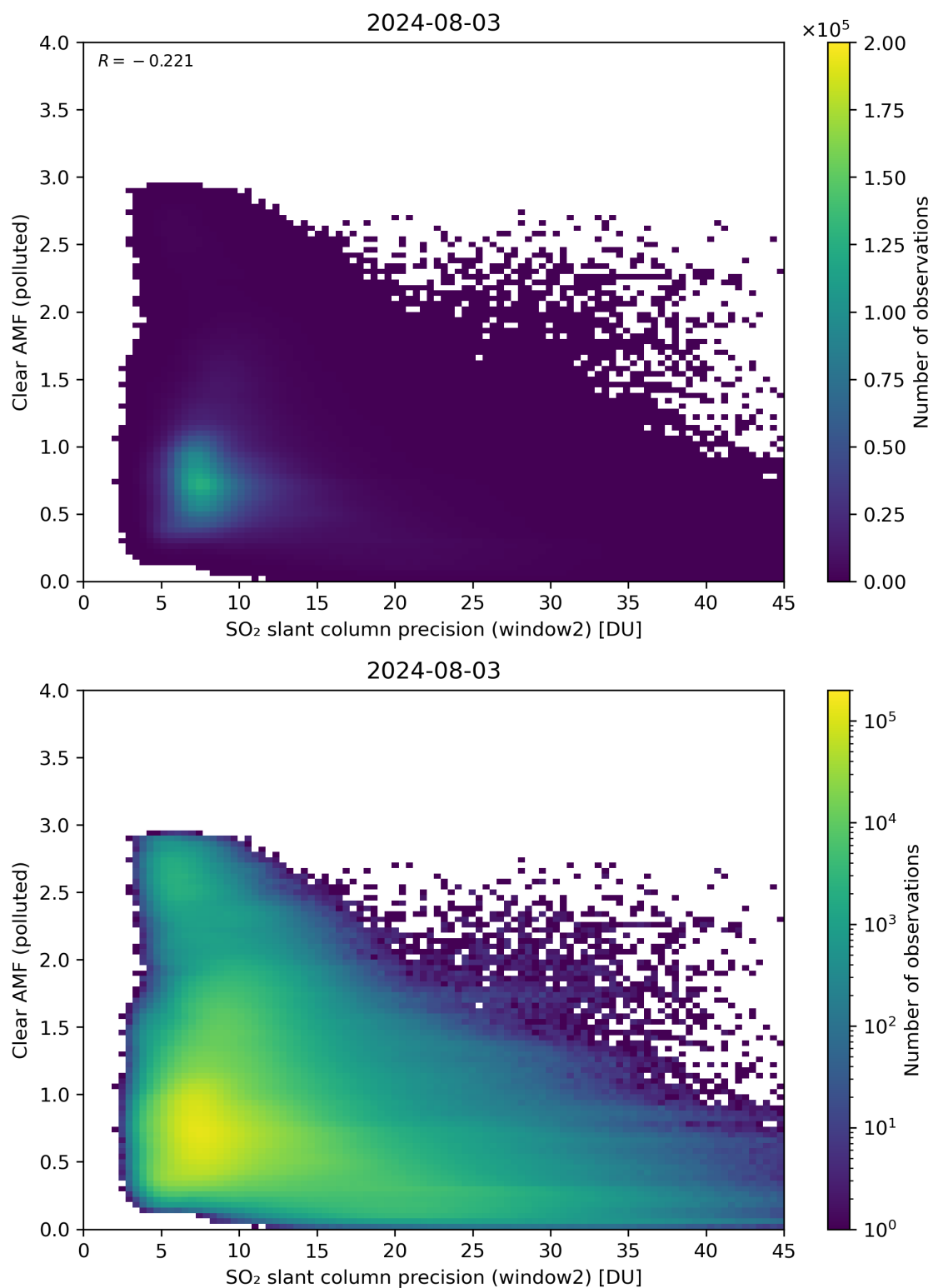
Figure 246: Scatter density plot of “SO 2 slant column precision (window2)” against “Clear AMF (polluted)” for 2024-08-02 to 2024-08-04.
