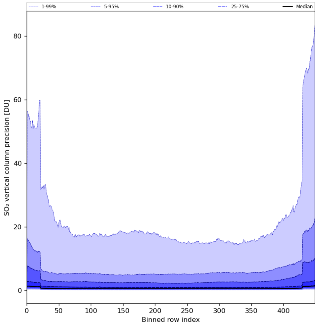
Figure 77: Along track statistics of “SO 2 vertical column precision” for 2024-08-02 to 2024-08-04
