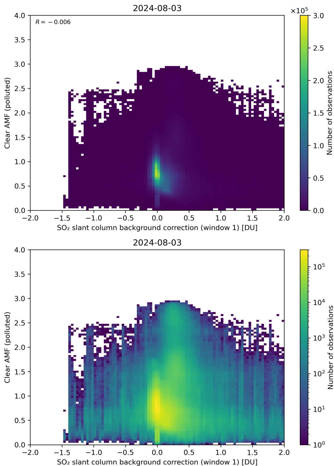
Figure 103: Scatter density plot of “SO 2 slant column background correction (window 1)” against “Clear AMF (polluted)” for 2024-08-02 to 2024-08-04.
