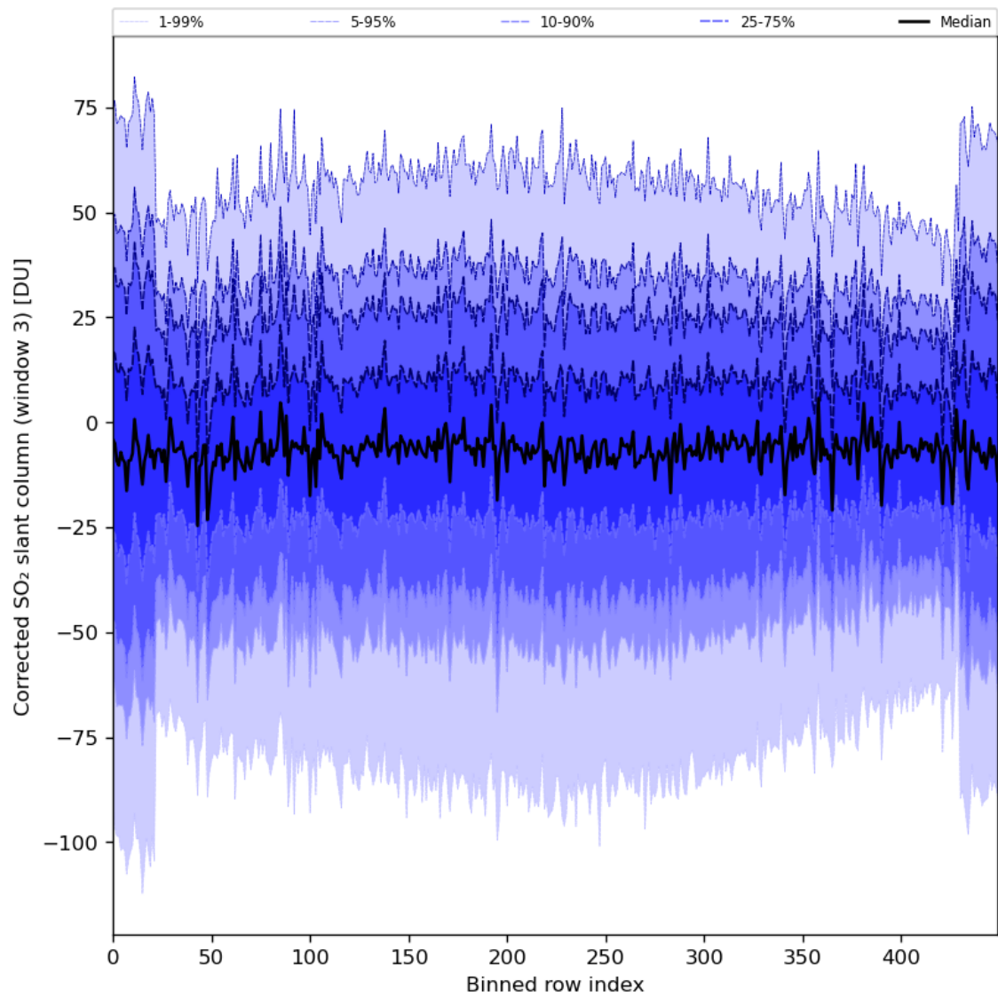
Figure 89: Along track statistics of “Corrected SO 2 slant column (window 3)” for 2024-08-02 to 2024-08-04
