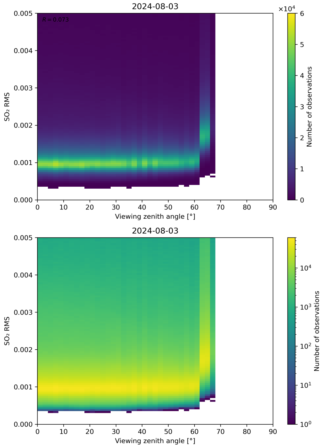
Figure 313: Scatter density plot of “Viewing zenith angle” against “SO 2 RMS” for 2024-08-02 to 2024-08-04.
