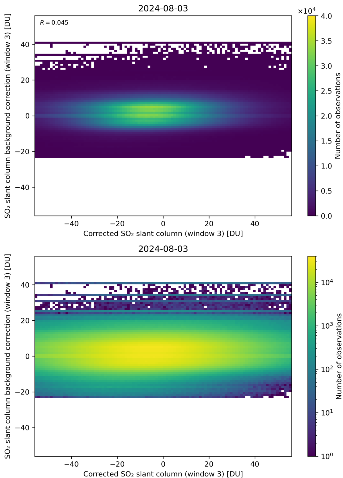
Figure 205: Scatter density plot of “Corrected SO 2 slant column (window 3)” against “SO 2 slant column background correction (window 3)” for 2024-08-02 to 2024-08-04.
