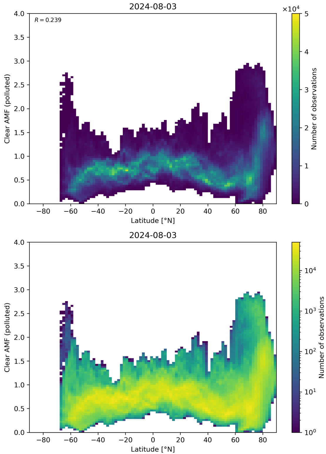
Figure 145: Scatter density plot of “Latitude” against “Clear AMF (polluted)” for 2024-08-02 to 2024-08-04.
