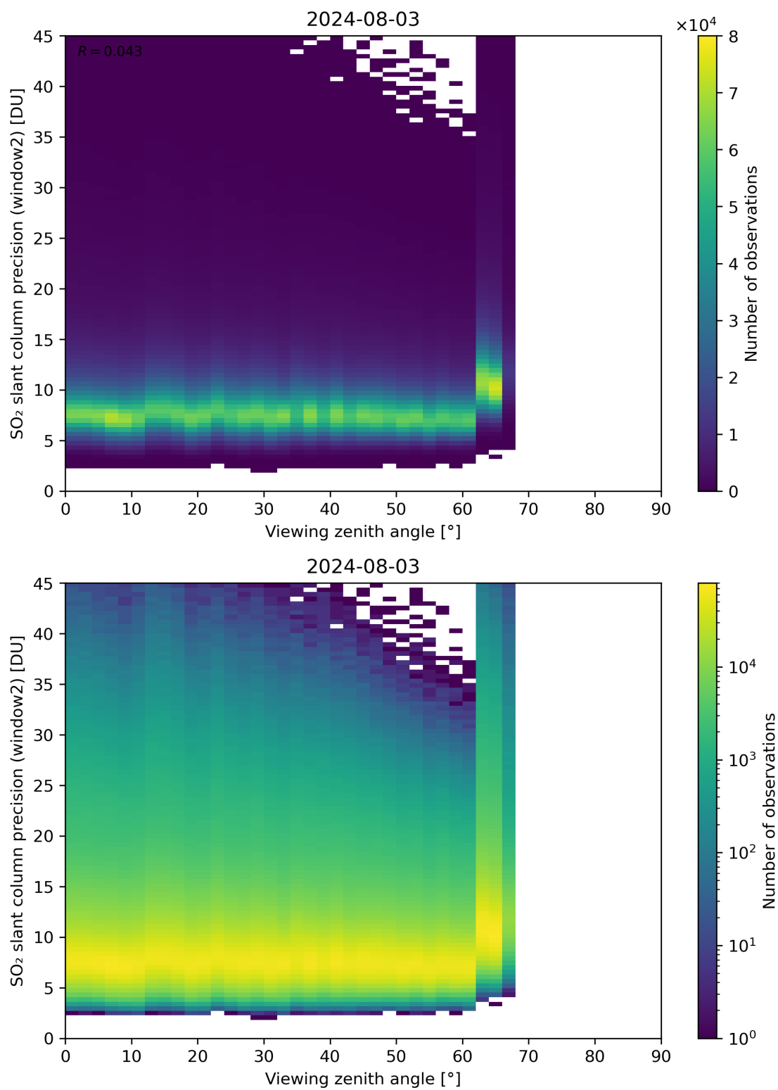
Figure 322: Scatter density plot of “Viewing zenith angle” against “SO 2 slant column precision (window2)” for 2024-08-02 to 2024-08-04.
