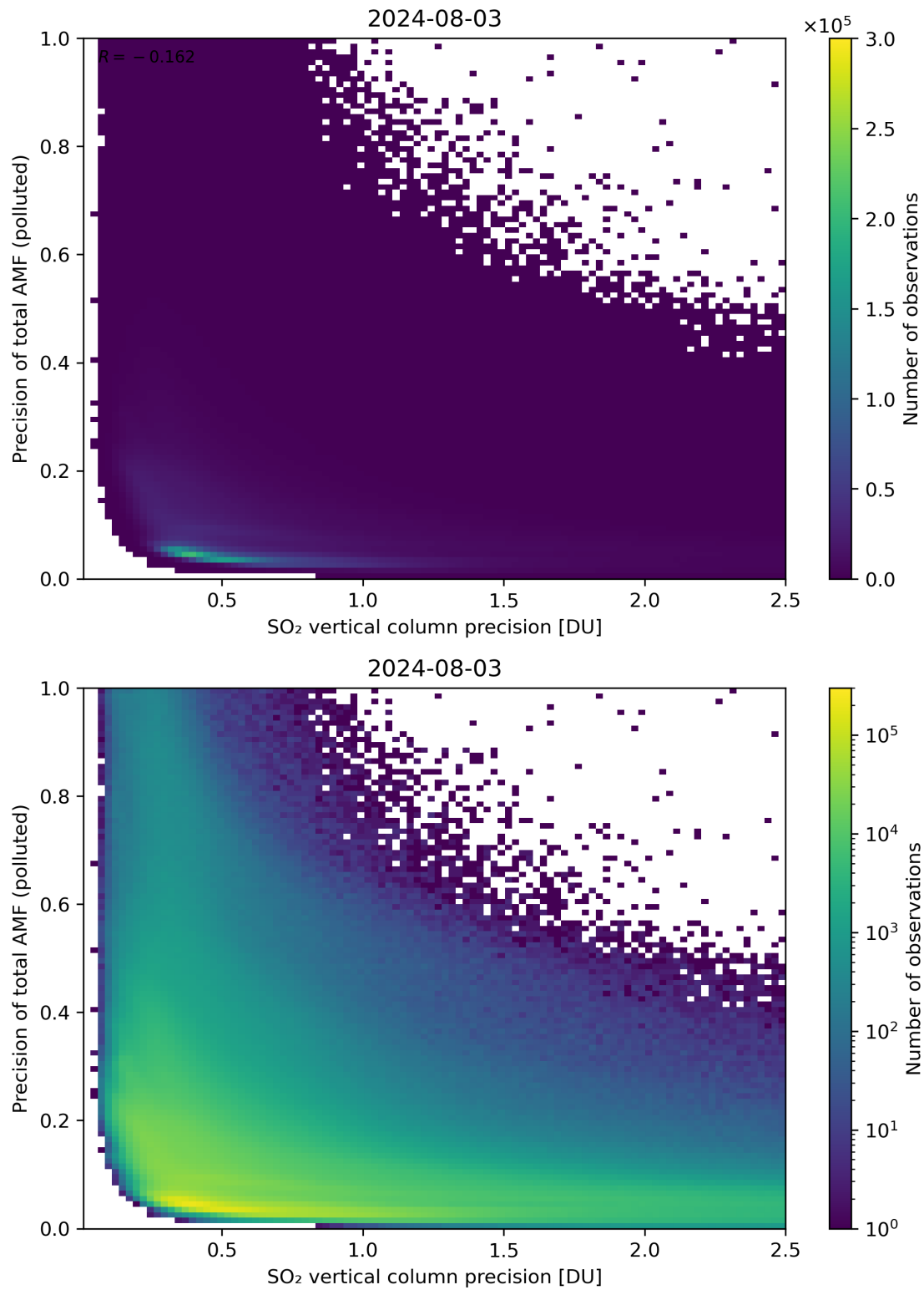
Figure 295: Scatter density plot of “SO 2 vertical column precision” against “Precision of total AMF (polluted)” for 2024-08-02 to 2024-08-04.
