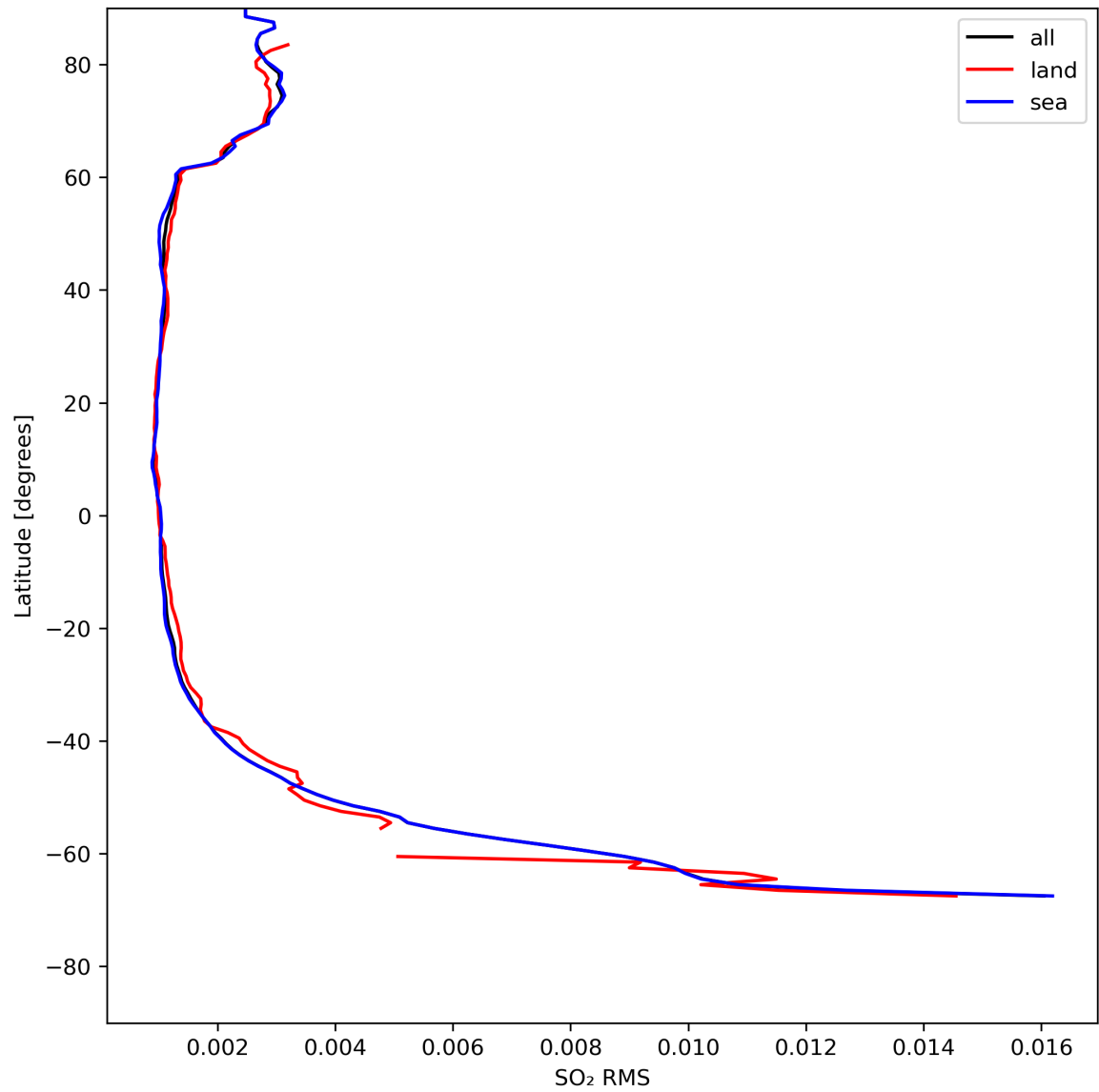
Figure 47: Zonal average of “SO 2 RMS” for 2024-08-02 to 2024-08-04.
