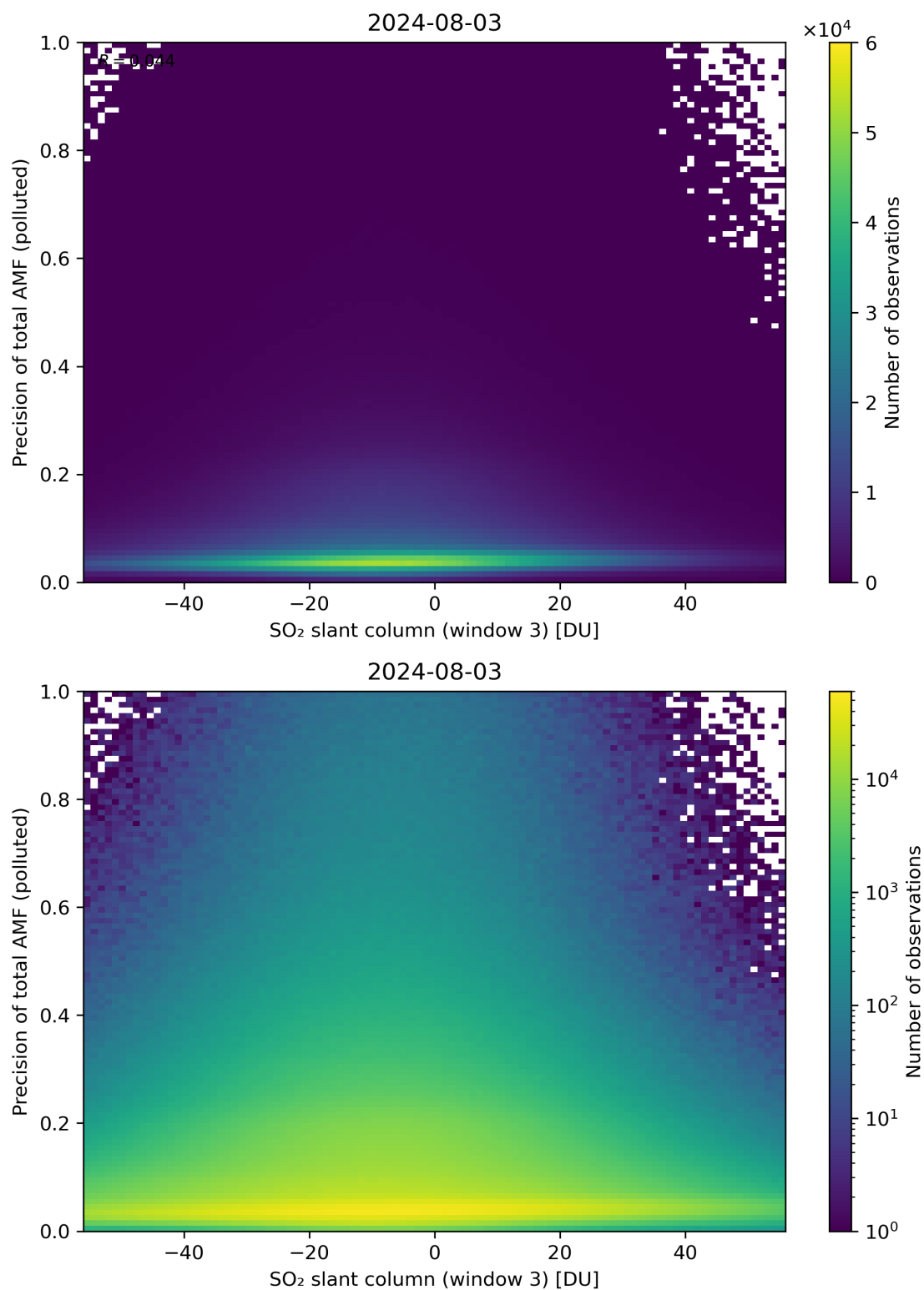
Figure 269: Scatter density plot of “SO 2 slant column (window 3)” against “Precision of total AMF (polluted)” for 2024-08-02 to 2024-08-04.
