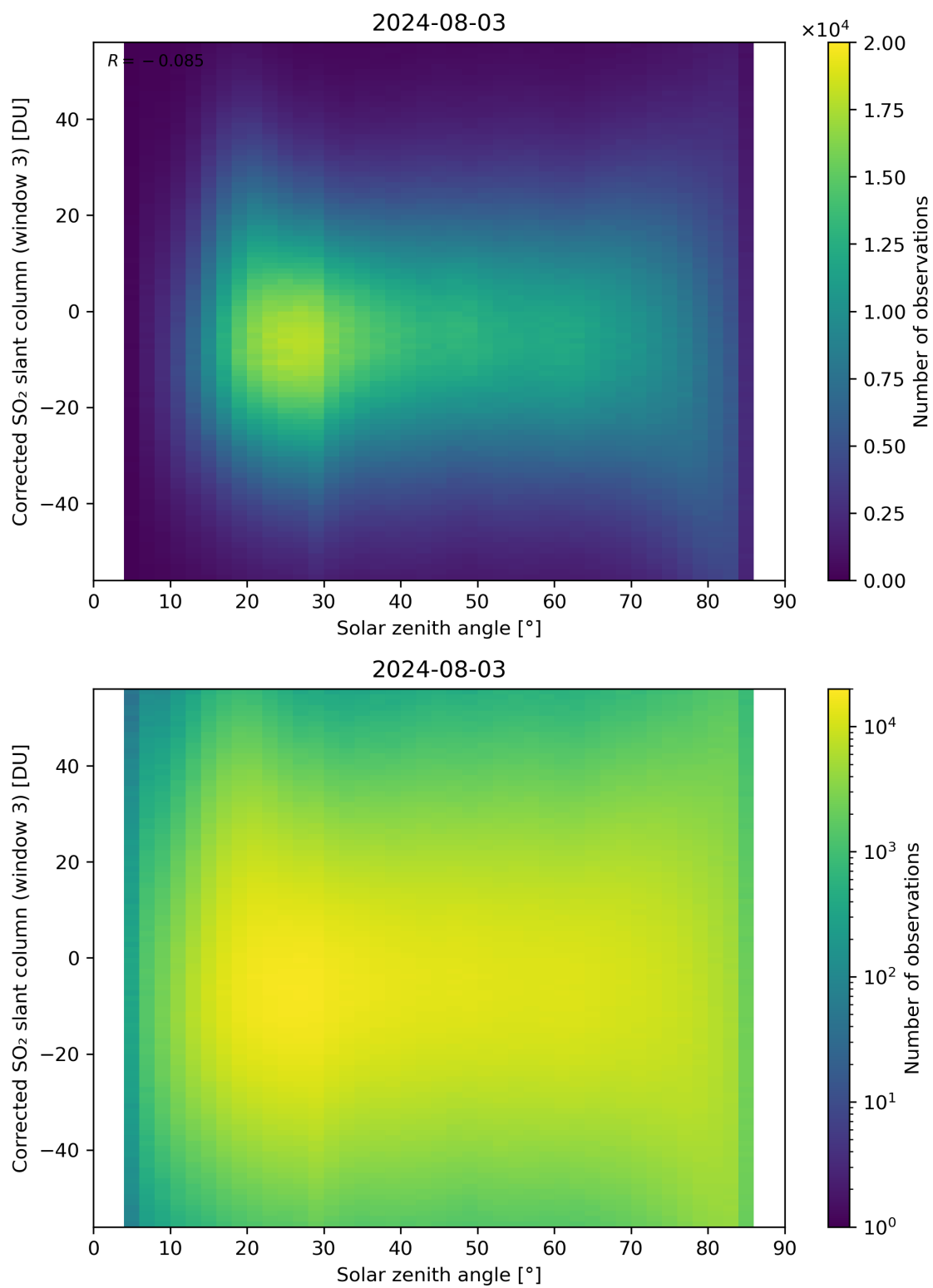
Figure 168: Scatter density plot of “Solar zenith angle” against “Corrected SO 2 slant column (window 3)” for 2024-08-02 to 2024-08-04.
