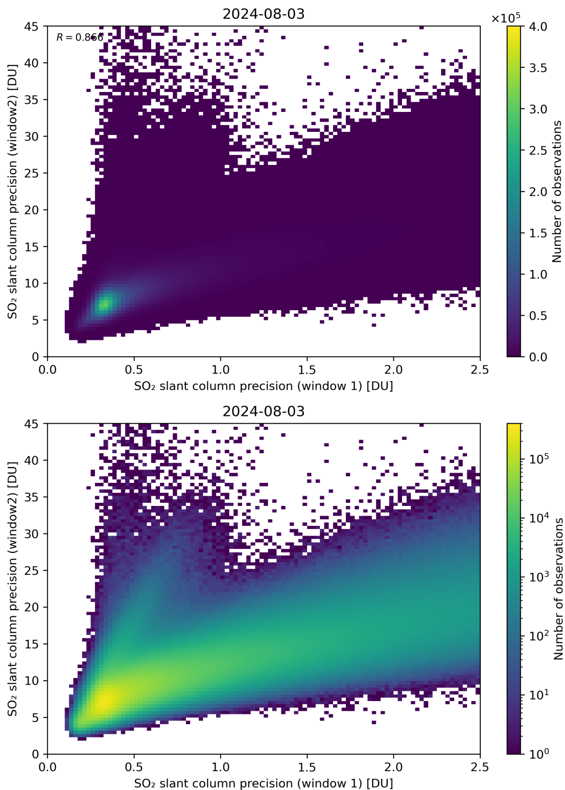
Figure 227: Scatter density plot of “SO 2 slant column precision (window 1)” against “SO 2 slant column precision (window2)” for 2024-08-02 to 2024-08-04.
