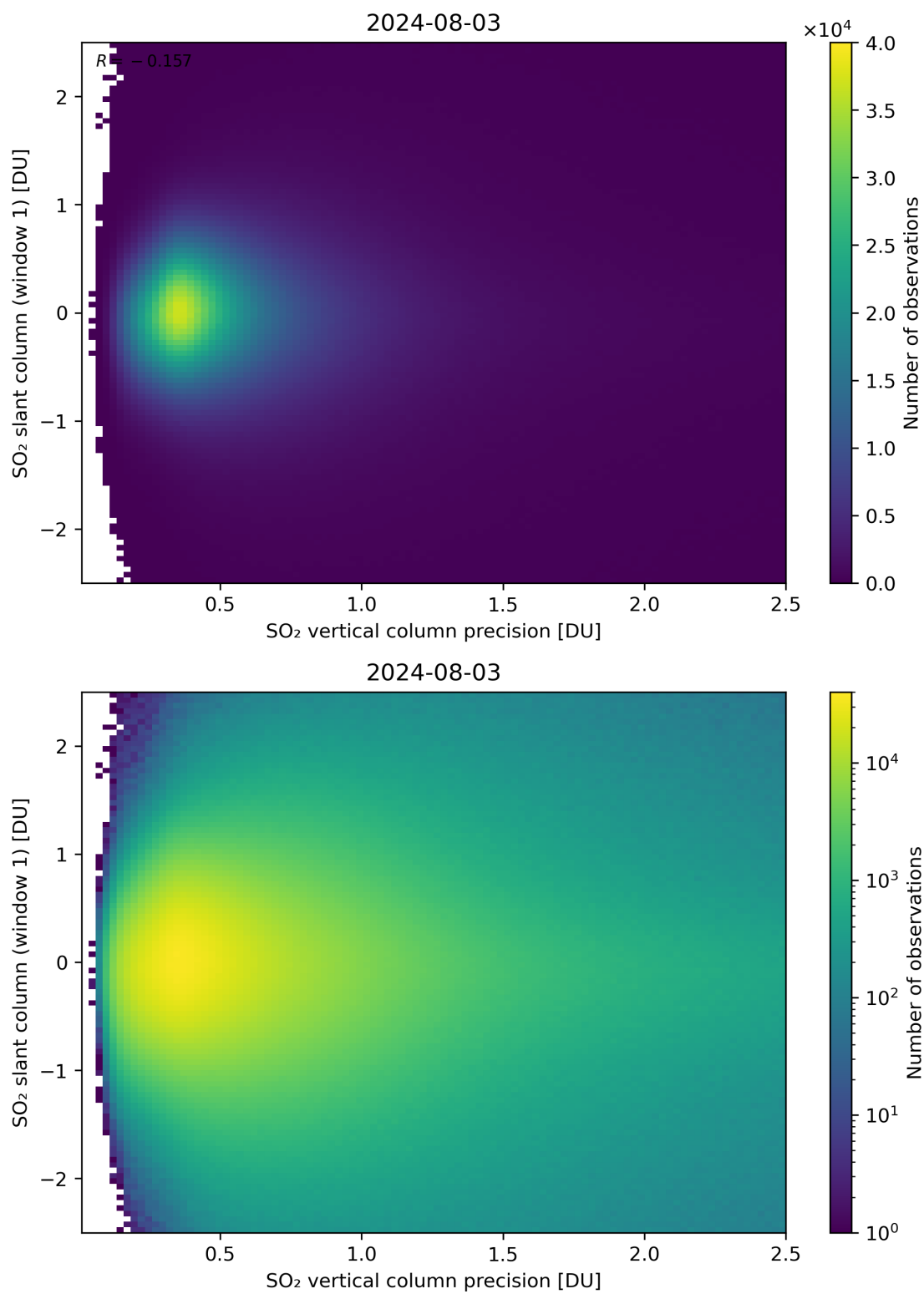
Figure 289: Scatter density plot of “SO 2 vertical column precision” against “SO 2 slant column (window 1)” for 2024-08-02 to 2024-08-04.
