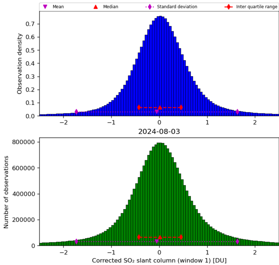
Figure 58: Histogram of “Corrected SO 2 slant column (window 1)” for 2024-08-02 to 2024-08-04
