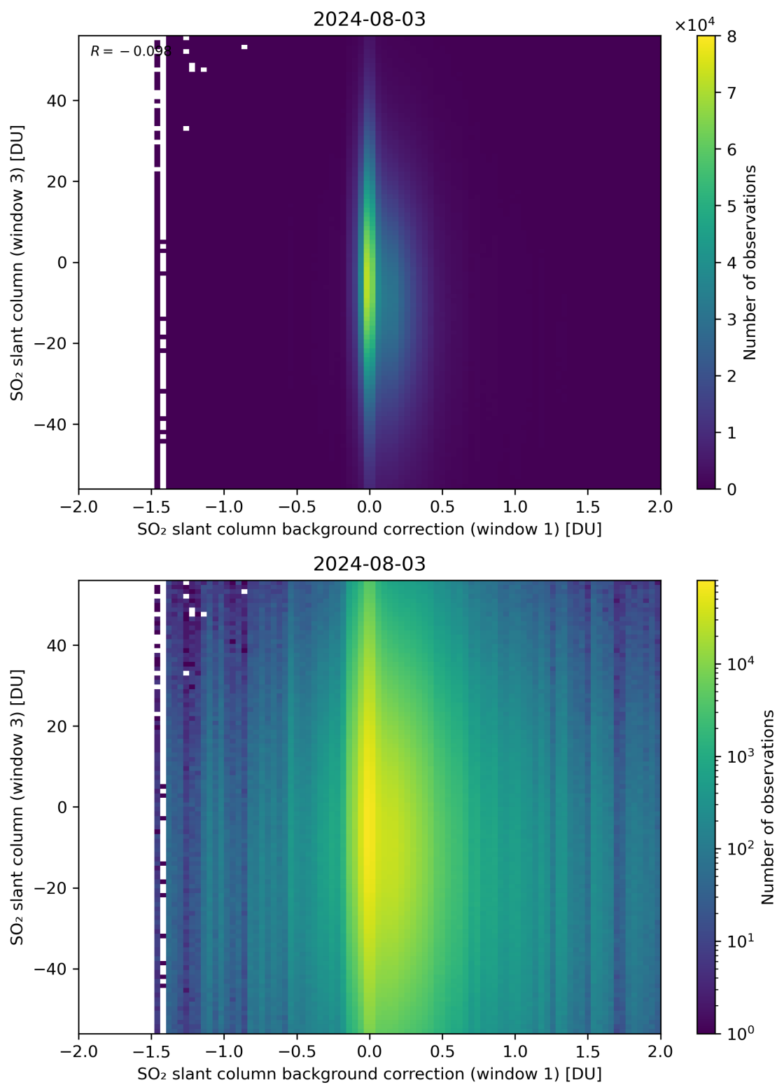
Figure 107: Scatter density plot of “SO 2 slant column background correction (window 1)” against “SO 2 slant column (window 3)” for 2024-08-02 to 2024-08-04.
