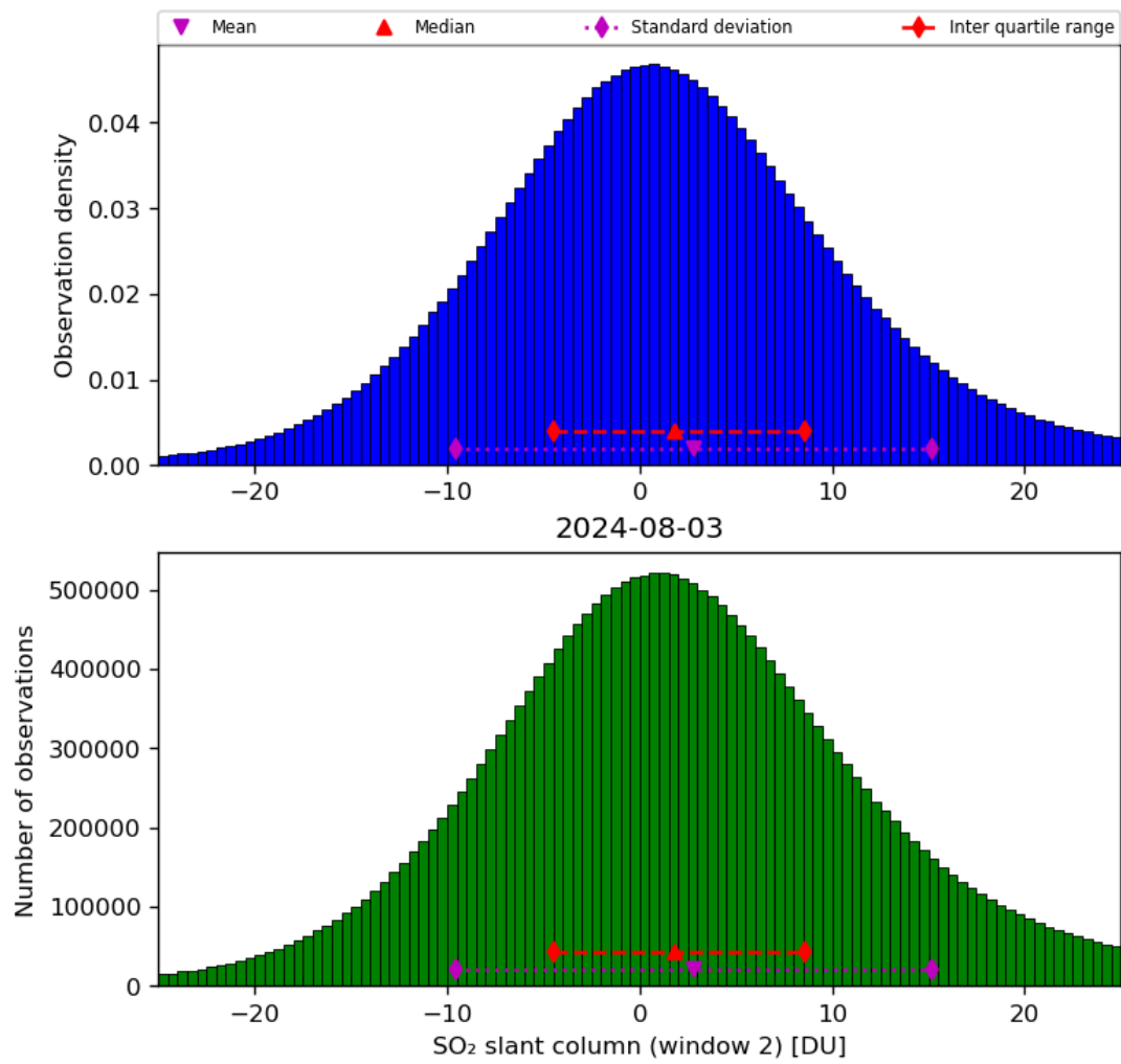
Figure 60: Histogram of “SO 2 slant column (window 2)” for 2024-08-02 to 2024-08-04
