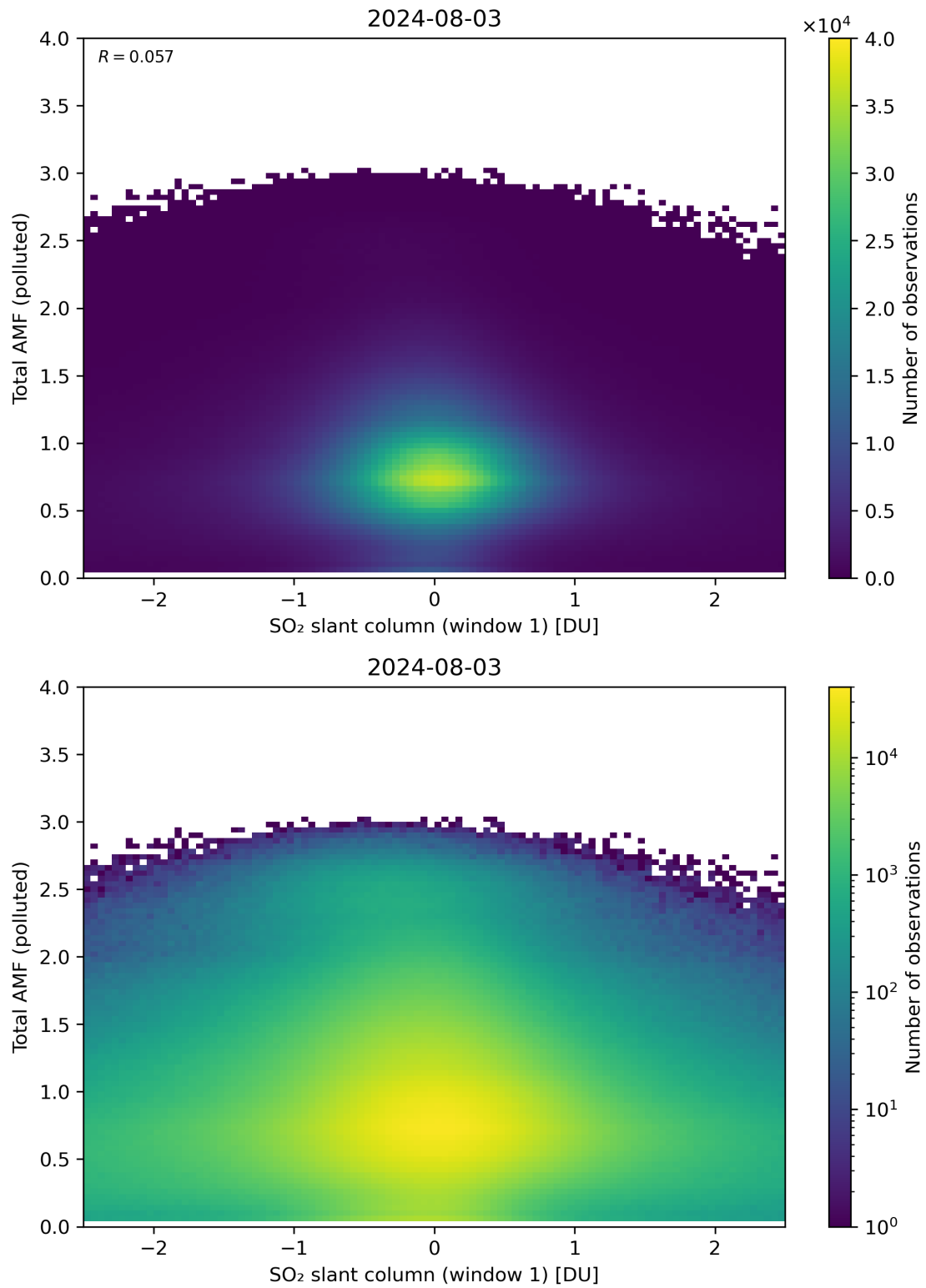
Figure 239: Scatter density plot of “SO 2 slant column (window 1)” against “Total AMF (polluted)” for 2024-08-02 to 2024-08-04.
