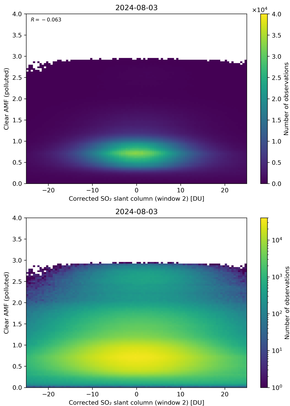
Figure 199: Scatter density plot of “Corrected SO 2 slant column (window 2)” against “Clear AMF (polluted)” for 2024-08-02 to 2024-08-04.
