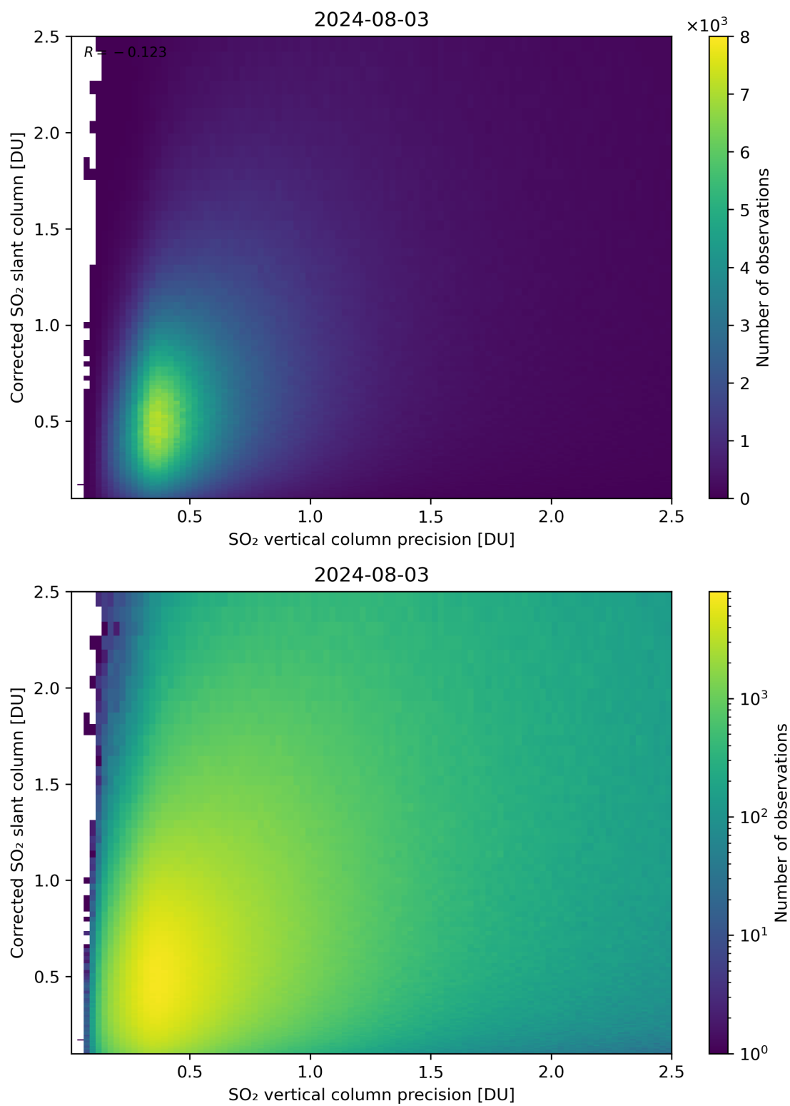
Figure 286: Scatter density plot of “SO 2 vertical column precision” against “Corrected SO 2 slant column” for 2024-08-02 to 2024-08-04.
