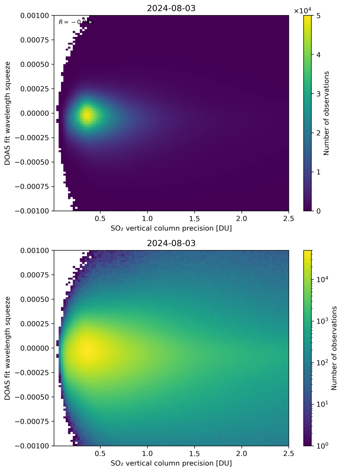
Figure 283: Scatter density plot of “SO 2 vertical column precision” against “DOAS fit wavelength squeeze” for 2024-08-02 to 2024-08-04.
