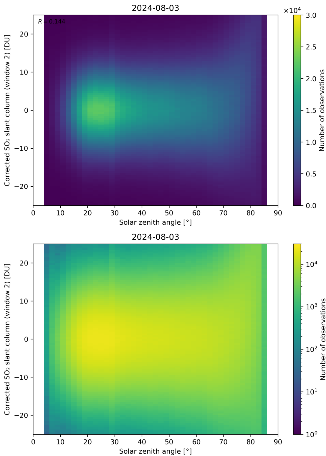
Figure 167: Scatter density plot of “Solar zenith angle” against “Corrected SO 2 slant column (window 2)” for 2024-08-02 to 2024-08-04.
