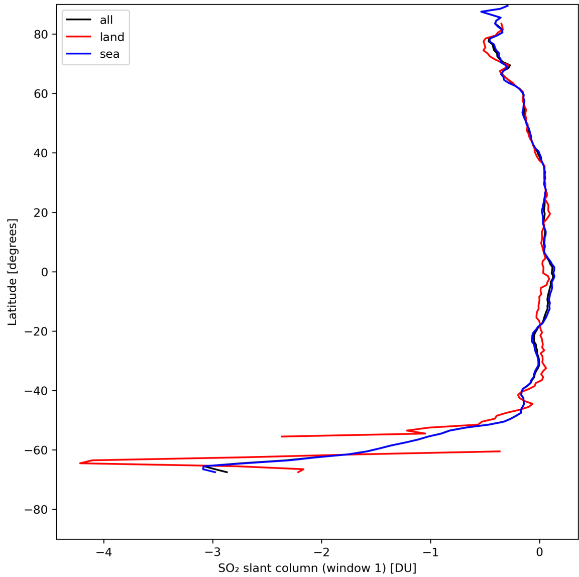
Figure 33: Zonal average of “SO 2 slant column (window 1)” for 2024-08-02 to 2024-08-04.
