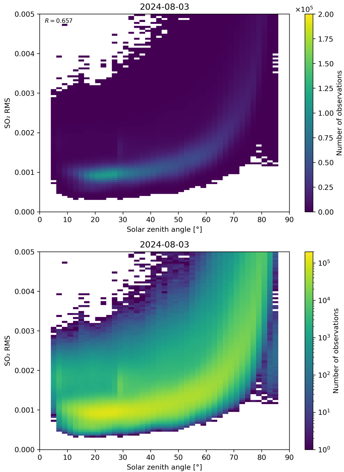
Figure 163: Scatter density plot of “Solar zenith angle” against “SO 2 RMS” for 2024-08-02 to 2024-08-04.
