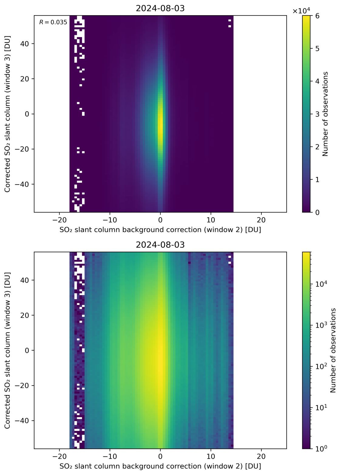
Figure 116: Scatter density plot of “SO 2 slant column background correction (window 2)” against “Corrected SO 2 slant column (window 3)” for 2024-08-02 to 2024-08-04.
