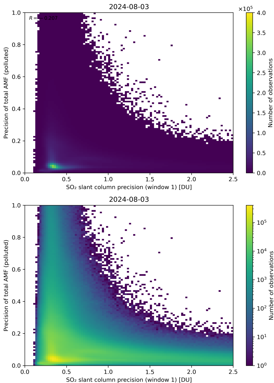
Figure 231: Scatter density plot of “SO 2 slant column precision (window 1)” against “Precision of total AMF (polluted)” for 2024-08-02 to 2024-08-04.
