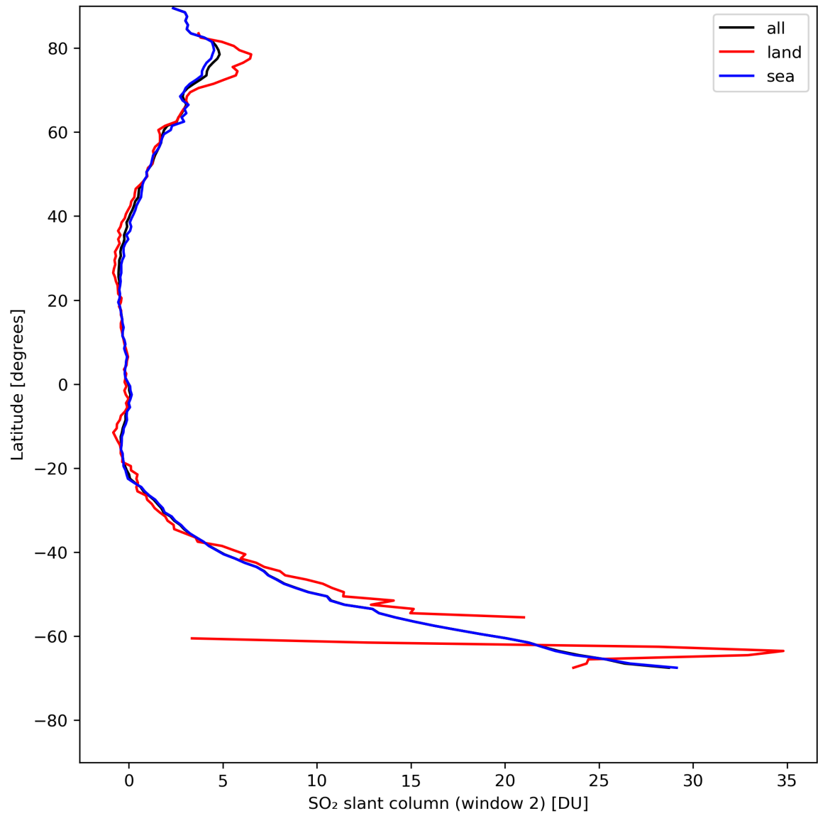
Figure 37: Zonal average of “SO 2 slant column (window 2)” for 2024-08-02 to 2024-08-04.
