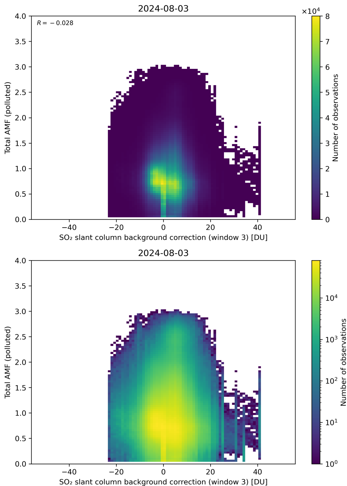
Figure 125: Scatter density plot of “SO 2 slant column background correction (window 3)” against “Total AMF (polluted)” for 2024-08-02 to 2024-08-04.
