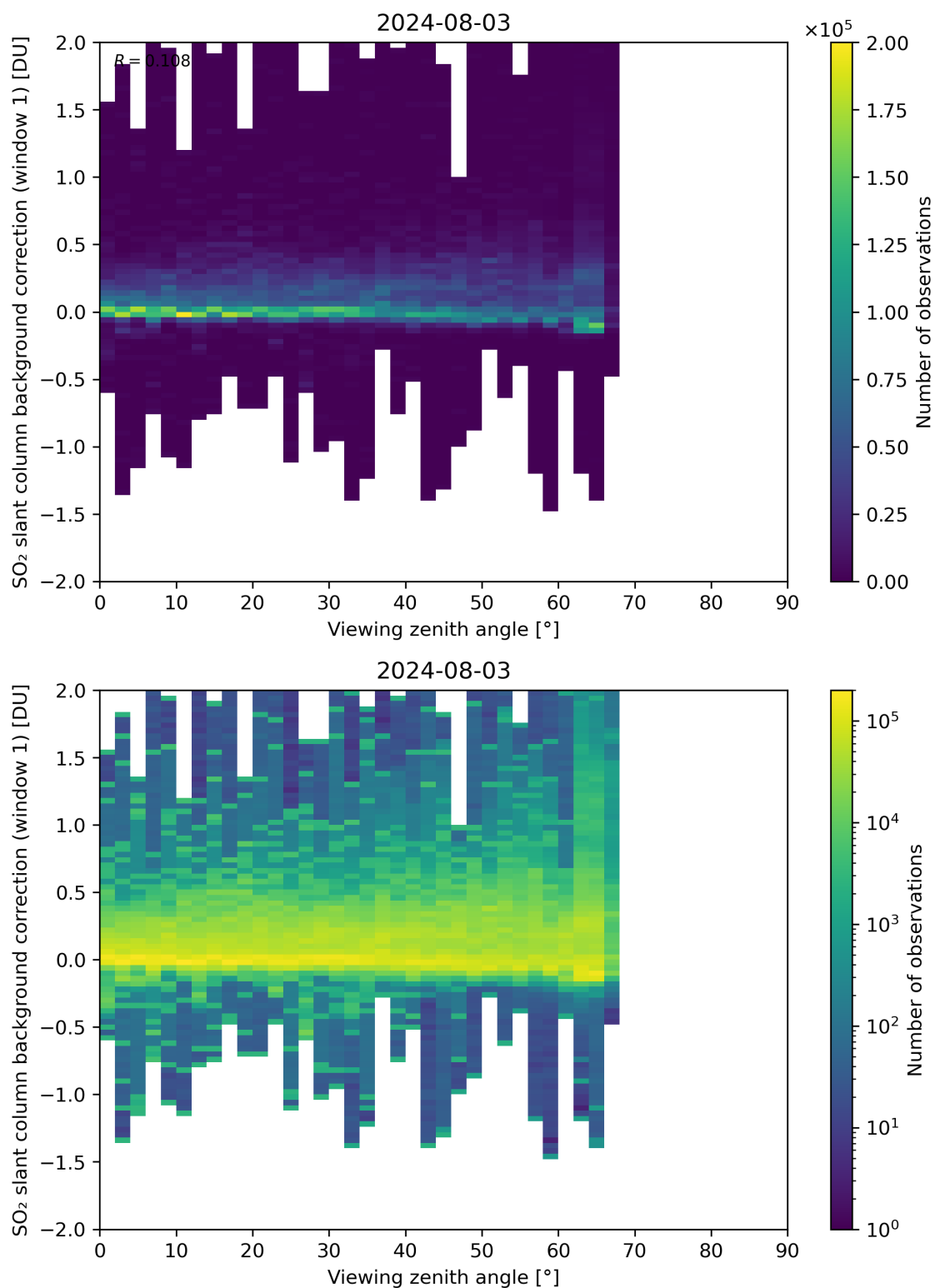
Figure 308: Scatter density plot of “Viewing zenith angle” against “SO 2 slant column background correction (window 1)” for 2024-08-02 to 2024-08-04.
