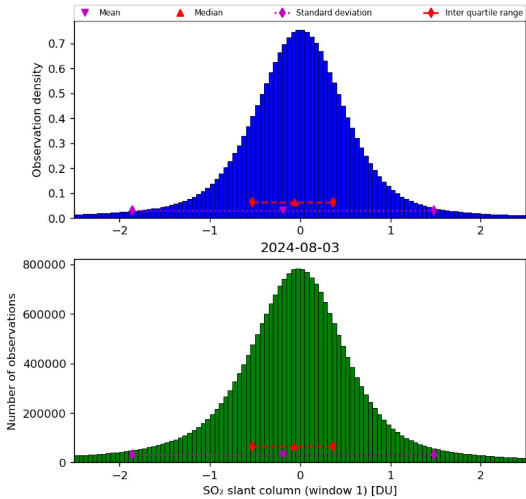
Figure 56: Histogram of “SO 2 slant column (window 1)” for 2024-08-02 to 2024-08-04
