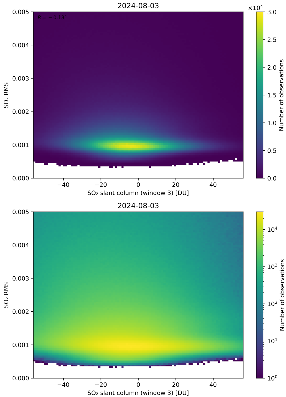
Figure 256: Scatter density plot of “SO 2 slant column (window 3)” against “SO 2 RMS” for 2024-08-02 to 2024-08-04.
