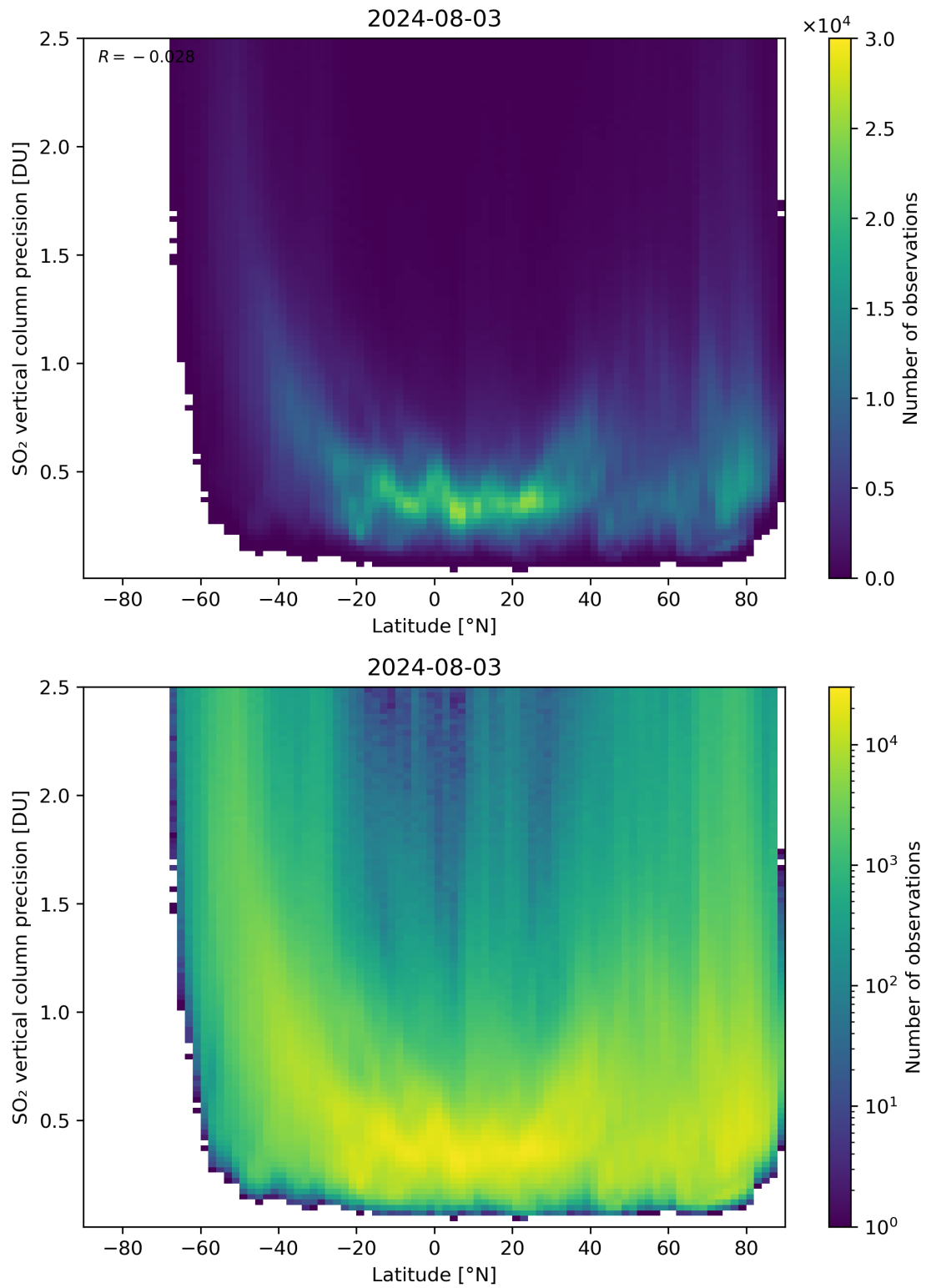
Figure 157: Scatter density plot of “Latitude” against “SO 2 vertical column precision” for 2024-08-02 to 2024-08-04.
