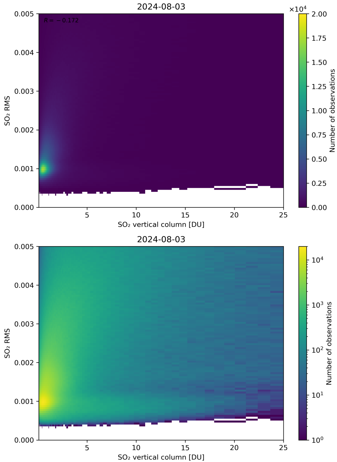
Figure 278: Scatter density plot of “SO 2 vertical column” against “SO 2 RMS” for 2024-08-02 to 2024-08-04.
