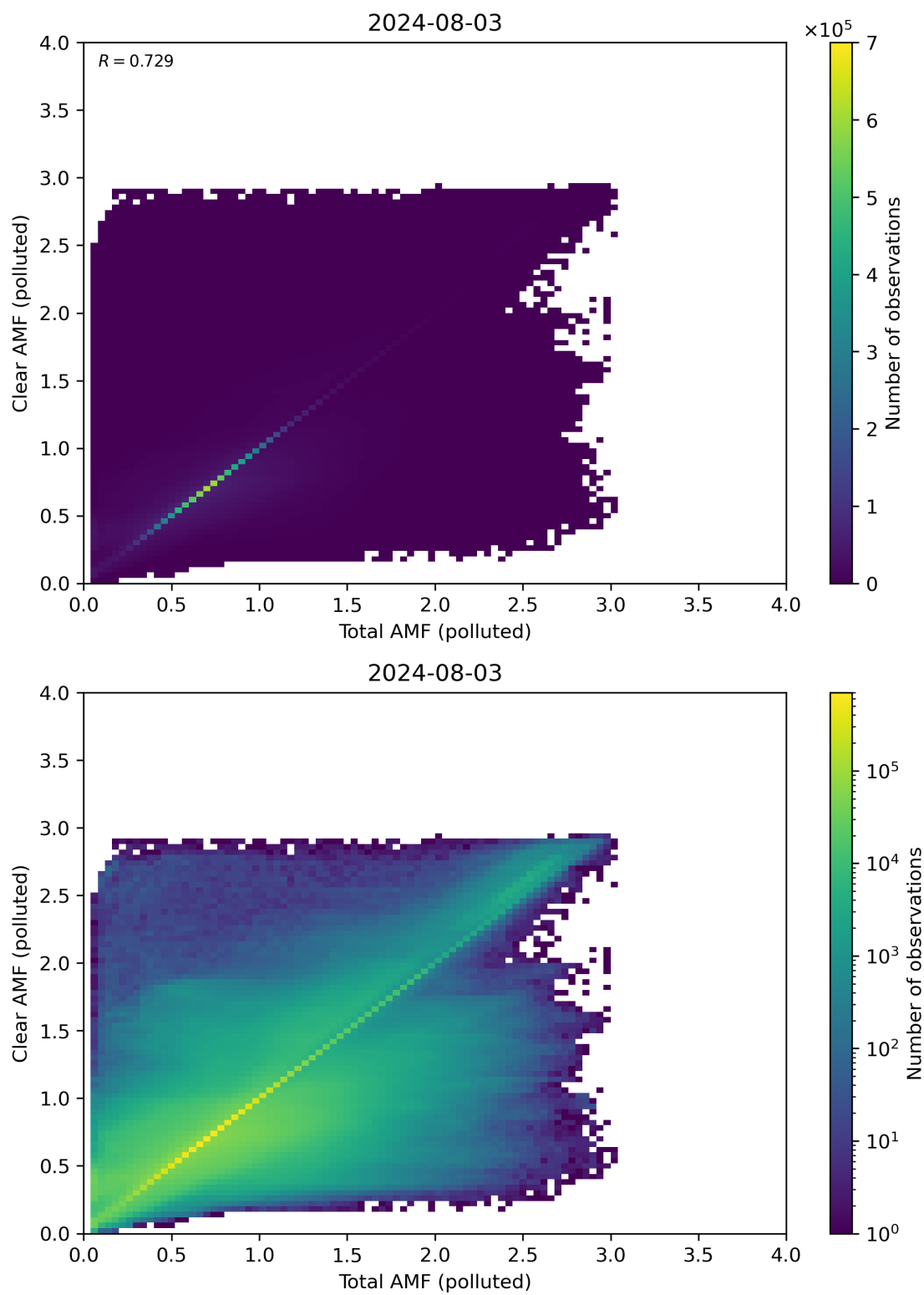
Figure 271: Scatter density plot of “Total AMF (polluted)” against “Clear AMF (polluted)” for 2024-08-02 to 2024-08-04.
