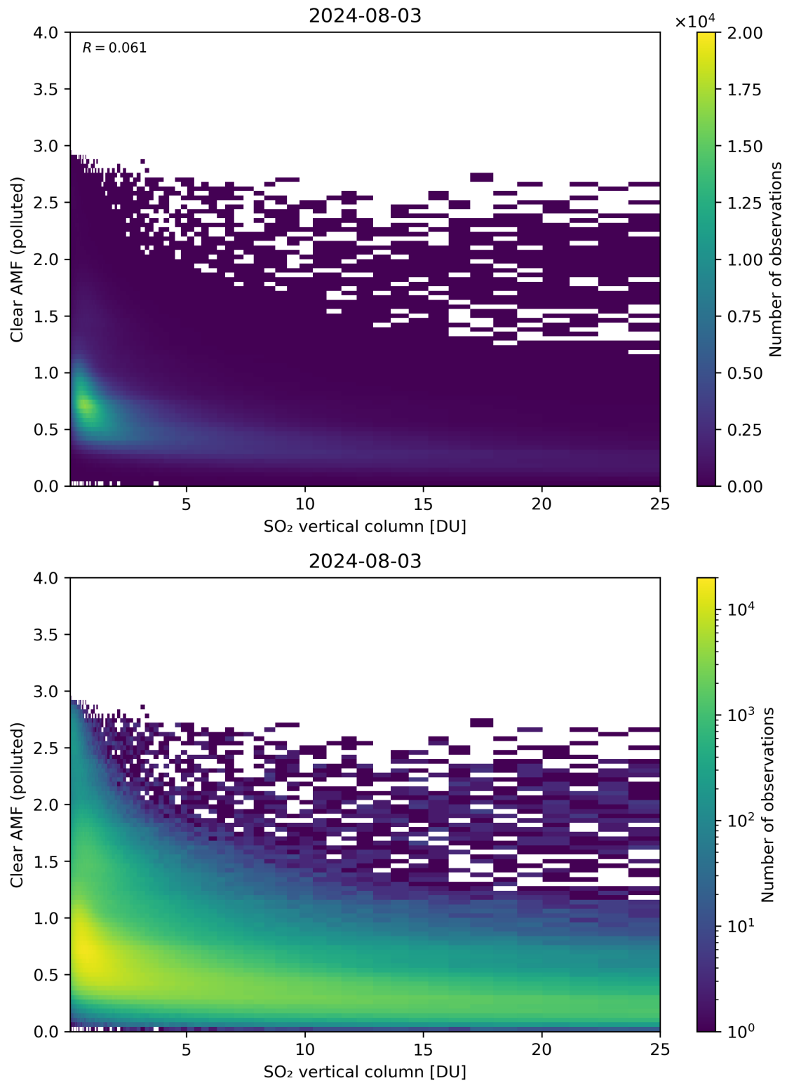
Figure 296: Scatter density plot of “SO 2 vertical column” against “Clear AMF (polluted)” for 2024-08-02 to 2024-08-04.
