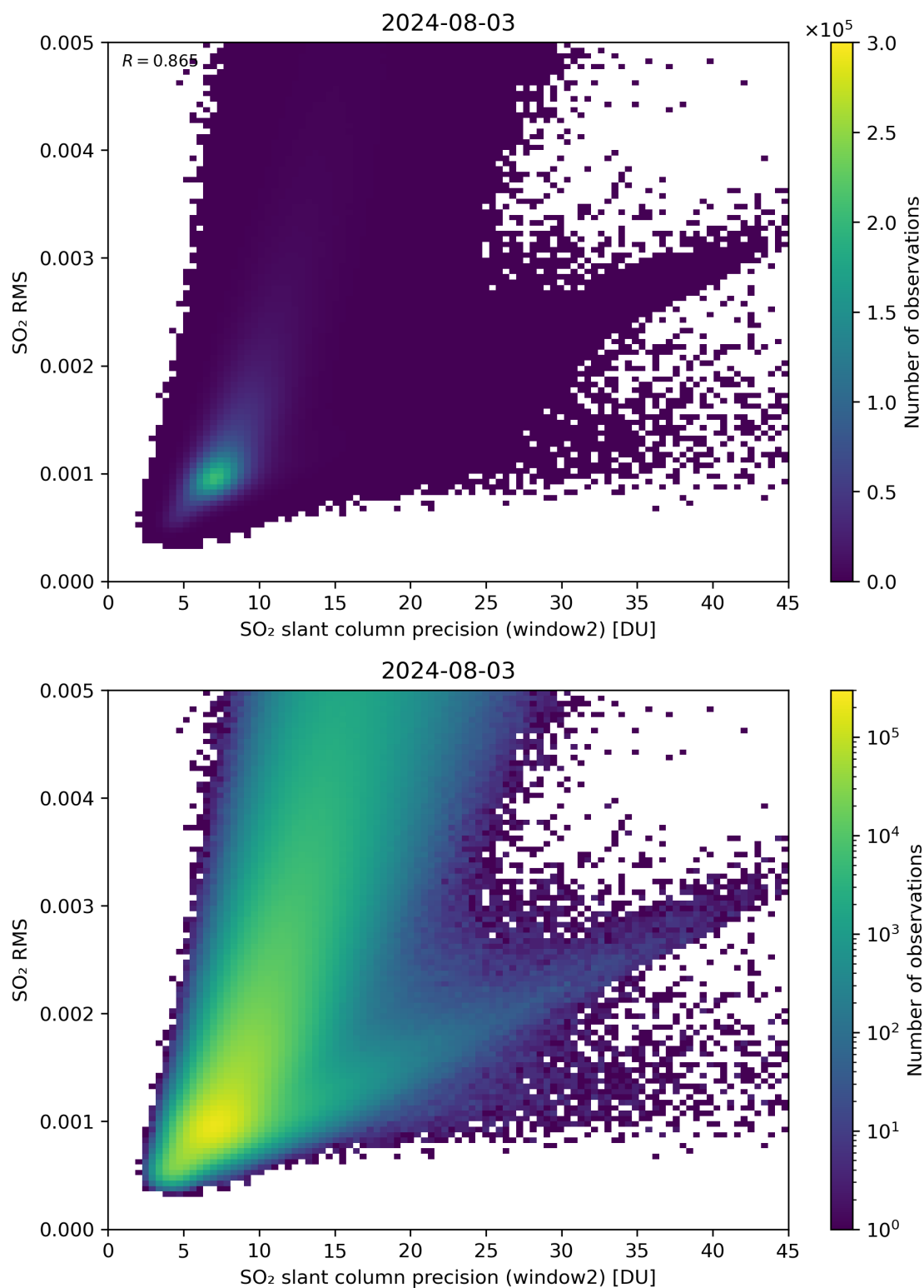
Figure 245: Scatter density plot of “SO 2 slant column precision (window2)” against “SO 2 RMS” for 2024-08-02 to 2024-08-04.
