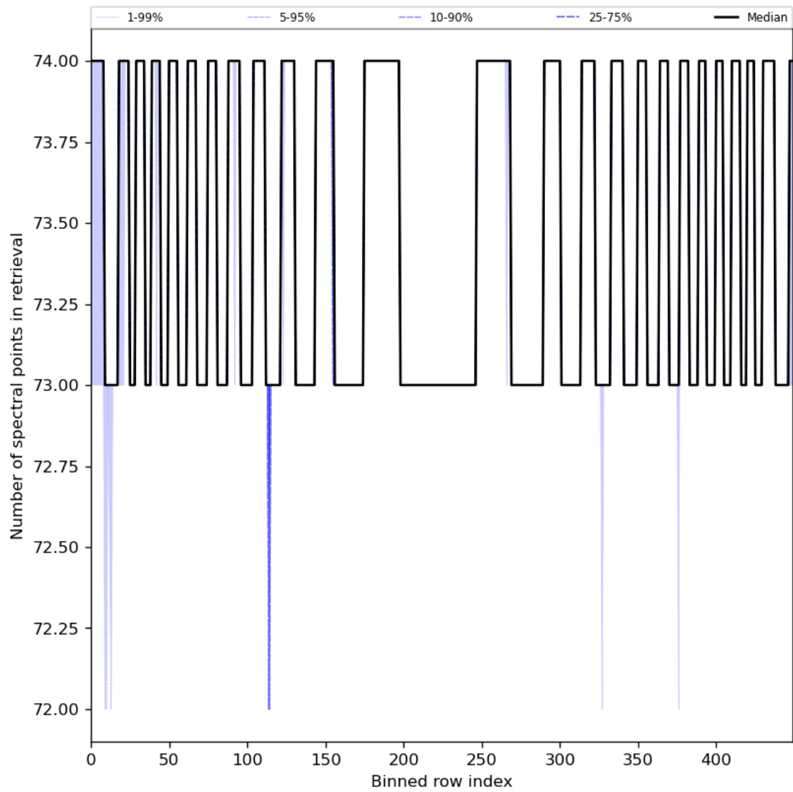
Figure 97: Along track statistics of “Number of spectral points in retrieval” for 2024-08-02 to 2024-08-04
