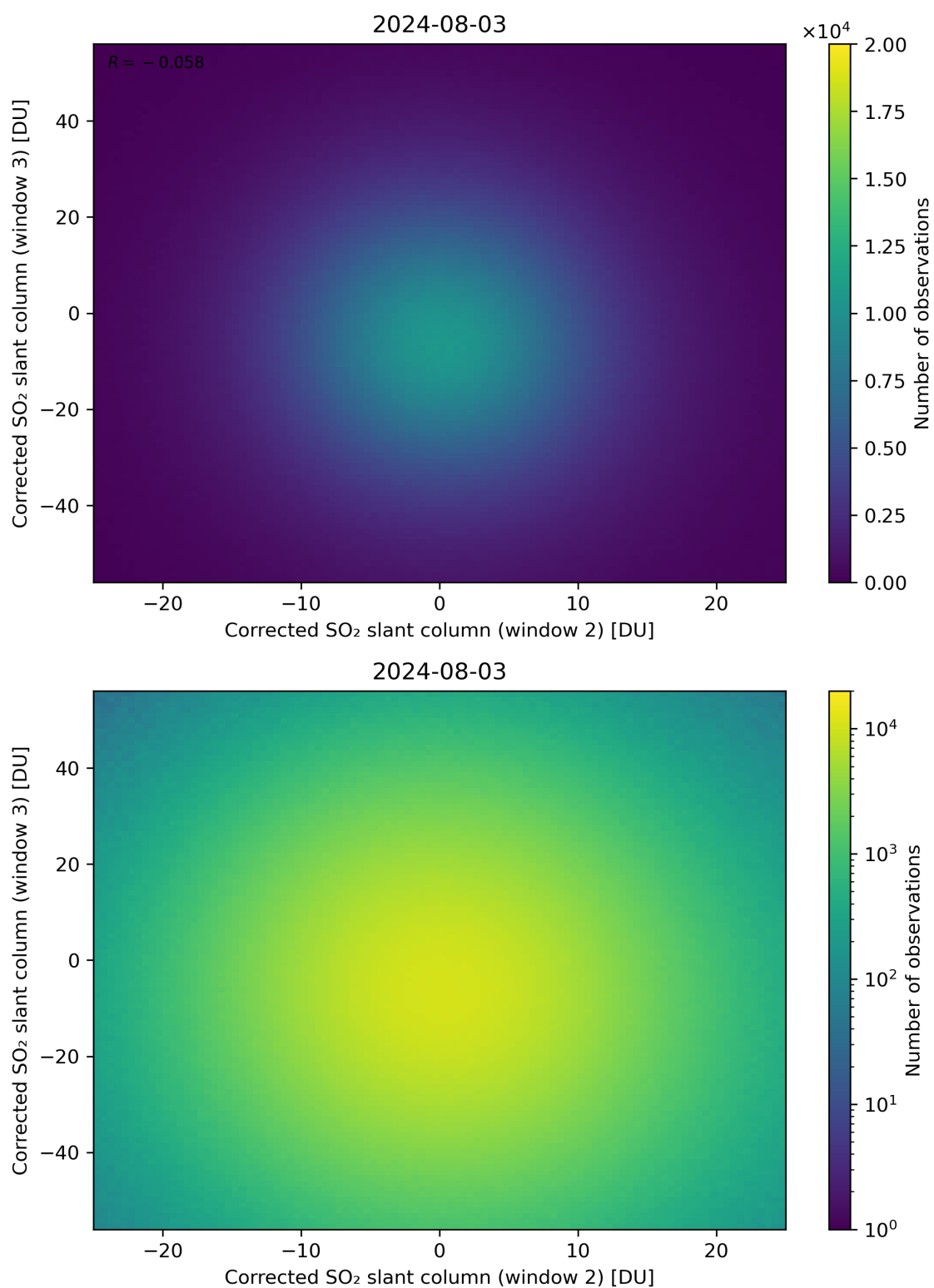
Figure 200: Scatter density plot of “Corrected SO 2 slant column (window 2)” against “Corrected SO 2 slant column (window 3)” for 2024-08-02 to 2024-08-04.
