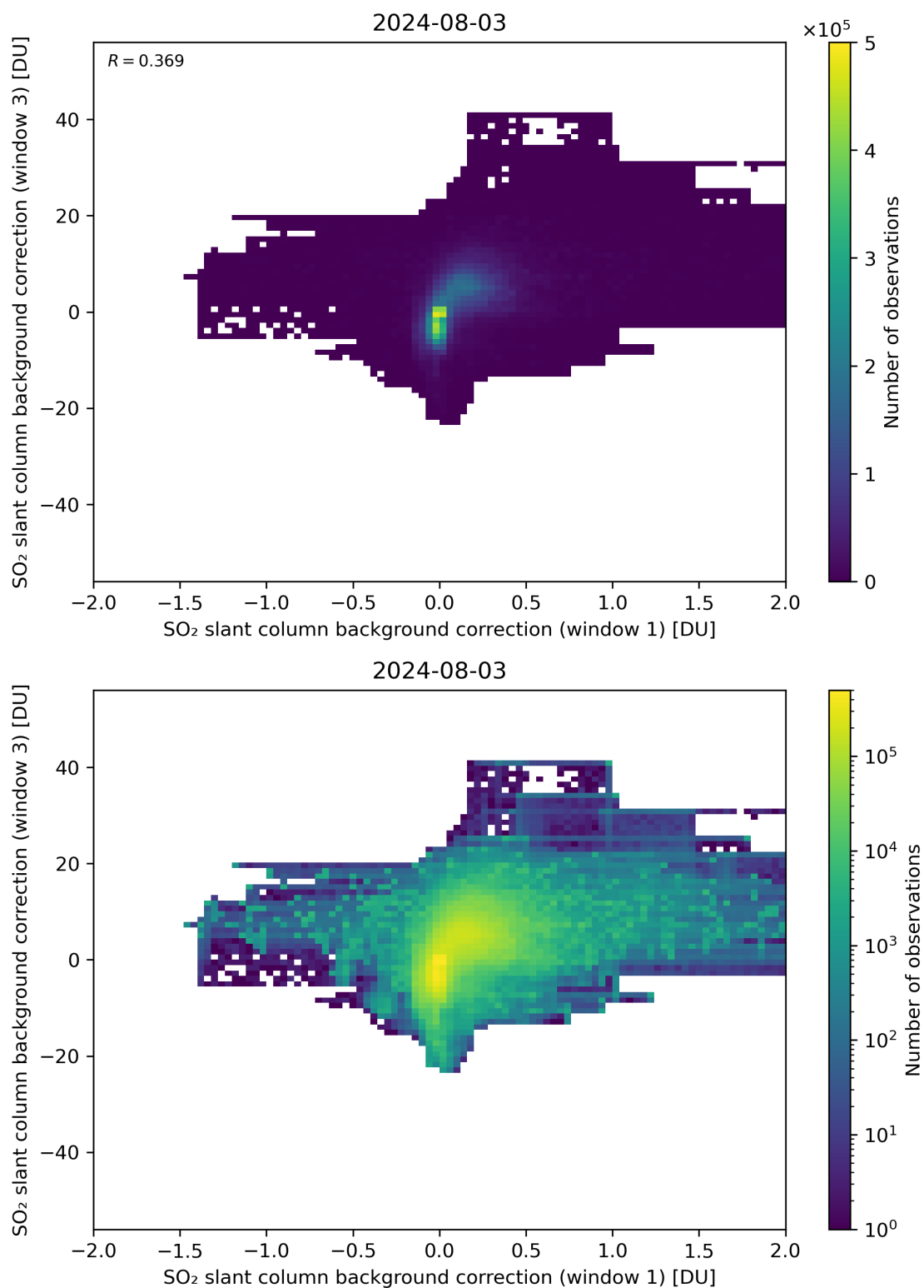
Figure 99: Scatter density plot of “SO 2 slant column background correction (window 1)” against “SO 2 slant column background correction (window 3)” for 2024-08-02 to 2024-08-04.
