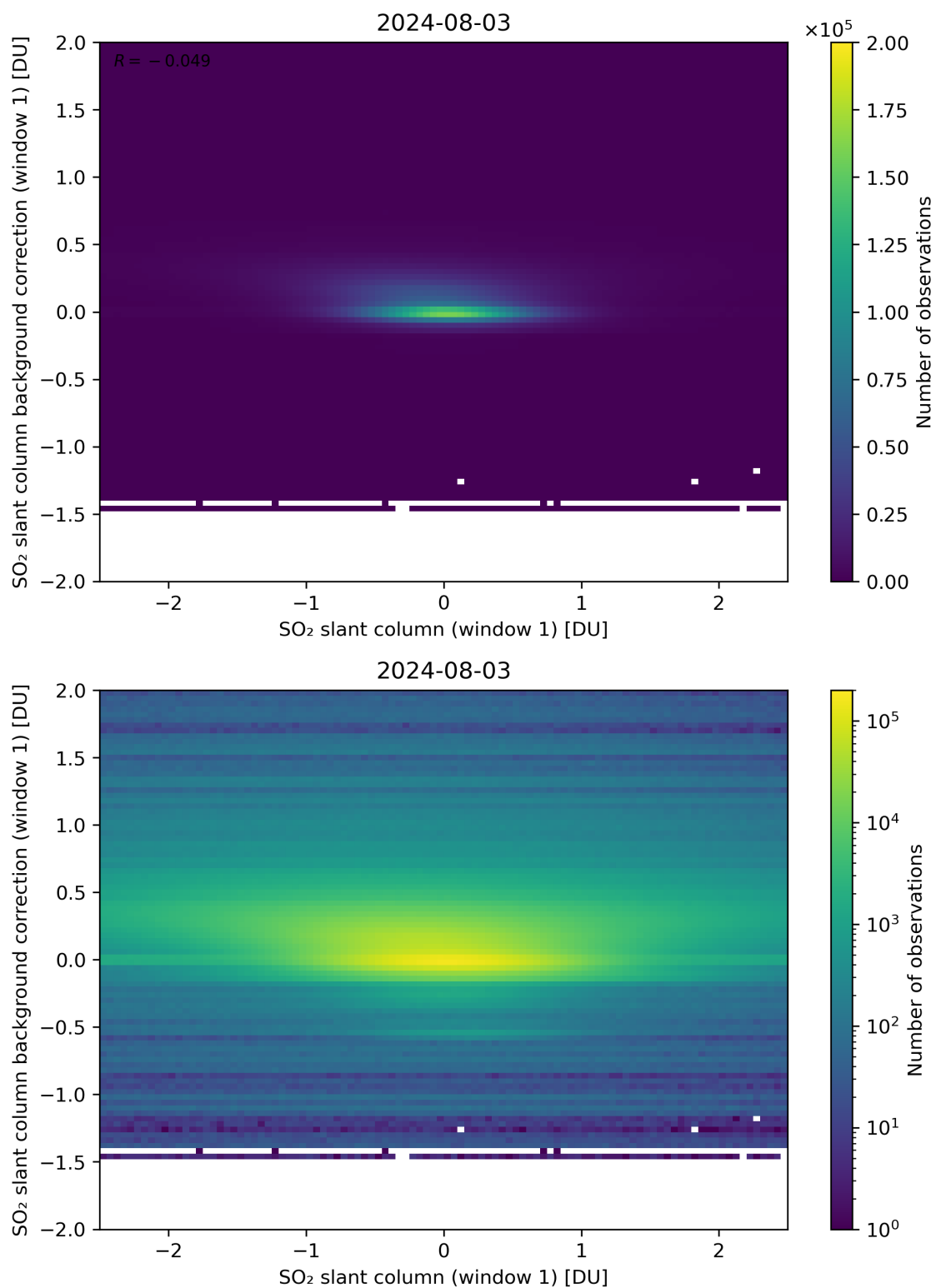
Figure 212: Scatter density plot of “SO 2 slant column (window 1)” against “SO 2 slant column background correction (window 1)” for 2024-08-02 to 2024-08-04.
