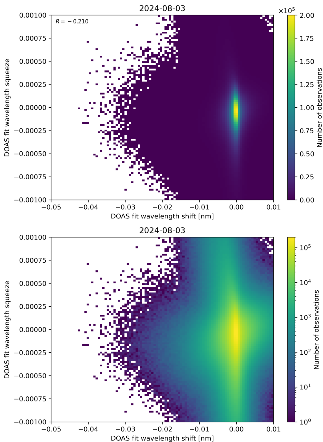
Figure 127: Scatter density plot of “DOAS fit wavelength shift” against “DOAS fit wavelength squeeze” for 2024-08-02 to 2024-08-04.
