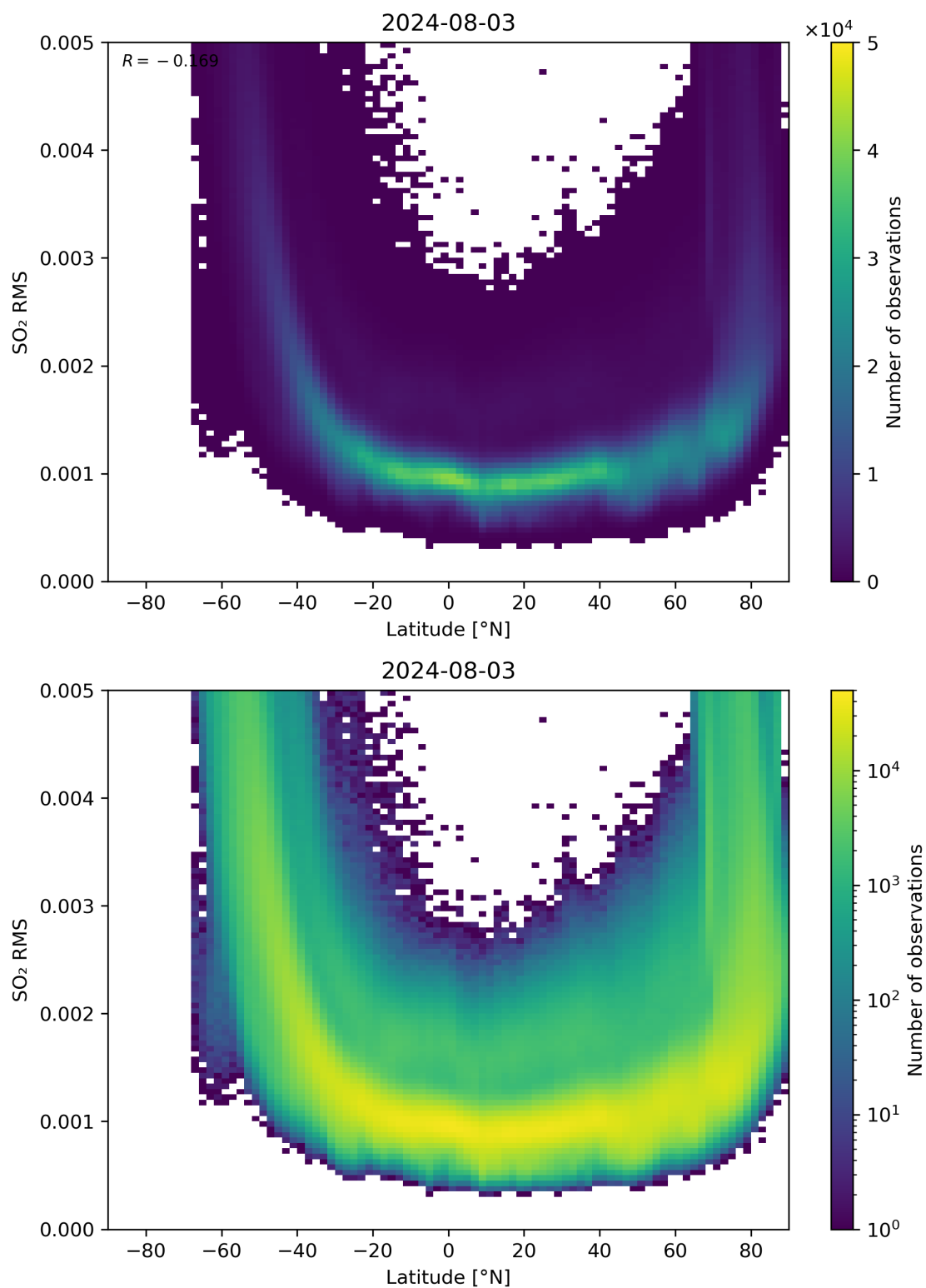
Figure 144: Scatter density plot of “Latitude” against “SO 2 RMS” for 2024-08-02 to 2024-08-04.
