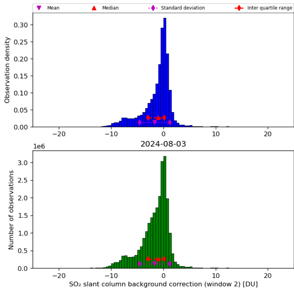
Figure 63: Histogram of “SO 2 slant column background correction (window 2)” for 2024-08-02 to 2024-08-04
