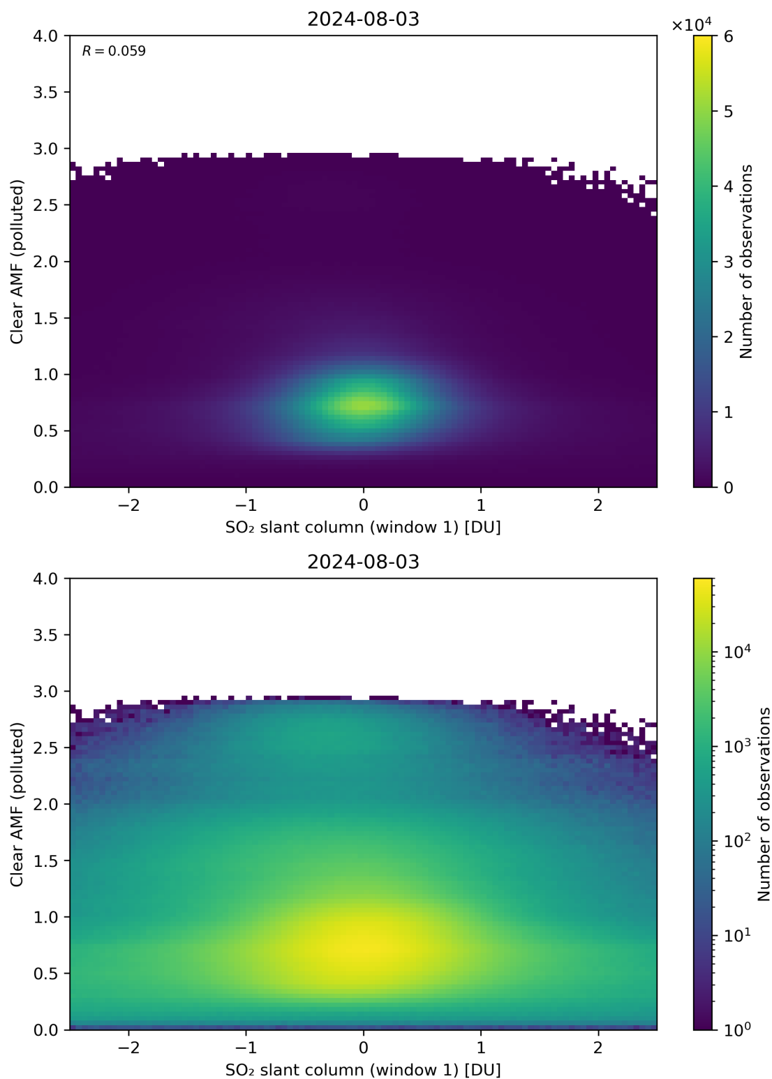
Figure 232: Scatter density plot of “SO 2 slant column (window 1)” against “Clear AMF (polluted)” for 2024-08-02 to 2024-08-04.
