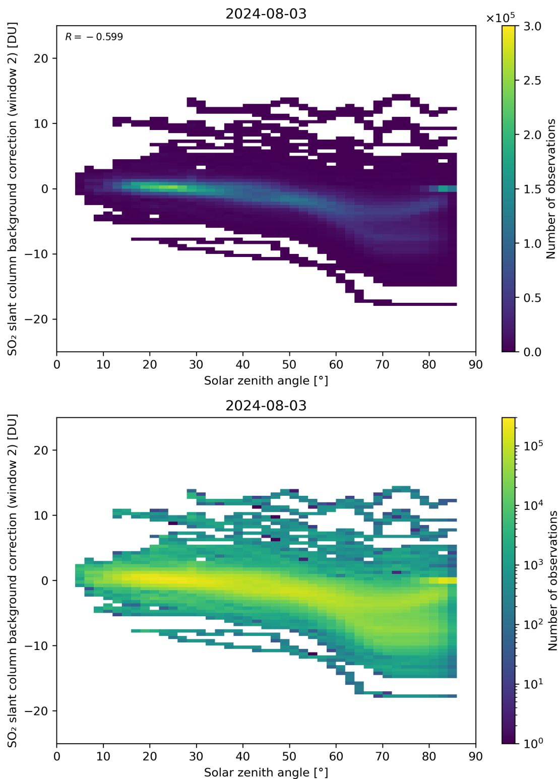
Figure 159: Scatter density plot of “Solar zenith angle” against “SO 2 slant column background correction (window 2)” for 2024-08-02 to 2024-08-04.
