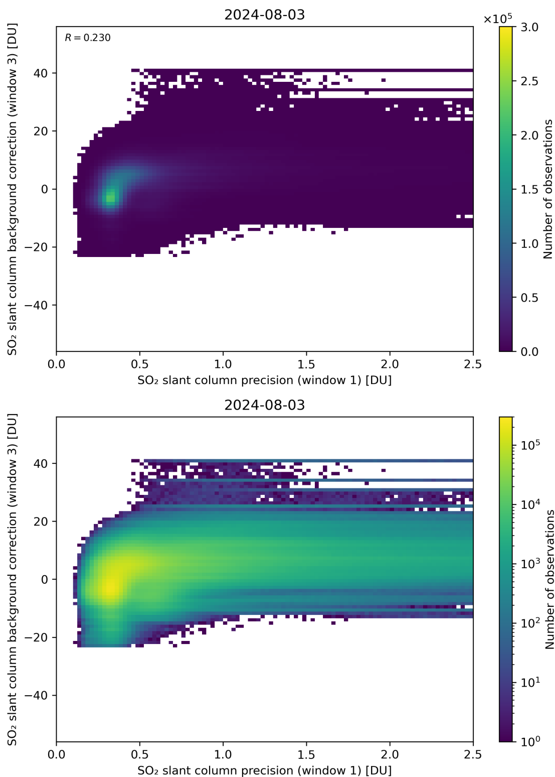
Figure 220: Scatter density plot of “SO 2 slant column precision (window 1)” against “SO 2 slant column background correction (window 3)” for 2024-08-02 to 2024-08-04.
