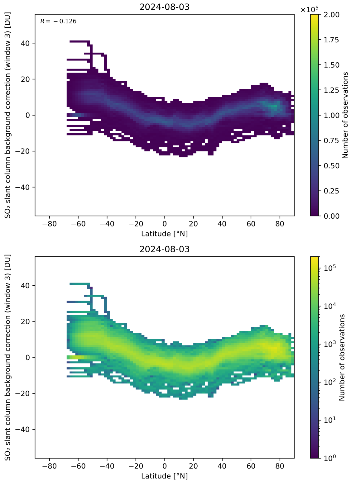
Figure 141: Scatter density plot of “Latitude” against “SO 2 slant column background correction (window 3)” for 2024-08-02 to 2024-08-04.
