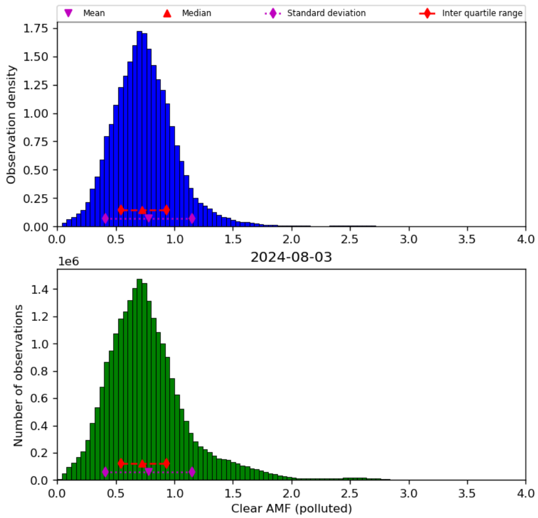
Figure 73: Histogram of “Clear AMF (polluted)” for 2024-08-02 to 2024-08-04
