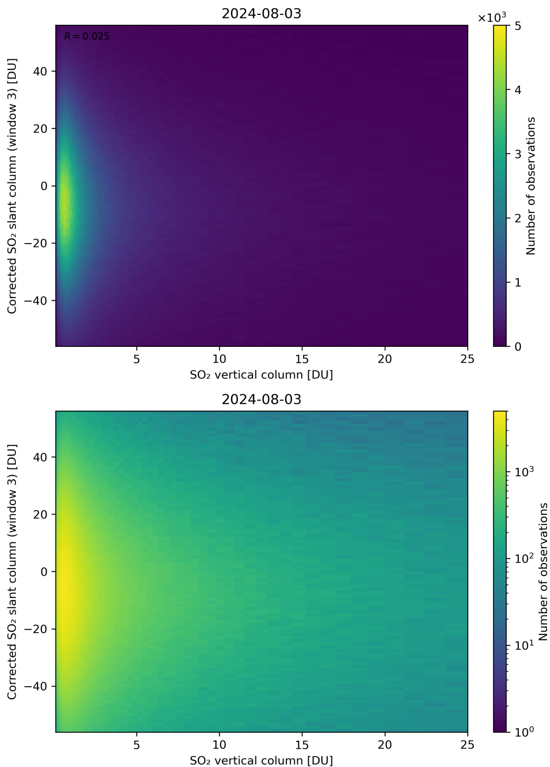
Figure 299: Scatter density plot of “SO 2 vertical column” against “Corrected SO 2 slant column (window 3)” for 2024-08-02 to 2024-08-04.
