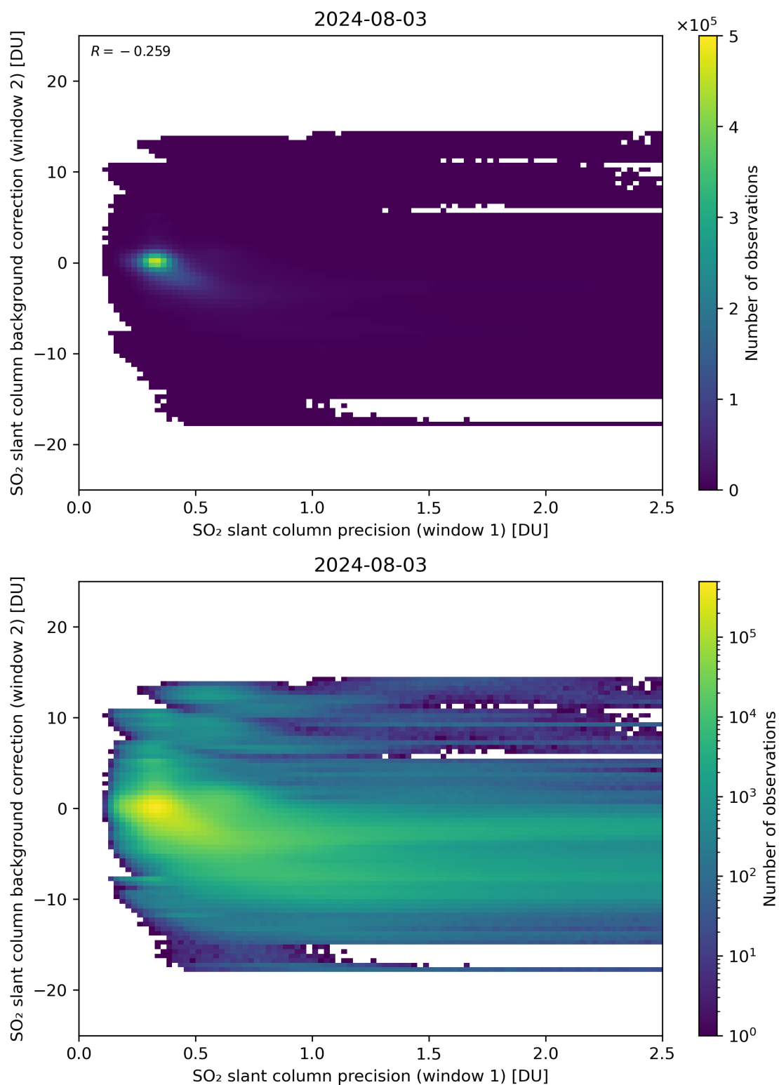
Figure 219: Scatter density plot of “SO 2 slant column precision (window 1)” against “SO 2 slant column background correction (window 2)” for 2024-08-02 to 2024-08-04.
