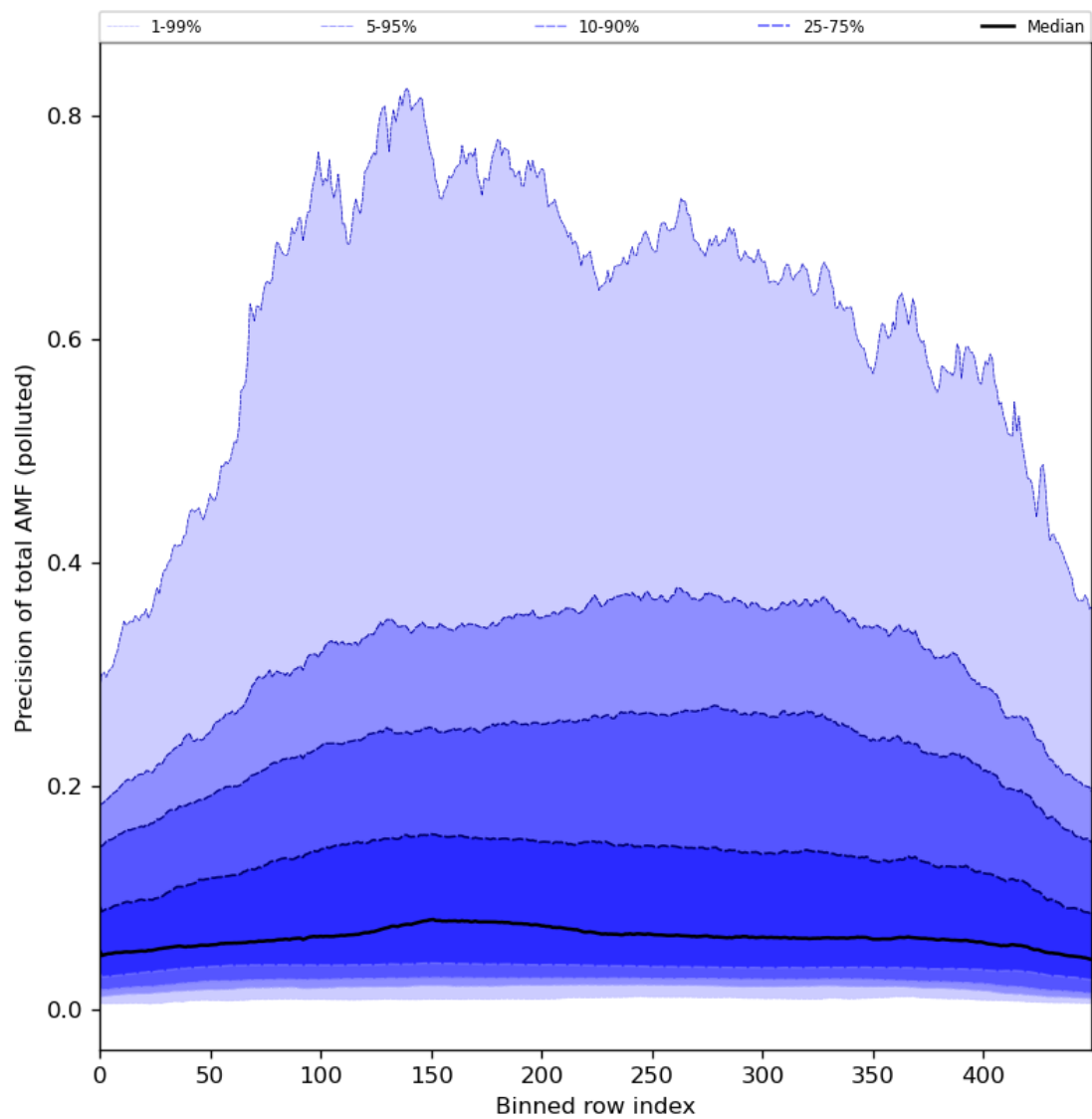
Figure 95: Along track statistics of “Precision of total AMF (polluted)” for 2024-08-02 to 2024-08-04
