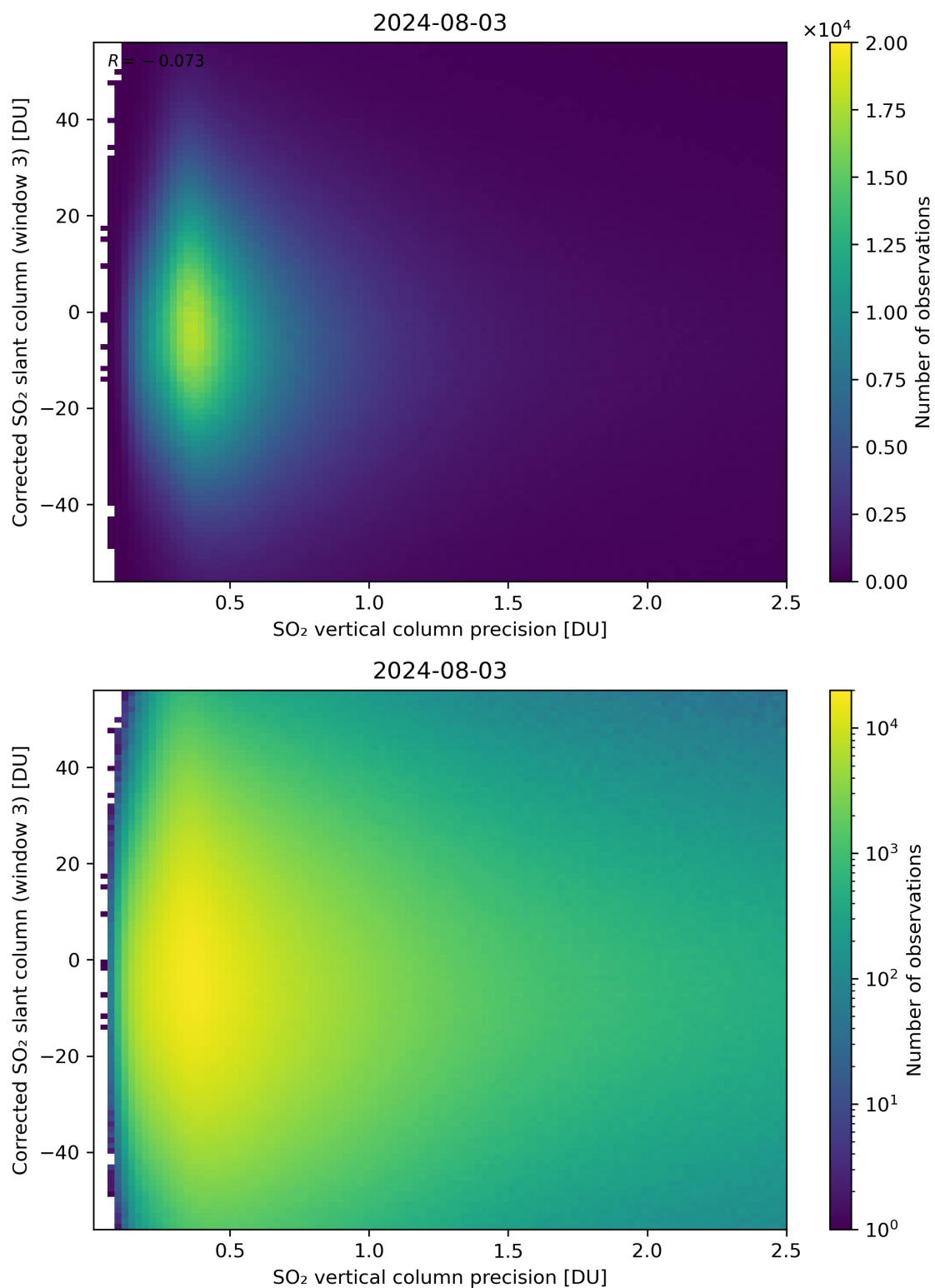
Figure 288: Scatter density plot of “SO 2 vertical column precision” against “Corrected SO 2 slant column (window 3)” for 2024-08-02 to 2024-08-04.
