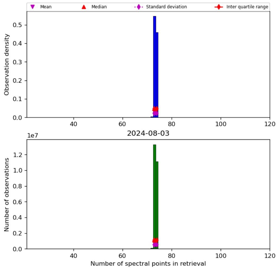
Figure 74: Histogram of “Number of spectral points in retrieval” for 2024-08-02 to 2024-08-04
