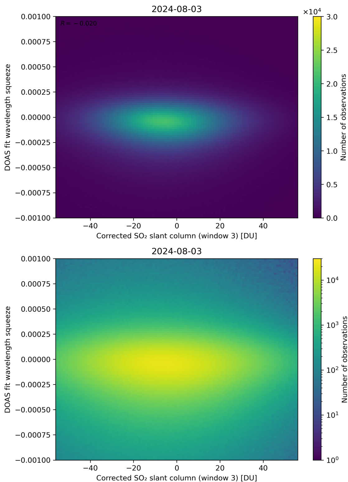
Figure 207: Scatter density plot of “Corrected SO 2 slant column (window 3)” against “DOAS fit wavelength squeeze” for 2024-08-02 to 2024-08-04.
