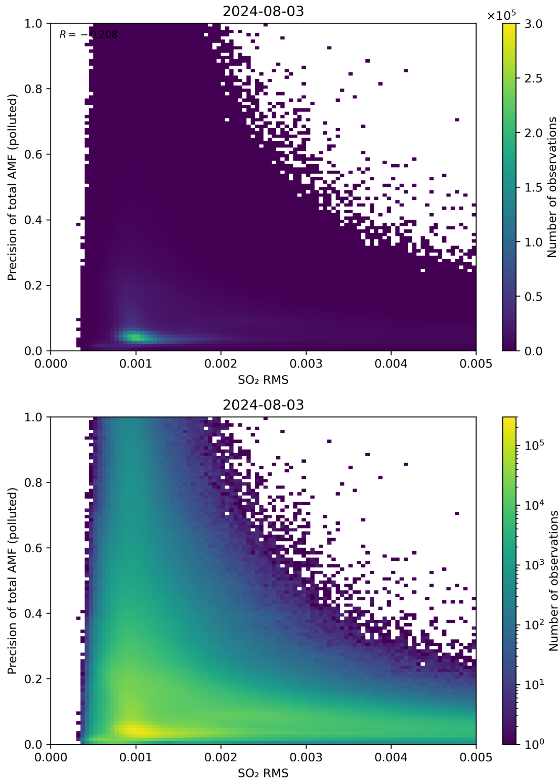
Figure 138: Scatter density plot of “SO 2 RMS” against “Precision of total AMF (polluted)” for 2024-08-02 to 2024-08-04.
