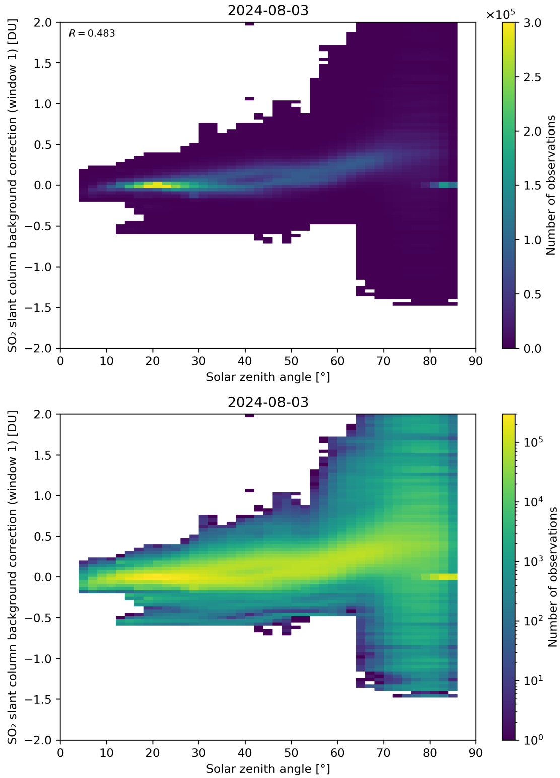
Figure 158: Scatter density plot of “Solar zenith angle” against “SO 2 slant column background correction (window 1)” for 2024-08-02 to 2024-08-04.
