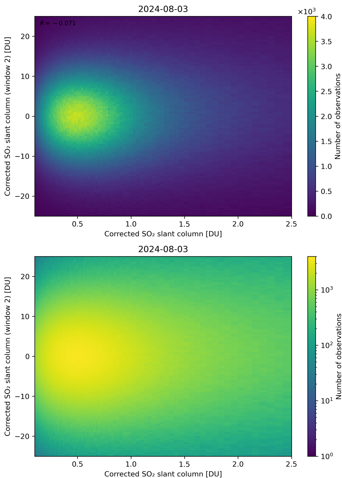
Figure 185: Scatter density plot of “Corrected SO 2 slant column” against “Corrected SO 2 slant column (window 2)” for 2024-08-02 to 2024-08-04.
