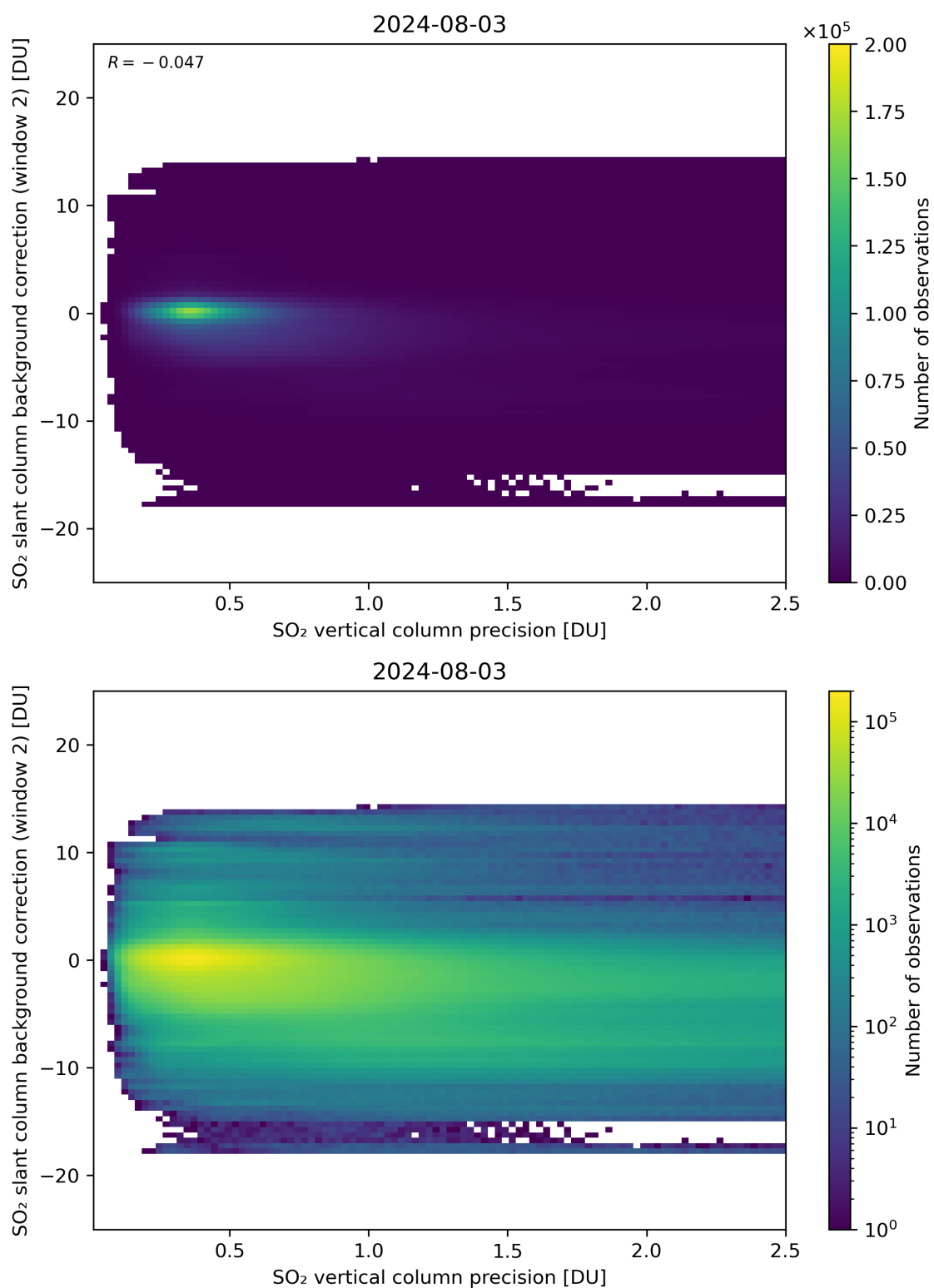
Figure 280: Scatter density plot of “SO 2 vertical column precision” against “SO 2 slant column background correction (window 2)” for 2024-08-02 to 2024-08-04.
