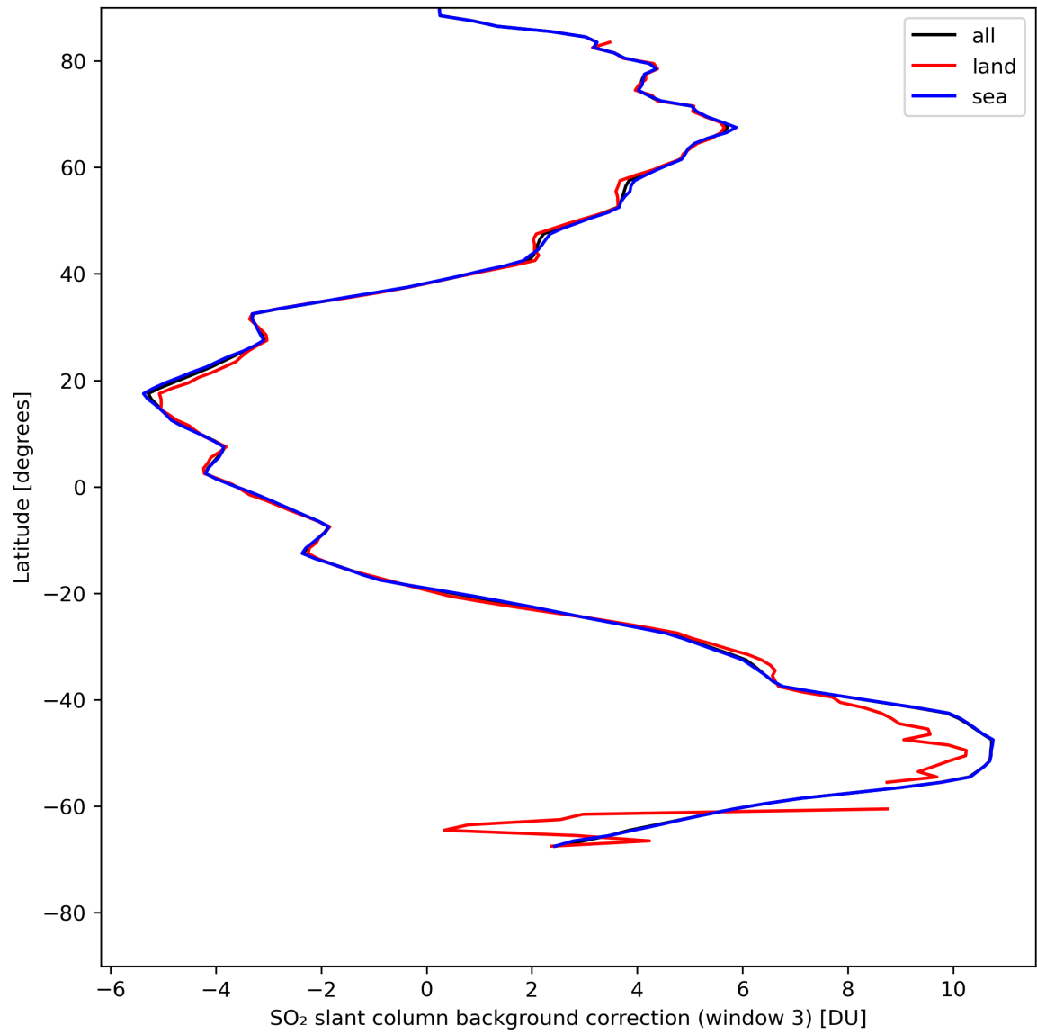
Figure 44: Zonal average of “SO 2 slant column background correction (window 3)” for 2024-08-02 to 2024-08-04.
