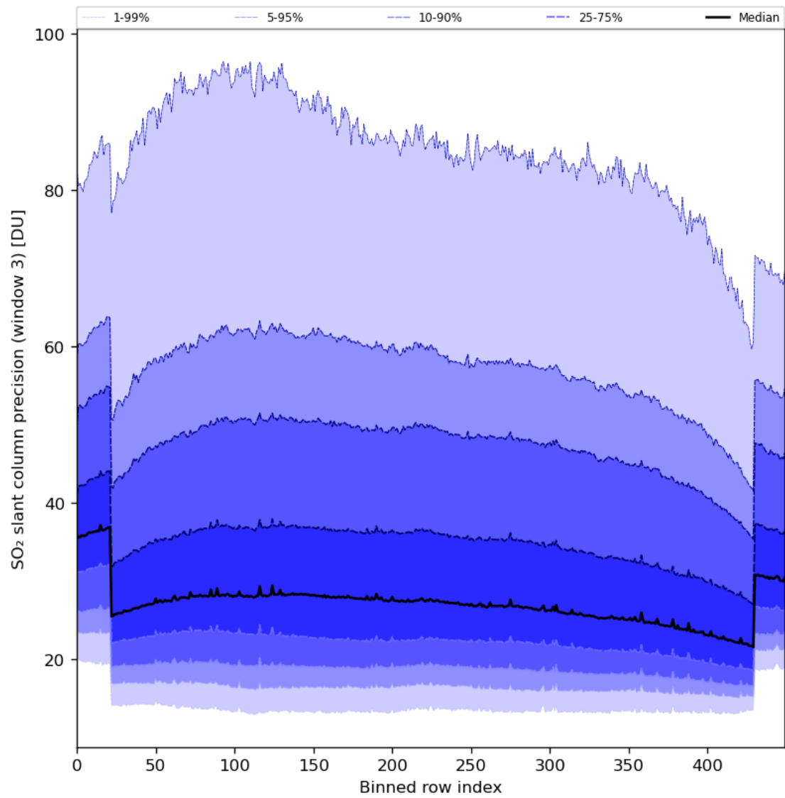
Figure 88: Along track statistics of “SO 2 slant column precision (window 3)” for 2024-08-02 to 2024-08-04
