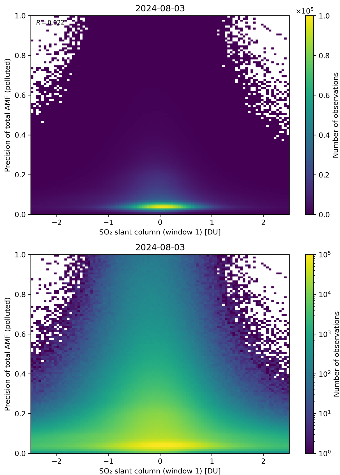
Figure 240: Scatter density plot of “SO 2 slant column (window 1)” against “Precision of total AMF (polluted)” for 2024-08-02 to 2024-08-04.
