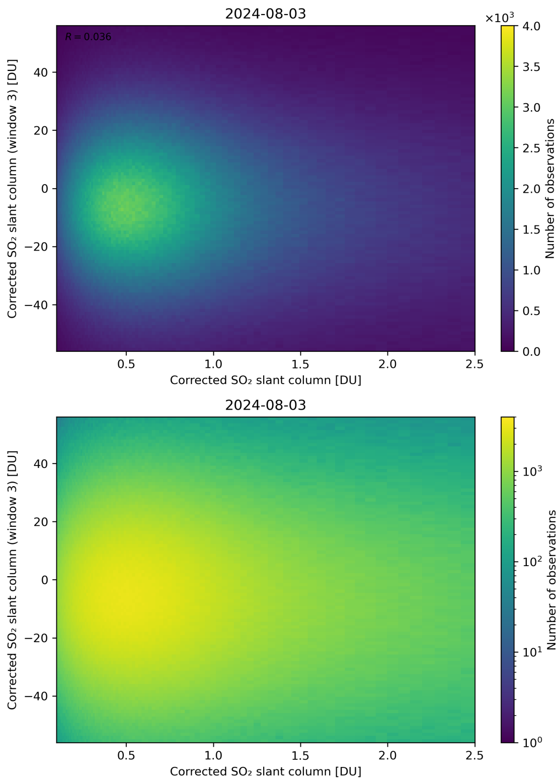
Figure 186: Scatter density plot of “Corrected SO 2 slant column” against “Corrected SO 2 slant column (window 3)” for 2024-08-02 to 2024-08-04.
