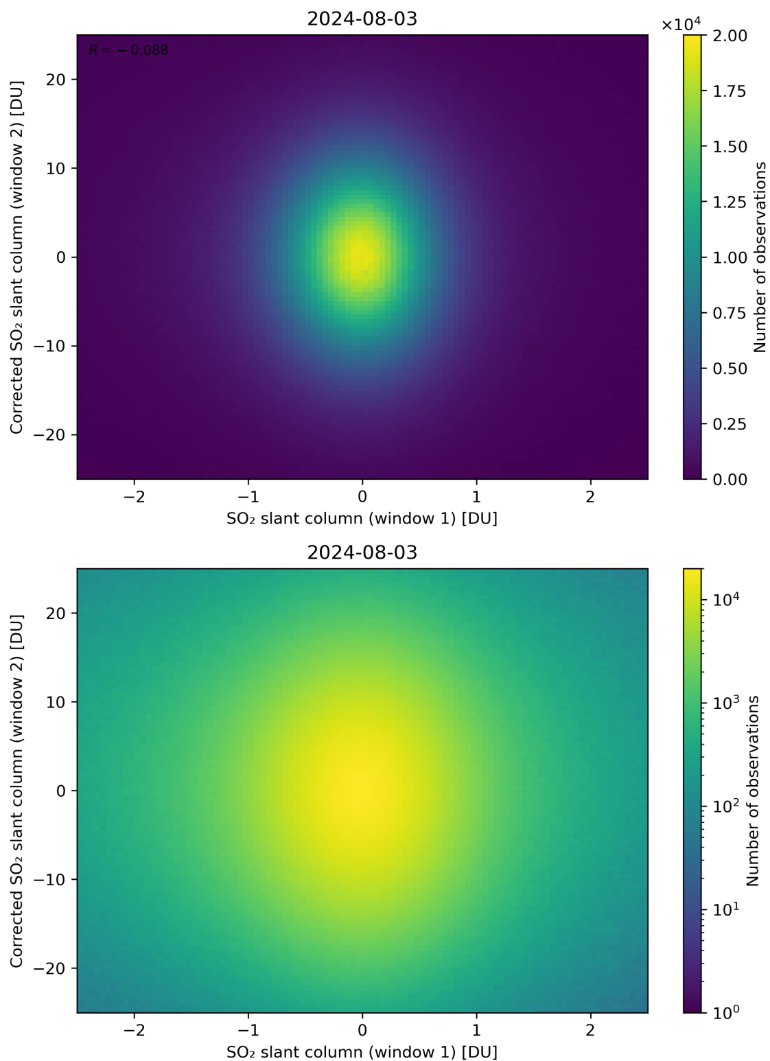
Figure 233: Scatter density plot of “SO 2 slant column (window 1)” against “Corrected SO 2 slant column (window 2)” for 2024-08-02 to 2024-08-04.
