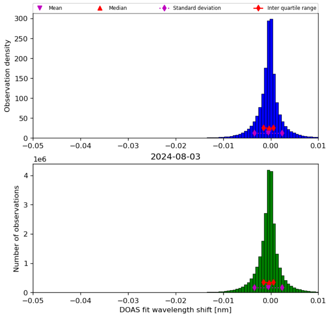
Figure 68: Histogram of “DOAS fit wavelength shift” for 2024-08-02 to 2024-08-04
