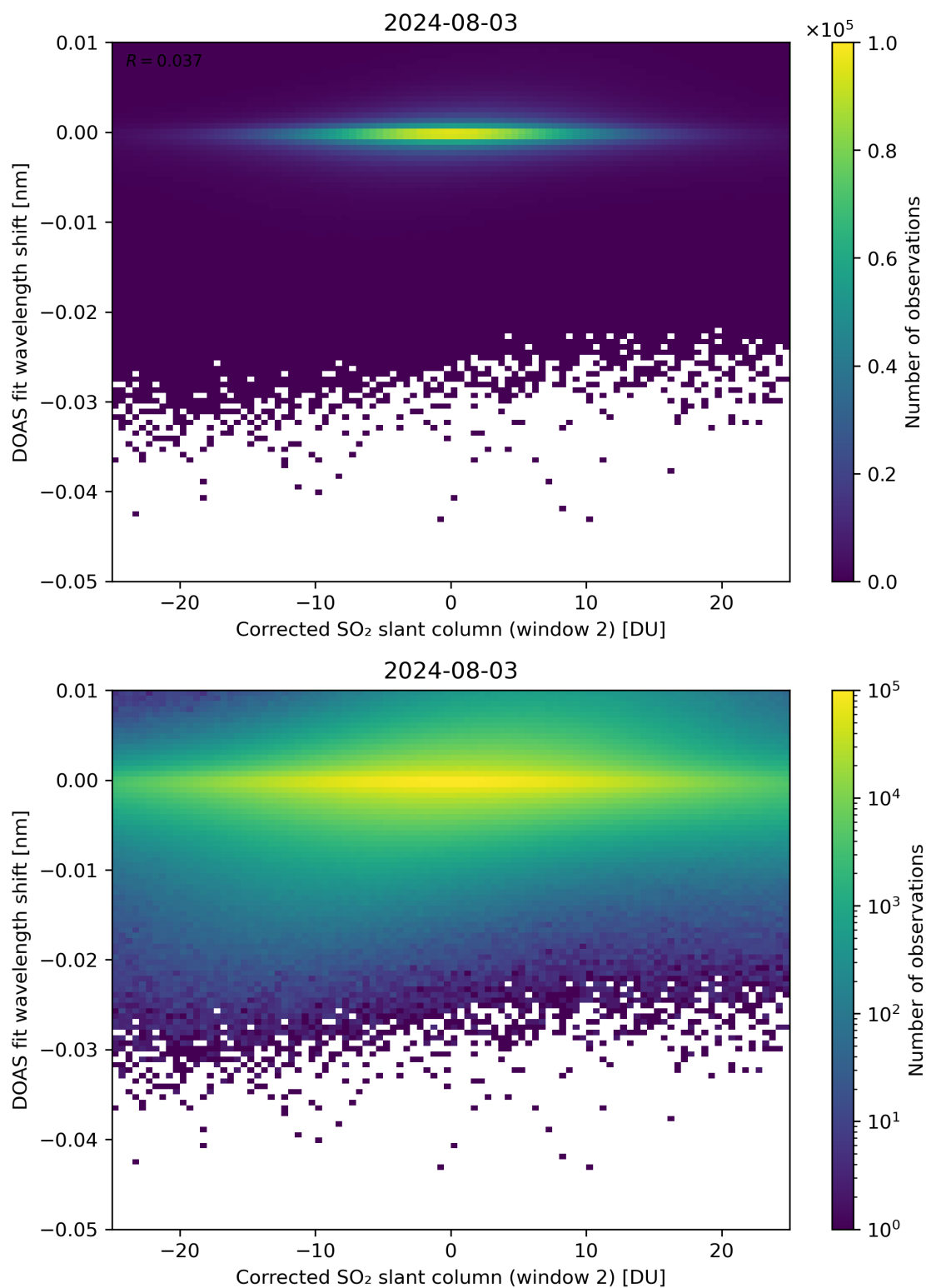
Figure 196: Scatter density plot of “Corrected SO 2 slant column (window 2)” against “DOAS fit wavelength shift” for 2024-08-02 to 2024-08-04.
