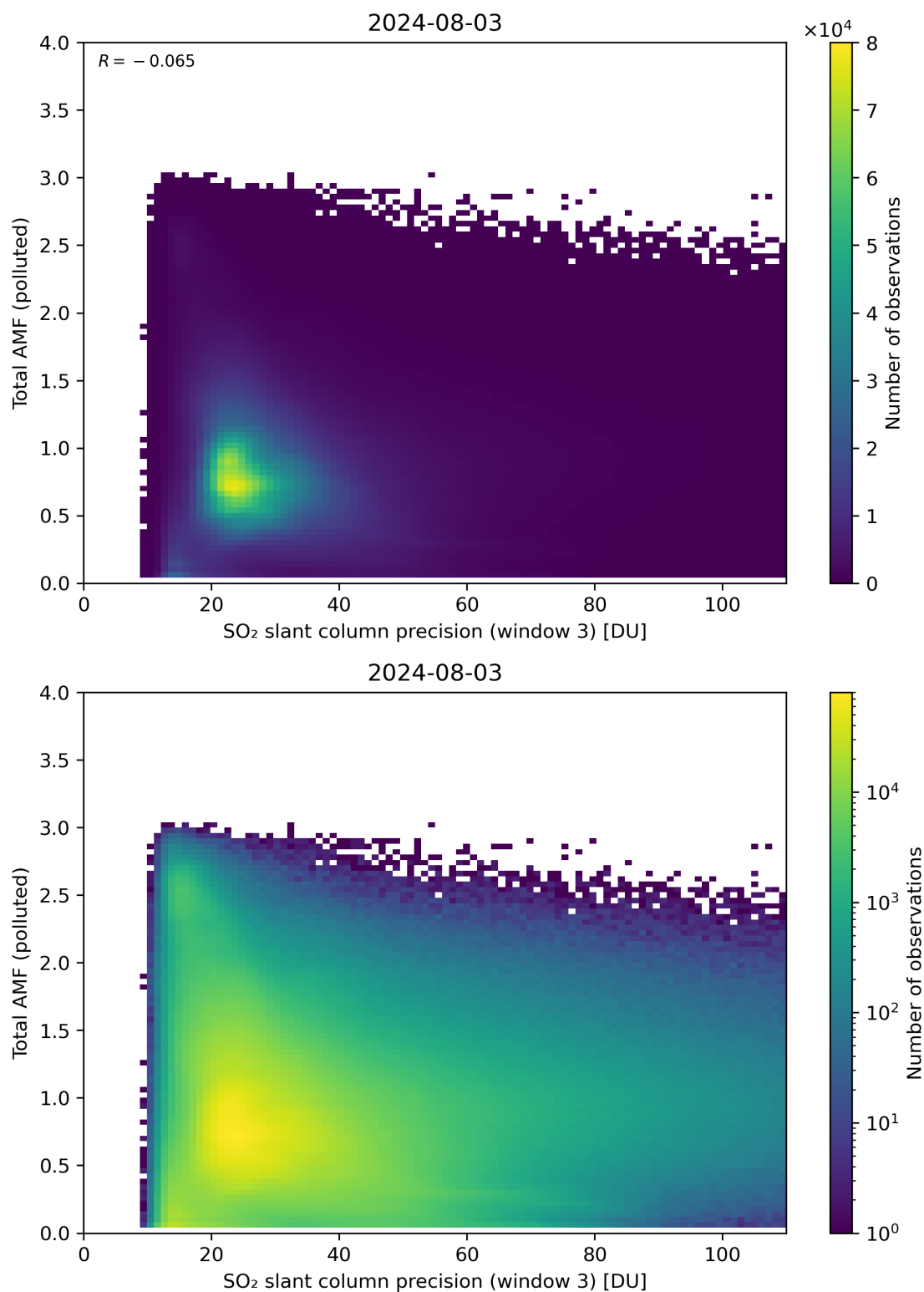
Figure 263: Scatter density plot of “SO 2 slant column precision (window 3)” against “Total AMF (polluted)” for 2024-08-02 to 2024-08-04.
