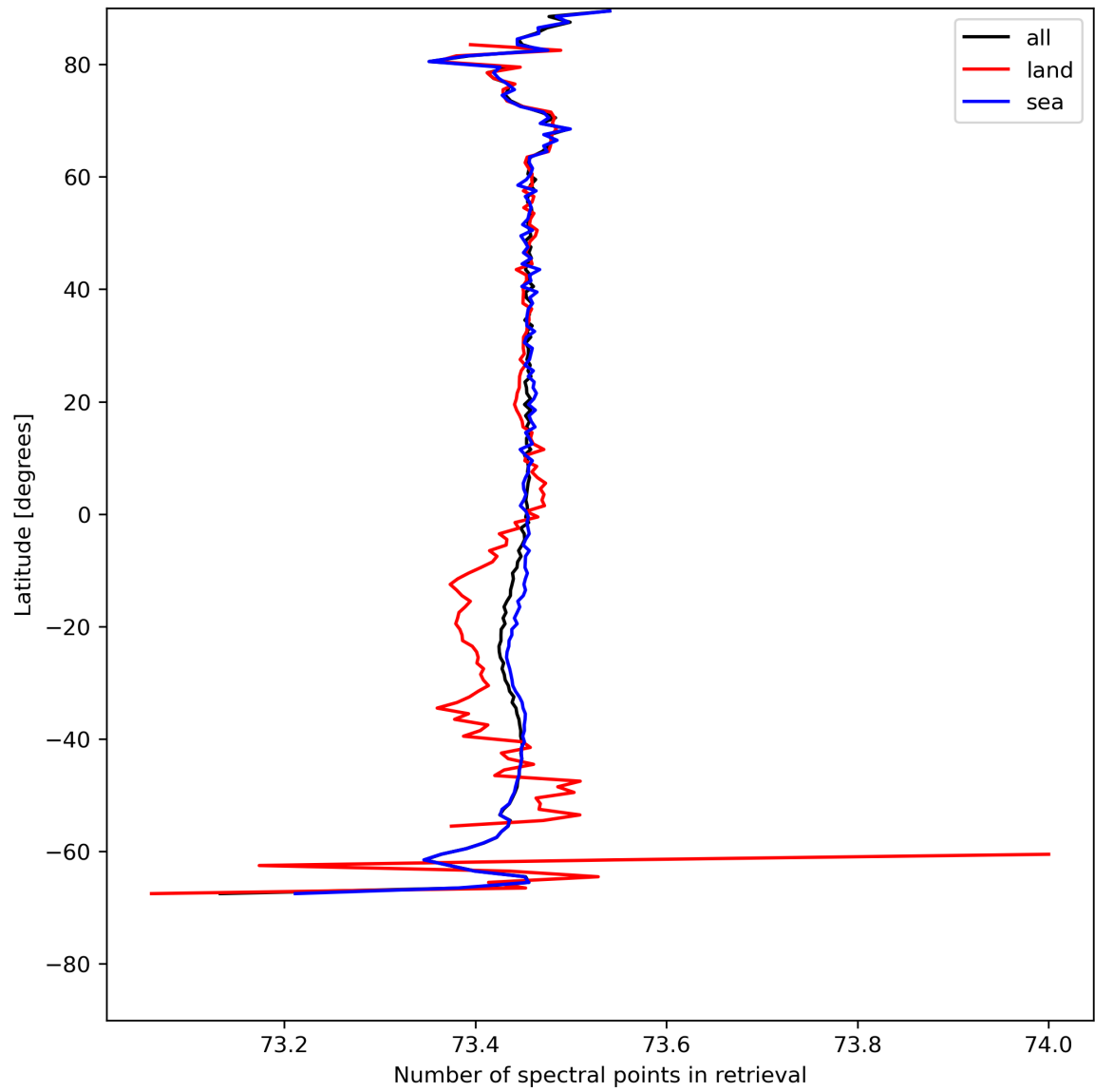
Figure 51: Zonal average of “Number of spectral points in retrieval” for 2024-08-02 to 2024-08-04.
