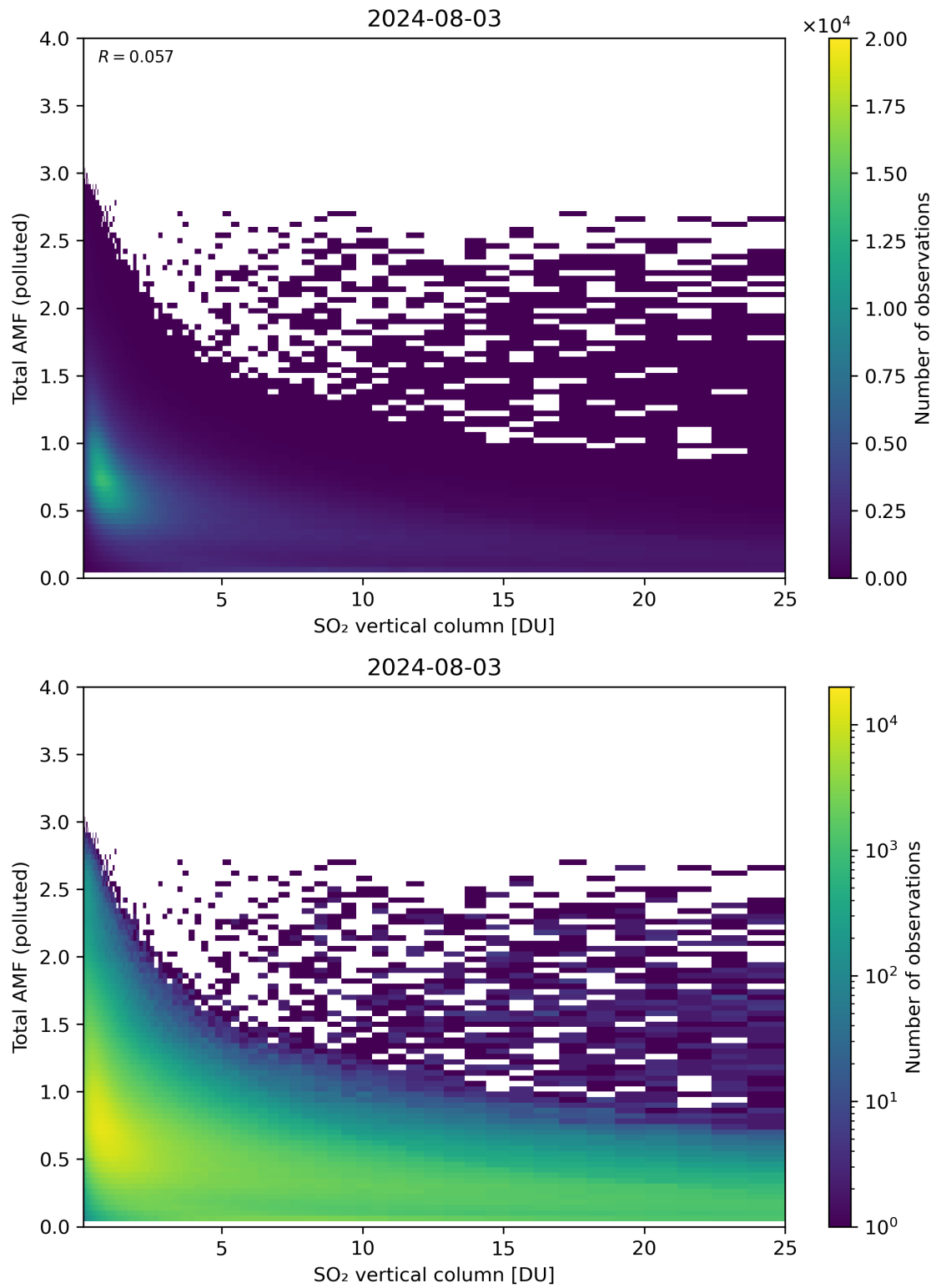
Figure 305: Scatter density plot of “SO 2 vertical column” against “Total AMF (polluted)” for 2024-08-02 to 2024-08-04.
