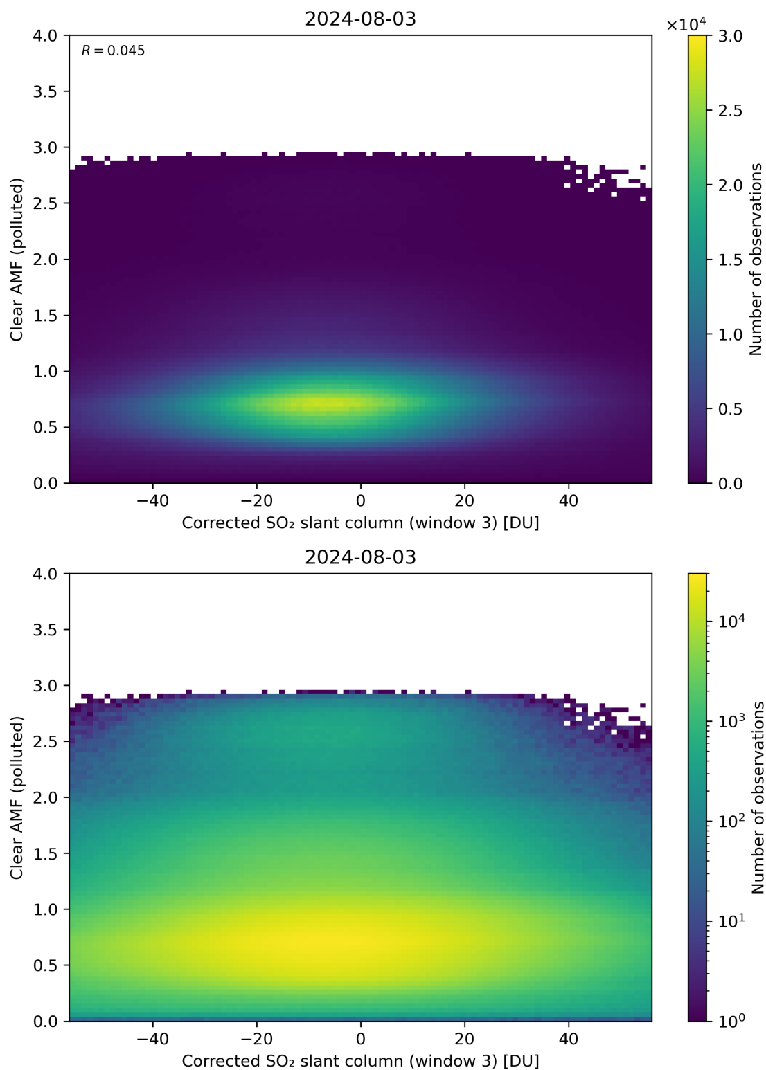
Figure 209: Scatter density plot of “Corrected SO 2 slant column (window 3)” against “Clear AMF (polluted)” for 2024-08-02 to 2024-08-04.
