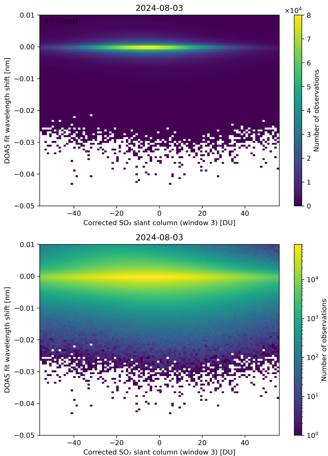
Figure 206: Scatter density plot of “Corrected SO 2 slant column (window 3)” against “DOAS fit wavelength shift” for 2024-08-02 to 2024-08-04.
