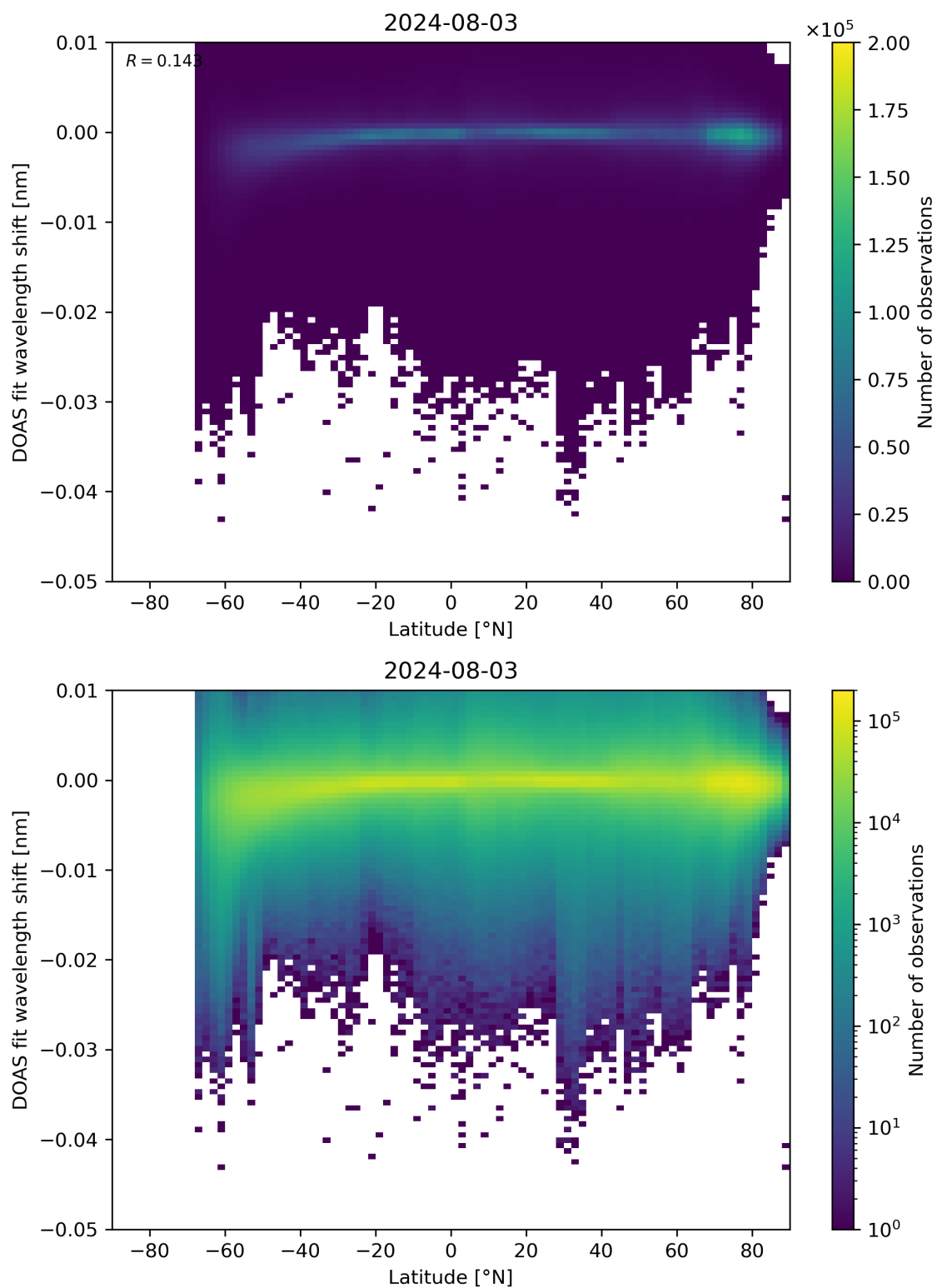
Figure 142: Scatter density plot of “Latitude” against “DOAS fit wavelength shift” for 2024-08-02 to 2024-08-04.
