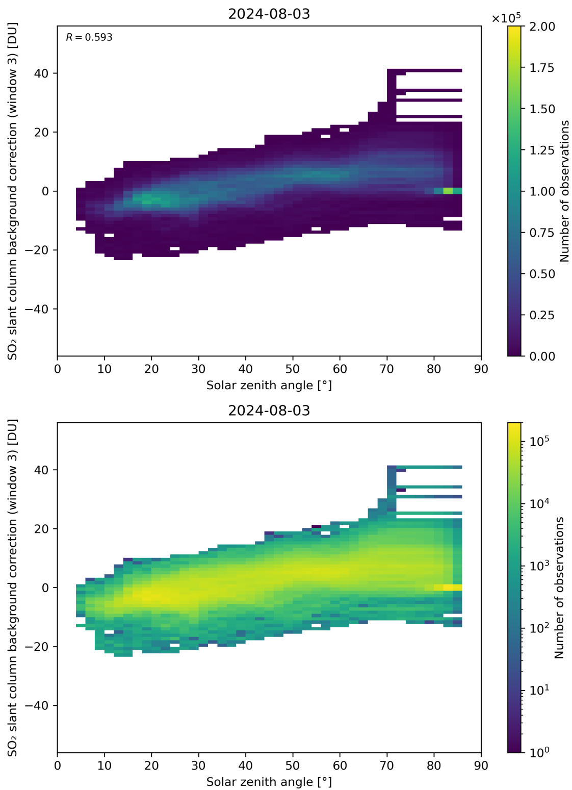
Figure 160: Scatter density plot of “Solar zenith angle” against “SO 2 slant column background correction (window 3)” for 2024-08-02 to 2024-08-04.
