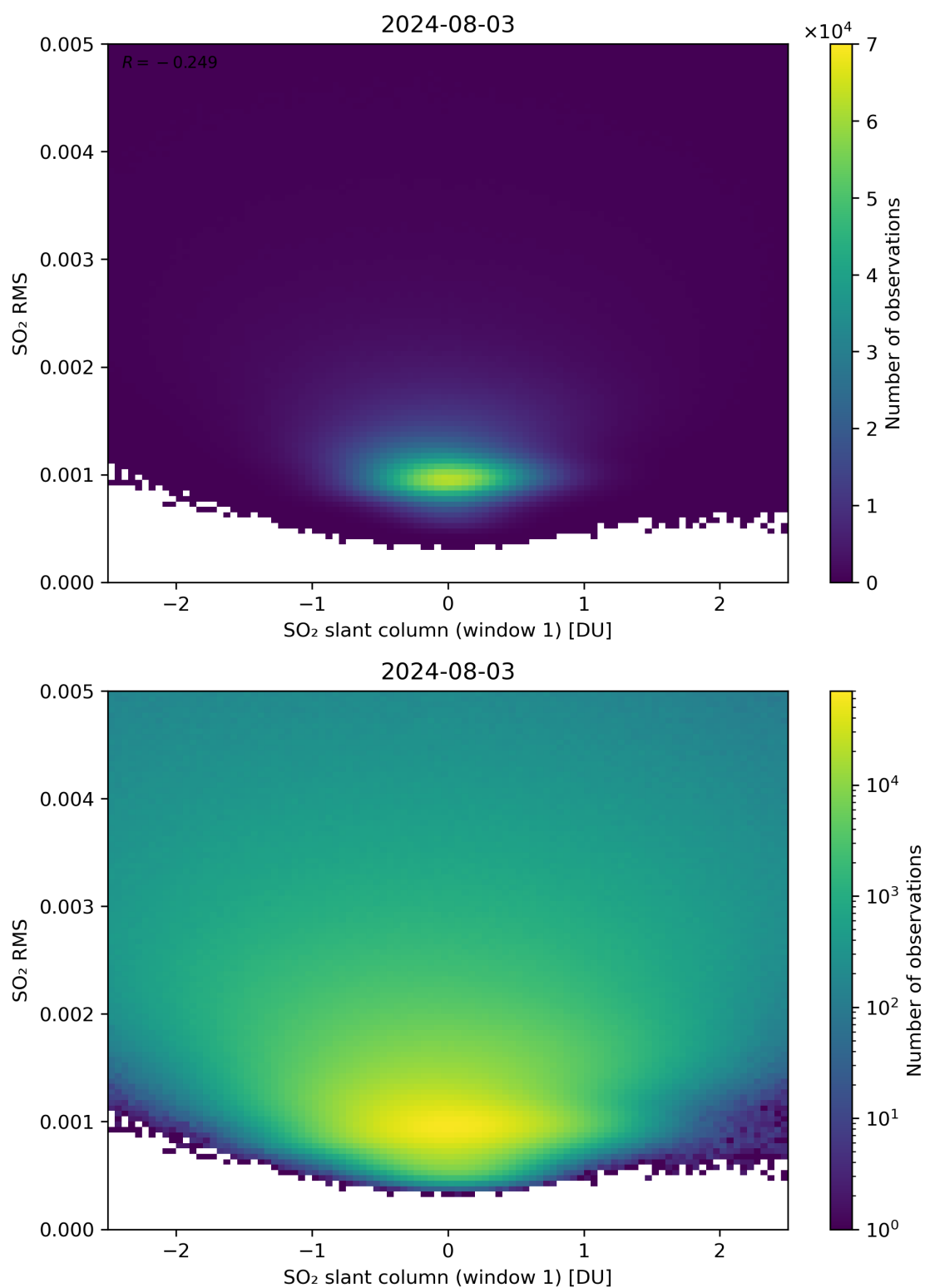
Figure 217: Scatter density plot of “SO 2 slant column (window 1)” against “SO 2 RMS” for 2024-08-02 to 2024-08-04.
