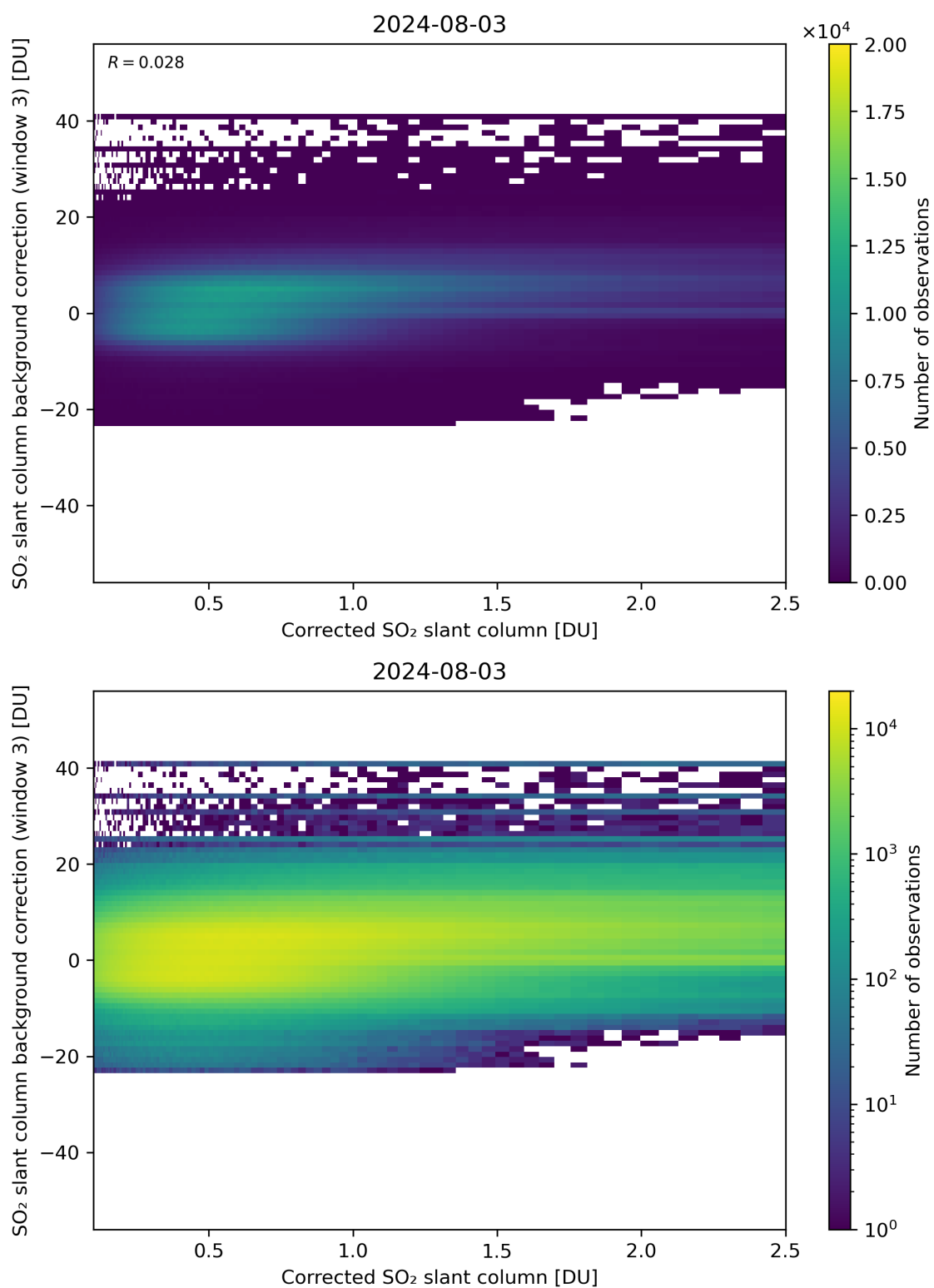
Figure 180: Scatter density plot of “Corrected SO 2 slant column” against “SO 2 slant column background correction (window 3)” for 2024-08-02 to 2024-08-04.
