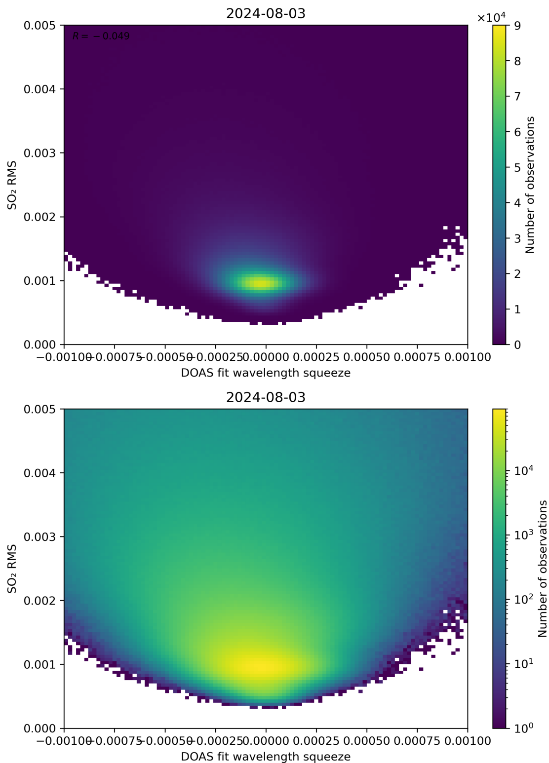
Figure 132: Scatter density plot of “DOAS fit wavelength squeeze” against “SO 2 RMS” for 2024-08-02 to 2024-08-04.
