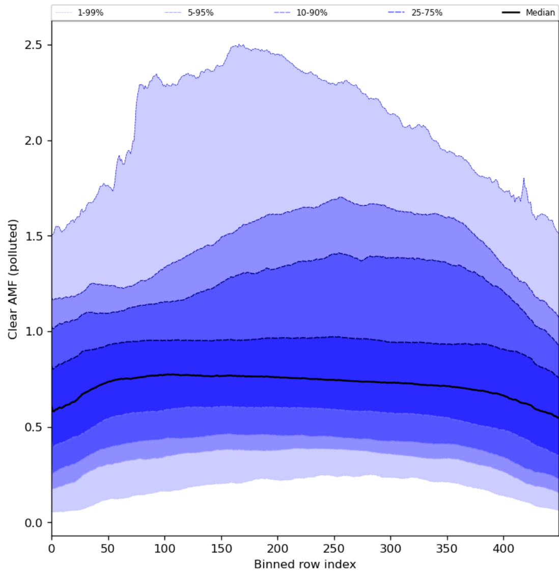
Figure 96: Along track statistics of “Clear AMF (polluted)” for 2024-08-02 to 2024-08-04
