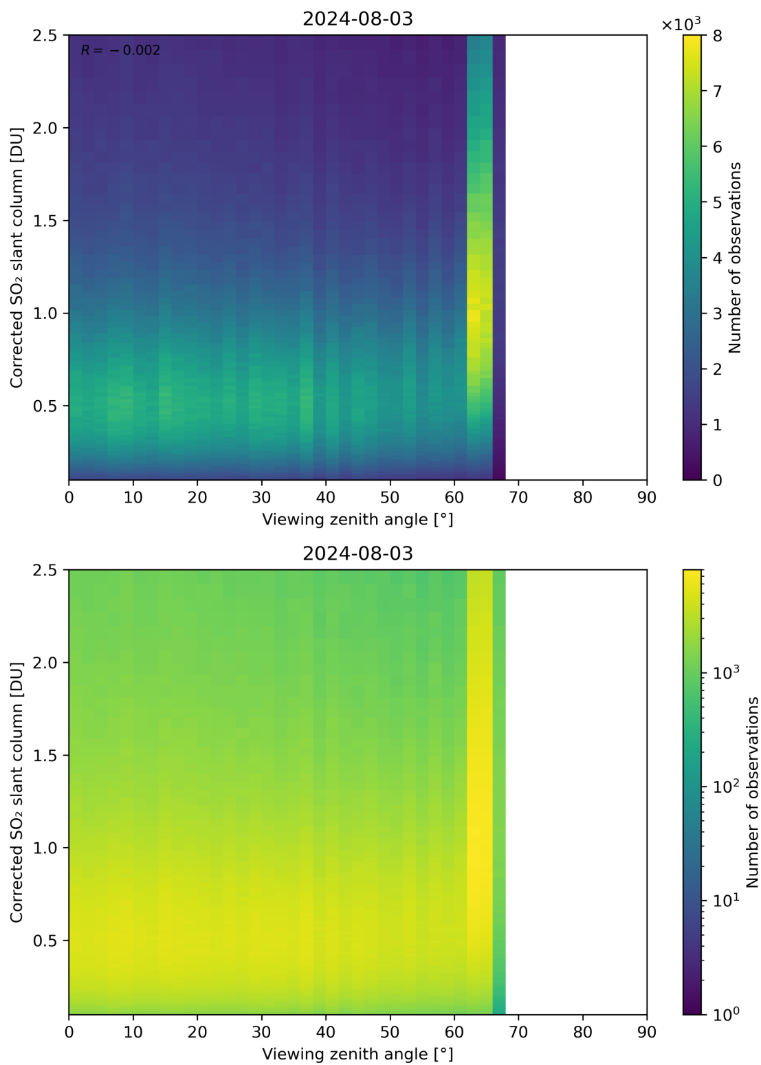
Figure 317: Scatter density plot of “Viewing zenith angle” against “Corrected SO 2 slant column” for 2024-08-02 to 2024-08-04.
