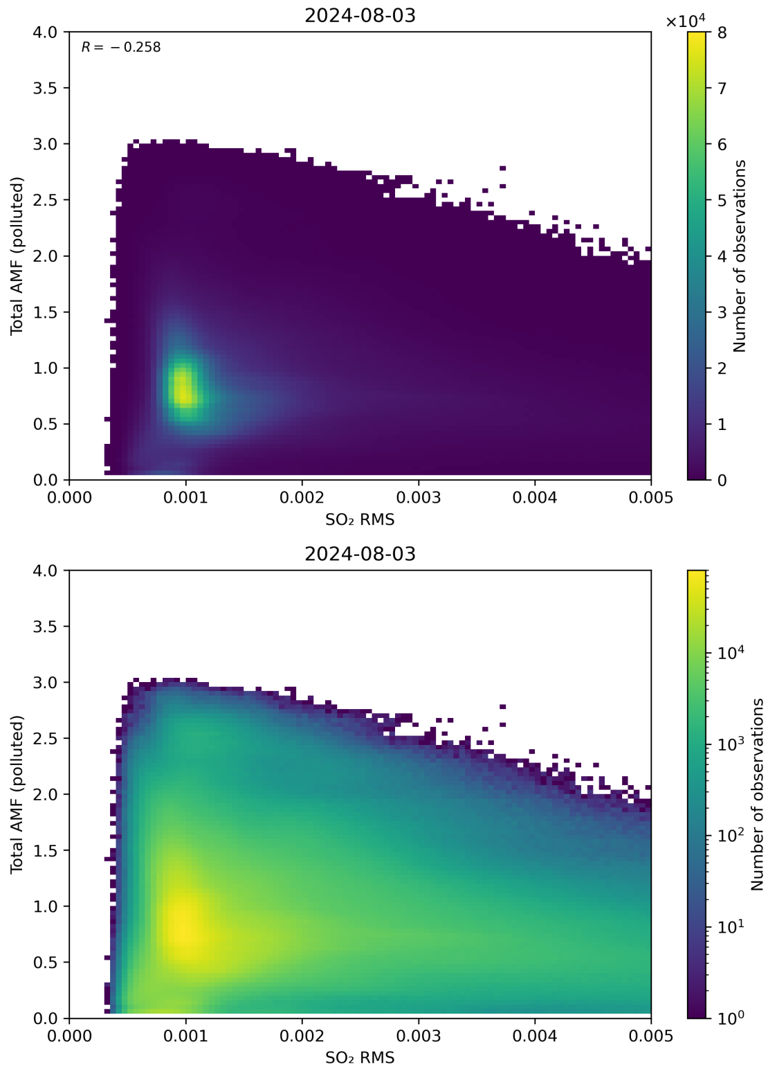
Figure 137: Scatter density plot of “SO 2 RMS” against “Total AMF (polluted)” for 2024-08-02 to 2024-08-04.
