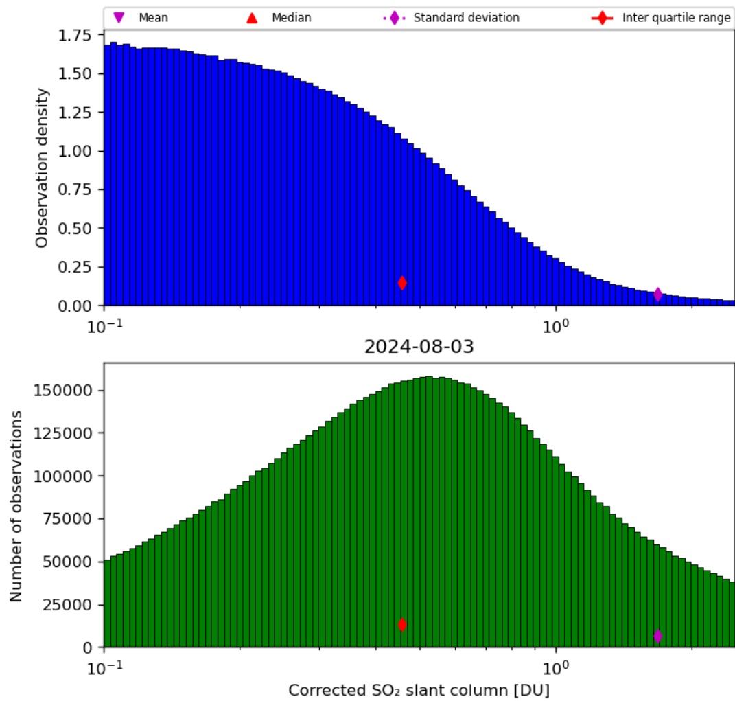
Figure 55: Histogram of “Corrected SO 2 slant column” for 2024-08-02 to 2024-08-04
