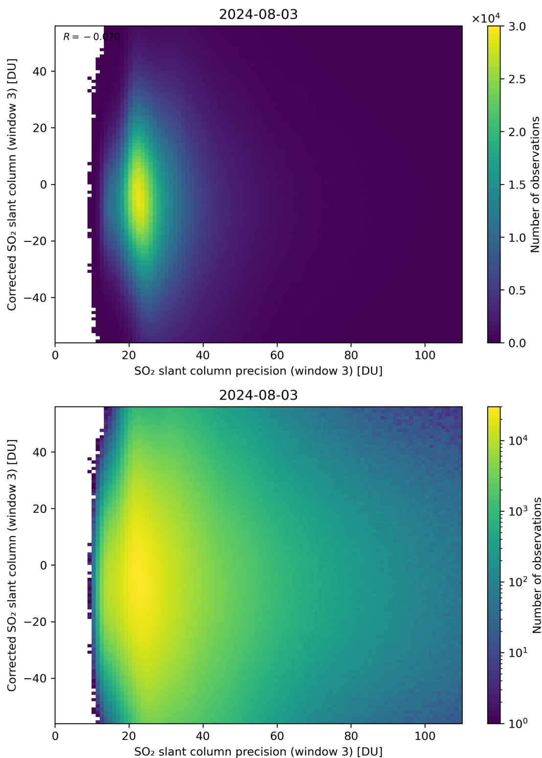
Figure 262: Scatter density plot of “SO 2 slant column precision (window 3)” against “Corrected SO 2 slant column (window 3)” for 2024-08-02 to 2024-08-04.
