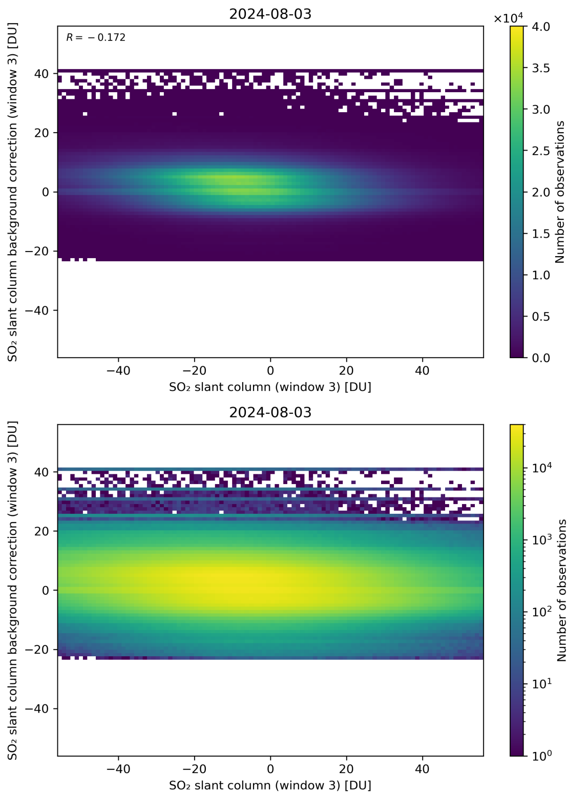
Figure 253: Scatter density plot of “SO 2 slant column (window 3)” against “SO 2 slant column background correction (window 3)” for 2024-08-02 to 2024-08-04.
