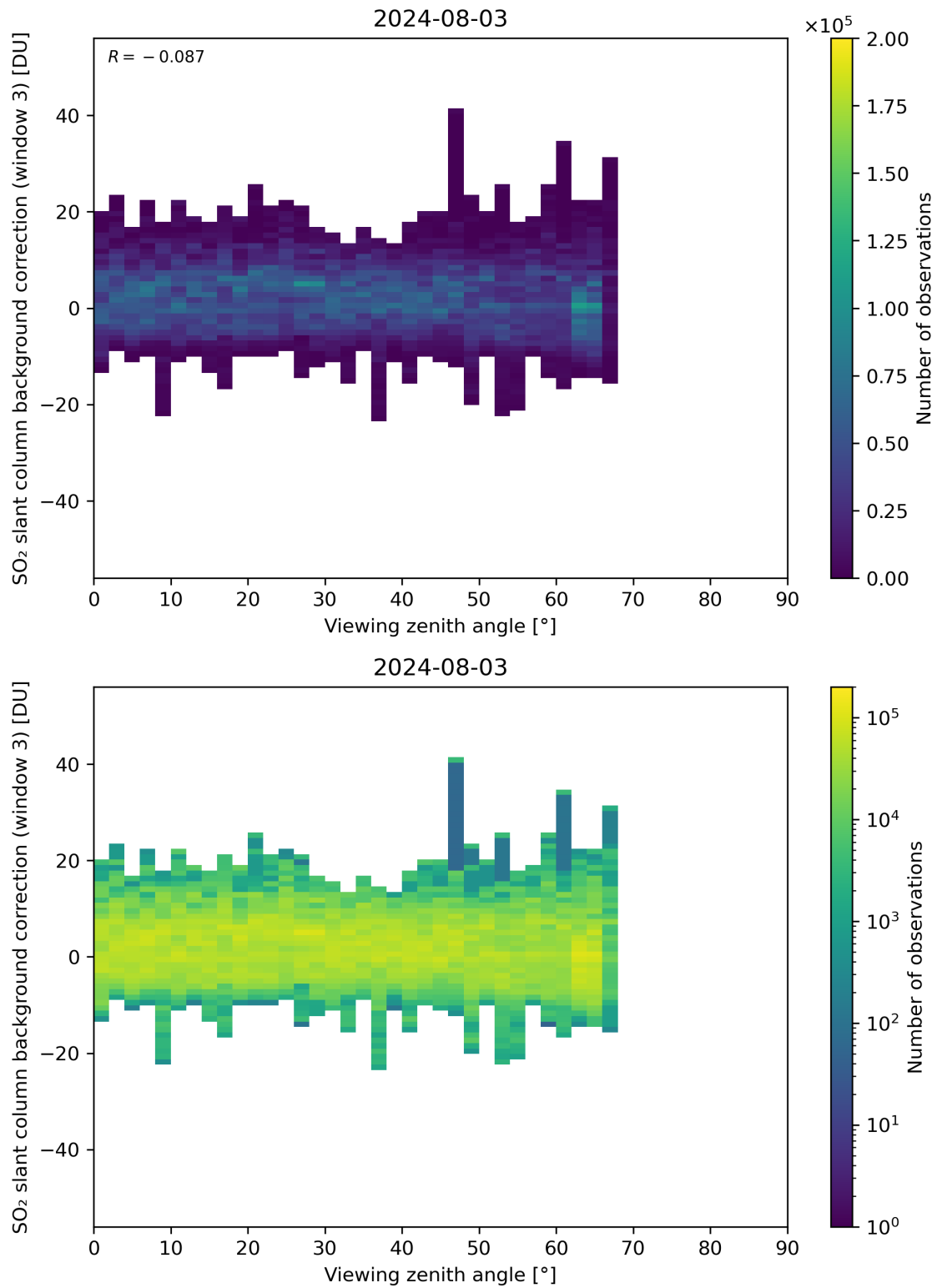
Figure 310: Scatter density plot of “Viewing zenith angle” against “SO 2 slant column background correction (window 3)” for 2024-08-02 to 2024-08-04.
