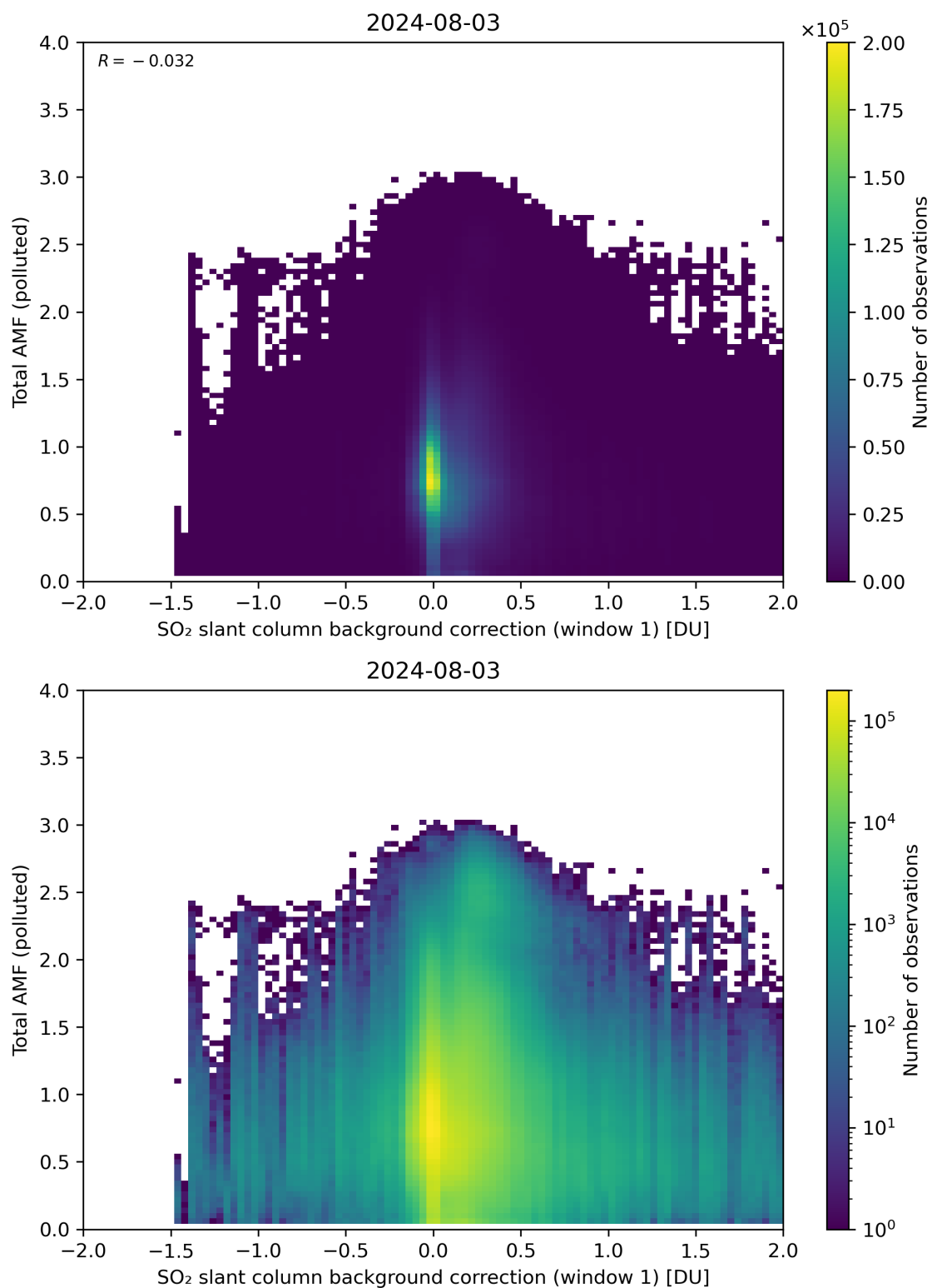
Figure 109: Scatter density plot of “SO 2 slant column background correction (window 1)” against “Total AMF (polluted)” for 2024-08-02 to 2024-08-04.
