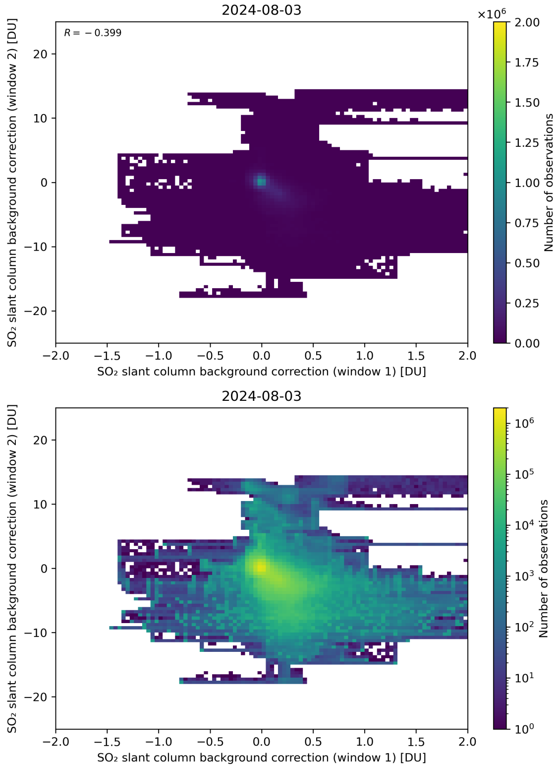
Figure 98: Scatter density plot of “SO 2 slant column background correction (window 1)” against “SO 2 slant column background correction (window 2)” for 2024-08-02 to 2024-08-04.
