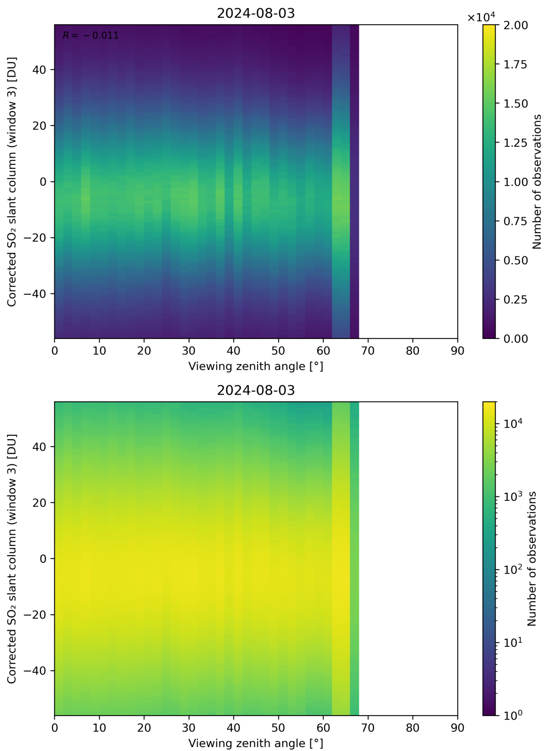
Figure 319: Scatter density plot of “Viewing zenith angle” against “Corrected SO 2 slant column (window 3)” for 2024-08-02 to 2024-08-04.
