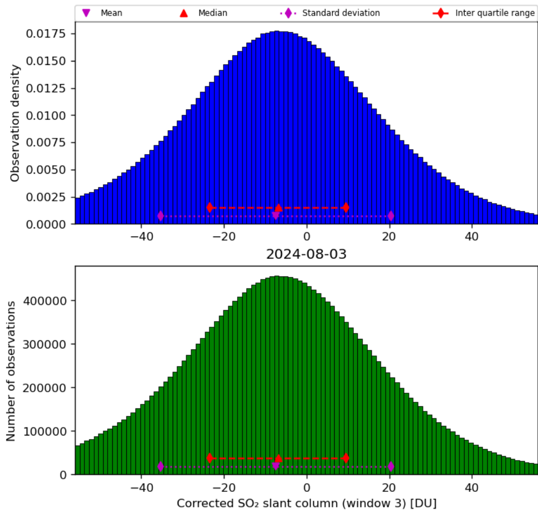
Figure 66: Histogram of “Corrected SO 2 slant column (window 3)” for 2024-08-02 to 2024-08-04
