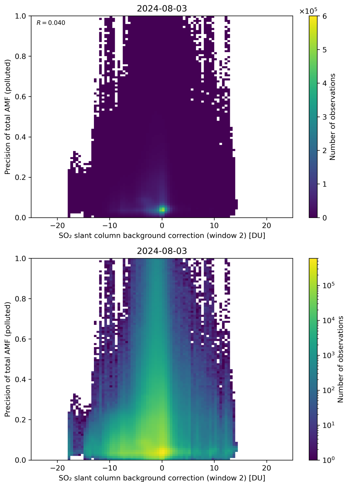
Figure 120: Scatter density plot of “SO 2 slant column background correction (window 2)” against “Precision of total AMF (polluted)” for 2024-08-02 to 2024-08-04.
