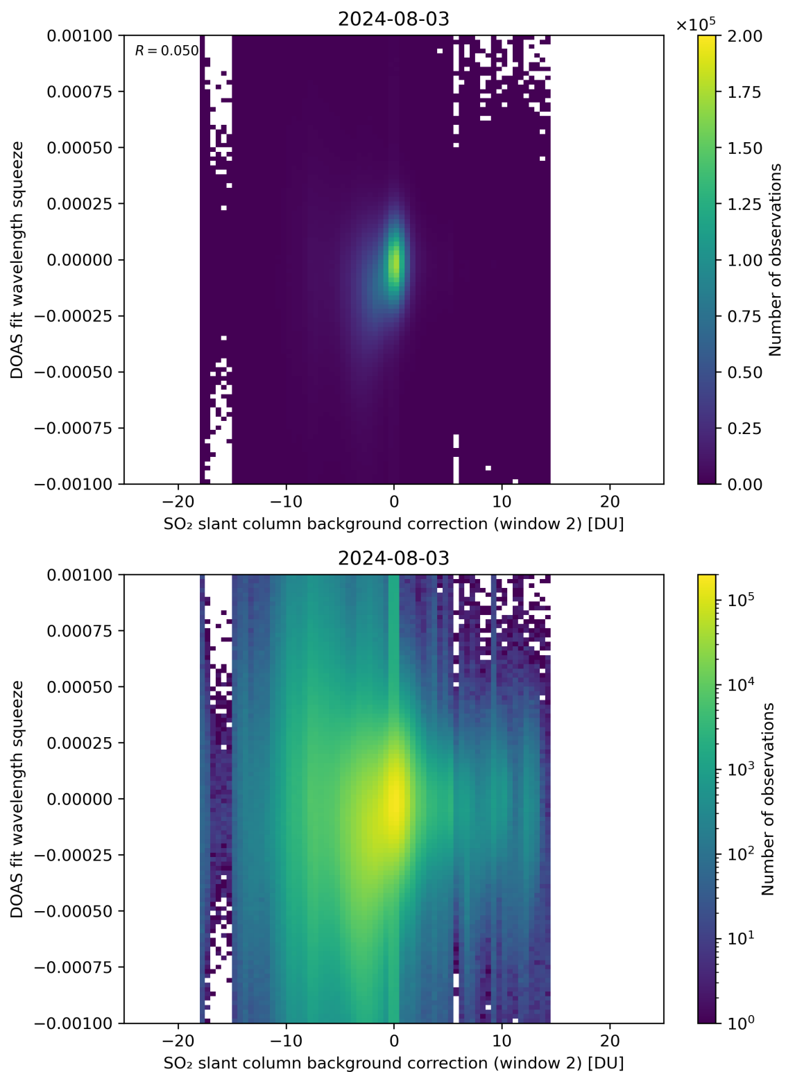
Figure 113: Scatter density plot of “SO 2 slant column background correction (window 2)” against “DOAS fit wavelength squeeze” for 2024-08-02 to 2024-08-04.
