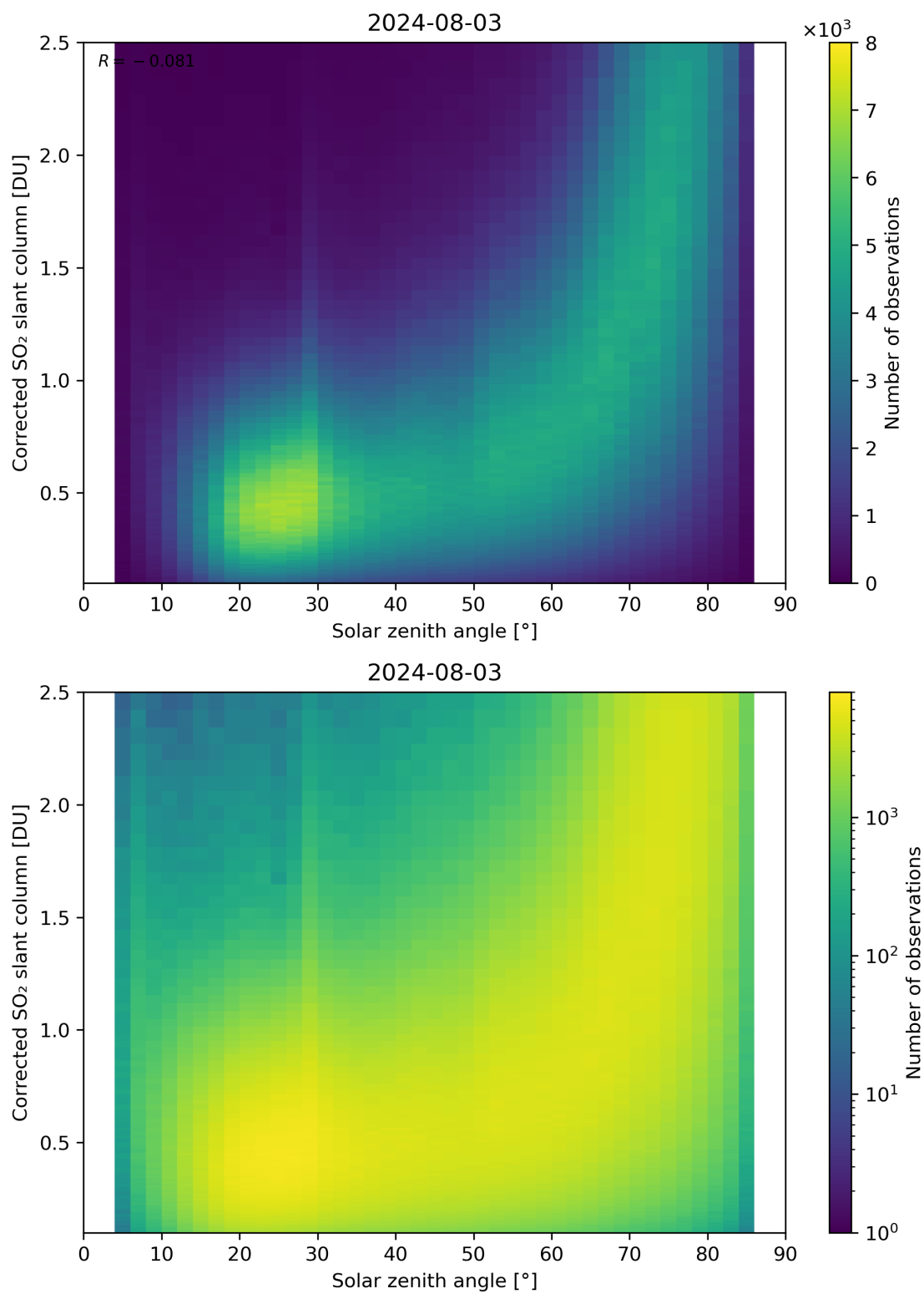
Figure 166: Scatter density plot of “Solar zenith angle” against “Corrected SO 2 slant column” for 2024-08-02 to 2024-08-04.
