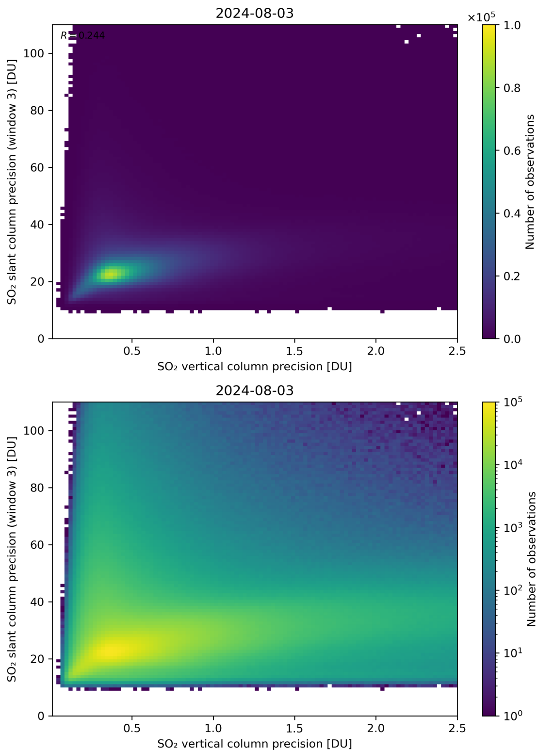
Figure 293: Scatter density plot of “SO 2 vertical column precision” against “SO 2 slant column precision (window 3)” for 2024-08-02 to 2024-08-04.
