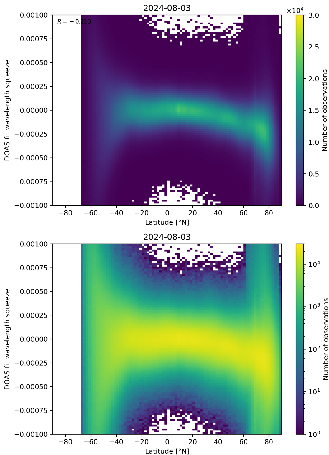
Figure 143: Scatter density plot of “Latitude” against “DOAS fit wavelength squeeze” for 2024-08-02 to 2024-08-04.
