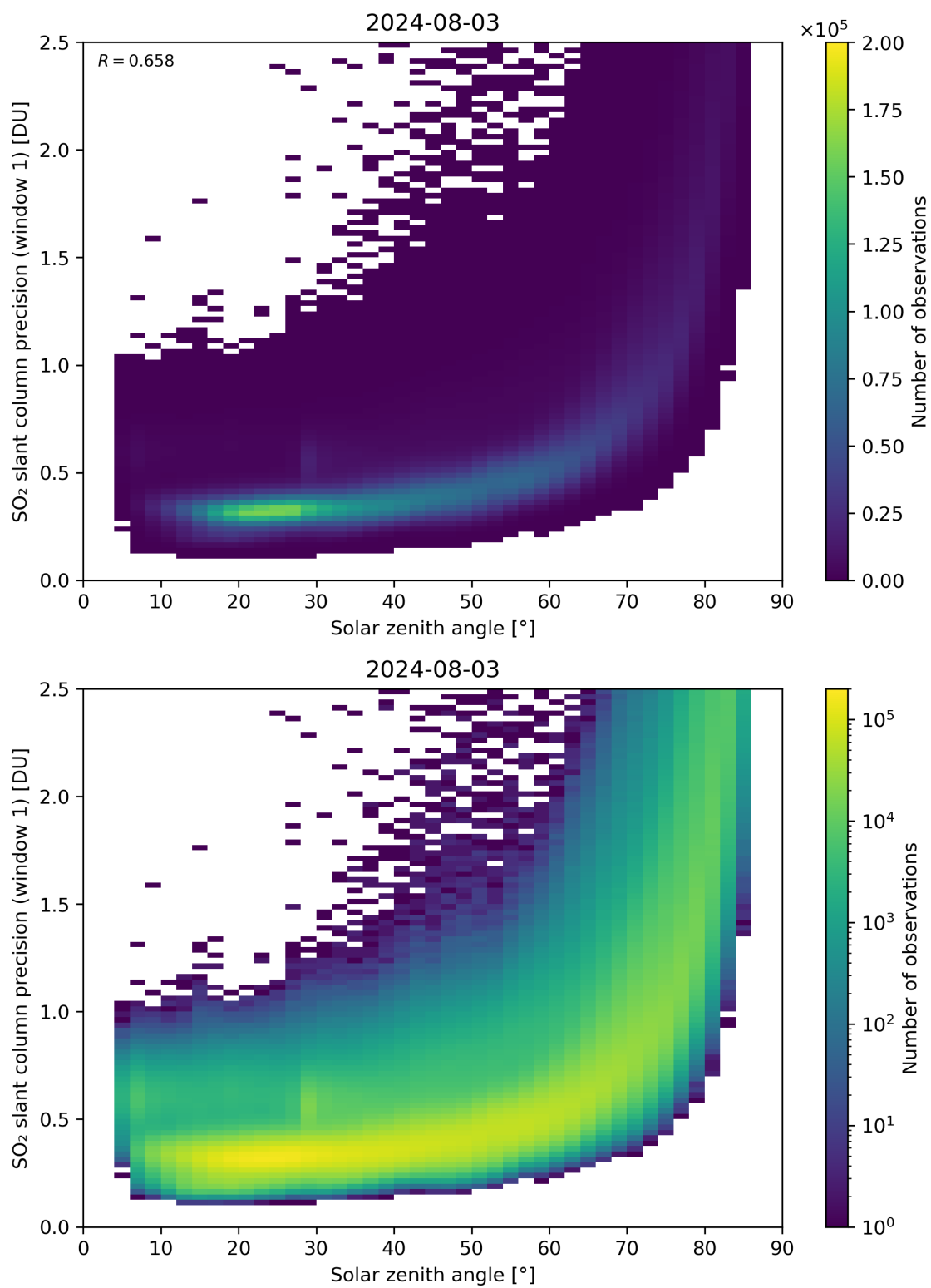
Figure 170: Scatter density plot of “Solar zenith angle” against “SO 2 slant column precision (window 1)” for 2024-08-02 to 2024-08-04.
