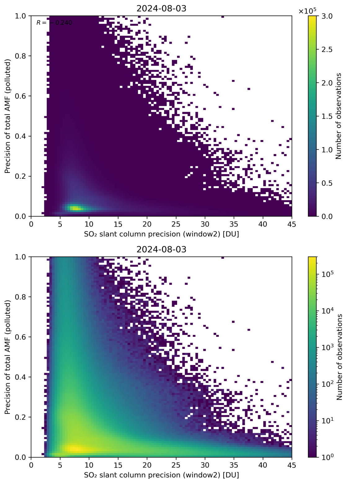
Figure 252: Scatter density plot of “SO 2 slant column precision (window2)” against “Precision of total AMF (polluted)” for 2024-08-02 to 2024-08-04.
