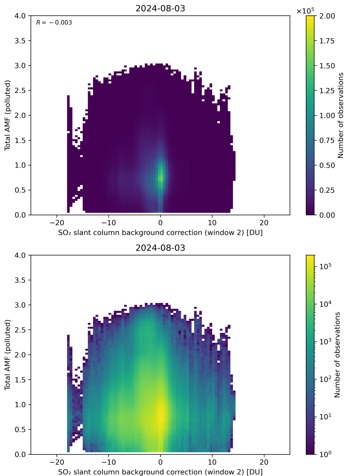
Figure 119: Scatter density plot of “SO 2 slant column background correction (window 2)” against “Total AMF (polluted)” for 2024-08-02 to 2024-08-04.
