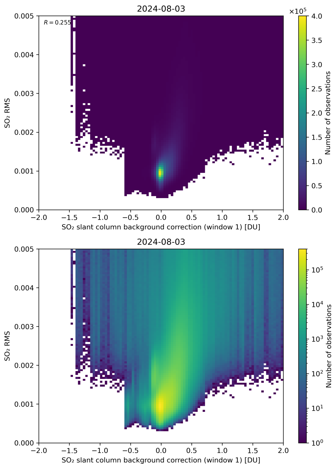
Figure 102: Scatter density plot of “SO 2 slant column background correction (window 1)” against “SO 2 RMS” for 2024-08-02 to 2024-08-04.
