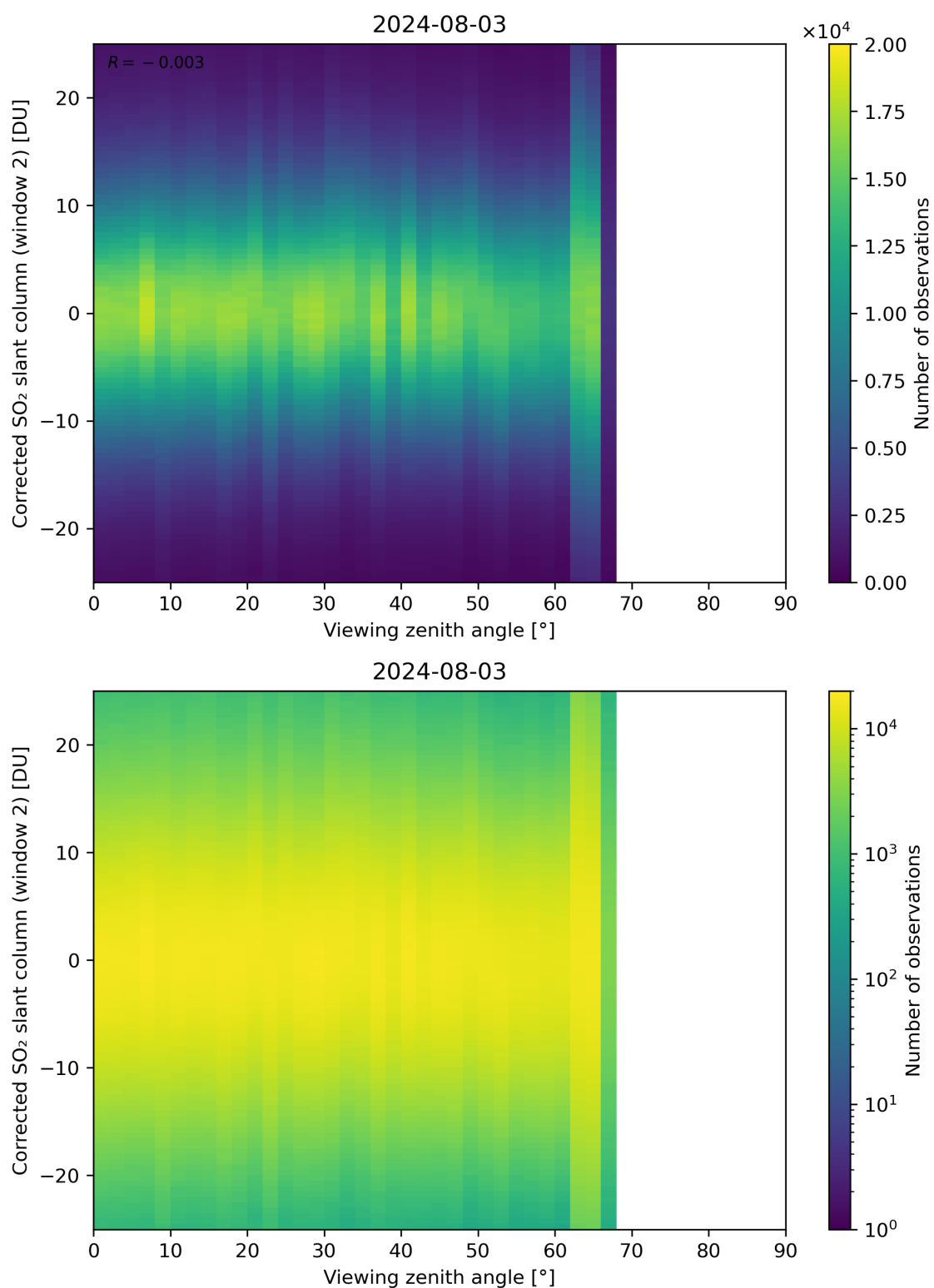
Figure 318: Scatter density plot of “Viewing zenith angle” against “Corrected SO 2 slant column (window 2)” for 2024-08-02 to 2024-08-04.
