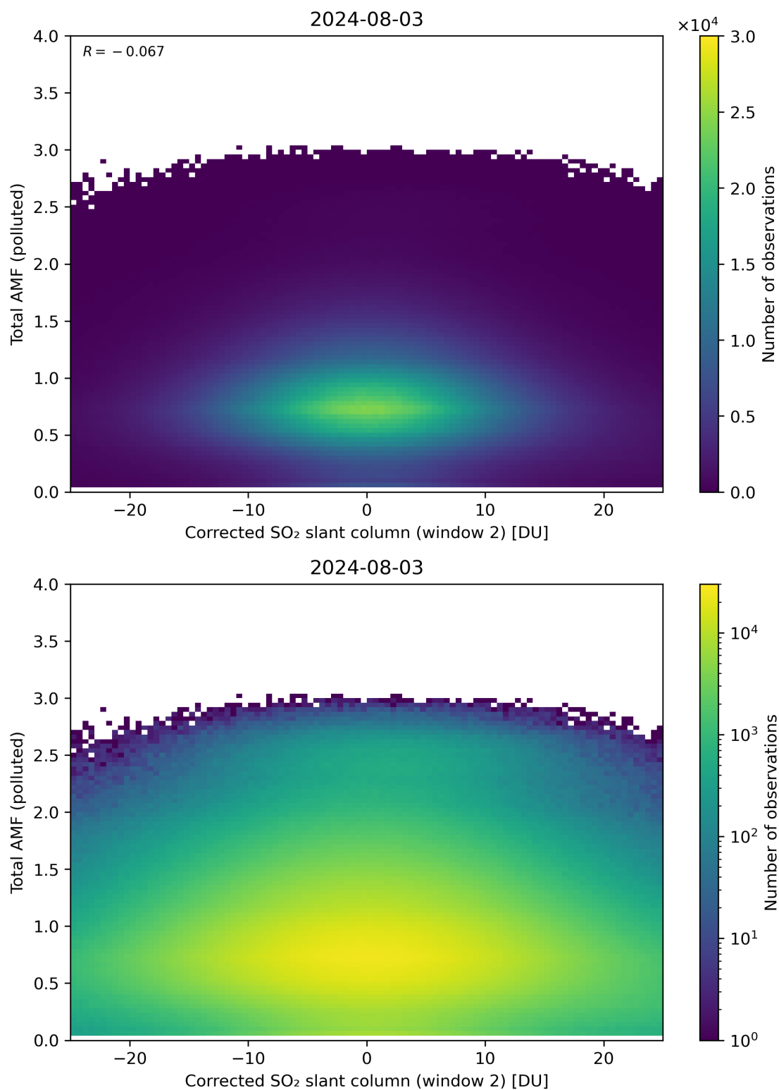
Figure 203: Scatter density plot of “Corrected SO 2 slant column (window 2)” against “Total AMF (polluted)” for 2024-08-02 to 2024-08-04.
