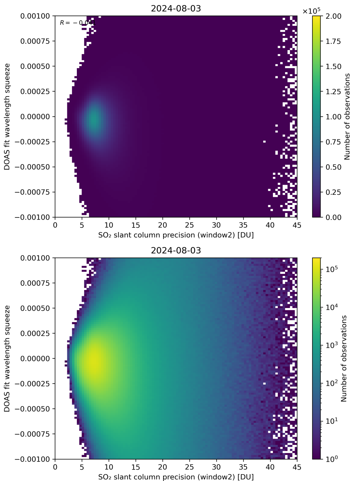
Figure 244: Scatter density plot of “SO 2 slant column precision (window2)” against “DOAS fit wavelength squeeze” for 2024-08-02 to 2024-08-04.
