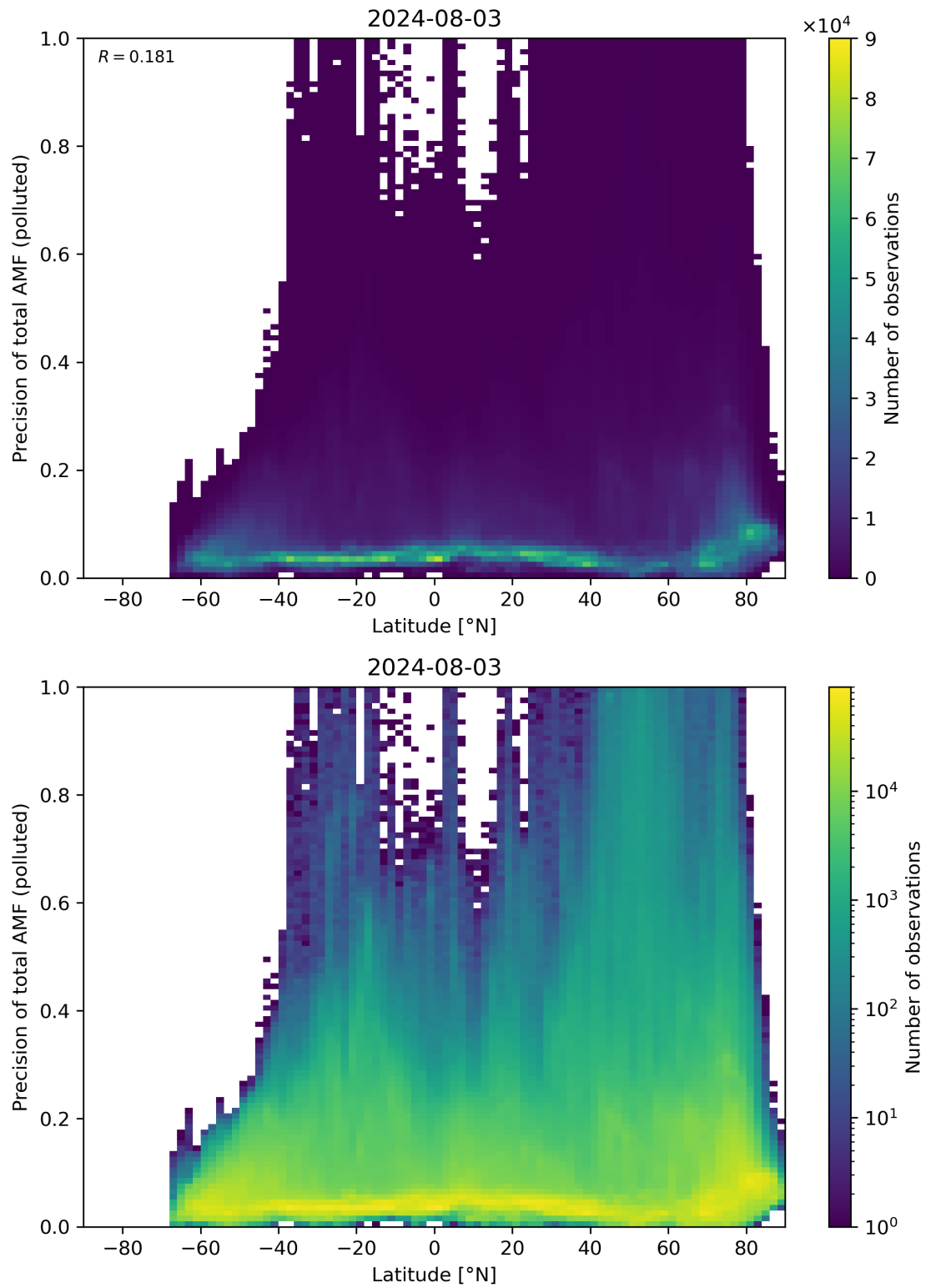
Figure 155: Scatter density plot of “Latitude” against “Precision of total AMF (polluted)” for 2024-08-02 to 2024-08-04.
