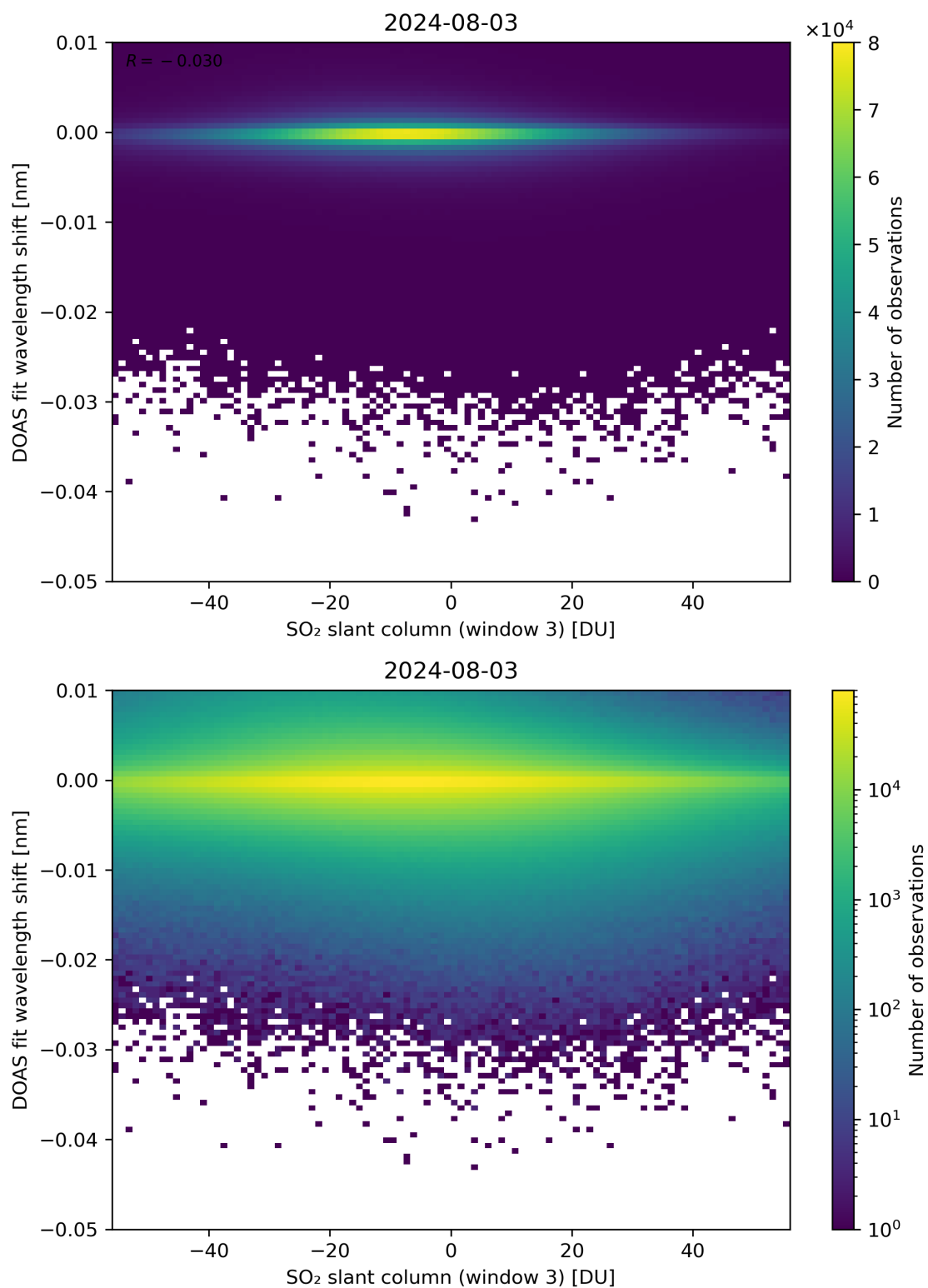
Figure 254: Scatter density plot of “SO 2 slant column (window 3)” against “DOAS fit wavelength shift” for 2024-08-02 to 2024-08-04.
