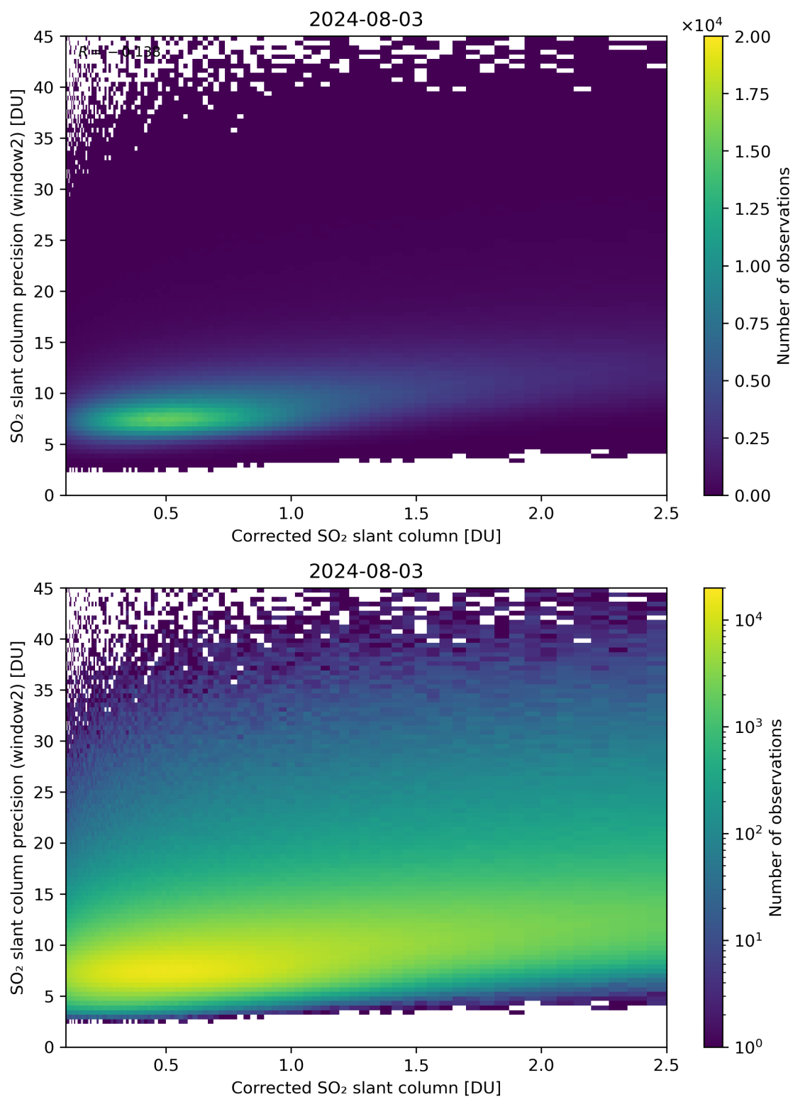
Figure 189: Scatter density plot of “Corrected SO 2 slant column” against “SO 2 slant column precision (window2)” for 2024-08-02 to 2024-08-04.
