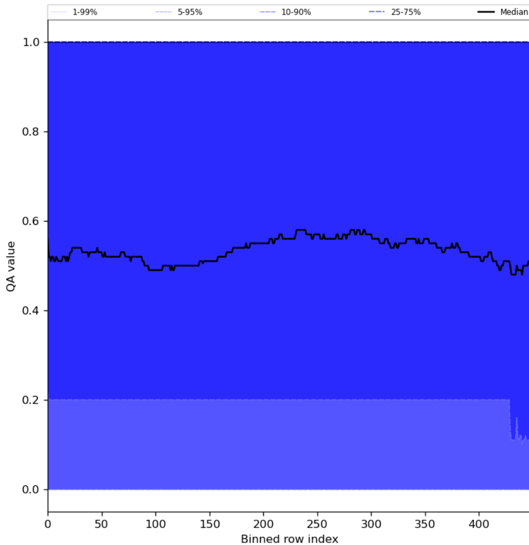
Figure 75: Along track statistics of “QA value” for 2024-08-02 to 2024-08-04
