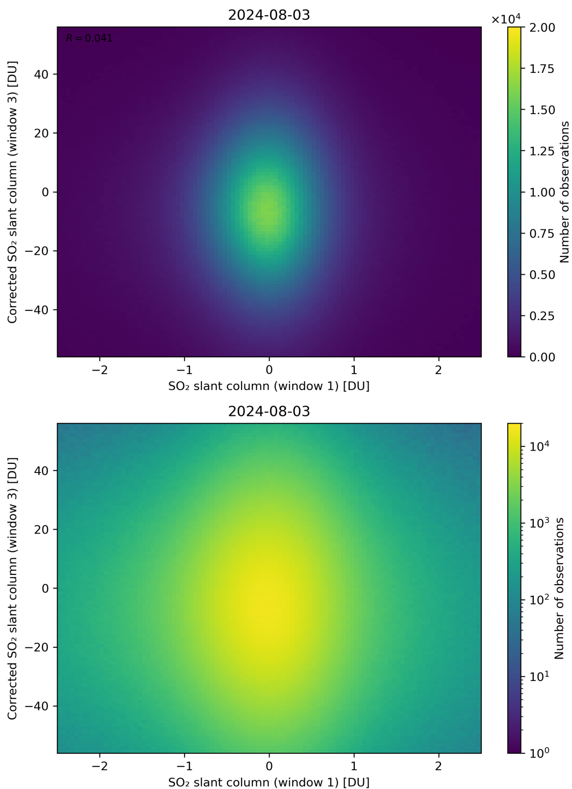
Figure 234: Scatter density plot of “SO 2 slant column (window 1)” against “Corrected SO 2 slant column (window 3)” for 2024-08-02 to 2024-08-04.
