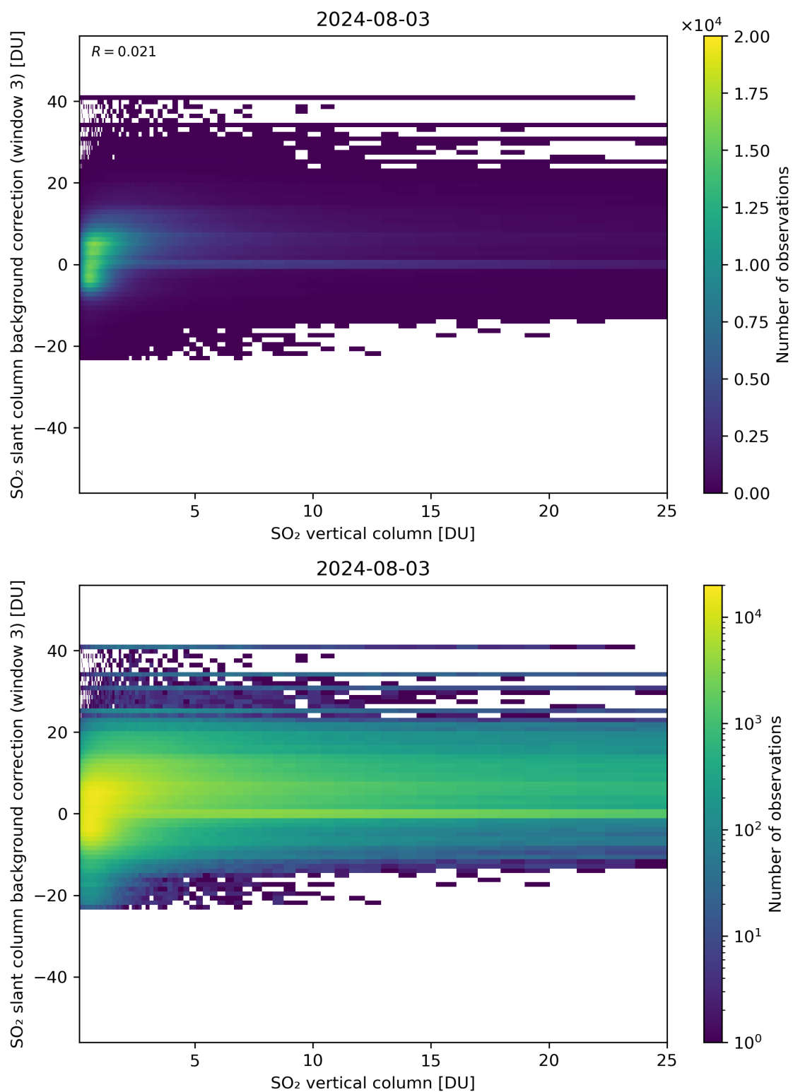
Figure 275: Scatter density plot of “SO 2 vertical column” against “SO 2 slant column background correction (window 3)” for 2024-08-02 to 2024-08-04.
