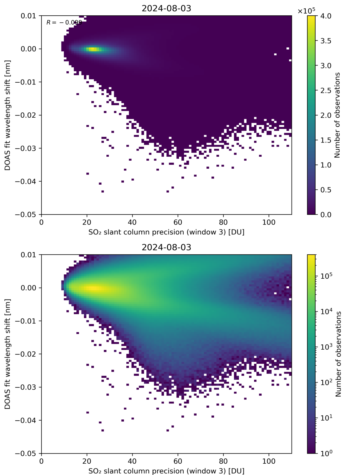
Figure 258: Scatter density plot of “SO 2 slant column precision (window 3)” against “DOAS fit wavelength shift” for 2024-08-02 to 2024-08-04.
