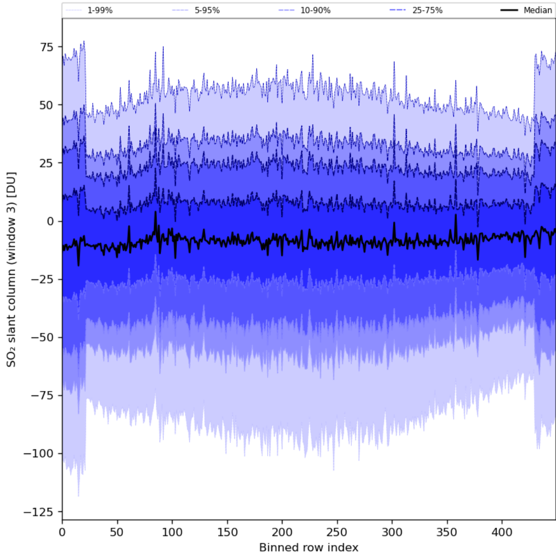
Figure 87: Along track statistics of “SO 2 slant column (window 3)” for 2024-08-02 to 2024-08-04
