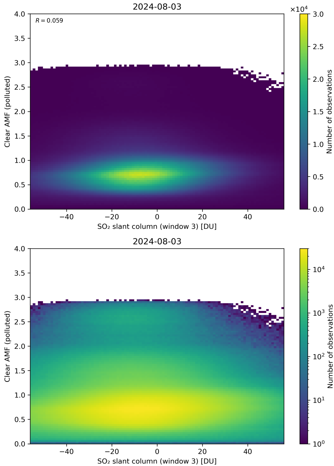
Figure 265: Scatter density plot of “SO 2 slant column (window 3)” against “Clear AMF (polluted)” for 2024-08-02 to 2024-08-04.
