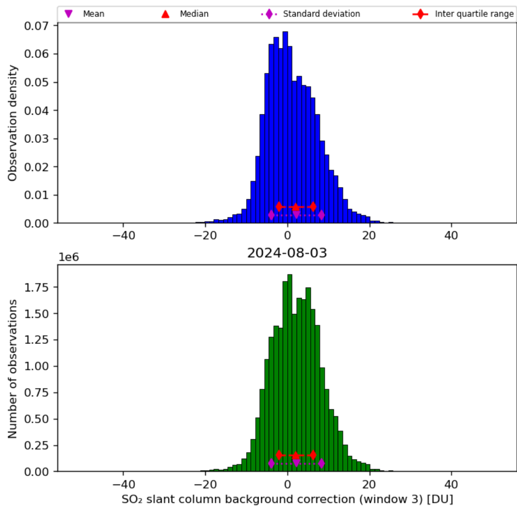
Figure 67: Histogram of “SO 2 slant column background correction (window 3)” for 2024-08-02 to 2024-08-04
