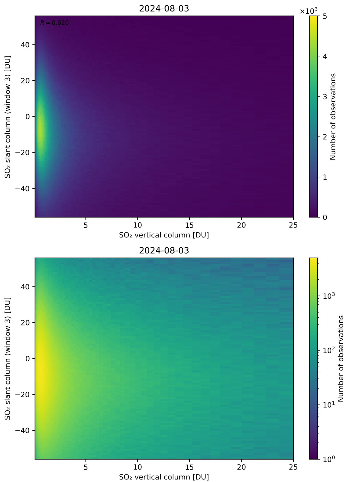
Figure 303: Scatter density plot of “SO 2 vertical column” against “SO 2 slant column (window 3)” for 2024-08-02 to 2024-08-04.
