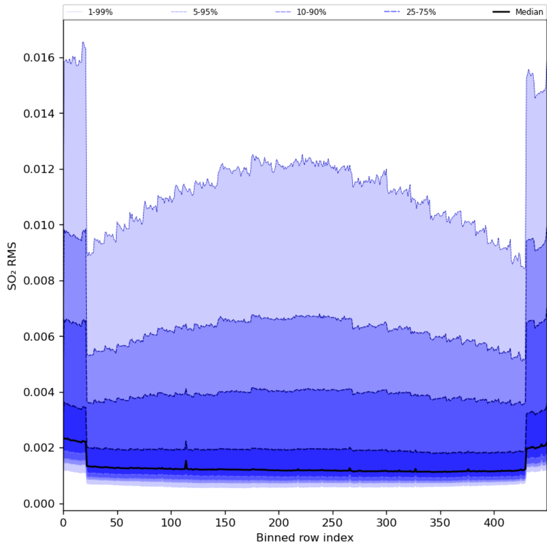
Figure 93: Along track statistics of “SO 2 RMS” for 2024-08-02 to 2024-08-04
