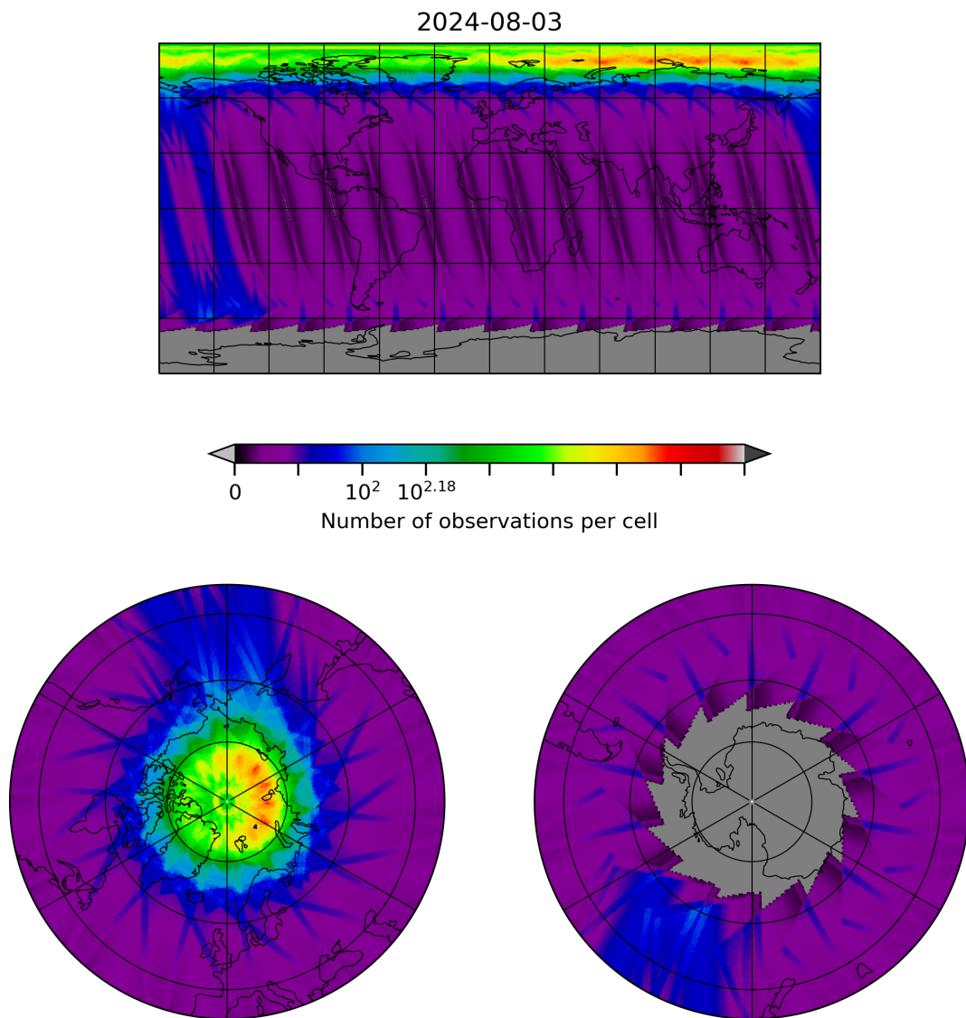
Figure 28: Map of the number of observations for 2024-08-02 to 2024-08-04
