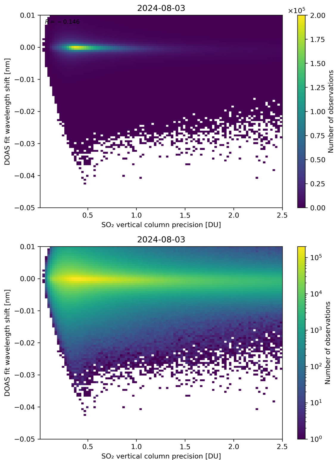
Figure 282: Scatter density plot of “SO 2 vertical column precision” against “DOAS fit wavelength shift” for 2024-08-02 to 2024-08-04.
