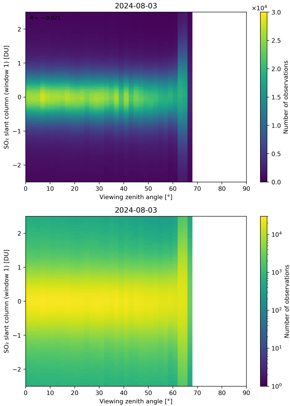
Figure 320: Scatter density plot of “Viewing zenith angle” against “SO 2 slant column (window 1)” for 2024-08-02 to 2024-08-04.
