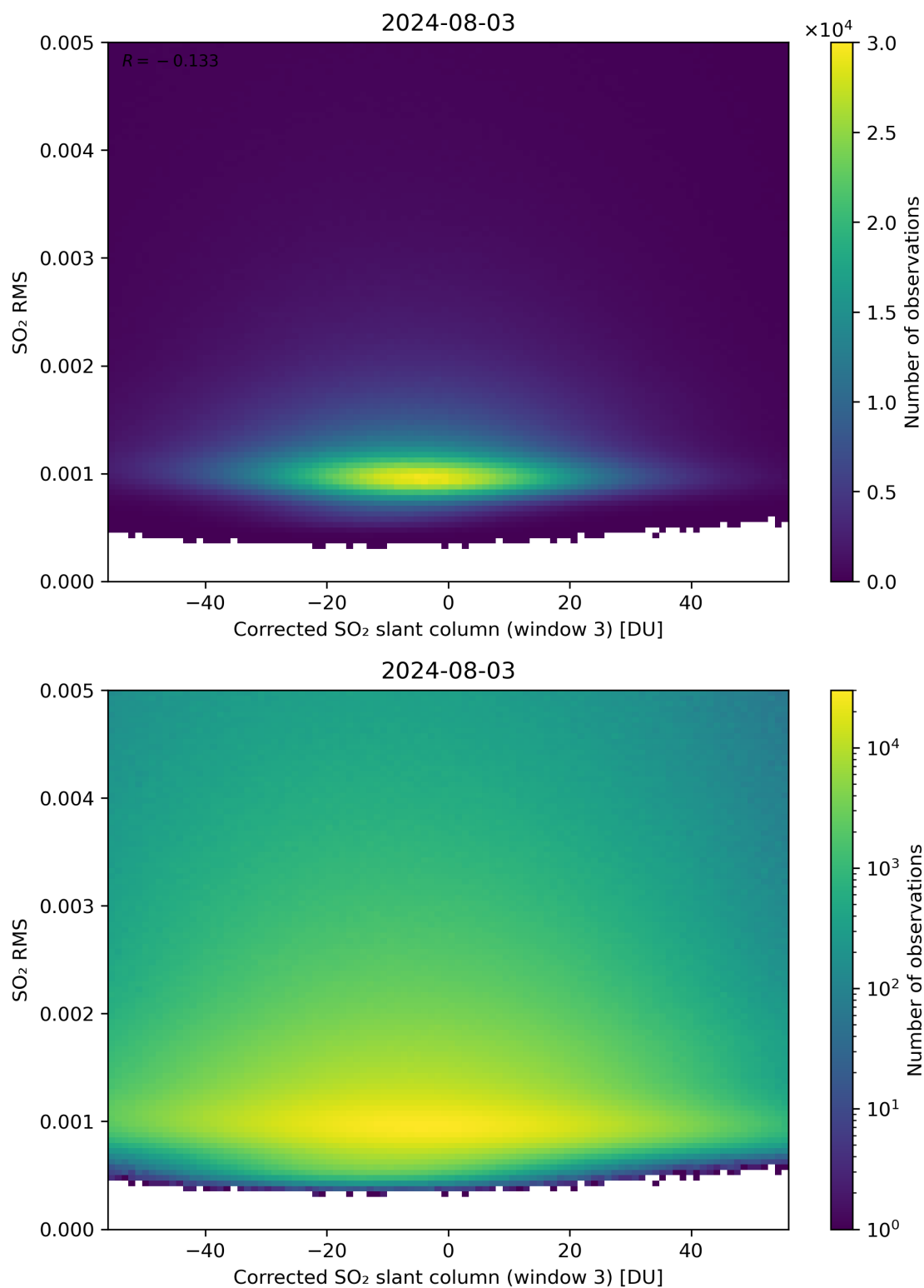
Figure 208: Scatter density plot of “Corrected SO 2 slant column (window 3)” against “SO 2 RMS” for 2024-08-02 to 2024-08-04.
