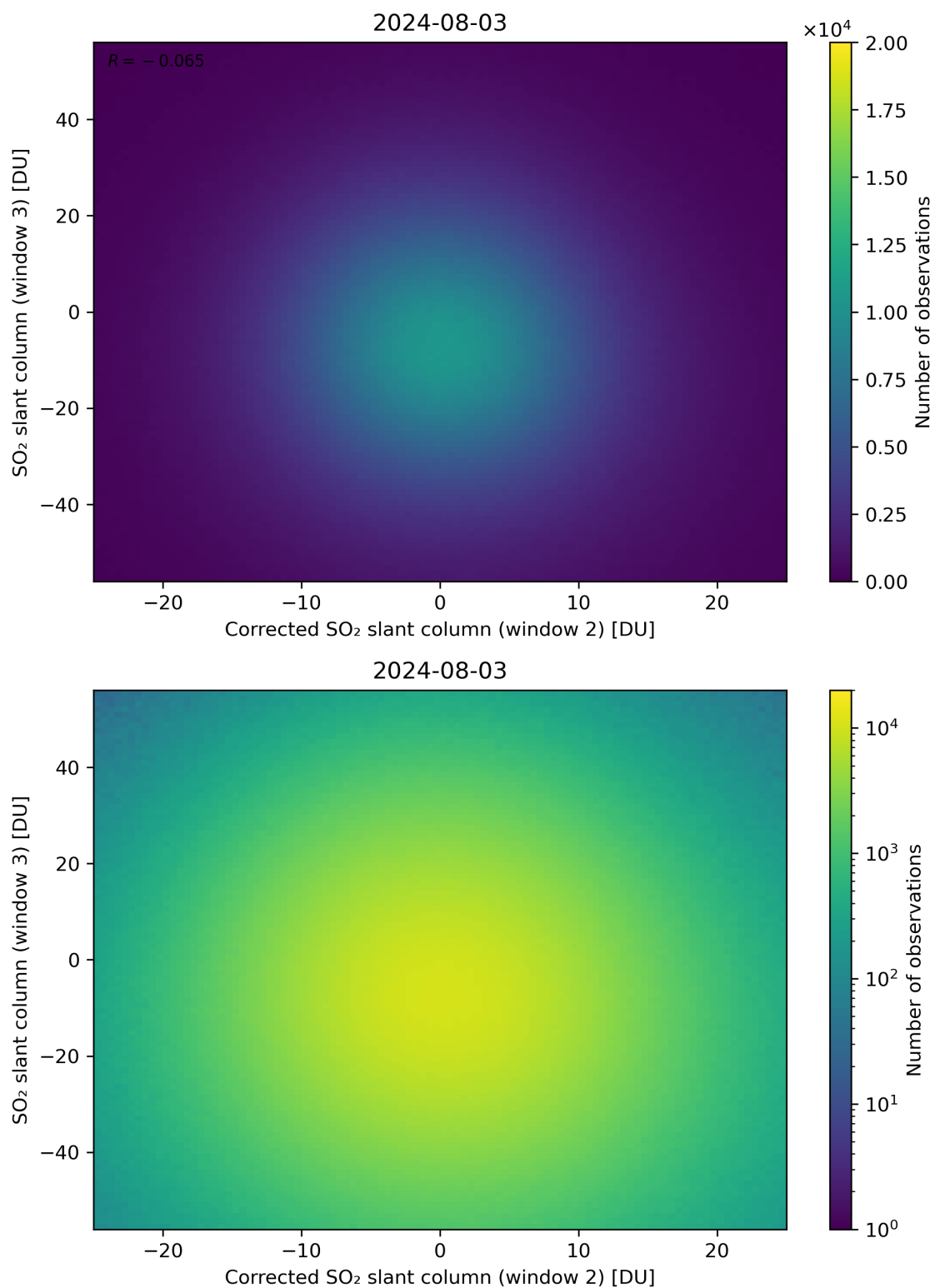
Figure 201: Scatter density plot of “Corrected SO 2 slant column (window 2)” against “SO 2 slant column (window 3)” for 2024-08-02 to 2024-08-04.
