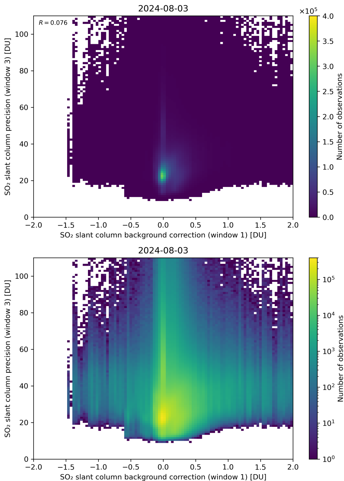
Figure 108: Scatter density plot of “SO 2 slant column background correction (window 1)” against “SO 2 slant column precision (window 3)” for 2024-08-02 to 2024-08-04.
