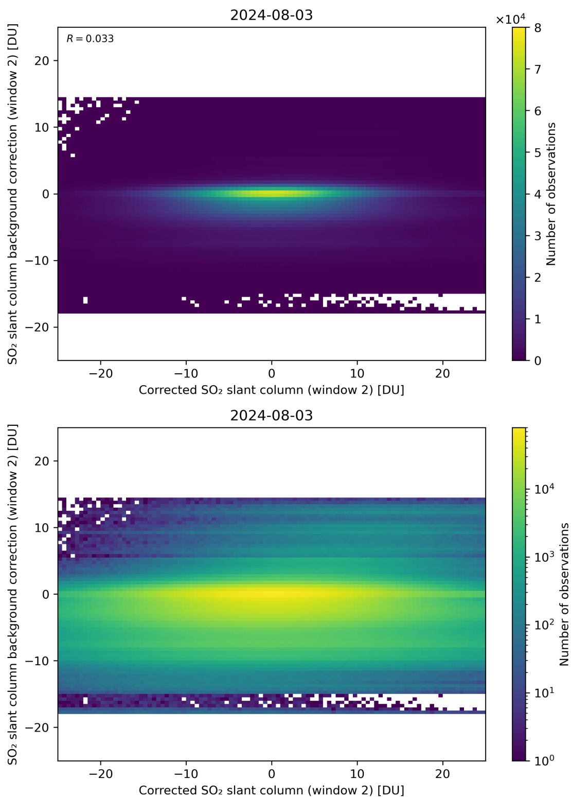
Figure 194: Scatter density plot of “Corrected SO 2 slant column (window 2)” against “SO 2 slant column background correction (window 2)” for 2024-08-02 to 2024-08-04.
