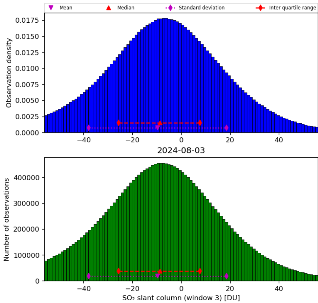
Figure 64: Histogram of “SO 2 slant column (window 3)” for 2024-08-02 to 2024-08-04
