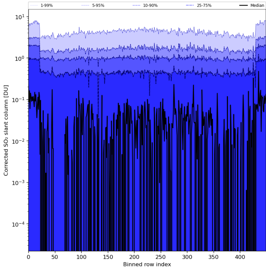
Figure 78: Along track statistics of “Corrected SO 2 slant column” for 2024-08-02 to 2024-08-04
