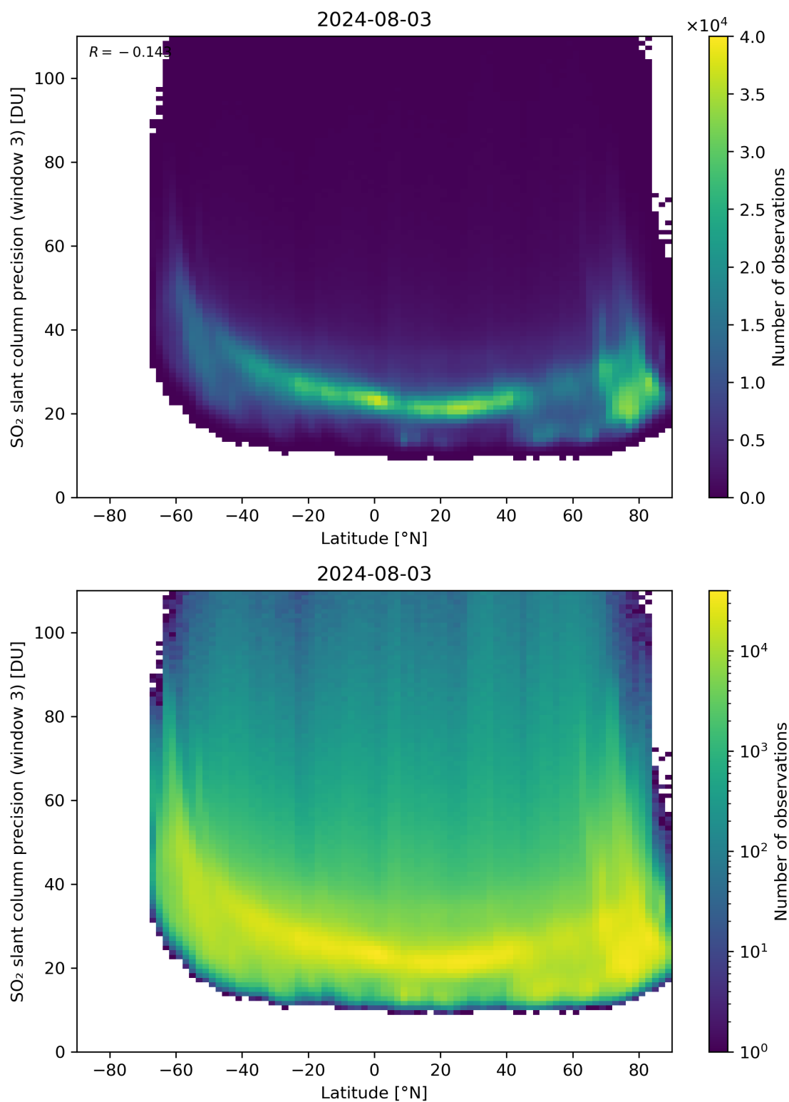
Figure 153: Scatter density plot of “Latitude” against “SO 2 slant column precision (window 3)” for 2024-08-02 to 2024-08-04.
