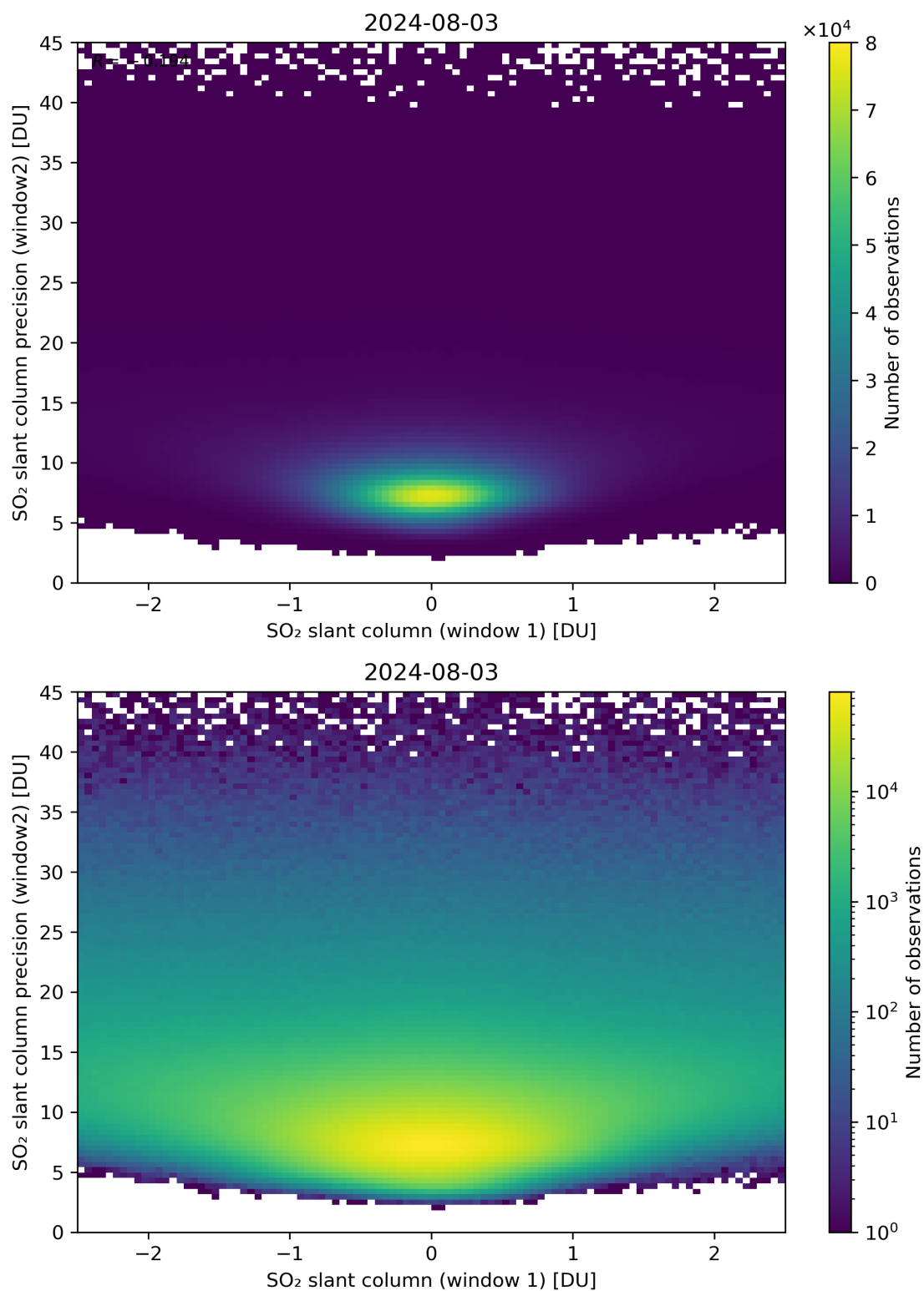
Figure 236: Scatter density plot of “SO 2 slant column (window 1)” against “SO 2 slant column precision (window2)” for 2024-08-02 to 2024-08-04.
