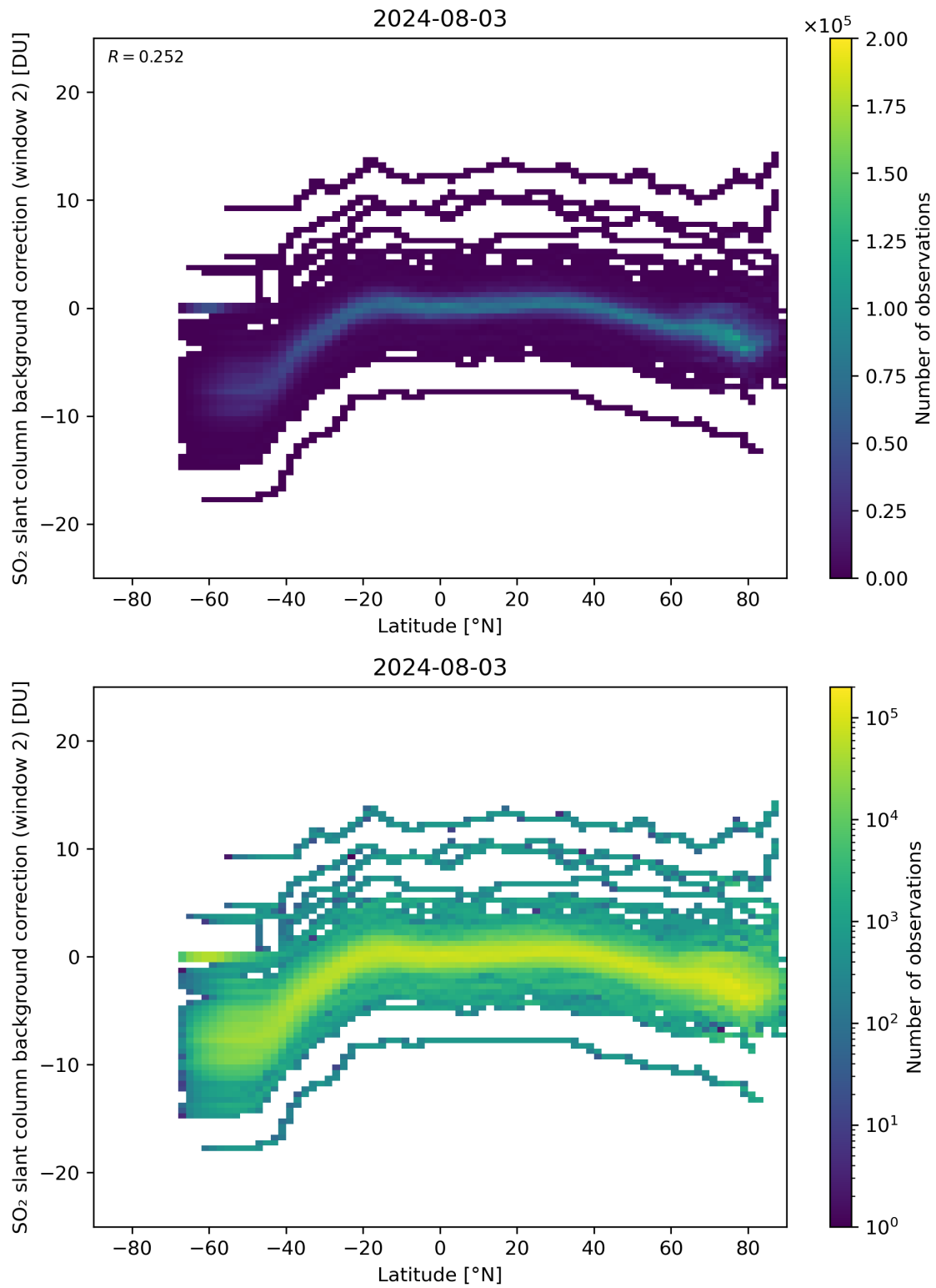
Figure 140: Scatter density plot of “Latitude” against “SO 2 slant column background correction (window 2)” for 2024-08-02 to 2024-08-04.
