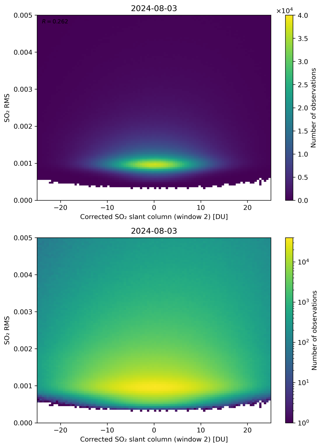
Figure 198: Scatter density plot of “Corrected SO 2 slant column (window 2)” against “SO 2 RMS” for 2024-08-02 to 2024-08-04.
