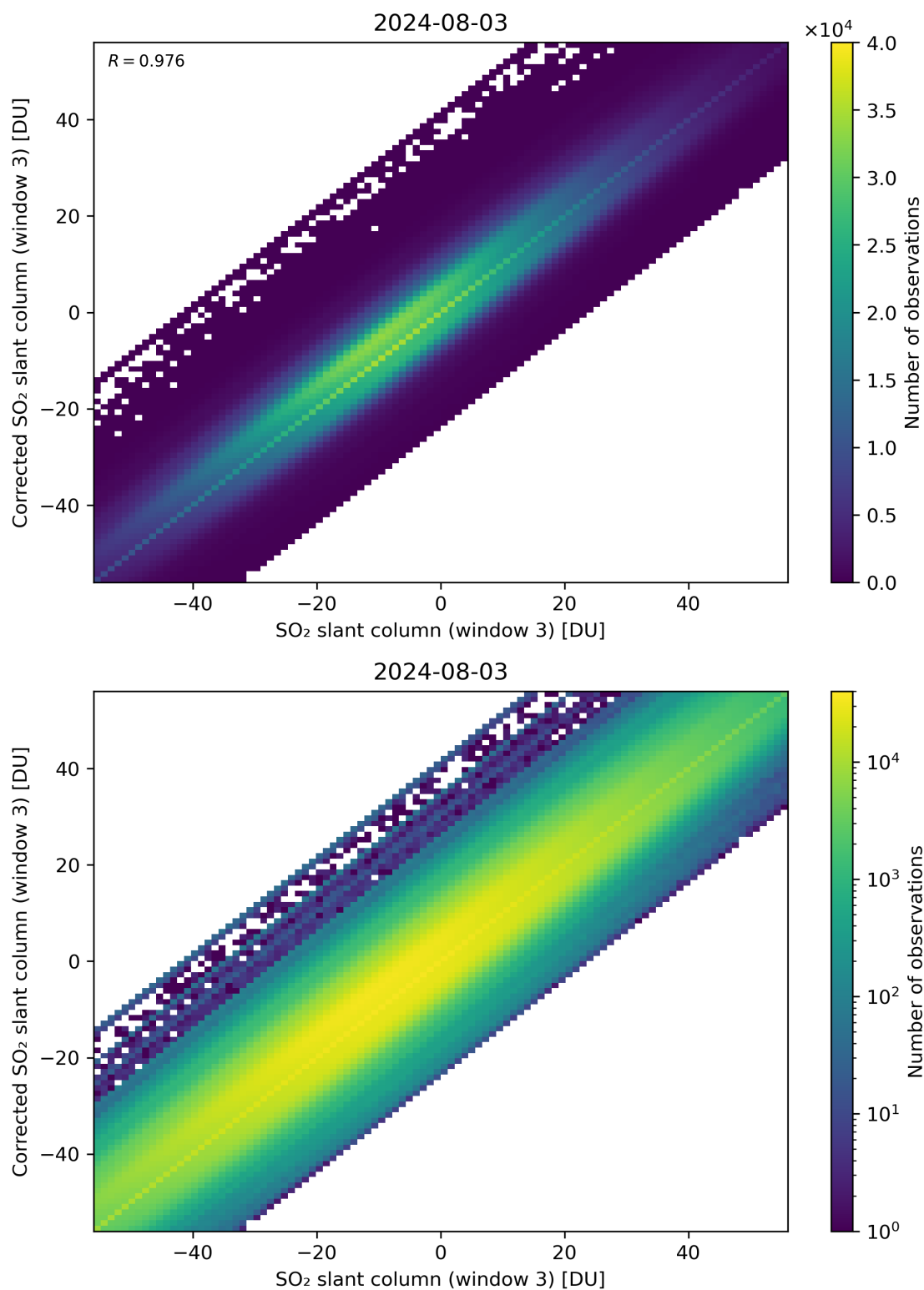
Figure 266: Scatter density plot of “SO 2 slant column (window 3)” against “Corrected SO 2 slant column (window 3)” for 2024-08-02 to 2024-08-04.
