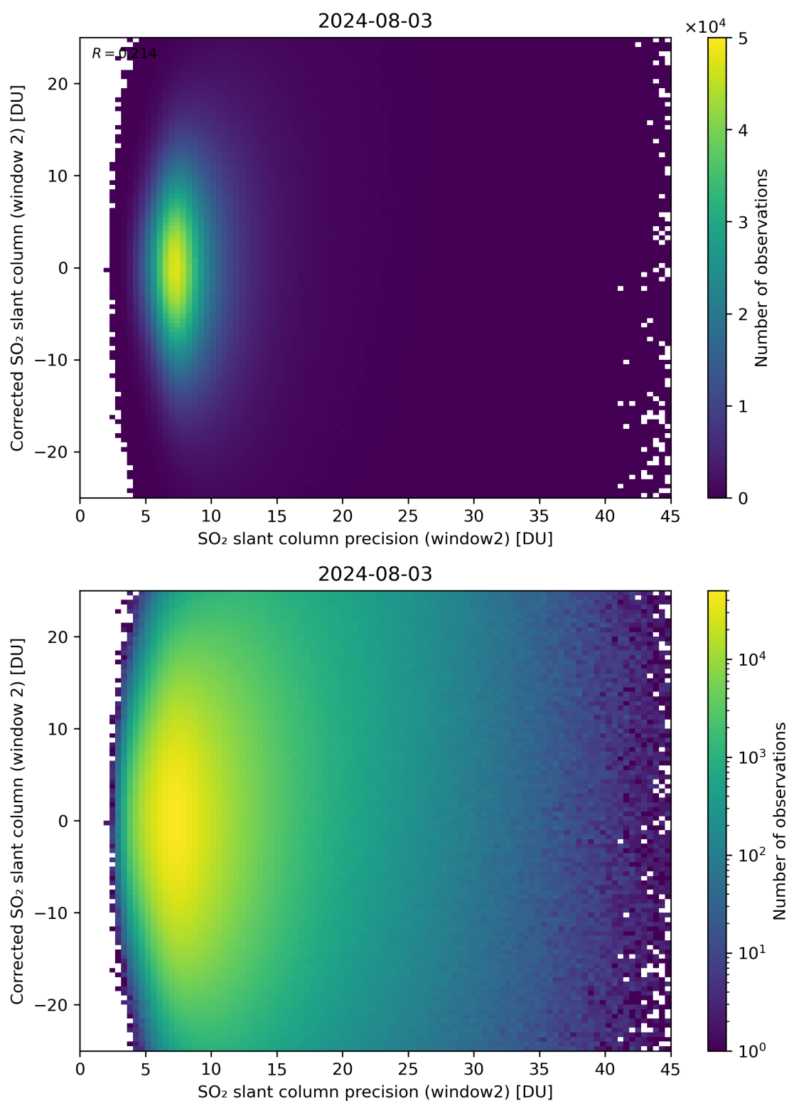
Figure 247: Scatter density plot of “SO 2 slant column precision (window2)” against “Corrected SO 2 slant column (window 2)” for 2024-08-02 to 2024-08-04.
