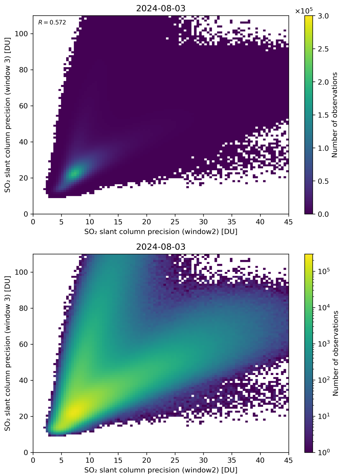
Figure 250: Scatter density plot of “SO 2 slant column precision (window2)” against “SO 2 slant column precision (window 3)” for 2024-08-02 to 2024-08-04.
