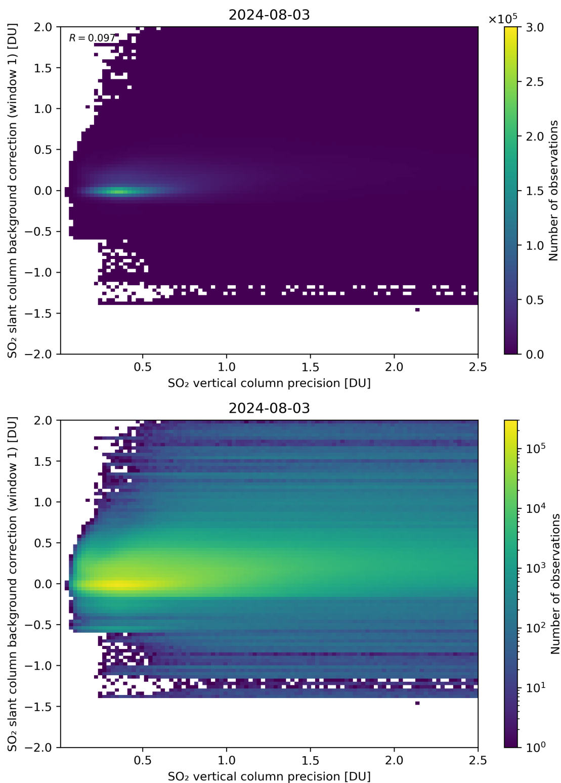
Figure 279: Scatter density plot of “SO 2 vertical column precision” against “SO 2 slant column background correction (window 1)” for 2024-08-02 to 2024-08-04.
