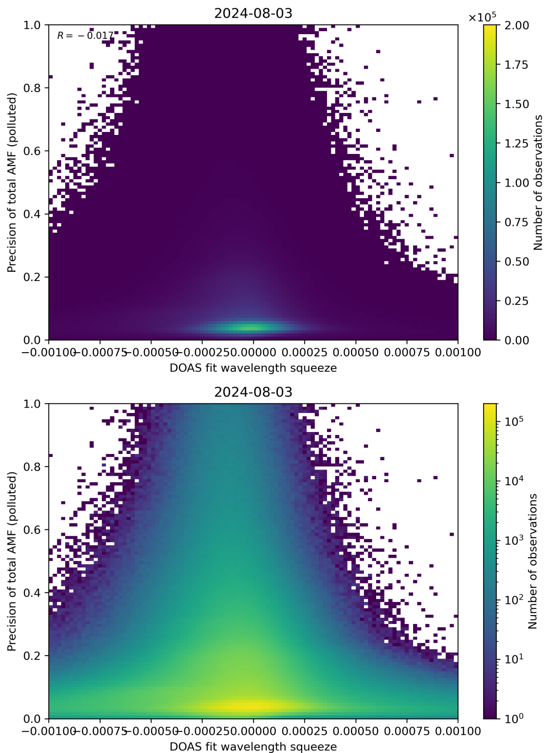
Figure 135: Scatter density plot of “DOAS fit wavelength squeeze” against “Precision of total AMF (polluted)” for 2024-08-02 to 2024-08-04.
