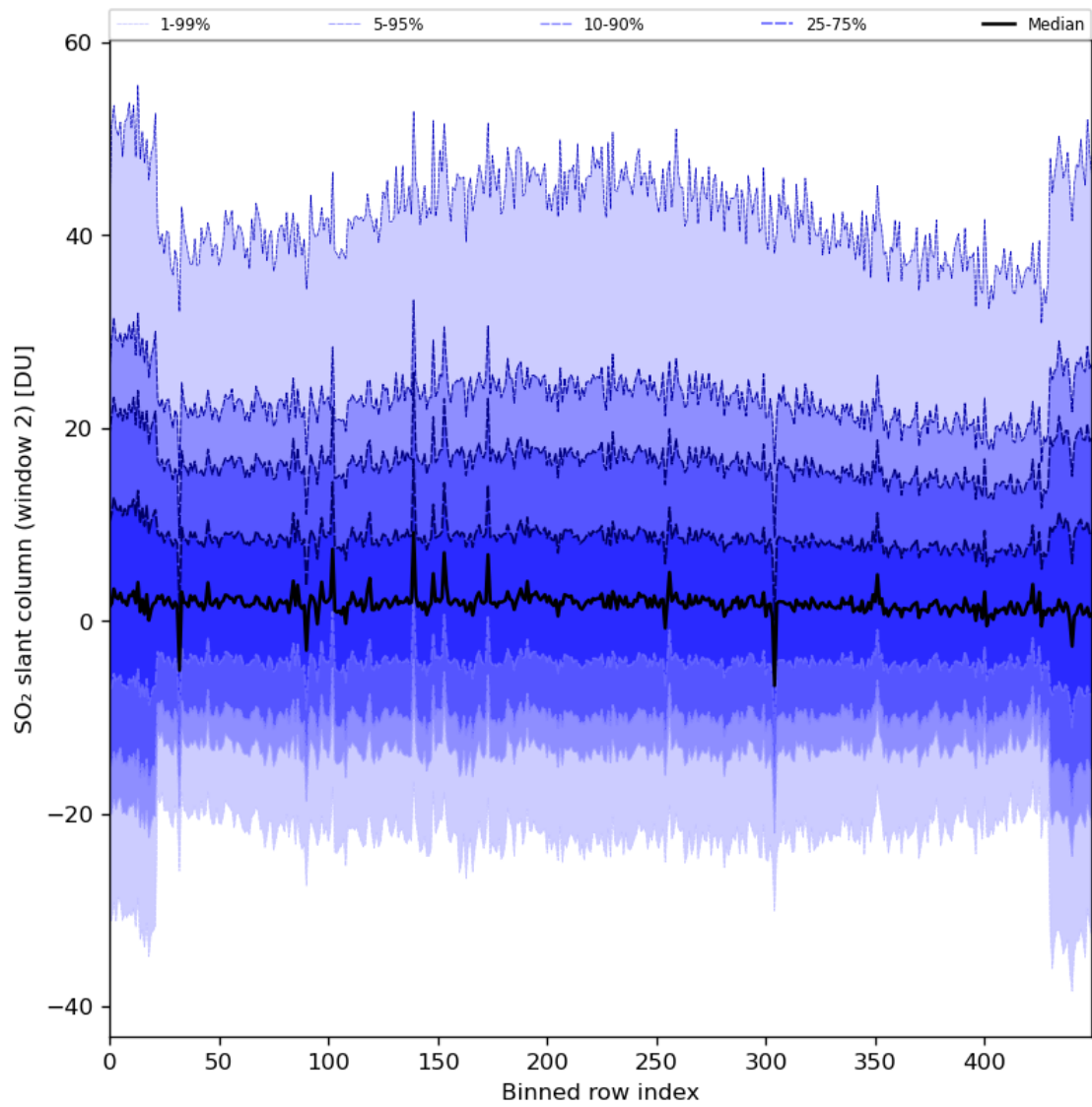
Figure 83: Along track statistics of “SO 2 slant column (window 2)” for 2024-08-02 to 2024-08-04
