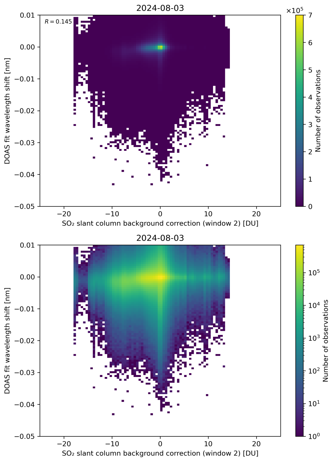
Figure 112: Scatter density plot of “SO 2 slant column background correction (window 2)” against “DOAS fit wavelength shift” for 2024-08-02 to 2024-08-04.
