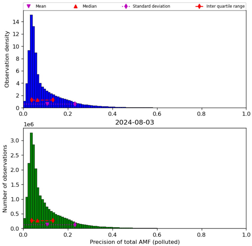
Figure 72: Histogram of “Precision of total AMF (polluted)” for 2024-08-02 to 2024-08-04
