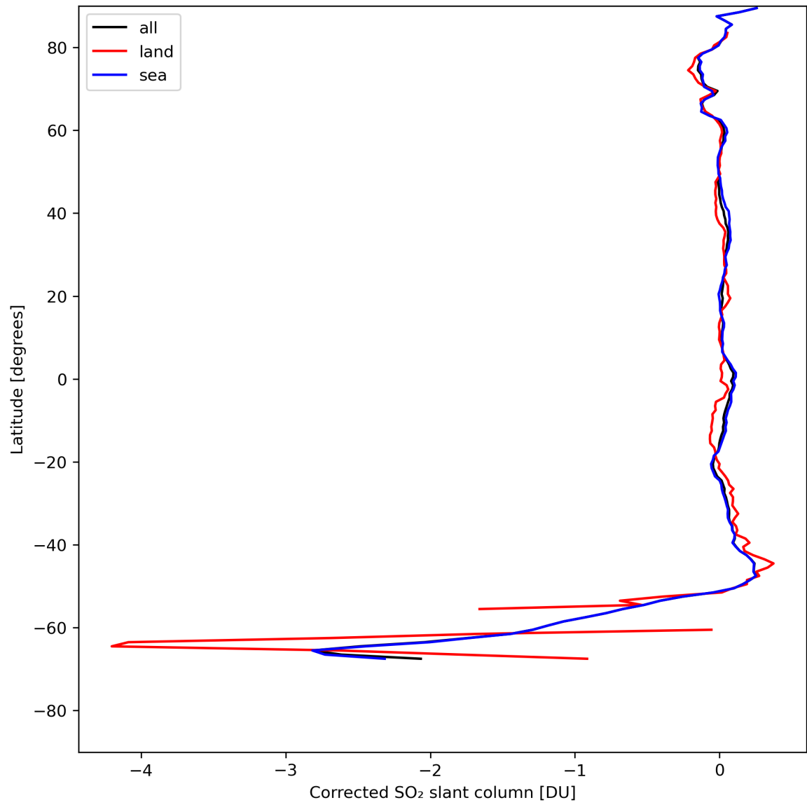
Figure 32: Zonal average of “Corrected SO 2 slant column” for 2024-08-02 to 2024-08-04.
