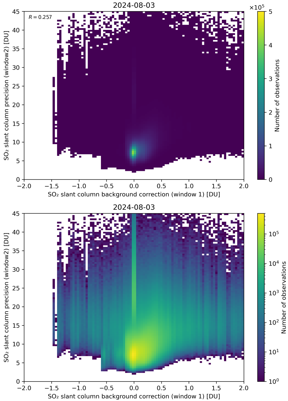
Figure 106: Scatter density plot of “SO 2 slant column background correction (window 1)” against “SO 2 slant column precision (window2)” for 2024-08-02 to 2024-08-04.
