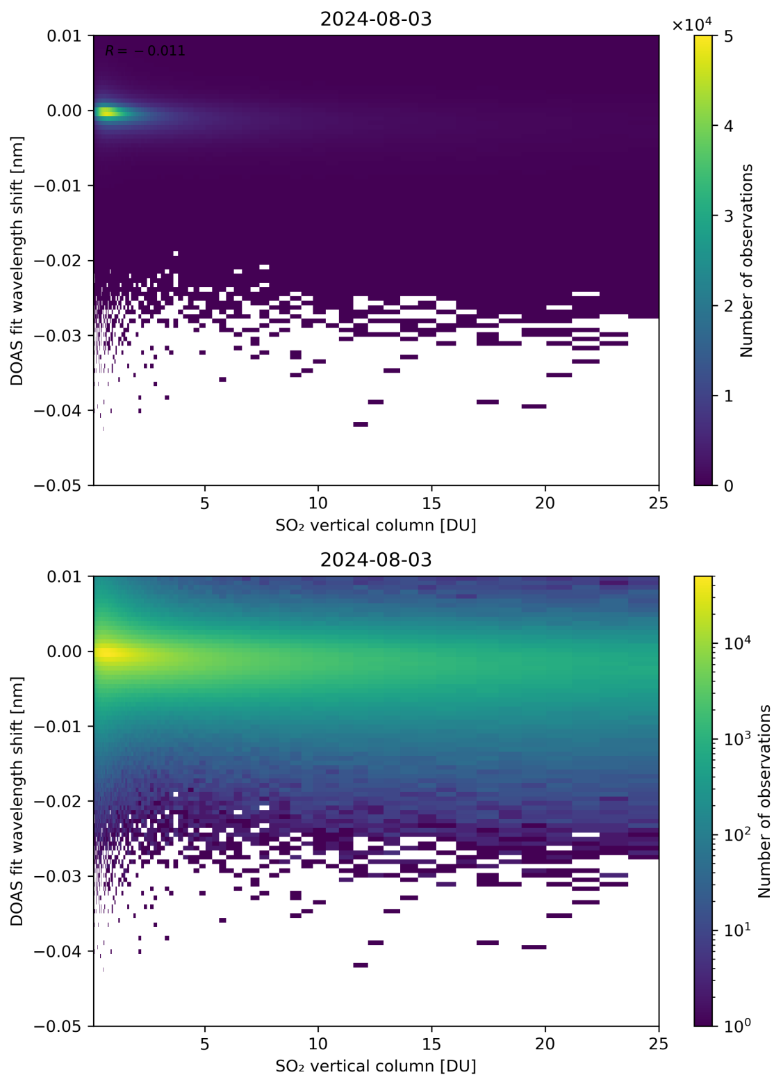
Figure 276: Scatter density plot of “SO 2 vertical column” against “DOAS fit wavelength shift” for 2024-08-02 to 2024-08-04.
