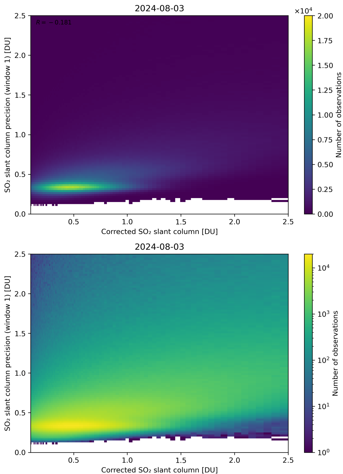
Figure 188: Scatter density plot of “Corrected SO 2 slant column” against “SO 2 slant column precision (window 1)” for 2024-08-02 to 2024-08-04.
