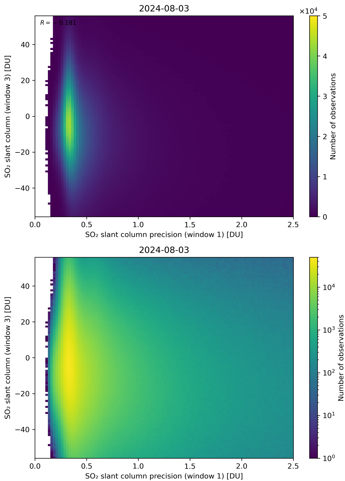
Figure 228: Scatter density plot of “SO 2 slant column precision (window 1)” against “SO 2 slant column (window 3)” for 2024-08-02 to 2024-08-04.
