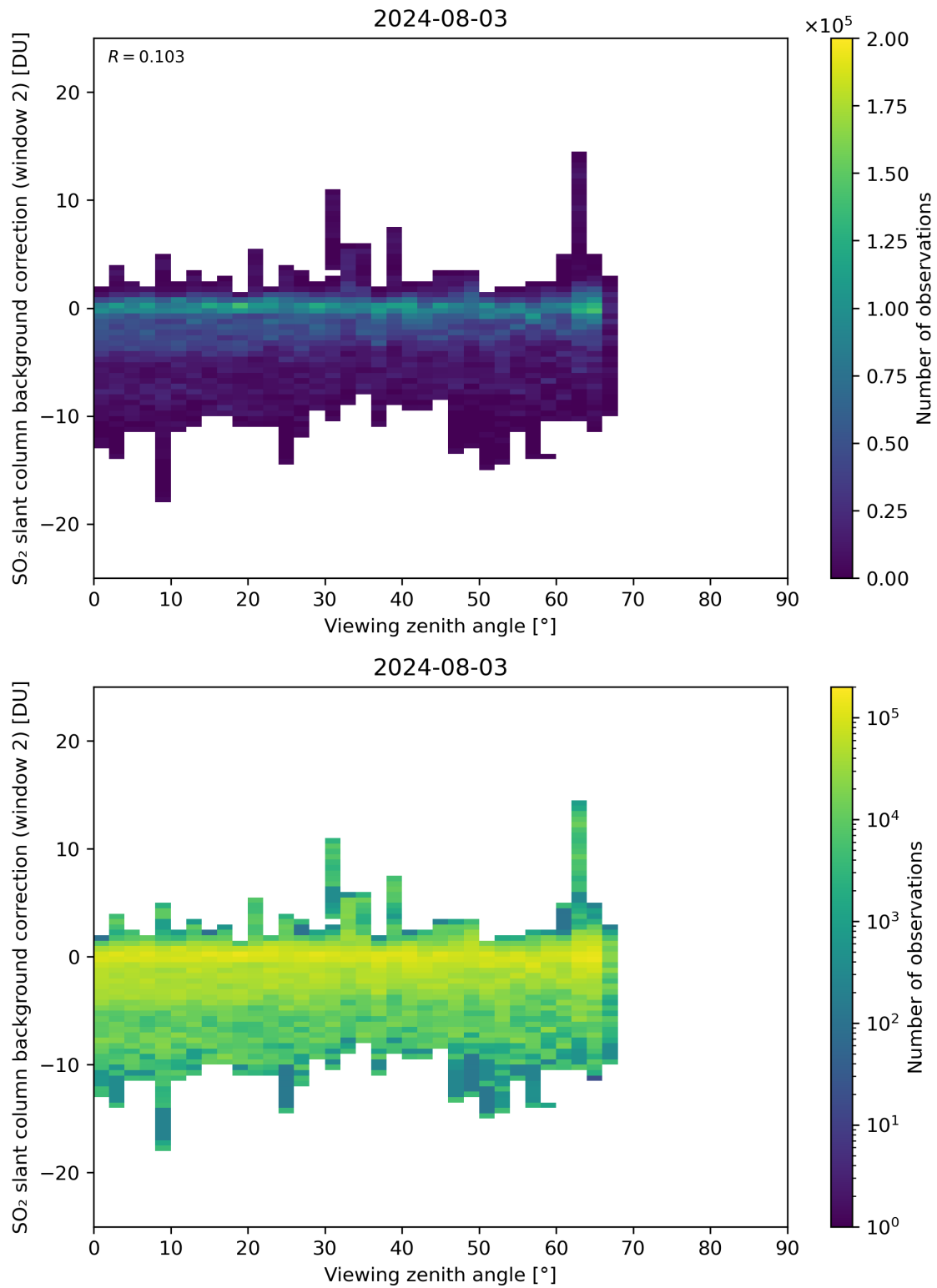
Figure 309: Scatter density plot of “Viewing zenith angle” against “SO 2 slant column background correction (window 2)” for 2024-08-02 to 2024-08-04.
