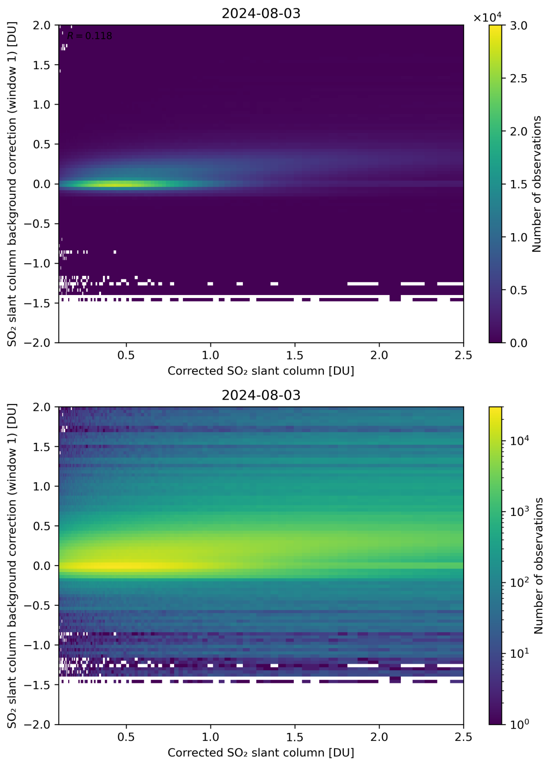
Figure 178: Scatter density plot of “Corrected SO 2 slant column” against “SO 2 slant column background correction (window 1)” for 2024-08-02 to 2024-08-04.
