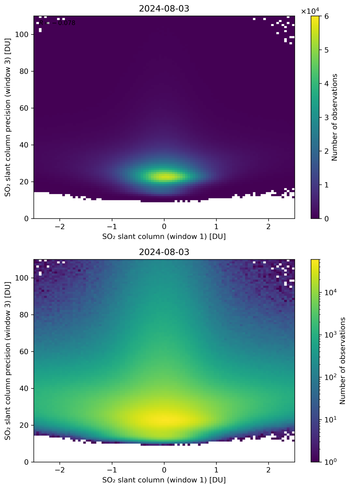
Figure 238: Scatter density plot of “SO 2 slant column (window 1)” against “SO 2 slant column precision (window 3)” for 2024-08-02 to 2024-08-04.
