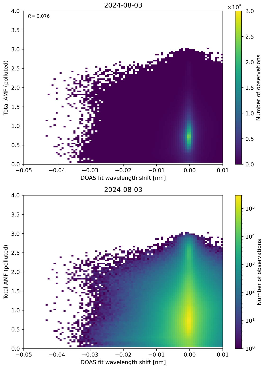
Figure 130: Scatter density plot of “DOAS fit wavelength shift” against “Total AMF (polluted)” for 2024-08-02 to 2024-08-04.
