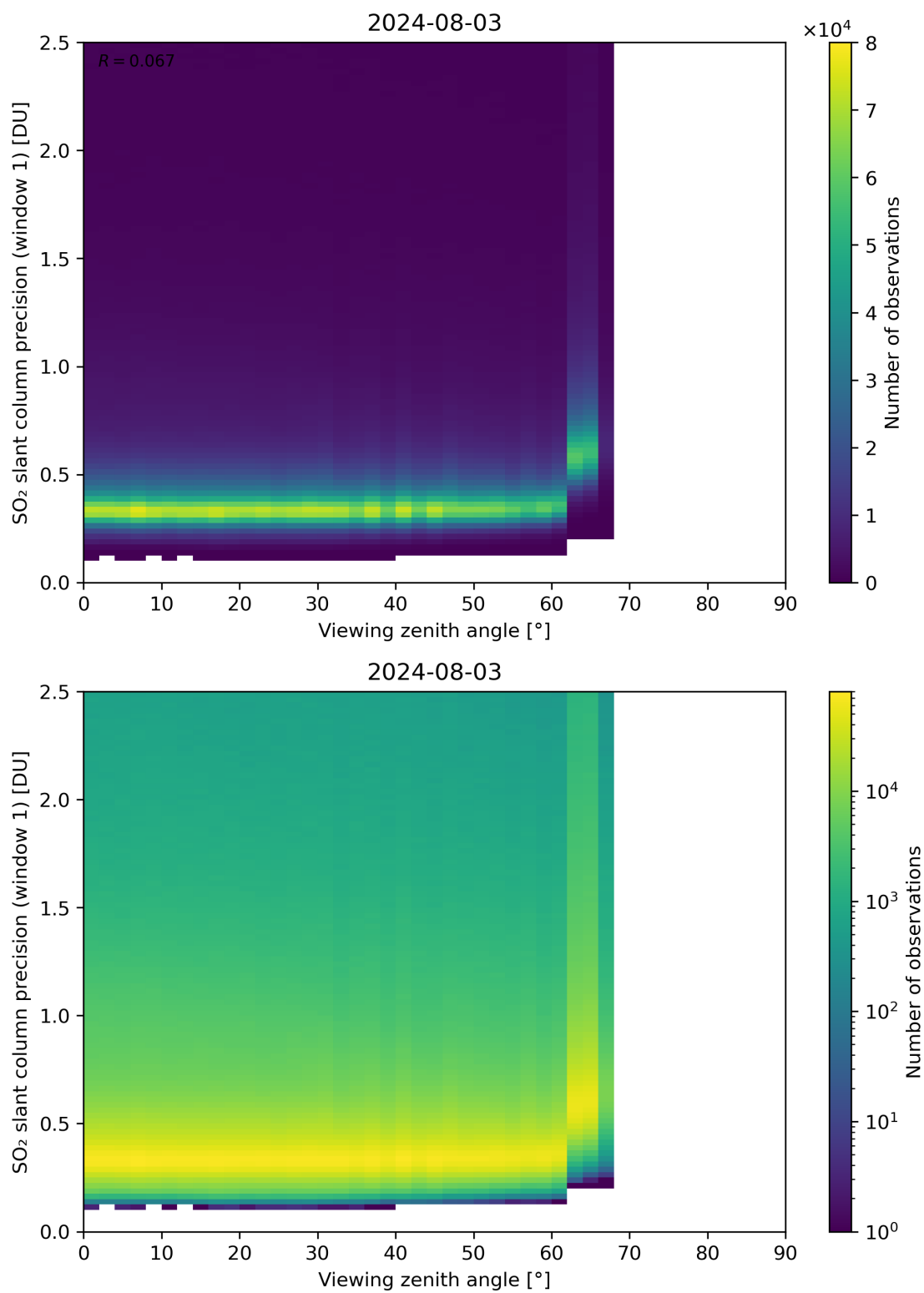
Figure 321: Scatter density plot of “Viewing zenith angle” against “SO 2 slant column precision (window 1)” for 2024-08-02 to 2024-08-04.
