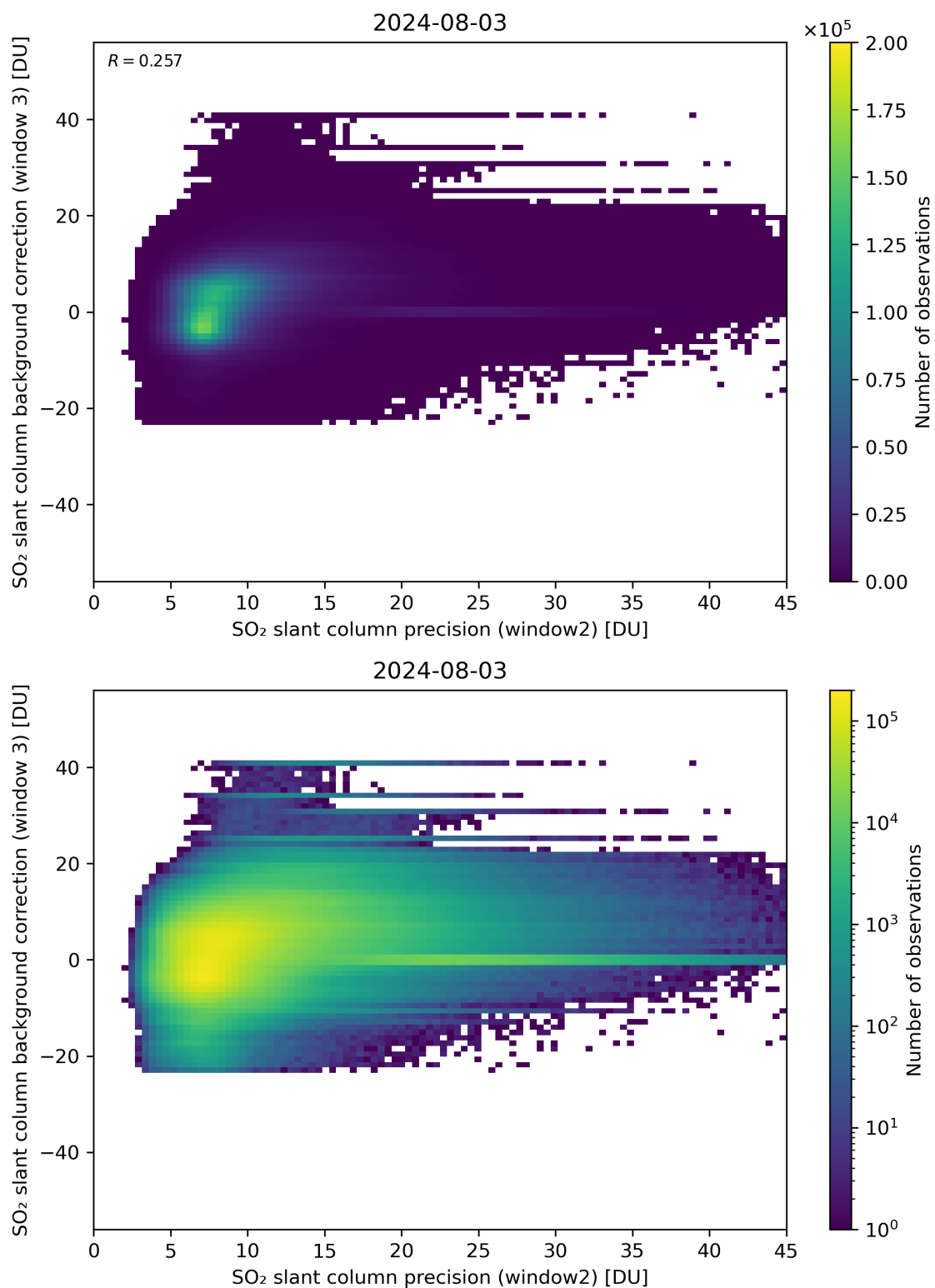
Figure 242: Scatter density plot of “SO 2 slant column precision (window2)” against “SO 2 slant column background correction (window 3)” for 2024-08-02 to 2024-08-04.
