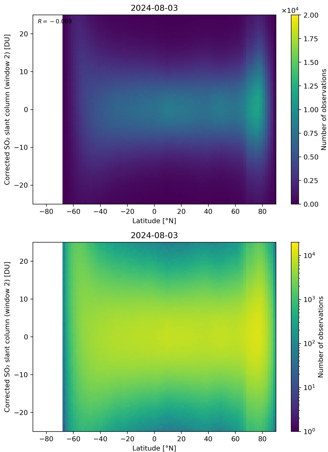
Figure 147: Scatter density plot of “Latitude” against “Corrected SO 2 slant column (window 2)” for 2024-08-02 to 2024-08-04.
