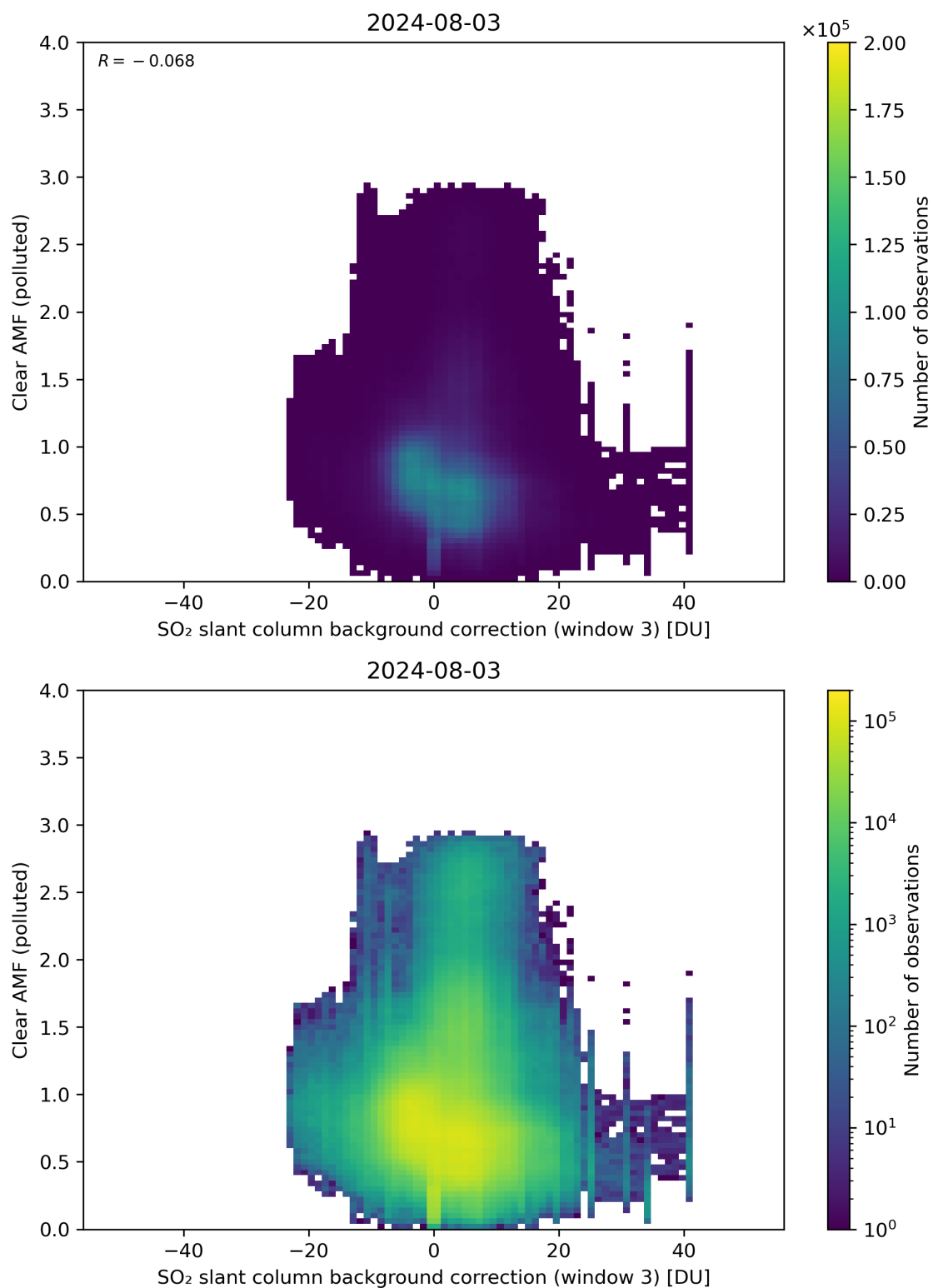
Figure 124: Scatter density plot of “SO 2 slant column background correction (window 3)” against “Clear AMF (polluted)” for 2024-08-02 to 2024-08-04.
