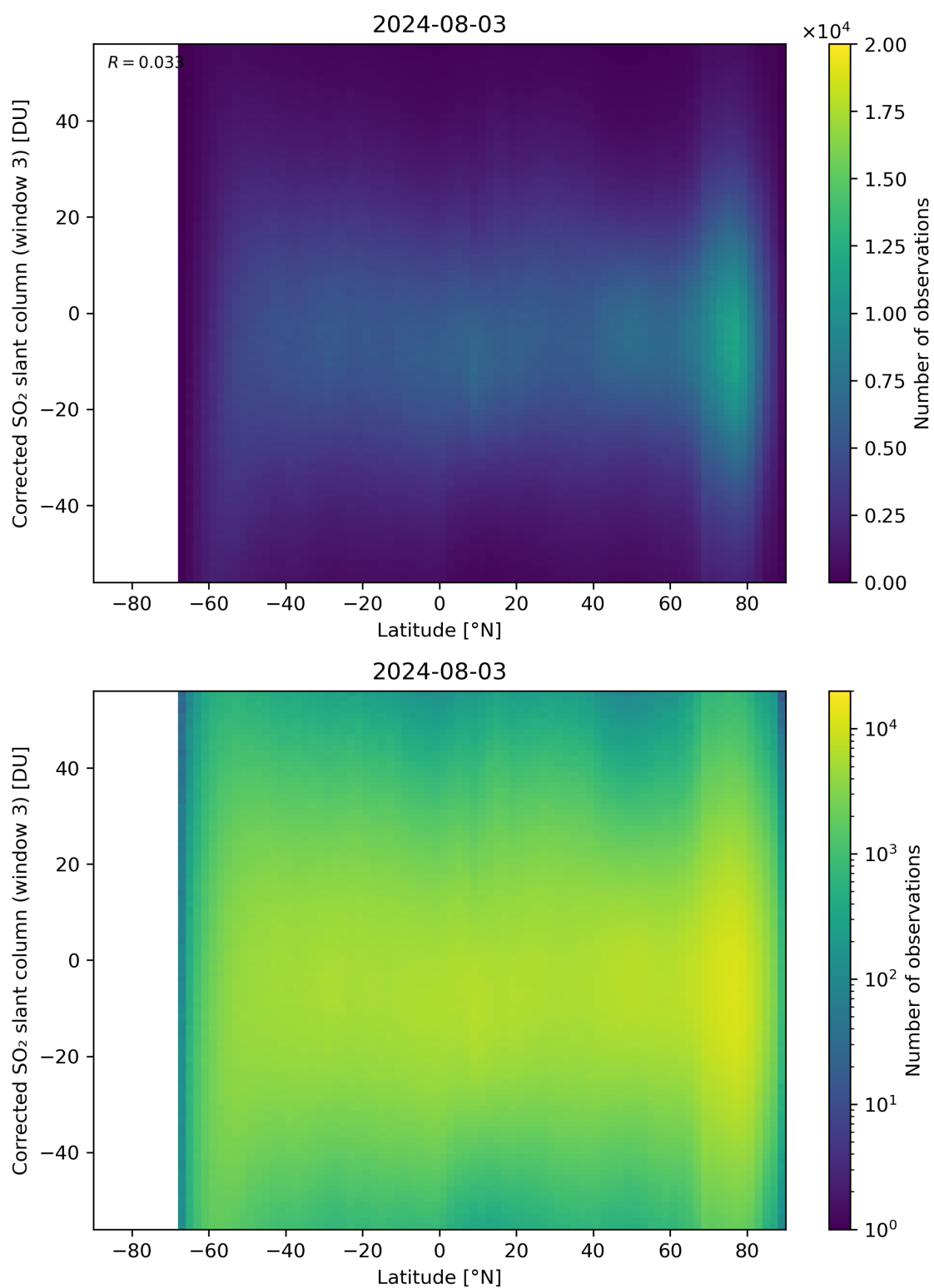
Figure 148: Scatter density plot of “Latitude” against “Corrected SO 2 slant column (window 3)” for 2024-08-02 to 2024-08-04.
