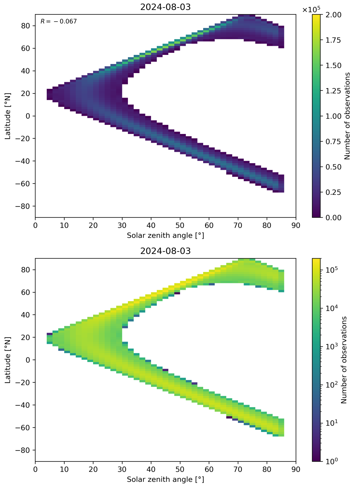
Figure 164: Scatter density plot of “Solar zenith angle” against “Latitude” for 2024-08-02 to 2024-08-04.
