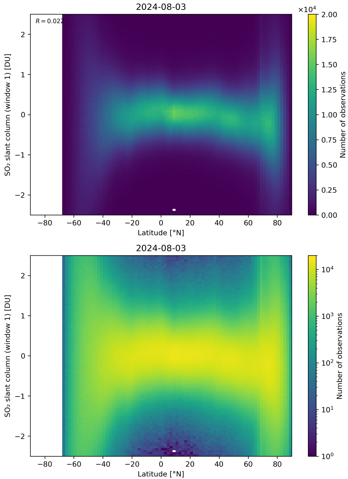
Figure 149: Scatter density plot of “Latitude” against “SO 2 slant column (window 1)” for 2024-08-02 to 2024-08-04.
