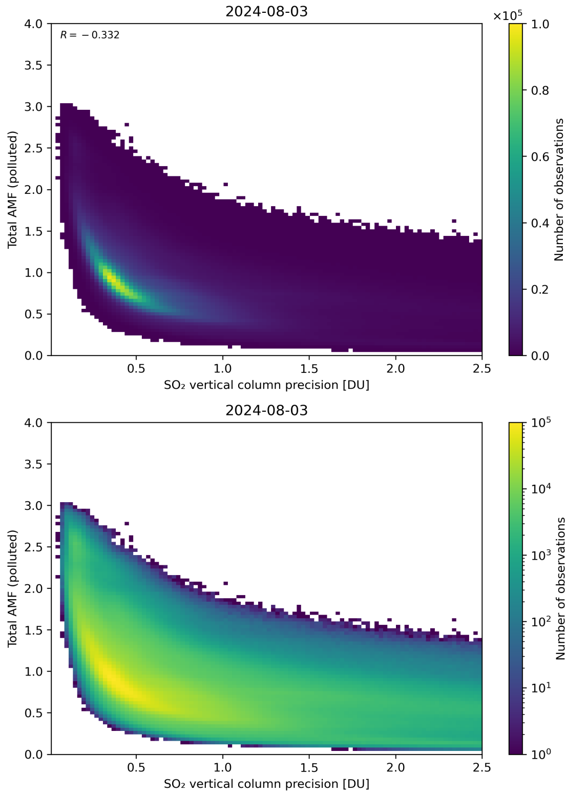
Figure 294: Scatter density plot of “SO 2 vertical column precision” against “Total AMF (polluted)” for 2024-08-02 to 2024-08-04.
