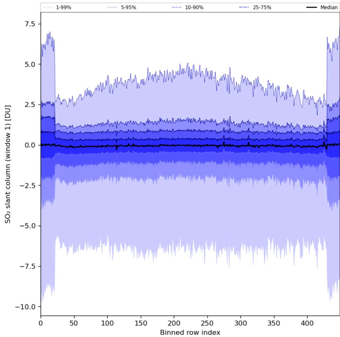
Figure 79: Along track statistics of “SO 2 slant column (window 1)” for 2024-08-02 to 2024-08-04
