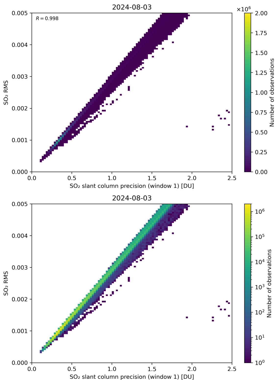
Figure 223: Scatter density plot of “SO 2 slant column precision (window 1)” against “SO 2 RMS” for 2024-08-02 to 2024-08-04.
