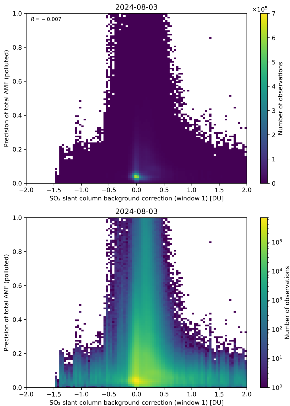
Figure 110: Scatter density plot of “SO 2 slant column background correction (window 1)” against “Precision of total AMF (polluted)” for 2024-08-02 to 2024-08-04.
