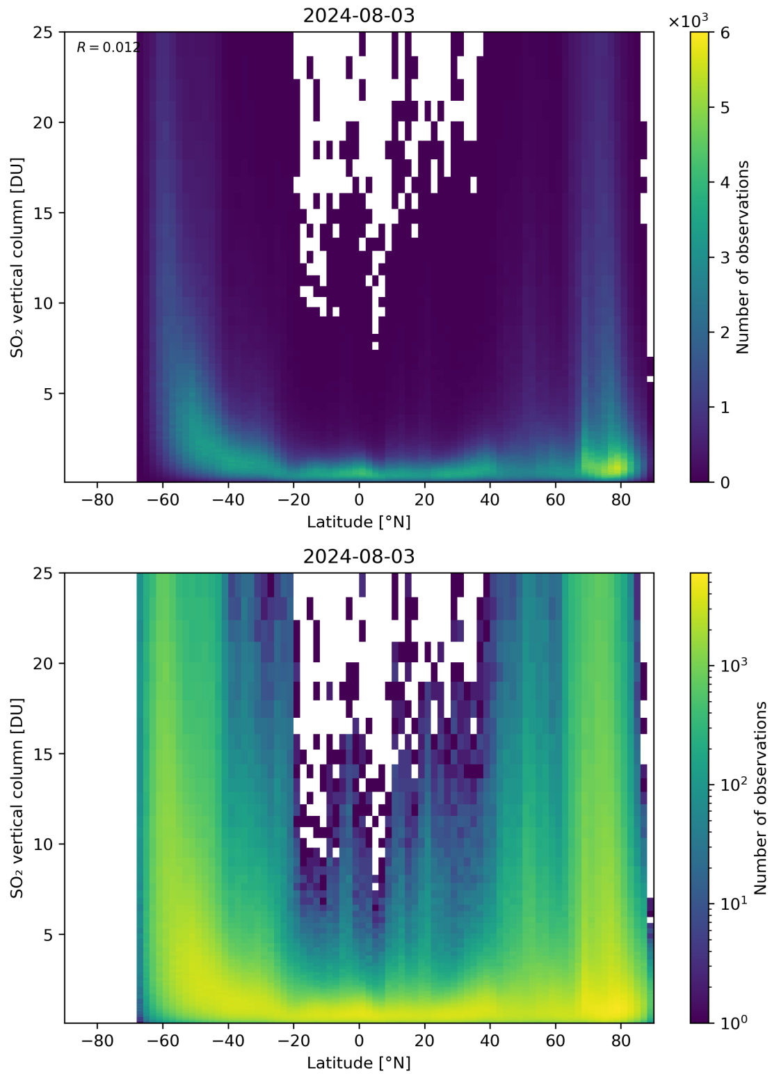
Figure 156: Scatter density plot of “Latitude” against “SO 2 vertical column” for 2024-08-02 to 2024-08-04.
