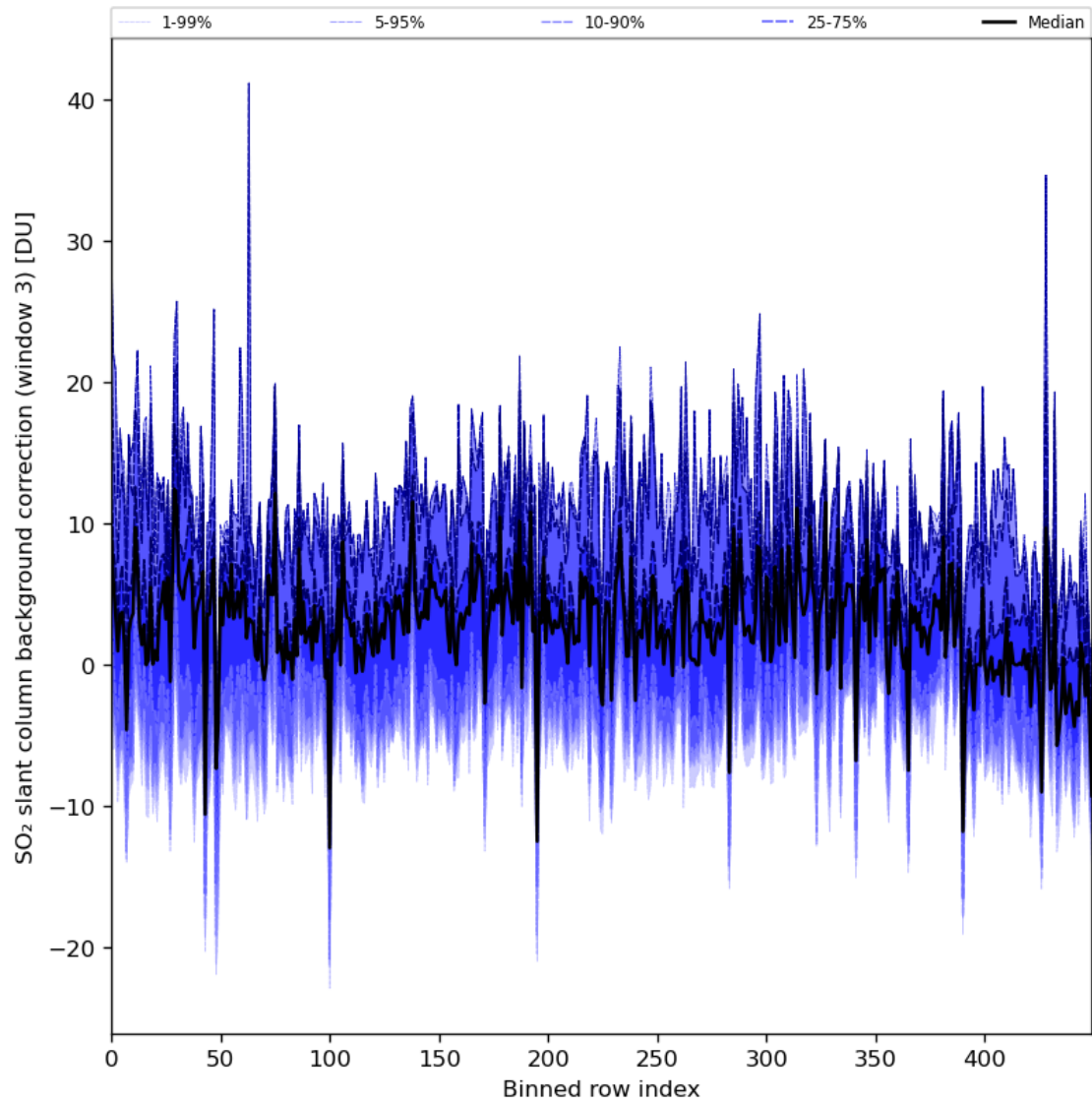
Figure 90: Along track statistics of “SO 2 slant column background correction (window 3)” for 2024-08-02 to 2024-08-04
