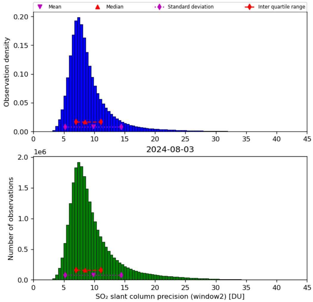
Figure 61: Histogram of “SO 2 slant column precision (window2)” for 2024-08-02 to 2024-08-04
