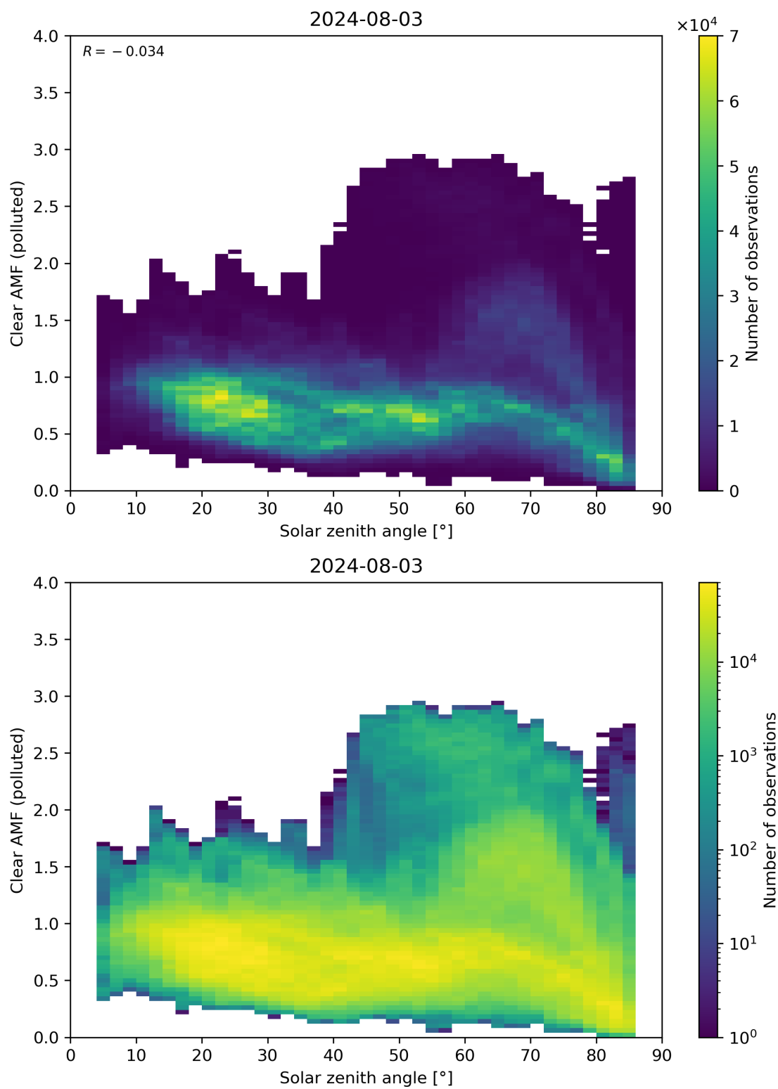
Figure 165: Scatter density plot of “Solar zenith angle” against “Clear AMF (polluted)” for 2024-08-02 to 2024-08-04.
