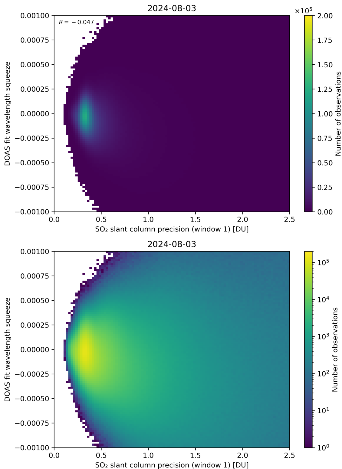
Figure 222: Scatter density plot of “SO 2 slant column precision (window 1)” against “DOAS fit wavelength squeeze” for 2024-08-02 to 2024-08-04.
