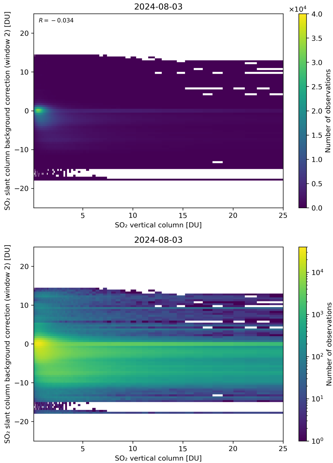
Figure 274: Scatter density plot of “SO 2 vertical column” against “SO 2 slant column background correction (window 2)” for 2024-08-02 to 2024-08-04.
