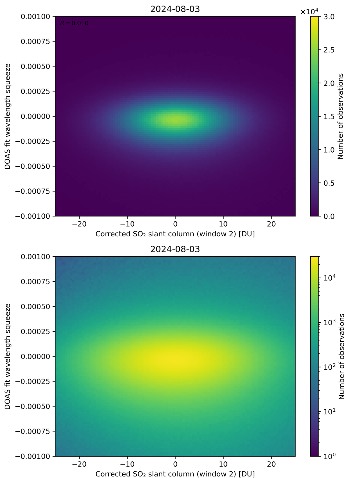
Figure 197: Scatter density plot of “Corrected SO 2 slant column (window 2)” against “DOAS fit wavelength squeeze” for 2024-08-02 to 2024-08-04.
