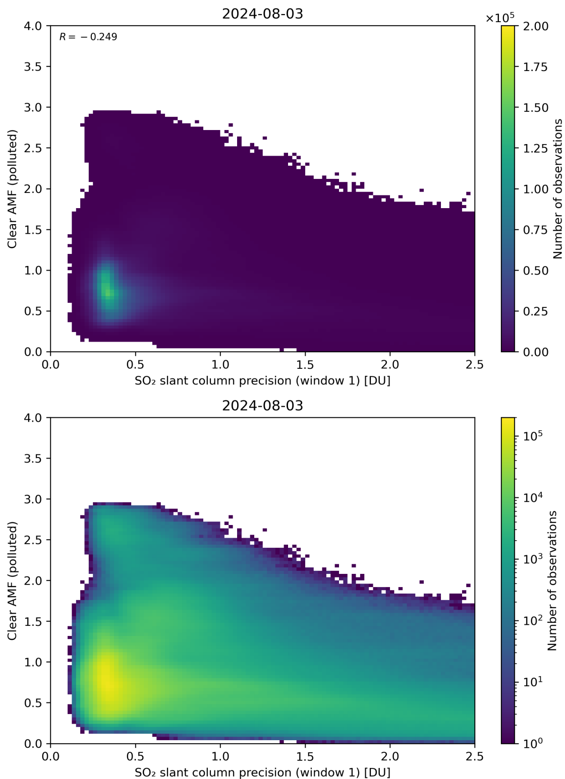
Figure 224: Scatter density plot of “SO 2 slant column precision (window 1)” against “Clear AMF (polluted)” for 2024-08-02 to 2024-08-04.
