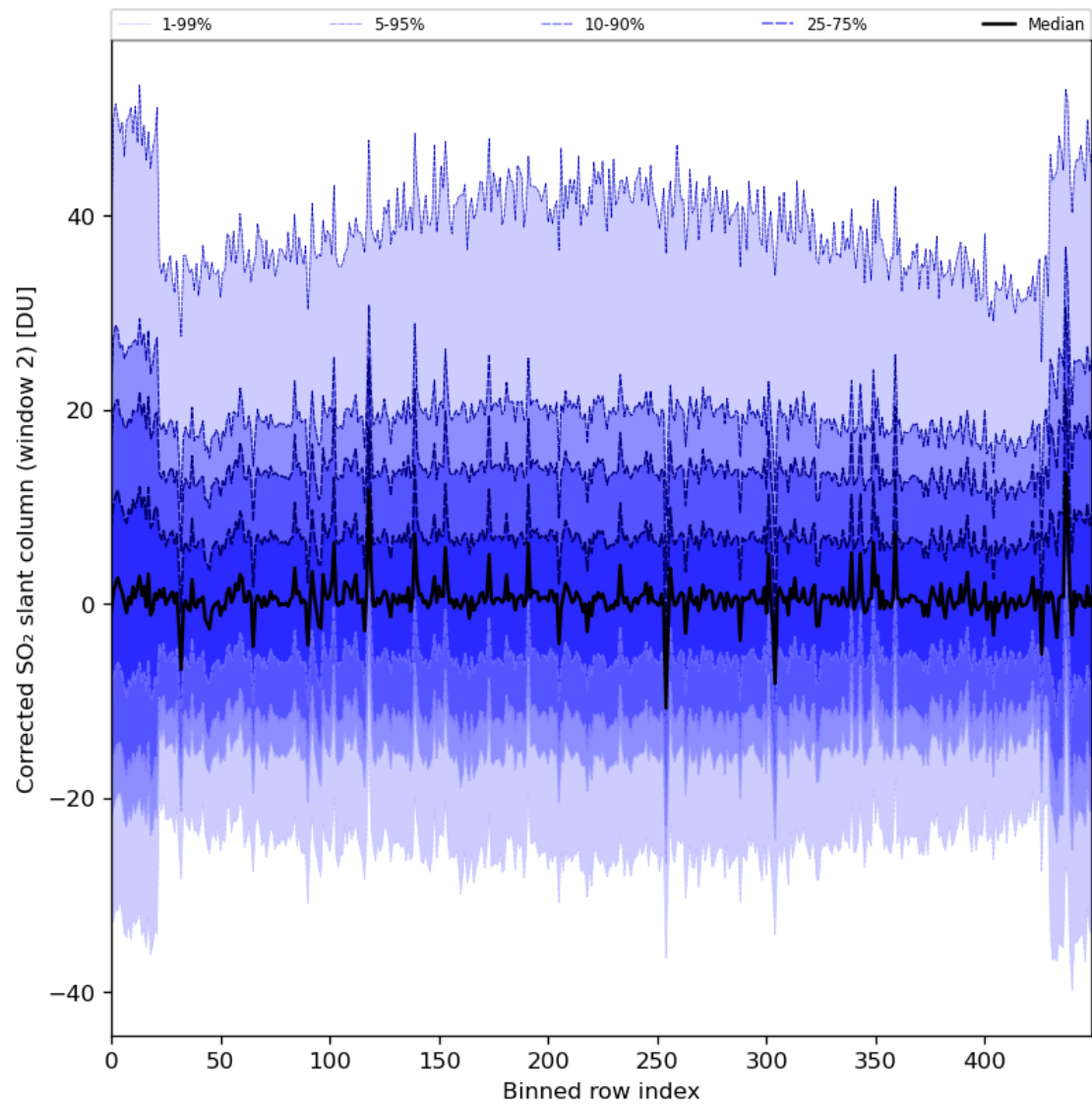
Figure 85: Along track statistics of “Corrected SO 2 slant column (window 2)” for 2024-08-02 to 2024-08-04
