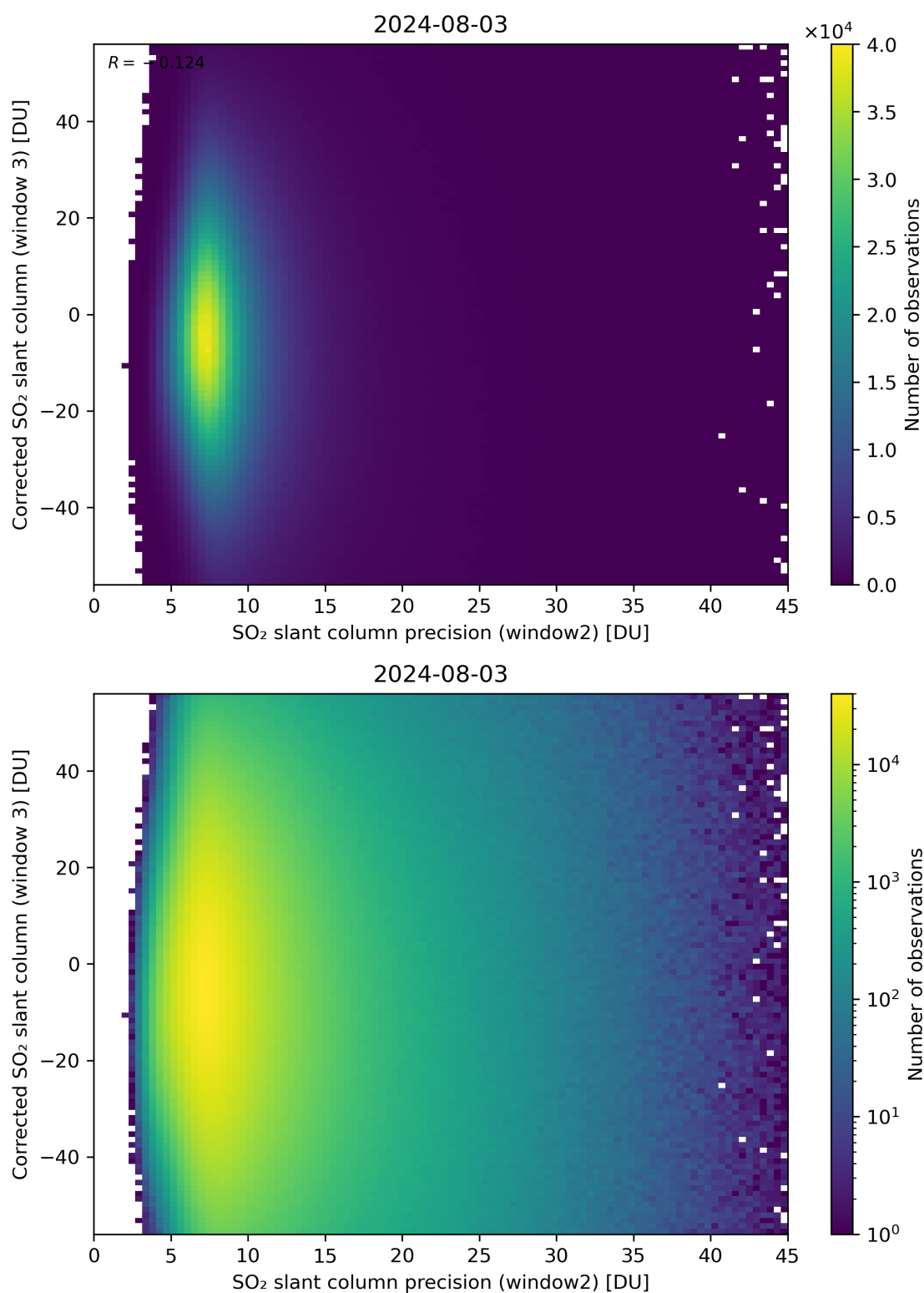
Figure 248: Scatter density plot of “SO 2 slant column precision (window2)” against “Corrected SO 2 slant column (window 3)” for 2024-08-02 to 2024-08-04.
