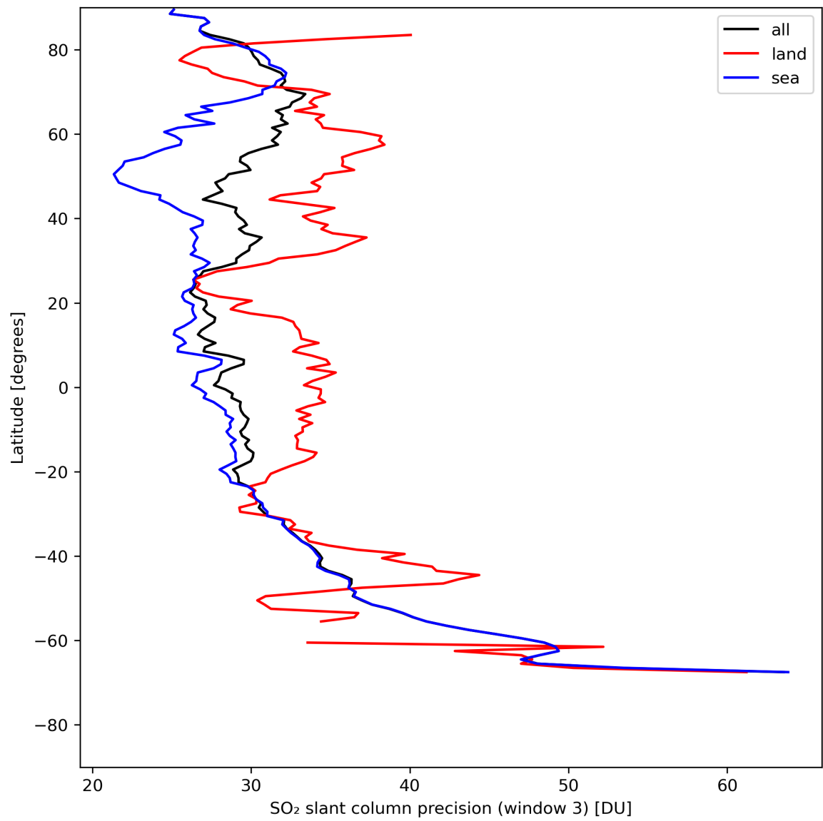
Figure 42: Zonal average of “SO 2 slant column precision (window 3)” for 2024-08-02 to 2024-08-04.
