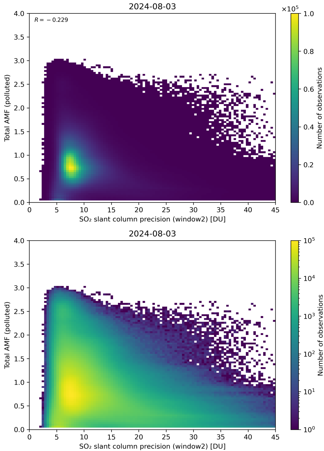
Figure 251: Scatter density plot of “SO 2 slant column precision (window2)” against “Total AMF (polluted)” for 2024-08-02 to 2024-08-04.
