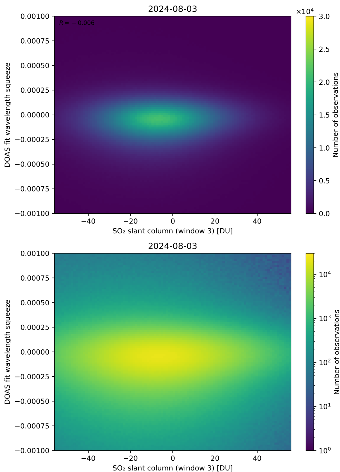
Figure 255: Scatter density plot of “SO 2 slant column (window 3)” against “DOAS fit wavelength squeeze” for 2024-08-02 to 2024-08-04.
