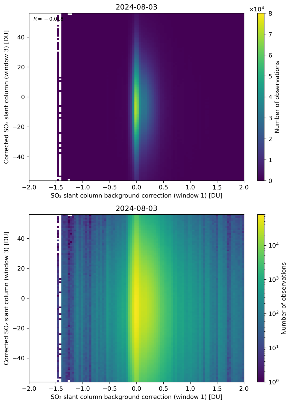
Figure 105: Scatter density plot of “SO 2 slant column background correction (window 1)” against “Corrected SO 2 slant column (window 3)” for 2024-08-02 to 2024-08-04.
