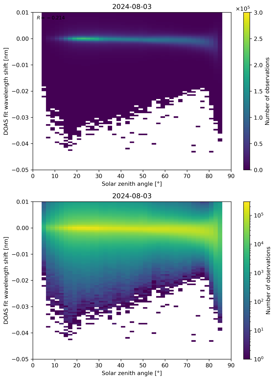
Figure 161: Scatter density plot of “Solar zenith angle” against “DOAS fit wavelength shift” for 2024-08-02 to 2024-08-04.
