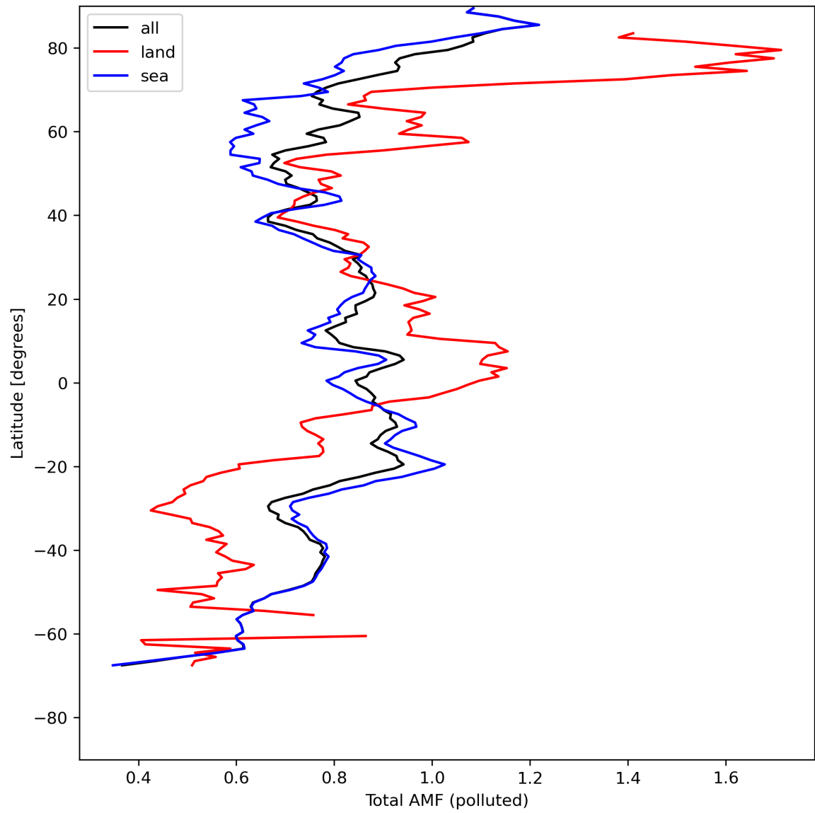
Figure 48: Zonal average of “Total AMF (polluted)” for 2024-08-02 to 2024-08-04.
