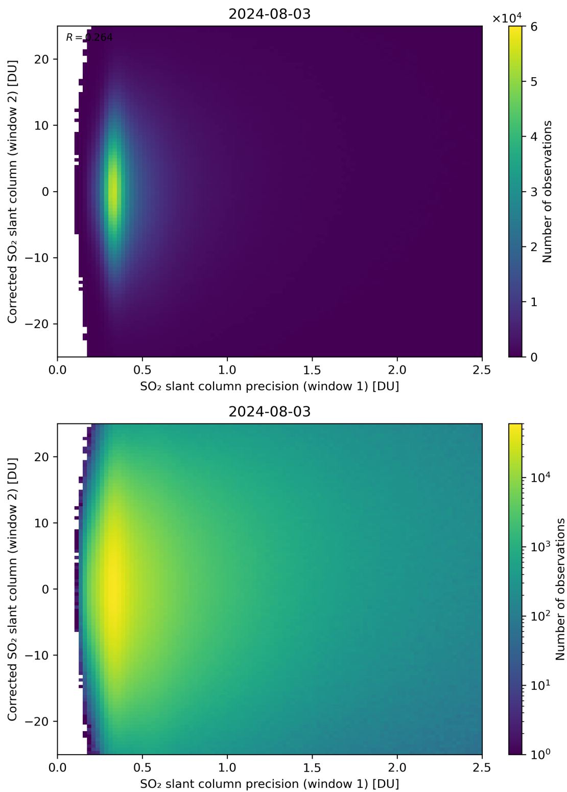
Figure 225: Scatter density plot of “SO 2 slant column precision (window 1)” against “Corrected SO 2 slant column (window 2)” for 2024-08-02 to 2024-08-04.
