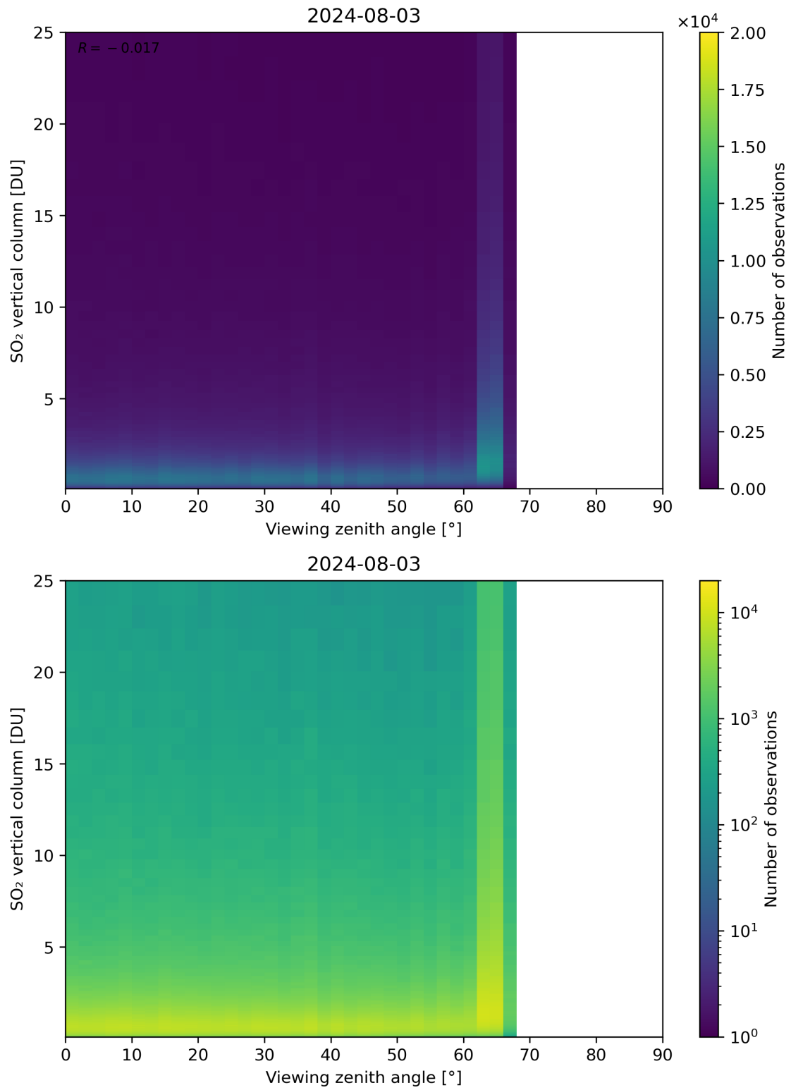
Figure 327: Scatter density plot of “Viewing zenith angle” against “SO 2 vertical column” for 2024-08-02 to 2024-08-04.
