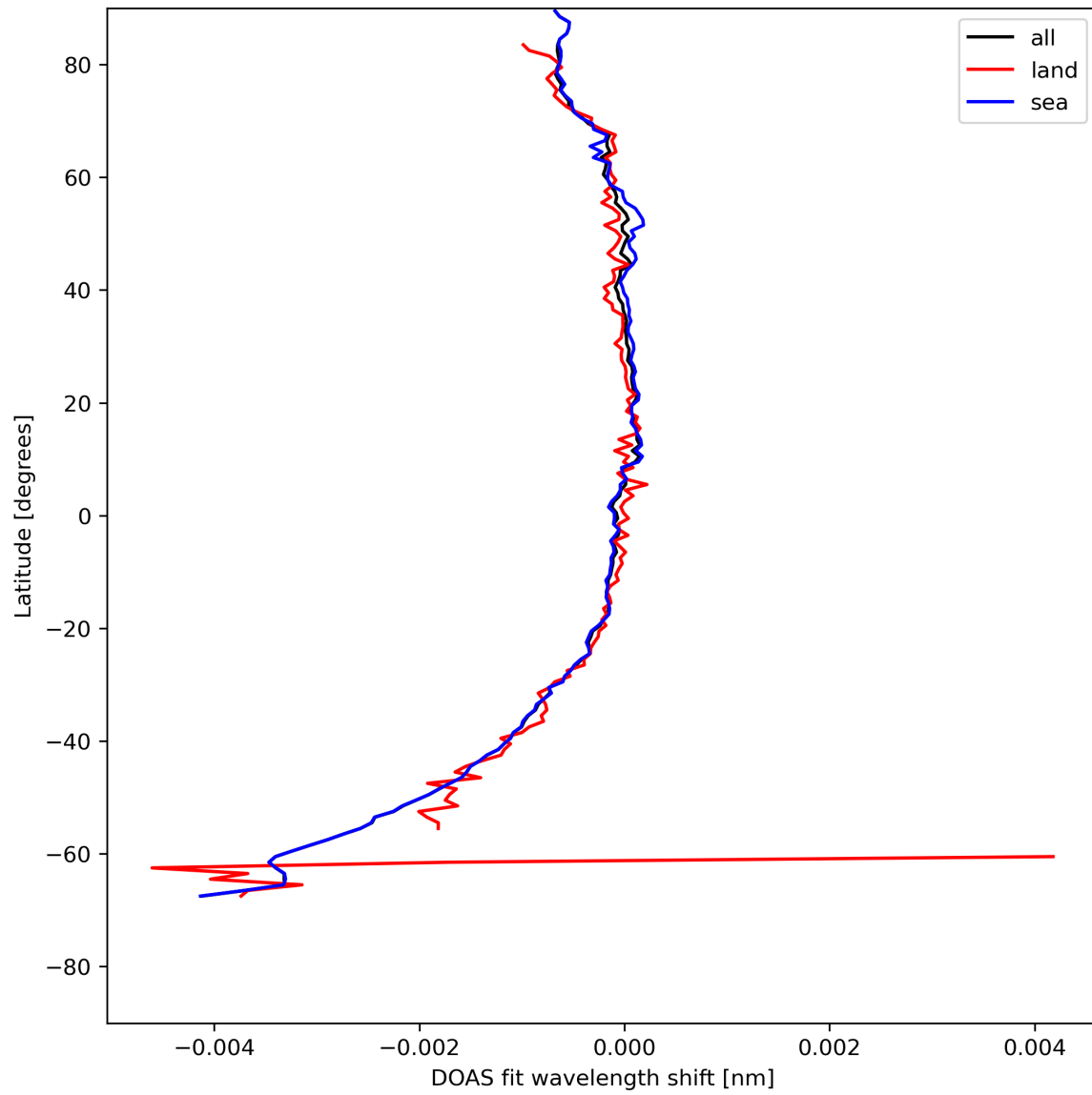
Figure 45: Zonal average of “DOAS fit wavelength shift” for 2024-08-02 to 2024-08-04.
