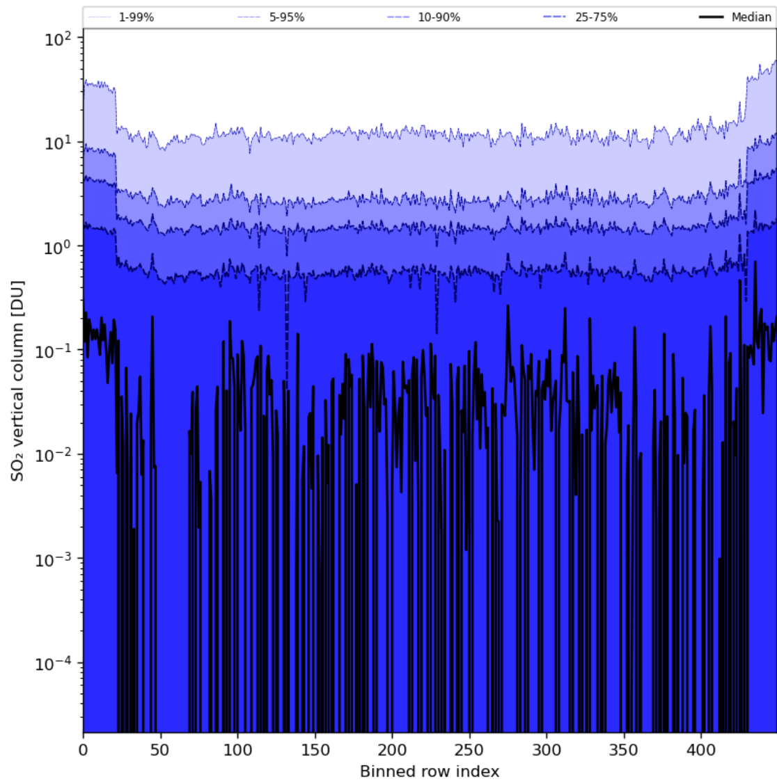
Figure 76: Along track statistics of “SO 2 vertical column” for 2024-08-02 to 2024-08-04
