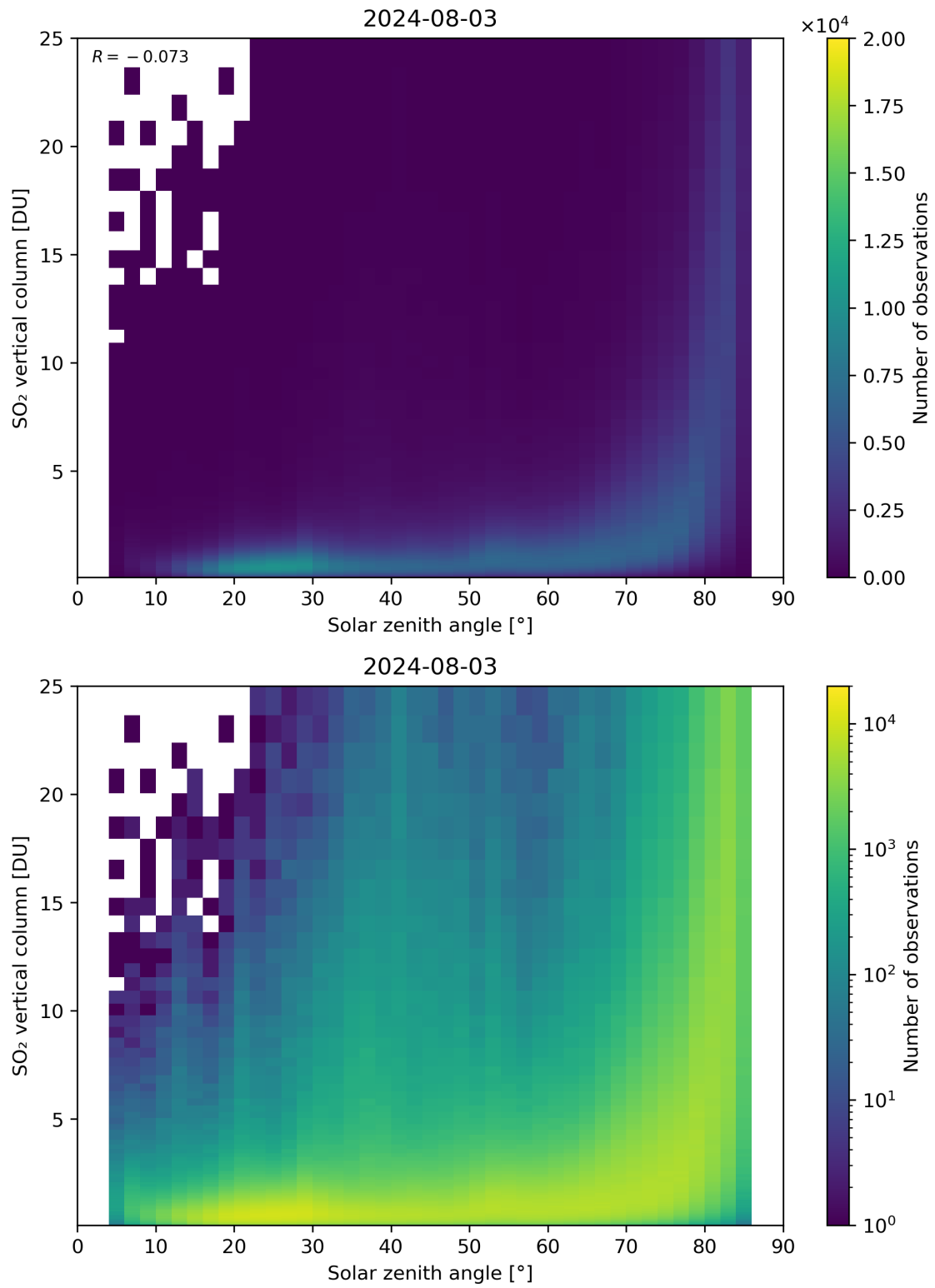
Figure 176: Scatter density plot of “Solar zenith angle” against “SO 2 vertical column” for 2024-08-02 to 2024-08-04.
