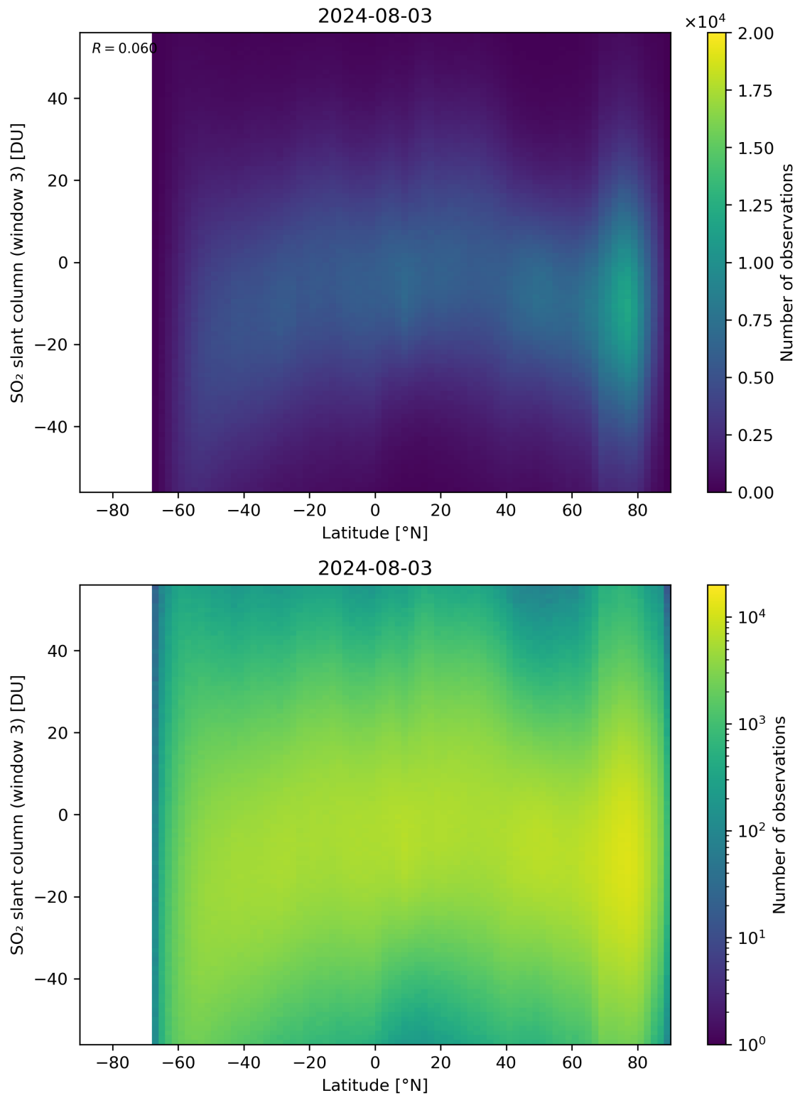
Figure 152: Scatter density plot of “Latitude” against “SO 2 slant column (window 3)” for 2024-08-02 to 2024-08-04.
