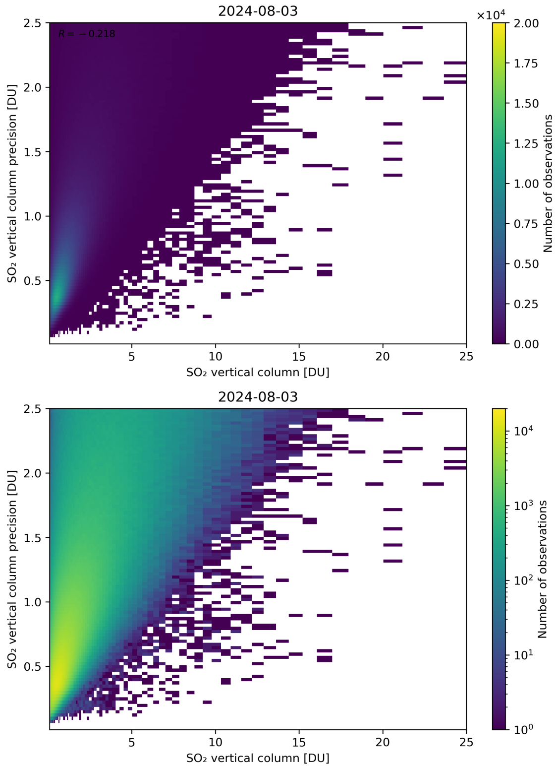
Figure 307: Scatter density plot of “SO 2 vertical column” against “SO 2 vertical column precision” for 2024-08-02 to 2024-08-04.
