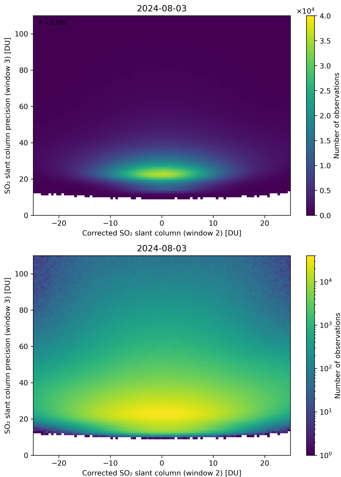
Figure 202: Scatter density plot of “Corrected SO 2 slant column (window 2)” against “SO 2 slant column precision (window 3)” for 2024-08-02 to 2024-08-04.
