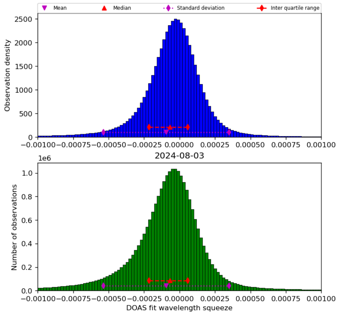
Figure 69: Histogram of “DOAS fit wavelength squeeze” for 2024-08-02 to 2024-08-04
