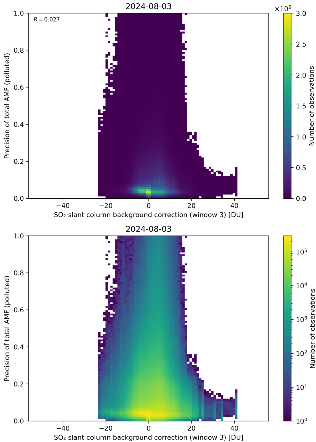
Figure 126: Scatter density plot of “SO 2 slant column background correction (window 3)” against “Precision of total AMF (polluted)” for 2024-08-02 to 2024-08-04.
