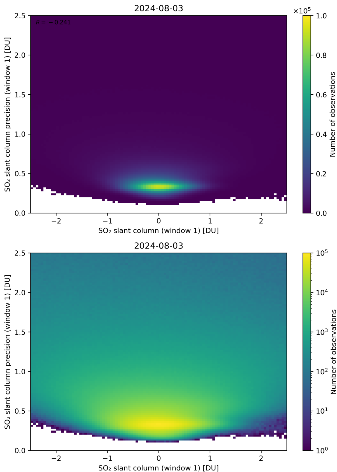
Figure 235: Scatter density plot of “SO 2 slant column (window 1)” against “SO 2 slant column precision (window 1)” for 2024-08-02 to 2024-08-04.
