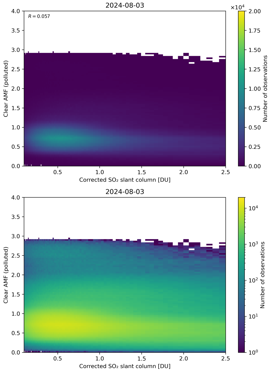
Figure 184: Scatter density plot of “Corrected SO 2 slant column” against “Clear AMF (polluted)” for 2024-08-02 to 2024-08-04.
