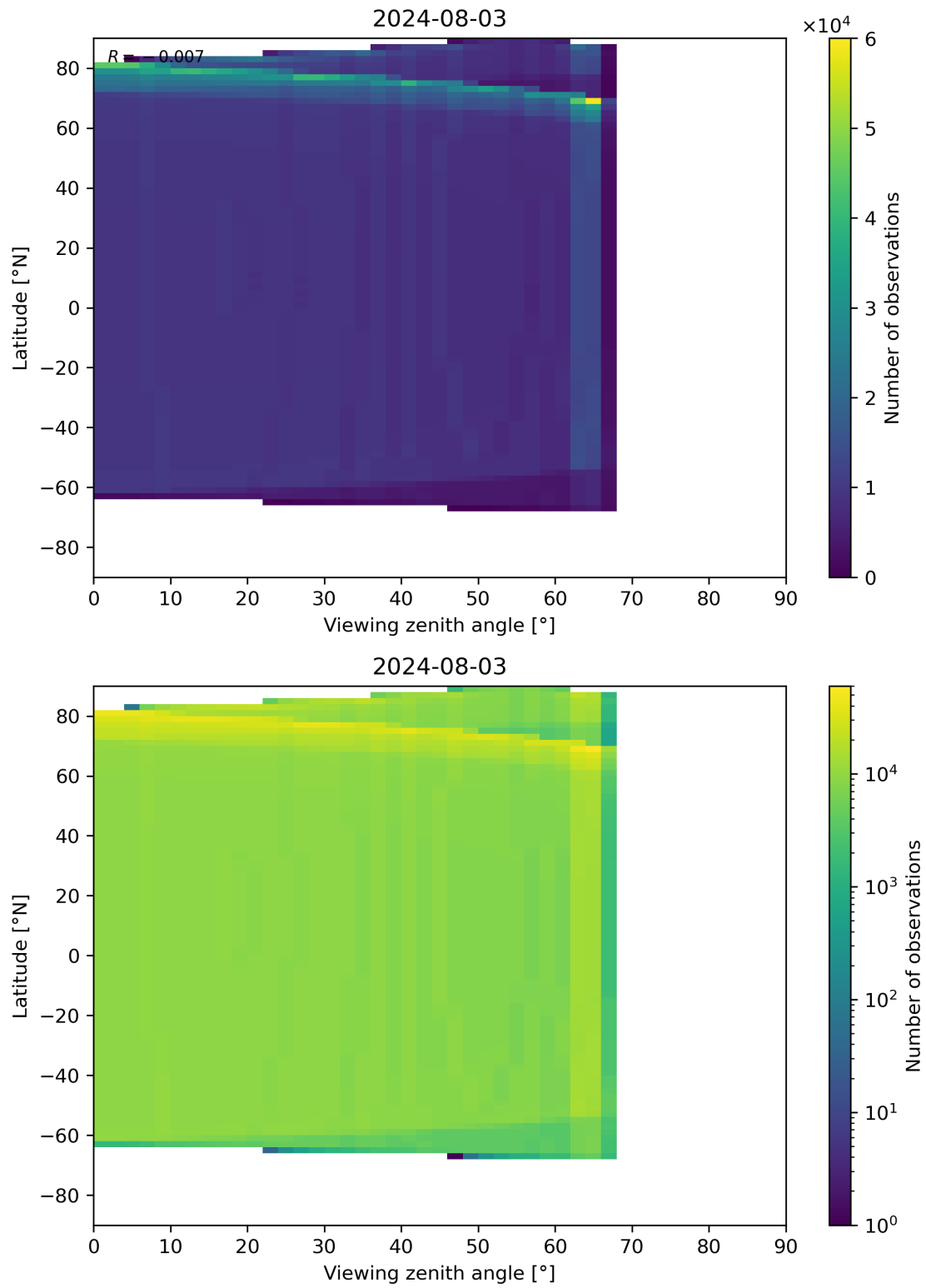
Figure 314: Scatter density plot of “Viewing zenith angle” against “Latitude” for 2024-08-02 to 2024-08-04.
