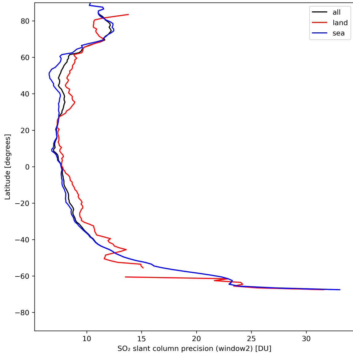
Figure 38: Zonal average of “SO 2 slant column precision (window2)” for 2024-08-02 to 2024-08-04.
