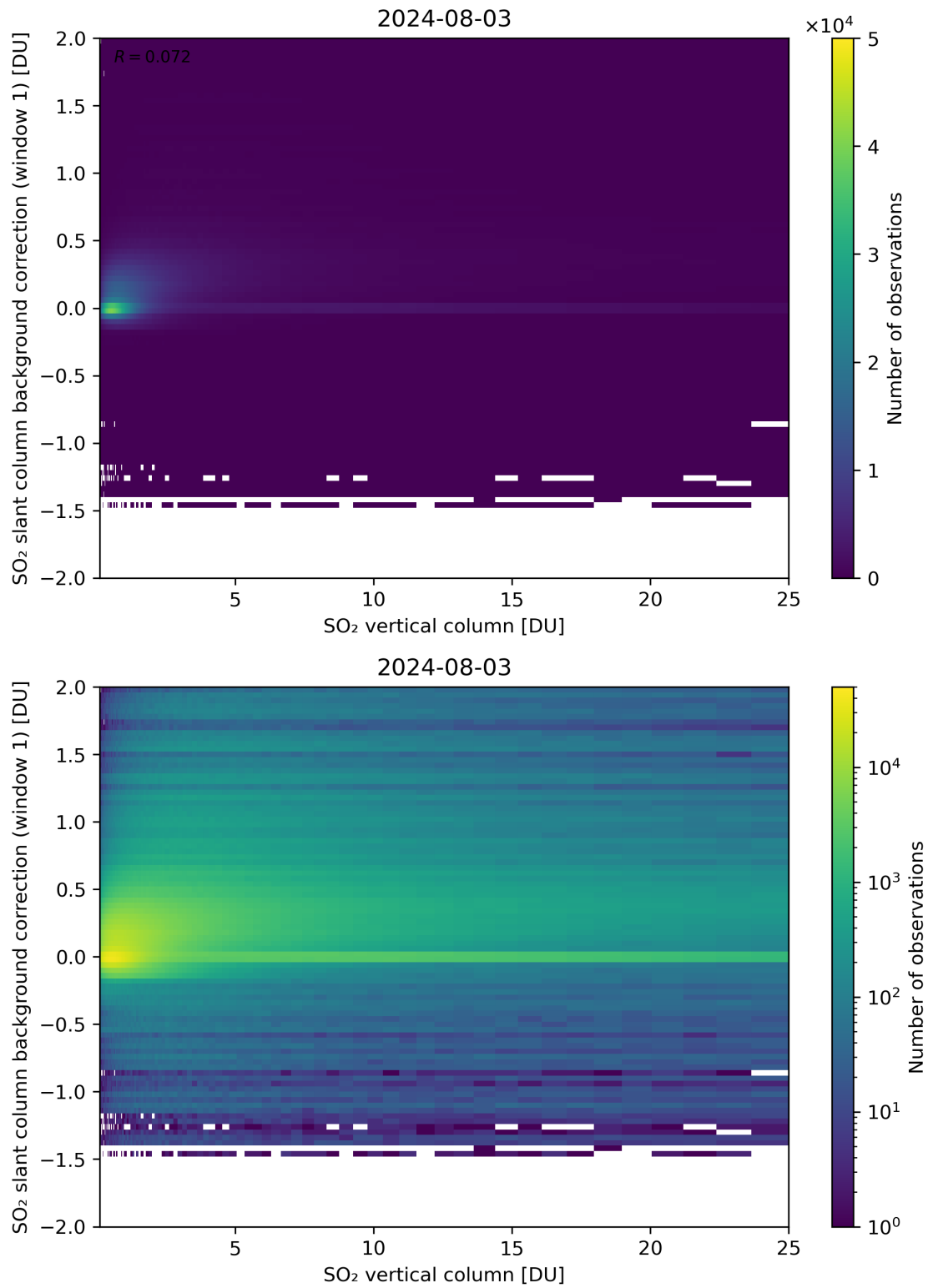
Figure 273: Scatter density plot of “SO 2 vertical column” against “SO 2 slant column background correction (window 1)” for 2024-08-02 to 2024-08-04.
