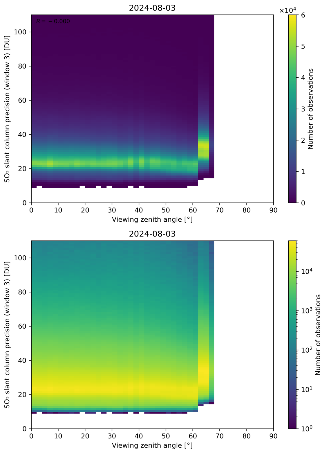
Figure 324: Scatter density plot of “Viewing zenith angle” against “SO 2 slant column precision (window 3)” for 2024-08-02 to 2024-08-04.
