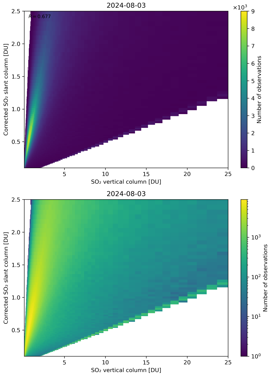
Figure 297: Scatter density plot of “SO 2 vertical column” against “Corrected SO 2 slant column” for 2024-08-02 to 2024-08-04.
