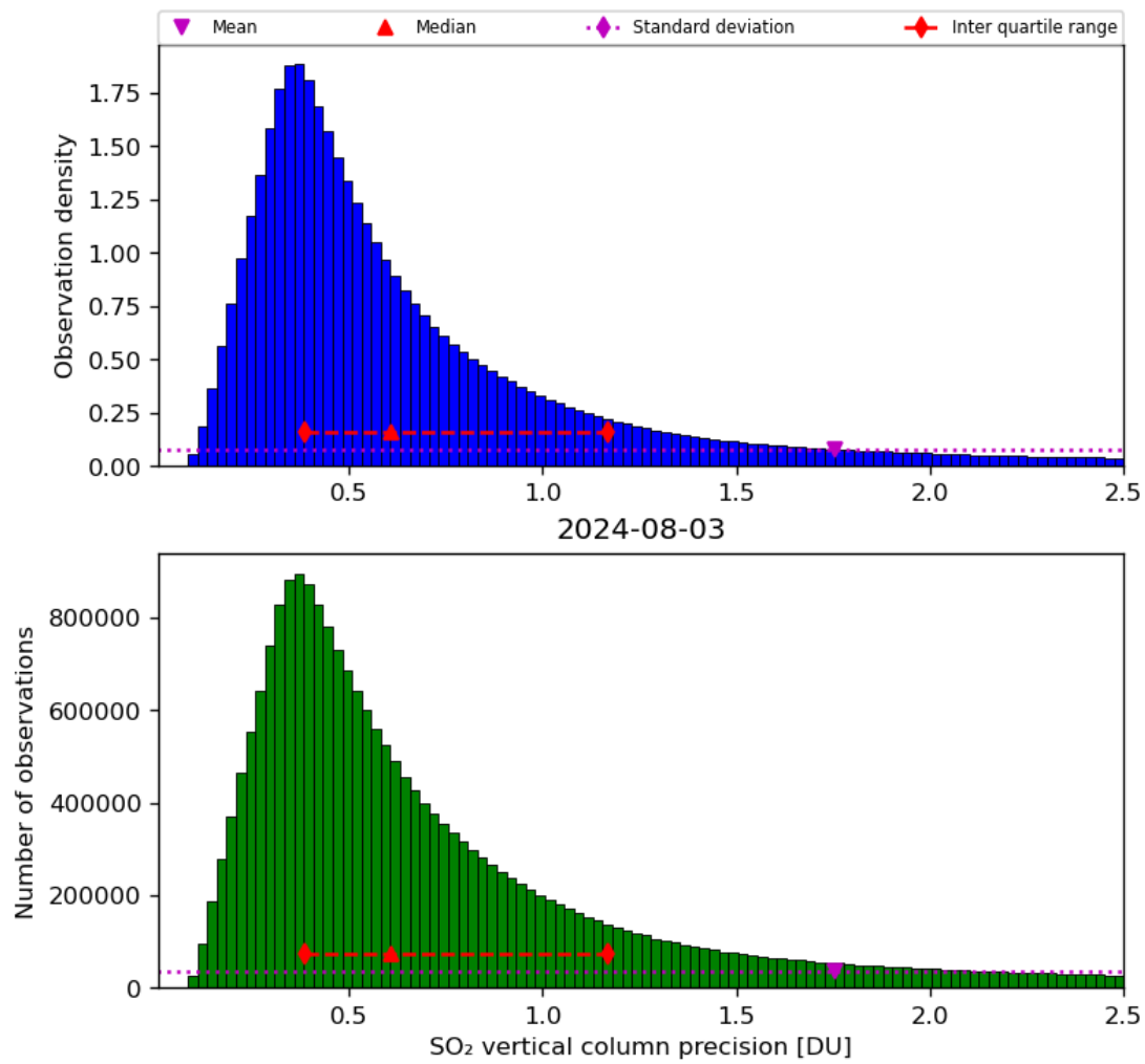
Figure 54: Histogram of “SO 2 vertical column precision” for 2024-08-02 to 2024-08-04
