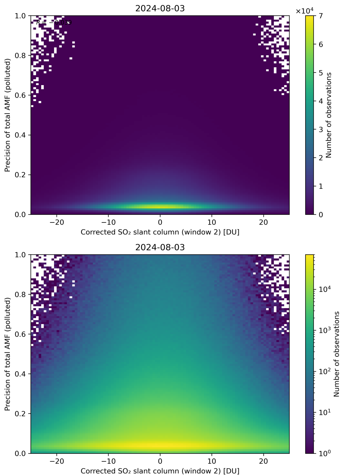
Figure 204: Scatter density plot of “Corrected SO 2 slant column (window 2)” against “Precision of total AMF (polluted)” for 2024-08-02 to 2024-08-04.
