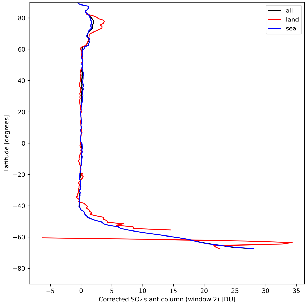
Figure 39: Zonal average of “Corrected SO 2 slant column (window 2)” for 2024-08-02 to 2024-08-04.
