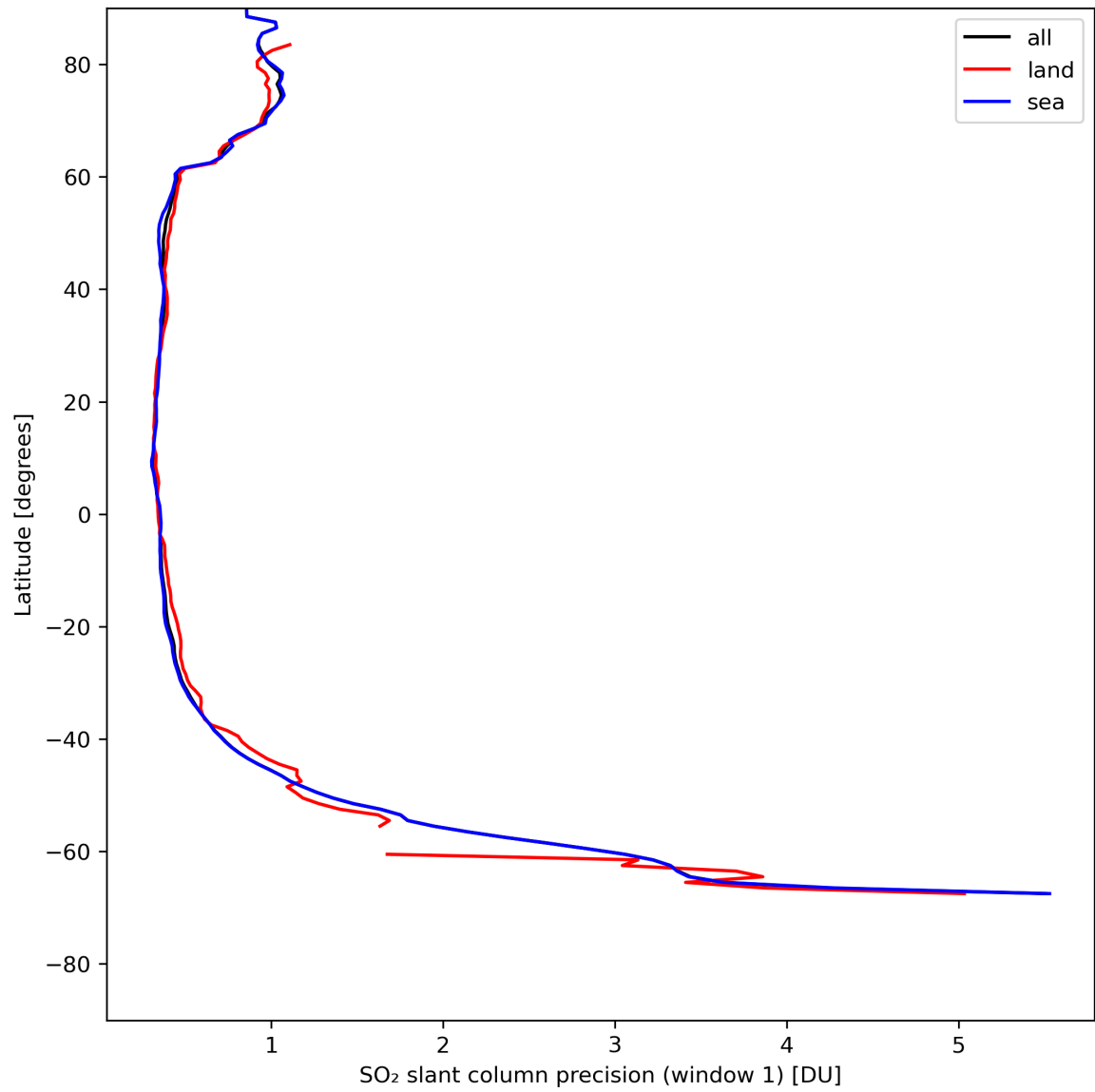
Figure 34: Zonal average of “SO 2 slant column precision (window 1)” for 2024-08-02 to 2024-08-04.
