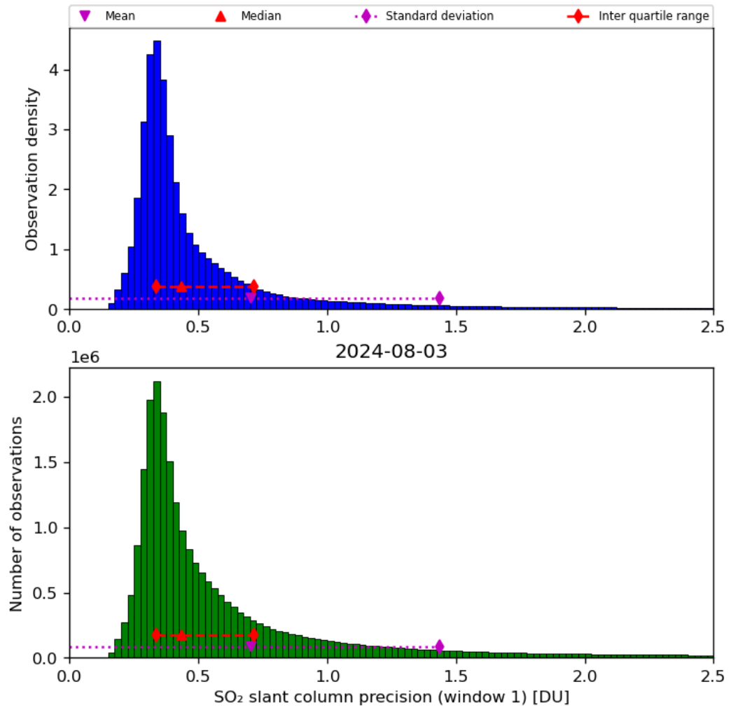
Figure 57: Histogram of “SO 2 slant column precision (window 1)” for 2024-08-02 to 2024-08-04
