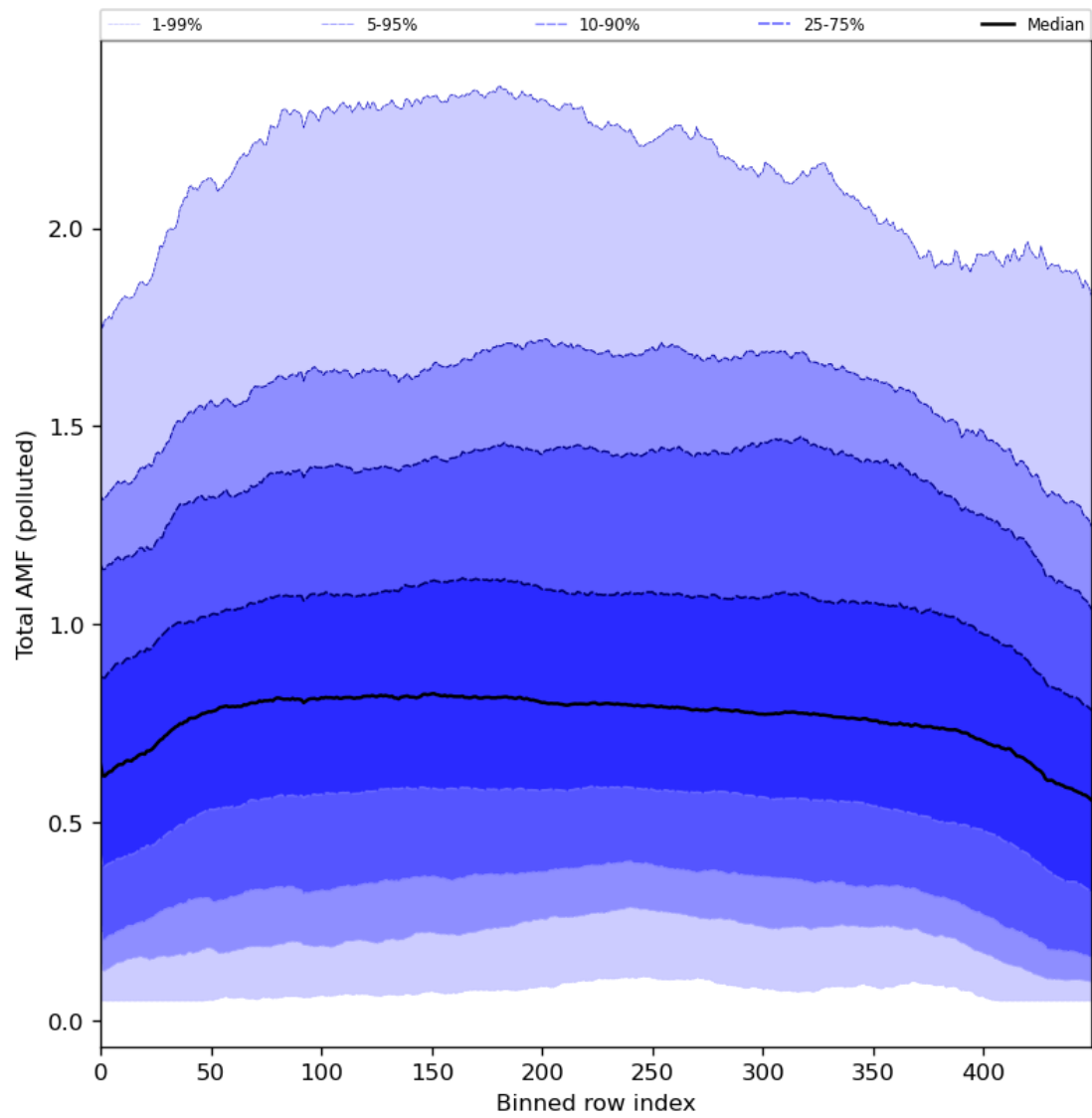
Figure 94: Along track statistics of “Total AMF (polluted)” for 2024-08-02 to 2024-08-04
