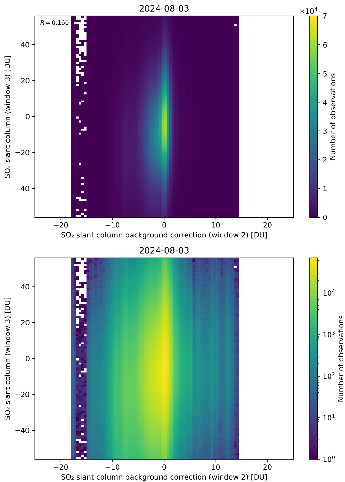
Figure 117: Scatter density plot of “SO 2 slant column background correction (window 2)” against “SO 2 slant column (window 3)” for 2024-08-02 to 2024-08-04.
