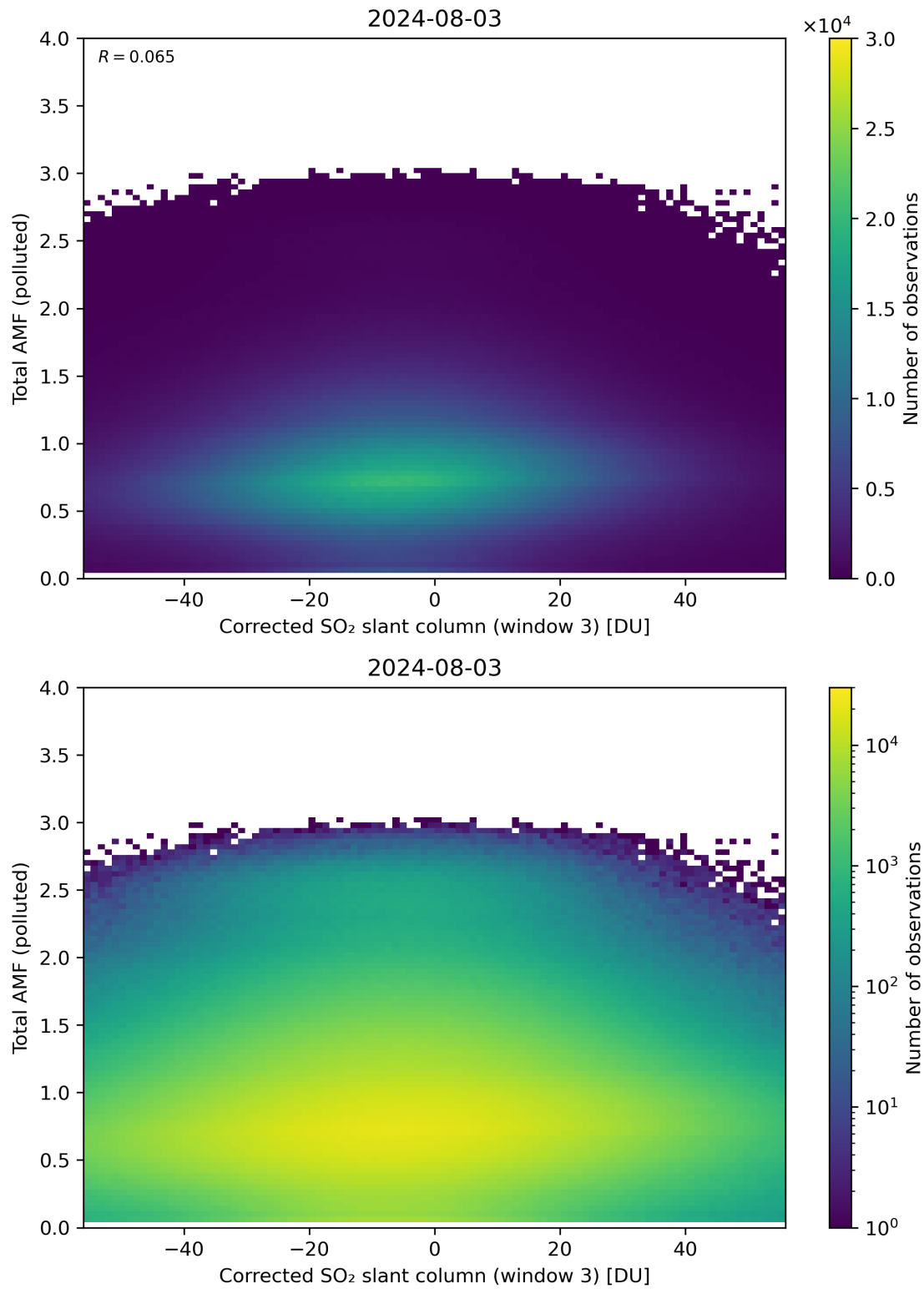
Figure 210: Scatter density plot of “Corrected SO 2 slant column (window 3)” against “Total AMF (polluted)” for 2024-08-02 to 2024-08-04.
