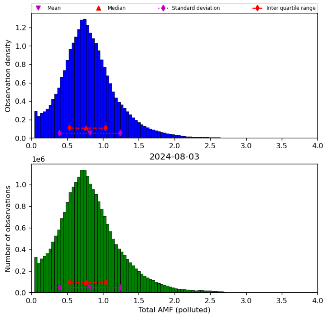
Figure 71: Histogram of “Total AMF (polluted)” for 2024-08-02 to 2024-08-04
