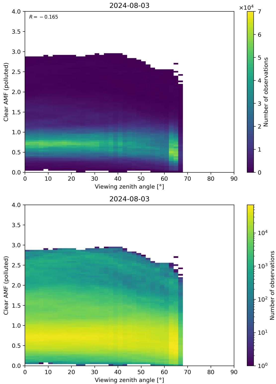
Figure 316: Scatter density plot of “Viewing zenith angle” against “Clear AMF (polluted)” for 2024-08-02 to 2024-08-04.
