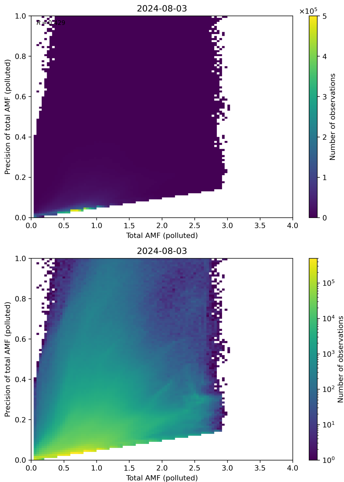
Figure 272: Scatter density plot of “Total AMF (polluted)” against “Precision of total AMF (polluted)” for 2024-08-02 to 2024-08-04.
