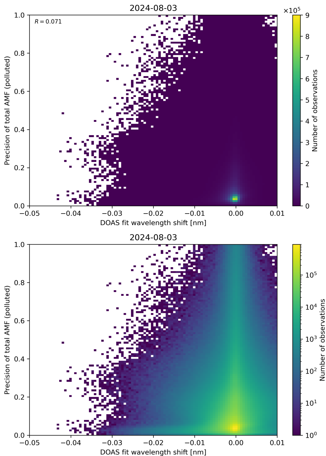
Figure 131: Scatter density plot of “DOAS fit wavelength shift” against “Precision of total AMF (polluted)” for 2024-08-02 to 2024-08-04.
