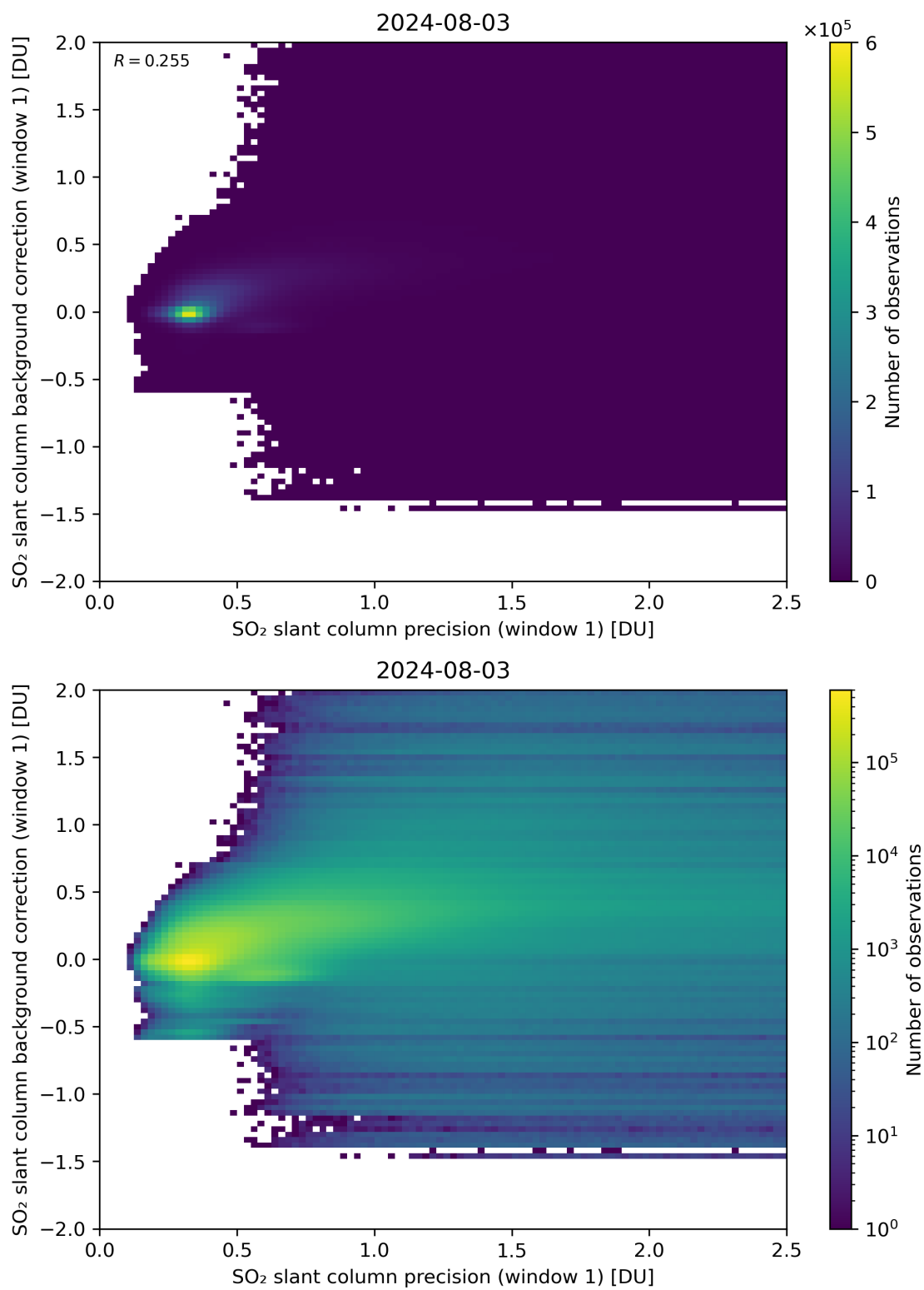
Figure 218: Scatter density plot of “SO 2 slant column precision (window 1)” against “SO 2 slant column background correction (window 1)” for 2024-08-02 to 2024-08-04.
