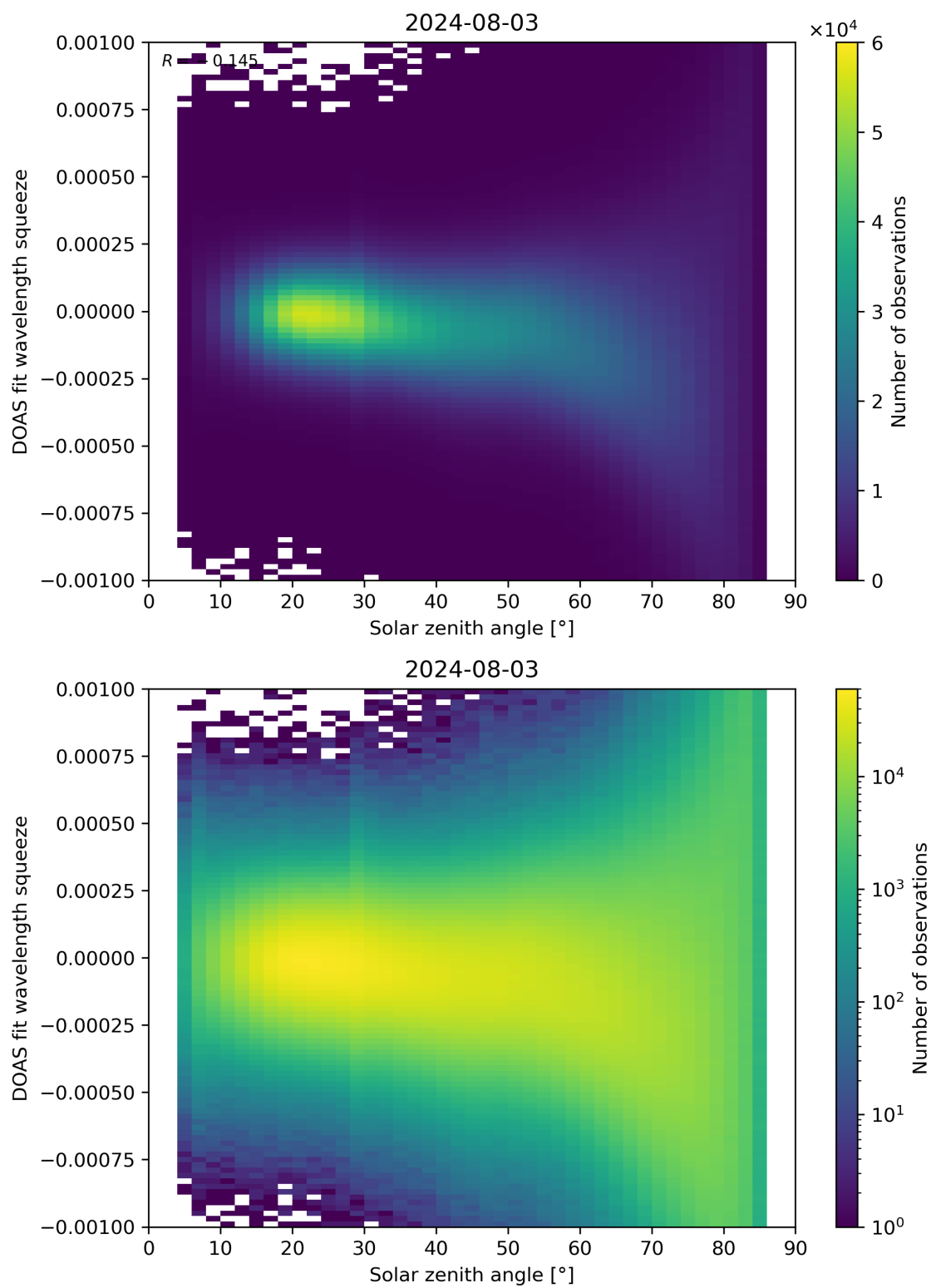
Figure 162: Scatter density plot of “Solar zenith angle” against “DOAS fit wavelength squeeze” for 2024-08-02 to 2024-08-04.
