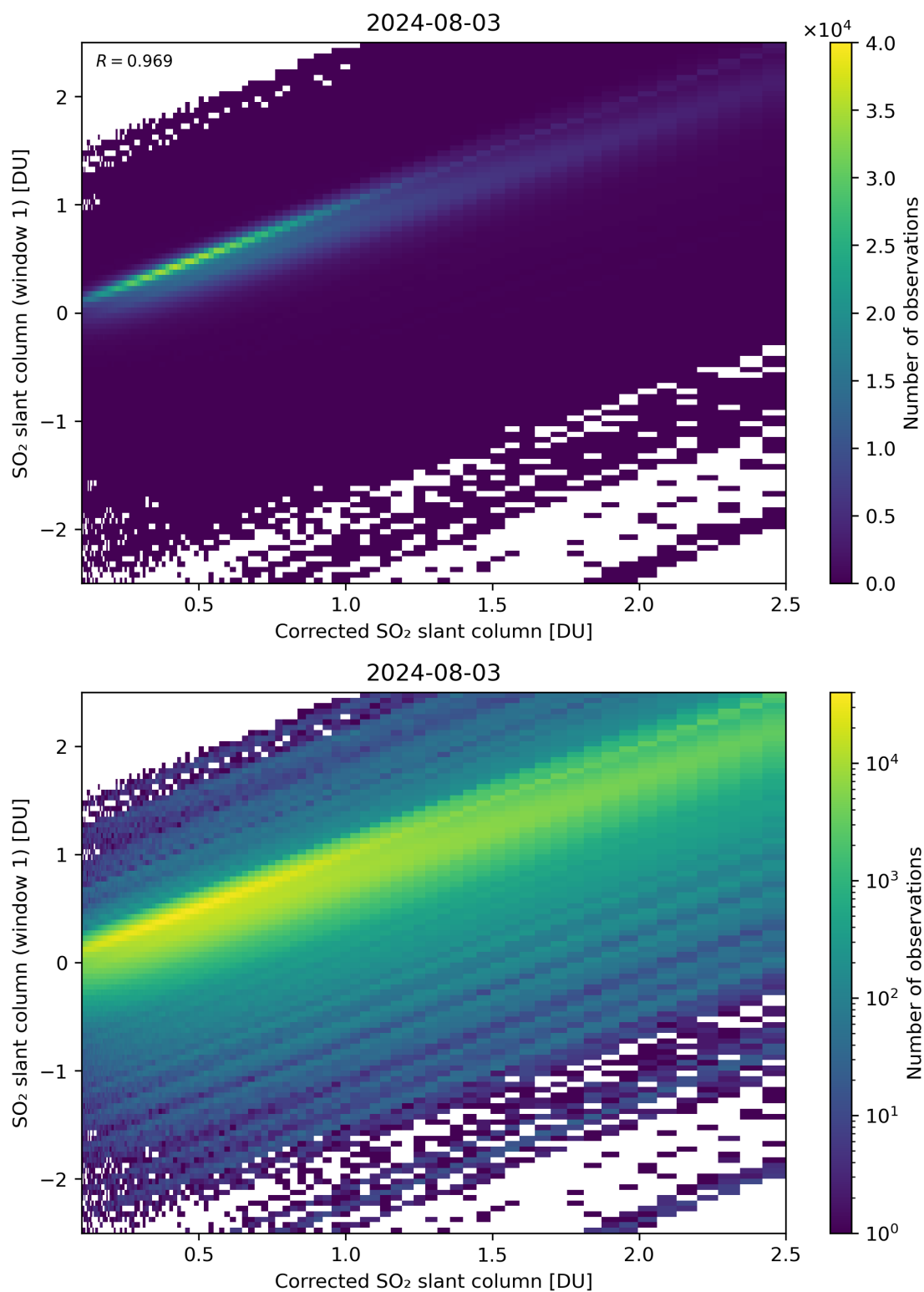
Figure 187: Scatter density plot of “Corrected SO 2 slant column” against “SO 2 slant column (window 1)” for 2024-08-02 to 2024-08-04.
