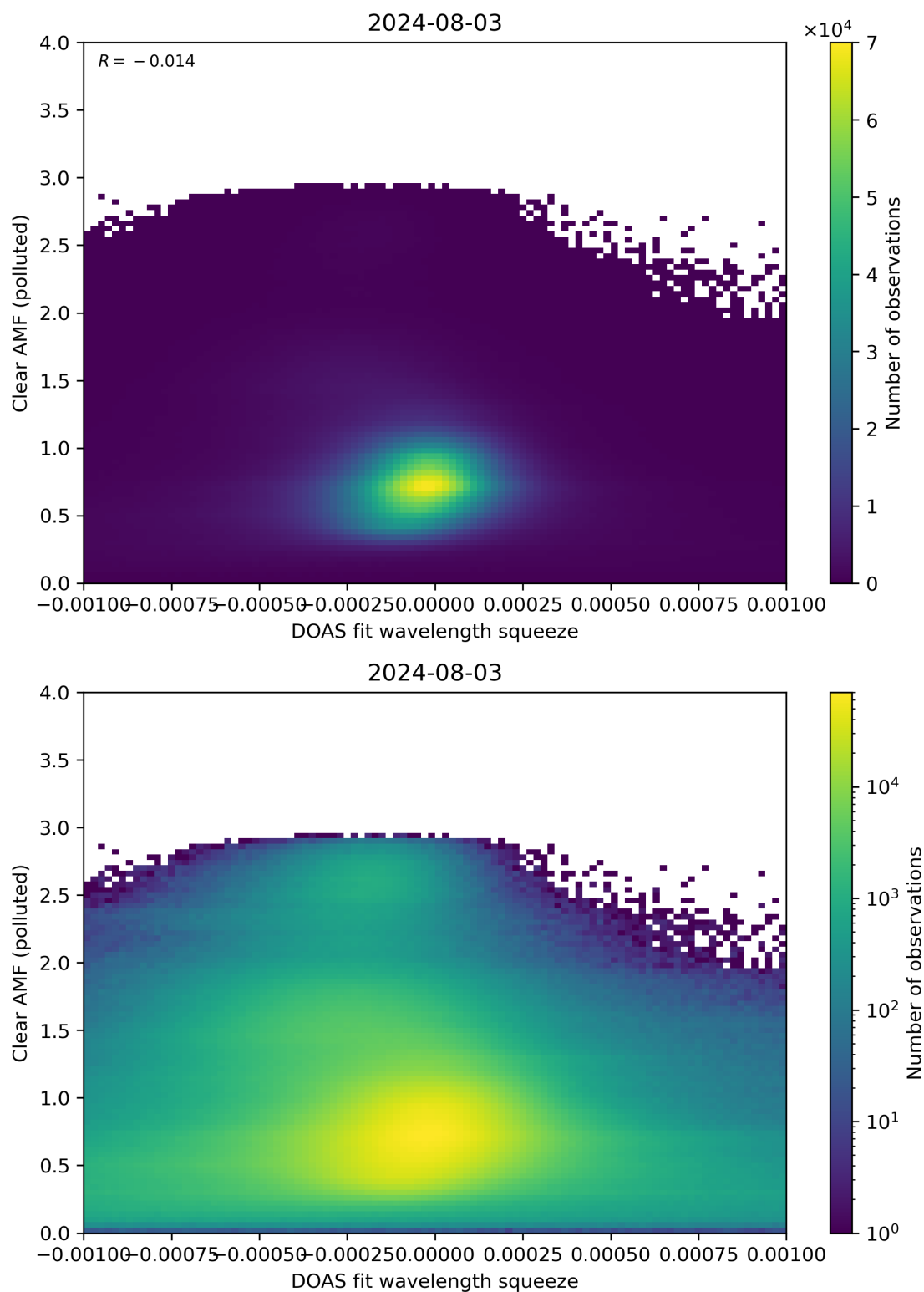
Figure 133: Scatter density plot of “DOAS fit wavelength squeeze” against “Clear AMF (polluted)” for 2024-08-02 to 2024-08-04.
