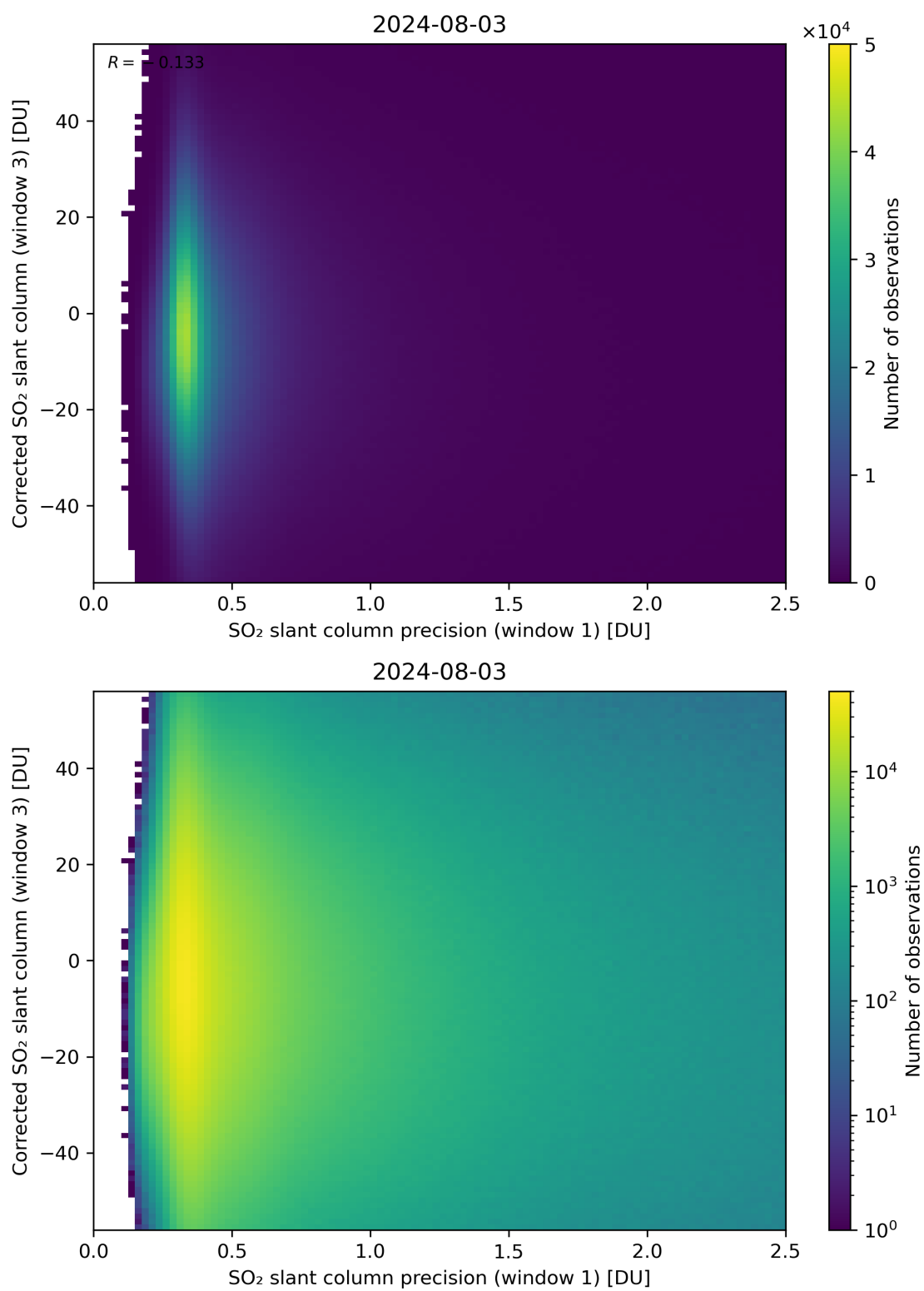
Figure 226: Scatter density plot of “SO 2 slant column precision (window 1)” against “Corrected SO 2 slant column (window 3)” for 2024-08-02 to 2024-08-04.
