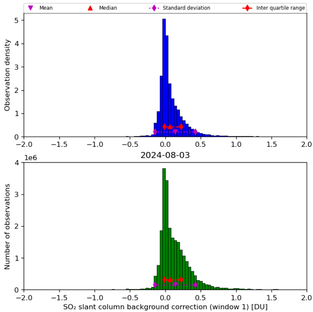
Figure 59: Histogram of “SO 2 slant column background correction (window 1)” for 2024-08-02 to 2024-08-04
