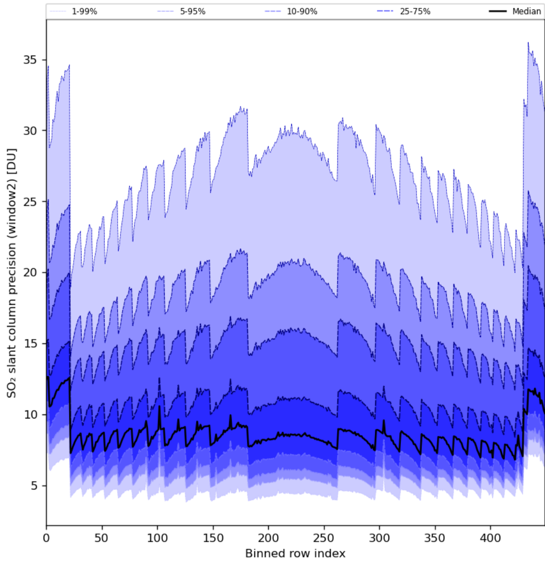
Figure 84: Along track statistics of “SO 2 slant column precision (window2)” for 2024-08-02 to 2024-08-04
