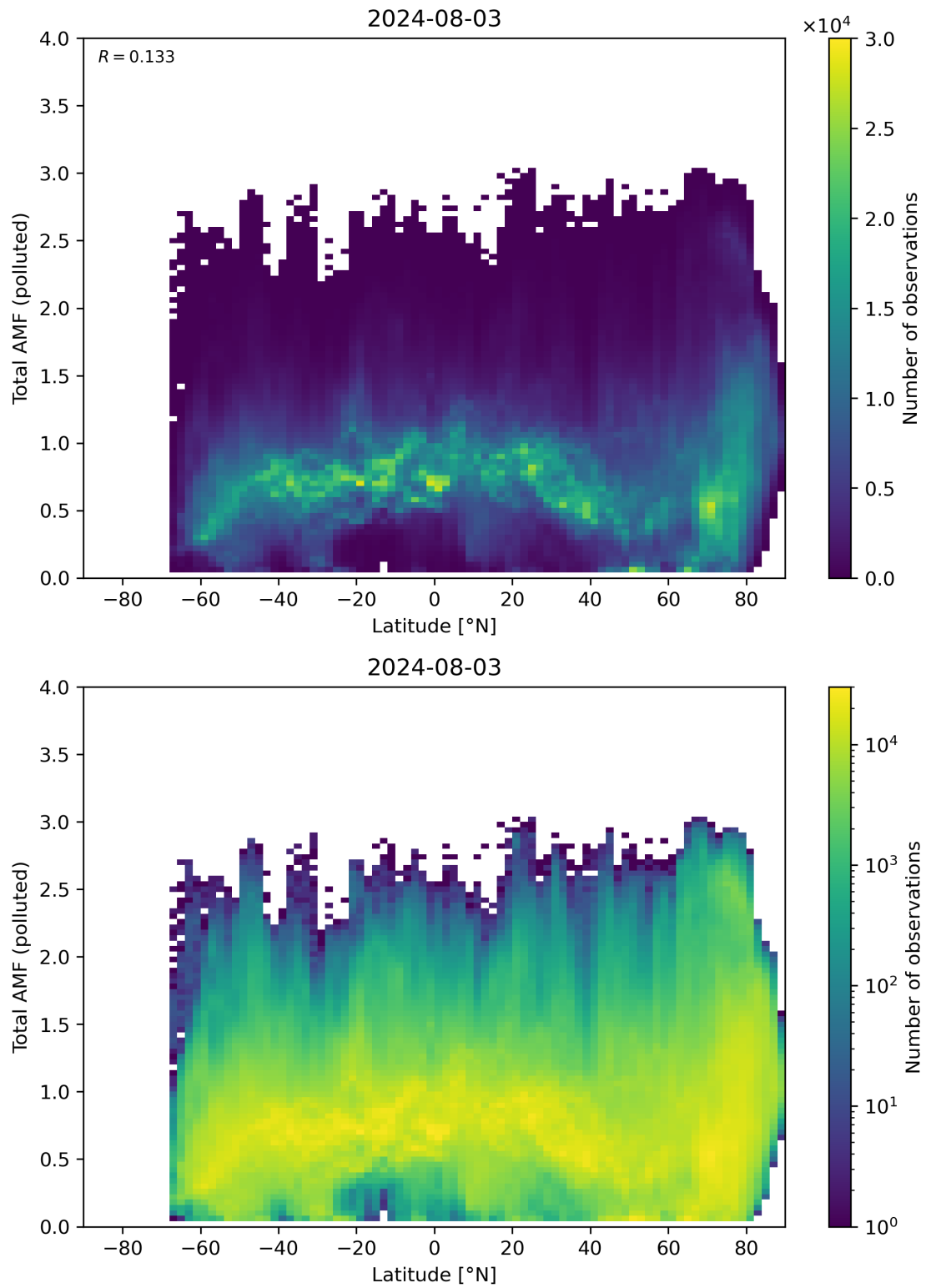
Figure 154: Scatter density plot of “Latitude” against “Total AMF (polluted)” for 2024-08-02 to 2024-08-04.
