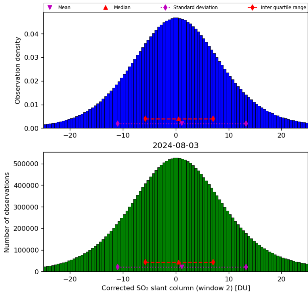
Figure 62: Histogram of “Corrected SO 2 slant column (window 2)” for 2024-08-02 to 2024-08-04
