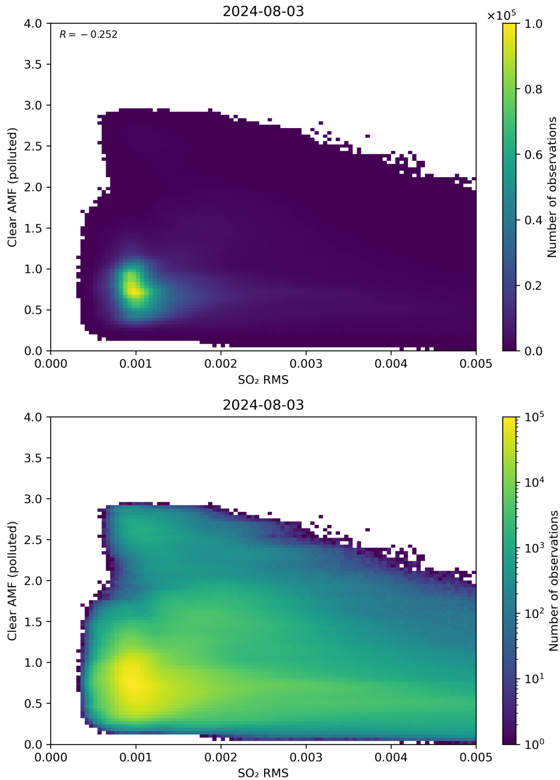
Figure 136: Scatter density plot of “SO 2 RMS” against “Clear AMF (polluted)” for 2024-08-02 to 2024-08-04.
