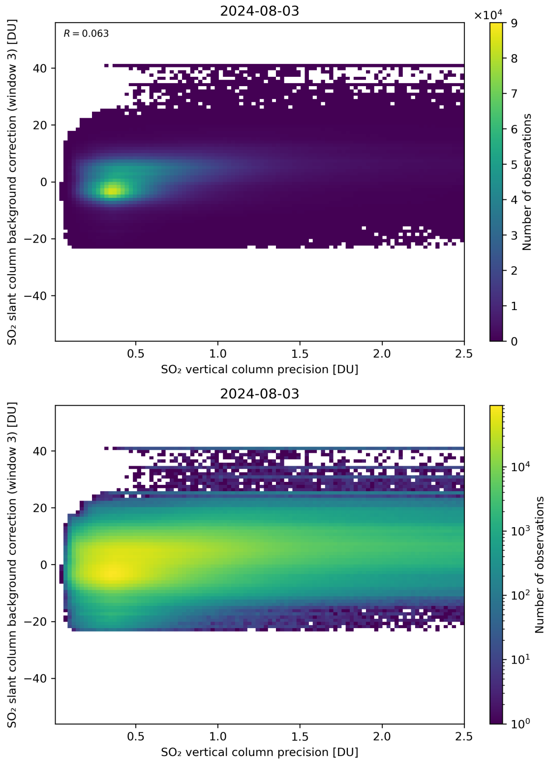
Figure 281: Scatter density plot of “SO 2 vertical column precision” against “SO 2 slant column background correction (window 3)” for 2024-08-02 to 2024-08-04.
