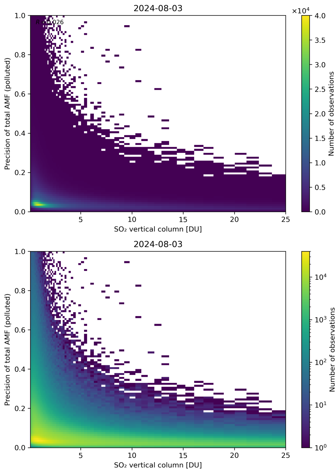
Figure 306: Scatter density plot of “SO 2 vertical column” against “Precision of total AMF (polluted)” for 2024-08-02 to 2024-08-04.
