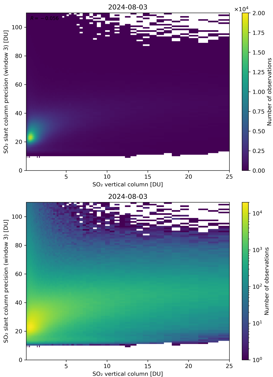
Figure 304: Scatter density plot of “SO 2 vertical column” against “SO 2 slant column precision (window 3)” for 2024-08-02 to 2024-08-04.
