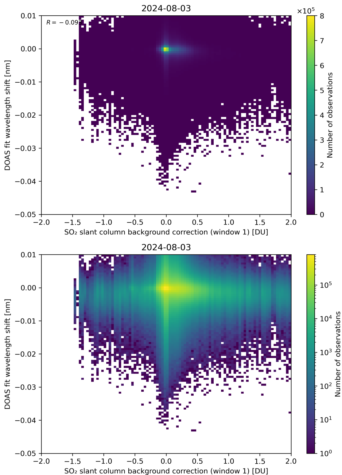
Figure 100: Scatter density plot of “SO 2 slant column background correction (window 1)” against “DOAS fit wavelength shift” for 2024-08-02 to 2024-08-04.
