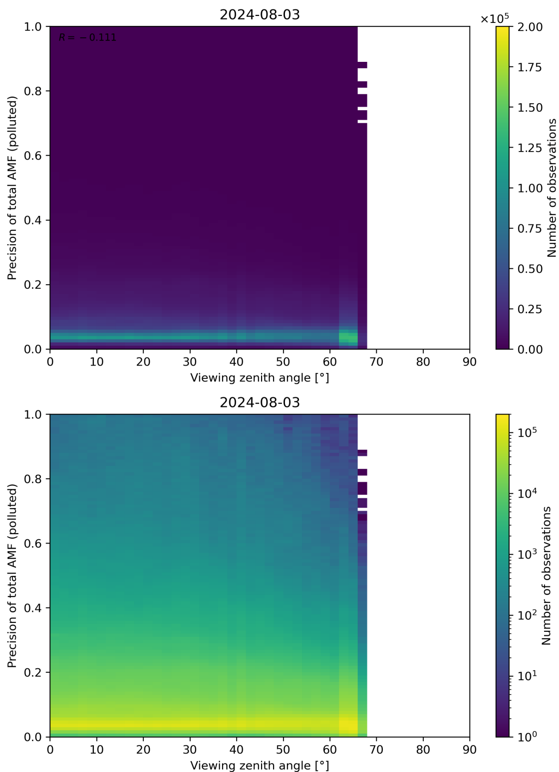
Figure 326: Scatter density plot of “Viewing zenith angle” against “Precision of total AMF (polluted)” for 2024-08-02 to 2024-08-04.
