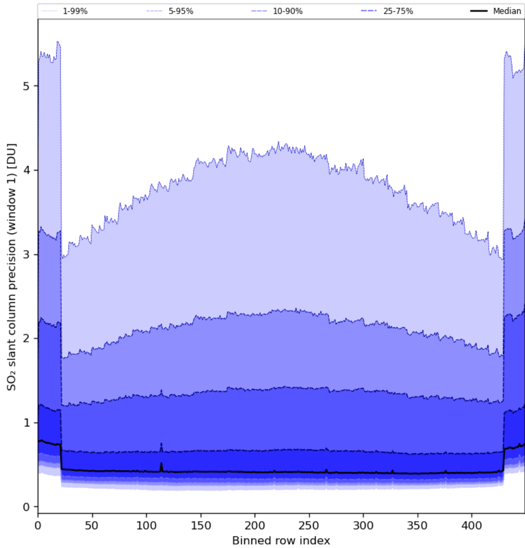
Figure 80: Along track statistics of “SO 2 slant column precision (window 1)” for 2024-08-02 to 2024-08-04
