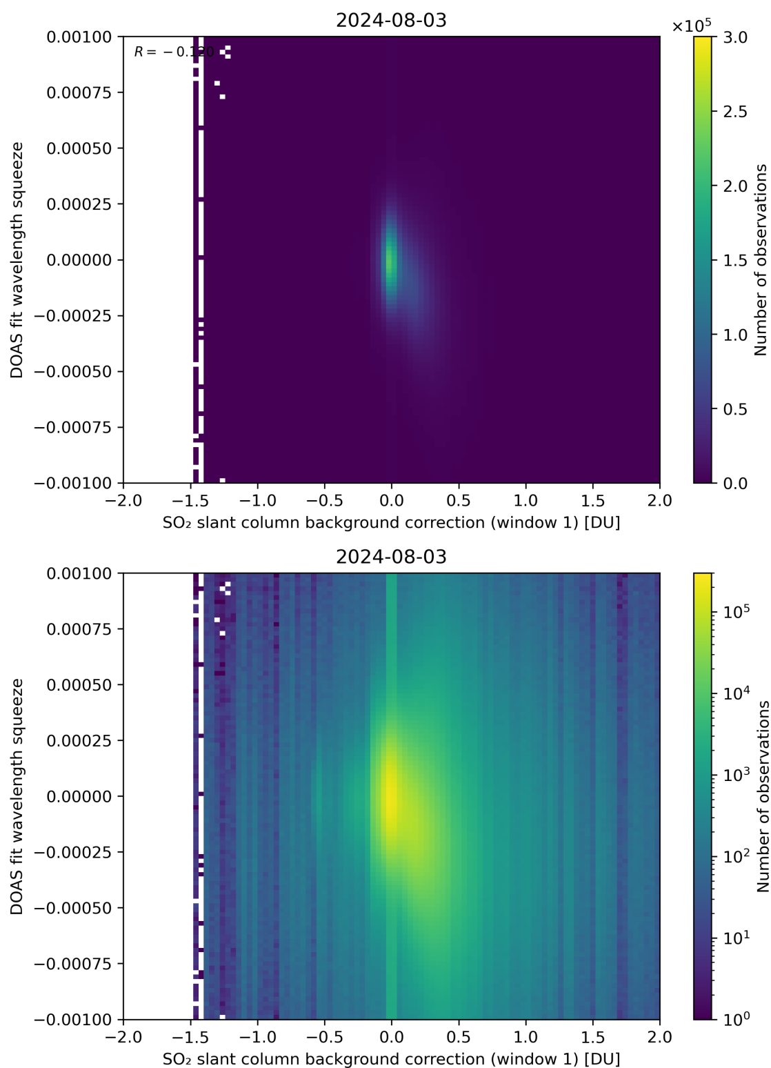
Figure 101: Scatter density plot of “SO 2 slant column background correction (window 1)” against “DOAS fit wavelength squeeze” for 2024-08-02 to 2024-08-04.
