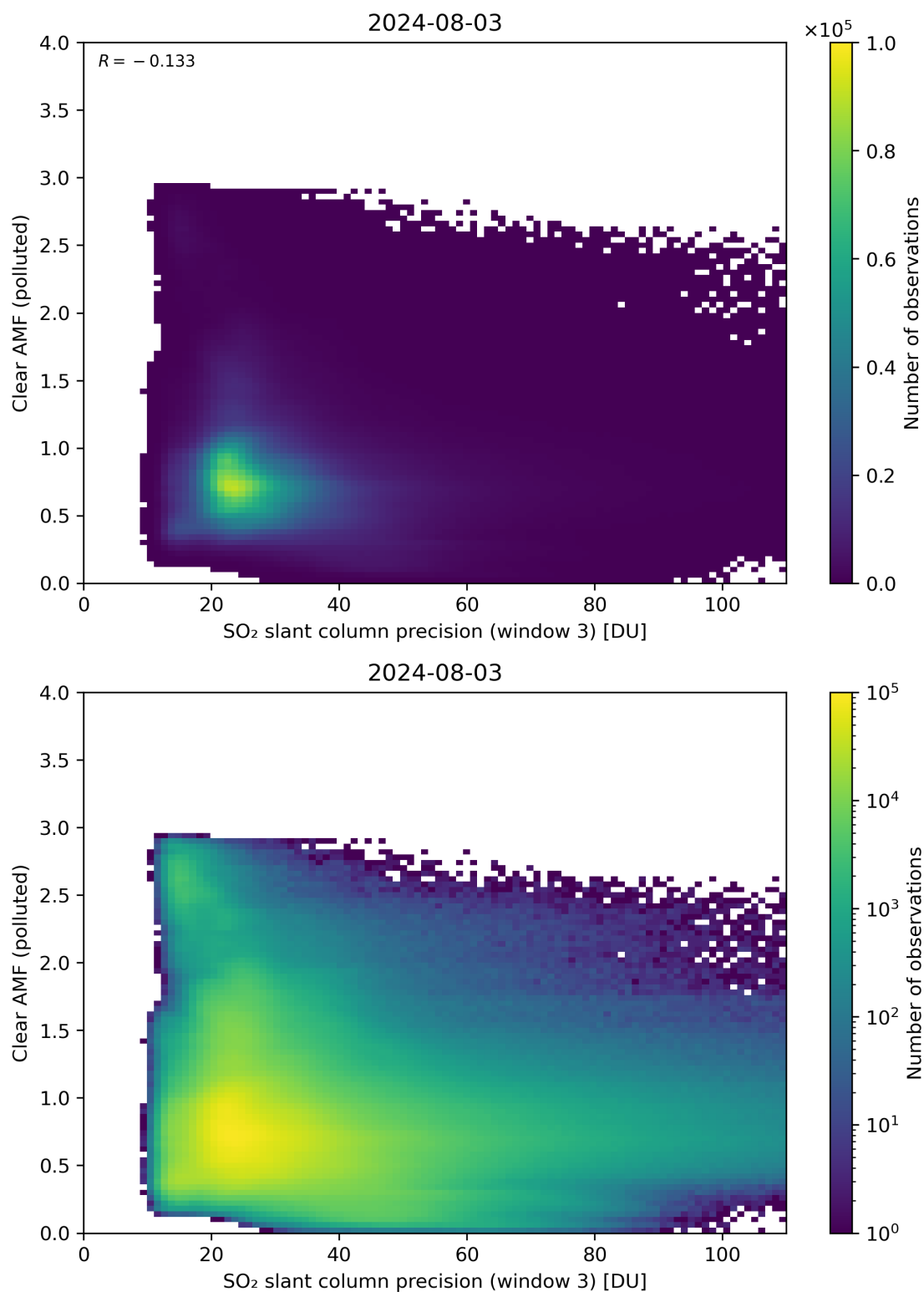
Figure 261: Scatter density plot of “SO 2 slant column precision (window 3)” against “Clear AMF (polluted)” for 2024-08-02 to 2024-08-04.
