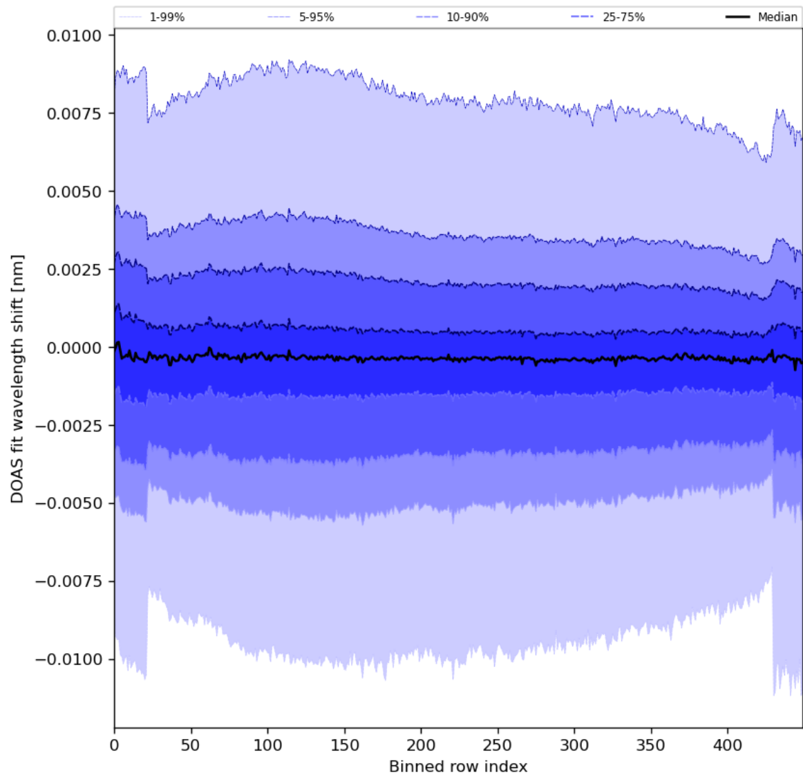
Figure 91: Along track statistics of “DOAS fit wavelength shift” for 2024-08-02 to 2024-08-04
