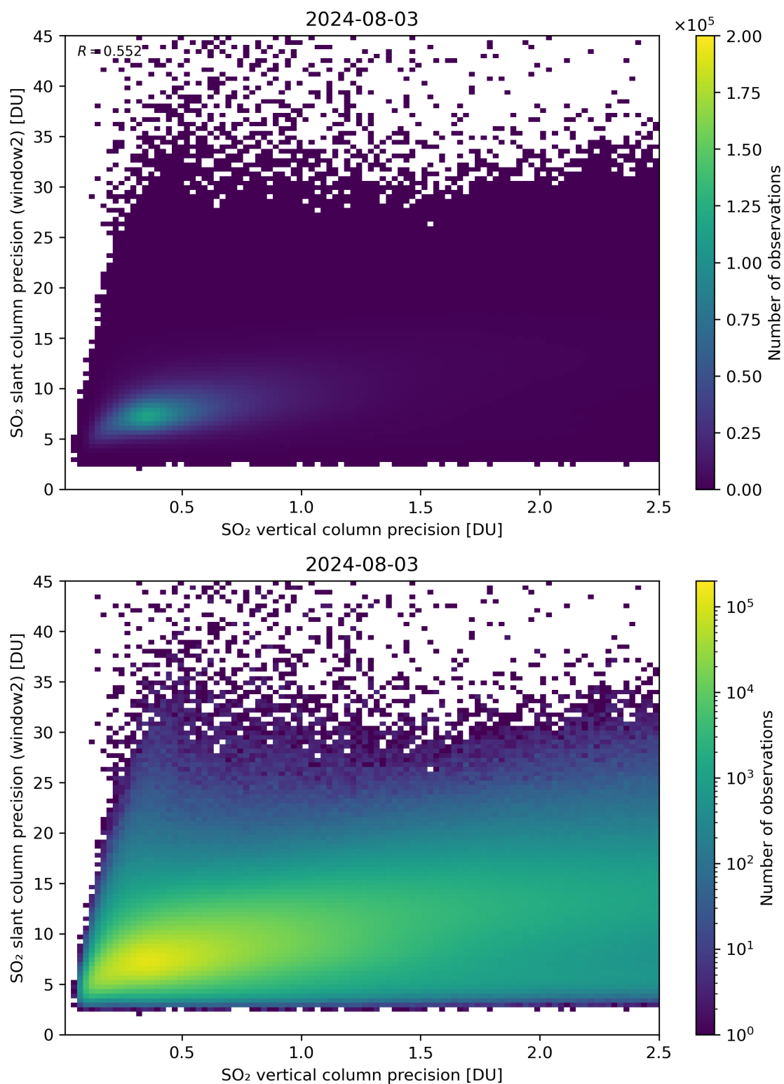
Figure 291: Scatter density plot of “SO 2 vertical column precision” against “SO 2 slant column precision (window2)” for 2024-08-02 to 2024-08-04.
