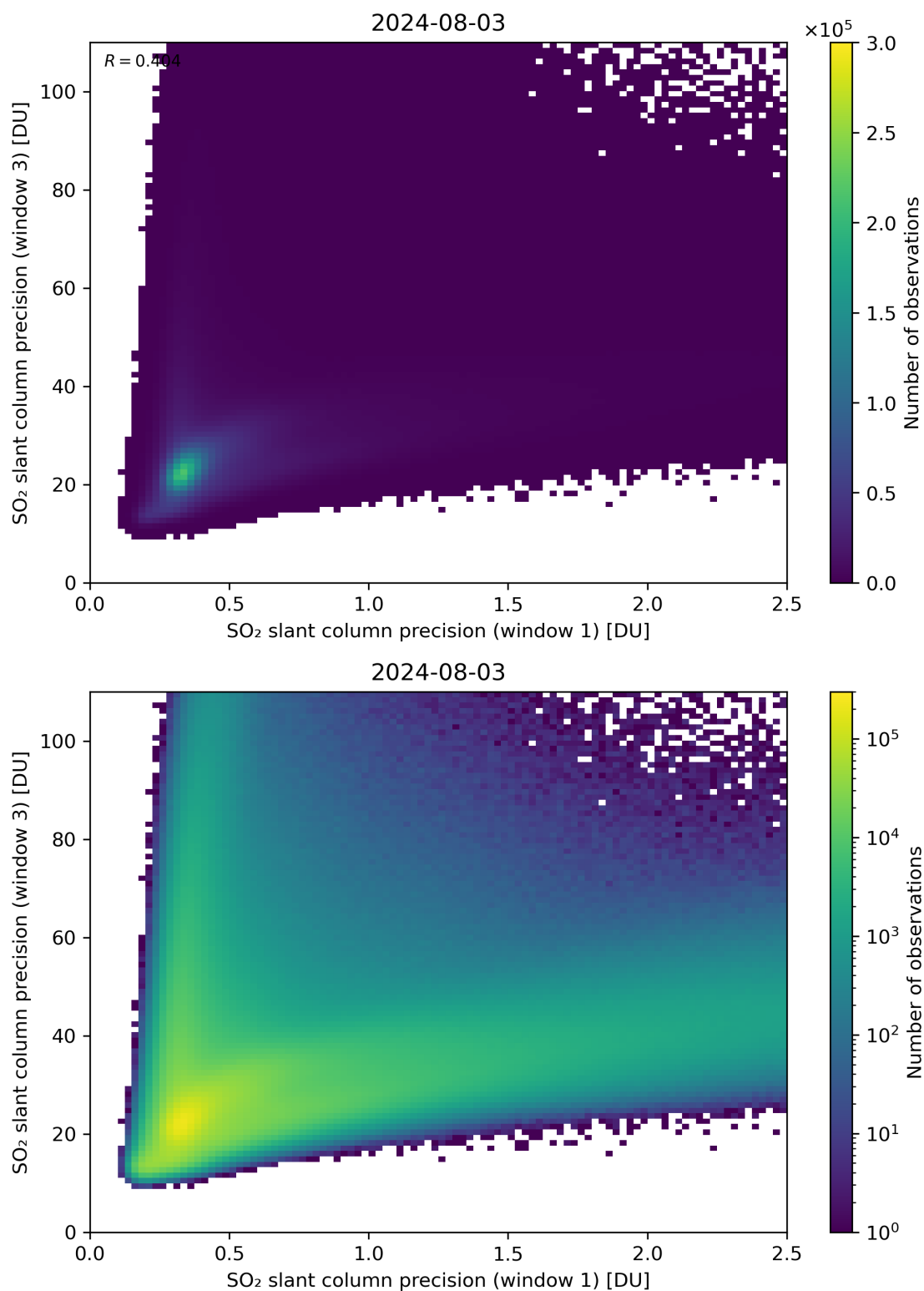
Figure 229: Scatter density plot of “SO 2 slant column precision (window 1)” against “SO 2 slant column precision (window 3)” for 2024-08-02 to 2024-08-04.
