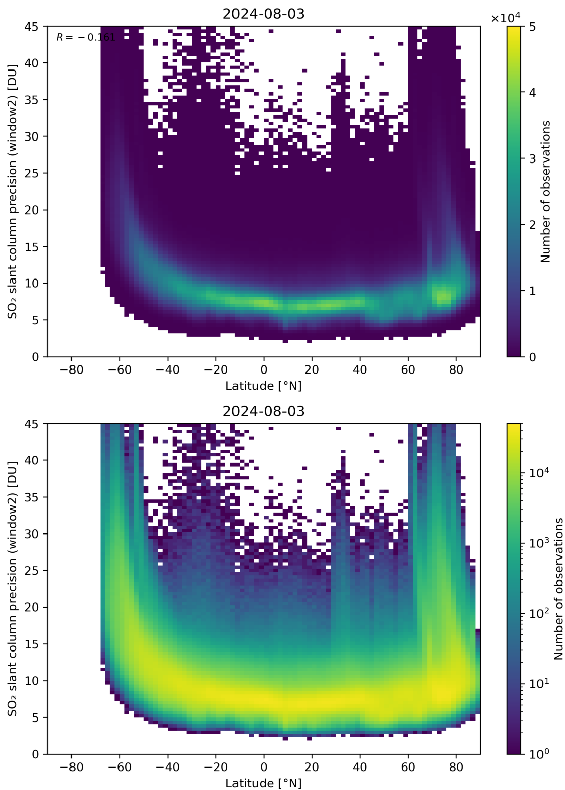
Figure 151: Scatter density plot of “Latitude” against “SO 2 slant column precision (window2)” for 2024-08-02 to 2024-08-04.
