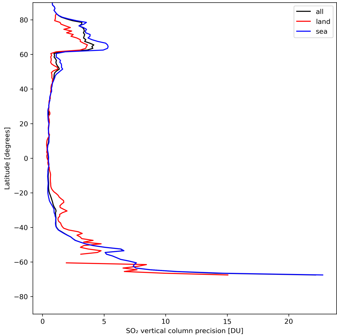
Figure 31: Zonal average of “SO 2 vertical column precision” for 2024-08-02 to 2024-08-04.
