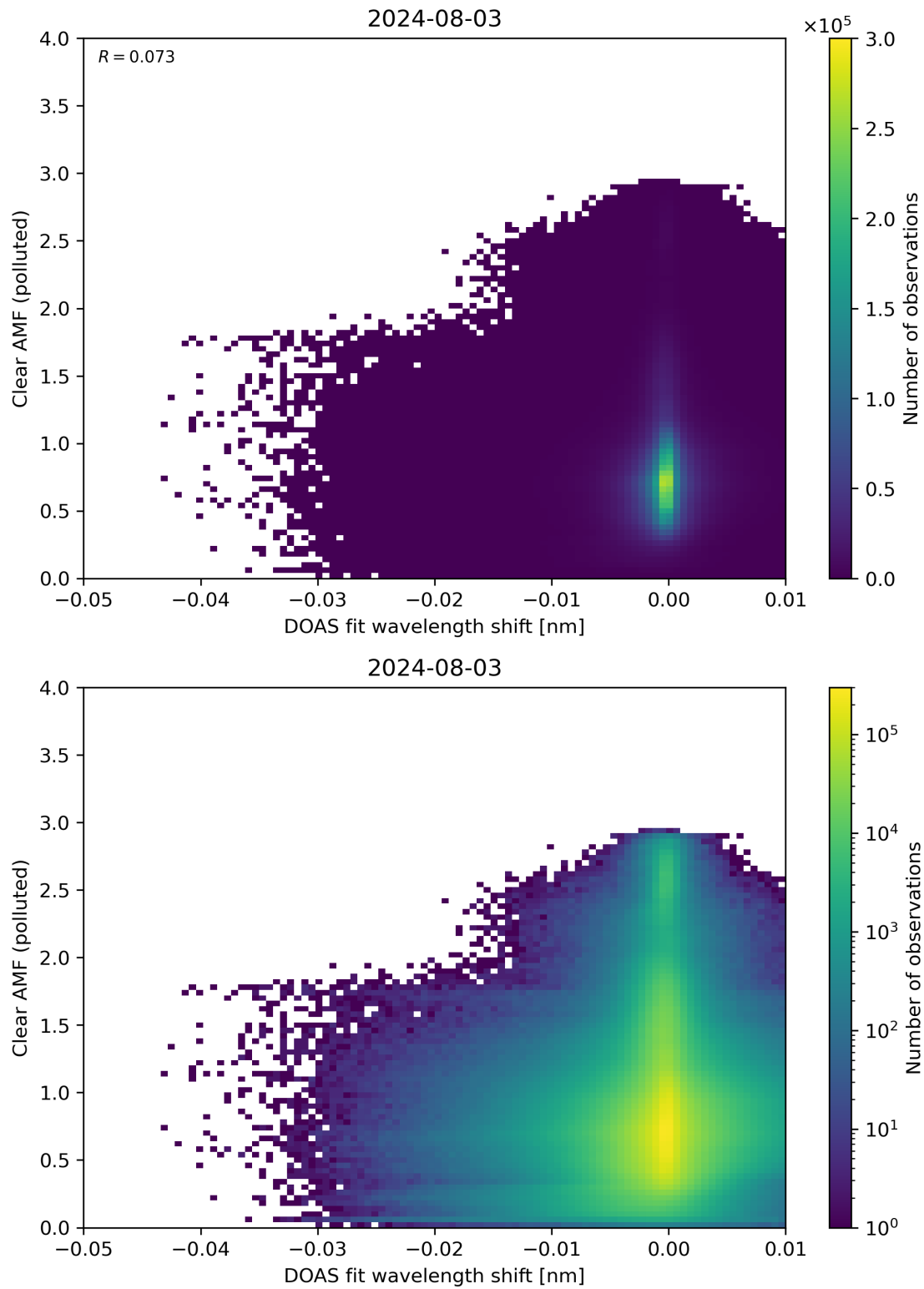
Figure 129: Scatter density plot of “DOAS fit wavelength shift” against “Clear AMF (polluted)” for 2024-08-02 to 2024-08-04.
