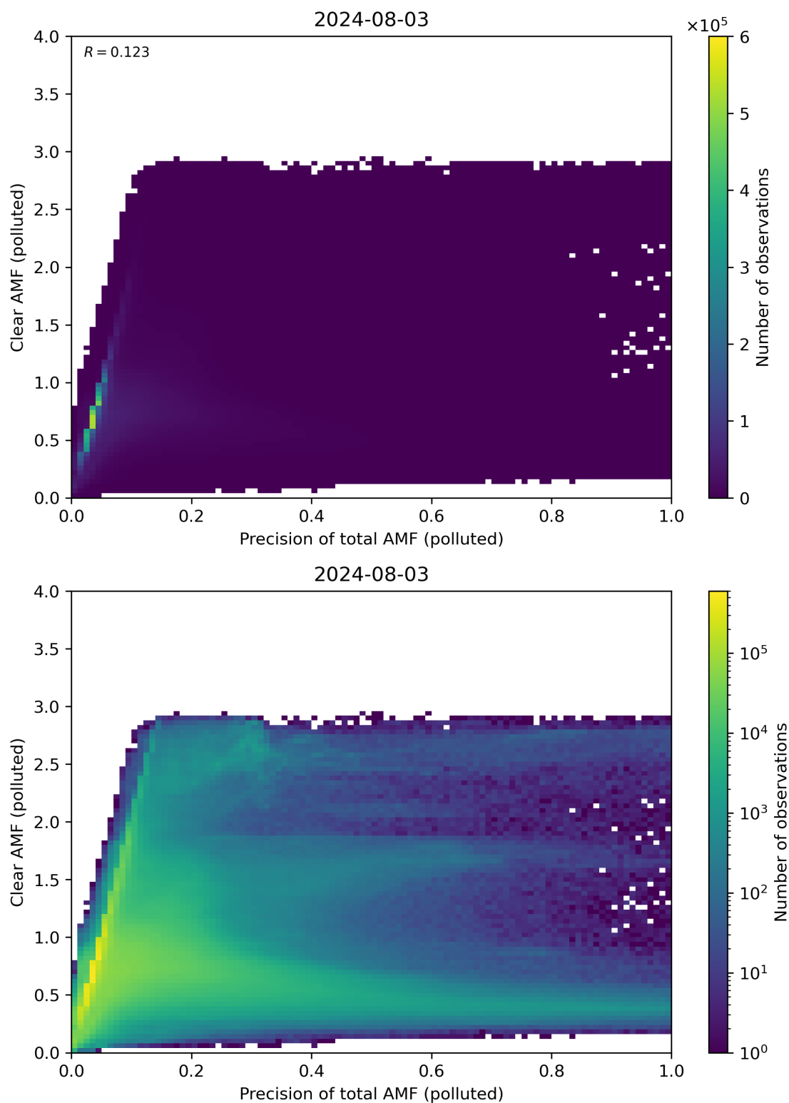
Figure 270: Scatter density plot of “Precision of total AMF (polluted)” against “Clear AMF (polluted)” for 2024-08-02 to 2024-08-04.
