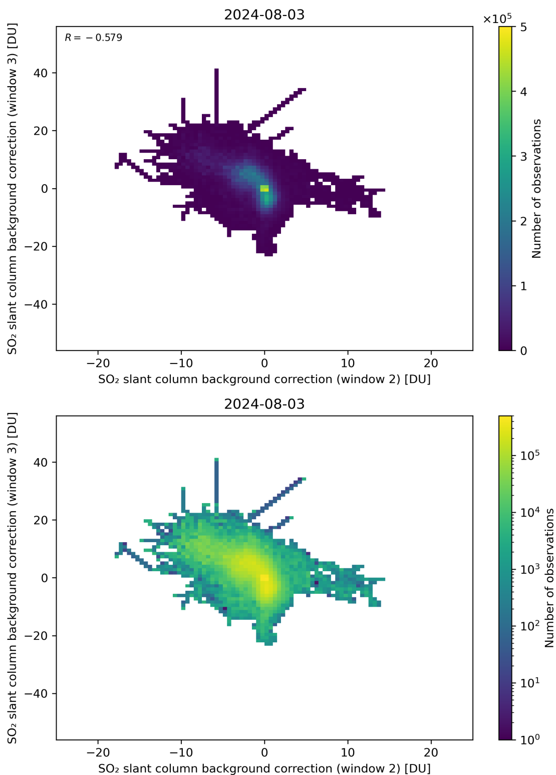
Figure 111: Scatter density plot of “SO 2 slant column background correction (window 2)” against “SO 2 slant column background correction (window 3)” for 2024-08-02 to 2024-08-04.
