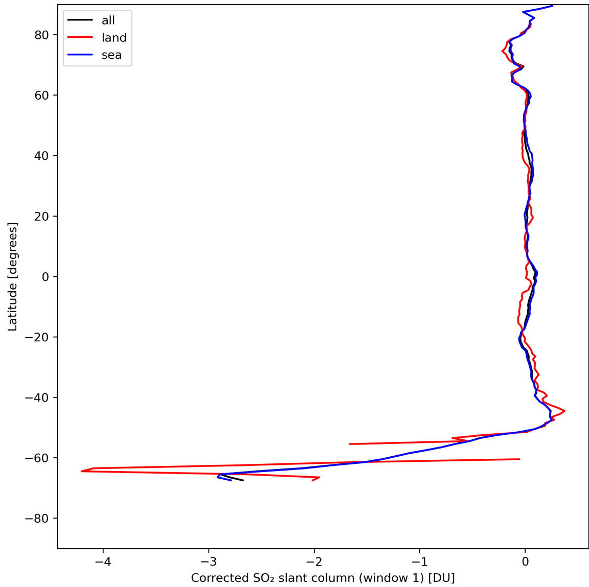
Figure 35: Zonal average of “Corrected SO 2 slant column (window 1)” for 2024-08-02 to 2024-08-04.
