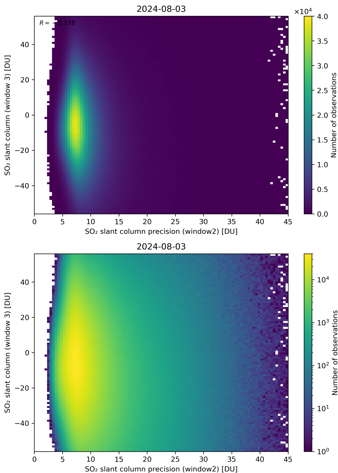
Figure 249: Scatter density plot of “SO 2 slant column precision (window2)” against “SO 2 slant column (window 3)” for 2024-08-02 to 2024-08-04.
