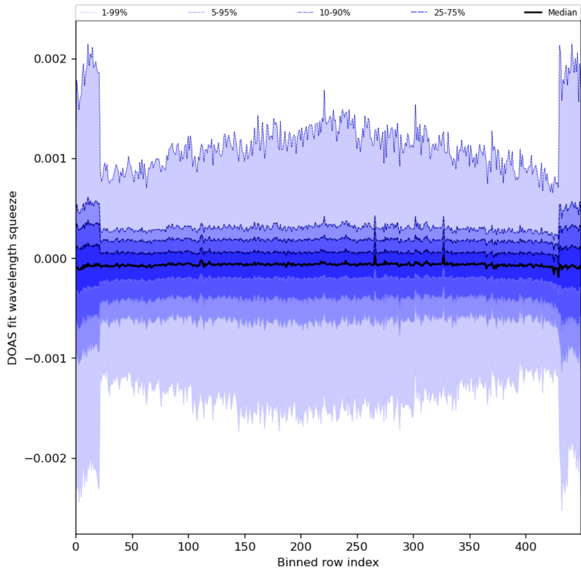
Figure 92: Along track statistics of “DOAS fit wavelength squeeze” for 2024-08-02 to 2024-08-04
