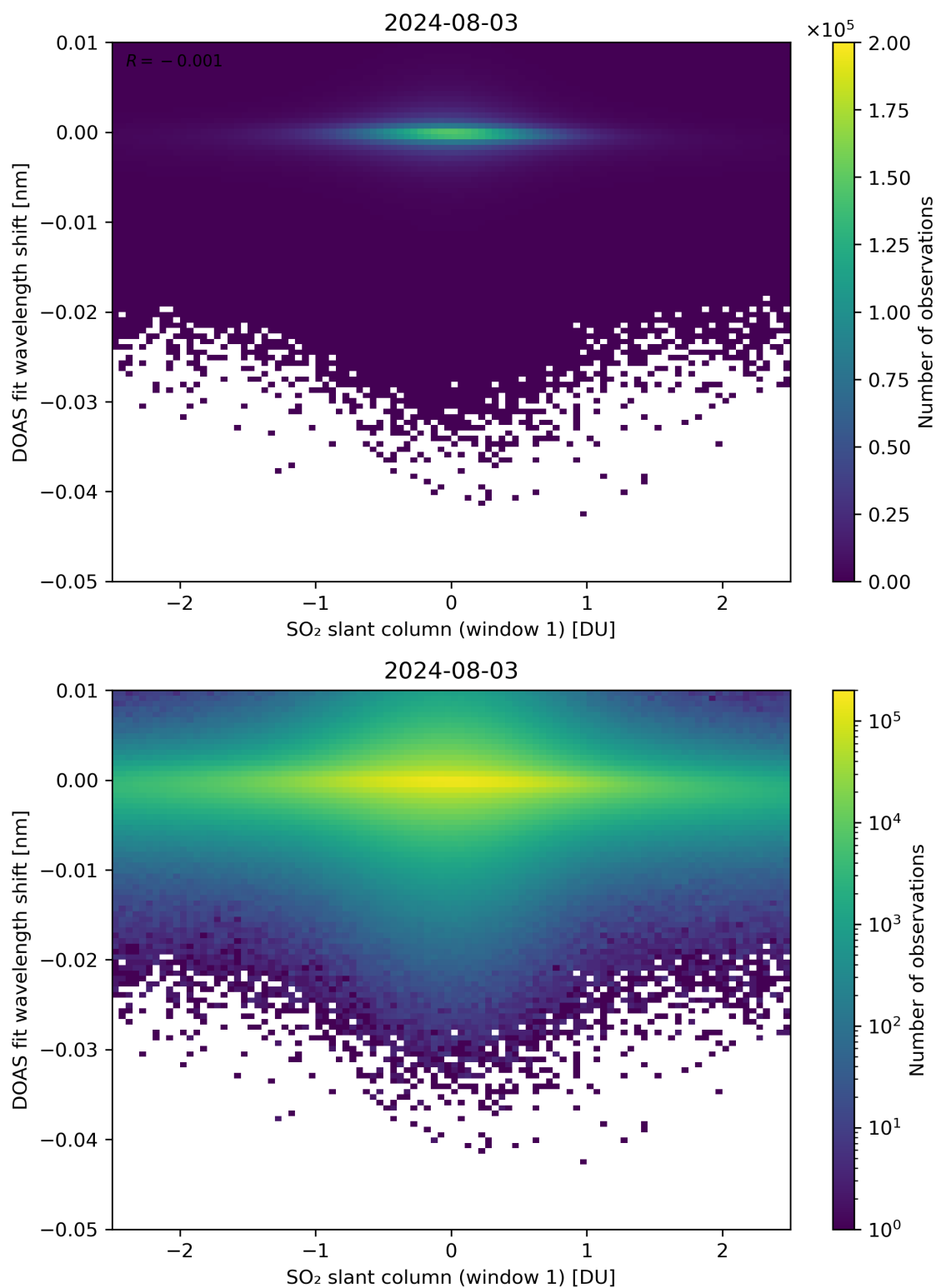
Figure 215: Scatter density plot of “SO 2 slant column (window 1)” against “DOAS fit wavelength shift” for 2024-08-02 to 2024-08-04.
