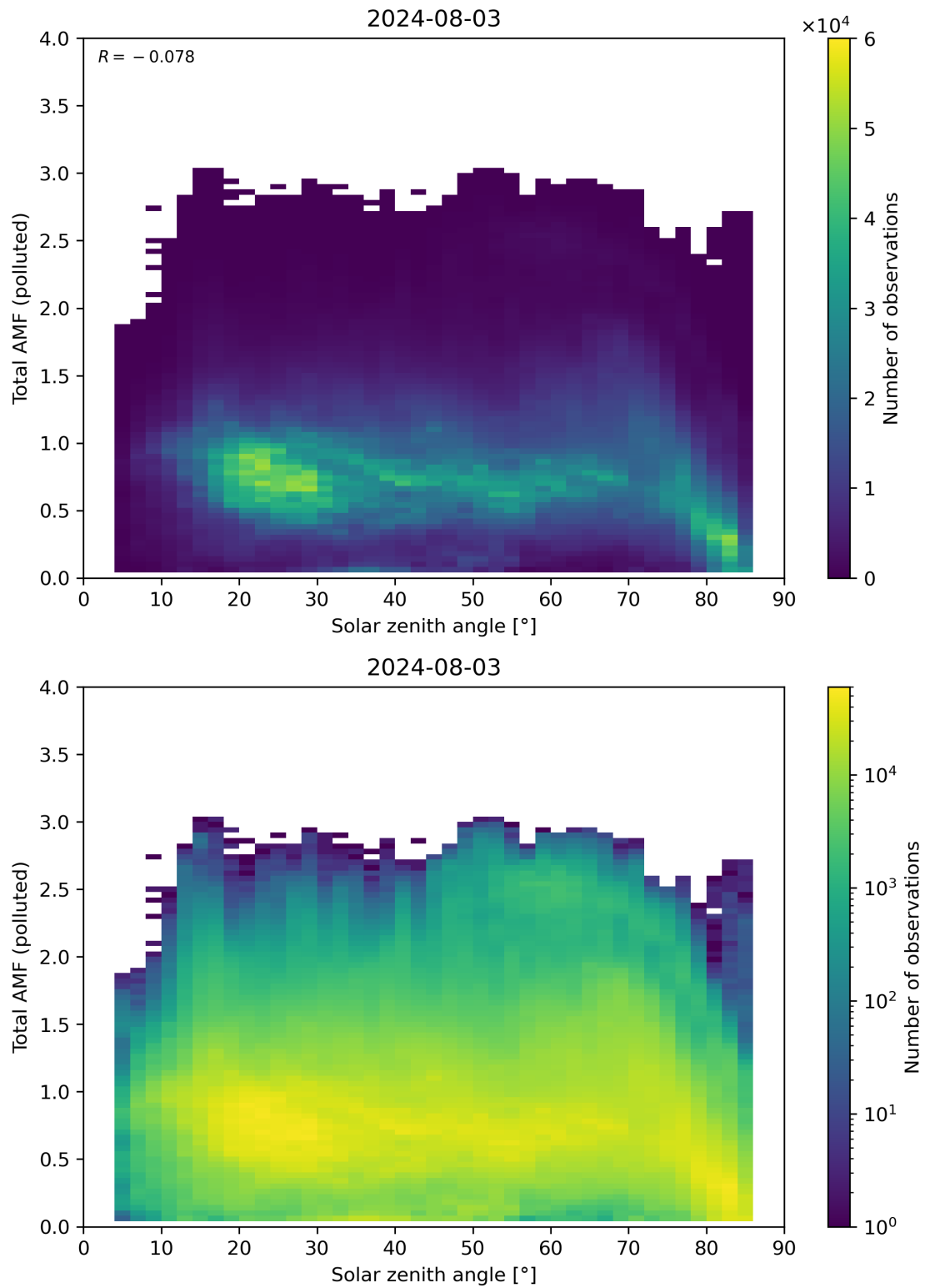
Figure 174: Scatter density plot of “Solar zenith angle” against “Total AMF (polluted)” for 2024-08-02 to 2024-08-04.
