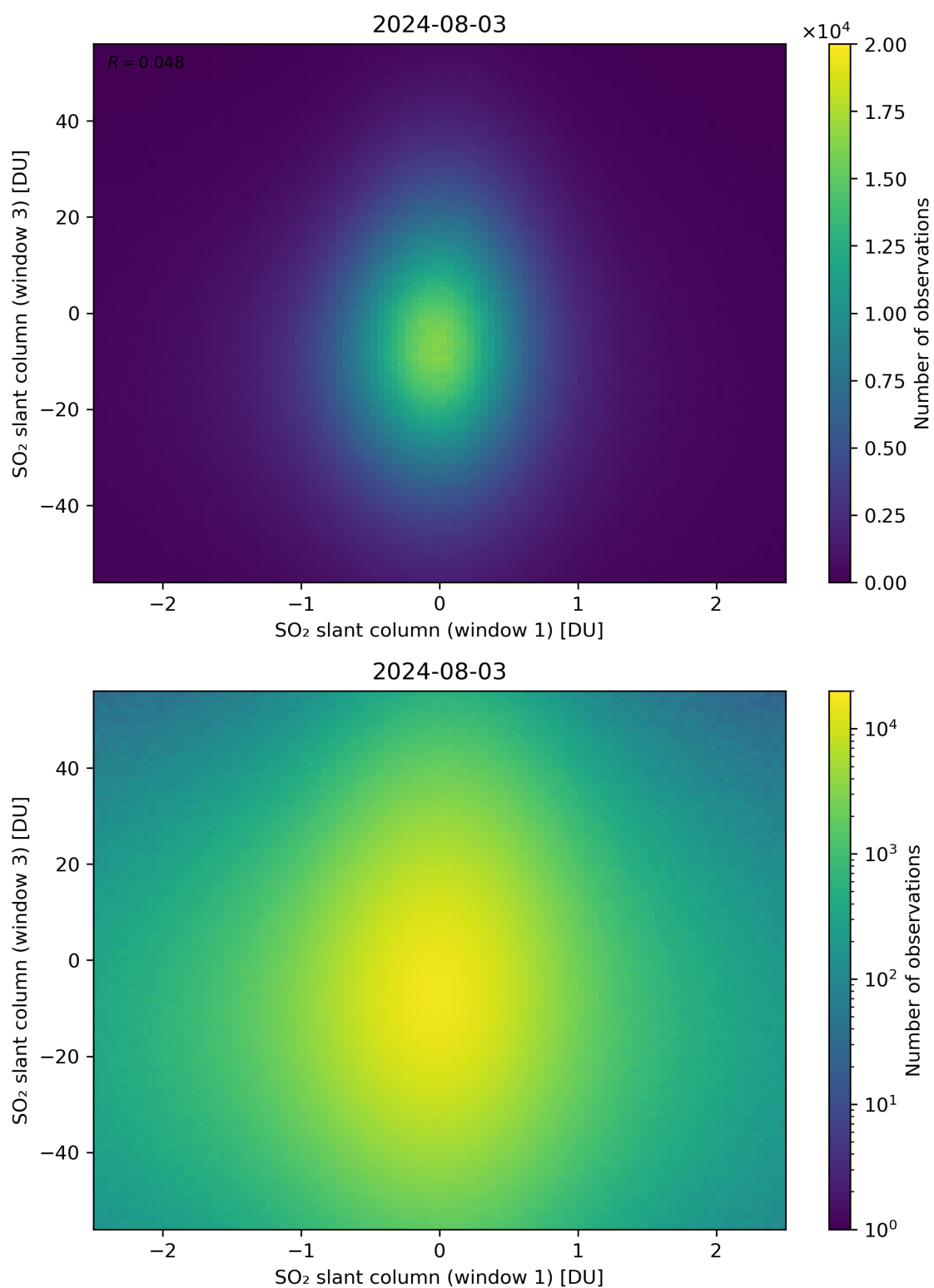
Figure 237: Scatter density plot of “SO 2 slant column (window 1)” against “SO 2 slant column (window 3)” for 2024-08-02 to 2024-08-04.
