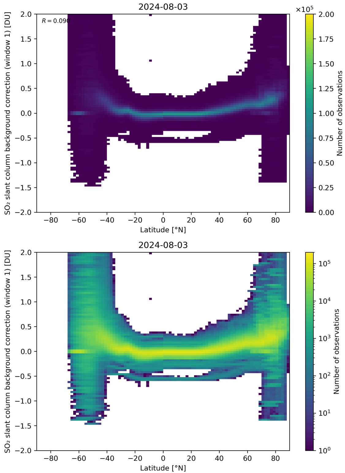
Figure 139: Scatter density plot of “Latitude” against “SO 2 slant column background correction (window 1)” for 2024-08-02 to 2024-08-04.
