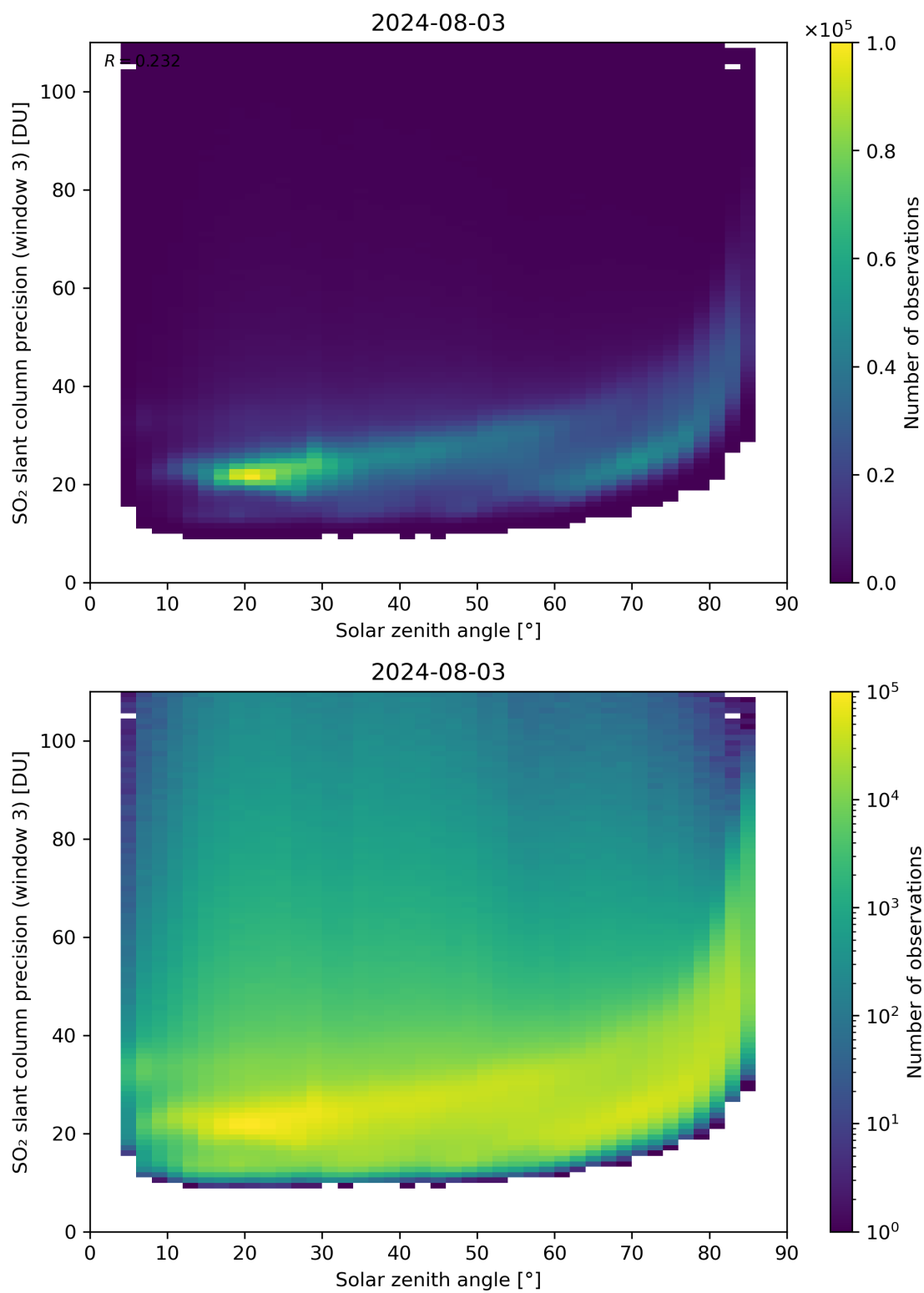
Figure 173: Scatter density plot of “Solar zenith angle” against “SO 2 slant column precision (window 3)” for 2024-08-02 to 2024-08-04.
