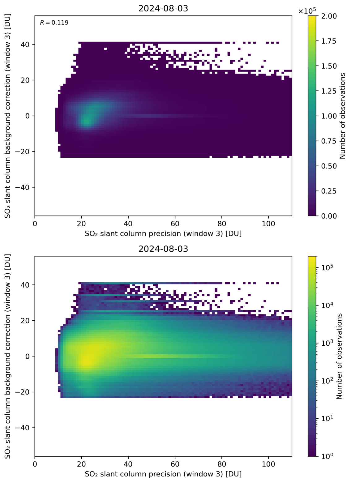
Figure 257: Scatter density plot of “SO 2 slant column precision (window 3)” against “SO 2 slant column background correction (window 3)” for 2024-08-02 to 2024-08-04.
