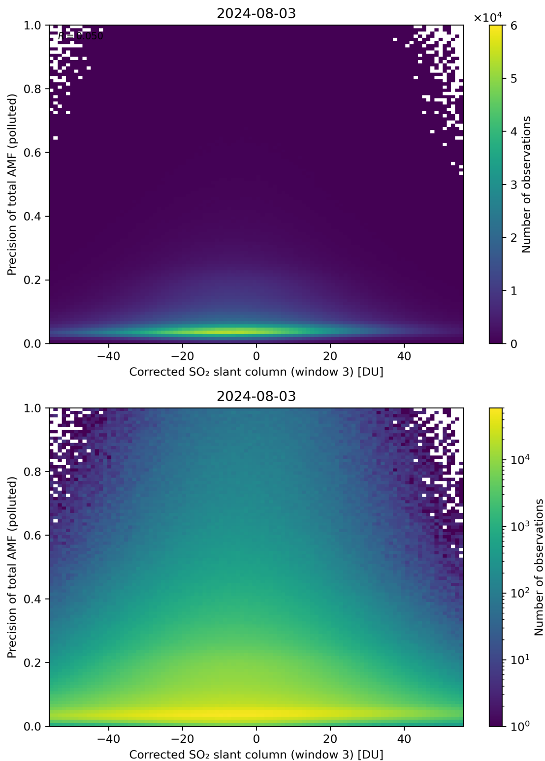
Figure 211: Scatter density plot of “Corrected SO 2 slant column (window 3)” against “Precision of total AMF (polluted)” for 2024-08-02 to 2024-08-04.
