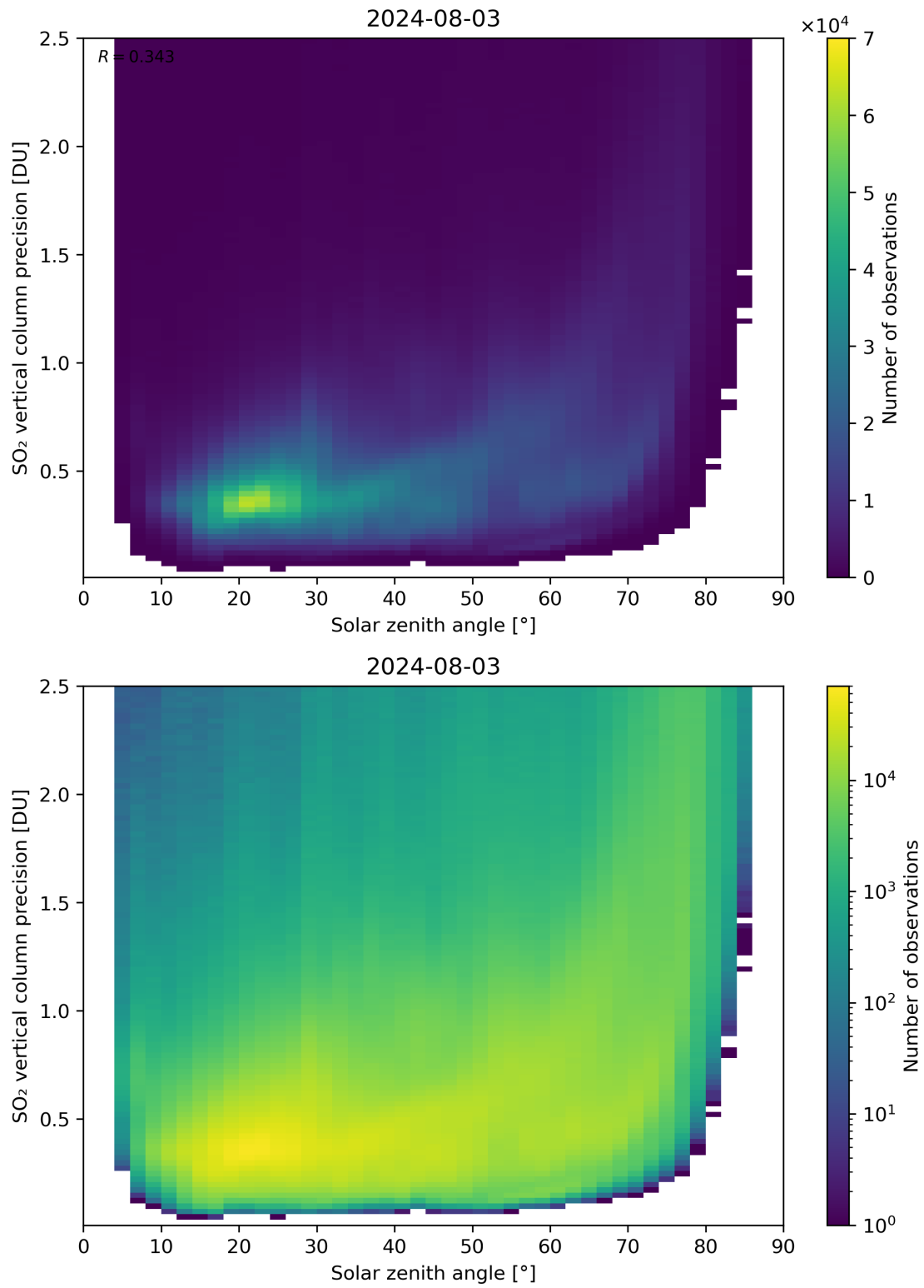
Figure 177: Scatter density plot of “Solar zenith angle” against “SO 2 vertical column precision” for 2024-08-02 to 2024-08-04.
