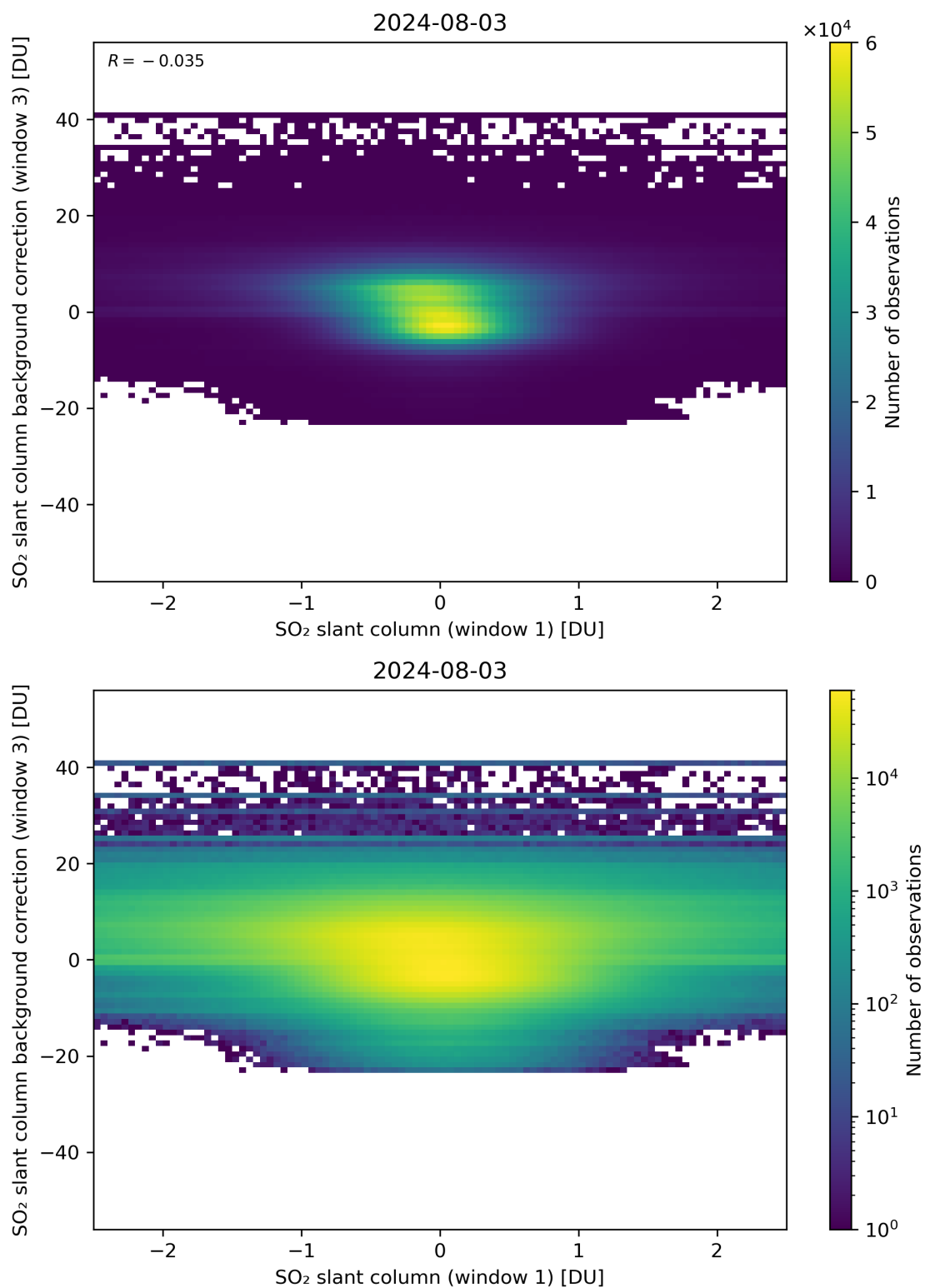
Figure 214: Scatter density plot of “SO 2 slant column (window 1)” against “SO 2 slant column background correction (window 3)” for 2024-08-02 to 2024-08-04.
