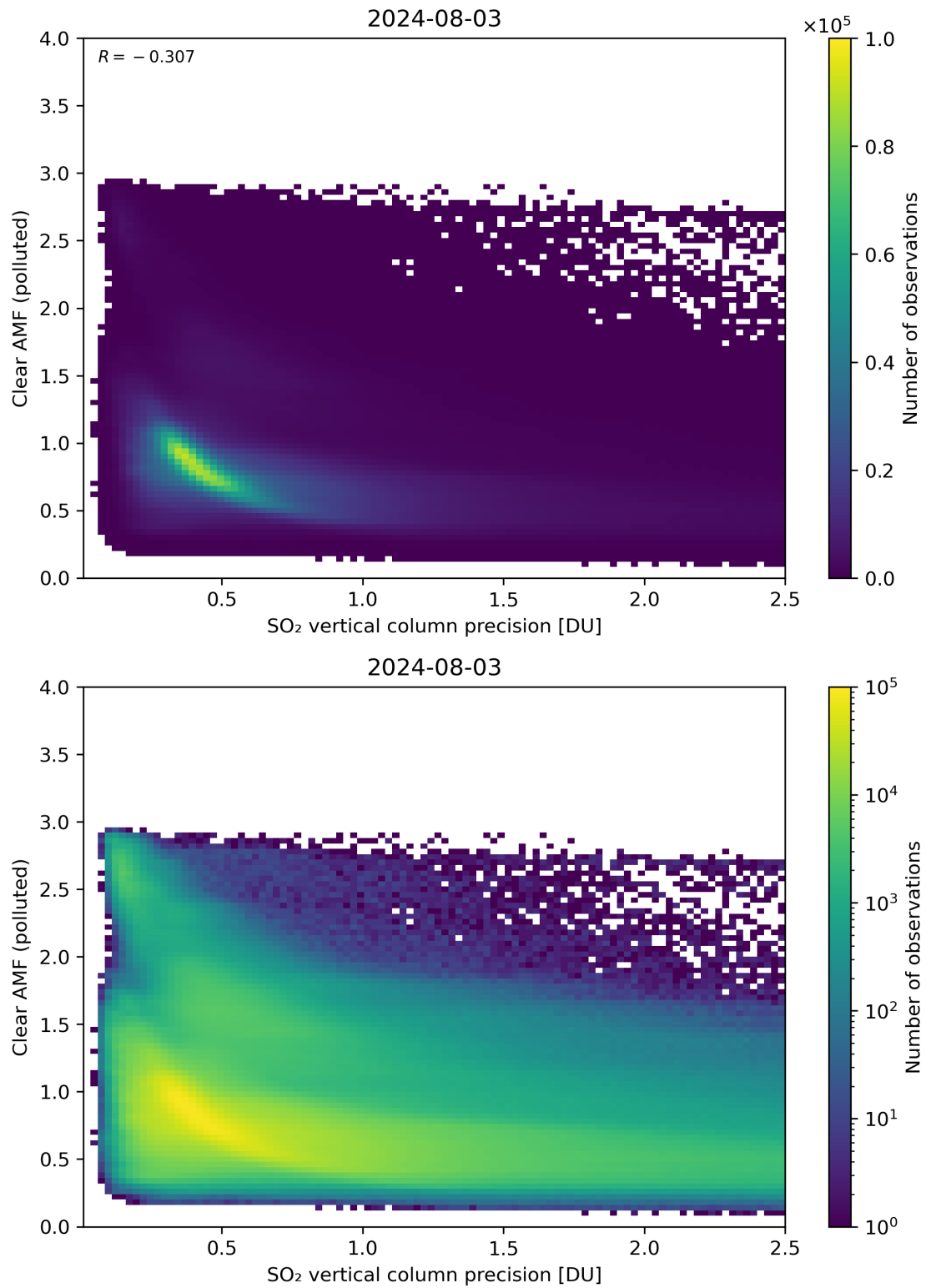
Figure 285: Scatter density plot of “SO 2 vertical column precision” against “Clear AMF (polluted)” for 2024-08-02 to 2024-08-04.
