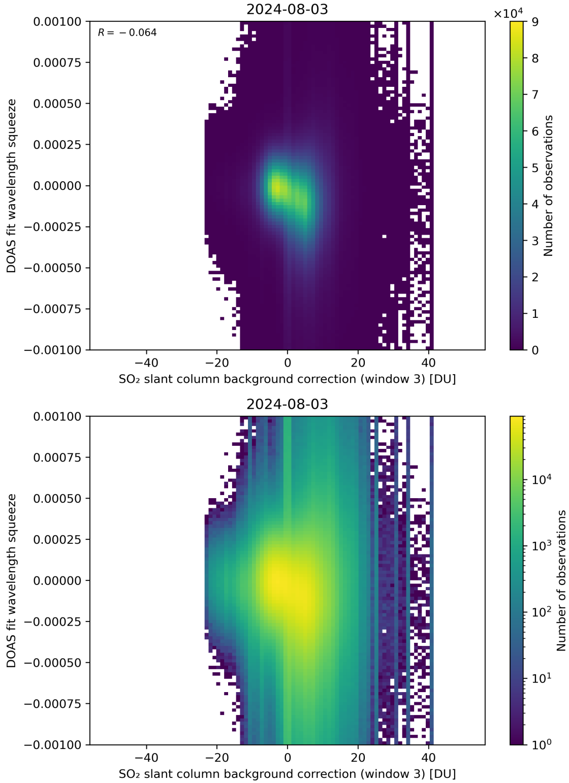
Figure 122: Scatter density plot of “SO 2 slant column background correction (window 3)” against “DOAS fit wavelength squeeze” for 2024-08-02 to 2024-08-04.
