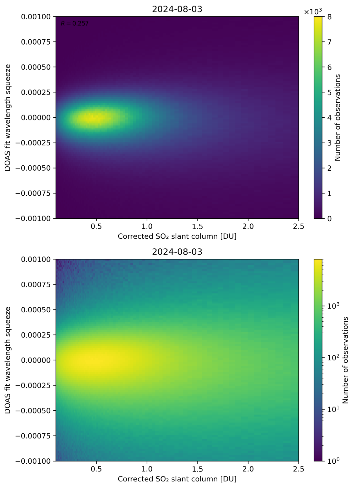
Figure 182: Scatter density plot of “Corrected SO 2 slant column” against “DOAS fit wavelength squeeze” for 2024-08-02 to 2024-08-04.
