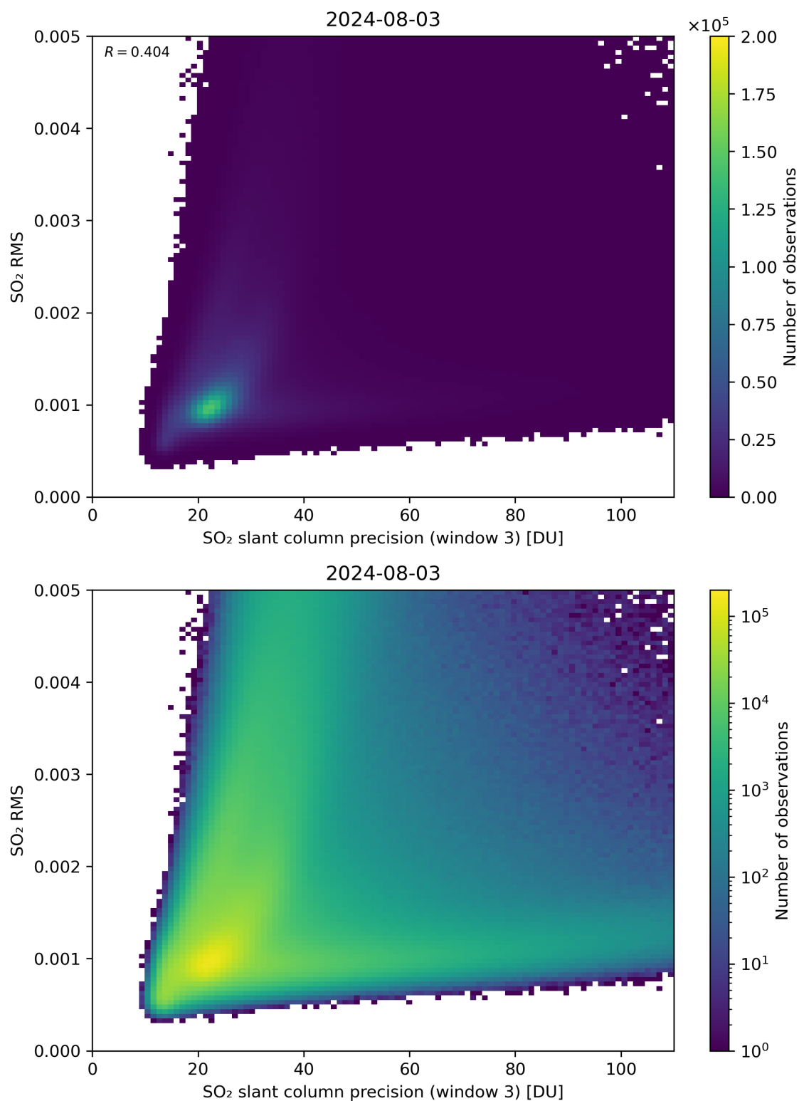
Figure 260: Scatter density plot of “SO 2 slant column precision (window 3)” against “SO 2 RMS” for 2024-08-02 to 2024-08-04.
