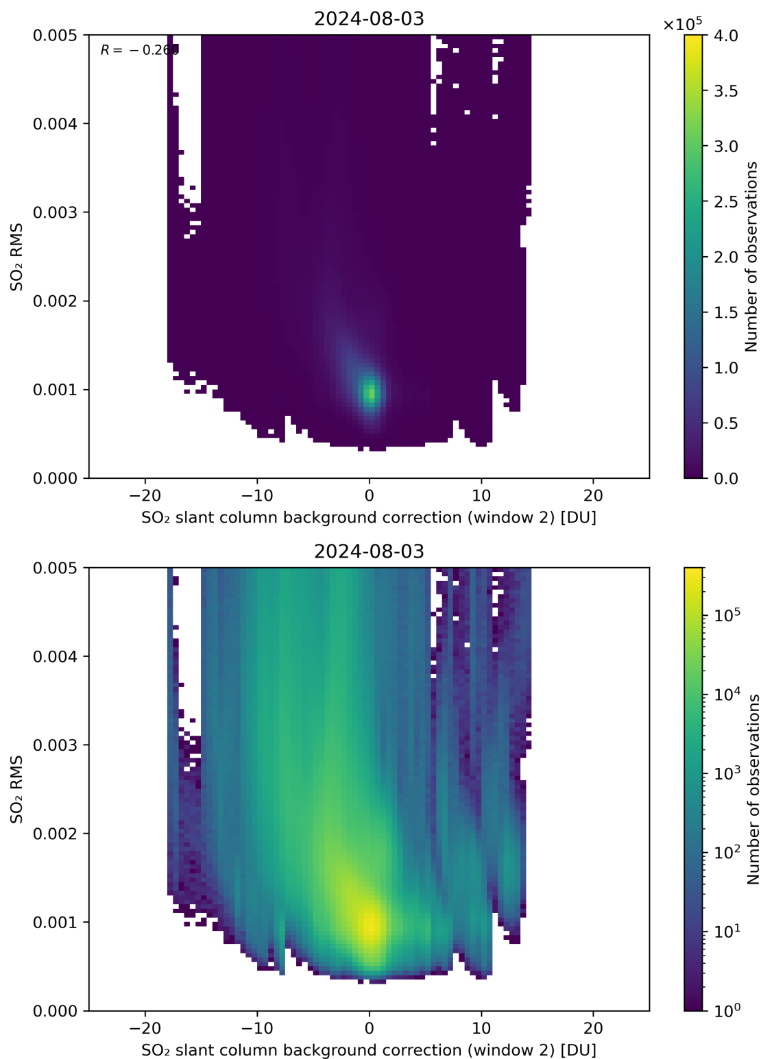
Figure 114: Scatter density plot of “SO 2 slant column background correction (window 2)” against “SO 2 RMS” for 2024-08-02 to 2024-08-04.
