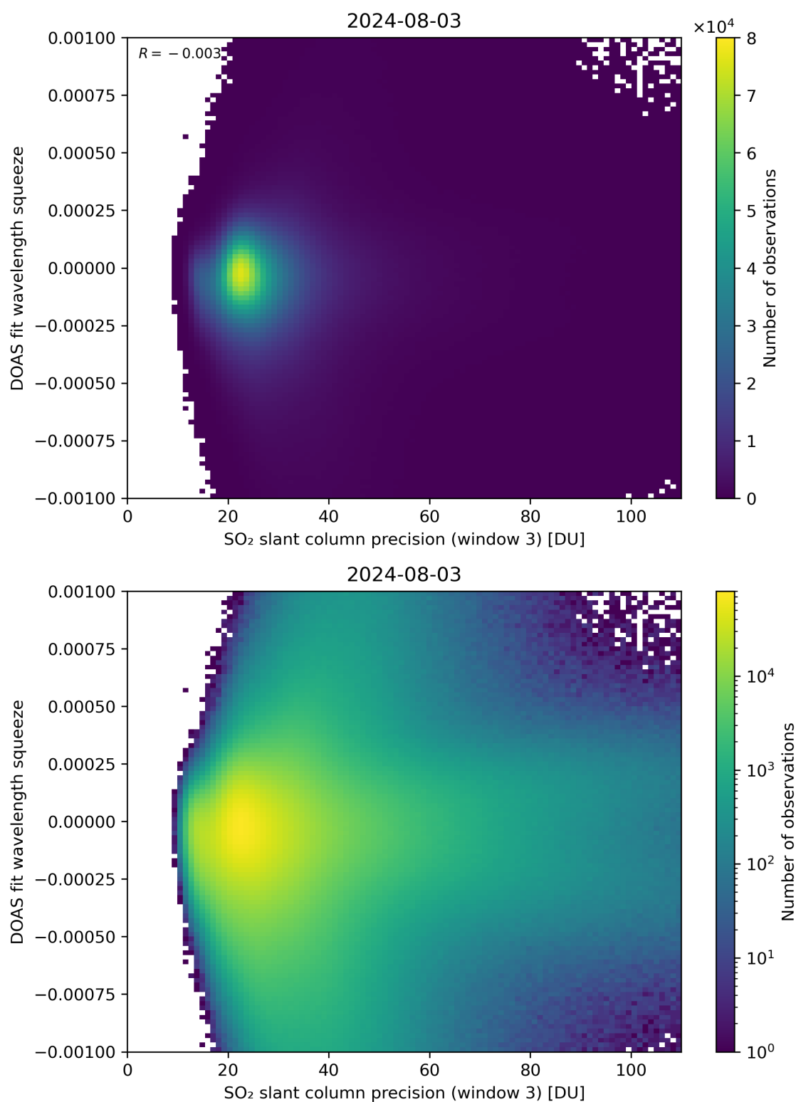
Figure 259: Scatter density plot of “SO 2 slant column precision (window 3)” against “DOAS fit wavelength squeeze” for 2024-08-02 to 2024-08-04.
