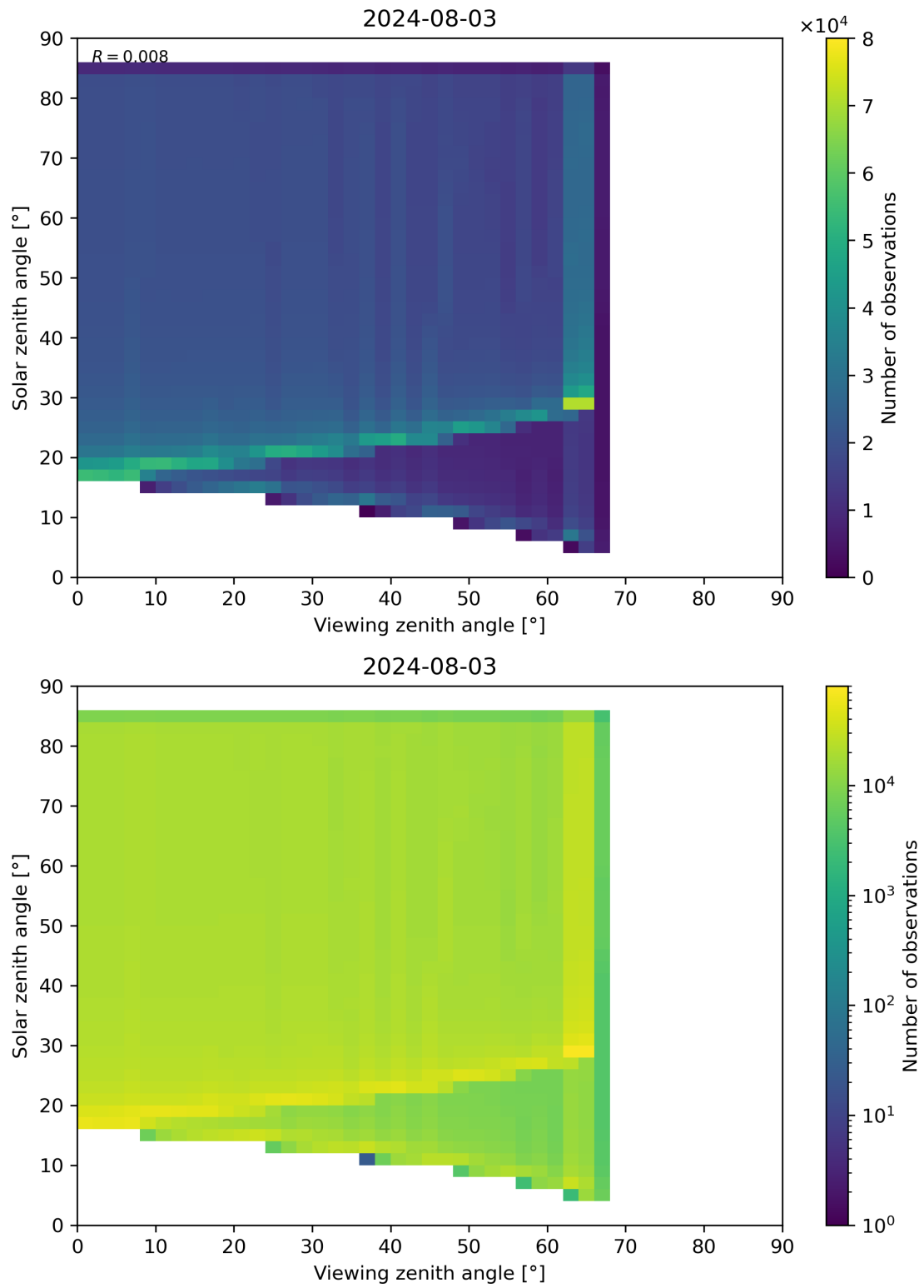
Figure 315: Scatter density plot of “Viewing zenith angle” against “Solar zenith angle” for 2024-08-02 to 2024-08-04.
