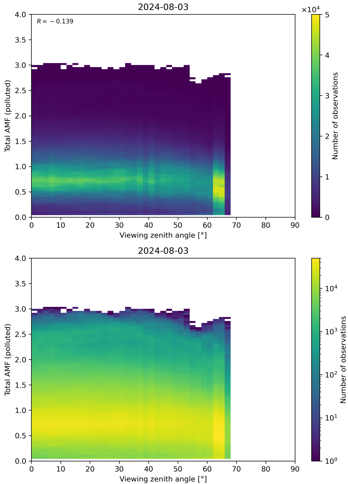
Figure 325: Scatter density plot of “Viewing zenith angle” against “Total AMF (polluted)” for 2024-08-02 to 2024-08-04.
