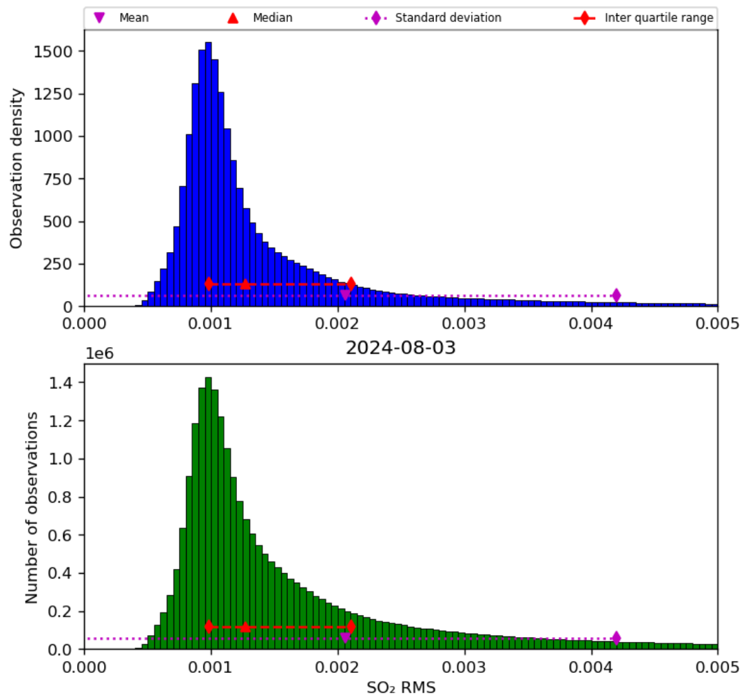
Figure 70: Histogram of “SO 2 RMS” for 2024-08-02 to 2024-08-04
