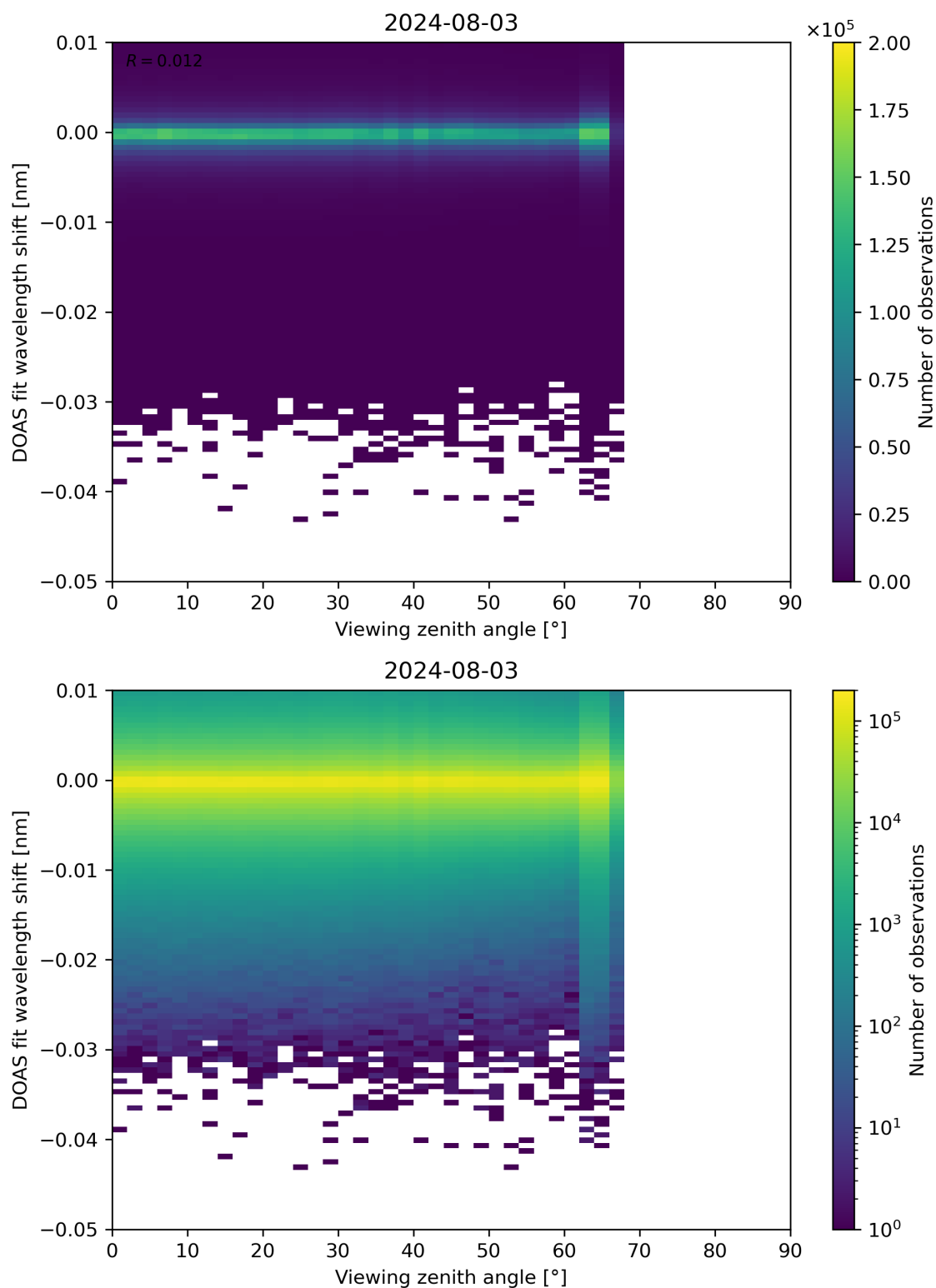
Figure 311: Scatter density plot of “Viewing zenith angle” against “DOAS fit wavelength shift” for 2024-08-02 to 2024-08-04.
