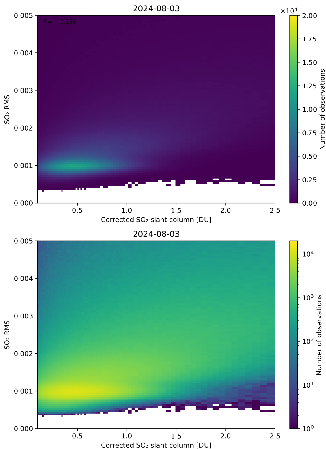
Figure 183: Scatter density plot of “Corrected SO 2 slant column” against “SO 2 RMS” for 2024-08-02 to 2024-08-04.
