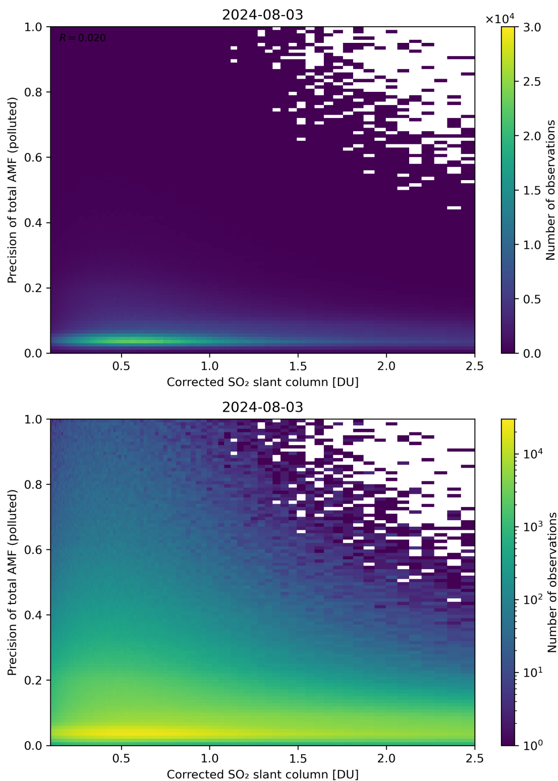
Figure 193: Scatter density plot of “Corrected SO 2 slant column” against “Precision of total AMF (polluted)” for 2024-08-02 to 2024-08-04.
