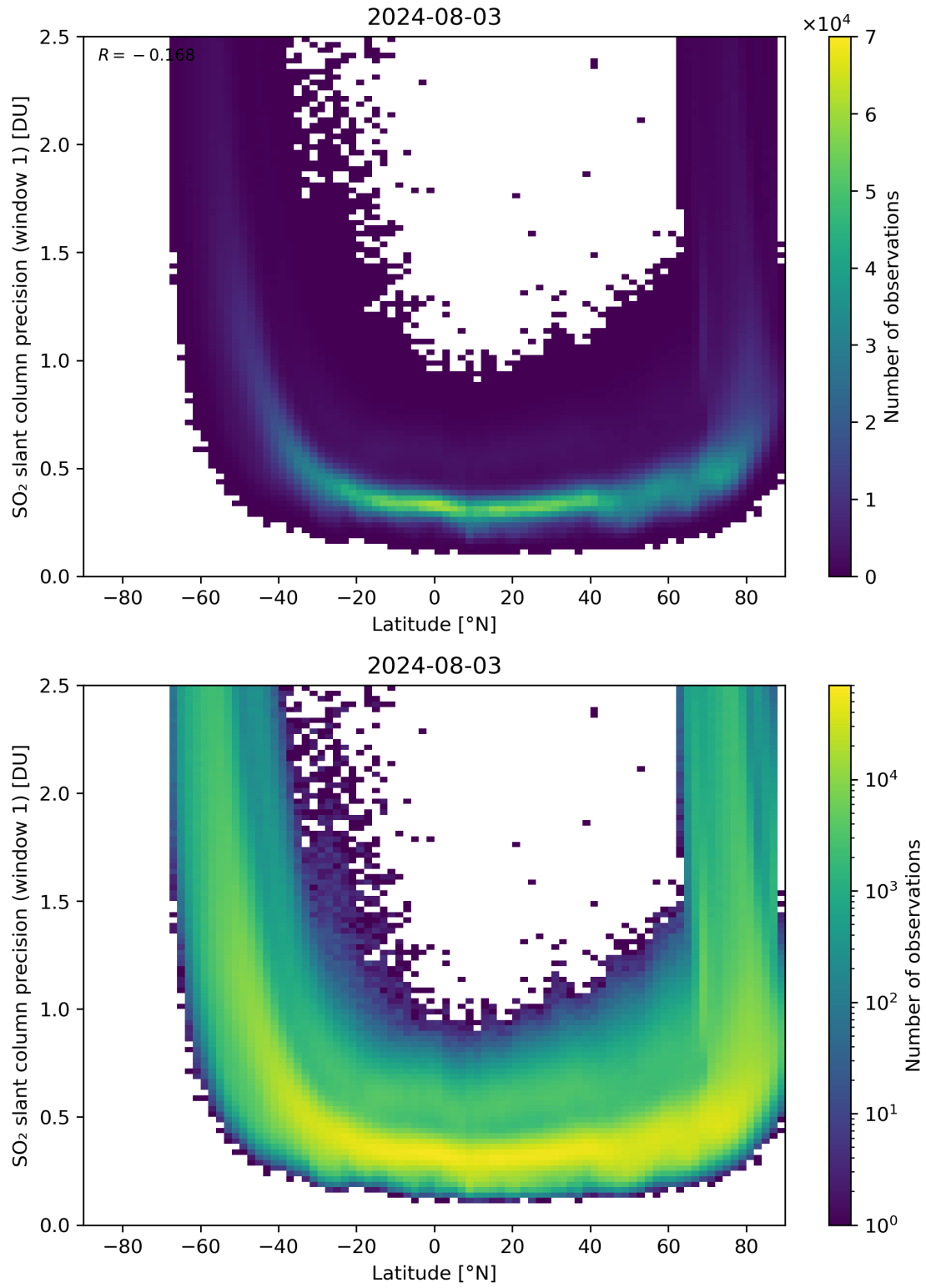
Figure 150: Scatter density plot of “Latitude” against “SO 2 slant column precision (window 1)” for 2024-08-02 to 2024-08-04.
