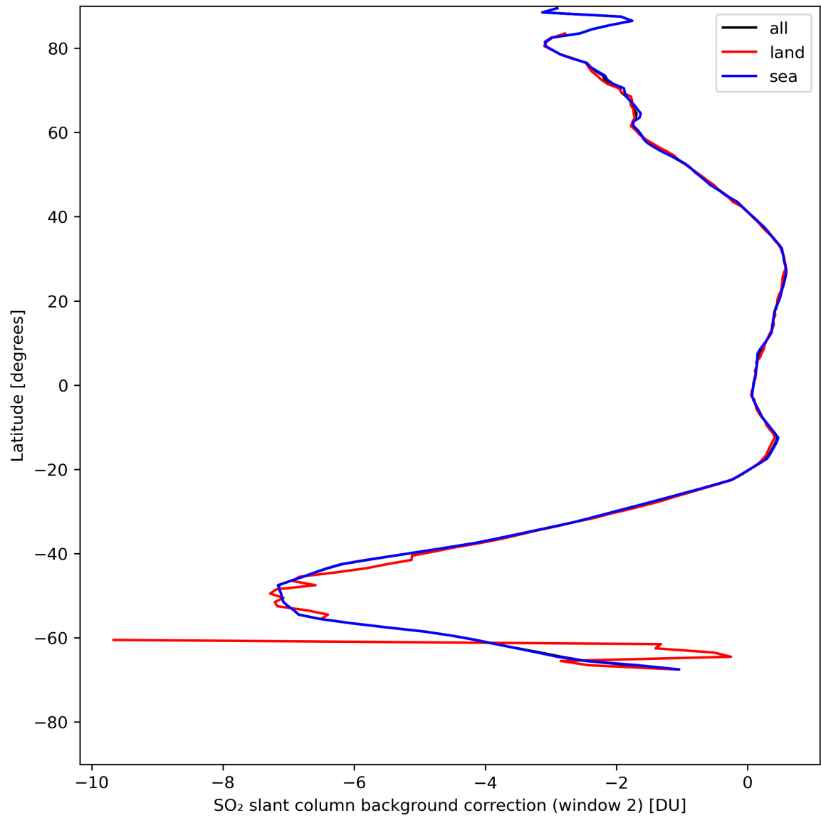
Figure 40: Zonal average of “SO 2 slant column background correction (window 2)” for 2024-08-02 to 2024-08-04.
