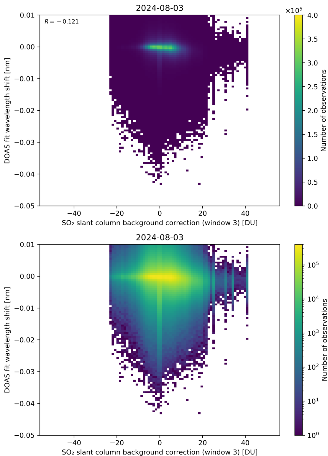
Figure 121: Scatter density plot of “SO 2 slant column background correction (window 3)” against “DOAS fit wavelength shift” for 2024-08-02 to 2024-08-04.
