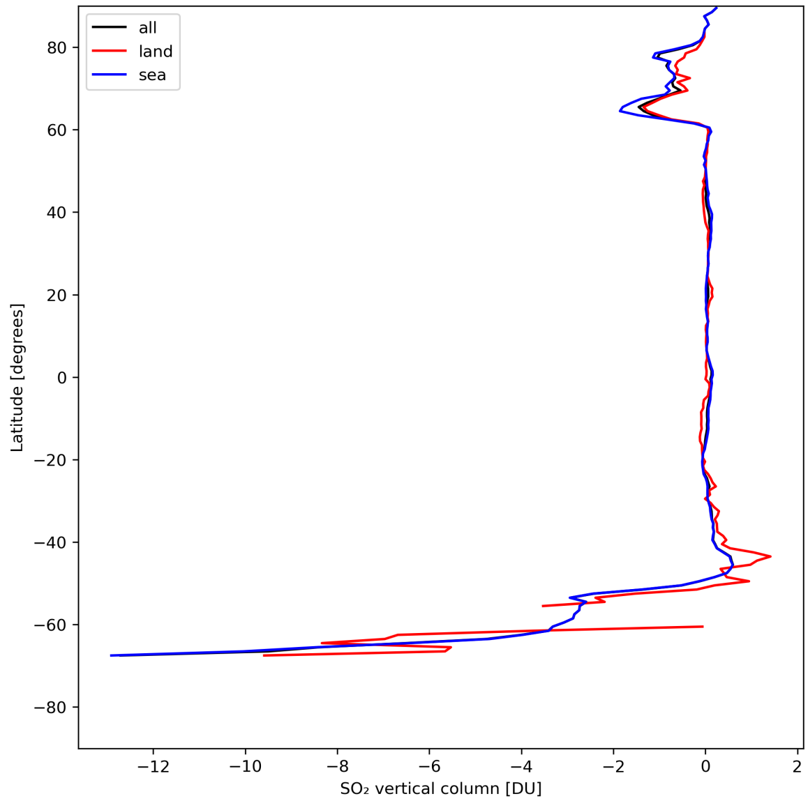
Figure 30: Zonal average of “SO 2 vertical column” for 2024-08-02 to 2024-08-04.
