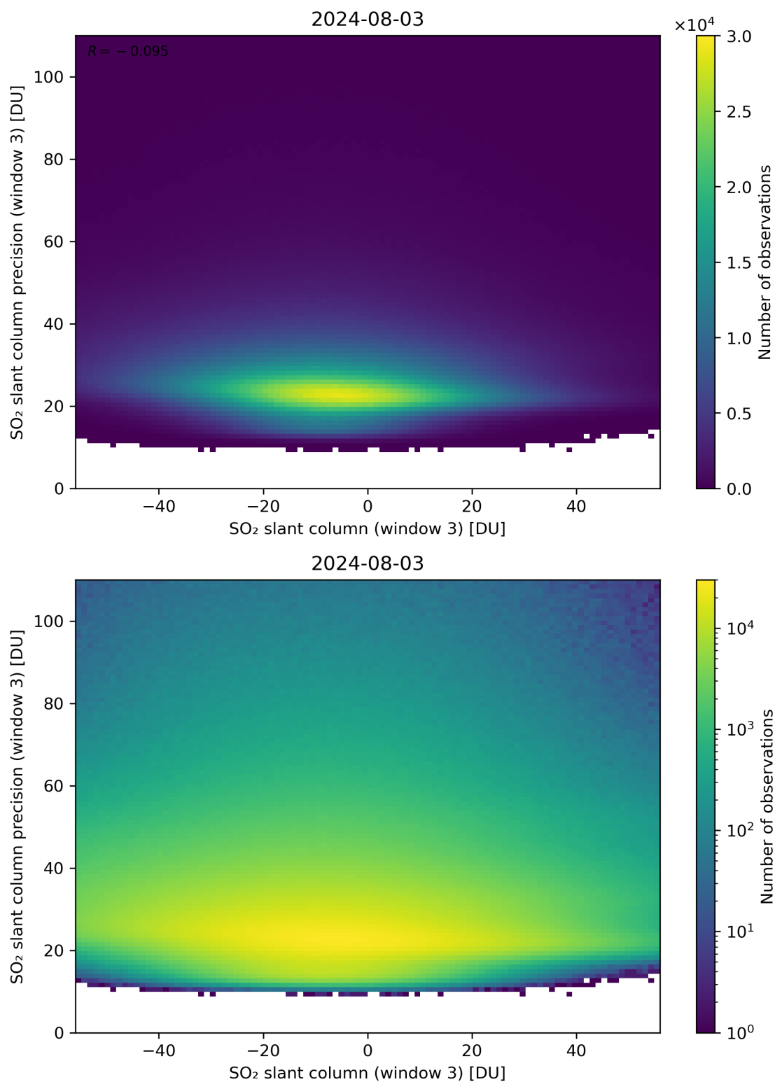
Figure 267: Scatter density plot of “SO 2 slant column (window 3)” against “SO 2 slant column precision (window 3)” for 2024-08-02 to 2024-08-04.
