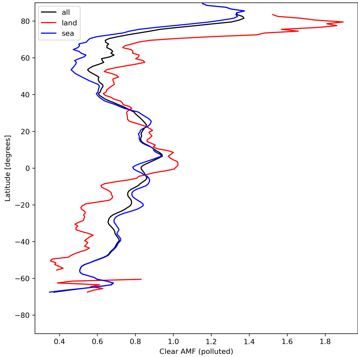
Figure 50: Zonal average of “Clear AMF (polluted)” for 2024-08-02 to 2024-08-04.
