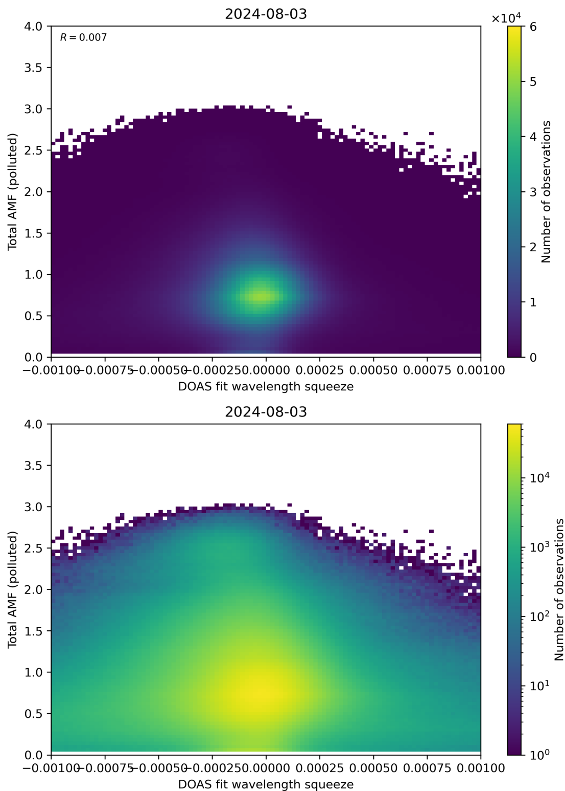
Figure 134: Scatter density plot of “DOAS fit wavelength squeeze” against “Total AMF (polluted)” for 2024-08-02 to 2024-08-04.
