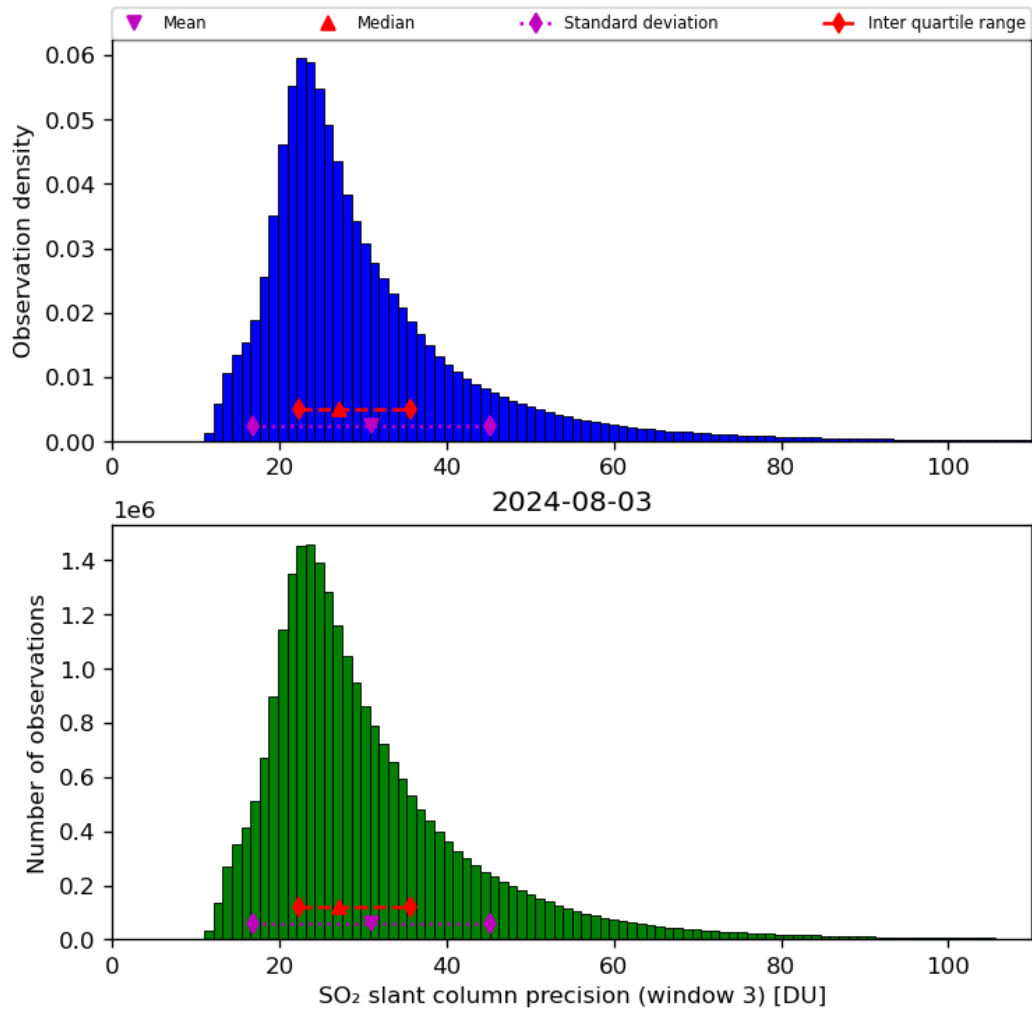
Figure 65: Histogram of “SO 2 slant column precision (window 3)” for 2024-08-02 to 2024-08-04
