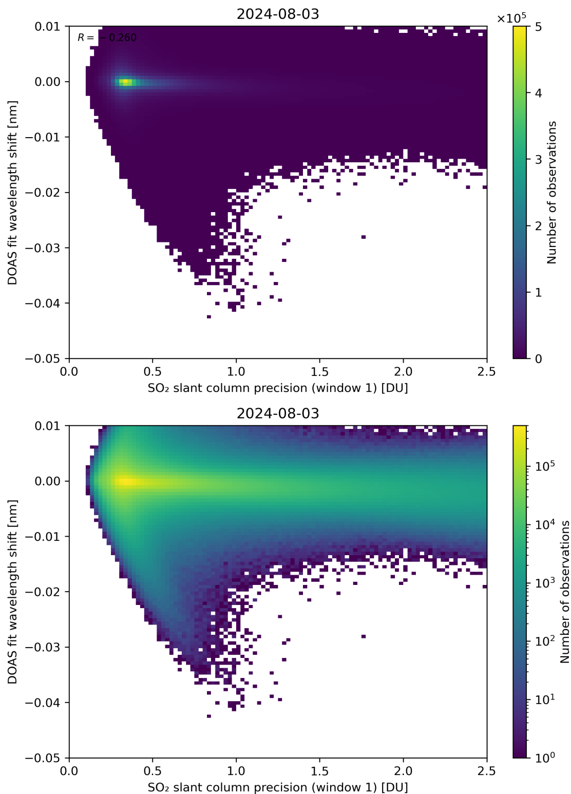
Figure 221: Scatter density plot of “SO 2 slant column precision (window 1)” against “DOAS fit wavelength shift” for 2024-08-02 to 2024-08-04.
