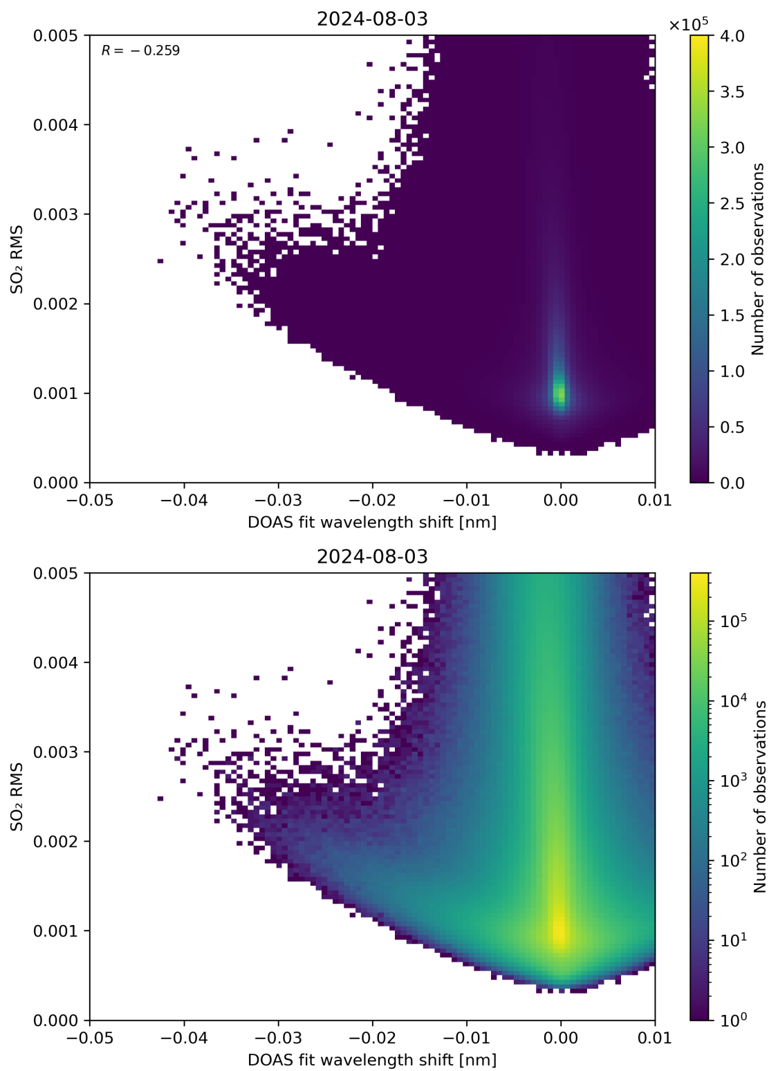
Figure 128: Scatter density plot of “DOAS fit wavelength shift” against “SO 2 RMS” for 2024-08-02 to 2024-08-04.
