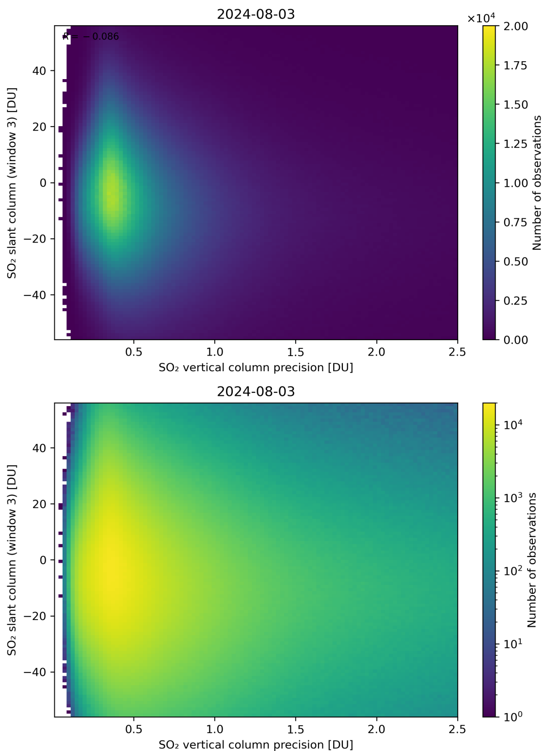
Figure 292: Scatter density plot of “SO 2 vertical column precision” against “SO 2 slant column (window 3)” for 2024-08-02 to 2024-08-04.
