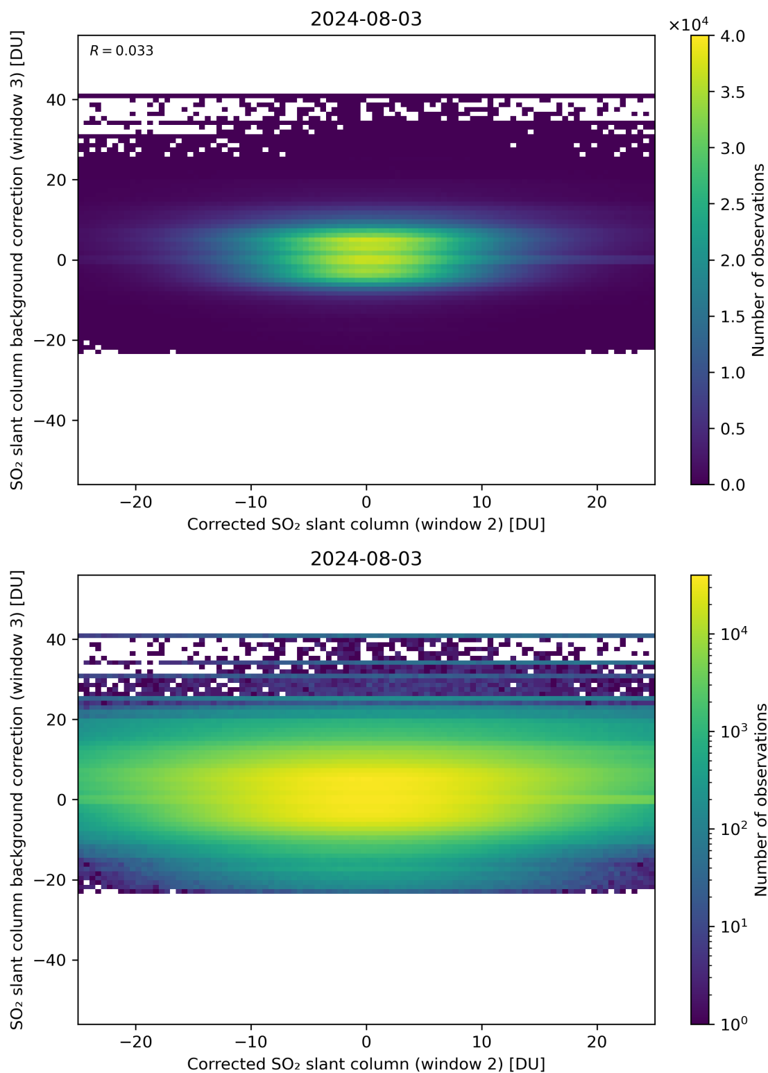
Figure 195: Scatter density plot of “Corrected SO 2 slant column (window 2)” against “SO 2 slant column background correction (window 3)” for 2024-08-02 to 2024-08-04.
