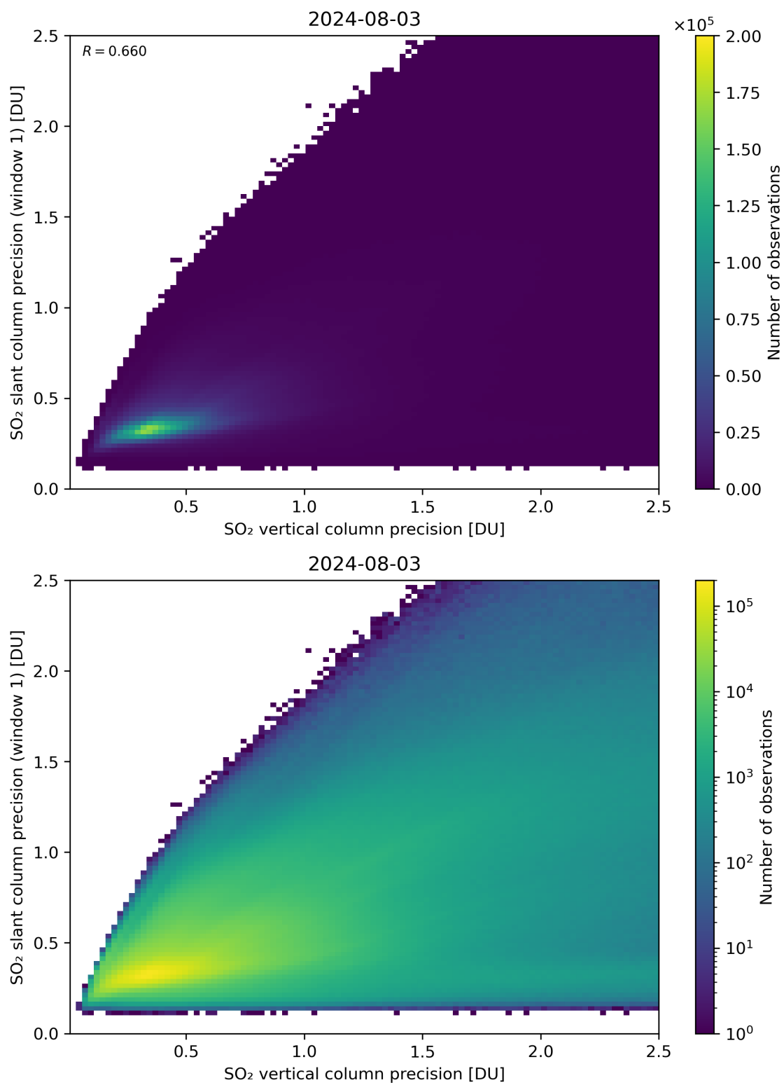
Figure 290: Scatter density plot of “SO 2 vertical column precision” against “SO 2 slant column precision (window 1)” for 2024-08-02 to 2024-08-04.
