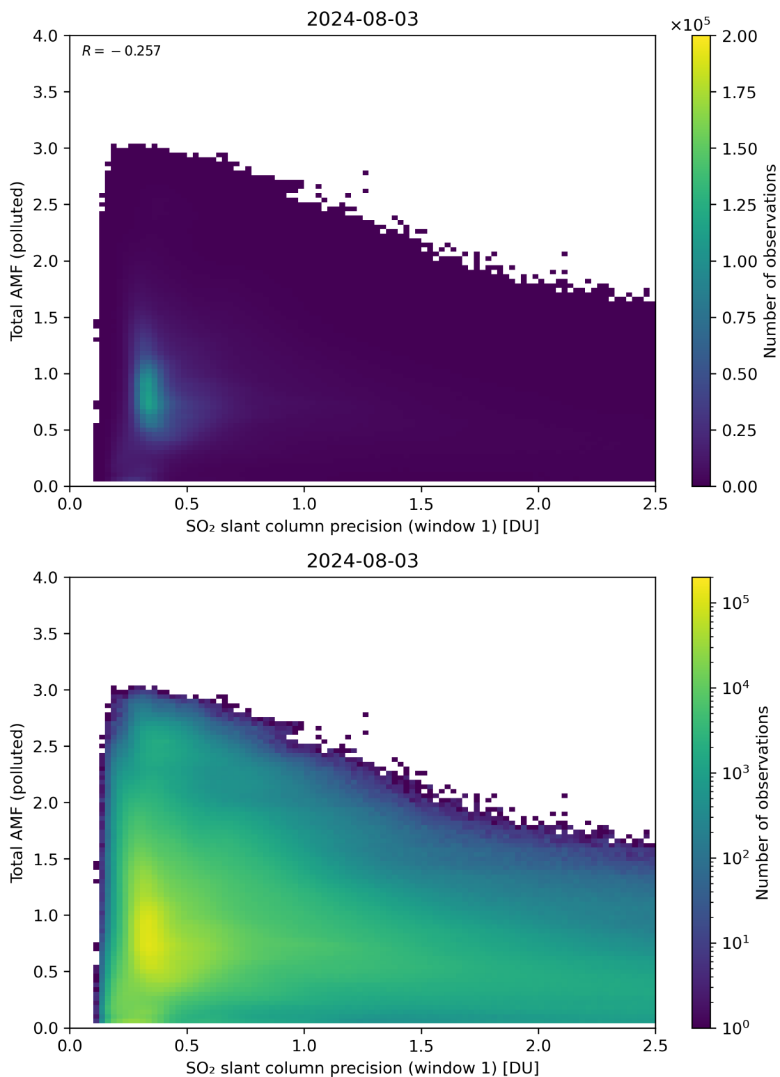
Figure 230: Scatter density plot of “SO 2 slant column precision (window 1)” against “Total AMF (polluted)” for 2024-08-02 to 2024-08-04.
