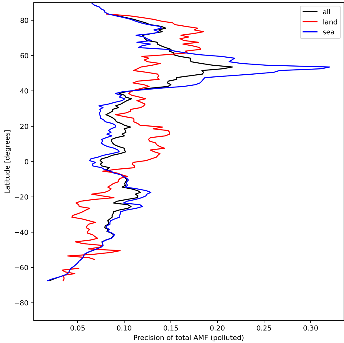
Figure 49: Zonal average of “Precision of total AMF (polluted)” for 2024-08-02 to 2024-08-04.
