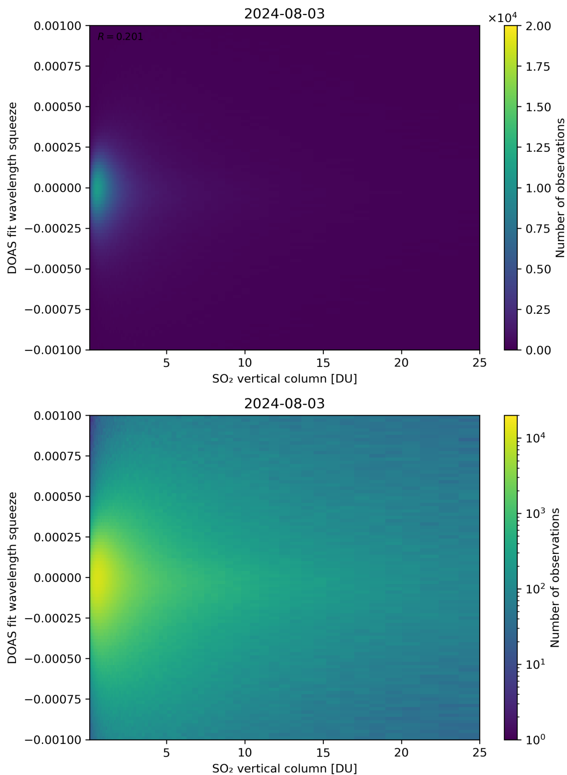
Figure 277: Scatter density plot of “SO 2 vertical column” against “DOAS fit wavelength squeeze” for 2024-08-02 to 2024-08-04.
