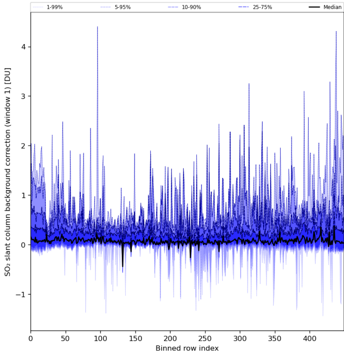
Figure 82: Along track statistics of “SO 2 slant column background correction (window 1)” for 2024-08-02 to 2024-08-04
