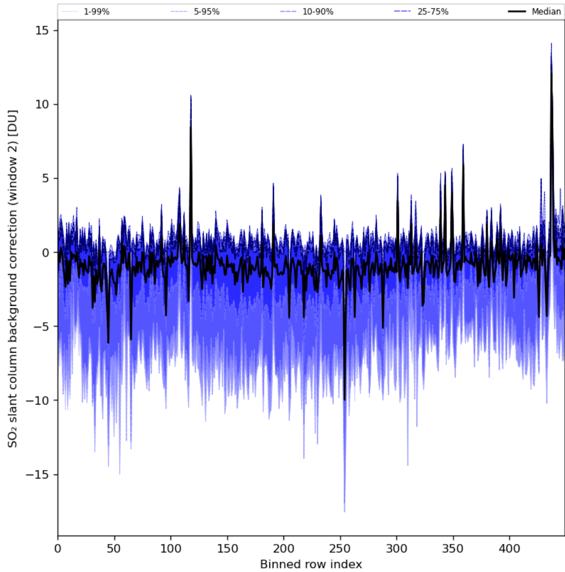
Figure 86: Along track statistics of “SO 2 slant column background correction (window 2)” for 2024-08-02 to 2024-08-04
