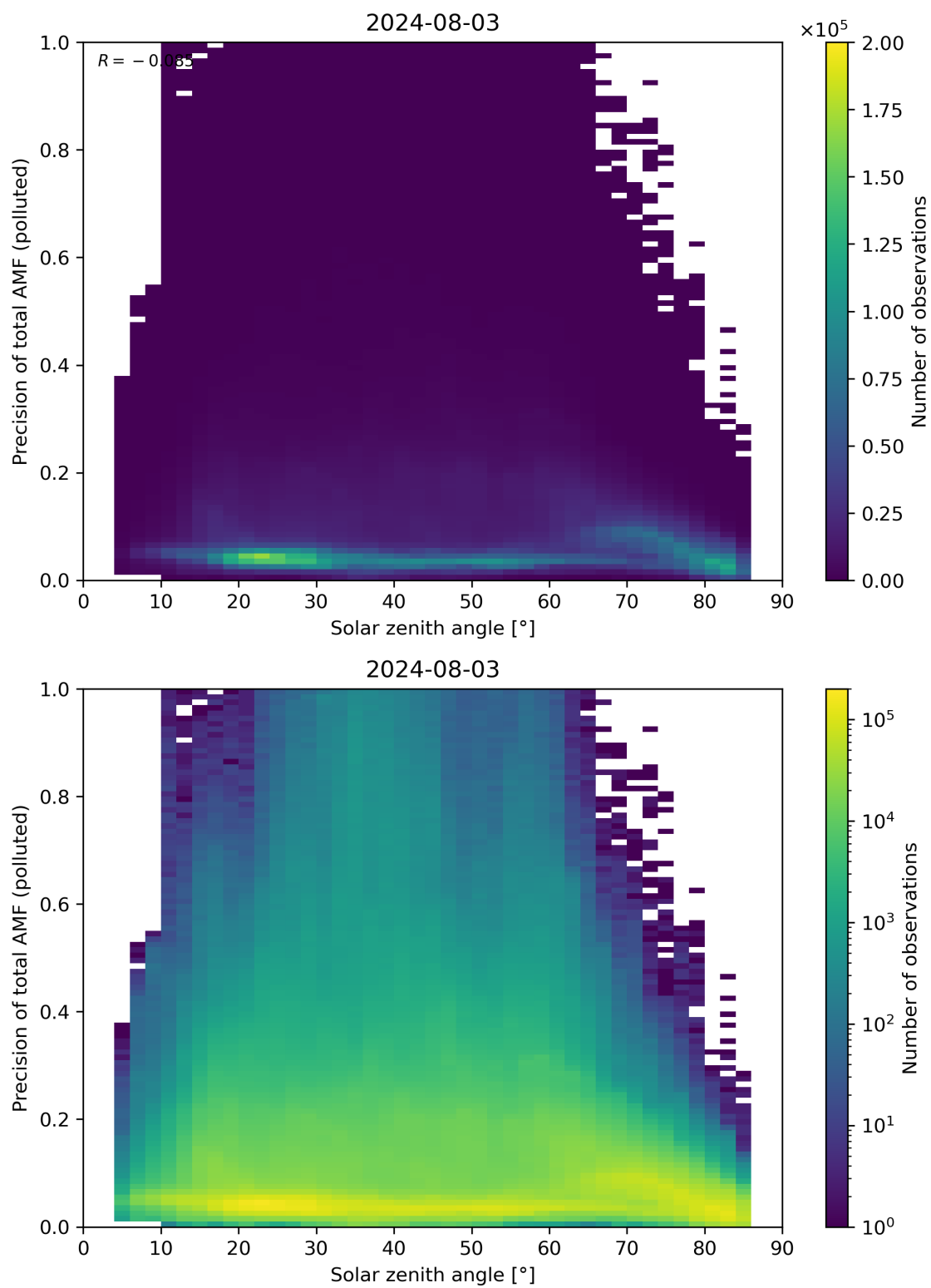
Figure 175: Scatter density plot of “Solar zenith angle” against “Precision of total AMF (polluted)” for 2024-08-02 to 2024-08-04.
