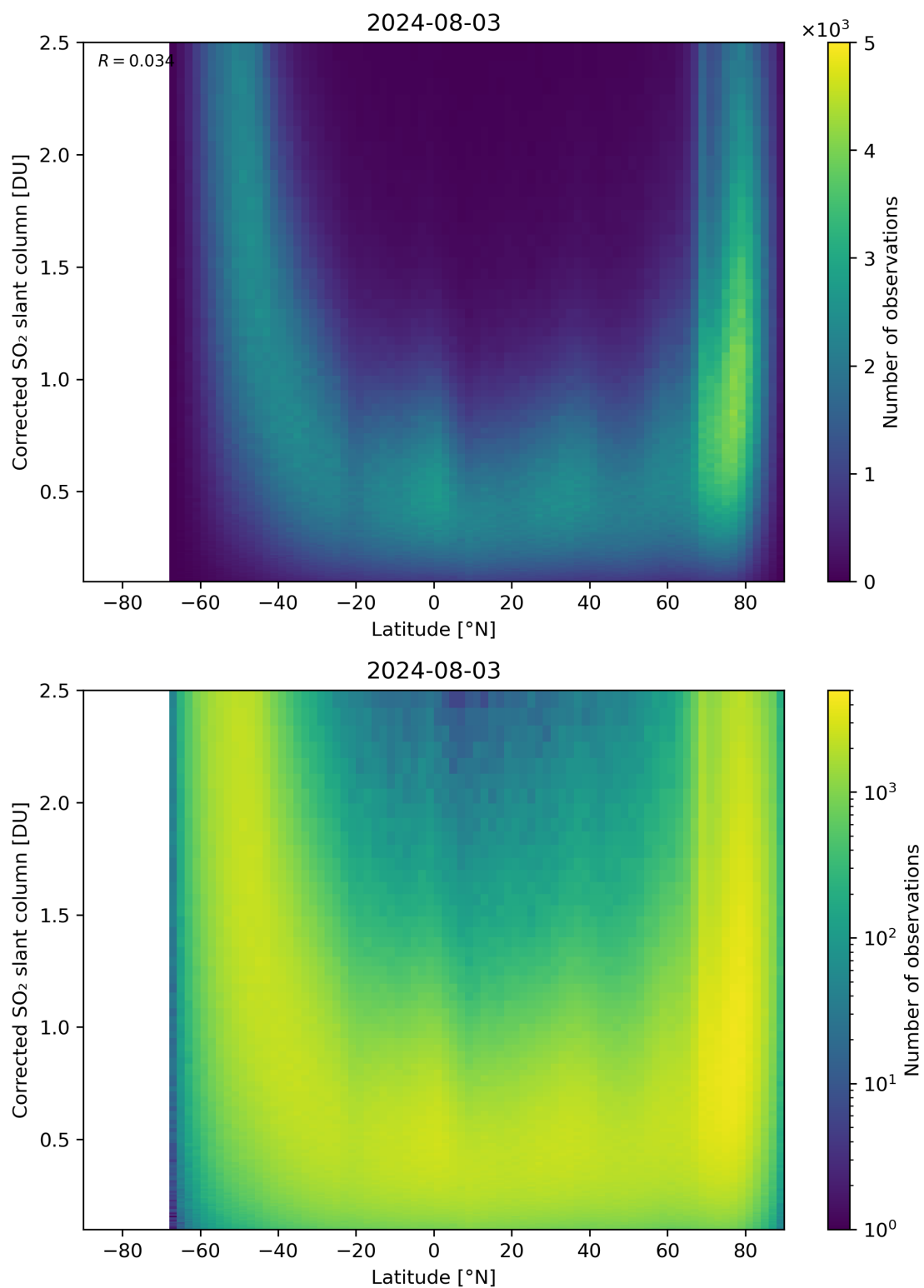
Figure 146: Scatter density plot of “Latitude” against “Corrected SO 2 slant column” for 2024-08-02 to 2024-08-04.
