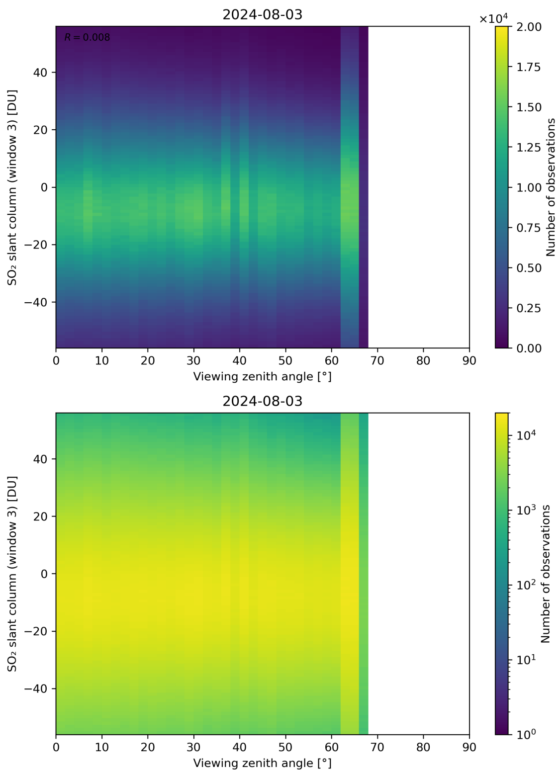
Figure 323: Scatter density plot of “Viewing zenith angle” against “SO 2 slant column (window 3)” for 2024-08-02 to 2024-08-04.
