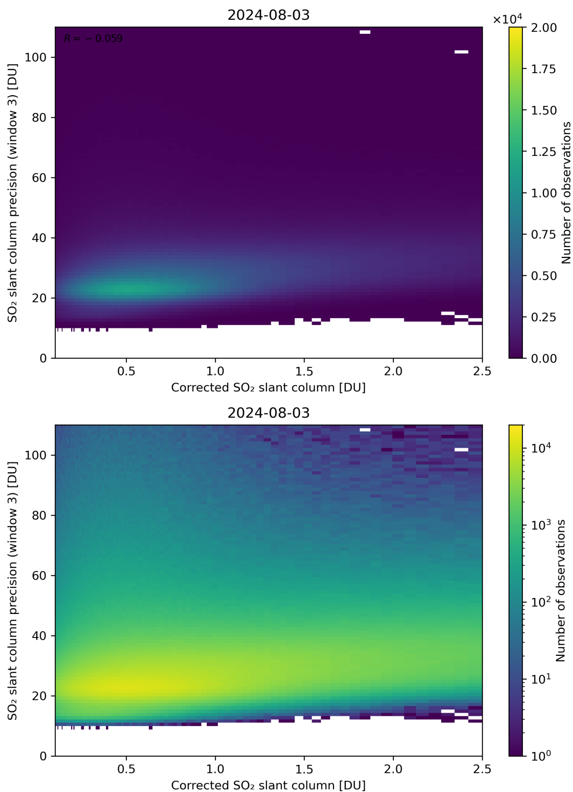
Figure 191: Scatter density plot of “Corrected SO 2 slant column” against “SO 2 slant column precision (window 3)” for 2024-08-02 to 2024-08-04.
