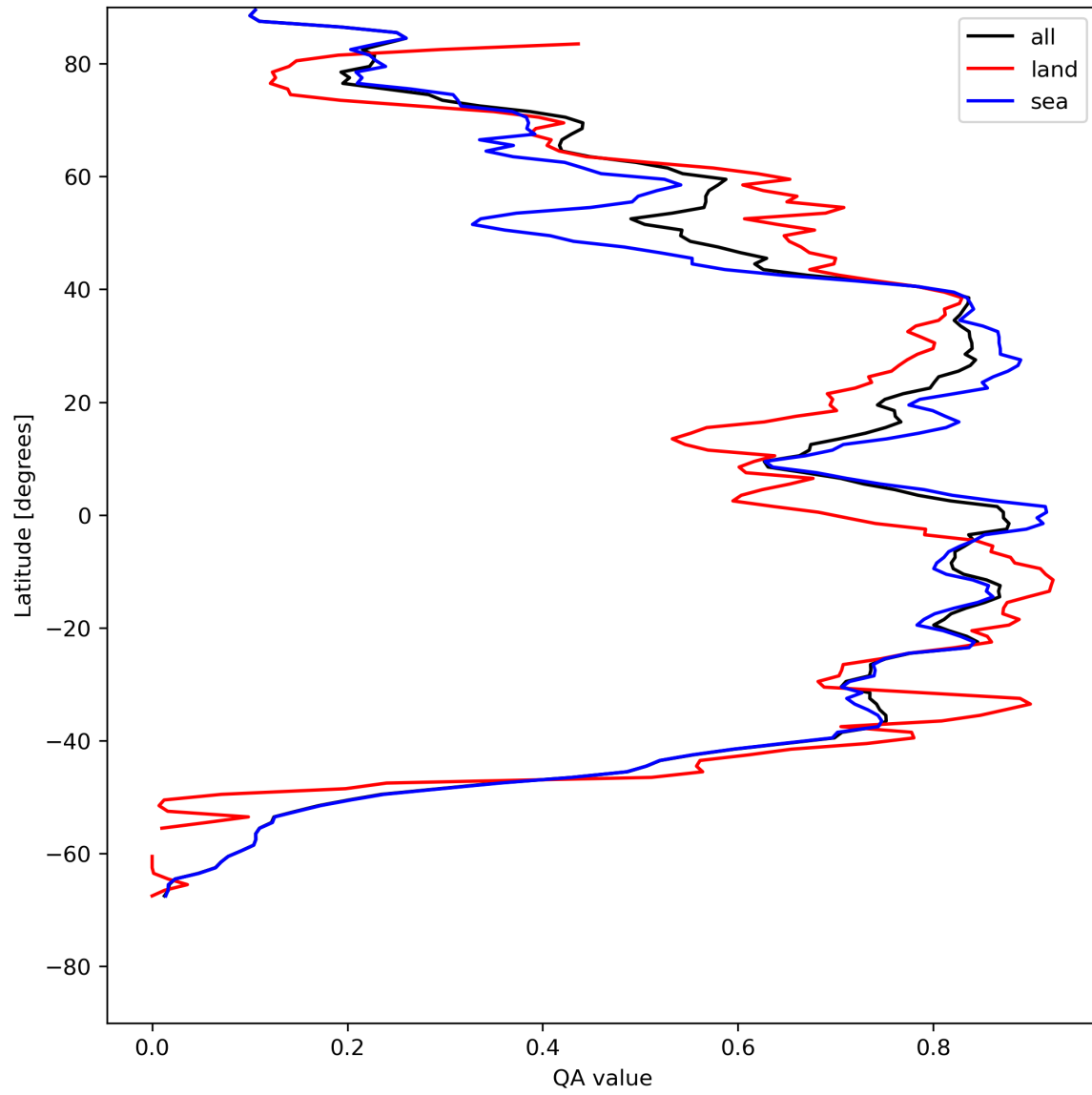
Figure 29: Zonal average of “QA value” for 2024-08-02 to 2024-08-04.
