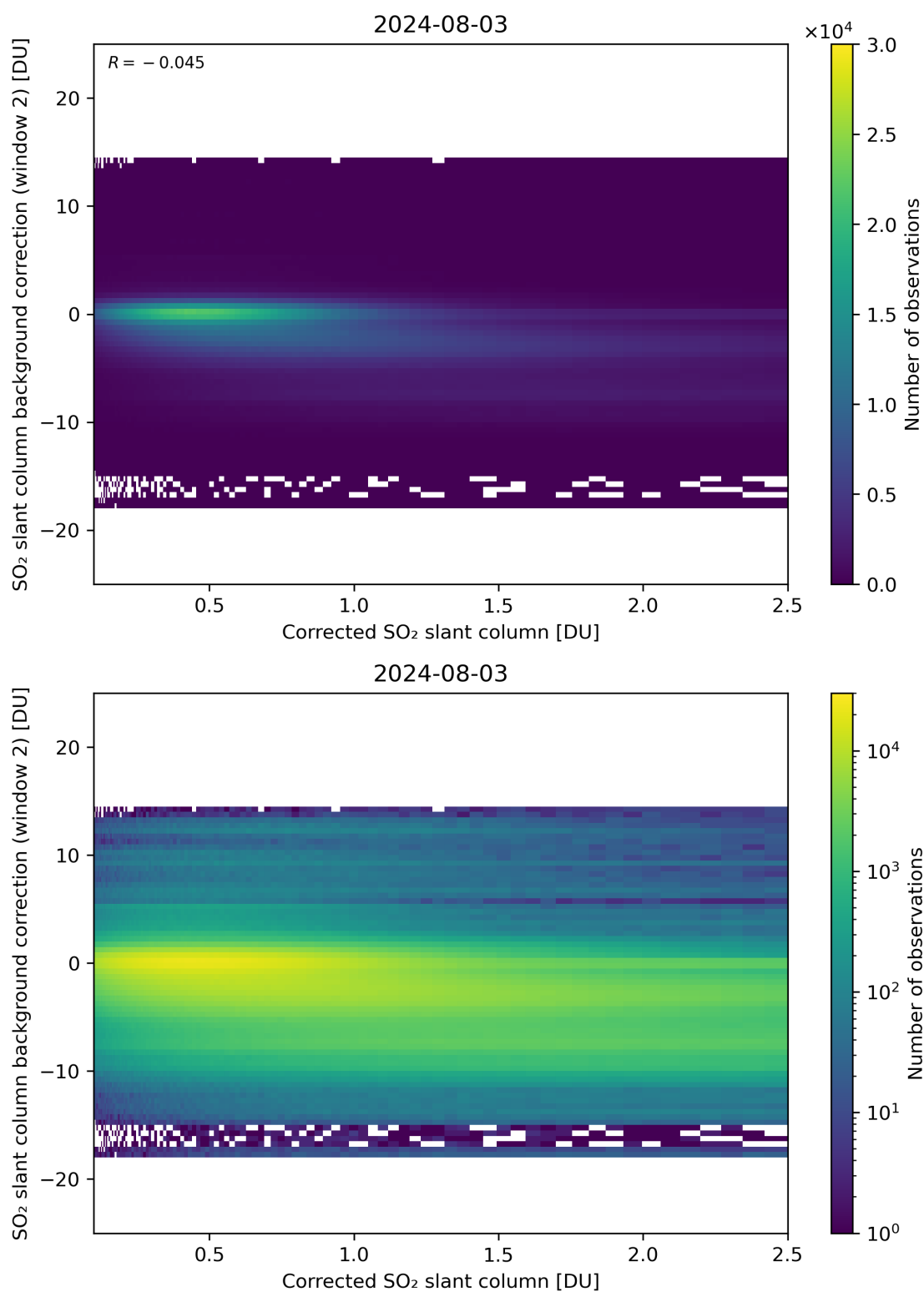
Figure 179: Scatter density plot of “Corrected SO 2 slant column” against “SO 2 slant column background correction (window 2)” for 2024-08-02 to 2024-08-04.
