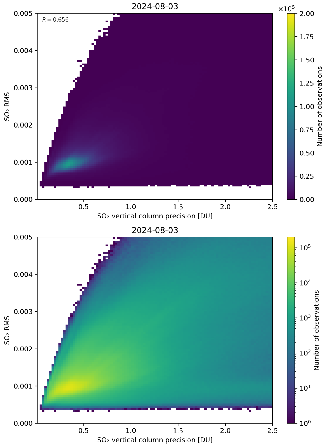
Figure 284: Scatter density plot of “SO 2 vertical column precision” against “SO 2 RMS” for 2024-08-02 to 2024-08-04.
