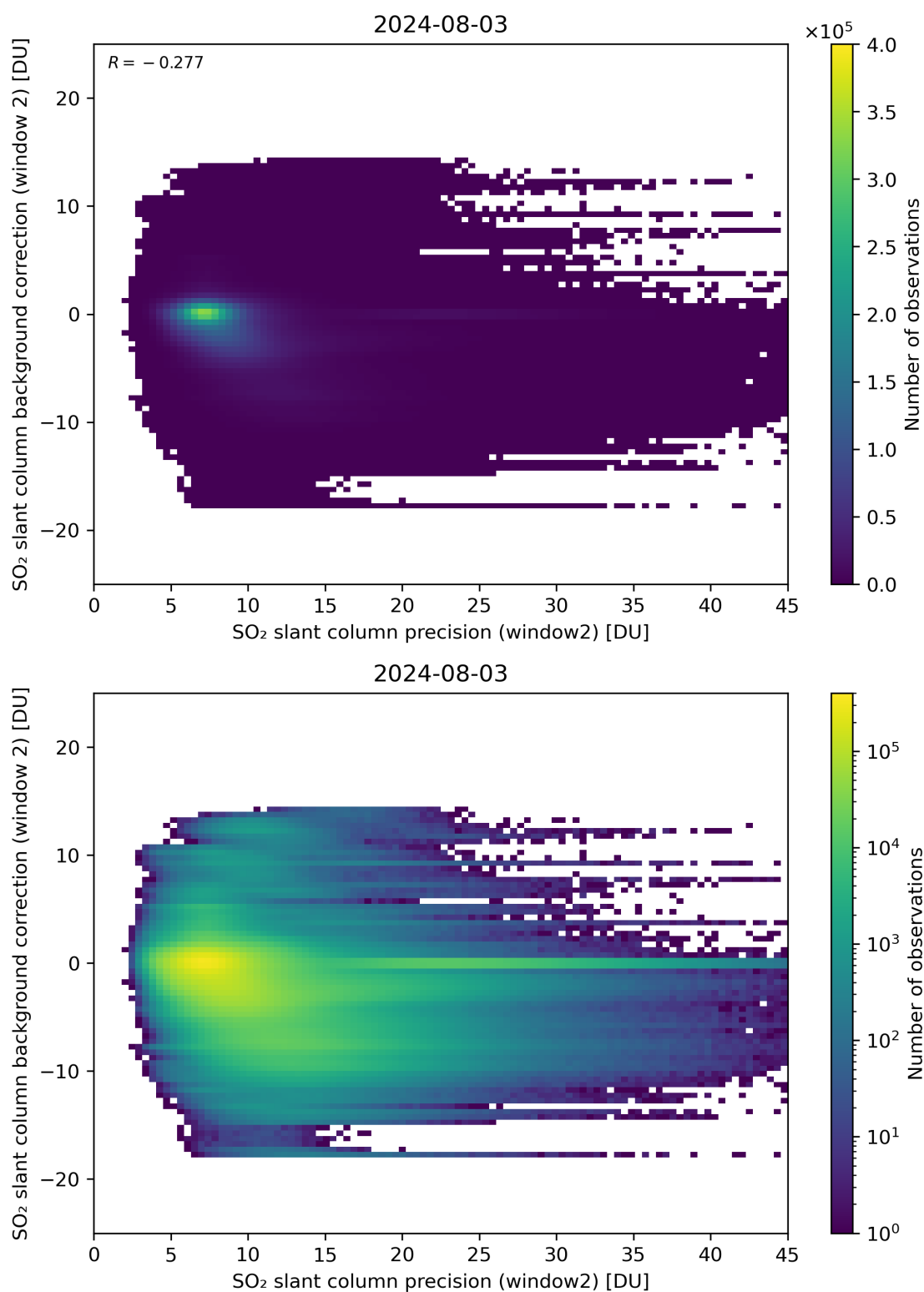
Figure 241: Scatter density plot of “SO 2 slant column precision (window2)” against “SO 2 slant column background correction (window 2)” for 2024-08-02 to 2024-08-04.
