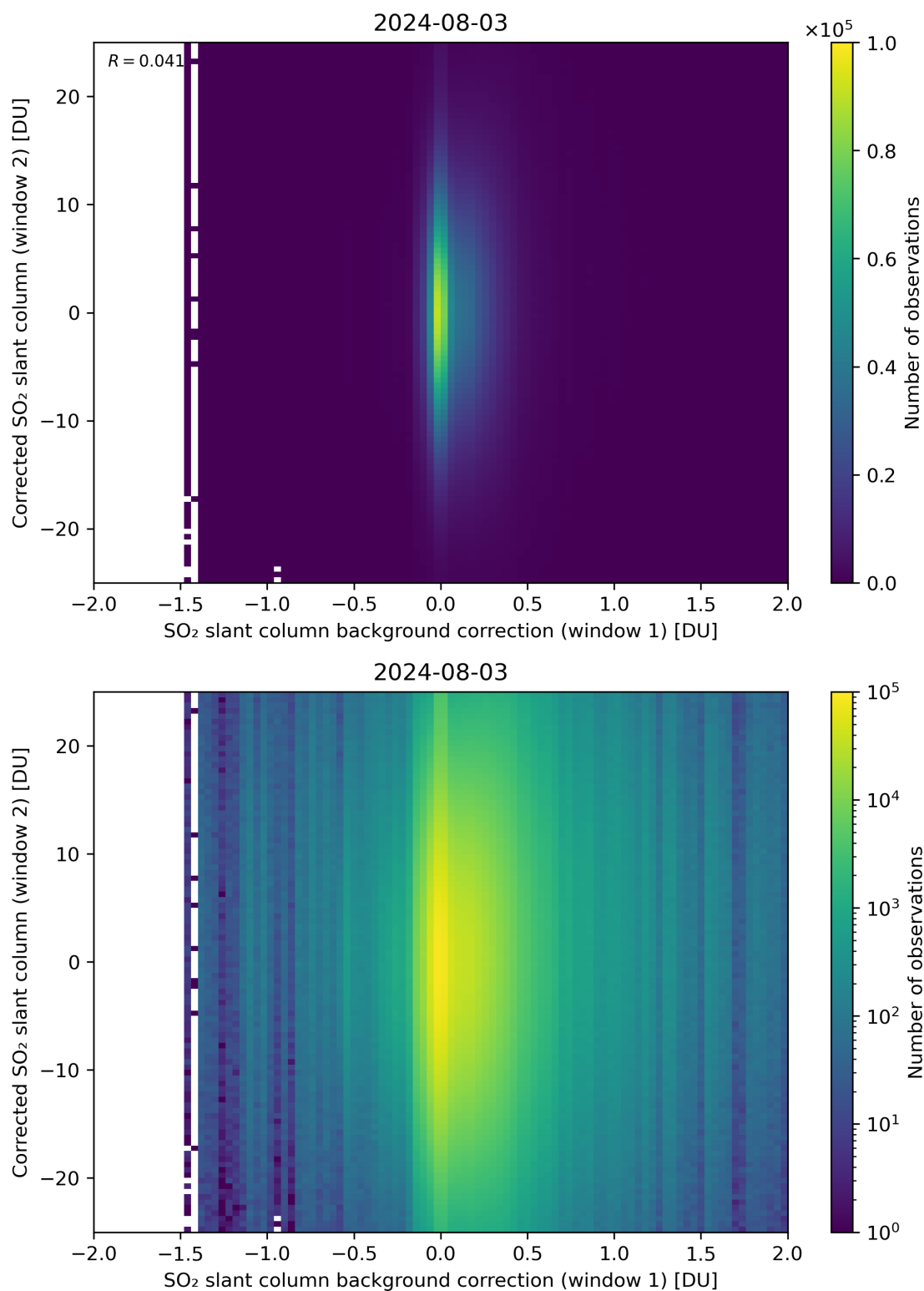
Figure 104: Scatter density plot of “SO 2 slant column background correction (window 1)” against “Corrected SO 2 slant column (window 2)” for 2024-08-02 to 2024-08-04.
