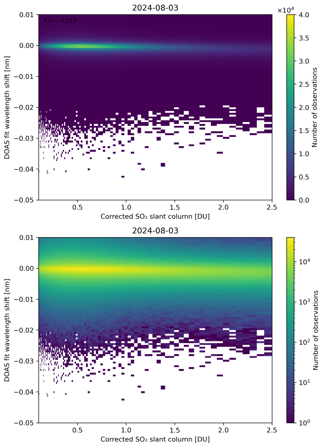
Figure 181: Scatter density plot of “Corrected SO 2 slant column” against “DOAS fit wavelength shift” for 2024-08-02 to 2024-08-04.
