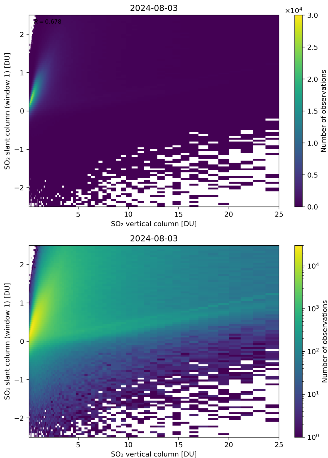
Figure 300: Scatter density plot of “SO 2 vertical column” against “SO 2 slant column (window 1)” for 2024-08-02 to 2024-08-04.
