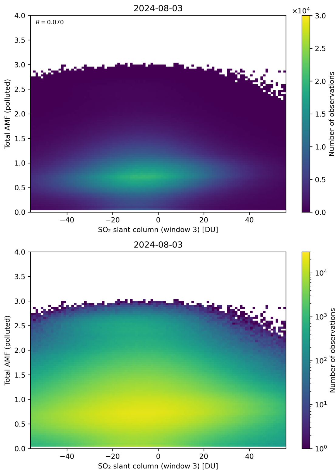
Figure 268: Scatter density plot of “SO 2 slant column (window 3)” against “Total AMF (polluted)” for 2024-08-02 to 2024-08-04.
