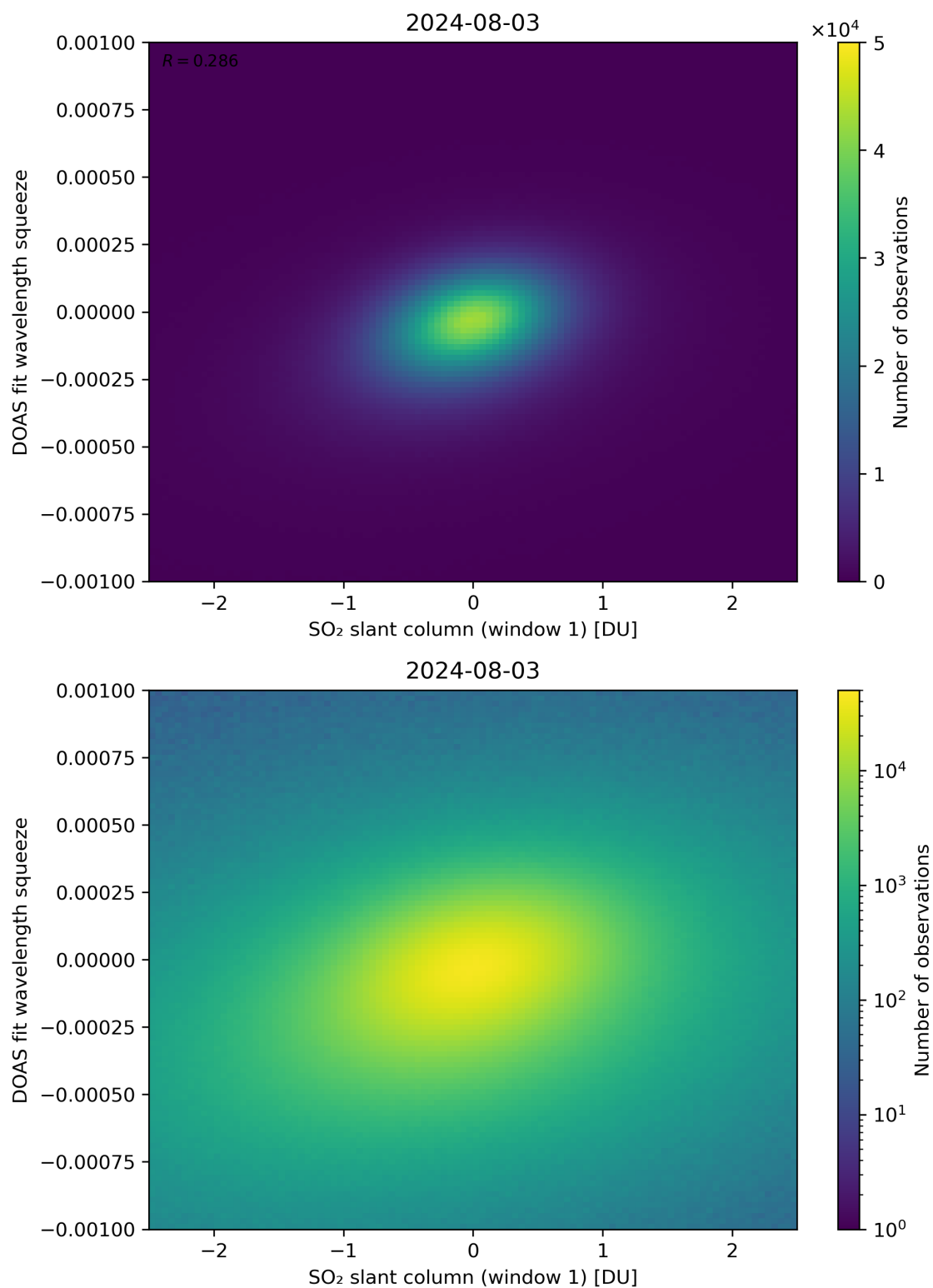
Figure 216: Scatter density plot of “SO 2 slant column (window 1)” against “DOAS fit wavelength squeeze” for 2024-08-02 to 2024-08-04.
