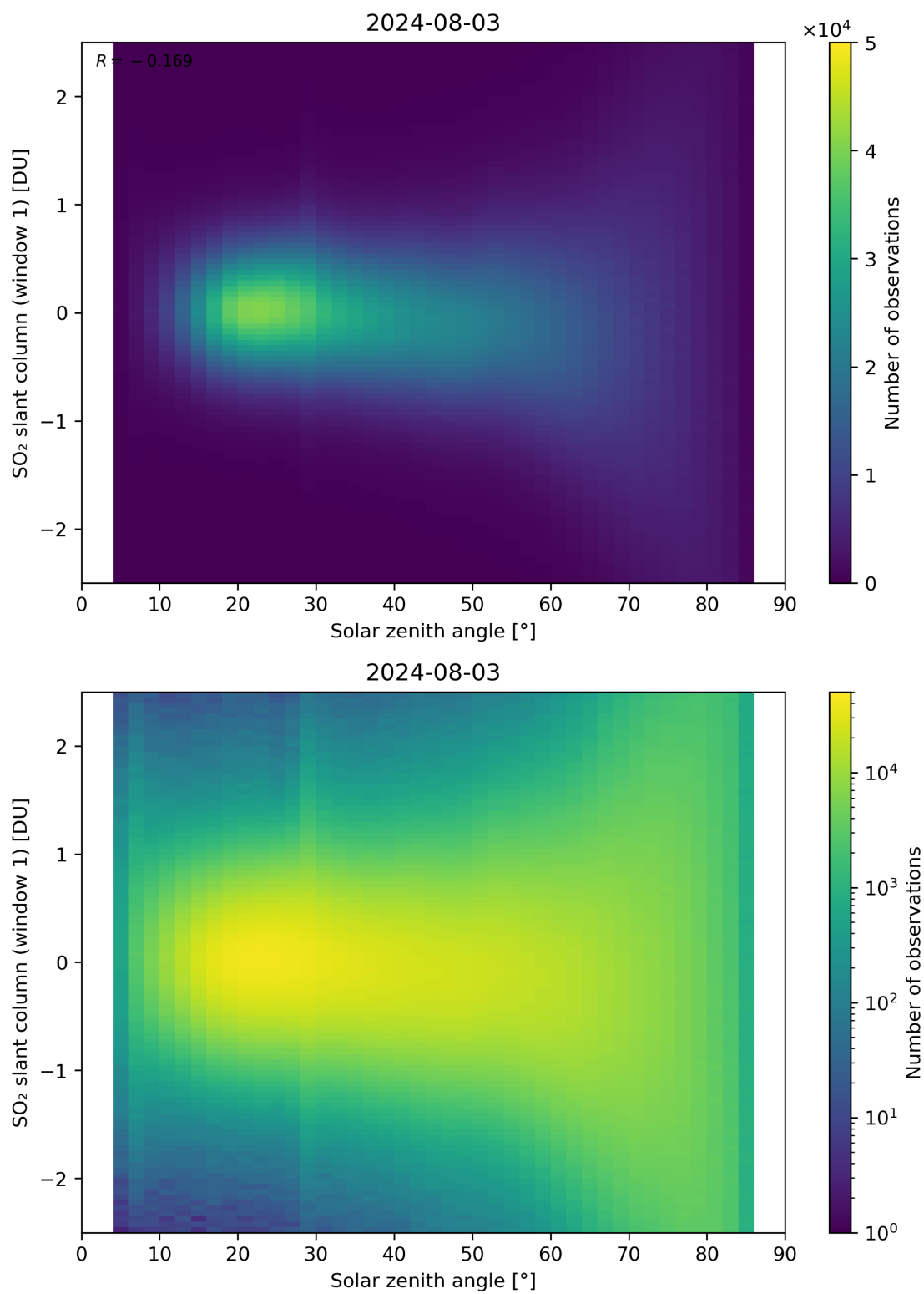
Figure 169: Scatter density plot of “Solar zenith angle” against “SO 2 slant column (window 1)” for 2024-08-02 to 2024-08-04.
