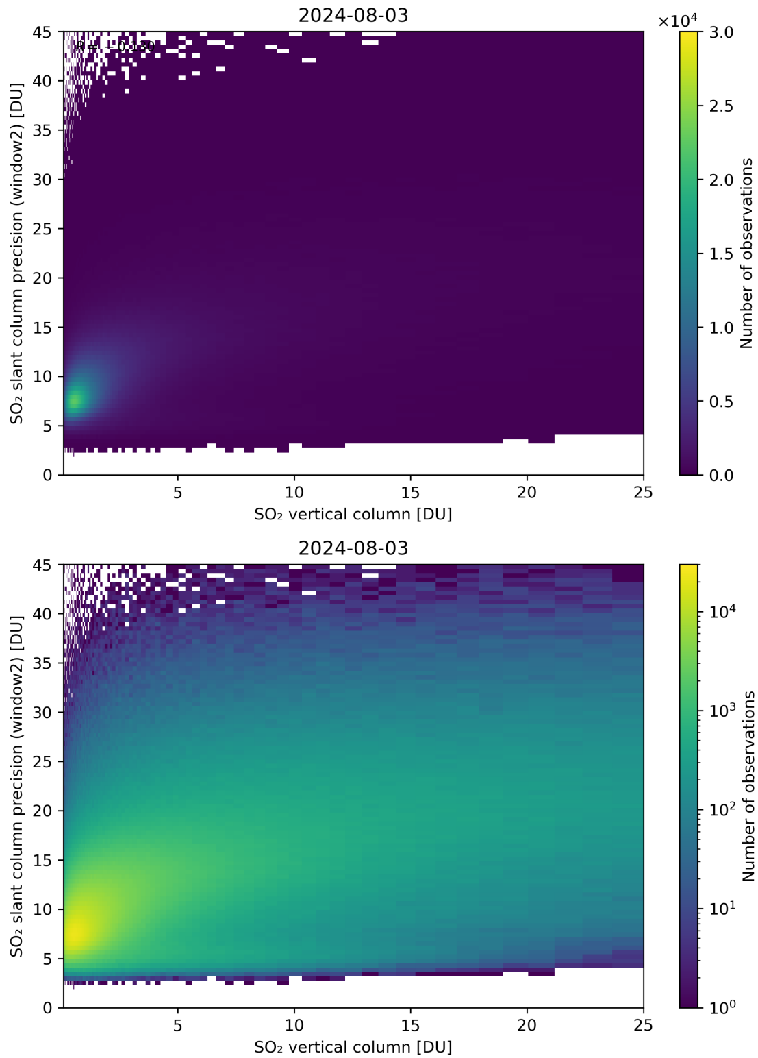
Figure 302: Scatter density plot of “SO 2 vertical column” against “SO 2 slant column precision (window2)” for 2024-08-02 to 2024-08-04.
