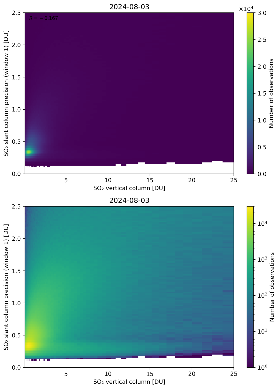
Figure 301: Scatter density plot of “SO 2 vertical column” against “SO 2 slant column precision (window 1)” for 2024-08-02 to 2024-08-04.
