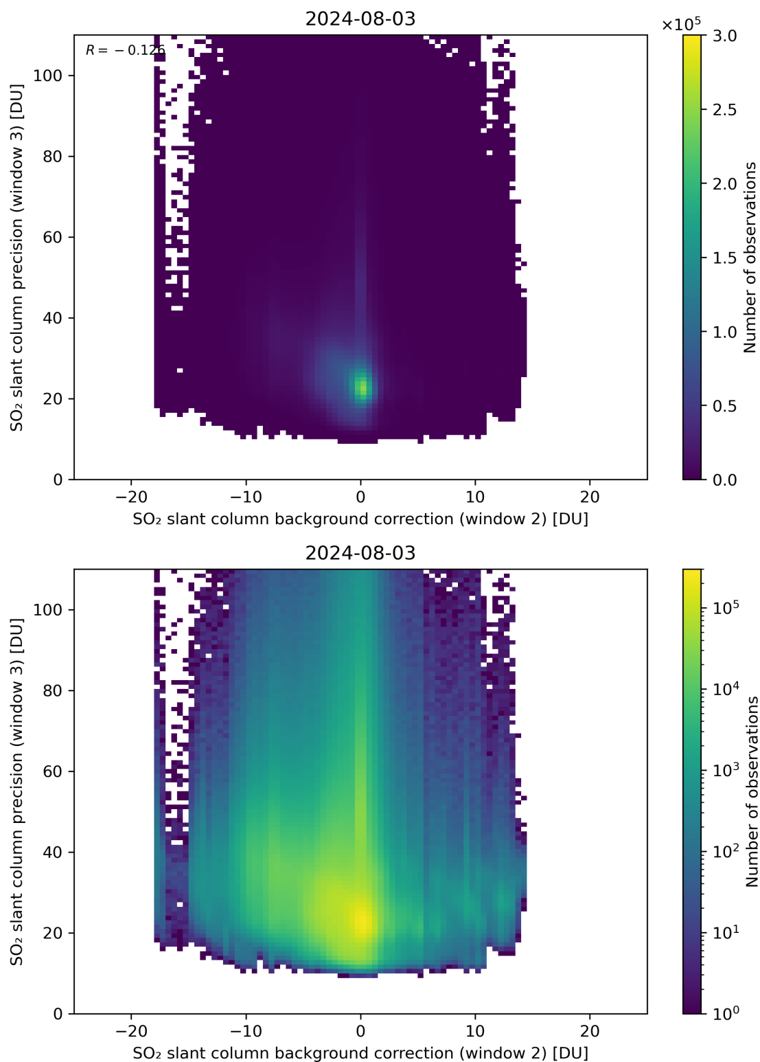
Figure 118: Scatter density plot of “SO 2 slant column background correction (window 2)” against “SO 2 slant column precision (window 3)” for 2024-08-02 to 2024-08-04.
