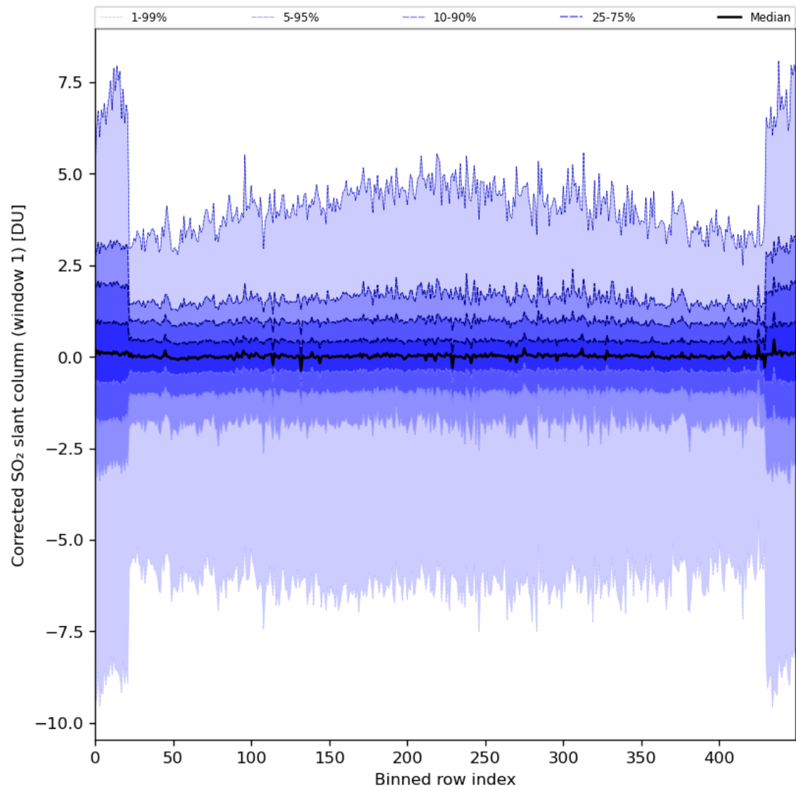
Figure 81: Along track statistics of “Corrected SO 2 slant column (window 1)” for 2024-08-02 to 2024-08-04
