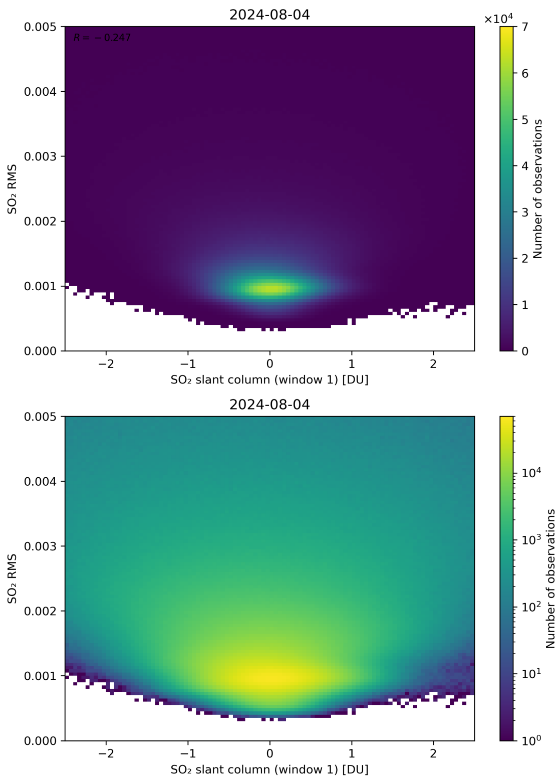
Figure 217: Scatter density plot of “SO 2 slant column (window 1)” against “SO 2 RMS” for 2024-08-03 to 2024-08-05.
