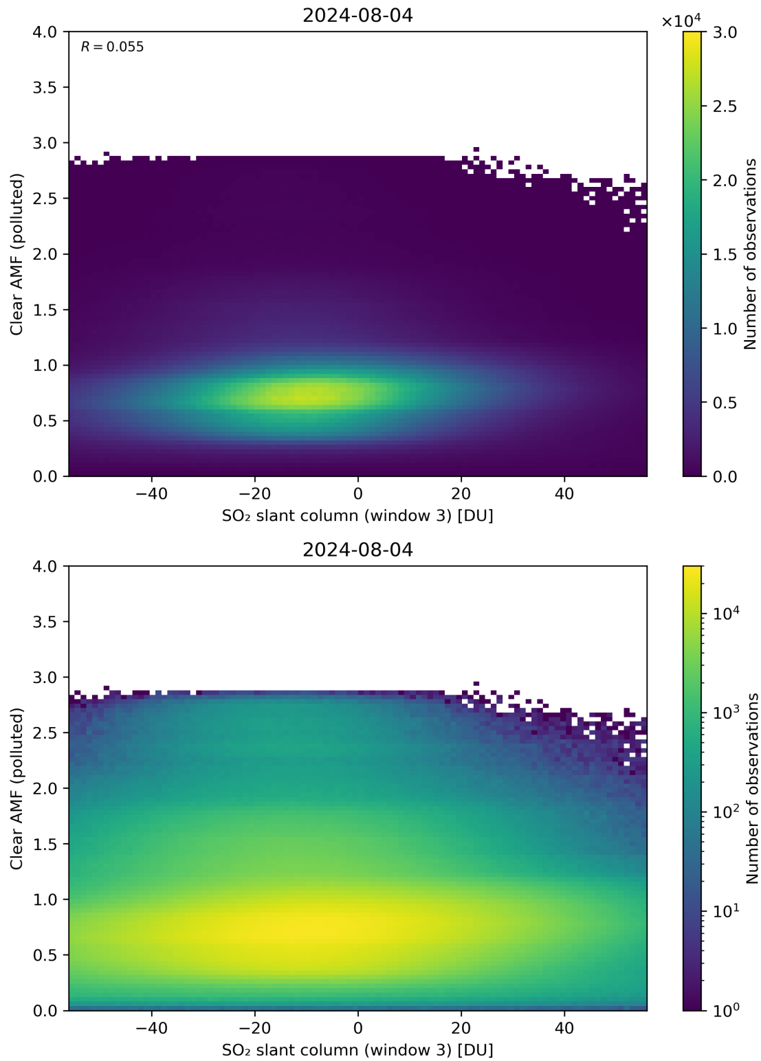
Figure 265: Scatter density plot of “SO 2 slant column (window 3)” against “Clear AMF (polluted)” for 2024-08-03 to 2024-08-05.
