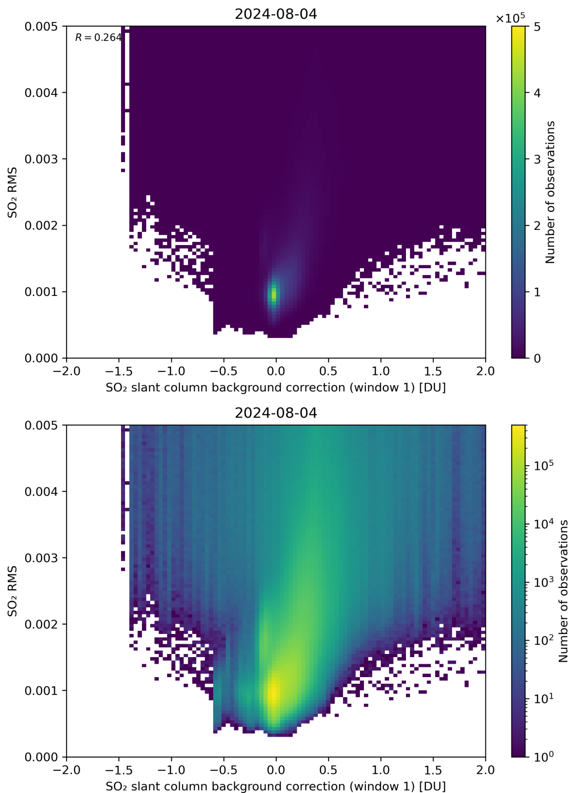
Figure 102: Scatter density plot of “SO 2 slant column background correction (window 1)” against “SO 2 RMS” for 2024-08-03 to 2024-08-05.
