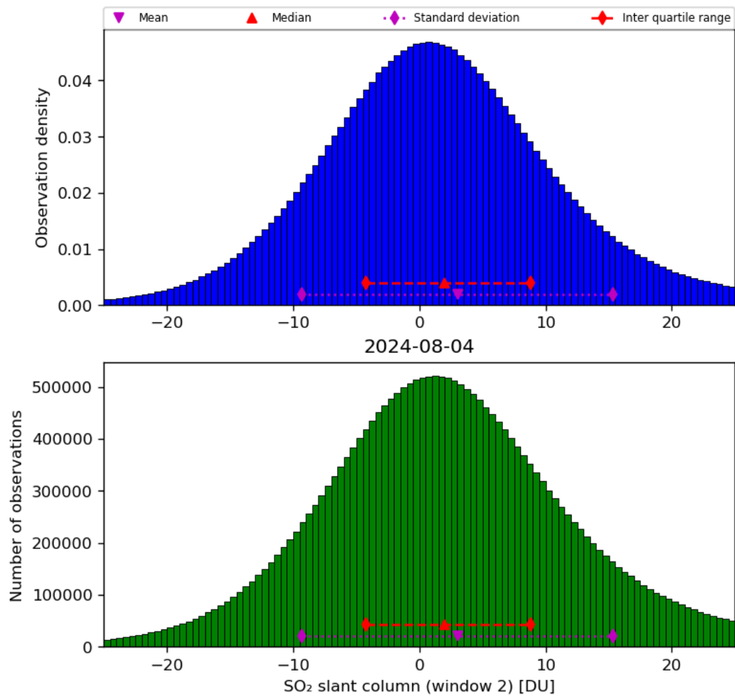
Figure 60: Histogram of “SO 2 slant column (window 2)” for 2024-08-03 to 2024-08-05
