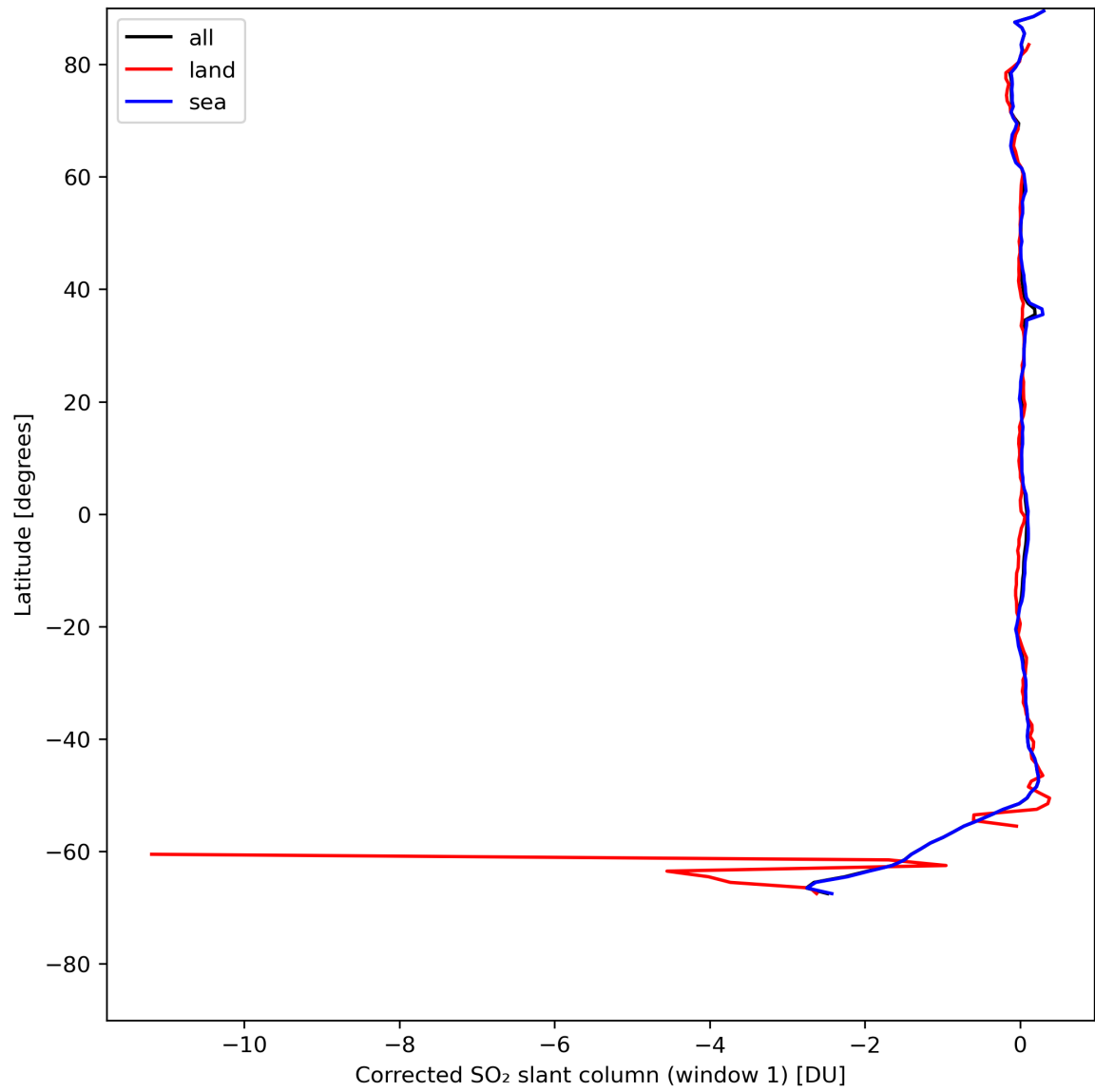
Figure 35: Zonal average of “Corrected SO 2 slant column (window 1)” for 2024-08-03 to 2024-08-05.
