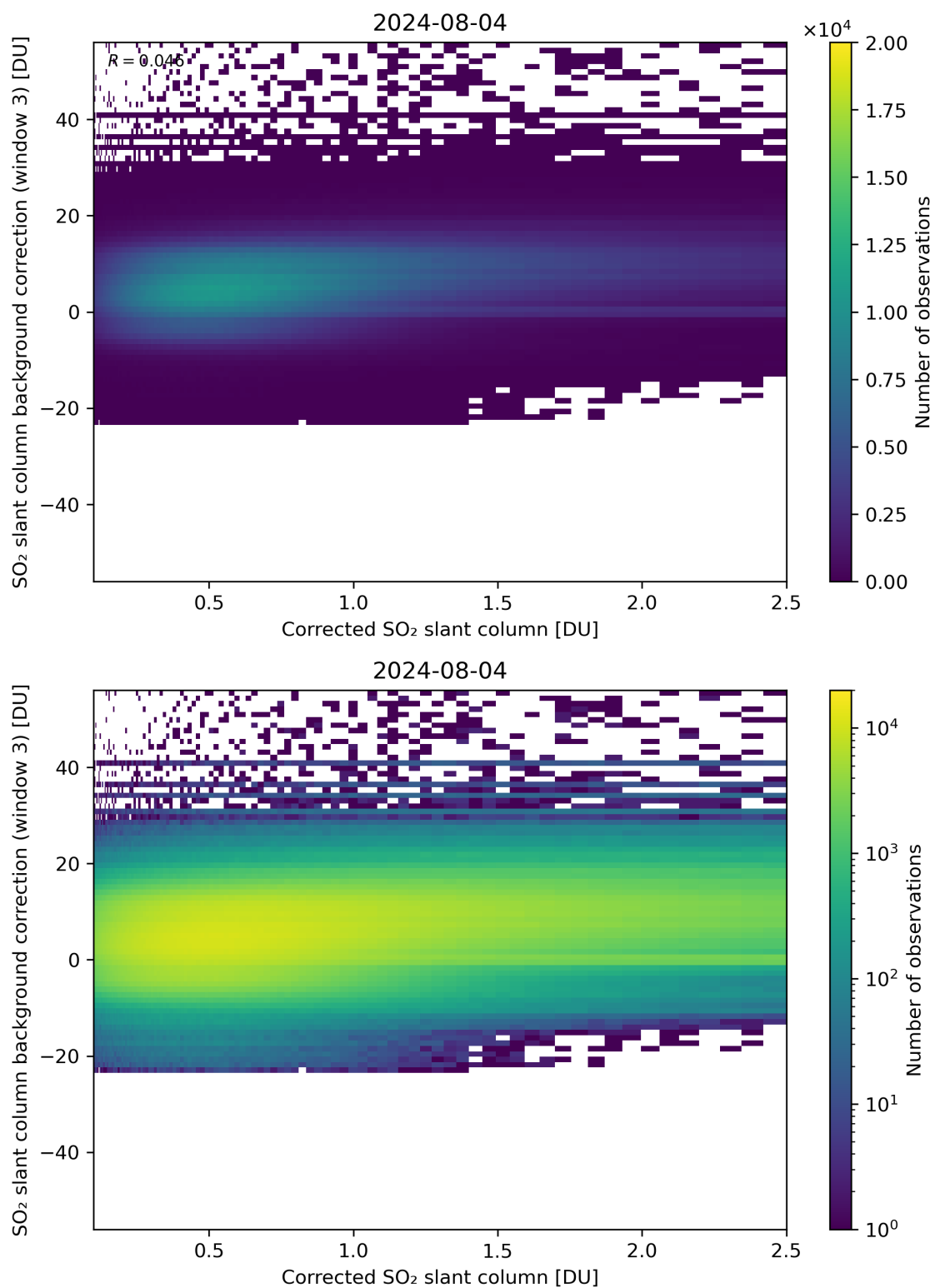
Figure 180: Scatter density plot of “Corrected SO 2 slant column” against “SO 2 slant column background correction (window 3)” for 2024-08-03 to 2024-08-05.
