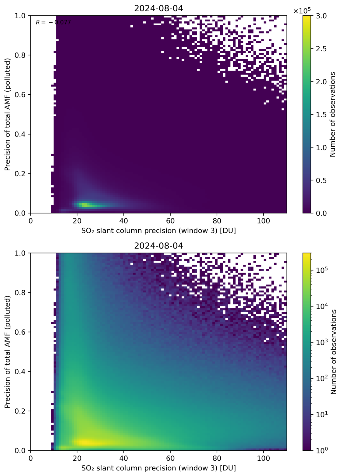
Figure 264: Scatter density plot of “SO 2 slant column precision (window 3)” against “Precision of total AMF (polluted)” for 2024-08-03 to 2024-08-05.
