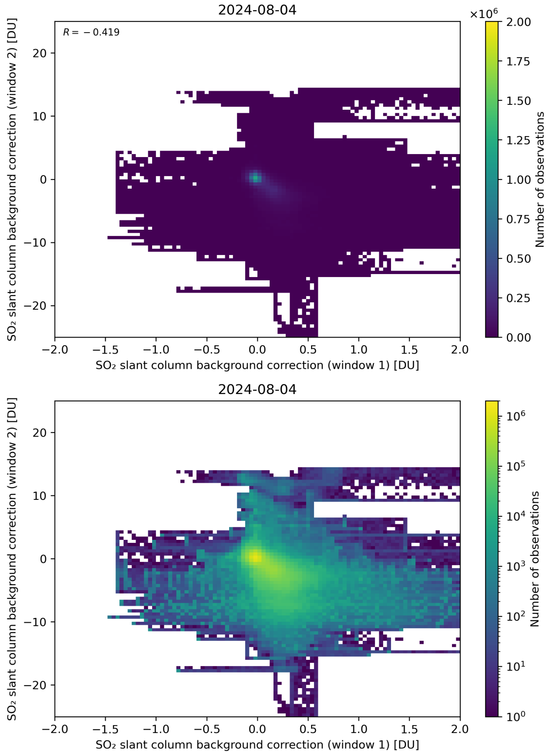
Figure 98: Scatter density plot of “SO 2 slant column background correction (window 1)” against “SO 2 slant column background correction (window 2)” for 2024-08-03 to 2024-08-05.
