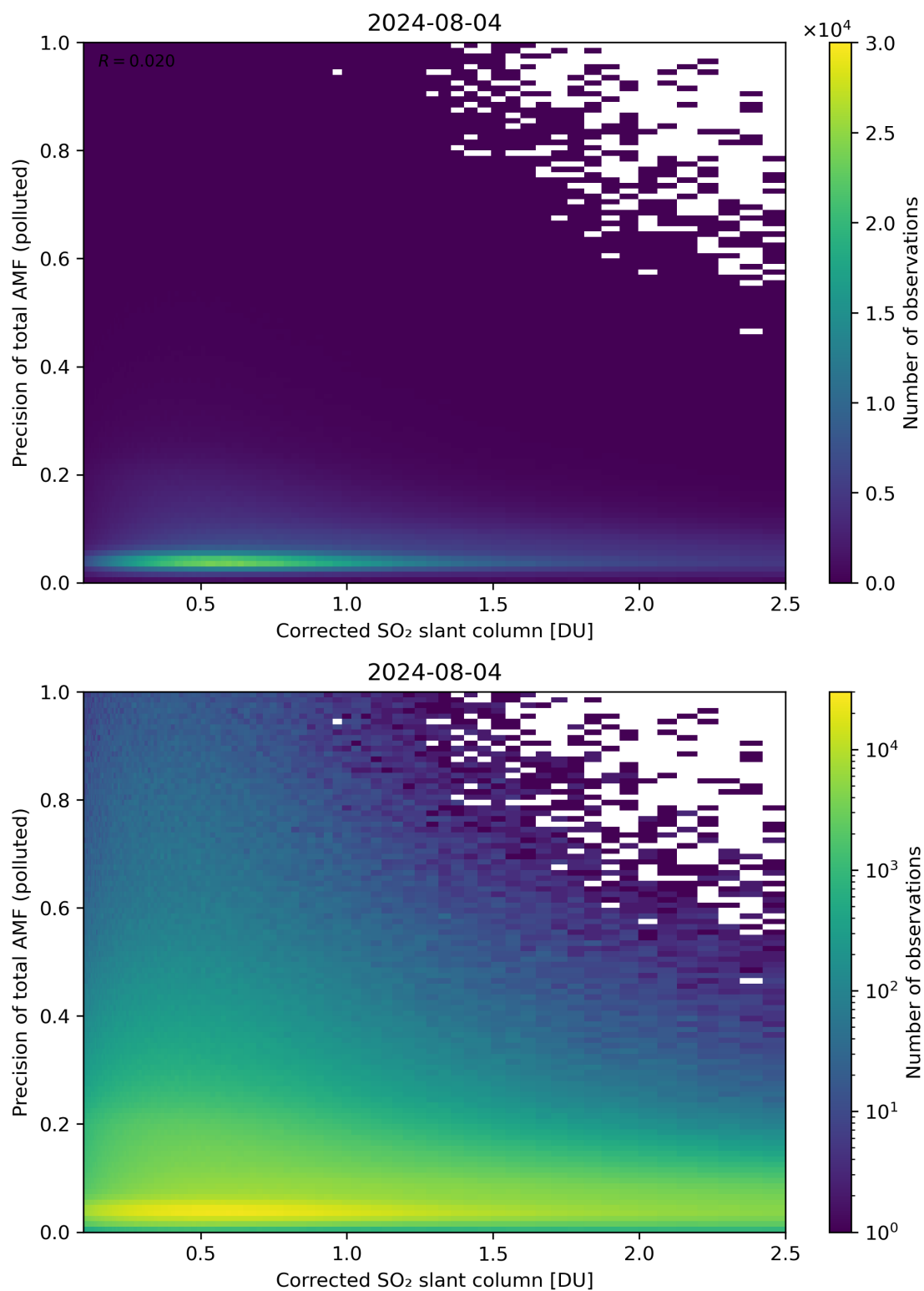
Figure 193: Scatter density plot of “Corrected SO 2 slant column” against “Precision of total AMF (polluted)” for 2024-08-03 to 2024-08-05.
