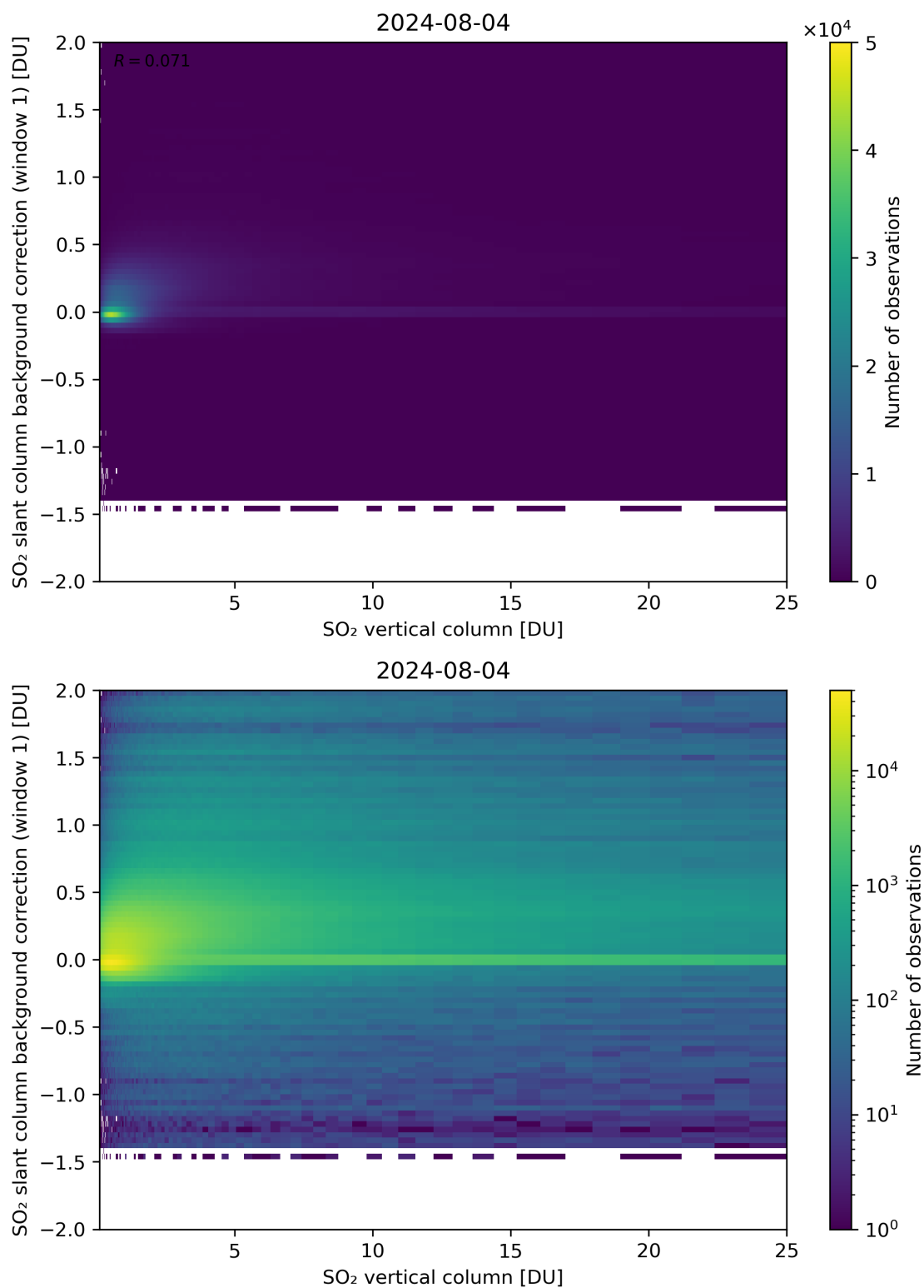
Figure 273: Scatter density plot of “SO 2 vertical column” against “SO 2 slant column background correction (window 1)” for 2024-08-03 to 2024-08-05.
