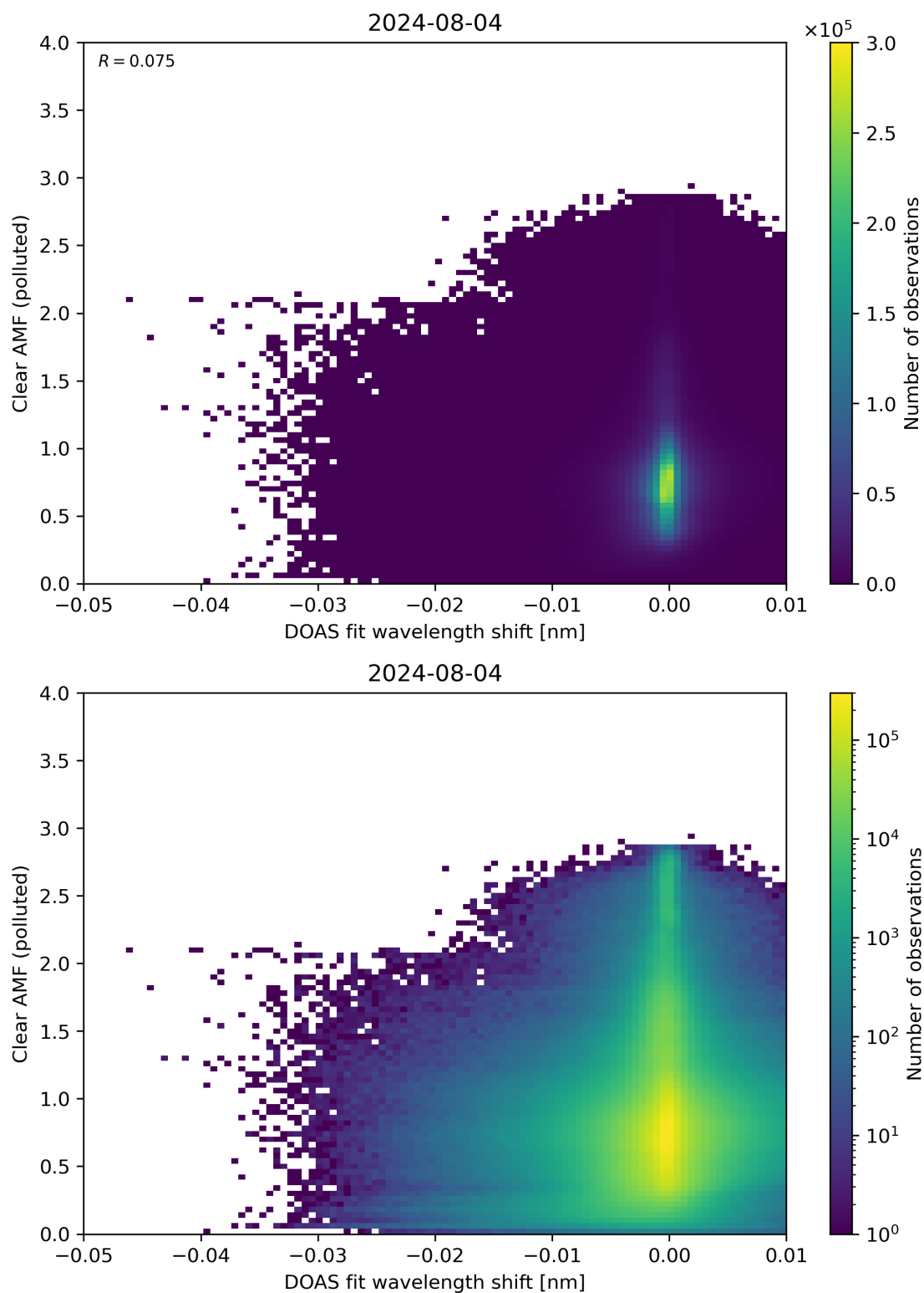
Figure 129: Scatter density plot of “DOAS fit wavelength shift” against “Clear AMF (polluted)” for 2024-08-03 to 2024-08-05.
