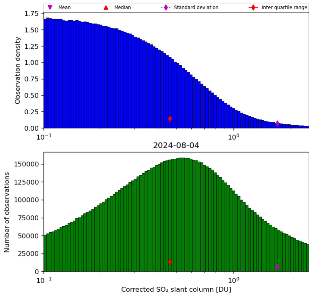
Figure 55: Histogram of “Corrected SO 2 slant column” for 2024-08-03 to 2024-08-05
