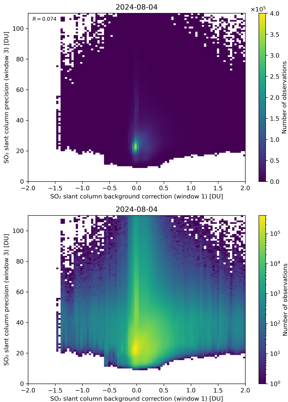
Figure 108: Scatter density plot of “SO 2 slant column background correction (window 1)” against “SO 2 slant column precision (window 3)” for 2024-08-03 to 2024-08-05.
