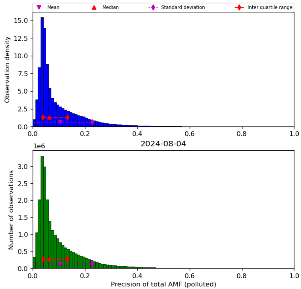
Figure 72: Histogram of “Precision of total AMF (polluted)” for 2024-08-03 to 2024-08-05
