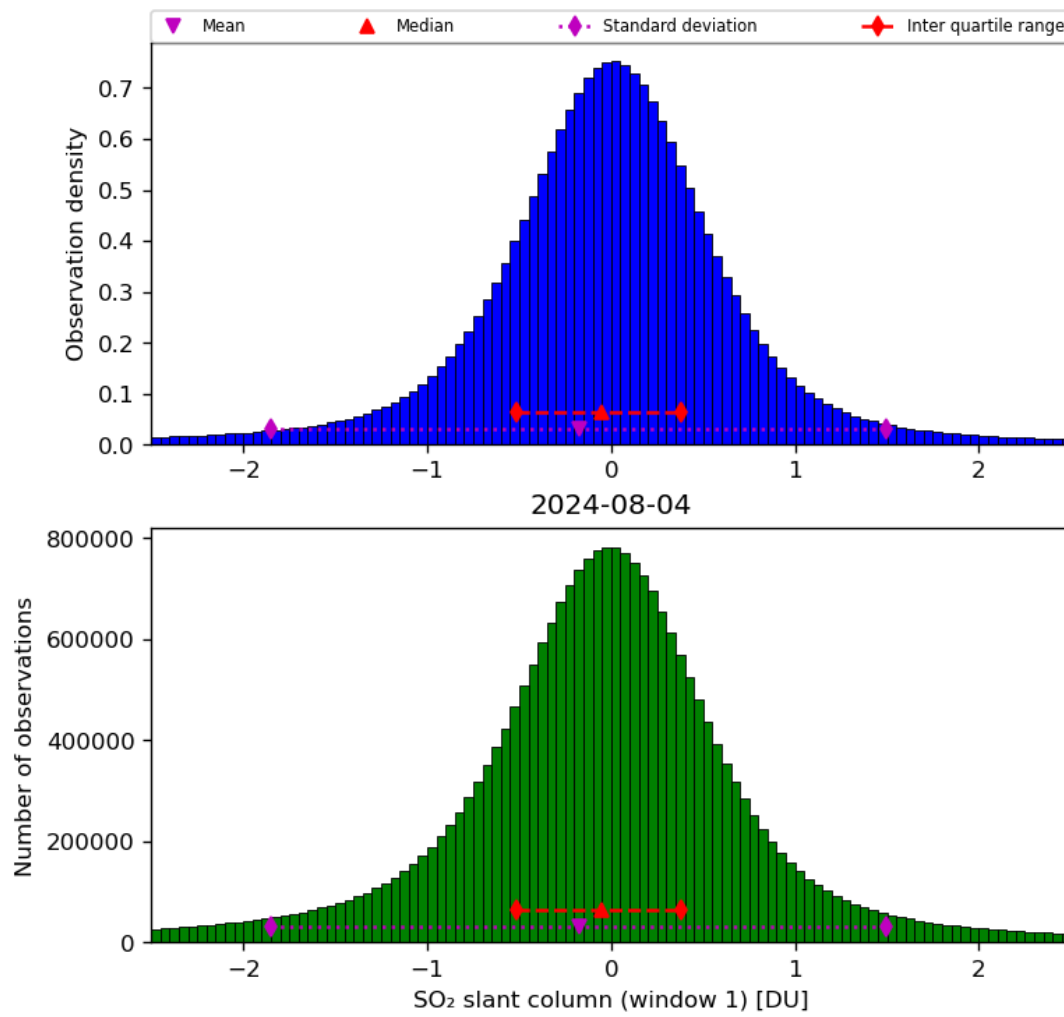
Figure 56: Histogram of “SO 2 slant column (window 1)” for 2024-08-03 to 2024-08-05
