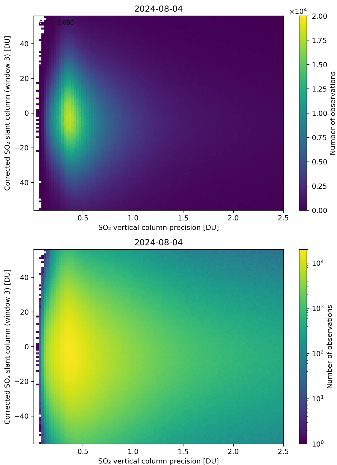
Figure 288: Scatter density plot of “SO 2 vertical column precision” against “Corrected SO 2 slant column (window 3)” for 2024-08-03 to 2024-08-05.
