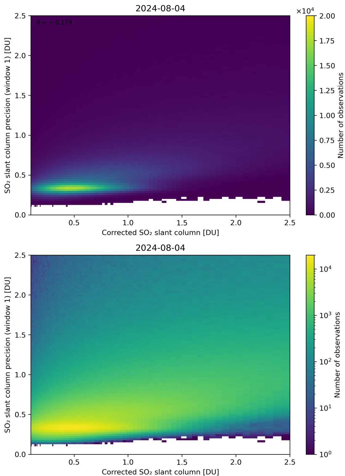
Figure 188: Scatter density plot of “Corrected SO 2 slant column” against “SO 2 slant column precision (window 1)” for 2024-08-03 to 2024-08-05.
