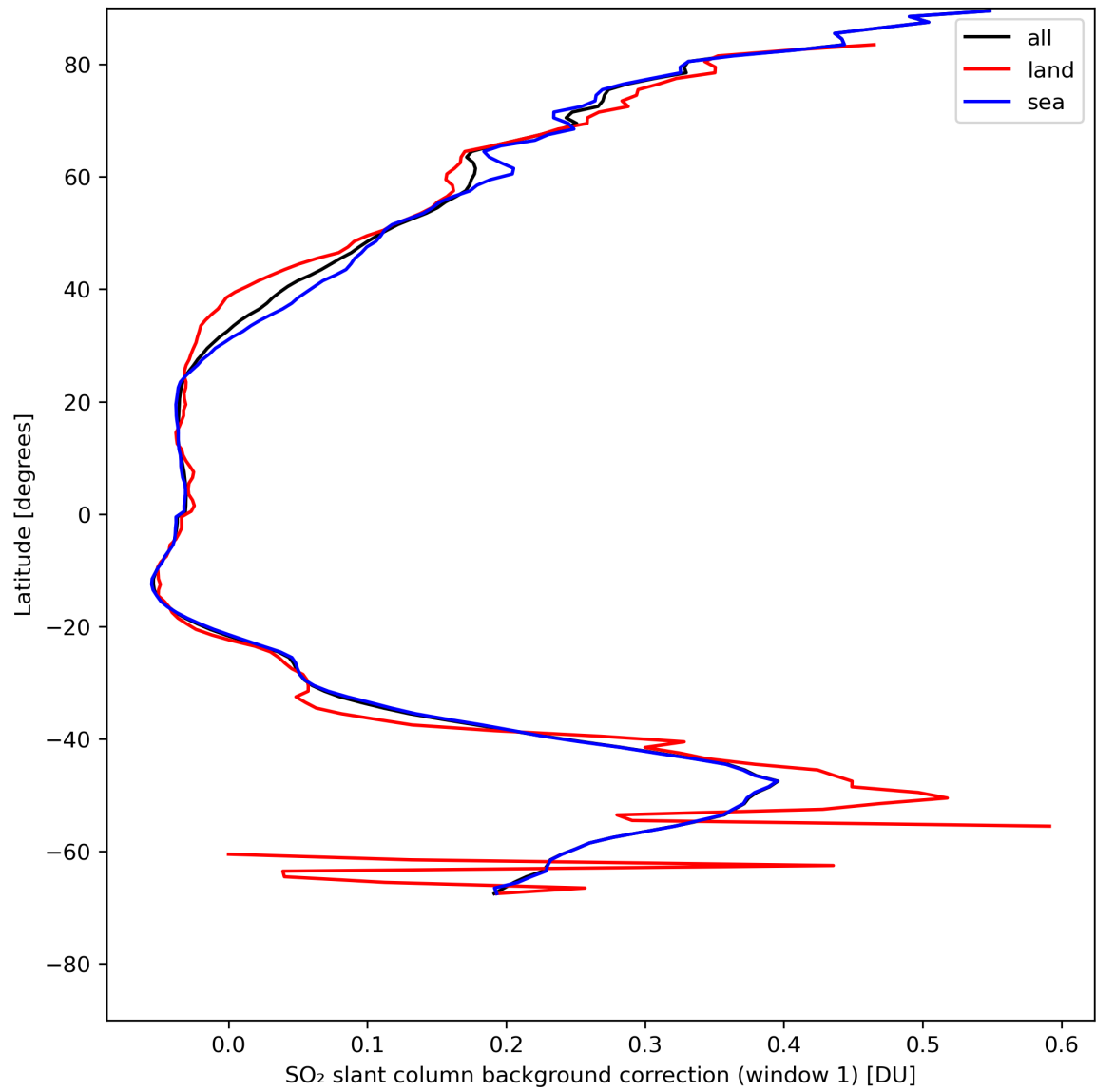
Figure 36: Zonal average of “SO 2 slant column background correction (window 1)” for 2024-08-03 to 2024-08-05.
