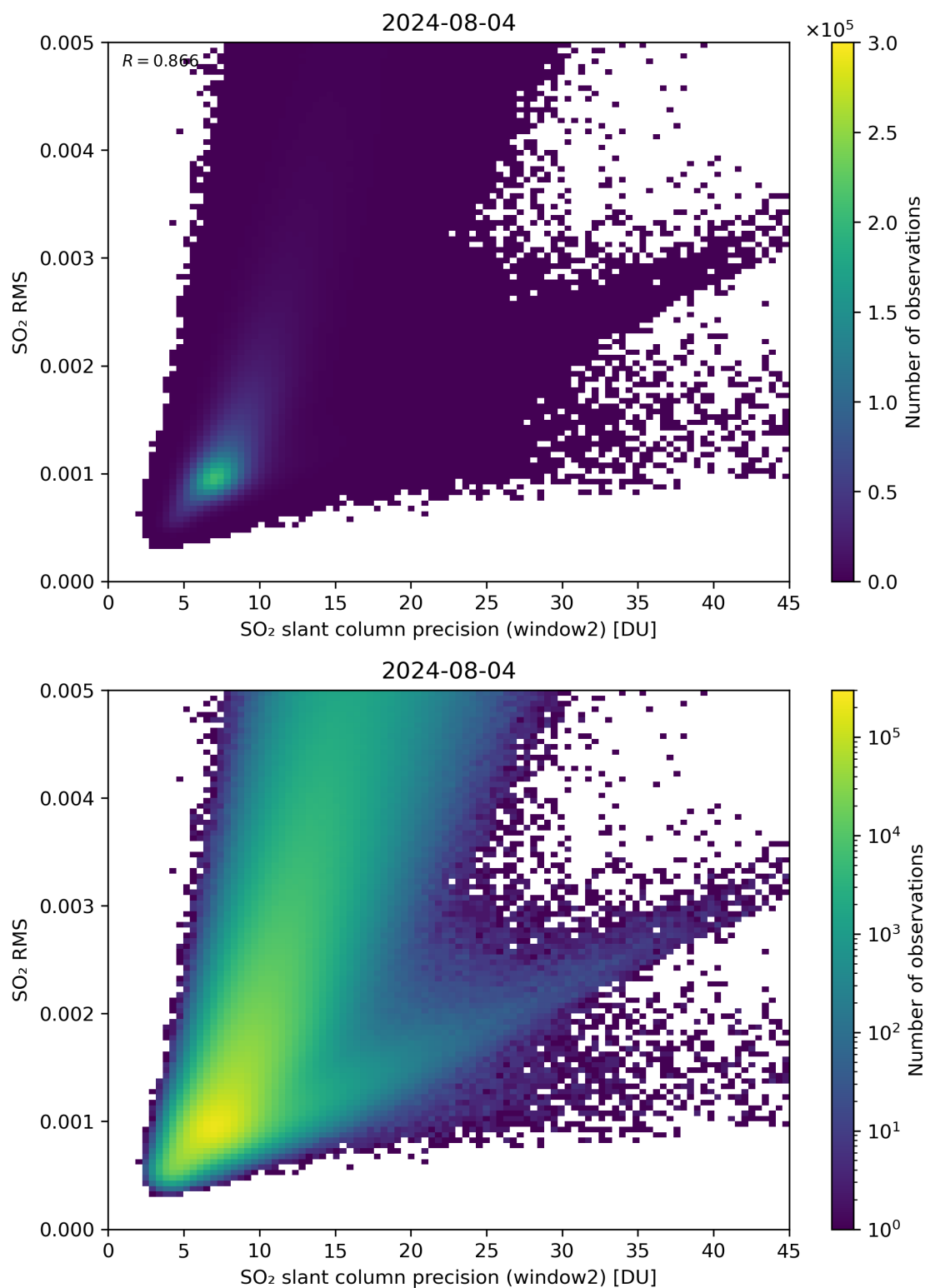
Figure 245: Scatter density plot of “SO 2 slant column precision (window2)” against “SO 2 RMS” for 2024-08-03 to 2024-08-05.
