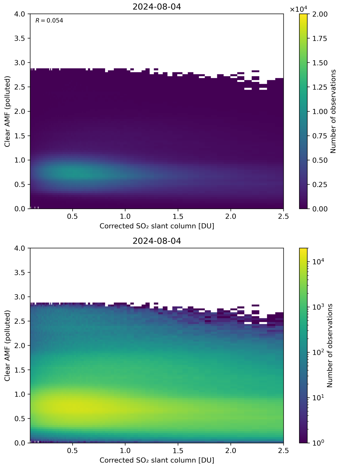
Figure 184: Scatter density plot of “Corrected SO 2 slant column” against “Clear AMF (polluted)” for 2024-08-03 to 2024-08-05.
