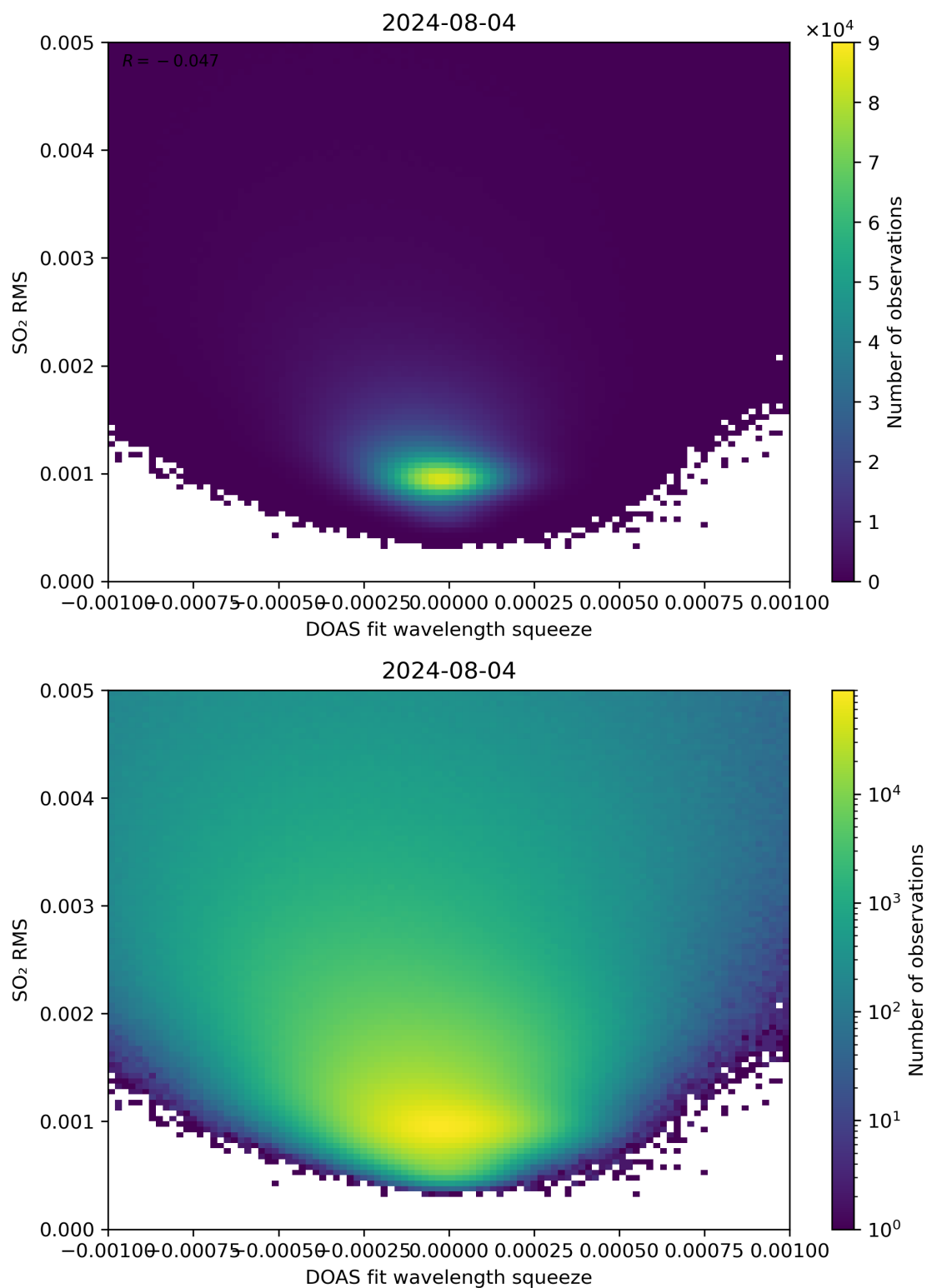
Figure 132: Scatter density plot of “DOAS fit wavelength squeeze” against “SO 2 RMS” for 2024-08-03 to 2024-08-05.
