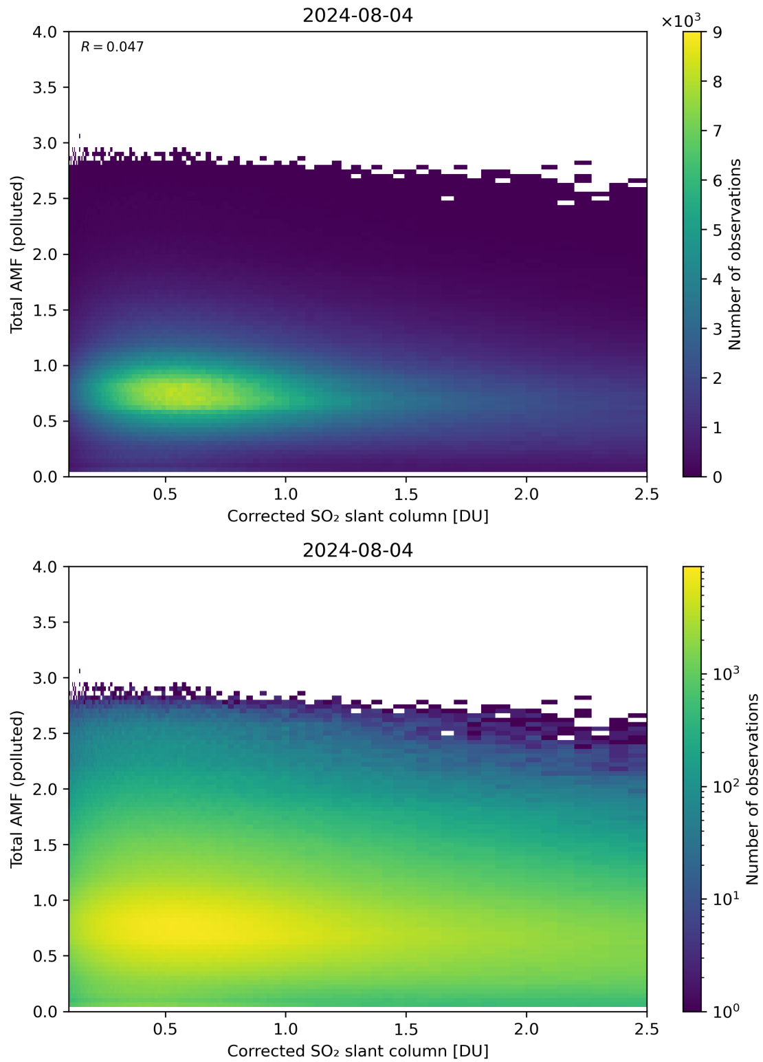
Figure 192: Scatter density plot of “Corrected SO 2 slant column” against “Total AMF (polluted)” for 2024-08-03 to 2024-08-05.
