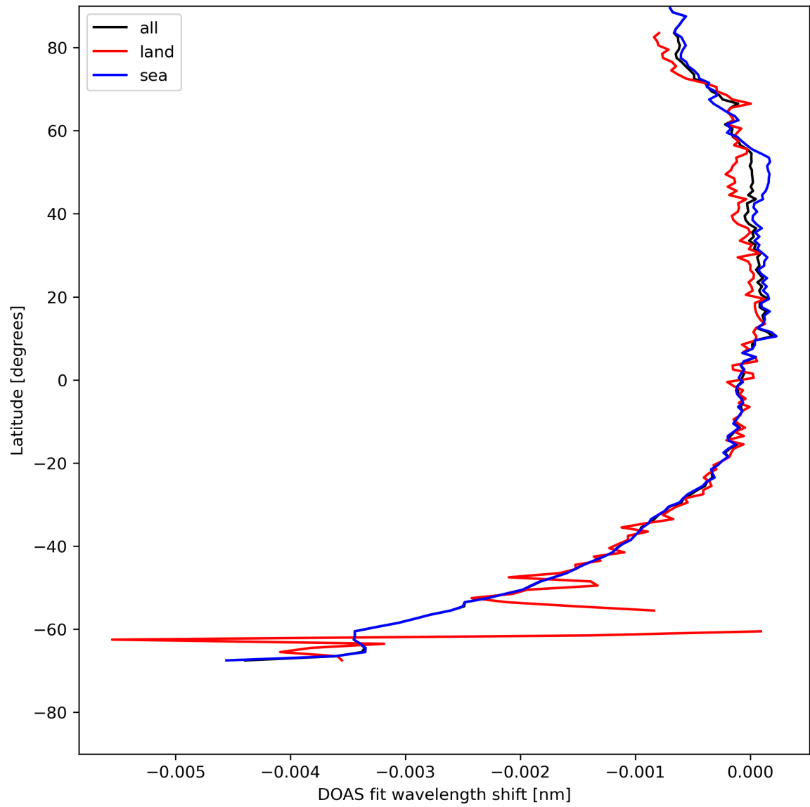
Figure 45: Zonal average of “DOAS fit wavelength shift” for 2024-08-03 to 2024-08-05.
