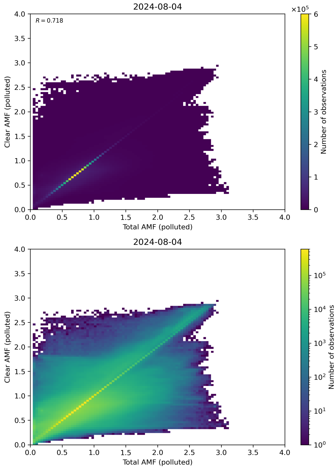
Figure 271: Scatter density plot of “Total AMF (polluted)” against “Clear AMF (polluted)” for 2024-08-03 to 2024-08-05.
