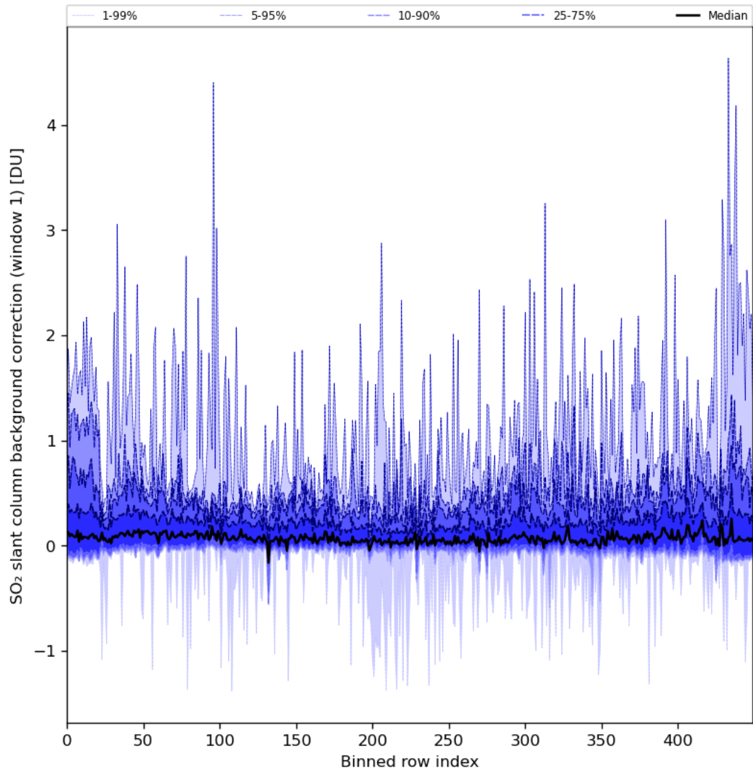
Figure 82: Along track statistics of “SO 2 slant column background correction (window 1)” for 2024-08-03 to 2024-08-05
