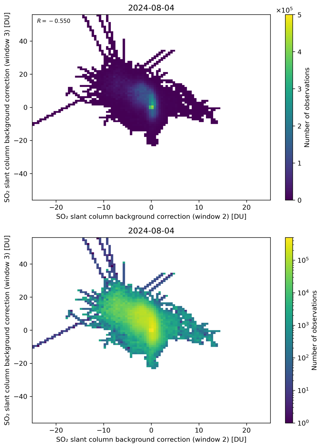
Figure 111: Scatter density plot of “SO 2 slant column background correction (window 2)” against “SO 2 slant column background correction (window 3)” for 2024-08-03 to 2024-08-05.
