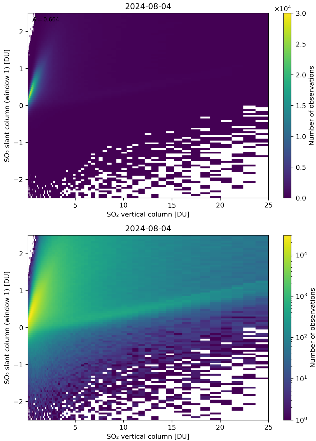
Figure 300: Scatter density plot of “SO 2 vertical column” against “SO 2 slant column (window 1)” for 2024-08-03 to 2024-08-05.
