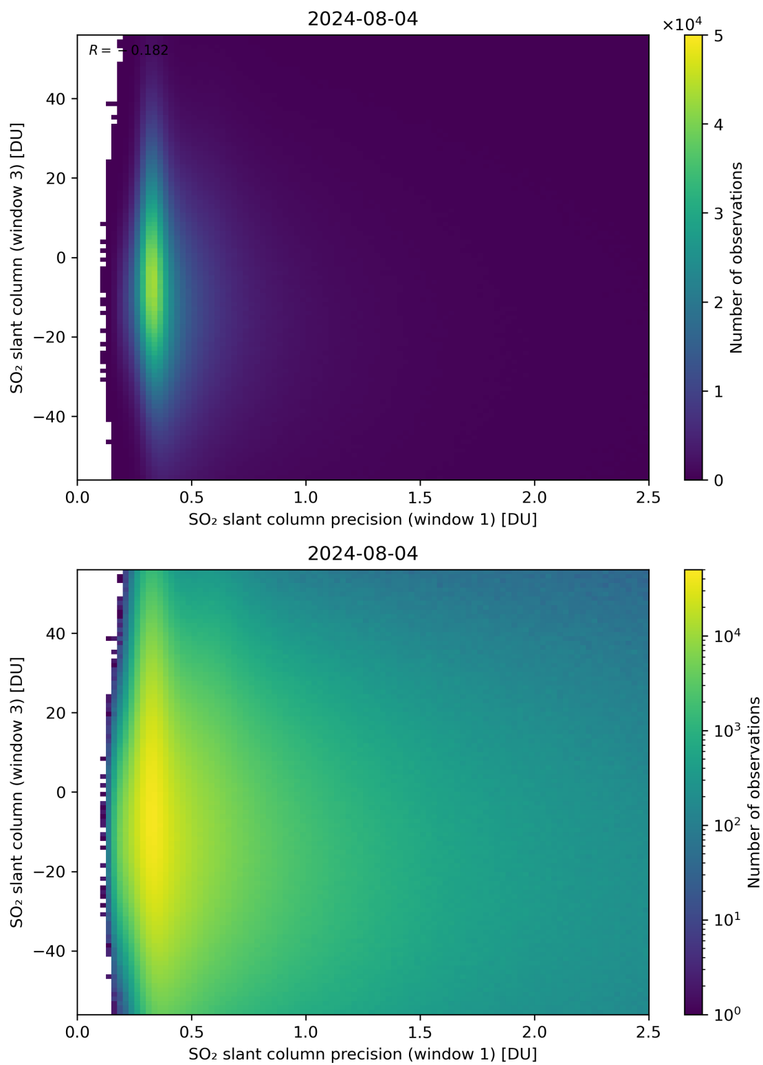
Figure 228: Scatter density plot of “SO 2 slant column precision (window 1)” against “SO 2 slant column (window 3)” for 2024-08-03 to 2024-08-05.
