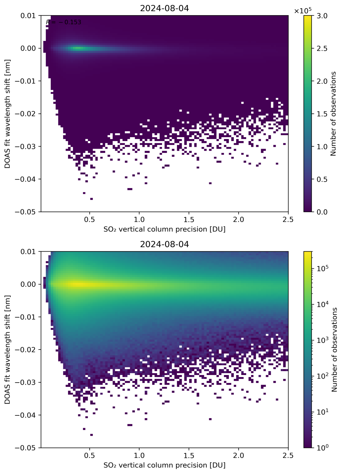
Figure 282: Scatter density plot of “SO 2 vertical column precision” against “DOAS fit wavelength shift” for 2024-08-03 to 2024-08-05.
