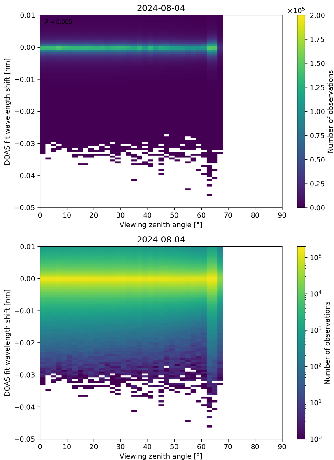
Figure 311: Scatter density plot of “Viewing zenith angle” against “DOAS fit wavelength shift” for 2024-08-03 to 2024-08-05.
