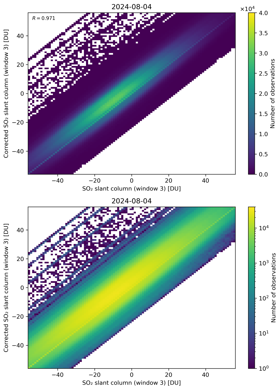
Figure 266: Scatter density plot of “SO 2 slant column (window 3)” against “Corrected SO 2 slant column (window 3)” for 2024-08-03 to 2024-08-05.
