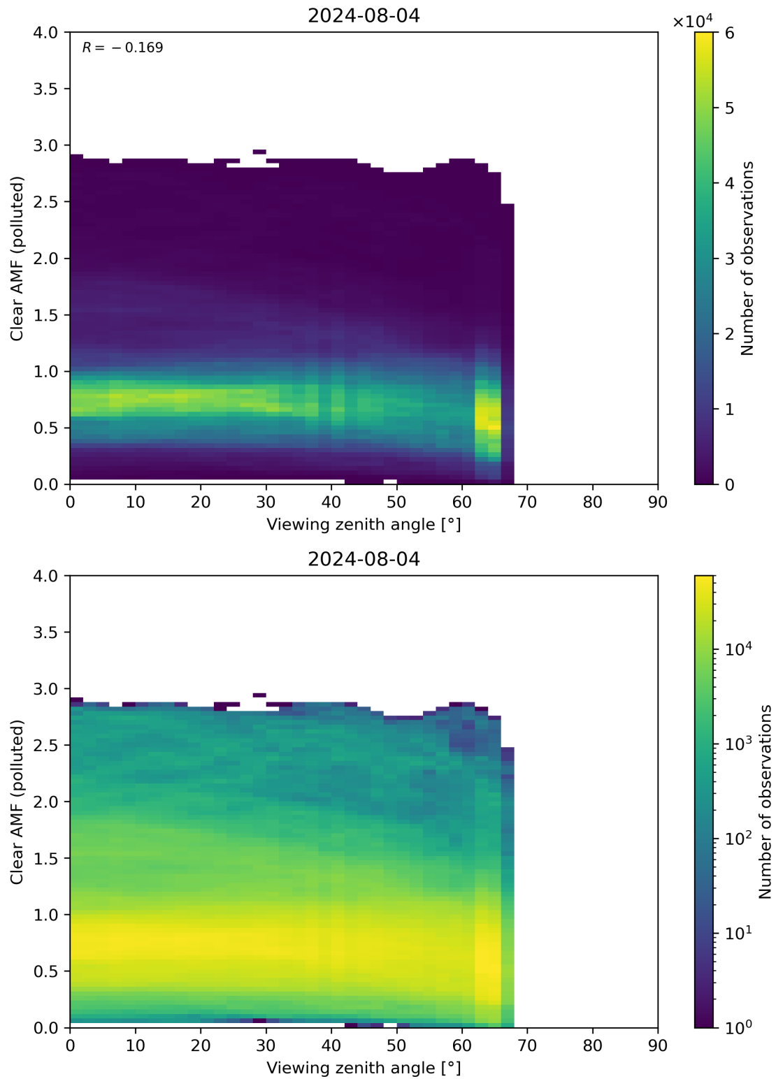
Figure 316: Scatter density plot of “Viewing zenith angle” against “Clear AMF (polluted)” for 2024-08-03 to 2024-08-05.
