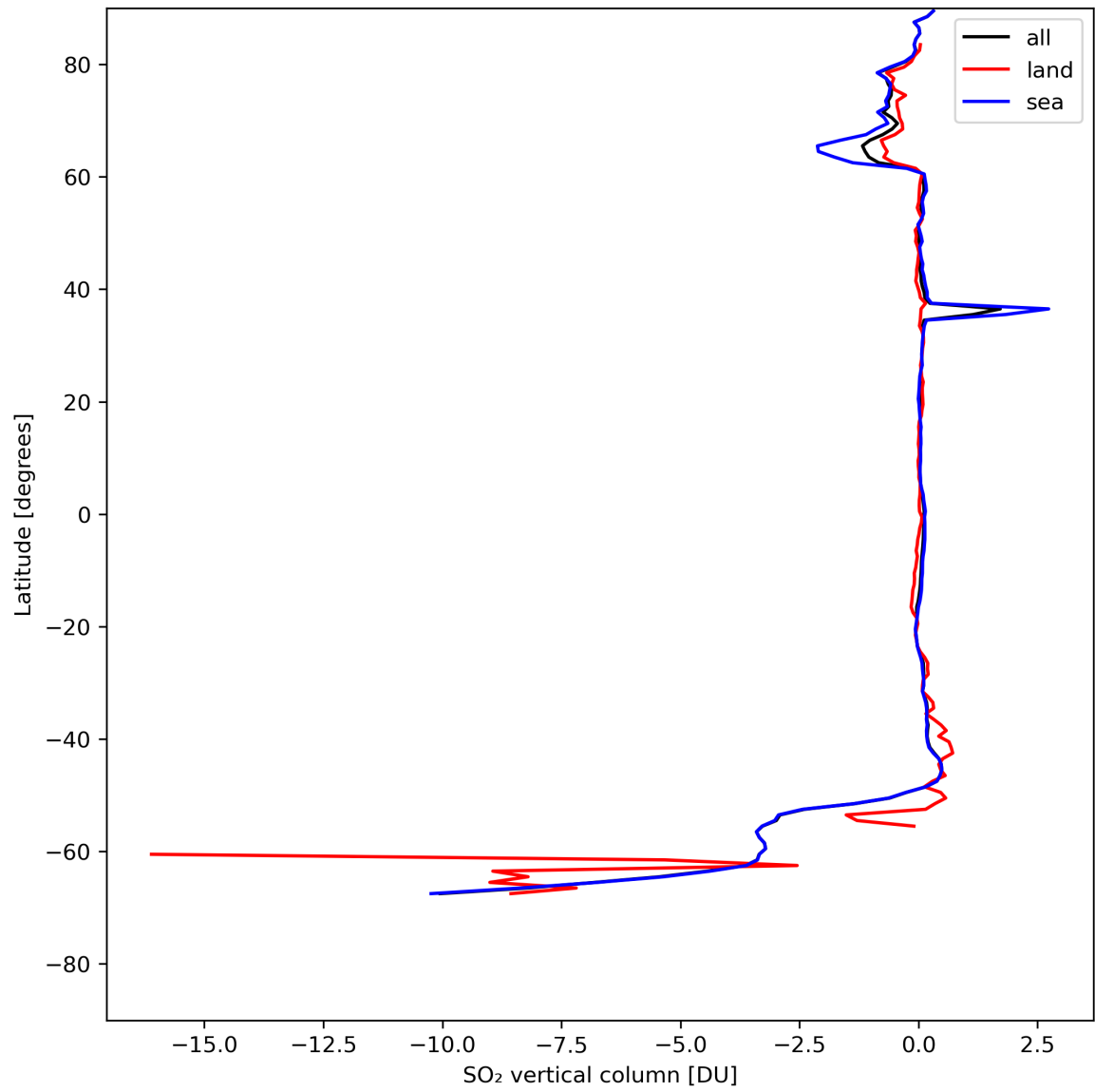
Figure 30: Zonal average of “SO 2 vertical column” for 2024-08-03 to 2024-08-05.
