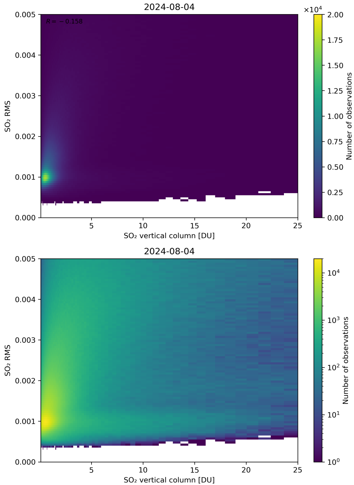
Figure 278: Scatter density plot of “SO 2 vertical column” against “SO 2 RMS” for 2024-08-03 to 2024-08-05.
