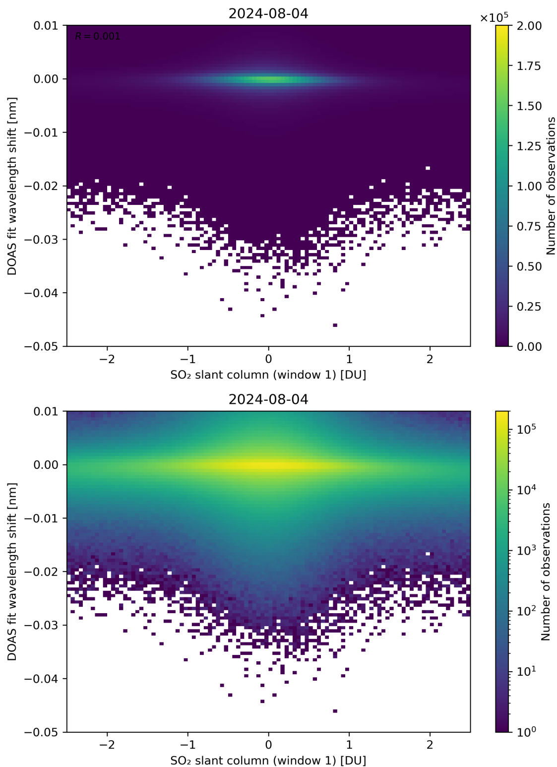
Figure 215: Scatter density plot of “SO 2 slant column (window 1)” against “DOAS fit wavelength shift” for 2024-08-03 to 2024-08-05.
