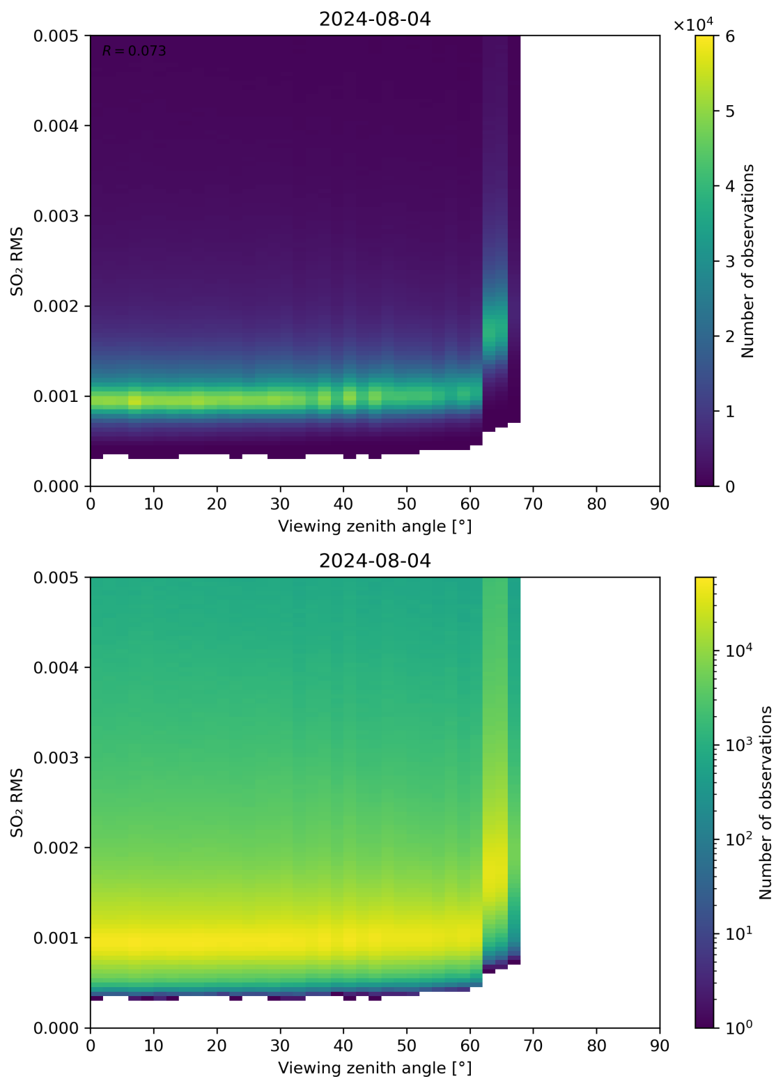
Figure 313: Scatter density plot of “Viewing zenith angle” against “SO 2 RMS” for 2024-08-03 to 2024-08-05.
