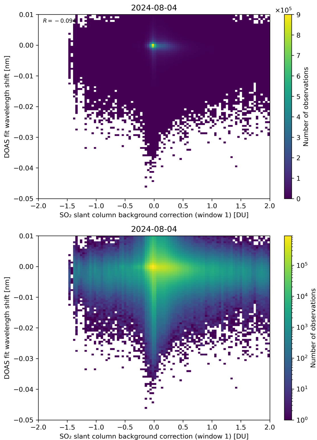
Figure 100: Scatter density plot of “SO 2 slant column background correction (window 1)” against “DOAS fit wavelength shift” for 2024-08-03 to 2024-08-05.
