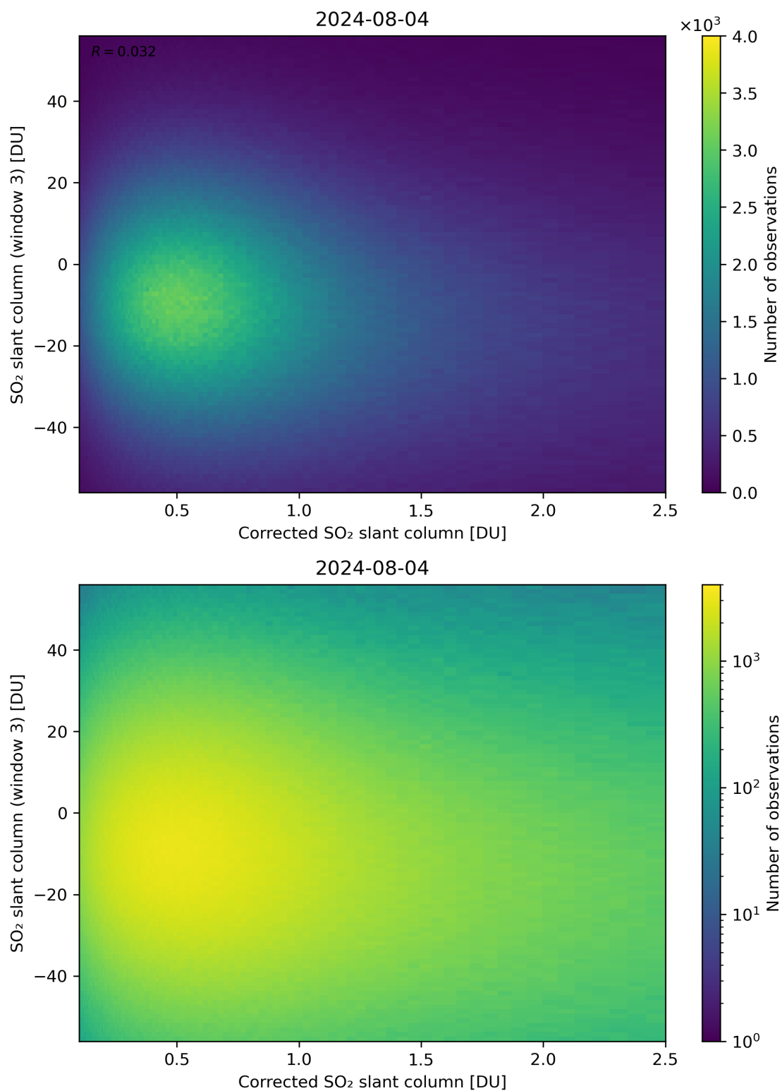
Figure 190: Scatter density plot of “Corrected SO 2 slant column” against “SO 2 slant column (window 3)” for 2024-08-03 to 2024-08-05.
