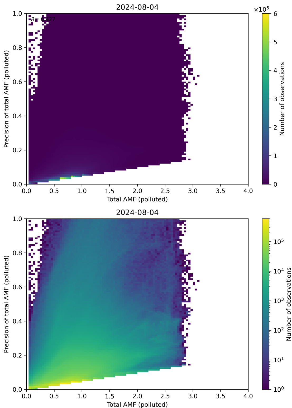
Figure 272: Scatter density plot of “Total AMF (polluted)” against “Precision of total AMF (polluted)” for 2024-08-03 to 2024-08-05.
