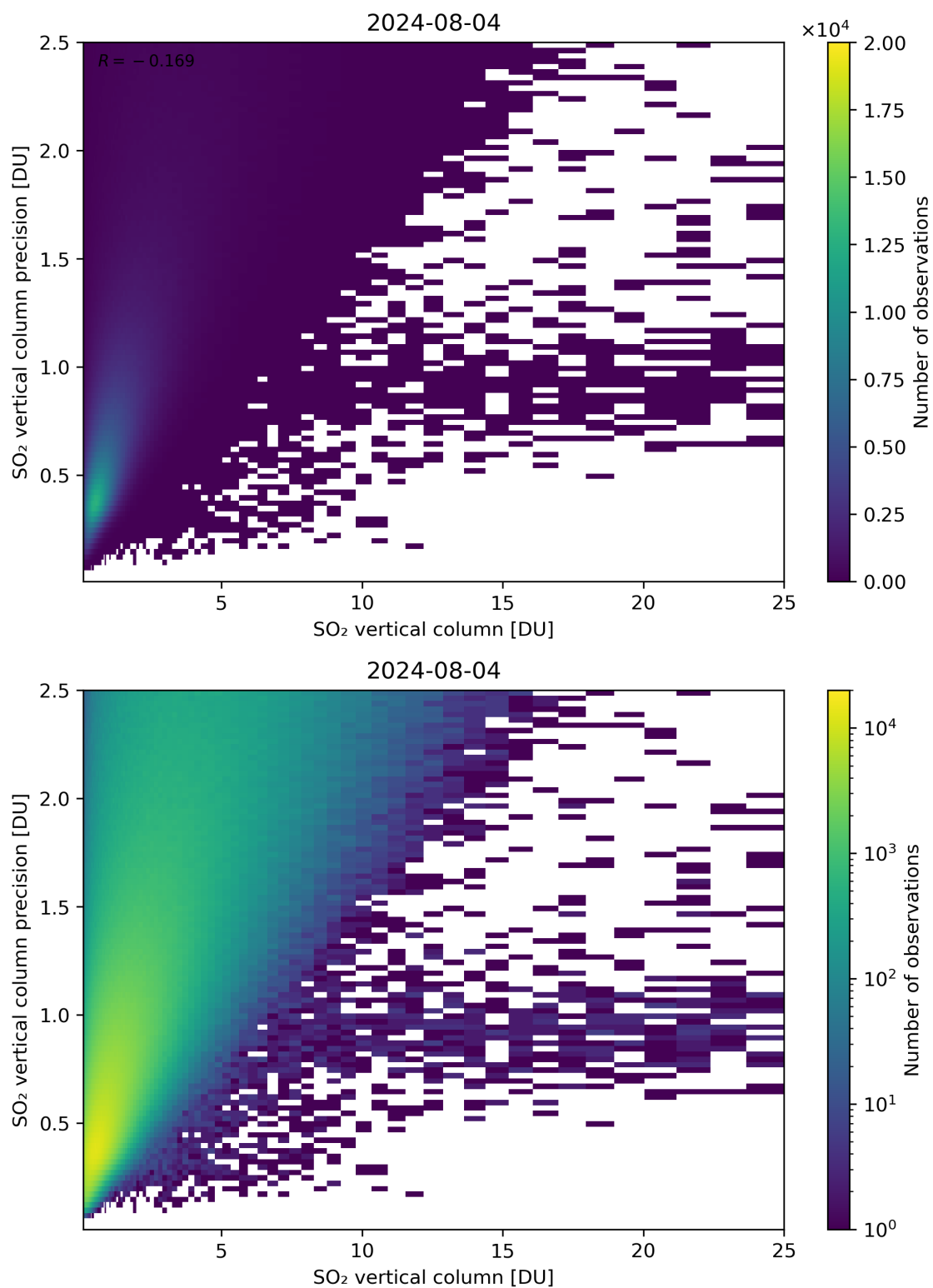
Figure 307: Scatter density plot of “SO 2 vertical column” against “SO 2 vertical column precision” for 2024-08-03 to 2024-08-05.
