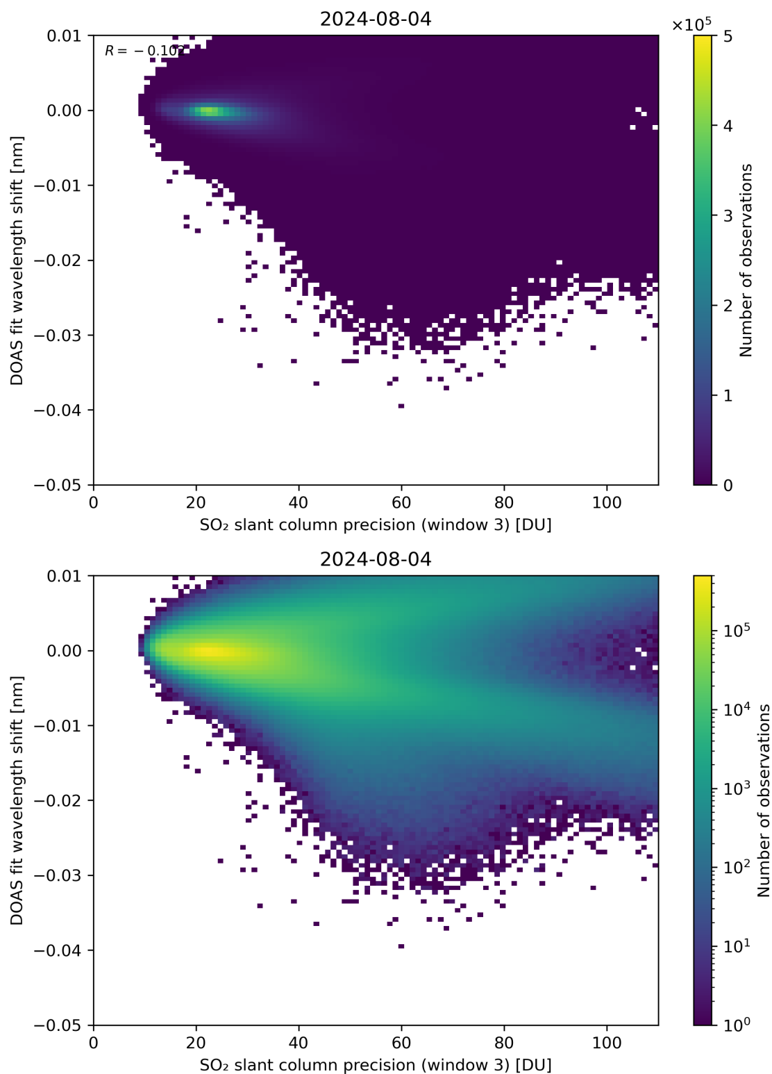
Figure 258: Scatter density plot of “SO 2 slant column precision (window 3)” against “DOAS fit wavelength shift” for 2024-08-03 to 2024-08-05.
