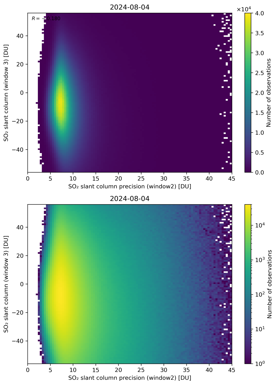
Figure 249: Scatter density plot of “SO 2 slant column precision (window2)” against “SO 2 slant column (window 3)” for 2024-08-03 to 2024-08-05.
