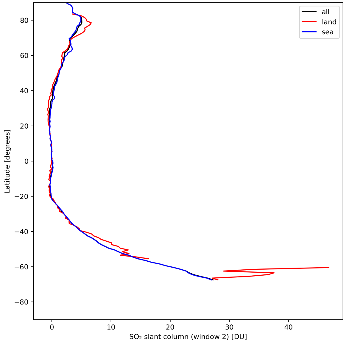
Figure 37: Zonal average of “SO 2 slant column (window 2)” for 2024-08-03 to 2024-08-05.
