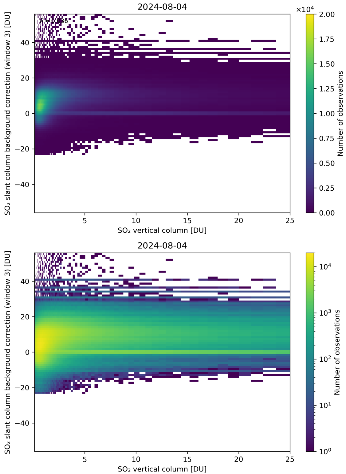
Figure 275: Scatter density plot of “SO 2 vertical column” against “SO 2 slant column background correction (window 3)” for 2024-08-03 to 2024-08-05.
