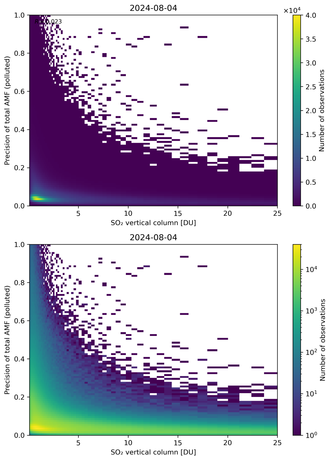
Figure 306: Scatter density plot of “SO 2 vertical column” against “Precision of total AMF (polluted)” for 2024-08-03 to 2024-08-05.
