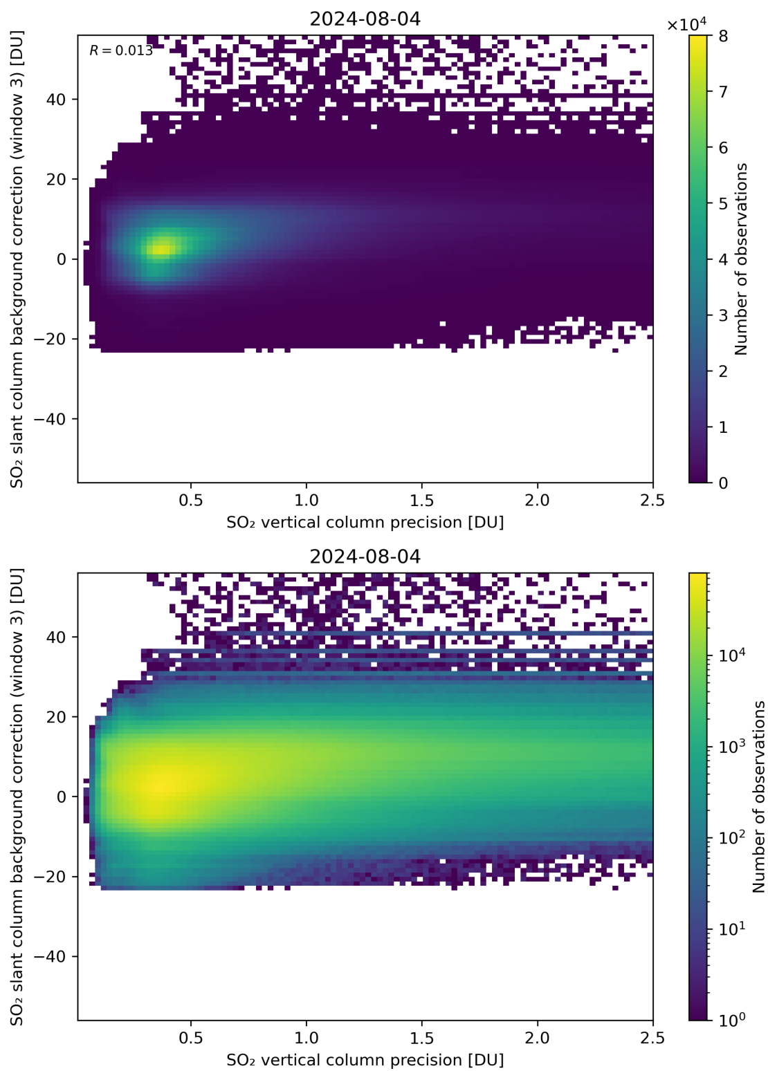
Figure 281: Scatter density plot of “SO 2 vertical column precision” against “SO 2 slant column background correction (window 3)” for 2024-08-03 to 2024-08-05.
