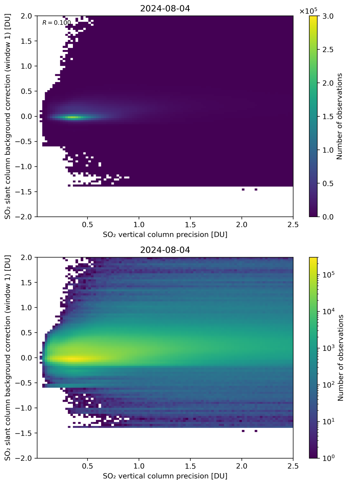
Figure 279: Scatter density plot of “SO 2 vertical column precision” against “SO 2 slant column background correction (window 1)” for 2024-08-03 to 2024-08-05.
