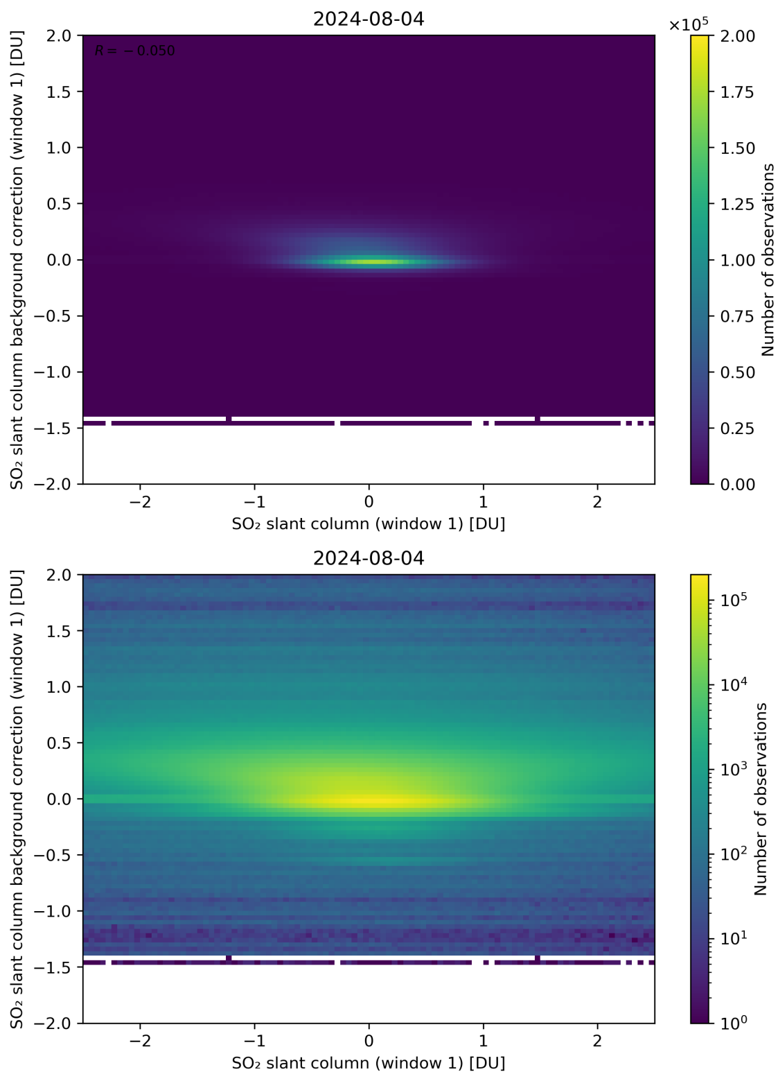
Figure 212: Scatter density plot of “SO 2 slant column (window 1)” against “SO 2 slant column background correction (window 1)” for 2024-08-03 to 2024-08-05.
