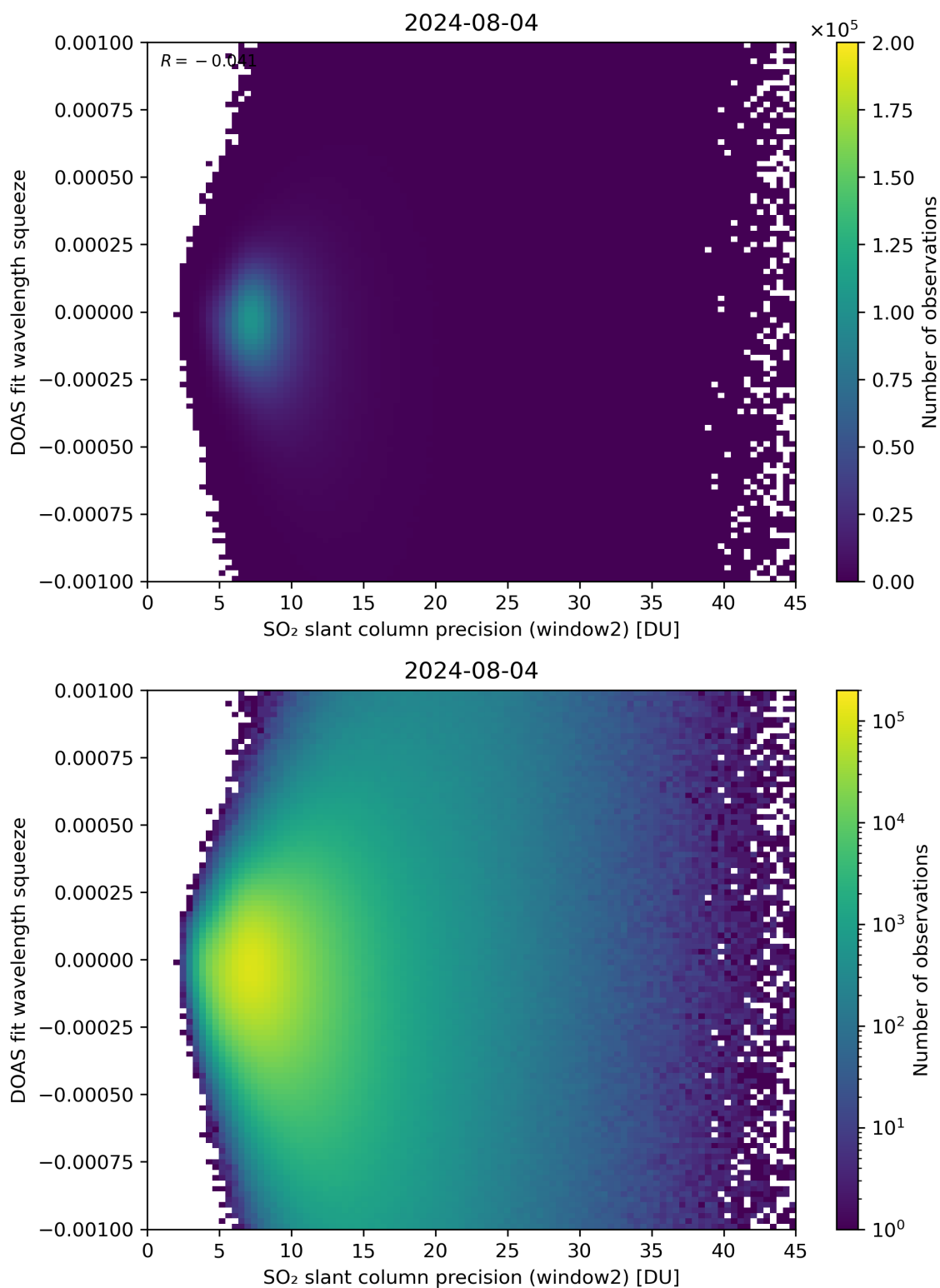
Figure 244: Scatter density plot of “SO 2 slant column precision (window2)” against “DOAS fit wavelength squeeze” for 2024-08-03 to 2024-08-05.
