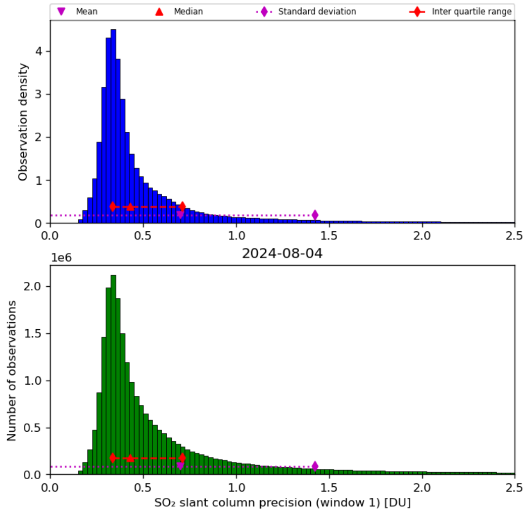
Figure 57: Histogram of “SO 2 slant column precision (window 1)” for 2024-08-03 to 2024-08-05
