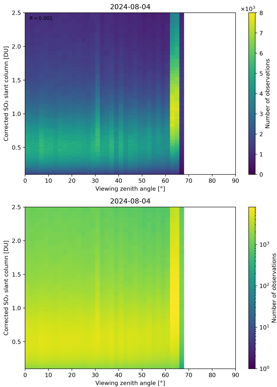
Figure 317: Scatter density plot of “Viewing zenith angle” against “Corrected SO 2 slant column” for 2024-08-03 to 2024-08-05.
