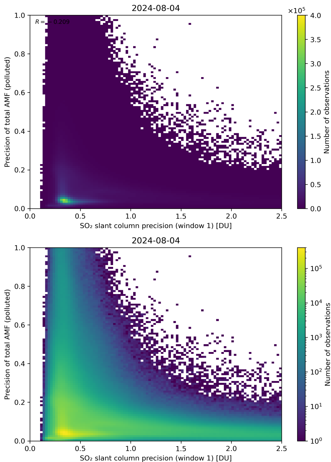
Figure 231: Scatter density plot of “SO 2 slant column precision (window 1)” against “Precision of total AMF (polluted)” for 2024-08-03 to 2024-08-05.
