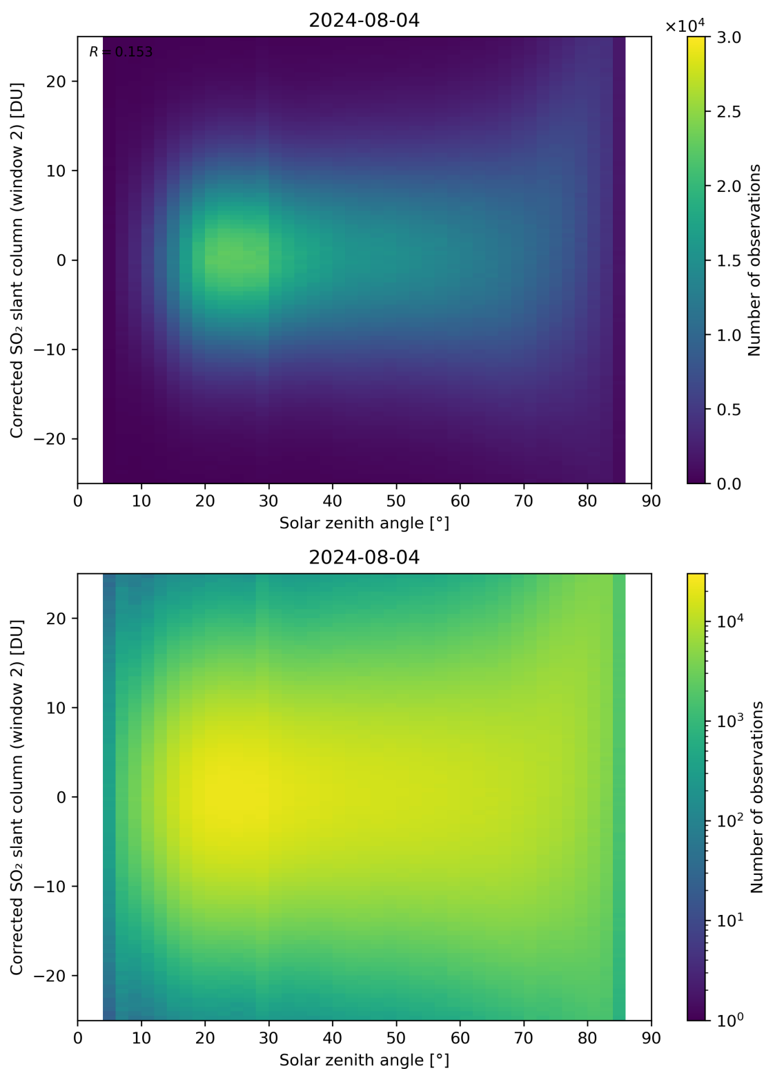
Figure 167: Scatter density plot of “Solar zenith angle” against “Corrected SO 2 slant column (window 2)” for 2024-08-03 to 2024-08-05.
