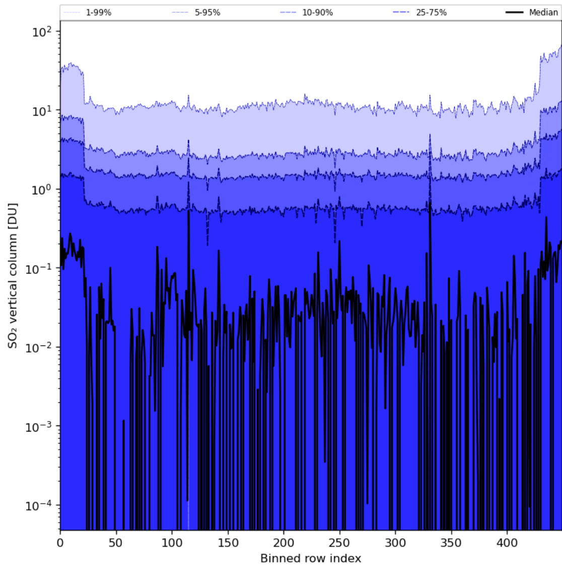
Figure 76: Along track statistics of “SO 2 vertical column” for 2024-08-03 to 2024-08-05
