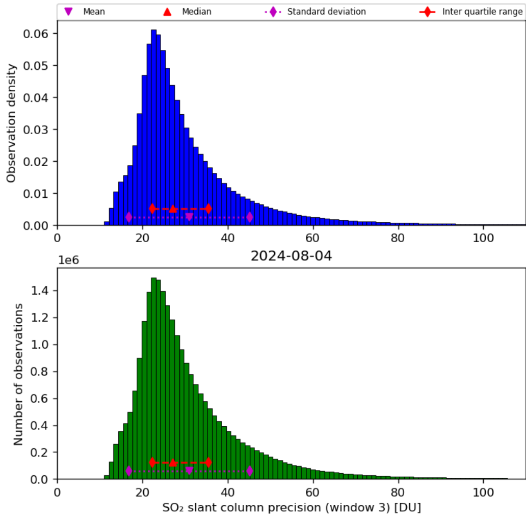
Figure 65: Histogram of “SO 2 slant column precision (window 3)” for 2024-08-03 to 2024-08-05
