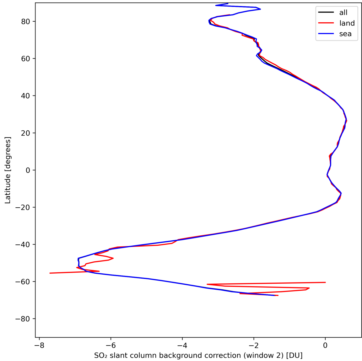
Figure 40: Zonal average of “SO 2 slant column background correction (window 2)” for 2024-08-03 to 2024-08-05.
