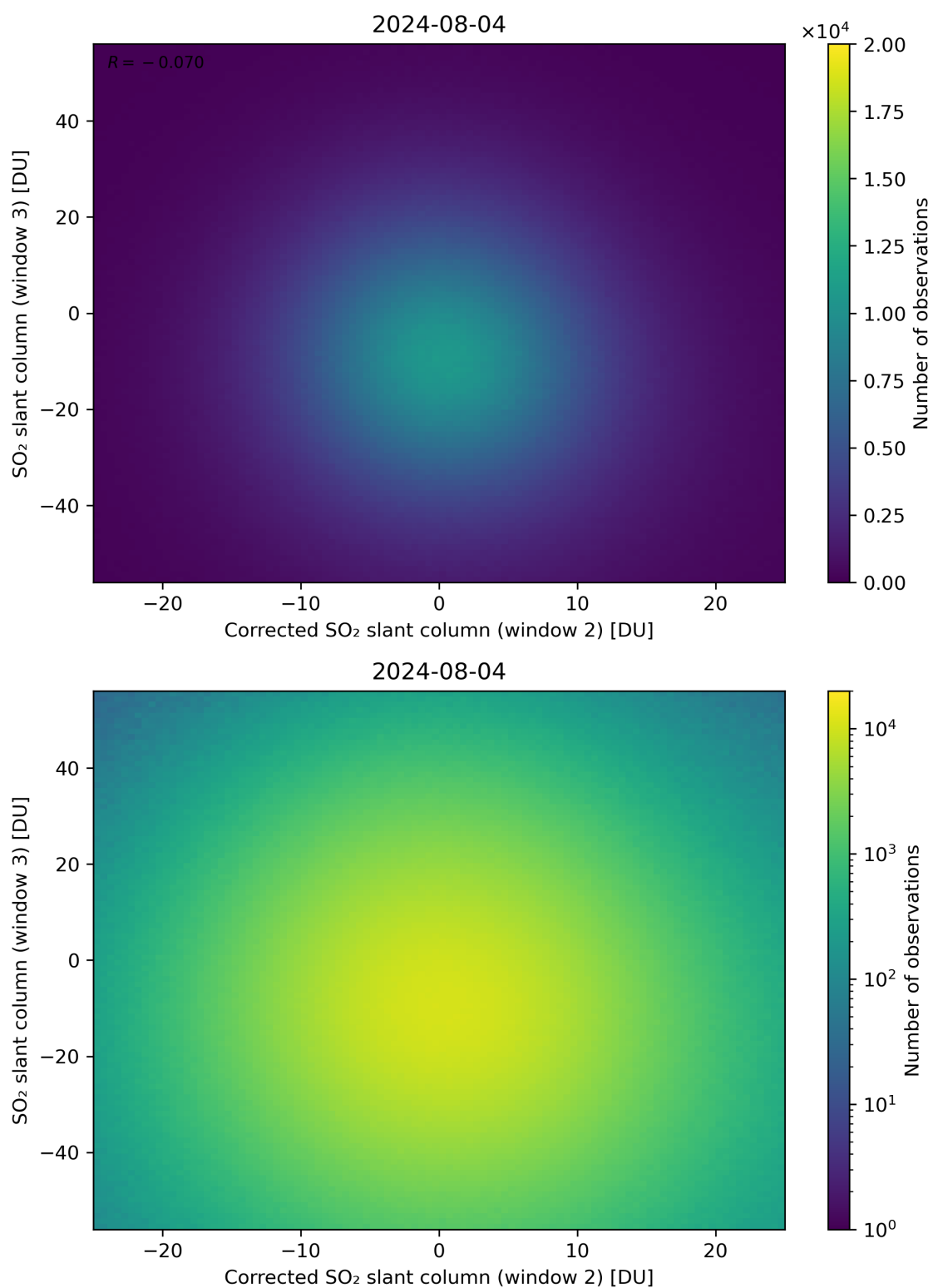
Figure 201: Scatter density plot of “Corrected SO 2 slant column (window 2)” against “SO 2 slant column (window 3)” for 2024-08-03 to 2024-08-05.
