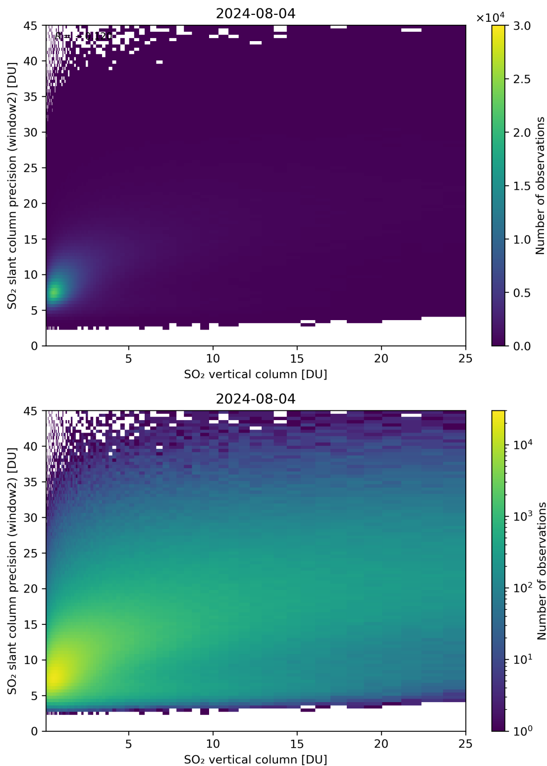
Figure 302: Scatter density plot of “SO 2 vertical column” against “SO 2 slant column precision (window2)” for 2024-08-03 to 2024-08-05.
