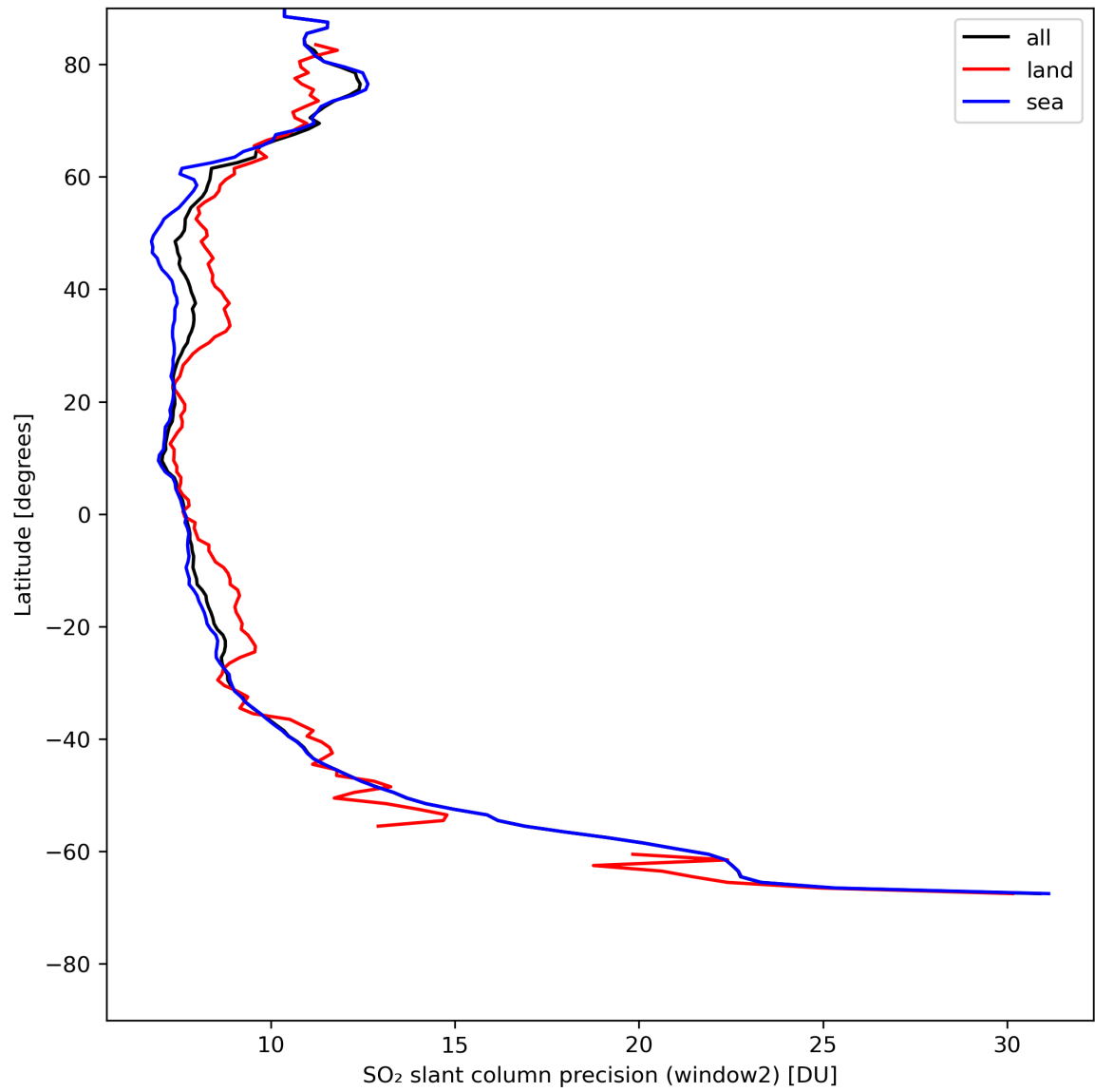
Figure 38: Zonal average of “SO 2 slant column precision (window2)” for 2024-08-03 to 2024-08-05.
