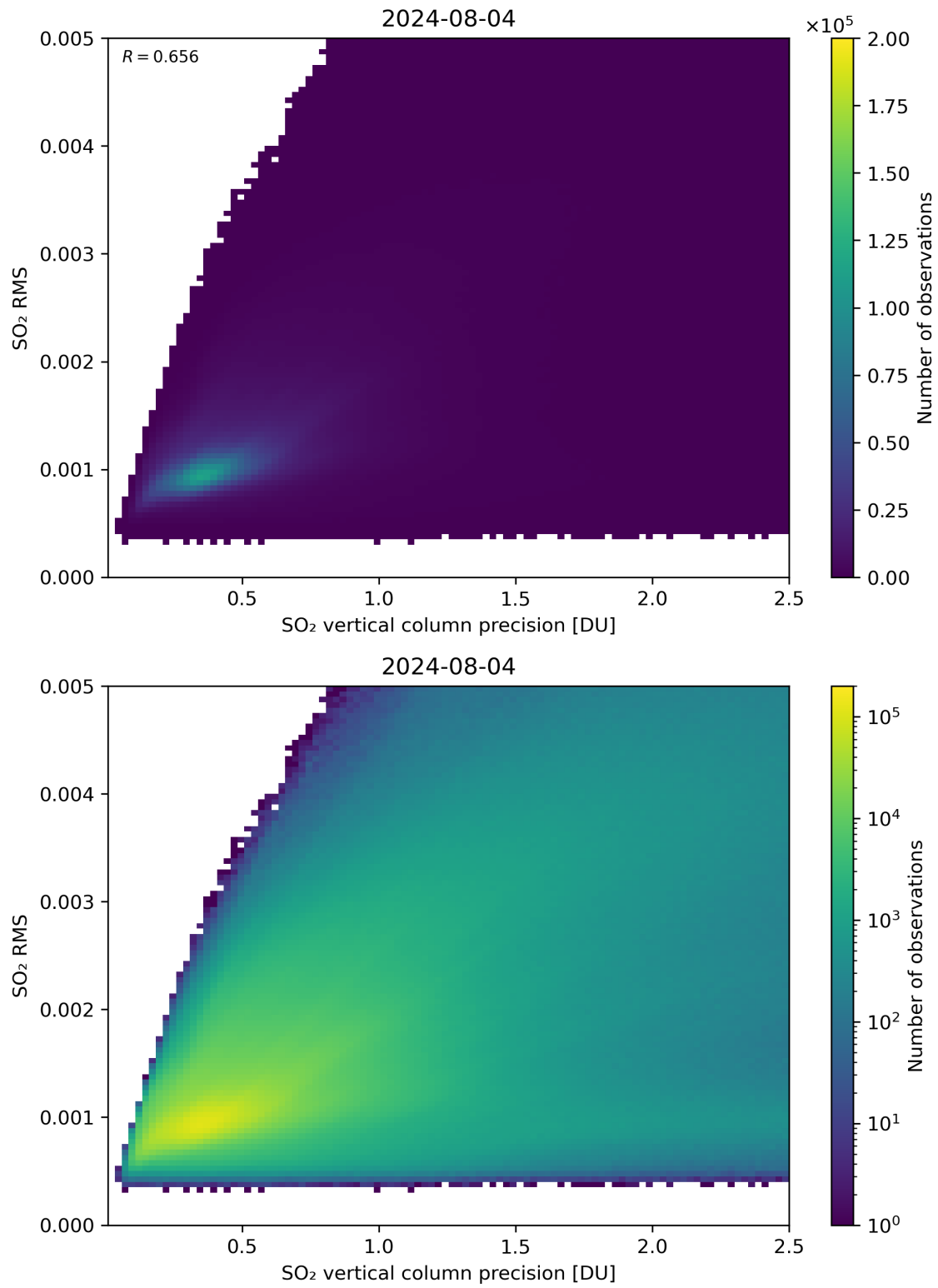
Figure 284: Scatter density plot of “SO 2 vertical column precision” against “SO 2 RMS” for 2024-08-03 to 2024-08-05.
