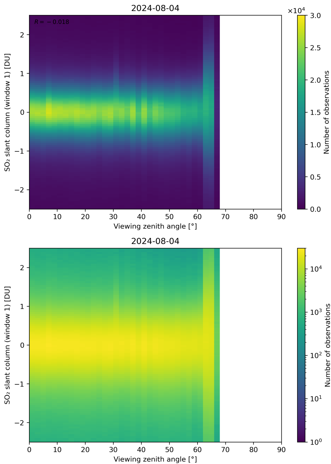
Figure 320: Scatter density plot of “Viewing zenith angle” against “SO 2 slant column (window 1)” for 2024-08-03 to 2024-08-05.
