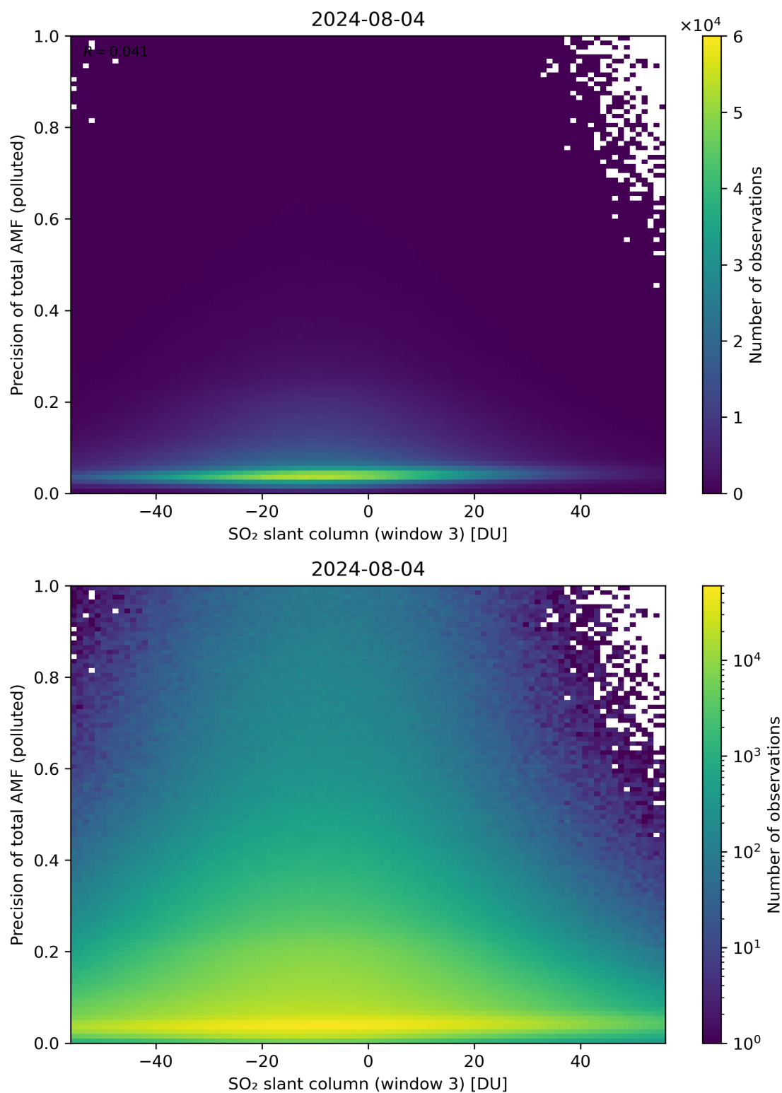
Figure 269: Scatter density plot of “SO 2 slant column (window 3)” against “Precision of total AMF (polluted)” for 2024-08-03 to 2024-08-05.
