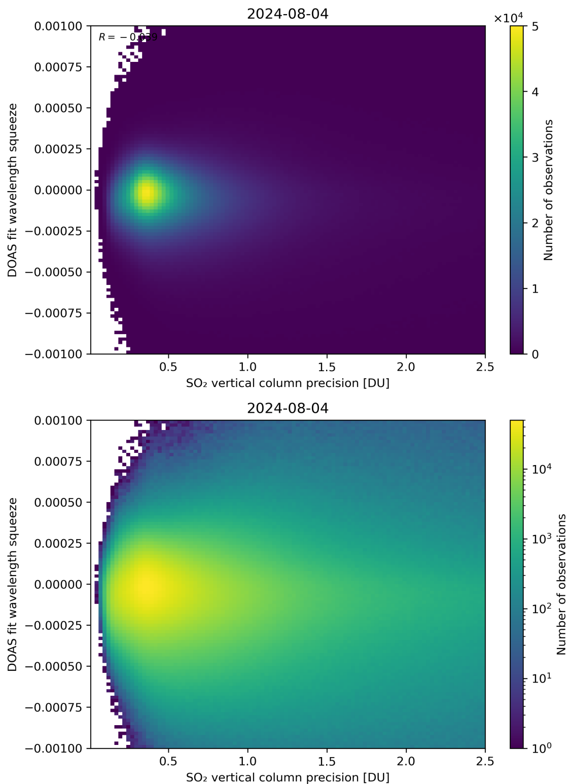
Figure 283: Scatter density plot of “SO 2 vertical column precision” against “DOAS fit wavelength squeeze” for 2024-08-03 to 2024-08-05.
