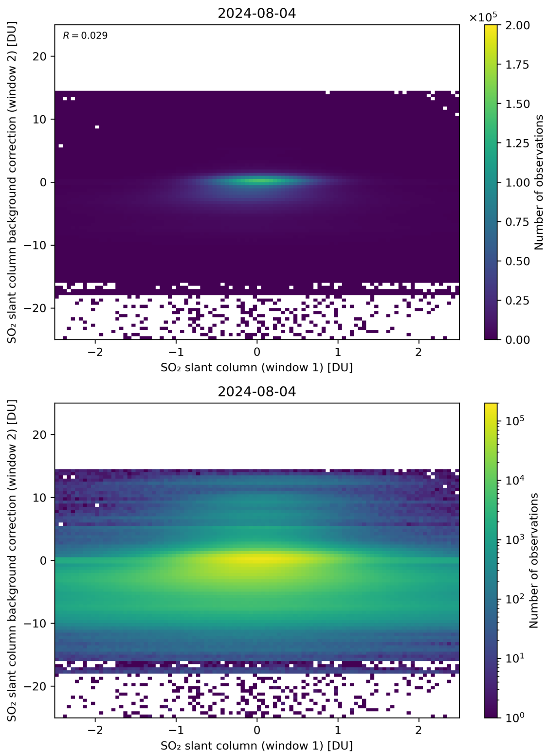
Figure 213: Scatter density plot of “SO 2 slant column (window 1)” against “SO 2 slant column background correction (window 2)” for 2024-08-03 to 2024-08-05.
