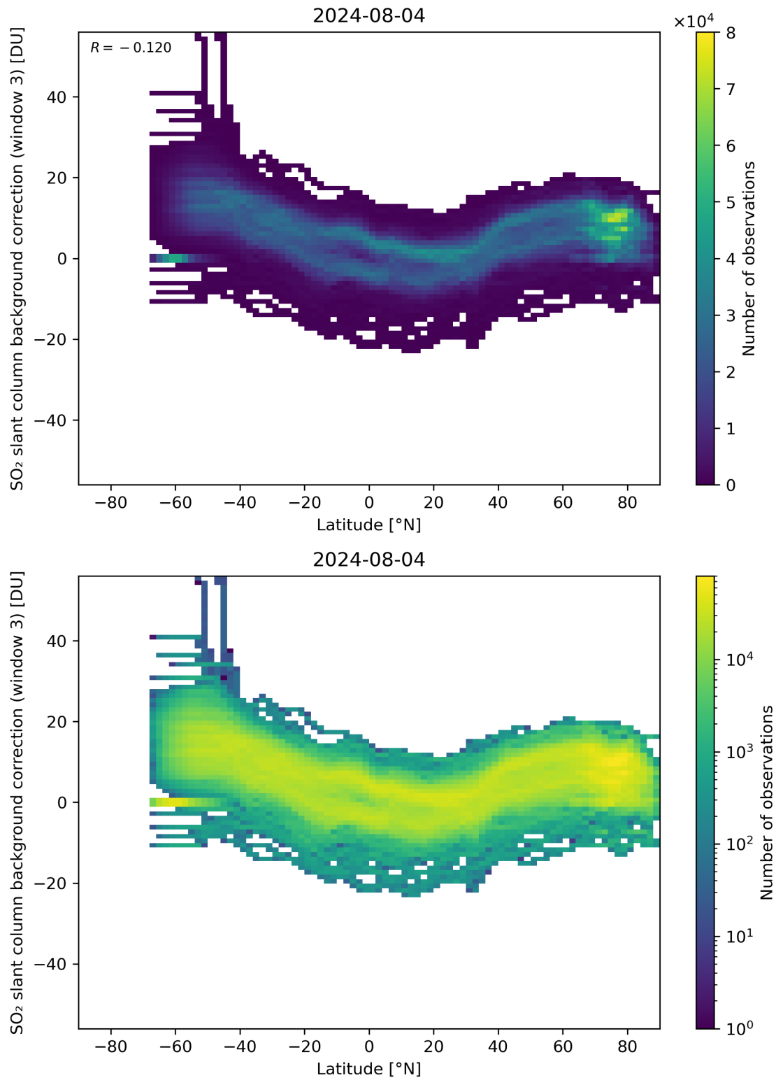
Figure 141: Scatter density plot of “Latitude” against “SO 2 slant column background correction (window 3)” for 2024-08-03 to 2024-08-05.
