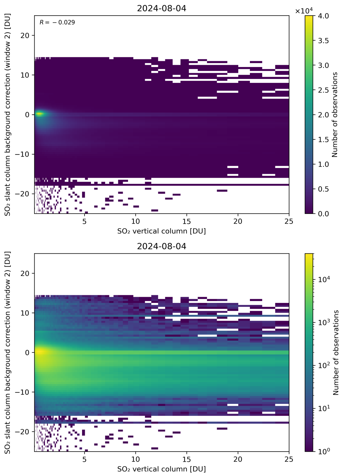
Figure 274: Scatter density plot of “SO 2 vertical column” against “SO 2 slant column background correction (window 2)” for 2024-08-03 to 2024-08-05.
