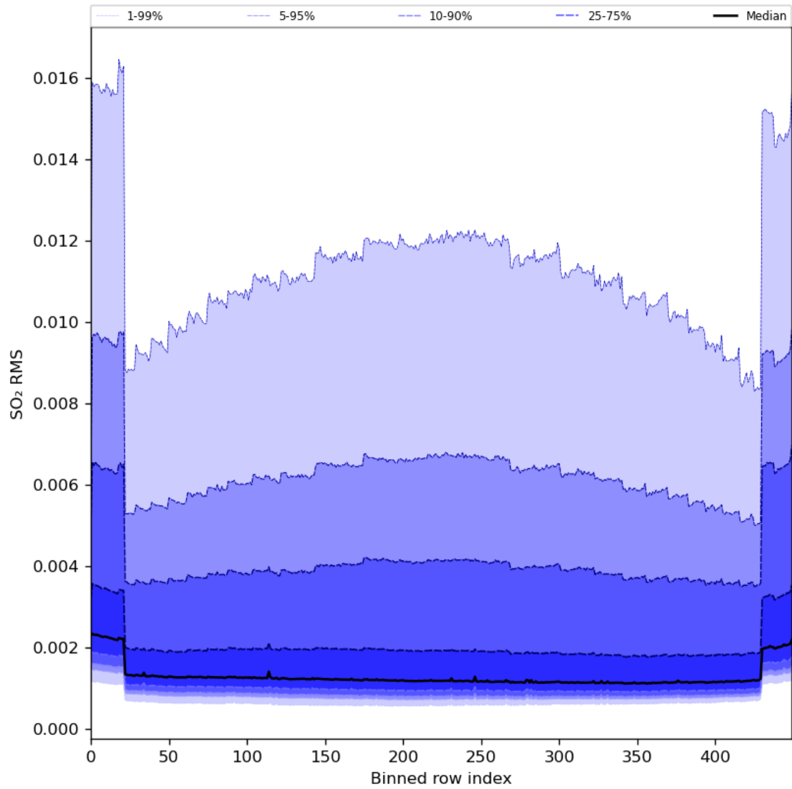
Figure 93: Along track statistics of “SO 2 RMS” for 2024-08-03 to 2024-08-05
