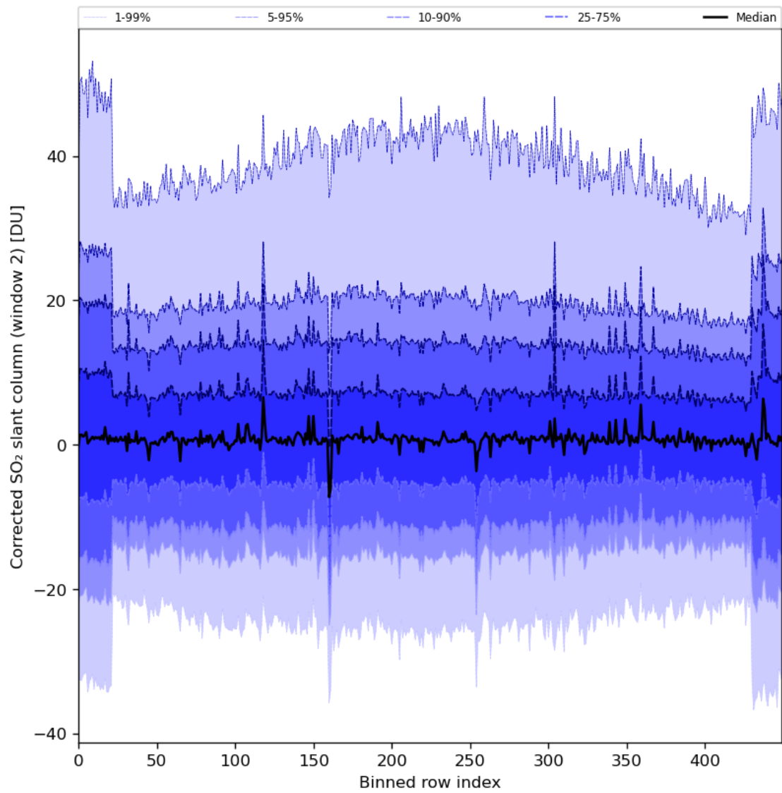
Figure 85: Along track statistics of “Corrected SO 2 slant column (window 2)” for 2024-08-03 to 2024-08-05
