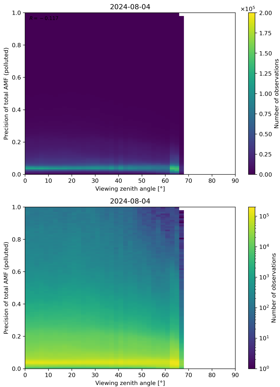
Figure 326: Scatter density plot of “Viewing zenith angle” against “Precision of total AMF (polluted)” for 2024-08-03 to 2024-08-05.
