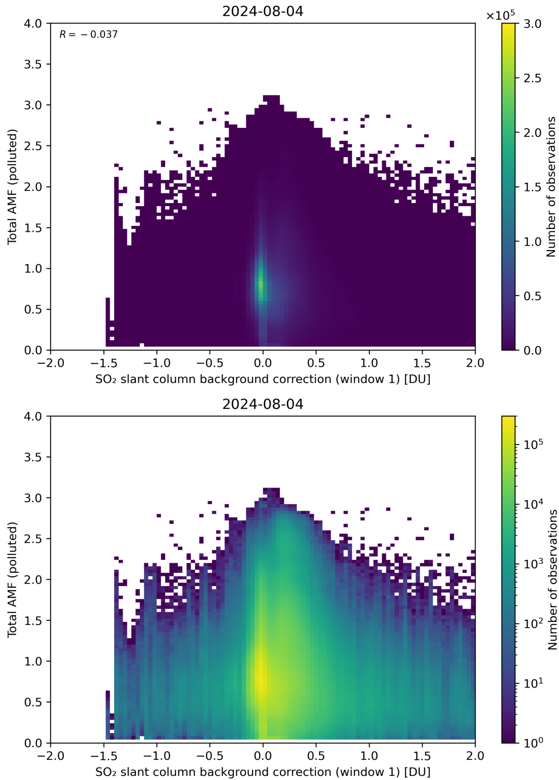
Figure 109: Scatter density plot of “SO 2 slant column background correction (window 1)” against “Total AMF (polluted)” for 2024-08-03 to 2024-08-05.
