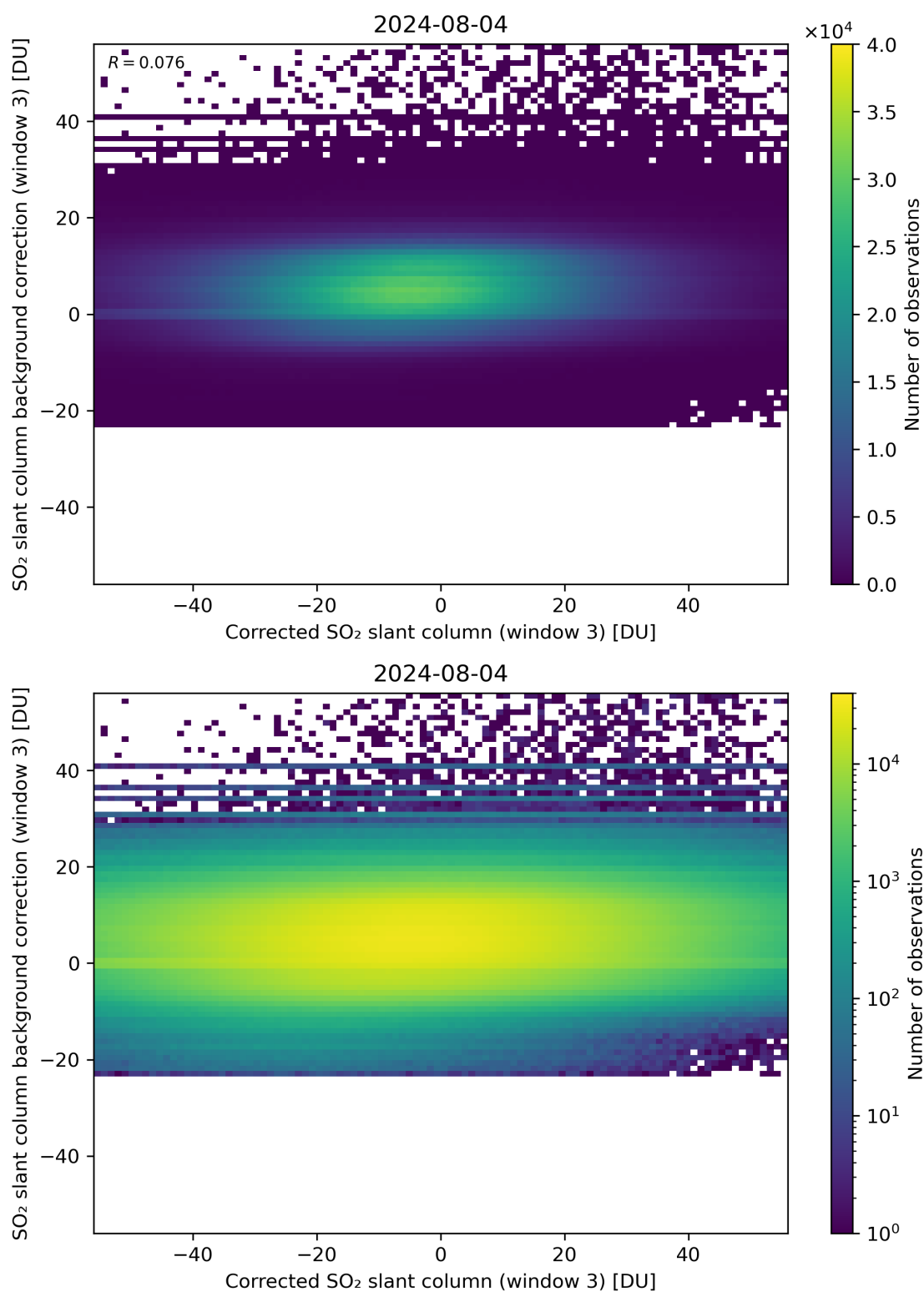
Figure 205: Scatter density plot of “Corrected SO 2 slant column (window 3)” against “SO 2 slant column background correction (window 3)” for 2024-08-03 to 2024-08-05.
