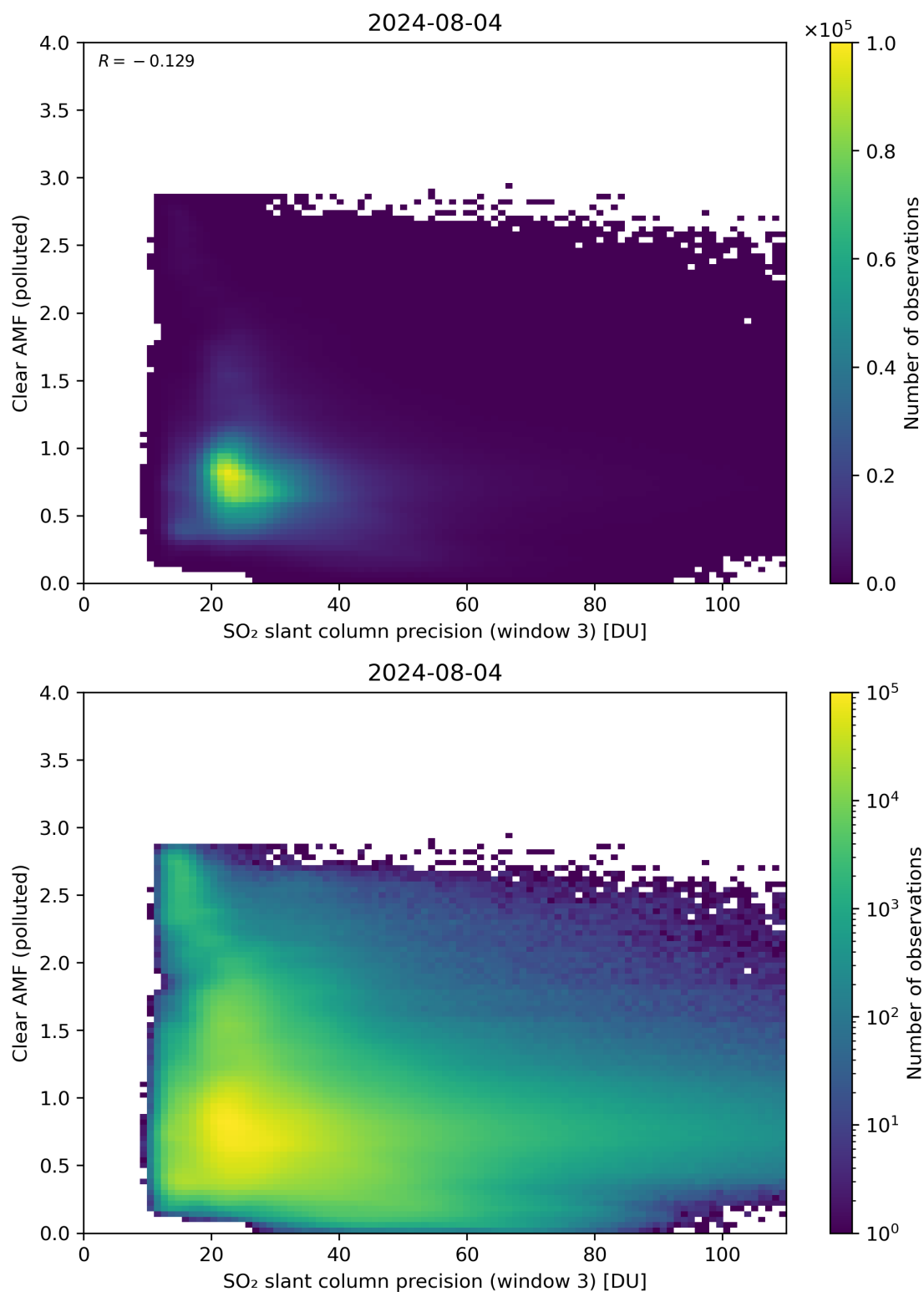
Figure 261: Scatter density plot of “SO 2 slant column precision (window 3)” against “Clear AMF (polluted)” for 2024-08-03 to 2024-08-05.
