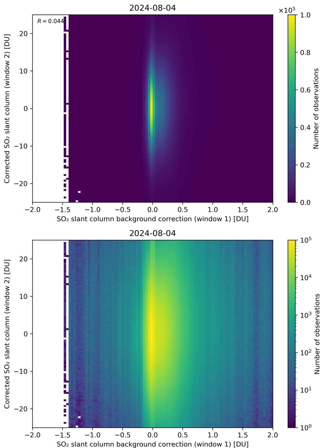
Figure 104: Scatter density plot of “SO 2 slant column background correction (window 1)” against “Corrected SO 2 slant column (window 2)” for 2024-08-03 to 2024-08-05.
