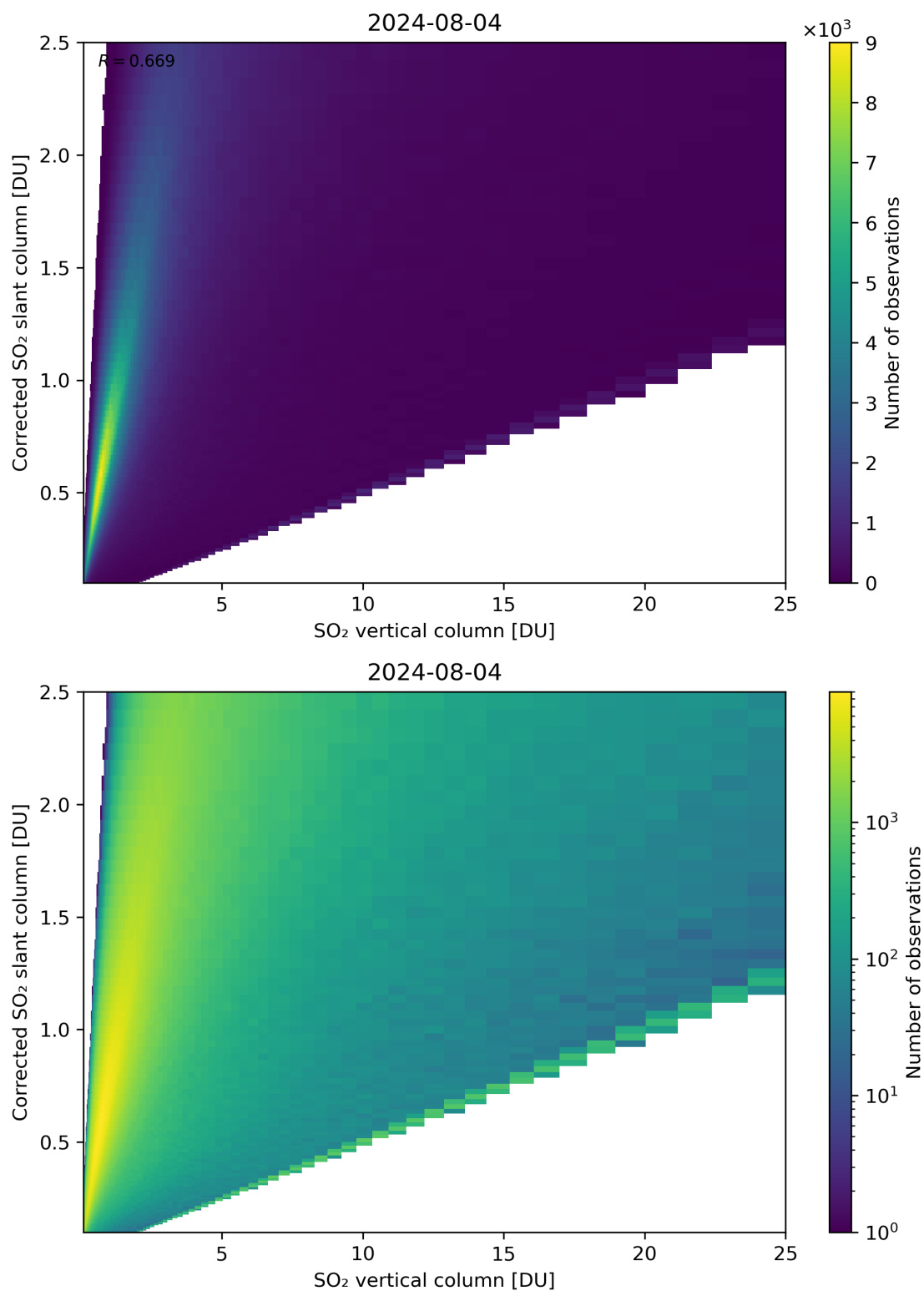
Figure 297: Scatter density plot of “SO 2 vertical column” against “Corrected SO 2 slant column” for 2024-08-03 to 2024-08-05.
