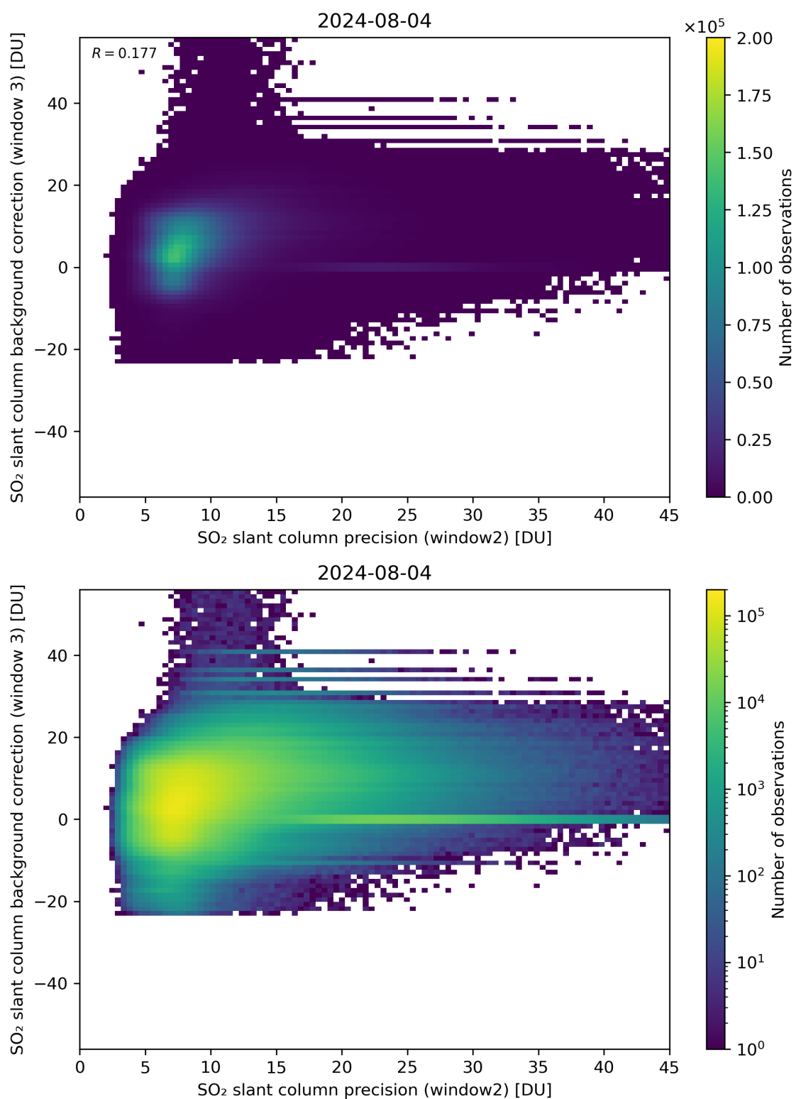
Figure 242: Scatter density plot of “SO 2 slant column precision (window2)” against “SO 2 slant column background correction (window 3)” for 2024-08-03 to 2024-08-05.
