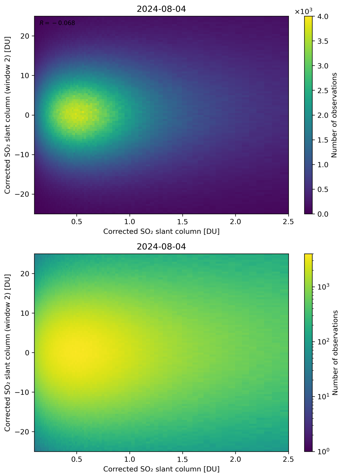
Figure 185: Scatter density plot of “Corrected SO 2 slant column” against “Corrected SO 2 slant column (window 2)” for 2024-08-03 to 2024-08-05.
