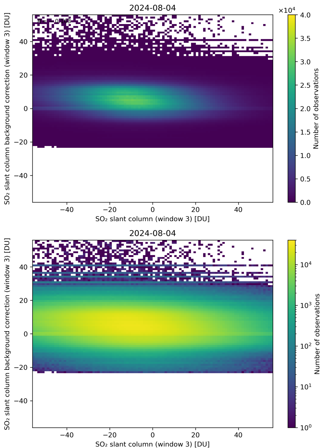
Figure 253: Scatter density plot of “SO 2 slant column (window 3)” against “SO 2 slant column background correction (window 3)” for 2024-08-03 to 2024-08-05.
