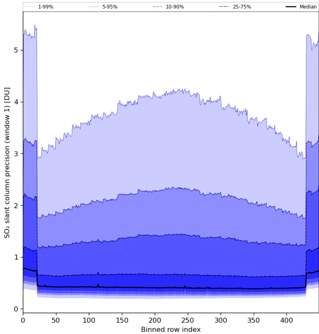
Figure 80: Along track statistics of “SO 2 slant column precision (window 1)” for 2024-08-03 to 2024-08-05
