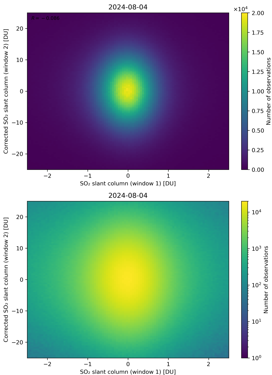
Figure 233: Scatter density plot of “SO 2 slant column (window 1)” against “Corrected SO 2 slant column (window 2)” for 2024-08-03 to 2024-08-05.
