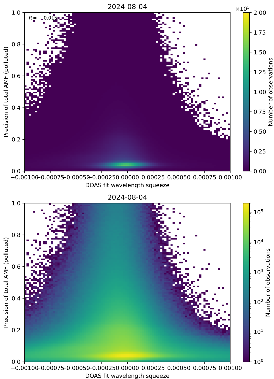
Figure 135: Scatter density plot of “DOAS fit wavelength squeeze” against “Precision of total AMF (polluted)” for 2024-08-03 to 2024-08-05.
