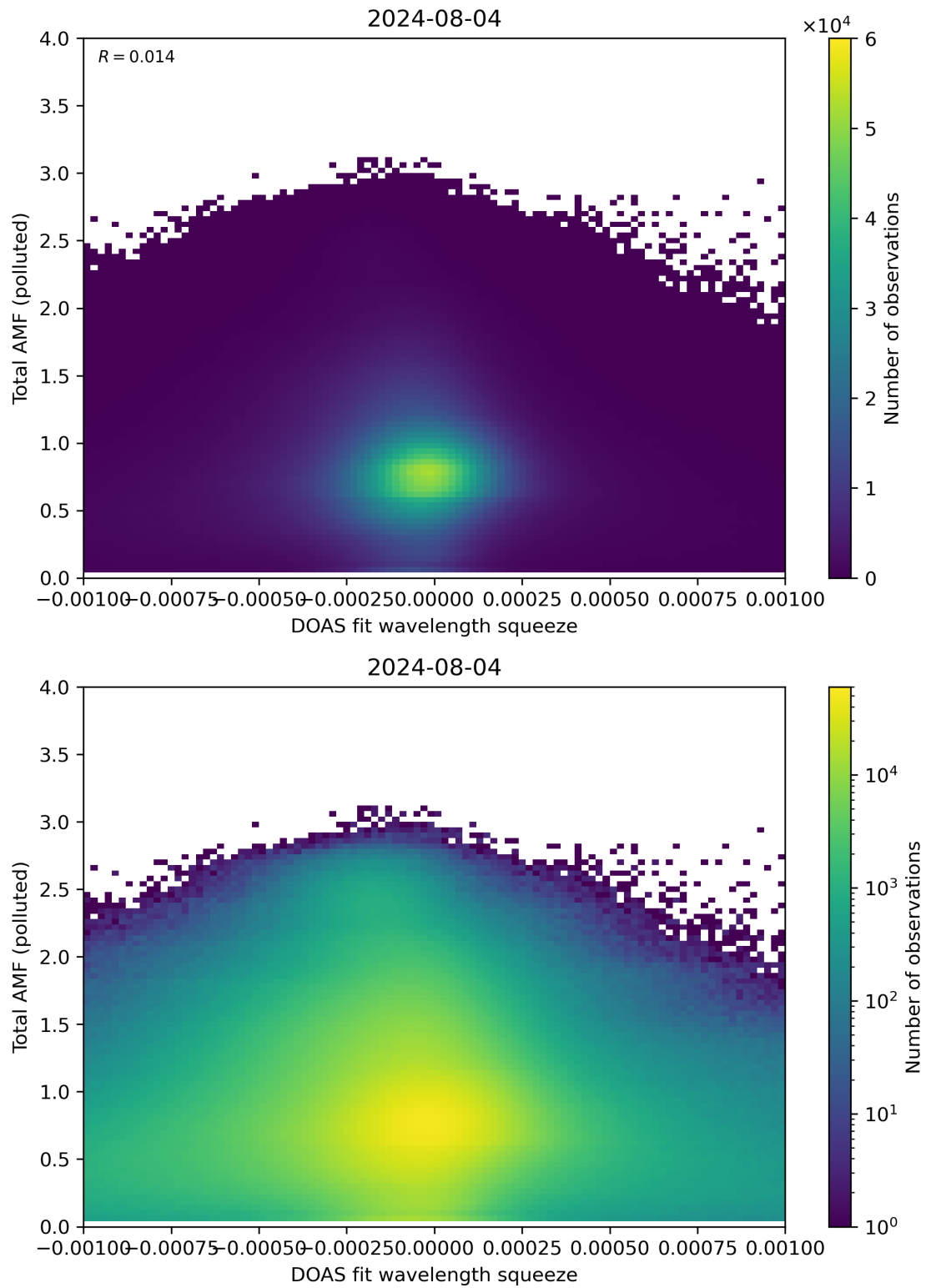
Figure 134: Scatter density plot of “DOAS fit wavelength squeeze” against “Total AMF (polluted)” for 2024-08-03 to 2024-08-05.
