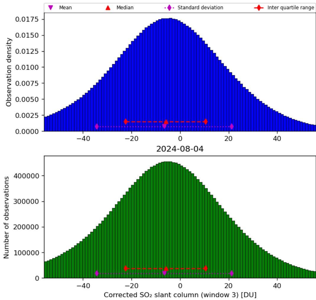
Figure 66: Histogram of “Corrected SO 2 slant column (window 3)” for 2024-08-03 to 2024-08-05
