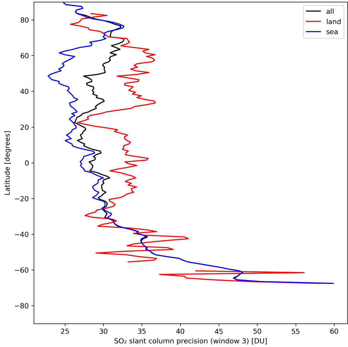
Figure 42: Zonal average of “SO 2 slant column precision (window 3)” for 2024-08-03 to 2024-08-05.
