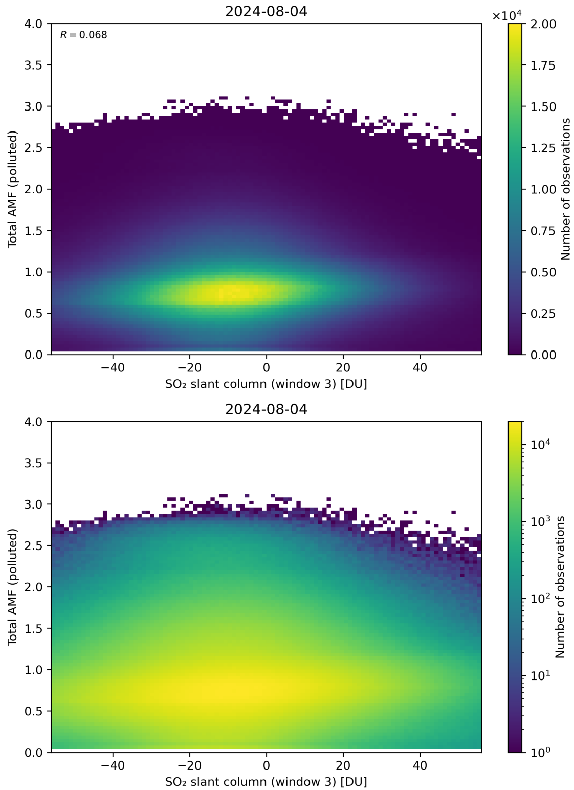
Figure 268: Scatter density plot of “SO 2 slant column (window 3)” against “Total AMF (polluted)” for 2024-08-03 to 2024-08-05.
