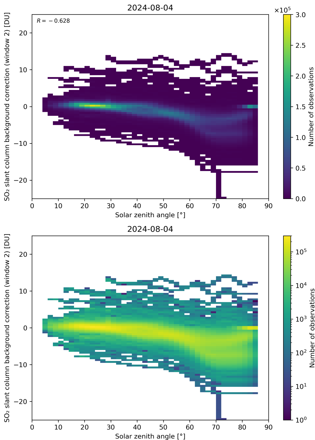
Figure 159: Scatter density plot of “Solar zenith angle” against “SO 2 slant column background correction (window 2)” for 2024-08-03 to 2024-08-05.
