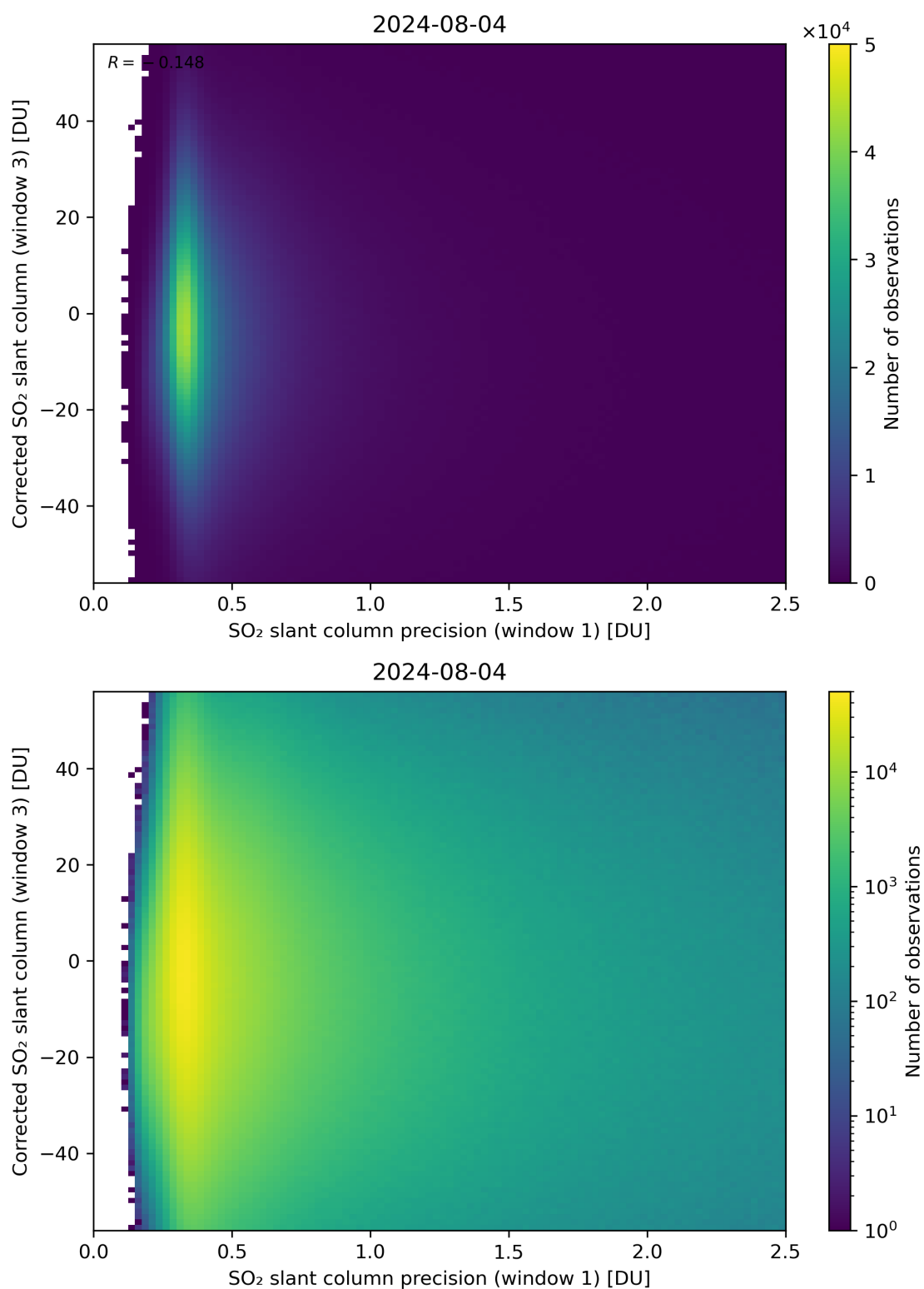
Figure 226: Scatter density plot of “SO 2 slant column precision (window 1)” against “Corrected SO 2 slant column (window 3)” for 2024-08-03 to 2024-08-05.
