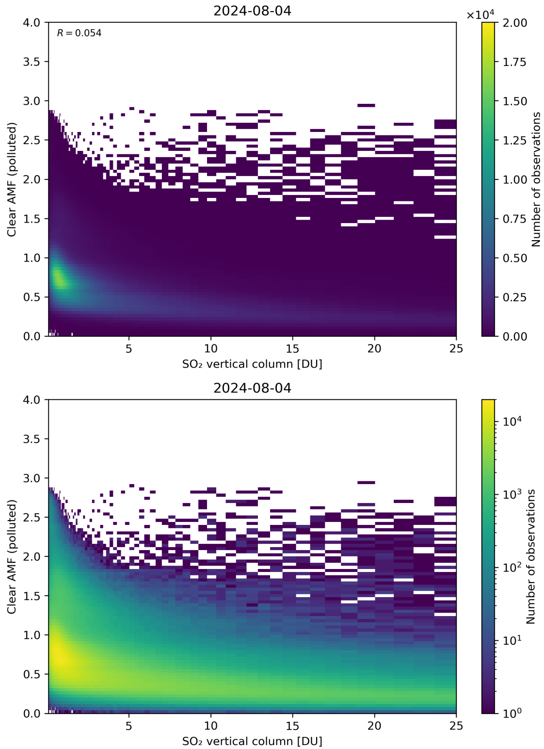
Figure 296: Scatter density plot of “SO 2 vertical column” against “Clear AMF (polluted)” for 2024-08-03 to 2024-08-05.
