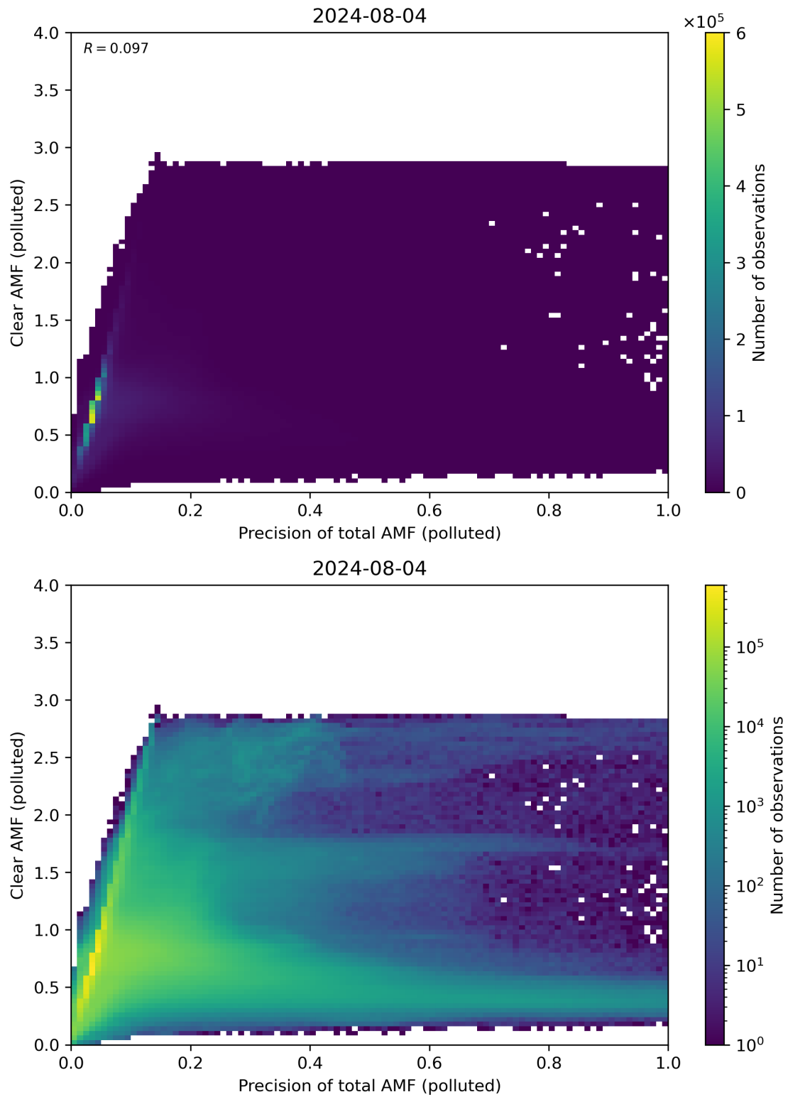
Figure 270: Scatter density plot of “Precision of total AMF (polluted)” against “Clear AMF (polluted)” for 2024-08-03 to 2024-08-05.
