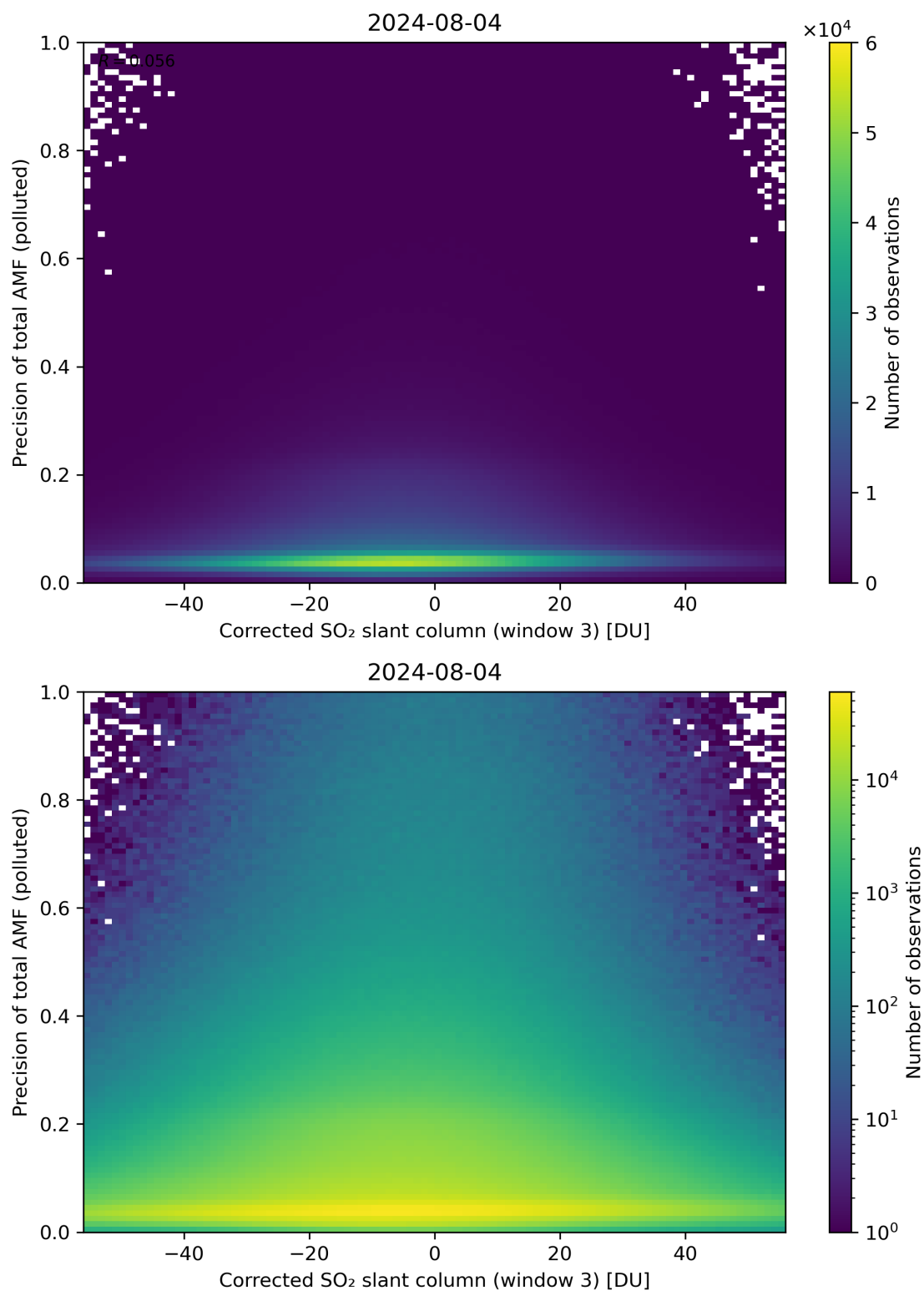
Figure 211: Scatter density plot of “Corrected SO 2 slant column (window 3)” against “Precision of total AMF (polluted)” for 2024-08-03 to 2024-08-05.
