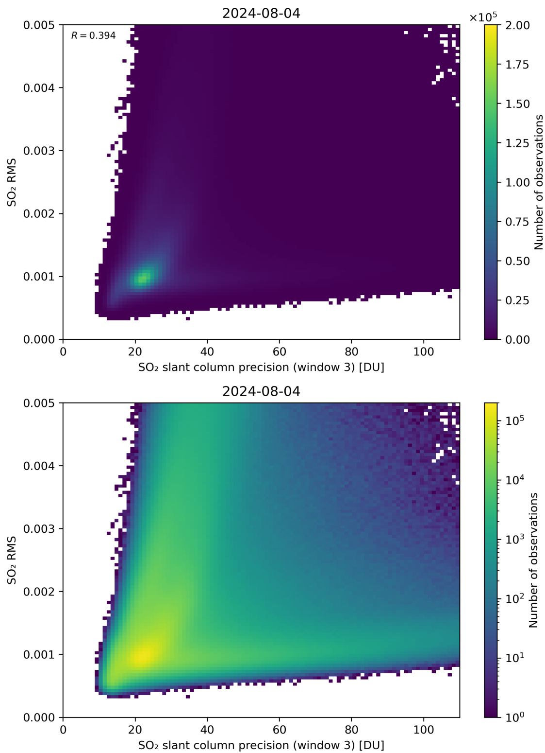
Figure 260: Scatter density plot of “SO 2 slant column precision (window 3)” against “SO 2 RMS” for 2024-08-03 to 2024-08-05.
