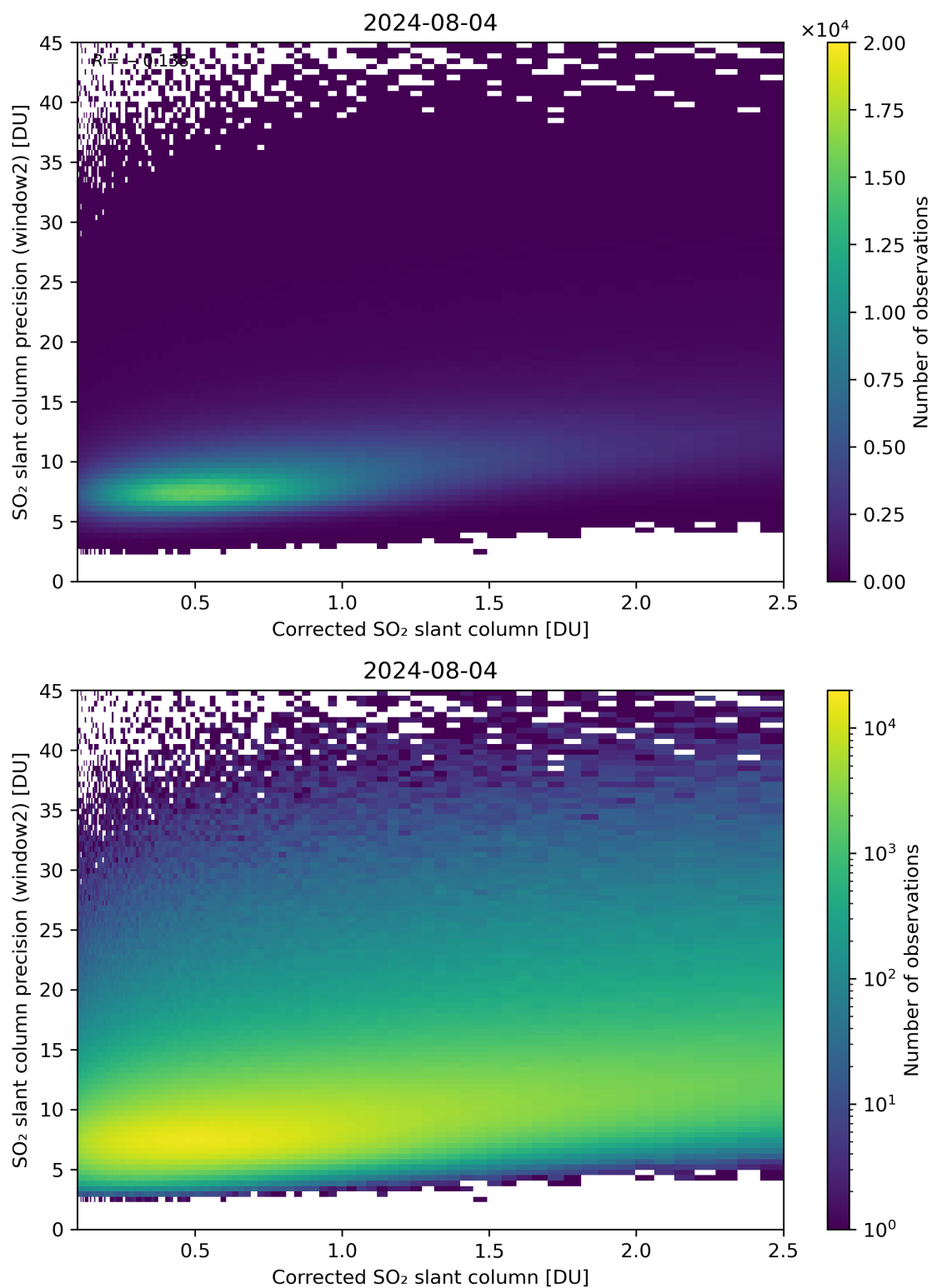
Figure 189: Scatter density plot of “Corrected SO 2 slant column” against “SO 2 slant column precision (window2)” for 2024-08-03 to 2024-08-05.
