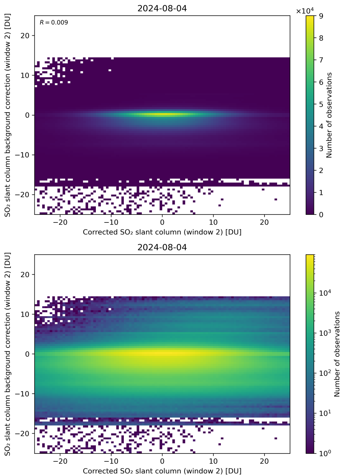
Figure 194: Scatter density plot of “Corrected SO 2 slant column (window 2)” against “SO 2 slant column background correction (window 2)” for 2024-08-03 to 2024-08-05.
