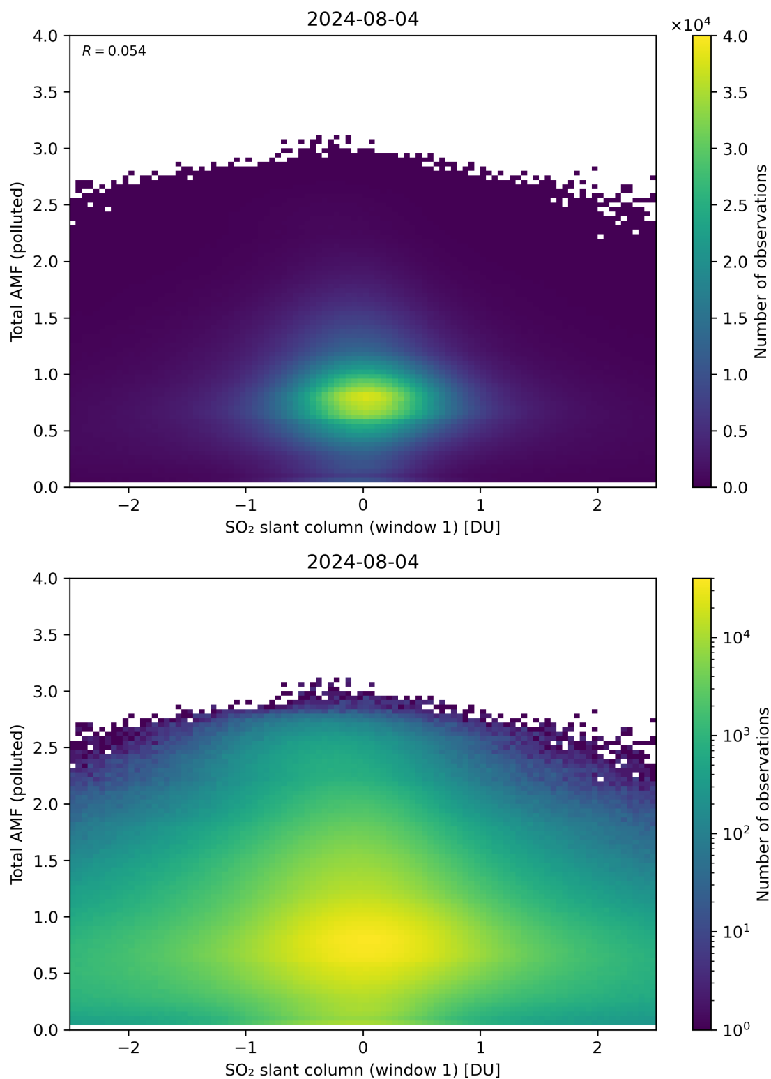
Figure 239: Scatter density plot of “SO 2 slant column (window 1)” against “Total AMF (polluted)” for 2024-08-03 to 2024-08-05.
