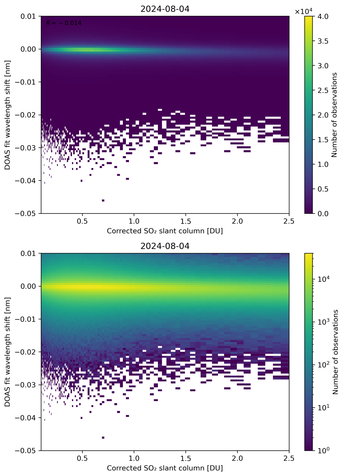
Figure 181: Scatter density plot of “Corrected SO 2 slant column” against “DOAS fit wavelength shift” for 2024-08-03 to 2024-08-05.
