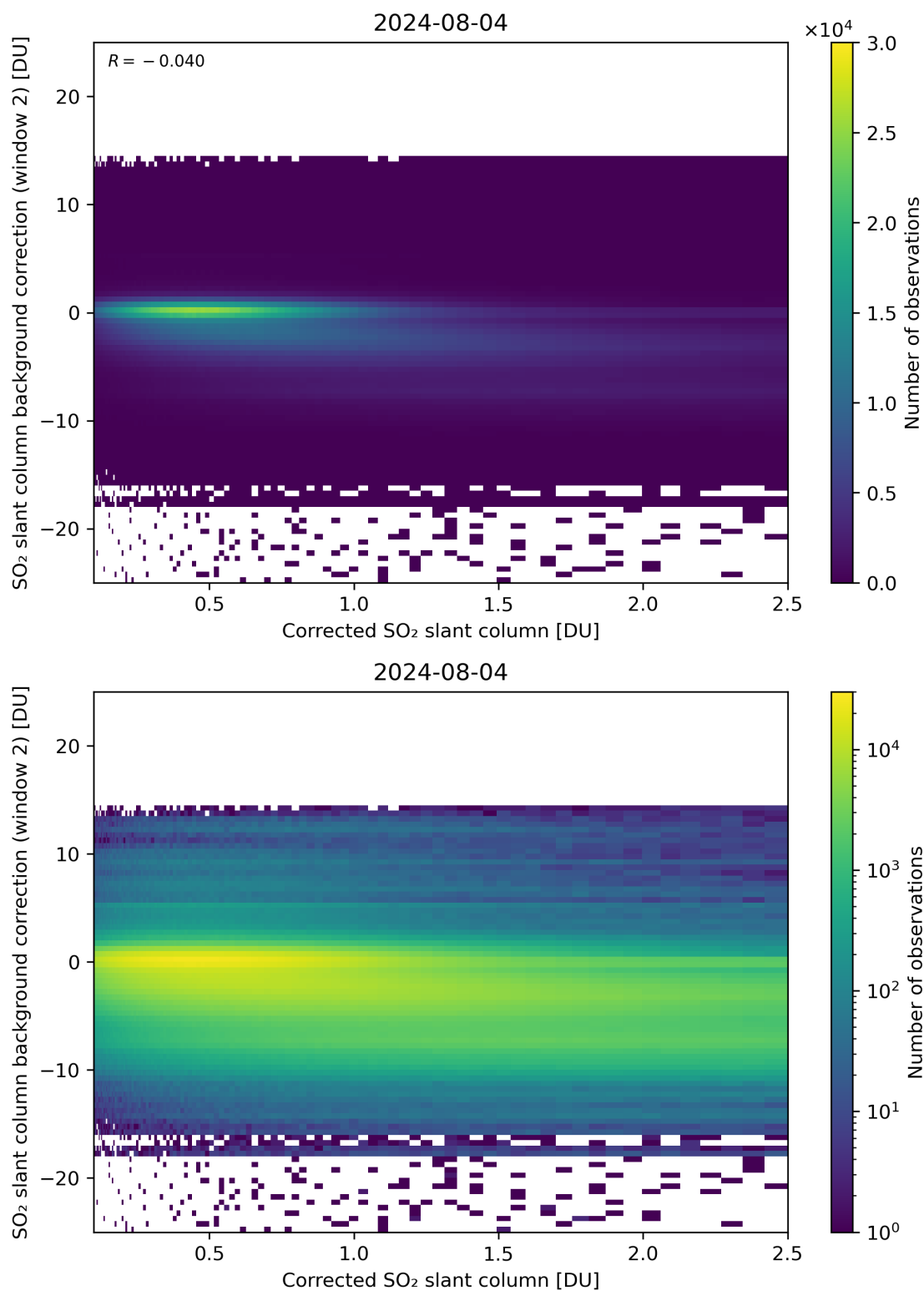
Figure 179: Scatter density plot of “Corrected SO 2 slant column” against “SO 2 slant column background correction (window 2)” for 2024-08-03 to 2024-08-05.
