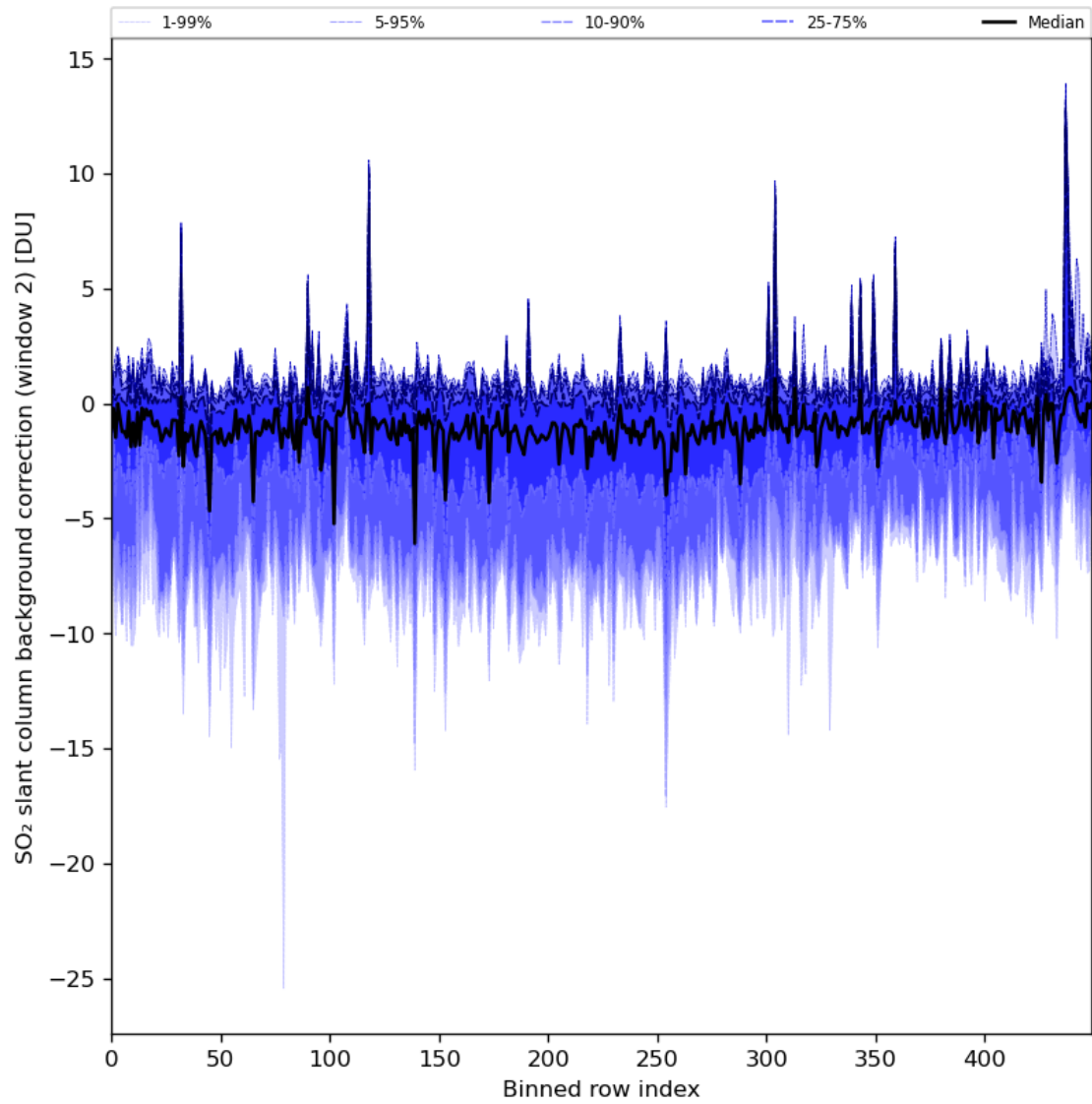
Figure 86: Along track statistics of “SO 2 slant column background correction (window 2)” for 2024-08-03 to 2024-08-05
