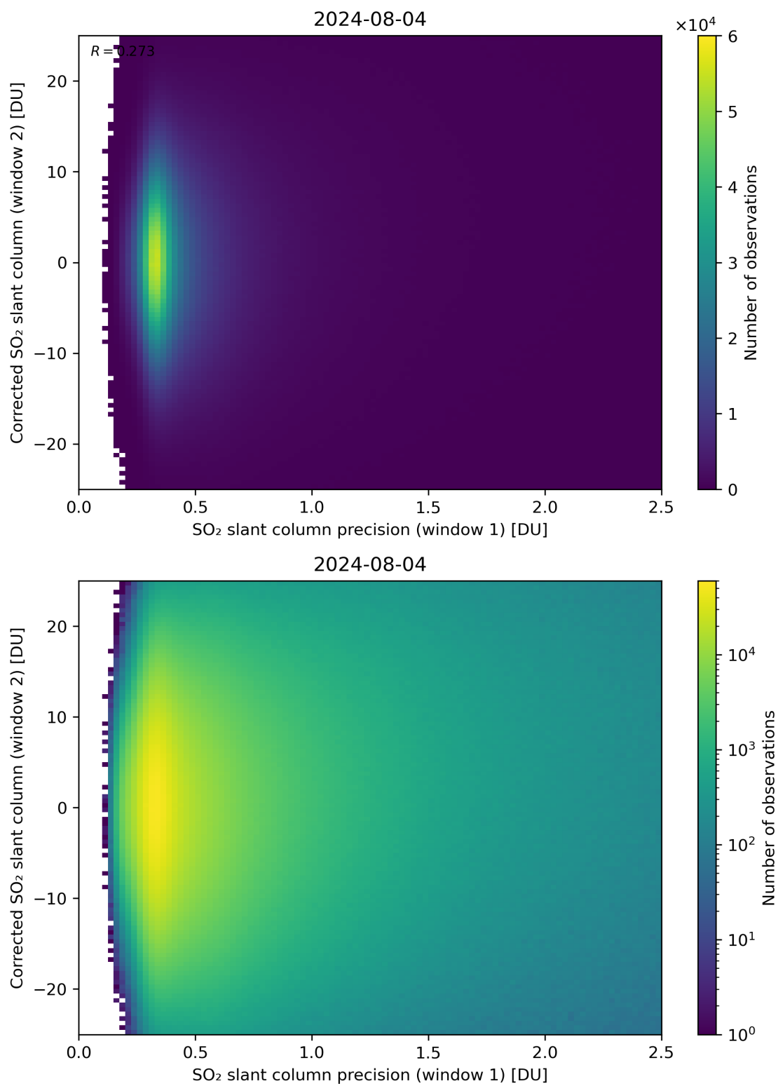
Figure 225: Scatter density plot of “SO 2 slant column precision (window 1)” against “Corrected SO 2 slant column (window 2)” for 2024-08-03 to 2024-08-05.
