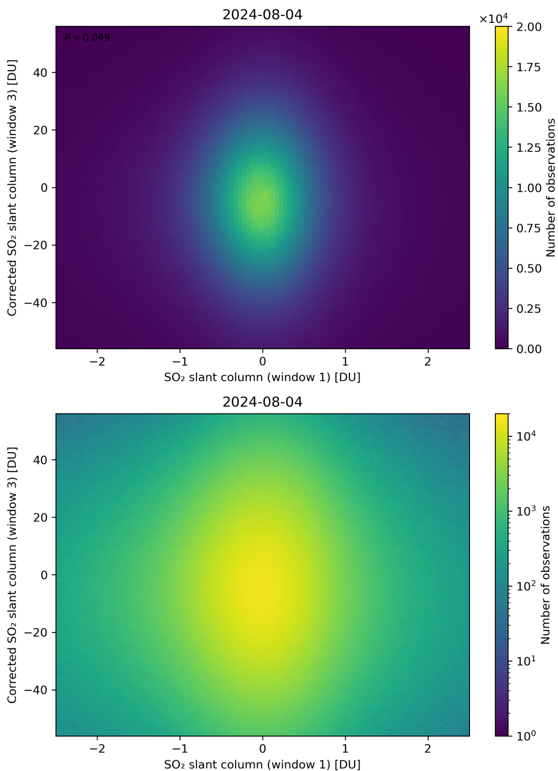
Figure 234: Scatter density plot of “SO 2 slant column (window 1)” against “Corrected SO 2 slant column (window 3)” for 2024-08-03 to 2024-08-05.
