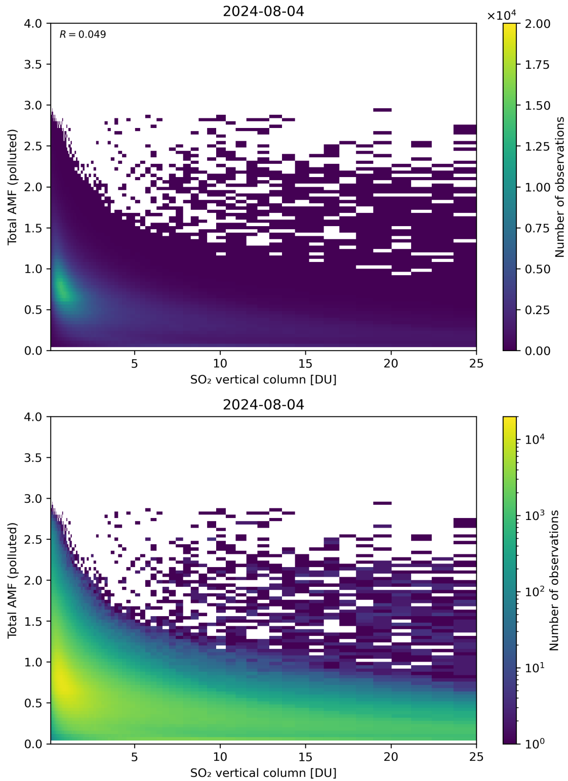
Figure 305: Scatter density plot of “SO 2 vertical column” against “Total AMF (polluted)” for 2024-08-03 to 2024-08-05.
