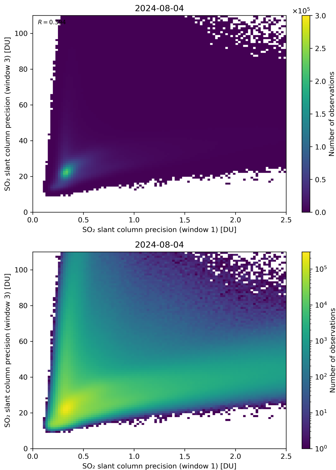
Figure 229: Scatter density plot of “SO 2 slant column precision (window 1)” against “SO 2 slant column precision (window 3)” for 2024-08-03 to 2024-08-05.
