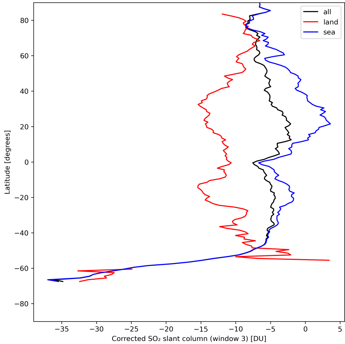
Figure 43: Zonal average of “Corrected SO 2 slant column (window 3)” for 2024-08-03 to 2024-08-05.
