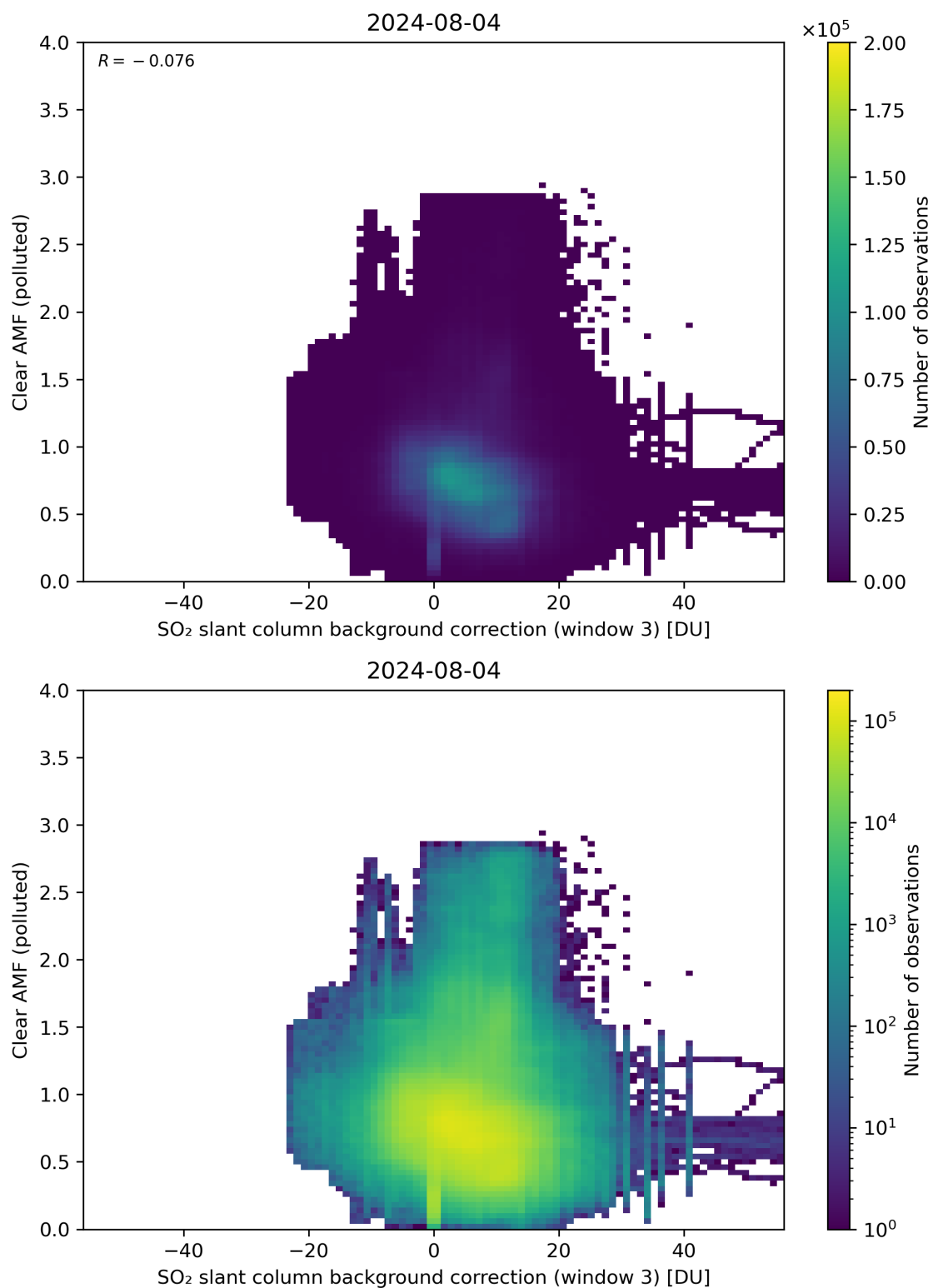
Figure 124: Scatter density plot of “SO 2 slant column background correction (window 3)” against “Clear AMF (polluted)” for 2024-08-03 to 2024-08-05.
