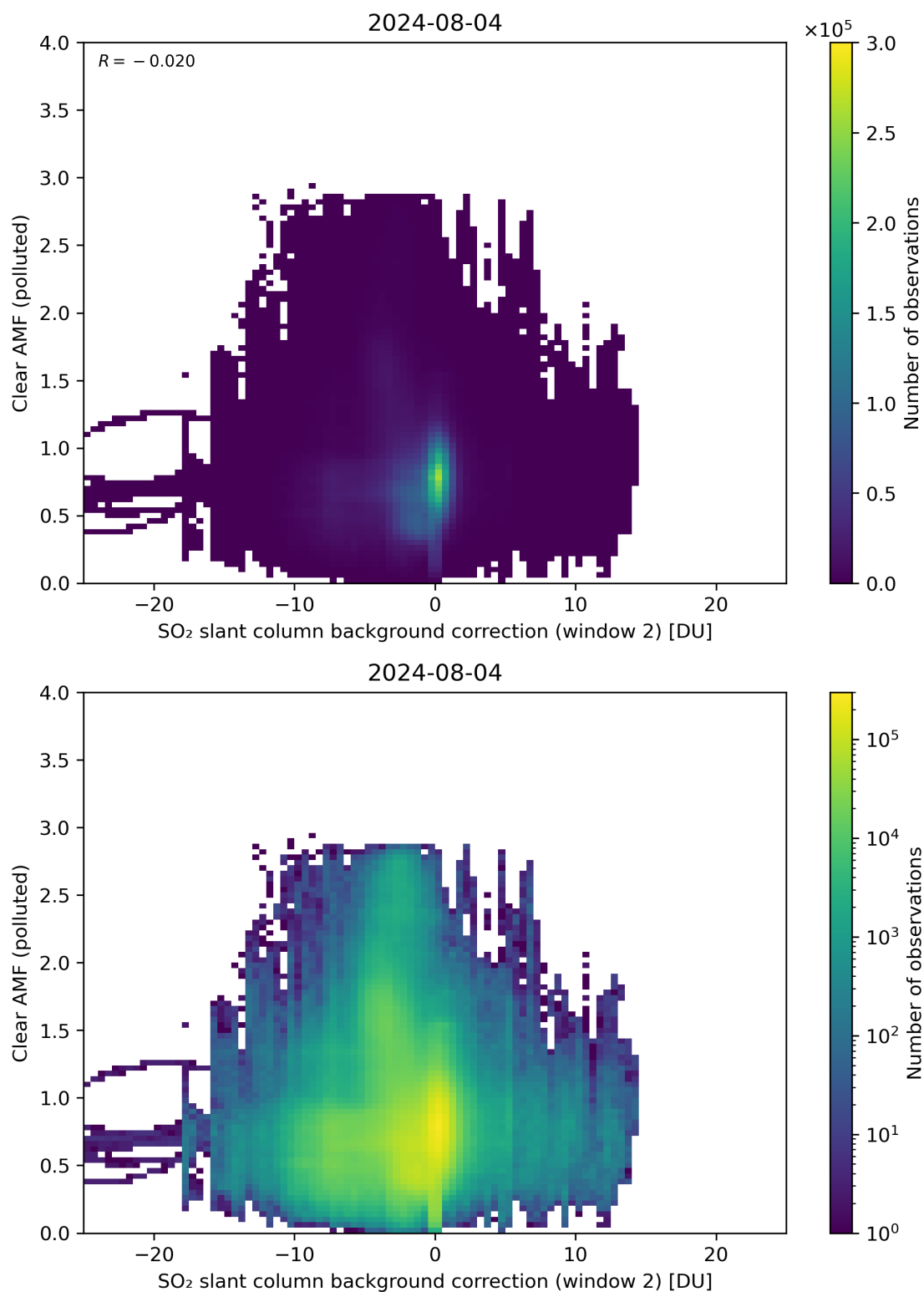
Figure 115: Scatter density plot of “SO 2 slant column background correction (window 2)” against “Clear AMF (polluted)” for 2024-08-03 to 2024-08-05.
