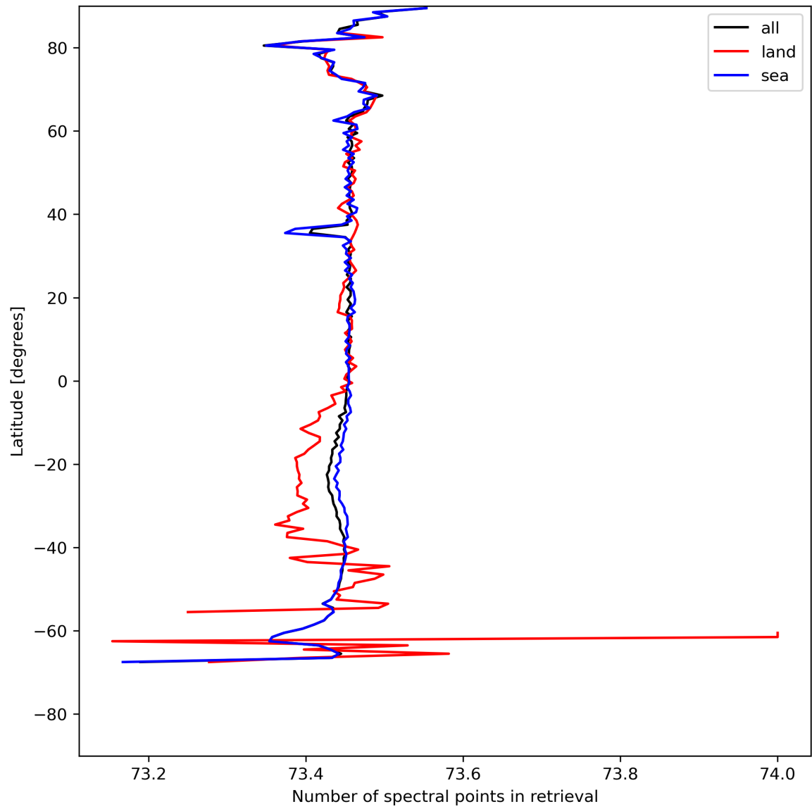
Figure 51: Zonal average of “Number of spectral points in retrieval” for 2024-08-03 to 2024-08-05.
