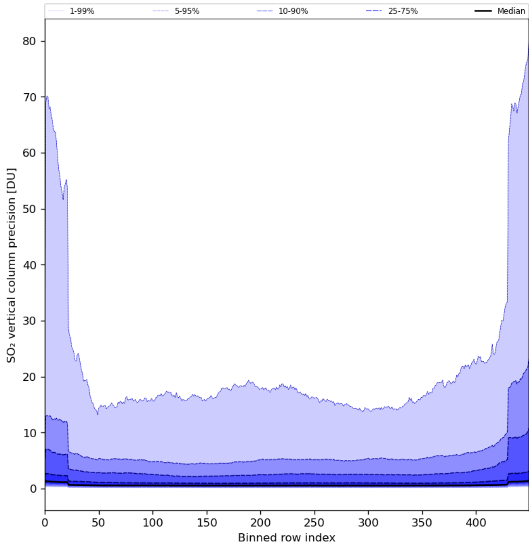
Figure 77: Along track statistics of “SO 2 vertical column precision” for 2024-08-03 to 2024-08-05
