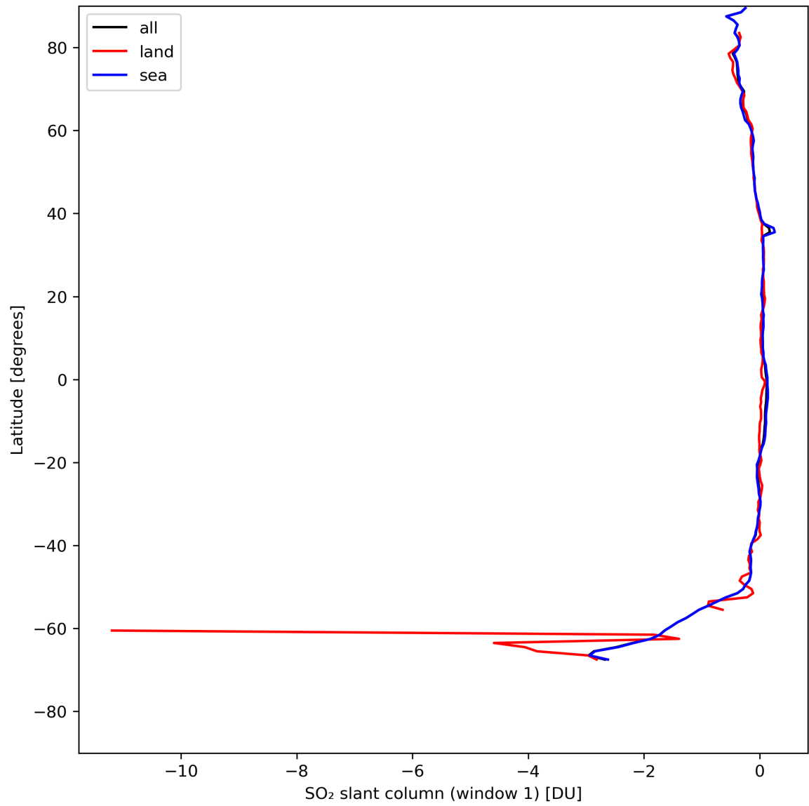
Figure 33: Zonal average of “SO 2 slant column (window 1)” for 2024-08-03 to 2024-08-05.
