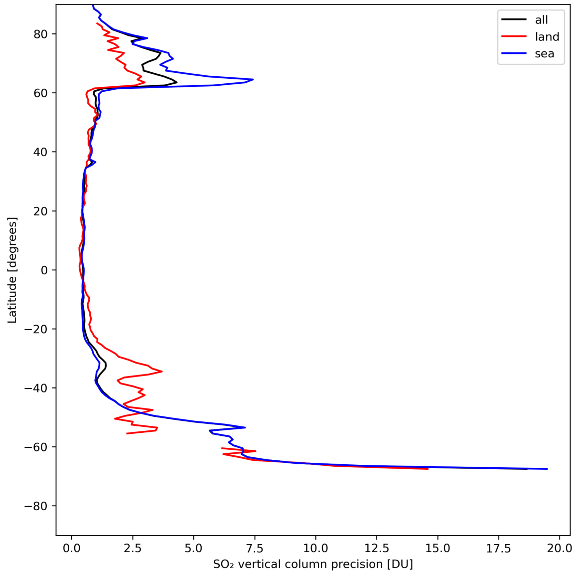
Figure 31: Zonal average of “SO 2 vertical column precision” for 2024-08-03 to 2024-08-05.
