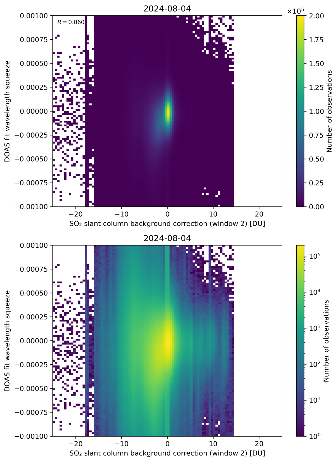
Figure 113: Scatter density plot of “SO 2 slant column background correction (window 2)” against “DOAS fit wavelength squeeze” for 2024-08-03 to 2024-08-05.
