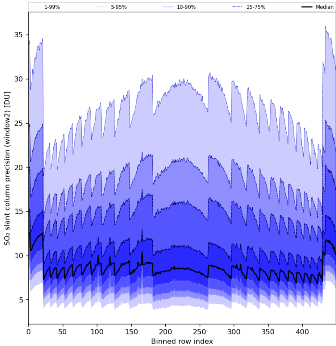
Figure 84: Along track statistics of “SO 2 slant column precision (window2)” for 2024-08-03 to 2024-08-05
