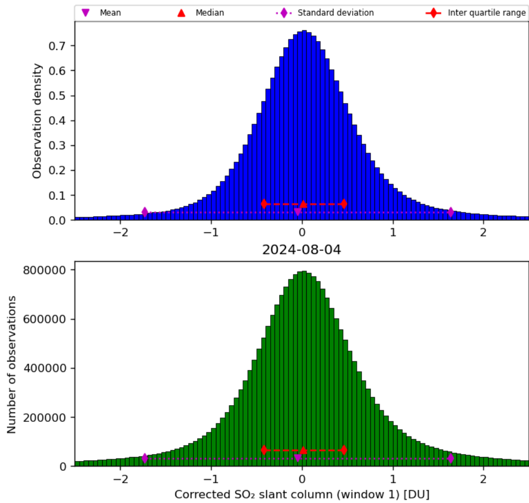
Figure 58: Histogram of “Corrected SO 2 slant column (window 1)” for 2024-08-03 to 2024-08-05
