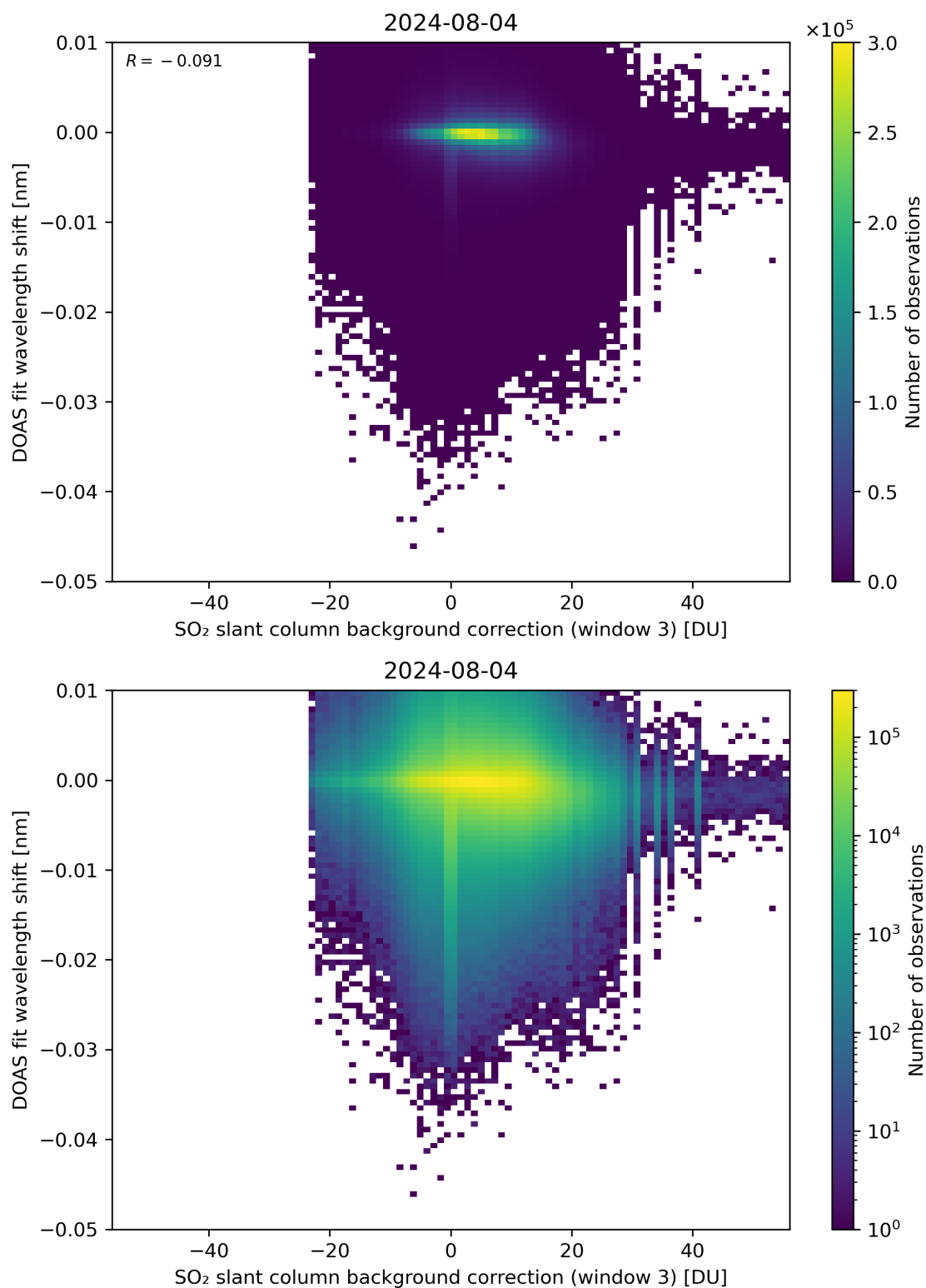
Figure 121: Scatter density plot of “SO 2 slant column background correction (window 3)” against “DOAS fit wavelength shift” for 2024-08-03 to 2024-08-05.
