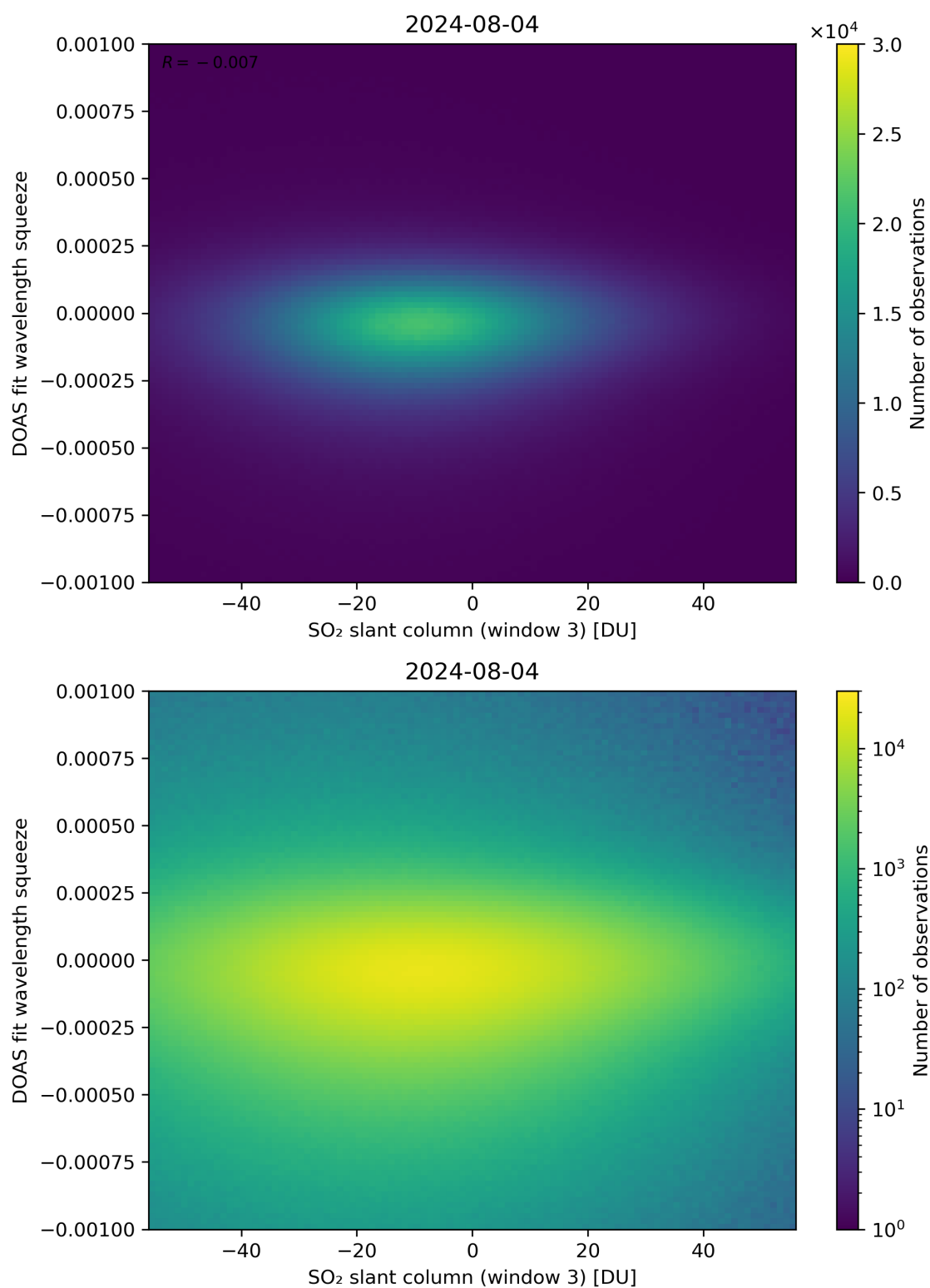
Figure 255: Scatter density plot of “SO 2 slant column (window 3)” against “DOAS fit wavelength squeeze” for 2024-08-03 to 2024-08-05.
