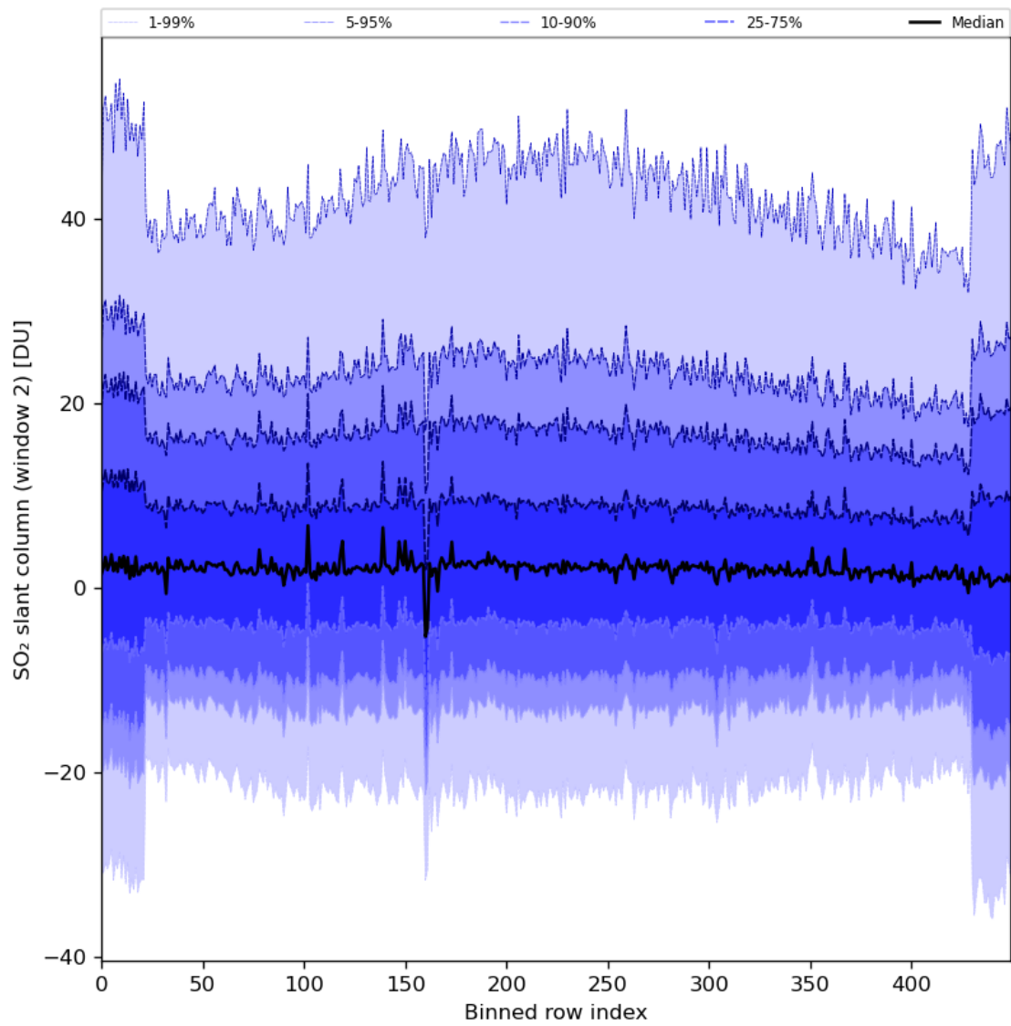
Figure 83: Along track statistics of “SO 2 slant column (window 2)” for 2024-08-03 to 2024-08-05
