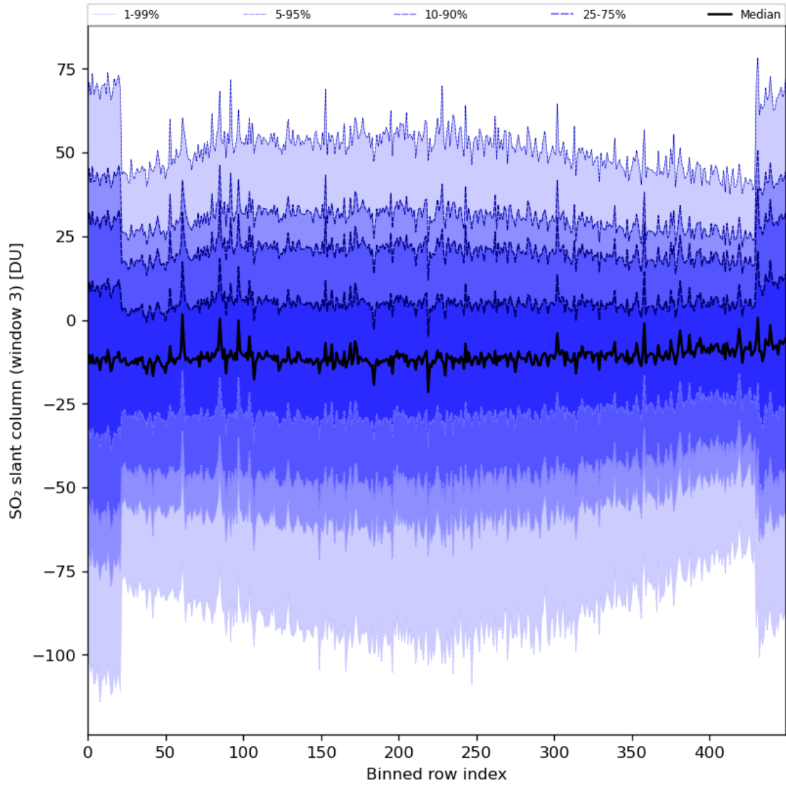
Figure 87: Along track statistics of “SO 2 slant column (window 3)” for 2024-08-03 to 2024-08-05
