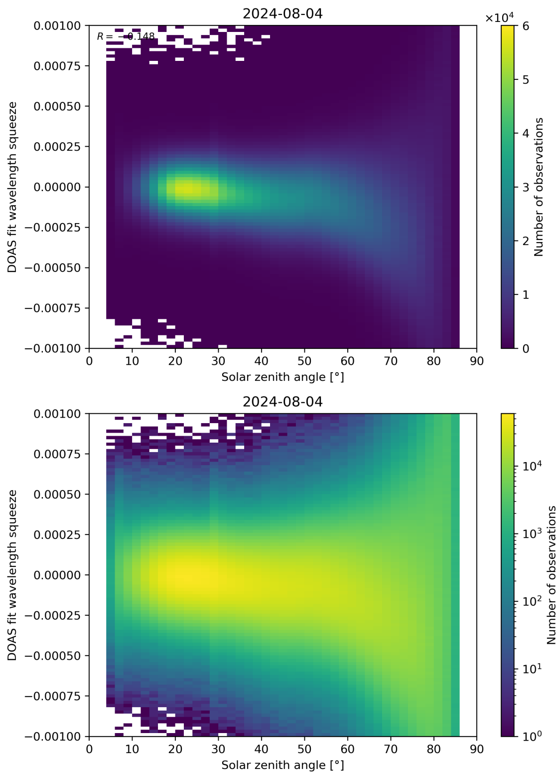
Figure 162: Scatter density plot of “Solar zenith angle” against “DOAS fit wavelength squeeze” for 2024-08-03 to 2024-08-05.
