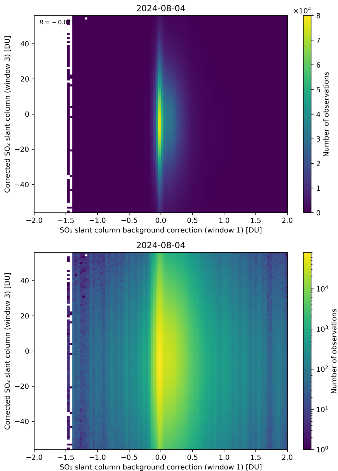
Figure 105: Scatter density plot of “SO 2 slant column background correction (window 1)” against “Corrected SO 2 slant column (window 3)” for 2024-08-03 to 2024-08-05.
