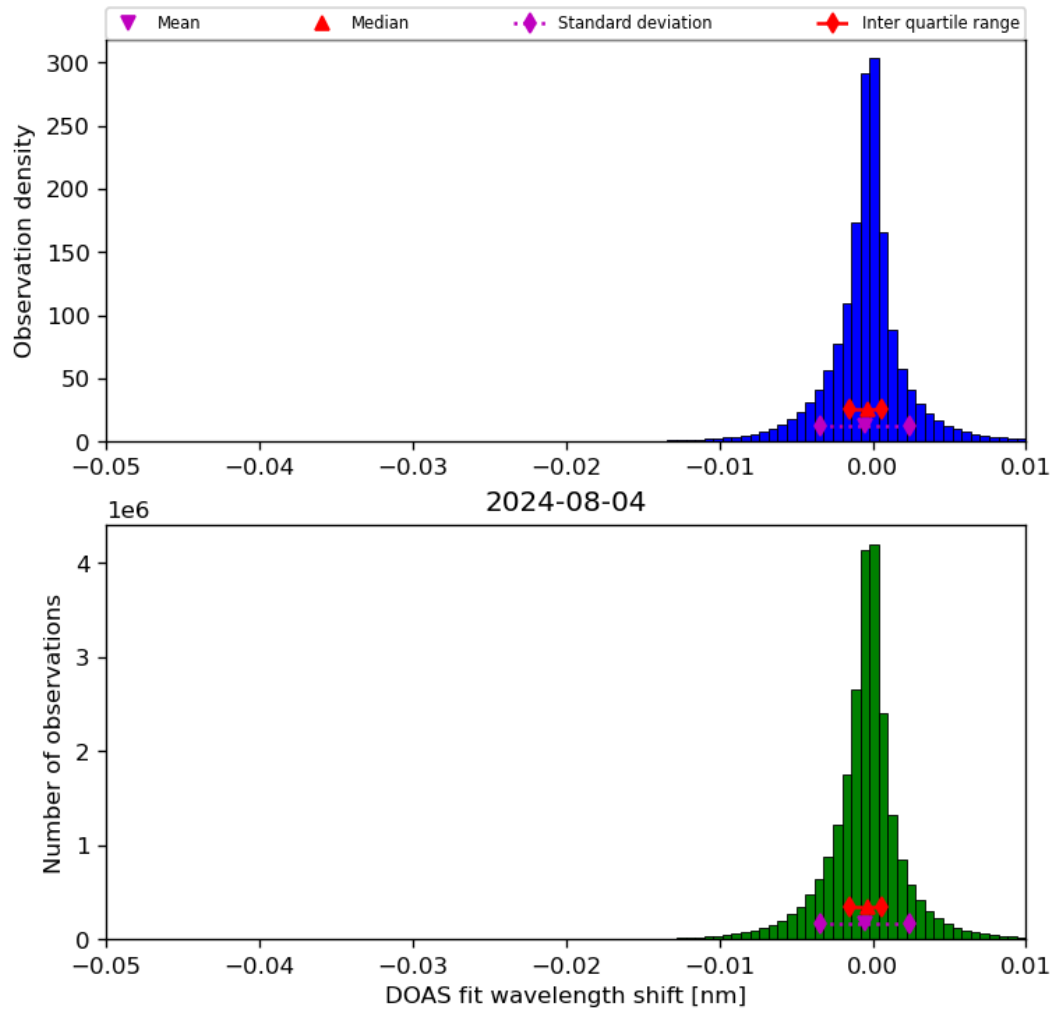
Figure 68: Histogram of “DOAS fit wavelength shift” for 2024-08-03 to 2024-08-05
