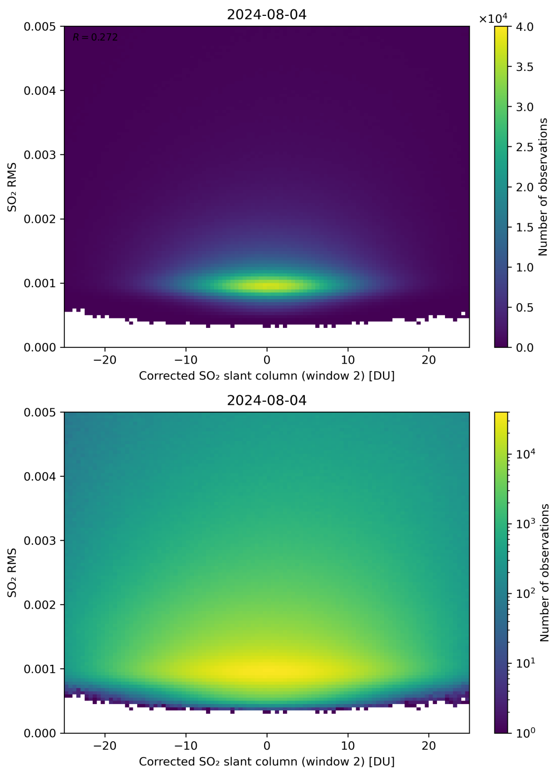
Figure 198: Scatter density plot of “Corrected SO 2 slant column (window 2)” against “SO 2 RMS” for 2024-08-03 to 2024-08-05.
