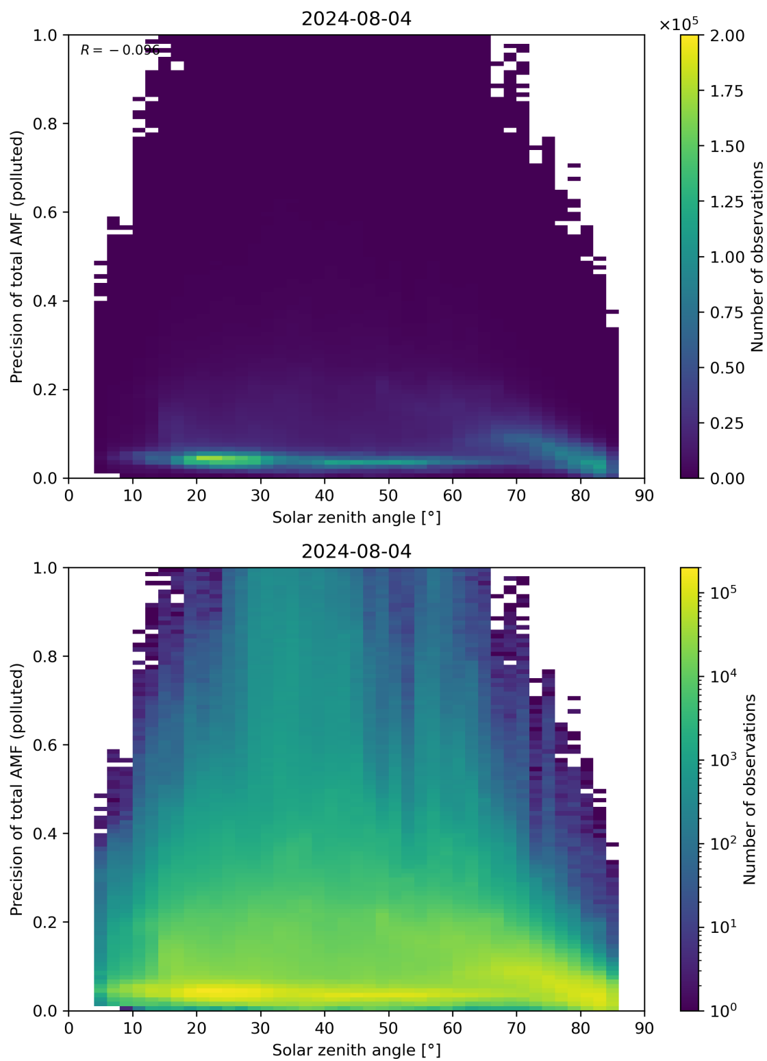
Figure 175: Scatter density plot of “Solar zenith angle” against “Precision of total AMF (polluted)” for 2024-08-03 to 2024-08-05.
