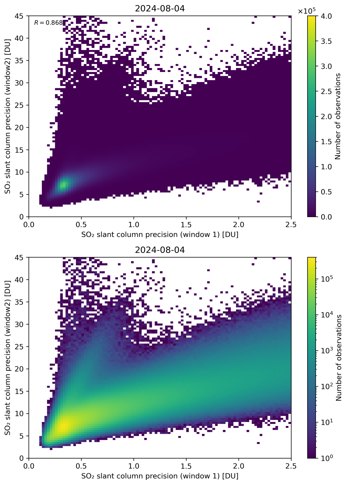
Figure 227: Scatter density plot of “SO 2 slant column precision (window 1)” against “SO 2 slant column precision (window2)” for 2024-08-03 to 2024-08-05.
