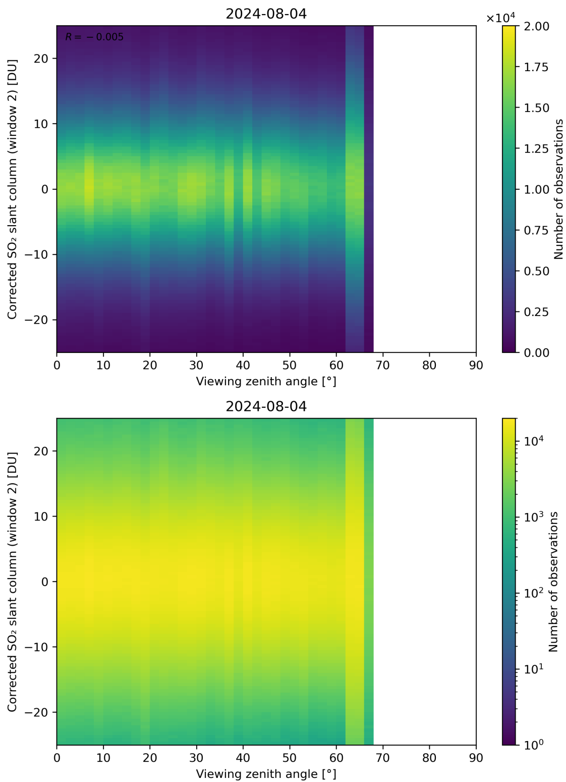
Figure 318: Scatter density plot of “Viewing zenith angle” against “Corrected SO 2 slant column (window 2)” for 2024-08-03 to 2024-08-05.
