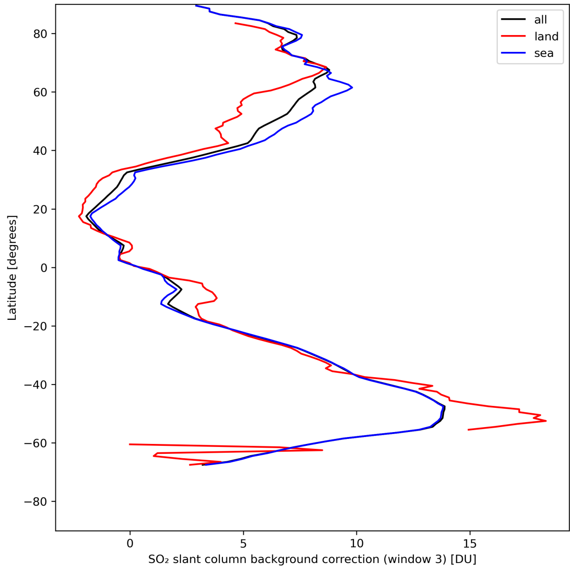
Figure 44: Zonal average of “SO 2 slant column background correction (window 3)” for 2024-08-03 to 2024-08-05.
