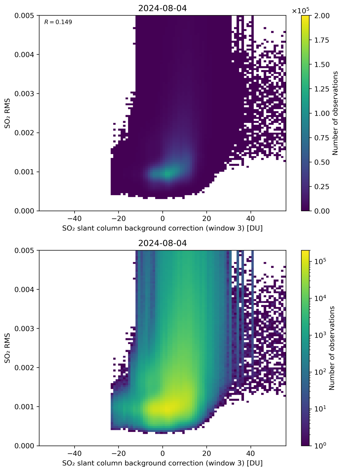
Figure 123: Scatter density plot of “SO 2 slant column background correction (window 3)” against “SO 2 RMS” for 2024-08-03 to 2024-08-05.
