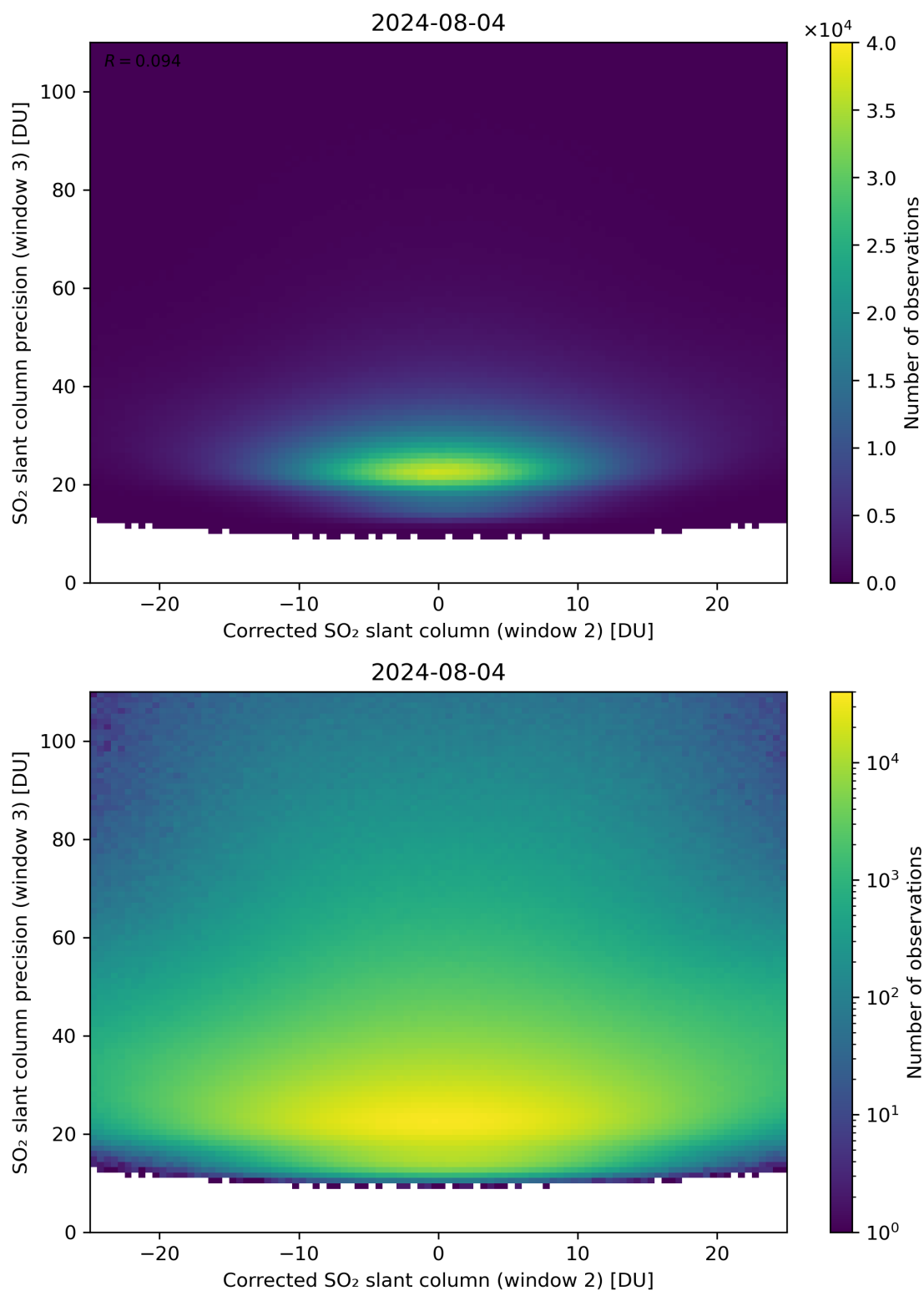
Figure 202: Scatter density plot of “Corrected SO 2 slant column (window 2)” against “SO 2 slant column precision (window 3)” for 2024-08-03 to 2024-08-05.
