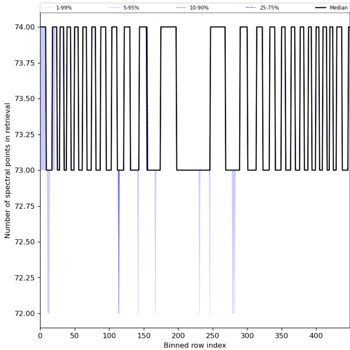
Figure 97: Along track statistics of “Number of spectral points in retrieval” for 2024-08-03 to 2024-08-05
