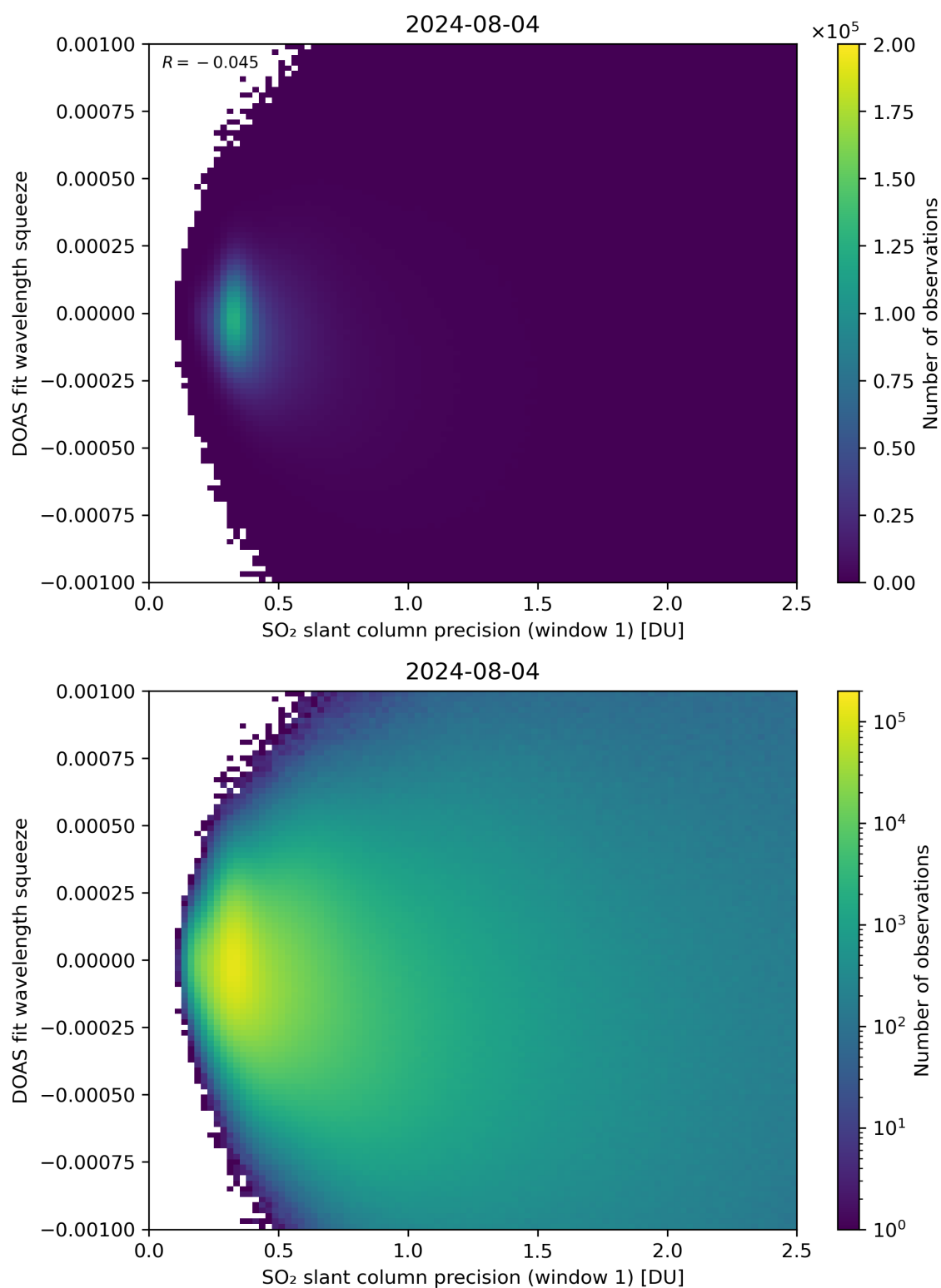
Figure 222: Scatter density plot of “SO 2 slant column precision (window 1)” against “DOAS fit wavelength squeeze” for 2024-08-03 to 2024-08-05.
