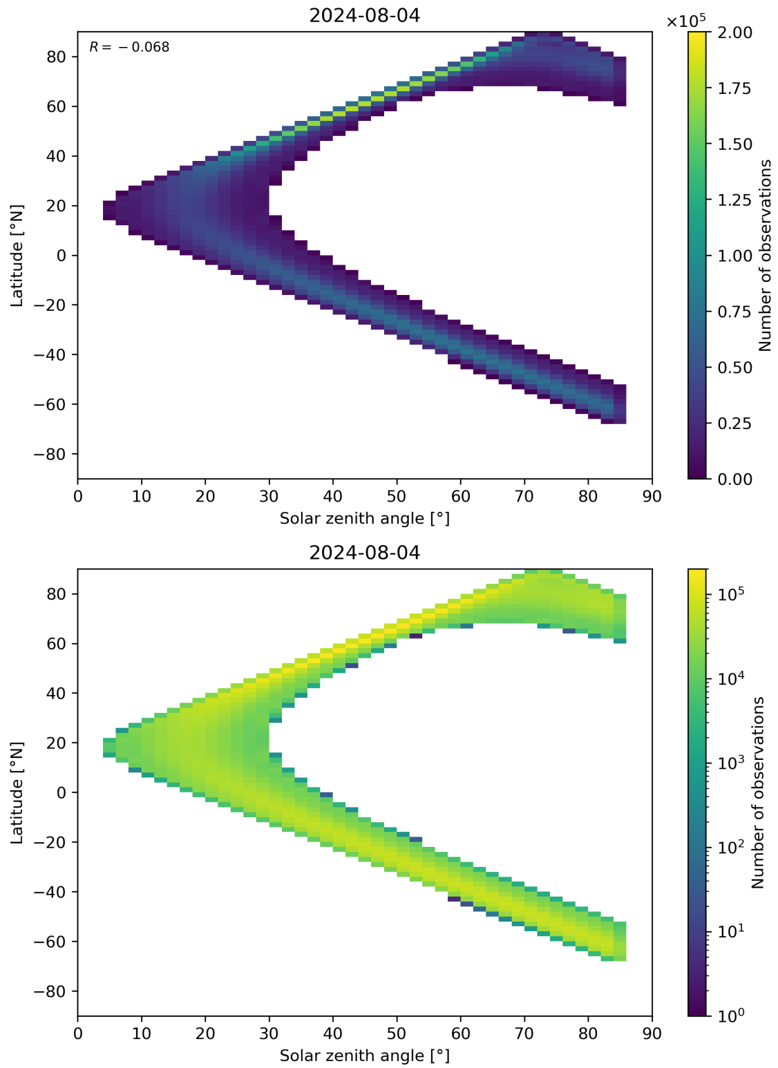
Figure 164: Scatter density plot of “Solar zenith angle” against “Latitude” for 2024-08-03 to 2024-08-05.
