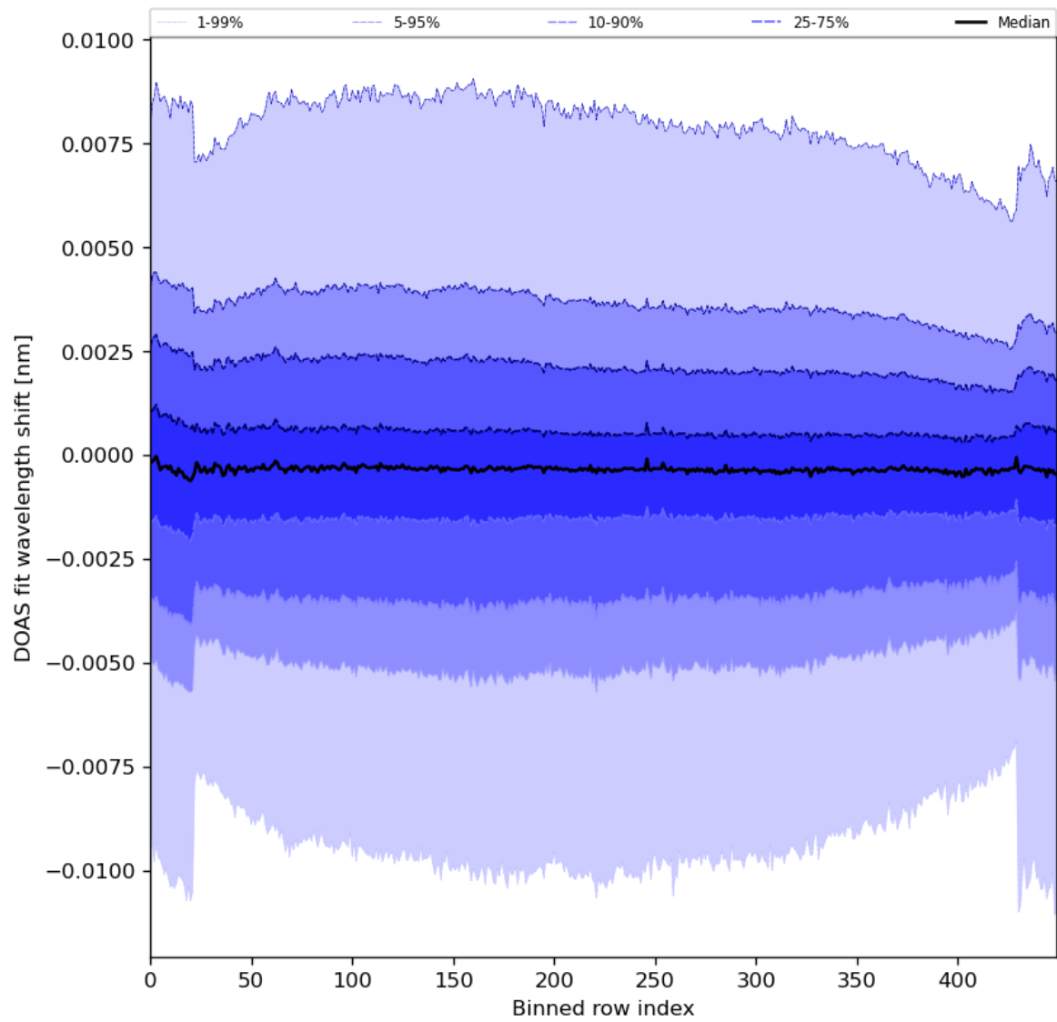
Figure 91: Along track statistics of “DOAS fit wavelength shift” for 2024-08-03 to 2024-08-05
