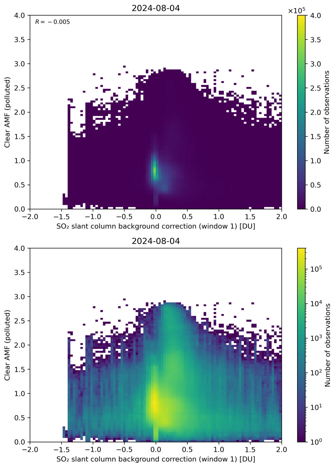
Figure 103: Scatter density plot of “SO 2 slant column background correction (window 1)” against “Clear AMF (polluted)” for 2024-08-03 to 2024-08-05.
