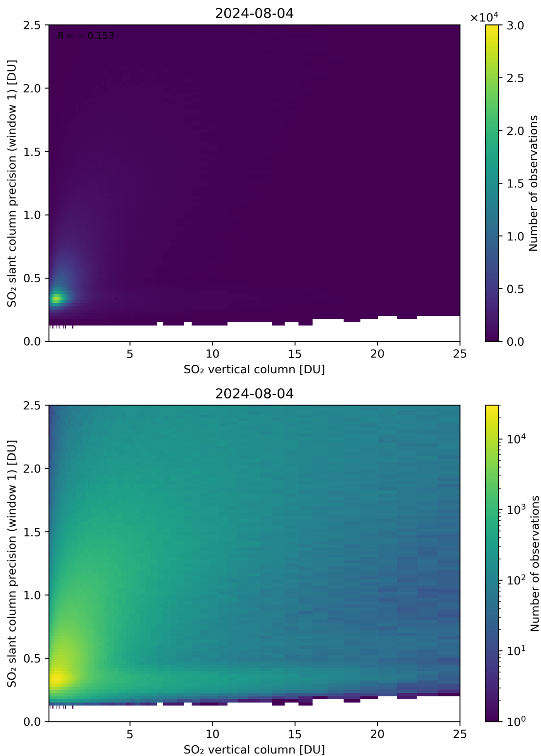
Figure 301: Scatter density plot of “SO 2 vertical column” against “SO 2 slant column precision (window 1)” for 2024-08-03 to 2024-08-05.
