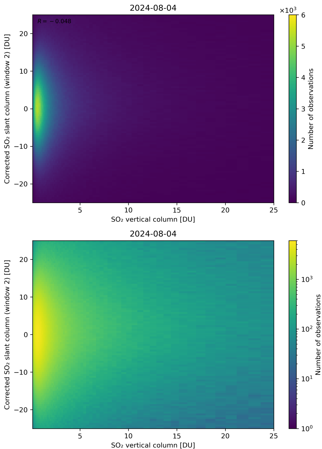
Figure 298: Scatter density plot of “SO 2 vertical column” against “Corrected SO 2 slant column (window 2)” for 2024-08-03 to 2024-08-05.
