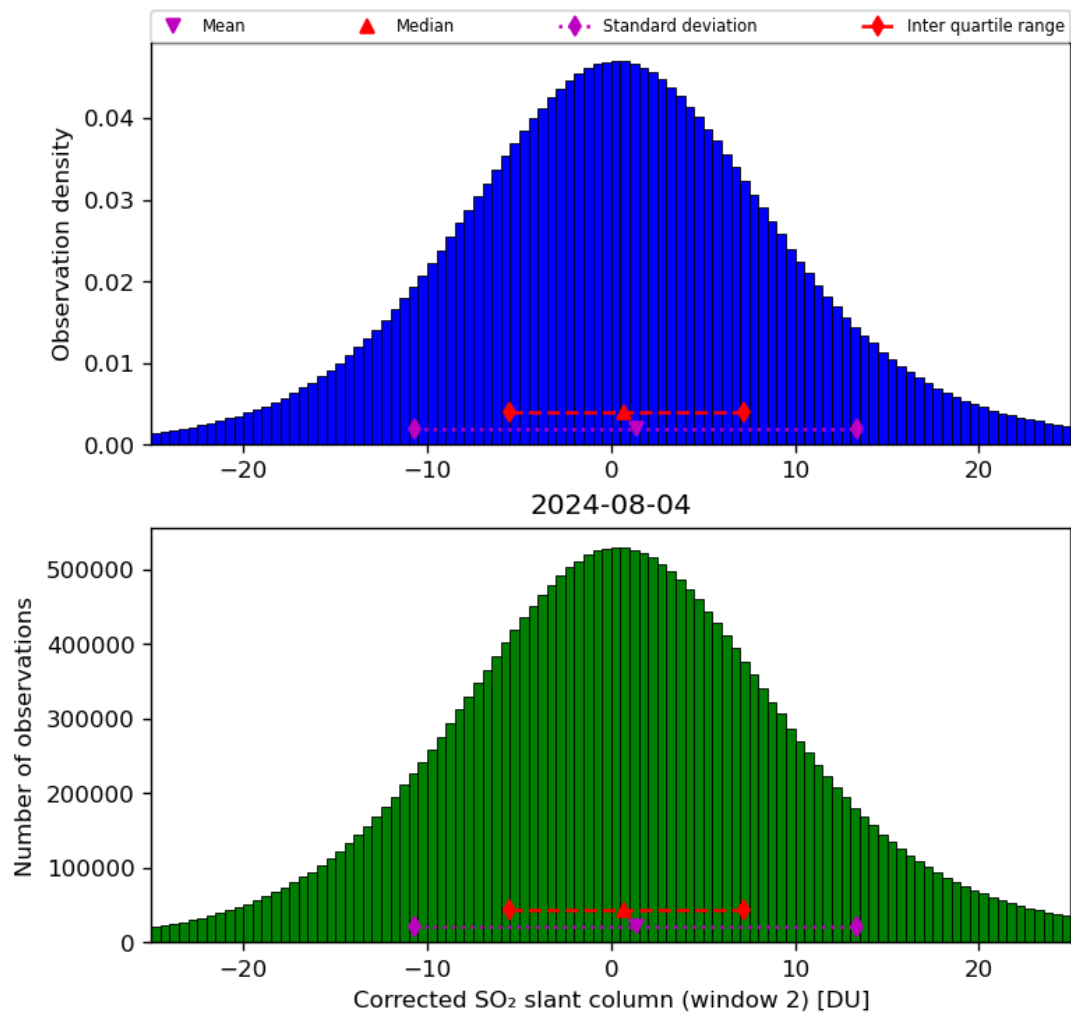
Figure 62: Histogram of “Corrected SO 2 slant column (window 2)” for 2024-08-03 to 2024-08-05
