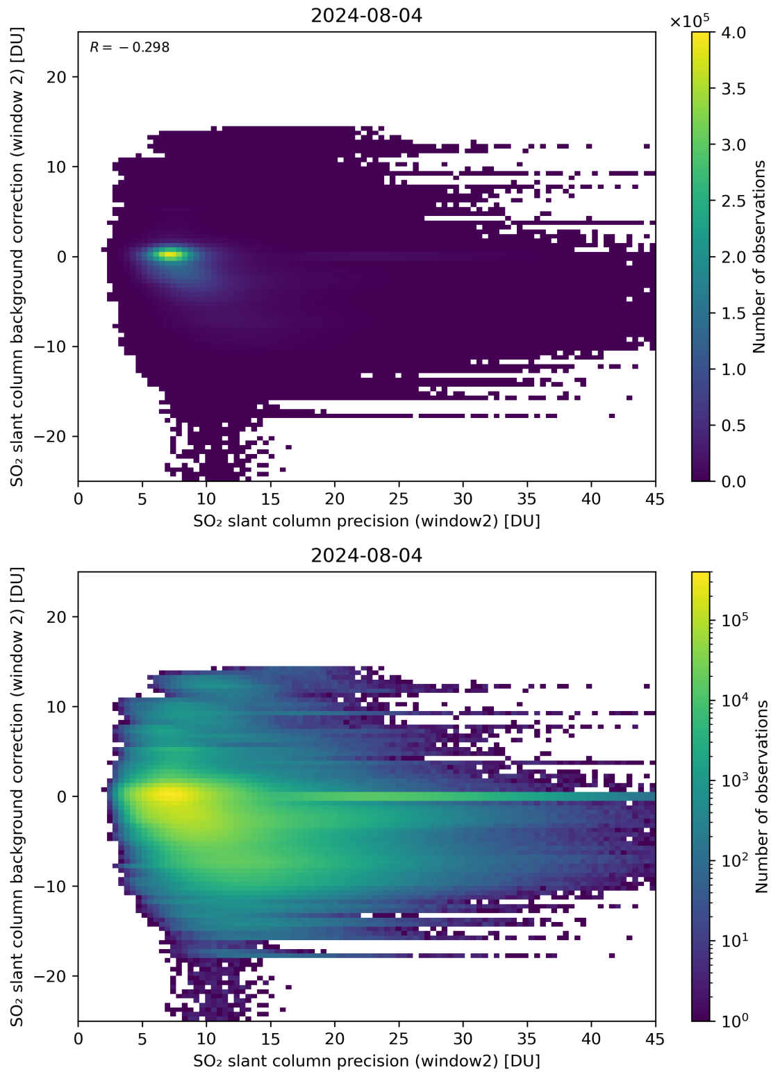
Figure 241: Scatter density plot of “SO 2 slant column precision (window2)” against “SO 2 slant column background correction (window 2)” for 2024-08-03 to 2024-08-05.
