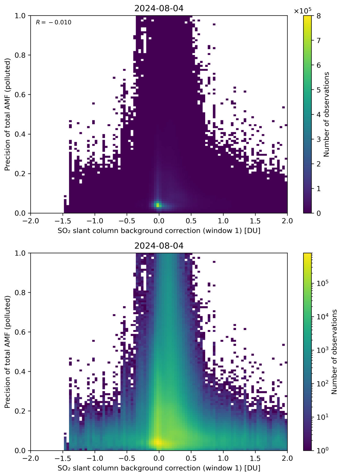
Figure 110: Scatter density plot of “SO 2 slant column background correction (window 1)” against “Precision of total AMF (polluted)” for 2024-08-03 to 2024-08-05.
