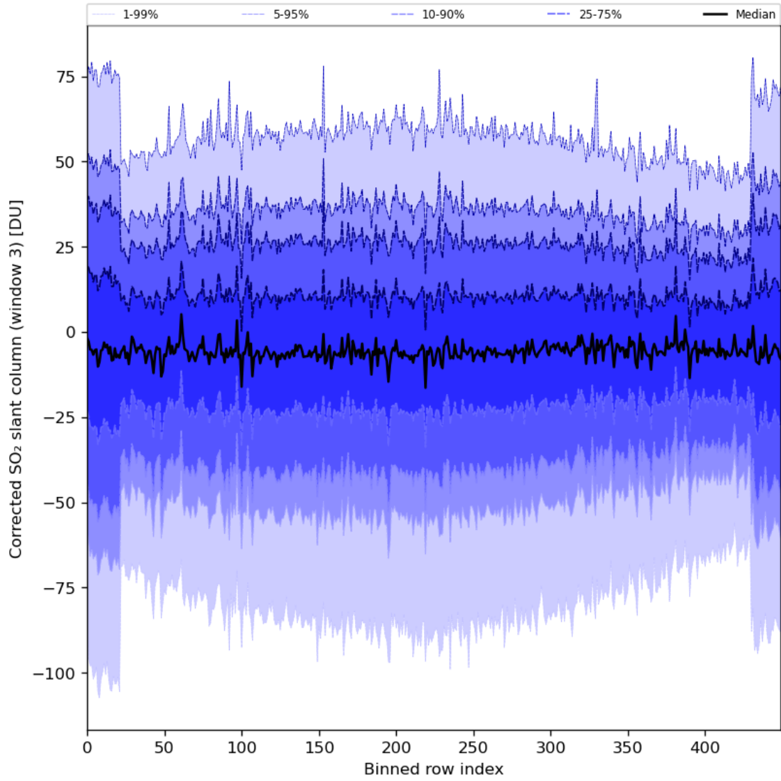
Figure 89: Along track statistics of “Corrected SO 2 slant column (window 3)” for 2024-08-03 to 2024-08-05
