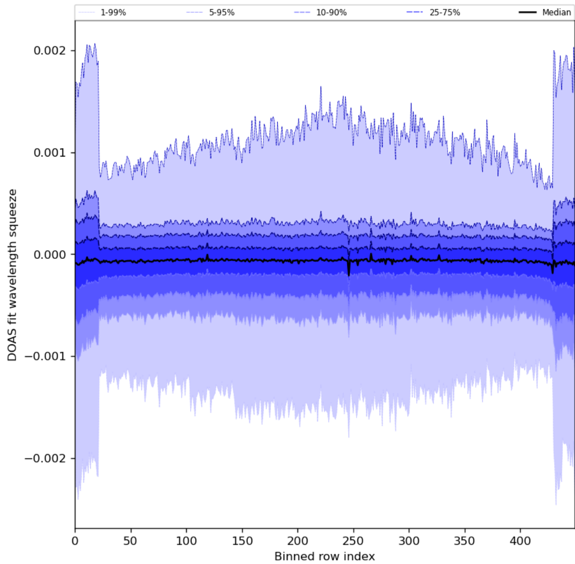
Figure 92: Along track statistics of “DOAS fit wavelength squeeze” for 2024-08-03 to 2024-08-05
