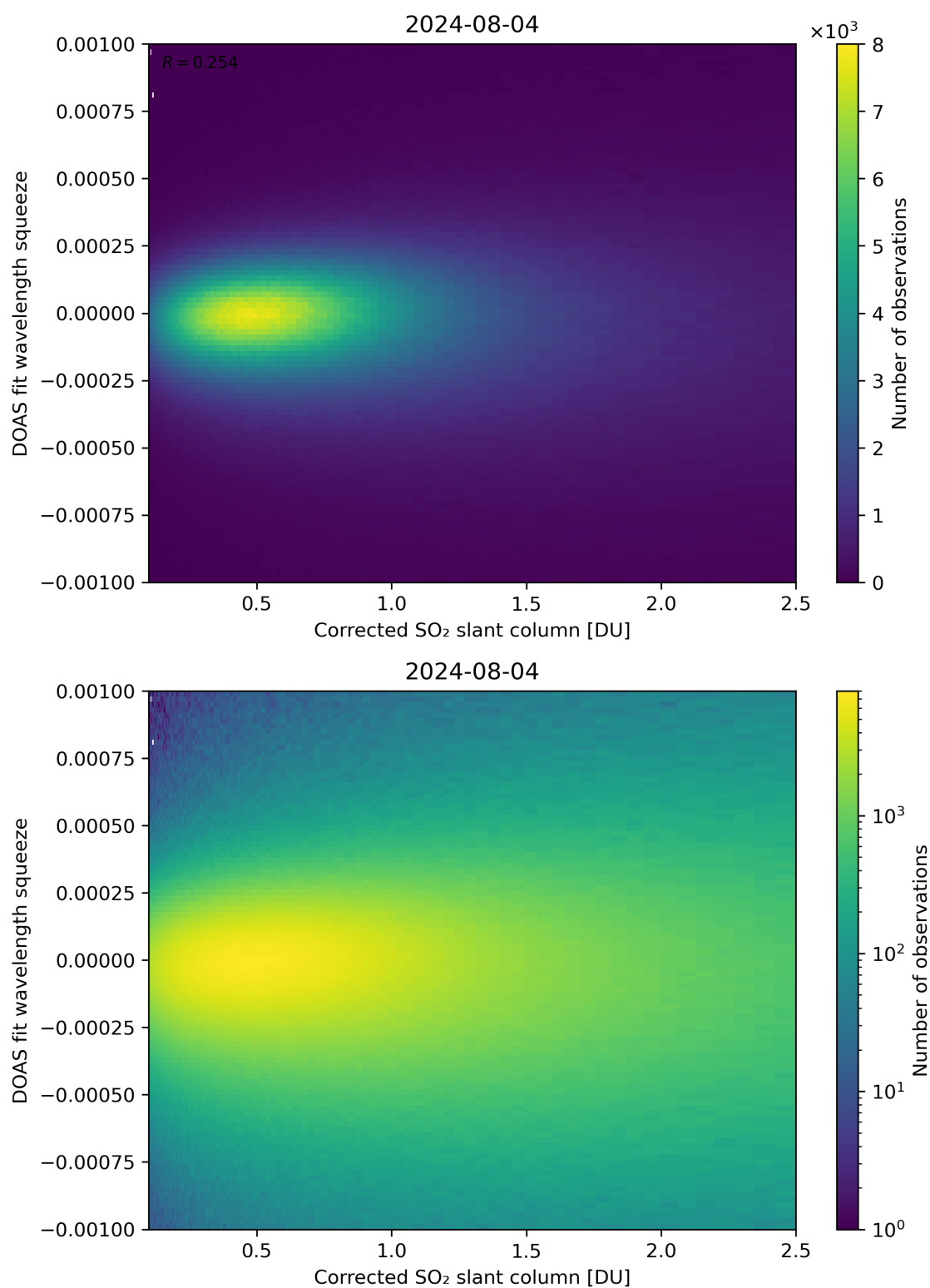
Figure 182: Scatter density plot of “Corrected SO 2 slant column” against “DOAS fit wavelength squeeze” for 2024-08-03 to 2024-08-05.
