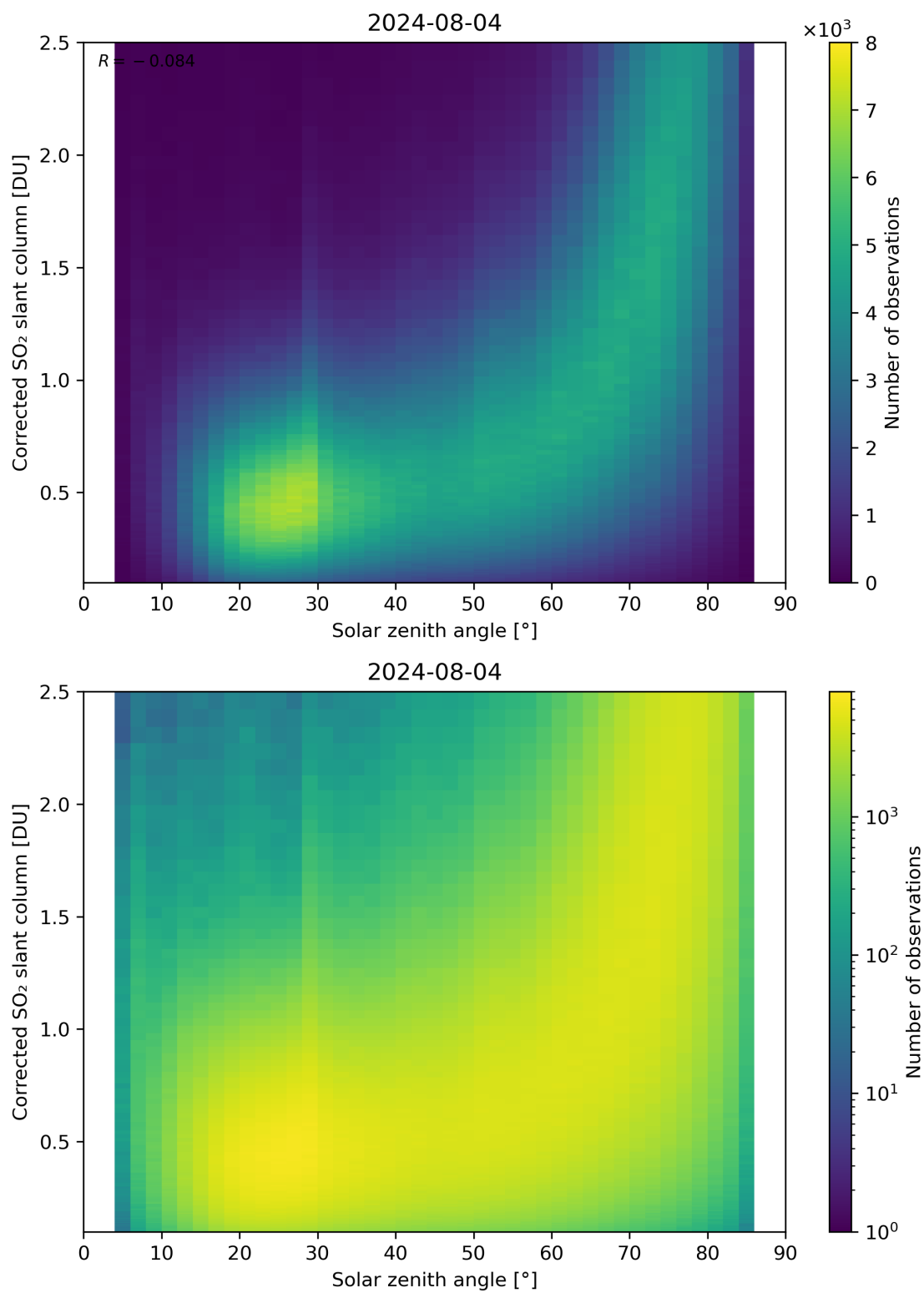
Figure 166: Scatter density plot of “Solar zenith angle” against “Corrected SO 2 slant column” for 2024-08-03 to 2024-08-05.
