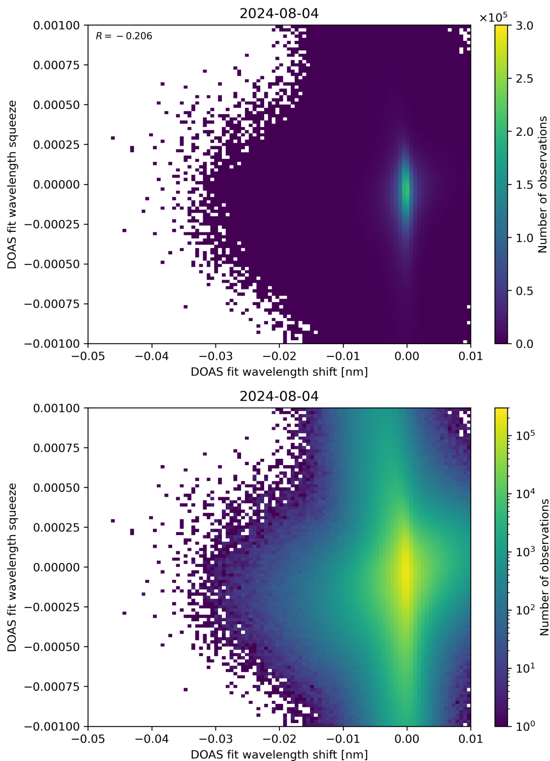
Figure 127: Scatter density plot of “DOAS fit wavelength shift” against “DOAS fit wavelength squeeze” for 2024-08-03 to 2024-08-05.
