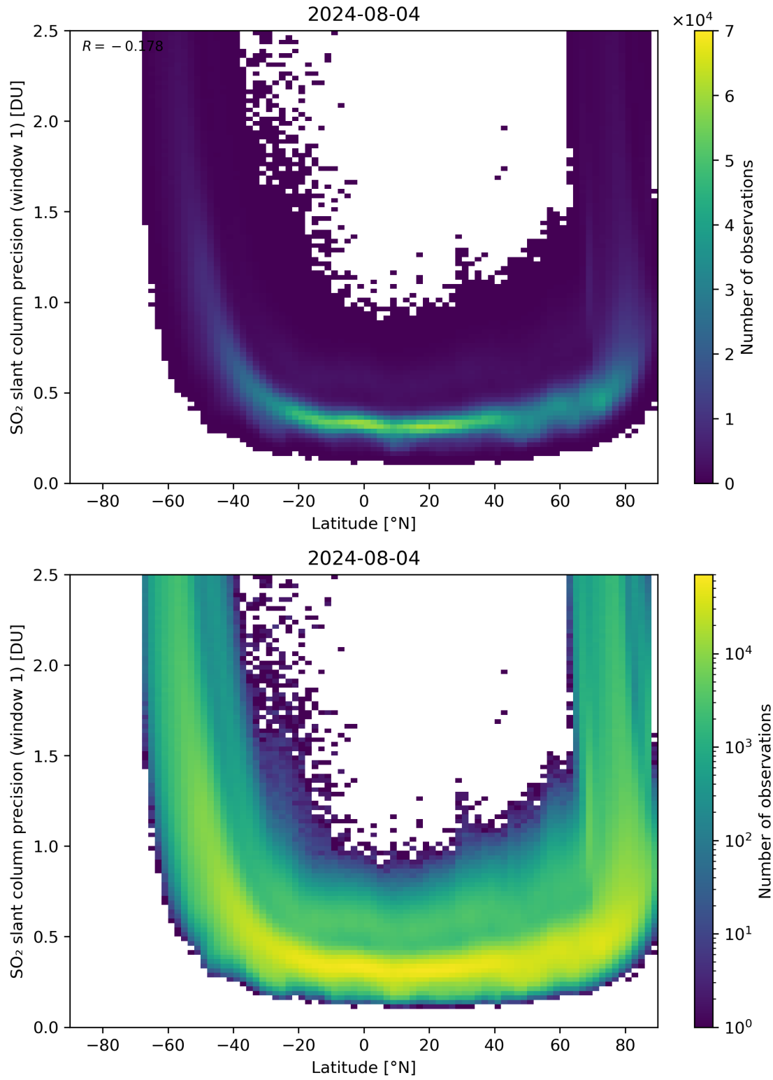
Figure 150: Scatter density plot of “Latitude” against “SO 2 slant column precision (window 1)” for 2024-08-03 to 2024-08-05.
