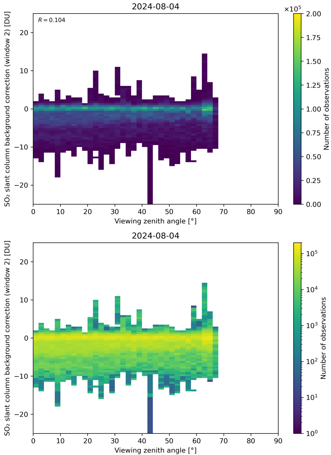
Figure 309: Scatter density plot of “Viewing zenith angle” against “SO 2 slant column background correction (window 2)” for 2024-08-03 to 2024-08-05.
