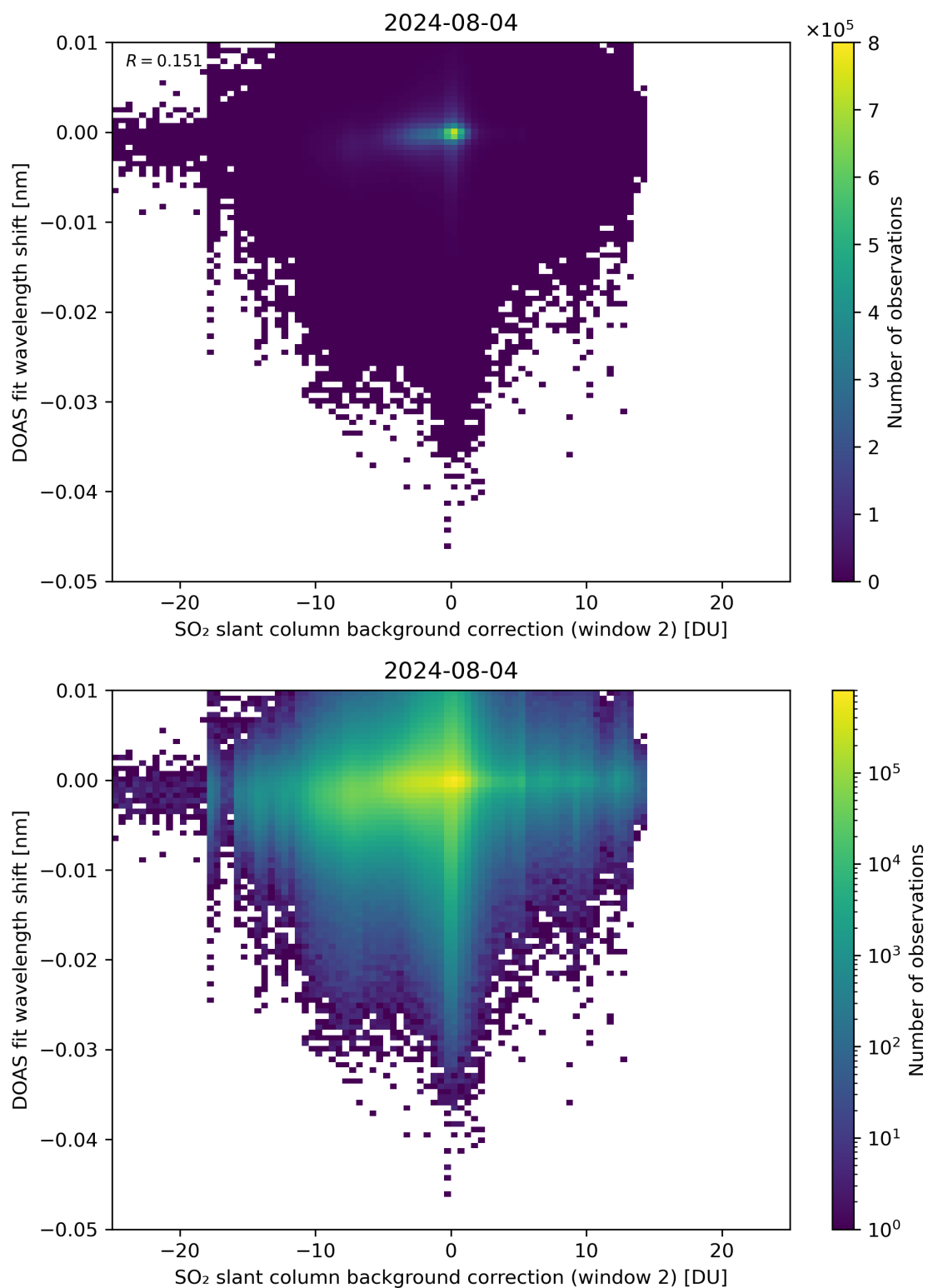
Figure 112: Scatter density plot of “SO 2 slant column background correction (window 2)” against “DOAS fit wavelength shift” for 2024-08-03 to 2024-08-05.
