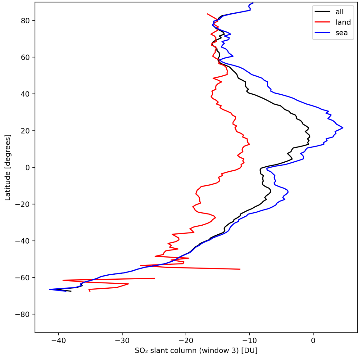
Figure 41: Zonal average of “SO 2 slant column (window 3)” for 2024-08-03 to 2024-08-05.
