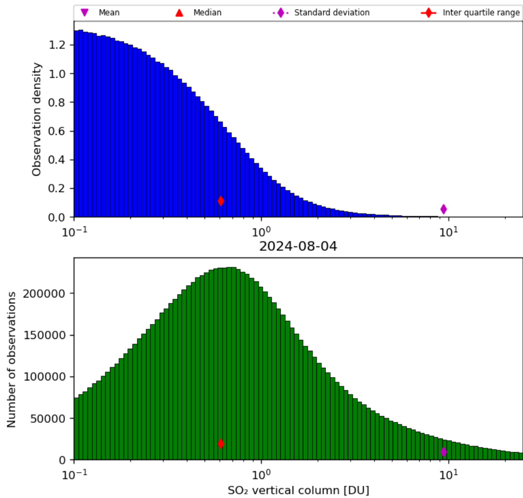
Figure 53: Histogram of “SO 2 vertical column” for 2024-08-03 to 2024-08-05
