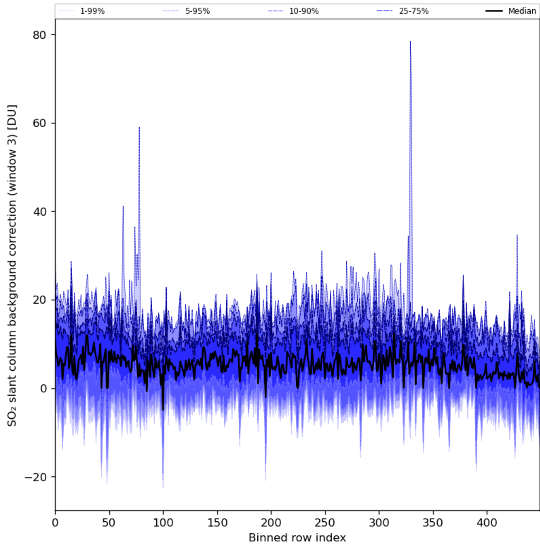
Figure 90: Along track statistics of “SO 2 slant column background correction (window 3)” for 2024-08-03 to 2024-08-05
