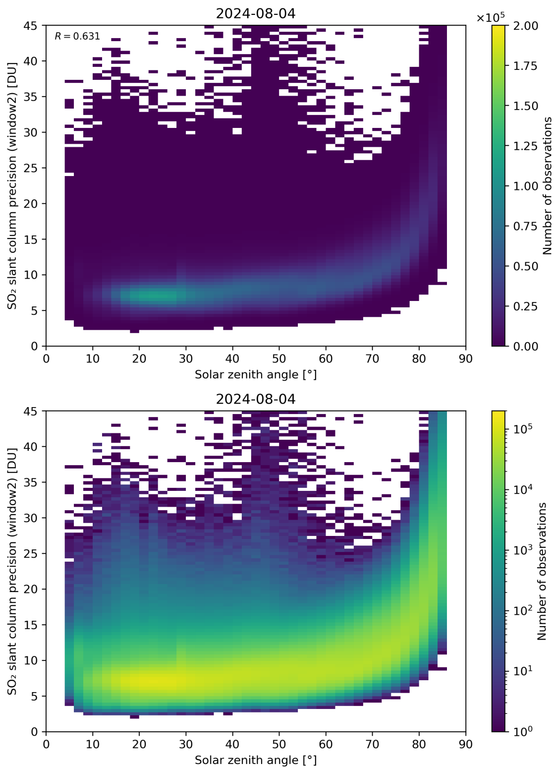
Figure 171: Scatter density plot of “Solar zenith angle” against “SO 2 slant column precision (window2)” for 2024-08-03 to 2024-08-05.
