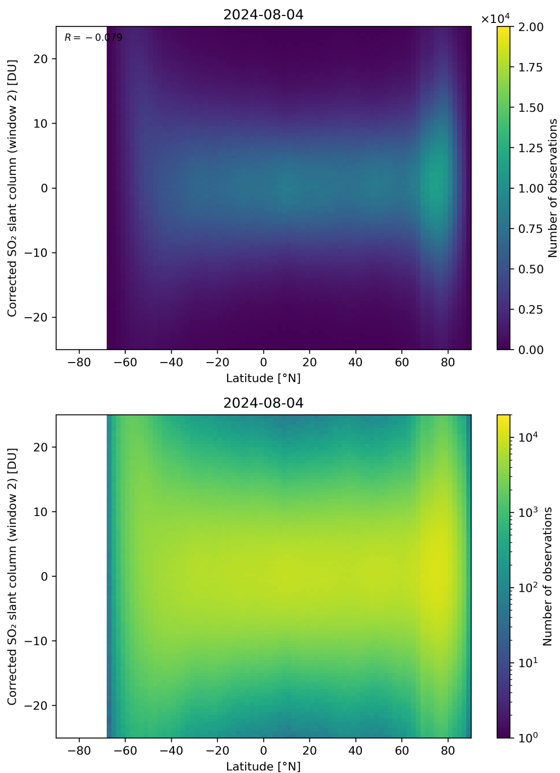
Figure 147: Scatter density plot of “Latitude” against “Corrected SO 2 slant column (window 2)” for 2024-08-03 to 2024-08-05.
