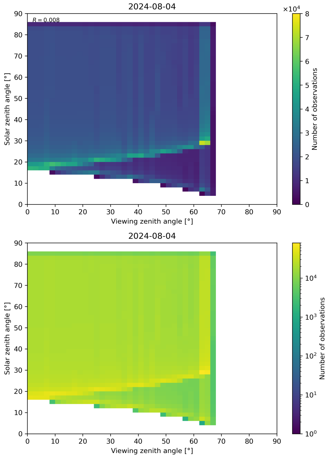
Figure 315: Scatter density plot of “Viewing zenith angle” against “Solar zenith angle” for 2024-08-03 to 2024-08-05.
