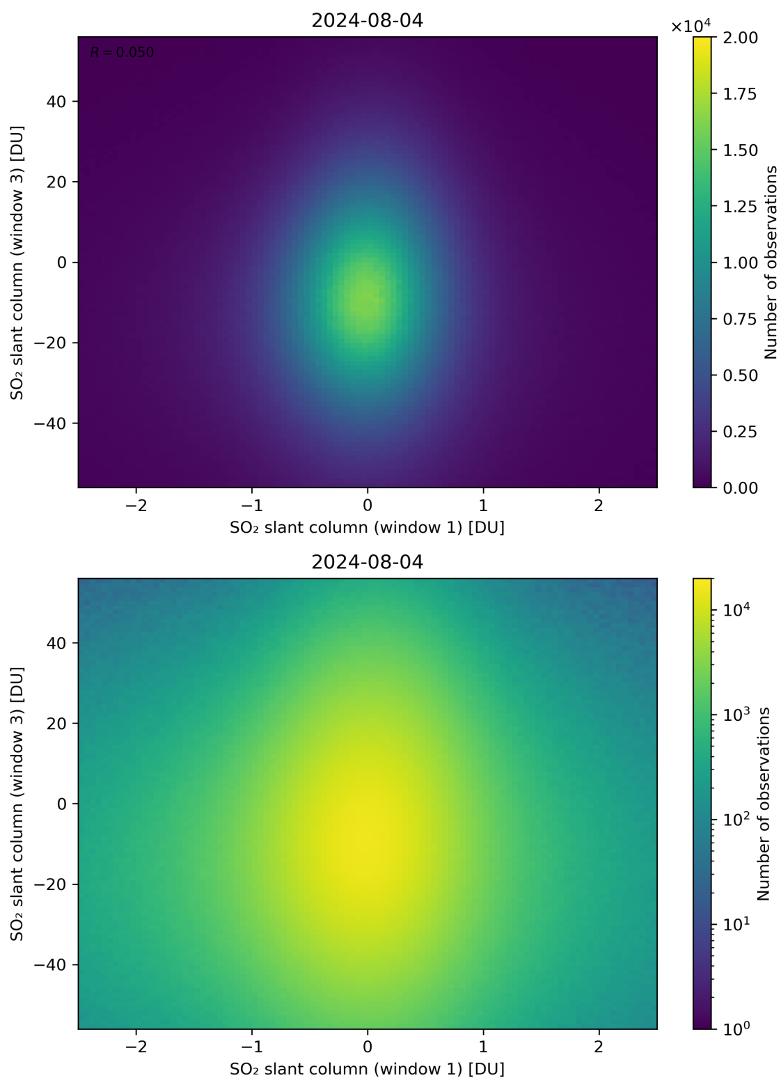
Figure 237: Scatter density plot of “SO 2 slant column (window 1)” against “SO 2 slant column (window 3)” for 2024-08-03 to 2024-08-05.
