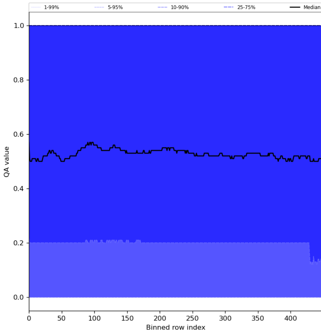
Figure 75: Along track statistics of “QA value” for 2024-08-03 to 2024-08-05
