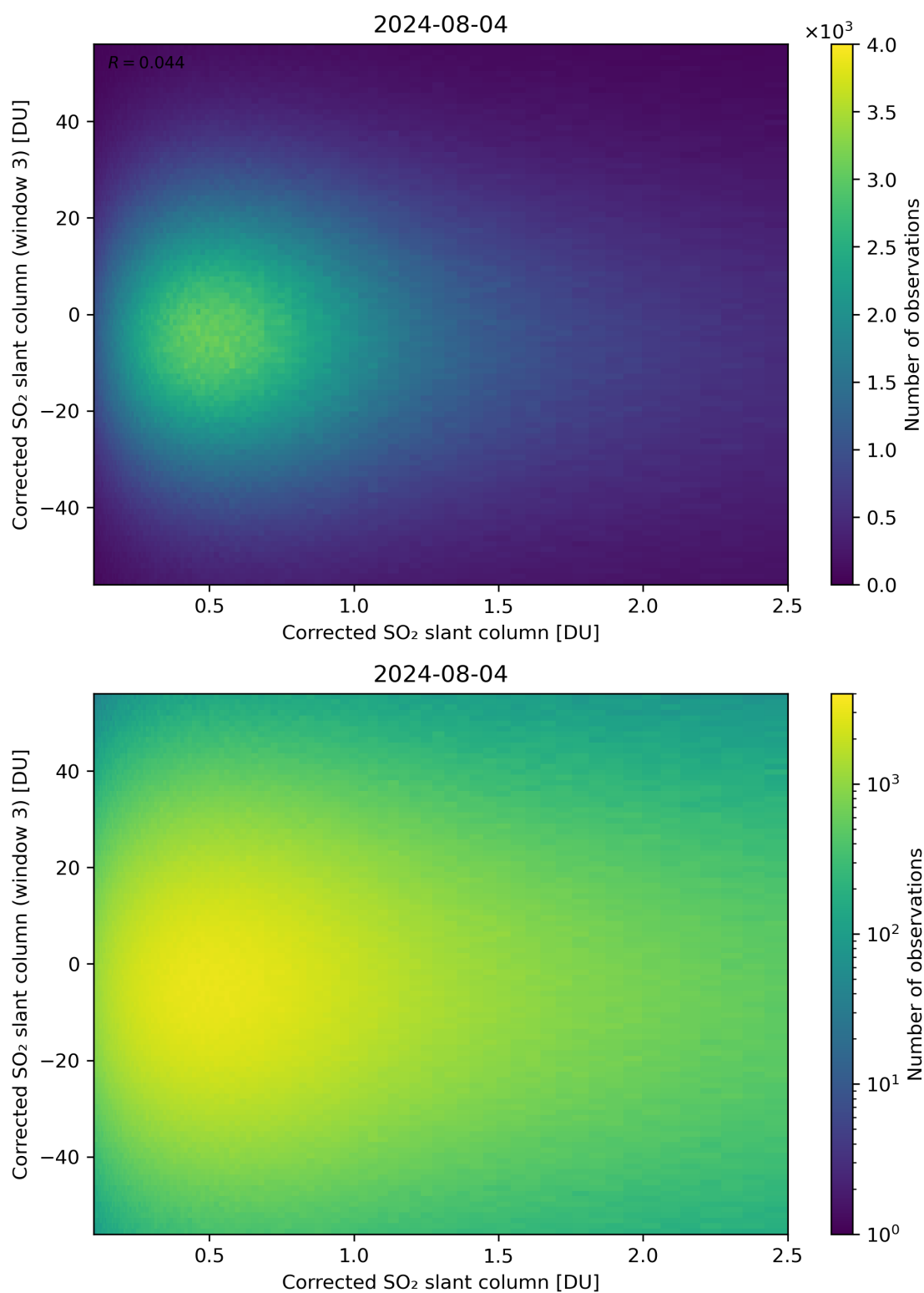
Figure 186: Scatter density plot of “Corrected SO 2 slant column” against “Corrected SO 2 slant column (window 3)” for 2024-08-03 to 2024-08-05.
