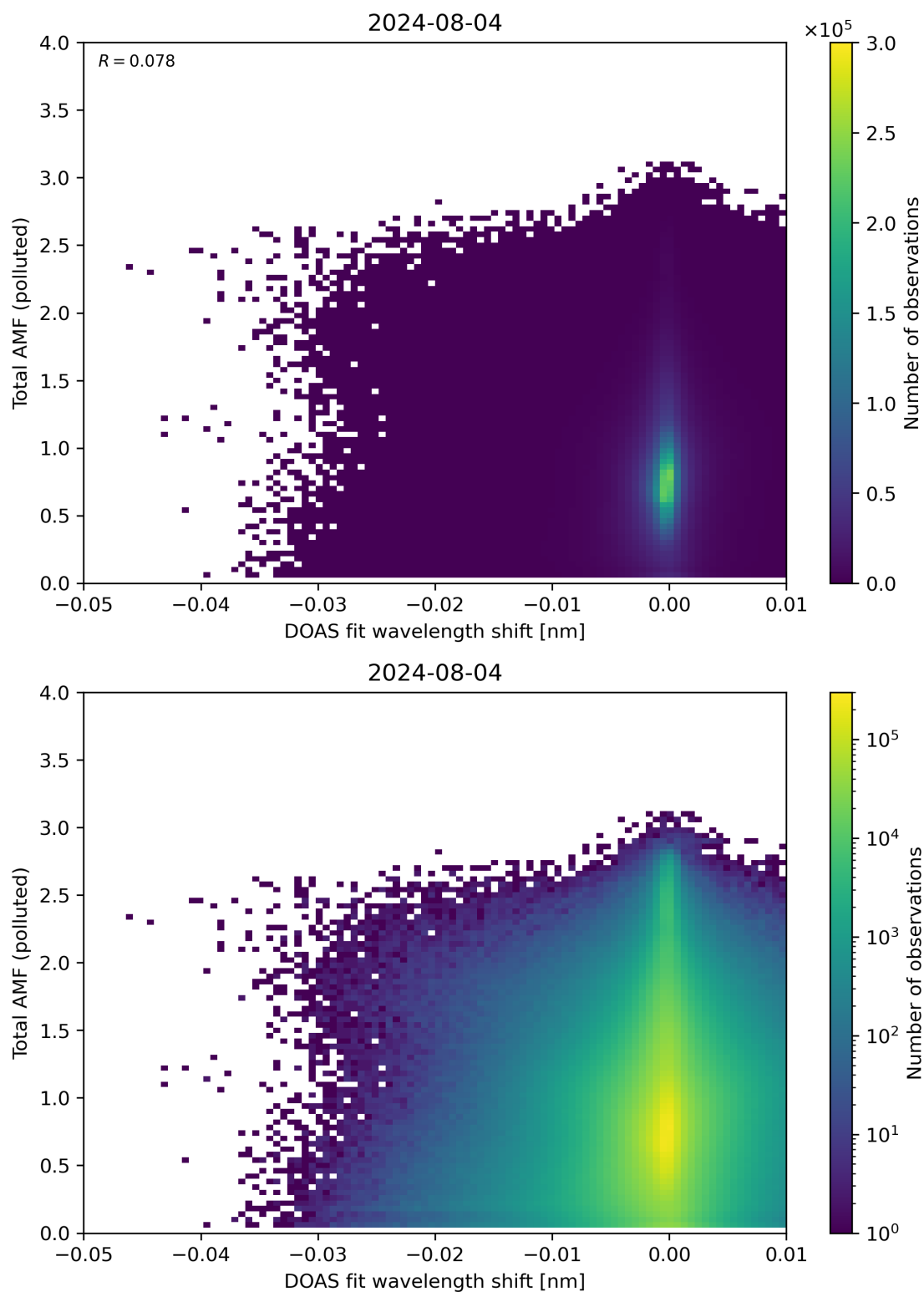
Figure 130: Scatter density plot of “DOAS fit wavelength shift” against “Total AMF (polluted)” for 2024-08-03 to 2024-08-05.
