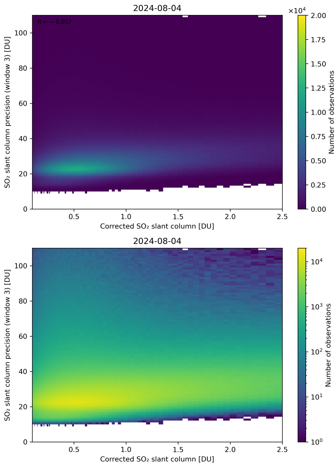
Figure 191: Scatter density plot of “Corrected SO 2 slant column” against “SO 2 slant column precision (window 3)” for 2024-08-03 to 2024-08-05.
