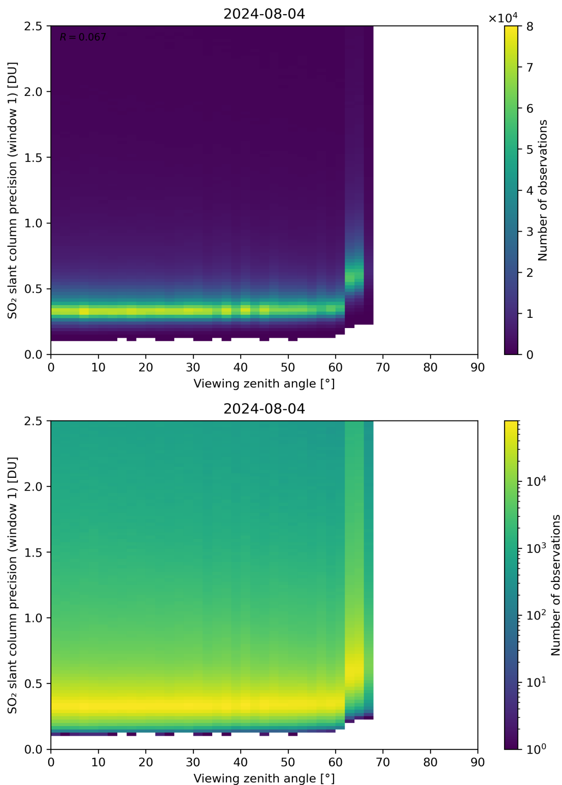
Figure 321: Scatter density plot of “Viewing zenith angle” against “SO 2 slant column precision (window 1)” for 2024-08-03 to 2024-08-05.
