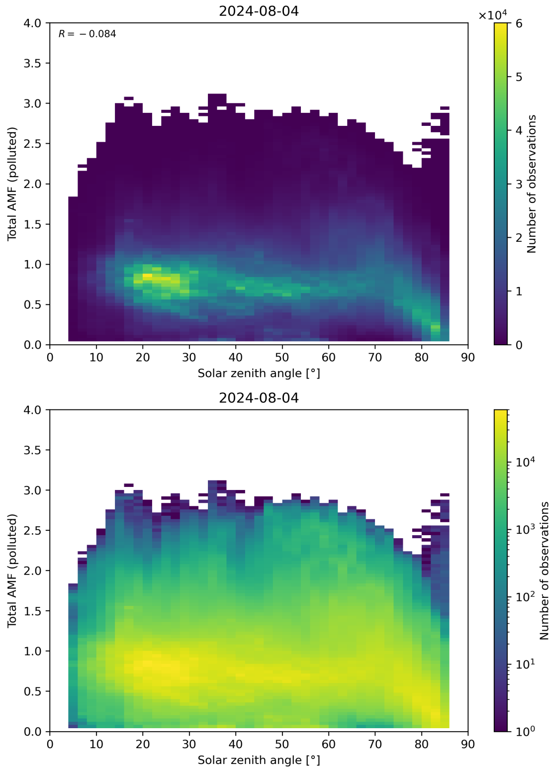
Figure 174: Scatter density plot of “Solar zenith angle” against “Total AMF (polluted)” for 2024-08-03 to 2024-08-05.
