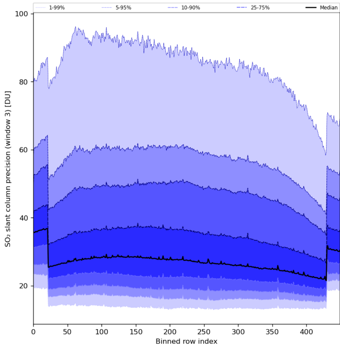
Figure 88: Along track statistics of “SO 2 slant column precision (window 3)” for 2024-08-03 to 2024-08-05
