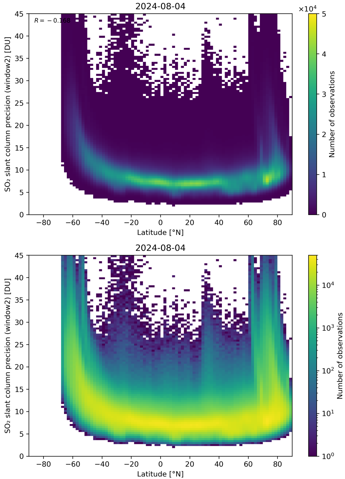
Figure 151: Scatter density plot of “Latitude” against “SO 2 slant column precision (window2)” for 2024-08-03 to 2024-08-05.
