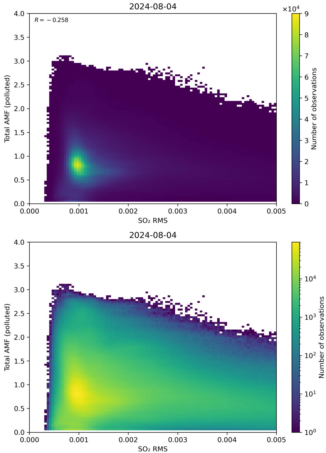
Figure 137: Scatter density plot of “SO 2 RMS” against “Total AMF (polluted)” for 2024-08-03 to 2024-08-05.
