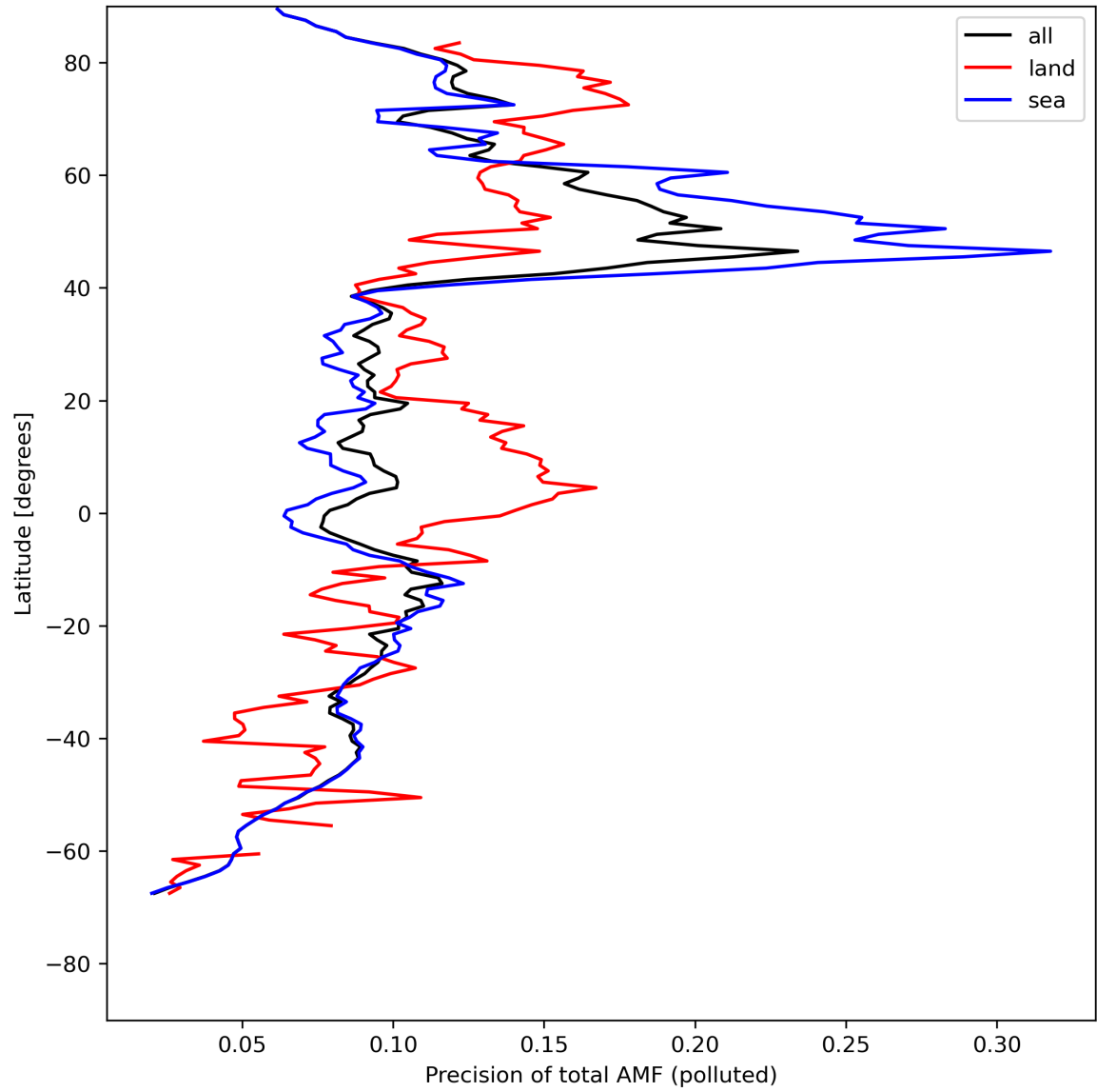
Figure 49: Zonal average of “Precision of total AMF (polluted)” for 2024-08-03 to 2024-08-05.
