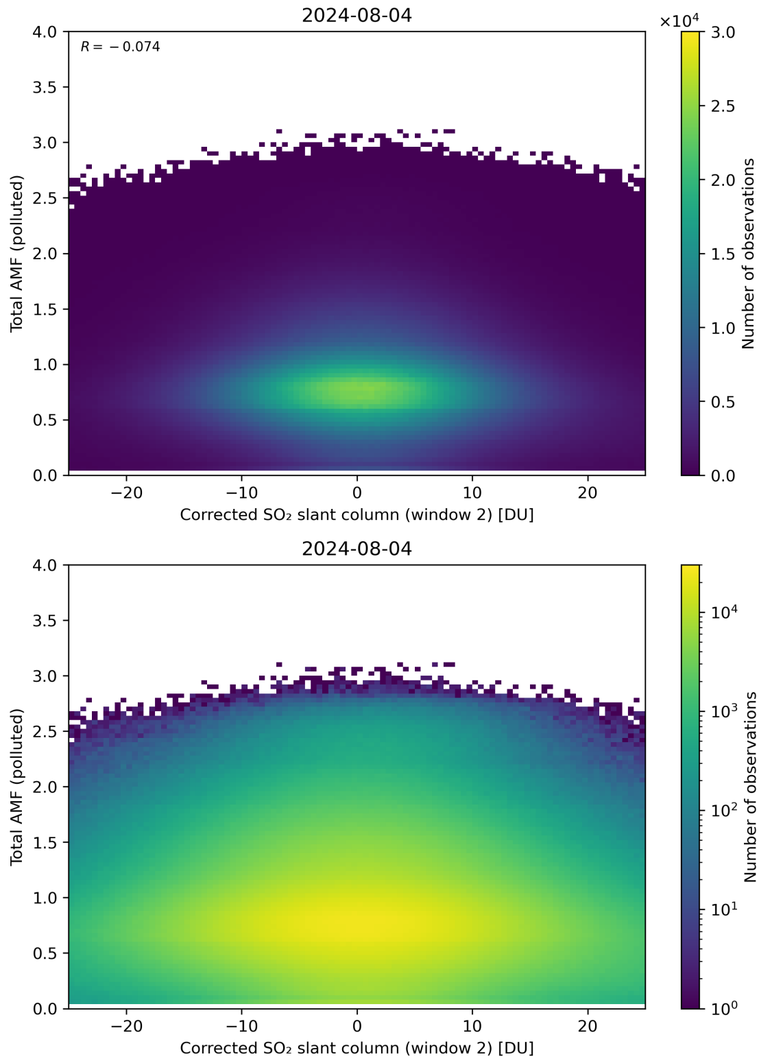
Figure 203: Scatter density plot of “Corrected SO 2 slant column (window 2)” against “Total AMF (polluted)” for 2024-08-03 to 2024-08-05.
