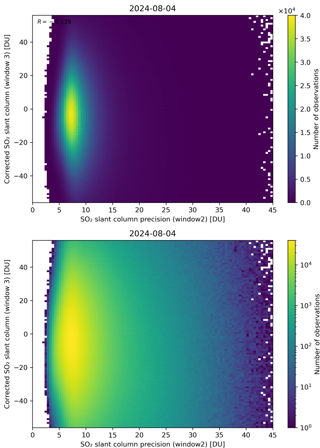
Figure 248: Scatter density plot of “SO 2 slant column precision (window2)” against “Corrected SO 2 slant column (window 3)” for 2024-08-03 to 2024-08-05.
