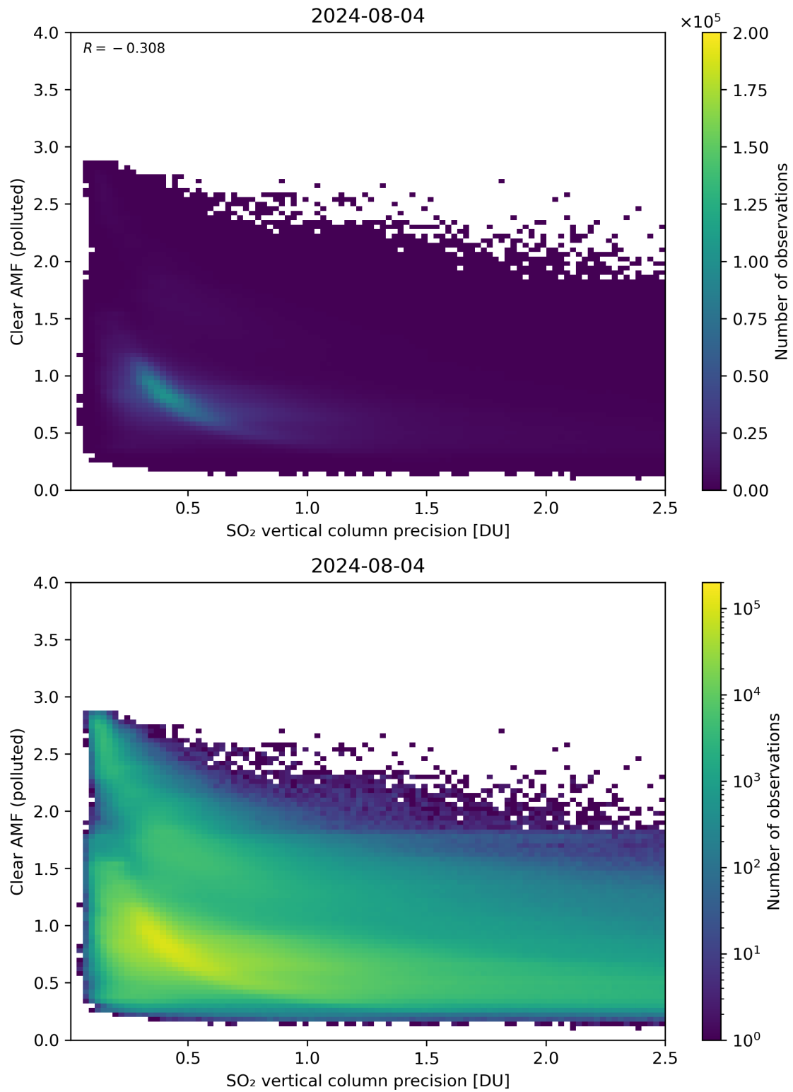
Figure 285: Scatter density plot of “SO 2 vertical column precision” against “Clear AMF (polluted)” for 2024-08-03 to 2024-08-05.
