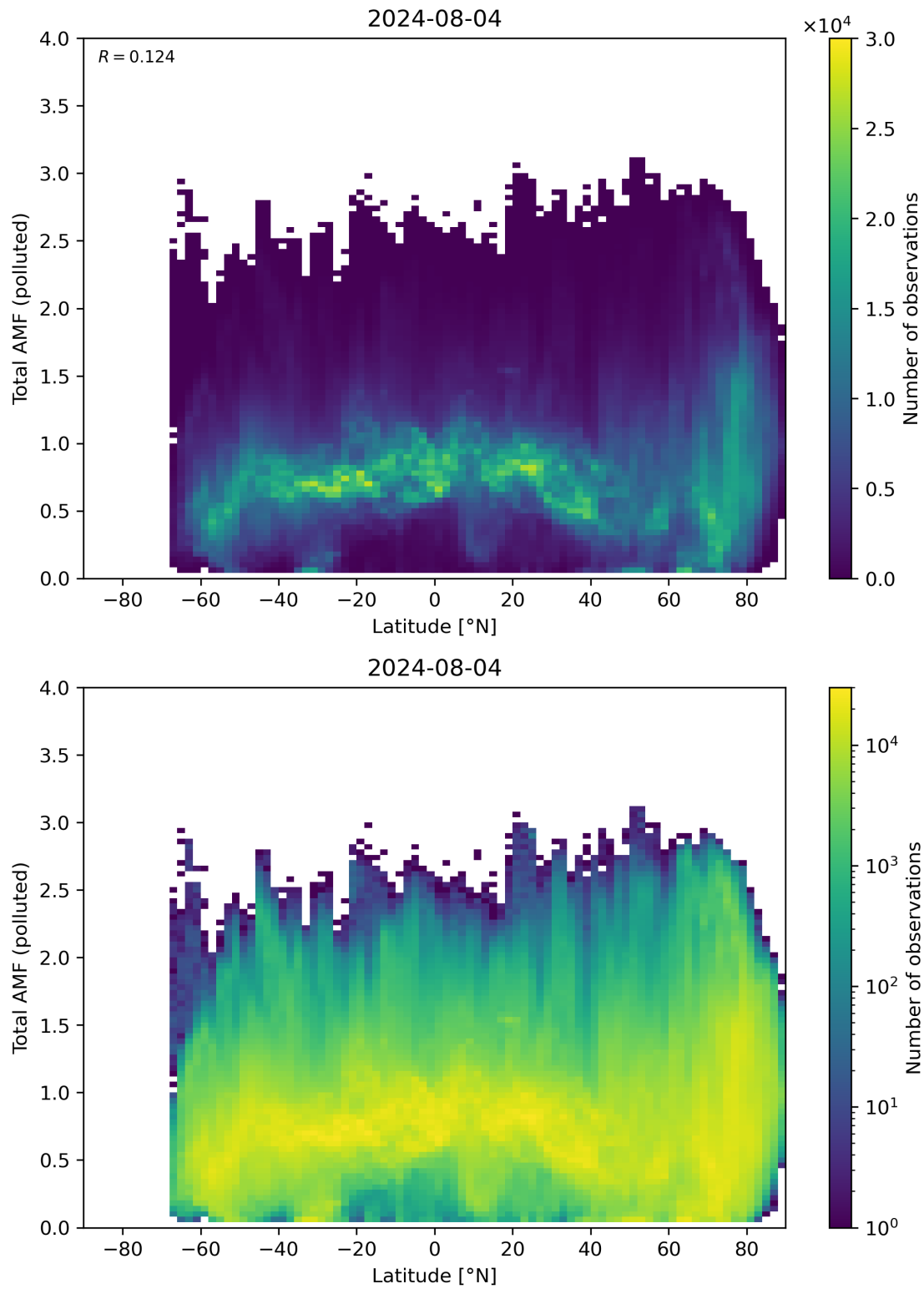
Figure 154: Scatter density plot of “Latitude” against “Total AMF (polluted)” for 2024-08-03 to 2024-08-05.
