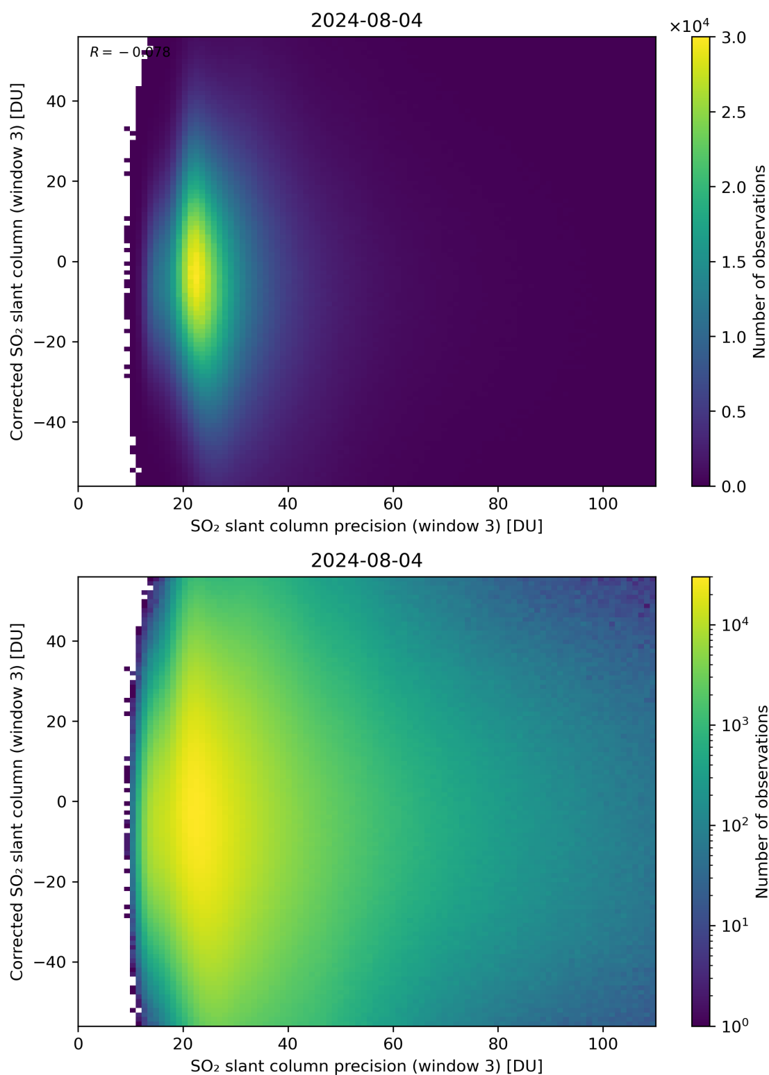
Figure 262: Scatter density plot of “SO 2 slant column precision (window 3)” against “Corrected SO 2 slant column (window 3)” for 2024-08-03 to 2024-08-05.
