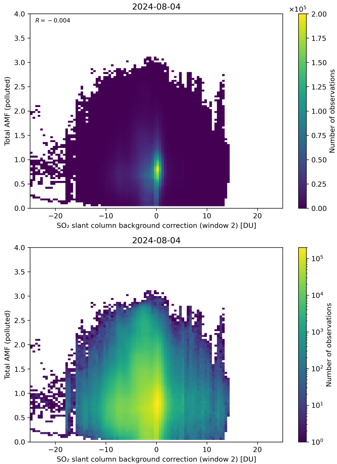
Figure 119: Scatter density plot of “SO 2 slant column background correction (window 2)” against “Total AMF (polluted)” for 2024-08-03 to 2024-08-05.
