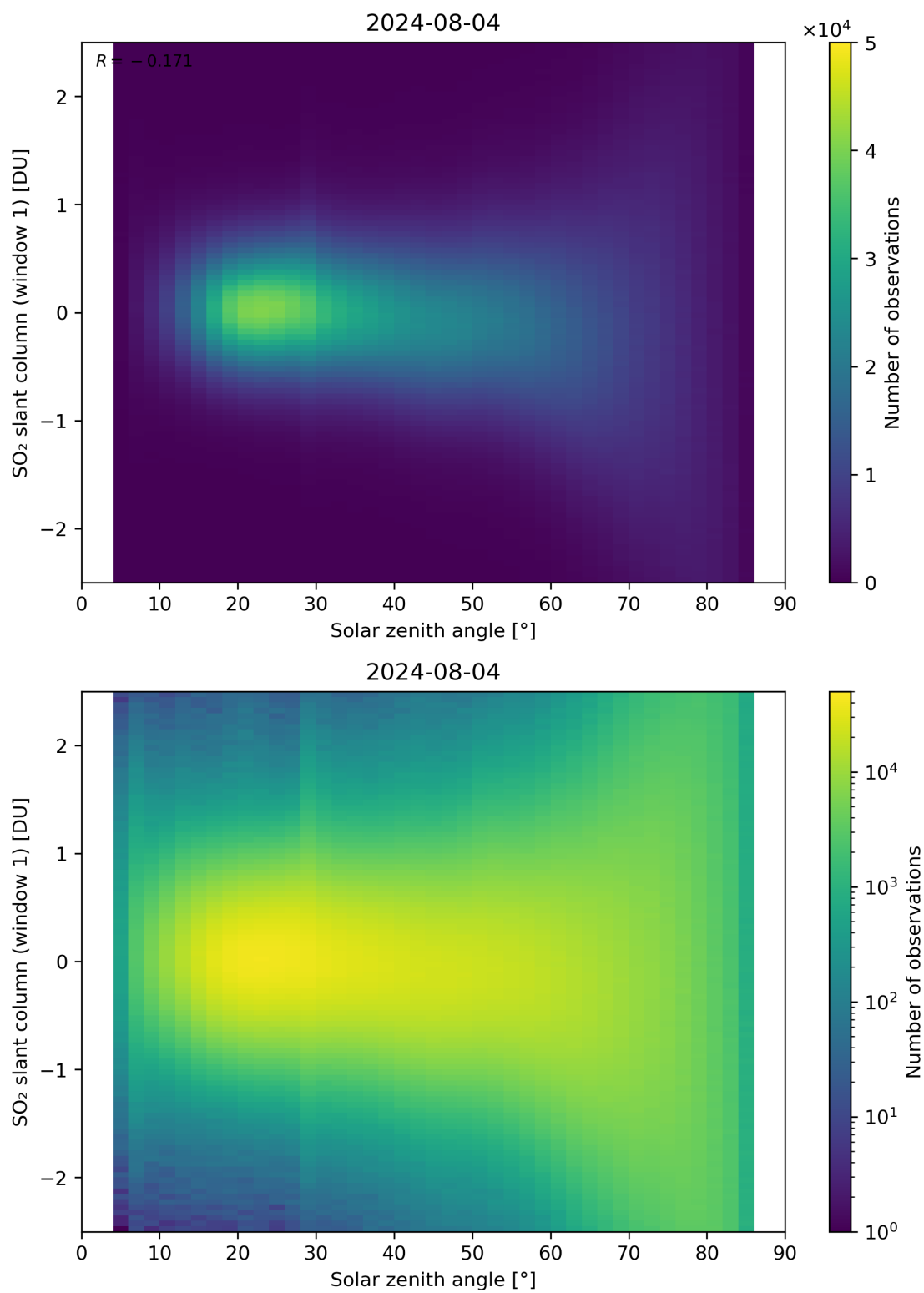
Figure 169: Scatter density plot of “Solar zenith angle” against “SO 2 slant column (window 1)” for 2024-08-03 to 2024-08-05.
