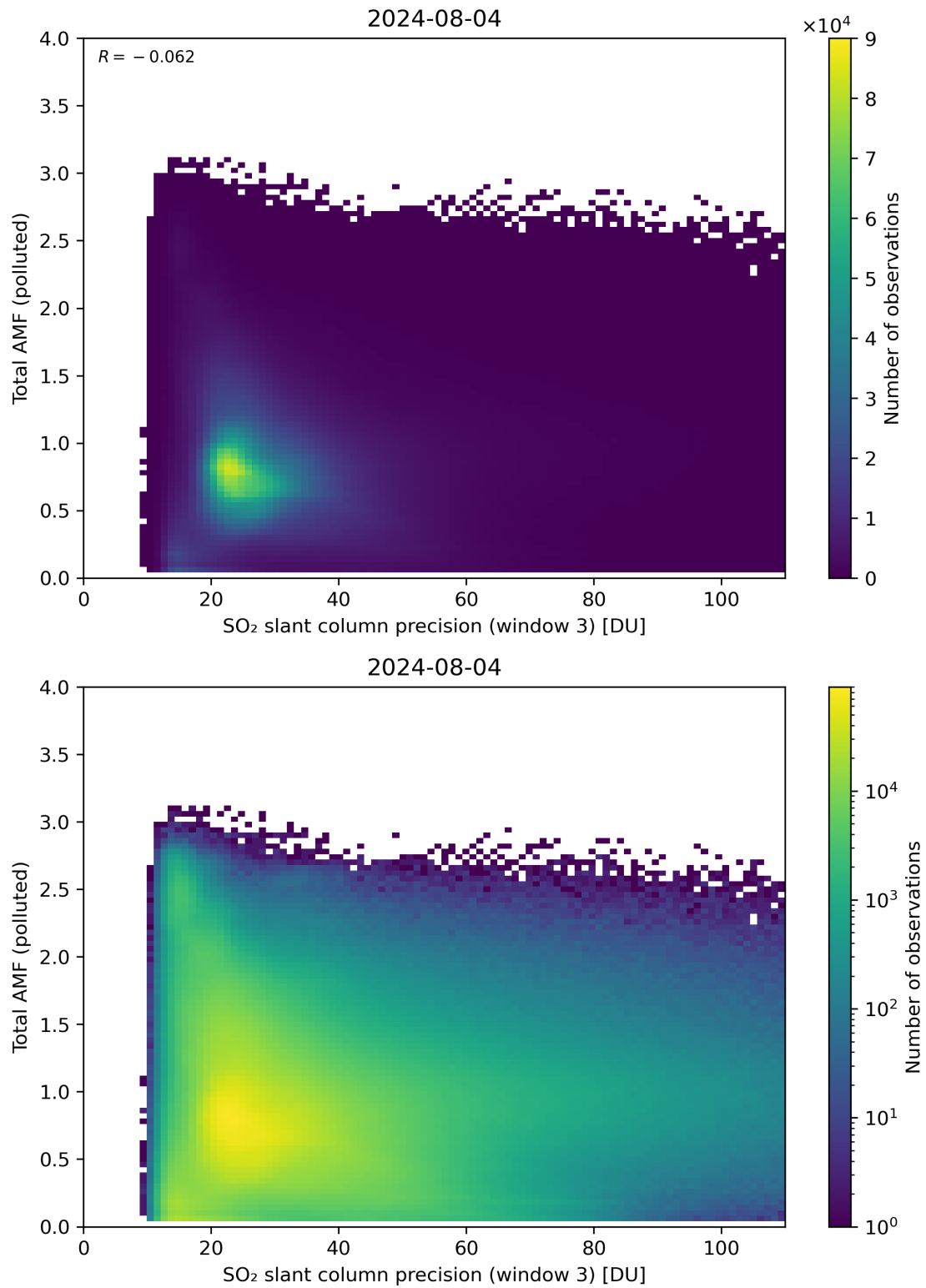
Figure 263: Scatter density plot of “SO 2 slant column precision (window 3)” against “Total AMF (polluted)” for 2024-08-03 to 2024-08-05.
