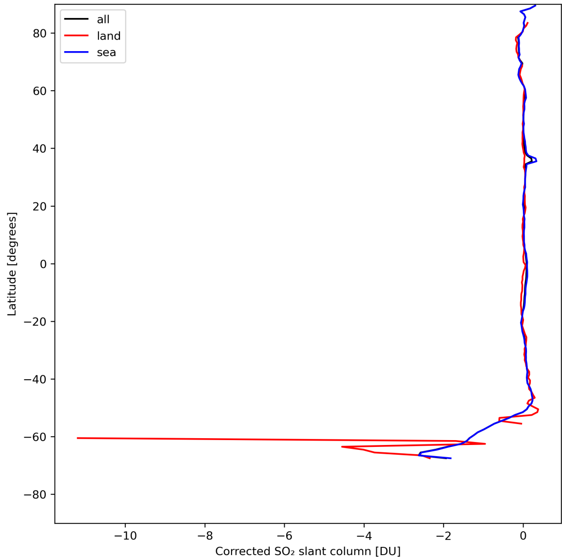
Figure 32: Zonal average of “Corrected SO 2 slant column” for 2024-08-03 to 2024-08-05.
