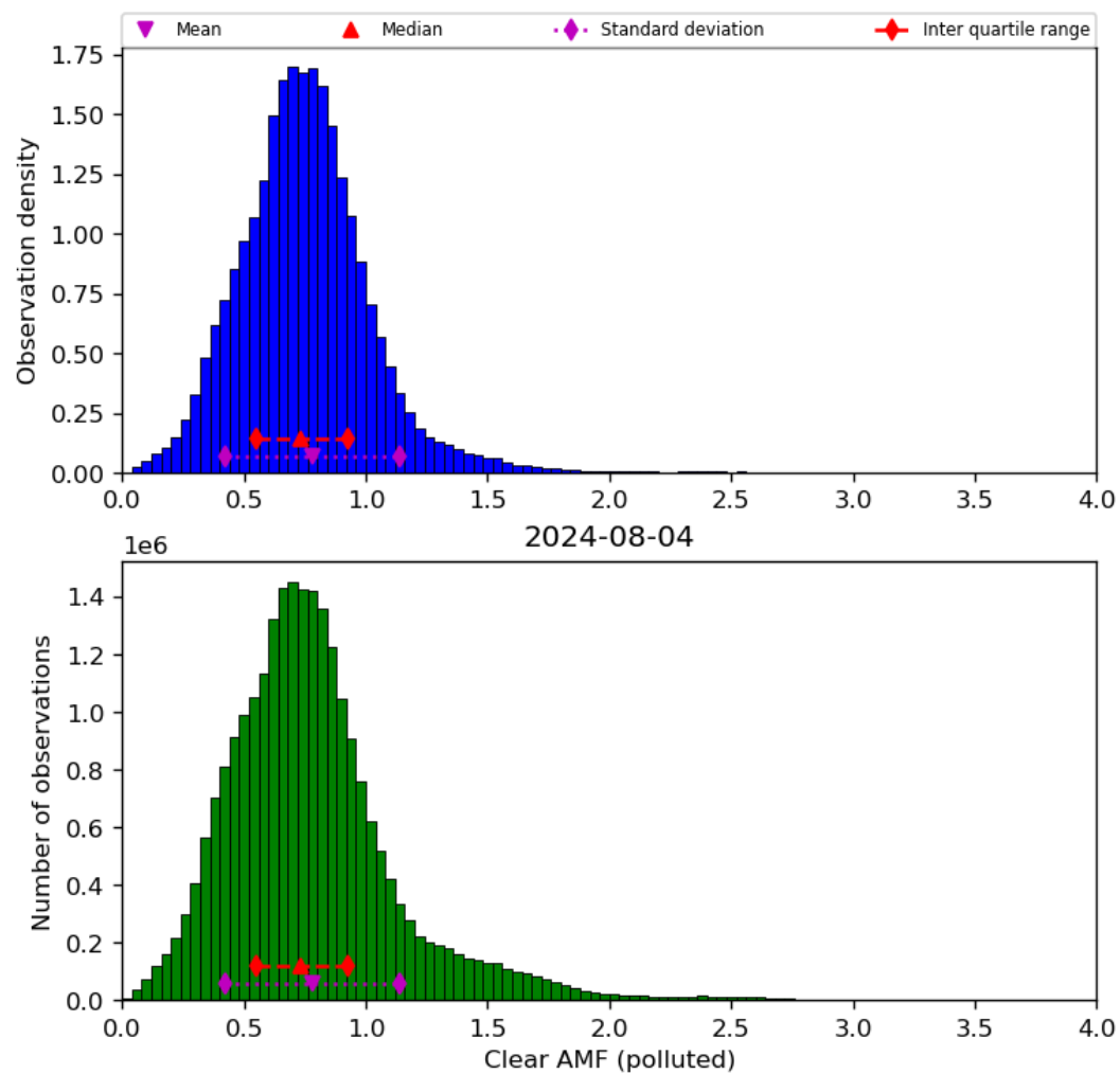
Figure 73: Histogram of “Clear AMF (polluted)” for 2024-08-03 to 2024-08-05
