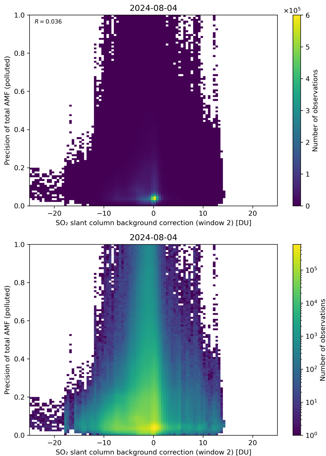
Figure 120: Scatter density plot of “SO 2 slant column background correction (window 2)” against “Precision of total AMF (polluted)” for 2024-08-03 to 2024-08-05.
