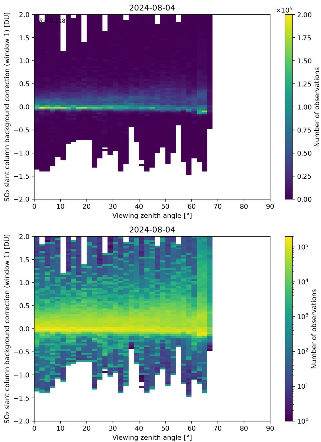
Figure 308: Scatter density plot of “Viewing zenith angle” against “SO 2 slant column background correction (window 1)” for 2024-08-03 to 2024-08-05.
