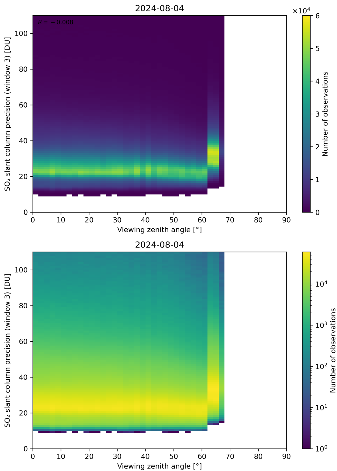
Figure 324: Scatter density plot of “Viewing zenith angle” against “SO 2 slant column precision (window 3)” for 2024-08-03 to 2024-08-05.
