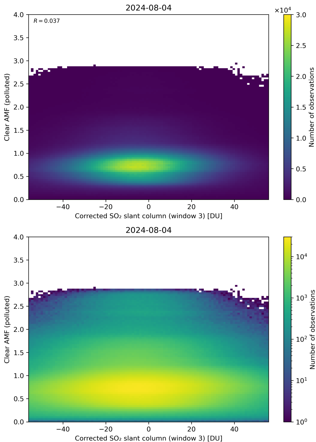
Figure 209: Scatter density plot of “Corrected SO 2 slant column (window 3)” against “Clear AMF (polluted)” for 2024-08-03 to 2024-08-05.
