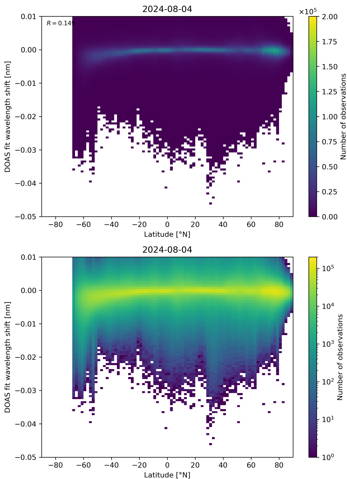
Figure 142: Scatter density plot of “Latitude” against “DOAS fit wavelength shift” for 2024-08-03 to 2024-08-05.
