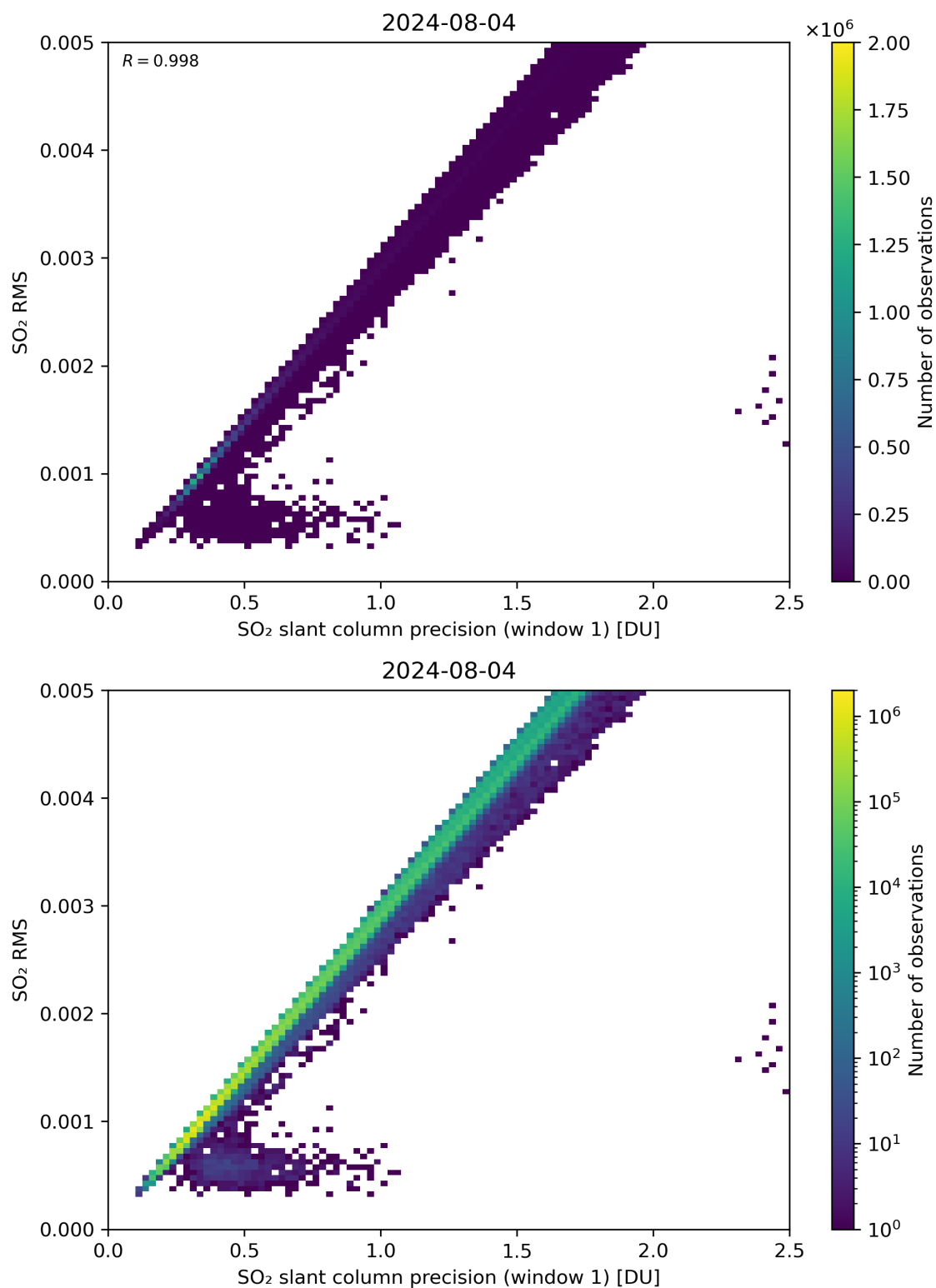
Figure 223: Scatter density plot of “SO 2 slant column precision (window 1)” against “SO 2 RMS” for 2024-08-03 to 2024-08-05.
