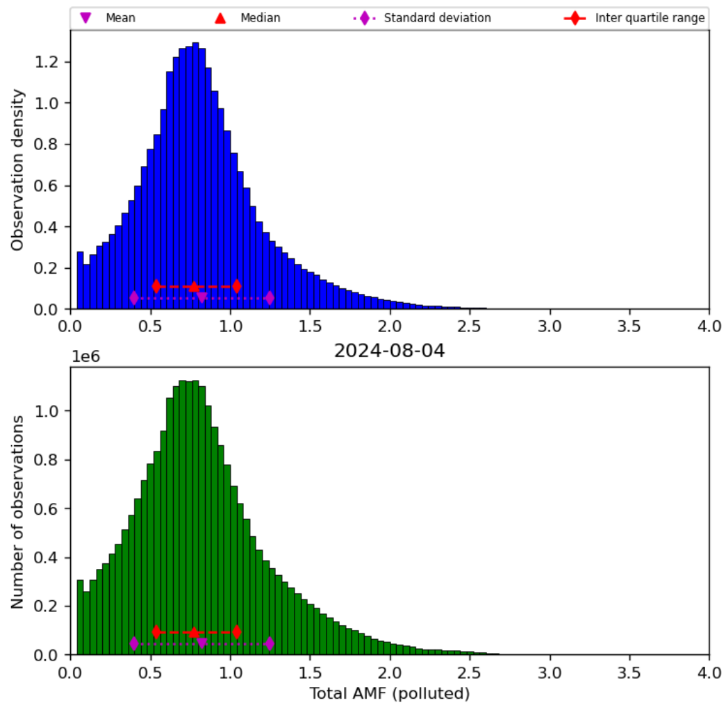
Figure 71: Histogram of “Total AMF (polluted)” for 2024-08-03 to 2024-08-05
