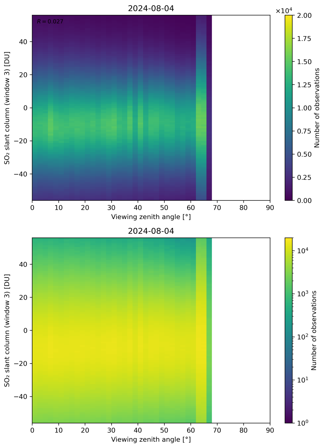
Figure 323: Scatter density plot of “Viewing zenith angle” against “SO 2 slant column (window 3)” for 2024-08-03 to 2024-08-05.
