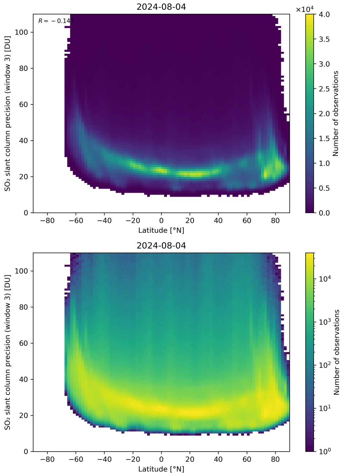
Figure 153: Scatter density plot of “Latitude” against “SO 2 slant column precision (window 3)” for 2024-08-03 to 2024-08-05.
