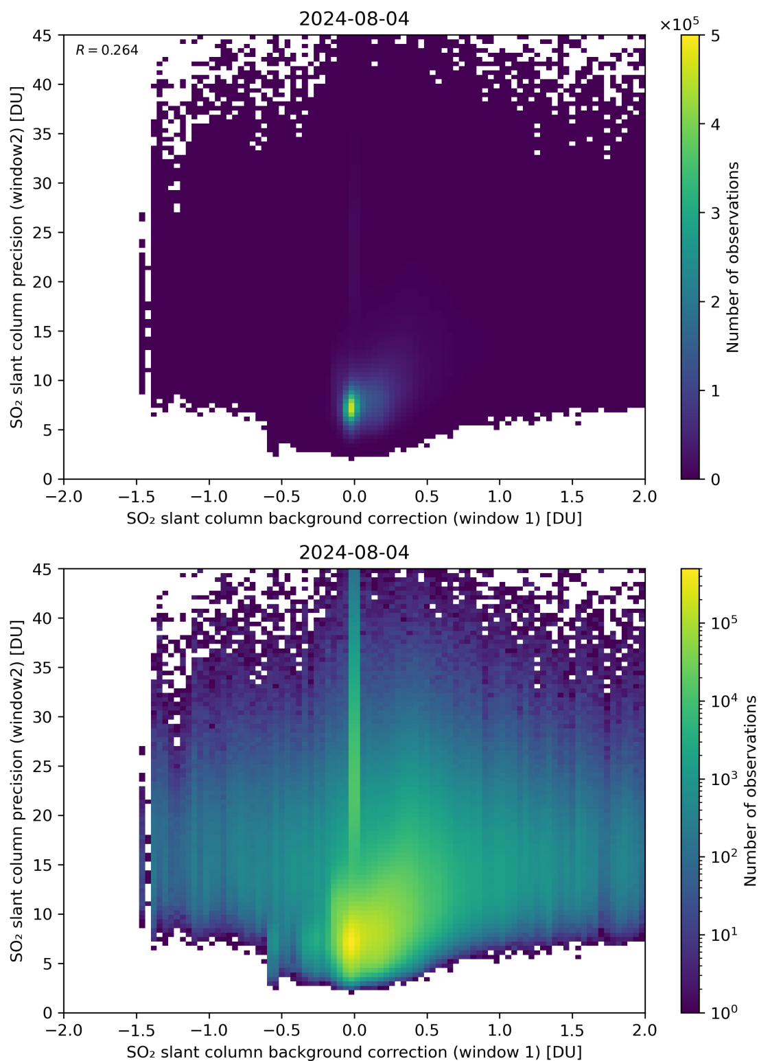
Figure 106: Scatter density plot of “SO 2 slant column background correction (window 1)” against “SO 2 slant column precision (window2)” for 2024-08-03 to 2024-08-05.
