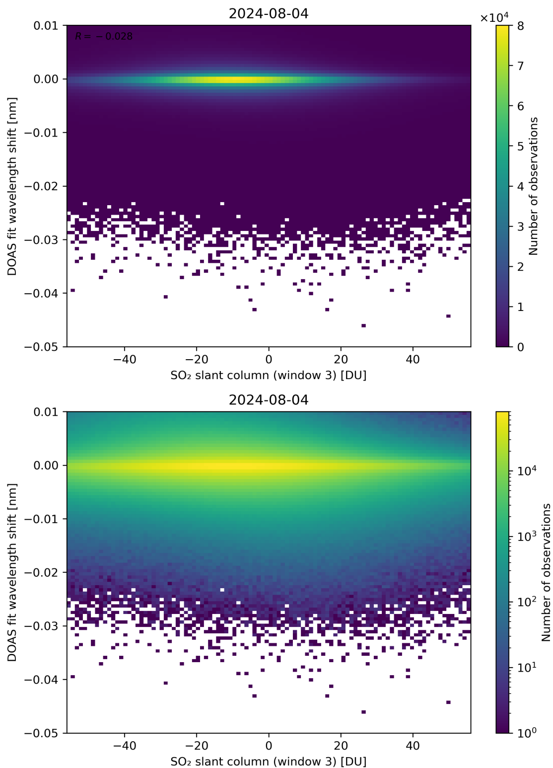
Figure 254: Scatter density plot of “SO 2 slant column (window 3)” against “DOAS fit wavelength shift” for 2024-08-03 to 2024-08-05.
