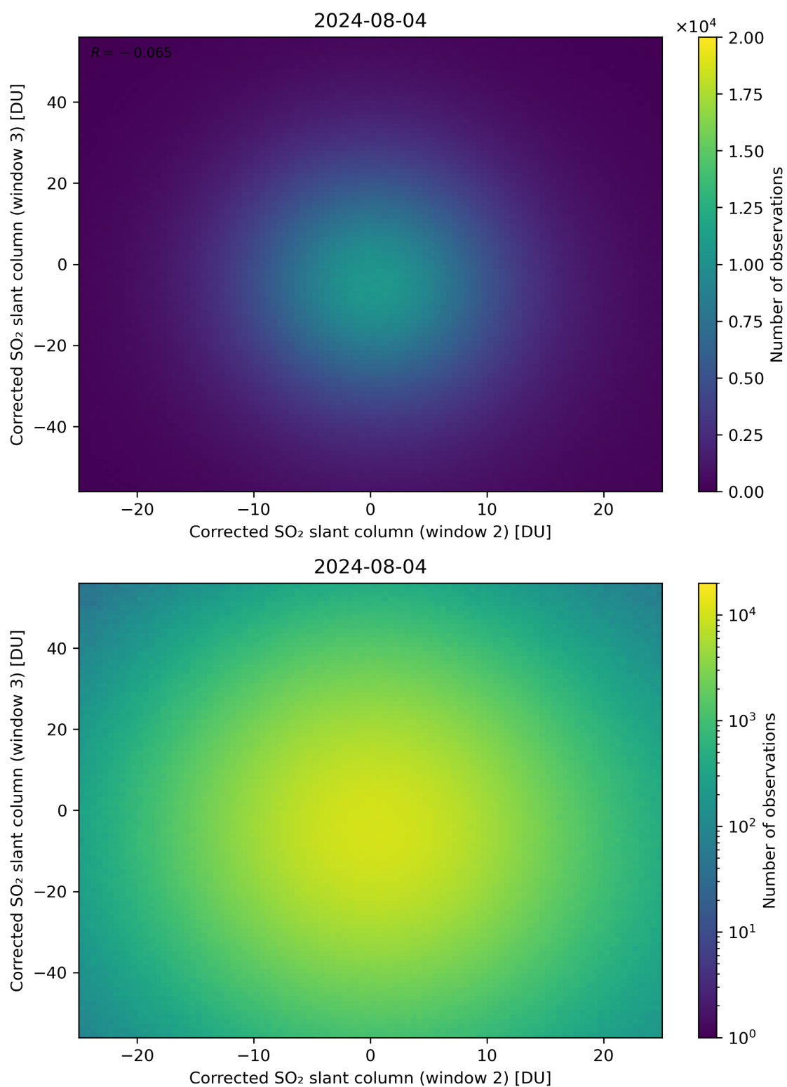
Figure 200: Scatter density plot of “Corrected SO 2 slant column (window 2)” against “Corrected SO 2 slant column (window 3)” for 2024-08-03 to 2024-08-05.
