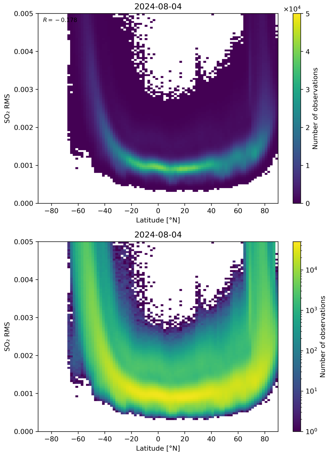
Figure 144: Scatter density plot of “Latitude” against “SO 2 RMS” for 2024-08-03 to 2024-08-05.
