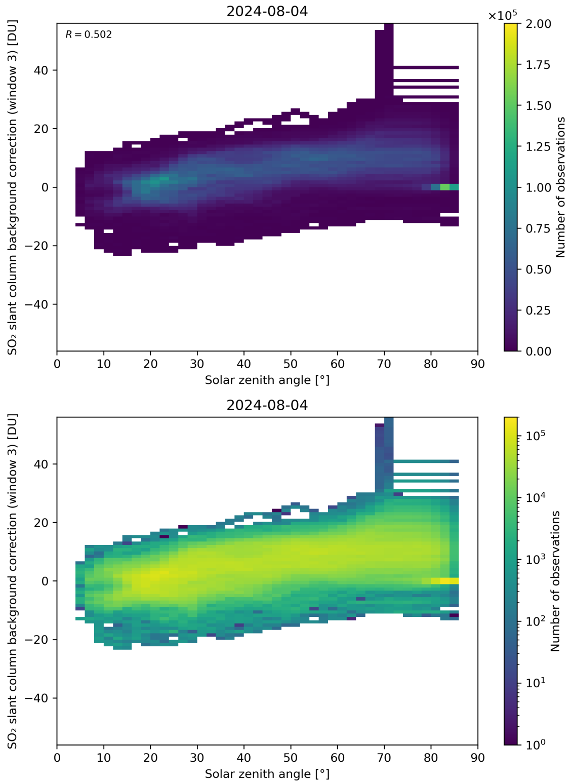
Figure 160: Scatter density plot of “Solar zenith angle” against “SO 2 slant column background correction (window 3)” for 2024-08-03 to 2024-08-05.
