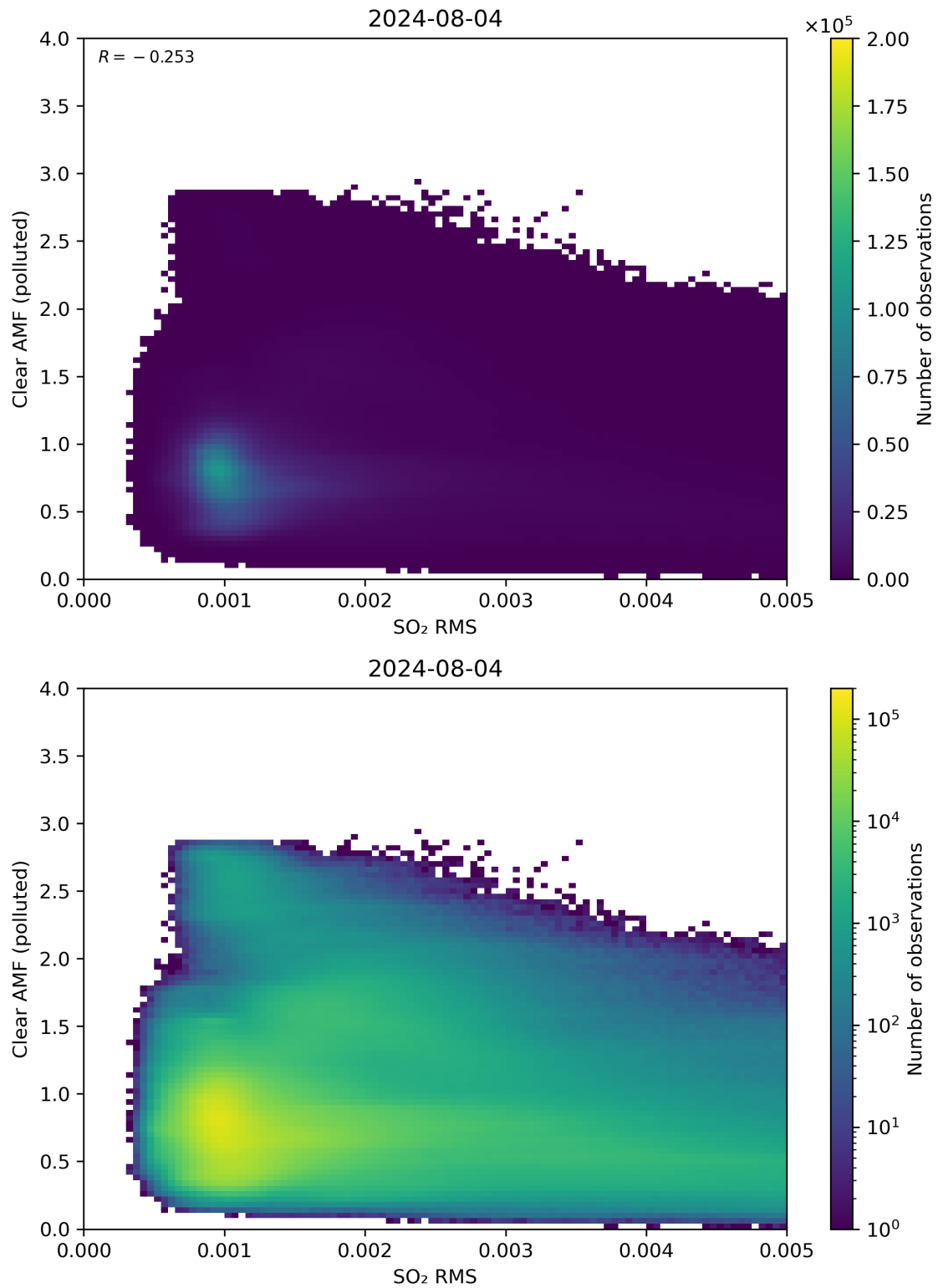
Figure 136: Scatter density plot of “SO 2 RMS” against “Clear AMF (polluted)” for 2024-08-03 to 2024-08-05.
