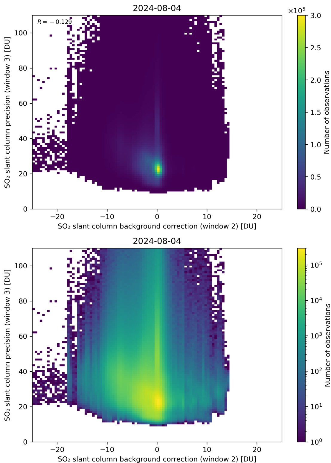
Figure 118: Scatter density plot of “SO 2 slant column background correction (window 2)” against “SO 2 slant column precision (window 3)” for 2024-08-03 to 2024-08-05.
