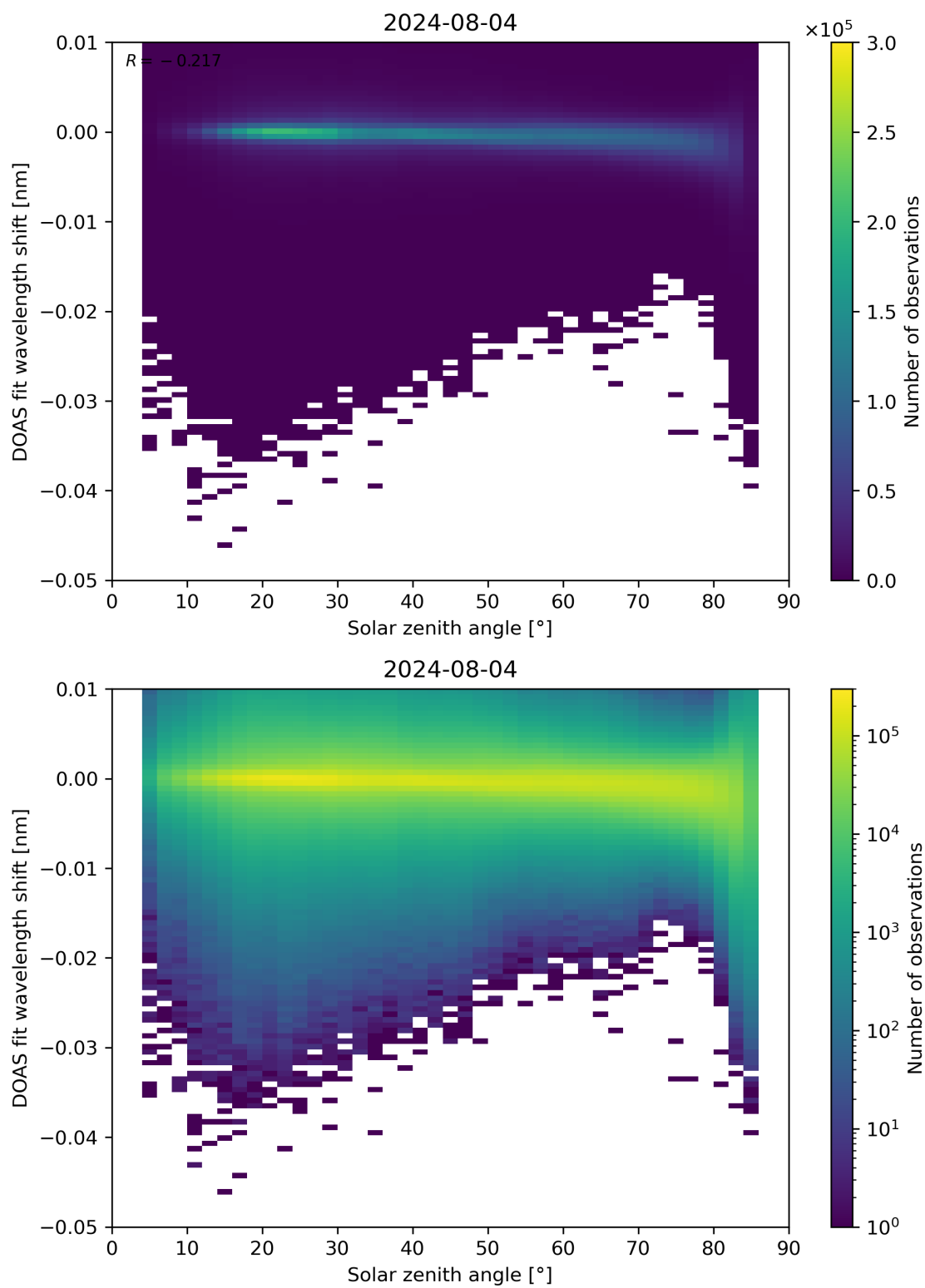
Figure 161: Scatter density plot of “Solar zenith angle” against “DOAS fit wavelength shift” for 2024-08-03 to 2024-08-05.
