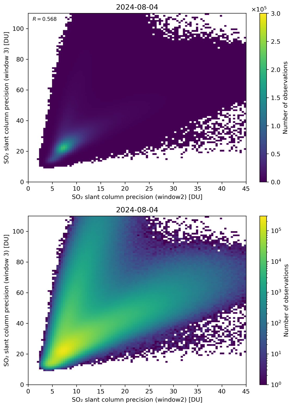
Figure 250: Scatter density plot of “SO 2 slant column precision (window2)” against “SO 2 slant column precision (window 3)” for 2024-08-03 to 2024-08-05.
