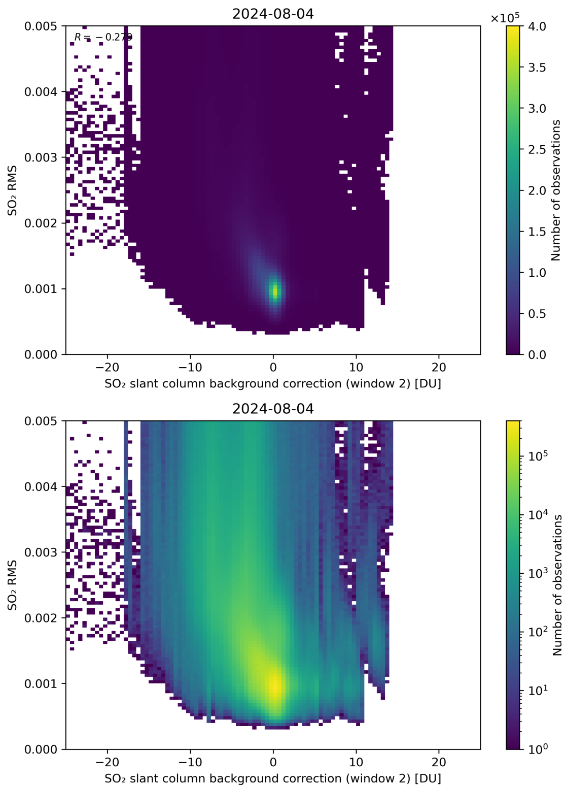
Figure 114: Scatter density plot of “SO 2 slant column background correction (window 2)” against “SO 2 RMS” for 2024-08-03 to 2024-08-05.
