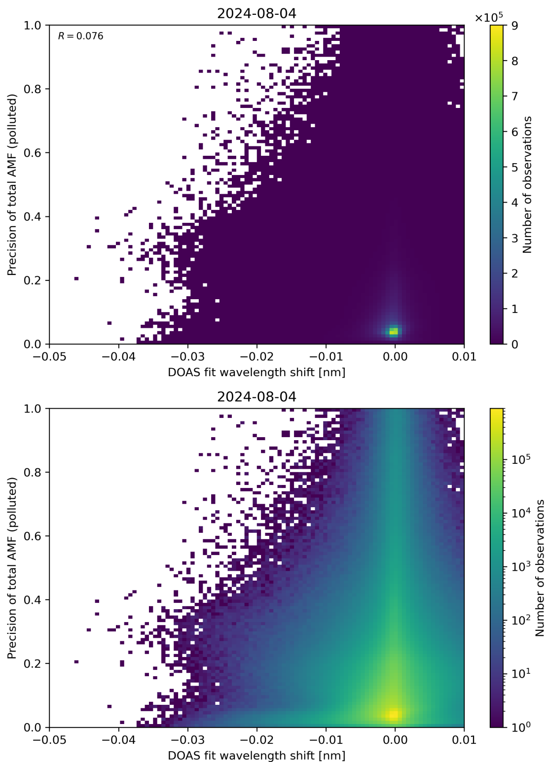
Figure 131: Scatter density plot of “DOAS fit wavelength shift” against “Precision of total AMF (polluted)” for 2024-08-03 to 2024-08-05.
