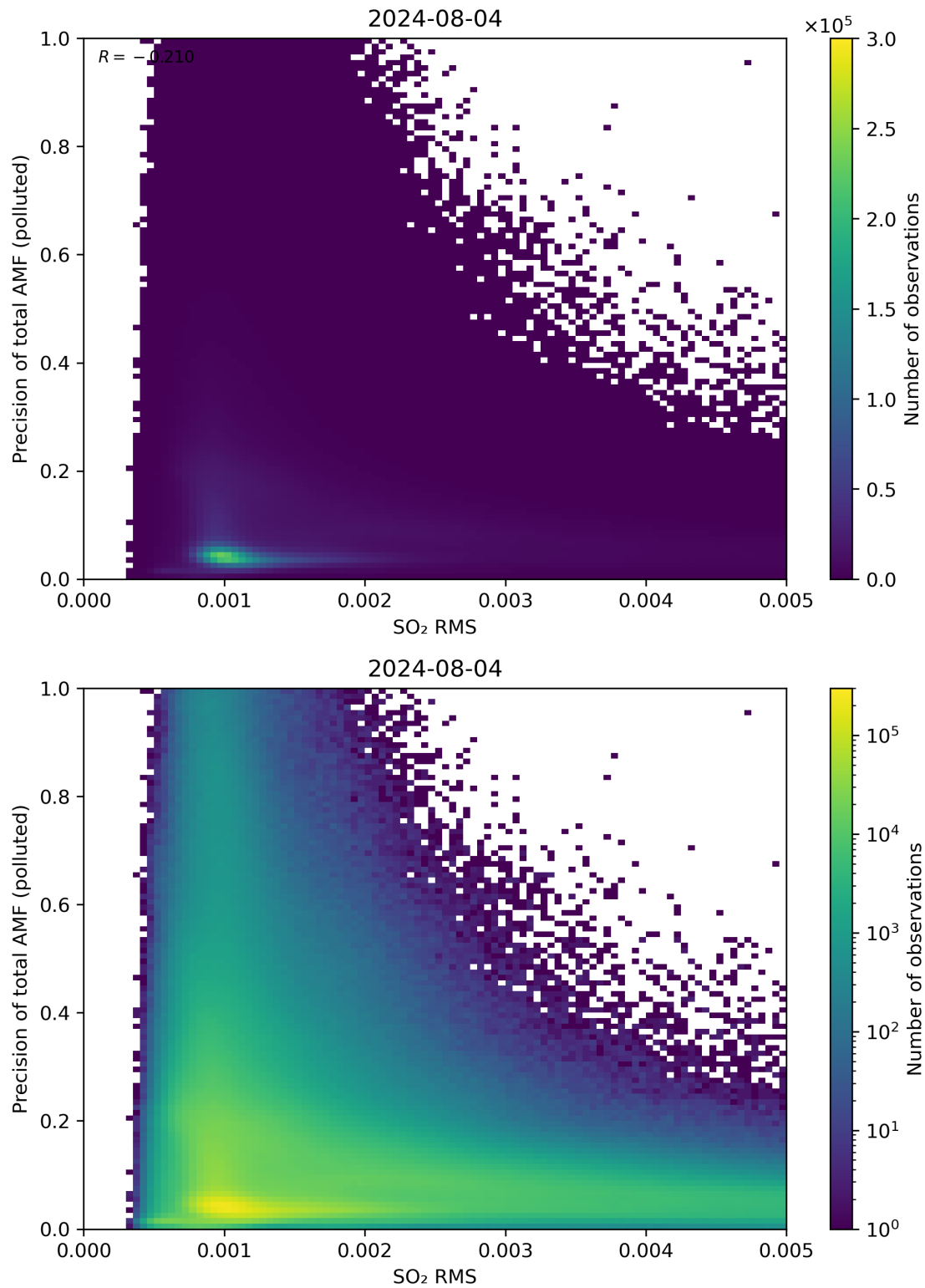
Figure 138: Scatter density plot of “SO 2 RMS” against “Precision of total AMF (polluted)” for 2024-08-03 to 2024-08-05.
