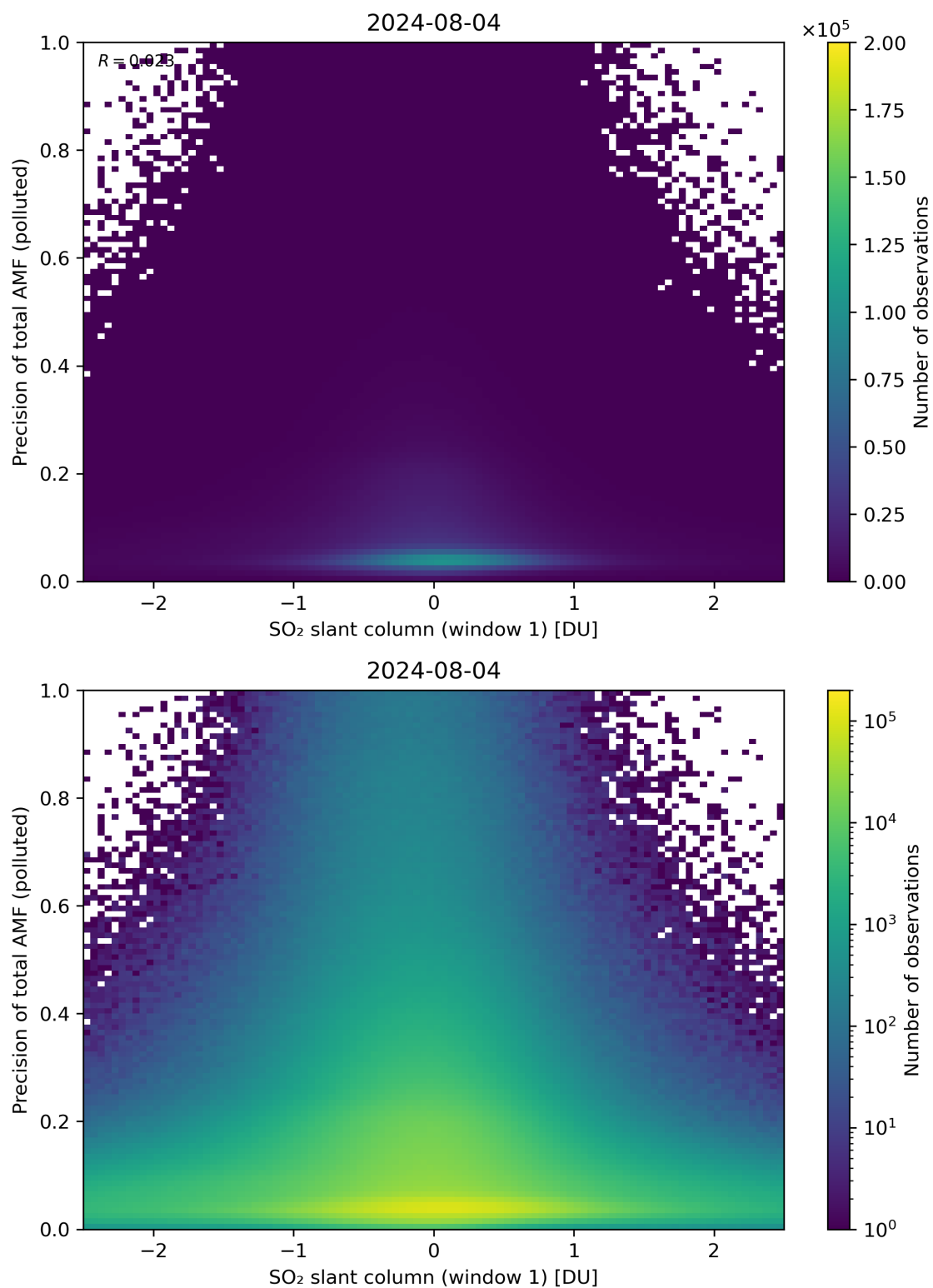
Figure 240: Scatter density plot of “SO 2 slant column (window 1)” against “Precision of total AMF (polluted)” for 2024-08-03 to 2024-08-05.
