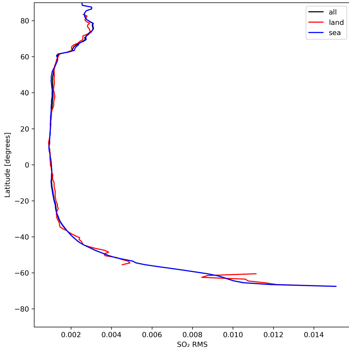
Figure 47: Zonal average of “SO 2 RMS” for 2024-08-03 to 2024-08-05.
