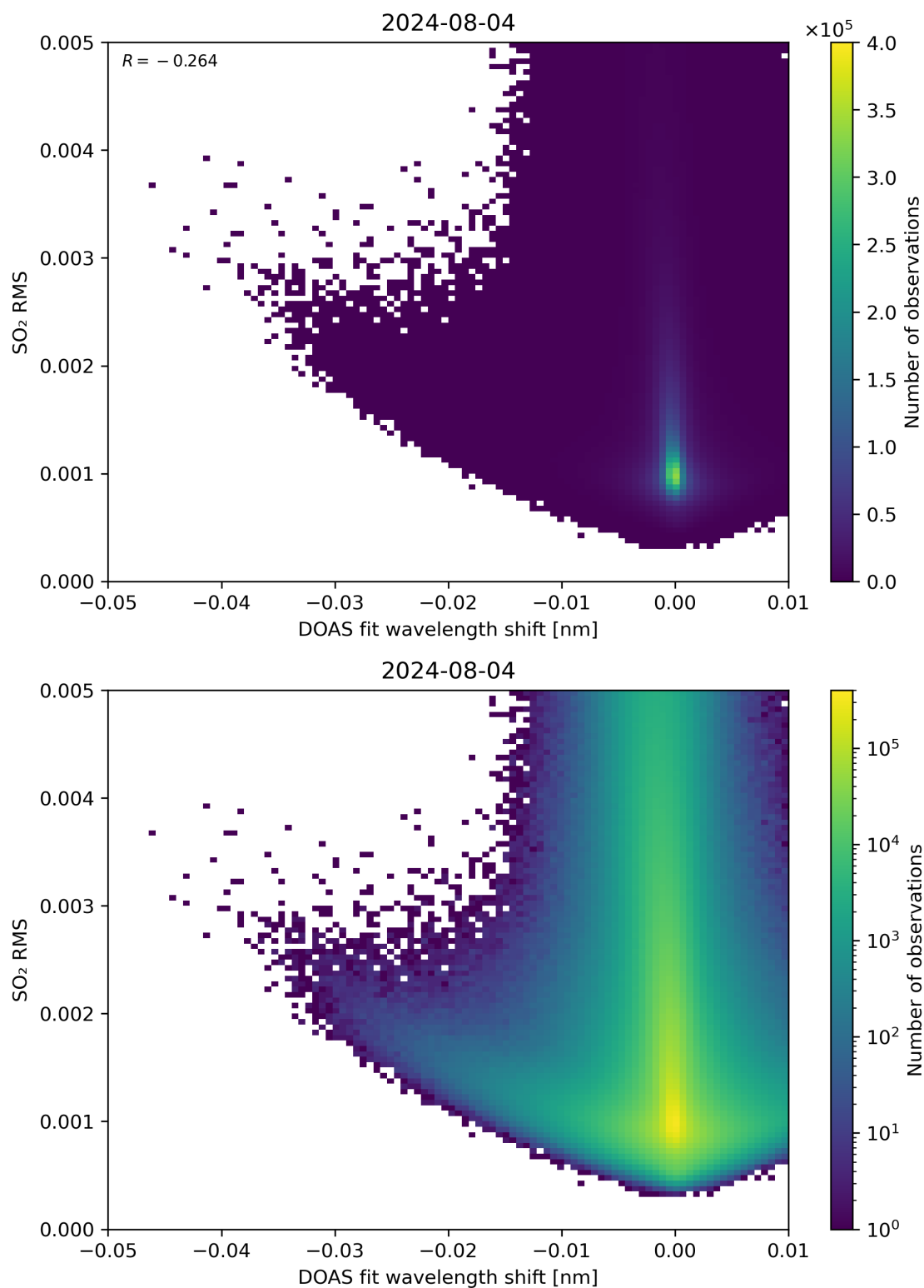
Figure 128: Scatter density plot of “DOAS fit wavelength shift” against “SO 2 RMS” for 2024-08-03 to 2024-08-05.
