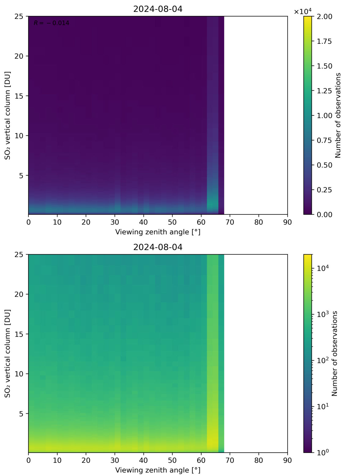
Figure 327: Scatter density plot of “Viewing zenith angle” against “SO 2 vertical column” for 2024-08-03 to 2024-08-05.
