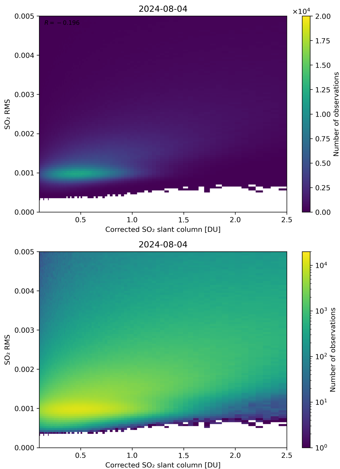
Figure 183: Scatter density plot of “Corrected SO 2 slant column” against “SO 2 RMS” for 2024-08-03 to 2024-08-05.
