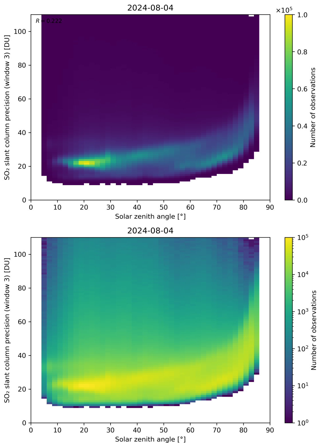
Figure 173: Scatter density plot of “Solar zenith angle” against “SO 2 slant column precision (window 3)” for 2024-08-03 to 2024-08-05.
