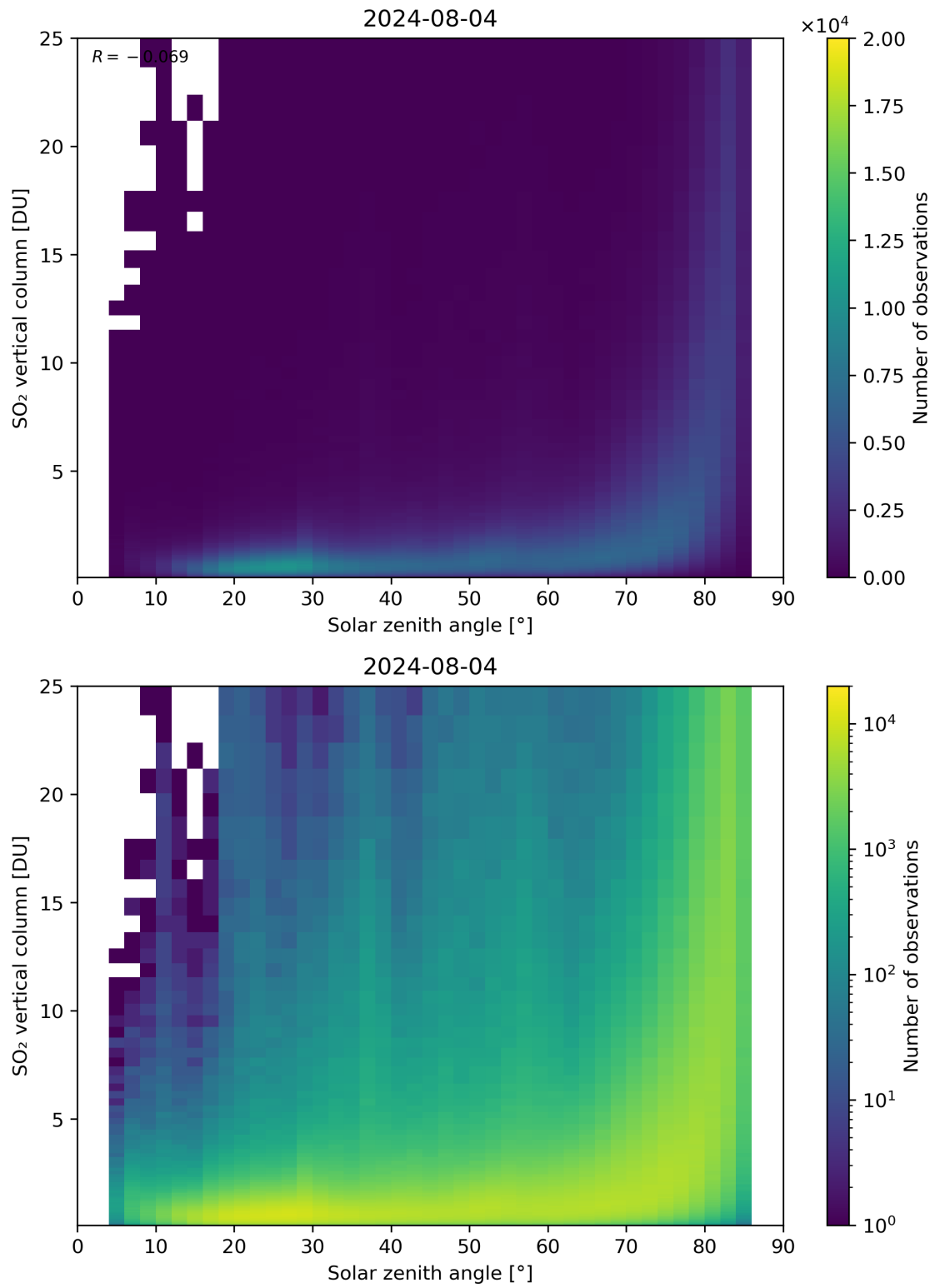
Figure 176: Scatter density plot of “Solar zenith angle” against “SO 2 vertical column” for 2024-08-03 to 2024-08-05.
