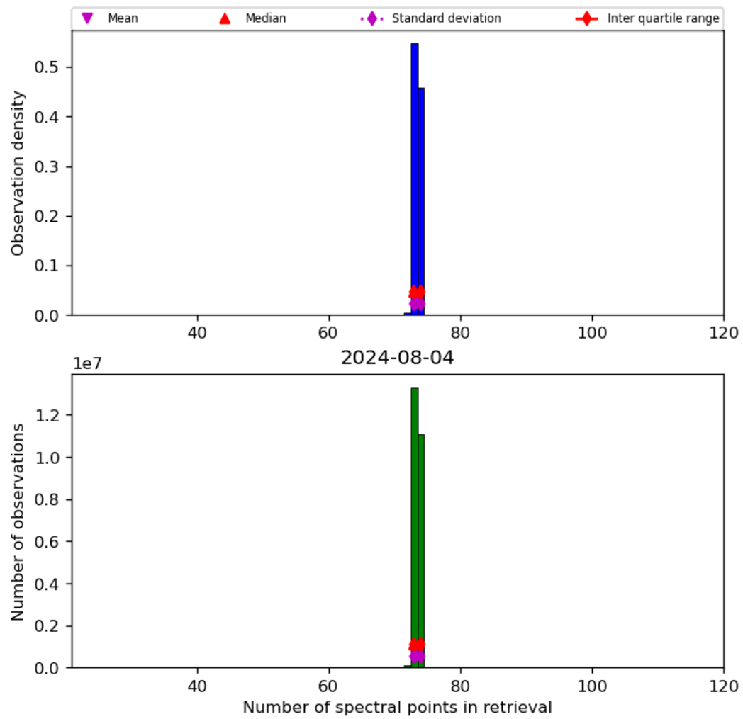
Figure 74: Histogram of “Number of spectral points in retrieval” for 2024-08-03 to 2024-08-05
