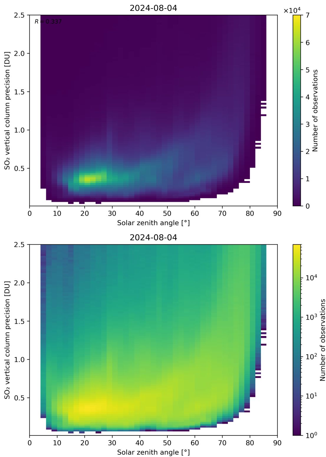
Figure 177: Scatter density plot of “Solar zenith angle” against “SO 2 vertical column precision” for 2024-08-03 to 2024-08-05.
