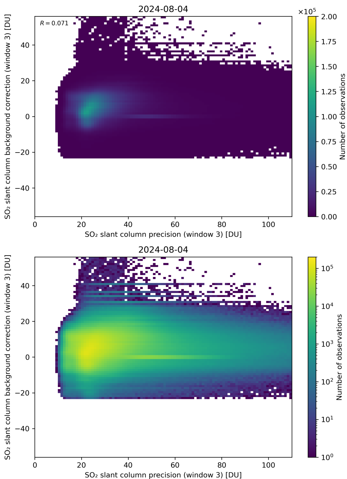
Figure 257: Scatter density plot of “SO 2 slant column precision (window 3)” against “SO 2 slant column background correction (window 3)” for 2024-08-03 to 2024-08-05.
