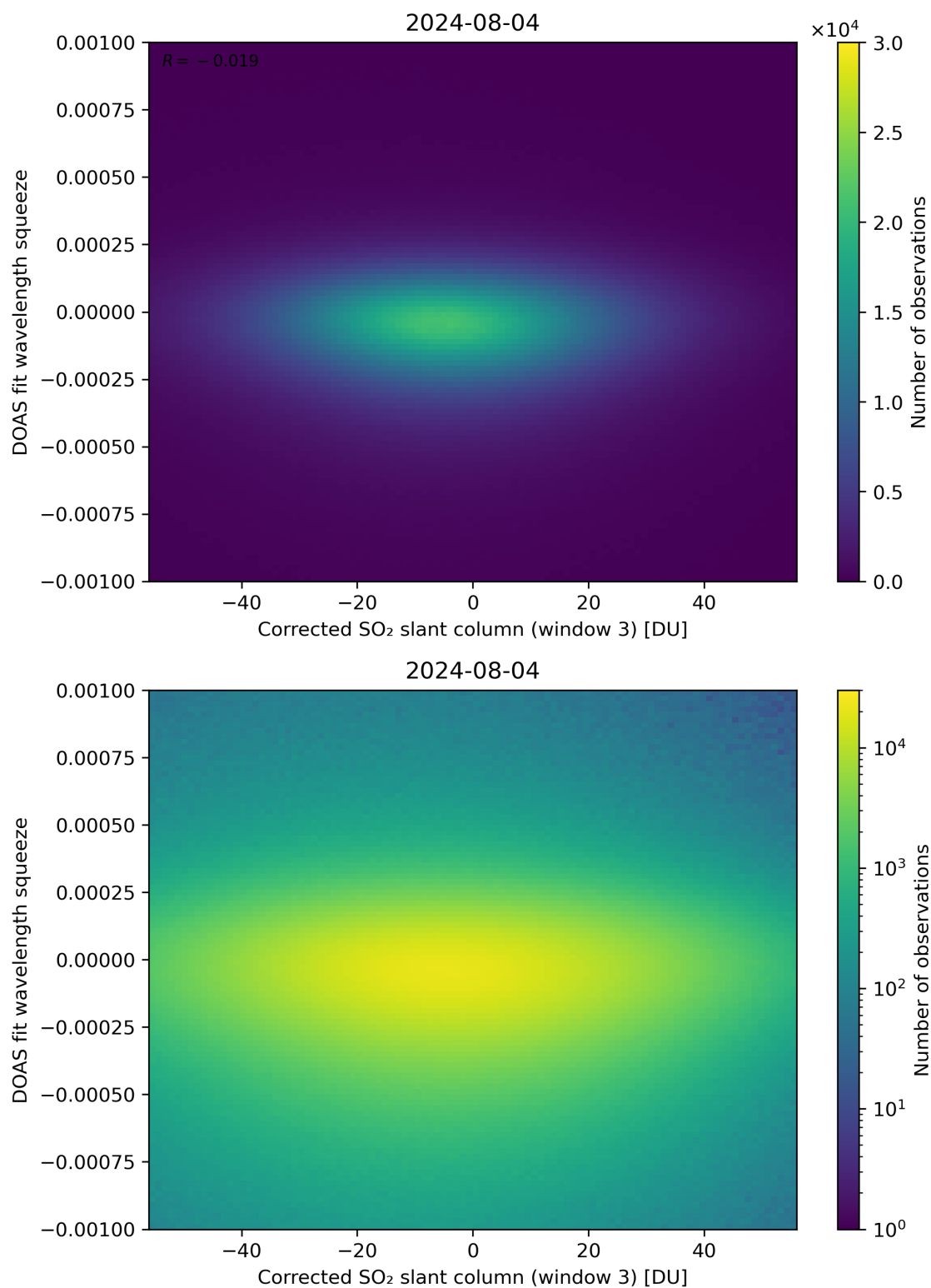
Figure 207: Scatter density plot of “Corrected SO 2 slant column (window 3)” against “DOAS fit wavelength squeeze” for 2024-08-03 to 2024-08-05.
