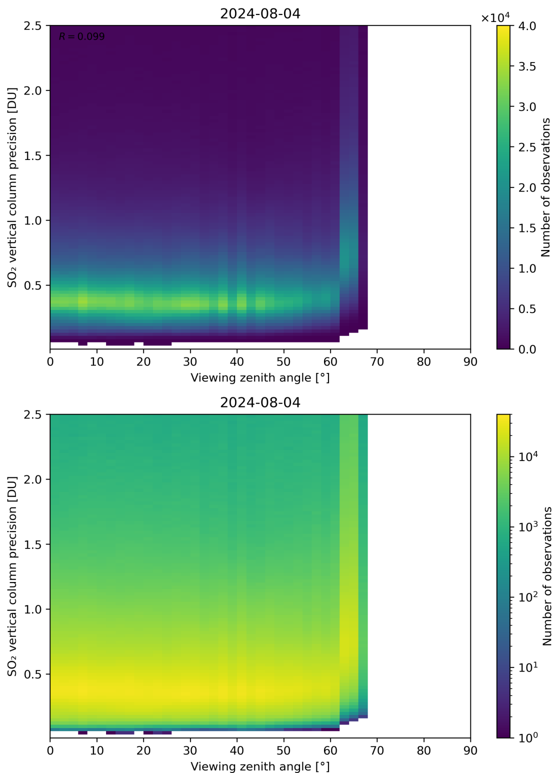
Figure 328: Scatter density plot of “Viewing zenith angle” against “SO 2 vertical column precision” for 2024-08-03 to 2024-08-05.
