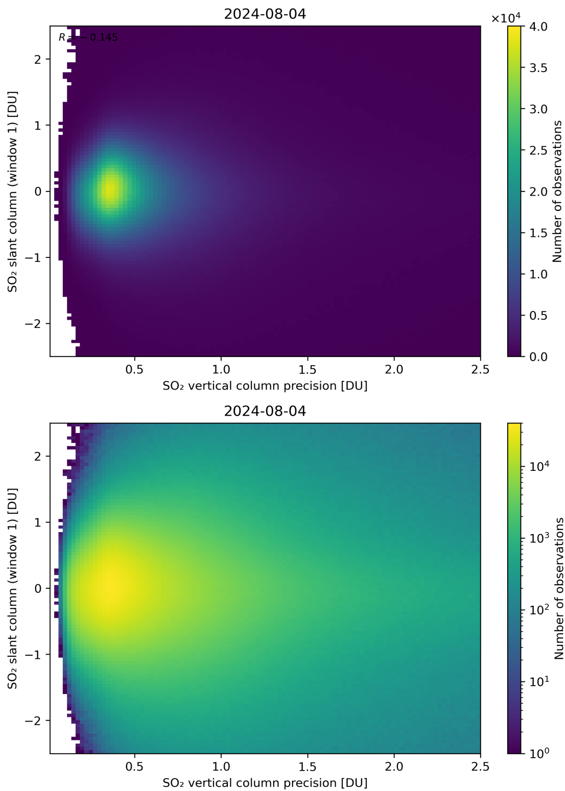
Figure 289: Scatter density plot of “SO 2 vertical column precision” against “SO 2 slant column (window 1)” for 2024-08-03 to 2024-08-05.
