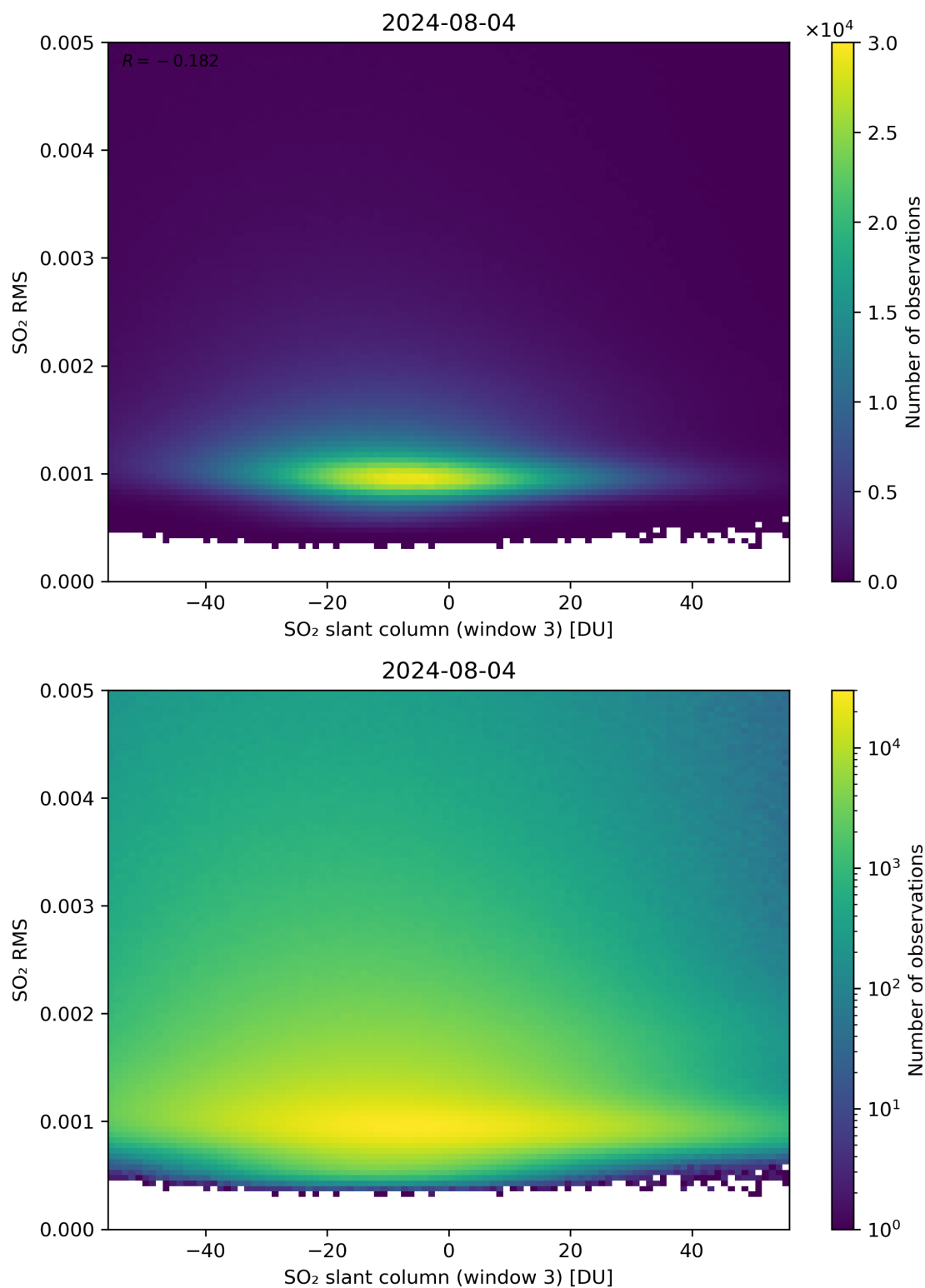
Figure 256: Scatter density plot of “SO 2 slant column (window 3)” against “SO 2 RMS” for 2024-08-03 to 2024-08-05.
