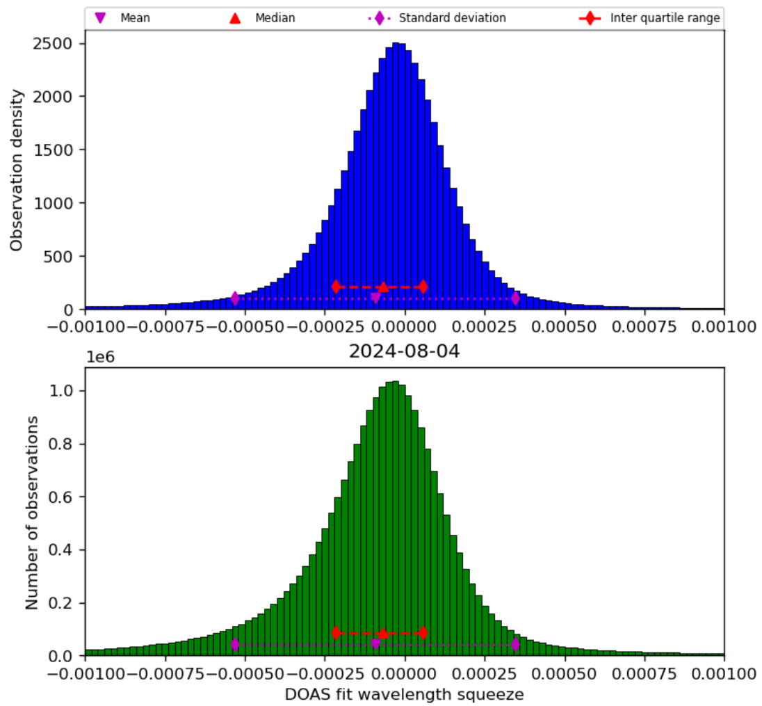
Figure 69: Histogram of “DOAS fit wavelength squeeze” for 2024-08-03 to 2024-08-05
