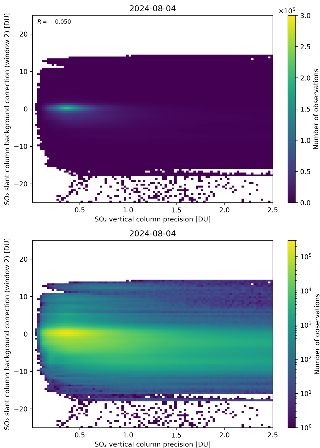
Figure 280: Scatter density plot of “SO 2 vertical column precision” against “SO 2 slant column background correction (window 2)” for 2024-08-03 to 2024-08-05.
