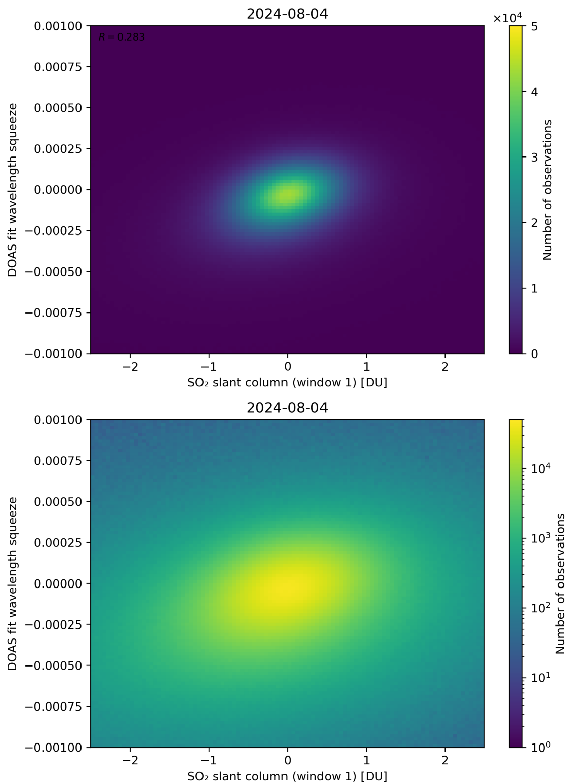
Figure 216: Scatter density plot of “SO 2 slant column (window 1)” against “DOAS fit wavelength squeeze” for 2024-08-03 to 2024-08-05.
