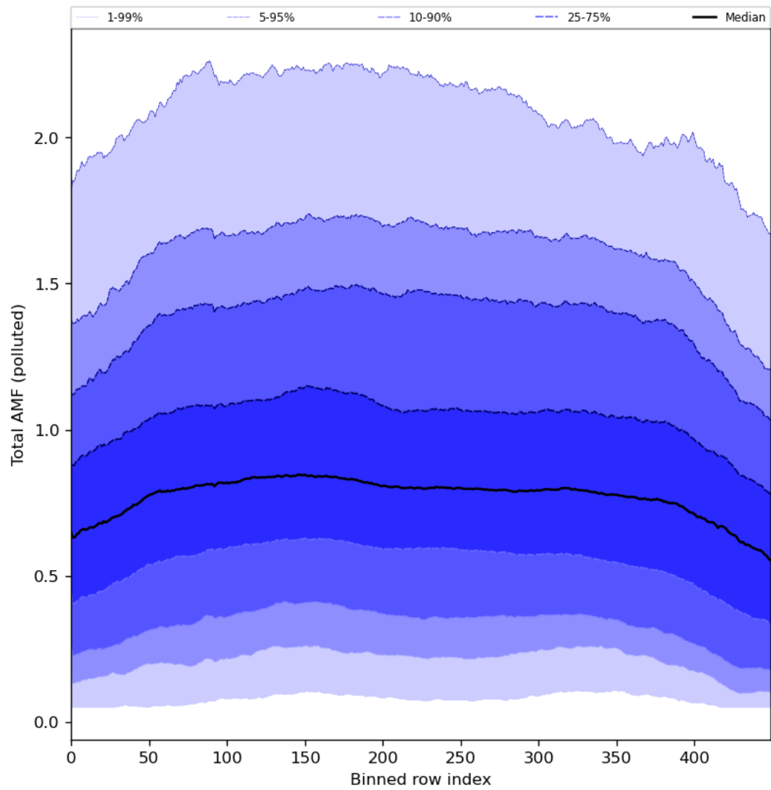
Figure 94: Along track statistics of “Total AMF (polluted)” for 2024-08-03 to 2024-08-05
