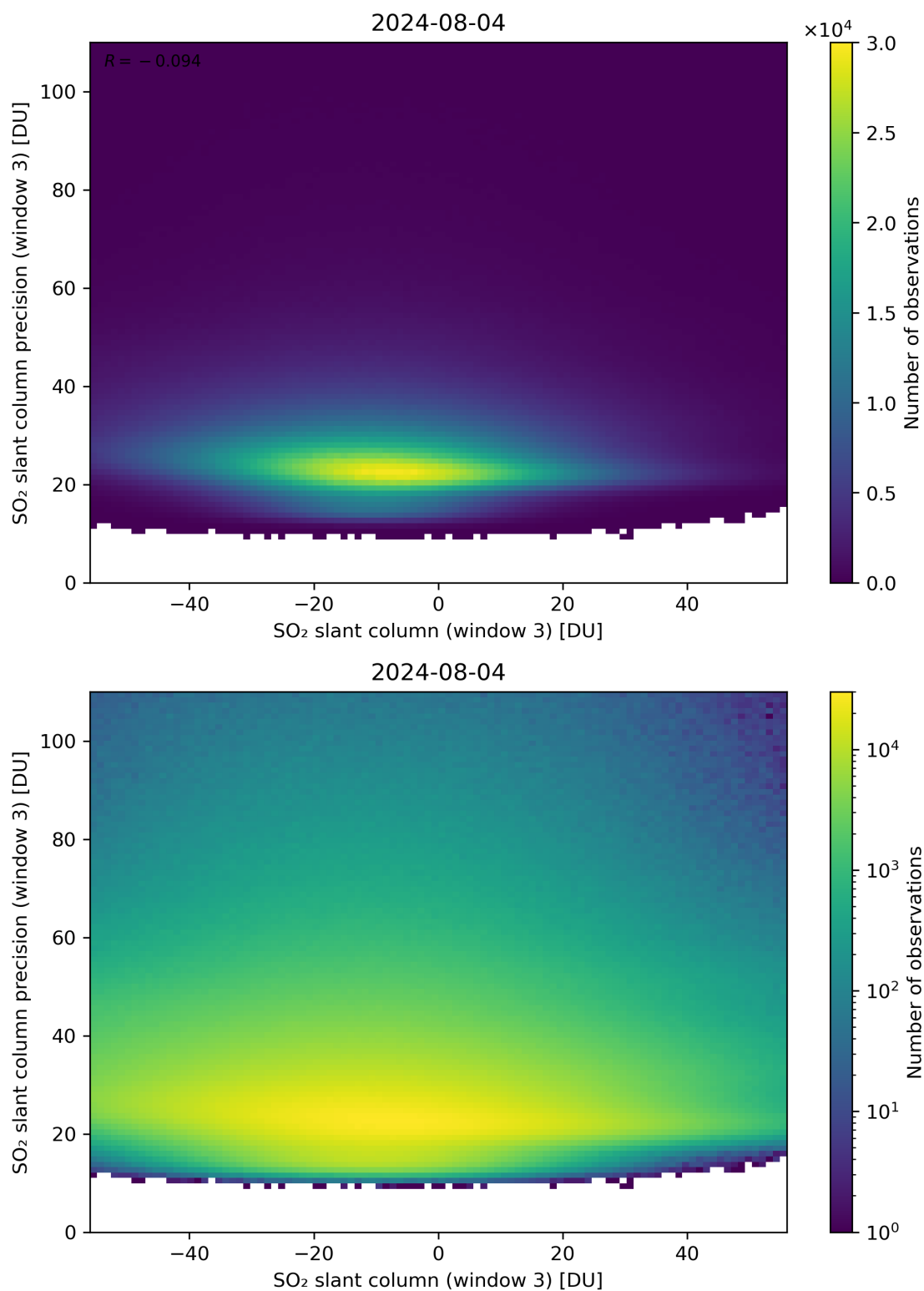
Figure 267: Scatter density plot of “SO 2 slant column (window 3)” against “SO 2 slant column precision (window 3)” for 2024-08-03 to 2024-08-05.
