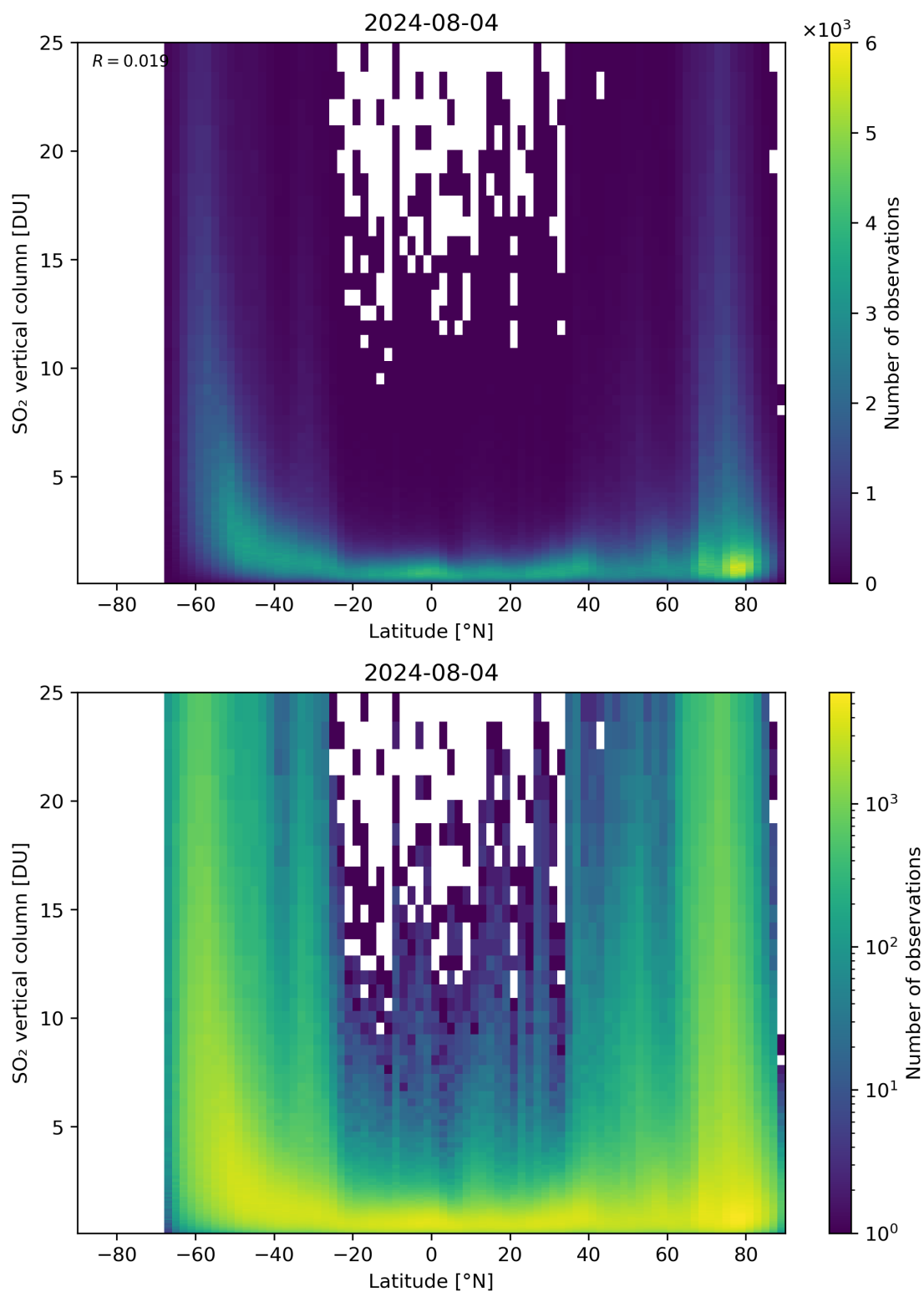
Figure 156: Scatter density plot of “Latitude” against “SO 2 vertical column” for 2024-08-03 to 2024-08-05.
