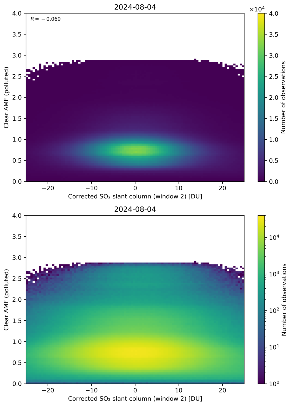
Figure 199: Scatter density plot of “Corrected SO 2 slant column (window 2)” against “Clear AMF (polluted)” for 2024-08-03 to 2024-08-05.
