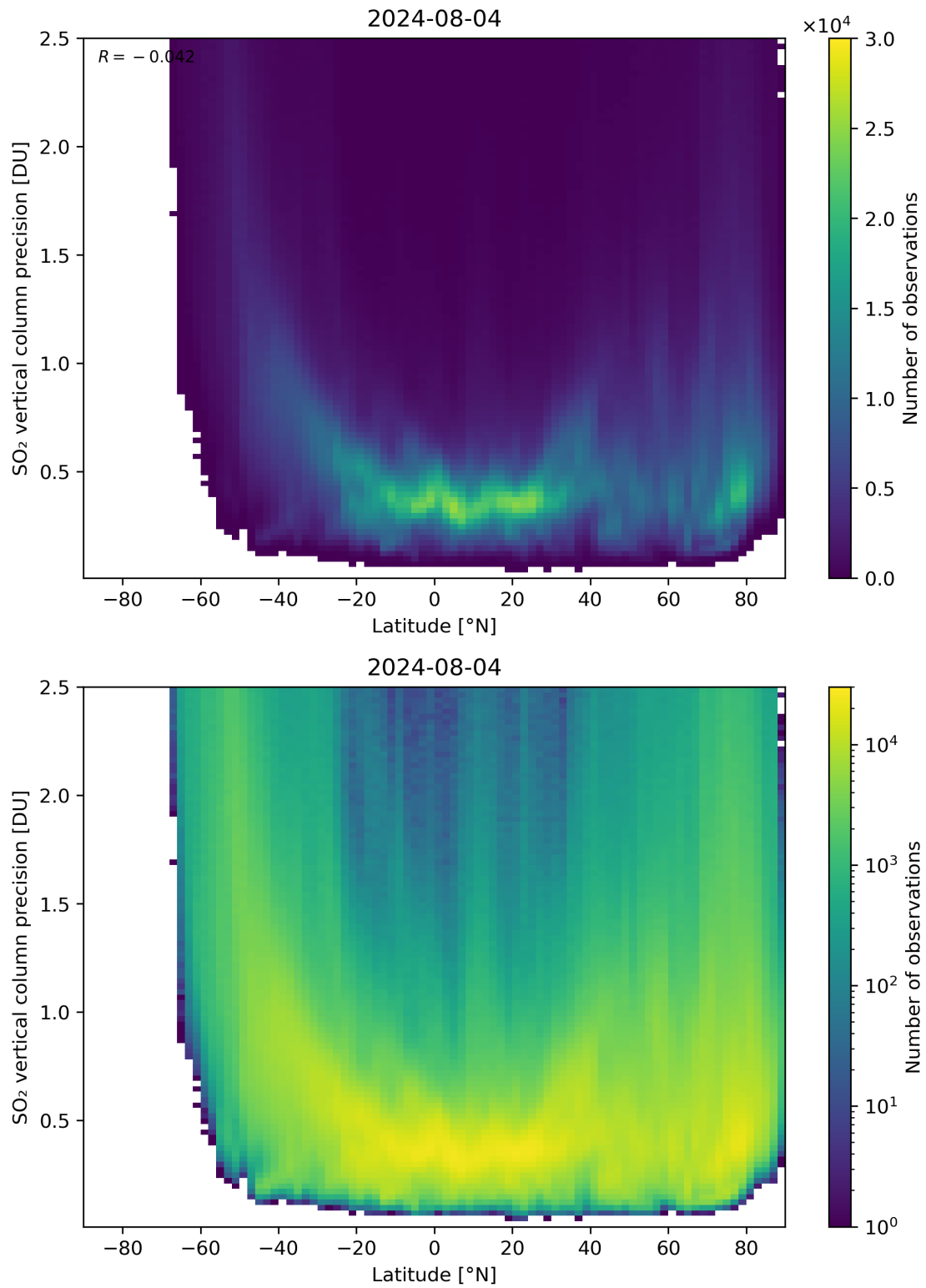
Figure 157: Scatter density plot of “Latitude” against “SO 2 vertical column precision” for 2024-08-03 to 2024-08-05.
