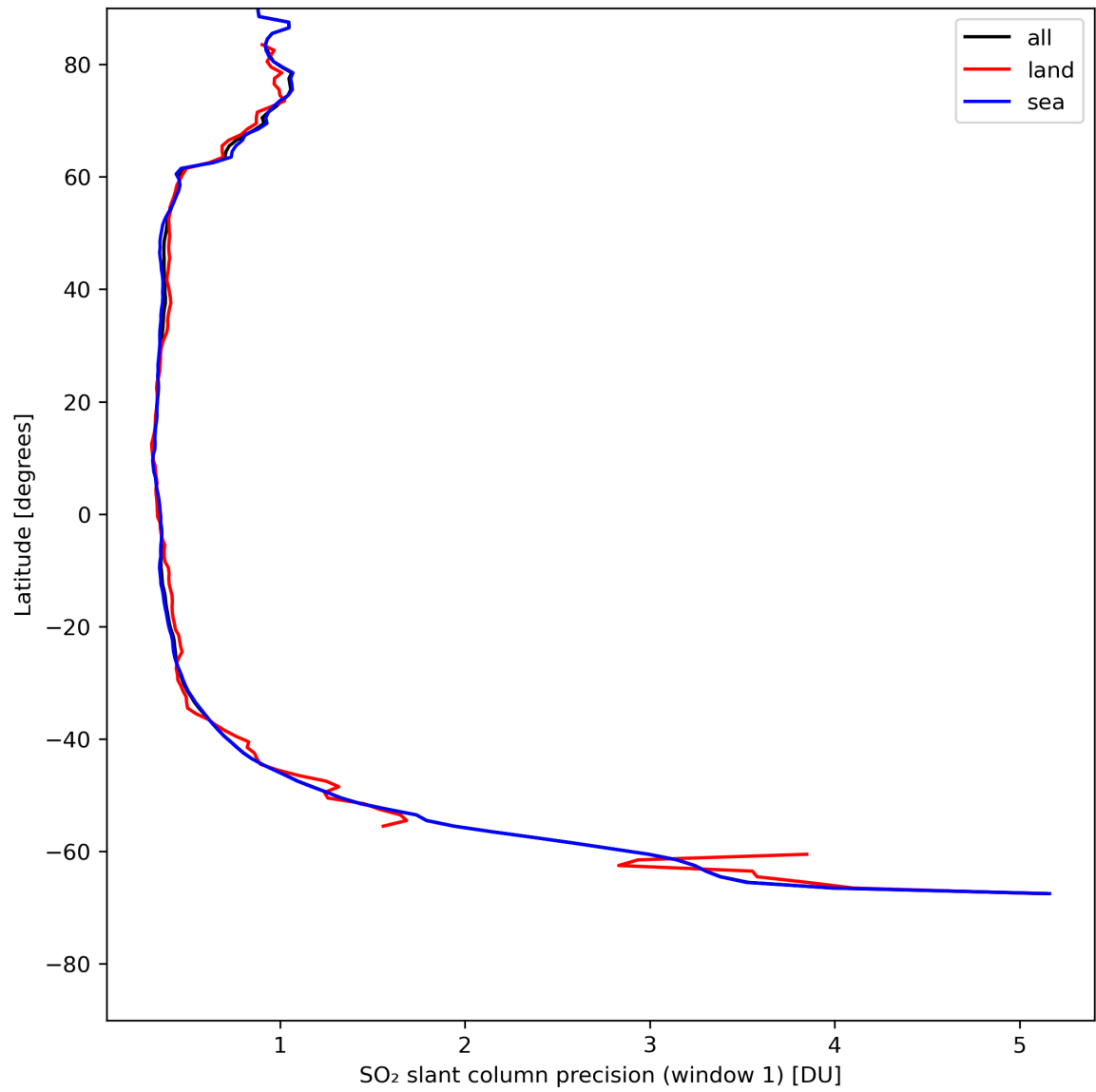
Figure 34: Zonal average of “SO 2 slant column precision (window 1)” for 2024-08-03 to 2024-08-05.
