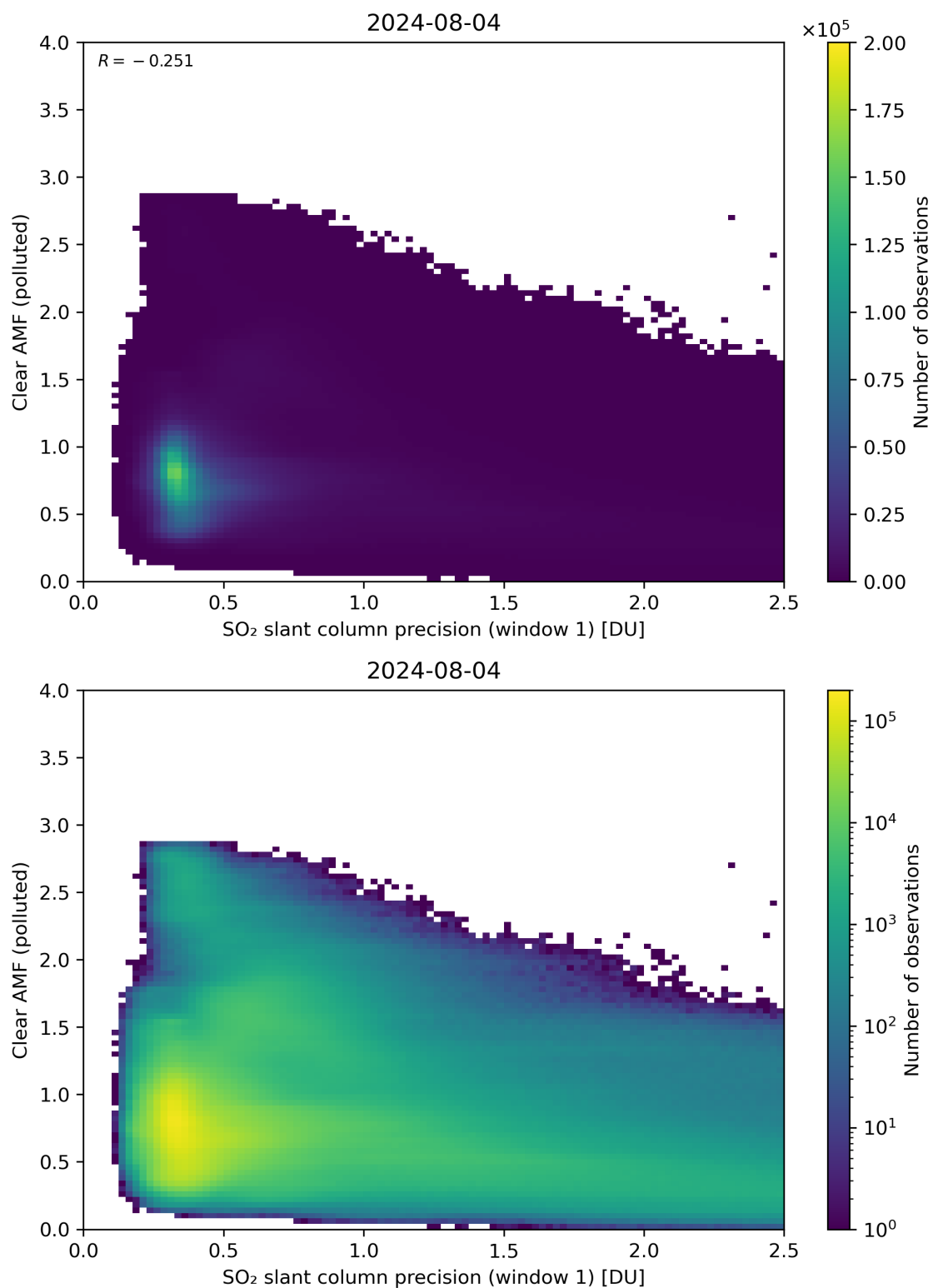
Figure 224: Scatter density plot of “SO 2 slant column precision (window 1)” against “Clear AMF (polluted)” for 2024-08-03 to 2024-08-05.
