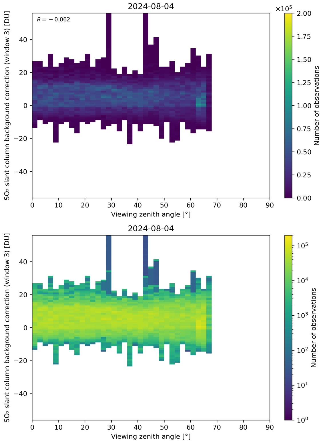
Figure 310: Scatter density plot of “Viewing zenith angle” against “SO 2 slant column background correction (window 3)” for 2024-08-03 to 2024-08-05.
