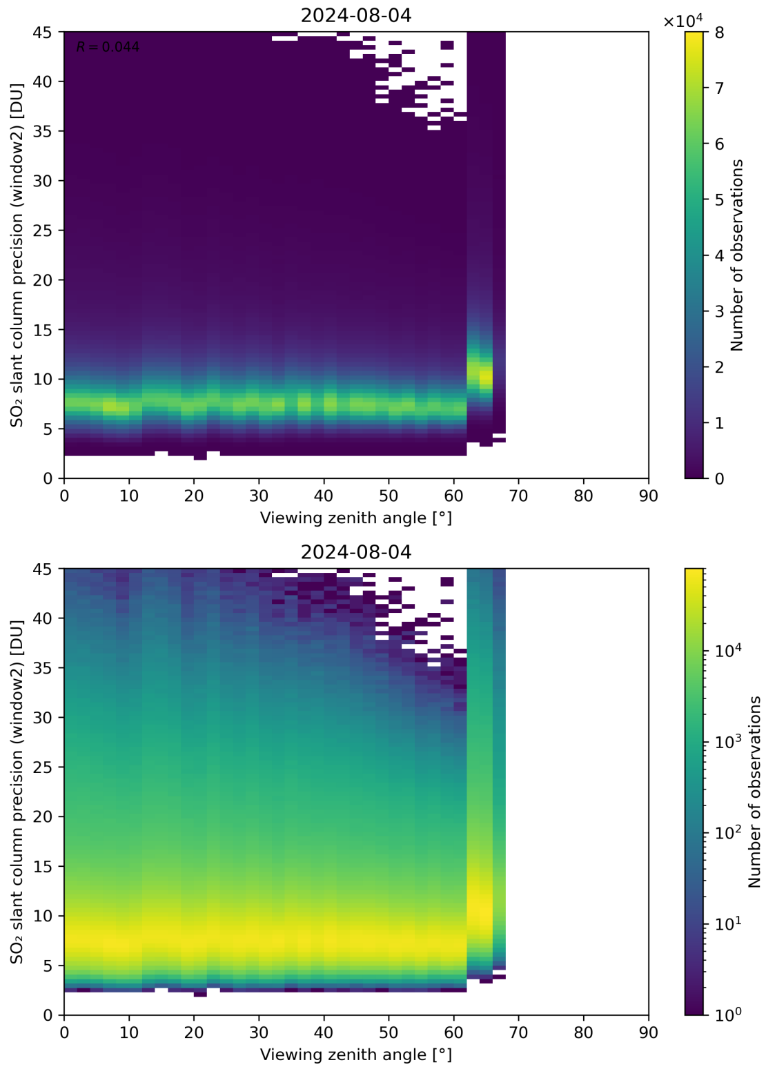
Figure 322: Scatter density plot of “Viewing zenith angle” against “SO 2 slant column precision (window2)” for 2024-08-03 to 2024-08-05.
