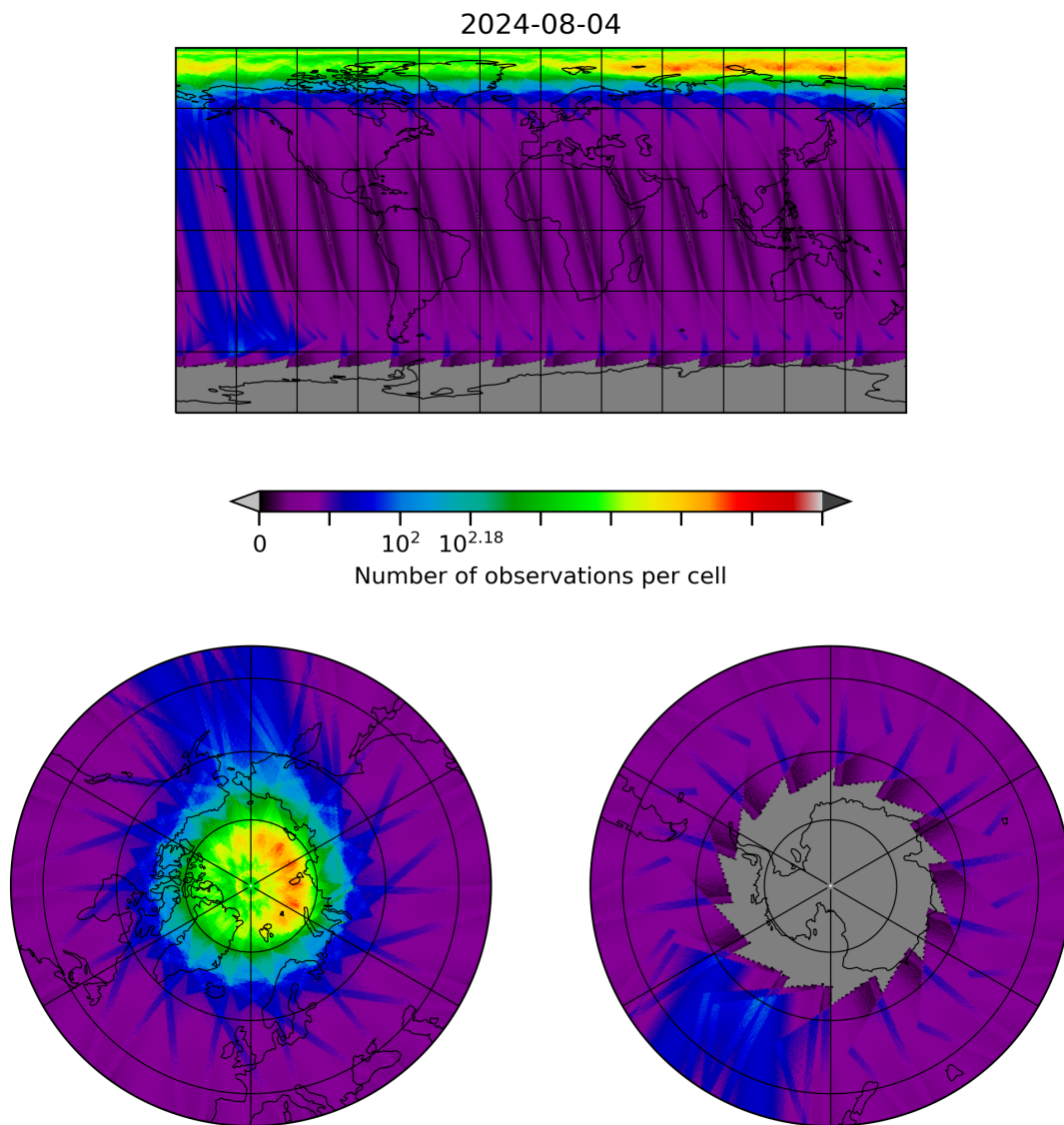
Figure 28: Map of the number of observations for 2024-08-03 to 2024-08-05
