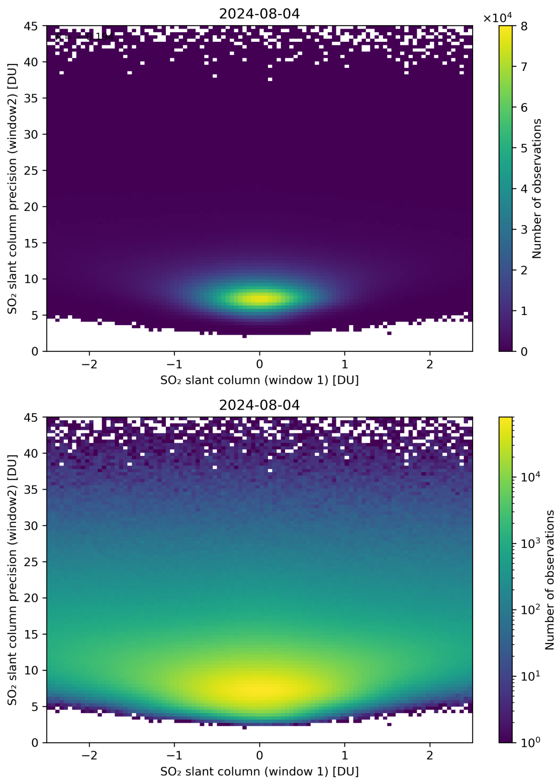
Figure 236: Scatter density plot of “SO 2 slant column (window 1)” against “SO 2 slant column precision (window2)” for 2024-08-03 to 2024-08-05.
