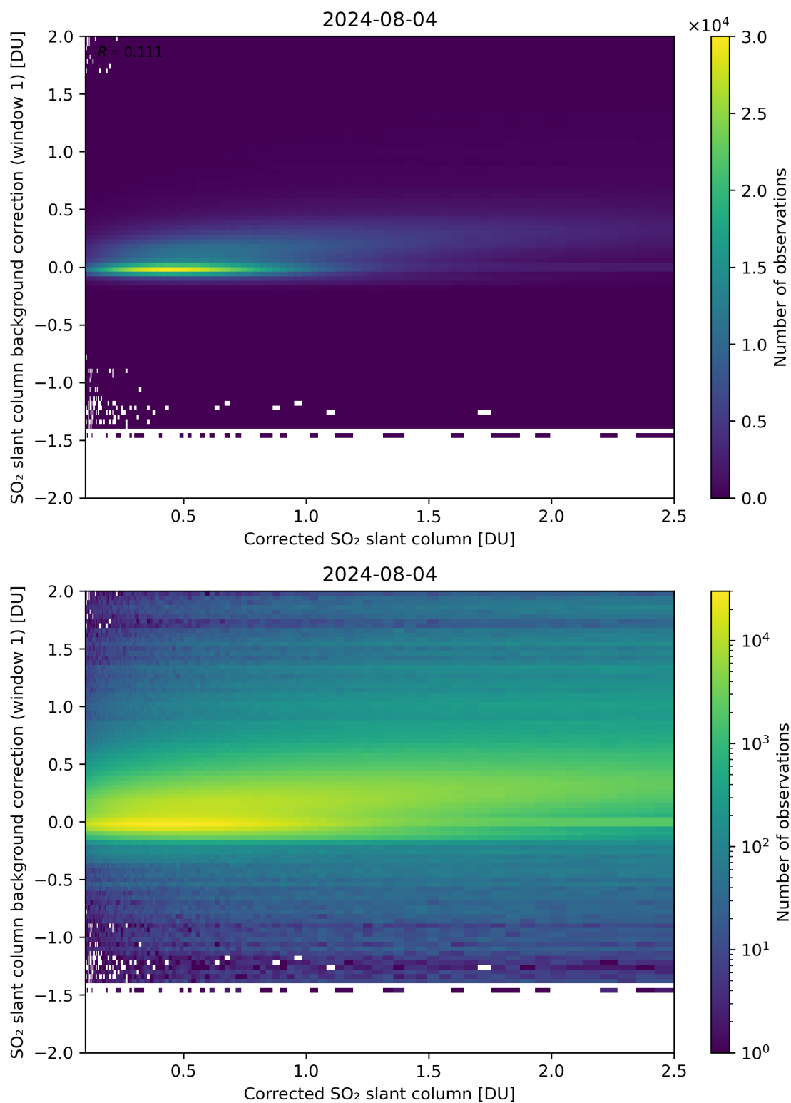
Figure 178: Scatter density plot of “Corrected SO 2 slant column” against “SO 2 slant column background correction (window 1)” for 2024-08-03 to 2024-08-05.
