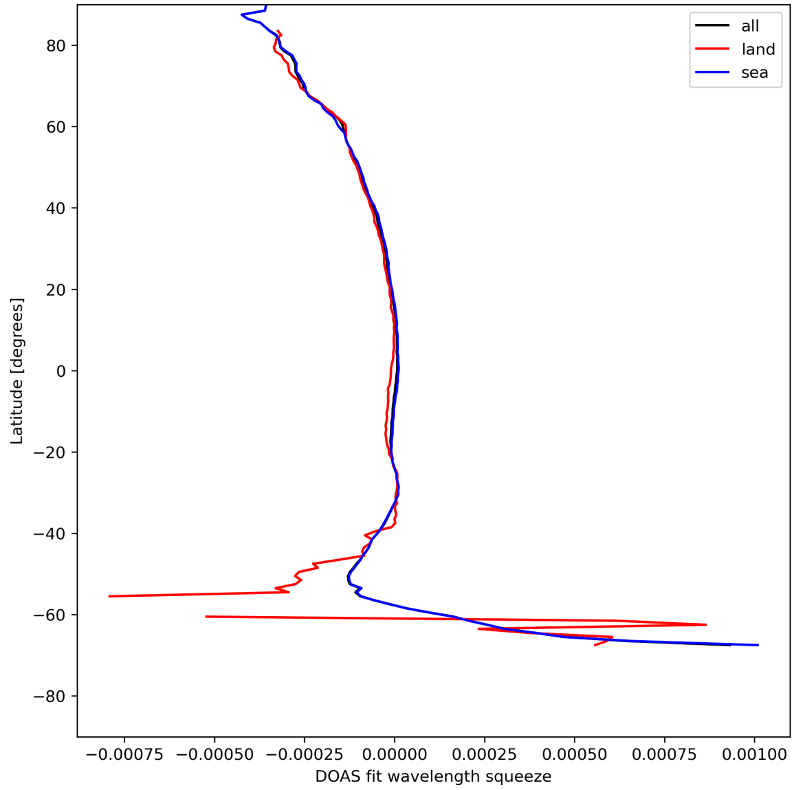
Figure 46: Zonal average of “DOAS fit wavelength squeeze” for 2024-08-03 to 2024-08-05.
