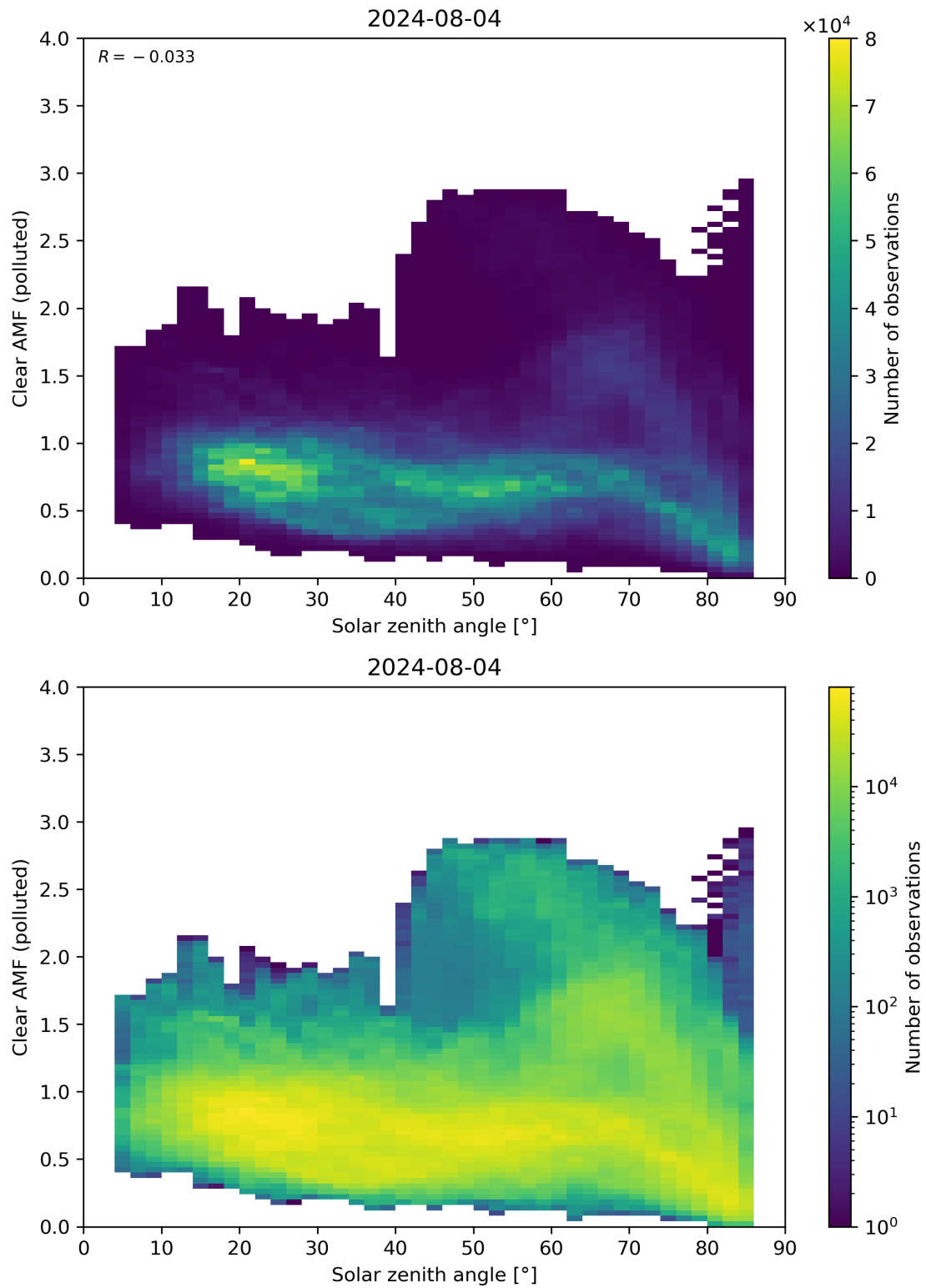
Figure 165: Scatter density plot of “Solar zenith angle” against “Clear AMF (polluted)” for 2024-08-03 to 2024-08-05.
