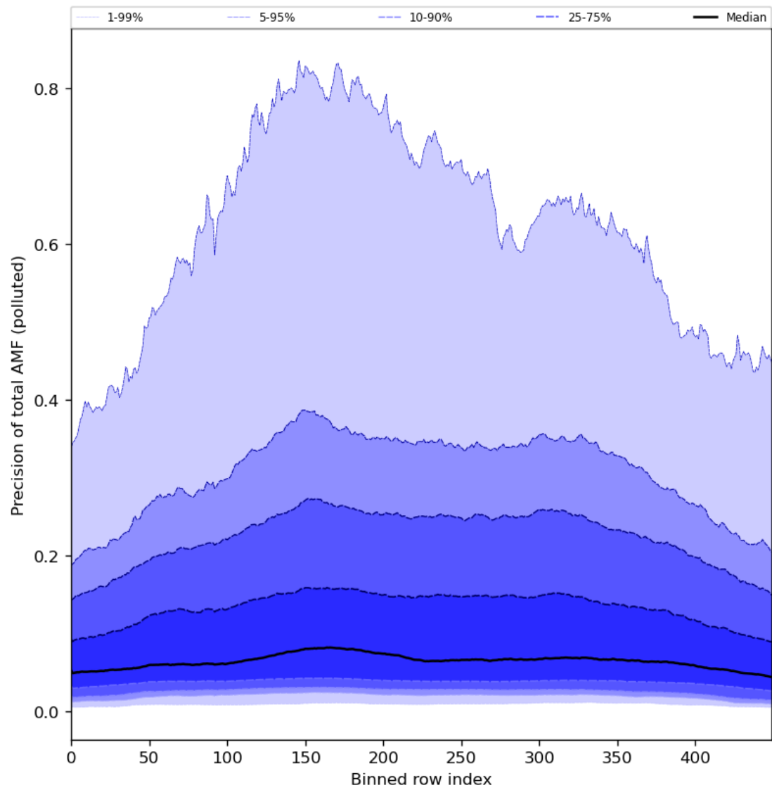
Figure 95: Along track statistics of “Precision of total AMF (polluted)” for 2024-08-03 to 2024-08-05
