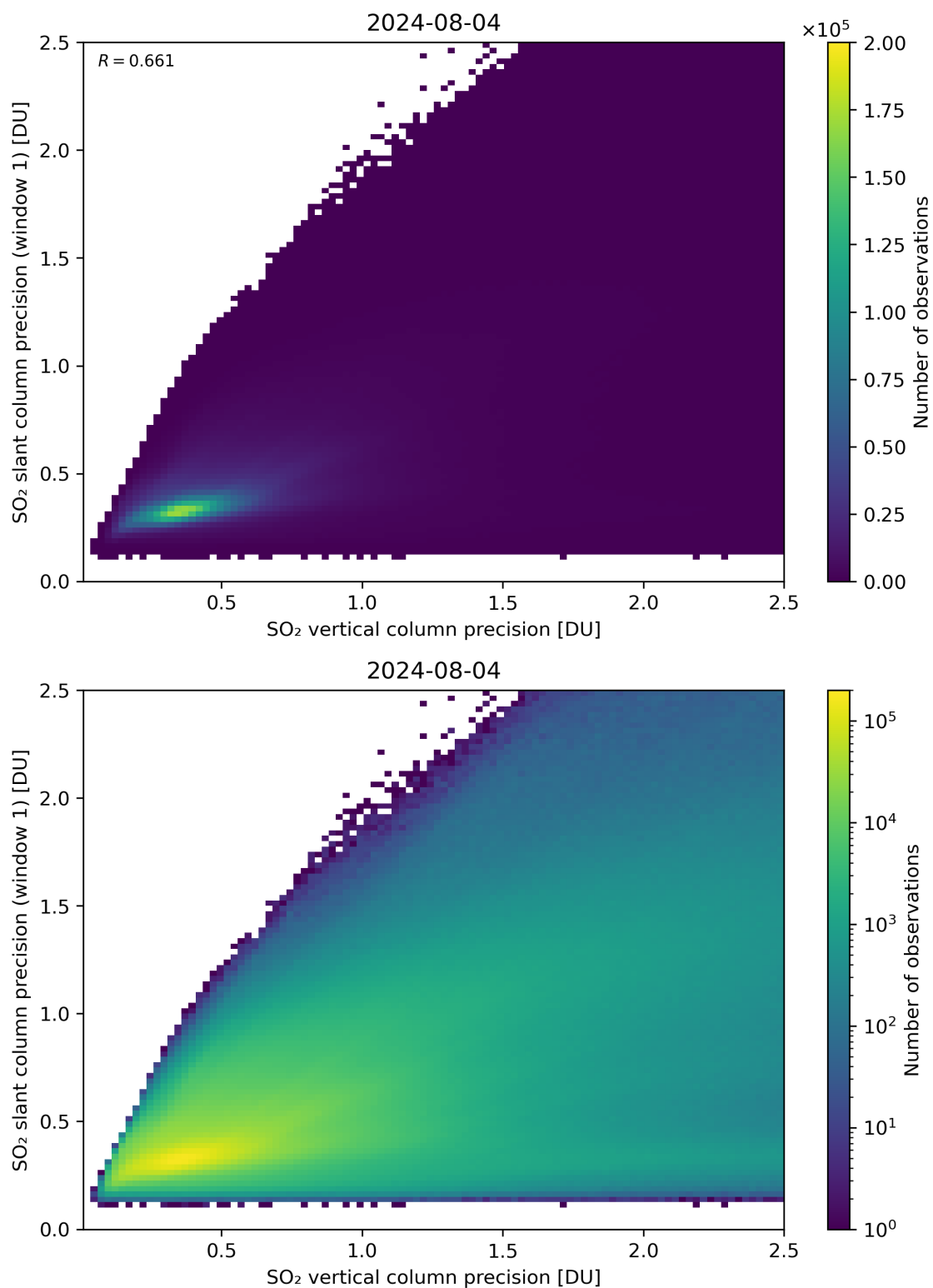
Figure 290: Scatter density plot of “SO 2 vertical column precision” against “SO 2 slant column precision (window 1)” for 2024-08-03 to 2024-08-05.
