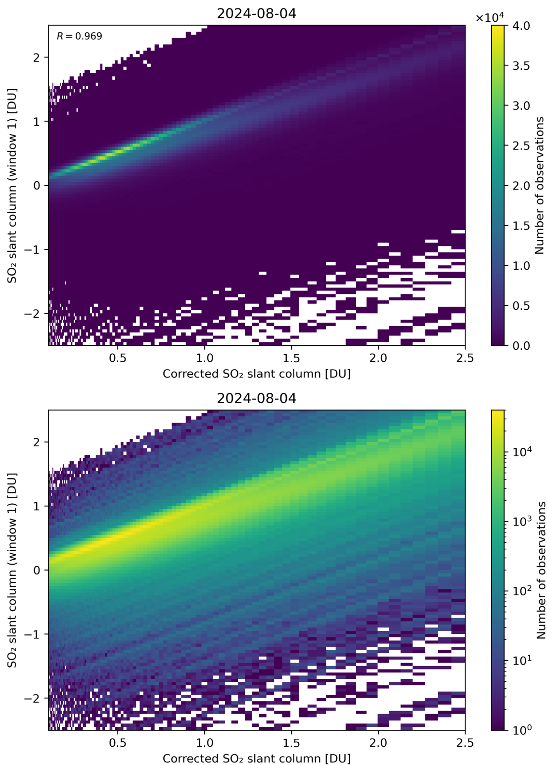
Figure 187: Scatter density plot of “Corrected SO 2 slant column” against “SO 2 slant column (window 1)” for 2024-08-03 to 2024-08-05.
