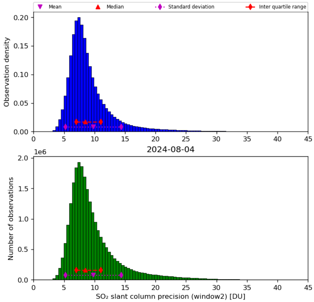
Figure 61: Histogram of “SO 2 slant column precision (window2)” for 2024-08-03 to 2024-08-05
