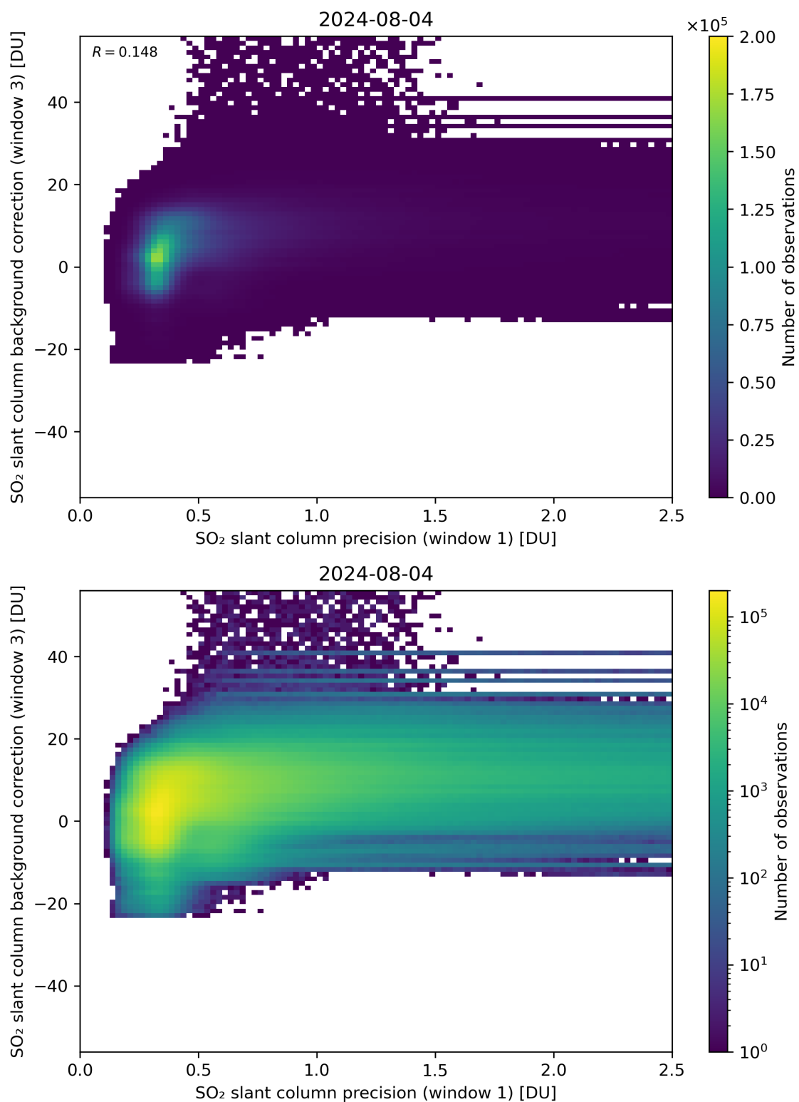
Figure 220: Scatter density plot of “SO 2 slant column precision (window 1)” against “SO 2 slant column background correction (window 3)” for 2024-08-03 to 2024-08-05.
