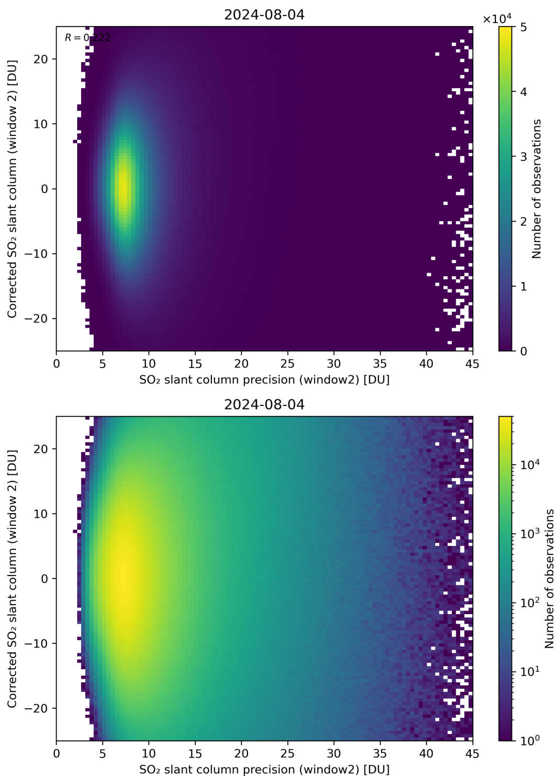
Figure 247: Scatter density plot of “SO 2 slant column precision (window2)” against “Corrected SO 2 slant column (window 2)” for 2024-08-03 to 2024-08-05.
