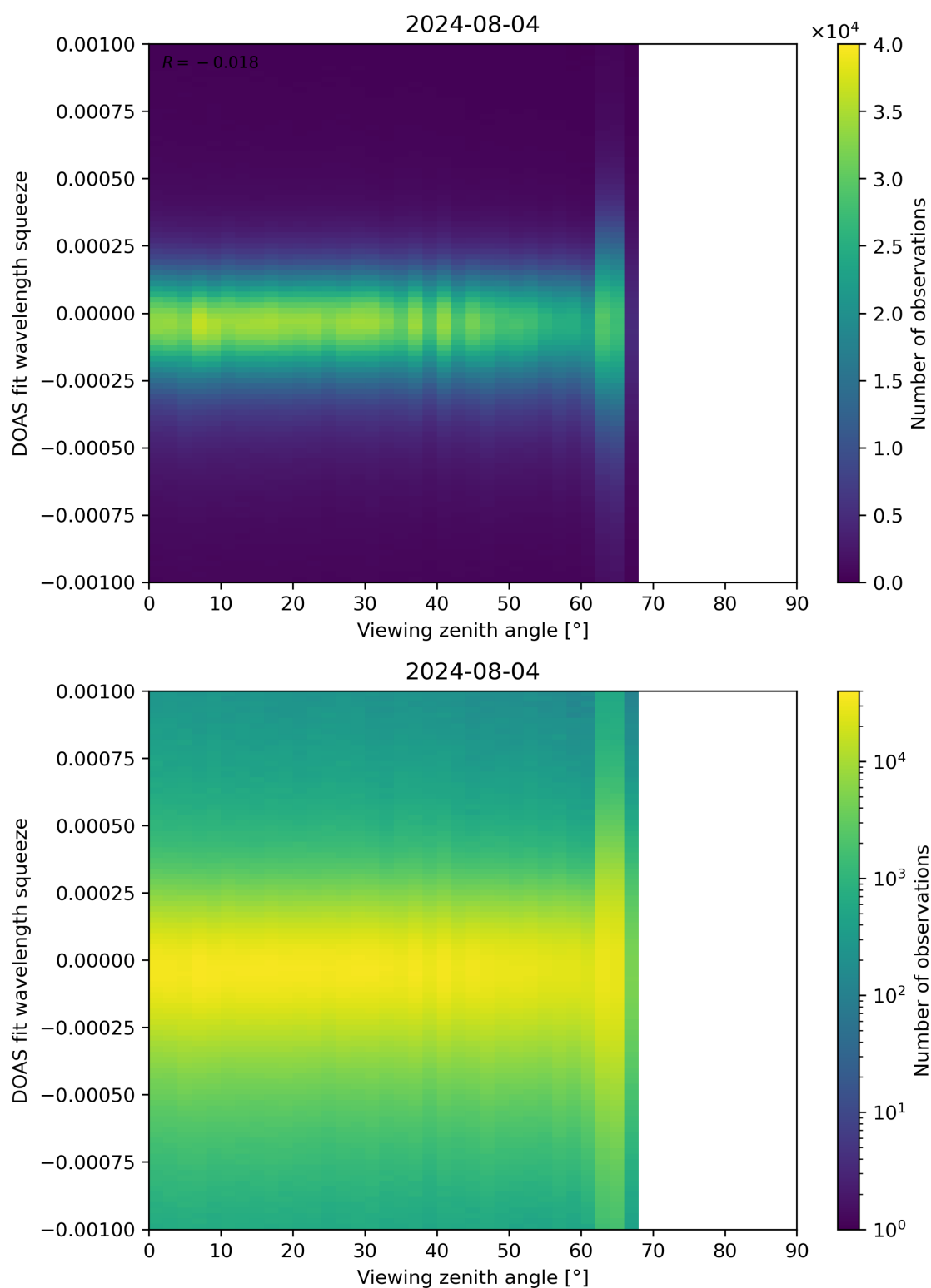
Figure 312: Scatter density plot of “Viewing zenith angle” against “DOAS fit wavelength squeeze” for 2024-08-03 to 2024-08-05.
