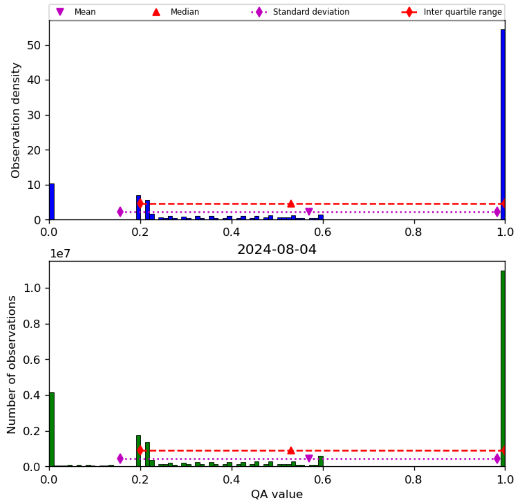
Figure 52: Histogram of “QA value” for 2024-08-03 to 2024-08-05
