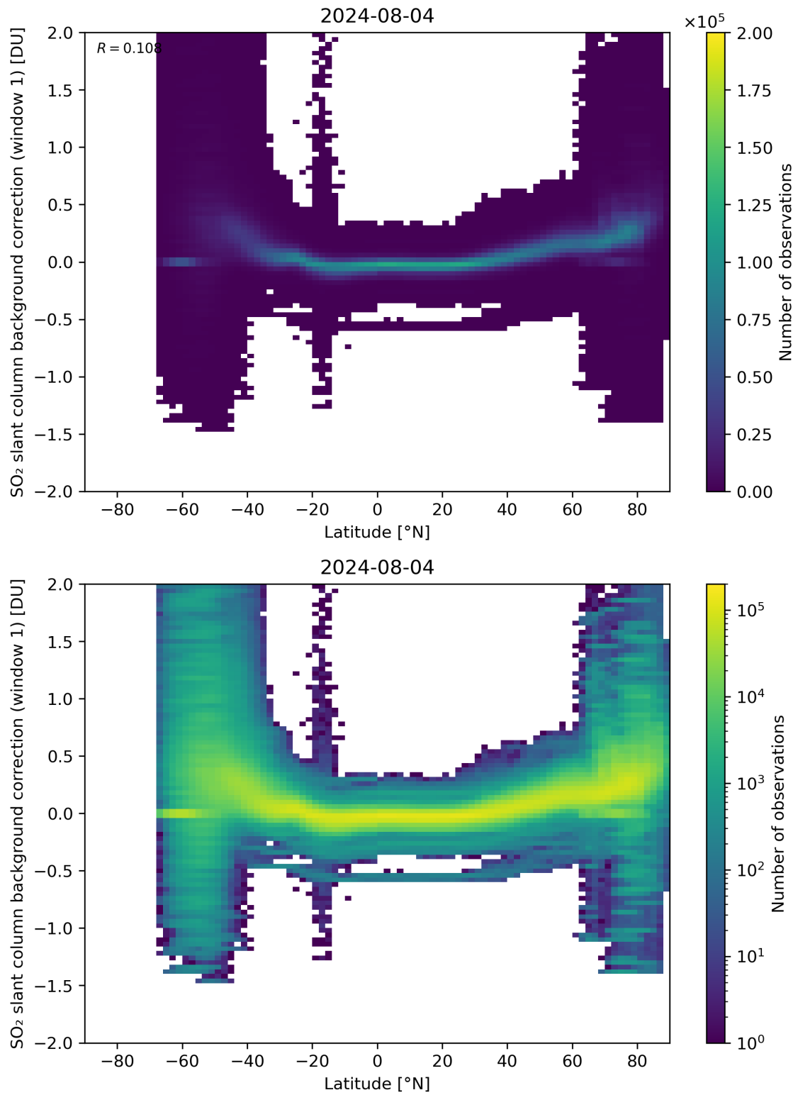
Figure 139: Scatter density plot of “Latitude” against “SO 2 slant column background correction (window 1)” for 2024-08-03 to 2024-08-05.
