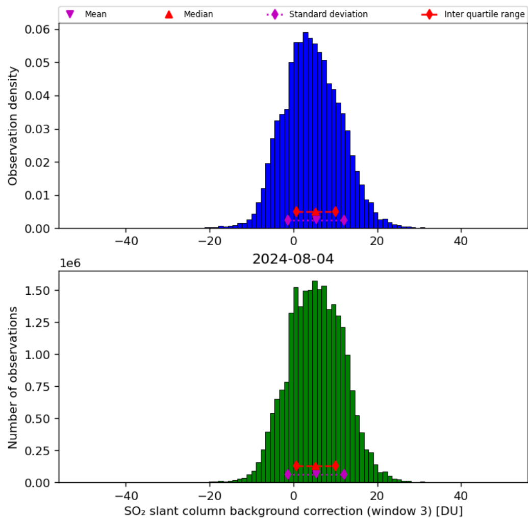
Figure 67: Histogram of “SO 2 slant column background correction (window 3)” for 2024-08-03 to 2024-08-05
