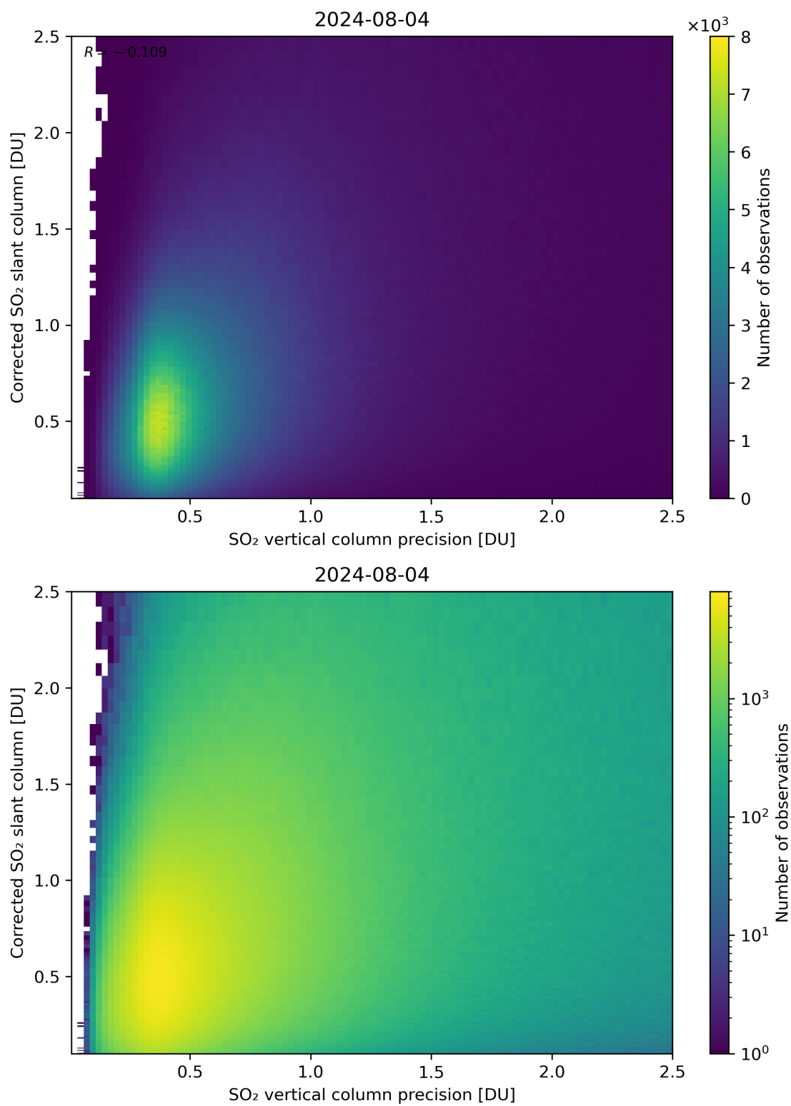
Figure 286: Scatter density plot of “SO 2 vertical column precision” against “Corrected SO 2 slant column” for 2024-08-03 to 2024-08-05.
