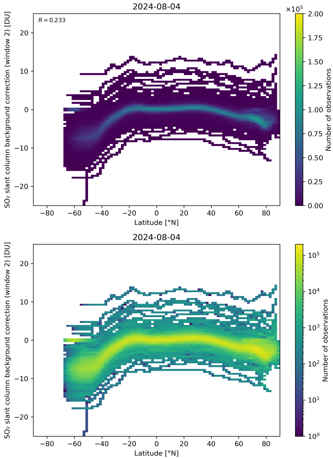
Figure 140: Scatter density plot of “Latitude” against “SO 2 slant column background correction (window 2)” for 2024-08-03 to 2024-08-05.
