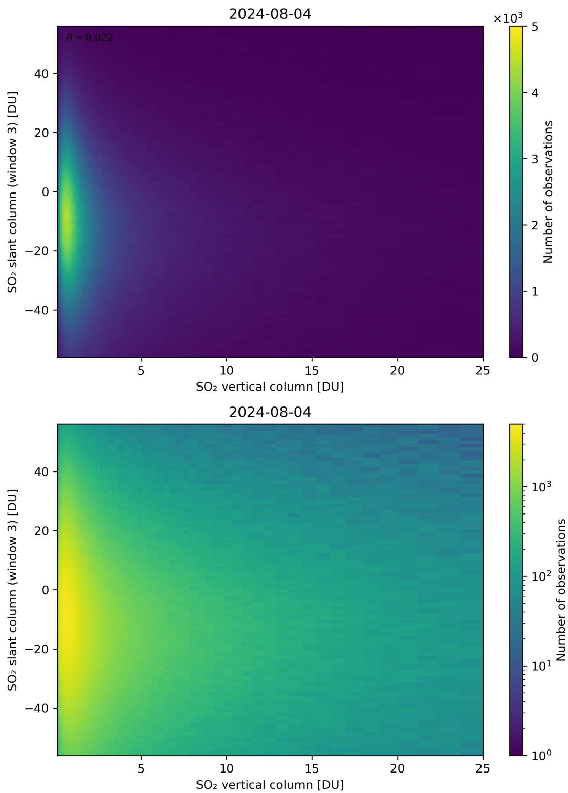
Figure 303: Scatter density plot of “SO 2 vertical column” against “SO 2 slant column (window 3)” for 2024-08-03 to 2024-08-05.
