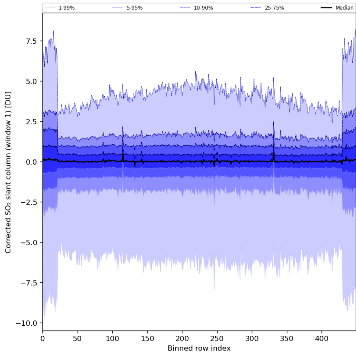
Figure 81: Along track statistics of “Corrected SO 2 slant column (window 1)” for 2024-08-03 to 2024-08-05
