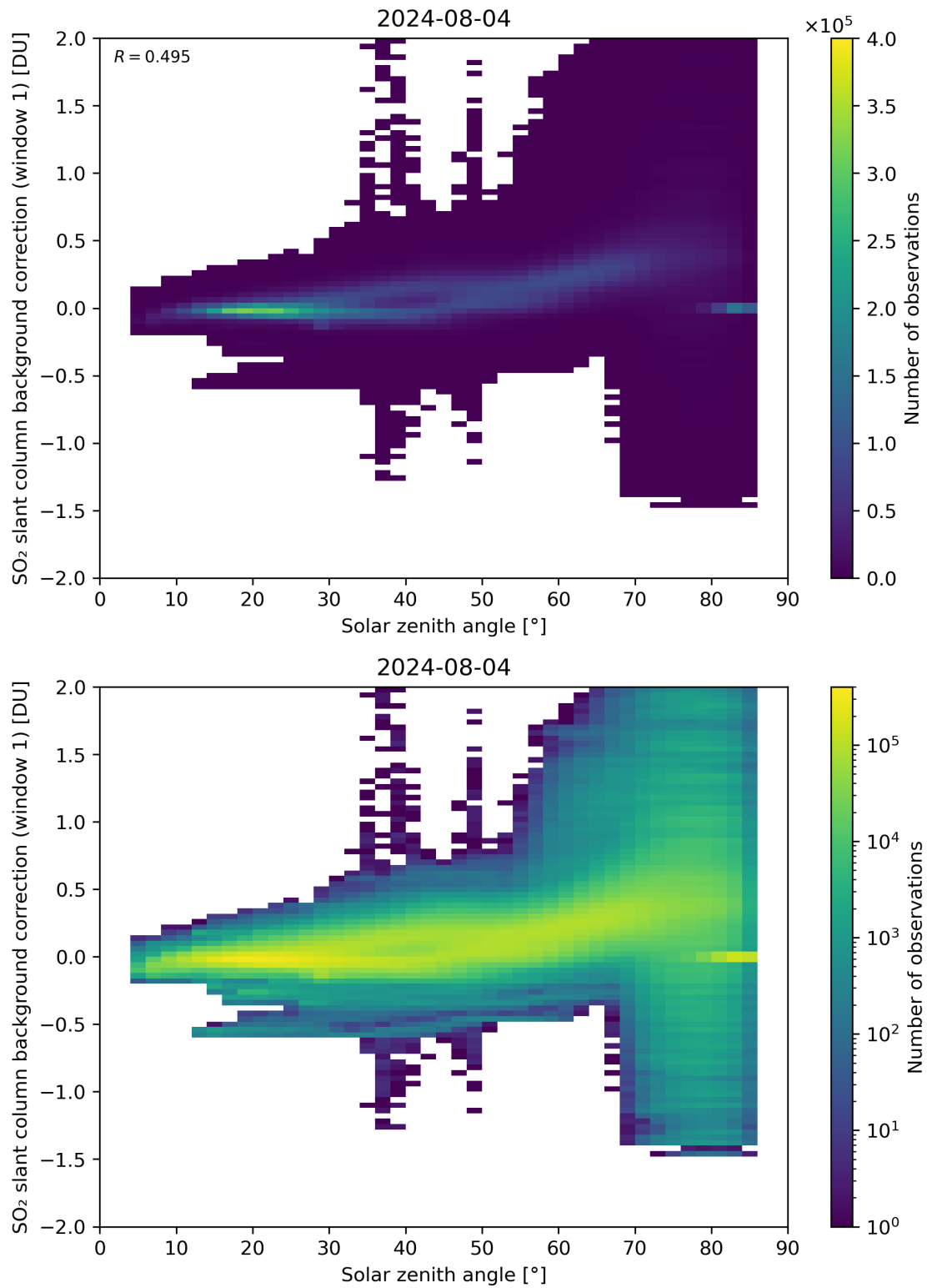
Figure 158: Scatter density plot of “Solar zenith angle” against “SO 2 slant column background correction (window 1)” for 2024-08-03 to 2024-08-05.
