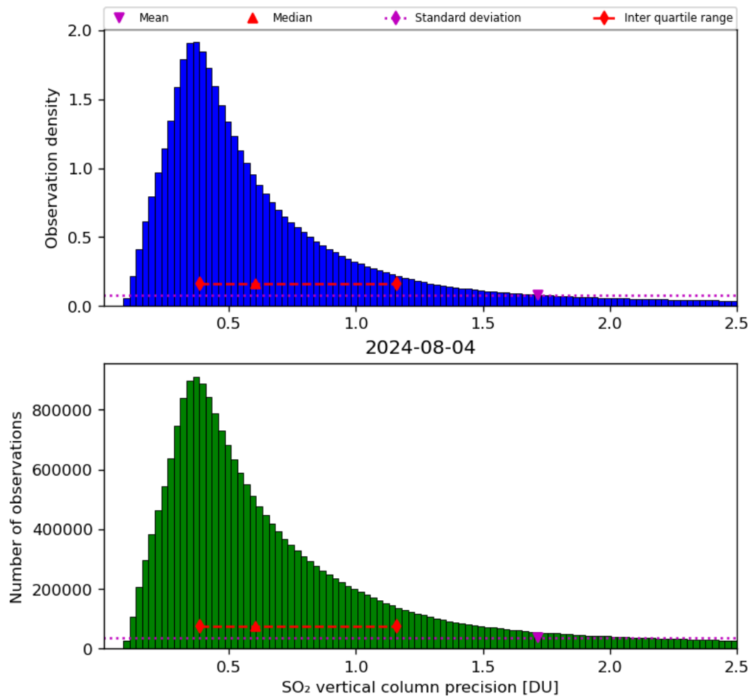
Figure 54: Histogram of “SO 2 vertical column precision” for 2024-08-03 to 2024-08-05
