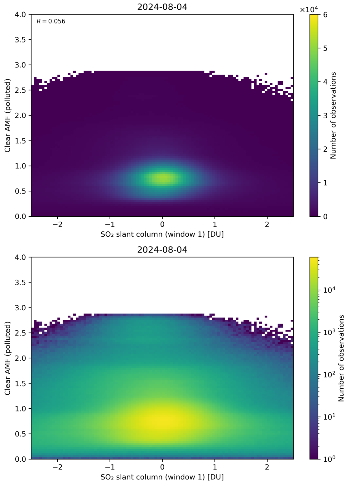
Figure 232: Scatter density plot of “SO 2 slant column (window 1)” against “Clear AMF (polluted)” for 2024-08-03 to 2024-08-05.
