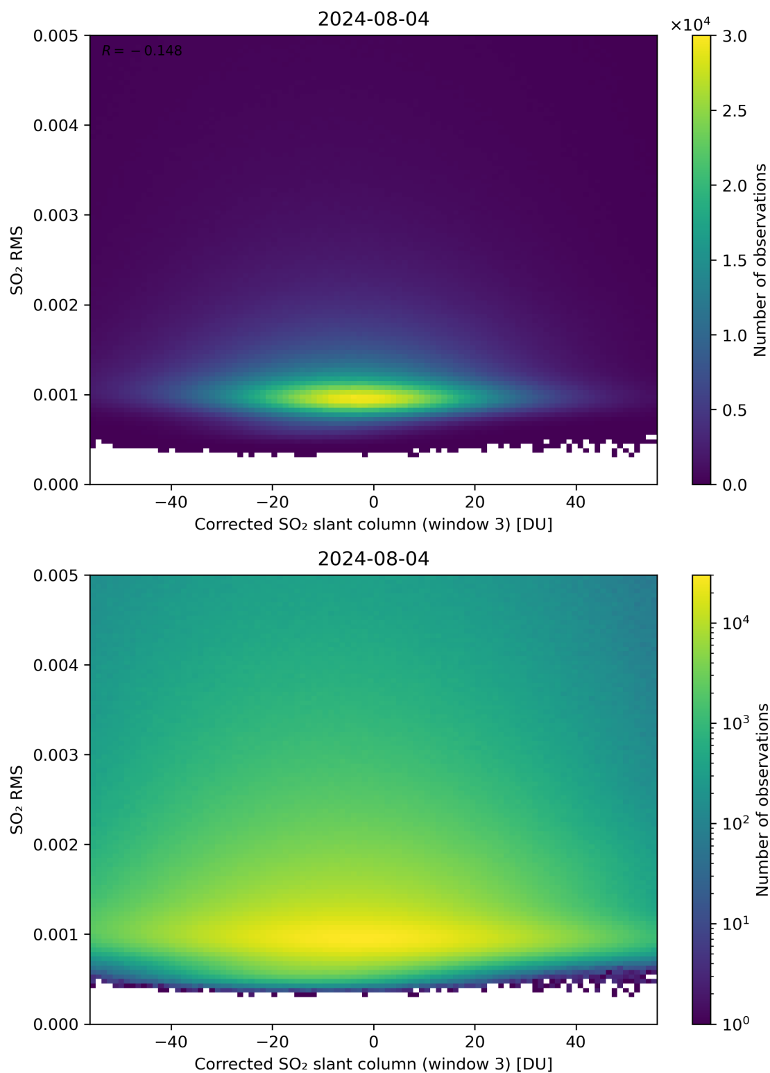
Figure 208: Scatter density plot of “Corrected SO 2 slant column (window 3)” against “SO 2 RMS” for 2024-08-03 to 2024-08-05.
