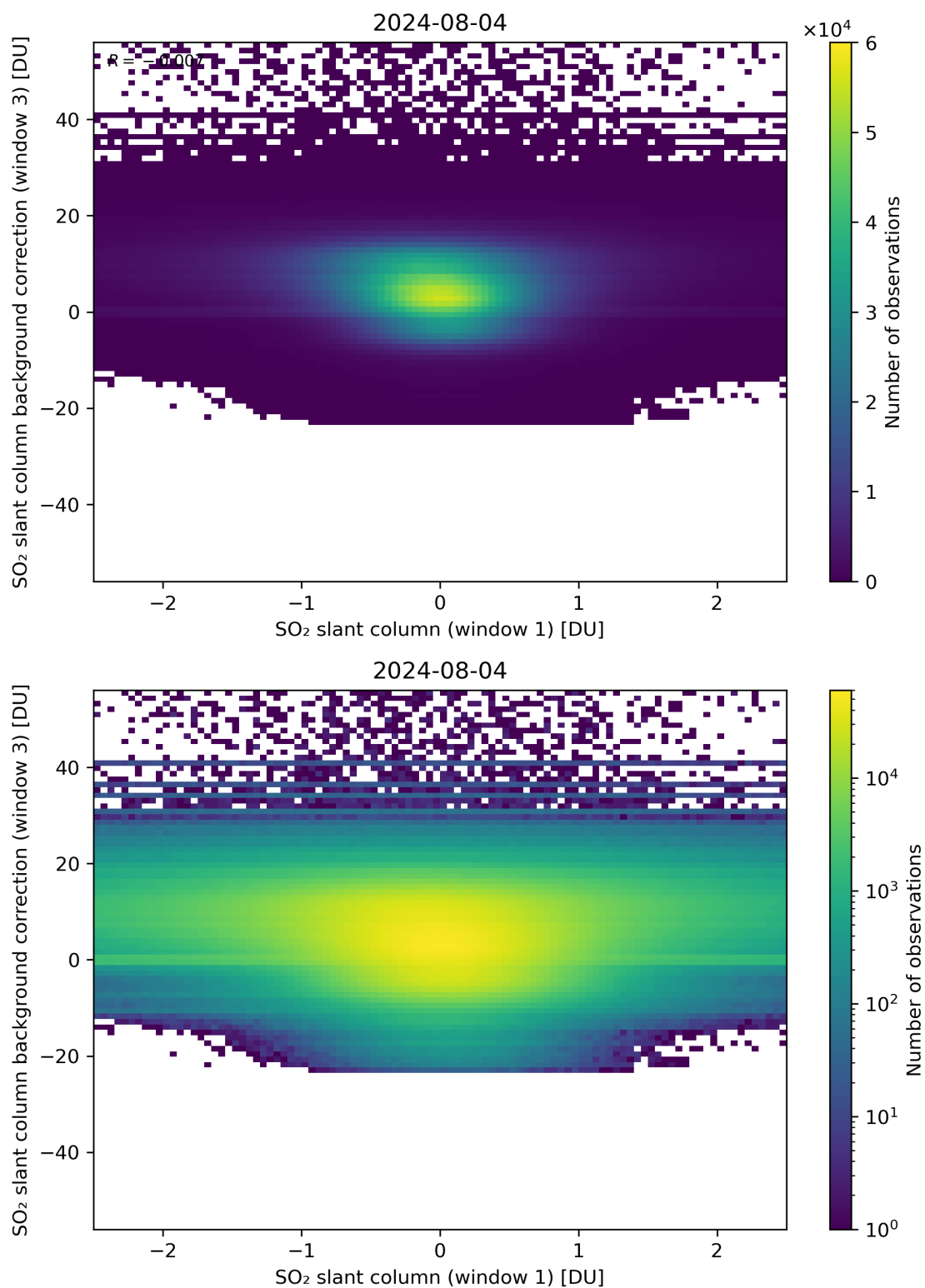
Figure 214: Scatter density plot of “SO 2 slant column (window 1)” against “SO 2 slant column background correction (window 3)” for 2024-08-03 to 2024-08-05.
