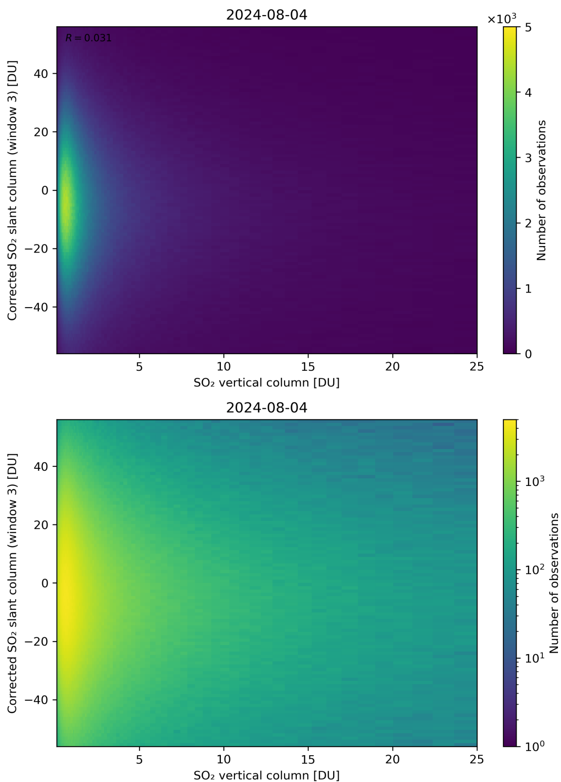
Figure 299: Scatter density plot of “SO 2 vertical column” against “Corrected SO 2 slant column (window 3)” for 2024-08-03 to 2024-08-05.
