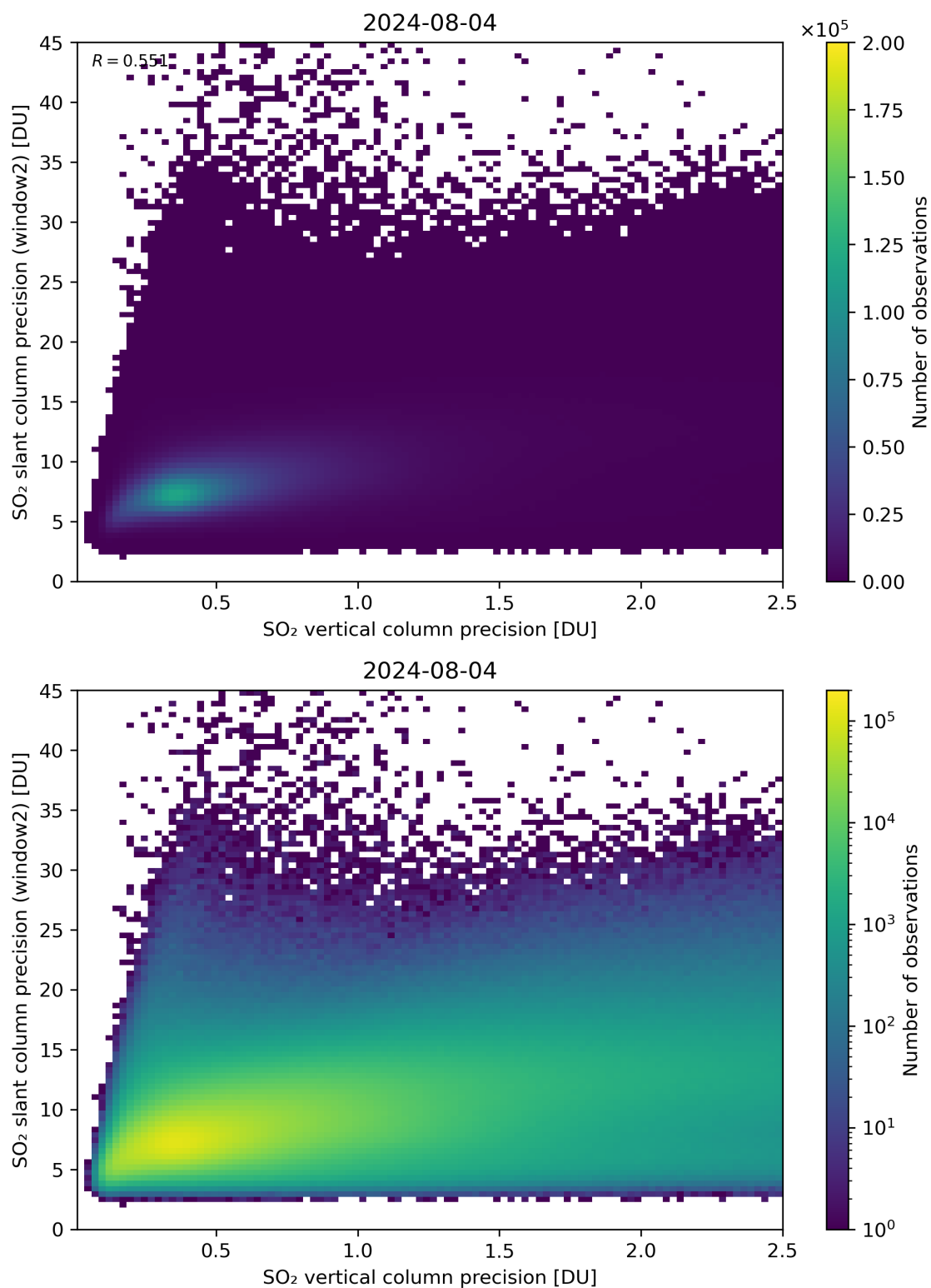
Figure 291: Scatter density plot of “SO 2 vertical column precision” against “SO 2 slant column precision (window2)” for 2024-08-03 to 2024-08-05.
