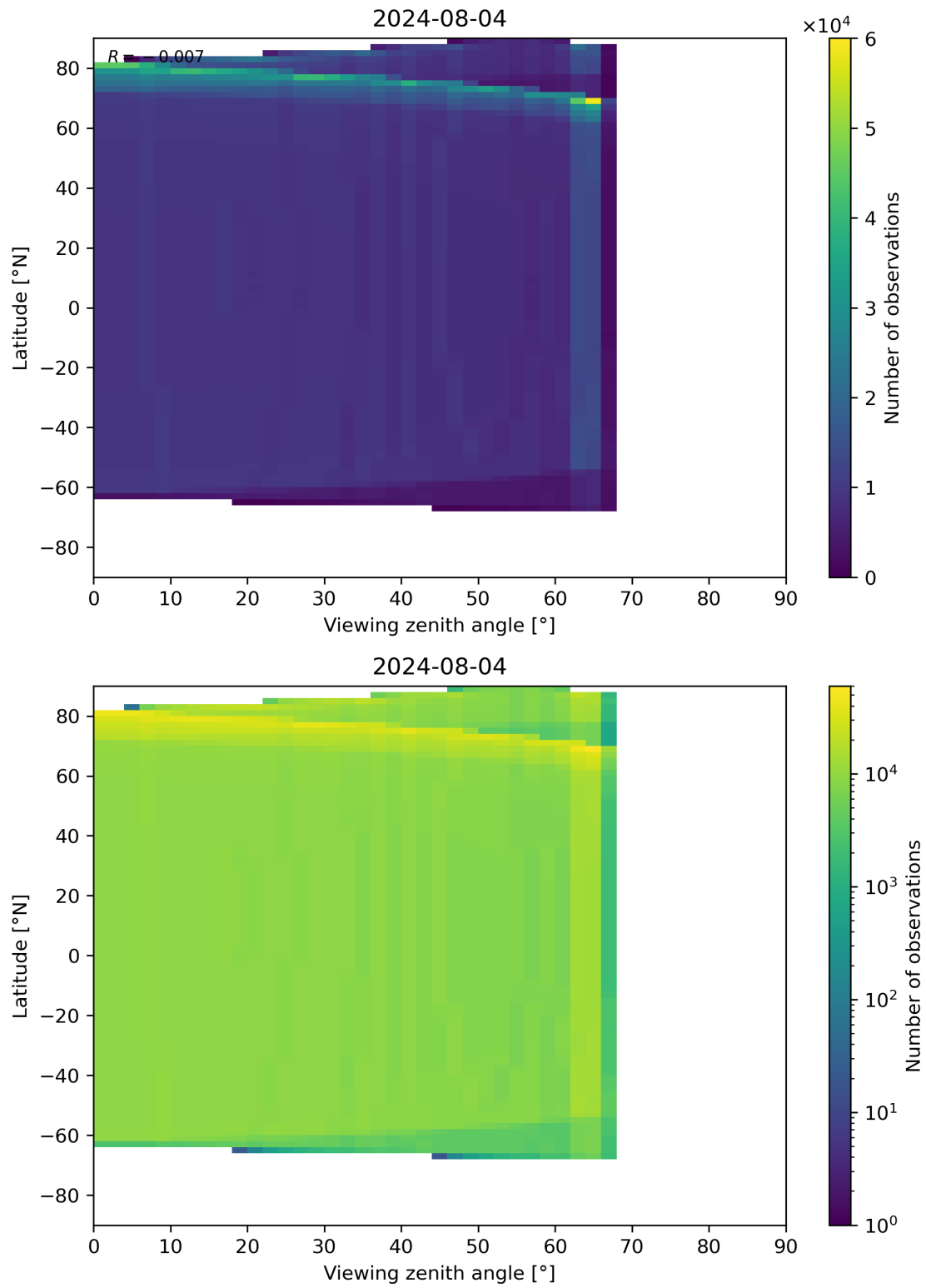
Figure 314: Scatter density plot of “Viewing zenith angle” against “Latitude” for 2024-08-03 to 2024-08-05.
