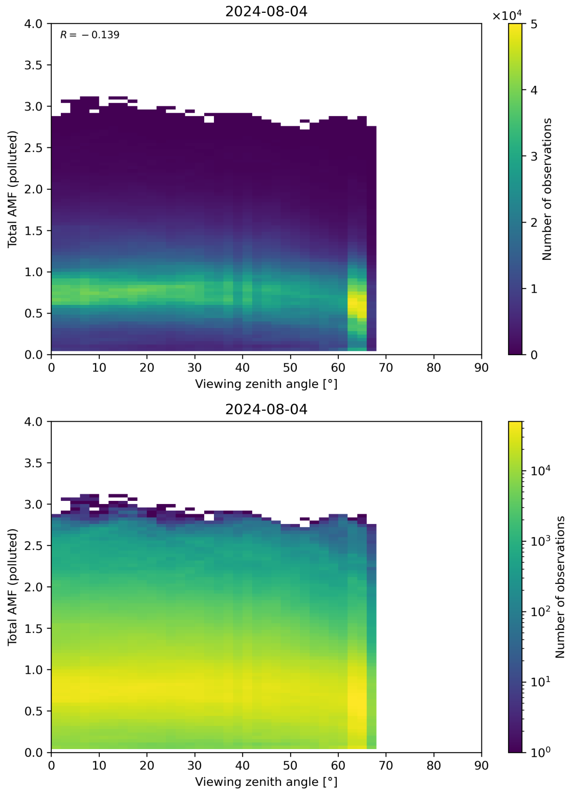
Figure 325: Scatter density plot of “Viewing zenith angle” against “Total AMF (polluted)” for 2024-08-03 to 2024-08-05.
