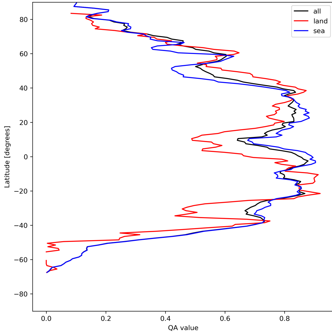
Figure 29: Zonal average of “QA value” for 2024-08-03 to 2024-08-05.
