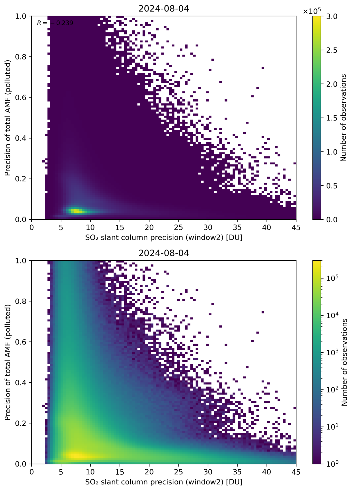
Figure 252: Scatter density plot of “SO 2 slant column precision (window2)” against “Precision of total AMF (polluted)” for 2024-08-03 to 2024-08-05.
