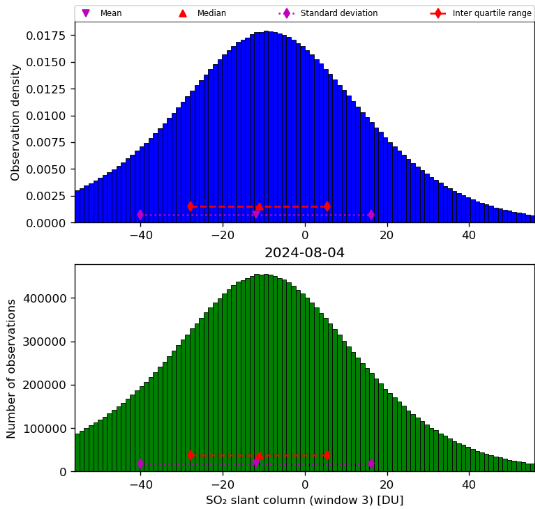
Figure 64: Histogram of “SO 2 slant column (window 3)” for 2024-08-03 to 2024-08-05
