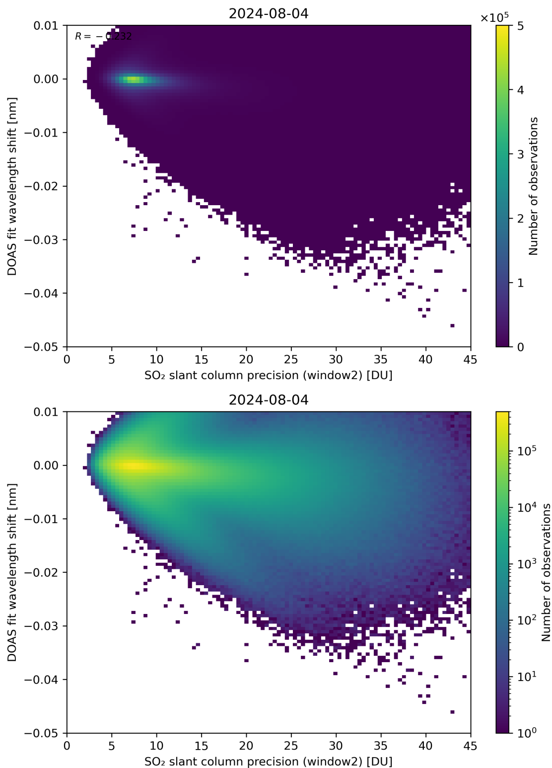
Figure 243: Scatter density plot of “SO 2 slant column precision (window2)” against “DOAS fit wavelength shift” for 2024-08-03 to 2024-08-05.
