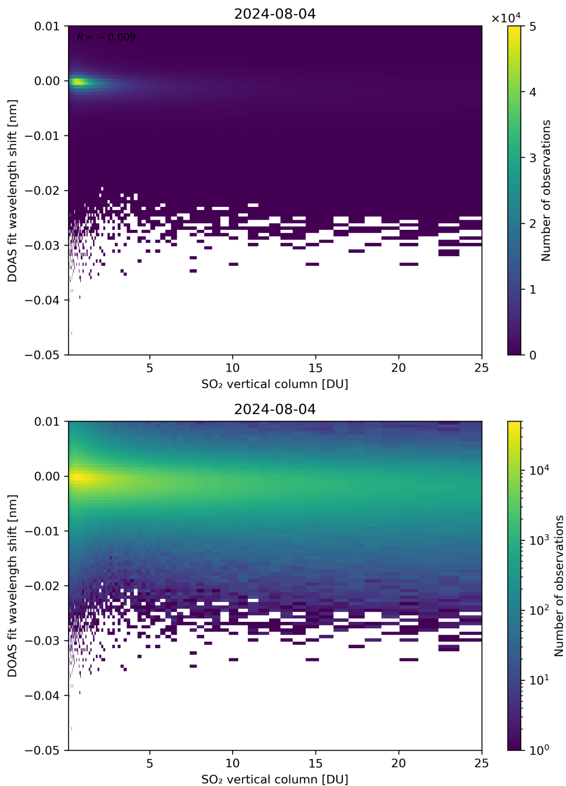
Figure 276: Scatter density plot of “SO 2 vertical column” against “DOAS fit wavelength shift” for 2024-08-03 to 2024-08-05.
