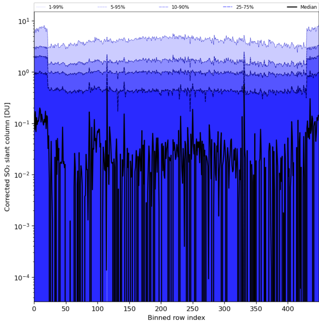
Figure 78: Along track statistics of “Corrected SO 2 slant column” for 2024-08-03 to 2024-08-05
