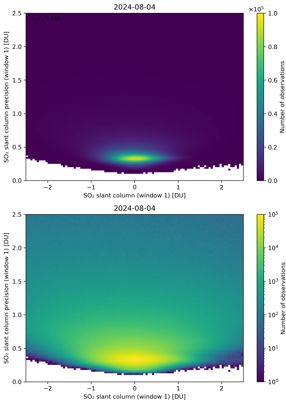
Figure 235: Scatter density plot of “SO 2 slant column (window 1)” against “SO 2 slant column precision (window 1)” for 2024-08-03 to 2024-08-05.
