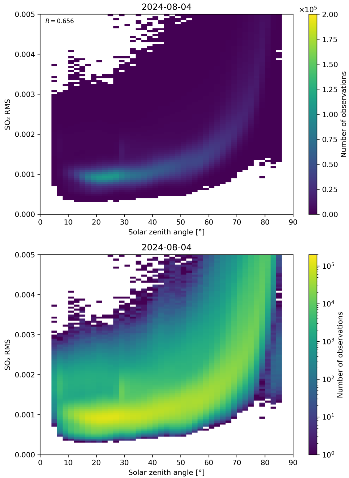
Figure 163: Scatter density plot of “Solar zenith angle” against “SO 2 RMS” for 2024-08-03 to 2024-08-05.
