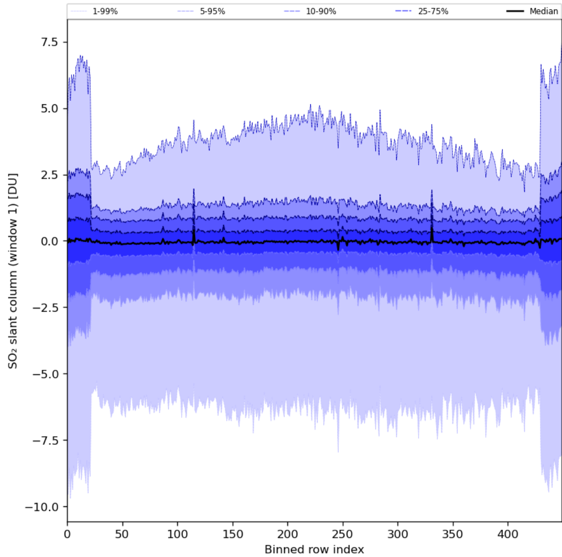
Figure 79: Along track statistics of “SO 2 slant column (window 1)” for 2024-08-03 to 2024-08-05
