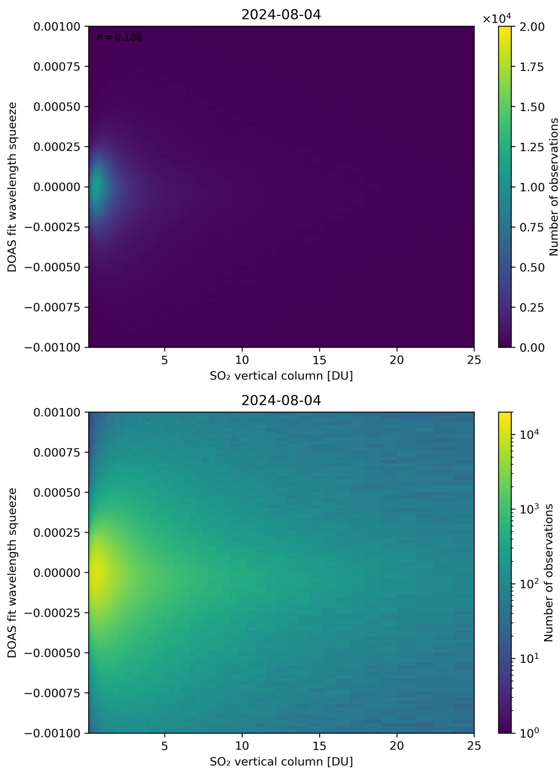
Figure 277: Scatter density plot of “SO 2 vertical column” against “DOAS fit wavelength squeeze” for 2024-08-03 to 2024-08-05.
