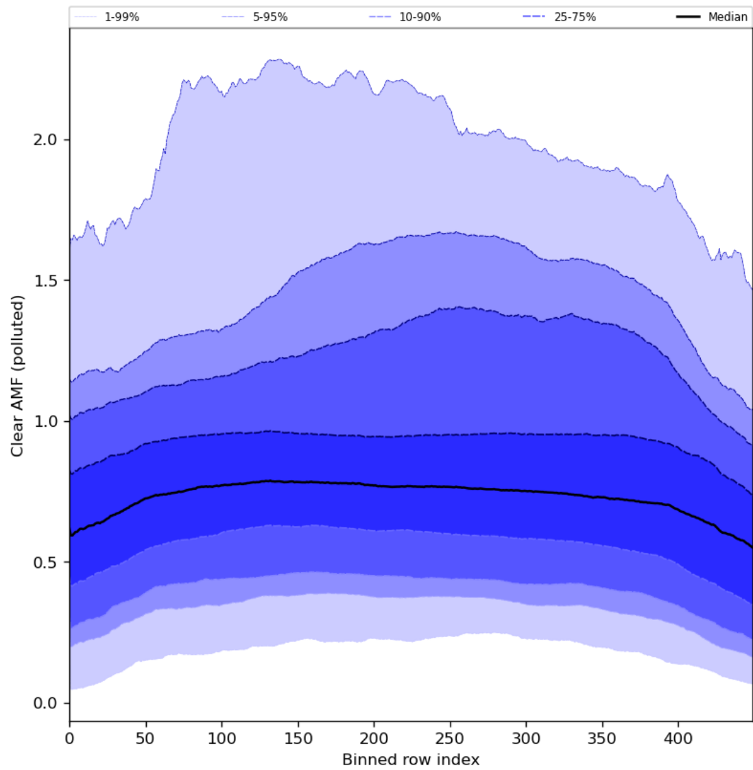
Figure 96: Along track statistics of “Clear AMF (polluted)” for 2024-08-03 to 2024-08-05
