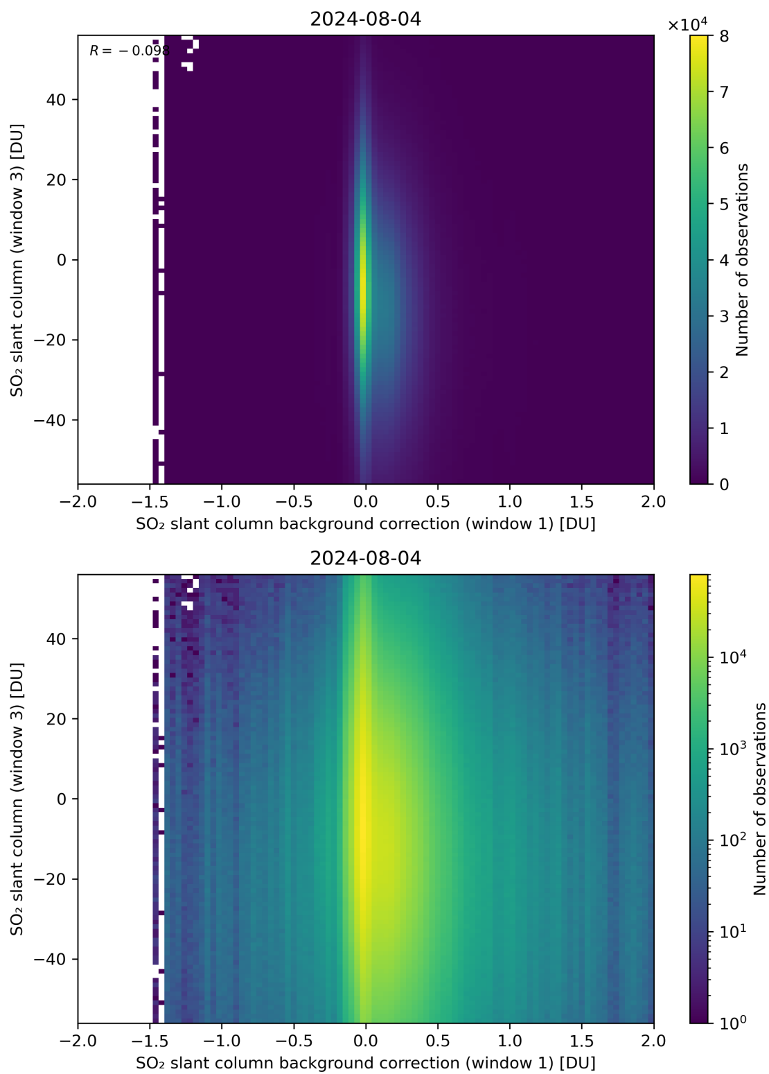
Figure 107: Scatter density plot of “SO 2 slant column background correction (window 1)” against “SO 2 slant column (window 3)” for 2024-08-03 to 2024-08-05.
