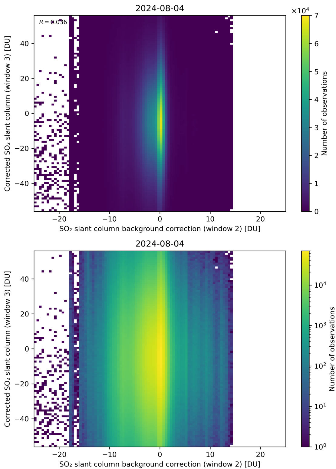
Figure 116: Scatter density plot of “SO 2 slant column background correction (window 2)” against “Corrected SO 2 slant column (window 3)” for 2024-08-03 to 2024-08-05.
