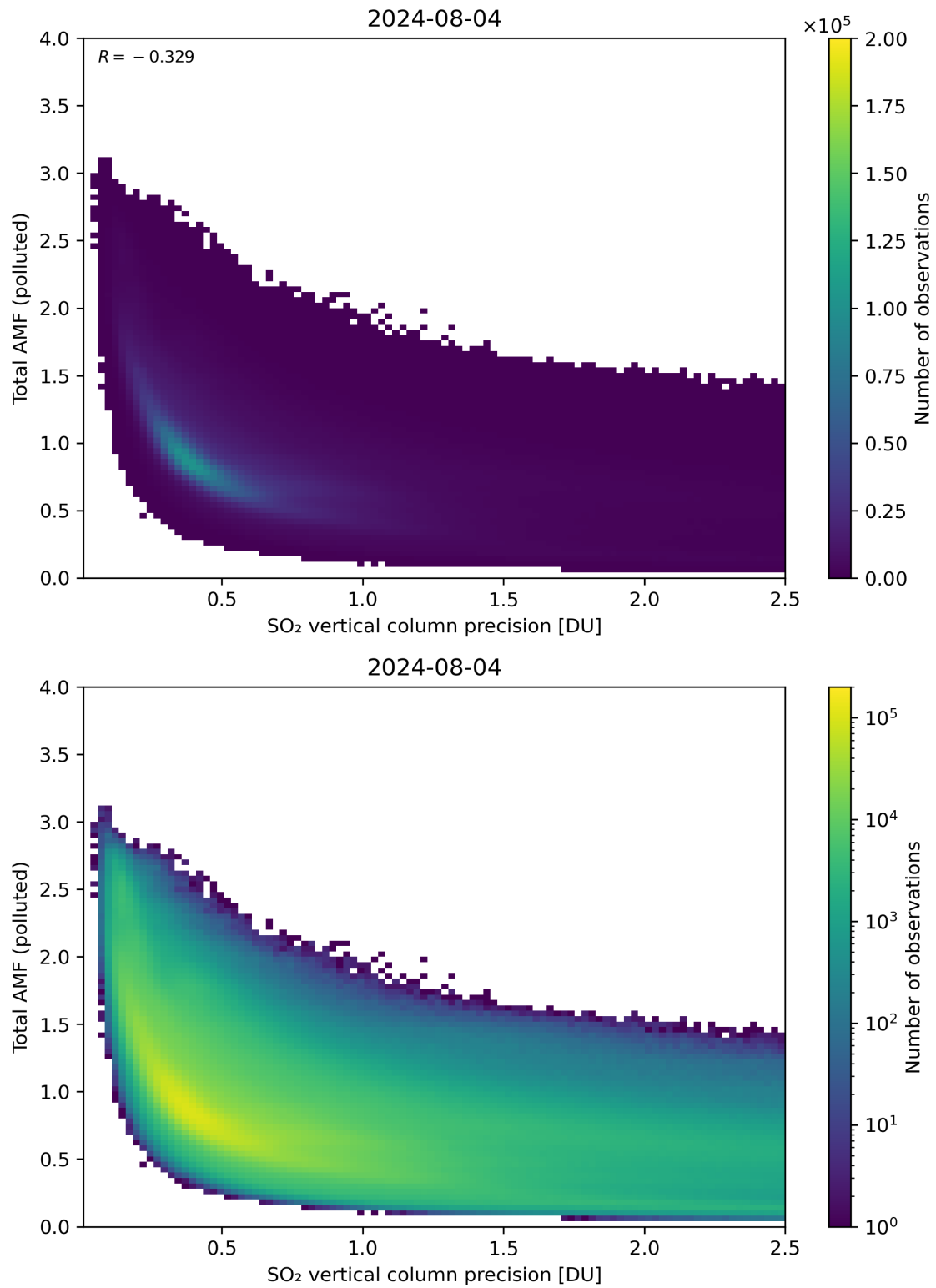
Figure 294: Scatter density plot of “SO 2 vertical column precision” against “Total AMF (polluted)” for 2024-08-03 to 2024-08-05.
