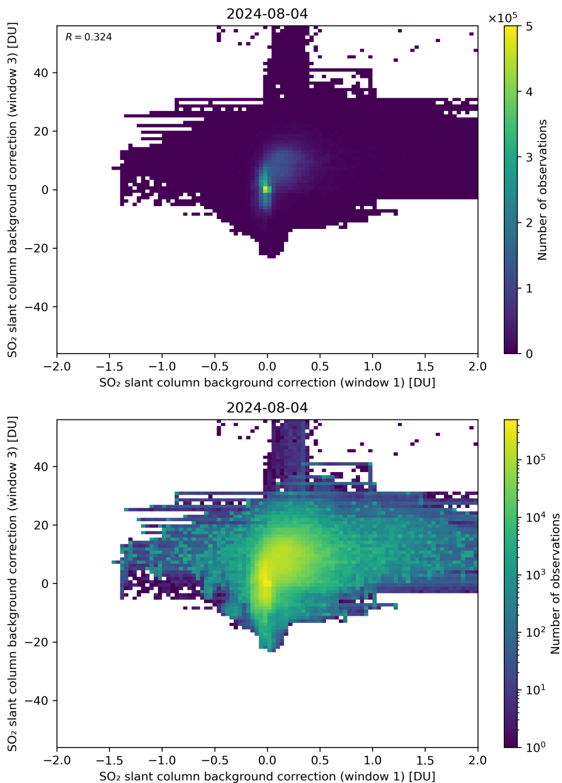
Figure 99: Scatter density plot of “SO 2 slant column background correction (window 1)” against “SO 2 slant column background correction (window 3)” for 2024-08-03 to 2024-08-05.
