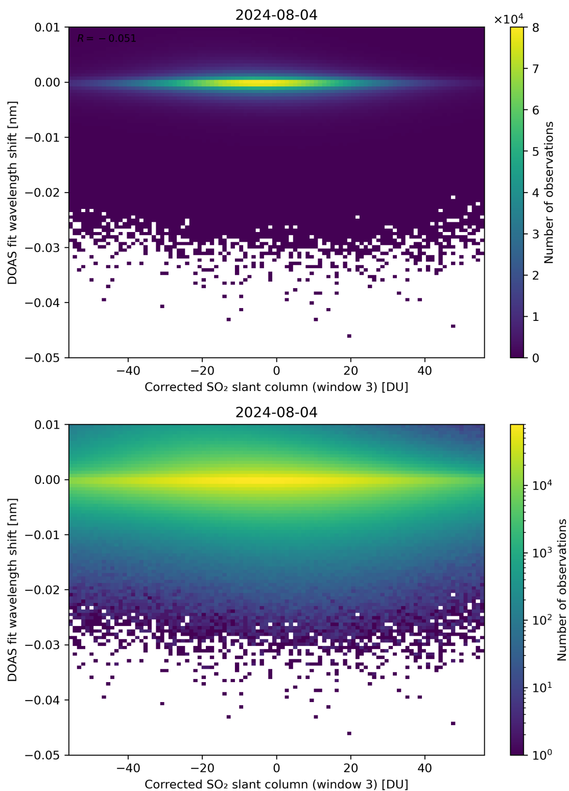
Figure 206: Scatter density plot of “Corrected SO 2 slant column (window 3)” against “DOAS fit wavelength shift” for 2024-08-03 to 2024-08-05.
