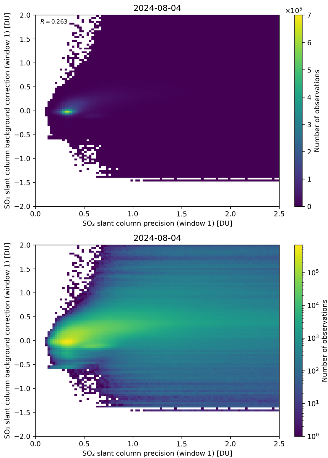
Figure 218: Scatter density plot of “SO 2 slant column precision (window 1)” against “SO 2 slant column background correction (window 1)” for 2024-08-03 to 2024-08-05.
