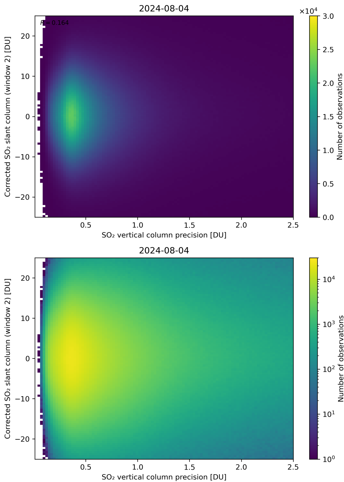
Figure 287: Scatter density plot of “SO 2 vertical column precision” against “Corrected SO 2 slant column (window 2)” for 2024-08-03 to 2024-08-05.
