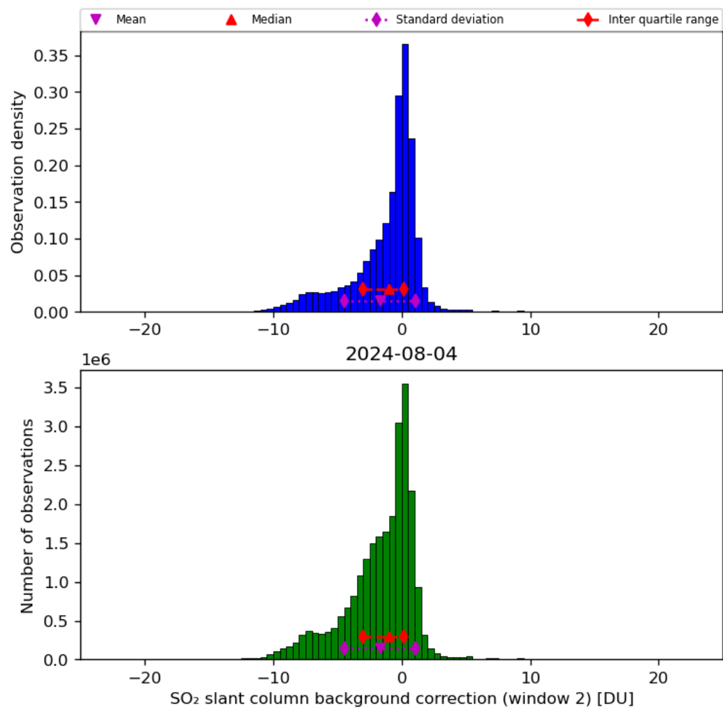
Figure 63: Histogram of “SO 2 slant column background correction (window 2)” for 2024-08-03 to 2024-08-05
