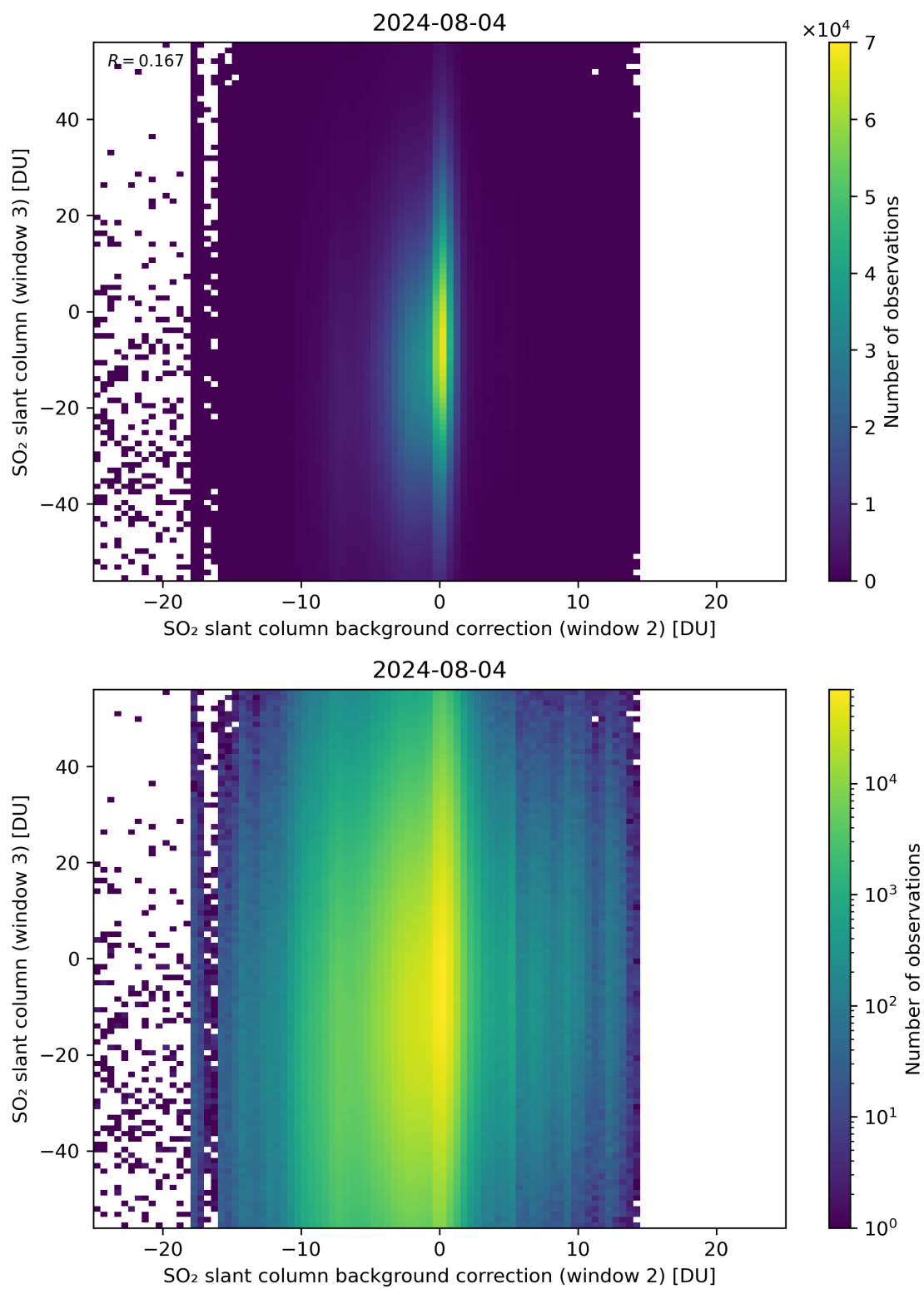
Figure 117: Scatter density plot of “SO 2 slant column background correction (window 2)” against “SO 2 slant column (window 3)” for 2024-08-03 to 2024-08-05.
