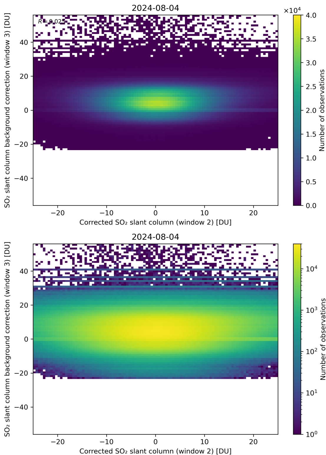
Figure 195: Scatter density plot of “Corrected SO 2 slant column (window 2)” against “SO 2 slant column background correction (window 3)” for 2024-08-03 to 2024-08-05.
