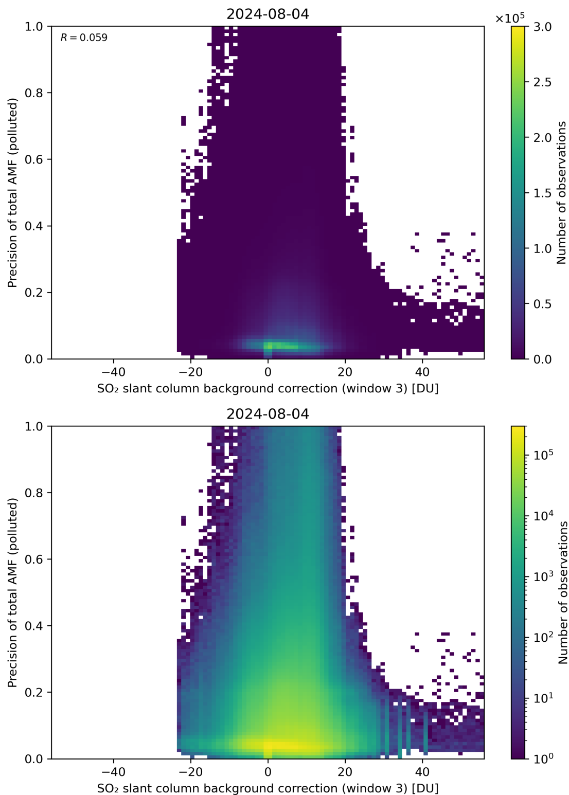
Figure 126: Scatter density plot of “SO 2 slant column background correction (window 3)” against “Precision of total AMF (polluted)” for 2024-08-03 to 2024-08-05.
