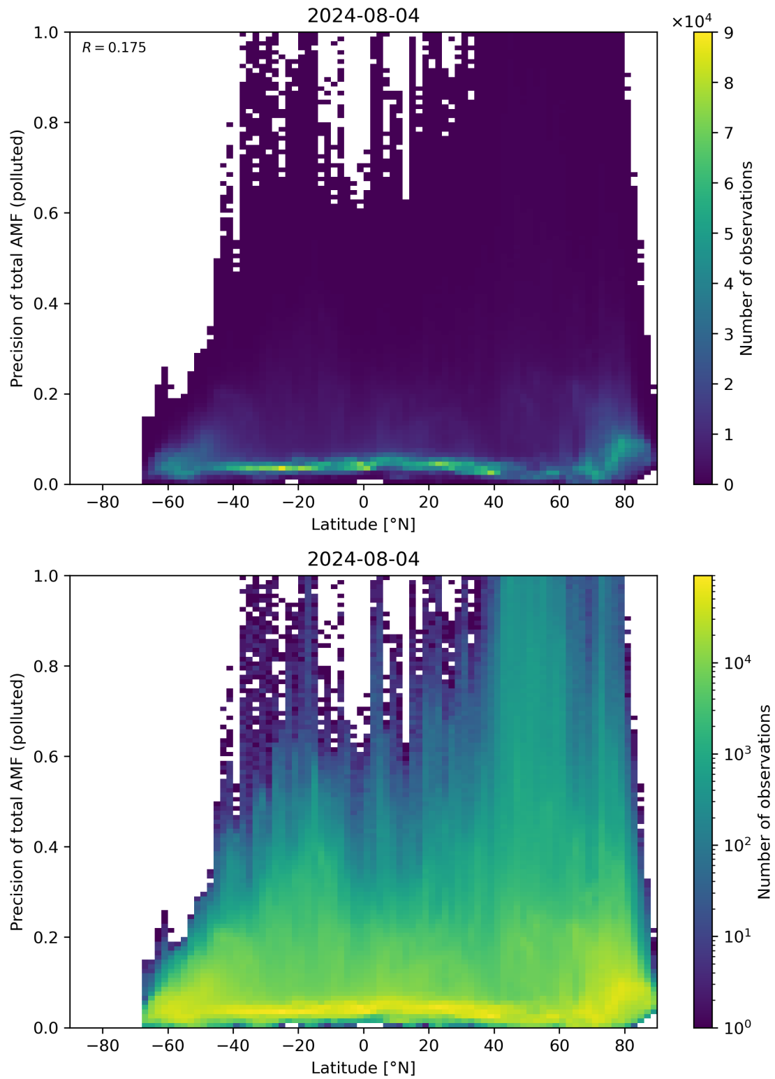
Figure 155: Scatter density plot of “Latitude” against “Precision of total AMF (polluted)” for 2024-08-03 to 2024-08-05.
