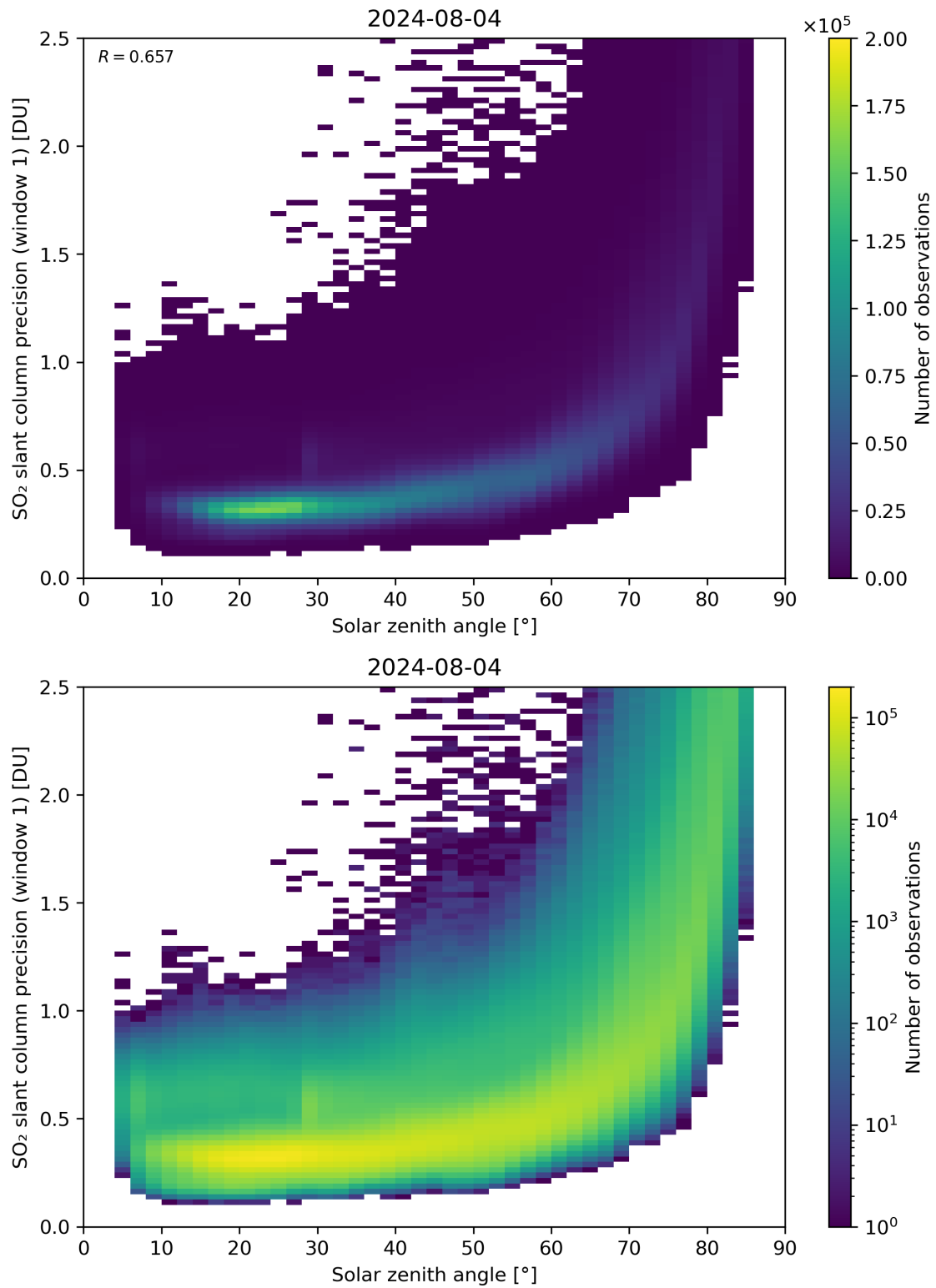
Figure 170: Scatter density plot of “Solar zenith angle” against “SO 2 slant column precision (window 1)” for 2024-08-03 to 2024-08-05.
