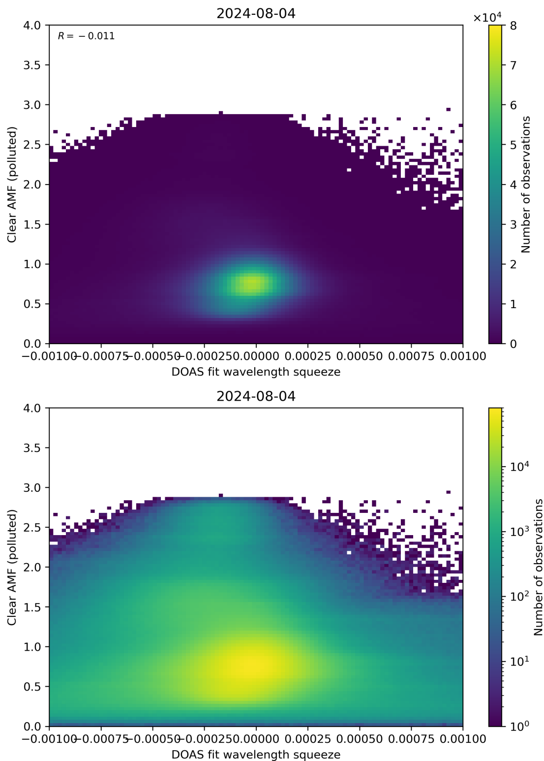
Figure 133: Scatter density plot of “DOAS fit wavelength squeeze” against “Clear AMF (polluted)” for 2024-08-03 to 2024-08-05.
