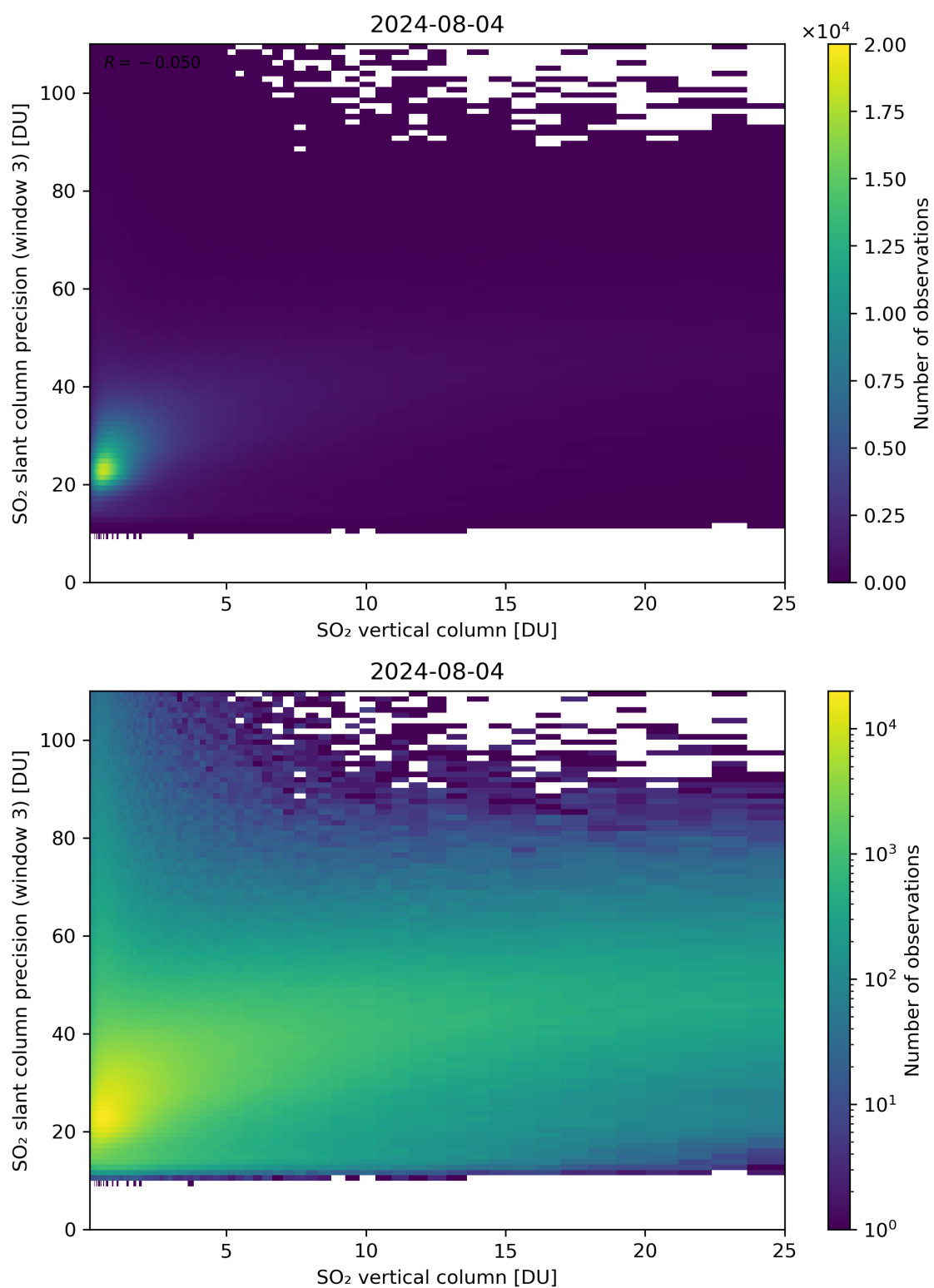
Figure 304: Scatter density plot of “SO 2 vertical column” against “SO 2 slant column precision (window 3)” for 2024-08-03 to 2024-08-05.
