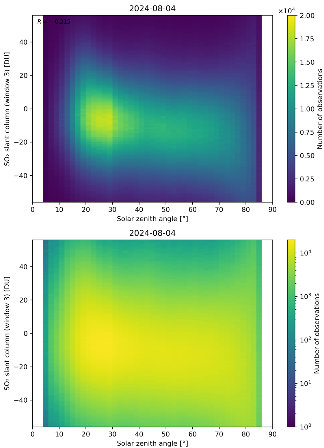
Figure 172: Scatter density plot of “Solar zenith angle” against “SO 2 slant column (window 3)” for 2024-08-03 to 2024-08-05.
