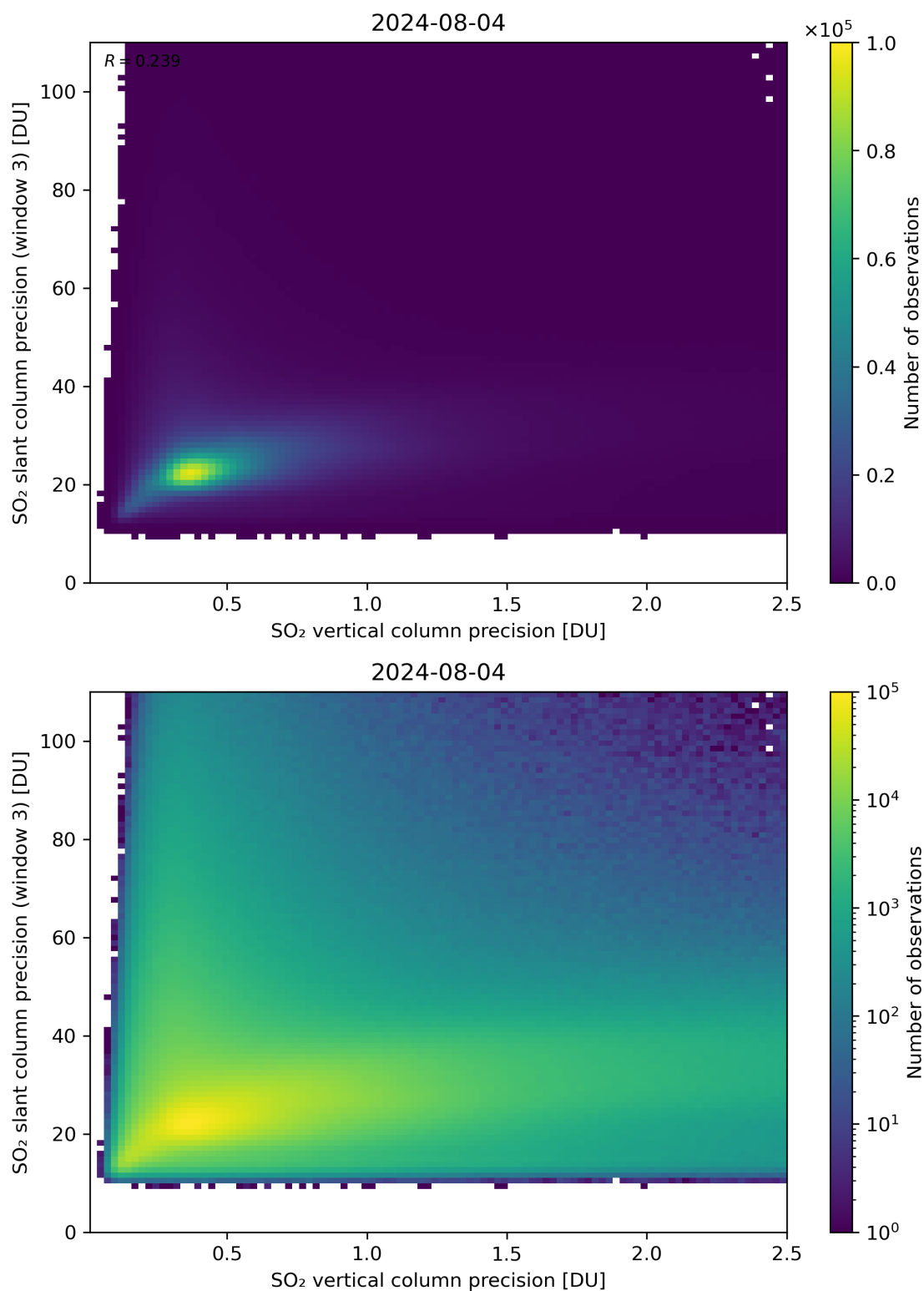
Figure 293: Scatter density plot of “SO 2 vertical column precision” against “SO 2 slant column precision (window 3)” for 2024-08-03 to 2024-08-05.
