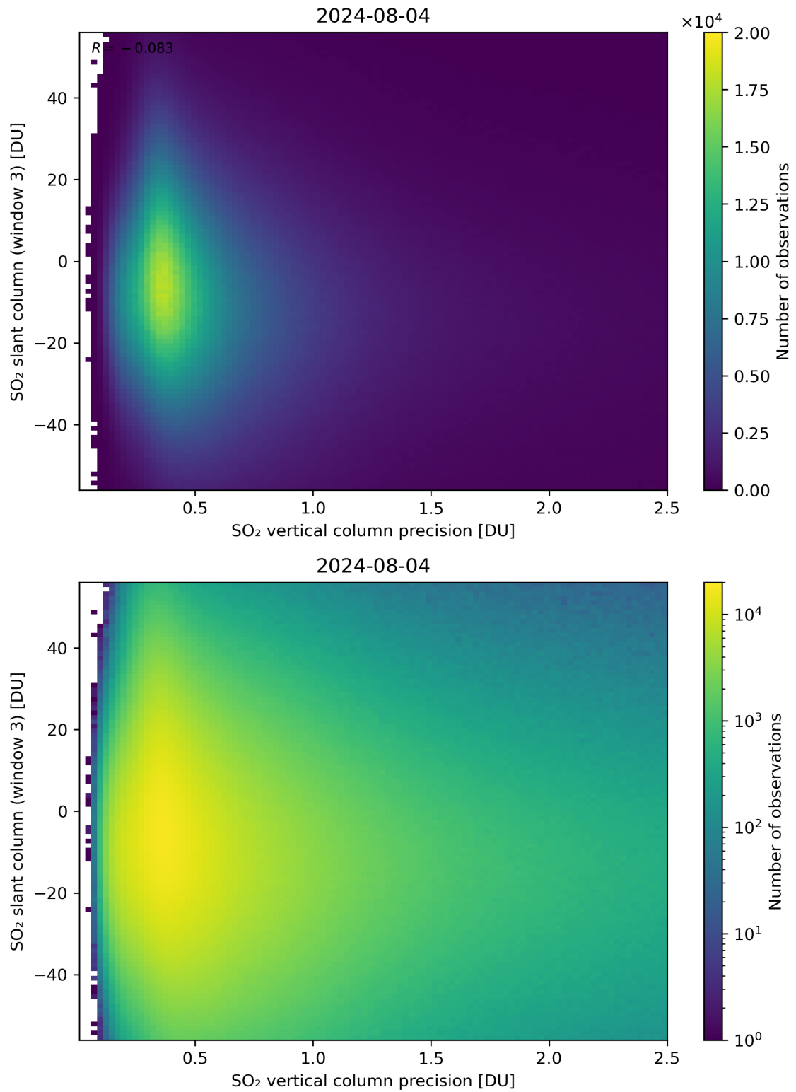
Figure 292: Scatter density plot of “SO 2 vertical column precision” against “SO 2 slant column (window 3)” for 2024-08-03 to 2024-08-05.
