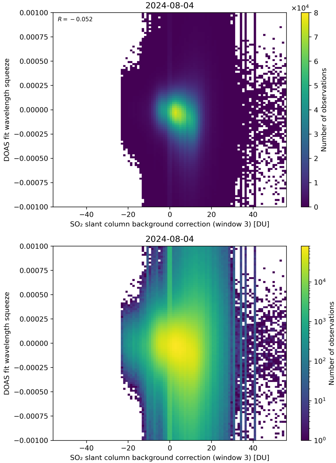
Figure 122: Scatter density plot of “SO 2 slant column background correction (window 3)” against “DOAS fit wavelength squeeze” for 2024-08-03 to 2024-08-05.
