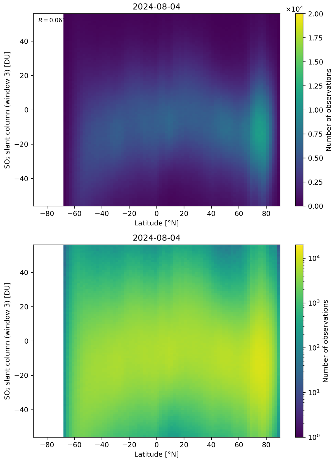
Figure 152: Scatter density plot of “Latitude” against “SO 2 slant column (window 3)” for 2024-08-03 to 2024-08-05.
