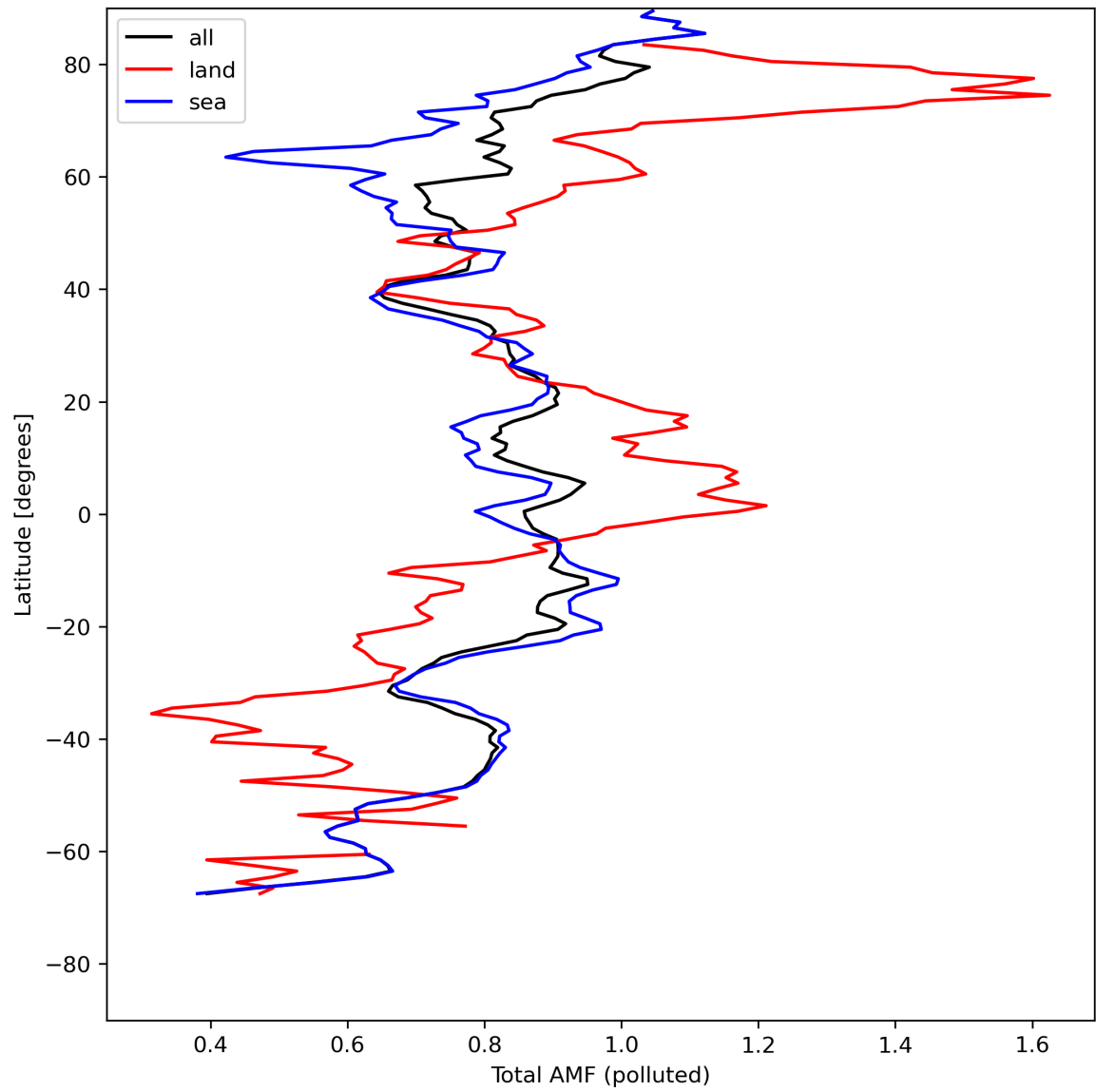
Figure 48: Zonal average of “Total AMF (polluted)” for 2024-08-03 to 2024-08-05.
