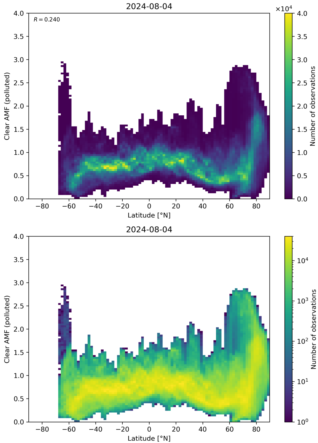
Figure 145: Scatter density plot of “Latitude” against “Clear AMF (polluted)” for 2024-08-03 to 2024-08-05.
