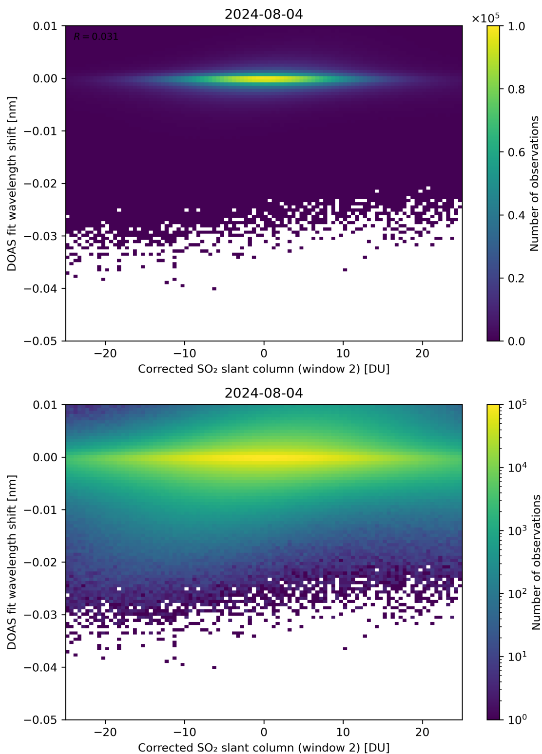
Figure 196: Scatter density plot of “Corrected SO 2 slant column (window 2)” against “DOAS fit wavelength shift” for 2024-08-03 to 2024-08-05.
