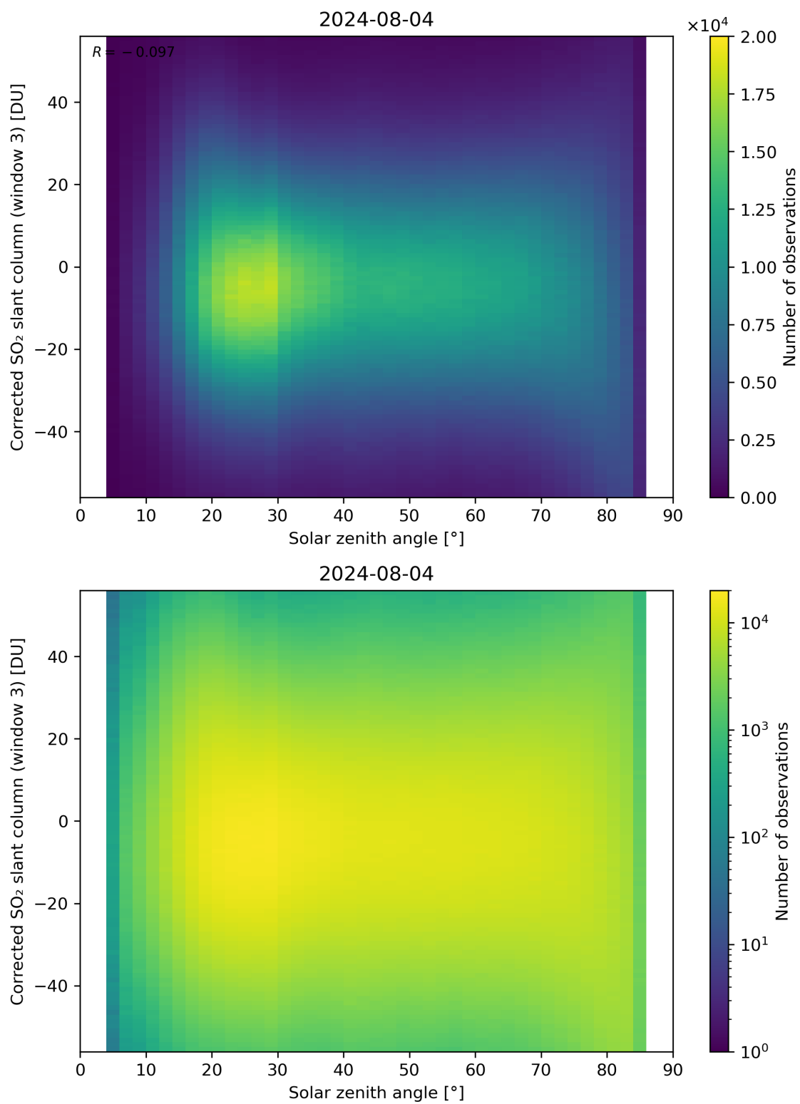
Figure 168: Scatter density plot of “Solar zenith angle” against “Corrected SO 2 slant column (window 3)” for 2024-08-03 to 2024-08-05.
