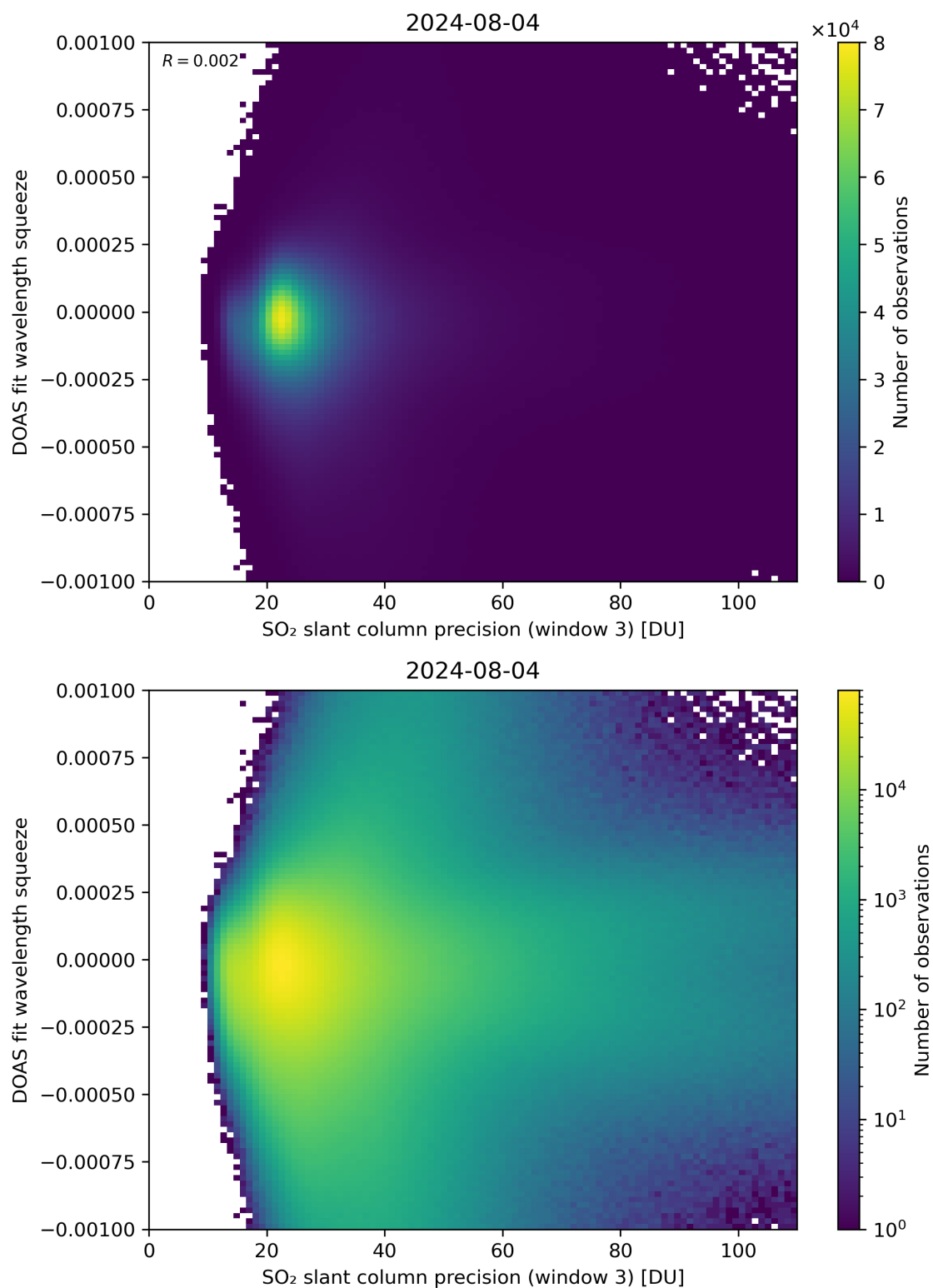
Figure 259: Scatter density plot of “SO 2 slant column precision (window 3)” against “DOAS fit wavelength squeeze” for 2024-08-03 to 2024-08-05.
