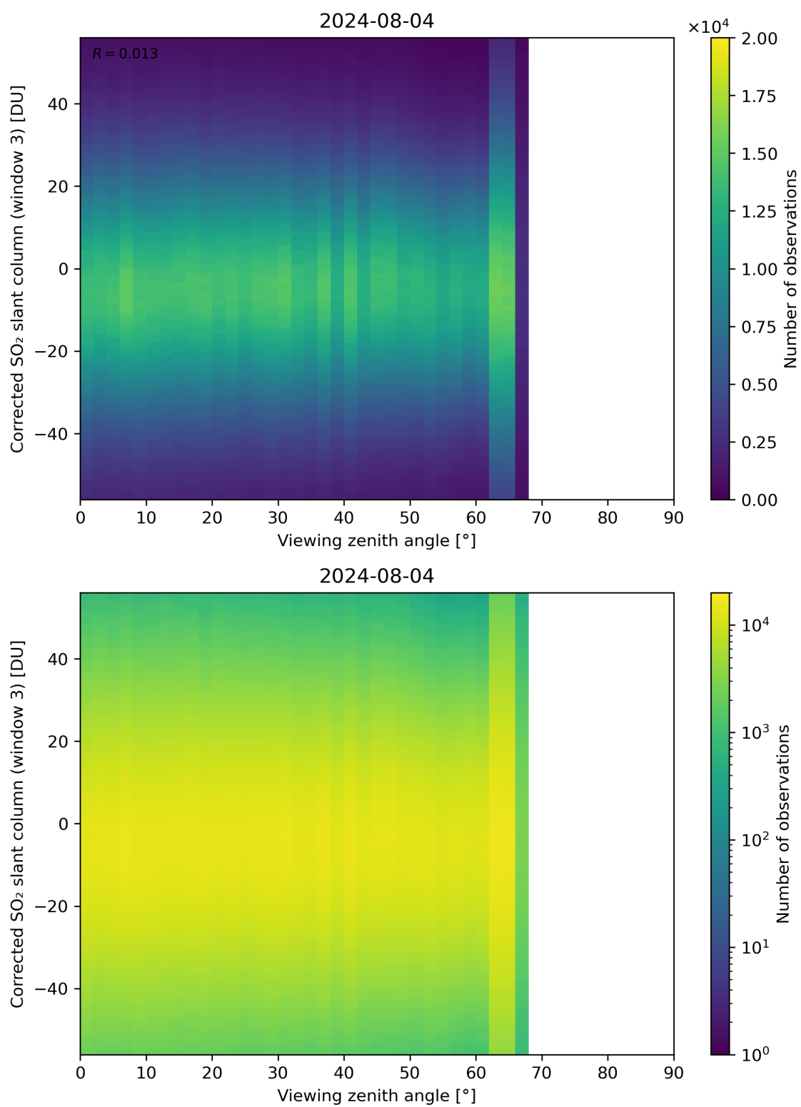
Figure 319: Scatter density plot of “Viewing zenith angle” against “Corrected SO 2 slant column (window 3)” for 2024-08-03 to 2024-08-05.
