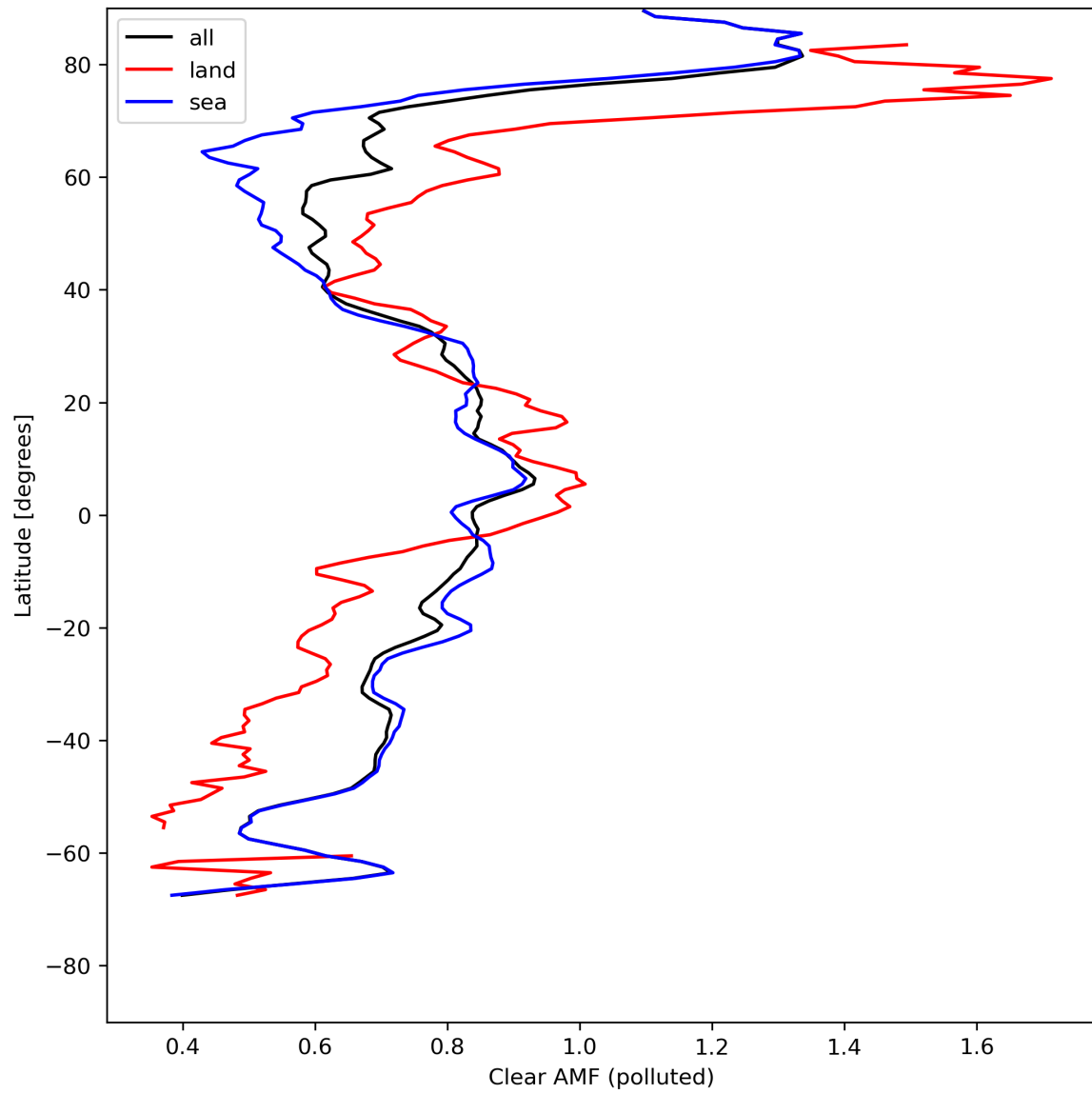
Figure 50: Zonal average of “Clear AMF (polluted)” for 2024-08-03 to 2024-08-05.
