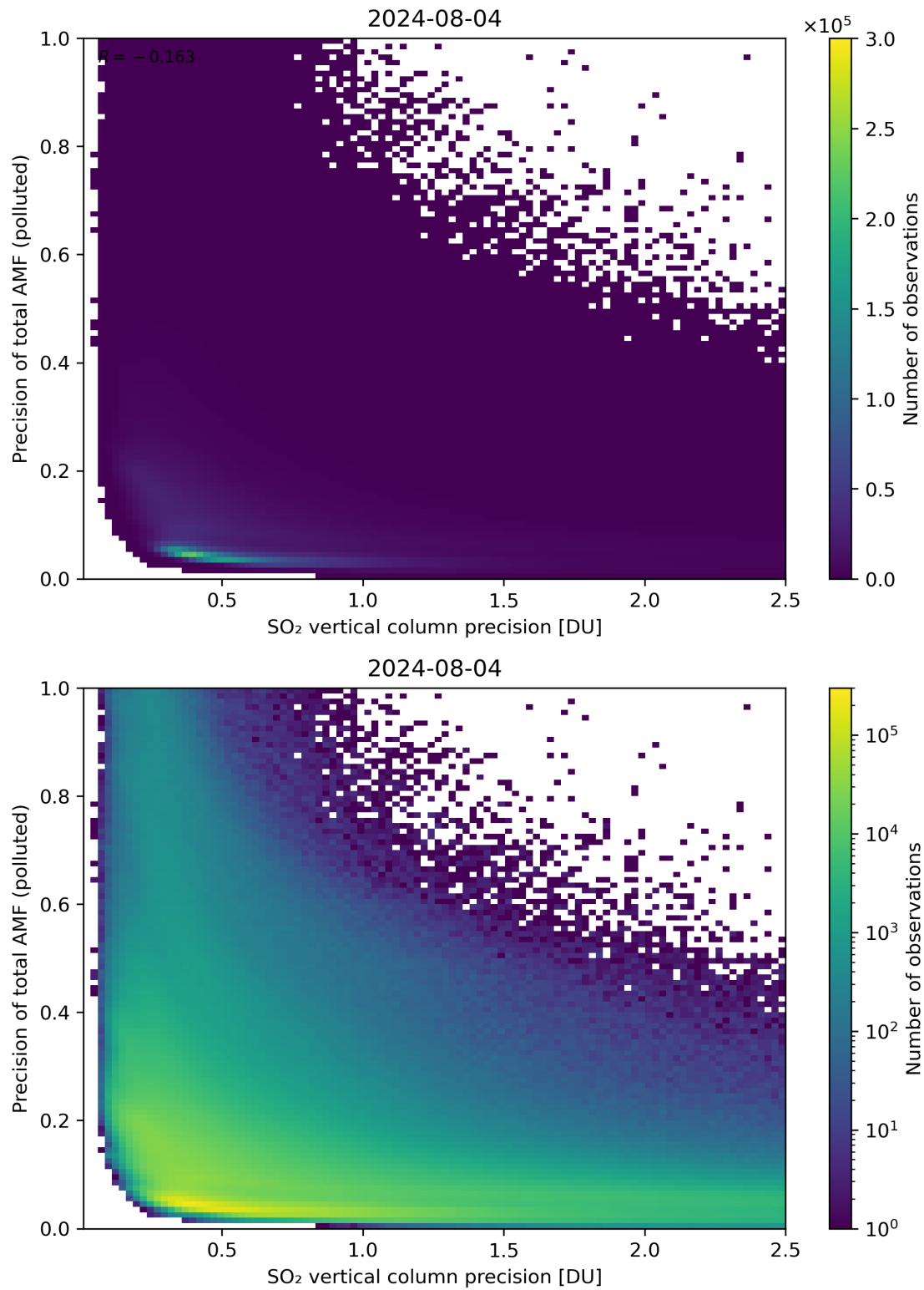
Figure 295: Scatter density plot of “SO 2 vertical column precision” against “Precision of total AMF (polluted)” for 2024-08-03 to 2024-08-05.
