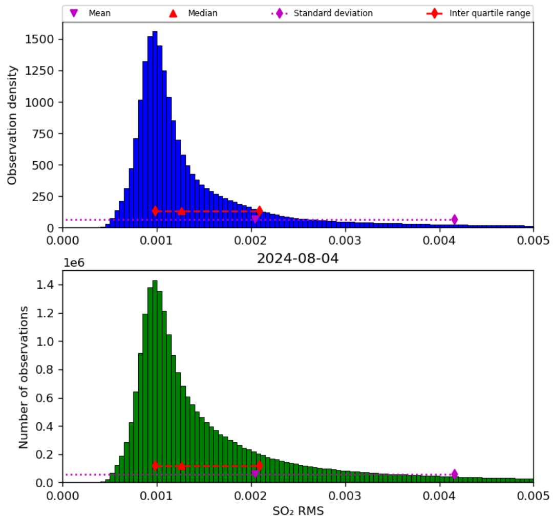
Figure 70: Histogram of “SO 2 RMS” for 2024-08-03 to 2024-08-05
