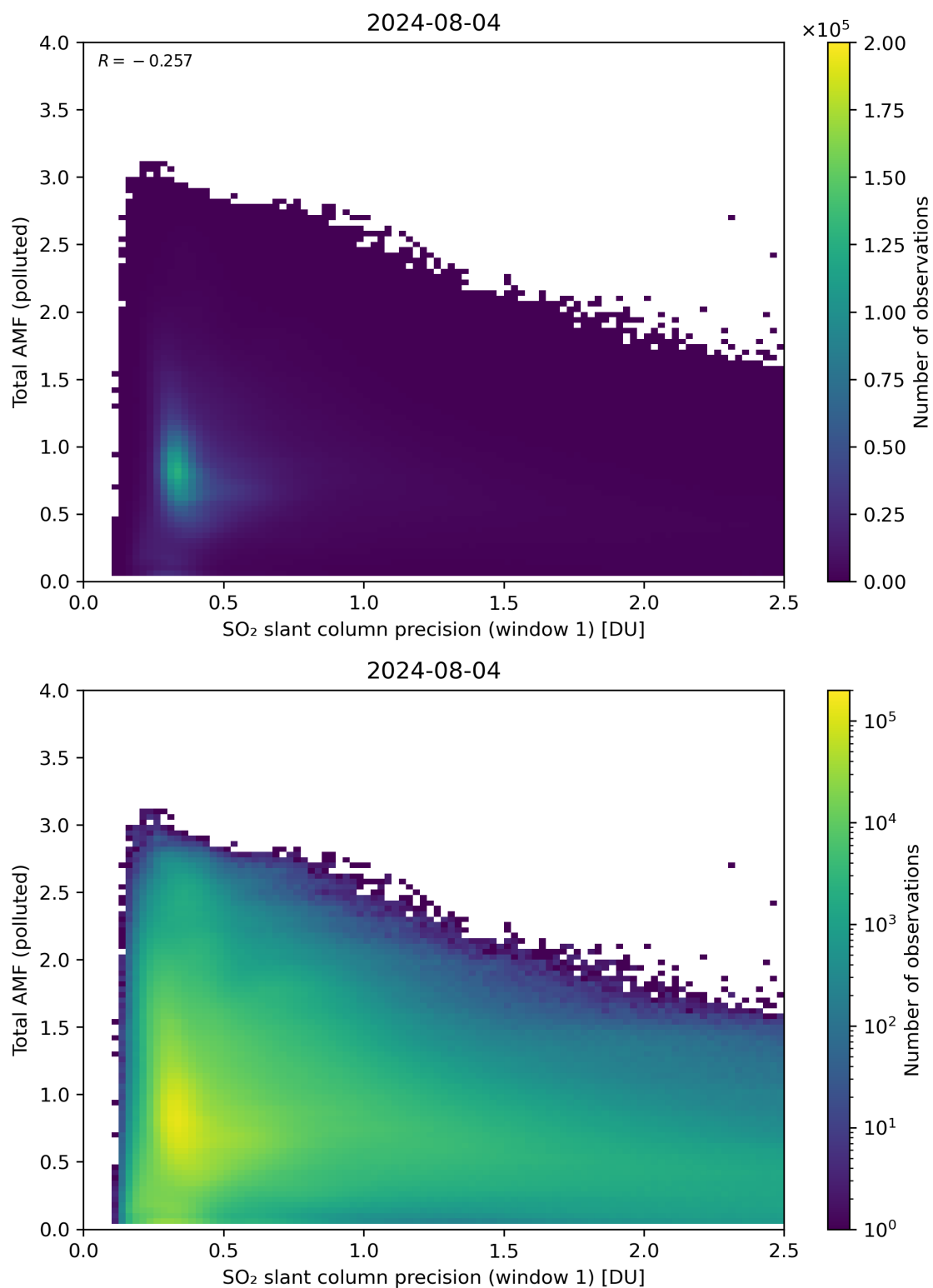
Figure 230: Scatter density plot of “SO 2 slant column precision (window 1)” against “Total AMF (polluted)” for 2024-08-03 to 2024-08-05.
