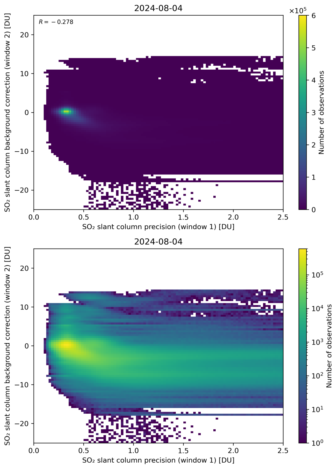
Figure 219: Scatter density plot of “SO 2 slant column precision (window 1)” against “SO 2 slant column background correction (window 2)” for 2024-08-03 to 2024-08-05.
