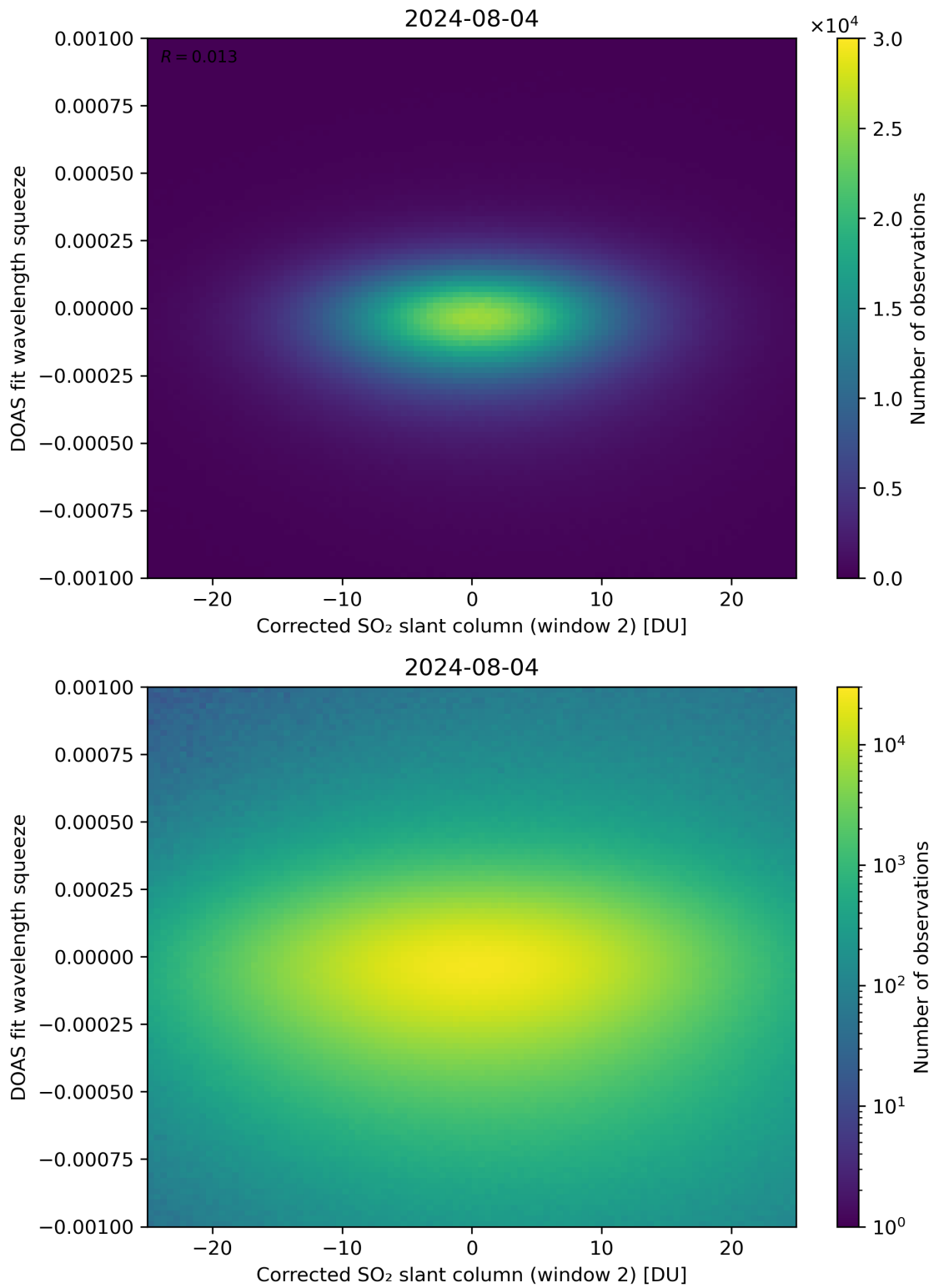
Figure 197: Scatter density plot of “Corrected SO 2 slant column (window 2)” against “DOAS fit wavelength squeeze” for 2024-08-03 to 2024-08-05.
