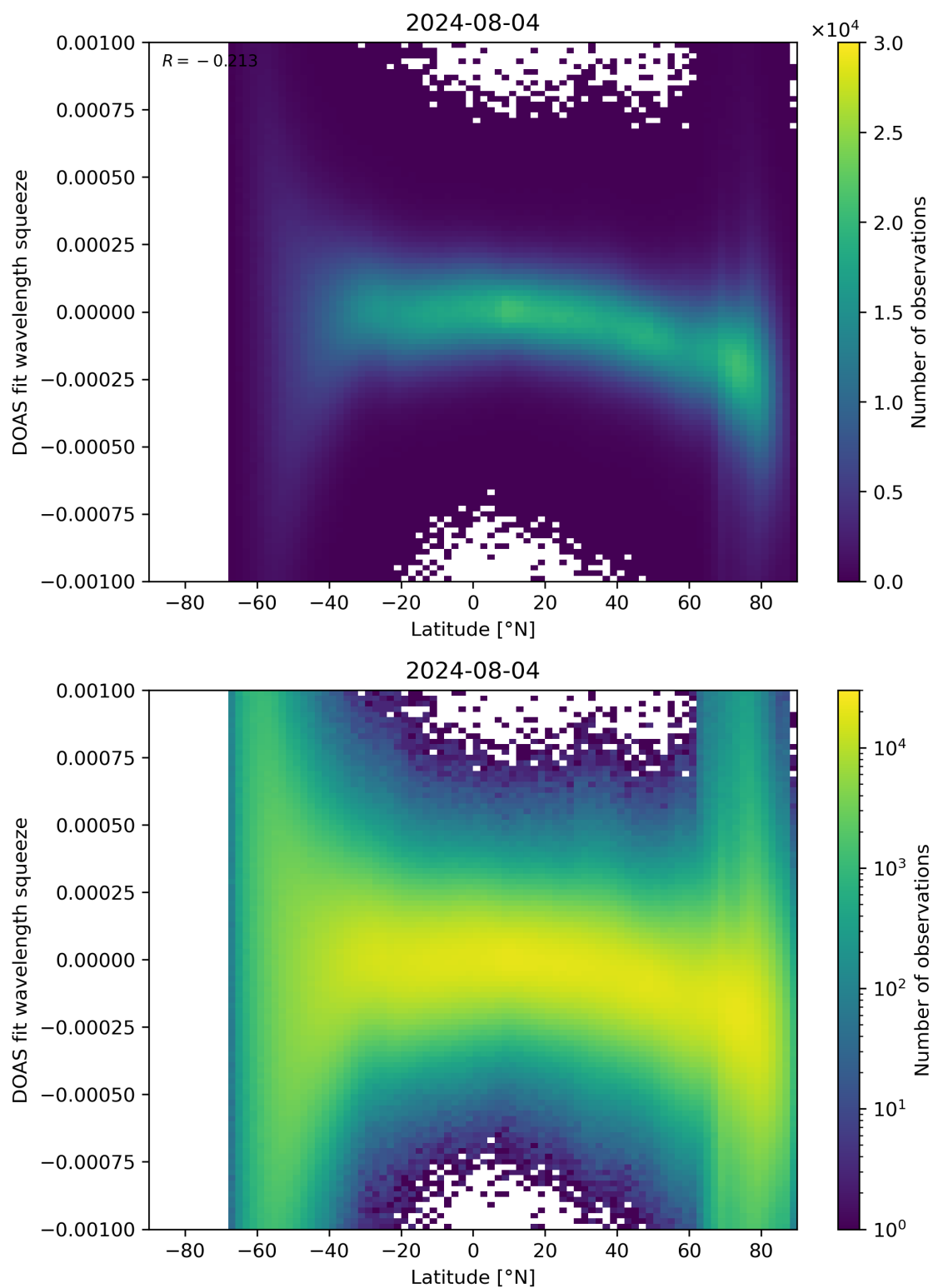
Figure 143: Scatter density plot of “Latitude” against “DOAS fit wavelength squeeze” for 2024-08-03 to 2024-08-05.
