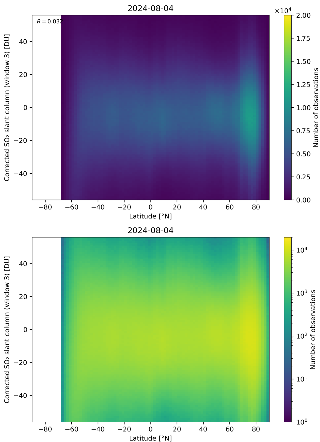
Figure 148: Scatter density plot of “Latitude” against “Corrected SO 2 slant column (window 3)” for 2024-08-03 to 2024-08-05.
