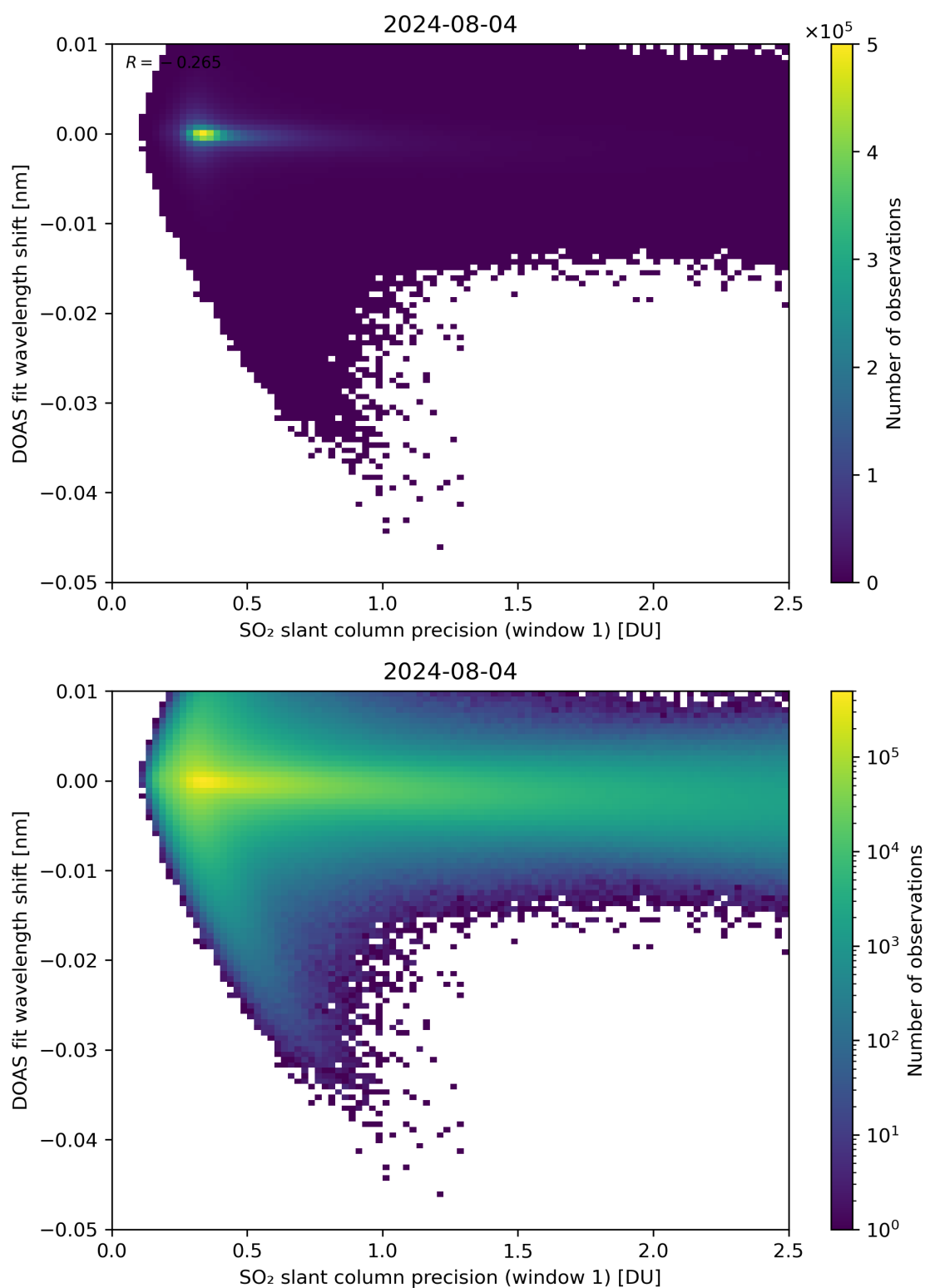
Figure 221: Scatter density plot of “SO 2 slant column precision (window 1)” against “DOAS fit wavelength shift” for 2024-08-03 to 2024-08-05.
