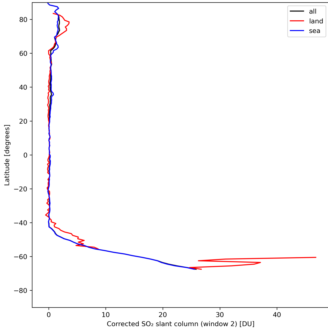
Figure 39: Zonal average of “Corrected SO 2 slant column (window 2)” for 2024-08-03 to 2024-08-05.
