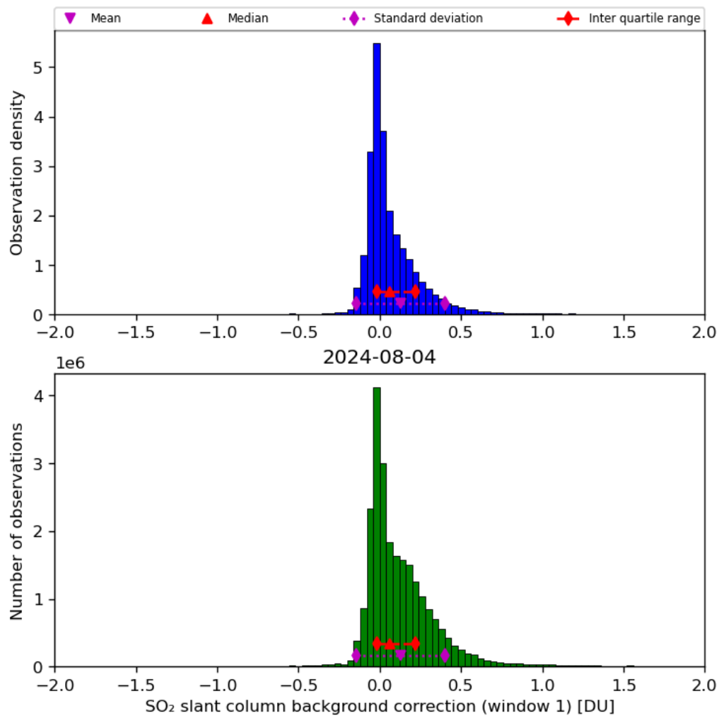
Figure 59: Histogram of “SO 2 slant column background correction (window 1)” for 2024-08-03 to 2024-08-05
