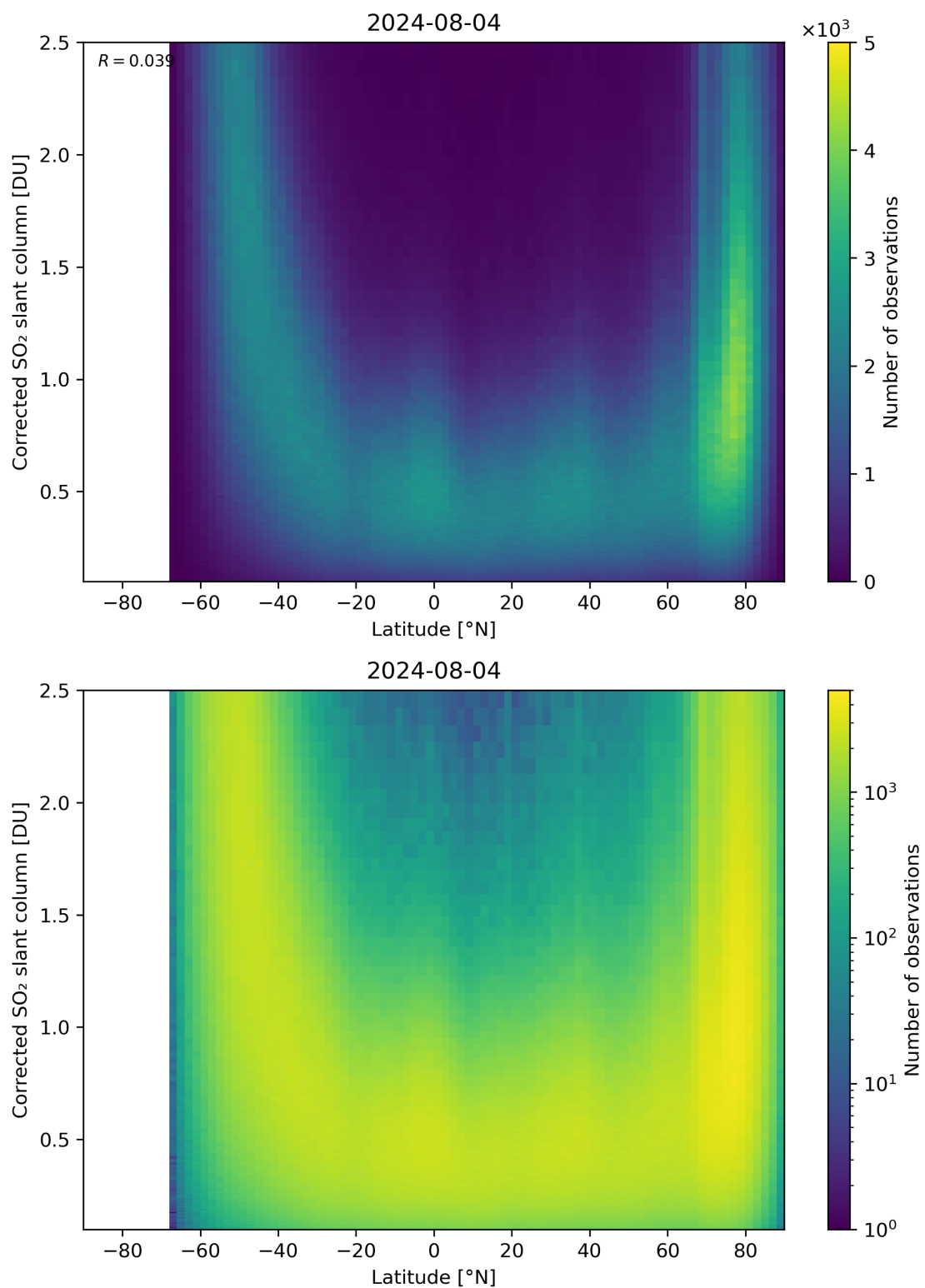
Figure 146: Scatter density plot of “Latitude” against “Corrected SO 2 slant column” for 2024-08-03 to 2024-08-05.
