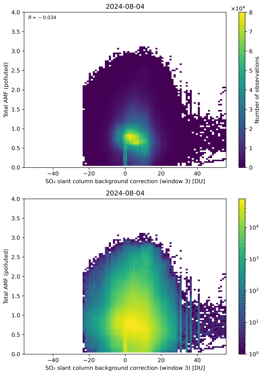
Figure 125: Scatter density plot of “SO 2 slant column background correction (window 3)” against “Total AMF (polluted)” for 2024-08-03 to 2024-08-05.
