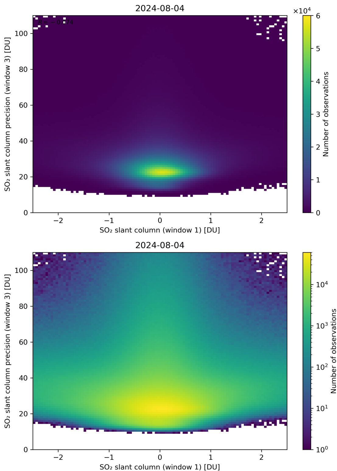
Figure 238: Scatter density plot of “SO 2 slant column (window 1)” against “SO 2 slant column precision (window 3)” for 2024-08-03 to 2024-08-05.
