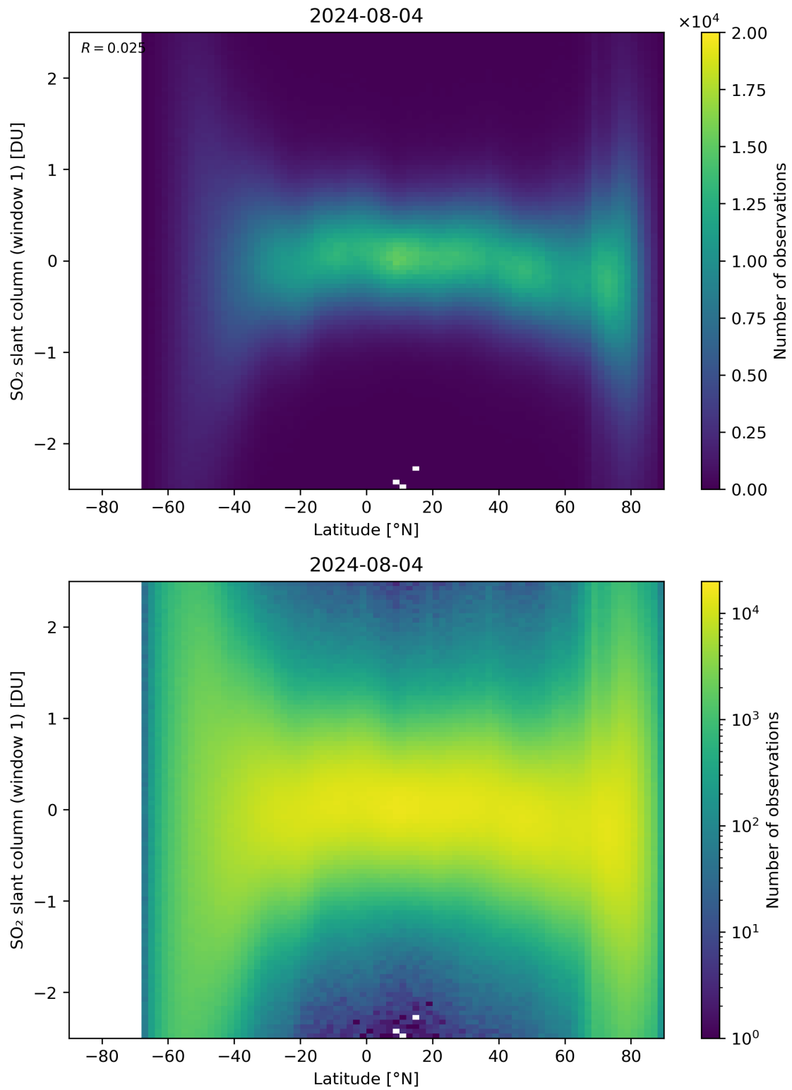
Figure 149: Scatter density plot of “Latitude” against “SO 2 slant column (window 1)” for 2024-08-03 to 2024-08-05.
