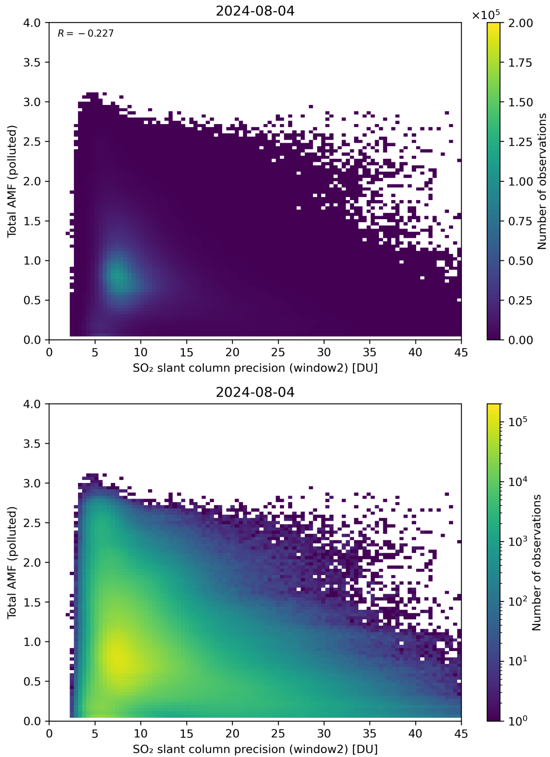
Figure 251: Scatter density plot of “SO 2 slant column precision (window2)” against “Total AMF (polluted)” for 2024-08-03 to 2024-08-05.
