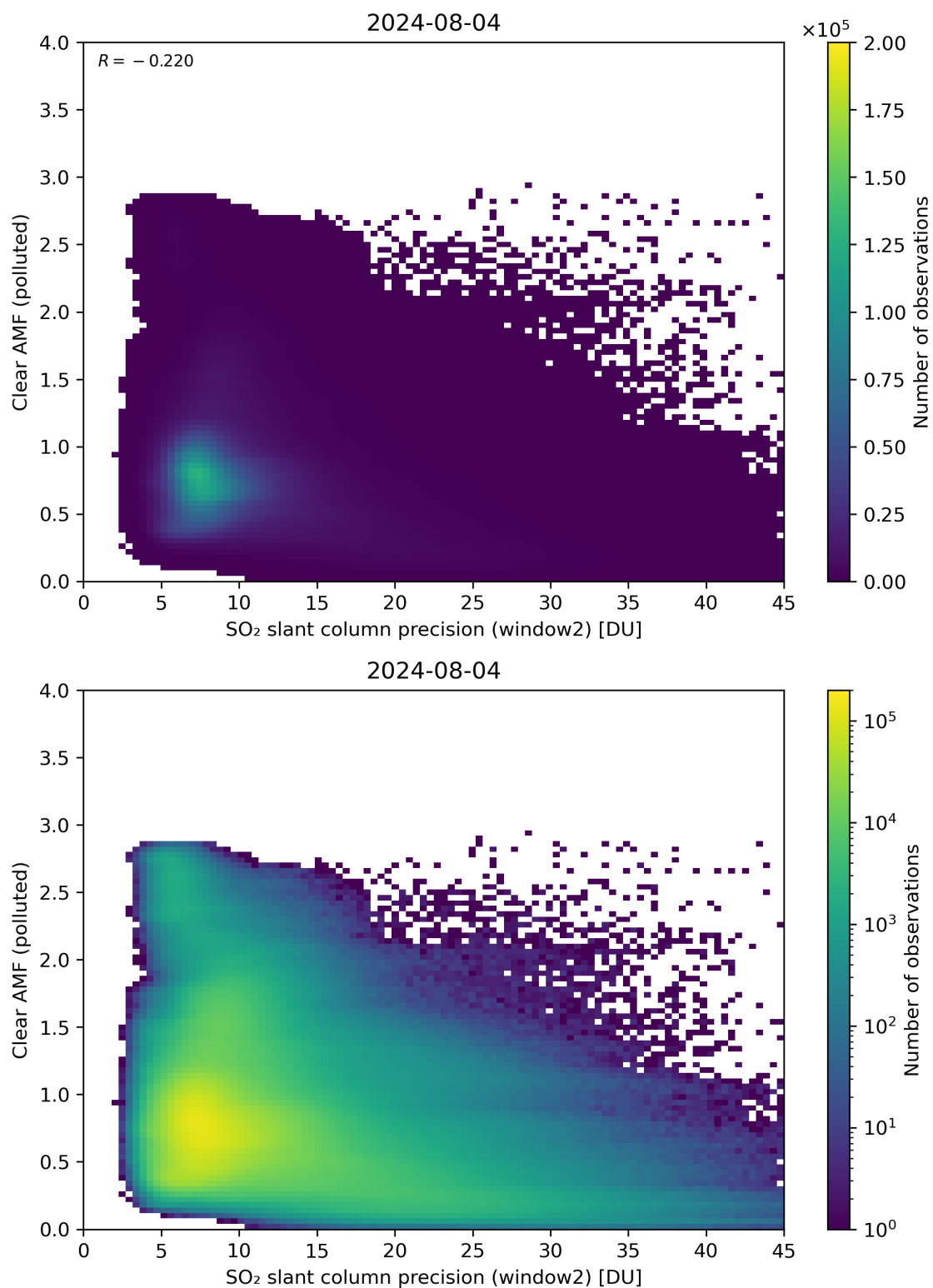
Figure 246: Scatter density plot of “SO 2 slant column precision (window2)” against “Clear AMF (polluted)” for 2024-08-03 to 2024-08-05.
