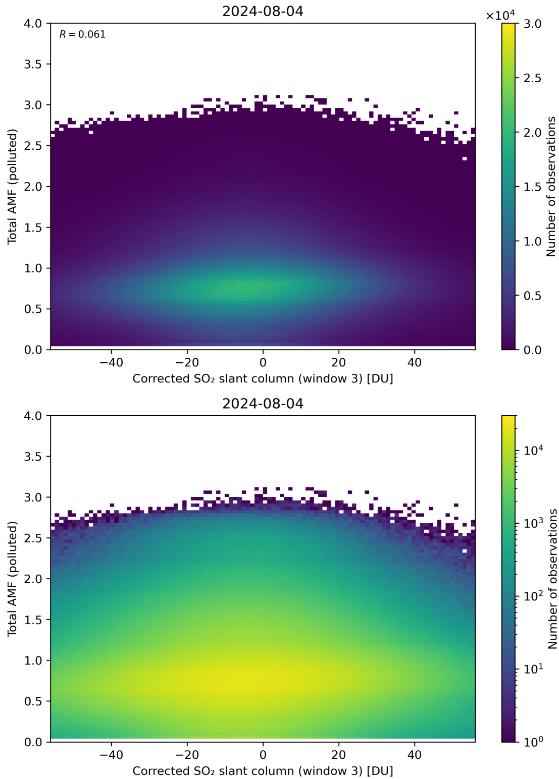
Figure 210: Scatter density plot of “Corrected SO 2 slant column (window 3)” against “Total AMF (polluted)” for 2024-08-03 to 2024-08-05.
