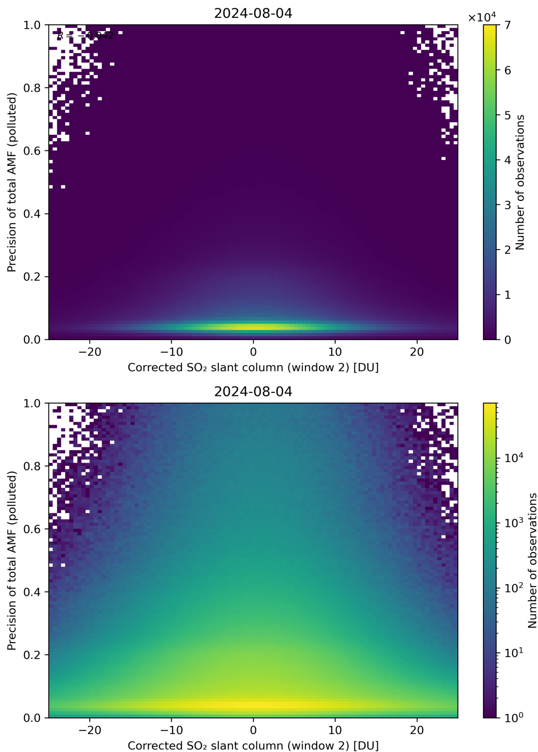
Figure 204: Scatter density plot of “Corrected SO 2 slant column (window 2)” against “Precision of total AMF (polluted)” for 2024-08-03 to 2024-08-05.
