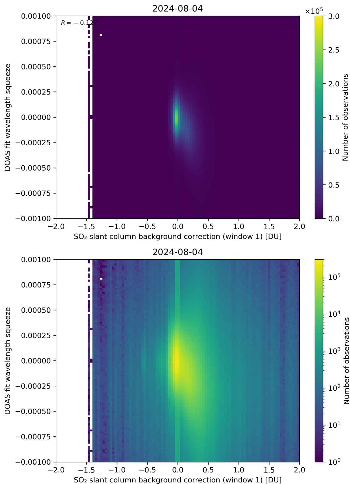
Figure 101: Scatter density plot of “SO 2 slant column background correction (window 1)” against “DOAS fit wavelength squeeze” for 2024-08-03 to 2024-08-05.
