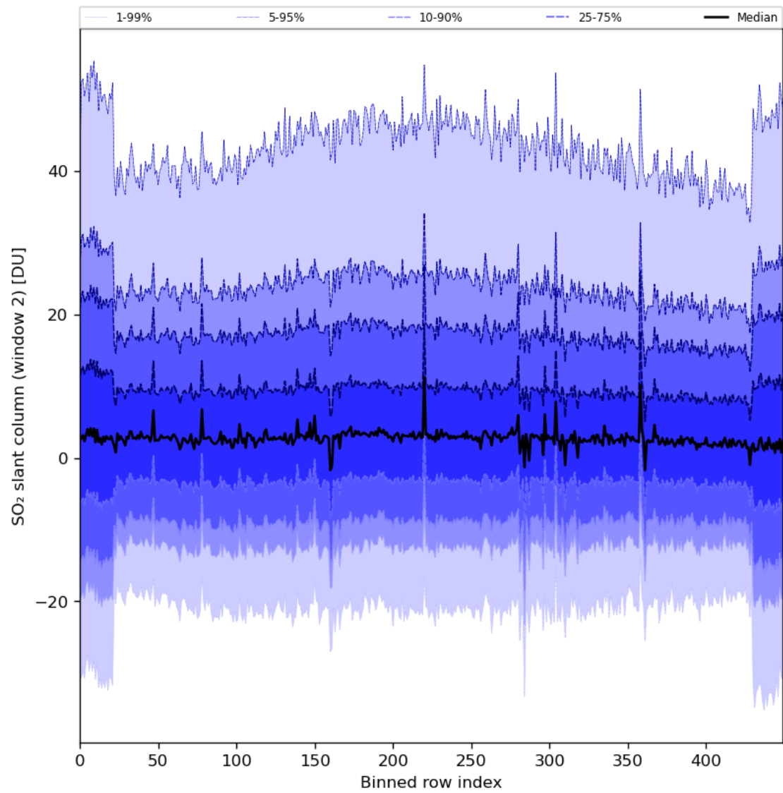
Figure 83: Along track statistics of “SO 2 slant column (window 2)” for 2024-08-04 to 2024-08-06
