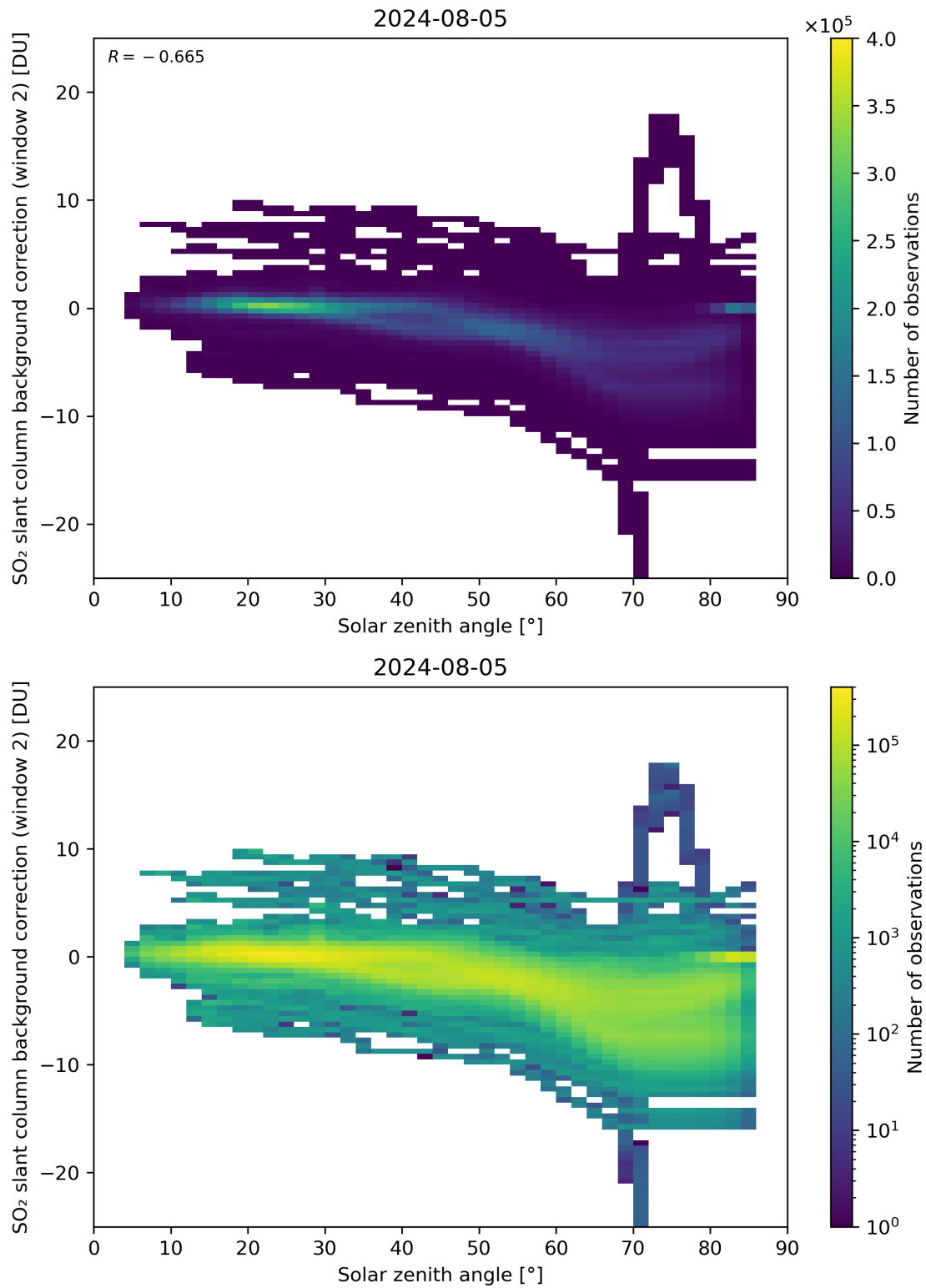
Figure 159: Scatter density plot of “Solar zenith angle” against “SO 2 slant column background correction (window 2)” for 2024-08-04 to 2024-08-06.
