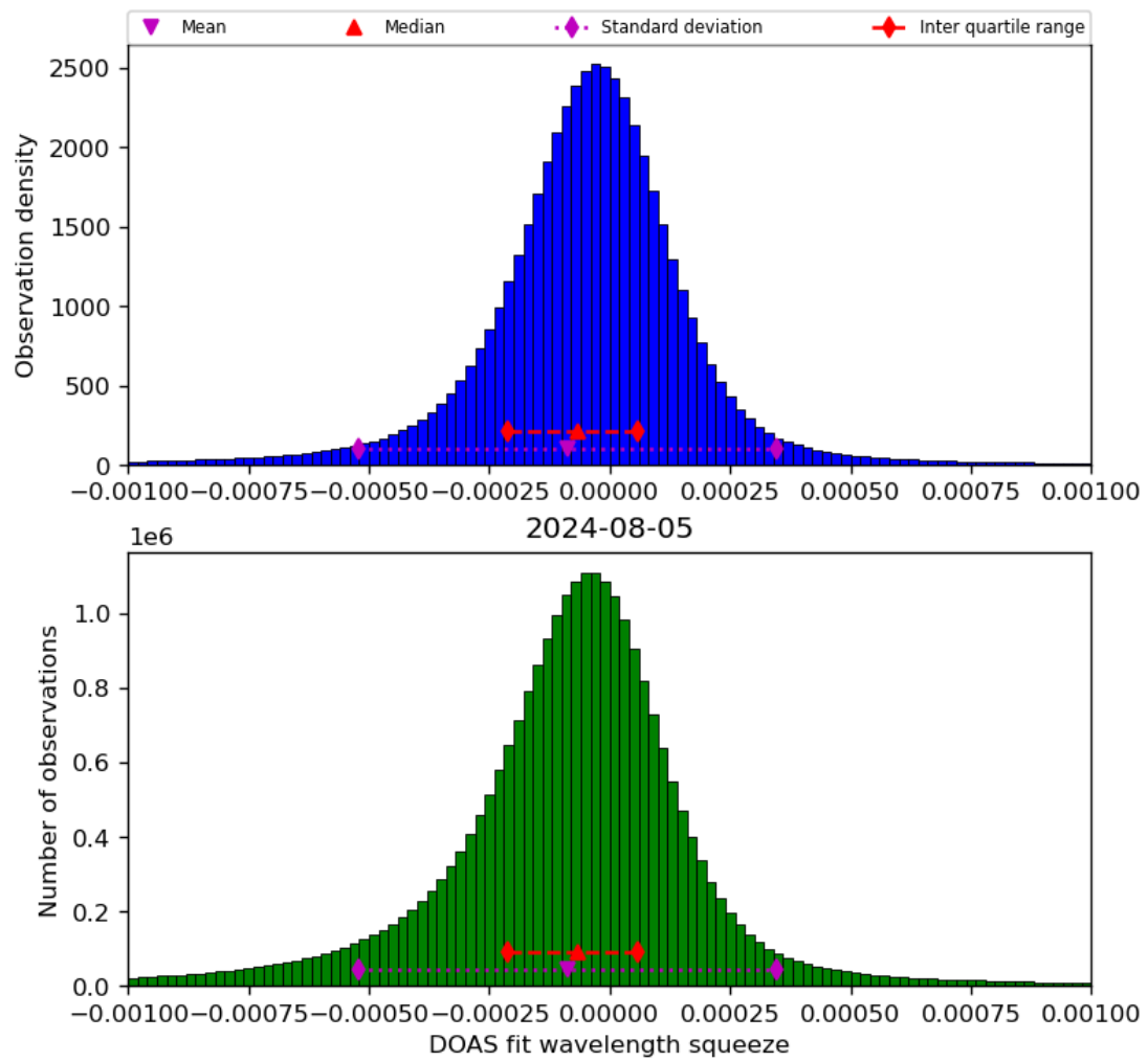
Figure 69: Histogram of “DOAS fit wavelength squeeze” for 2024-08-04 to 2024-08-06
