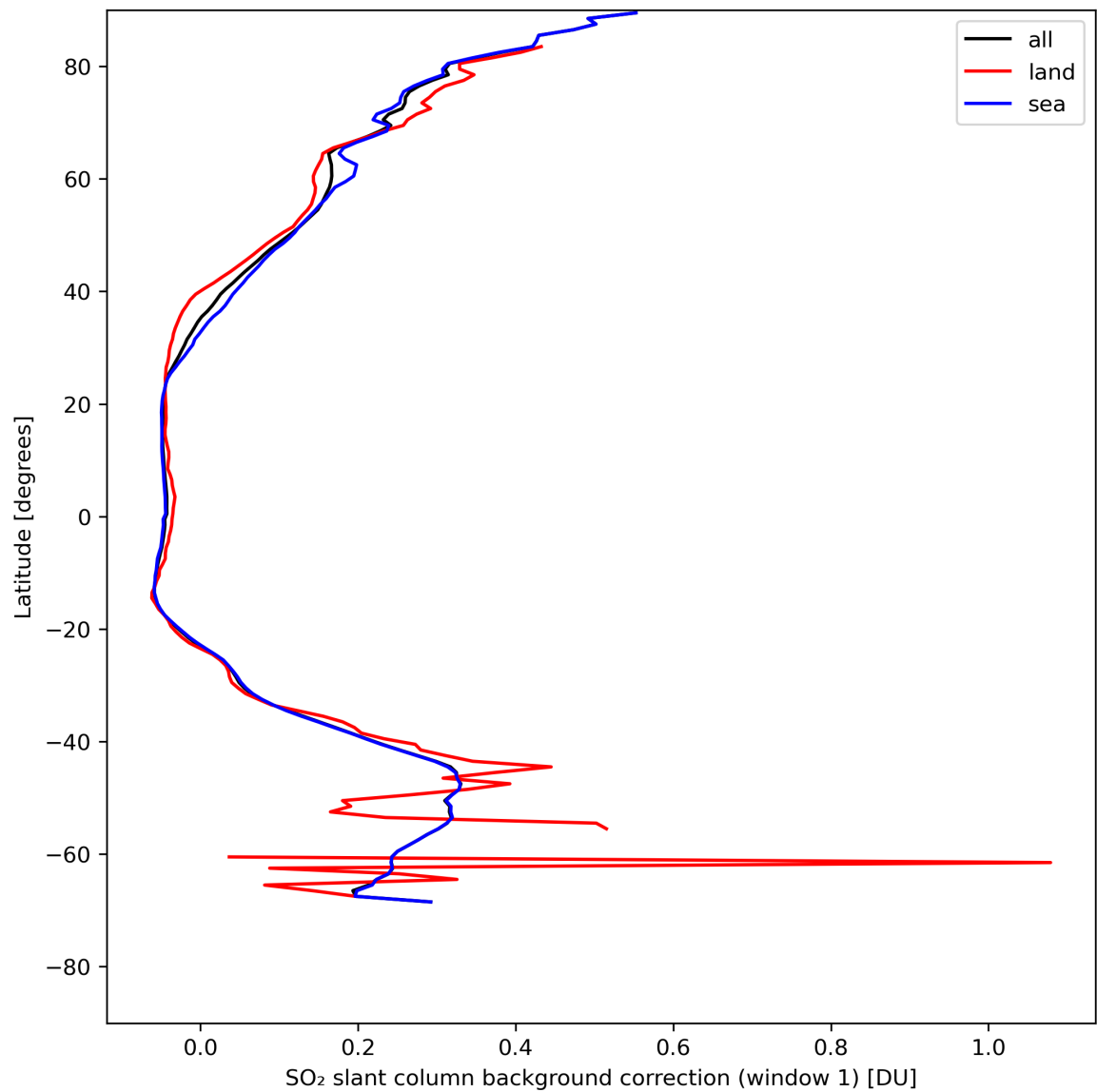
Figure 36: Zonal average of “SO 2 slant column background correction (window 1)” for 2024-08-04 to 2024-08-06.
