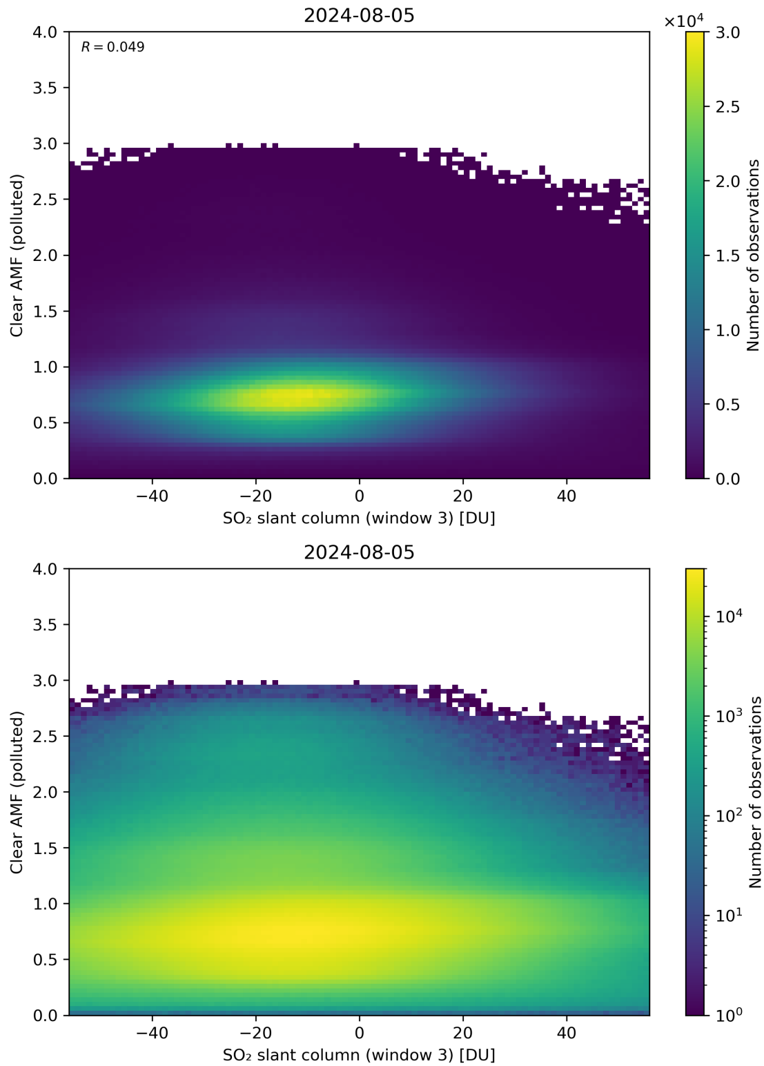
Figure 265: Scatter density plot of “SO 2 slant column (window 3)” against “Clear AMF (polluted)” for 2024-08-04 to 2024-08-06.
