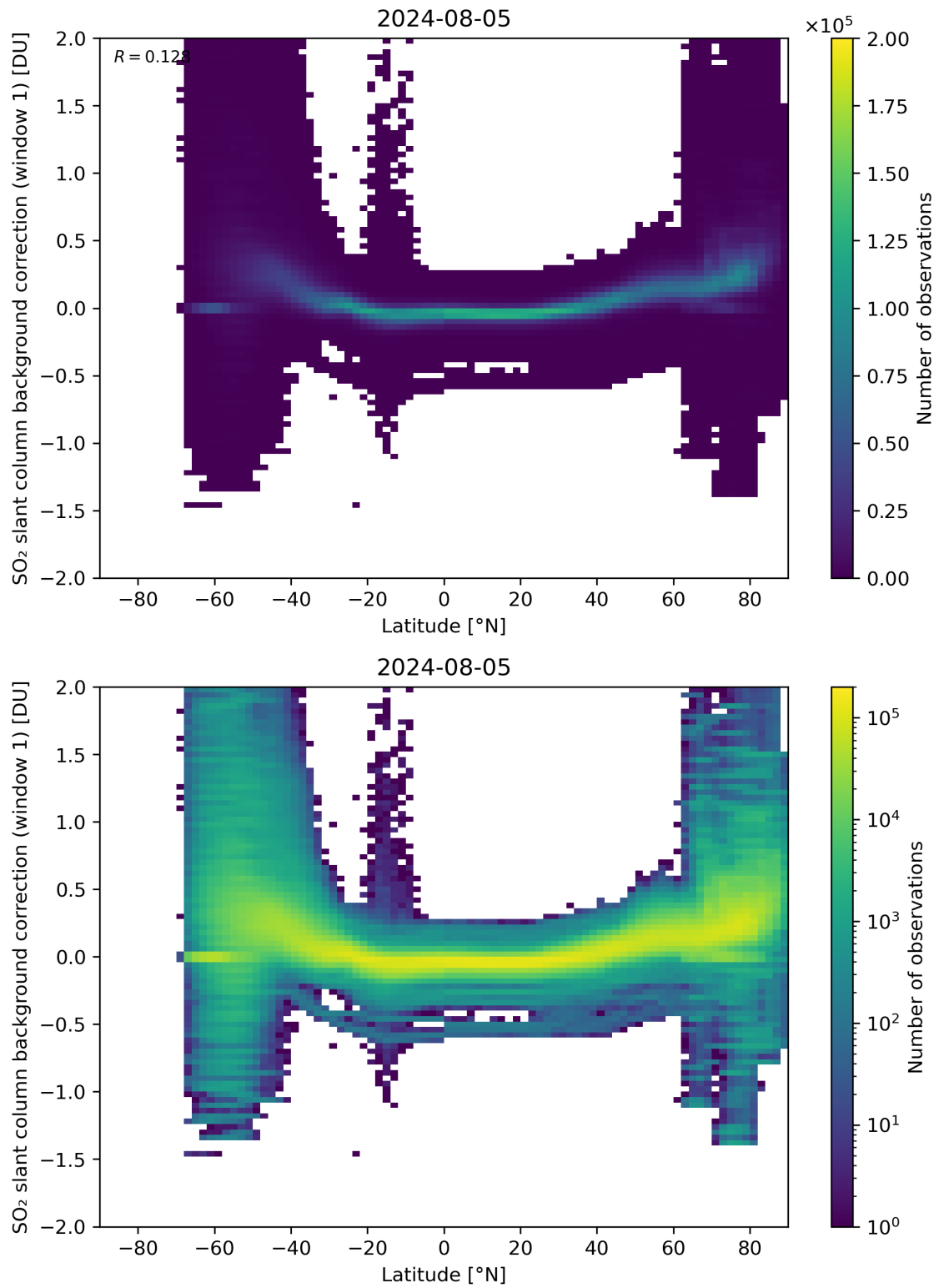
Figure 139: Scatter density plot of “Latitude” against “SO 2 slant column background correction (window 1)” for 2024-08-04 to 2024-08-06.
