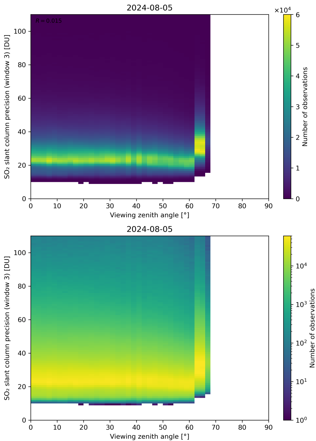
Figure 324: Scatter density plot of “Viewing zenith angle” against “SO 2 slant column precision (window 3)” for 2024-08-04 to 2024-08-06.
