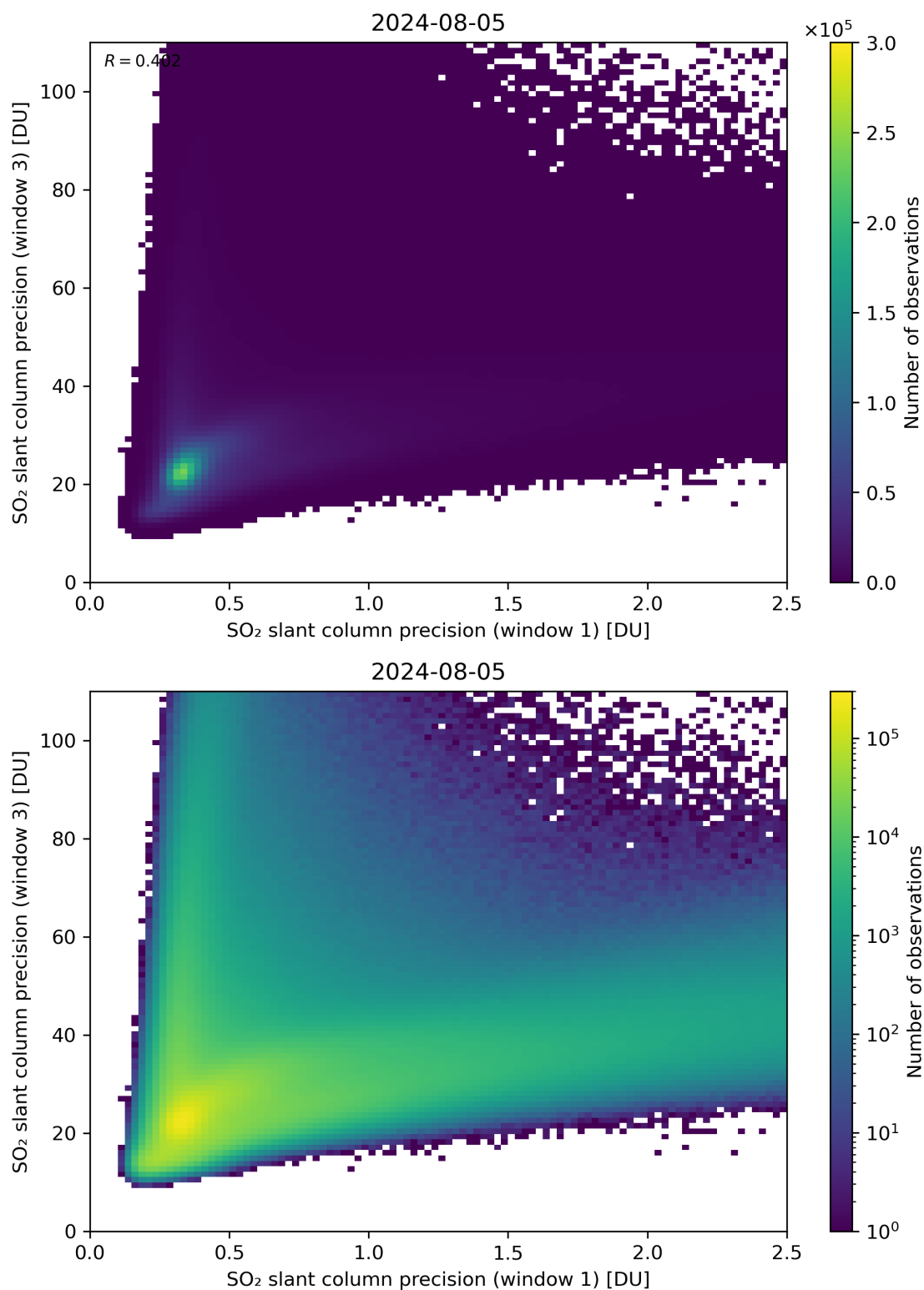
Figure 229: Scatter density plot of “SO 2 slant column precision (window 1)” against “SO 2 slant column precision (window 3)” for 2024-08-04 to 2024-08-06.
