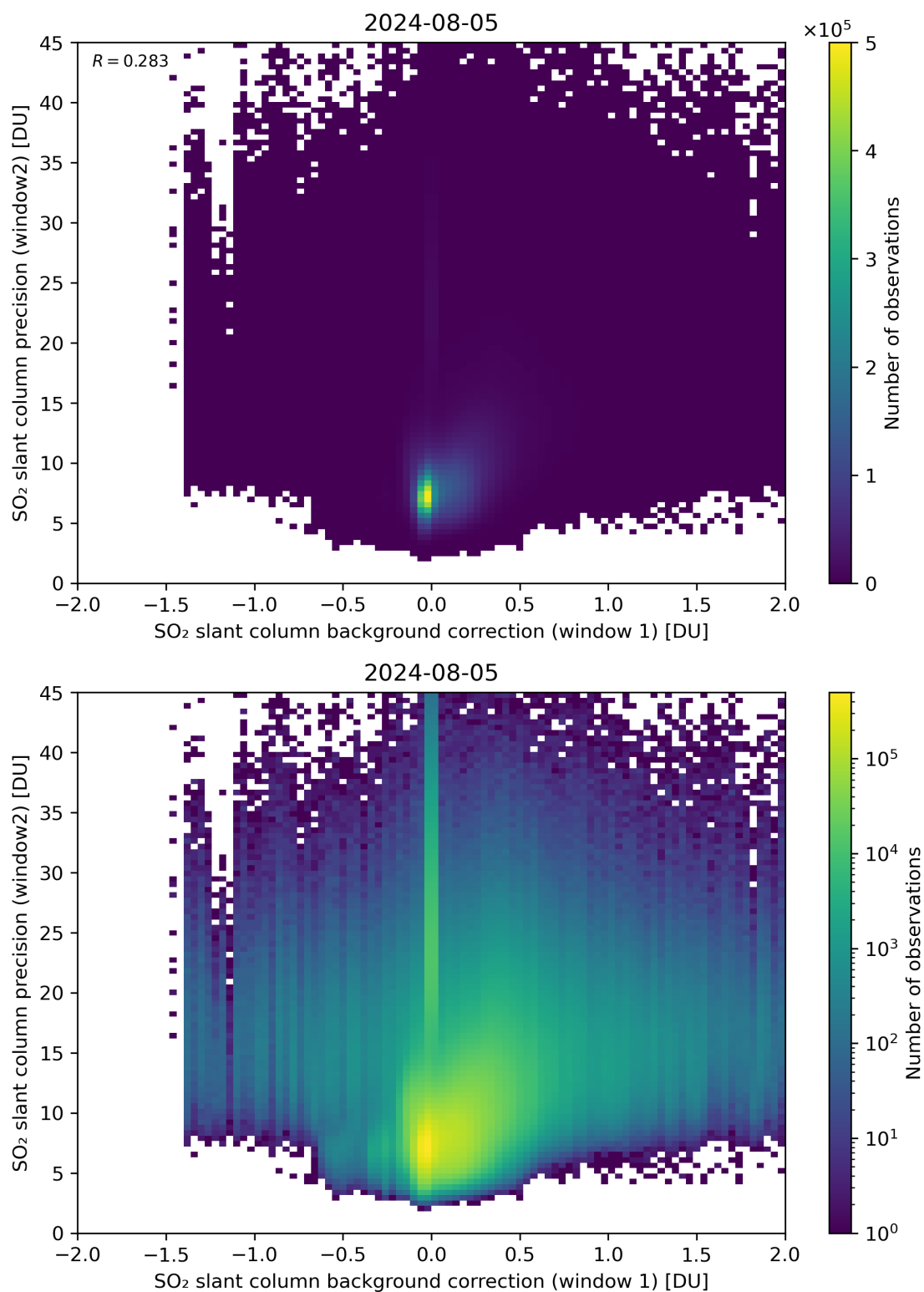
Figure 106: Scatter density plot of “SO 2 slant column background correction (window 1)” against “SO 2 slant column precision (window2)” for 2024-08-04 to 2024-08-06.
