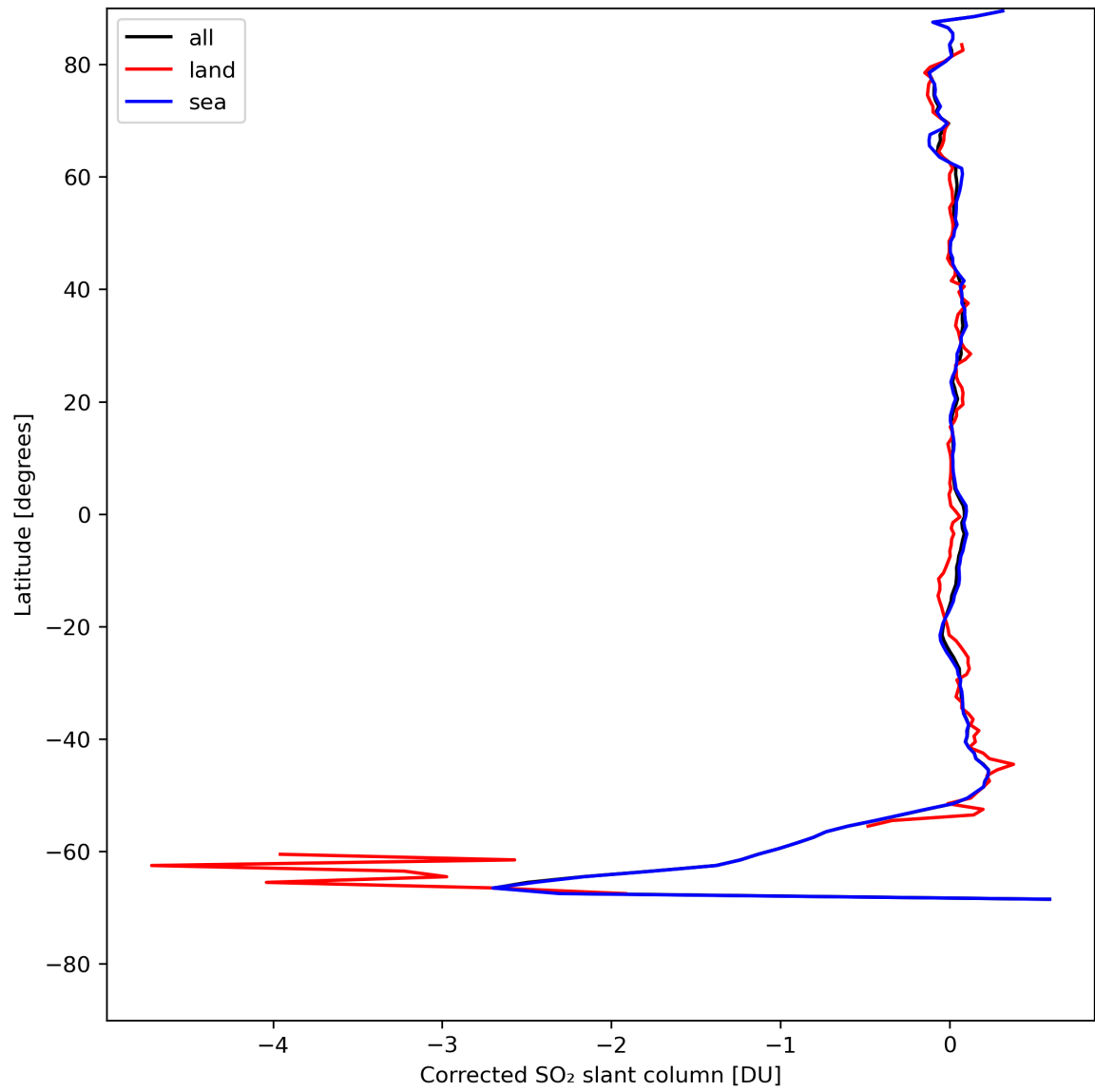
Figure 32: Zonal average of “Corrected SO 2 slant column” for 2024-08-04 to 2024-08-06.
