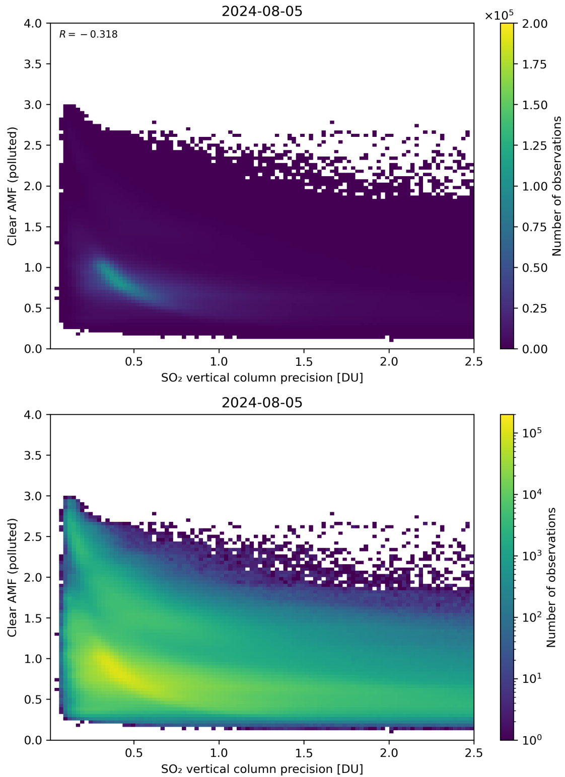
Figure 285: Scatter density plot of “SO 2 vertical column precision” against “Clear AMF (polluted)” for 2024-08-04 to 2024-08-06.
