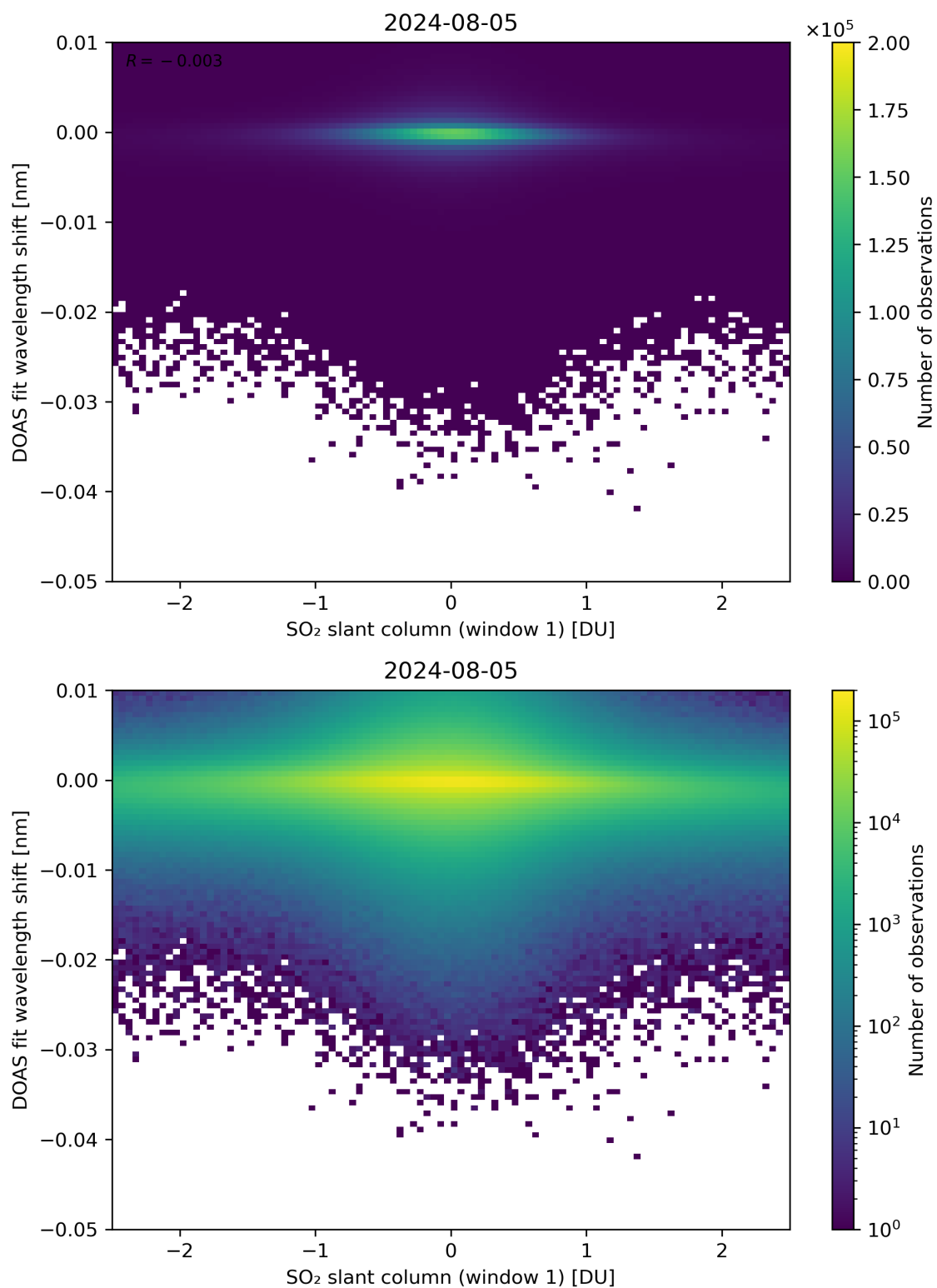
Figure 215: Scatter density plot of “SO 2 slant column (window 1)” against “DOAS fit wavelength shift” for 2024-08-04 to 2024-08-06.
