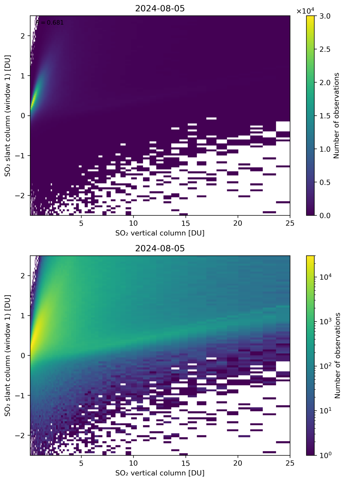
Figure 300: Scatter density plot of “SO 2 vertical column” against “SO 2 slant column (window 1)” for 2024-08-04 to 2024-08-06.
