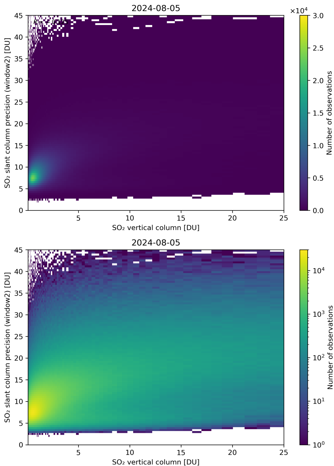
Figure 302: Scatter density plot of “SO 2 vertical column” against “SO 2 slant column precision (window2)” for 2024-08-04 to 2024-08-06.
