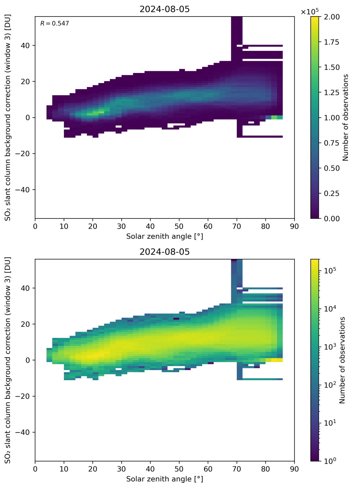
Figure 160: Scatter density plot of “Solar zenith angle” against “SO 2 slant column background correction (window 3)” for 2024-08-04 to 2024-08-06.
