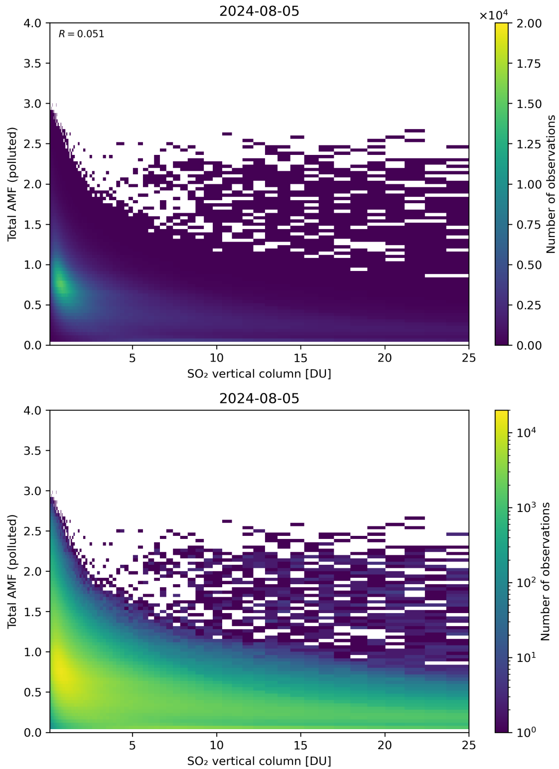
Figure 305: Scatter density plot of “SO 2 vertical column” against “Total AMF (polluted)” for 2024-08-04 to 2024-08-06.
