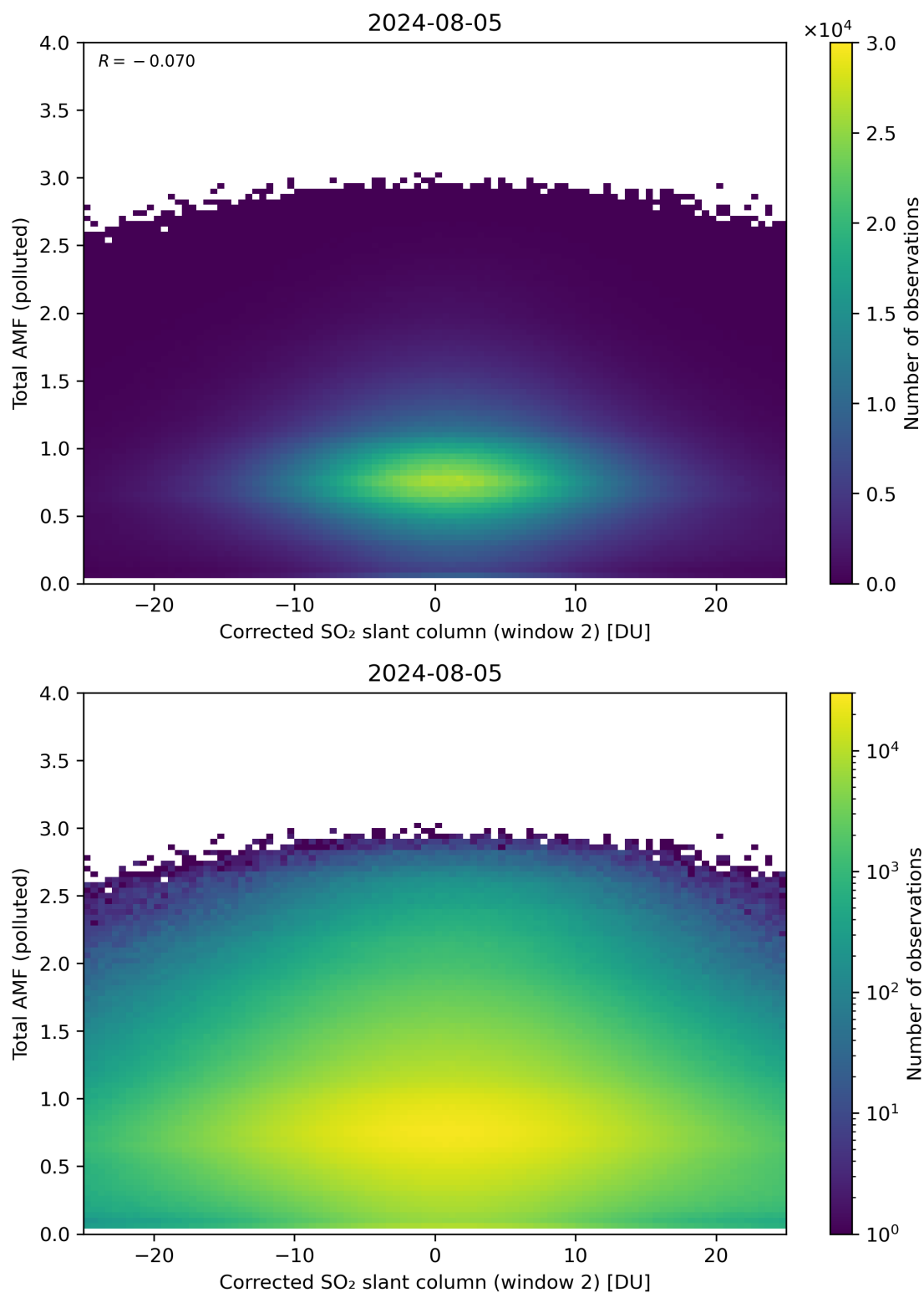
Figure 203: Scatter density plot of “Corrected SO 2 slant column (window 2)” against “Total AMF (polluted)” for 2024-08-04 to 2024-08-06.
