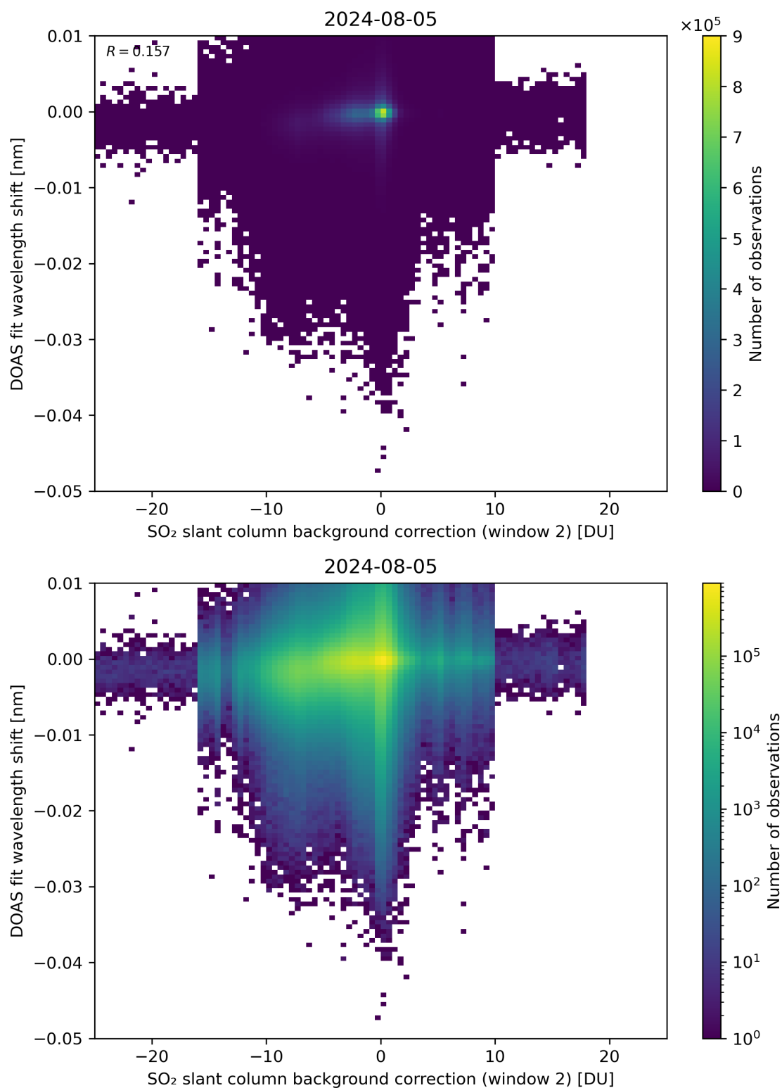
Figure 112: Scatter density plot of “SO 2 slant column background correction (window 2)” against “DOAS fit wavelength shift” for 2024-08-04 to 2024-08-06.
