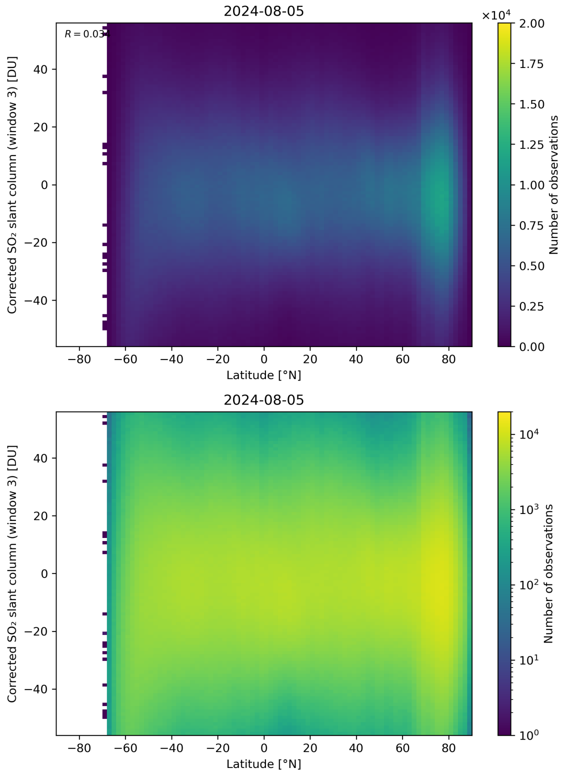
Figure 148: Scatter density plot of “Latitude” against “Corrected SO 2 slant column (window 3)” for 2024-08-04 to 2024-08-06.
