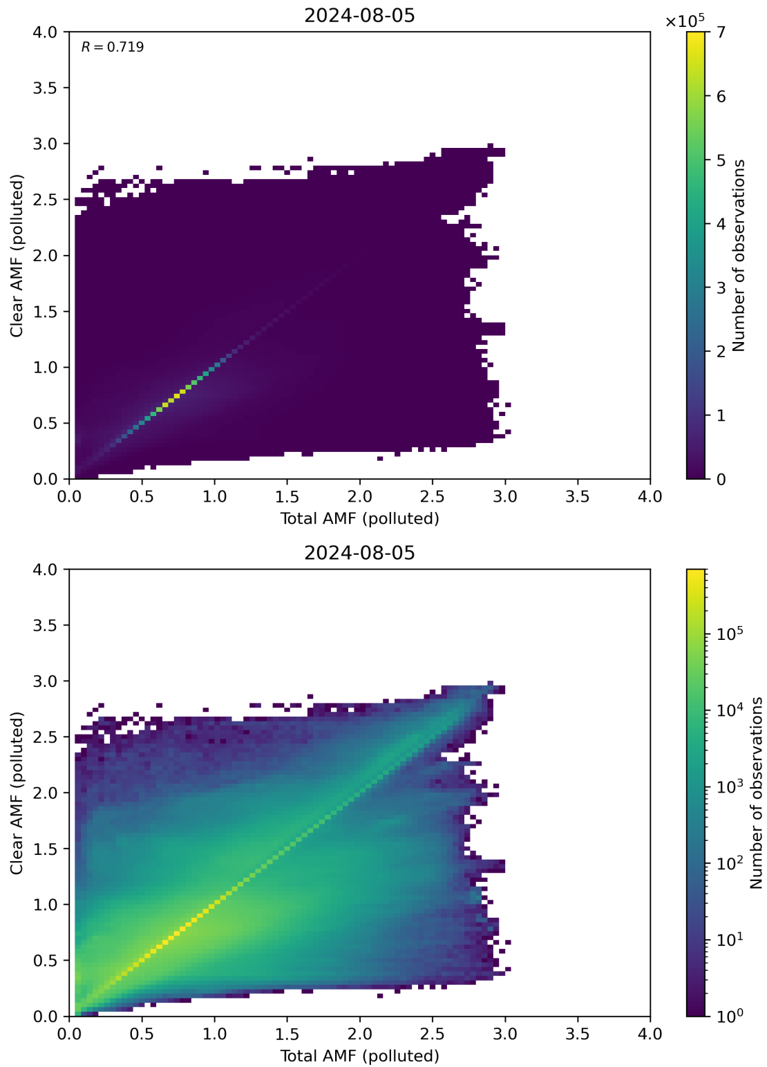
Figure 271: Scatter density plot of “Total AMF (polluted)” against “Clear AMF (polluted)” for 2024-08-04 to 2024-08-06.
