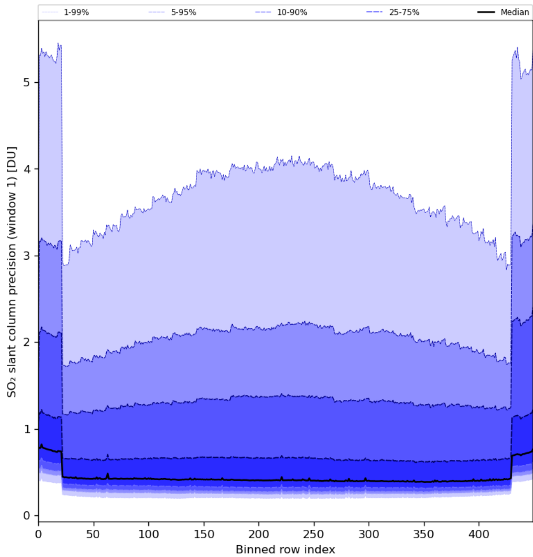
Figure 80: Along track statistics of “SO 2 slant column precision (window 1)” for 2024-08-04 to 2024-08-06
