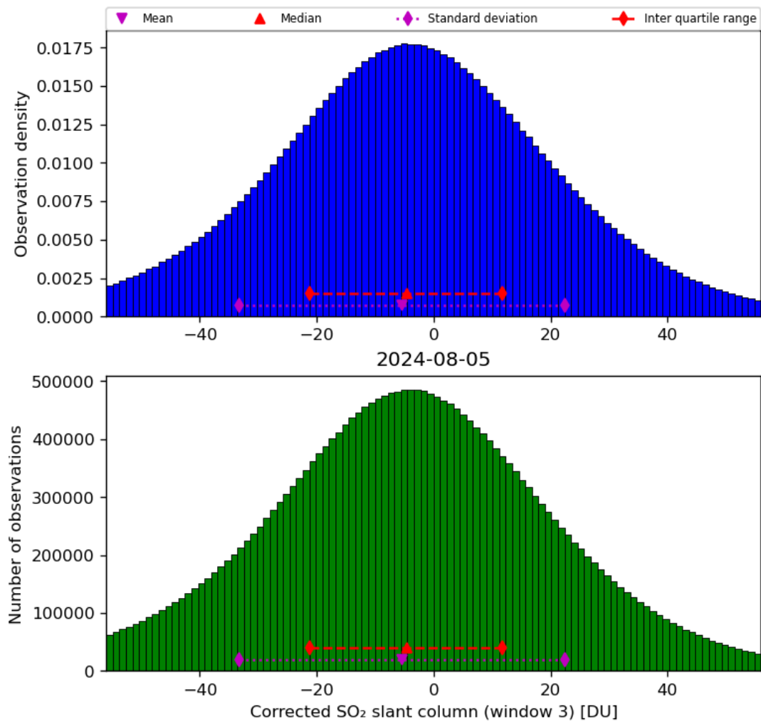
Figure 66: Histogram of “Corrected SO 2 slant column (window 3)” for 2024-08-04 to 2024-08-06
