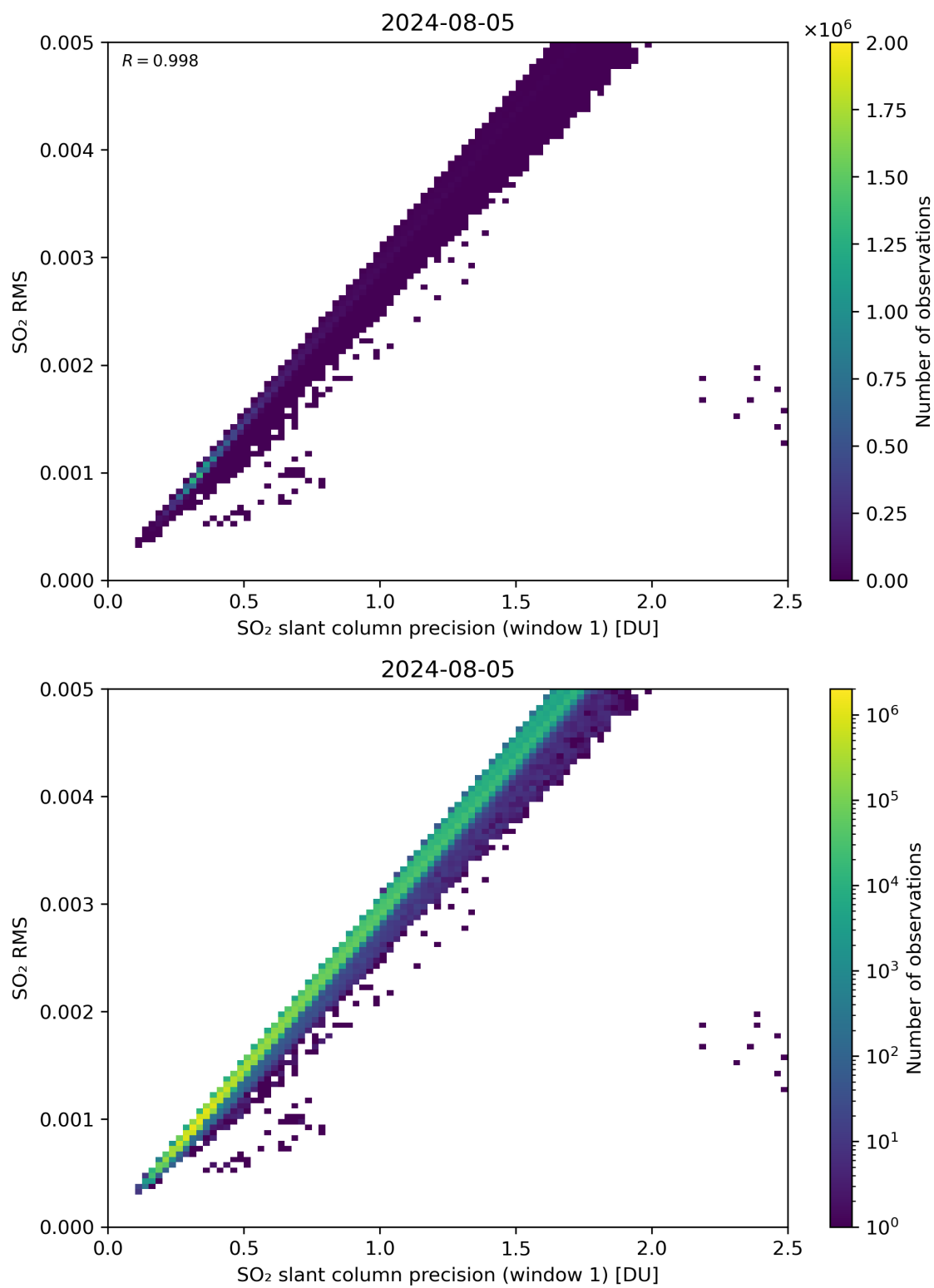
Figure 223: Scatter density plot of “SO 2 slant column precision (window 1)” against “SO 2 RMS” for 2024-08-04 to 2024-08-06.
