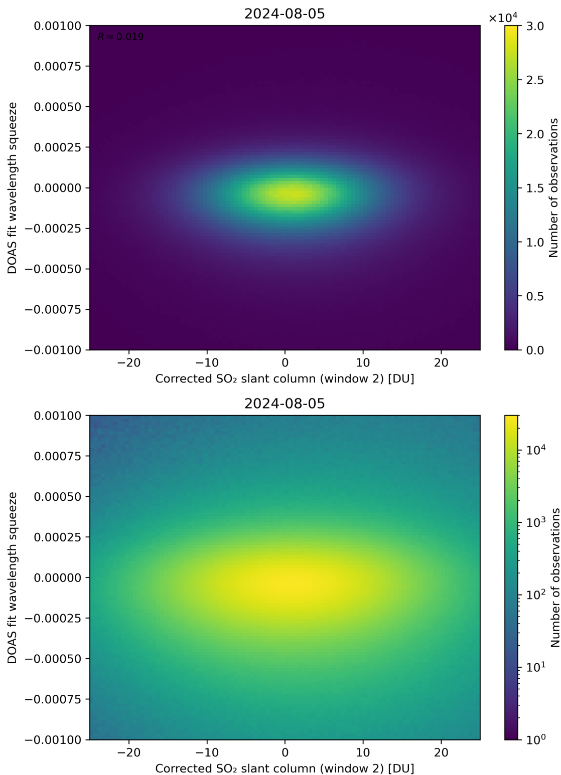
Figure 197: Scatter density plot of “Corrected SO 2 slant column (window 2)” against “DOAS fit wavelength squeeze” for 2024-08-04 to 2024-08-06.
