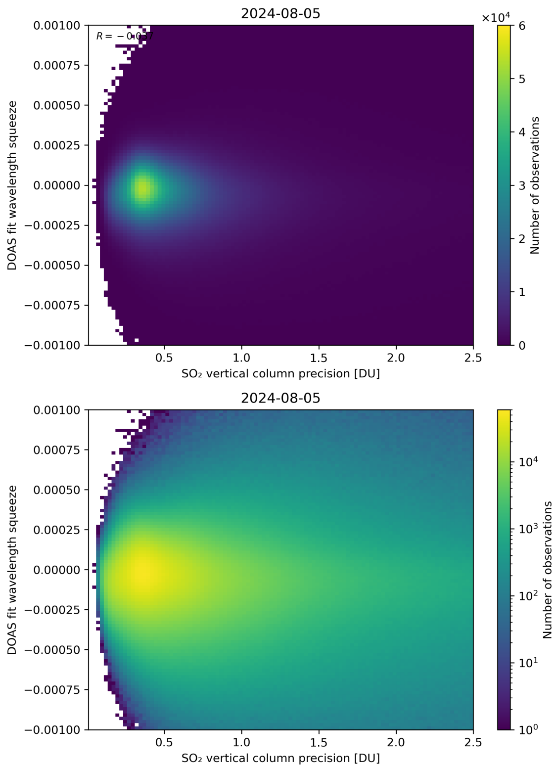
Figure 283: Scatter density plot of “SO 2 vertical column precision” against “DOAS fit wavelength squeeze” for 2024-08-04 to 2024-08-06.
