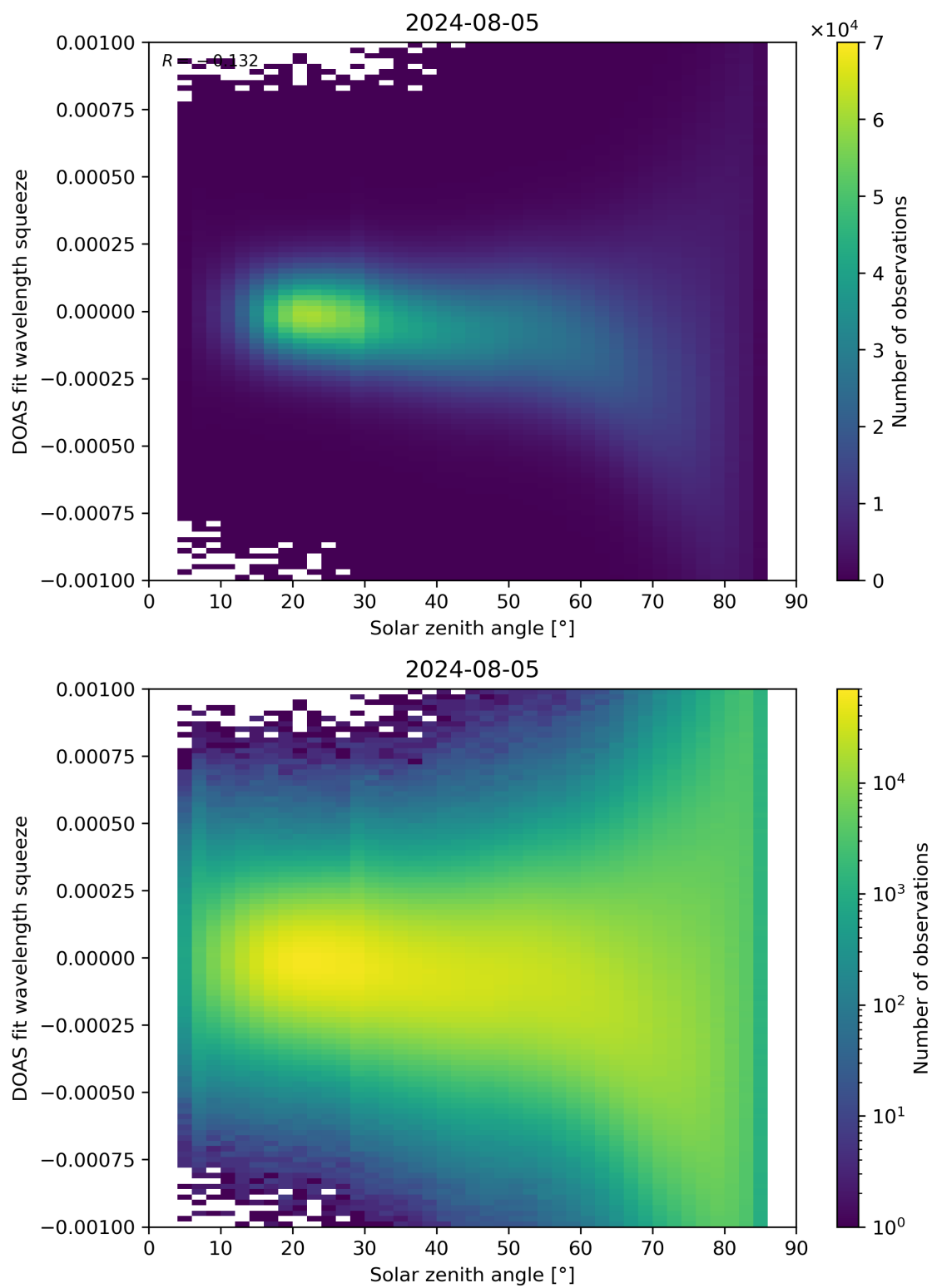
Figure 162: Scatter density plot of “Solar zenith angle” against “DOAS fit wavelength squeeze” for 2024-08-04 to 2024-08-06.
