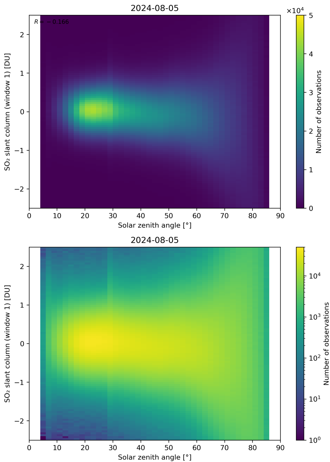
Figure 169: Scatter density plot of “Solar zenith angle” against “SO 2 slant column (window 1)” for 2024-08-04 to 2024-08-06.
