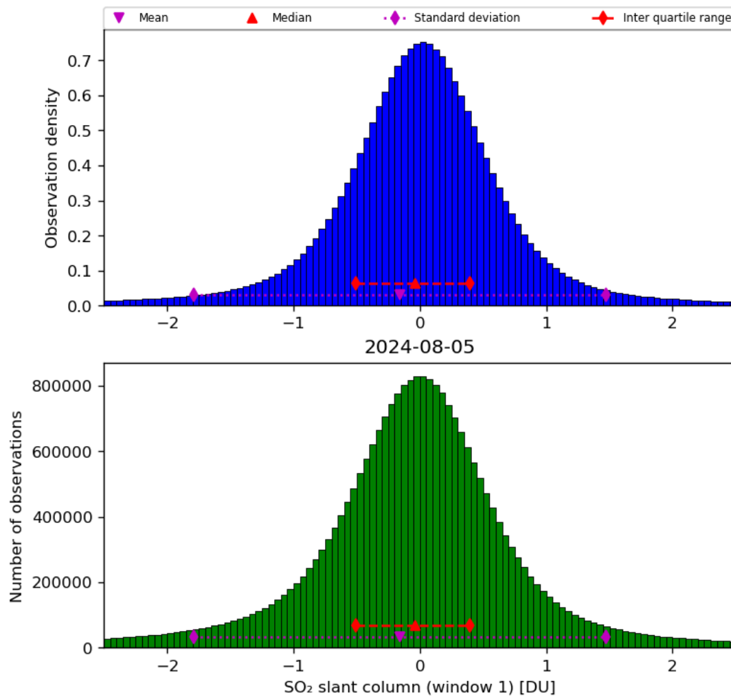
Figure 56: Histogram of “SO 2 slant column (window 1)” for 2024-08-04 to 2024-08-06
