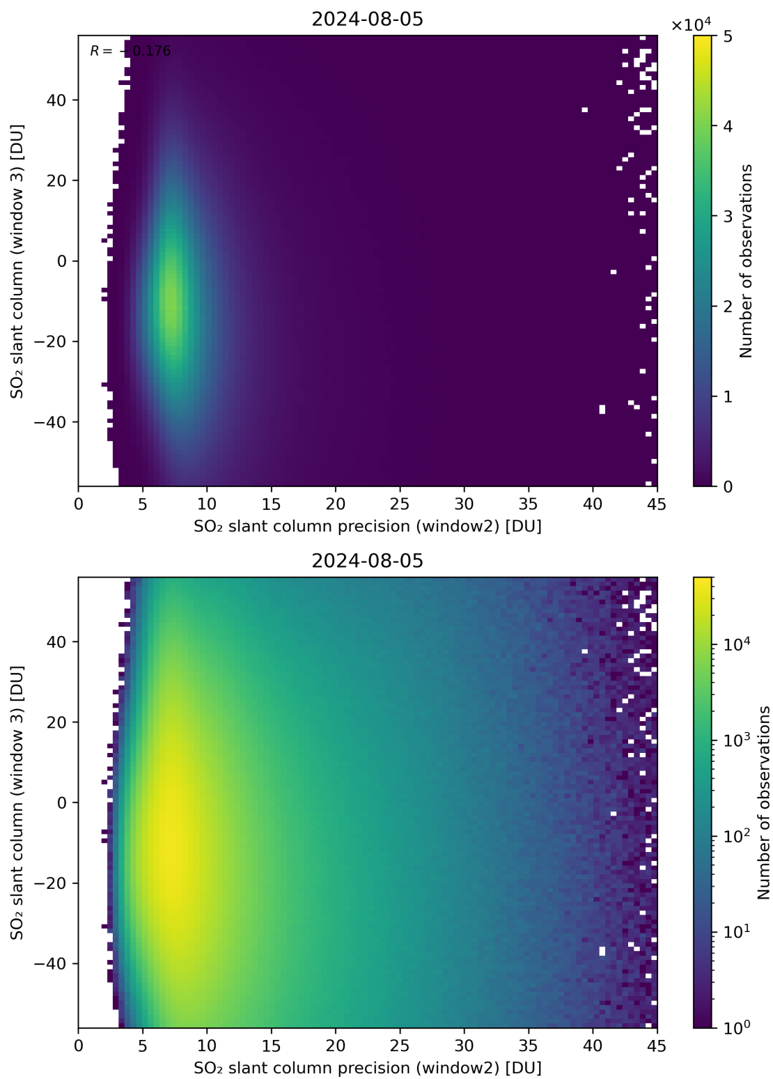
Figure 249: Scatter density plot of “SO 2 slant column precision (window2)” against “SO 2 slant column (window 3)” for 2024-08-04 to 2024-08-06.
