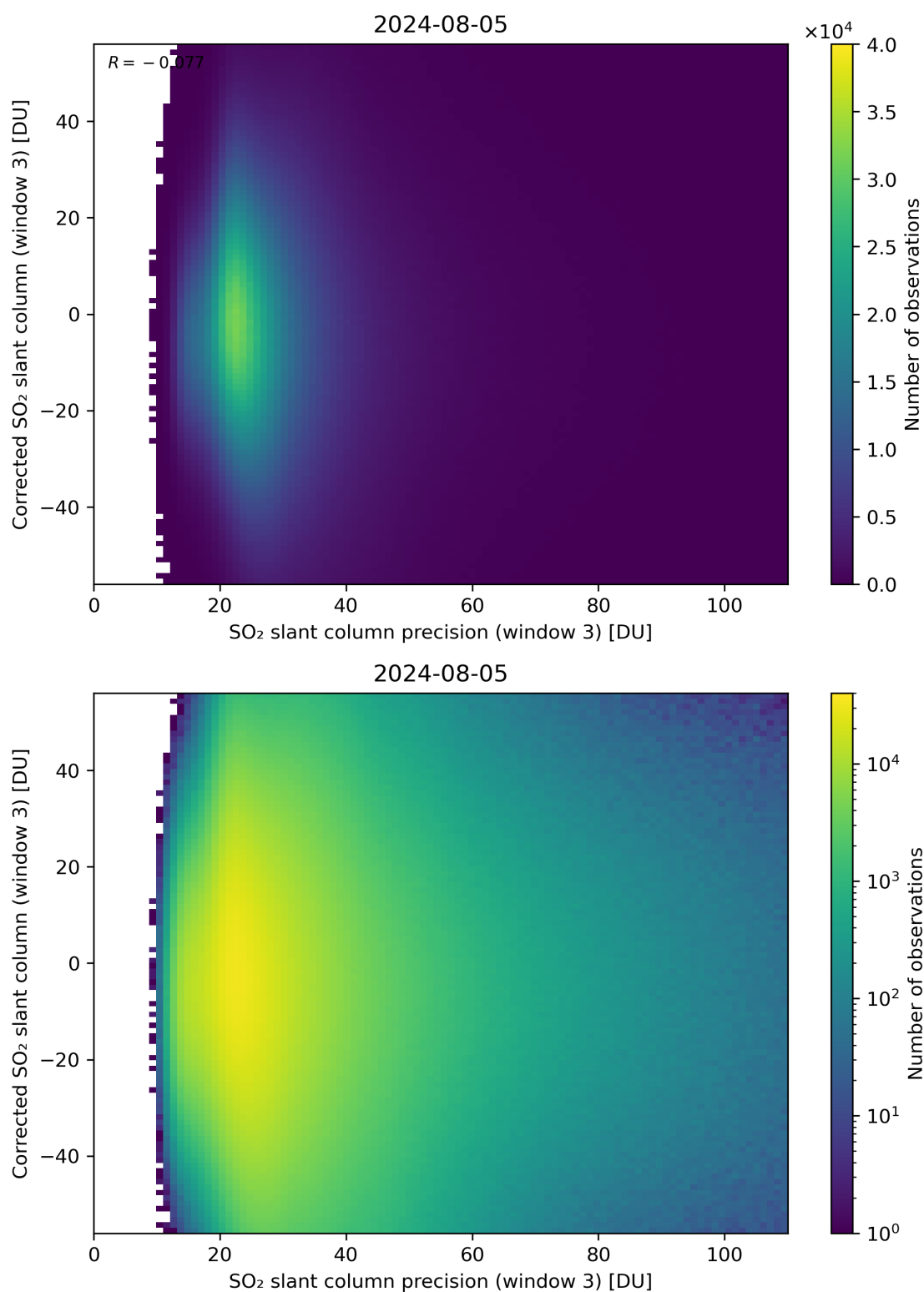
Figure 262: Scatter density plot of “SO 2 slant column precision (window 3)” against “Corrected SO 2 slant column (window 3)” for 2024-08-04 to 2024-08-06.
