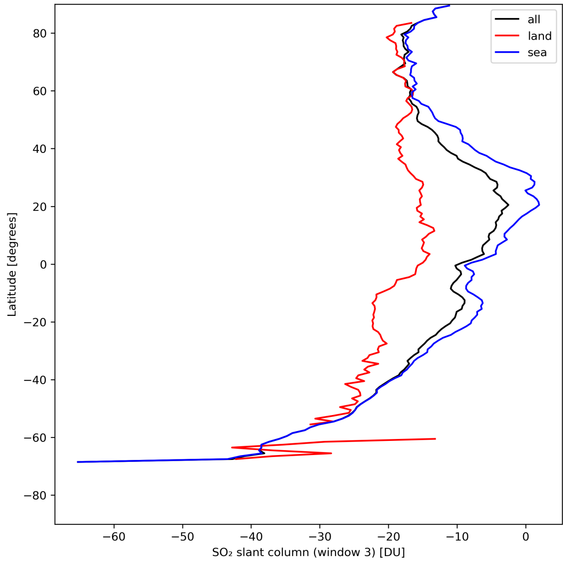
Figure 41: Zonal average of “SO 2 slant column (window 3)” for 2024-08-04 to 2024-08-06.
