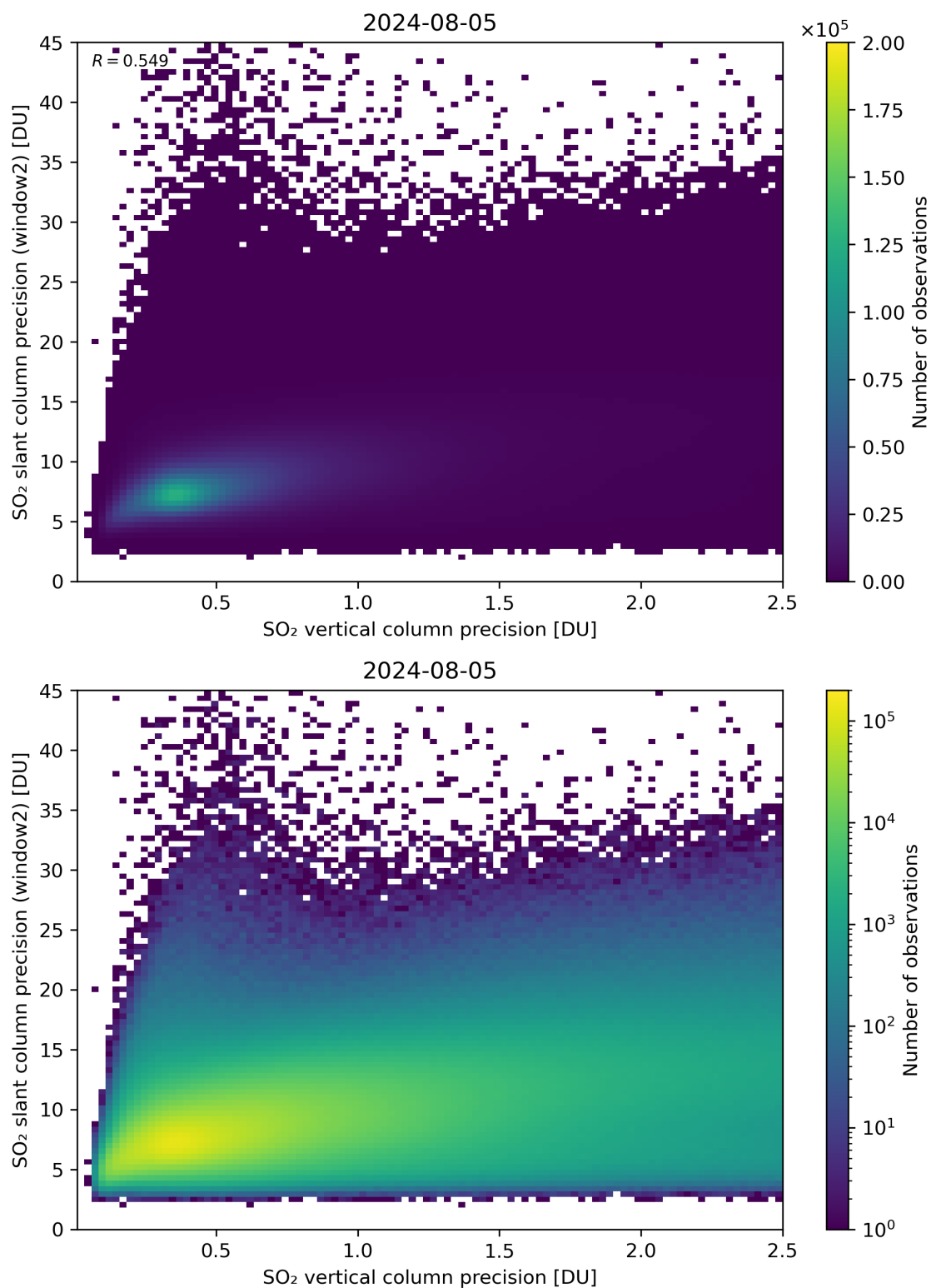
Figure 291: Scatter density plot of “SO 2 vertical column precision” against “SO 2 slant column precision (window2)” for 2024-08-04 to 2024-08-06.
