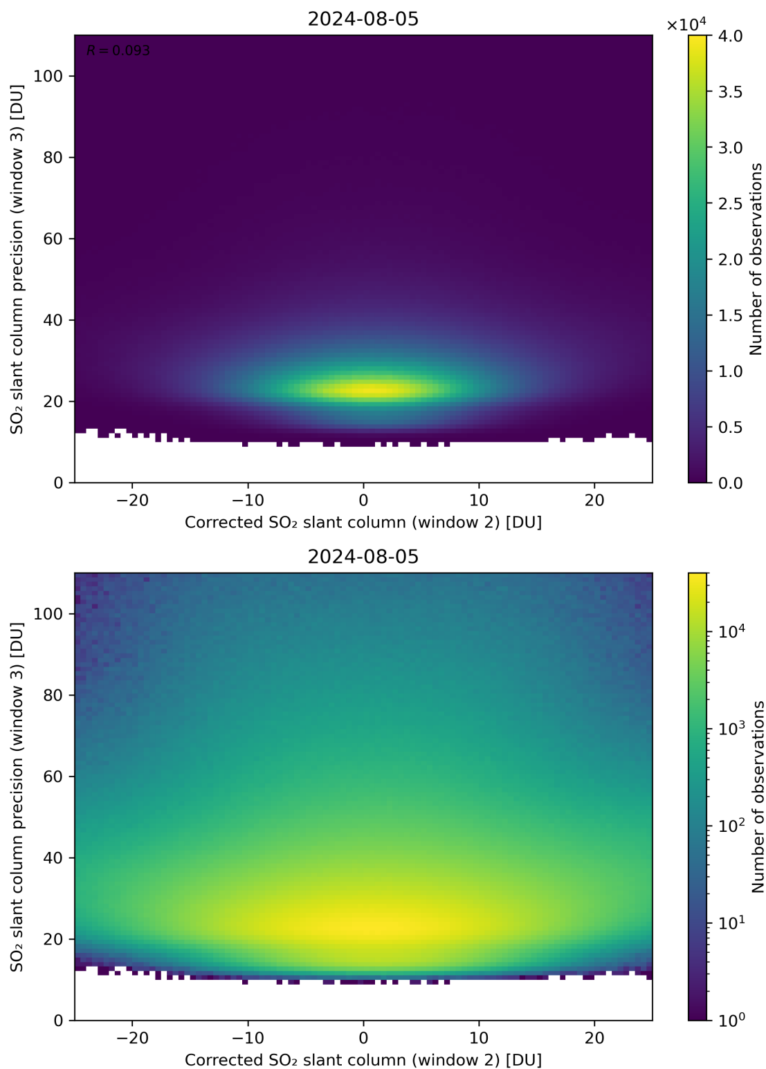
Figure 202: Scatter density plot of “Corrected SO 2 slant column (window 2)” against “SO 2 slant column precision (window 3)” for 2024-08-04 to 2024-08-06.
