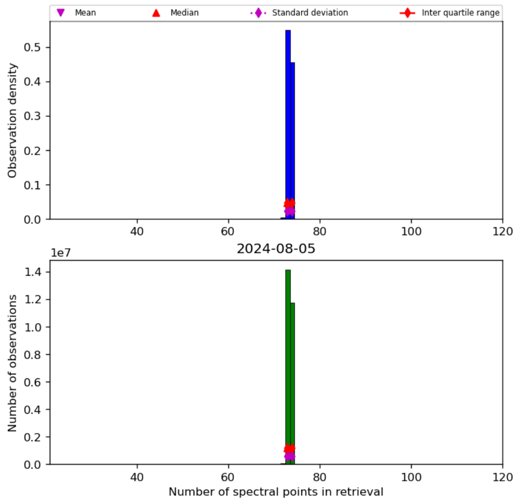
Figure 74: Histogram of “Number of spectral points in retrieval” for 2024-08-04 to 2024-08-06
