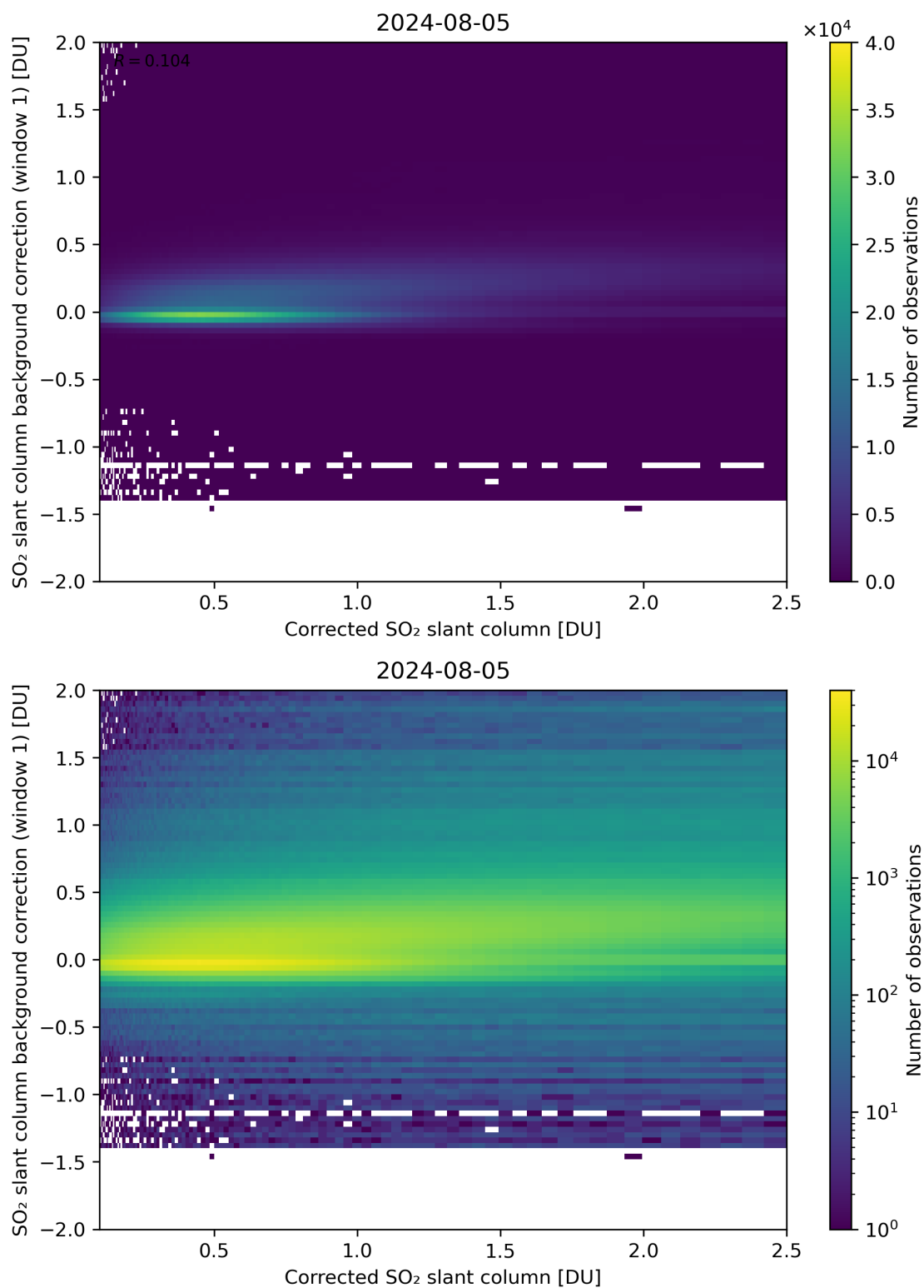
Figure 178: Scatter density plot of “Corrected SO 2 slant column” against “SO 2 slant column background correction (window 1)” for 2024-08-04 to 2024-08-06.
