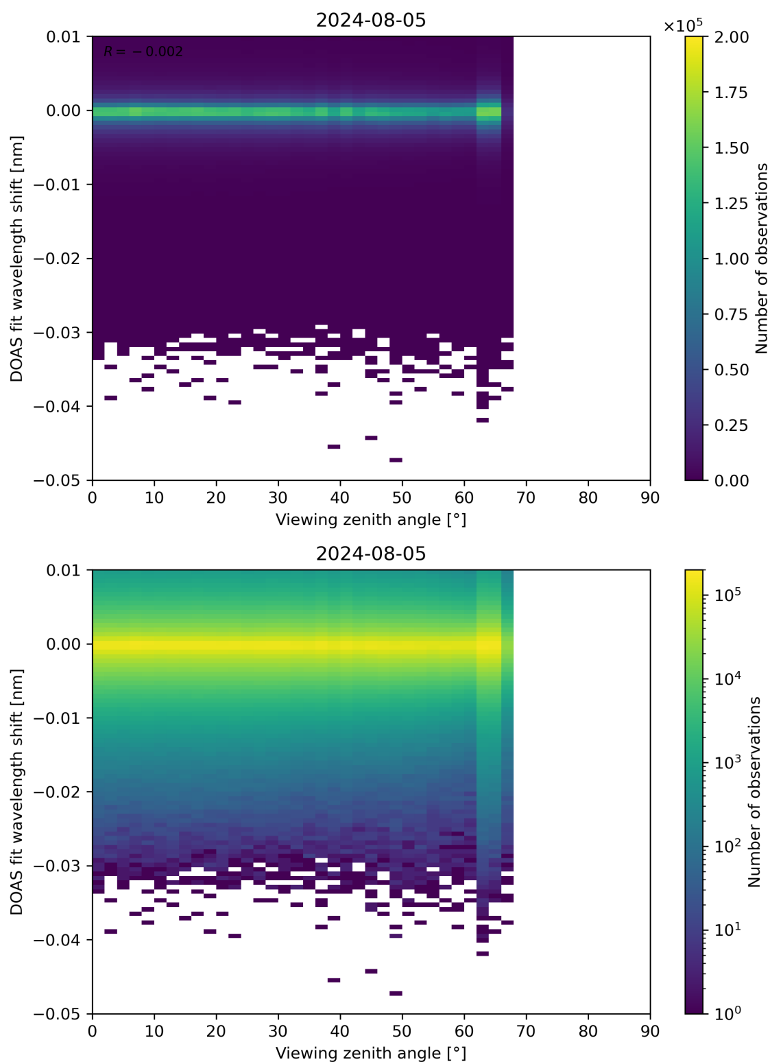
Figure 311: Scatter density plot of “Viewing zenith angle” against “DOAS fit wavelength shift” for 2024-08-04 to 2024-08-06.
