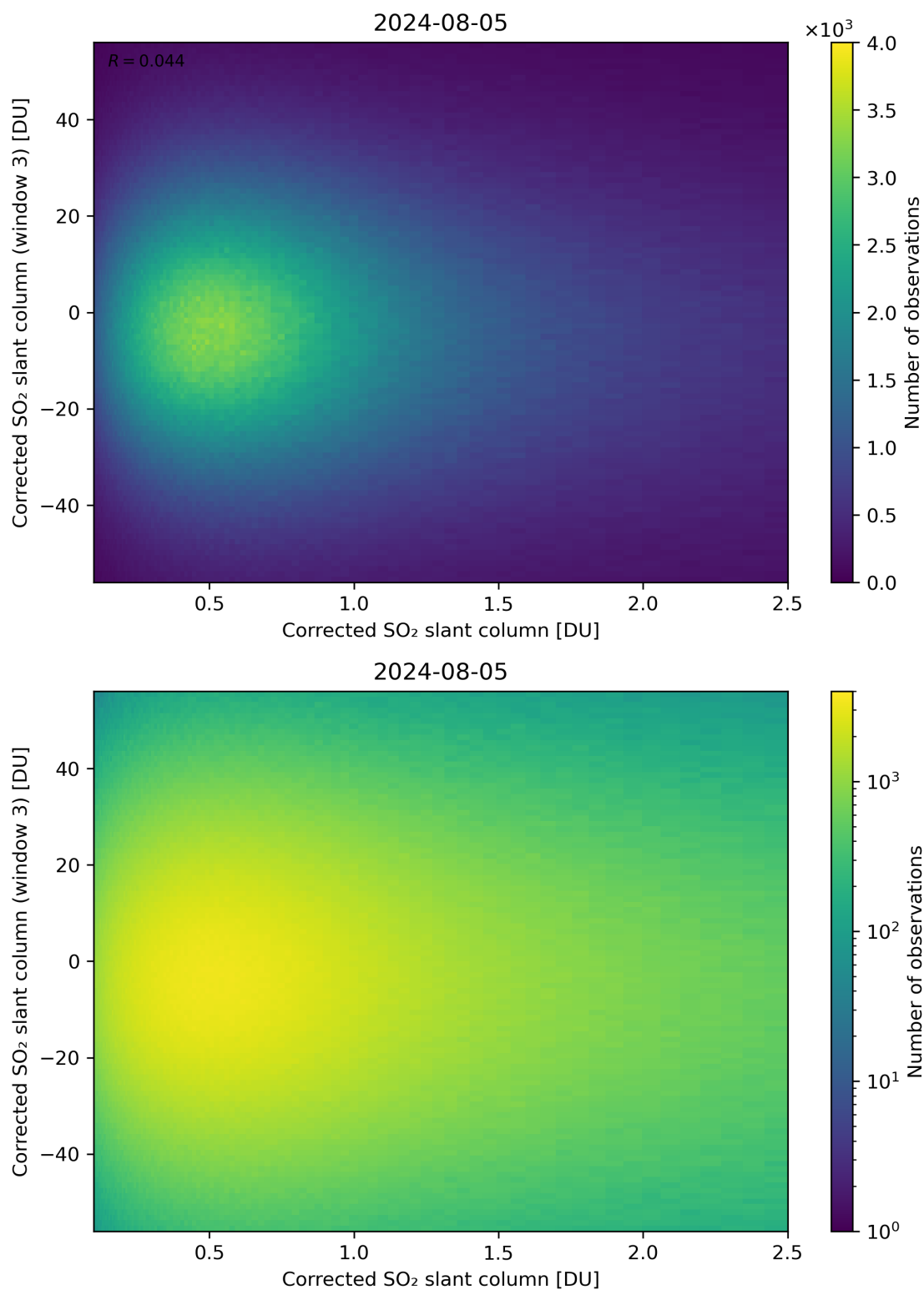
Figure 186: Scatter density plot of “Corrected SO 2 slant column” against “Corrected SO 2 slant column (window 3)” for 2024-08-04 to 2024-08-06.
