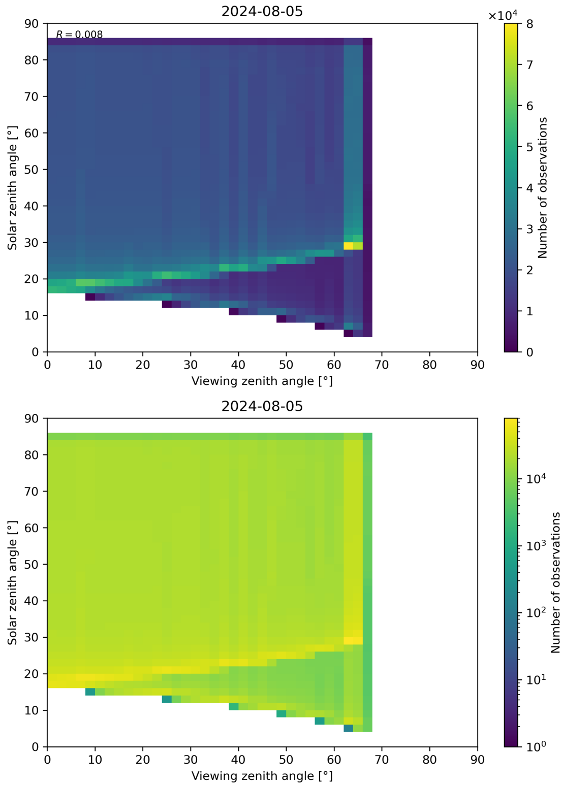
Figure 315: Scatter density plot of “Viewing zenith angle” against “Solar zenith angle” for 2024-08-04 to 2024-08-06.
