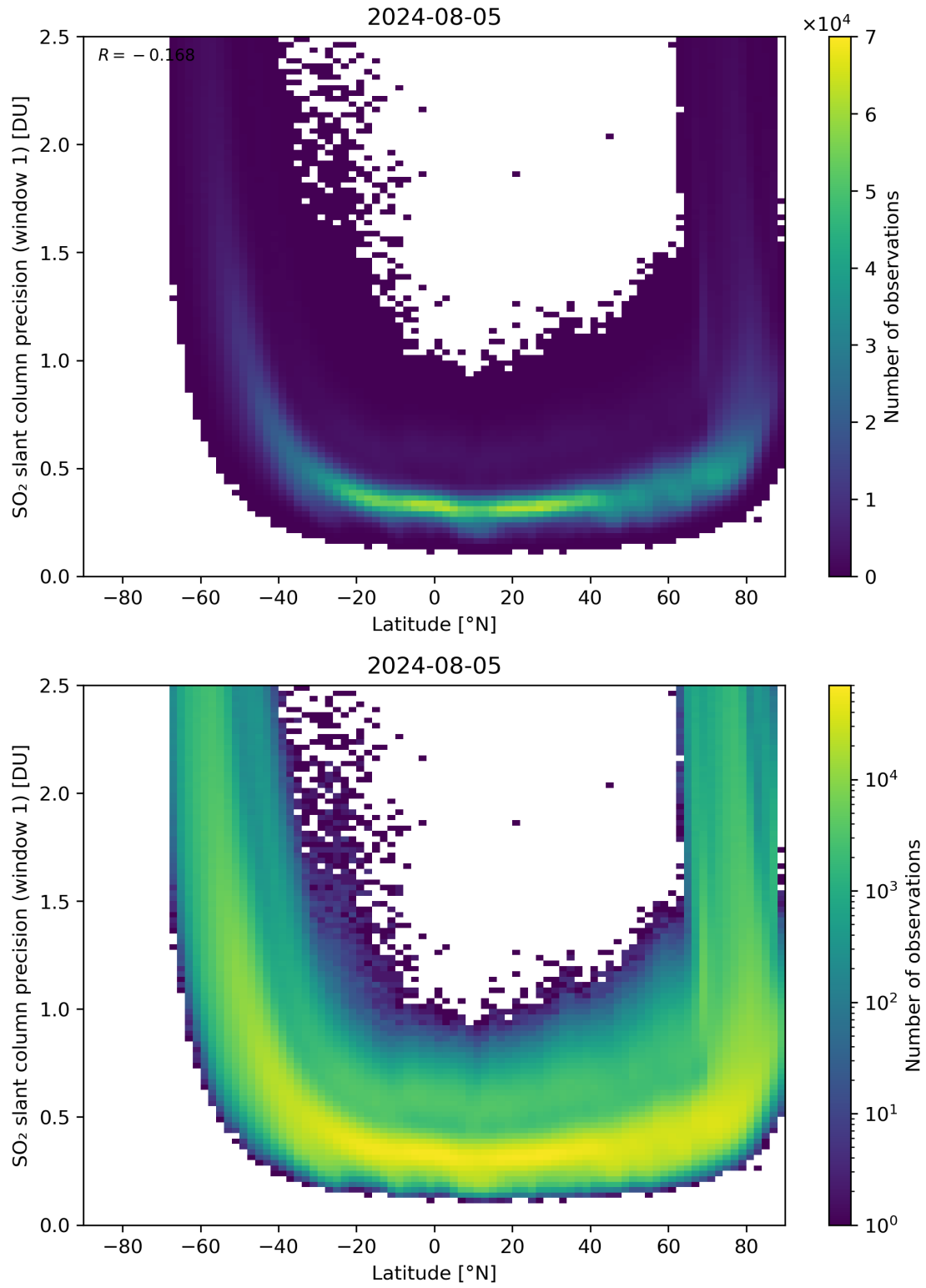
Figure 150: Scatter density plot of “Latitude” against “SO 2 slant column precision (window 1)” for 2024-08-04 to 2024-08-06.
