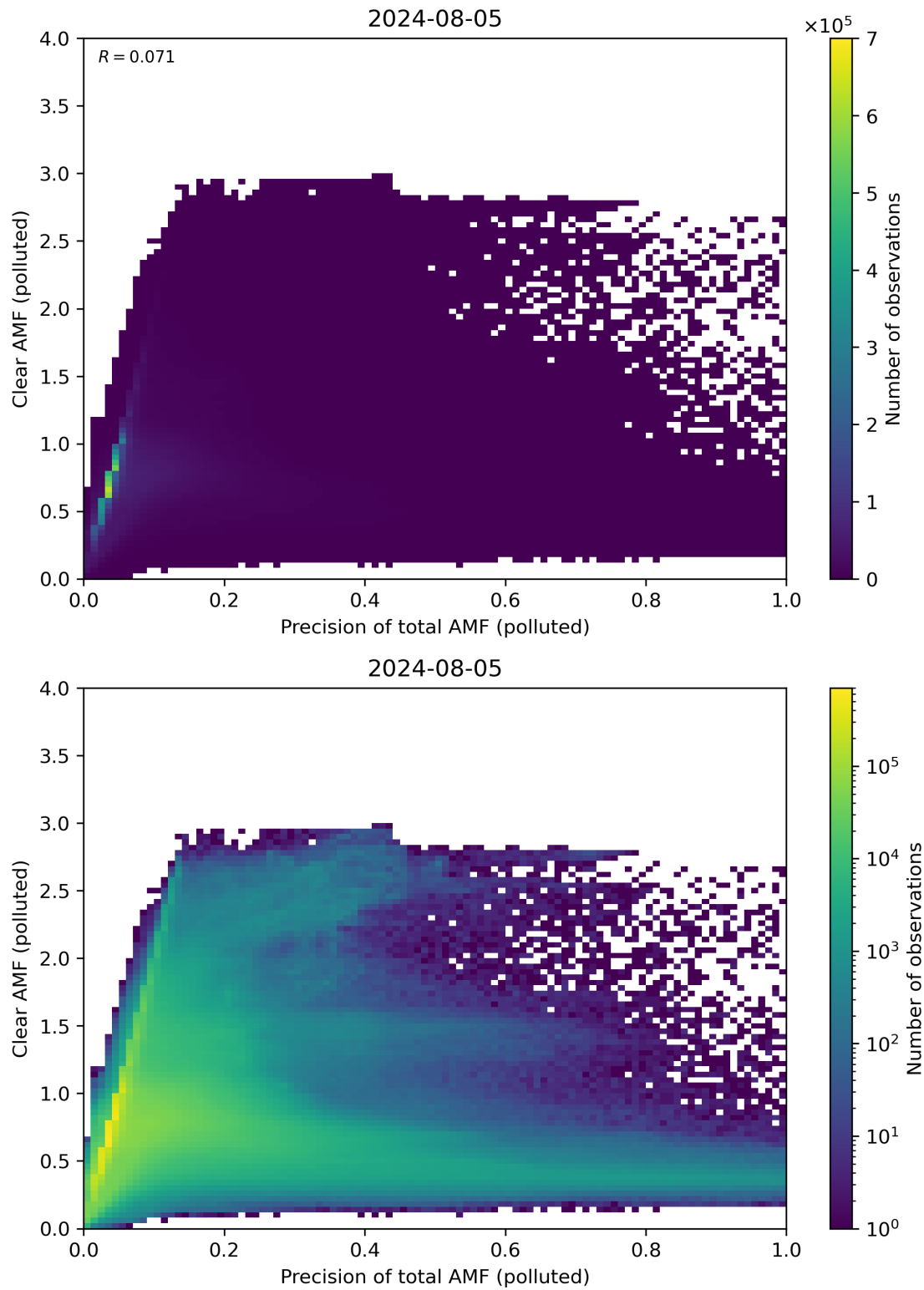
Figure 270: Scatter density plot of “Precision of total AMF (polluted)” against “Clear AMF (polluted)” for 2024-08-04 to 2024-08-06.
