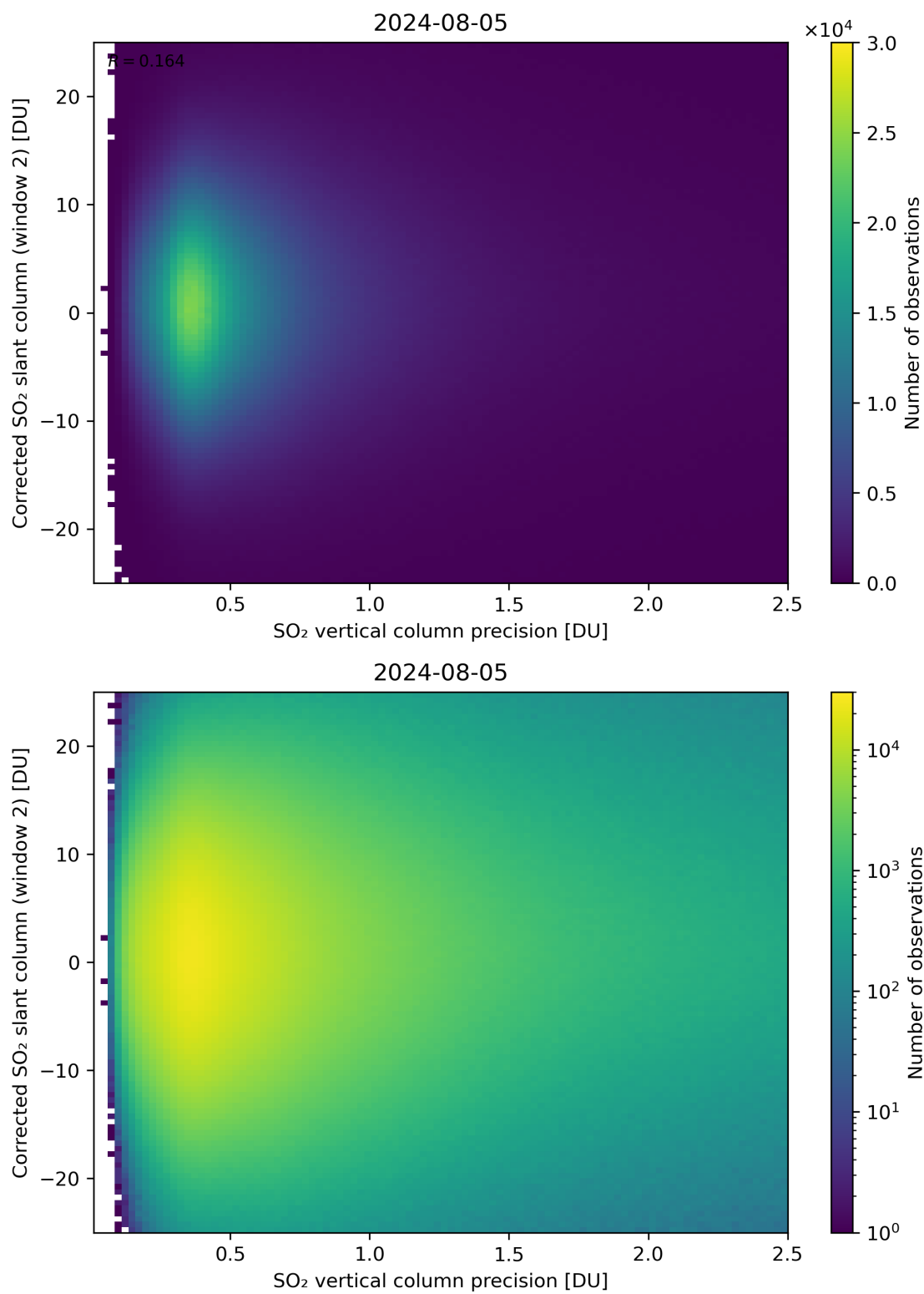
Figure 287: Scatter density plot of “SO 2 vertical column precision” against “Corrected SO 2 slant column (window 2)” for 2024-08-04 to 2024-08-06.
