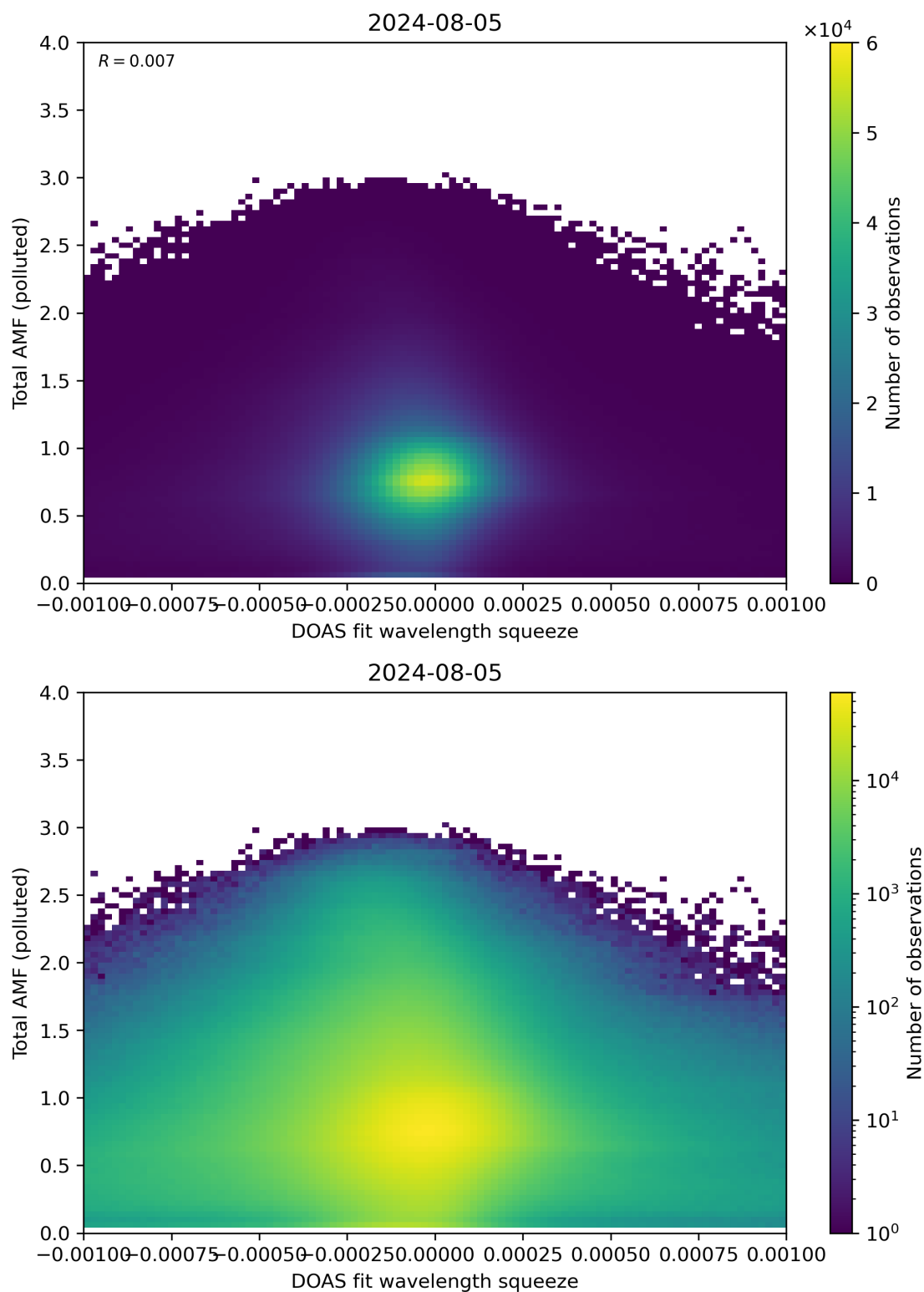
Figure 134: Scatter density plot of “DOAS fit wavelength squeeze” against “Total AMF (polluted)” for 2024-08-04 to 2024-08-06.
