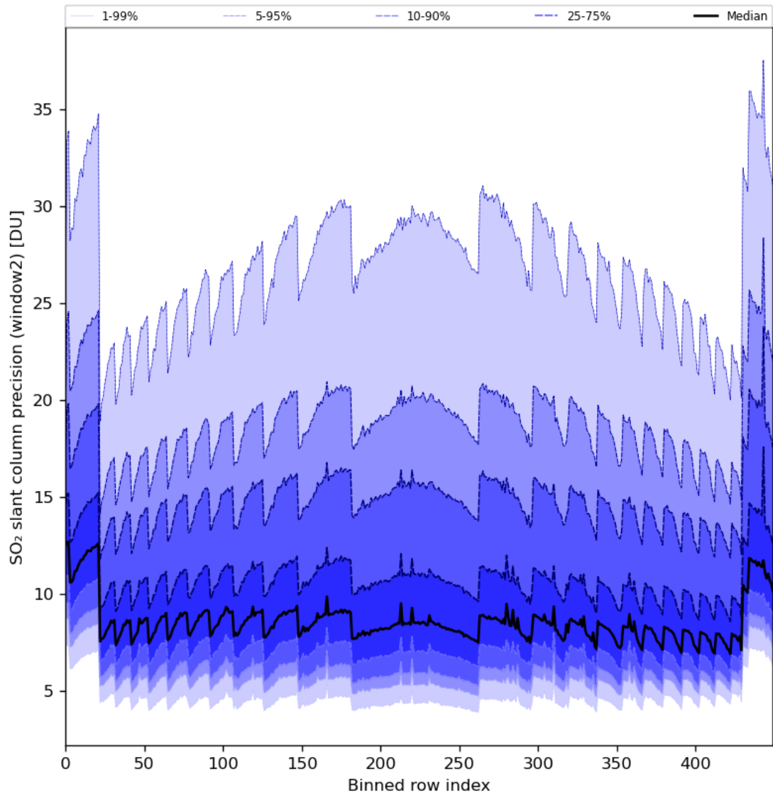
Figure 84: Along track statistics of “SO 2 slant column precision (window2)” for 2024-08-04 to 2024-08-06
