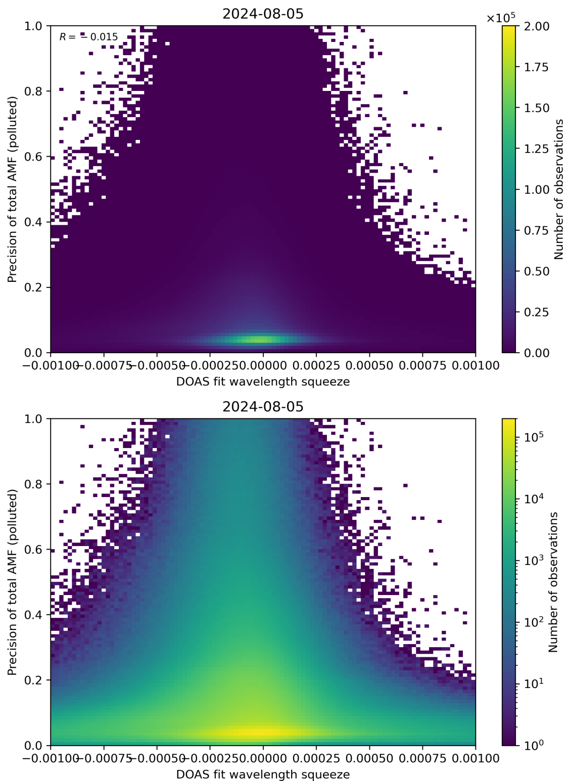
Figure 135: Scatter density plot of “DOAS fit wavelength squeeze” against “Precision of total AMF (polluted)” for 2024-08-04 to 2024-08-06.
