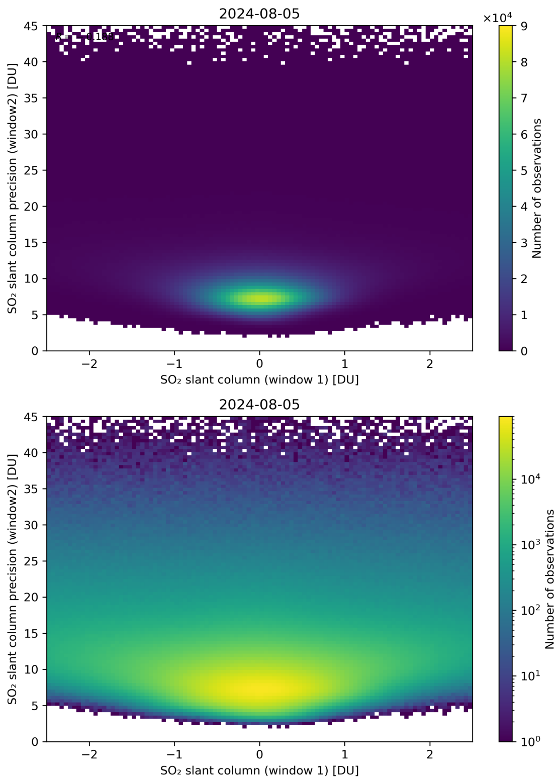
Figure 236: Scatter density plot of “SO 2 slant column (window 1)” against “SO 2 slant column precision (window2)” for 2024-08-04 to 2024-08-06.
