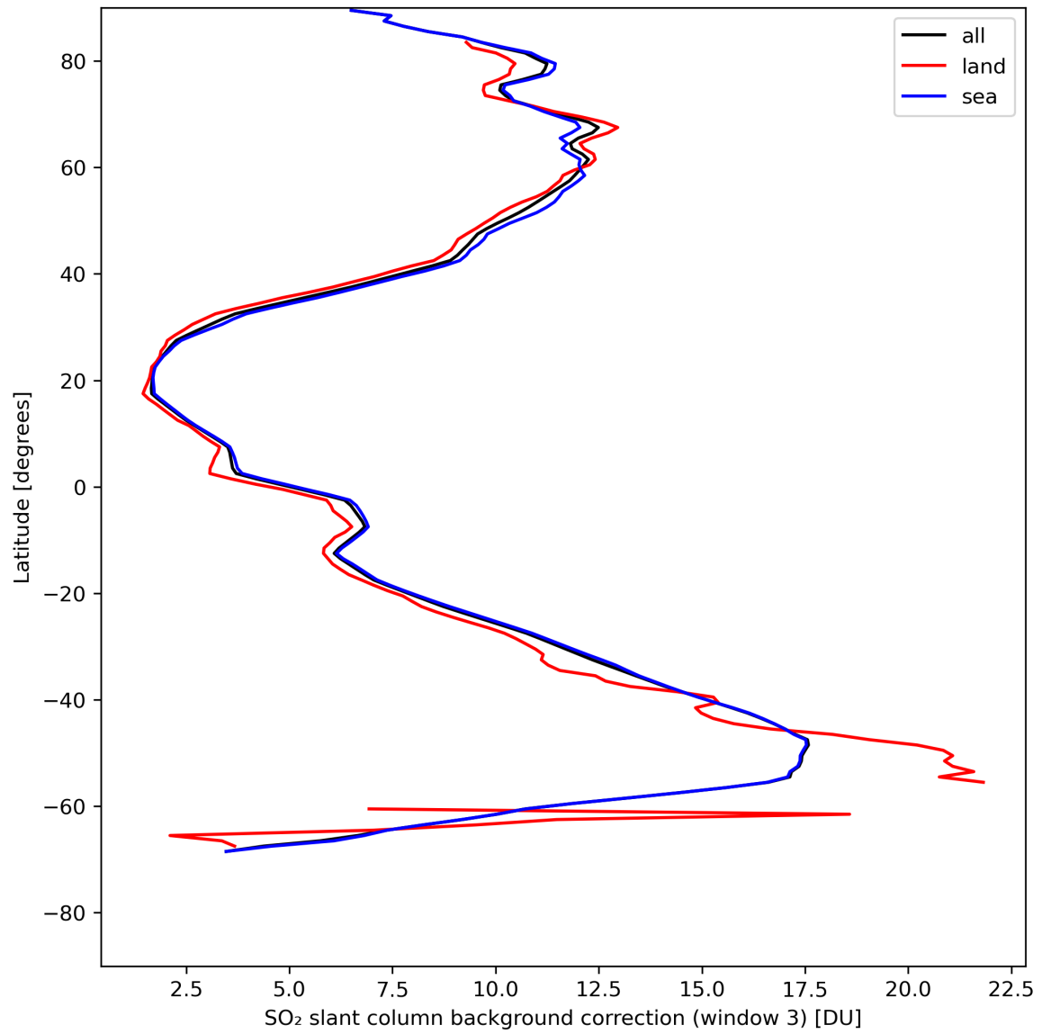
Figure 44: Zonal average of “SO 2 slant column background correction (window 3)” for 2024-08-04 to 2024-08-06.
