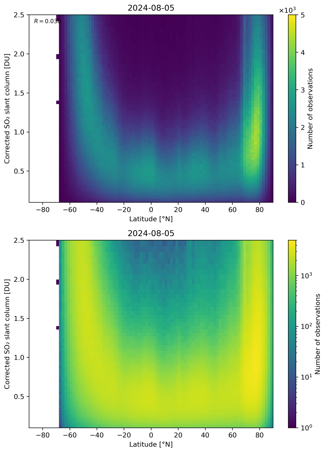
Figure 146: Scatter density plot of “Latitude” against “Corrected SO 2 slant column” for 2024-08-04 to 2024-08-06.
