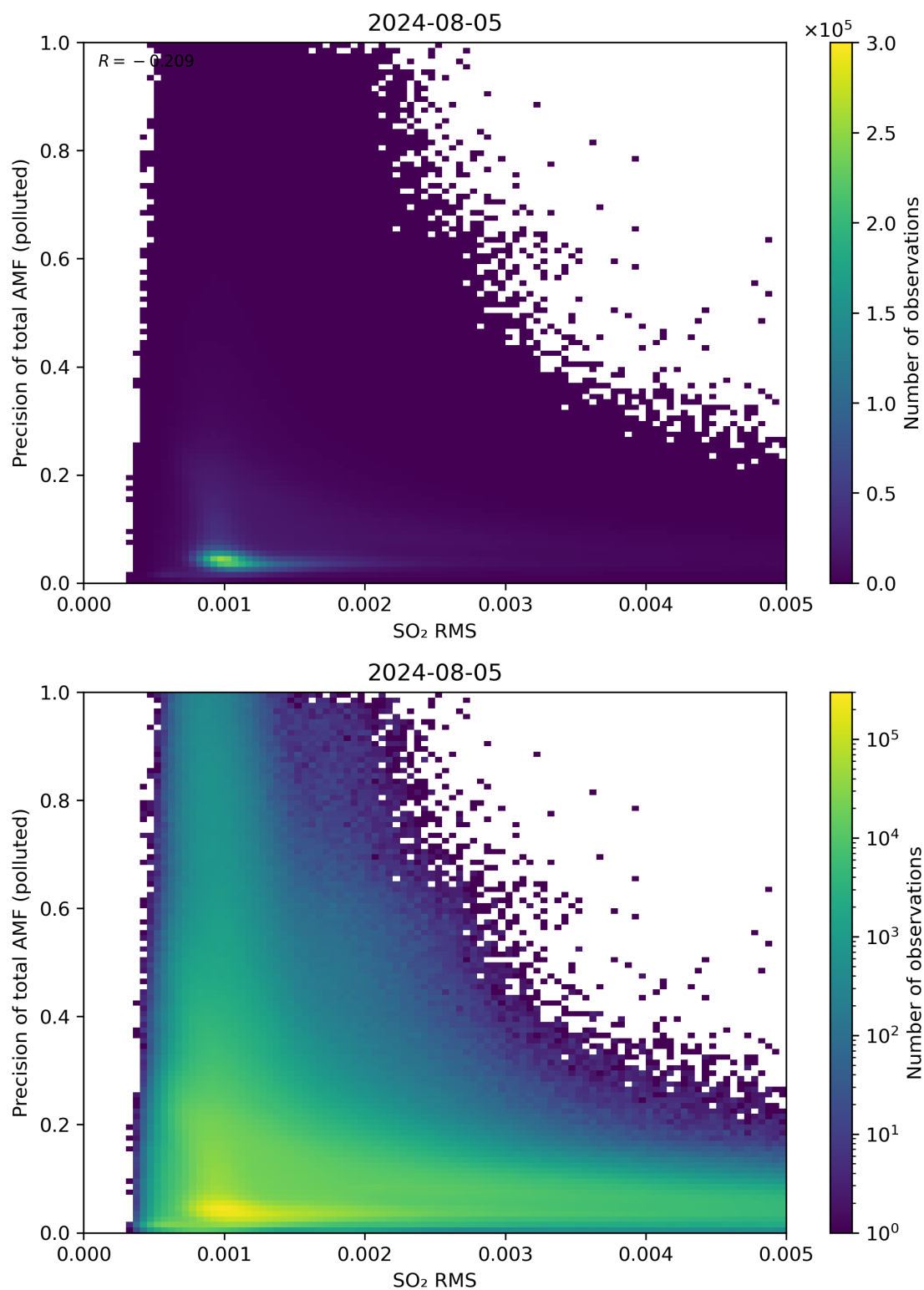
Figure 138: Scatter density plot of “SO 2 RMS” against “Precision of total AMF (polluted)” for 2024-08-04 to 2024-08-06.
