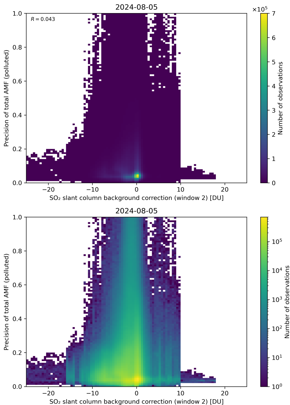
Figure 120: Scatter density plot of “SO 2 slant column background correction (window 2)” against “Precision of total AMF (polluted)” for 2024-08-04 to 2024-08-06.
