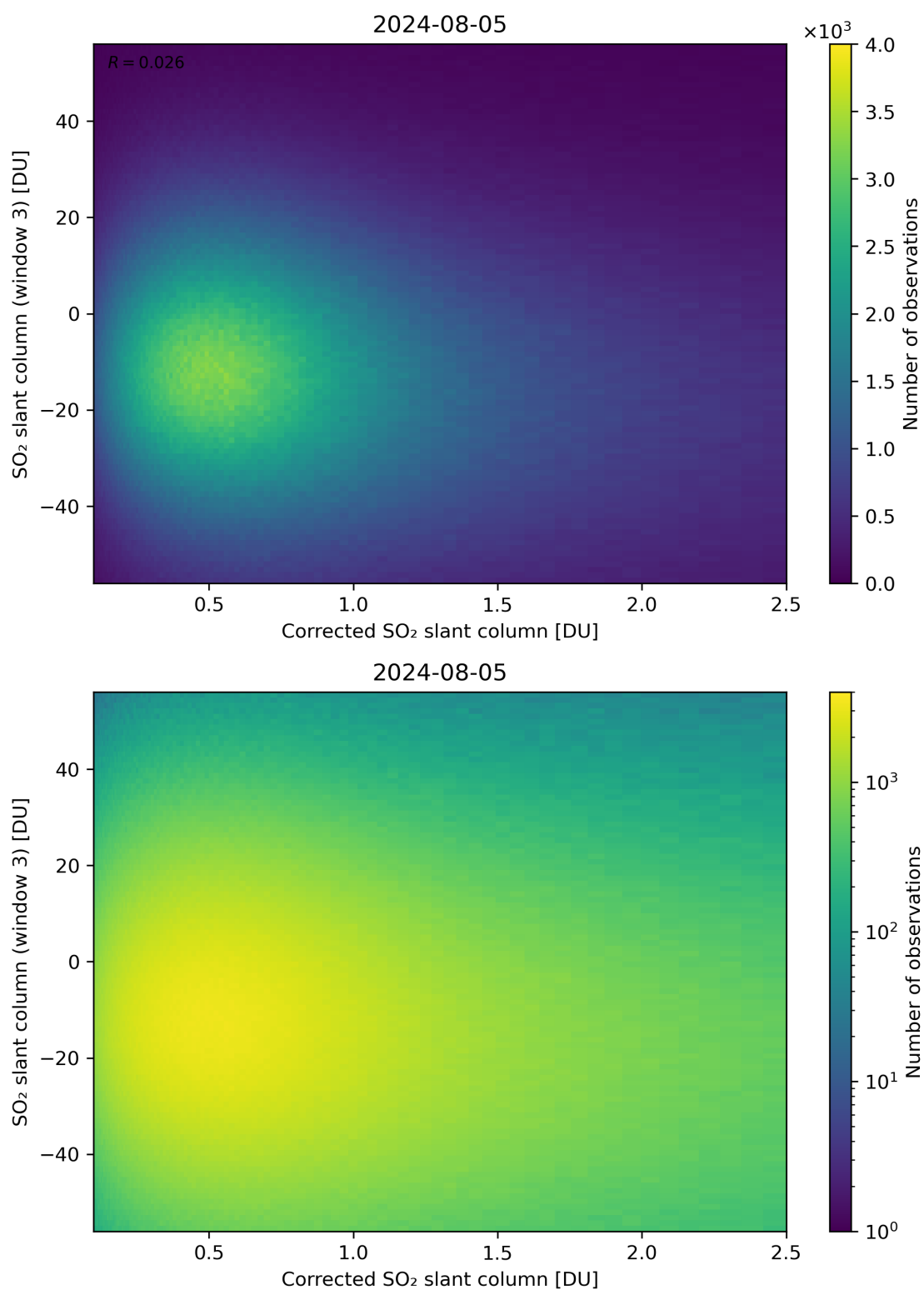
Figure 190: Scatter density plot of “Corrected SO 2 slant column” against “SO 2 slant column (window 3)” for 2024-08-04 to 2024-08-06.
