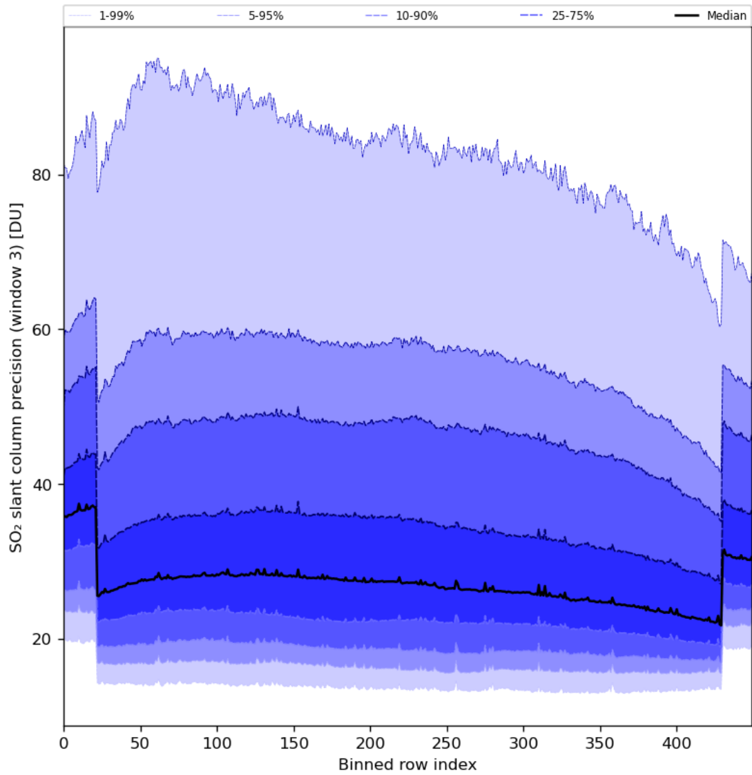
Figure 88: Along track statistics of “SO 2 slant column precision (window 3)” for 2024-08-04 to 2024-08-06
