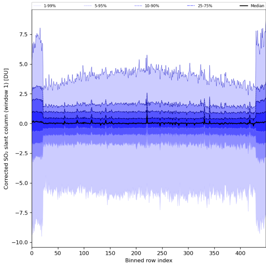
Figure 81: Along track statistics of “Corrected SO 2 slant column (window 1)” for 2024-08-04 to 2024-08-06
