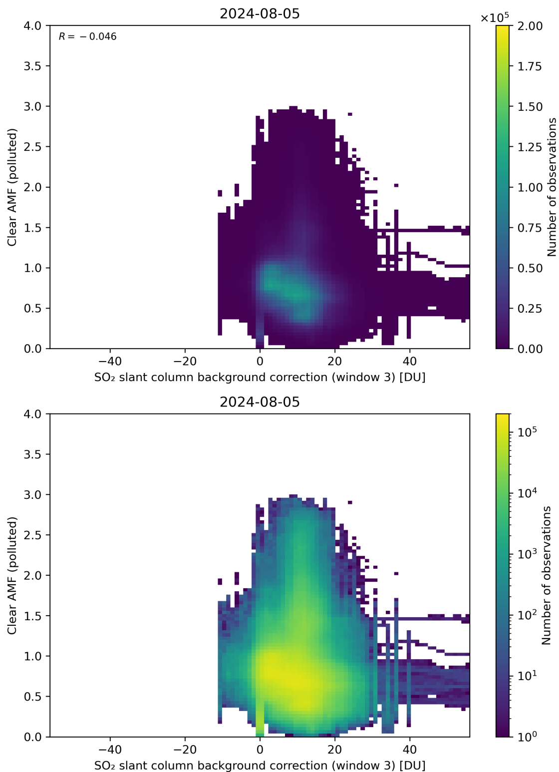
Figure 124: Scatter density plot of “SO 2 slant column background correction (window 3)” against “Clear AMF (polluted)” for 2024-08-04 to 2024-08-06.
