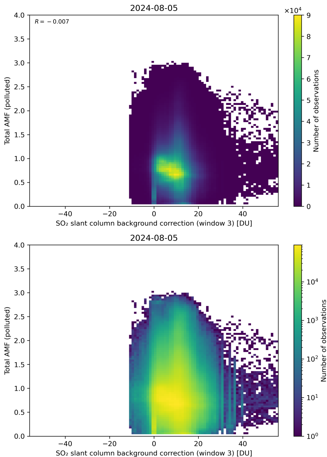
Figure 125: Scatter density plot of “SO 2 slant column background correction (window 3)” against “Total AMF (polluted)” for 2024-08-04 to 2024-08-06.
