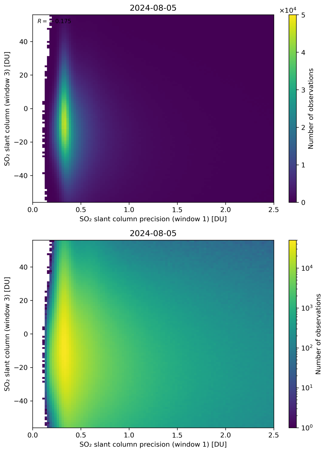
Figure 228: Scatter density plot of “SO 2 slant column precision (window 1)” against “SO 2 slant column (window 3)” for 2024-08-04 to 2024-08-06.
