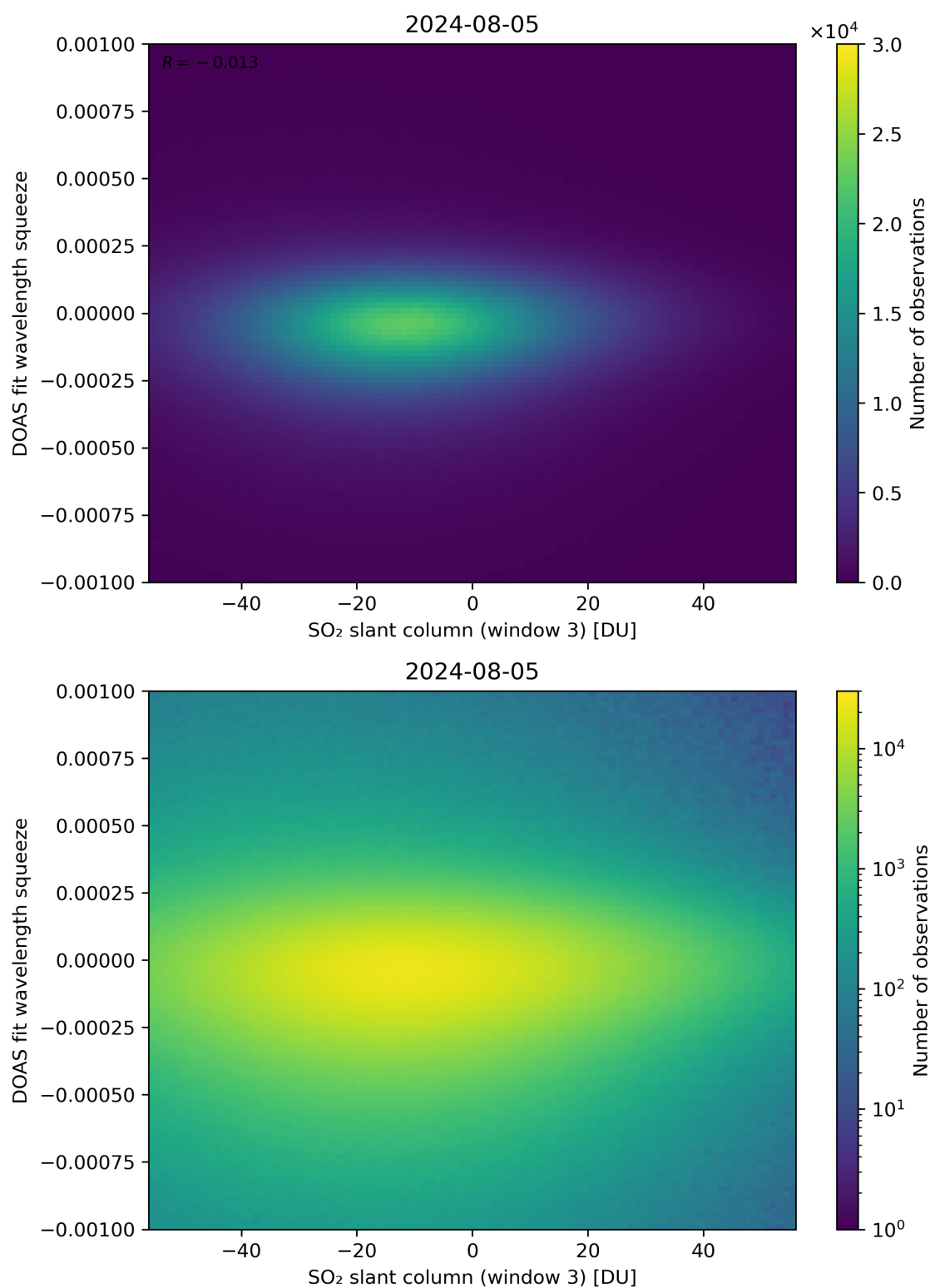
Figure 255: Scatter density plot of “SO 2 slant column (window 3)” against “DOAS fit wavelength squeeze” for 2024-08-04 to 2024-08-06.
