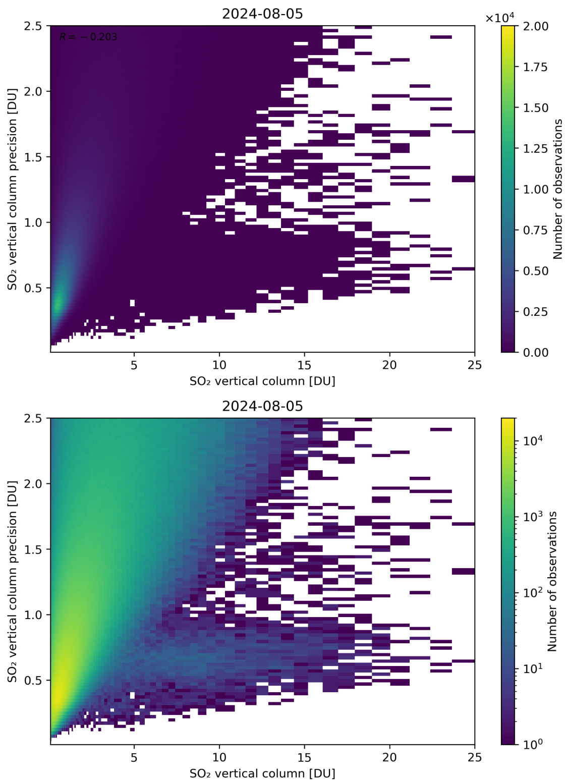
Figure 307: Scatter density plot of “SO 2 vertical column” against “SO 2 vertical column precision” for 2024-08-04 to 2024-08-06.
