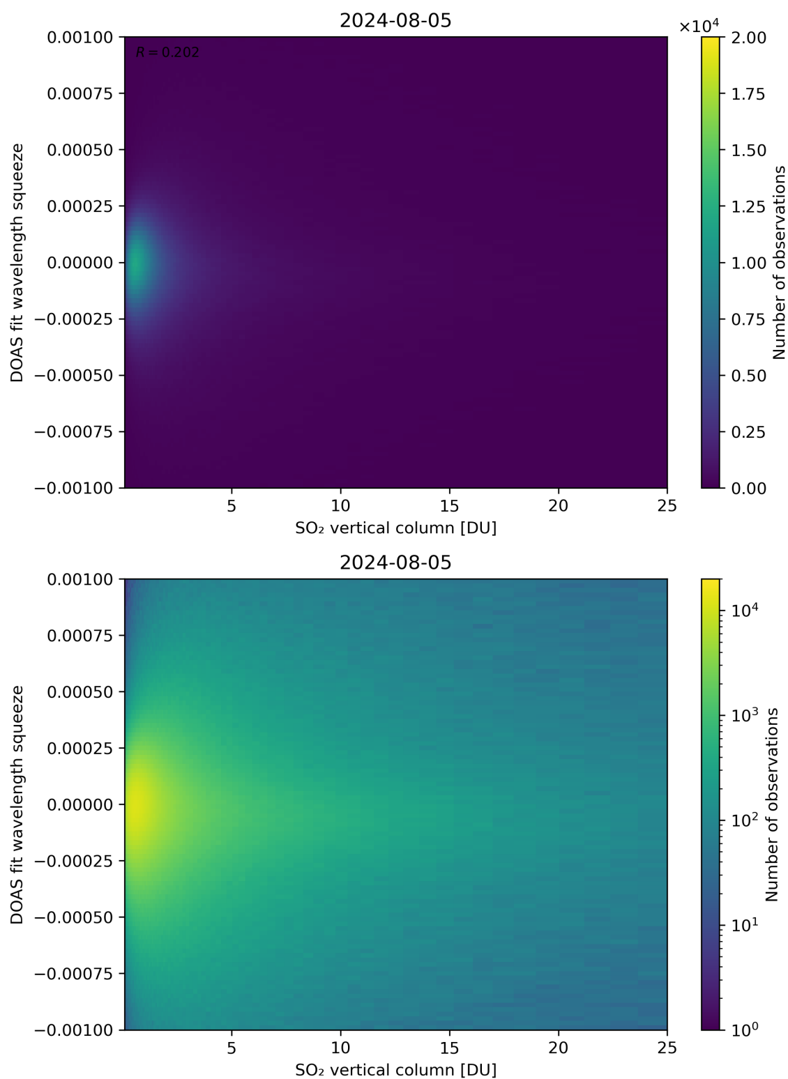
Figure 277: Scatter density plot of “SO 2 vertical column” against “DOAS fit wavelength squeeze” for 2024-08-04 to 2024-08-06.
