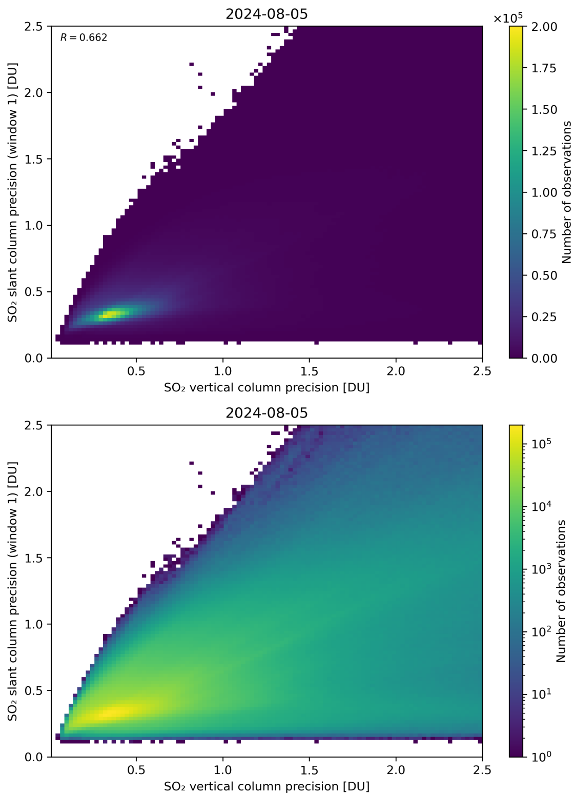
Figure 290: Scatter density plot of “SO 2 vertical column precision” against “SO 2 slant column precision (window 1)” for 2024-08-04 to 2024-08-06.
