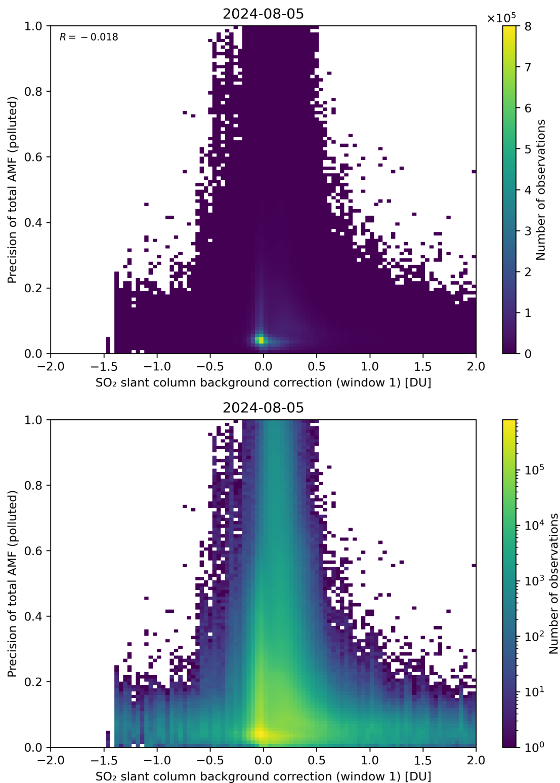
Figure 110: Scatter density plot of “SO 2 slant column background correction (window 1)” against “Precision of total AMF (polluted)” for 2024-08-04 to 2024-08-06.
