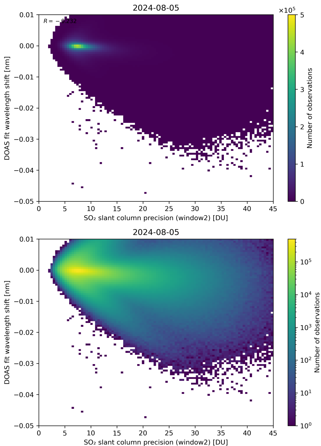
Figure 243: Scatter density plot of “SO 2 slant column precision (window2)” against “DOAS fit wavelength shift” for 2024-08-04 to 2024-08-06.
