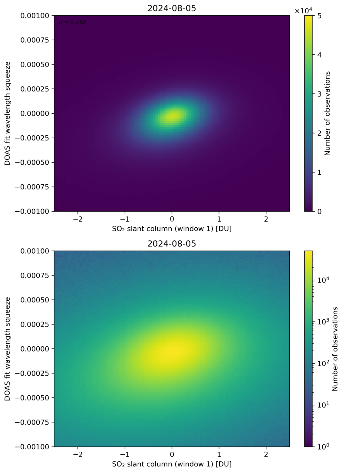
Figure 216: Scatter density plot of “SO 2 slant column (window 1)” against “DOAS fit wavelength squeeze” for 2024-08-04 to 2024-08-06.
