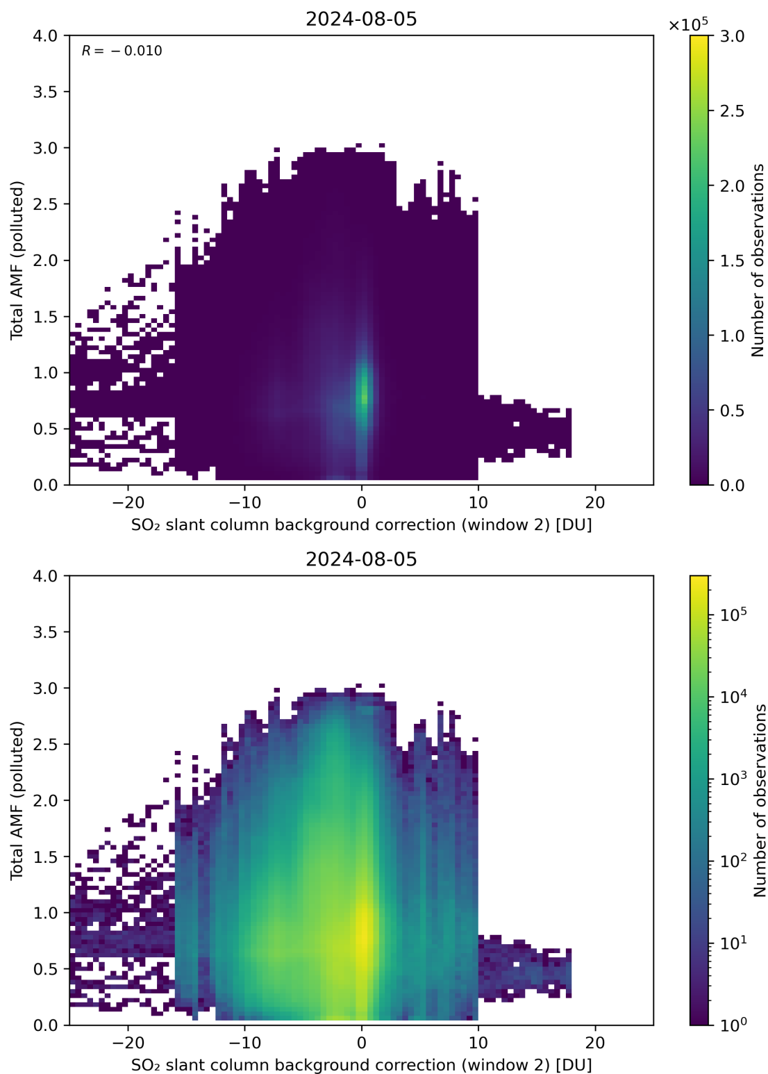
Figure 119: Scatter density plot of “SO 2 slant column background correction (window 2)” against “Total AMF (polluted)” for 2024-08-04 to 2024-08-06.
