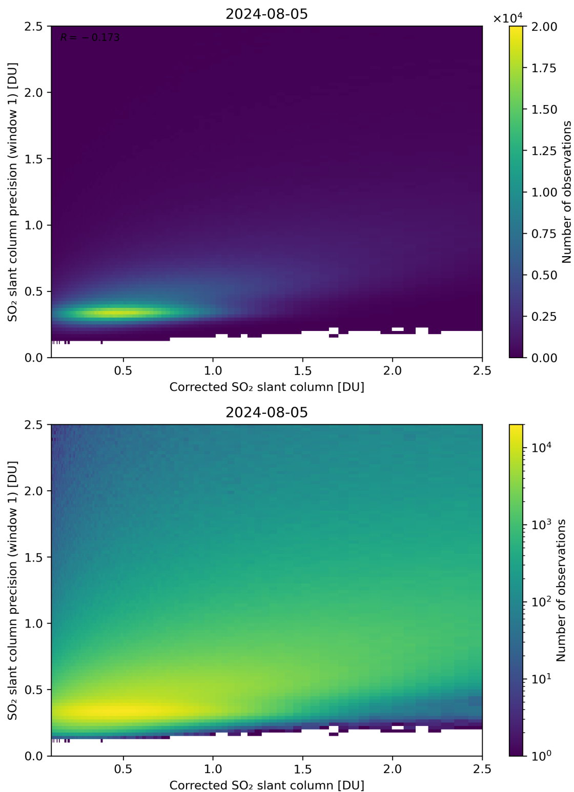
Figure 188: Scatter density plot of “Corrected SO 2 slant column” against “SO 2 slant column precision (window 1)” for 2024-08-04 to 2024-08-06.
