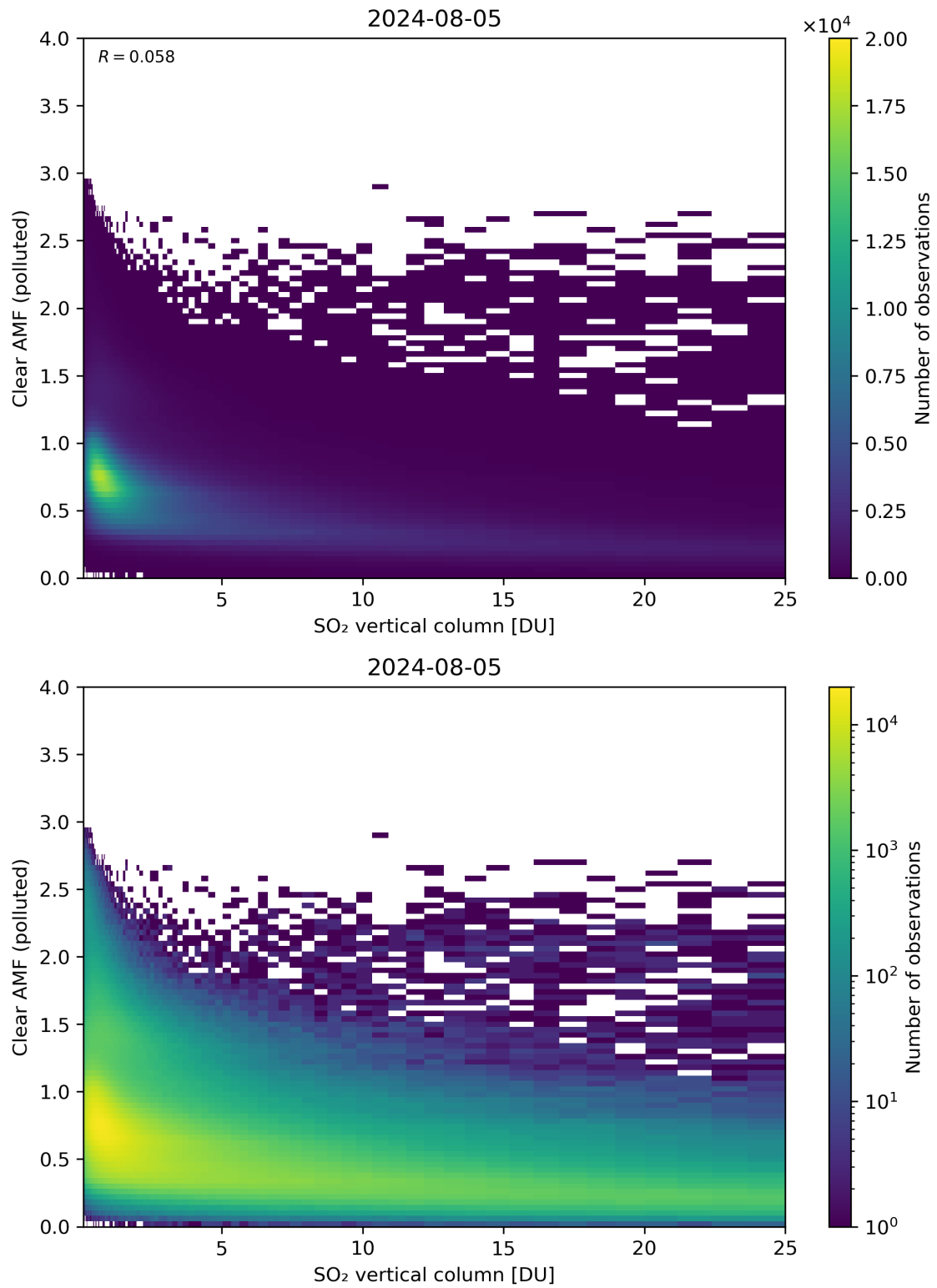
Figure 296: Scatter density plot of “SO 2 vertical column” against “Clear AMF (polluted)” for 2024-08-04 to 2024-08-06.
