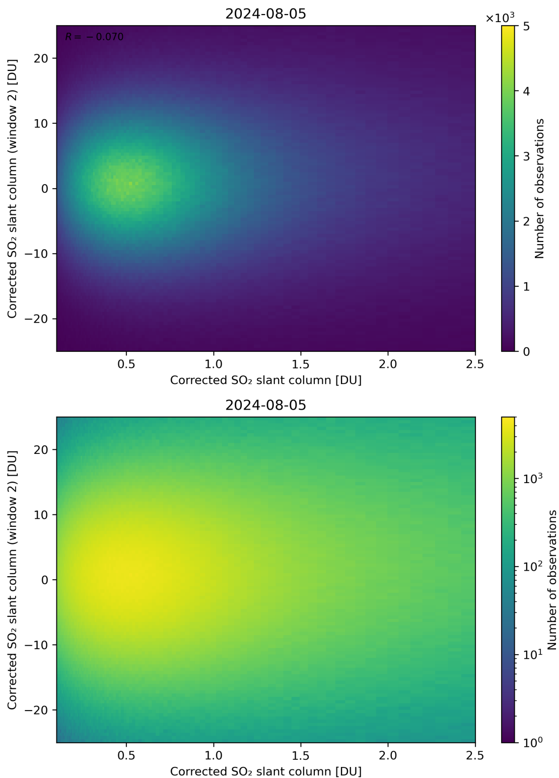
Figure 185: Scatter density plot of “Corrected SO 2 slant column” against “Corrected SO 2 slant column (window 2)” for 2024-08-04 to 2024-08-06.
