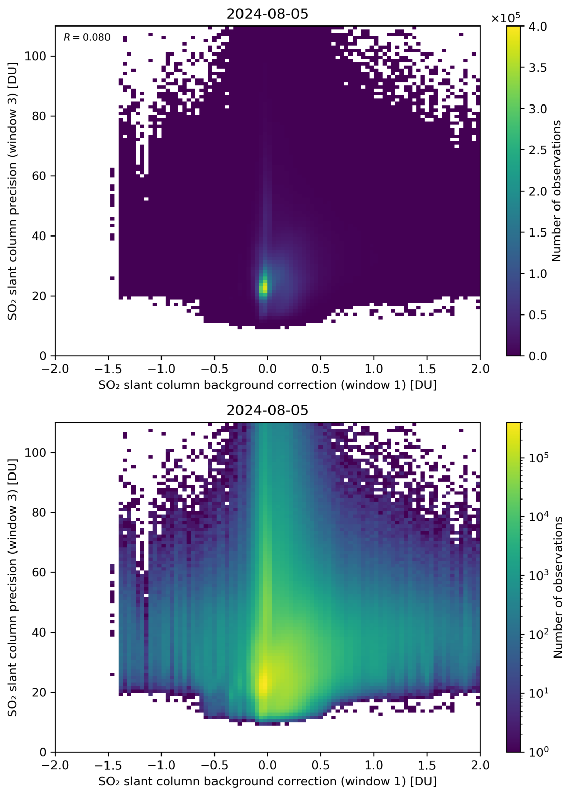
Figure 108: Scatter density plot of “SO 2 slant column background correction (window 1)” against “SO 2 slant column precision (window 3)” for 2024-08-04 to 2024-08-06.
