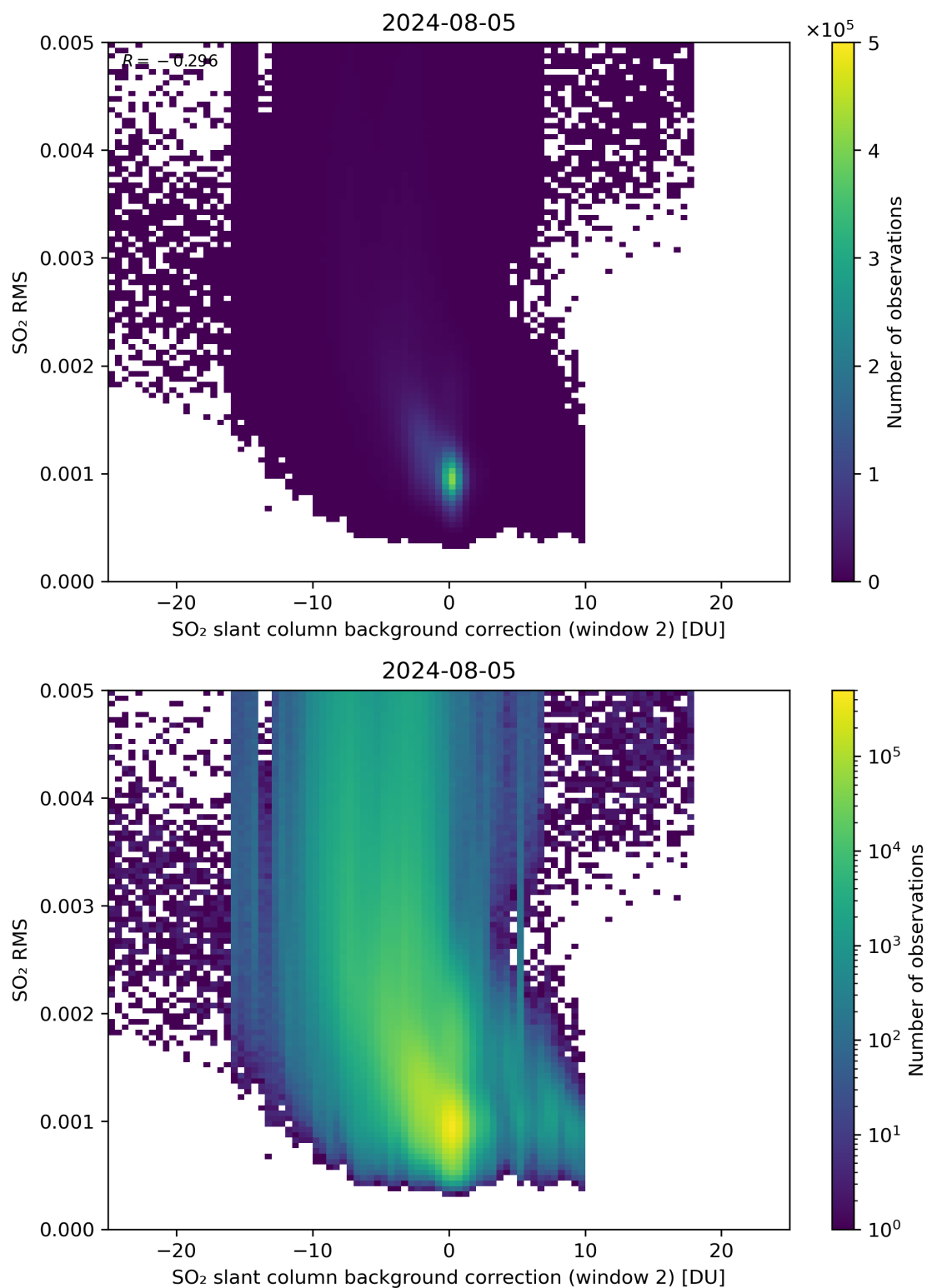
Figure 114: Scatter density plot of “SO 2 slant column background correction (window 2)” against “SO 2 RMS” for 2024-08-04 to 2024-08-06.
