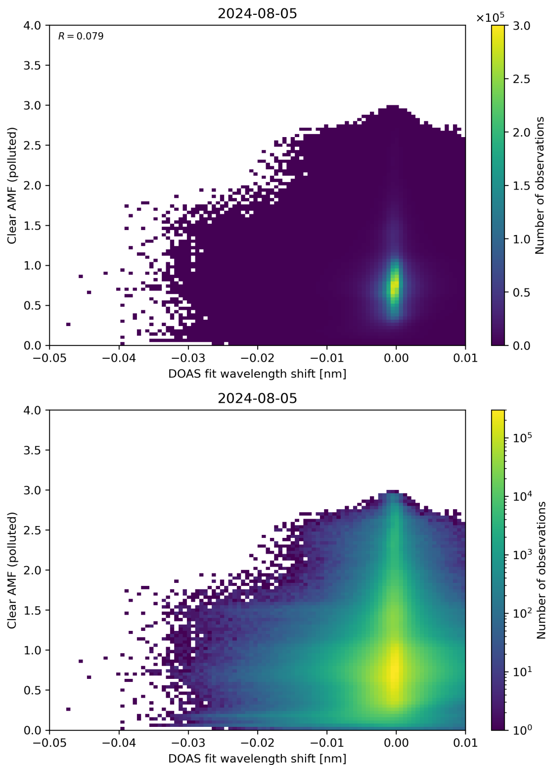
Figure 129: Scatter density plot of “DOAS fit wavelength shift” against “Clear AMF (polluted)” for 2024-08-04 to 2024-08-06.
