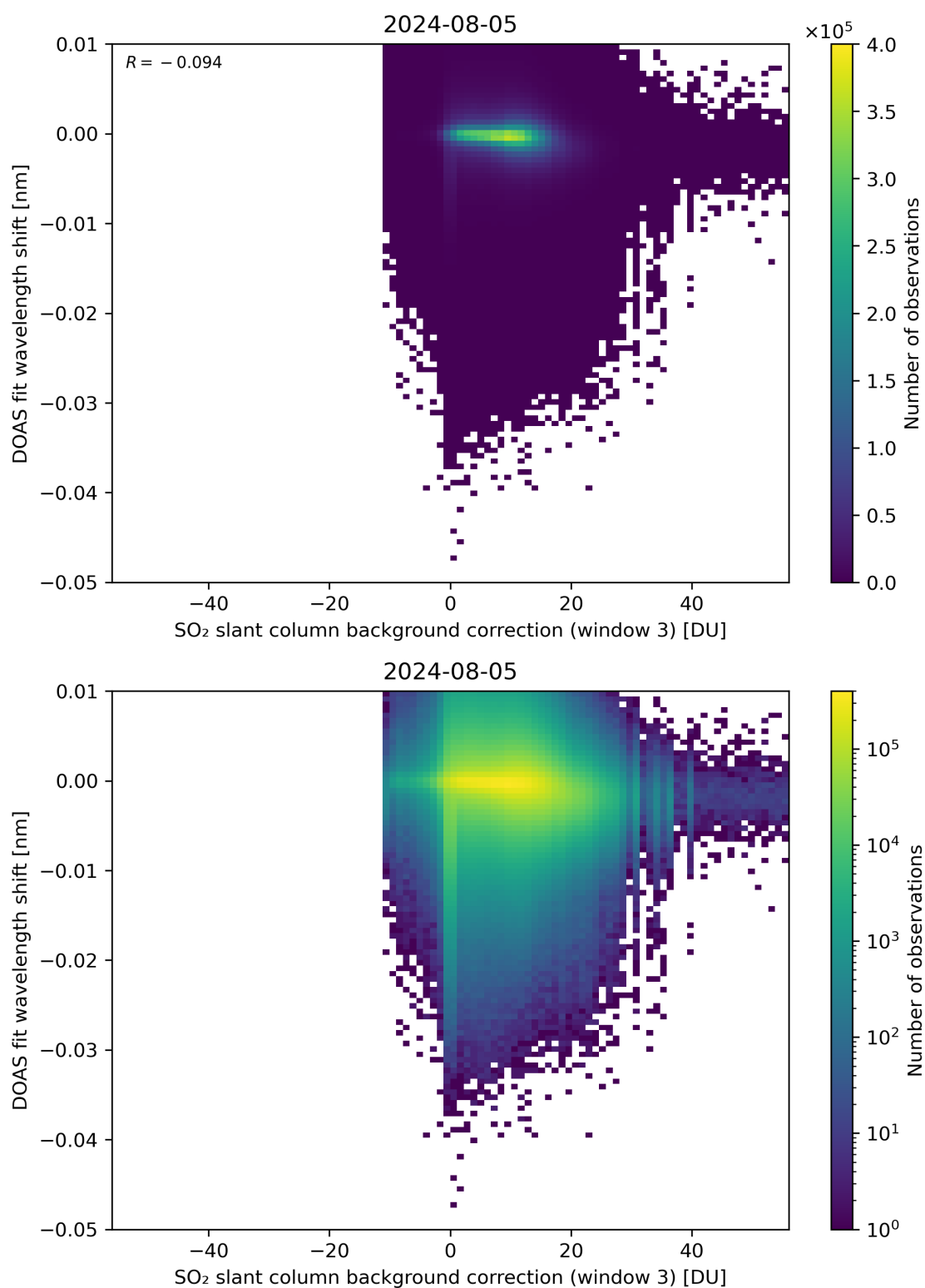
Figure 121: Scatter density plot of “SO 2 slant column background correction (window 3)” against “DOAS fit wavelength shift” for 2024-08-04 to 2024-08-06.
