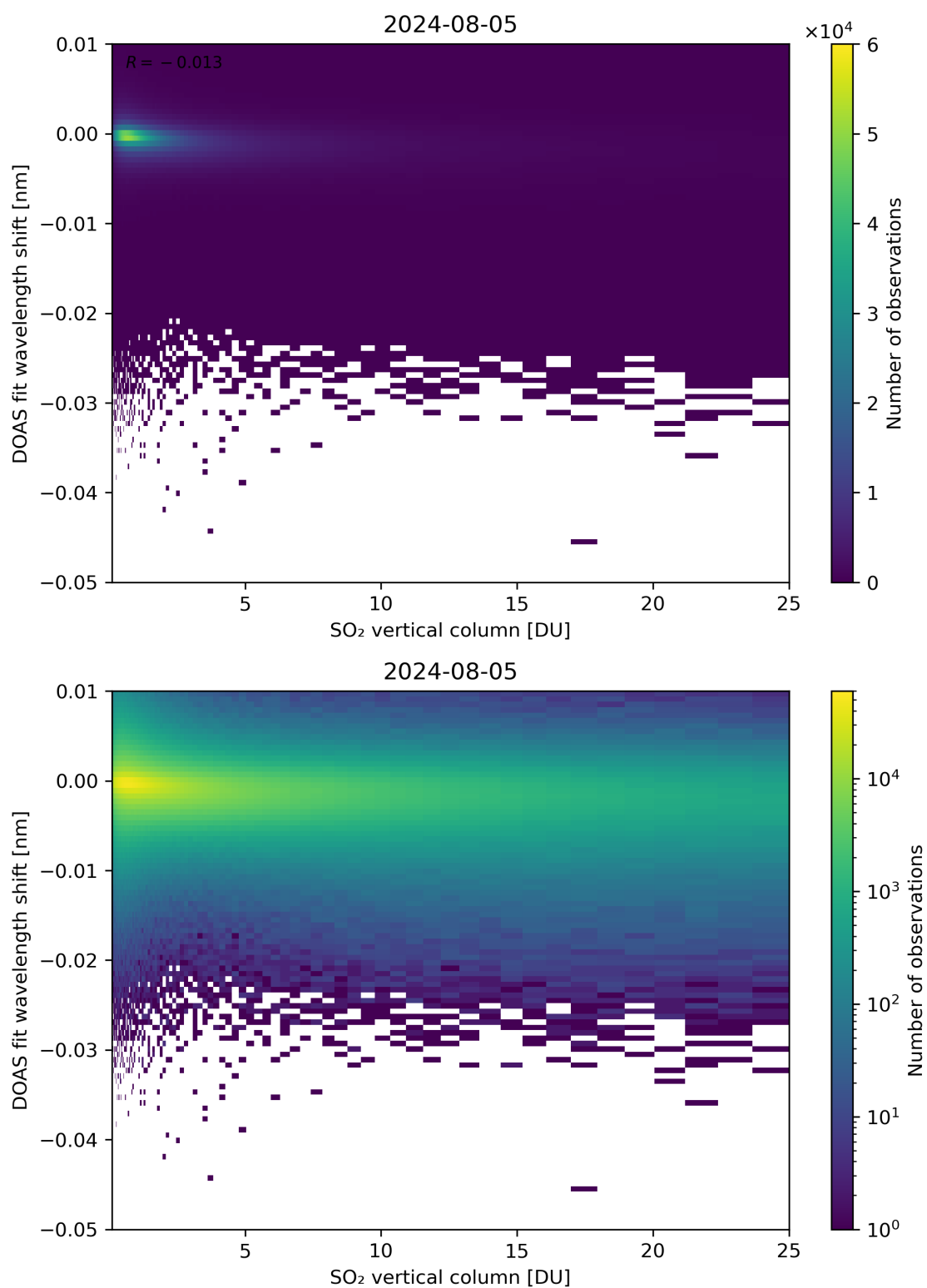
Figure 276: Scatter density plot of “SO 2 vertical column” against “DOAS fit wavelength shift” for 2024-08-04 to 2024-08-06.
