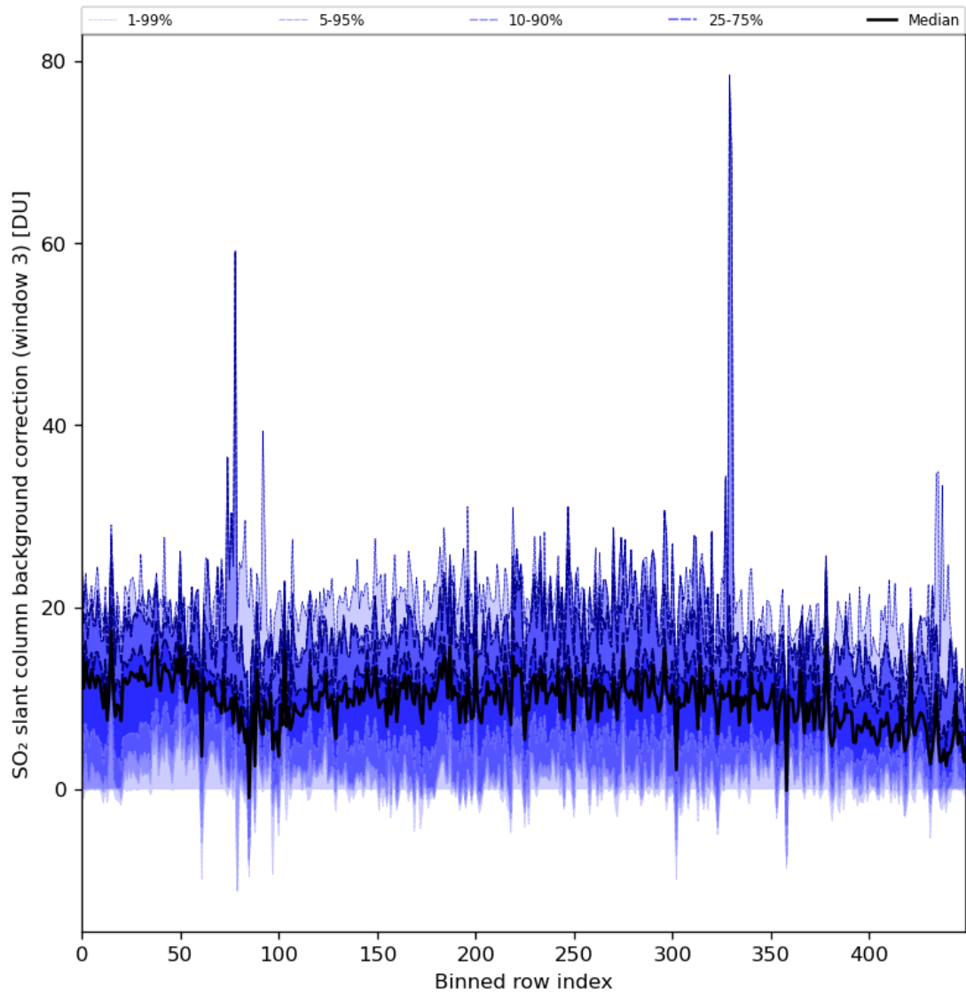
Figure 90: Along track statistics of “SO 2 slant column background correction (window 3)” for 2024-08-04 to 2024-08-06
