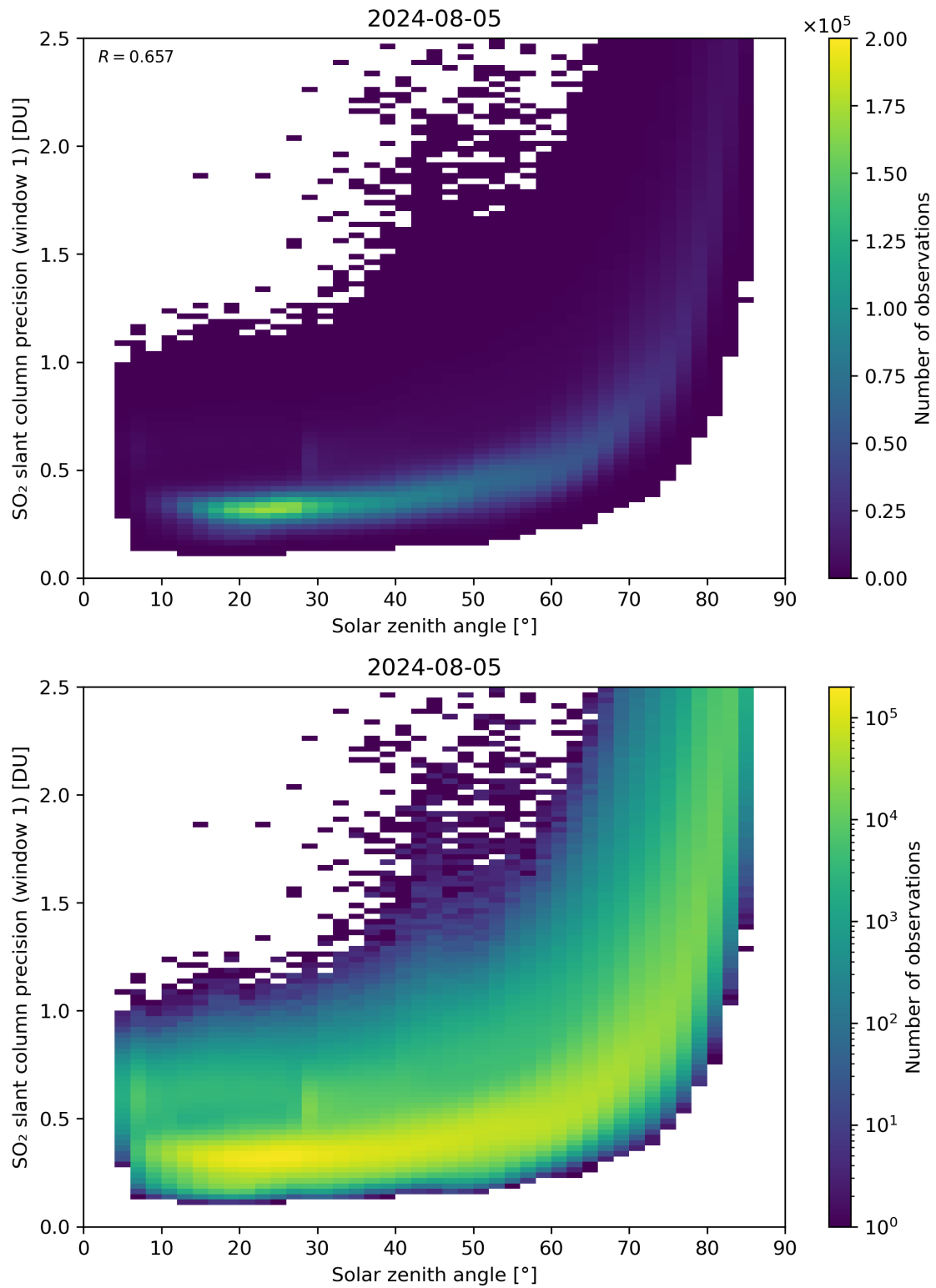
Figure 170: Scatter density plot of “Solar zenith angle” against “SO 2 slant column precision (window 1)” for 2024-08-04 to 2024-08-06.
