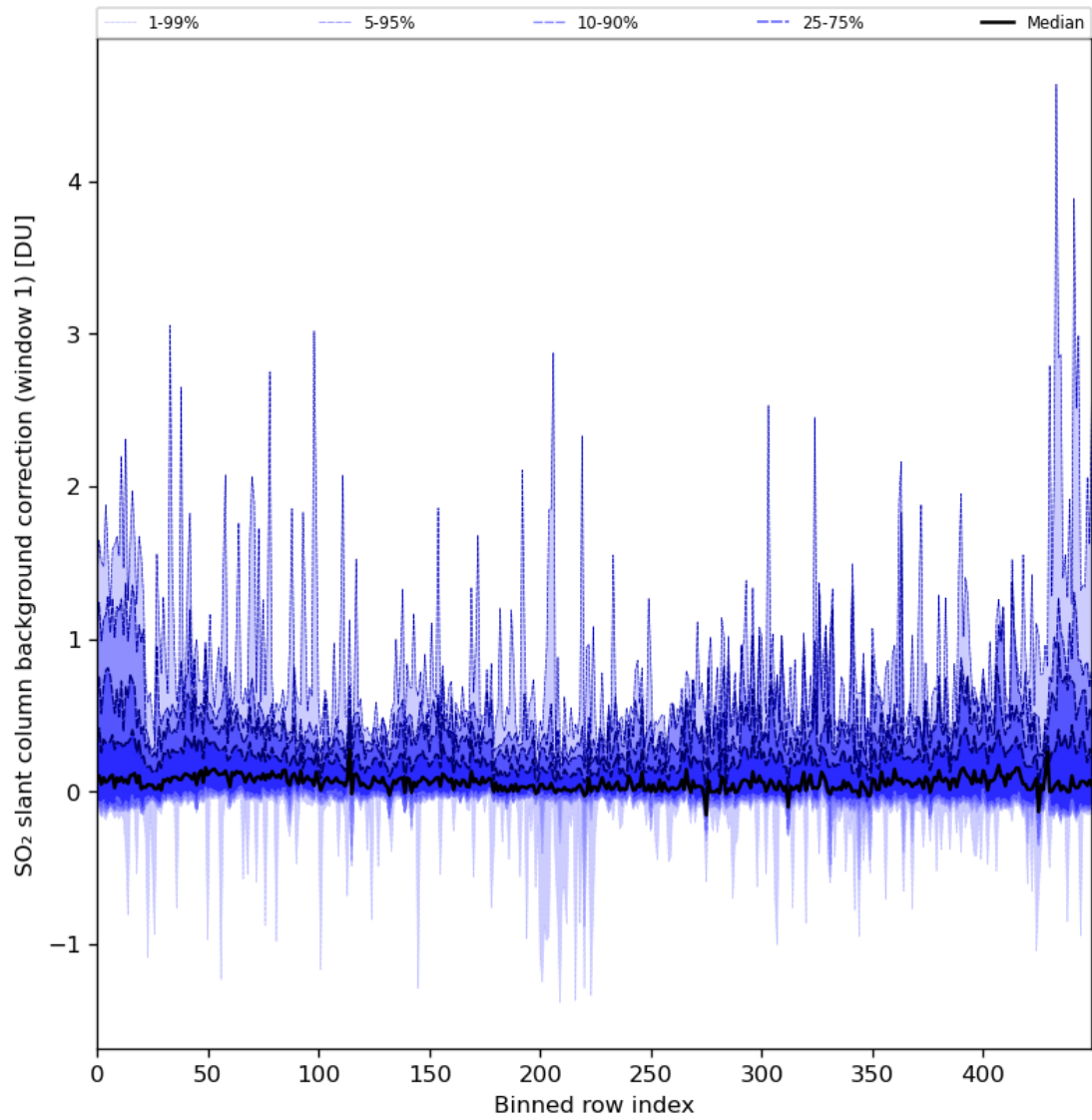
Figure 82: Along track statistics of “SO 2 slant column background correction (window 1)” for 2024-08-04 to 2024-08-06
