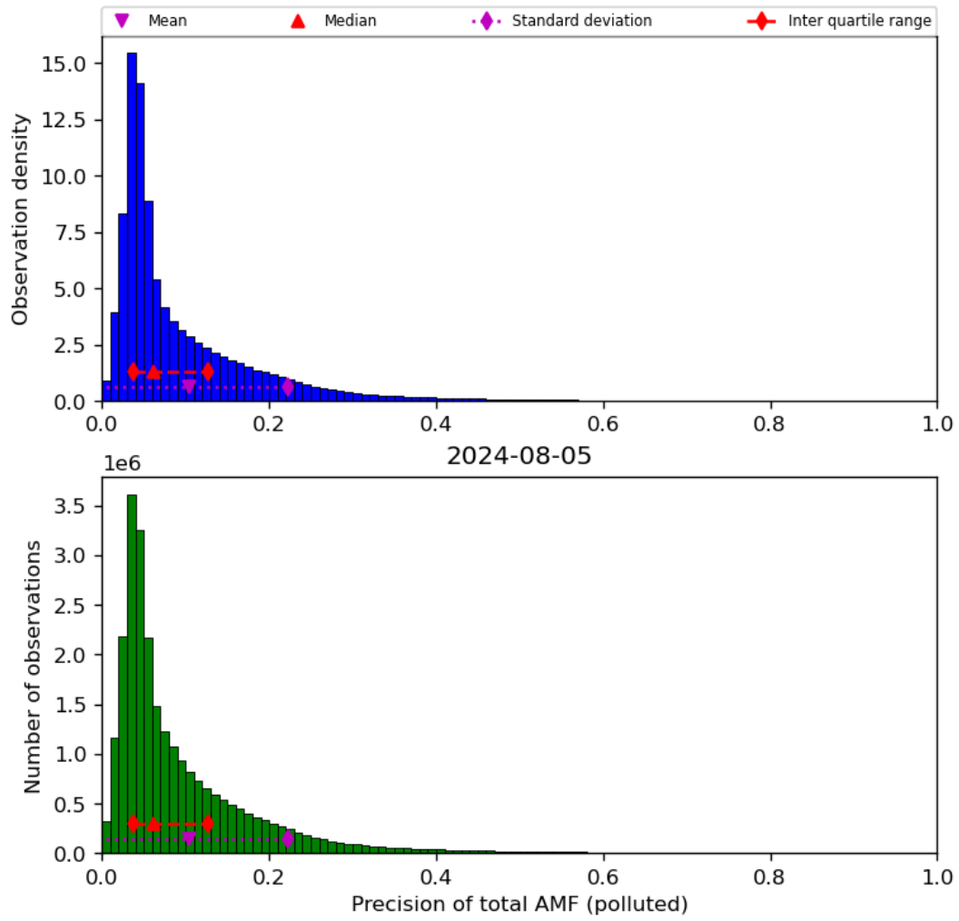
Figure 72: Histogram of “Precision of total AMF (polluted)” for 2024-08-04 to 2024-08-06
