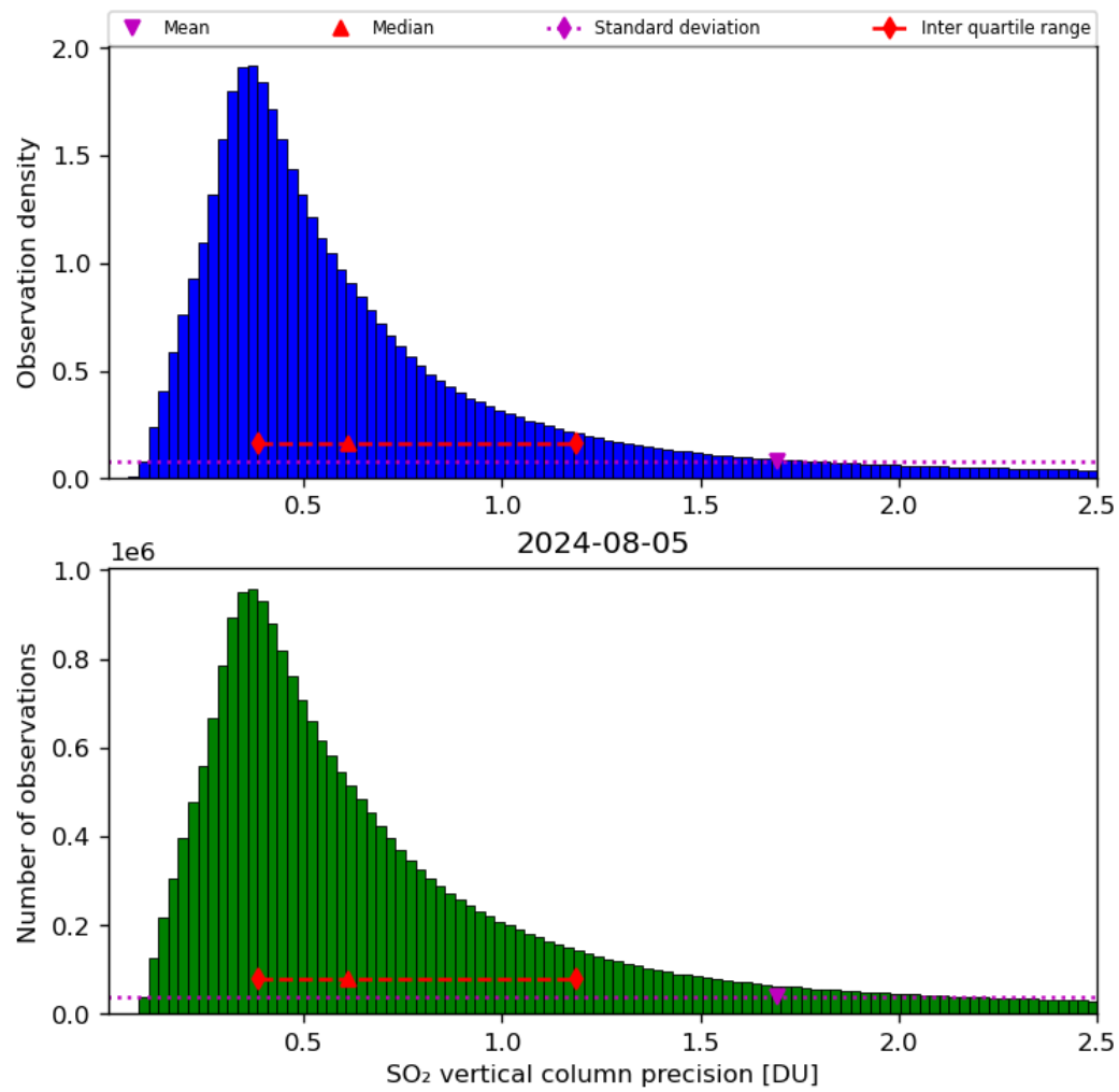
Figure 54: Histogram of “SO 2 vertical column precision” for 2024-08-04 to 2024-08-06
