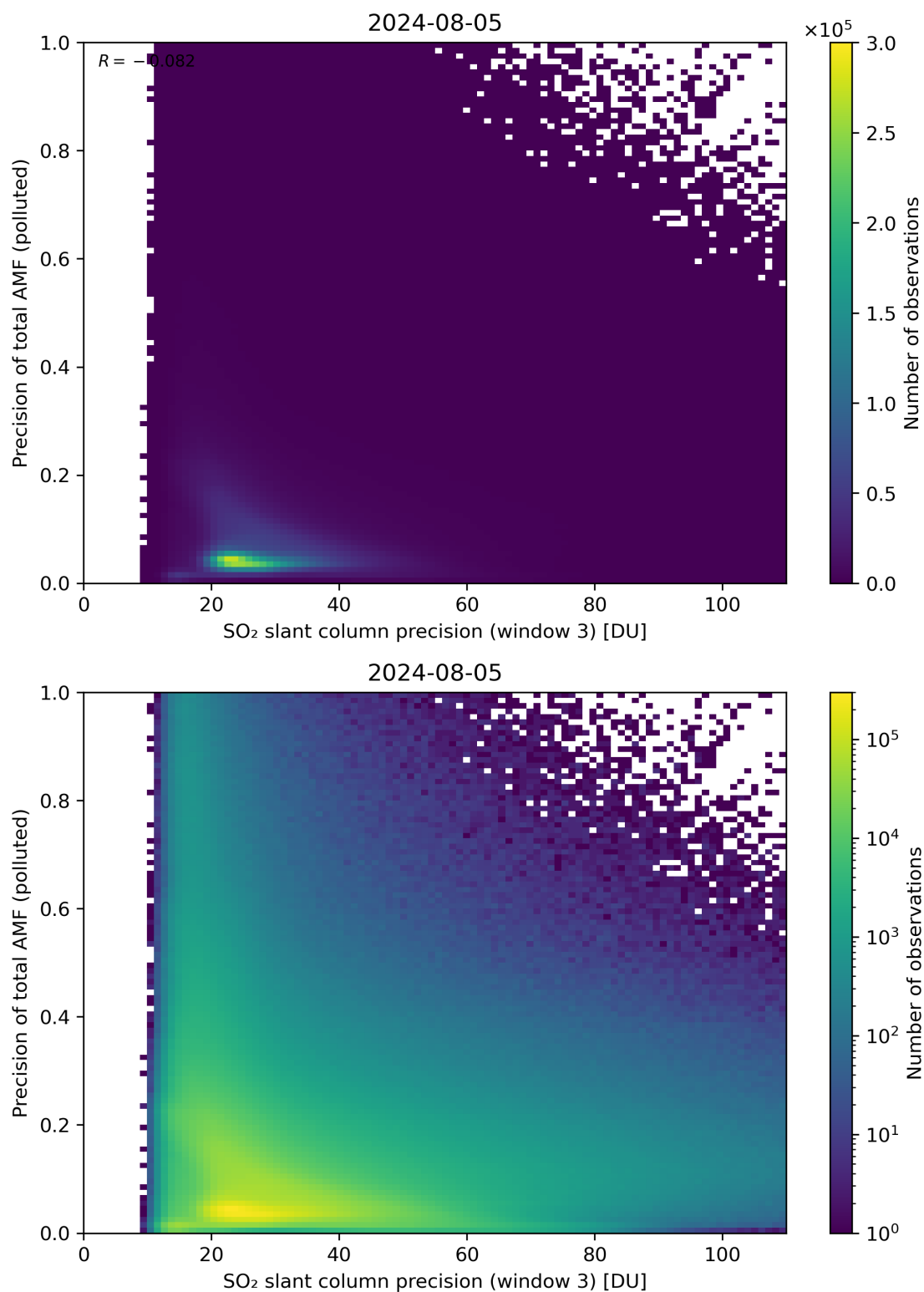
Figure 264: Scatter density plot of “SO 2 slant column precision (window 3)” against “Precision of total AMF (polluted)” for 2024-08-04 to 2024-08-06.
