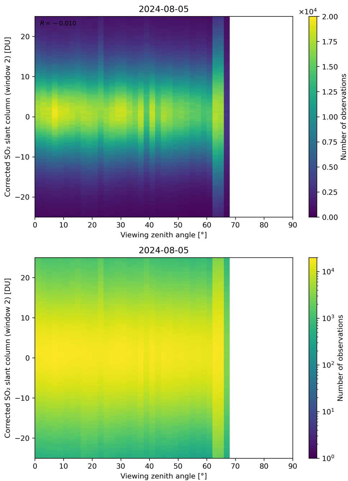
Figure 318: Scatter density plot of “Viewing zenith angle” against “Corrected SO 2 slant column (window 2)” for 2024-08-04 to 2024-08-06.
