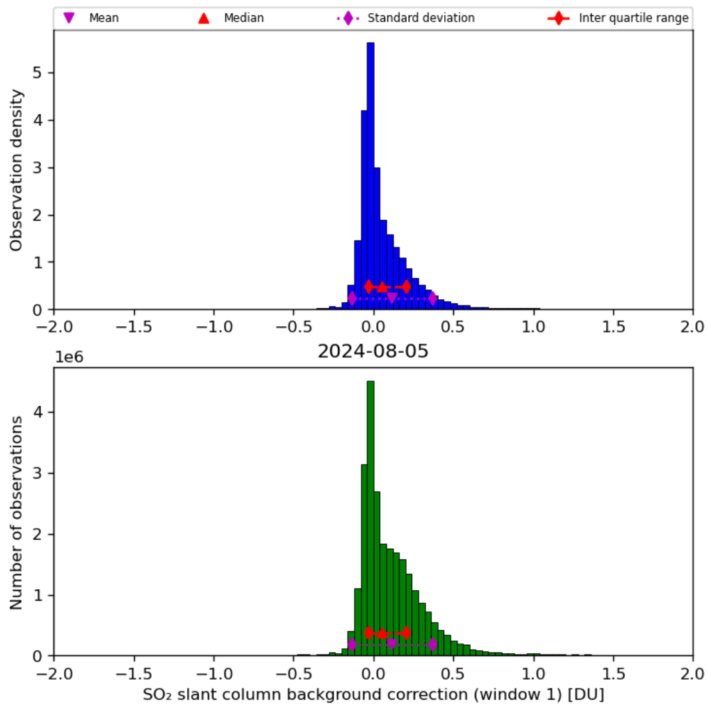
Figure 59: Histogram of “SO 2 slant column background correction (window 1)” for 2024-08-04 to 2024-08-06
