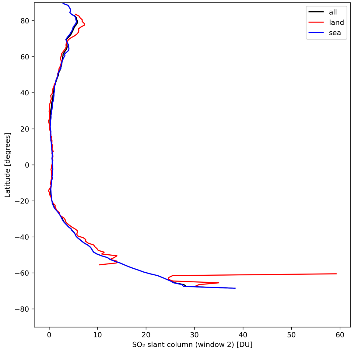
Figure 37: Zonal average of “SO 2 slant column (window 2)” for 2024-08-04 to 2024-08-06.
