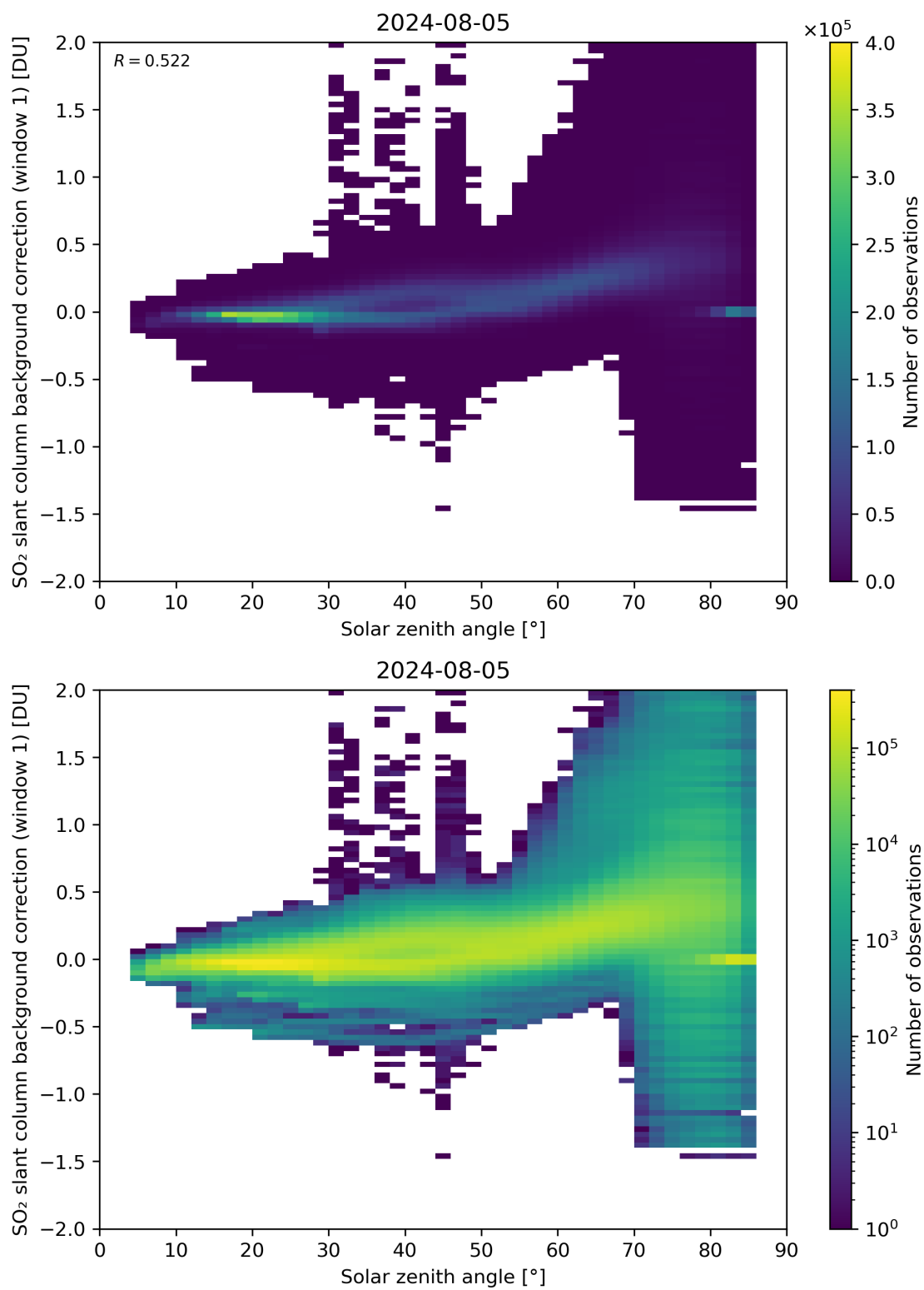
Figure 158: Scatter density plot of “Solar zenith angle” against “SO 2 slant column background correction (window 1)” for 2024-08-04 to 2024-08-06.
