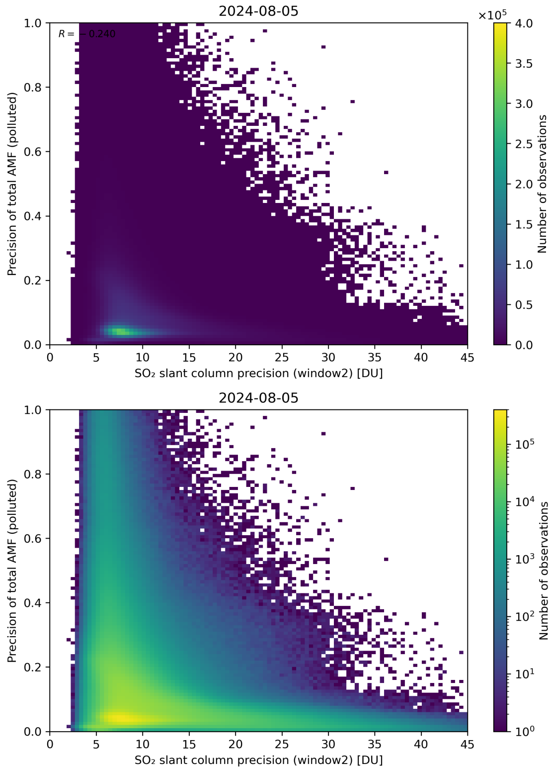
Figure 252: Scatter density plot of “SO 2 slant column precision (window2)” against “Precision of total AMF (polluted)” for 2024-08-04 to 2024-08-06.
