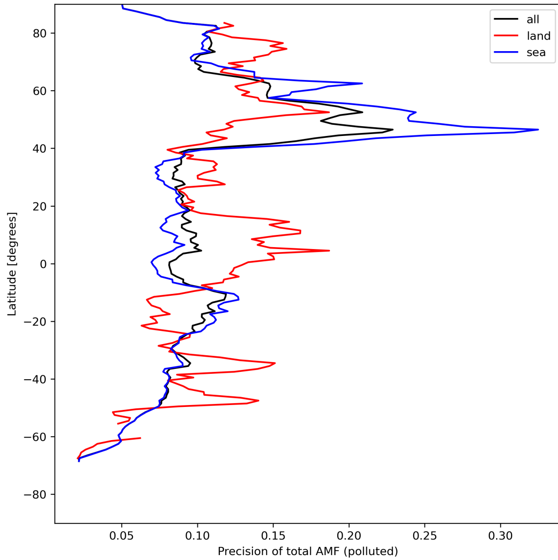
Figure 49: Zonal average of “Precision of total AMF (polluted)” for 2024-08-04 to 2024-08-06.
