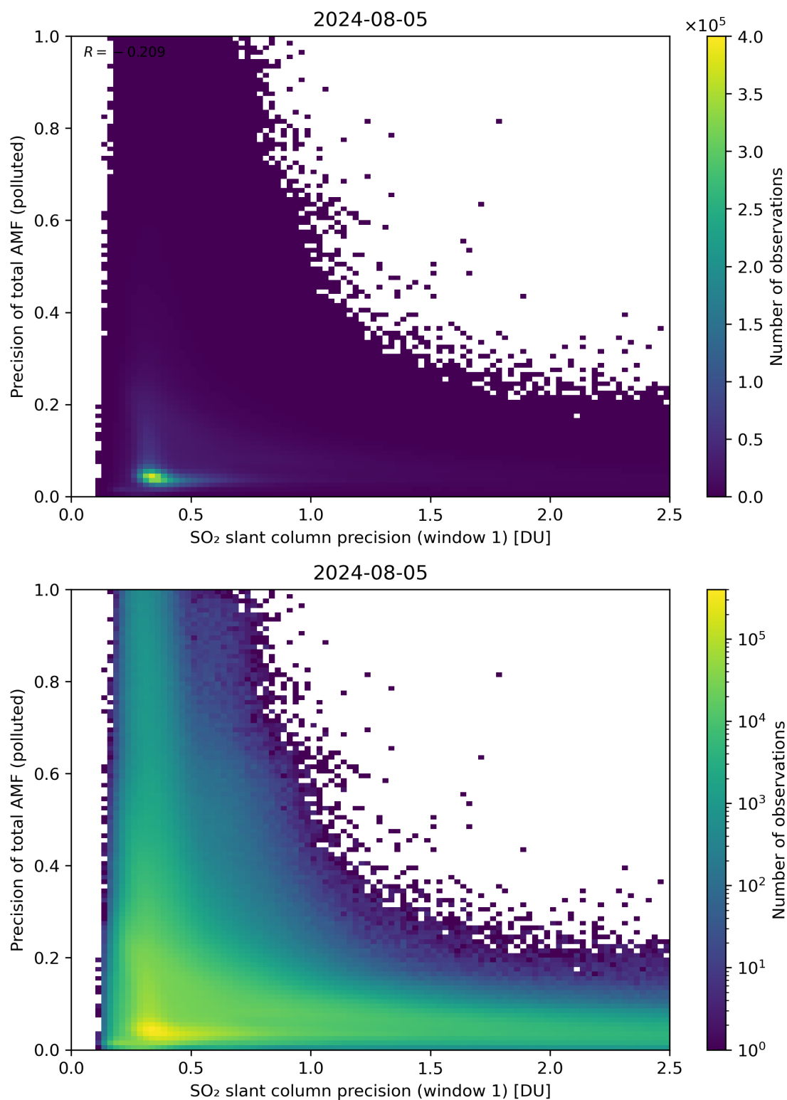
Figure 231: Scatter density plot of “SO 2 slant column precision (window 1)” against “Precision of total AMF (polluted)” for 2024-08-04 to 2024-08-06.
