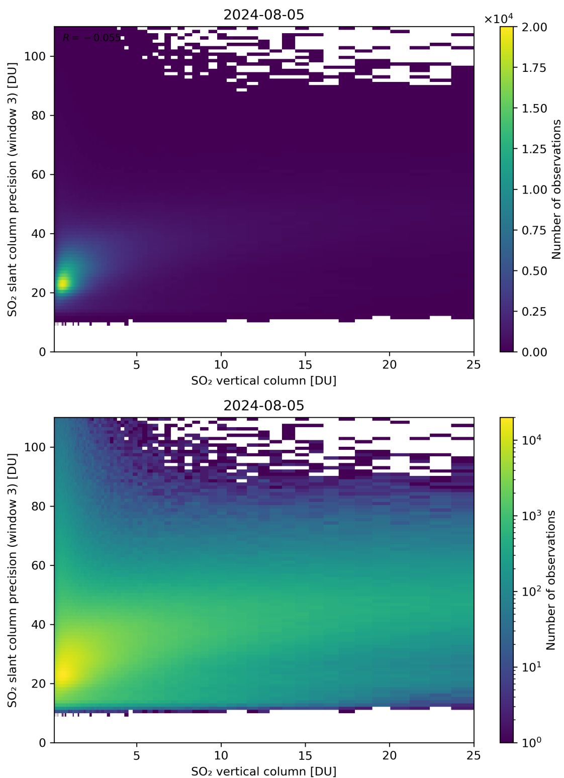
Figure 304: Scatter density plot of “SO 2 vertical column” against “SO 2 slant column precision (window 3)” for 2024-08-04 to 2024-08-06.
