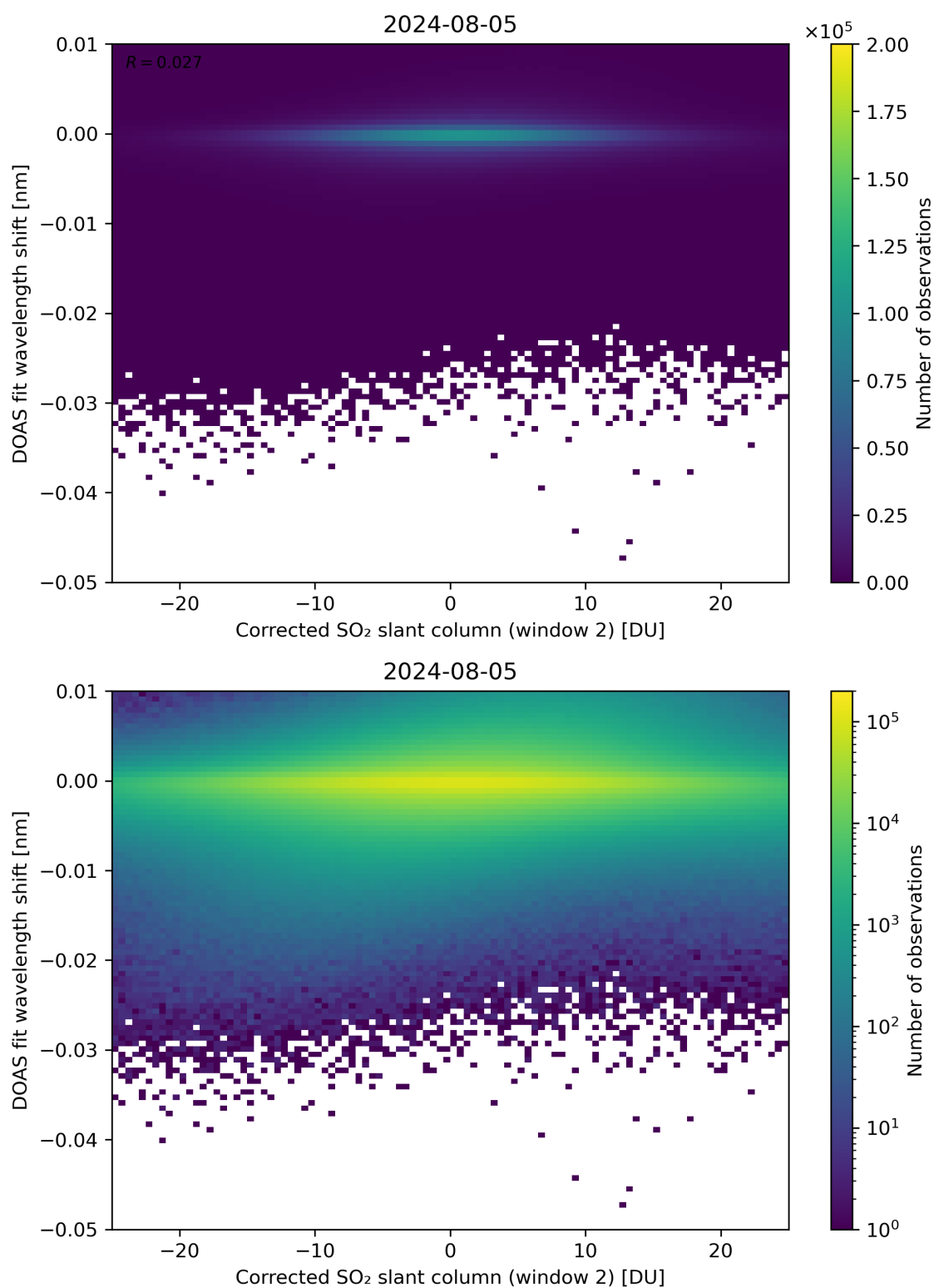
Figure 196: Scatter density plot of “Corrected SO 2 slant column (window 2)” against “DOAS fit wavelength shift” for 2024-08-04 to 2024-08-06.
