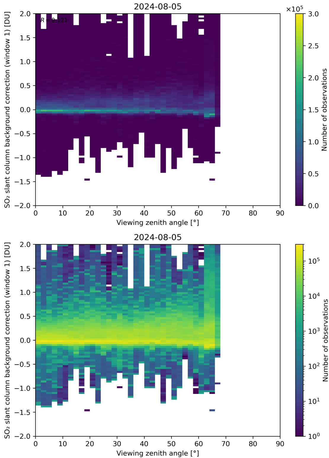
Figure 308: Scatter density plot of “Viewing zenith angle” against “SO 2 slant column background correction (window 1)” for 2024-08-04 to 2024-08-06.
