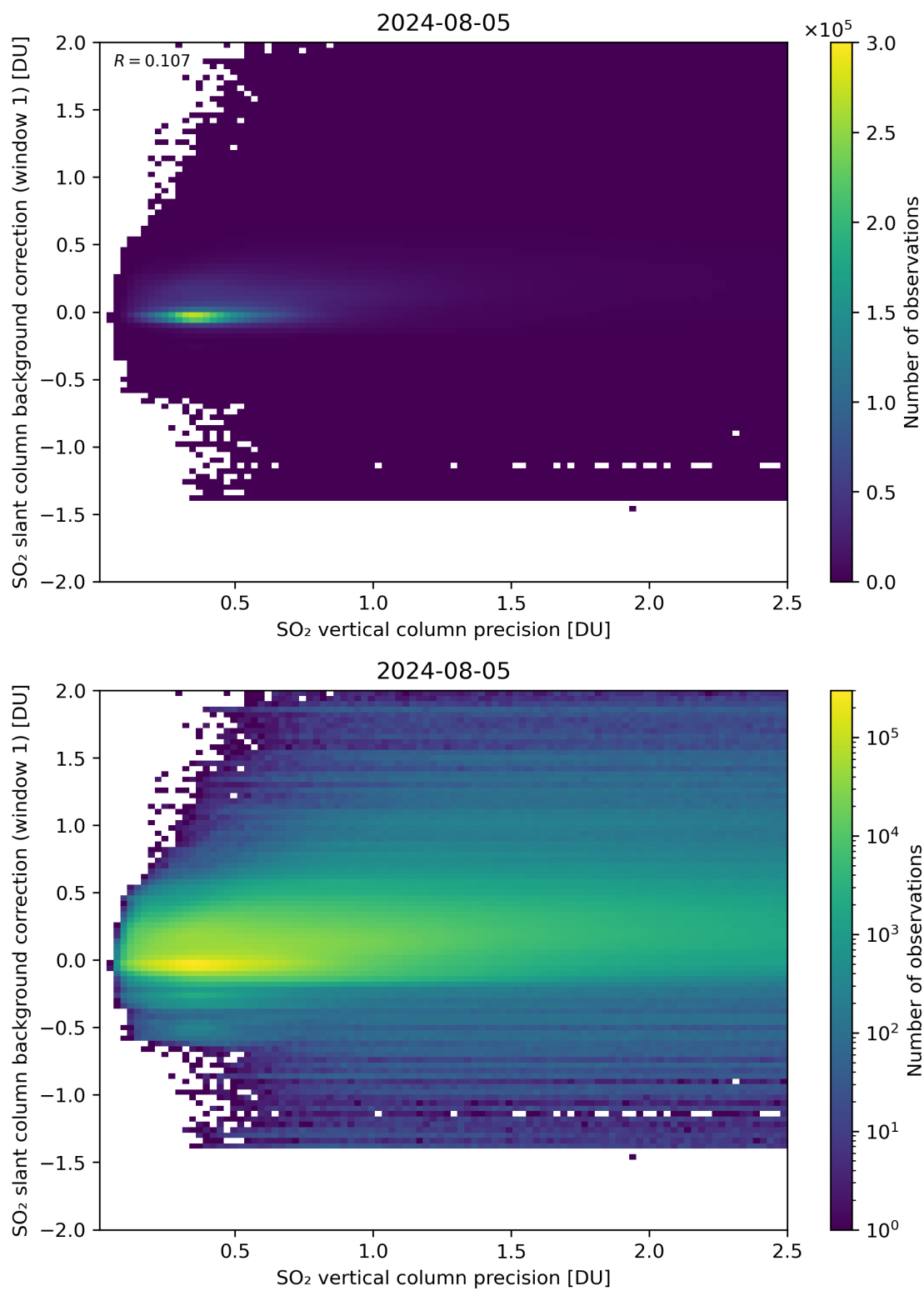
Figure 279: Scatter density plot of “SO 2 vertical column precision” against “SO 2 slant column background correction (window 1)” for 2024-08-04 to 2024-08-06.
