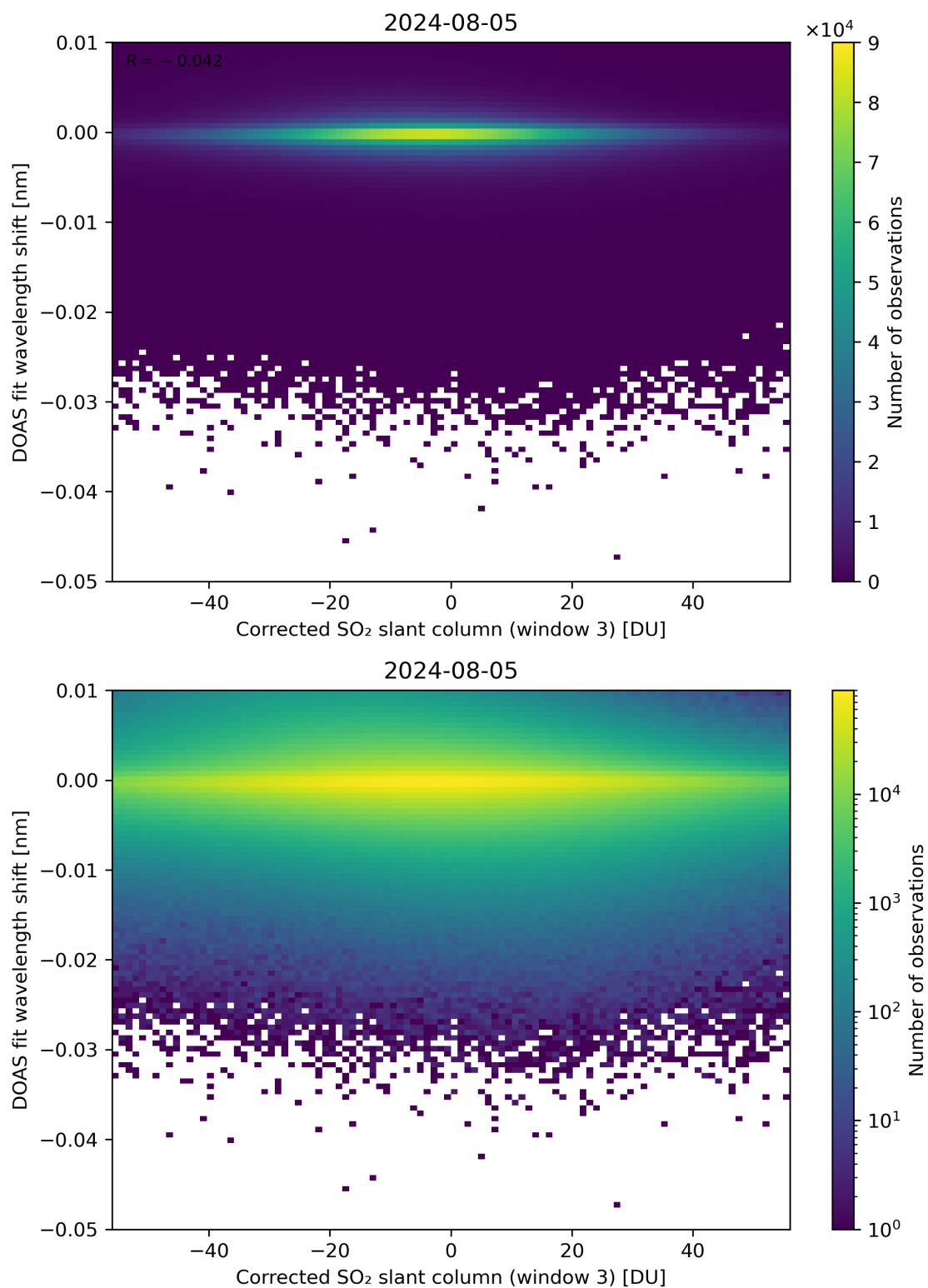
Figure 206: Scatter density plot of “Corrected SO 2 slant column (window 3)” against “DOAS fit wavelength shift” for 2024-08-04 to 2024-08-06.
