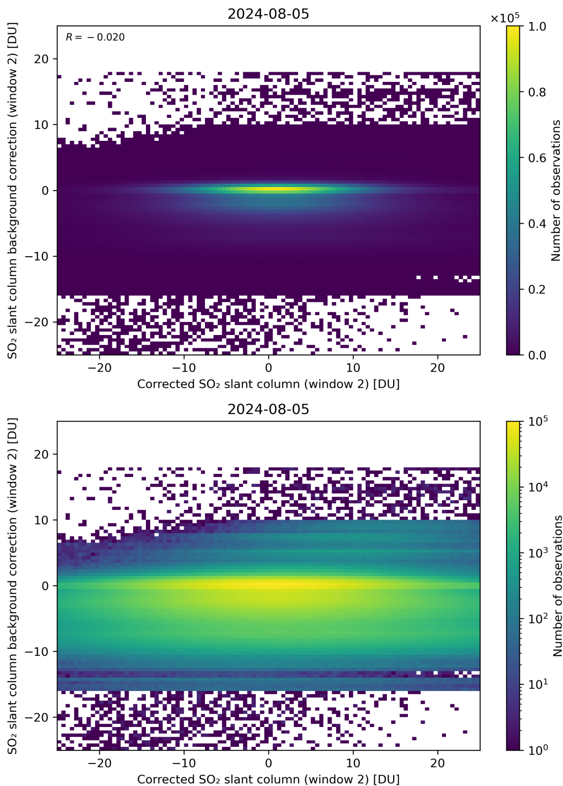
Figure 194: Scatter density plot of “Corrected SO 2 slant column (window 2)” against “SO 2 slant column background correction (window 2)” for 2024-08-04 to 2024-08-06.
