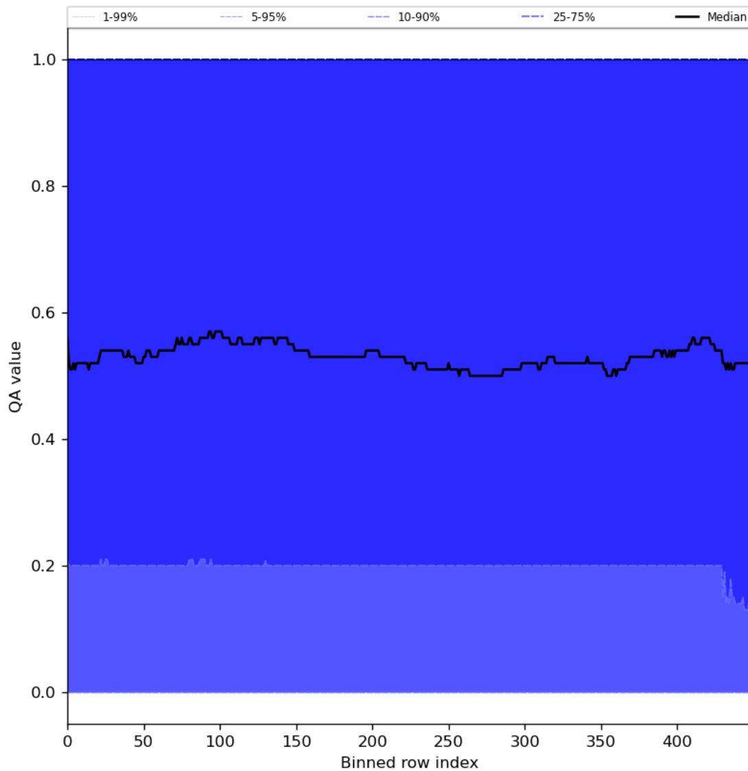
Figure 75: Along track statistics of “QA value” for 2024-08-04 to 2024-08-06
