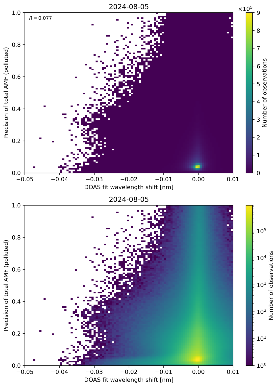
Figure 131: Scatter density plot of “DOAS fit wavelength shift” against “Precision of total AMF (polluted)” for 2024-08-04 to 2024-08-06.
