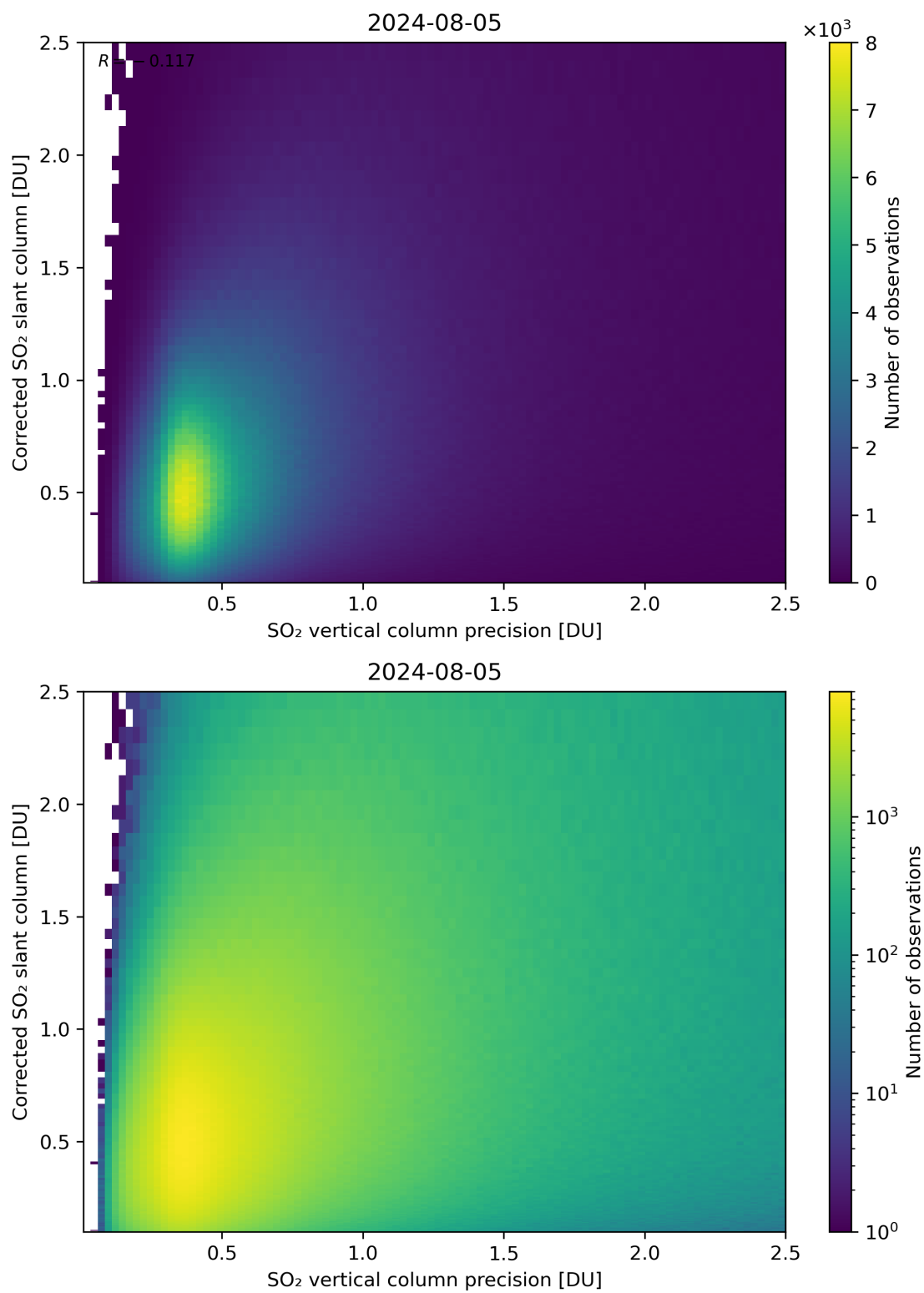
Figure 286: Scatter density plot of “SO 2 vertical column precision” against “Corrected SO 2 slant column” for 2024-08-04 to 2024-08-06.
