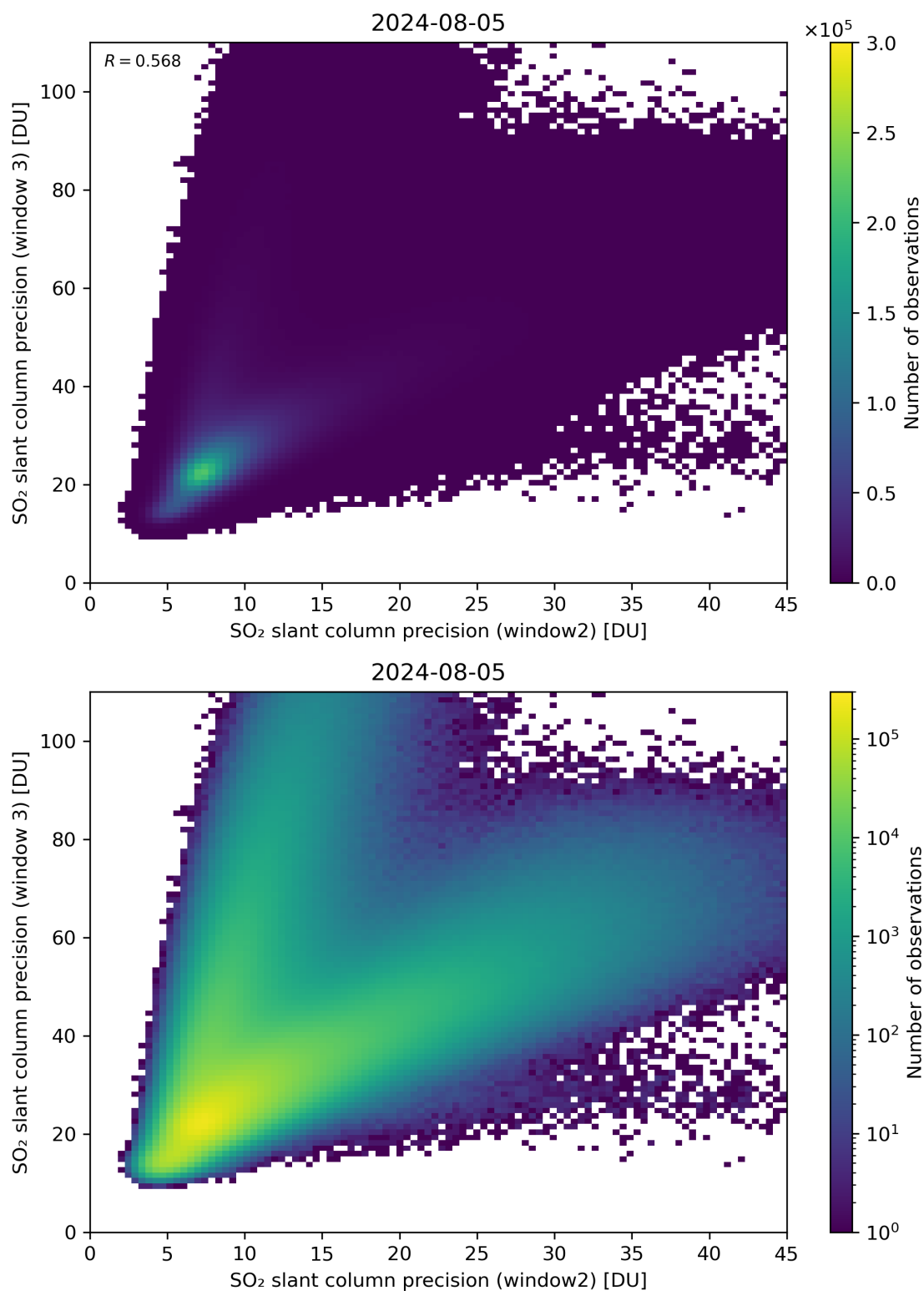
Figure 250: Scatter density plot of “SO 2 slant column precision (window2)” against “SO 2 slant column precision (window 3)” for 2024-08-04 to 2024-08-06.
