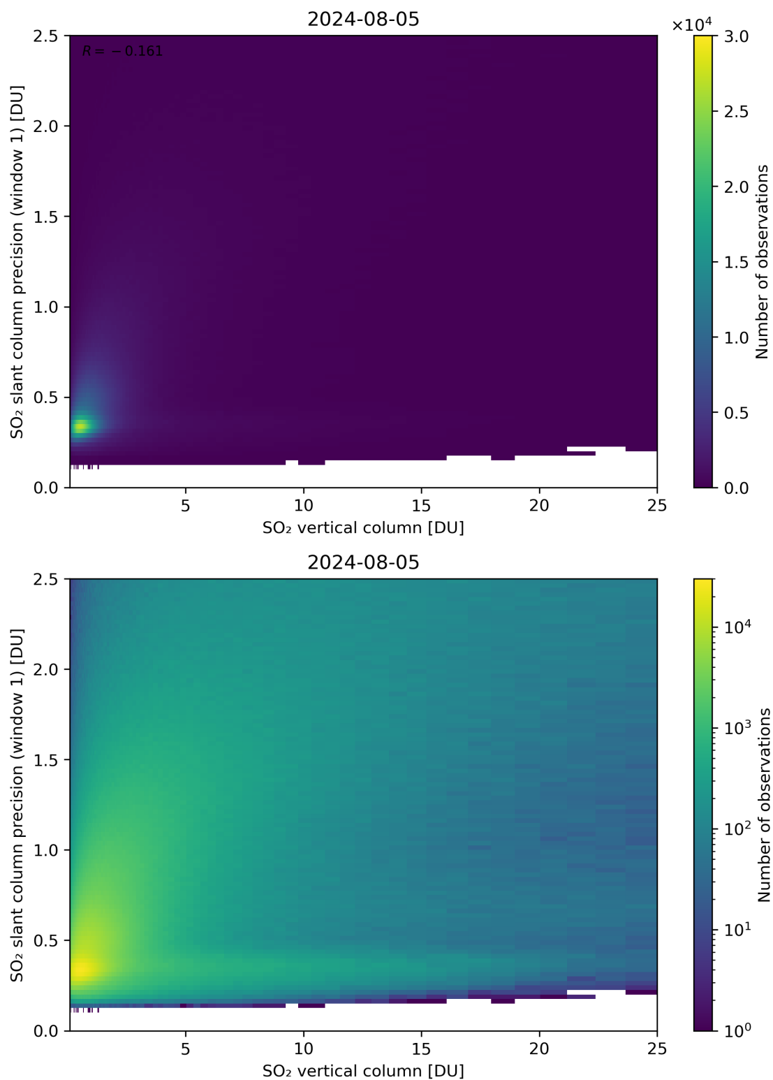
Figure 301: Scatter density plot of “SO 2 vertical column” against “SO 2 slant column precision (window 1)” for 2024-08-04 to 2024-08-06.
