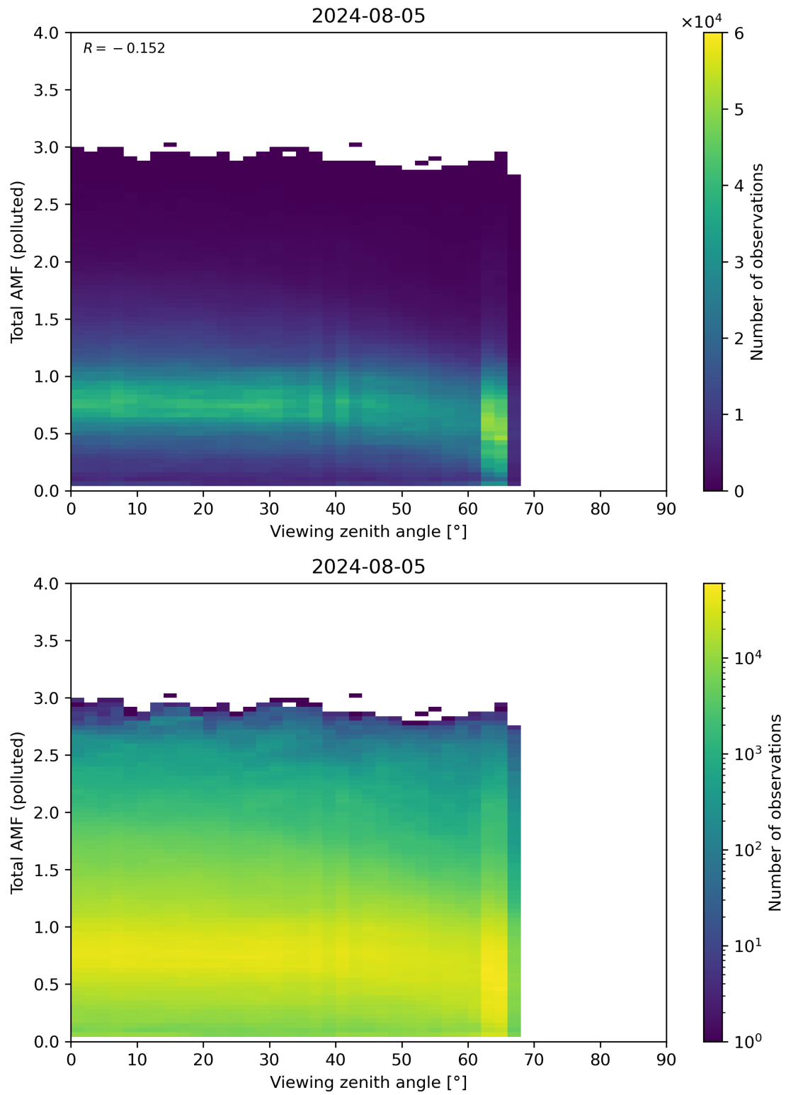
Figure 325: Scatter density plot of “Viewing zenith angle” against “Total AMF (polluted)” for 2024-08-04 to 2024-08-06.
