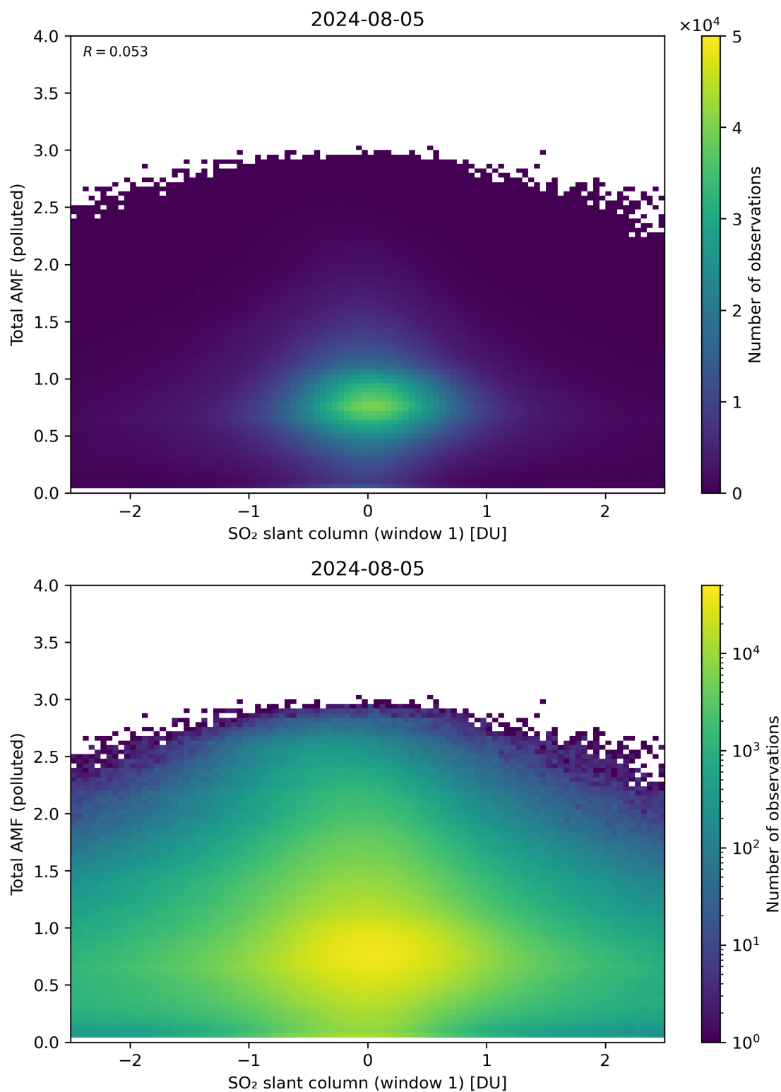
Figure 239: Scatter density plot of “SO 2 slant column (window 1)” against “Total AMF (polluted)” for 2024-08-04 to 2024-08-06.
