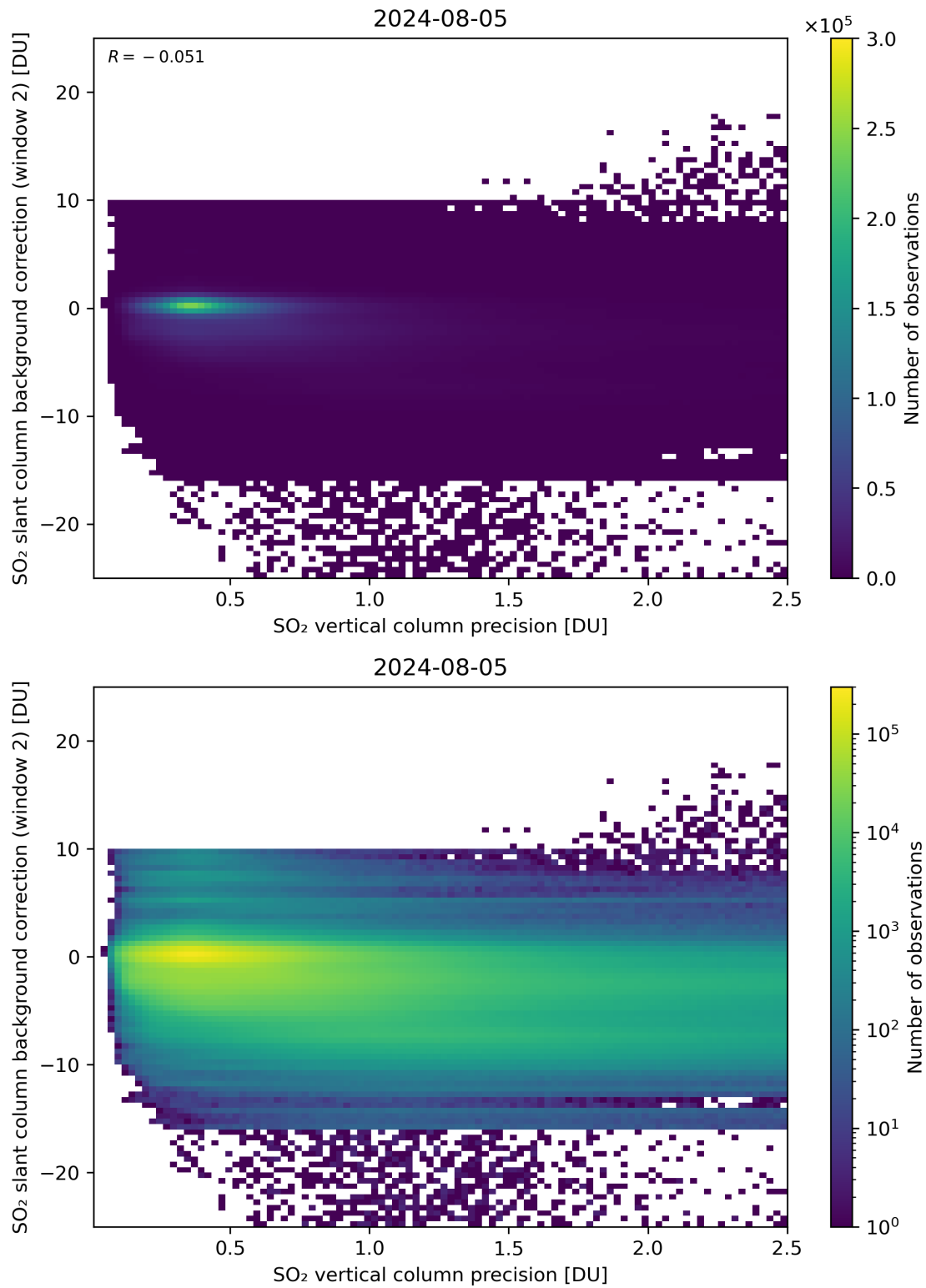
Figure 280: Scatter density plot of “SO 2 vertical column precision” against “SO 2 slant column background correction (window 2)” for 2024-08-04 to 2024-08-06.
