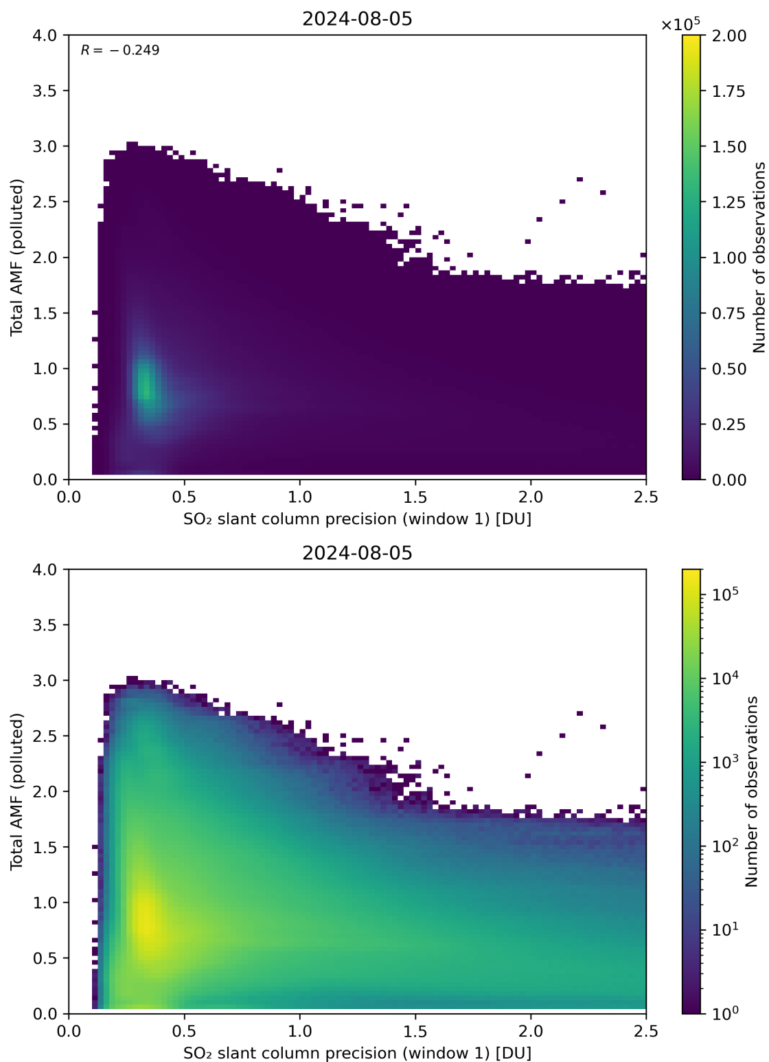
Figure 230: Scatter density plot of “SO 2 slant column precision (window 1)” against “Total AMF (polluted)” for 2024-08-04 to 2024-08-06.
