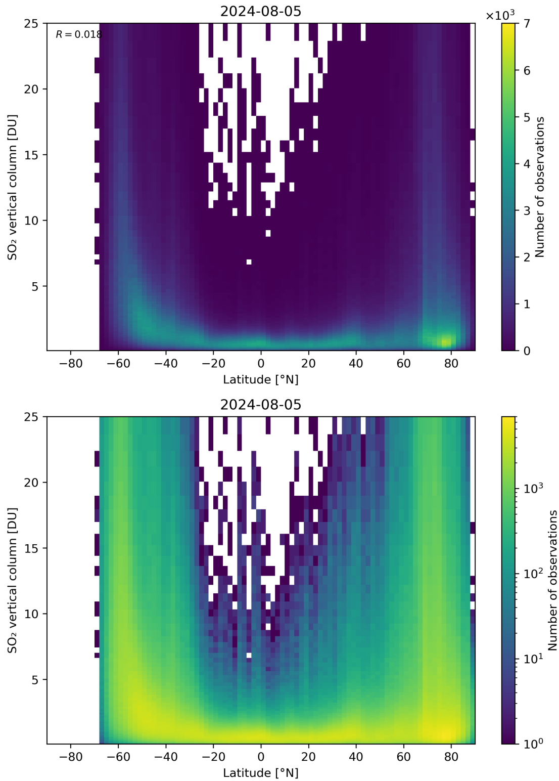
Figure 156: Scatter density plot of “Latitude” against “SO 2 vertical column” for 2024-08-04 to 2024-08-06.
