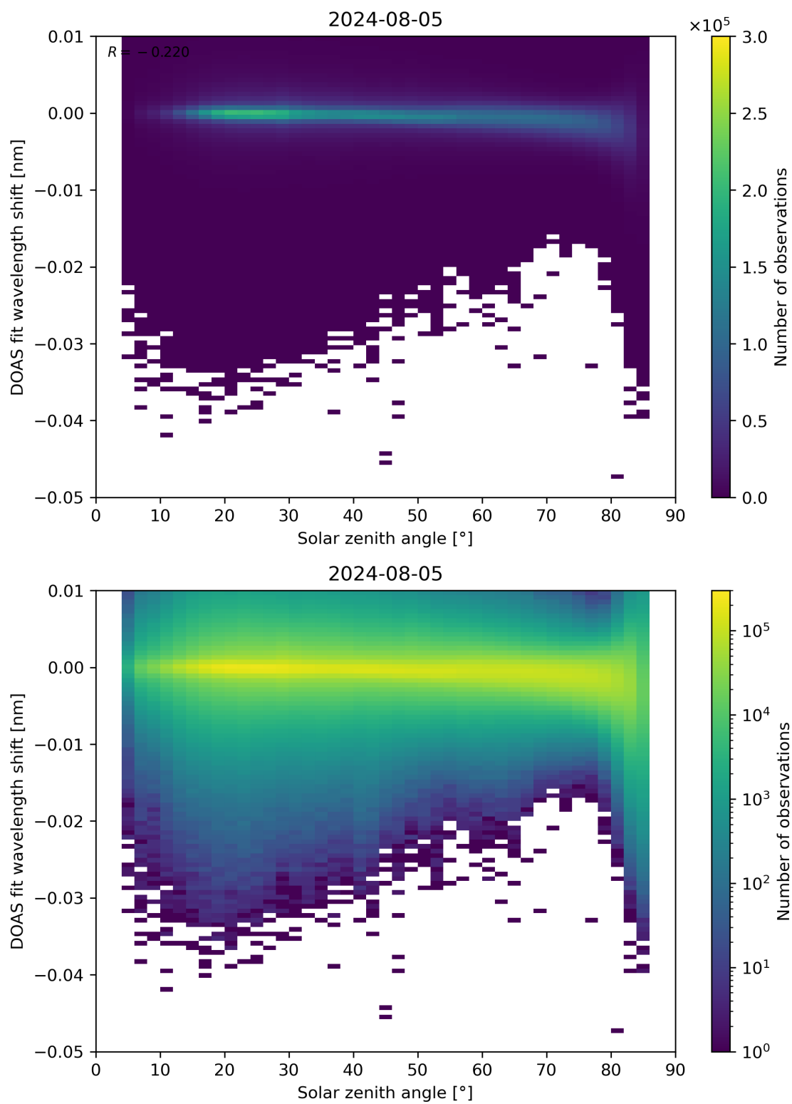
Figure 161: Scatter density plot of “Solar zenith angle” against “DOAS fit wavelength shift” for 2024-08-04 to 2024-08-06.
