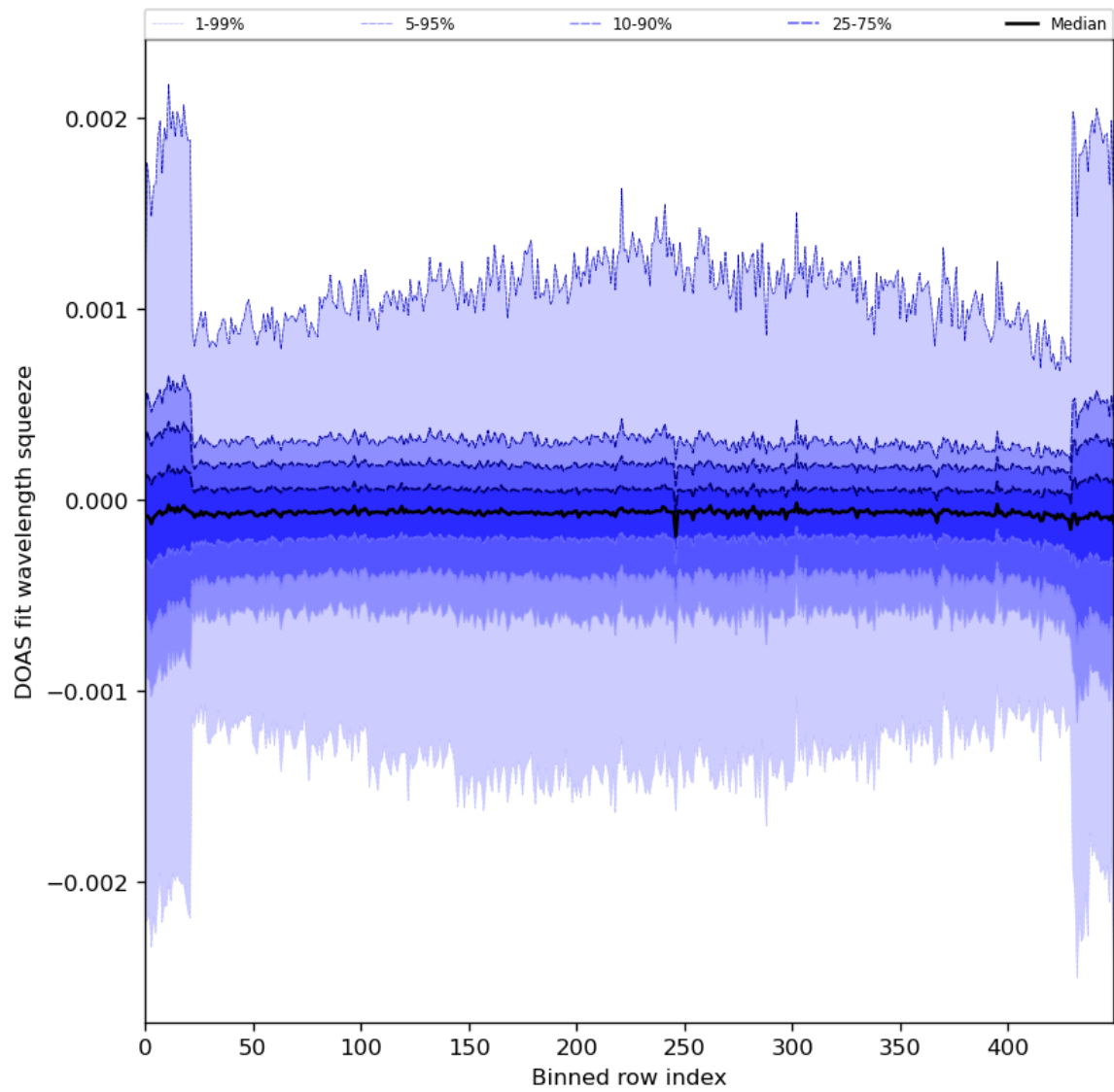
Figure 92: Along track statistics of “DOAS fit wavelength squeeze” for 2024-08-04 to 2024-08-06
