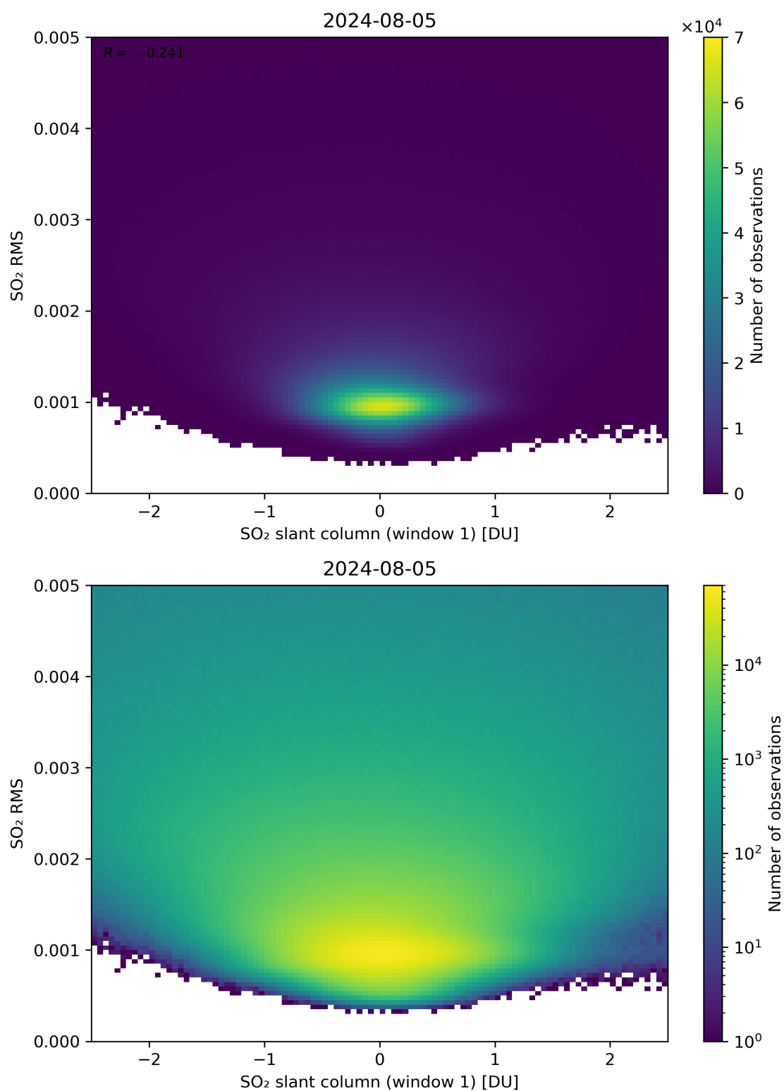
Figure 217: Scatter density plot of “SO 2 slant column (window 1)” against “SO 2 RMS” for 2024-08-04 to 2024-08-06.
