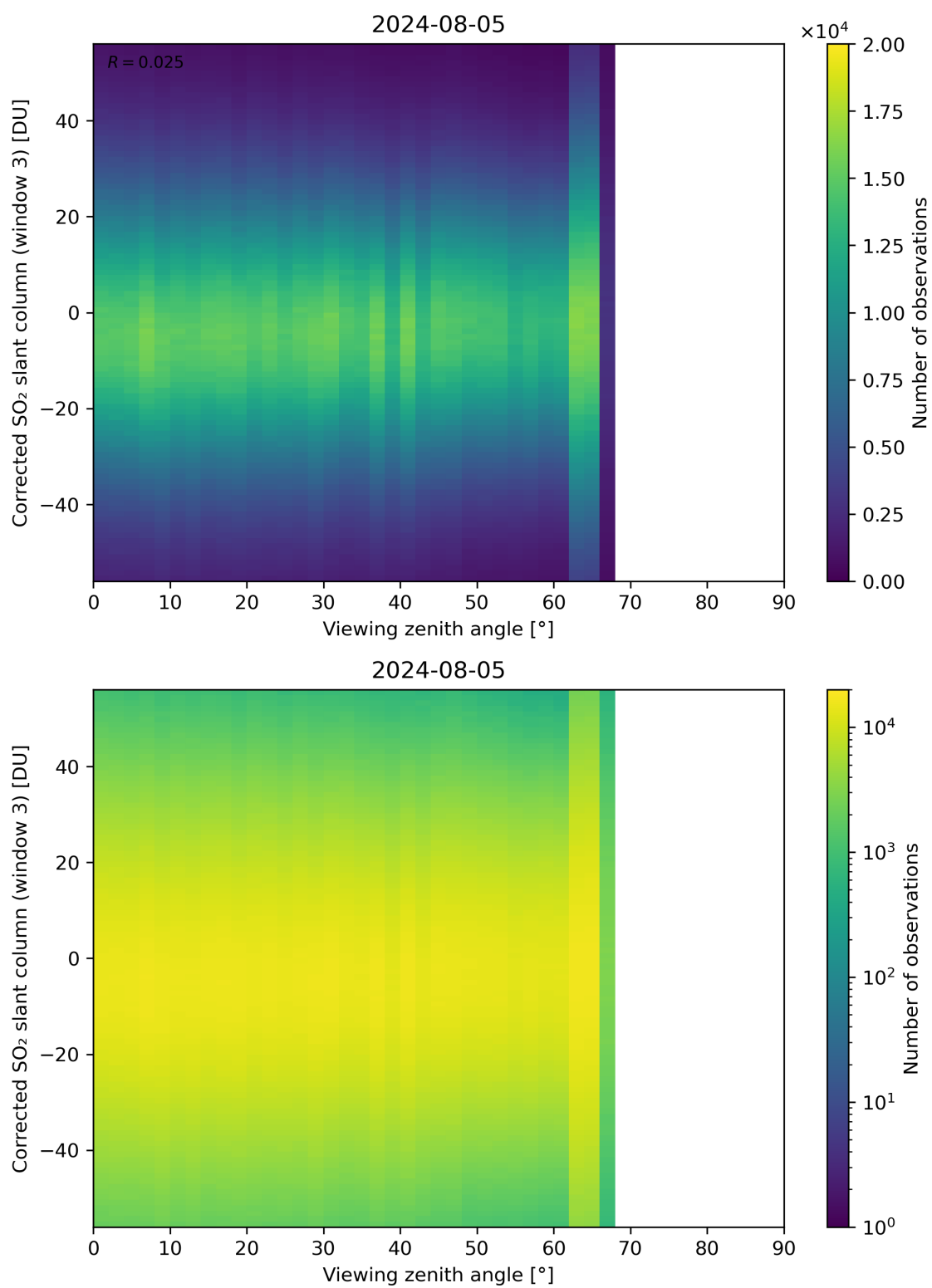
Figure 319: Scatter density plot of “Viewing zenith angle” against “Corrected SO 2 slant column (window 3)” for 2024-08-04 to 2024-08-06.
