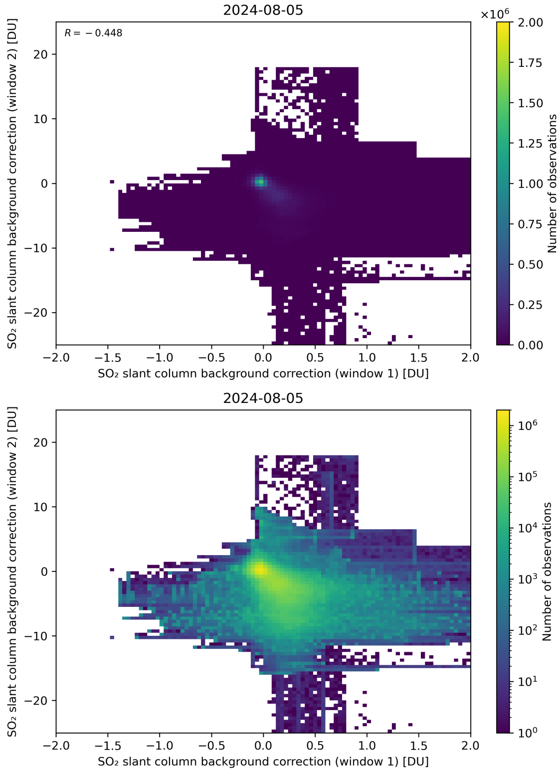
Figure 98: Scatter density plot of “SO 2 slant column background correction (window 1)” against “SO 2 slant column background correction (window 2)” for 2024-08-04 to 2024-08-06.
