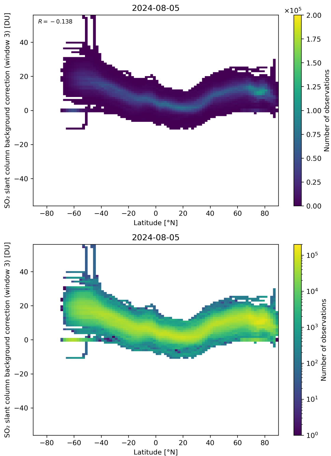
Figure 141: Scatter density plot of “Latitude” against “SO 2 slant column background correction (window 3)” for 2024-08-04 to 2024-08-06.
