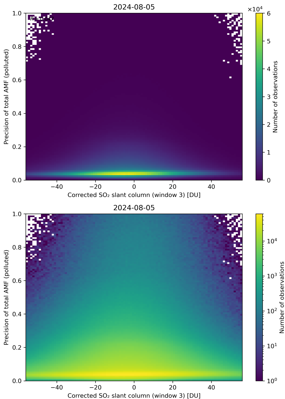
Figure 211: Scatter density plot of “Corrected SO 2 slant column (window 3)” against “Precision of total AMF (polluted)” for 2024-08-04 to 2024-08-06.
