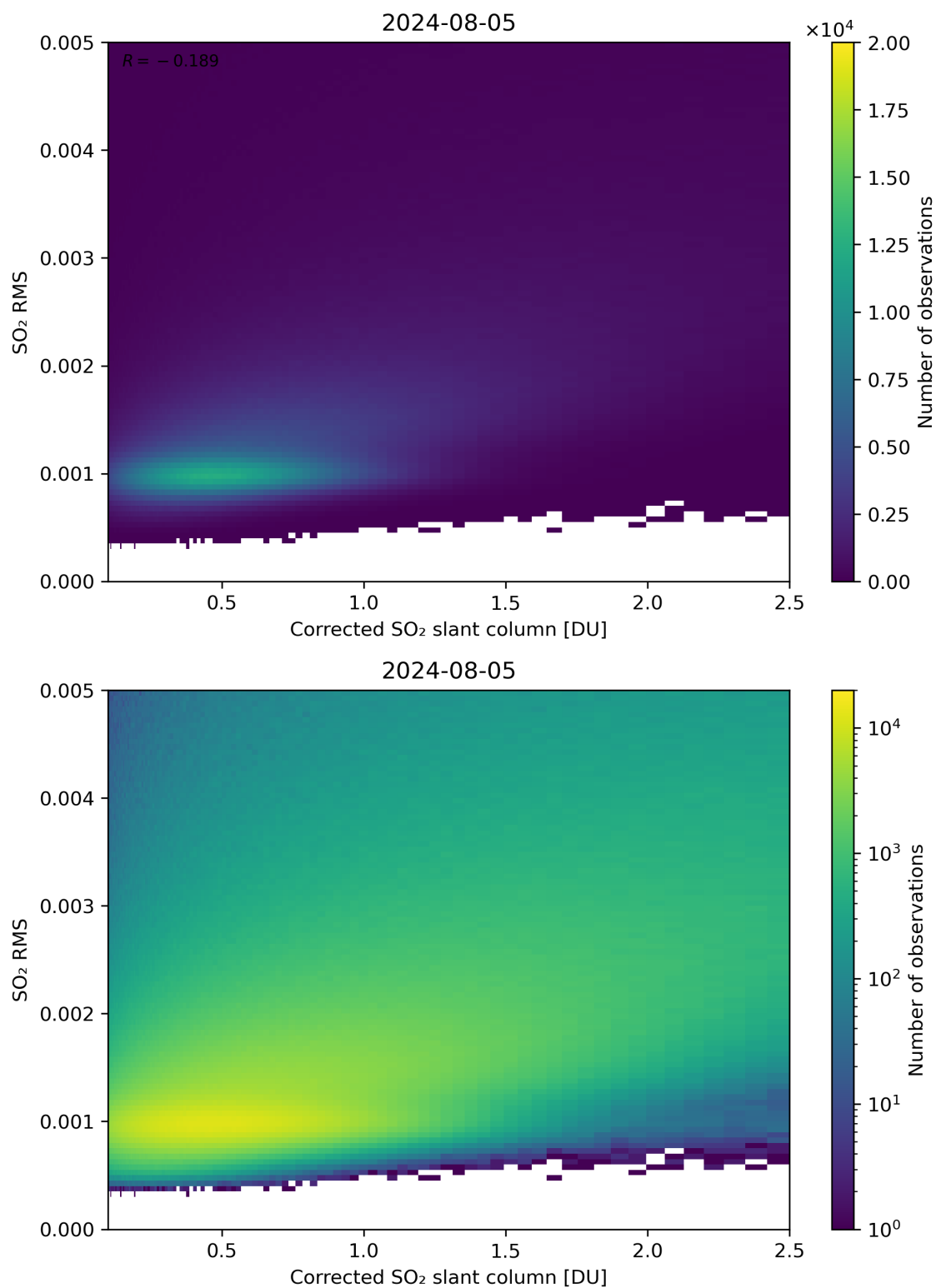
Figure 183: Scatter density plot of “Corrected SO 2 slant column” against “SO 2 RMS” for 2024-08-04 to 2024-08-06.
