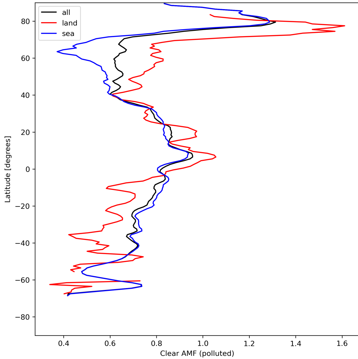
Figure 50: Zonal average of “Clear AMF (polluted)” for 2024-08-04 to 2024-08-06.
