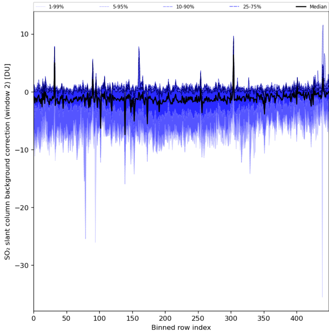
Figure 86: Along track statistics of “SO 2 slant column background correction (window 2)” for 2024-08-04 to 2024-08-06
