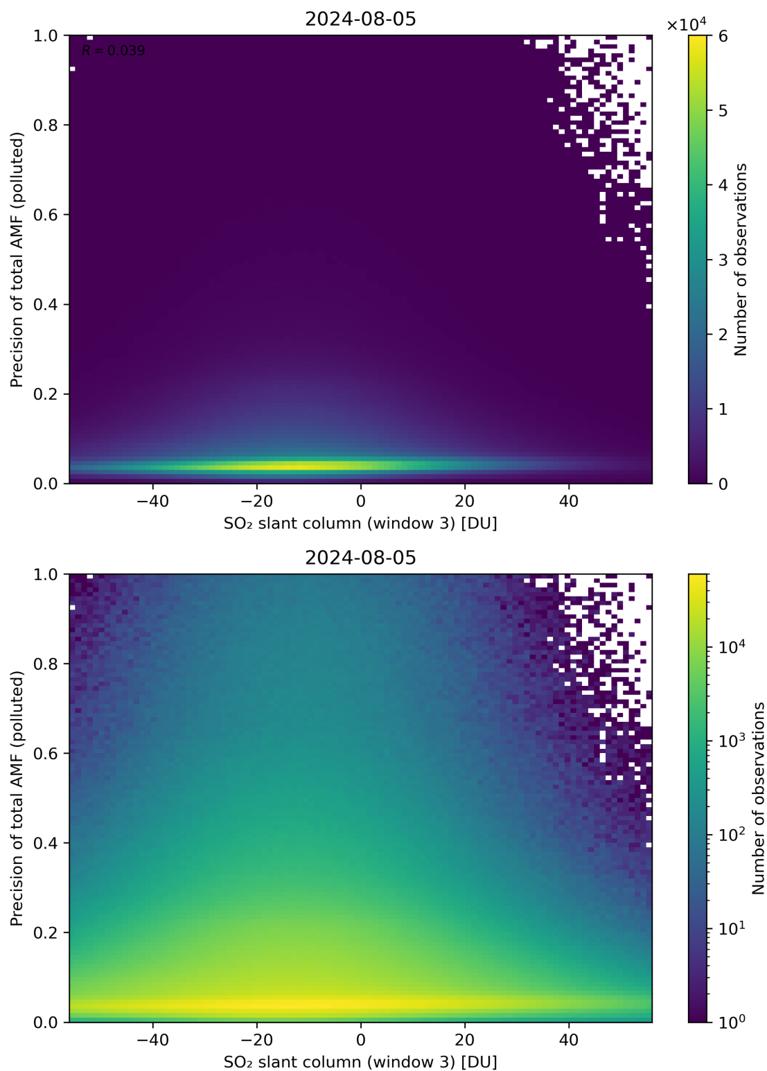
Figure 269: Scatter density plot of “SO 2 slant column (window 3)” against “Precision of total AMF (polluted)” for 2024-08-04 to 2024-08-06.
