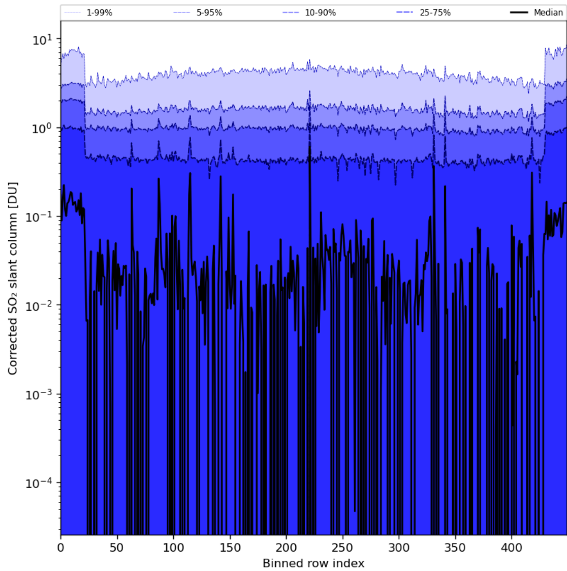
Figure 78: Along track statistics of “Corrected SO 2 slant column” for 2024-08-04 to 2024-08-06
