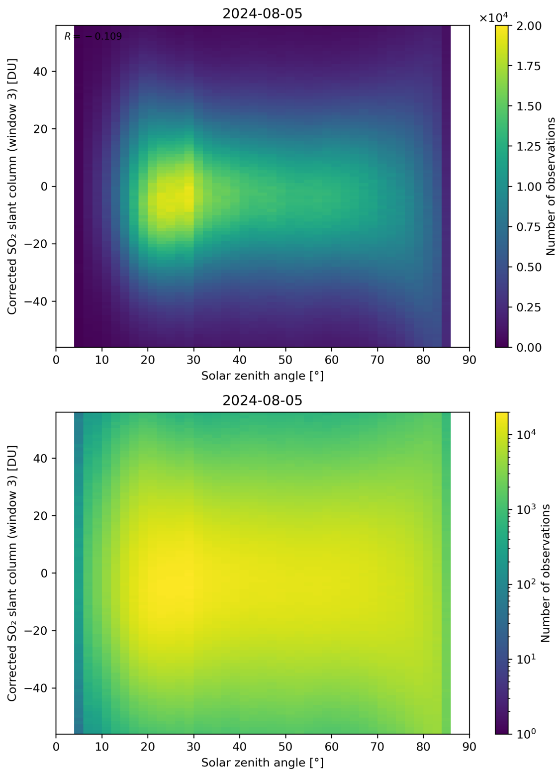
Figure 168: Scatter density plot of “Solar zenith angle” against “Corrected SO 2 slant column (window 3)” for 2024-08-04 to 2024-08-06.
