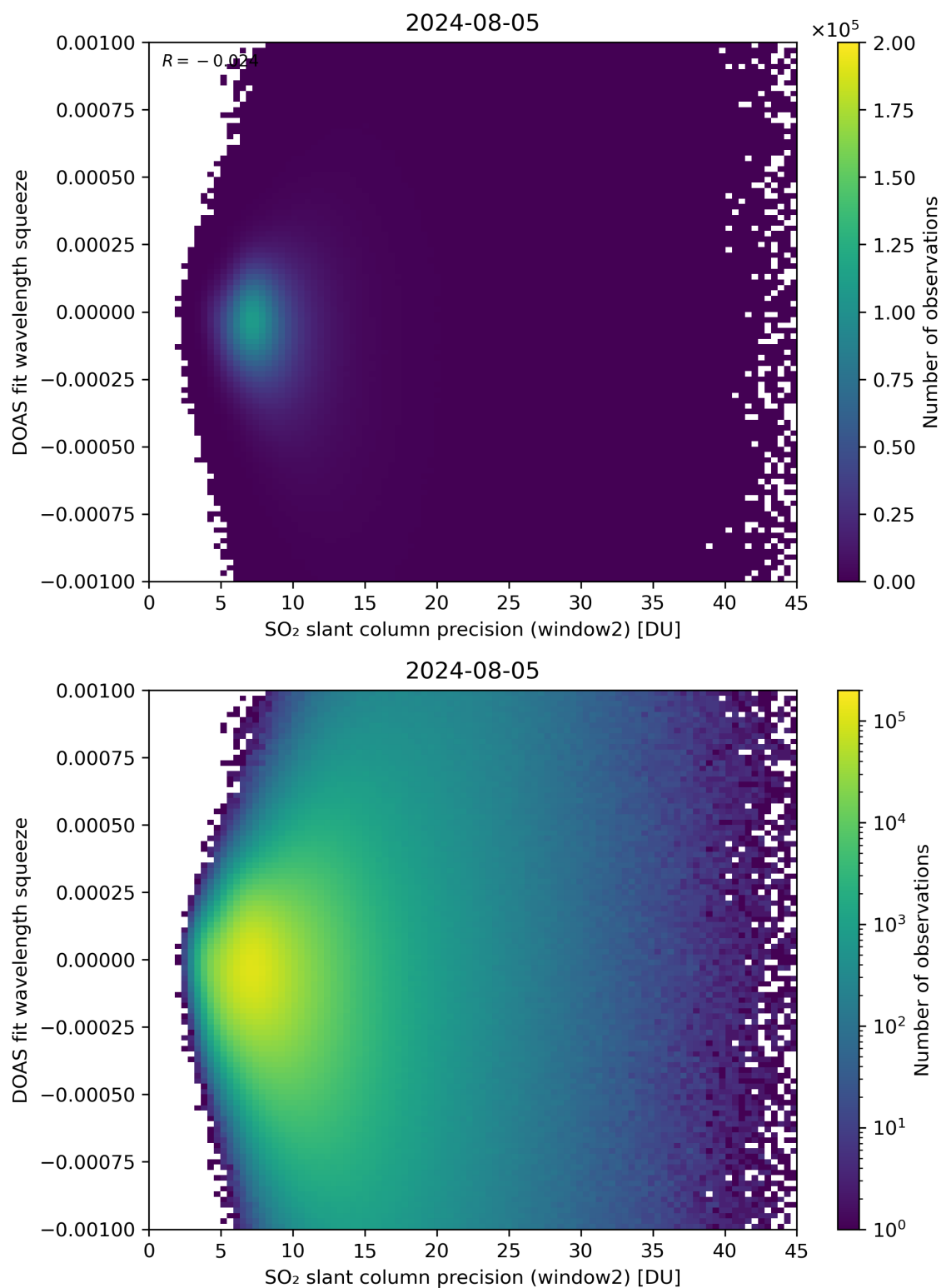
Figure 244: Scatter density plot of “SO 2 slant column precision (window2)” against “DOAS fit wavelength squeeze” for 2024-08-04 to 2024-08-06.
