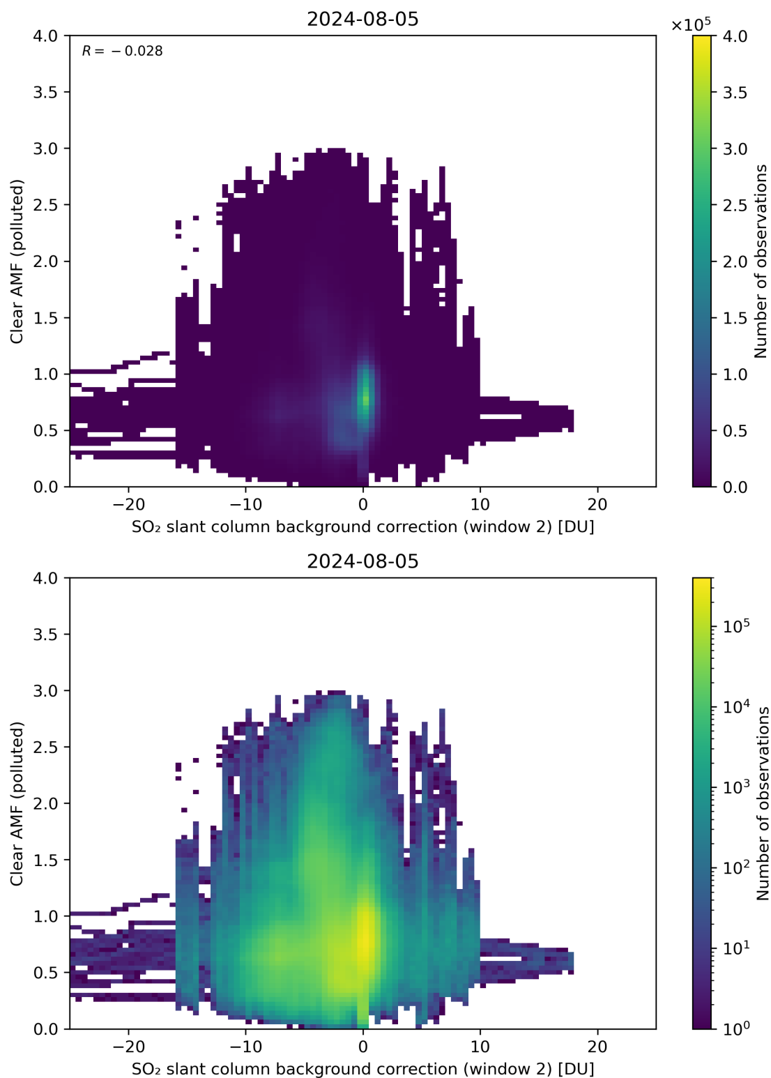
Figure 115: Scatter density plot of “SO 2 slant column background correction (window 2)” against “Clear AMF (polluted)” for 2024-08-04 to 2024-08-06.
