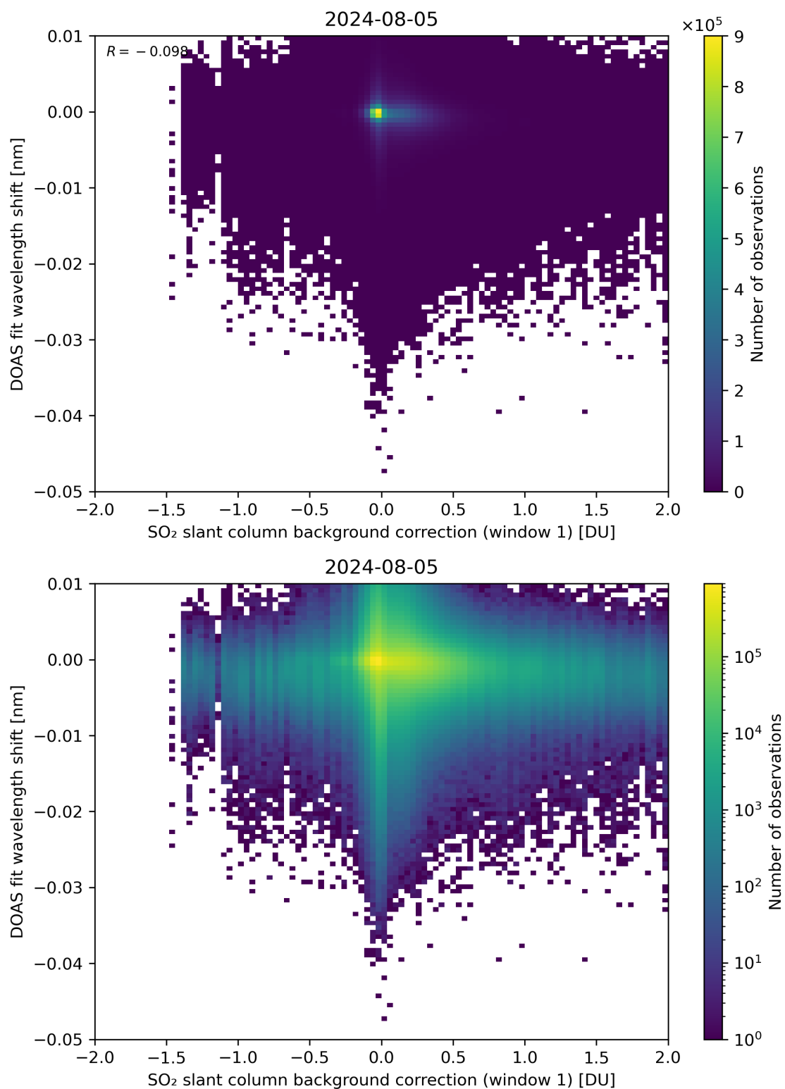
Figure 100: Scatter density plot of “SO 2 slant column background correction (window 1)” against “DOAS fit wavelength shift” for 2024-08-04 to 2024-08-06.
