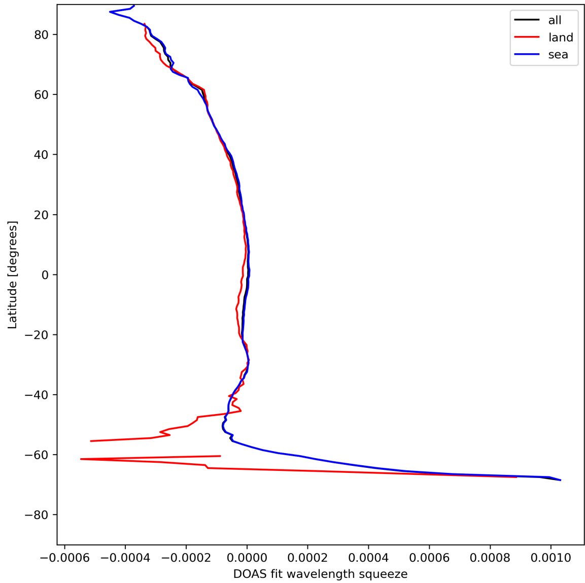
Figure 46: Zonal average of “DOAS fit wavelength squeeze” for 2024-08-04 to 2024-08-06.
