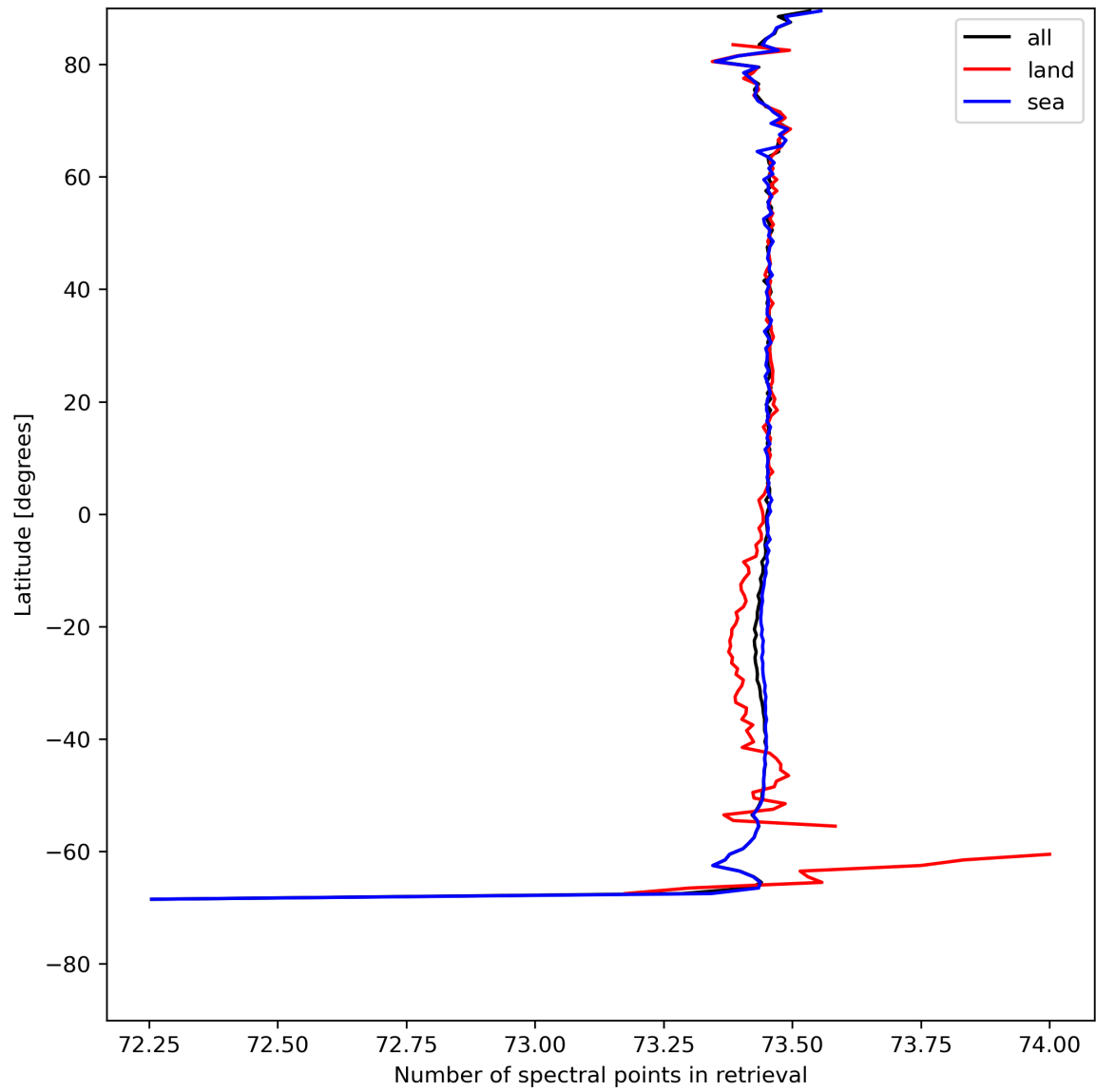
Figure 51: Zonal average of “Number of spectral points in retrieval” for 2024-08-04 to 2024-08-06.
