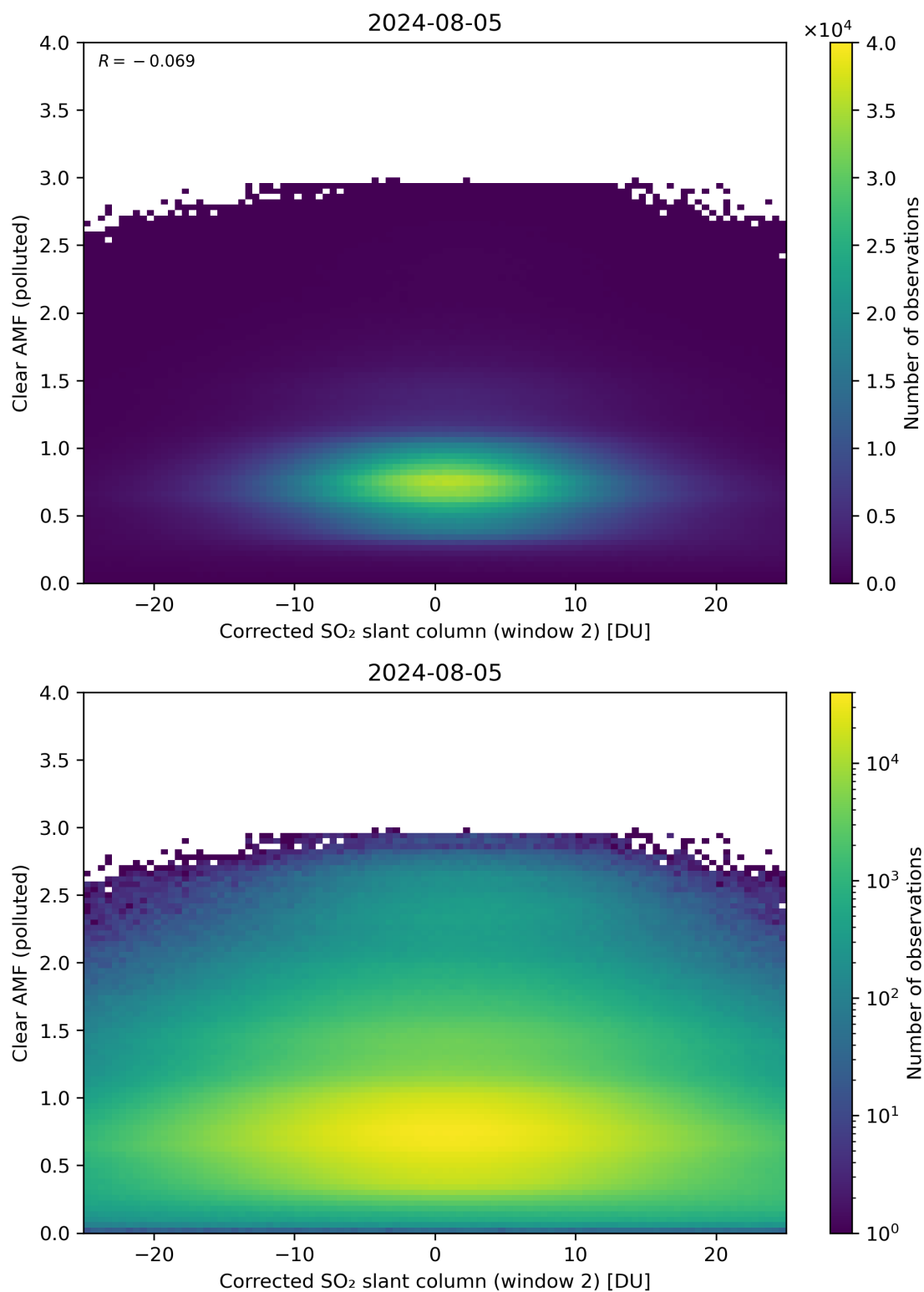
Figure 199: Scatter density plot of “Corrected SO 2 slant column (window 2)” against “Clear AMF (polluted)” for 2024-08-04 to 2024-08-06.
