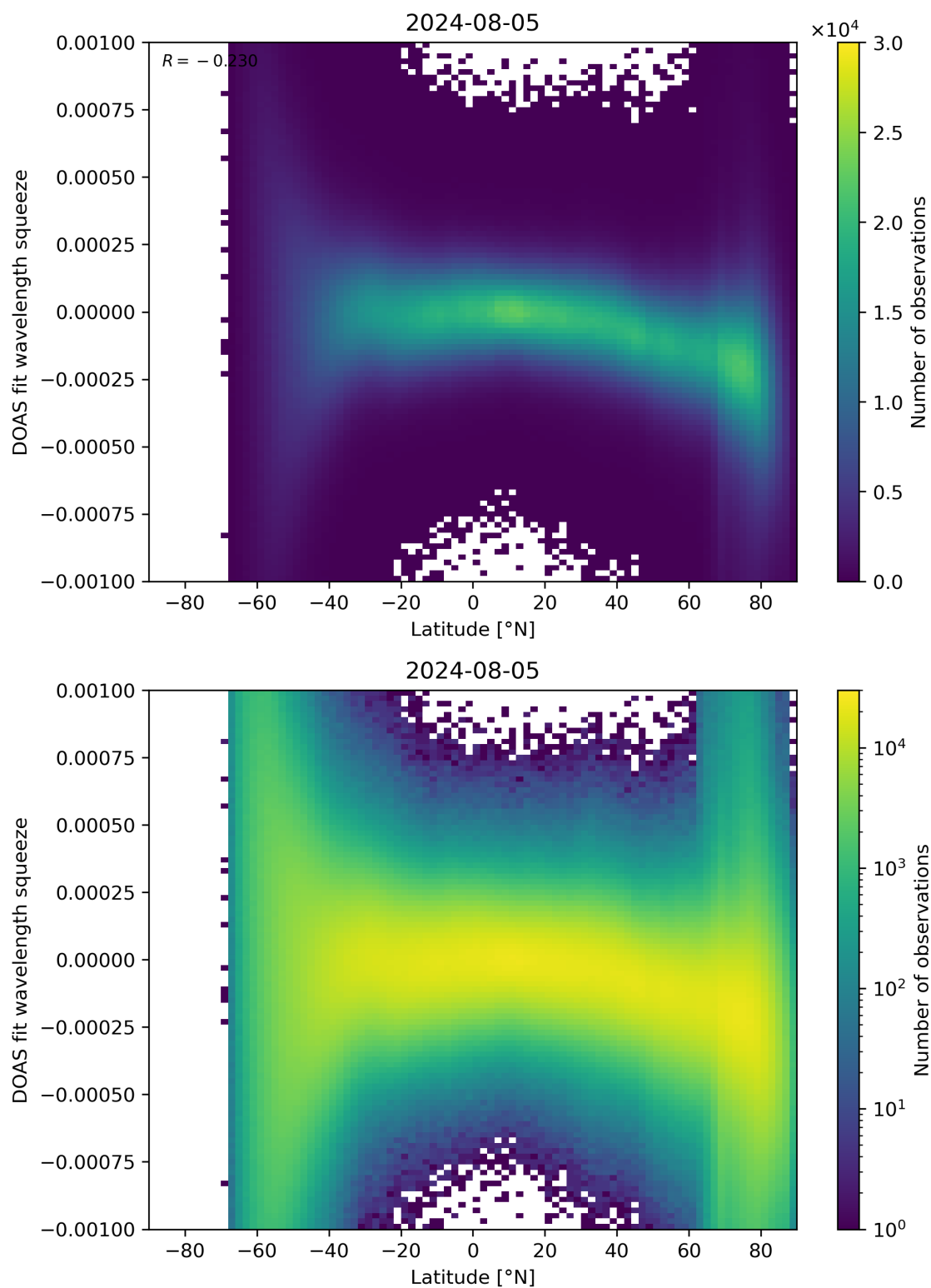
Figure 143: Scatter density plot of “Latitude” against “DOAS fit wavelength squeeze” for 2024-08-04 to 2024-08-06.
