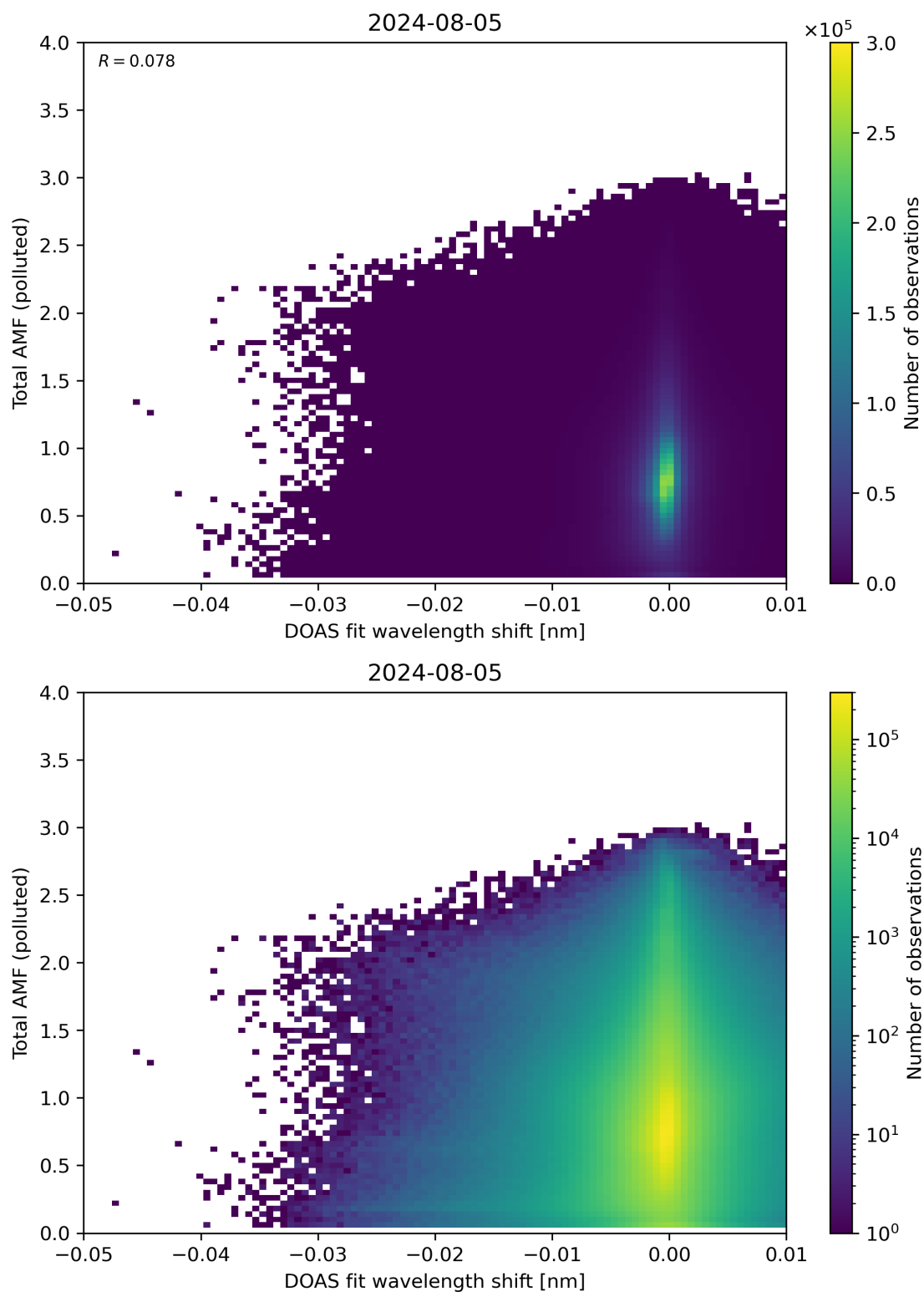
Figure 130: Scatter density plot of “DOAS fit wavelength shift” against “Total AMF (polluted)” for 2024-08-04 to 2024-08-06.
