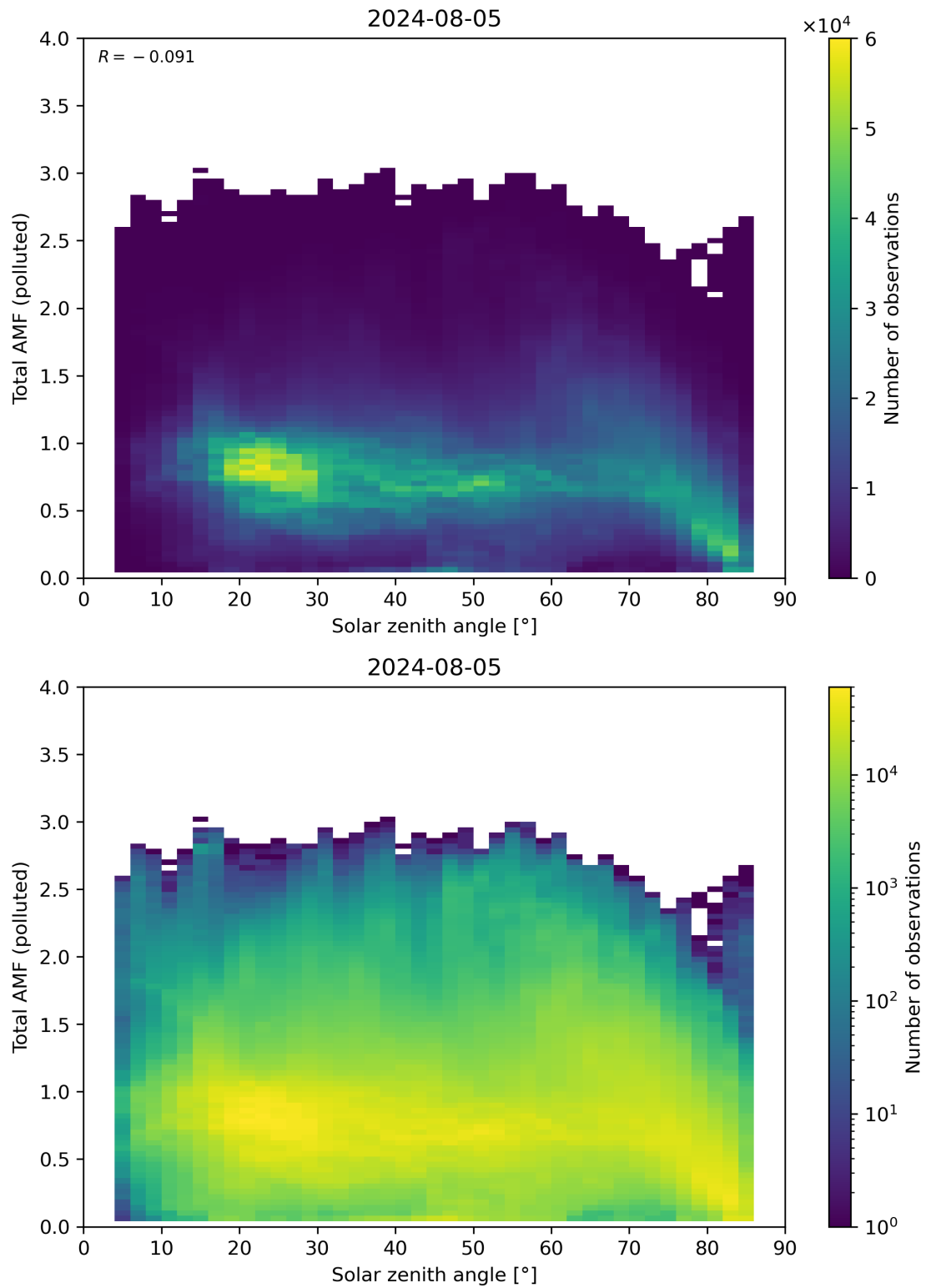
Figure 174: Scatter density plot of “Solar zenith angle” against “Total AMF (polluted)” for 2024-08-04 to 2024-08-06.
