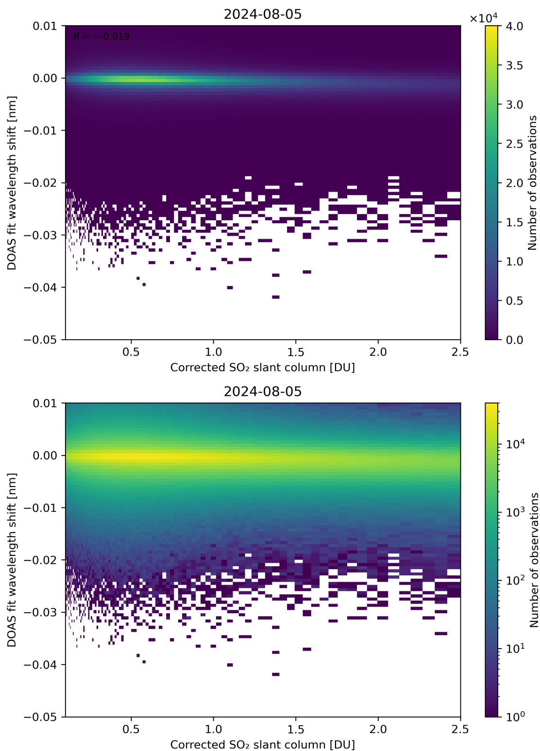
Figure 181: Scatter density plot of “Corrected SO 2 slant column” against “DOAS fit wavelength shift” for 2024-08-04 to 2024-08-06.
