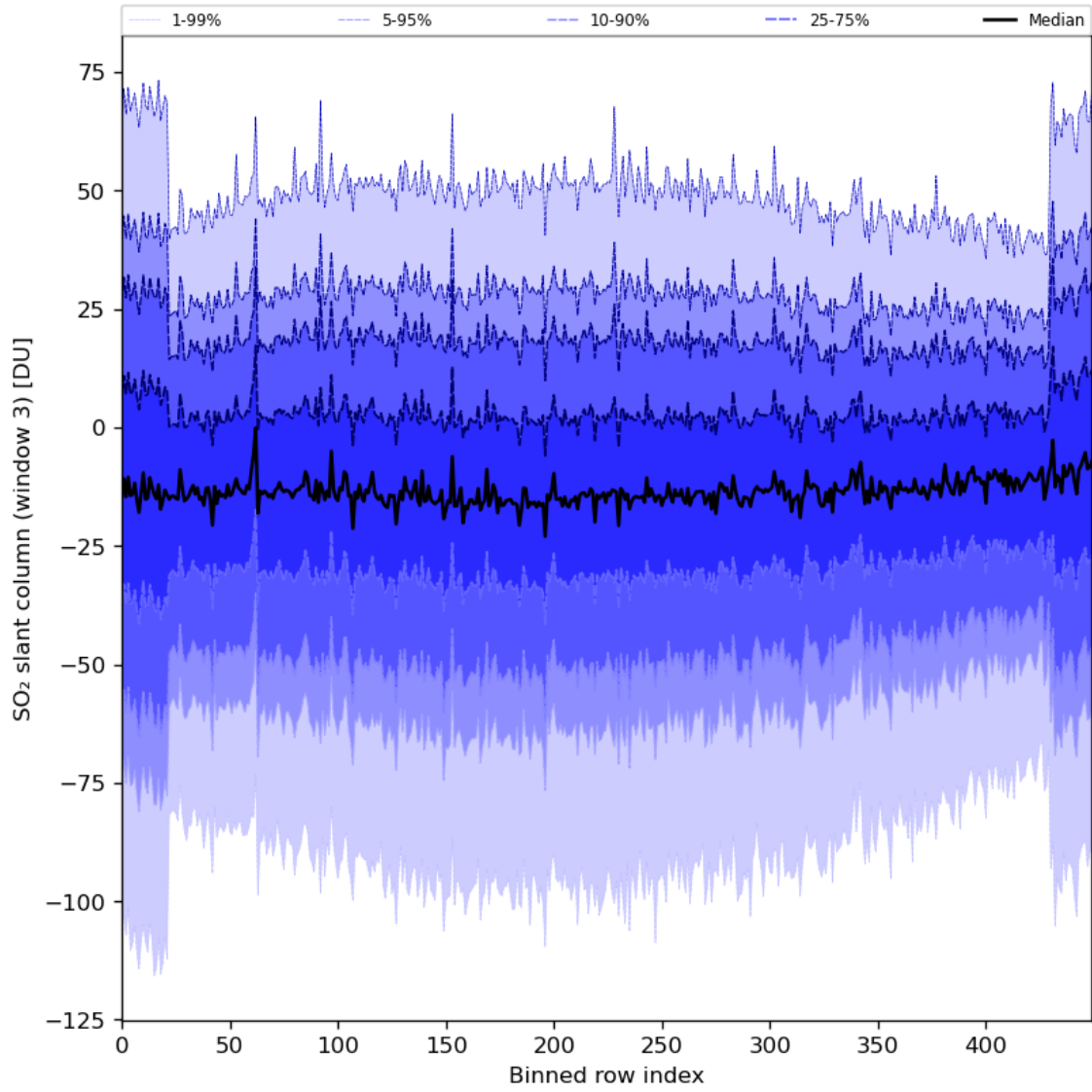
Figure 87: Along track statistics of “SO 2 slant column (window 3)” for 2024-08-04 to 2024-08-06
