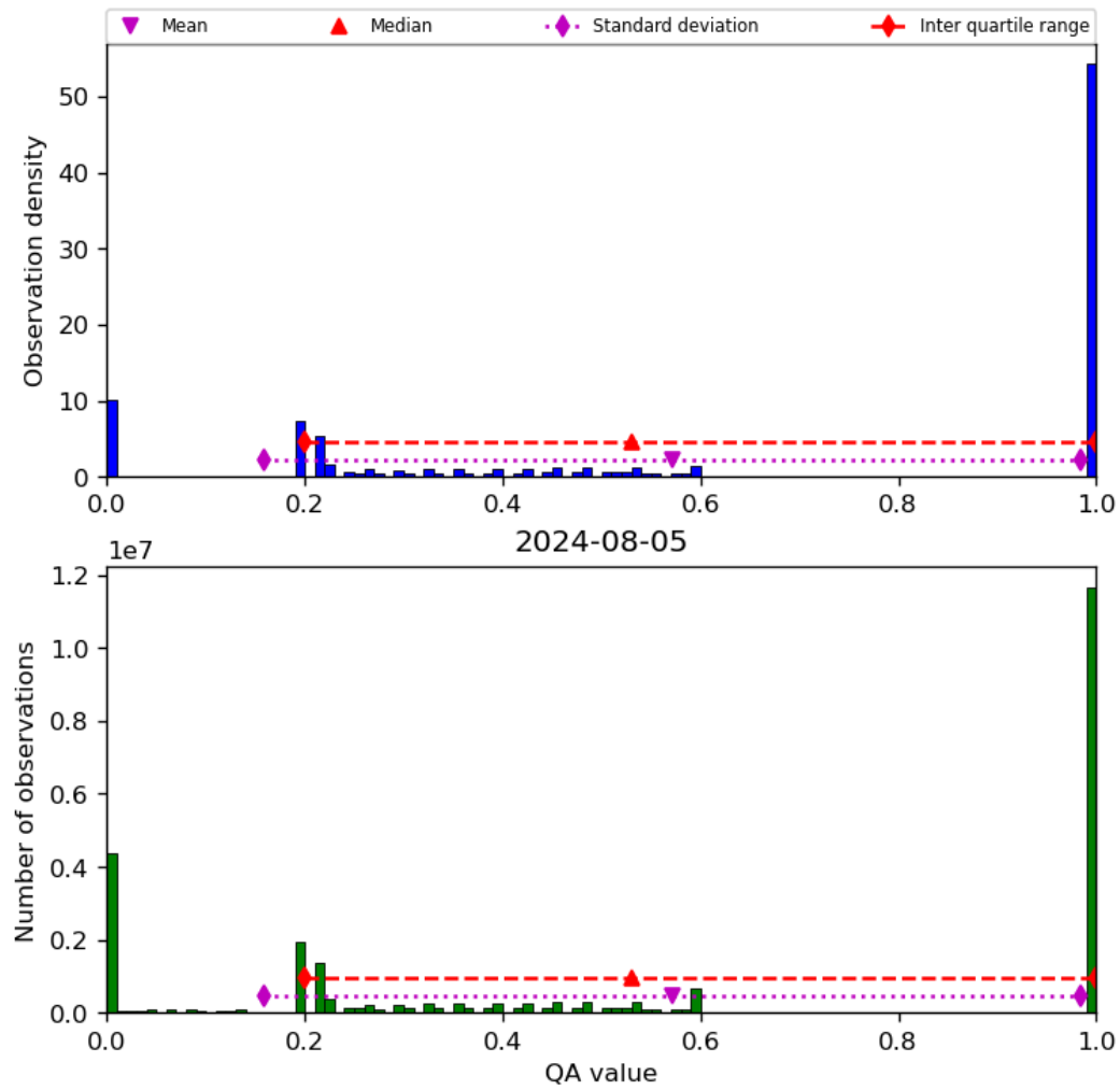
Figure 52: Histogram of “QA value” for 2024-08-04 to 2024-08-06
