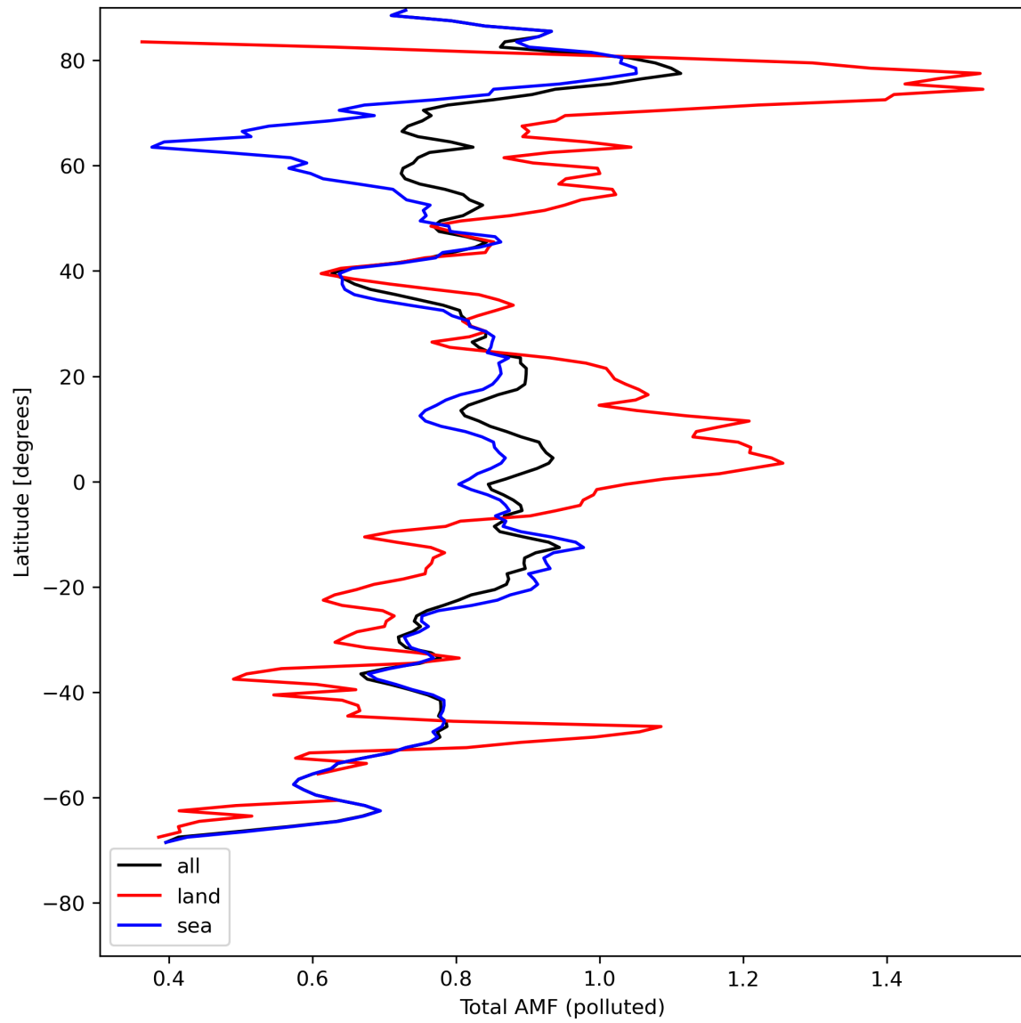
Figure 48: Zonal average of “Total AMF (polluted)” for 2024-08-04 to 2024-08-06.
