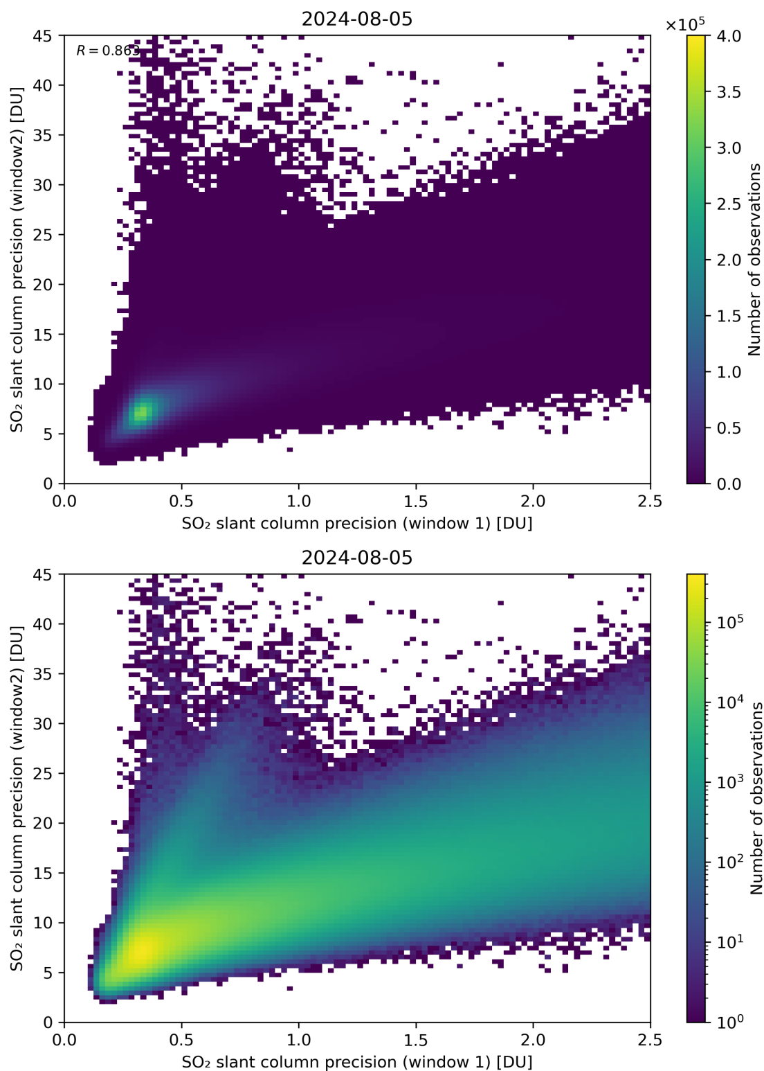
Figure 227: Scatter density plot of “SO 2 slant column precision (window 1)” against “SO 2 slant column precision (window2)” for 2024-08-04 to 2024-08-06.
