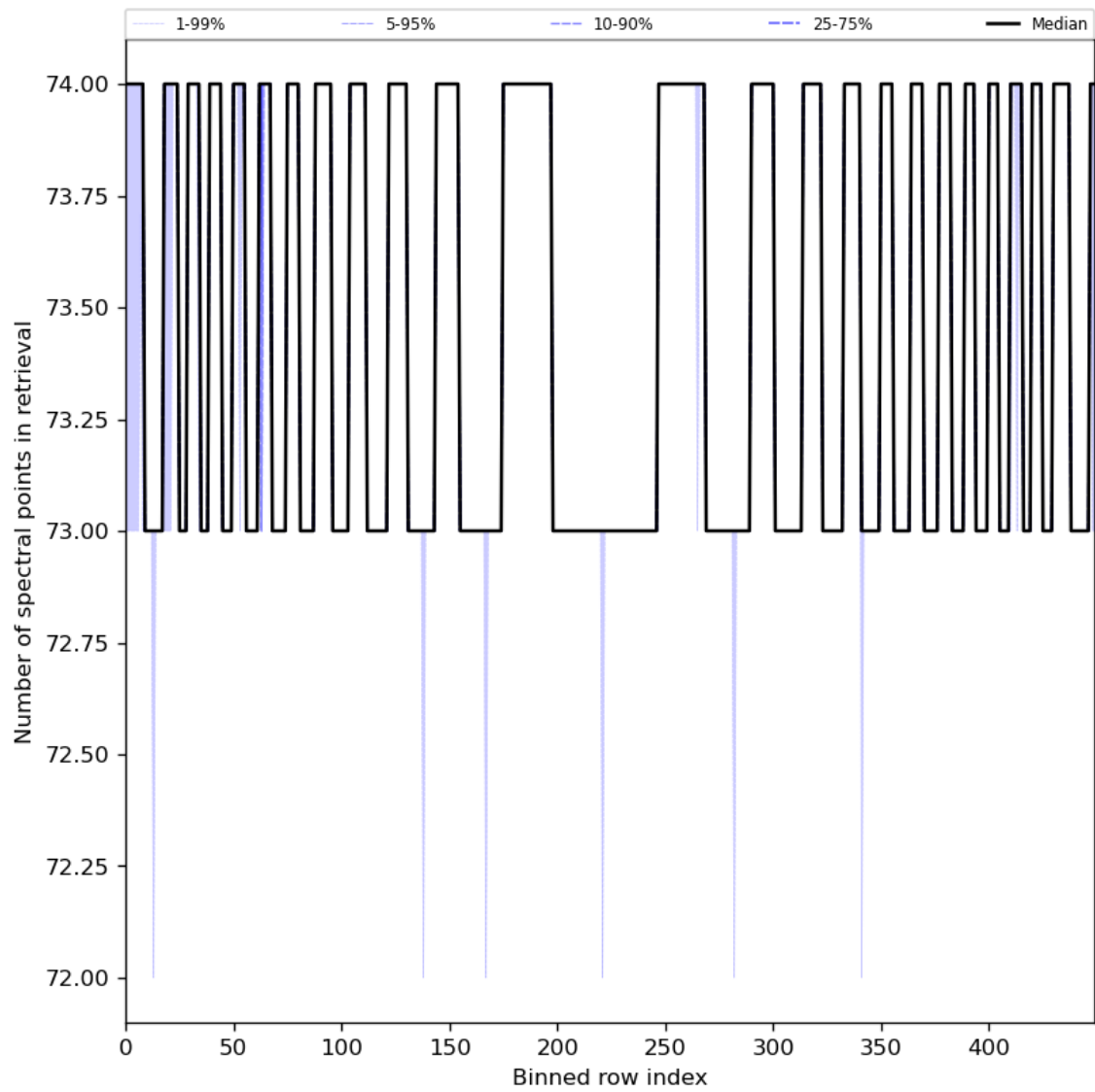
Figure 97: Along track statistics of “Number of spectral points in retrieval” for 2024-08-04 to 2024-08-06
