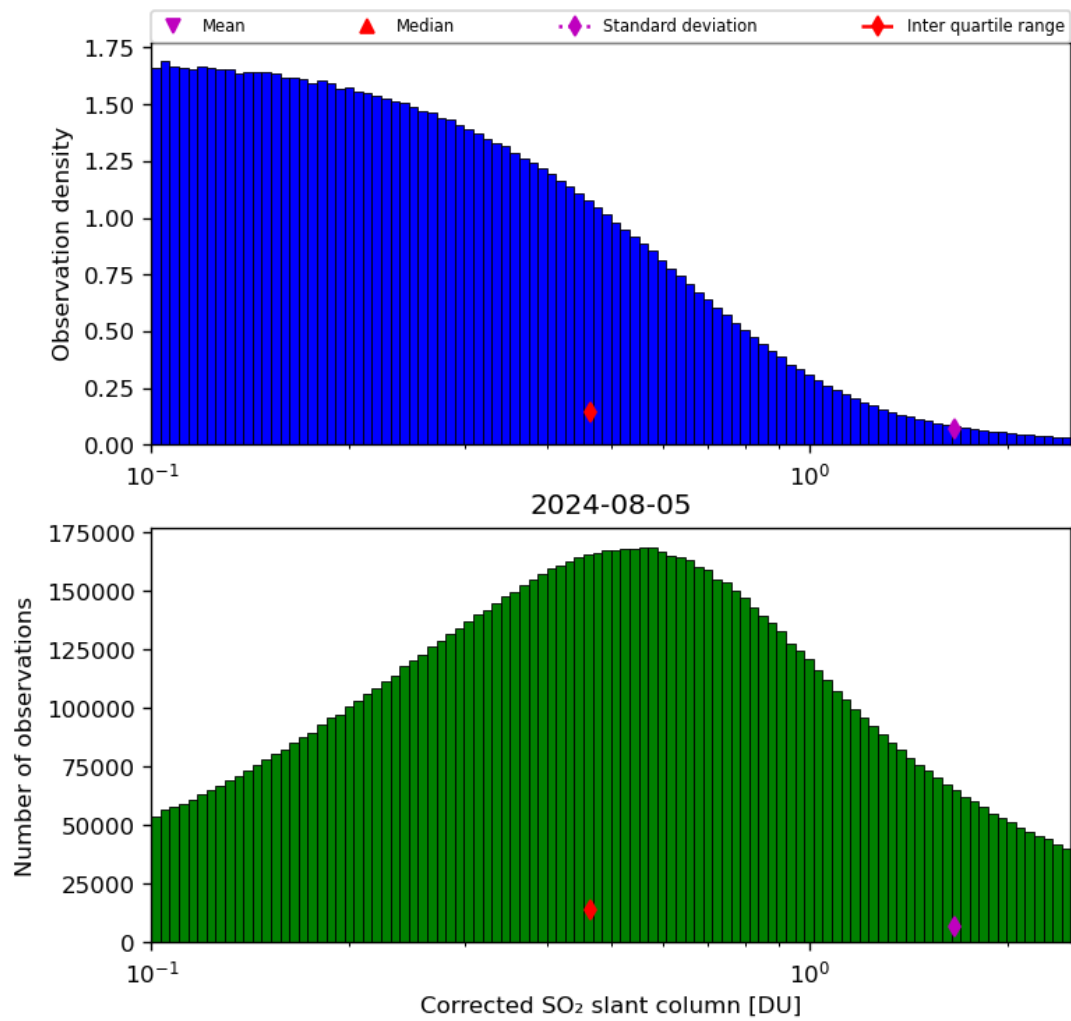
Figure 55: Histogram of “Corrected SO 2 slant column” for 2024-08-04 to 2024-08-06
