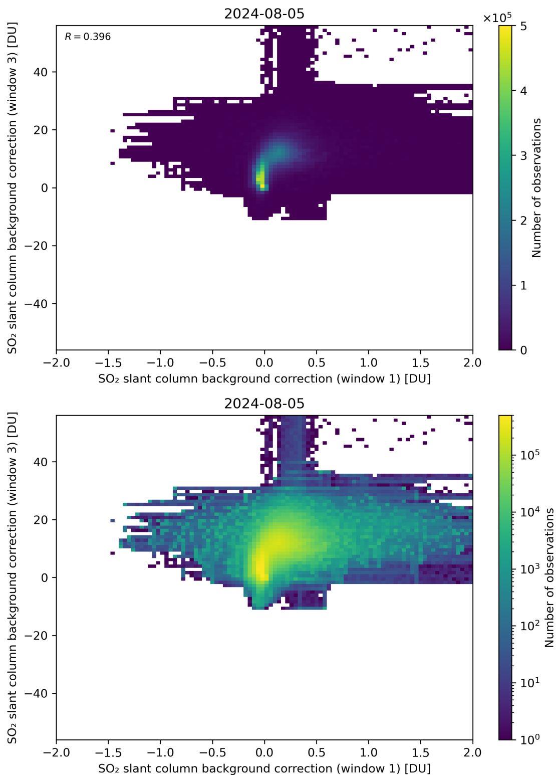
Figure 99: Scatter density plot of “SO 2 slant column background correction (window 1)” against “SO 2 slant column background correction (window 3)” for 2024-08-04 to 2024-08-06.
