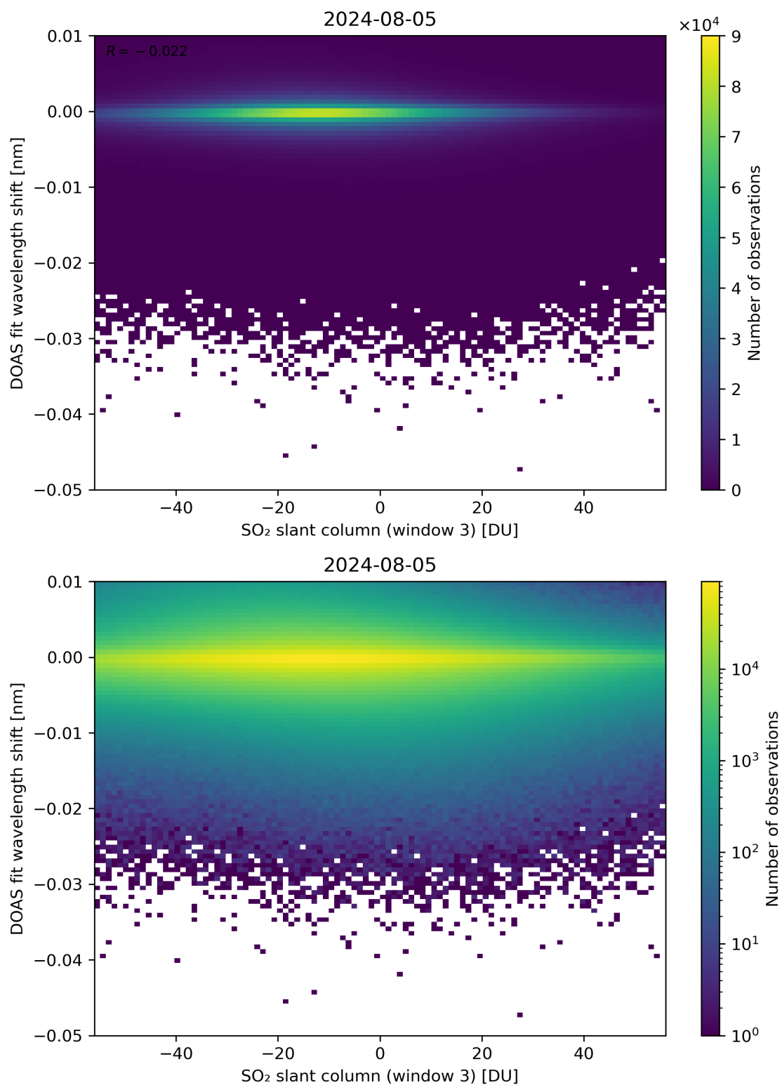
Figure 254: Scatter density plot of “SO 2 slant column (window 3)” against “DOAS fit wavelength shift” for 2024-08-04 to 2024-08-06.
