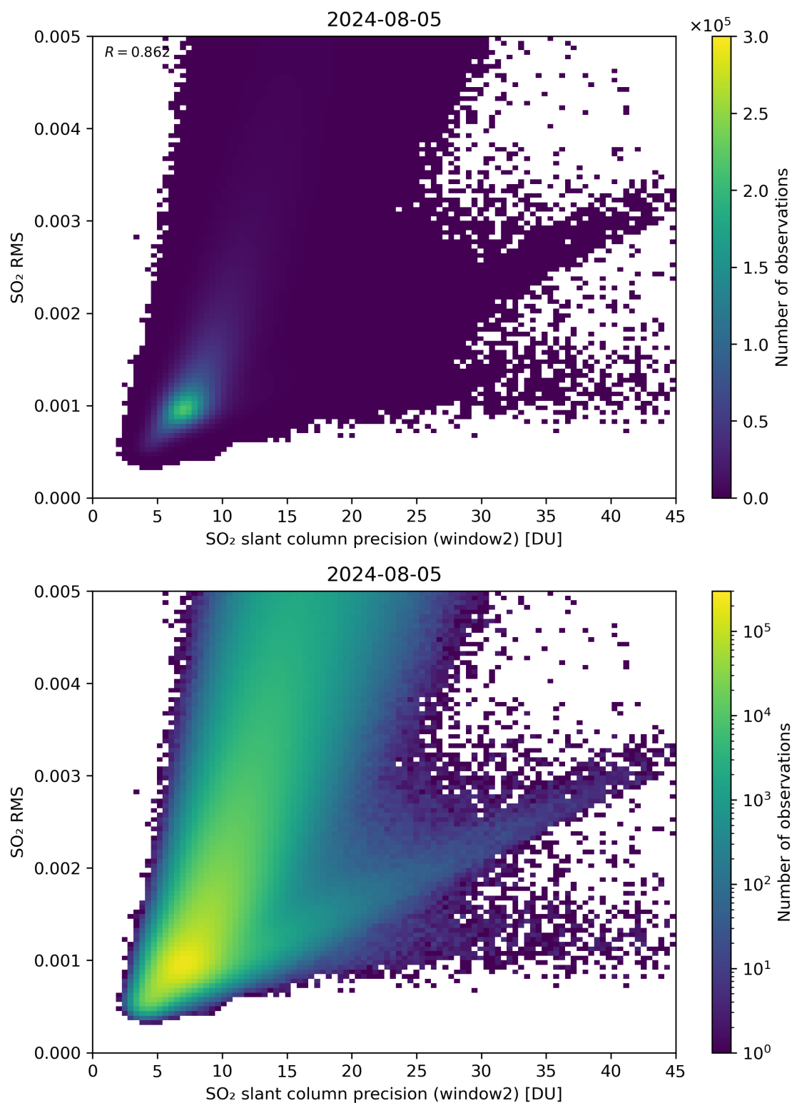
Figure 245: Scatter density plot of “SO 2 slant column precision (window2)” against “SO 2 RMS” for 2024-08-04 to 2024-08-06.
