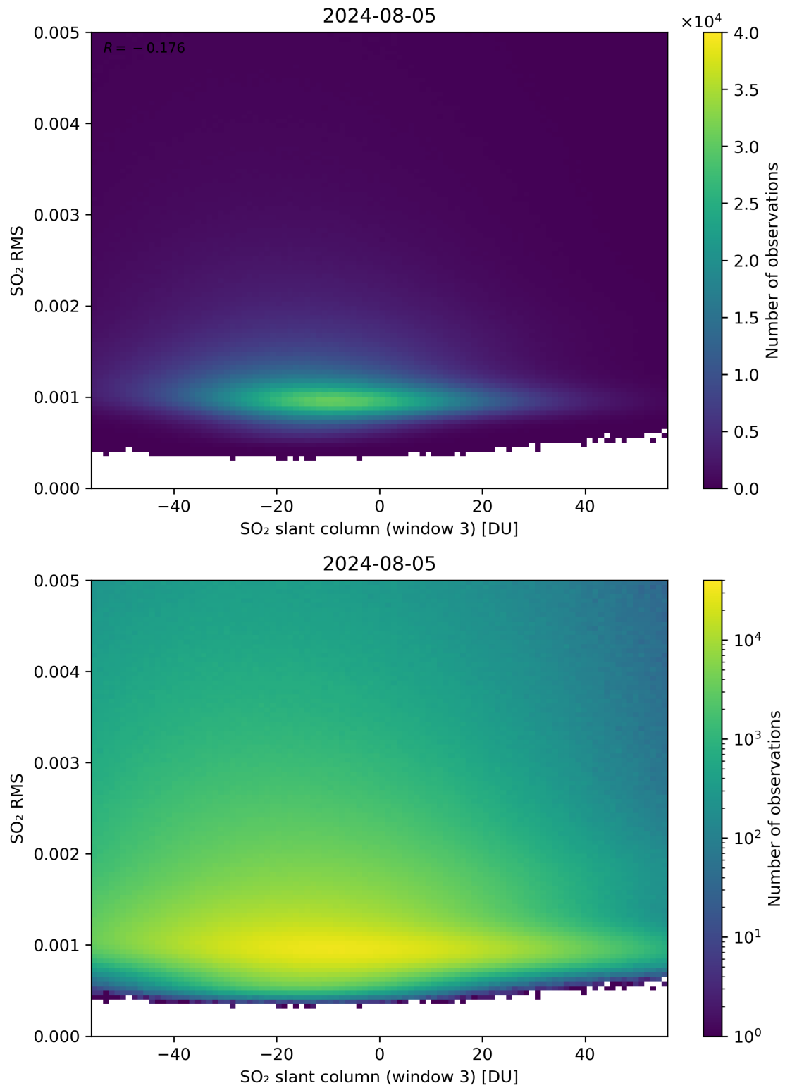
Figure 256: Scatter density plot of “SO 2 slant column (window 3)” against “SO 2 RMS” for 2024-08-04 to 2024-08-06.
