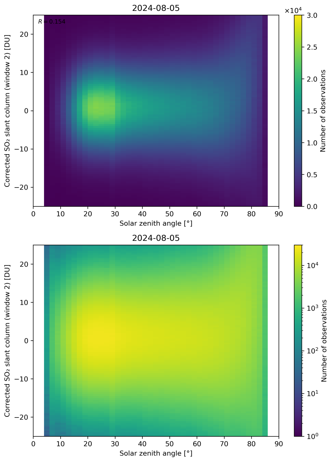
Figure 167: Scatter density plot of “Solar zenith angle” against “Corrected SO 2 slant column (window 2)” for 2024-08-04 to 2024-08-06.
