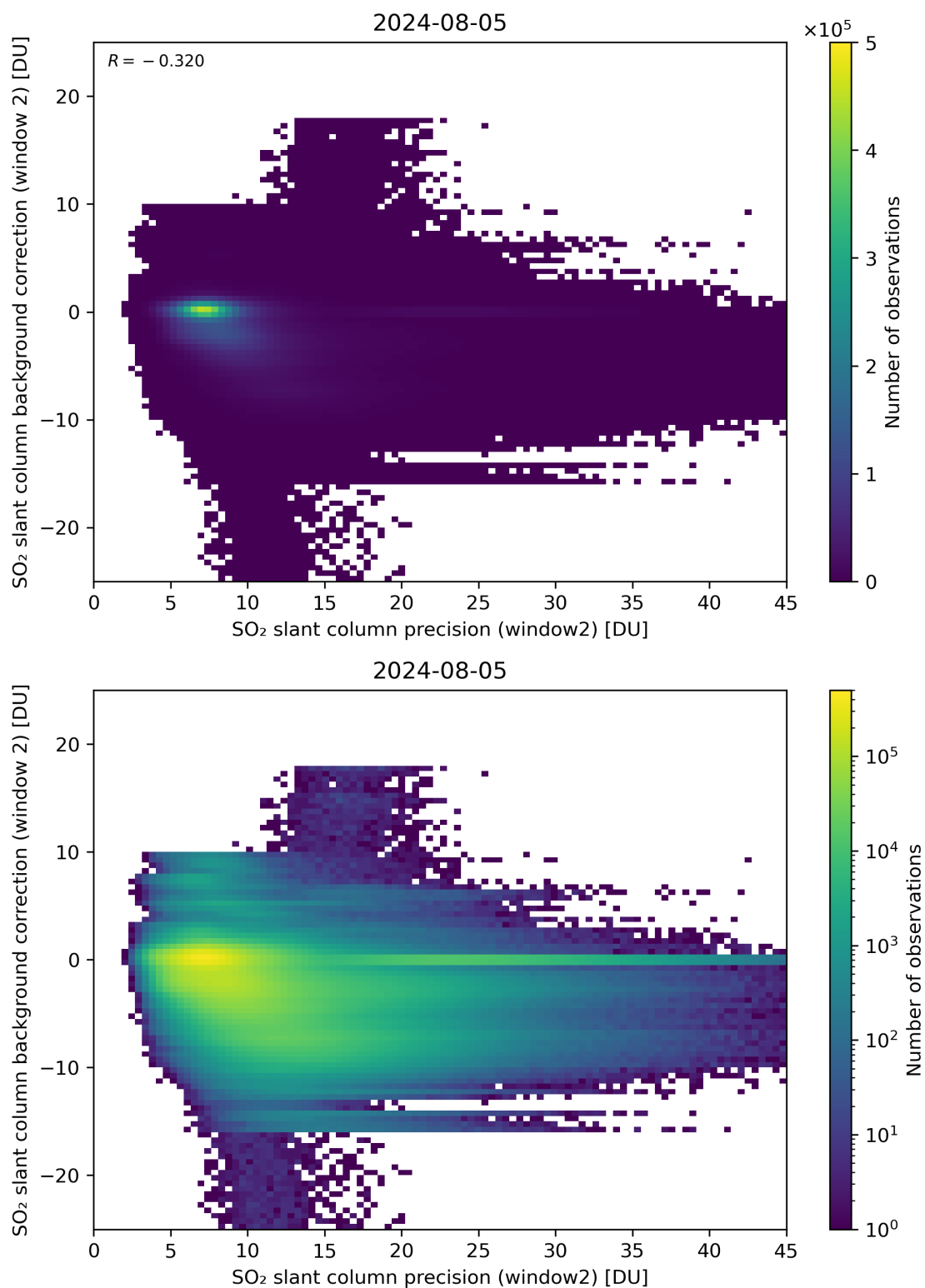
Figure 241: Scatter density plot of “SO 2 slant column precision (window2)” against “SO 2 slant column background correction (window 2)” for 2024-08-04 to 2024-08-06.
