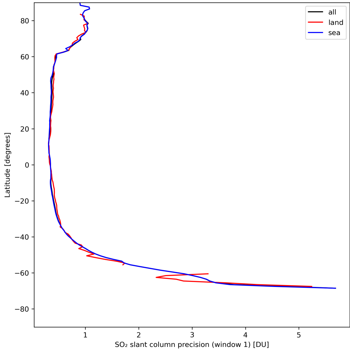
Figure 34: Zonal average of “SO 2 slant column precision (window 1)” for 2024-08-04 to 2024-08-06.
