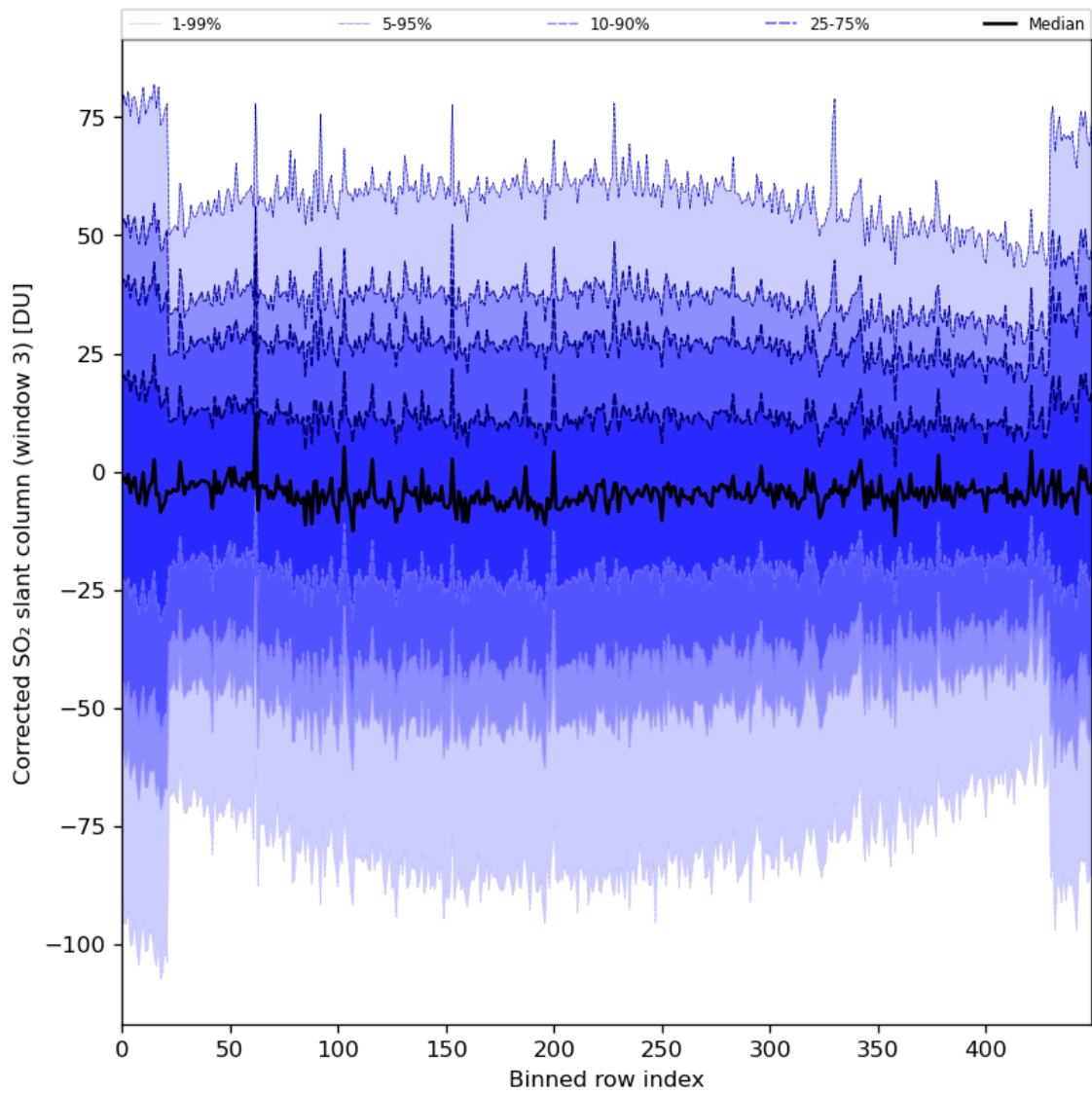
Figure 89: Along track statistics of “Corrected SO 2 slant column (window 3)” for 2024-08-04 to 2024-08-06
