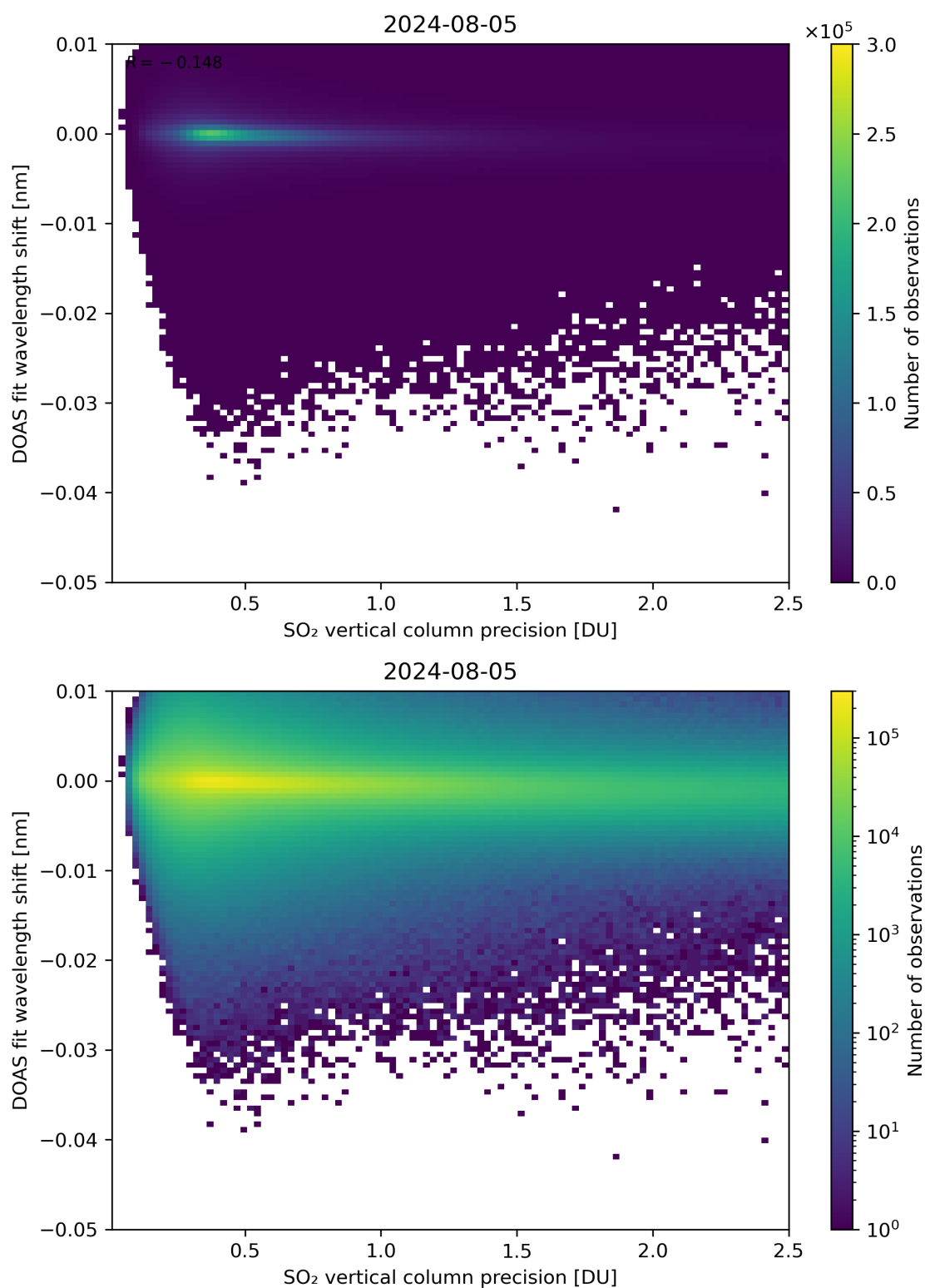
Figure 282: Scatter density plot of “SO 2 vertical column precision” against “DOAS fit wavelength shift” for 2024-08-04 to 2024-08-06.
