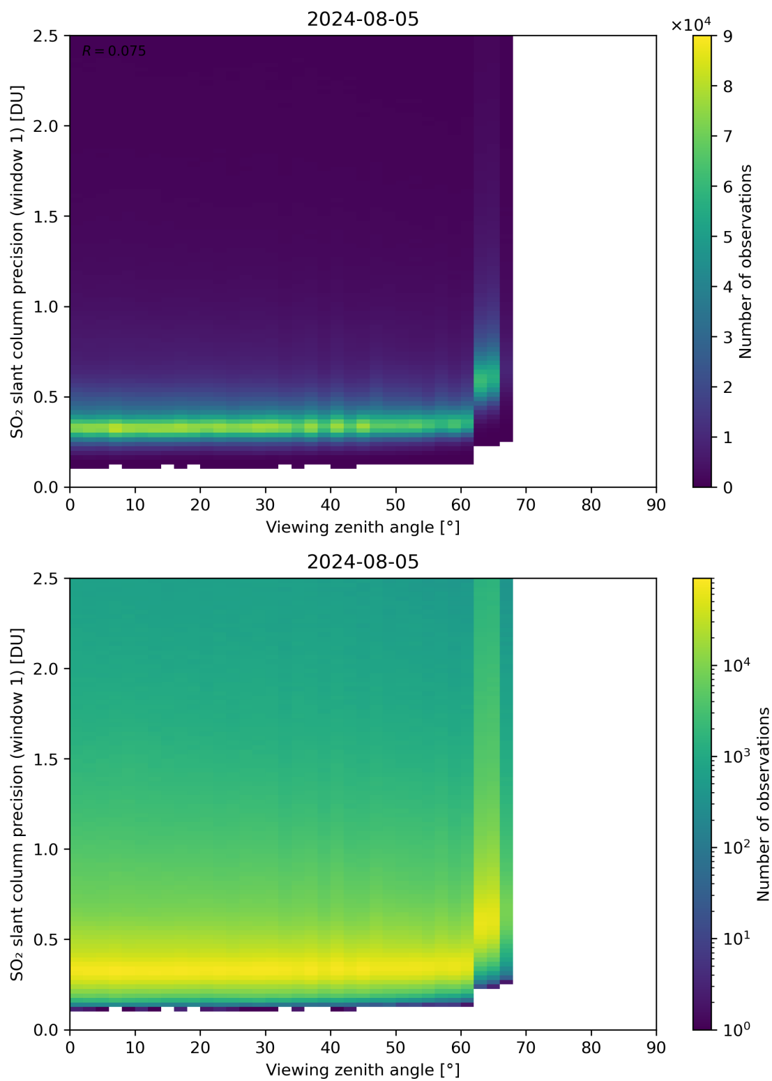
Figure 321: Scatter density plot of “Viewing zenith angle” against “SO 2 slant column precision (window 1)” for 2024-08-04 to 2024-08-06.
