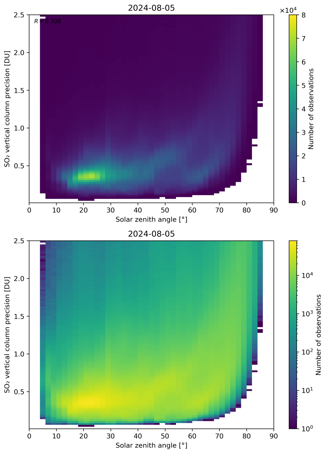
Figure 177: Scatter density plot of “Solar zenith angle” against “SO 2 vertical column precision” for 2024-08-04 to 2024-08-06.
