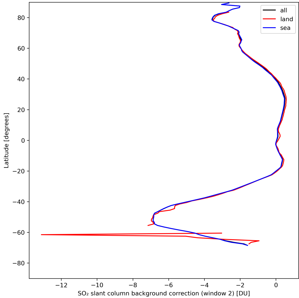
Figure 40: Zonal average of “SO 2 slant column background correction (window 2)” for 2024-08-04 to 2024-08-06.
