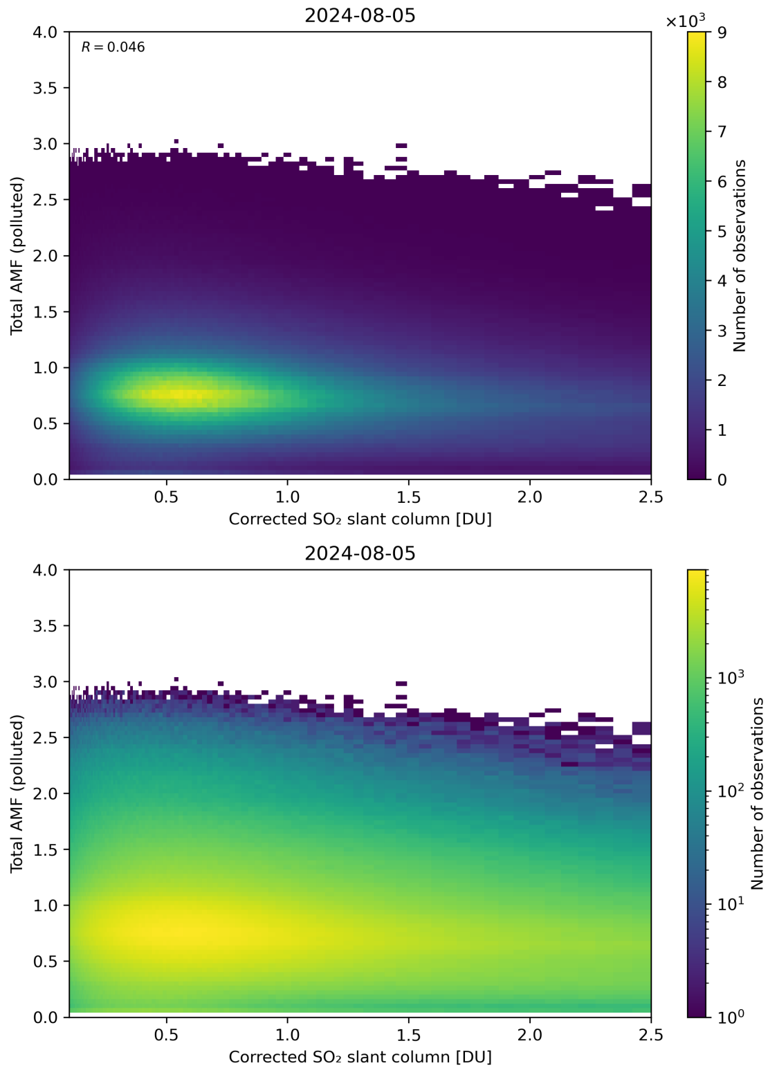
Figure 192: Scatter density plot of “Corrected SO 2 slant column” against “Total AMF (polluted)” for 2024-08-04 to 2024-08-06.
