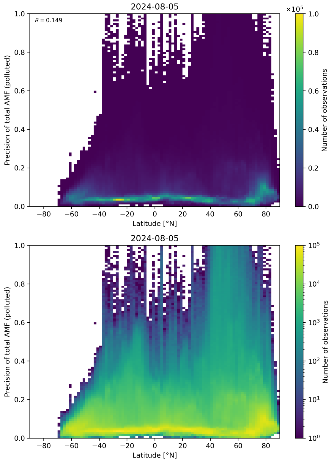
Figure 155: Scatter density plot of “Latitude” against “Precision of total AMF (polluted)” for 2024-08-04 to 2024-08-06.
