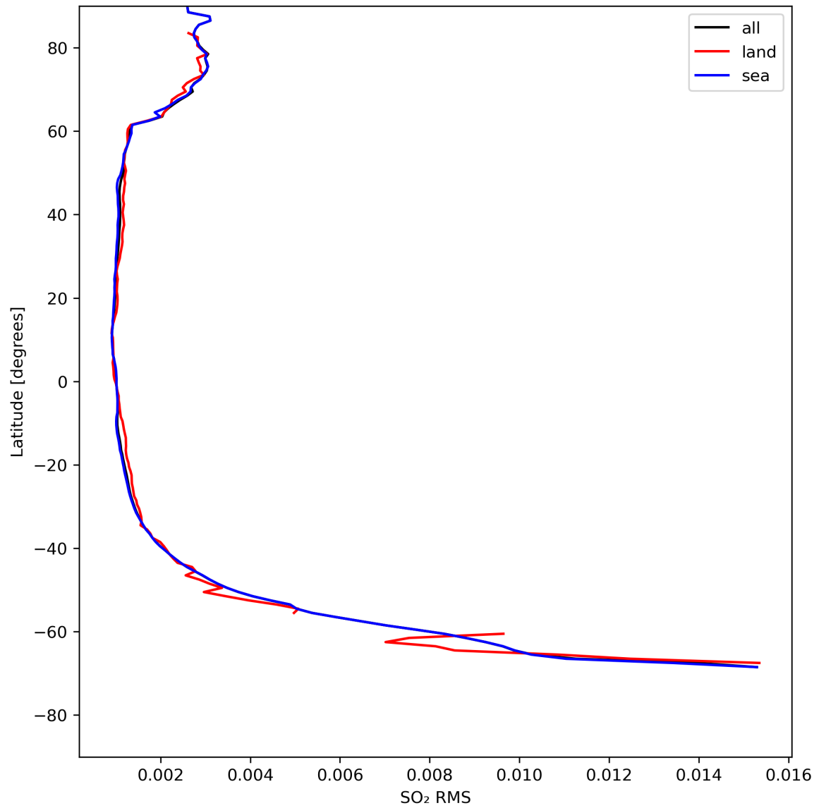
Figure 47: Zonal average of “SO 2 RMS” for 2024-08-04 to 2024-08-06.
