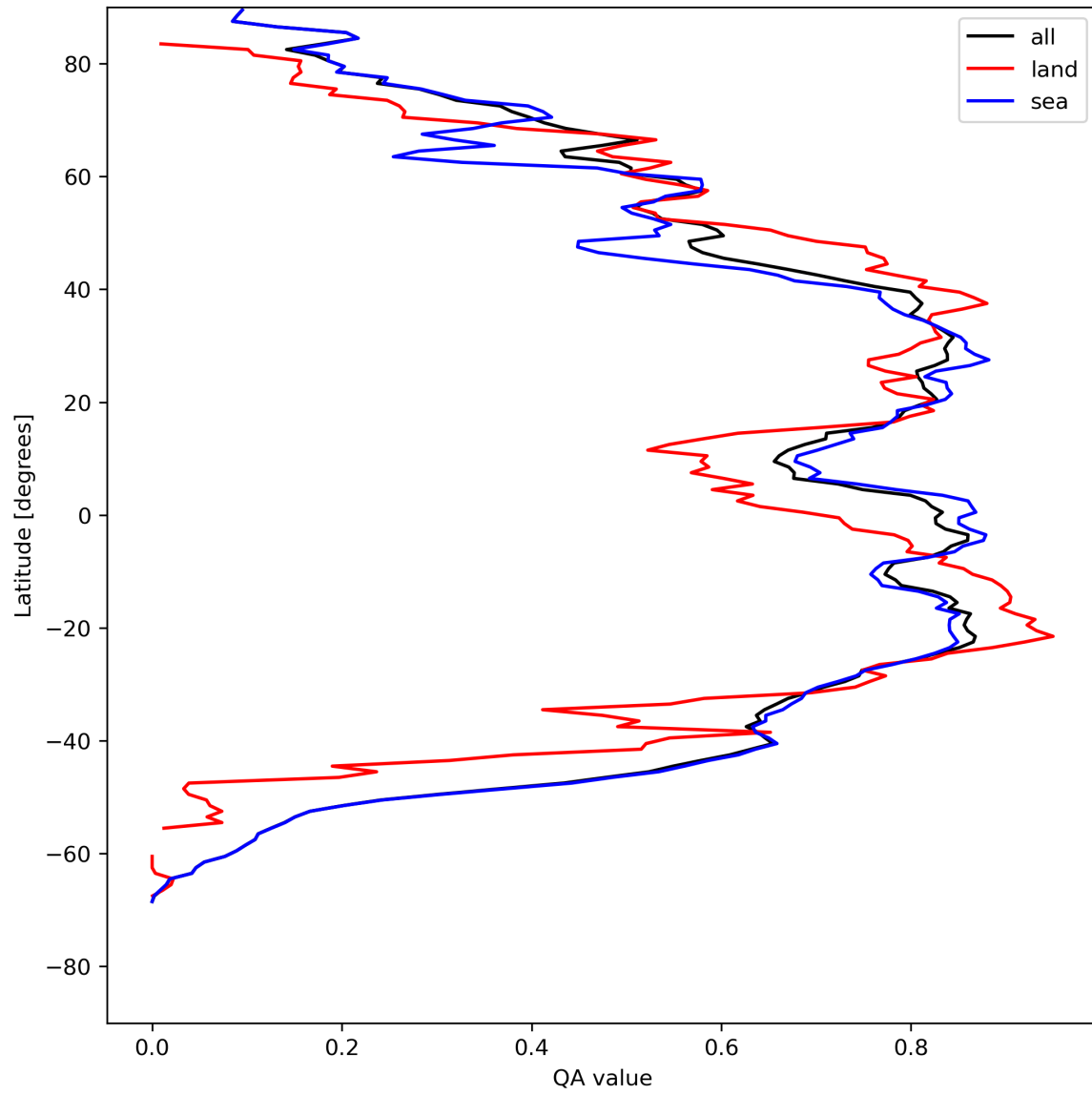
Figure 29: Zonal average of “QA value” for 2024-08-04 to 2024-08-06.
