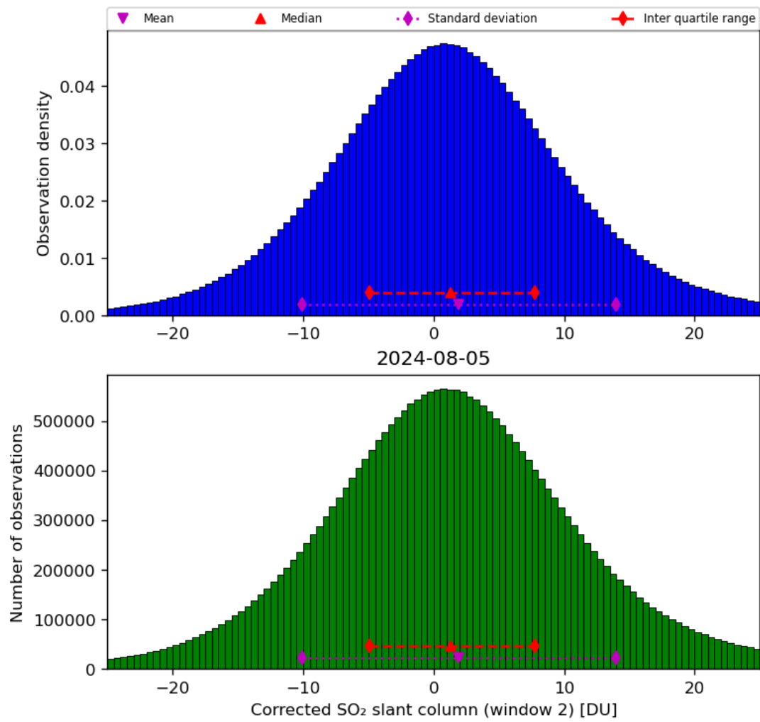
Figure 62: Histogram of “Corrected SO 2 slant column (window 2)” for 2024-08-04 to 2024-08-06
