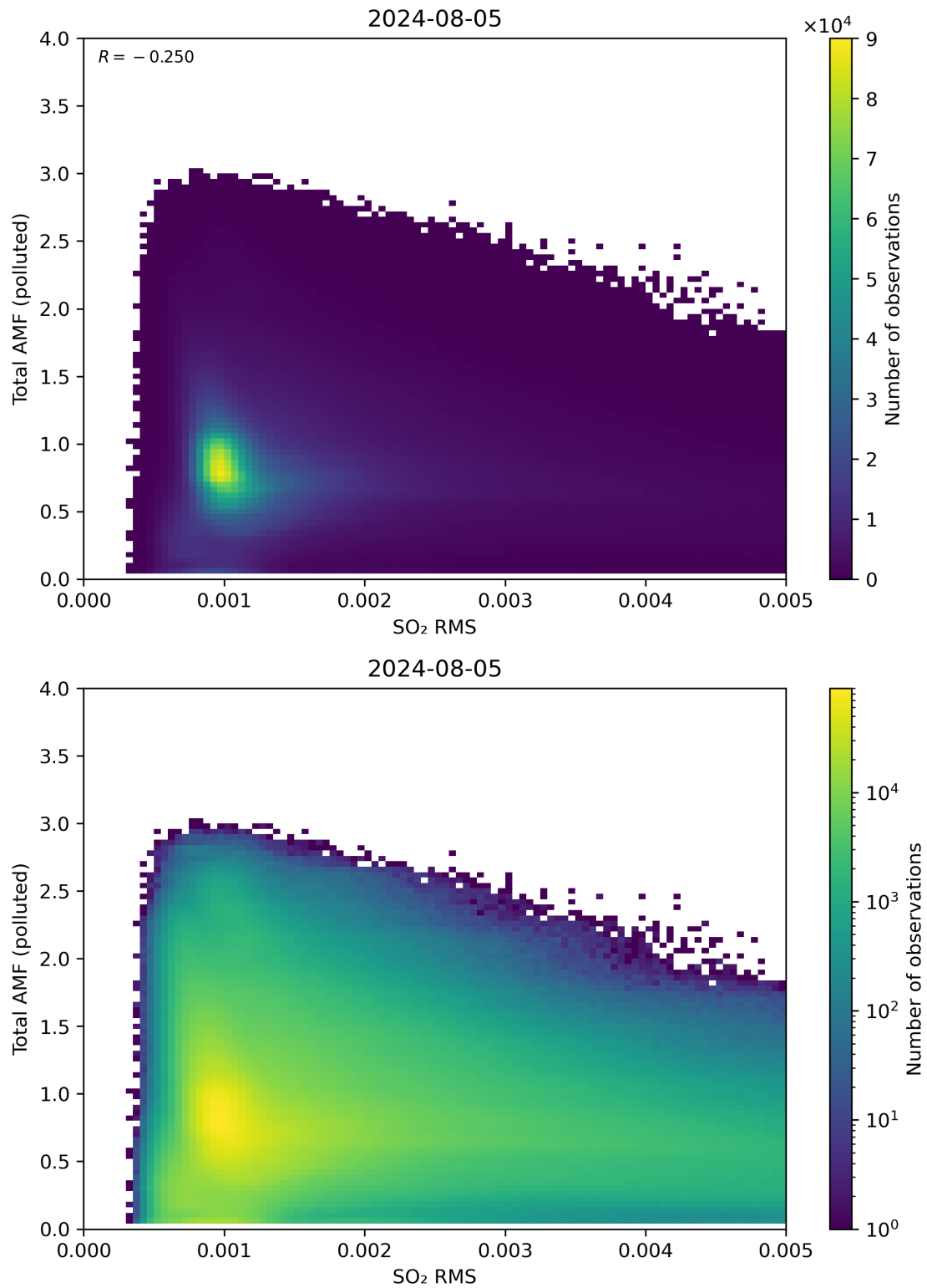
Figure 137: Scatter density plot of “SO 2 RMS” against “Total AMF (polluted)” for 2024-08-04 to 2024-08-06.
