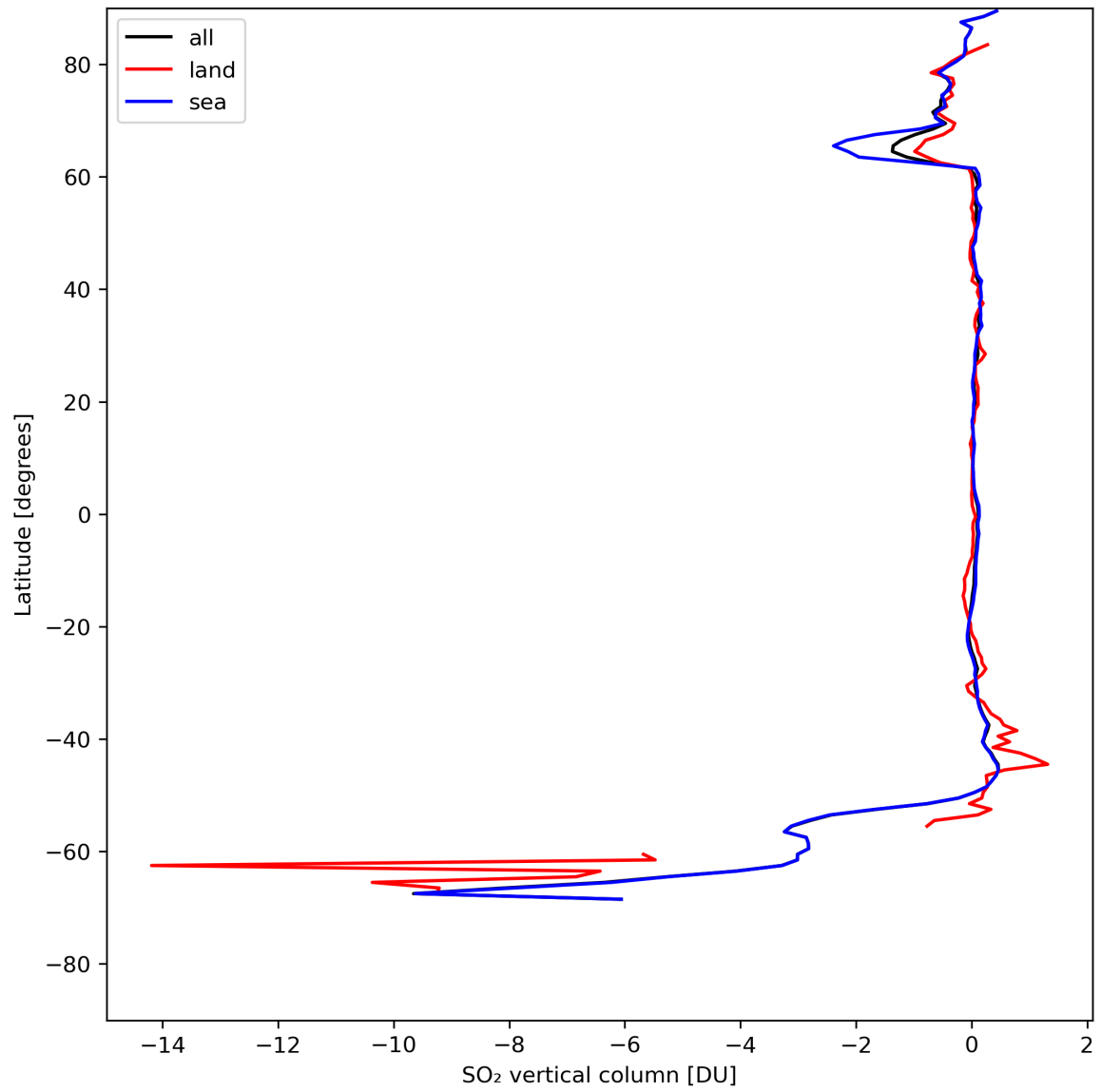
Figure 30: Zonal average of “SO 2 vertical column” for 2024-08-04 to 2024-08-06.
