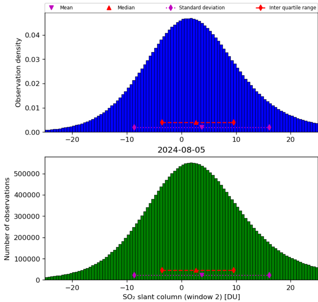
Figure 60: Histogram of “SO 2 slant column (window 2)” for 2024-08-04 to 2024-08-06
