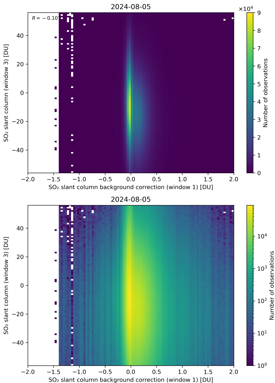
Figure 107: Scatter density plot of “SO 2 slant column background correction (window 1)” against “SO 2 slant column (window 3)” for 2024-08-04 to 2024-08-06.
