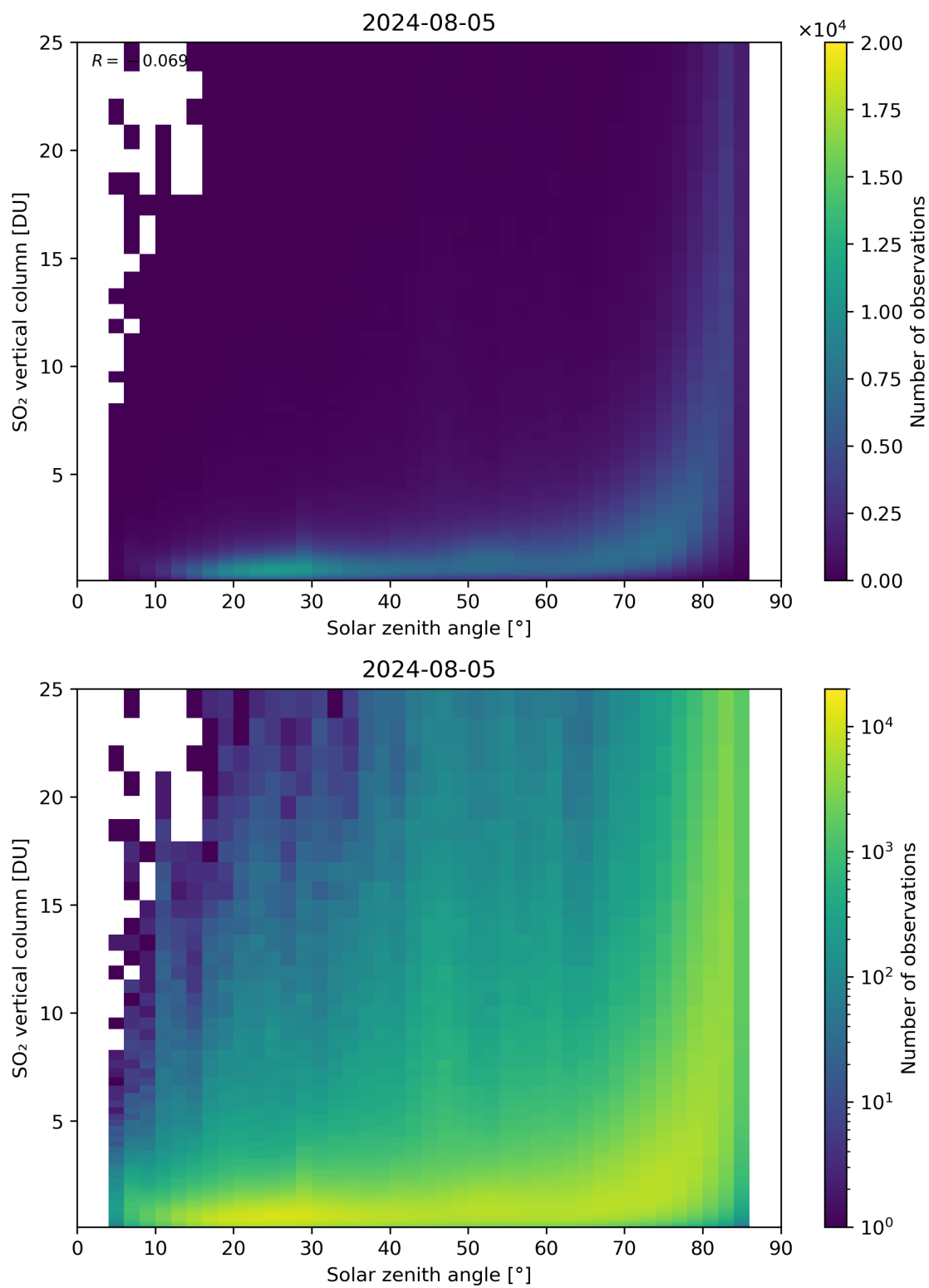
Figure 176: Scatter density plot of “Solar zenith angle” against “SO 2 vertical column” for 2024-08-04 to 2024-08-06.
