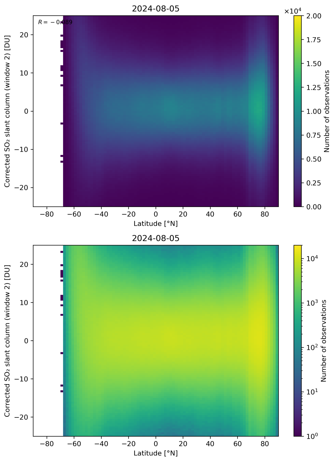
Figure 147: Scatter density plot of “Latitude” against “Corrected SO 2 slant column (window 2)” for 2024-08-04 to 2024-08-06.
