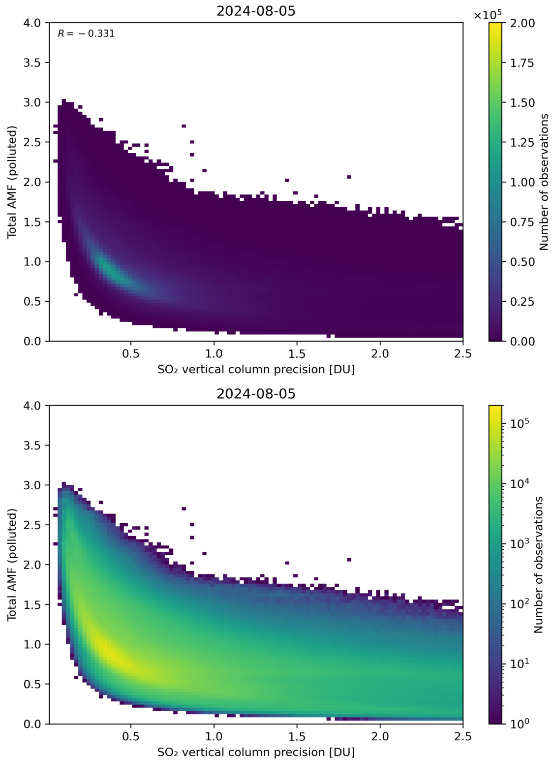
Figure 294: Scatter density plot of “SO 2 vertical column precision” against “Total AMF (polluted)” for 2024-08-04 to 2024-08-06.
