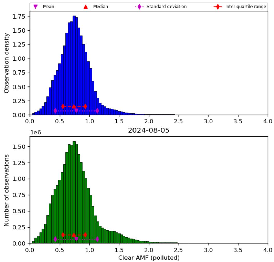
Figure 73: Histogram of “Clear AMF (polluted)” for 2024-08-04 to 2024-08-06
