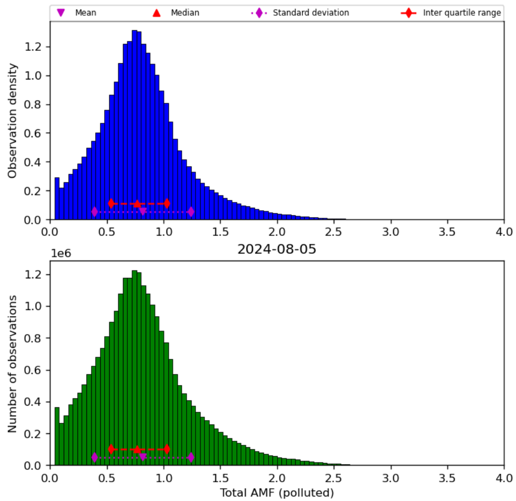
Figure 71: Histogram of “Total AMF (polluted)” for 2024-08-04 to 2024-08-06
