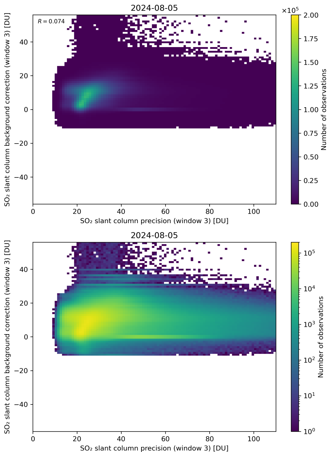
Figure 257: Scatter density plot of “SO 2 slant column precision (window 3)” against “SO 2 slant column background correction (window 3)” for 2024-08-04 to 2024-08-06.
