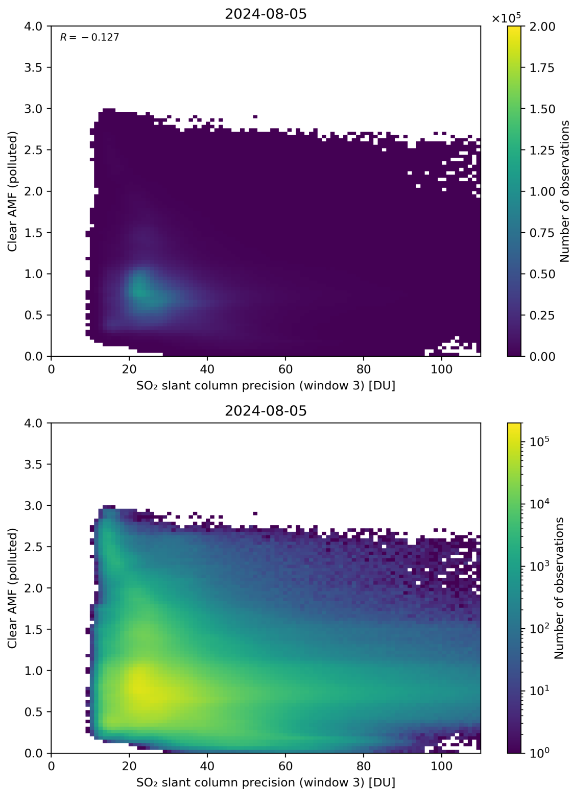
Figure 261: Scatter density plot of “SO 2 slant column precision (window 3)” against “Clear AMF (polluted)” for 2024-08-04 to 2024-08-06.
