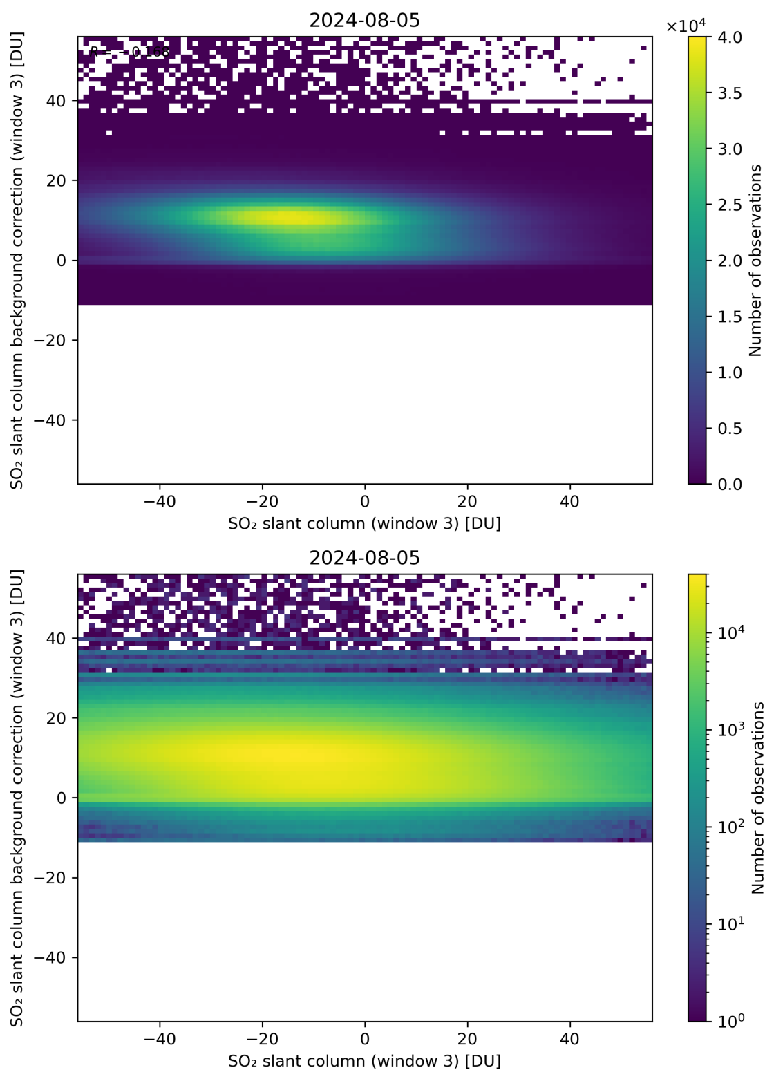
Figure 253: Scatter density plot of “SO 2 slant column (window 3)” against “SO 2 slant column background correction (window 3)” for 2024-08-04 to 2024-08-06.
