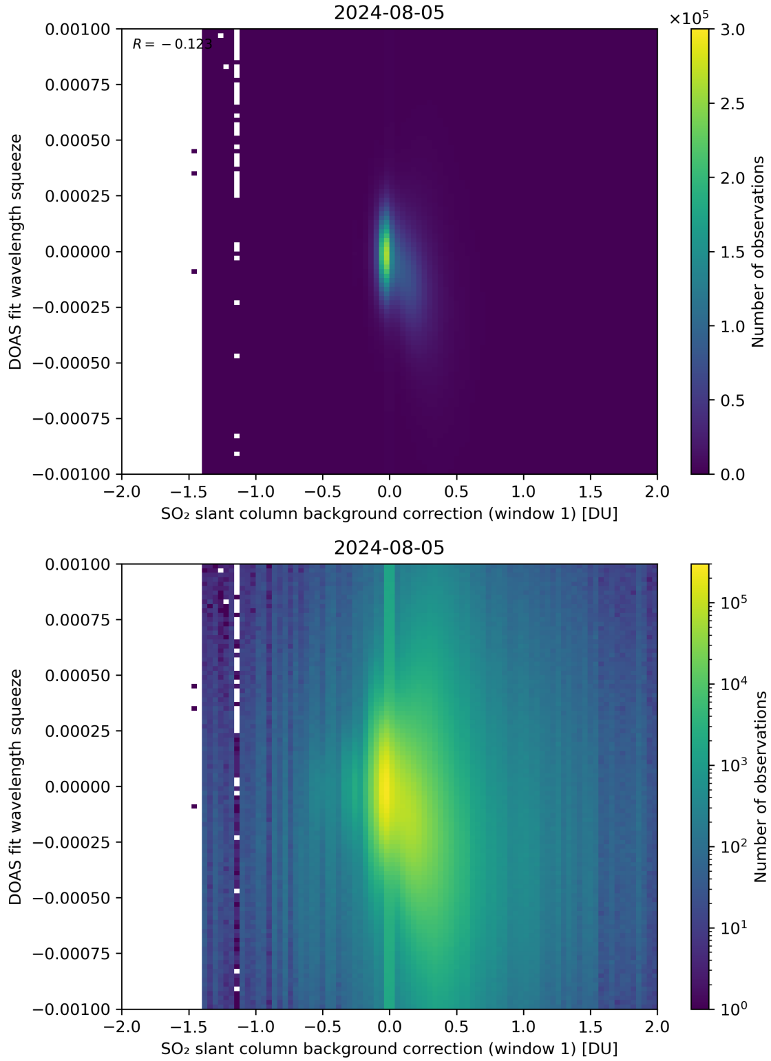
Figure 101: Scatter density plot of “SO 2 slant column background correction (window 1)” against “DOAS fit wavelength squeeze” for 2024-08-04 to 2024-08-06.
