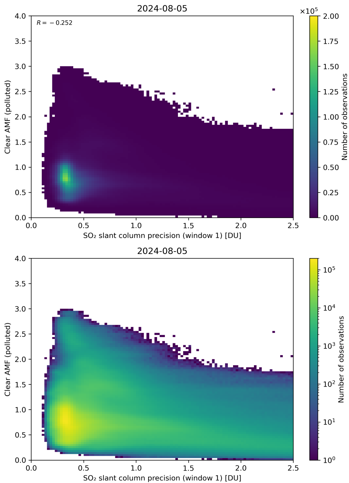
Figure 224: Scatter density plot of “SO 2 slant column precision (window 1)” against “Clear AMF (polluted)” for 2024-08-04 to 2024-08-06.
