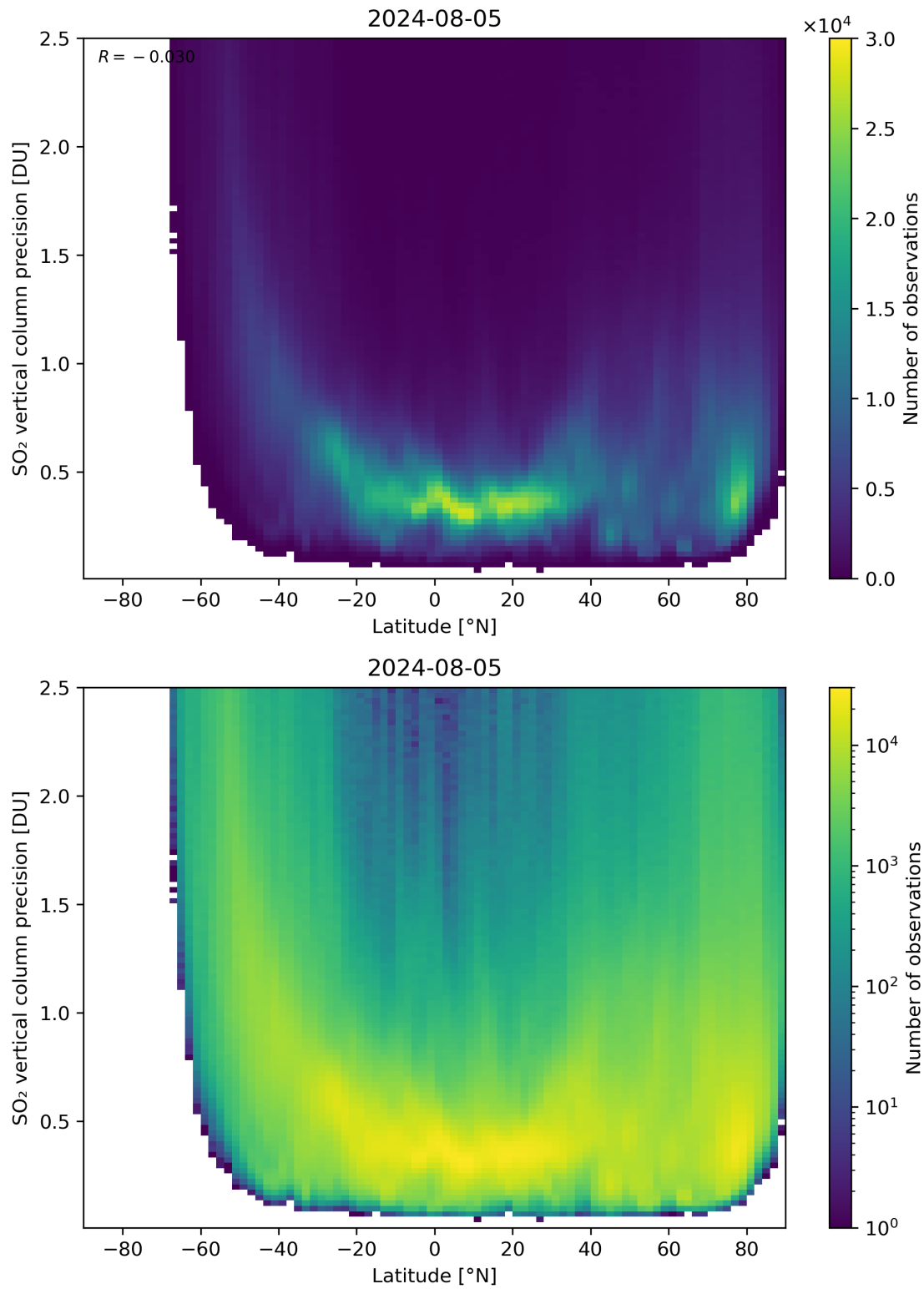
Figure 157: Scatter density plot of “Latitude” against “SO 2 vertical column precision” for 2024-08-04 to 2024-08-06.
