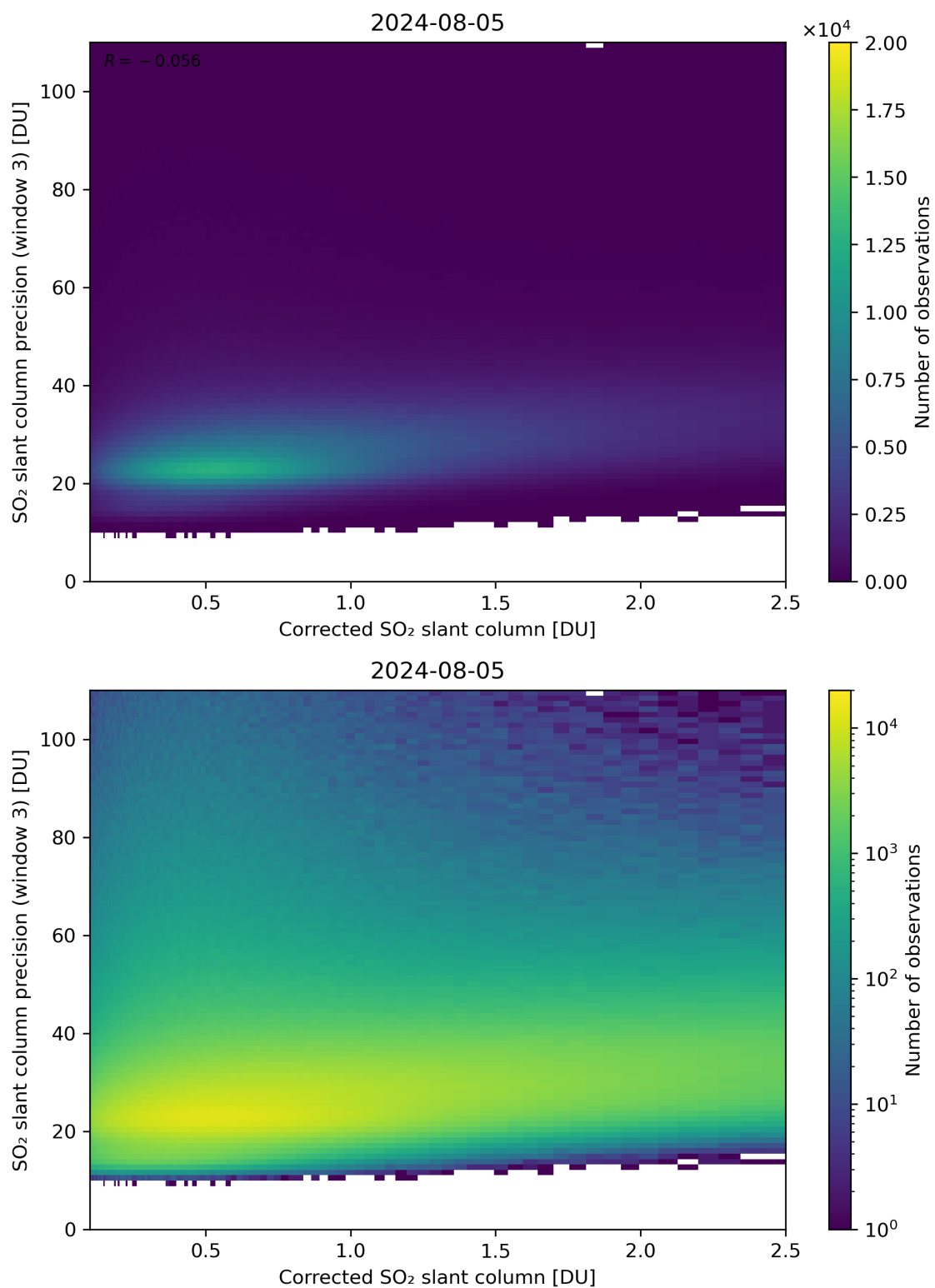
Figure 191: Scatter density plot of “Corrected SO 2 slant column” against “SO 2 slant column precision (window 3)” for 2024-08-04 to 2024-08-06.
