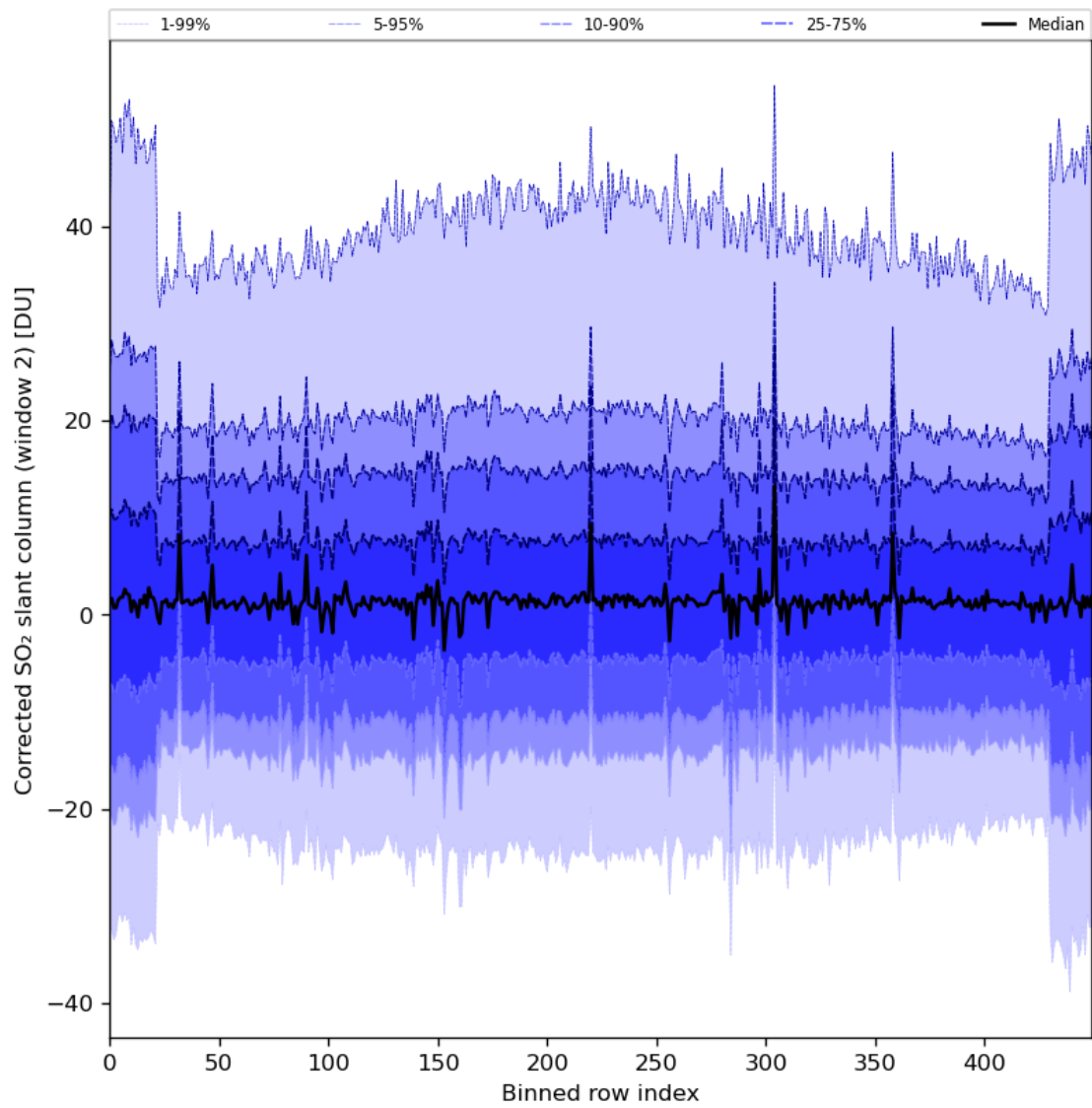
Figure 85: Along track statistics of “Corrected SO 2 slant column (window 2)” for 2024-08-04 to 2024-08-06
