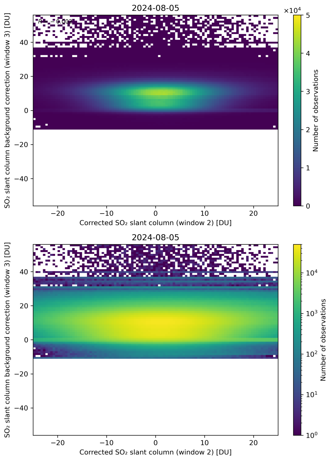
Figure 195: Scatter density plot of “Corrected SO 2 slant column (window 2)” against “SO 2 slant column background correction (window 3)” for 2024-08-04 to 2024-08-06.
