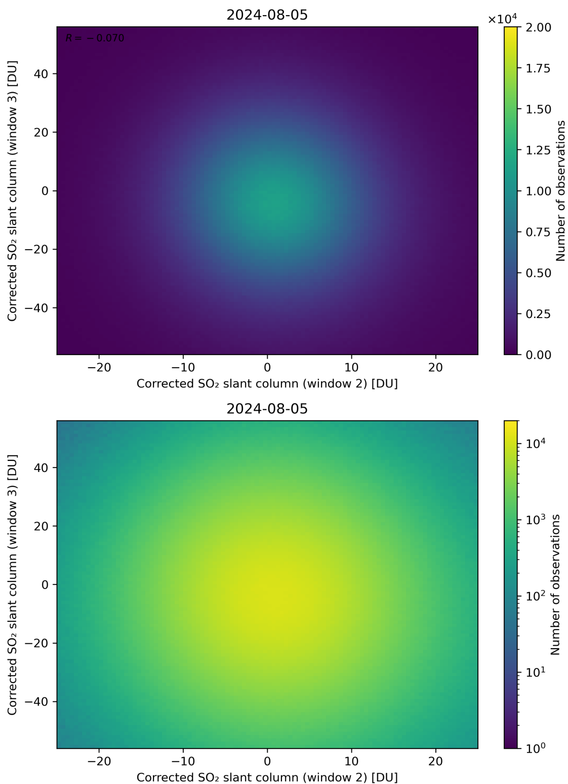
Figure 200: Scatter density plot of “Corrected SO 2 slant column (window 2)” against “Corrected SO 2 slant column (window 3)” for 2024-08-04 to 2024-08-06.
