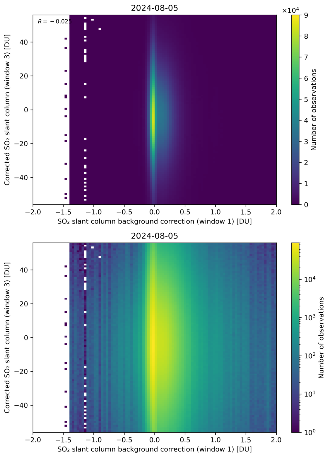
Figure 105: Scatter density plot of “SO 2 slant column background correction (window 1)” against “Corrected SO 2 slant column (window 3)” for 2024-08-04 to 2024-08-06.
