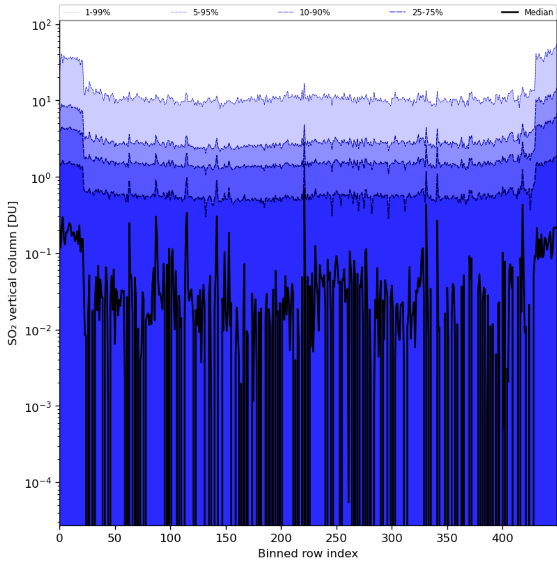
Figure 76: Along track statistics of “SO 2 vertical column” for 2024-08-04 to 2024-08-06
