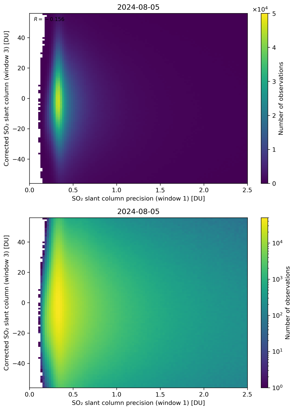
Figure 226: Scatter density plot of “SO 2 slant column precision (window 1)” against “Corrected SO 2 slant column (window 3)” for 2024-08-04 to 2024-08-06.
