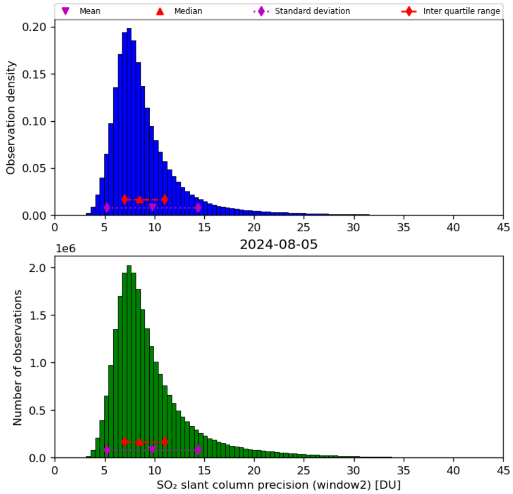
Figure 61: Histogram of “SO 2 slant column precision (window2)” for 2024-08-04 to 2024-08-06
