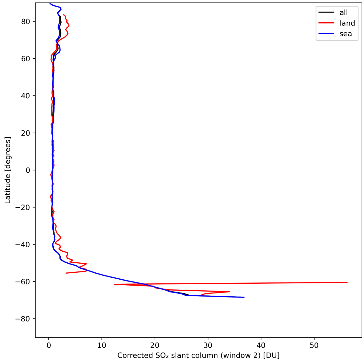
Figure 39: Zonal average of “Corrected SO 2 slant column (window 2)” for 2024-08-04 to 2024-08-06.
