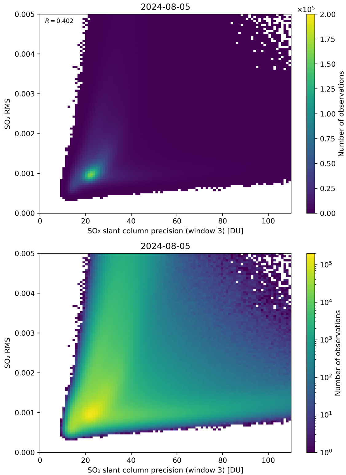
Figure 260: Scatter density plot of “SO 2 slant column precision (window 3)” against “SO 2 RMS” for 2024-08-04 to 2024-08-06.
