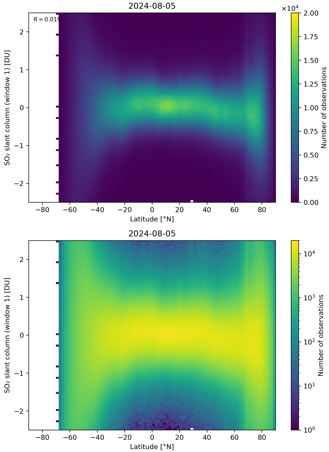
Figure 149: Scatter density plot of “Latitude” against “SO 2 slant column (window 1)” for 2024-08-04 to 2024-08-06.
