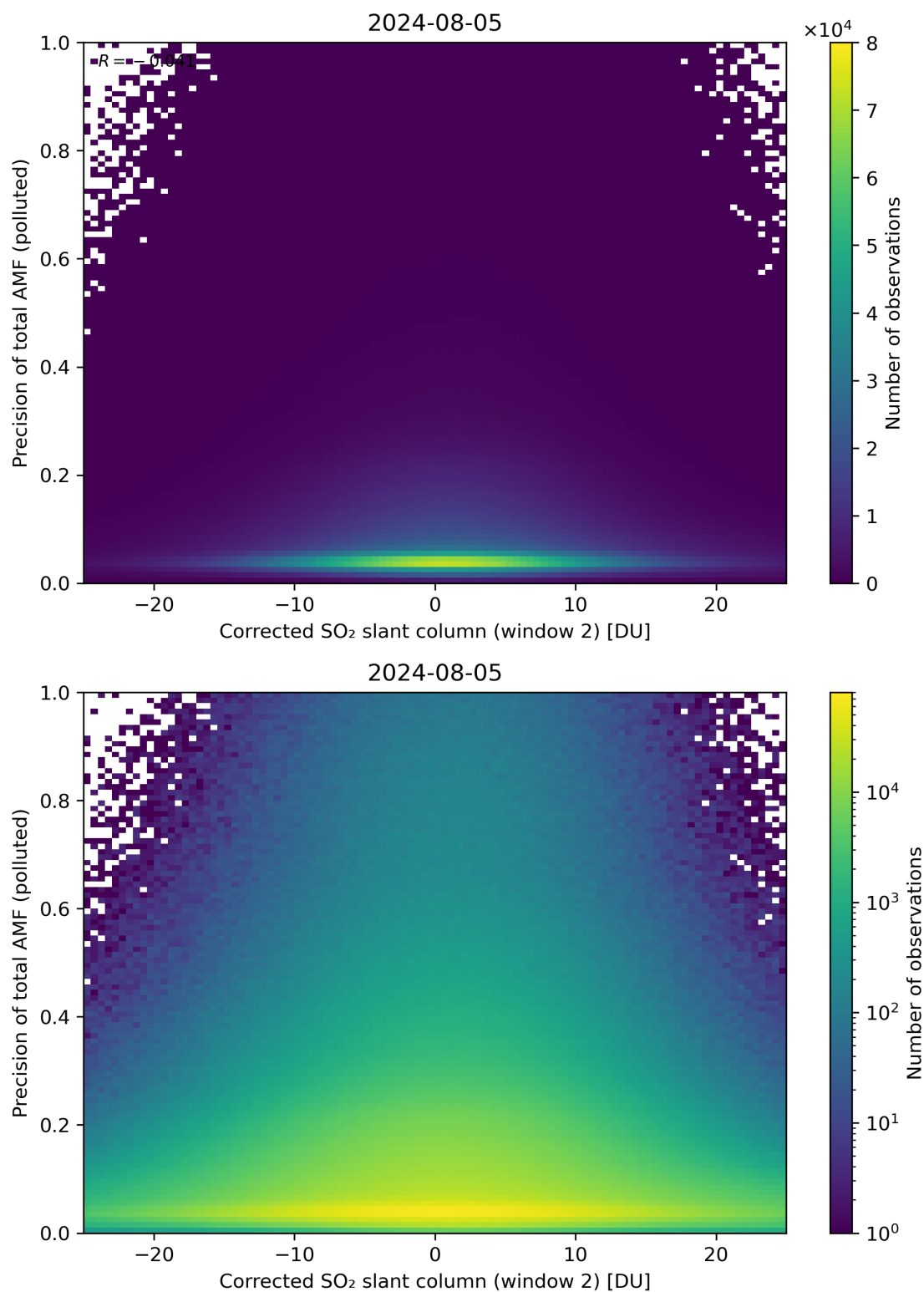
Figure 204: Scatter density plot of “Corrected SO 2 slant column (window 2)” against “Precision of total AMF (polluted)” for 2024-08-04 to 2024-08-06.
