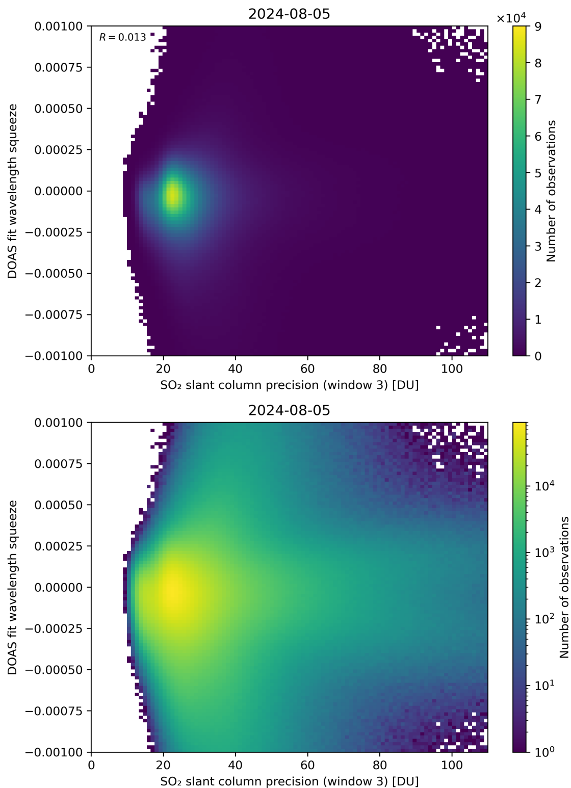
Figure 259: Scatter density plot of “SO 2 slant column precision (window 3)” against “DOAS fit wavelength squeeze” for 2024-08-04 to 2024-08-06.
