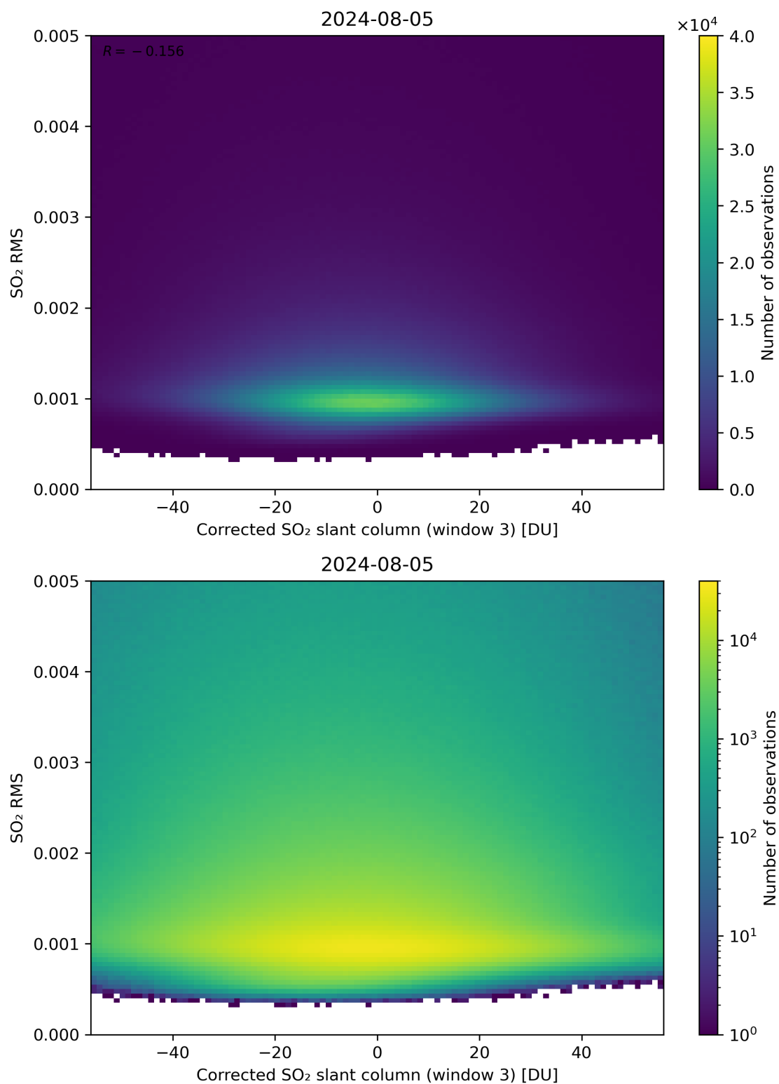
Figure 208: Scatter density plot of “Corrected SO 2 slant column (window 3)” against “SO 2 RMS” for 2024-08-04 to 2024-08-06.
