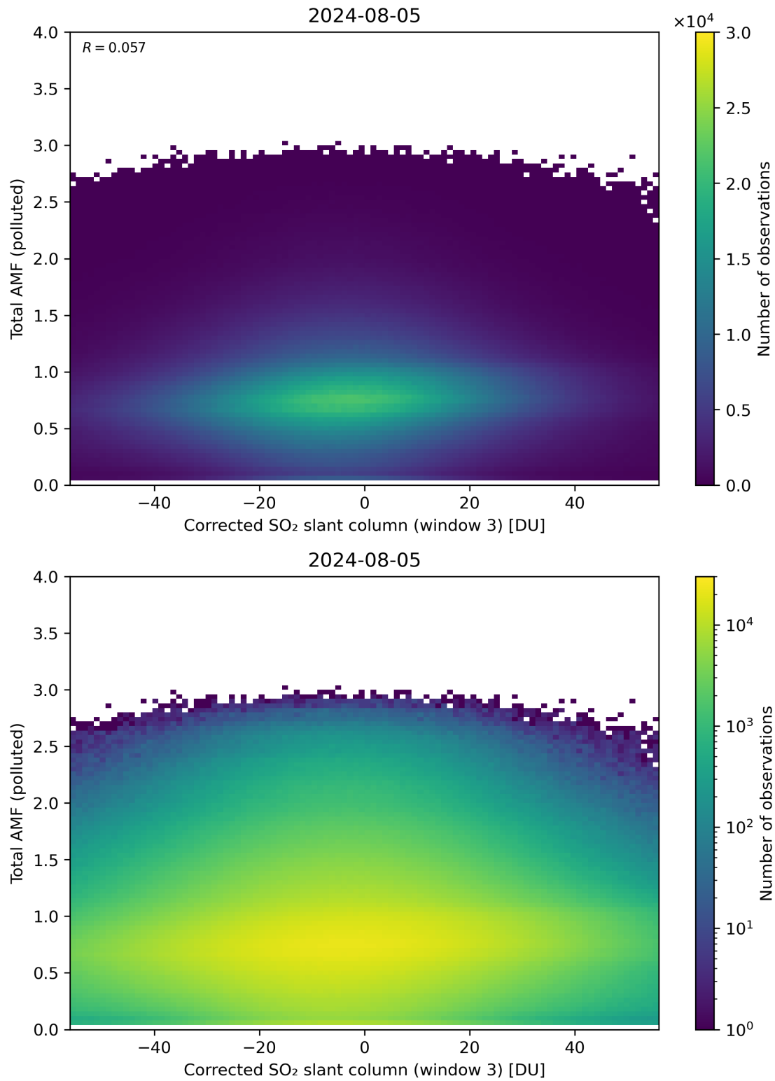
Figure 210: Scatter density plot of “Corrected SO 2 slant column (window 3)” against “Total AMF (polluted)” for 2024-08-04 to 2024-08-06.
