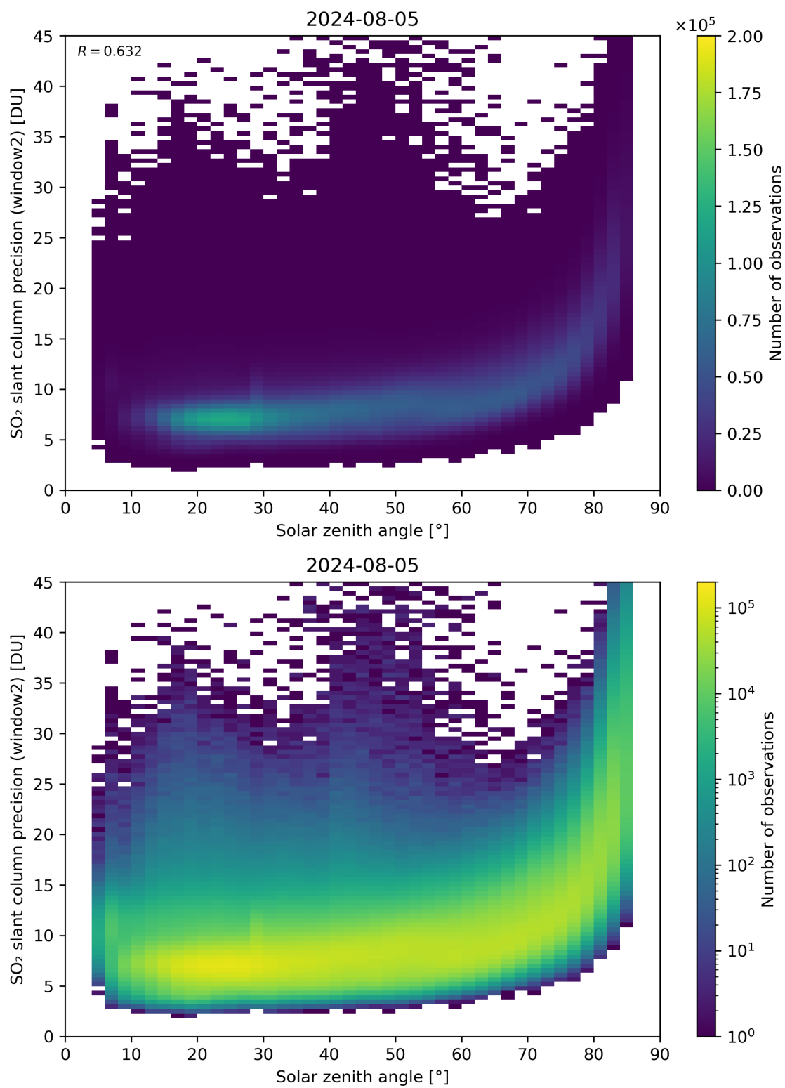
Figure 171: Scatter density plot of “Solar zenith angle” against “SO 2 slant column precision (window2)” for 2024-08-04 to 2024-08-06.
