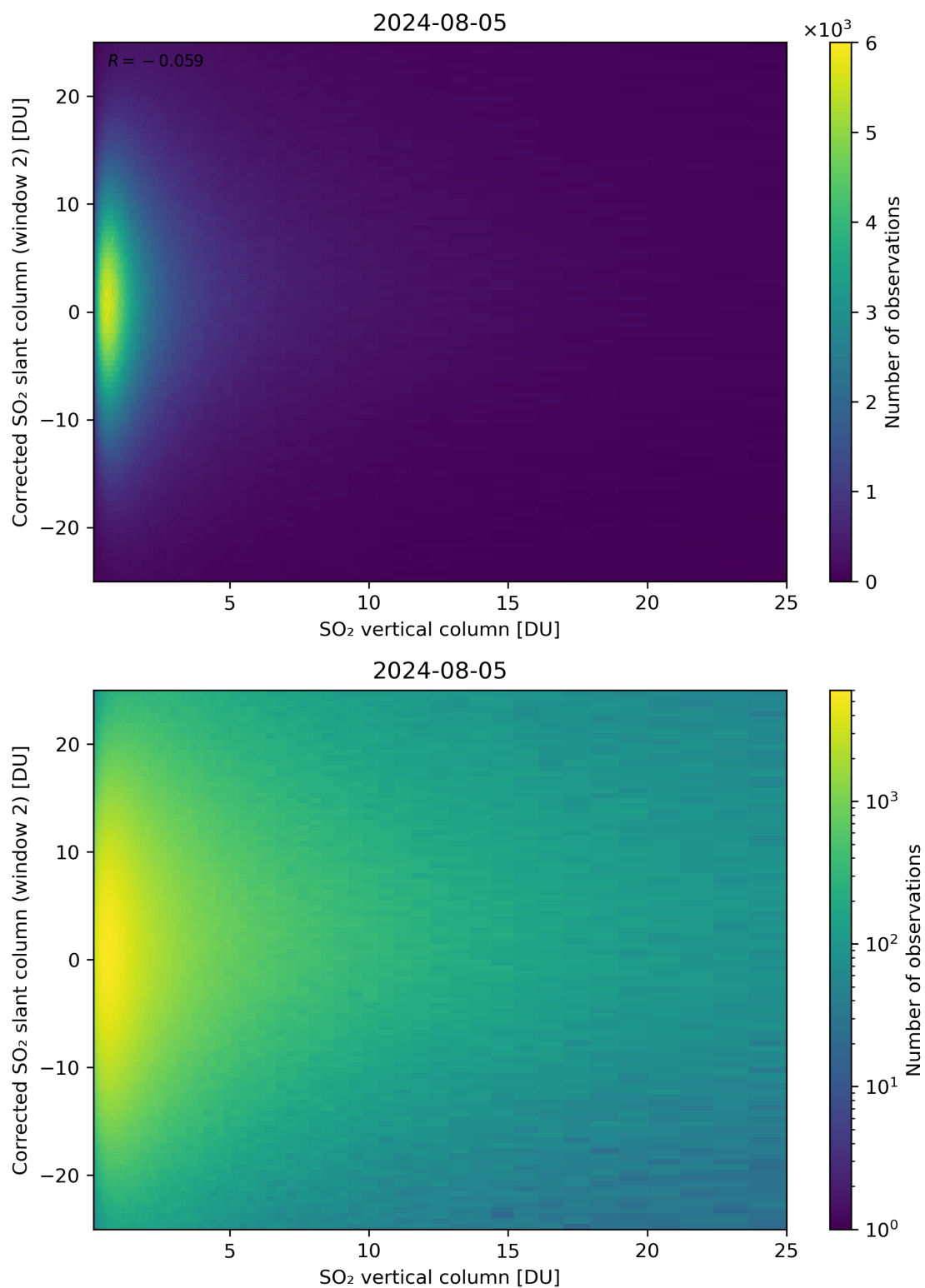
Figure 298: Scatter density plot of “SO 2 vertical column” against “Corrected SO 2 slant column (window 2)” for 2024-08-04 to 2024-08-06.
