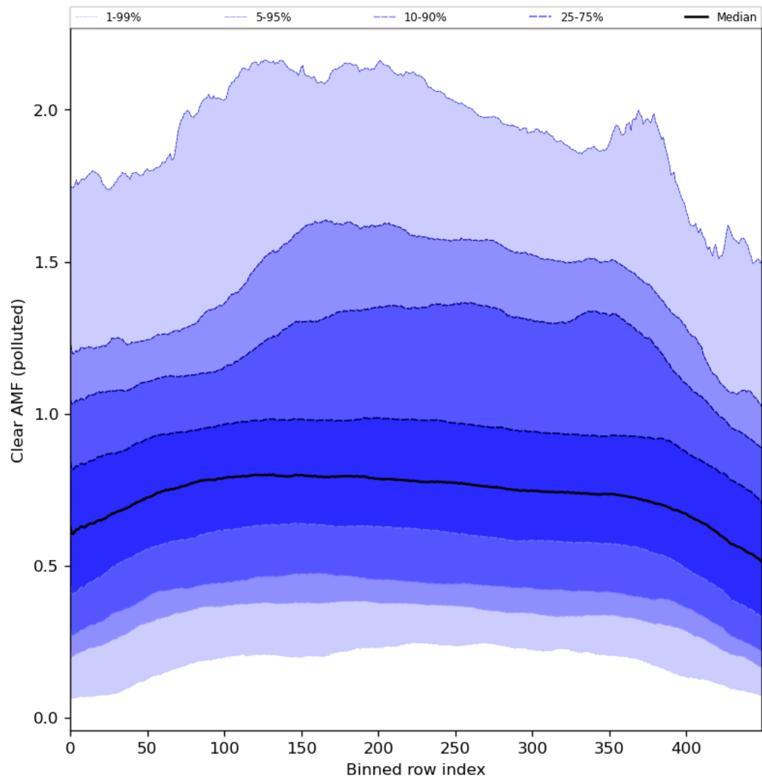
Figure 96: Along track statistics of “Clear AMF (polluted)” for 2024-08-04 to 2024-08-06
