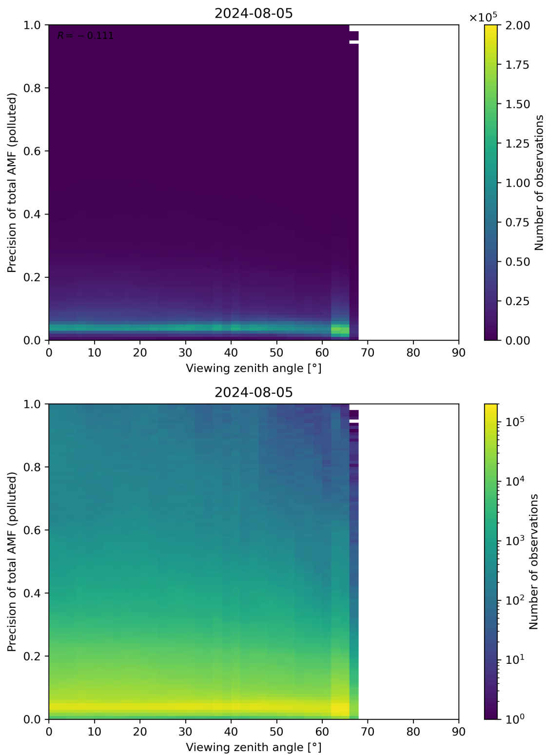
Figure 326: Scatter density plot of “Viewing zenith angle” against “Precision of total AMF (polluted)” for 2024-08-04 to 2024-08-06.
