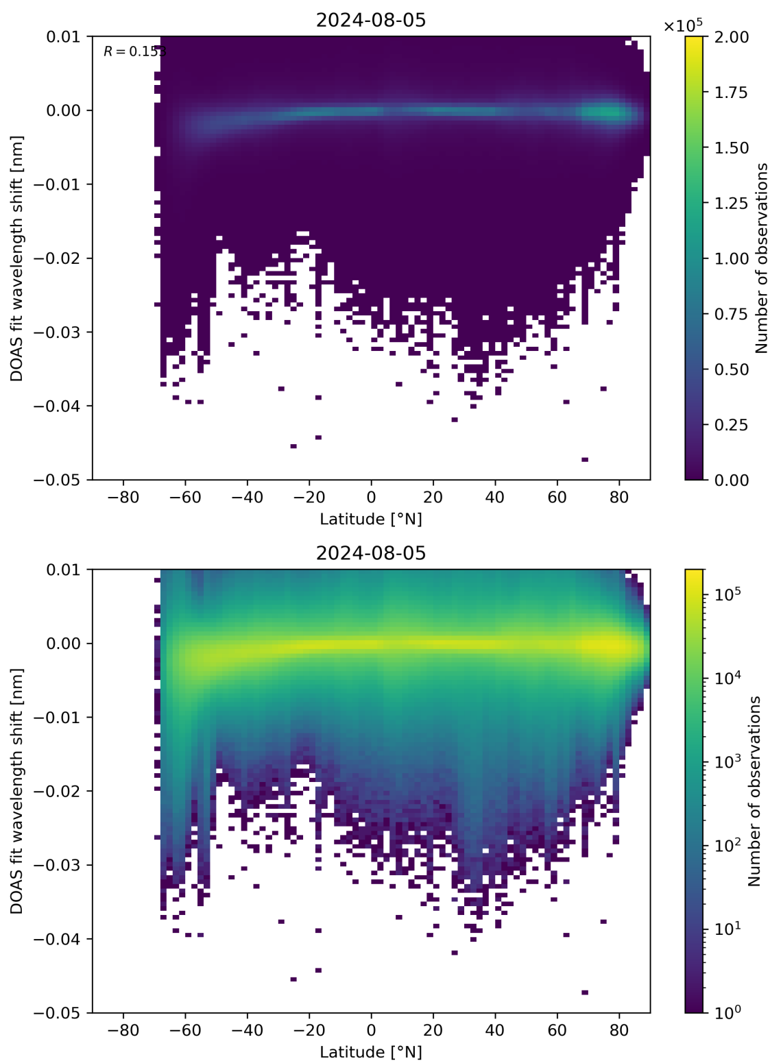
Figure 142: Scatter density plot of “Latitude” against “DOAS fit wavelength shift” for 2024-08-04 to 2024-08-06.
