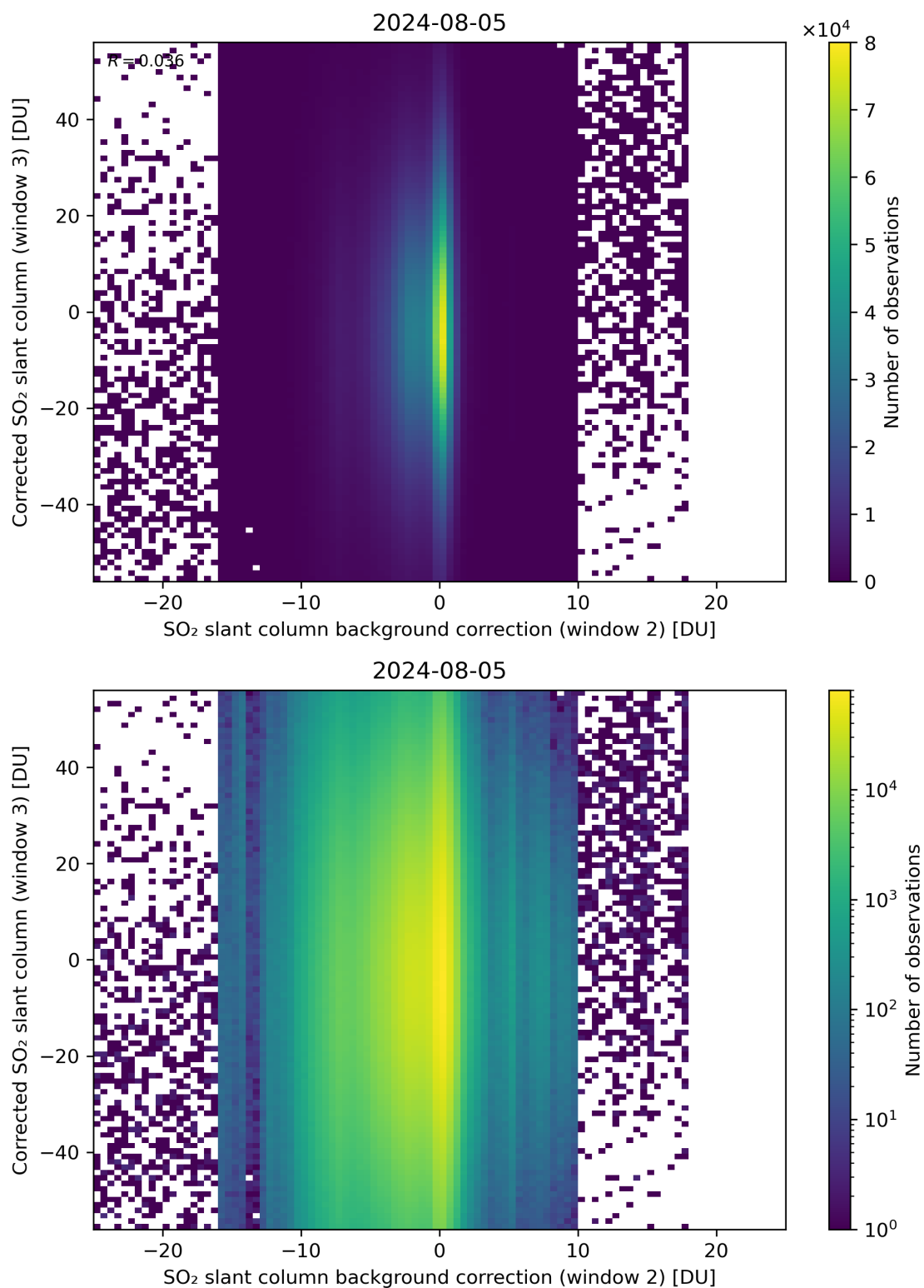
Figure 116: Scatter density plot of “SO 2 slant column background correction (window 2)” against “Corrected SO 2 slant column (window 3)” for 2024-08-04 to 2024-08-06.
