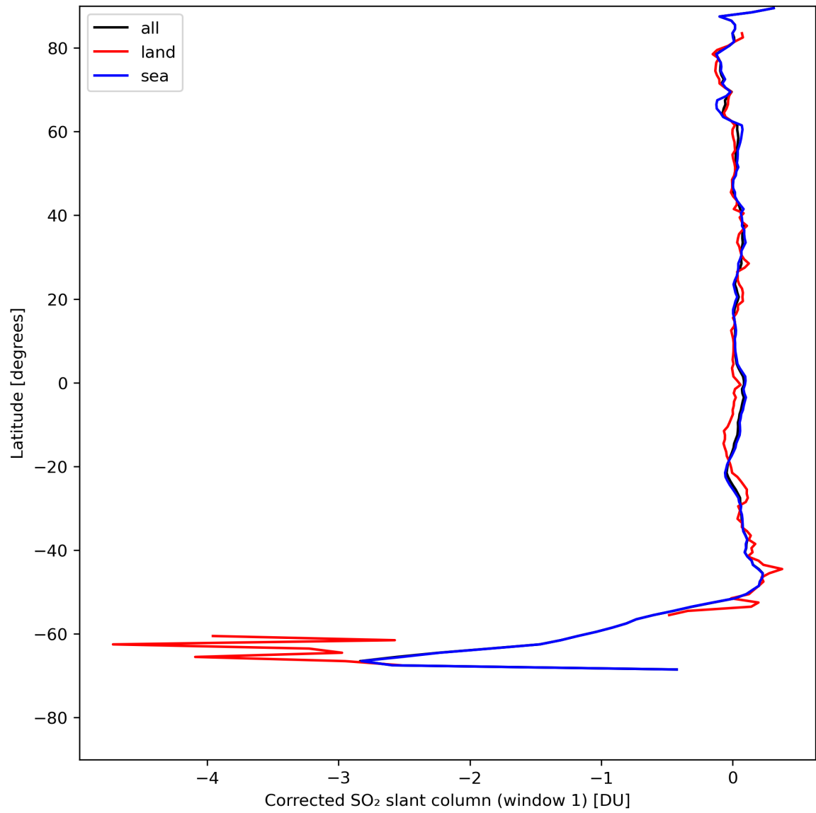
Figure 35: Zonal average of “Corrected SO 2 slant column (window 1)” for 2024-08-04 to 2024-08-06.
