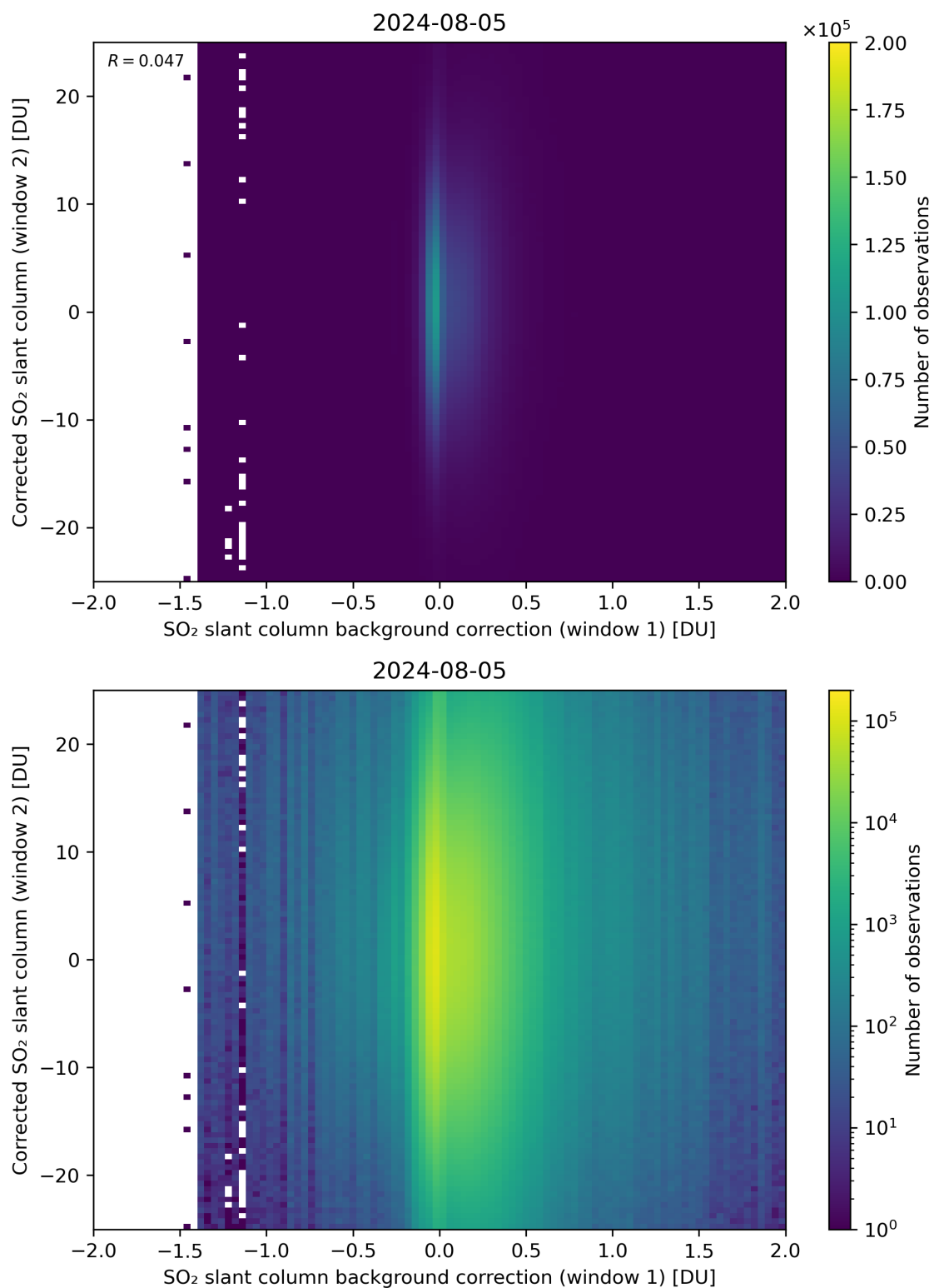
Figure 104: Scatter density plot of “SO 2 slant column background correction (window 1)” against “Corrected SO 2 slant column (window 2)” for 2024-08-04 to 2024-08-06.
