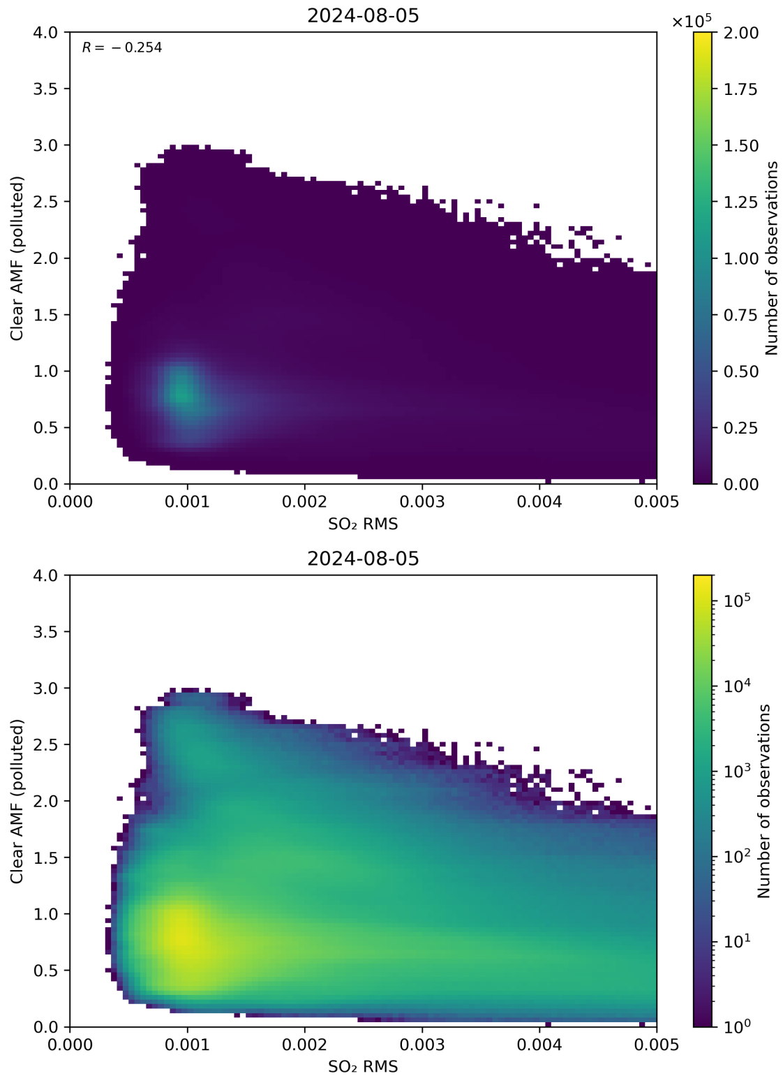
Figure 136: Scatter density plot of “SO 2 RMS” against “Clear AMF (polluted)” for 2024-08-04 to 2024-08-06.
