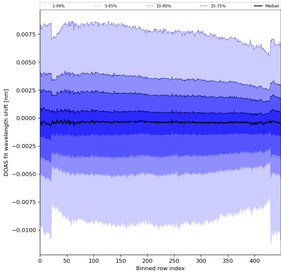
Figure 91: Along track statistics of “DOAS fit wavelength shift” for 2024-08-04 to 2024-08-06
