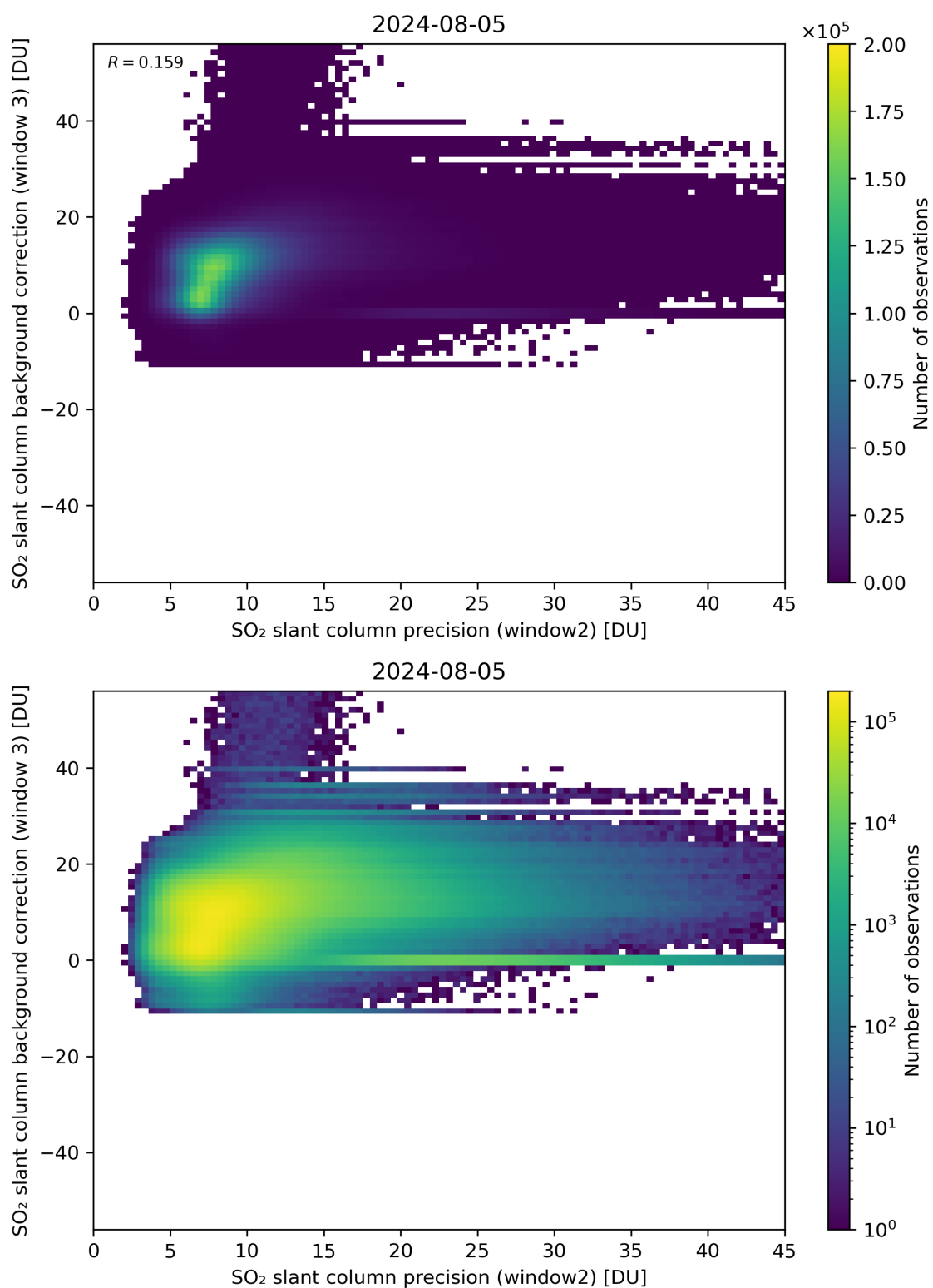
Figure 242: Scatter density plot of “SO 2 slant column precision (window2)” against “SO 2 slant column background correction (window 3)” for 2024-08-04 to 2024-08-06.
