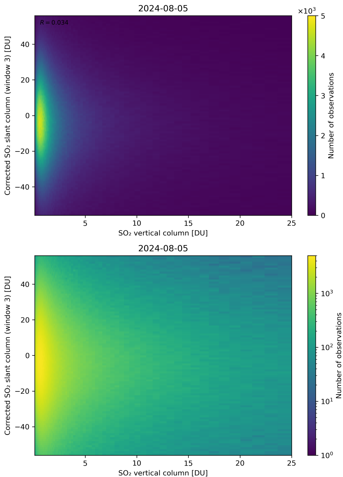
Figure 299: Scatter density plot of “SO 2 vertical column” against “Corrected SO 2 slant column (window 3)” for 2024-08-04 to 2024-08-06.
