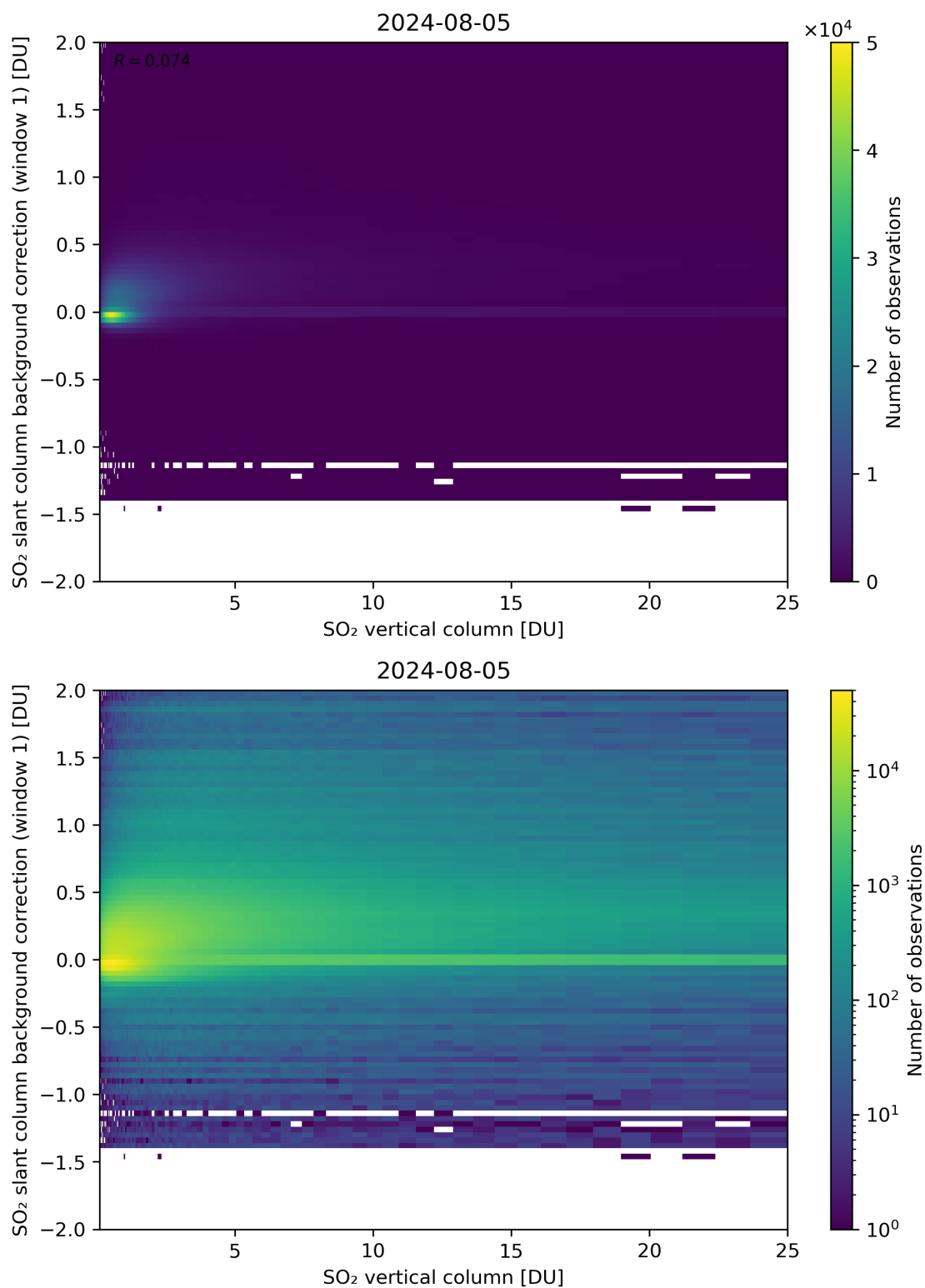
Figure 273: Scatter density plot of “SO 2 vertical column” against “SO 2 slant column background correction (window 1)” for 2024-08-04 to 2024-08-06.
