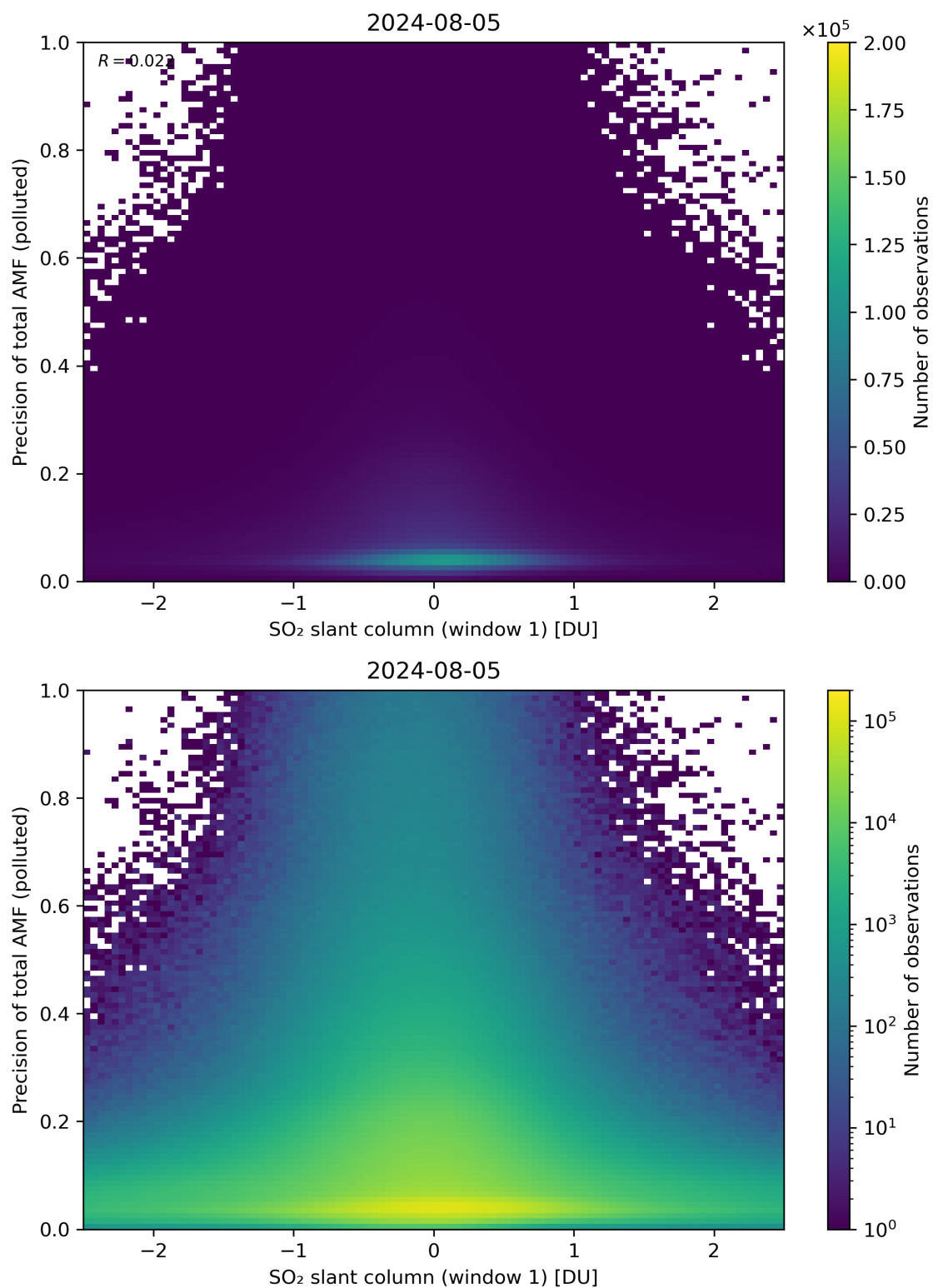
Figure 240: Scatter density plot of “SO 2 slant column (window 1)” against “Precision of total AMF (polluted)” for 2024-08-04 to 2024-08-06.
