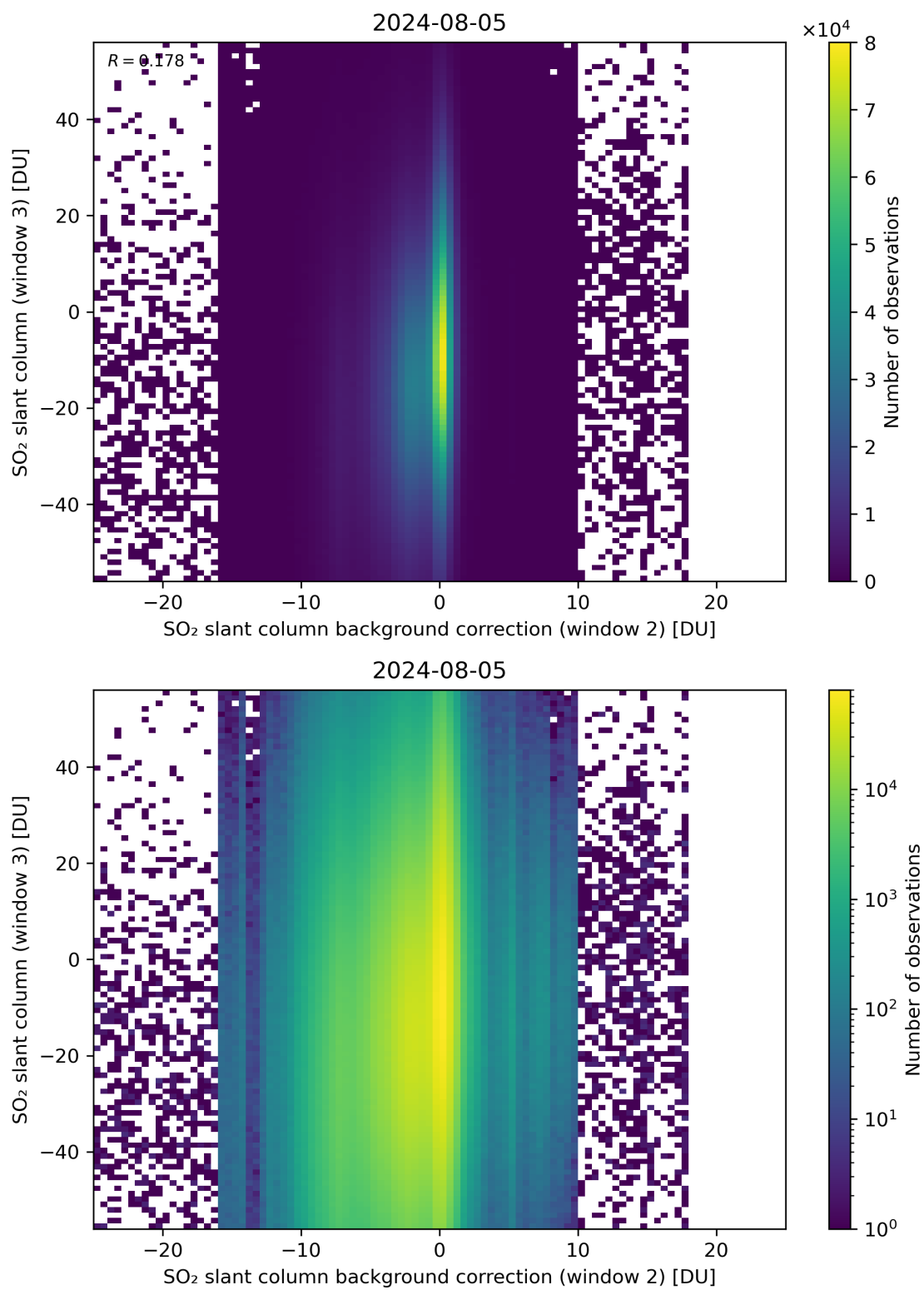
Figure 117: Scatter density plot of “SO 2 slant column background correction (window 2)” against “SO 2 slant column (window 3)” for 2024-08-04 to 2024-08-06.
