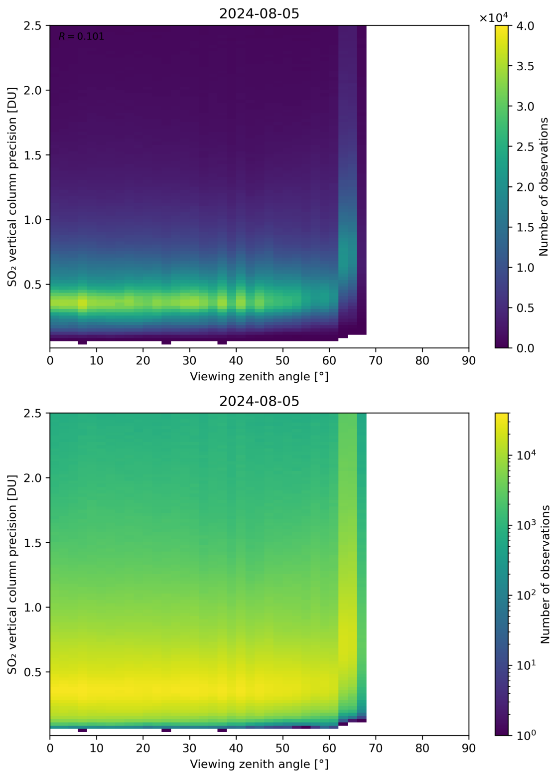
Figure 328: Scatter density plot of “Viewing zenith angle” against “SO 2 vertical column precision” for 2024-08-04 to 2024-08-06.
