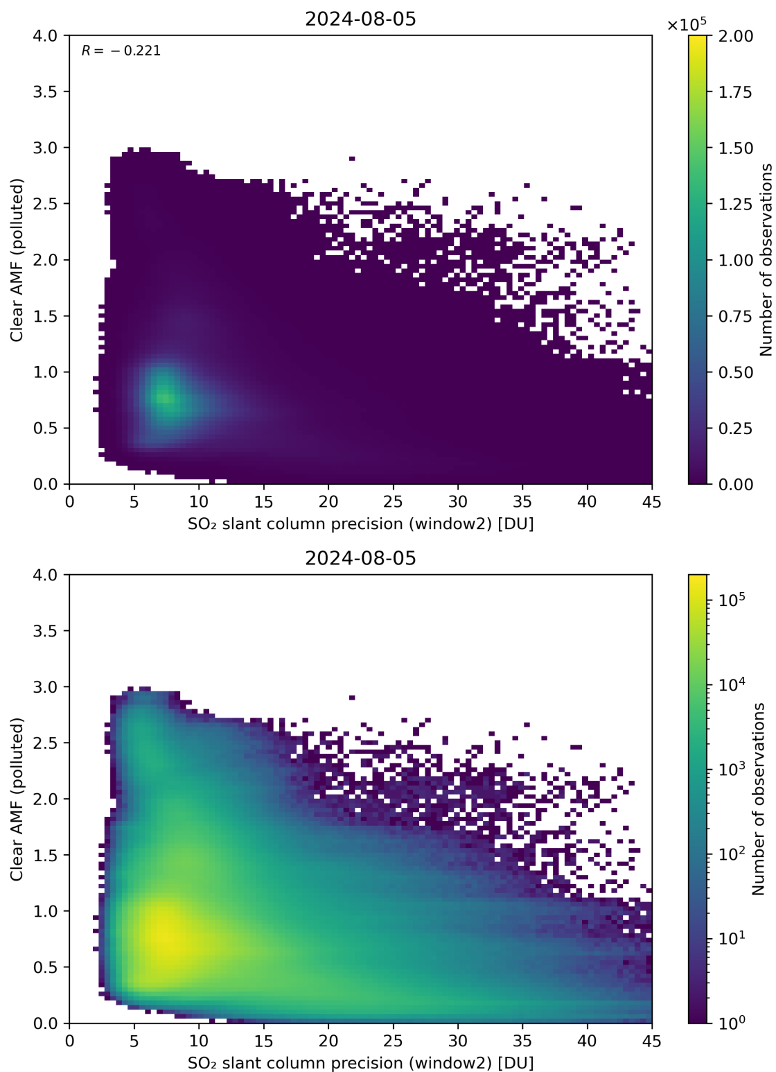
Figure 246: Scatter density plot of “SO 2 slant column precision (window2)” against “Clear AMF (polluted)” for 2024-08-04 to 2024-08-06.
