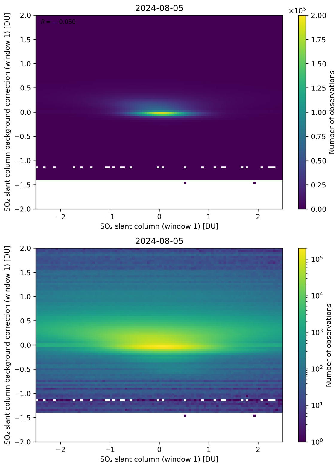
Figure 212: Scatter density plot of “SO 2 slant column (window 1)” against “SO 2 slant column background correction (window 1)” for 2024-08-04 to 2024-08-06.
