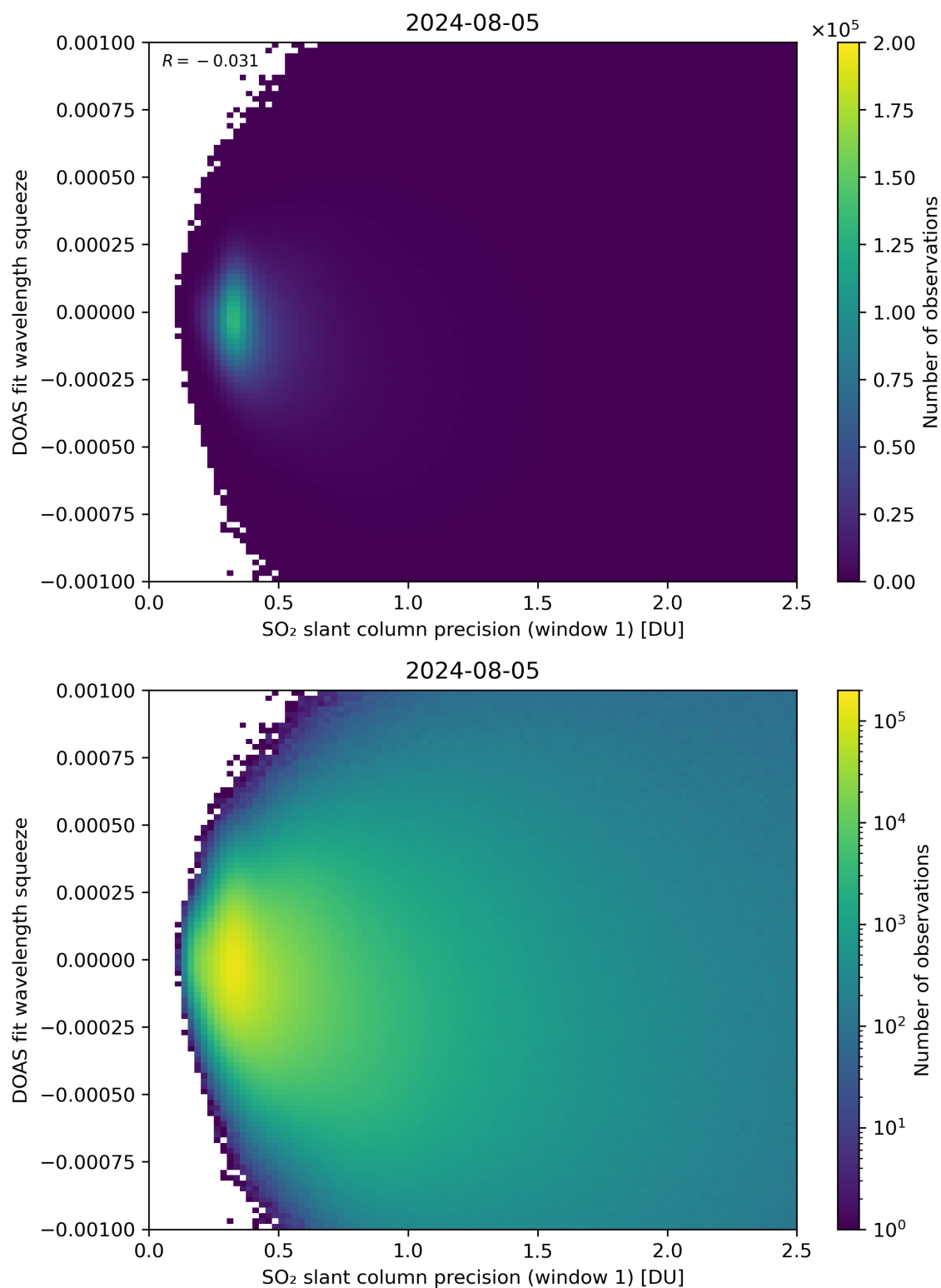
Figure 222: Scatter density plot of “SO 2 slant column precision (window 1)” against “DOAS fit wavelength squeeze” for 2024-08-04 to 2024-08-06.
