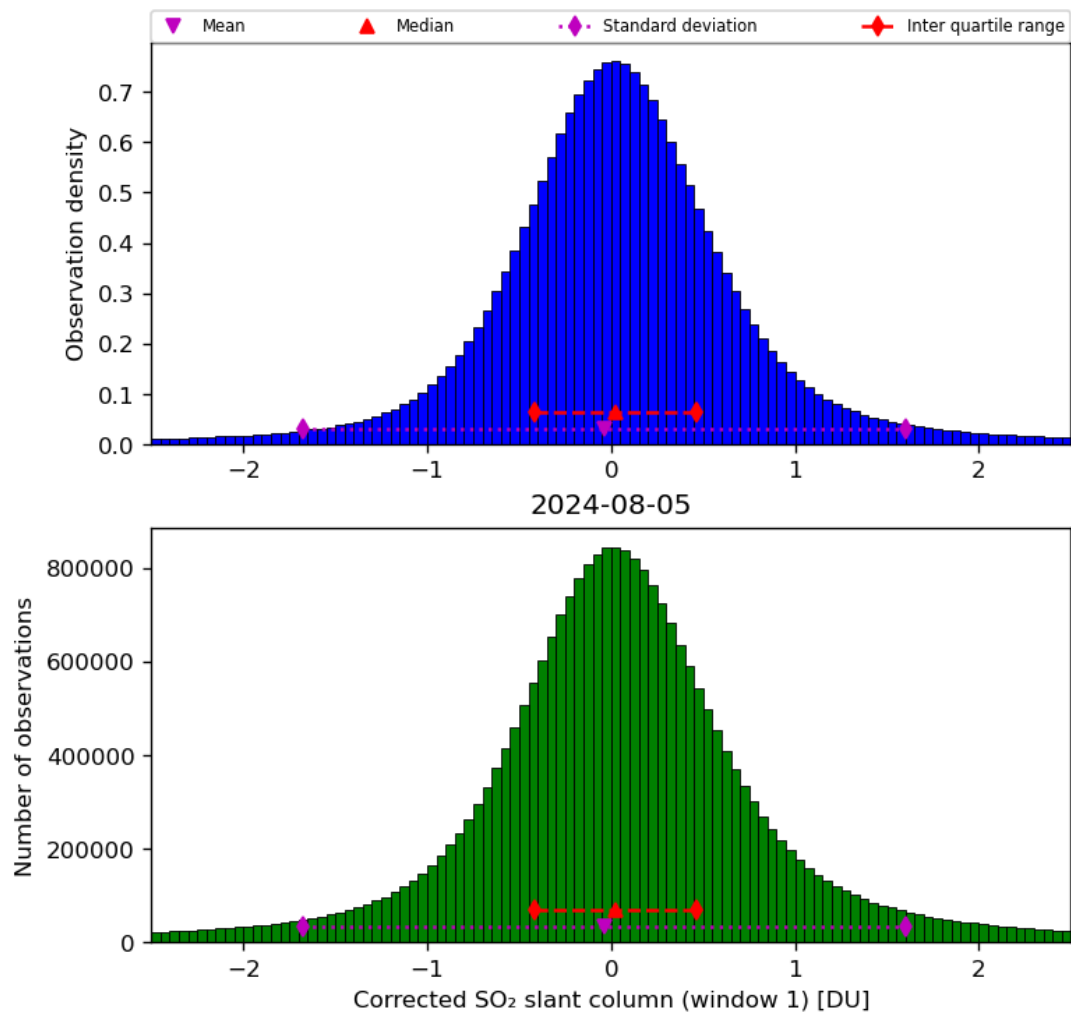
Figure 58: Histogram of “Corrected SO 2 slant column (window 1)” for 2024-08-04 to 2024-08-06
