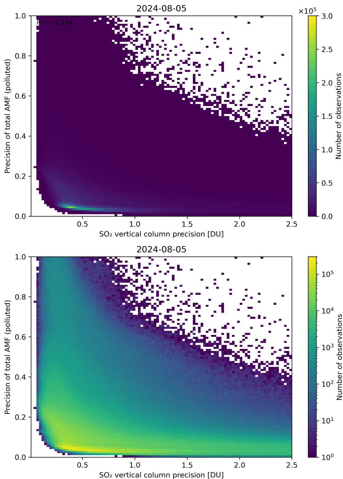
Figure 295: Scatter density plot of “SO 2 vertical column precision” against “Precision of total AMF (polluted)” for 2024-08-04 to 2024-08-06.
