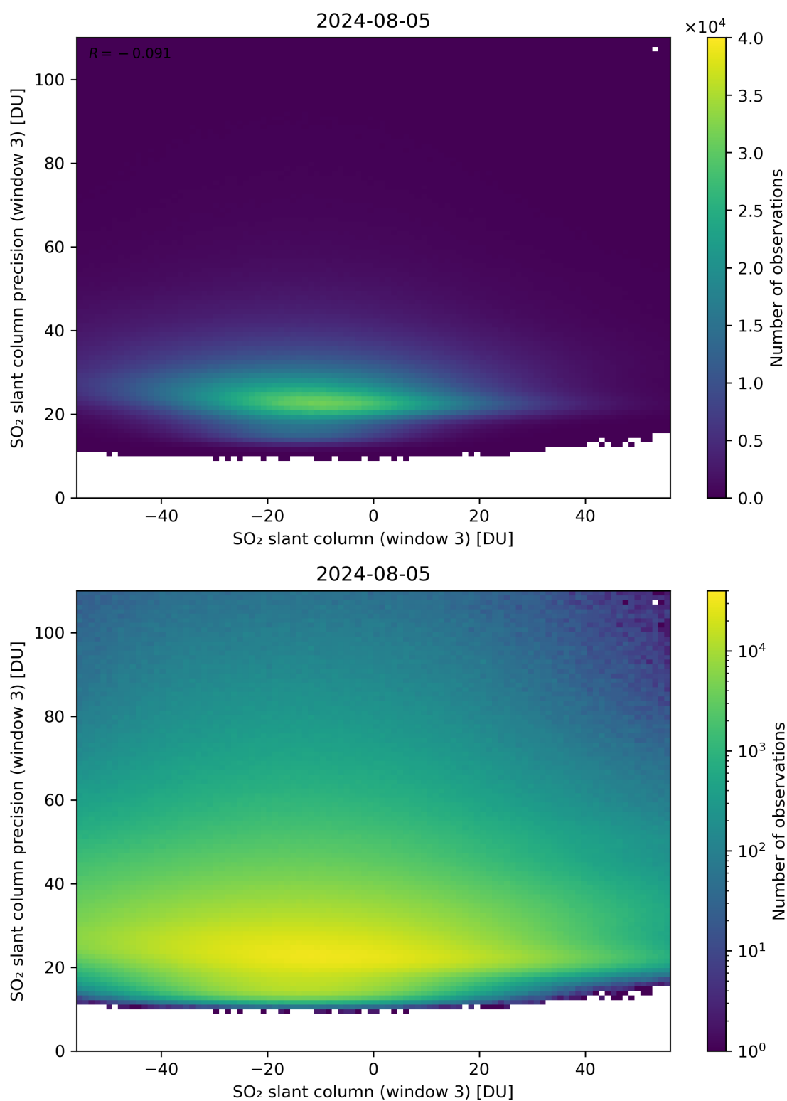
Figure 267: Scatter density plot of “SO 2 slant column (window 3)” against “SO 2 slant column precision (window 3)” for 2024-08-04 to 2024-08-06.
