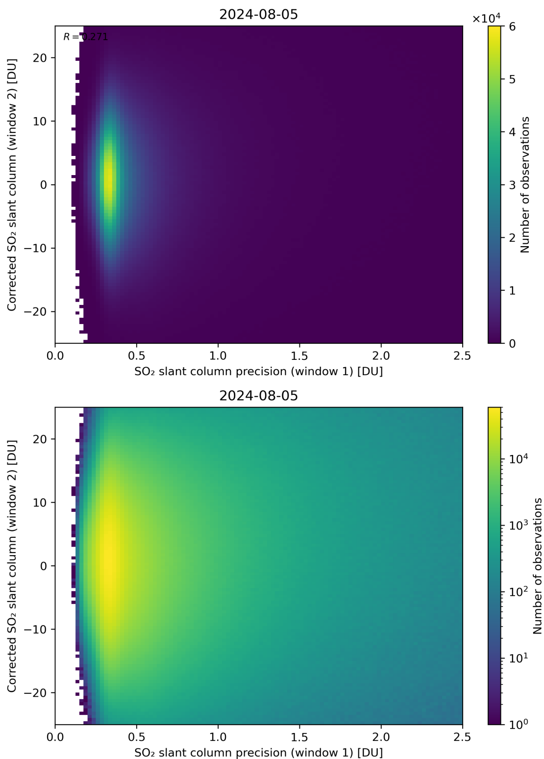
Figure 225: Scatter density plot of “SO 2 slant column precision (window 1)” against “Corrected SO 2 slant column (window 2)” for 2024-08-04 to 2024-08-06.
