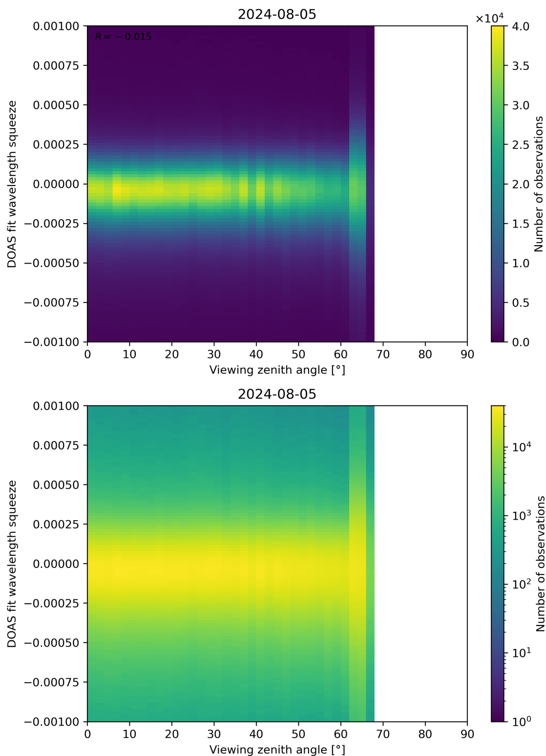
Figure 312: Scatter density plot of “Viewing zenith angle” against “DOAS fit wavelength squeeze” for 2024-08-04 to 2024-08-06.
