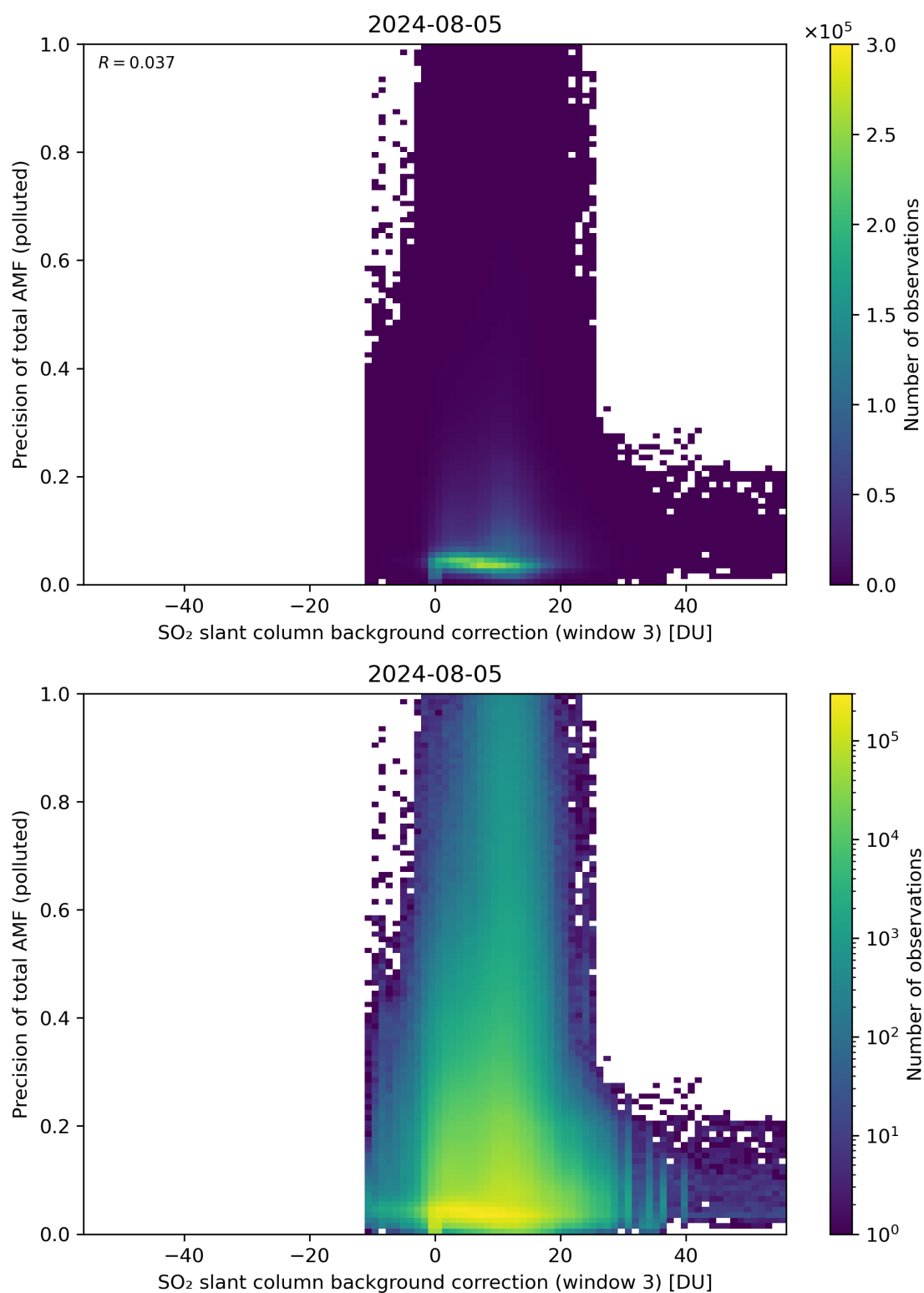
Figure 126: Scatter density plot of “SO 2 slant column background correction (window 3)” against “Precision of total AMF (polluted)” for 2024-08-04 to 2024-08-06.
