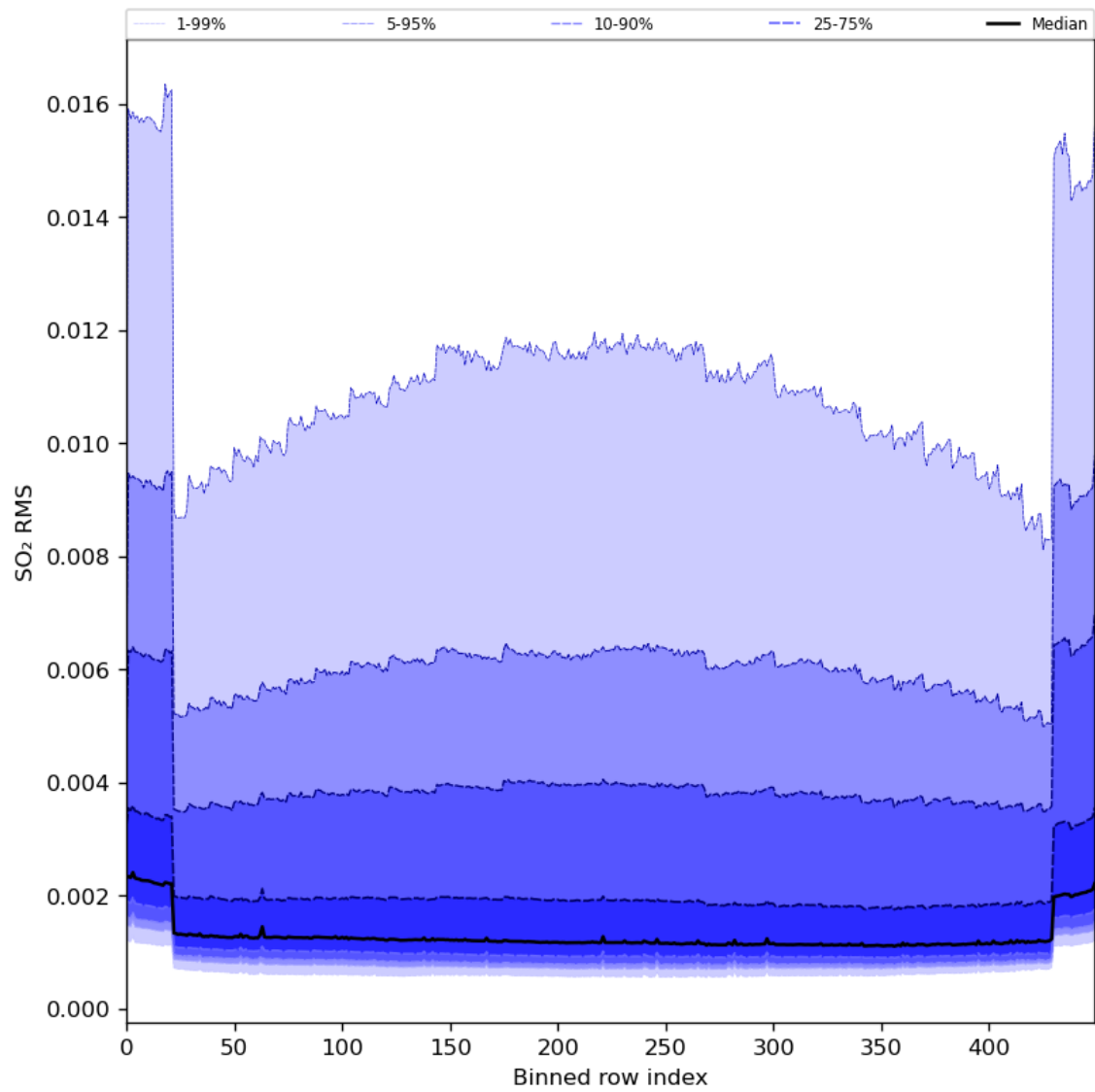
Figure 93: Along track statistics of “SO 2 RMS” for 2024-08-04 to 2024-08-06
