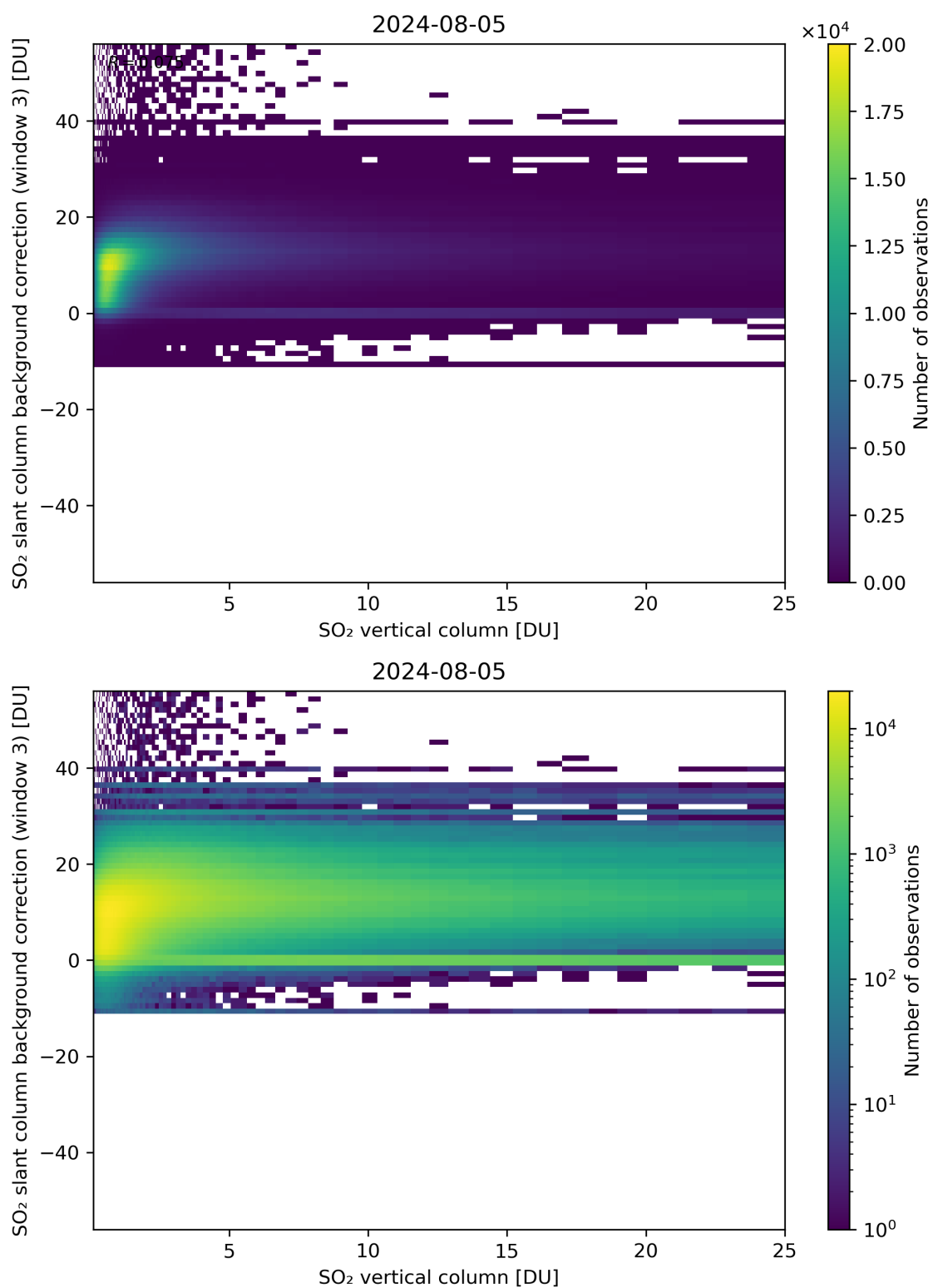
Figure 275: Scatter density plot of “SO 2 vertical column” against “SO 2 slant column background correction (window 3)” for 2024-08-04 to 2024-08-06.
