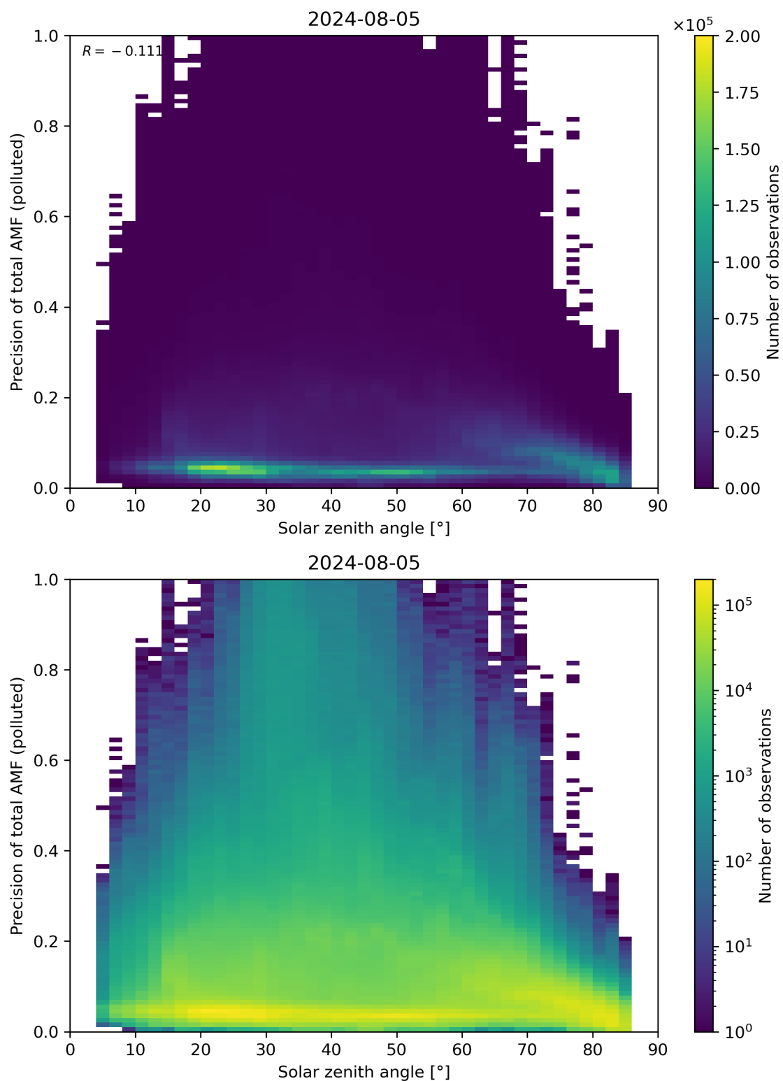
Figure 175: Scatter density plot of “Solar zenith angle” against “Precision of total AMF (polluted)” for 2024-08-04 to 2024-08-06.
