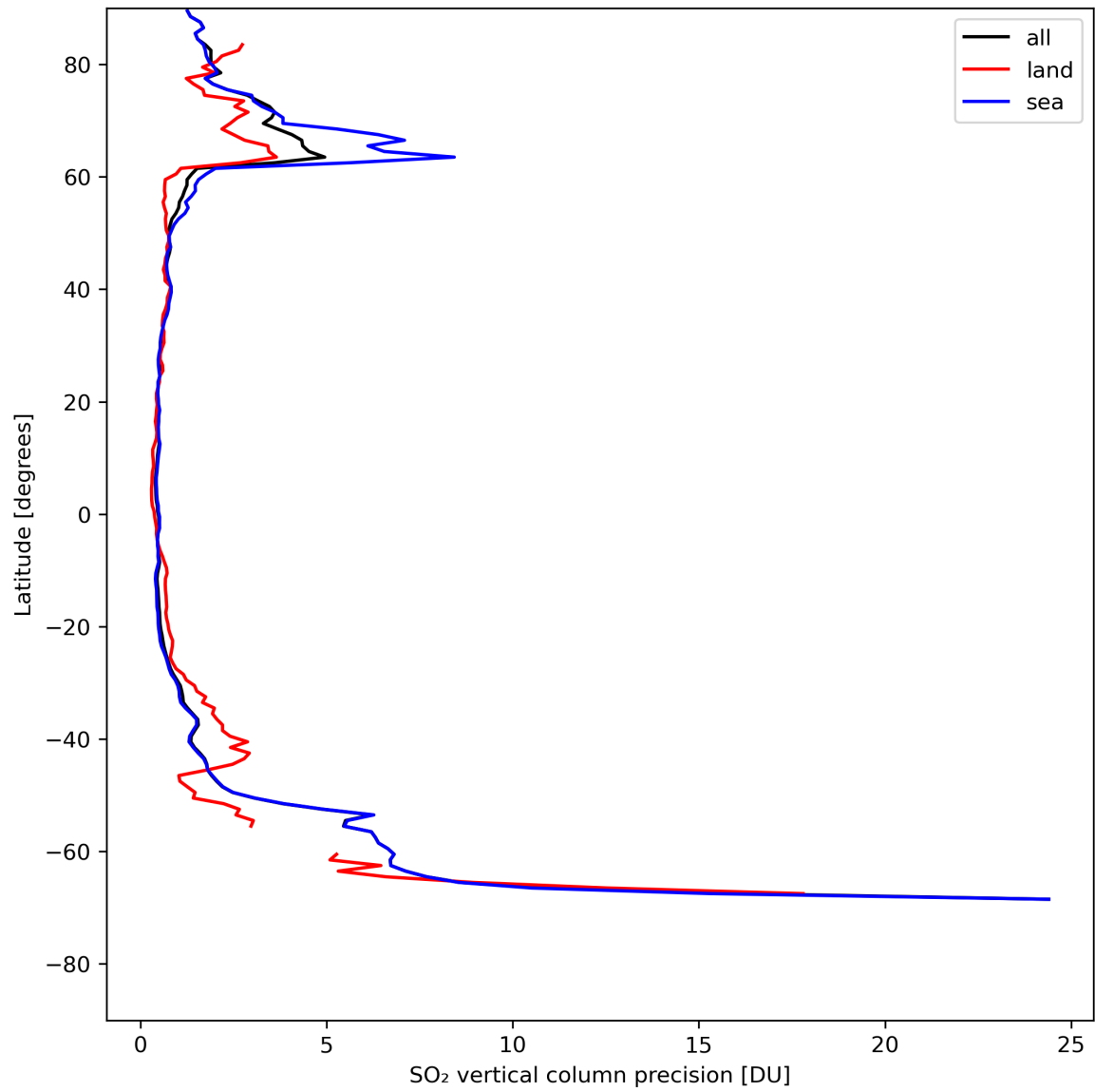
Figure 31: Zonal average of “SO 2 vertical column precision” for 2024-08-04 to 2024-08-06.
