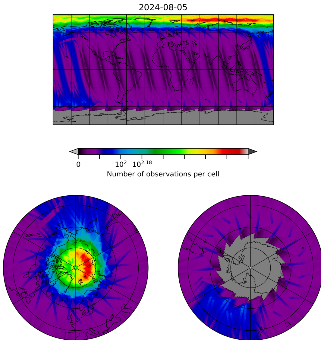
Figure 28: Map of the number of observations for 2024-08-04 to 2024-08-06
