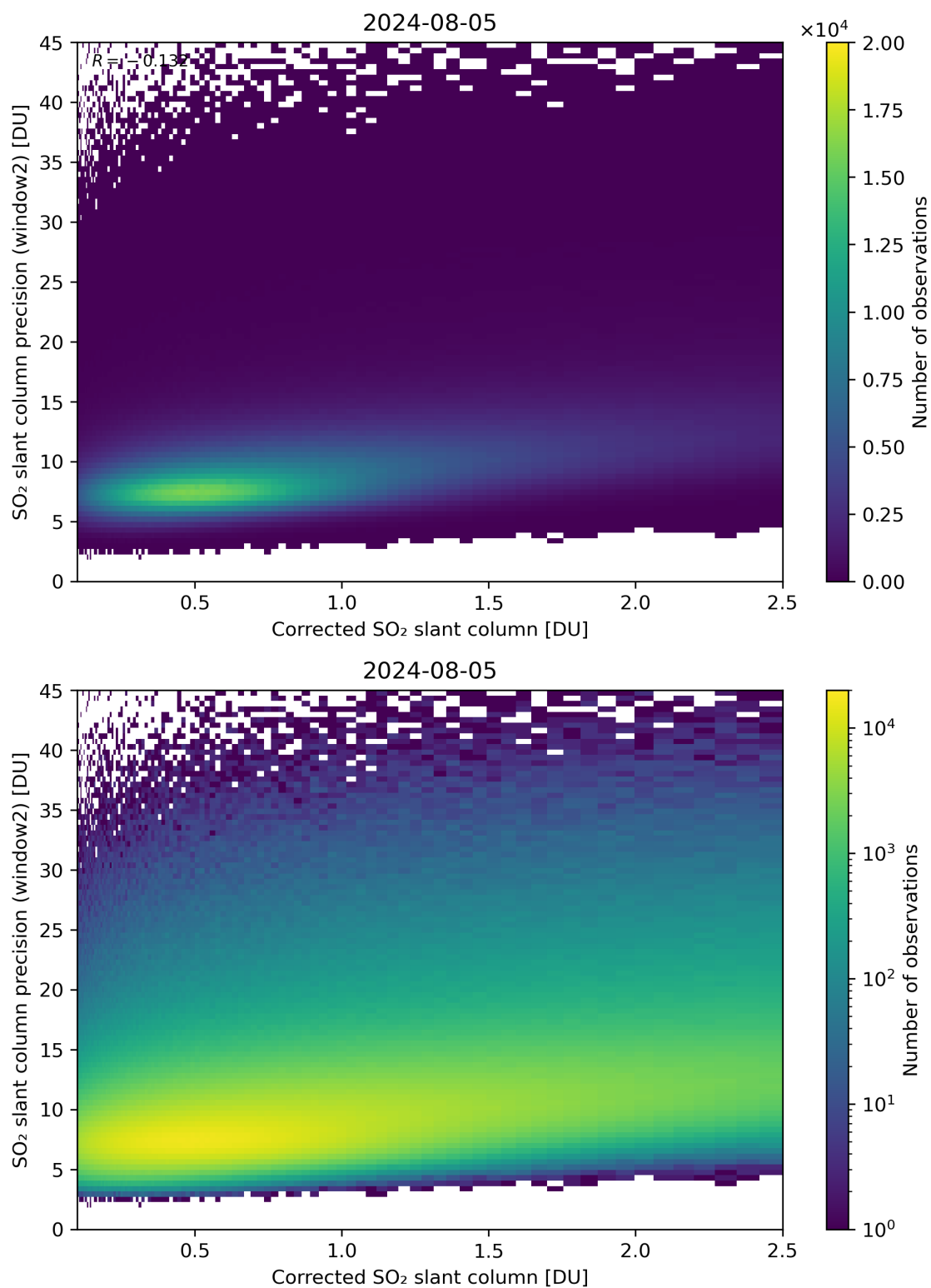
Figure 189: Scatter density plot of “Corrected SO 2 slant column” against “SO 2 slant column precision (window2)” for 2024-08-04 to 2024-08-06.
