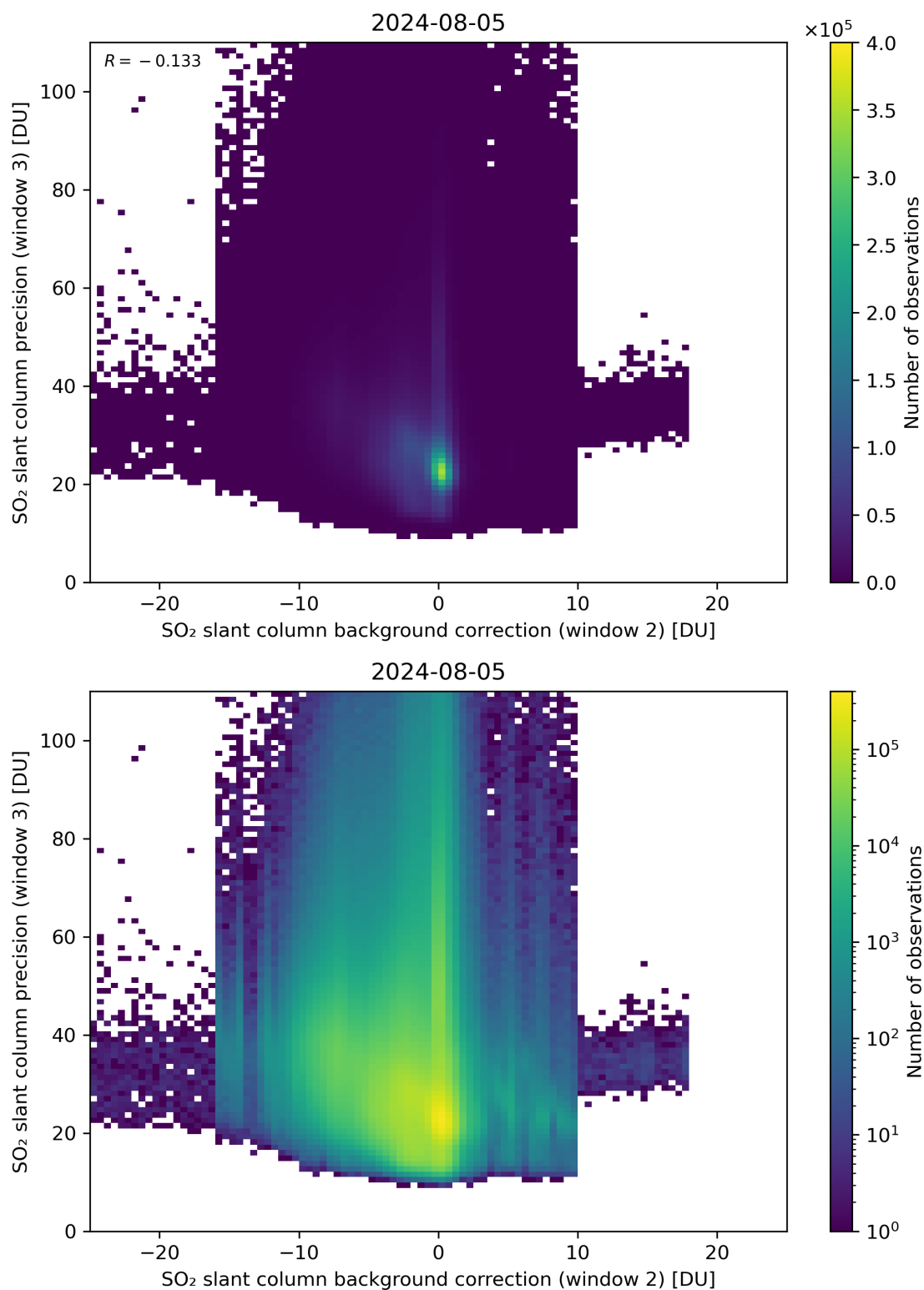
Figure 118: Scatter density plot of “SO 2 slant column background correction (window 2)” against “SO 2 slant column precision (window 3)” for 2024-08-04 to 2024-08-06.
