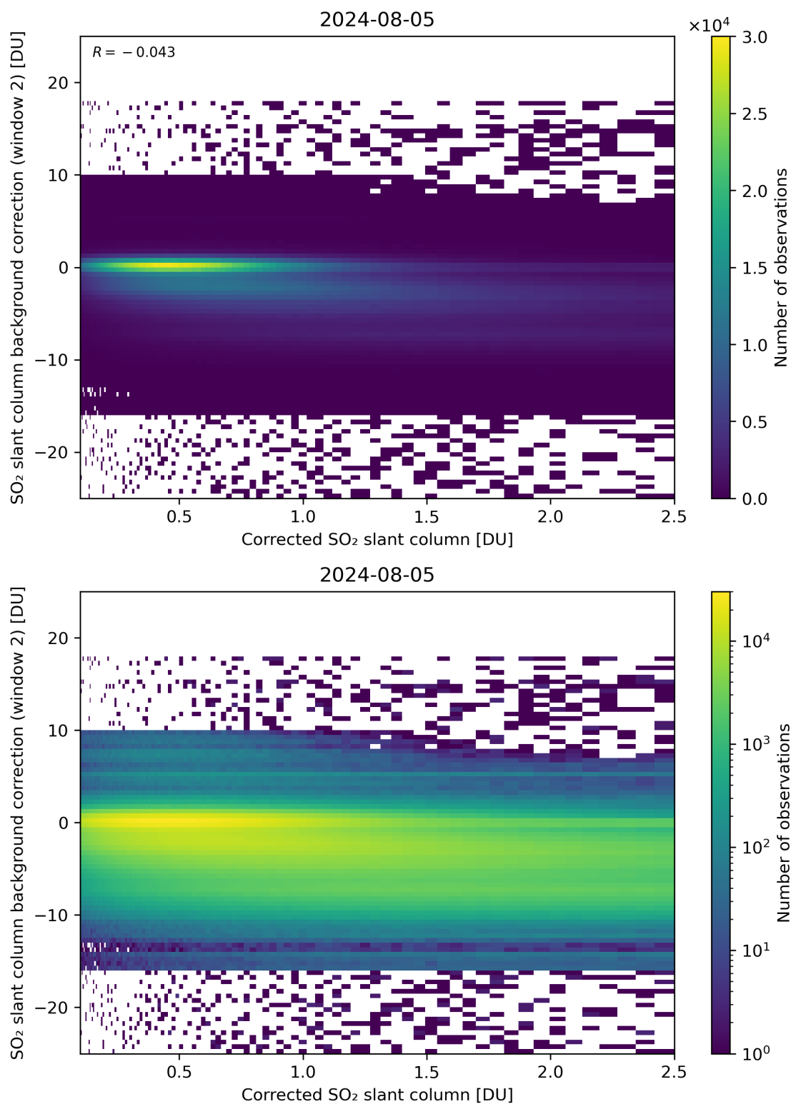
Figure 179: Scatter density plot of “Corrected SO 2 slant column” against “SO 2 slant column background correction (window 2)” for 2024-08-04 to 2024-08-06.
