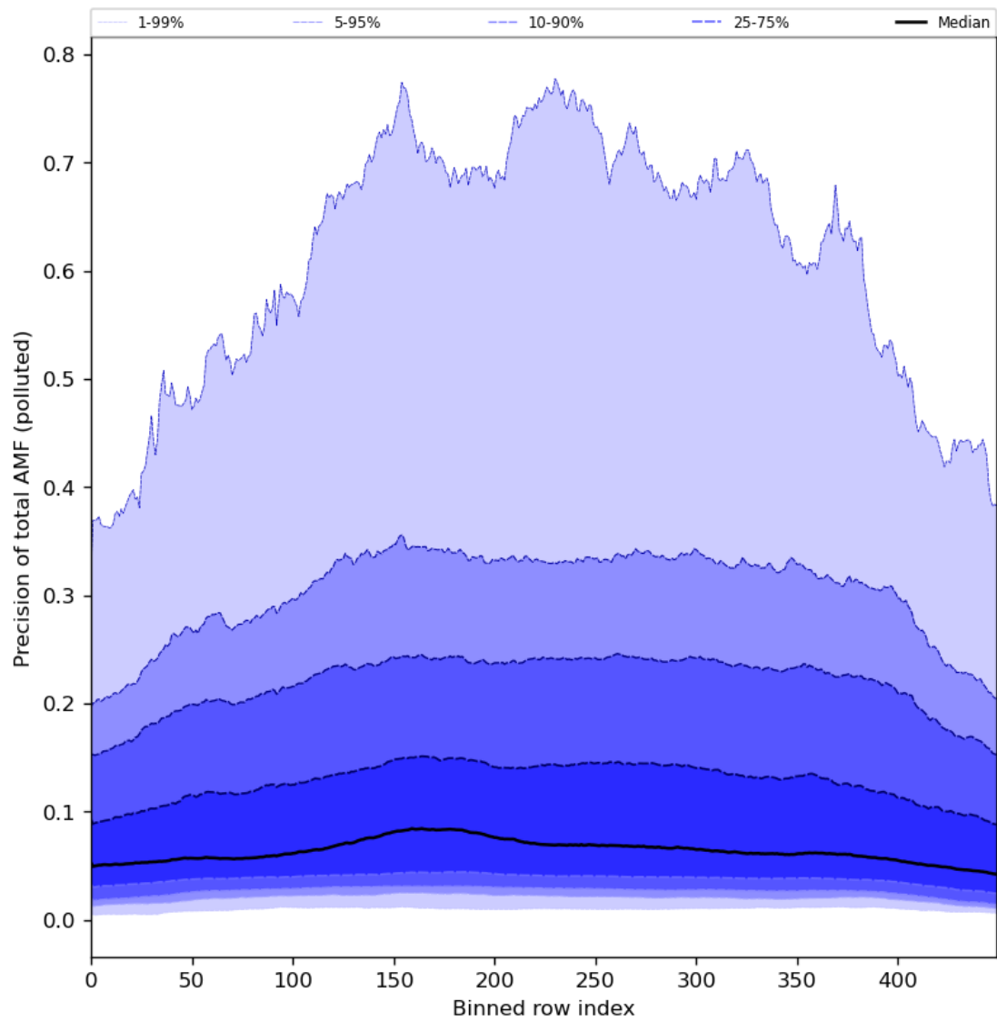
Figure 95: Along track statistics of “Precision of total AMF (polluted)” for 2024-08-04 to 2024-08-06
