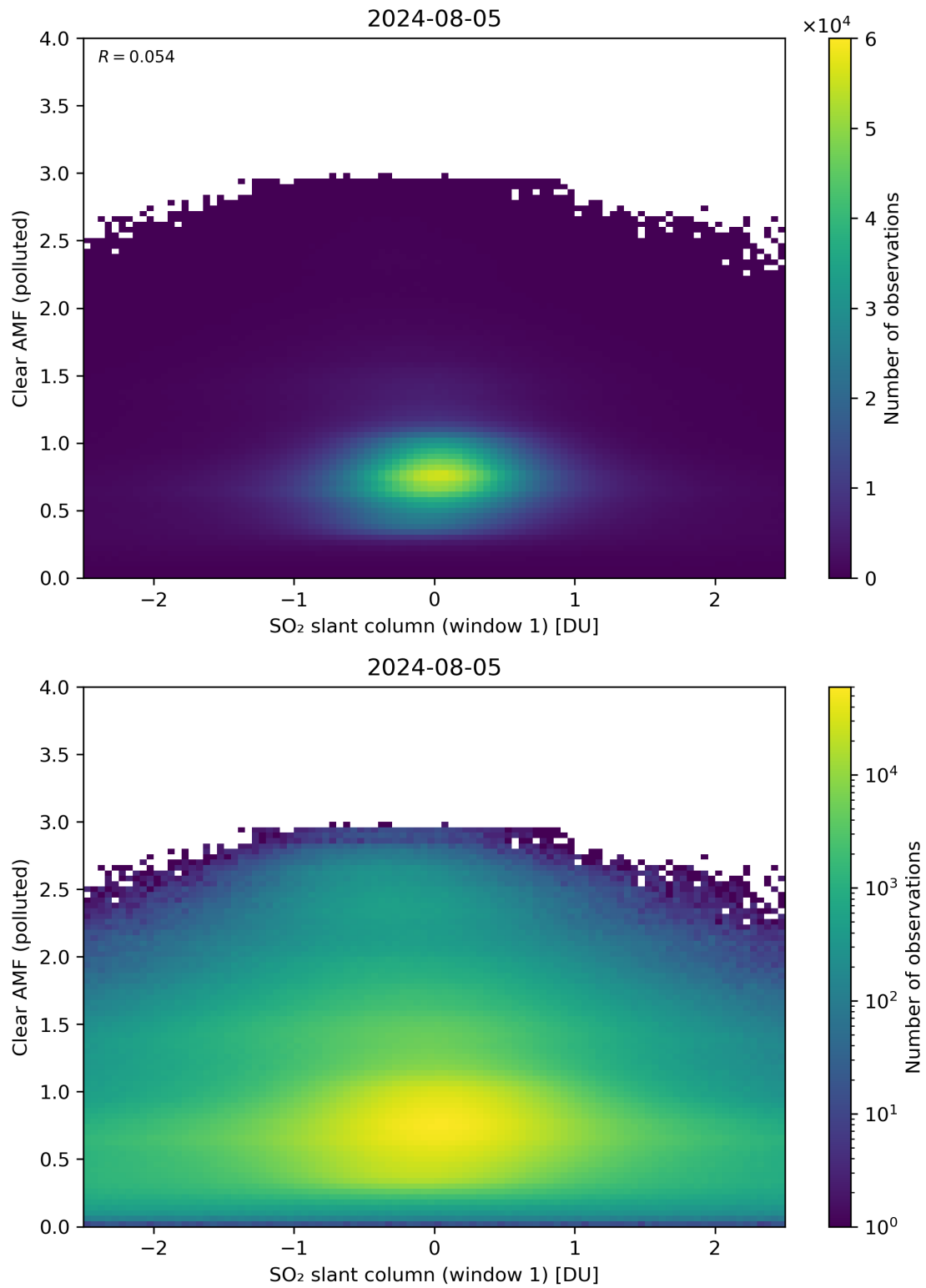
Figure 232: Scatter density plot of “SO 2 slant column (window 1)” against “Clear AMF (polluted)” for 2024-08-04 to 2024-08-06.
