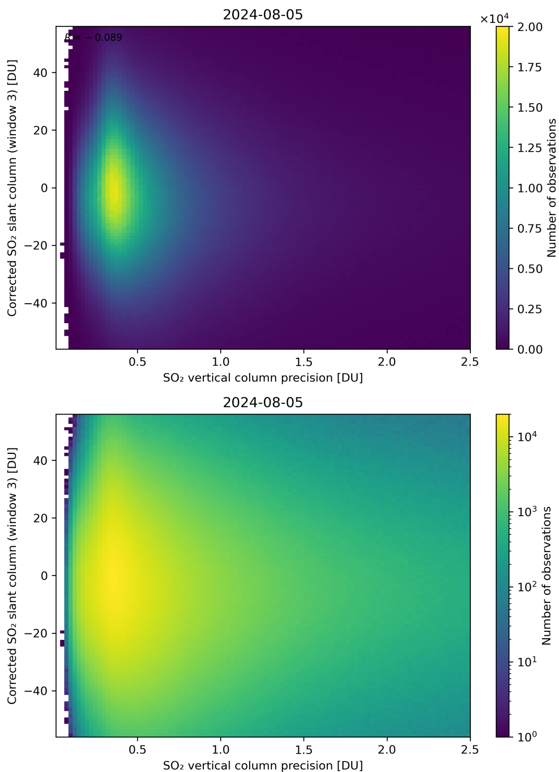
Figure 288: Scatter density plot of “SO 2 vertical column precision” against “Corrected SO 2 slant column (window 3)” for 2024-08-04 to 2024-08-06.
