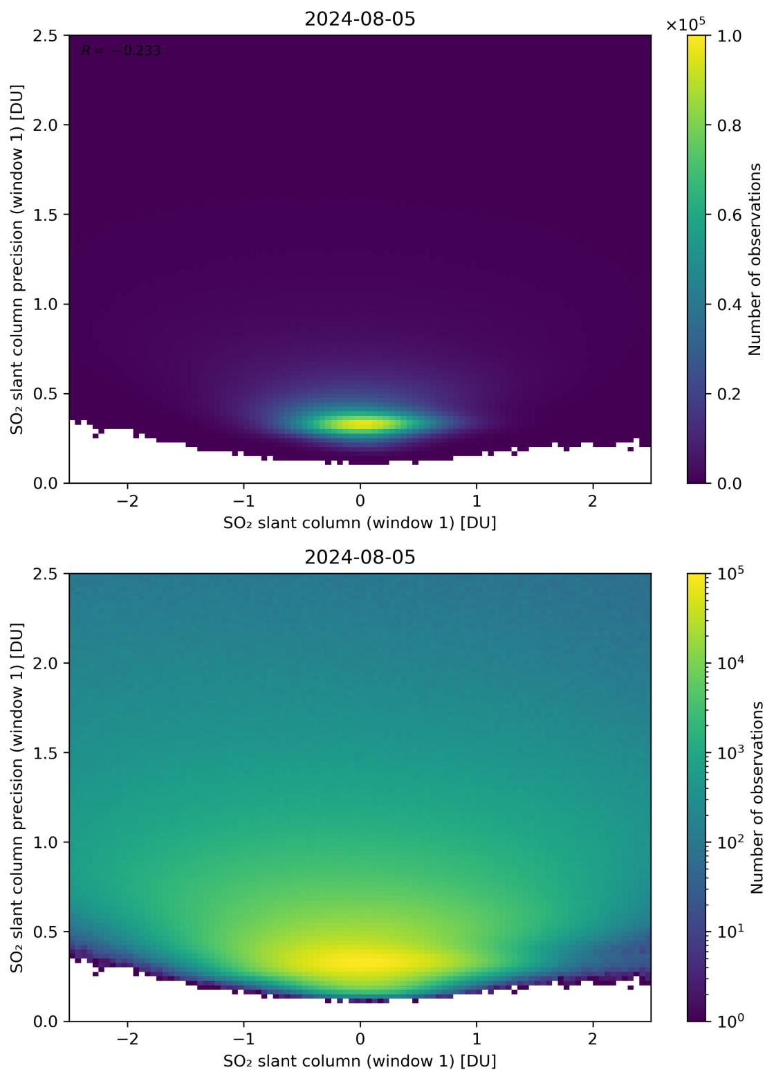
Figure 235: Scatter density plot of “SO 2 slant column (window 1)” against “SO 2 slant column precision (window 1)” for 2024-08-04 to 2024-08-06.
