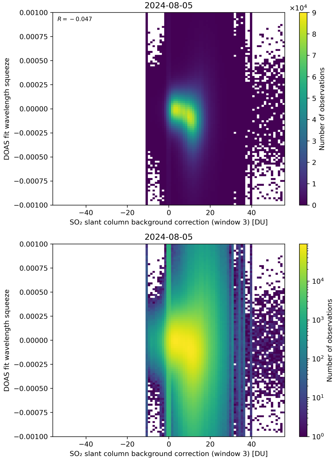
Figure 122: Scatter density plot of “SO 2 slant column background correction (window 3)” against “DOAS fit wavelength squeeze” for 2024-08-04 to 2024-08-06.
