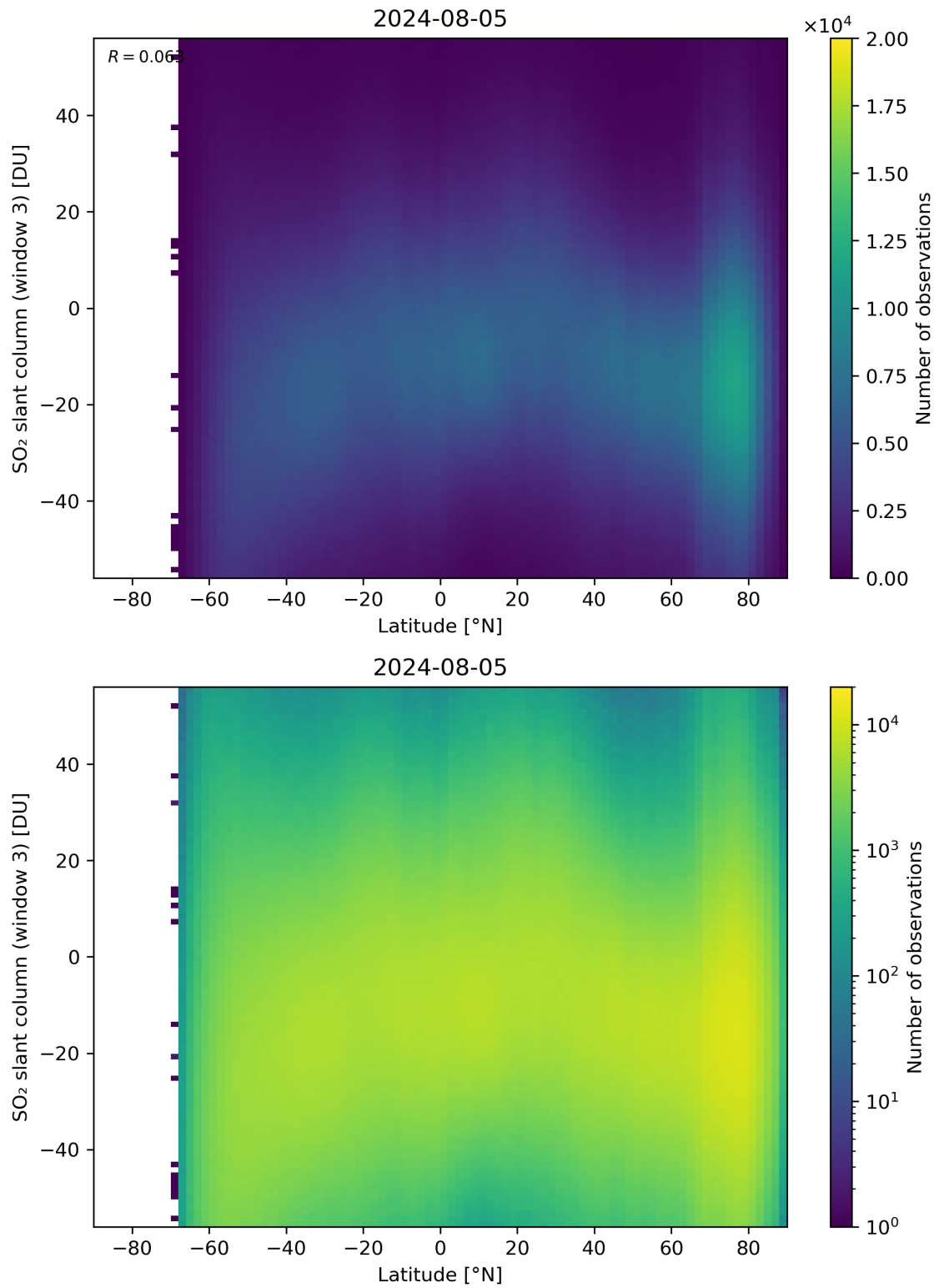
Figure 152: Scatter density plot of “Latitude” against “SO 2 slant column (window 3)” for 2024-08-04 to 2024-08-06.
