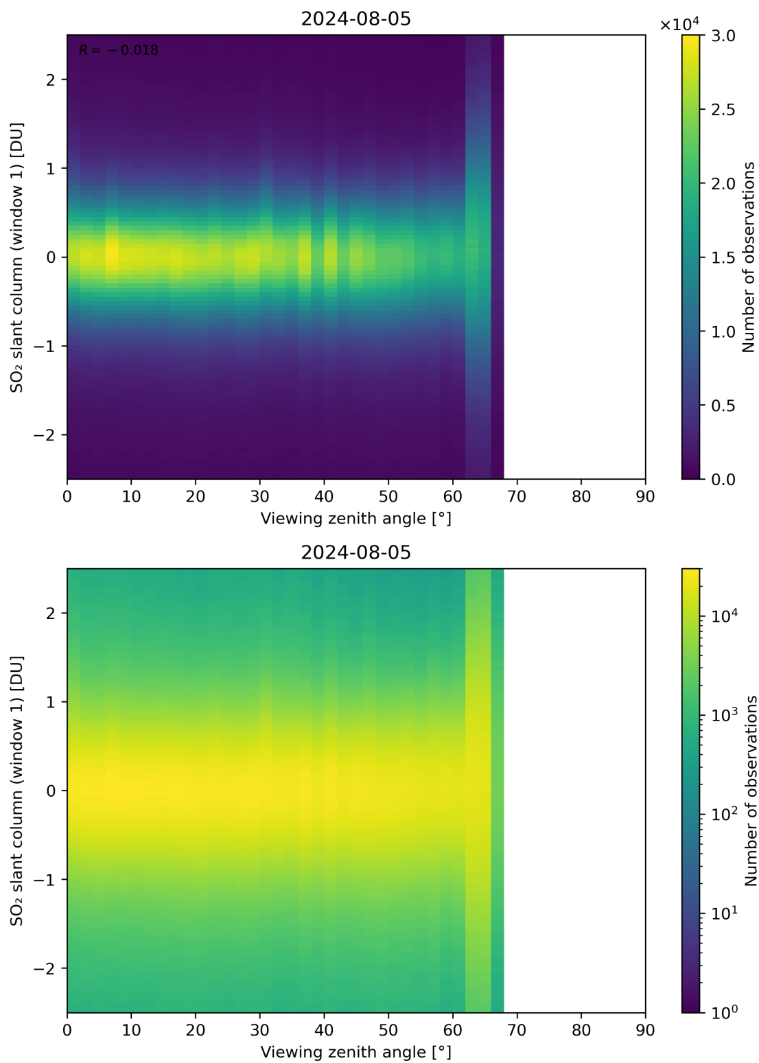
Figure 320: Scatter density plot of “Viewing zenith angle” against “SO 2 slant column (window 1)” for 2024-08-04 to 2024-08-06.
