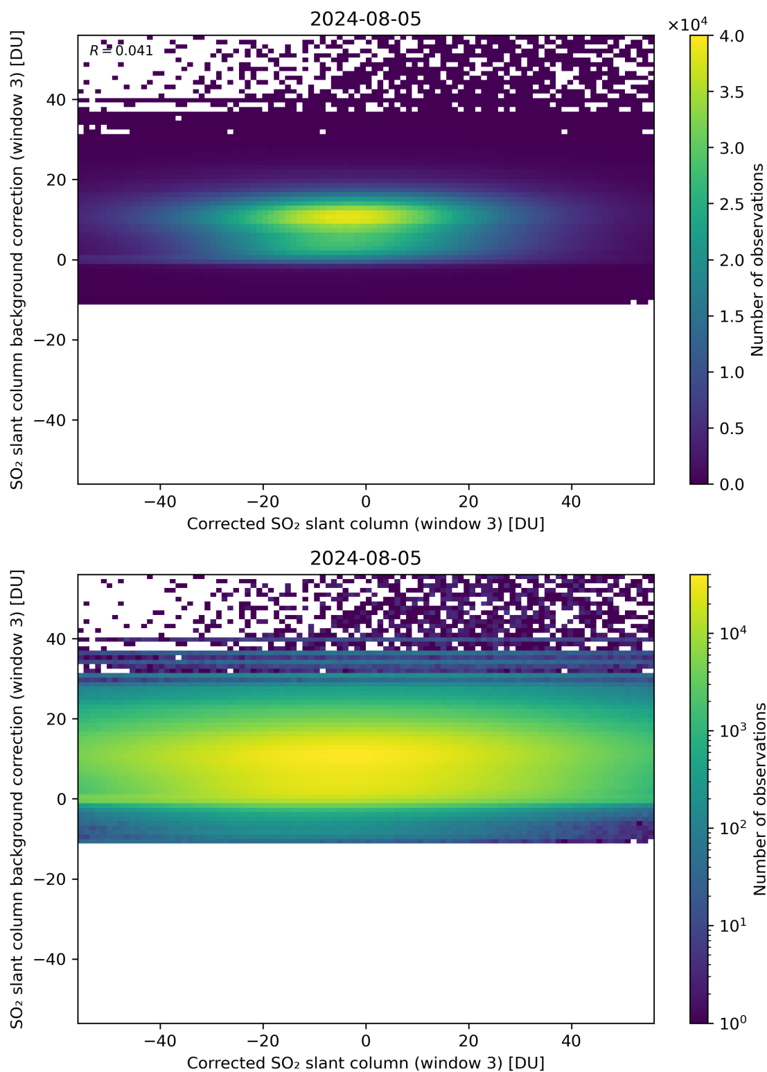
Figure 205: Scatter density plot of “Corrected SO 2 slant column (window 3)” against “SO 2 slant column background correction (window 3)” for 2024-08-04 to 2024-08-06.
