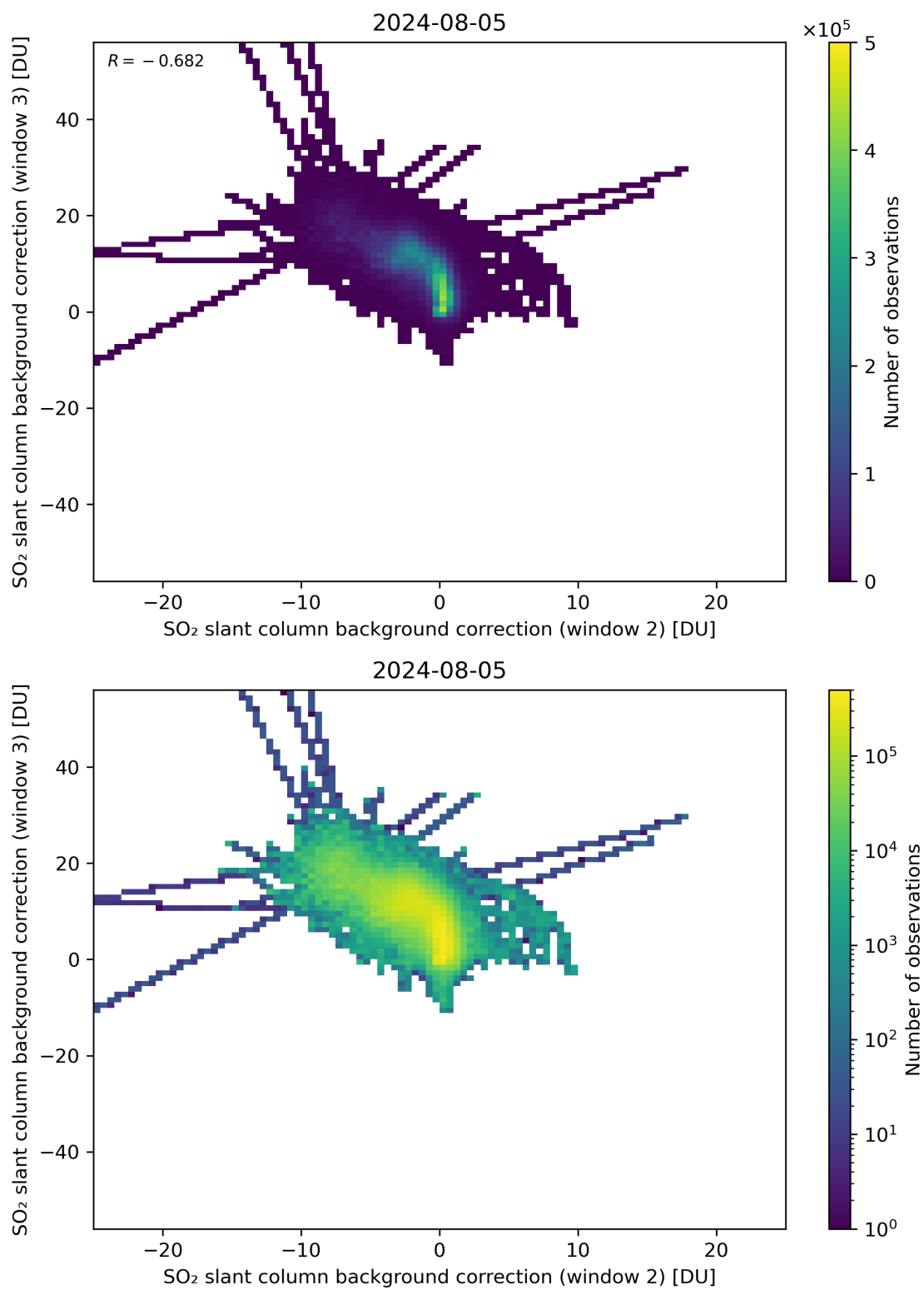
Figure 111: Scatter density plot of “SO 2 slant column background correction (window 2)” against “SO 2 slant column background correction (window 3)” for 2024-08-04 to 2024-08-06.
