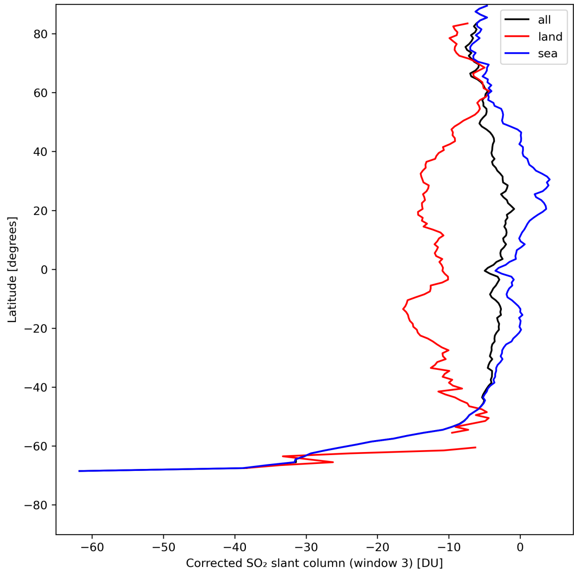
Figure 43: Zonal average of “Corrected SO 2 slant column (window 3)” for 2024-08-04 to 2024-08-06.
