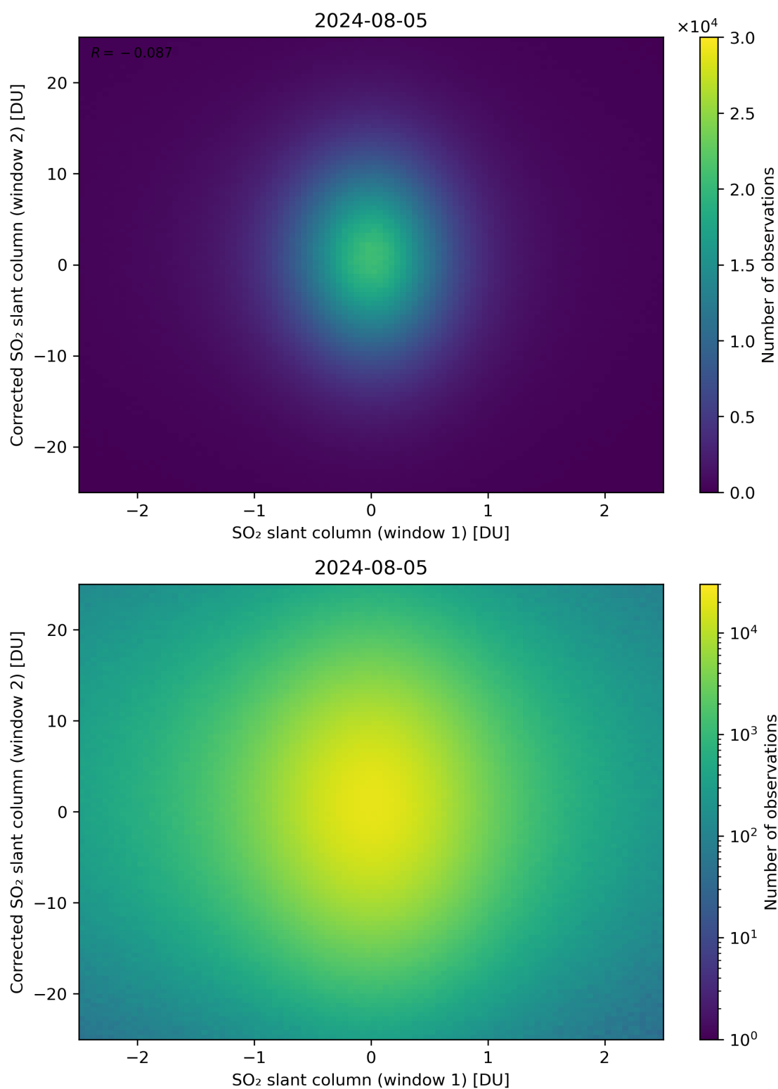
Figure 233: Scatter density plot of “SO 2 slant column (window 1)” against “Corrected SO 2 slant column (window 2)” for 2024-08-04 to 2024-08-06.
