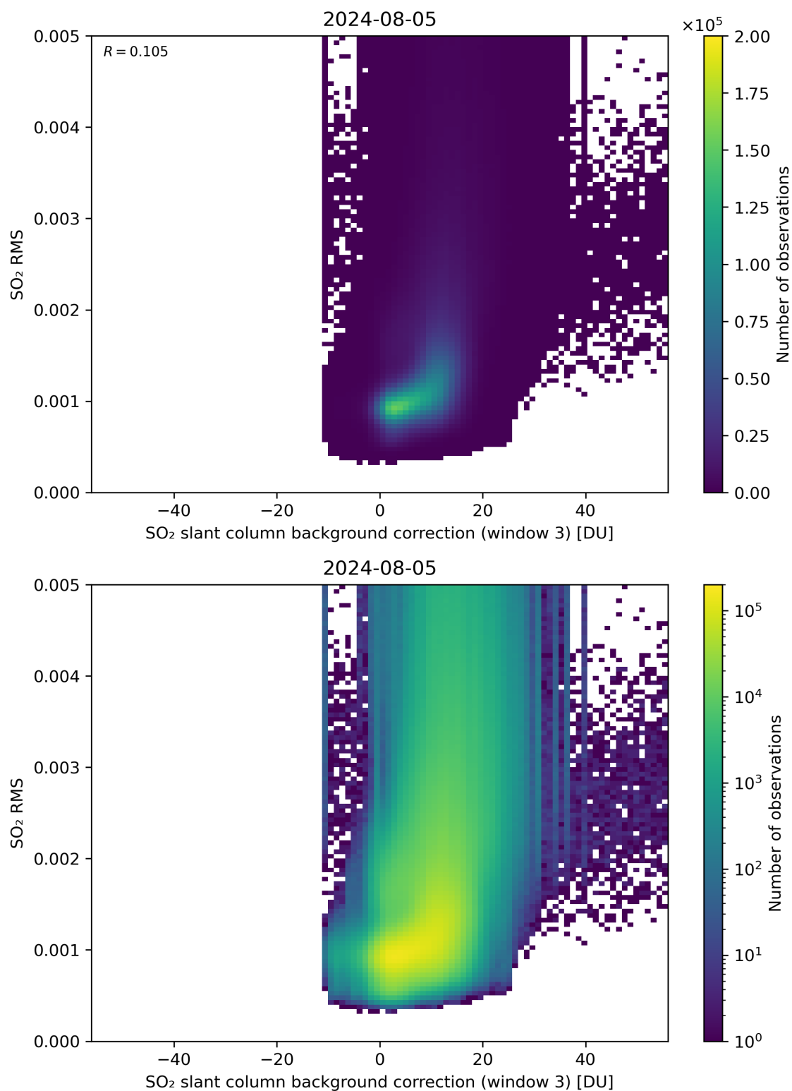
Figure 123: Scatter density plot of “SO 2 slant column background correction (window 3)” against “SO 2 RMS” for 2024-08-04 to 2024-08-06.
