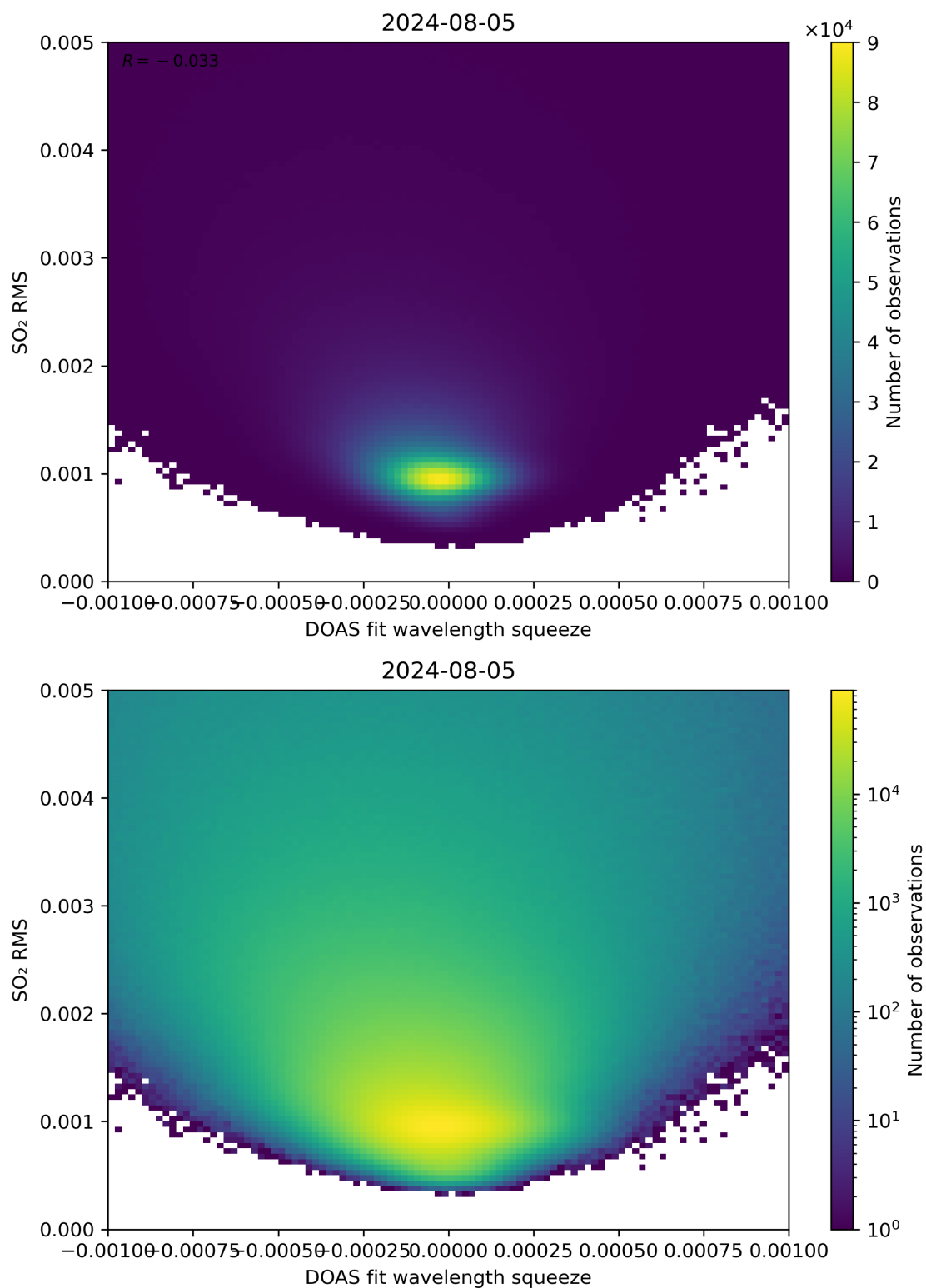
Figure 132: Scatter density plot of “DOAS fit wavelength squeeze” against “SO 2 RMS” for 2024-08-04 to 2024-08-06.
