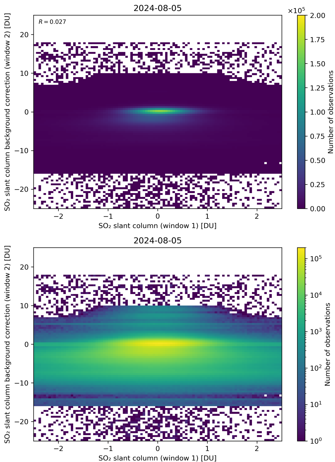
Figure 213: Scatter density plot of “SO 2 slant column (window 1)” against “SO 2 slant column background correction (window 2)” for 2024-08-04 to 2024-08-06.
