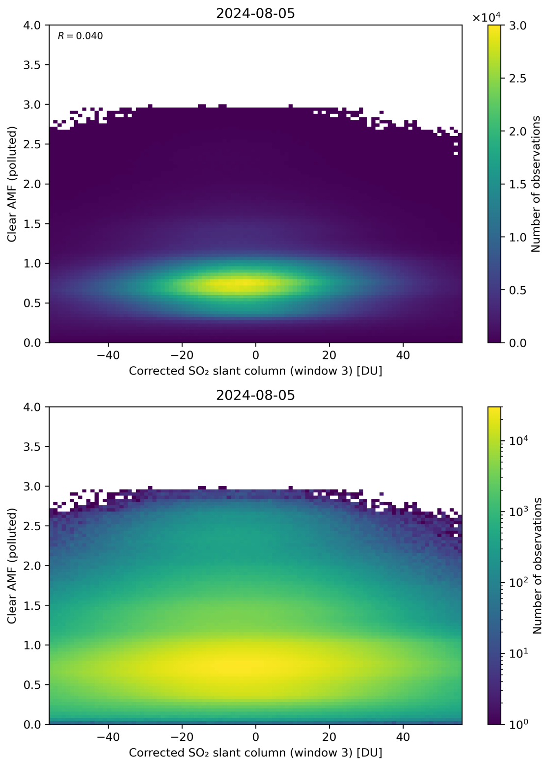
Figure 209: Scatter density plot of “Corrected SO 2 slant column (window 3)” against “Clear AMF (polluted)” for 2024-08-04 to 2024-08-06.
