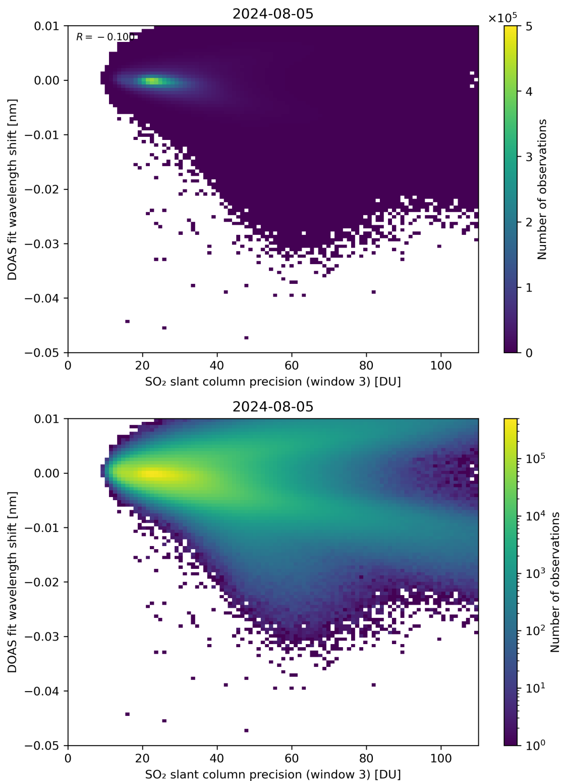
Figure 258: Scatter density plot of “SO 2 slant column precision (window 3)” against “DOAS fit wavelength shift” for 2024-08-04 to 2024-08-06.
