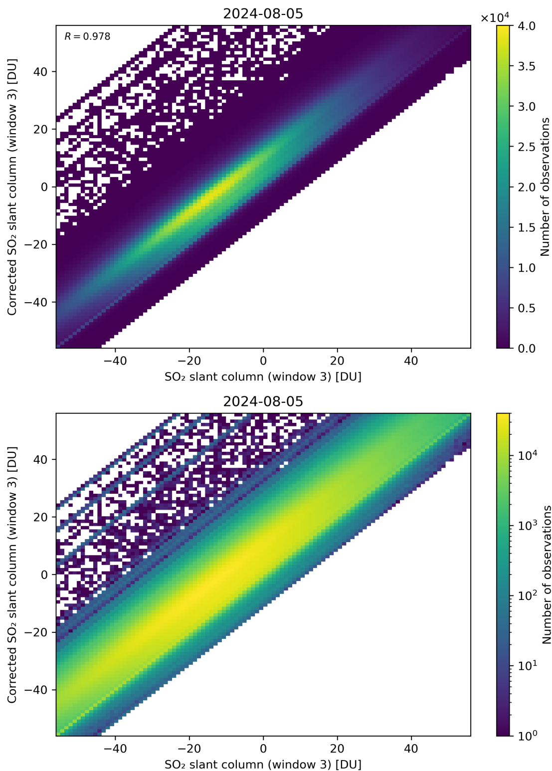
Figure 266: Scatter density plot of “SO 2 slant column (window 3)” against “Corrected SO 2 slant column (window 3)” for 2024-08-04 to 2024-08-06.
