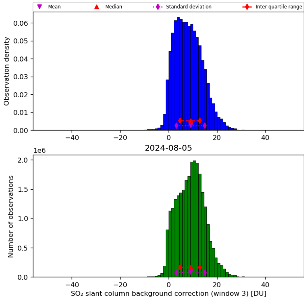
Figure 67: Histogram of “SO 2 slant column background correction (window 3)” for 2024-08-04 to 2024-08-06
