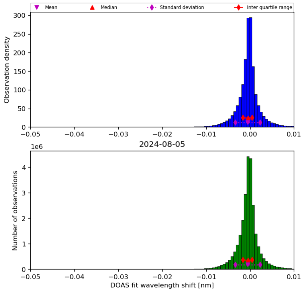
Figure 68: Histogram of “DOAS fit wavelength shift” for 2024-08-04 to 2024-08-06
