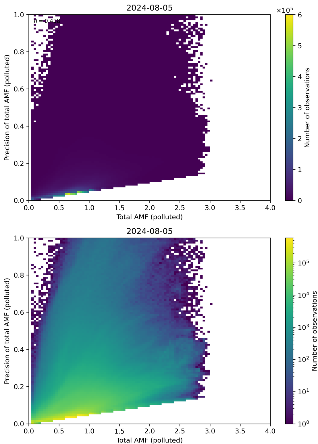
Figure 272: Scatter density plot of “Total AMF (polluted)” against “Precision of total AMF (polluted)” for 2024-08-04 to 2024-08-06.
