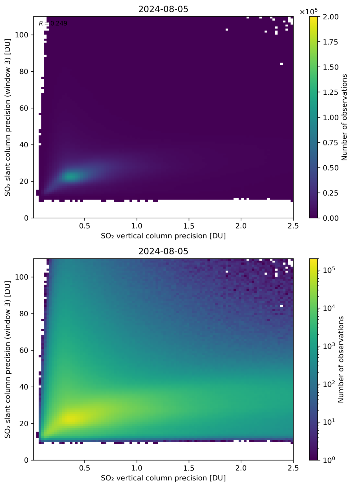
Figure 293: Scatter density plot of “SO 2 vertical column precision” against “SO 2 slant column precision (window 3)” for 2024-08-04 to 2024-08-06.
