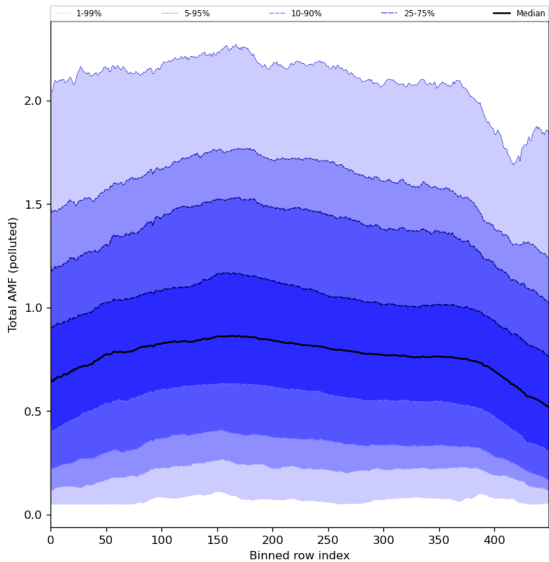
Figure 94: Along track statistics of “Total AMF (polluted)” for 2024-08-04 to 2024-08-06
