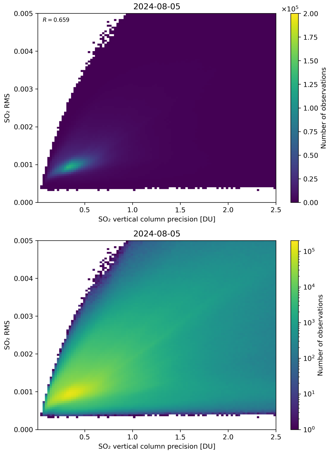
Figure 284: Scatter density plot of “SO 2 vertical column precision” against “SO 2 RMS” for 2024-08-04 to 2024-08-06.
