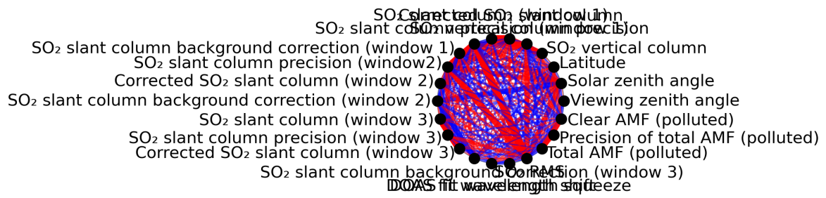
Figure 1: Map of correlation graph for 2024-08-04 to 2024-08-06.
