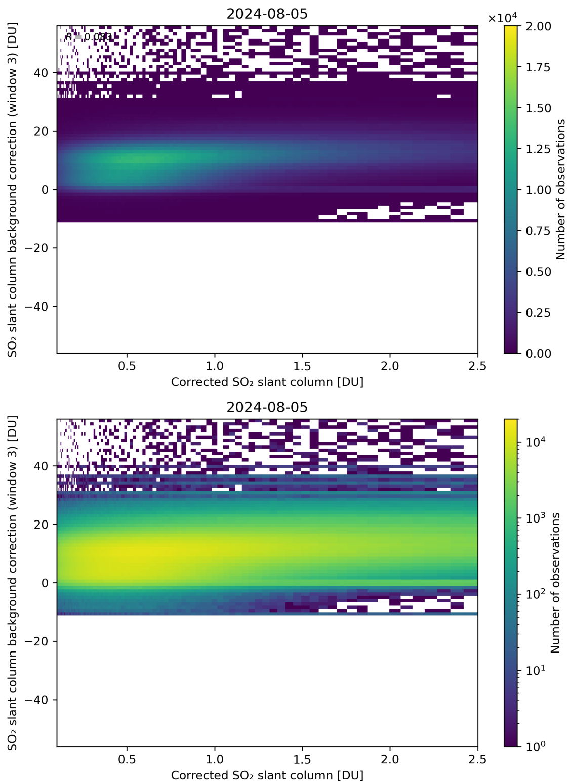
Figure 180: Scatter density plot of “Corrected SO 2 slant column” against “SO 2 slant column background correction (window 3)” for 2024-08-04 to 2024-08-06.
