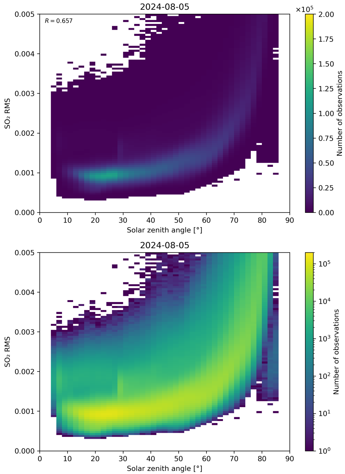
Figure 163: Scatter density plot of “Solar zenith angle” against “SO 2 RMS” for 2024-08-04 to 2024-08-06.
