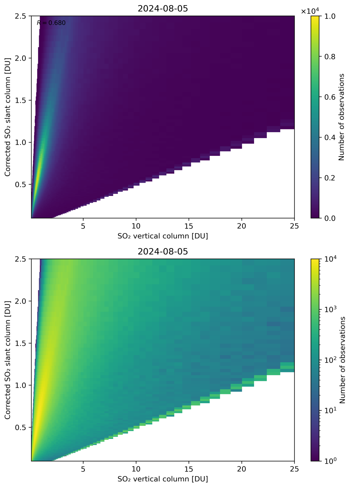
Figure 297: Scatter density plot of “SO 2 vertical column” against “Corrected SO 2 slant column” for 2024-08-04 to 2024-08-06.
