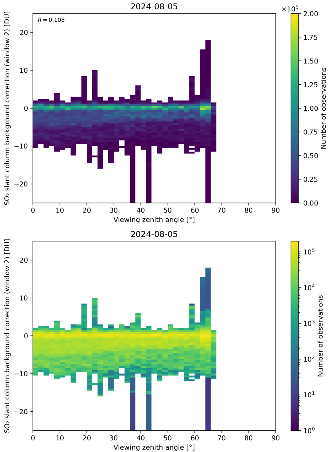
Figure 309: Scatter density plot of “Viewing zenith angle” against “SO 2 slant column background correction (window 2)” for 2024-08-04 to 2024-08-06.
