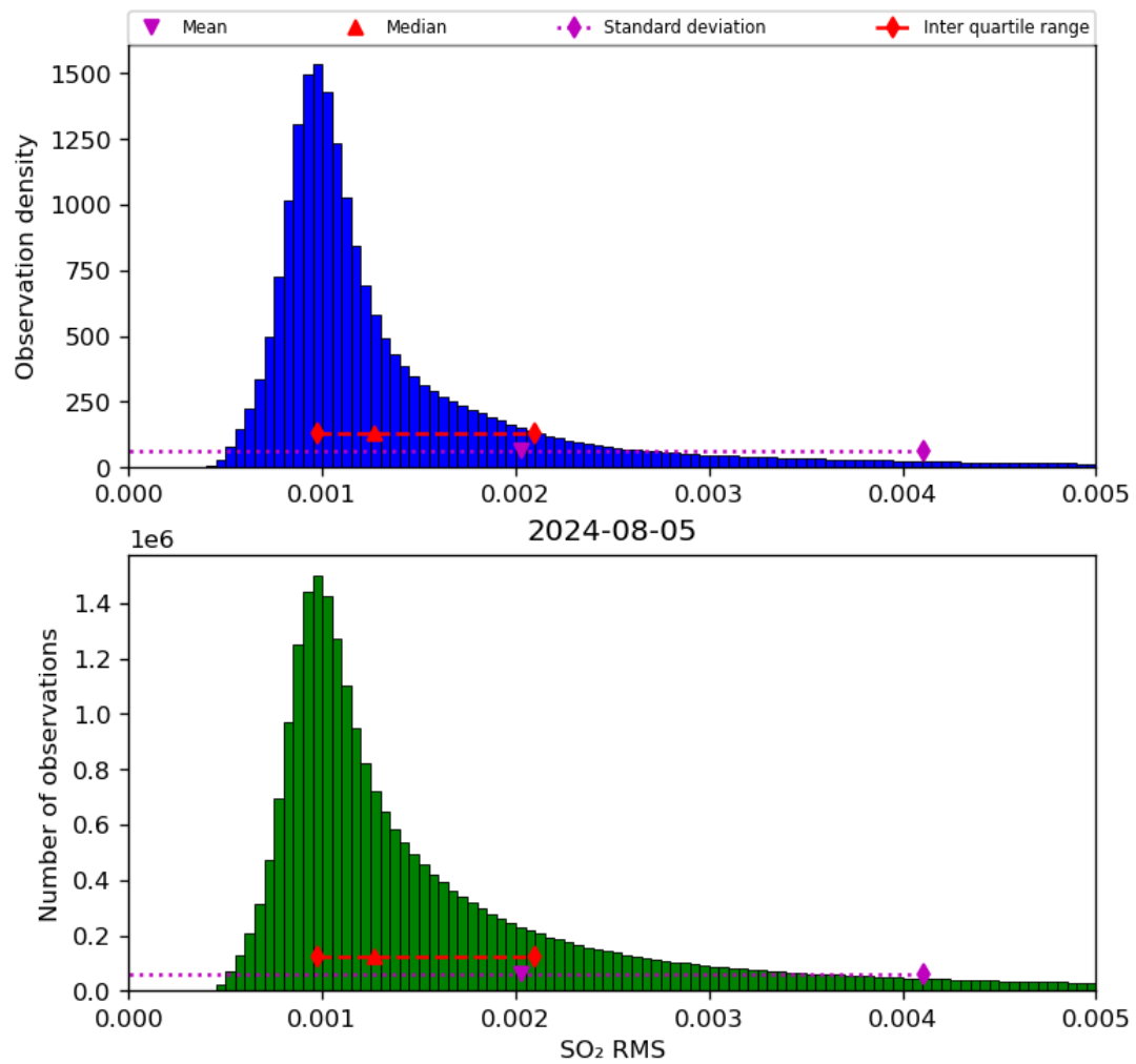
Figure 70: Histogram of “SO 2 RMS” for 2024-08-04 to 2024-08-06
