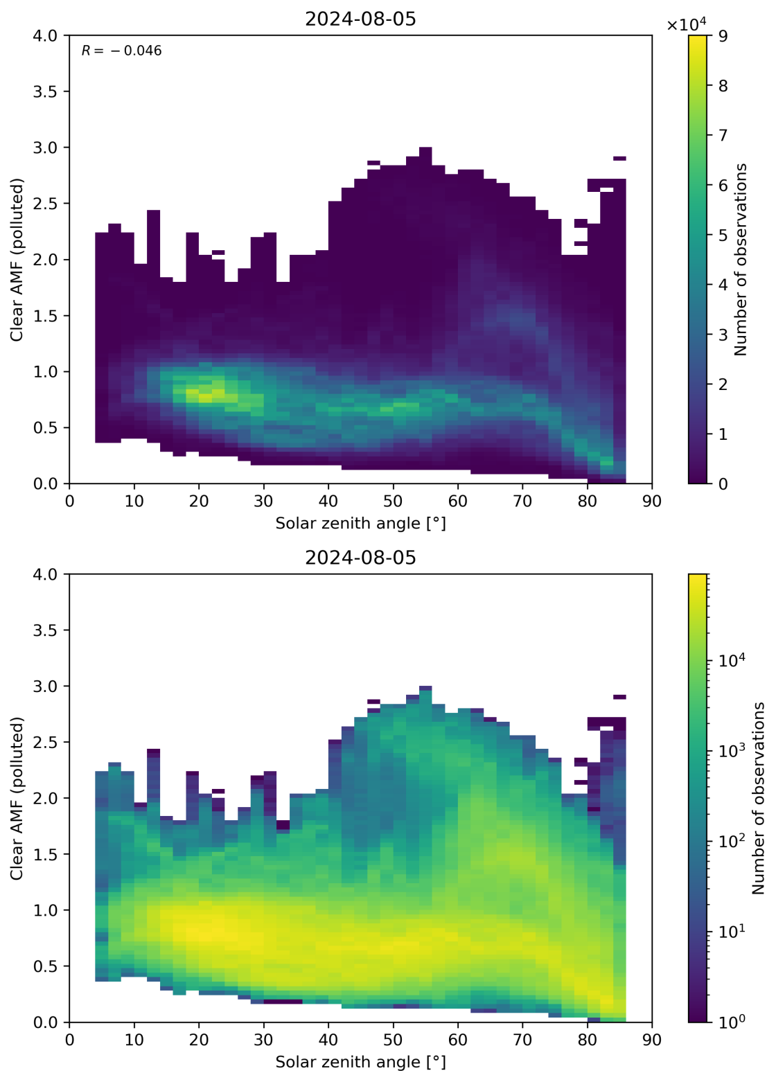
Figure 165: Scatter density plot of “Solar zenith angle” against “Clear AMF (polluted)” for 2024-08-04 to 2024-08-06.
