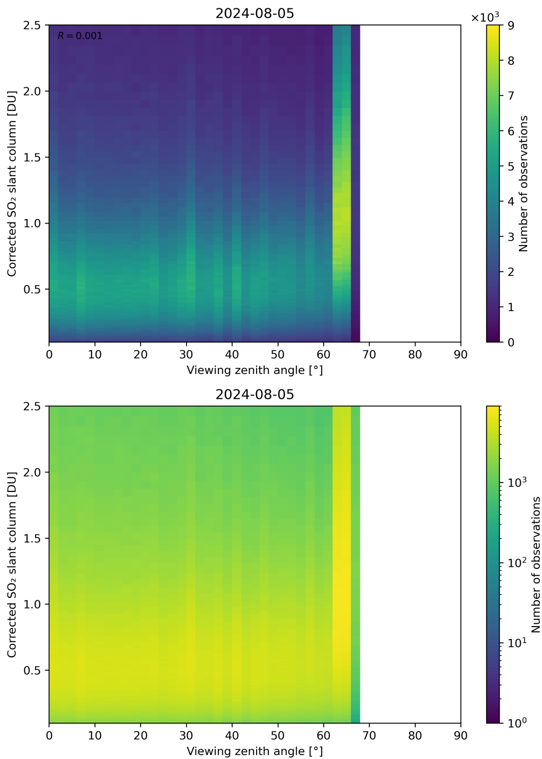
Figure 317: Scatter density plot of “Viewing zenith angle” against “Corrected SO 2 slant column” for 2024-08-04 to 2024-08-06.
