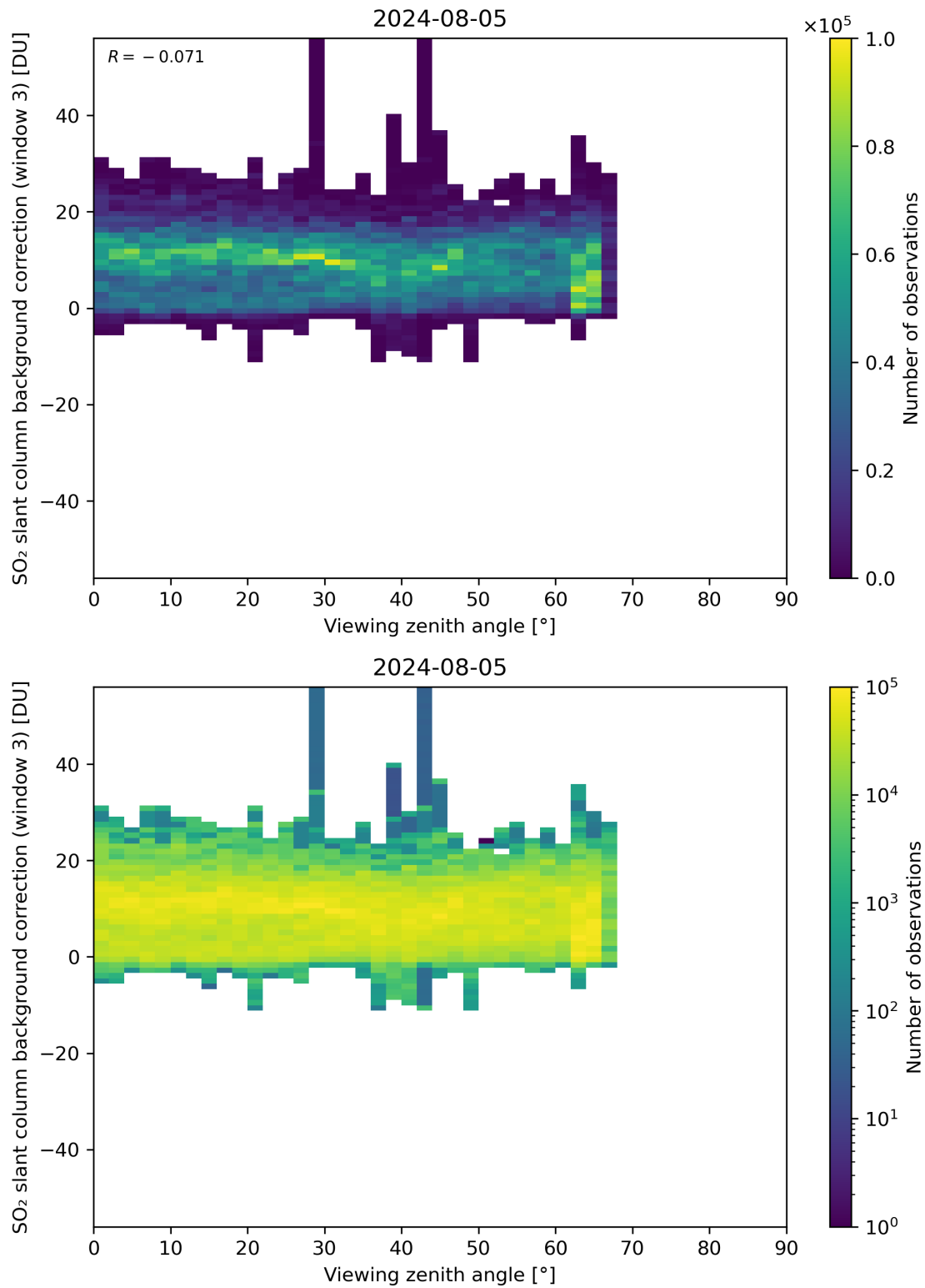
Figure 310: Scatter density plot of “Viewing zenith angle” against “SO 2 slant column background correction (window 3)” for 2024-08-04 to 2024-08-06.
