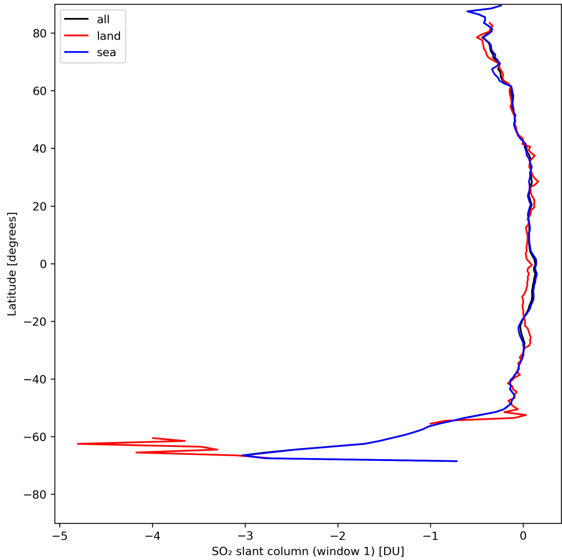
Figure 33: Zonal average of “SO 2 slant column (window 1)” for 2024-08-04 to 2024-08-06.
