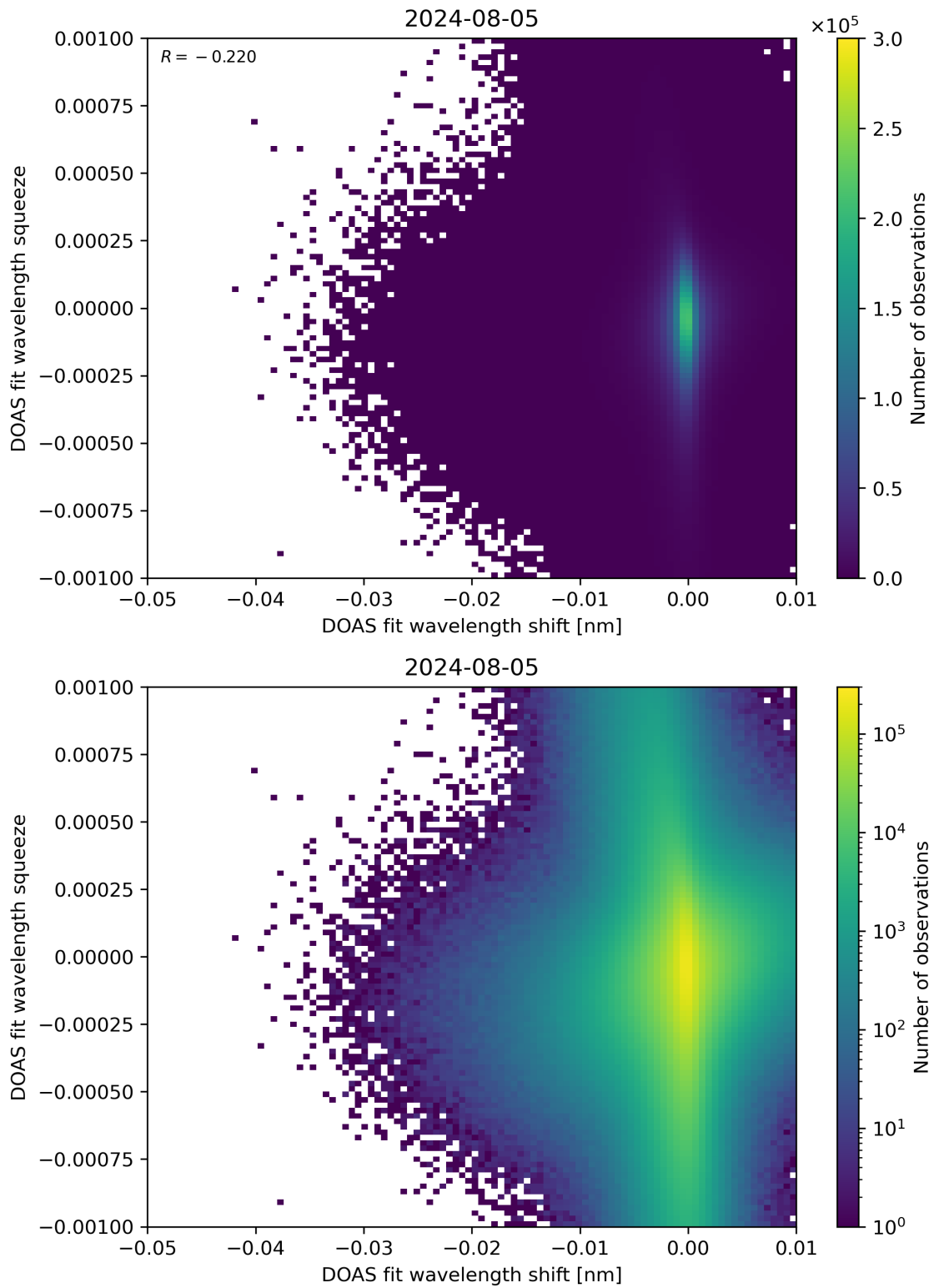
Figure 127: Scatter density plot of “DOAS fit wavelength shift” against “DOAS fit wavelength squeeze” for 2024-08-04 to 2024-08-06.
