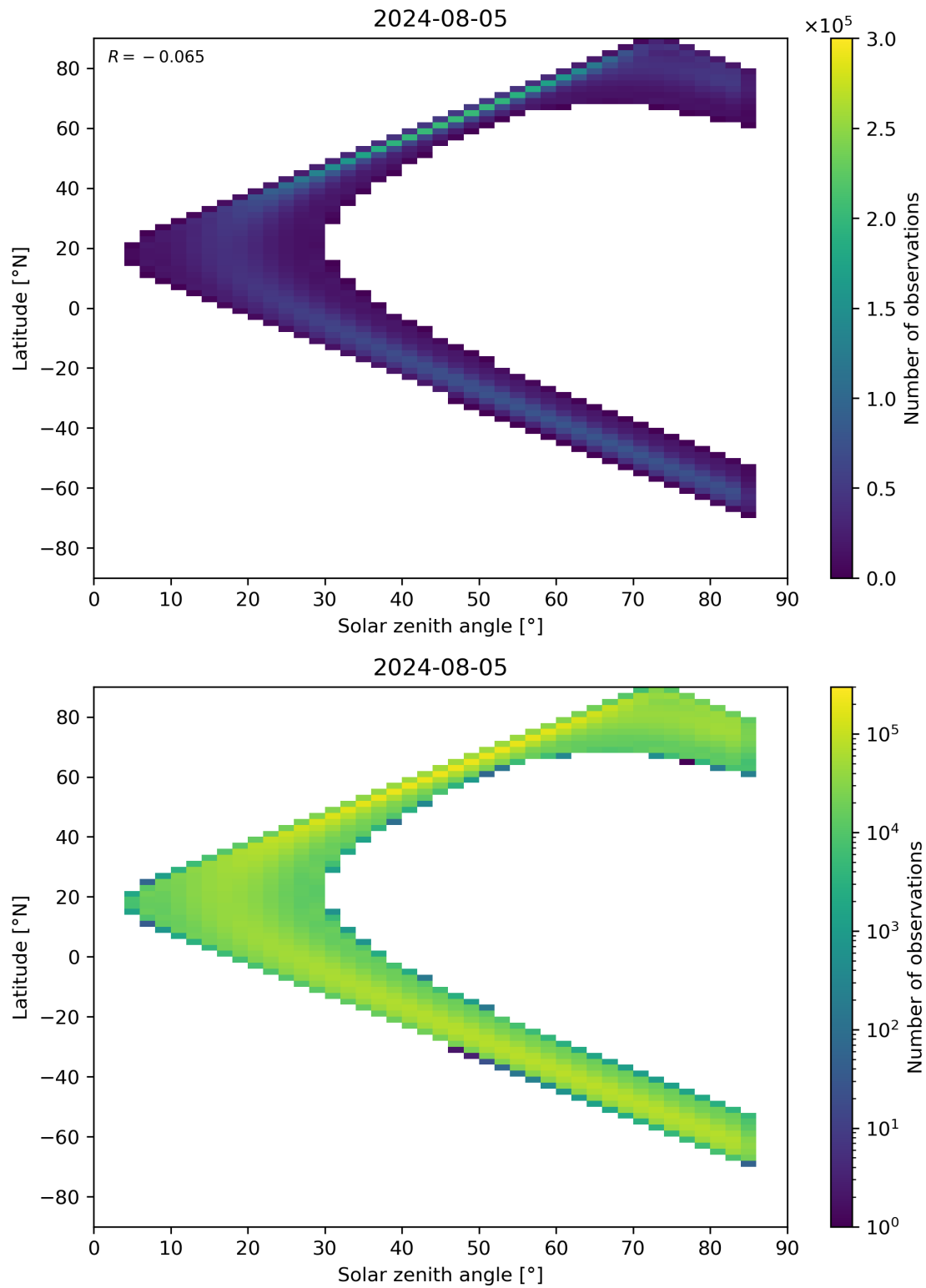
Figure 164: Scatter density plot of “Solar zenith angle” against “Latitude” for 2024-08-04 to 2024-08-06.
