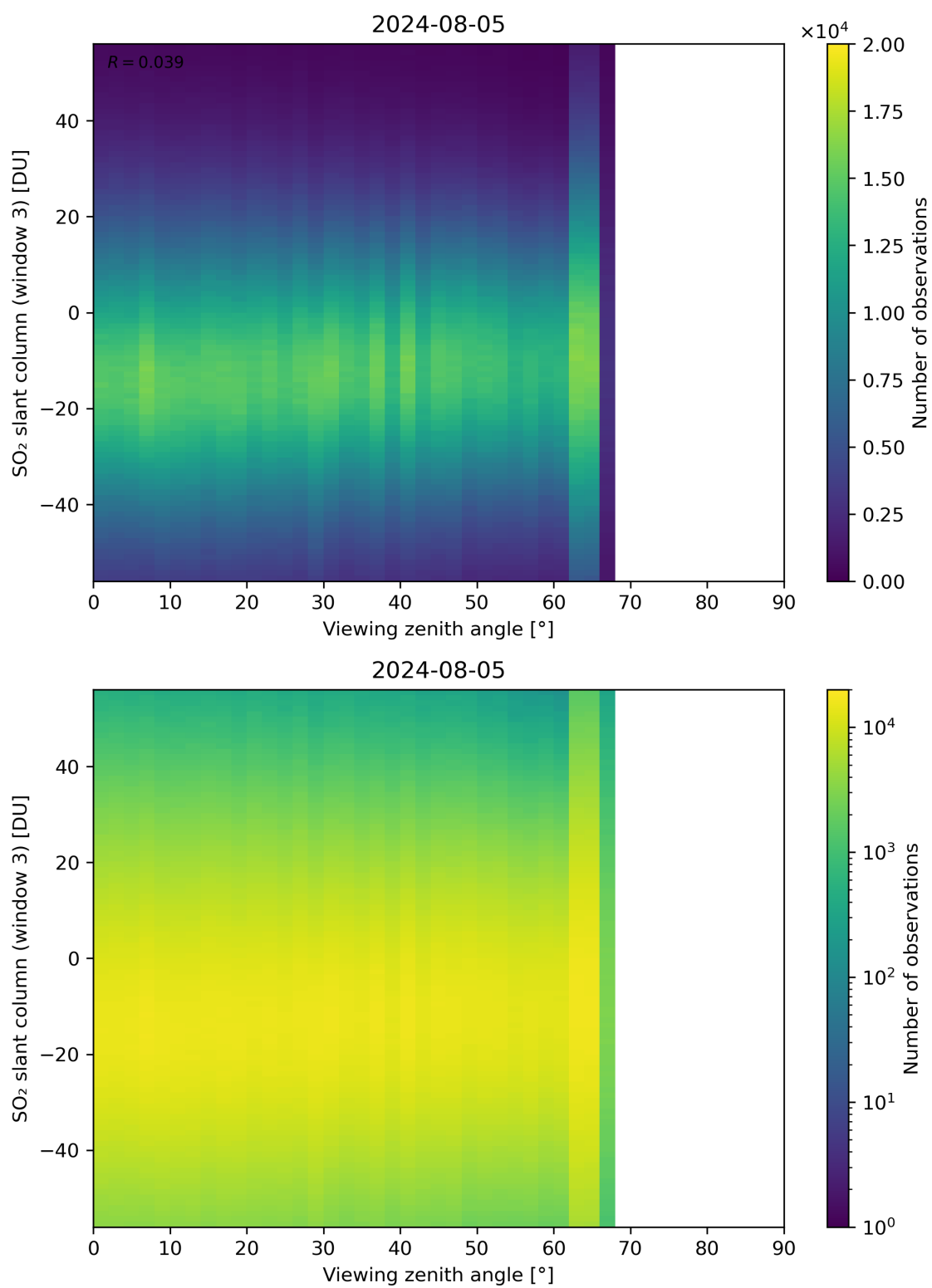
Figure 323: Scatter density plot of “Viewing zenith angle” against “SO 2 slant column (window 3)” for 2024-08-04 to 2024-08-06.
