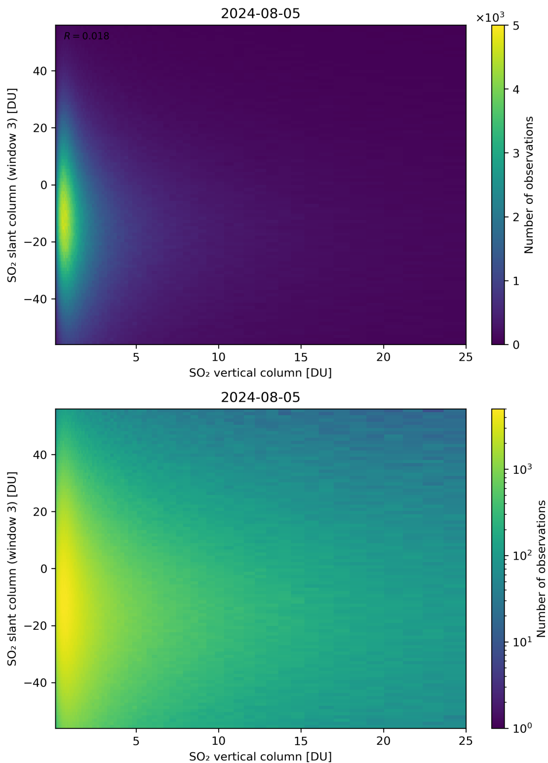
Figure 303: Scatter density plot of “SO 2 vertical column” against “SO 2 slant column (window 3)” for 2024-08-04 to 2024-08-06.
