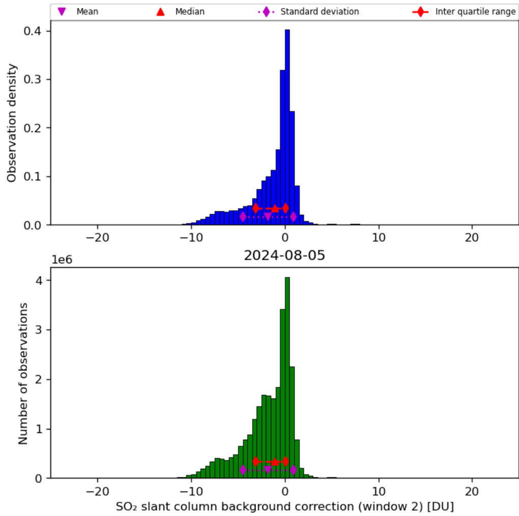
Figure 63: Histogram of “SO 2 slant column background correction (window 2)” for 2024-08-04 to 2024-08-06
