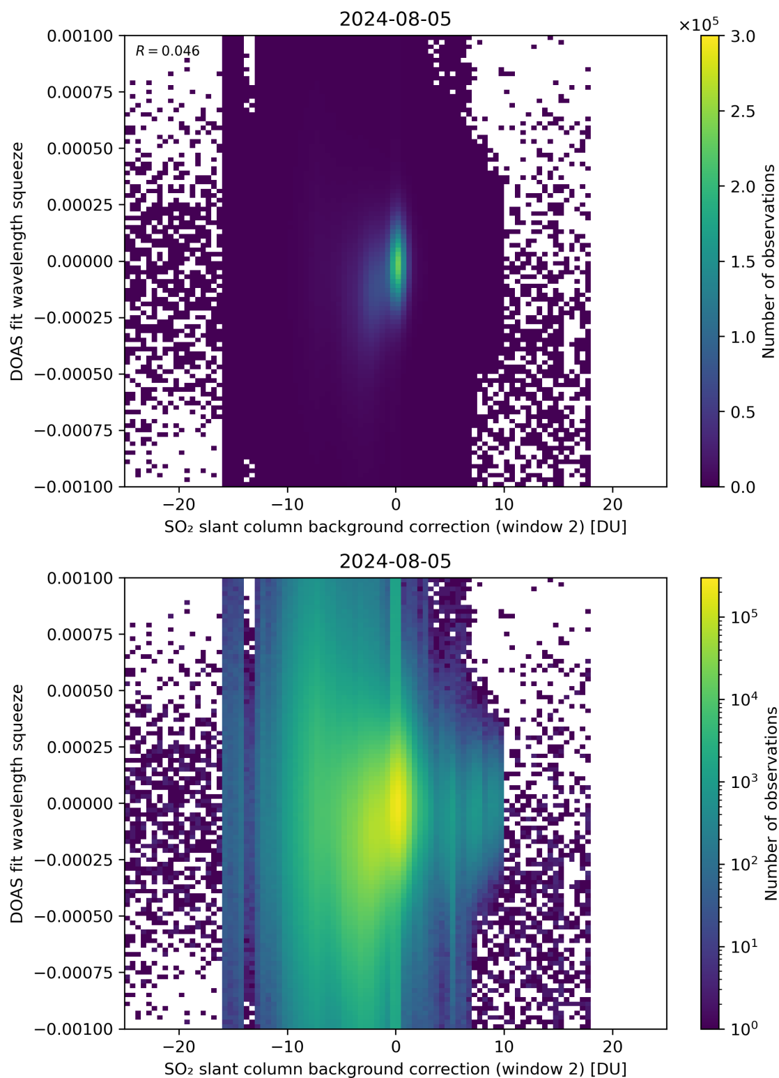
Figure 113: Scatter density plot of “SO 2 slant column background correction (window 2)” against “DOAS fit wavelength squeeze” for 2024-08-04 to 2024-08-06.
