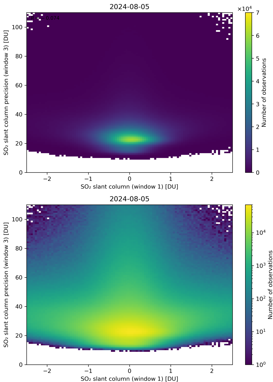
Figure 238: Scatter density plot of “SO 2 slant column (window 1)” against “SO 2 slant column precision (window 3)” for 2024-08-04 to 2024-08-06.
