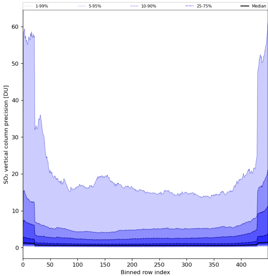
Figure 77: Along track statistics of “SO 2 vertical column precision” for 2024-08-04 to 2024-08-06
