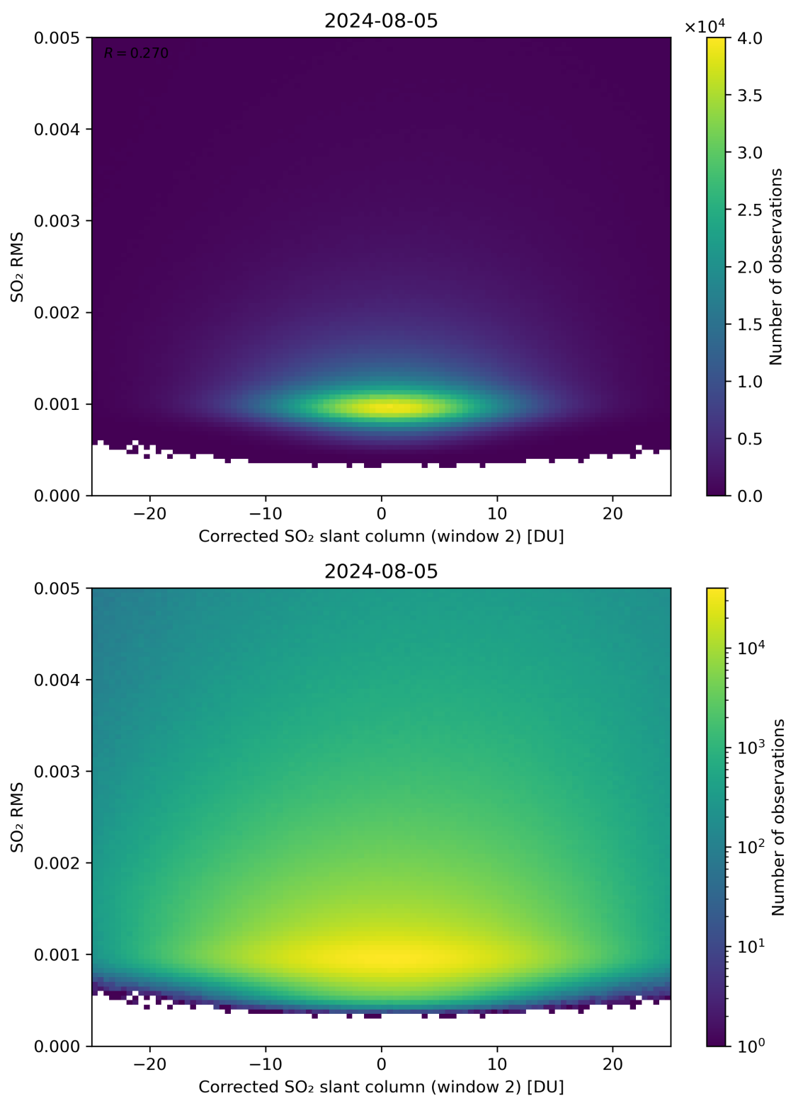
Figure 198: Scatter density plot of “Corrected SO 2 slant column (window 2)” against “SO 2 RMS” for 2024-08-04 to 2024-08-06.
