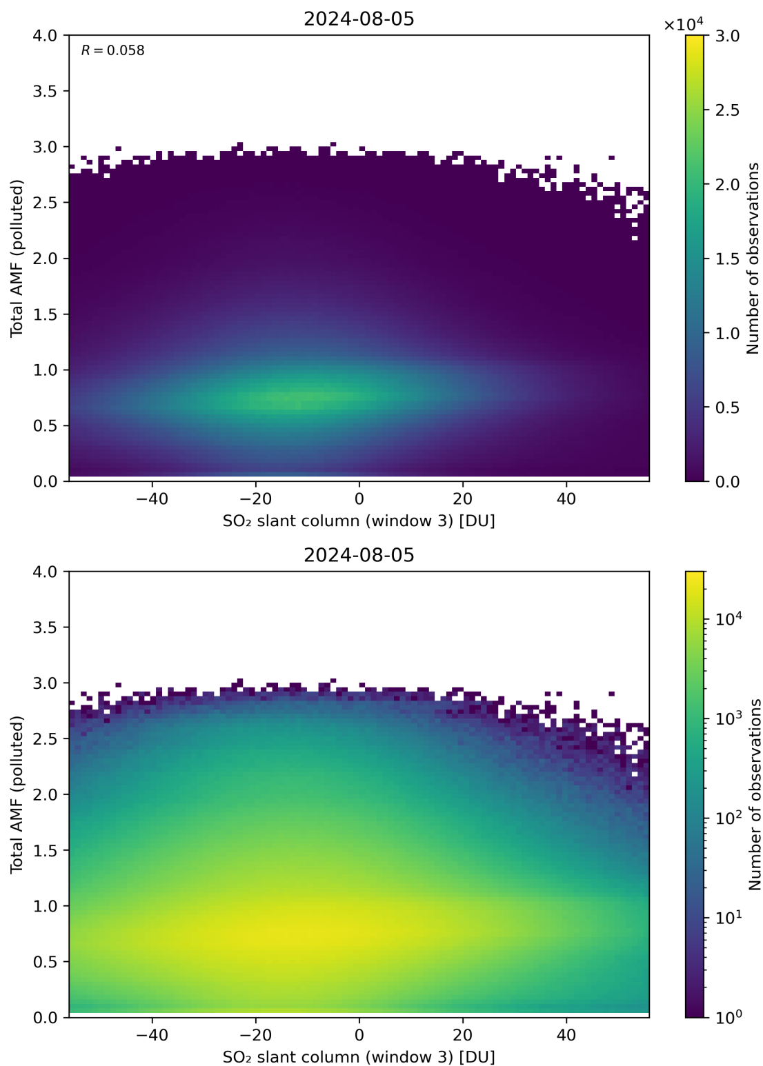
Figure 268: Scatter density plot of “SO 2 slant column (window 3)” against “Total AMF (polluted)” for 2024-08-04 to 2024-08-06.
