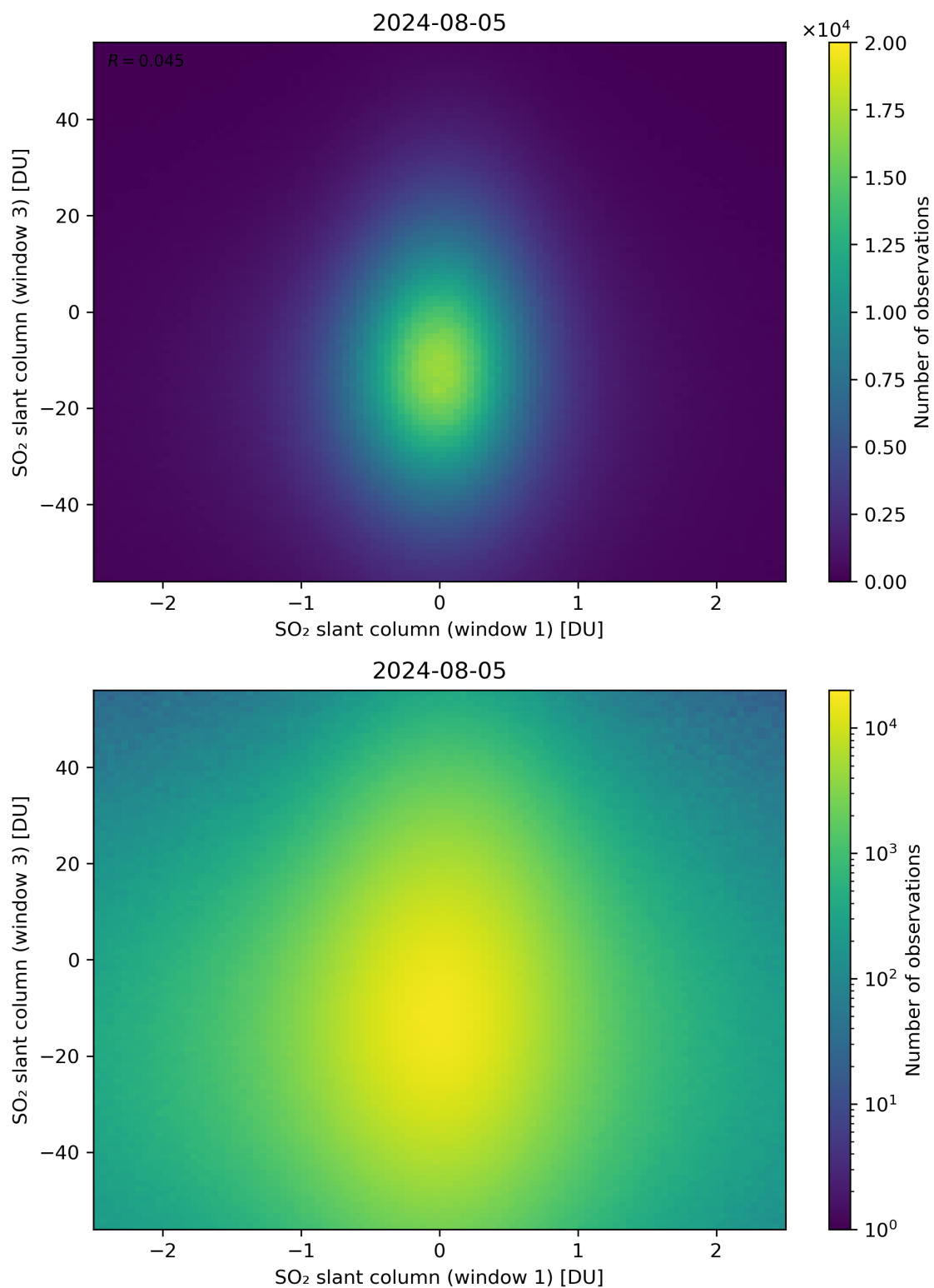
Figure 237: Scatter density plot of “SO 2 slant column (window 1)” against “SO 2 slant column (window 3)” for 2024-08-04 to 2024-08-06.
