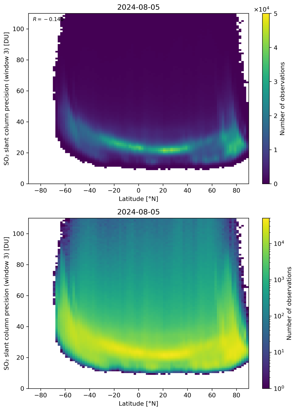
Figure 153: Scatter density plot of “Latitude” against “SO 2 slant column precision (window 3)” for 2024-08-04 to 2024-08-06.
