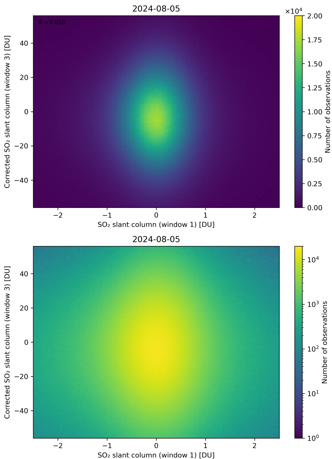
Figure 234: Scatter density plot of “SO 2 slant column (window 1)” against “Corrected SO 2 slant column (window 3)” for 2024-08-04 to 2024-08-06.
