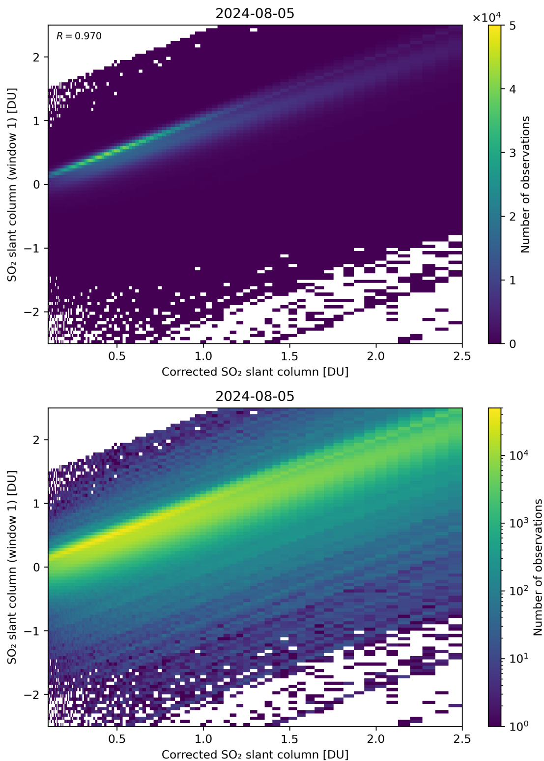
Figure 187: Scatter density plot of “Corrected SO 2 slant column” against “SO 2 slant column (window 1)” for 2024-08-04 to 2024-08-06.
