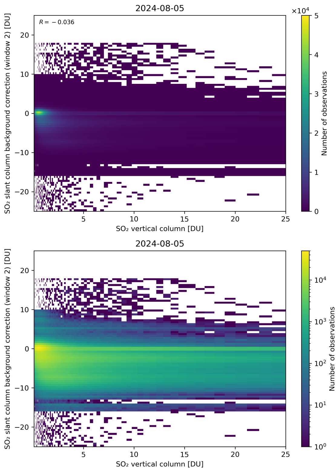
Figure 274: Scatter density plot of “SO 2 vertical column” against “SO 2 slant column background correction (window 2)” for 2024-08-04 to 2024-08-06.
