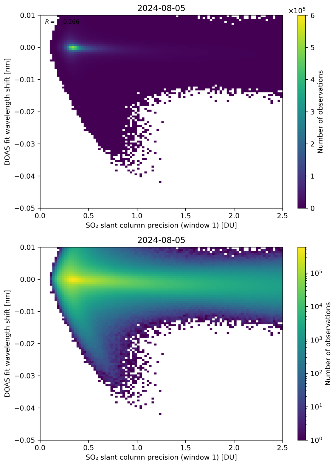
Figure 221: Scatter density plot of “SO 2 slant column precision (window 1)” against “DOAS fit wavelength shift” for 2024-08-04 to 2024-08-06.
