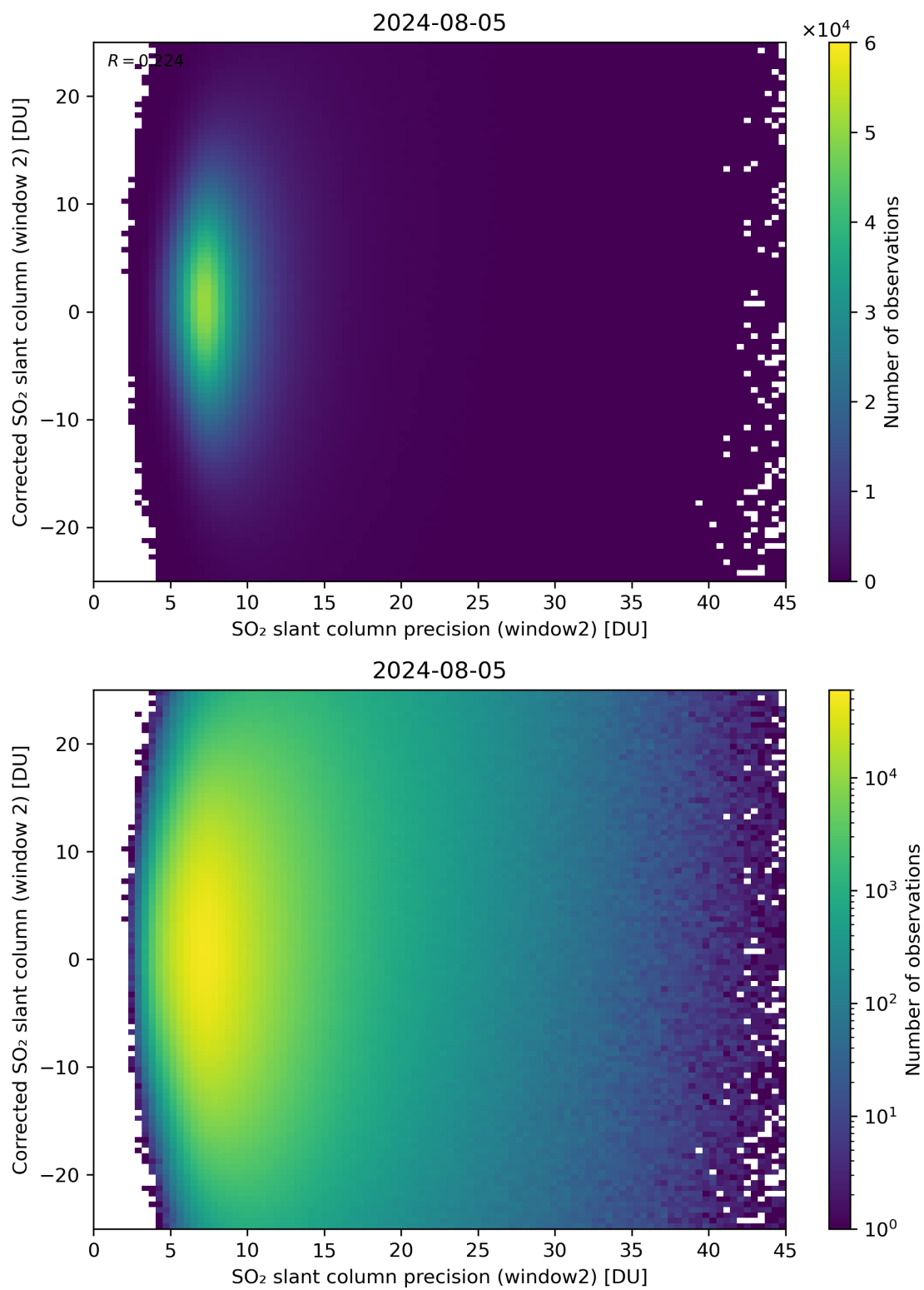
Figure 247: Scatter density plot of “SO 2 slant column precision (window2)” against “Corrected SO 2 slant column (window 2)” for 2024-08-04 to 2024-08-06.
