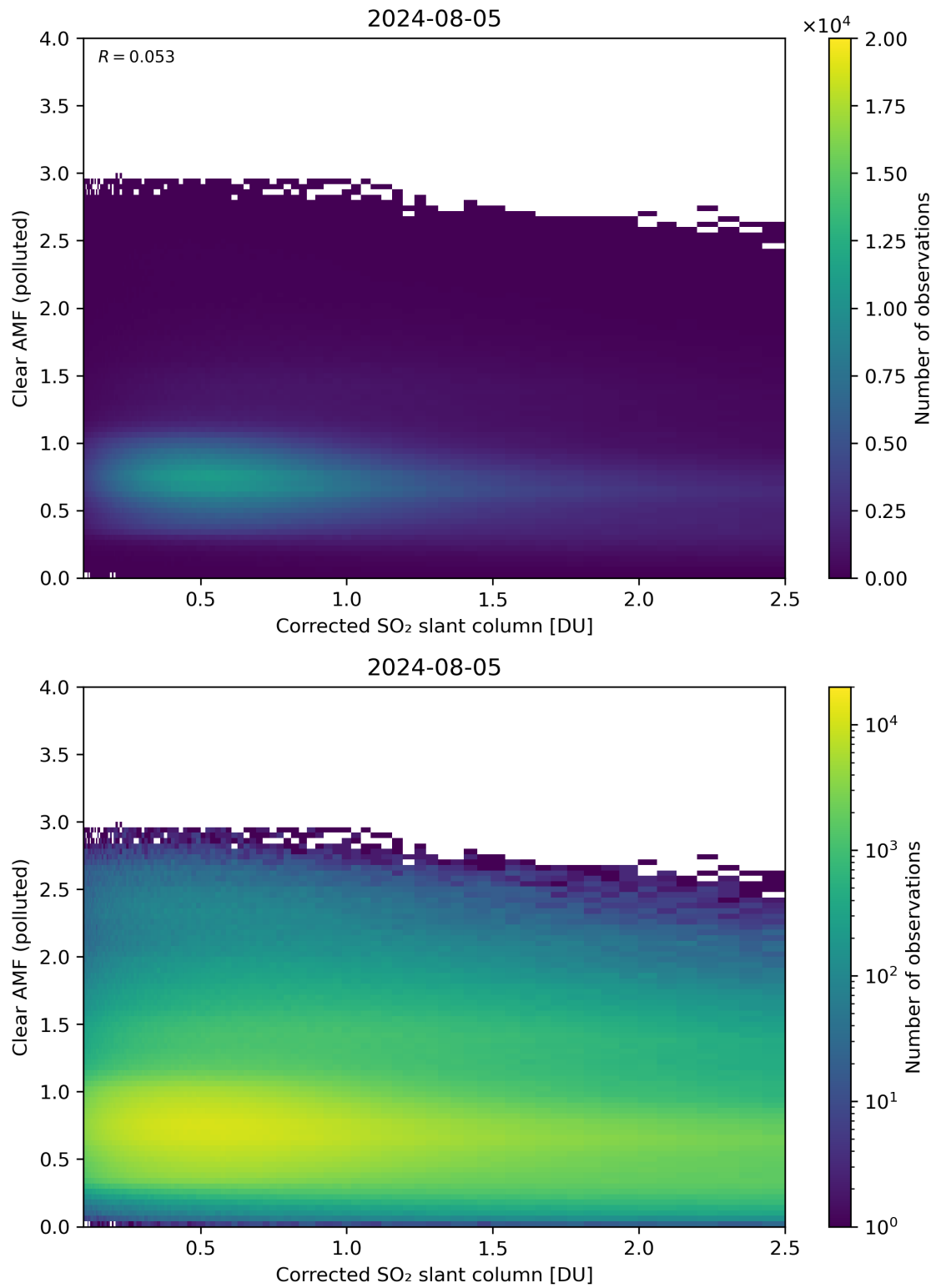
Figure 184: Scatter density plot of “Corrected SO 2 slant column” against “Clear AMF (polluted)” for 2024-08-04 to 2024-08-06.
