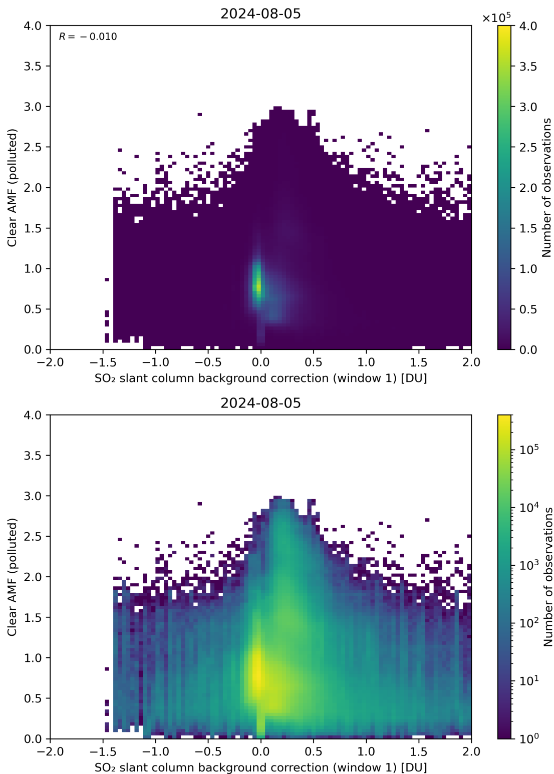
Figure 103: Scatter density plot of “SO 2 slant column background correction (window 1)” against “Clear AMF (polluted)” for 2024-08-04 to 2024-08-06.
