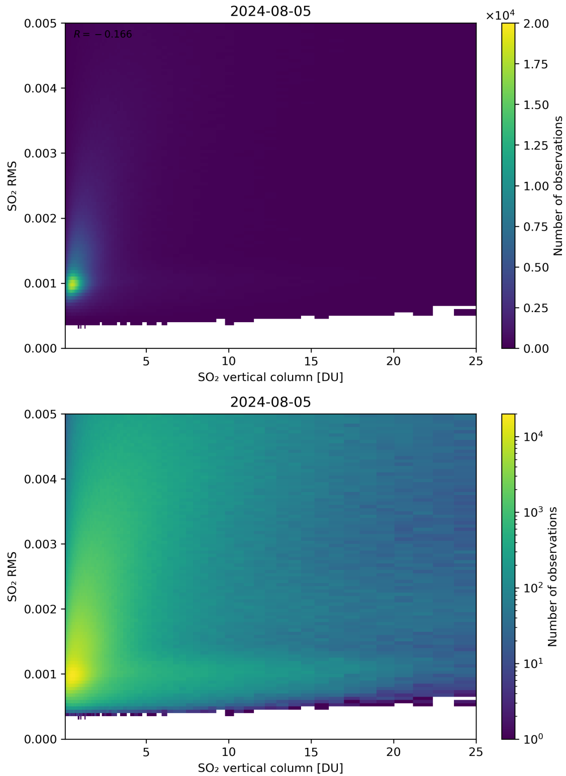
Figure 278: Scatter density plot of “SO 2 vertical column” against “SO 2 RMS” for 2024-08-04 to 2024-08-06.
