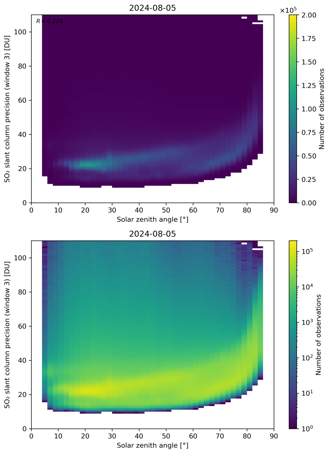
Figure 173: Scatter density plot of “Solar zenith angle” against “SO 2 slant column precision (window 3)” for 2024-08-04 to 2024-08-06.
