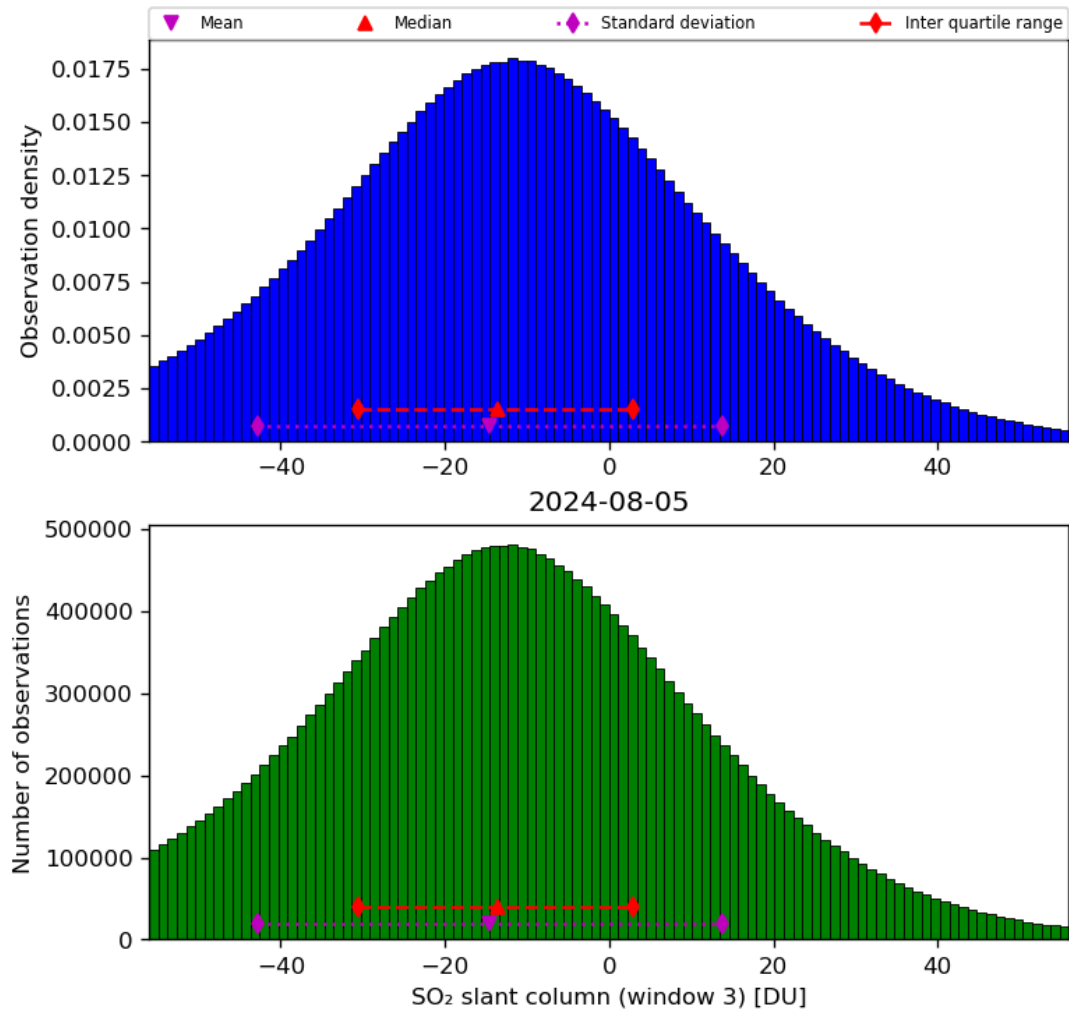
Figure 64: Histogram of “SO 2 slant column (window 3)” for 2024-08-04 to 2024-08-06
