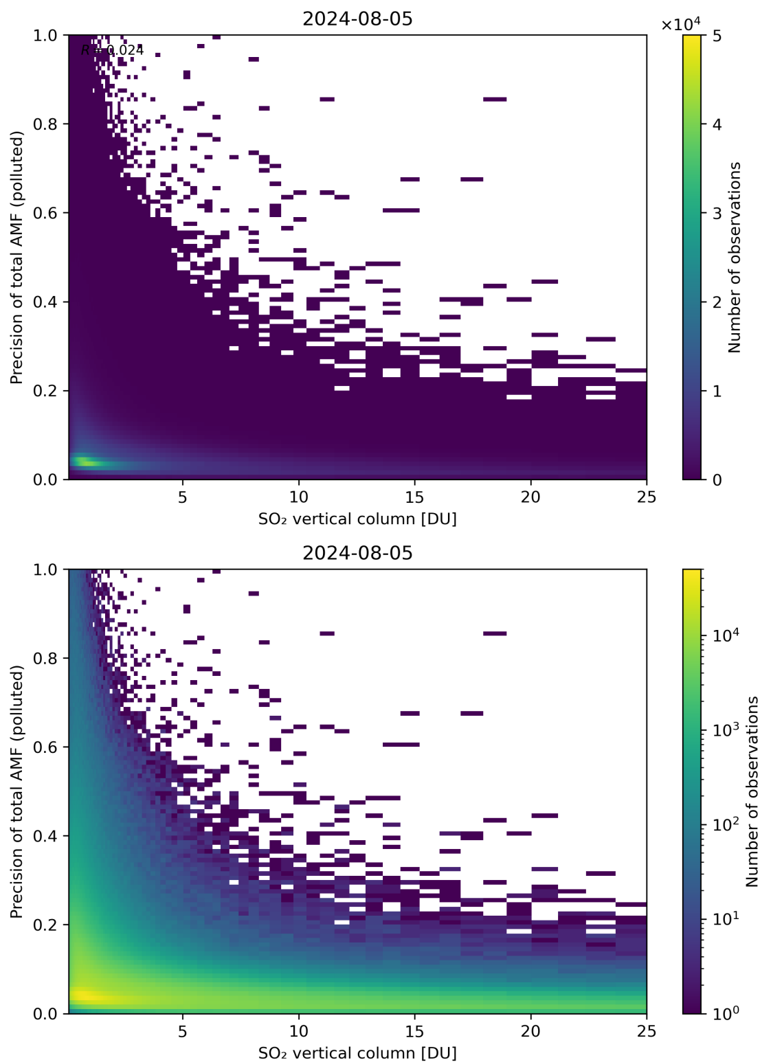
Figure 306: Scatter density plot of “SO 2 vertical column” against “Precision of total AMF (polluted)” for 2024-08-04 to 2024-08-06.
