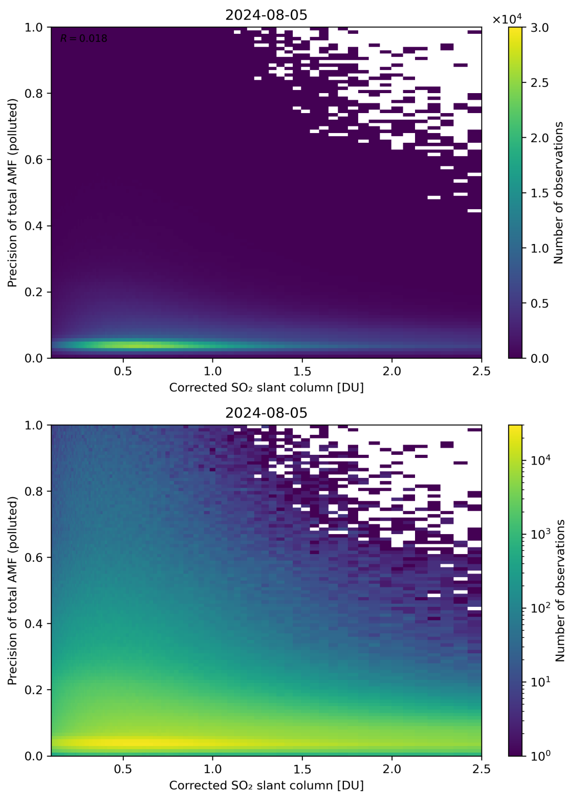
Figure 193: Scatter density plot of “Corrected SO 2 slant column” against “Precision of total AMF (polluted)” for 2024-08-04 to 2024-08-06.
