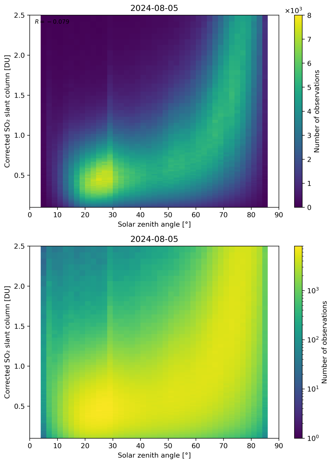
Figure 166: Scatter density plot of “Solar zenith angle” against “Corrected SO 2 slant column” for 2024-08-04 to 2024-08-06.
