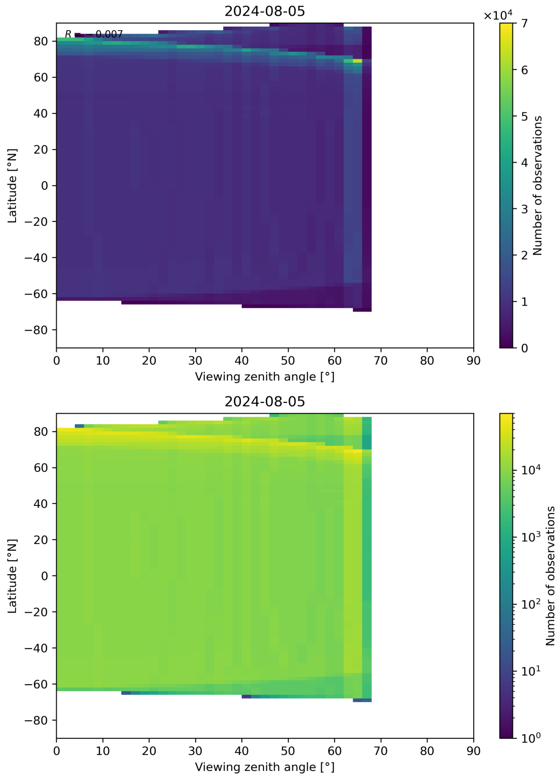
Figure 314: Scatter density plot of “Viewing zenith angle” against “Latitude” for 2024-08-04 to 2024-08-06.
