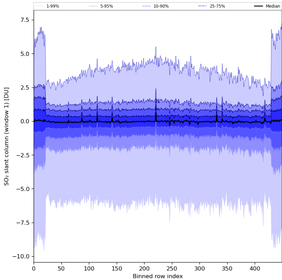
Figure 79: Along track statistics of “SO 2 slant column (window 1)” for 2024-08-04 to 2024-08-06
