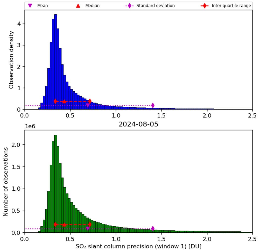
Figure 57: Histogram of “SO 2 slant column precision (window 1)” for 2024-08-04 to 2024-08-06
