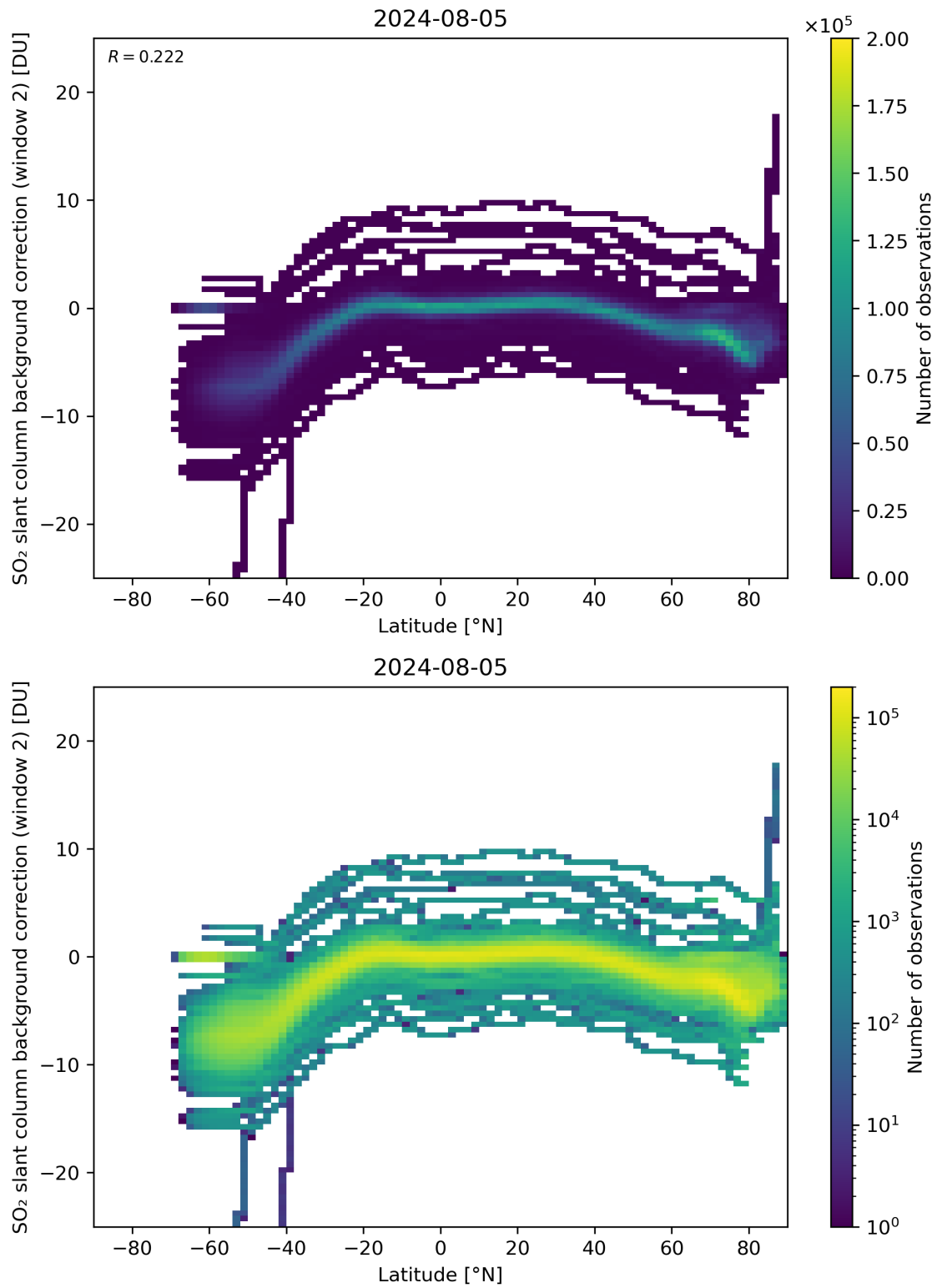
Figure 140: Scatter density plot of “Latitude” against “SO 2 slant column background correction (window 2)” for 2024-08-04 to 2024-08-06.
