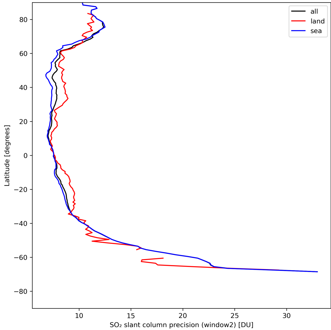
Figure 38: Zonal average of “SO 2 slant column precision (window2)” for 2024-08-04 to 2024-08-06.
