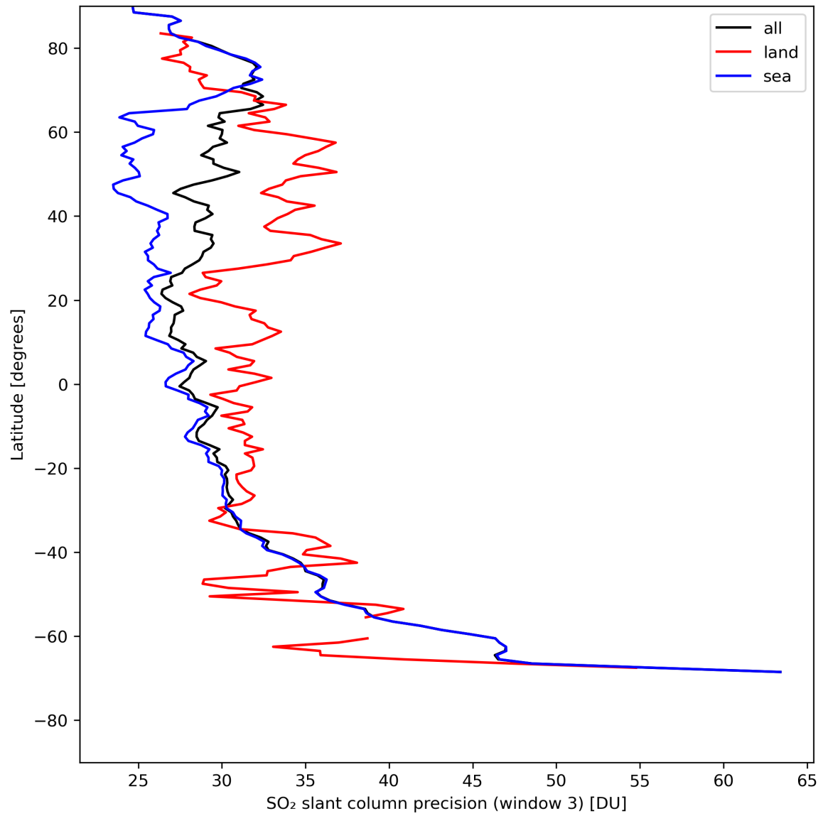
Figure 42: Zonal average of “SO 2 slant column precision (window 3)” for 2024-08-04 to 2024-08-06.
