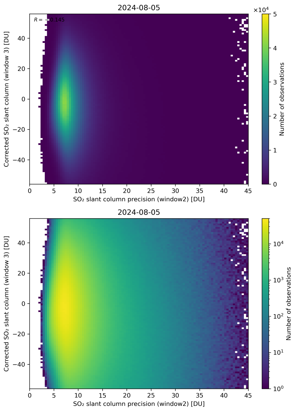
Figure 248: Scatter density plot of “SO 2 slant column precision (window2)” against “Corrected SO 2 slant column (window 3)” for 2024-08-04 to 2024-08-06.
