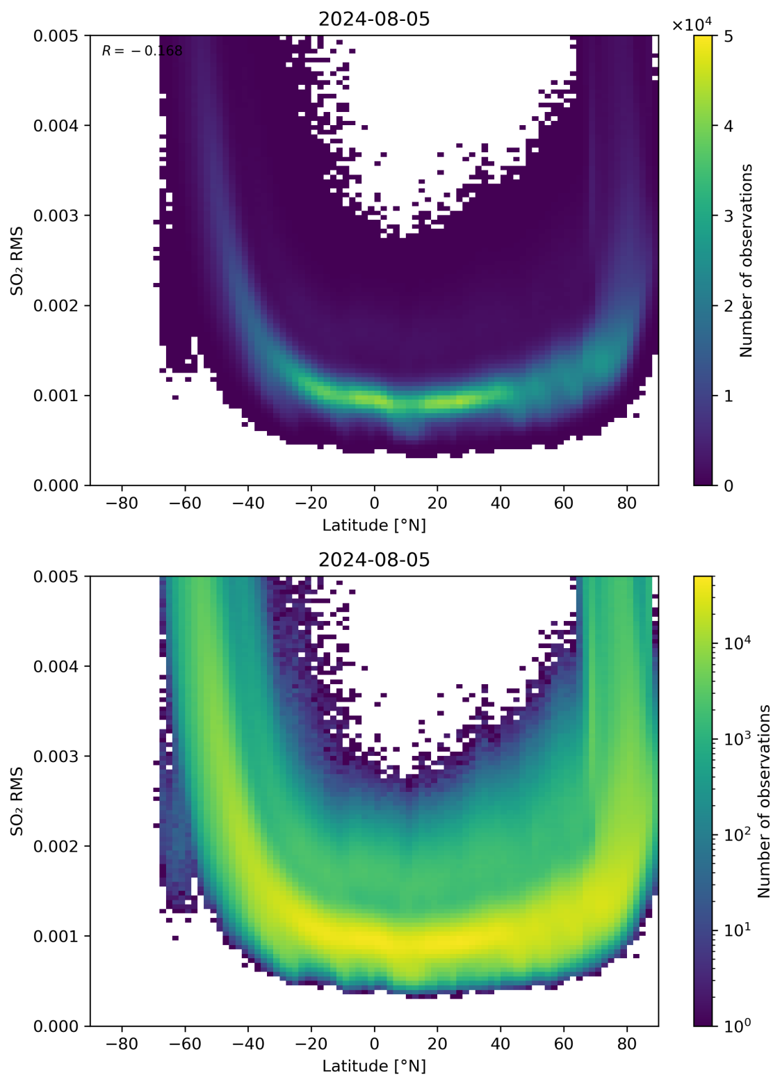
Figure 144: Scatter density plot of “Latitude” against “SO 2 RMS” for 2024-08-04 to 2024-08-06.
