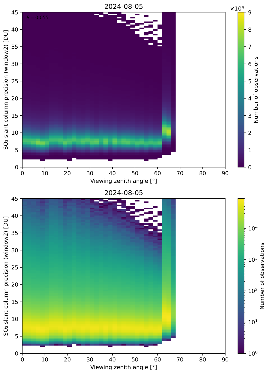
Figure 322: Scatter density plot of “Viewing zenith angle” against “SO 2 slant column precision (window2)” for 2024-08-04 to 2024-08-06.
