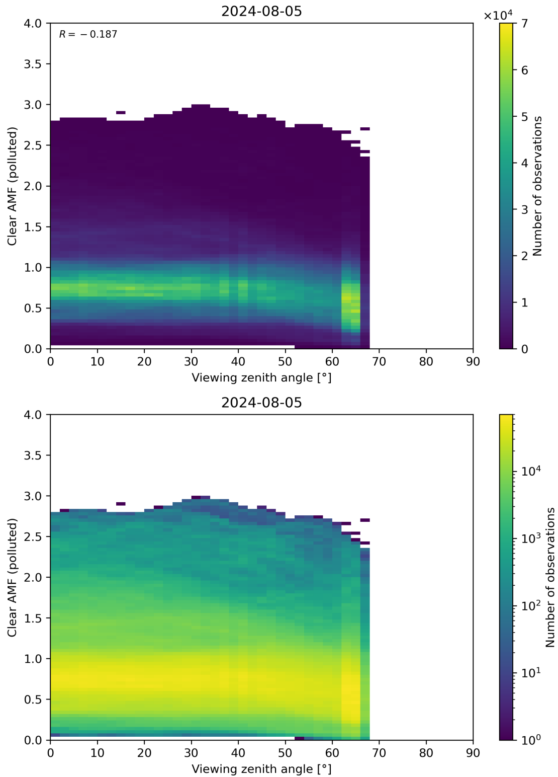
Figure 316: Scatter density plot of “Viewing zenith angle” against “Clear AMF (polluted)” for 2024-08-04 to 2024-08-06.
