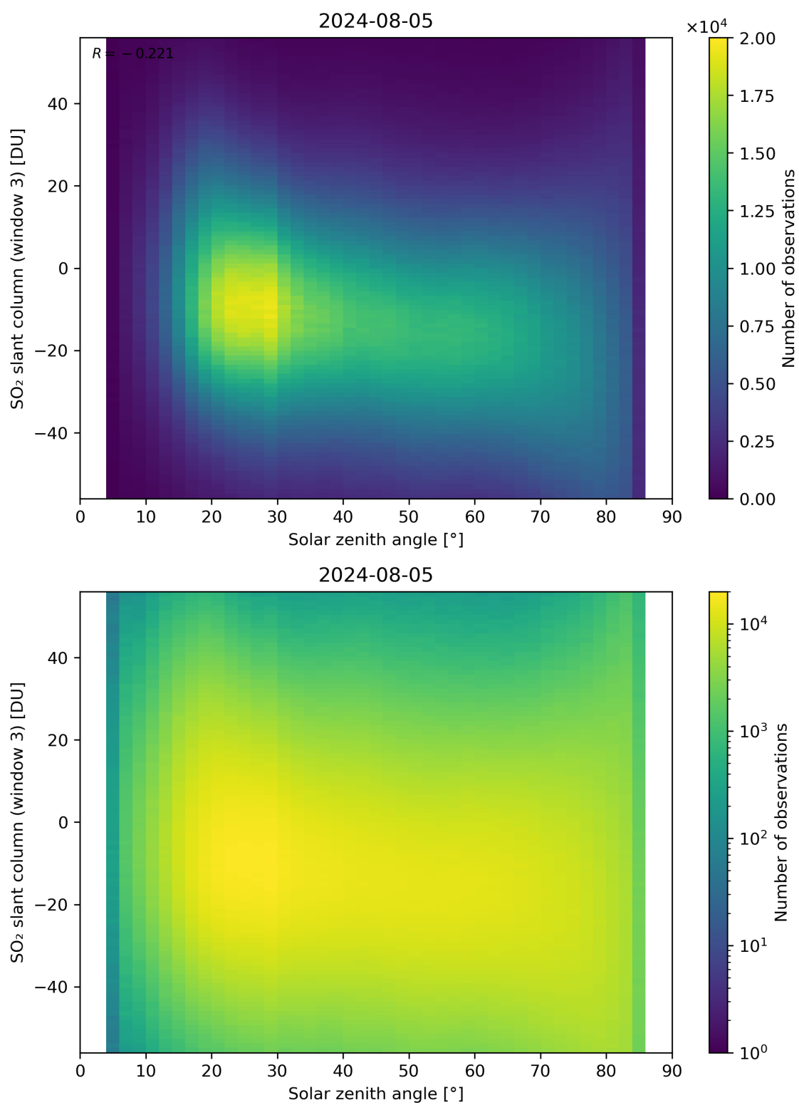
Figure 172: Scatter density plot of “Solar zenith angle” against “SO 2 slant column (window 3)” for 2024-08-04 to 2024-08-06.
