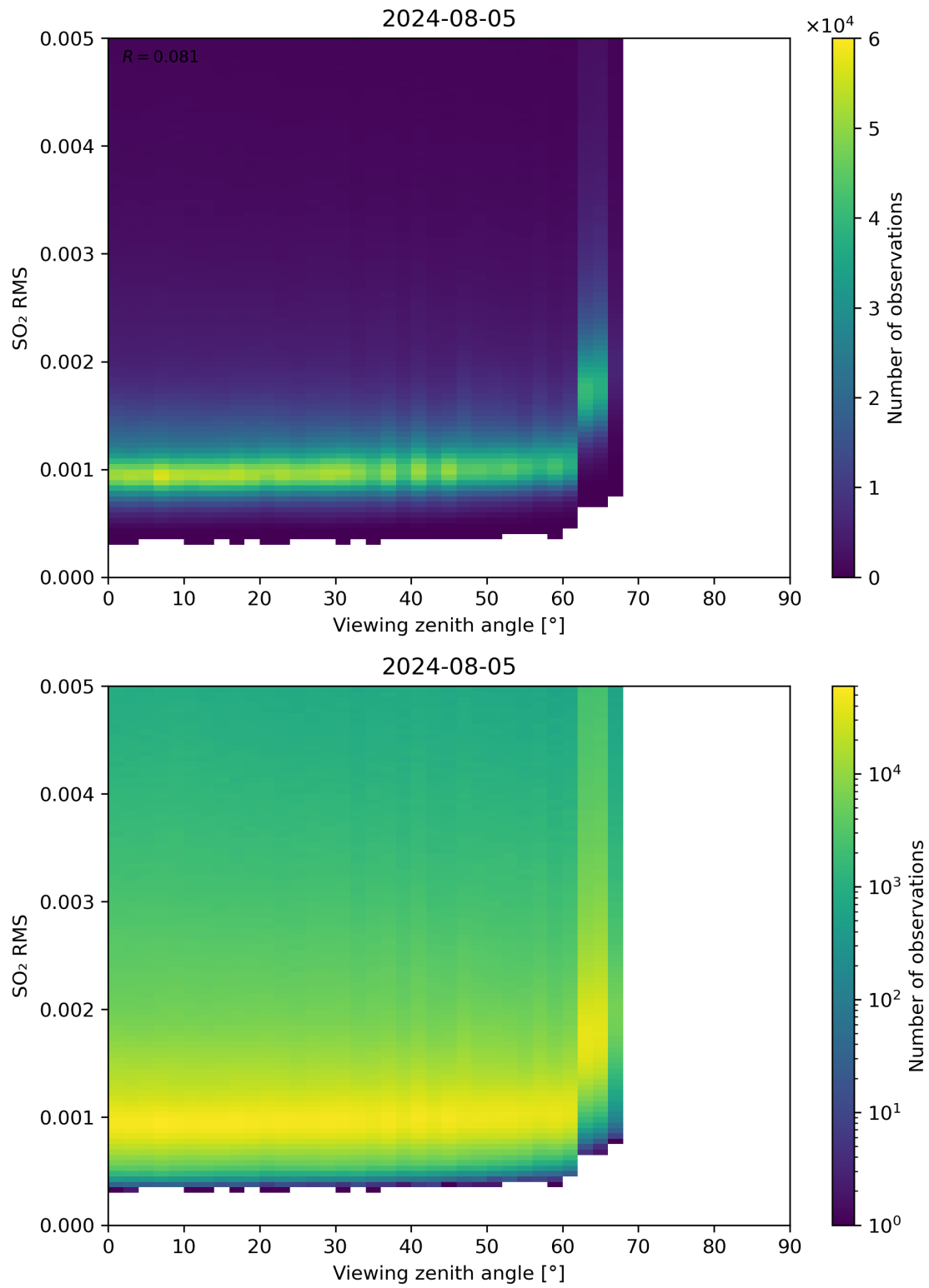
Figure 313: Scatter density plot of “Viewing zenith angle” against “SO 2 RMS” for 2024-08-04 to 2024-08-06.
