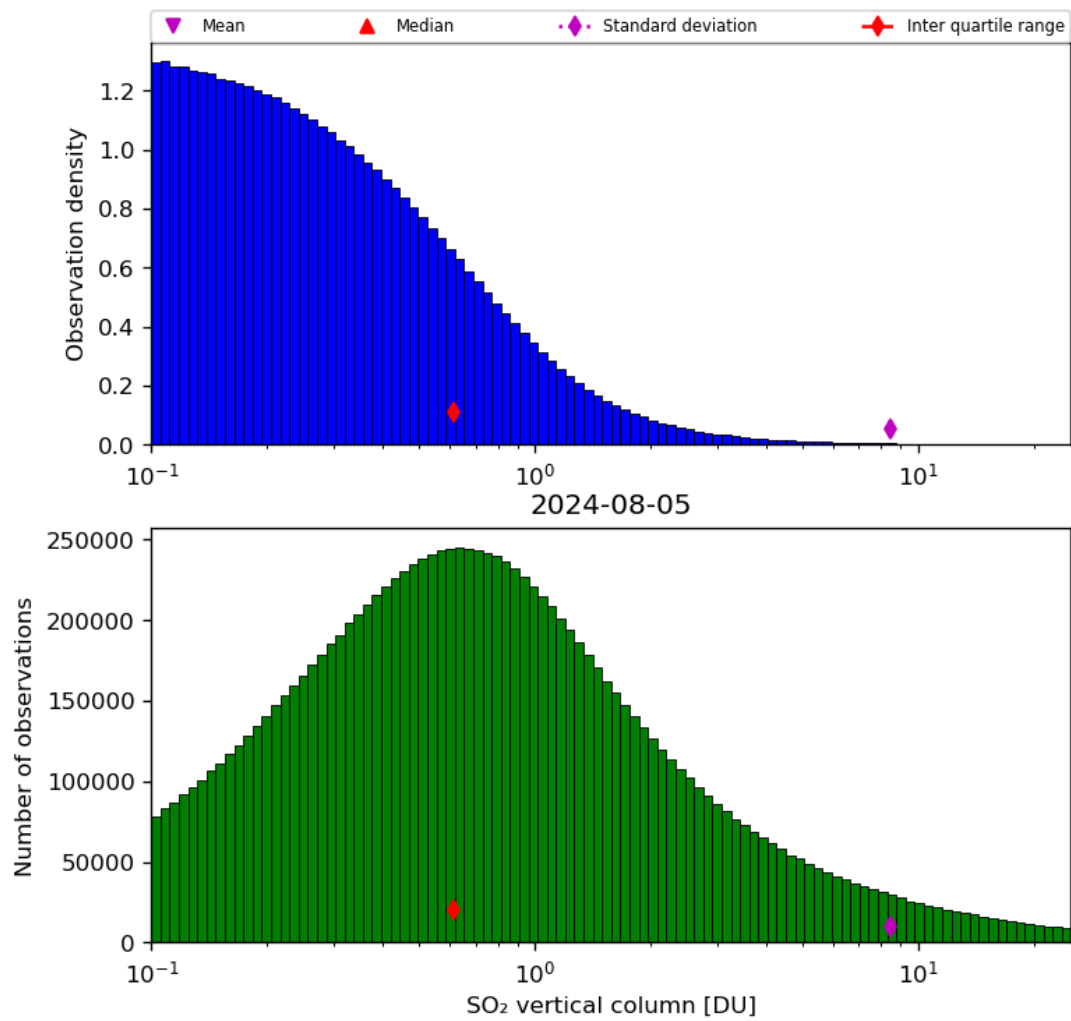
Figure 53: Histogram of “SO 2 vertical column” for 2024-08-04 to 2024-08-06
