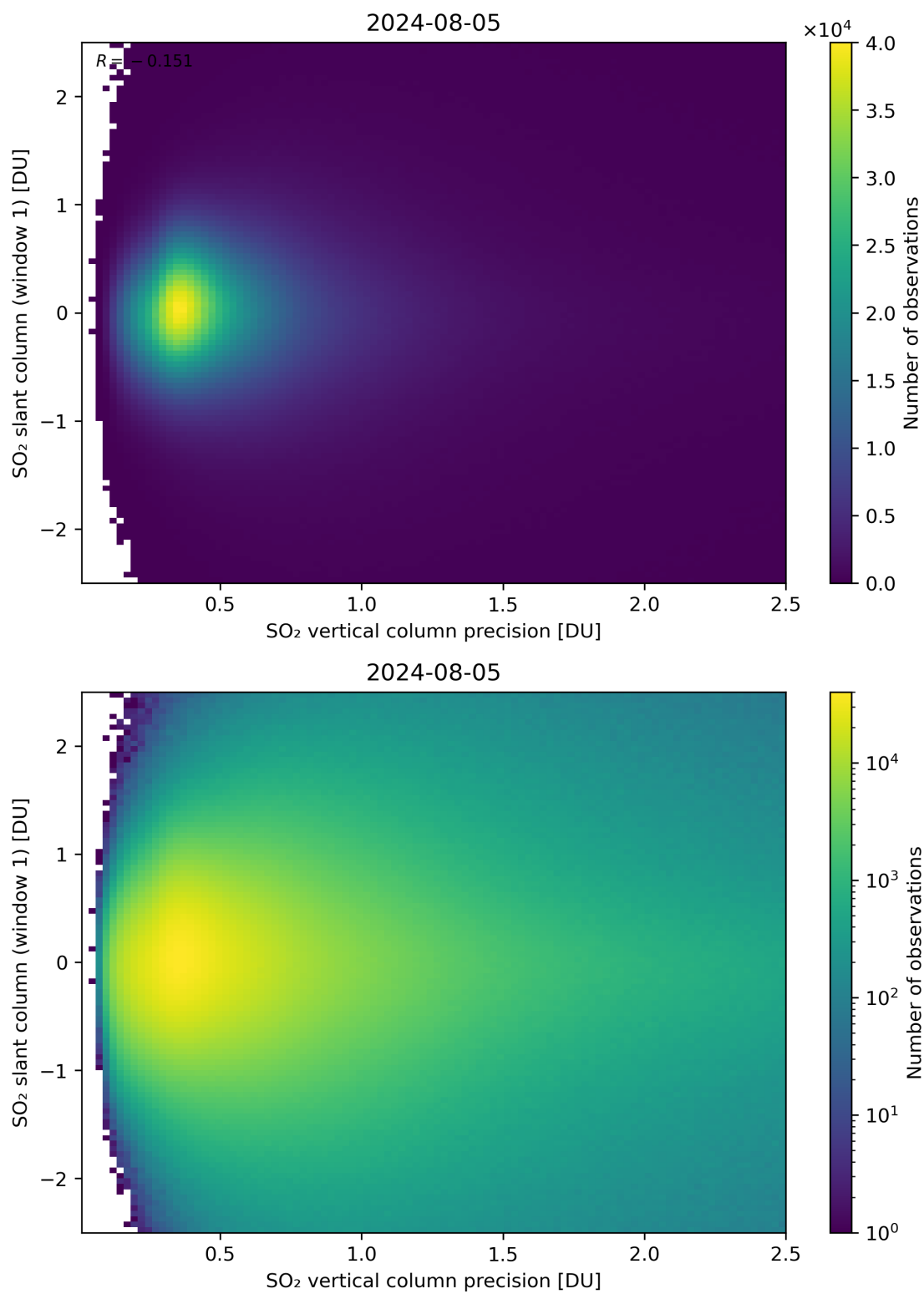
Figure 289: Scatter density plot of “SO 2 vertical column precision” against “SO 2 slant column (window 1)” for 2024-08-04 to 2024-08-06.
