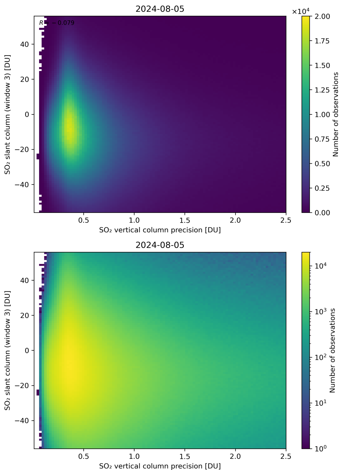
Figure 292: Scatter density plot of “SO 2 vertical column precision” against “SO 2 slant column (window 3)” for 2024-08-04 to 2024-08-06.
