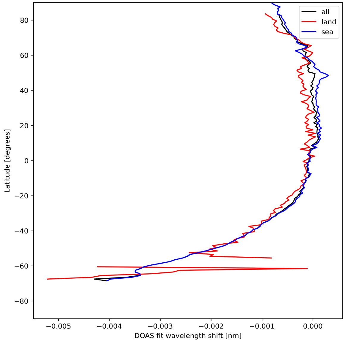
Figure 45: Zonal average of “DOAS fit wavelength shift” for 2024-08-04 to 2024-08-06.
