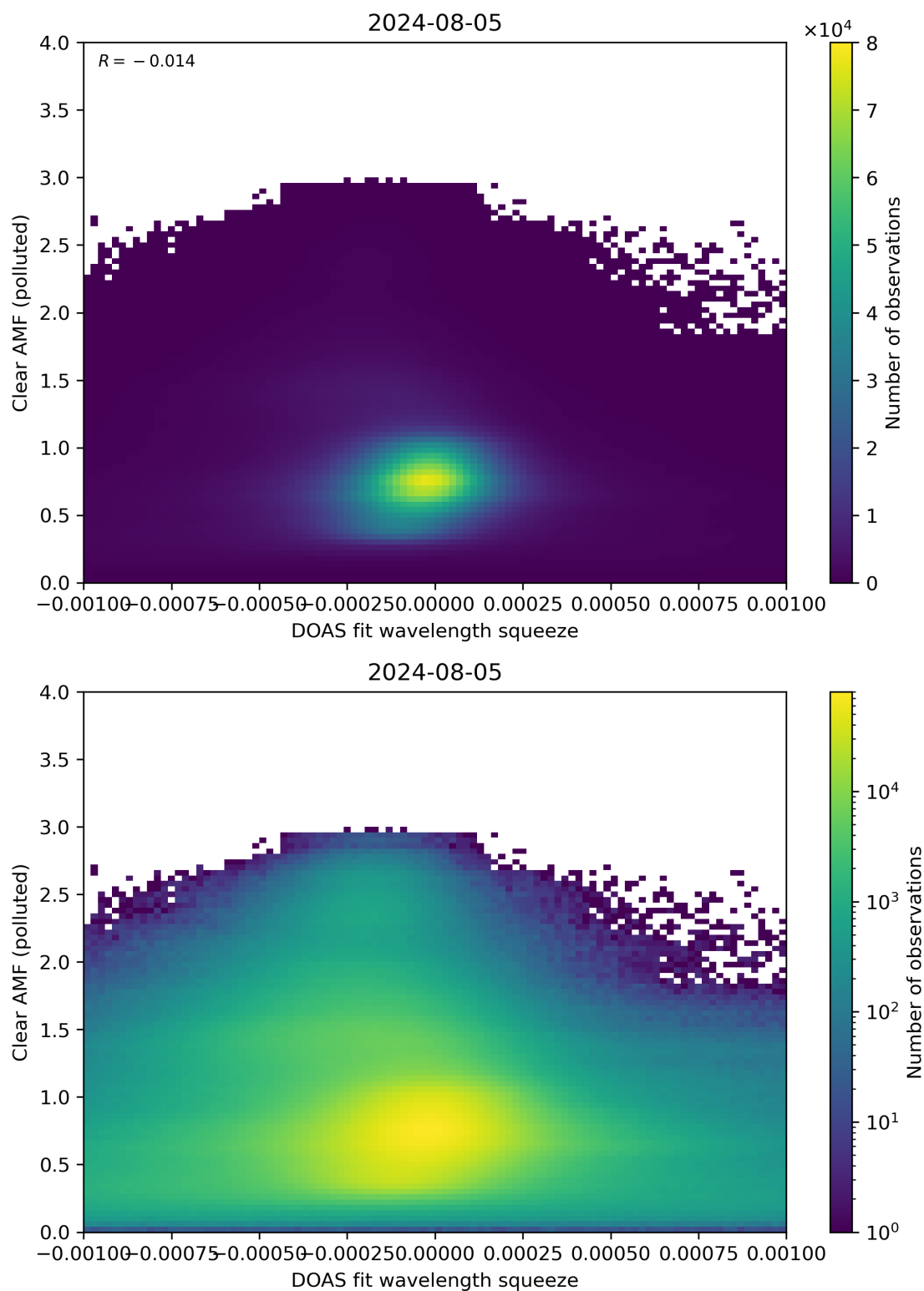
Figure 133: Scatter density plot of “DOAS fit wavelength squeeze” against “Clear AMF (polluted)” for 2024-08-04 to 2024-08-06.
