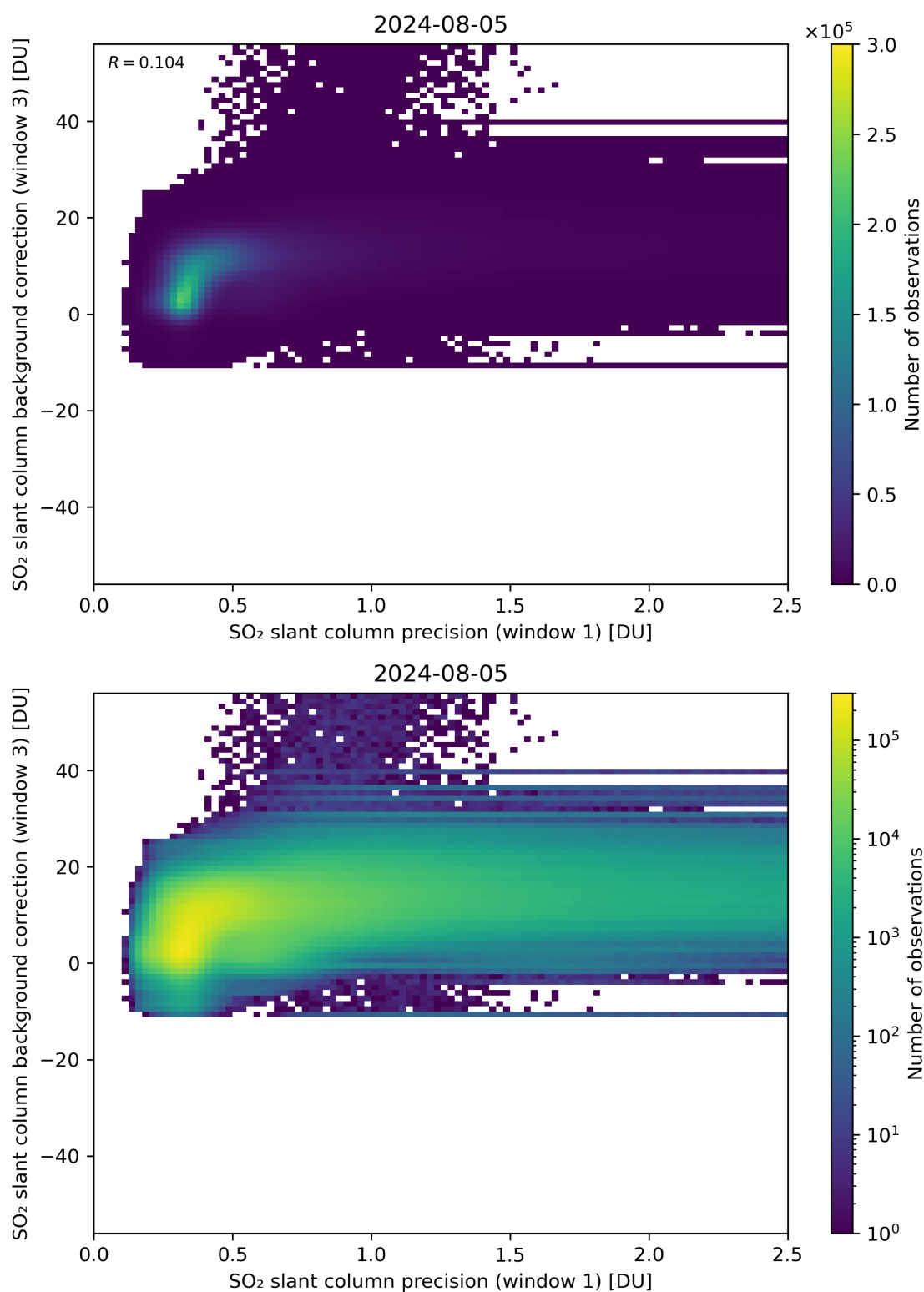
Figure 220: Scatter density plot of “SO 2 slant column precision (window 1)” against “SO 2 slant column background correction (window 3)” for 2024-08-04 to 2024-08-06.
