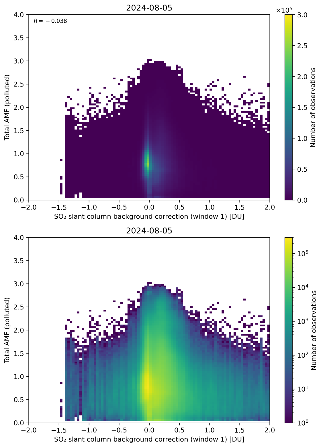
Figure 109: Scatter density plot of “SO 2 slant column background correction (window 1)” against “Total AMF (polluted)” for 2024-08-04 to 2024-08-06.
