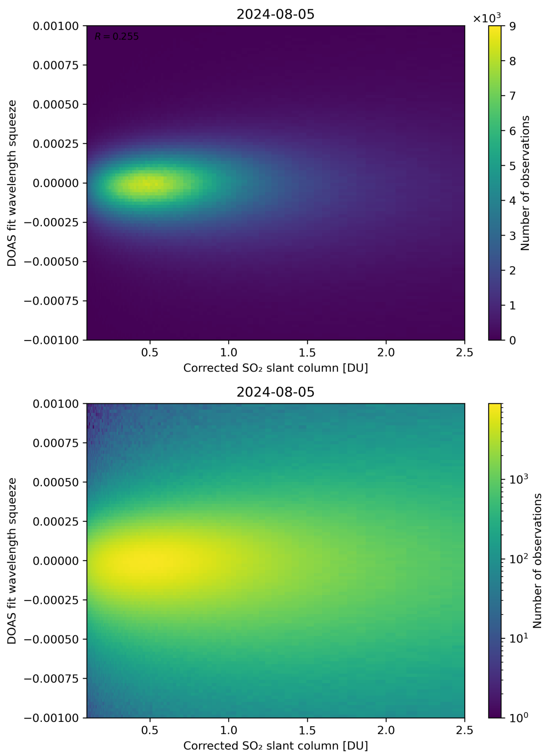
Figure 182: Scatter density plot of “Corrected SO 2 slant column” against “DOAS fit wavelength squeeze” for 2024-08-04 to 2024-08-06.
