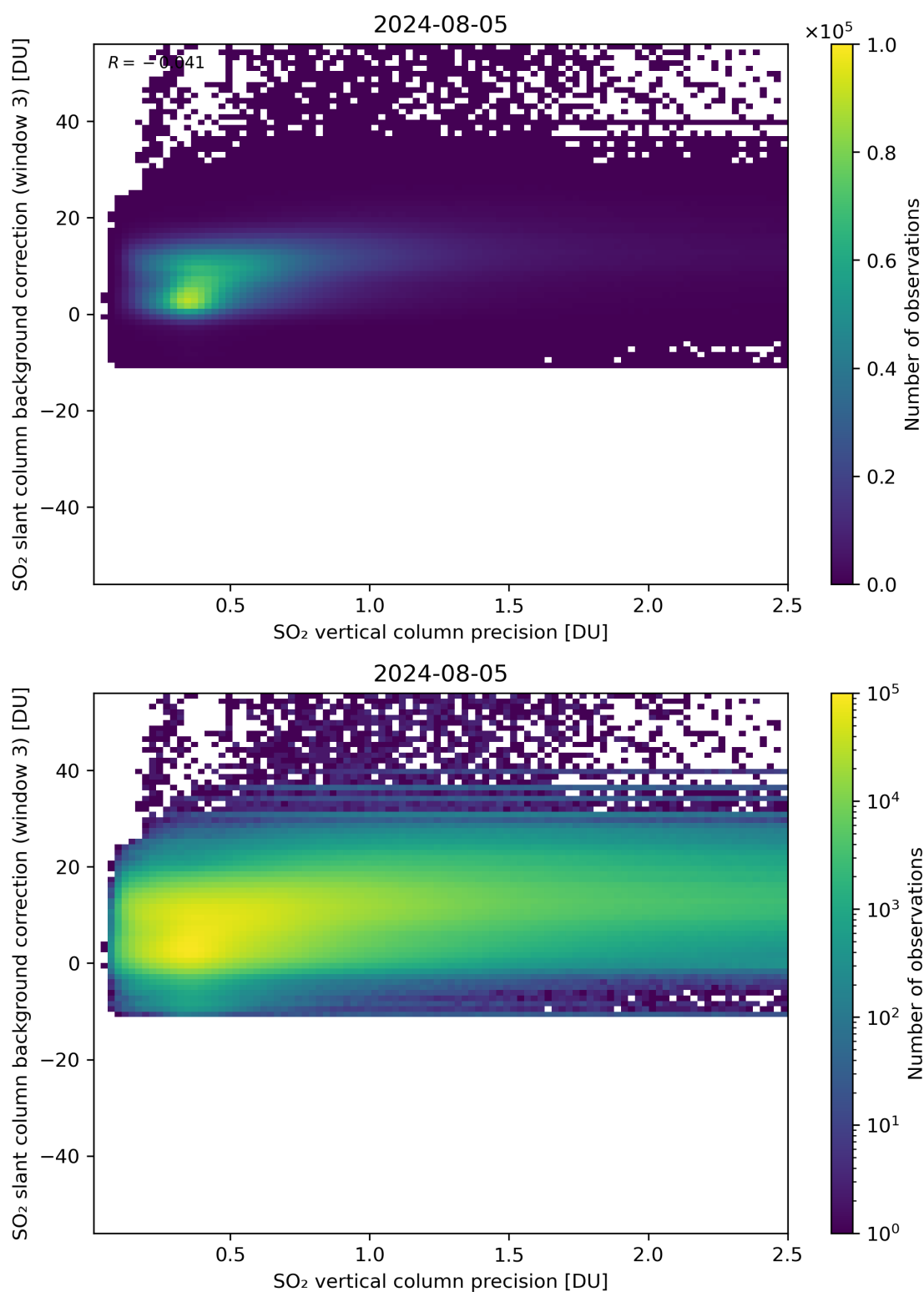
Figure 281: Scatter density plot of “SO 2 vertical column precision” against “SO 2 slant column background correction (window 3)” for 2024-08-04 to 2024-08-06.
