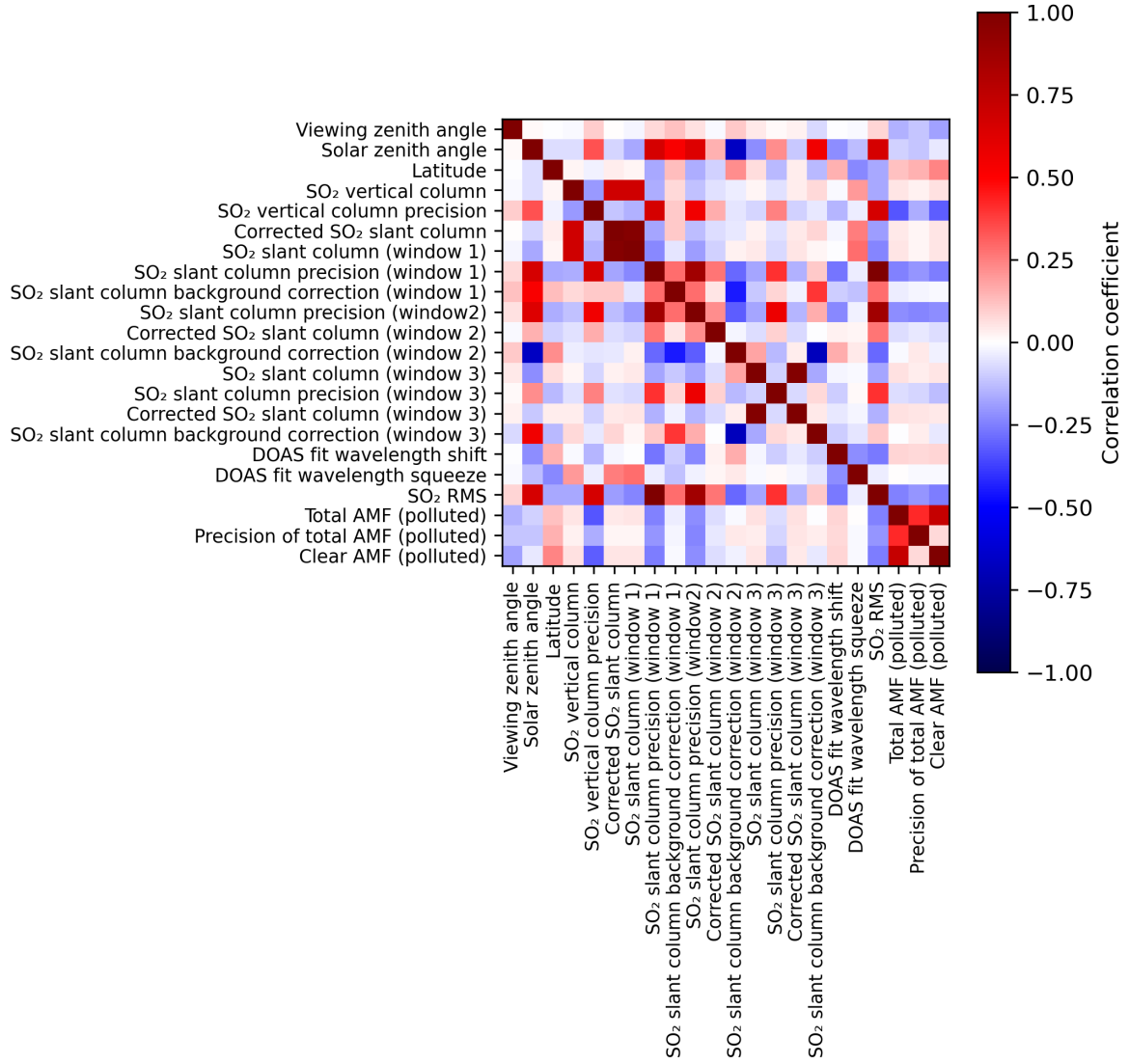
Figure 2: Map of correlation matrix for 2024-08-04 to 2024-08-06.
