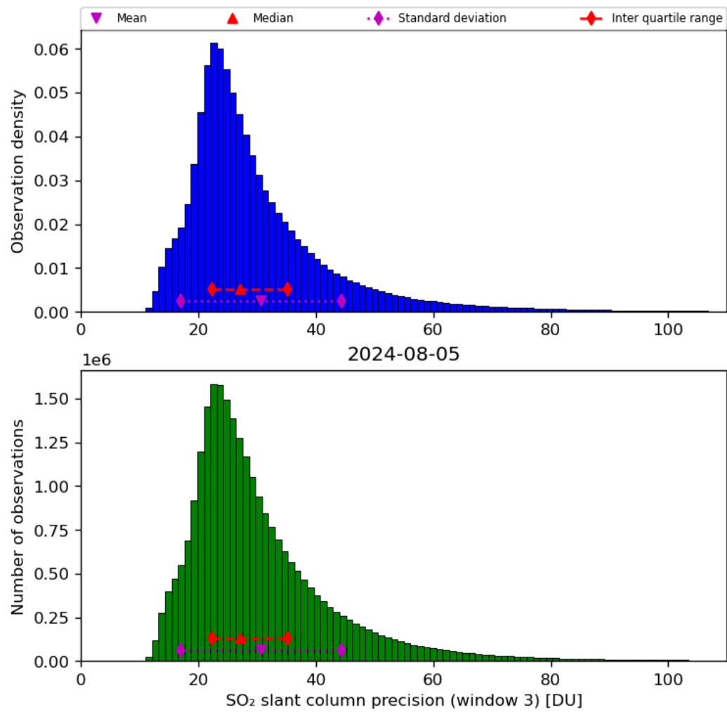
Figure 65: Histogram of “SO 2 slant column precision (window 3)” for 2024-08-04 to 2024-08-06
