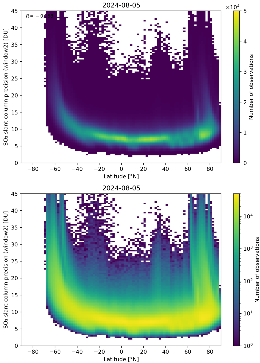
Figure 151: Scatter density plot of “Latitude” against “SO 2 slant column precision (window2)” for 2024-08-04 to 2024-08-06.
