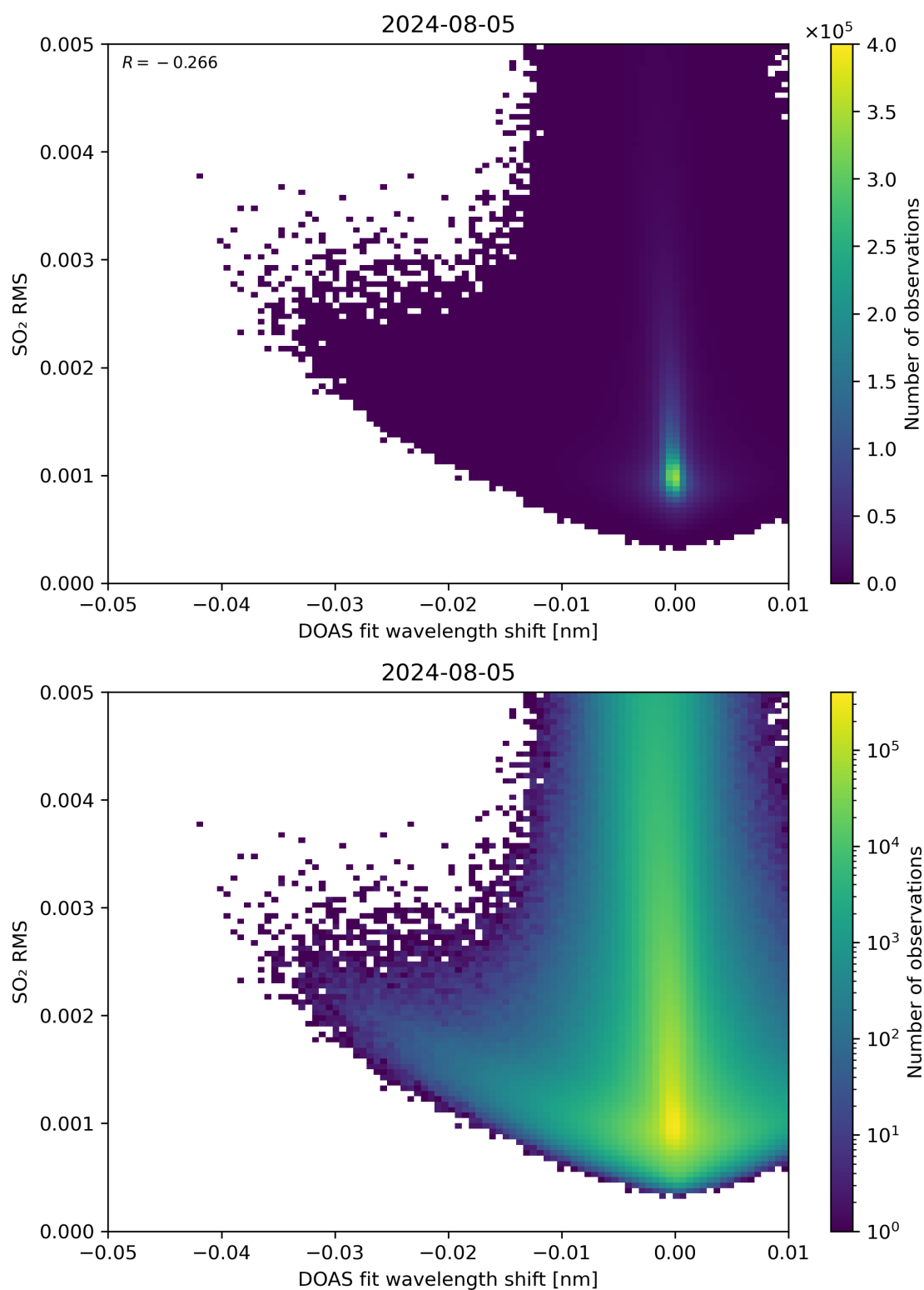
Figure 128: Scatter density plot of “DOAS fit wavelength shift” against “SO 2 RMS” for 2024-08-04 to 2024-08-06.
