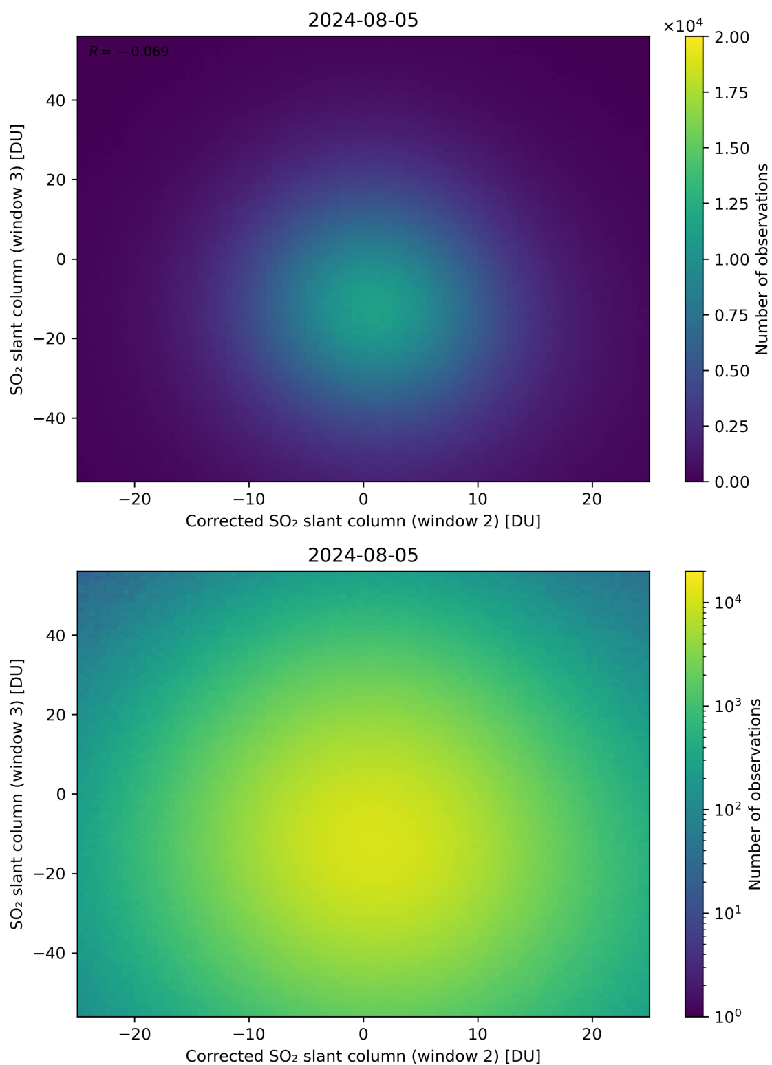
Figure 201: Scatter density plot of “Corrected SO 2 slant column (window 2)” against “SO 2 slant column (window 3)” for 2024-08-04 to 2024-08-06.
