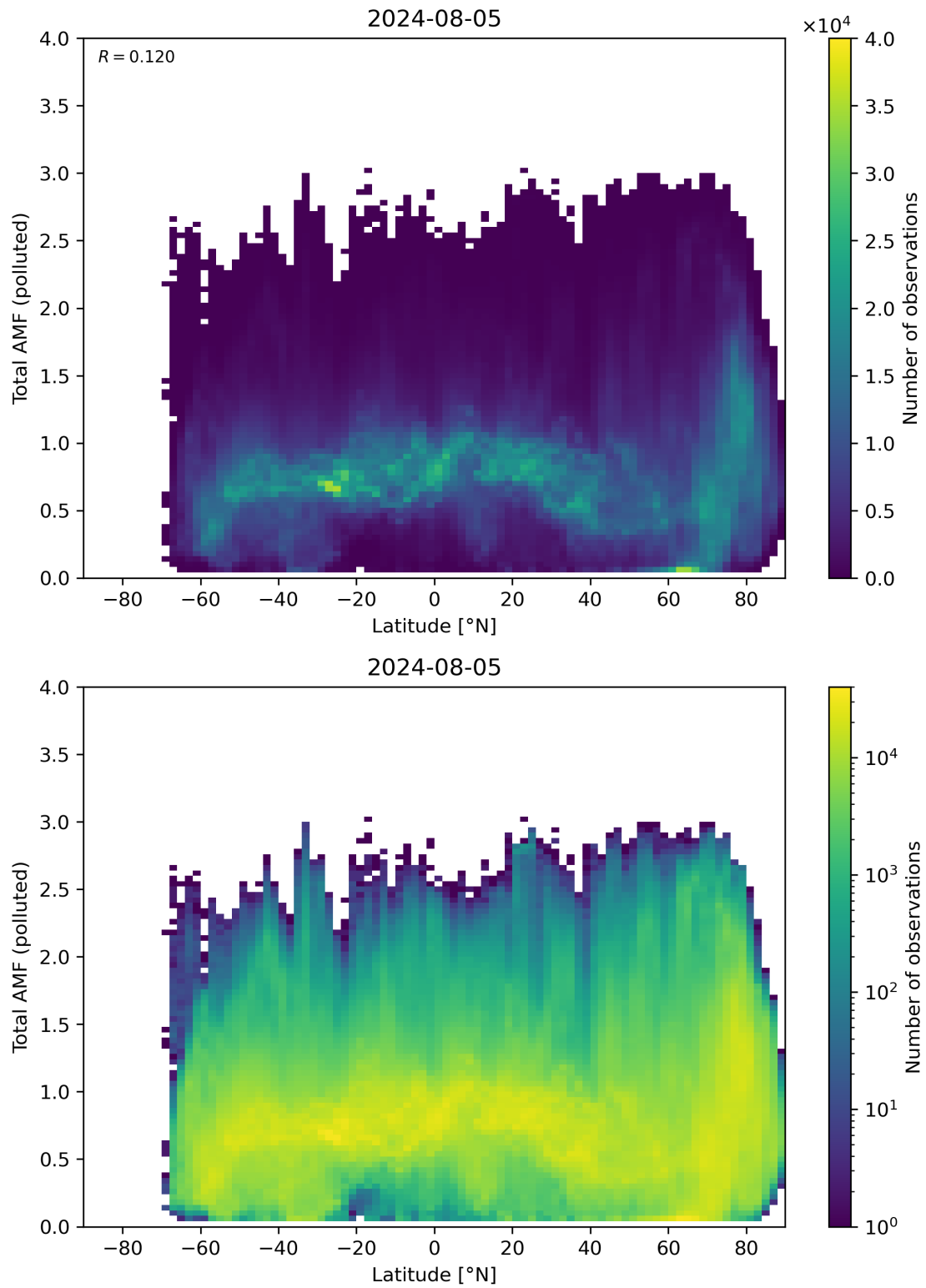
Figure 154: Scatter density plot of “Latitude” against “Total AMF (polluted)” for 2024-08-04 to 2024-08-06.
