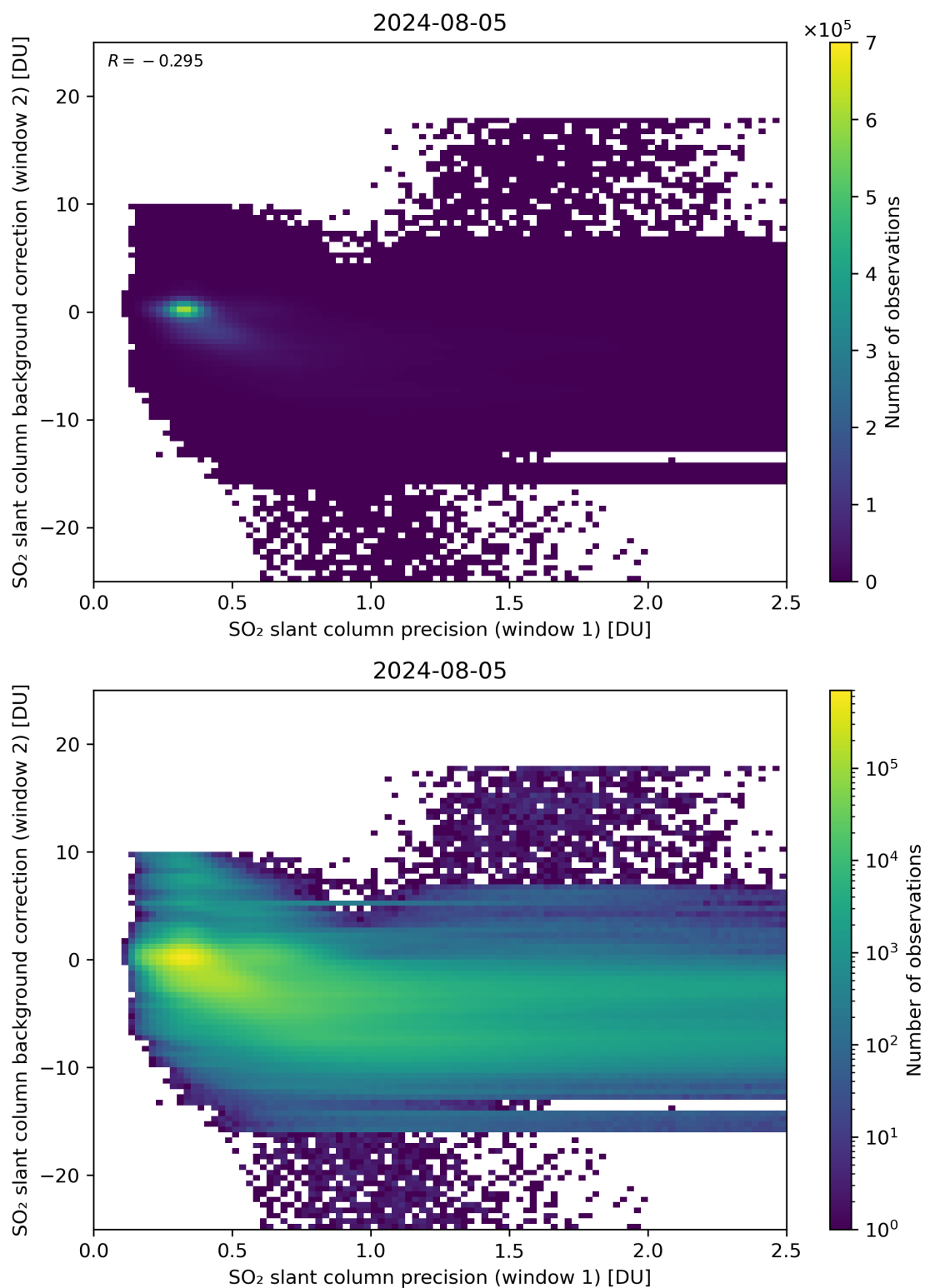
Figure 219: Scatter density plot of “SO 2 slant column precision (window 1)” against “SO 2 slant column background correction (window 2)” for 2024-08-04 to 2024-08-06.
