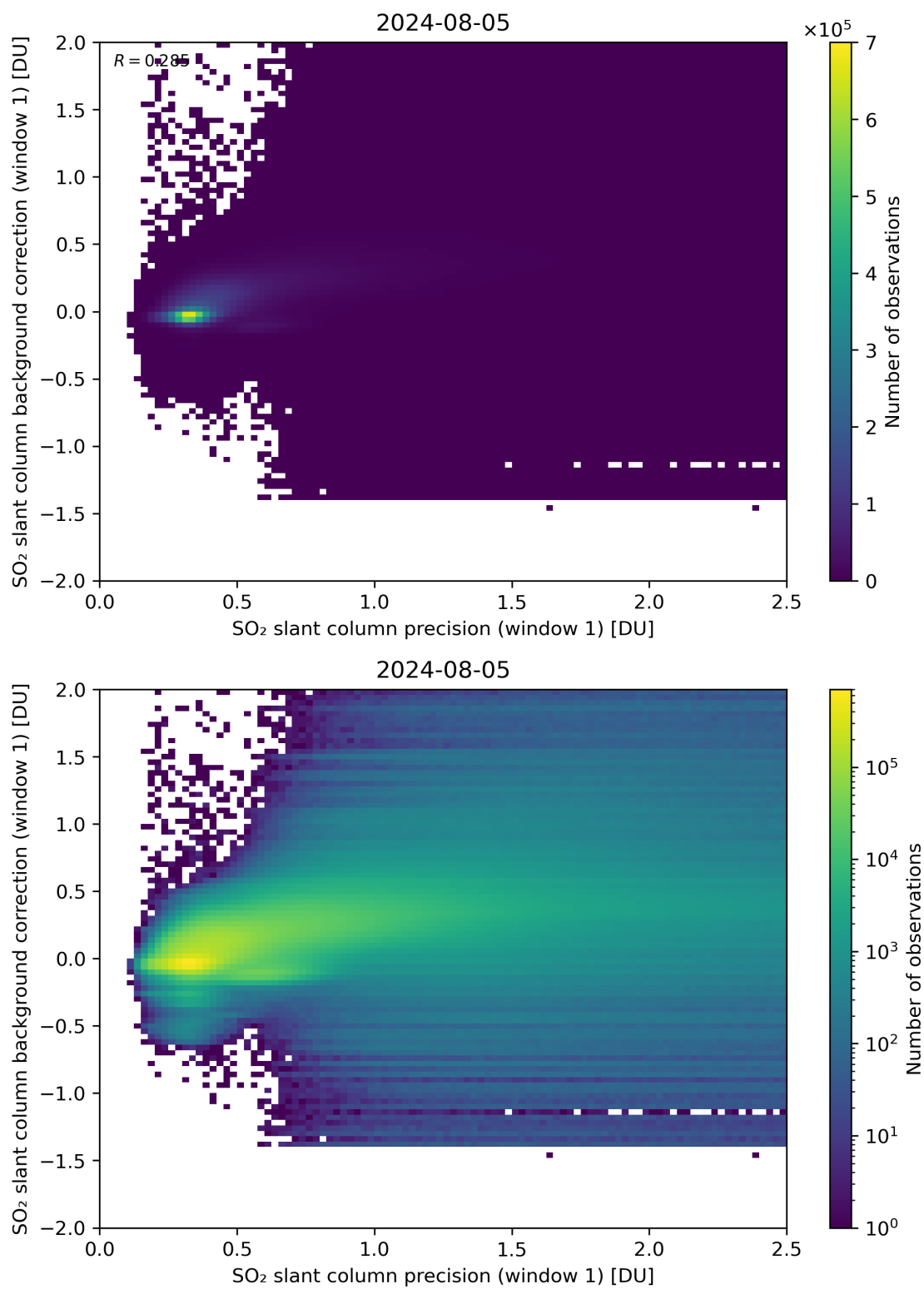
Figure 218: Scatter density plot of “SO 2 slant column precision (window 1)” against “SO 2 slant column background correction (window 1)” for 2024-08-04 to 2024-08-06.
