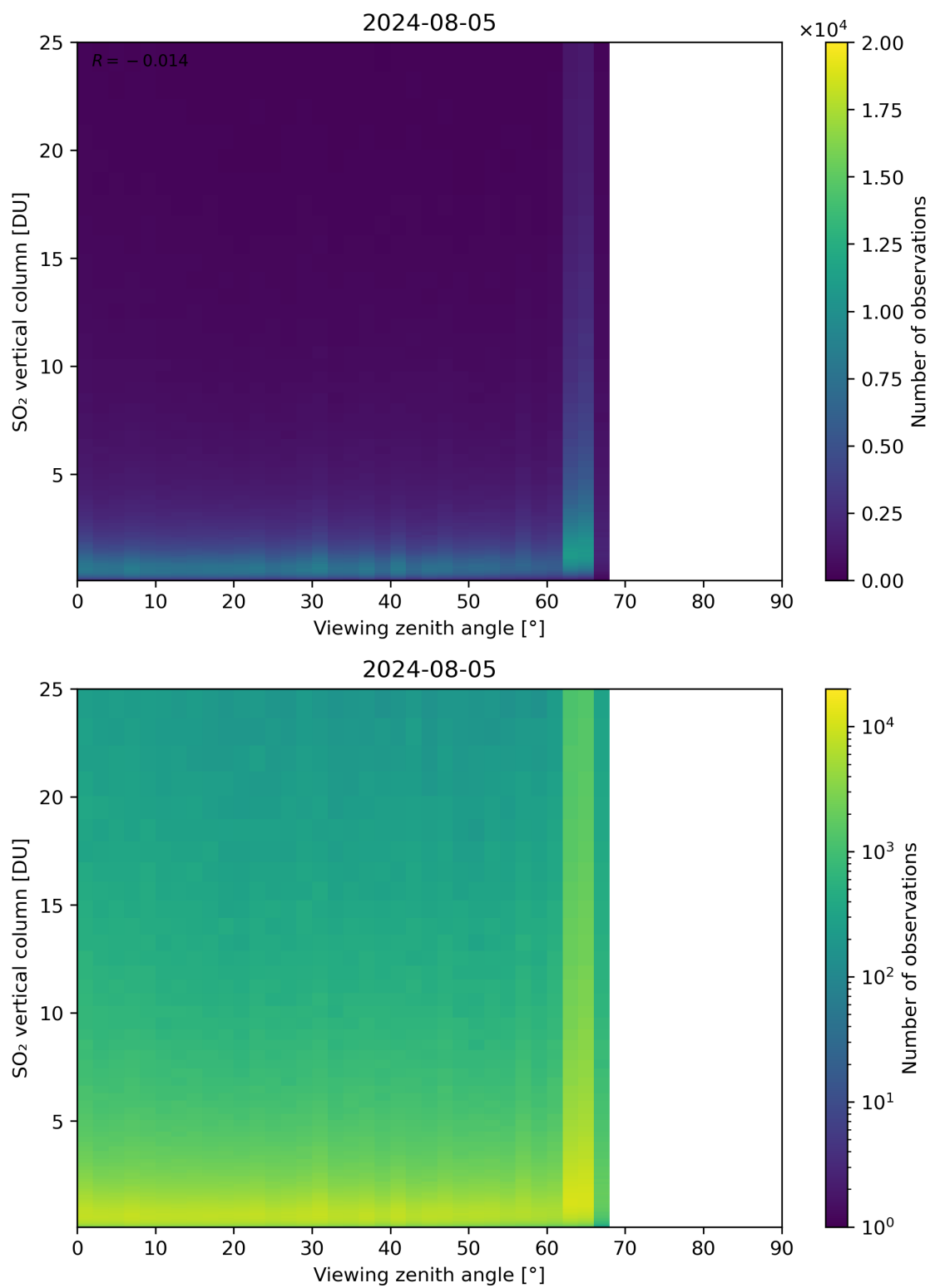
Figure 327: Scatter density plot of “Viewing zenith angle” against “SO 2 vertical column” for 2024-08-04 to 2024-08-06.
