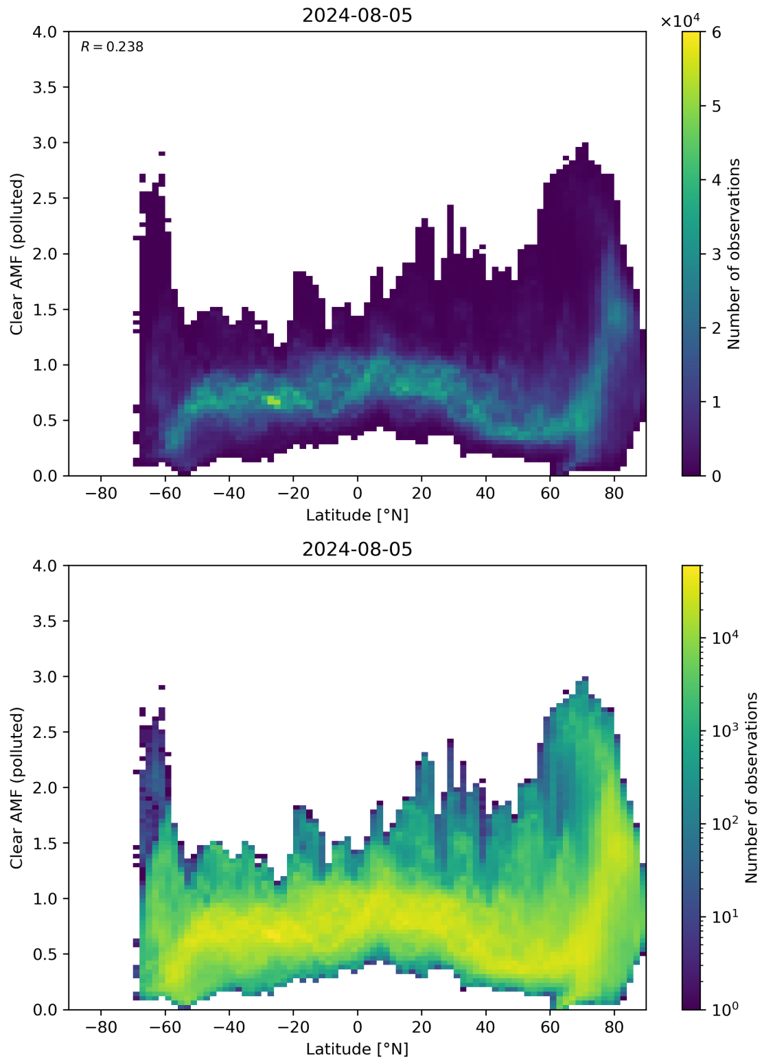
Figure 145: Scatter density plot of “Latitude” against “Clear AMF (polluted)” for 2024-08-04 to 2024-08-06.
