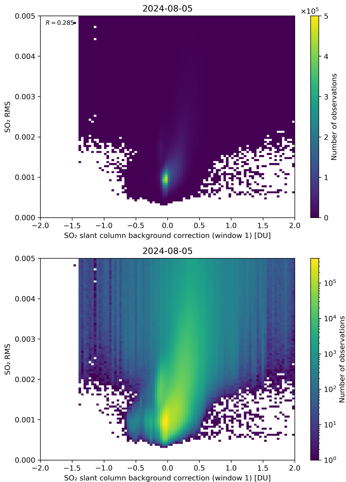
Figure 102: Scatter density plot of “SO 2 slant column background correction (window 1)” against “SO 2 RMS” for 2024-08-04 to 2024-08-06.
