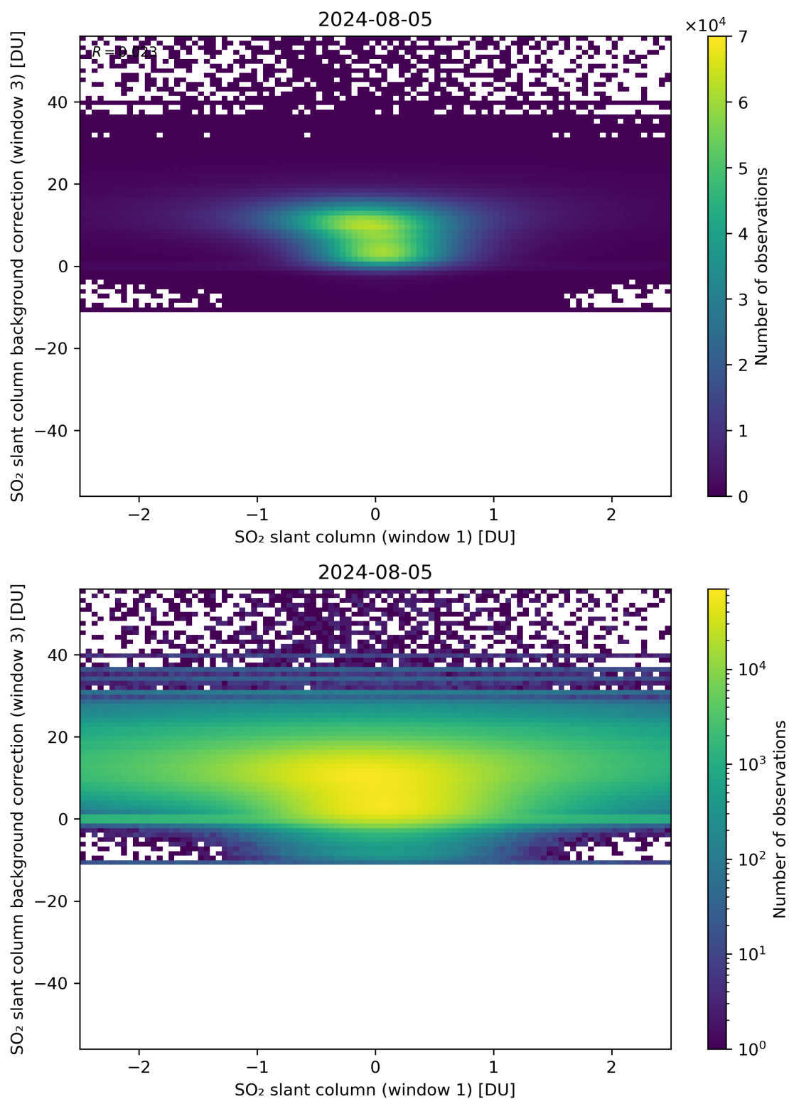
Figure 214: Scatter density plot of “SO 2 slant column (window 1)” against “SO 2 slant column background correction (window 3)” for 2024-08-04 to 2024-08-06.
