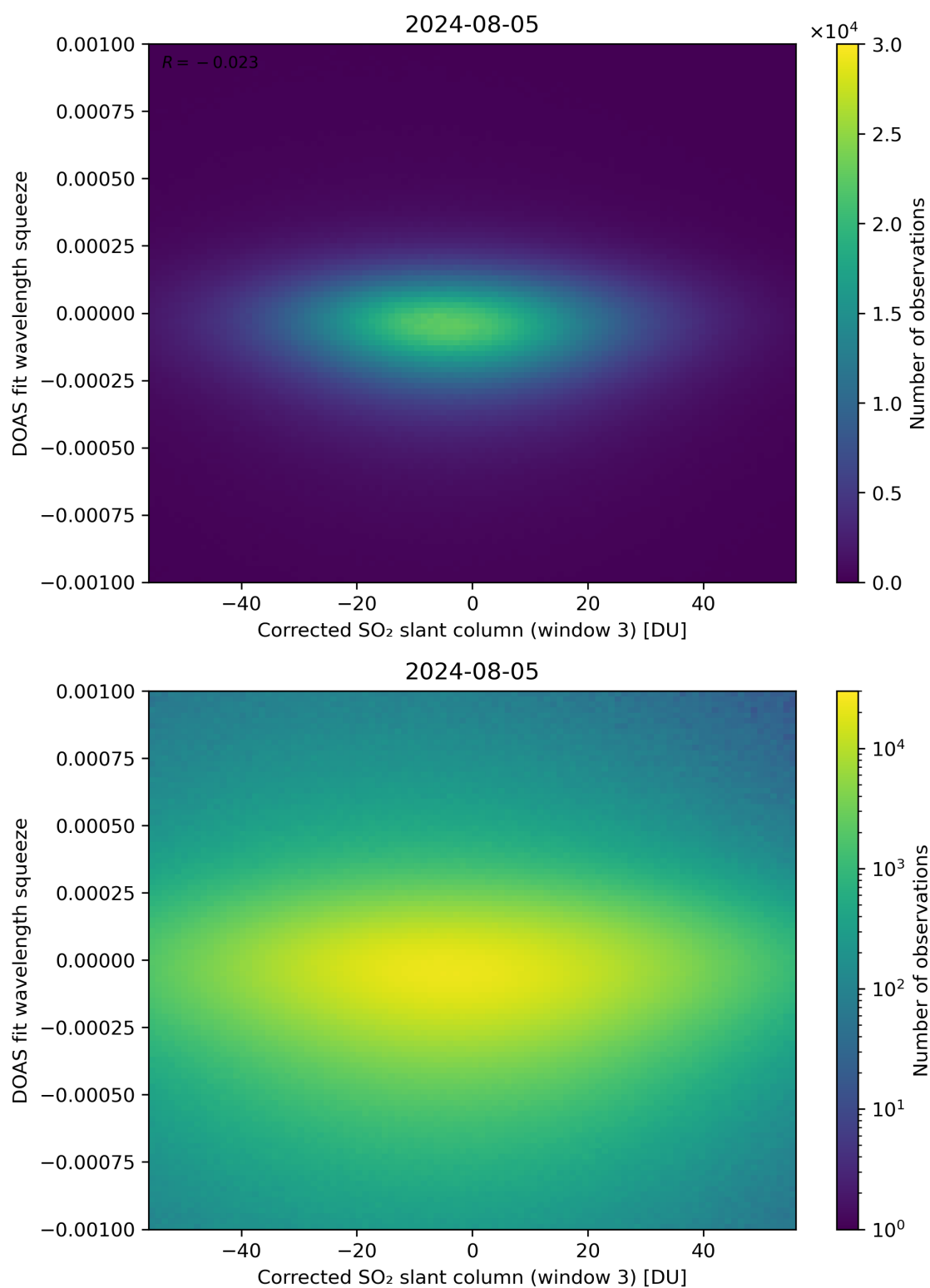
Figure 207: Scatter density plot of “Corrected SO 2 slant column (window 3)” against “DOAS fit wavelength squeeze” for 2024-08-04 to 2024-08-06.
