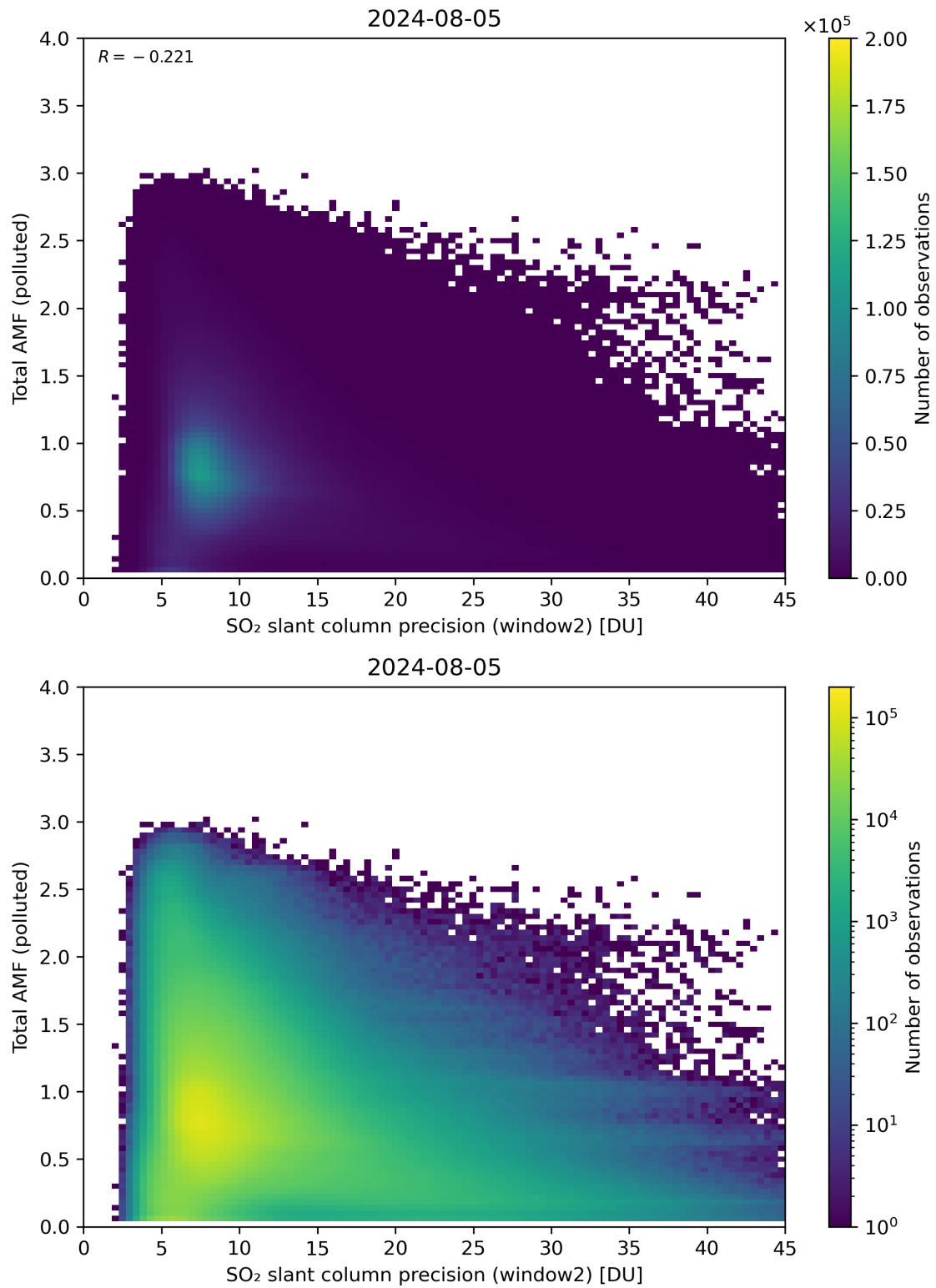
Figure 251: Scatter density plot of “SO 2 slant column precision (window2)” against “Total AMF (polluted)” for 2024-08-04 to 2024-08-06.
