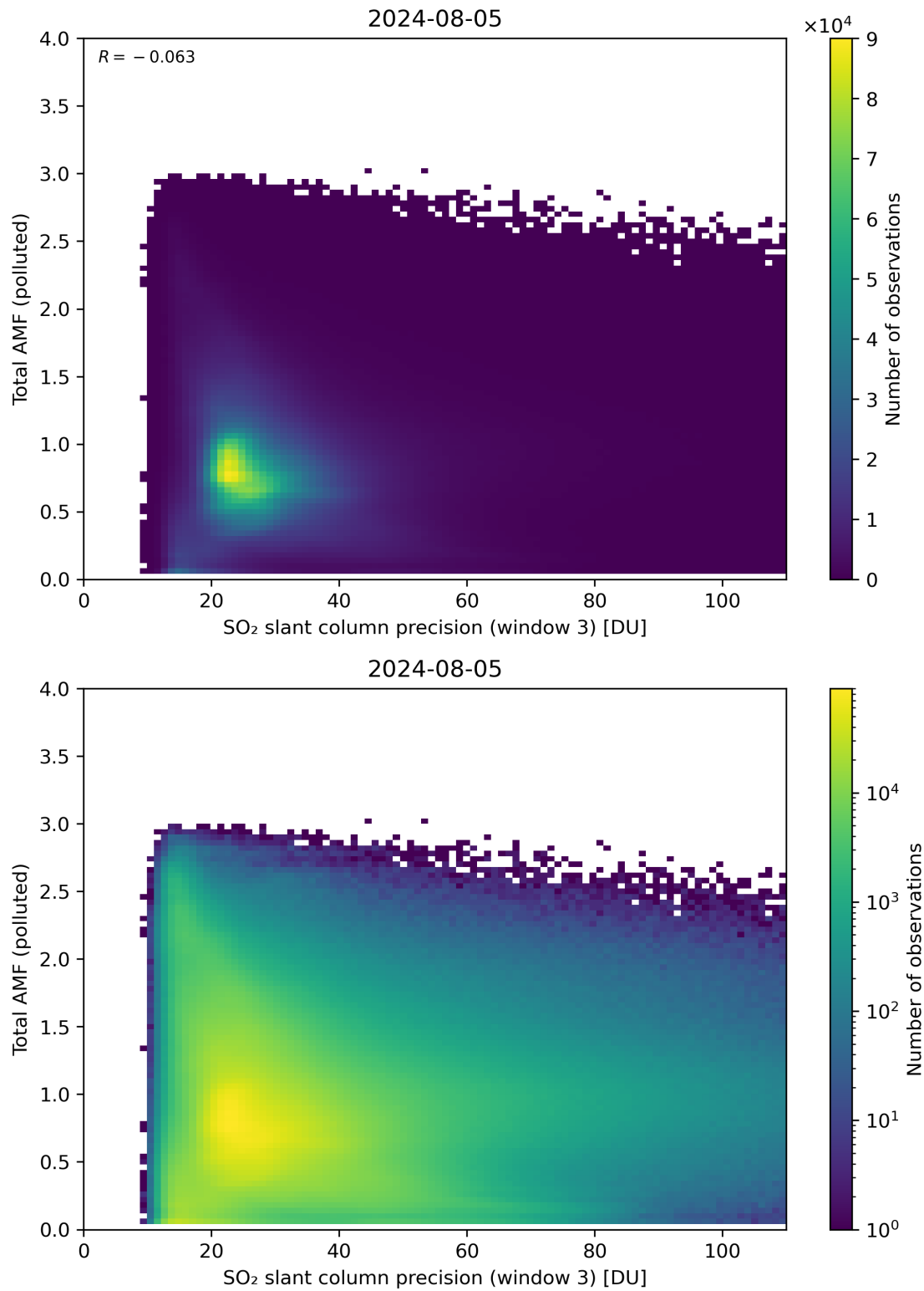
Figure 263: Scatter density plot of “SO 2 slant column precision (window 3)” against “Total AMF (polluted)” for 2024-08-04 to 2024-08-06.
