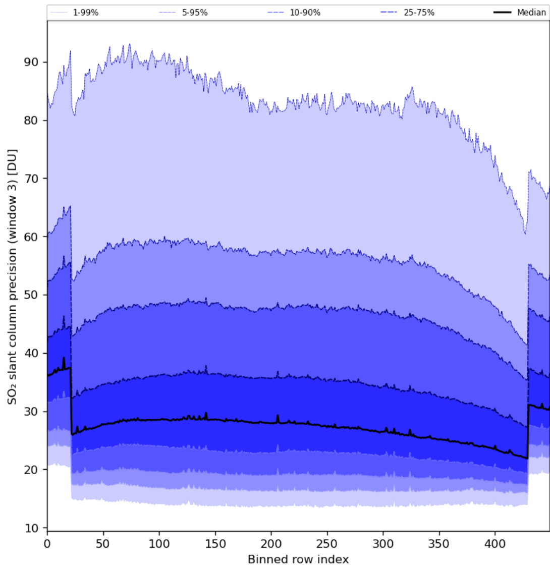
Figure 88: Along track statistics of “SO 2 slant column precision (window 3)” for 2024-08-06 to 2024-08-07
