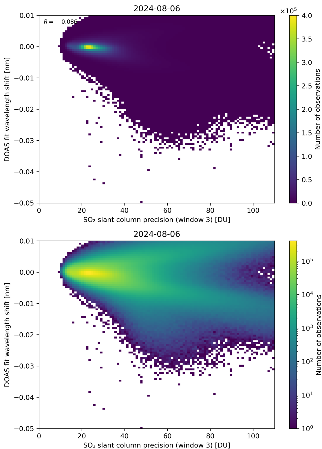
Figure 258: Scatter density plot of “SO 2 slant column precision (window 3)” against “DOAS fit wavelength shift” for 2024-08-06 to 2024-08-07.
