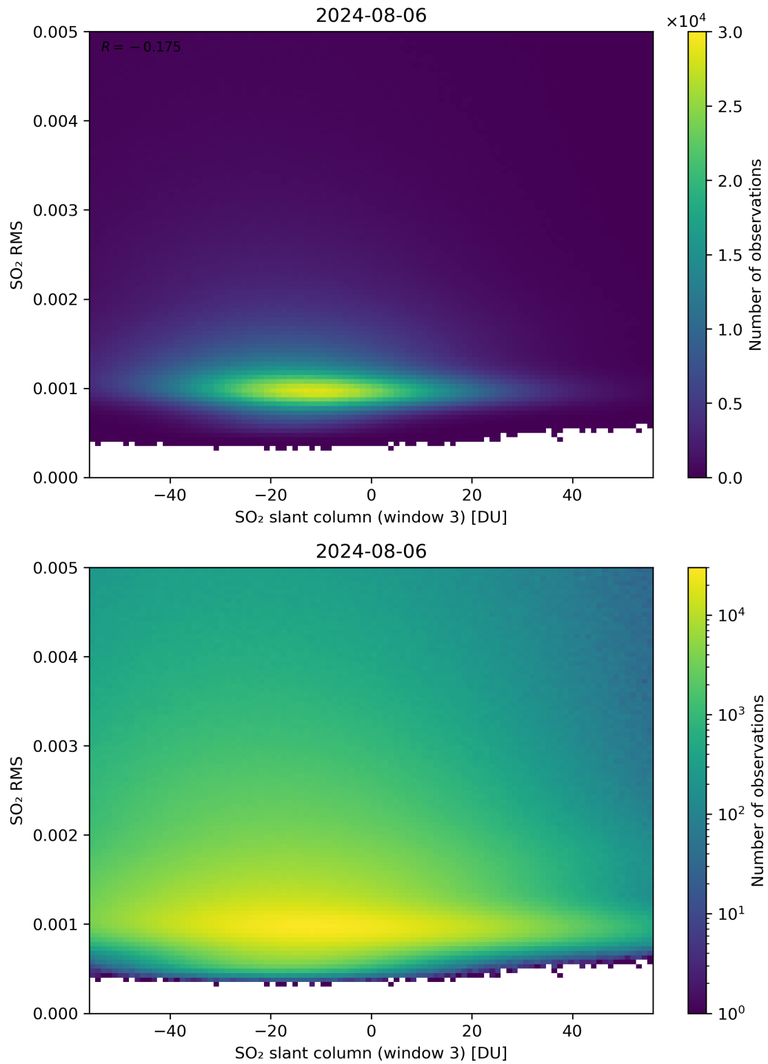
Figure 256: Scatter density plot of “SO 2 slant column (window 3)” against “SO 2 RMS” for 2024-08-06 to 2024-08-07.
