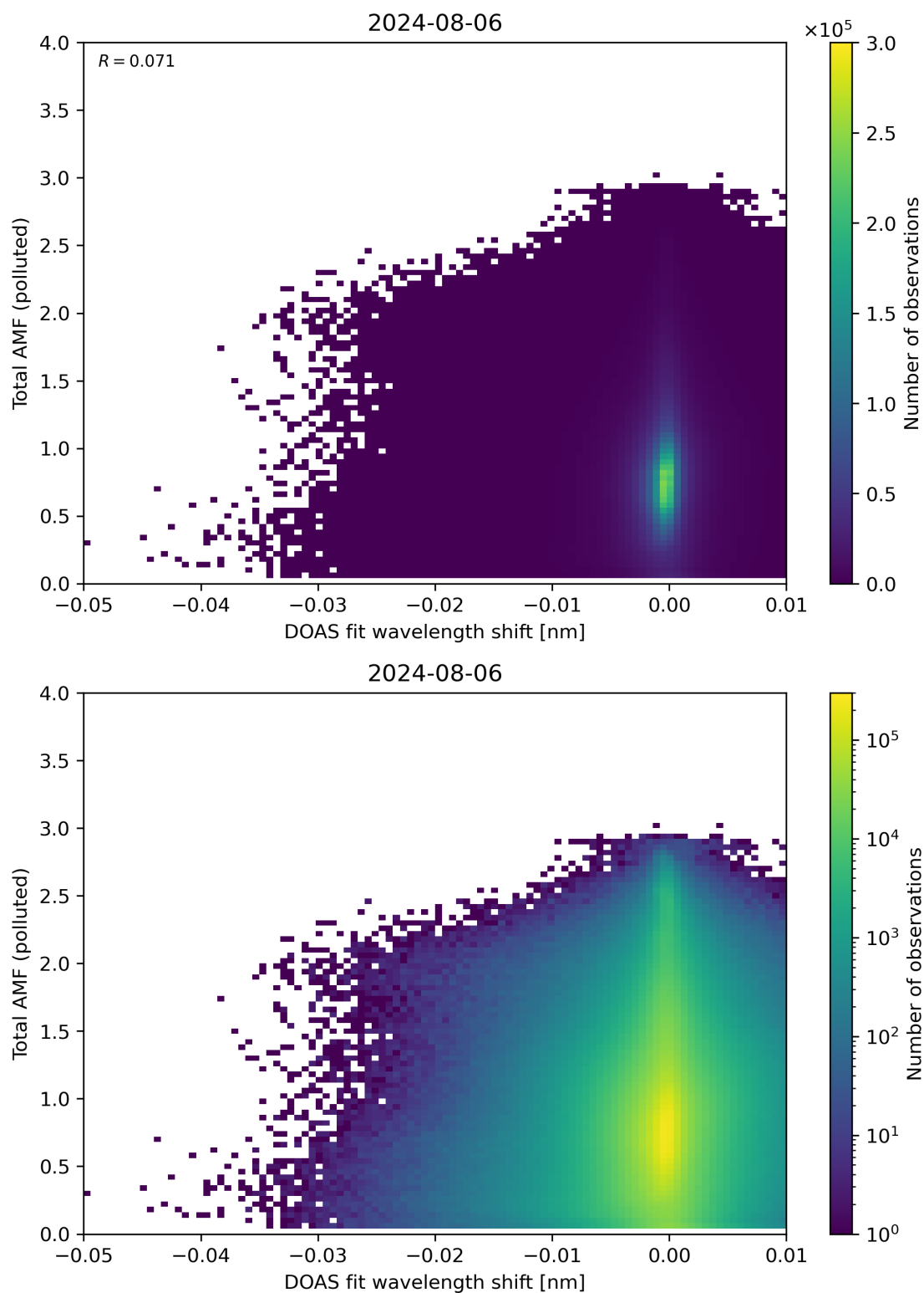
Figure 130: Scatter density plot of “DOAS fit wavelength shift” against “Total AMF (polluted)” for 2024-08-06 to 2024-08-07.
