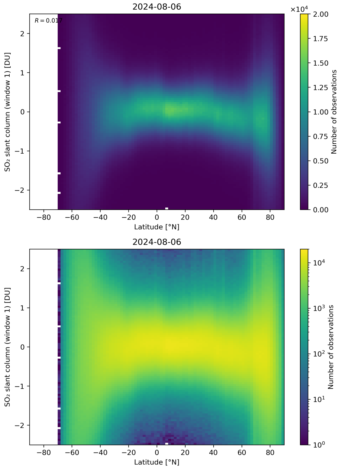
Figure 149: Scatter density plot of “Latitude” against “SO 2 slant column (window 1)” for 2024-08-06 to 2024-08-07.
