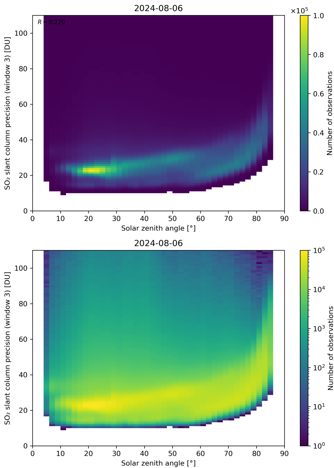
Figure 173: Scatter density plot of “Solar zenith angle” against “SO 2 slant column precision (window 3)” for 2024-08-06 to 2024-08-07.
