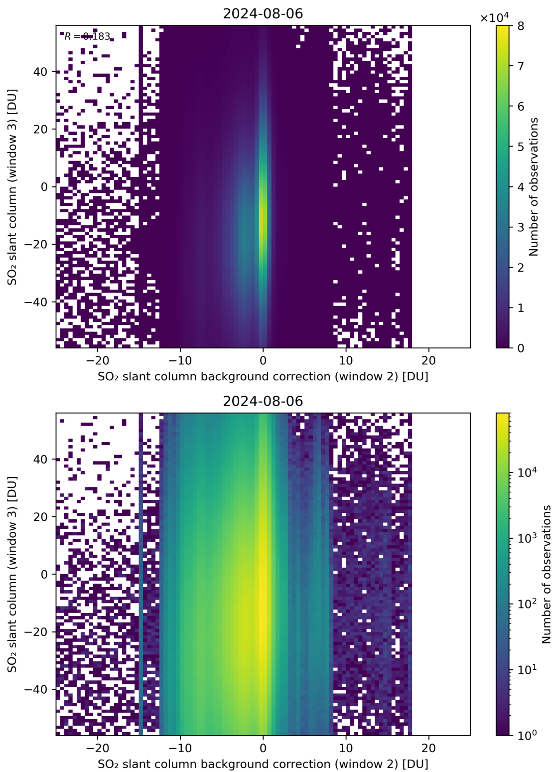
Figure 117: Scatter density plot of “SO 2 slant column background correction (window 2)” against “SO 2 slant column (window 3)” for 2024-08-06 to 2024-08-07.
