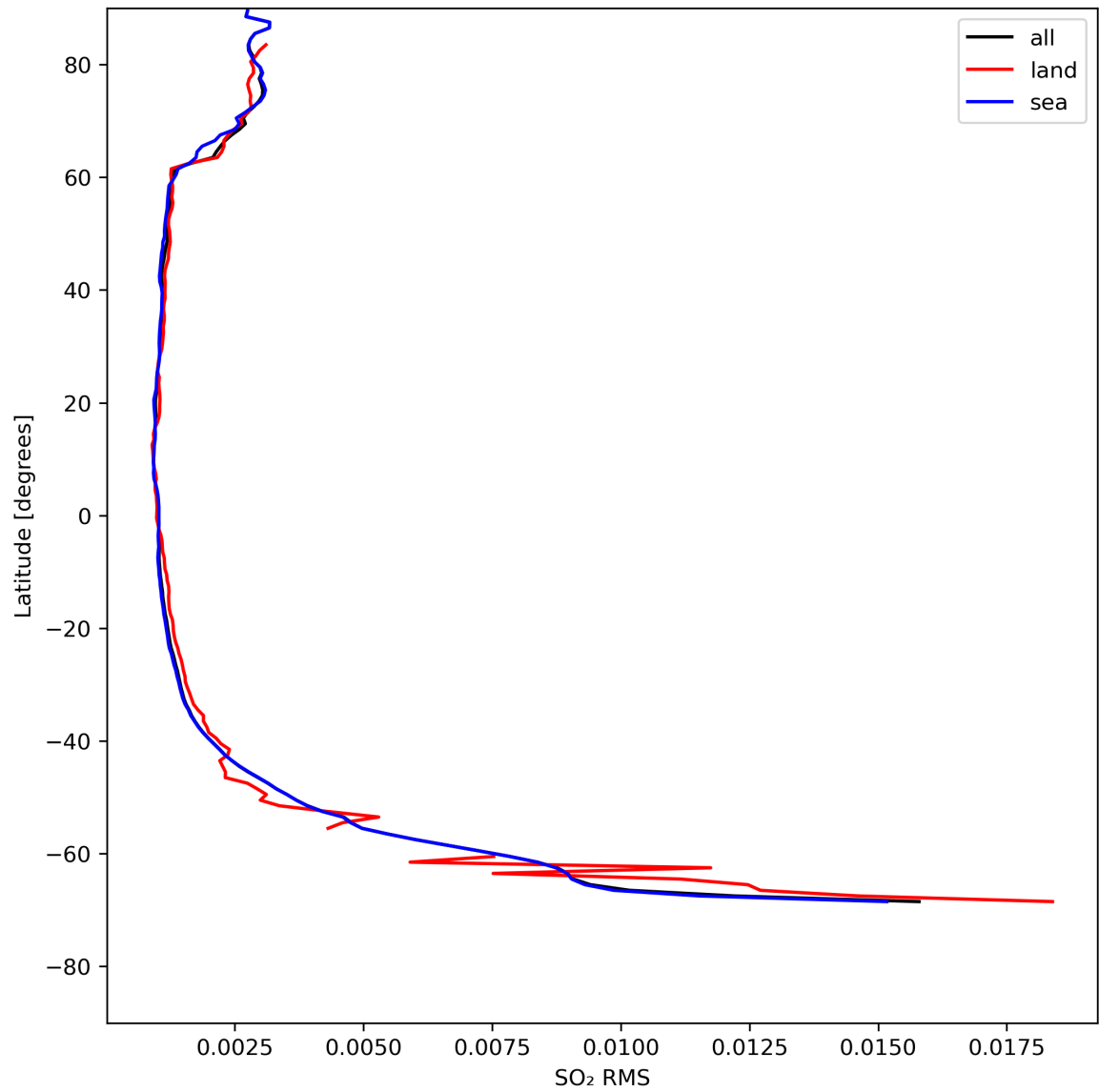
Figure 47: Zonal average of “SO 2 RMS” for 2024-08-06 to 2024-08-07.
