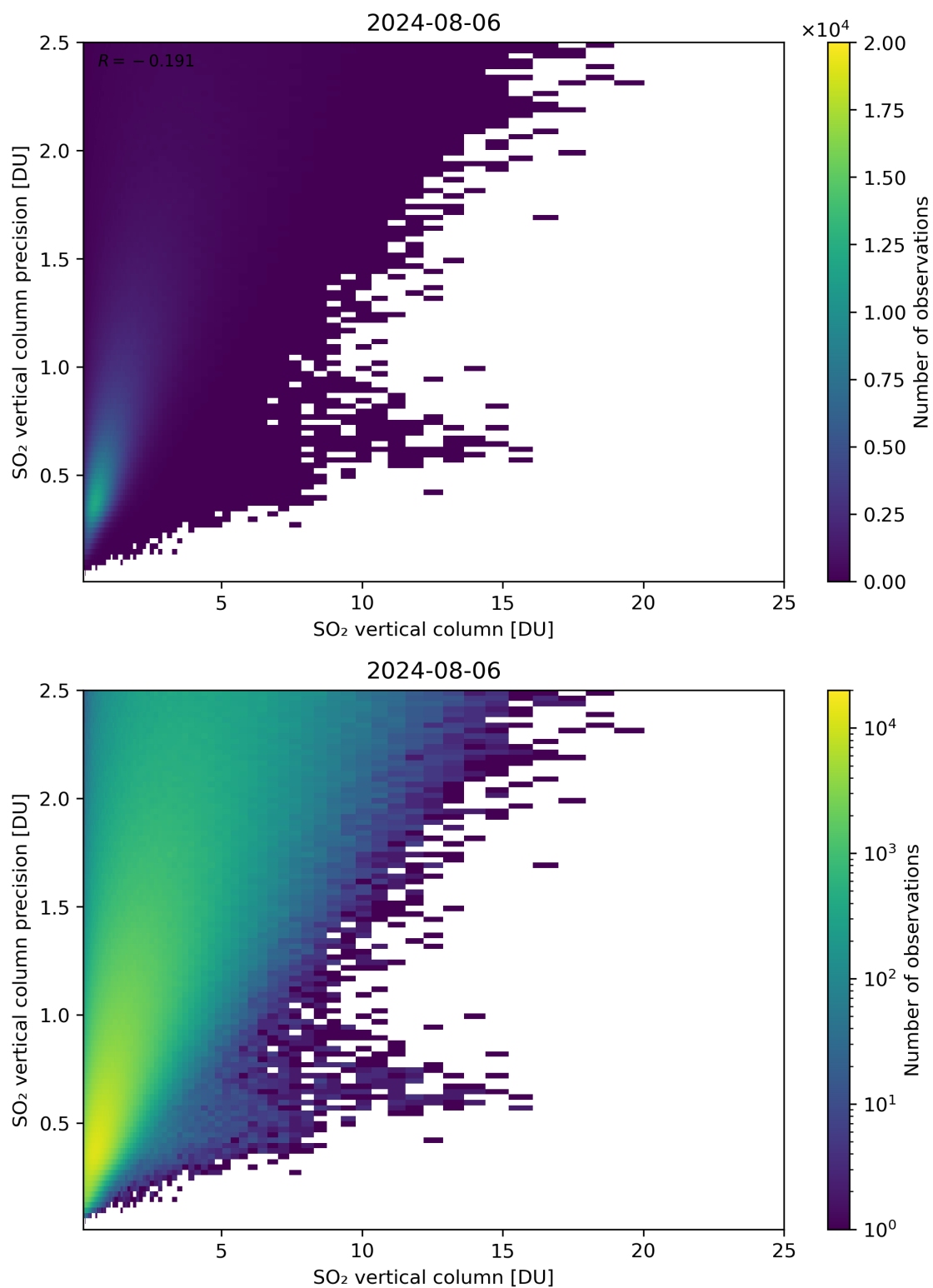
Figure 307: Scatter density plot of “SO 2 vertical column” against “SO 2 vertical column precision” for 2024-08-06 to 2024-08-07.
