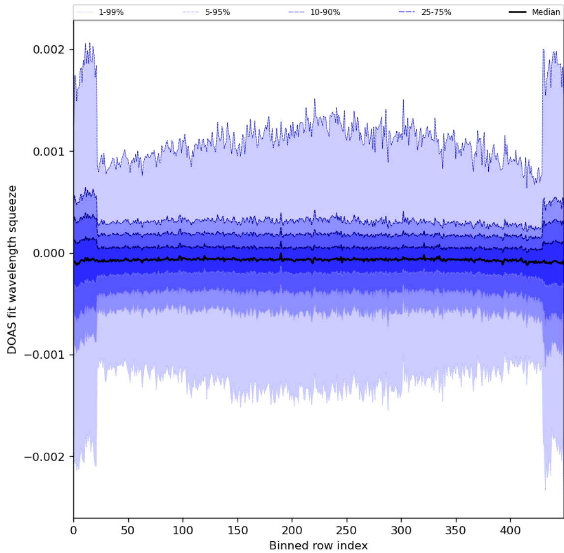
Figure 92: Along track statistics of “DOAS fit wavelength squeeze” for 2024-08-06 to 2024-08-07
