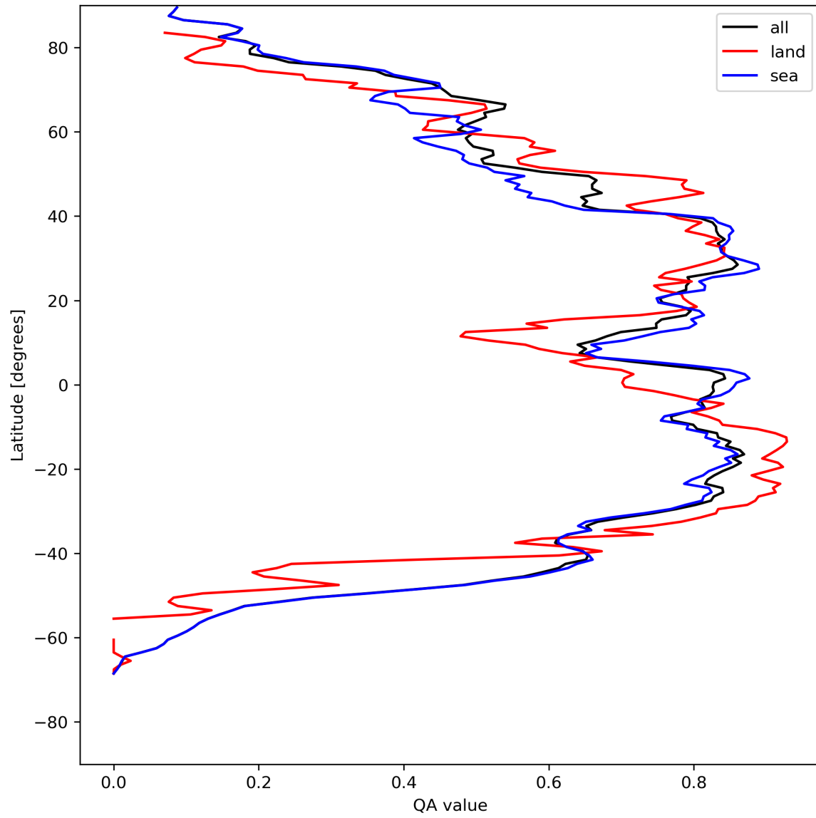
Figure 29: Zonal average of “QA value” for 2024-08-06 to 2024-08-07.
