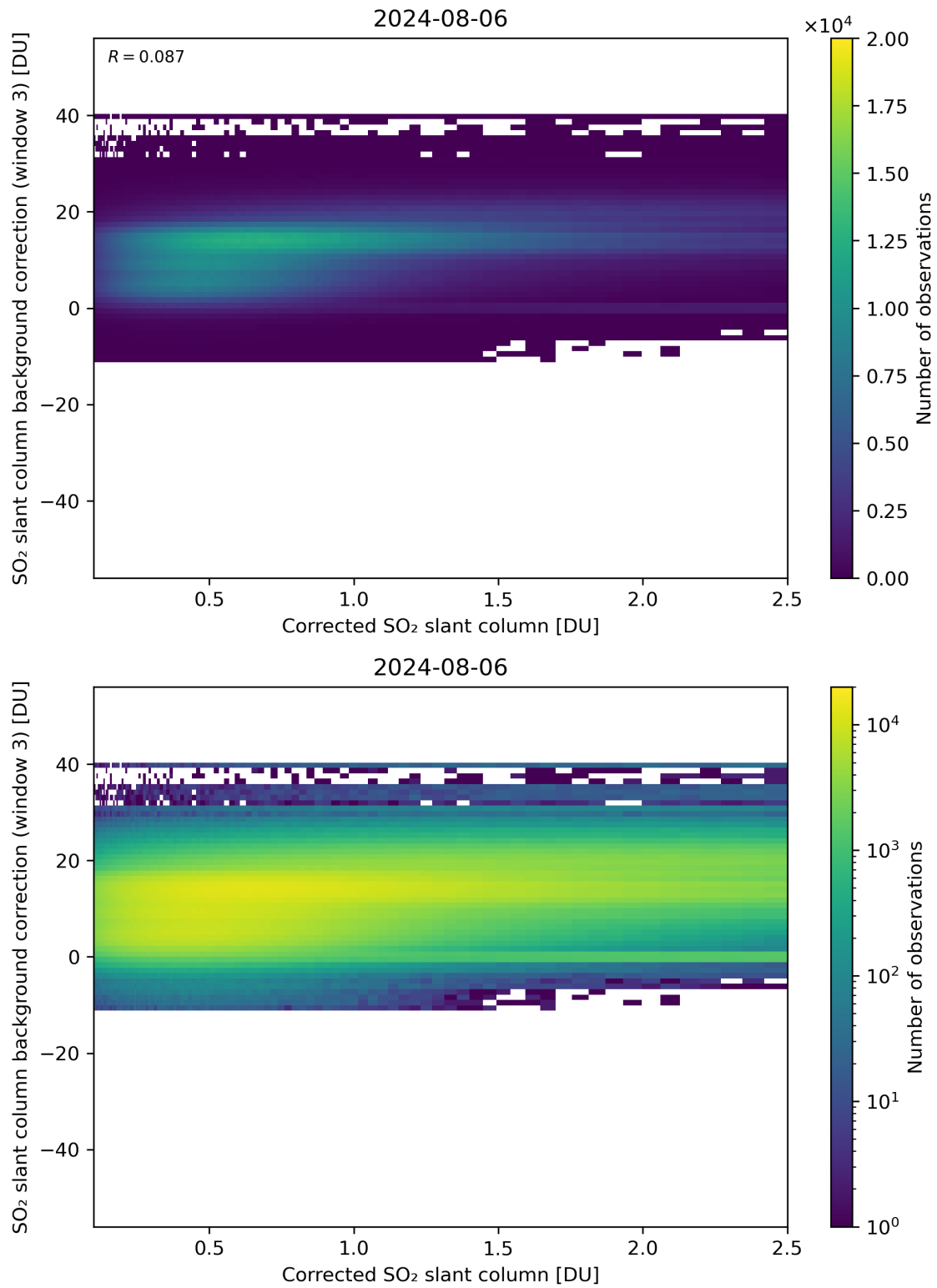
Figure 180: Scatter density plot of “Corrected SO 2 slant column” against “SO 2 slant column background correction (window 3)” for 2024-08-06 to 2024-08-07.
