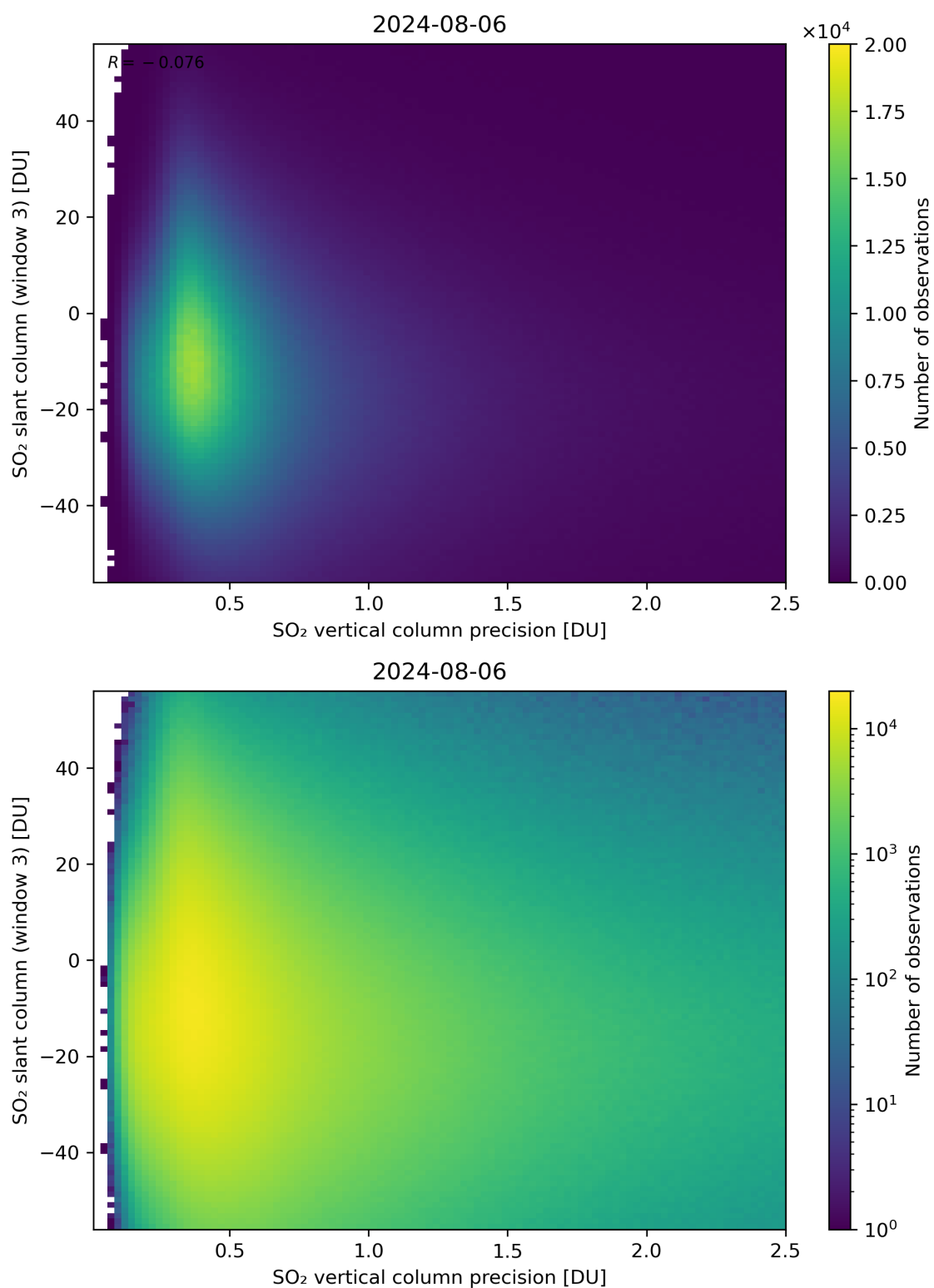
Figure 292: Scatter density plot of “SO 2 vertical column precision” against “SO 2 slant column (window 3)” for 2024-08-06 to 2024-08-07.
