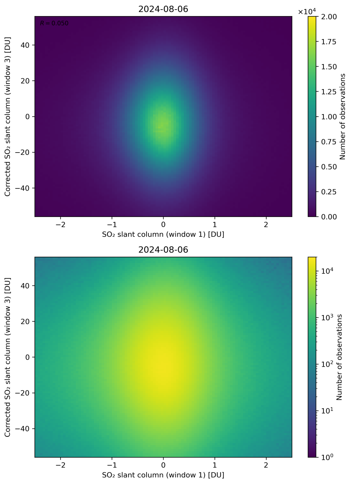
Figure 234: Scatter density plot of “SO 2 slant column (window 1)” against “Corrected SO 2 slant column (window 3)” for 2024-08-06 to 2024-08-07.
