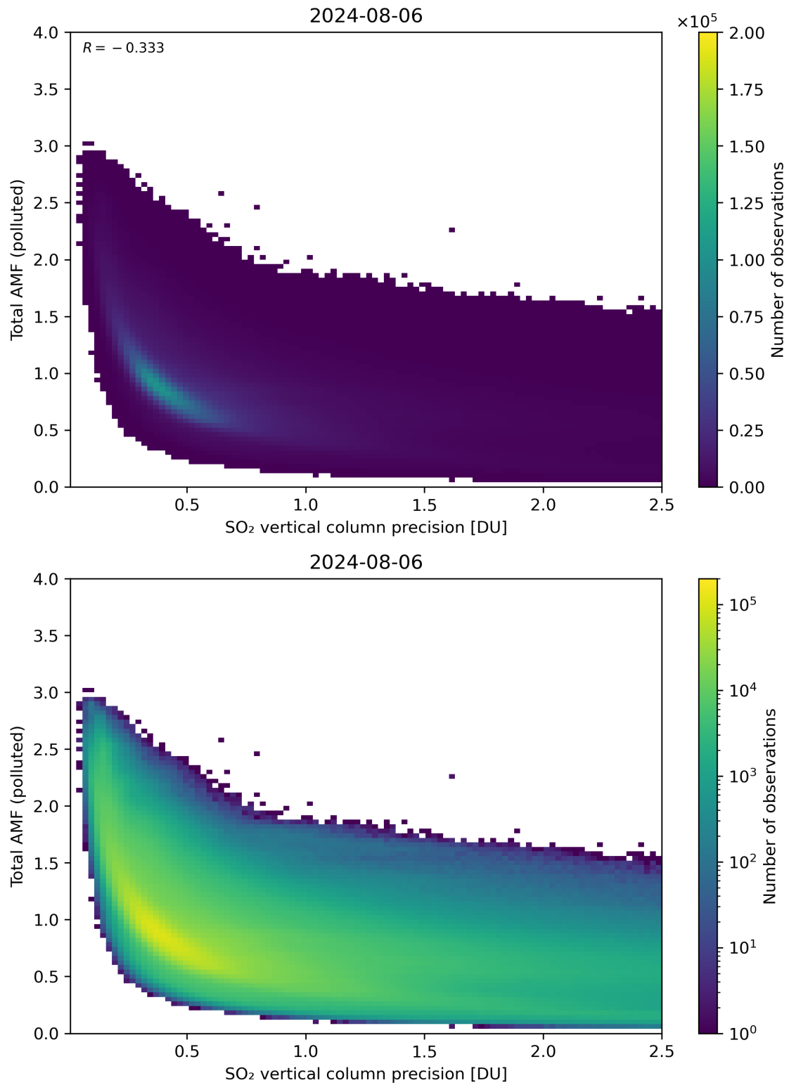
Figure 294: Scatter density plot of “SO 2 vertical column precision” against “Total AMF (polluted)” for 2024-08-06 to 2024-08-07.
