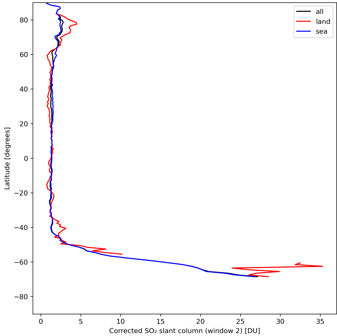
Figure 39: Zonal average of “Corrected SO 2 slant column (window 2)” for 2024-08-06 to 2024-08-07.
