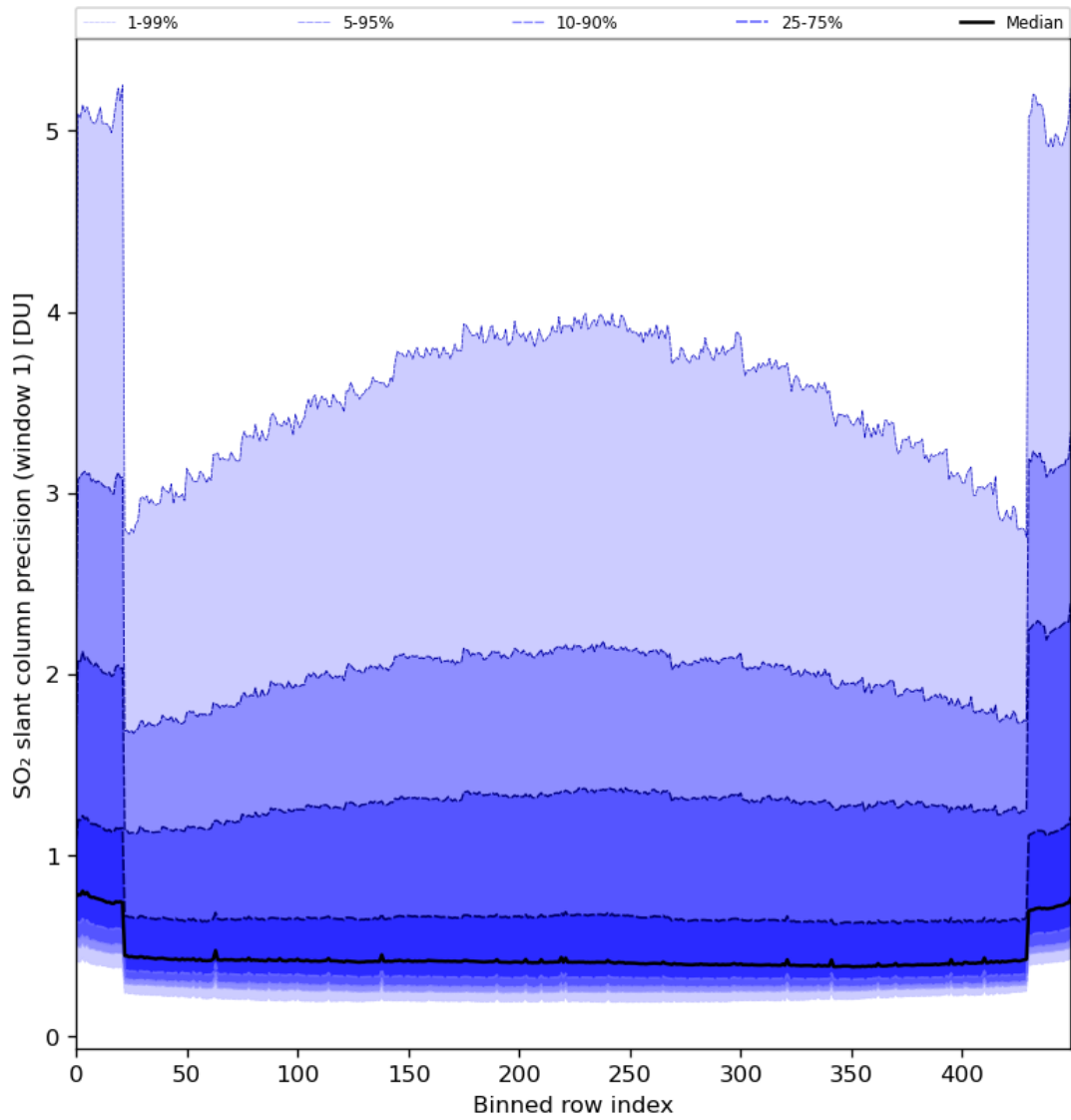
Figure 80: Along track statistics of “SO 2 slant column precision (window 1)” for 2024-08-06 to 2024-08-07
