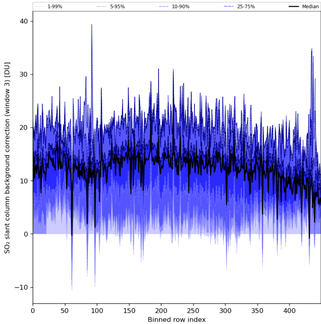
Figure 90: Along track statistics of “SO 2 slant column background correction (window 3)” for 2024-08-06 to 2024-08-07
