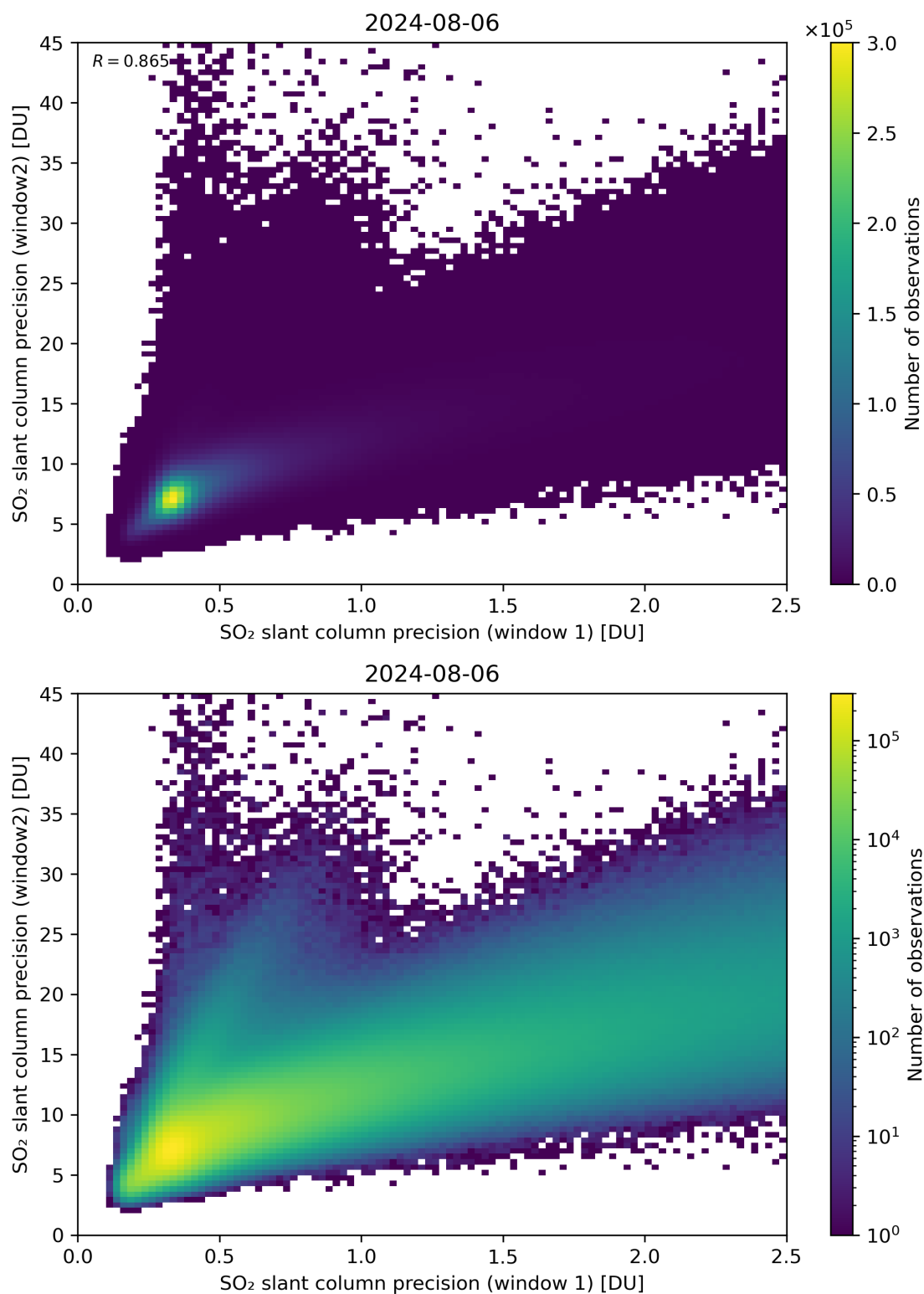
Figure 227: Scatter density plot of “SO 2 slant column precision (window 1)” against “SO 2 slant column precision (window2)” for 2024-08-06 to 2024-08-07.
