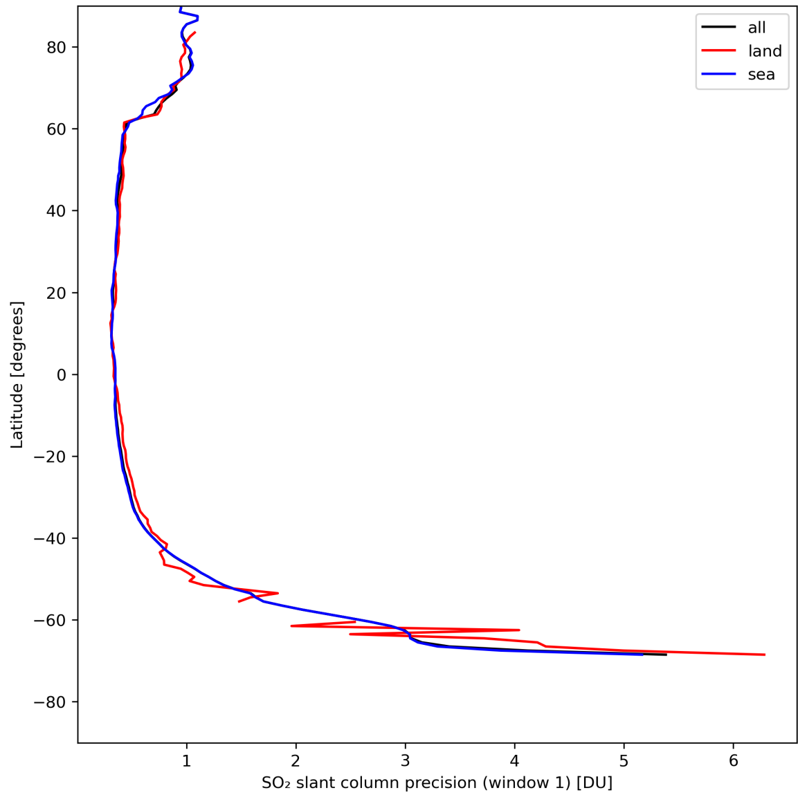
Figure 34: Zonal average of “SO 2 slant column precision (window 1)” for 2024-08-06 to 2024-08-07.
