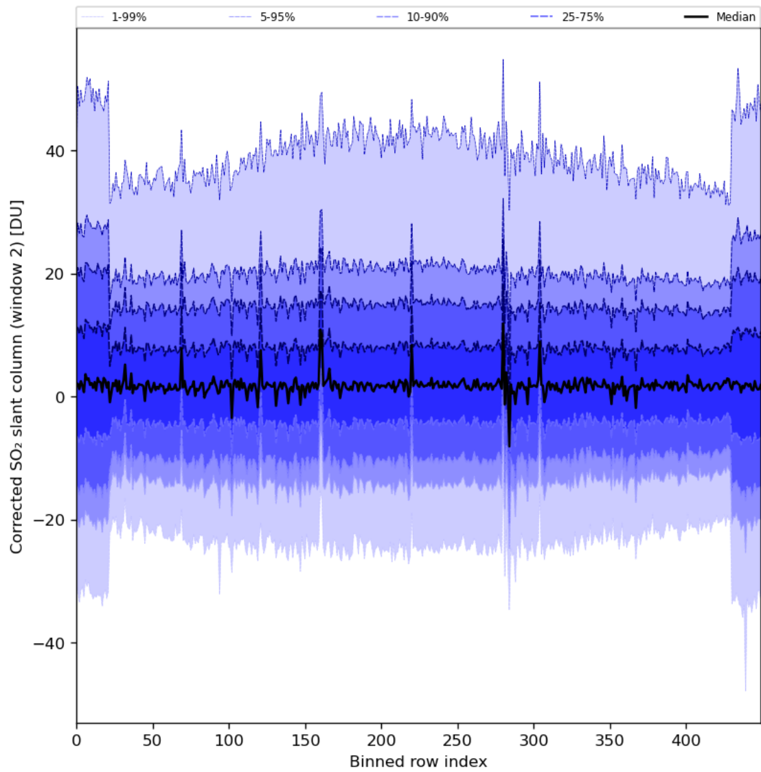
Figure 85: Along track statistics of “Corrected SO 2 slant column (window 2)” for 2024-08-06 to 2024-08-07
