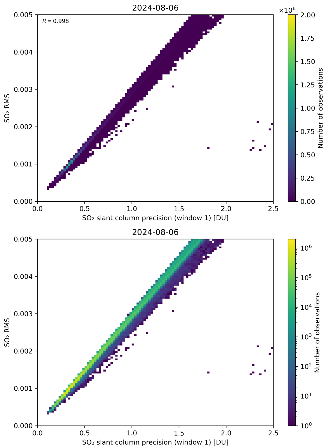
Figure 223: Scatter density plot of “SO 2 slant column precision (window 1)” against “SO 2 RMS” for 2024-08-06 to 2024-08-07.
