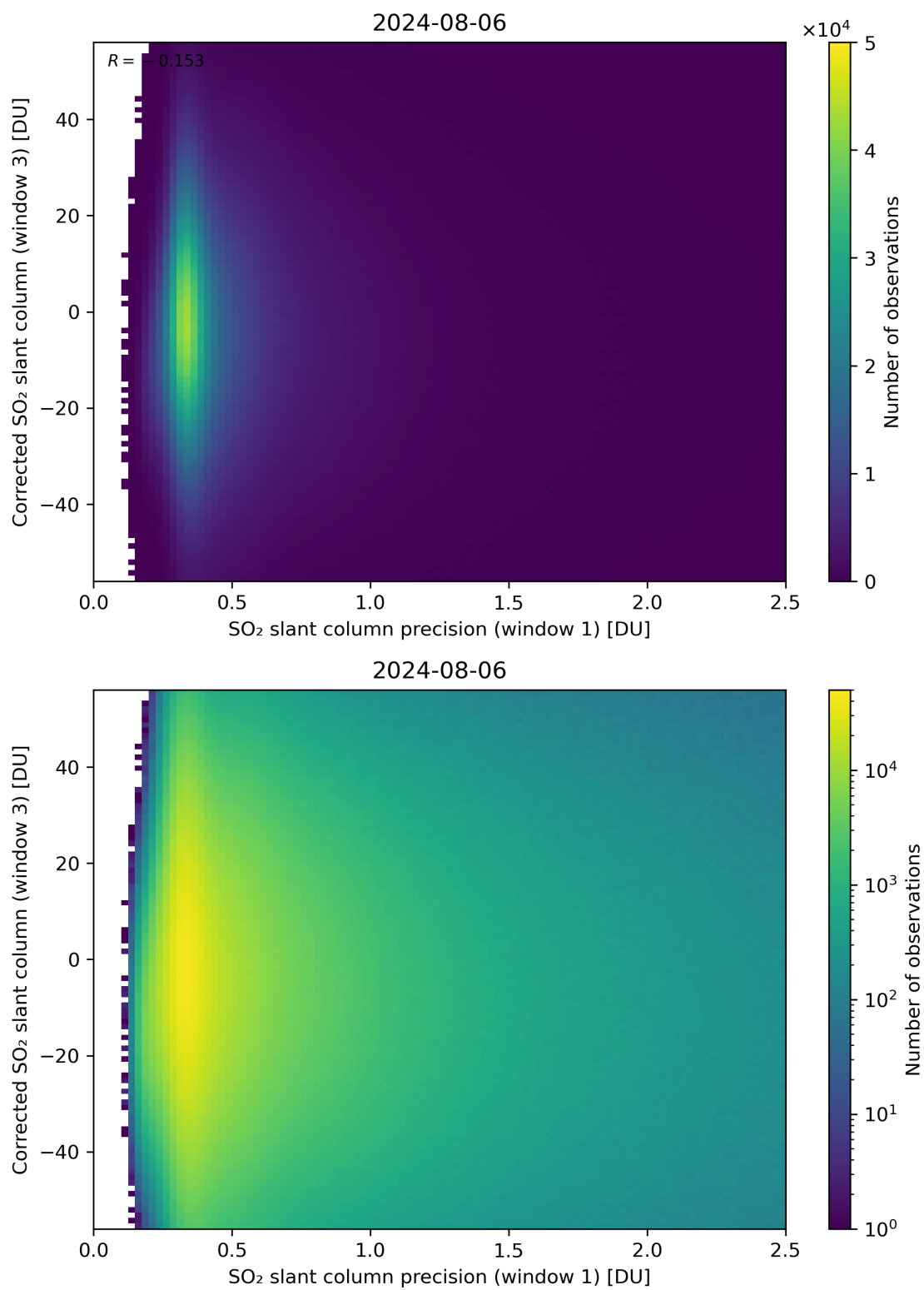
Figure 226: Scatter density plot of “SO 2 slant column precision (window 1)” against “Corrected SO 2 slant column (window 3)” for 2024-08-06 to 2024-08-07.
