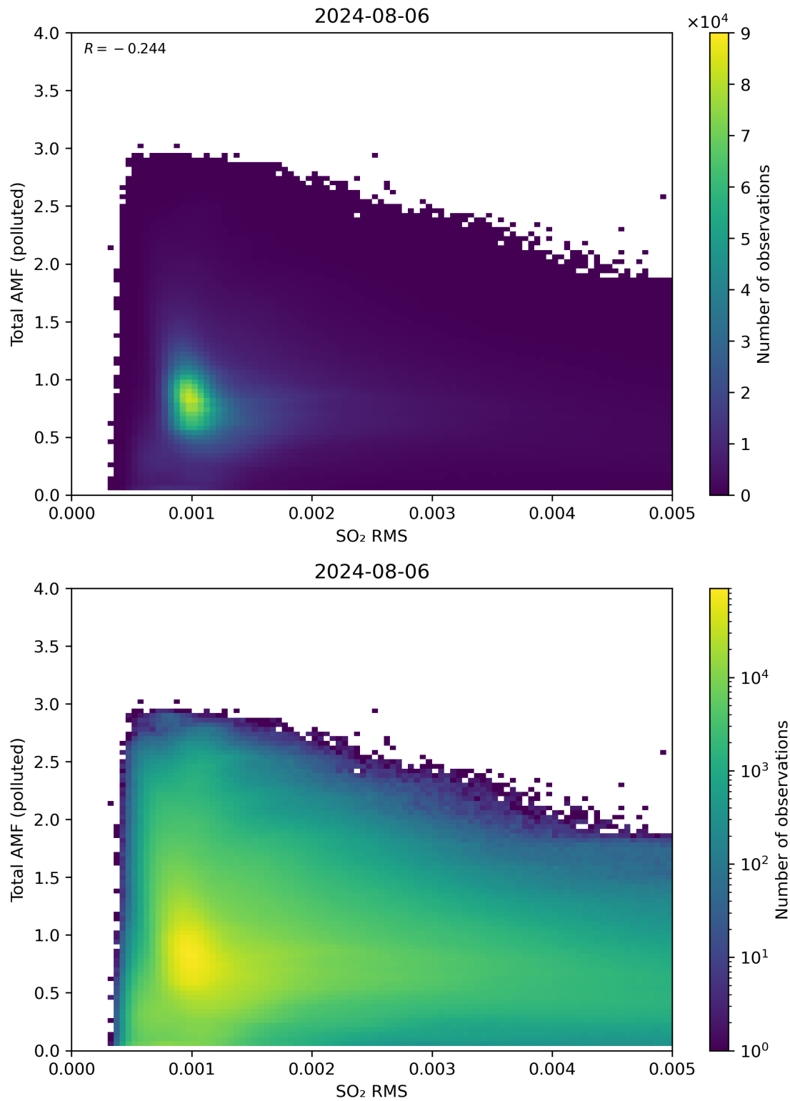
Figure 137: Scatter density plot of “SO 2 RMS” against “Total AMF (polluted)” for 2024-08-06 to 2024-08-07.
