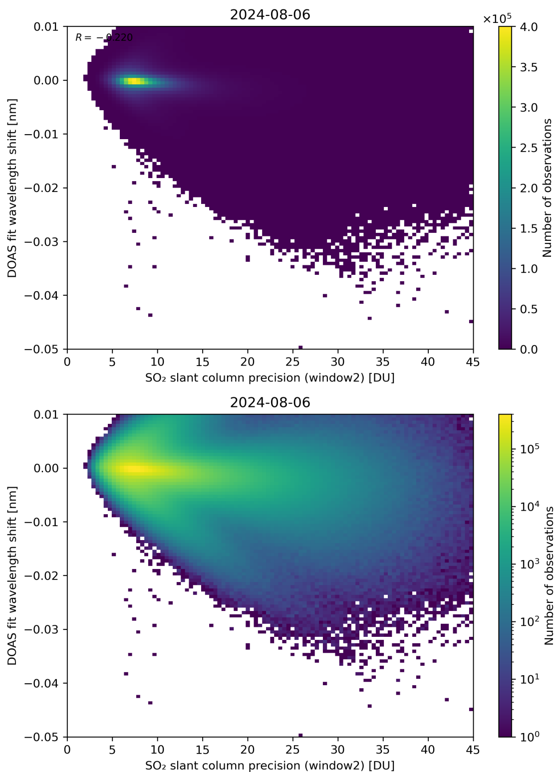
Figure 243: Scatter density plot of “SO 2 slant column precision (window2)” against “DOAS fit wavelength shift” for 2024-08-06 to 2024-08-07.
