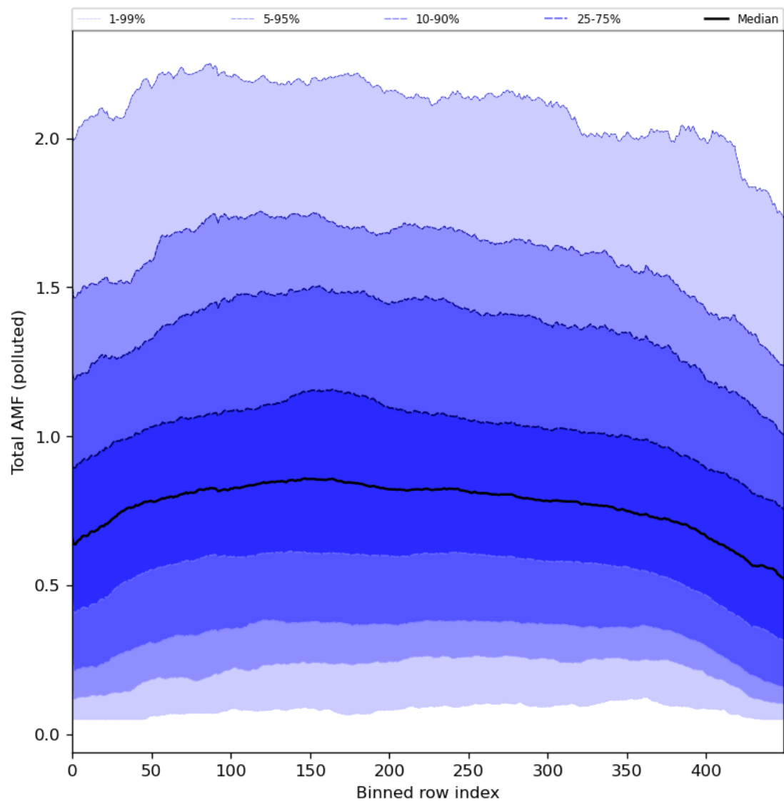
Figure 94: Along track statistics of “Total AMF (polluted)” for 2024-08-06 to 2024-08-07
