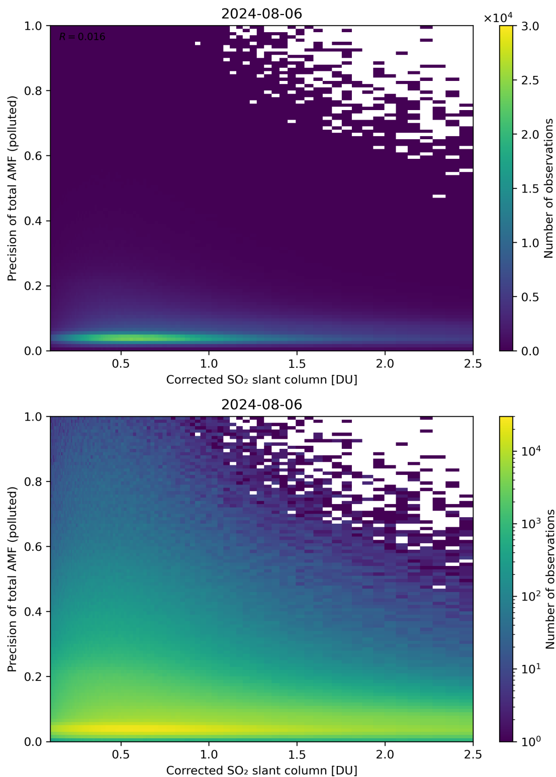
Figure 193: Scatter density plot of “Corrected SO 2 slant column” against “Precision of total AMF (polluted)” for 2024-08-06 to 2024-08-07.
