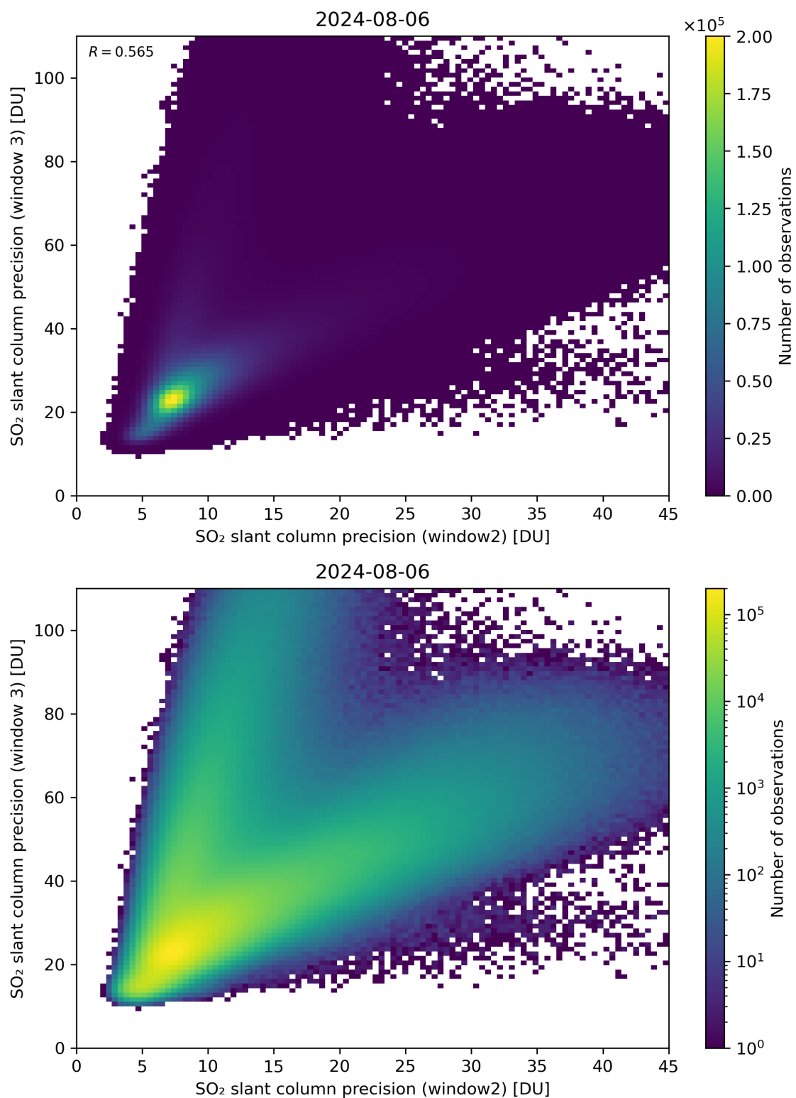
Figure 250: Scatter density plot of “SO 2 slant column precision (window2)” against “SO 2 slant column precision (window 3)” for 2024-08-06 to 2024-08-07.
