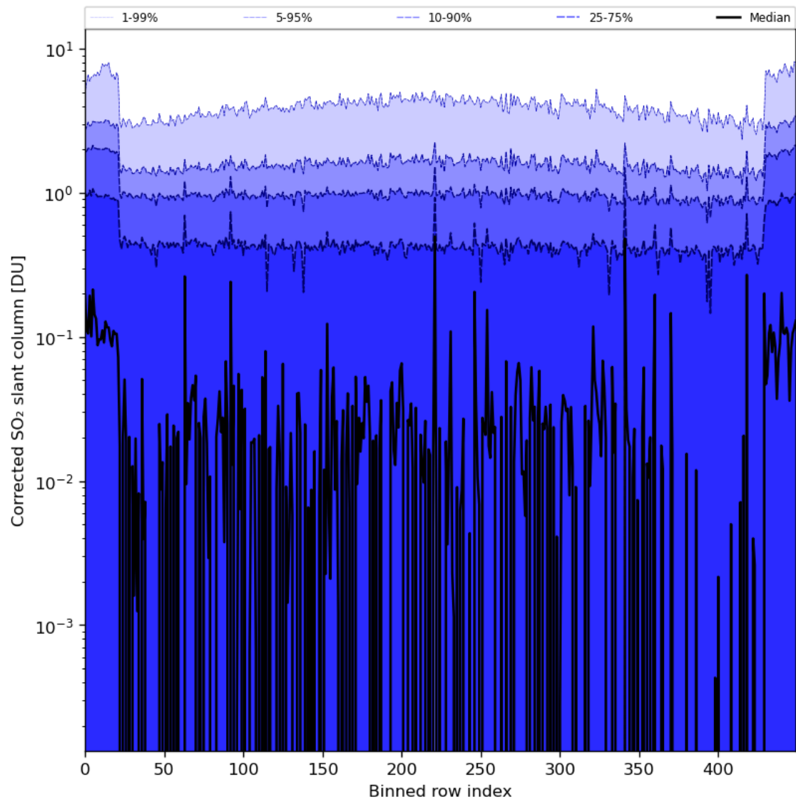
Figure 78: Along track statistics of “Corrected SO 2 slant column” for 2024-08-06 to 2024-08-07
