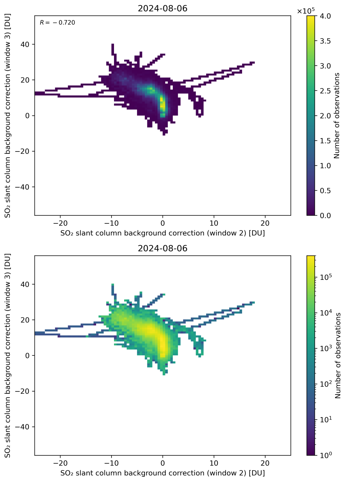
Figure 111: Scatter density plot of “SO 2 slant column background correction (window 2)” against “SO 2 slant column background correction (window 3)” for 2024-08-06 to 2024-08-07.
