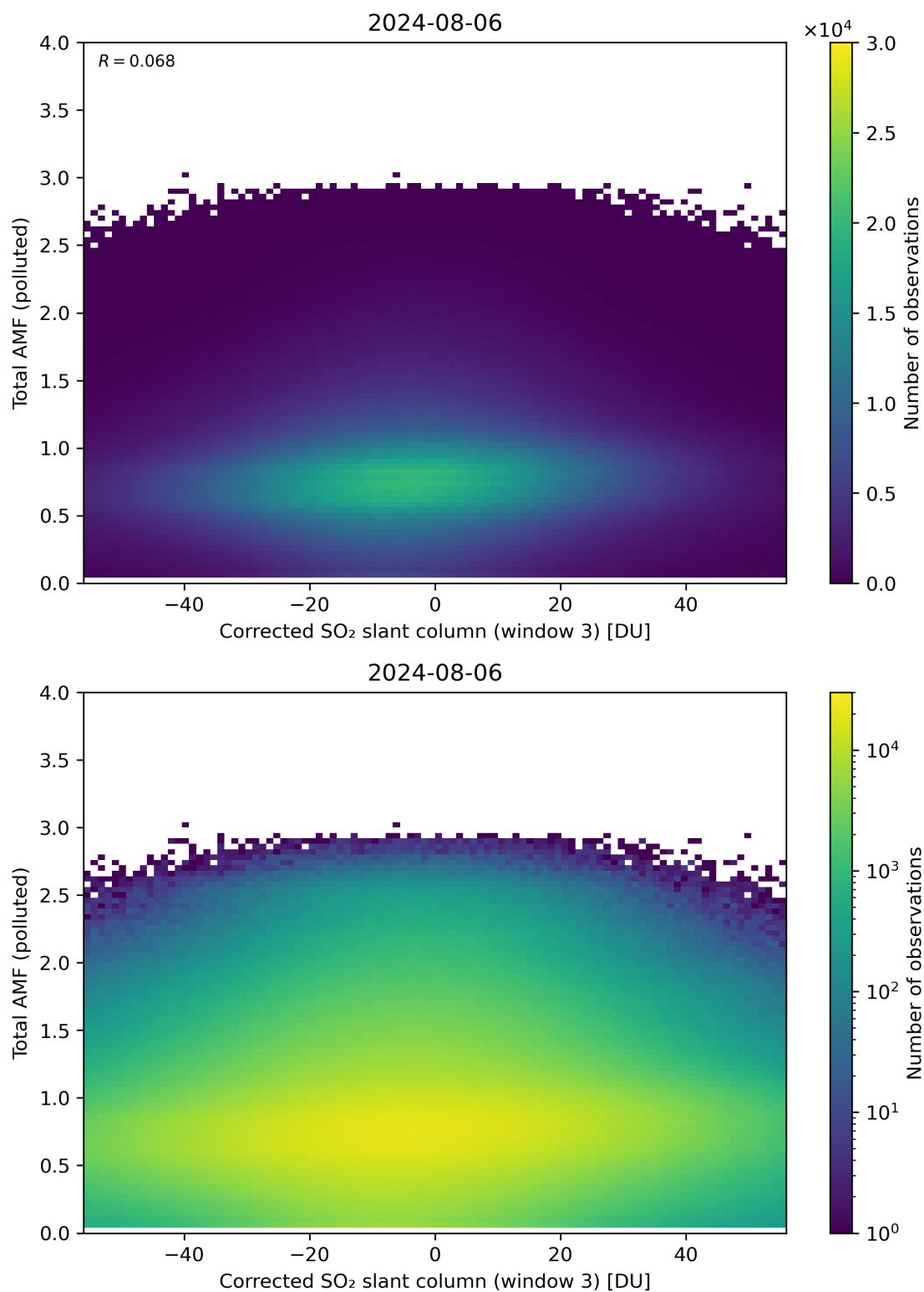
Figure 210: Scatter density plot of “Corrected SO 2 slant column (window 3)” against “Total AMF (polluted)” for 2024-08-06 to 2024-08-07.
