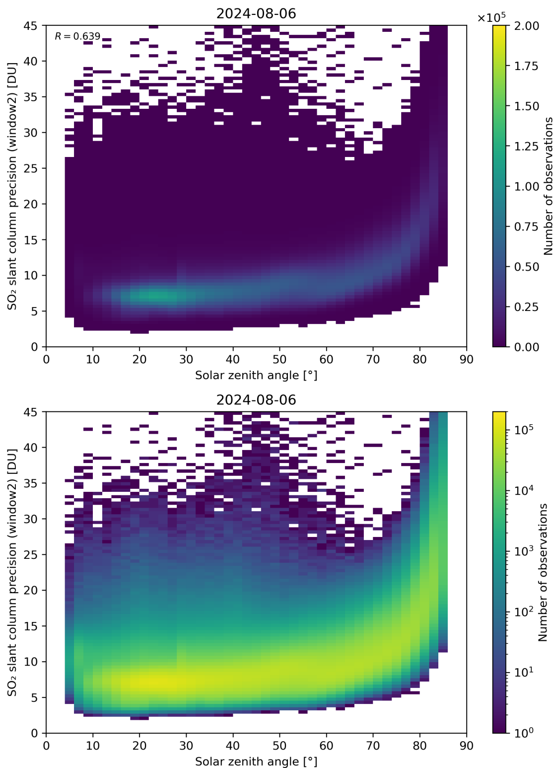
Figure 171: Scatter density plot of “Solar zenith angle” against “SO 2 slant column precision (window2)” for 2024-08-06 to 2024-08-07.
