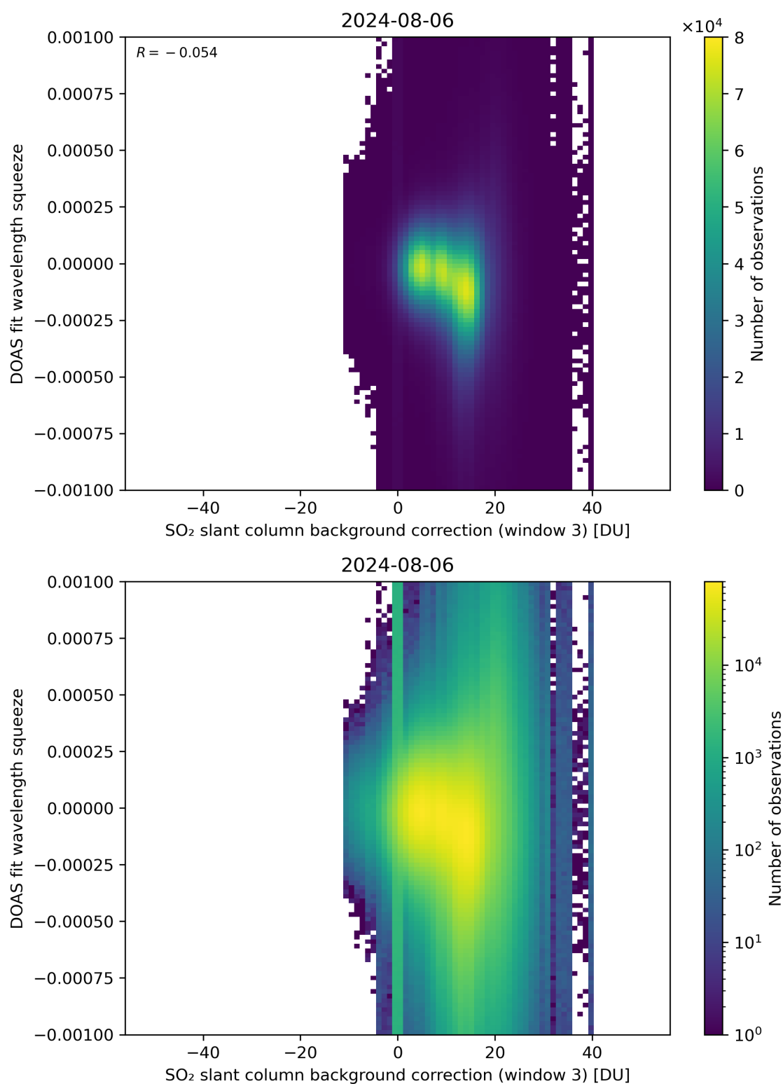
Figure 122: Scatter density plot of “SO 2 slant column background correction (window 3)” against “DOAS fit wavelength squeeze” for 2024-08-06 to 2024-08-07.
