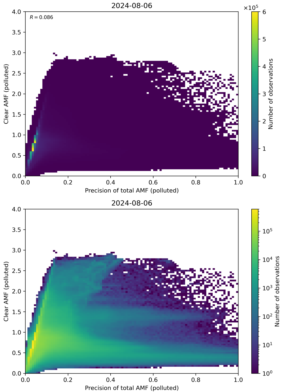
Figure 270: Scatter density plot of “Precision of total AMF (polluted)” against “Clear AMF (polluted)” for 2024-08-06 to 2024-08-07.
