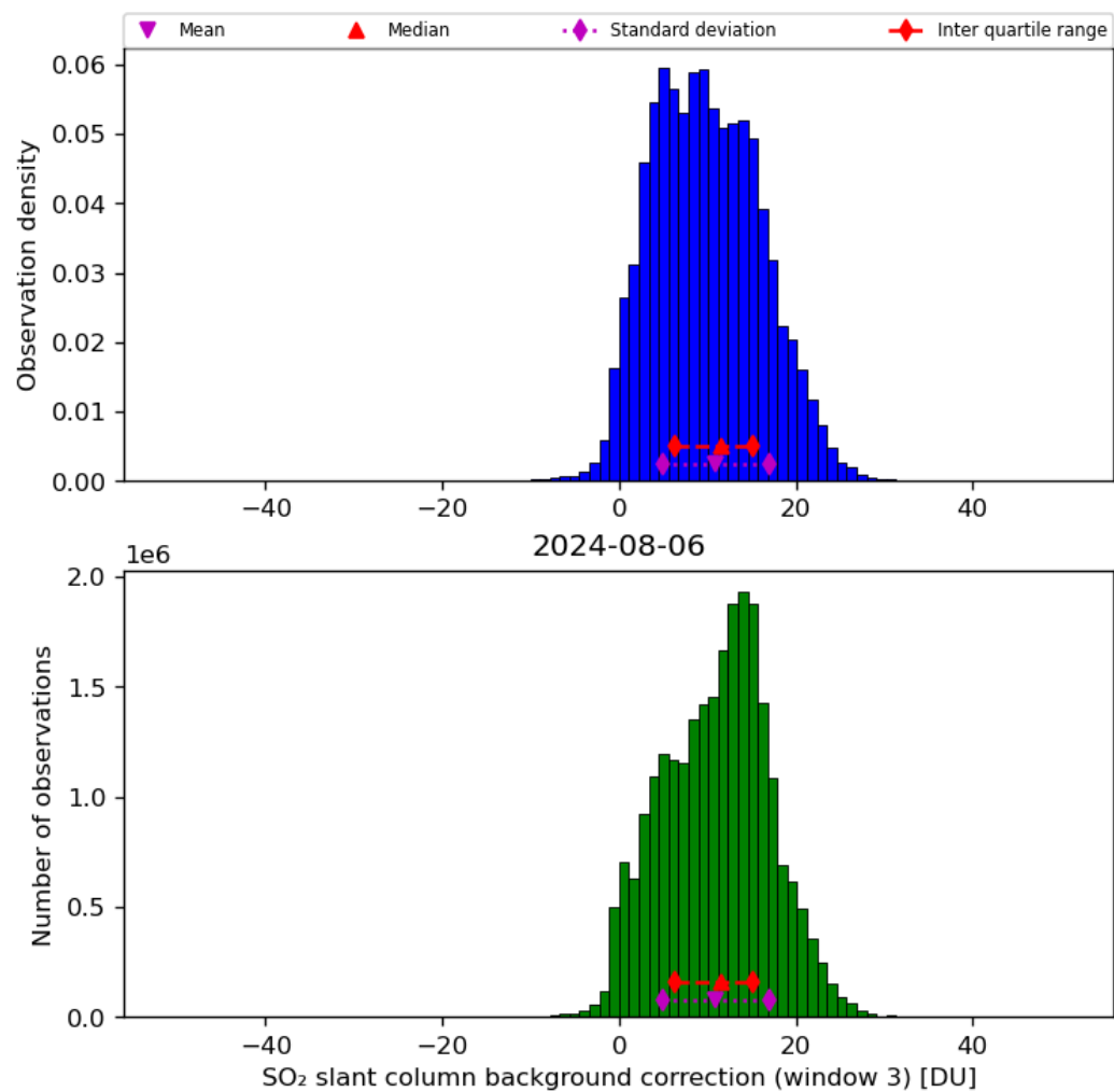
Figure 67: Histogram of “SO 2 slant column background correction (window 3)” for 2024-08-06 to 2024-08-07
