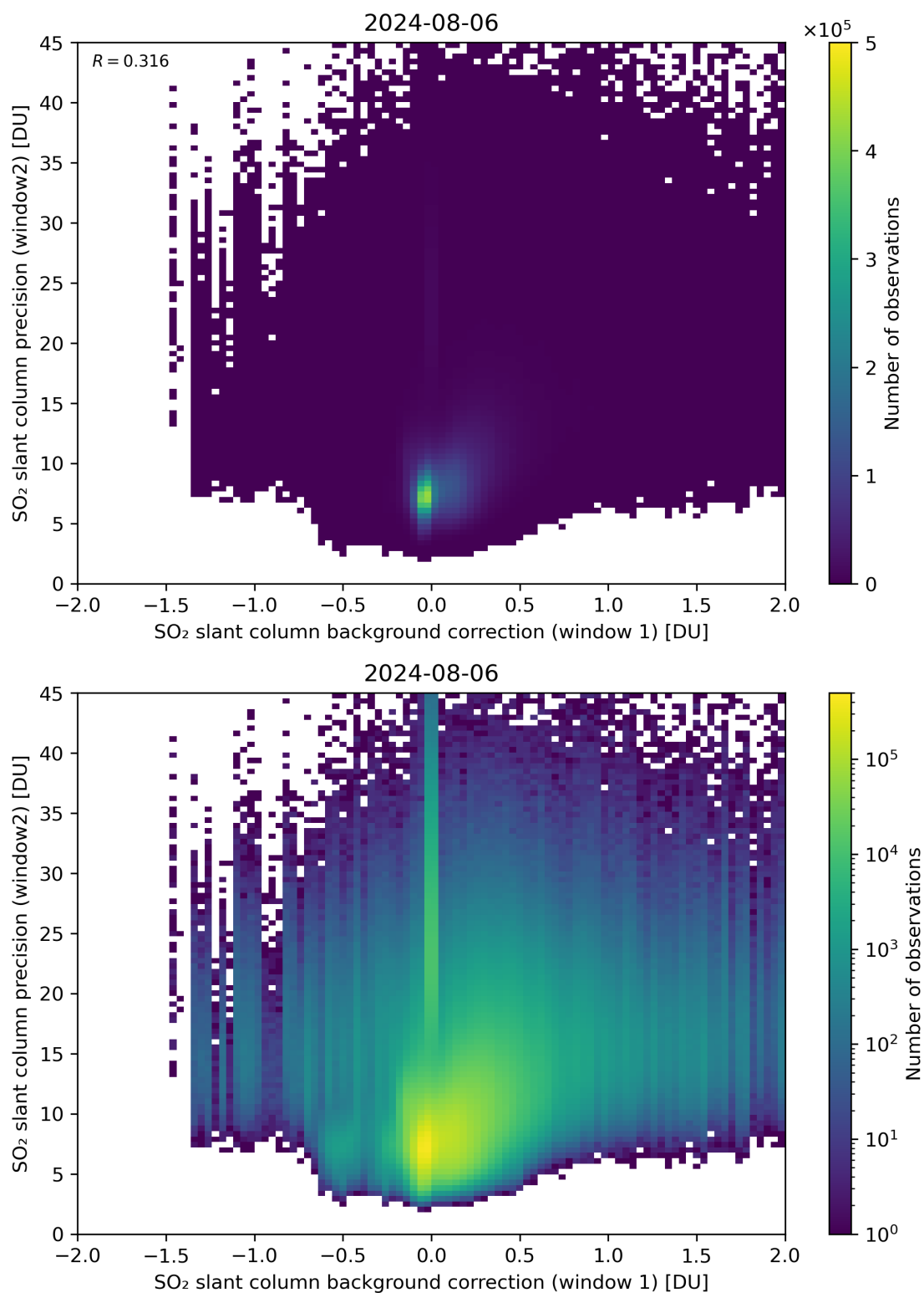
Figure 106: Scatter density plot of “SO 2 slant column background correction (window 1)” against “SO 2 slant column precision (window2)” for 2024-08-06 to 2024-08-07.
