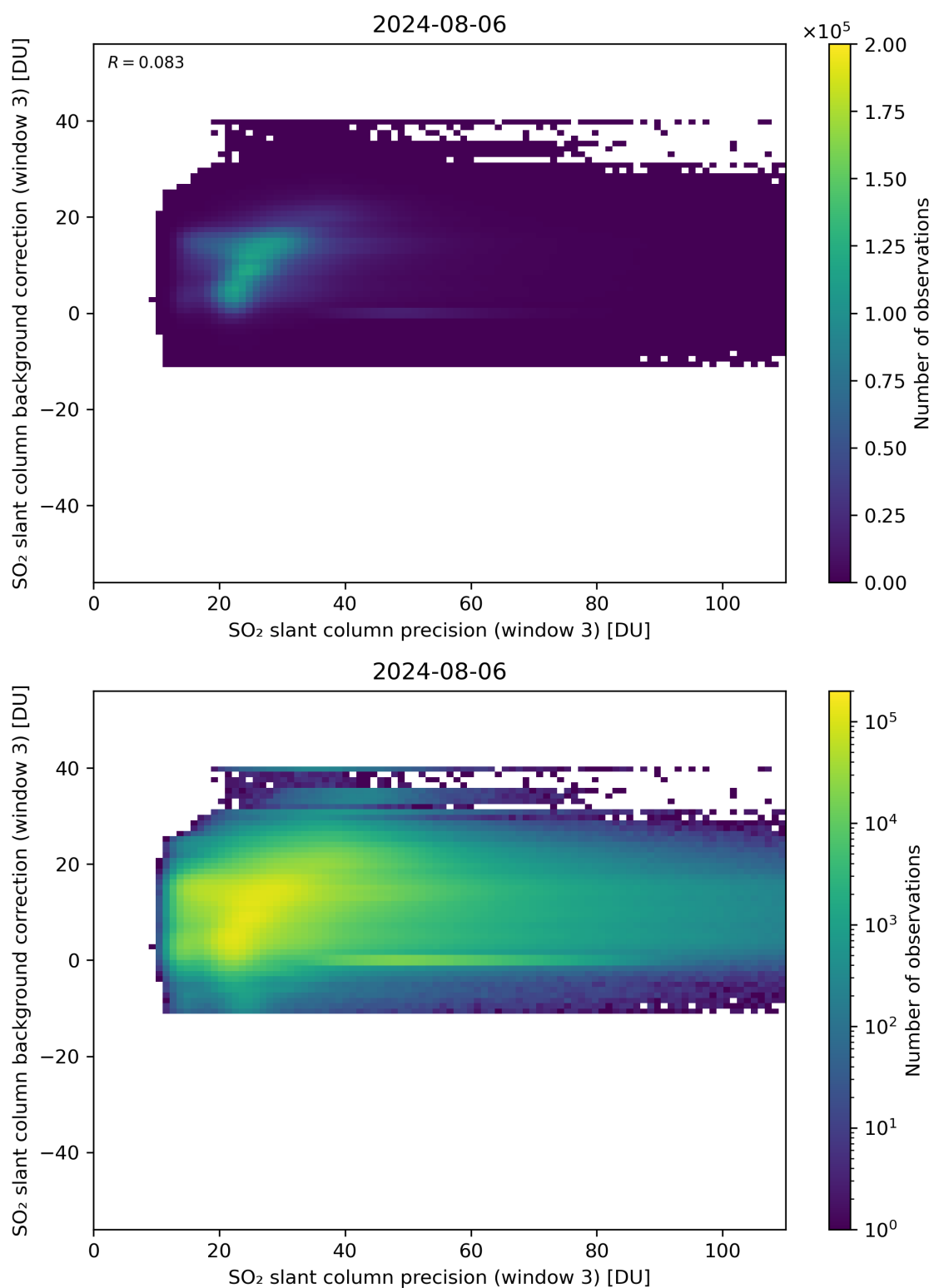
Figure 257: Scatter density plot of “SO 2 slant column precision (window 3)” against “SO 2 slant column background correction (window 3)” for 2024-08-06 to 2024-08-07.
