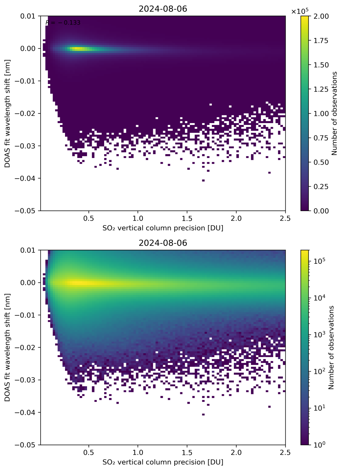
Figure 282: Scatter density plot of “SO 2 vertical column precision” against “DOAS fit wavelength shift” for 2024-08-06 to 2024-08-07.
