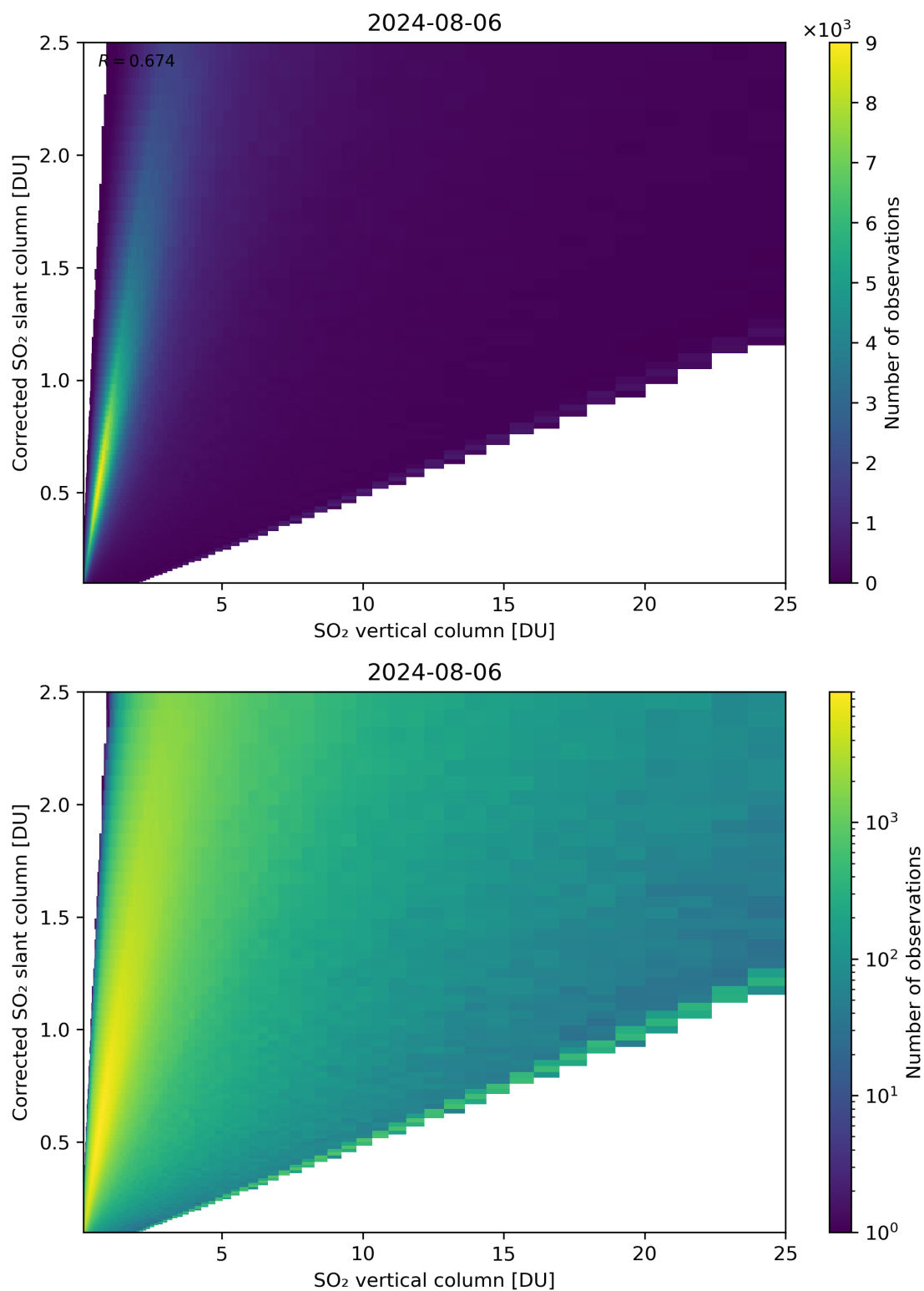
Figure 297: Scatter density plot of “SO 2 vertical column” against “Corrected SO 2 slant column” for 2024-08-06 to 2024-08-07.
