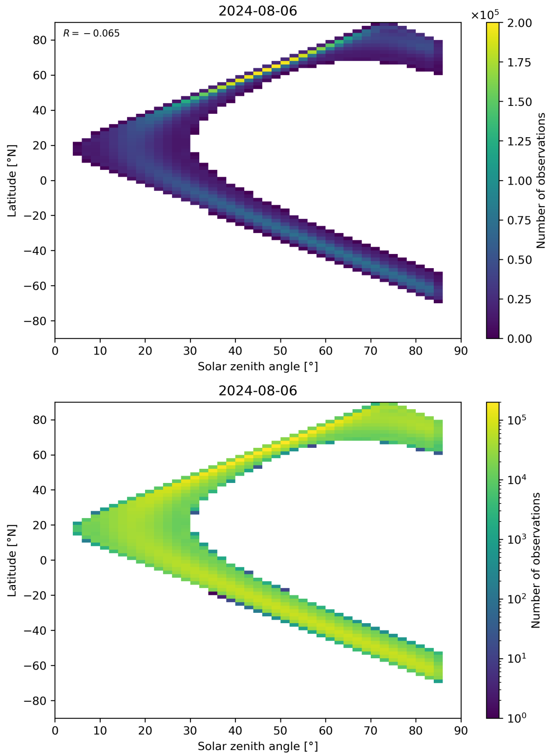
Figure 164: Scatter density plot of “Solar zenith angle” against “Latitude” for 2024-08-06 to 2024-08-07.
