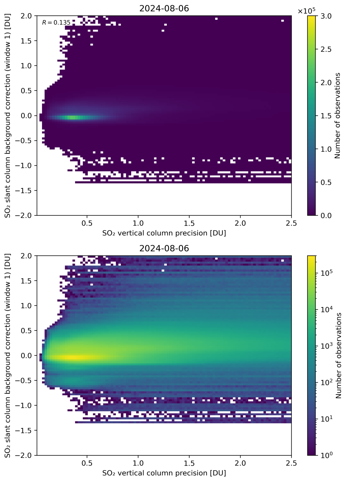
Figure 279: Scatter density plot of “SO 2 vertical column precision” against “SO 2 slant column background correction (window 1)” for 2024-08-06 to 2024-08-07.
