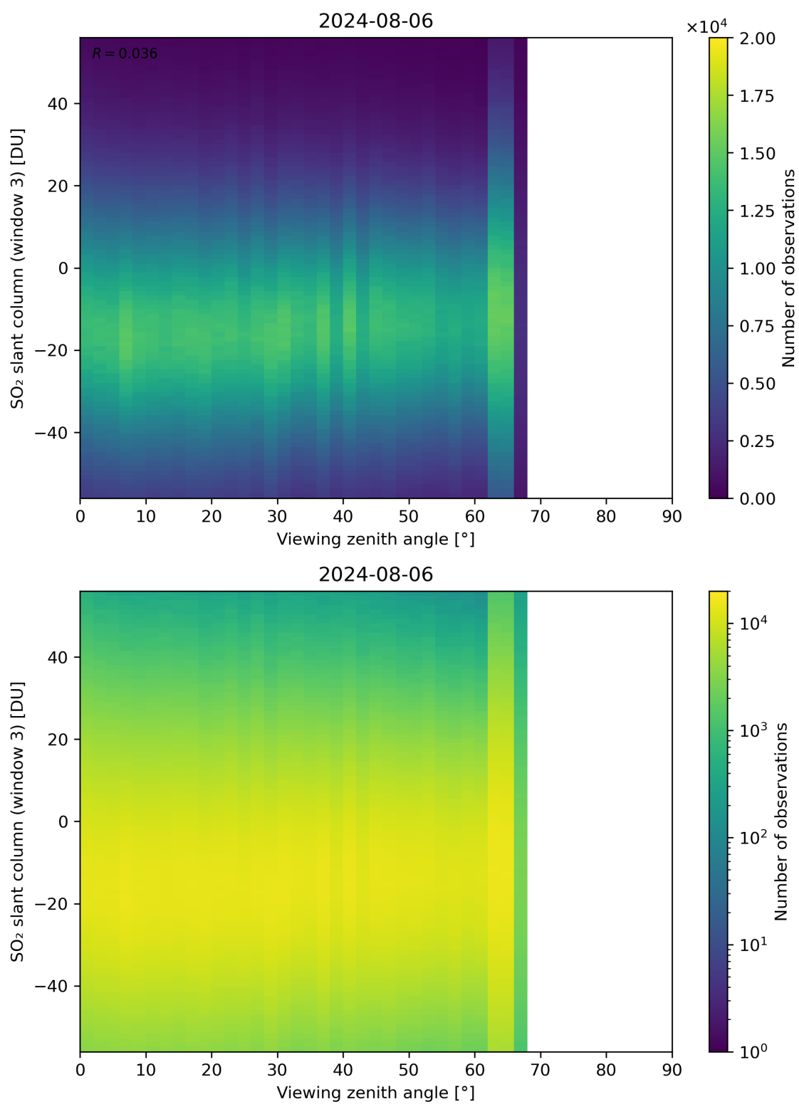
Figure 323: Scatter density plot of “Viewing zenith angle” against “SO 2 slant column (window 3)” for 2024-08-06 to 2024-08-07.
