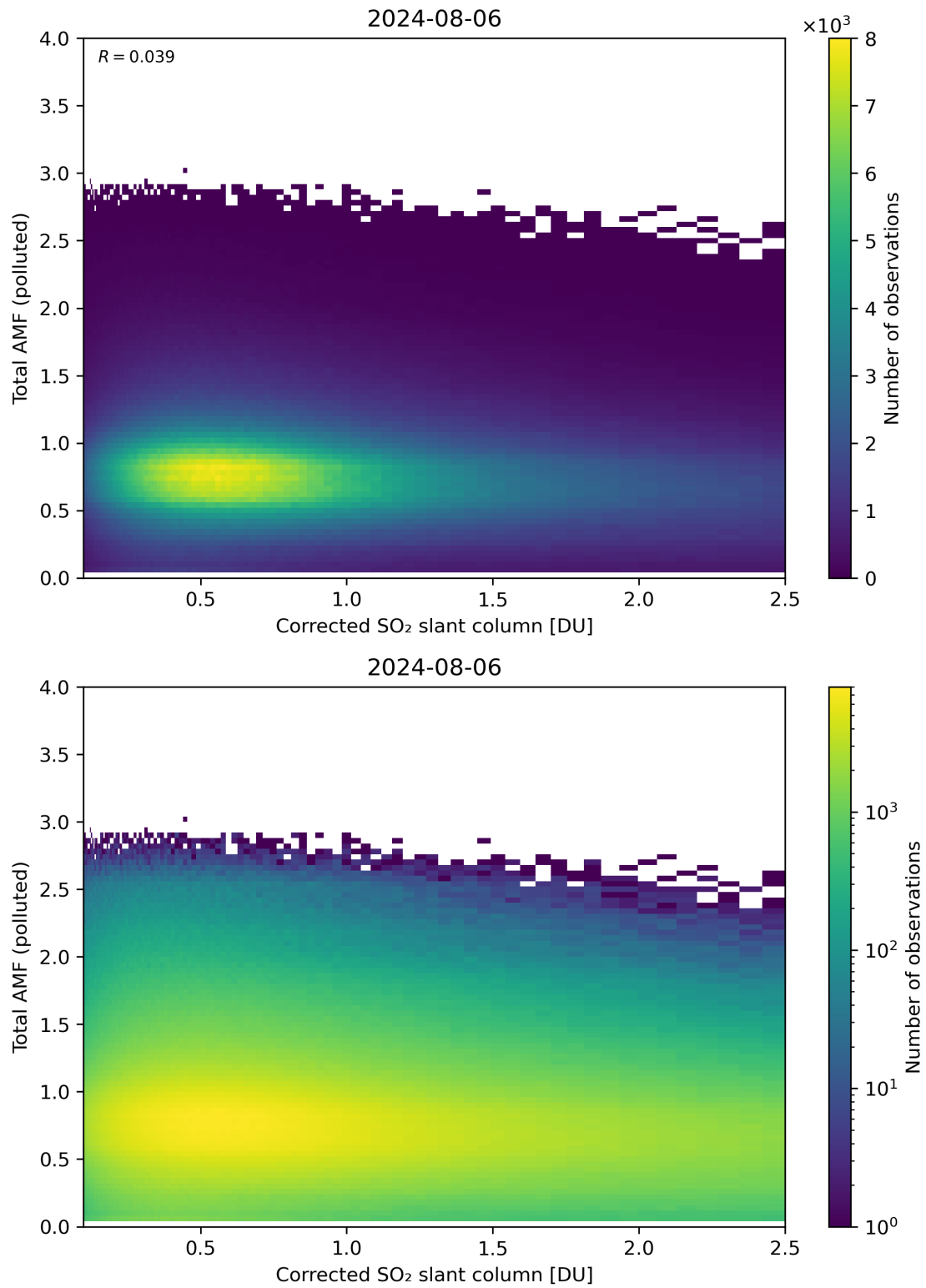
Figure 192: Scatter density plot of “Corrected SO 2 slant column” against “Total AMF (polluted)” for 2024-08-06 to 2024-08-07.
