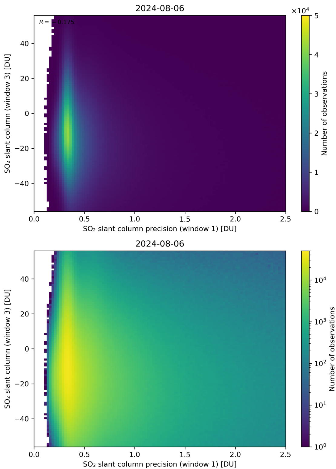
Figure 228: Scatter density plot of “SO 2 slant column precision (window 1)” against “SO 2 slant column (window 3)” for 2024-08-06 to 2024-08-07.
