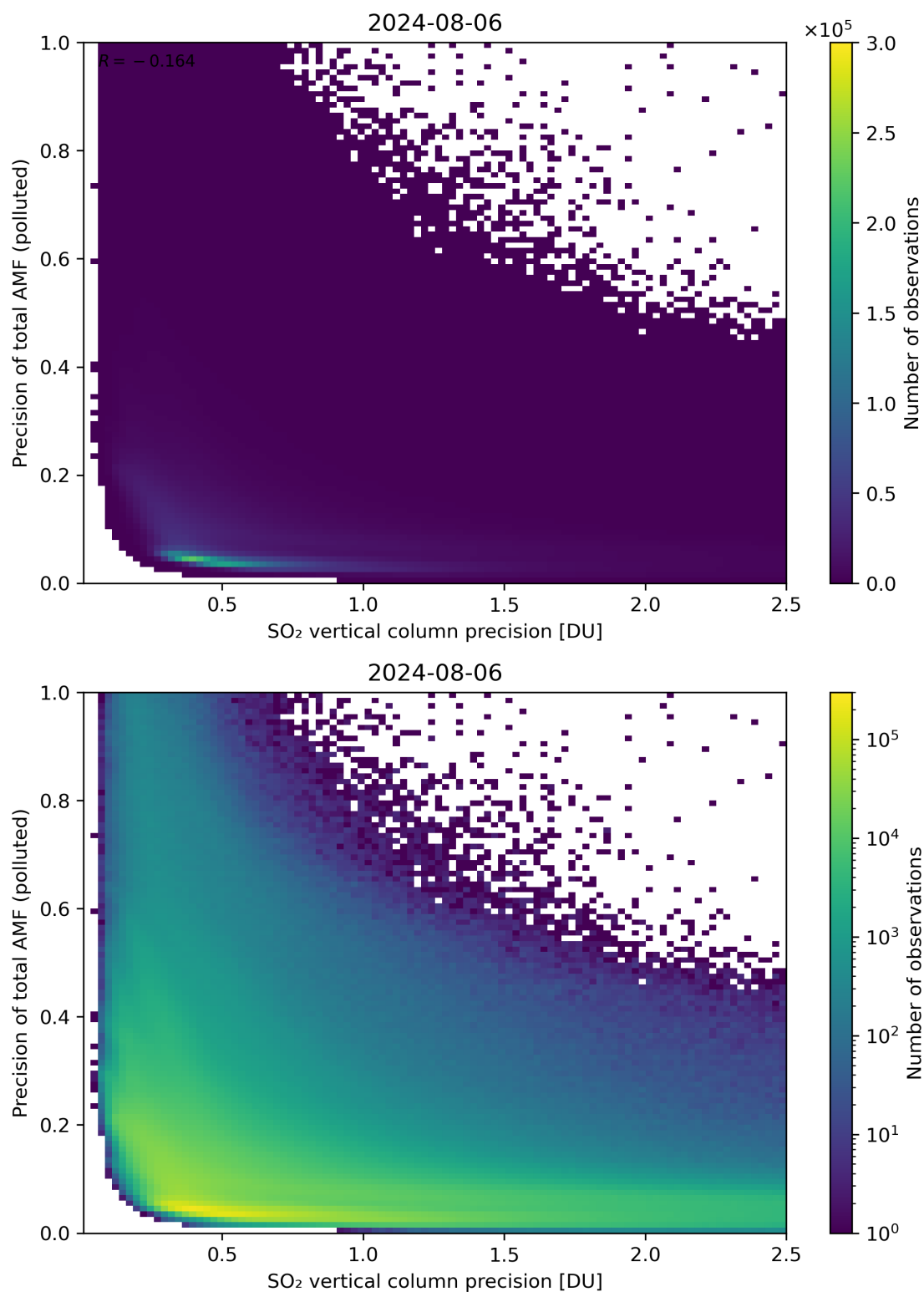
Figure 295: Scatter density plot of “SO 2 vertical column precision” against “Precision of total AMF (polluted)” for 2024-08-06 to 2024-08-07.
