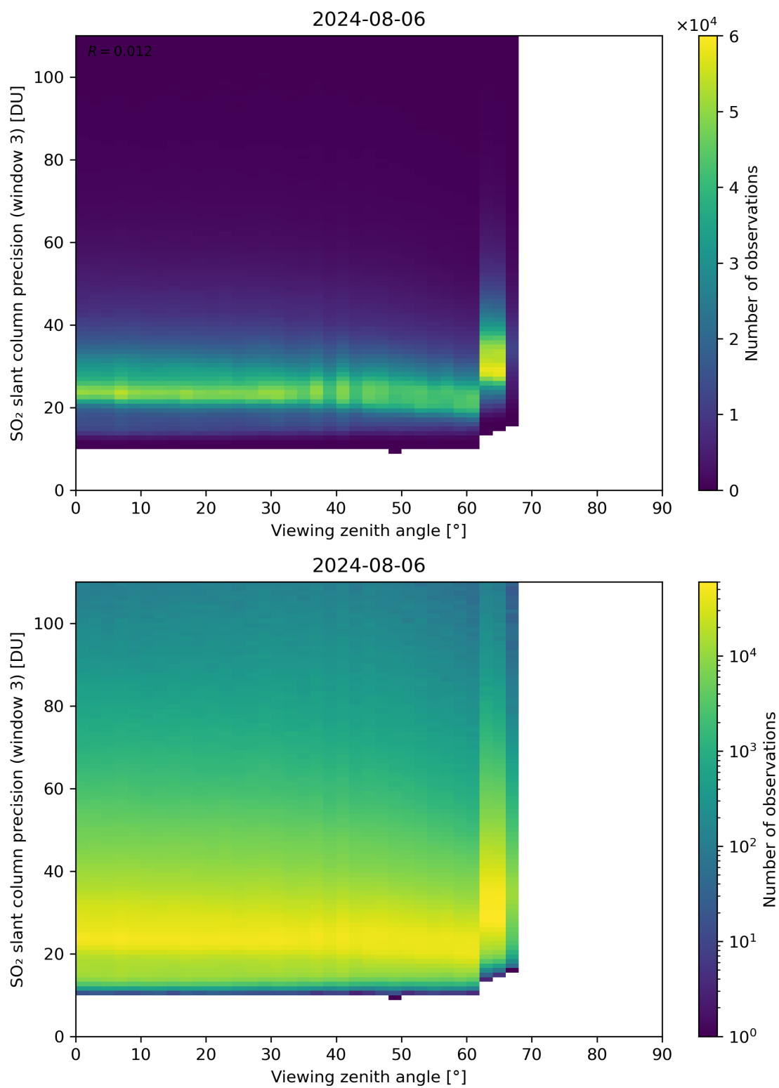
Figure 324: Scatter density plot of “Viewing zenith angle” against “SO 2 slant column precision (window 3)” for 2024-08-06 to 2024-08-07.
