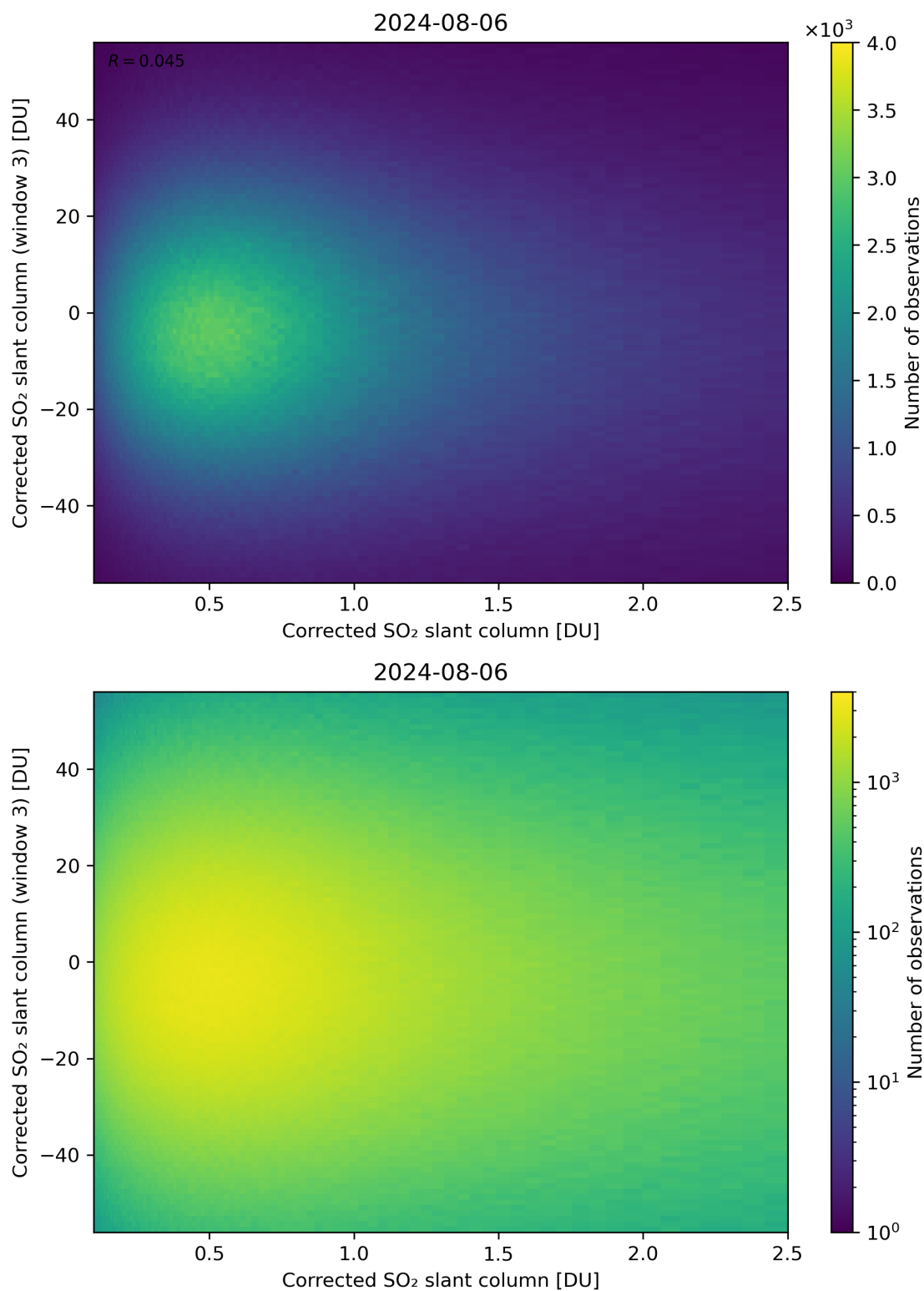
Figure 186: Scatter density plot of “Corrected SO 2 slant column” against “Corrected SO 2 slant column (window 3)” for 2024-08-06 to 2024-08-07.
