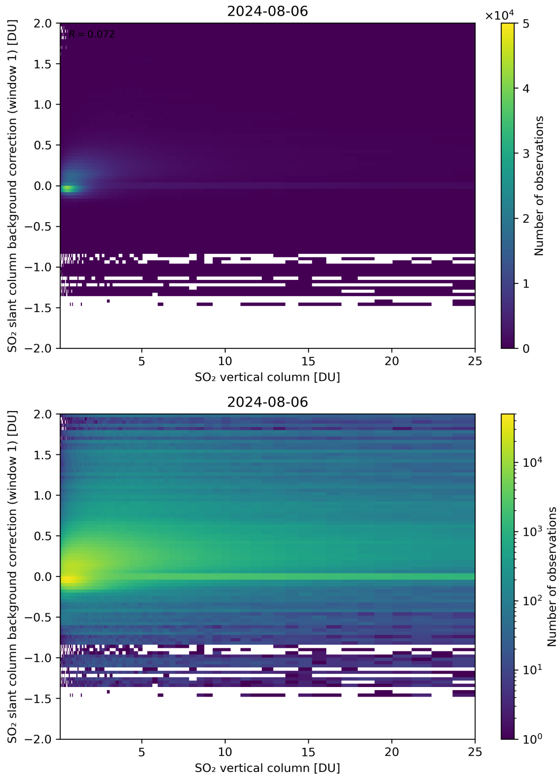
Figure 273: Scatter density plot of “SO 2 vertical column” against “SO 2 slant column background correction (window 1)” for 2024-08-06 to 2024-08-07.
