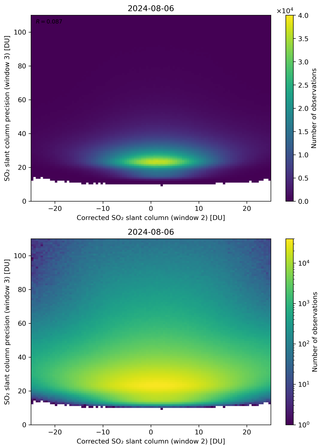
Figure 202: Scatter density plot of “Corrected SO 2 slant column (window 2)” against “SO 2 slant column precision (window 3)” for 2024-08-06 to 2024-08-07.
