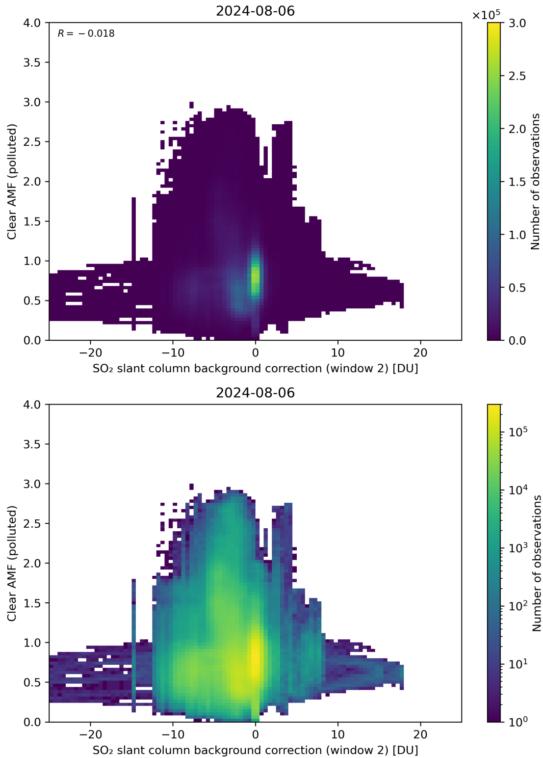
Figure 115: Scatter density plot of “SO 2 slant column background correction (window 2)” against “Clear AMF (polluted)” for 2024-08-06 to 2024-08-07.
