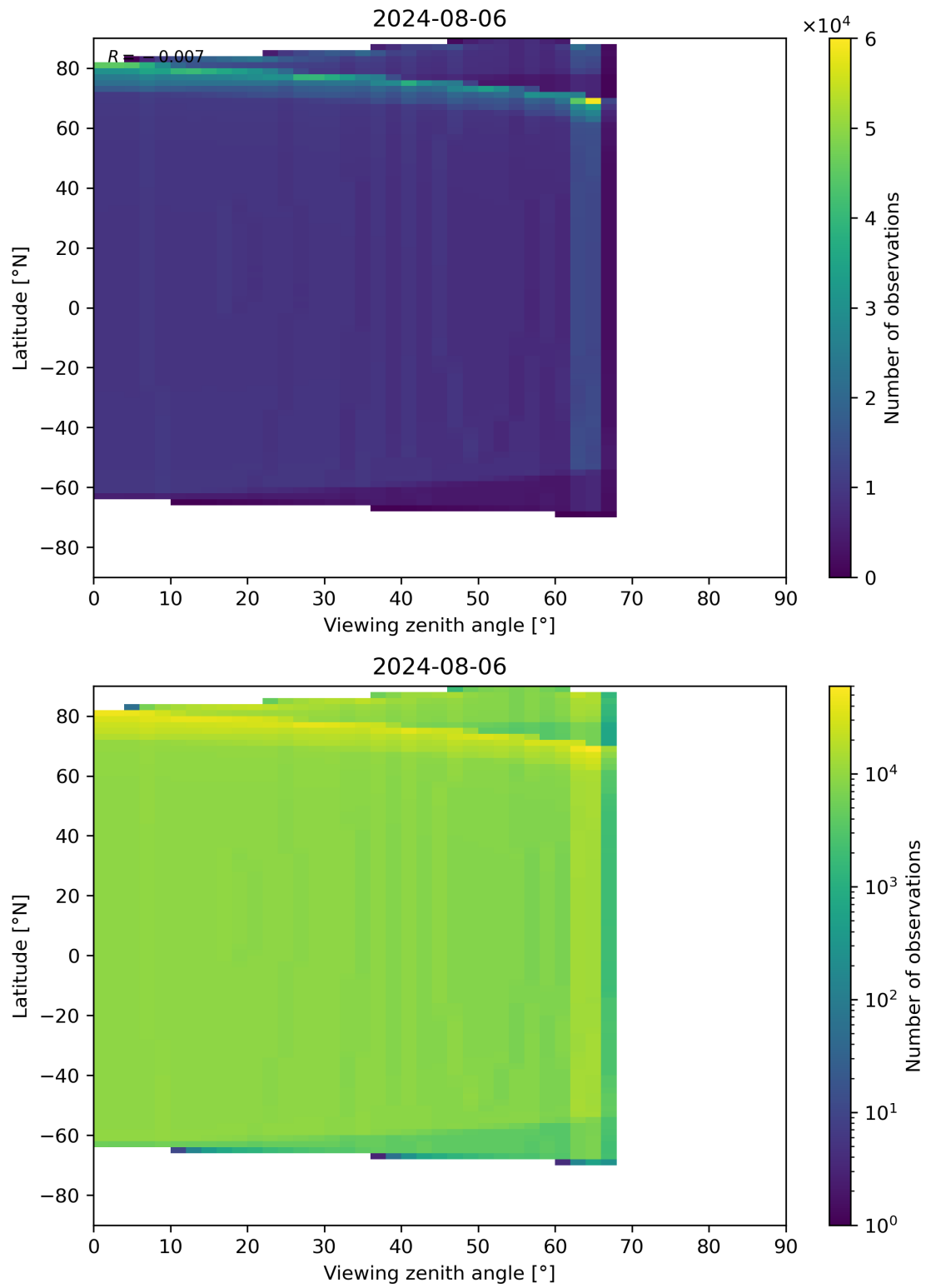
Figure 314: Scatter density plot of “Viewing zenith angle” against “Latitude” for 2024-08-06 to 2024-08-07.
