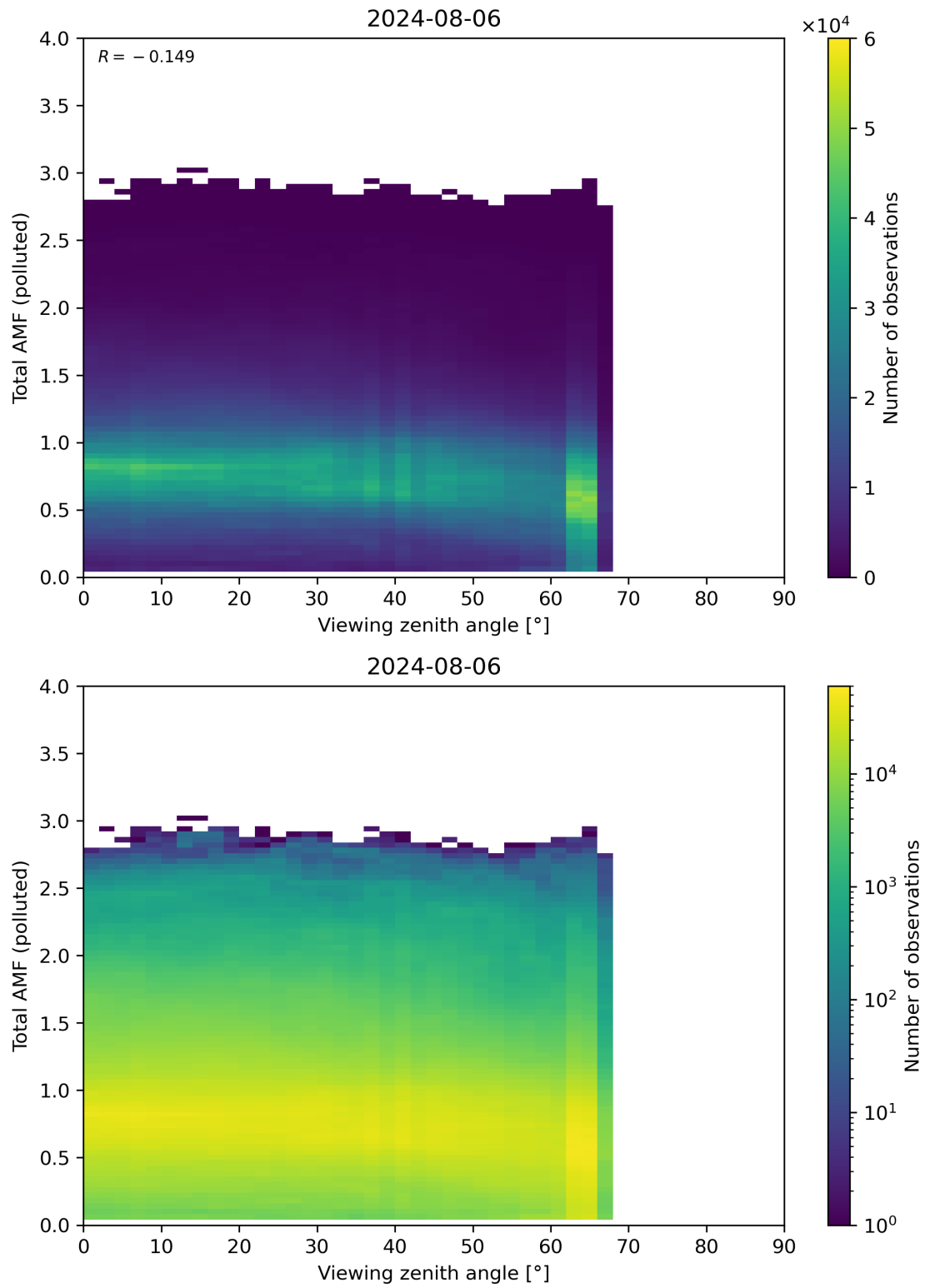
Figure 325: Scatter density plot of “Viewing zenith angle” against “Total AMF (polluted)” for 2024-08-06 to 2024-08-07.
