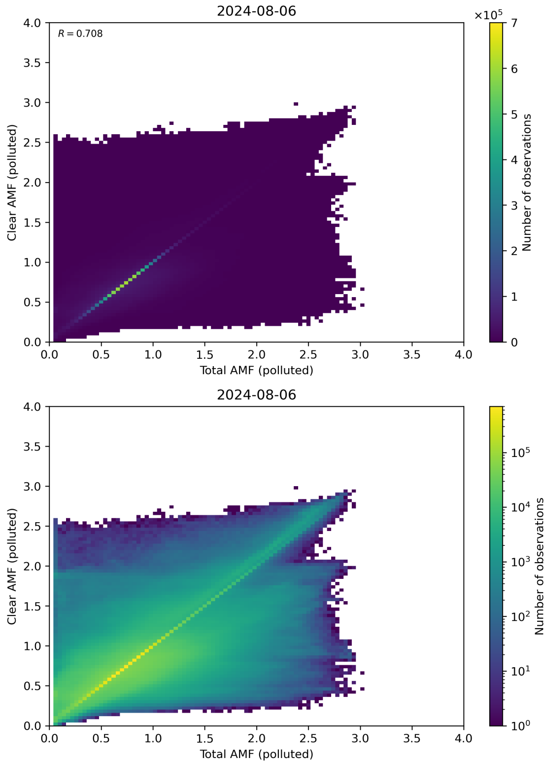
Figure 271: Scatter density plot of “Total AMF (polluted)” against “Clear AMF (polluted)” for 2024-08-06 to 2024-08-07.
