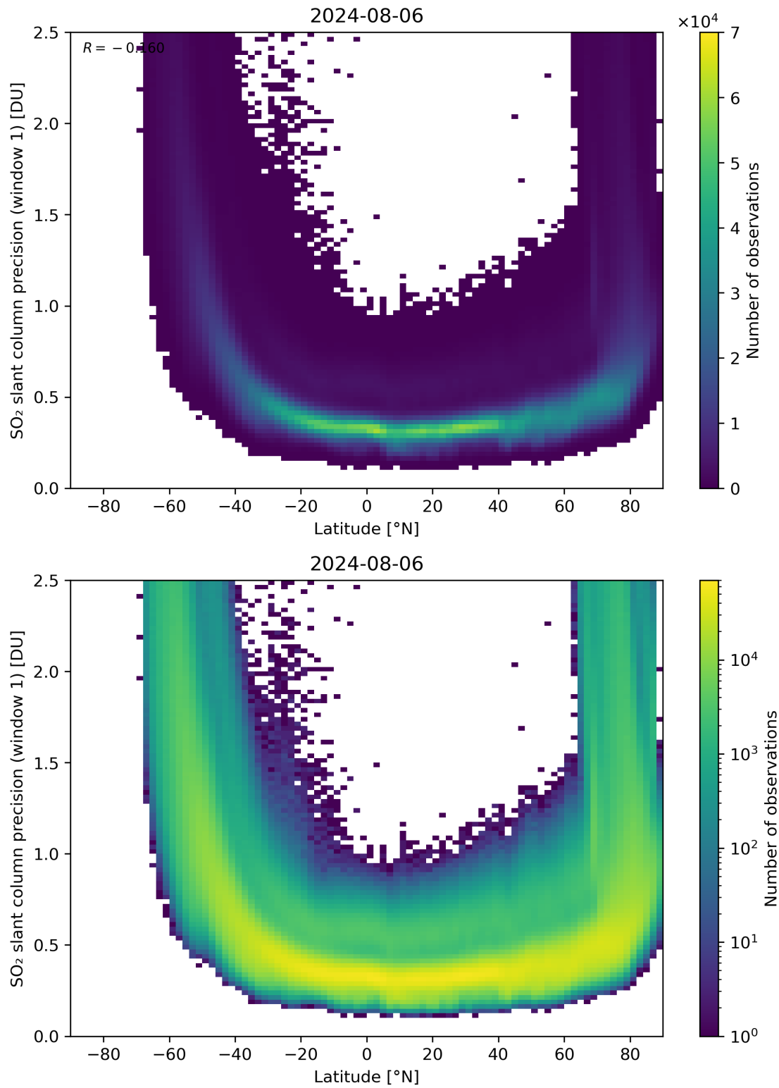
Figure 150: Scatter density plot of “Latitude” against “SO 2 slant column precision (window 1)” for 2024-08-06 to 2024-08-07.
