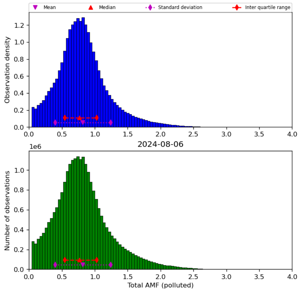
Figure 71: Histogram of “Total AMF (polluted)” for 2024-08-06 to 2024-08-07
