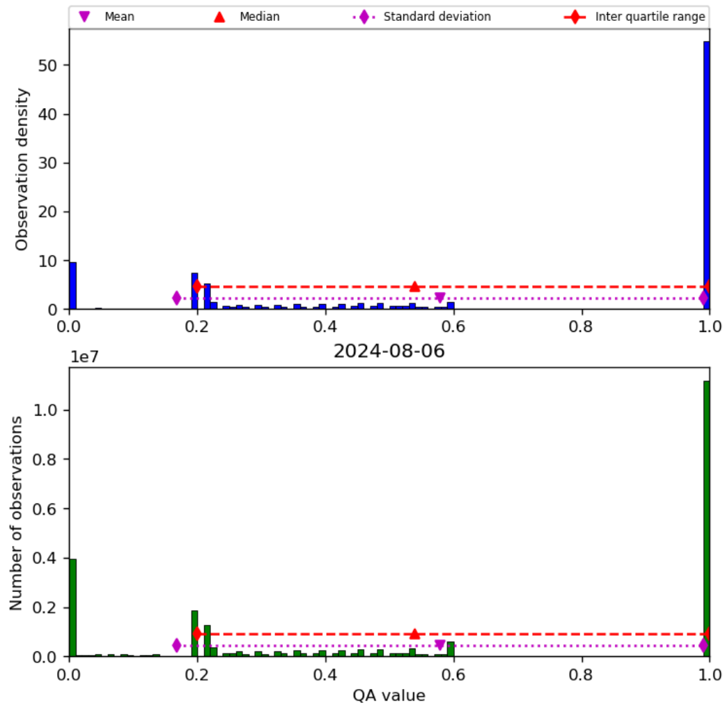
Figure 52: Histogram of “QA value” for 2024-08-06 to 2024-08-07
