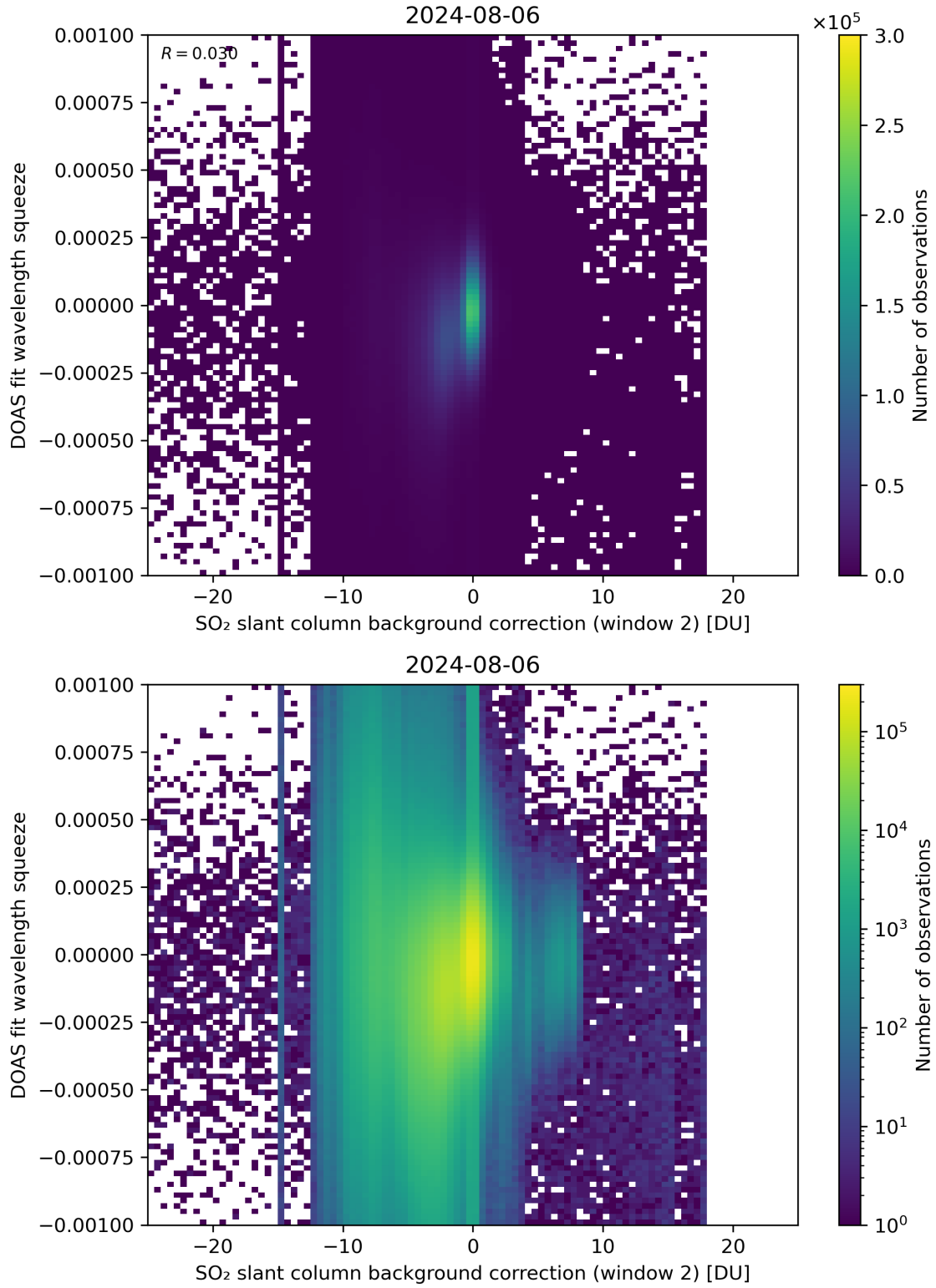
Figure 113: Scatter density plot of “SO 2 slant column background correction (window 2)” against “DOAS fit wavelength squeeze” for 2024-08-06 to 2024-08-07.
