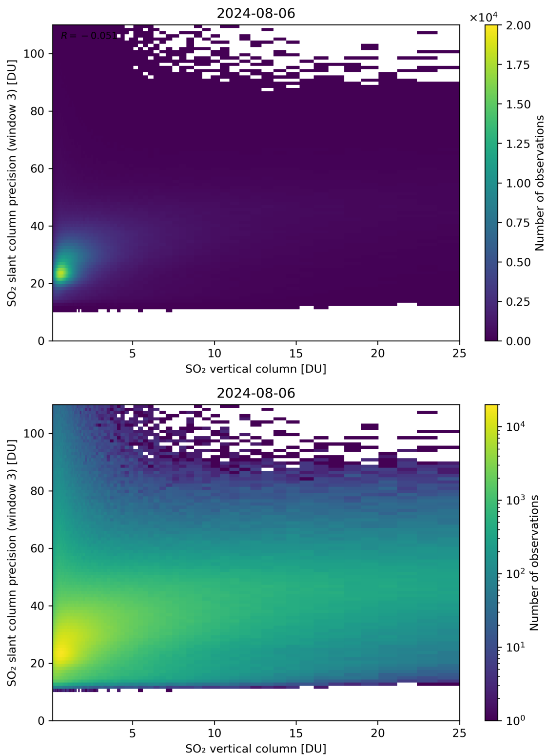
Figure 304: Scatter density plot of “SO 2 vertical column” against “SO 2 slant column precision (window 3)” for 2024-08-06 to 2024-08-07.
