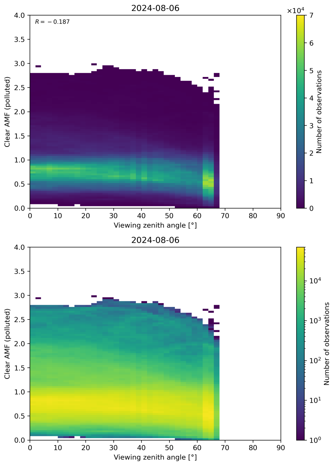
Figure 316: Scatter density plot of “Viewing zenith angle” against “Clear AMF (polluted)” for 2024-08-06 to 2024-08-07.
