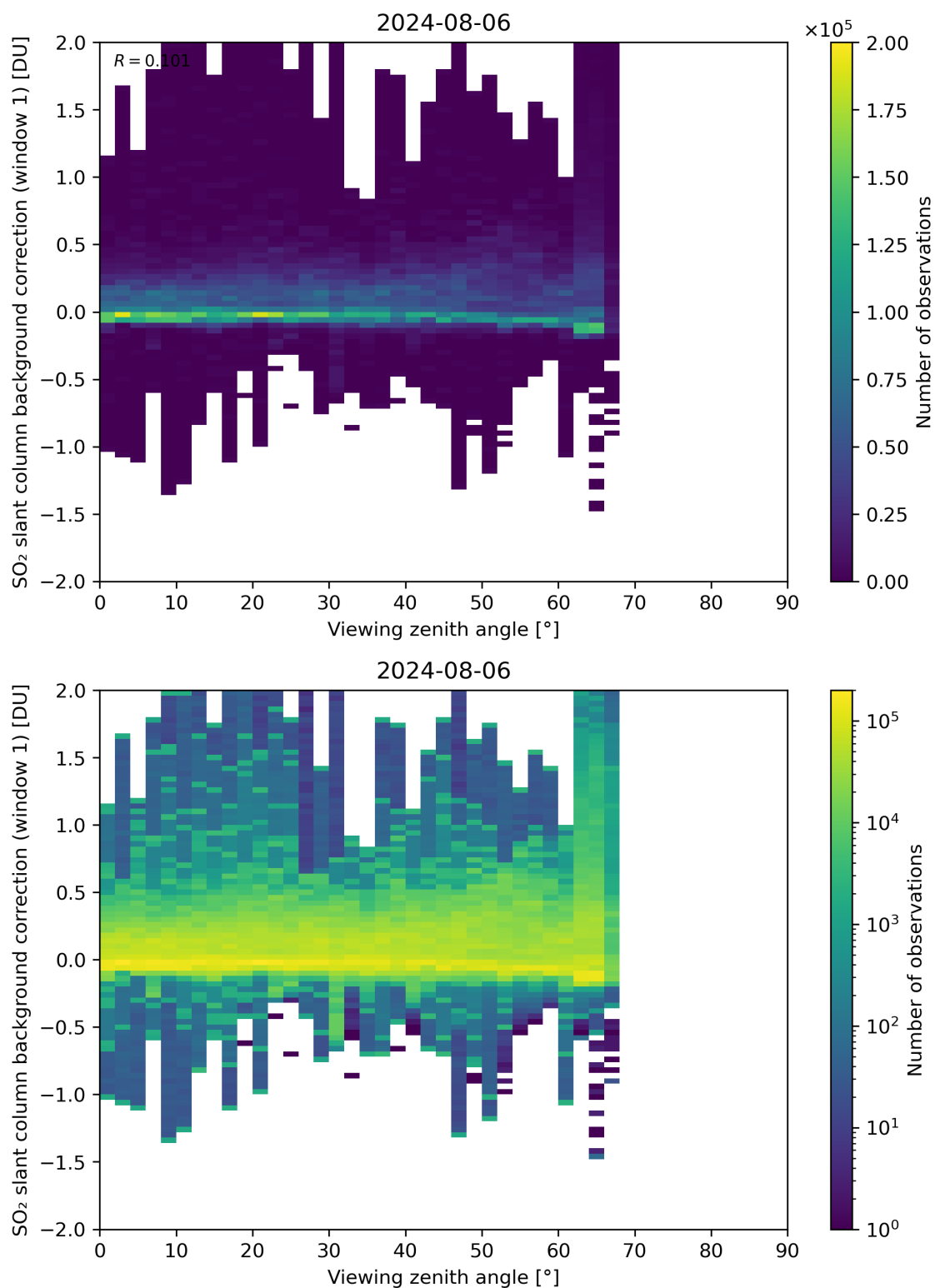
Figure 308: Scatter density plot of “Viewing zenith angle” against “SO 2 slant column background correction (window 1)” for 2024-08-06 to 2024-08-07.
