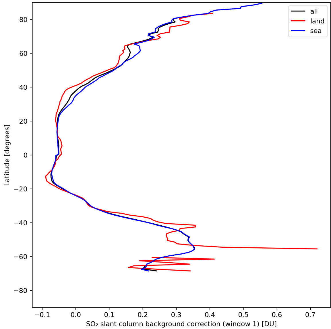
Figure 36: Zonal average of “SO 2 slant column background correction (window 1)” for 2024-08-06 to 2024-08-07.
