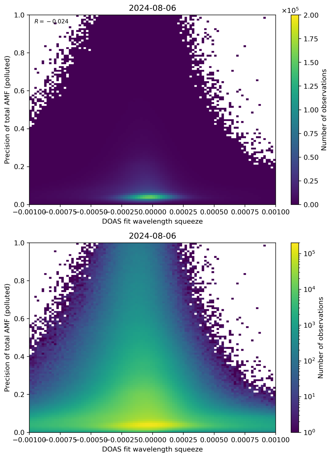
Figure 135: Scatter density plot of “DOAS fit wavelength squeeze” against “Precision of total AMF (polluted)” for 2024-08-06 to 2024-08-07.
