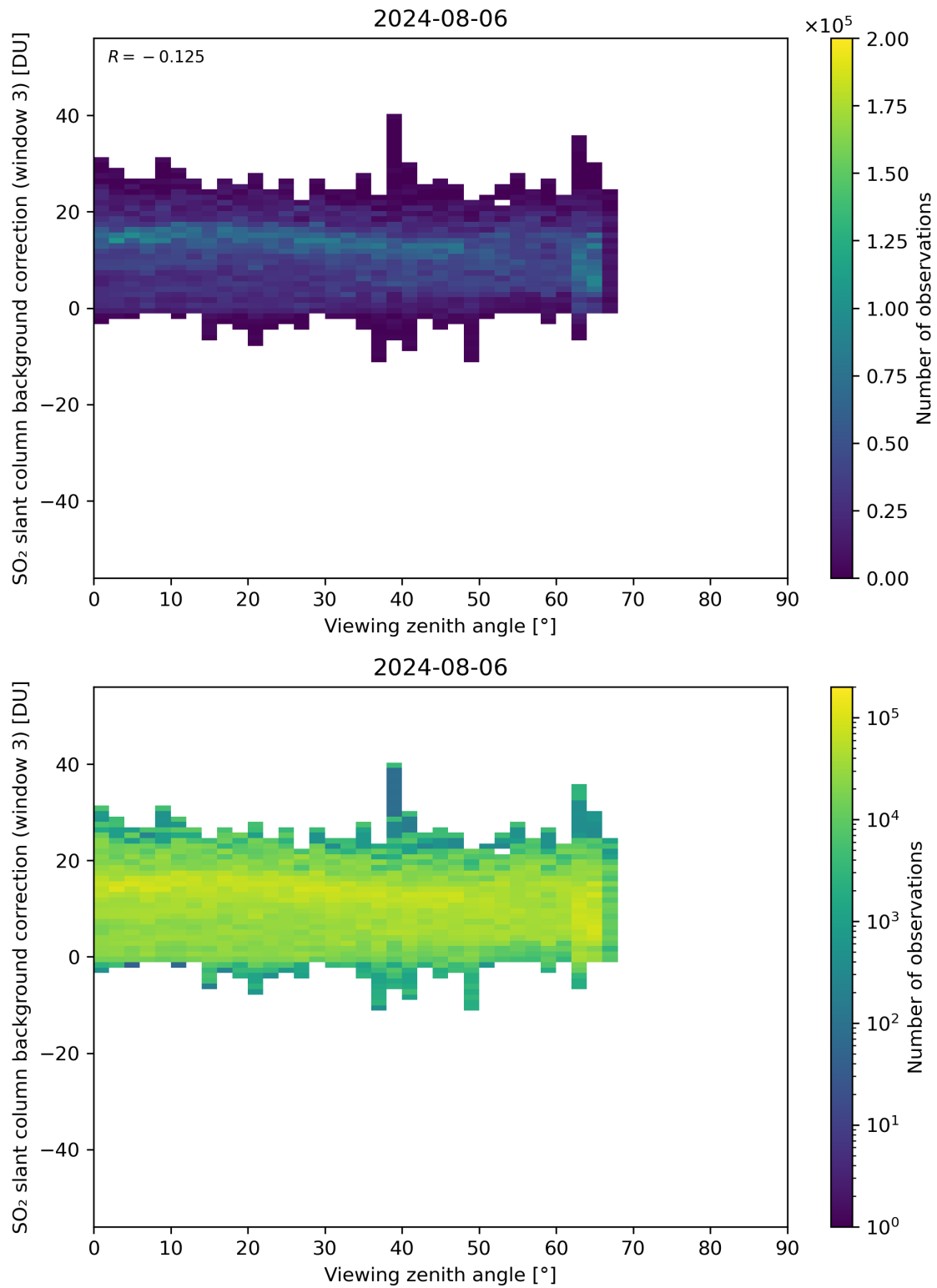
Figure 310: Scatter density plot of “Viewing zenith angle” against “SO 2 slant column background correction (window 3)” for 2024-08-06 to 2024-08-07.
