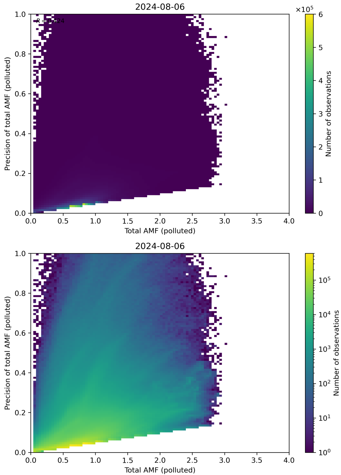
Figure 272: Scatter density plot of “Total AMF (polluted)” against “Precision of total AMF (polluted)” for 2024-08-06 to 2024-08-07.
