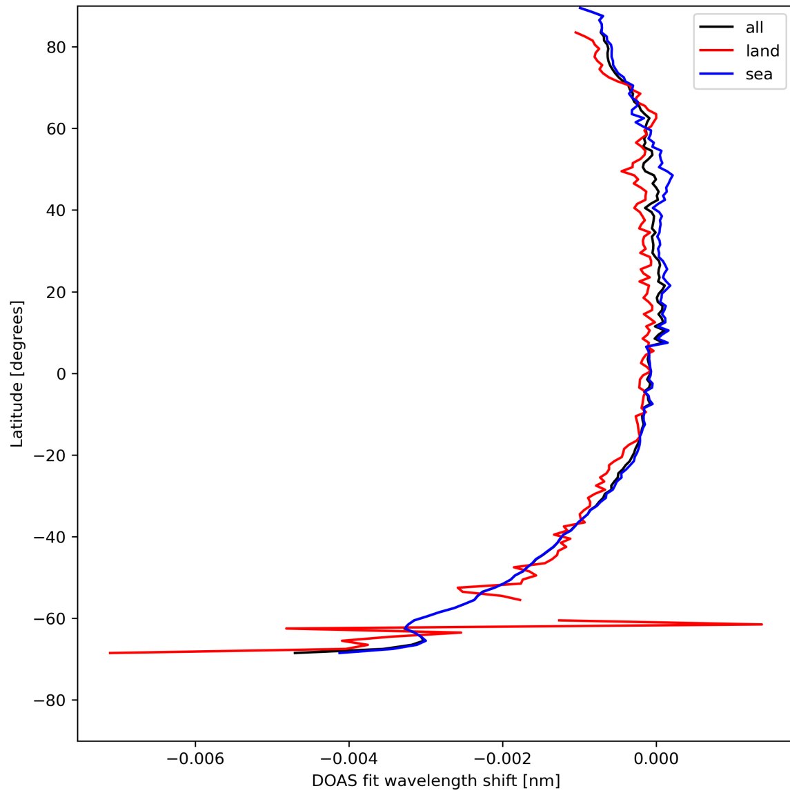
Figure 45: Zonal average of “DOAS fit wavelength shift” for 2024-08-06 to 2024-08-07.
