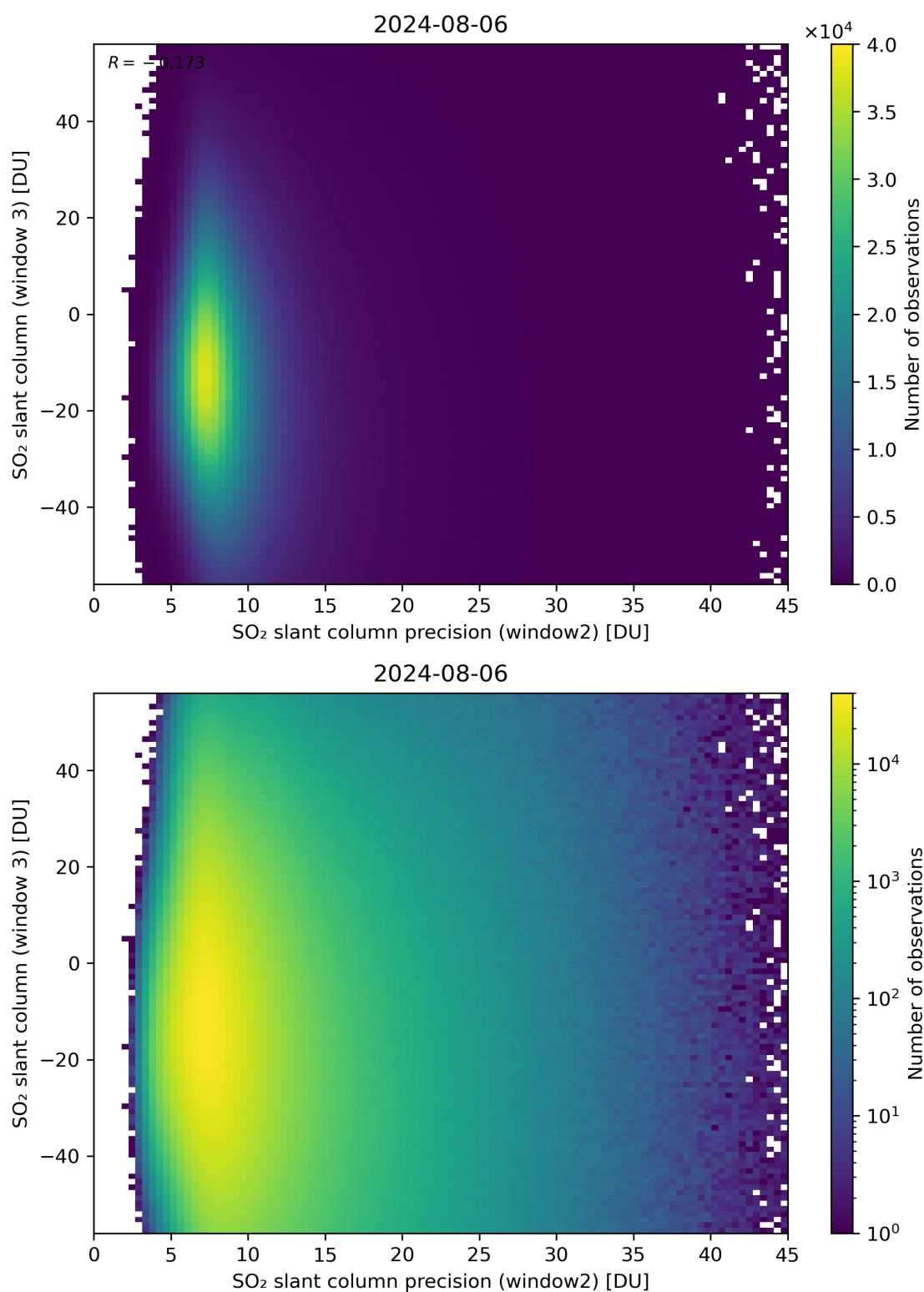
Figure 249: Scatter density plot of “SO 2 slant column precision (window2)” against “SO 2 slant column (window 3)” for 2024-08-06 to 2024-08-07.
