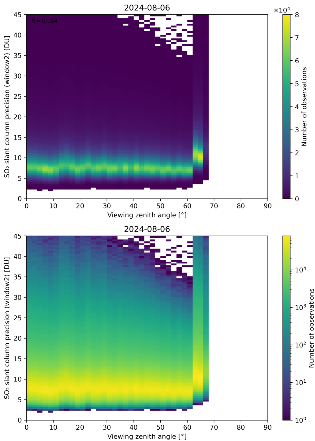
Figure 322: Scatter density plot of “Viewing zenith angle” against “SO 2 slant column precision (window2)” for 2024-08-06 to 2024-08-07.
