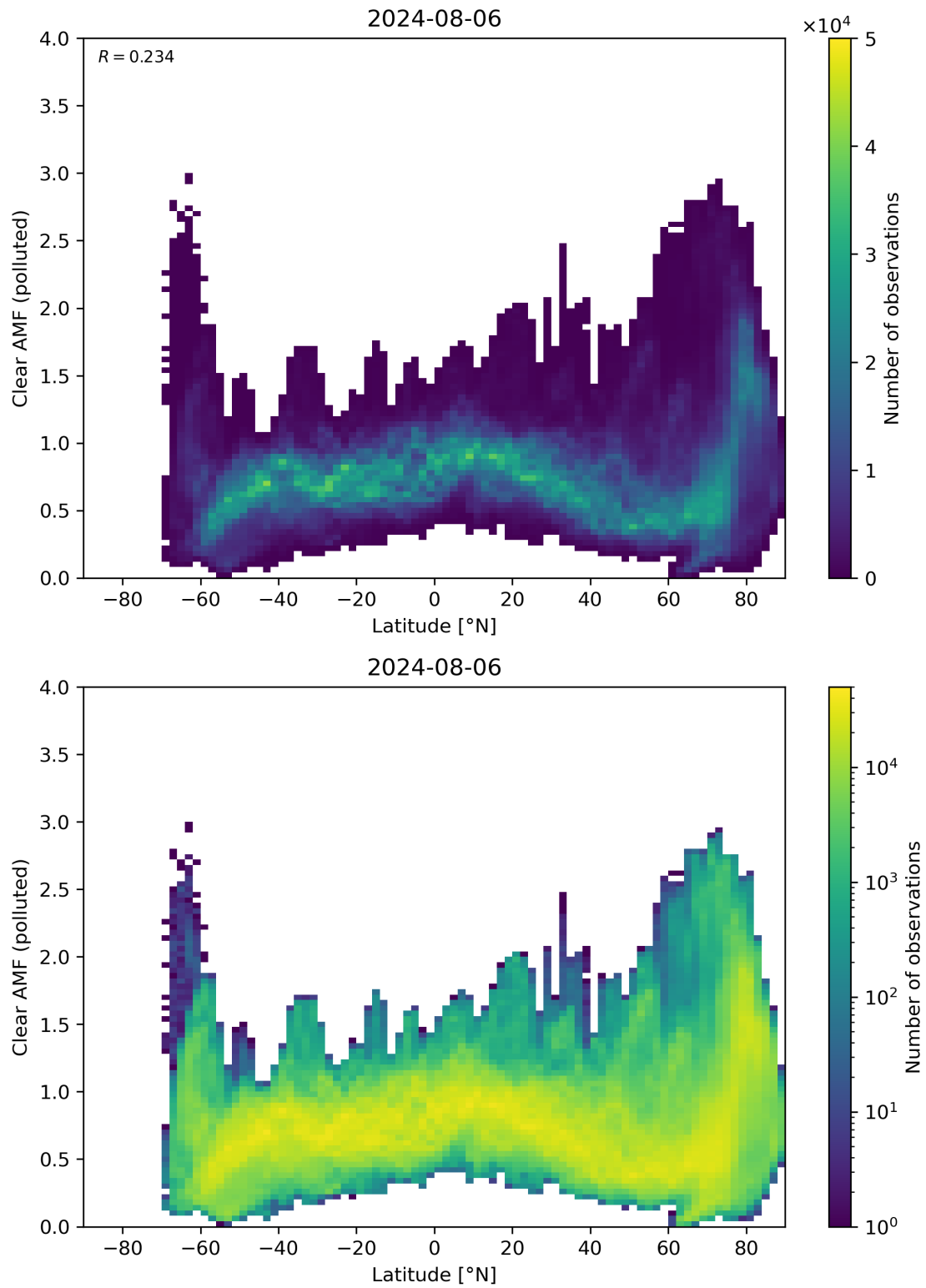
Figure 145: Scatter density plot of “Latitude” against “Clear AMF (polluted)” for 2024-08-06 to 2024-08-07.
