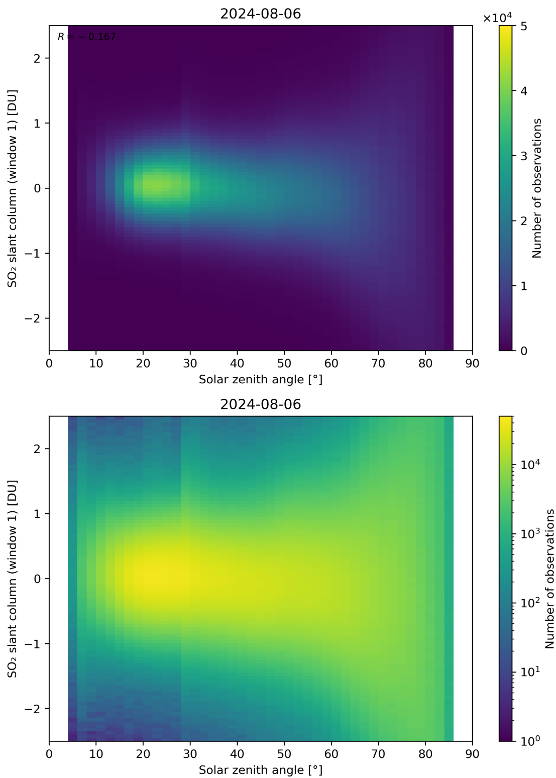
Figure 169: Scatter density plot of “Solar zenith angle” against “SO 2 slant column (window 1)” for 2024-08-06 to 2024-08-07.
