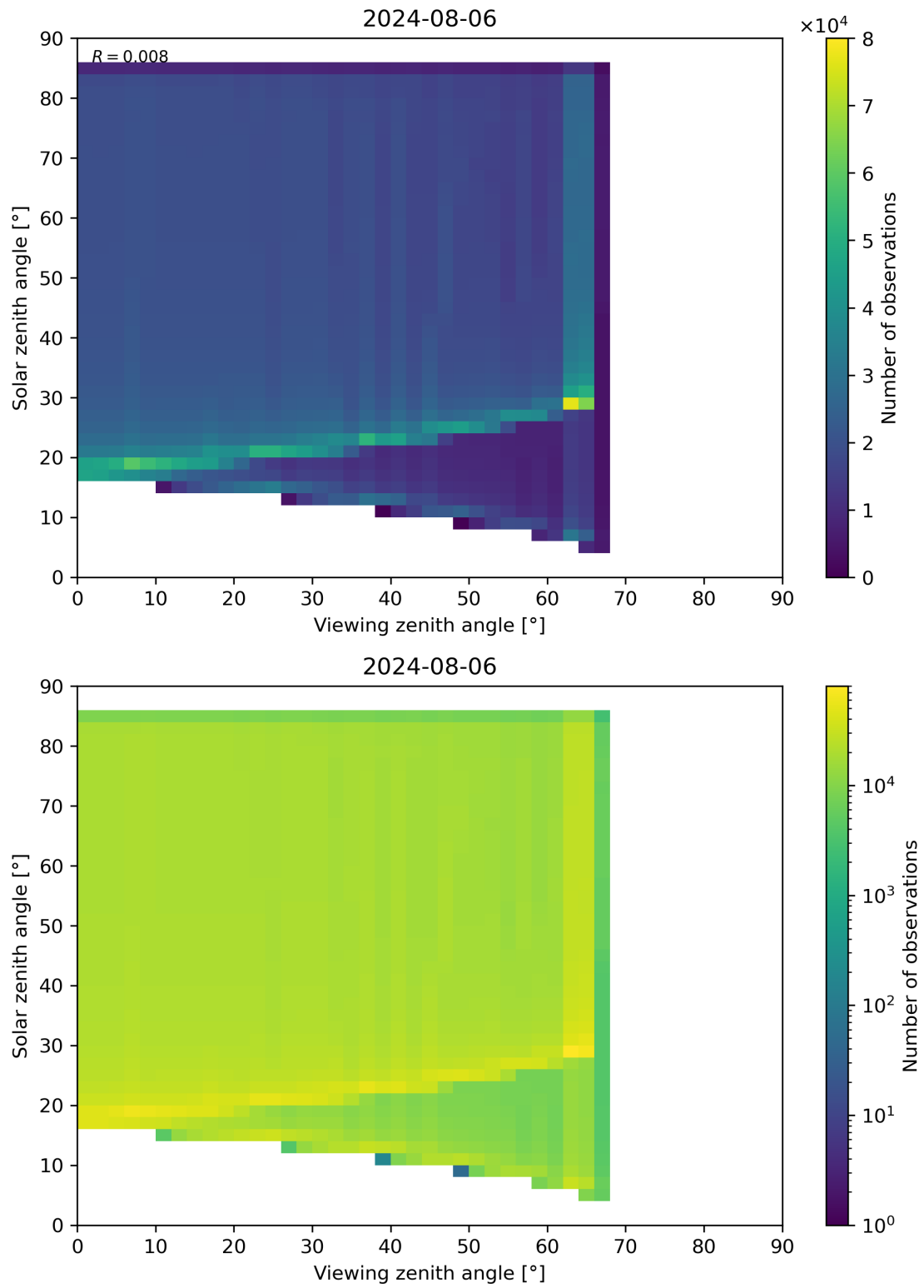
Figure 315: Scatter density plot of “Viewing zenith angle” against “Solar zenith angle” for 2024-08-06 to 2024-08-07.
