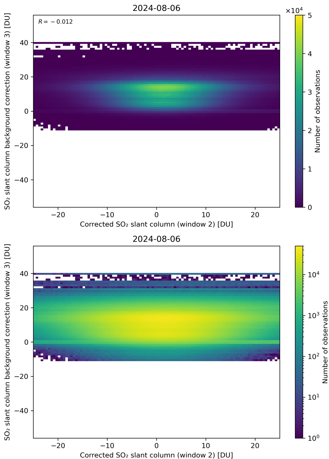
Figure 195: Scatter density plot of “Corrected SO 2 slant column (window 2)” against “SO 2 slant column background correction (window 3)” for 2024-08-06 to 2024-08-07.
