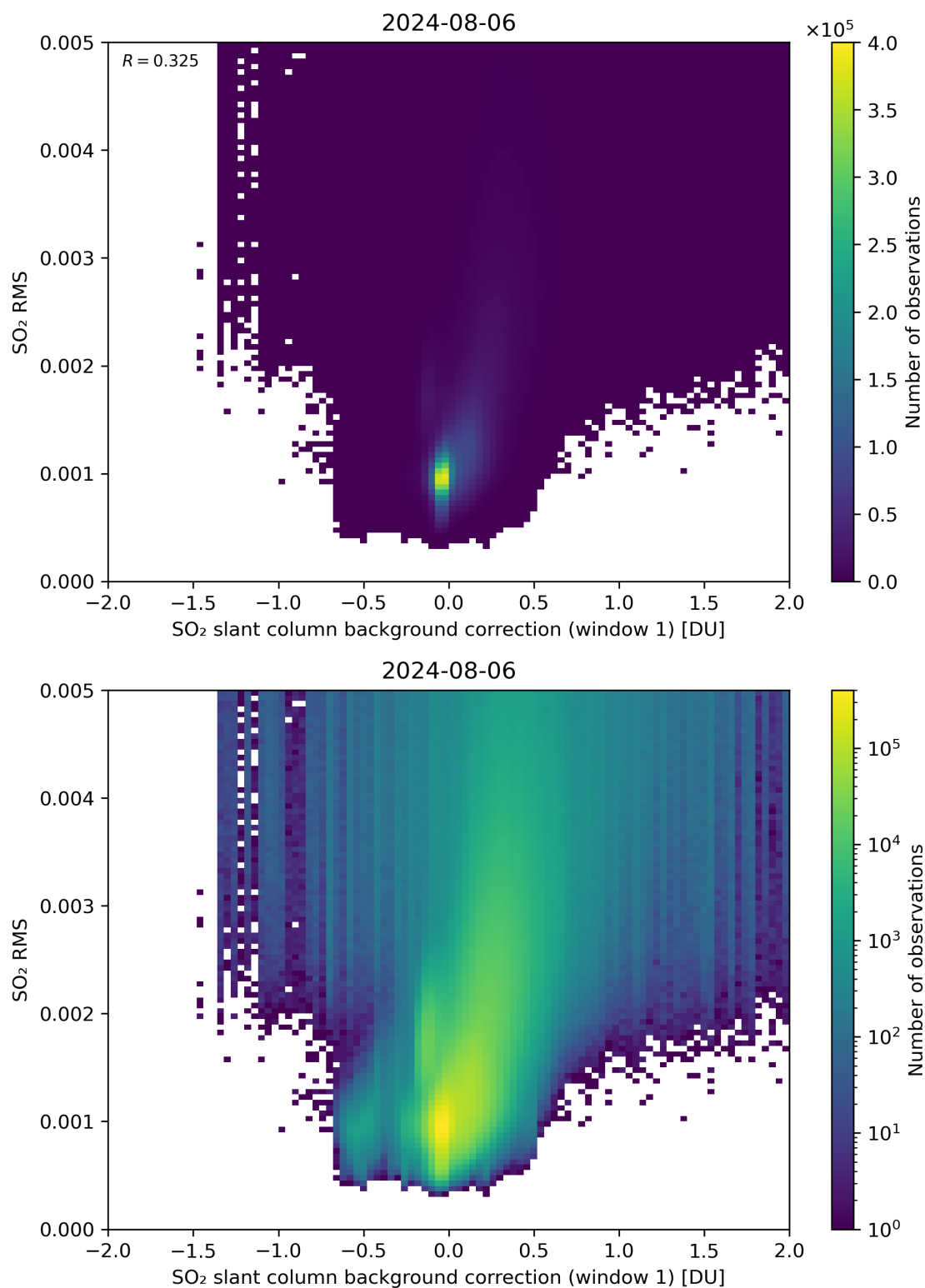
Figure 102: Scatter density plot of “SO 2 slant column background correction (window 1)” against “SO 2 RMS” for 2024-08-06 to 2024-08-07.
