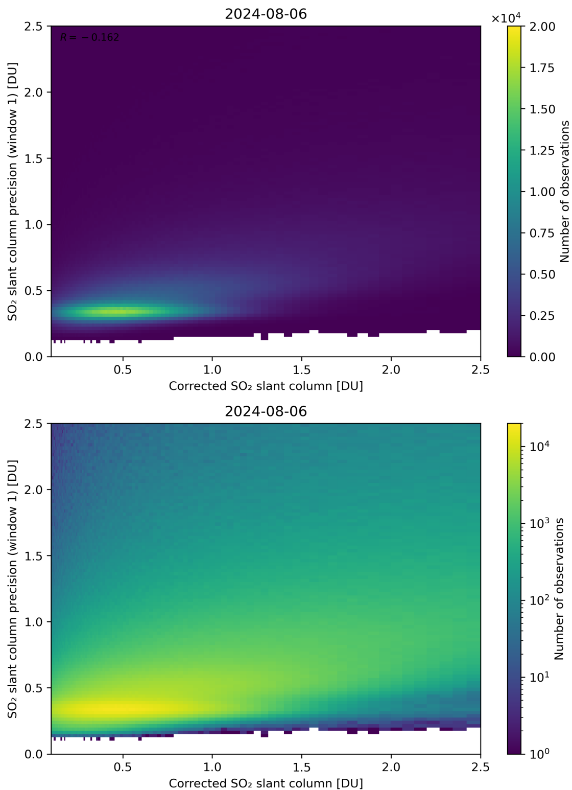
Figure 188: Scatter density plot of “Corrected SO 2 slant column” against “SO 2 slant column precision (window 1)” for 2024-08-06 to 2024-08-07.
