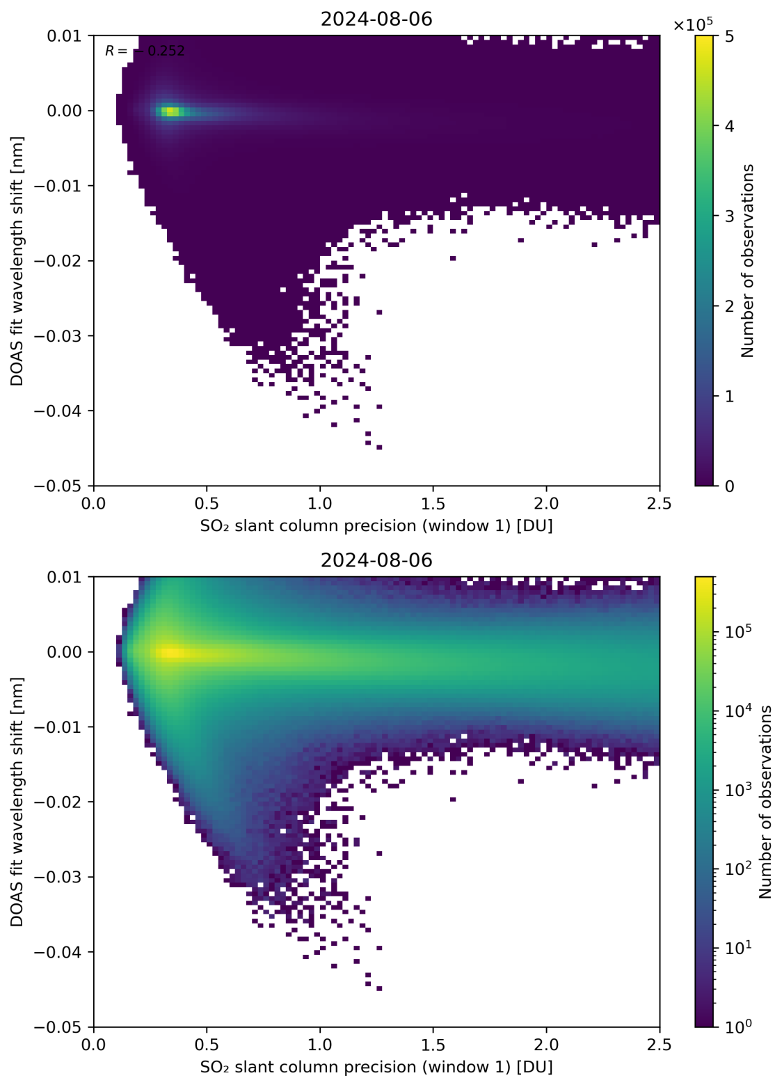
Figure 221: Scatter density plot of “SO 2 slant column precision (window 1)” against “DOAS fit wavelength shift” for 2024-08-06 to 2024-08-07.
