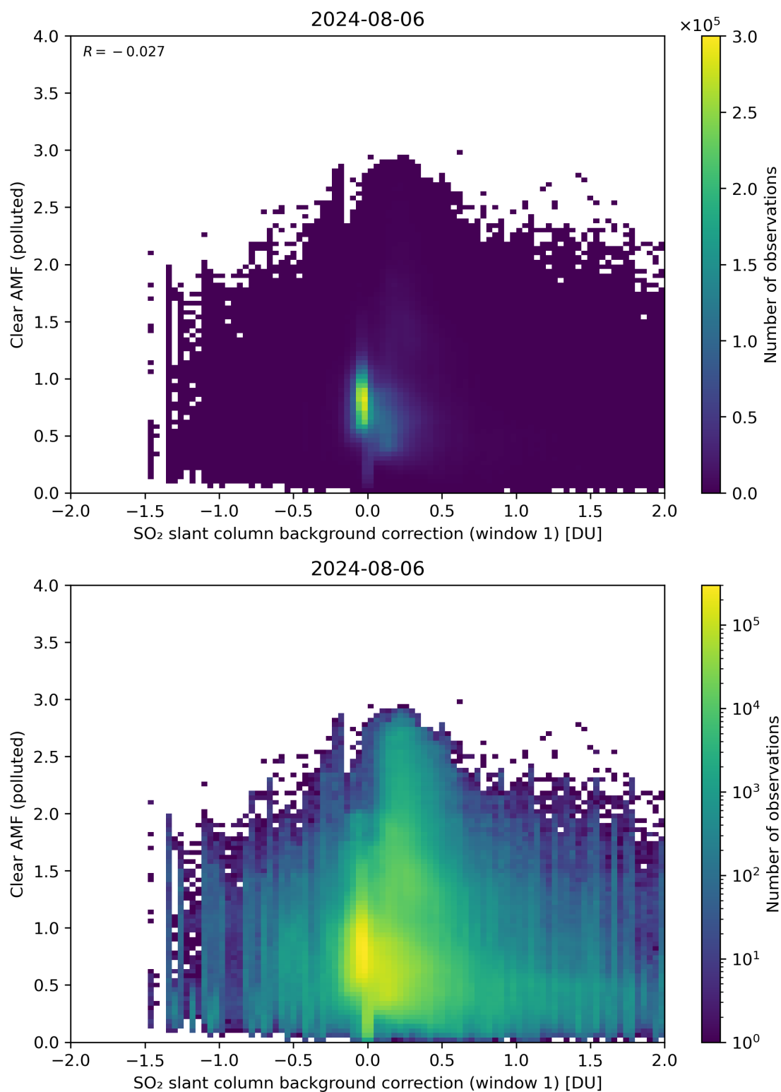
Figure 103: Scatter density plot of “SO 2 slant column background correction (window 1)” against “Clear AMF (polluted)” for 2024-08-06 to 2024-08-07.
