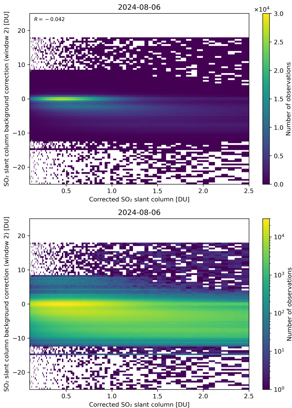
Figure 179: Scatter density plot of “Corrected SO 2 slant column” against “SO 2 slant column background correction (window 2)” for 2024-08-06 to 2024-08-07.
