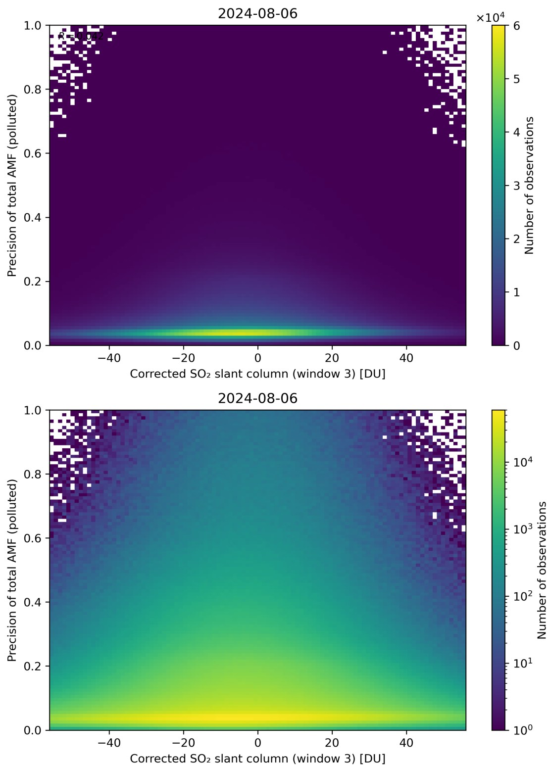
Figure 211: Scatter density plot of “Corrected SO 2 slant column (window 3)” against “Precision of total AMF (polluted)” for 2024-08-06 to 2024-08-07.
