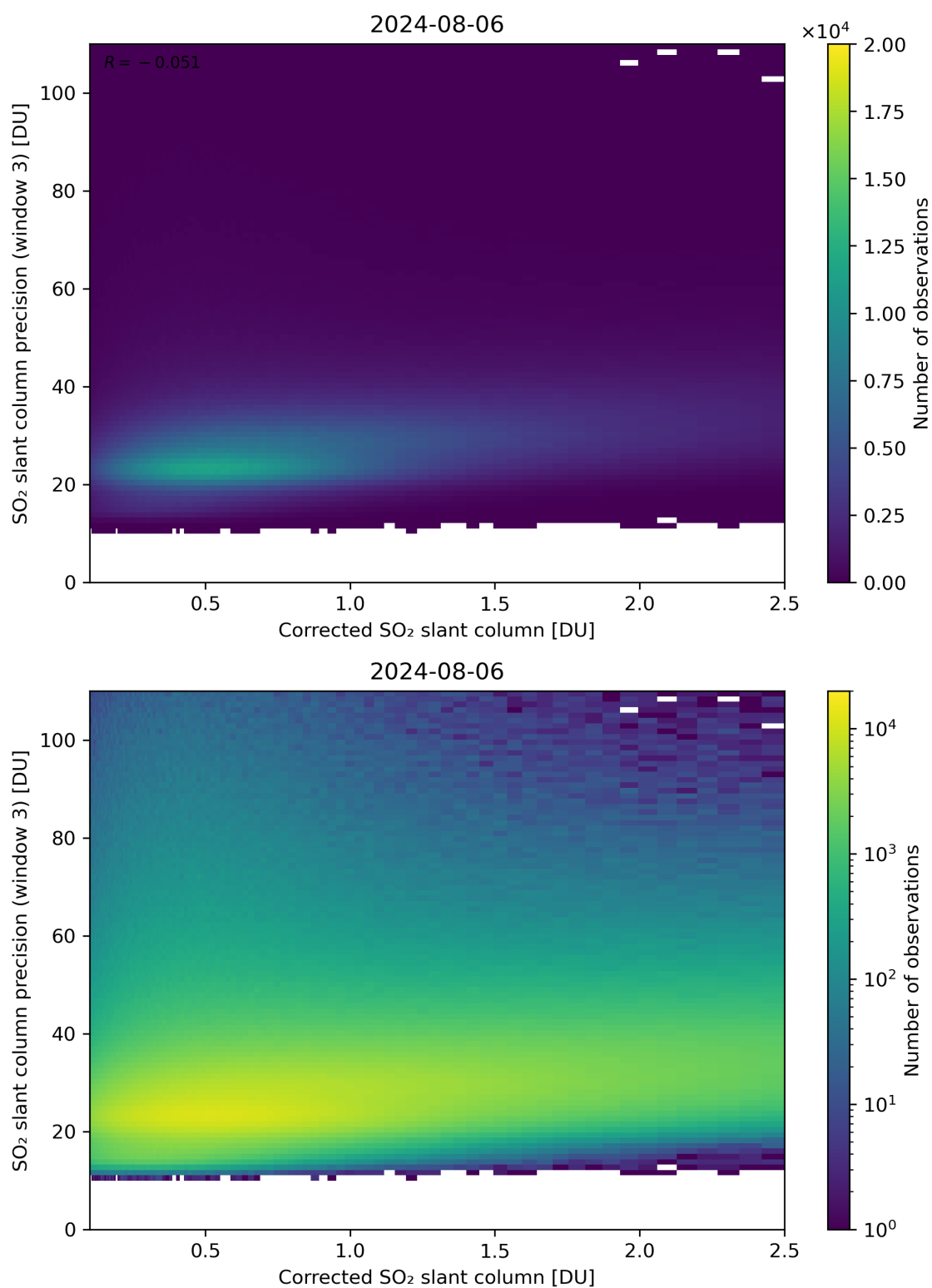
Figure 191: Scatter density plot of “Corrected SO 2 slant column” against “SO 2 slant column precision (window 3)” for 2024-08-06 to 2024-08-07.
