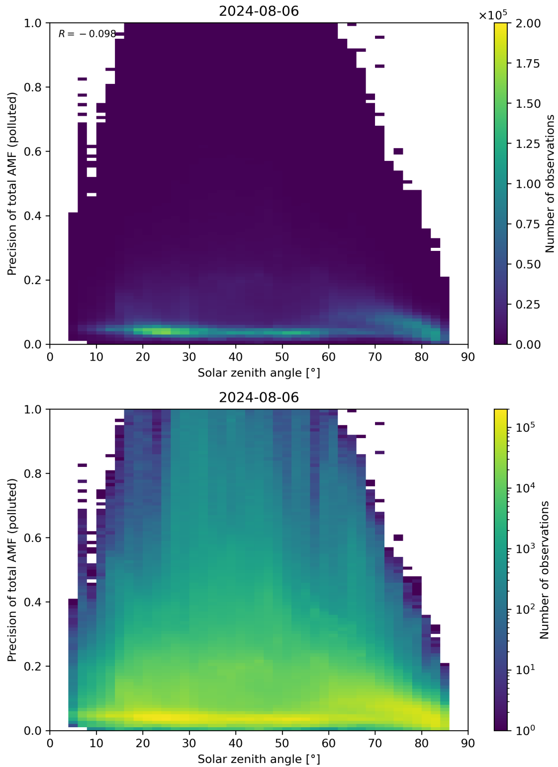
Figure 175: Scatter density plot of “Solar zenith angle” against “Precision of total AMF (polluted)” for 2024-08-06 to 2024-08-07.
