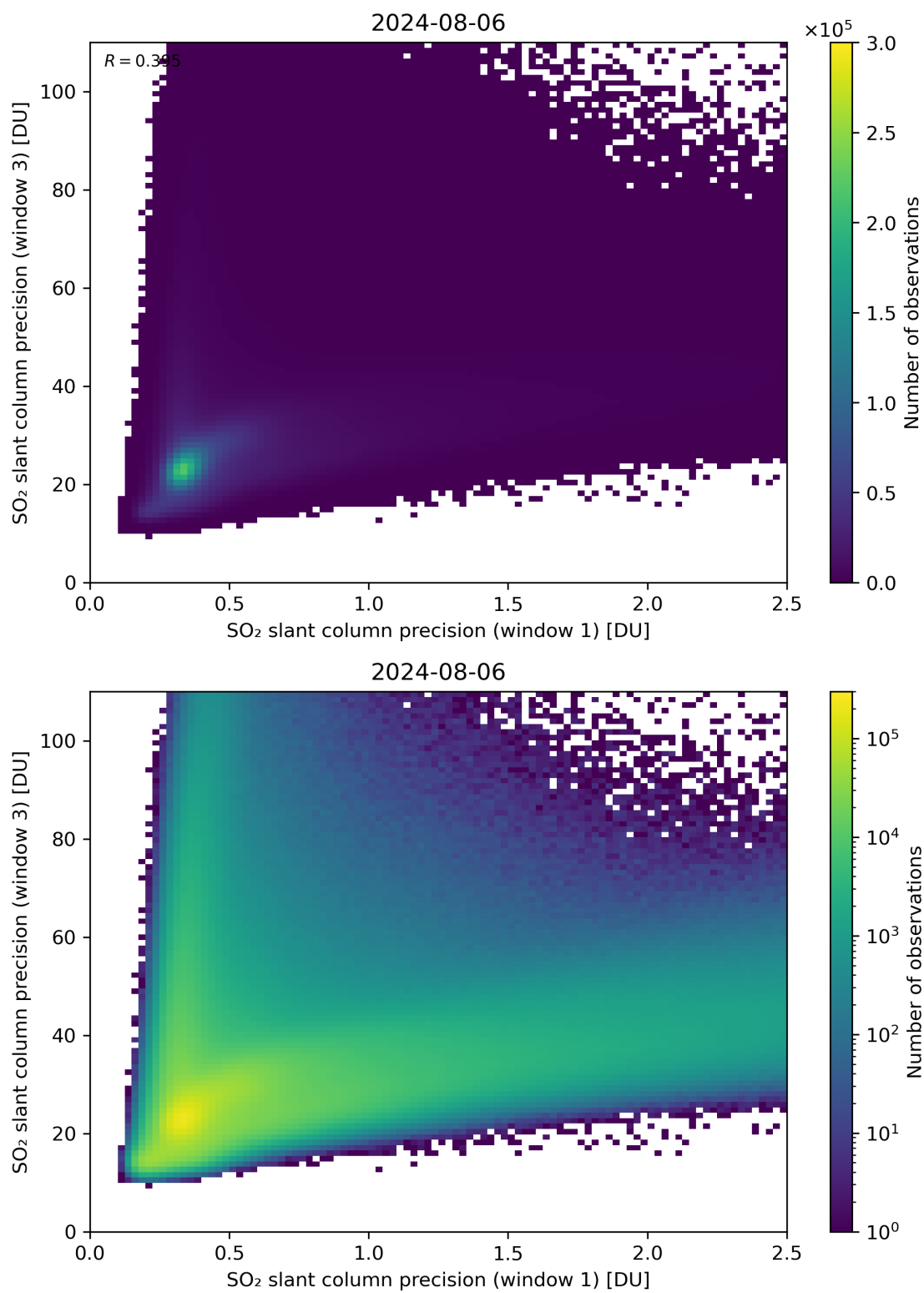
Figure 229: Scatter density plot of “SO 2 slant column precision (window 1)” against “SO 2 slant column precision (window 3)” for 2024-08-06 to 2024-08-07.
