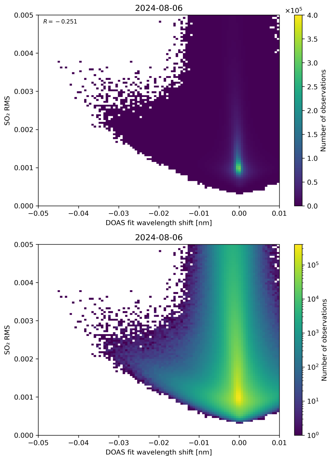
Figure 128: Scatter density plot of “DOAS fit wavelength shift” against “SO 2 RMS” for 2024-08-06 to 2024-08-07.
