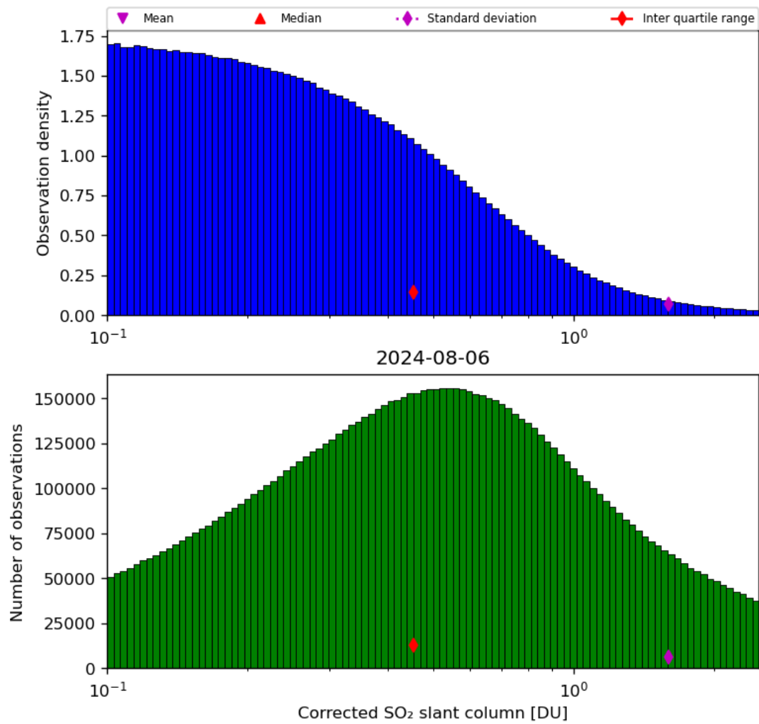
Figure 55: Histogram of “Corrected SO 2 slant column” for 2024-08-06 to 2024-08-07
