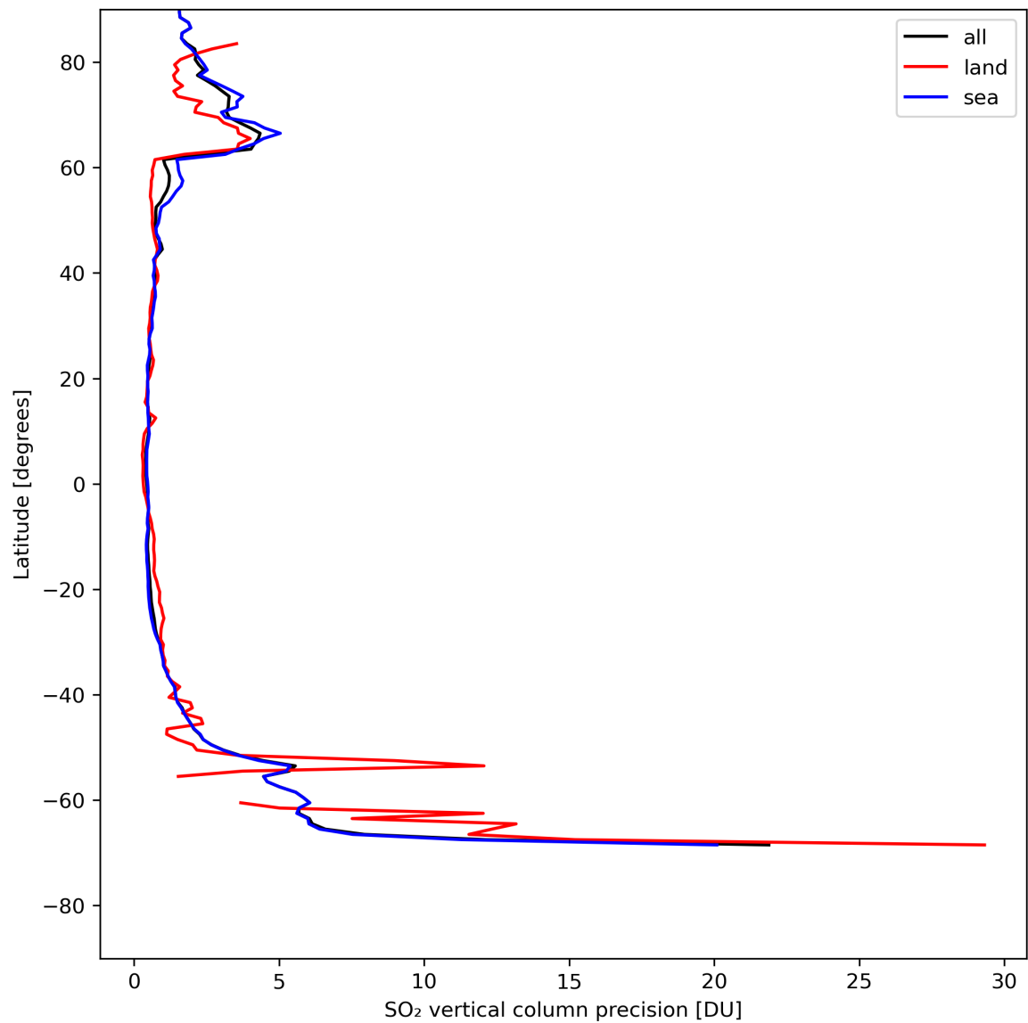
Figure 31: Zonal average of “SO 2 vertical column precision” for 2024-08-06 to 2024-08-07.
