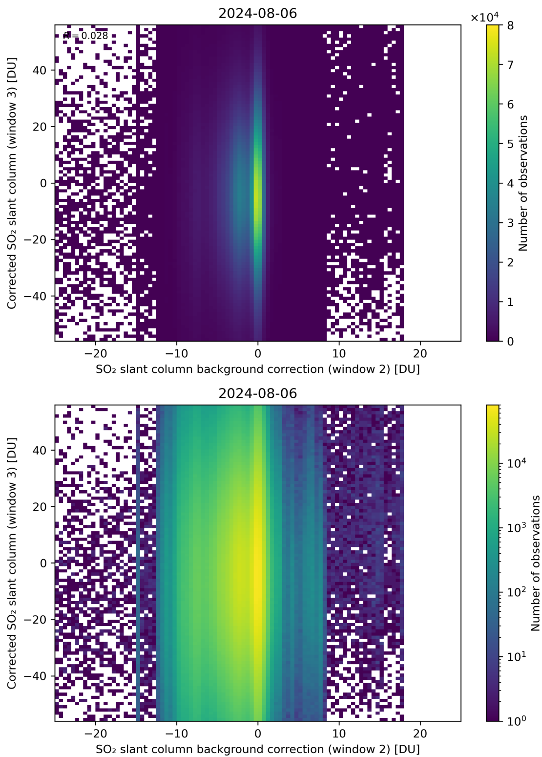
Figure 116: Scatter density plot of “SO 2 slant column background correction (window 2)” against “Corrected SO 2 slant column (window 3)” for 2024-08-06 to 2024-08-07.
