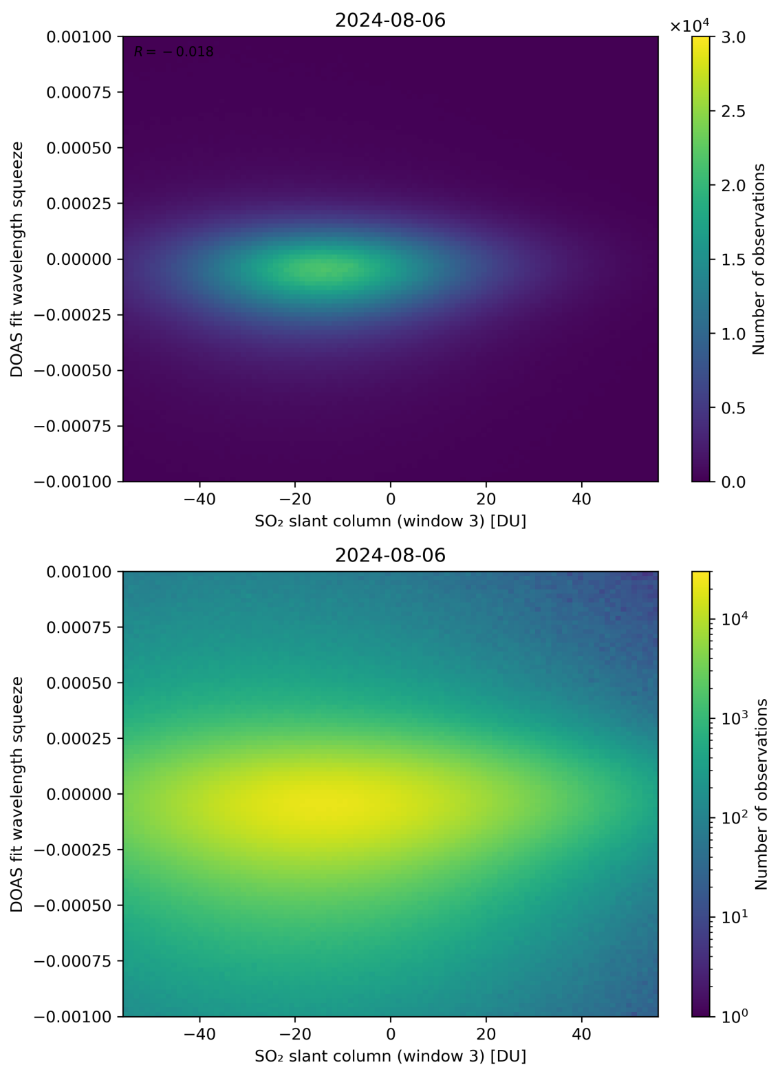
Figure 255: Scatter density plot of “SO 2 slant column (window 3)” against “DOAS fit wavelength squeeze” for 2024-08-06 to 2024-08-07.
