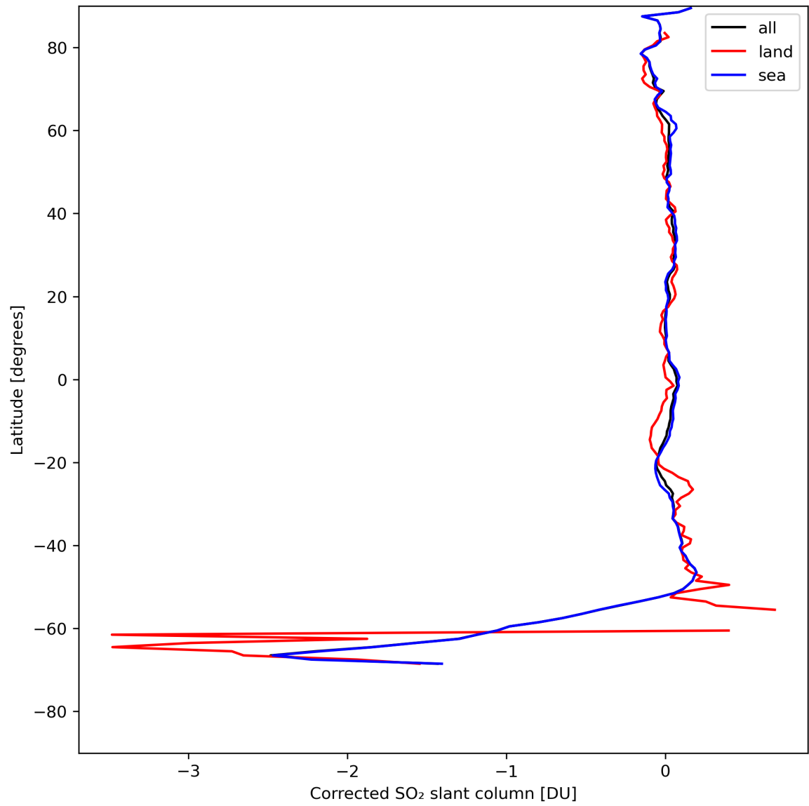
Figure 32: Zonal average of “Corrected SO 2 slant column” for 2024-08-06 to 2024-08-07.
