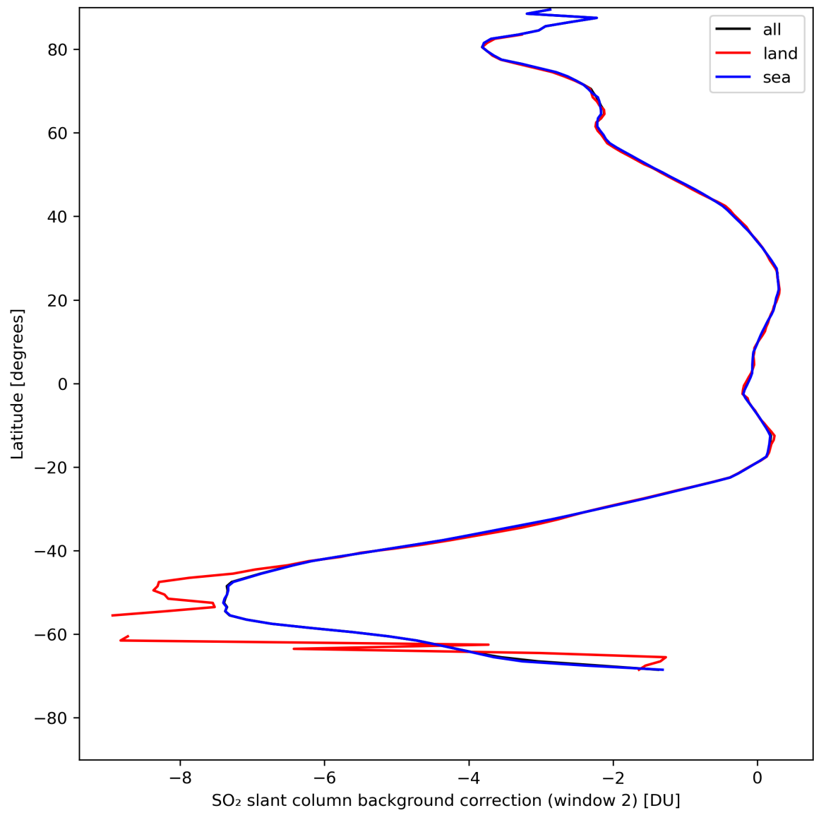
Figure 40: Zonal average of “SO 2 slant column background correction (window 2)” for 2024-08-06 to 2024-08-07.
