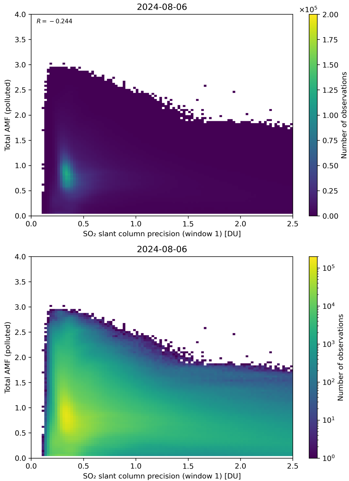
Figure 230: Scatter density plot of “SO 2 slant column precision (window 1)” against “Total AMF (polluted)” for 2024-08-06 to 2024-08-07.
