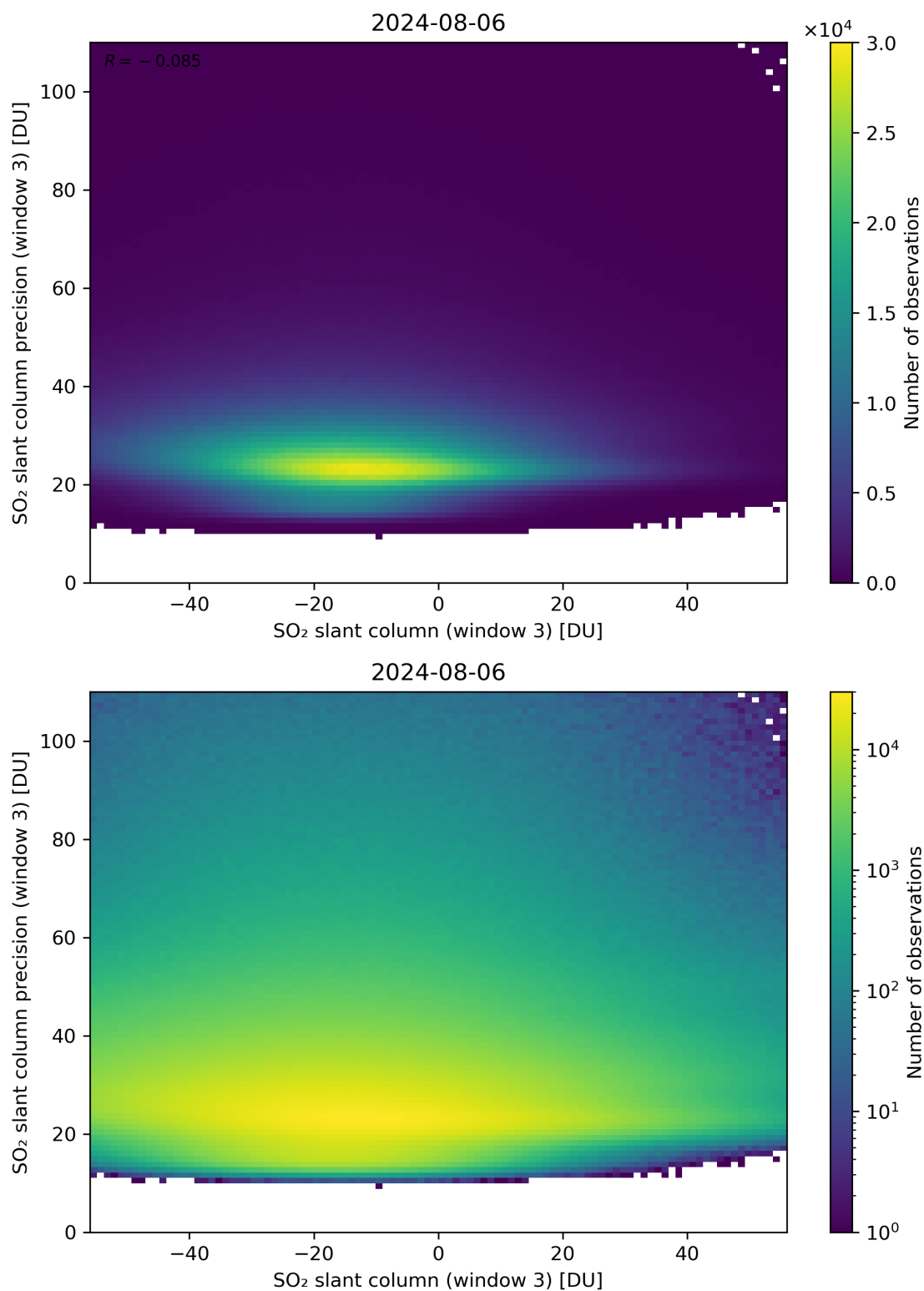
Figure 267: Scatter density plot of “SO 2 slant column (window 3)” against “SO 2 slant column precision (window 3)” for 2024-08-06 to 2024-08-07.
