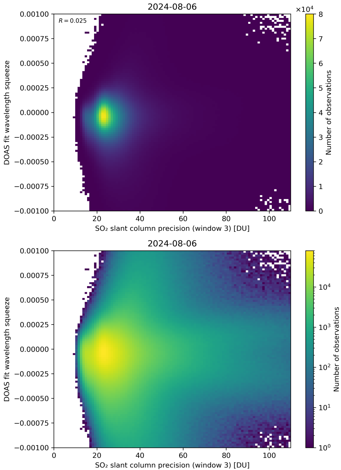
Figure 259: Scatter density plot of “SO 2 slant column precision (window 3)” against “DOAS fit wavelength squeeze” for 2024-08-06 to 2024-08-07.
