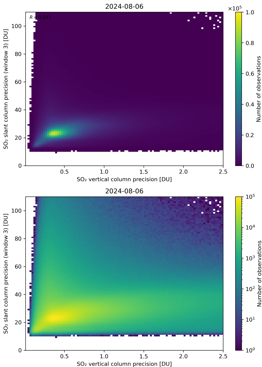
Figure 293: Scatter density plot of “SO 2 vertical column precision” against “SO 2 slant column precision (window 3)” for 2024-08-06 to 2024-08-07.
