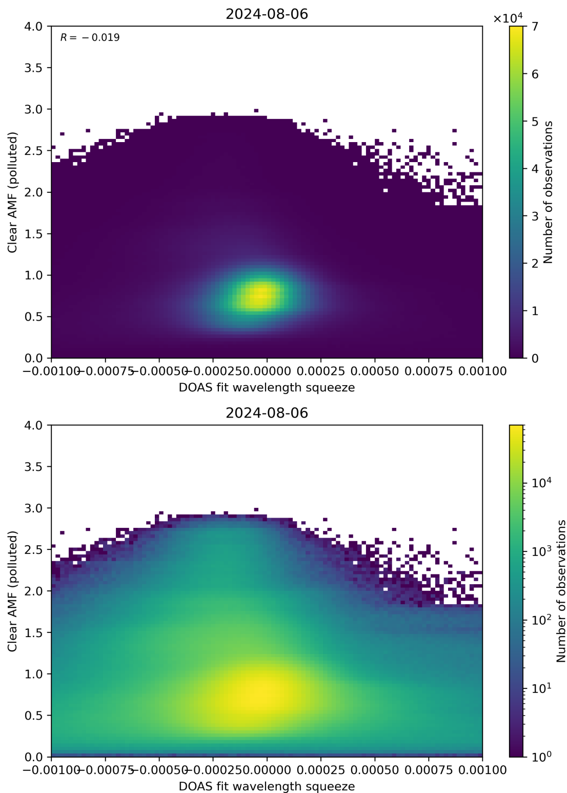
Figure 133: Scatter density plot of “DOAS fit wavelength squeeze” against “Clear AMF (polluted)” for 2024-08-06 to 2024-08-07.
