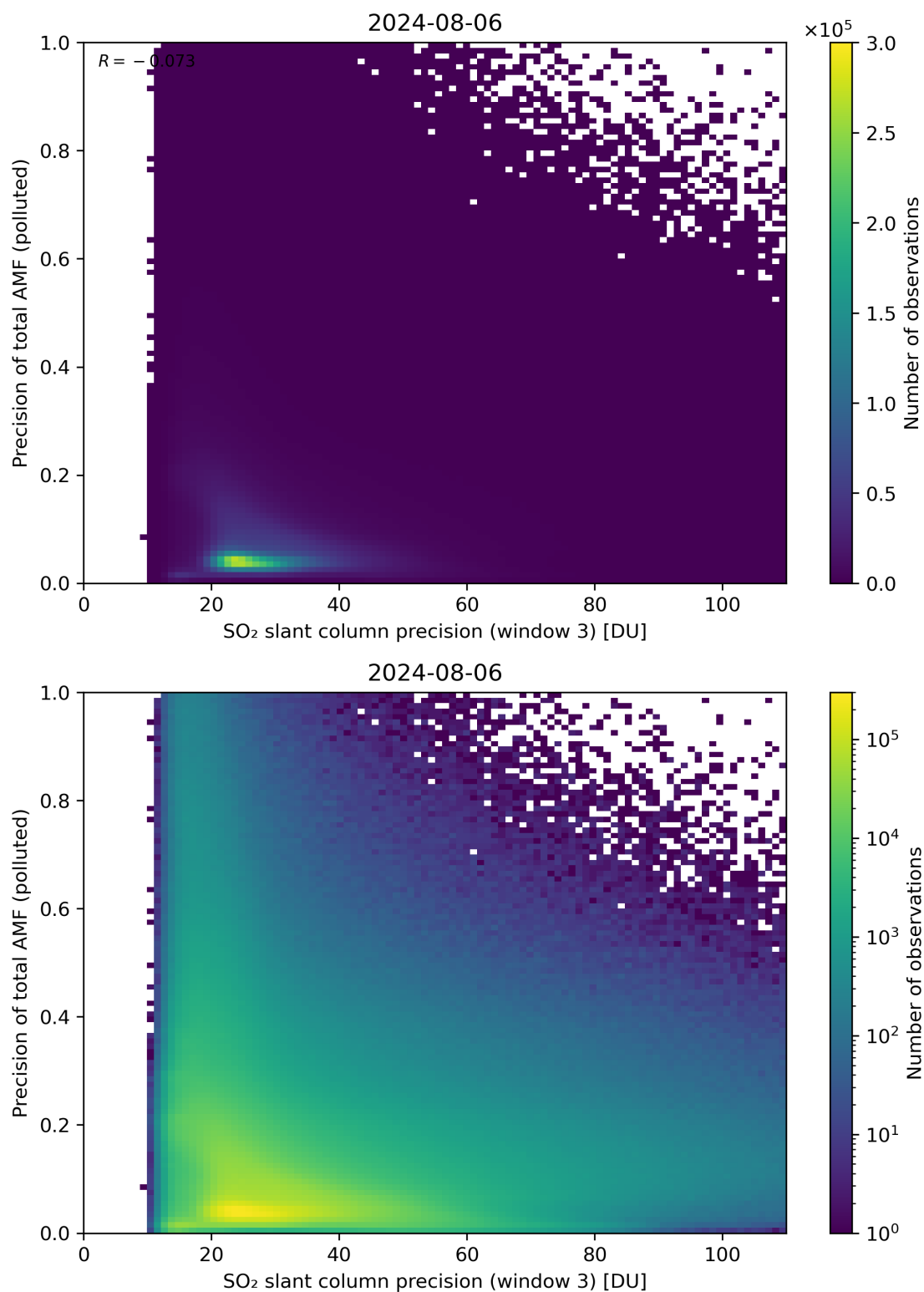
Figure 264: Scatter density plot of “SO 2 slant column precision (window 3)” against “Precision of total AMF (polluted)” for 2024-08-06 to 2024-08-07.
