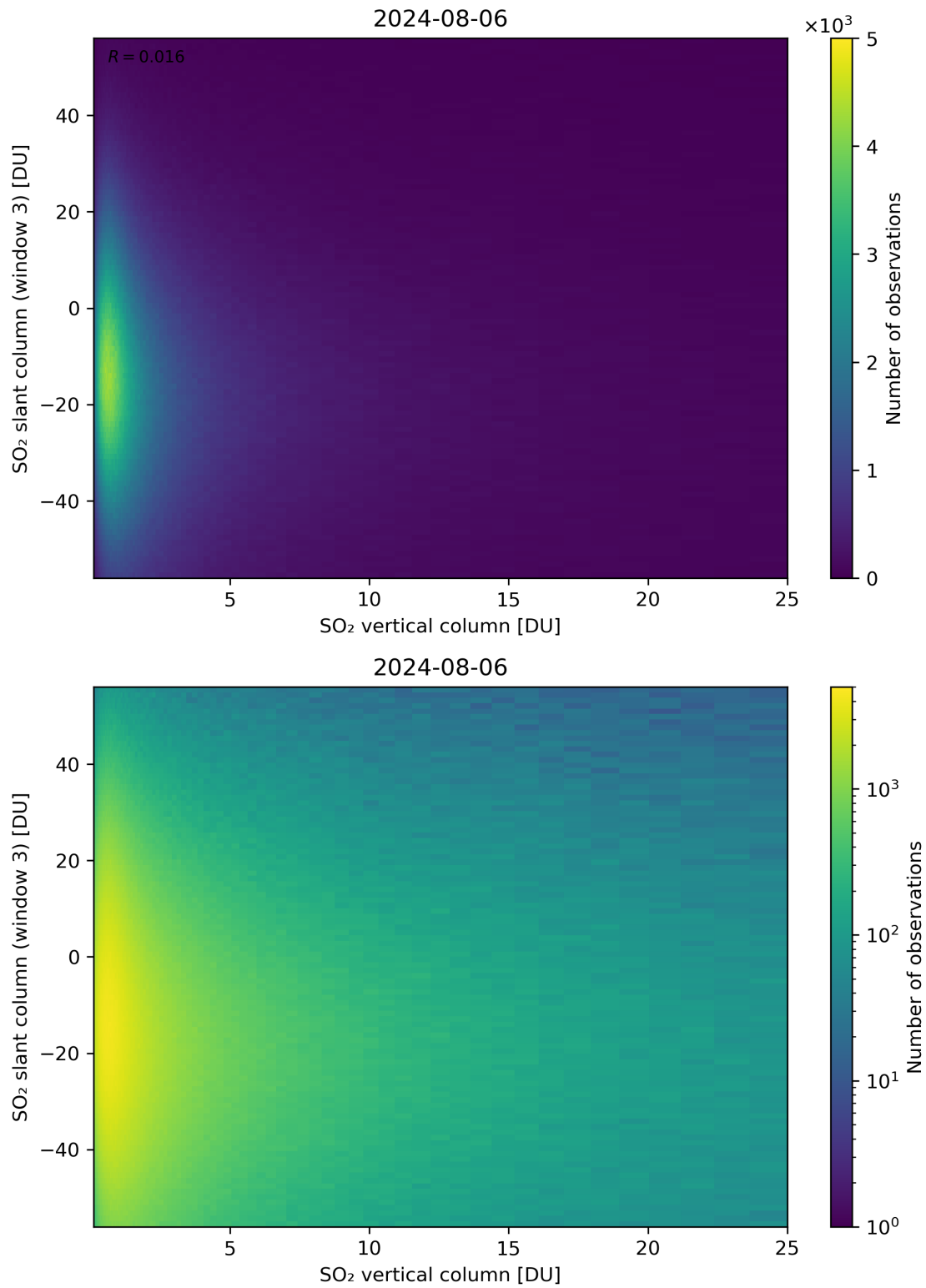
Figure 303: Scatter density plot of “SO 2 vertical column” against “SO 2 slant column (window 3)” for 2024-08-06 to 2024-08-07.
