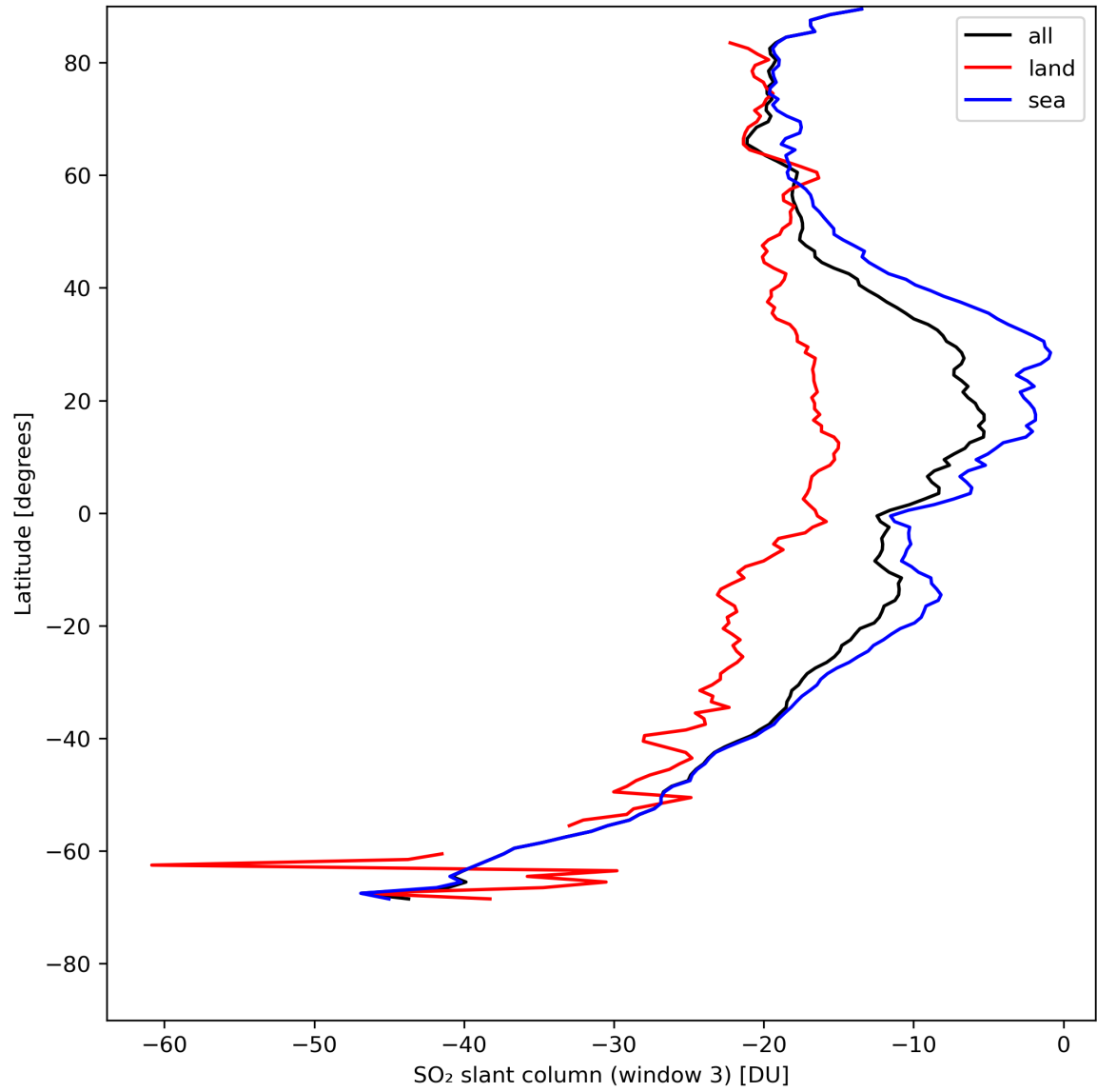
Figure 41: Zonal average of “SO 2 slant column (window 3)” for 2024-08-06 to 2024-08-07.
