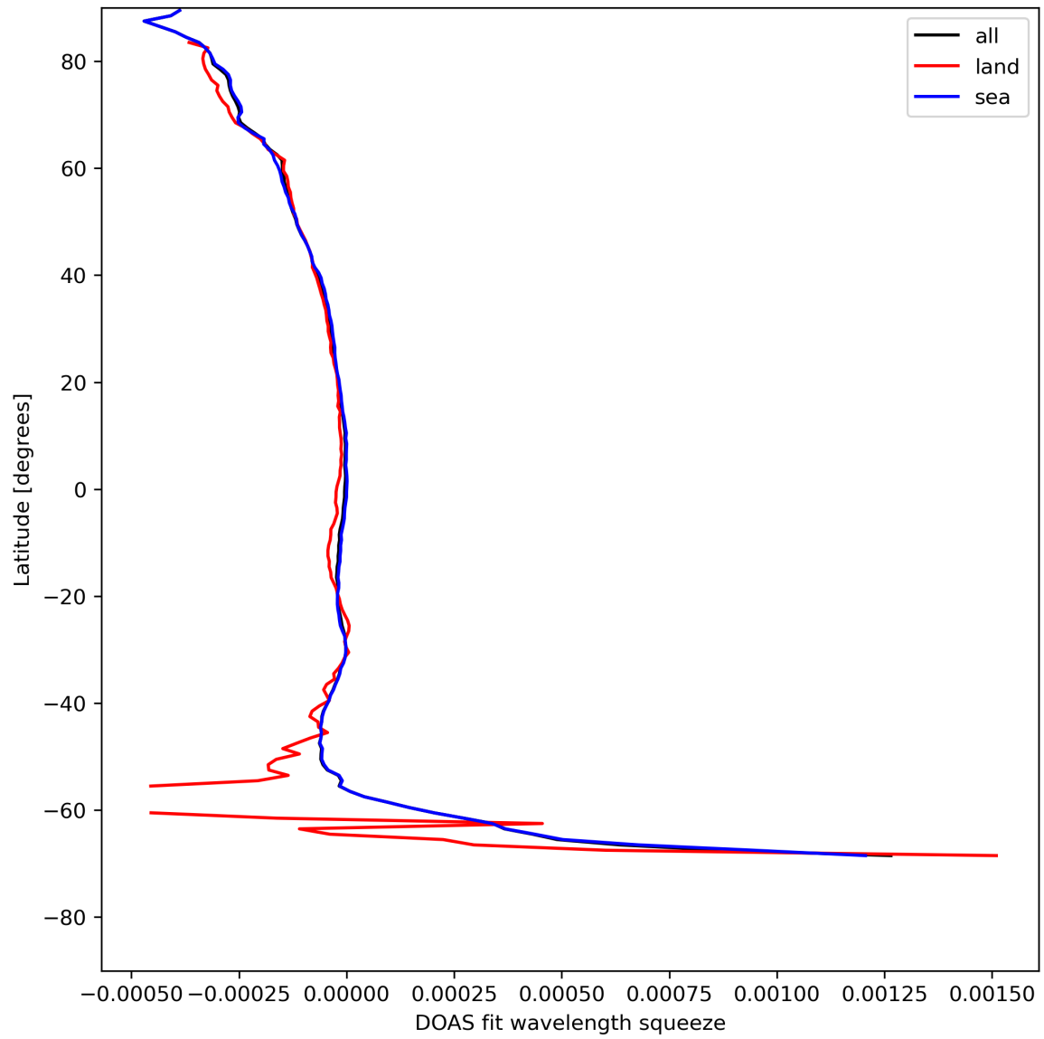
Figure 46: Zonal average of “DOAS fit wavelength squeeze” for 2024-08-06 to 2024-08-07.
