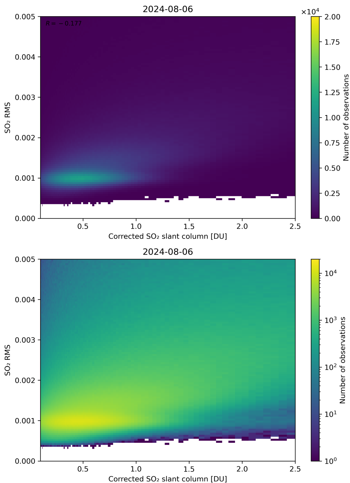
Figure 183: Scatter density plot of “Corrected SO 2 slant column” against “SO 2 RMS” for 2024-08-06 to 2024-08-07.
