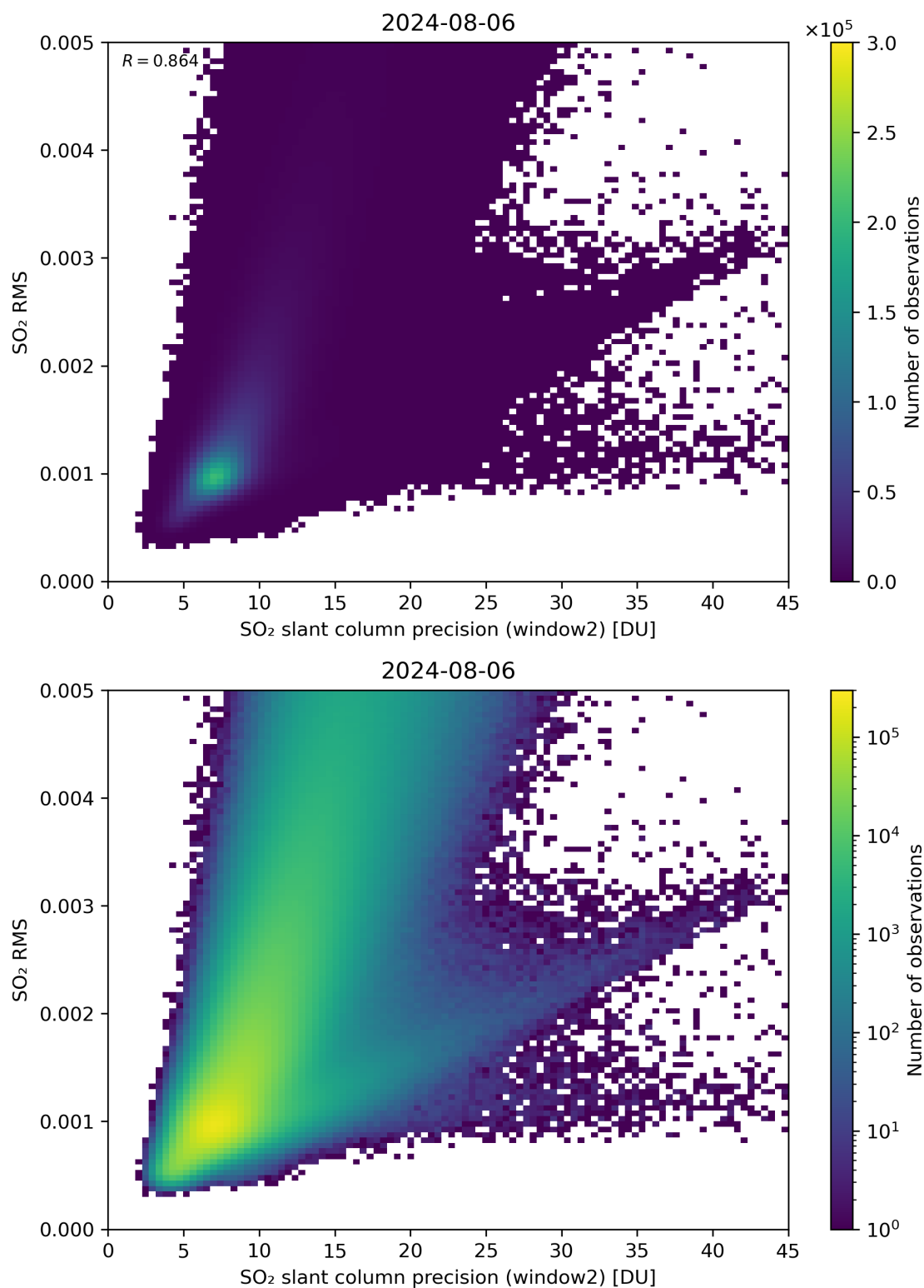
Figure 245: Scatter density plot of “SO 2 slant column precision (window2)” against “SO 2 RMS” for 2024-08-06 to 2024-08-07.
