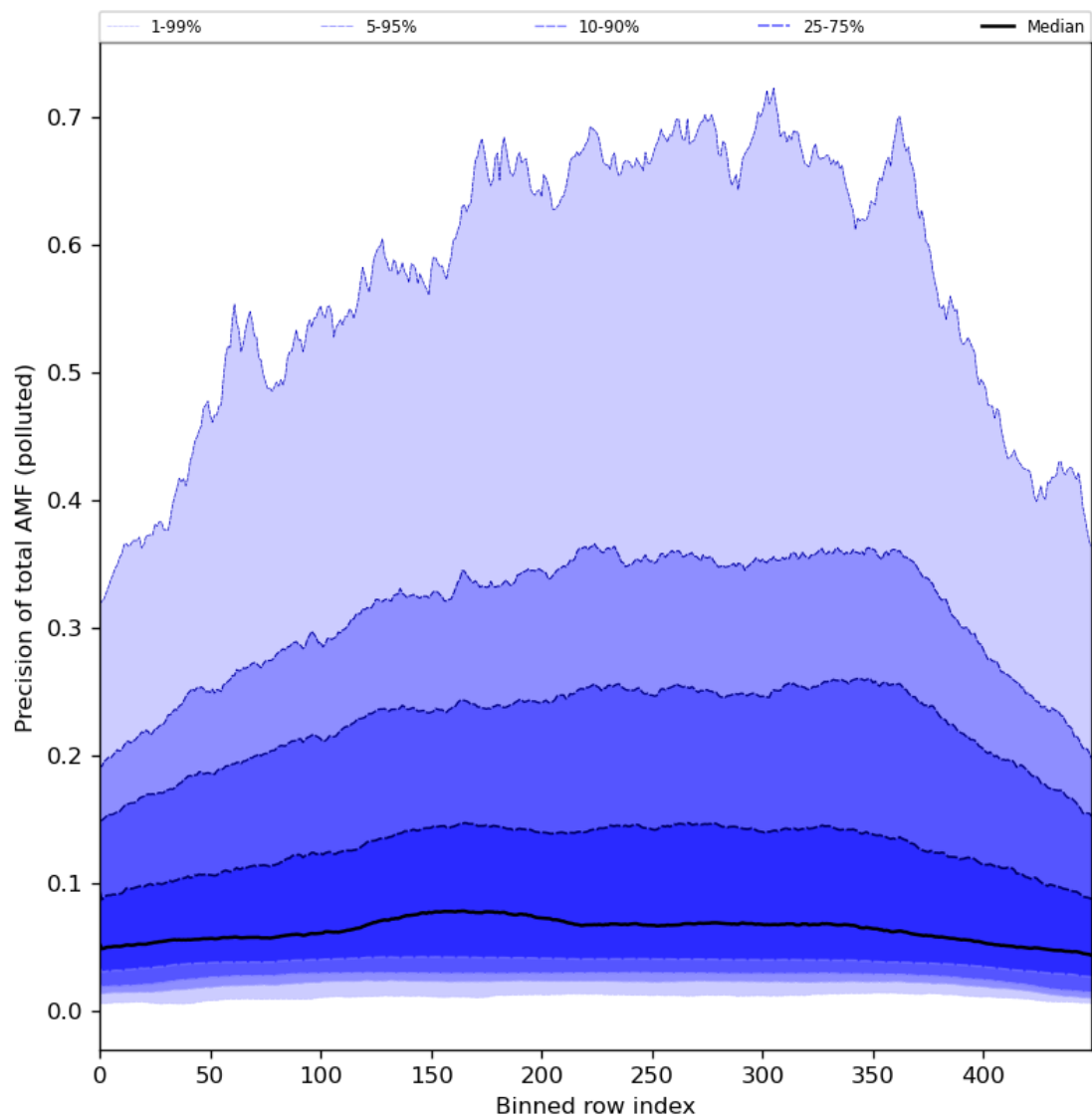
Figure 95: Along track statistics of “Precision of total AMF (polluted)” for 2024-08-06 to 2024-08-07
