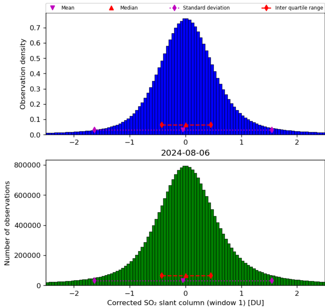
Figure 58: Histogram of “Corrected SO 2 slant column (window 1)” for 2024-08-06 to 2024-08-07
