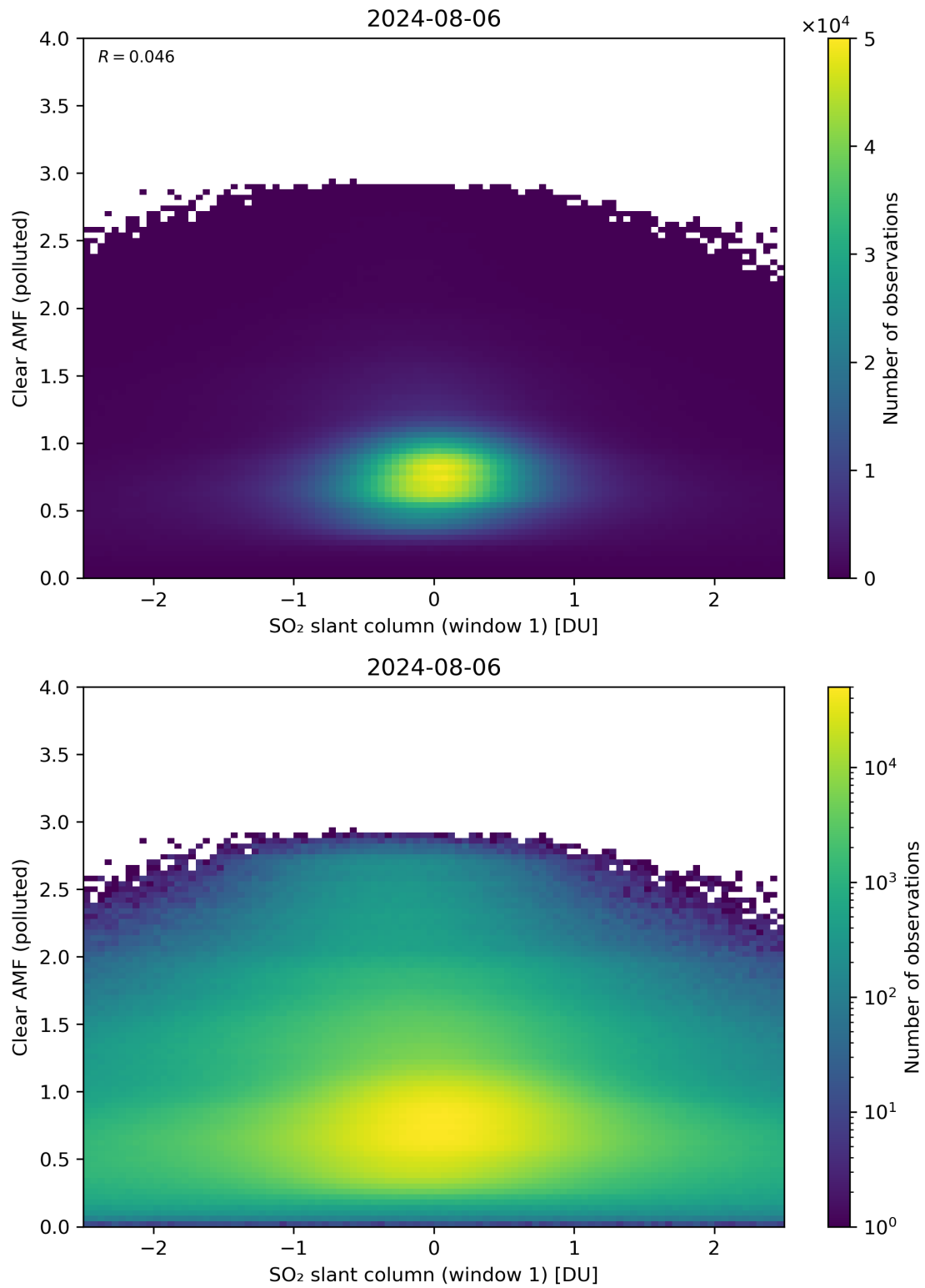
Figure 232: Scatter density plot of “SO 2 slant column (window 1)” against “Clear AMF (polluted)” for 2024-08-06 to 2024-08-07.
