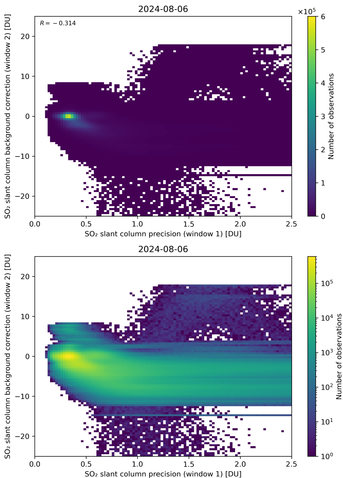
Figure 219: Scatter density plot of “SO 2 slant column precision (window 1)” against “SO 2 slant column background correction (window 2)” for 2024-08-06 to 2024-08-07.
