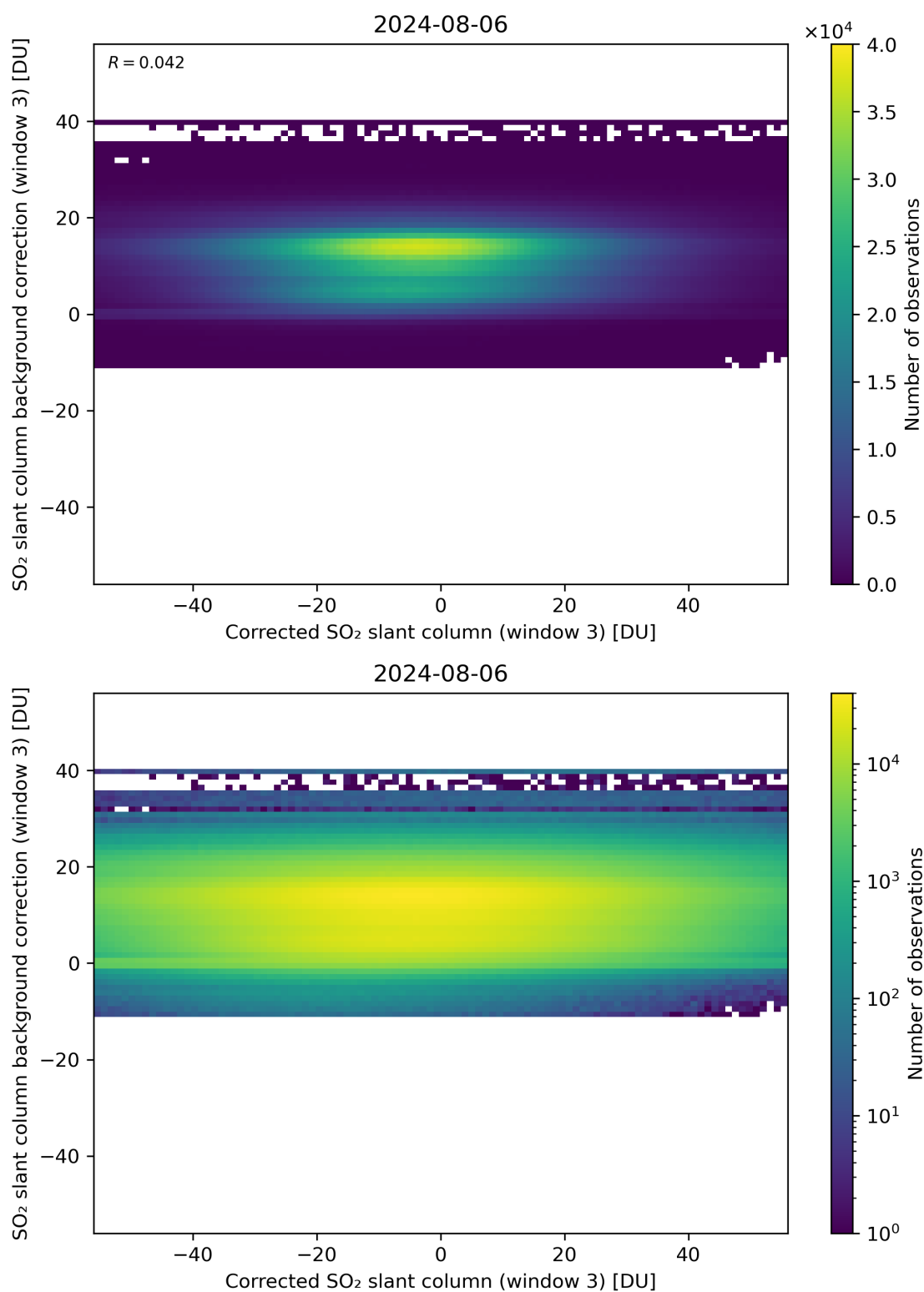
Figure 205: Scatter density plot of “Corrected SO 2 slant column (window 3)” against “SO 2 slant column background correction (window 3)” for 2024-08-06 to 2024-08-07.
