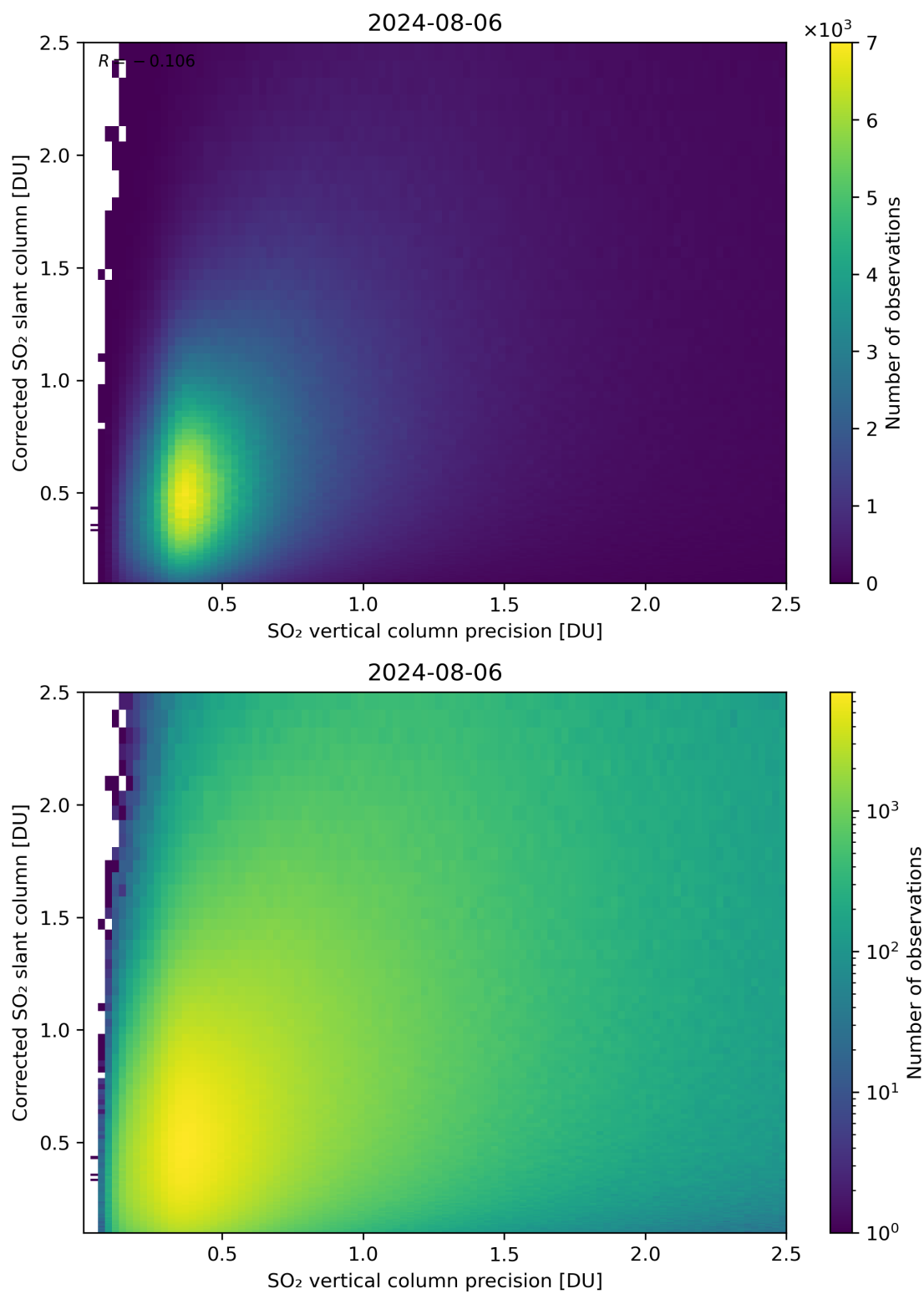
Figure 286: Scatter density plot of “SO 2 vertical column precision” against “Corrected SO 2 slant column” for 2024-08-06 to 2024-08-07.
