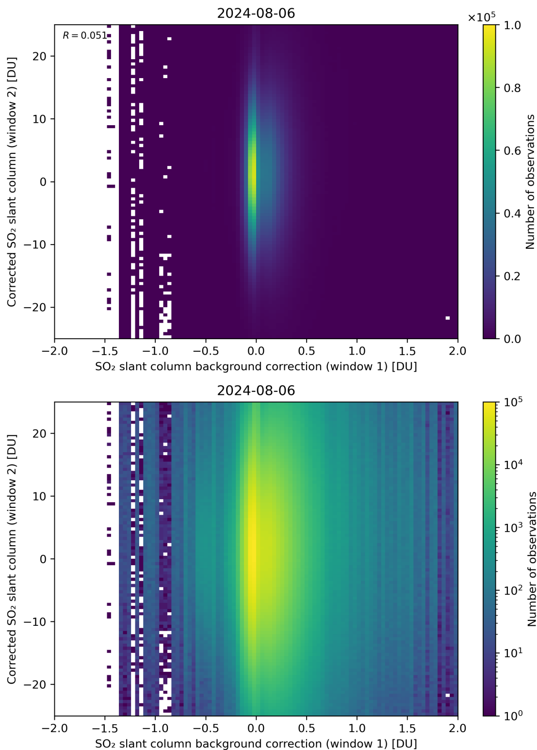
Figure 104: Scatter density plot of “SO 2 slant column background correction (window 1)” against “Corrected SO 2 slant column (window 2)” for 2024-08-06 to 2024-08-07.
