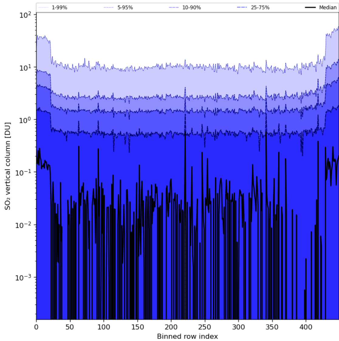
Figure 76: Along track statistics of “SO 2 vertical column” for 2024-08-06 to 2024-08-07
