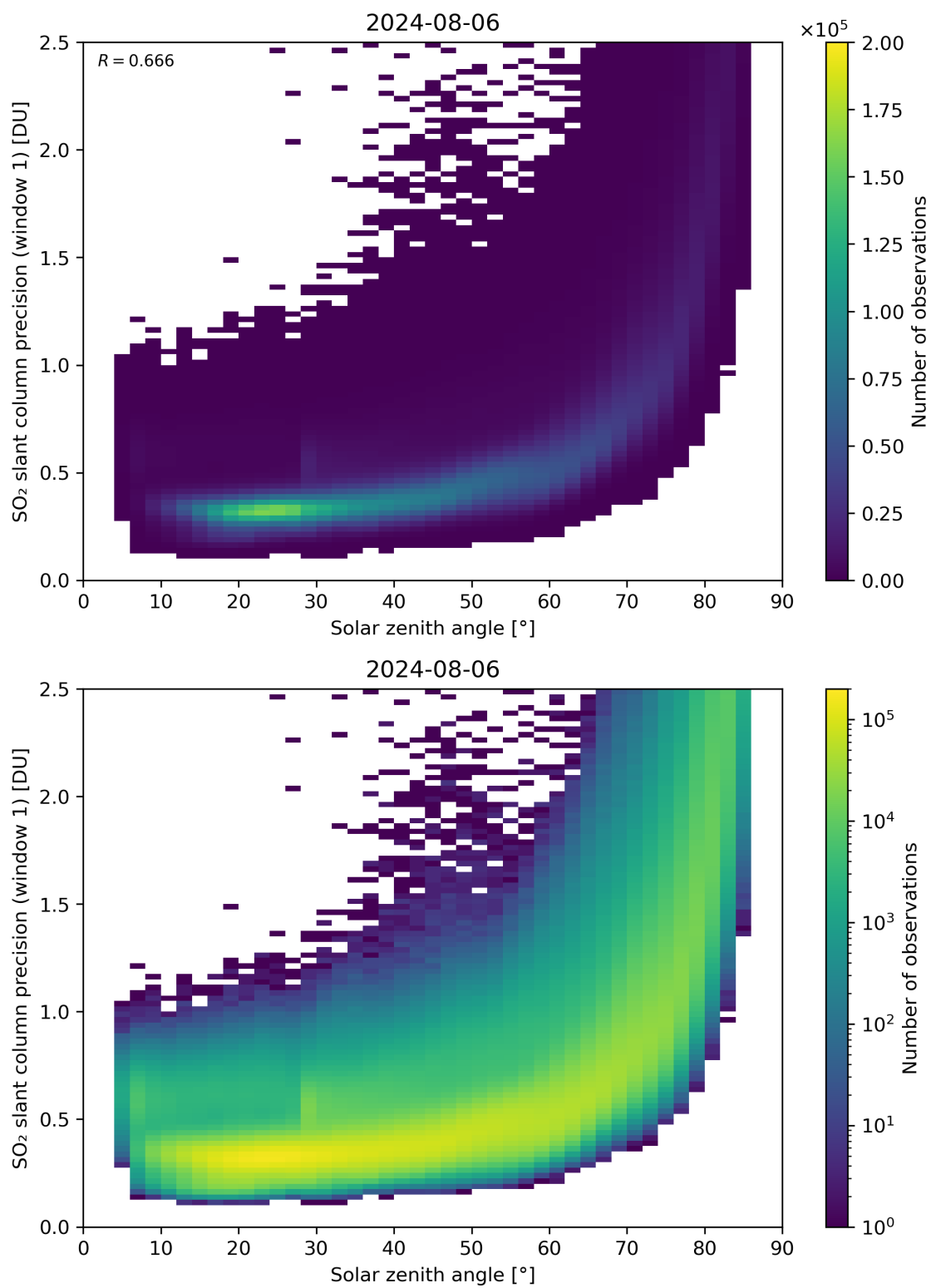
Figure 170: Scatter density plot of “Solar zenith angle” against “SO 2 slant column precision (window 1)” for 2024-08-06 to 2024-08-07.
