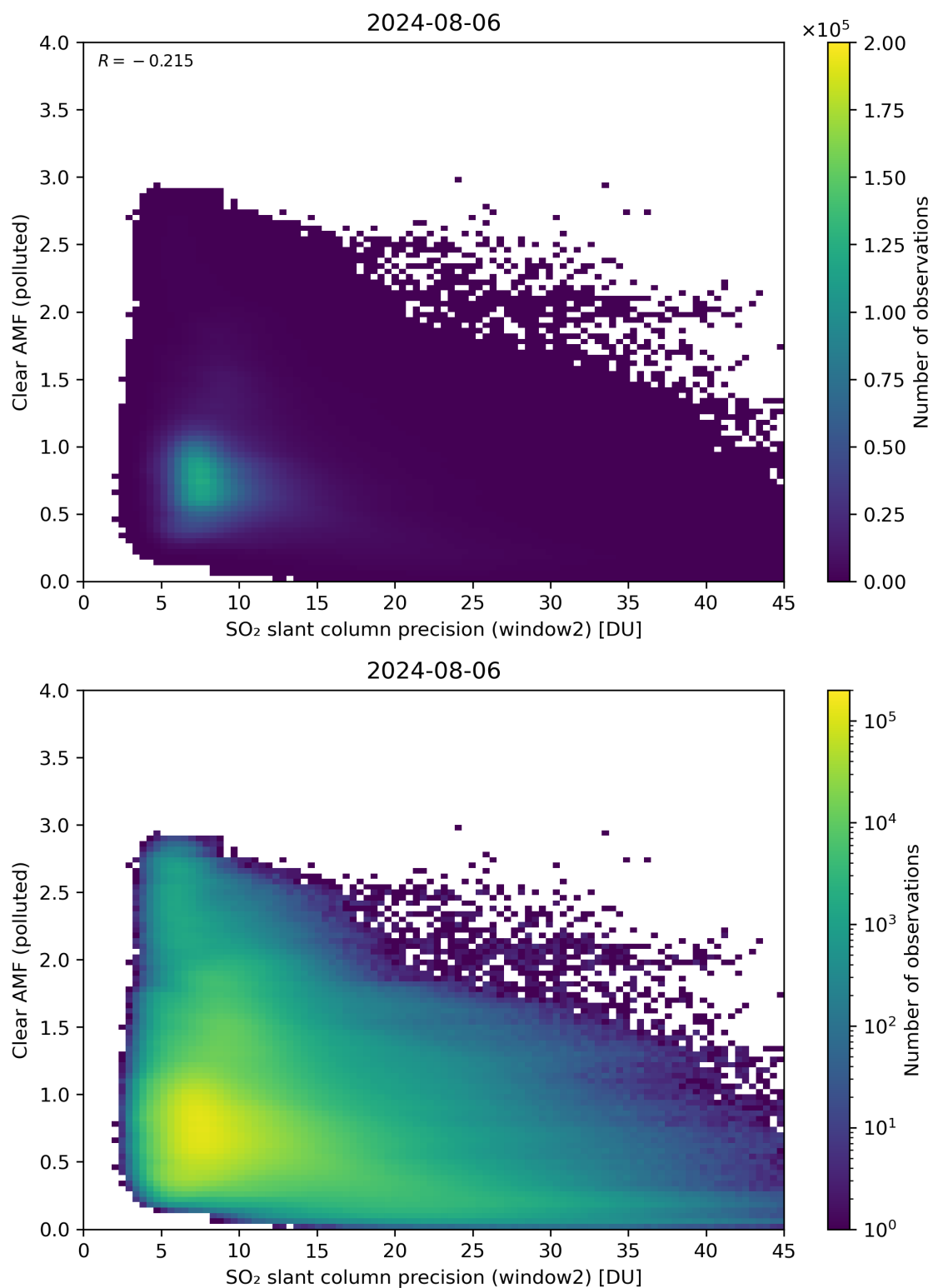
Figure 246: Scatter density plot of “SO 2 slant column precision (window2)” against “Clear AMF (polluted)” for 2024-08-06 to 2024-08-07.
