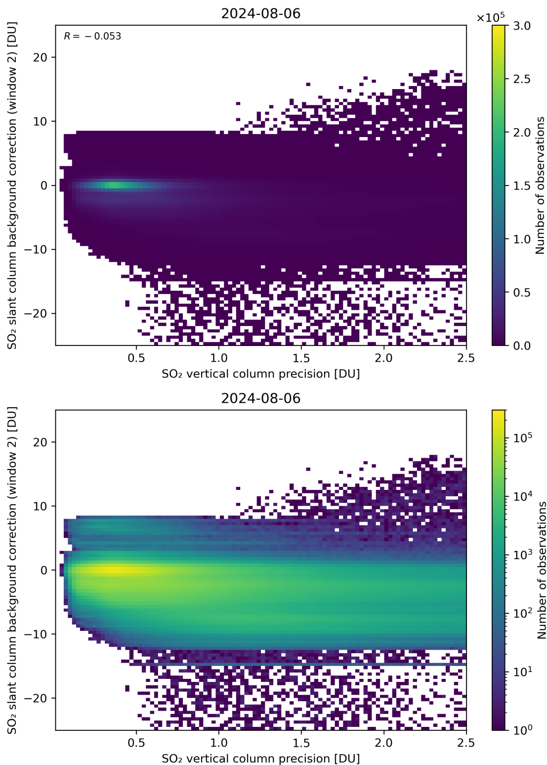
Figure 280: Scatter density plot of “SO 2 vertical column precision” against “SO 2 slant column background correction (window 2)” for 2024-08-06 to 2024-08-07.
