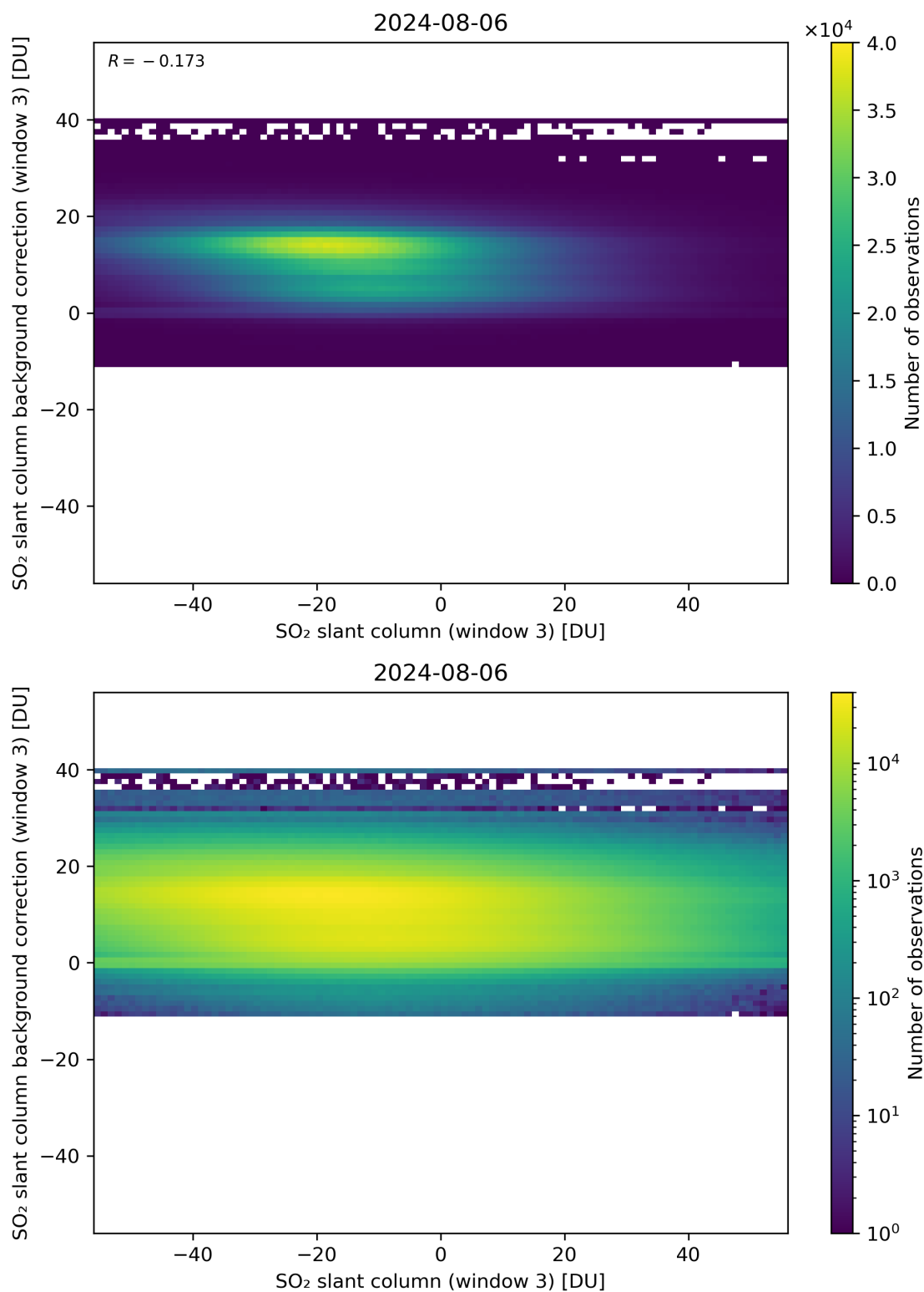
Figure 253: Scatter density plot of “SO 2 slant column (window 3)” against “SO 2 slant column background correction (window 3)” for 2024-08-06 to 2024-08-07.
