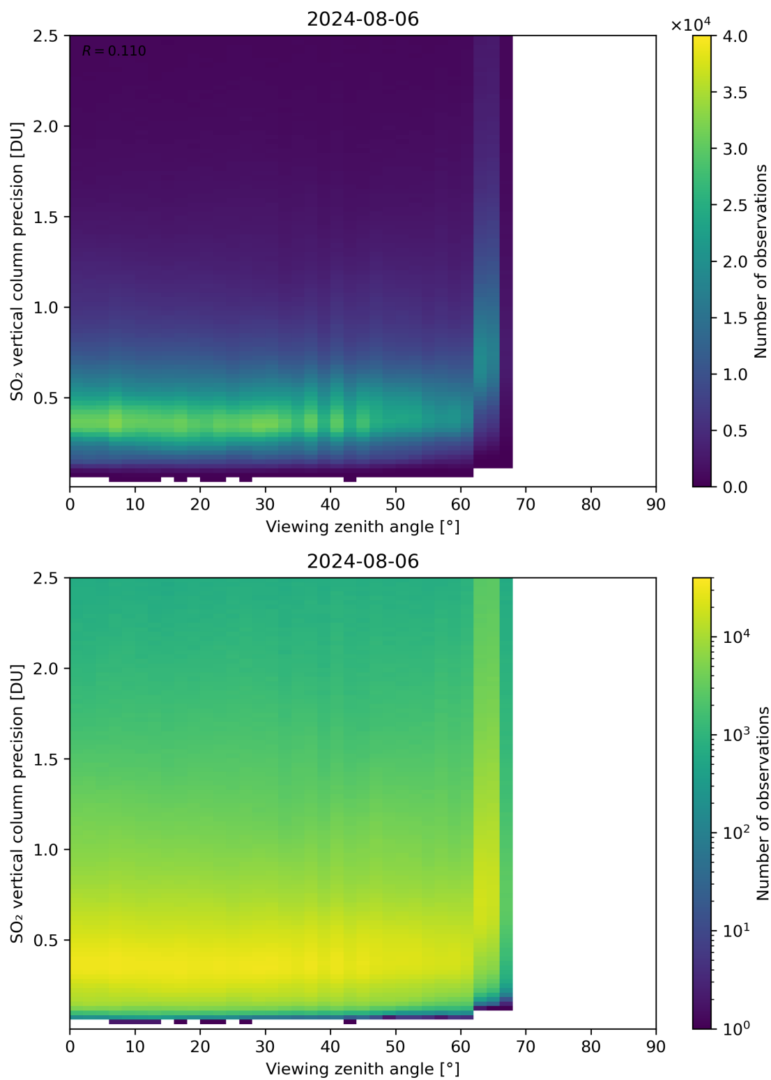
Figure 328: Scatter density plot of “Viewing zenith angle” against “SO 2 vertical column precision” for 2024-08-06 to 2024-08-07.
