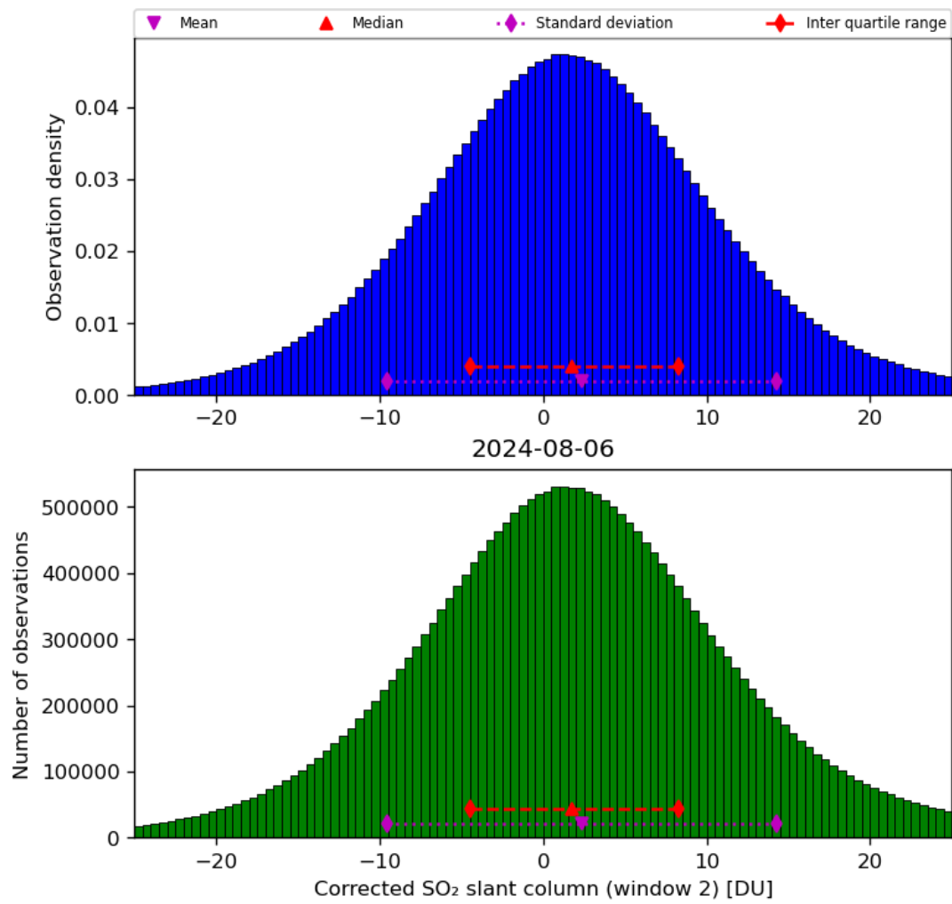
Figure 62: Histogram of “Corrected SO 2 slant column (window 2)” for 2024-08-06 to 2024-08-07
