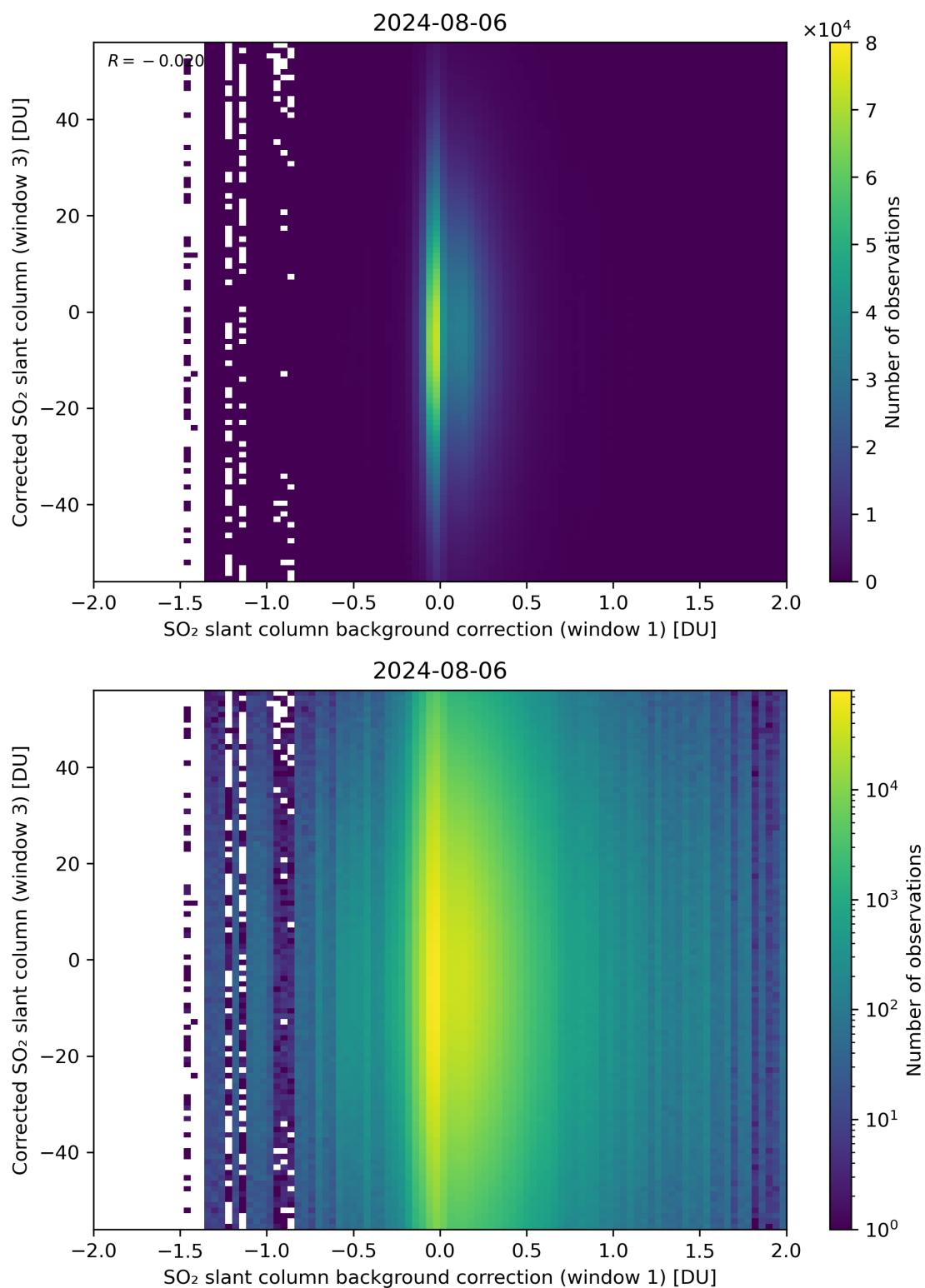
Figure 105: Scatter density plot of “SO 2 slant column background correction (window 1)” against “Corrected SO 2 slant column (window 3)” for 2024-08-06 to 2024-08-07.
