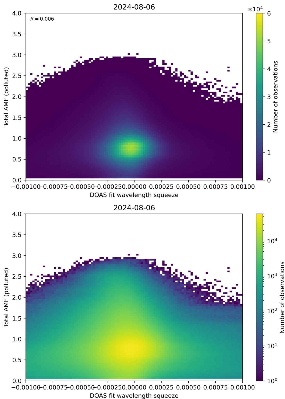
Figure 134: Scatter density plot of “DOAS fit wavelength squeeze” against “Total AMF (polluted)” for 2024-08-06 to 2024-08-07.
