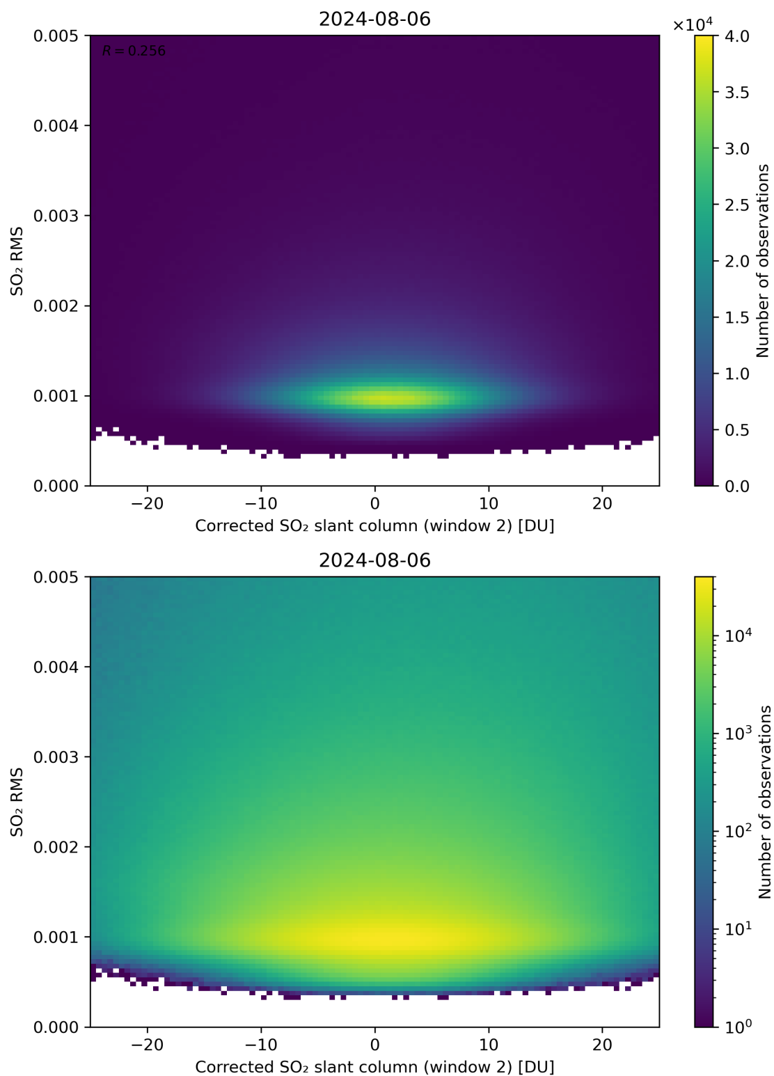
Figure 198: Scatter density plot of “Corrected SO 2 slant column (window 2)” against “SO 2 RMS” for 2024-08-06 to 2024-08-07.
