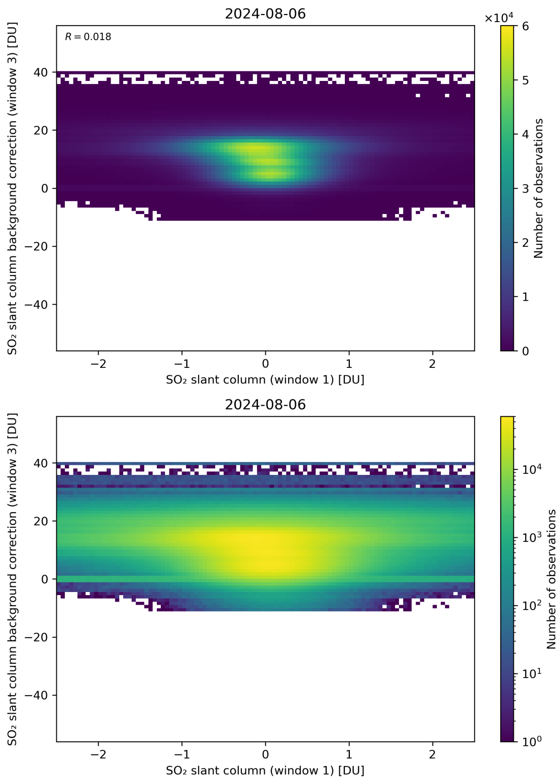
Figure 214: Scatter density plot of “SO 2 slant column (window 1)” against “SO 2 slant column background correction (window 3)” for 2024-08-06 to 2024-08-07.
