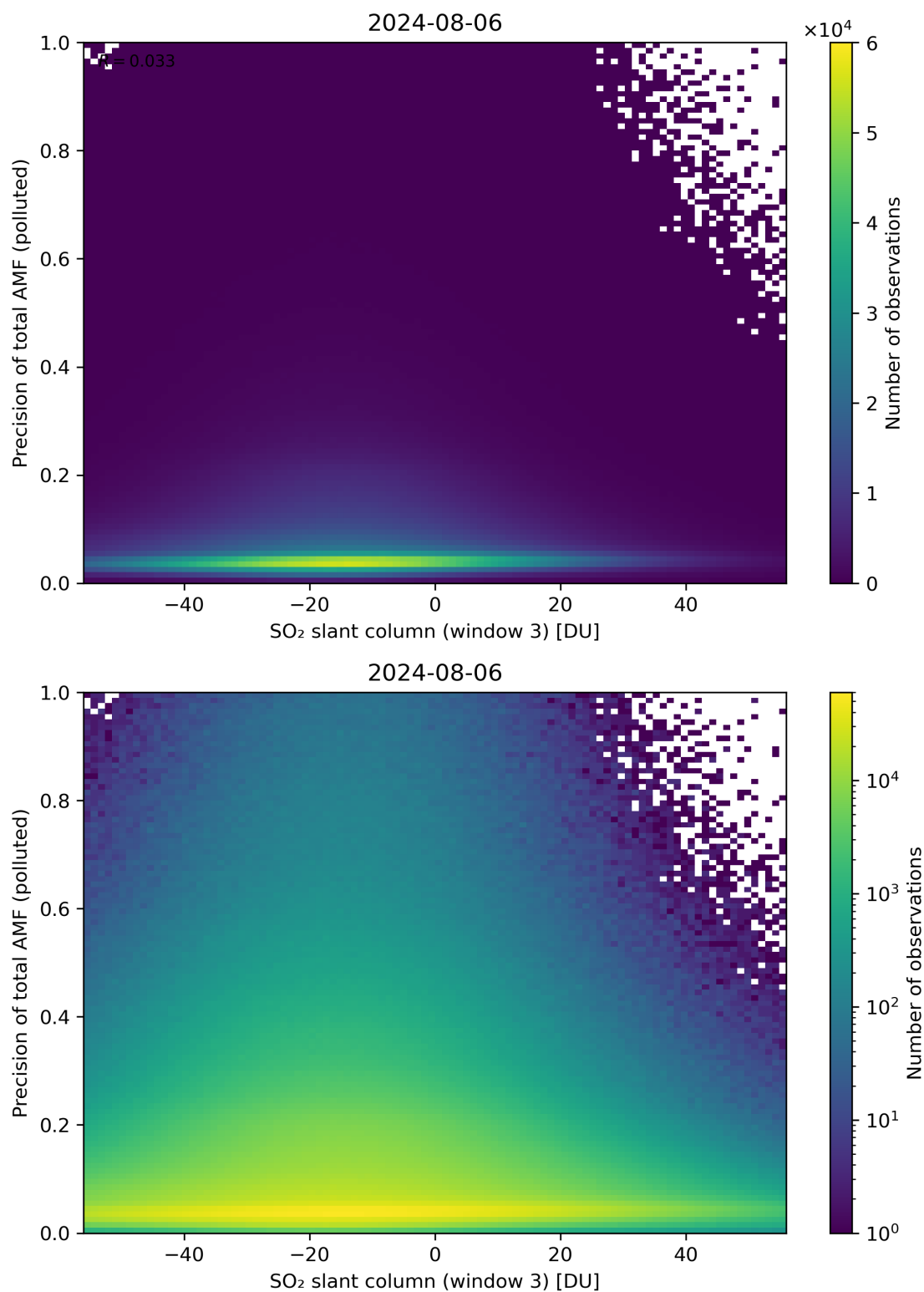
Figure 269: Scatter density plot of “SO 2 slant column (window 3)” against “Precision of total AMF (polluted)” for 2024-08-06 to 2024-08-07.
