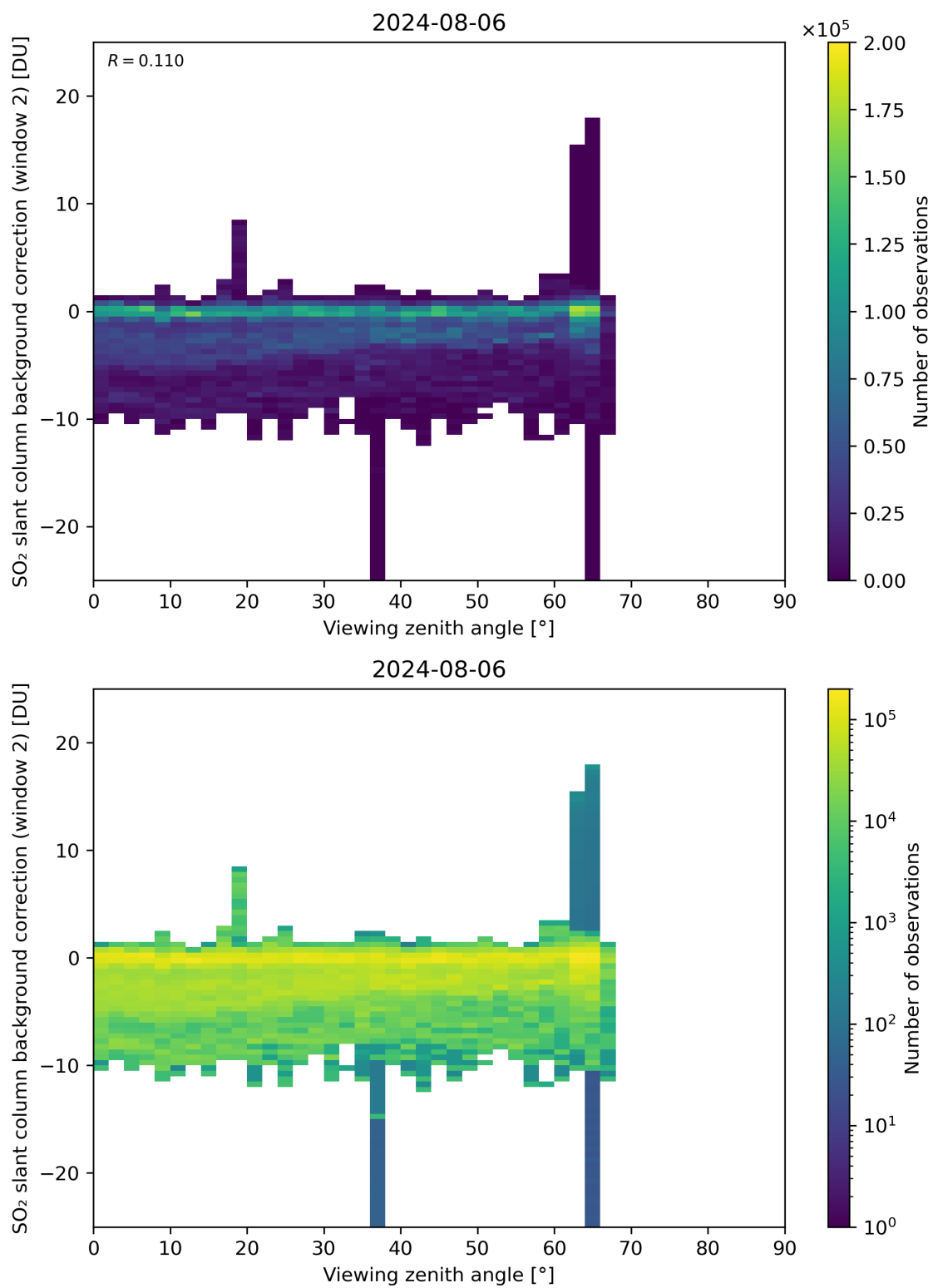
Figure 309: Scatter density plot of “Viewing zenith angle” against “SO 2 slant column background correction (window 2)” for 2024-08-06 to 2024-08-07.
