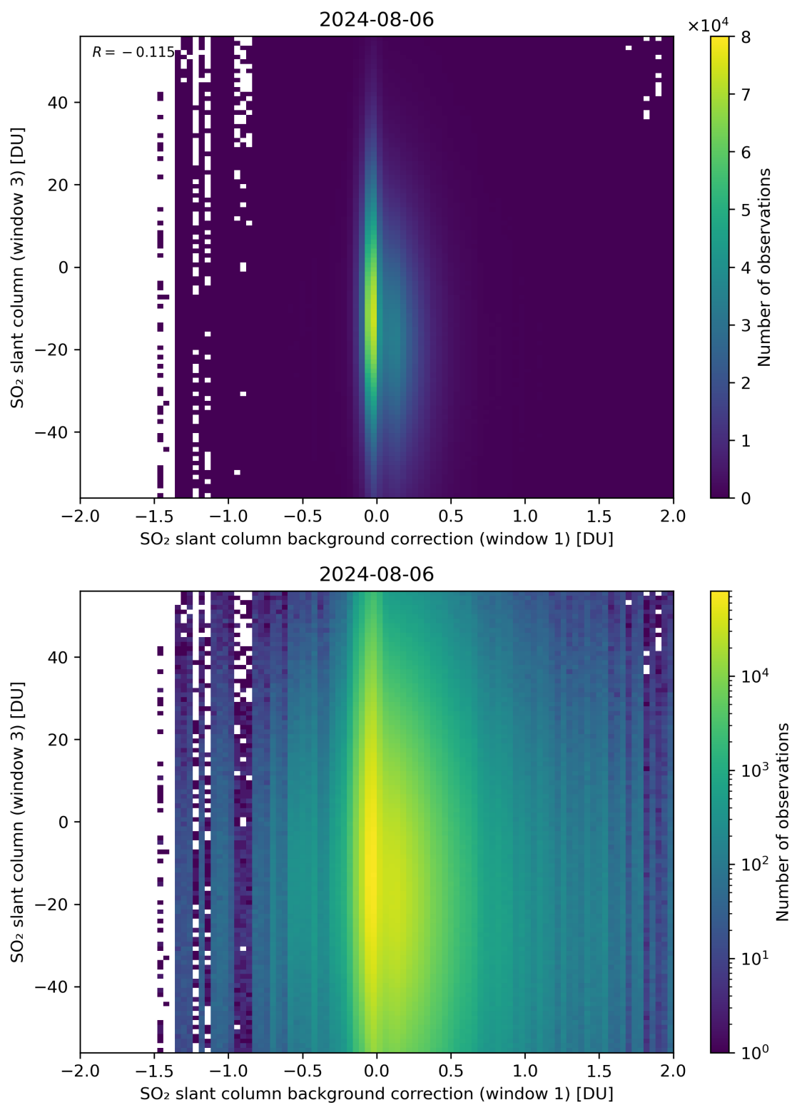
Figure 107: Scatter density plot of “SO 2 slant column background correction (window 1)” against “SO 2 slant column (window 3)” for 2024-08-06 to 2024-08-07.
