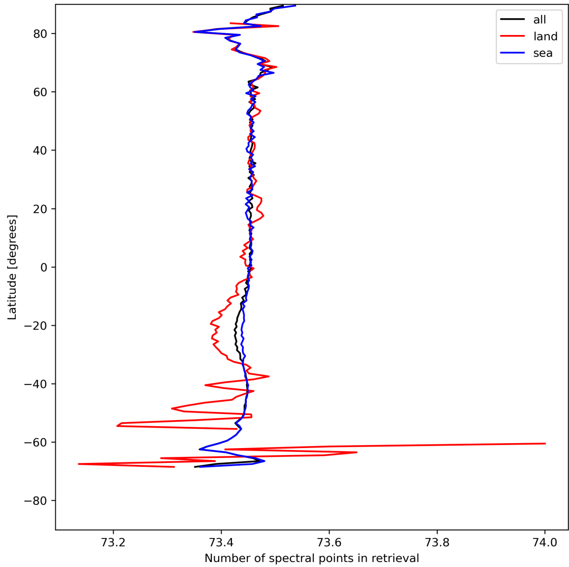
Figure 51: Zonal average of “Number of spectral points in retrieval” for 2024-08-06 to 2024-08-07.
