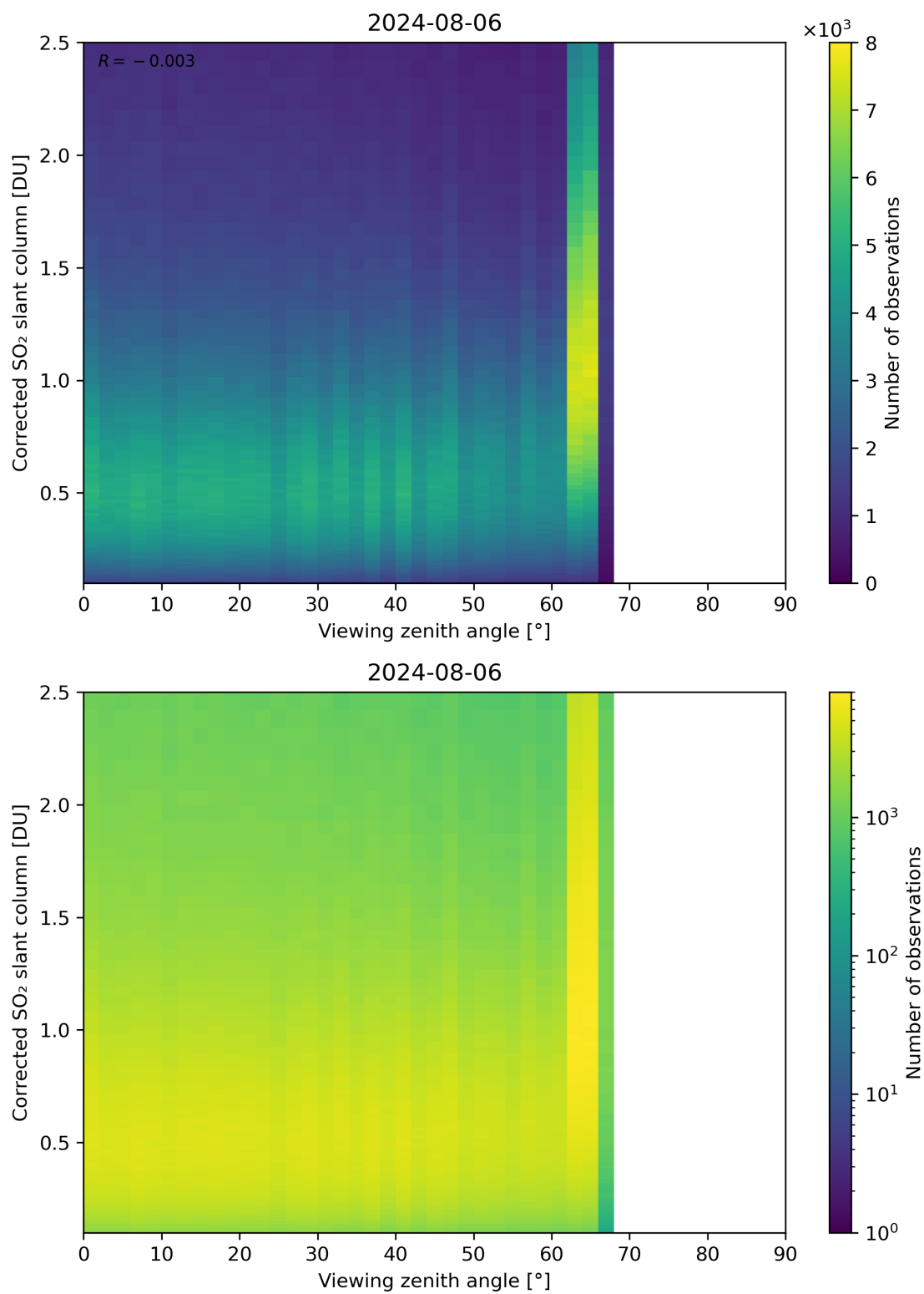
Figure 317: Scatter density plot of “Viewing zenith angle” against “Corrected SO 2 slant column” for 2024-08-06 to 2024-08-07.
