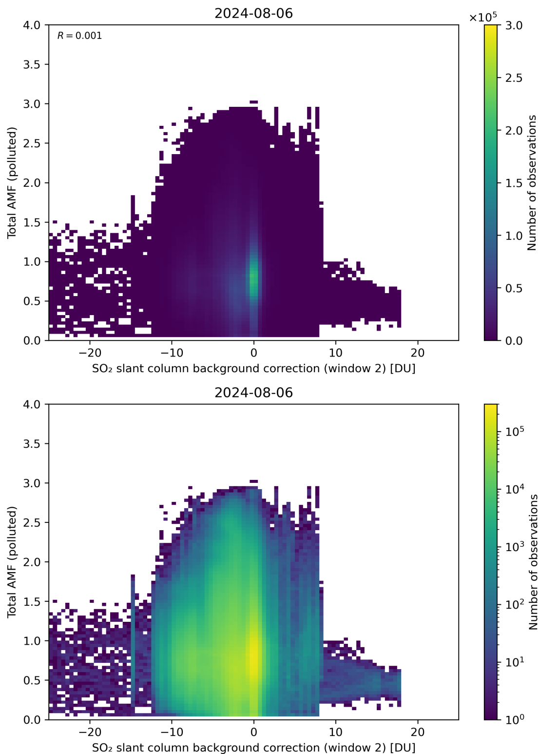
Figure 119: Scatter density plot of “SO 2 slant column background correction (window 2)” against “Total AMF (polluted)” for 2024-08-06 to 2024-08-07.
