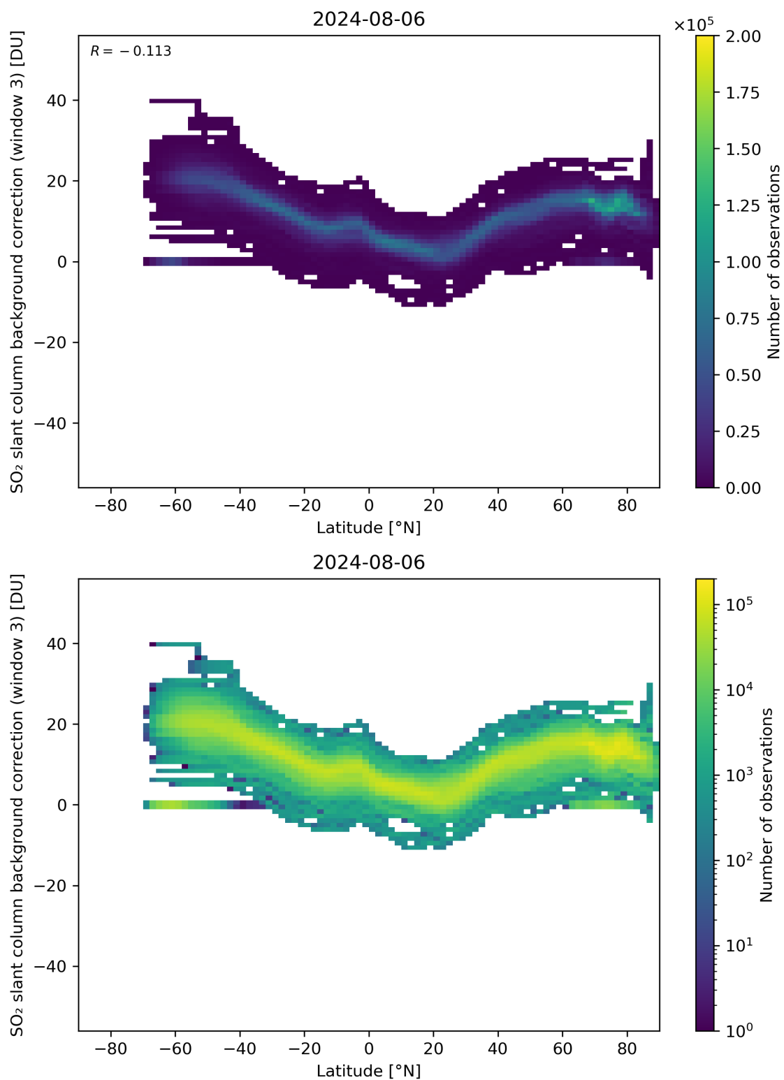
Figure 141: Scatter density plot of “Latitude” against “SO 2 slant column background correction (window 3)” for 2024-08-06 to 2024-08-07.
