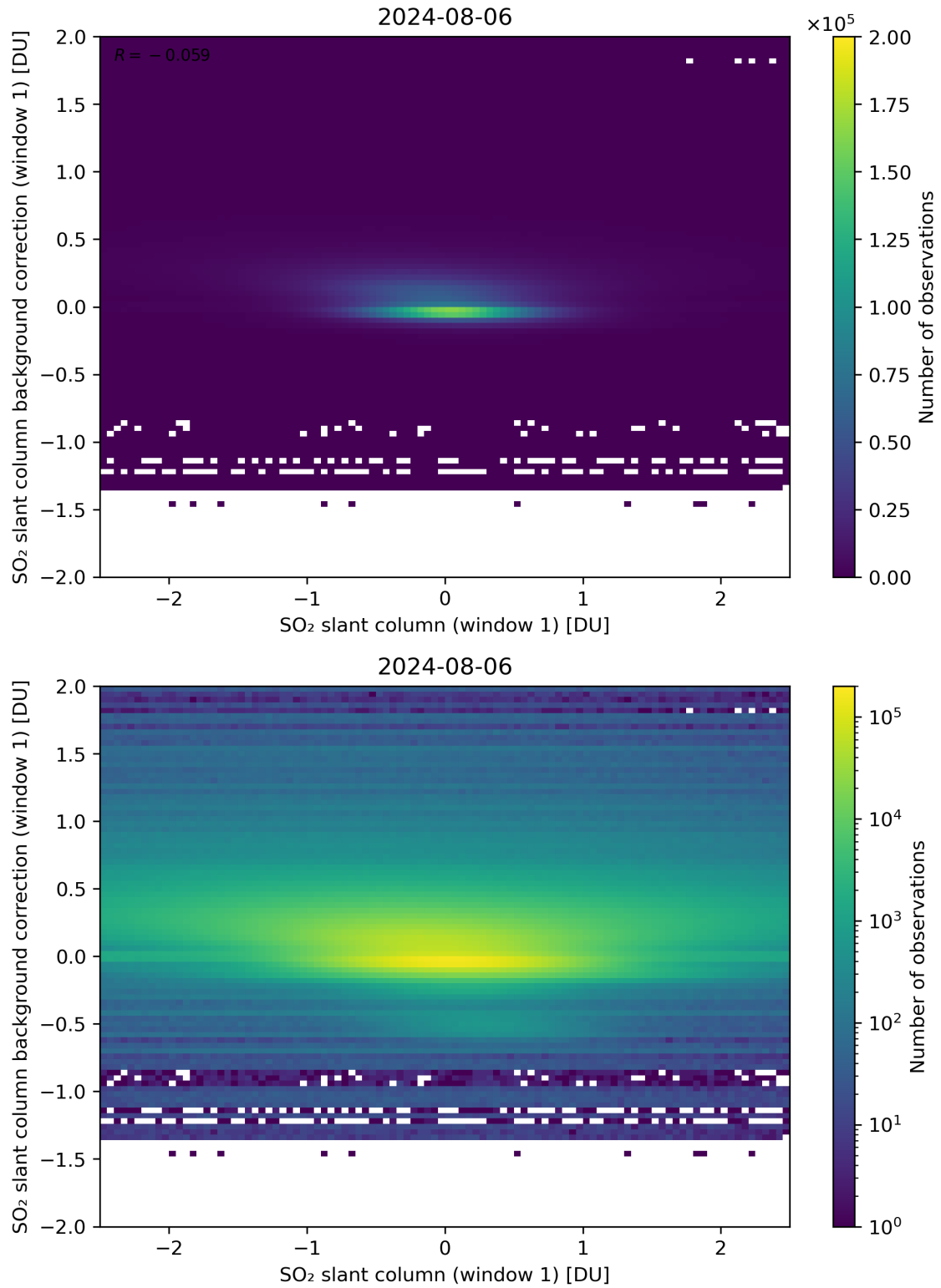
Figure 212: Scatter density plot of “SO 2 slant column (window 1)” against “SO 2 slant column background correction (window 1)” for 2024-08-06 to 2024-08-07.
