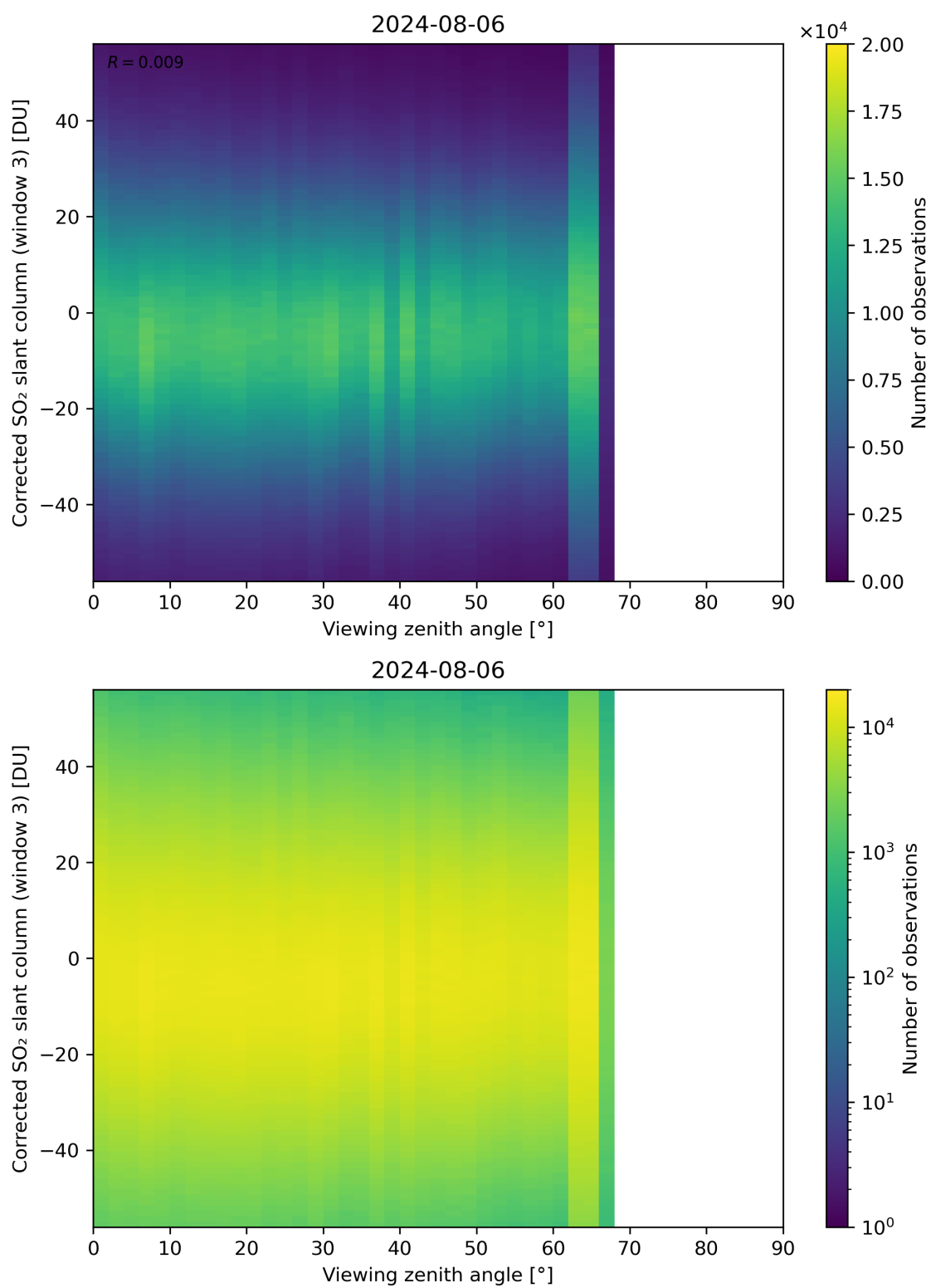
Figure 319: Scatter density plot of “Viewing zenith angle” against “Corrected SO 2 slant column (window 3)” for 2024-08-06 to 2024-08-07.
