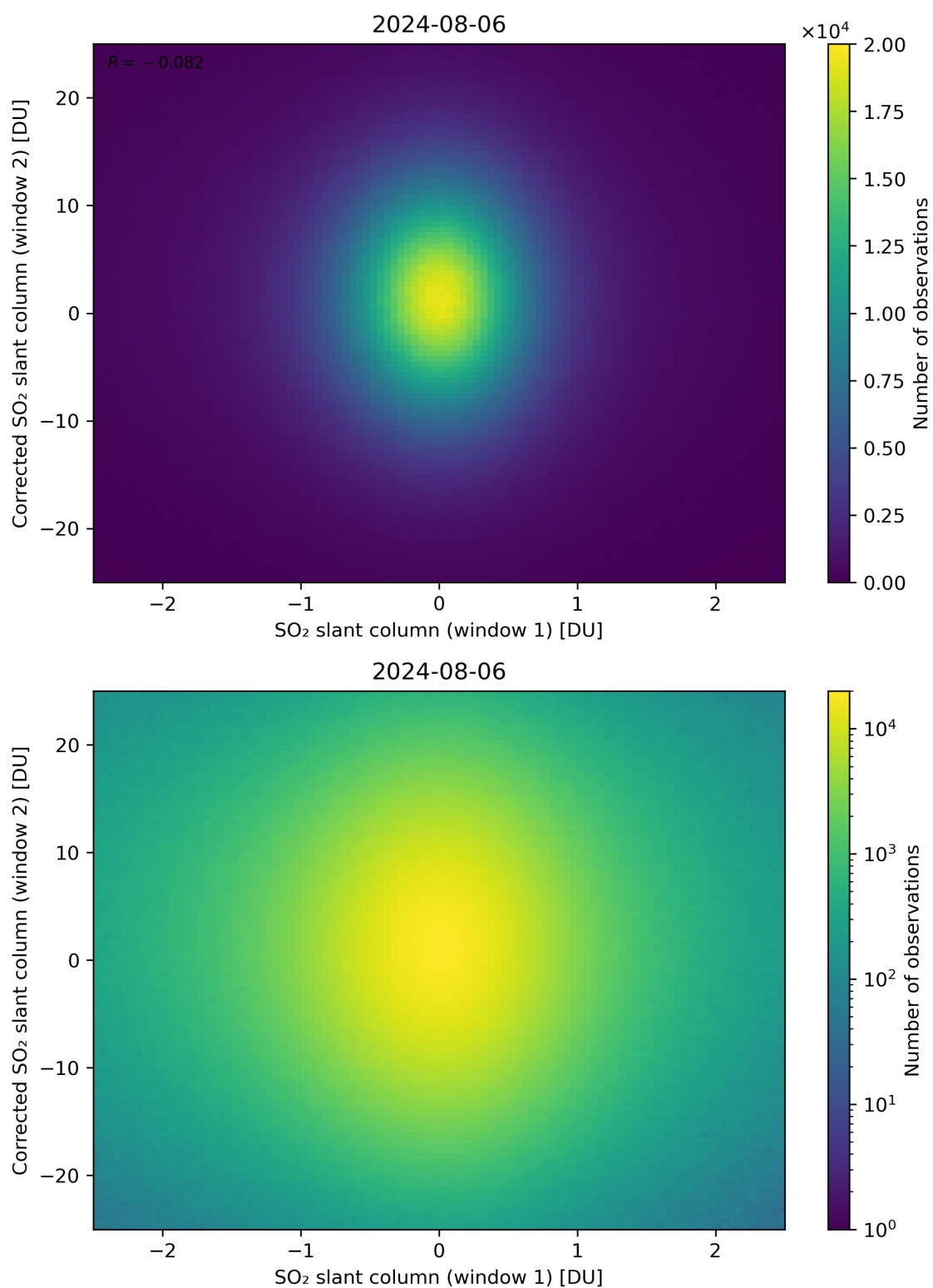
Figure 233: Scatter density plot of “SO 2 slant column (window 1)” against “Corrected SO 2 slant column (window 2)” for 2024-08-06 to 2024-08-07.
