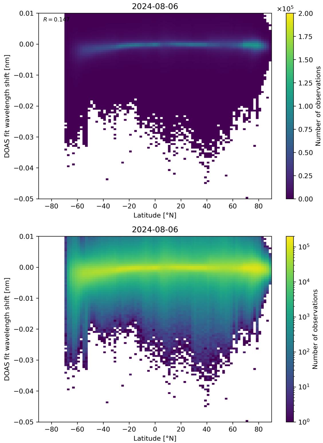
Figure 142: Scatter density plot of “Latitude” against “DOAS fit wavelength shift” for 2024-08-06 to 2024-08-07.
