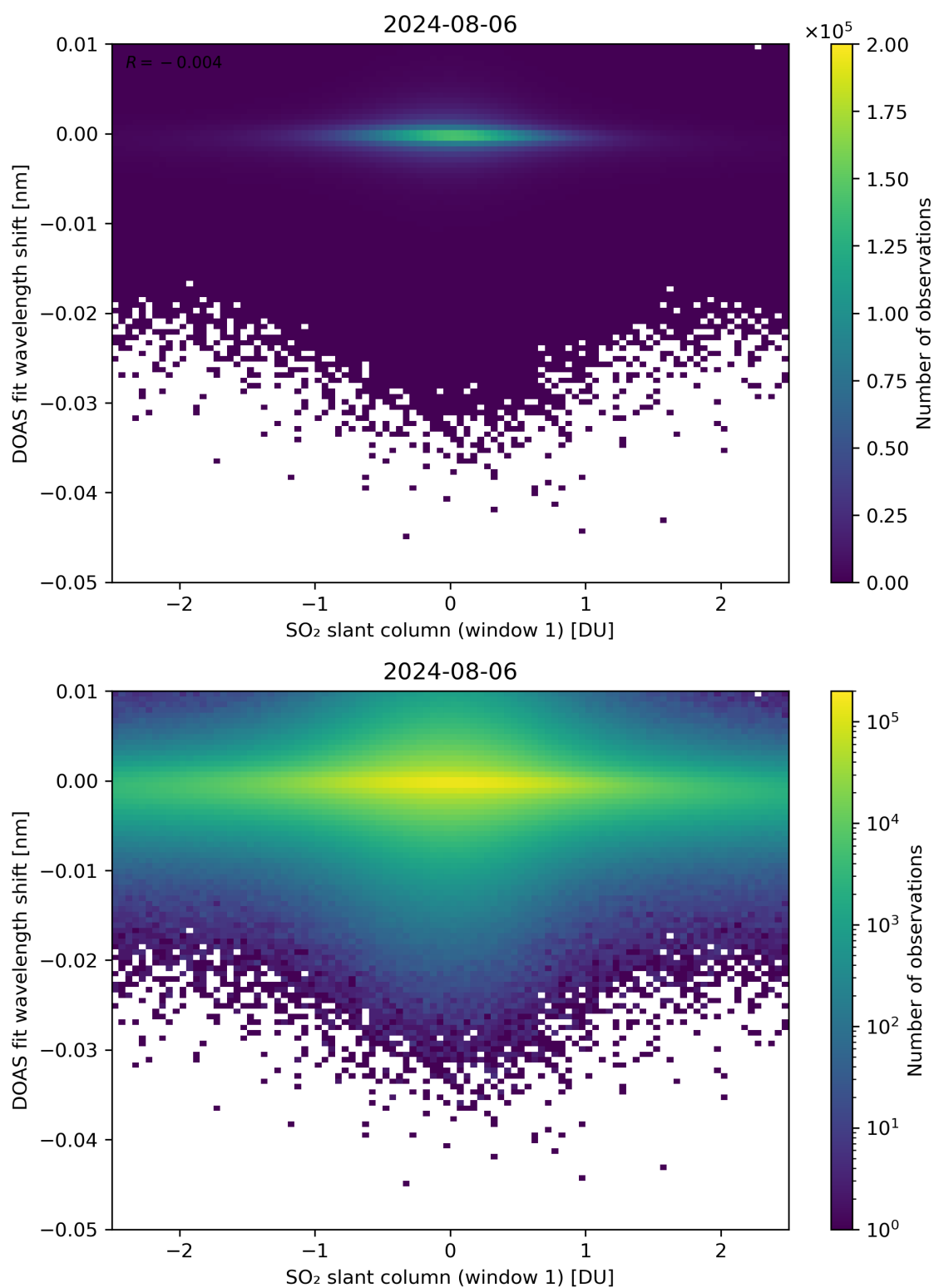
Figure 215: Scatter density plot of “SO 2 slant column (window 1)” against “DOAS fit wavelength shift” for 2024-08-06 to 2024-08-07.
