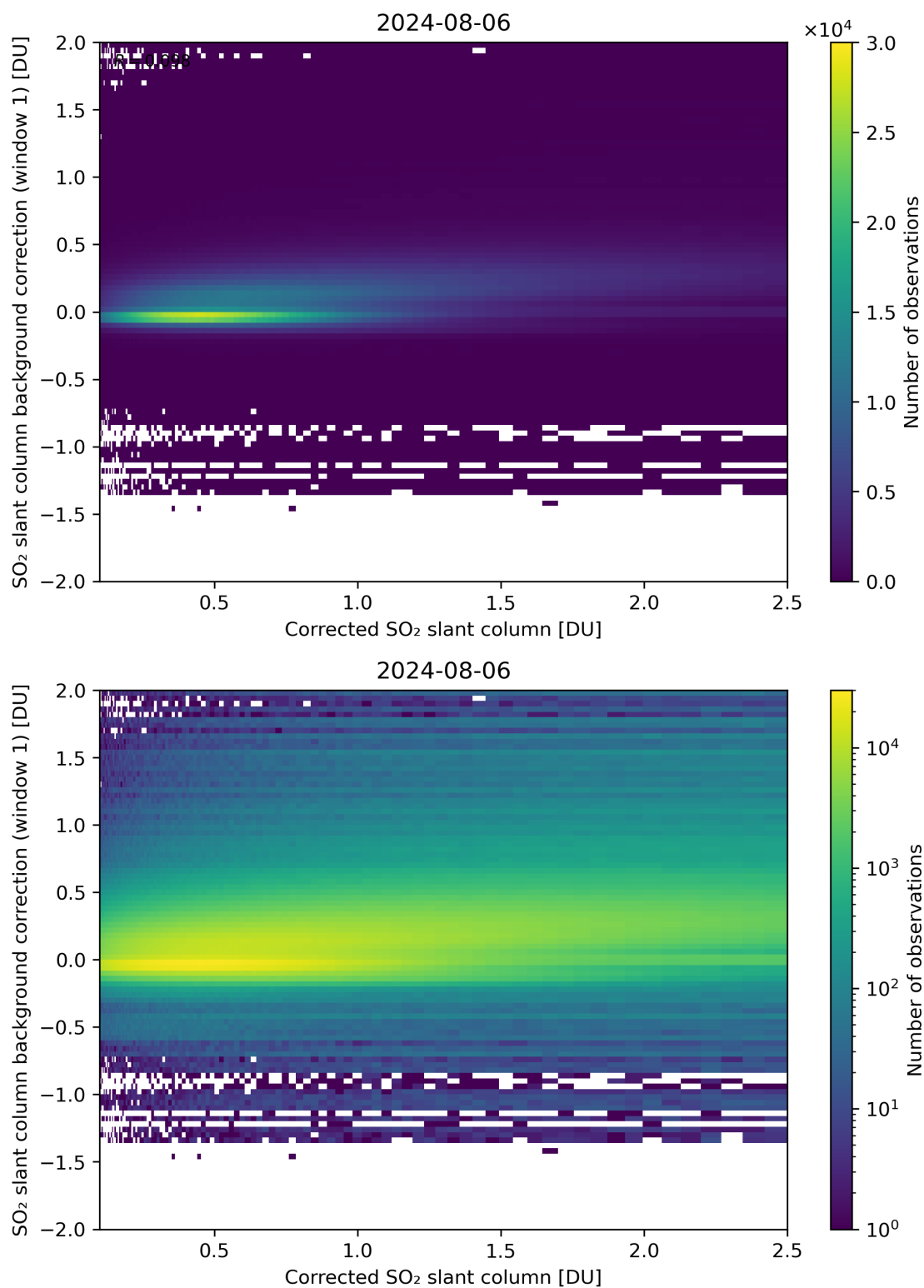
Figure 178: Scatter density plot of “Corrected SO 2 slant column” against “SO 2 slant column background correction (window 1)” for 2024-08-06 to 2024-08-07.
