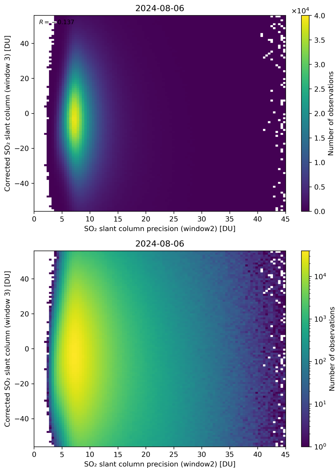
Figure 248: Scatter density plot of “SO 2 slant column precision (window2)” against “Corrected SO 2 slant column (window 3)” for 2024-08-06 to 2024-08-07.
