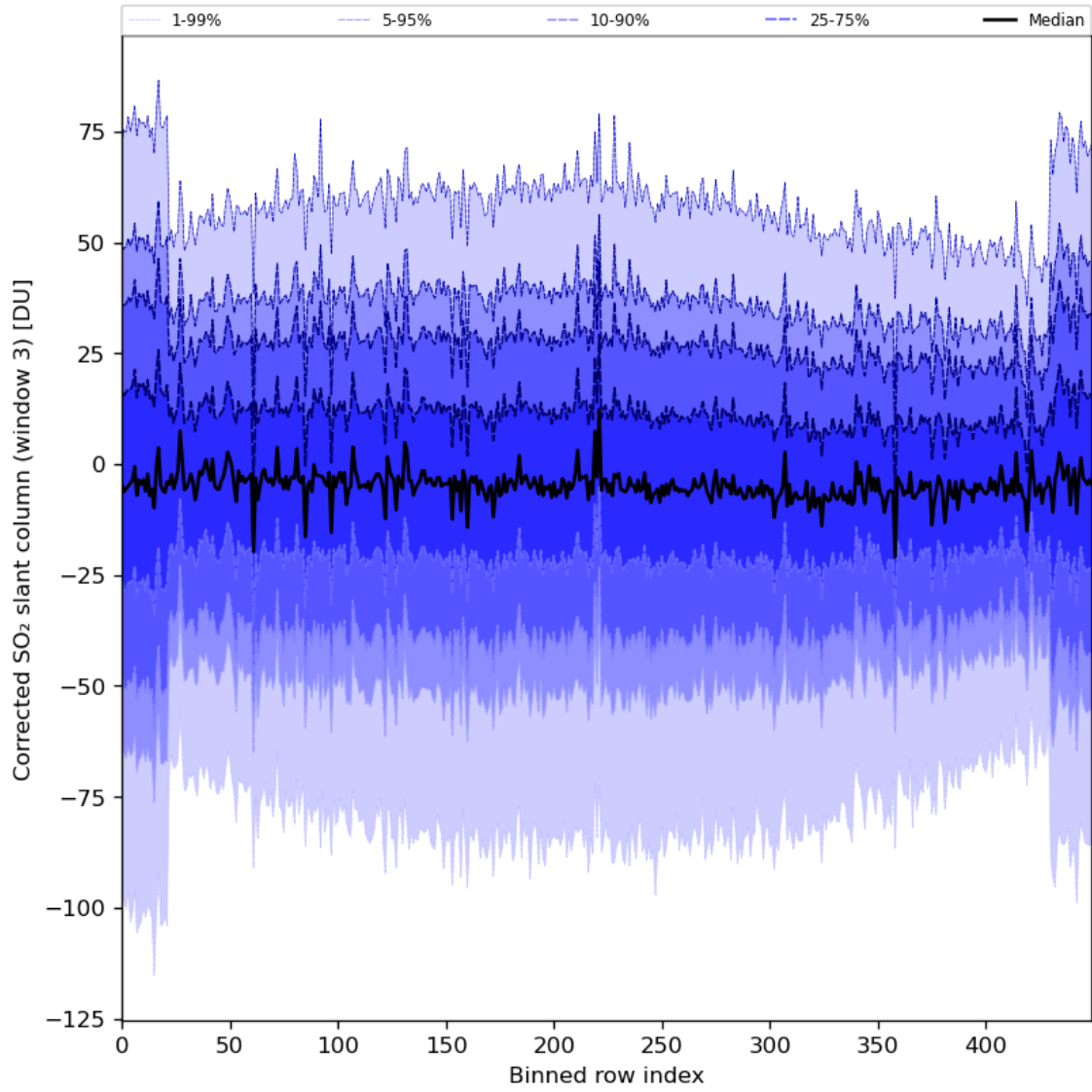
Figure 89: Along track statistics of “Corrected SO 2 slant column (window 3)” for 2024-08-06 to 2024-08-07
