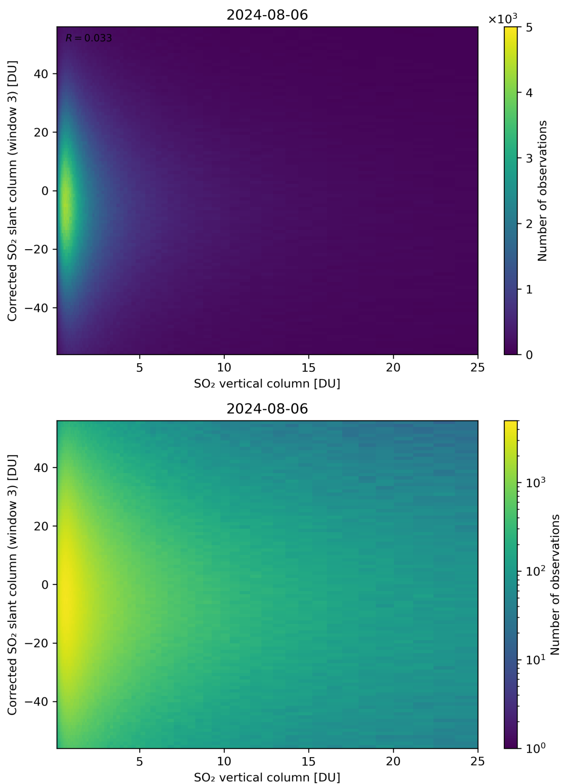
Figure 299: Scatter density plot of “SO 2 vertical column” against “Corrected SO 2 slant column (window 3)” for 2024-08-06 to 2024-08-07.
