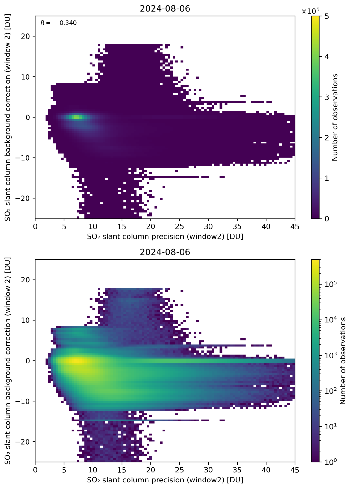
Figure 241: Scatter density plot of “SO 2 slant column precision (window2)” against “SO 2 slant column background correction (window 2)” for 2024-08-06 to 2024-08-07.
