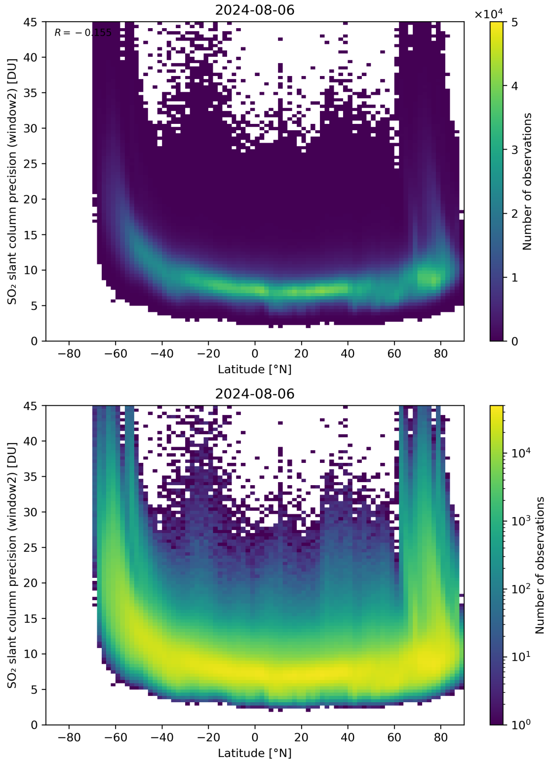
Figure 151: Scatter density plot of “Latitude” against “SO 2 slant column precision (window2)” for 2024-08-06 to 2024-08-07.
