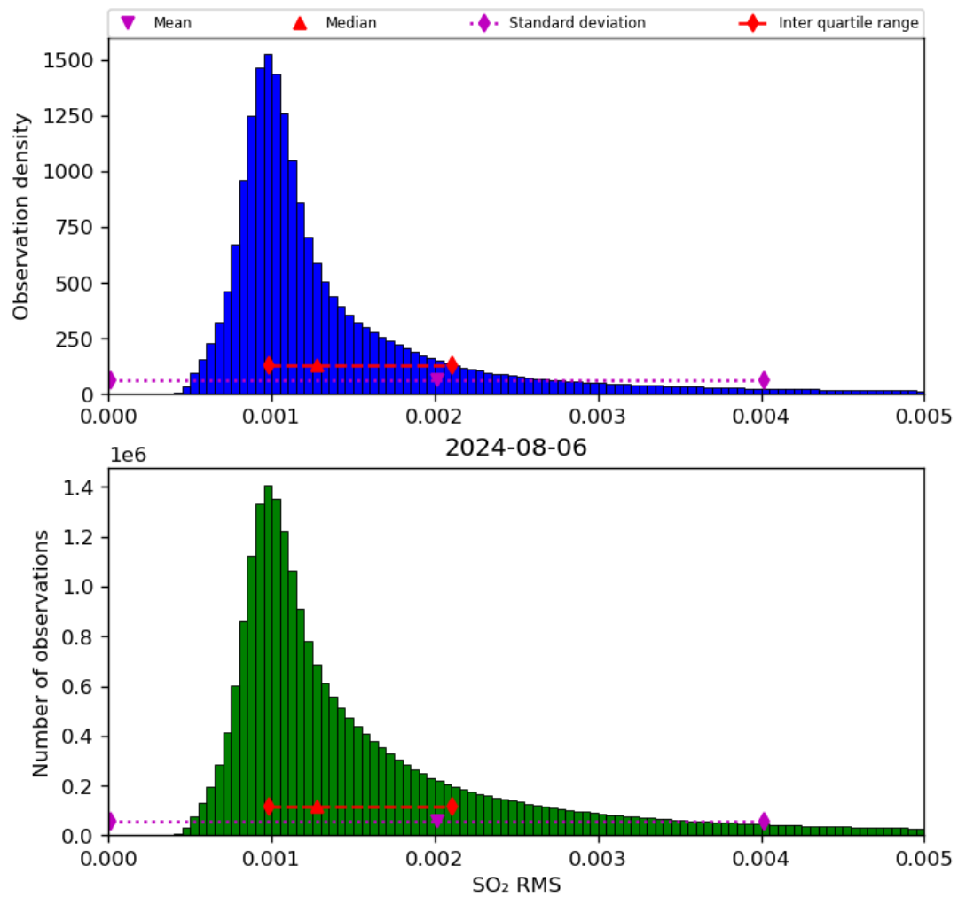
Figure 70: Histogram of “SO 2 RMS” for 2024-08-06 to 2024-08-07
