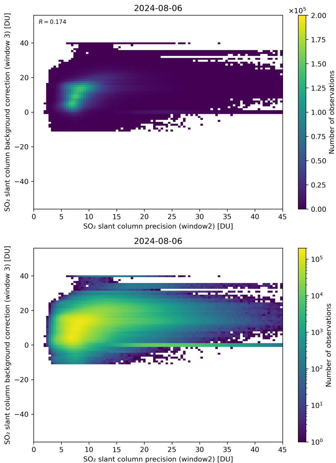
Figure 242: Scatter density plot of “SO 2 slant column precision (window2)” against “SO 2 slant column background correction (window 3)” for 2024-08-06 to 2024-08-07.
