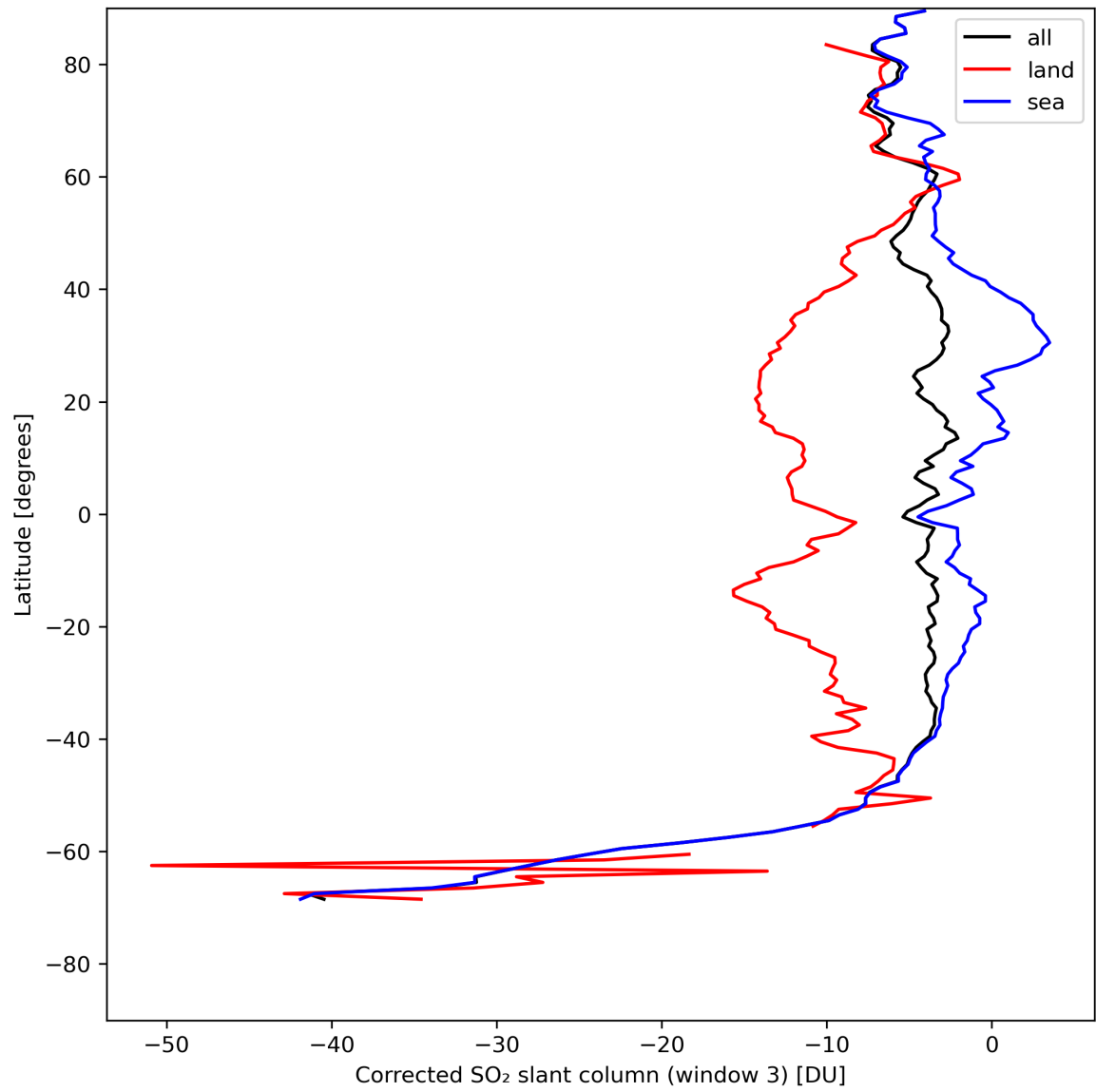
Figure 43: Zonal average of “Corrected SO 2 slant column (window 3)” for 2024-08-06 to 2024-08-07.
