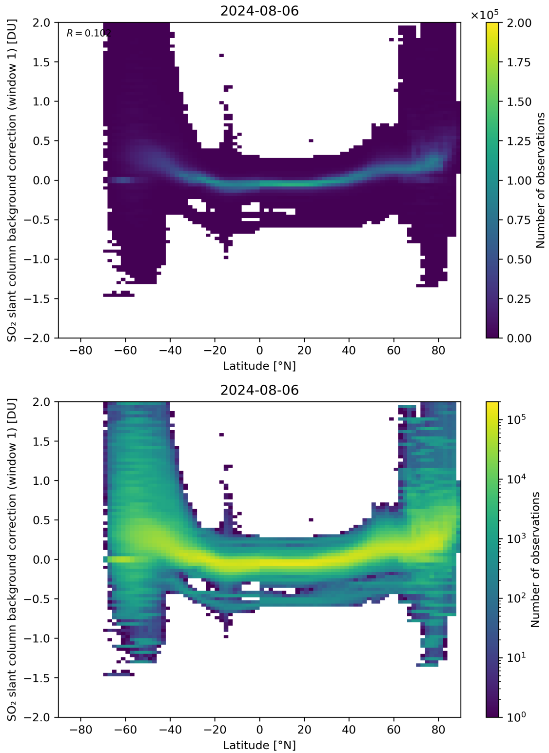
Figure 139: Scatter density plot of “Latitude” against “SO 2 slant column background correction (window 1)” for 2024-08-06 to 2024-08-07.
