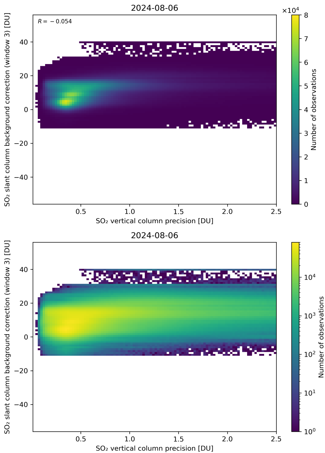
Figure 281: Scatter density plot of “SO 2 vertical column precision” against “SO 2 slant column background correction (window 3)” for 2024-08-06 to 2024-08-07.
