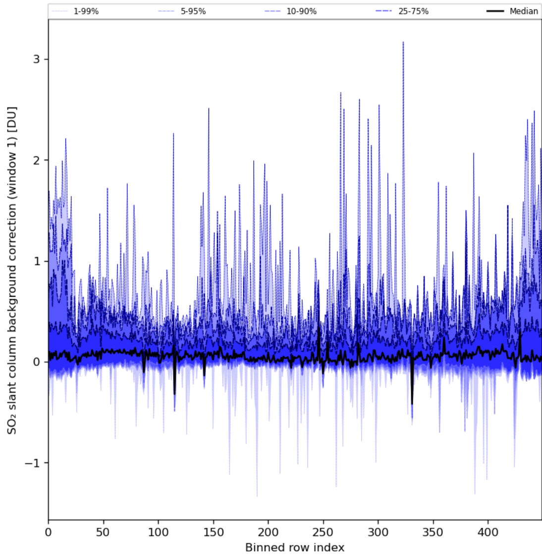
Figure 82: Along track statistics of “SO 2 slant column background correction (window 1)” for 2024-08-06 to 2024-08-07
