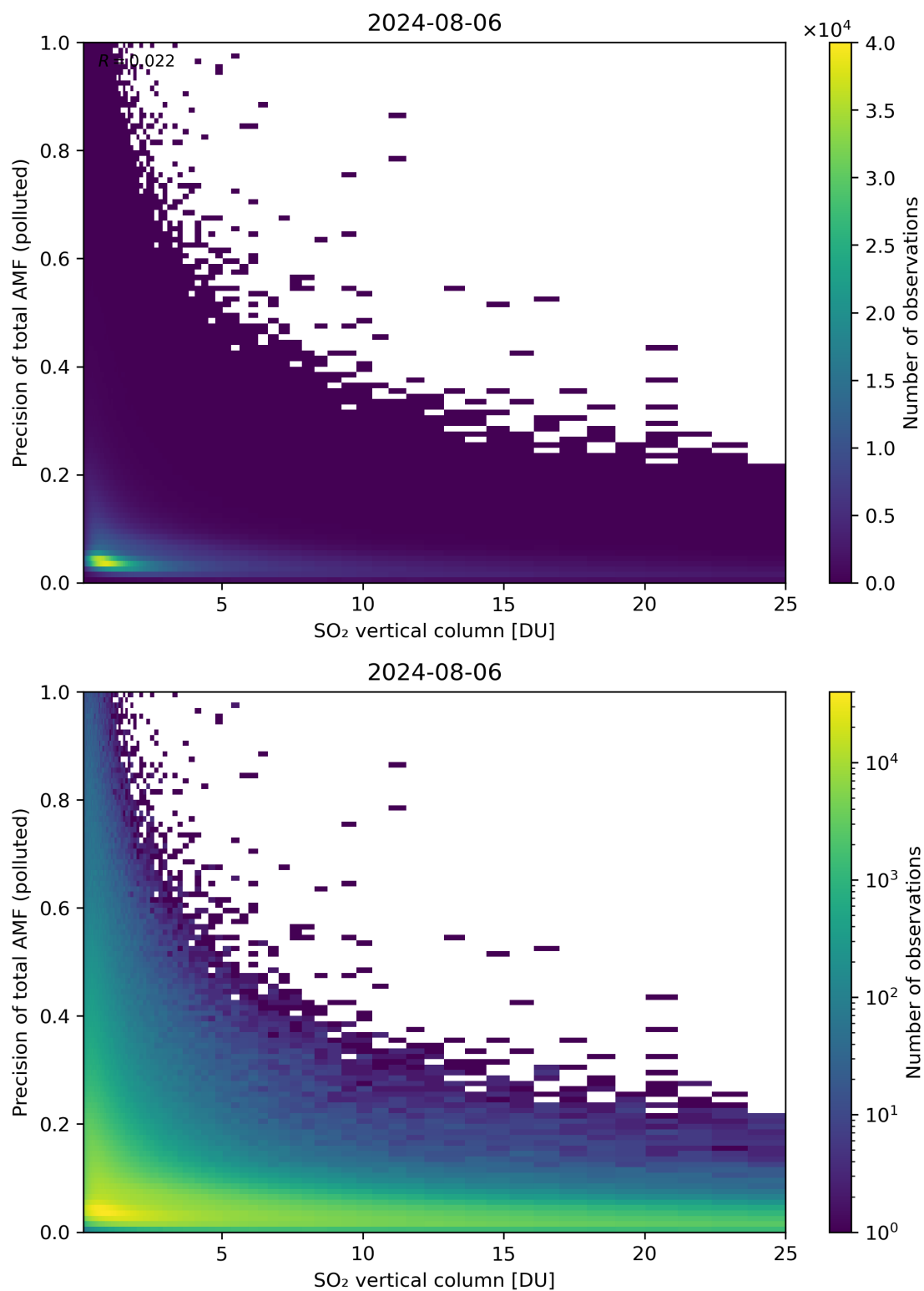
Figure 306: Scatter density plot of “SO 2 vertical column” against “Precision of total AMF (polluted)” for 2024-08-06 to 2024-08-07.
