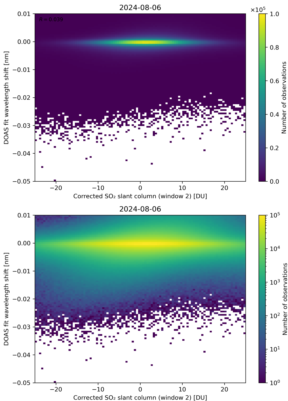
Figure 196: Scatter density plot of “Corrected SO 2 slant column (window 2)” against “DOAS fit wavelength shift” for 2024-08-06 to 2024-08-07.
