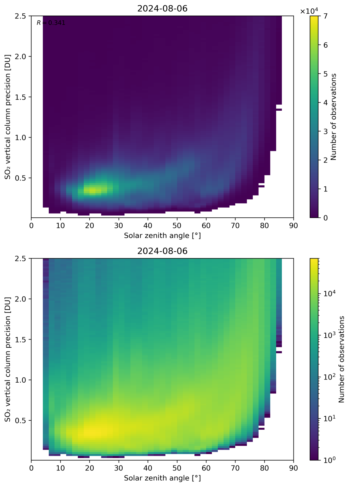
Figure 177: Scatter density plot of “Solar zenith angle” against “SO 2 vertical column precision” for 2024-08-06 to 2024-08-07.
