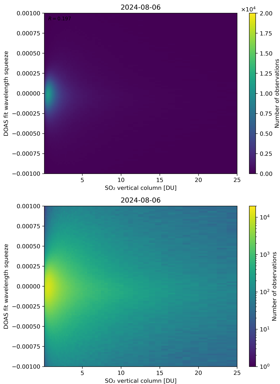
Figure 277: Scatter density plot of “SO 2 vertical column” against “DOAS fit wavelength squeeze” for 2024-08-06 to 2024-08-07.
