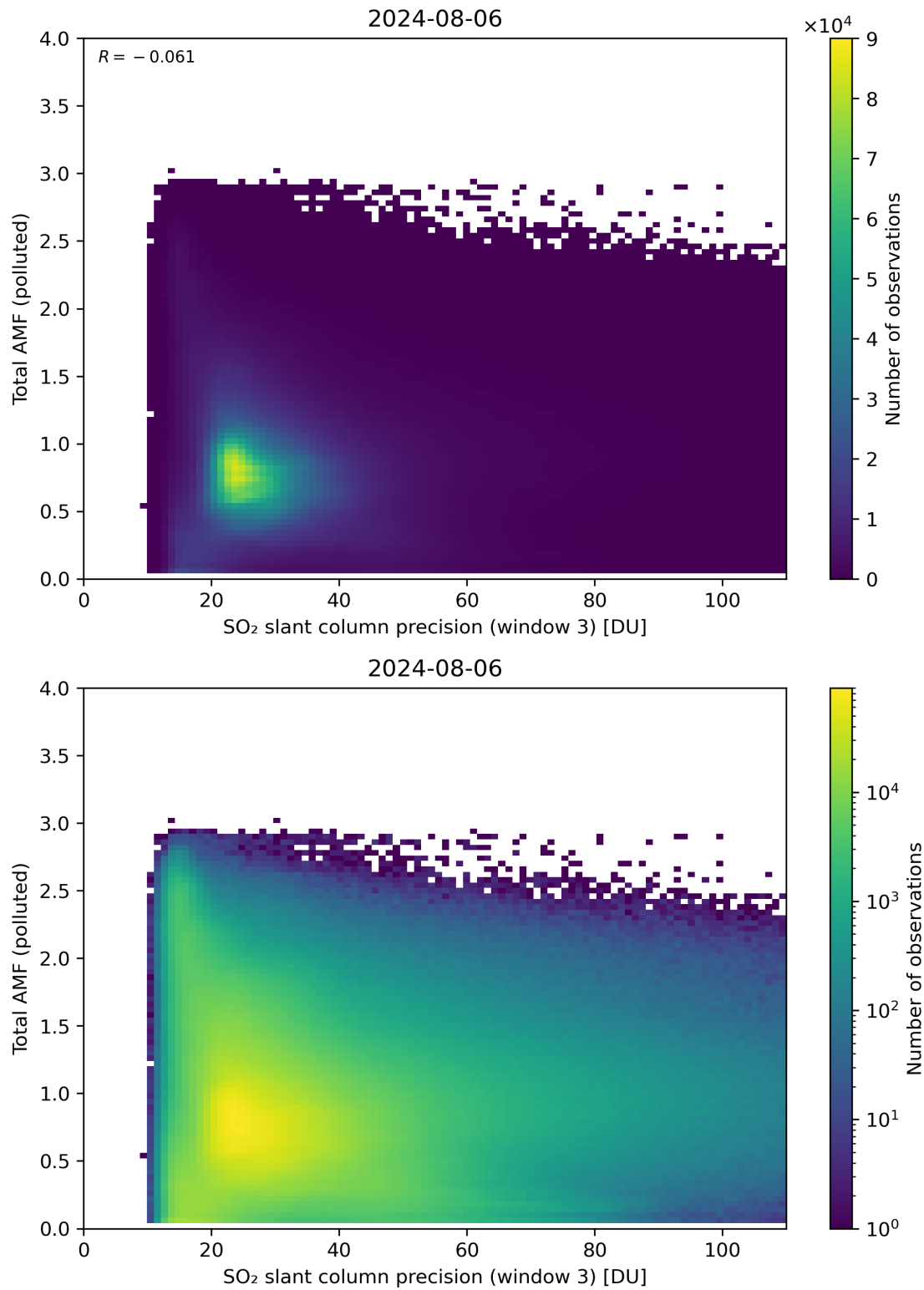
Figure 263: Scatter density plot of “SO 2 slant column precision (window 3)” against “Total AMF (polluted)” for 2024-08-06 to 2024-08-07.
