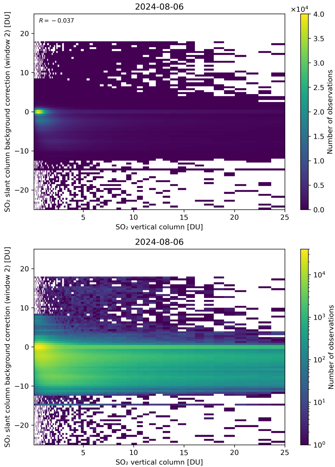
Figure 274: Scatter density plot of “SO 2 vertical column” against “SO 2 slant column background correction (window 2)” for 2024-08-06 to 2024-08-07.
