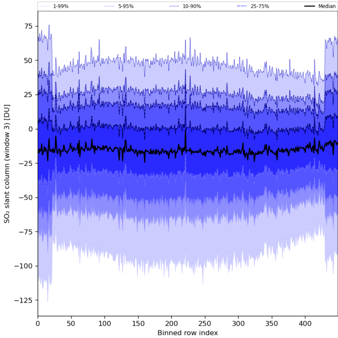
Figure 87: Along track statistics of “SO 2 slant column (window 3)” for 2024-08-06 to 2024-08-07
