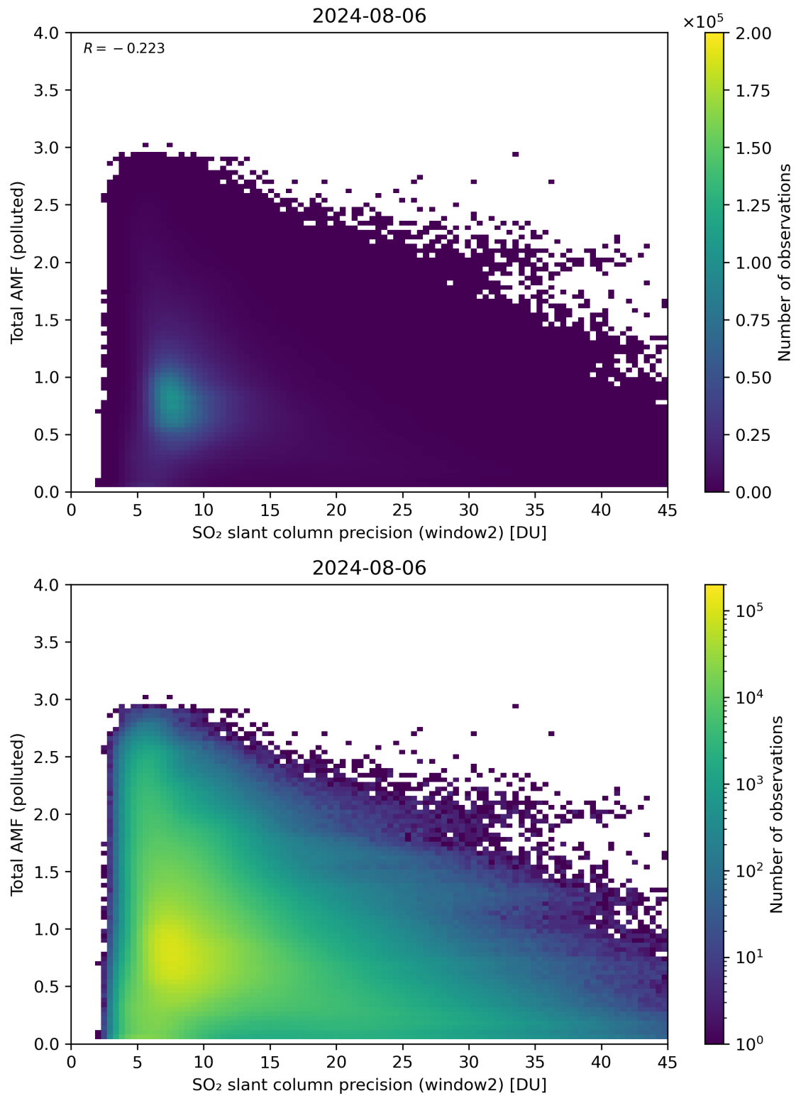
Figure 251: Scatter density plot of “SO 2 slant column precision (window2)” against “Total AMF (polluted)” for 2024-08-06 to 2024-08-07.
