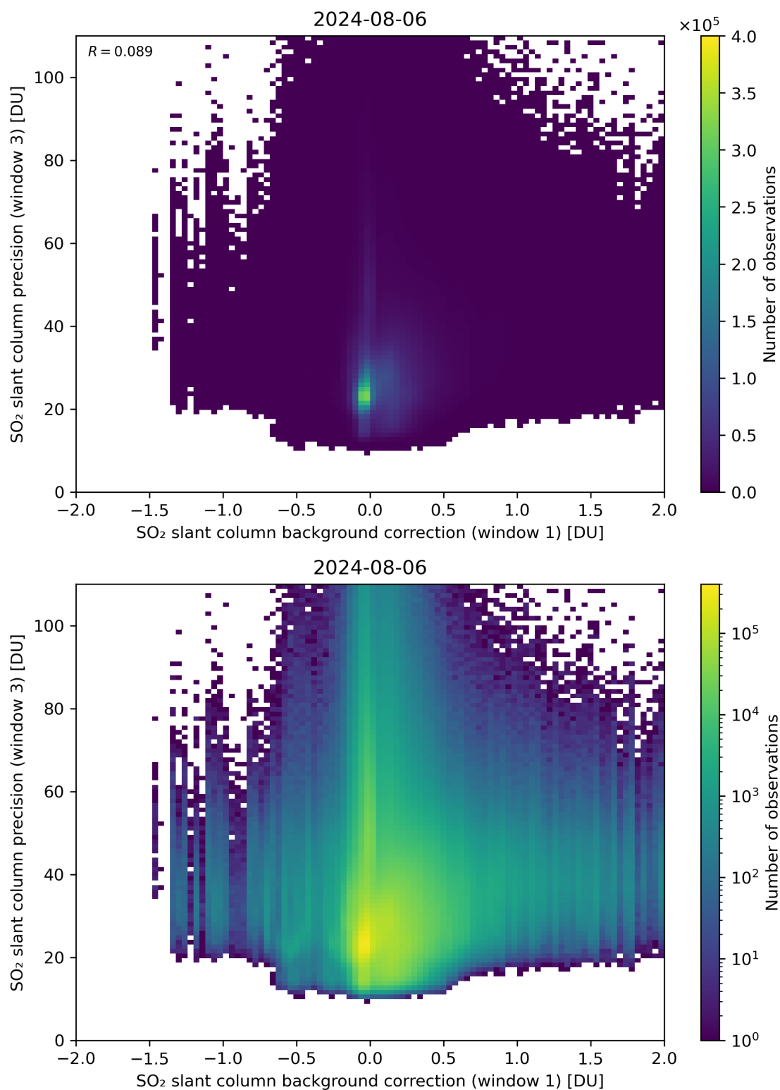
Figure 108: Scatter density plot of “SO 2 slant column background correction (window 1)” against “SO 2 slant column precision (window 3)” for 2024-08-06 to 2024-08-07.
