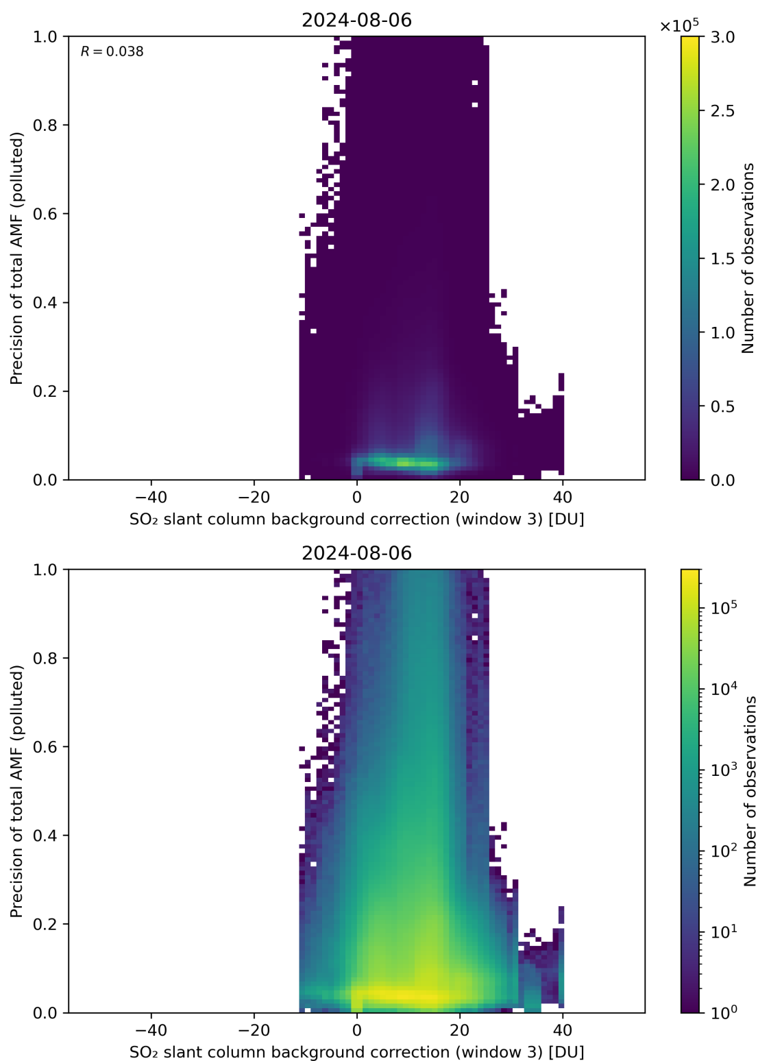
Figure 126: Scatter density plot of “SO 2 slant column background correction (window 3)” against “Precision of total AMF (polluted)” for 2024-08-06 to 2024-08-07.
