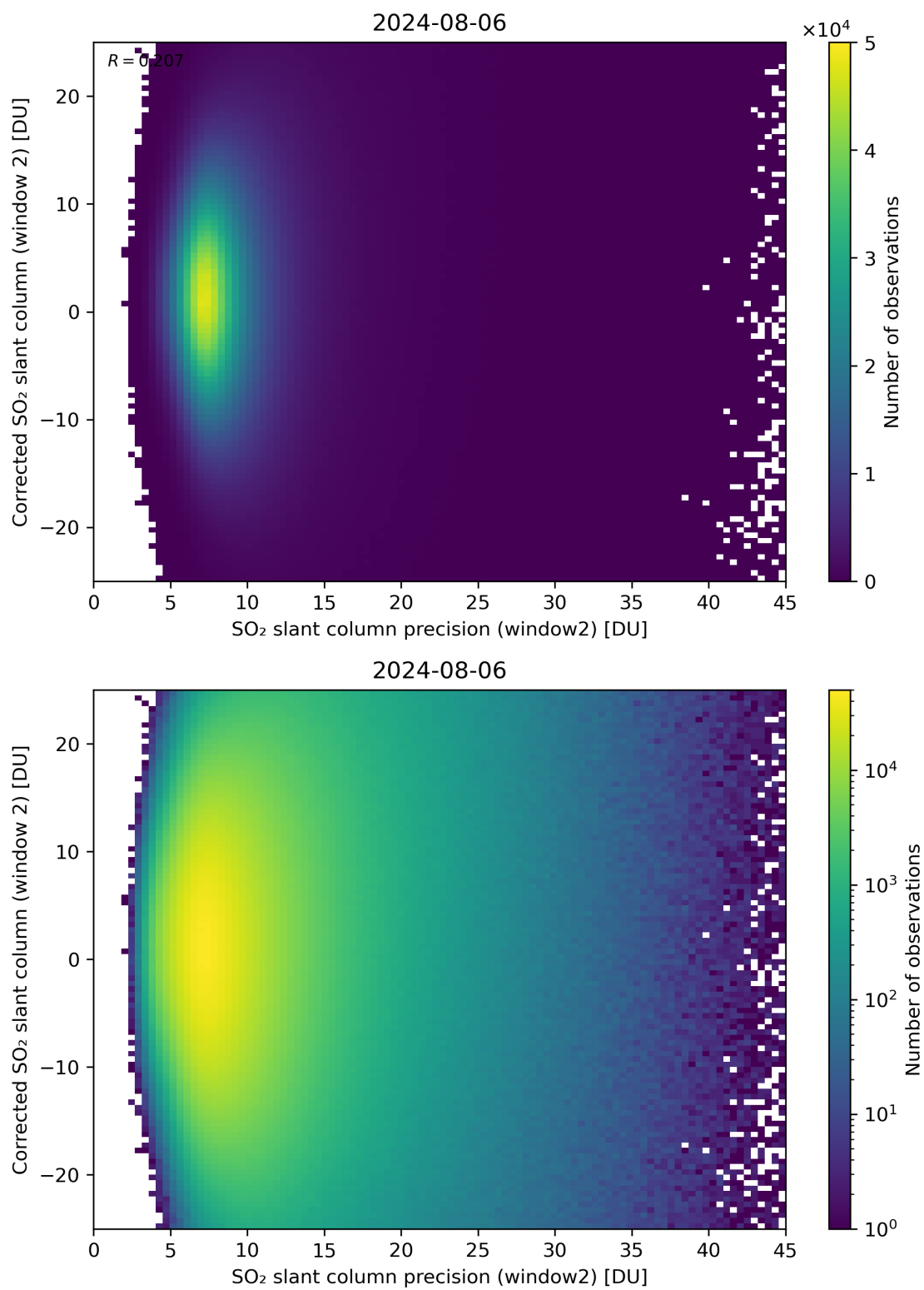
Figure 247: Scatter density plot of “SO 2 slant column precision (window2)” against “Corrected SO 2 slant column (window 2)” for 2024-08-06 to 2024-08-07.
