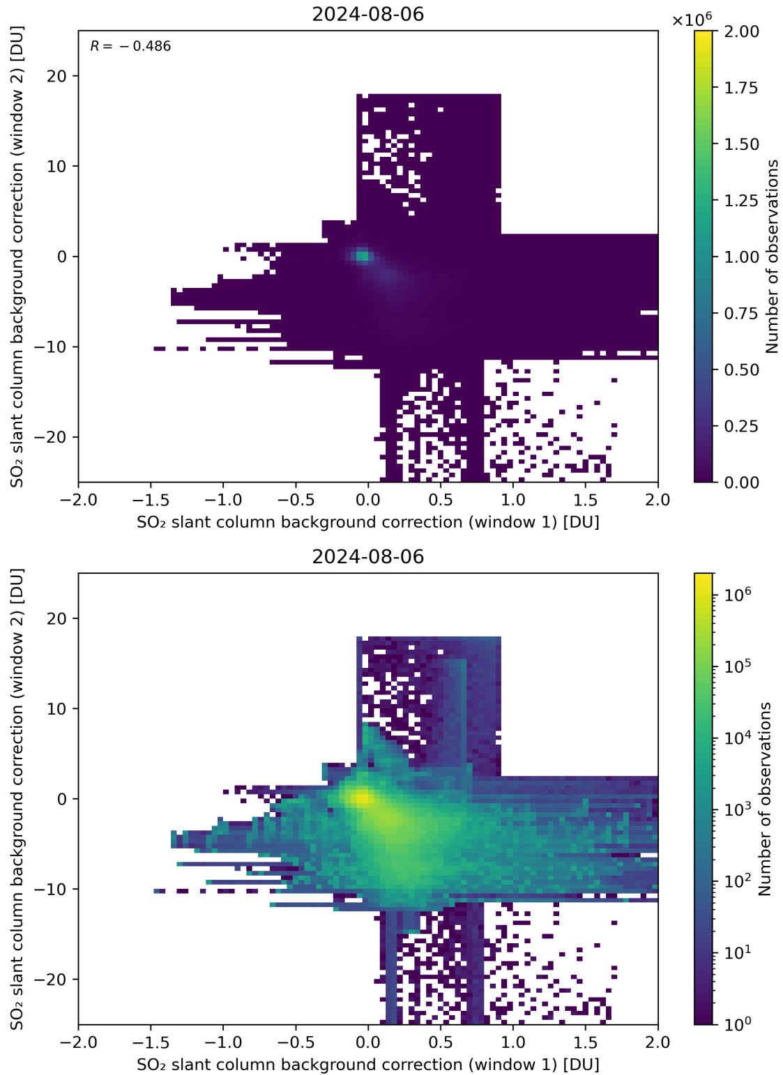
Figure 98: Scatter density plot of “SO 2 slant column background correction (window 1)” against “SO 2 slant column background correction (window 2)” for 2024-08-06 to 2024-08-07.
