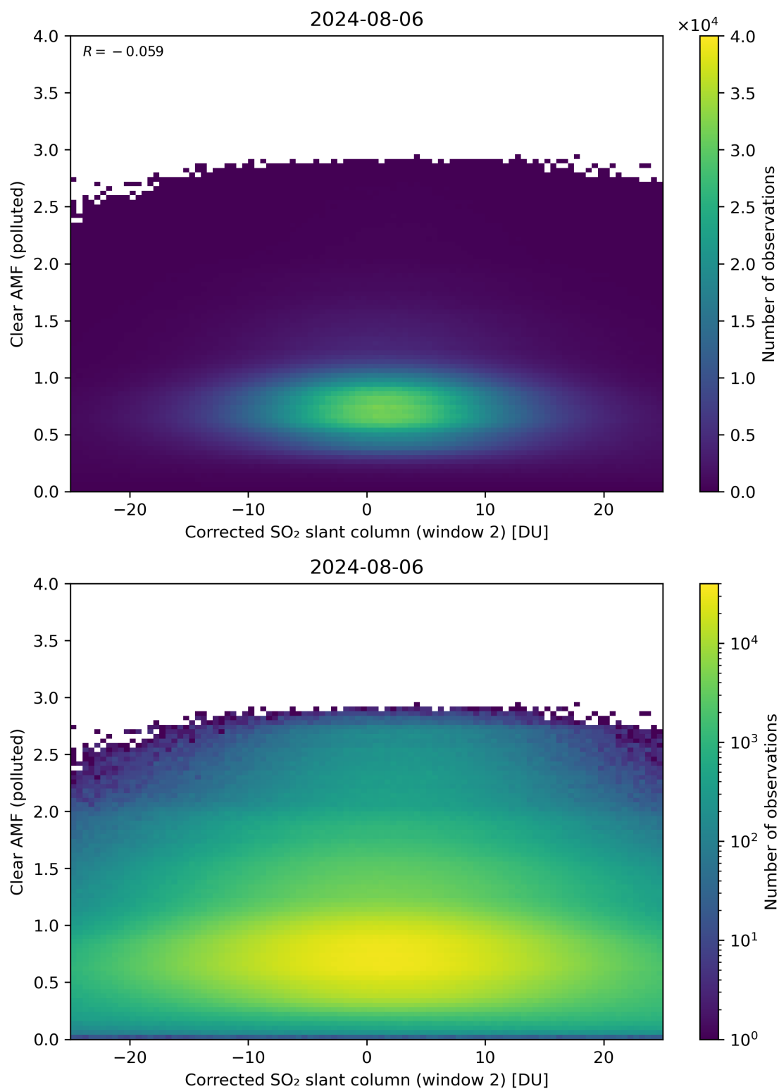
Figure 199: Scatter density plot of “Corrected SO 2 slant column (window 2)” against “Clear AMF (polluted)” for 2024-08-06 to 2024-08-07.
