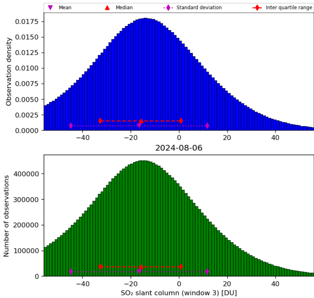
Figure 64: Histogram of “SO 2 slant column (window 3)” for 2024-08-06 to 2024-08-07
