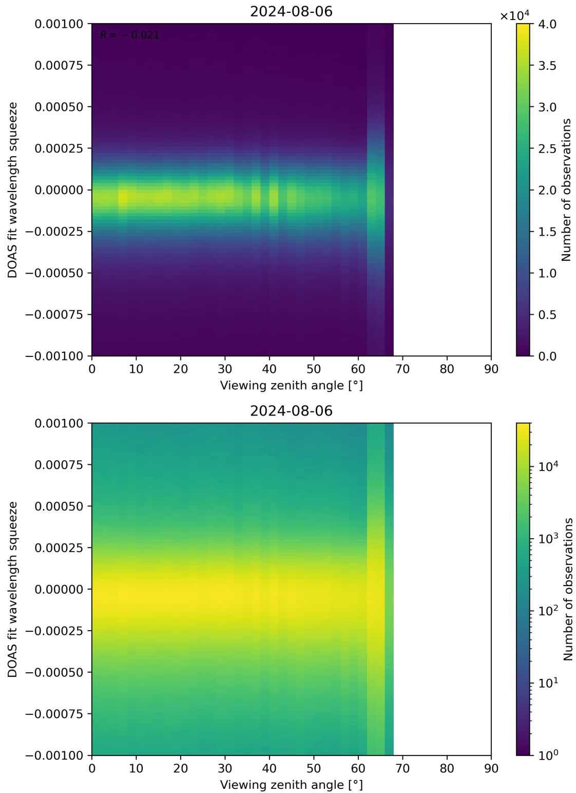
Figure 312: Scatter density plot of “Viewing zenith angle” against “DOAS fit wavelength squeeze” for 2024-08-06 to 2024-08-07.
