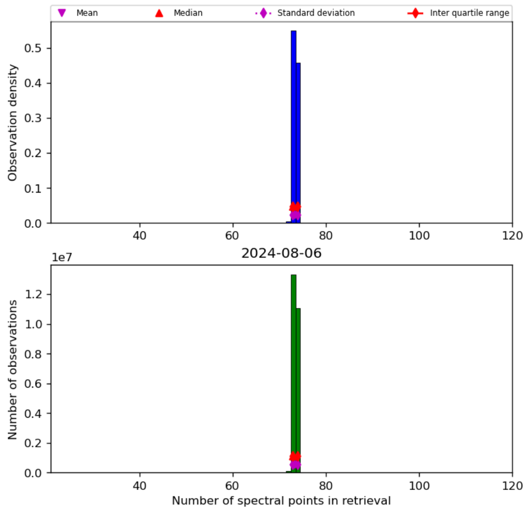
Figure 74: Histogram of “Number of spectral points in retrieval” for 2024-08-06 to 2024-08-07
