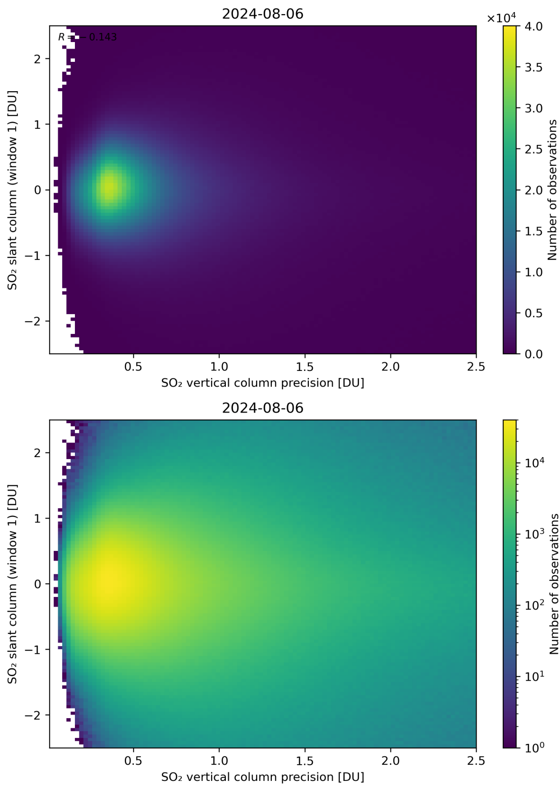
Figure 289: Scatter density plot of “SO 2 vertical column precision” against “SO 2 slant column (window 1)” for 2024-08-06 to 2024-08-07.
