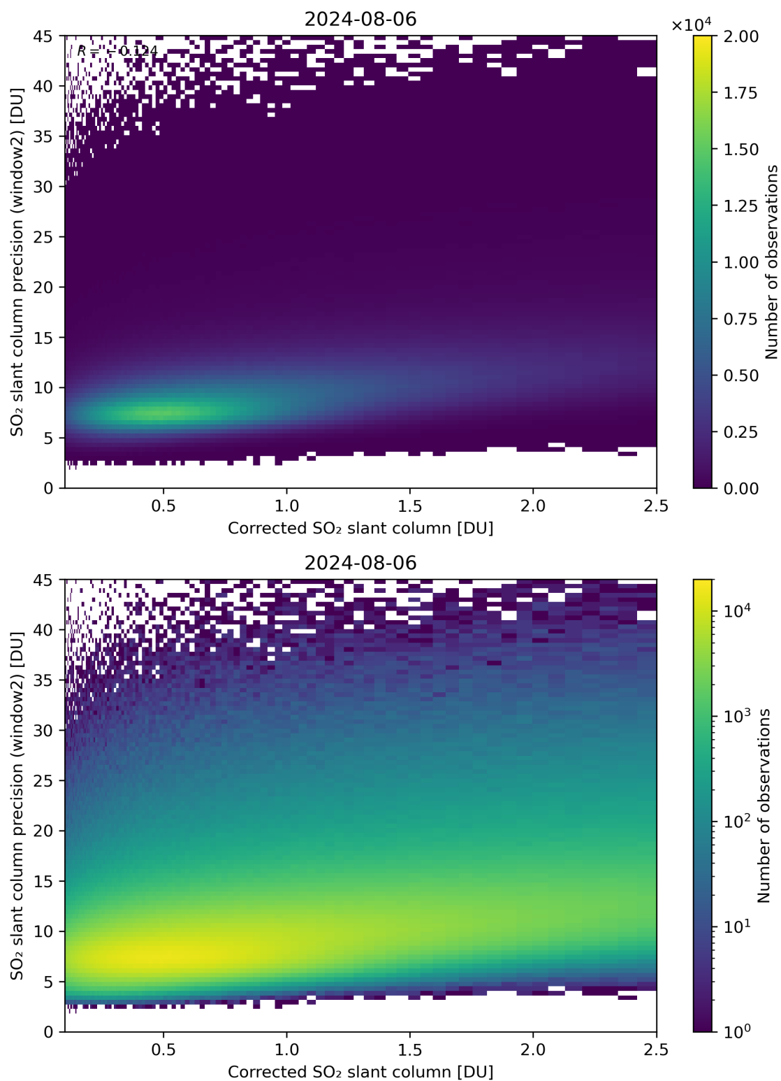
Figure 189: Scatter density plot of “Corrected SO 2 slant column” against “SO 2 slant column precision (window2)” for 2024-08-06 to 2024-08-07.
