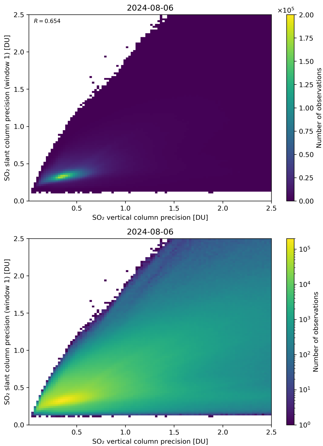
Figure 290: Scatter density plot of “SO 2 vertical column precision” against “SO 2 slant column precision (window 1)” for 2024-08-06 to 2024-08-07.
