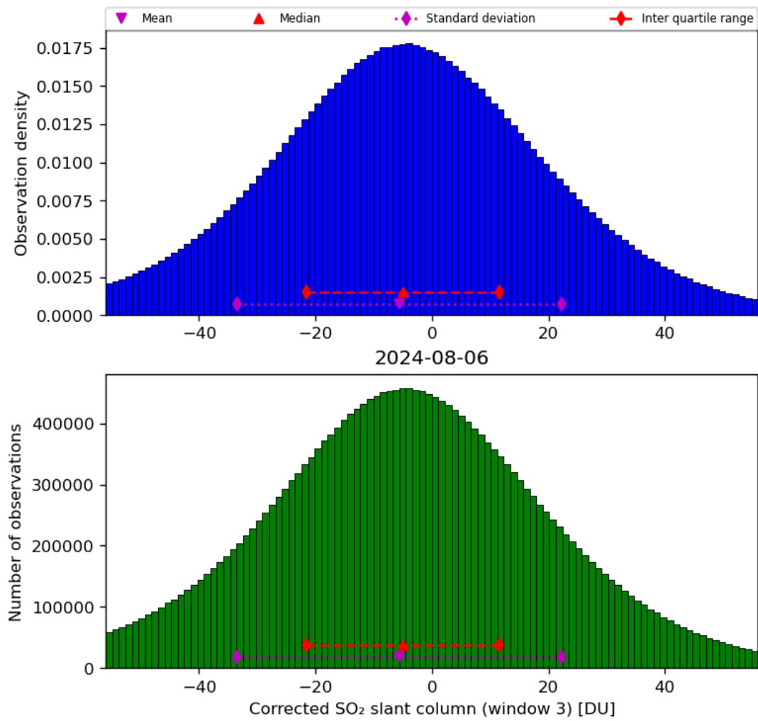
Figure 66: Histogram of “Corrected SO 2 slant column (window 3)” for 2024-08-06 to 2024-08-07
