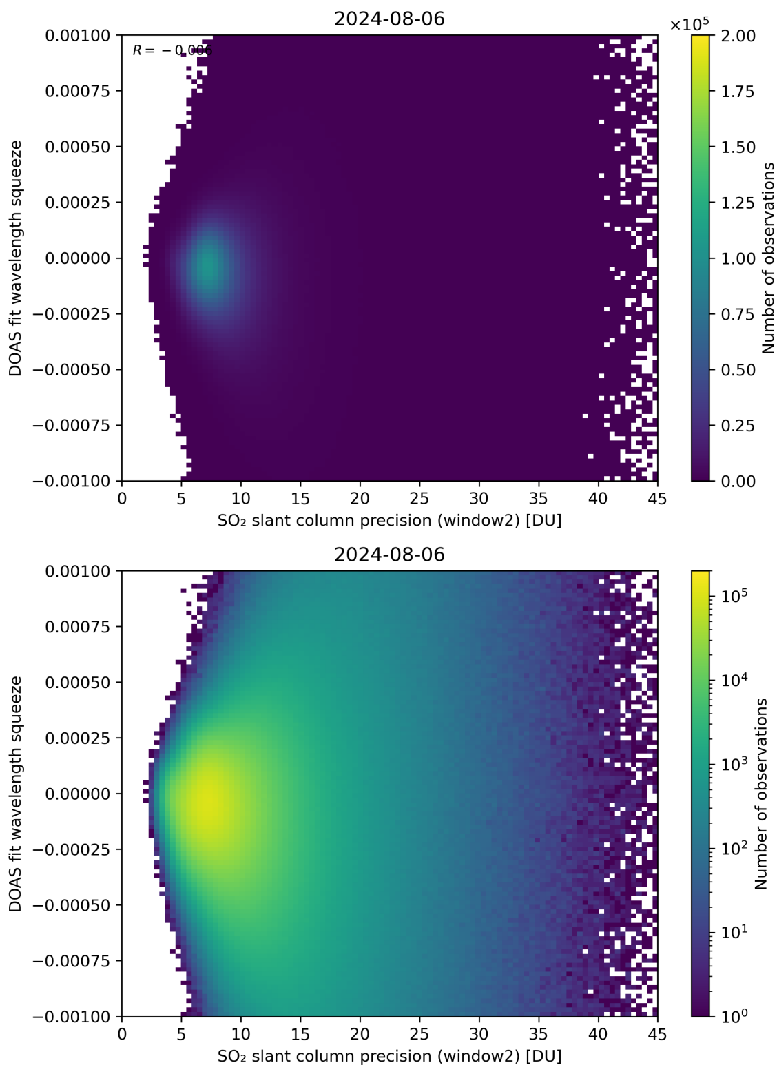
Figure 244: Scatter density plot of “SO 2 slant column precision (window2)” against “DOAS fit wavelength squeeze” for 2024-08-06 to 2024-08-07.
