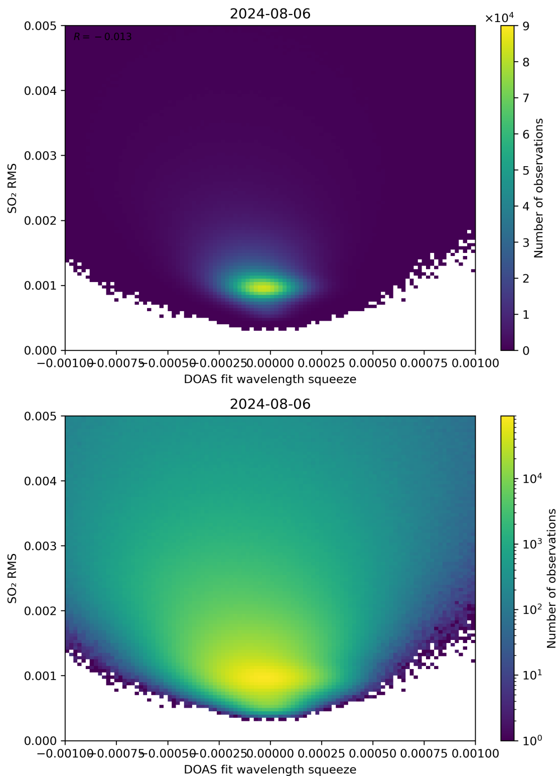
Figure 132: Scatter density plot of “DOAS fit wavelength squeeze” against “SO 2 RMS” for 2024-08-06 to 2024-08-07.
