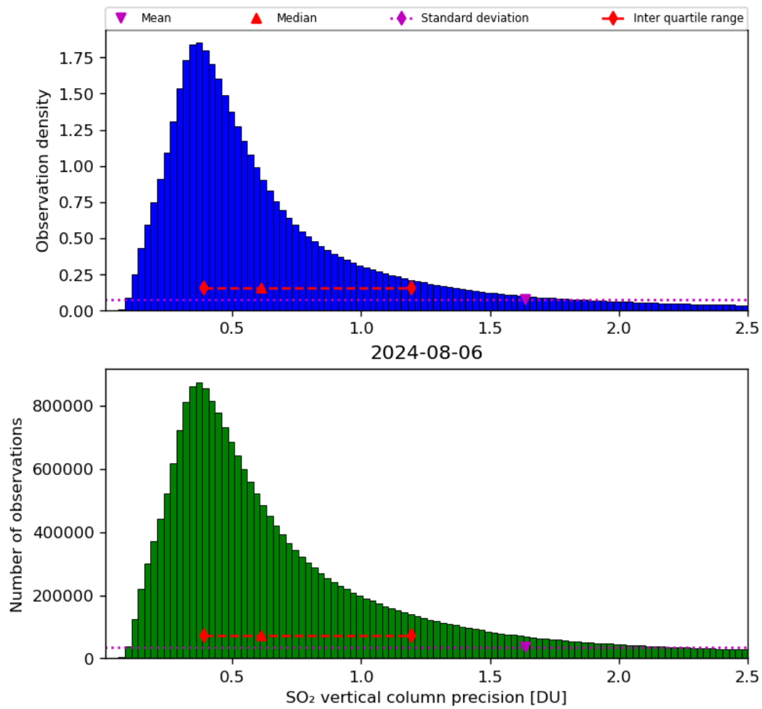
Figure 54: Histogram of “SO 2 vertical column precision” for 2024-08-06 to 2024-08-07
