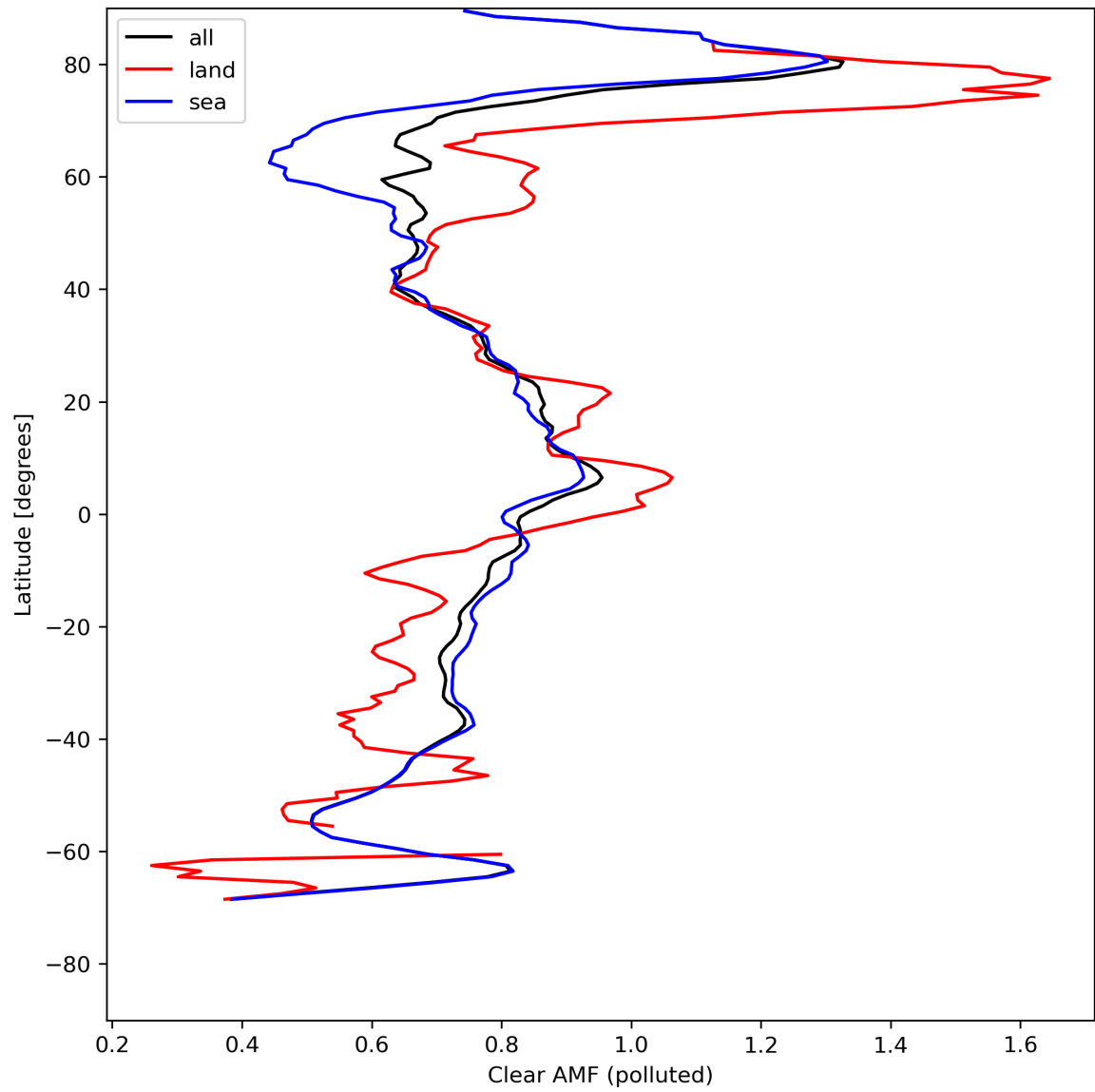
Figure 50: Zonal average of “Clear AMF (polluted)” for 2024-08-06 to 2024-08-07.
