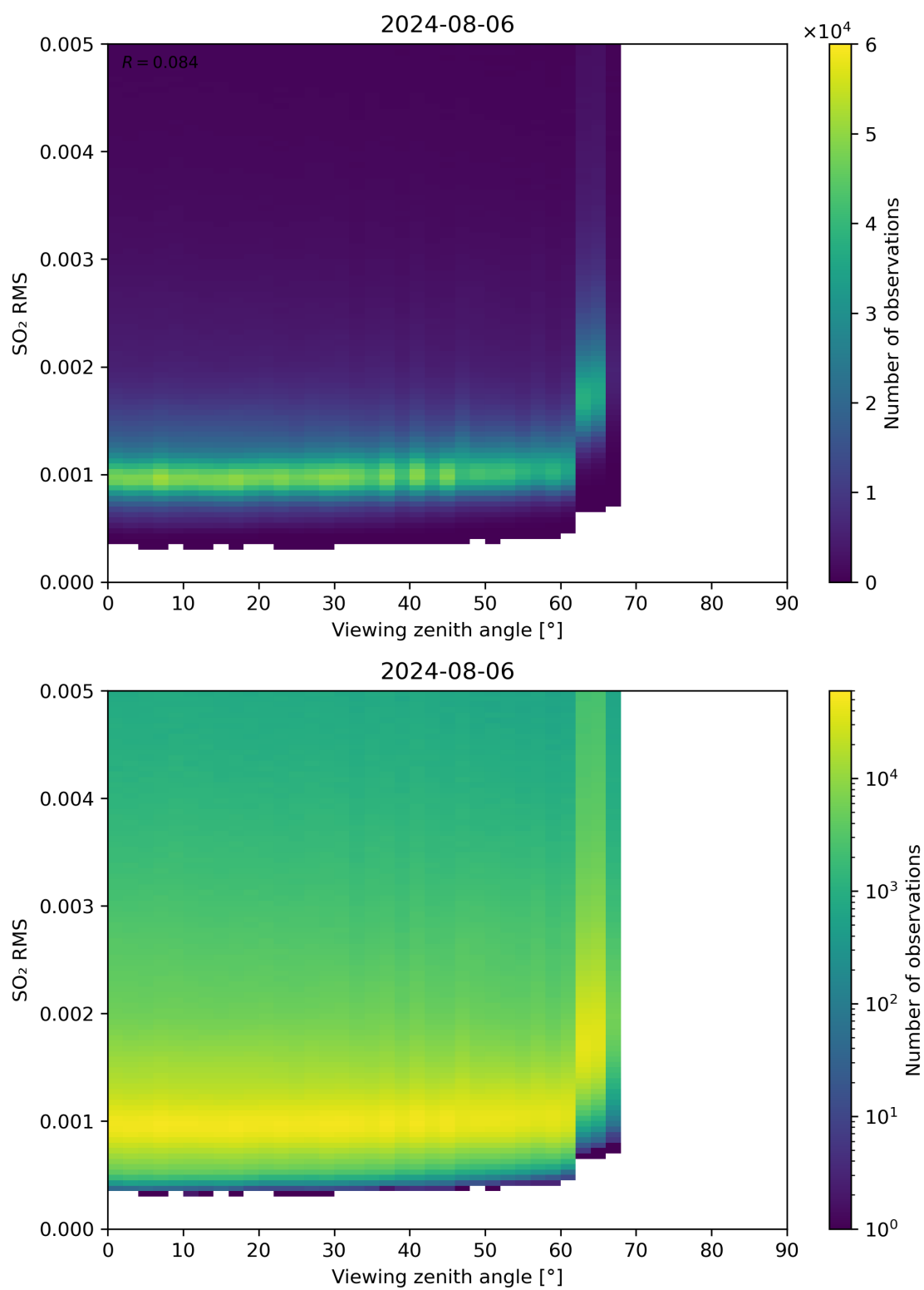
Figure 313: Scatter density plot of “Viewing zenith angle” against “SO 2 RMS” for 2024-08-06 to 2024-08-07.
