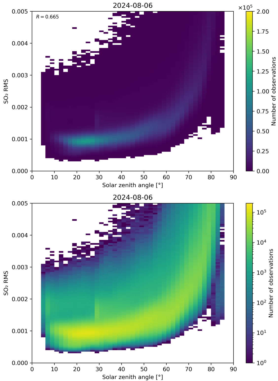
Figure 163: Scatter density plot of “Solar zenith angle” against “SO 2 RMS” for 2024-08-06 to 2024-08-07.
