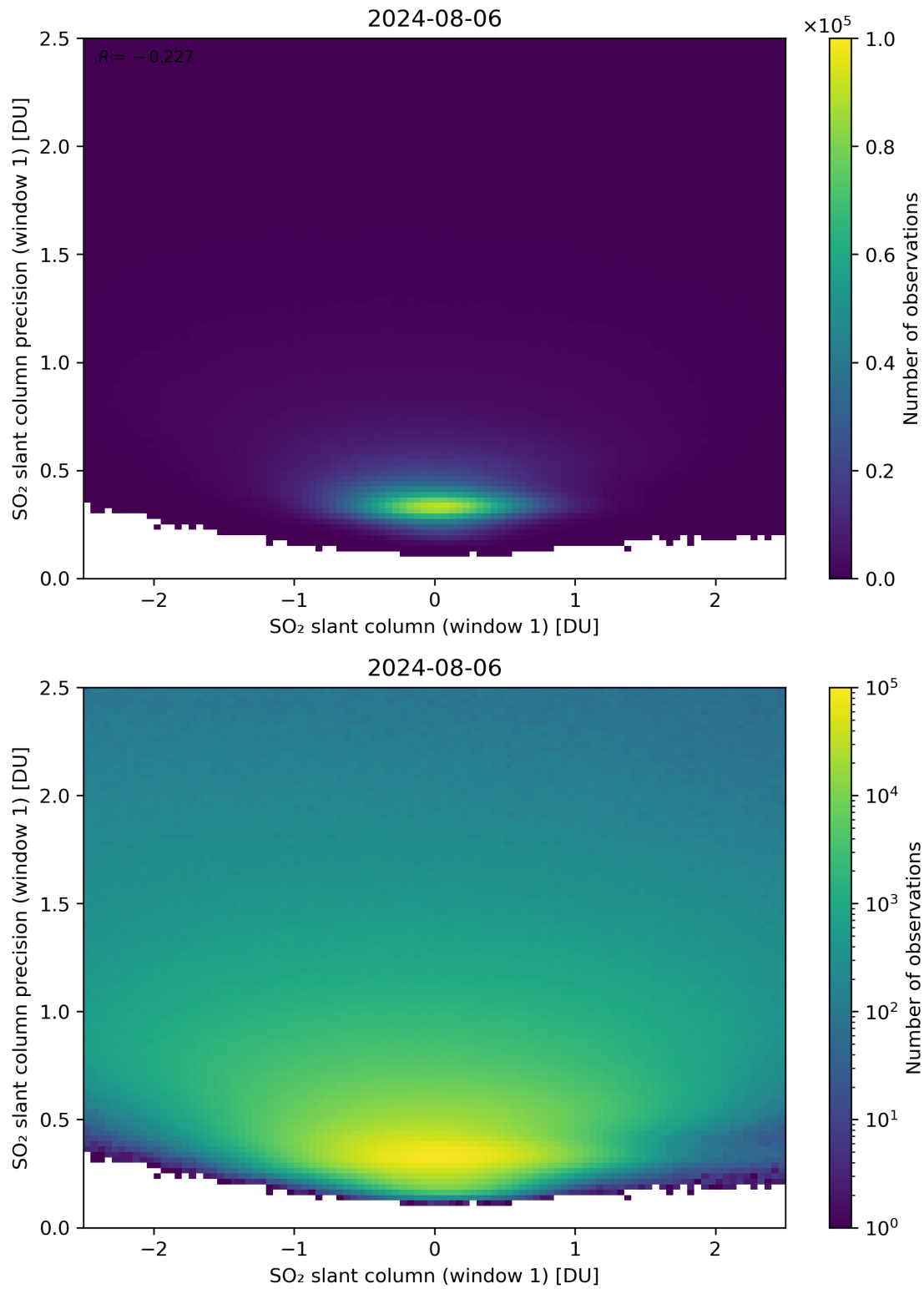
Figure 235: Scatter density plot of “SO 2 slant column (window 1)” against “SO 2 slant column precision (window 1)” for 2024-08-06 to 2024-08-07.
