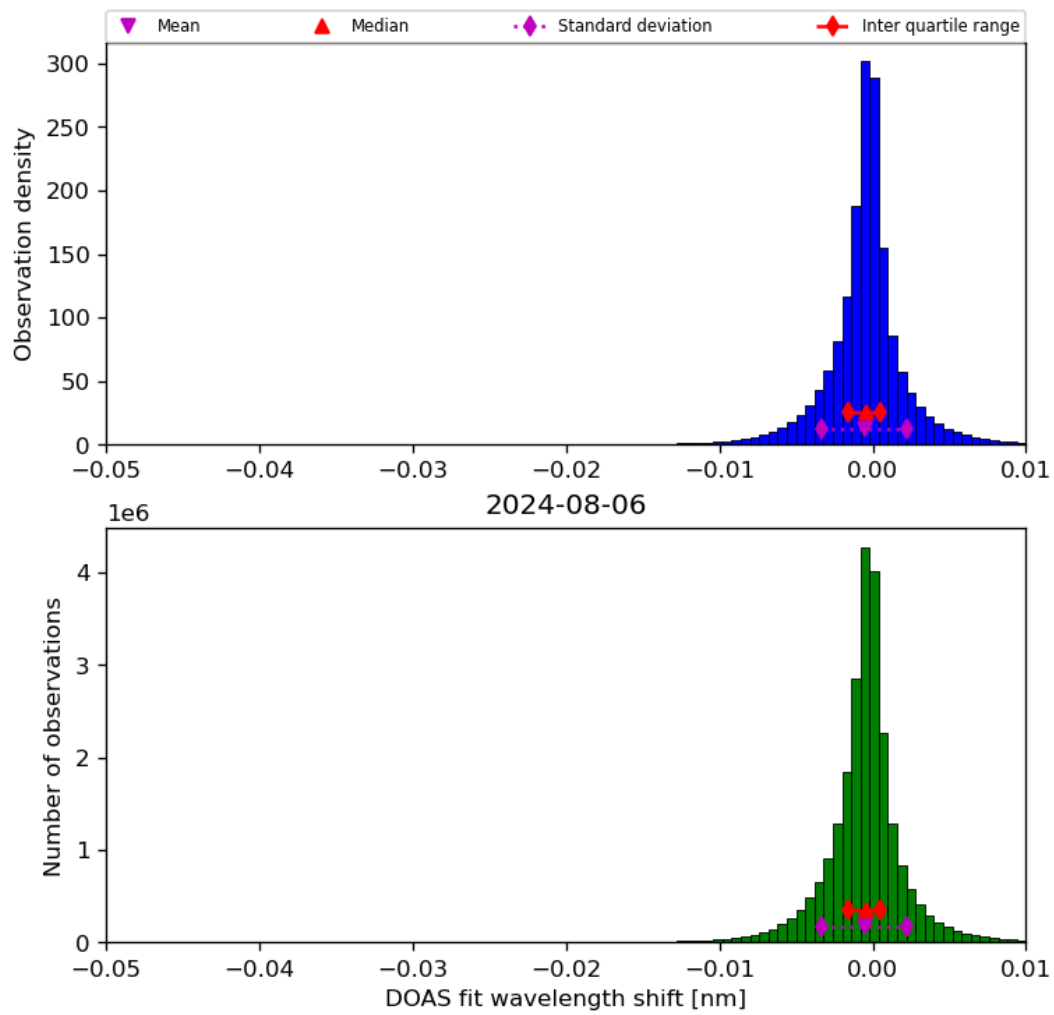
Figure 68: Histogram of “DOAS fit wavelength shift” for 2024-08-06 to 2024-08-07
