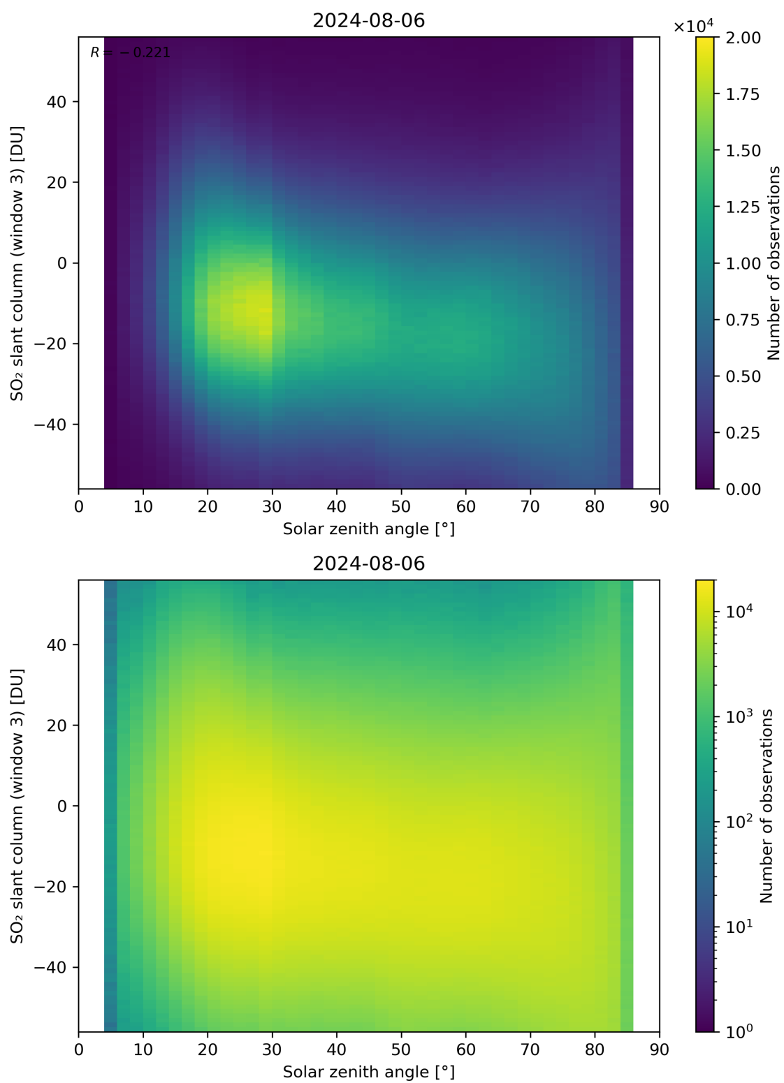
Figure 172: Scatter density plot of “Solar zenith angle” against “SO 2 slant column (window 3)” for 2024-08-06 to 2024-08-07.
