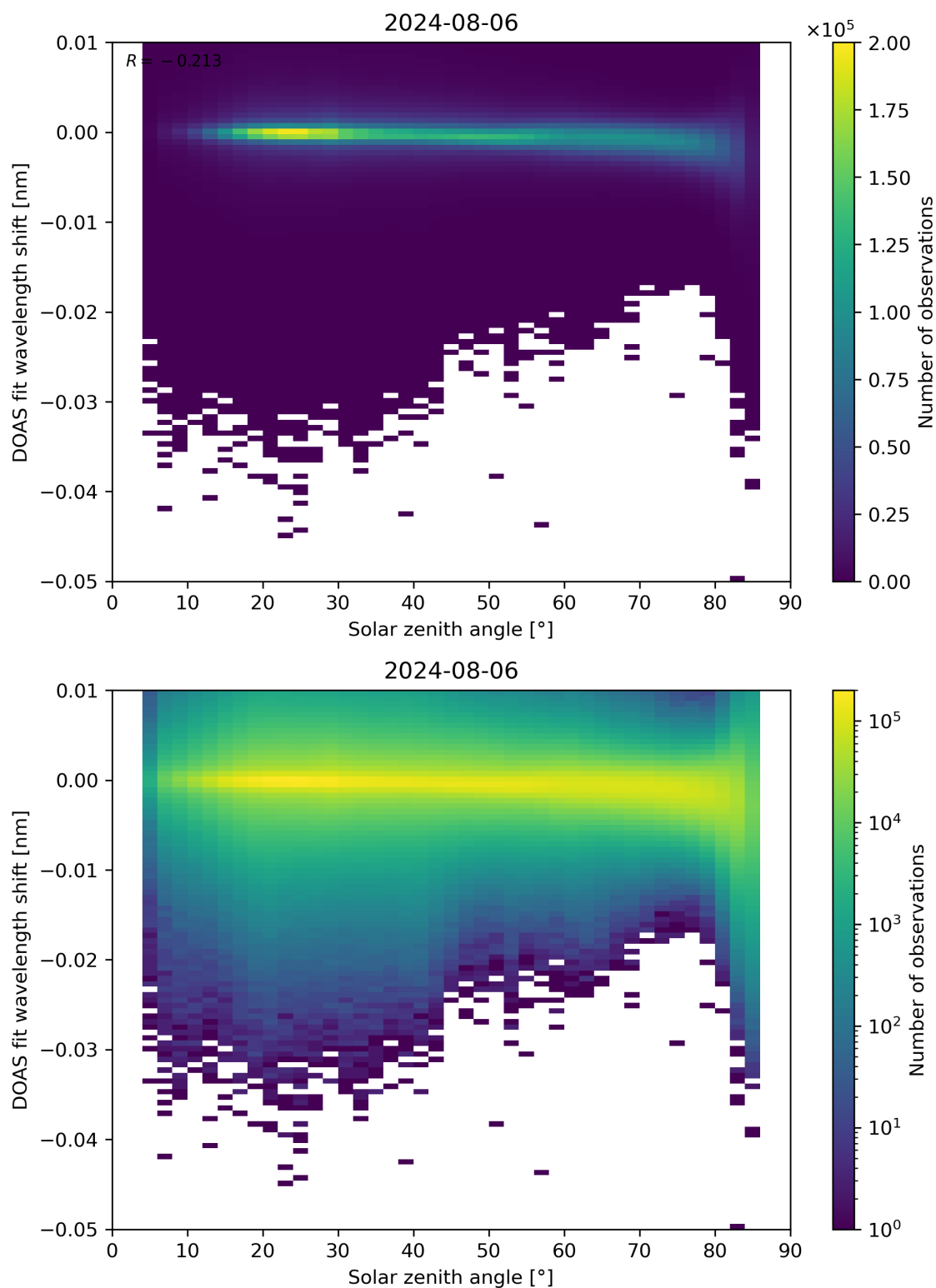
Figure 161: Scatter density plot of “Solar zenith angle” against “DOAS fit wavelength shift” for 2024-08-06 to 2024-08-07.
