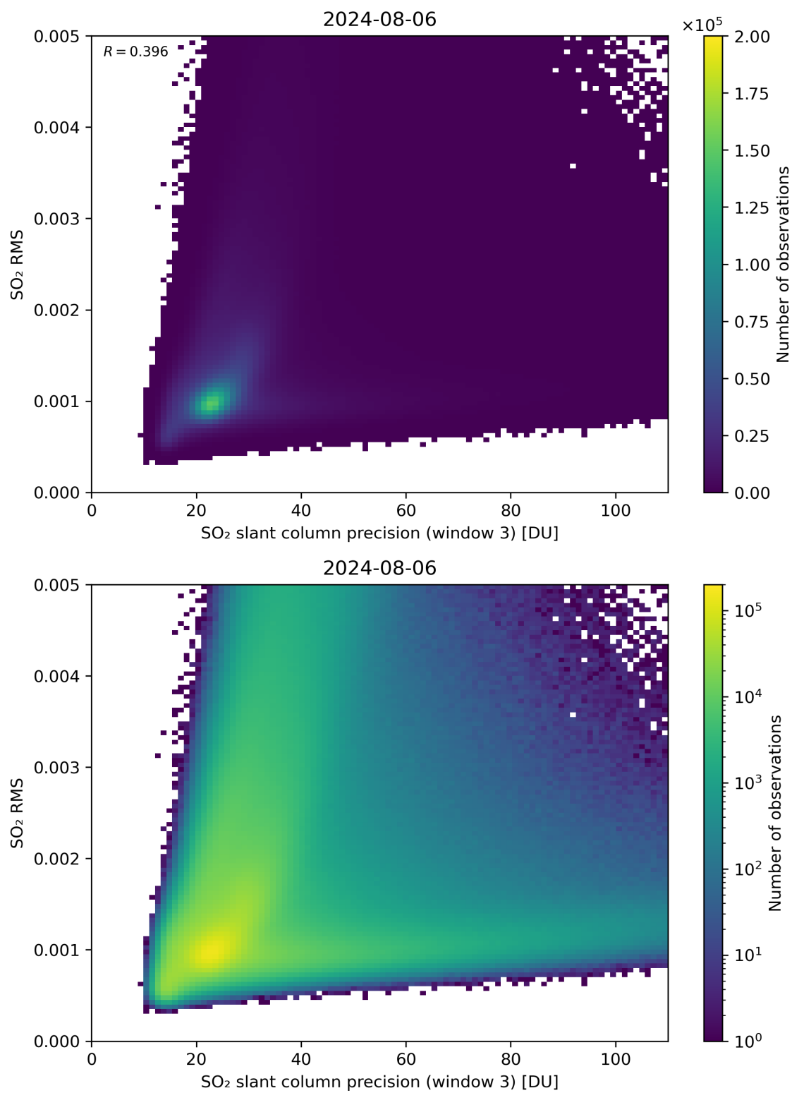
Figure 260: Scatter density plot of “SO 2 slant column precision (window 3)” against “SO 2 RMS” for 2024-08-06 to 2024-08-07.
