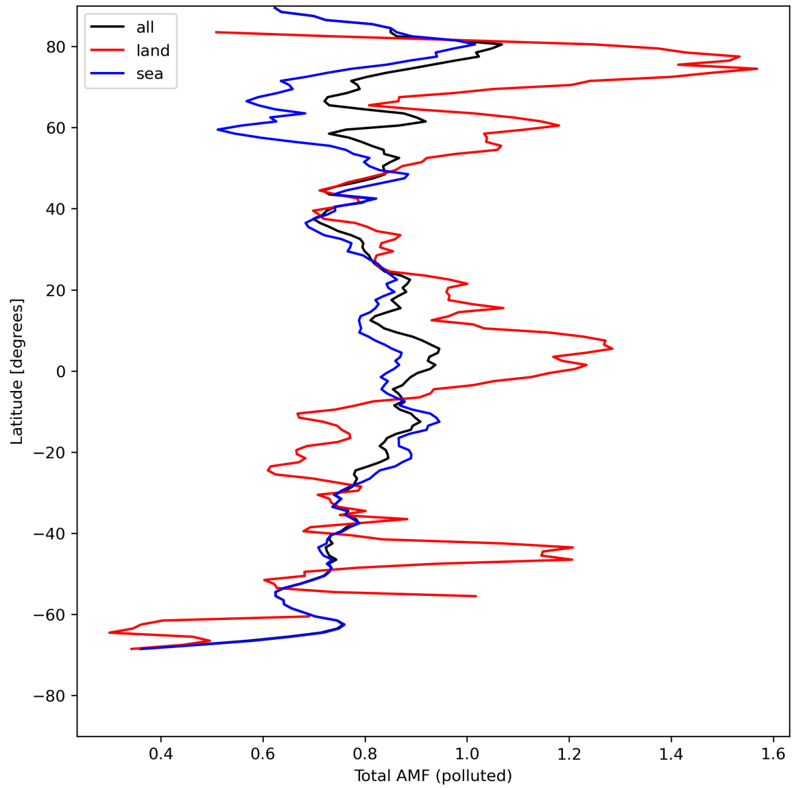
Figure 48: Zonal average of “Total AMF (polluted)” for 2024-08-06 to 2024-08-07.
