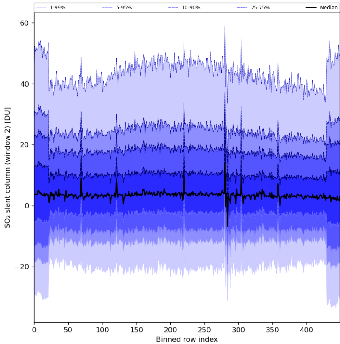
Figure 83: Along track statistics of “SO 2 slant column (window 2)” for 2024-08-06 to 2024-08-07
