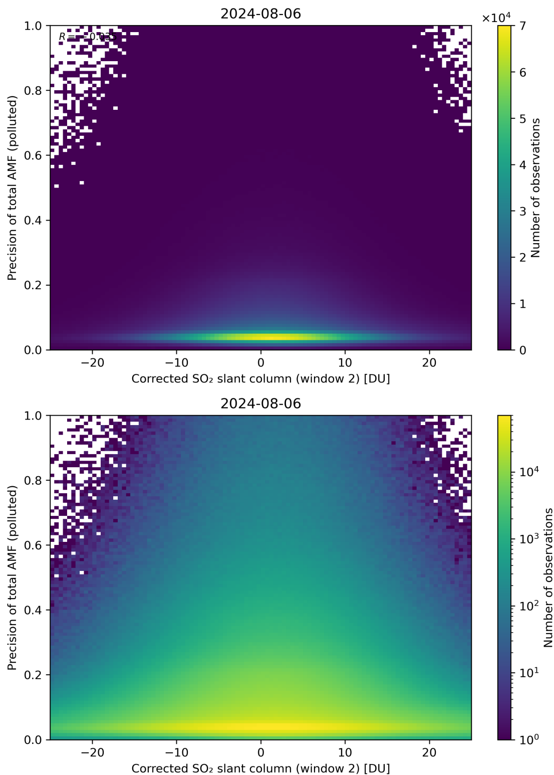
Figure 204: Scatter density plot of “Corrected SO 2 slant column (window 2)” against “Precision of total AMF (polluted)” for 2024-08-06 to 2024-08-07.
