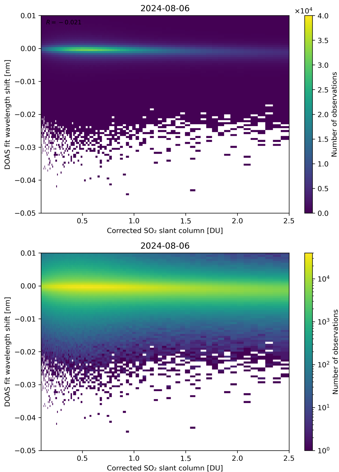
Figure 181: Scatter density plot of “Corrected SO 2 slant column” against “DOAS fit wavelength shift” for 2024-08-06 to 2024-08-07.
