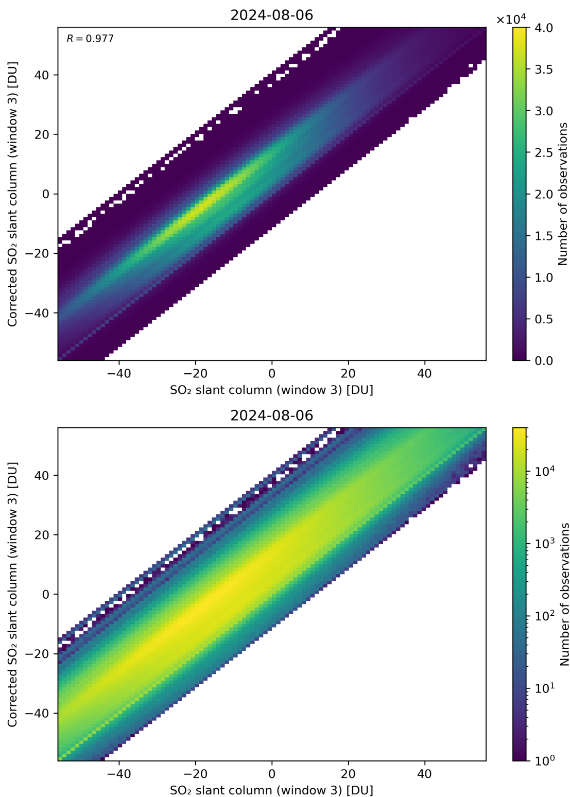
Figure 266: Scatter density plot of “SO 2 slant column (window 3)” against “Corrected SO 2 slant column (window 3)” for 2024-08-06 to 2024-08-07.
