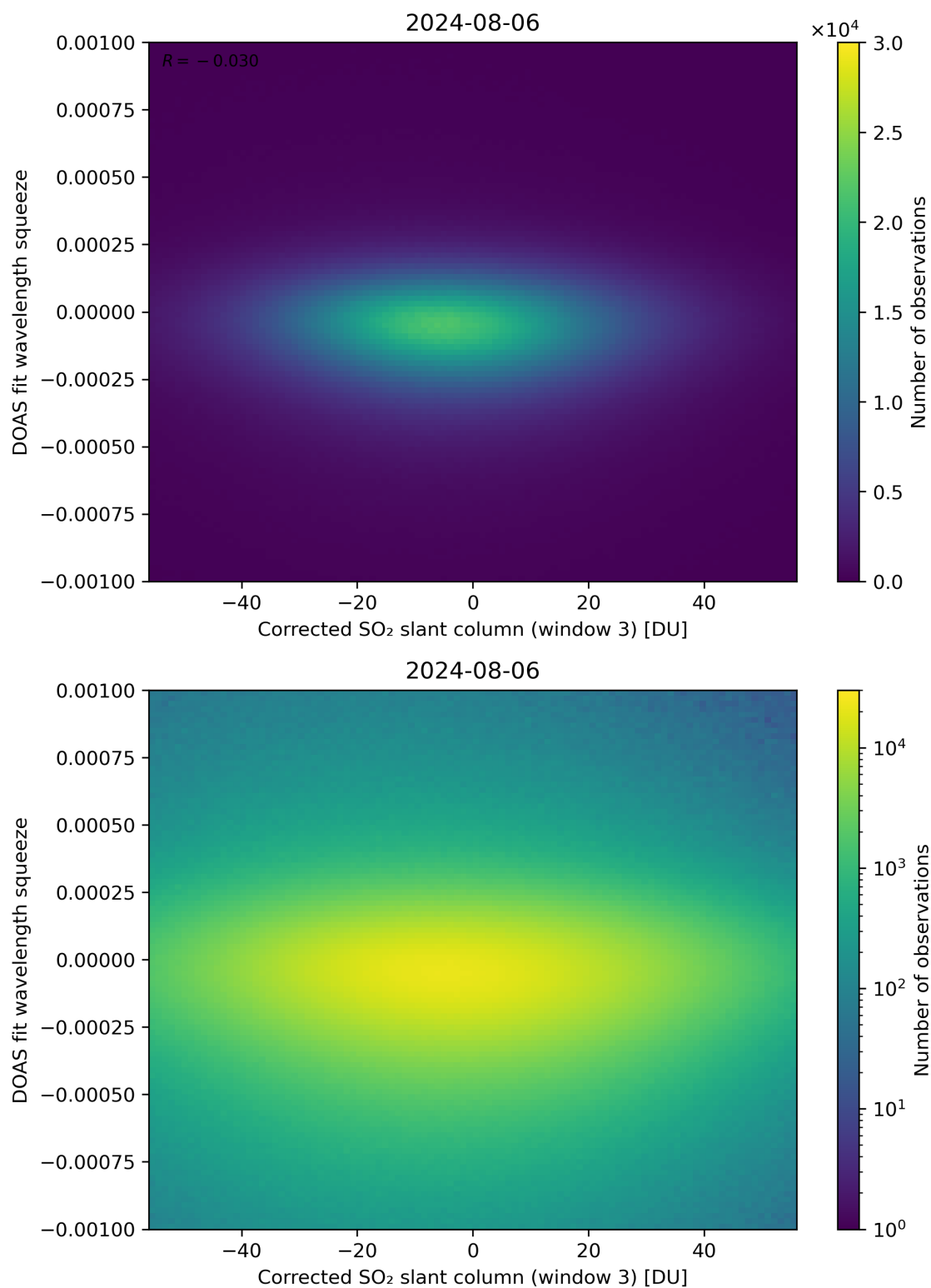
Figure 207: Scatter density plot of “Corrected SO 2 slant column (window 3)” against “DOAS fit wavelength squeeze” for 2024-08-06 to 2024-08-07.
