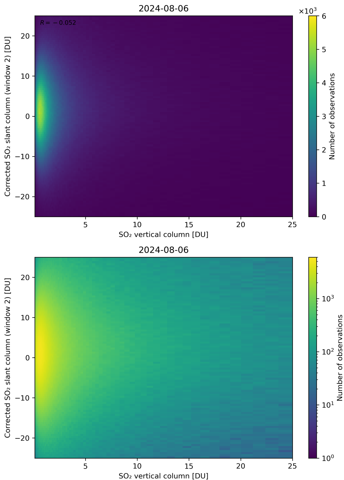
Figure 298: Scatter density plot of “SO 2 vertical column” against “Corrected SO 2 slant column (window 2)” for 2024-08-06 to 2024-08-07.
