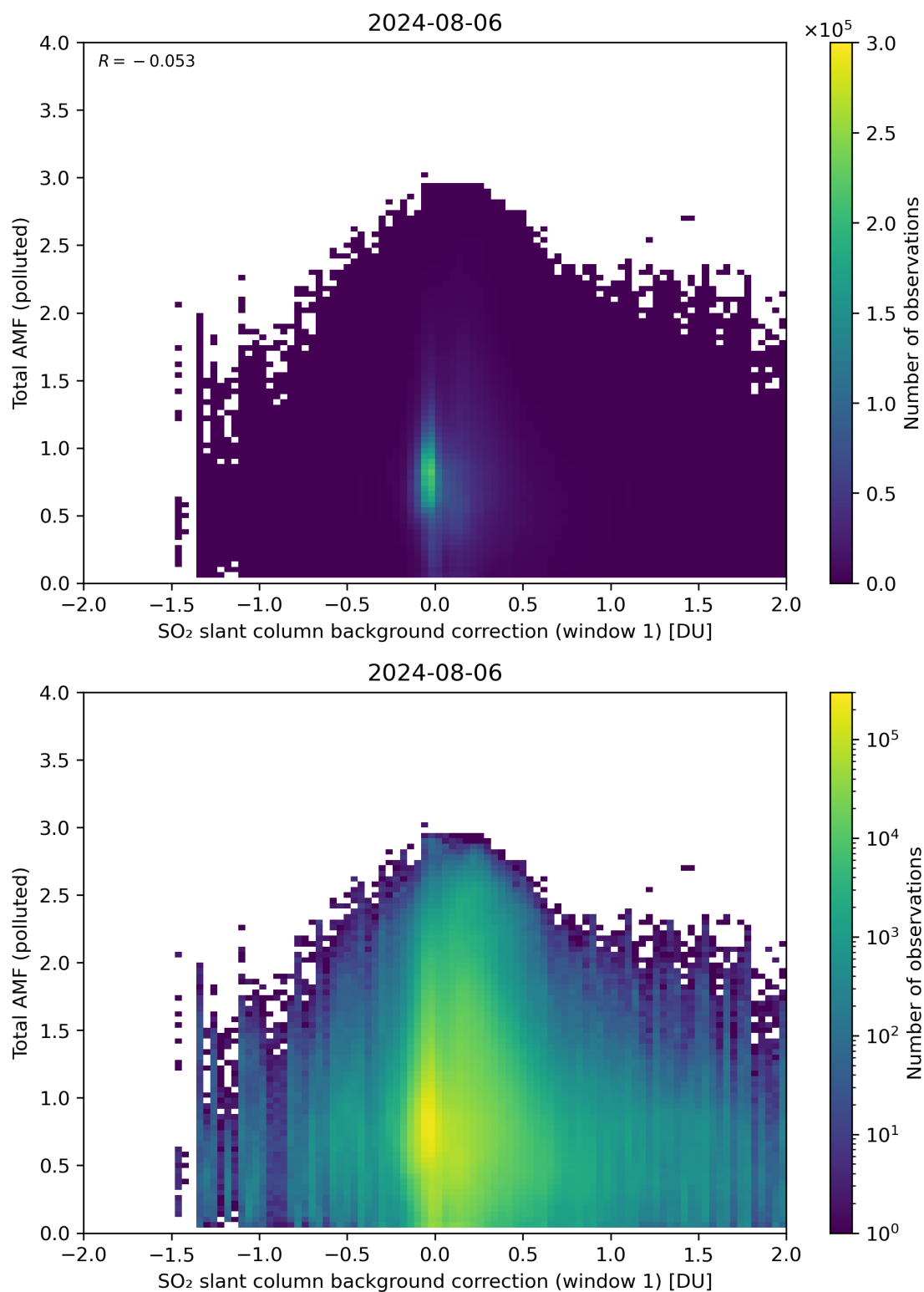
Figure 109: Scatter density plot of “SO 2 slant column background correction (window 1)” against “Total AMF (polluted)” for 2024-08-06 to 2024-08-07.
