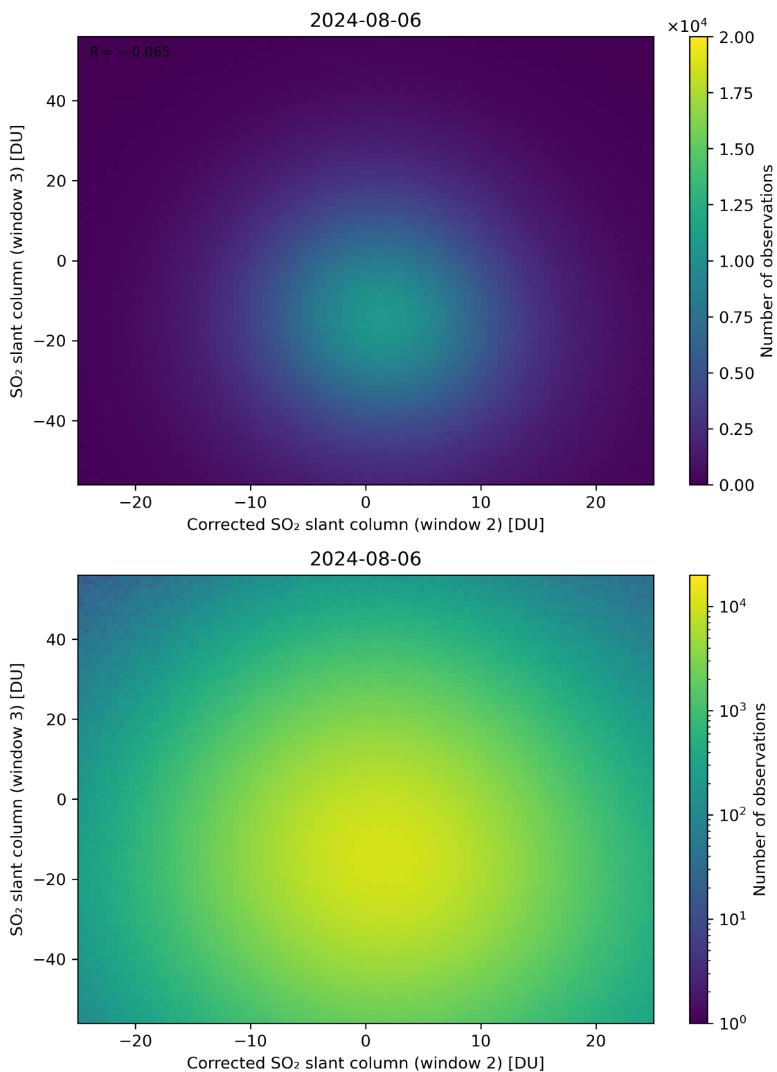
Figure 201: Scatter density plot of “Corrected SO 2 slant column (window 2)” against “SO 2 slant column (window 3)” for 2024-08-06 to 2024-08-07.
