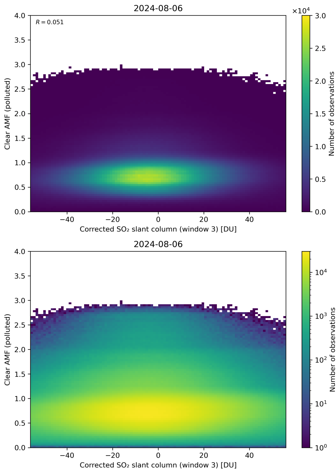
Figure 209: Scatter density plot of “Corrected SO 2 slant column (window 3)” against “Clear AMF (polluted)” for 2024-08-06 to 2024-08-07.
