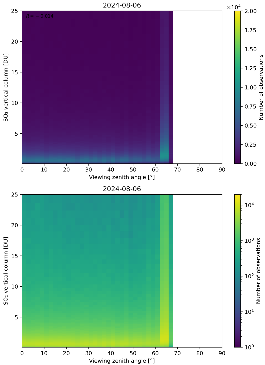
Figure 327: Scatter density plot of “Viewing zenith angle” against “SO 2 vertical column” for 2024-08-06 to 2024-08-07.
