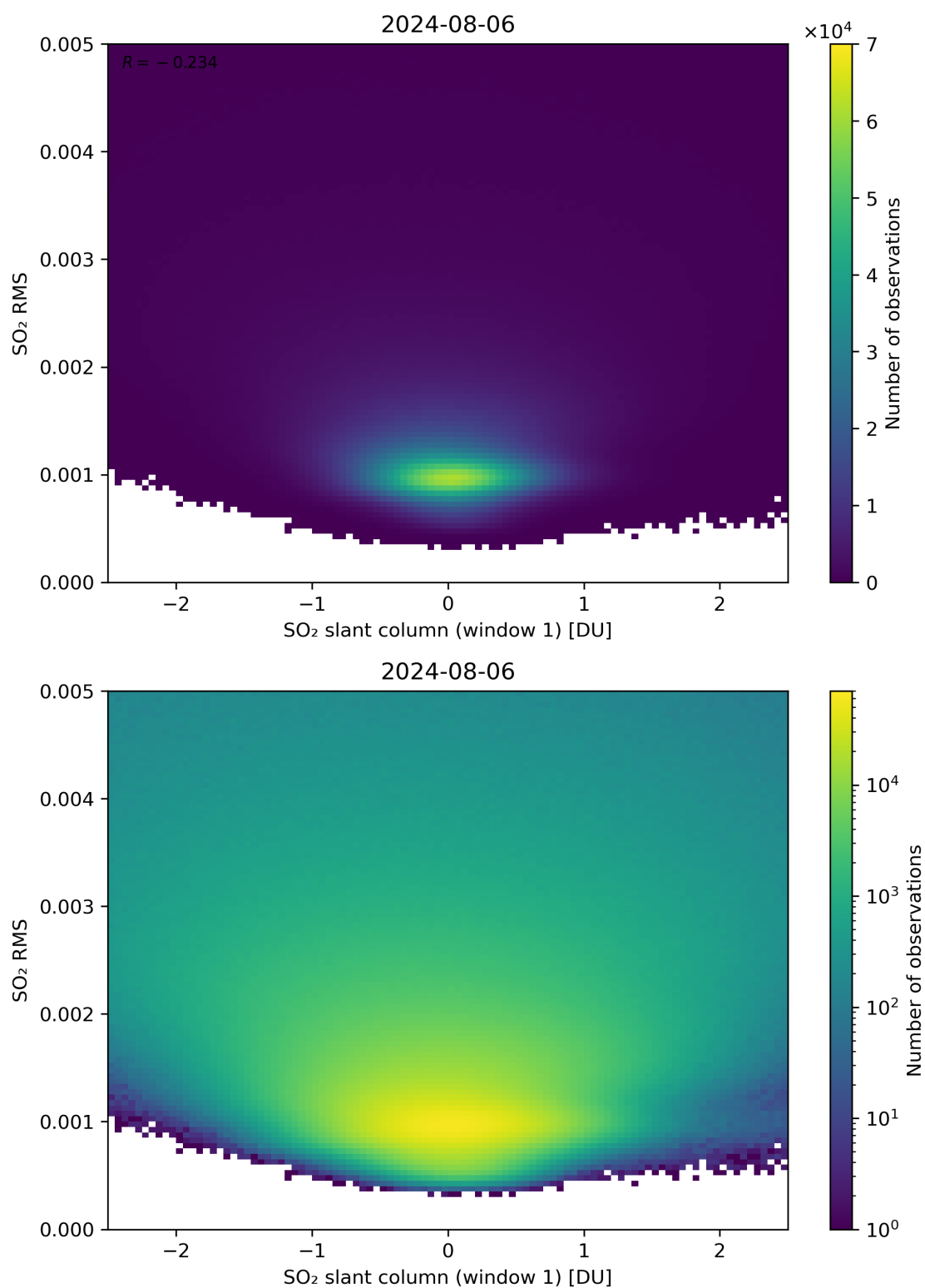
Figure 217: Scatter density plot of “SO 2 slant column (window 1)” against “SO 2 RMS” for 2024-08-06 to 2024-08-07.
