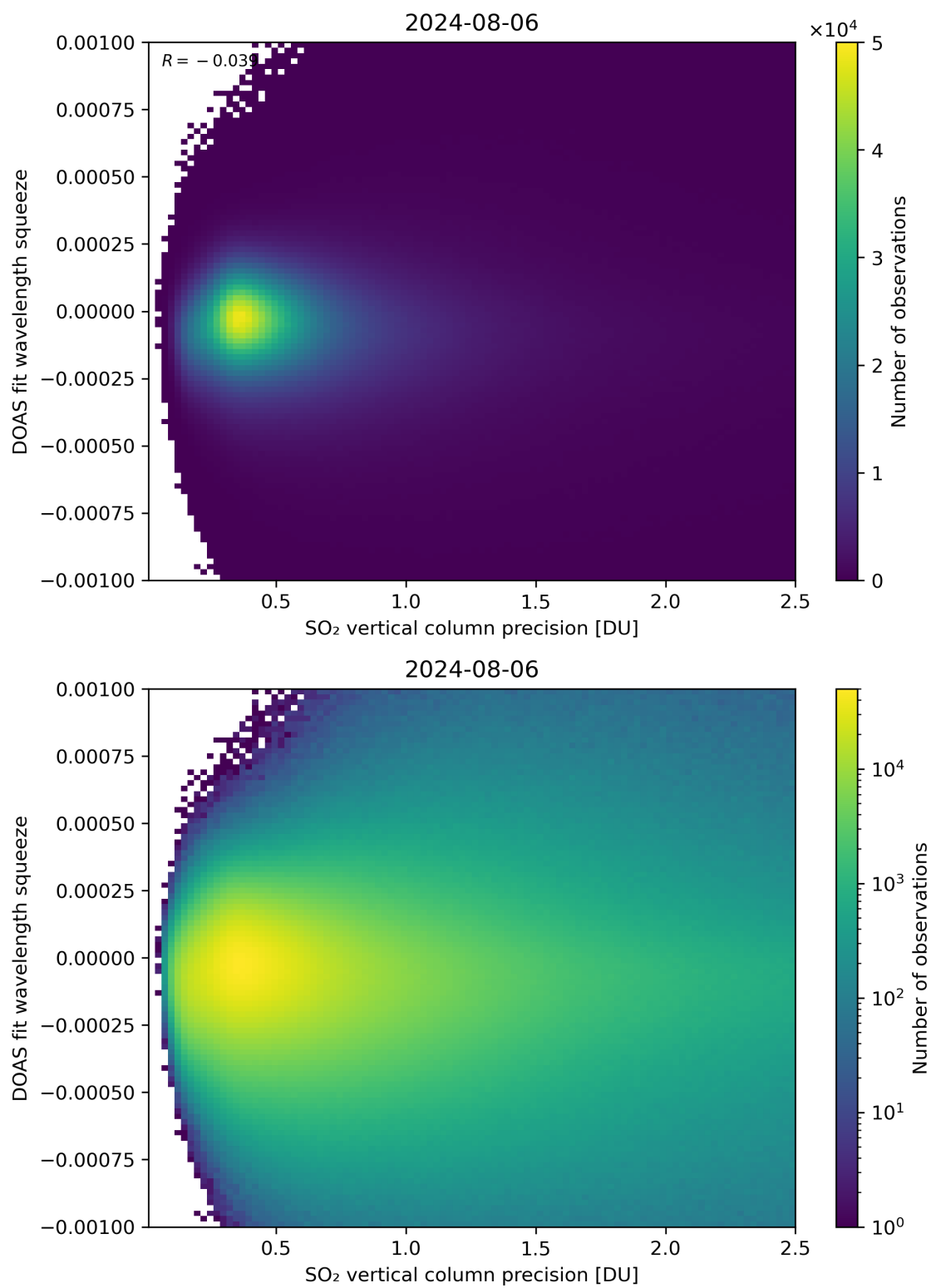
Figure 283: Scatter density plot of “SO 2 vertical column precision” against “DOAS fit wavelength squeeze” for 2024-08-06 to 2024-08-07.
