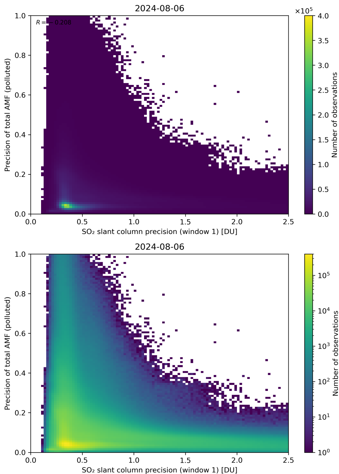
Figure 231: Scatter density plot of “SO 2 slant column precision (window 1)” against “Precision of total AMF (polluted)” for 2024-08-06 to 2024-08-07.
