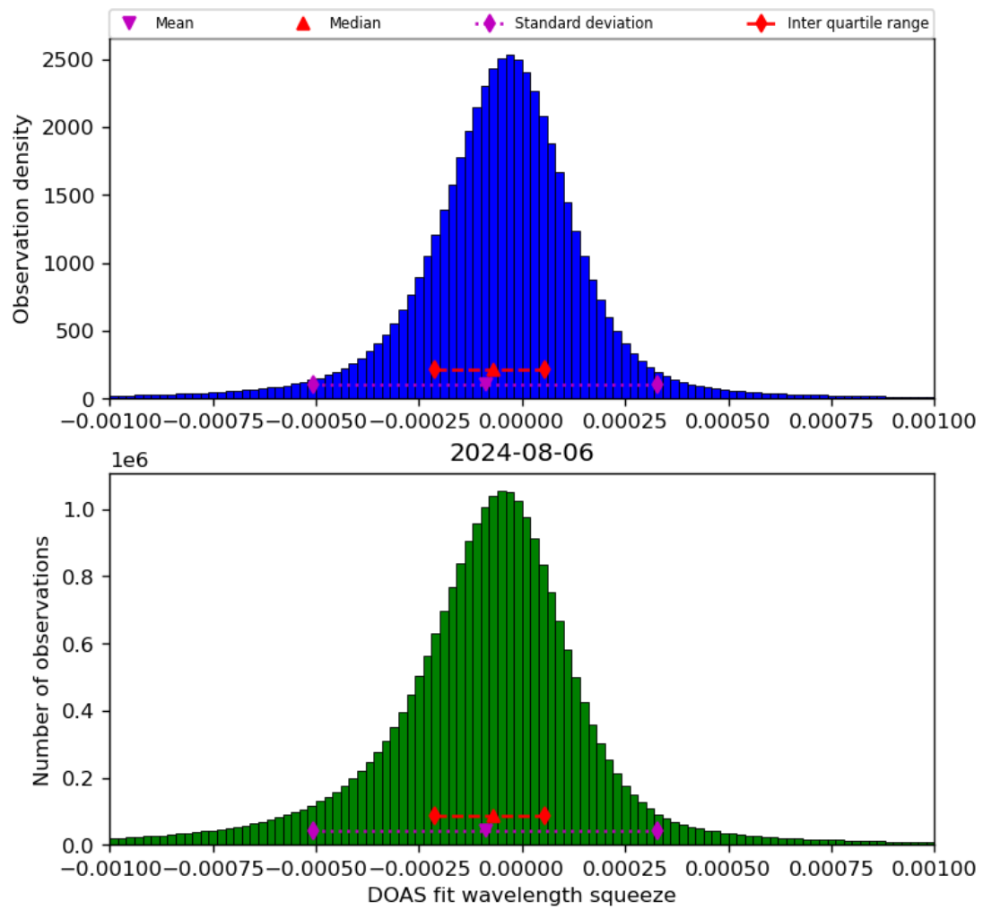
Figure 69: Histogram of “DOAS fit wavelength squeeze” for 2024-08-06 to 2024-08-07
