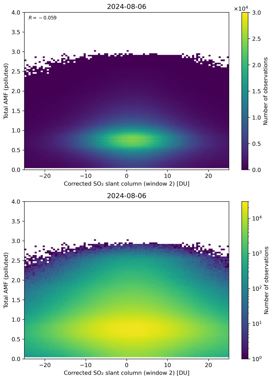
Figure 203: Scatter density plot of “Corrected SO 2 slant column (window 2)” against “Total AMF (polluted)” for 2024-08-06 to 2024-08-07.
