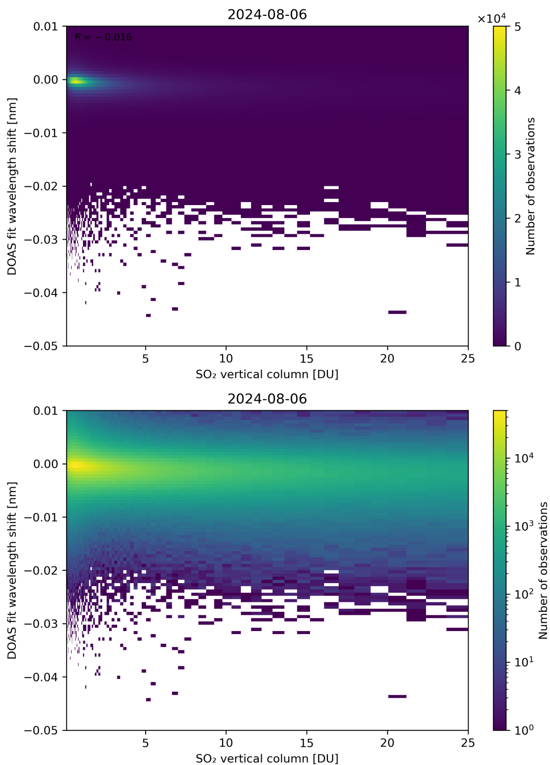
Figure 276: Scatter density plot of “SO 2 vertical column” against “DOAS fit wavelength shift” for 2024-08-06 to 2024-08-07.
