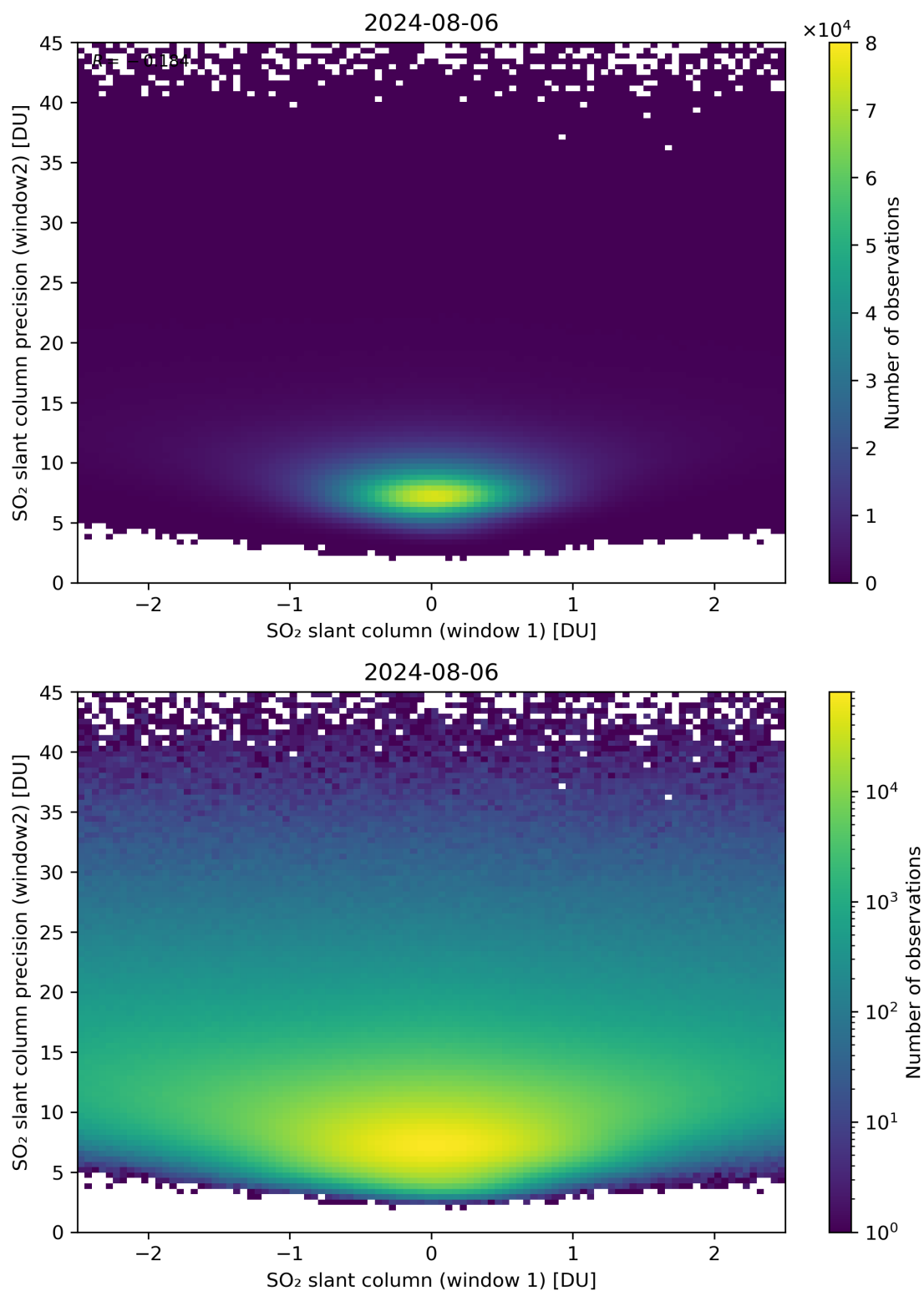
Figure 236: Scatter density plot of “SO 2 slant column (window 1)” against “SO 2 slant column precision (window2)” for 2024-08-06 to 2024-08-07.
