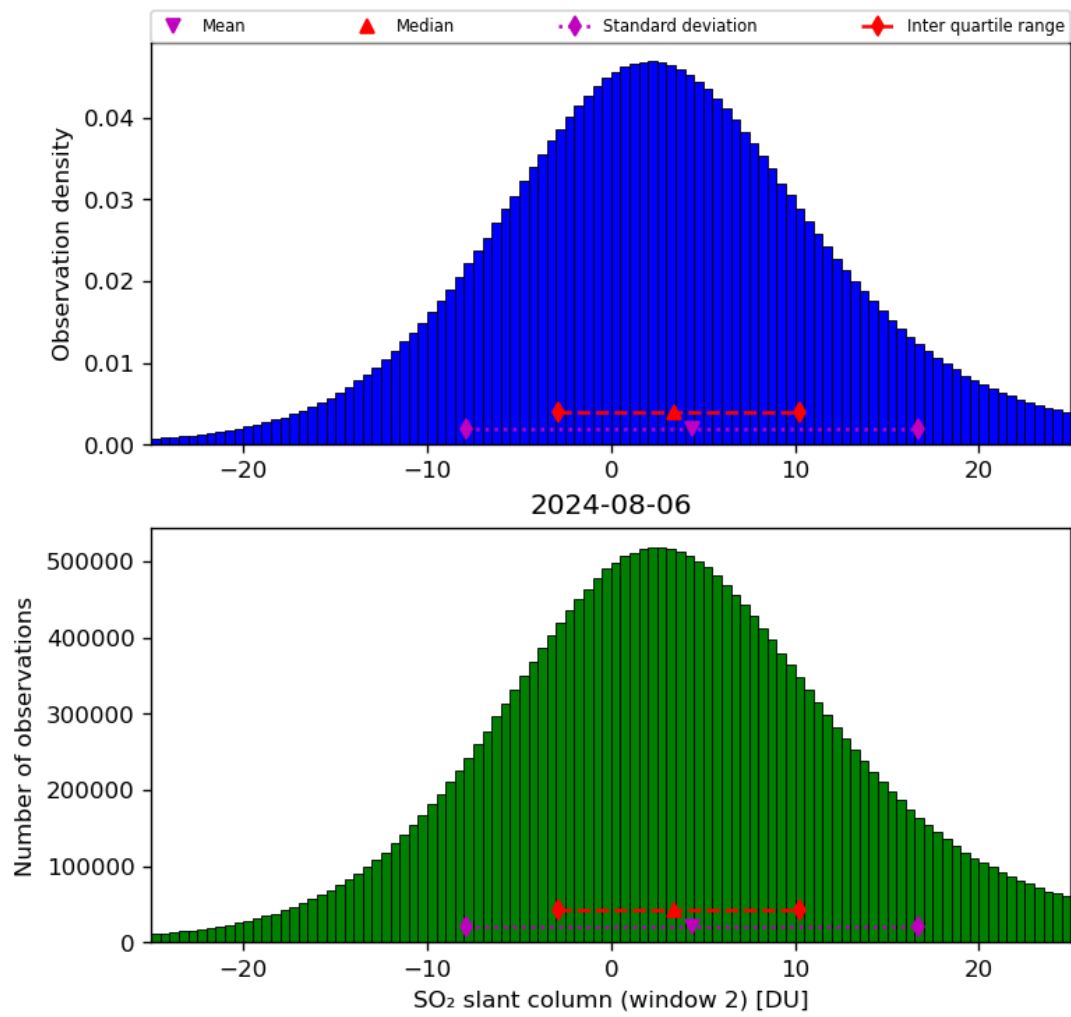
Figure 60: Histogram of “SO 2 slant column (window 2)” for 2024-08-06 to 2024-08-07
