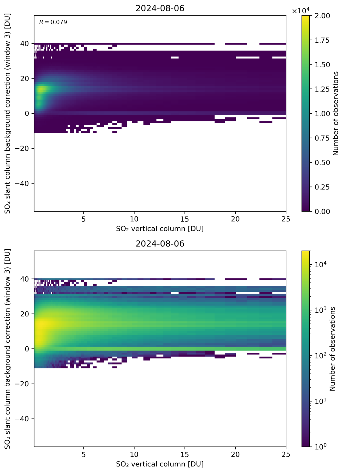
Figure 275: Scatter density plot of “SO 2 vertical column” against “SO 2 slant column background correction (window 3)” for 2024-08-06 to 2024-08-07.
