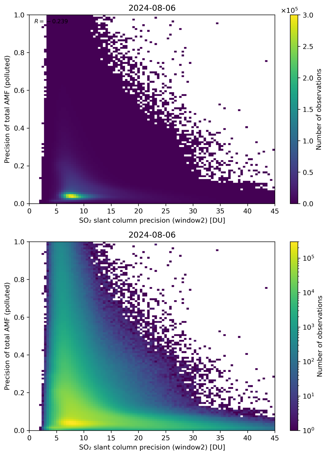
Figure 252: Scatter density plot of “SO 2 slant column precision (window2)” against “Precision of total AMF (polluted)” for 2024-08-06 to 2024-08-07.
