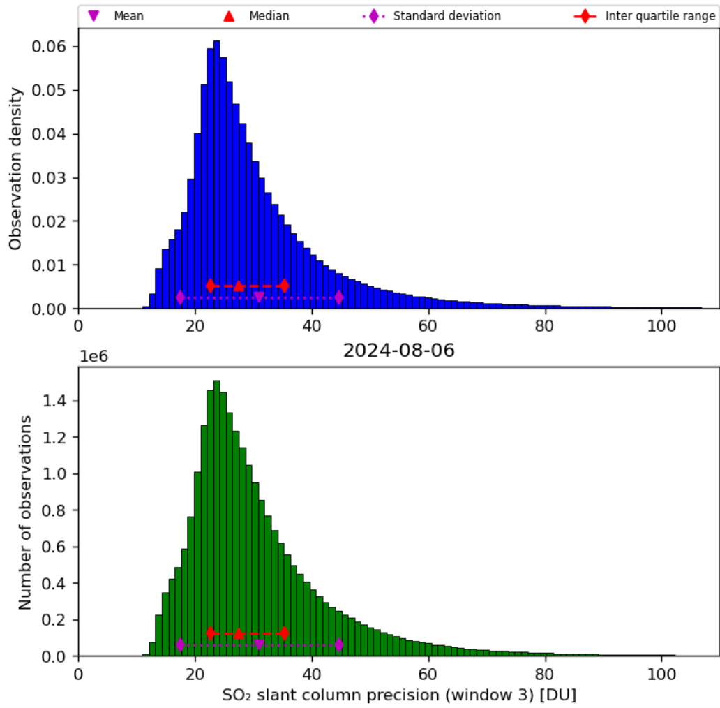
Figure 65: Histogram of “SO 2 slant column precision (window 3)” for 2024-08-06 to 2024-08-07
