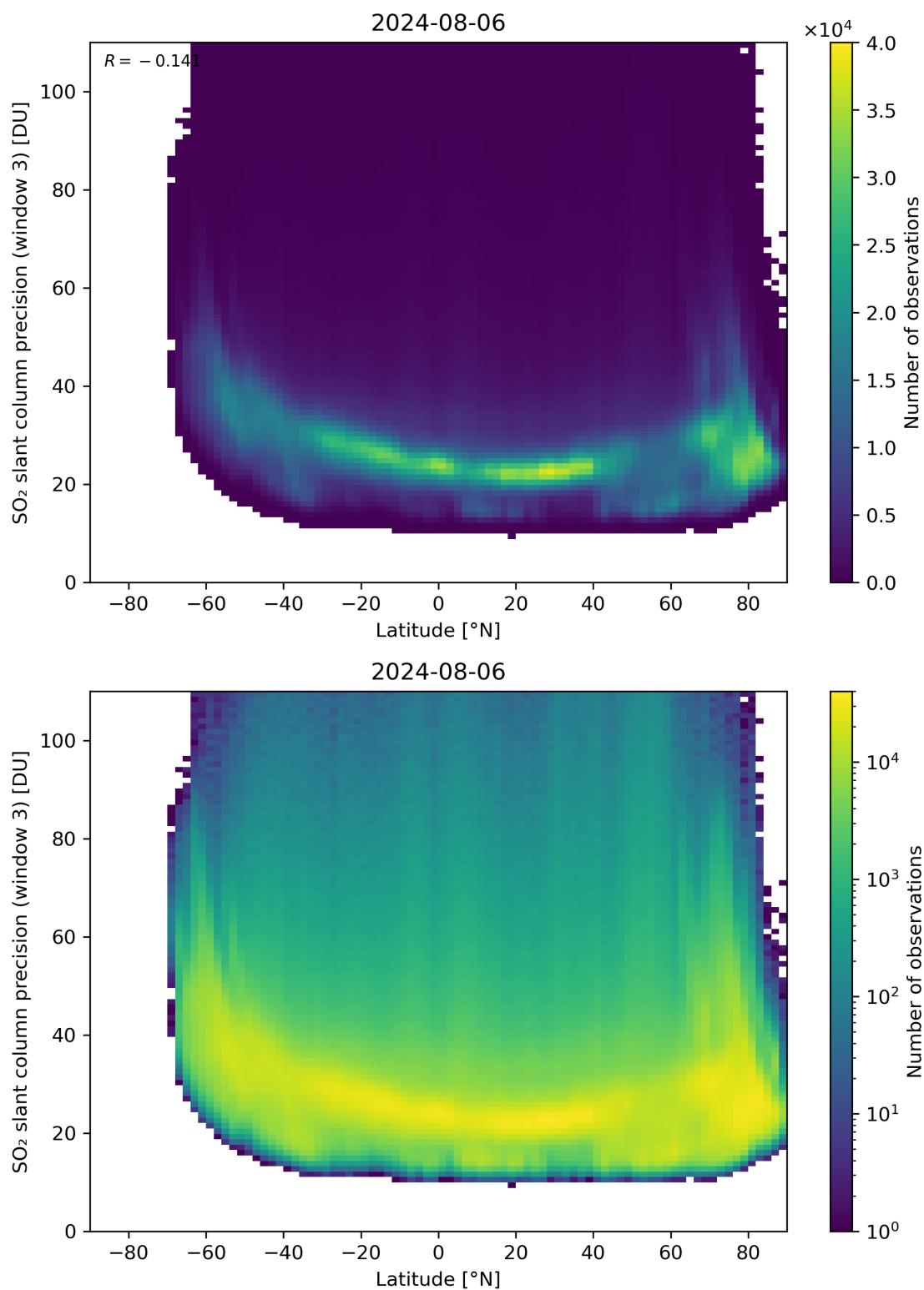
Figure 153: Scatter density plot of “Latitude” against “SO 2 slant column precision (window 3)” for 2024-08-06 to 2024-08-07.
