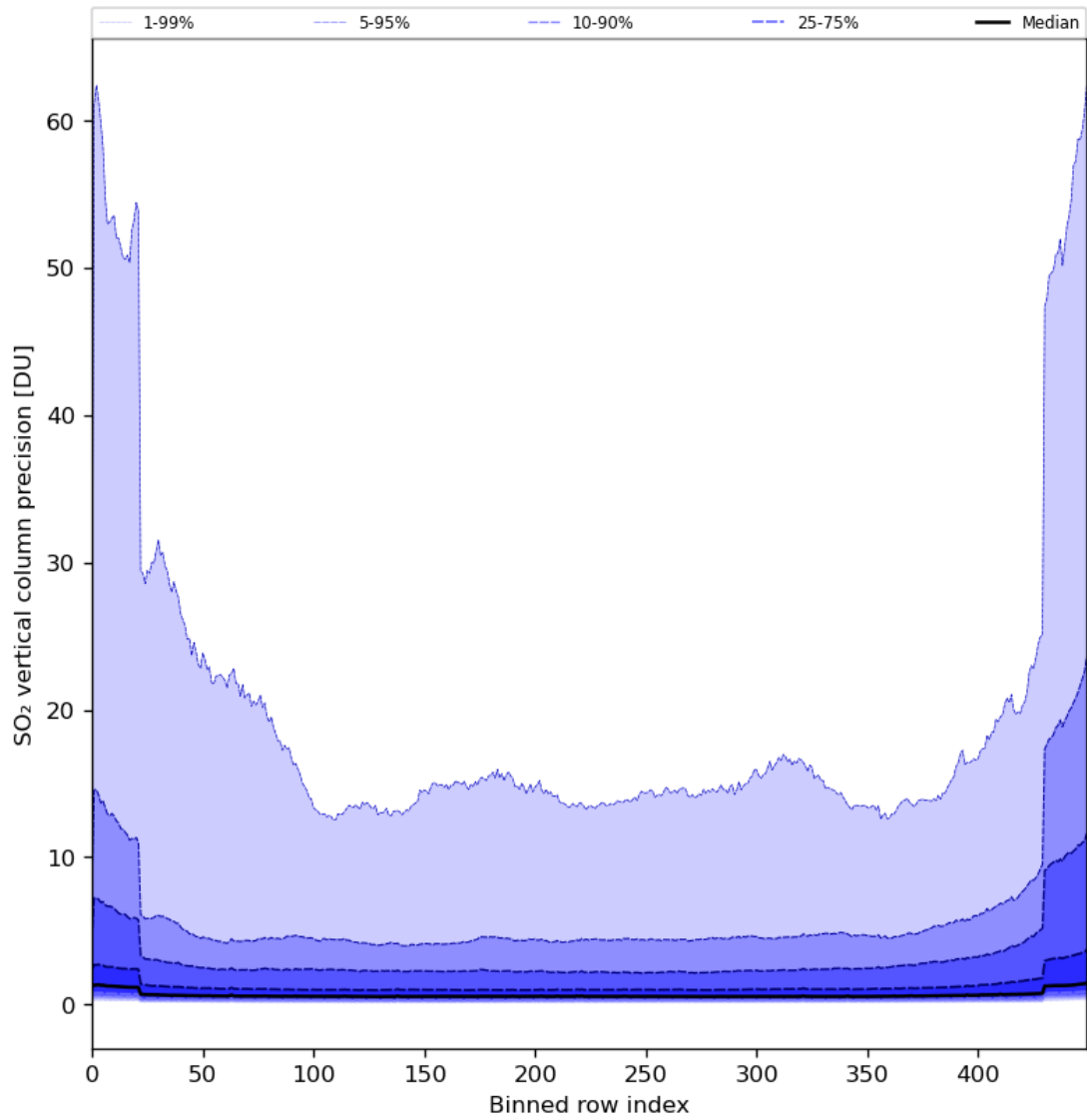
Figure 77: Along track statistics of “SO 2 vertical column precision” for 2024-08-06 to 2024-08-07
