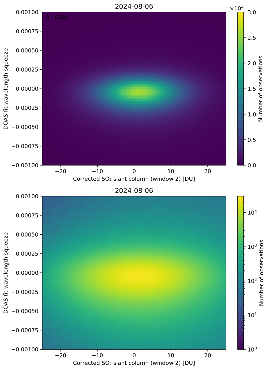
Figure 197: Scatter density plot of “Corrected SO 2 slant column (window 2)” against “DOAS fit wavelength squeeze” for 2024-08-06 to 2024-08-07.
