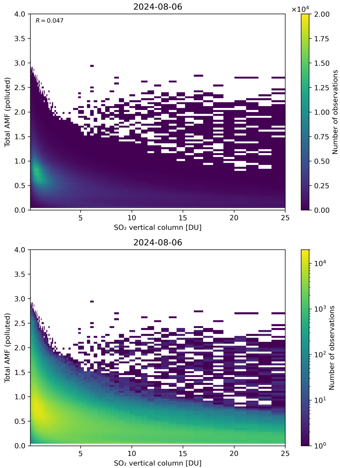
Figure 305: Scatter density plot of “SO 2 vertical column” against “Total AMF (polluted)” for 2024-08-06 to 2024-08-07.
