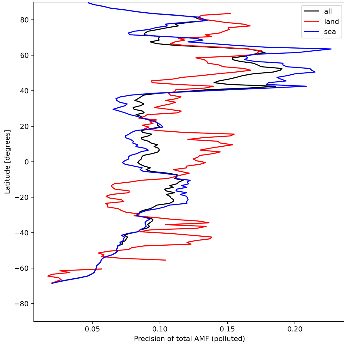
Figure 49: Zonal average of “Precision of total AMF (polluted)” for 2024-08-06 to 2024-08-07.
