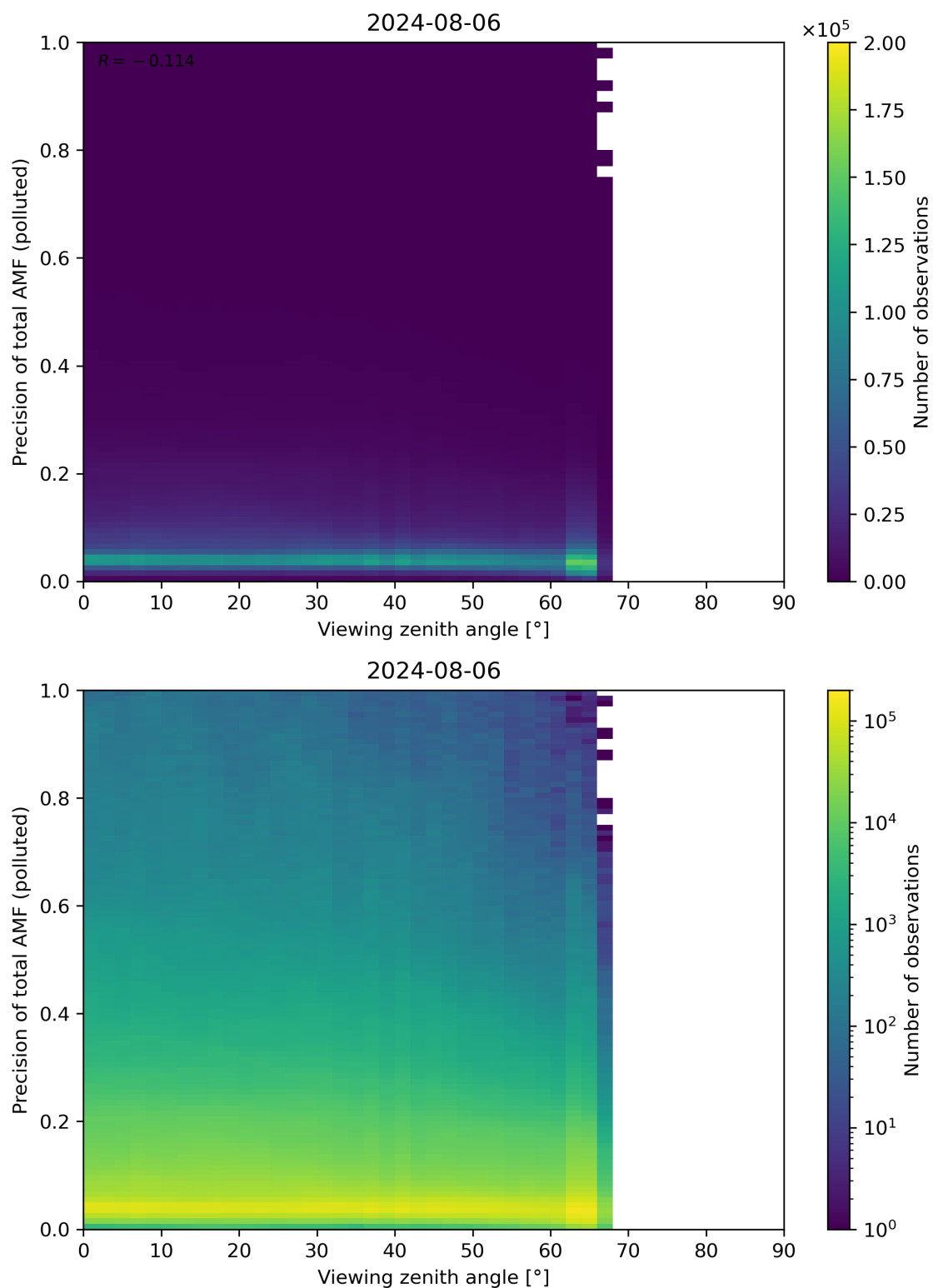
Figure 326: Scatter density plot of “Viewing zenith angle” against “Precision of total AMF (polluted)” for 2024-08-06 to 2024-08-07.
