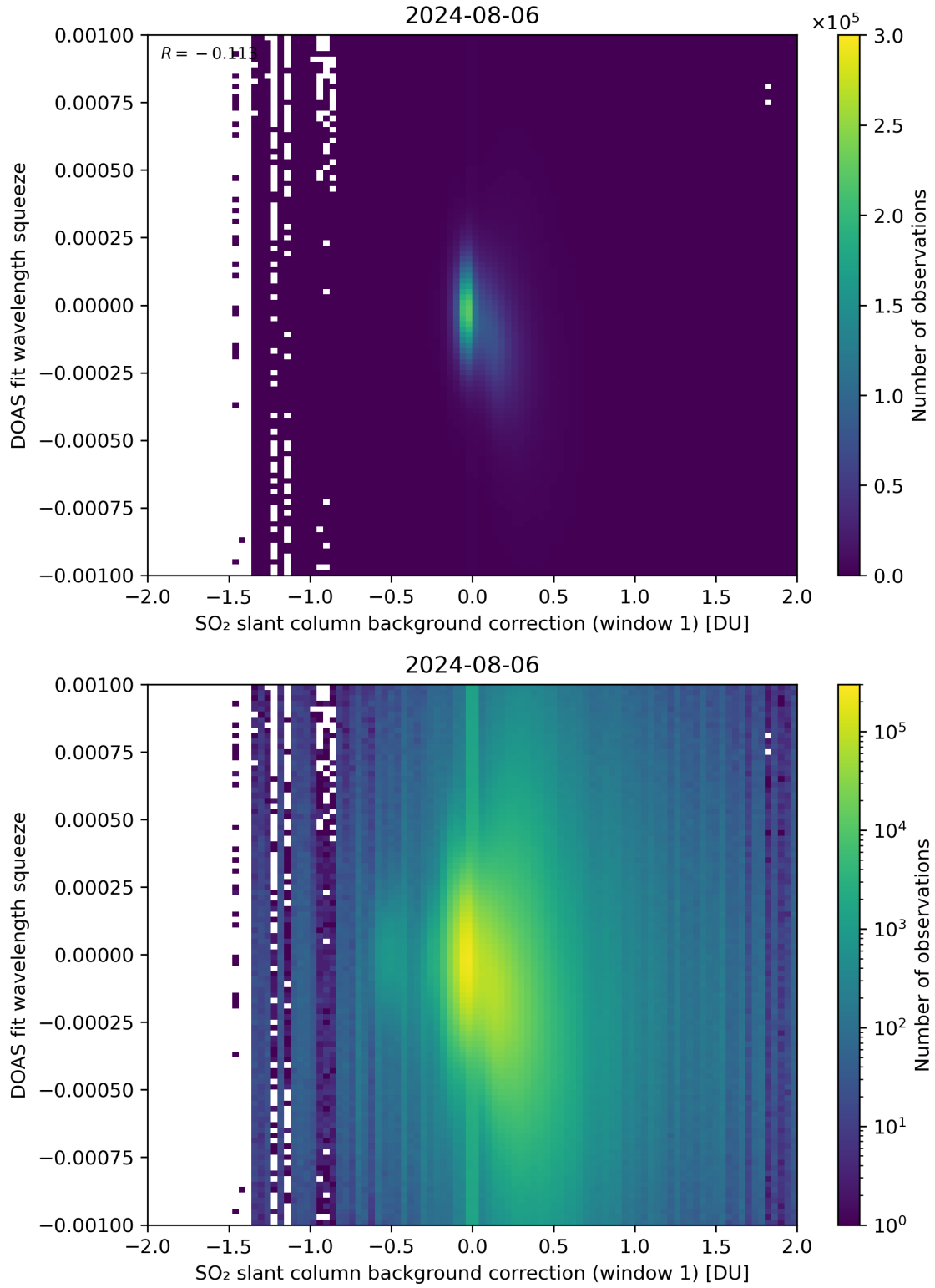
Figure 101: Scatter density plot of “SO 2 slant column background correction (window 1)” against “DOAS fit wavelength squeeze” for 2024-08-06 to 2024-08-07.
