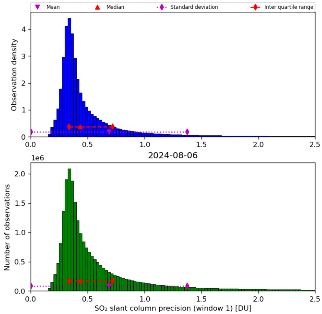
Figure 57: Histogram of “SO 2 slant column precision (window 1)” for 2024-08-06 to 2024-08-07
