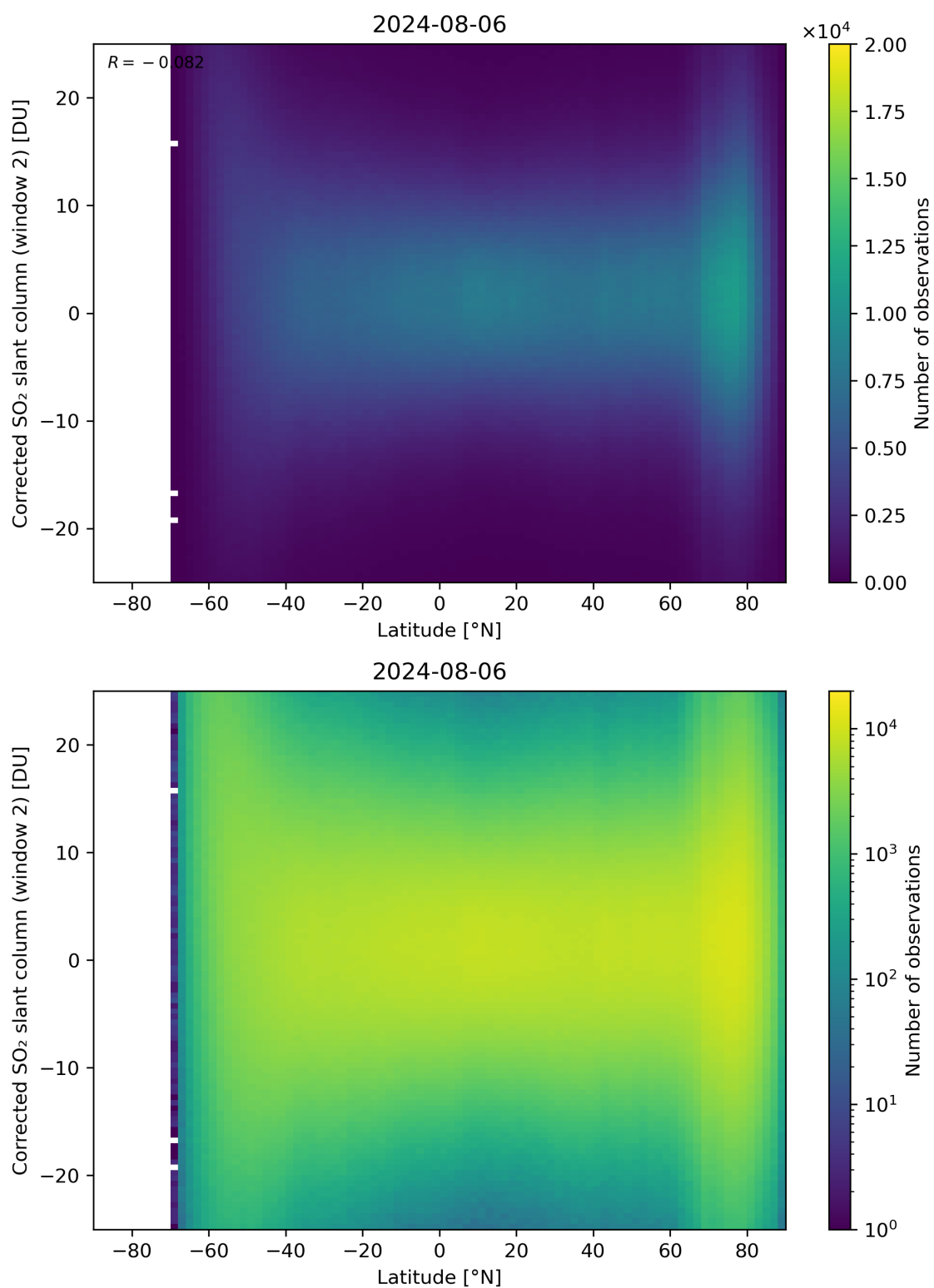
Figure 147: Scatter density plot of “Latitude” against “Corrected SO 2 slant column (window 2)” for 2024-08-06 to 2024-08-07.
