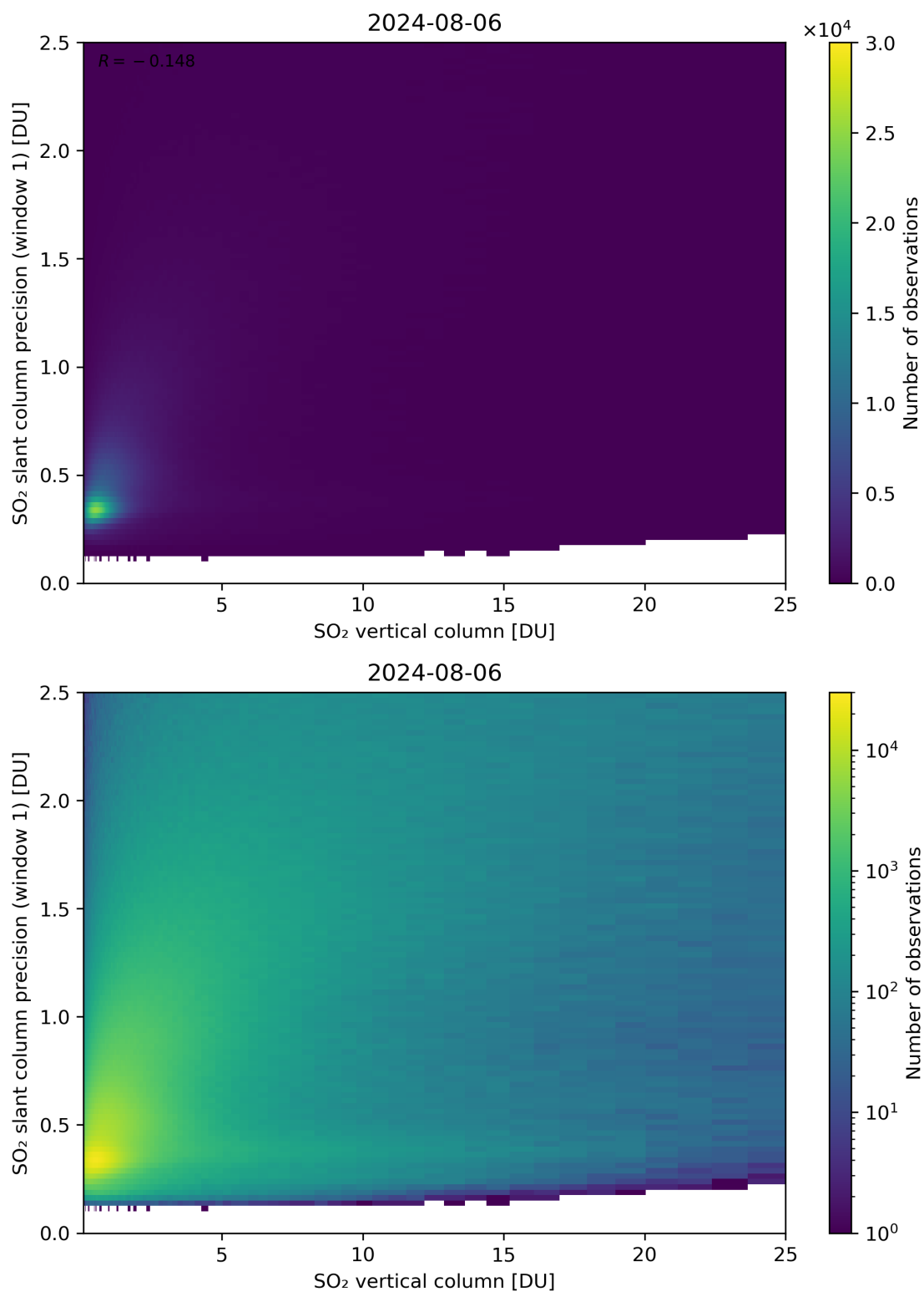
Figure 301: Scatter density plot of “SO 2 vertical column” against “SO 2 slant column precision (window 1)” for 2024-08-06 to 2024-08-07.
