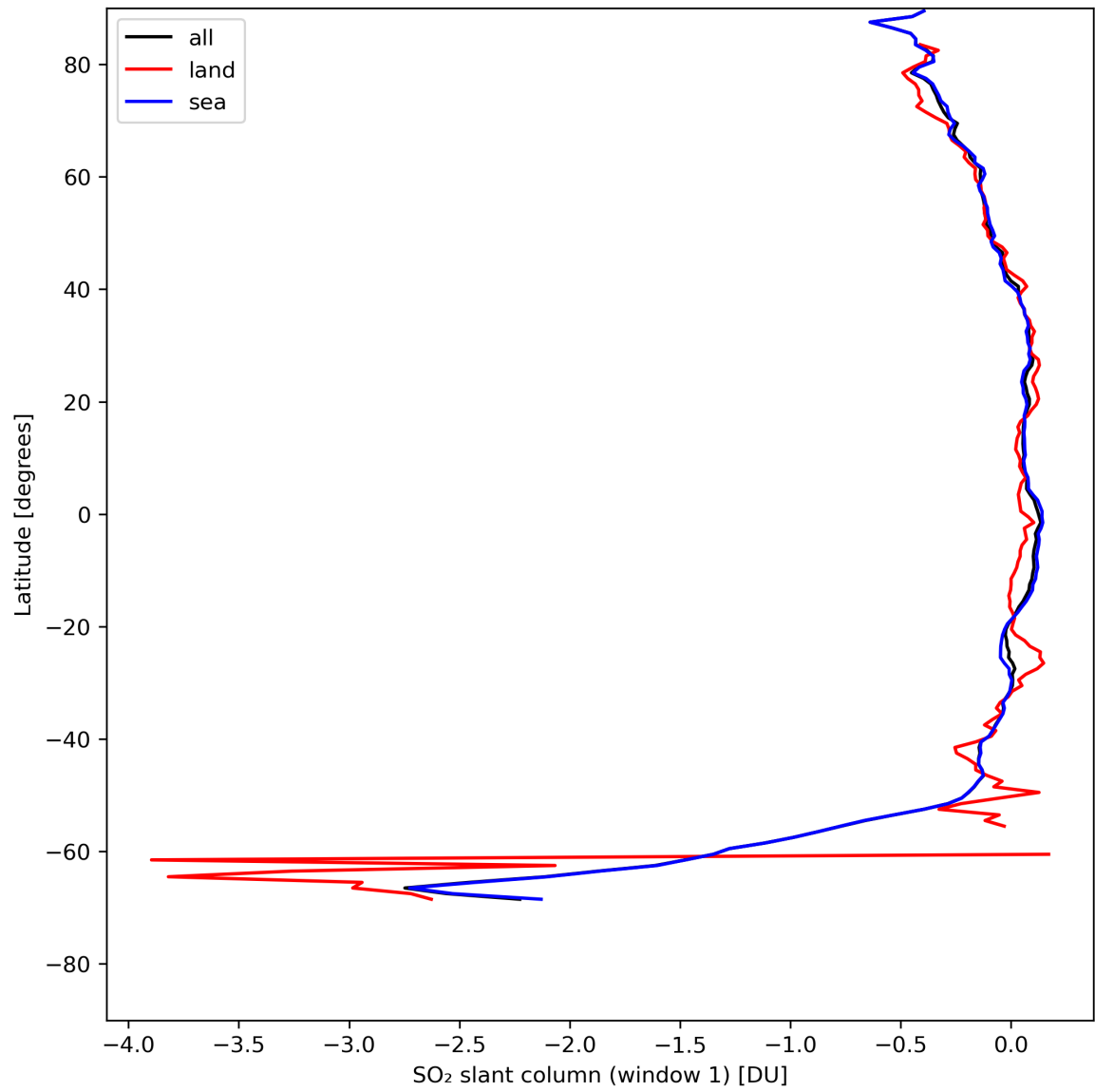
Figure 33: Zonal average of “SO 2 slant column (window 1)” for 2024-08-06 to 2024-08-07.
