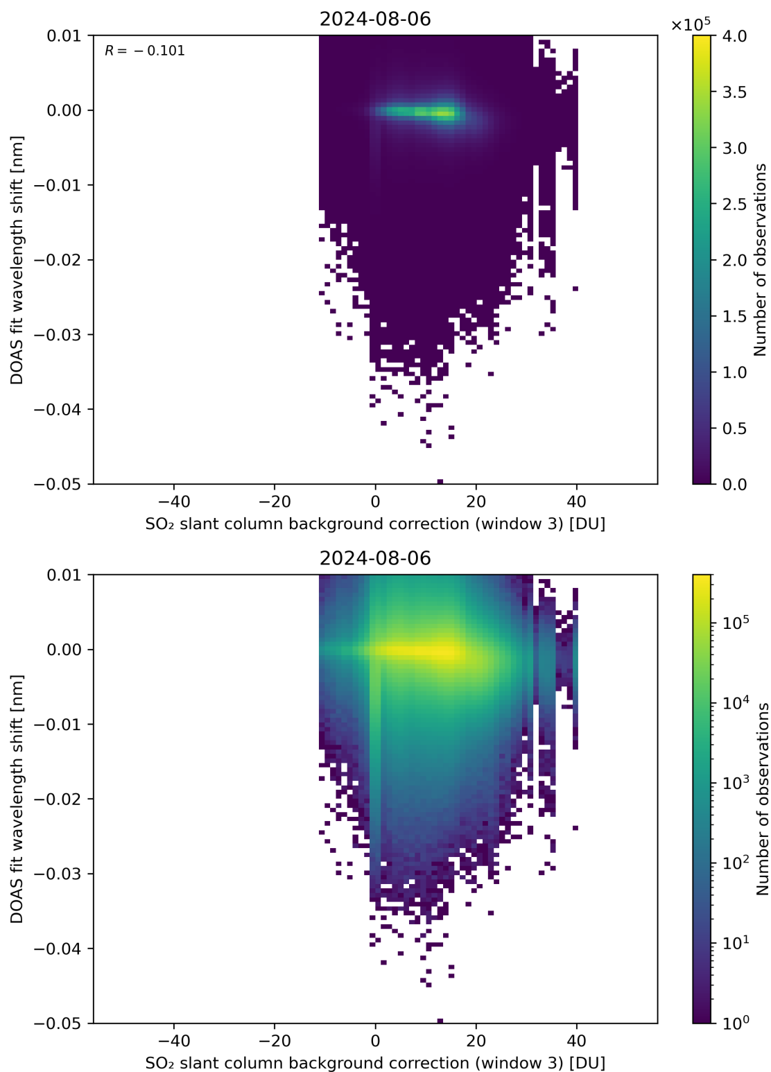
Figure 121: Scatter density plot of “SO 2 slant column background correction (window 3)” against “DOAS fit wavelength shift” for 2024-08-06 to 2024-08-07.
