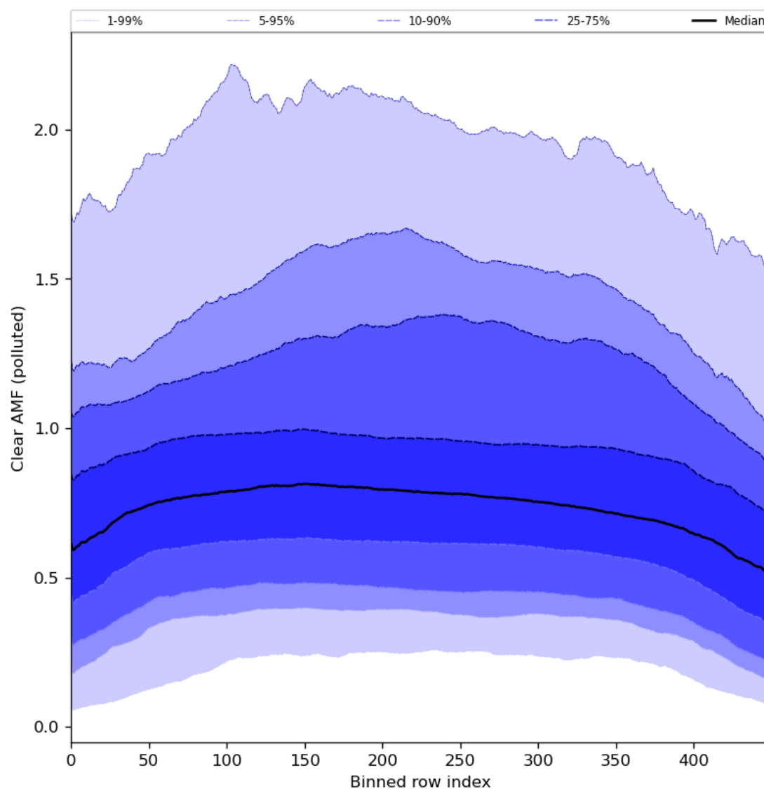
Figure 96: Along track statistics of “Clear AMF (polluted)” for 2024-08-06 to 2024-08-07
