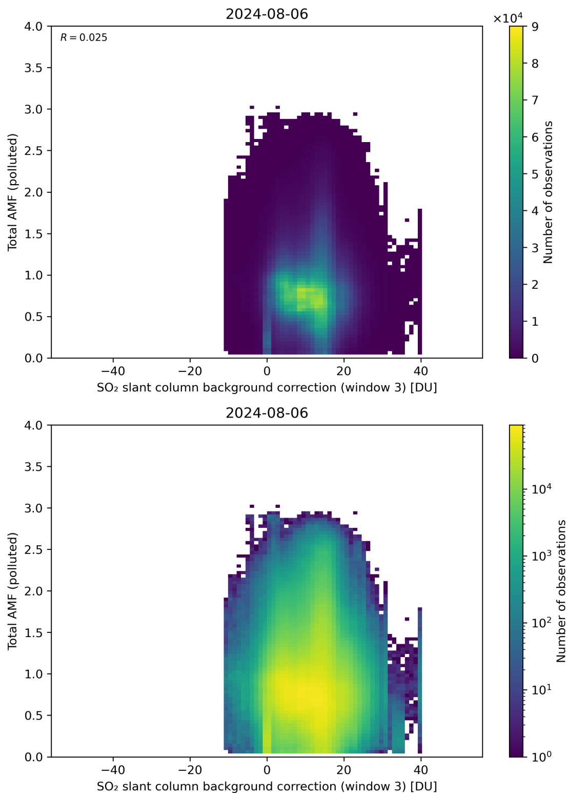
Figure 125: Scatter density plot of “SO 2 slant column background correction (window 3)” against “Total AMF (polluted)” for 2024-08-06 to 2024-08-07.
