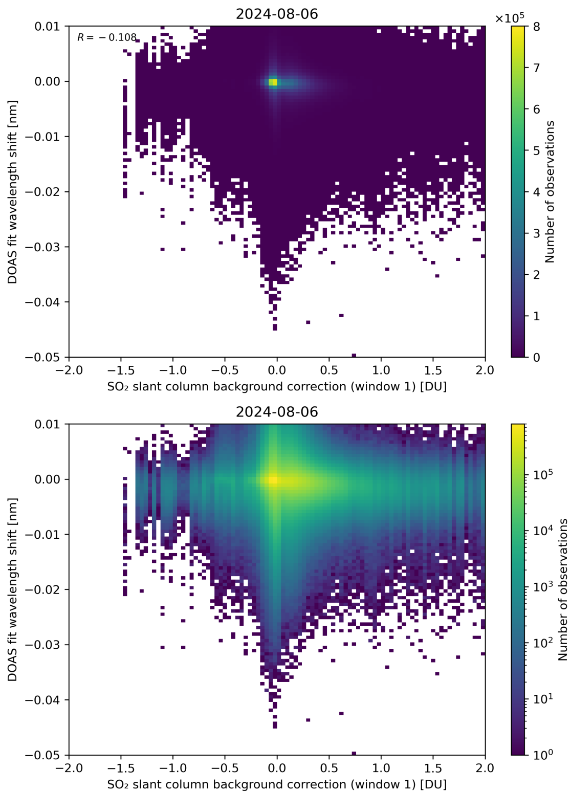
Figure 100: Scatter density plot of “SO 2 slant column background correction (window 1)” against “DOAS fit wavelength shift” for 2024-08-06 to 2024-08-07.
