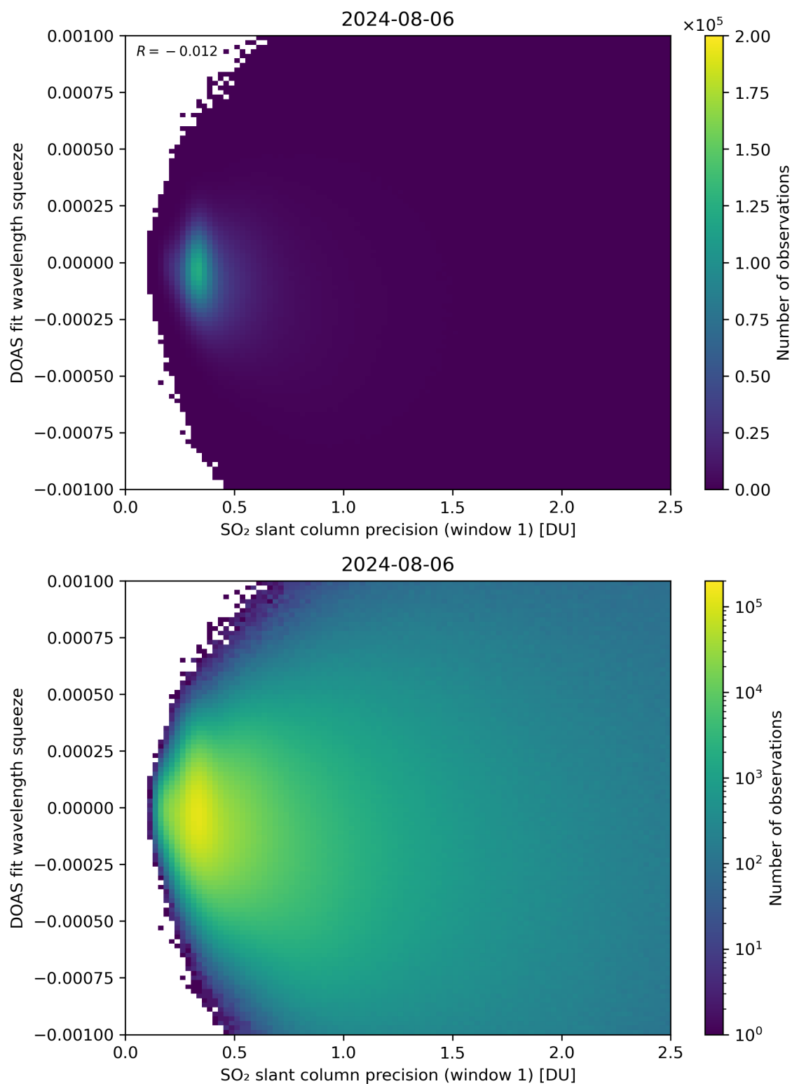
Figure 222: Scatter density plot of “SO 2 slant column precision (window 1)” against “DOAS fit wavelength squeeze” for 2024-08-06 to 2024-08-07.
