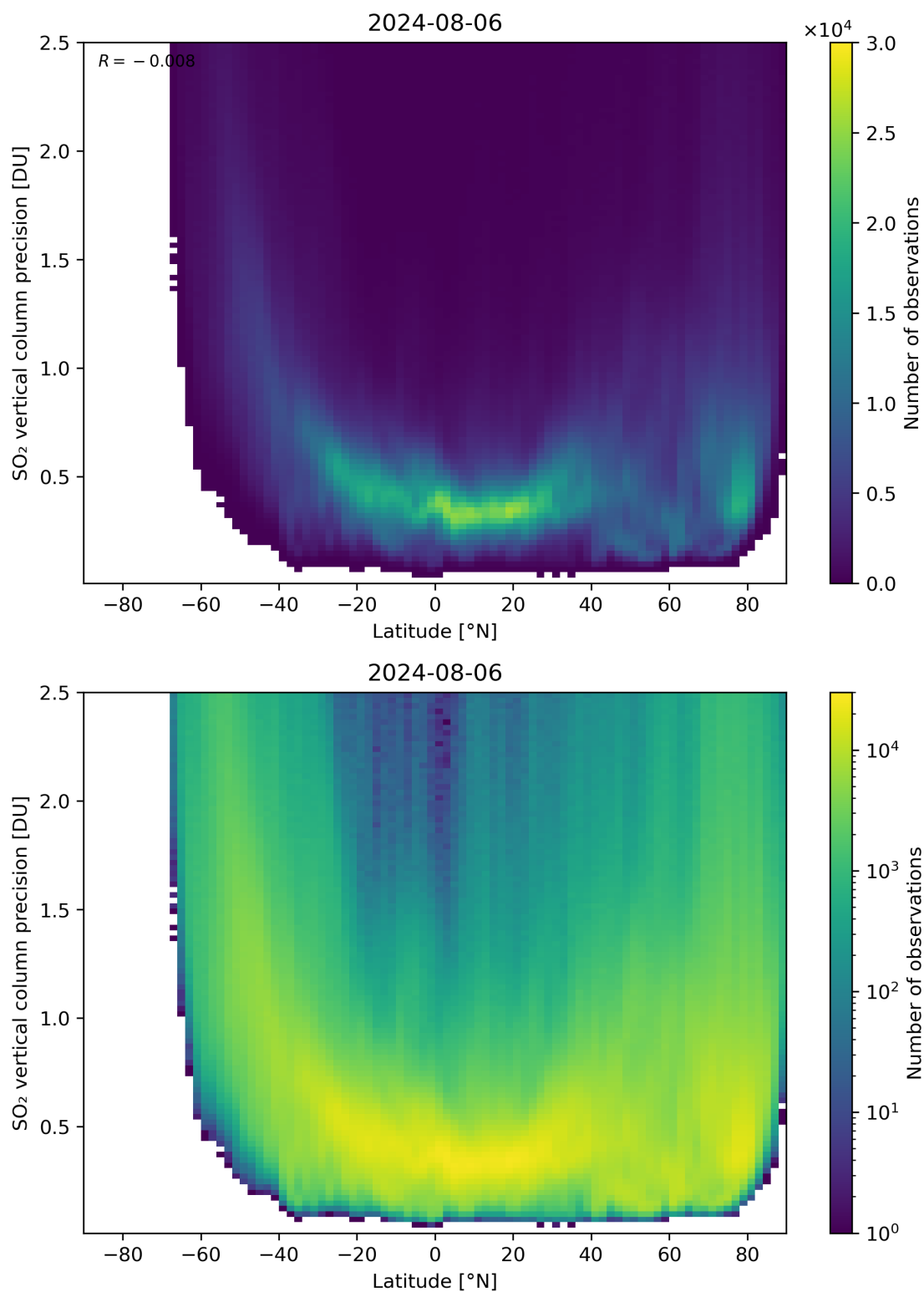
Figure 157: Scatter density plot of “Latitude” against “SO 2 vertical column precision” for 2024-08-06 to 2024-08-07.
