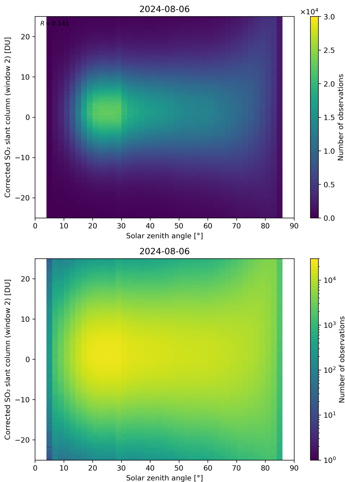
Figure 167: Scatter density plot of “Solar zenith angle” against “Corrected SO 2 slant column (window 2)” for 2024-08-06 to 2024-08-07.
