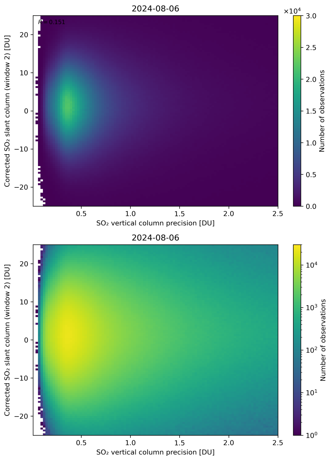
Figure 287: Scatter density plot of “SO 2 vertical column precision” against “Corrected SO 2 slant column (window 2)” for 2024-08-06 to 2024-08-07.
