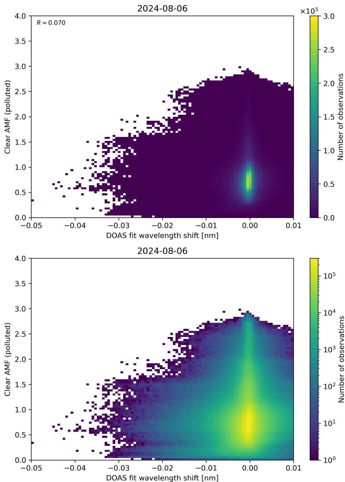
Figure 129: Scatter density plot of “DOAS fit wavelength shift” against “Clear AMF (polluted)” for 2024-08-06 to 2024-08-07.
