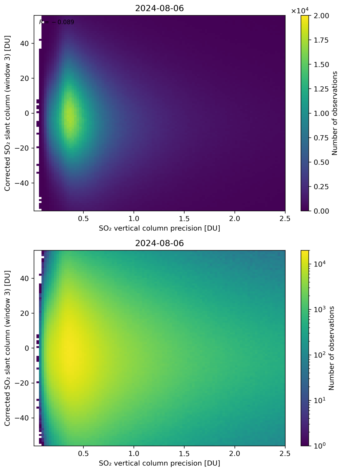
Figure 288: Scatter density plot of “SO 2 vertical column precision” against “Corrected SO 2 slant column (window 3)” for 2024-08-06 to 2024-08-07.
