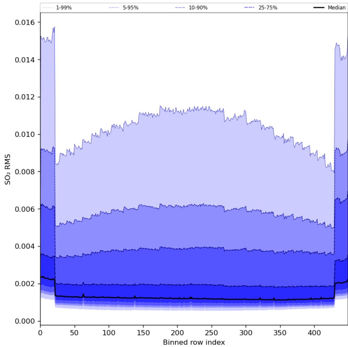
Figure 93: Along track statistics of “SO 2 RMS” for 2024-08-06 to 2024-08-07
