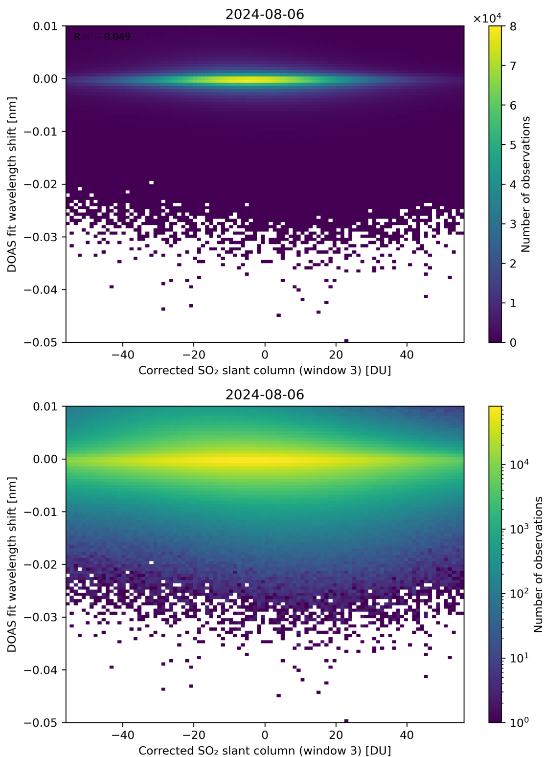
Figure 206: Scatter density plot of “Corrected SO 2 slant column (window 3)” against “DOAS fit wavelength shift” for 2024-08-06 to 2024-08-07.
