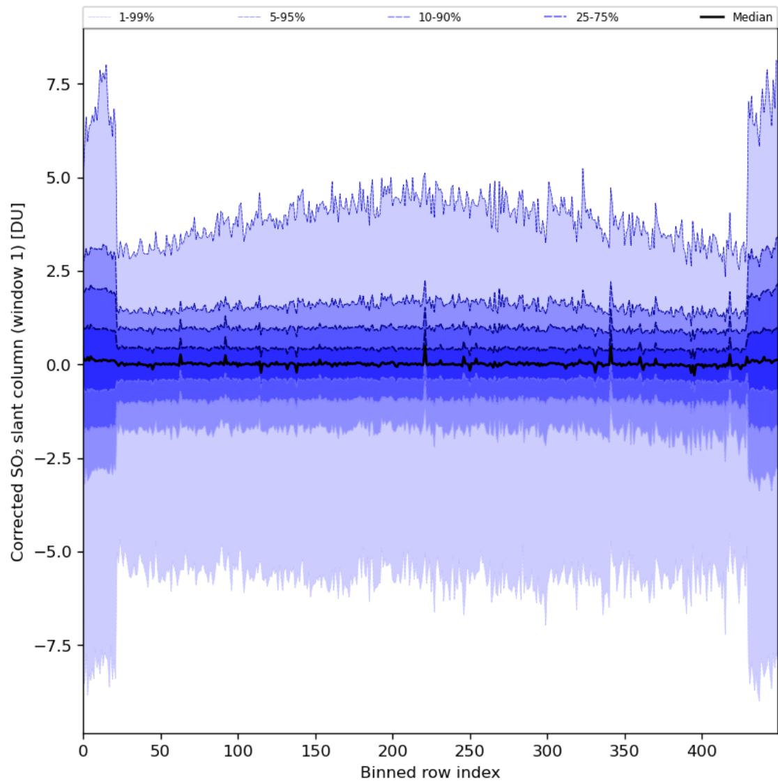
Figure 81: Along track statistics of “Corrected SO 2 slant column (window 1)” for 2024-08-06 to 2024-08-07
