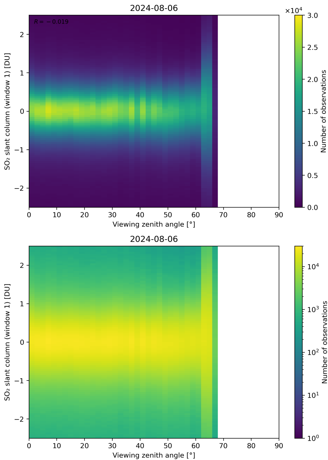
Figure 320: Scatter density plot of “Viewing zenith angle” against “SO 2 slant column (window 1)” for 2024-08-06 to 2024-08-07.
