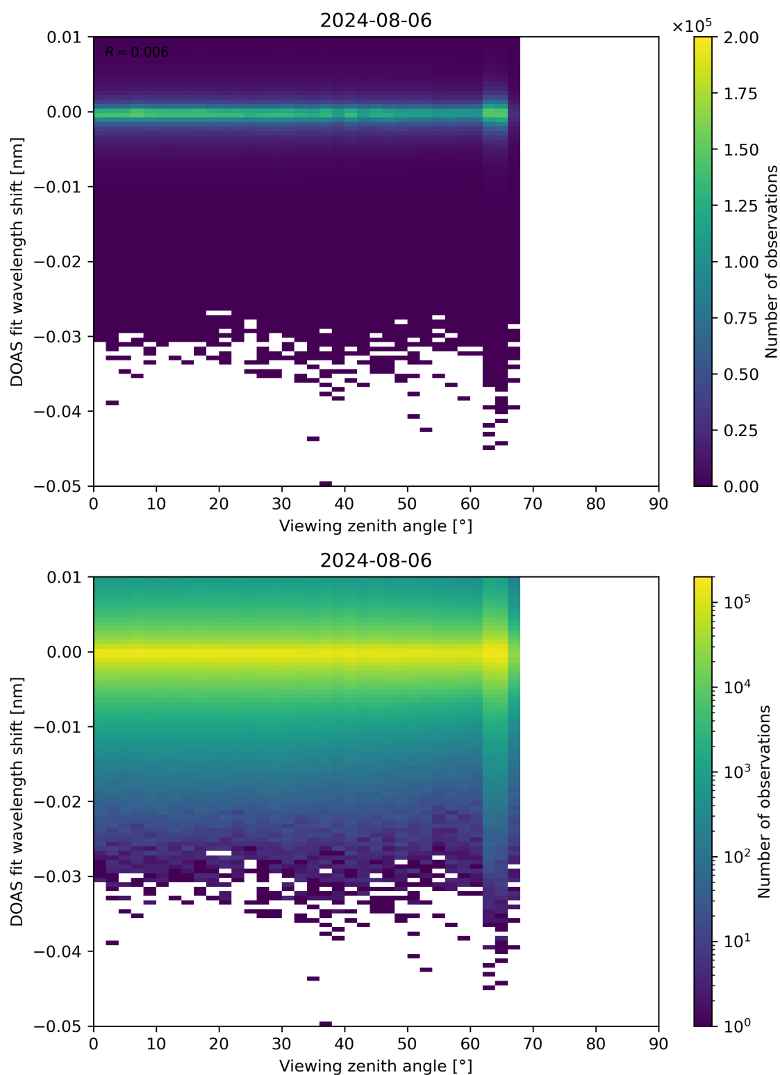
Figure 311: Scatter density plot of “Viewing zenith angle” against “DOAS fit wavelength shift” for 2024-08-06 to 2024-08-07.
