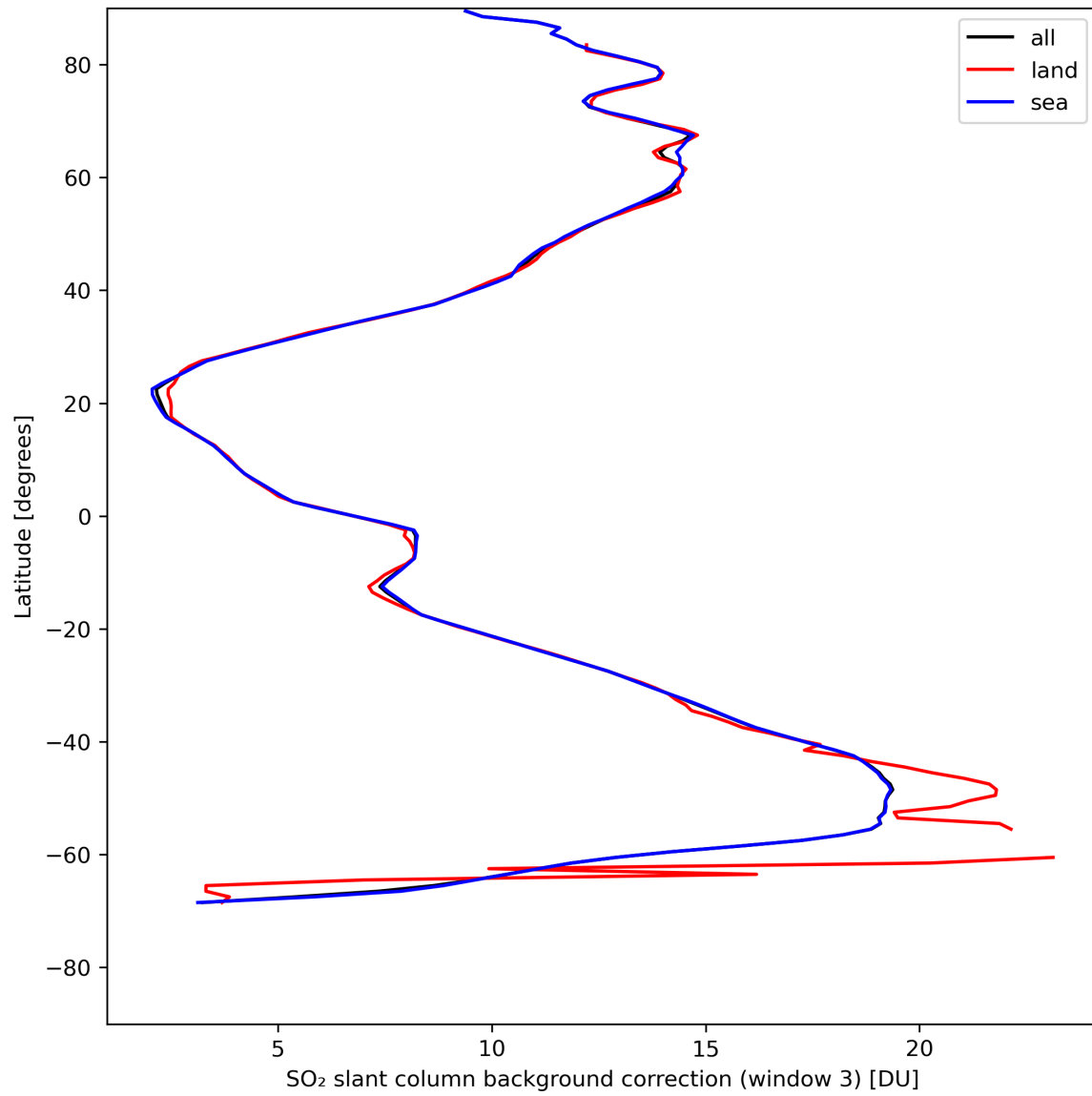
Figure 44: Zonal average of “SO 2 slant column background correction (window 3)” for 2024-08-06 to 2024-08-07.
