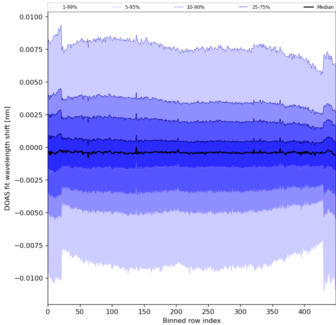
Figure 91: Along track statistics of “DOAS fit wavelength shift” for 2024-08-06 to 2024-08-07
