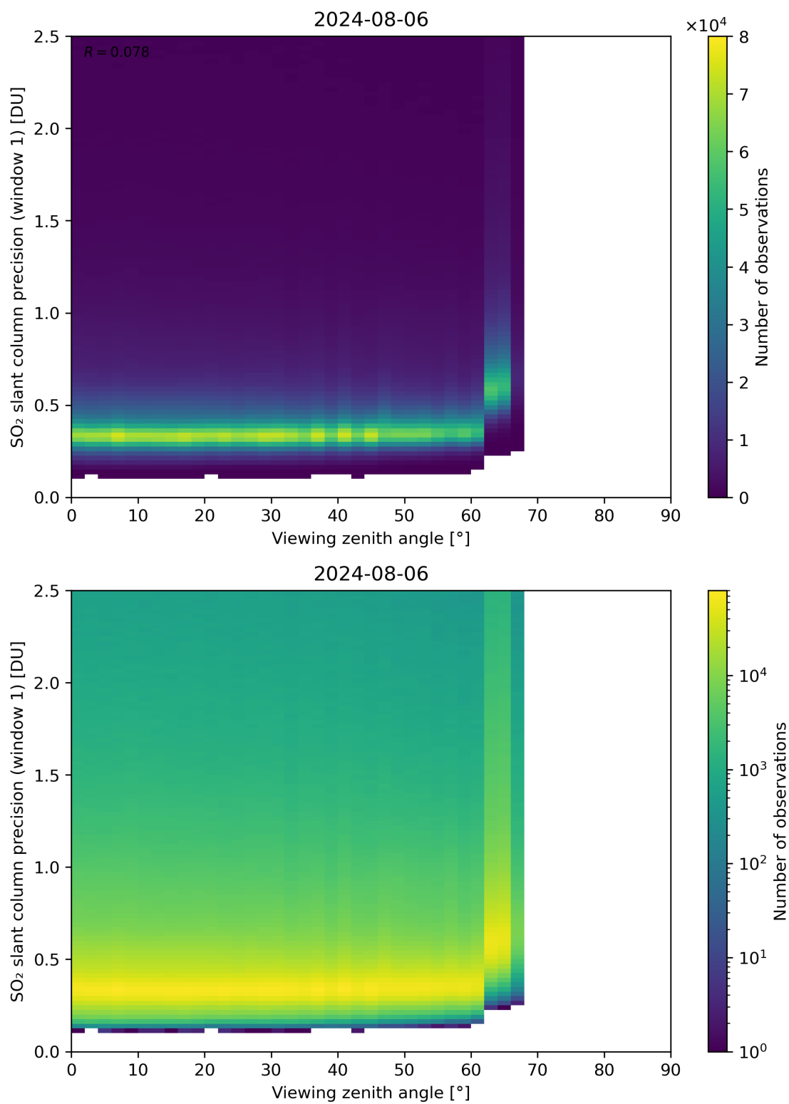
Figure 321: Scatter density plot of “Viewing zenith angle” against “SO 2 slant column precision (window 1)” for 2024-08-06 to 2024-08-07.
