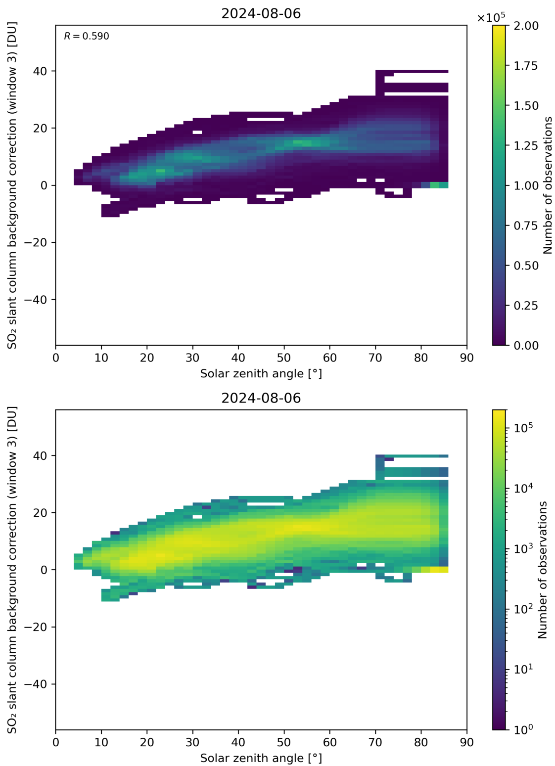
Figure 160: Scatter density plot of “Solar zenith angle” against “SO 2 slant column background correction (window 3)” for 2024-08-06 to 2024-08-07.
