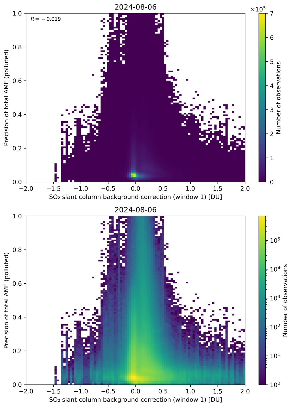
Figure 110: Scatter density plot of “SO 2 slant column background correction (window 1)” against “Precision of total AMF (polluted)” for 2024-08-06 to 2024-08-07.
