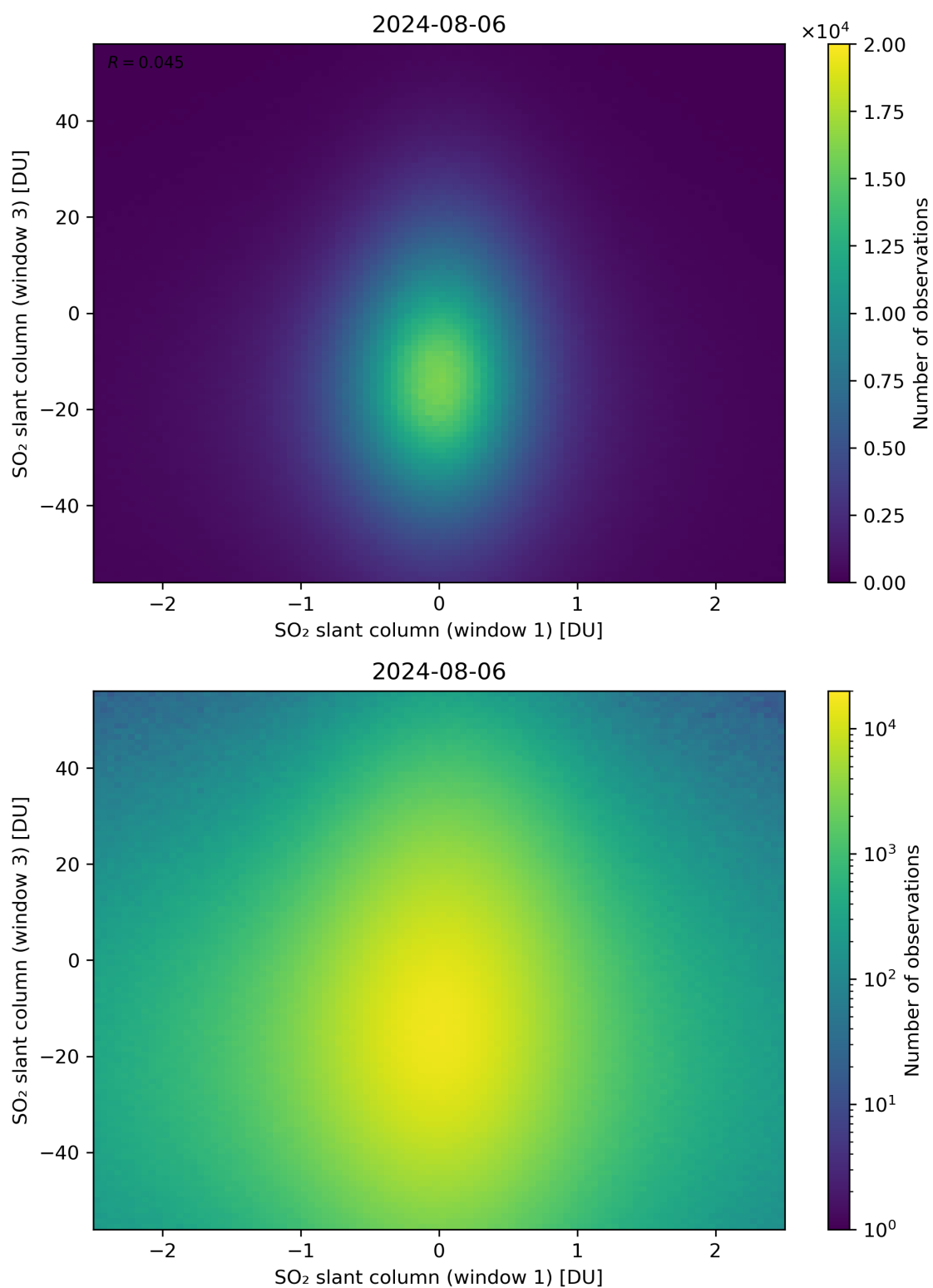
Figure 237: Scatter density plot of “SO 2 slant column (window 1)” against “SO 2 slant column (window 3)” for 2024-08-06 to 2024-08-07.
