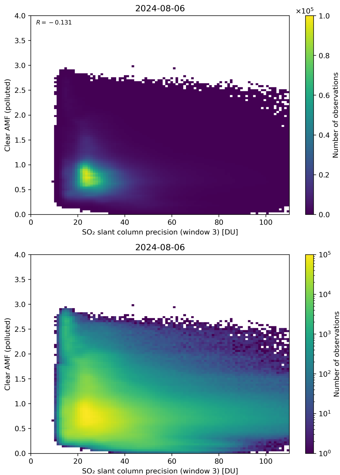
Figure 261: Scatter density plot of “SO 2 slant column precision (window 3)” against “Clear AMF (polluted)” for 2024-08-06 to 2024-08-07.
