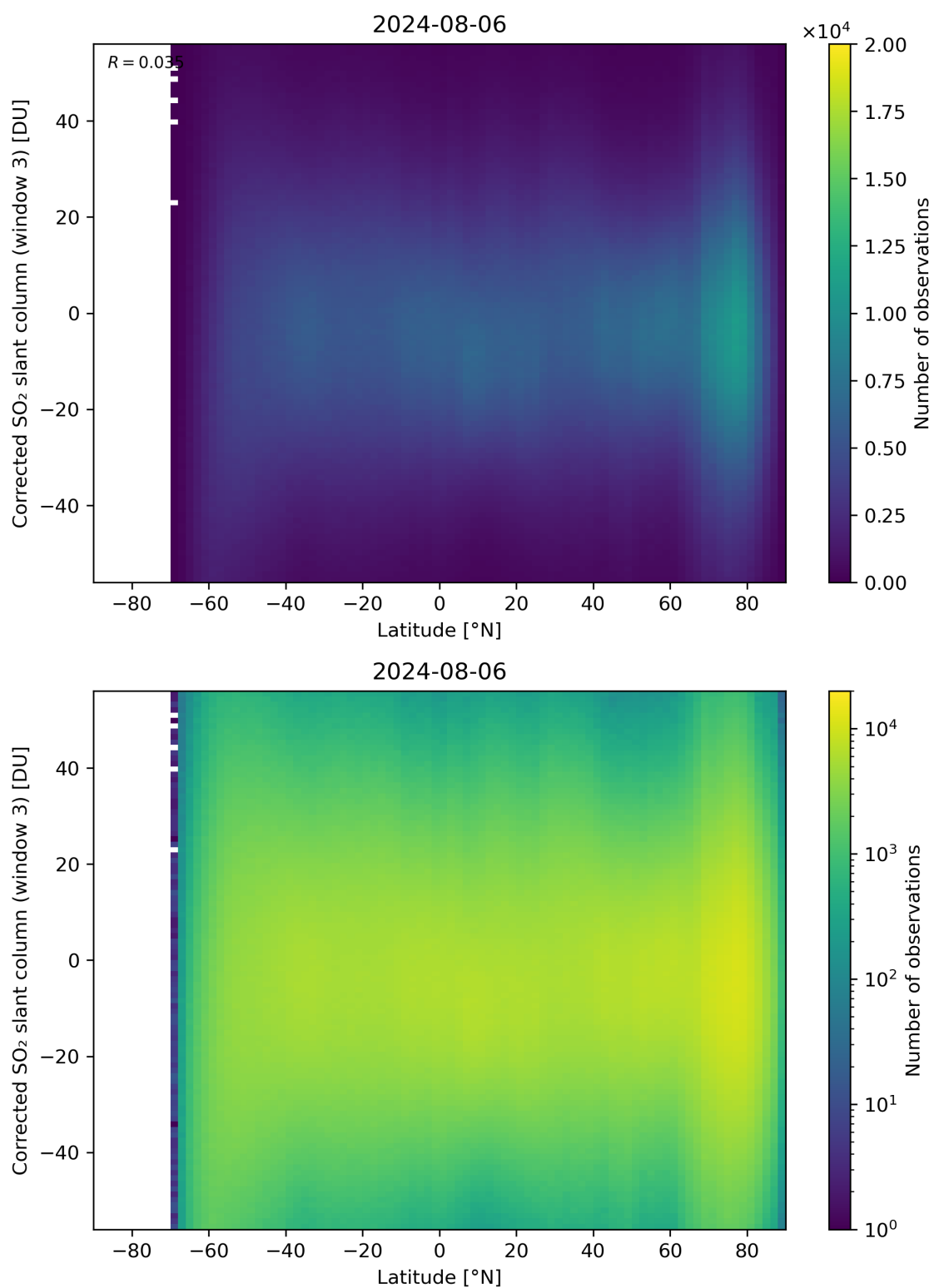
Figure 148: Scatter density plot of “Latitude” against “Corrected SO 2 slant column (window 3)” for 2024-08-06 to 2024-08-07.
