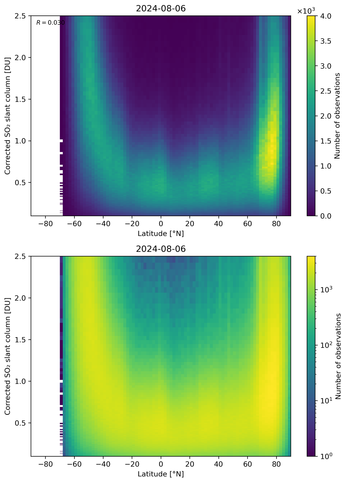
Figure 146: Scatter density plot of “Latitude” against “Corrected SO 2 slant column” for 2024-08-06 to 2024-08-07.
