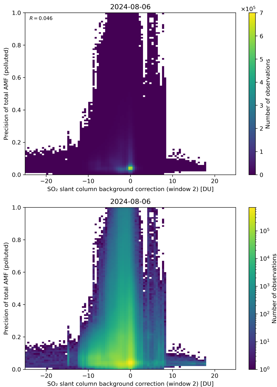
Figure 120: Scatter density plot of “SO 2 slant column background correction (window 2)” against “Precision of total AMF (polluted)” for 2024-08-06 to 2024-08-07.
