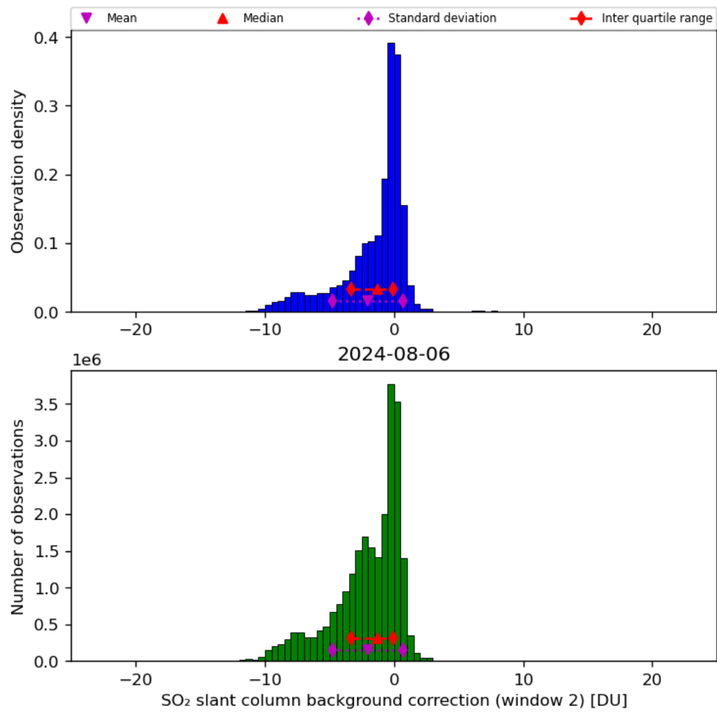
Figure 63: Histogram of “SO 2 slant column background correction (window 2)” for 2024-08-06 to 2024-08-07
