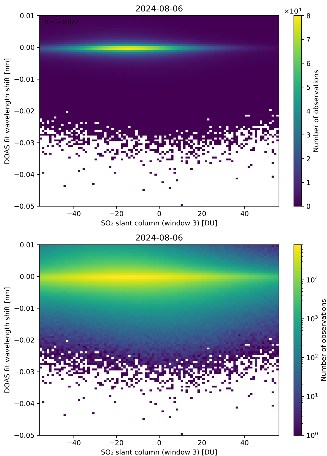
Figure 254: Scatter density plot of “SO 2 slant column (window 3)” against “DOAS fit wavelength shift” for 2024-08-06 to 2024-08-07.
