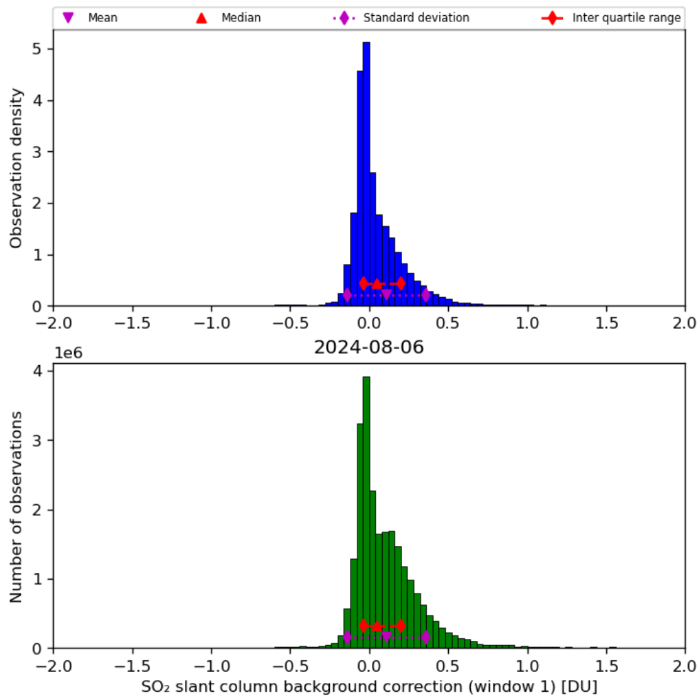
Figure 59: Histogram of “SO 2 slant column background correction (window 1)” for 2024-08-06 to 2024-08-07
