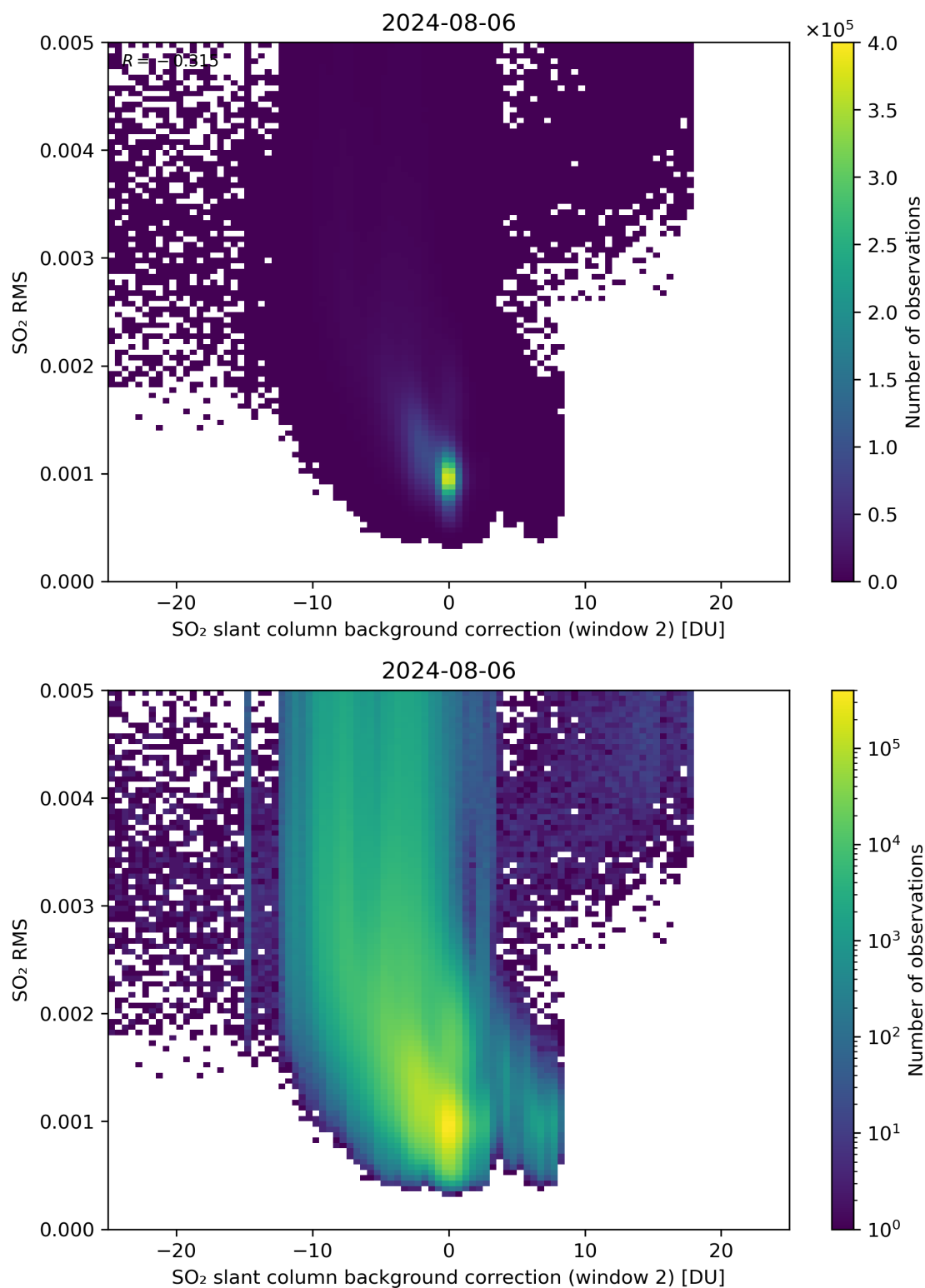
Figure 114: Scatter density plot of “SO 2 slant column background correction (window 2)” against “SO 2 RMS” for 2024-08-06 to 2024-08-07.
