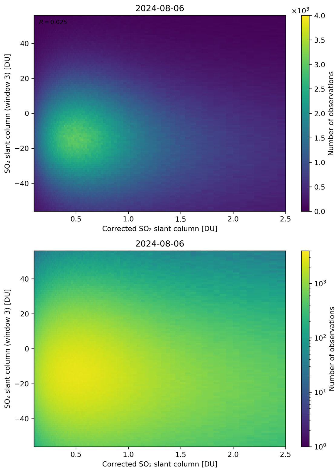
Figure 190: Scatter density plot of “Corrected SO 2 slant column” against “SO 2 slant column (window 3)” for 2024-08-06 to 2024-08-07.
