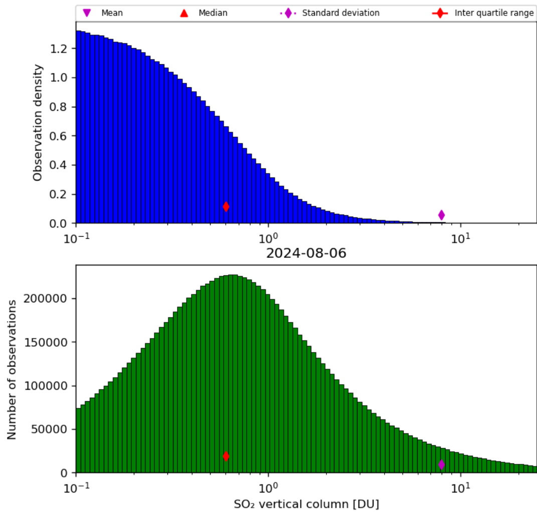
Figure 53: Histogram of “SO 2 vertical column” for 2024-08-06 to 2024-08-07
