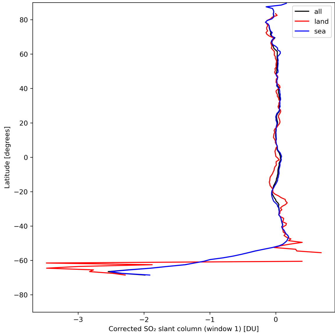
Figure 35: Zonal average of “Corrected SO 2 slant column (window 1)” for 2024-08-06 to 2024-08-07.
