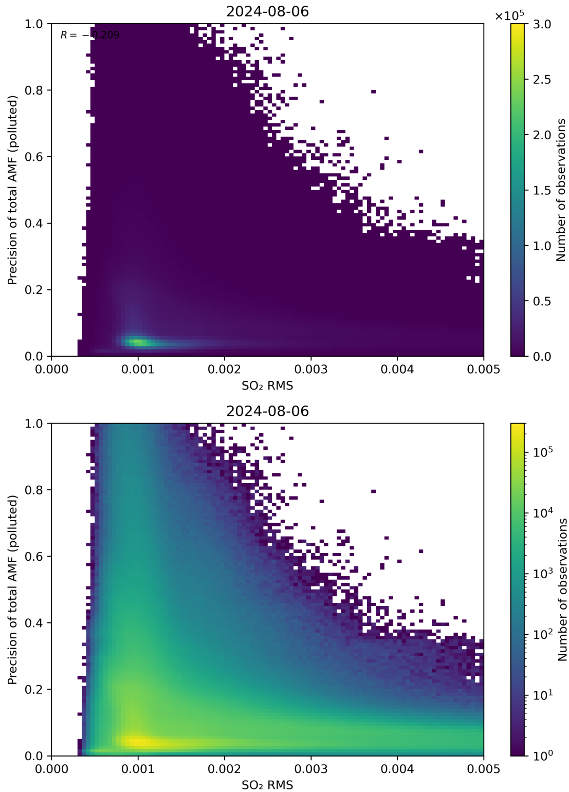
Figure 138: Scatter density plot of “SO 2 RMS” against “Precision of total AMF (polluted)” for 2024-08-06 to 2024-08-07.
