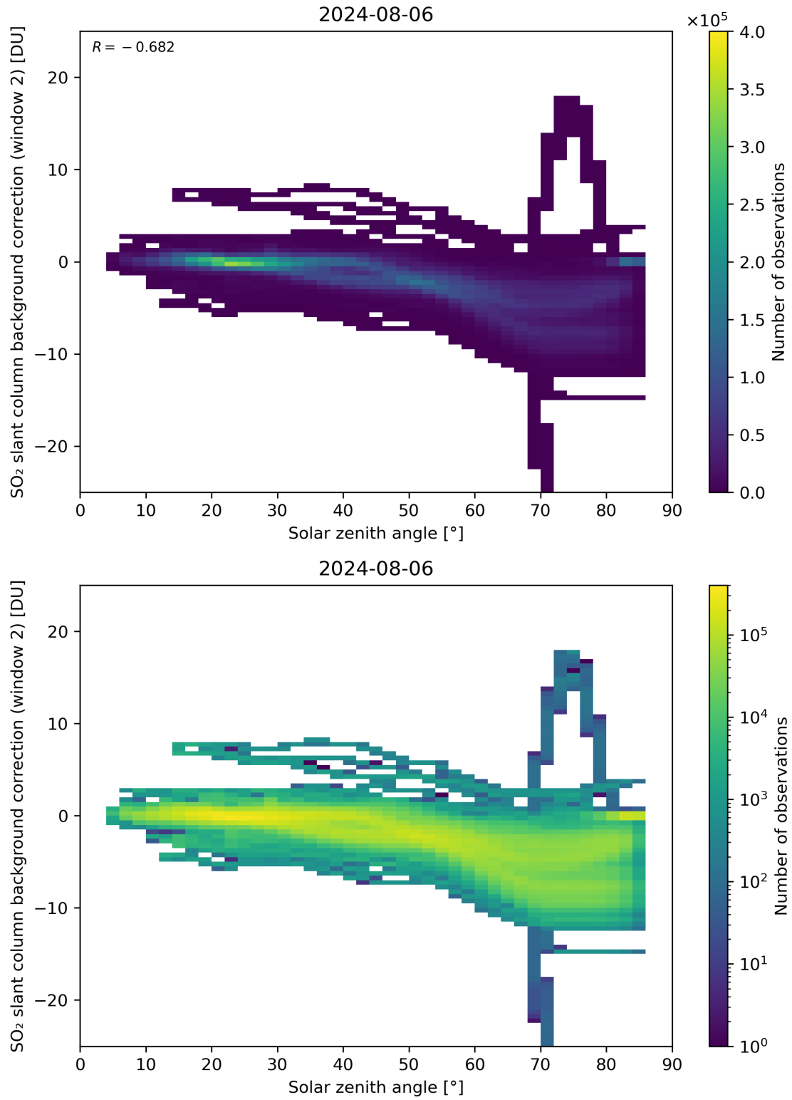
Figure 159: Scatter density plot of “Solar zenith angle” against “SO 2 slant column background correction (window 2)” for 2024-08-06 to 2024-08-07.
