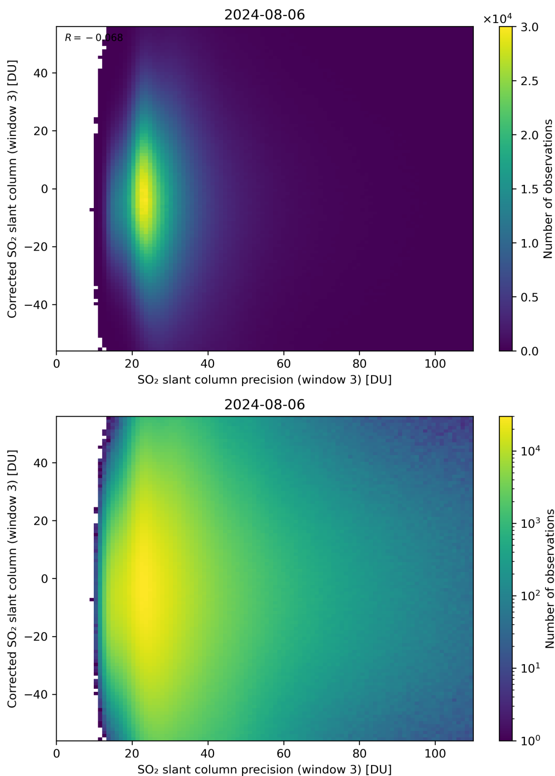
Figure 262: Scatter density plot of “SO 2 slant column precision (window 3)” against “Corrected SO 2 slant column (window 3)” for 2024-08-06 to 2024-08-07.
