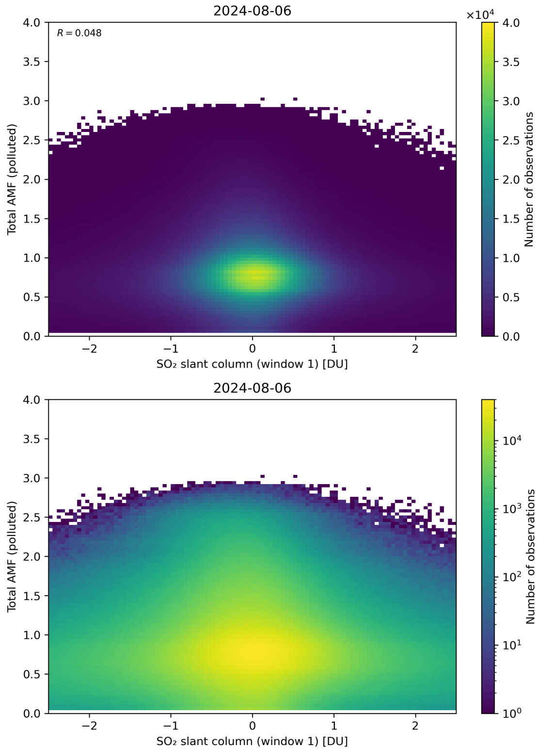
Figure 239: Scatter density plot of “SO 2 slant column (window 1)” against “Total AMF (polluted)” for 2024-08-06 to 2024-08-07.
