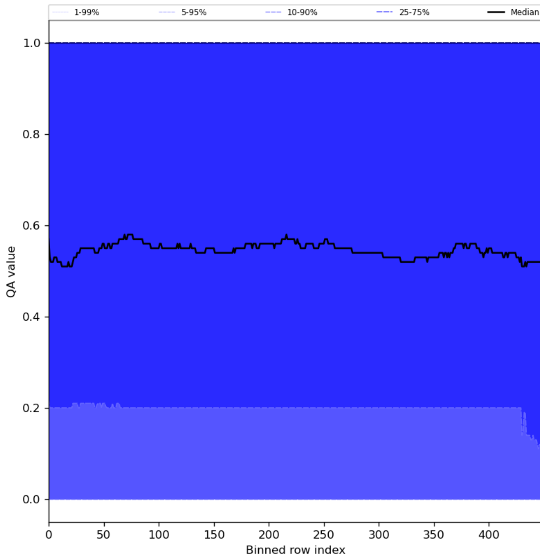
Figure 75: Along track statistics of “QA value” for 2024-08-06 to 2024-08-07
