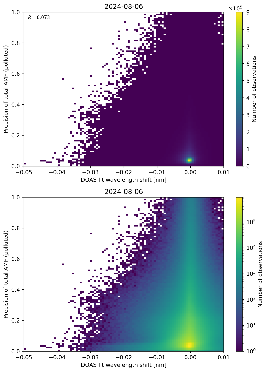
Figure 131: Scatter density plot of “DOAS fit wavelength shift” against “Precision of total AMF (polluted)” for 2024-08-06 to 2024-08-07.
