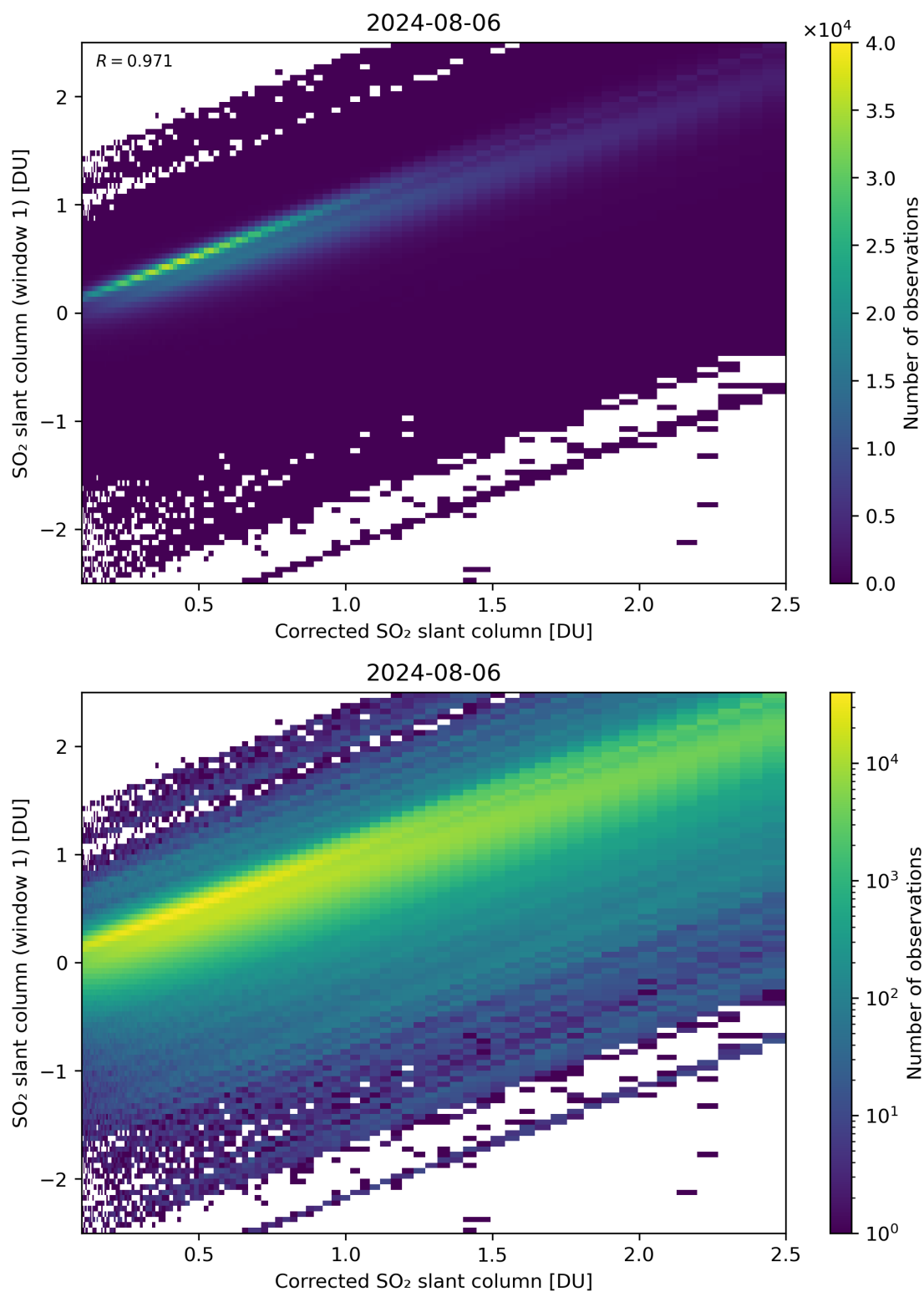
Figure 187: Scatter density plot of “Corrected SO 2 slant column” against “SO 2 slant column (window 1)” for 2024-08-06 to 2024-08-07.
