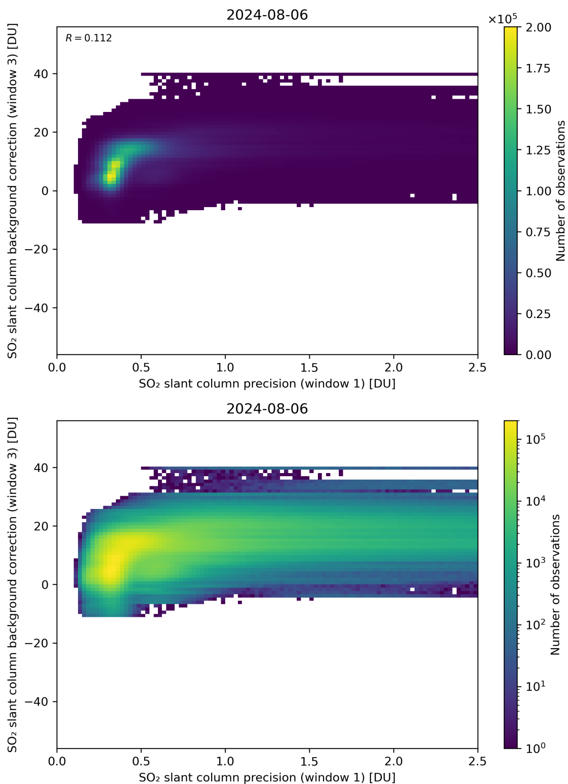
Figure 220: Scatter density plot of “SO 2 slant column precision (window 1)” against “SO 2 slant column background correction (window 3)” for 2024-08-06 to 2024-08-07.
