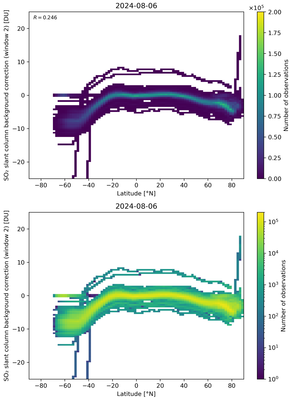
Figure 140: Scatter density plot of “Latitude” against “SO 2 slant column background correction (window 2)” for 2024-08-06 to 2024-08-07.
