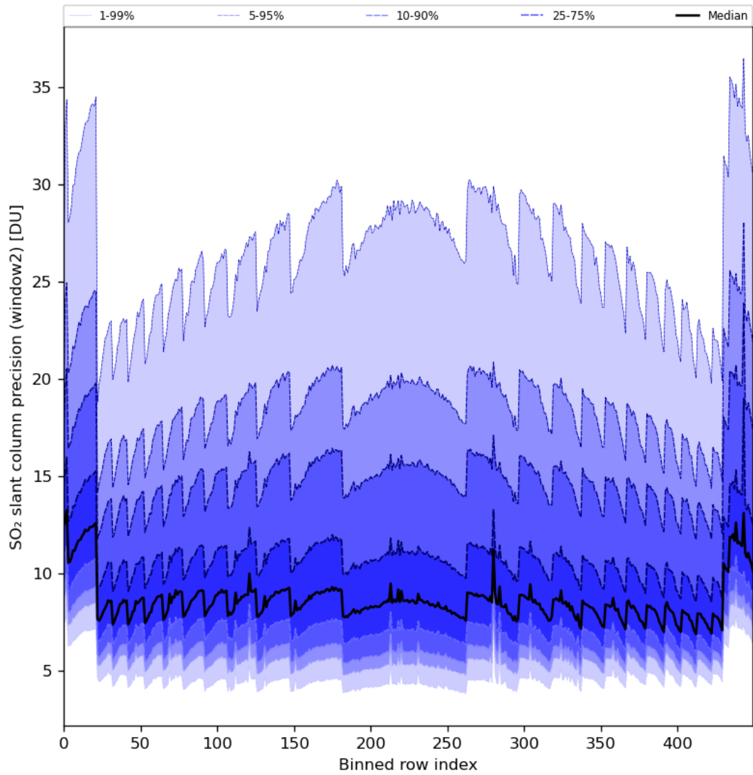
Figure 84: Along track statistics of “SO 2 slant column precision (window2)” for 2024-08-06 to 2024-08-07
