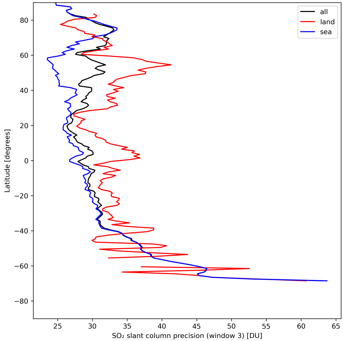
Figure 42: Zonal average of “SO 2 slant column precision (window 3)” for 2024-08-06 to 2024-08-07.
