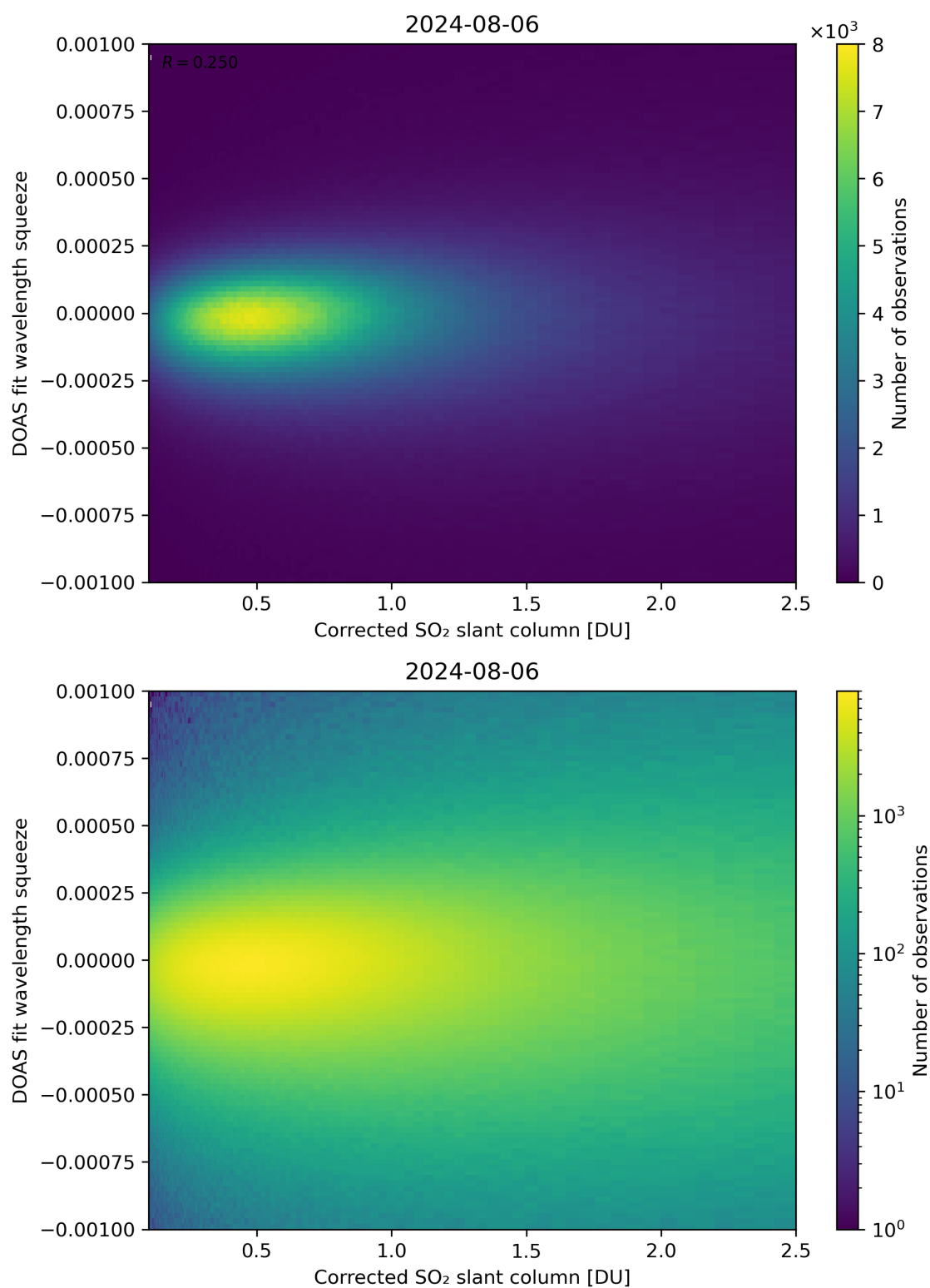
Figure 182: Scatter density plot of “Corrected SO 2 slant column” against “DOAS fit wavelength squeeze” for 2024-08-06 to 2024-08-07.
