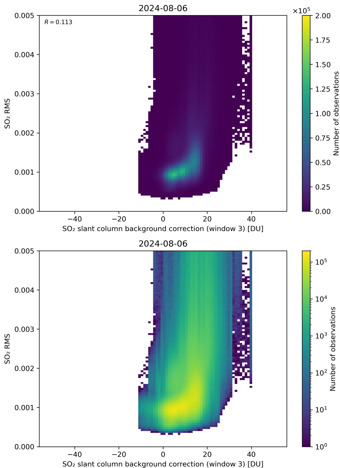
Figure 123: Scatter density plot of “SO 2 slant column background correction (window 3)” against “SO 2 RMS” for 2024-08-06 to 2024-08-07.
