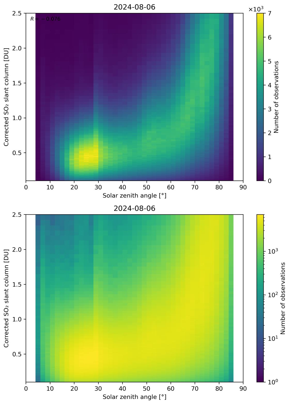
Figure 166: Scatter density plot of “Solar zenith angle” against “Corrected SO 2 slant column” for 2024-08-06 to 2024-08-07.
