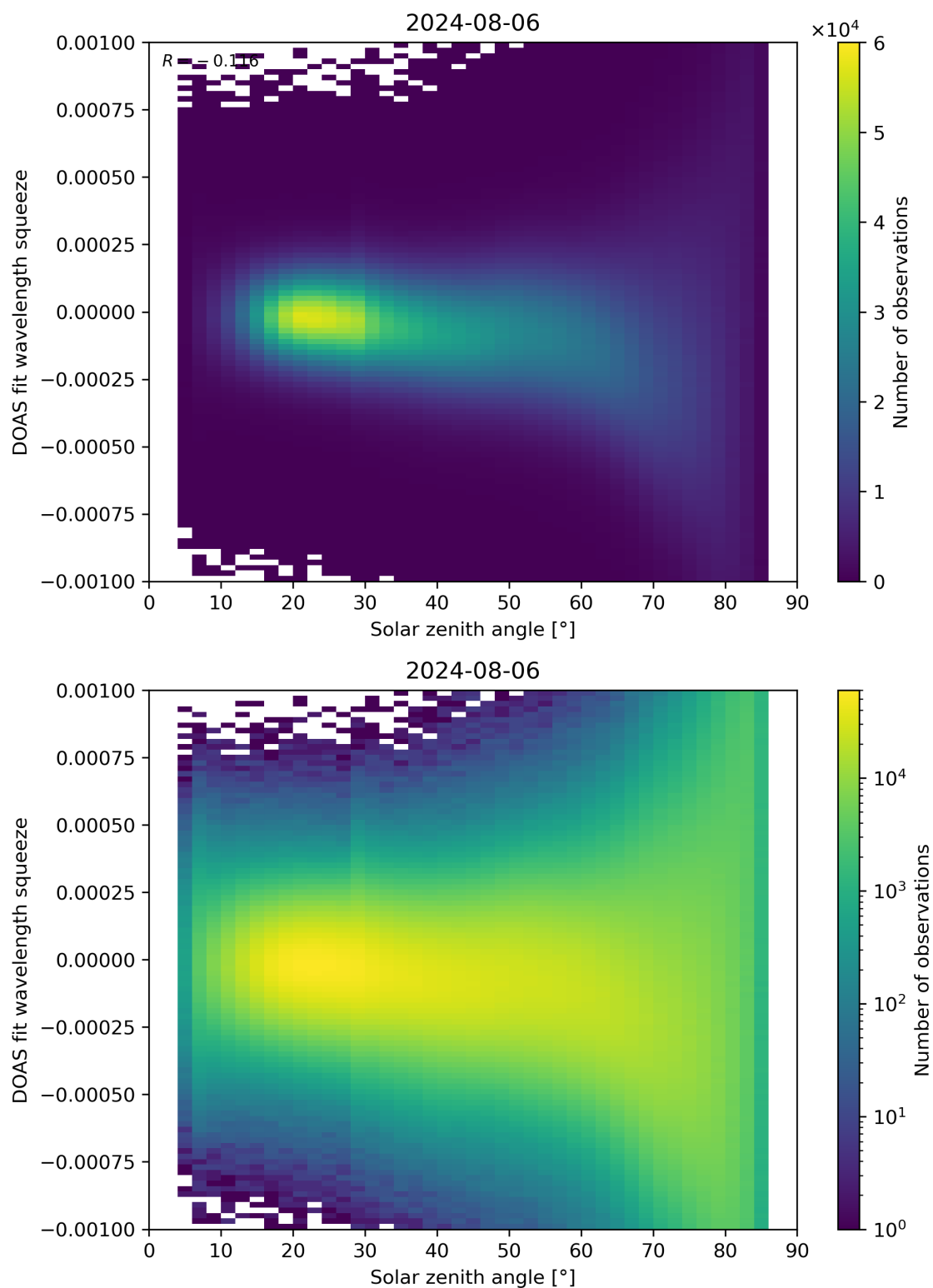
Figure 162: Scatter density plot of “Solar zenith angle” against “DOAS fit wavelength squeeze” for 2024-08-06 to 2024-08-07.
