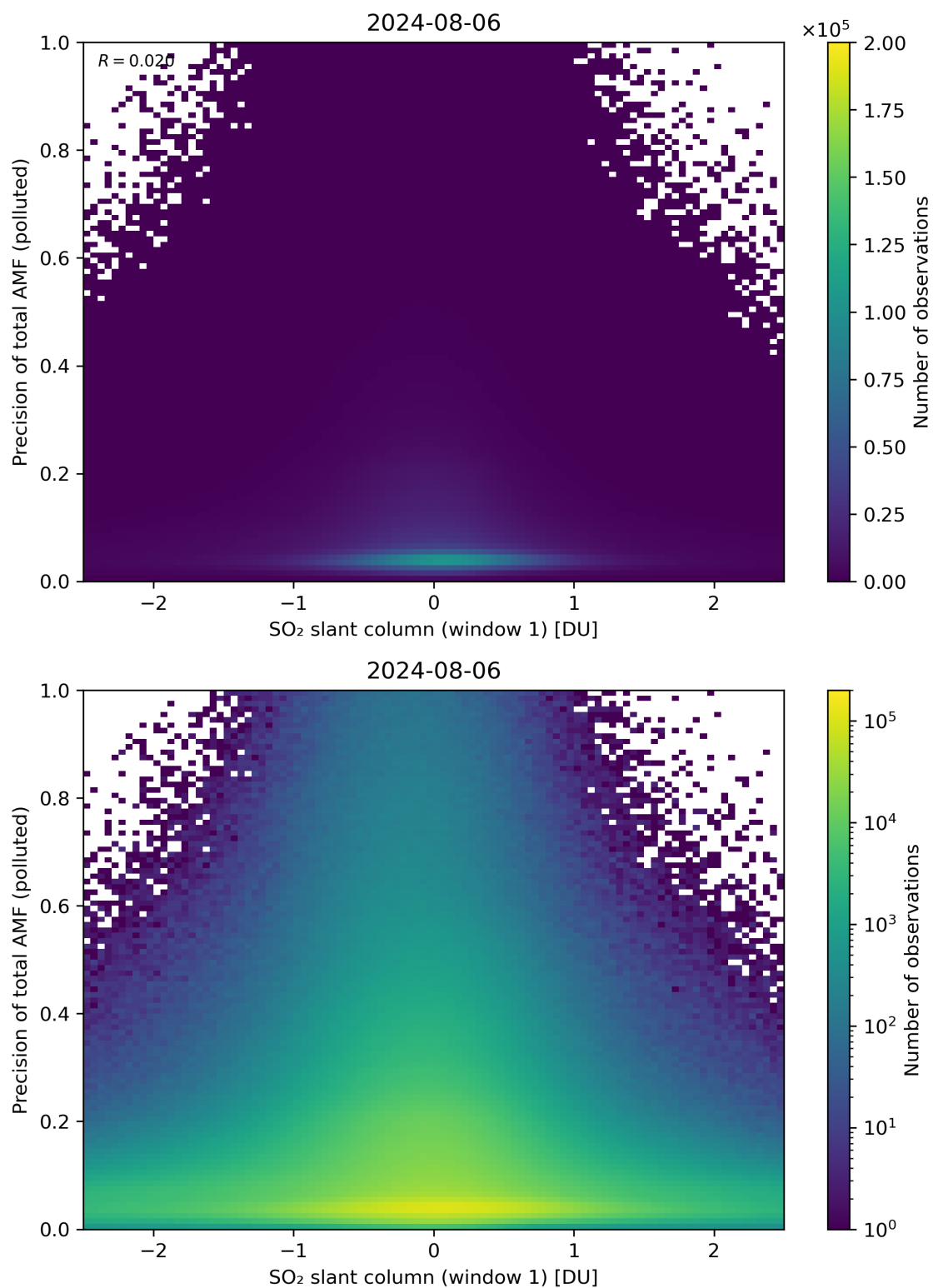
Figure 240: Scatter density plot of “SO 2 slant column (window 1)” against “Precision of total AMF (polluted)” for 2024-08-06 to 2024-08-07.
