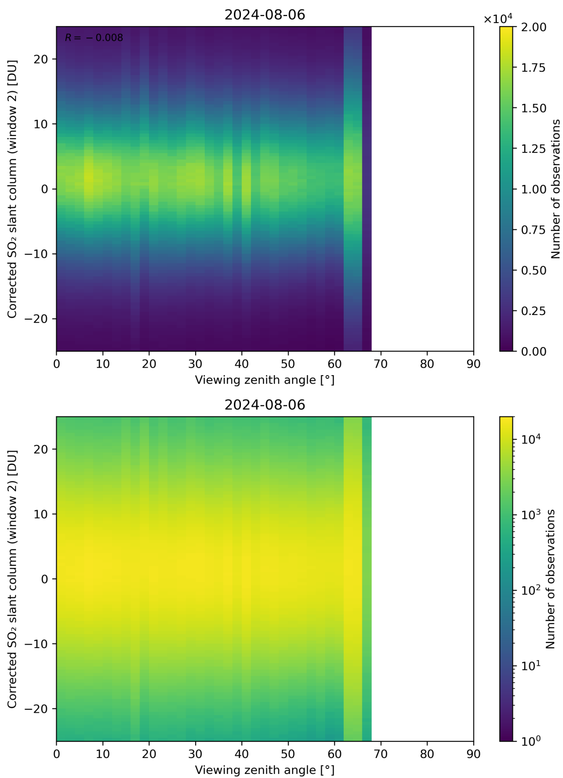
Figure 318: Scatter density plot of “Viewing zenith angle” against “Corrected SO 2 slant column (window 2)” for 2024-08-06 to 2024-08-07.
