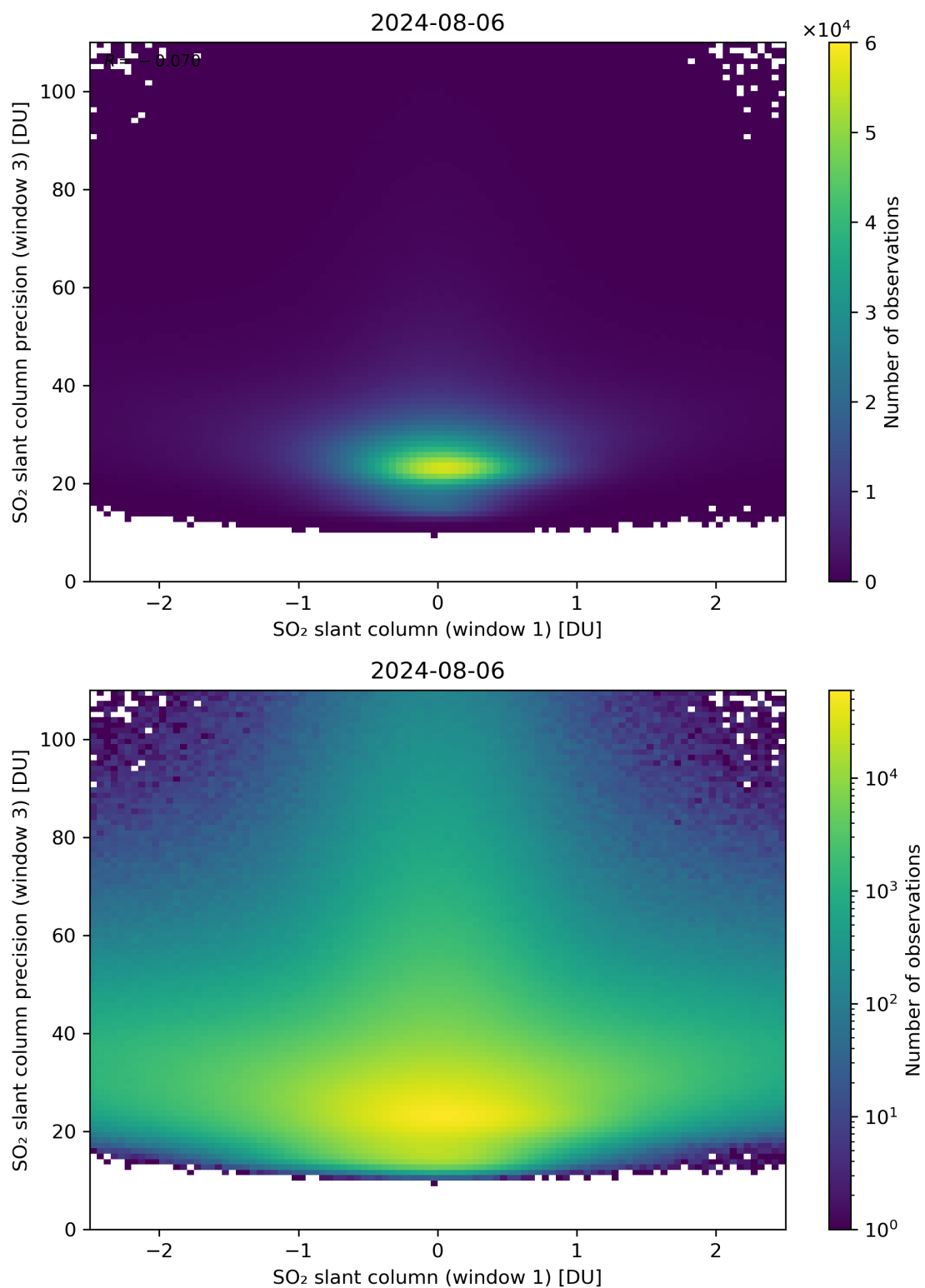
Figure 238: Scatter density plot of “SO 2 slant column (window 1)” against “SO 2 slant column precision (window 3)” for 2024-08-06 to 2024-08-07.
