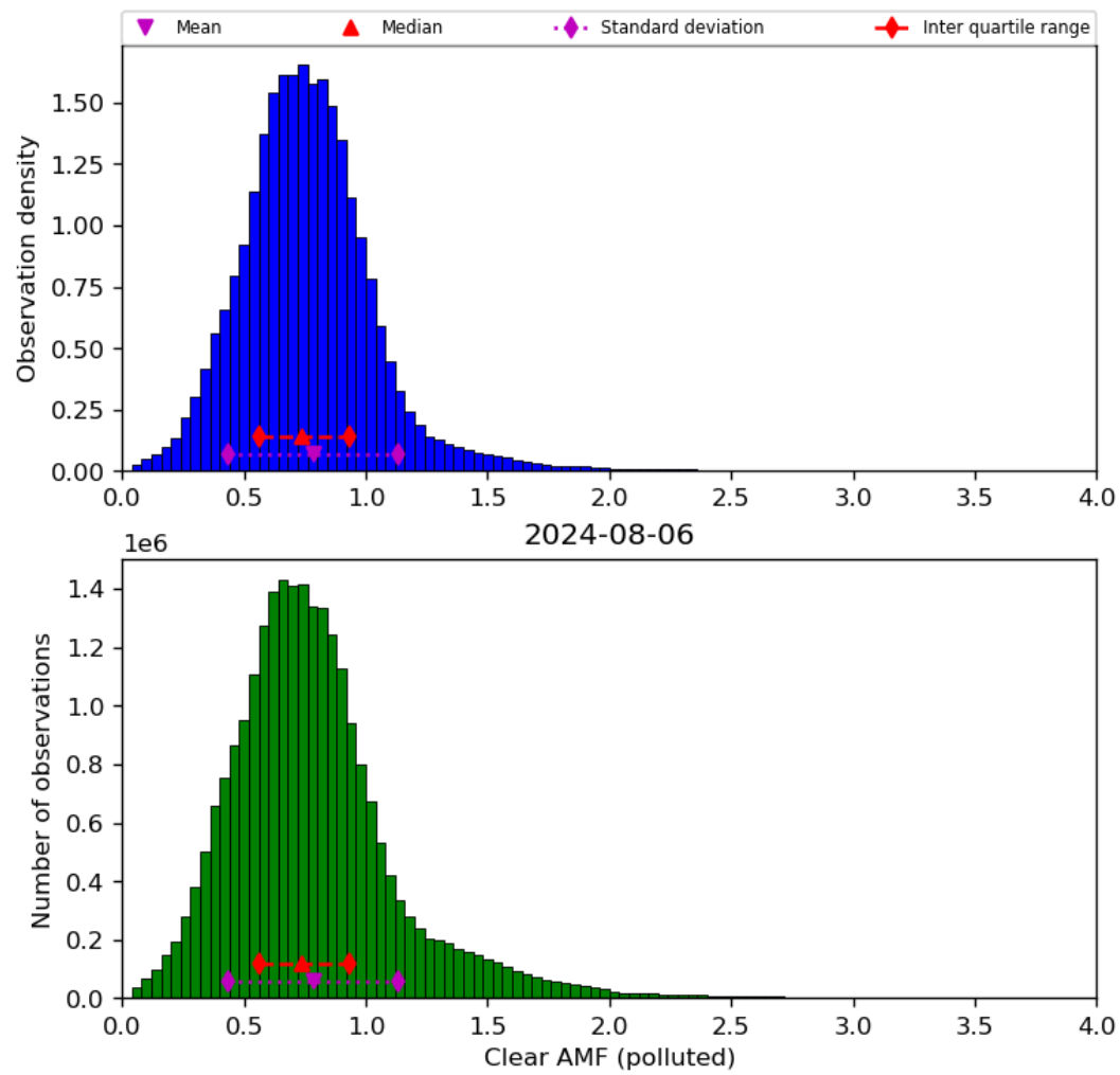
Figure 73: Histogram of “Clear AMF (polluted)” for 2024-08-06 to 2024-08-07
