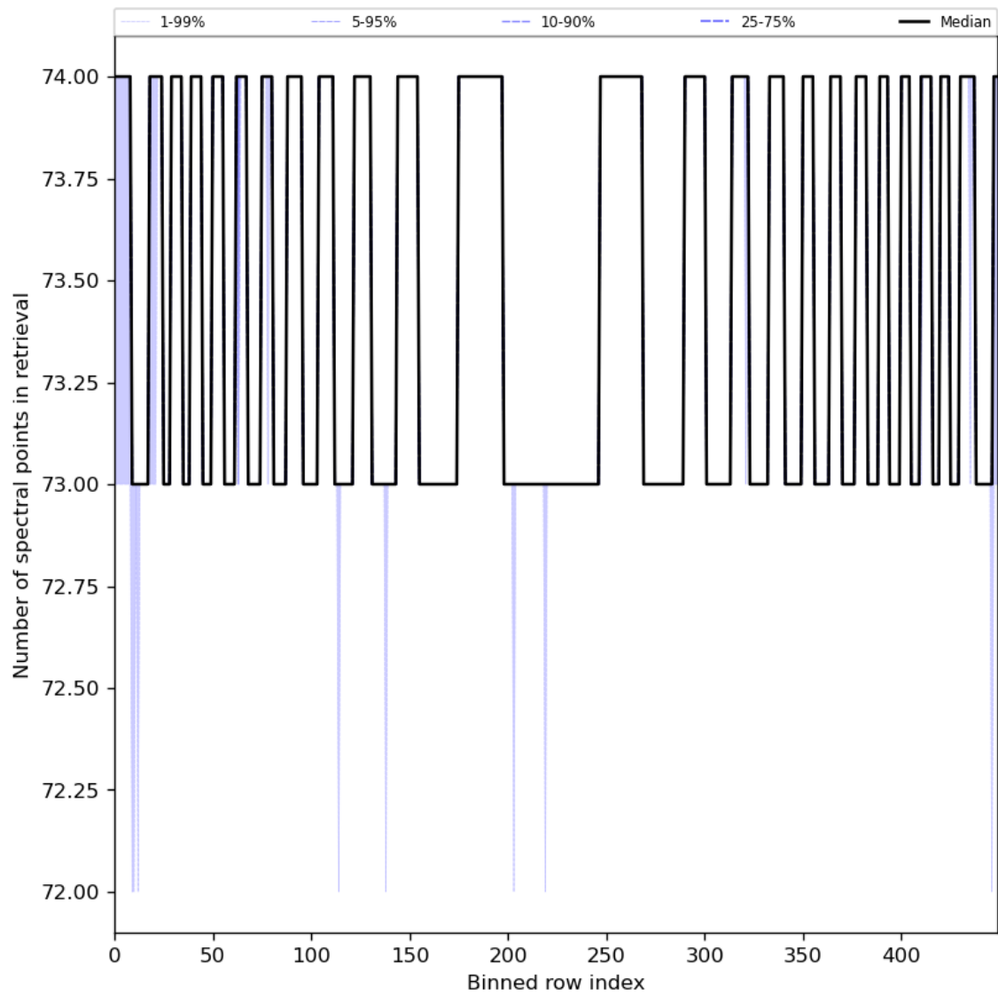
Figure 97: Along track statistics of “Number of spectral points in retrieval” for 2024-08-06 to 2024-08-07
