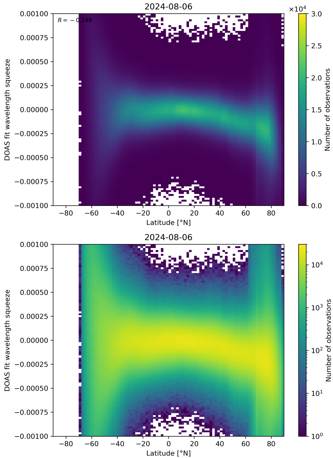
Figure 143: Scatter density plot of “Latitude” against “DOAS fit wavelength squeeze” for 2024-08-06 to 2024-08-07.
