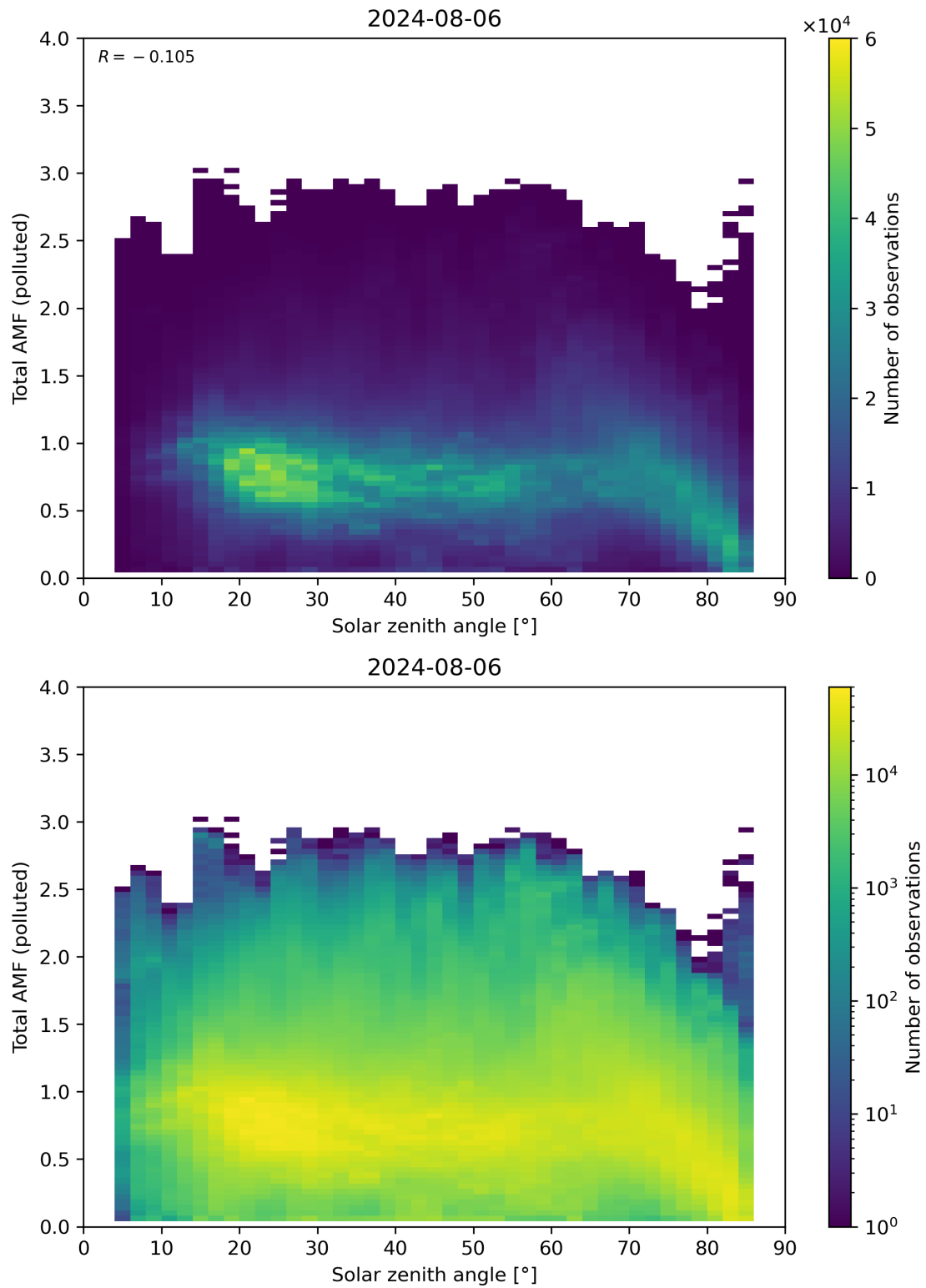
Figure 174: Scatter density plot of “Solar zenith angle” against “Total AMF (polluted)” for 2024-08-06 to 2024-08-07.
