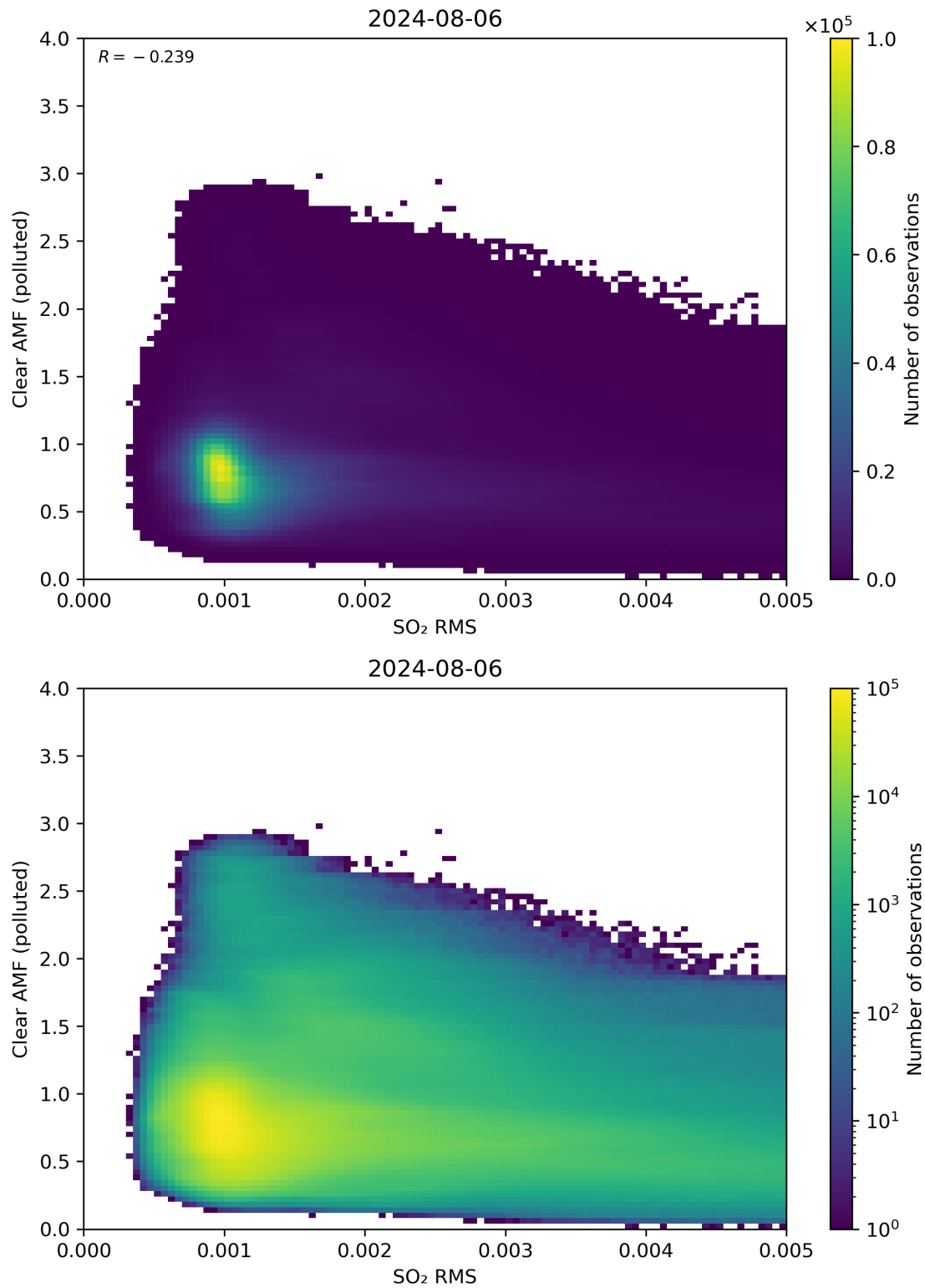
Figure 136: Scatter density plot of “SO 2 RMS” against “Clear AMF (polluted)” for 2024-08-06 to 2024-08-07.
