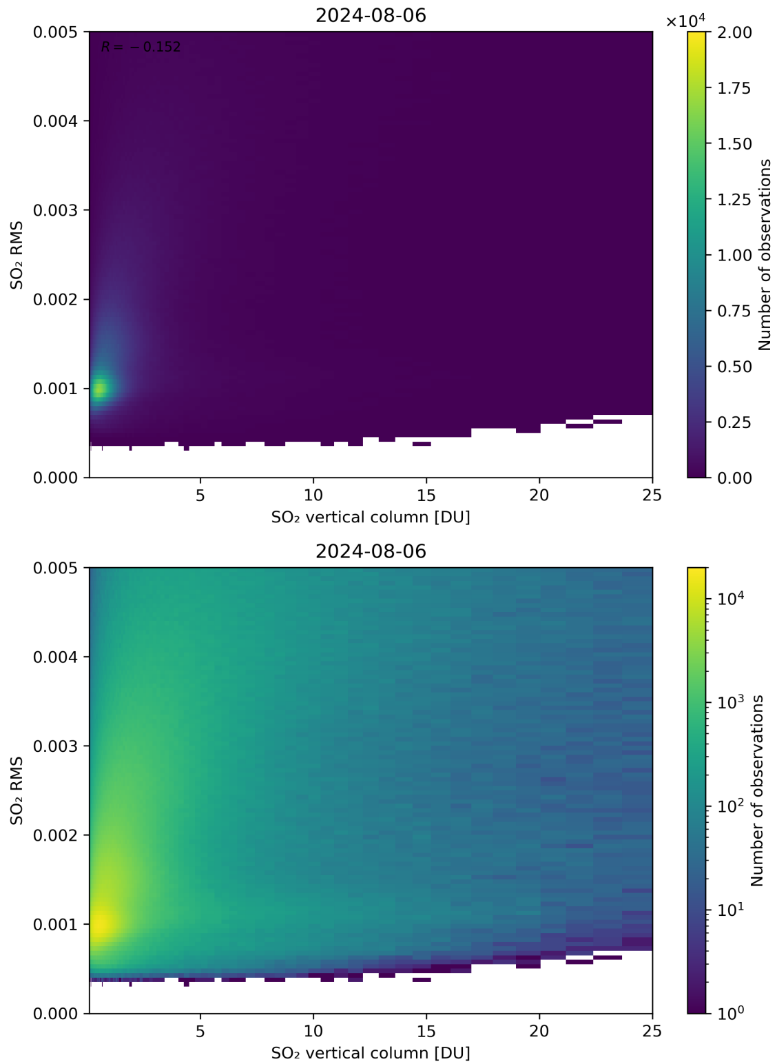
Figure 278: Scatter density plot of “SO 2 vertical column” against “SO 2 RMS” for 2024-08-06 to 2024-08-07.
