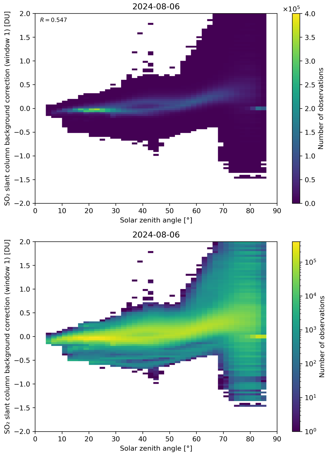
Figure 158: Scatter density plot of “Solar zenith angle” against “SO 2 slant column background correction (window 1)” for 2024-08-06 to 2024-08-07.
