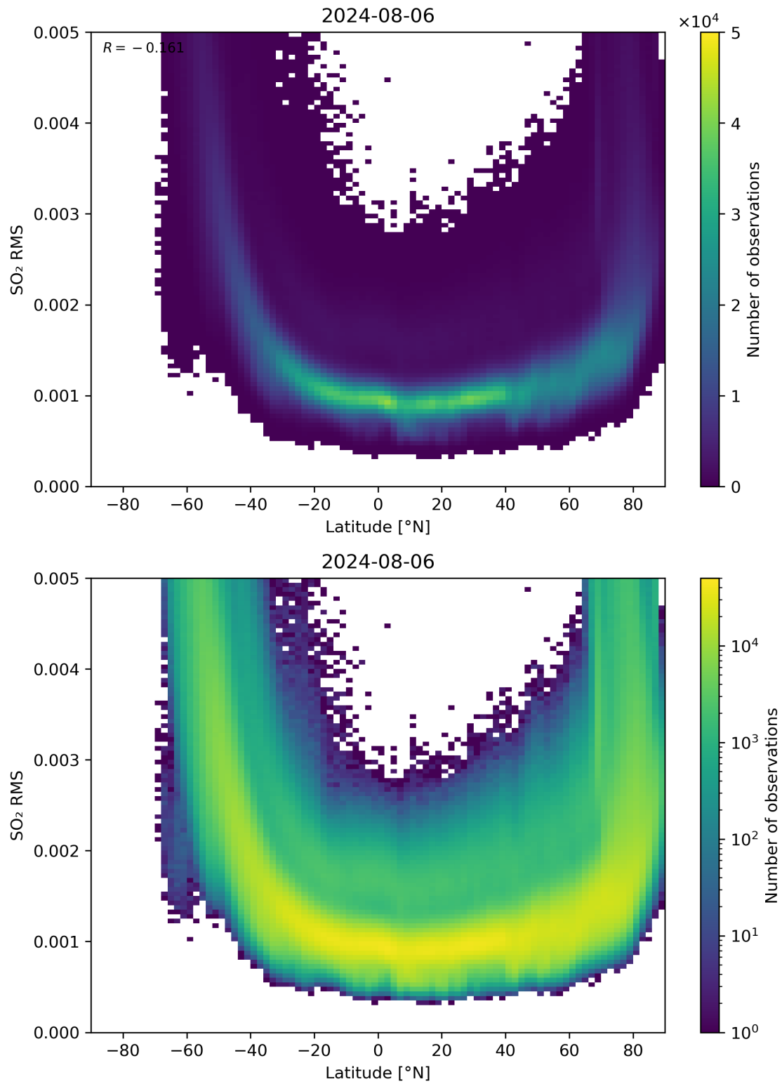
Figure 144: Scatter density plot of “Latitude” against “SO 2 RMS” for 2024-08-06 to 2024-08-07.
