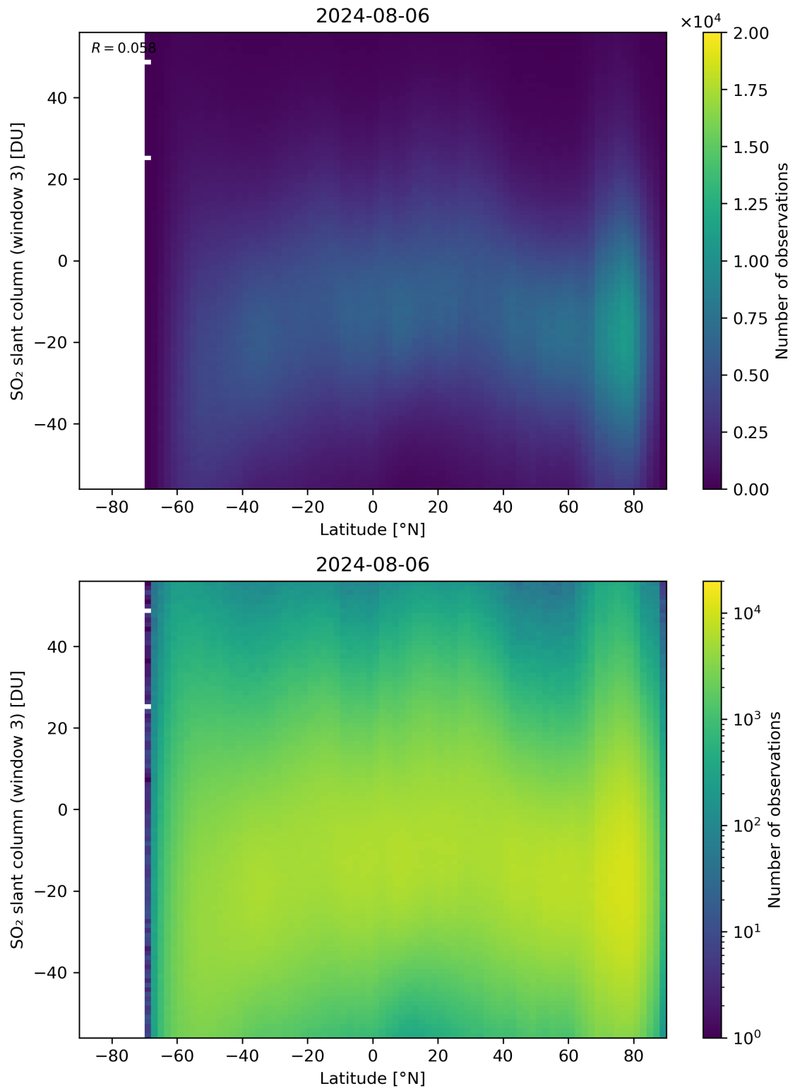
Figure 152: Scatter density plot of “Latitude” against “SO 2 slant column (window 3)” for 2024-08-06 to 2024-08-07.
