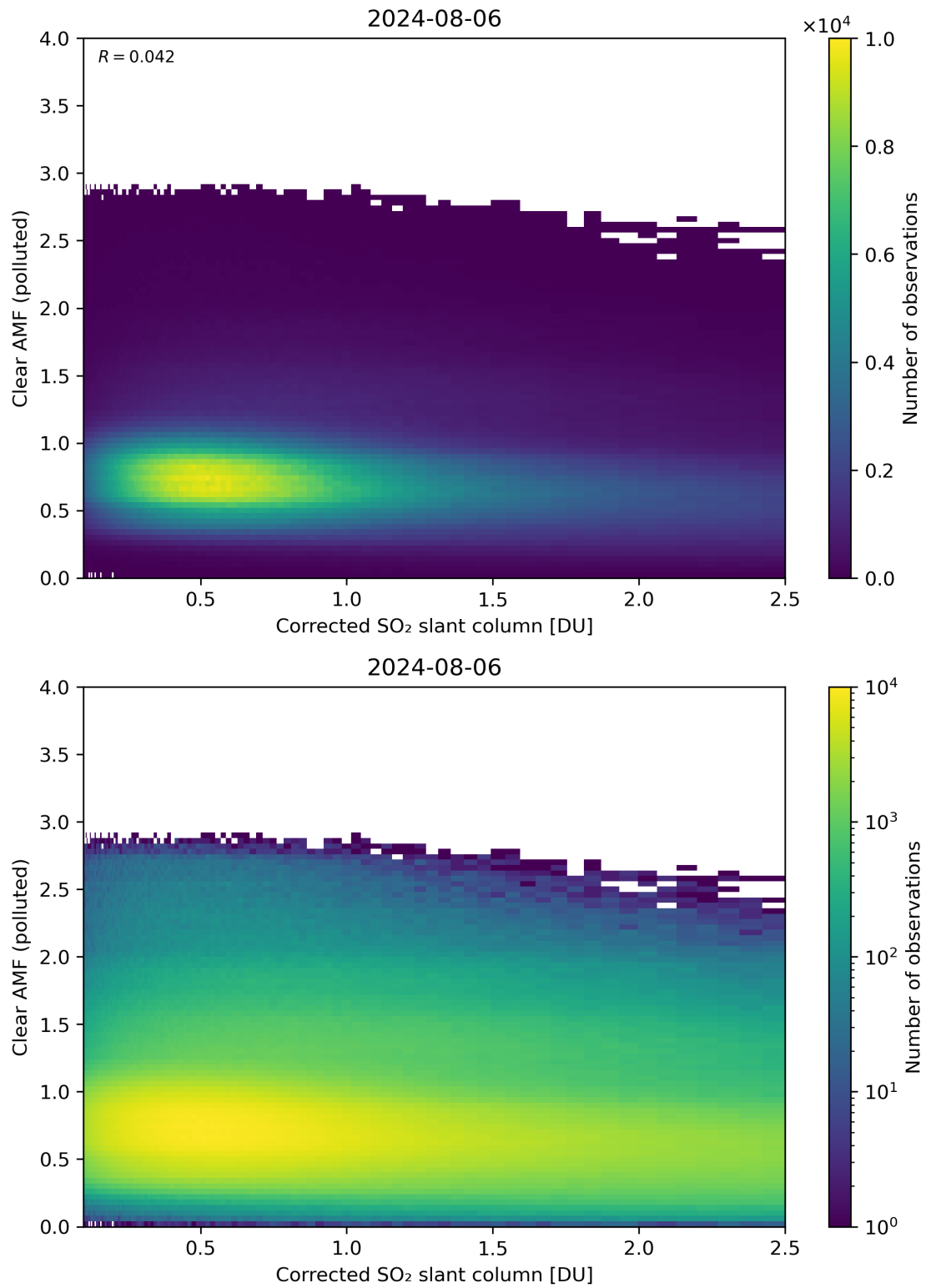
Figure 184: Scatter density plot of “Corrected SO 2 slant column” against “Clear AMF (polluted)” for 2024-08-06 to 2024-08-07.
