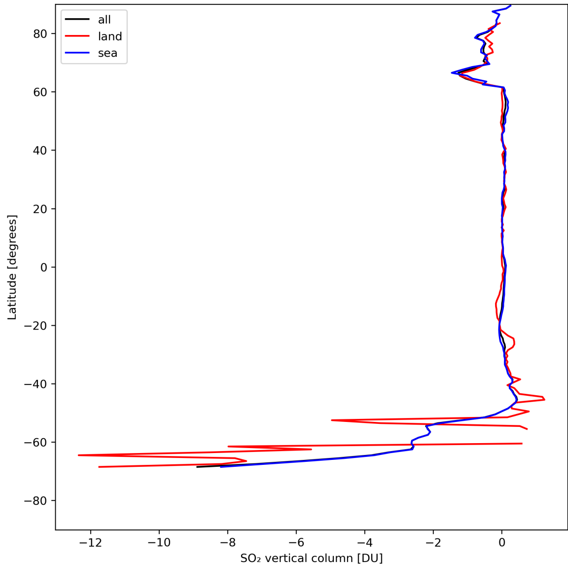
Figure 30: Zonal average of “SO 2 vertical column” for 2024-08-06 to 2024-08-07.
