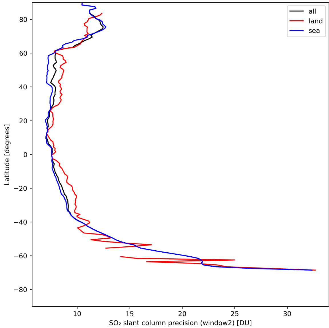
Figure 38: Zonal average of “SO 2 slant column precision (window2)” for 2024-08-06 to 2024-08-07.
