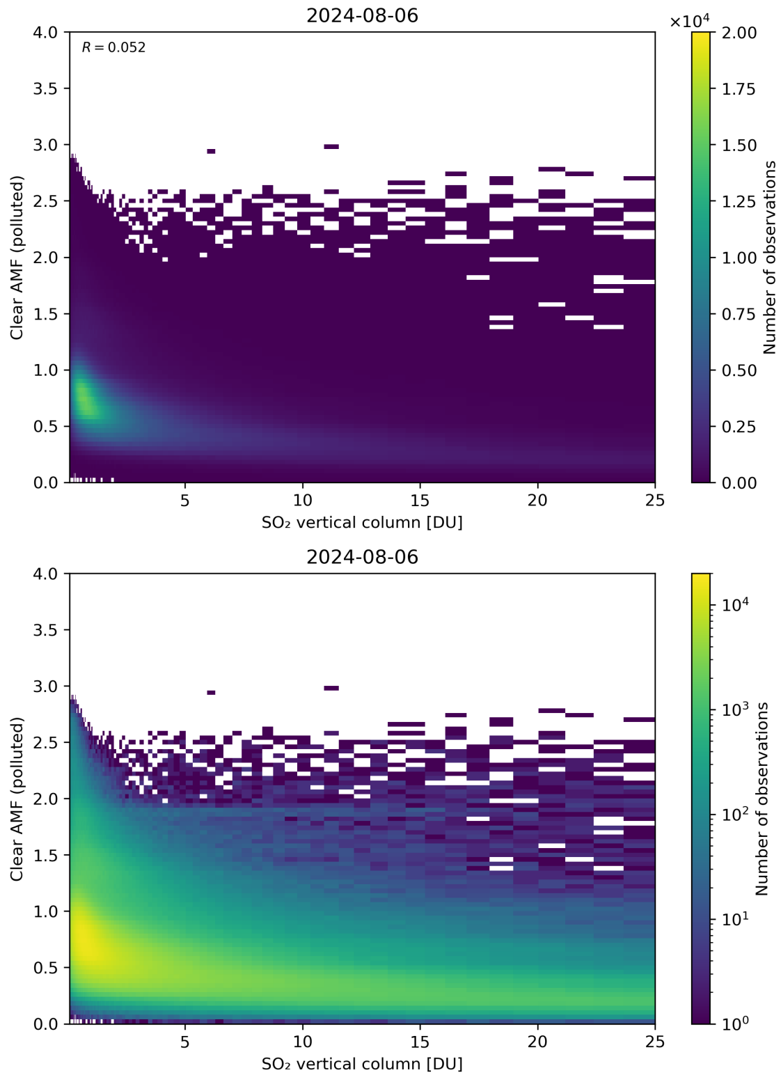
Figure 296: Scatter density plot of “SO 2 vertical column” against “Clear AMF (polluted)” for 2024-08-06 to 2024-08-07.
