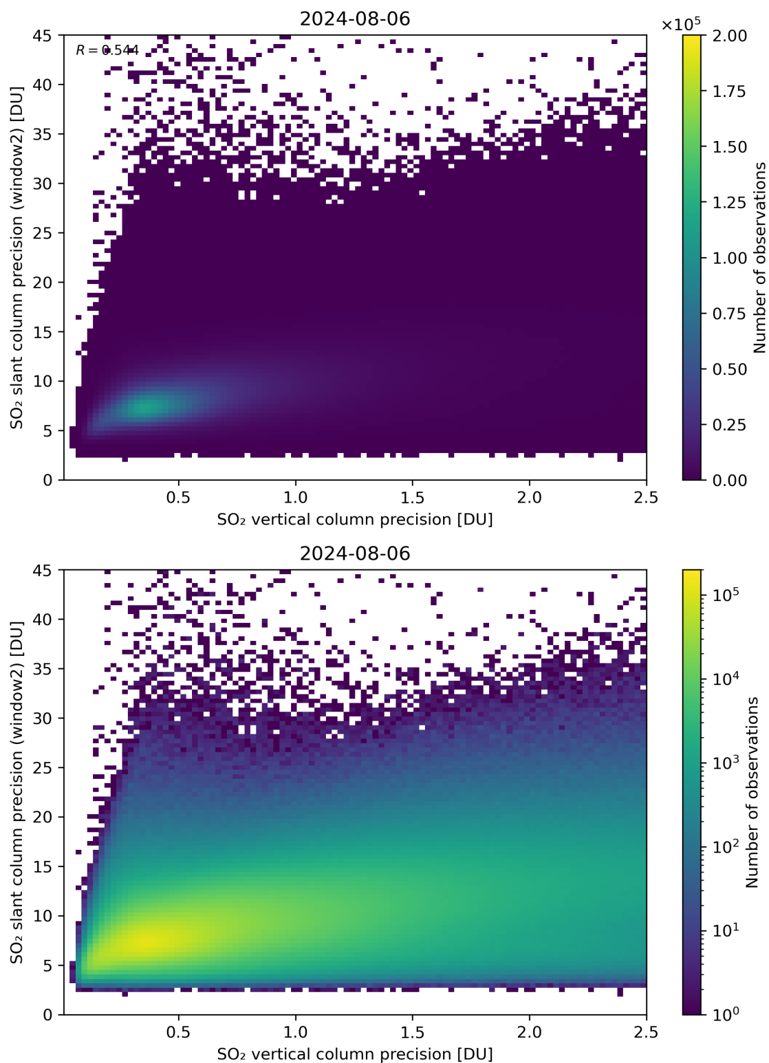
Figure 291: Scatter density plot of “SO 2 vertical column precision” against “SO 2 slant column precision (window2)” for 2024-08-06 to 2024-08-07.
