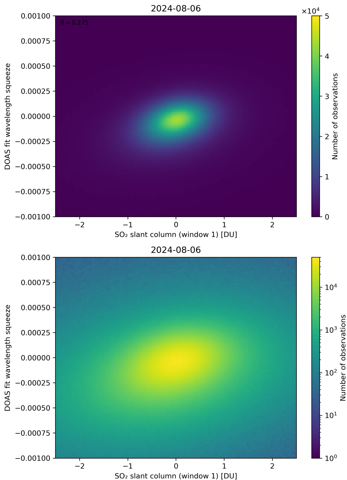
Figure 216: Scatter density plot of “SO 2 slant column (window 1)” against “DOAS fit wavelength squeeze” for 2024-08-06 to 2024-08-07.
