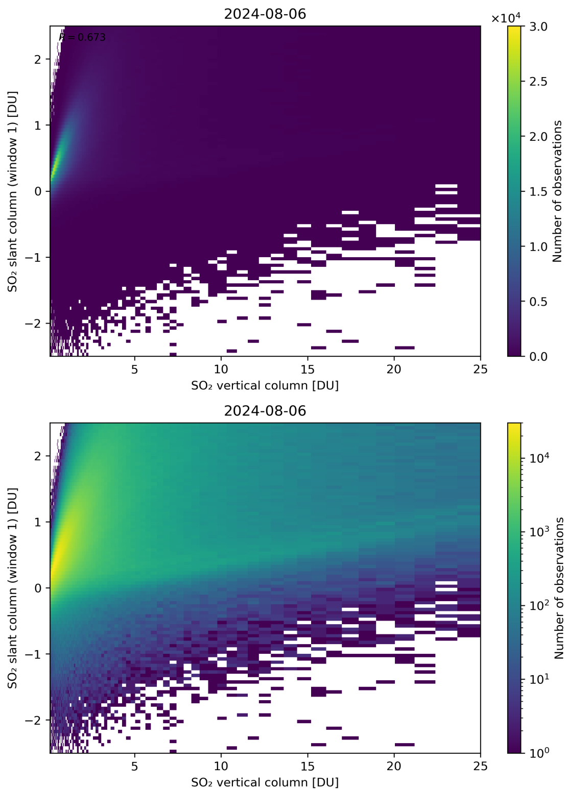
Figure 300: Scatter density plot of “SO 2 vertical column” against “SO 2 slant column (window 1)” for 2024-08-06 to 2024-08-07.
