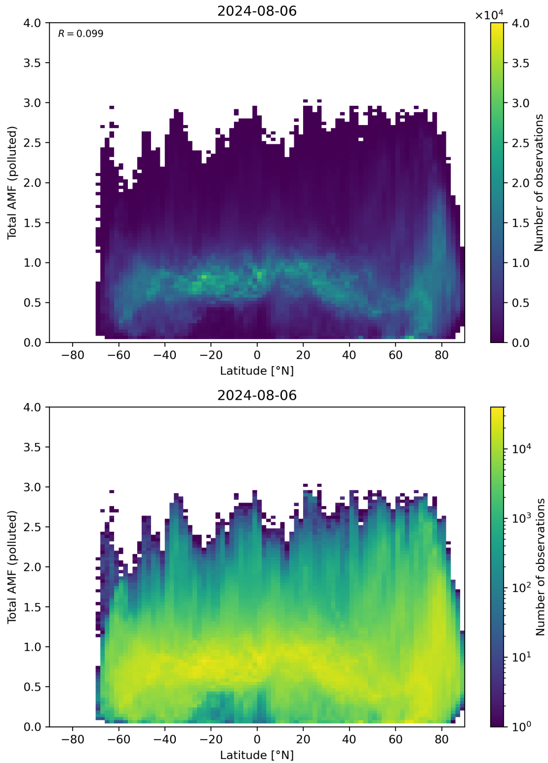
Figure 154: Scatter density plot of “Latitude” against “Total AMF (polluted)” for 2024-08-06 to 2024-08-07.
