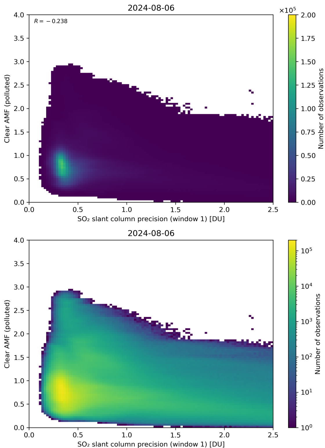
Figure 224: Scatter density plot of “SO 2 slant column precision (window 1)” against “Clear AMF (polluted)” for 2024-08-06 to 2024-08-07.
