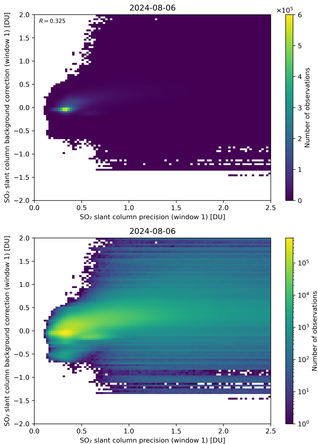
Figure 218: Scatter density plot of “SO 2 slant column precision (window 1)” against “SO 2 slant column background correction (window 1)” for 2024-08-06 to 2024-08-07.
