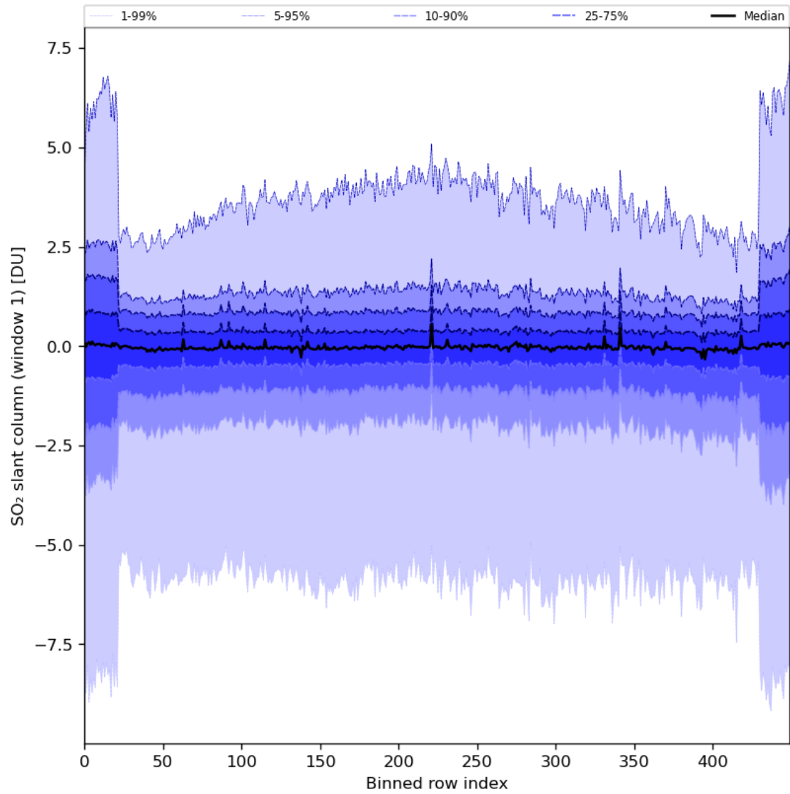
Figure 79: Along track statistics of “SO 2 slant column (window 1)” for 2024-08-06 to 2024-08-07
