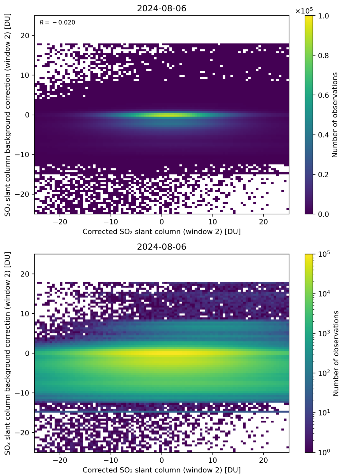
Figure 194: Scatter density plot of “Corrected SO 2 slant column (window 2)” against “SO 2 slant column background correction (window 2)” for 2024-08-06 to 2024-08-07.
