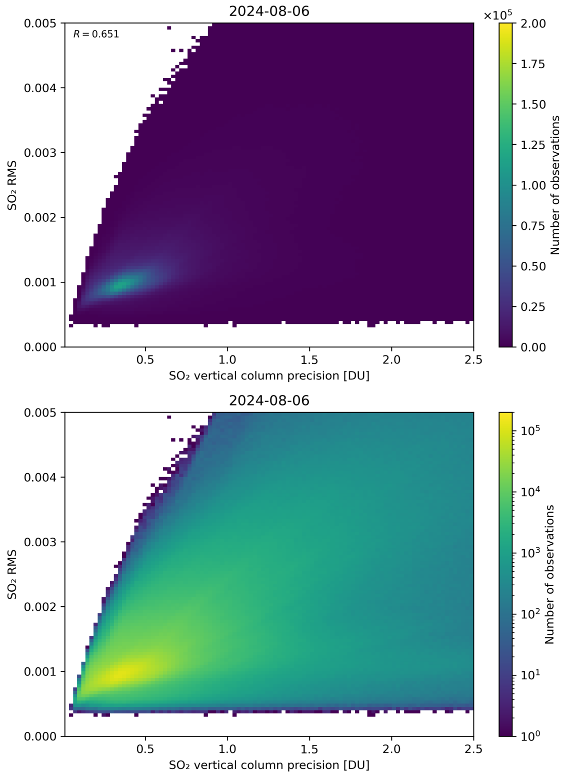
Figure 284: Scatter density plot of “SO 2 vertical column precision” against “SO 2 RMS” for 2024-08-06 to 2024-08-07.
