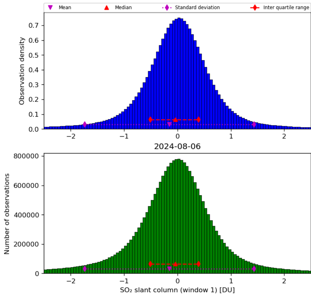
Figure 56: Histogram of “SO 2 slant column (window 1)” for 2024-08-06 to 2024-08-07
