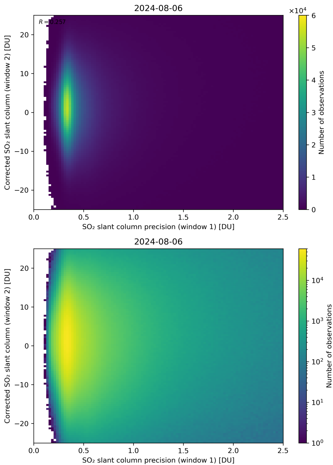
Figure 225: Scatter density plot of “SO 2 slant column precision (window 1)” against “Corrected SO 2 slant column (window 2)” for 2024-08-06 to 2024-08-07.
