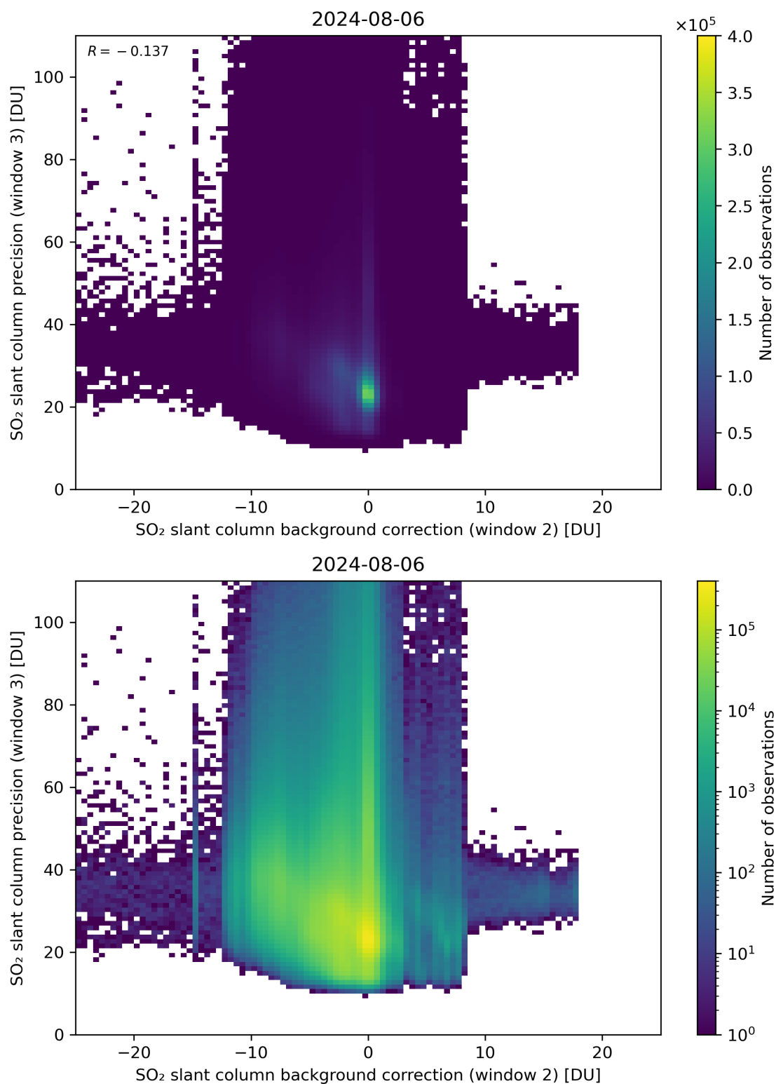
Figure 118: Scatter density plot of “SO 2 slant column background correction (window 2)” against “SO 2 slant column precision (window 3)” for 2024-08-06 to 2024-08-07.
