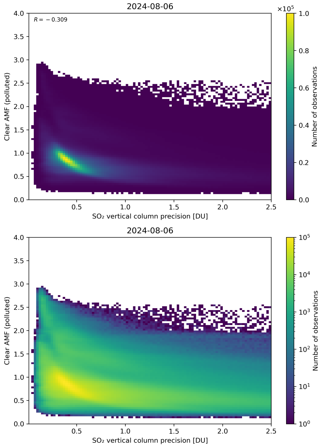
Figure 285: Scatter density plot of “SO 2 vertical column precision” against “Clear AMF (polluted)” for 2024-08-06 to 2024-08-07.
