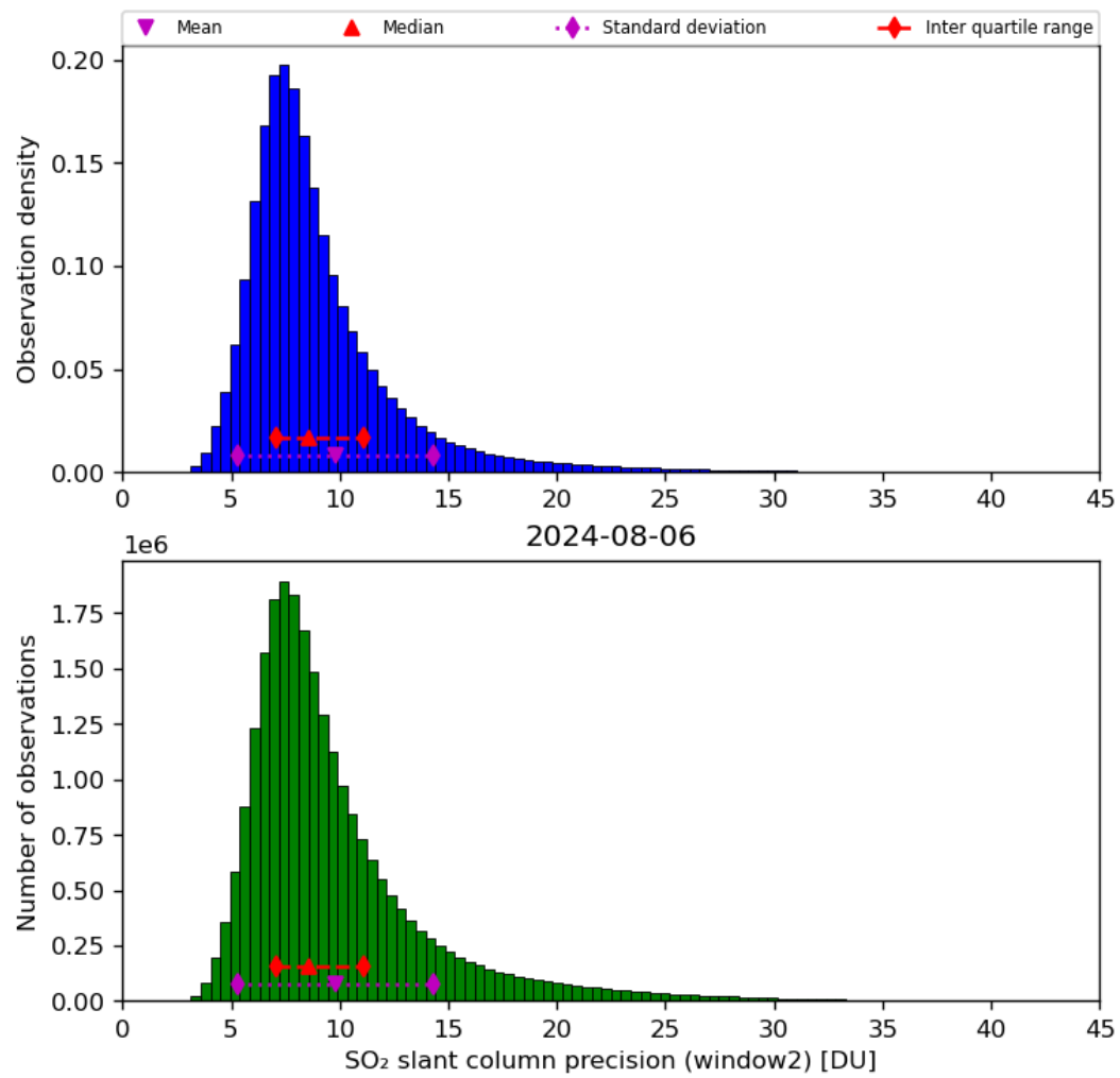
Figure 61: Histogram of “SO 2 slant column precision (window2)” for 2024-08-06 to 2024-08-07
