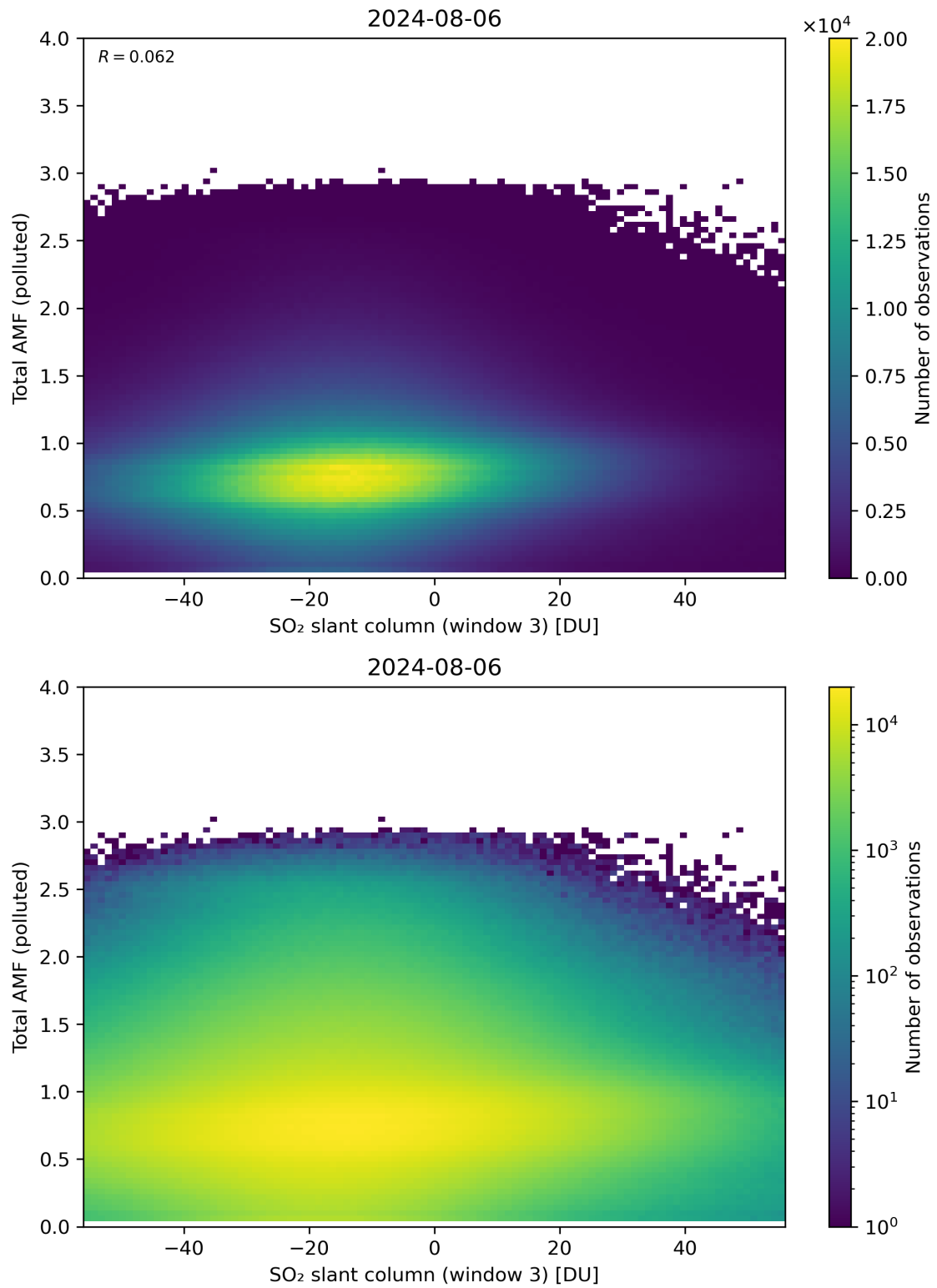
Figure 268: Scatter density plot of “SO 2 slant column (window 3)” against “Total AMF (polluted)” for 2024-08-06 to 2024-08-07.
