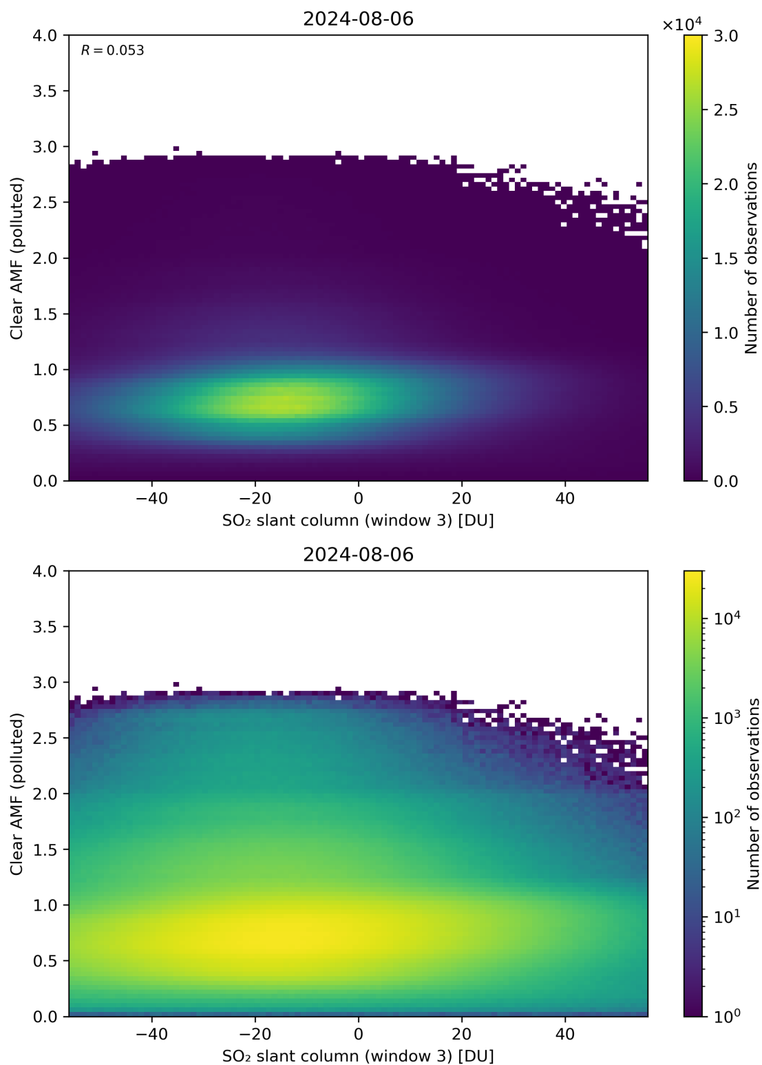
Figure 265: Scatter density plot of “SO 2 slant column (window 3)” against “Clear AMF (polluted)” for 2024-08-06 to 2024-08-07.
