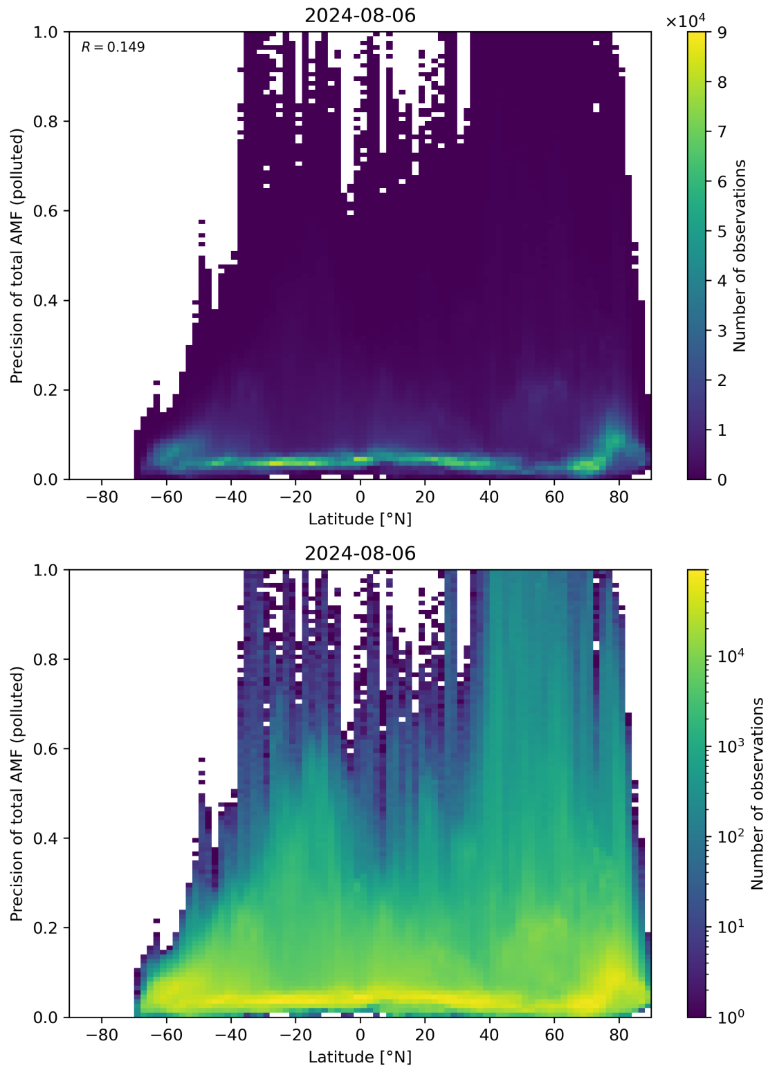
Figure 155: Scatter density plot of “Latitude” against “Precision of total AMF (polluted)” for 2024-08-06 to 2024-08-07.
