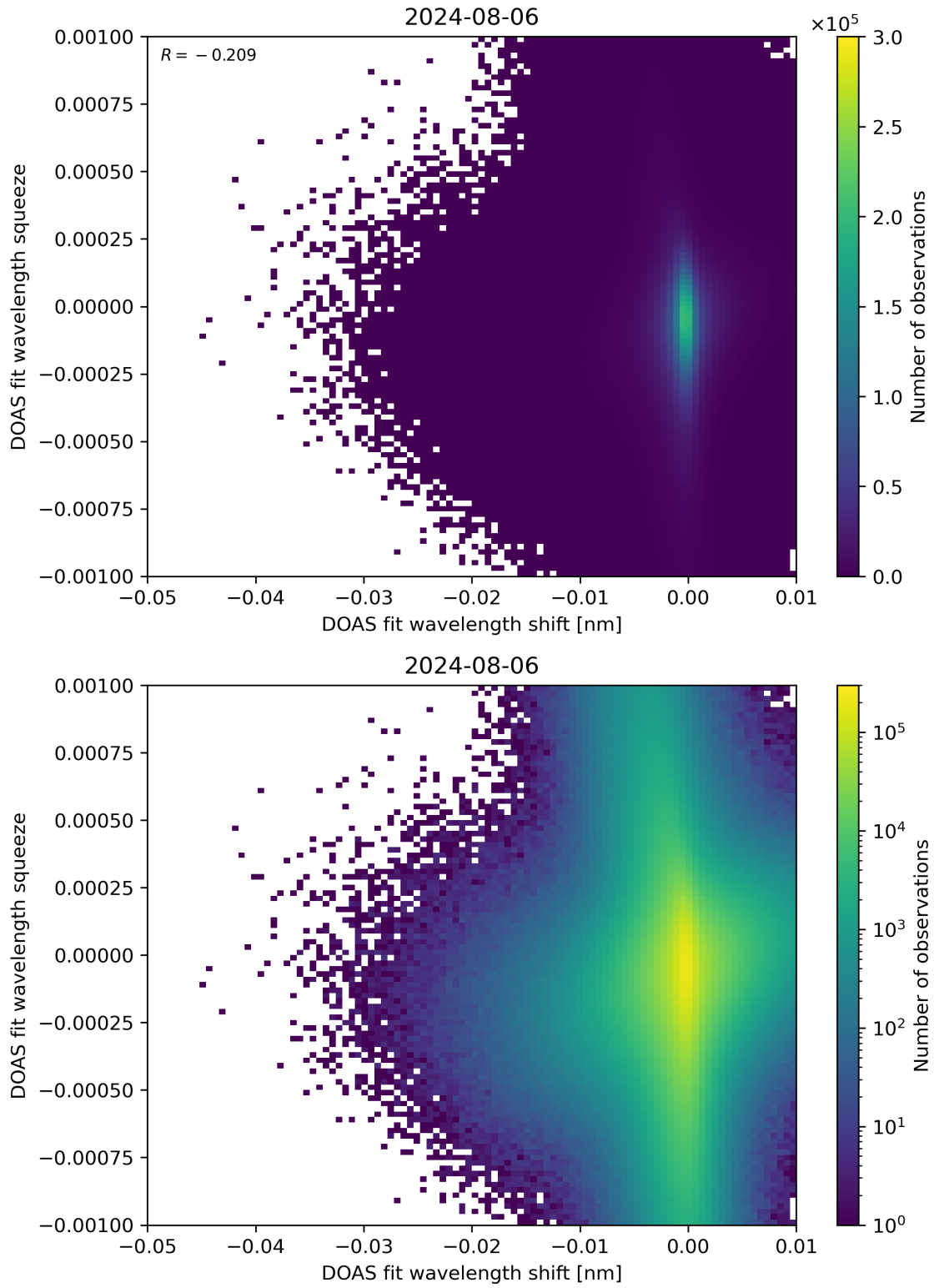
Figure 127: Scatter density plot of “DOAS fit wavelength shift” against “DOAS fit wavelength squeeze” for 2024-08-06 to 2024-08-07.
