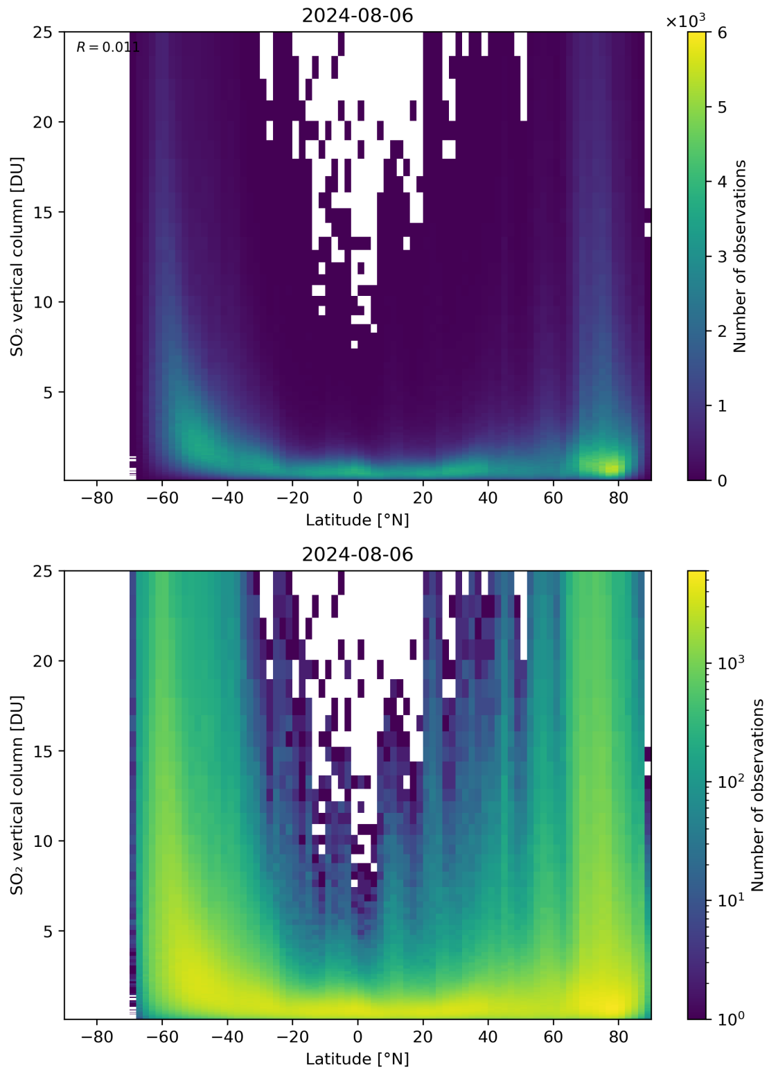
Figure 156: Scatter density plot of “Latitude” against “SO 2 vertical column” for 2024-08-06 to 2024-08-07.
