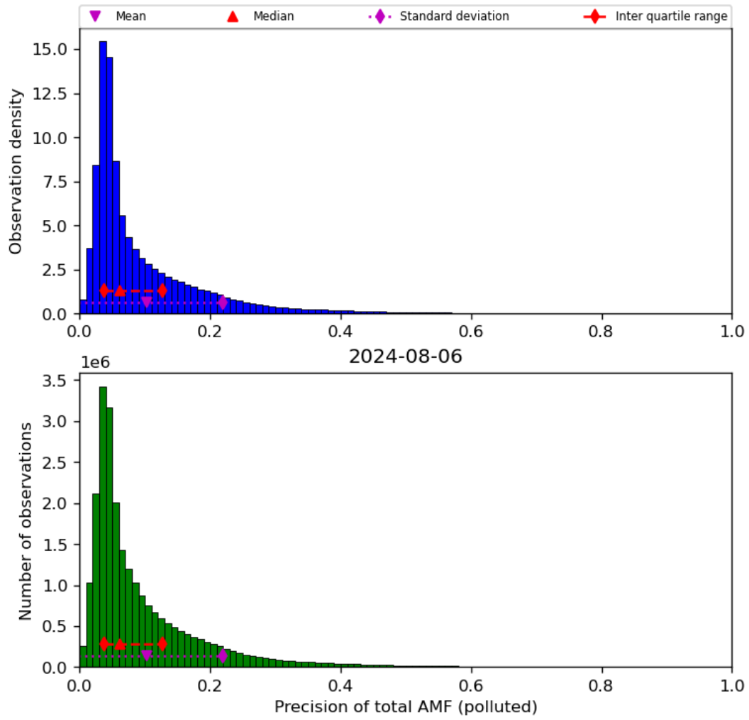
Figure 72: Histogram of “Precision of total AMF (polluted)” for 2024-08-06 to 2024-08-07
