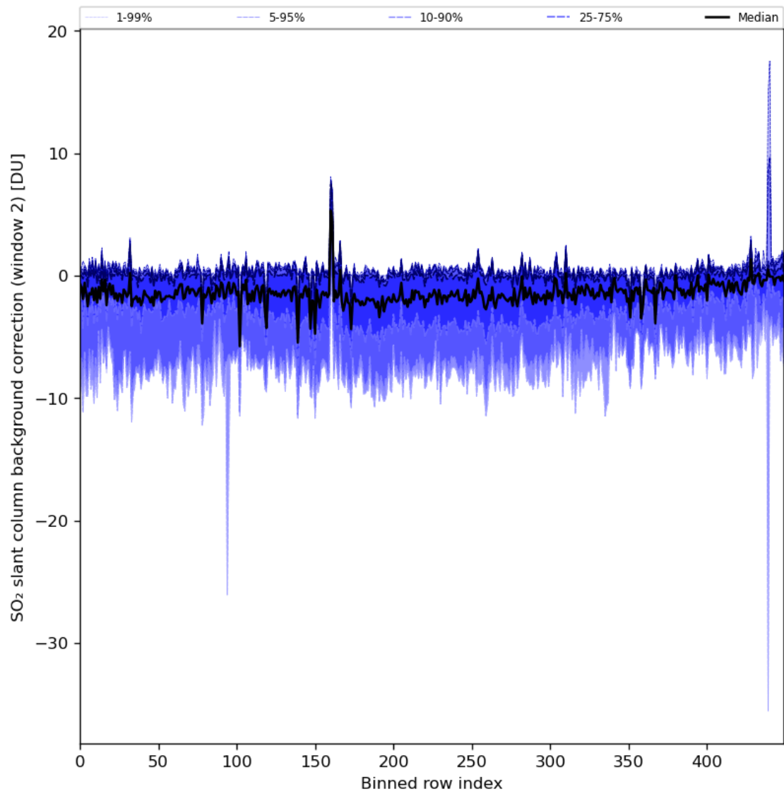
Figure 86: Along track statistics of “SO 2 slant column background correction (window 2)” for 2024-08-06 to 2024-08-07
