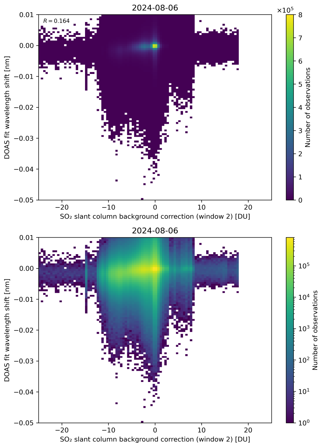
Figure 112: Scatter density plot of “SO 2 slant column background correction (window 2)” against “DOAS fit wavelength shift” for 2024-08-06 to 2024-08-07.
