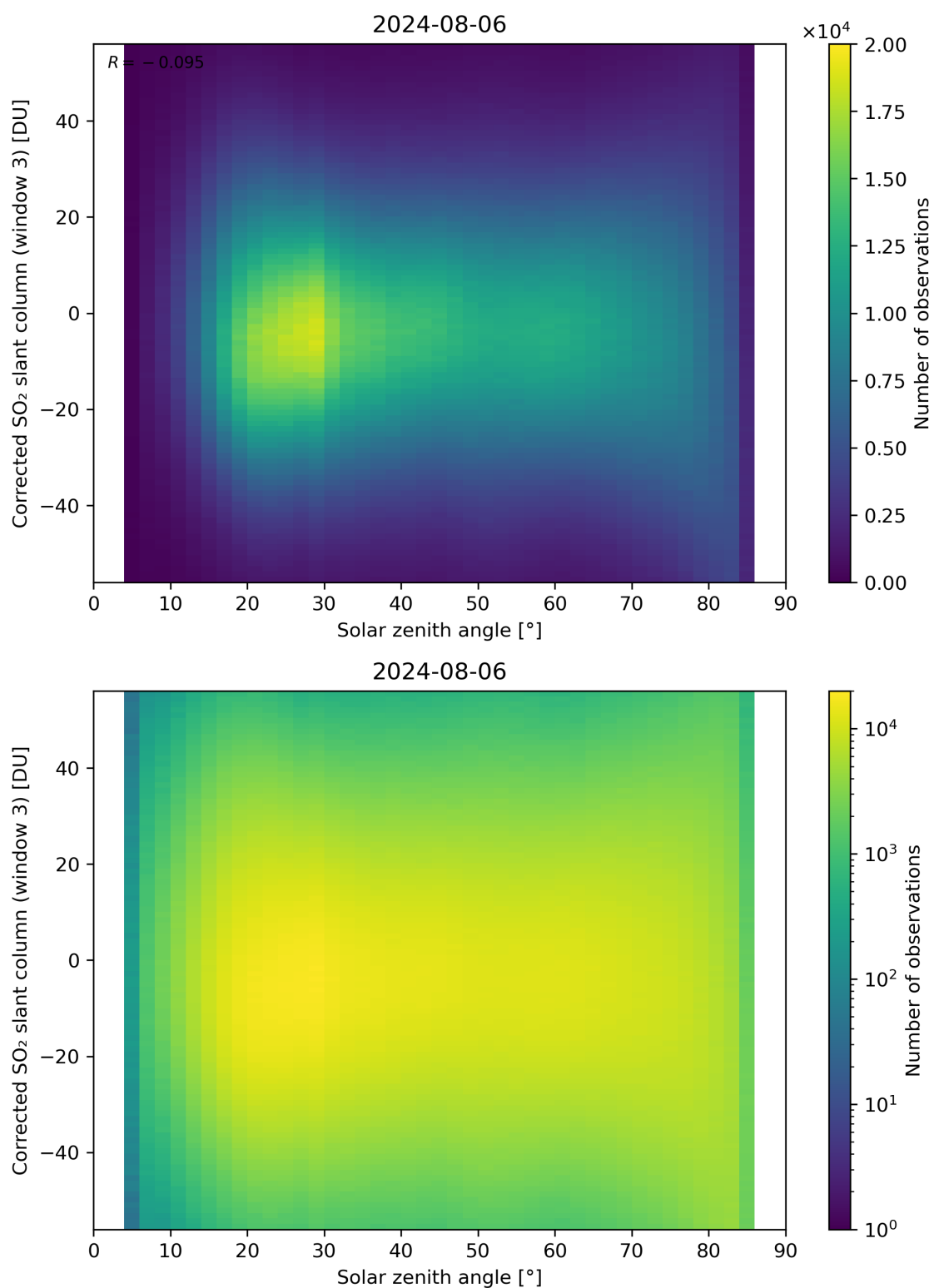
Figure 168: Scatter density plot of “Solar zenith angle” against “Corrected SO 2 slant column (window 3)” for 2024-08-06 to 2024-08-07.
