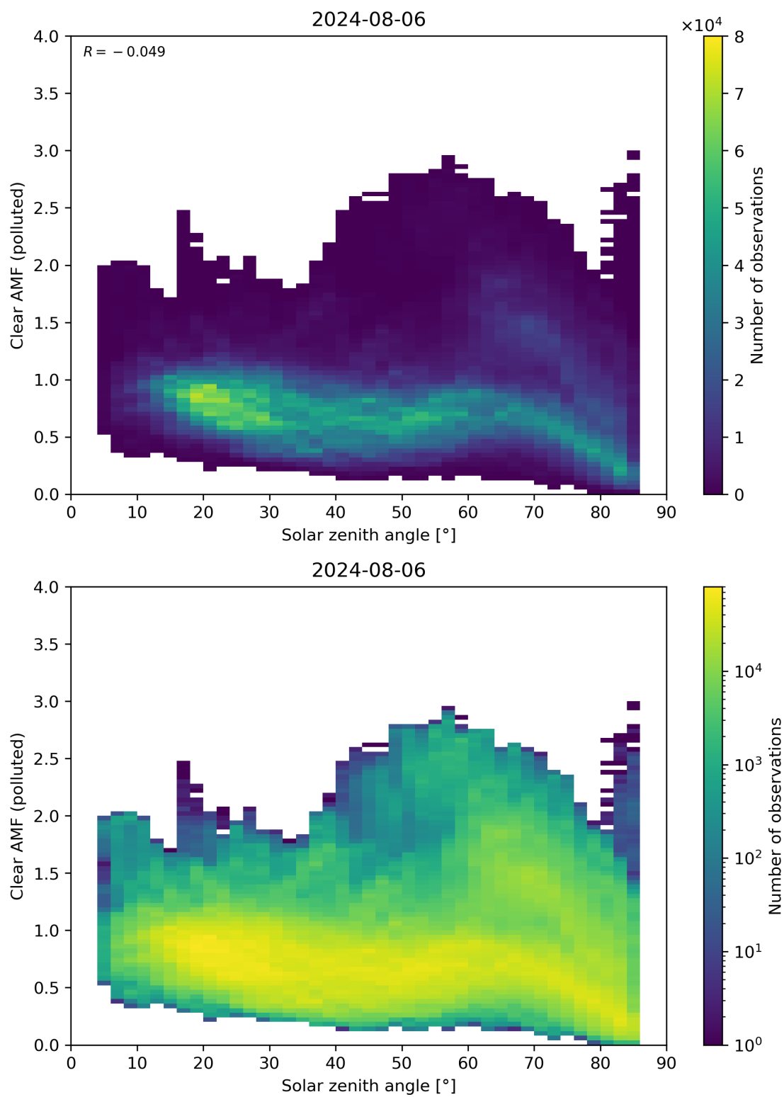
Figure 165: Scatter density plot of “Solar zenith angle” against “Clear AMF (polluted)” for 2024-08-06 to 2024-08-07.
