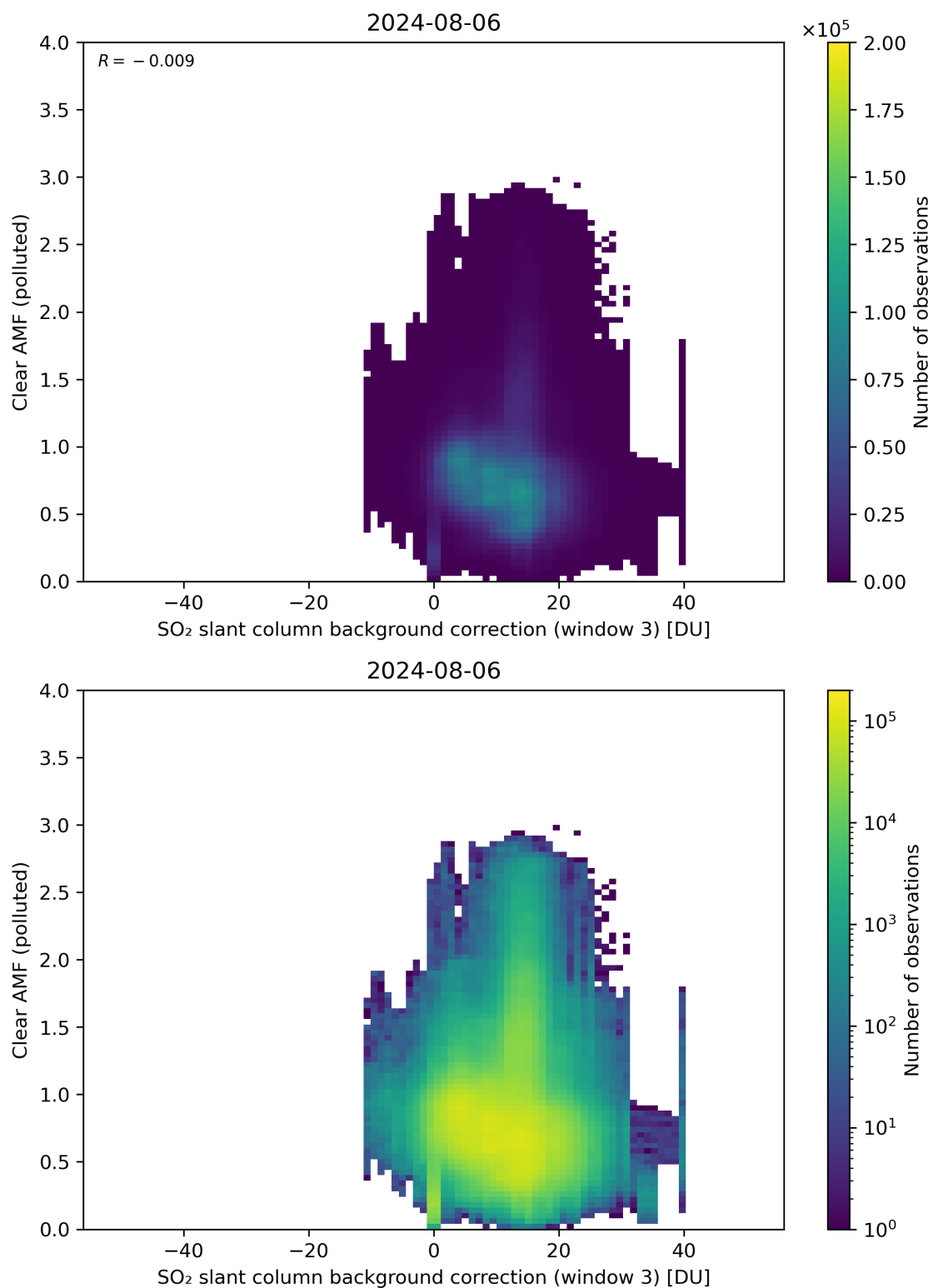
Figure 124: Scatter density plot of “SO 2 slant column background correction (window 3)” against “Clear AMF (polluted)” for 2024-08-06 to 2024-08-07.
