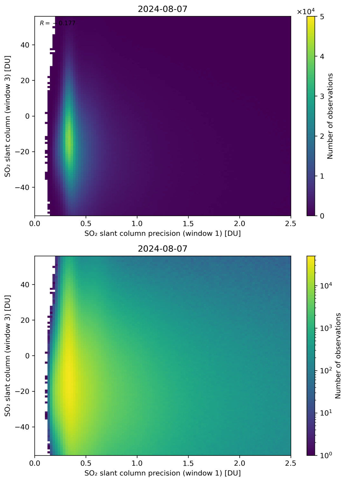
Figure 228: Scatter density plot of “SO 2 slant column precision (window 1)” against “SO 2 slant column (window 3)” for 2024-08-06 to 2024-08-08.
