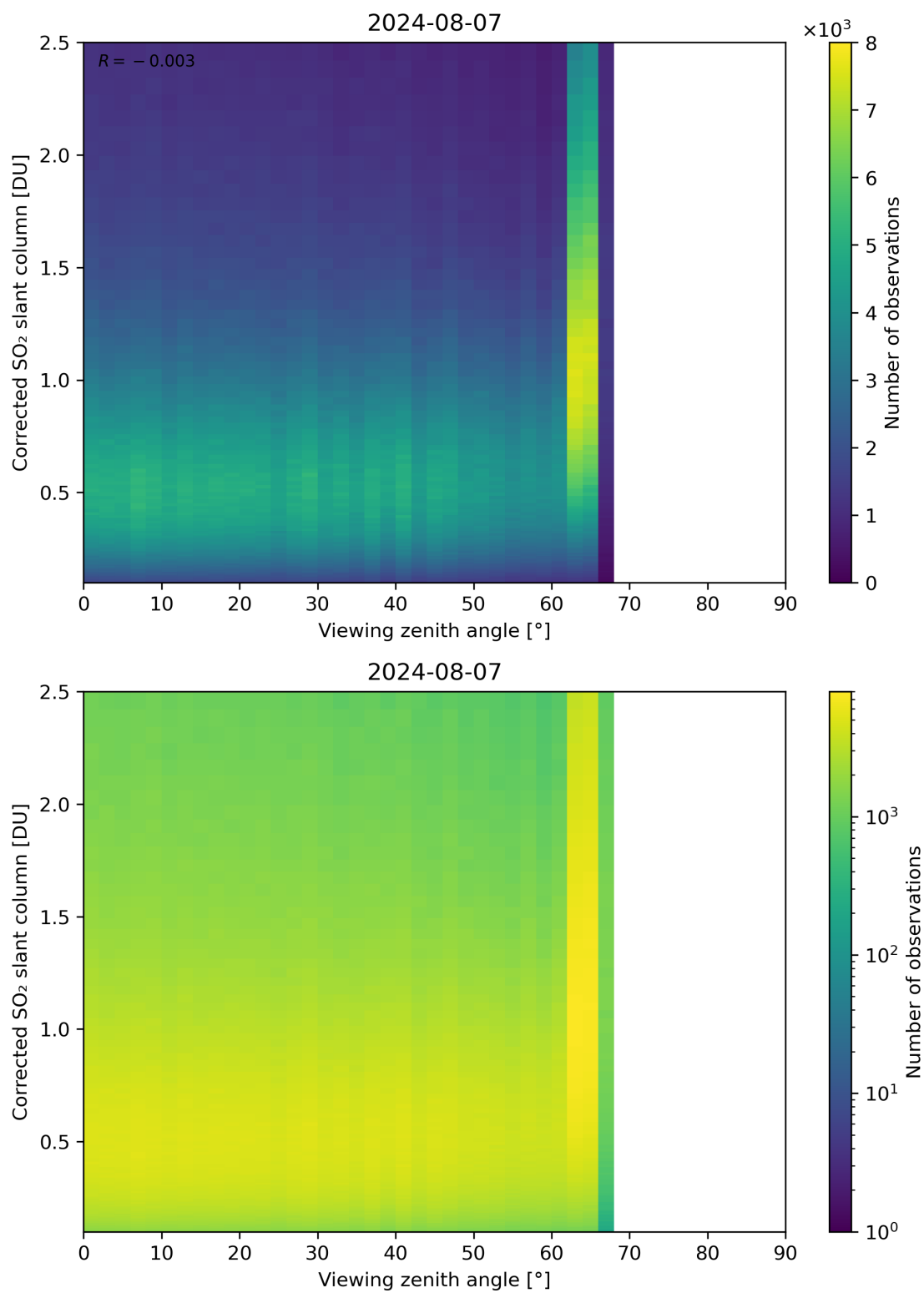
Figure 317: Scatter density plot of “Viewing zenith angle” against “Corrected SO 2 slant column” for 2024-08-06 to 2024-08-08.
