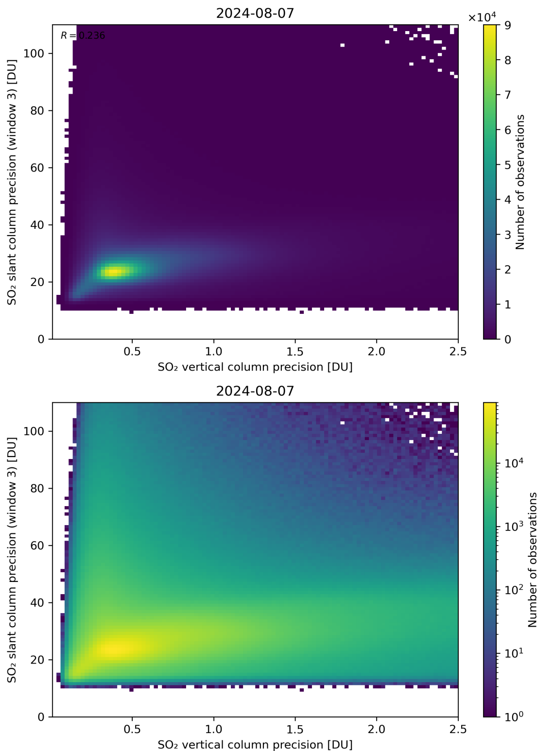
Figure 293: Scatter density plot of “SO 2 vertical column precision” against “SO 2 slant column precision (window 3)” for 2024-08-06 to 2024-08-08.
