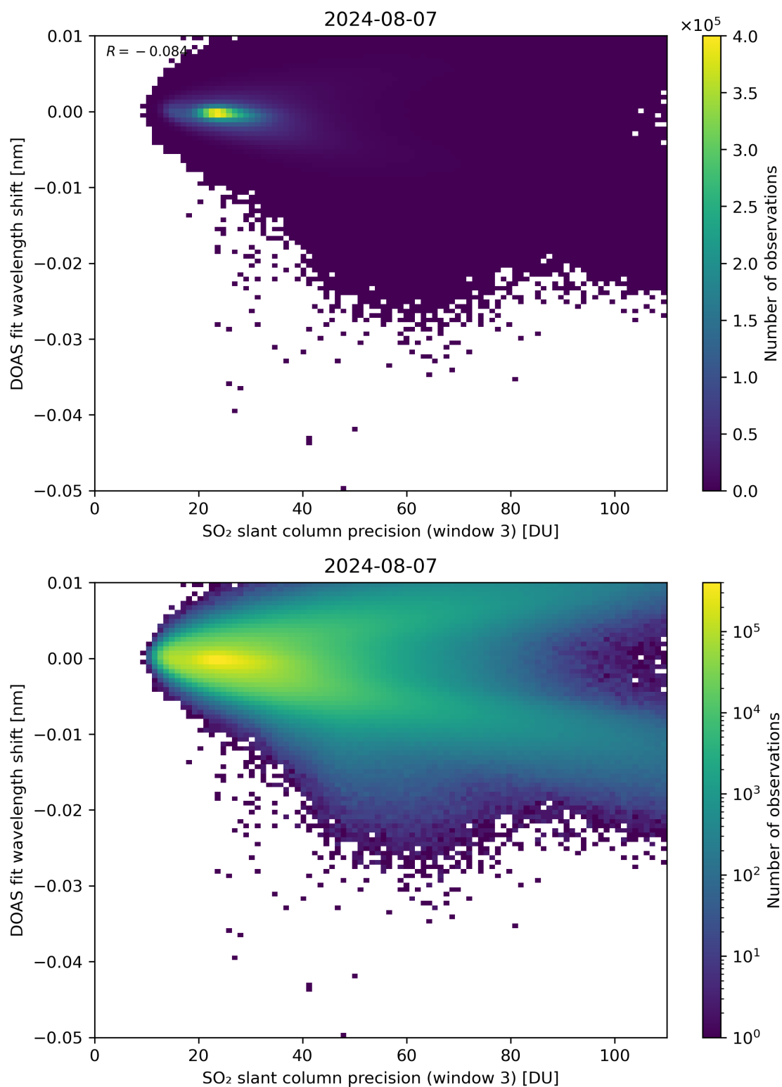
Figure 258: Scatter density plot of “SO 2 slant column precision (window 3)” against “DOAS fit wavelength shift” for 2024-08-06 to 2024-08-08.
