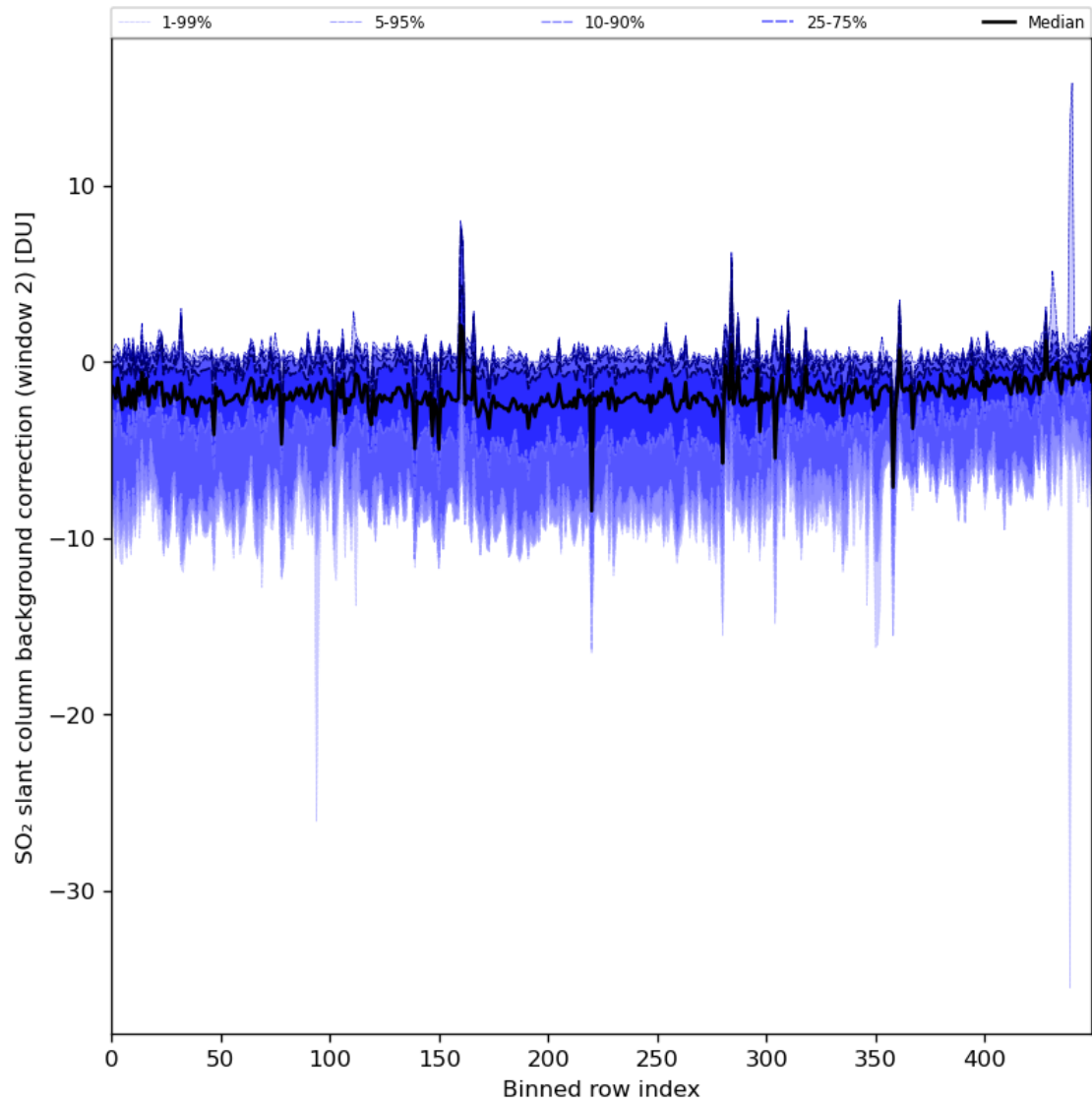
Figure 86: Along track statistics of “SO 2 slant column background correction (window 2)” for 2024-08-06 to 2024-08-08
