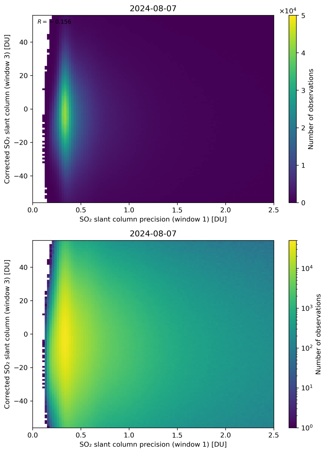
Figure 226: Scatter density plot of “SO 2 slant column precision (window 1)” against “Corrected SO 2 slant column (window 3)” for 2024-08-06 to 2024-08-08.
