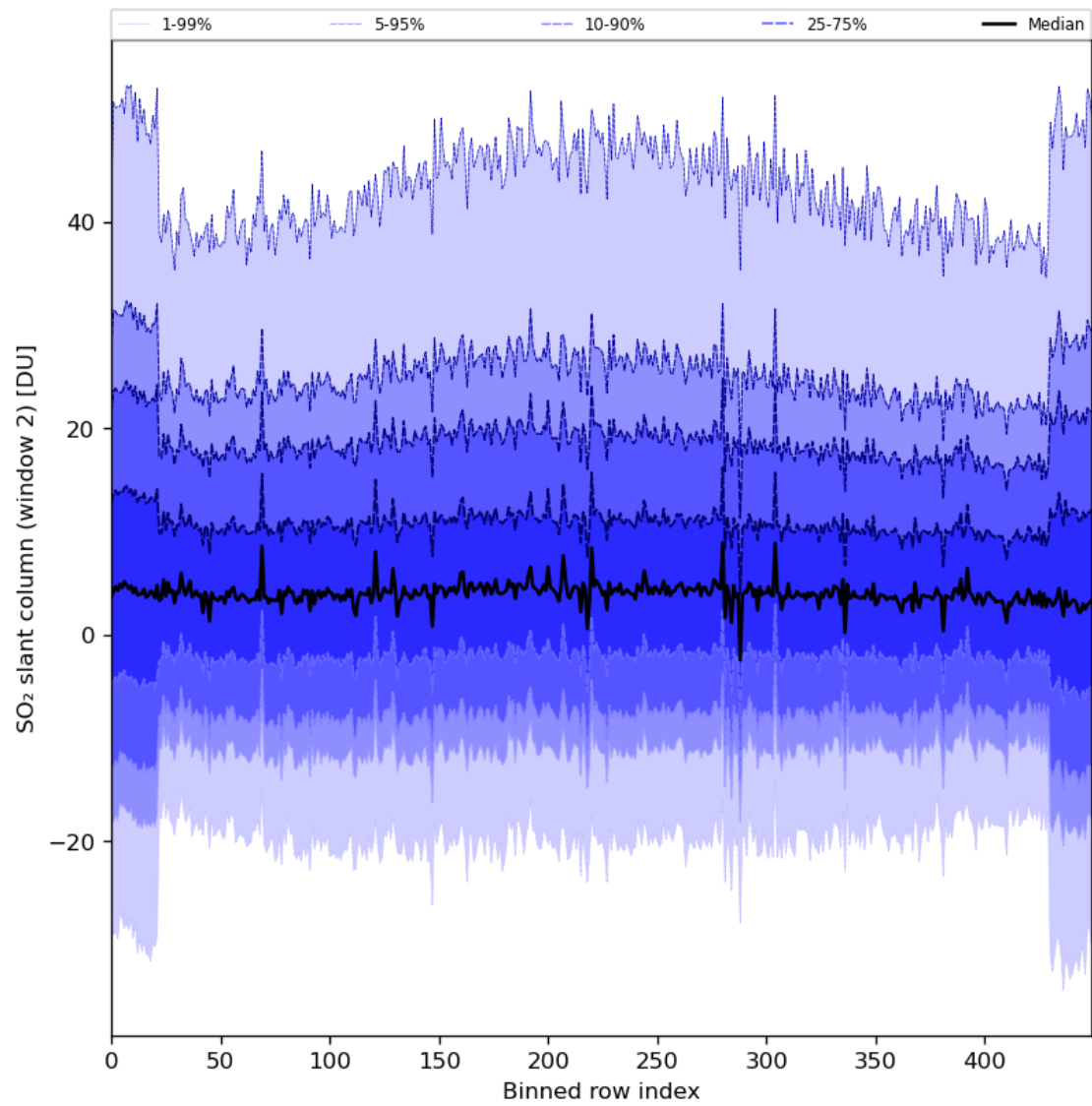
Figure 83: Along track statistics of “SO 2 slant column (window 2)” for 2024-08-06 to 2024-08-08
