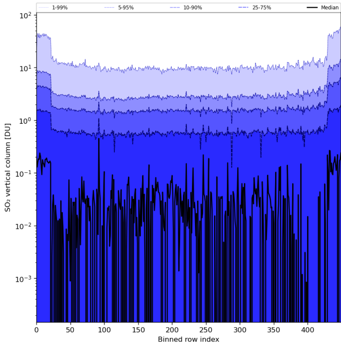
Figure 76: Along track statistics of “SO 2 vertical column” for 2024-08-06 to 2024-08-08
