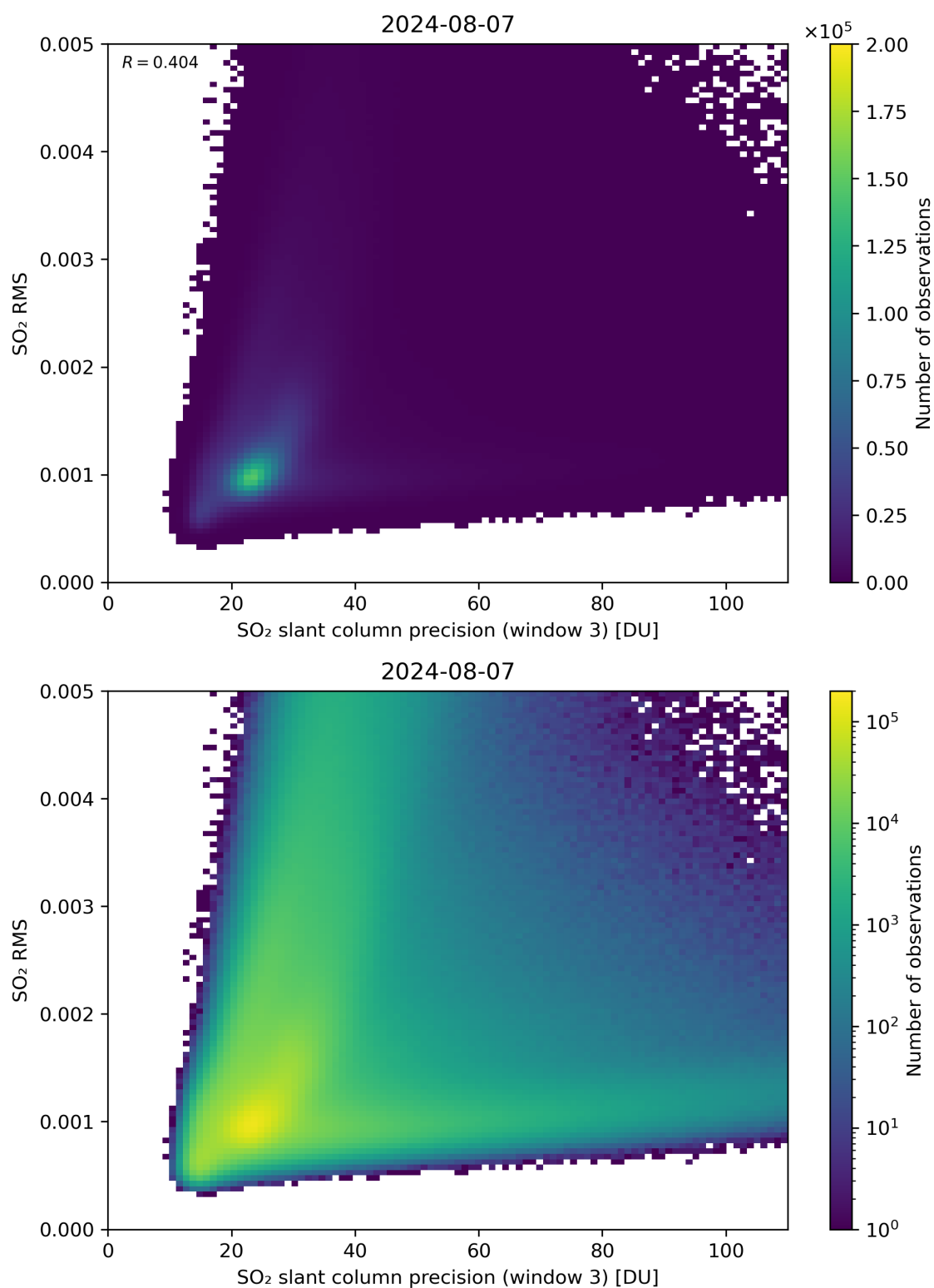
Figure 260: Scatter density plot of “SO 2 slant column precision (window 3)” against “SO 2 RMS” for 2024-08-06 to 2024-08-08.
