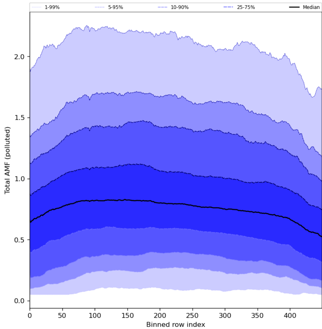
Figure 94: Along track statistics of “Total AMF (polluted)” for 2024-08-06 to 2024-08-08
