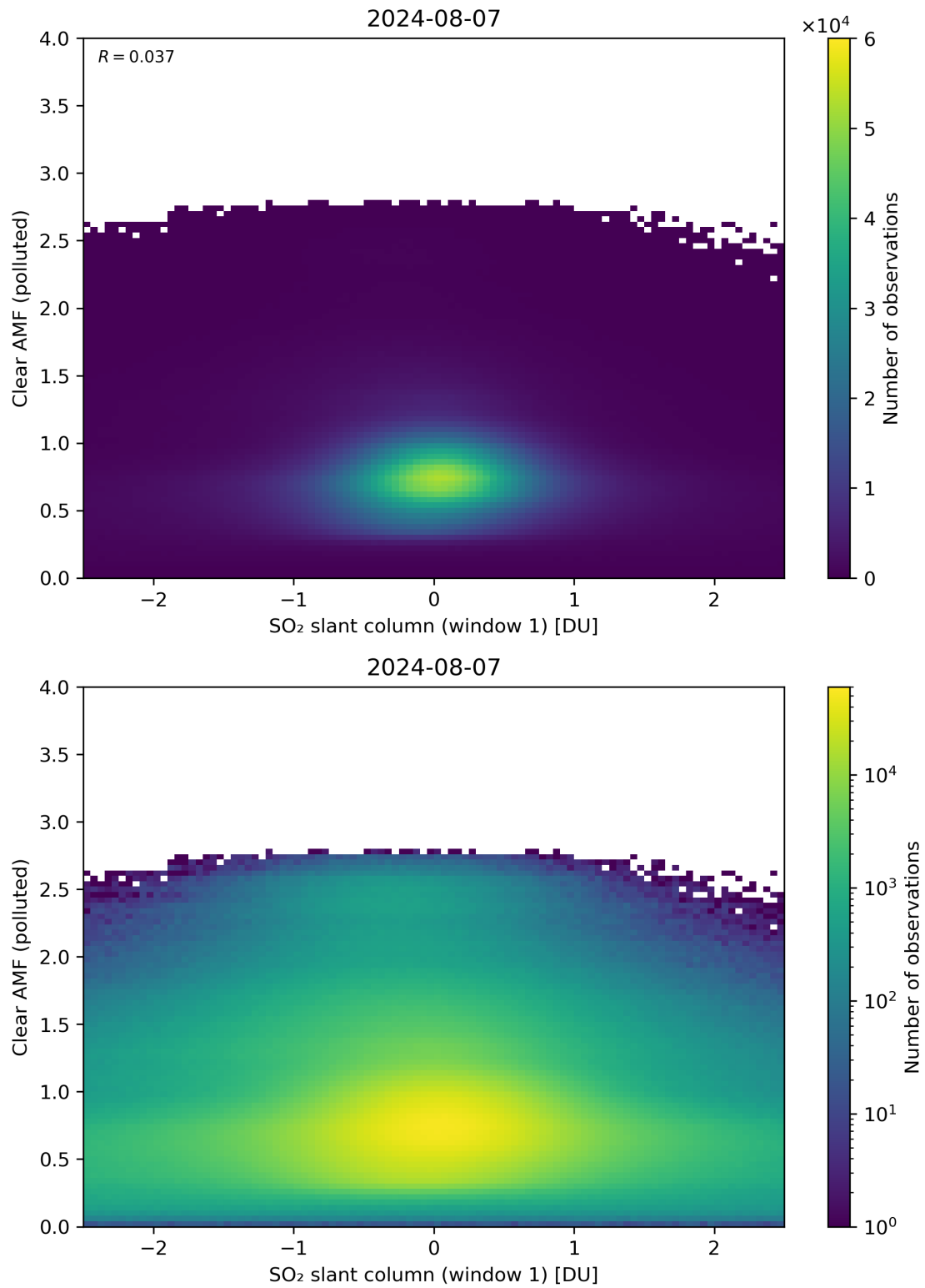
Figure 232: Scatter density plot of “SO 2 slant column (window 1)” against “Clear AMF (polluted)” for 2024-08-06 to 2024-08-08.
