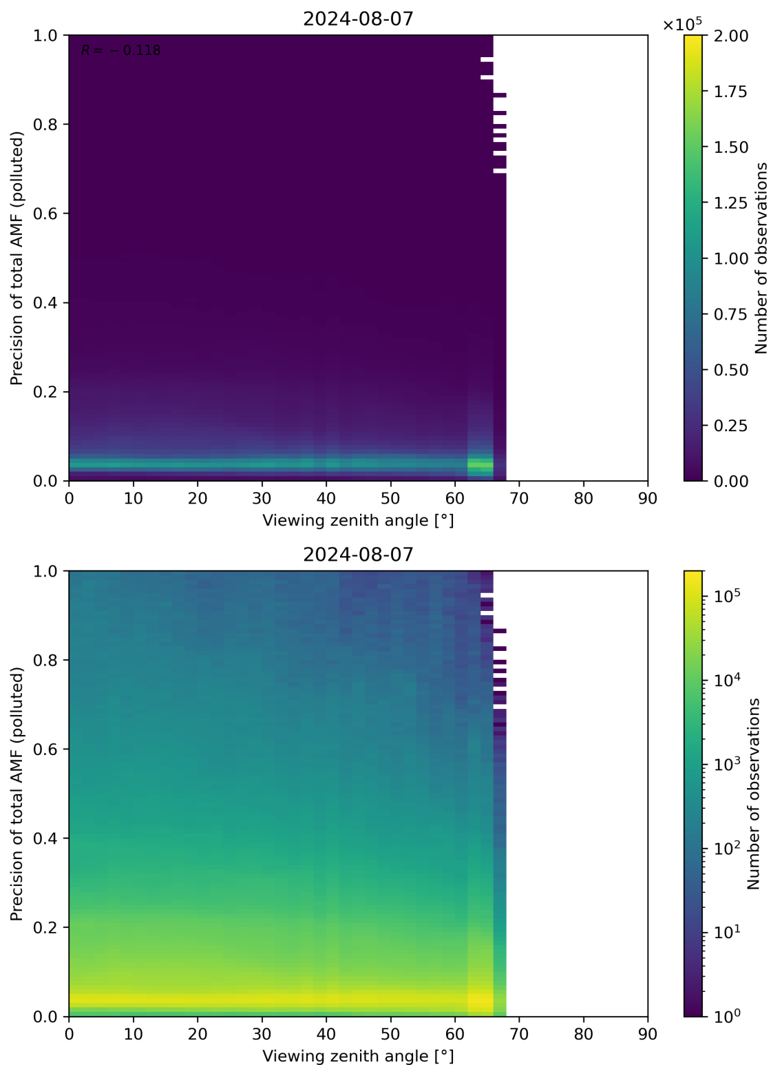
Figure 326: Scatter density plot of “Viewing zenith angle” against “Precision of total AMF (polluted)” for 2024-08-06 to 2024-08-08.
