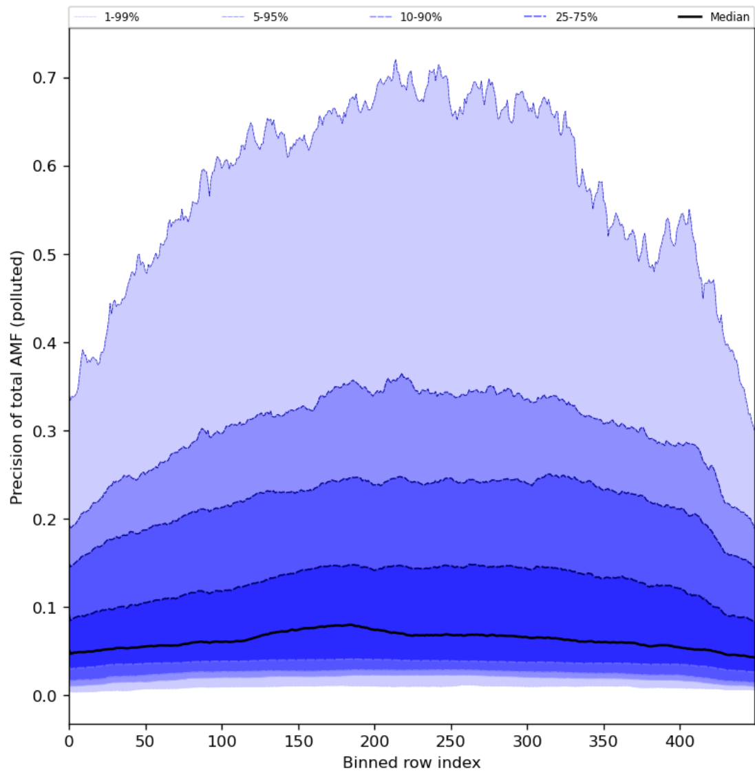
Figure 95: Along track statistics of “Precision of total AMF (polluted)” for 2024-08-06 to 2024-08-08
