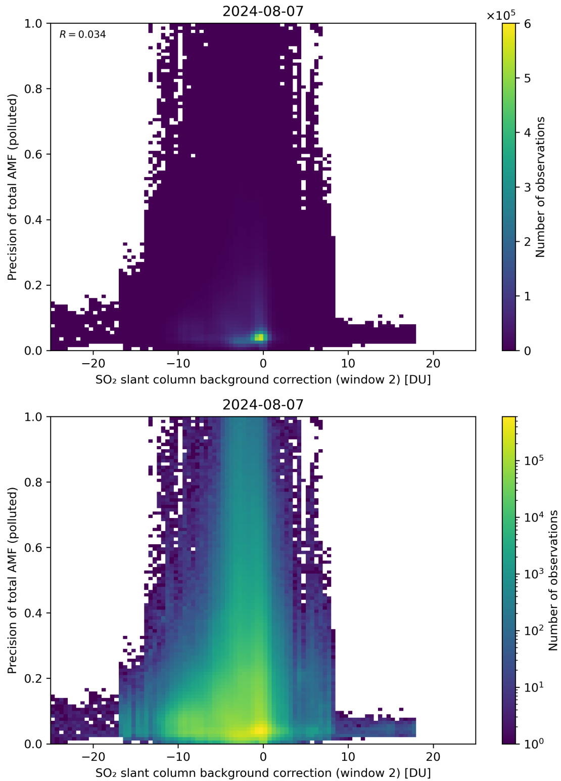
Figure 120: Scatter density plot of “SO 2 slant column background correction (window 2)” against “Precision of total AMF (polluted)” for 2024-08-06 to 2024-08-08.
