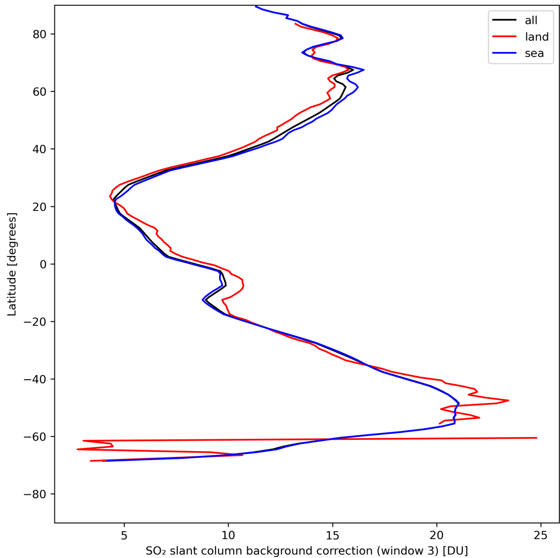
Figure 44: Zonal average of “SO 2 slant column background correction (window 3)” for 2024-08-06 to 2024-08-08.
