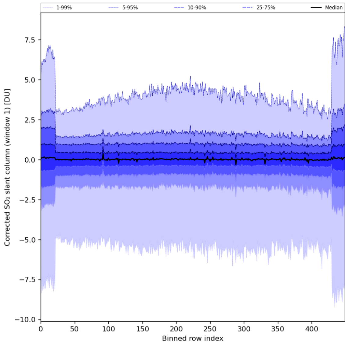
Figure 81: Along track statistics of “Corrected SO 2 slant column (window 1)” for 2024-08-06 to 2024-08-08
