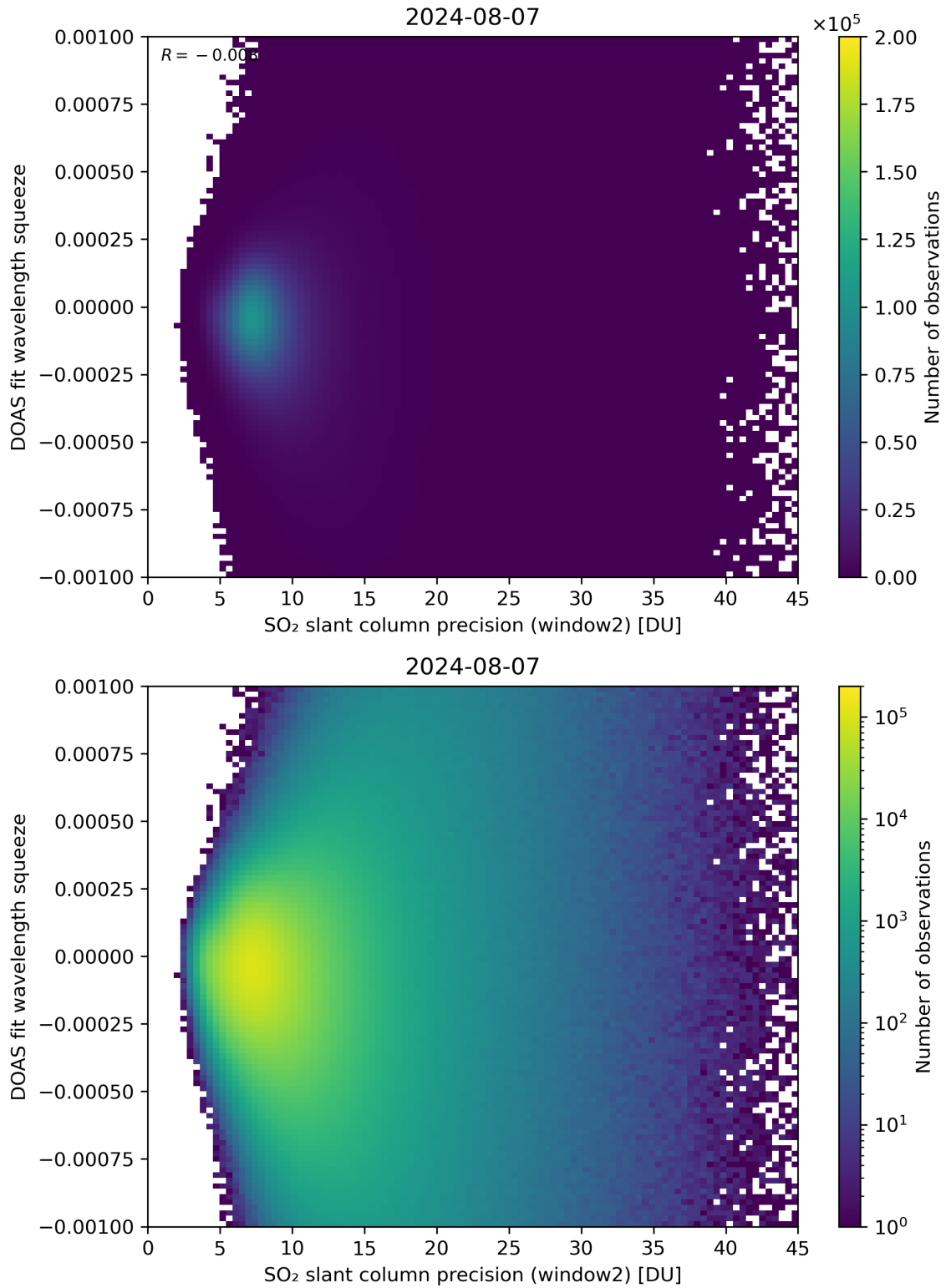
Figure 244: Scatter density plot of “SO 2 slant column precision (window2)” against “DOAS fit wavelength squeeze” for 2024-08-06 to 2024-08-08.
