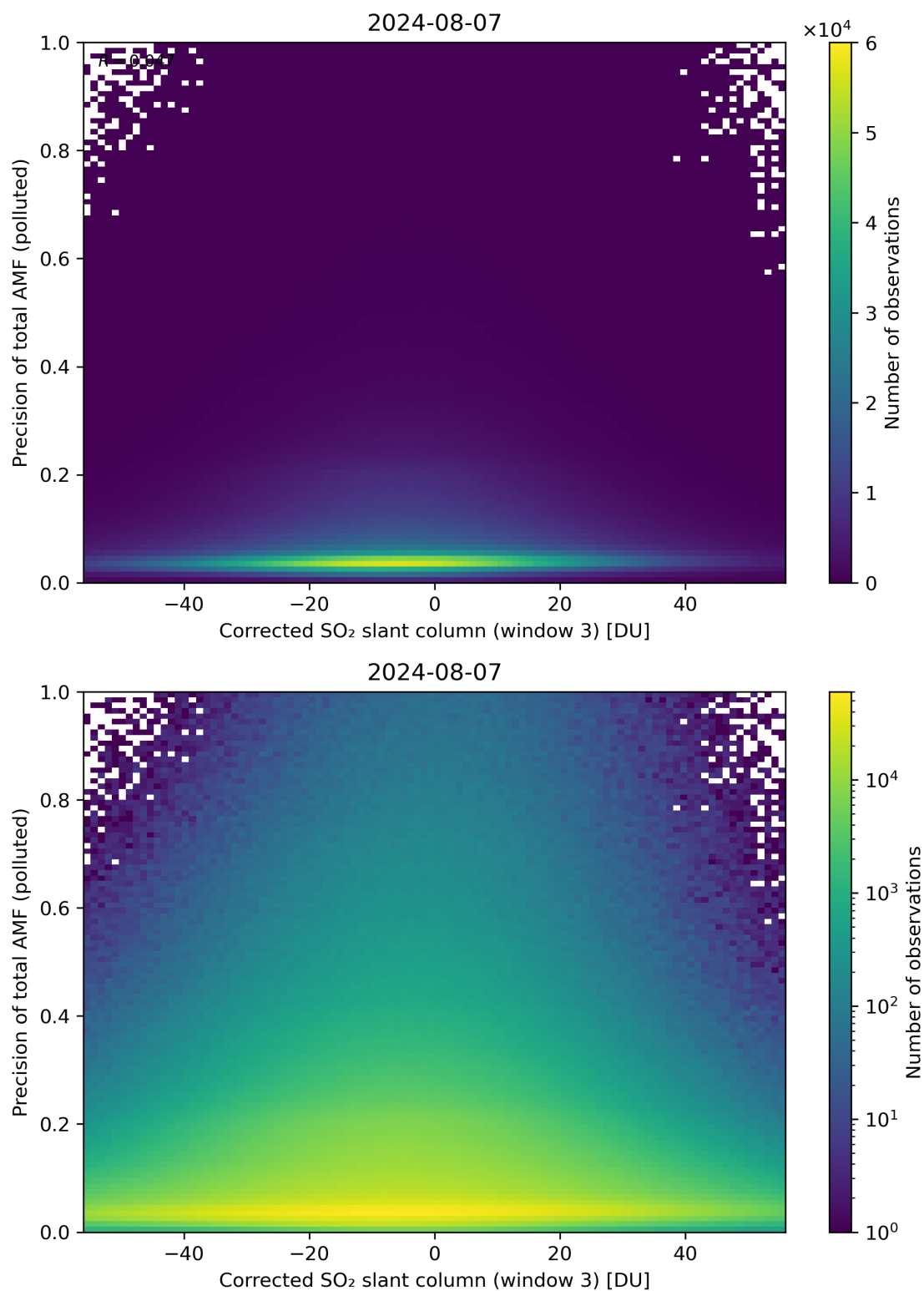
Figure 211: Scatter density plot of “Corrected SO 2 slant column (window 3)” against “Precision of total AMF (polluted)” for 2024-08-06 to 2024-08-08.
