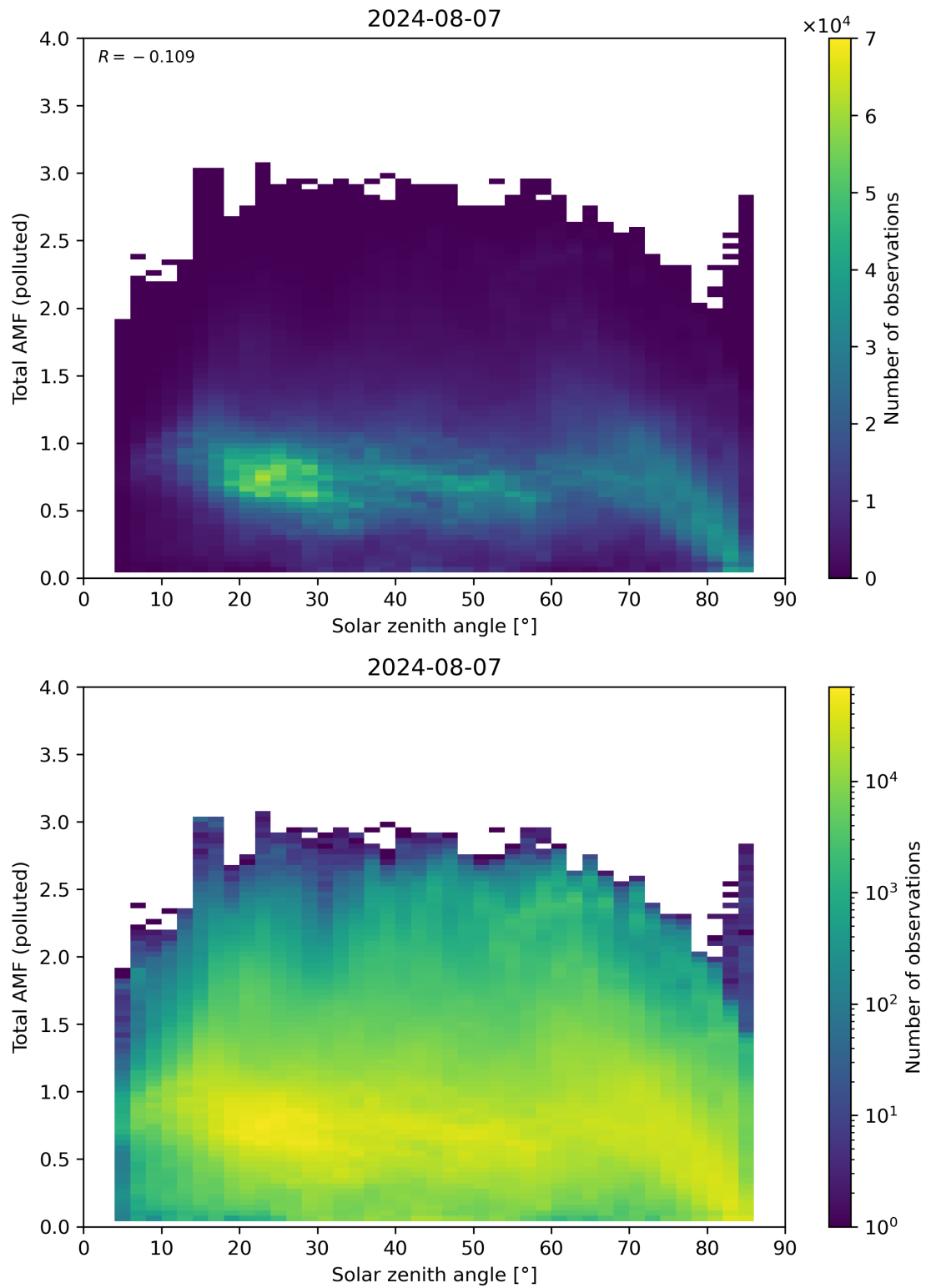
Figure 174: Scatter density plot of “Solar zenith angle” against “Total AMF (polluted)” for 2024-08-06 to 2024-08-08.
