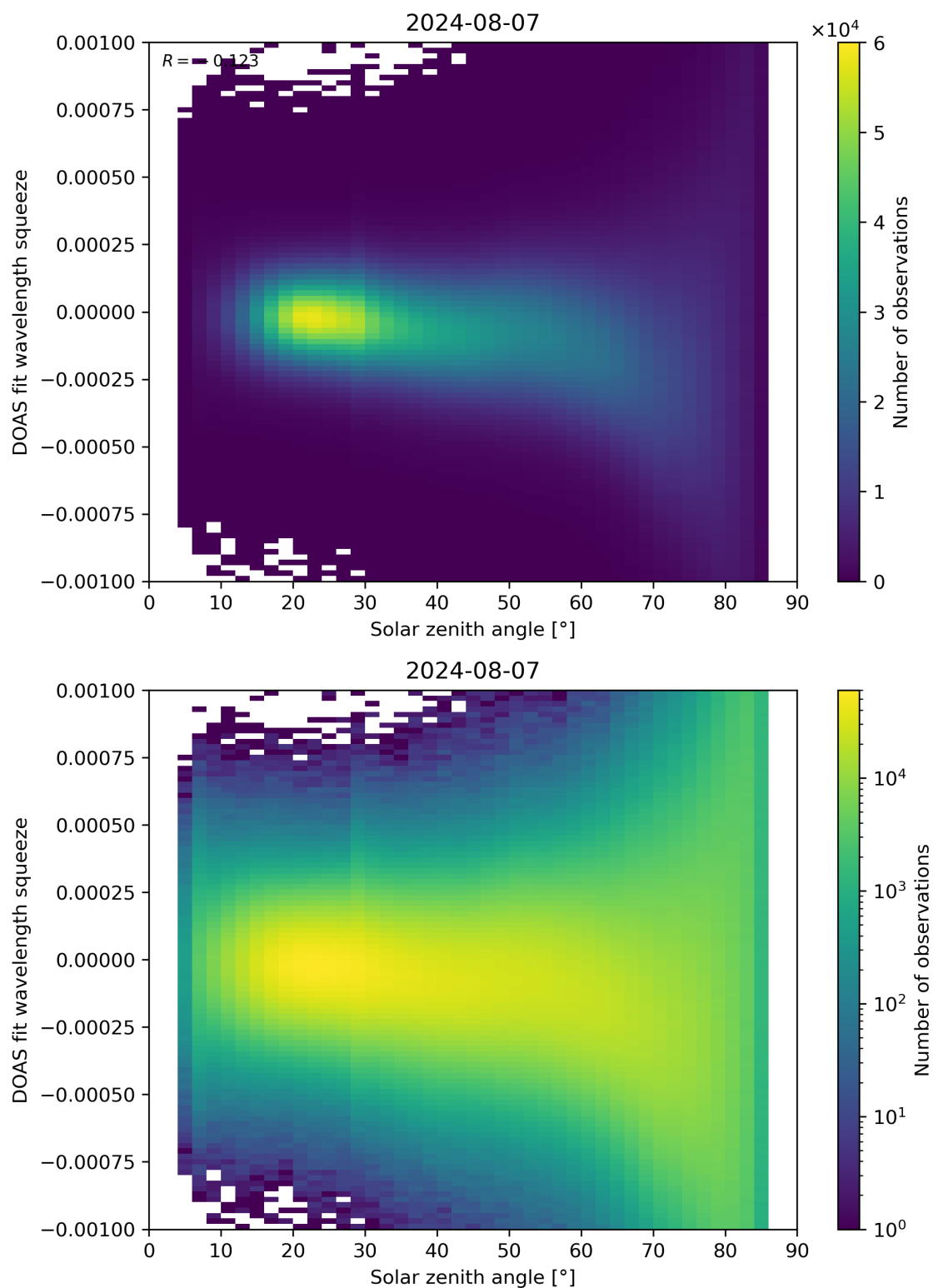
Figure 162: Scatter density plot of “Solar zenith angle” against “DOAS fit wavelength squeeze” for 2024-08-06 to 2024-08-08.
