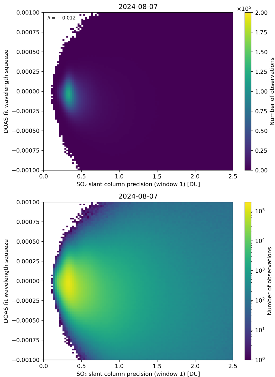
Figure 222: Scatter density plot of “SO 2 slant column precision (window 1)” against “DOAS fit wavelength squeeze” for 2024-08-06 to 2024-08-08.
