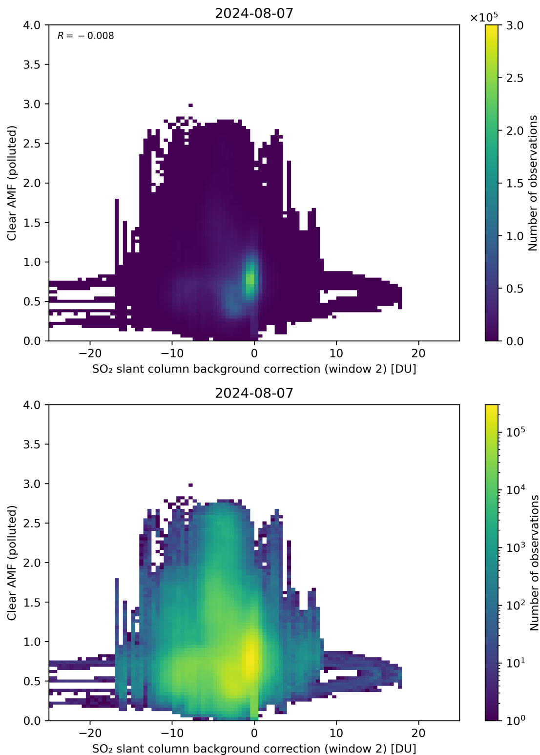
Figure 115: Scatter density plot of “SO 2 slant column background correction (window 2)” against “Clear AMF (polluted)” for 2024-08-06 to 2024-08-08.
