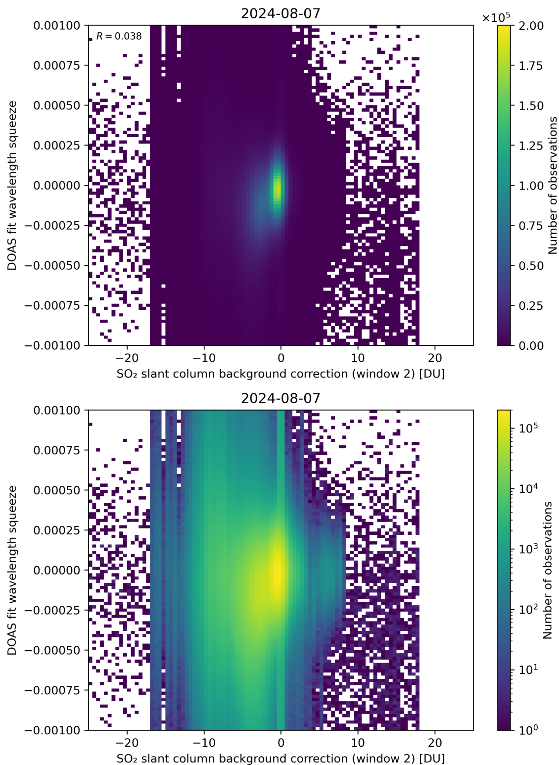
Figure 113: Scatter density plot of “SO 2 slant column background correction (window 2)” against “DOAS fit wavelength squeeze” for 2024-08-06 to 2024-08-08.
