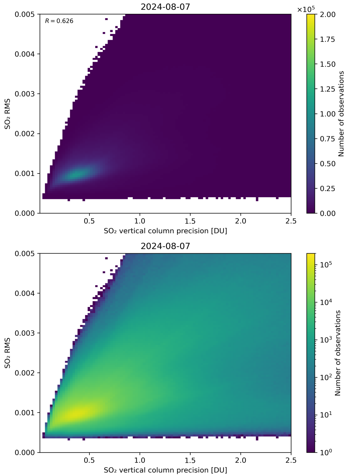
Figure 284: Scatter density plot of “SO 2 vertical column precision” against “SO 2 RMS” for 2024-08-06 to 2024-08-08.
