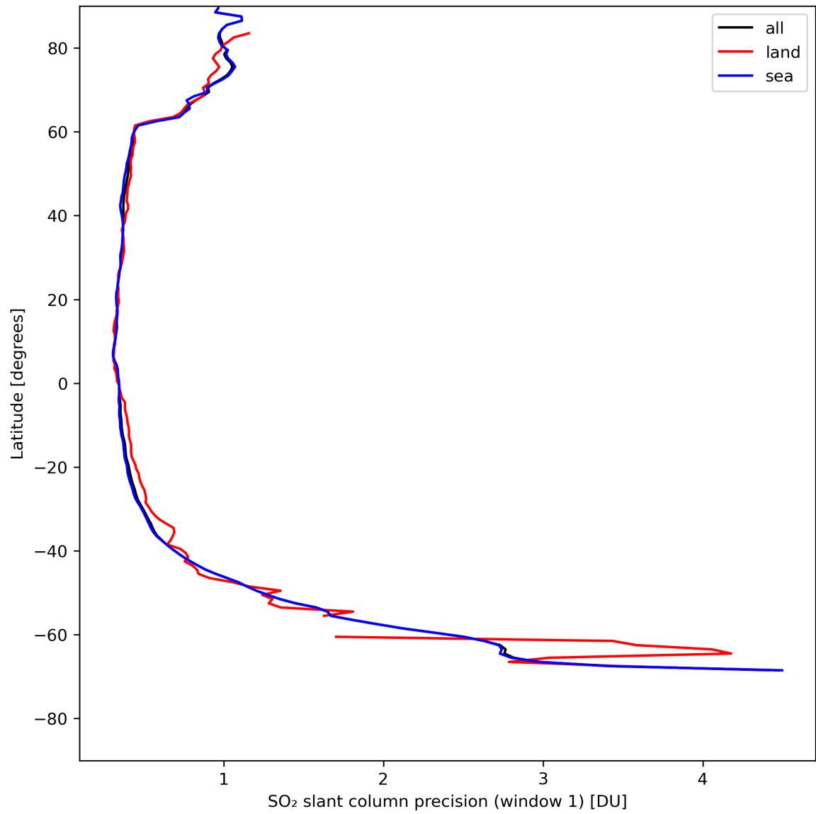
Figure 34: Zonal average of “SO 2 slant column precision (window 1)” for 2024-08-06 to 2024-08-08.
