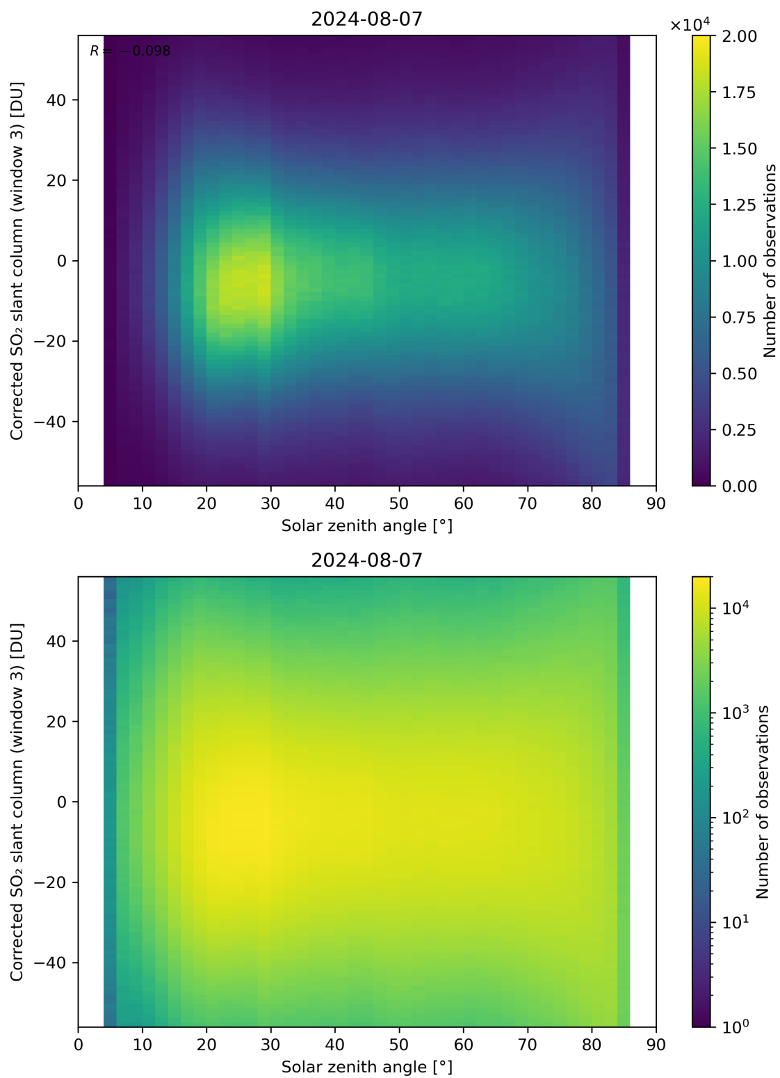
Figure 168: Scatter density plot of “Solar zenith angle” against “Corrected SO 2 slant column (window 3)” for 2024-08-06 to 2024-08-08.
