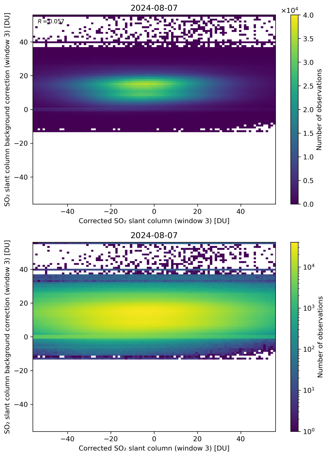
Figure 205: Scatter density plot of “Corrected SO 2 slant column (window 3)” against “SO 2 slant column background correction (window 3)” for 2024-08-06 to 2024-08-08.
