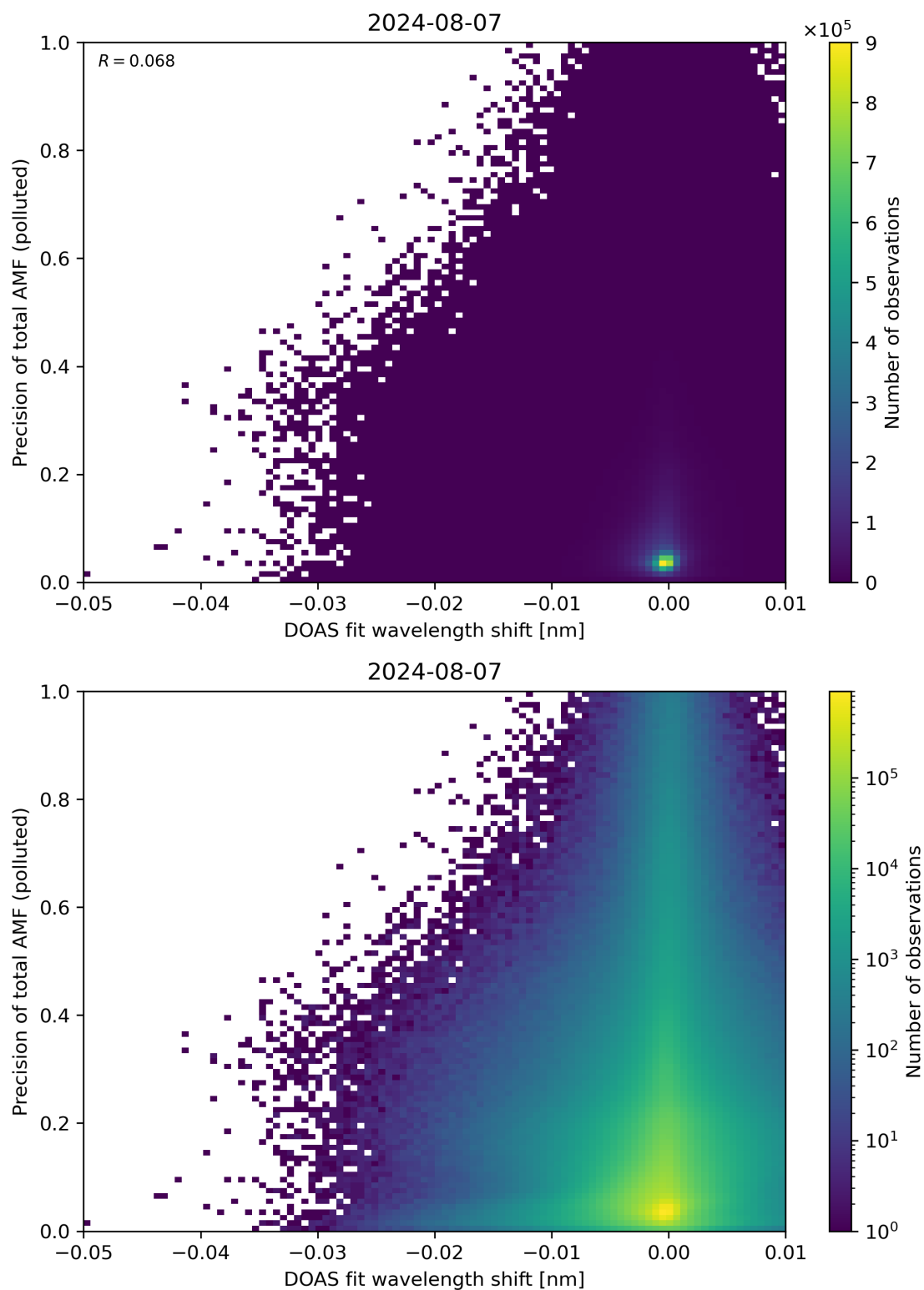
Figure 131: Scatter density plot of “DOAS fit wavelength shift” against “Precision of total AMF (polluted)” for 2024-08-06 to 2024-08-08.
