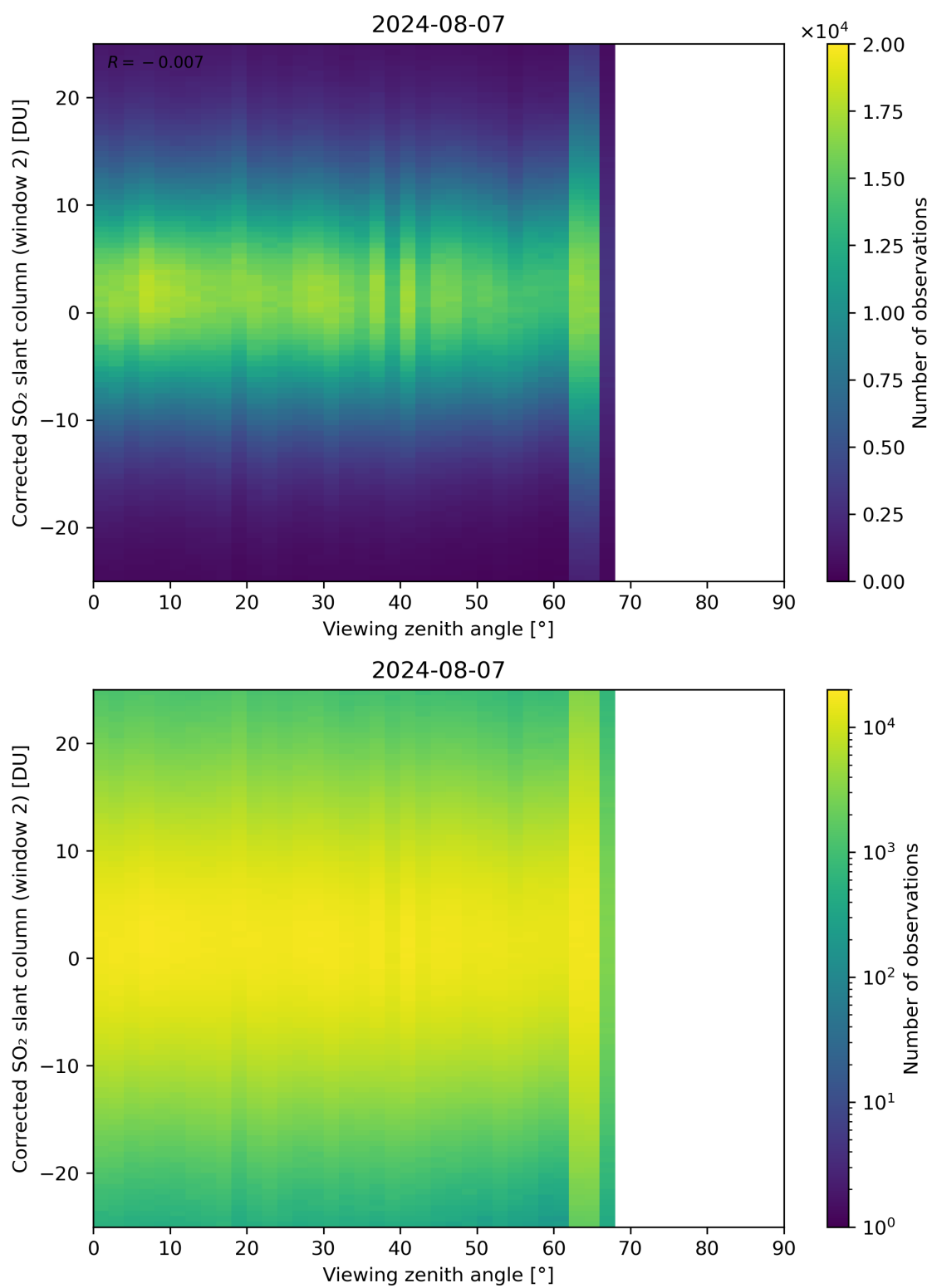
Figure 318: Scatter density plot of “Viewing zenith angle” against “Corrected SO 2 slant column (window 2)” for 2024-08-06 to 2024-08-08.
