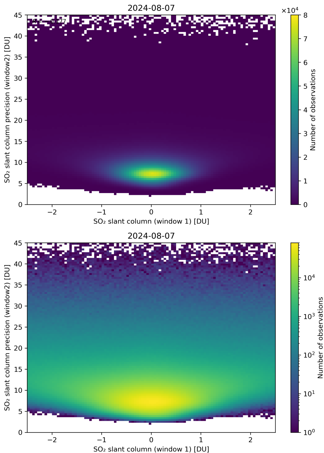
Figure 236: Scatter density plot of “SO 2 slant column (window 1)” against “SO 2 slant column precision (window2)” for 2024-08-06 to 2024-08-08.
