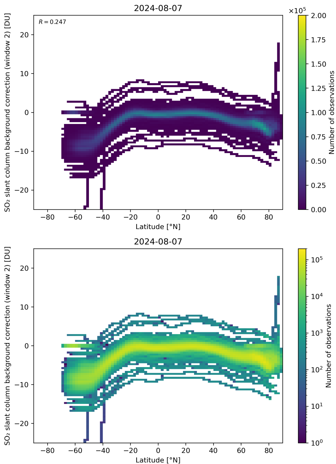
Figure 140: Scatter density plot of “Latitude” against “SO 2 slant column background correction (window 2)” for 2024-08-06 to 2024-08-08.
