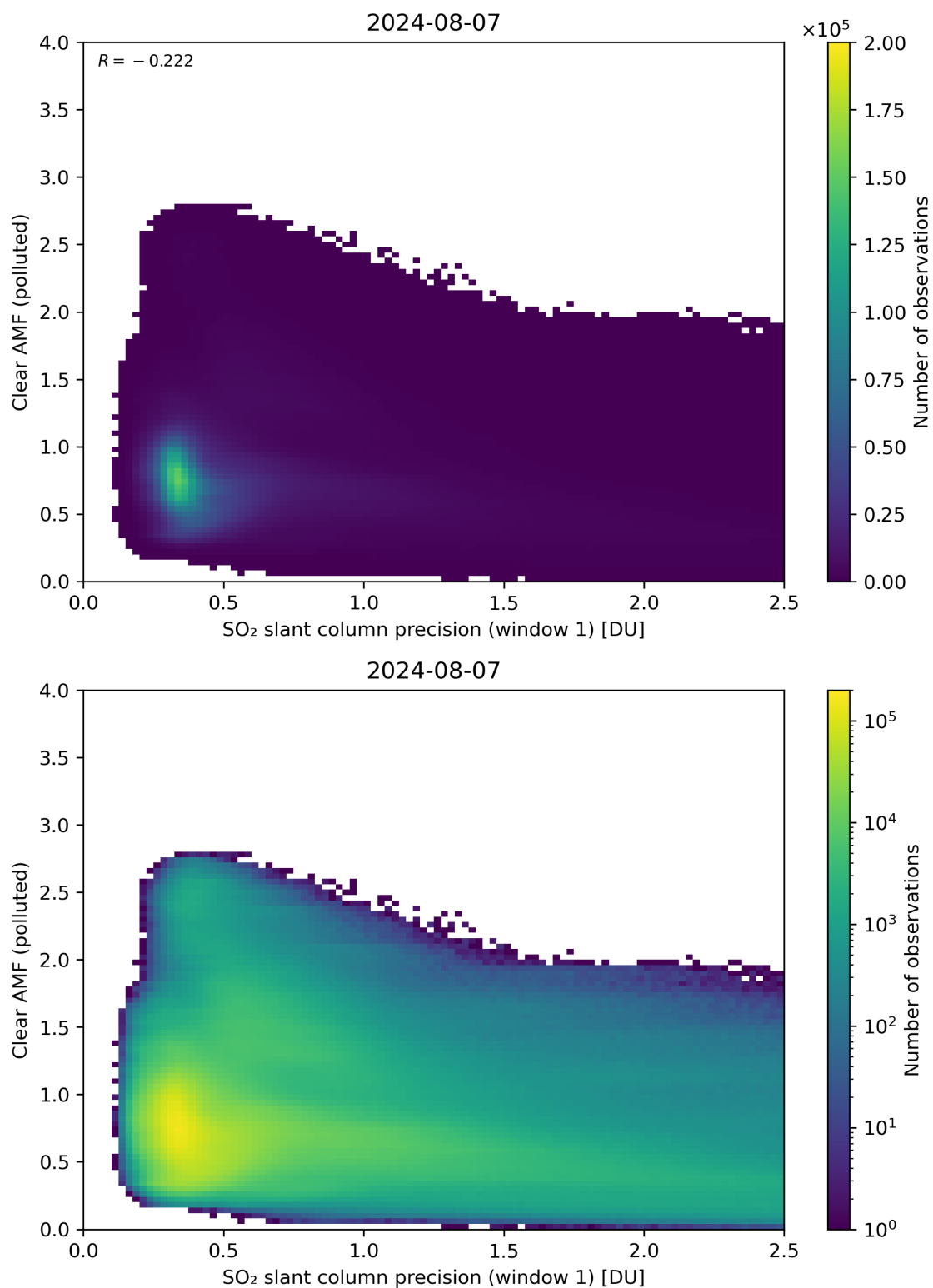
Figure 224: Scatter density plot of “SO 2 slant column precision (window 1)” against “Clear AMF (polluted)” for 2024-08-06 to 2024-08-08.
