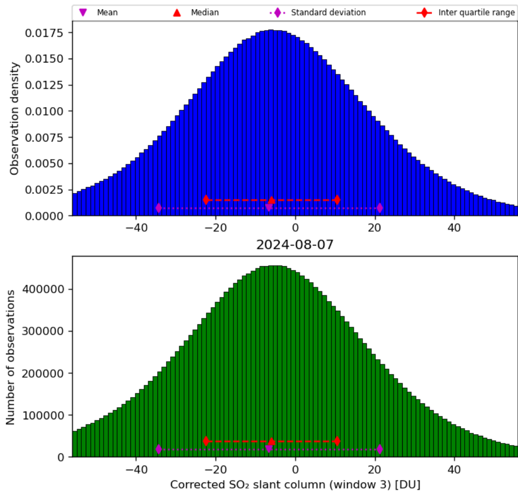
Figure 66: Histogram of “Corrected SO 2 slant column (window 3)” for 2024-08-06 to 2024-08-08
