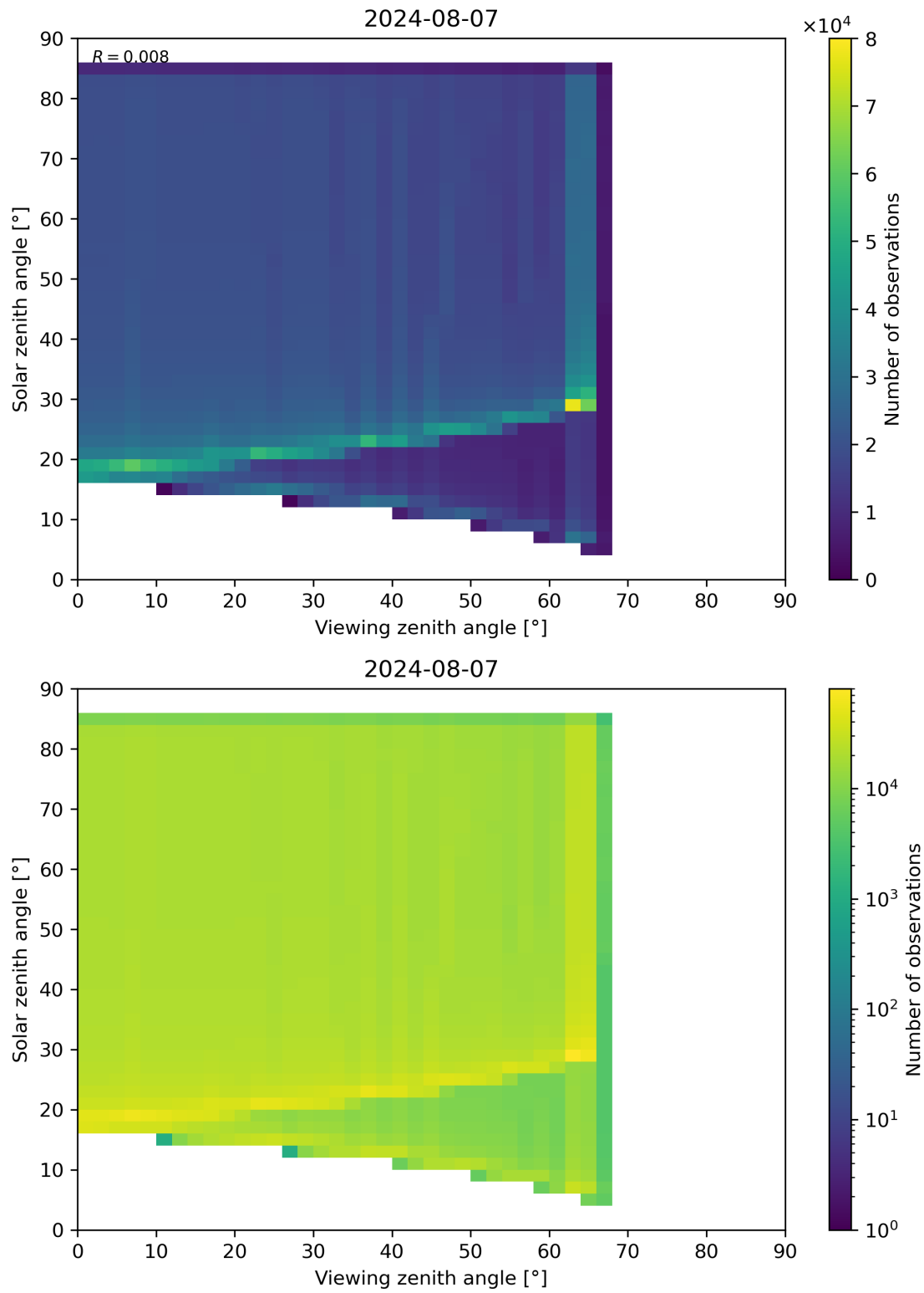
Figure 315: Scatter density plot of “Viewing zenith angle” against “Solar zenith angle” for 2024-08-06 to 2024-08-08.
