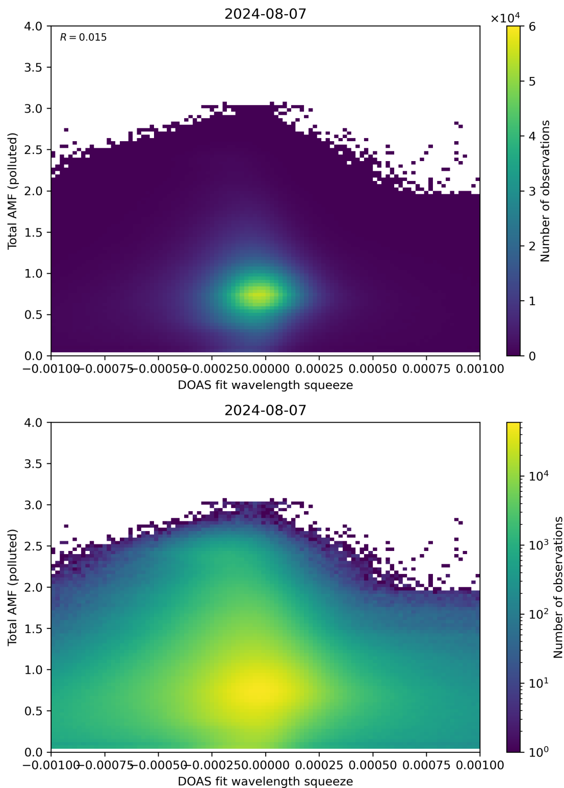
Figure 134: Scatter density plot of “DOAS fit wavelength squeeze” against “Total AMF (polluted)” for 2024-08-06 to 2024-08-08.
