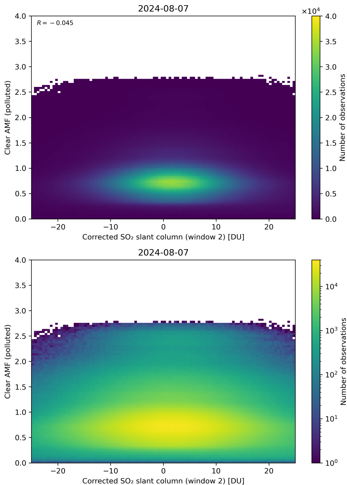
Figure 199: Scatter density plot of “Corrected SO 2 slant column (window 2)” against “Clear AMF (polluted)” for 2024-08-06 to 2024-08-08.
