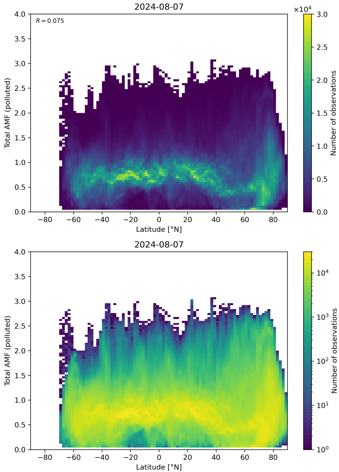
Figure 154: Scatter density plot of “Latitude” against “Total AMF (polluted)” for 2024-08-06 to 2024-08-08.
