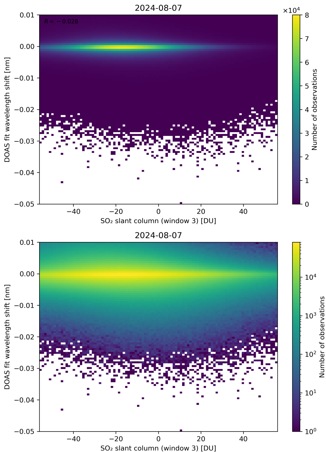
Figure 254: Scatter density plot of “SO 2 slant column (window 3)” against “DOAS fit wavelength shift” for 2024-08-06 to 2024-08-08.
