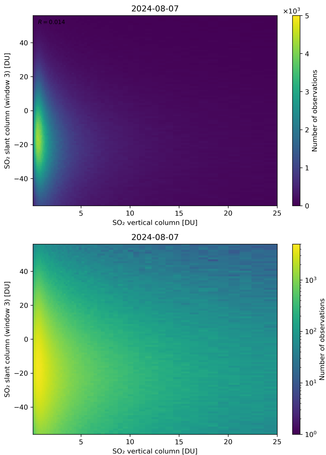
Figure 303: Scatter density plot of “SO 2 vertical column” against “SO 2 slant column (window 3)” for 2024-08-06 to 2024-08-08.
