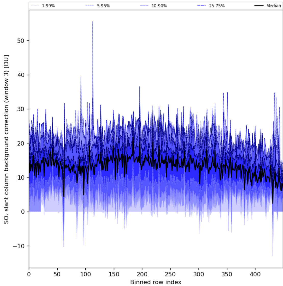
Figure 90: Along track statistics of “SO 2 slant column background correction (window 3)” for 2024-08-06 to 2024-08-08
