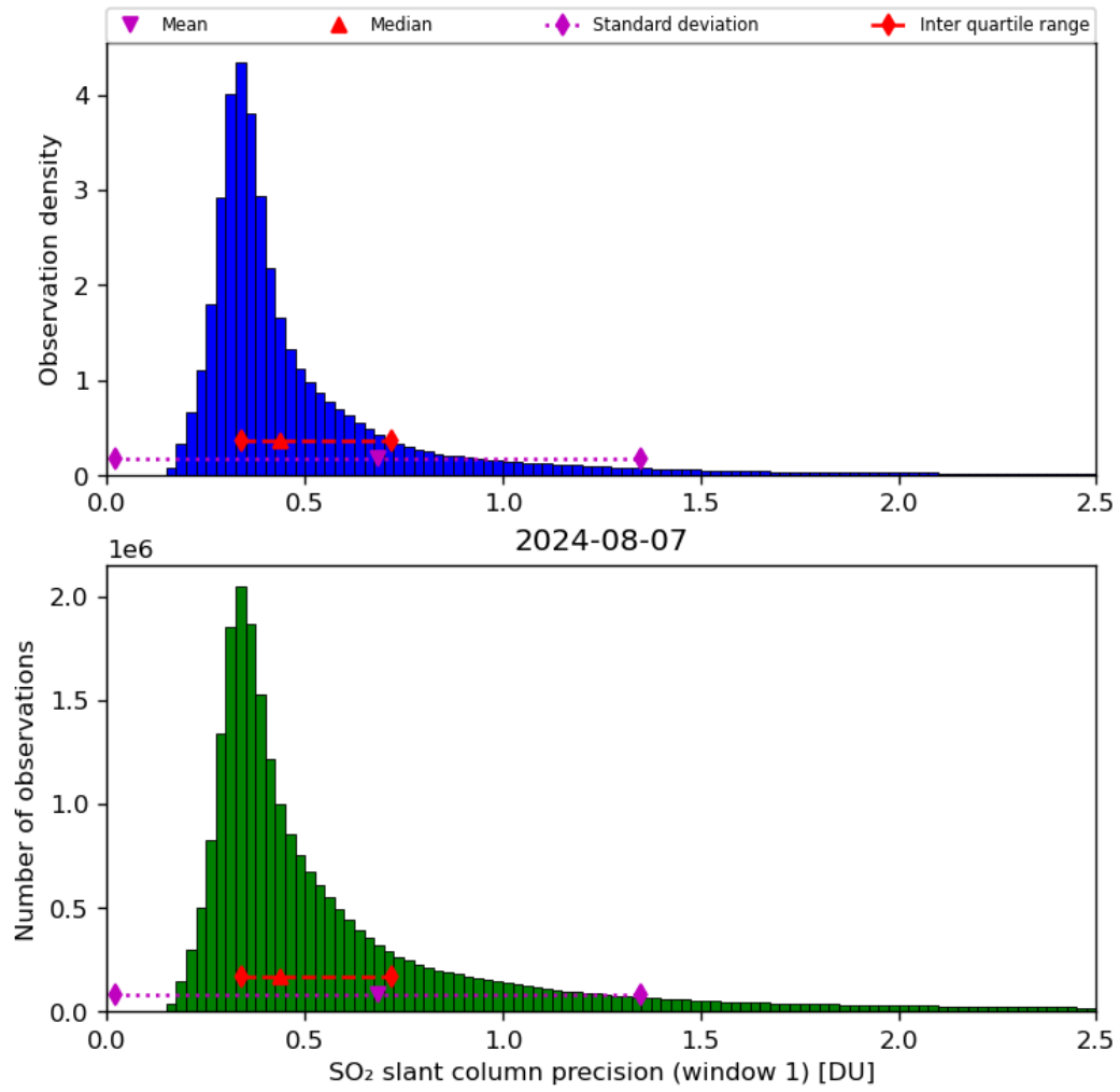
Figure 57: Histogram of “SO 2 slant column precision (window 1)” for 2024-08-06 to 2024-08-08
