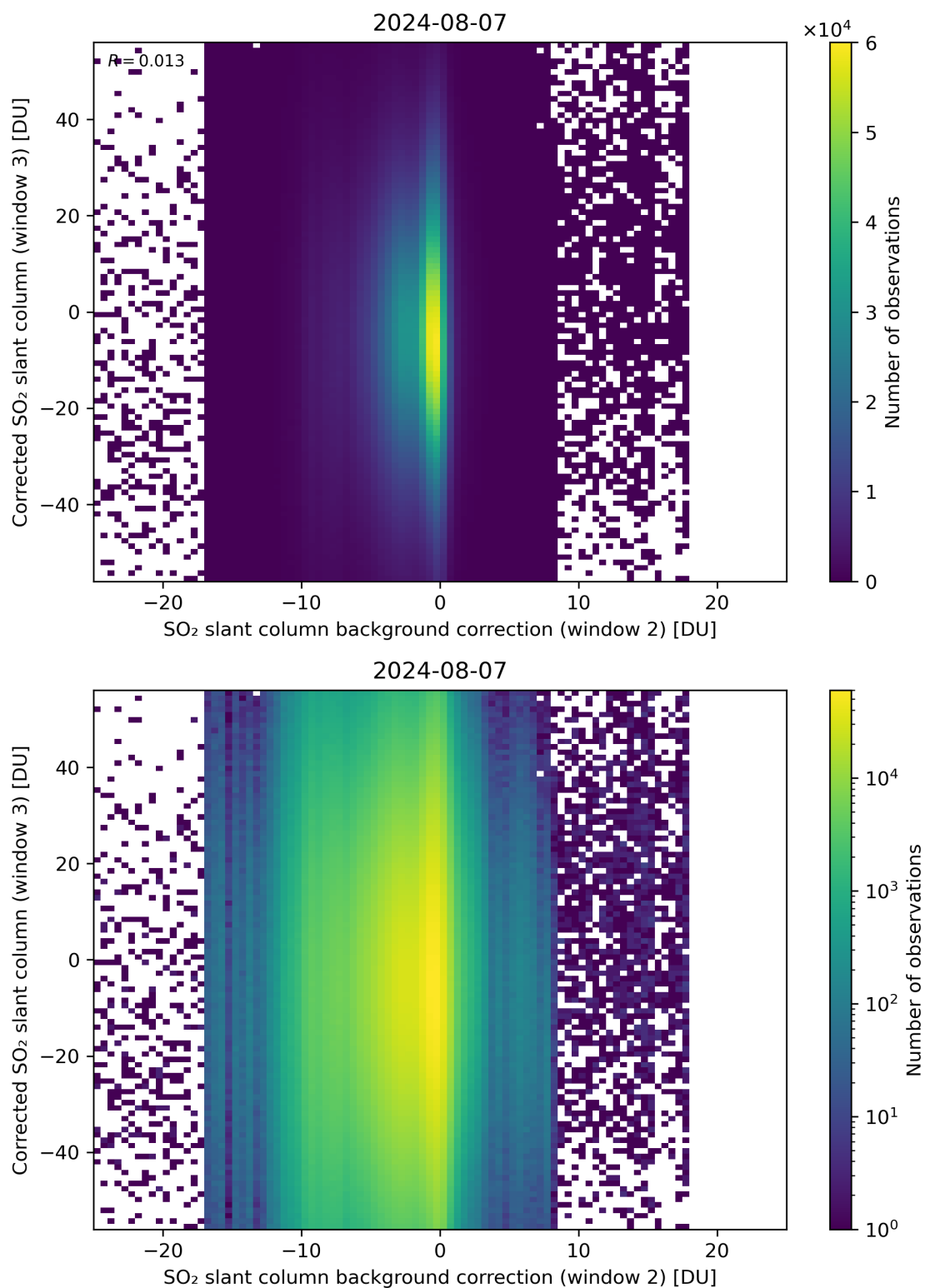
Figure 116: Scatter density plot of “SO 2 slant column background correction (window 2)” against “Corrected SO 2 slant column (window 3)” for 2024-08-06 to 2024-08-08.
