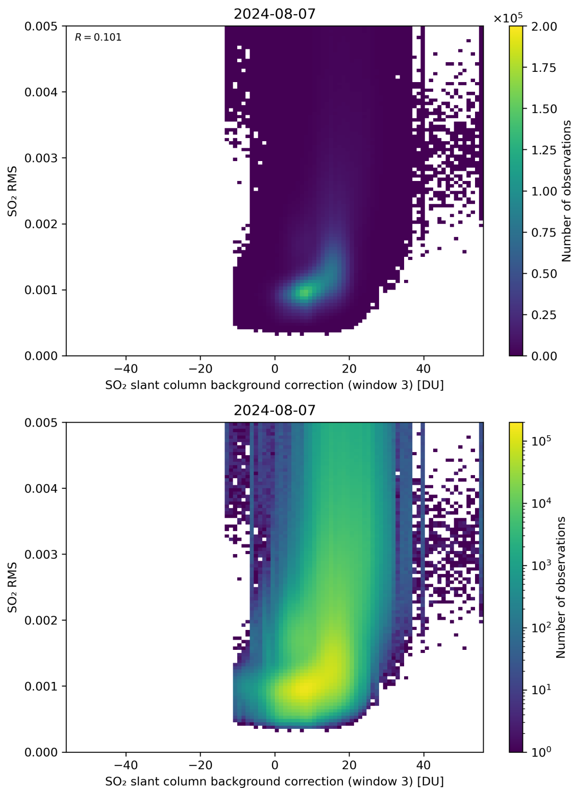
Figure 123: Scatter density plot of “SO 2 slant column background correction (window 3)” against “SO 2 RMS” for 2024-08-06 to 2024-08-08.
