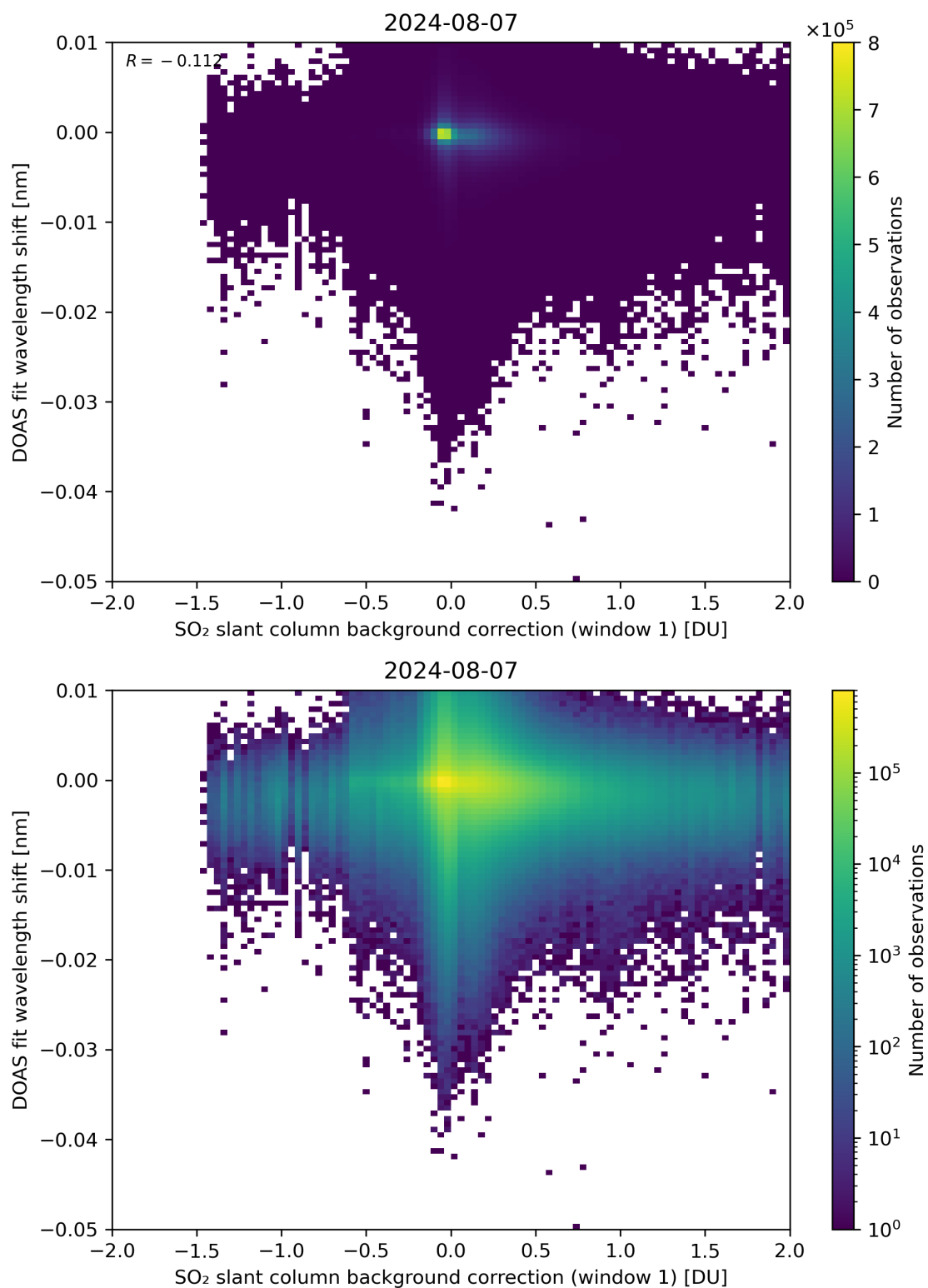
Figure 100: Scatter density plot of “SO 2 slant column background correction (window 1)” against “DOAS fit wavelength shift” for 2024-08-06 to 2024-08-08.
