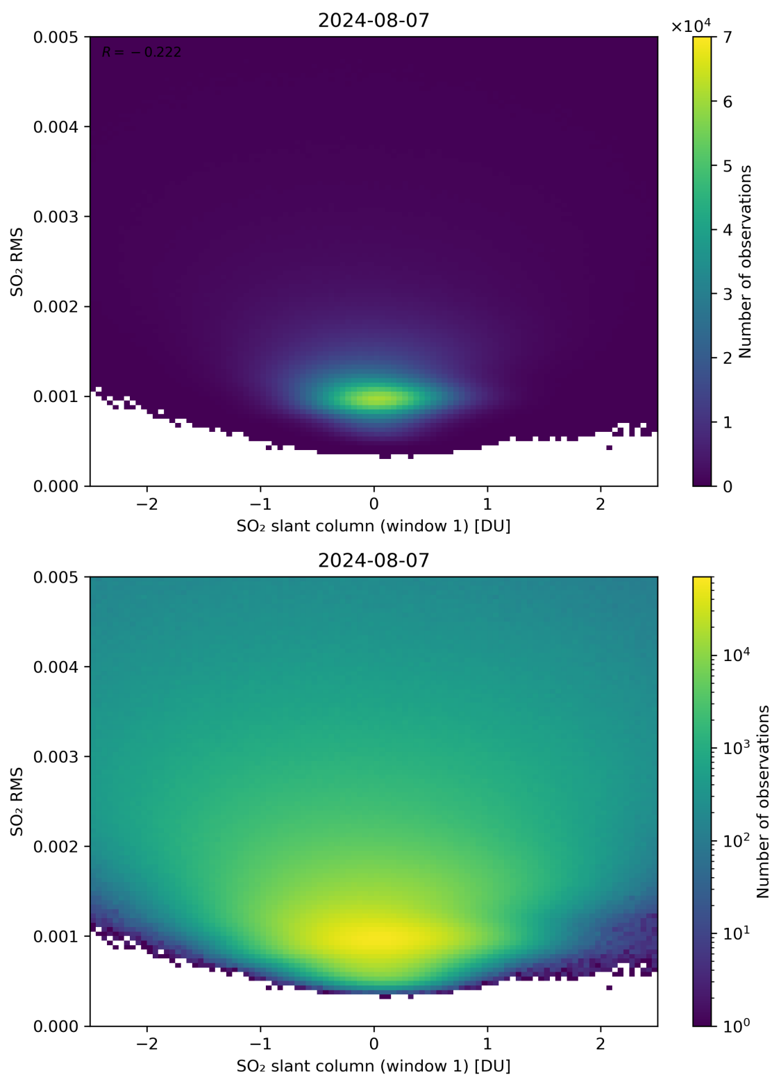
Figure 217: Scatter density plot of “SO 2 slant column (window 1)” against “SO 2 RMS” for 2024-08-06 to 2024-08-08.
