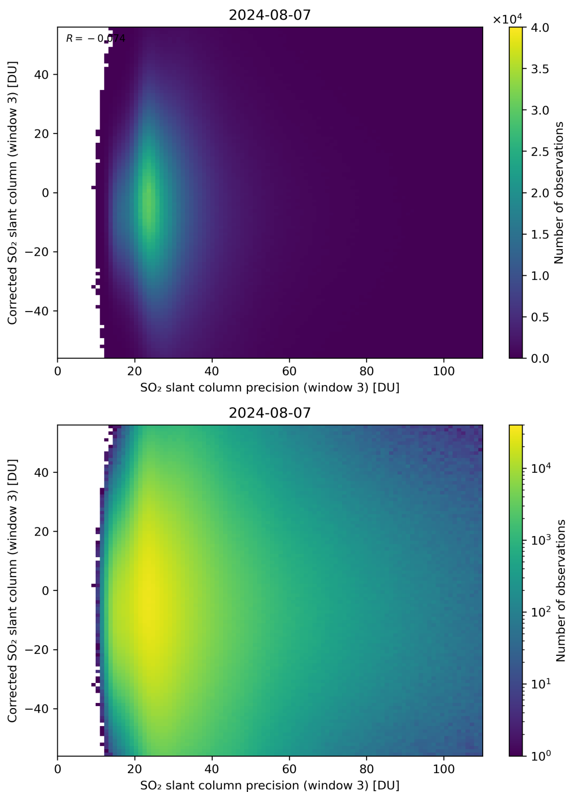
Figure 262: Scatter density plot of “SO 2 slant column precision (window 3)” against “Corrected SO 2 slant column (window 3)” for 2024-08-06 to 2024-08-08.
