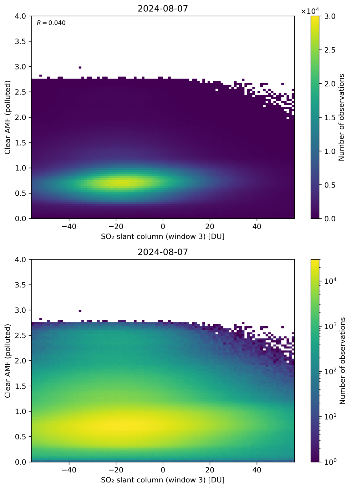
Figure 265: Scatter density plot of “SO 2 slant column (window 3)” against “Clear AMF (polluted)” for 2024-08-06 to 2024-08-08.
