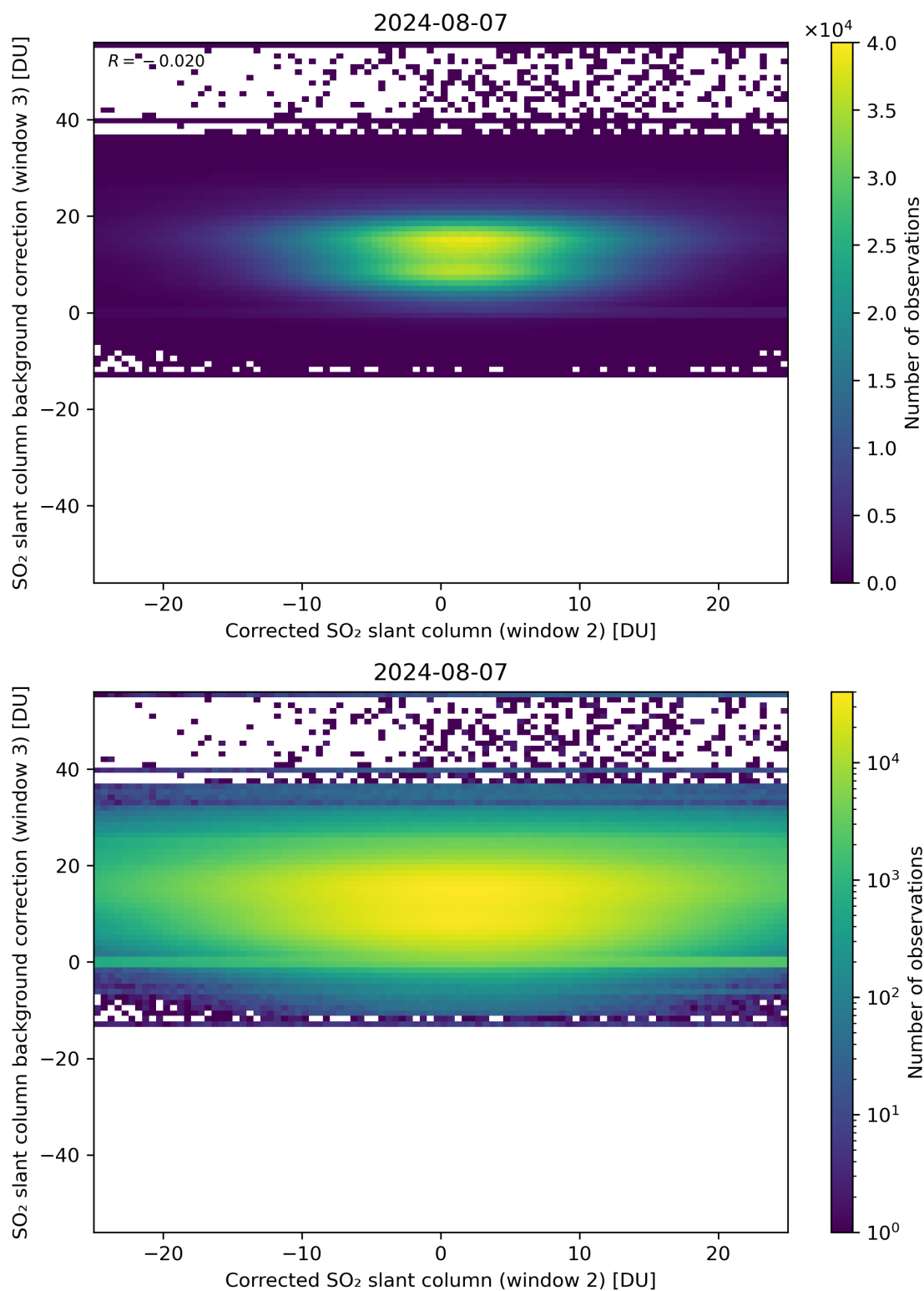
Figure 195: Scatter density plot of “Corrected SO 2 slant column (window 2)” against “SO 2 slant column background correction (window 3)” for 2024-08-06 to 2024-08-08.
