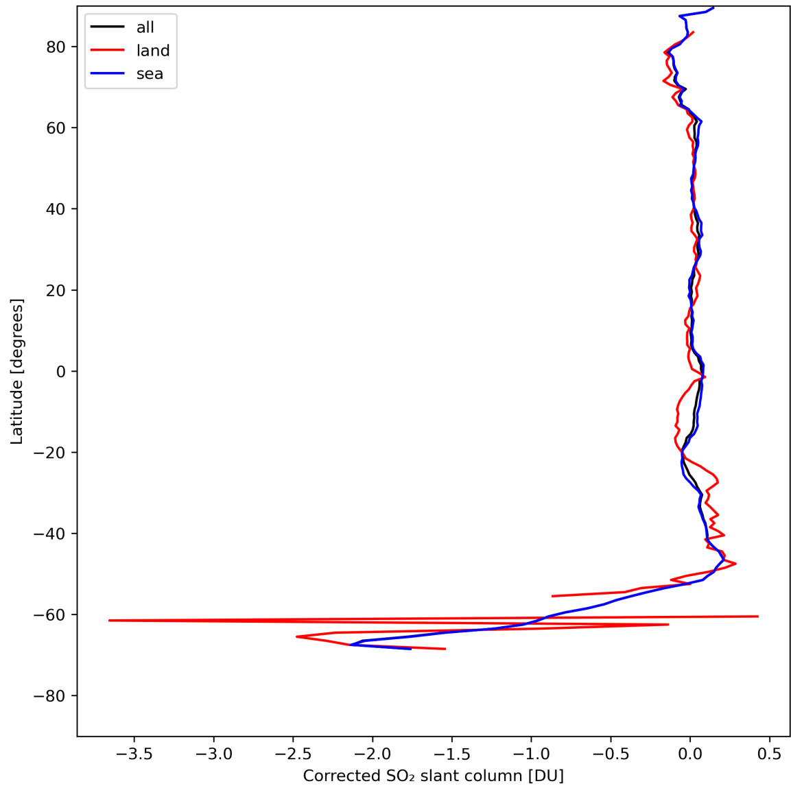
Figure 32: Zonal average of “Corrected SO 2 slant column” for 2024-08-06 to 2024-08-08.
