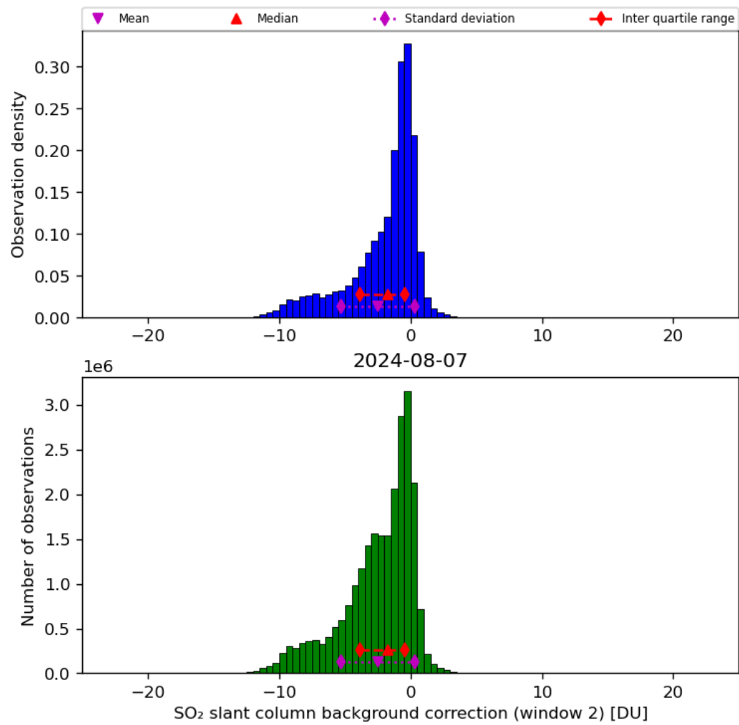
Figure 63: Histogram of “SO 2 slant column background correction (window 2)” for 2024-08-06 to 2024-08-08
