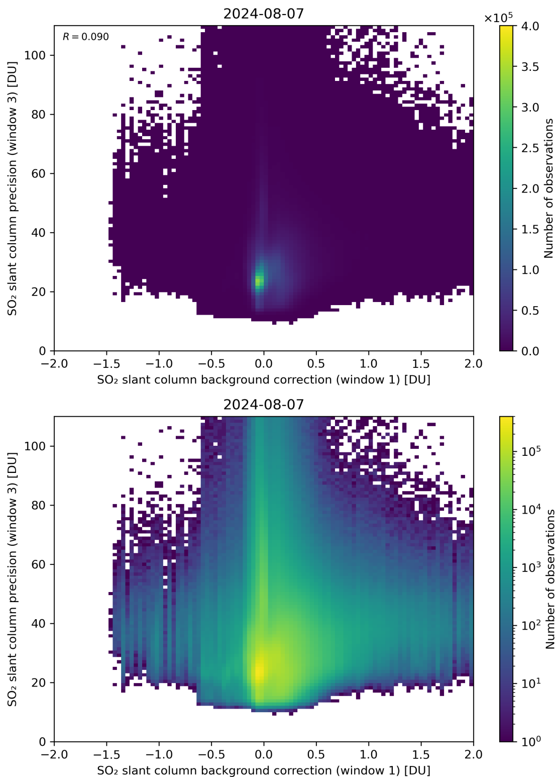
Figure 108: Scatter density plot of “SO 2 slant column background correction (window 1)” against “SO 2 slant column precision (window 3)” for 2024-08-06 to 2024-08-08.
