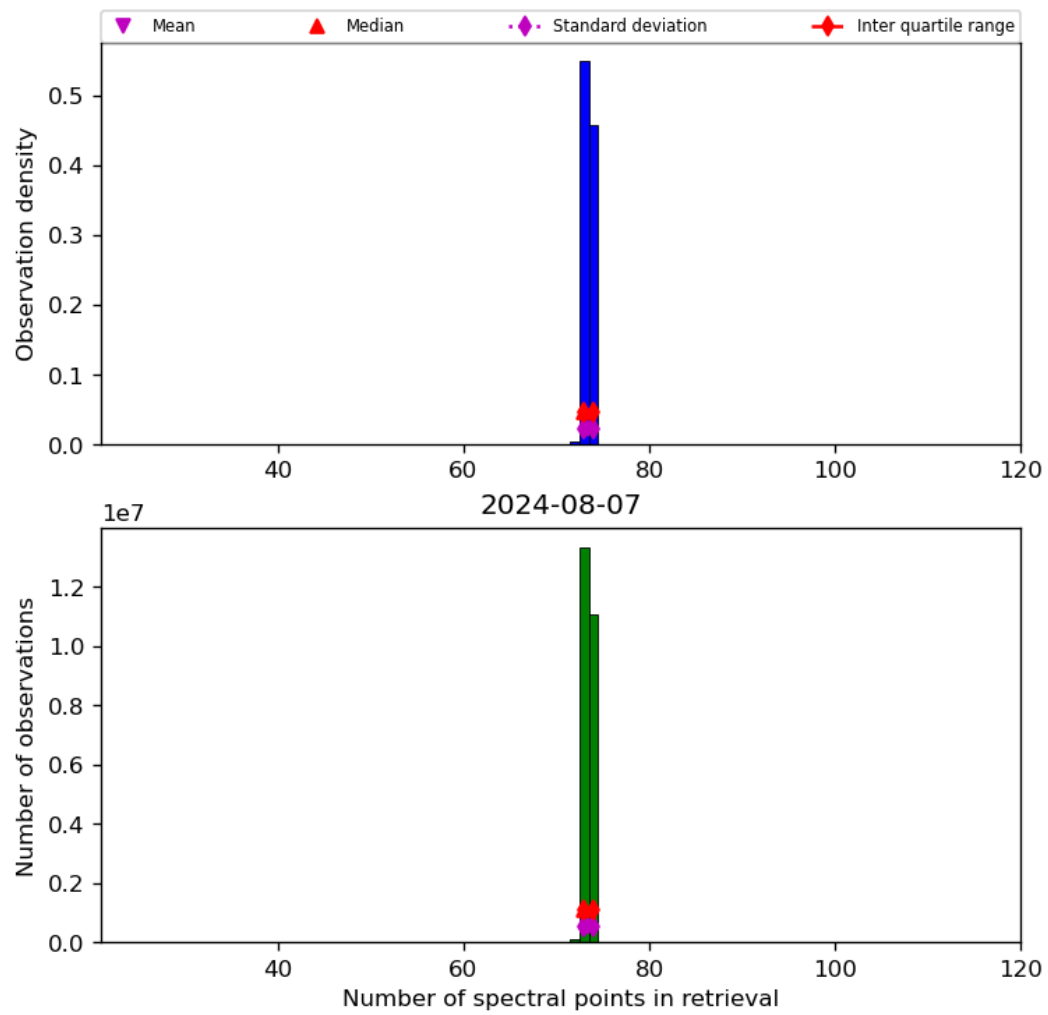
Figure 74: Histogram of “Number of spectral points in retrieval” for 2024-08-06 to 2024-08-08
