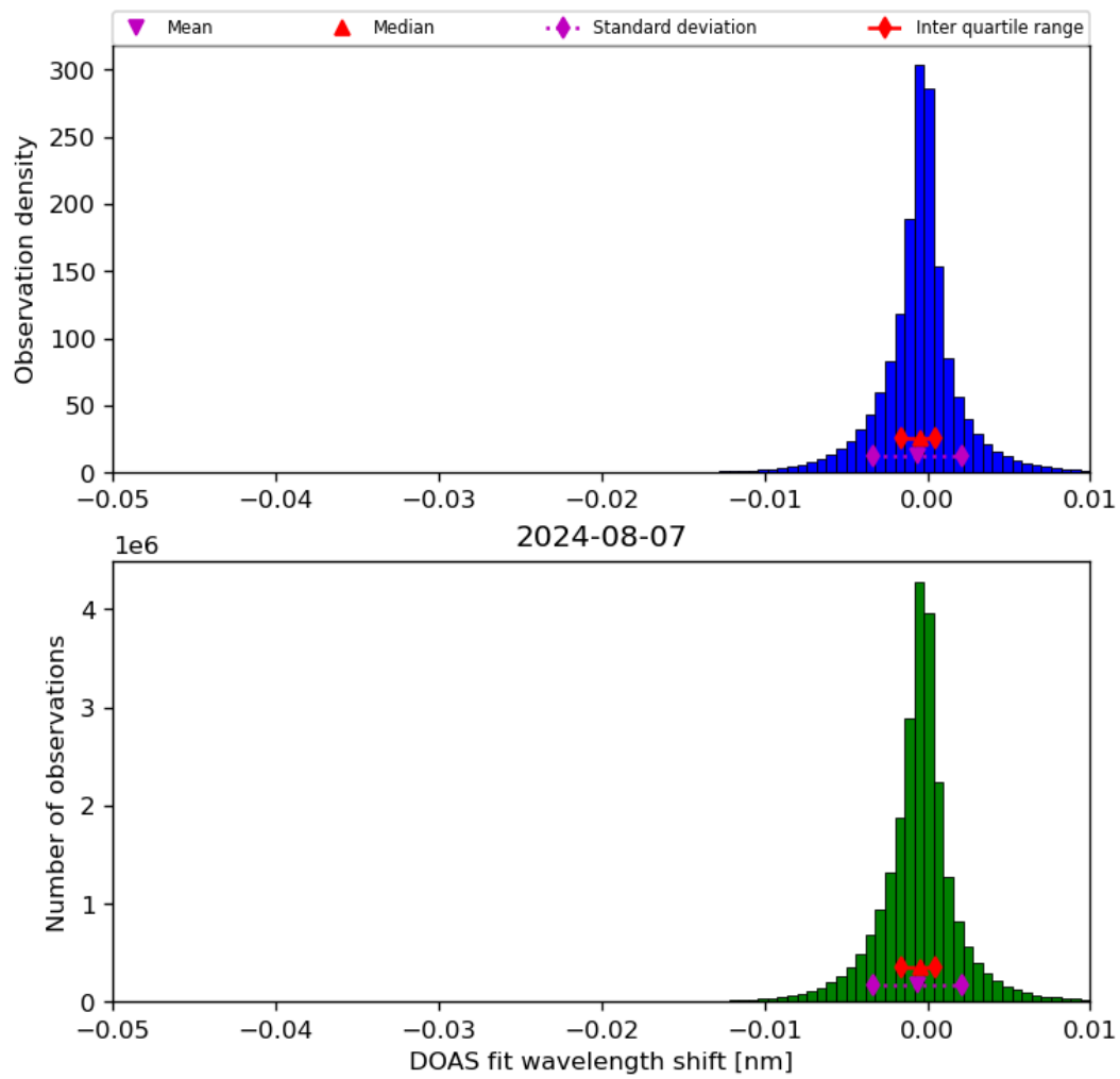
Figure 68: Histogram of “DOAS fit wavelength shift” for 2024-08-06 to 2024-08-08
