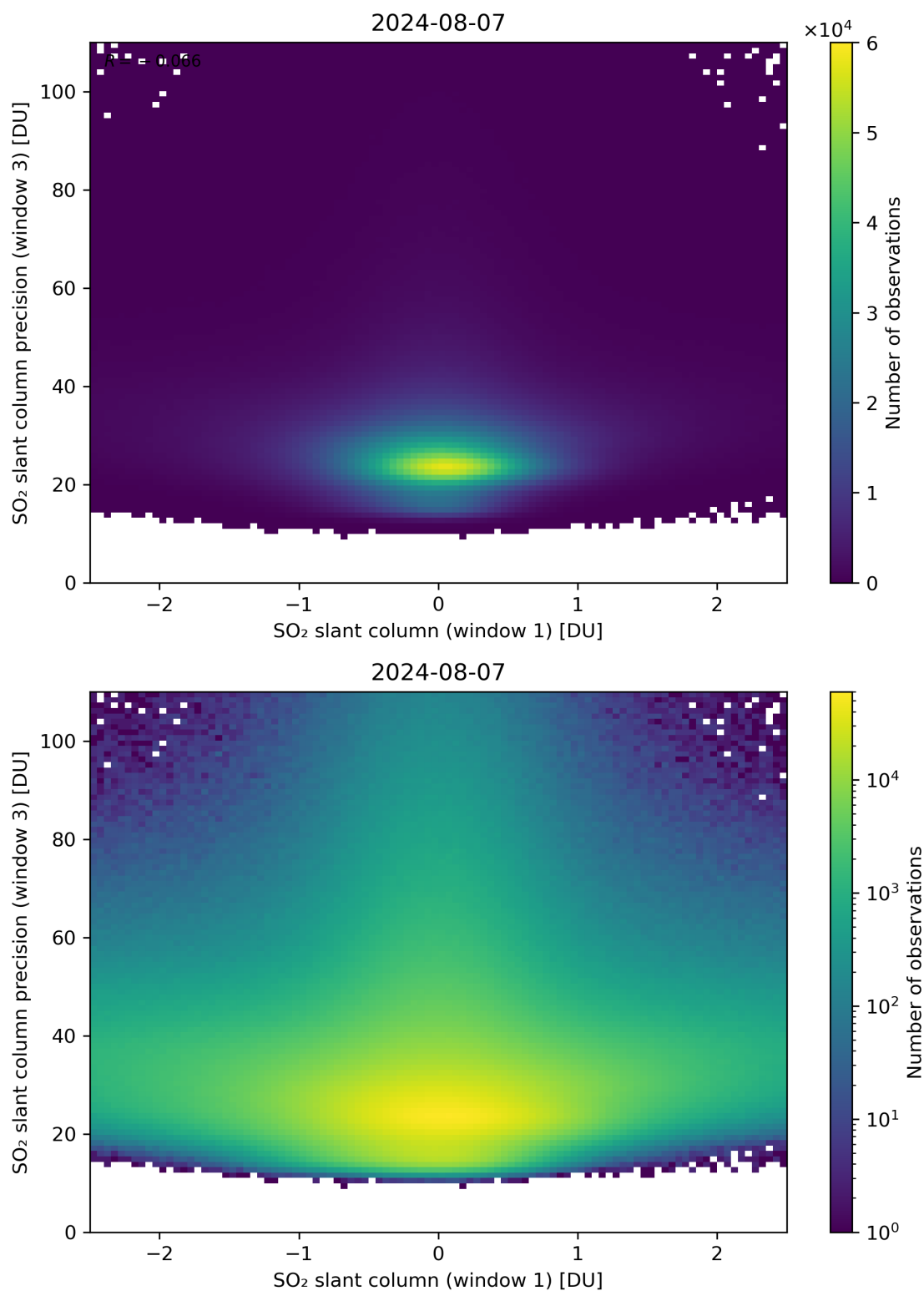
Figure 238: Scatter density plot of “SO 2 slant column (window 1)” against “SO 2 slant column precision (window 3)” for 2024-08-06 to 2024-08-08.
