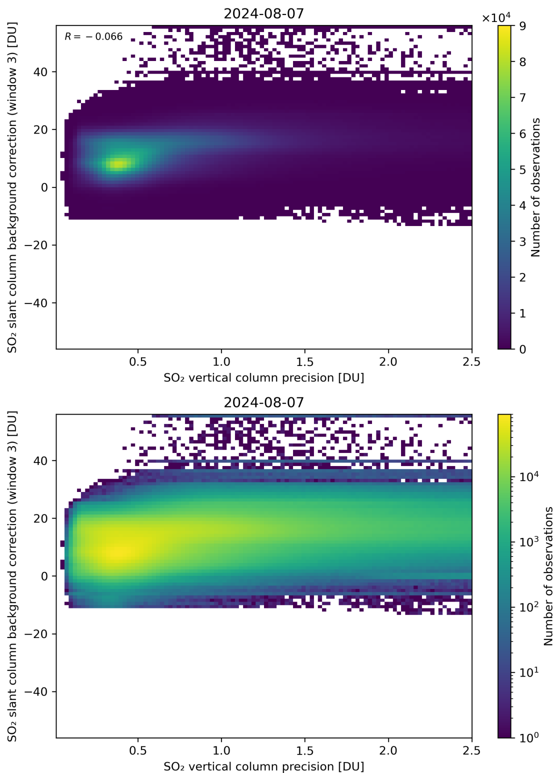
Figure 281: Scatter density plot of “SO 2 vertical column precision” against “SO 2 slant column background correction (window 3)” for 2024-08-06 to 2024-08-08.
