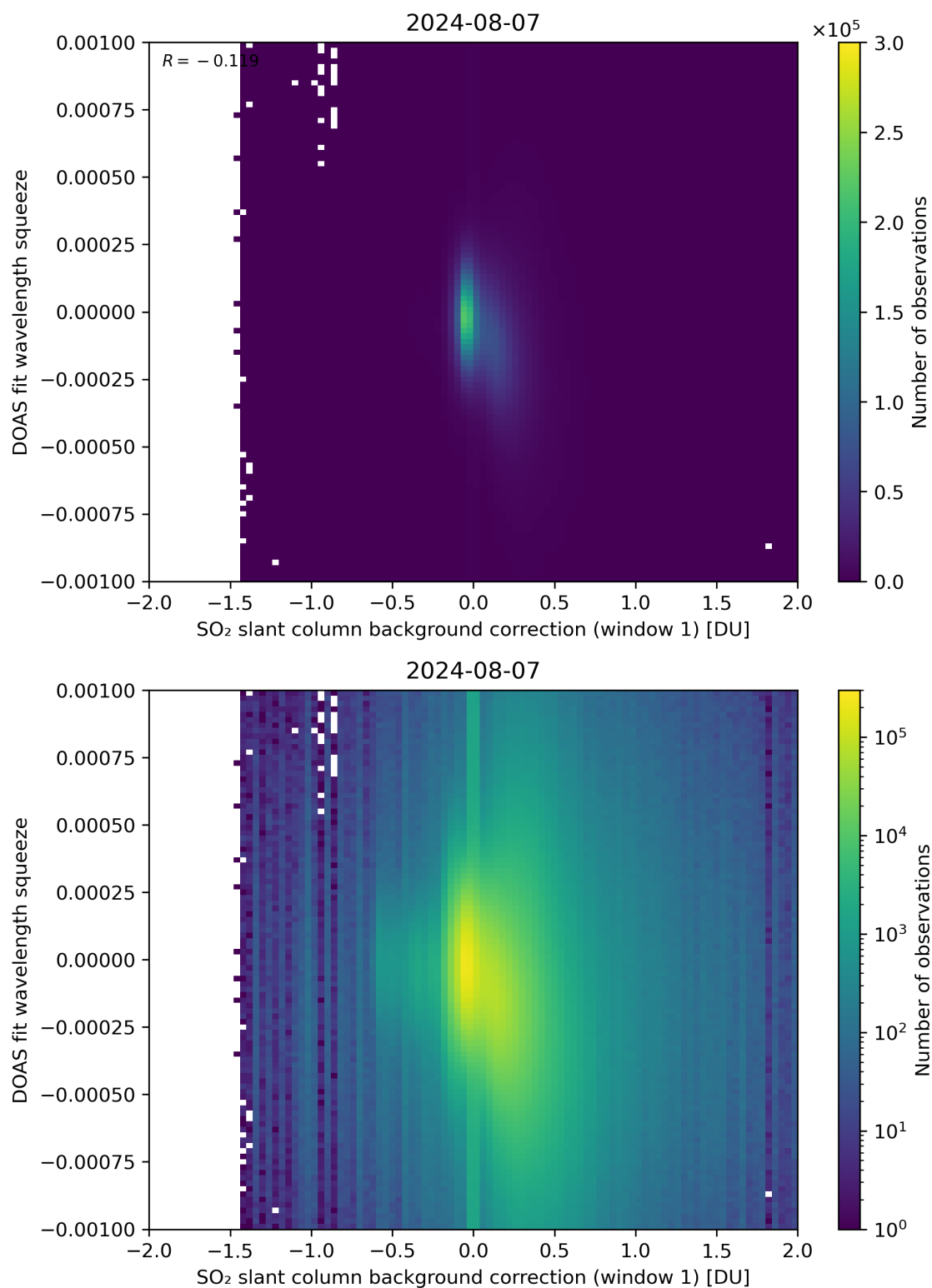
Figure 101: Scatter density plot of “SO 2 slant column background correction (window 1)” against “DOAS fit wavelength squeeze” for 2024-08-06 to 2024-08-08.
