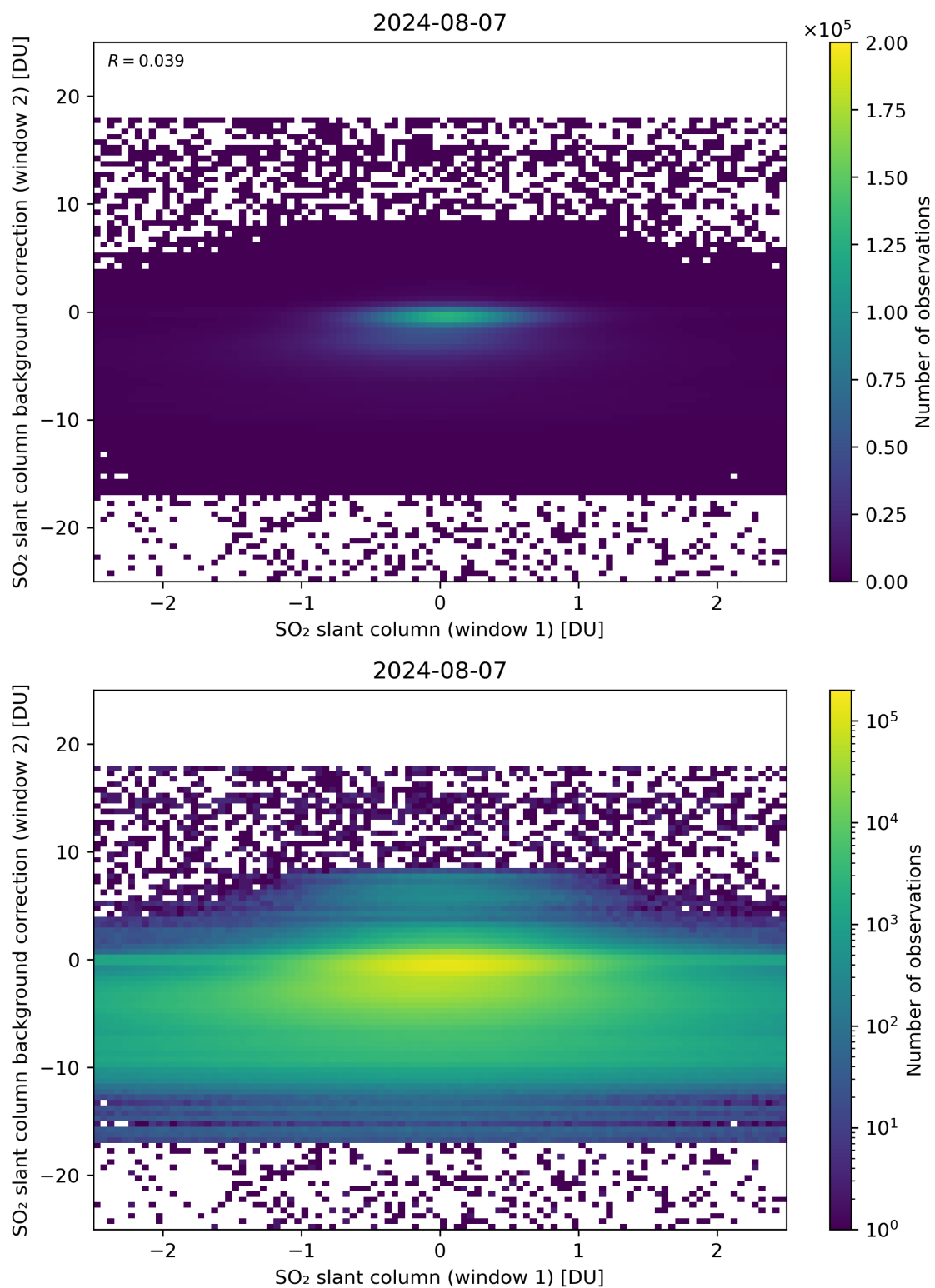
Figure 213: Scatter density plot of “SO 2 slant column (window 1)” against “SO 2 slant column background correction (window 2)” for 2024-08-06 to 2024-08-08.
