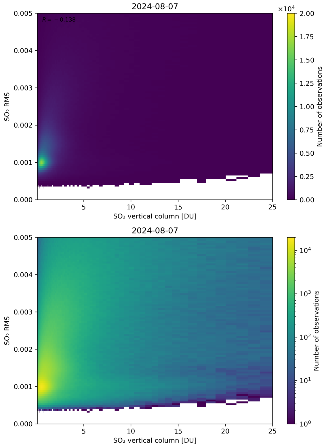
Figure 278: Scatter density plot of “SO 2 vertical column” against “SO 2 RMS” for 2024-08-06 to 2024-08-08.
