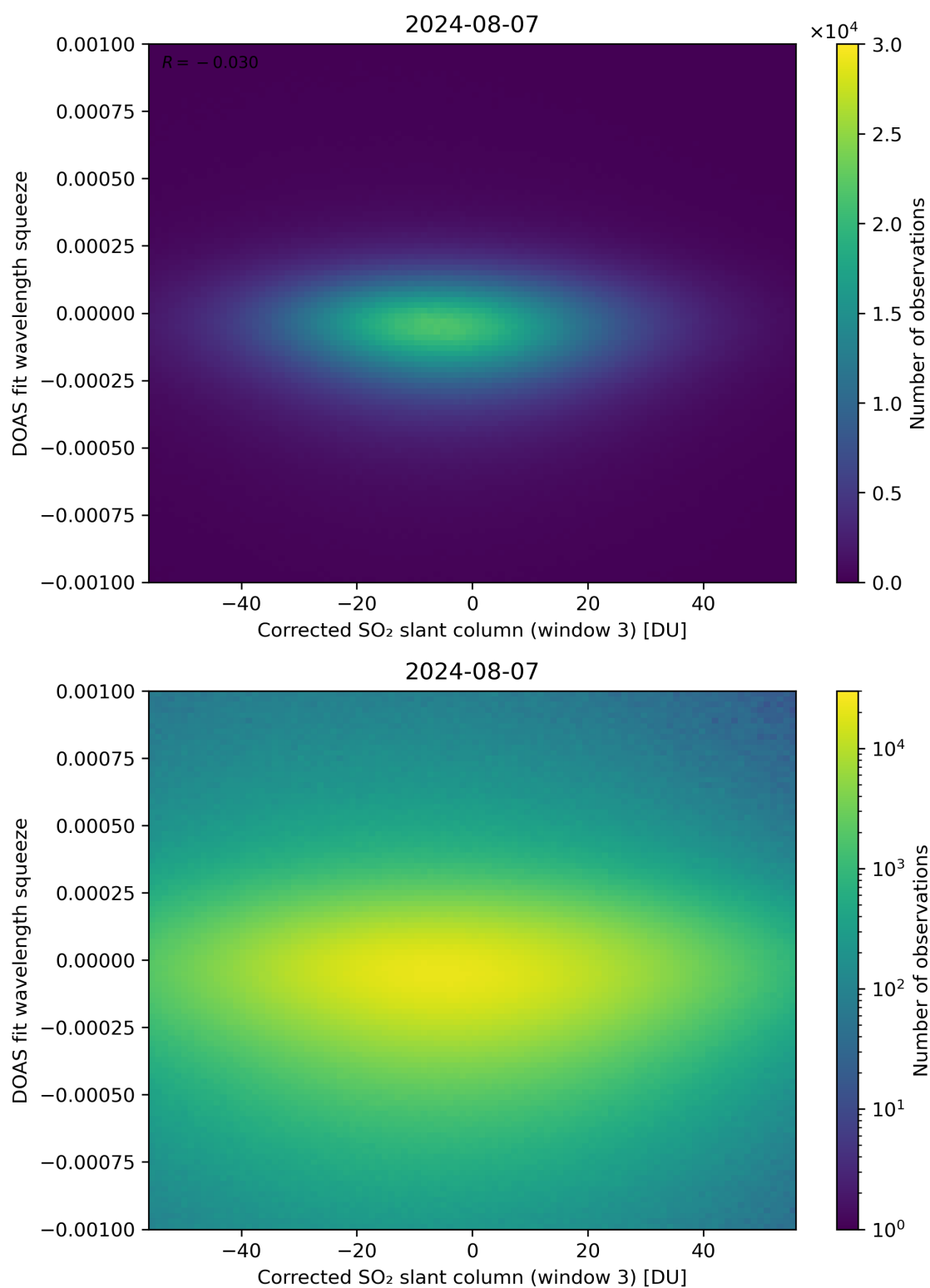
Figure 207: Scatter density plot of “Corrected SO 2 slant column (window 3)” against “DOAS fit wavelength squeeze” for 2024-08-06 to 2024-08-08.
