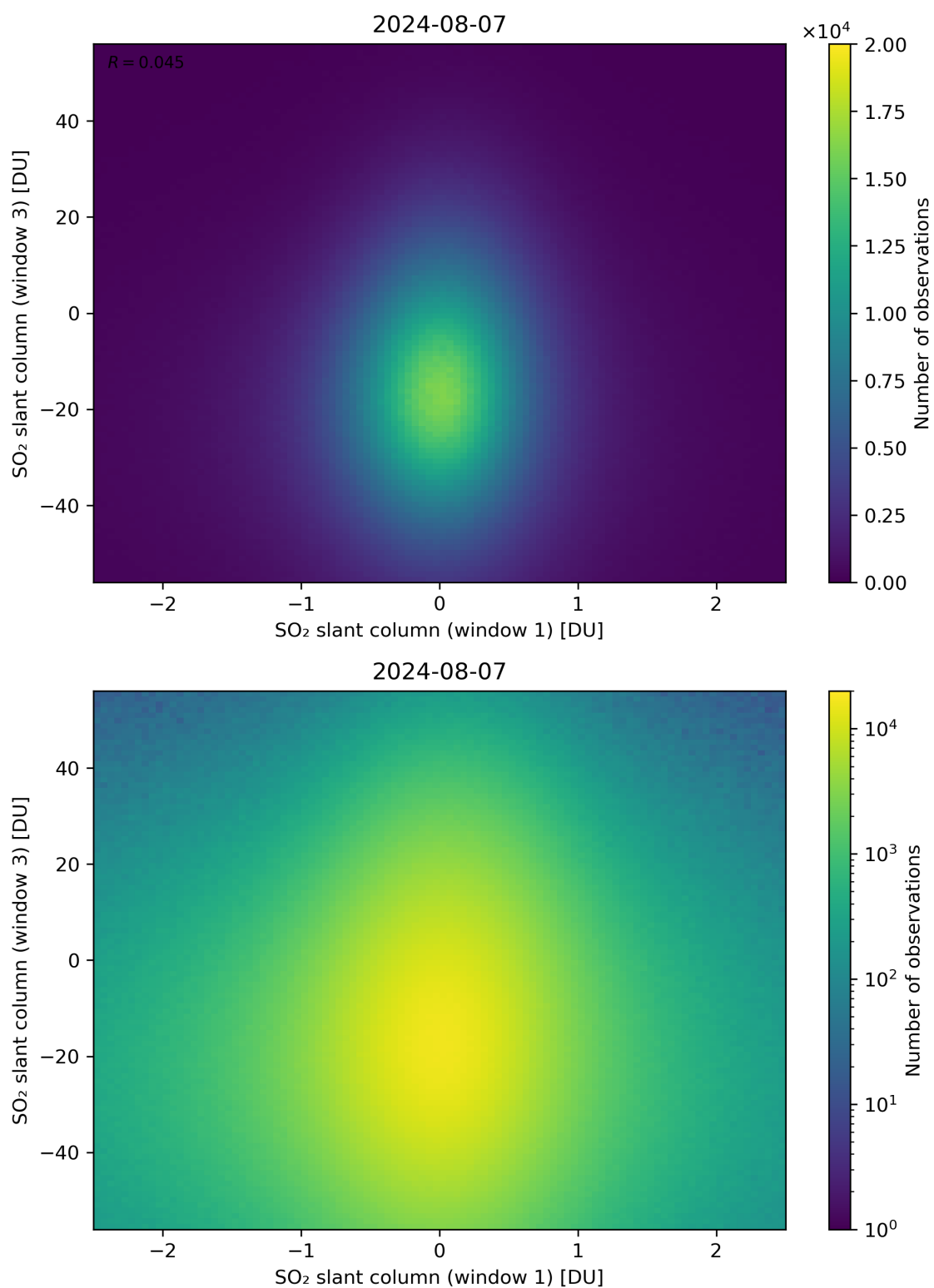
Figure 237: Scatter density plot of “SO 2 slant column (window 1)” against “SO 2 slant column (window 3)” for 2024-08-06 to 2024-08-08.
