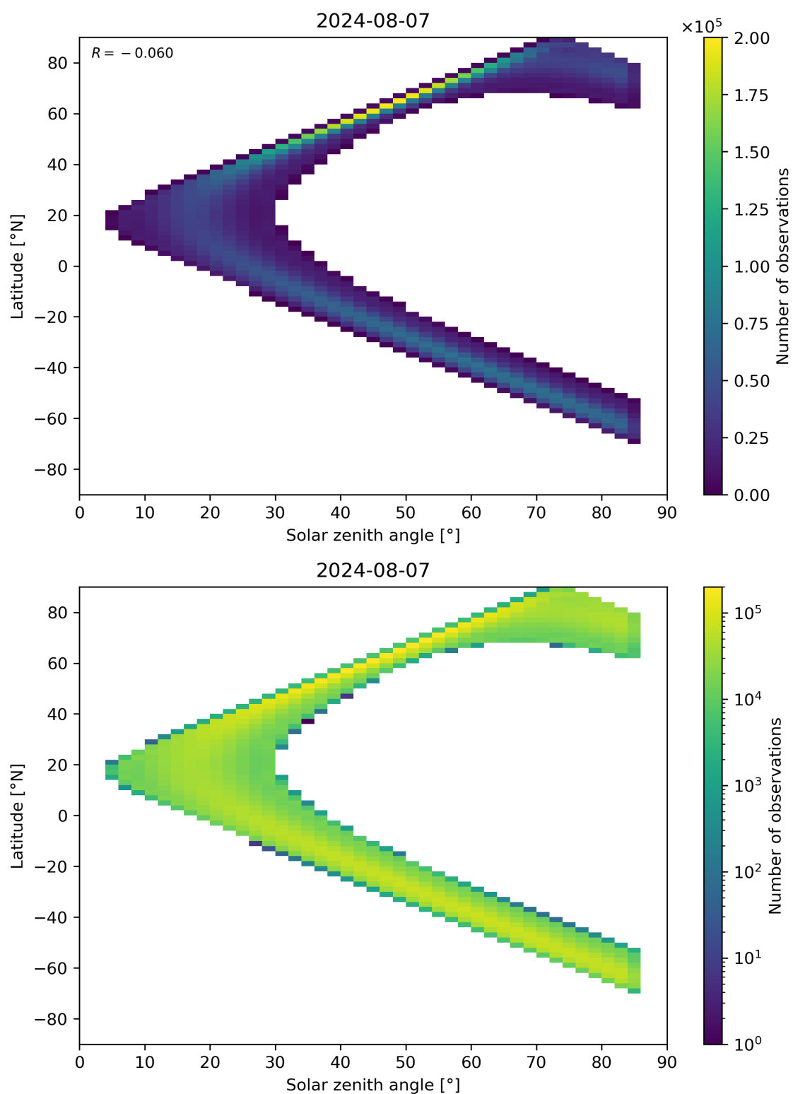
Figure 164: Scatter density plot of “Solar zenith angle” against “Latitude” for 2024-08-06 to 2024-08-08.
