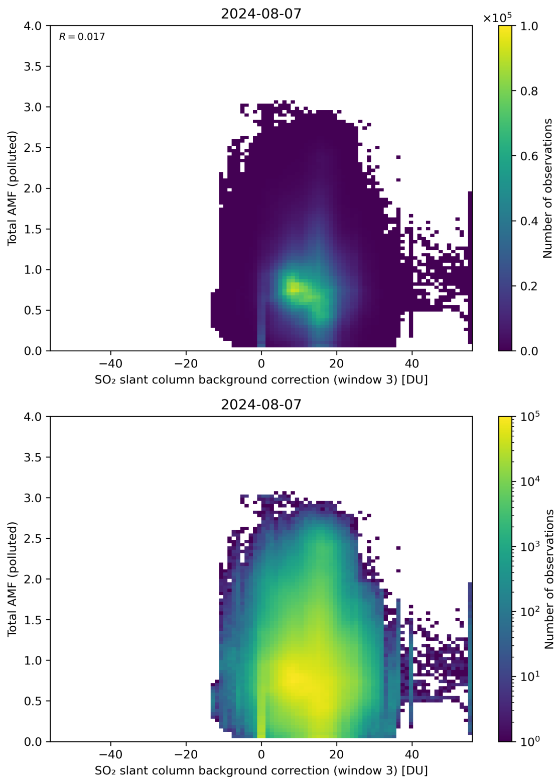
Figure 125: Scatter density plot of “SO 2 slant column background correction (window 3)” against “Total AMF (polluted)” for 2024-08-06 to 2024-08-08.
