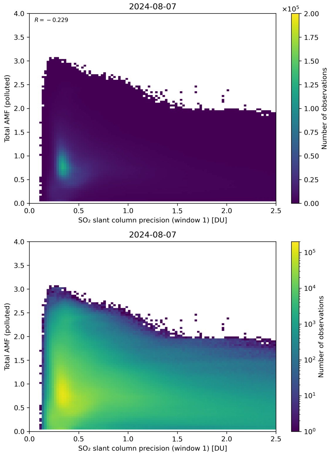
Figure 230: Scatter density plot of “SO 2 slant column precision (window 1)” against “Total AMF (polluted)” for 2024-08-06 to 2024-08-08.
