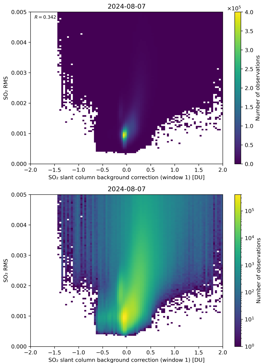
Figure 102: Scatter density plot of “SO 2 slant column background correction (window 1)” against “SO 2 RMS” for 2024-08-06 to 2024-08-08.
