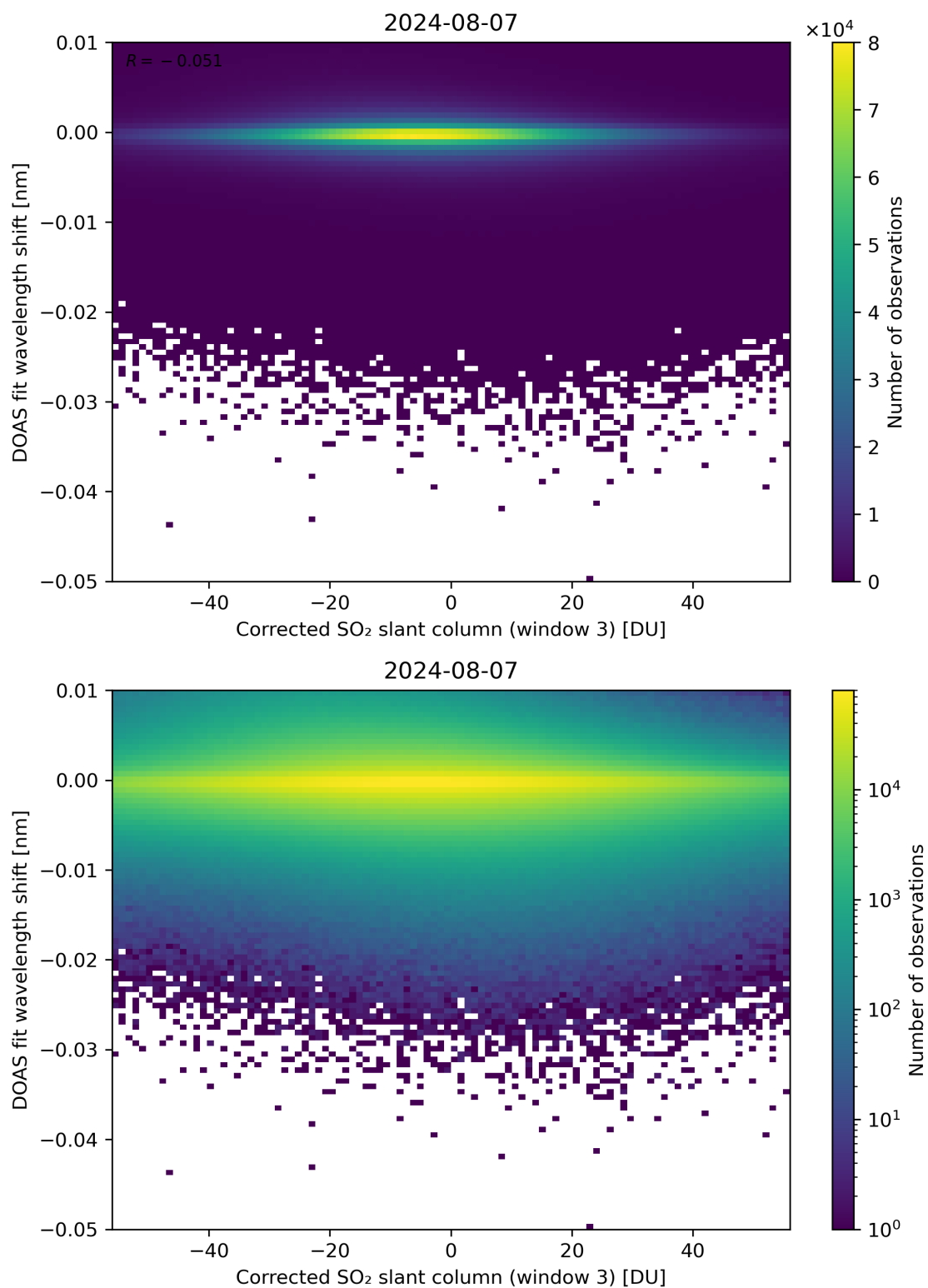
Figure 206: Scatter density plot of “Corrected SO 2 slant column (window 3)” against “DOAS fit wavelength shift” for 2024-08-06 to 2024-08-08.
