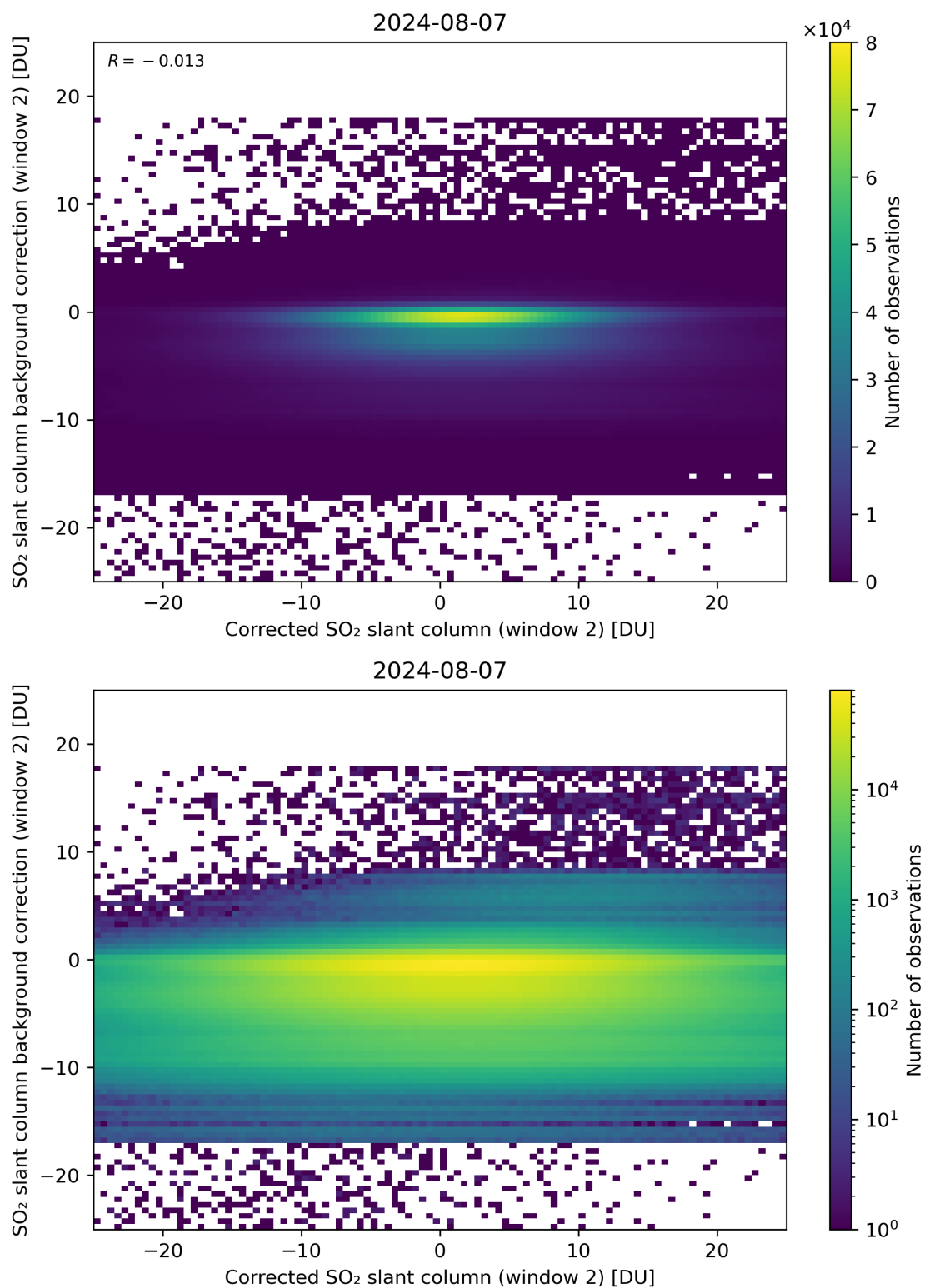
Figure 194: Scatter density plot of “Corrected SO 2 slant column (window 2)” against “SO 2 slant column background correction (window 2)” for 2024-08-06 to 2024-08-08.
