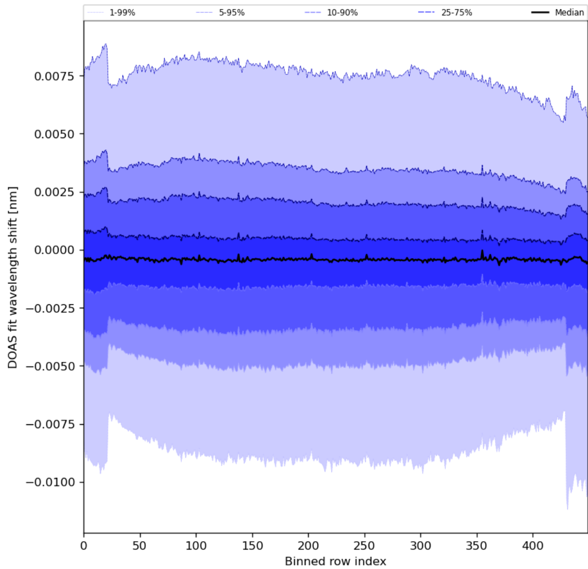
Figure 91: Along track statistics of “DOAS fit wavelength shift” for 2024-08-06 to 2024-08-08
