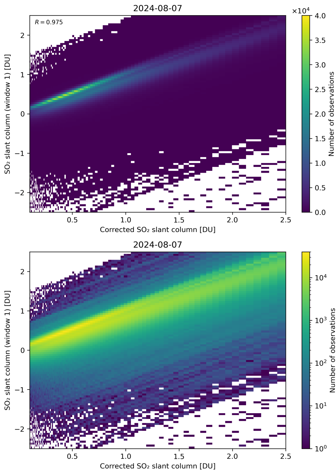
Figure 187: Scatter density plot of “Corrected SO 2 slant column” against “SO 2 slant column (window 1)” for 2024-08-06 to 2024-08-08.
