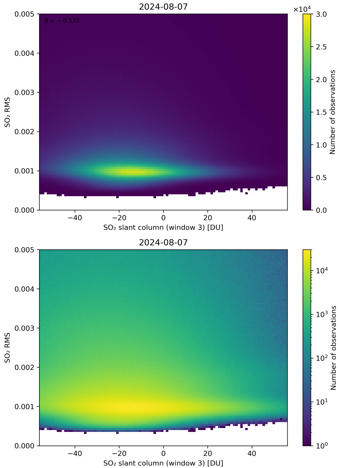
Figure 256: Scatter density plot of “SO 2 slant column (window 3)” against “SO 2 RMS” for 2024-08-06 to 2024-08-08.
