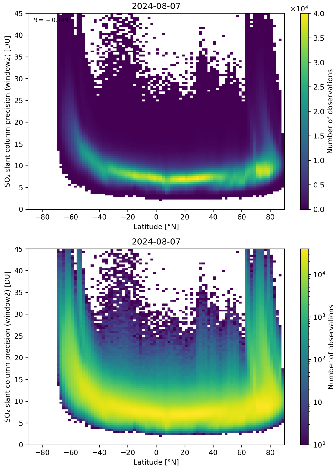
Figure 151: Scatter density plot of “Latitude” against “SO 2 slant column precision (window2)” for 2024-08-06 to 2024-08-08.
