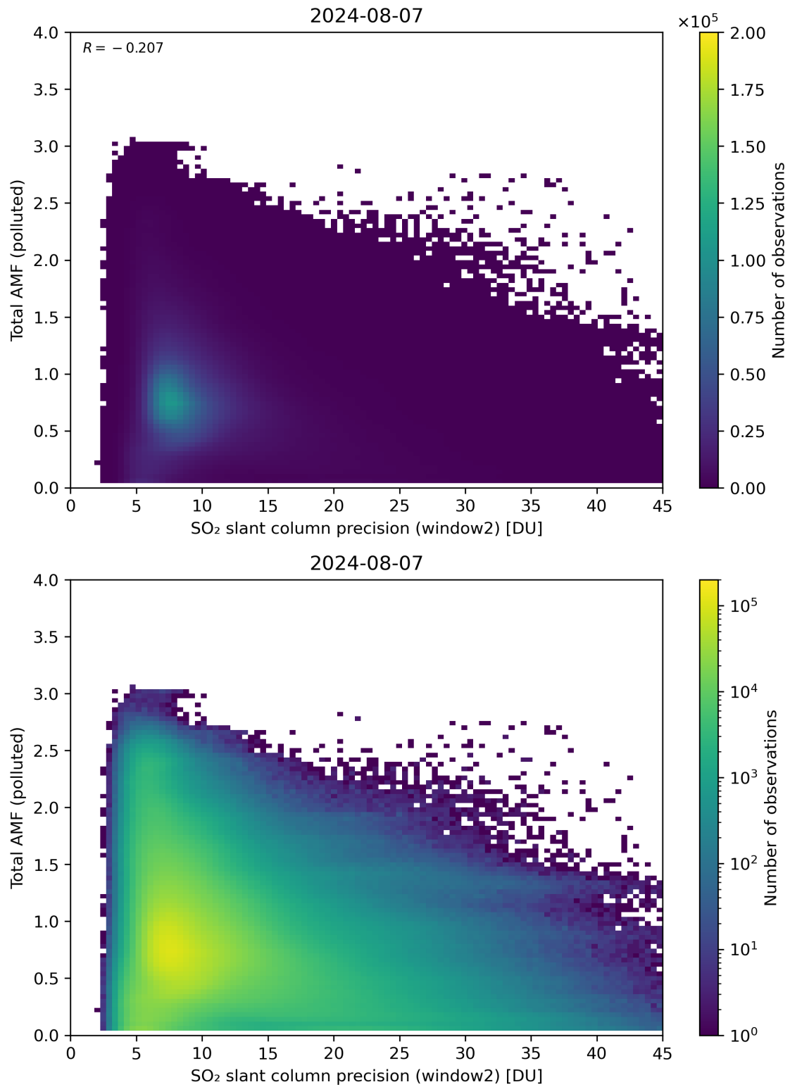
Figure 251: Scatter density plot of “SO 2 slant column precision (window2)” against “Total AMF (polluted)” for 2024-08-06 to 2024-08-08.
