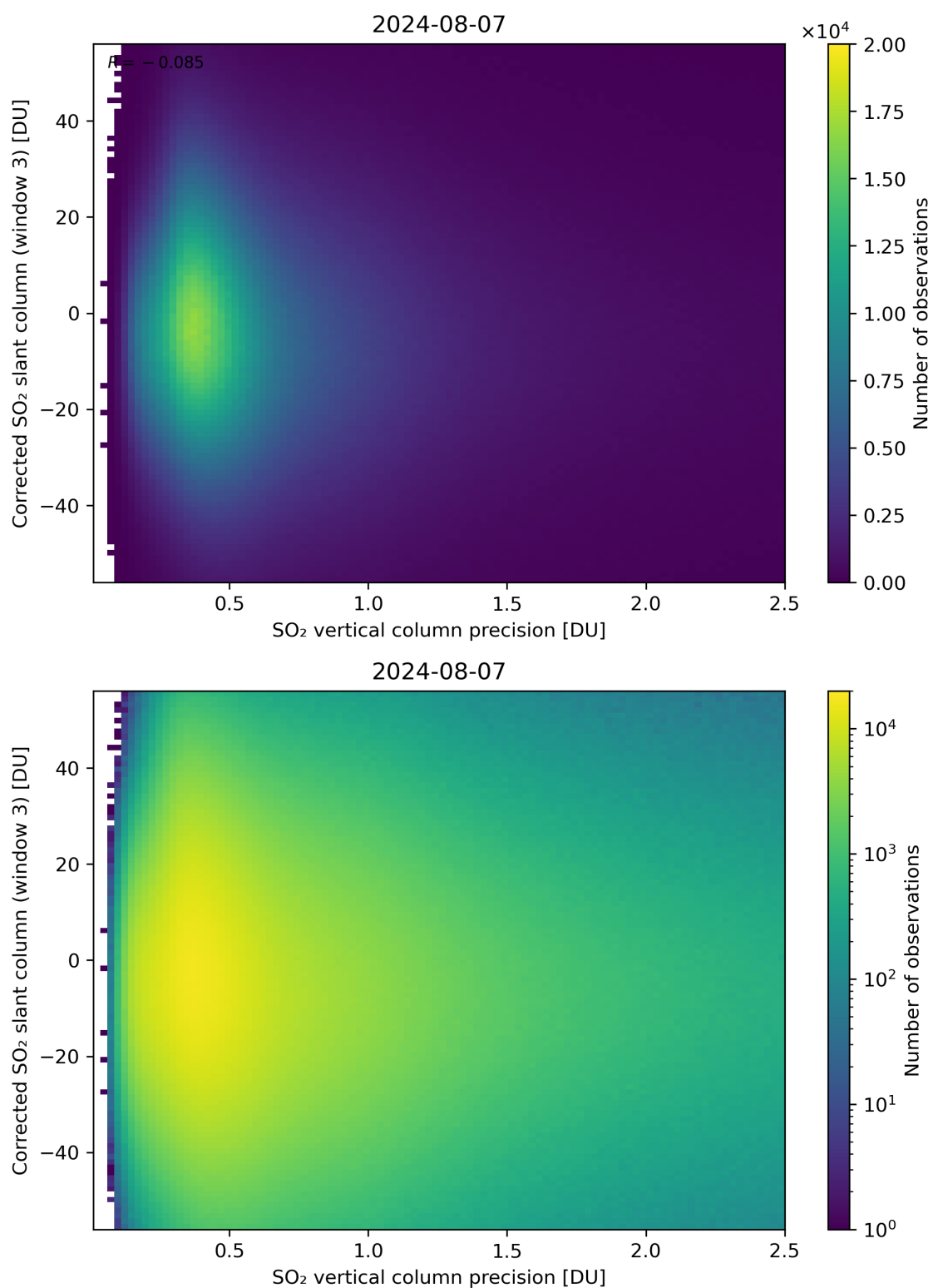
Figure 288: Scatter density plot of “SO 2 vertical column precision” against “Corrected SO 2 slant column (window 3)” for 2024-08-06 to 2024-08-08.
