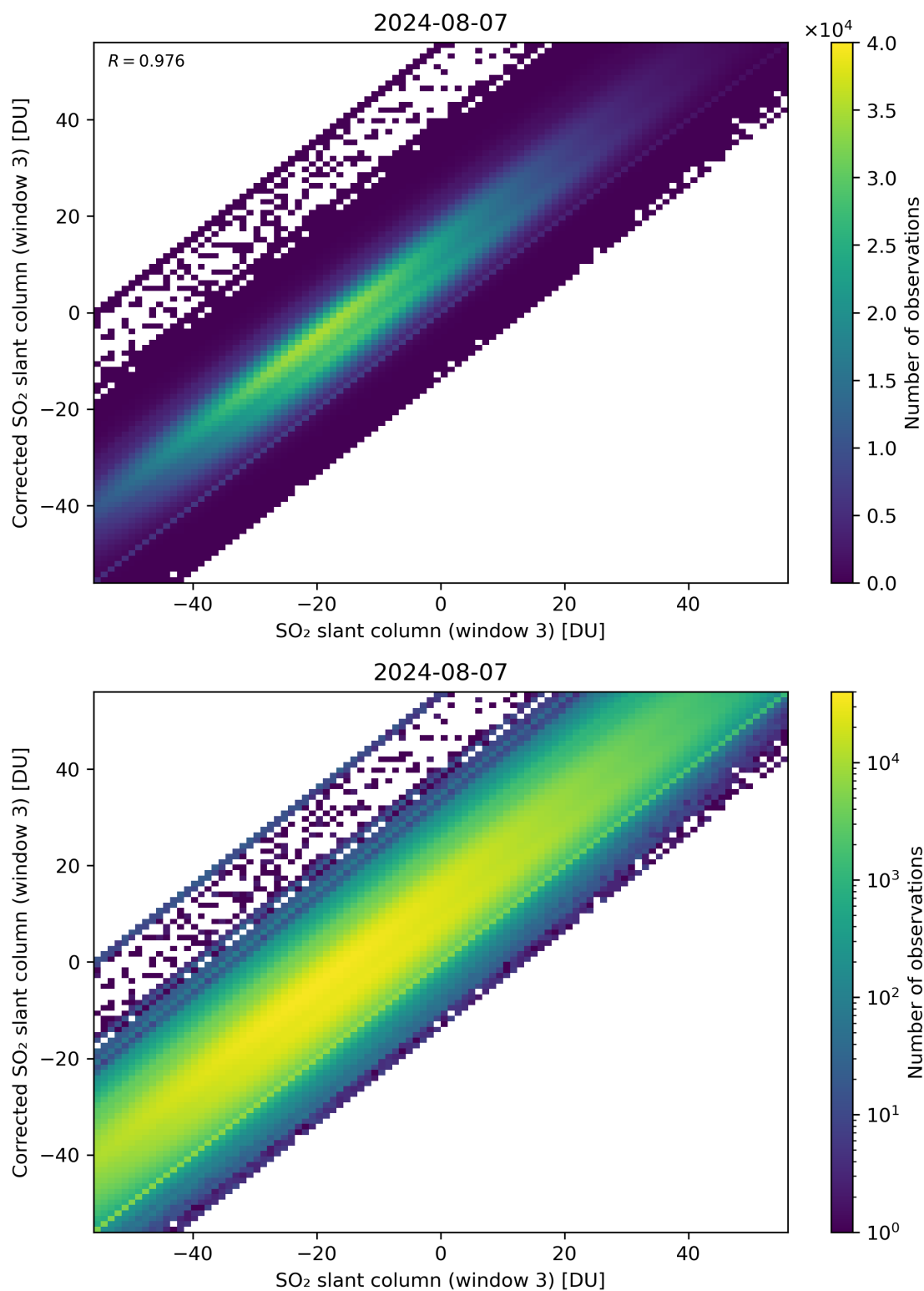
Figure 266: Scatter density plot of “SO 2 slant column (window 3)” against “Corrected SO 2 slant column (window 3)” for 2024-08-06 to 2024-08-08.
