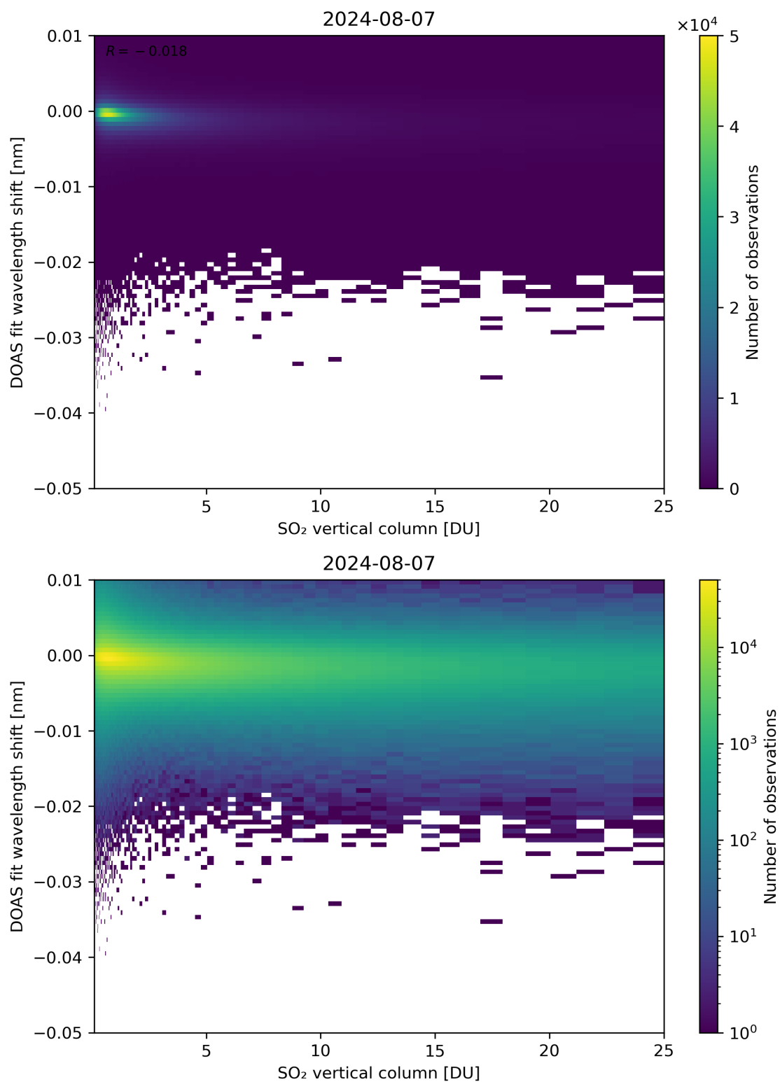
Figure 276: Scatter density plot of “SO 2 vertical column” against “DOAS fit wavelength shift” for 2024-08-06 to 2024-08-08.
