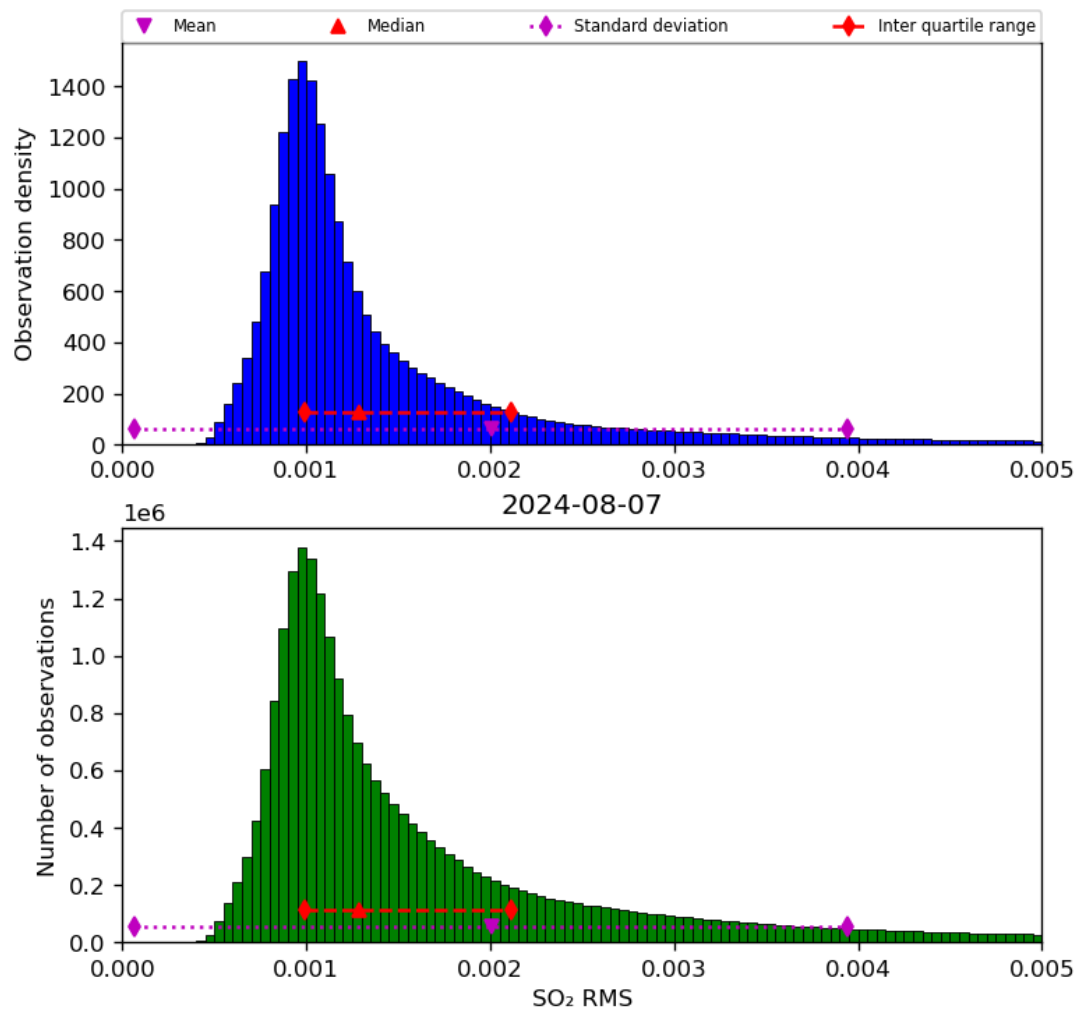
Figure 70: Histogram of “SO 2 RMS” for 2024-08-06 to 2024-08-08
