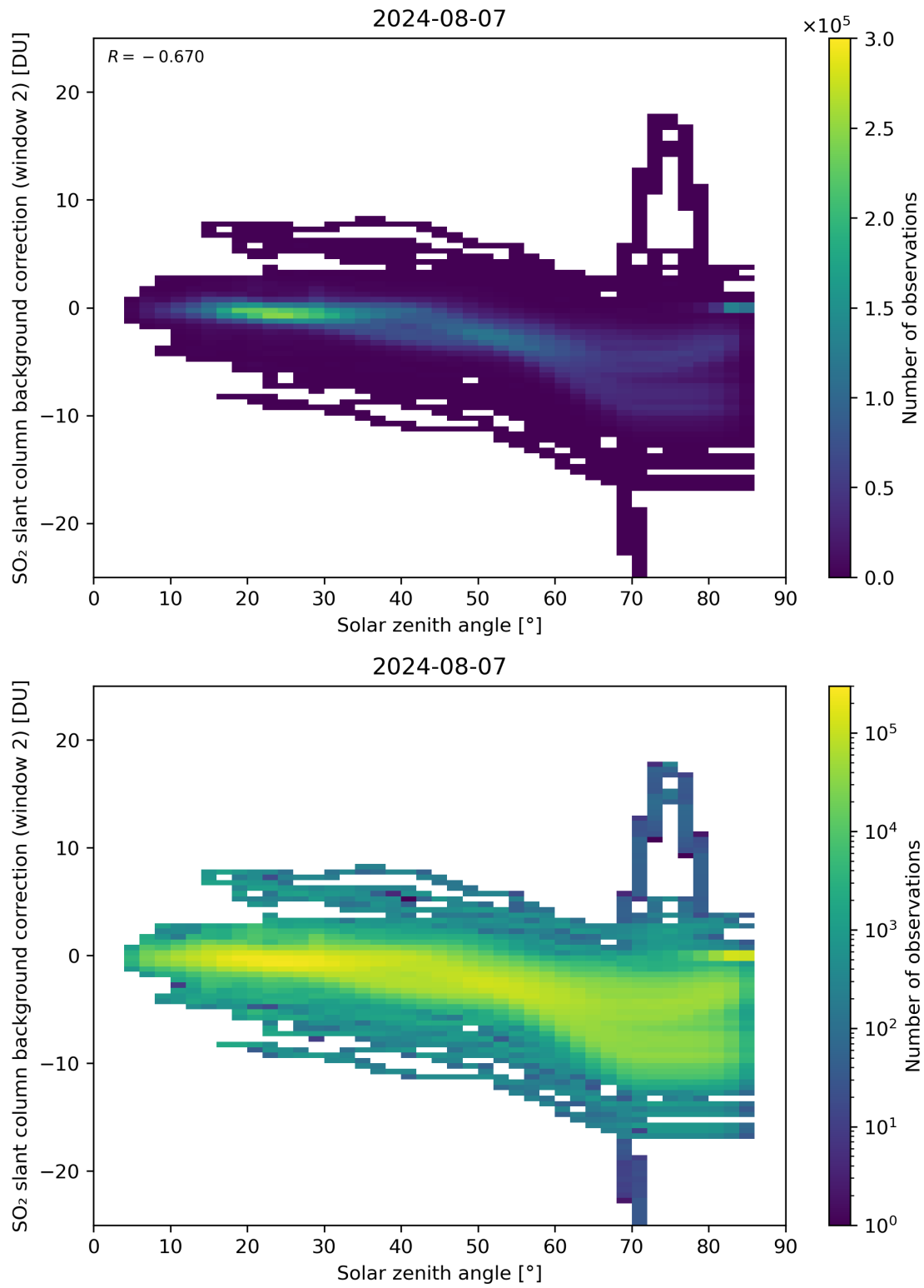
Figure 159: Scatter density plot of “Solar zenith angle” against “SO 2 slant column background correction (window 2)” for 2024-08-06 to 2024-08-08.
