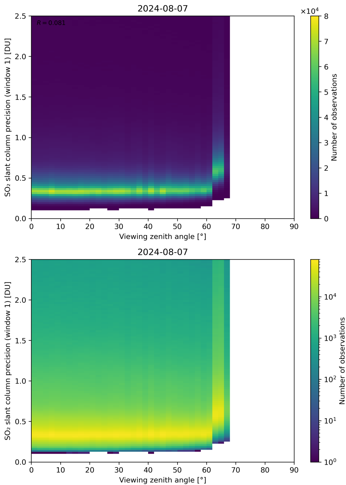
Figure 321: Scatter density plot of “Viewing zenith angle” against “SO 2 slant column precision (window 1)” for 2024-08-06 to 2024-08-08.
