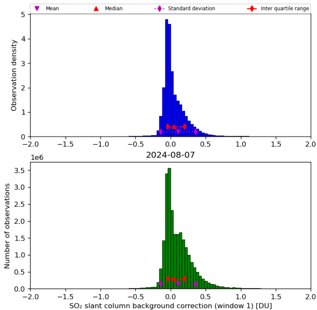
Figure 59: Histogram of “SO 2 slant column background correction (window 1)” for 2024-08-06 to 2024-08-08
