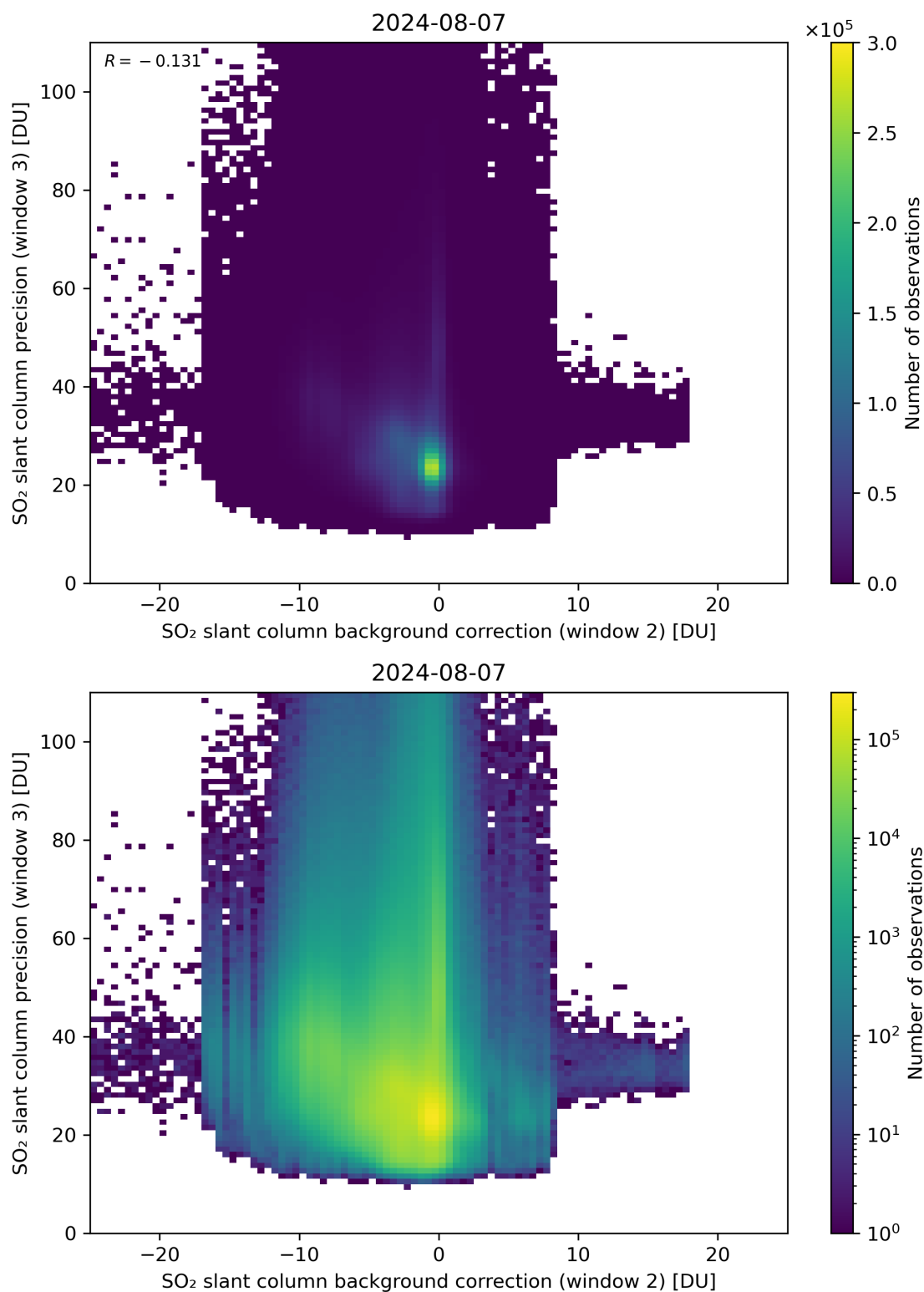
Figure 118: Scatter density plot of “SO 2 slant column background correction (window 2)” against “SO 2 slant column precision (window 3)” for 2024-08-06 to 2024-08-08.
