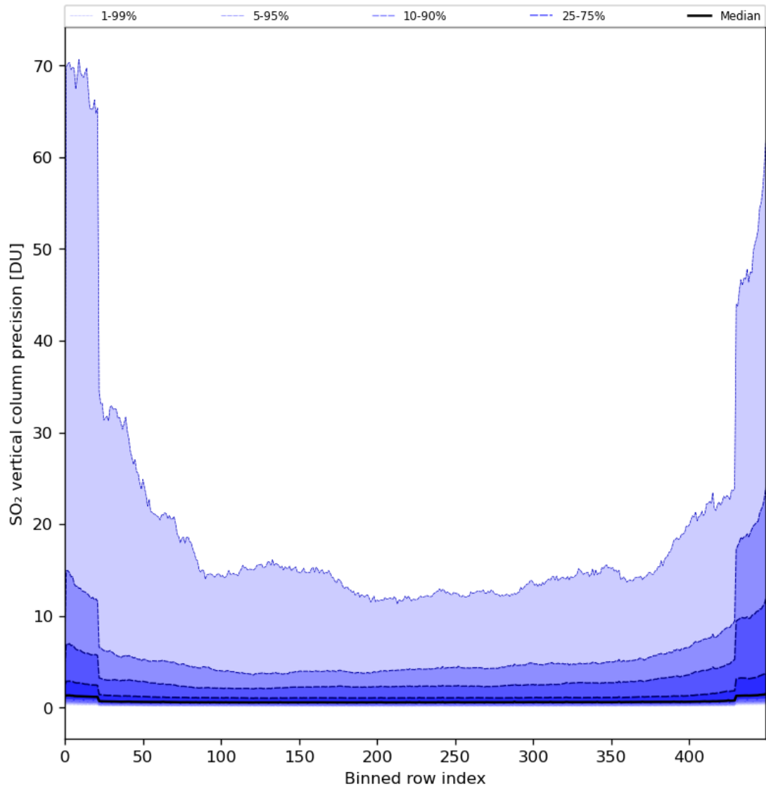
Figure 77: Along track statistics of “SO 2 vertical column precision” for 2024-08-06 to 2024-08-08
