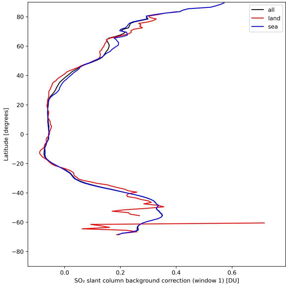
Figure 36: Zonal average of “SO 2 slant column background correction (window 1)” for 2024-08-06 to 2024-08-08.
