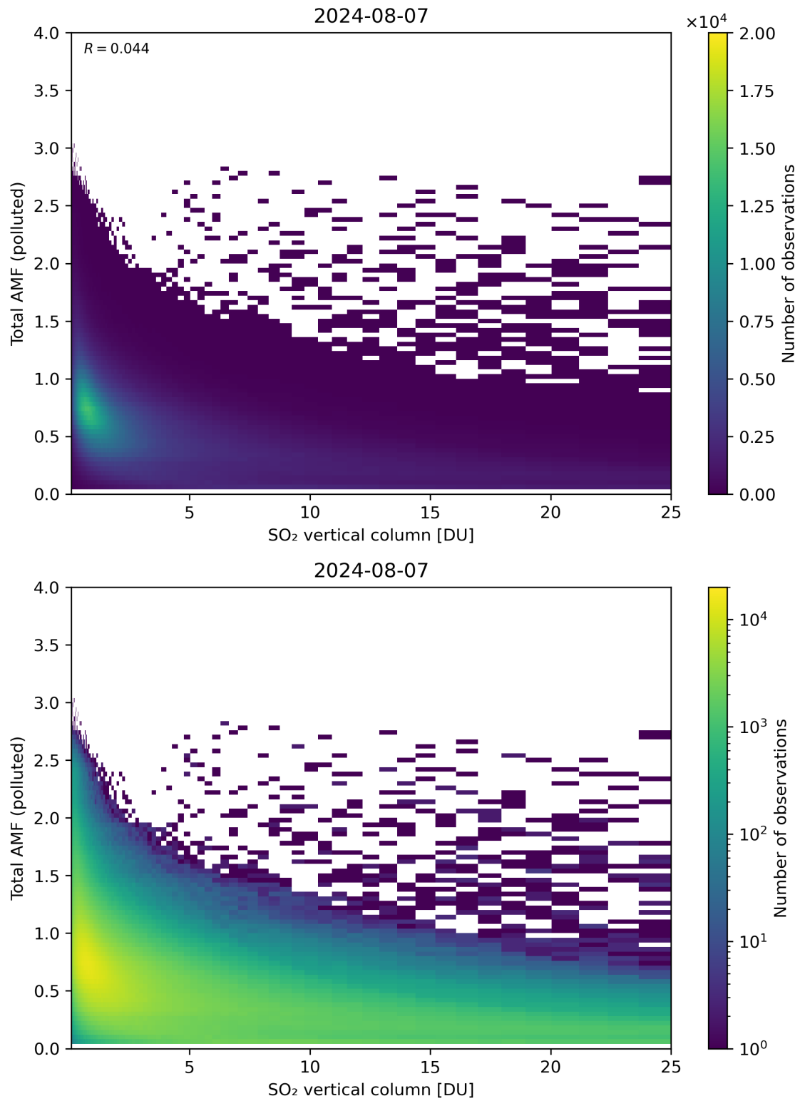
Figure 305: Scatter density plot of “SO 2 vertical column” against “Total AMF (polluted)” for 2024-08-06 to 2024-08-08.
