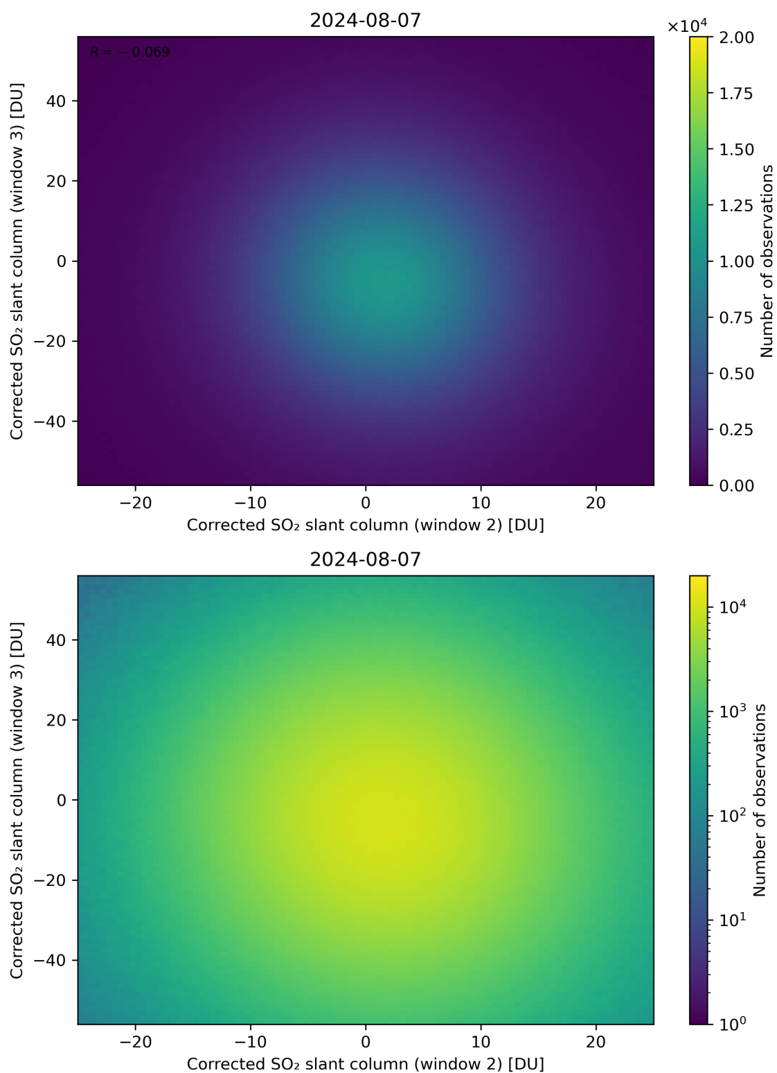
Figure 200: Scatter density plot of “Corrected SO 2 slant column (window 2)” against “Corrected SO 2 slant column (window 3)” for 2024-08-06 to 2024-08-08.
