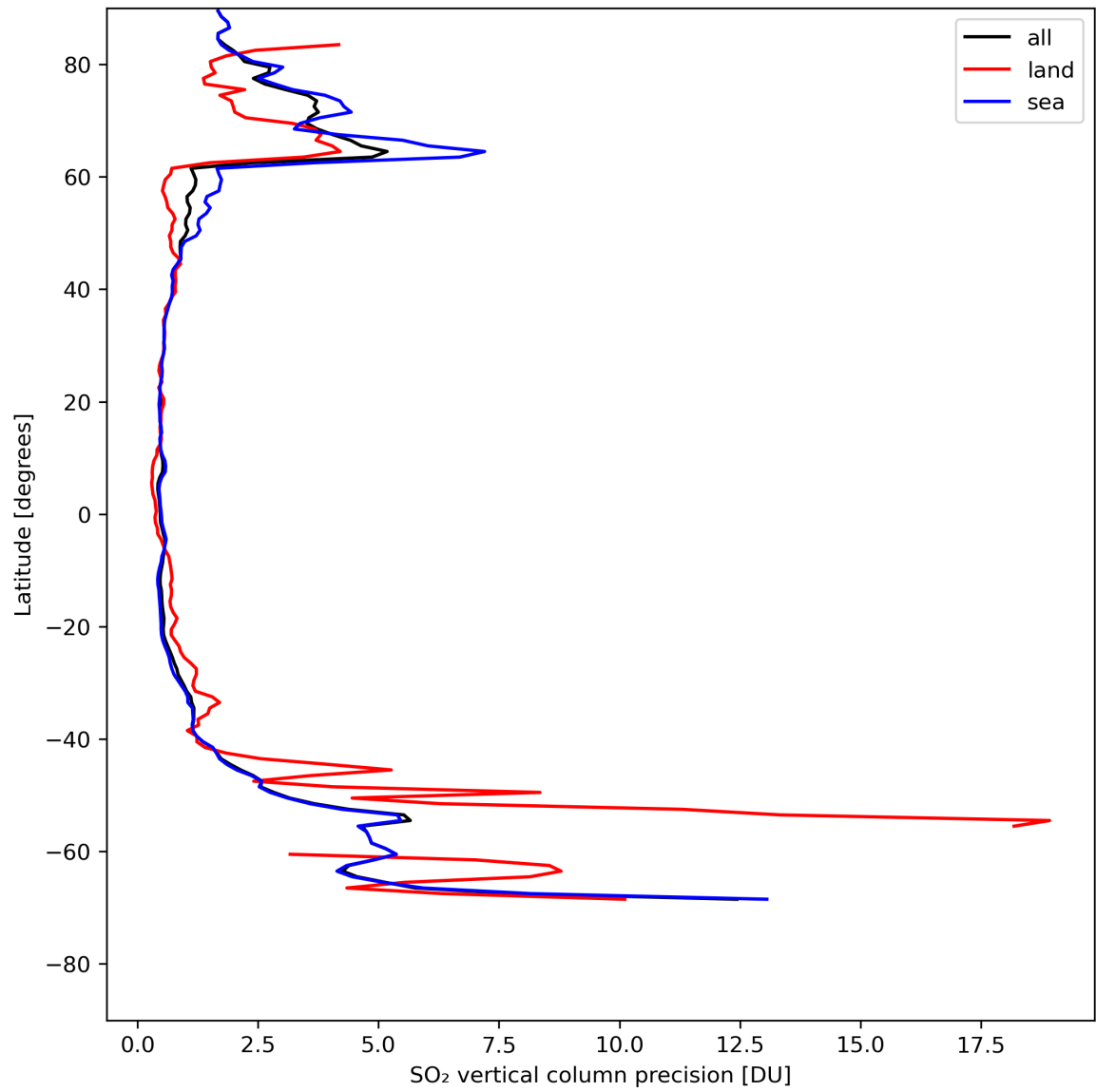
Figure 31: Zonal average of “SO 2 vertical column precision” for 2024-08-06 to 2024-08-08.
