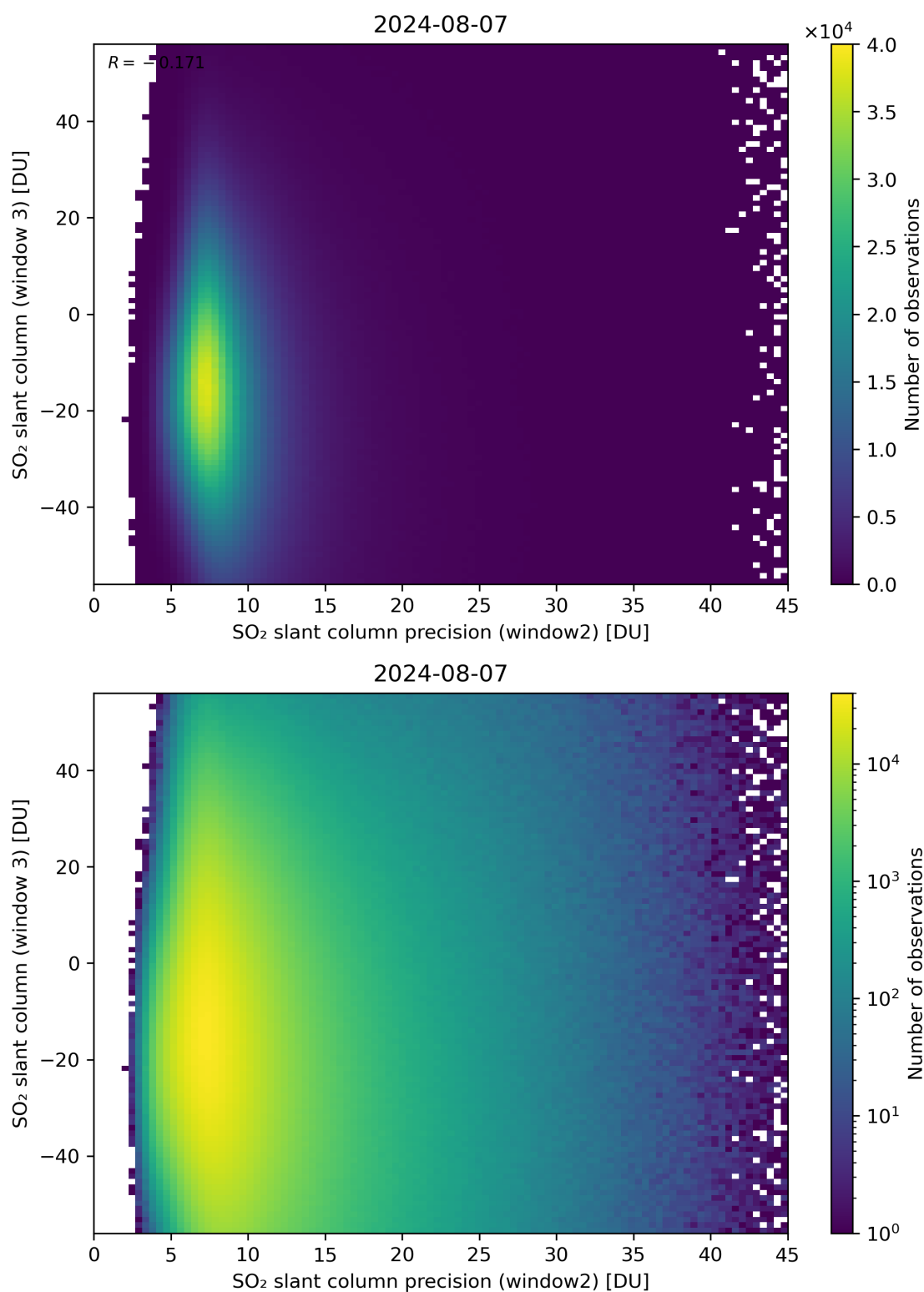
Figure 249: Scatter density plot of “SO 2 slant column precision (window2)” against “SO 2 slant column (window 3)” for 2024-08-06 to 2024-08-08.
