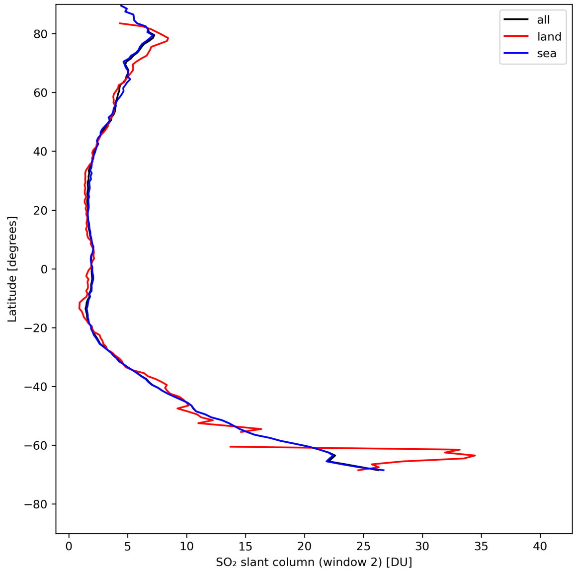
Figure 37: Zonal average of “SO 2 slant column (window 2)” for 2024-08-06 to 2024-08-08.
