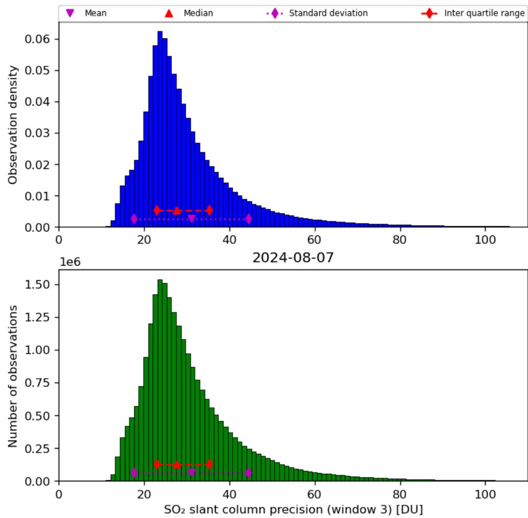
Figure 65: Histogram of “SO 2 slant column precision (window 3)” for 2024-08-06 to 2024-08-08
