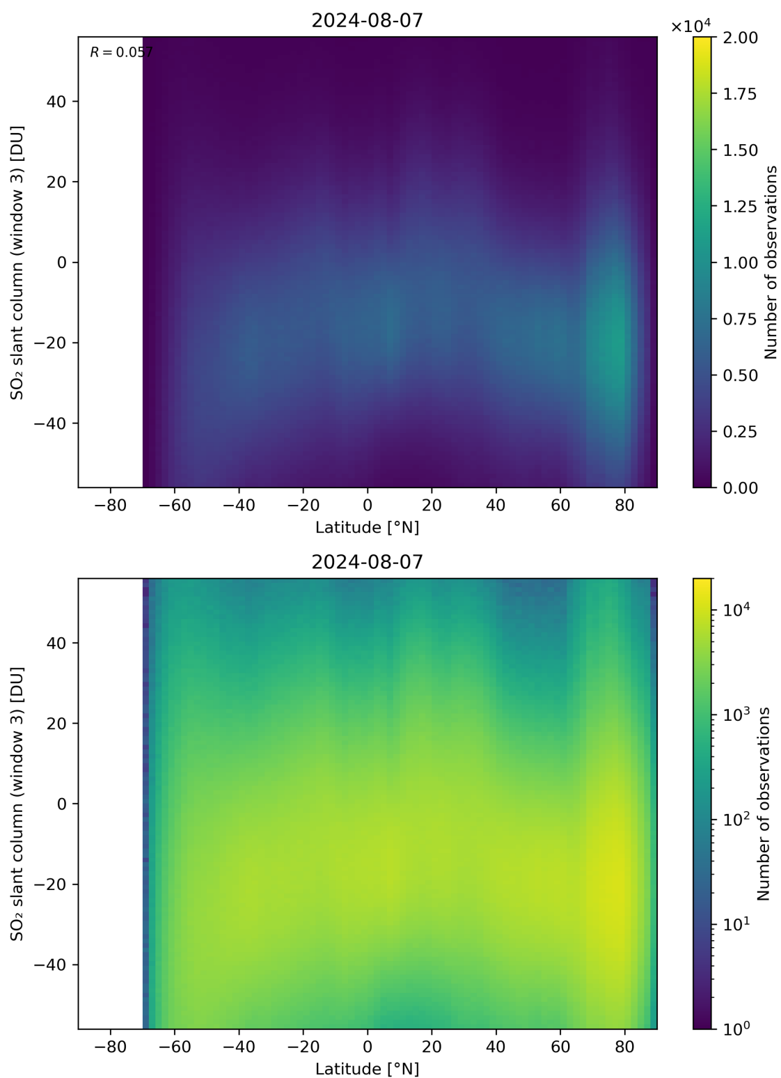
Figure 152: Scatter density plot of “Latitude” against “SO 2 slant column (window 3)” for 2024-08-06 to 2024-08-08.
