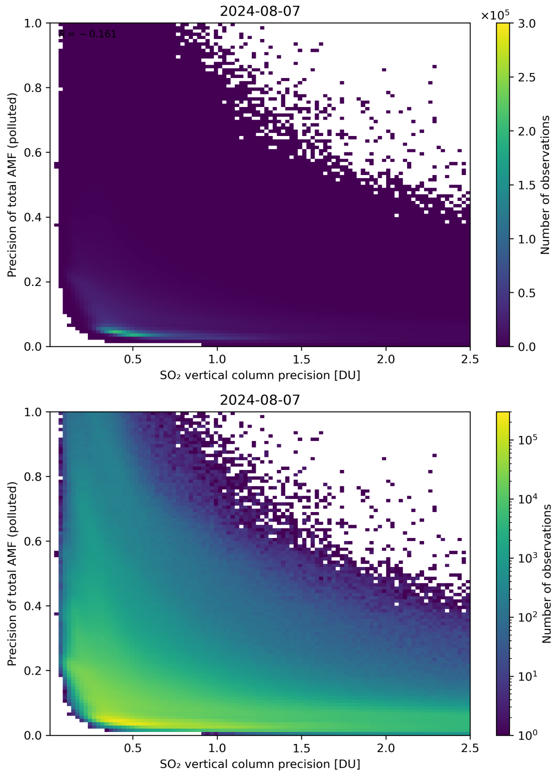
Figure 295: Scatter density plot of “SO 2 vertical column precision” against “Precision of total AMF (polluted)” for 2024-08-06 to 2024-08-08.
