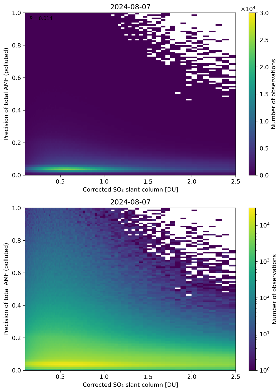
Figure 193: Scatter density plot of “Corrected SO 2 slant column” against “Precision of total AMF (polluted)” for 2024-08-06 to 2024-08-08.
