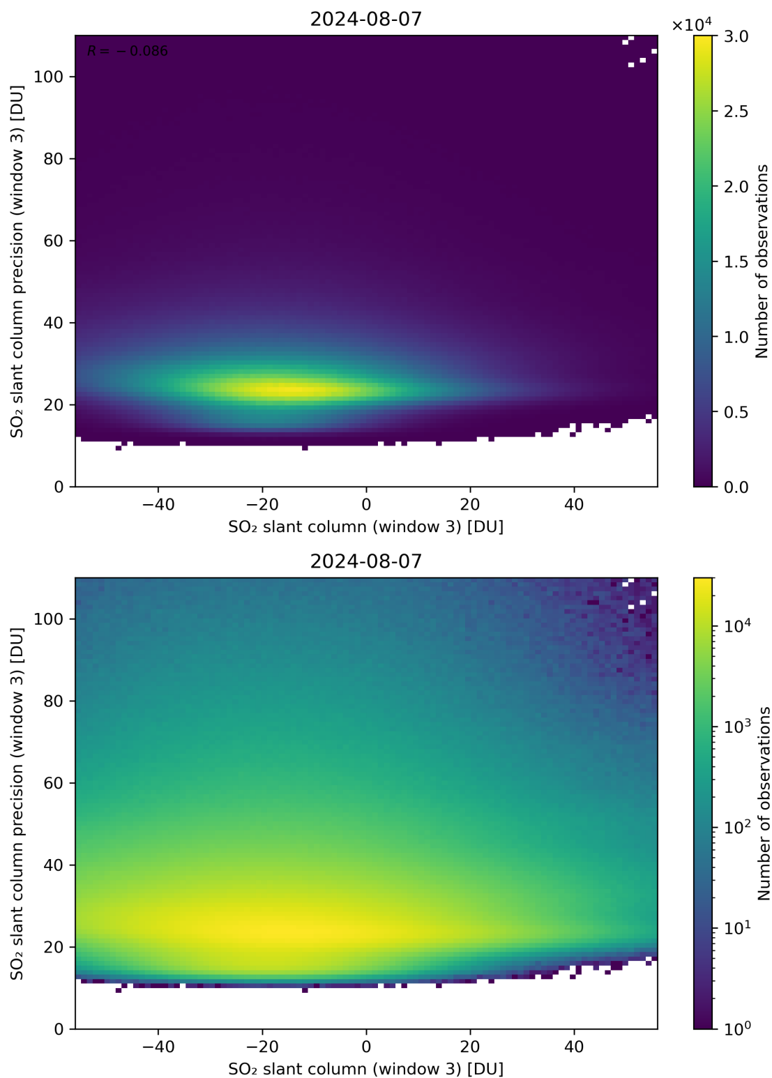
Figure 267: Scatter density plot of “SO 2 slant column (window 3)” against “SO 2 slant column precision (window 3)” for 2024-08-06 to 2024-08-08.
