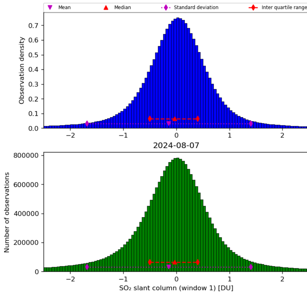
Figure 56: Histogram of “SO 2 slant column (window 1)” for 2024-08-06 to 2024-08-08
