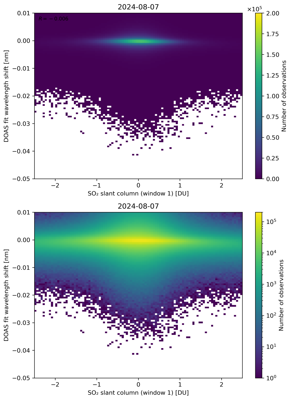
Figure 215: Scatter density plot of “SO 2 slant column (window 1)” against “DOAS fit wavelength shift” for 2024-08-06 to 2024-08-08.
