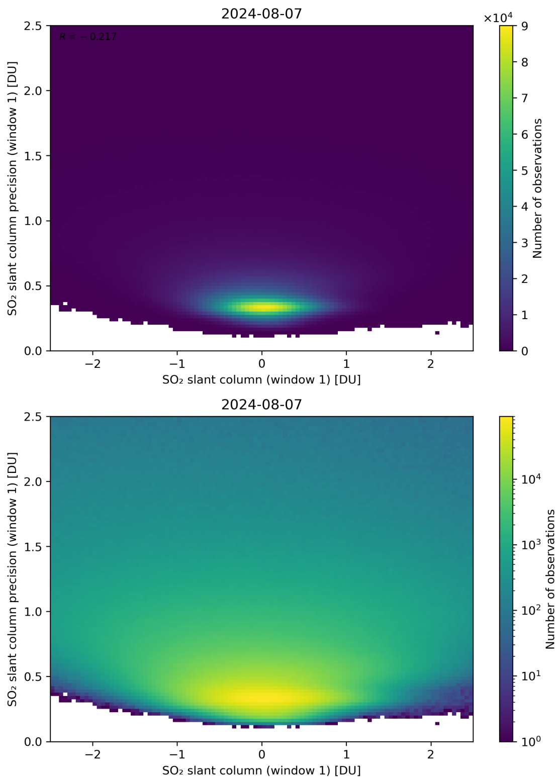
Figure 235: Scatter density plot of “SO 2 slant column (window 1)” against “SO 2 slant column precision (window 1)” for 2024-08-06 to 2024-08-08.
