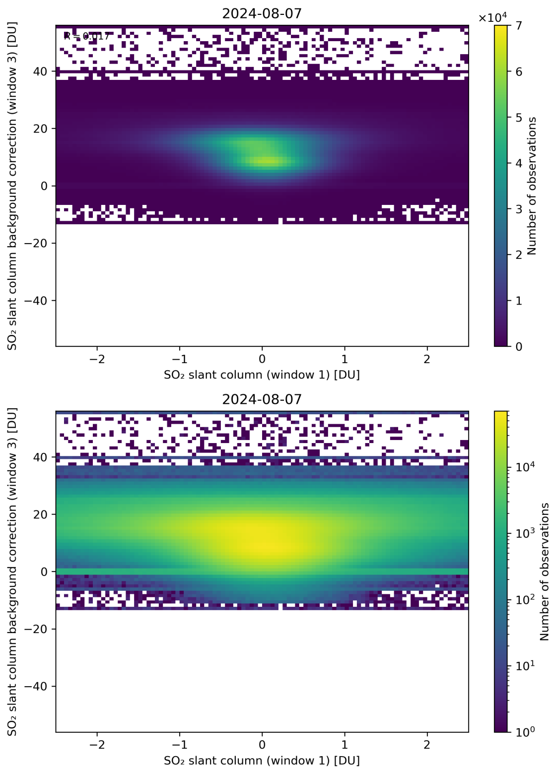
Figure 214: Scatter density plot of “SO 2 slant column (window 1)” against “SO 2 slant column background correction (window 3)” for 2024-08-06 to 2024-08-08.
