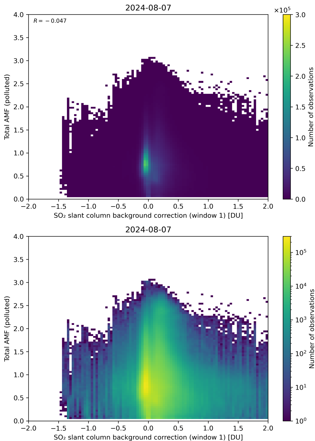
Figure 109: Scatter density plot of “SO 2 slant column background correction (window 1)” against “Total AMF (polluted)” for 2024-08-06 to 2024-08-08.
