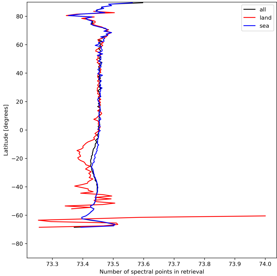
Figure 51: Zonal average of “Number of spectral points in retrieval” for 2024-08-06 to 2024-08-08.
