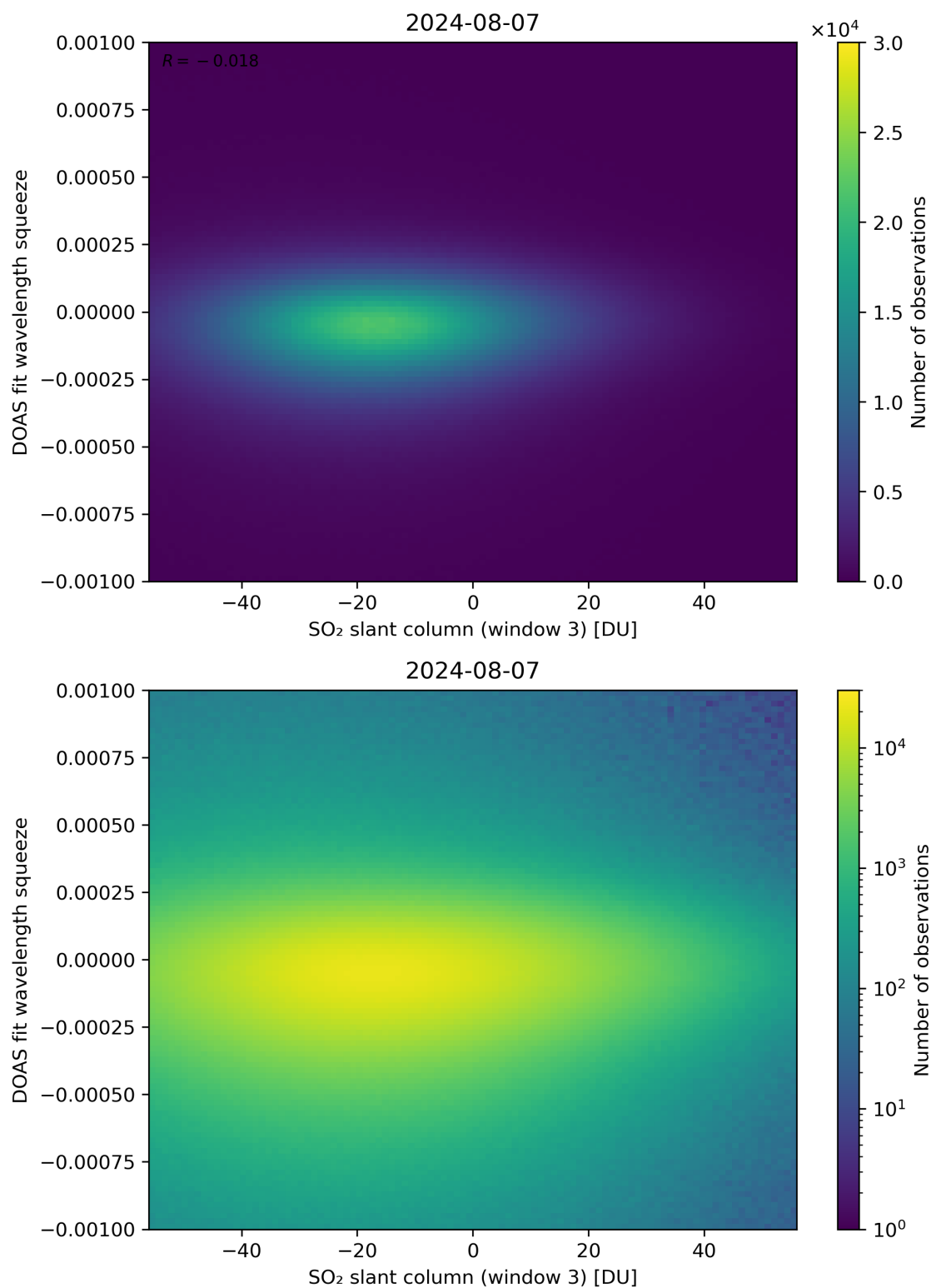
Figure 255: Scatter density plot of “SO 2 slant column (window 3)” against “DOAS fit wavelength squeeze” for 2024-08-06 to 2024-08-08.
