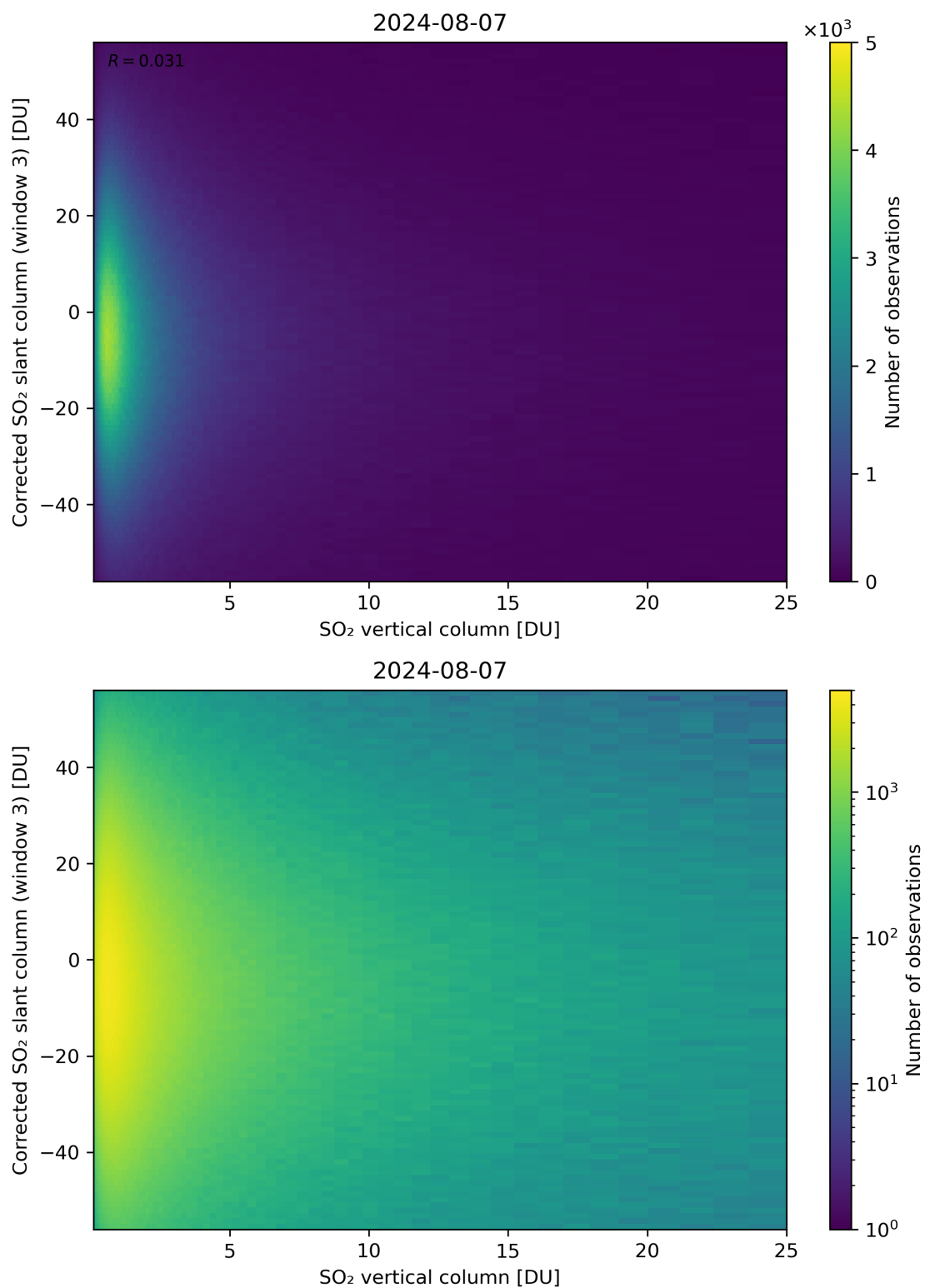
Figure 299: Scatter density plot of “SO 2 vertical column” against “Corrected SO 2 slant column (window 3)” for 2024-08-06 to 2024-08-08.
