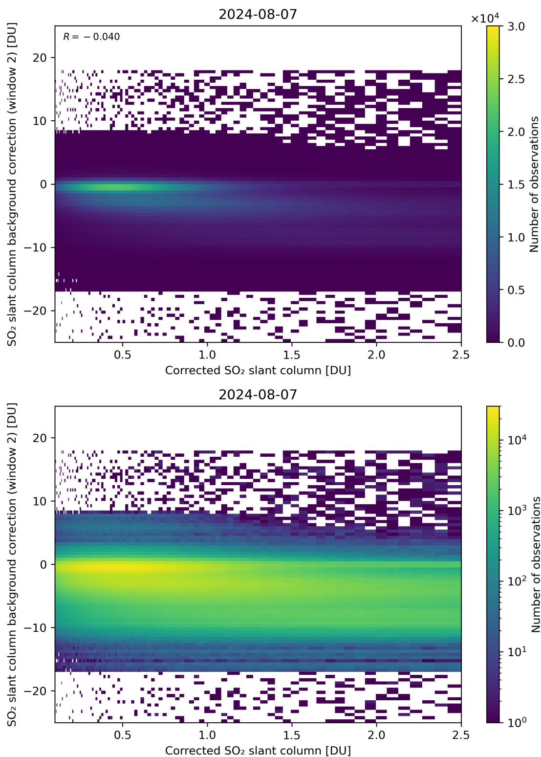
Figure 179: Scatter density plot of “Corrected SO 2 slant column” against “SO 2 slant column background correction (window 2)” for 2024-08-06 to 2024-08-08.
