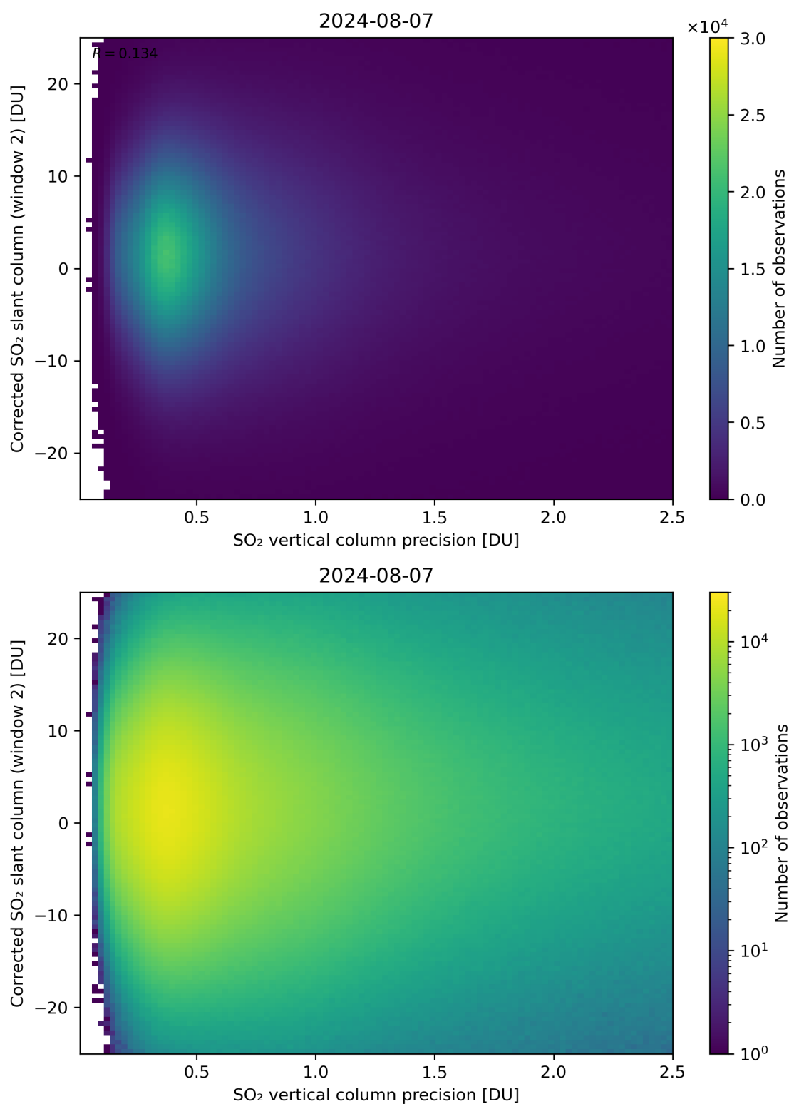
Figure 287: Scatter density plot of “SO 2 vertical column precision” against “Corrected SO 2 slant column (window 2)” for 2024-08-06 to 2024-08-08.
