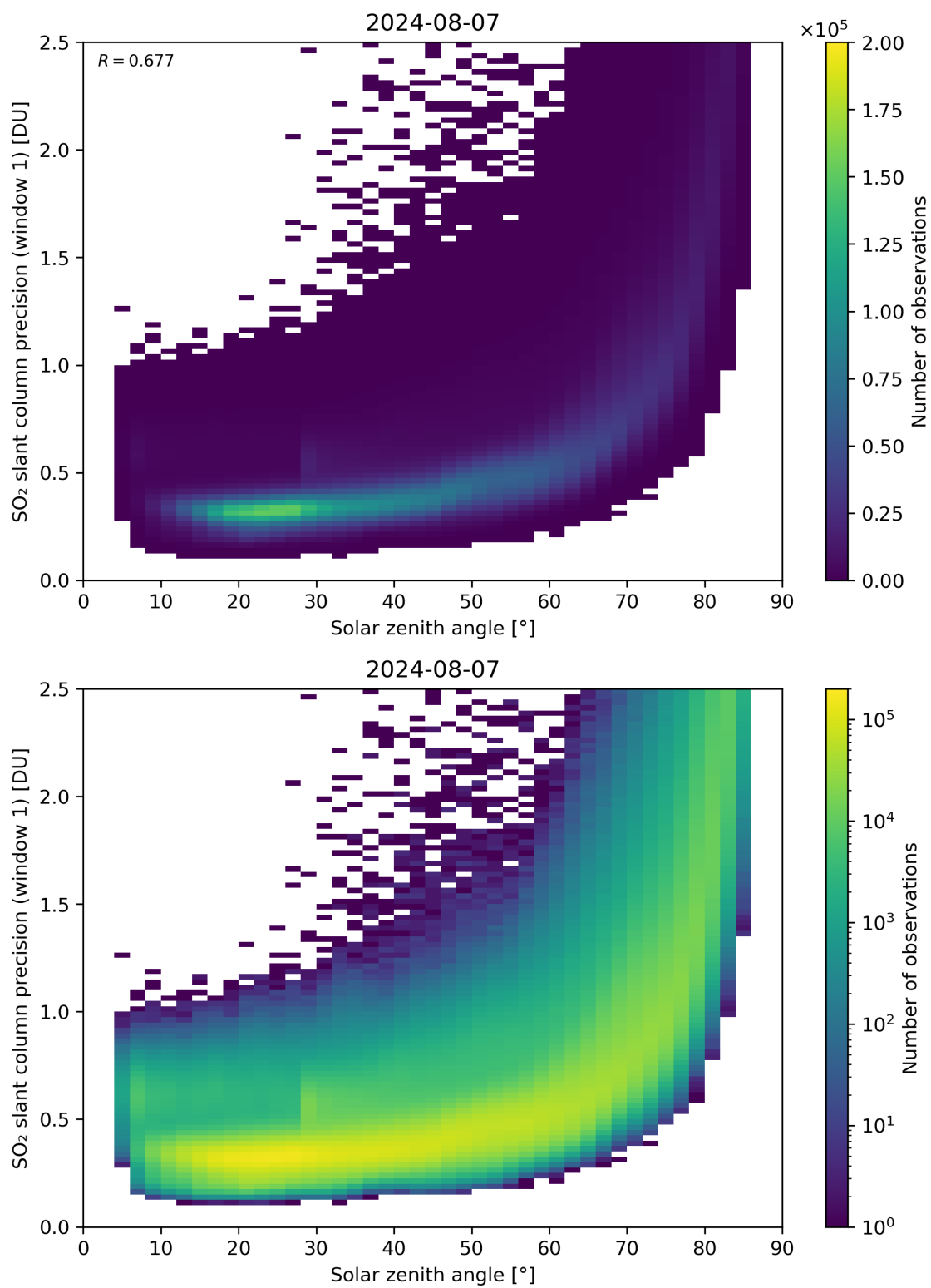
Figure 170: Scatter density plot of “Solar zenith angle” against “SO 2 slant column precision (window 1)” for 2024-08-06 to 2024-08-08.
