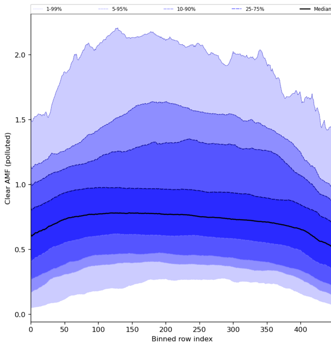
Figure 96: Along track statistics of “Clear AMF (polluted)” for 2024-08-06 to 2024-08-08
