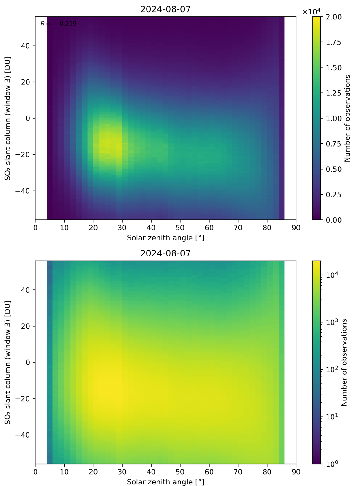
Figure 172: Scatter density plot of “Solar zenith angle” against “SO 2 slant column (window 3)” for 2024-08-06 to 2024-08-08.
