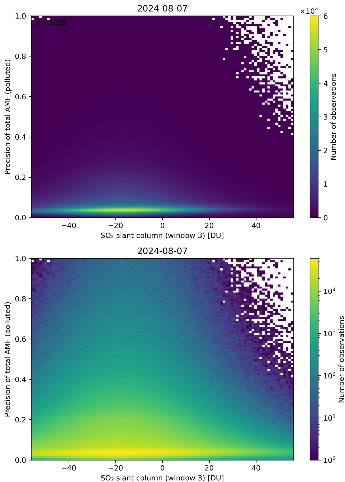
Figure 269: Scatter density plot of “SO 2 slant column (window 3)” against “Precision of total AMF (polluted)” for 2024-08-06 to 2024-08-08.
