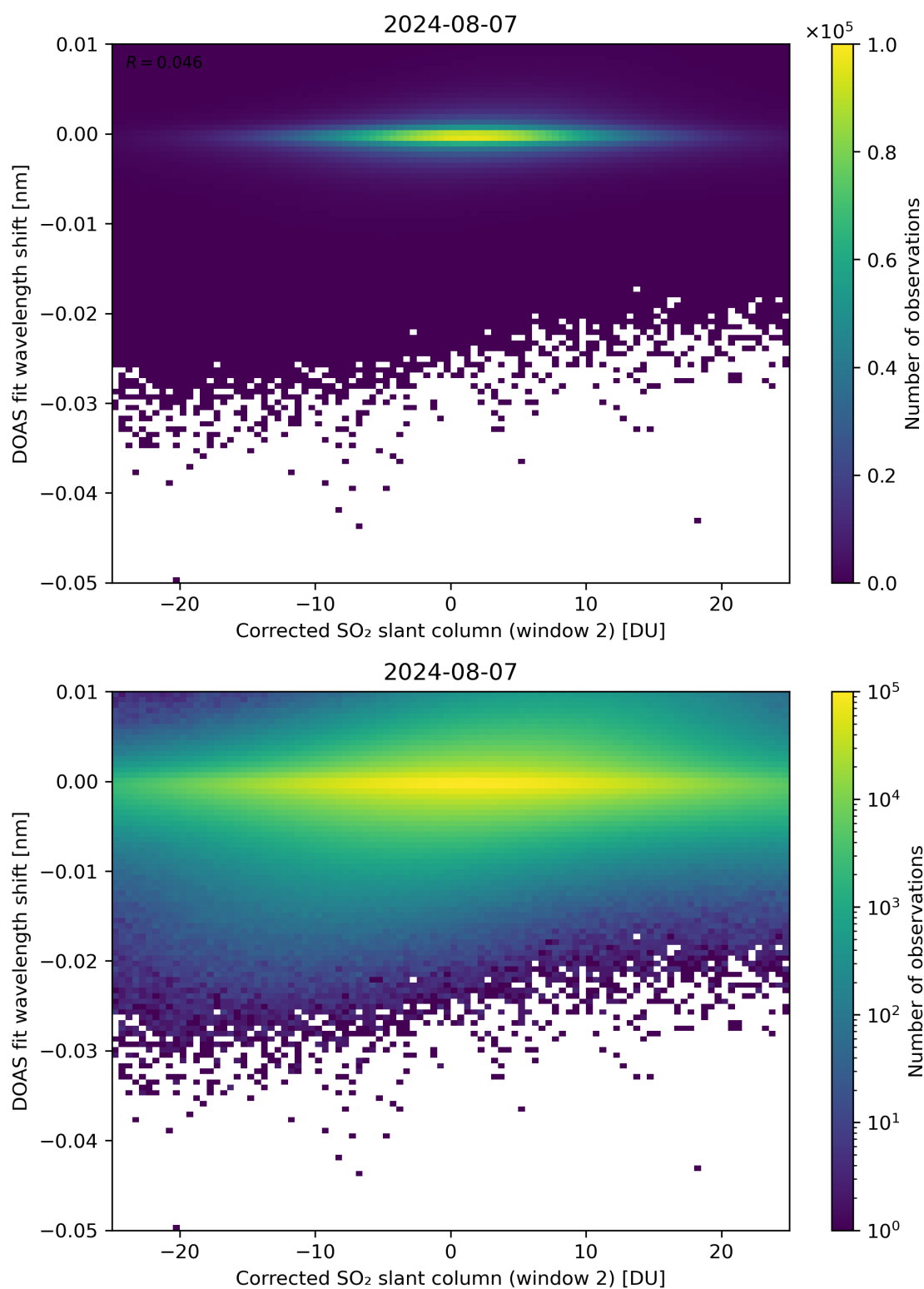
Figure 196: Scatter density plot of “Corrected SO 2 slant column (window 2)” against “DOAS fit wavelength shift” for 2024-08-06 to 2024-08-08.
