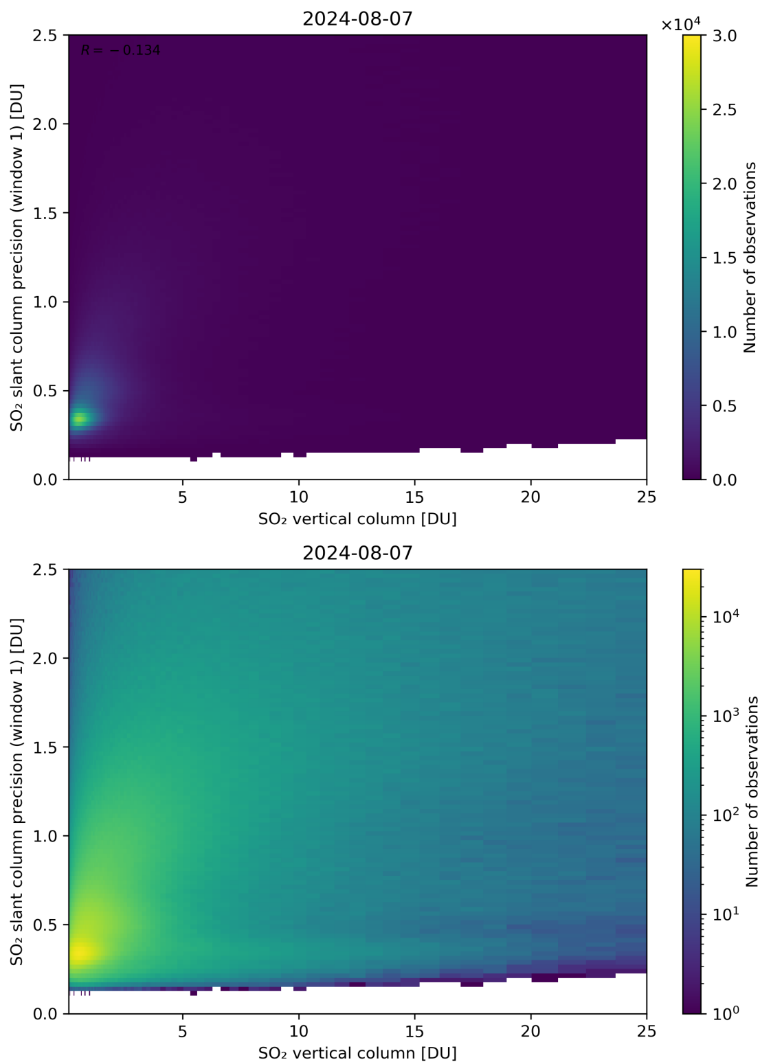
Figure 301: Scatter density plot of “SO 2 vertical column” against “SO 2 slant column precision (window 1)” for 2024-08-06 to 2024-08-08.
