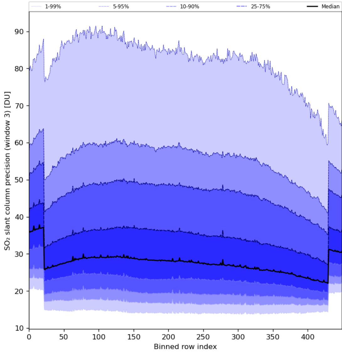
Figure 88: Along track statistics of “SO 2 slant column precision (window 3)” for 2024-08-06 to 2024-08-08
