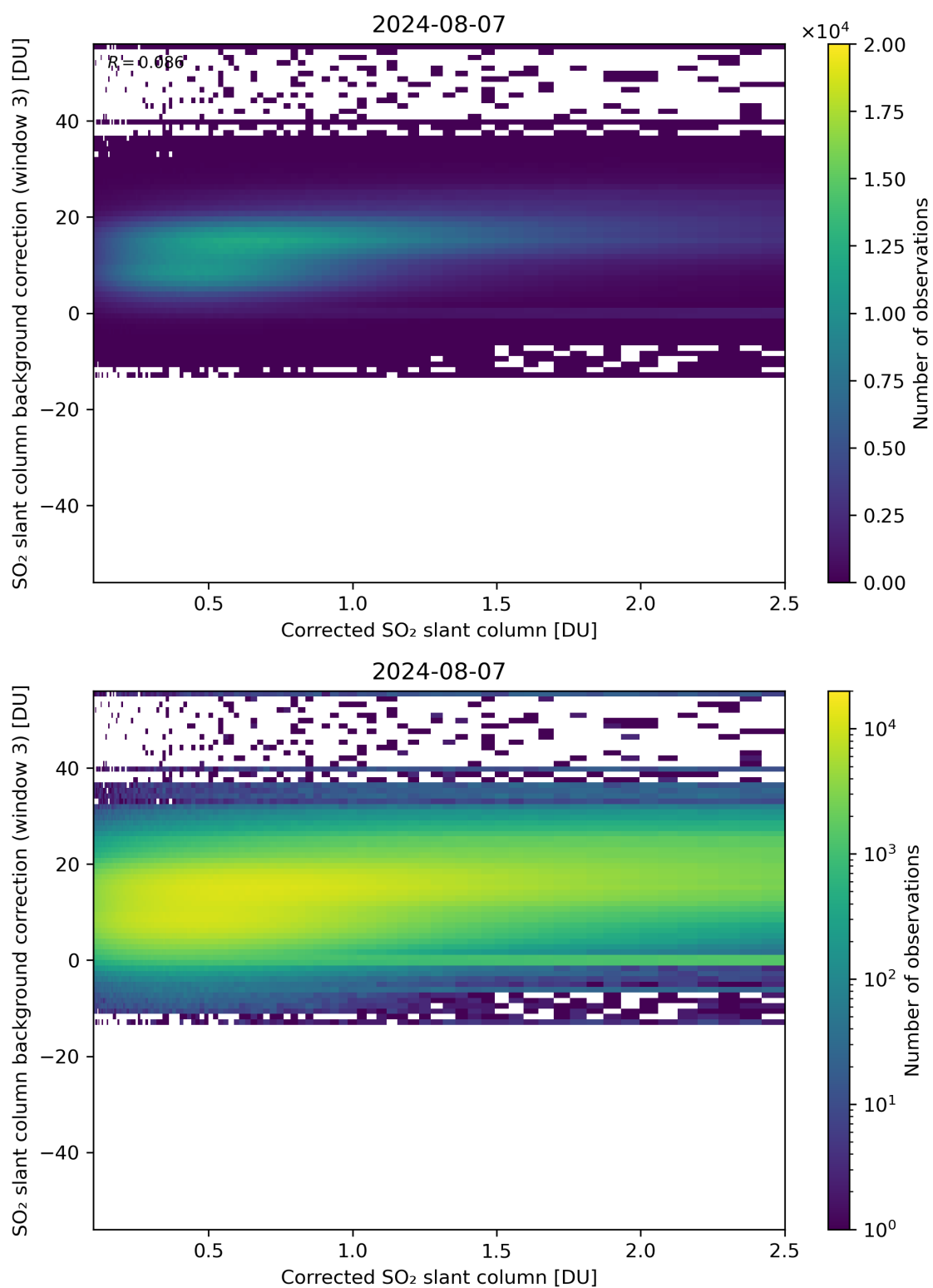
Figure 180: Scatter density plot of “Corrected SO 2 slant column” against “SO 2 slant column background correction (window 3)” for 2024-08-06 to 2024-08-08.
