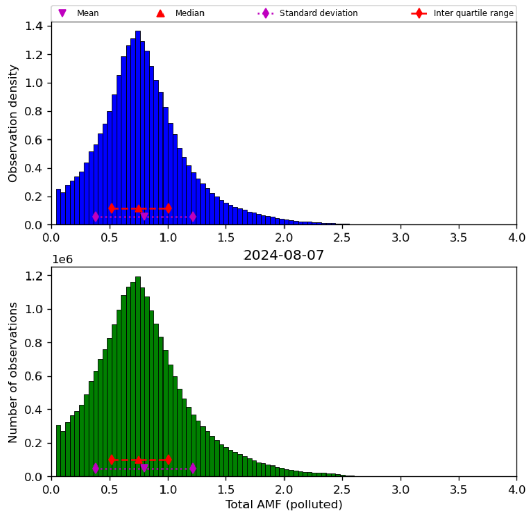
Figure 71: Histogram of “Total AMF (polluted)” for 2024-08-06 to 2024-08-08
