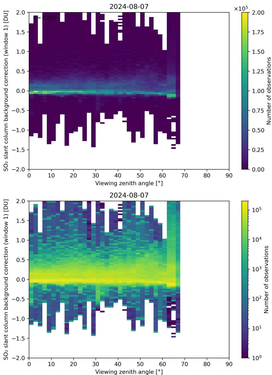
Figure 308: Scatter density plot of “Viewing zenith angle” against “SO 2 slant column background correction (window 1)” for 2024-08-06 to 2024-08-08.
