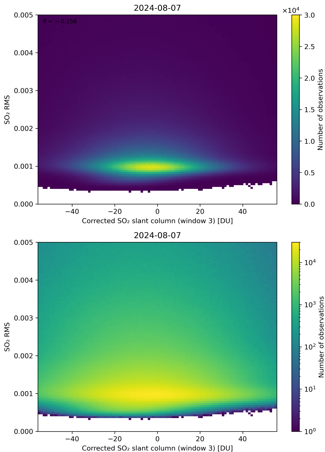
Figure 208: Scatter density plot of “Corrected SO 2 slant column (window 3)” against “SO 2 RMS” for 2024-08-06 to 2024-08-08.
