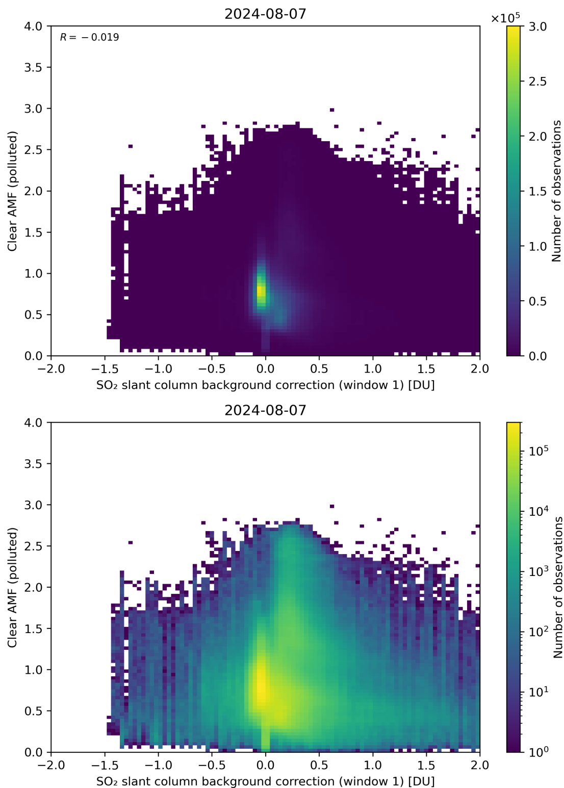
Figure 103: Scatter density plot of “SO 2 slant column background correction (window 1)” against “Clear AMF (polluted)” for 2024-08-06 to 2024-08-08.
