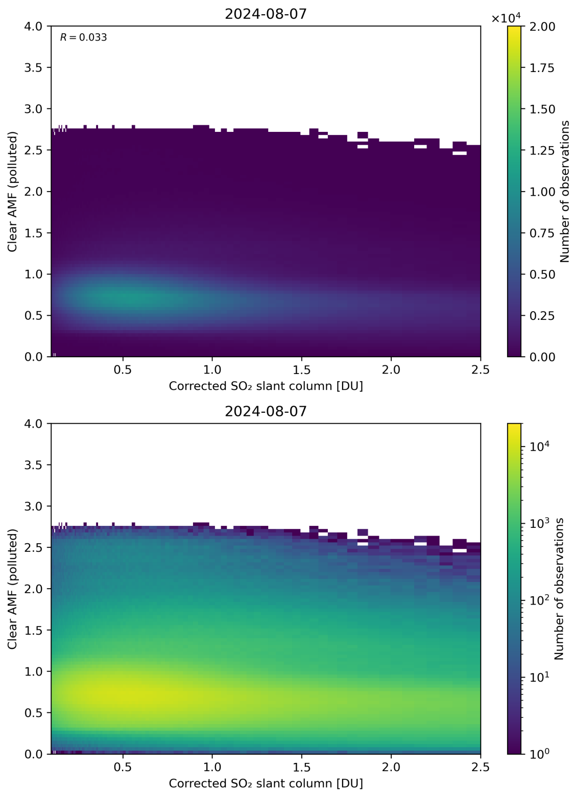
Figure 184: Scatter density plot of “Corrected SO 2 slant column” against “Clear AMF (polluted)” for 2024-08-06 to 2024-08-08.
