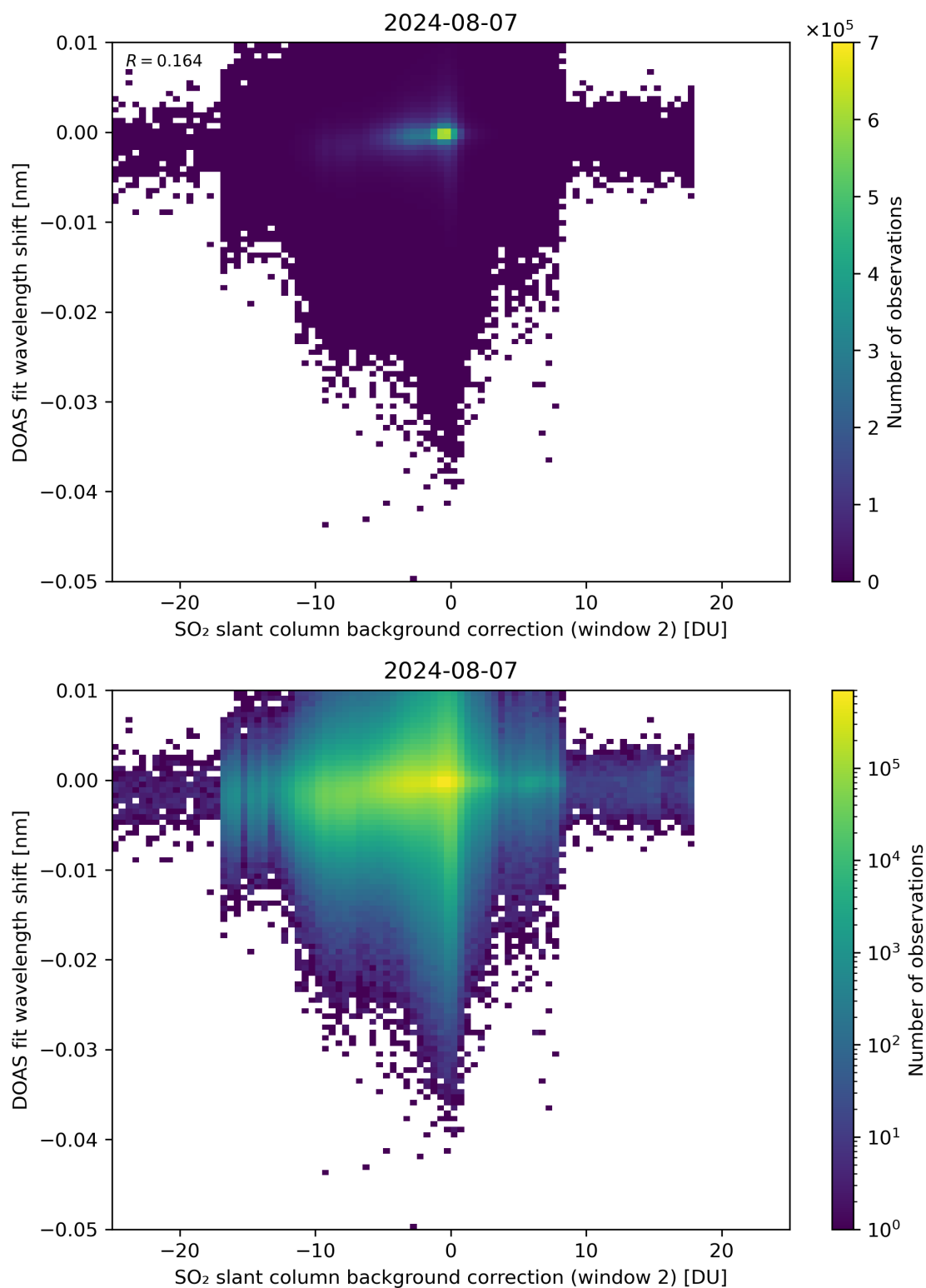
Figure 112: Scatter density plot of “SO 2 slant column background correction (window 2)” against “DOAS fit wavelength shift” for 2024-08-06 to 2024-08-08.
