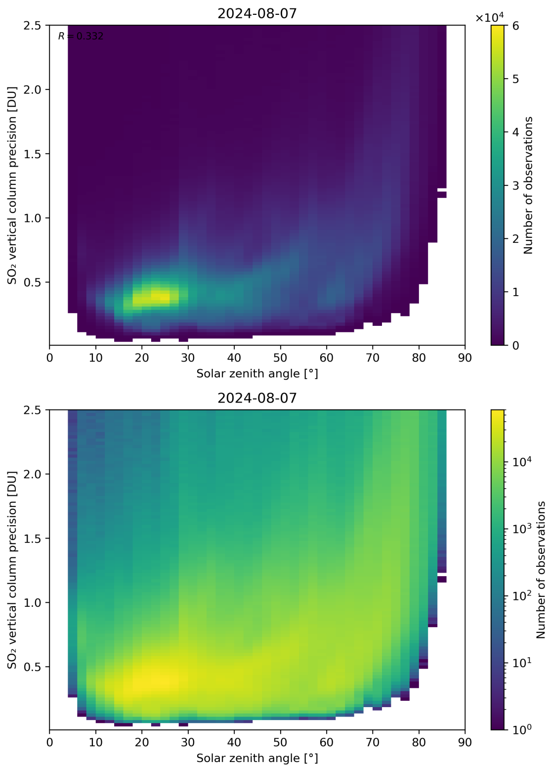
Figure 177: Scatter density plot of “Solar zenith angle” against “SO 2 vertical column precision” for 2024-08-06 to 2024-08-08.
