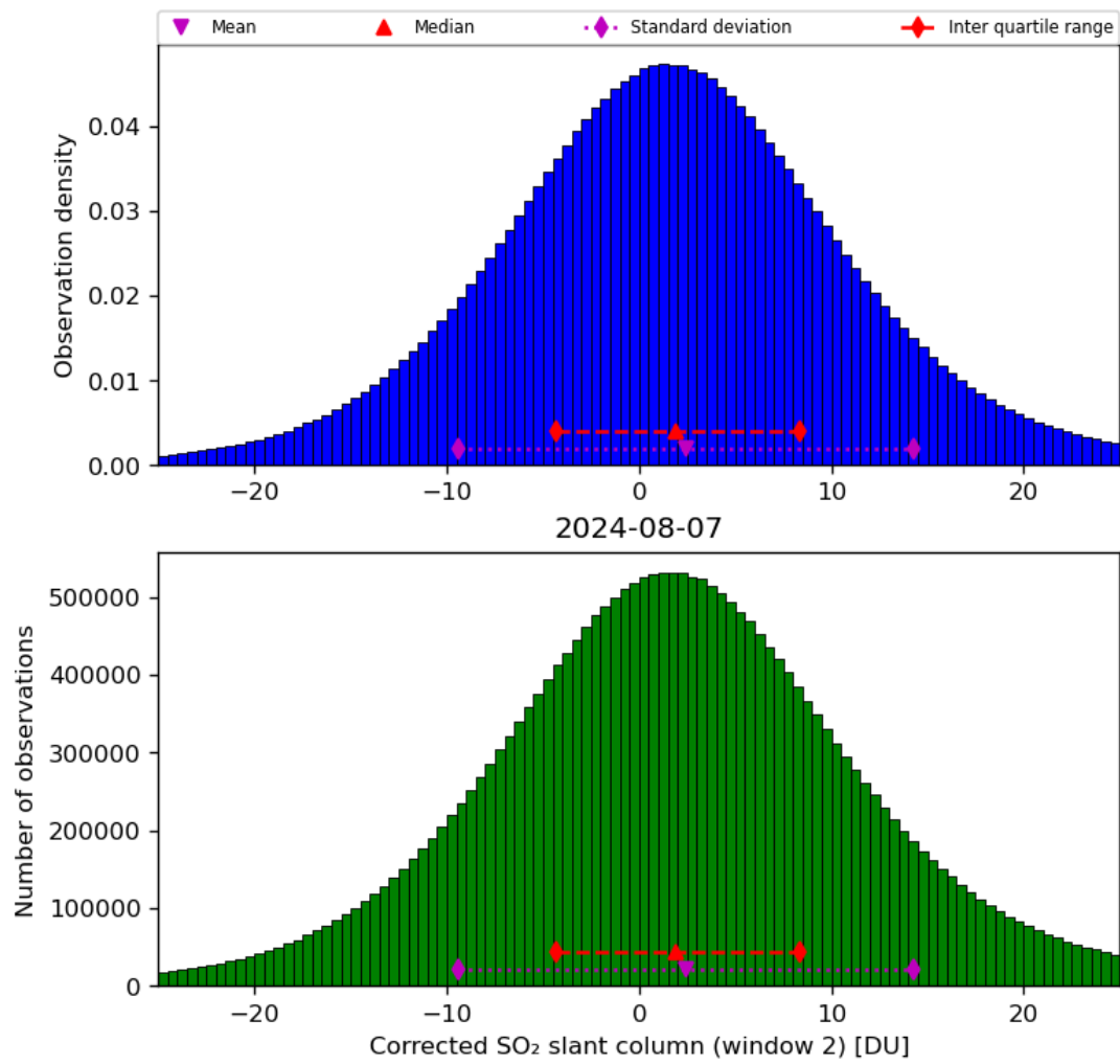
Figure 62: Histogram of “Corrected SO 2 slant column (window 2)” for 2024-08-06 to 2024-08-08
