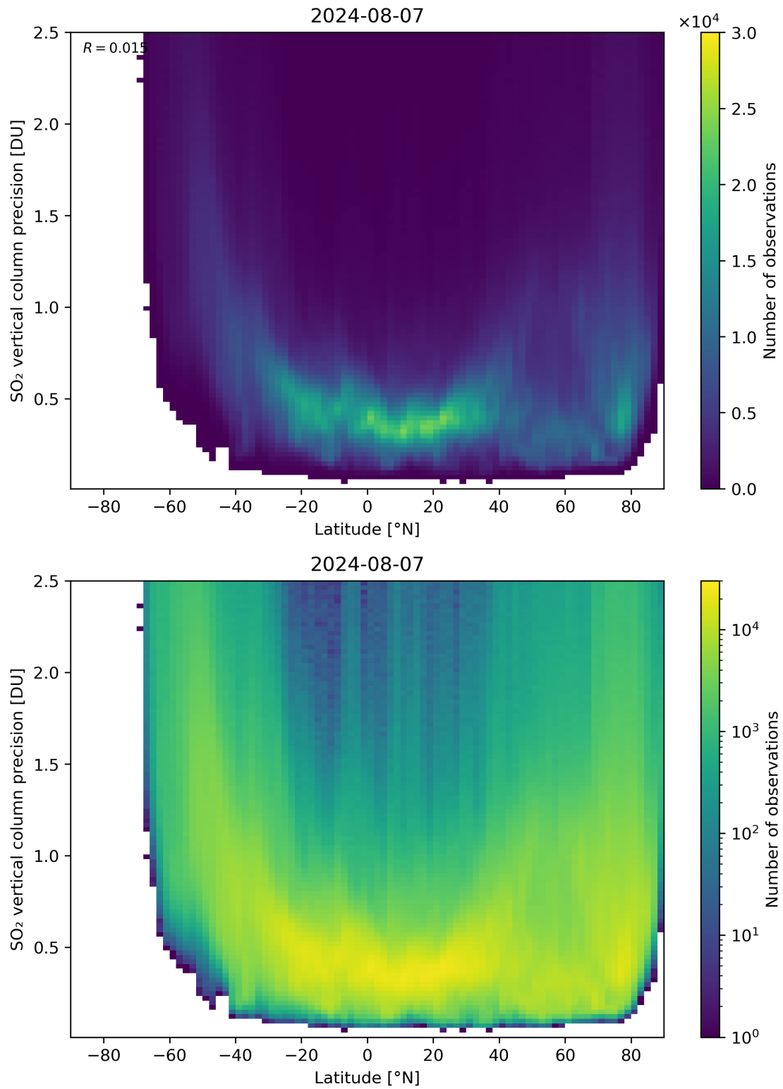
Figure 157: Scatter density plot of “Latitude” against “SO 2 vertical column precision” for 2024-08-06 to 2024-08-08.
