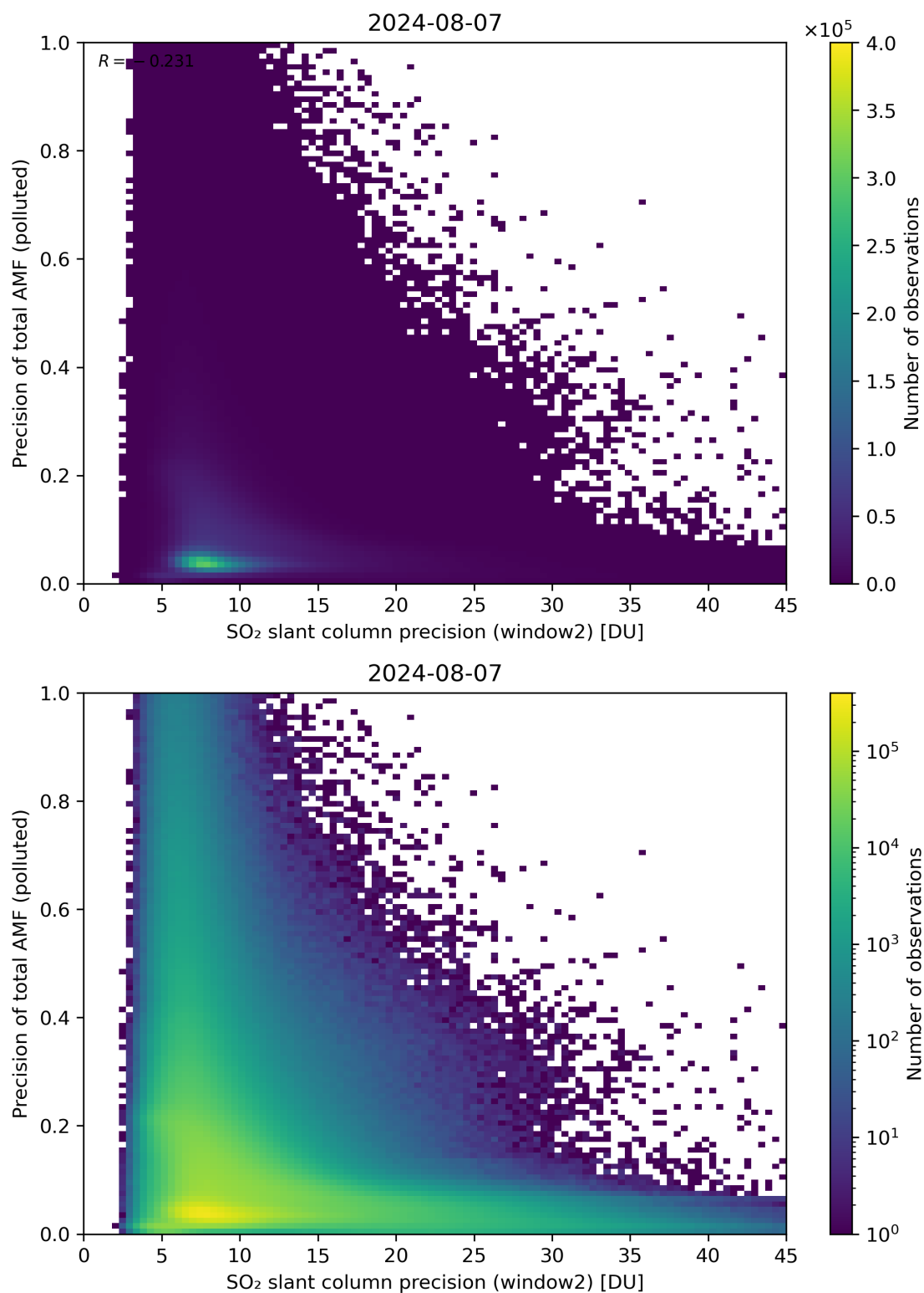
Figure 252: Scatter density plot of “SO 2 slant column precision (window2)” against “Precision of total AMF (polluted)” for 2024-08-06 to 2024-08-08.
