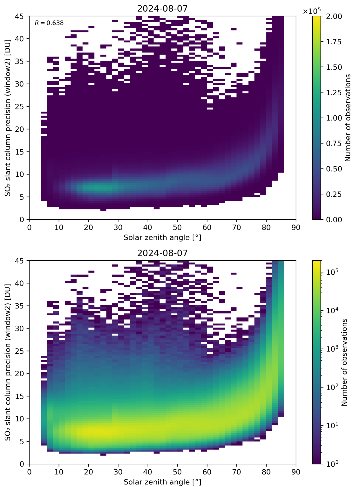
Figure 171: Scatter density plot of “Solar zenith angle” against “SO 2 slant column precision (window2)” for 2024-08-06 to 2024-08-08.
