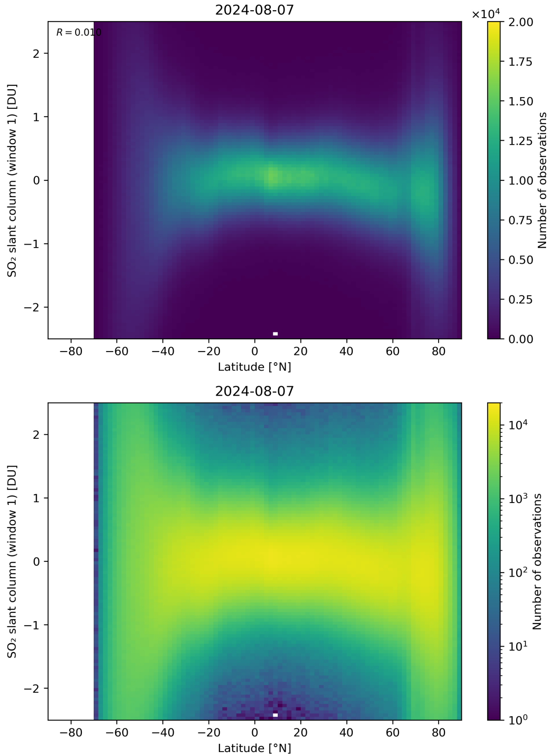
Figure 149: Scatter density plot of “Latitude” against “SO 2 slant column (window 1)” for 2024-08-06 to 2024-08-08.
