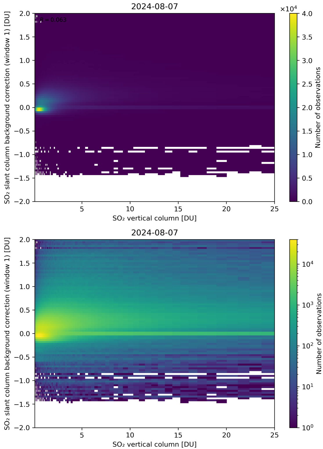
Figure 273: Scatter density plot of “SO 2 vertical column” against “SO 2 slant column background correction (window 1)” for 2024-08-06 to 2024-08-08.
