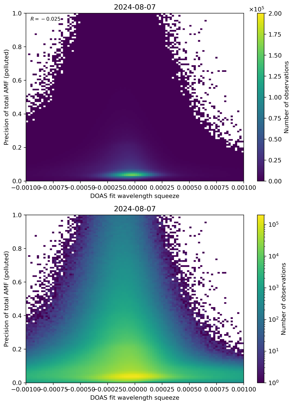
Figure 135: Scatter density plot of “DOAS fit wavelength squeeze” against “Precision of total AMF (polluted)” for 2024-08-06 to 2024-08-08.
