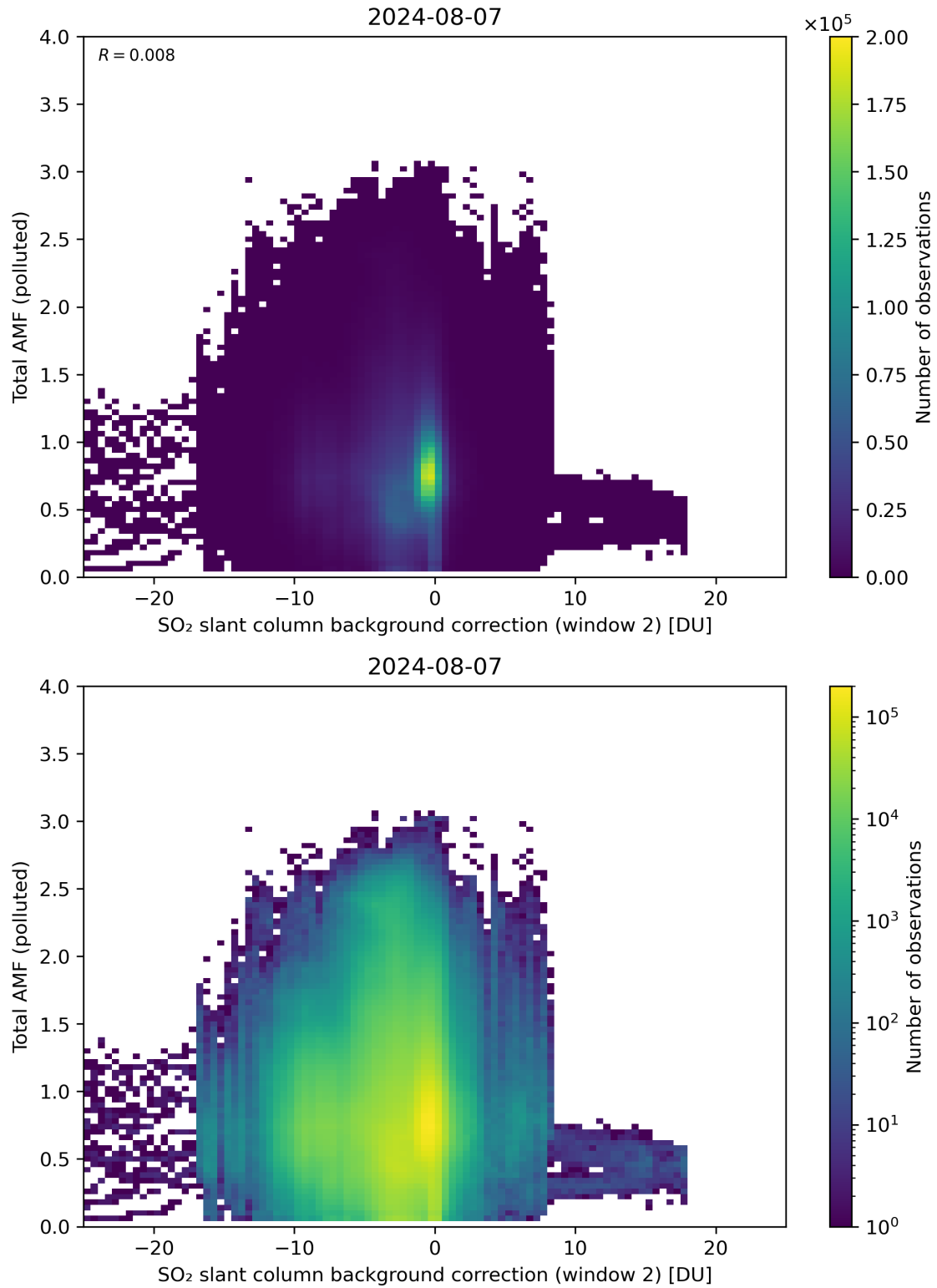
Figure 119: Scatter density plot of “SO 2 slant column background correction (window 2)” against “Total AMF (polluted)” for 2024-08-06 to 2024-08-08.
