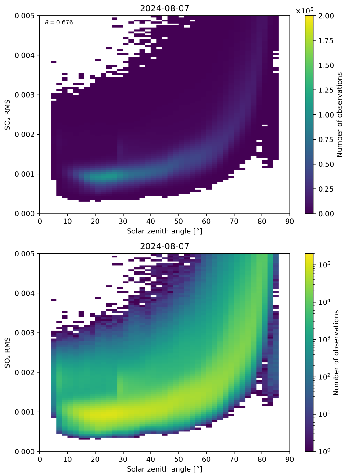
Figure 163: Scatter density plot of “Solar zenith angle” against “SO 2 RMS” for 2024-08-06 to 2024-08-08.
