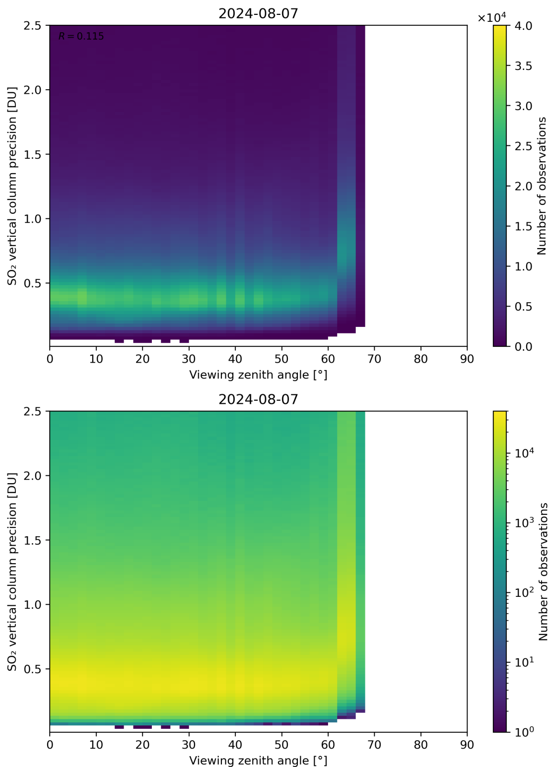
Figure 328: Scatter density plot of “Viewing zenith angle” against “SO 2 vertical column precision” for 2024-08-06 to 2024-08-08.
