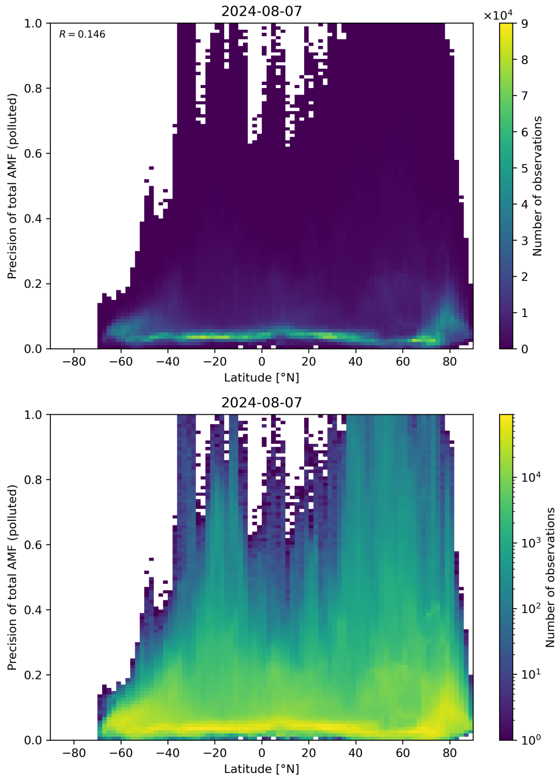
Figure 155: Scatter density plot of “Latitude” against “Precision of total AMF (polluted)” for 2024-08-06 to 2024-08-08.
