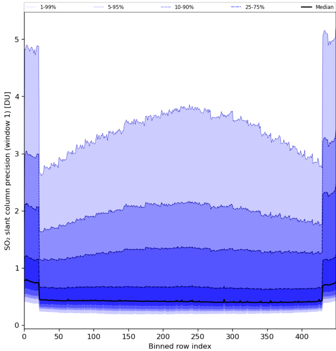
Figure 80: Along track statistics of “SO 2 slant column precision (window 1)” for 2024-08-06 to 2024-08-08
