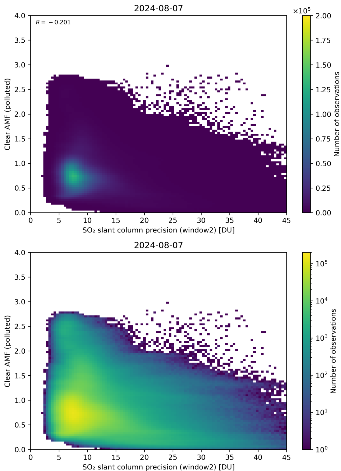
Figure 246: Scatter density plot of “SO 2 slant column precision (window2)” against “Clear AMF (polluted)” for 2024-08-06 to 2024-08-08.
