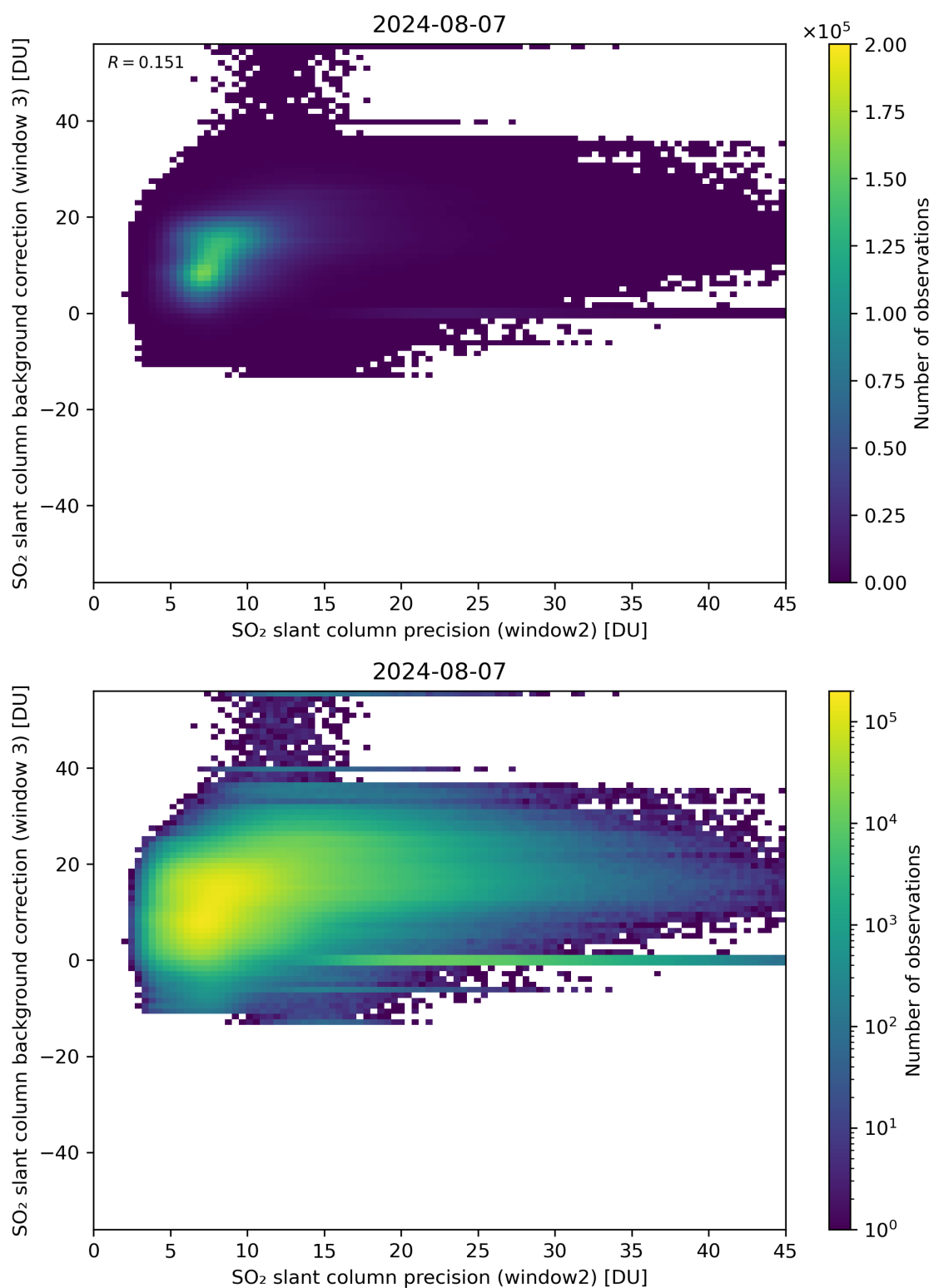
Figure 242: Scatter density plot of “SO 2 slant column precision (window2)” against “SO 2 slant column background correction (window 3)” for 2024-08-06 to 2024-08-08.
