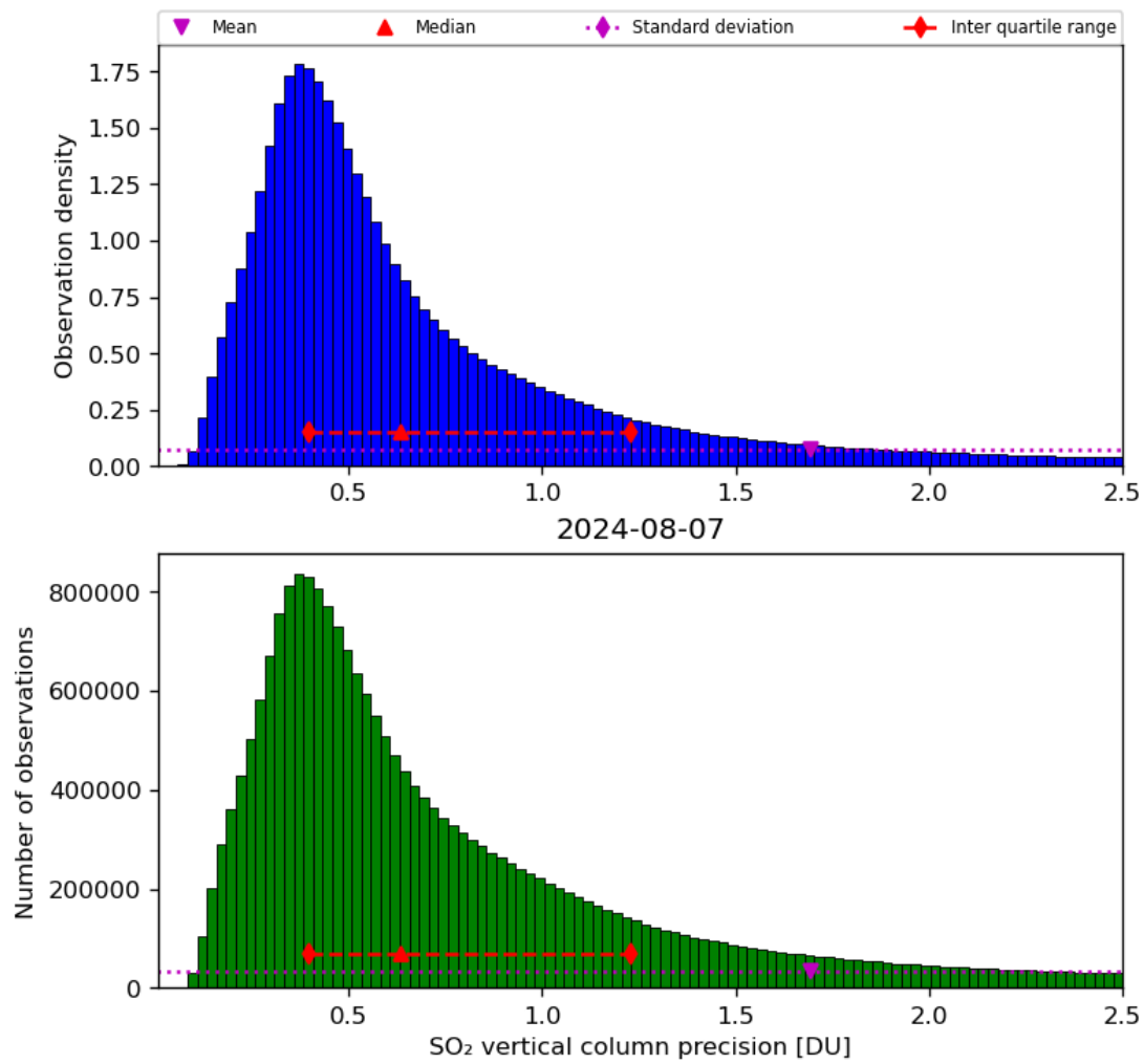
Figure 54: Histogram of “SO 2 vertical column precision” for 2024-08-06 to 2024-08-08
