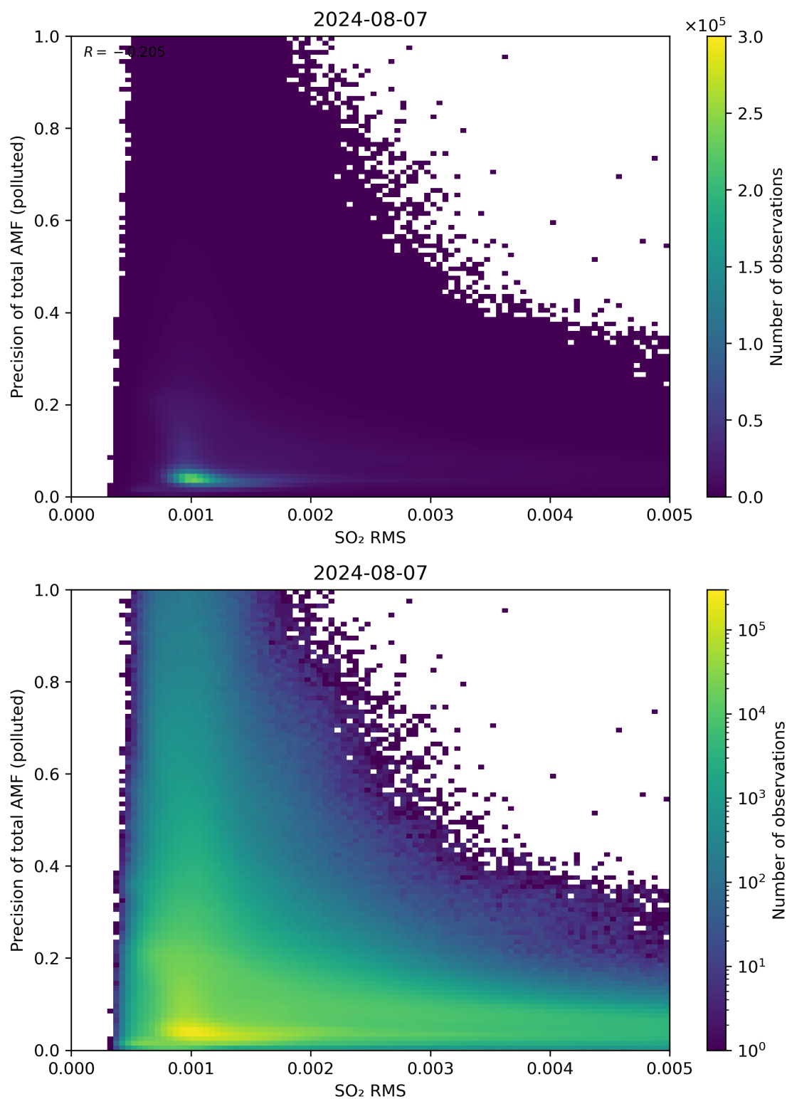
Figure 138: Scatter density plot of “SO 2 RMS” against “Precision of total AMF (polluted)” for 2024-08-06 to 2024-08-08.
