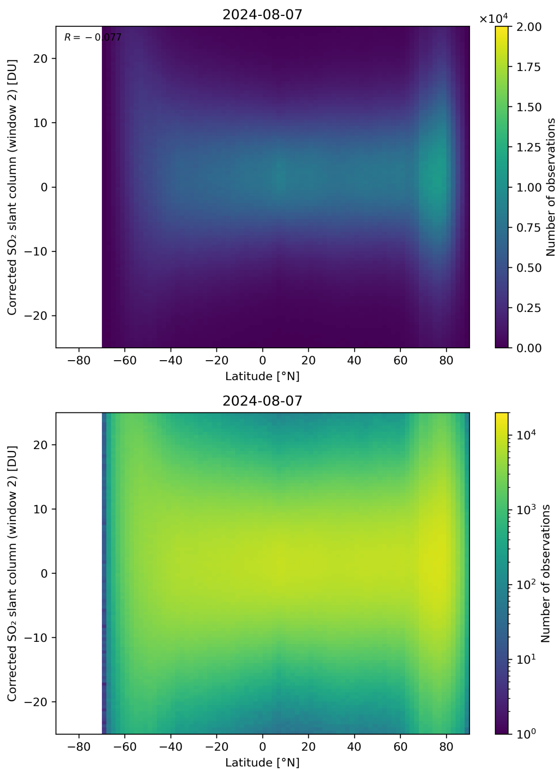
Figure 147: Scatter density plot of “Latitude” against “Corrected SO 2 slant column (window 2)” for 2024-08-06 to 2024-08-08.
