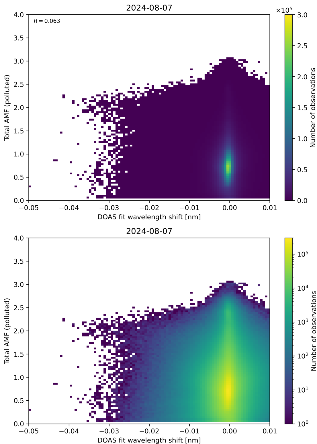
Figure 130: Scatter density plot of “DOAS fit wavelength shift” against “Total AMF (polluted)” for 2024-08-06 to 2024-08-08.
