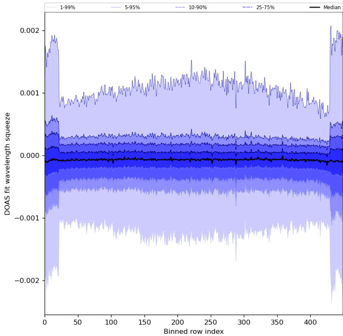
Figure 92: Along track statistics of “DOAS fit wavelength squeeze” for 2024-08-06 to 2024-08-08
