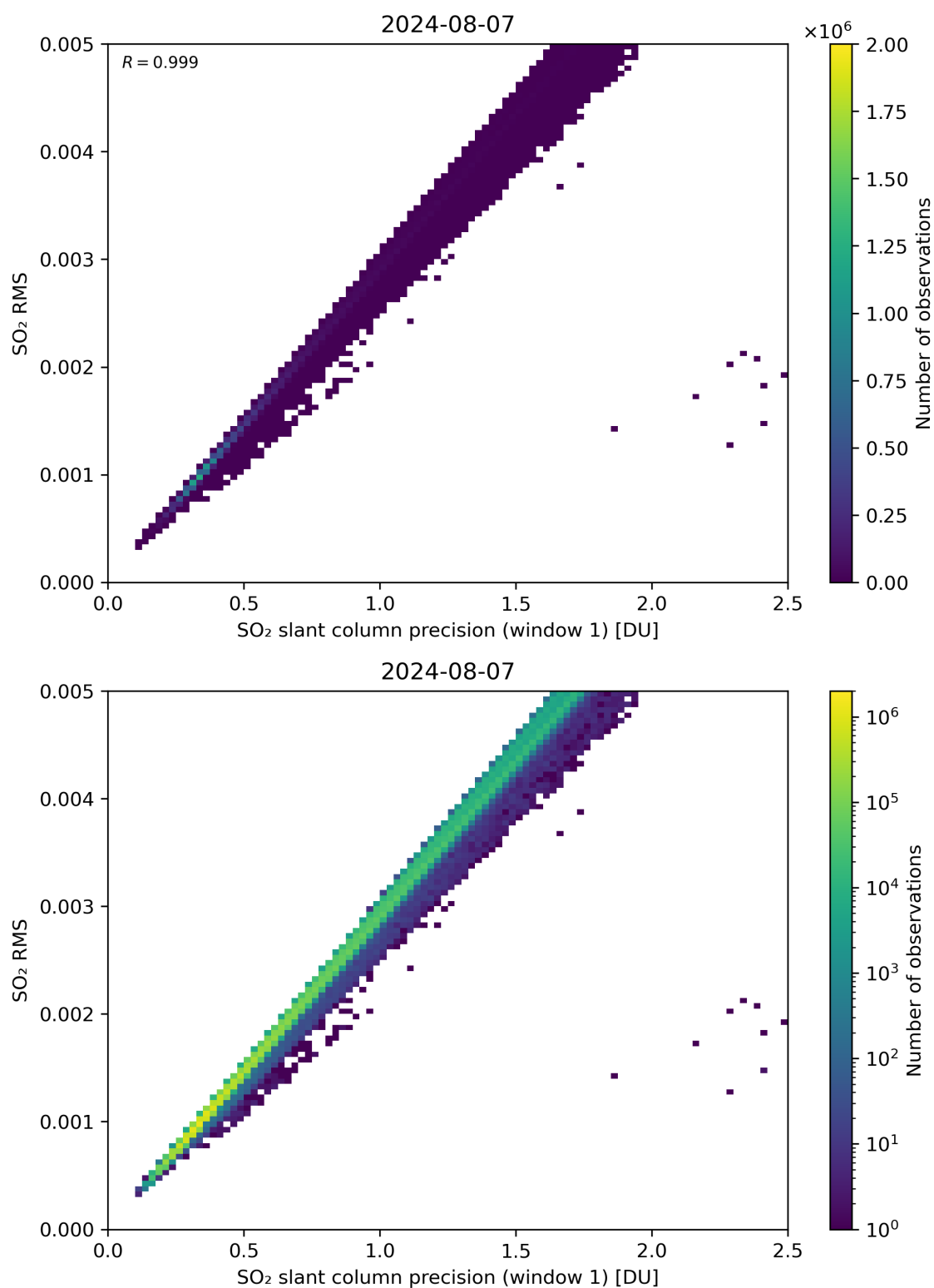
Figure 223: Scatter density plot of “SO 2 slant column precision (window 1)” against “SO 2 RMS” for 2024-08-06 to 2024-08-08.
