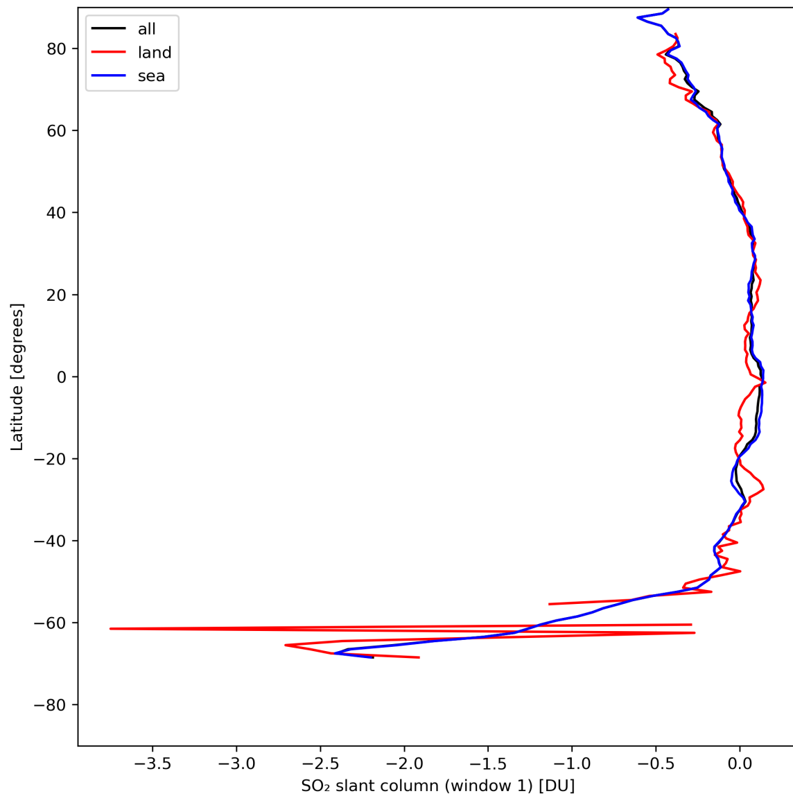
Figure 33: Zonal average of “SO 2 slant column (window 1)” for 2024-08-06 to 2024-08-08.
