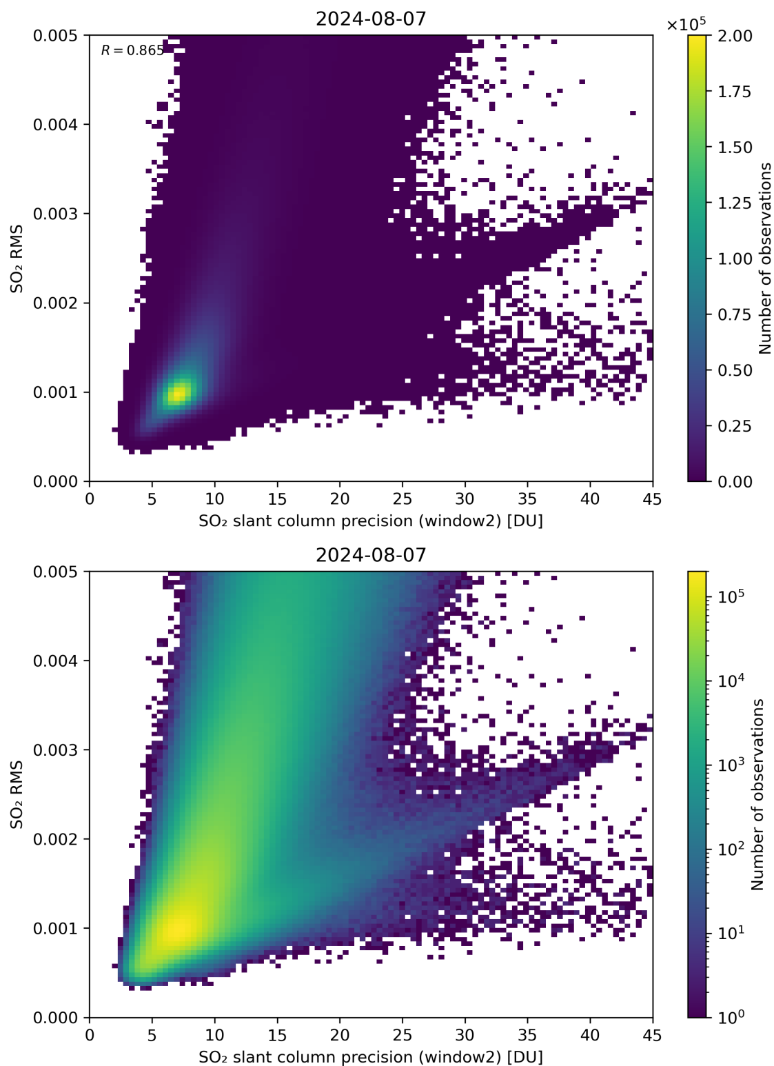
Figure 245: Scatter density plot of “SO 2 slant column precision (window2)” against “SO 2 RMS” for 2024-08-06 to 2024-08-08.
