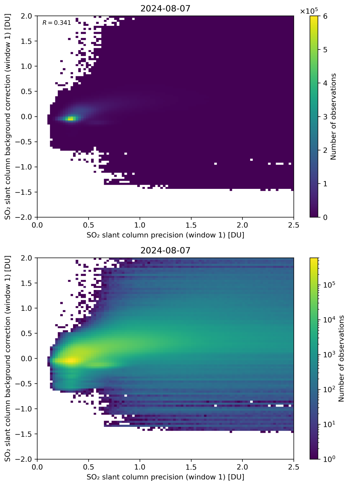
Figure 218: Scatter density plot of “SO 2 slant column precision (window 1)” against “SO 2 slant column background correction (window 1)” for 2024-08-06 to 2024-08-08.
