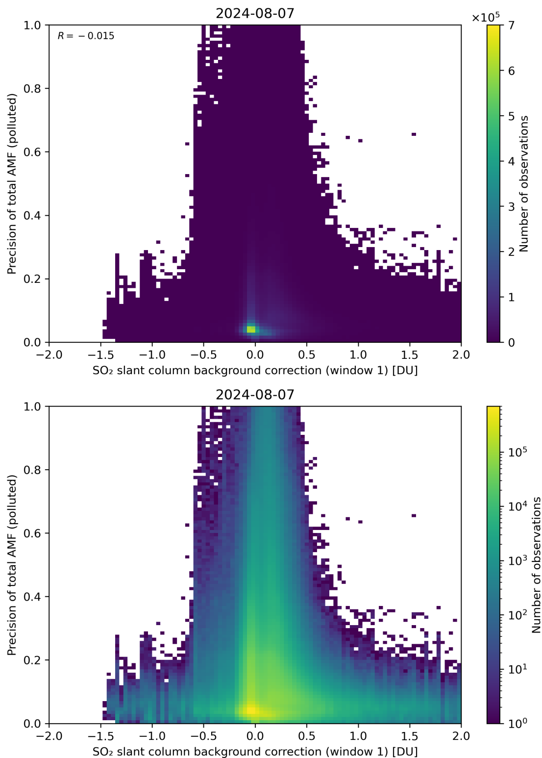
Figure 110: Scatter density plot of “SO 2 slant column background correction (window 1)” against “Precision of total AMF (polluted)” for 2024-08-06 to 2024-08-08.
