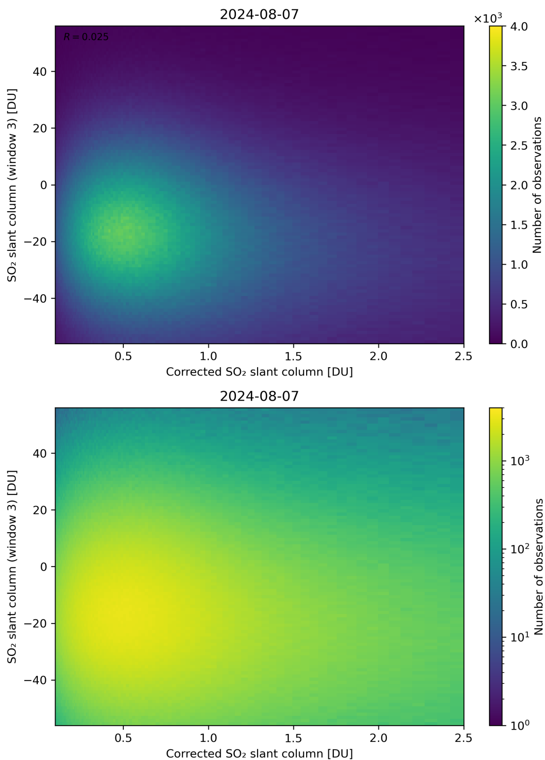
Figure 190: Scatter density plot of “Corrected SO 2 slant column” against “SO 2 slant column (window 3)” for 2024-08-06 to 2024-08-08.
