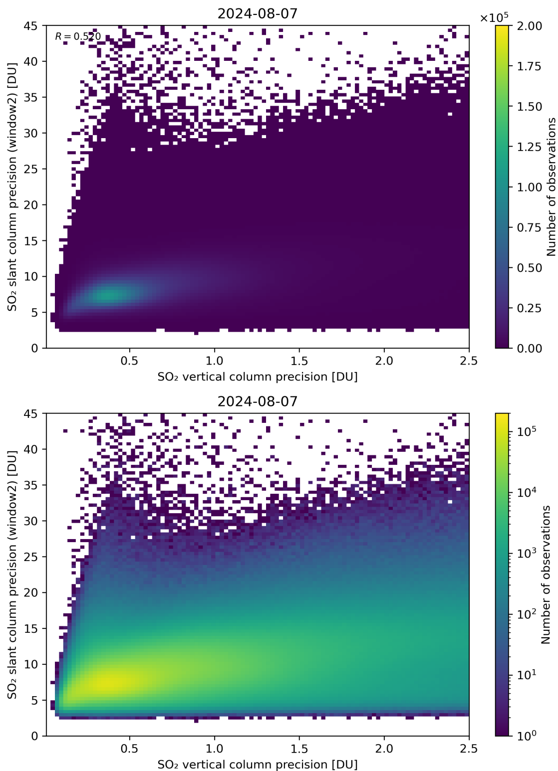
Figure 291: Scatter density plot of “SO 2 vertical column precision” against “SO 2 slant column precision (window2)” for 2024-08-06 to 2024-08-08.
