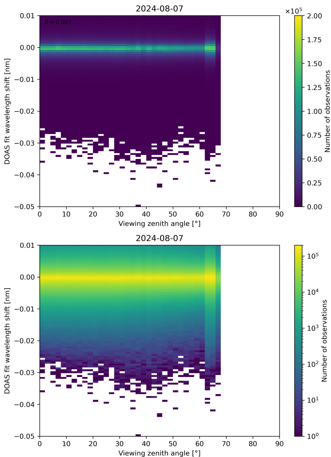
Figure 311: Scatter density plot of “Viewing zenith angle” against “DOAS fit wavelength shift” for 2024-08-06 to 2024-08-08.
