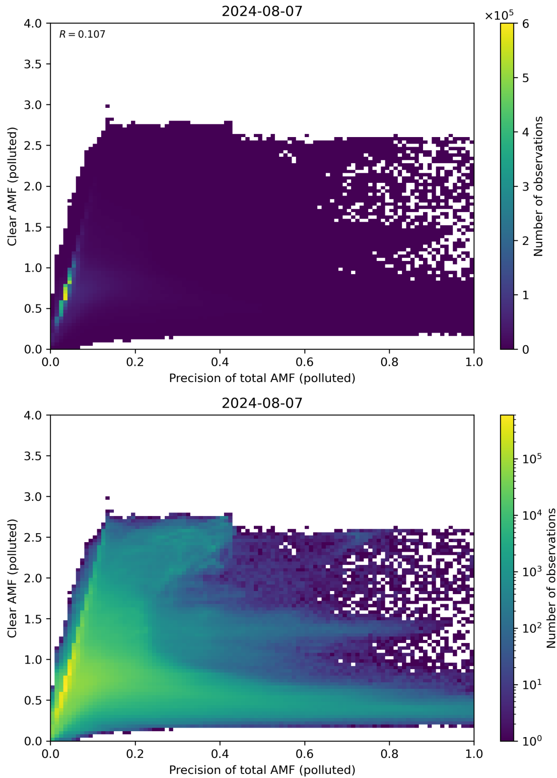
Figure 270: Scatter density plot of “Precision of total AMF (polluted)” against “Clear AMF (polluted)” for 2024-08-06 to 2024-08-08.
