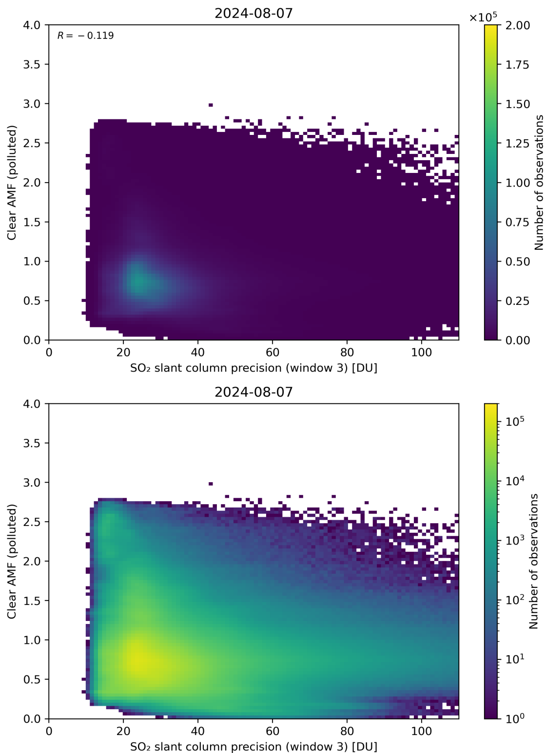
Figure 261: Scatter density plot of “SO 2 slant column precision (window 3)” against “Clear AMF (polluted)” for 2024-08-06 to 2024-08-08.
