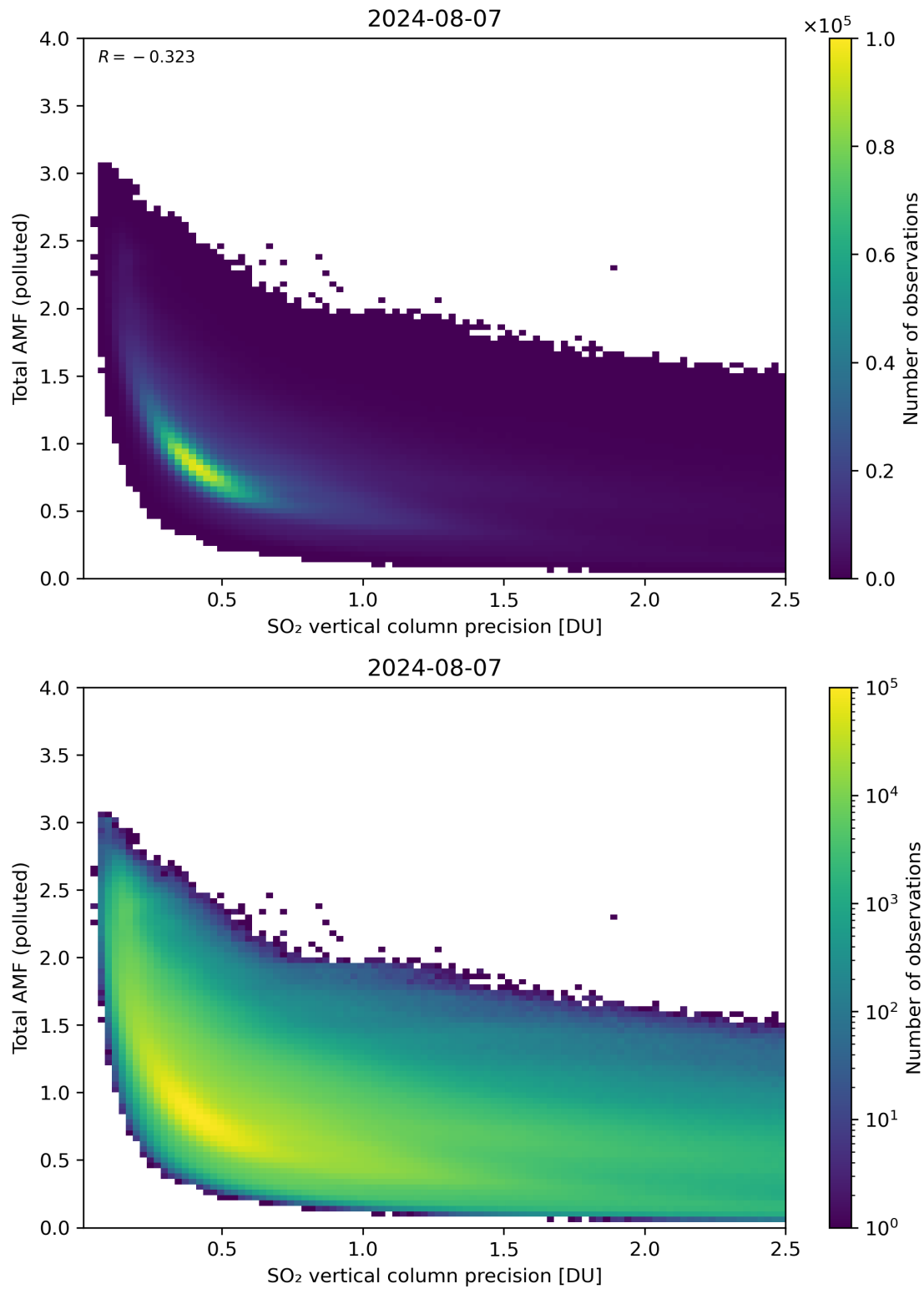
Figure 294: Scatter density plot of “SO 2 vertical column precision” against “Total AMF (polluted)” for 2024-08-06 to 2024-08-08.
