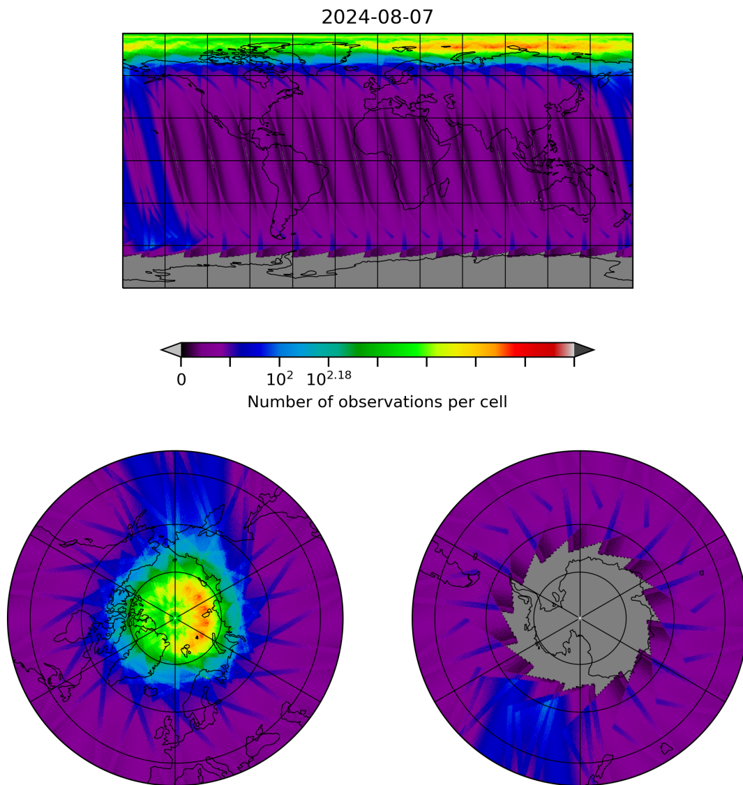
Figure 28: Map of the number of observations for 2024-08-06 to 2024-08-08
