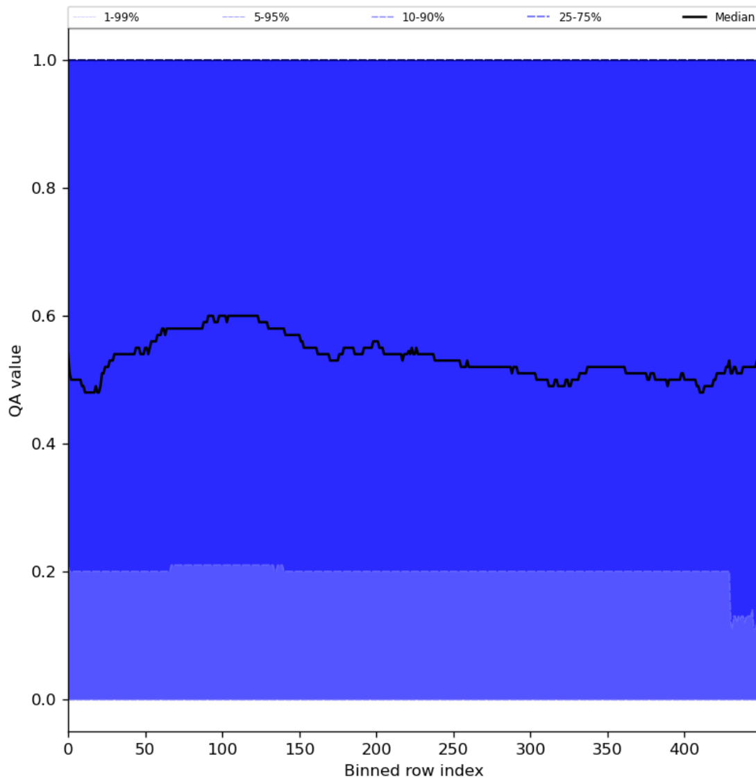
Figure 75: Along track statistics of “QA value” for 2024-08-06 to 2024-08-08
