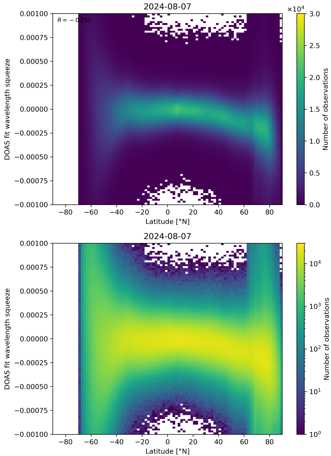
Figure 143: Scatter density plot of “Latitude” against “DOAS fit wavelength squeeze” for 2024-08-06 to 2024-08-08.
