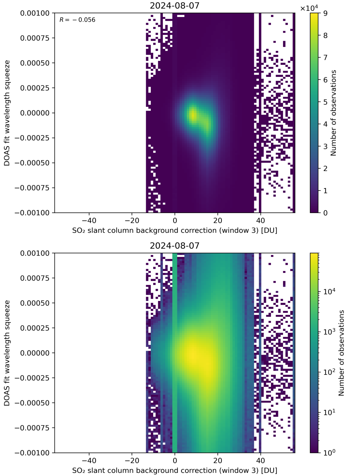
Figure 122: Scatter density plot of “SO 2 slant column background correction (window 3)” against “DOAS fit wavelength squeeze” for 2024-08-06 to 2024-08-08.
