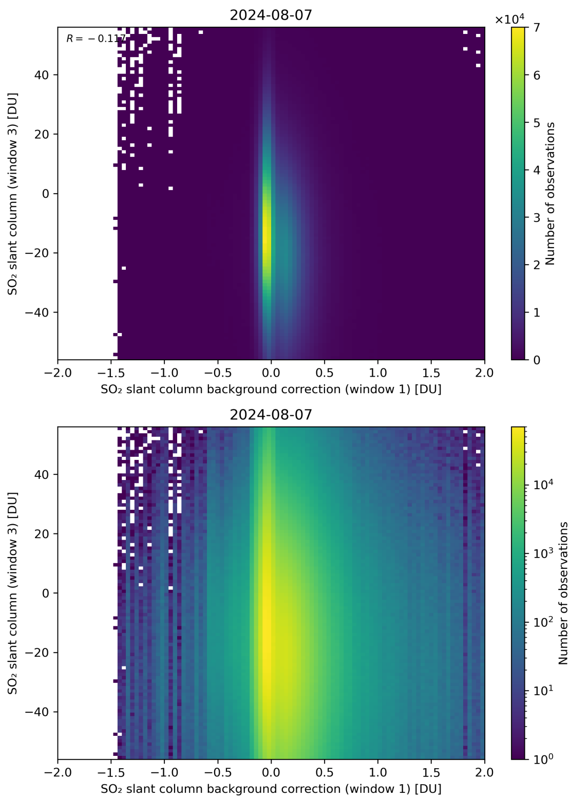
Figure 107: Scatter density plot of “SO 2 slant column background correction (window 1)” against “SO 2 slant column (window 3)” for 2024-08-06 to 2024-08-08.
