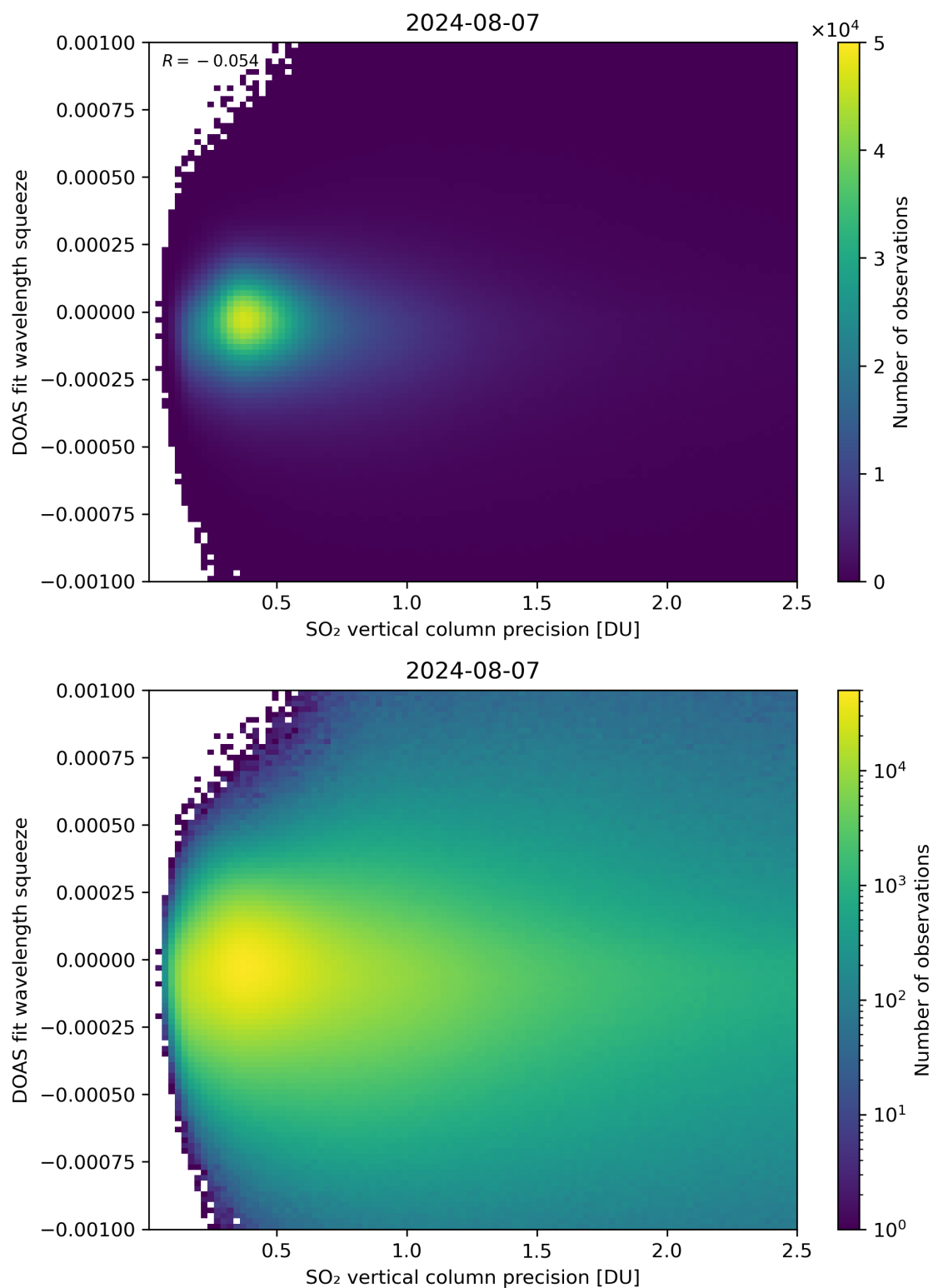
Figure 283: Scatter density plot of “SO 2 vertical column precision” against “DOAS fit wavelength squeeze” for 2024-08-06 to 2024-08-08.
