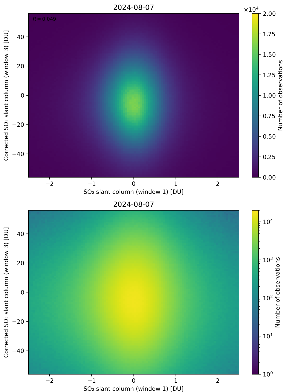
Figure 234: Scatter density plot of “SO 2 slant column (window 1)” against “Corrected SO 2 slant column (window 3)” for 2024-08-06 to 2024-08-08.
