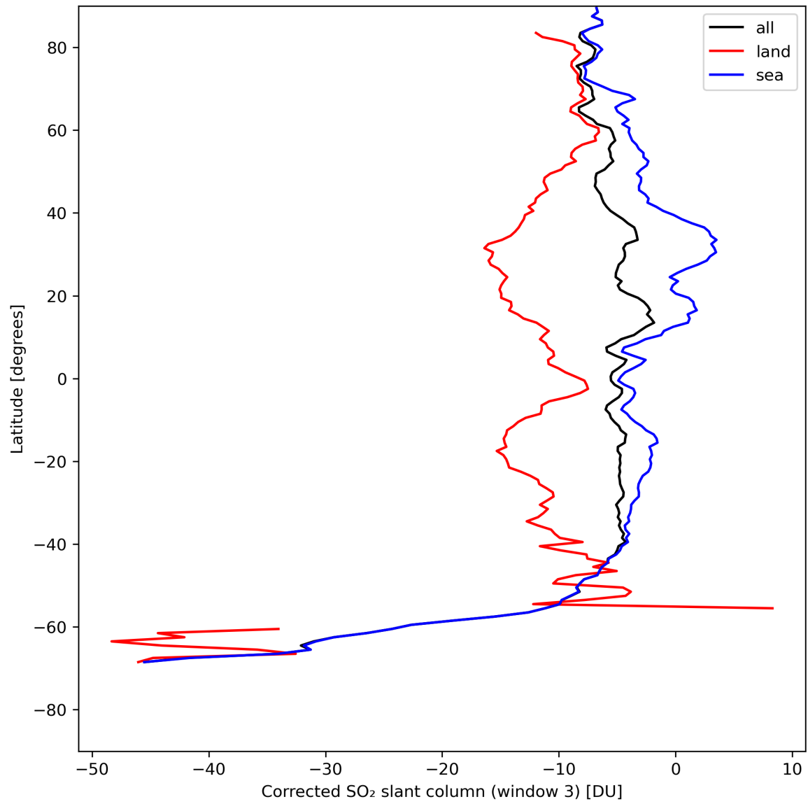
Figure 43: Zonal average of “Corrected SO 2 slant column (window 3)” for 2024-08-06 to 2024-08-08.
