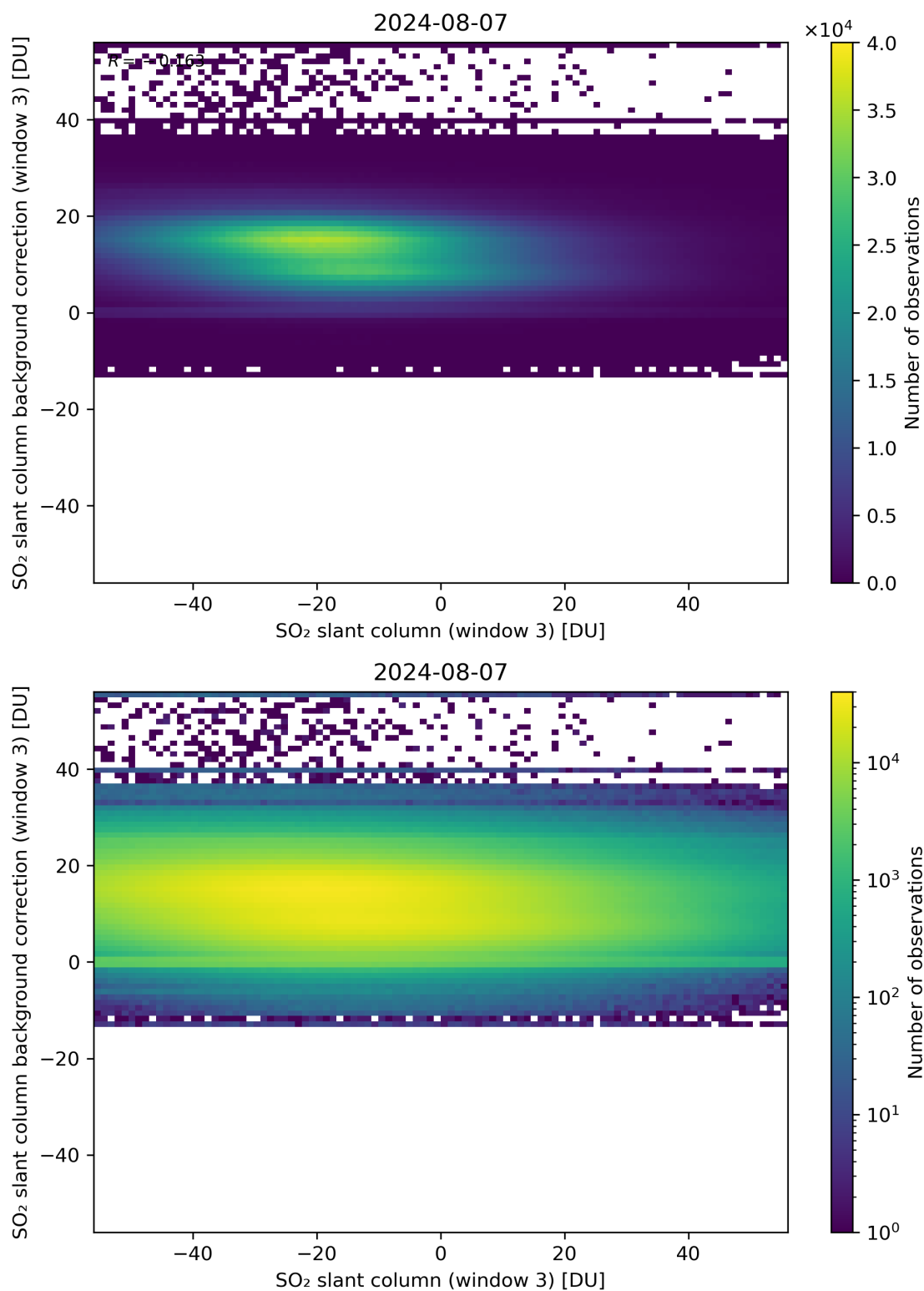
Figure 253: Scatter density plot of “SO 2 slant column (window 3)” against “SO 2 slant column background correction (window 3)” for 2024-08-06 to 2024-08-08.
