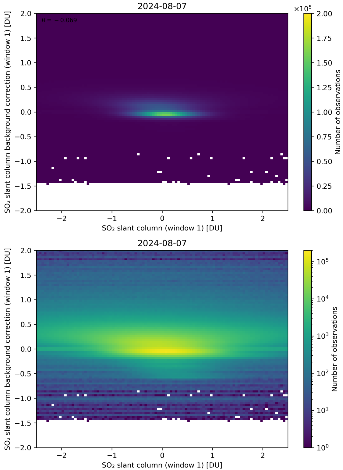
Figure 212: Scatter density plot of “SO 2 slant column (window 1)” against “SO 2 slant column background correction (window 1)” for 2024-08-06 to 2024-08-08.
