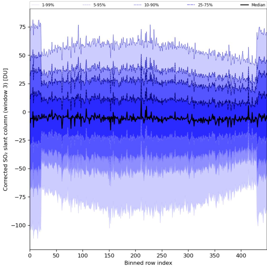
Figure 89: Along track statistics of “Corrected SO 2 slant column (window 3)” for 2024-08-06 to 2024-08-08
