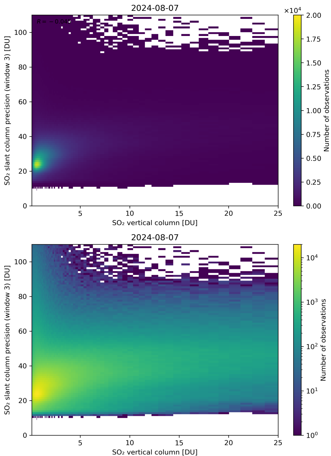
Figure 304: Scatter density plot of “SO 2 vertical column” against “SO 2 slant column precision (window 3)” for 2024-08-06 to 2024-08-08.
