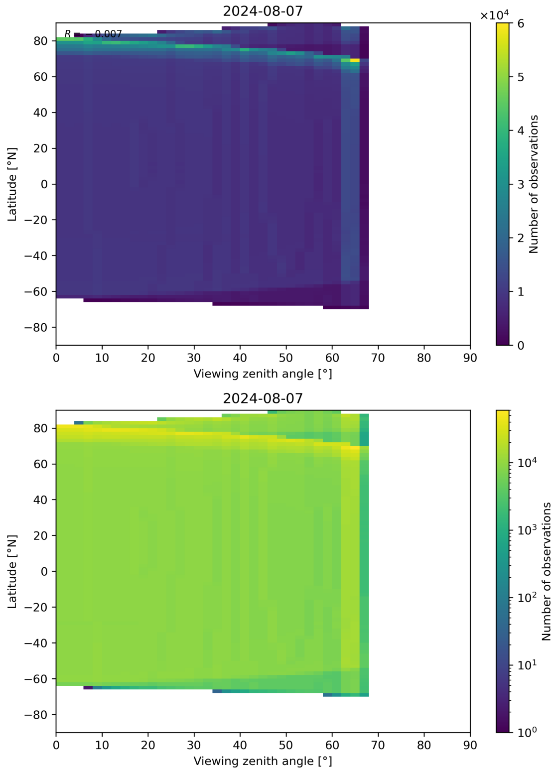
Figure 314: Scatter density plot of “Viewing zenith angle” against “Latitude” for 2024-08-06 to 2024-08-08.
