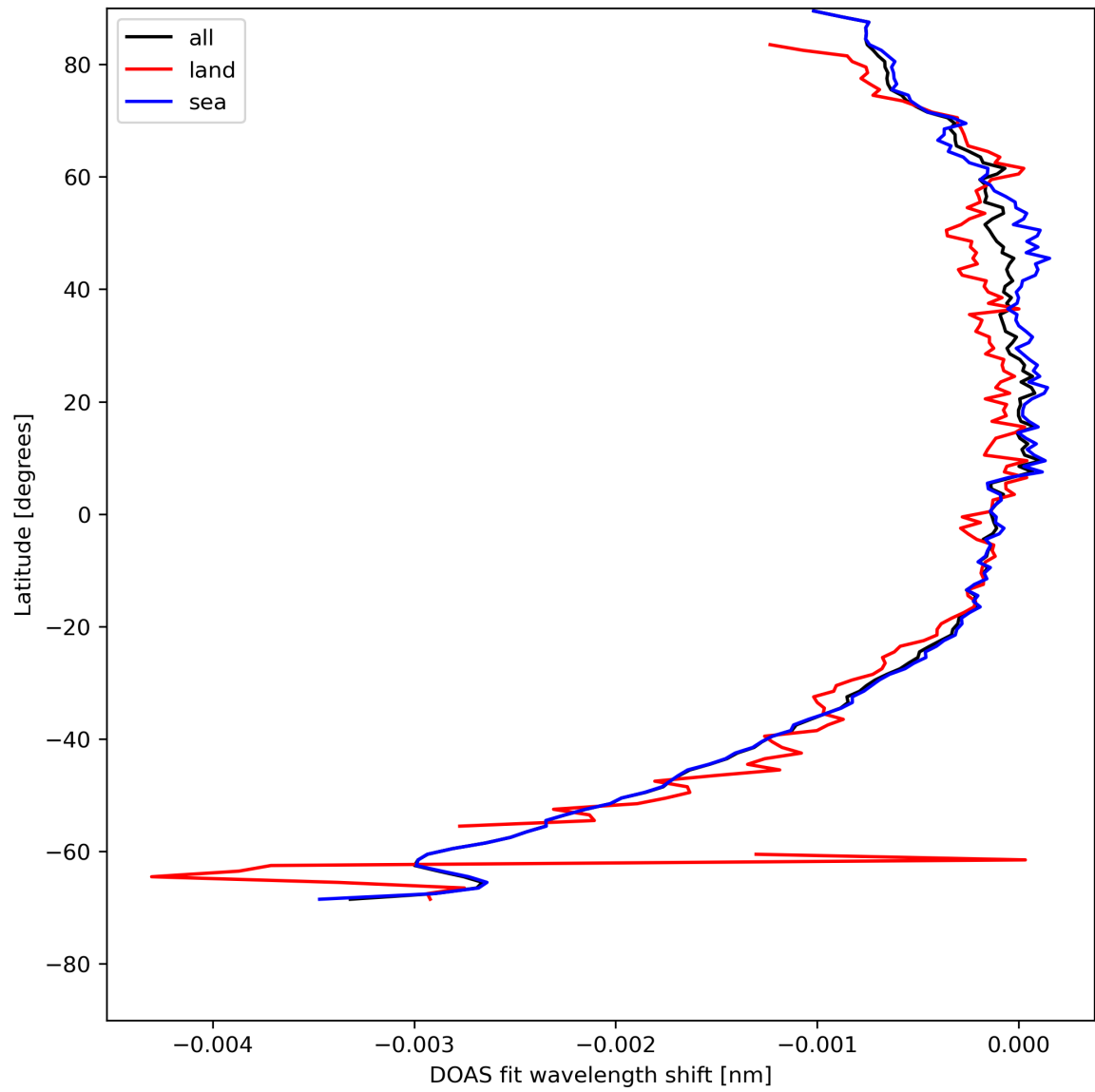
Figure 45: Zonal average of “DOAS fit wavelength shift” for 2024-08-06 to 2024-08-08.
