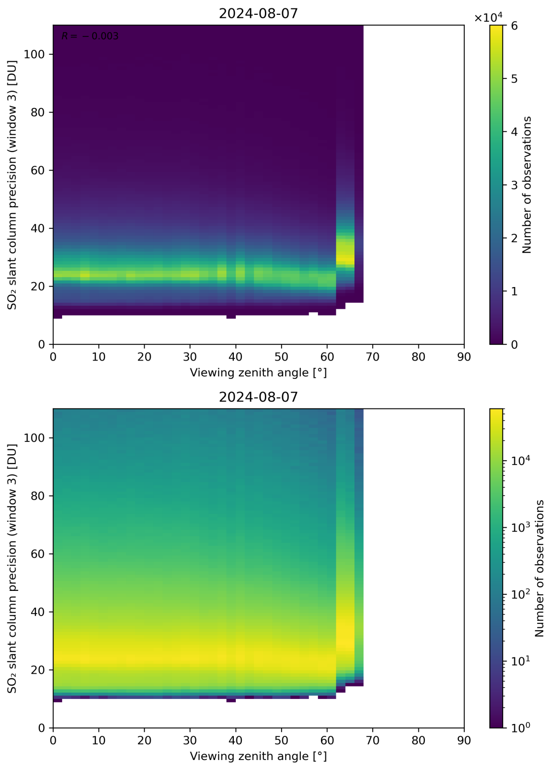
Figure 324: Scatter density plot of “Viewing zenith angle” against “SO 2 slant column precision (window 3)” for 2024-08-06 to 2024-08-08.
