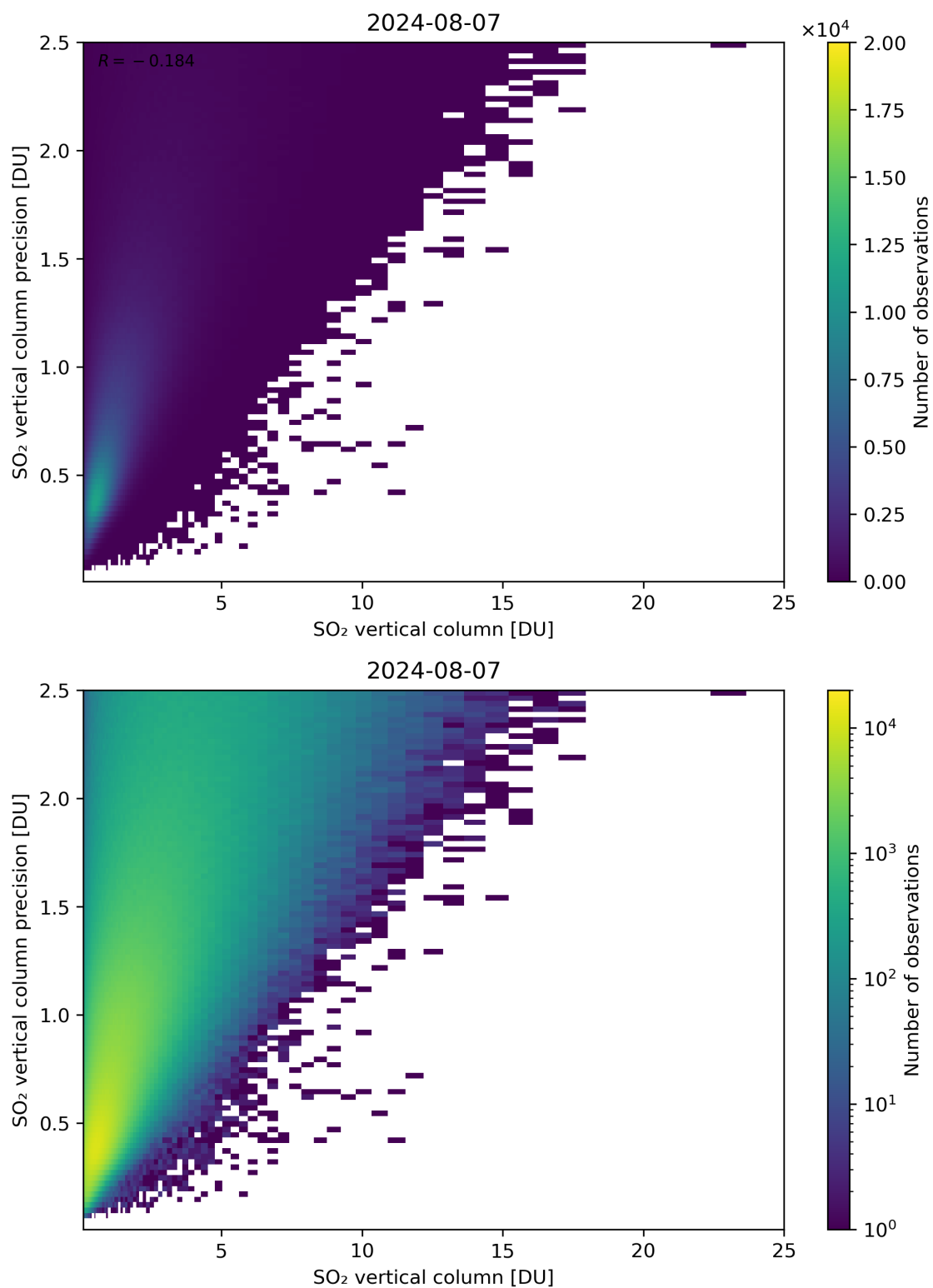
Figure 307: Scatter density plot of “SO 2 vertical column” against “SO 2 vertical column precision” for 2024-08-06 to 2024-08-08.
