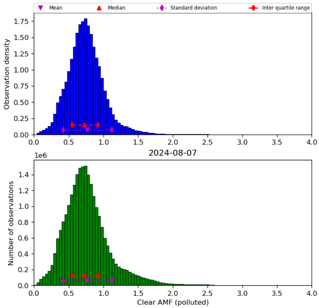
Figure 73: Histogram of “Clear AMF (polluted)” for 2024-08-06 to 2024-08-08
