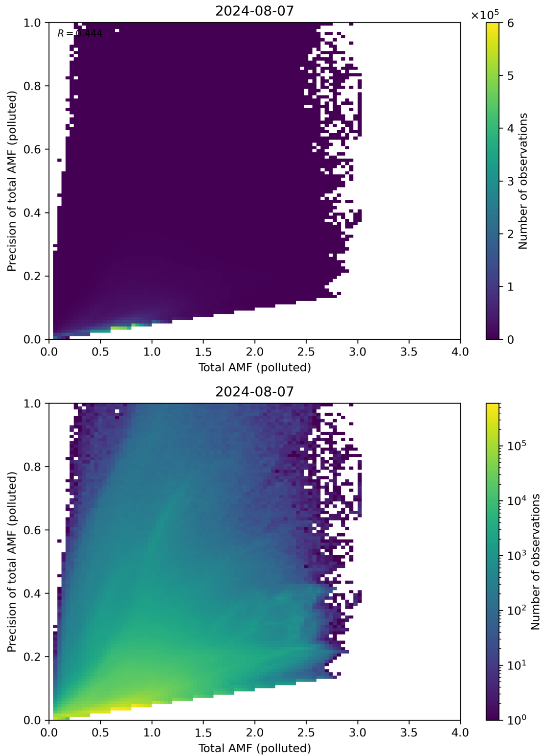
Figure 272: Scatter density plot of “Total AMF (polluted)” against “Precision of total AMF (polluted)” for 2024-08-06 to 2024-08-08.
