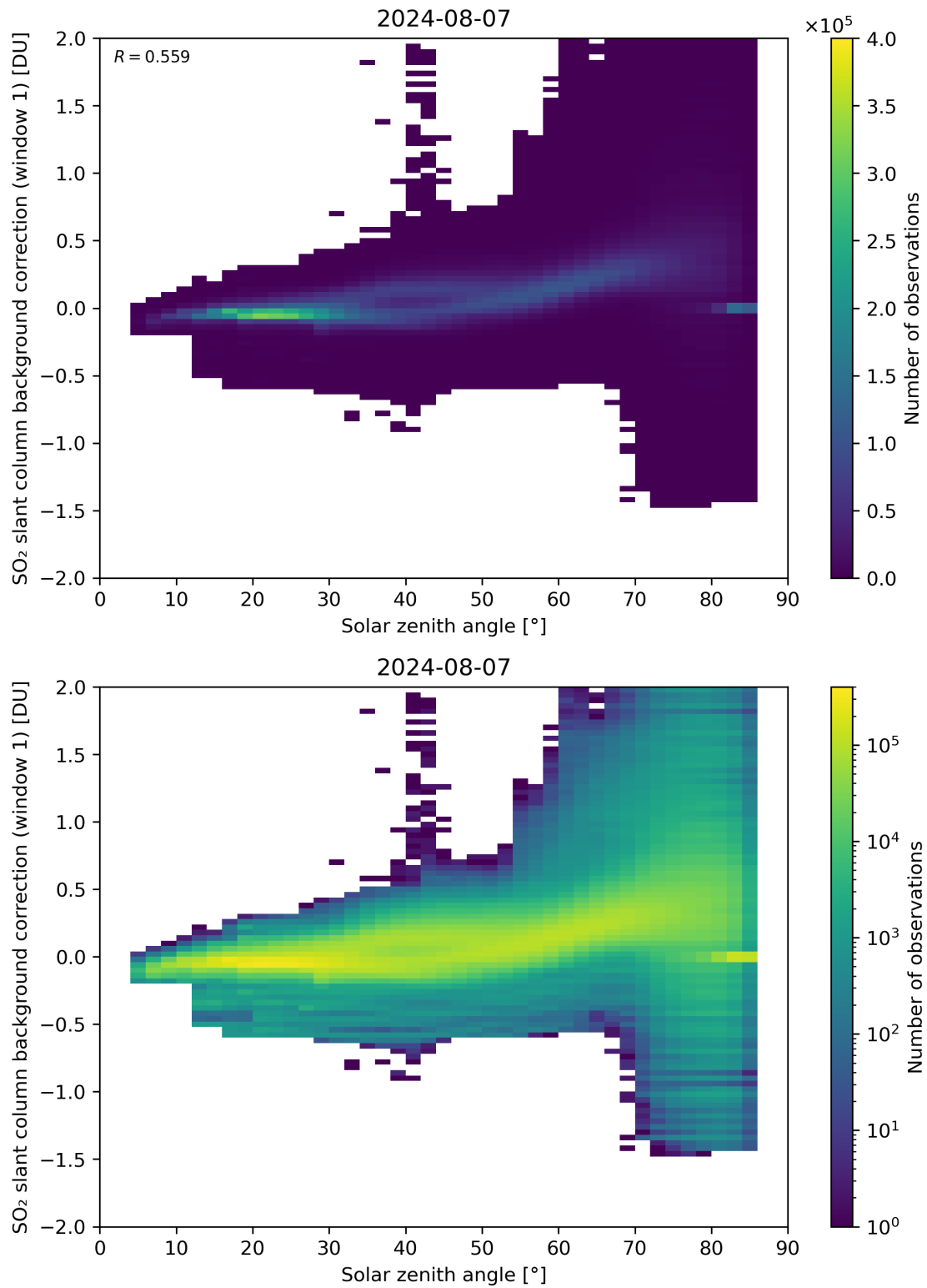
Figure 158: Scatter density plot of “Solar zenith angle” against “SO 2 slant column background correction (window 1)” for 2024-08-06 to 2024-08-08.
