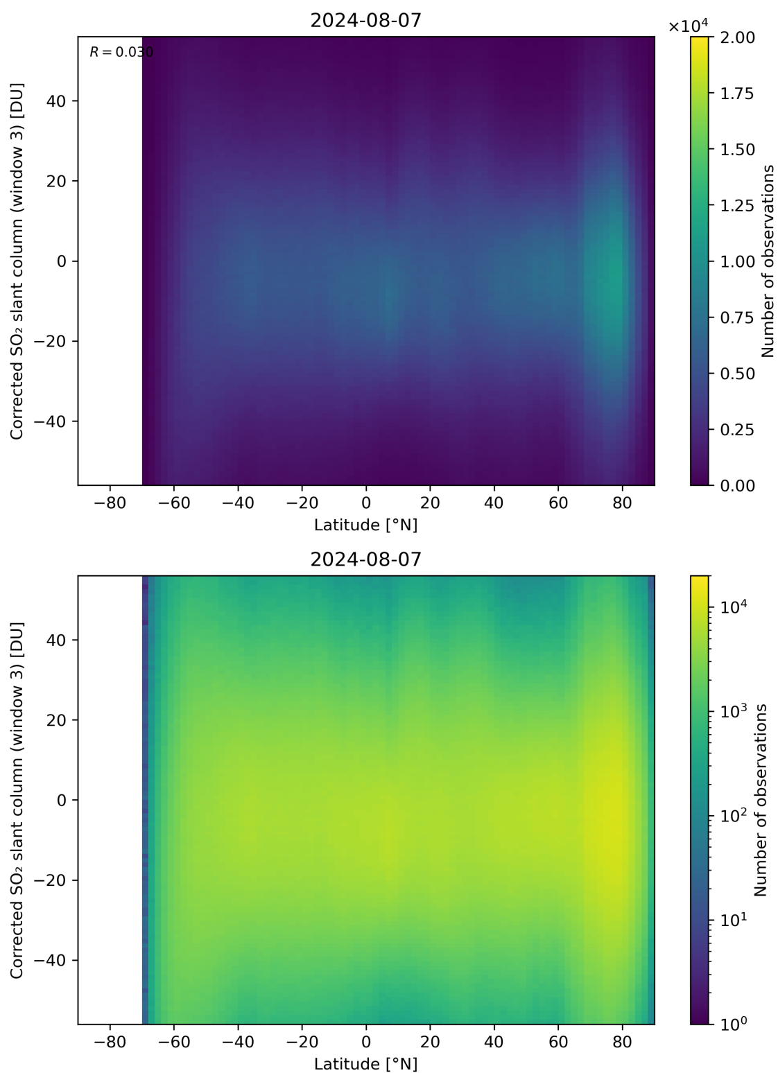
Figure 148: Scatter density plot of “Latitude” against “Corrected SO 2 slant column (window 3)” for 2024-08-06 to 2024-08-08.
