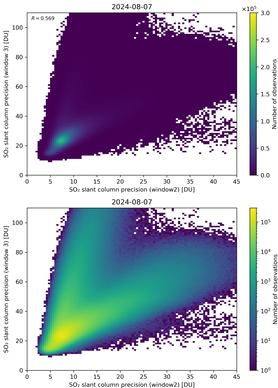
Figure 250: Scatter density plot of “SO 2 slant column precision (window2)” against “SO 2 slant column precision (window 3)” for 2024-08-06 to 2024-08-08.
