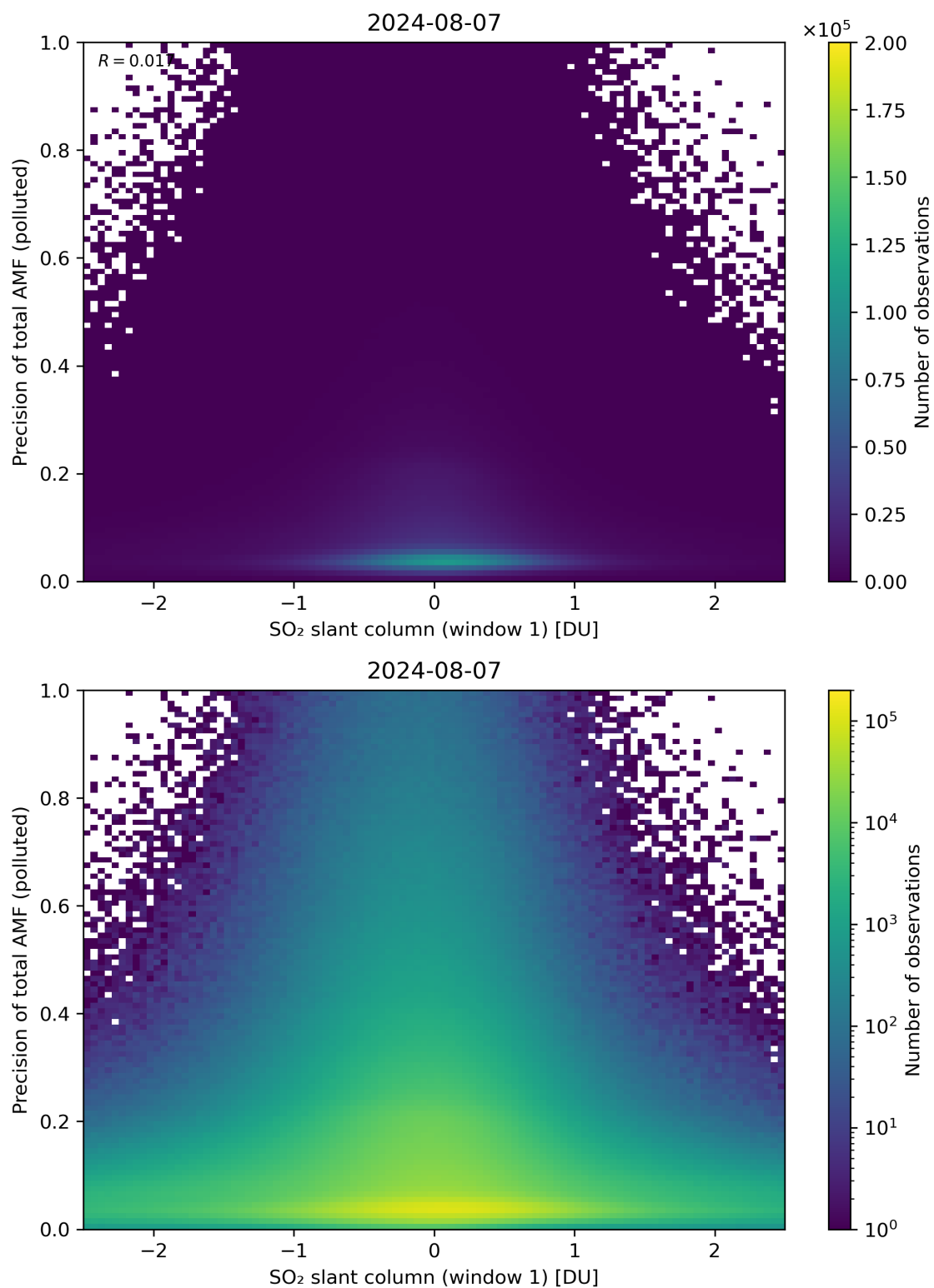
Figure 240: Scatter density plot of “SO 2 slant column (window 1)” against “Precision of total AMF (polluted)” for 2024-08-06 to 2024-08-08.
