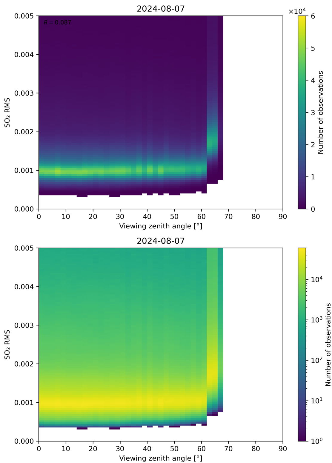
Figure 313: Scatter density plot of “Viewing zenith angle” against “SO 2 RMS” for 2024-08-06 to 2024-08-08.
