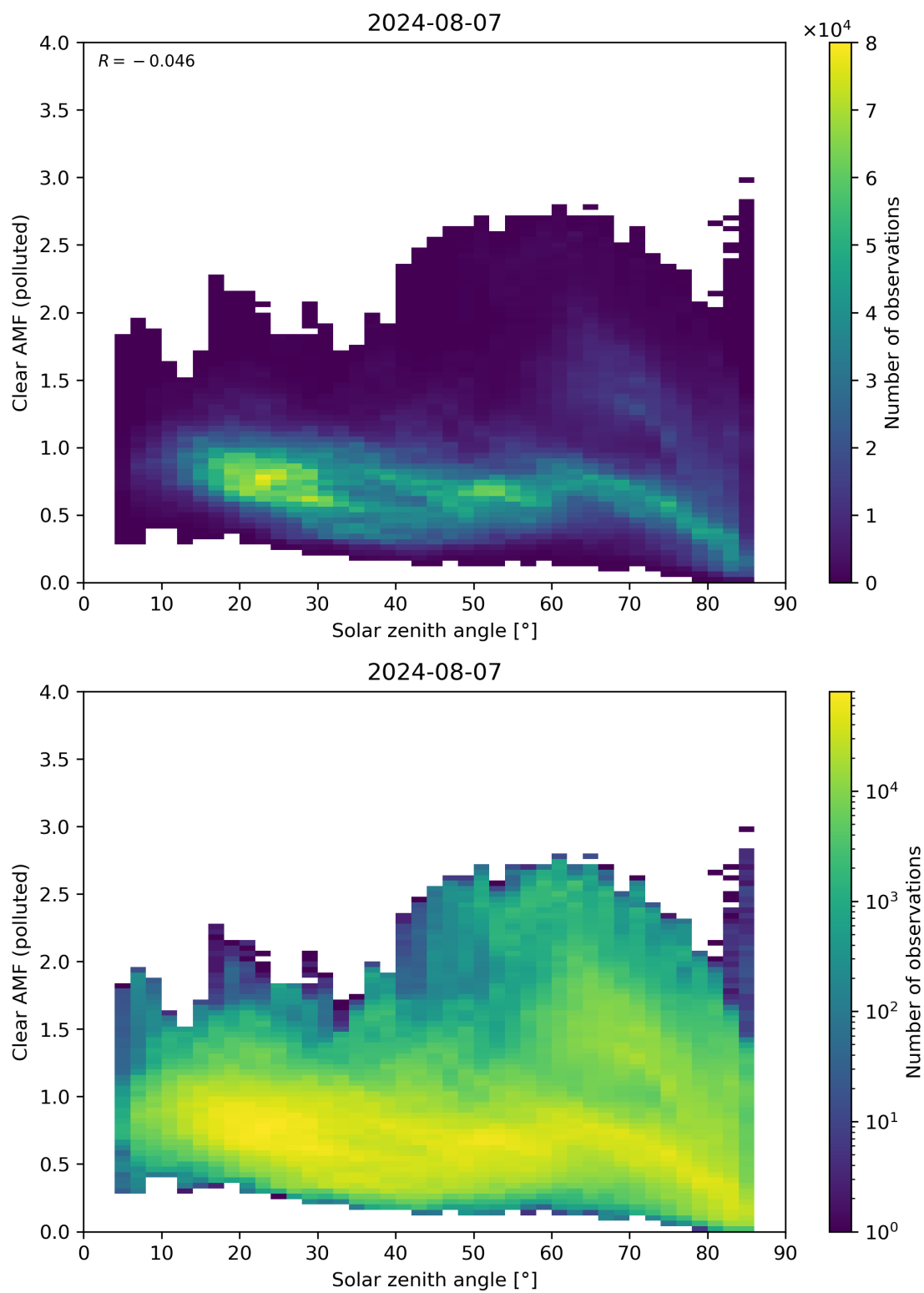
Figure 165: Scatter density plot of “Solar zenith angle” against “Clear AMF (polluted)” for 2024-08-06 to 2024-08-08.
