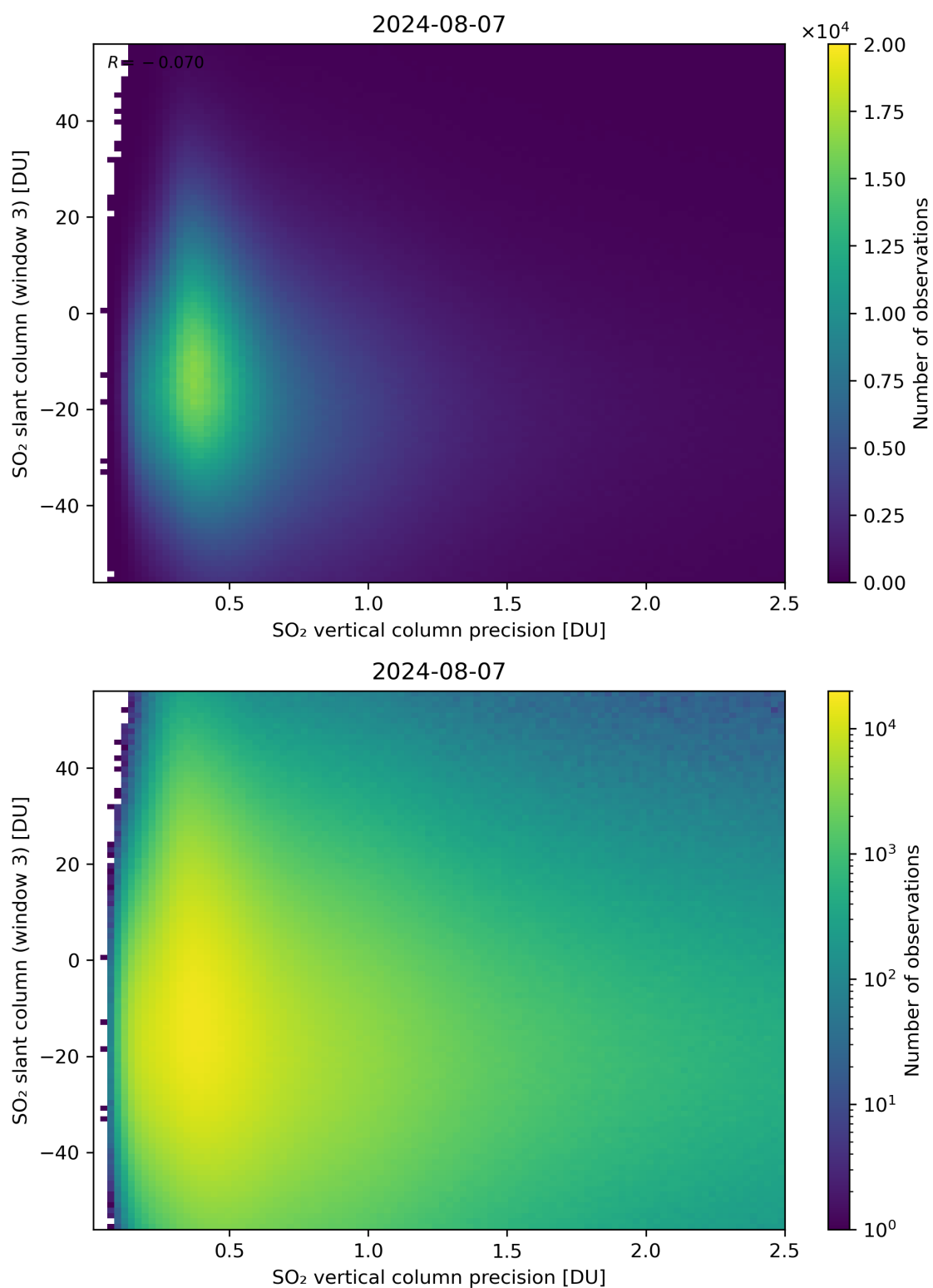
Figure 292: Scatter density plot of “SO 2 vertical column precision” against “SO 2 slant column (window 3)” for 2024-08-06 to 2024-08-08.
