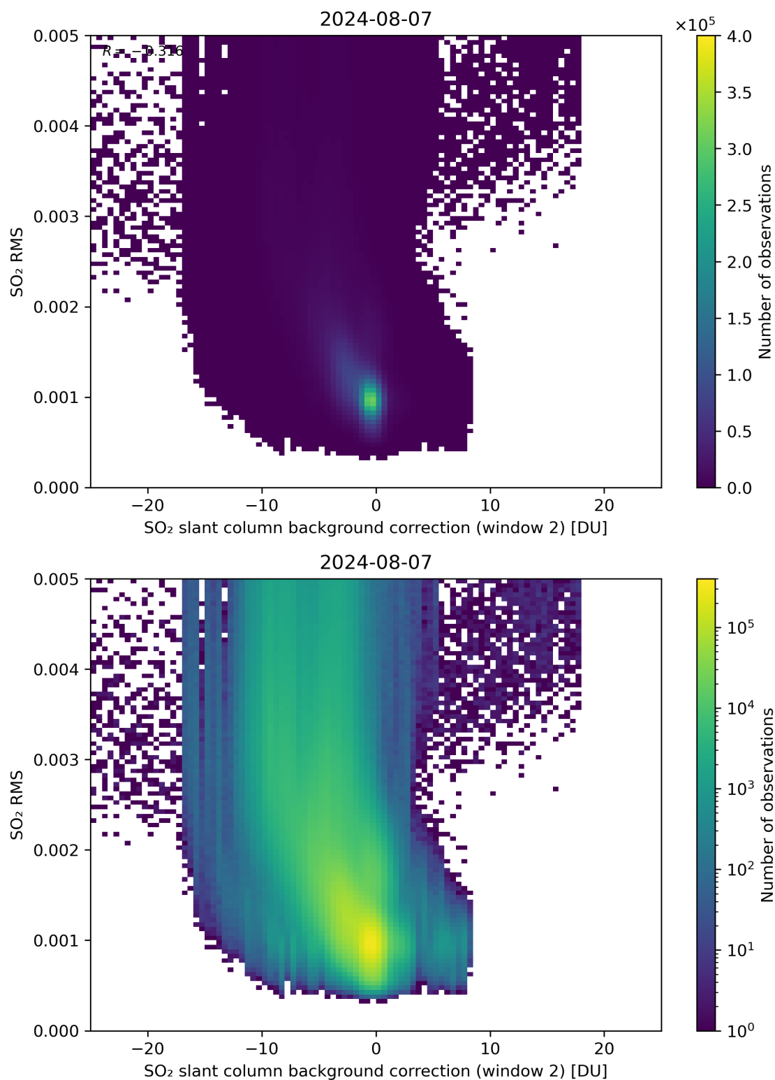
Figure 114: Scatter density plot of “SO 2 slant column background correction (window 2)” against “SO 2 RMS” for 2024-08-06 to 2024-08-08.
