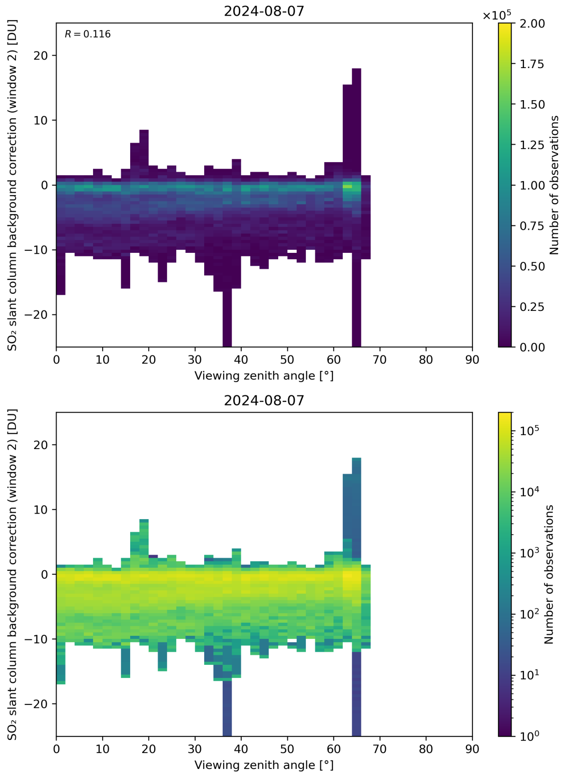
Figure 309: Scatter density plot of “Viewing zenith angle” against “SO 2 slant column background correction (window 2)” for 2024-08-06 to 2024-08-08.
