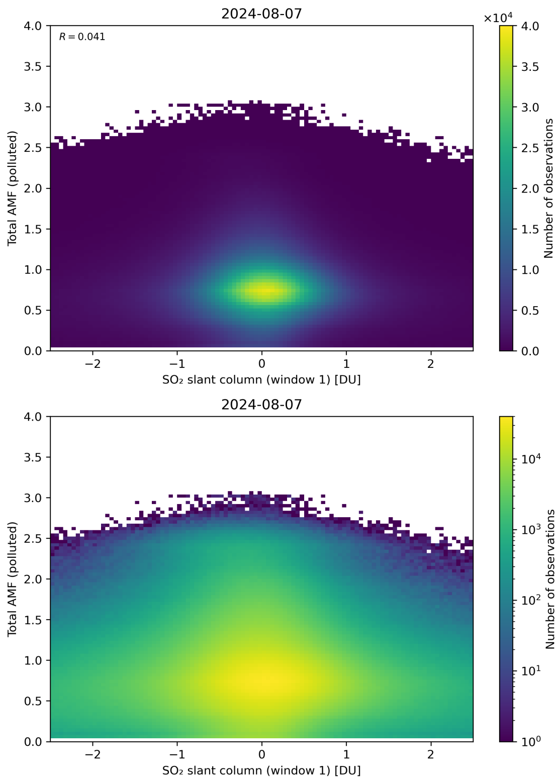
Figure 239: Scatter density plot of “SO 2 slant column (window 1)” against “Total AMF (polluted)” for 2024-08-06 to 2024-08-08.
