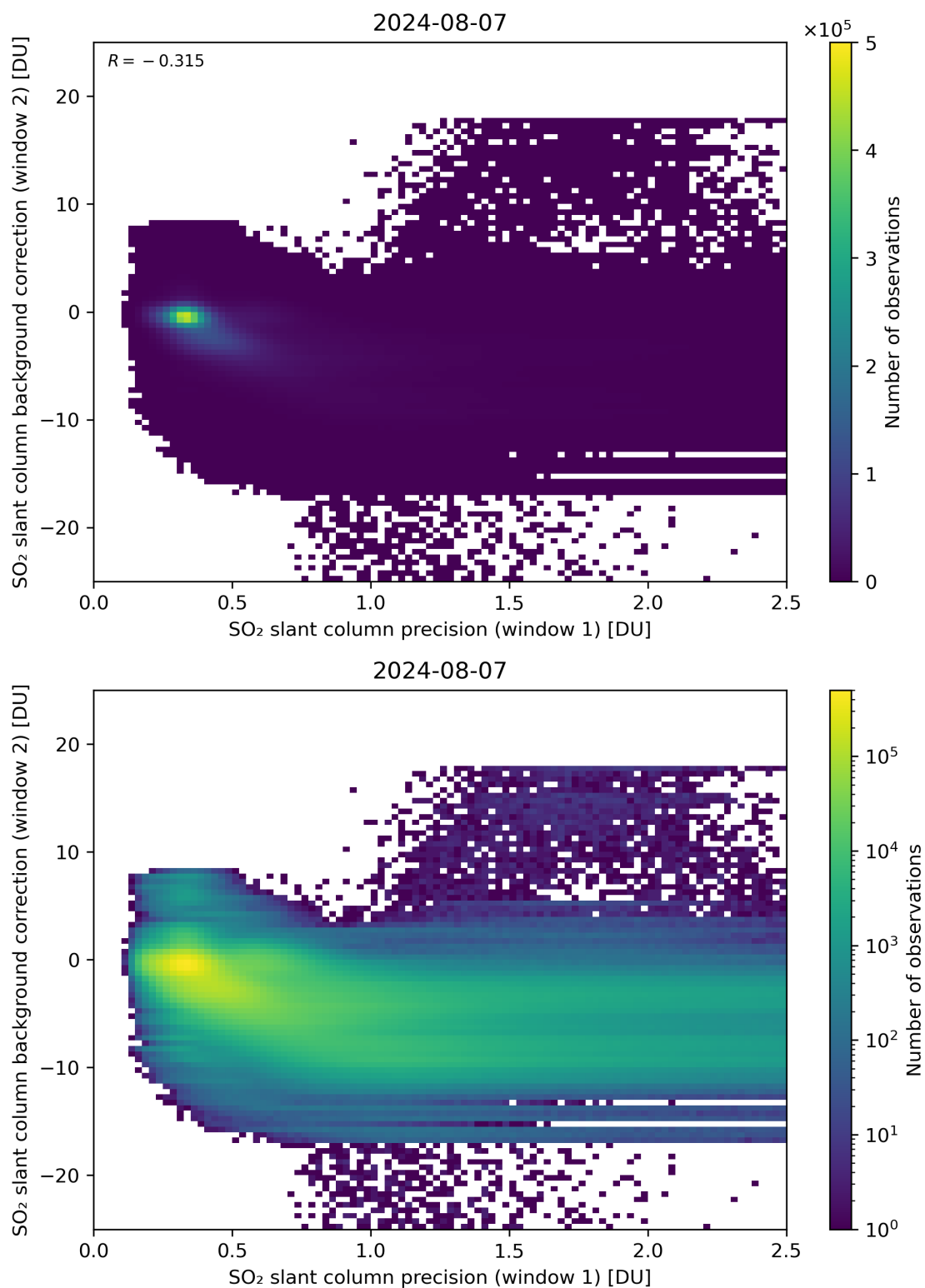
Figure 219: Scatter density plot of “SO 2 slant column precision (window 1)” against “SO 2 slant column background correction (window 2)” for 2024-08-06 to 2024-08-08.
