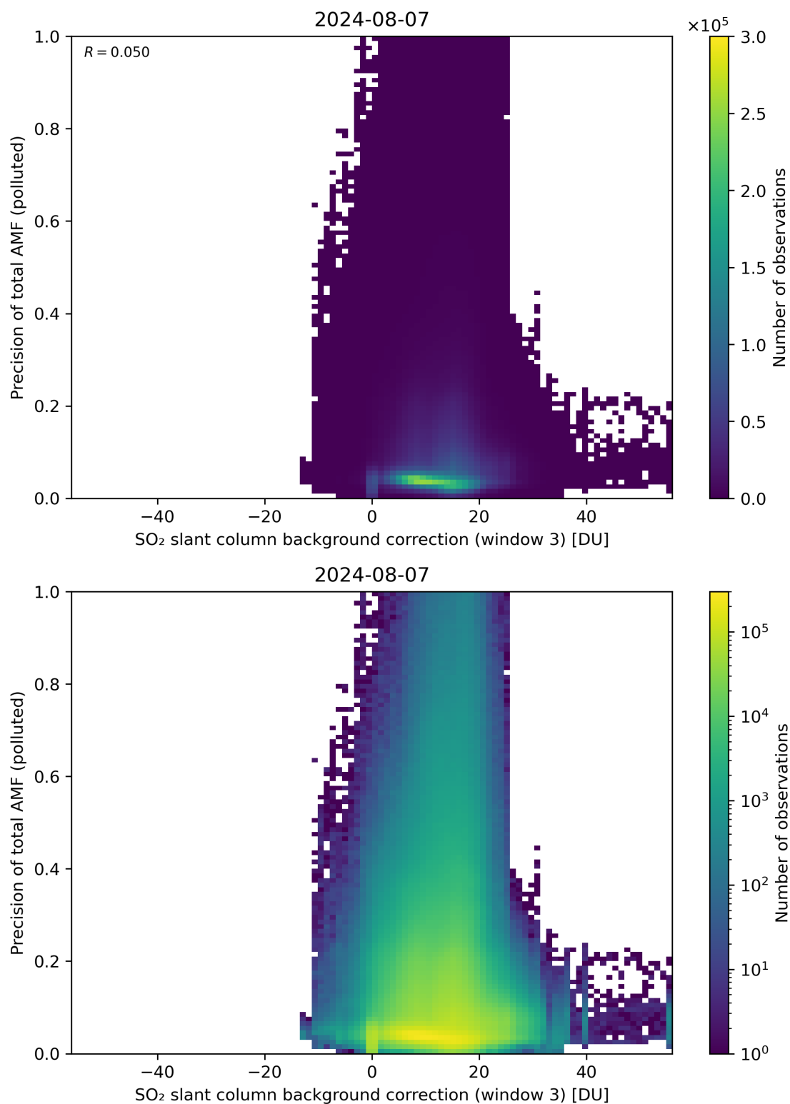
Figure 126: Scatter density plot of “SO 2 slant column background correction (window 3)” against “Precision of total AMF (polluted)” for 2024-08-06 to 2024-08-08.
