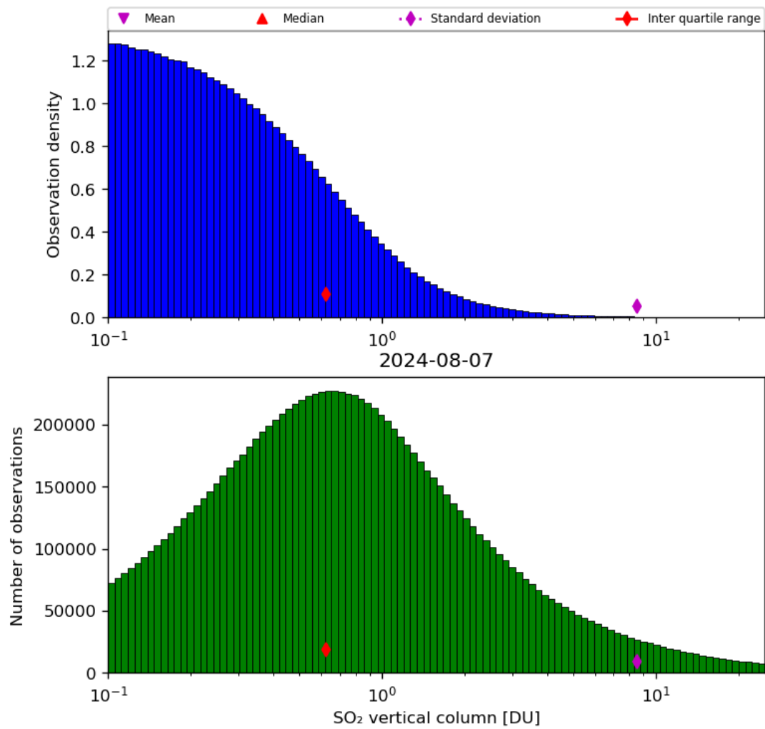
Figure 53: Histogram of “SO 2 vertical column” for 2024-08-06 to 2024-08-08
