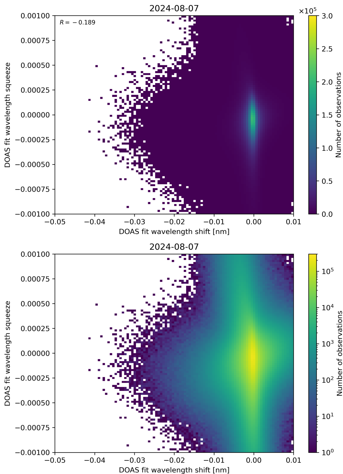
Figure 127: Scatter density plot of “DOAS fit wavelength shift” against “DOAS fit wavelength squeeze” for 2024-08-06 to 2024-08-08.
