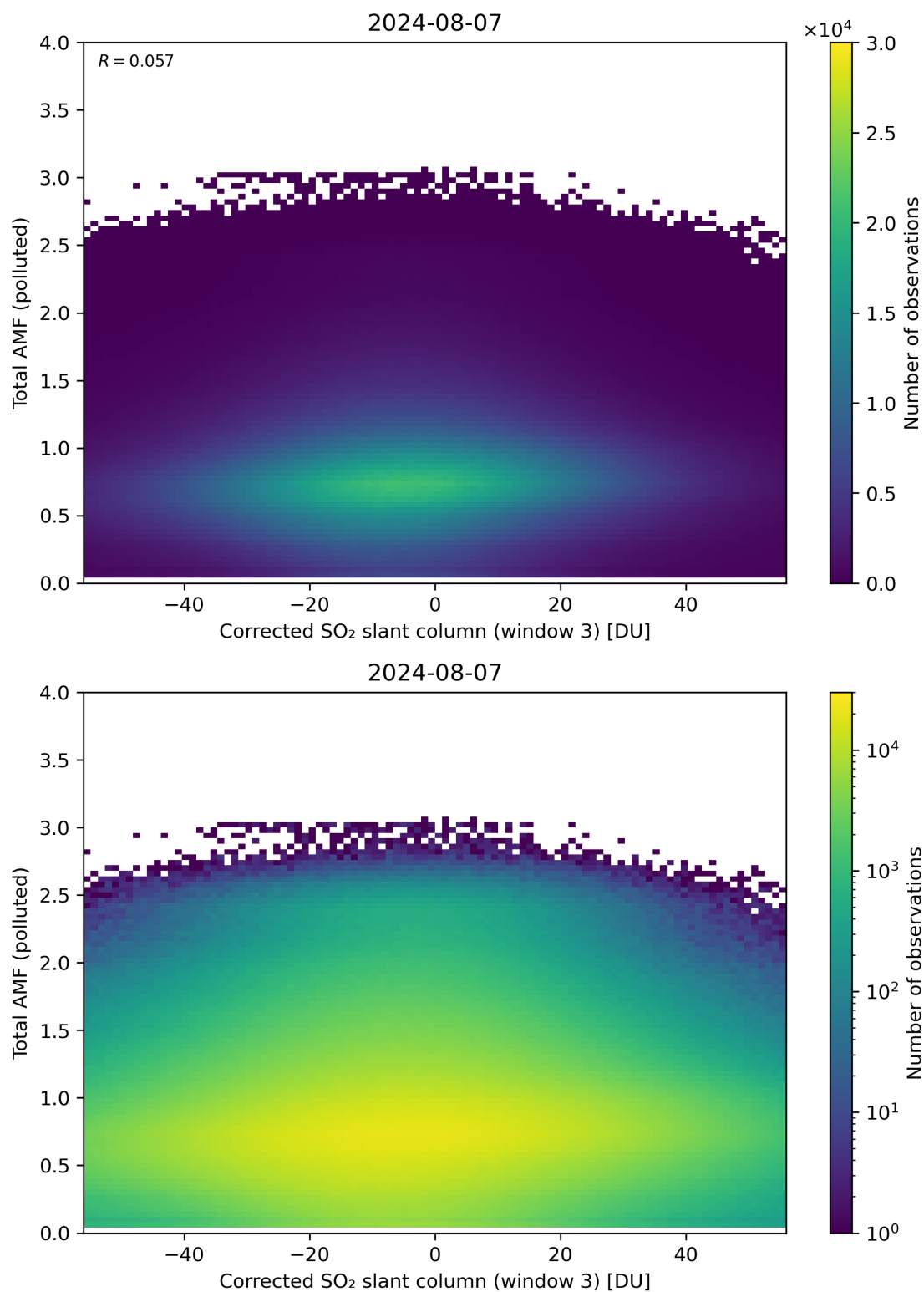
Figure 210: Scatter density plot of “Corrected SO 2 slant column (window 3)” against “Total AMF (polluted)” for 2024-08-06 to 2024-08-08.
