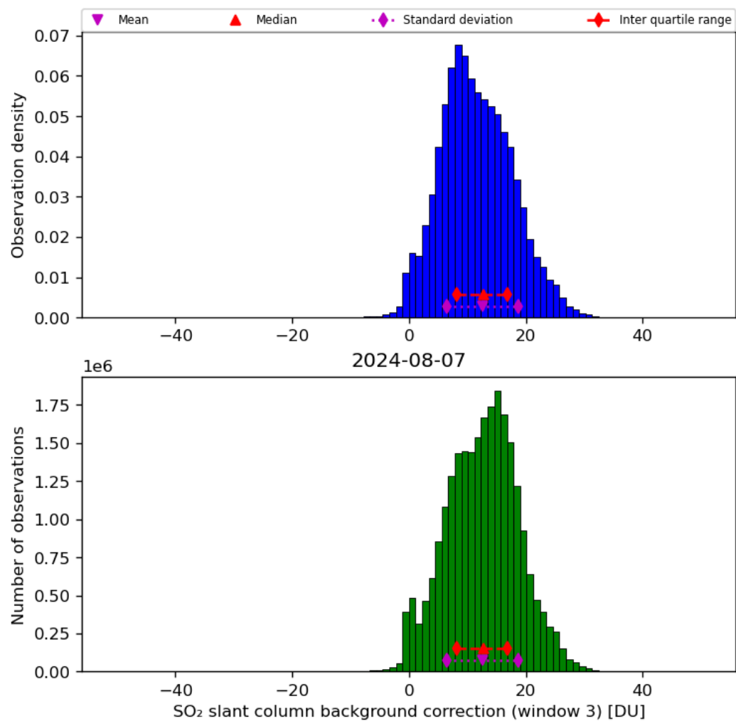
Figure 67: Histogram of “SO 2 slant column background correction (window 3)” for 2024-08-06 to 2024-08-08
