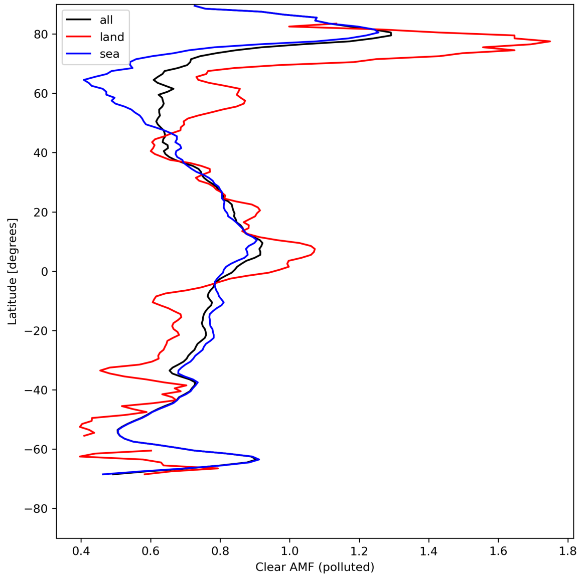
Figure 50: Zonal average of “Clear AMF (polluted)” for 2024-08-06 to 2024-08-08.
