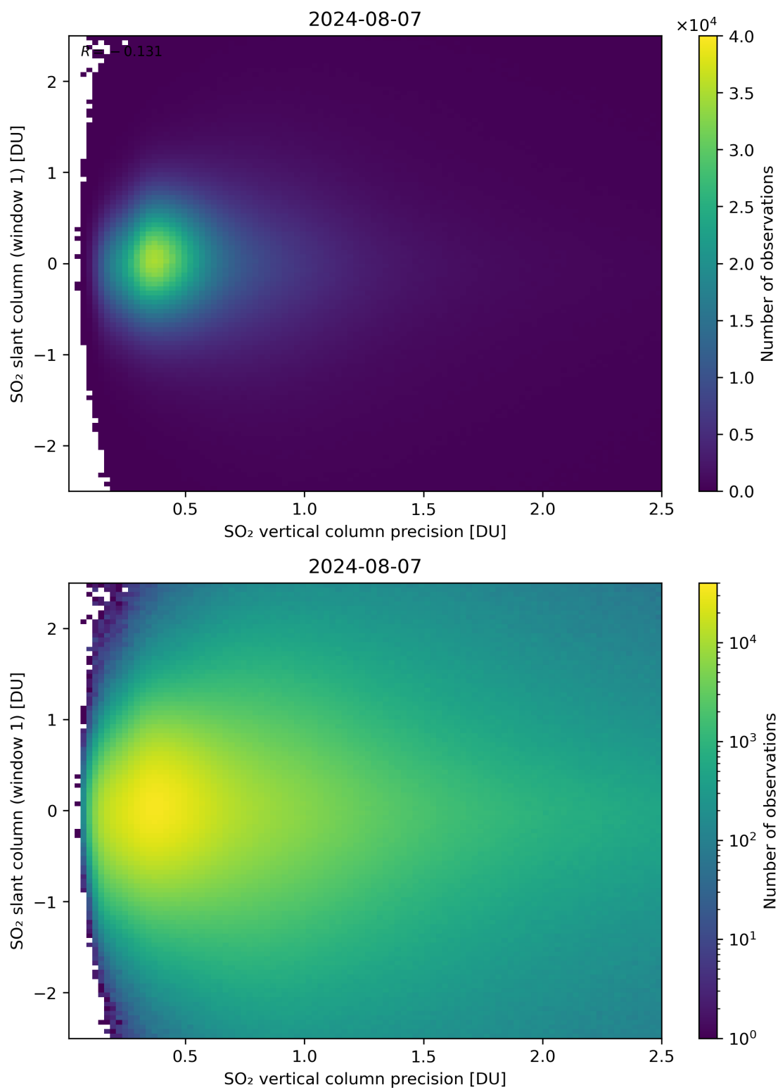
Figure 289: Scatter density plot of “SO 2 vertical column precision” against “SO 2 slant column (window 1)” for 2024-08-06 to 2024-08-08.
