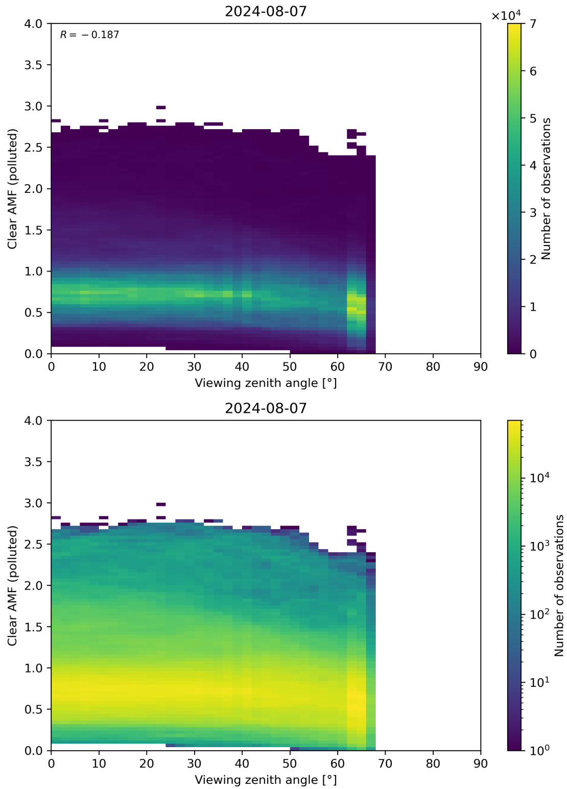
Figure 316: Scatter density plot of “Viewing zenith angle” against “Clear AMF (polluted)” for 2024-08-06 to 2024-08-08.
