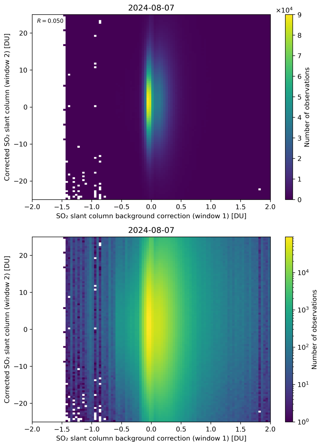
Figure 104: Scatter density plot of “SO 2 slant column background correction (window 1)” against “Corrected SO 2 slant column (window 2)” for 2024-08-06 to 2024-08-08.
