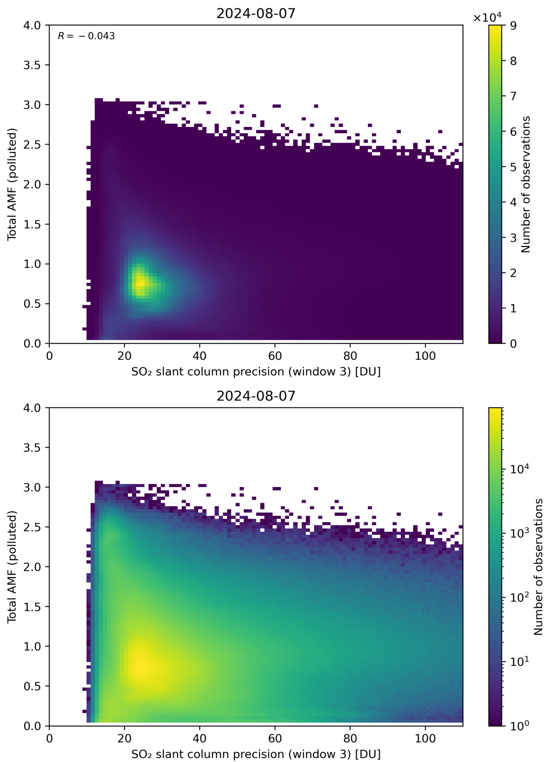
Figure 263: Scatter density plot of “SO 2 slant column precision (window 3)” against “Total AMF (polluted)” for 2024-08-06 to 2024-08-08.
