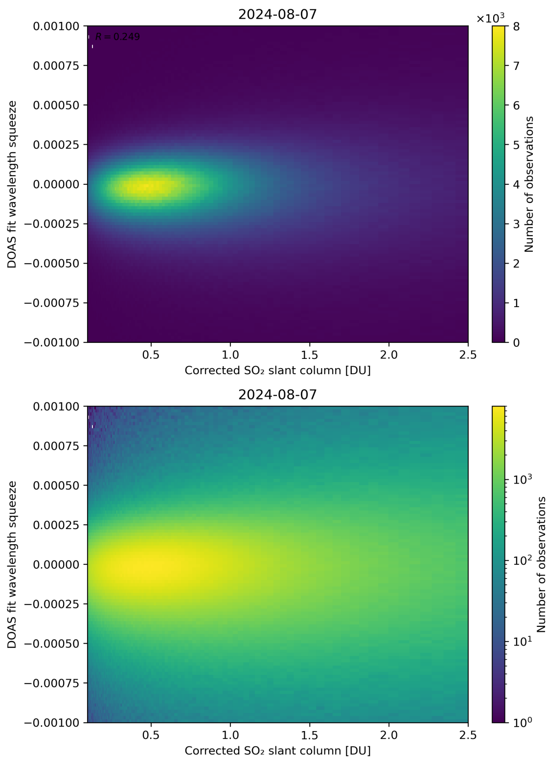
Figure 182: Scatter density plot of “Corrected SO 2 slant column” against “DOAS fit wavelength squeeze” for 2024-08-06 to 2024-08-08.
