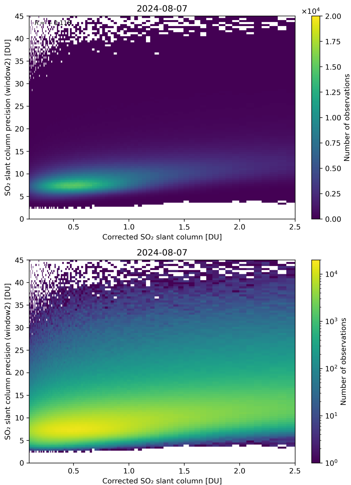
Figure 189: Scatter density plot of “Corrected SO 2 slant column” against “SO 2 slant column precision (window2)” for 2024-08-06 to 2024-08-08.
