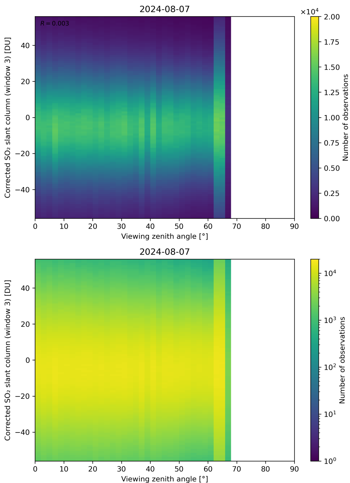
Figure 319: Scatter density plot of “Viewing zenith angle” against “Corrected SO 2 slant column (window 3)” for 2024-08-06 to 2024-08-08.
