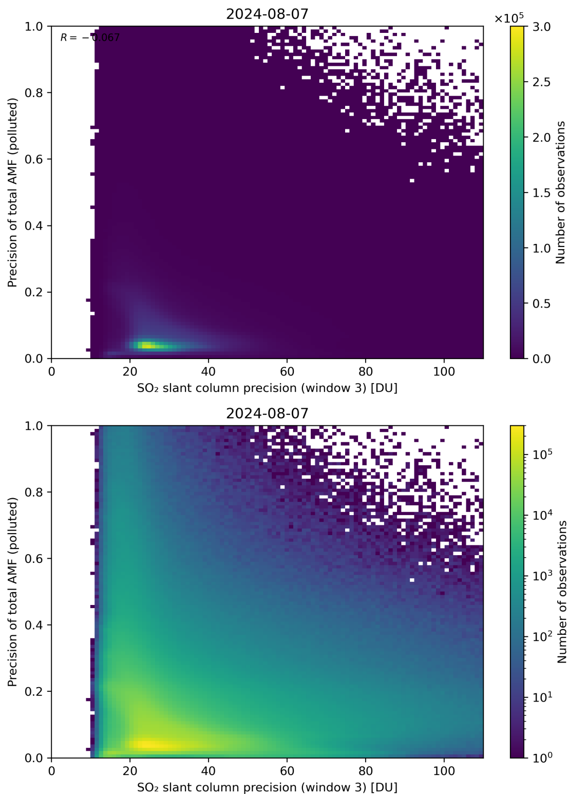
Figure 264: Scatter density plot of “SO 2 slant column precision (window 3)” against “Precision of total AMF (polluted)” for 2024-08-06 to 2024-08-08.
