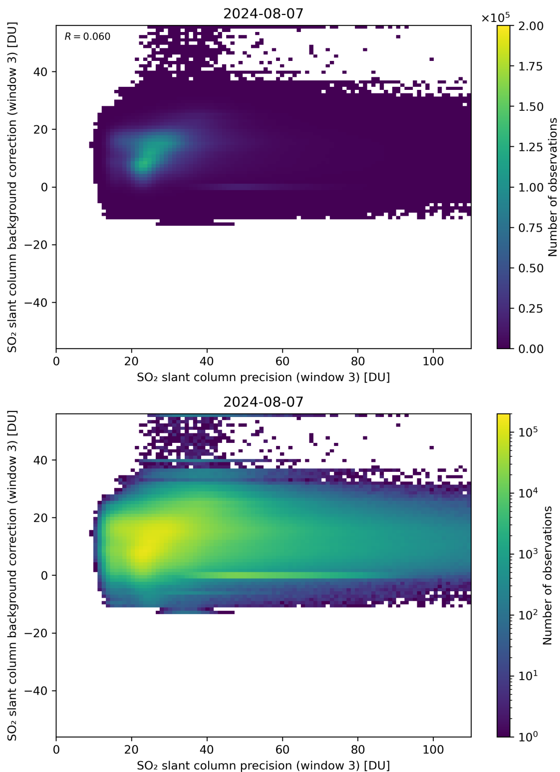
Figure 257: Scatter density plot of “SO 2 slant column precision (window 3)” against “SO 2 slant column background correction (window 3)” for 2024-08-06 to 2024-08-08.
