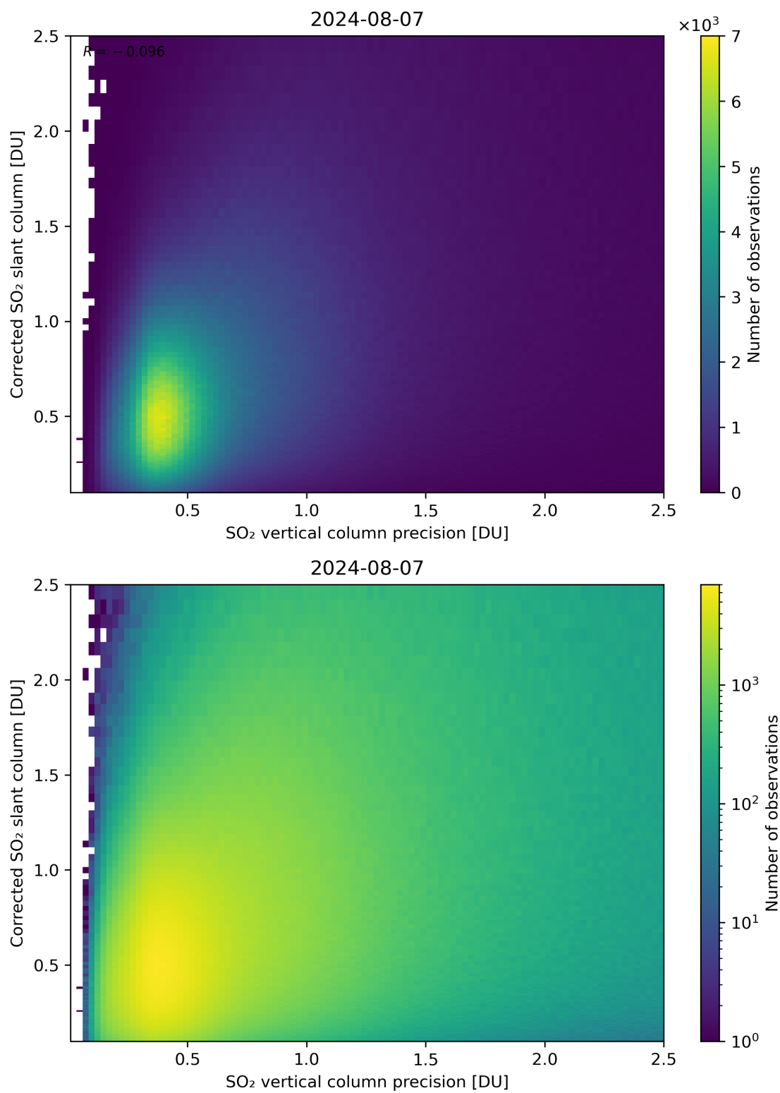
Figure 286: Scatter density plot of “SO 2 vertical column precision” against “Corrected SO 2 slant column” for 2024-08-06 to 2024-08-08.
