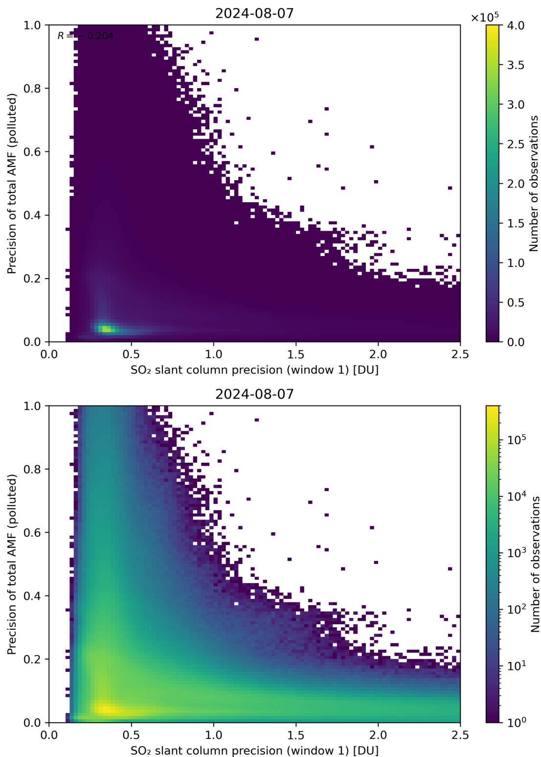
Figure 231: Scatter density plot of “SO 2 slant column precision (window 1)” against “Precision of total AMF (polluted)” for 2024-08-06 to 2024-08-08.
