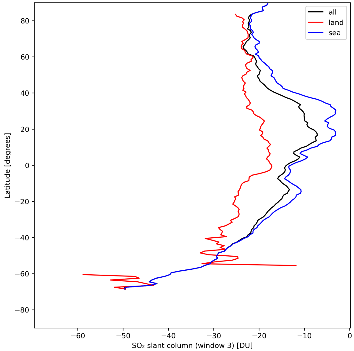
Figure 41: Zonal average of “SO 2 slant column (window 3)” for 2024-08-06 to 2024-08-08.
