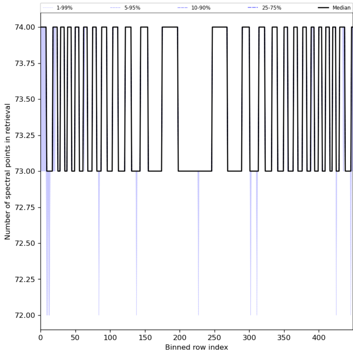
Figure 97: Along track statistics of “Number of spectral points in retrieval” for 2024-08-06 to 2024-08-08
