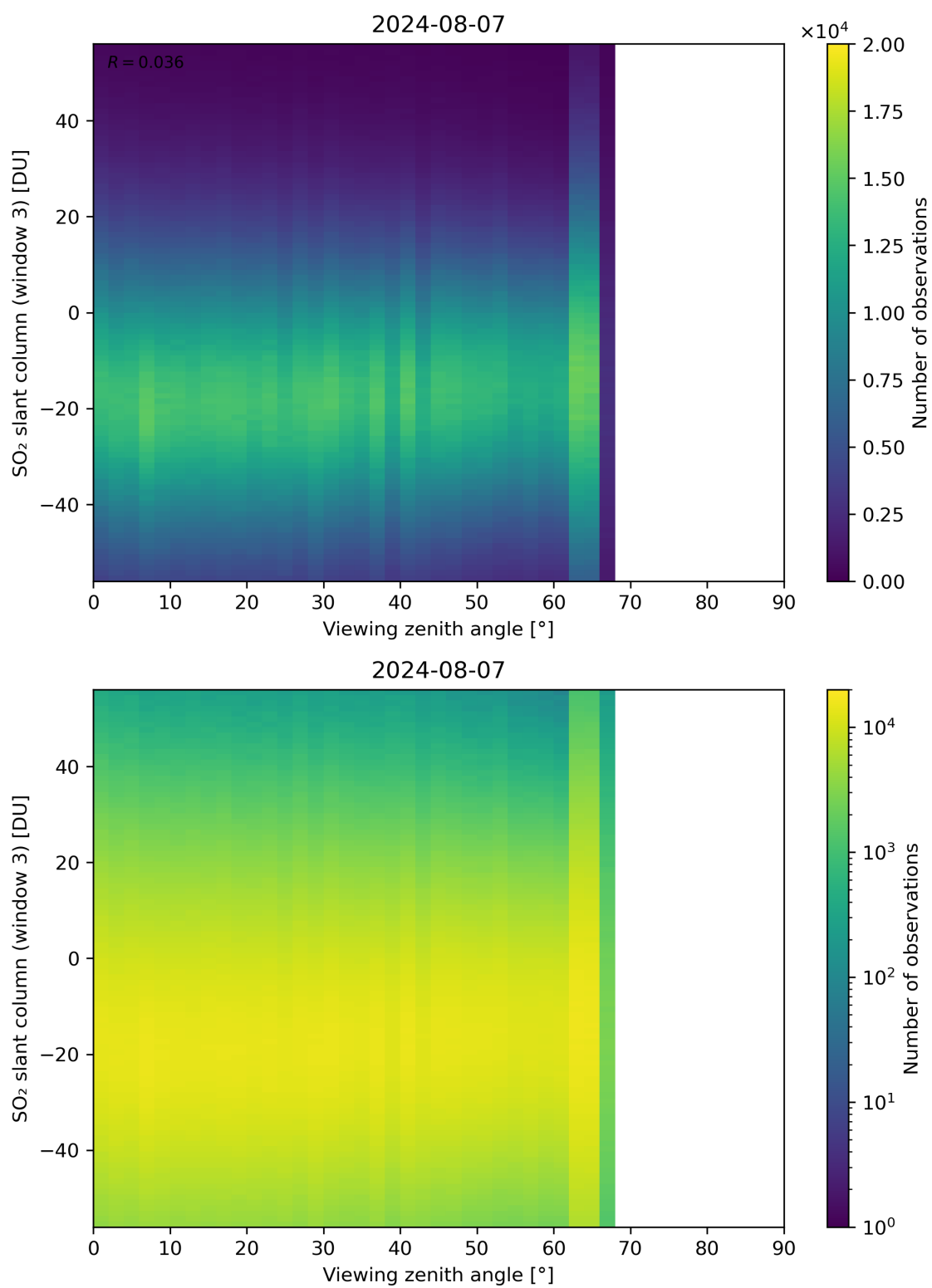
Figure 323: Scatter density plot of “Viewing zenith angle” against “SO 2 slant column (window 3)” for 2024-08-06 to 2024-08-08.
