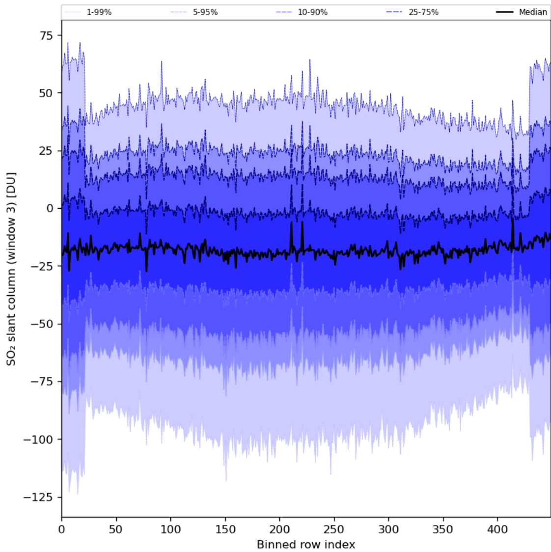
Figure 87: Along track statistics of “SO 2 slant column (window 3)” for 2024-08-06 to 2024-08-08
