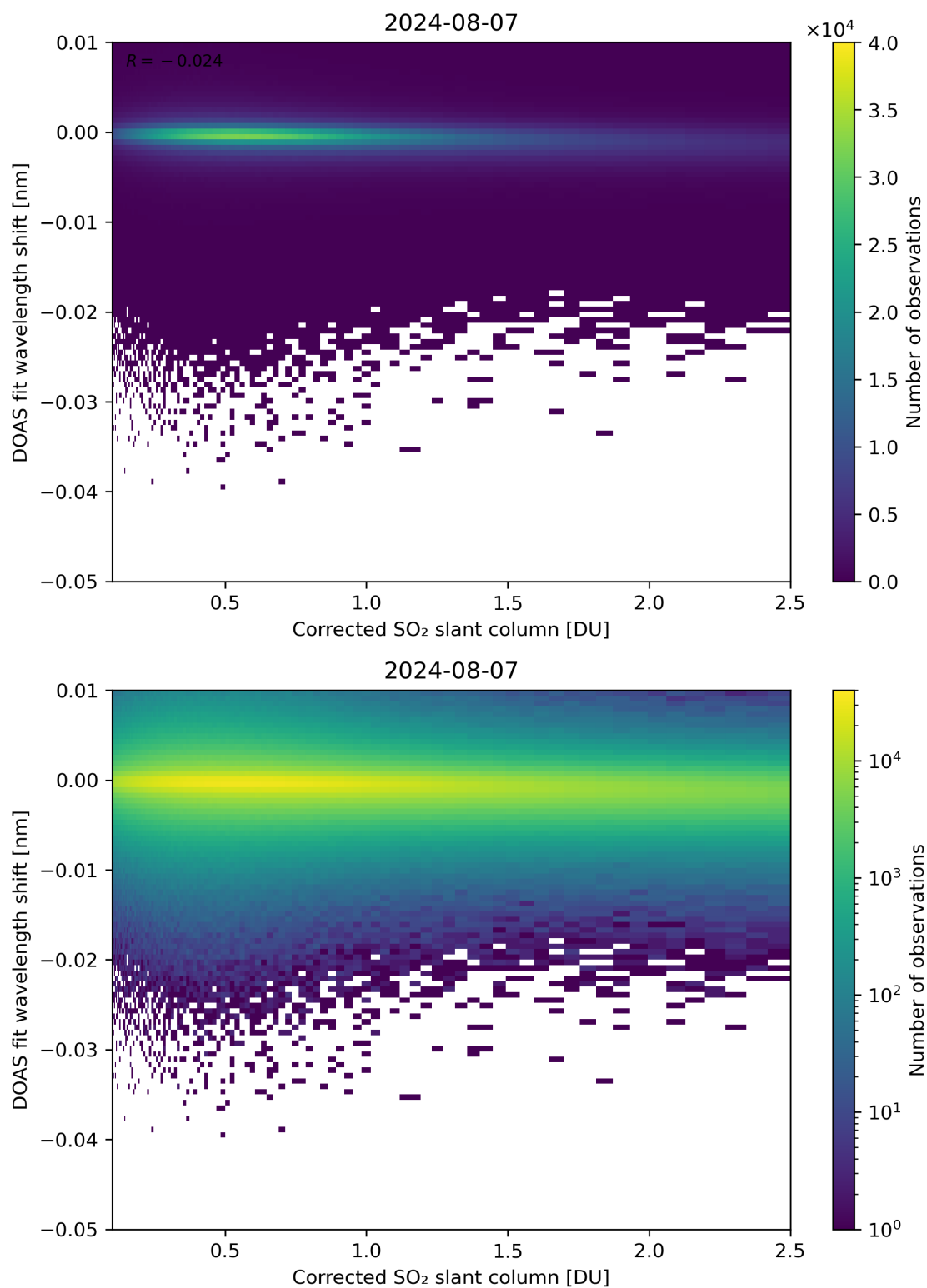
Figure 181: Scatter density plot of “Corrected SO 2 slant column” against “DOAS fit wavelength shift” for 2024-08-06 to 2024-08-08.
