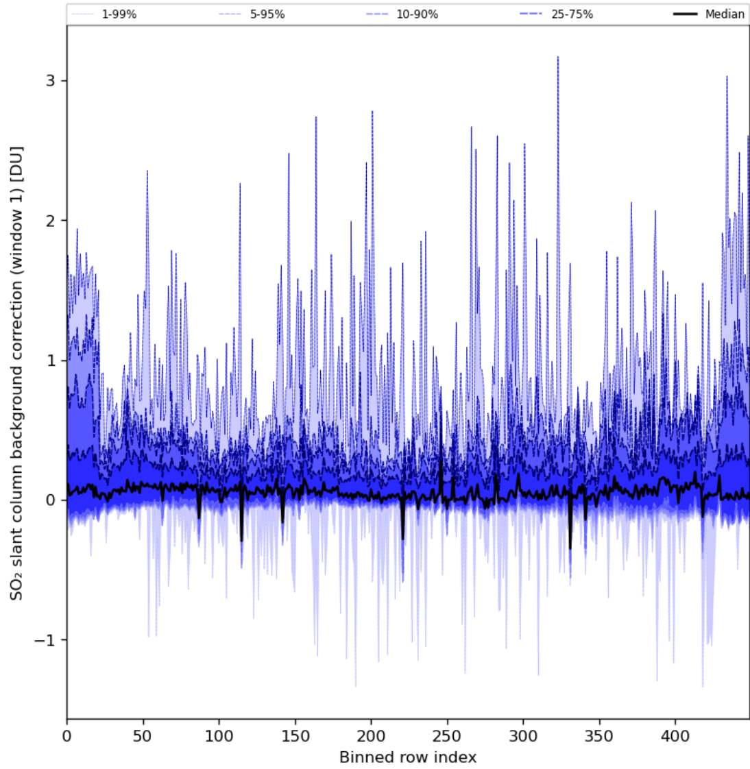
Figure 82: Along track statistics of “SO 2 slant column background correction (window 1)” for 2024-08-06 to 2024-08-08
