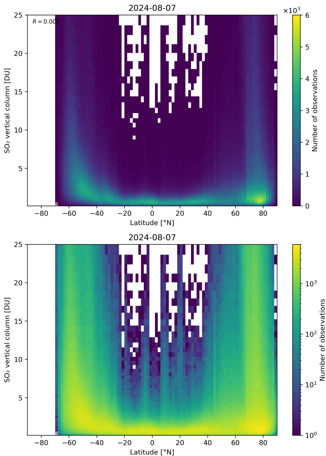
Figure 156: Scatter density plot of “Latitude” against “SO 2 vertical column” for 2024-08-06 to 2024-08-08.
