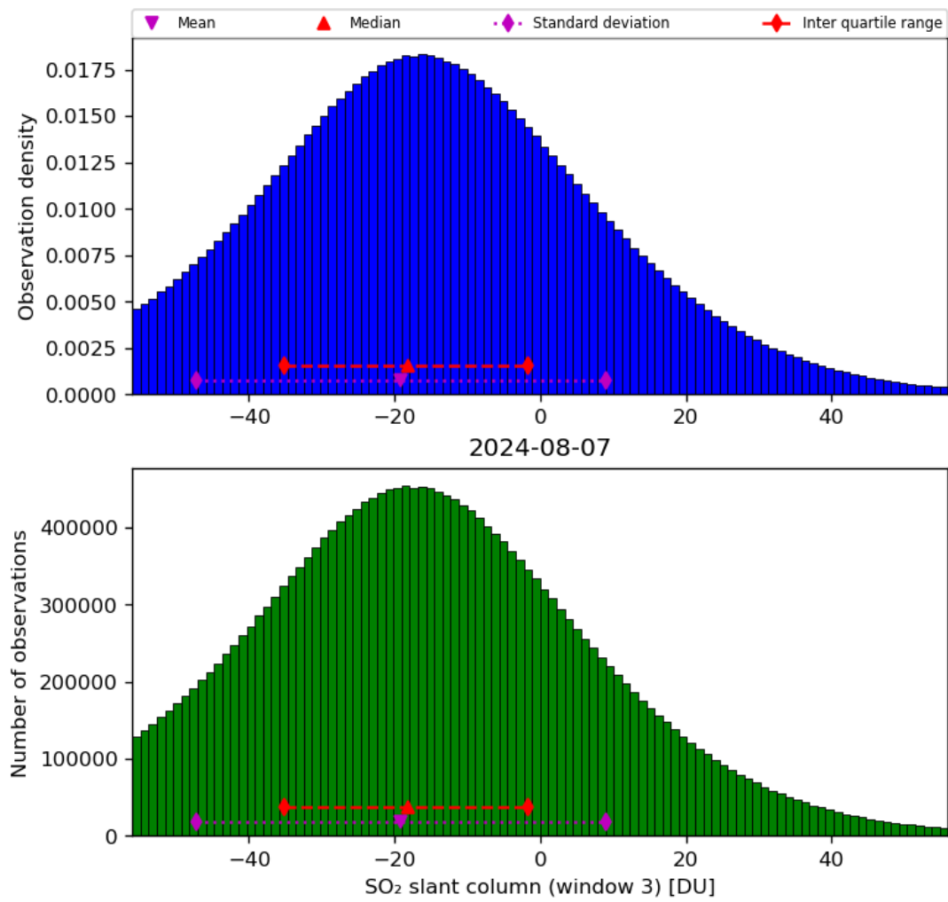
Figure 64: Histogram of “SO 2 slant column (window 3)” for 2024-08-06 to 2024-08-08
