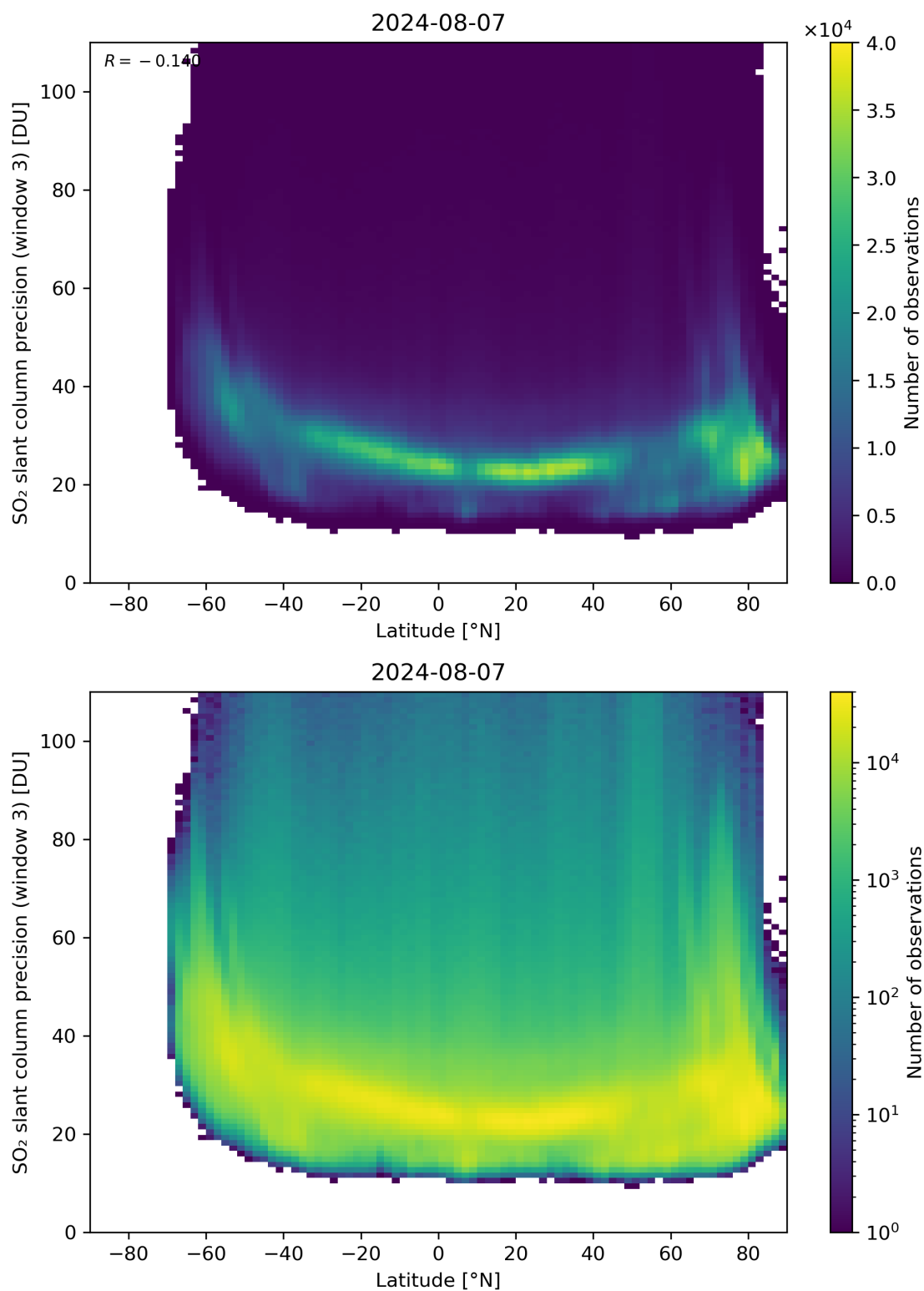
Figure 153: Scatter density plot of “Latitude” against “SO 2 slant column precision (window 3)” for 2024-08-06 to 2024-08-08.
