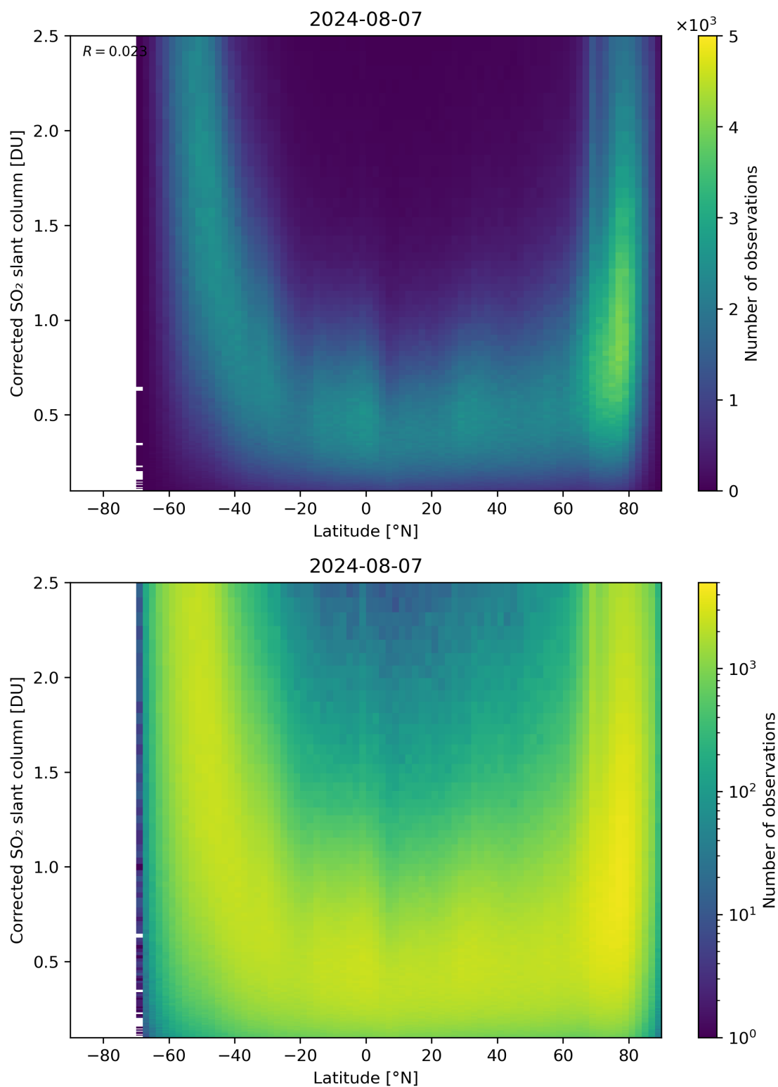
Figure 146: Scatter density plot of “Latitude” against “Corrected SO 2 slant column” for 2024-08-06 to 2024-08-08.
