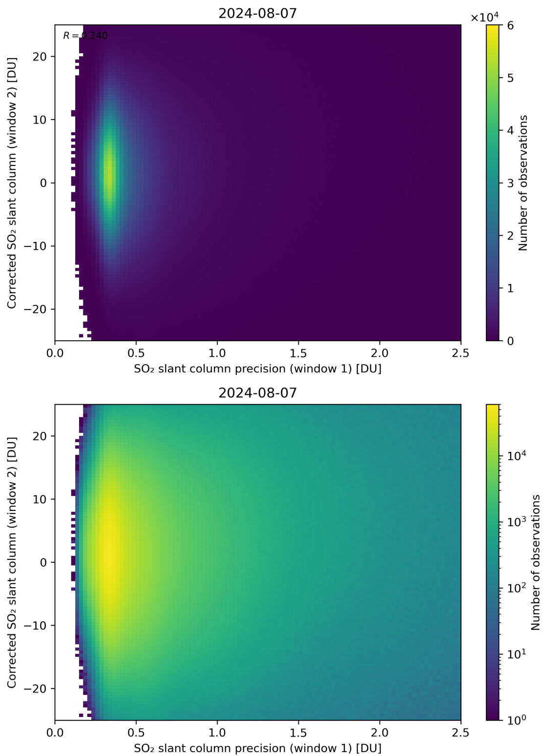
Figure 225: Scatter density plot of “SO 2 slant column precision (window 1)” against “Corrected SO 2 slant column (window 2)” for 2024-08-06 to 2024-08-08.
