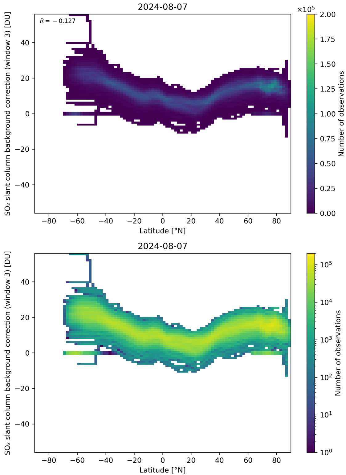
Figure 141: Scatter density plot of “Latitude” against “SO 2 slant column background correction (window 3)” for 2024-08-06 to 2024-08-08.
