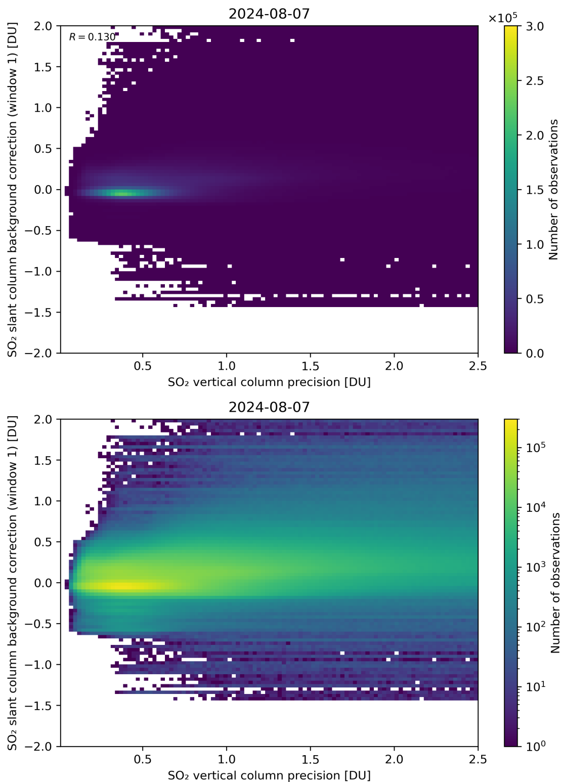
Figure 279: Scatter density plot of “SO 2 vertical column precision” against “SO 2 slant column background correction (window 1)” for 2024-08-06 to 2024-08-08.
