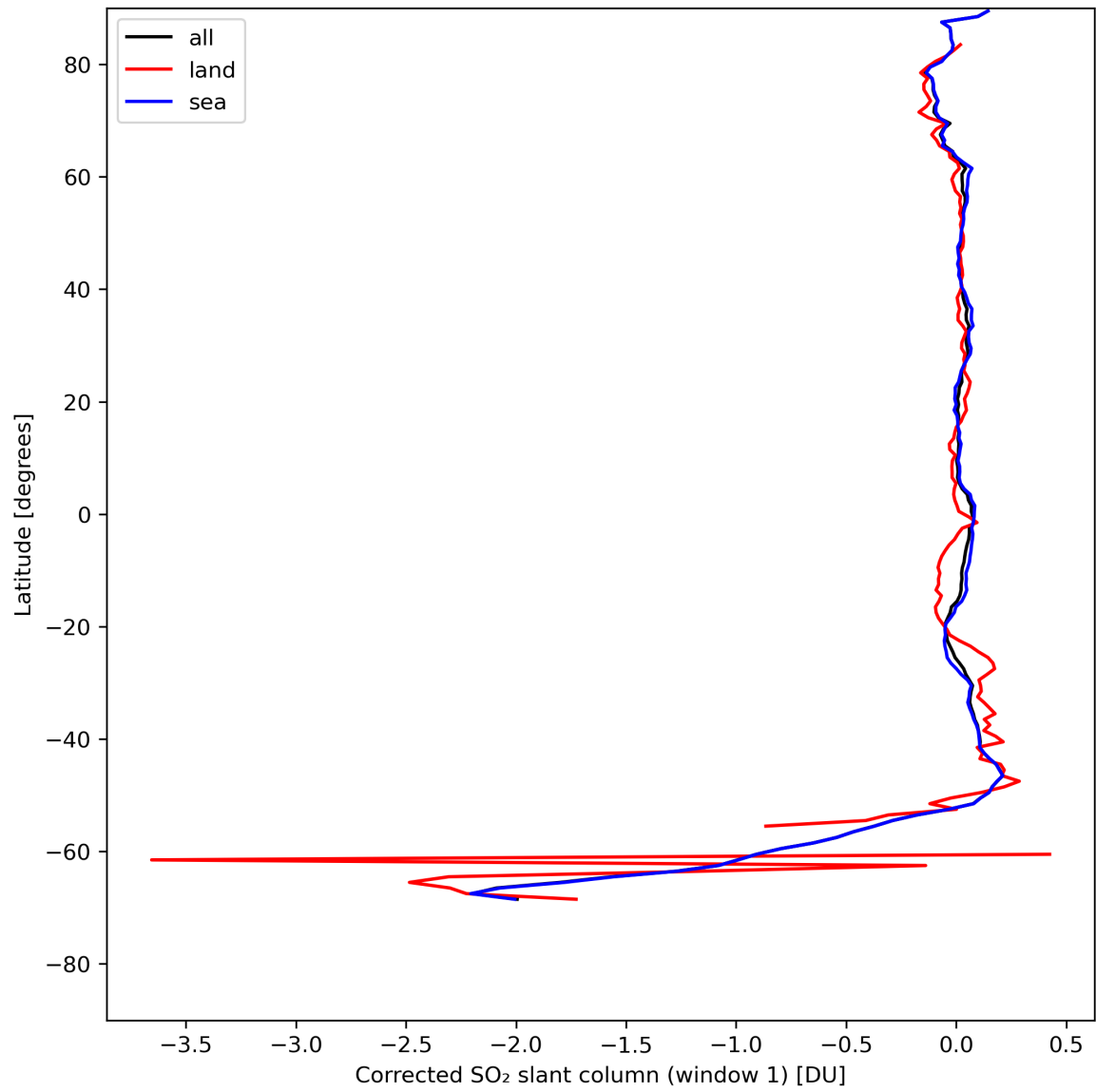
Figure 35: Zonal average of “Corrected SO 2 slant column (window 1)” for 2024-08-06 to 2024-08-08.
