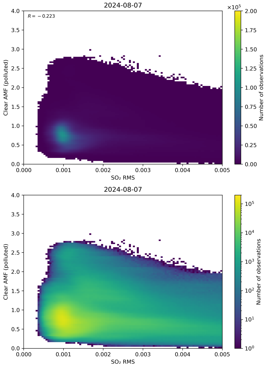
Figure 136: Scatter density plot of “SO 2 RMS” against “Clear AMF (polluted)” for 2024-08-06 to 2024-08-08.
