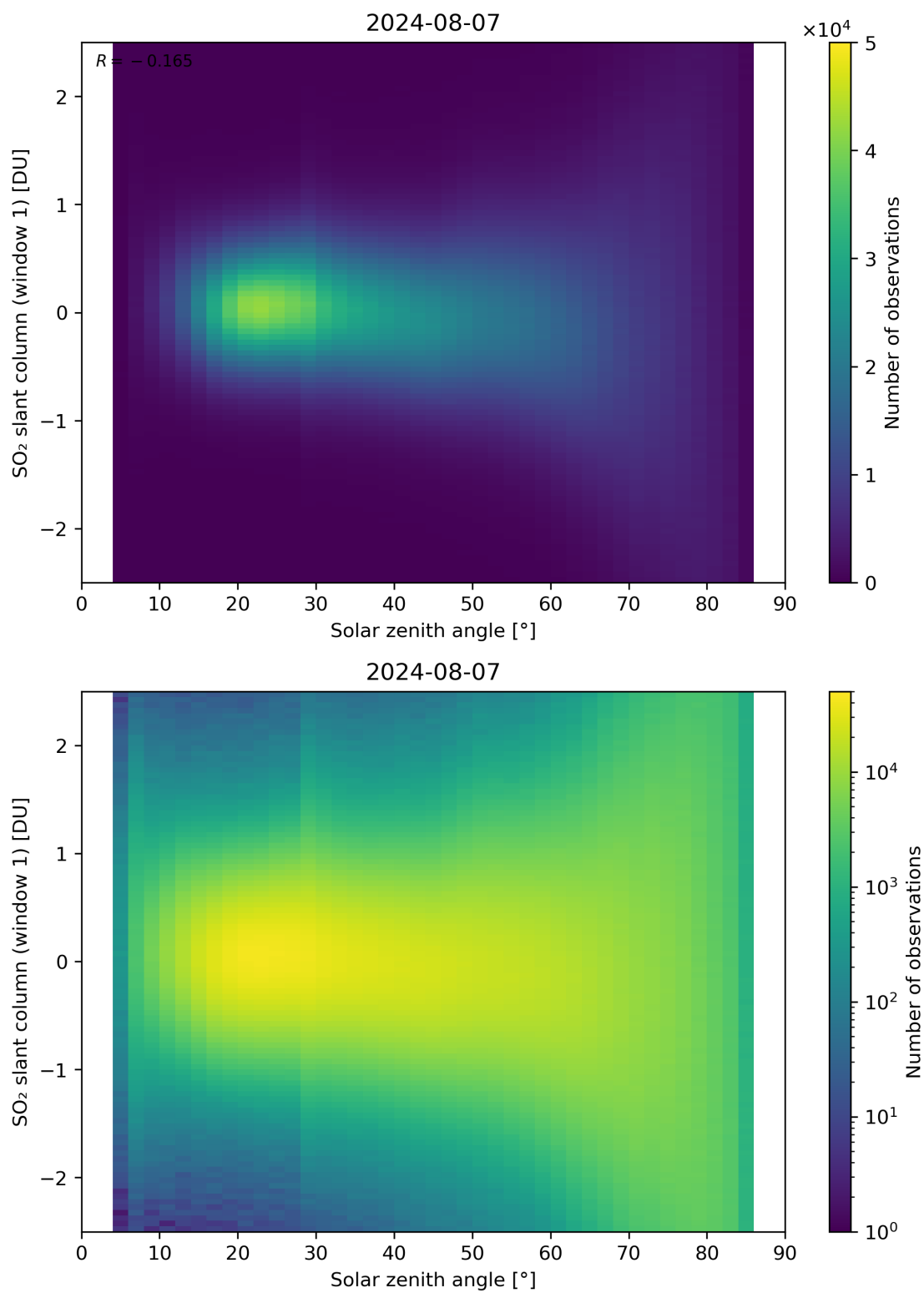
Figure 169: Scatter density plot of “Solar zenith angle” against “SO 2 slant column (window 1)” for 2024-08-06 to 2024-08-08.
