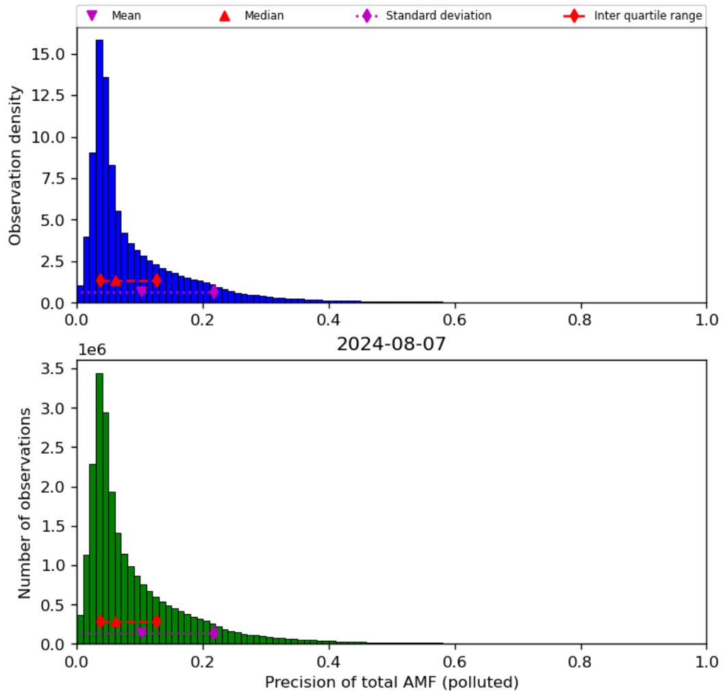
Figure 72: Histogram of “Precision of total AMF (polluted)” for 2024-08-06 to 2024-08-08
