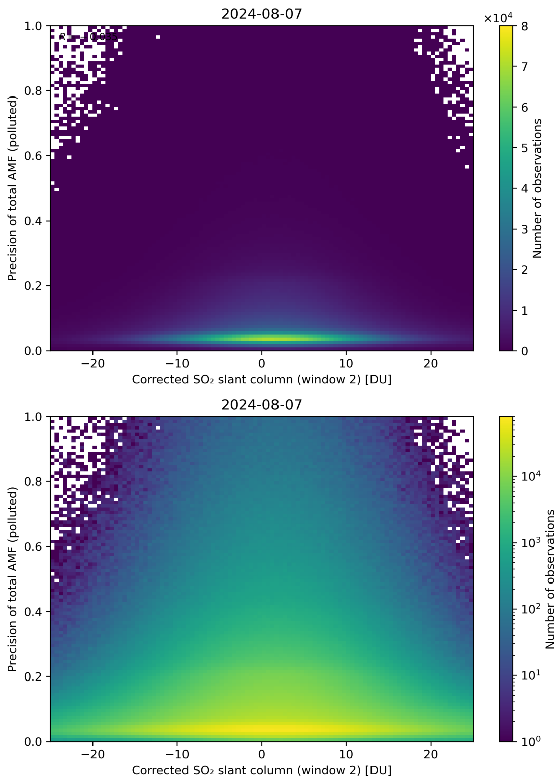
Figure 204: Scatter density plot of “Corrected SO 2 slant column (window 2)” against “Precision of total AMF (polluted)” for 2024-08-06 to 2024-08-08.
