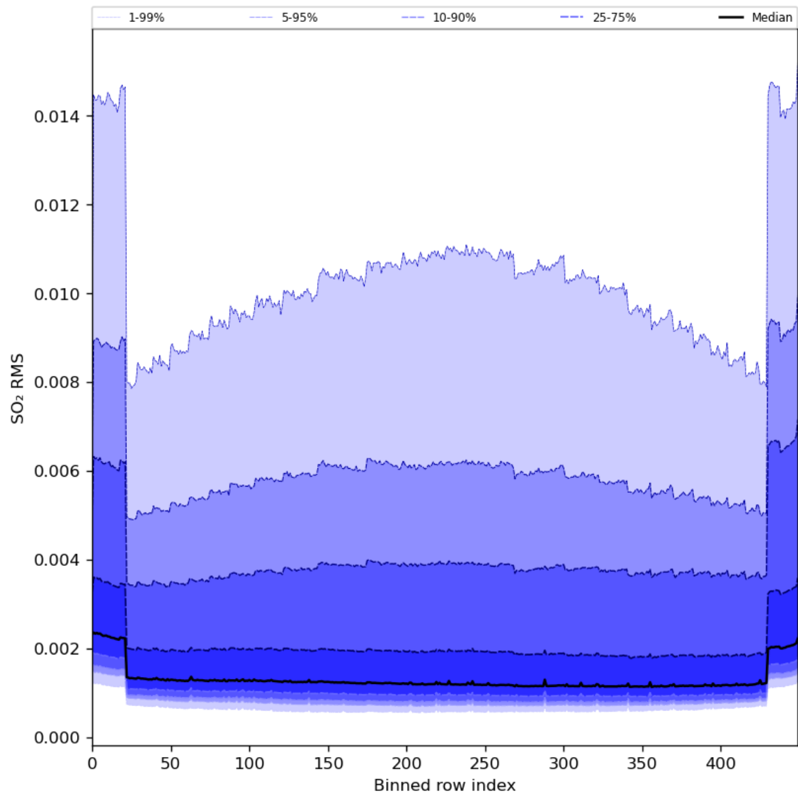
Figure 93: Along track statistics of “SO 2 RMS” for 2024-08-06 to 2024-08-08
