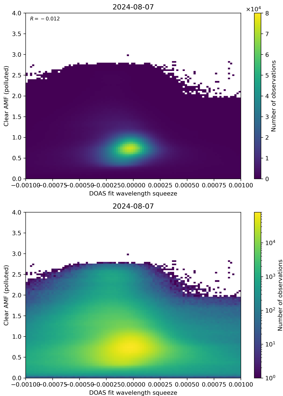
Figure 133: Scatter density plot of “DOAS fit wavelength squeeze” against “Clear AMF (polluted)” for 2024-08-06 to 2024-08-08.
