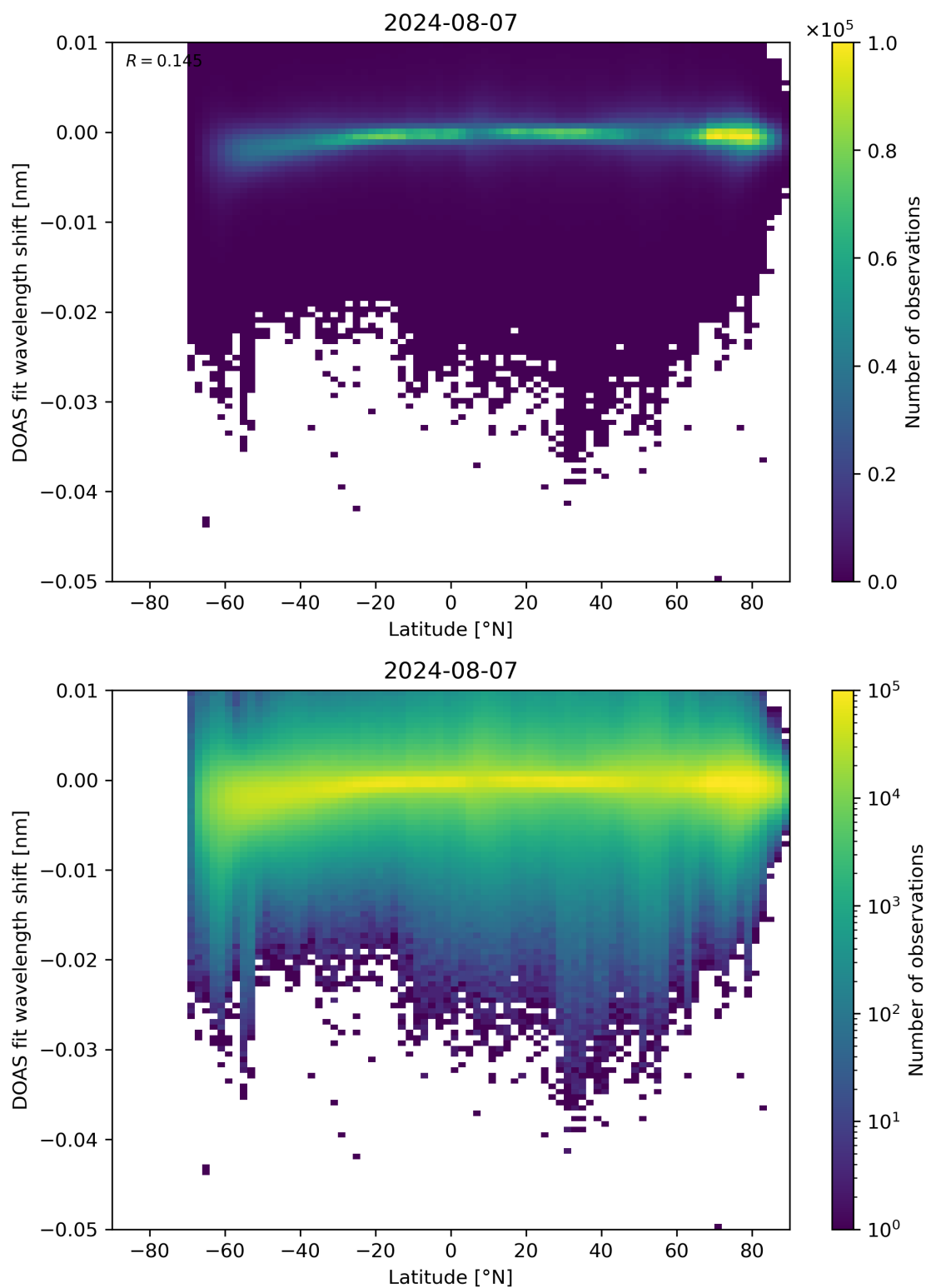
Figure 142: Scatter density plot of “Latitude” against “DOAS fit wavelength shift” for 2024-08-06 to 2024-08-08.
