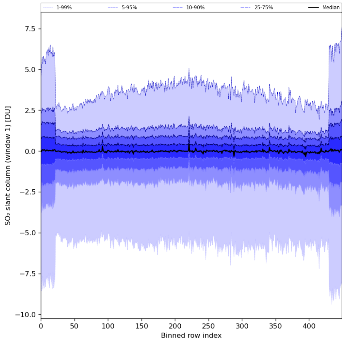
Figure 79: Along track statistics of “SO 2 slant column (window 1)” for 2024-08-06 to 2024-08-08
