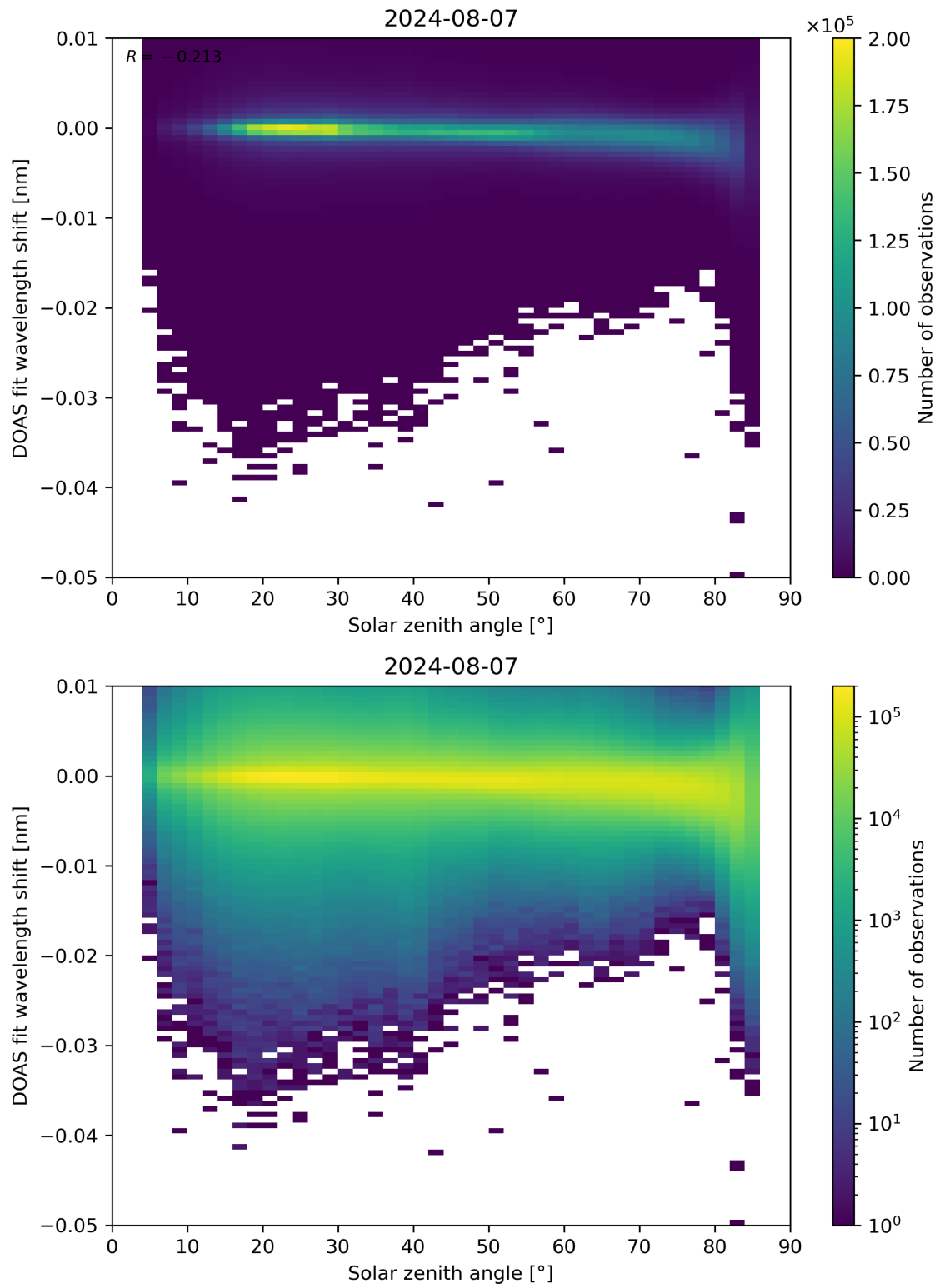
Figure 161: Scatter density plot of “Solar zenith angle” against “DOAS fit wavelength shift” for 2024-08-06 to 2024-08-08.
