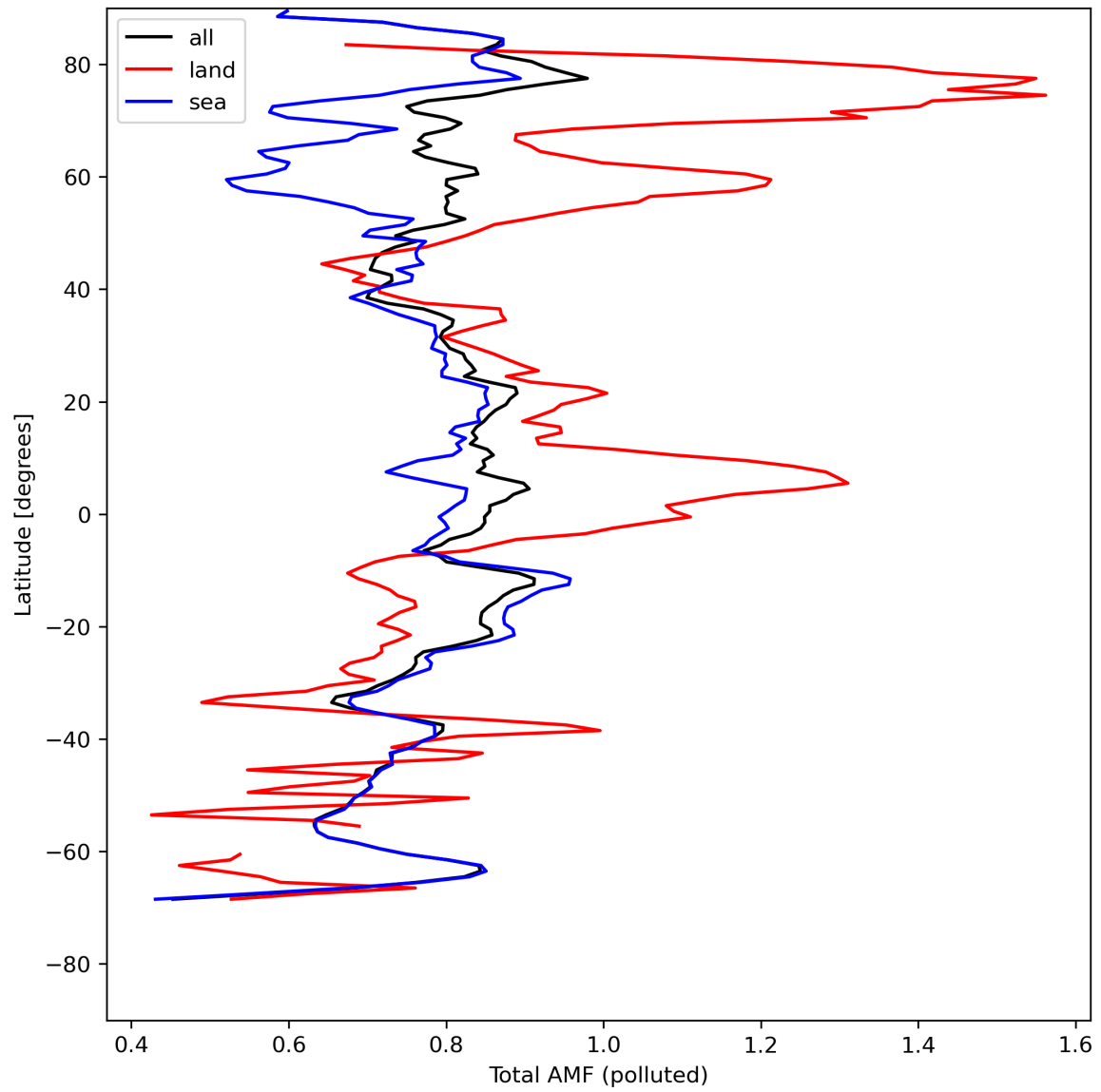
Figure 48: Zonal average of “Total AMF (polluted)” for 2024-08-06 to 2024-08-08.
