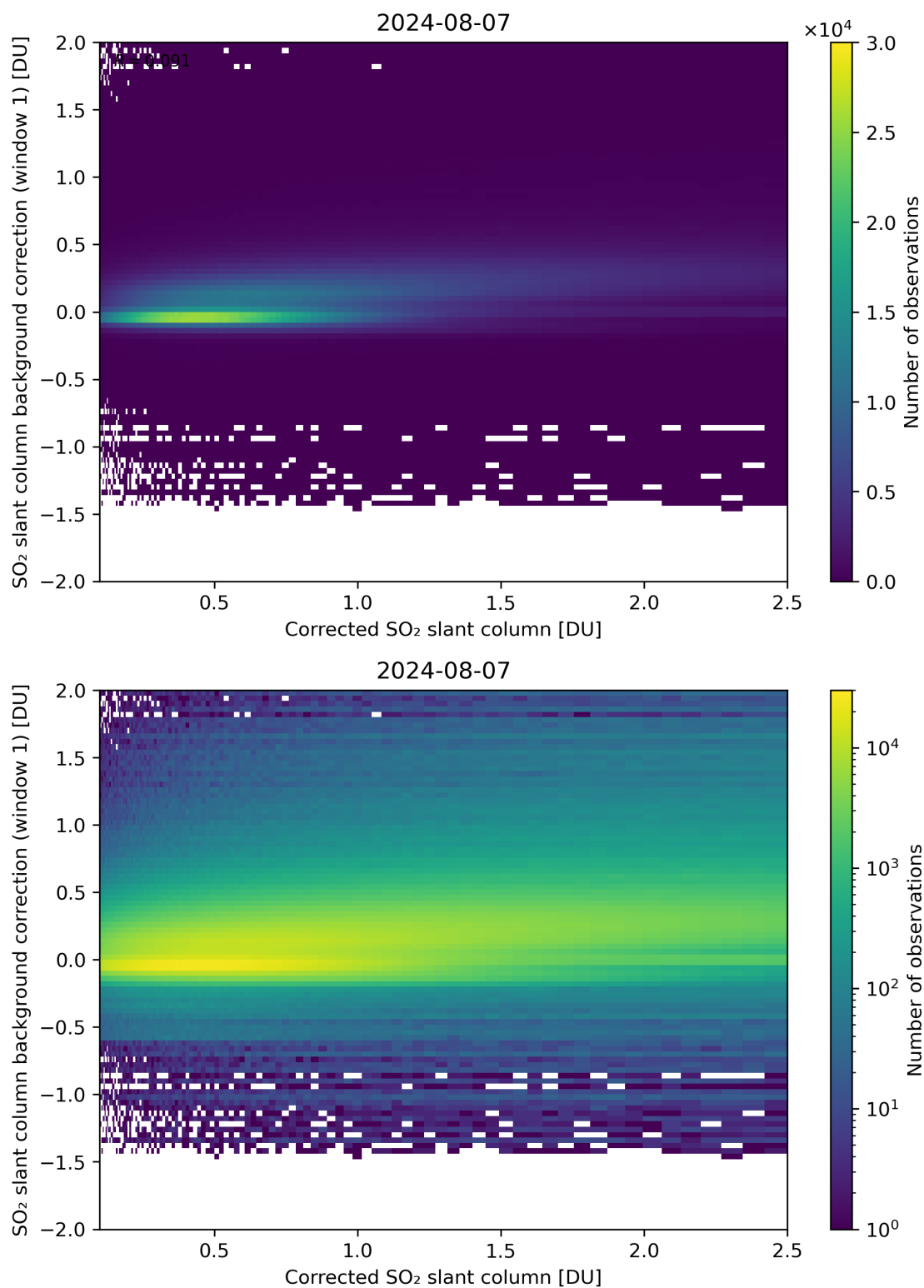
Figure 178: Scatter density plot of “Corrected SO 2 slant column” against “SO 2 slant column background correction (window 1)” for 2024-08-06 to 2024-08-08.
