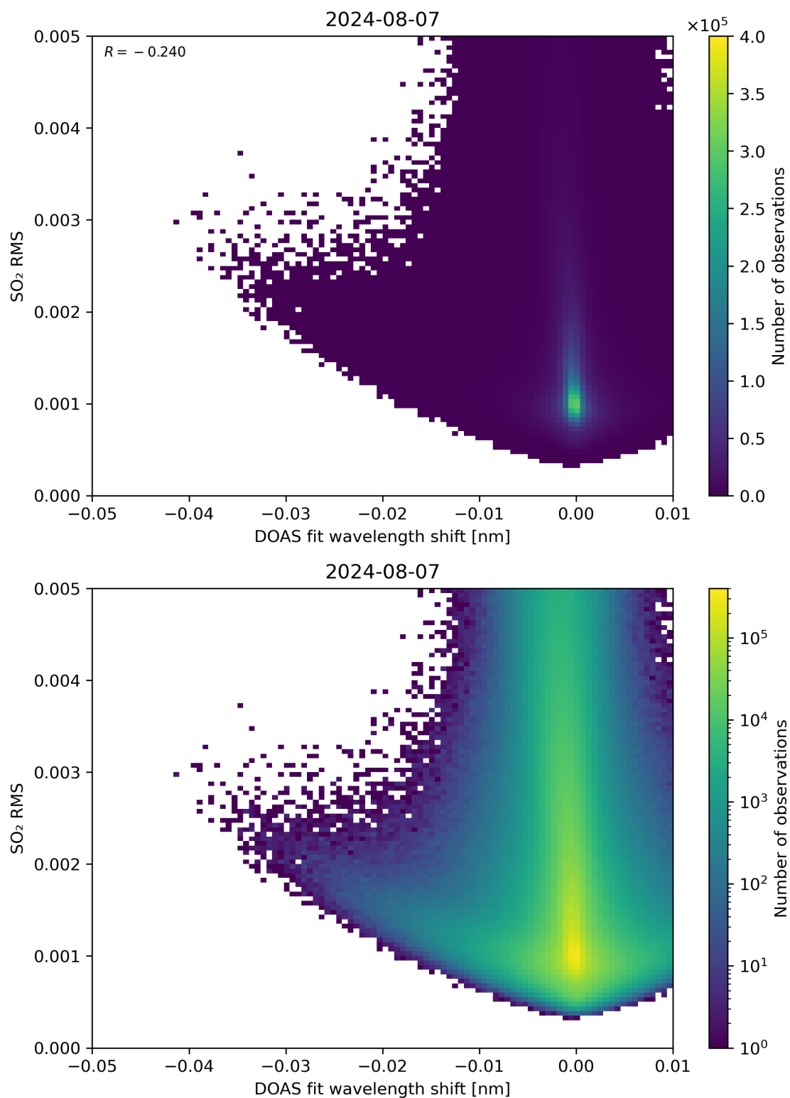
Figure 128: Scatter density plot of “DOAS fit wavelength shift” against “SO 2 RMS” for 2024-08-06 to 2024-08-08.
