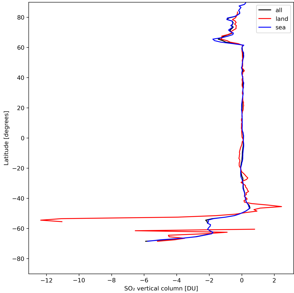
Figure 30: Zonal average of “SO 2 vertical column” for 2024-08-06 to 2024-08-08.
