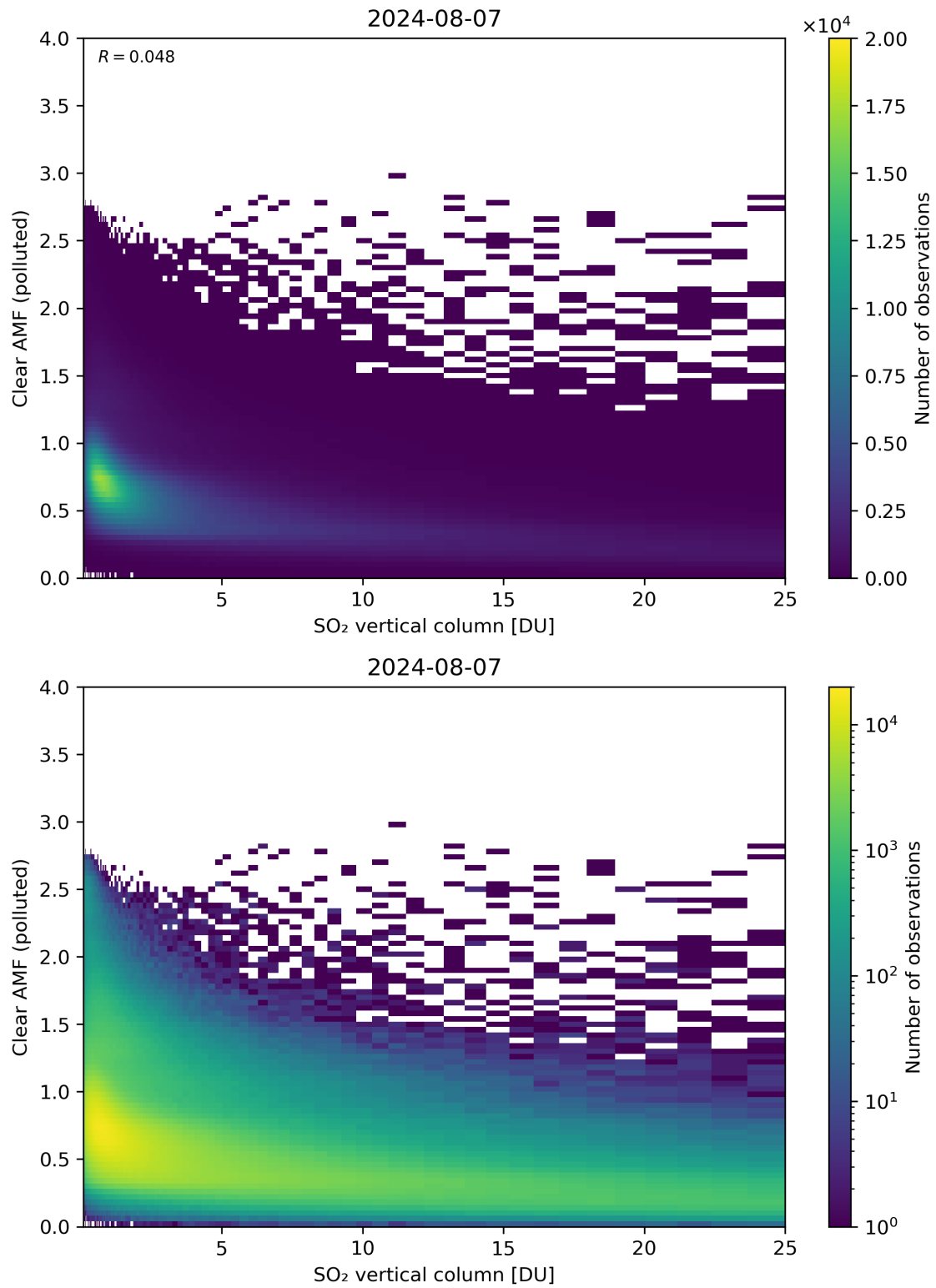
Figure 296: Scatter density plot of “SO 2 vertical column” against “Clear AMF (polluted)” for 2024-08-06 to 2024-08-08.
