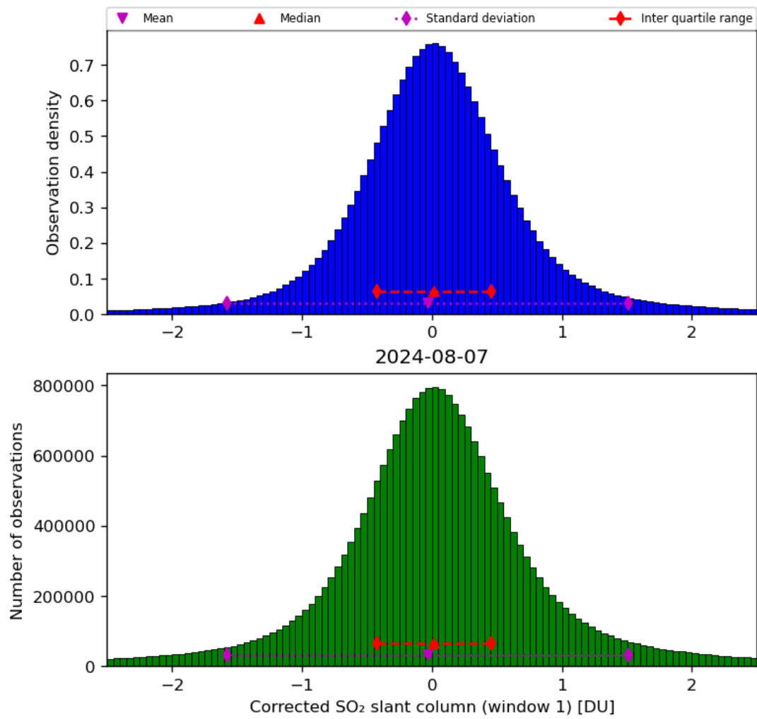
Figure 58: Histogram of “Corrected SO 2 slant column (window 1)” for 2024-08-06 to 2024-08-08
