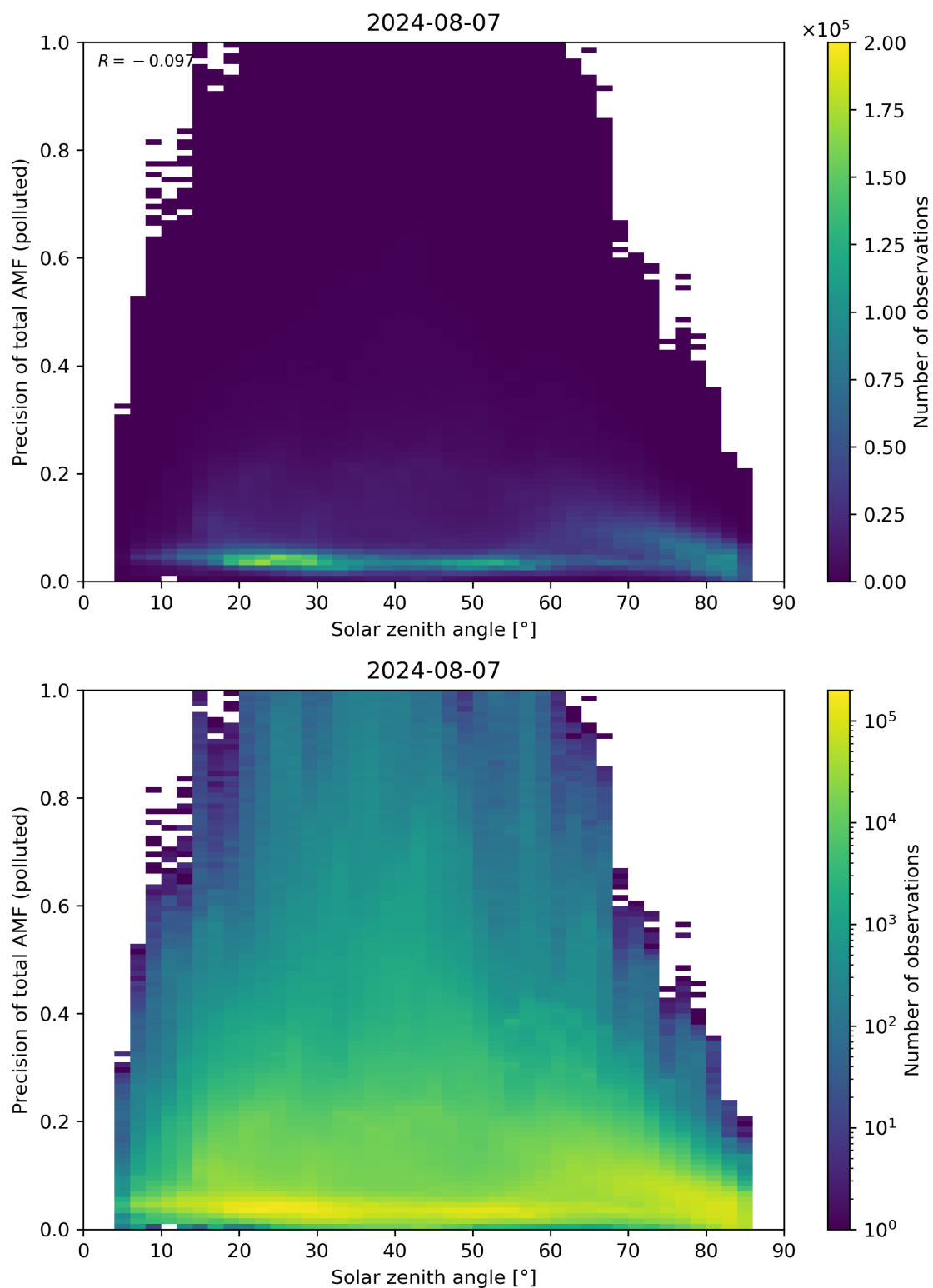
Figure 175: Scatter density plot of “Solar zenith angle” against “Precision of total AMF (polluted)” for 2024-08-06 to 2024-08-08.
