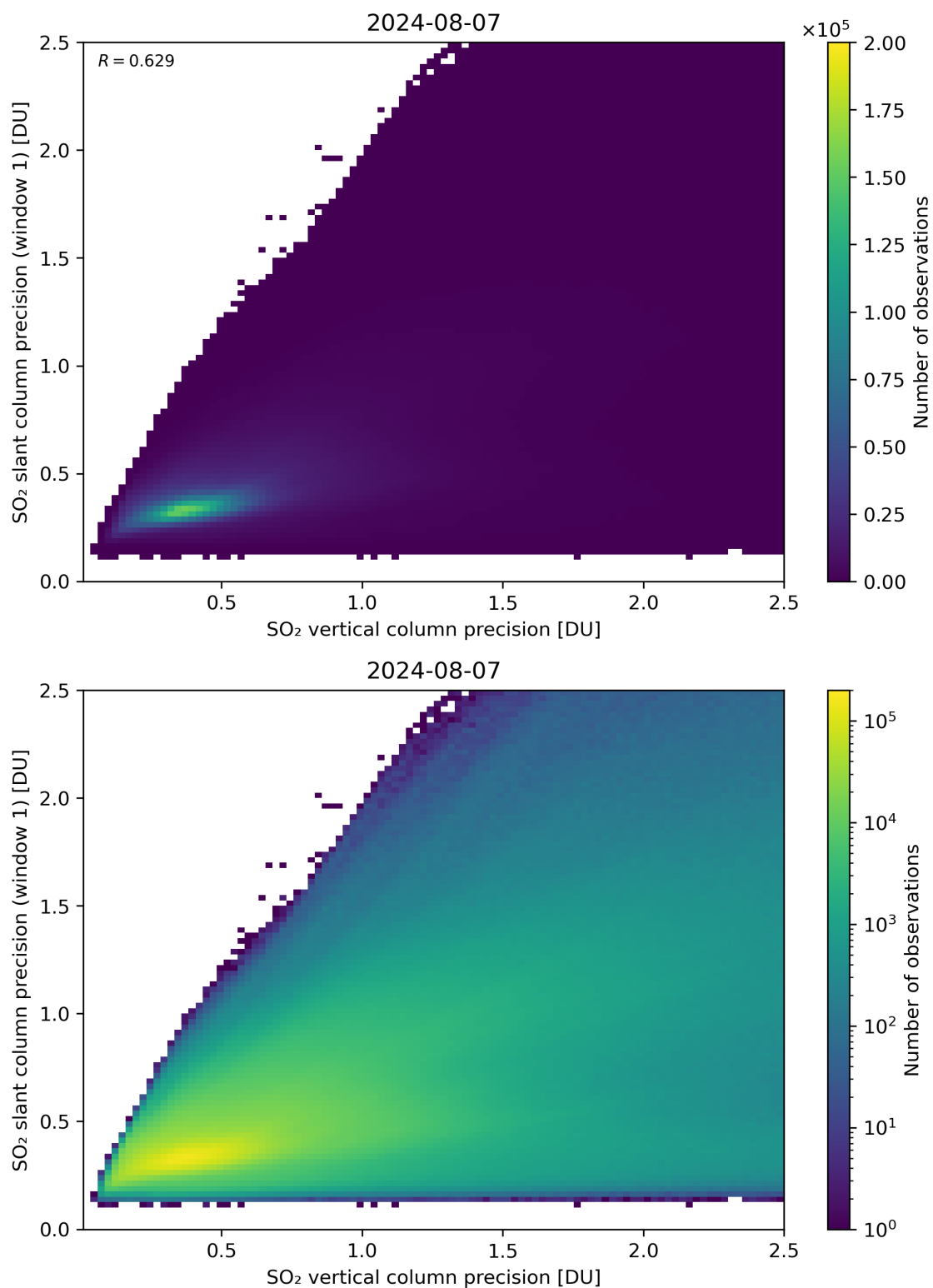
Figure 290: Scatter density plot of “SO 2 vertical column precision” against “SO 2 slant column precision (window 1)” for 2024-08-06 to 2024-08-08.
