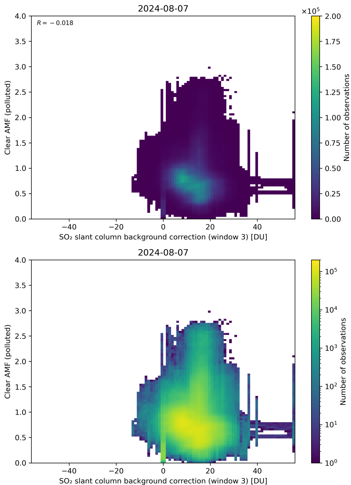
Figure 124: Scatter density plot of “SO 2 slant column background correction (window 3)” against “Clear AMF (polluted)” for 2024-08-06 to 2024-08-08.
