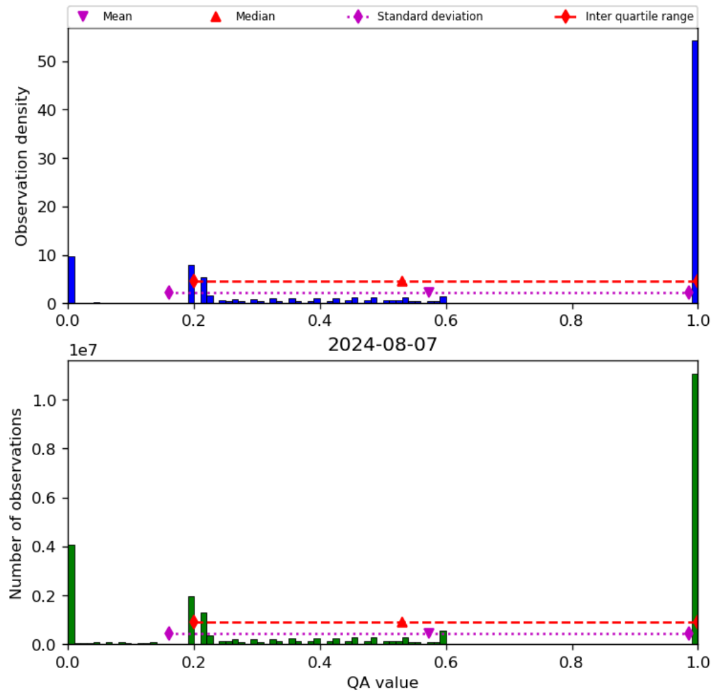
Figure 52: Histogram of “QA value” for 2024-08-06 to 2024-08-08
