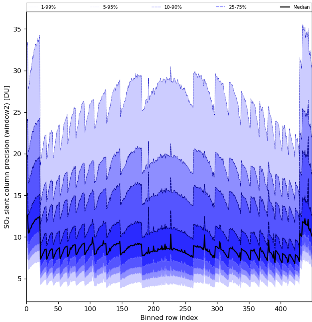
Figure 84: Along track statistics of “SO 2 slant column precision (window2)” for 2024-08-06 to 2024-08-08
