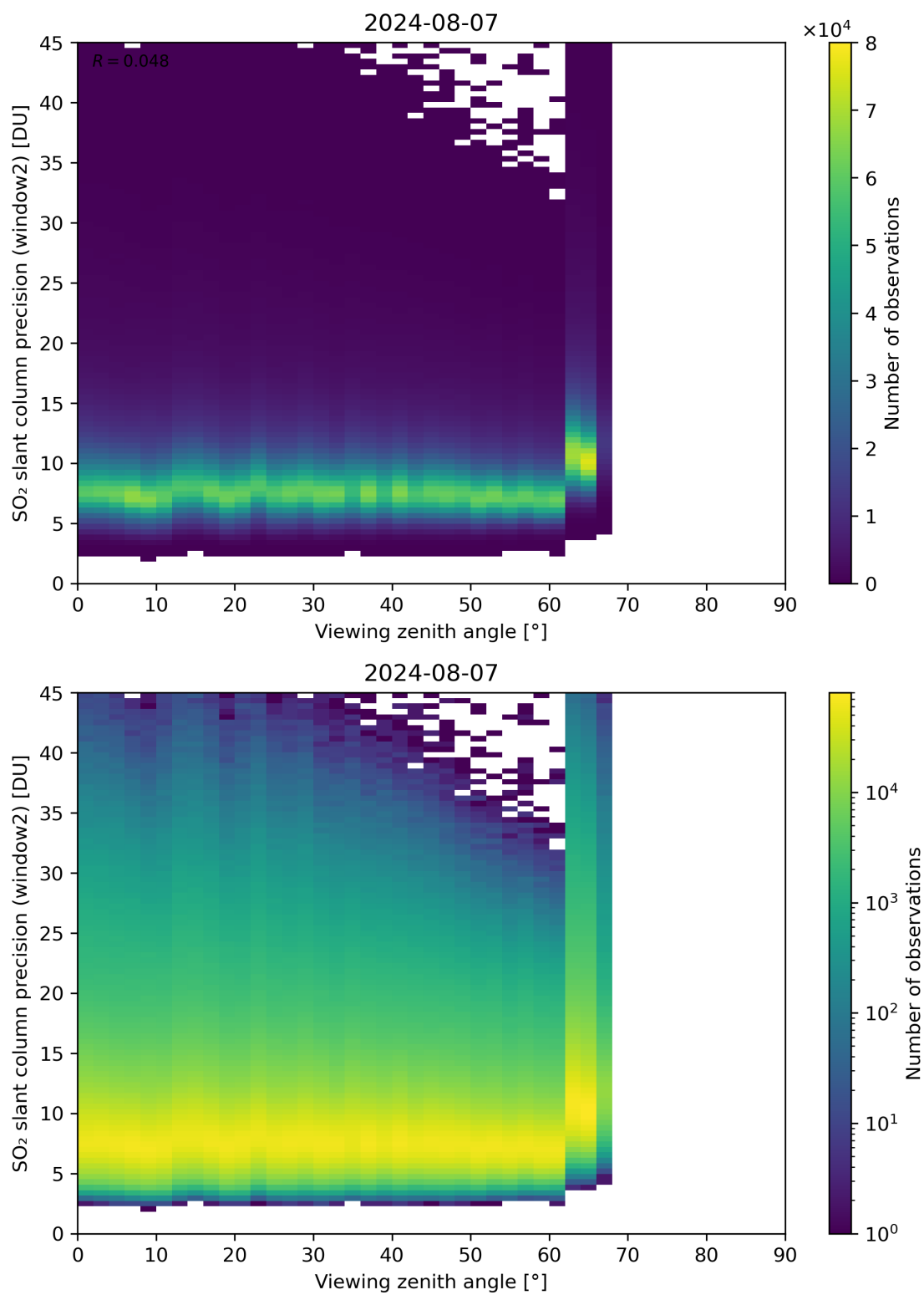
Figure 322: Scatter density plot of “Viewing zenith angle” against “SO 2 slant column precision (window2)” for 2024-08-06 to 2024-08-08.
