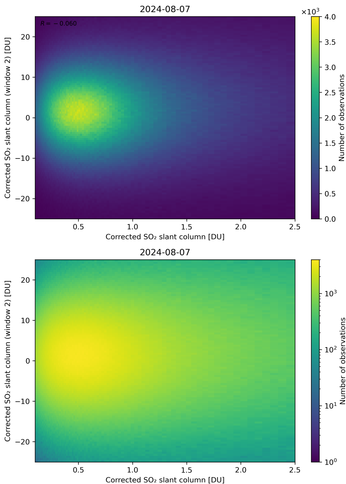
Figure 185: Scatter density plot of “Corrected SO 2 slant column” against “Corrected SO 2 slant column (window 2)” for 2024-08-06 to 2024-08-08.
