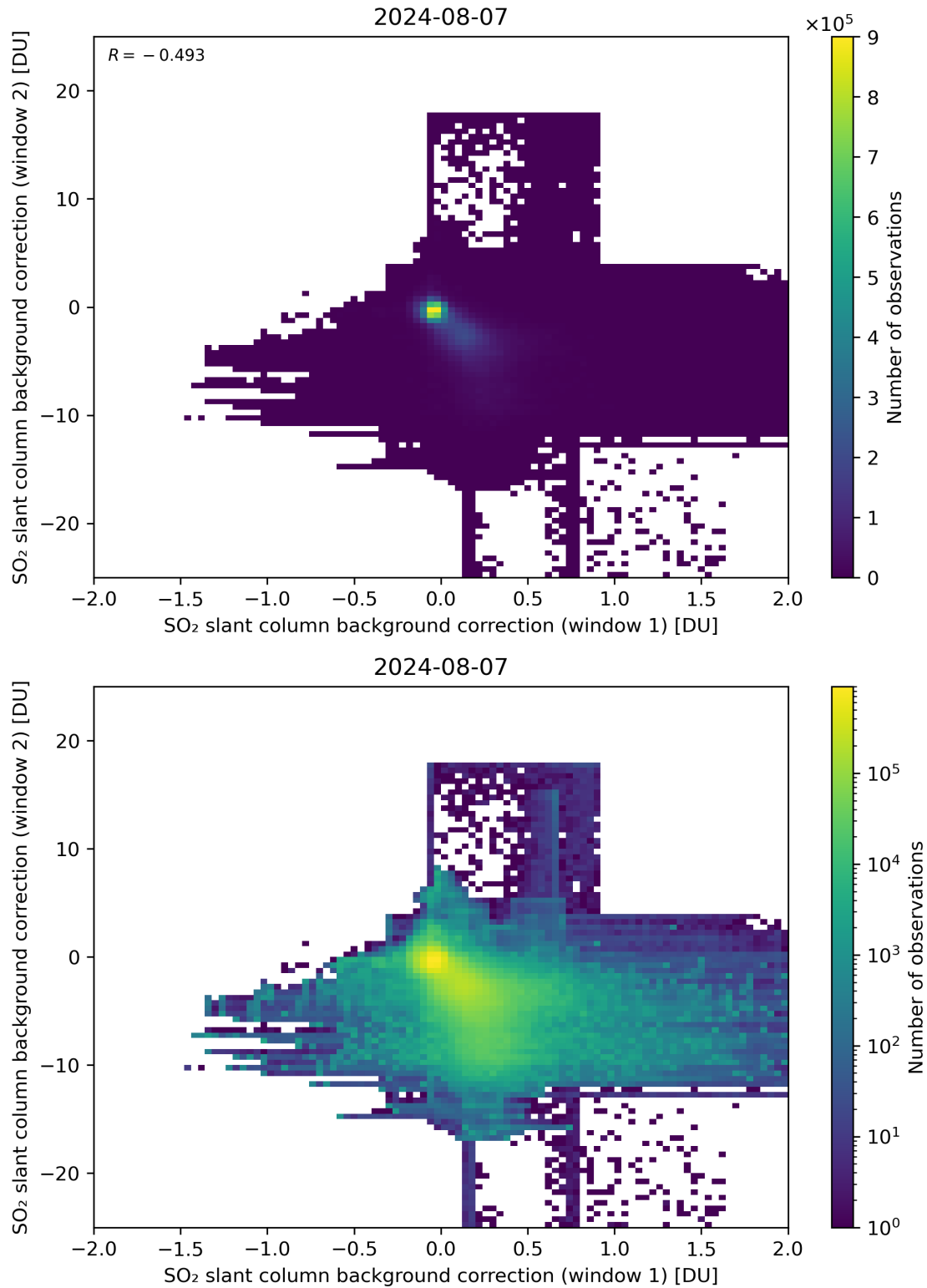
Figure 98: Scatter density plot of “SO 2 slant column background correction (window 1)” against “SO 2 slant column background correction (window 2)” for 2024-08-06 to 2024-08-08.
