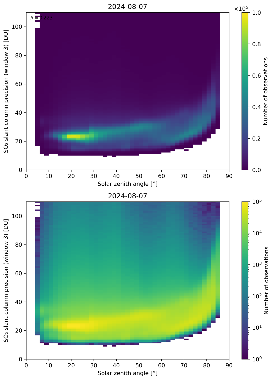
Figure 173: Scatter density plot of “Solar zenith angle” against “SO 2 slant column precision (window 3)” for 2024-08-06 to 2024-08-08.
