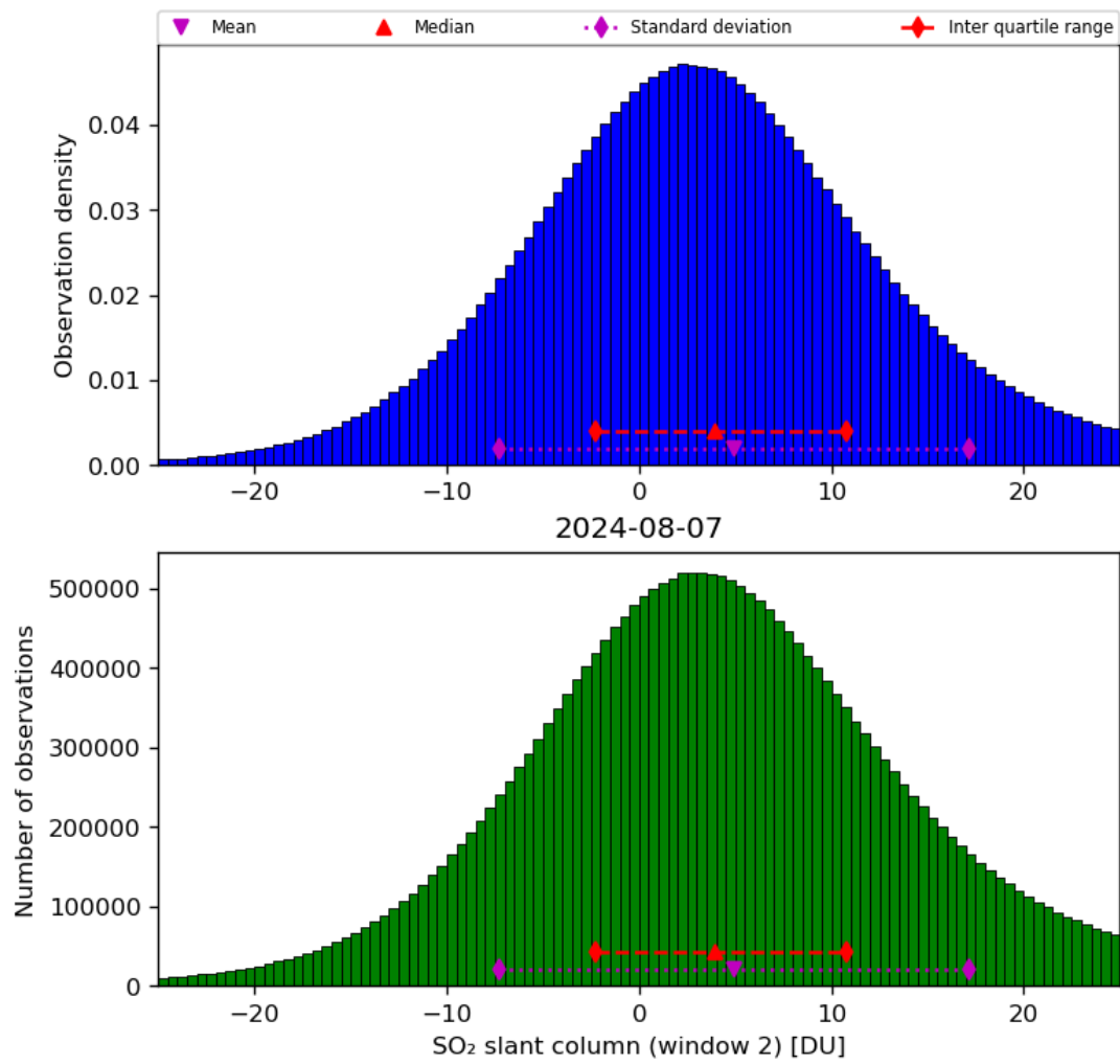
Figure 60: Histogram of “SO 2 slant column (window 2)” for 2024-08-06 to 2024-08-08
