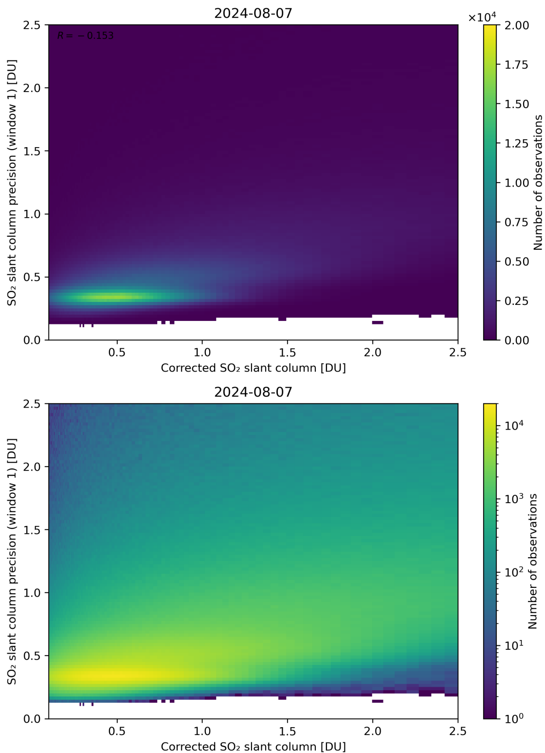
Figure 188: Scatter density plot of “Corrected SO 2 slant column” against “SO 2 slant column precision (window 1)” for 2024-08-06 to 2024-08-08.
