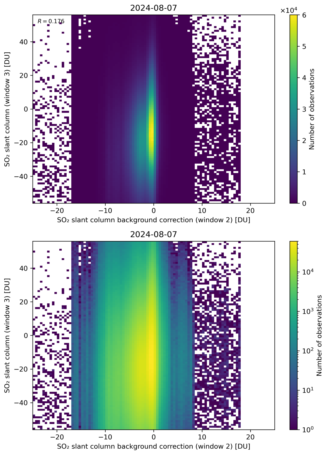
Figure 117: Scatter density plot of “SO 2 slant column background correction (window 2)” against “SO 2 slant column (window 3)” for 2024-08-06 to 2024-08-08.
