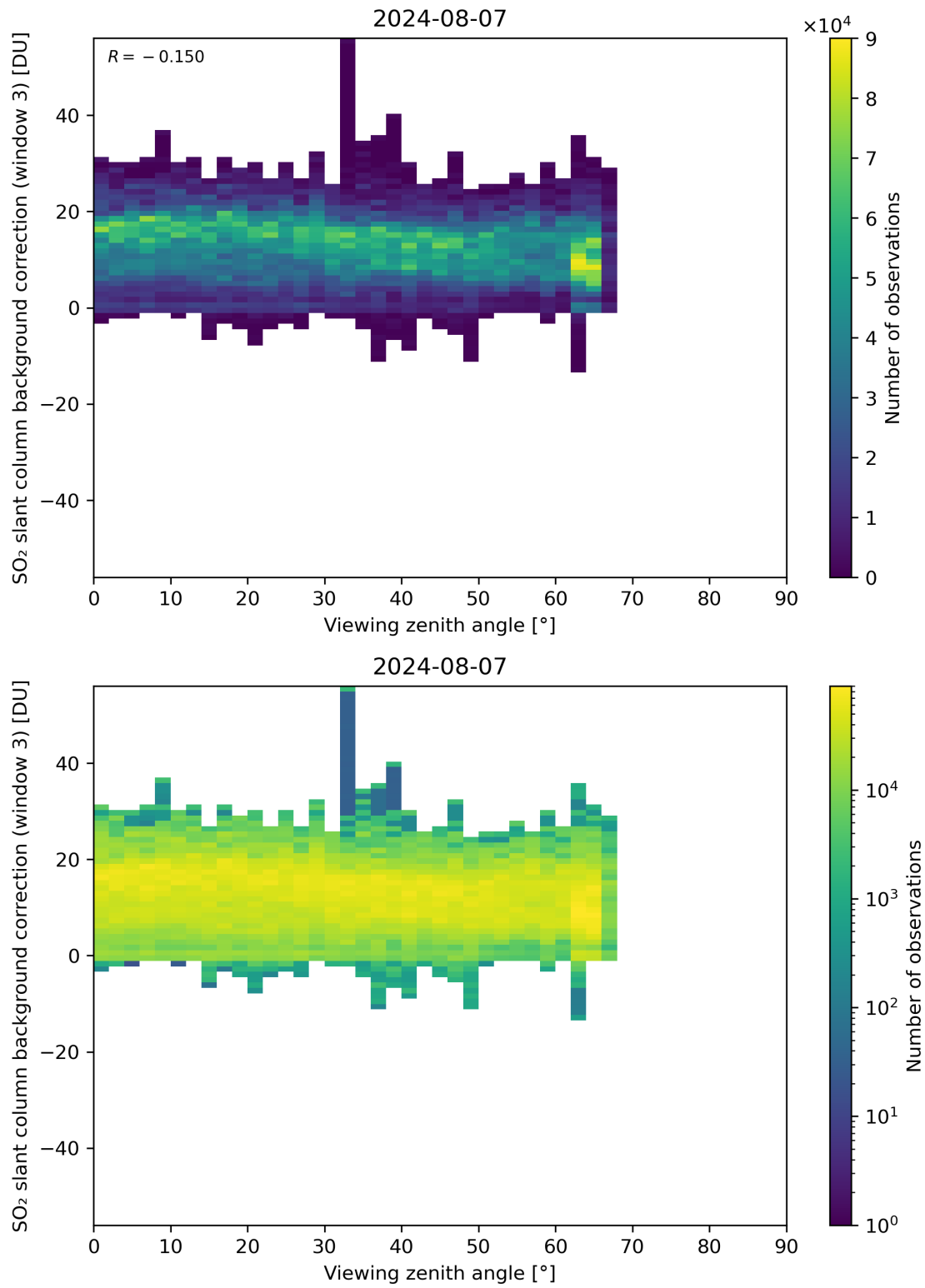
Figure 310: Scatter density plot of “Viewing zenith angle” against “SO 2 slant column background correction (window 3)” for 2024-08-06 to 2024-08-08.
