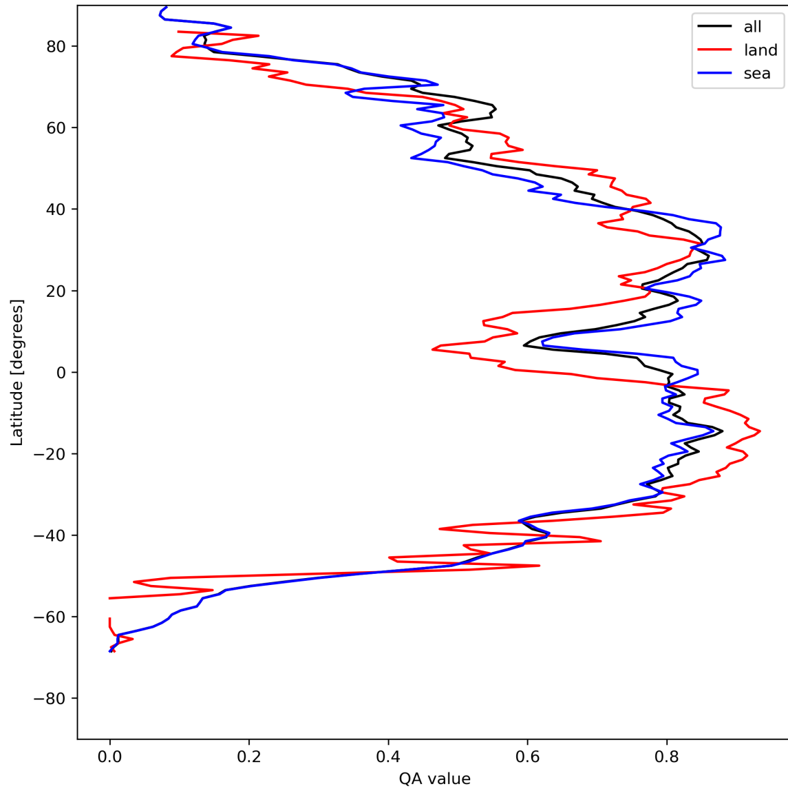
Figure 29: Zonal average of “QA value” for 2024-08-06 to 2024-08-08.
