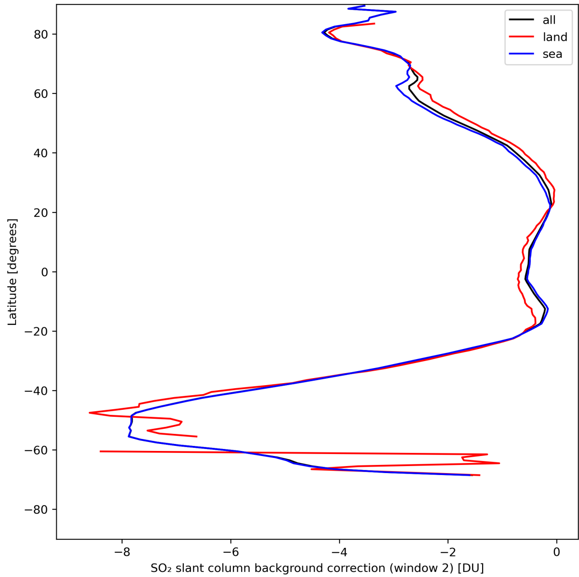
Figure 40: Zonal average of "SO 2 slant column background correction (window 2)" for 2024-08-06 to 2024-08-08.
