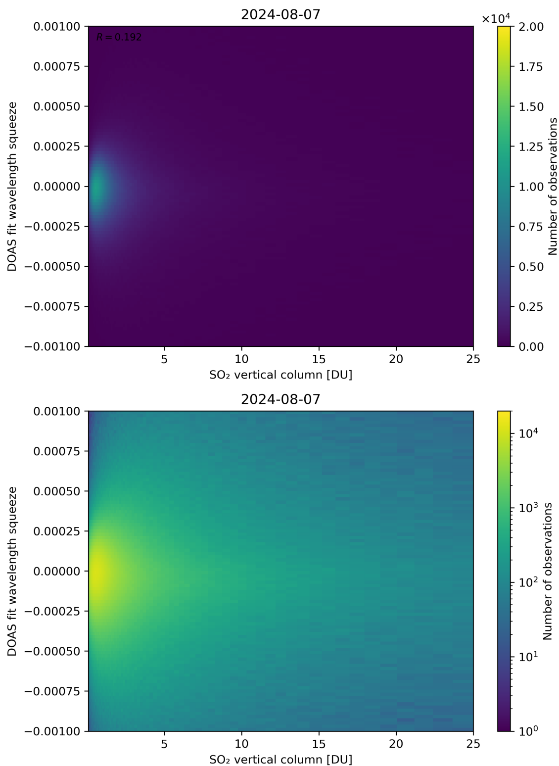
Figure 277: Scatter density plot of “SO 2 vertical column” against “DOAS fit wavelength squeeze” for 2024-08-06 to 2024-08-08.
