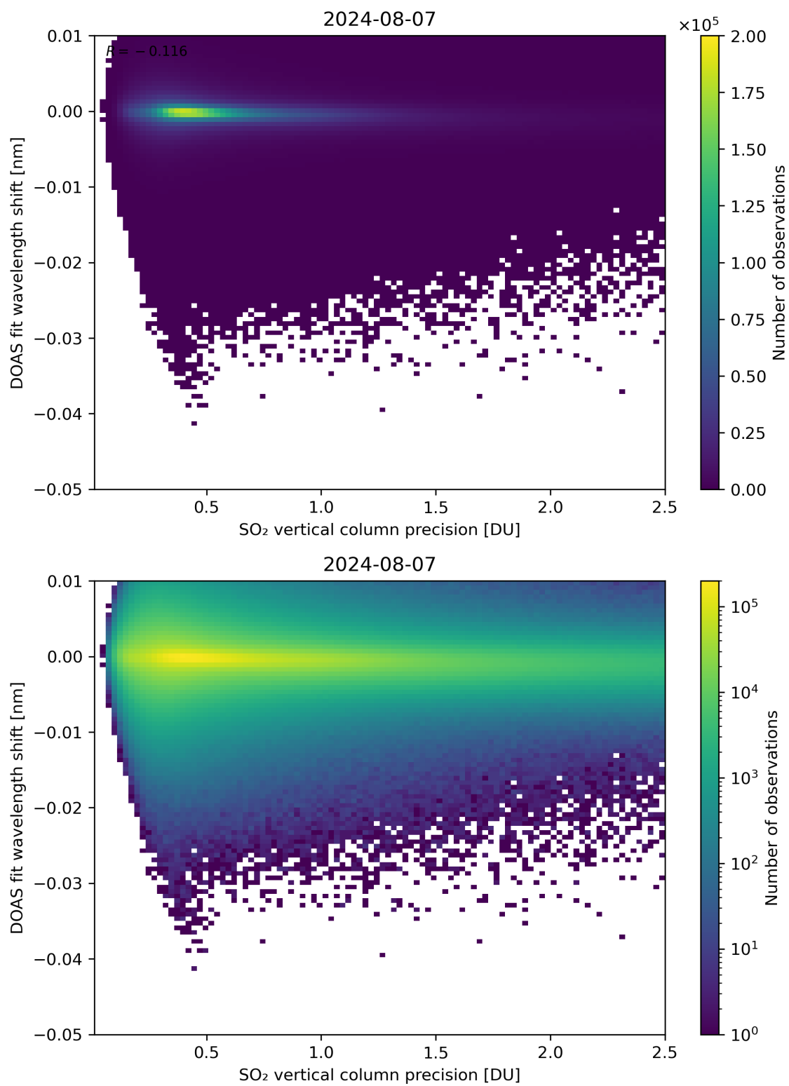
Figure 282: Scatter density plot of “SO 2 vertical column precision” against “DOAS fit wavelength shift” for 2024-08-06 to 2024-08-08.
