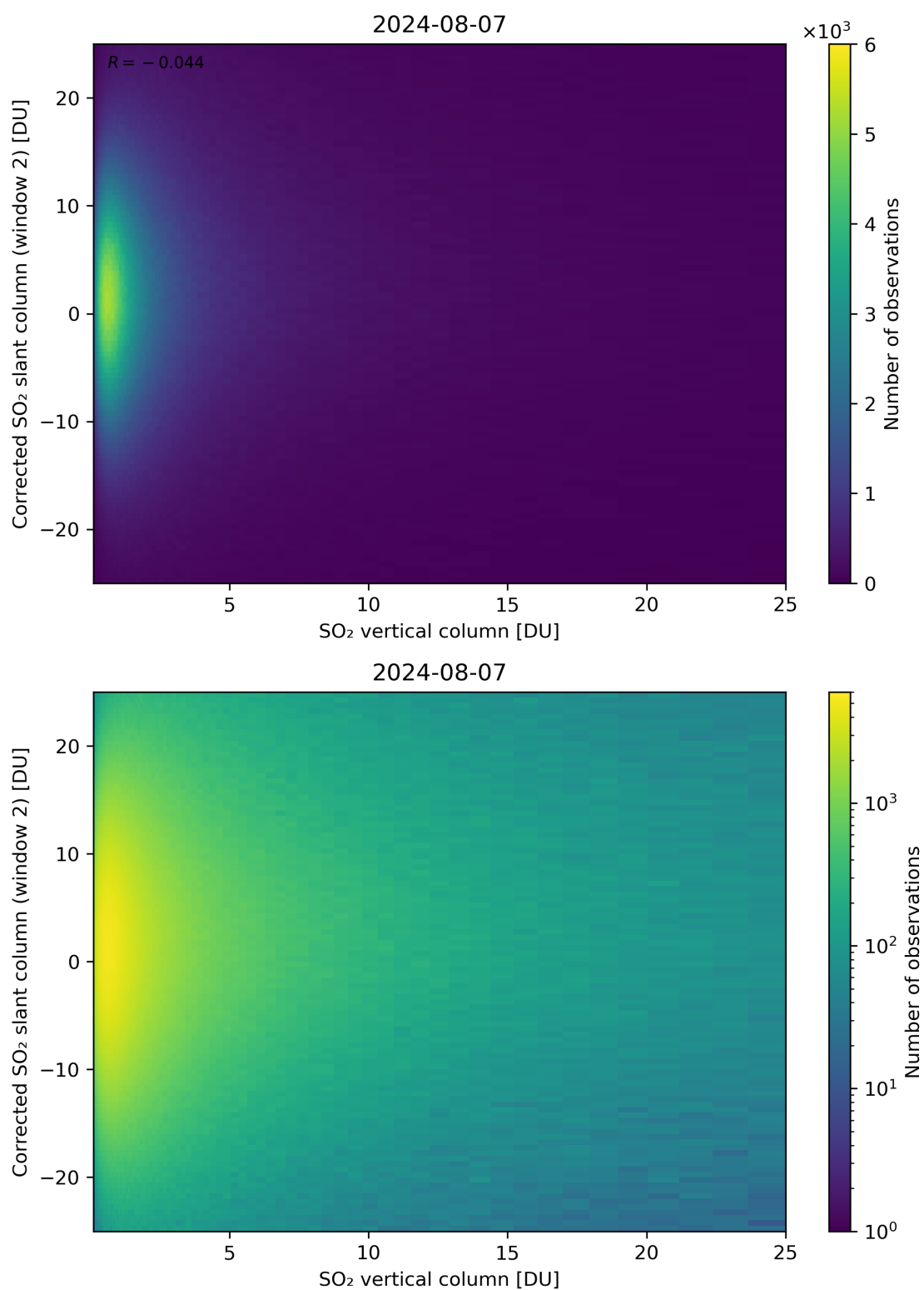
Figure 298: Scatter density plot of “SO 2 vertical column” against “Corrected SO 2 slant column (window 2)” for 2024-08-06 to 2024-08-08.
