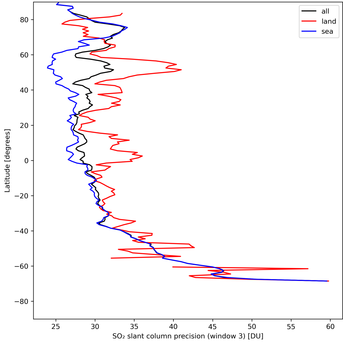
Figure 42: Zonal average of “SO 2 slant column precision (window 3)” for 2024-08-06 to 2024-08-08.
