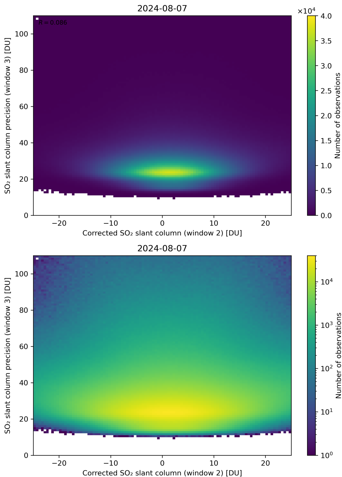
Figure 202: Scatter density plot of “Corrected SO 2 slant column (window 2)” against “SO 2 slant column precision (window 3)” for 2024-08-06 to 2024-08-08.
