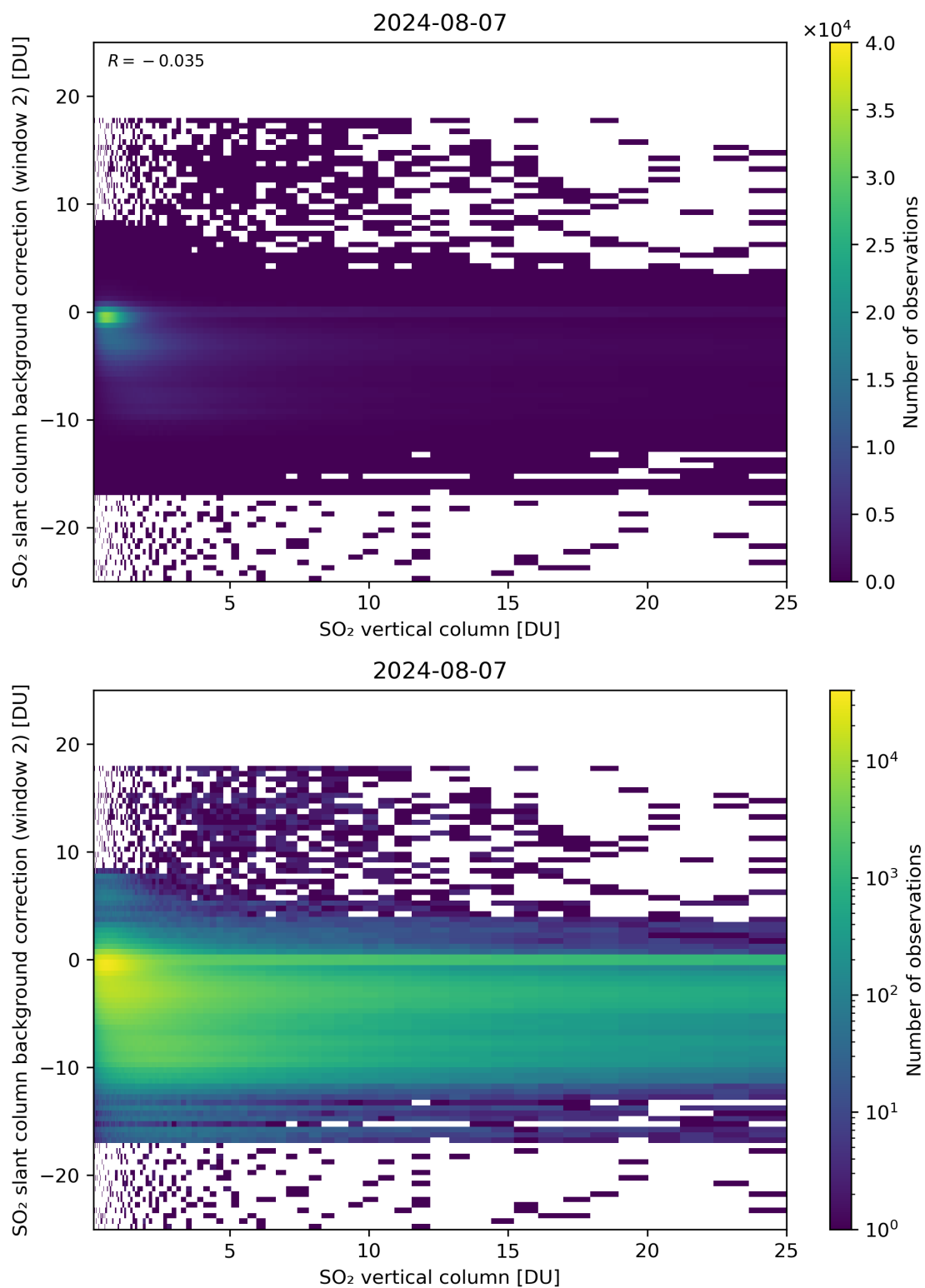
Figure 274: Scatter density plot of “SO 2 vertical column” against “SO 2 slant column background correction (window 2)” for 2024-08-06 to 2024-08-08.
