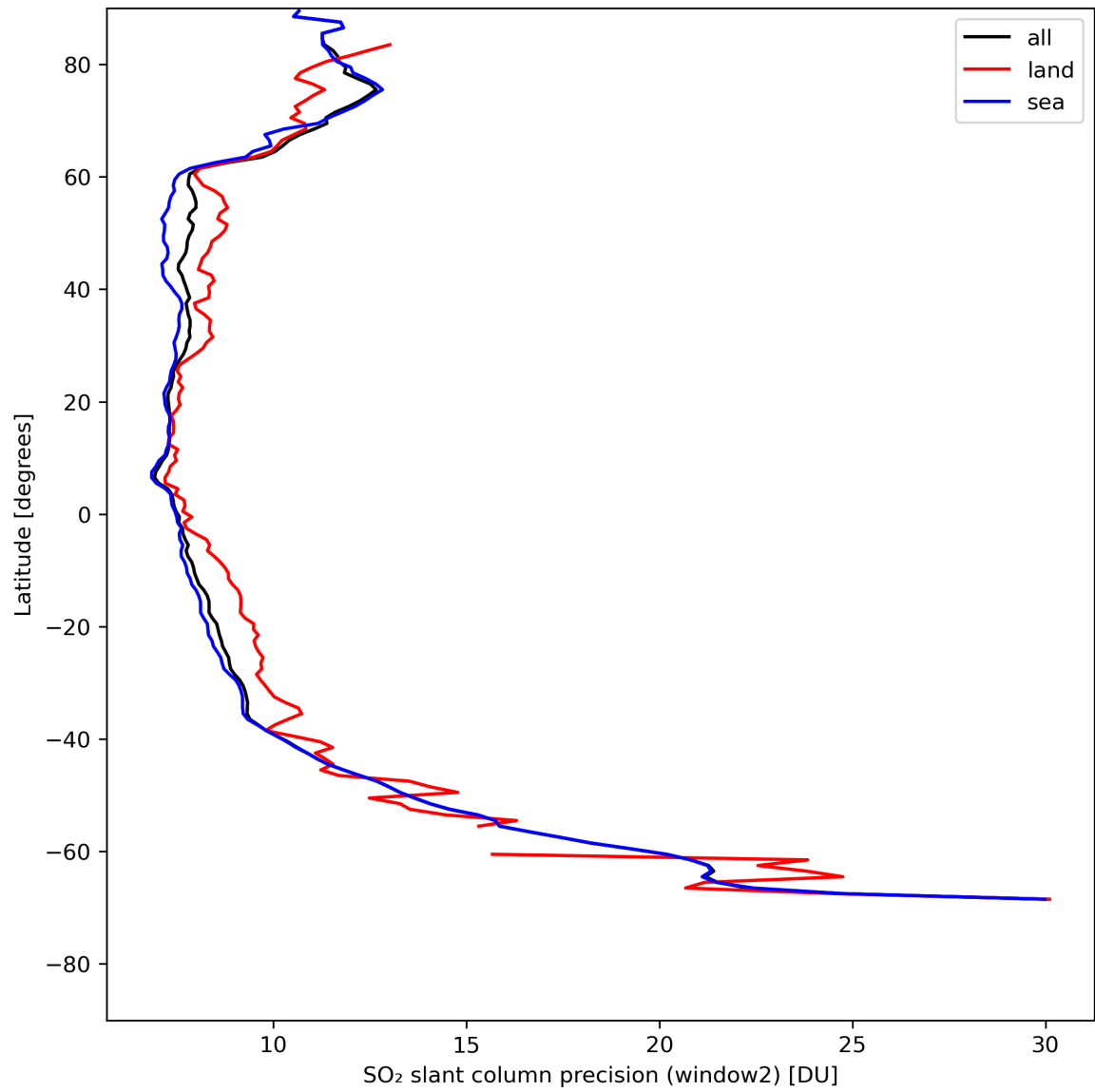
Figure 38: Zonal average of “SO 2 slant column precision (window2)” for 2024-08-06 to 2024-08-08.
