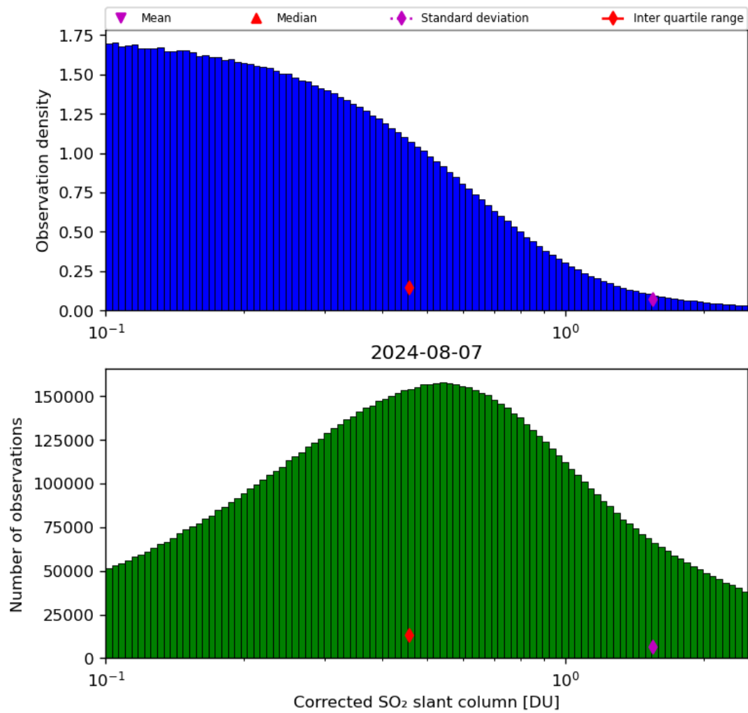
Figure 55: Histogram of “Corrected SO 2 slant column” for 2024-08-06 to 2024-08-08
