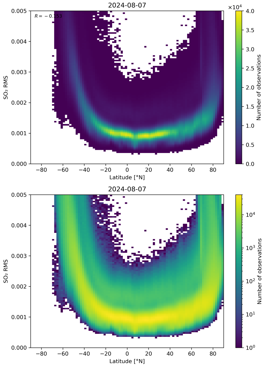
Figure 144: Scatter density plot of “Latitude” against “SO 2 RMS” for 2024-08-06 to 2024-08-08.
