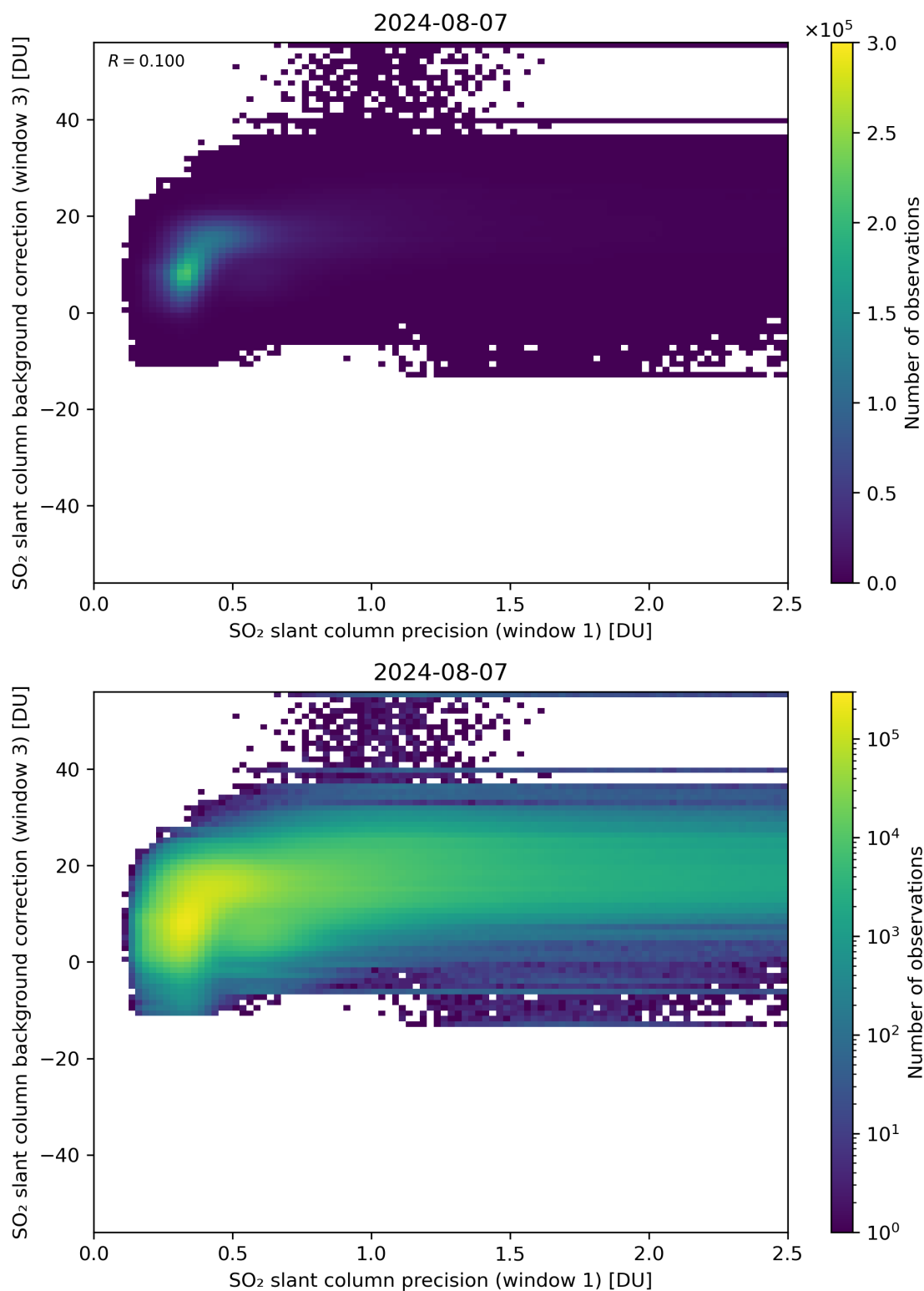
Figure 220: Scatter density plot of “SO 2 slant column precision (window 1)” against “SO 2 slant column background correction (window 3)” for 2024-08-06 to 2024-08-08.
