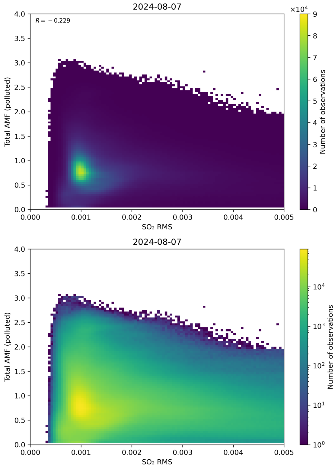
Figure 137: Scatter density plot of “SO 2 RMS” against “Total AMF (polluted)” for 2024-08-06 to 2024-08-08.
