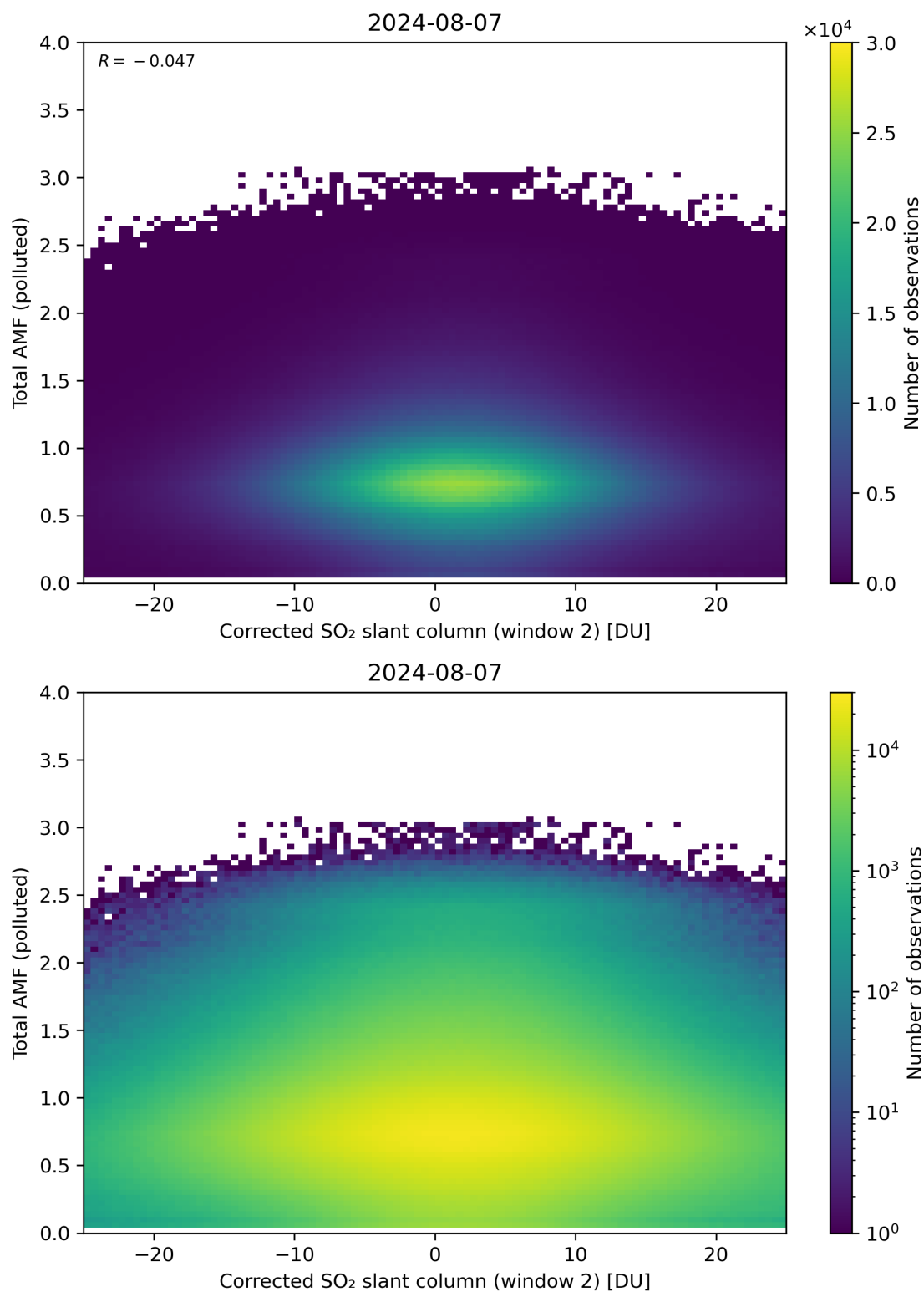
Figure 203: Scatter density plot of “Corrected SO 2 slant column (window 2)” against “Total AMF (polluted)” for 2024-08-06 to 2024-08-08.
