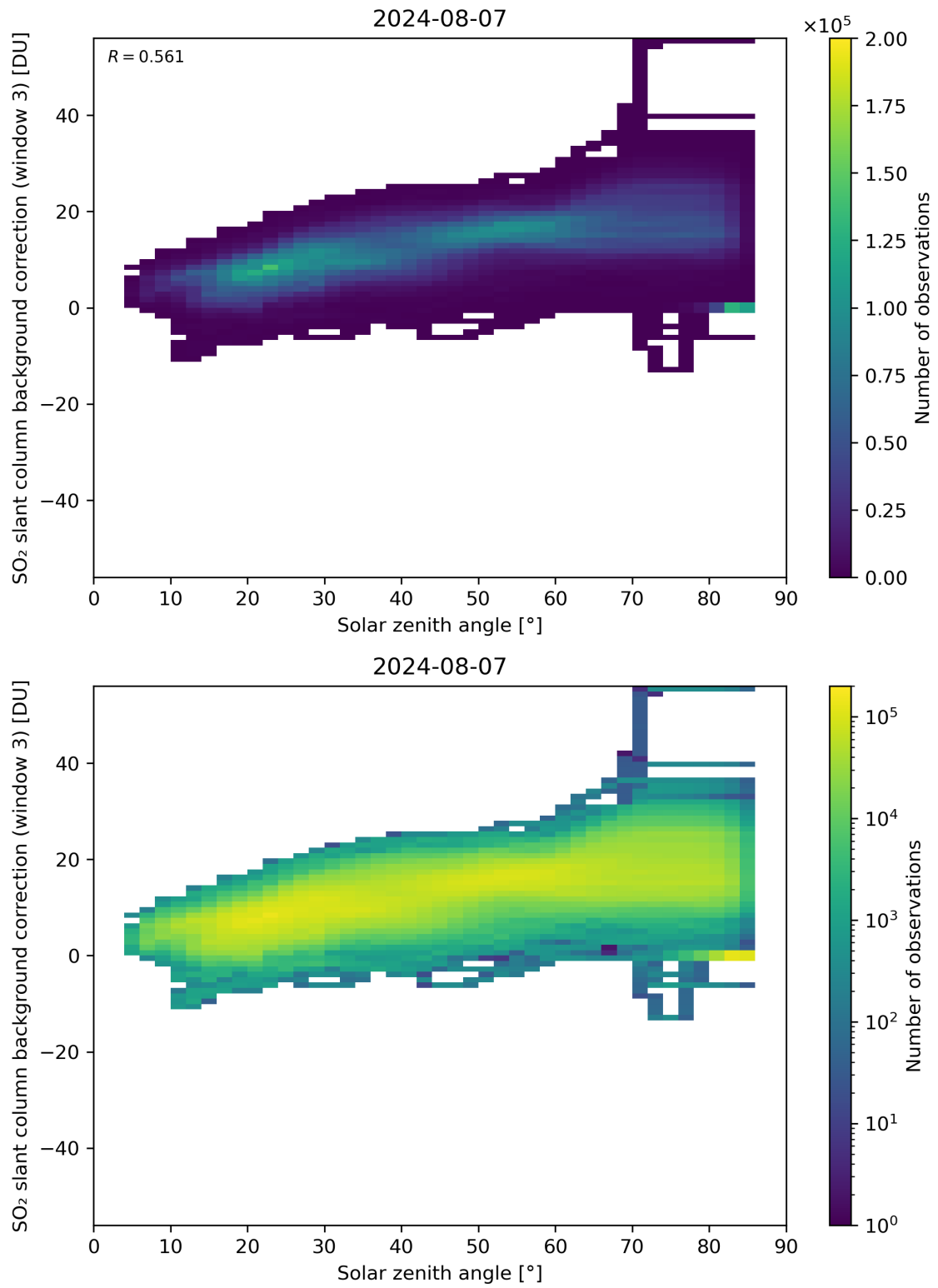
Figure 160: Scatter density plot of “Solar zenith angle” against “SO 2 slant column background correction (window 3)” for 2024-08-06 to 2024-08-08.
