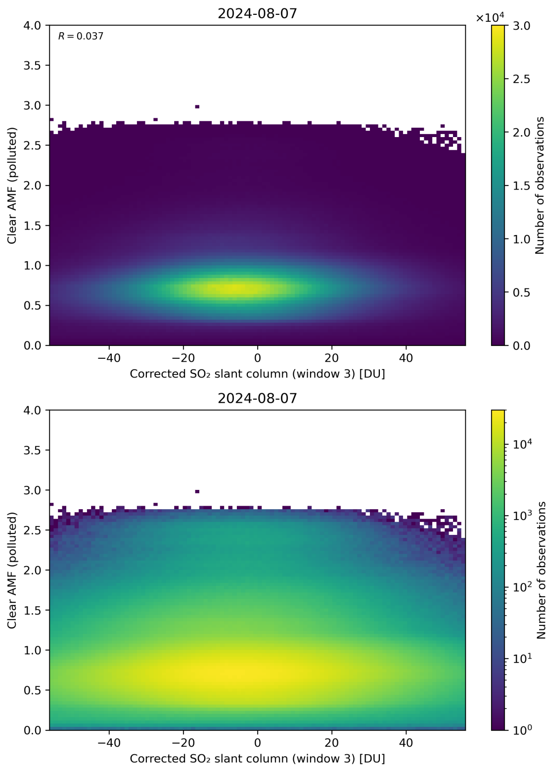
Figure 209: Scatter density plot of “Corrected SO 2 slant column (window 3)” against “Clear AMF (polluted)” for 2024-08-06 to 2024-08-08.
