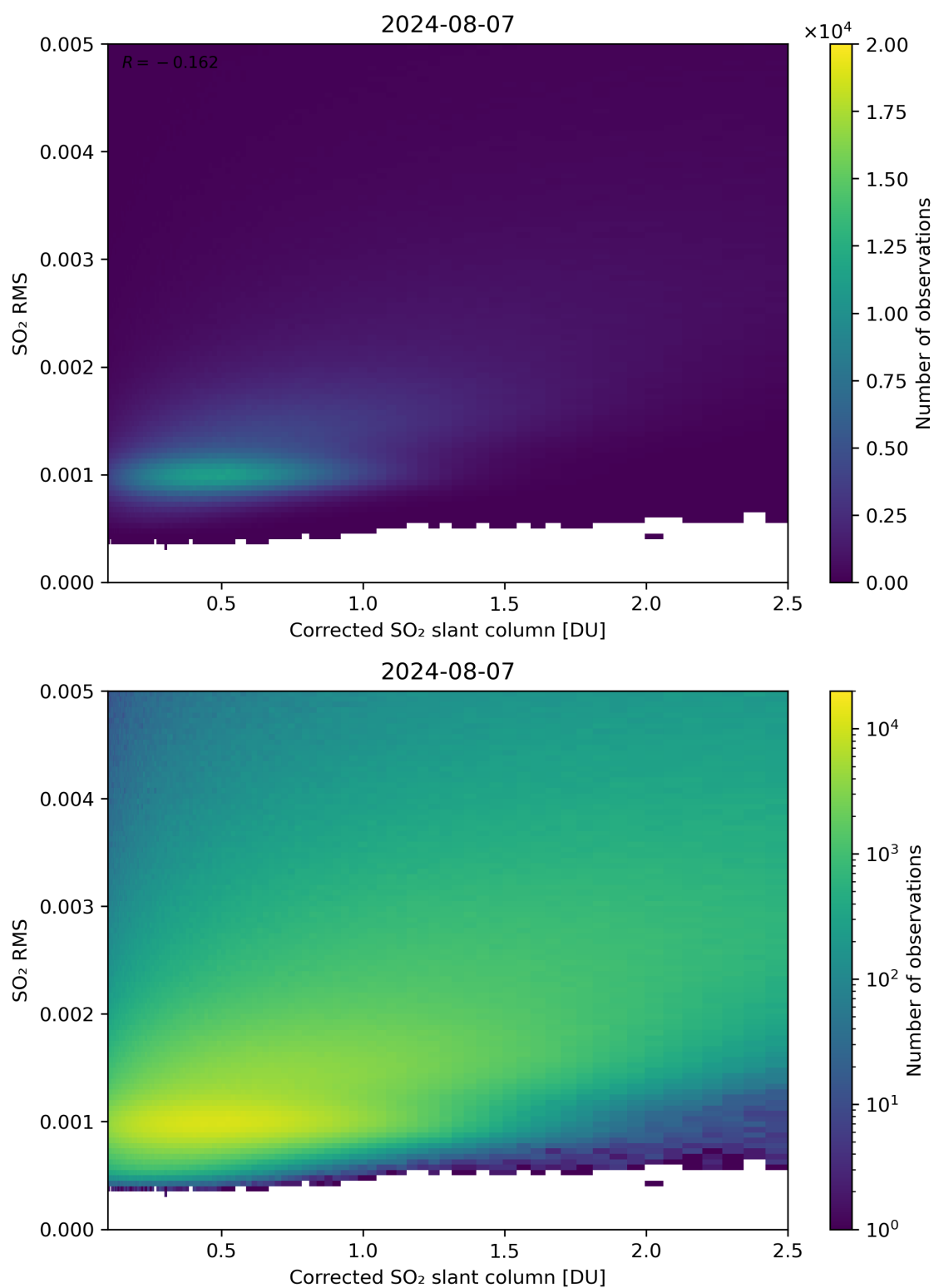
Figure 183: Scatter density plot of “Corrected SO 2 slant column” against “SO 2 RMS” for 2024-08-06 to 2024-08-08.
