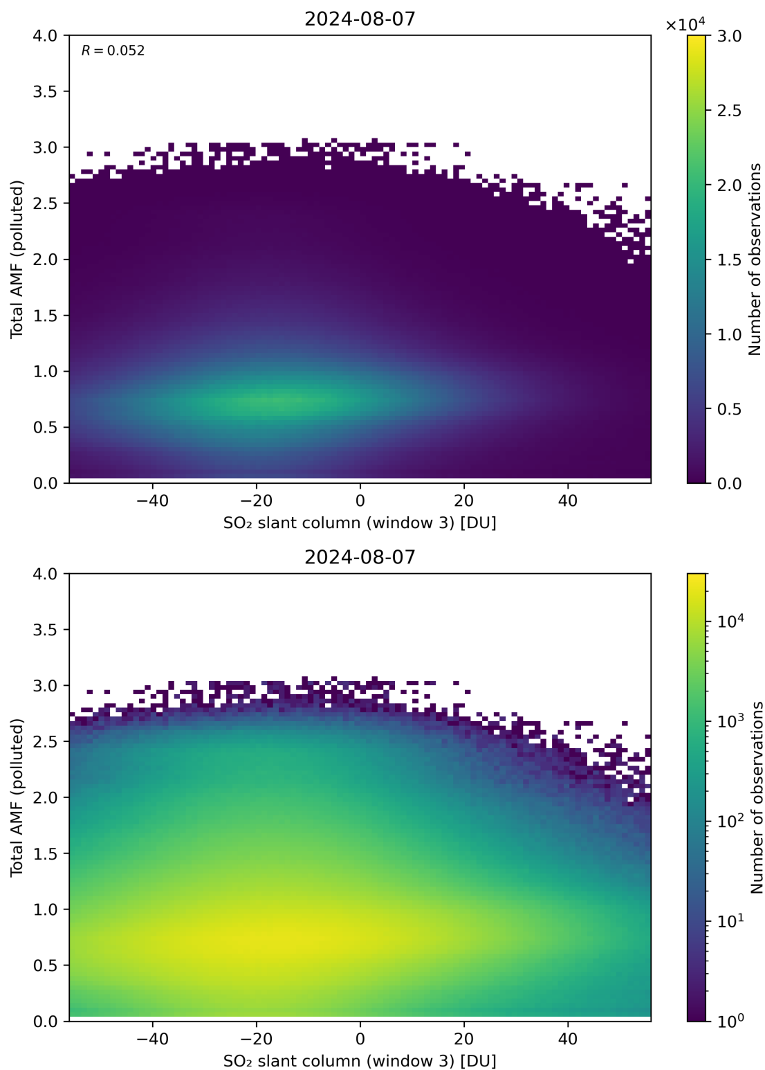
Figure 268: Scatter density plot of “SO 2 slant column (window 3)” against “Total AMF (polluted)” for 2024-08-06 to 2024-08-08.
