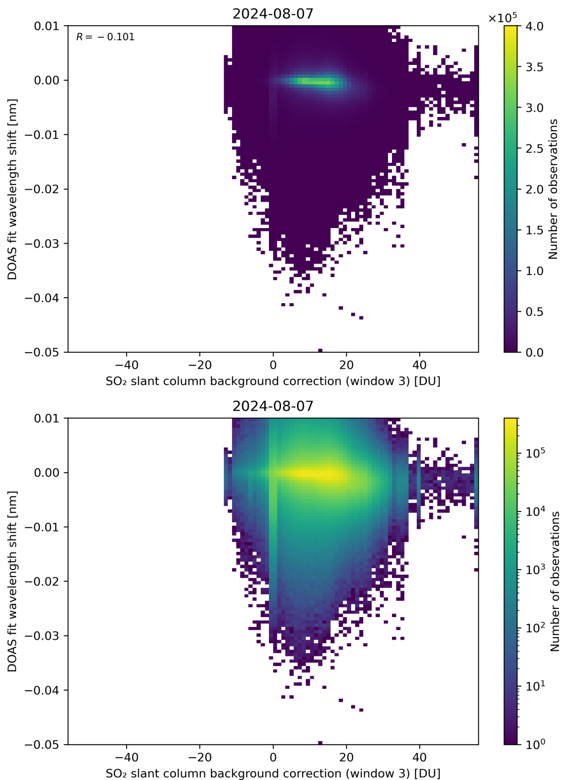
Figure 121: Scatter density plot of “SO 2 slant column background correction (window 3)” against “DOAS fit wavelength shift” for 2024-08-06 to 2024-08-08.
