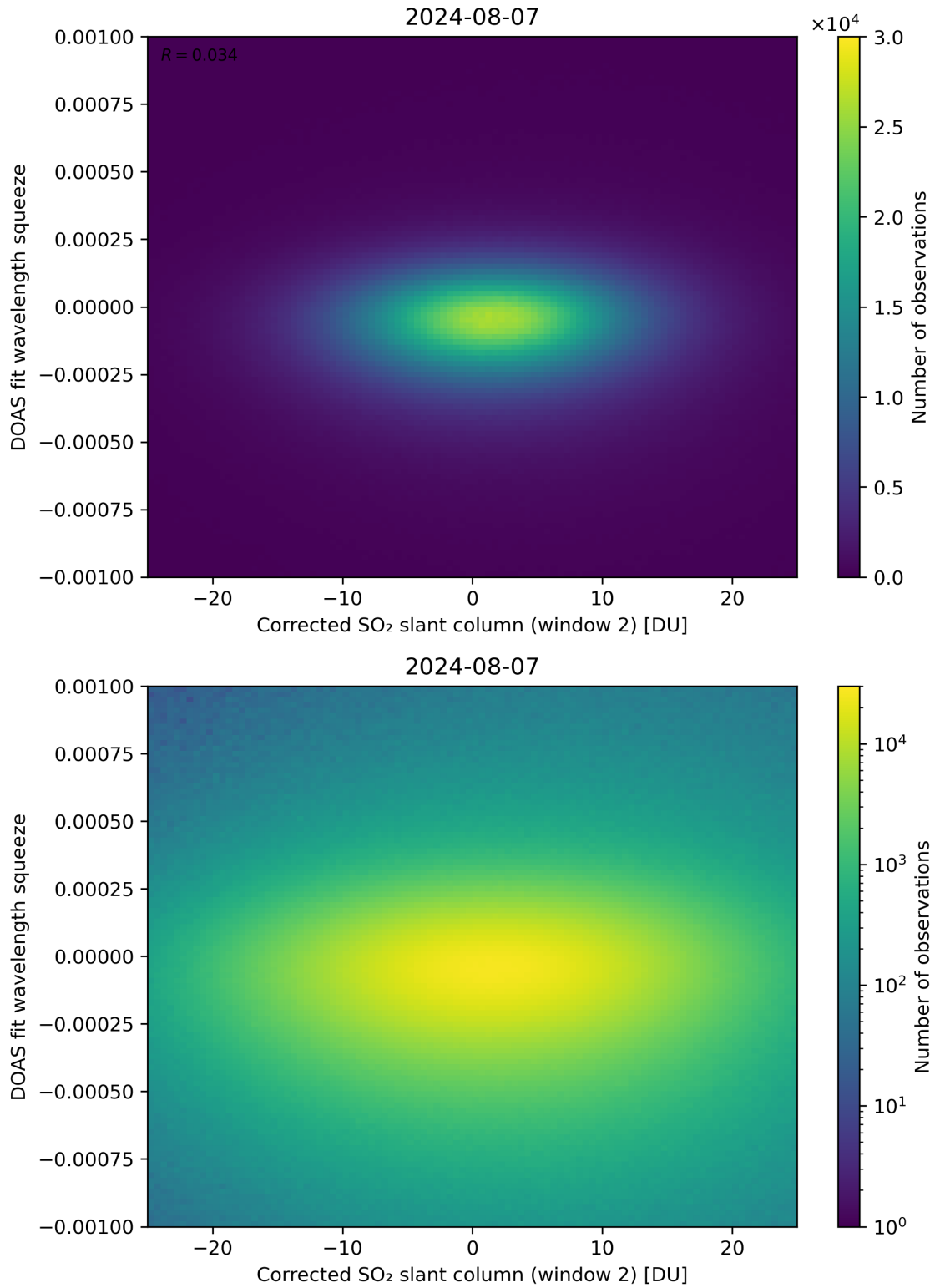
Figure 197: Scatter density plot of “Corrected SO 2 slant column (window 2)” against “DOAS fit wavelength squeeze” for 2024-08-06 to 2024-08-08.
