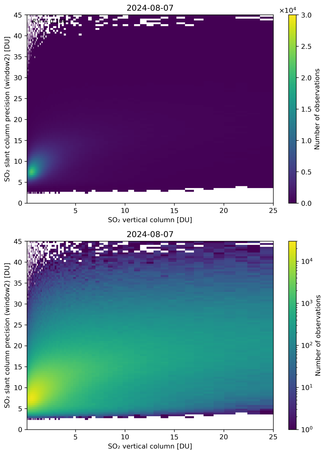
Figure 302: Scatter density plot of “SO 2 vertical column” against “SO 2 slant column precision (window2)” for 2024-08-06 to 2024-08-08.
