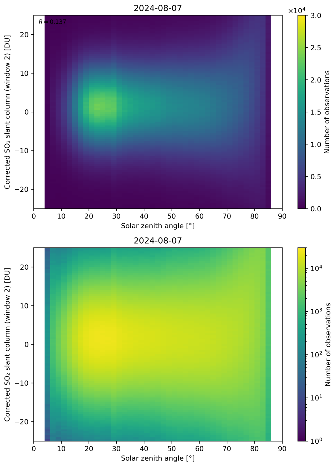
Figure 167: Scatter density plot of “Solar zenith angle” against “Corrected SO 2 slant column (window 2)” for 2024-08-06 to 2024-08-08.
