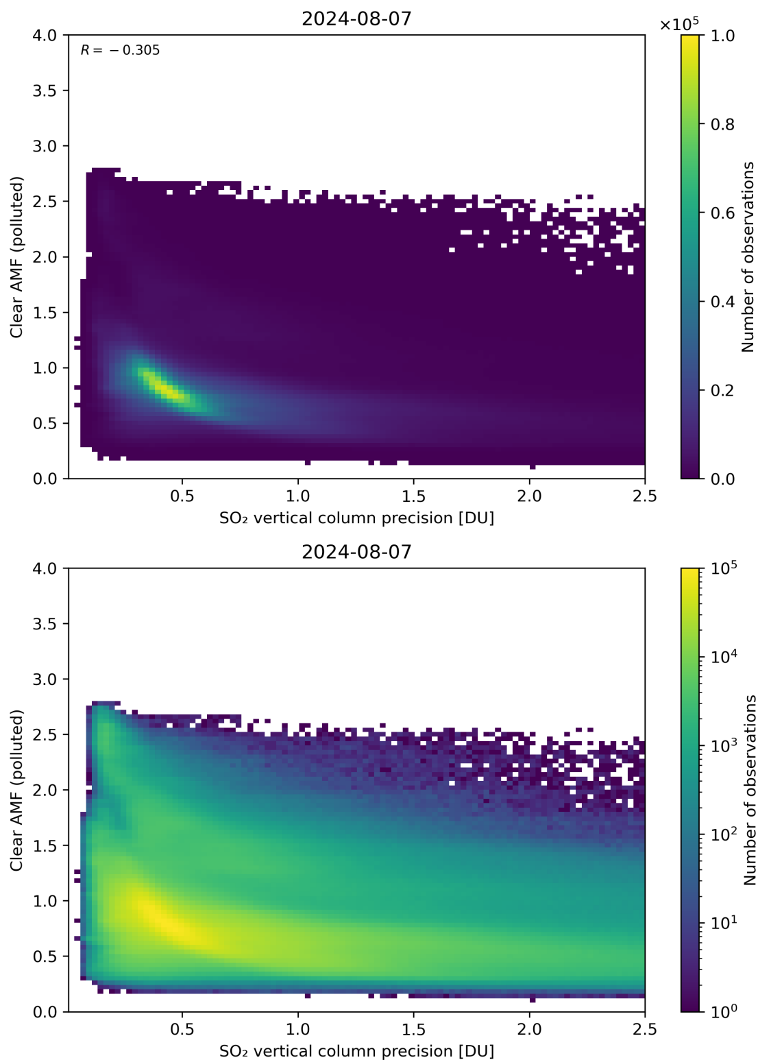
Figure 285: Scatter density plot of “SO 2 vertical column precision” against “Clear AMF (polluted)” for 2024-08-06 to 2024-08-08.
