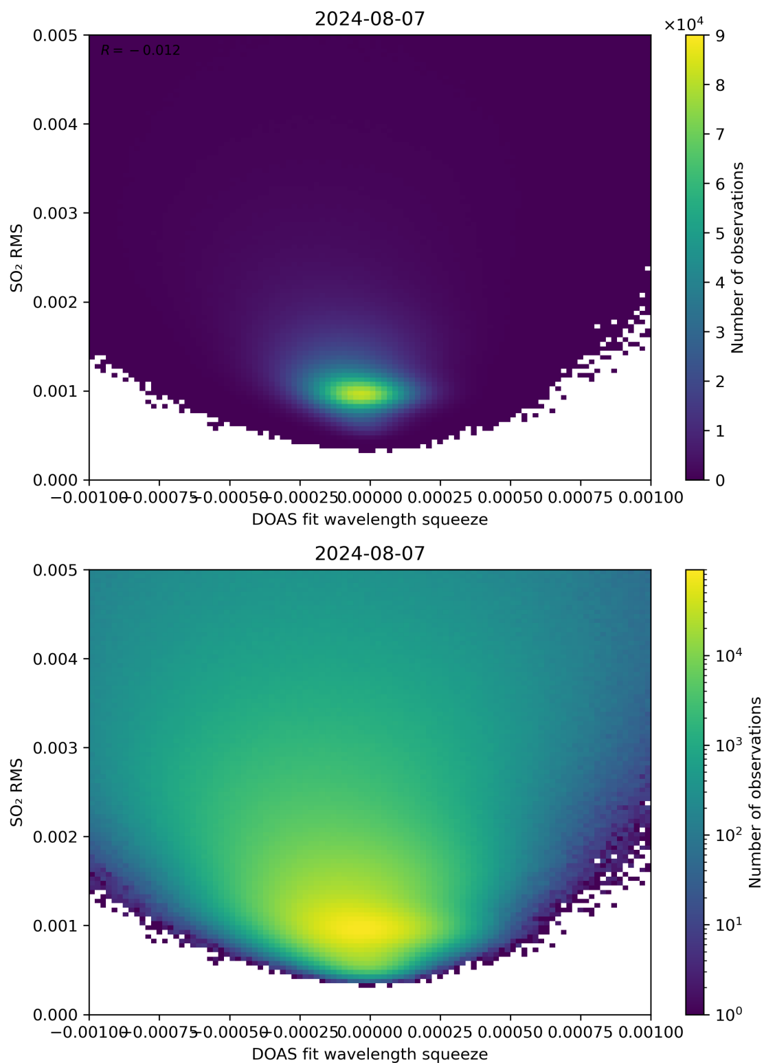
Figure 132: Scatter density plot of “DOAS fit wavelength squeeze” against “SO 2 RMS” for 2024-08-06 to 2024-08-08.
