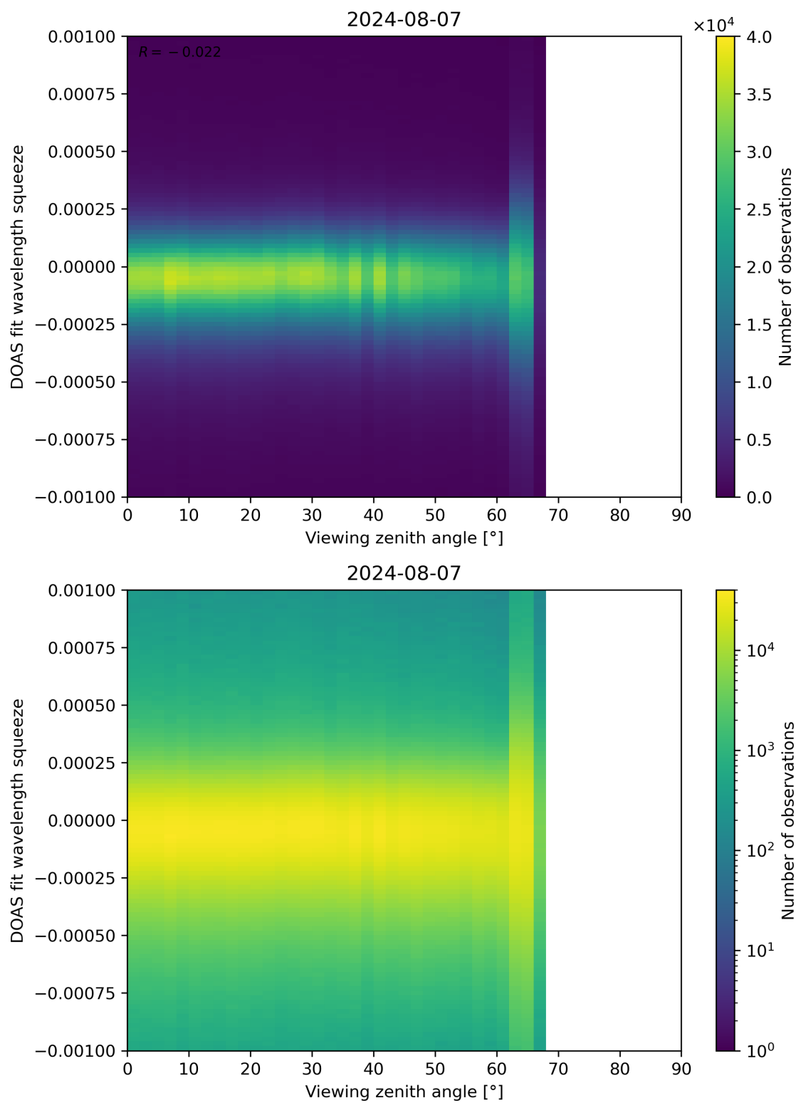
Figure 312: Scatter density plot of “Viewing zenith angle” against “DOAS fit wavelength squeeze” for 2024-08-06 to 2024-08-08.
