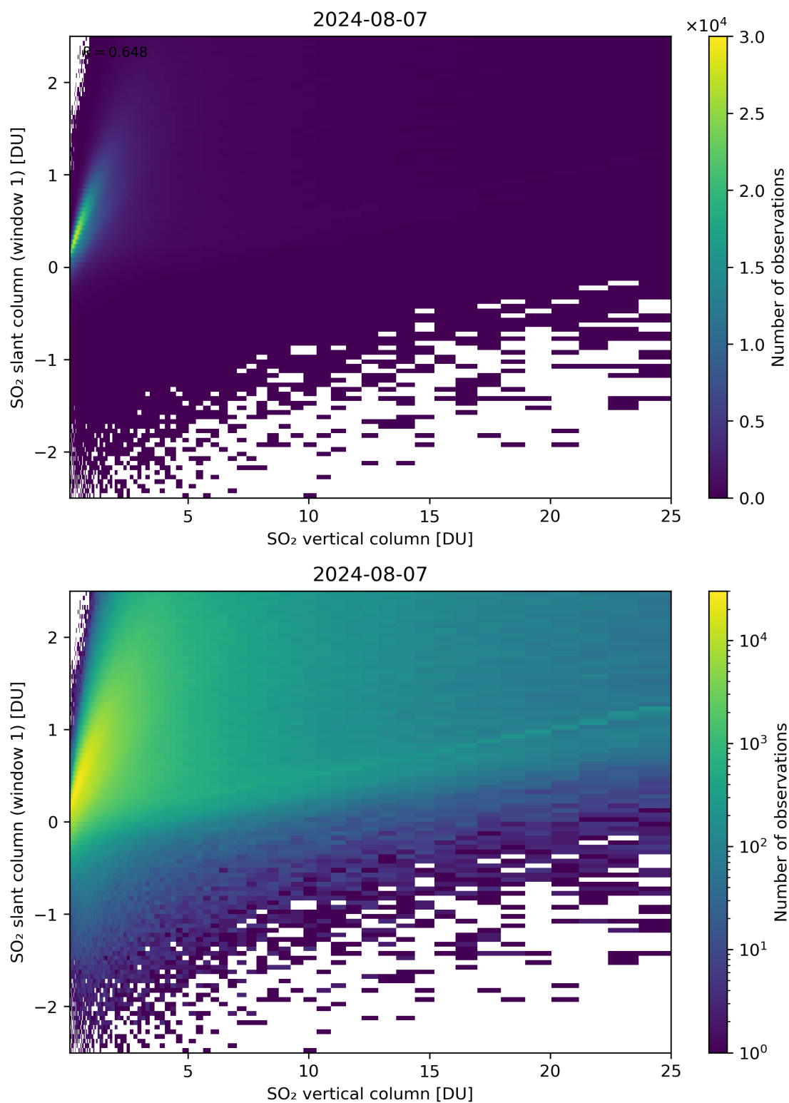
Figure 300: Scatter density plot of “SO 2 vertical column” against “SO 2 slant column (window 1)” for 2024-08-06 to 2024-08-08.
