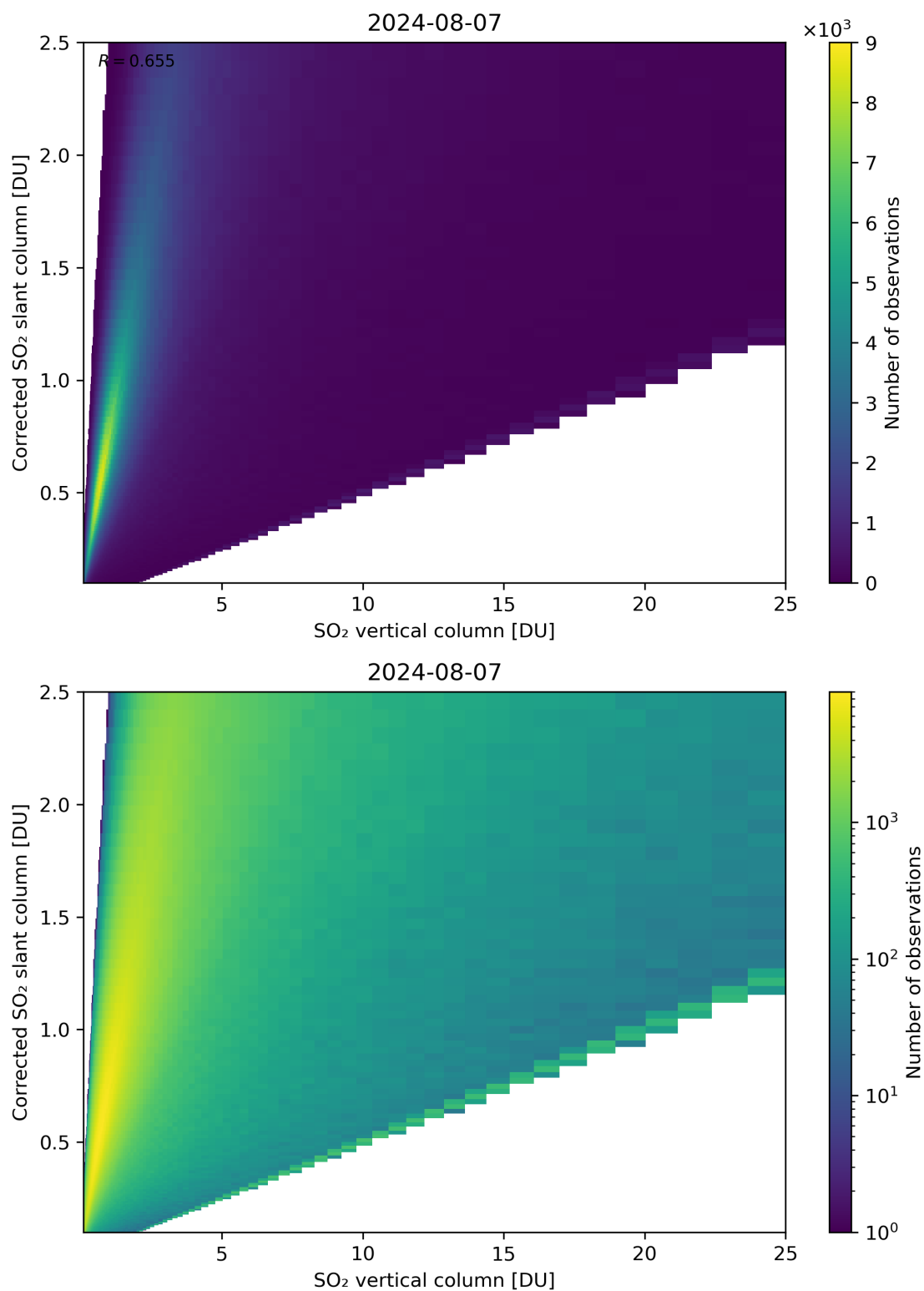
Figure 297: Scatter density plot of “SO 2 vertical column” against “Corrected SO 2 slant column” for 2024-08-06 to 2024-08-08.
