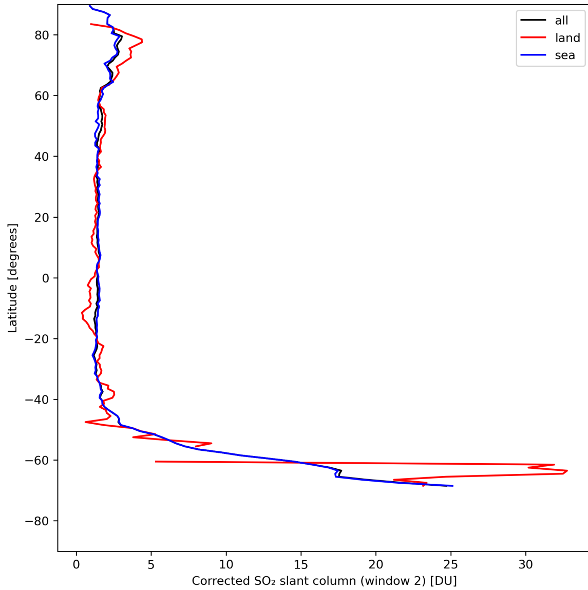
Figure 39: Zonal average of “Corrected SO 2 slant column (window 2)” for 2024-08-06 to 2024-08-08.
