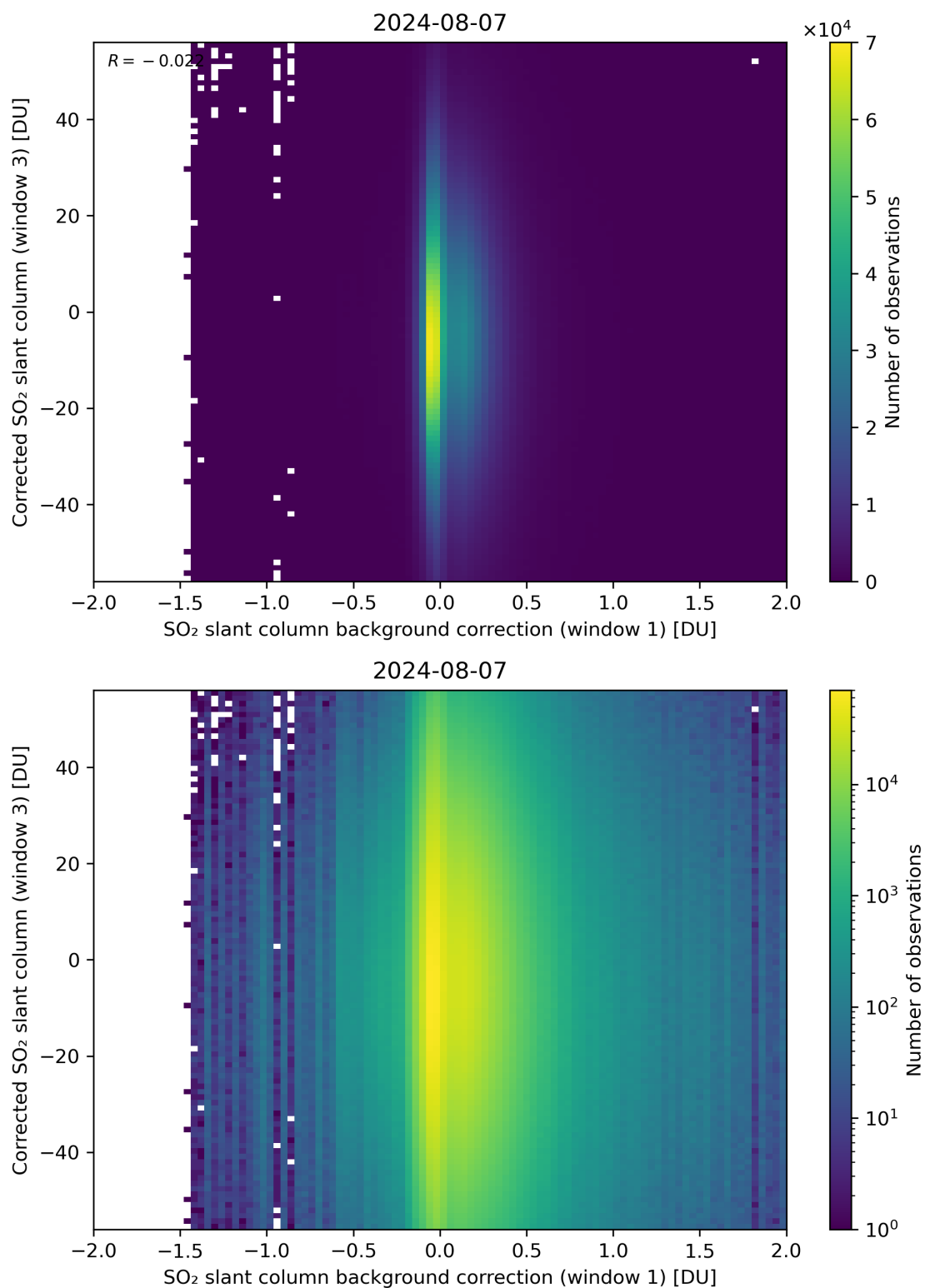
Figure 105: Scatter density plot of “SO 2 slant column background correction (window 1)” against “Corrected SO 2 slant column (window 3)” for 2024-08-06 to 2024-08-08.
