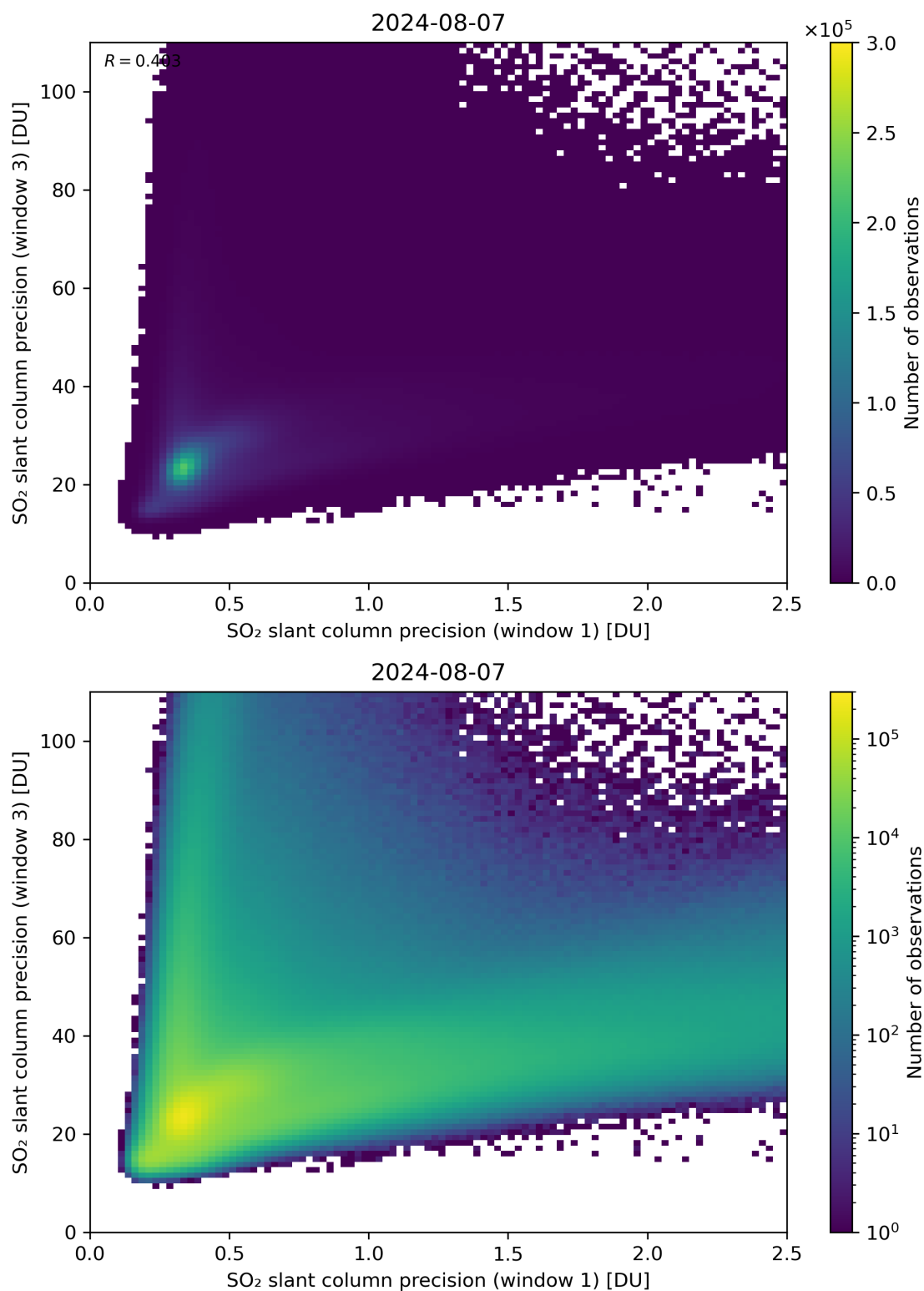
Figure 229: Scatter density plot of “SO 2 slant column precision (window 1)” against “SO 2 slant column precision (window 3)” for 2024-08-06 to 2024-08-08.
