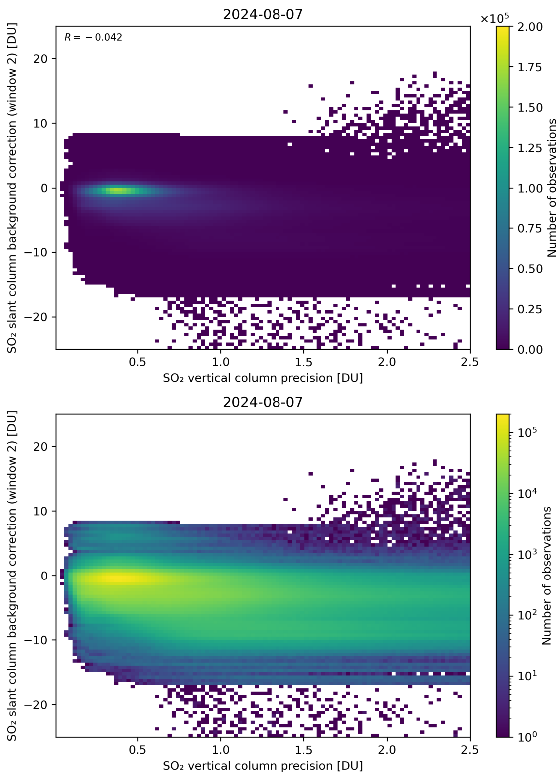
Figure 280: Scatter density plot of “SO 2 vertical column precision” against “SO 2 slant column background correction (window 2)” for 2024-08-06 to 2024-08-08.
