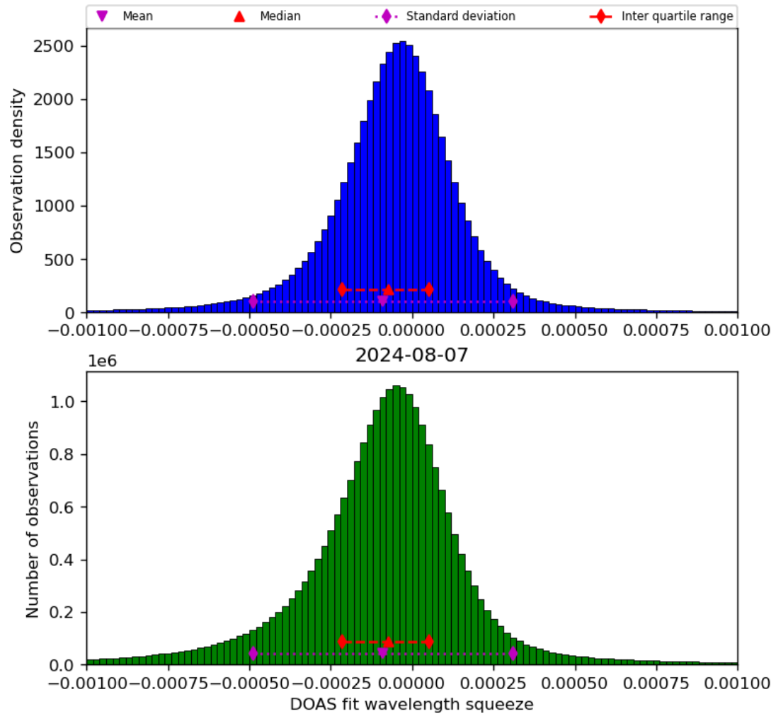
Figure 69: Histogram of “DOAS fit wavelength squeeze” for 2024-08-06 to 2024-08-08
