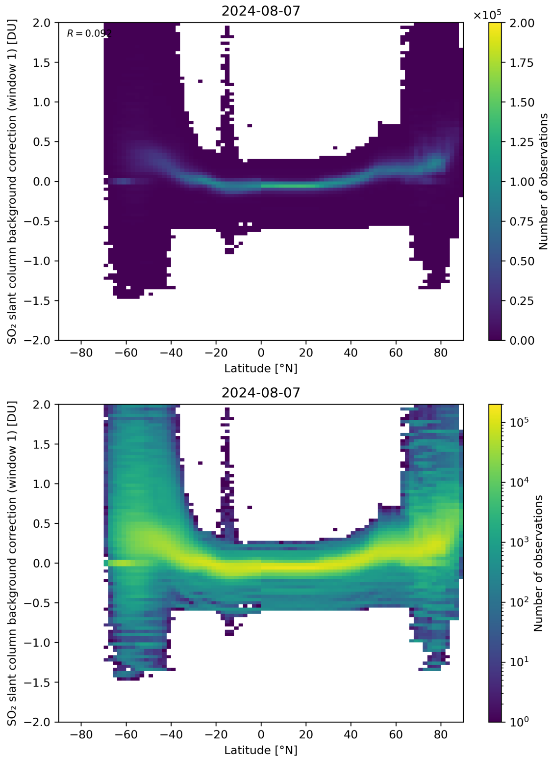
Figure 139: Scatter density plot of “Latitude” against “SO 2 slant column background correction (window 1)” for 2024-08-06 to 2024-08-08.
