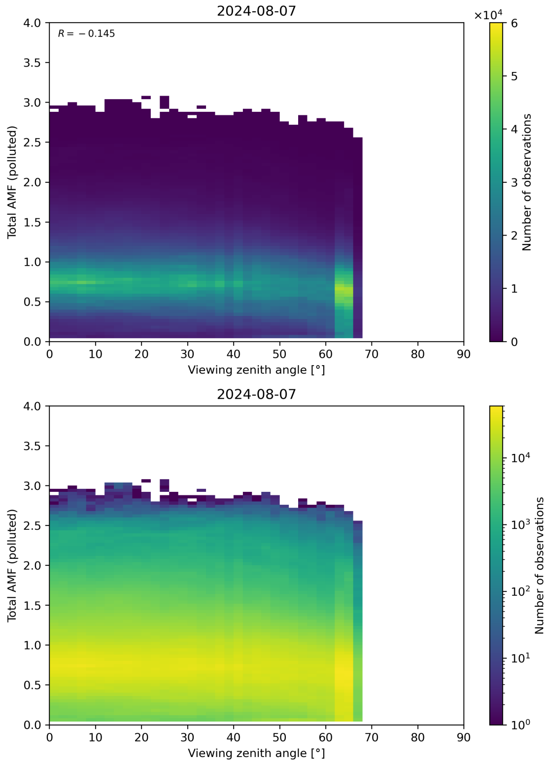
Figure 325: Scatter density plot of “Viewing zenith angle” against “Total AMF (polluted)” for 2024-08-06 to 2024-08-08.
