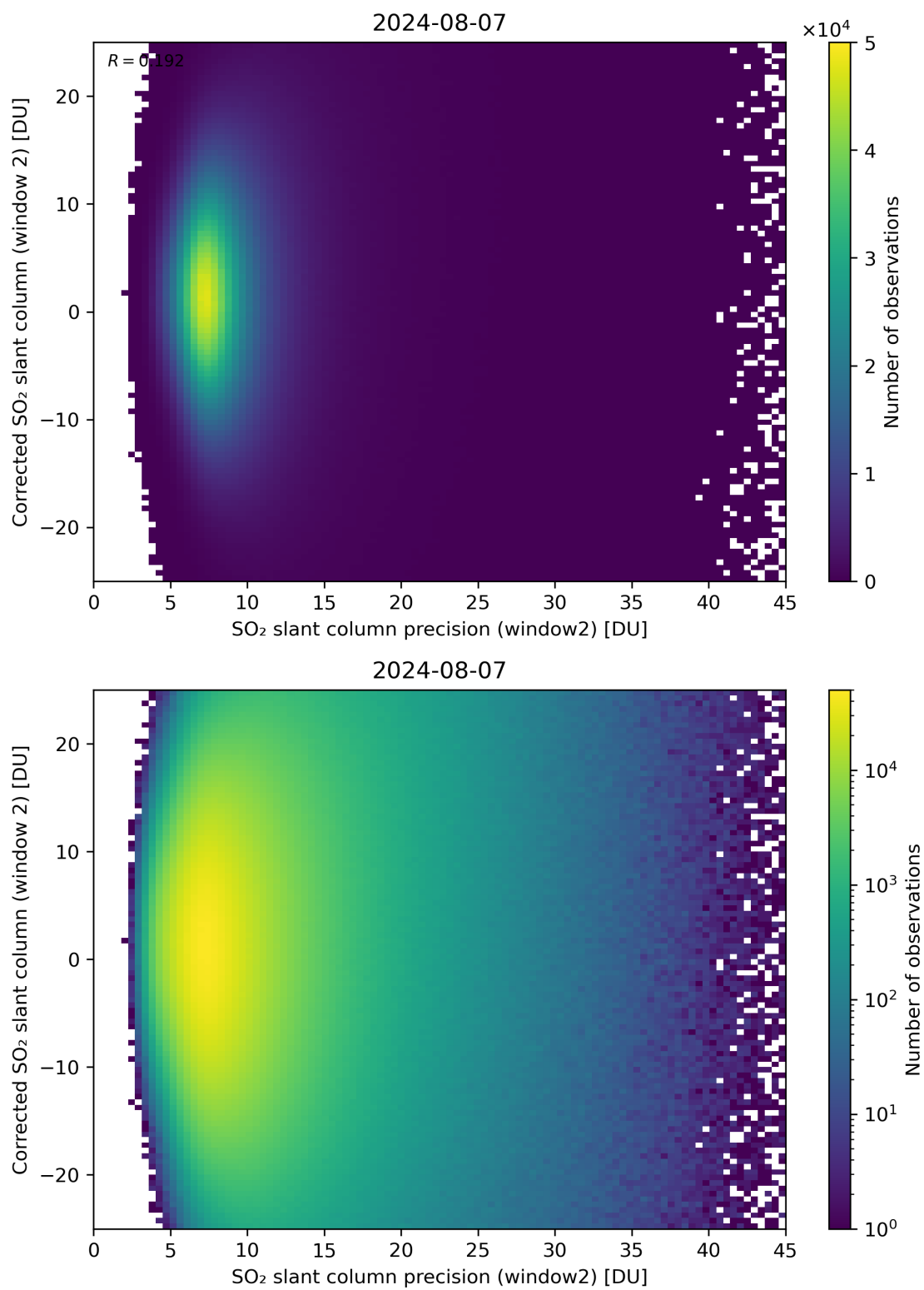
Figure 247: Scatter density plot of “SO 2 slant column precision (window2)” against “Corrected SO 2 slant column (window 2)” for 2024-08-06 to 2024-08-08.
