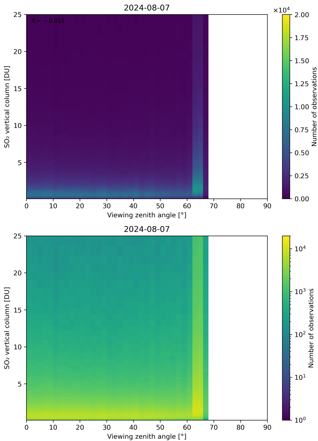
Figure 327: Scatter density plot of “Viewing zenith angle” against “SO 2 vertical column” for 2024-08-06 to 2024-08-08.
