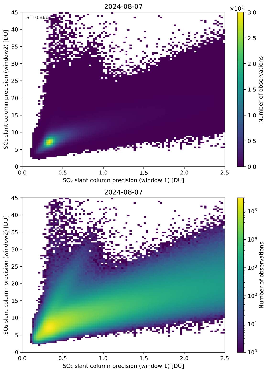
Figure 227: Scatter density plot of “SO 2 slant column precision (window 1)” against “SO 2 slant column precision (window 2)” for 2024-08-06 to 2024-08-08.
