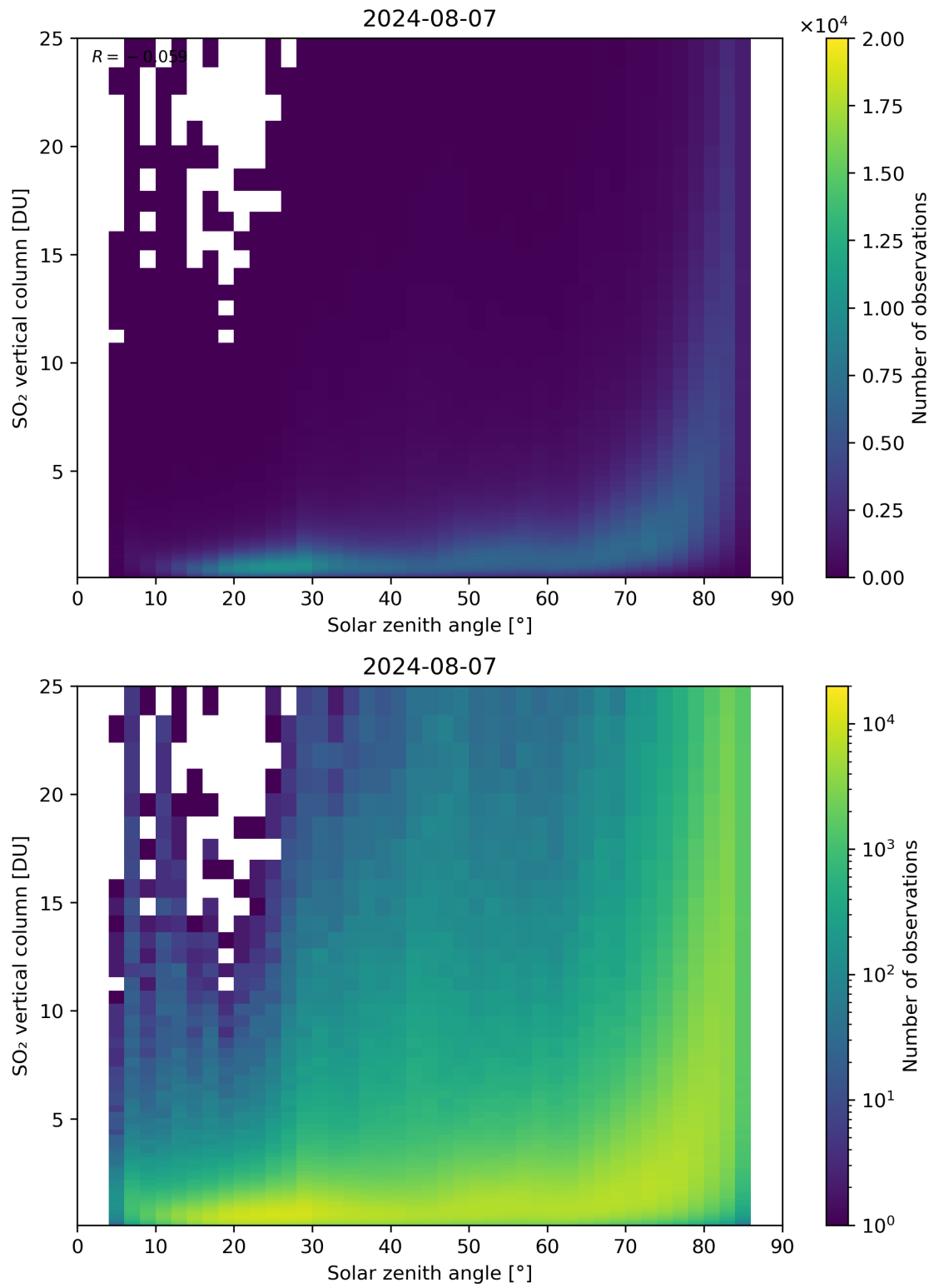
Figure 176: Scatter density plot of “Solar zenith angle” against “SO 2 vertical column” for 2024-08-06 to 2024-08-08.
