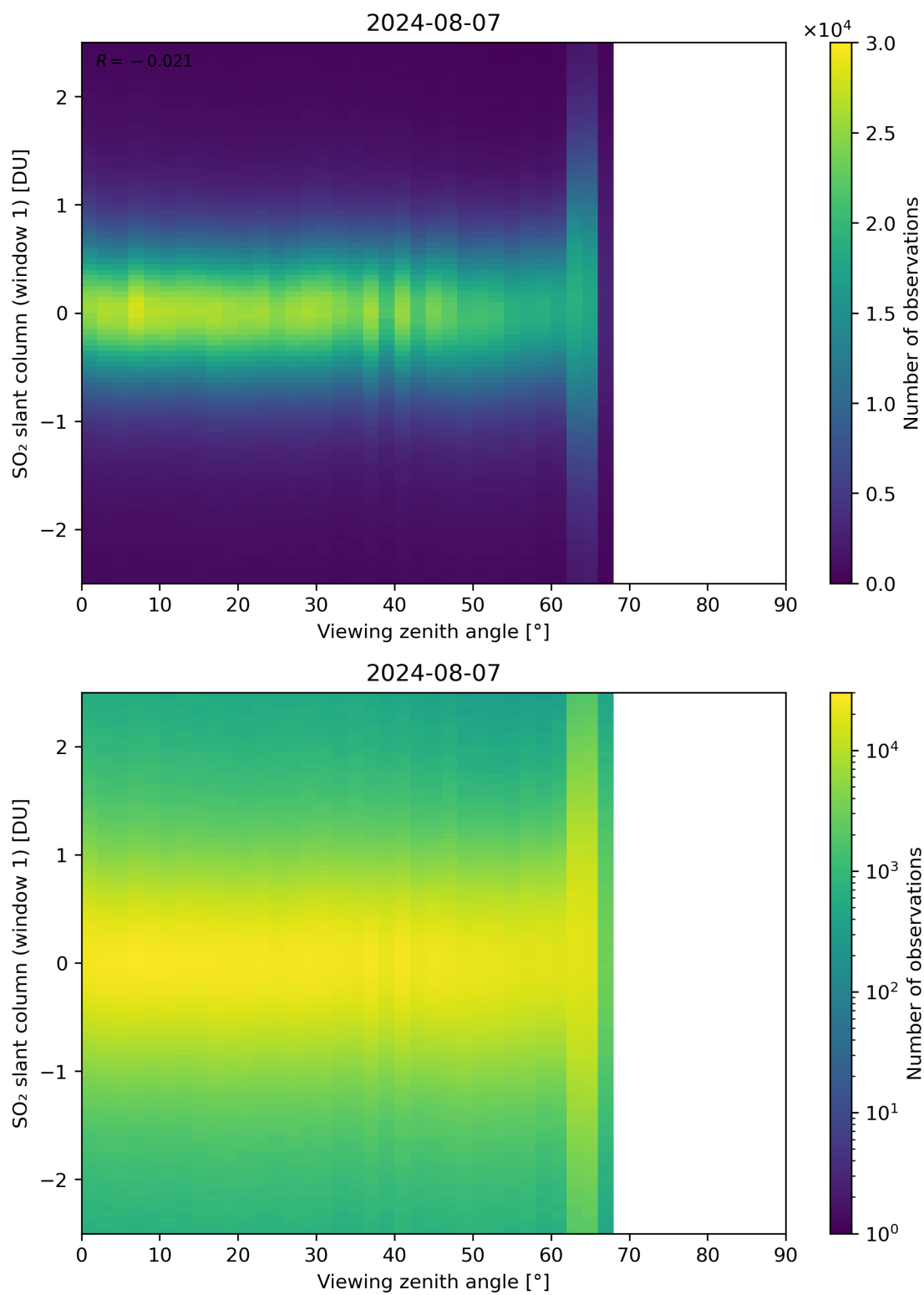
Figure 320: Scatter density plot of “Viewing zenith angle” against “SO 2 slant column (window 1)” for 2024-08-06 to 2024-08-08.
