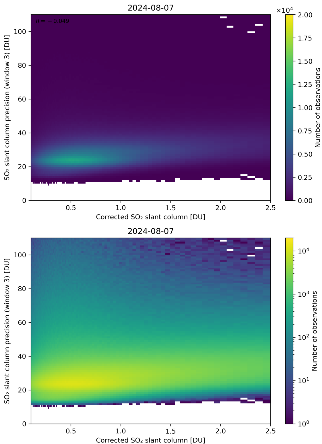
Figure 191: Scatter density plot of “Corrected SO 2 slant column” against “SO 2 slant column precision (window 3)” for 2024-08-06 to 2024-08-08.
