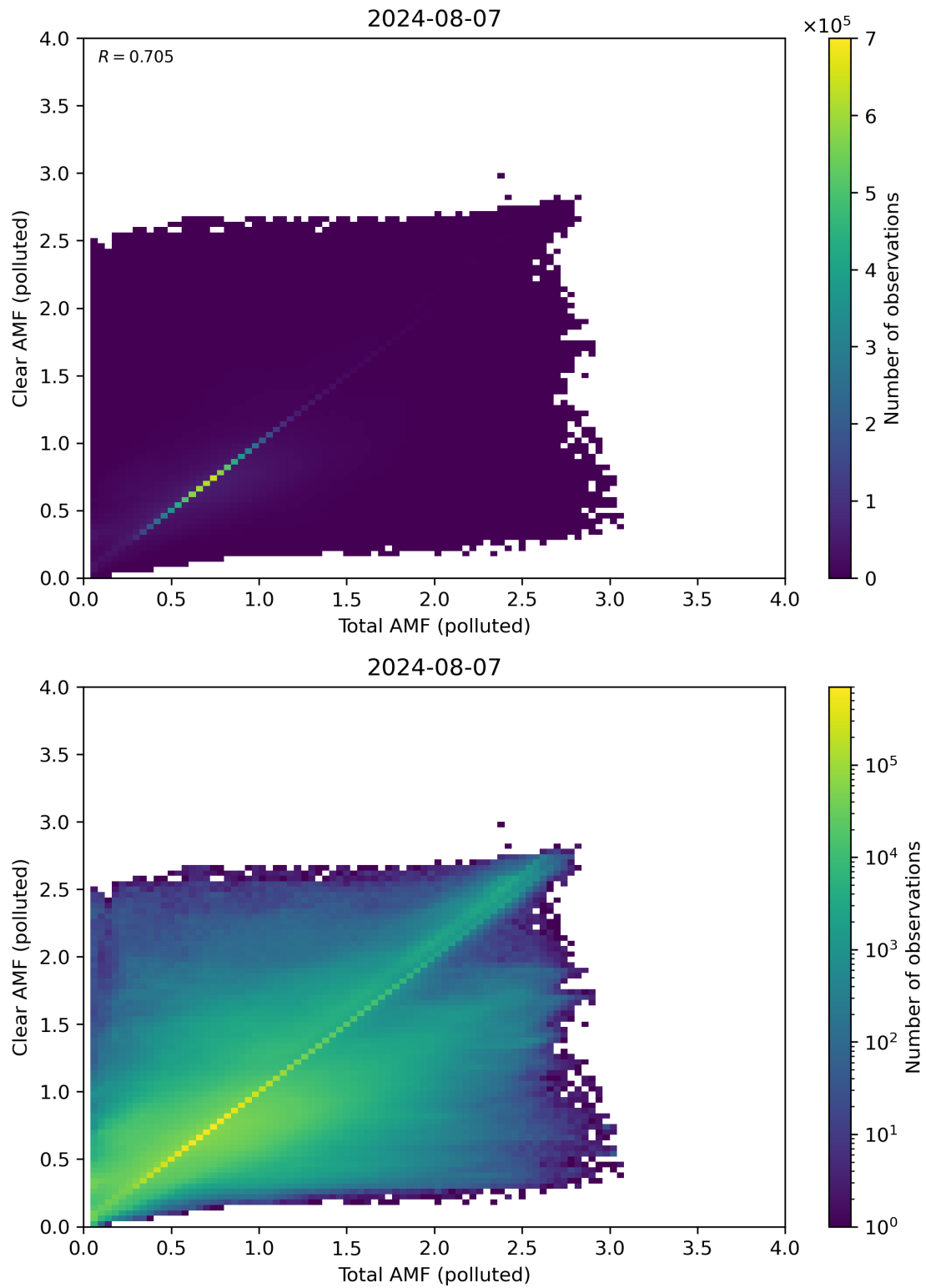
Figure 271: Scatter density plot of “Total AMF (polluted)” against “Clear AMF (polluted)” for 2024-08-06 to 2024-08-08.
