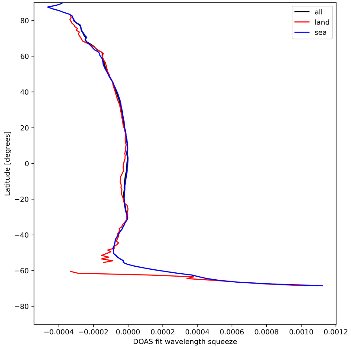
Figure 46: Zonal average of “DOAS fit wavelength squeeze” for 2024-08-06 to 2024-08-08.
