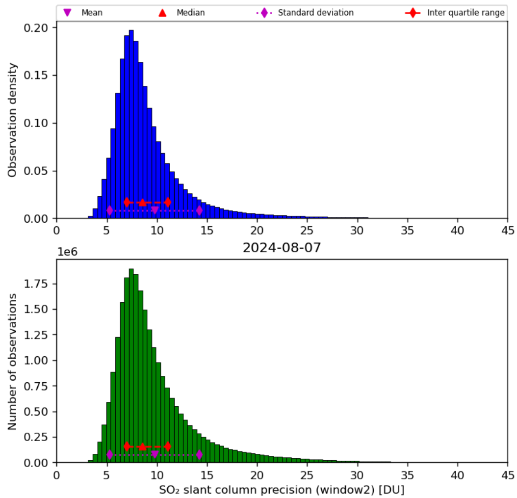
Figure 61: Histogram of “SO 2 slant column precision (window2)” for 2024-08-06 to 2024-08-08
