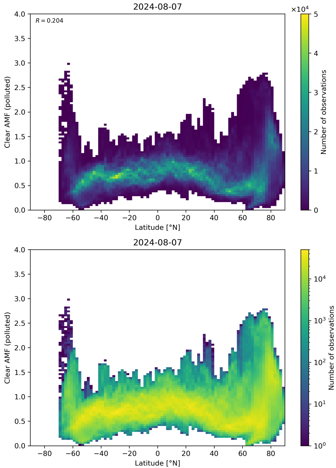
Figure 145: Scatter density plot of “Latitude” against “Clear AMF (polluted)” for 2024-08-06 to 2024-08-08.
