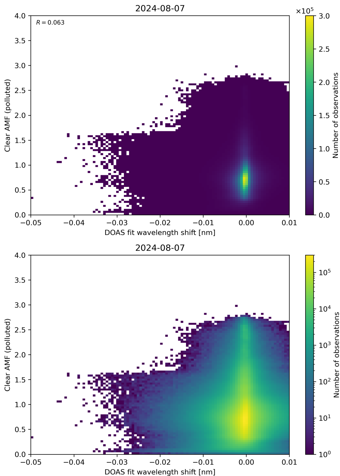
Figure 129: Scatter density plot of “DOAS fit wavelength shift” against “Clear AMF (polluted)” for 2024-08-06 to 2024-08-08.
