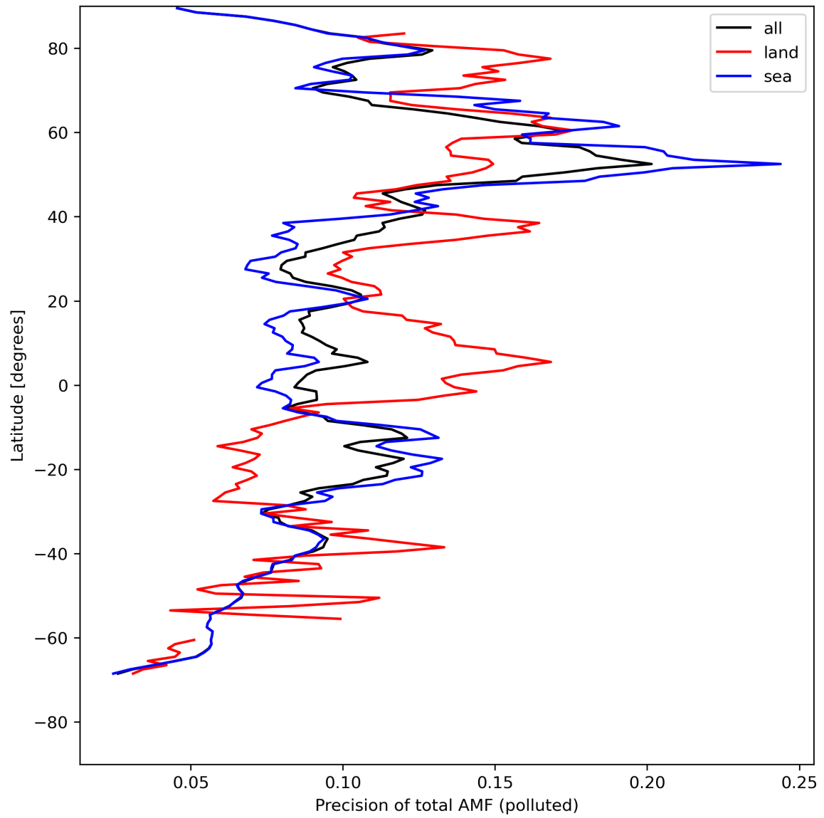
Figure 49: Zonal average of “Precision of total AMF (polluted)” for 2024-08-06 to 2024-08-08.
