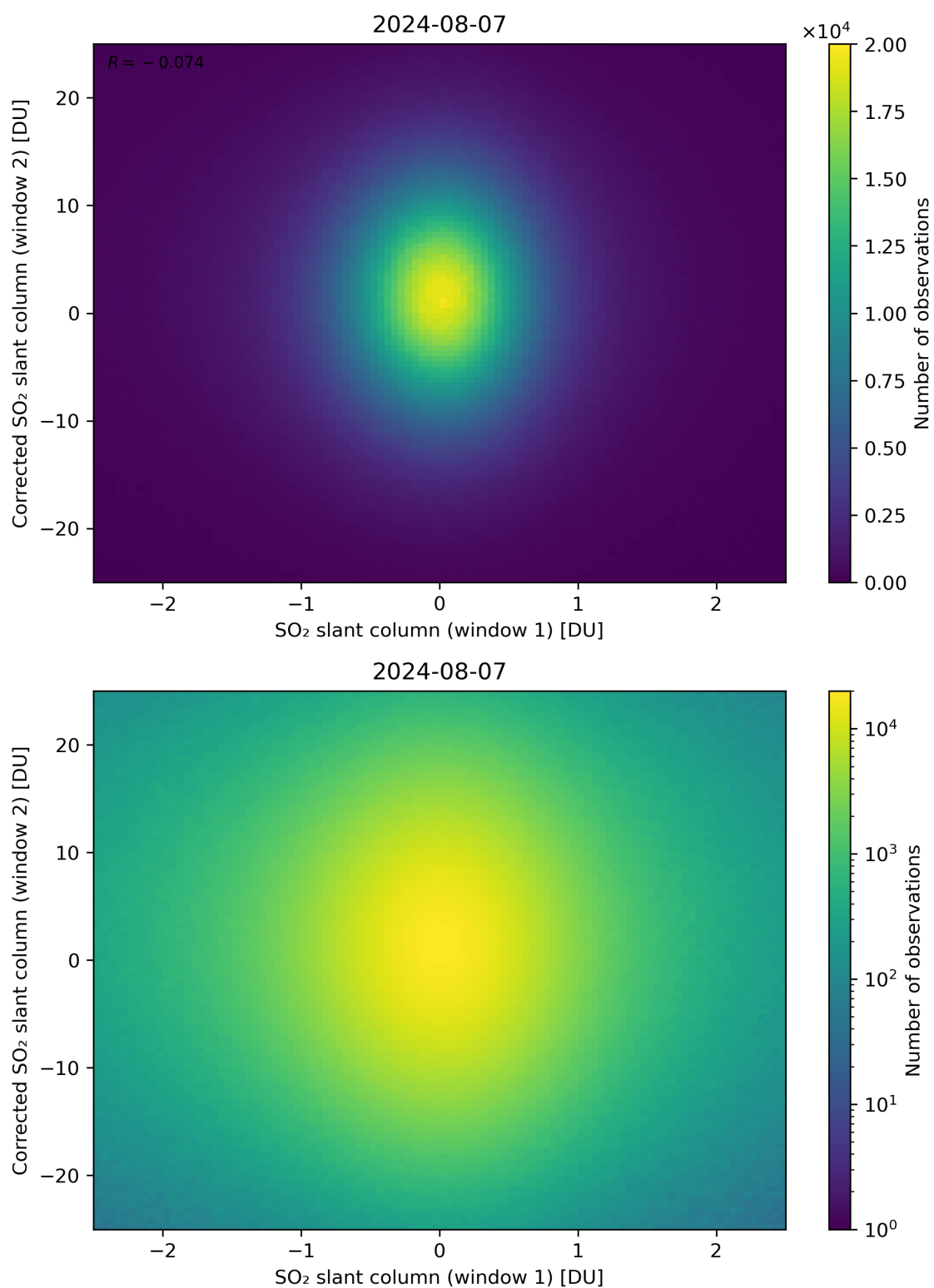
Figure 233: Scatter density plot of “SO 2 slant column (window 1)” against “Corrected SO 2 slant column (window 2)” for 2024-08-06 to 2024-08-08.
