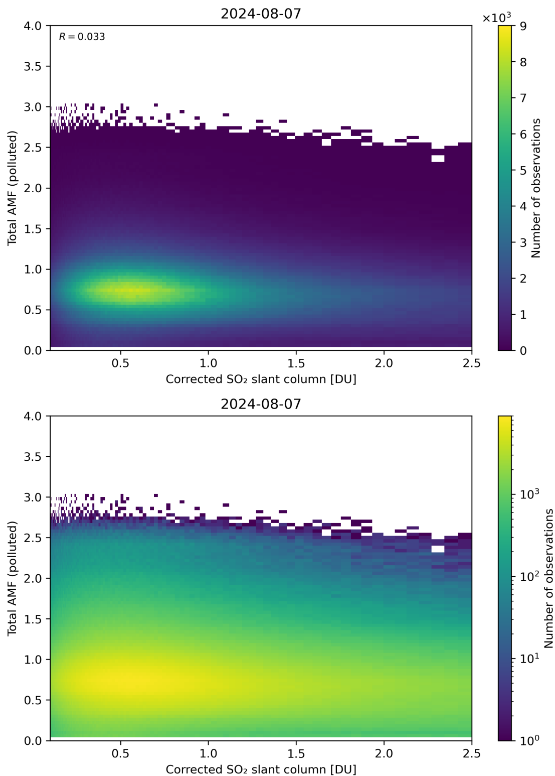
Figure 192: Scatter density plot of “Corrected SO 2 slant column” against “Total AMF (polluted)” for 2024-08-06 to 2024-08-08.
