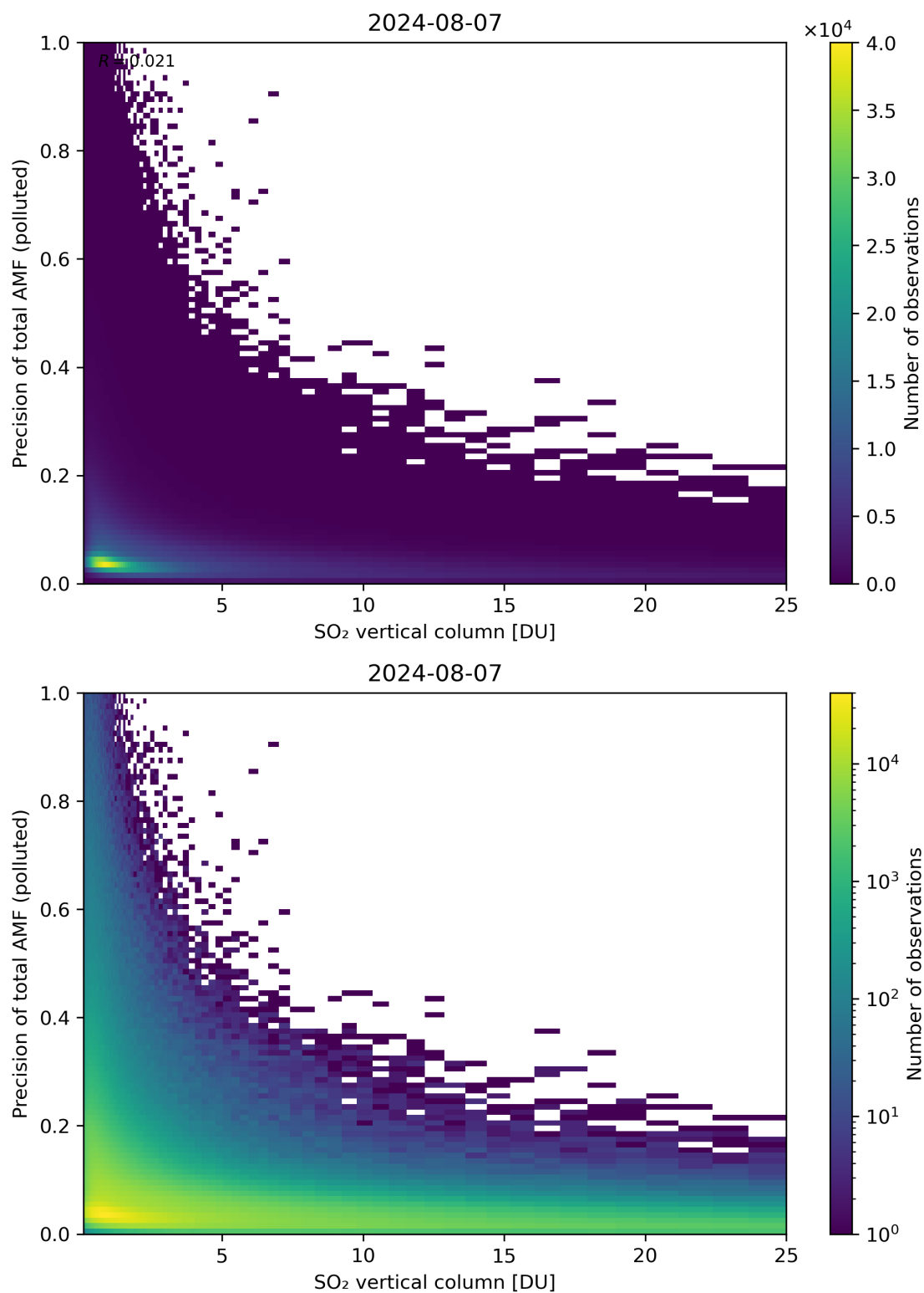
Figure 306: Scatter density plot of “SO 2 vertical column” against “Precision of total AMF (polluted)” for 2024-08-06 to 2024-08-08.
