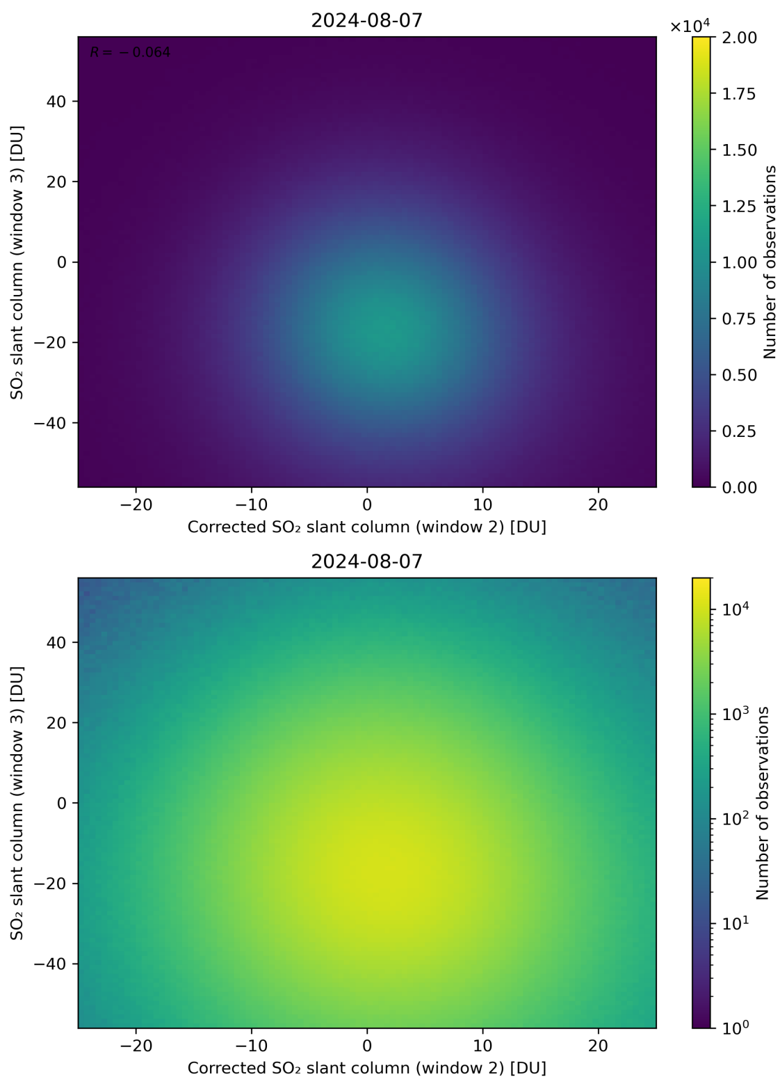
Figure 201: Scatter density plot of “Corrected SO 2 slant column (window 2)” against “SO 2 slant column (window 3)” for 2024-08-06 to 2024-08-08.
