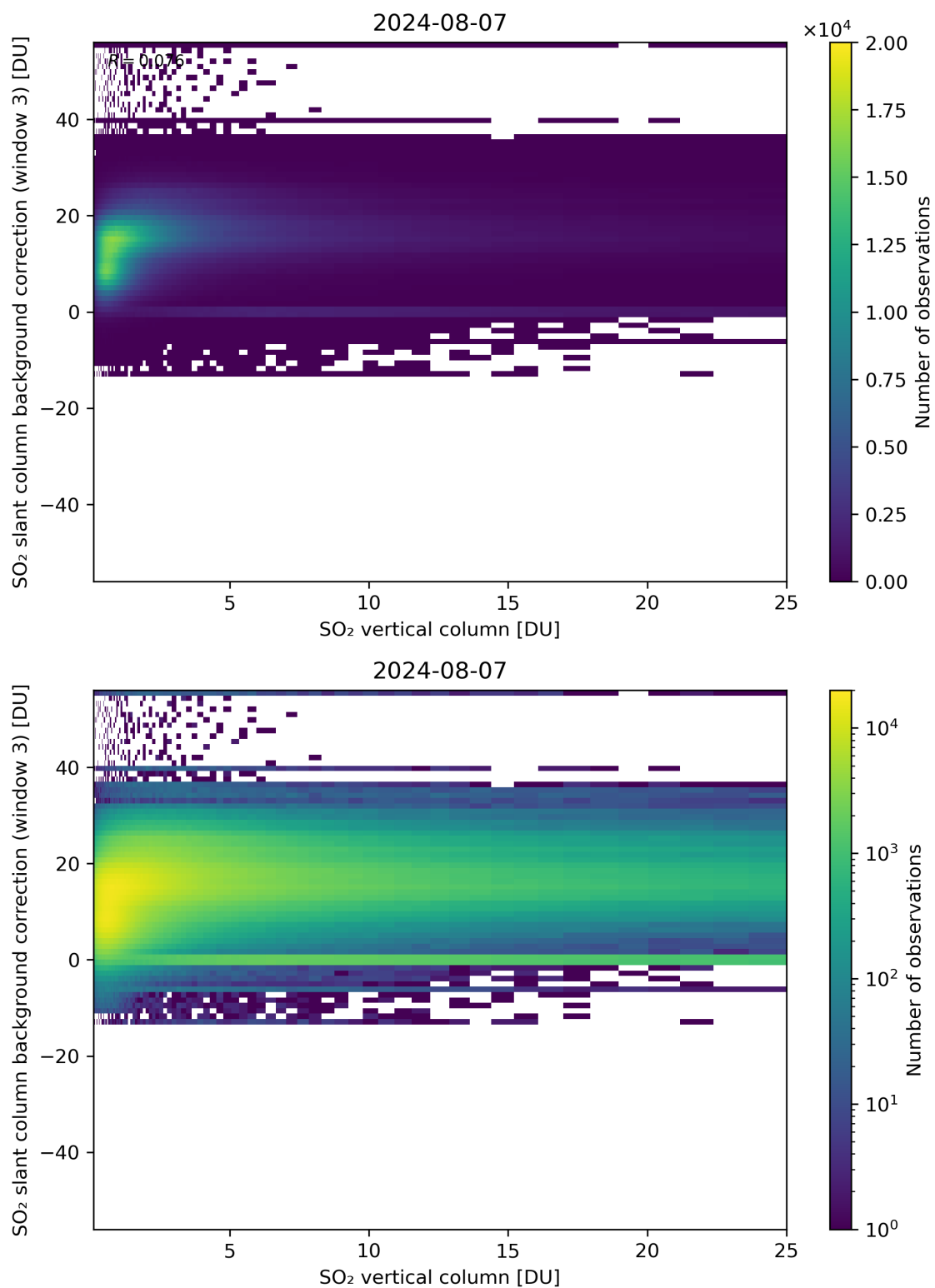
Figure 275: Scatter density plot of “SO 2 vertical column” against “SO 2 slant column background correction (window 3)” for 2024-08-06 to 2024-08-08.
