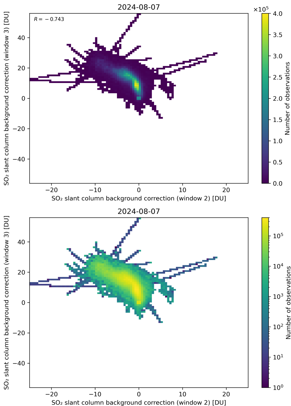
Figure 111: Scatter density plot of “SO 2 slant column background correction (window 2)” against “SO 2 slant column background correction (window 3)” for 2024-08-06 to 2024-08-08.
