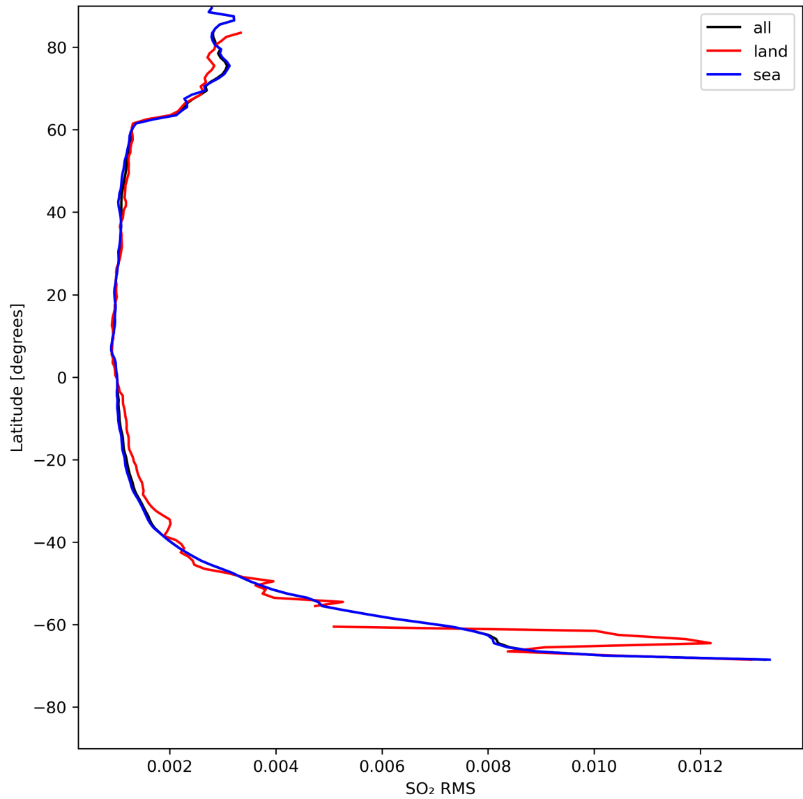
Figure 47: Zonal average of “SO 2 RMS” for 2024-08-06 to 2024-08-08.
