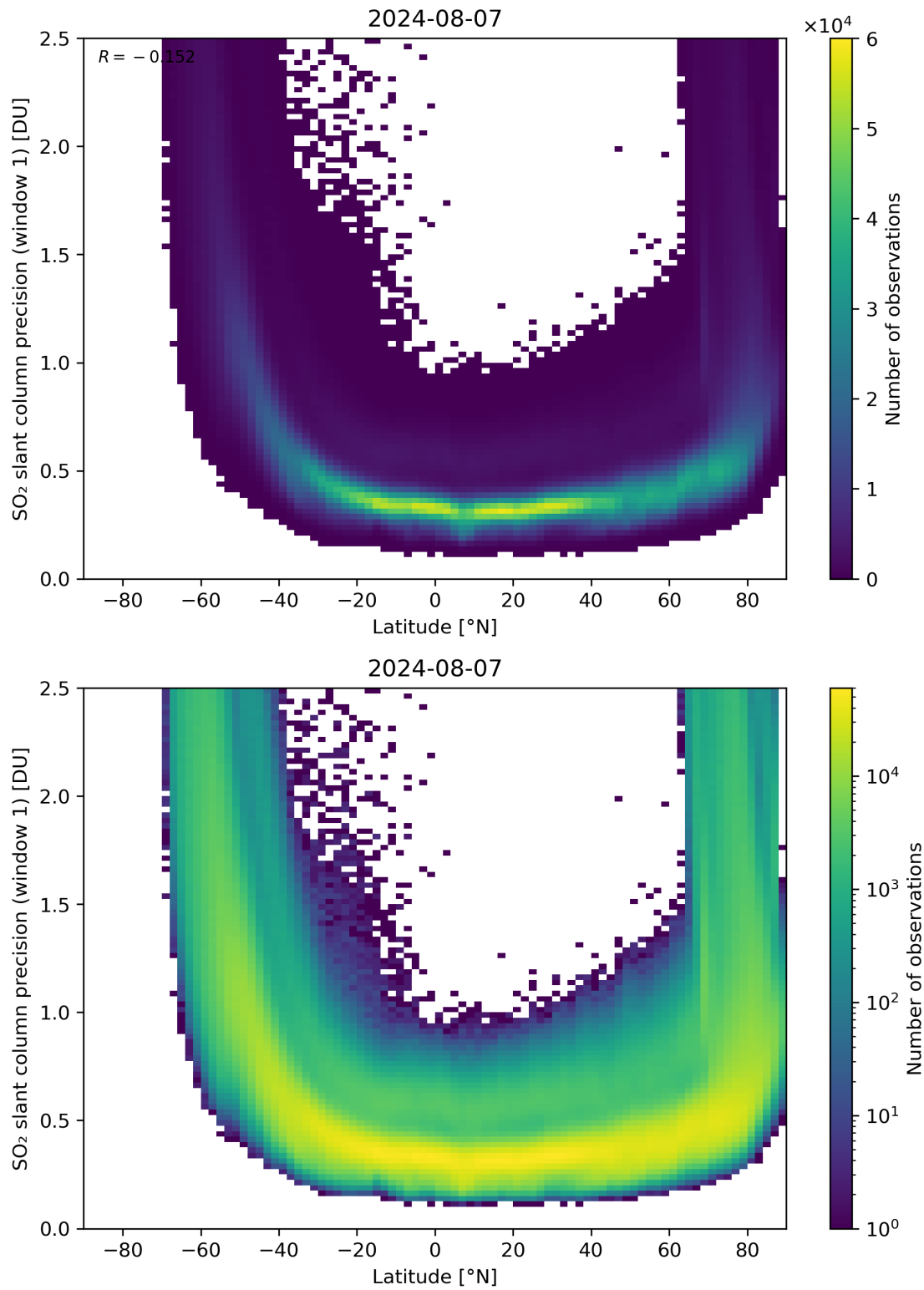
Figure 150: Scatter density plot of “Latitude” against “SO 2 slant column precision (window 1)” for 2024-08-06 to 2024-08-08.
