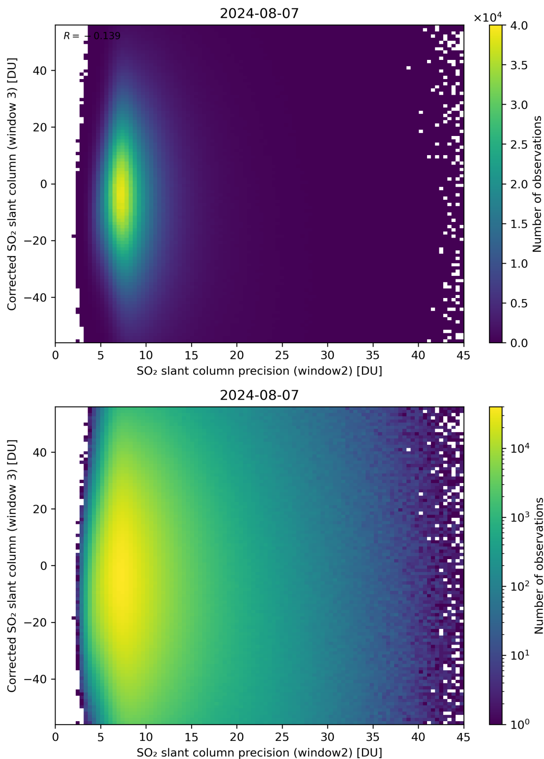
Figure 248: Scatter density plot of “SO 2 slant column precision (window2)” against “Corrected SO 2 slant column (window 3)” for 2024-08-06 to 2024-08-08.
