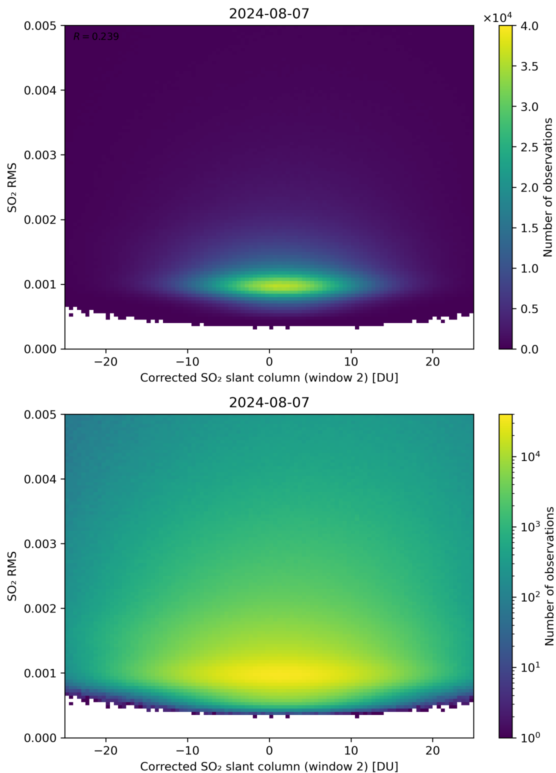
Figure 198: Scatter density plot of “Corrected SO 2 slant column (window 2)” against “SO 2 RMS” for 2024-08-06 to 2024-08-08.
