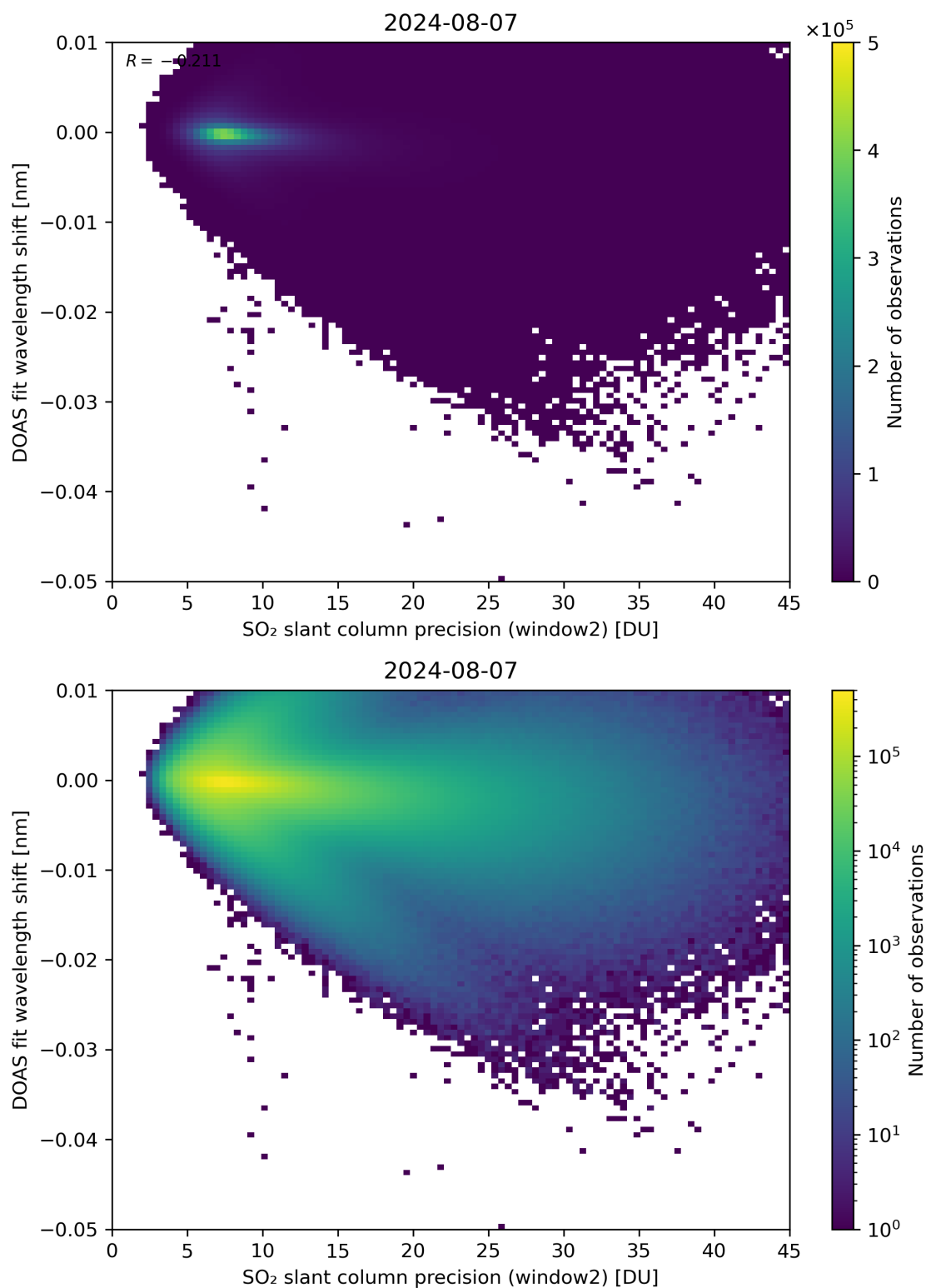
Figure 243: Scatter density plot of “SO 2 slant column precision (window2)” against “DOAS fit wavelength shift” for 2024-08-06 to 2024-08-08.
