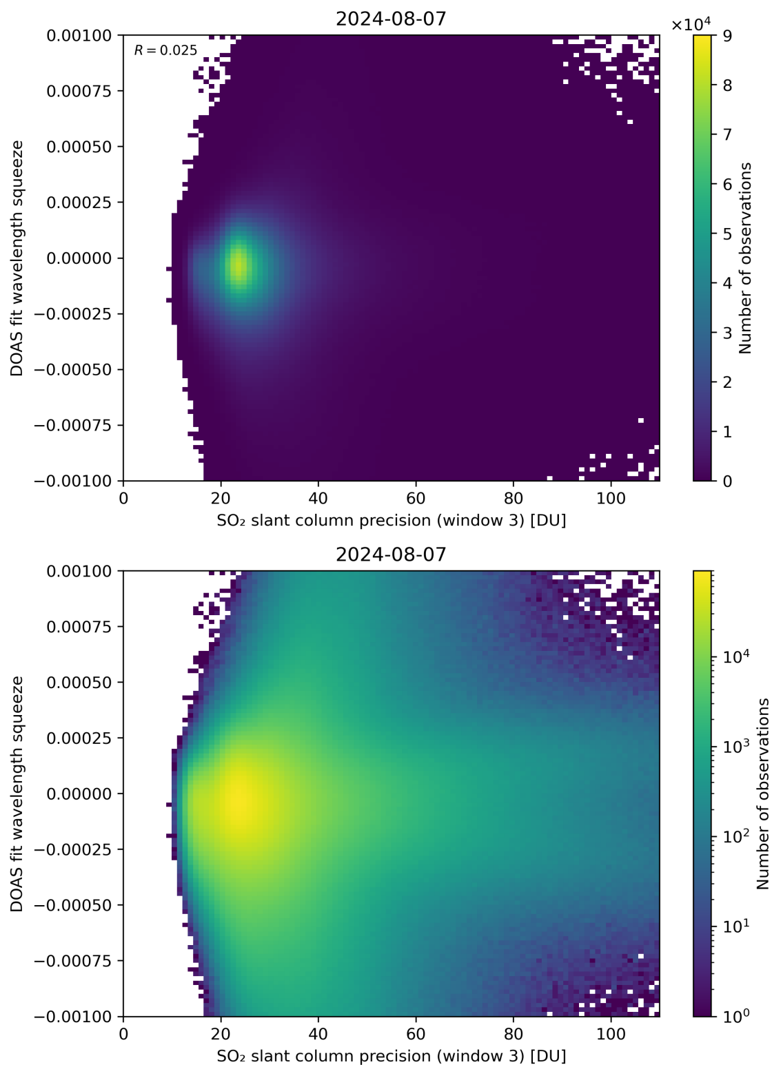
Figure 259: Scatter density plot of “SO 2 slant column precision (window 3)” against “DOAS fit wavelength squeeze” for 2024-08-06 to 2024-08-08.
