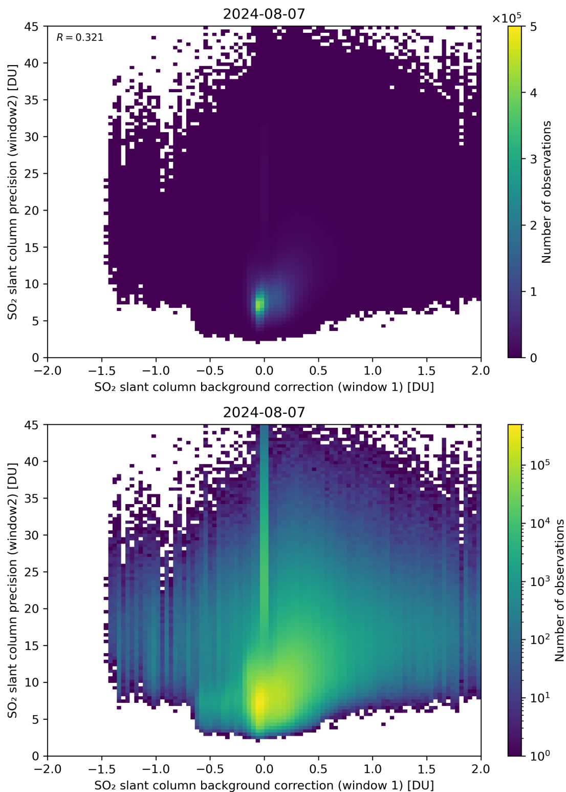
Figure 106: Scatter density plot of “SO 2 slant column background correction (window 1)” against “SO 2 slant column precision (window2)” for 2024-08-06 to 2024-08-08.
