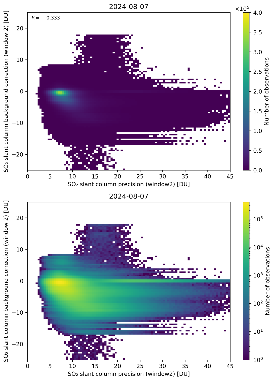
Figure 241: Scatter density plot of “SO 2 slant column precision (window2)” against “SO 2 slant column background correction (window 2)” for 2024-08-06 to 2024-08-08.
