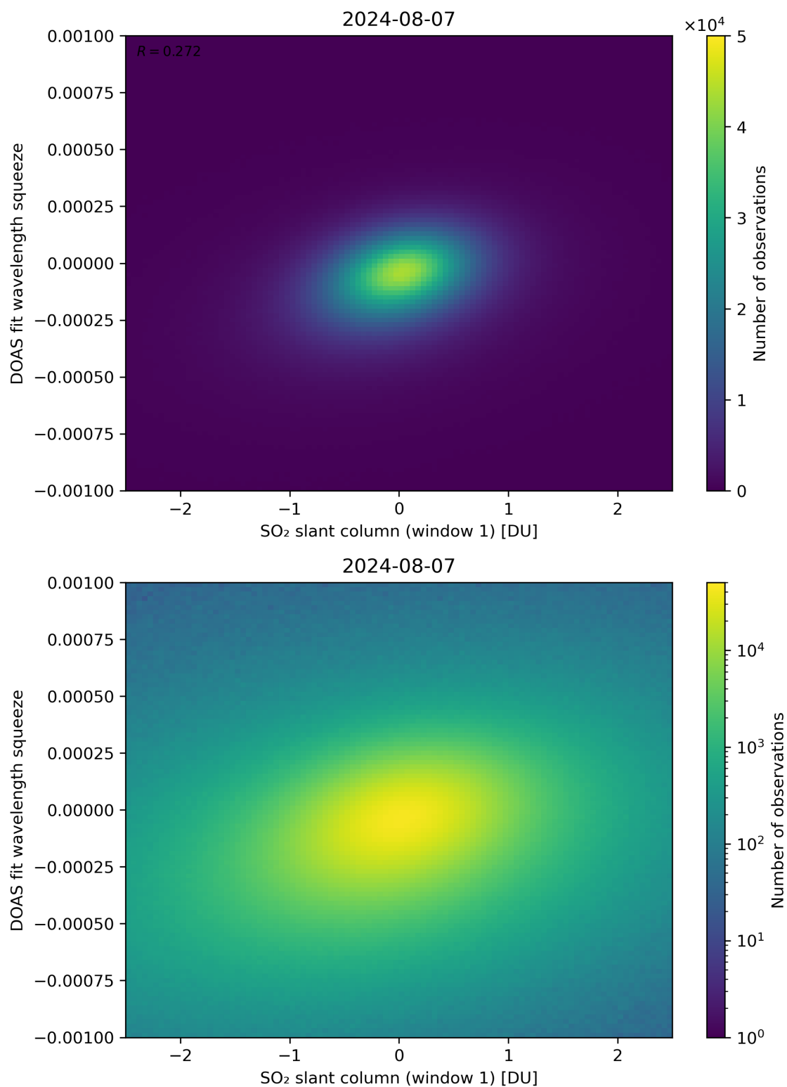
Figure 216: Scatter density plot of “SO 2 slant column (window 1)” against “DOAS fit wavelength squeeze” for 2024-08-06 to 2024-08-08.
