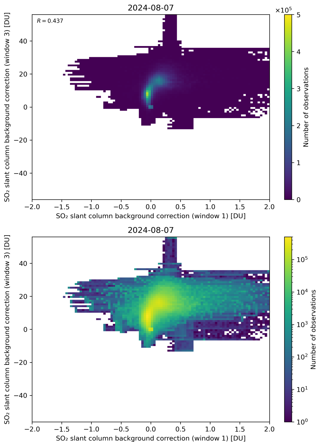
Figure 99: Scatter density plot of “SO 2 slant column background correction (window 1)” against “SO 2 slant column background correction (window 3)” for 2024-08-06 to 2024-08-08.
