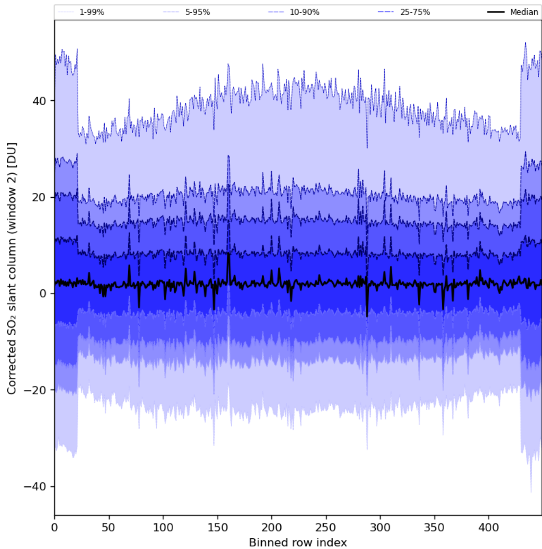
Figure 85: Along track statistics of “Corrected SO 2 slant column (window 2)” for 2024-08-06 to 2024-08-08
