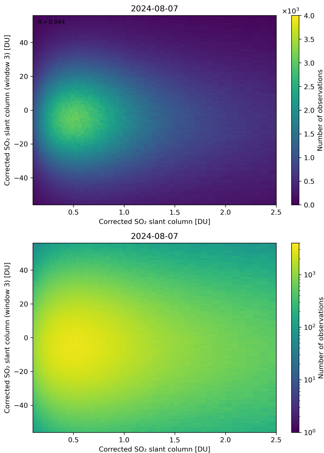
Figure 186: Scatter density plot of “Corrected SO 2 slant column” against “Corrected SO 2 slant column (window 3)” for 2024-08-06 to 2024-08-08.
