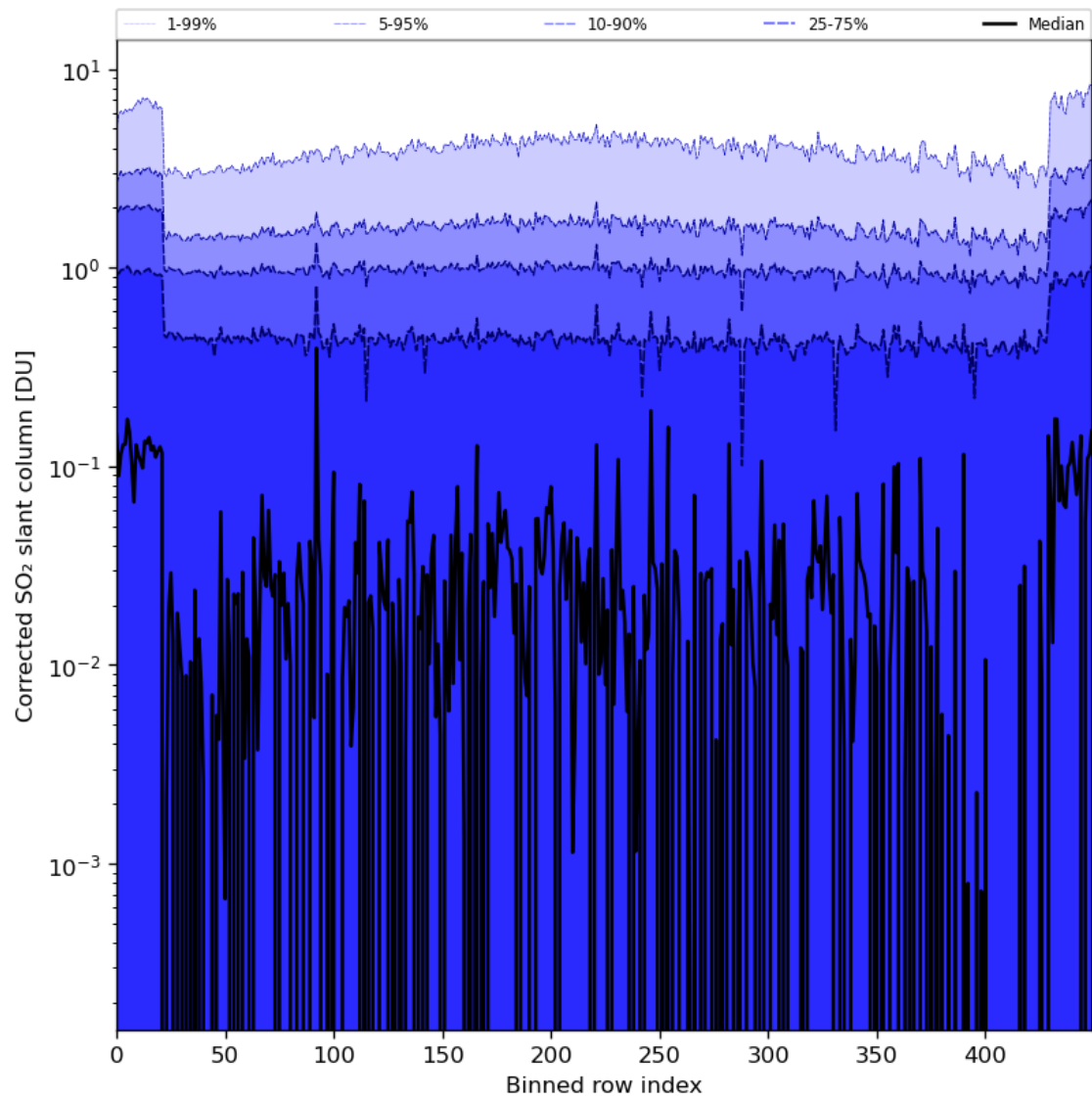
Figure 78: Along track statistics of “Corrected SO 2 slant column” for 2024-08-06 to 2024-08-08
