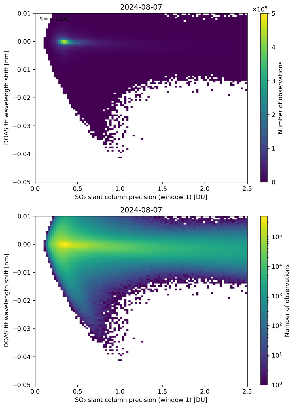
Figure 221: Scatter density plot of “SO 2 slant column precision (window 1)” against “DOAS fit wavelength shift” for 2024-08-06 to 2024-08-08.
