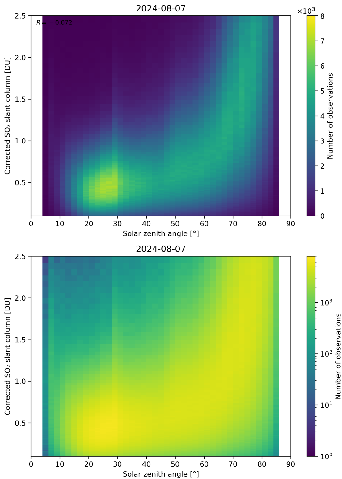
Figure 166: Scatter density plot of “Solar zenith angle” against “Corrected SO 2 slant column” for 2024-08-06 to 2024-08-08.
