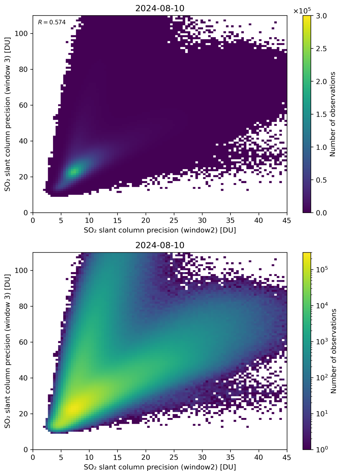
Figure 250: Scatter density plot of “SO 2 slant column precision (window2)” against “SO 2 slant column precision (window 3)” for 2024-08-09 to 2024-08-11.
