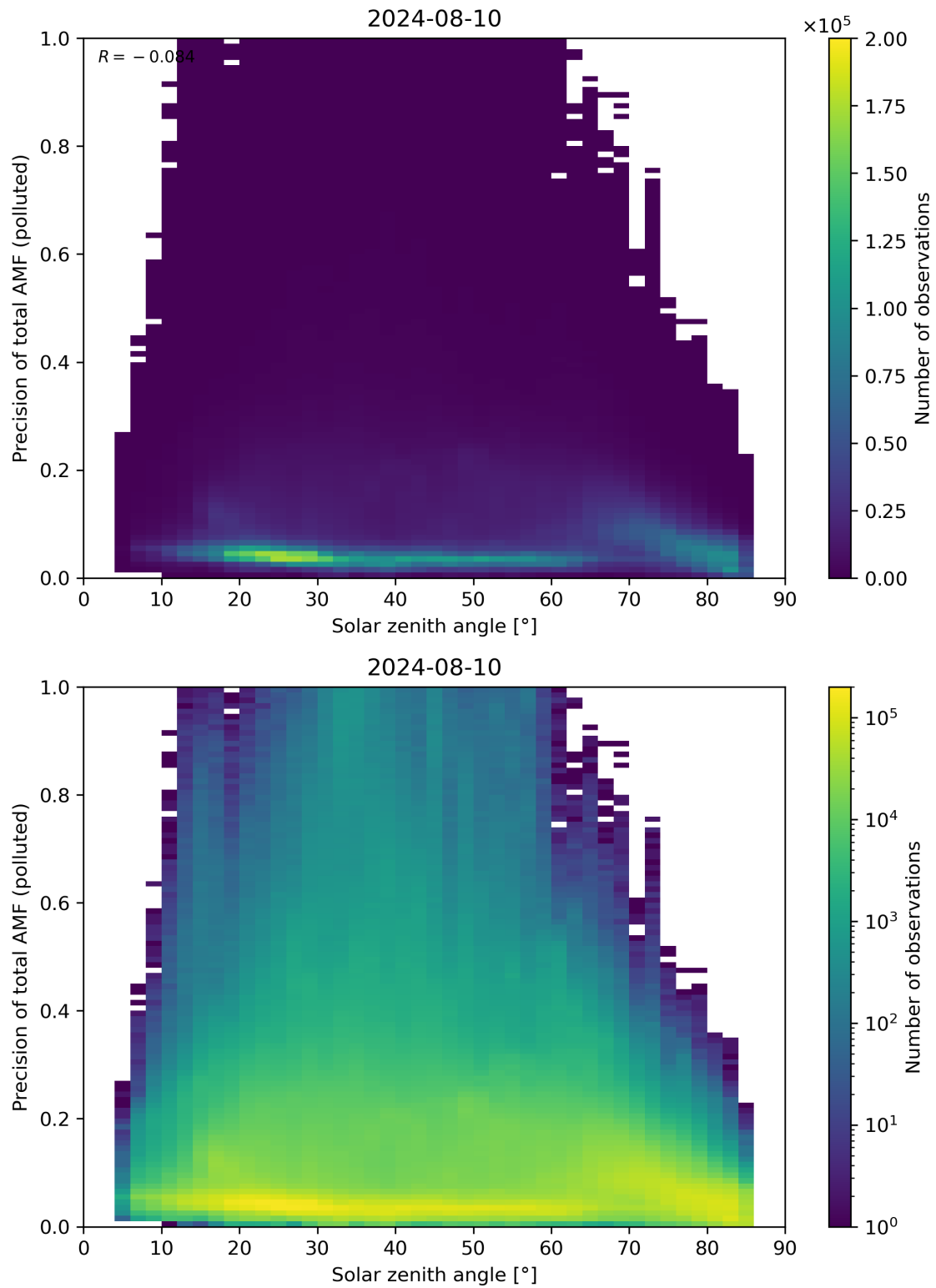
Figure 175: Scatter density plot of “Solar zenith angle” against “Precision of total AMF (polluted)” for 2024-08-09 to 2024-08-11.
