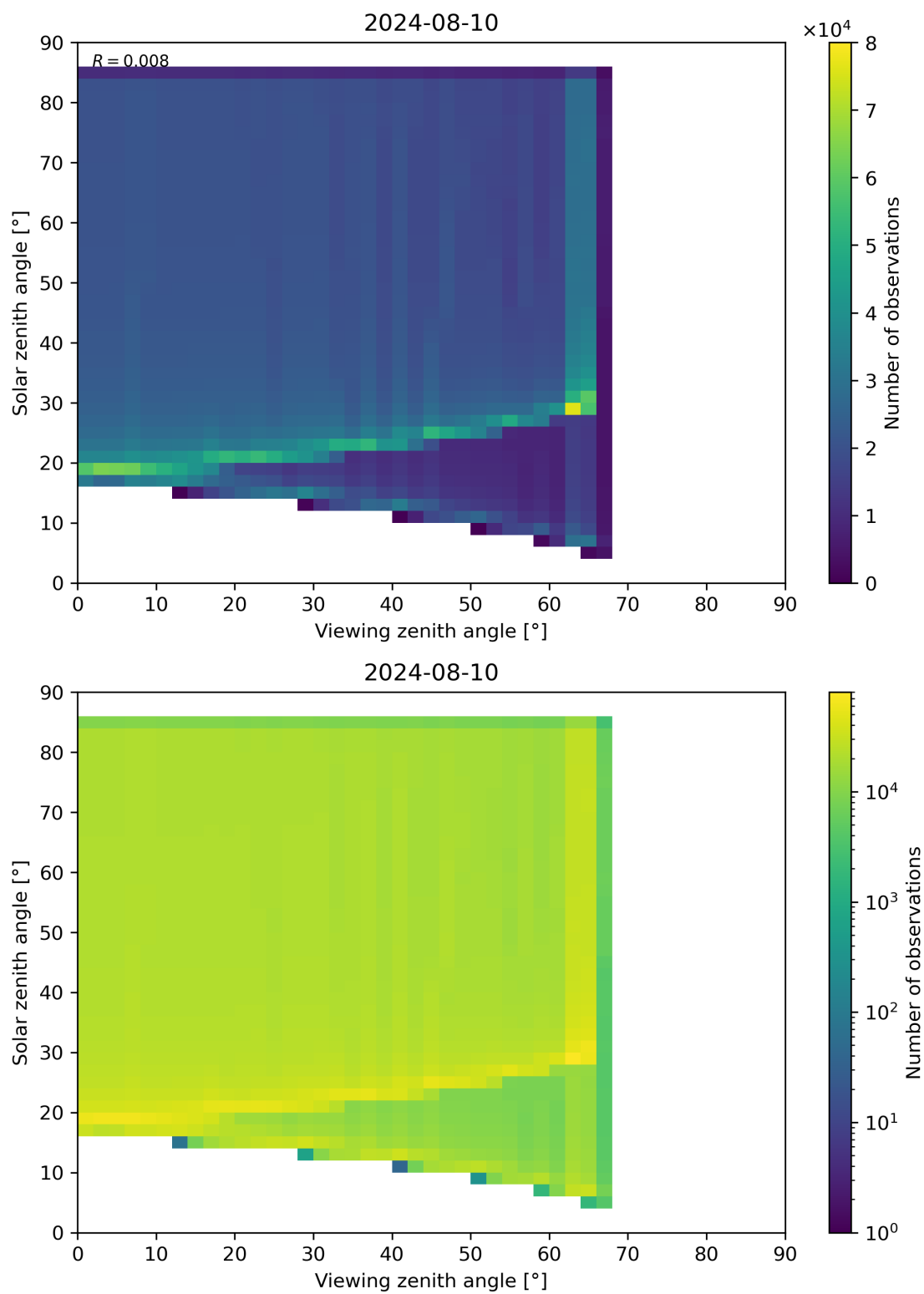
Figure 315: Scatter density plot of “Viewing zenith angle” against “Solar zenith angle” for 2024-08-09 to 2024-08-11.
