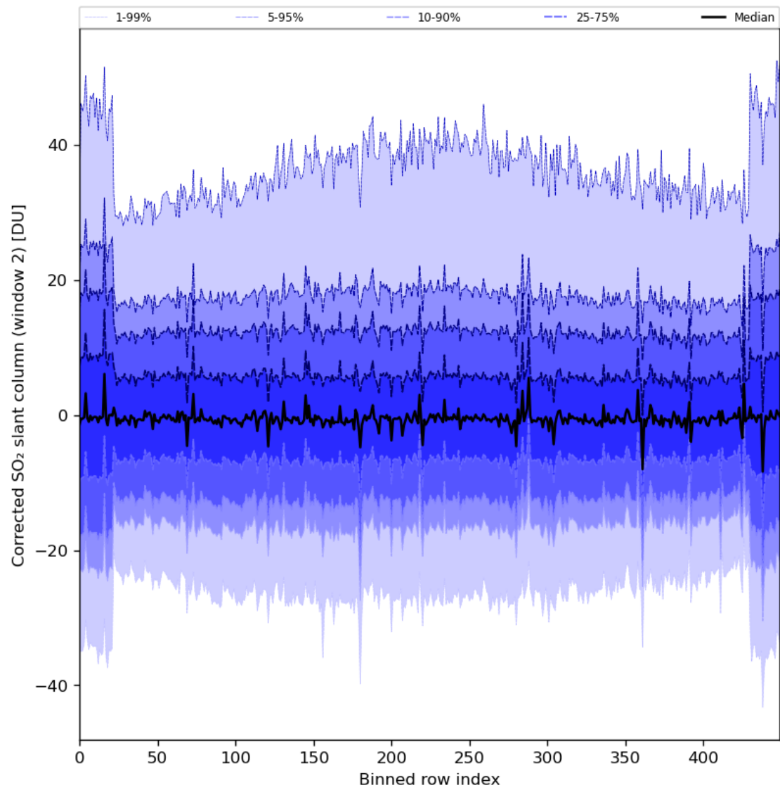
Figure 85: Along track statistics of “Corrected SO 2 slant column (window 2)” for 2024-08-09 to 2024-08-11
