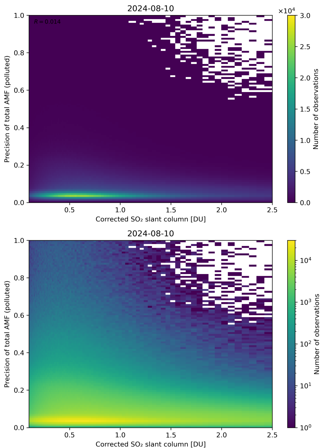
Figure 193: Scatter density plot of “Corrected SO 2 slant column” against “Precision of total AMF (polluted)” for 2024-08-09 to 2024-08-11.
