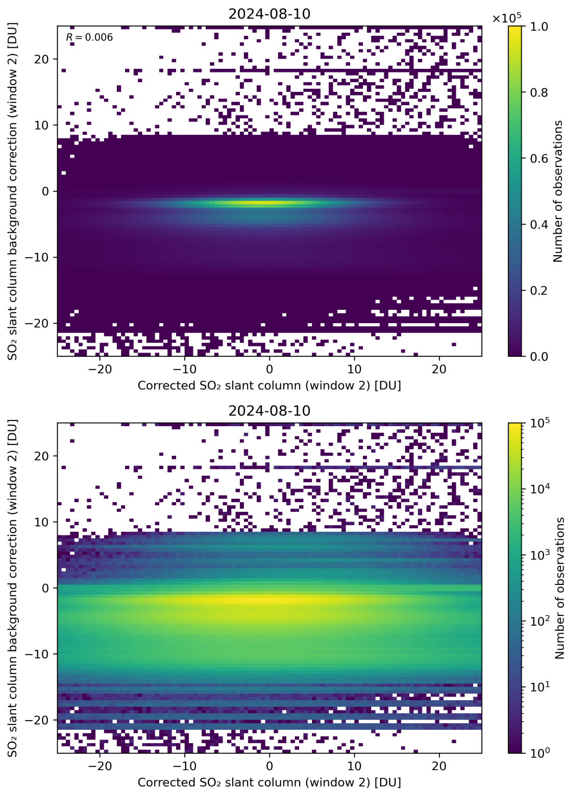
Figure 194: Scatter density plot of “Corrected SO 2 slant column (window 2)” against “SO 2 slant column background correction (window 2)” for 2024-08-09 to 2024-08-11.
