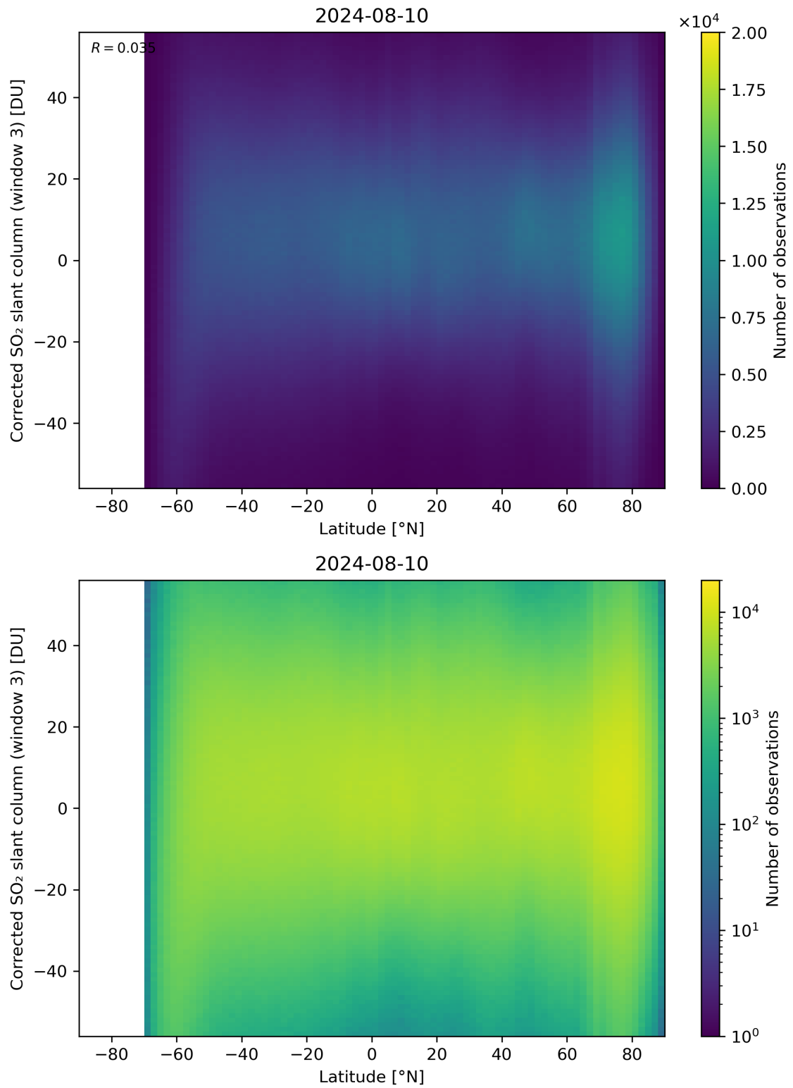
Figure 148: Scatter density plot of “Latitude” against “Corrected SO 2 slant column (window 3)” for 2024-08-09 to 2024-08-11.
