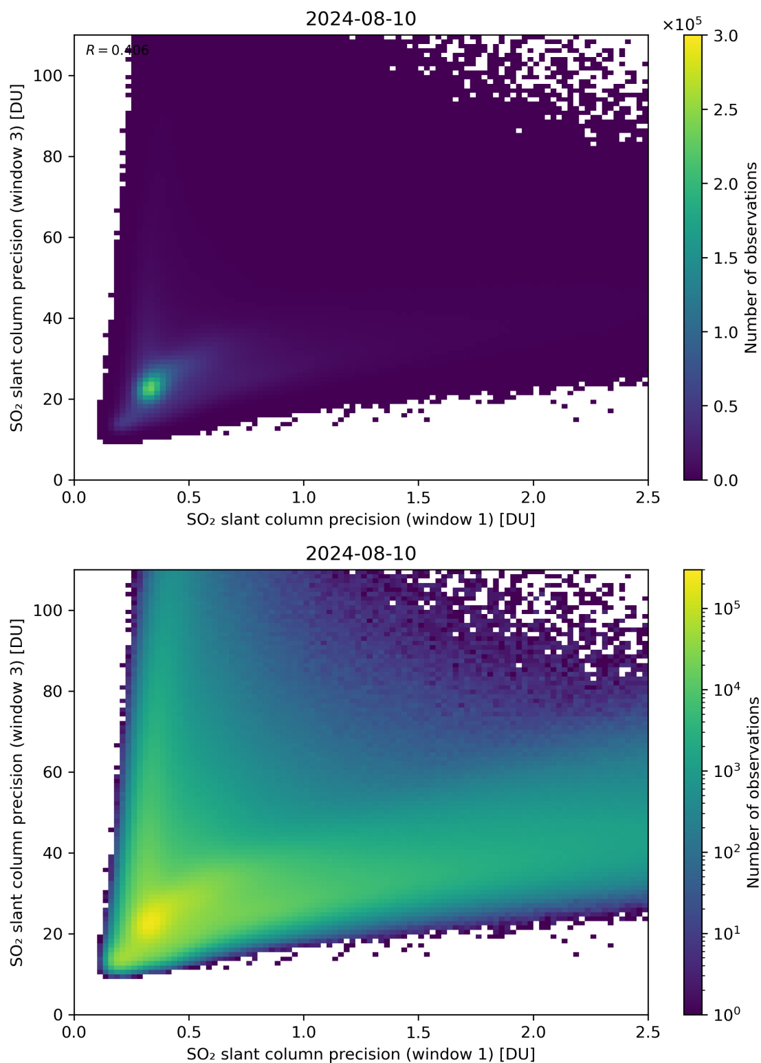
Figure 229: Scatter density plot of “SO 2 slant column precision (window 1)” against “SO 2 slant column precision (window 3)” for 2024-08-09 to 2024-08-11.
