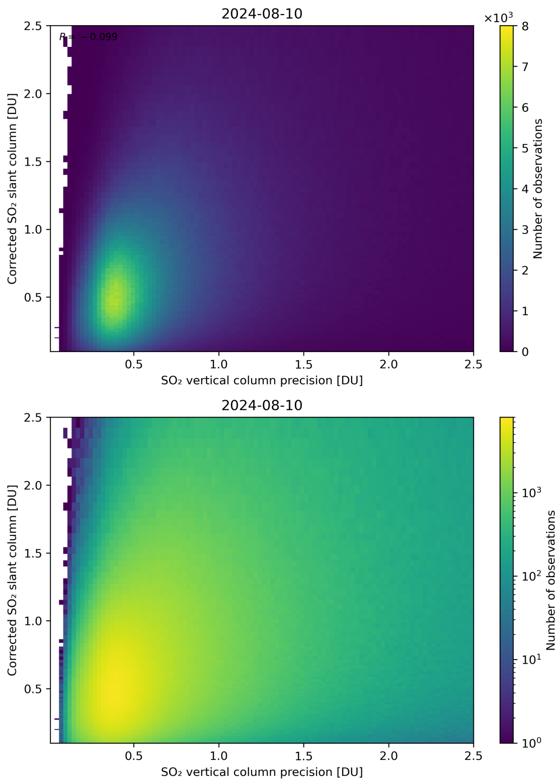
Figure 286: Scatter density plot of “SO 2 vertical column precision” against “Corrected SO 2 slant column” for 2024-08-09 to 2024-08-11.
