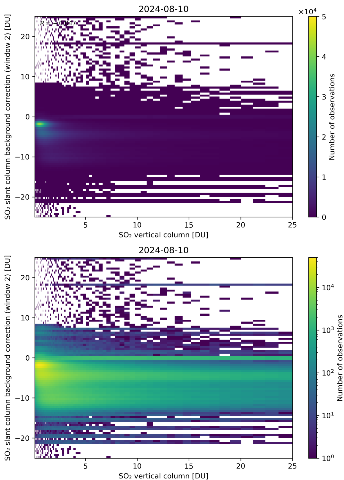
Figure 274: Scatter density plot of “SO 2 vertical column” against “SO 2 slant column background correction (window 2)” for 2024-08-09 to 2024-08-11.
