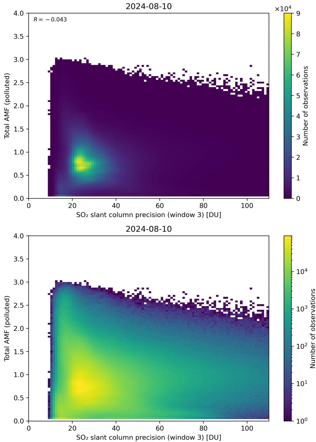
Figure 263: Scatter density plot of “SO 2 slant column precision (window 3)” against “Total AMF (polluted)” for 2024-08-09 to 2024-08-11.
