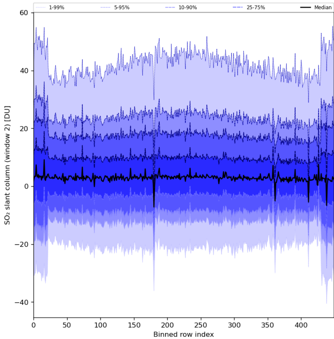
Figure 83: Along track statistics of “SO 2 slant column (window 2)” for 2024-08-09 to 2024-08-11
