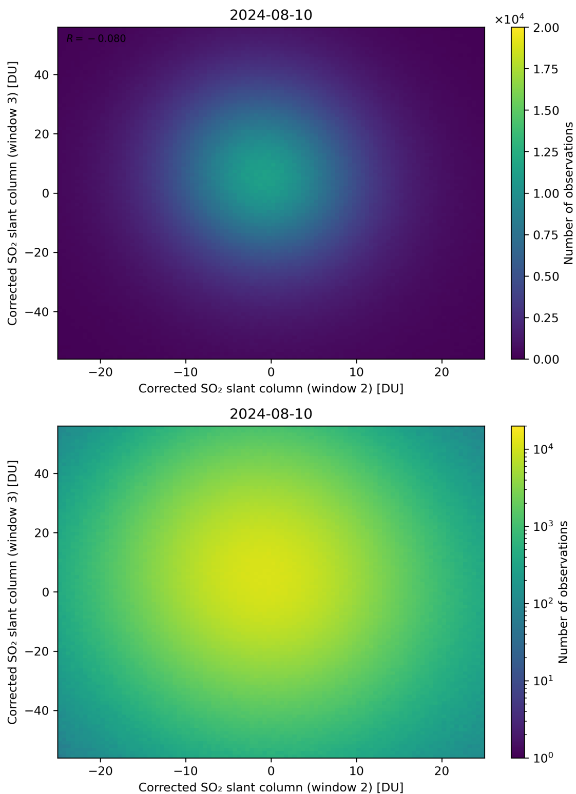
Figure 200: Scatter density plot of “Corrected SO 2 slant column (window 2)” against “Corrected SO 2 slant column (window 3)” for 2024-08-09 to 2024-08-11.
