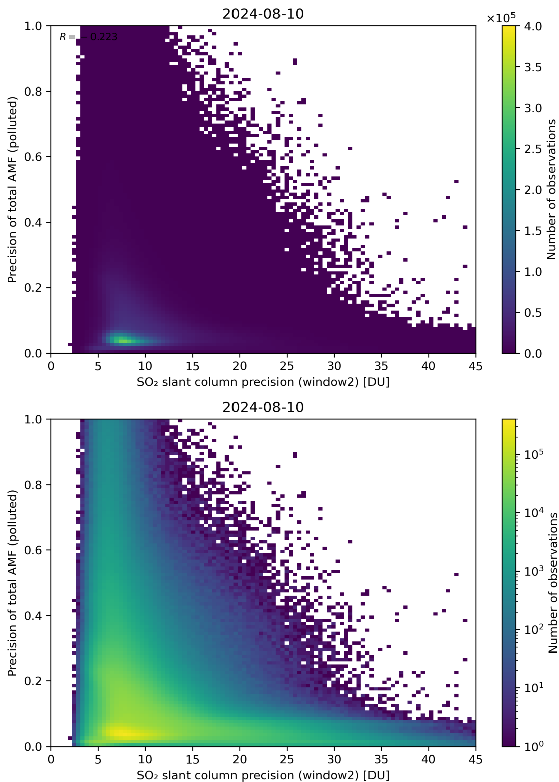
Figure 252: Scatter density plot of “SO 2 slant column precision (window2)” against “Precision of total AMF (polluted)” for 2024-08-09 to 2024-08-11.
