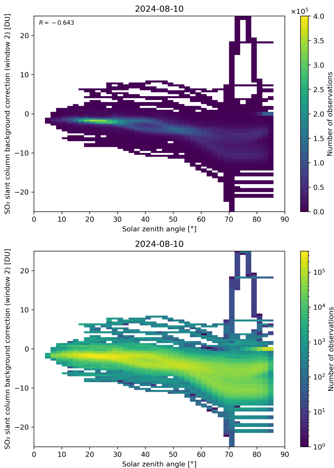
Figure 159: Scatter density plot of “Solar zenith angle” against “SO 2 slant column background correction (window 2)” for 2024-08-09 to 2024-08-11.
