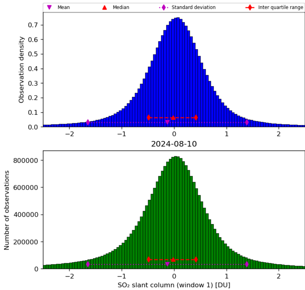
Figure 56: Histogram of “SO 2 slant column (window 1)” for 2024-08-09 to 2024-08-11
