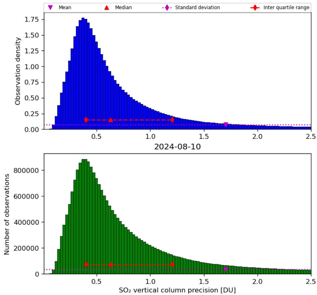
Figure 54: Histogram of “SO 2 vertical column precision” for 2024-08-09 to 2024-08-11
