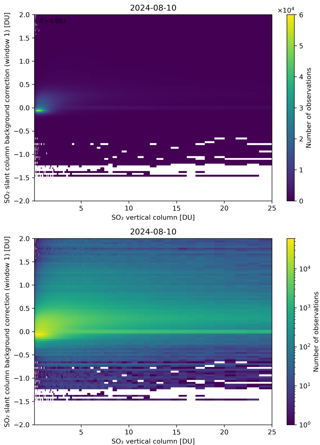
Figure 273: Scatter density plot of “SO 2 vertical column” against “SO 2 slant column background correction (window 1)” for 2024-08-09 to 2024-08-11.
