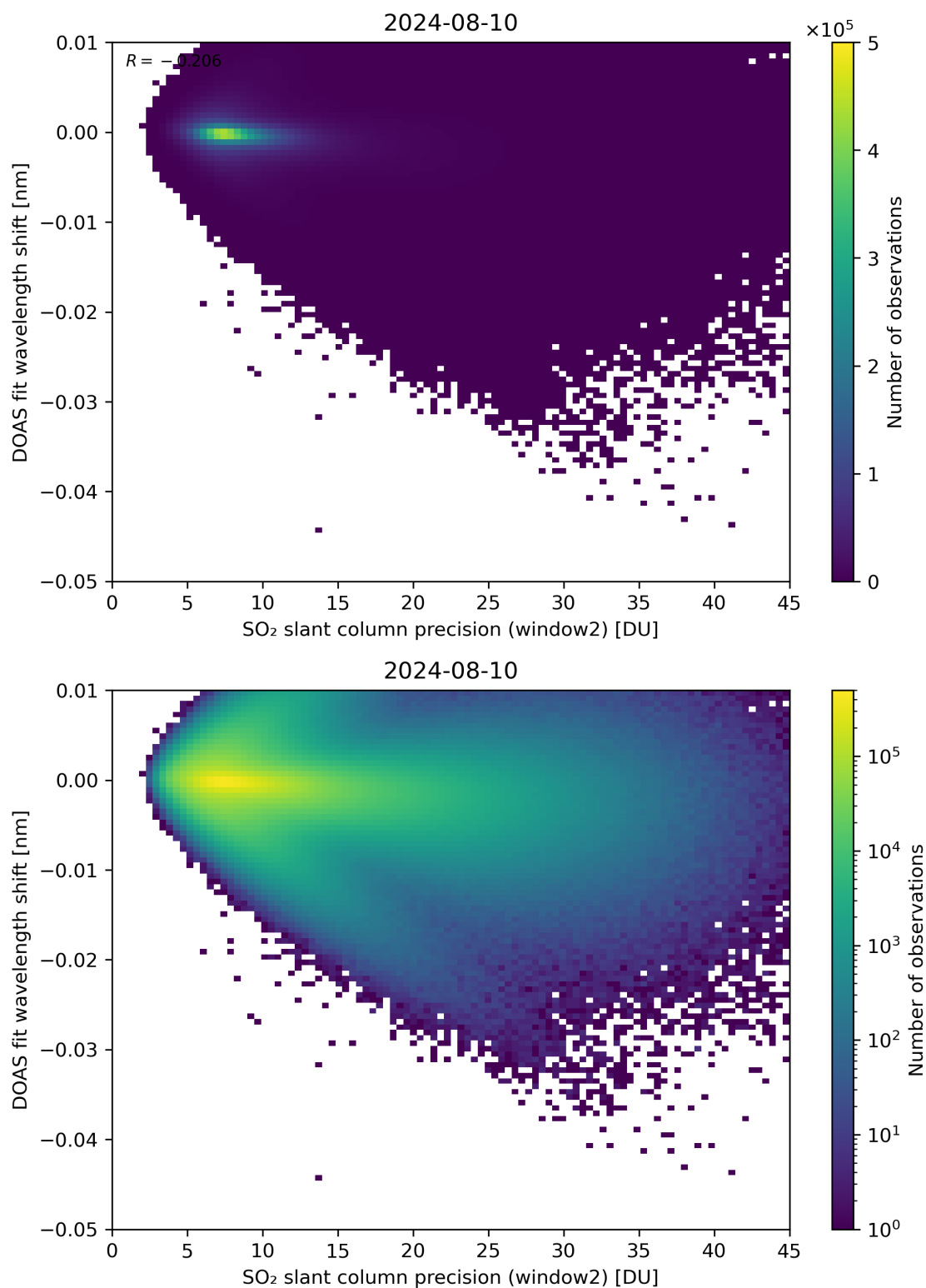
Figure 243: Scatter density plot of “SO 2 slant column precision (window2)” against “DOAS fit wavelength shift” for 2024-08-09 to 2024-08-11.
