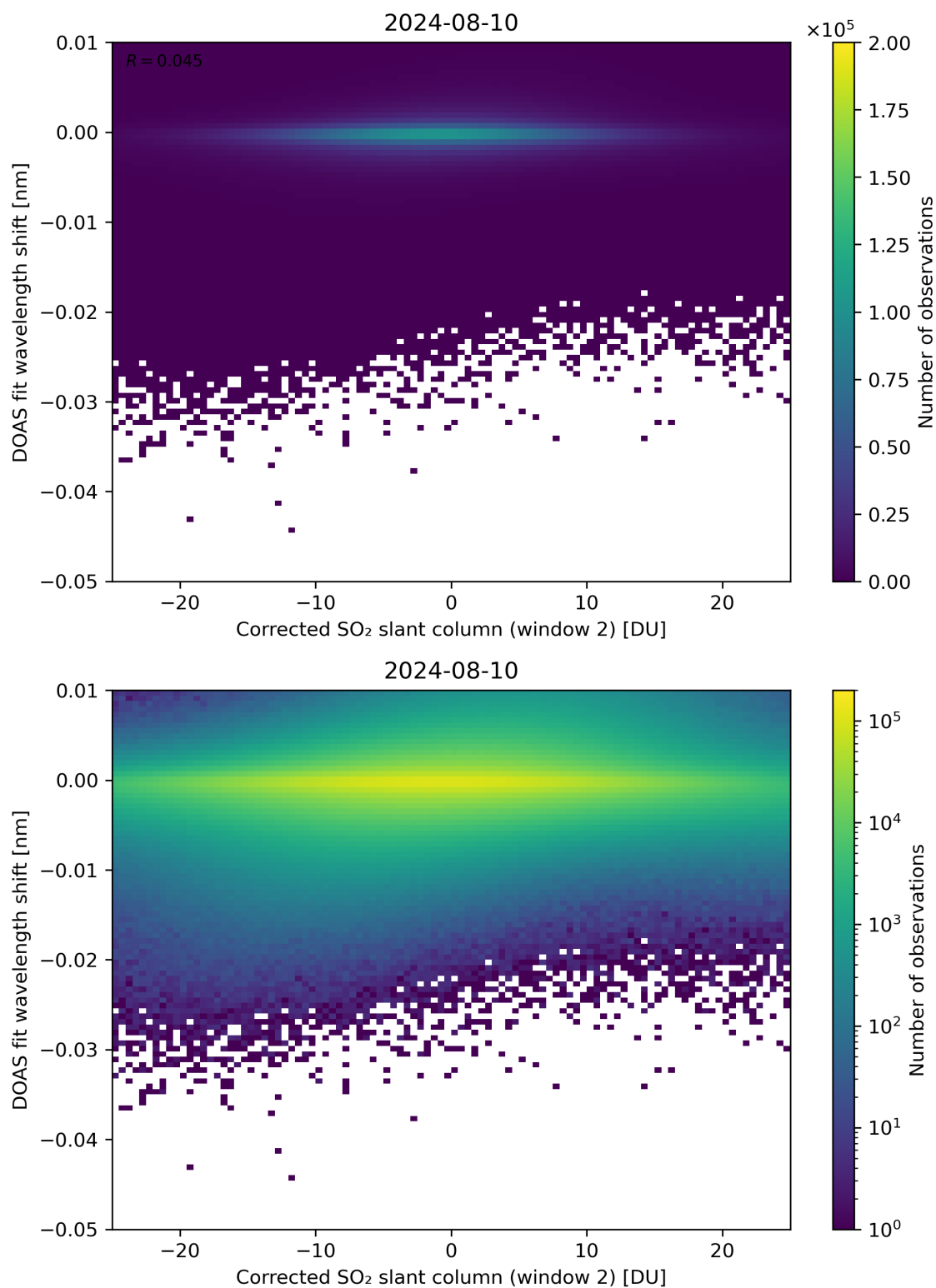
Figure 196: Scatter density plot of “Corrected SO 2 slant column (window 2)” against “DOAS fit wavelength shift” for 2024-08-09 to 2024-08-11.
