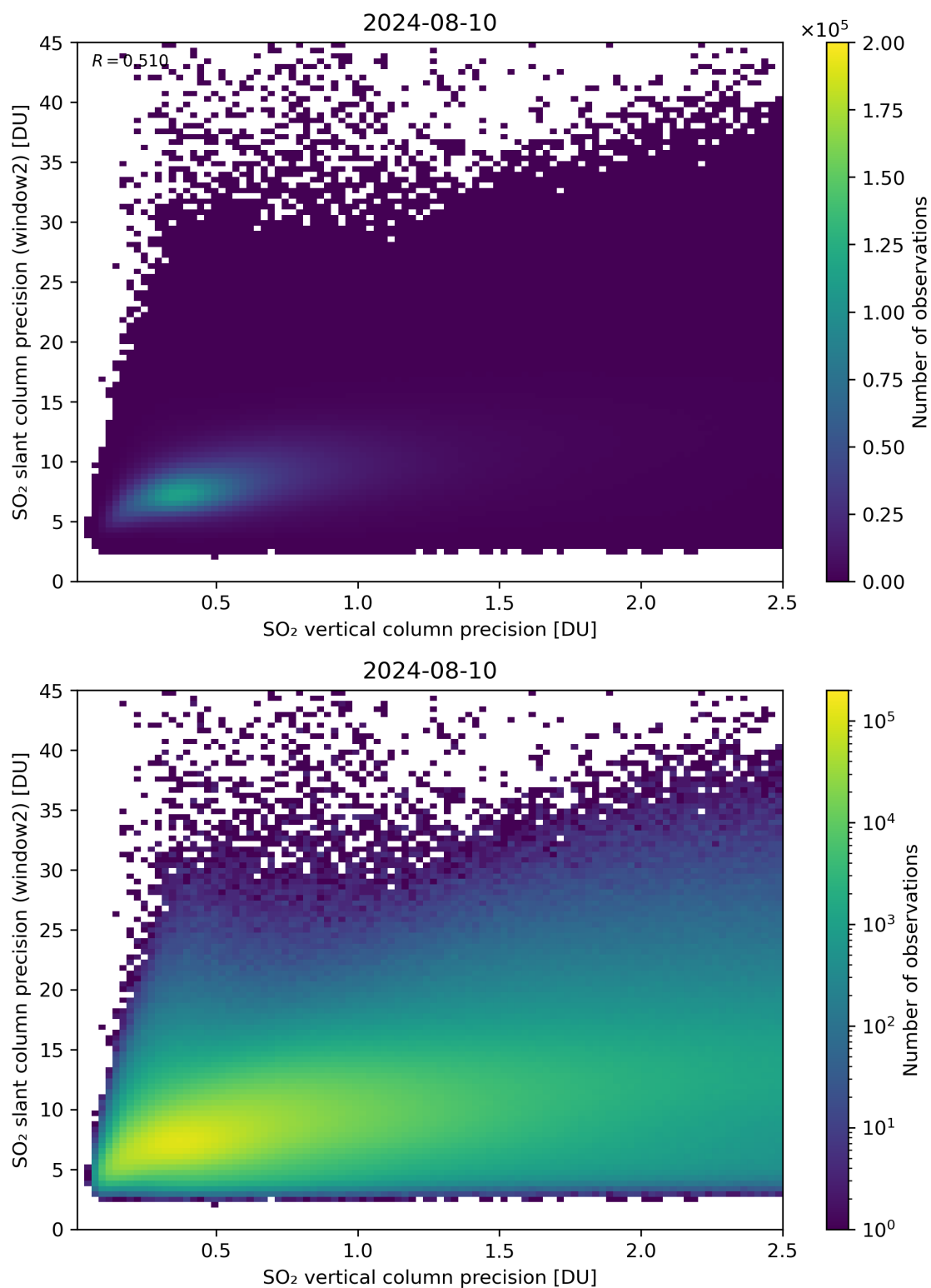
Figure 291: Scatter density plot of “SO 2 vertical column precision” against “SO 2 slant column precision (window2)” for 2024-08-09 to 2024-08-11.
