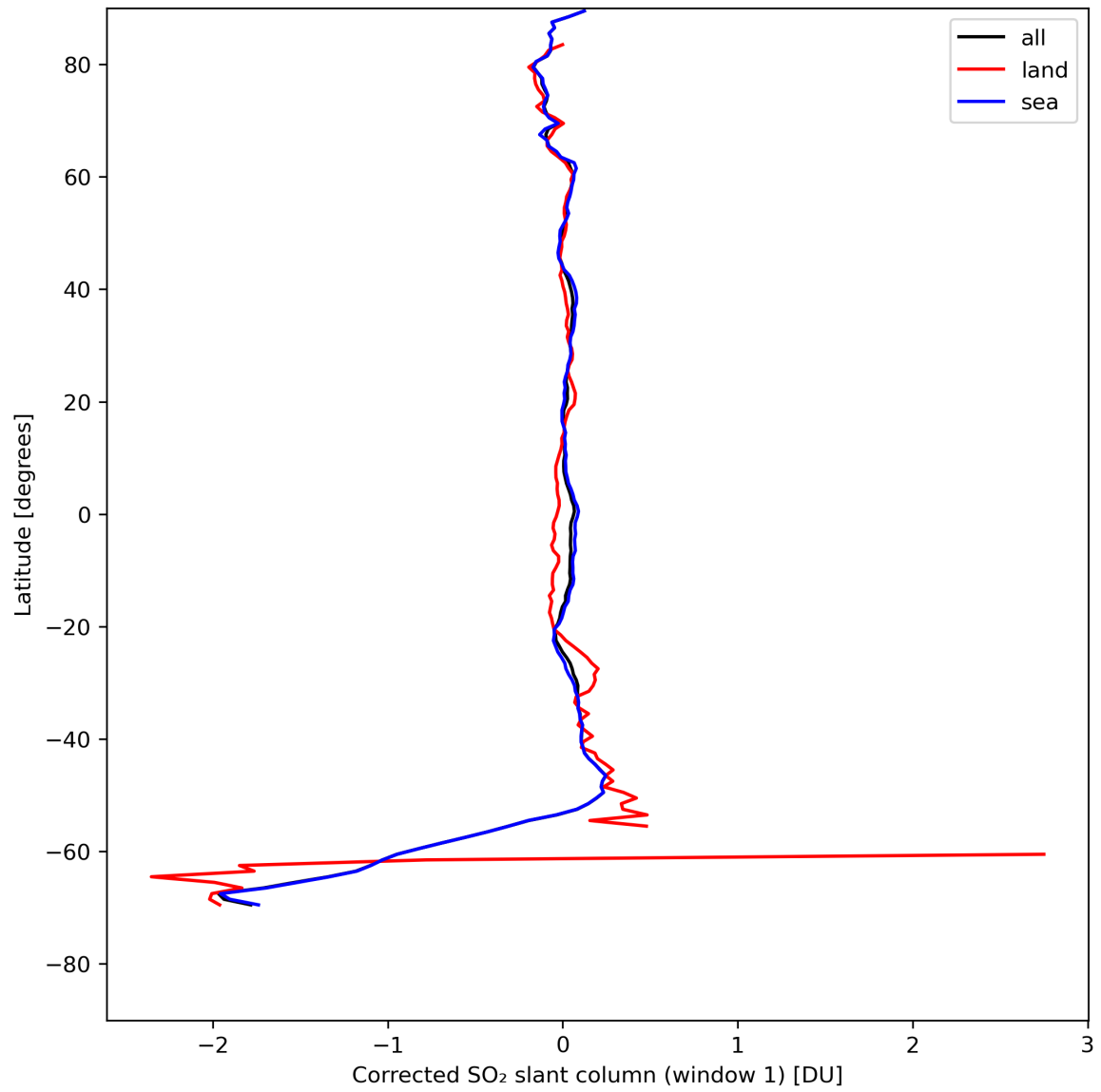
Figure 35: Zonal average of “Corrected SO 2 slant column (window 1)” for 2024-08-09 to 2024-08-11.
