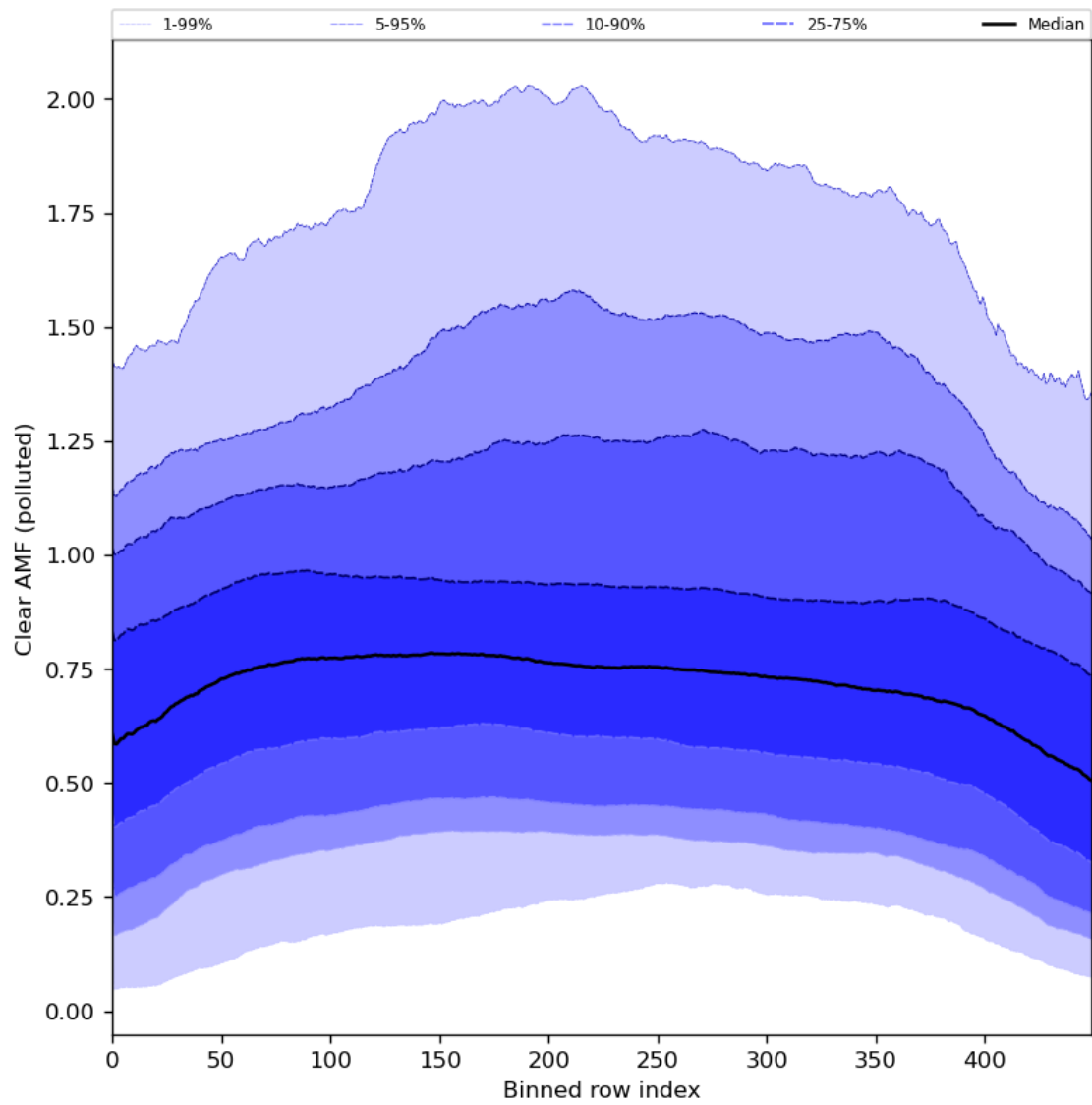
Figure 96: Along track statistics of “Clear AMF (polluted)” for 2024-08-09 to 2024-08-11
