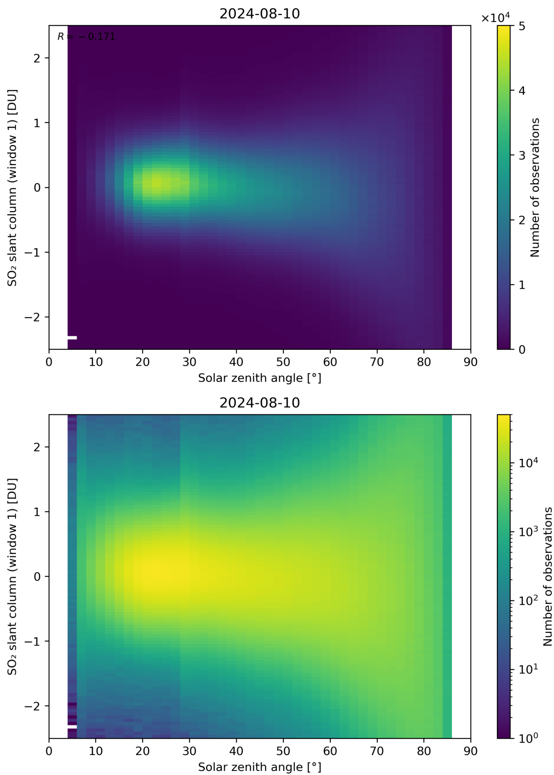
Figure 169: Scatter density plot of “Solar zenith angle” against “SO 2 slant column (window 1)” for 2024-08-09 to 2024-08-11.
