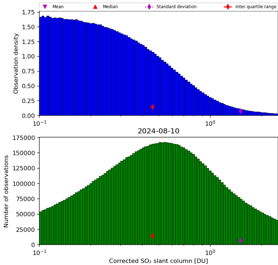
Figure 55: Histogram of “Corrected SO 2 slant column” for 2024-08-09 to 2024-08-11
