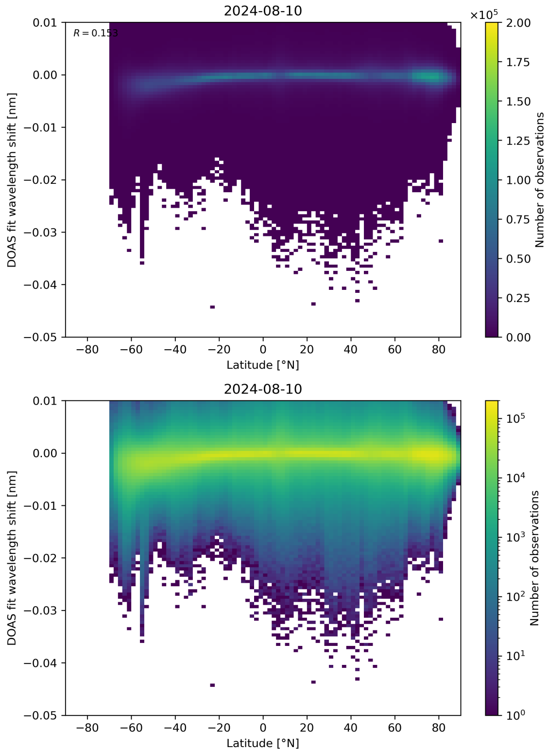
Figure 142: Scatter density plot of “Latitude” against “DOAS fit wavelength shift” for 2024-08-09 to 2024-08-11.
