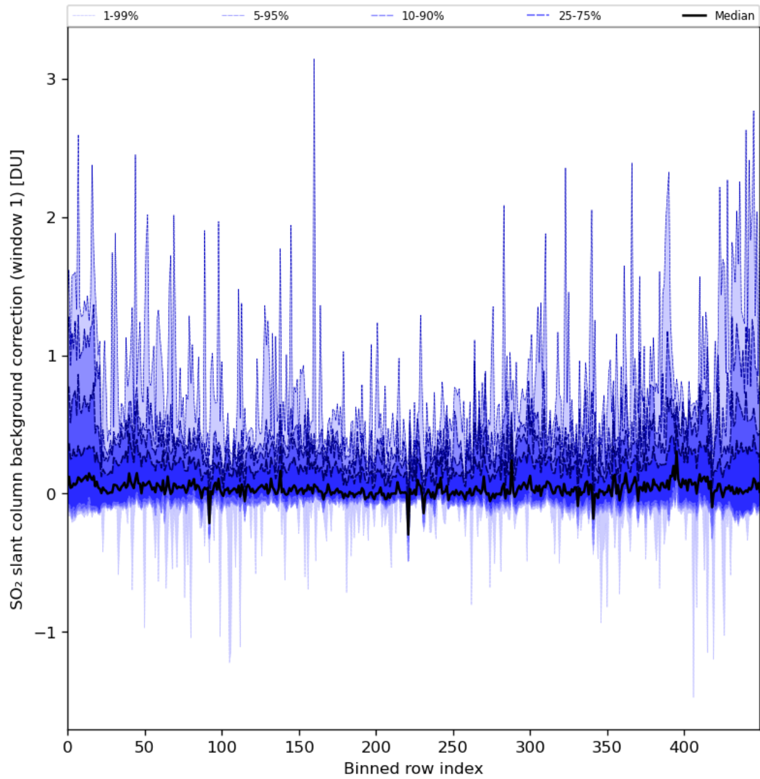
Figure 82: Along track statistics of “SO 2 slant column background correction (window 1)” for 2024-08-09 to 2024-08-11
