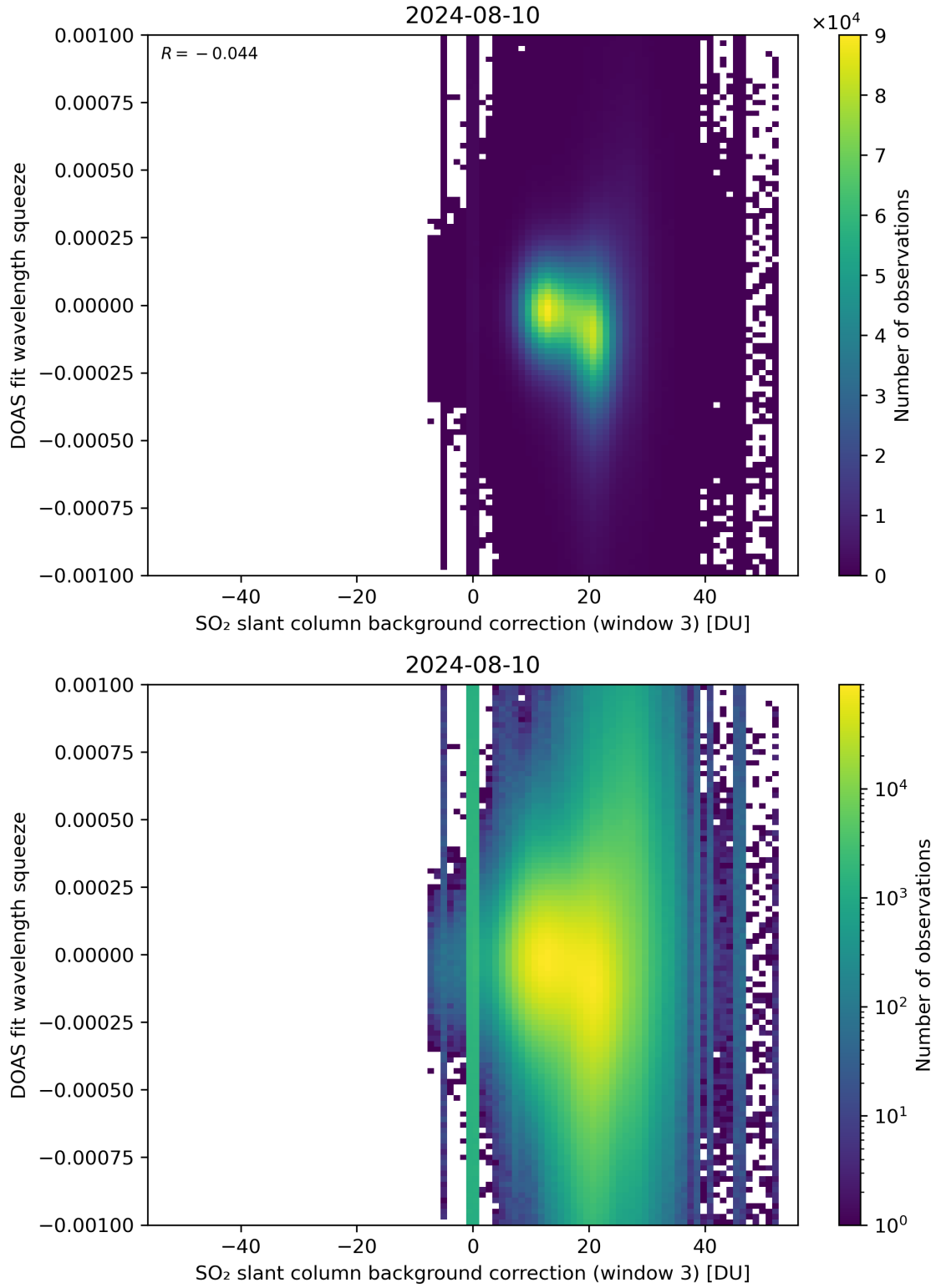
Figure 122: Scatter density plot of “SO 2 slant column background correction (window 3)” against “DOAS fit wavelength squeeze” for 2024-08-09 to 2024-08-11.
