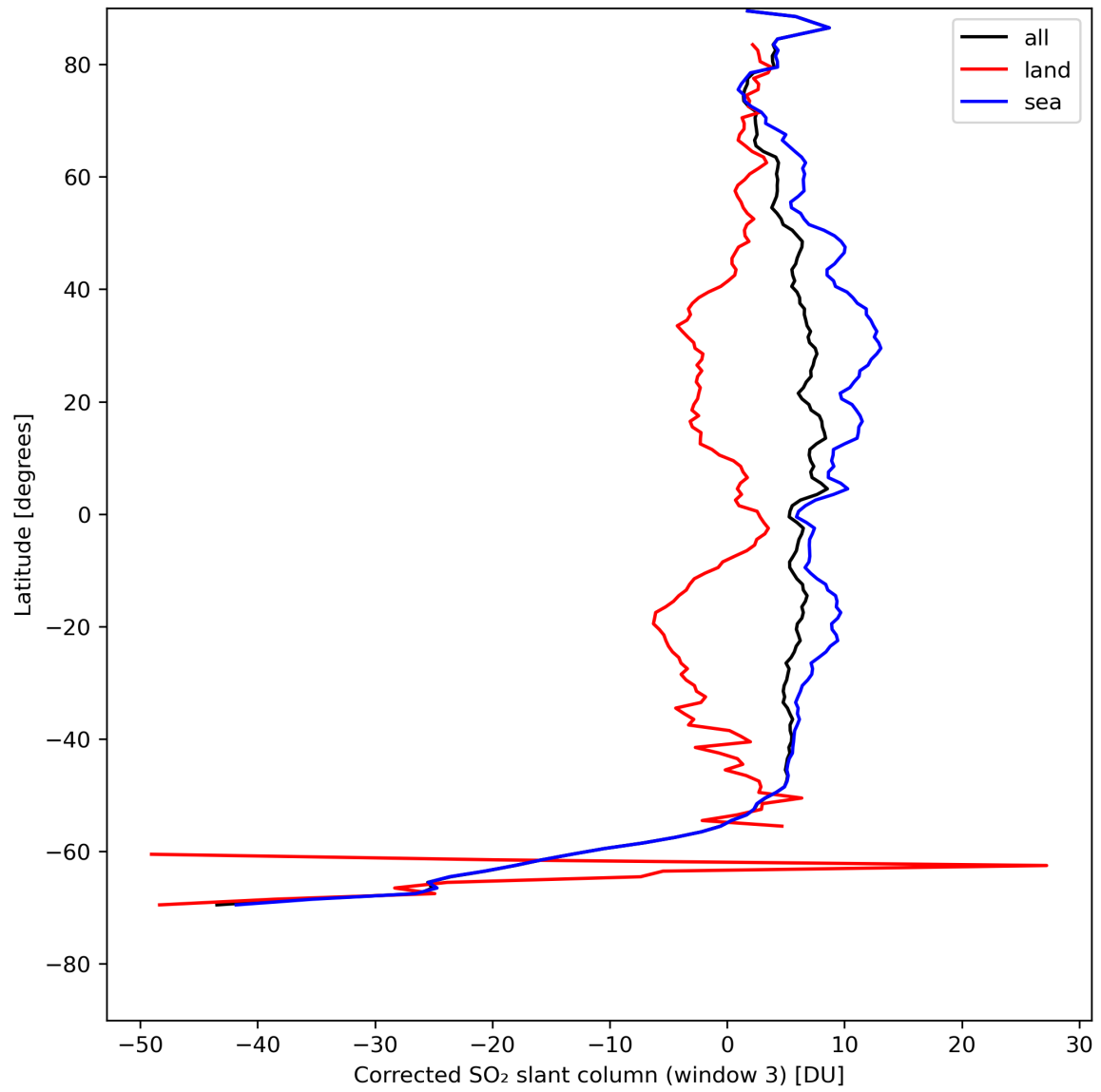
Figure 43: Zonal average of “Corrected SO 2 slant column (window 3)” for 2024-08-09 to 2024-08-11.
