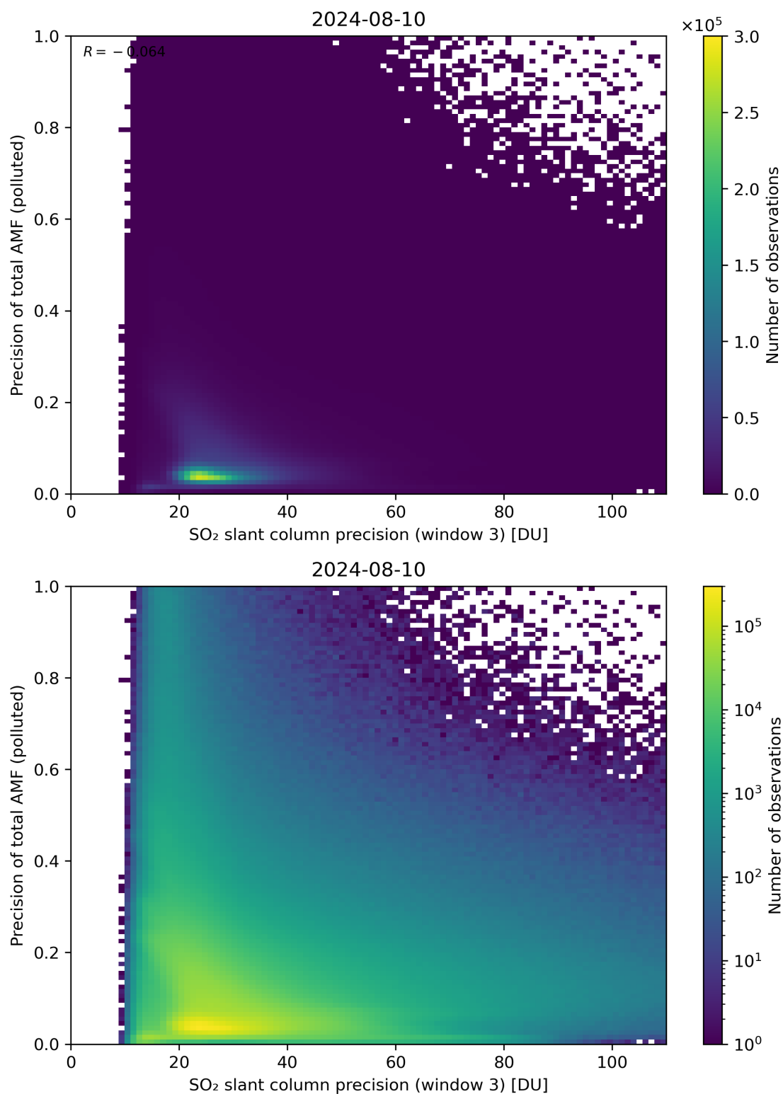
Figure 264: Scatter density plot of “SO 2 slant column precision (window 3)” against “Precision of total AMF (polluted)” for 2024-08-09 to 2024-08-11.
