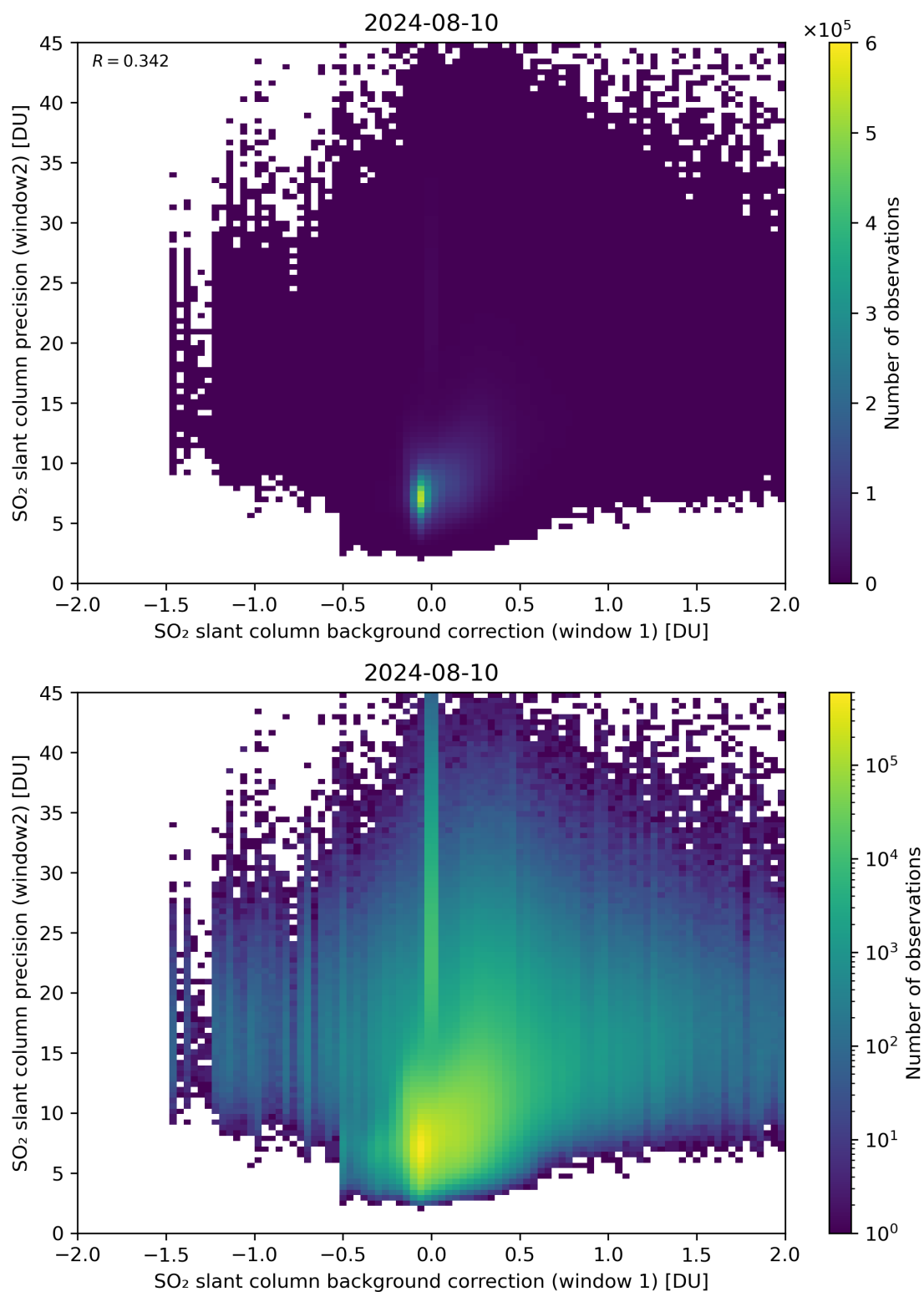
Figure 106: Scatter density plot of “SO 2 slant column background correction (window 1)” against “SO 2 slant column precision (window2)” for 2024-08-09 to 2024-08-11.
