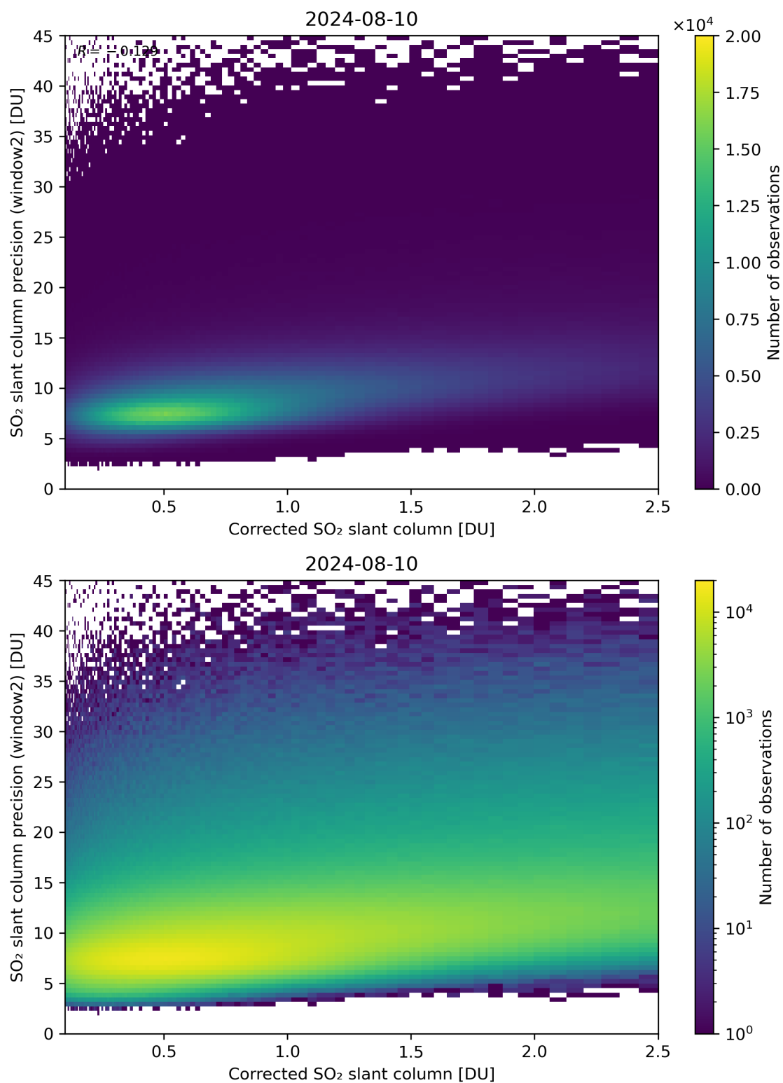
Figure 189: Scatter density plot of “Corrected SO 2 slant column” against “SO 2 slant column precision (window2)” for 2024-08-09 to 2024-08-11.
