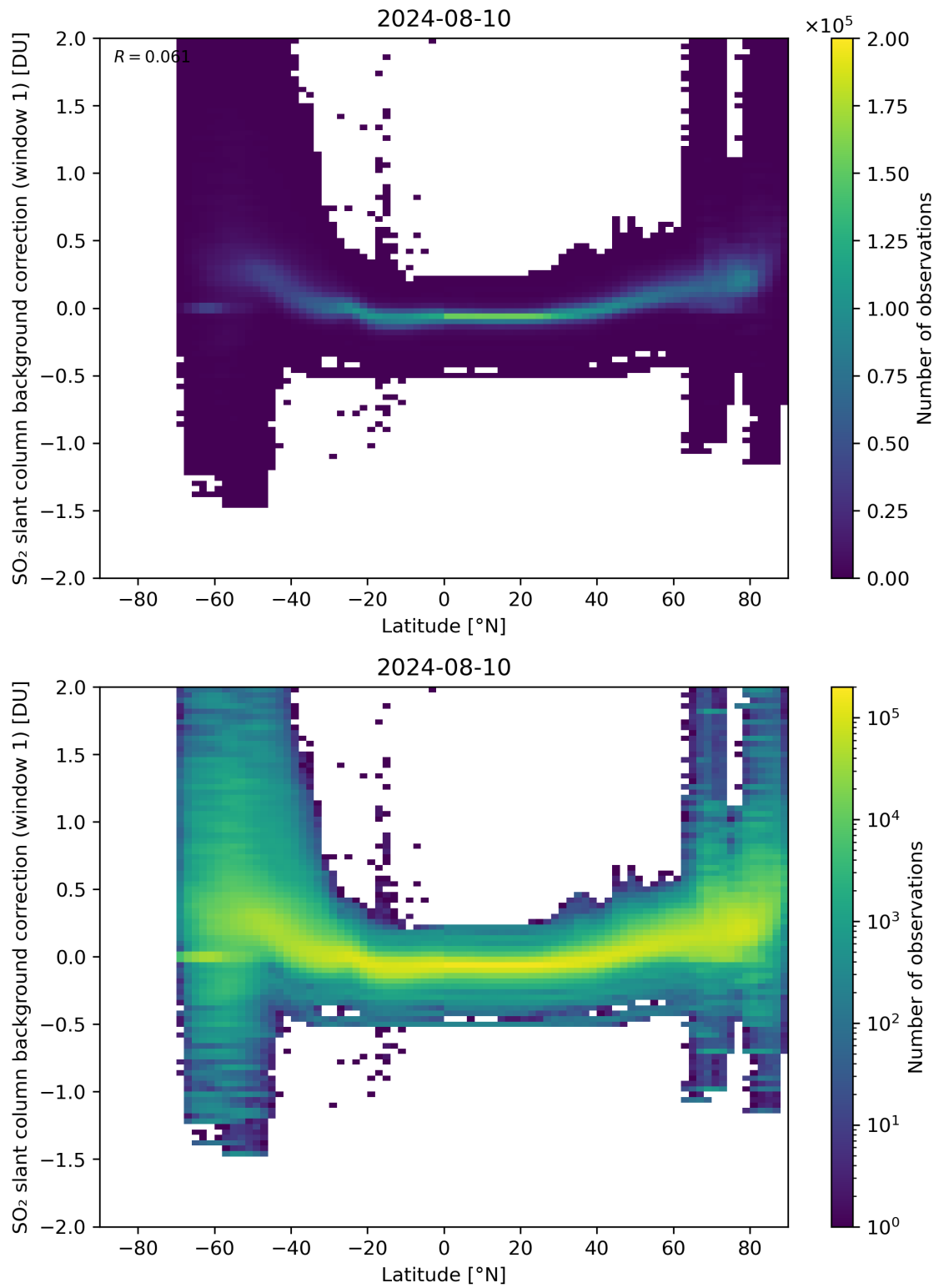
Figure 139: Scatter density plot of “Latitude” against “SO 2 slant column background correction (window 1)” for 2024-08-09 to 2024-08-11.
