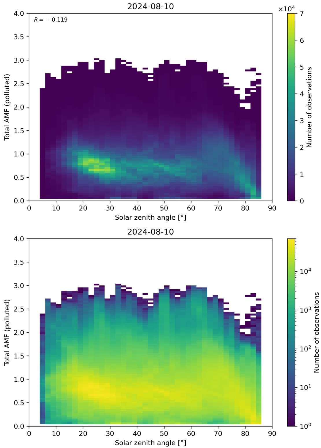
Figure 174: Scatter density plot of “Solar zenith angle” against “Total AMF (polluted)” for 2024-08-09 to 2024-08-11.
