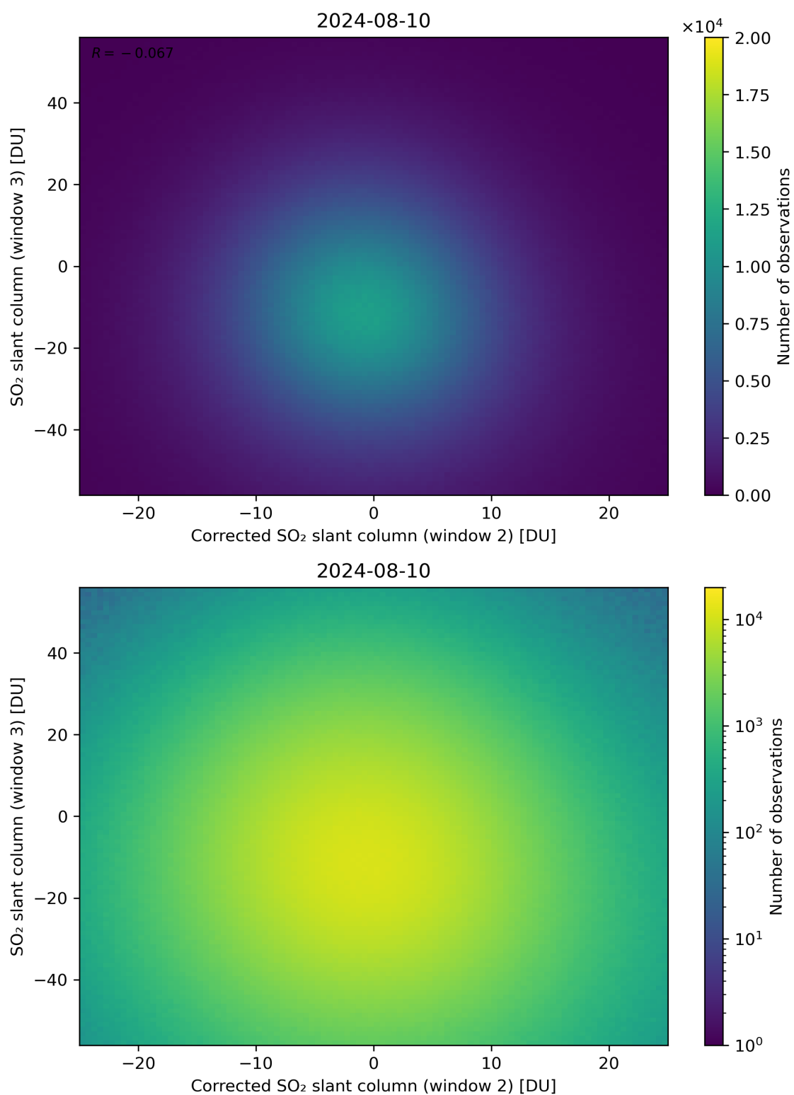
Figure 201: Scatter density plot of “Corrected SO 2 slant column (window 2)” against “SO 2 slant column (window 3)” for 2024-08-09 to 2024-08-11.
