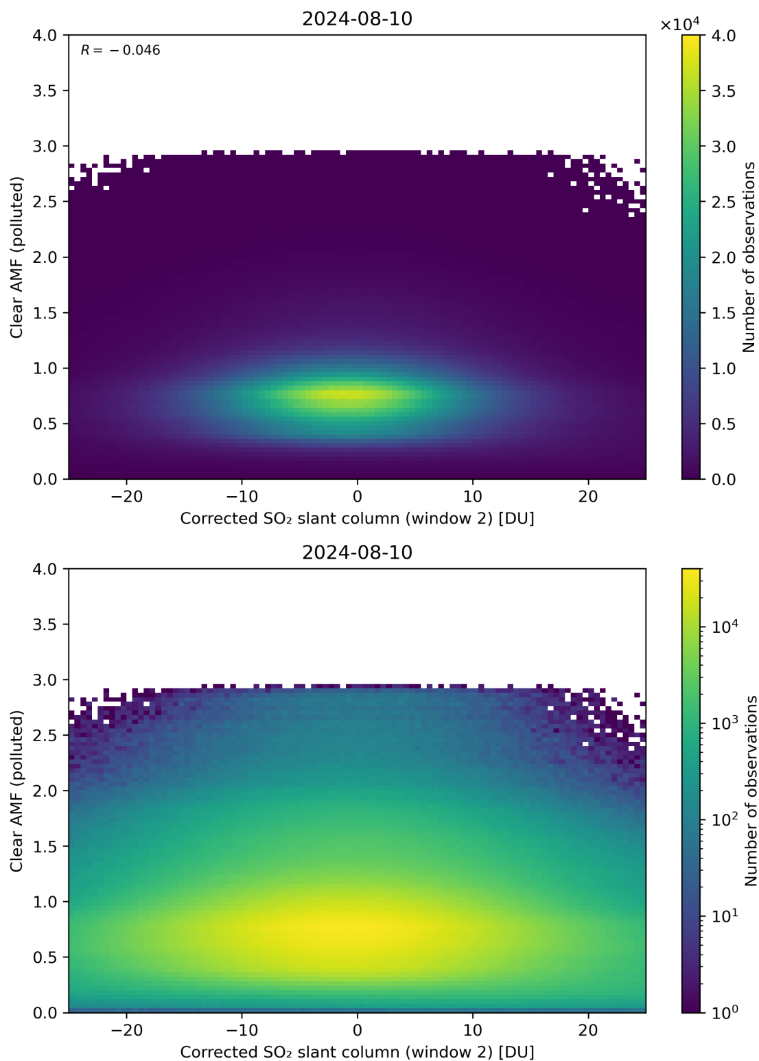
Figure 199: Scatter density plot of “Corrected SO 2 slant column (window 2)” against “Clear AMF (polluted)” for 2024-08-09 to 2024-08-11.
