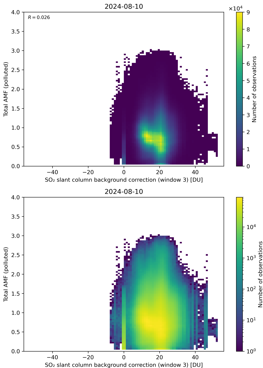
Figure 125: Scatter density plot of “SO 2 slant column background correction (window 3)” against “Total AMF (polluted)” for 2024-08-09 to 2024-08-11.
