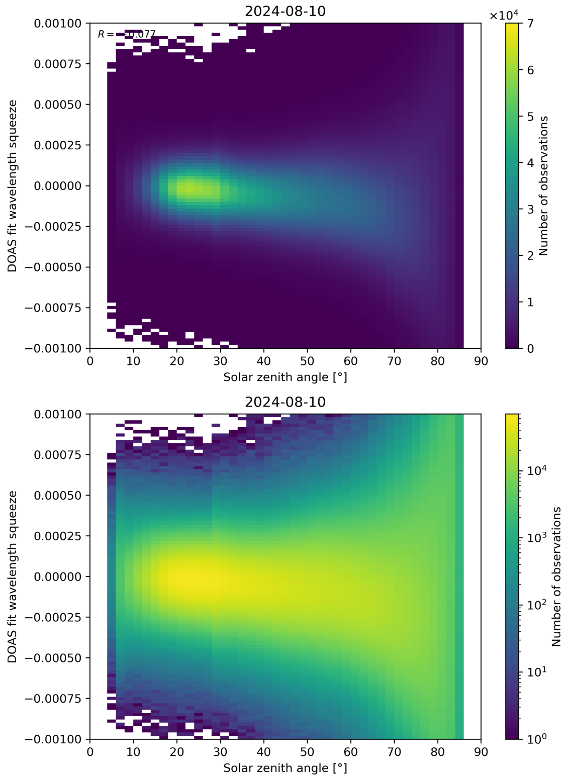
Figure 162: Scatter density plot of “Solar zenith angle” against “DOAS fit wavelength squeeze” for 2024-08-09 to 2024-08-11.
