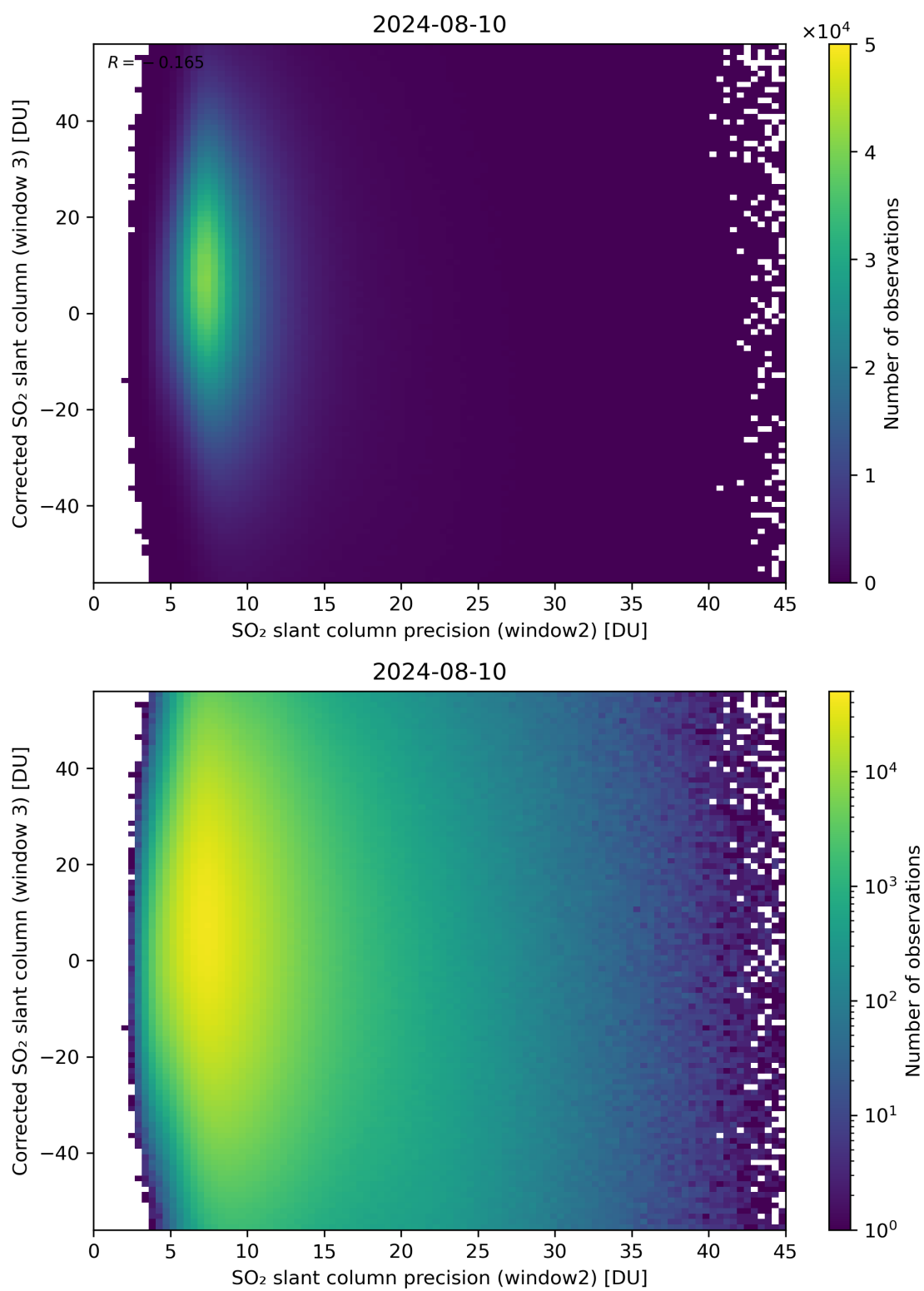
Figure 248: Scatter density plot of “SO 2 slant column precision (window2)” against “Corrected SO 2 slant column (window 3)” for 2024-08-09 to 2024-08-11.
