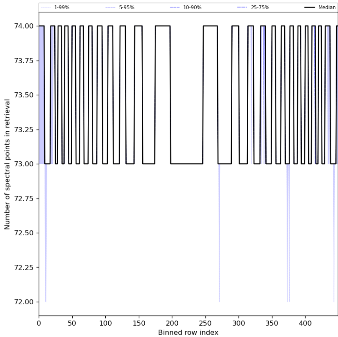
Figure 97: Along track statistics of “Number of spectral points in retrieval” for 2024-08-09 to 2024-08-11
