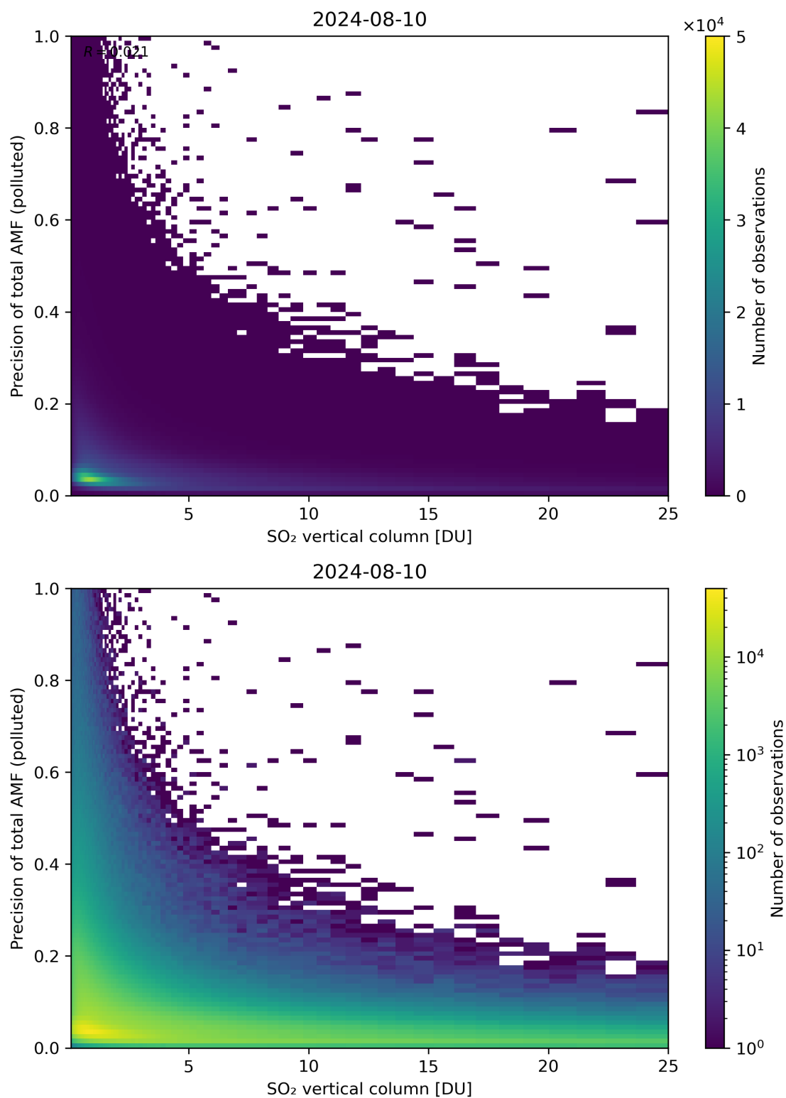
Figure 306: Scatter density plot of “SO 2 vertical column” against “Precision of total AMF (polluted)” for 2024-08-09 to 2024-08-11.
