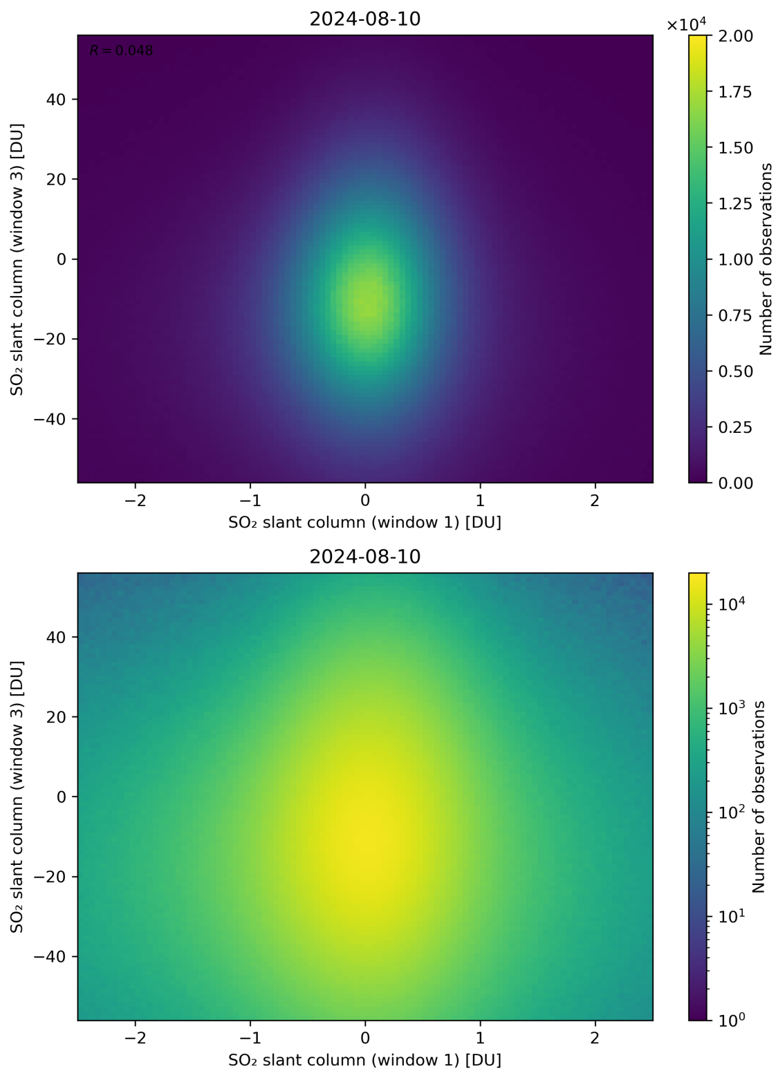
Figure 237: Scatter density plot of “SO 2 slant column (window 1)” against “SO 2 slant column (window 3)” for 2024-08-09 to 2024-08-11.
