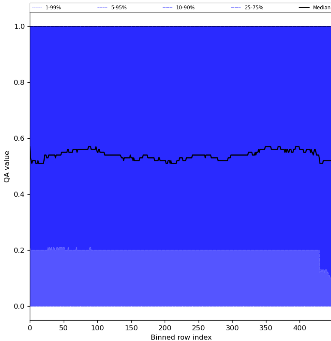
Figure 75: Along track statistics of “QA value” for 2024-08-09 to 2024-08-11
