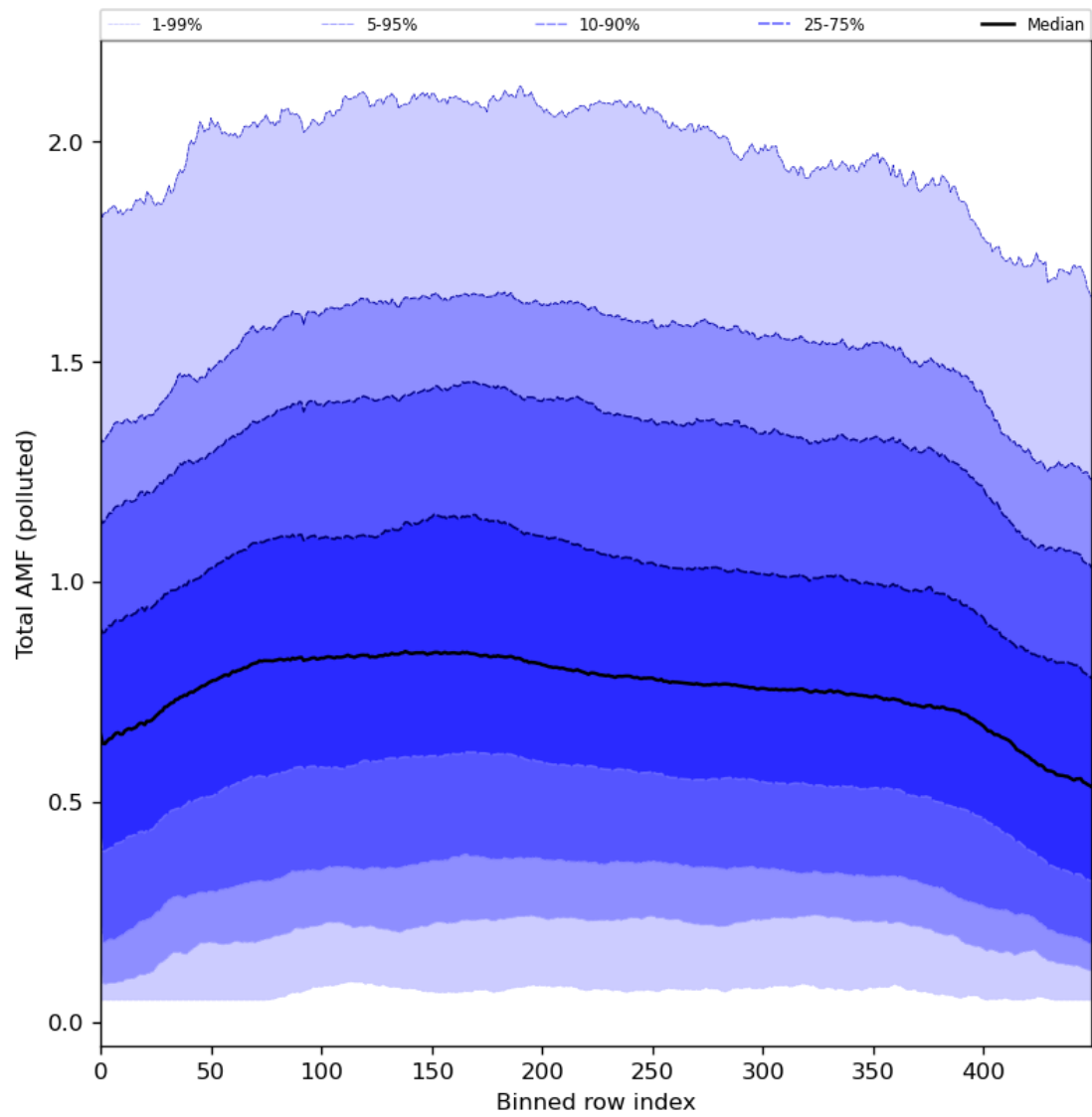
Figure 94: Along track statistics of “Total AMF (polluted)” for 2024-08-09 to 2024-08-11
