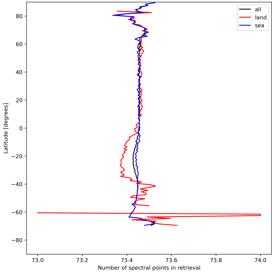
Figure 51: Zonal average of “Number of spectral points in retrieval” for 2024-08-09 to 2024-08-11.
