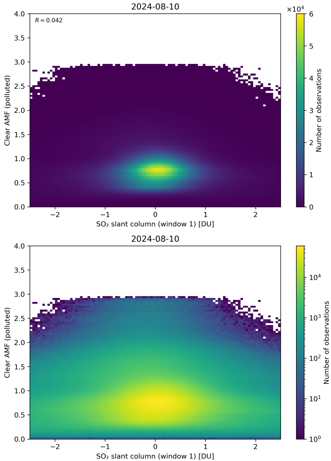
Figure 232: Scatter density plot of “SO 2 slant column (window 1)” against “Clear AMF (polluted)” for 2024-08-09 to 2024-08-11.
