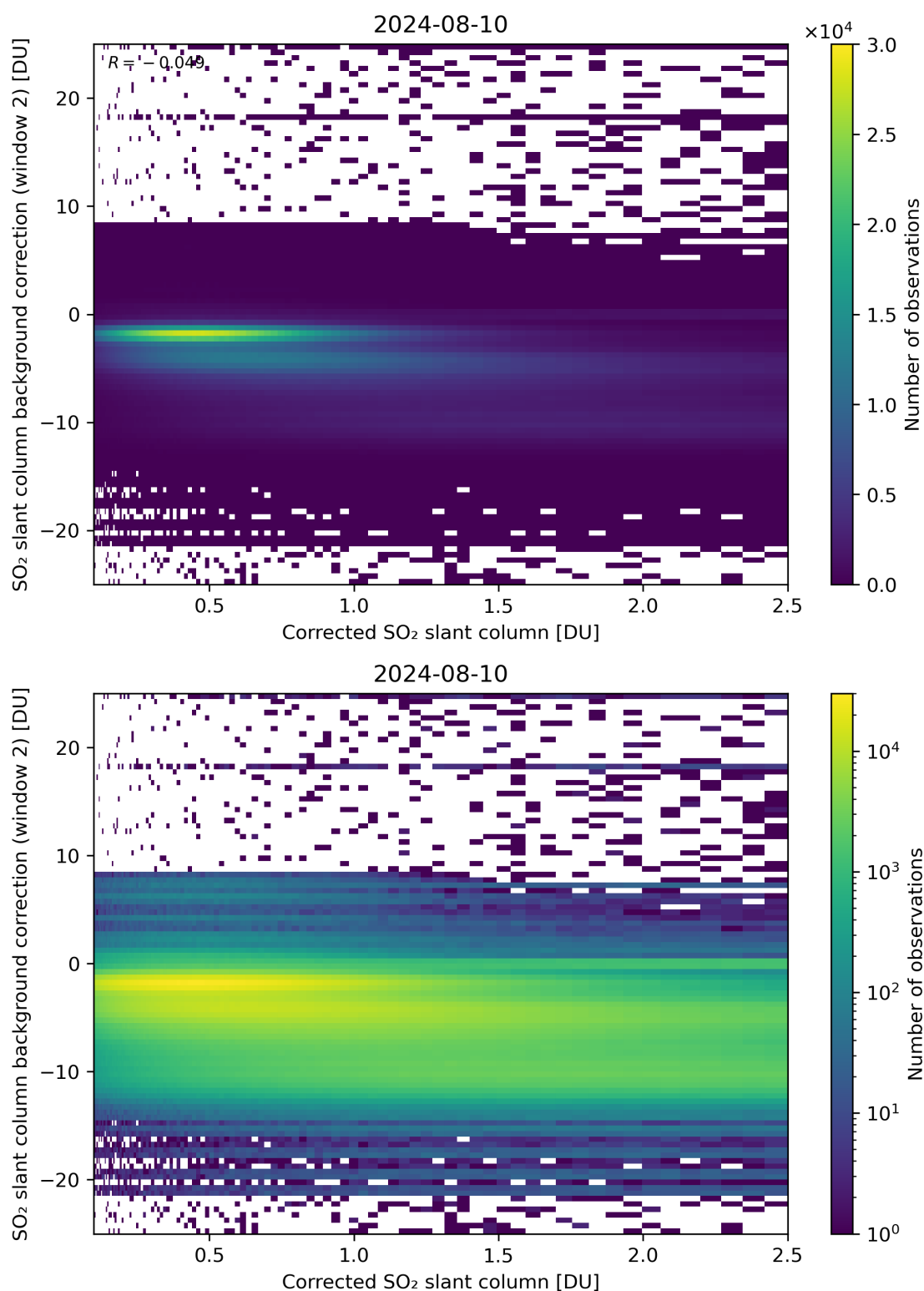
Figure 179: Scatter density plot of “Corrected SO 2 slant column” against “SO 2 slant column background correction (window 2)” for 2024-08-09 to 2024-08-11.
