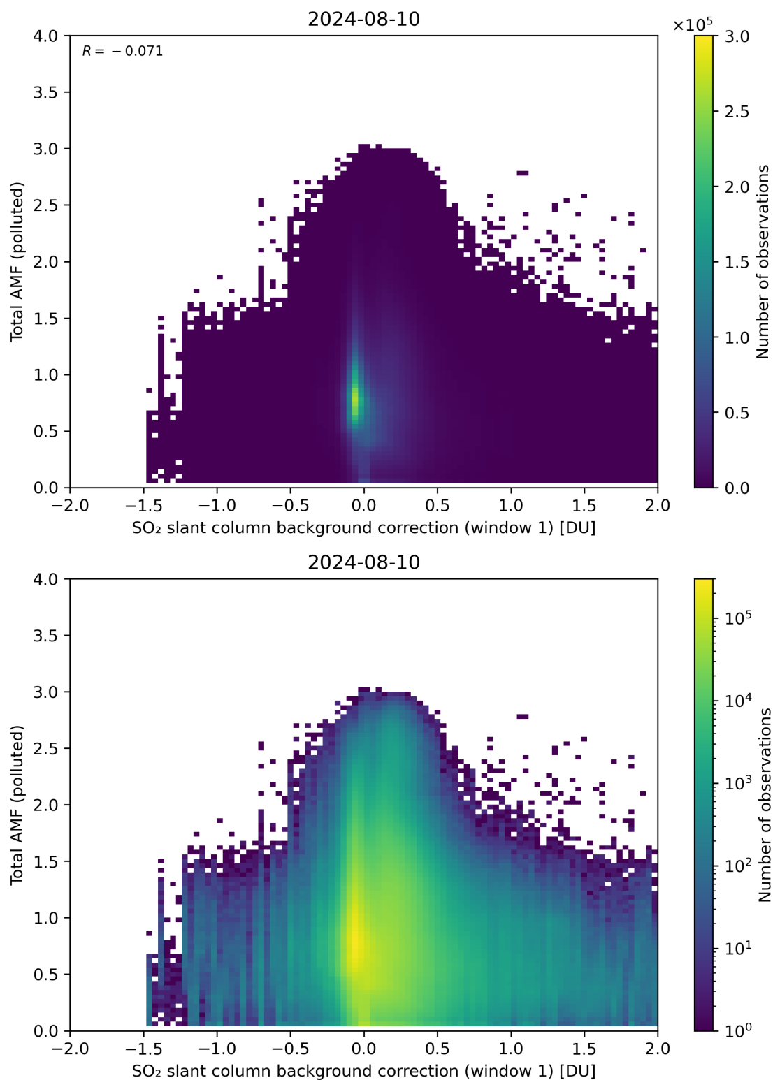
Figure 109: Scatter density plot of “SO 2 slant column background correction (window 1)” against “Total AMF (polluted)” for 2024-08-09 to 2024-08-11.
