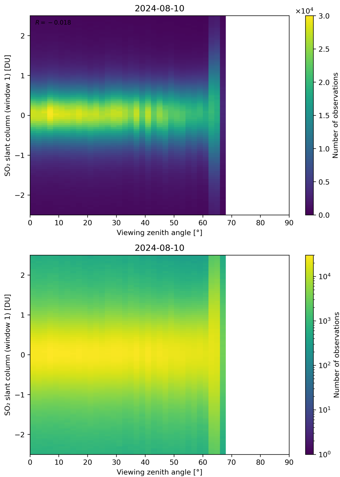
Figure 320: Scatter density plot of “Viewing zenith angle” against “SO 2 slant column (window 1)” for 2024-08-09 to 2024-08-11.
