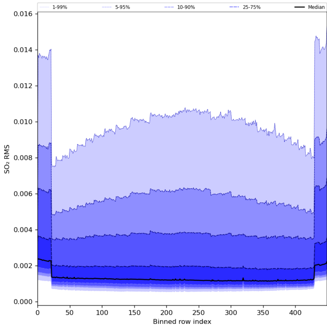
Figure 93: Along track statistics of "SO 2 RMS" for 2024-08-09 to 2024-08-11
