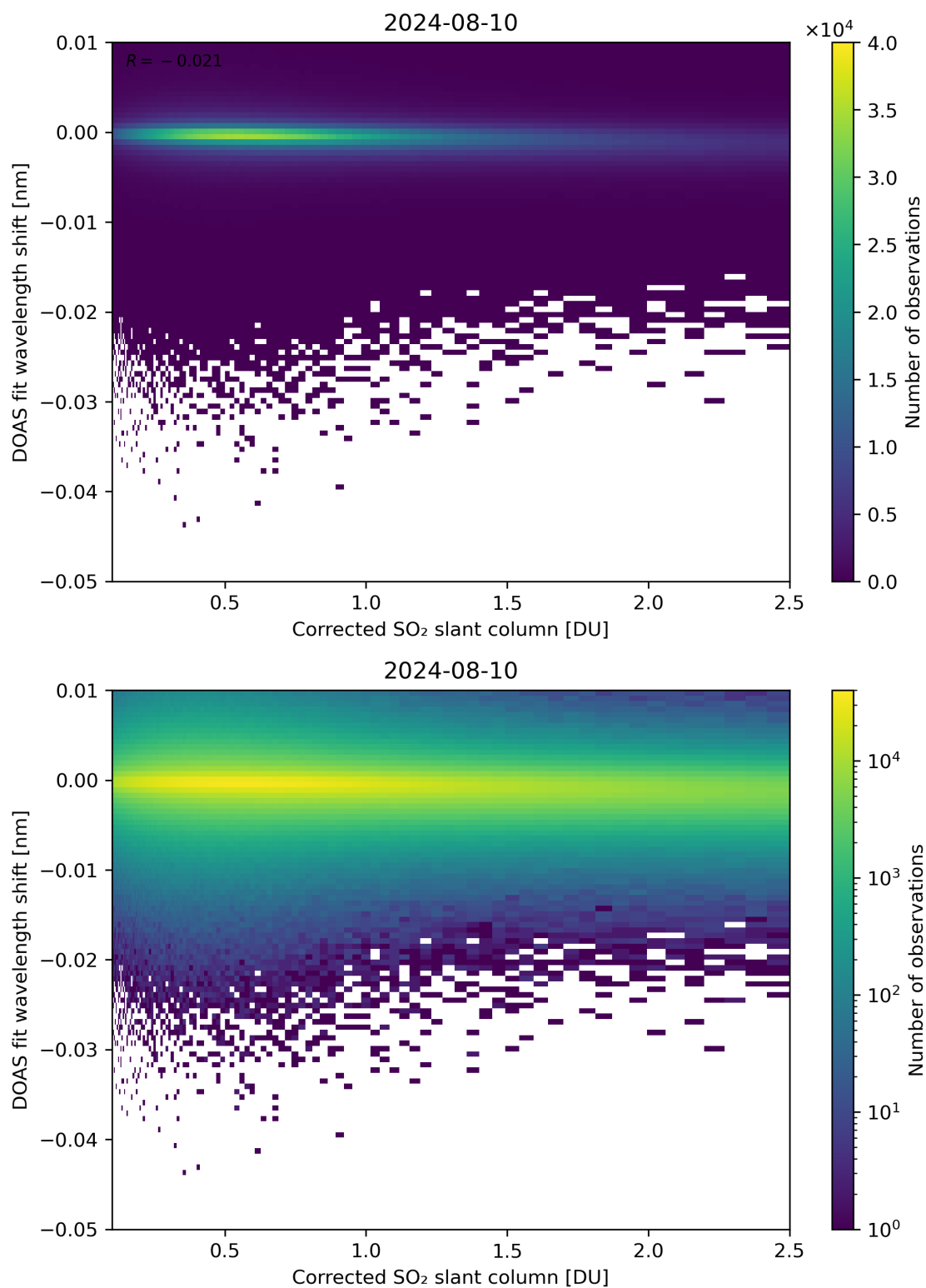
Figure 181: Scatter density plot of “Corrected SO 2 slant column” against “DOAS fit wavelength shift” for 2024-08-09 to 2024-08-11.
