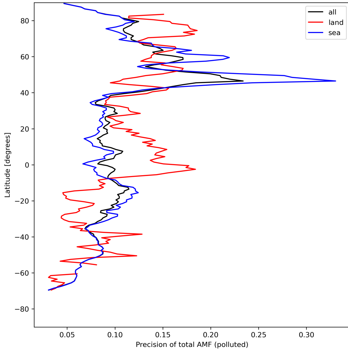
Figure 49: Zonal average of “Precision of total AMF (polluted)” for 2024-08-09 to 2024-08-11.
