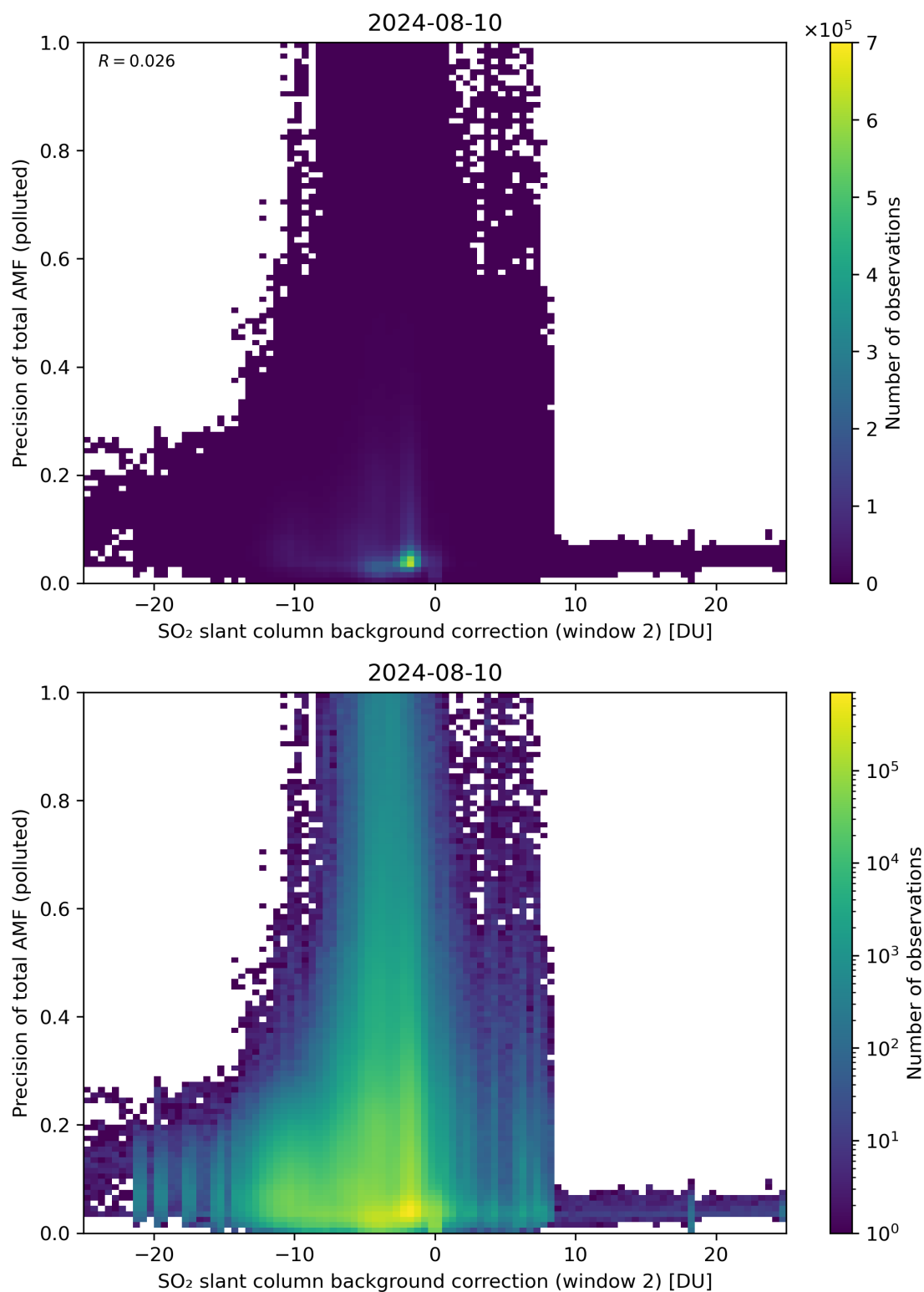
Figure 120: Scatter density plot of “SO 2 slant column background correction (window 2)” against “Precision of total AMF (polluted)” for 2024-08-09 to 2024-08-11.
