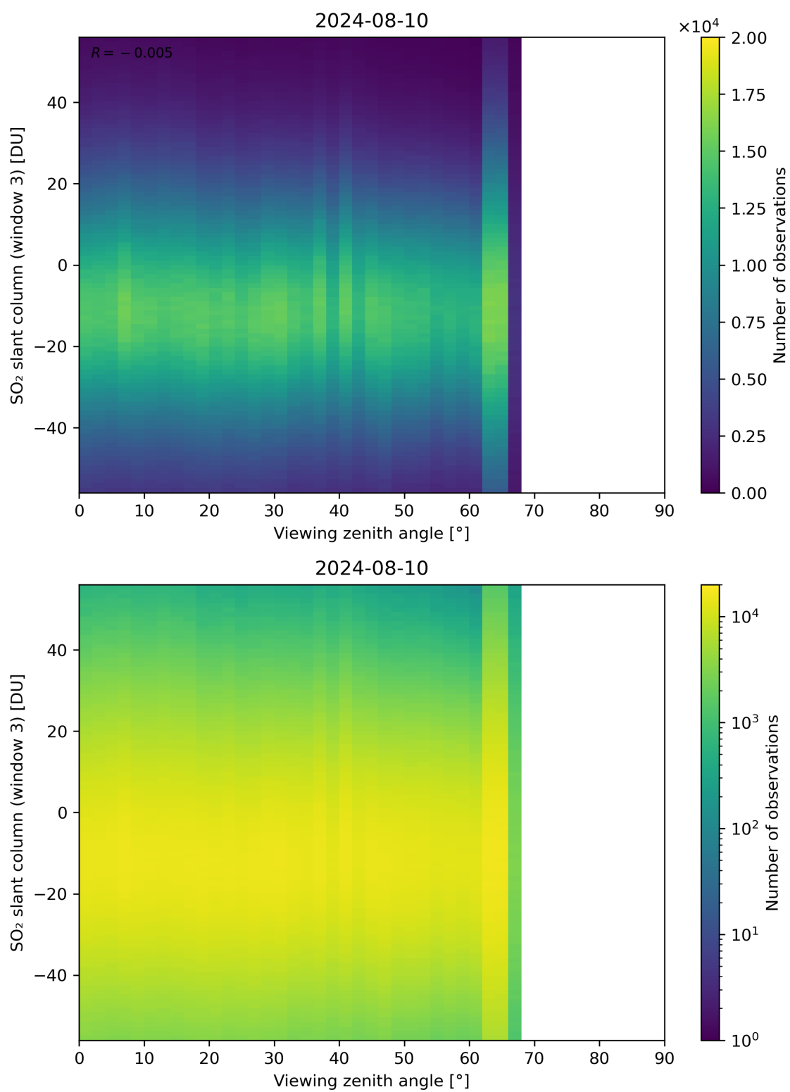
Figure 323: Scatter density plot of “Viewing zenith angle” against “SO 2 slant column (window 3)” for 2024-08-09 to 2024-08-11.
