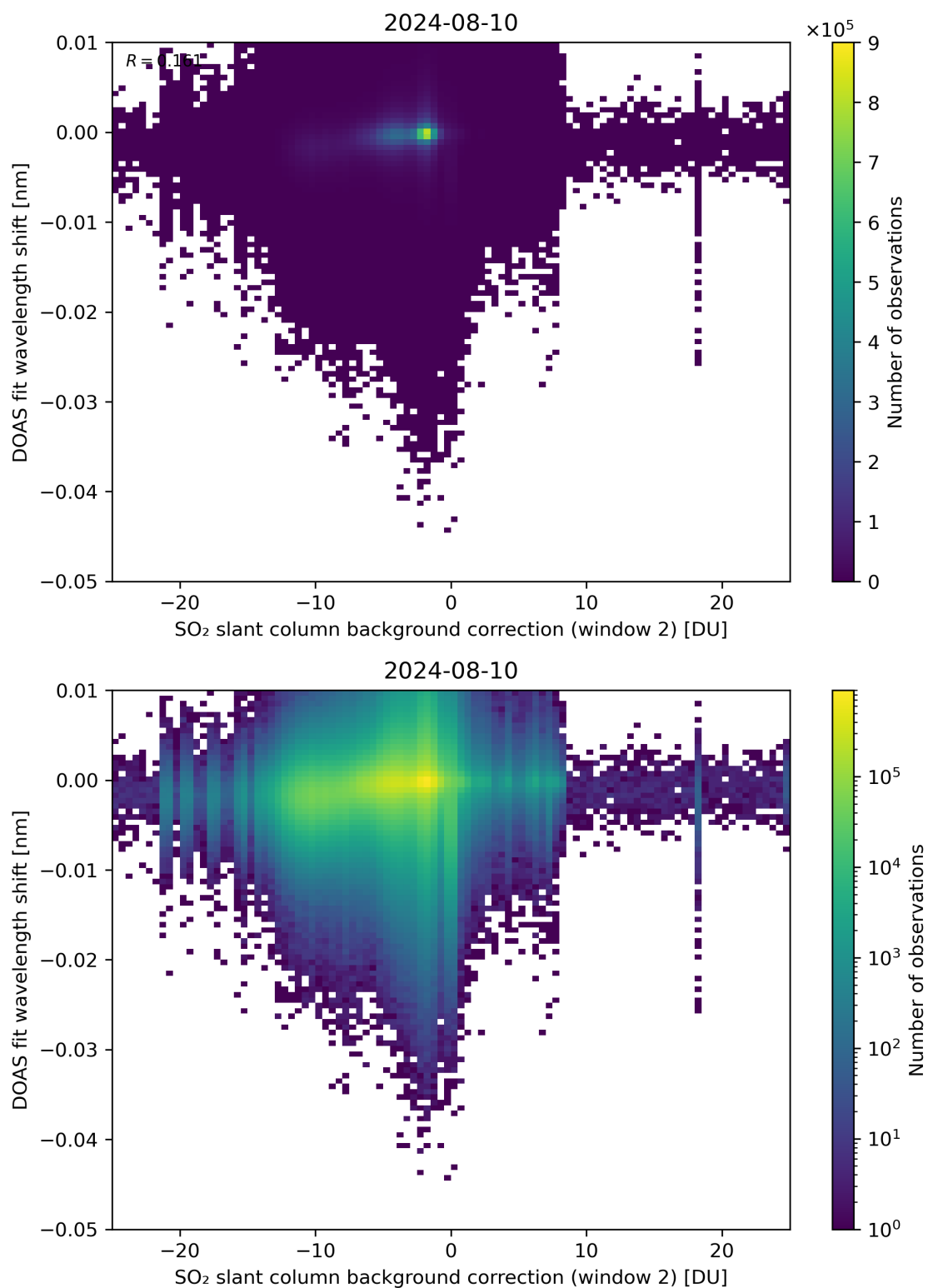
Figure 112: Scatter density plot of “SO 2 slant column background correction (window 2)” against “DOAS fit wavelength shift” for 2024-08-09 to 2024-08-11.
