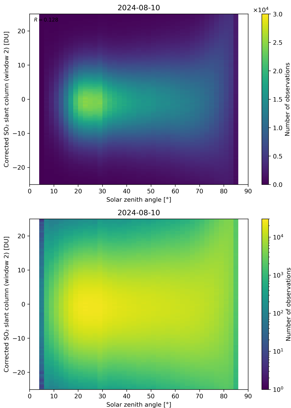
Figure 167: Scatter density plot of “Solar zenith angle” against “Corrected SO 2 slant column (window 2)” for 2024-08-09 to 2024-08-11.
