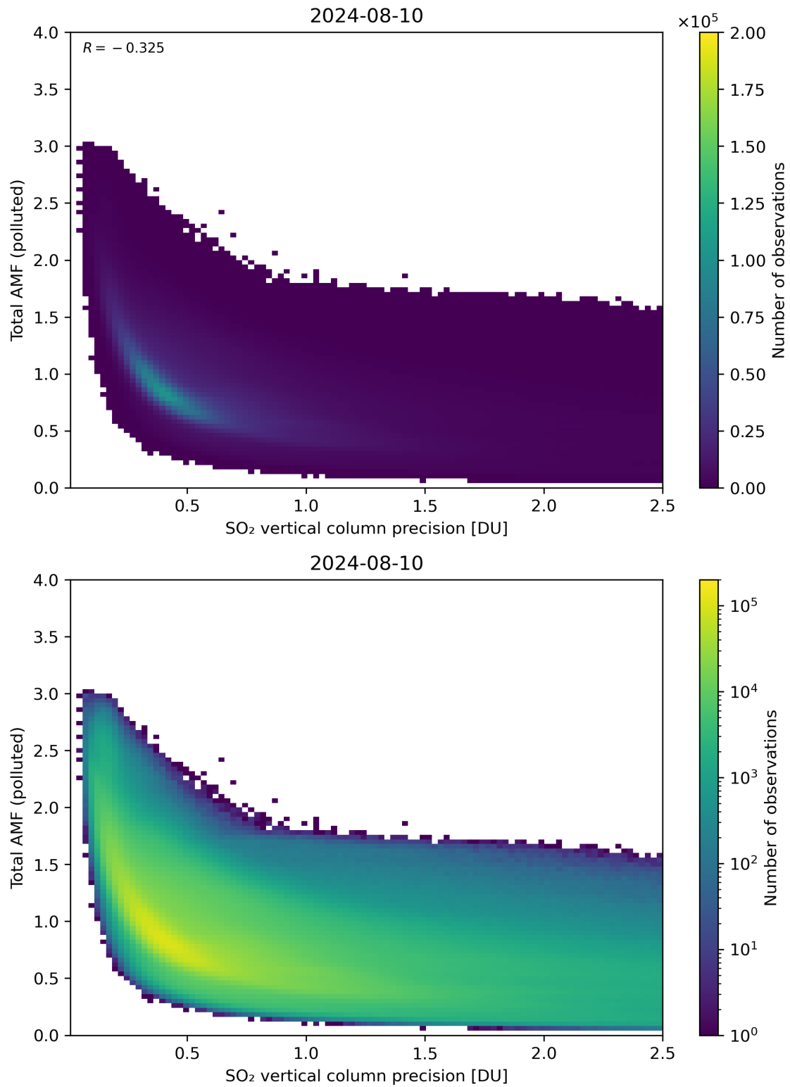
Figure 294: Scatter density plot of “SO 2 vertical column precision” against “Total AMF (polluted)” for 2024-08-09 to 2024-08-11.
