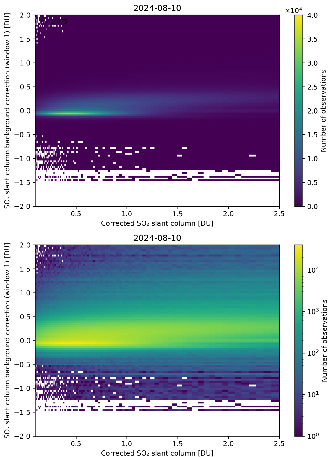
Figure 178: Scatter density plot of “Corrected SO 2 slant column” against “SO 2 slant column background correction (window 1)” for 2024-08-09 to 2024-08-11.
