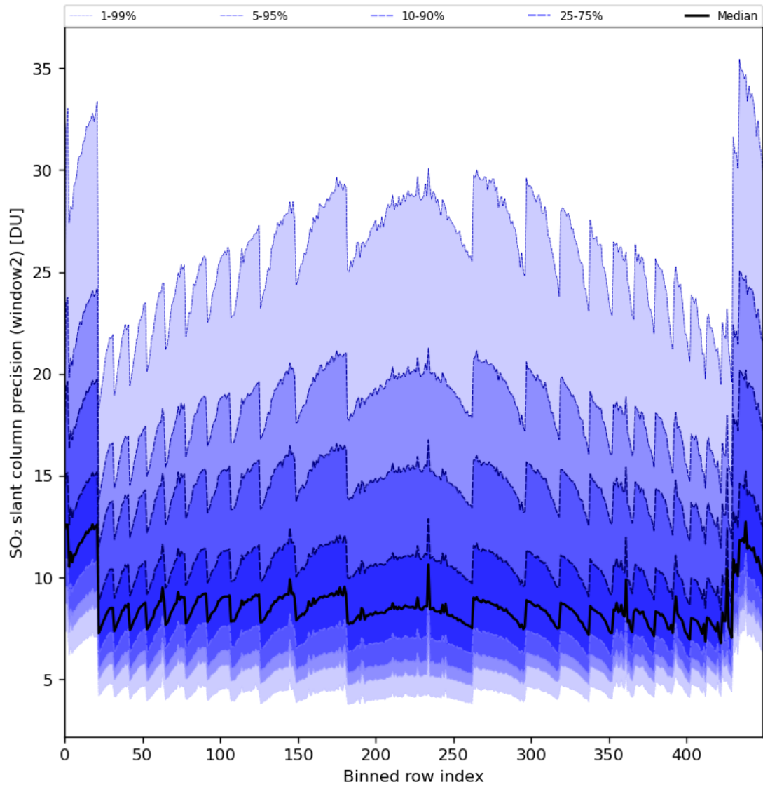
Figure 84: Along track statistics of “SO 2 slant column precision (window2)” for 2024-08-09 to 2024-08-11
