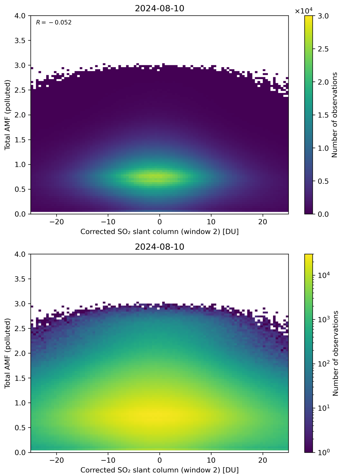
Figure 203: Scatter density plot of “Corrected SO 2 slant column (window 2)” against “Total AMF (polluted)” for 2024-08-09 to 2024-08-11.
