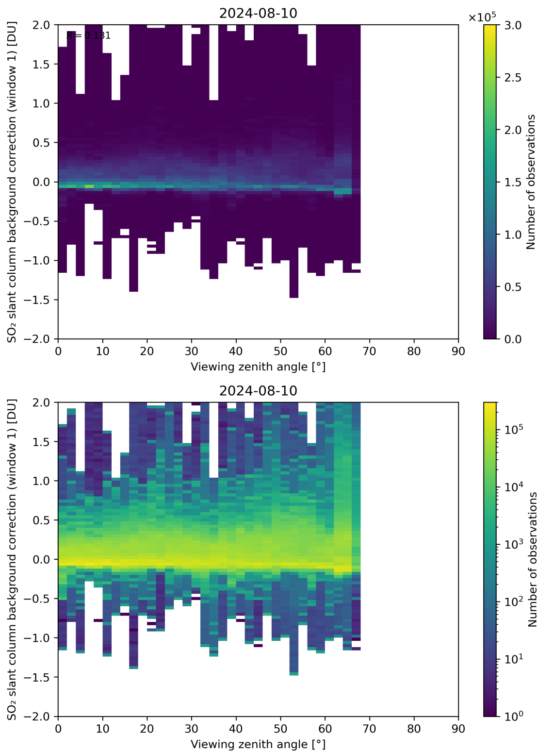
Figure 308: Scatter density plot of “Viewing zenith angle” against “SO 2 slant column background correction (window 1)” for 2024-08-09 to 2024-08-11.
