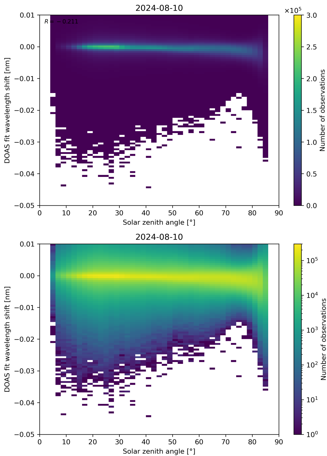
Figure 161: Scatter density plot of “Solar zenith angle” against “DOAS fit wavelength shift” for 2024-08-09 to 2024-08-11.
