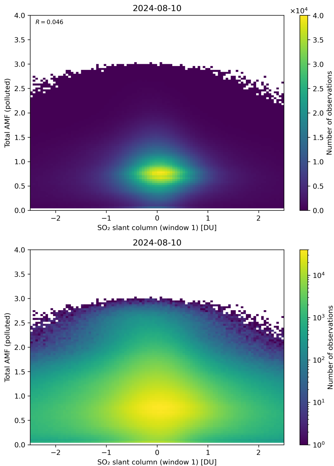
Figure 239: Scatter density plot of “SO 2 slant column (window 1)” against “Total AMF (polluted)” for 2024-08-09 to 2024-08-11.
