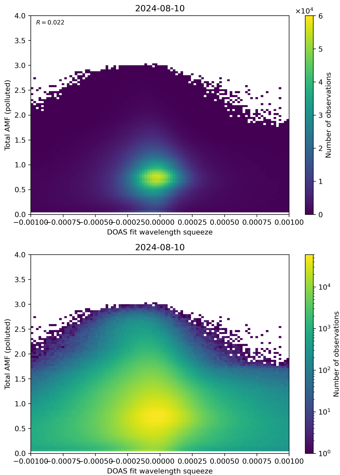
Figure 134: Scatter density plot of “DOAS fit wavelength squeeze” against “Total AMF (polluted)” for 2024-08-09 to 2024-08-11.
