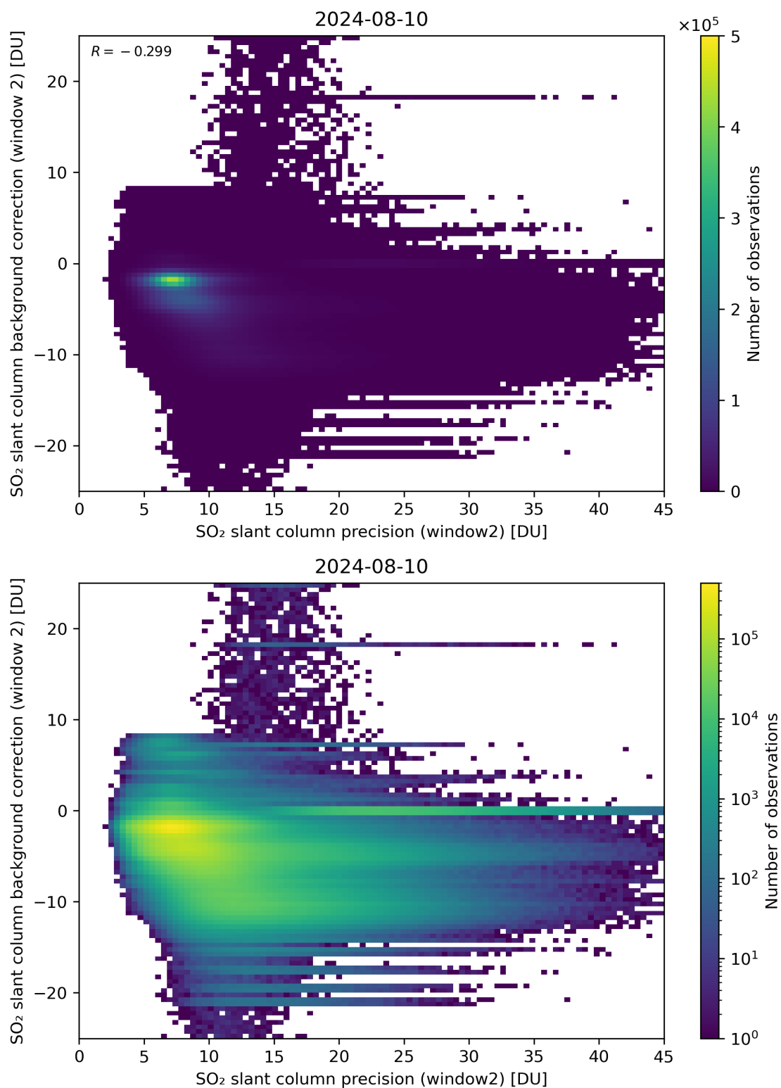
Figure 241: Scatter density plot of “SO 2 slant column precision (window2)” against “SO 2 slant column background correction (window 2)” for 2024-08-09 to 2024-08-11.
