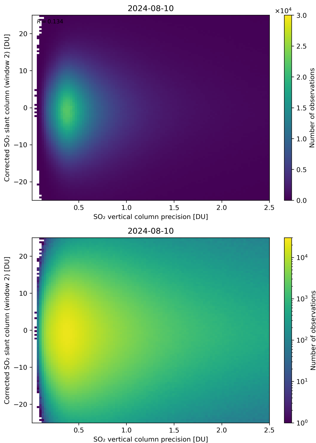
Figure 287: Scatter density plot of “SO 2 vertical column precision” against “Corrected SO 2 slant column (window 2)” for 2024-08-09 to 2024-08-11.
