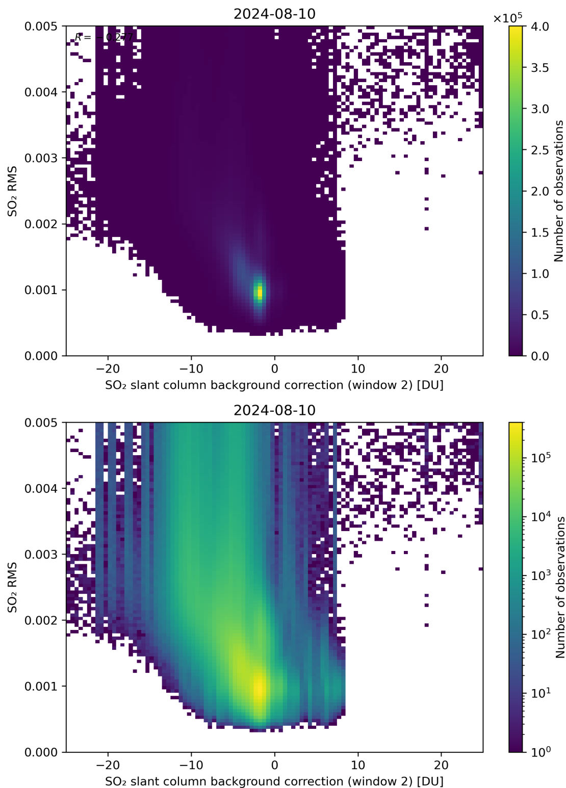
Figure 114: Scatter density plot of “SO 2 slant column background correction (window 2)” against “SO 2 RMS” for 2024-08-09 to 2024-08-11.
