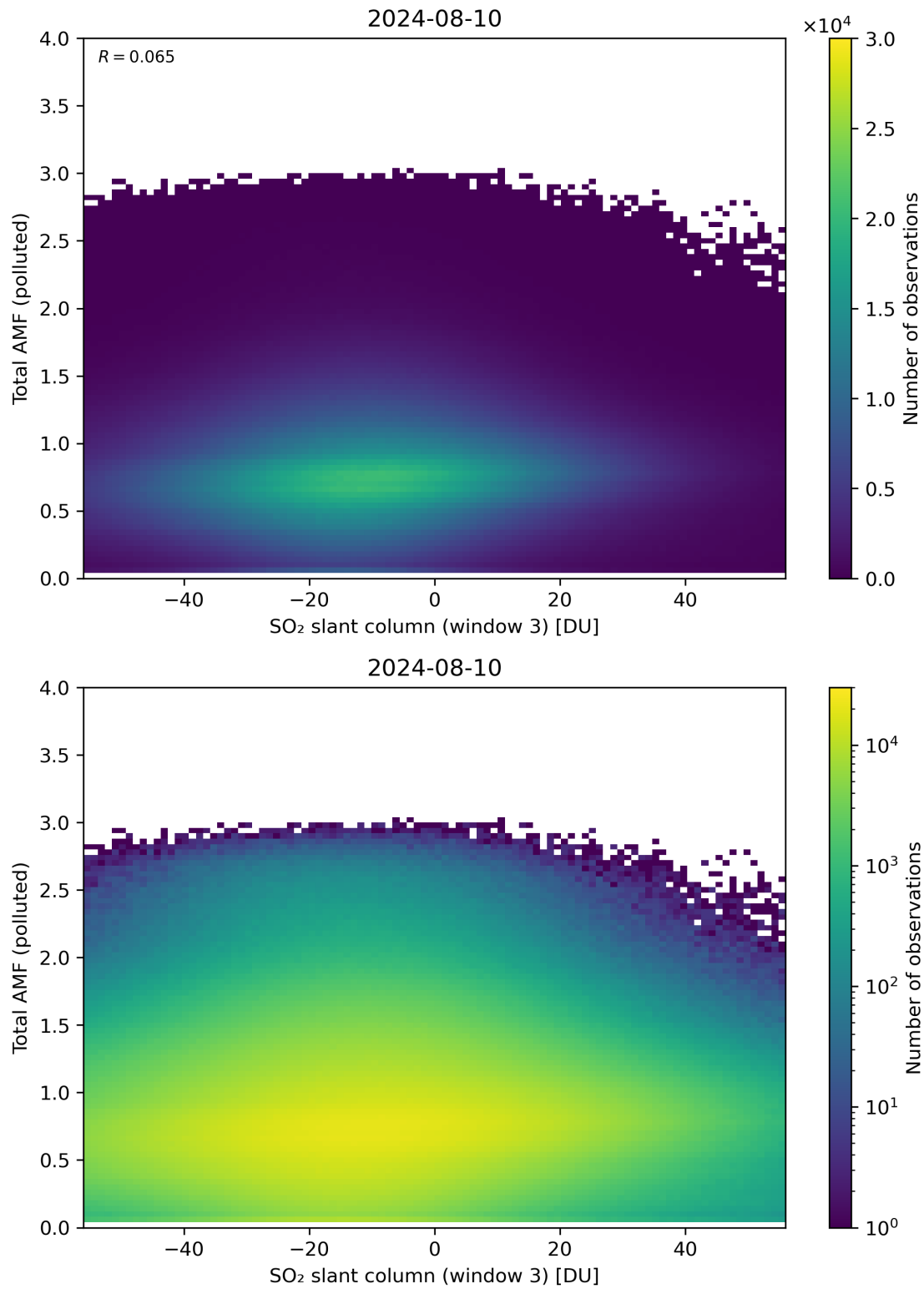
Figure 268: Scatter density plot of “SO 2 slant column (window 3)” against “Total AMF (polluted)” for 2024-08-09 to 2024-08-11.
