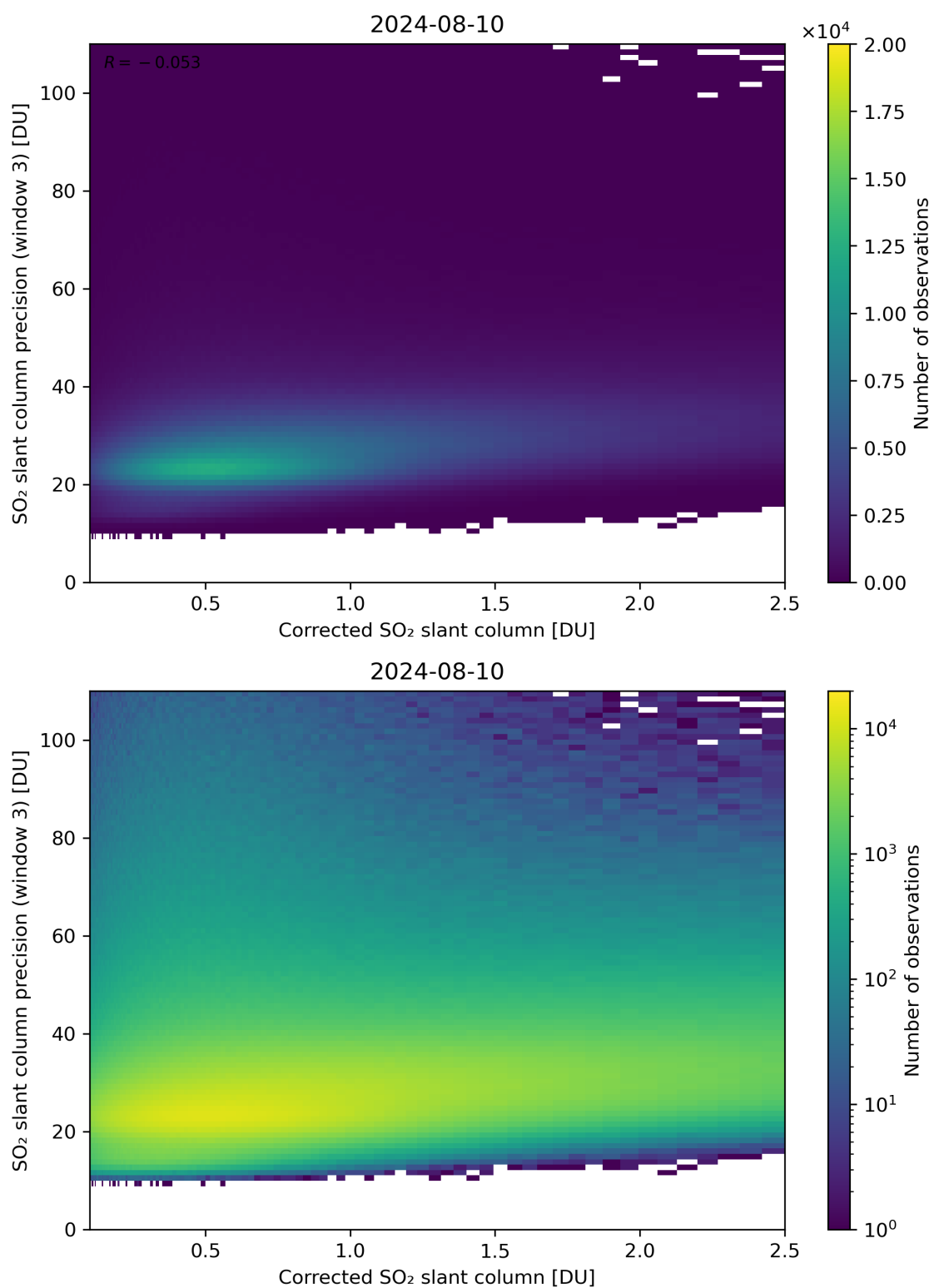
Figure 191: Scatter density plot of “Corrected SO 2 slant column” against “SO 2 slant column precision (window 3)” for 2024-08-09 to 2024-08-11.
