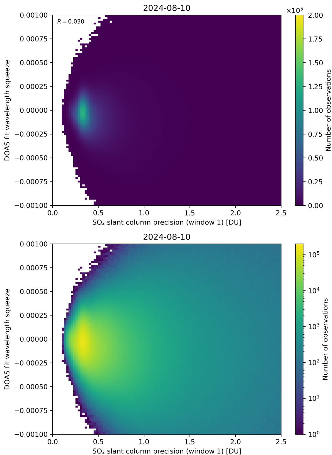
Figure 222: Scatter density plot of “SO 2 slant column precision (window 1)” against “DOAS fit wavelength squeeze” for 2024-08-09 to 2024-08-11.
