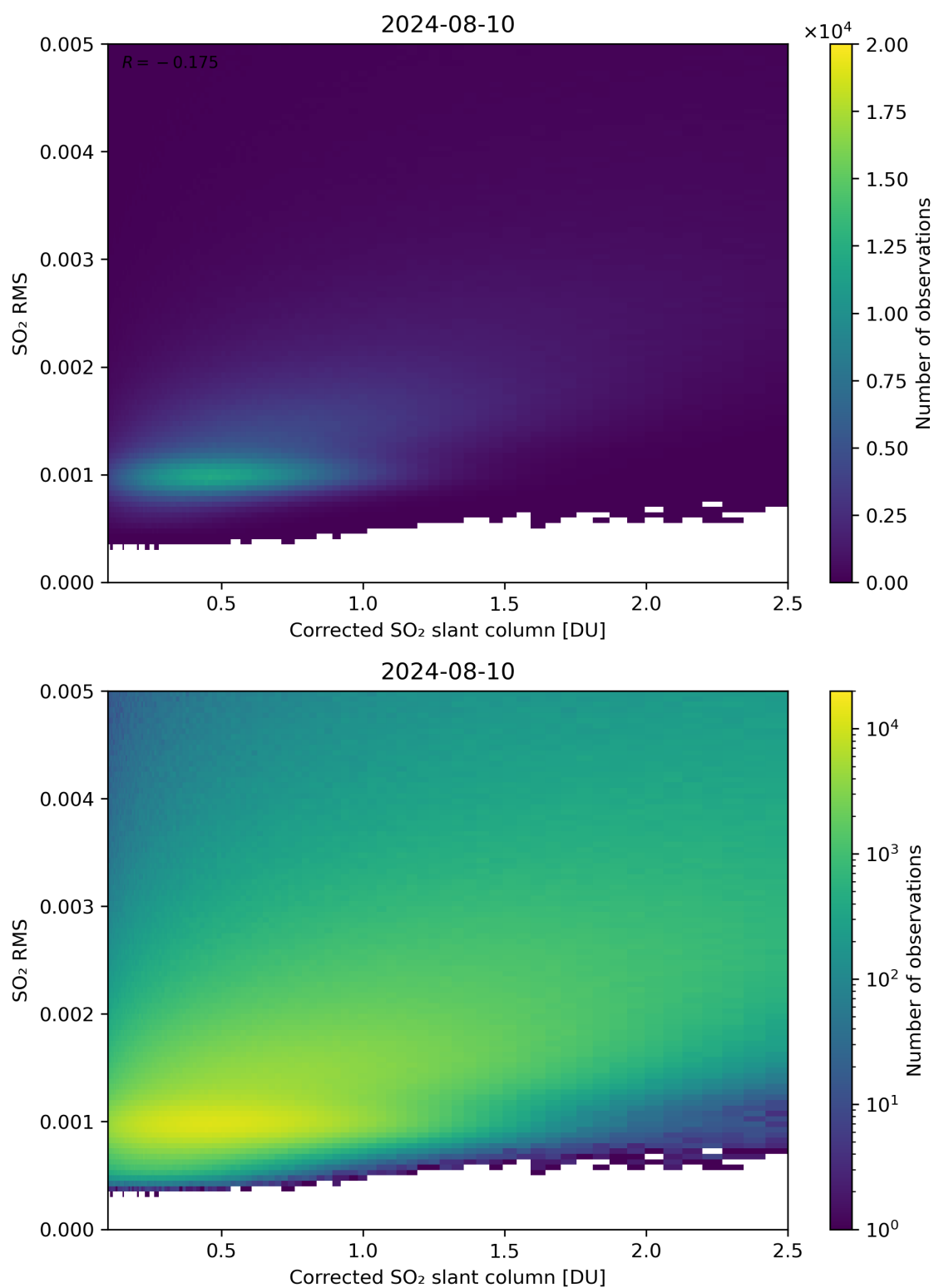
Figure 183: Scatter density plot of “Corrected SO 2 slant column” against “SO 2 RMS” for 2024-08-09 to 2024-08-11.
