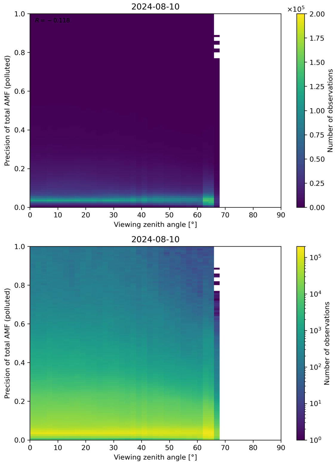
Figure 326: Scatter density plot of “Viewing zenith angle” against “Precision of total AMF (polluted)” for 2024-08-09 to 2024-08-11.
