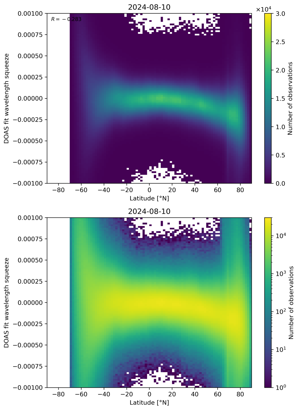
Figure 143: Scatter density plot of “Latitude” against “DOAS fit wavelength squeeze” for 2024-08-09 to 2024-08-11.
