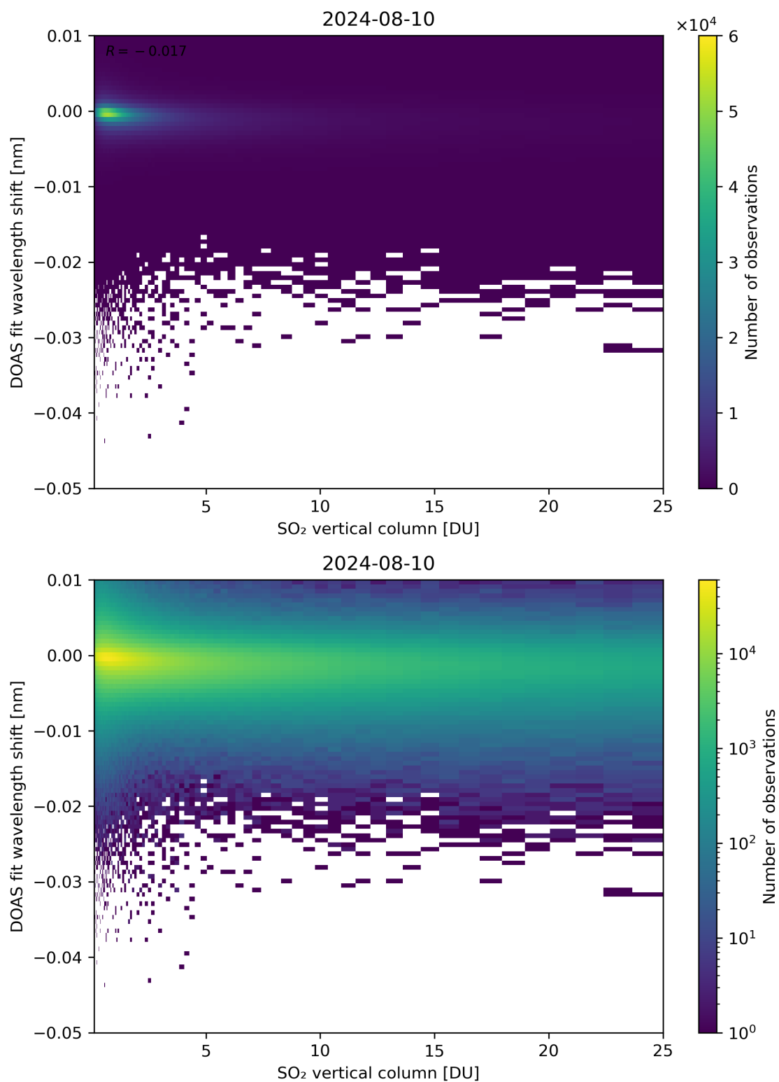
Figure 276: Scatter density plot of “SO 2 vertical column” against “DOAS fit wavelength shift” for 2024-08-09 to 2024-08-11.
