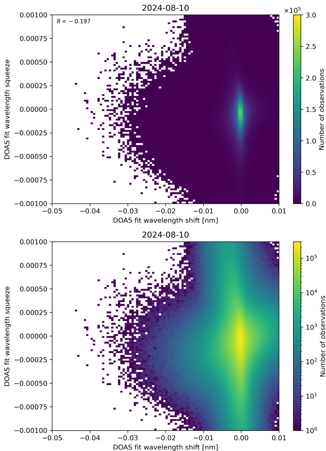
Figure 127: Scatter density plot of “DOAS fit wavelength shift” against “DOAS fit wavelength squeeze” for 2024-08-09 to 2024-08-11.
