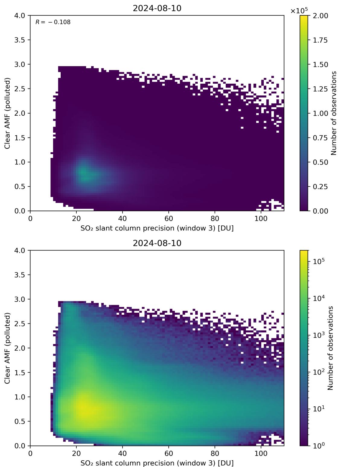
Figure 261: Scatter density plot of “SO 2 slant column precision (window 3)” against “Clear AMF (polluted)” for 2024-08-09 to 2024-08-11.
