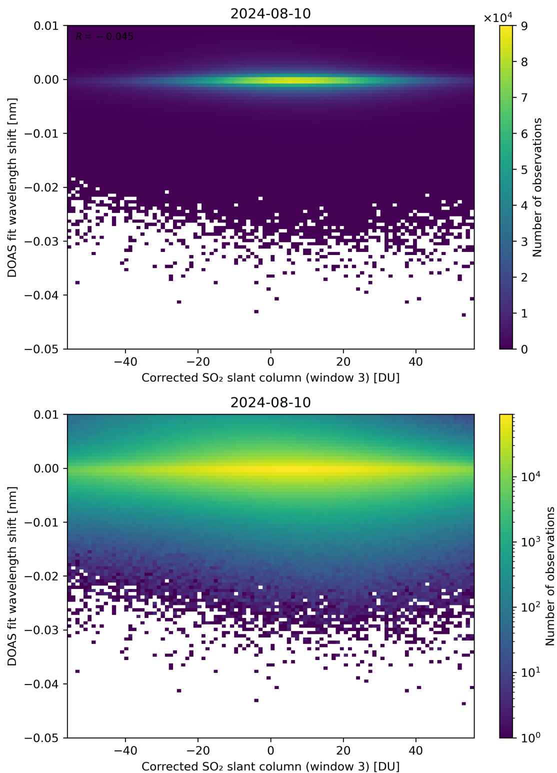
Figure 206: Scatter density plot of “Corrected SO 2 slant column (window 3)” against “DOAS fit wavelength shift” for 2024-08-09 to 2024-08-11.
