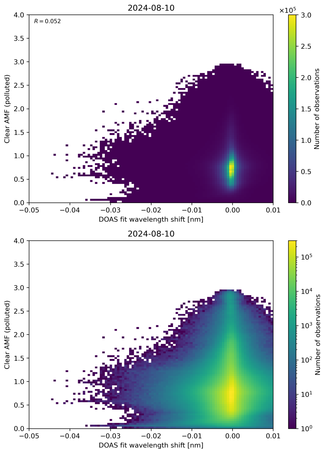
Figure 129: Scatter density plot of “DOAS fit wavelength shift” against “Clear AMF (polluted)” for 2024-08-09 to 2024-08-11.
