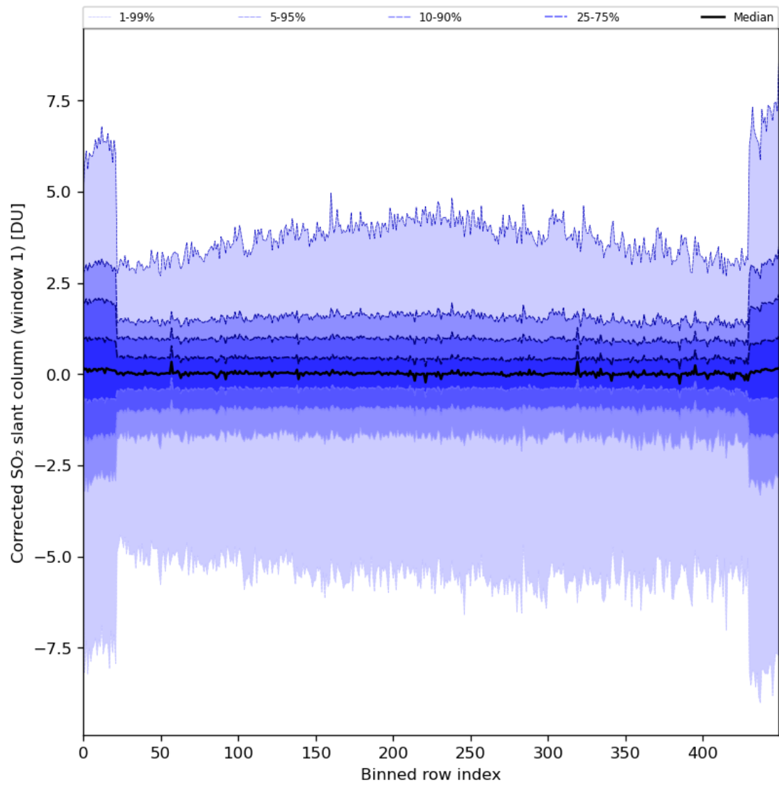
Figure 81: Along track statistics of “Corrected SO 2 slant column (window 1)” for 2024-08-09 to 2024-08-11
