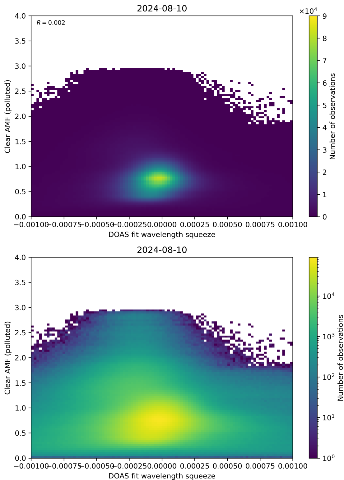
Figure 133: Scatter density plot of “DOAS fit wavelength squeeze” against “Clear AMF (polluted)” for 2024-08-09 to 2024-08-11.
