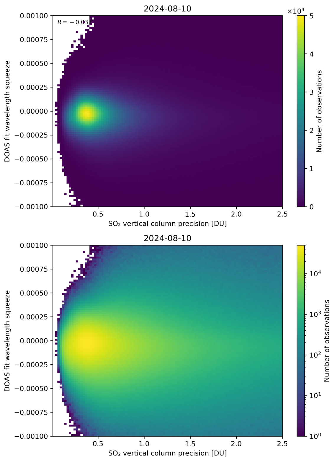
Figure 283: Scatter density plot of “SO 2 vertical column precision” against “DOAS fit wavelength squeeze” for 2024-08-09 to 2024-08-11.
