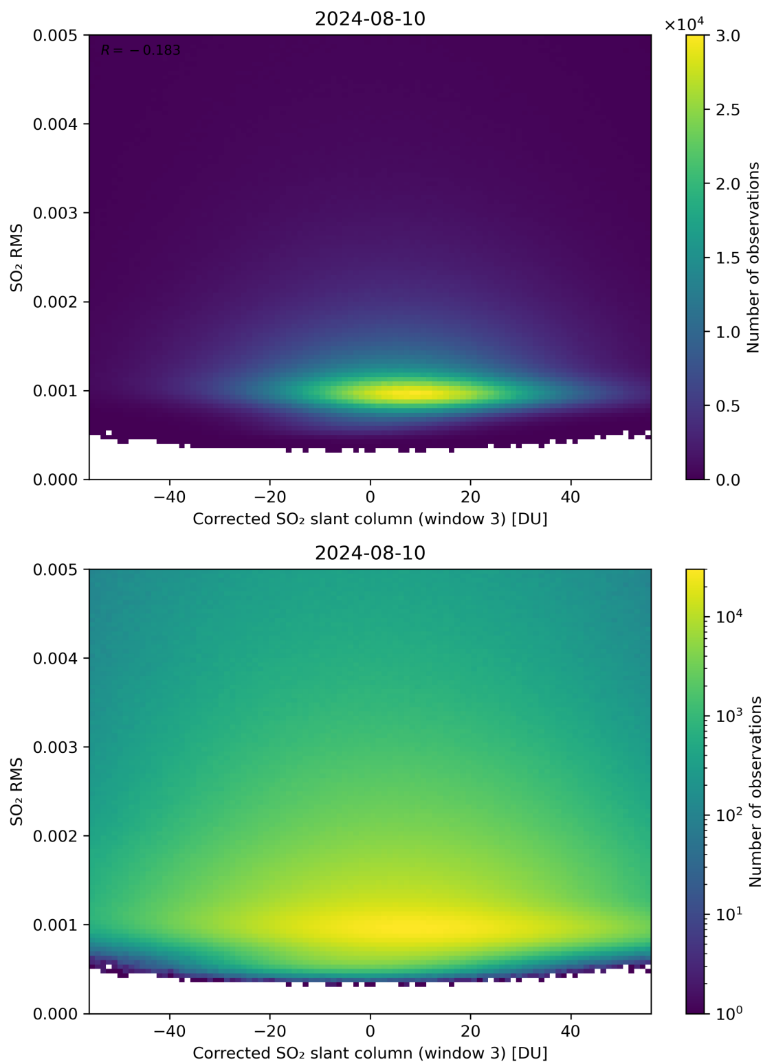
Figure 208: Scatter density plot of “Corrected SO 2 slant column (window 3)” against “SO 2 RMS” for 2024-08-09 to 2024-08-11.
