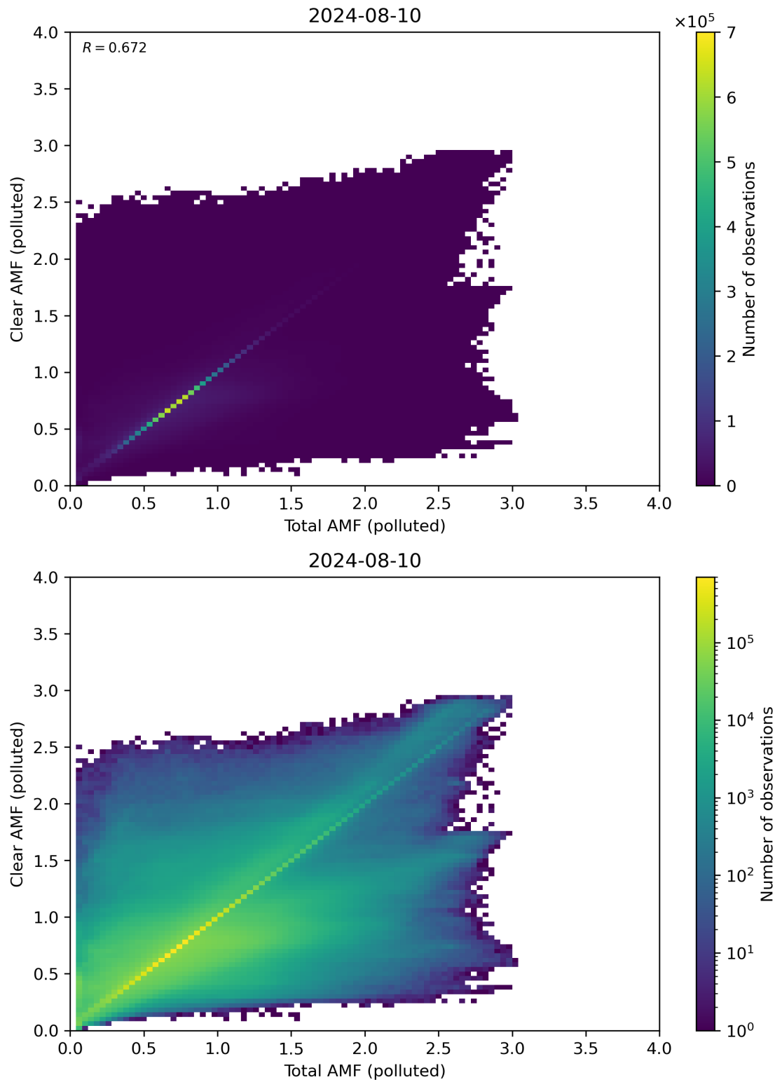
Figure 271: Scatter density plot of “Total AMF (polluted)” against “Clear AMF (polluted)” for 2024-08-09 to 2024-08-11.
