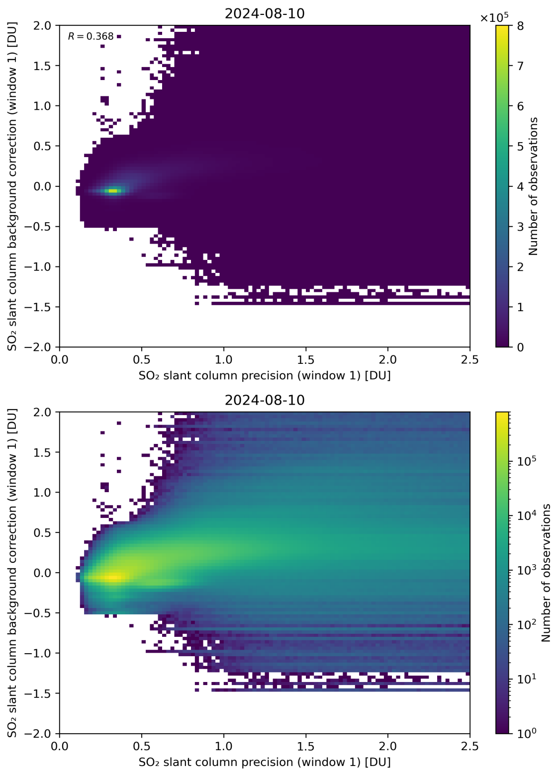
Figure 218: Scatter density plot of “SO 2 slant column precision (window 1)” against “SO 2 slant column background correction (window 1)” for 2024-08-09 to 2024-08-11.
