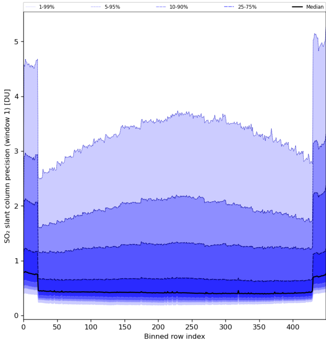
Figure 80: Along track statistics of “SO 2 slant column precision (window 1)” for 2024-08-09 to 2024-08-11
