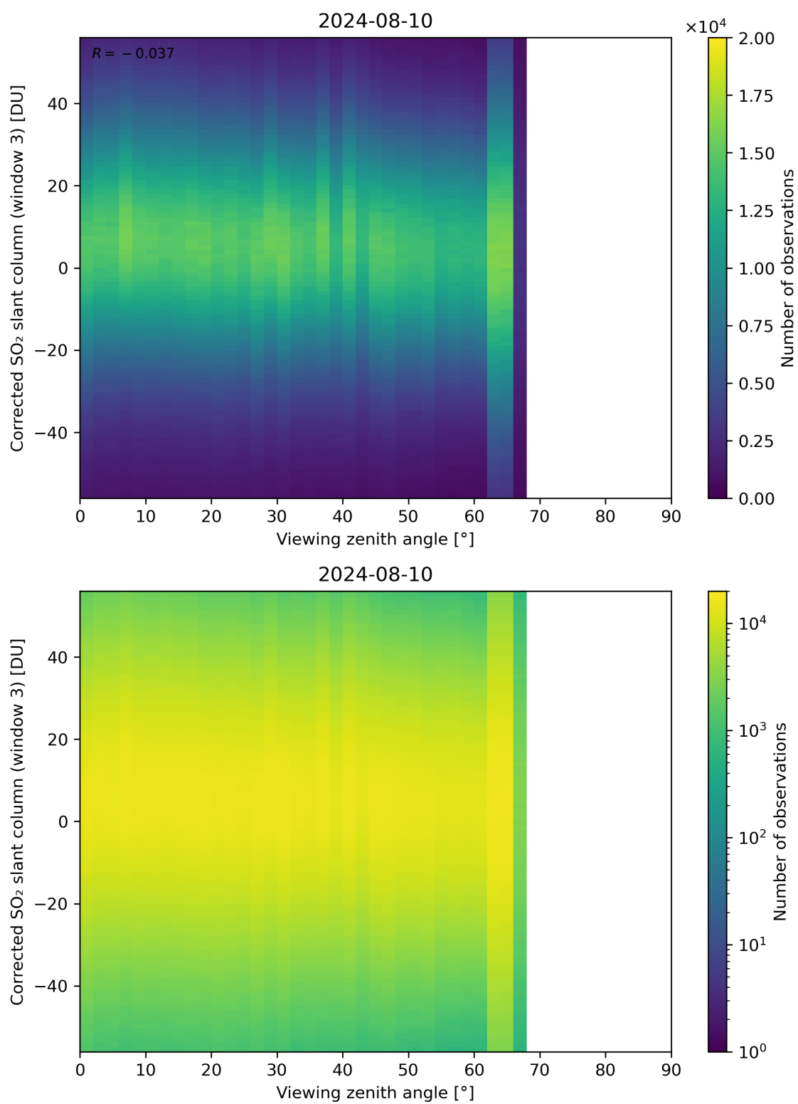
Figure 319: Scatter density plot of “Viewing zenith angle” against “Corrected SO 2 slant column (window 3)” for 2024-08-09 to 2024-08-11.
