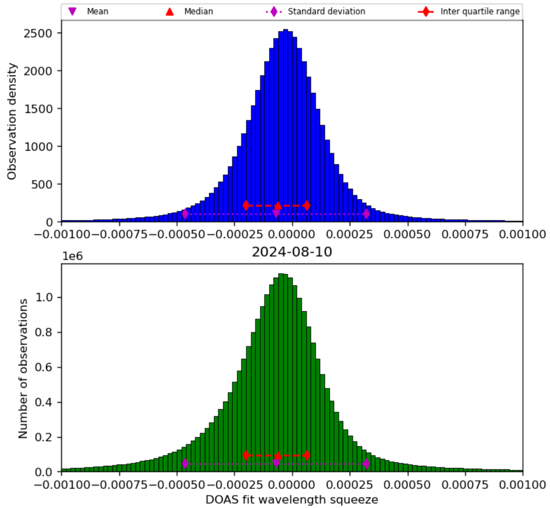
Figure 69: Histogram of “DOAS fit wavelength squeeze” for 2024-08-09 to 2024-08-11
