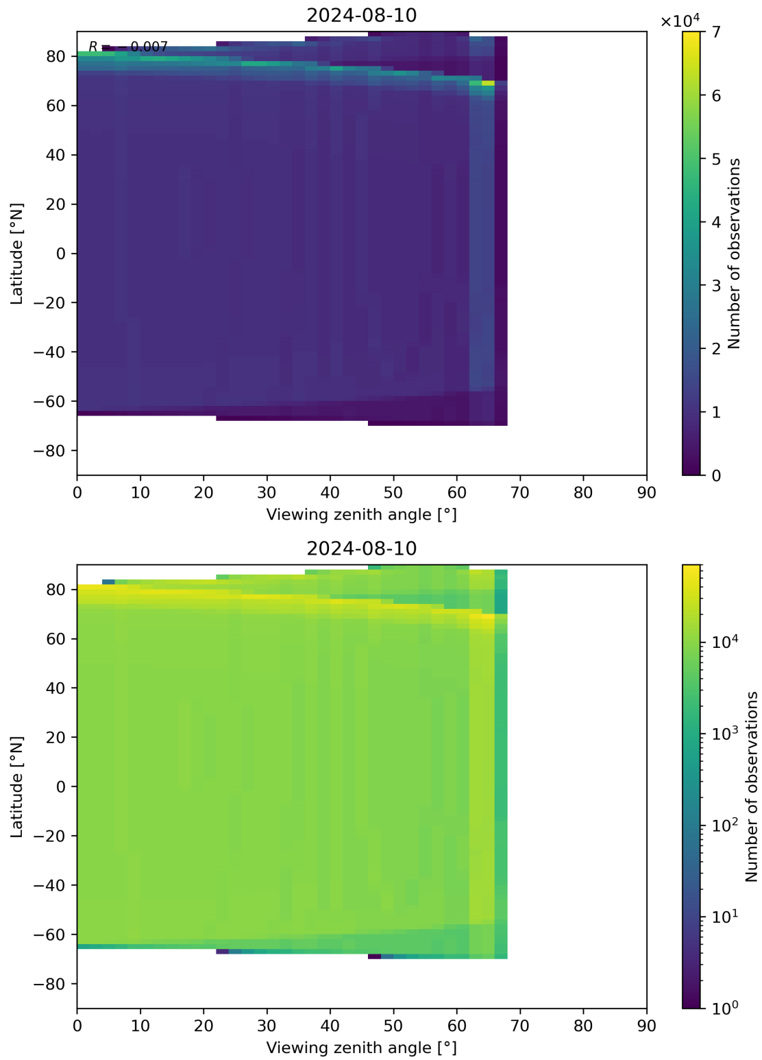
Figure 314: Scatter density plot of “Viewing zenith angle” against “Latitude” for 2024-08-09 to 2024-08-11.
