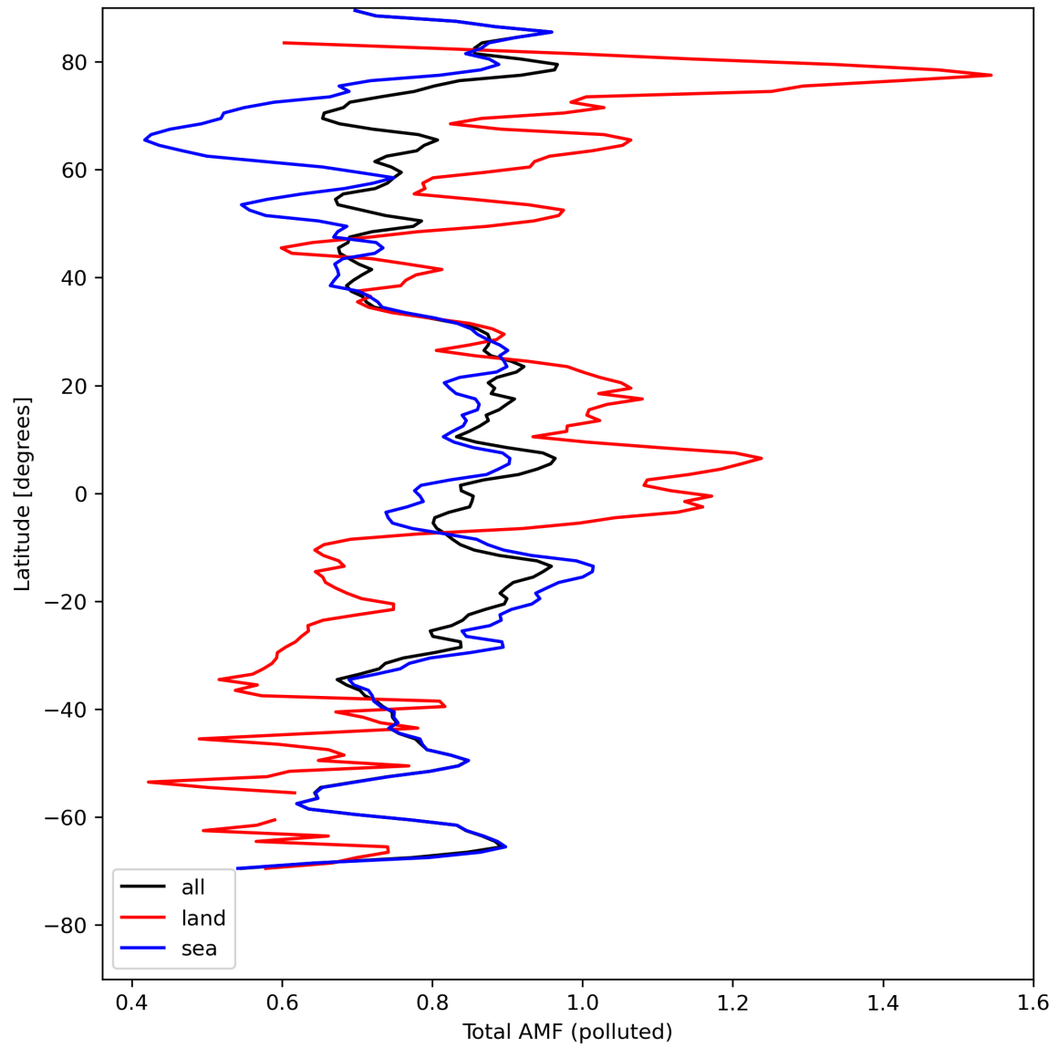
Figure 48: Zonal average of “Total AMF (polluted)” for 2024-08-09 to 2024-08-11.
