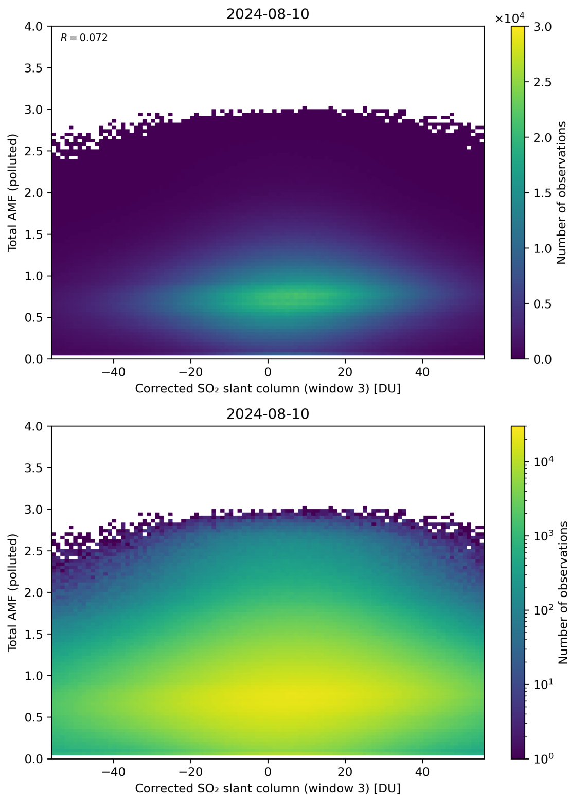
Figure 210: Scatter density plot of “Corrected SO 2 slant column (window 3)” against “Total AMF (polluted)” for 2024-08-09 to 2024-08-11.
