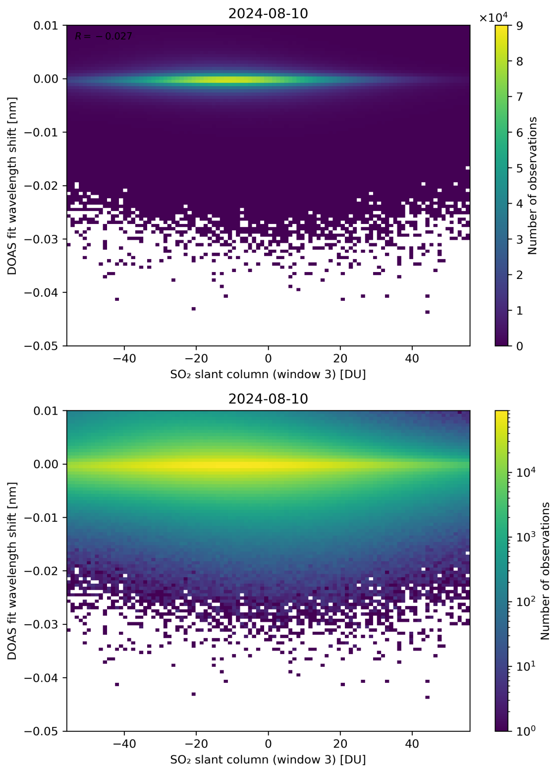
Figure 254: Scatter density plot of “SO 2 slant column (window 3)” against “DOAS fit wavelength shift” for 2024-08-09 to 2024-08-11.
