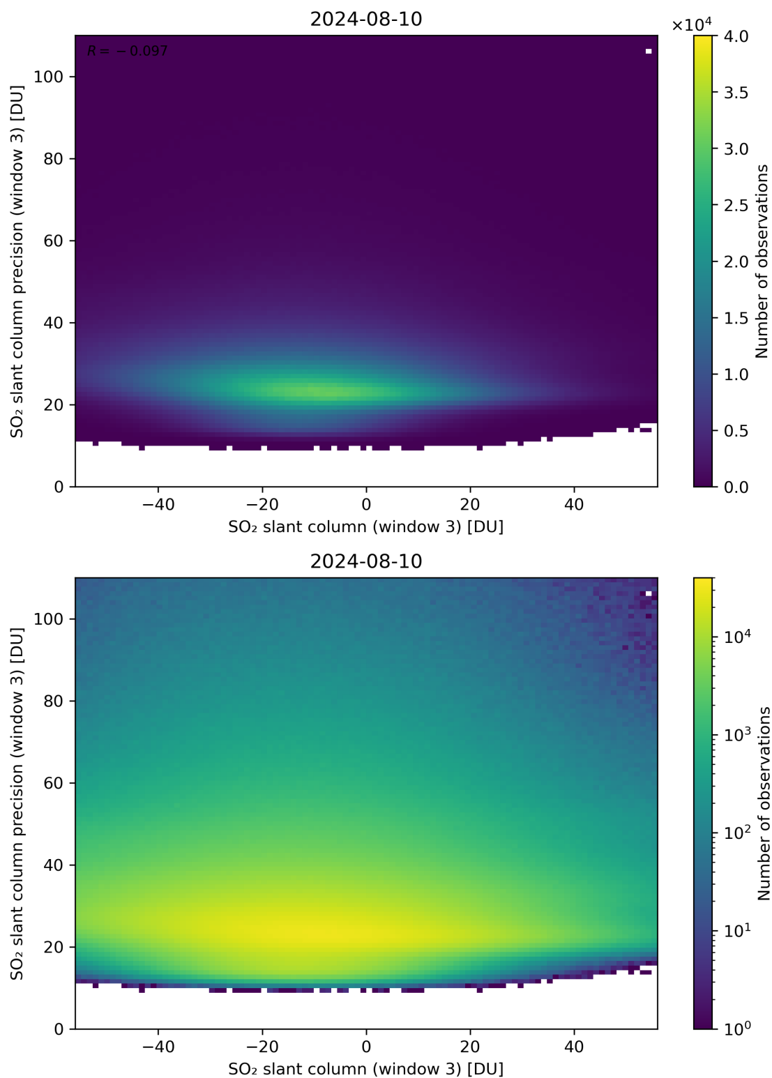
Figure 267: Scatter density plot of “SO 2 slant column (window 3)” against “SO 2 slant column precision (window 3)” for 2024-08-09 to 2024-08-11.
