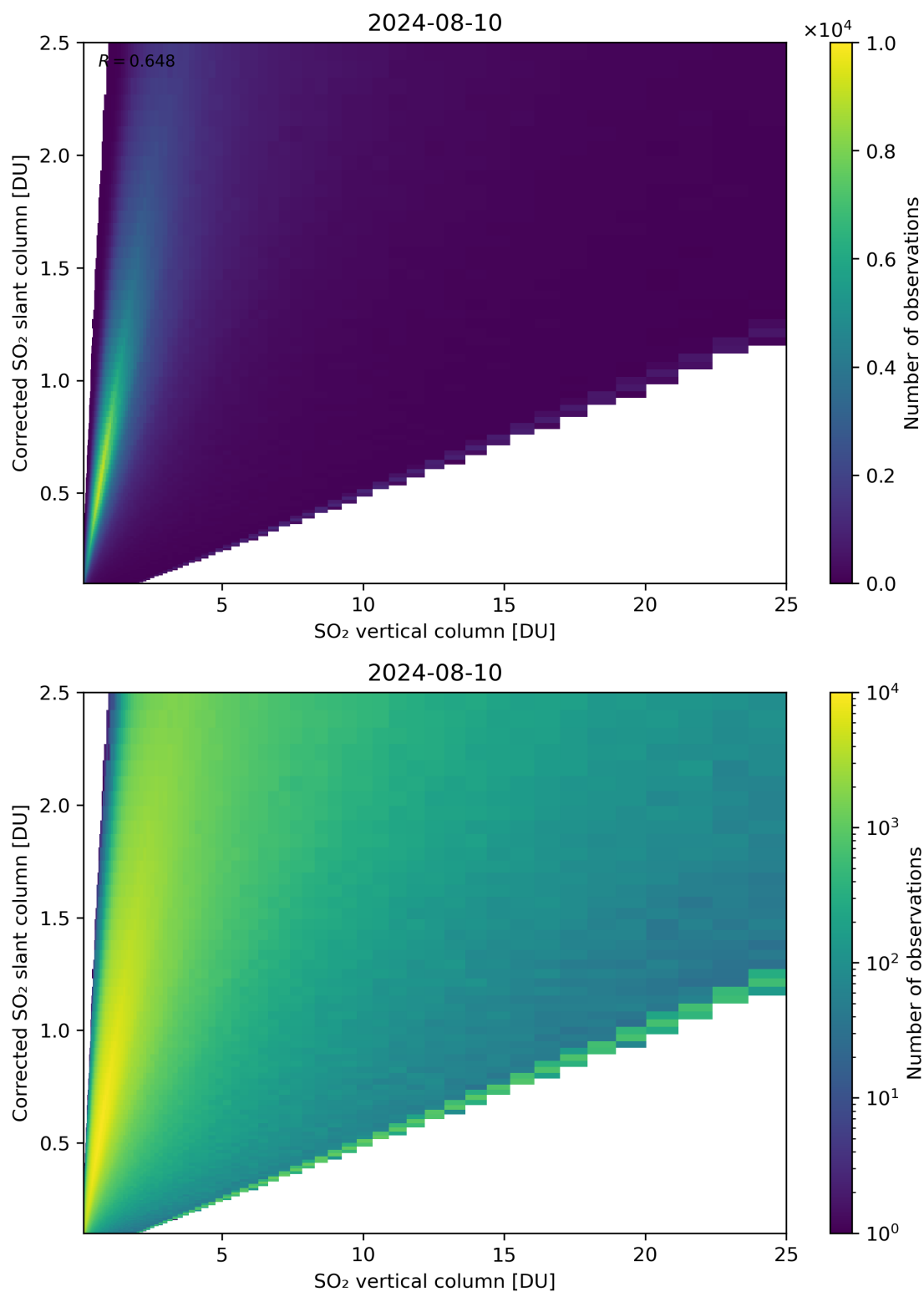
Figure 297: Scatter density plot of “SO 2 vertical column” against “Corrected SO 2 slant column” for 2024-08-09 to 2024-08-11.
