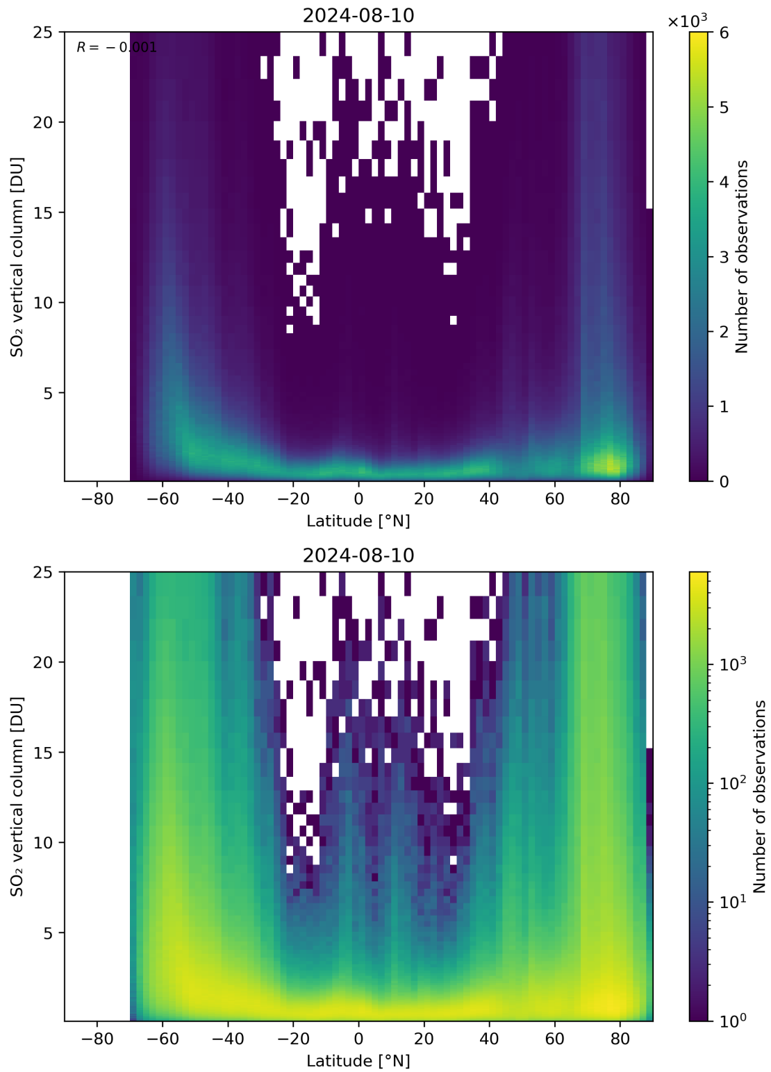
Figure 156: Scatter density plot of “Latitude” against “SO 2 vertical column” for 2024-08-09 to 2024-08-11.
