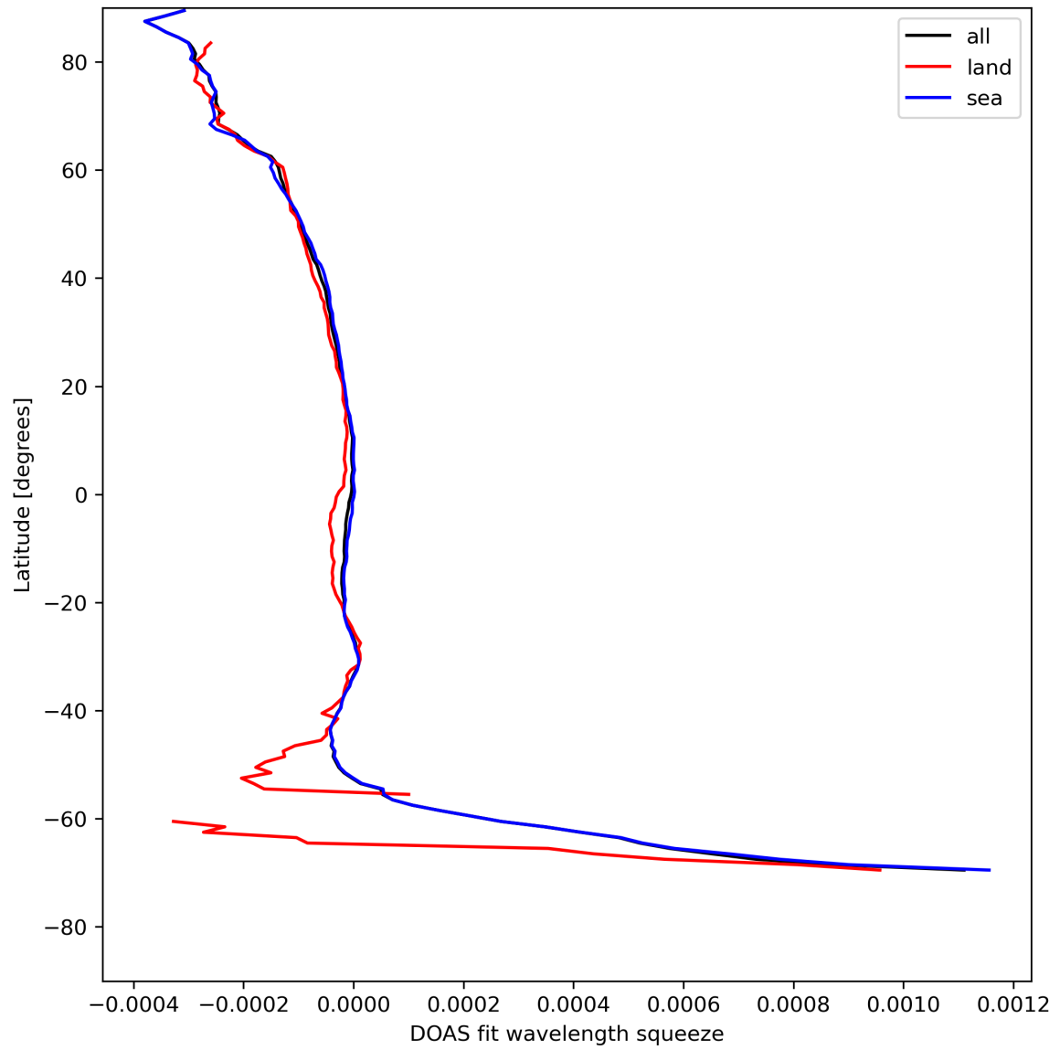
Figure 46: Zonal average of “DOAS fit wavelength squeeze” for 2024-08-09 to 2024-08-11.
