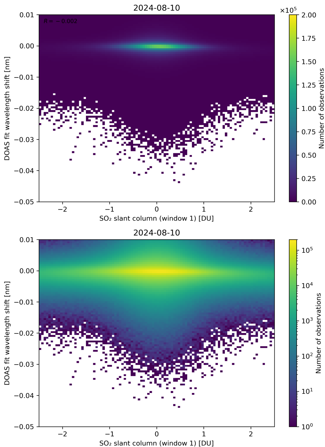
Figure 215: Scatter density plot of “SO 2 slant column (window 1)” against “DOAS fit wavelength shift” for 2024-08-09 to 2024-08-11.
