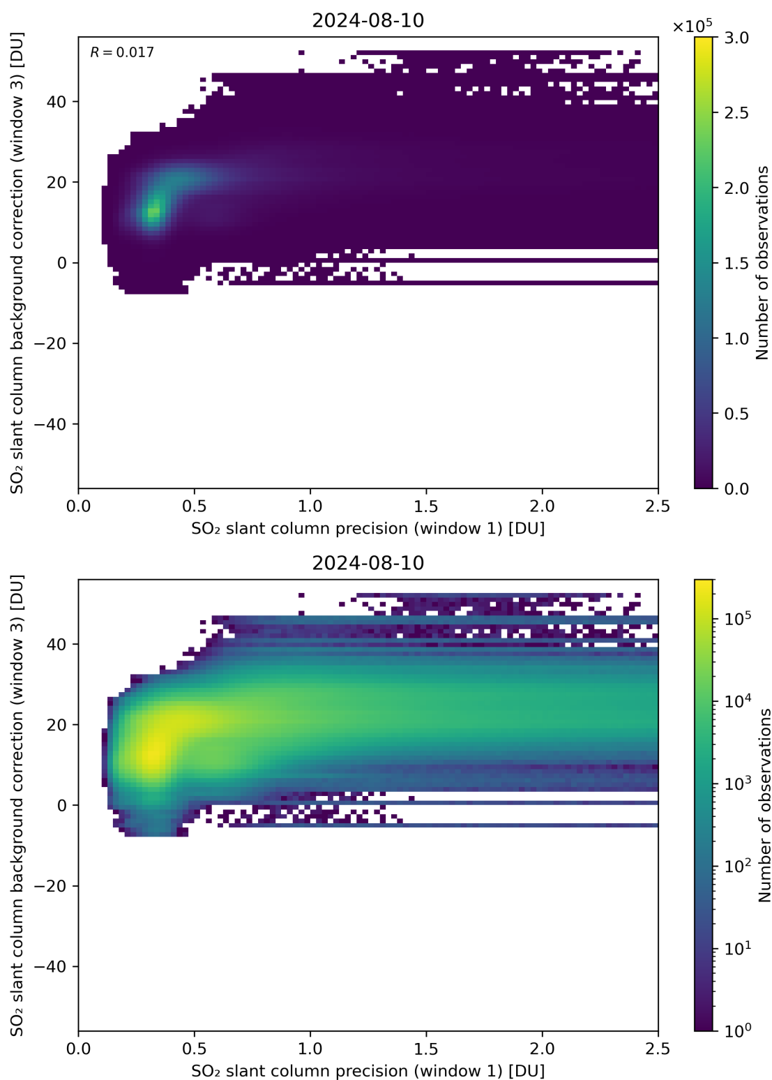
Figure 220: Scatter density plot of “SO 2 slant column precision (window 1)” against “SO 2 slant column background correction (window 3)” for 2024-08-09 to 2024-08-11.
