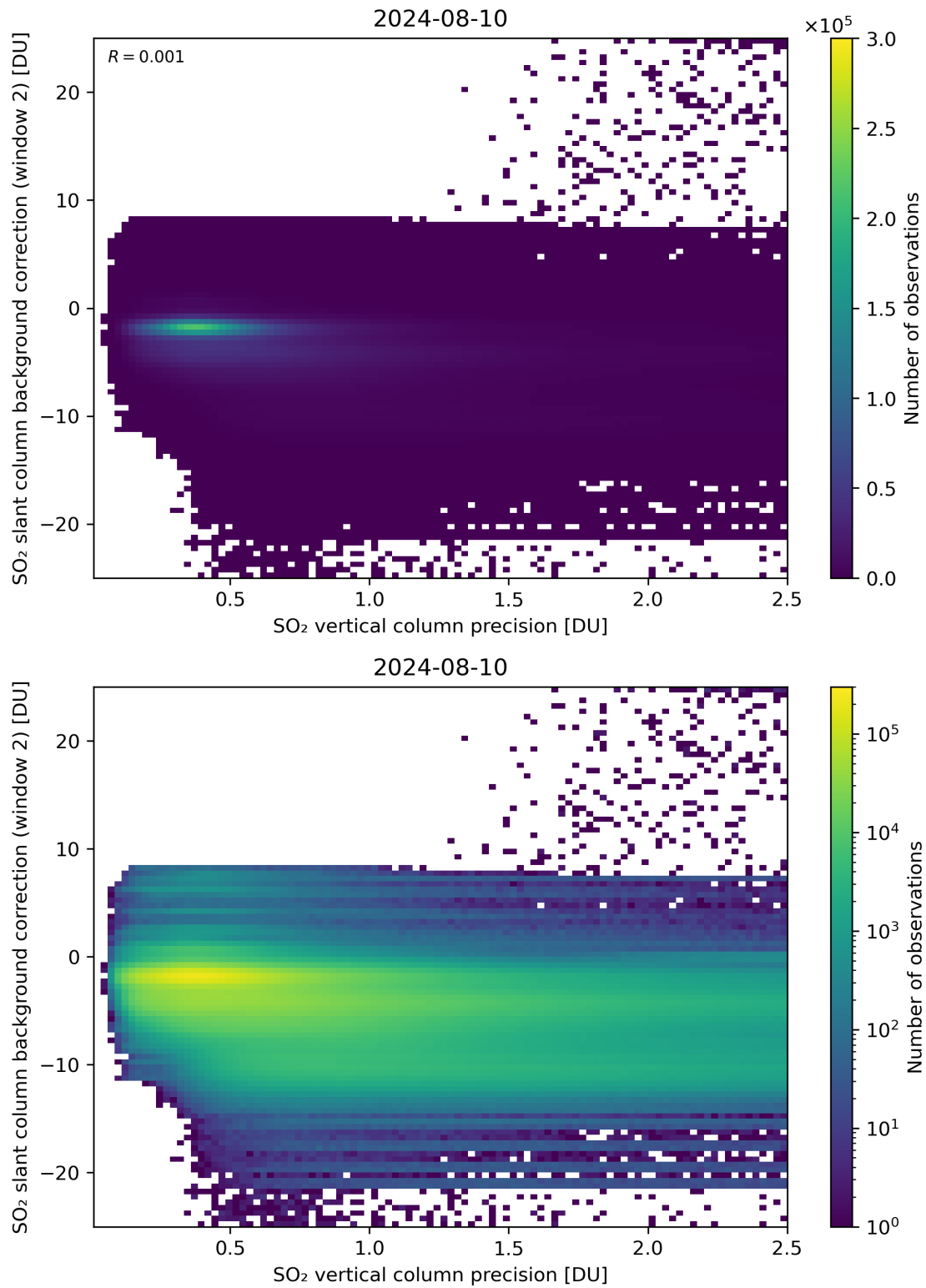
Figure 280: Scatter density plot of “SO 2 vertical column precision” against “SO 2 slant column background correction (window 2)” for 2024-08-09 to 2024-08-11.
