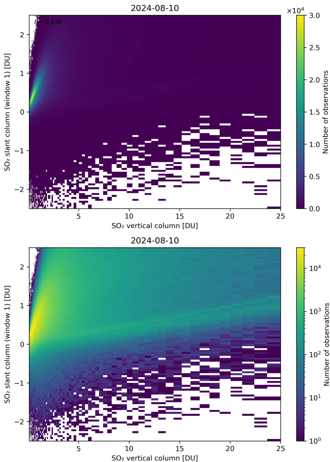
Figure 300: Scatter density plot of “SO 2 vertical column” against “SO 2 slant column (window 1)” for 2024-08-09 to 2024-08-11.
