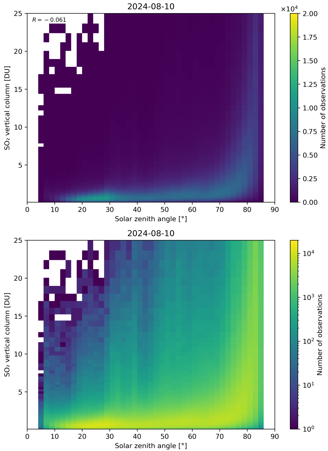
Figure 176: Scatter density plot of “Solar zenith angle” against “SO 2 vertical column” for 2024-08-09 to 2024-08-11.
