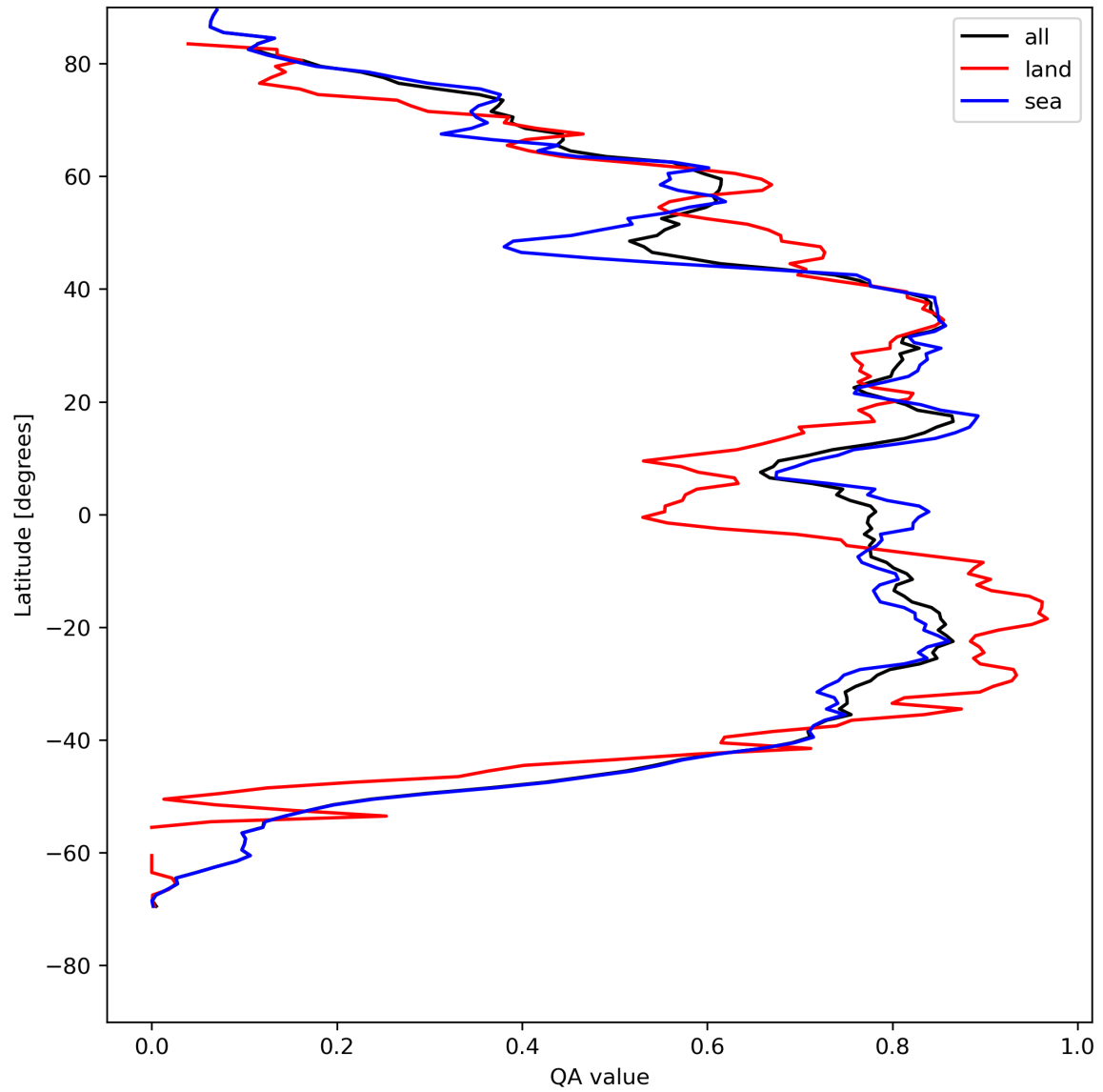
Figure 29: Zonal average of “QA value” for 2024-08-09 to 2024-08-11.
