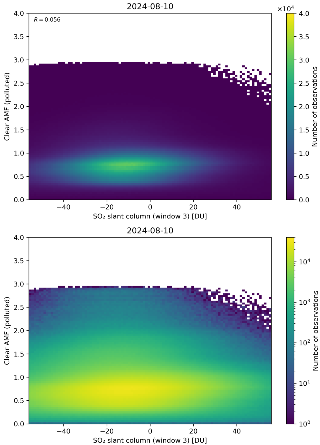
Figure 265: Scatter density plot of “SO 2 slant column (window 3)” against “Clear AMF (polluted)” for 2024-08-09 to 2024-08-11.
