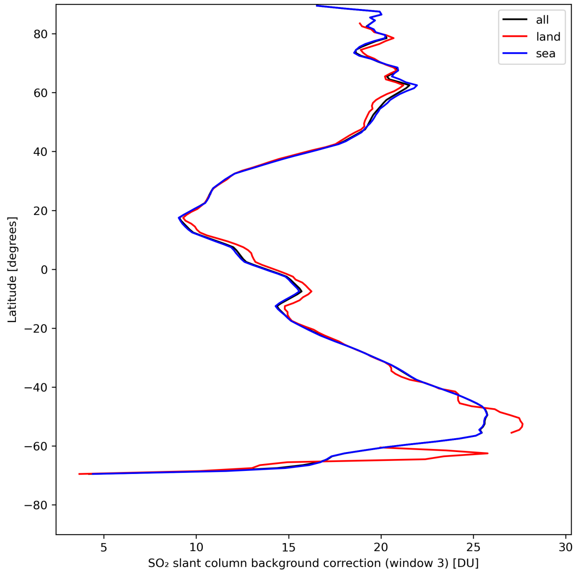
Figure 44: Zonal average of “SO 2 slant column background correction (window 3)” for 2024-08-09 to 2024-08-11.
