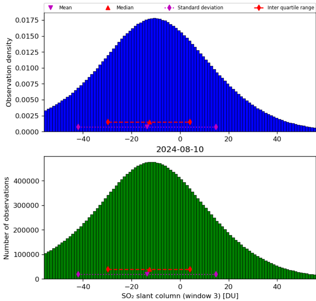
Figure 64: Histogram of “SO 2 slant column (window 3)” for 2024-08-09 to 2024-08-11
