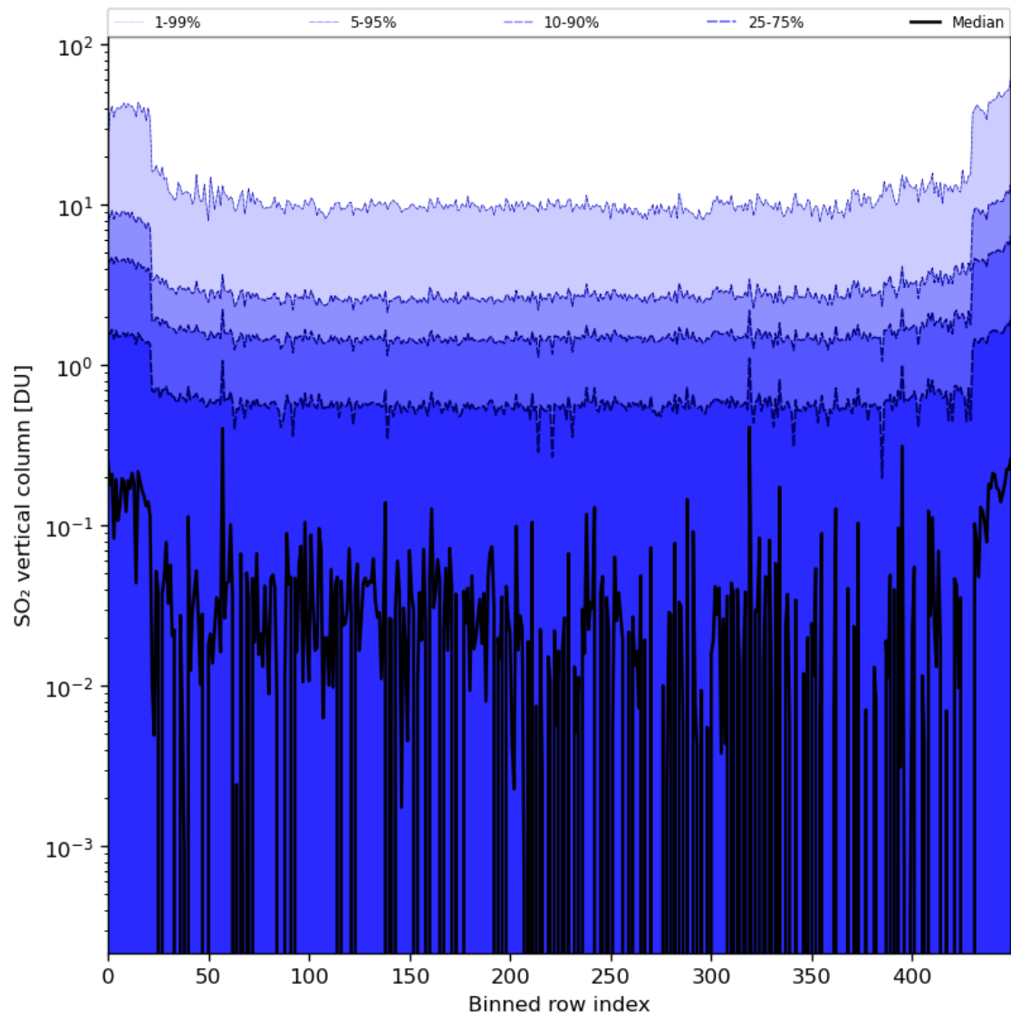
Figure 76: Along track statistics of “SO 2 vertical column” for 2024-08-09 to 2024-08-11
