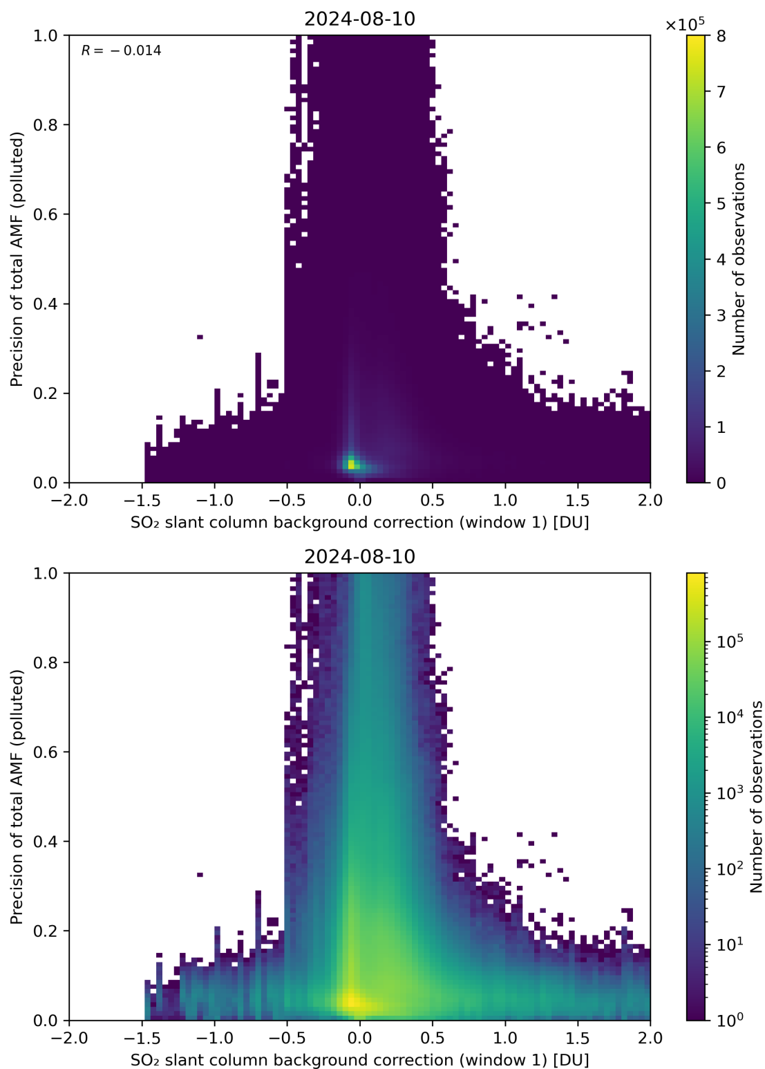
Figure 110: Scatter density plot of “SO 2 slant column background correction (window 1)” against “Precision of total AMF (polluted)” for 2024-08-09 to 2024-08-11.
