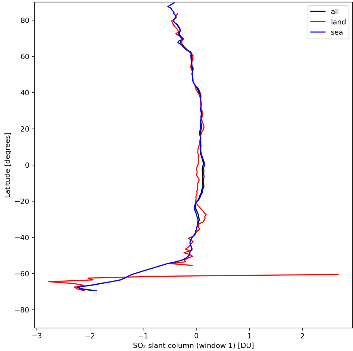
Figure 33: Zonal average of “SO 2 slant column (window 1)” for 2024-08-09 to 2024-08-11.
