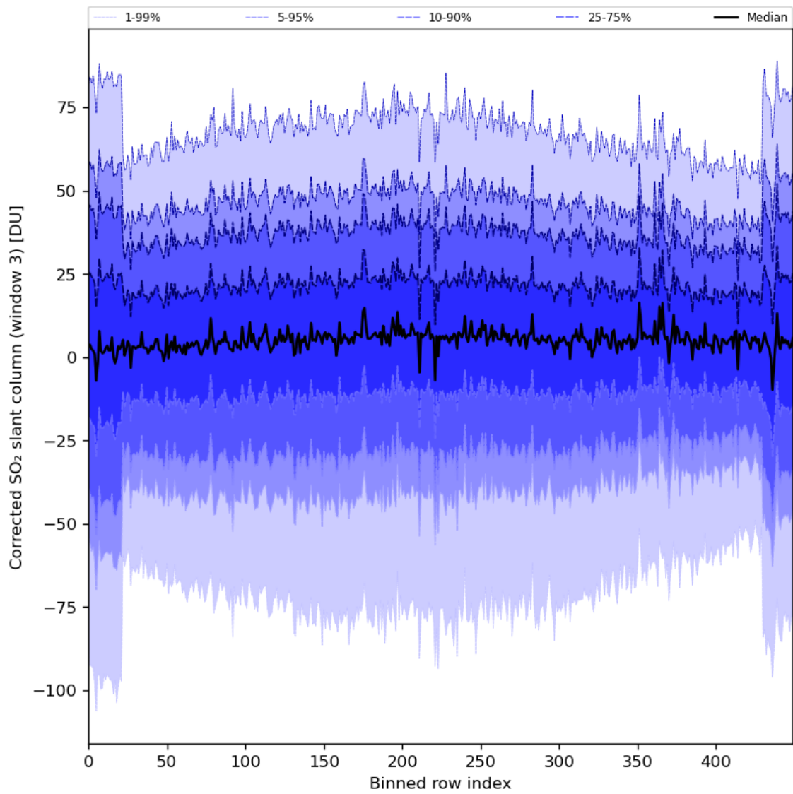
Figure 89: Along track statistics of “Corrected SO 2 slant column (window 3)” for 2024-08-09 to 2024-08-11
