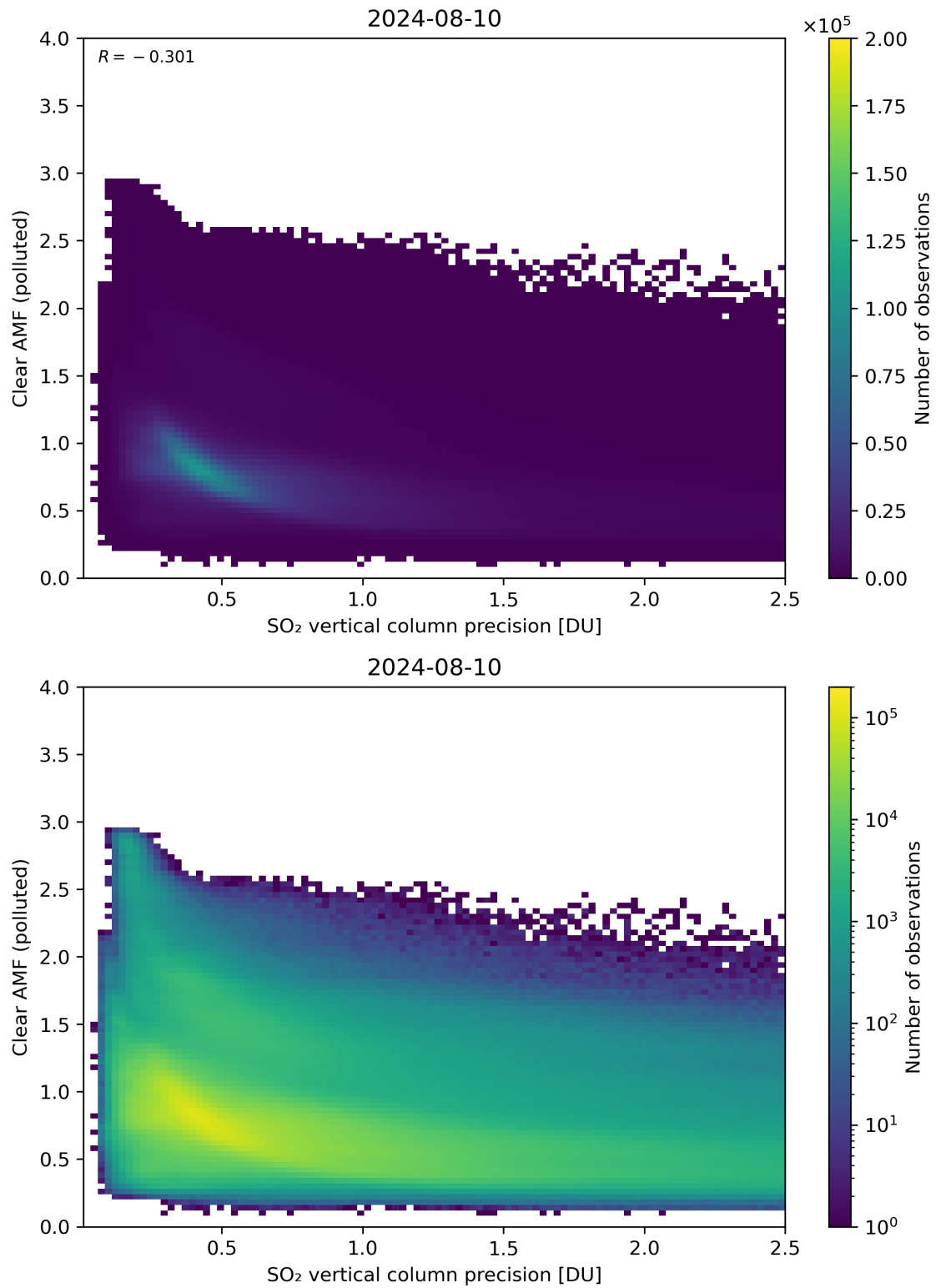
Figure 285: Scatter density plot of “SO 2 vertical column precision” against “Clear AMF (polluted)” for 2024-08-09 to 2024-08-11.
