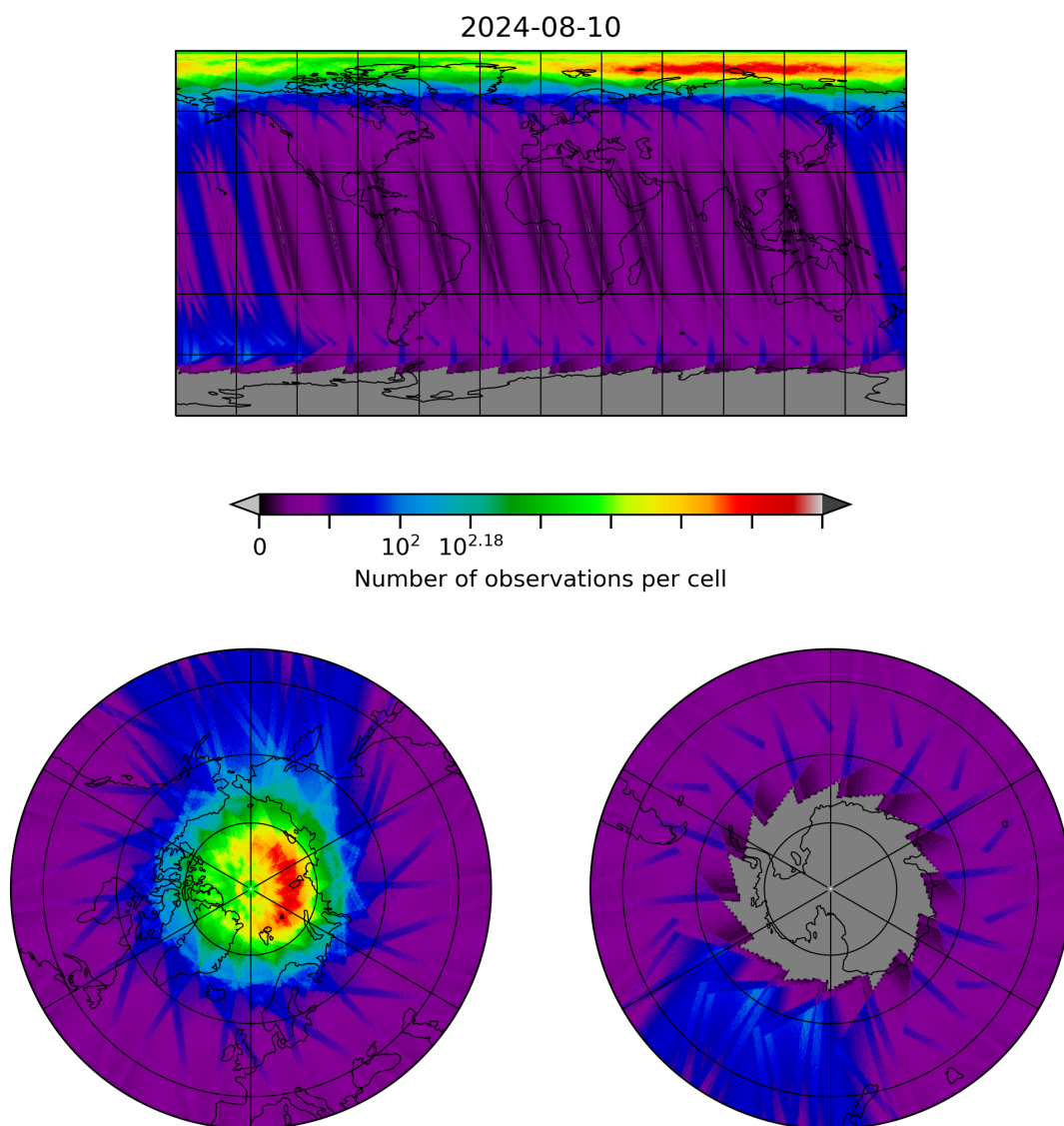
Figure 28: Map of the number of observations for 2024-08-09 to 2024-08-11
