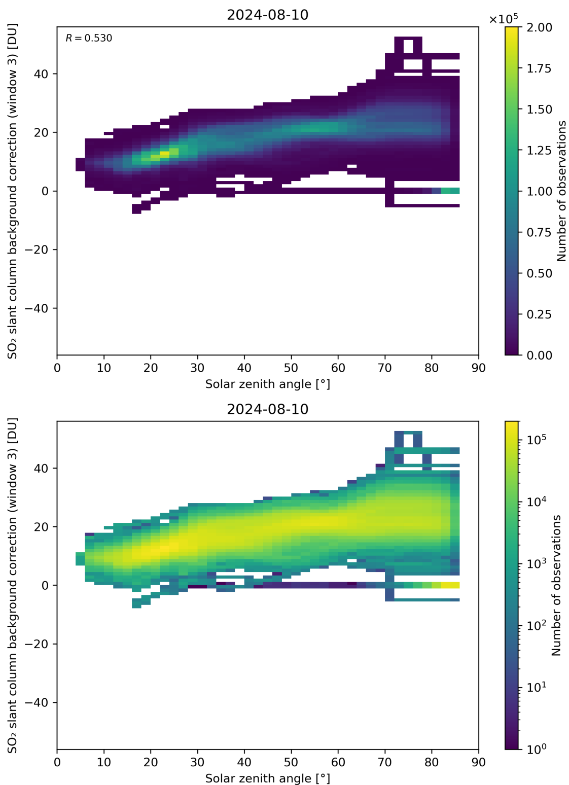
Figure 160: Scatter density plot of “Solar zenith angle” against “SO 2 slant column background correction (window 3)” for 2024-08-09 to 2024-08-11.
