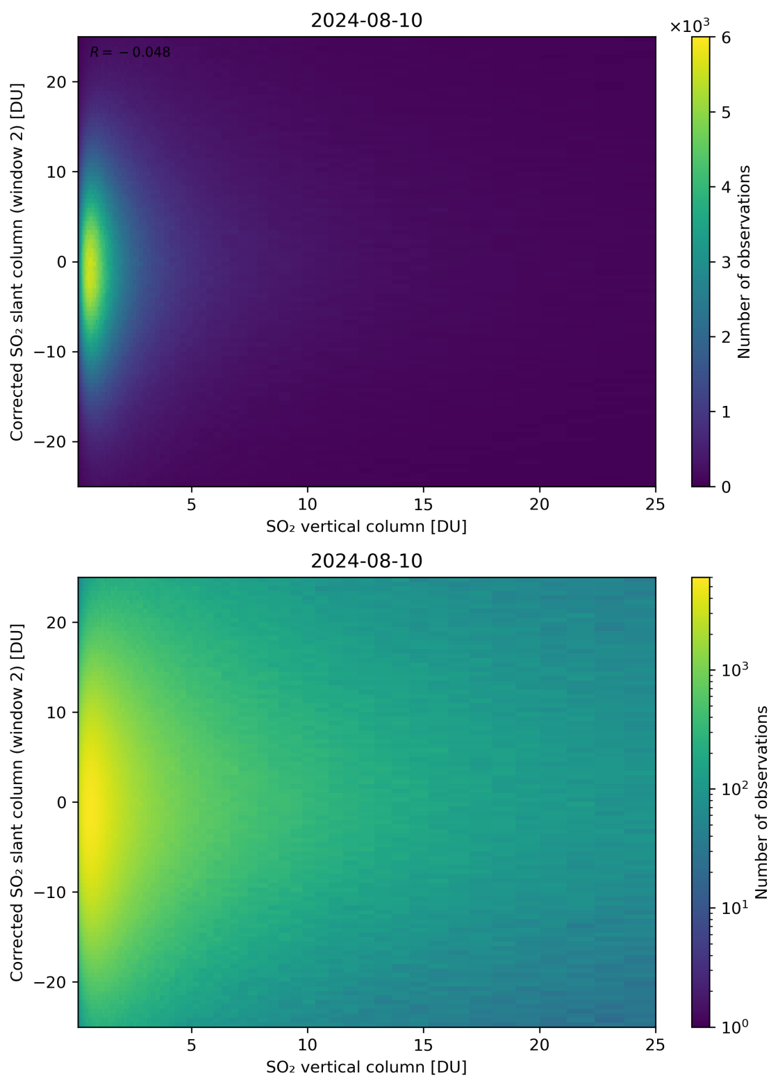
Figure 298: Scatter density plot of “SO 2 vertical column” against “Corrected SO 2 slant column (window 2)” for 2024-08-09 to 2024-08-11.
