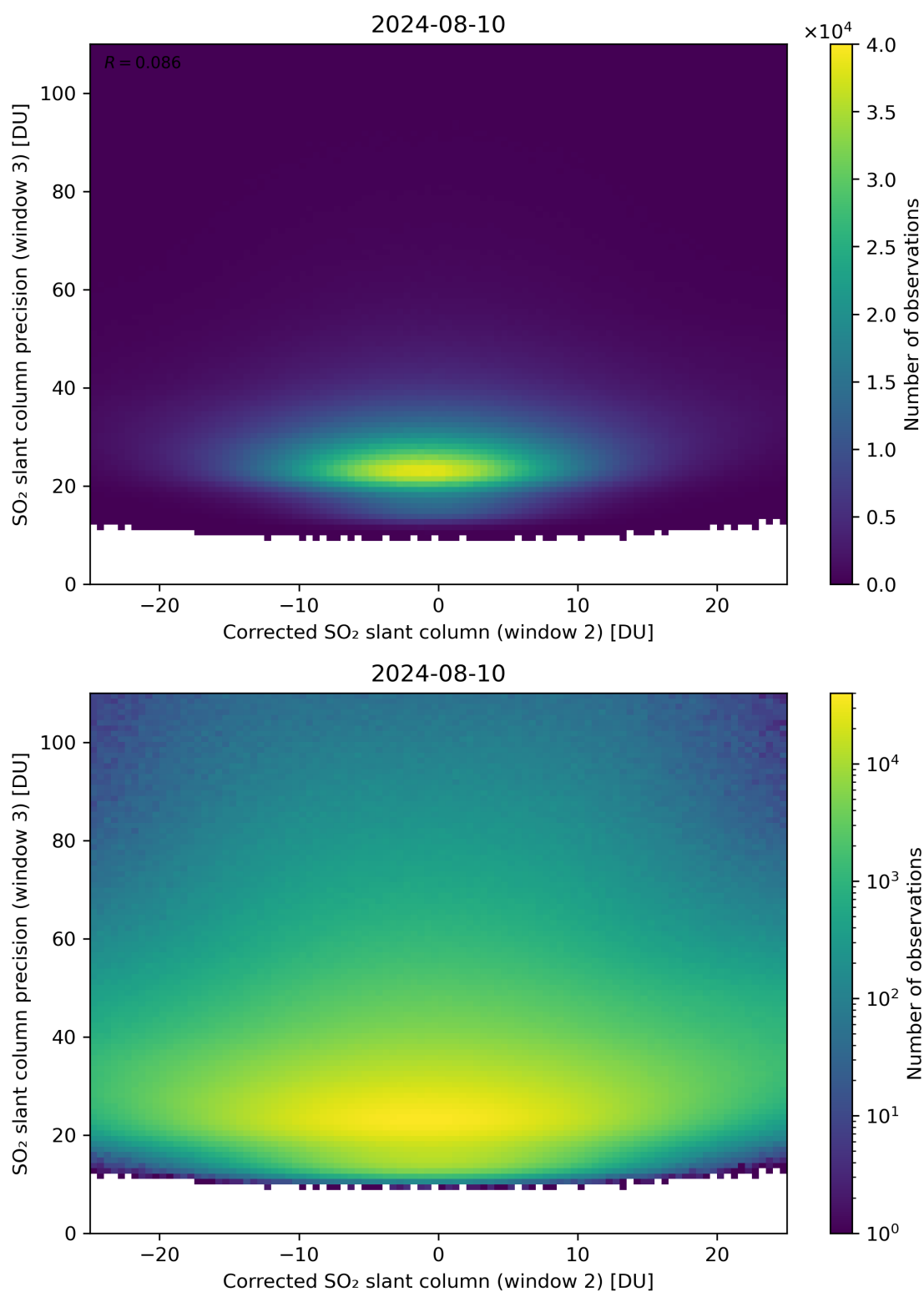
Figure 202: Scatter density plot of “Corrected SO 2 slant column (window 2)” against “SO 2 slant column precision (window 3)” for 2024-08-09 to 2024-08-11.
