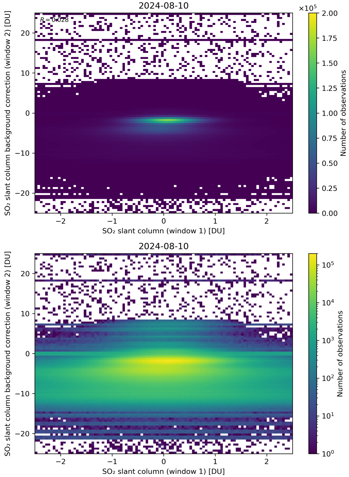
Figure 213: Scatter density plot of “SO 2 slant column (window 1)” against “SO 2 slant column background correction (window 2)” for 2024-08-09 to 2024-08-11.
