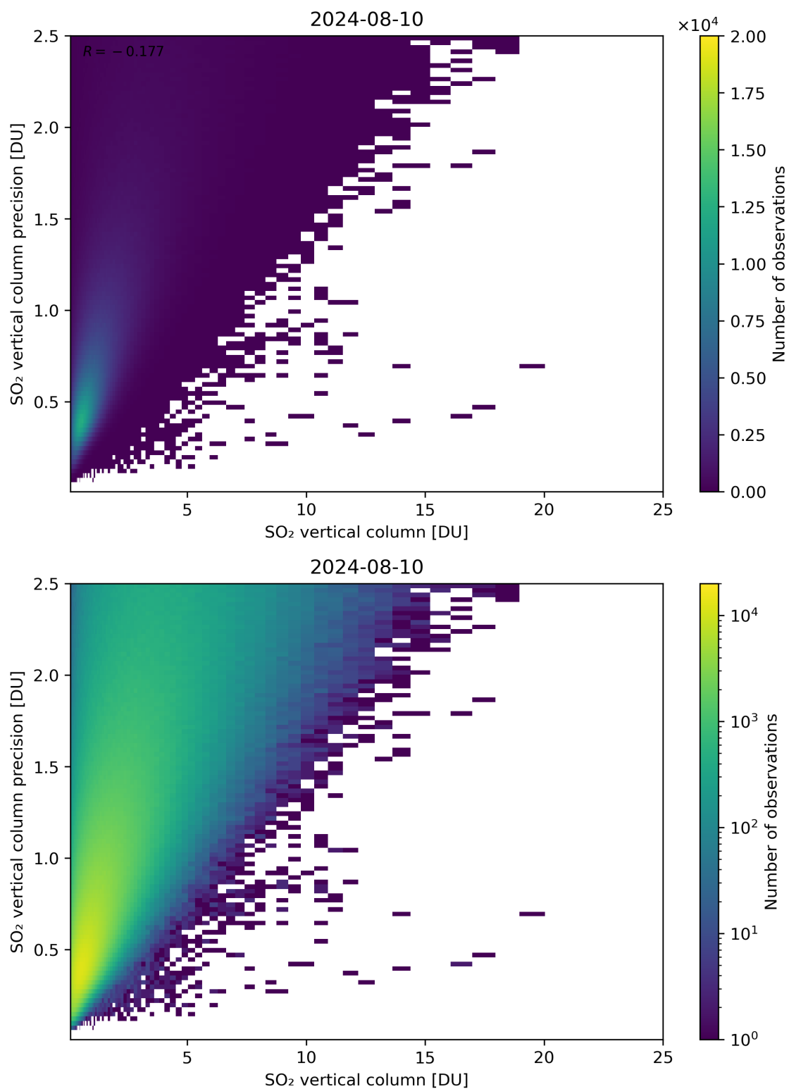
Figure 307: Scatter density plot of “SO 2 vertical column” against “SO 2 vertical column precision” for 2024-08-09 to 2024-08-11.
