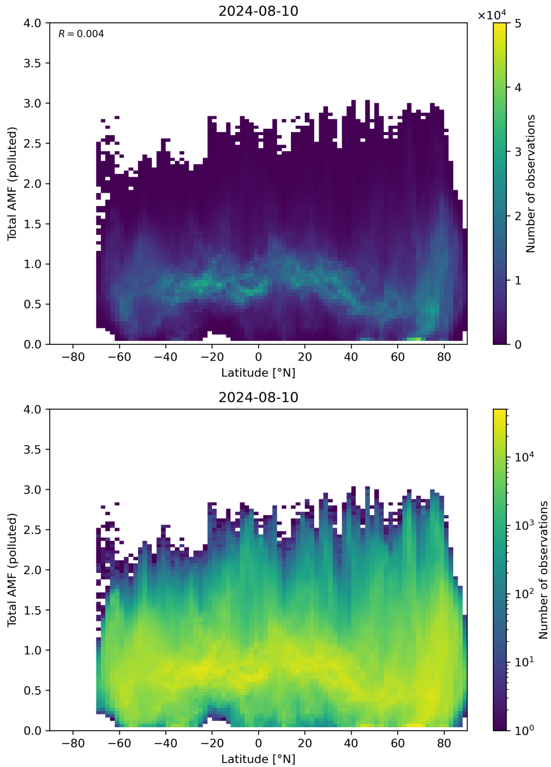
Figure 154: Scatter density plot of “Latitude” against “Total AMF (polluted)” for 2024-08-09 to 2024-08-11.
