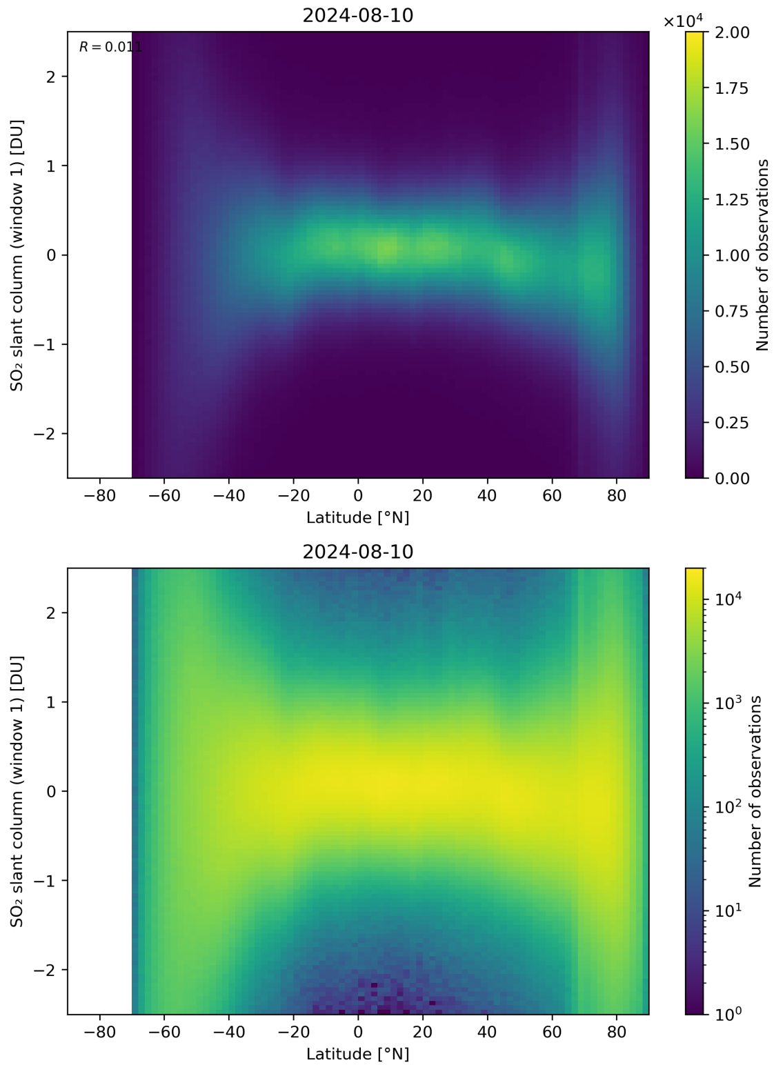
Figure 149: Scatter density plot of “Latitude” against “SO 2 slant column (window 1)” for 2024-08-09 to 2024-08-11.
