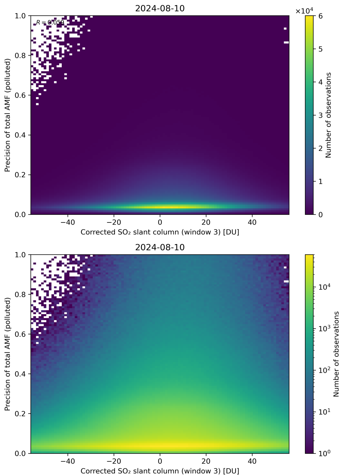
Figure 211: Scatter density plot of “Corrected SO 2 slant column (window 3)” against “Precision of total AMF (polluted)” for 2024-08-09 to 2024-08-11.
