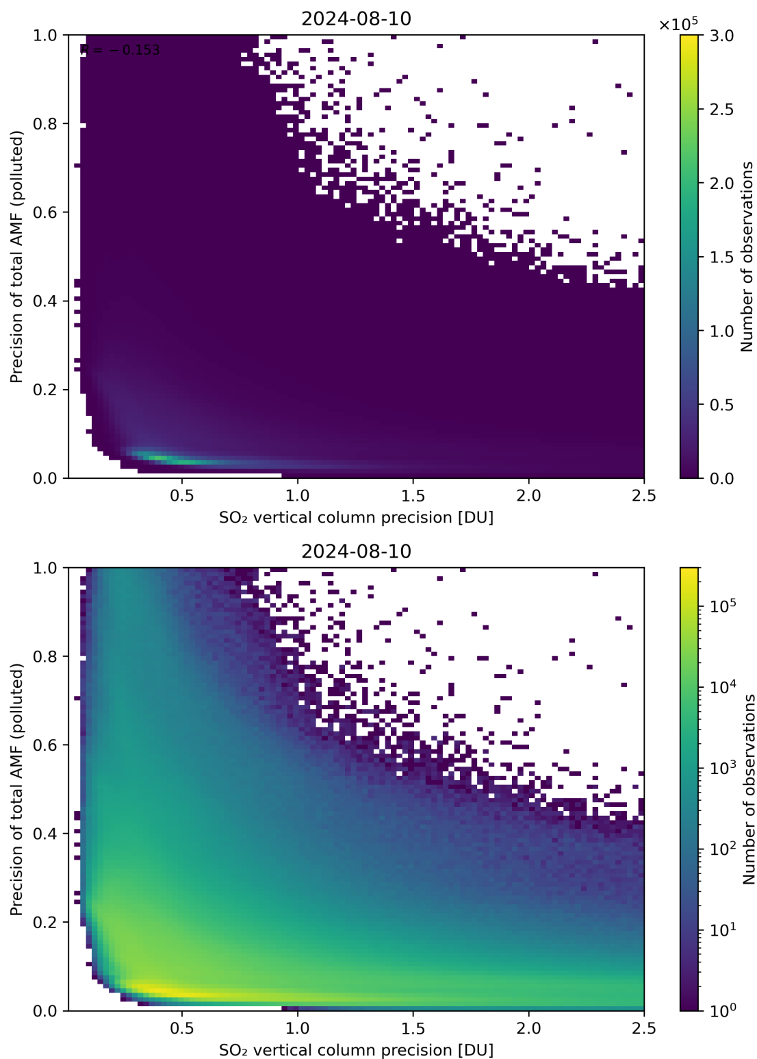
Figure 295: Scatter density plot of “SO 2 vertical column precision” against “Precision of total AMF (polluted)” for 2024-08-09 to 2024-08-11.
