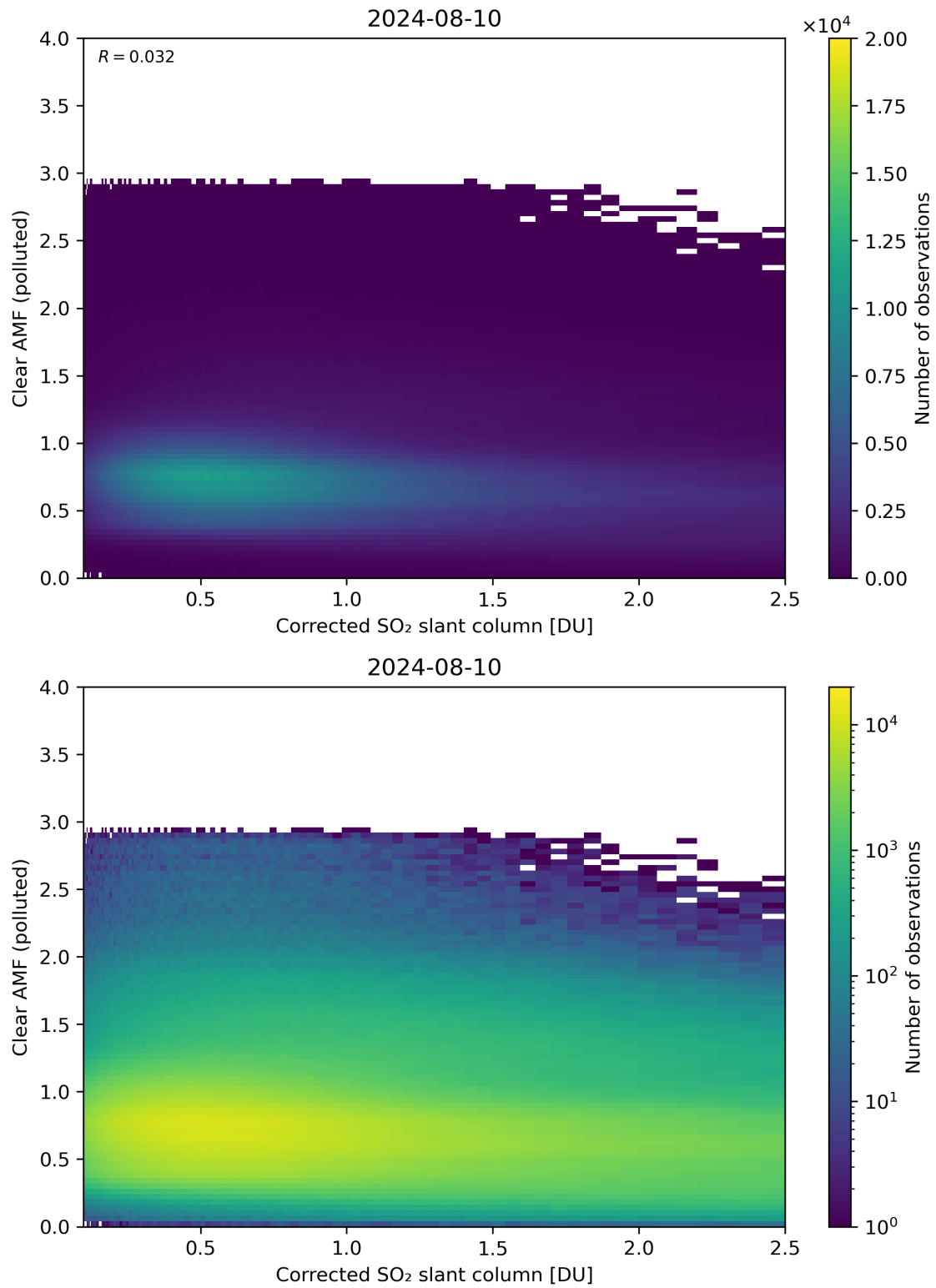
Figure 184: Scatter density plot of “Corrected SO 2 slant column” against “Clear AMF (polluted)” for 2024-08-09 to 2024-08-11.
