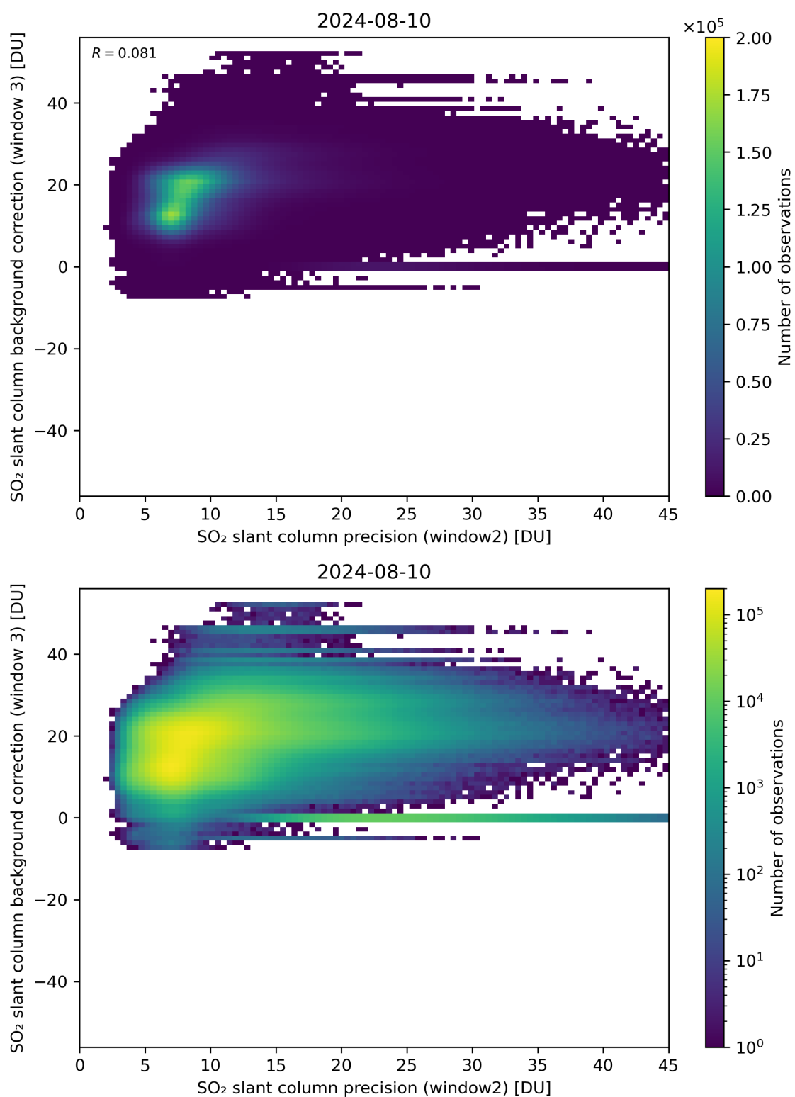
Figure 242: Scatter density plot of “SO 2 slant column precision (window2)” against “SO 2 slant column background correction (window 3)” for 2024-08-09 to 2024-08-11.
