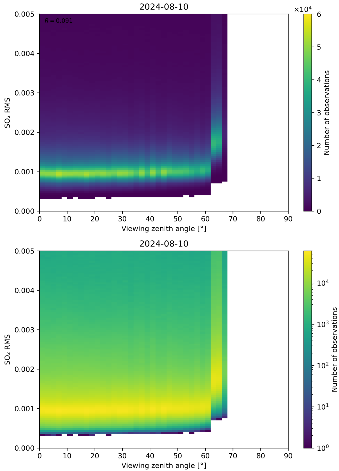
Figure 313: Scatter density plot of “Viewing zenith angle” against “SO 2 RMS” for 2024-08-09 to 2024-08-11.
