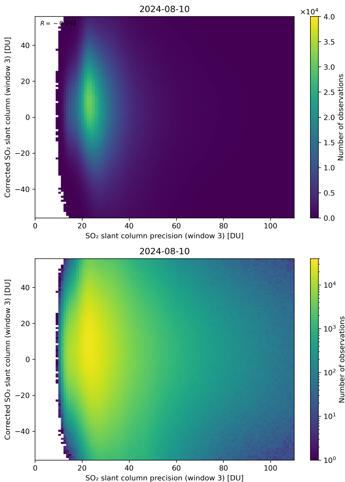
Figure 262: Scatter density plot of “SO 2 slant column precision (window 3)” against “Corrected SO 2 slant column (window 3)” for 2024-08-09 to 2024-08-11.
