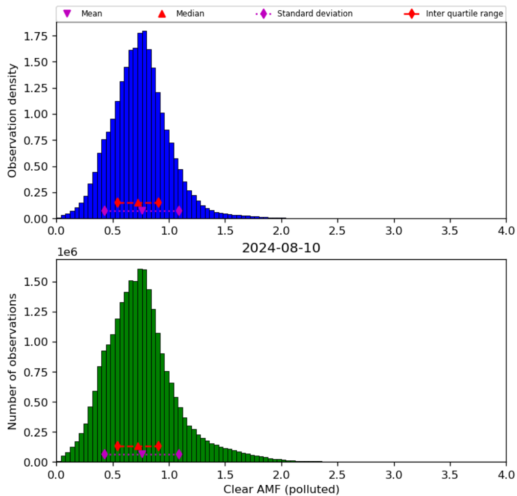
Figure 73: Histogram of “Clear AMF (polluted)” for 2024-08-09 to 2024-08-11
