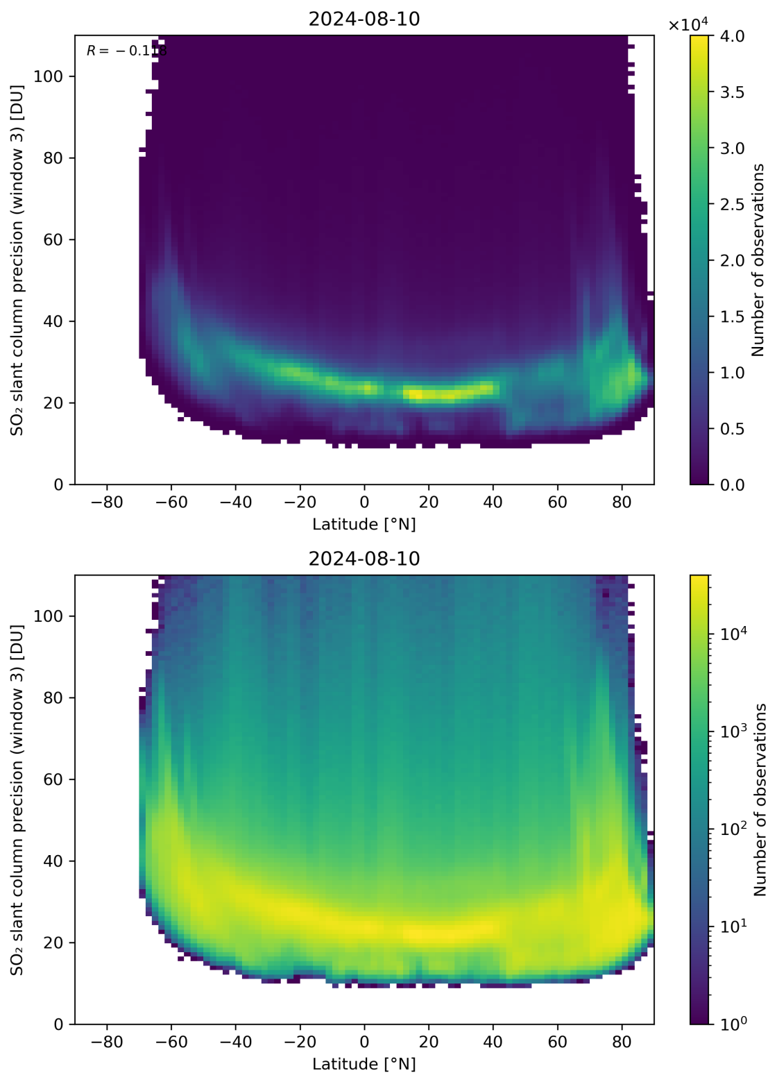
Figure 153: Scatter density plot of “Latitude” against “SO 2 slant column precision (window 3)” for 2024-08-09 to 2024-08-11.
