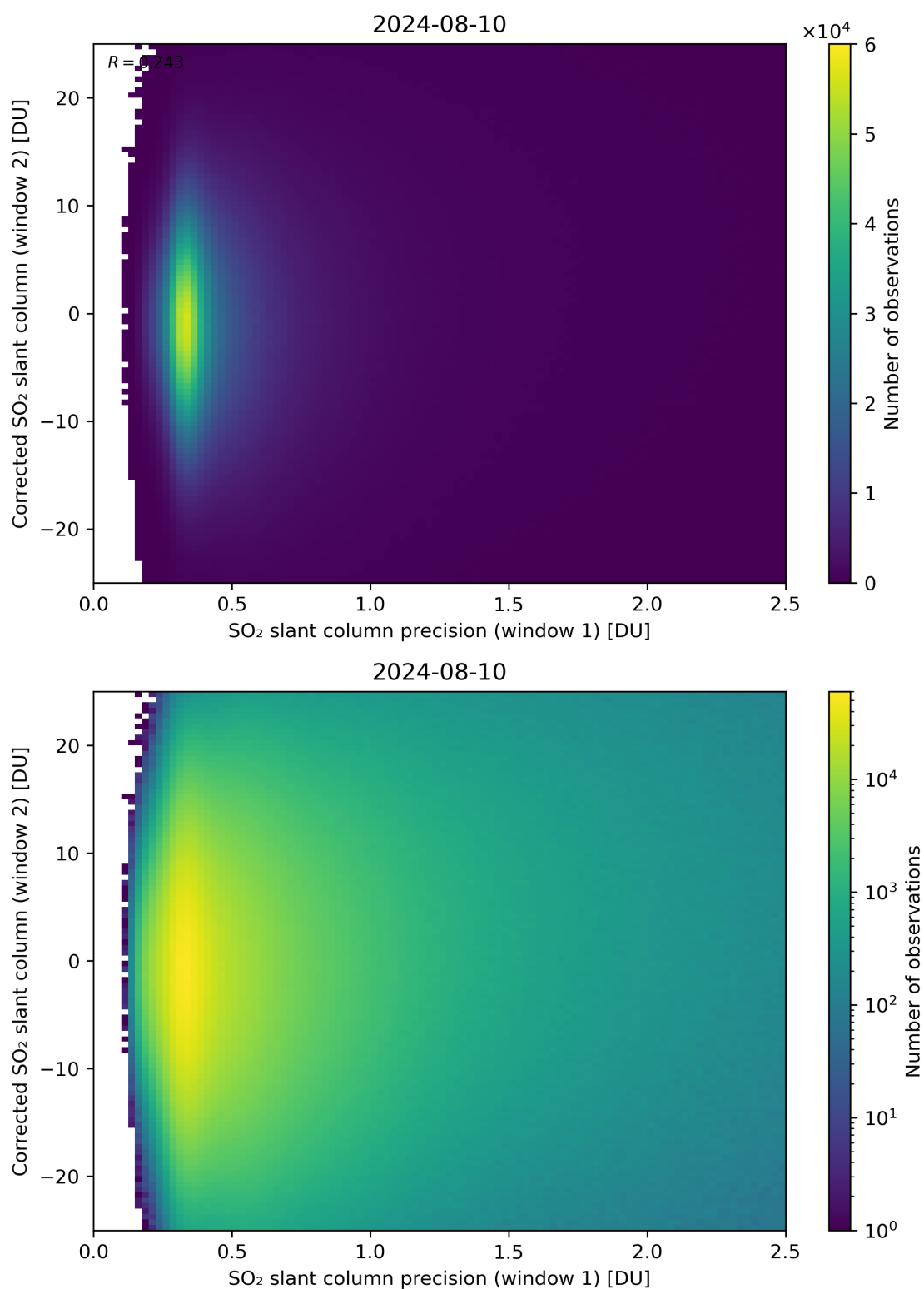
Figure 225: Scatter density plot of “SO 2 slant column precision (window 1)” against “Corrected SO 2 slant column (window 2)” for 2024-08-09 to 2024-08-11.
