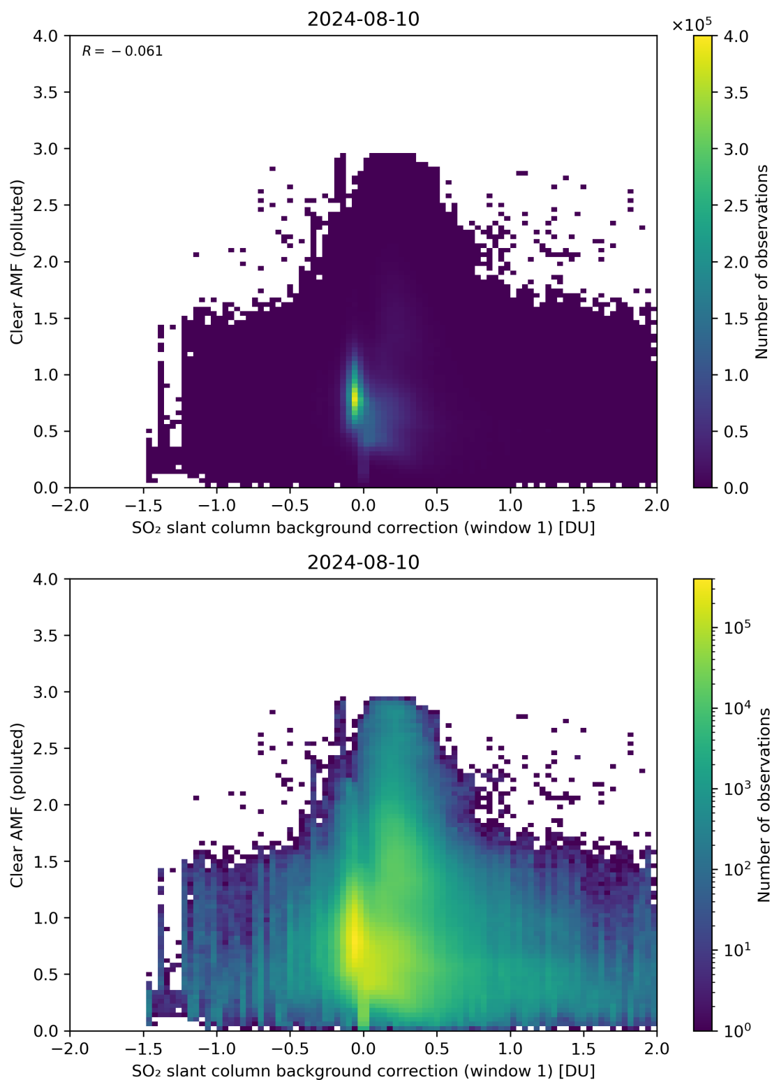
Figure 103: Scatter density plot of “SO 2 slant column background correction (window 1)” against “Clear AMF (polluted)” for 2024-08-09 to 2024-08-11.
