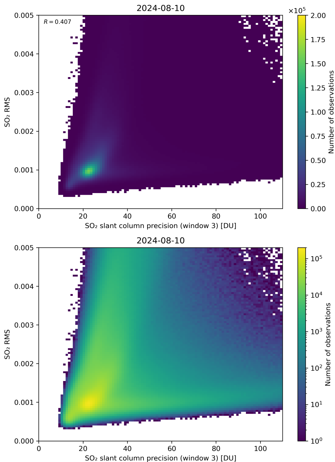
Figure 260: Scatter density plot of “SO 2 slant column precision (window 3)” against “SO 2 RMS” for 2024-08-09 to 2024-08-11.
