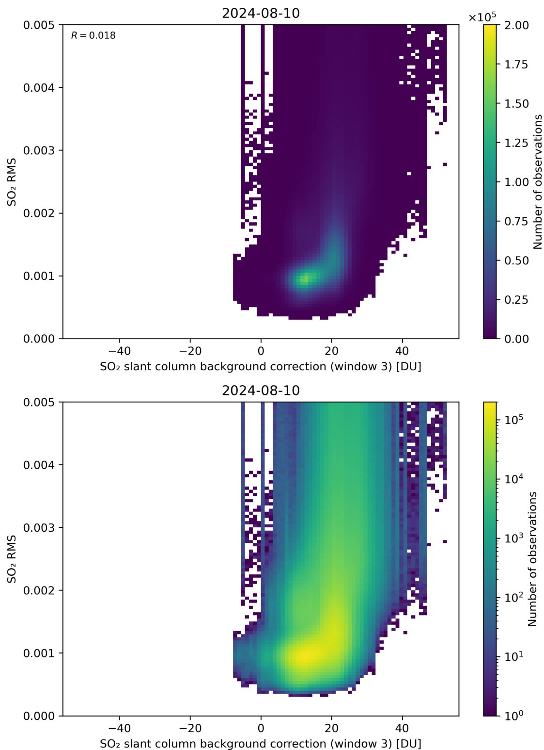
Figure 123: Scatter density plot of “SO 2 slant column background correction (window 3)” against “SO 2 RMS” for 2024-08-09 to 2024-08-11.
