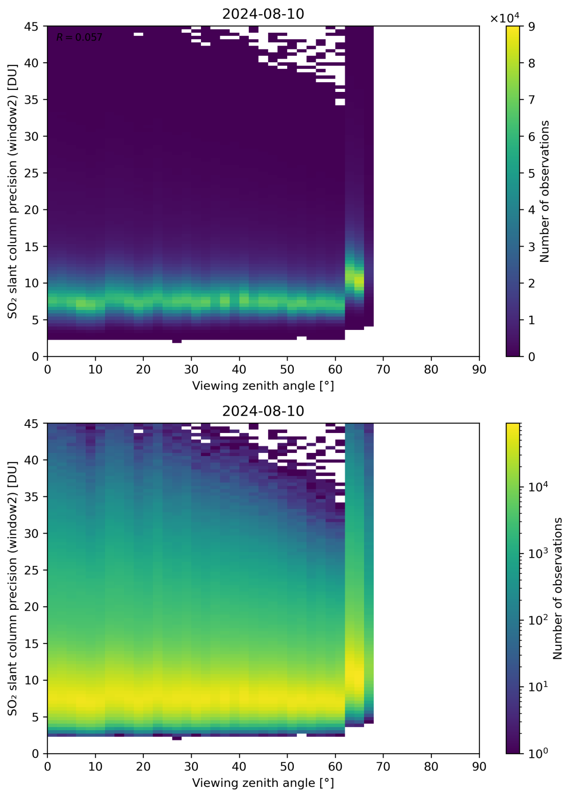
Figure 322: Scatter density plot of “Viewing zenith angle” against “SO 2 slant column precision (window2)” for 2024-08-09 to 2024-08-11.
