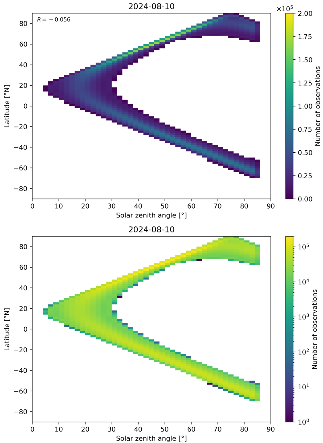
Figure 164: Scatter density plot of “Solar zenith angle” against “Latitude” for 2024-08-09 to 2024-08-11.
