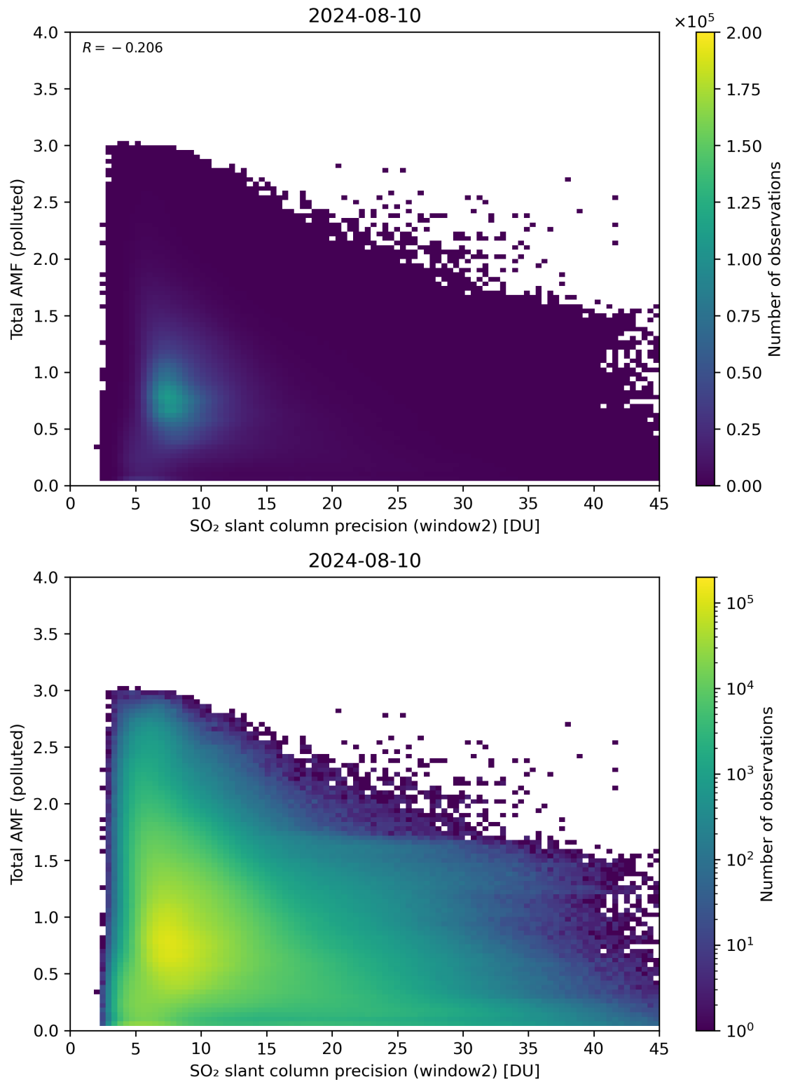
Figure 251: Scatter density plot of “SO 2 slant column precision (window2)” against “Total AMF (polluted)” for 2024-08-09 to 2024-08-11.
