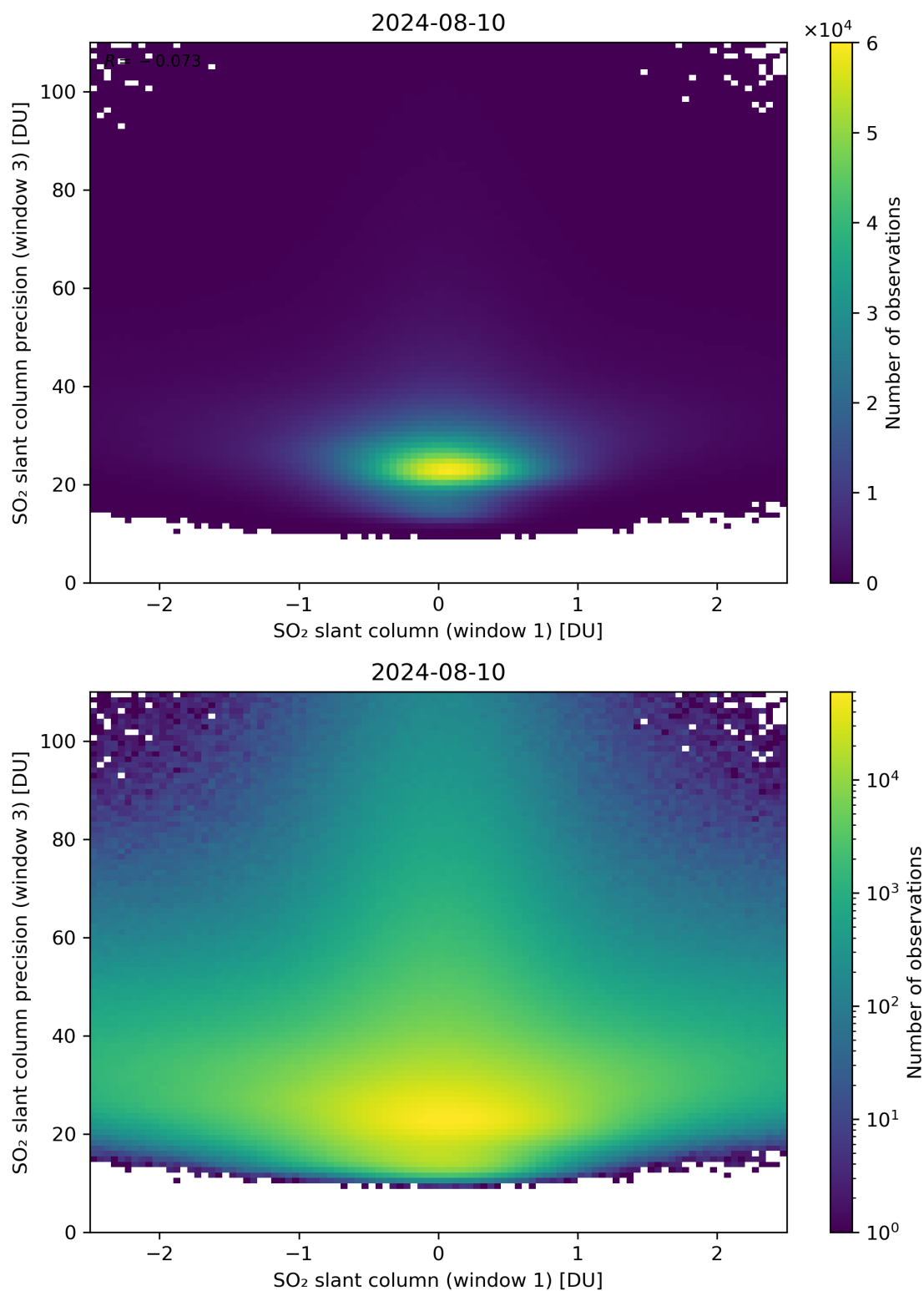
Figure 238: Scatter density plot of “SO 2 slant column (window 1)” against “SO 2 slant column precision (window 3)” for 2024-08-09 to 2024-08-11.
