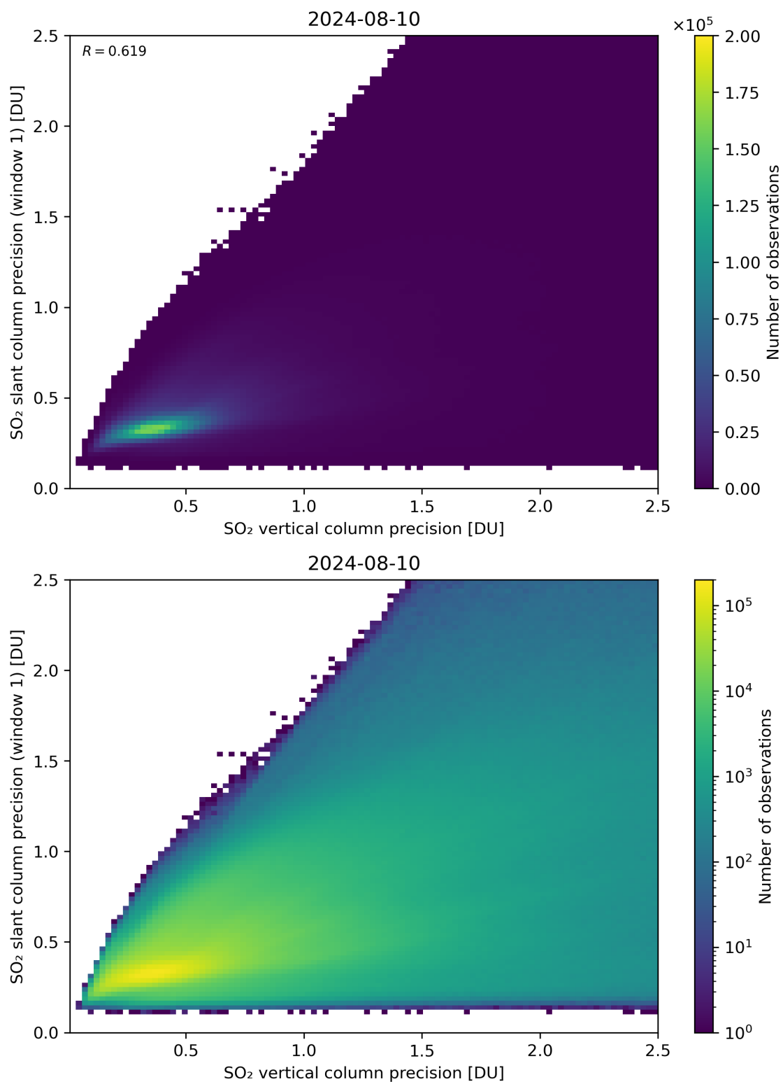
Figure 290: Scatter density plot of “SO 2 vertical column precision” against “SO 2 slant column precision (window 1)” for 2024-08-09 to 2024-08-11.
