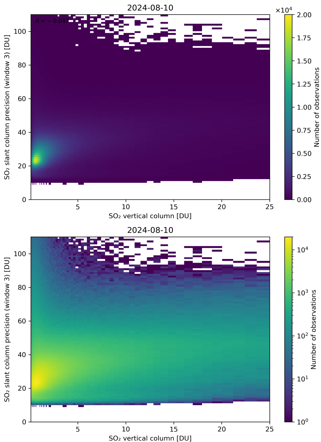
Figure 304: Scatter density plot of “SO 2 vertical column” against “SO 2 slant column precision (window 3)” for 2024-08-09 to 2024-08-11.
