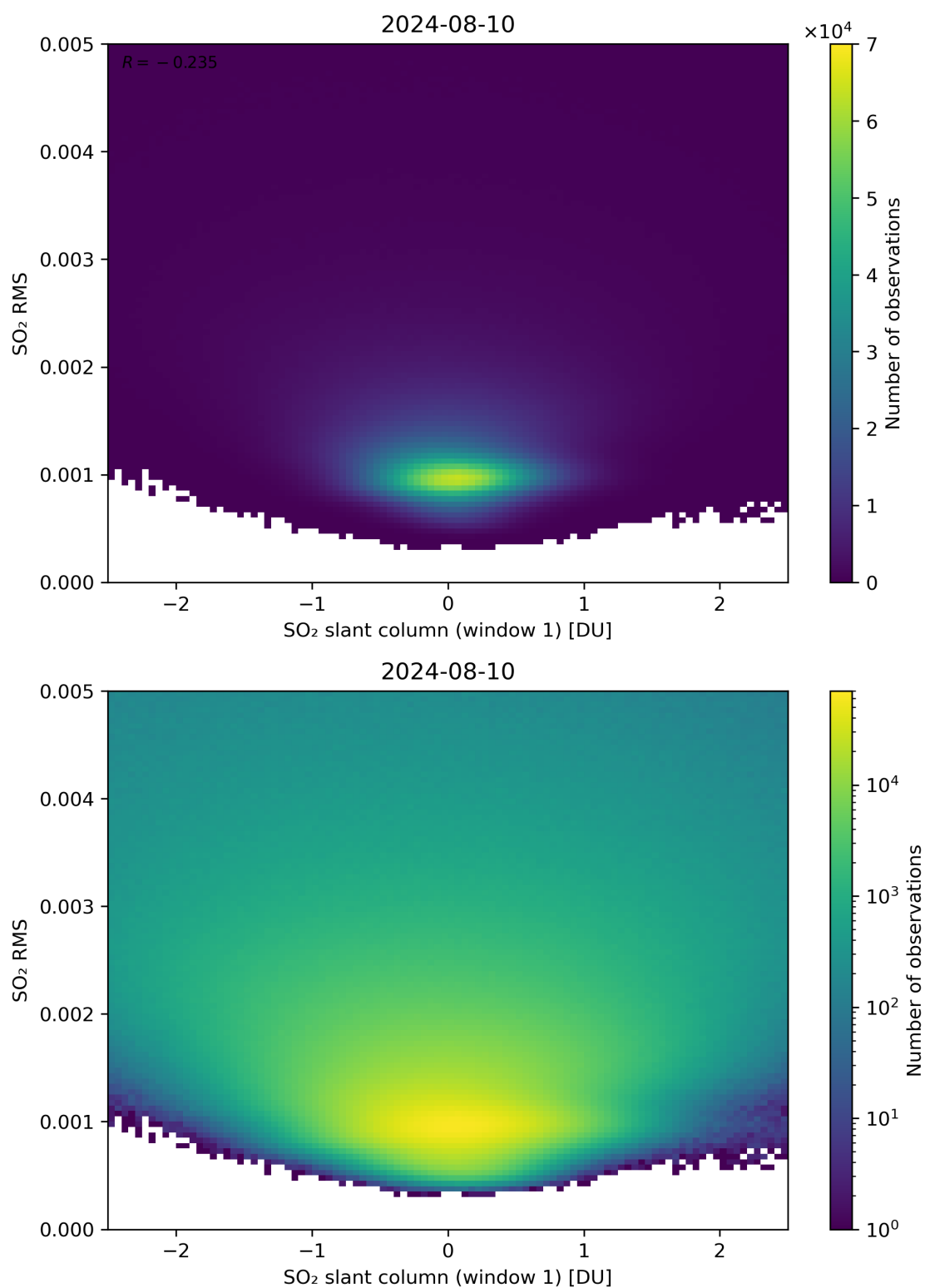
Figure 217: Scatter density plot of “SO 2 slant column (window 1)” against “SO 2 RMS” for 2024-08-09 to 2024-08-11.
