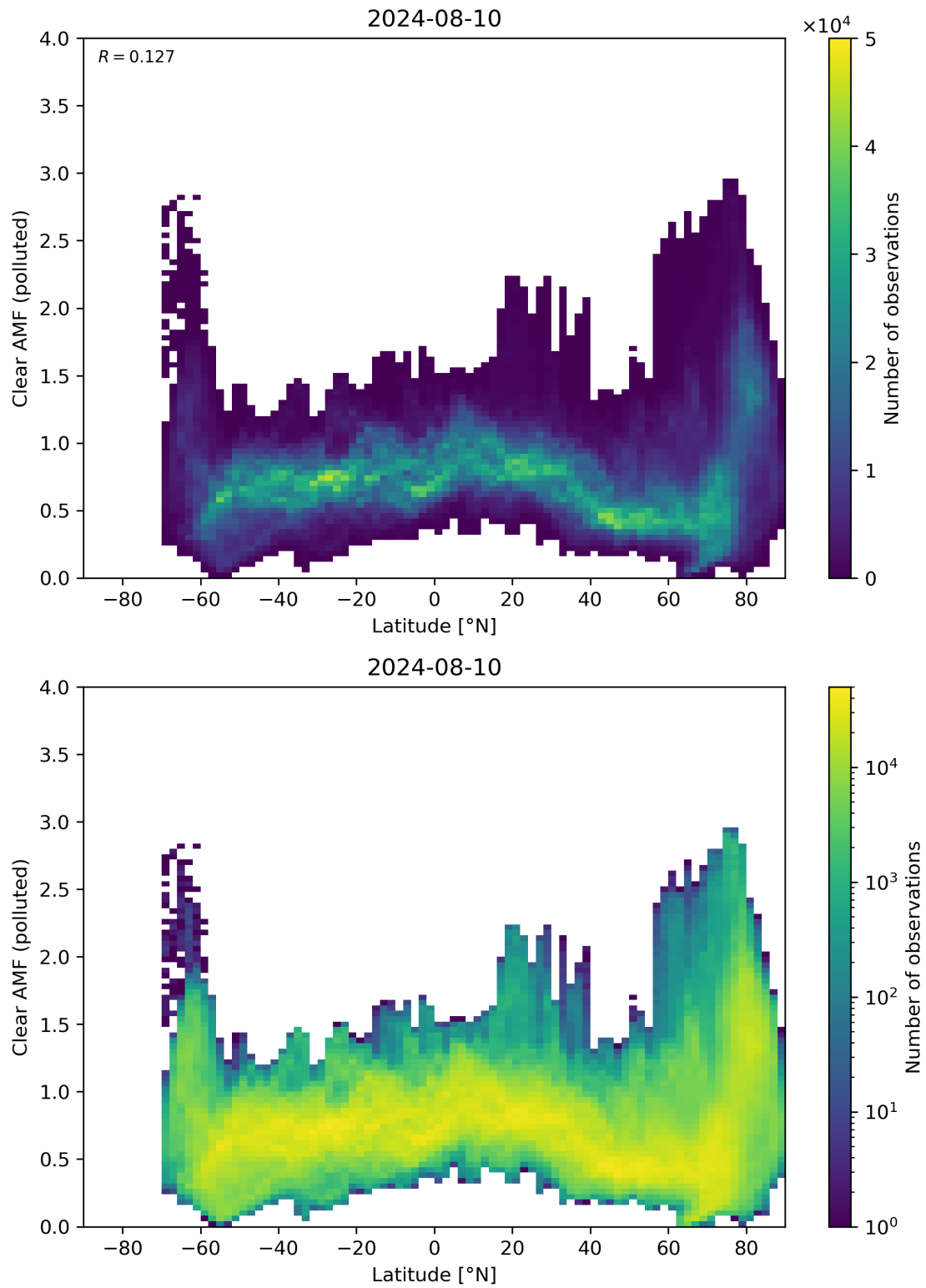
Figure 145: Scatter density plot of “Latitude” against “Clear AMF (polluted)” for 2024-08-09 to 2024-08-11.
