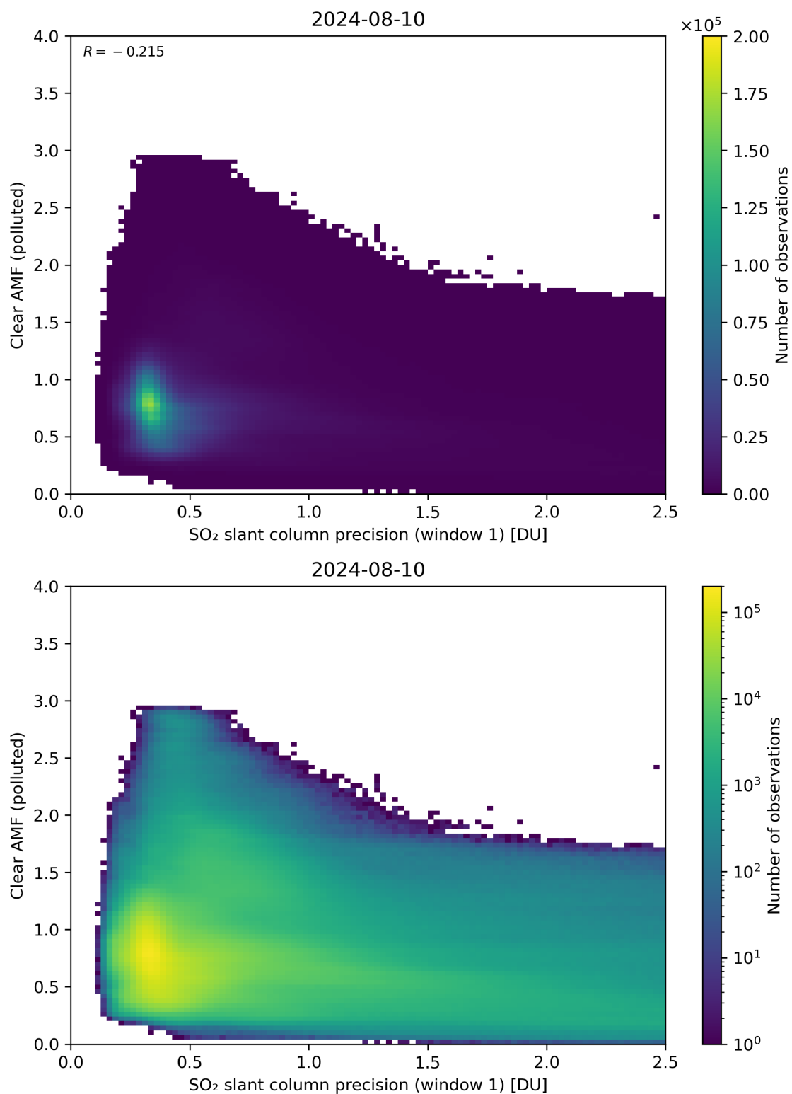
Figure 224: Scatter density plot of “SO 2 slant column precision (window 1)” against “Clear AMF (polluted)” for 2024-08-09 to 2024-08-11.
