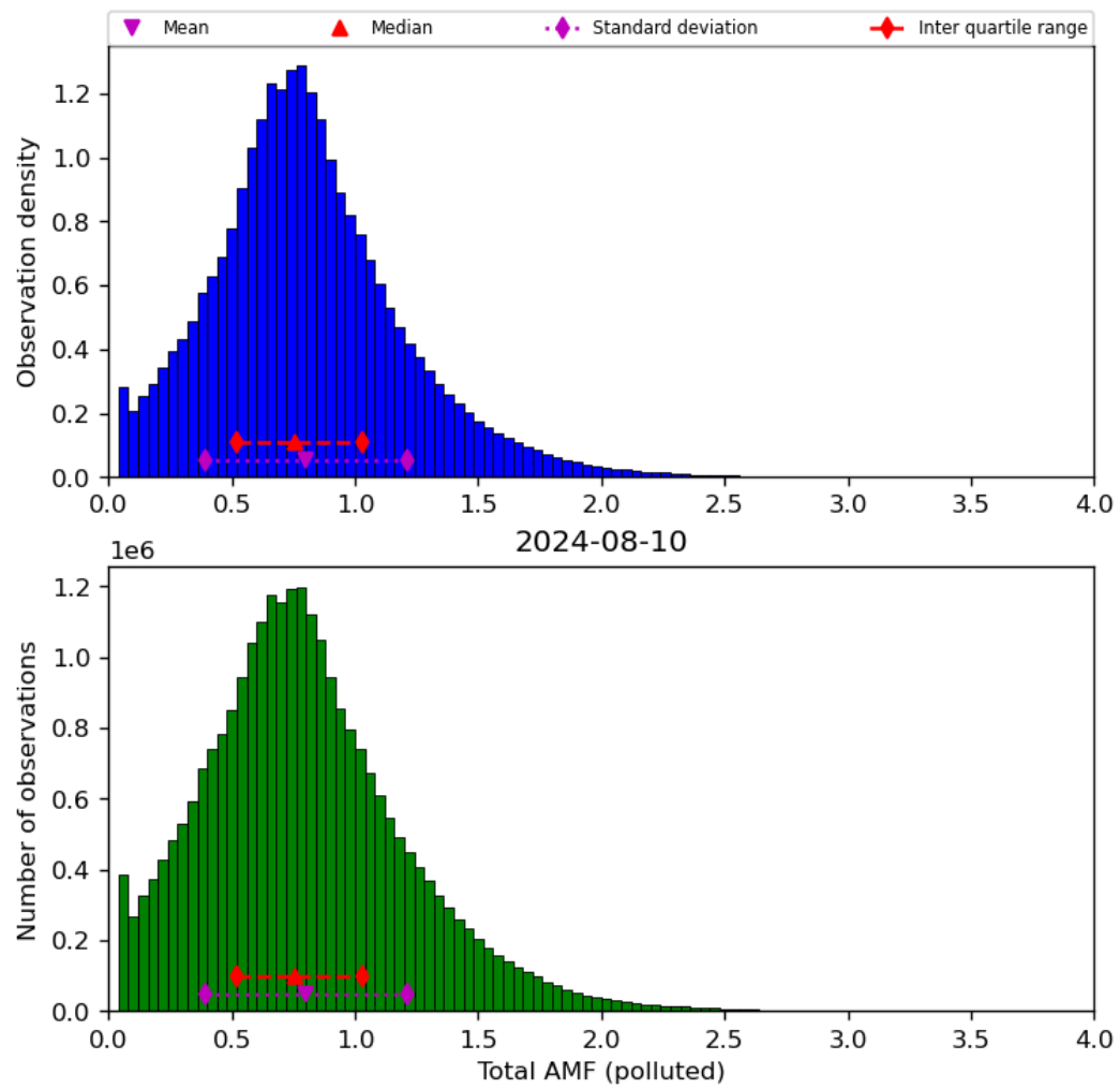
Figure 71: Histogram of “Total AMF (polluted)” for 2024-08-09 to 2024-08-11
