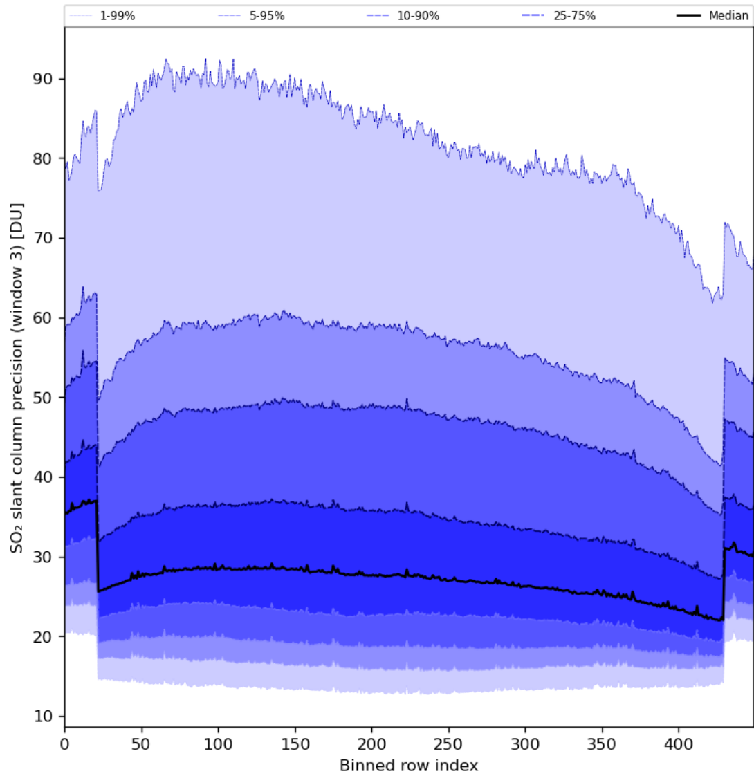
Figure 88: Along track statistics of “SO 2 slant column precision (window 3)” for 2024-08-09 to 2024-08-11
