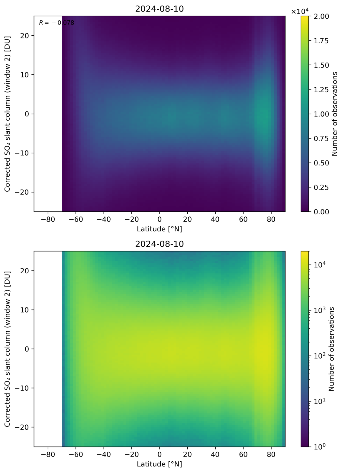
Figure 147: Scatter density plot of “Latitude” against “Corrected SO 2 slant column (window 2)” for 2024-08-09 to 2024-08-11.
