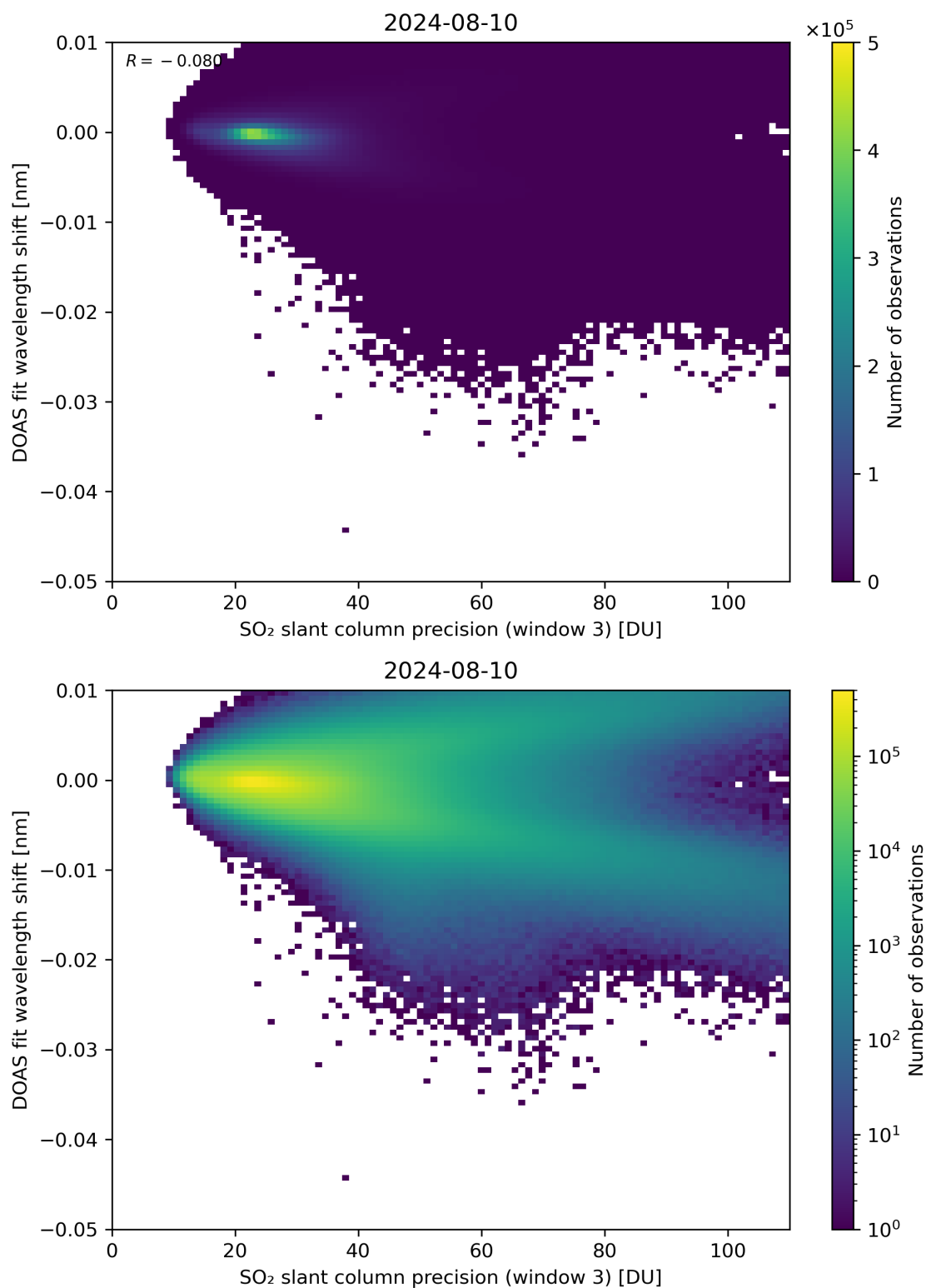
Figure 258: Scatter density plot of “SO 2 slant column precision (window 3)” against “DOAS fit wavelength shift” for 2024-08-09 to 2024-08-11.
