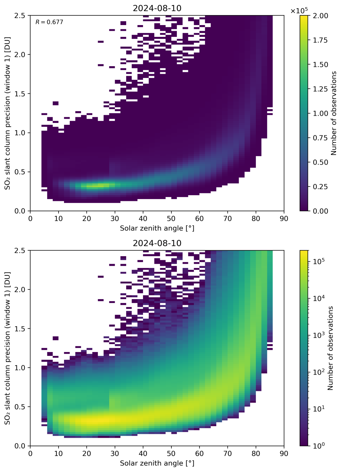
Figure 170: Scatter density plot of “Solar zenith angle” against “SO 2 slant column precision (window 1)” for 2024-08-09 to 2024-08-11.
