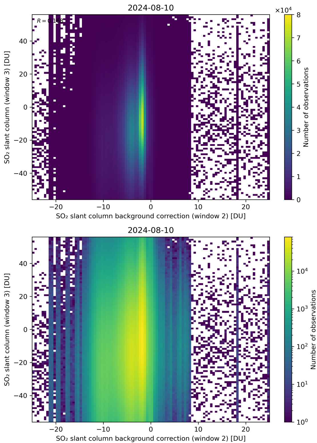
Figure 117: Scatter density plot of “SO 2 slant column background correction (window 2)” against “SO 2 slant column (window 3)” for 2024-08-09 to 2024-08-11.
