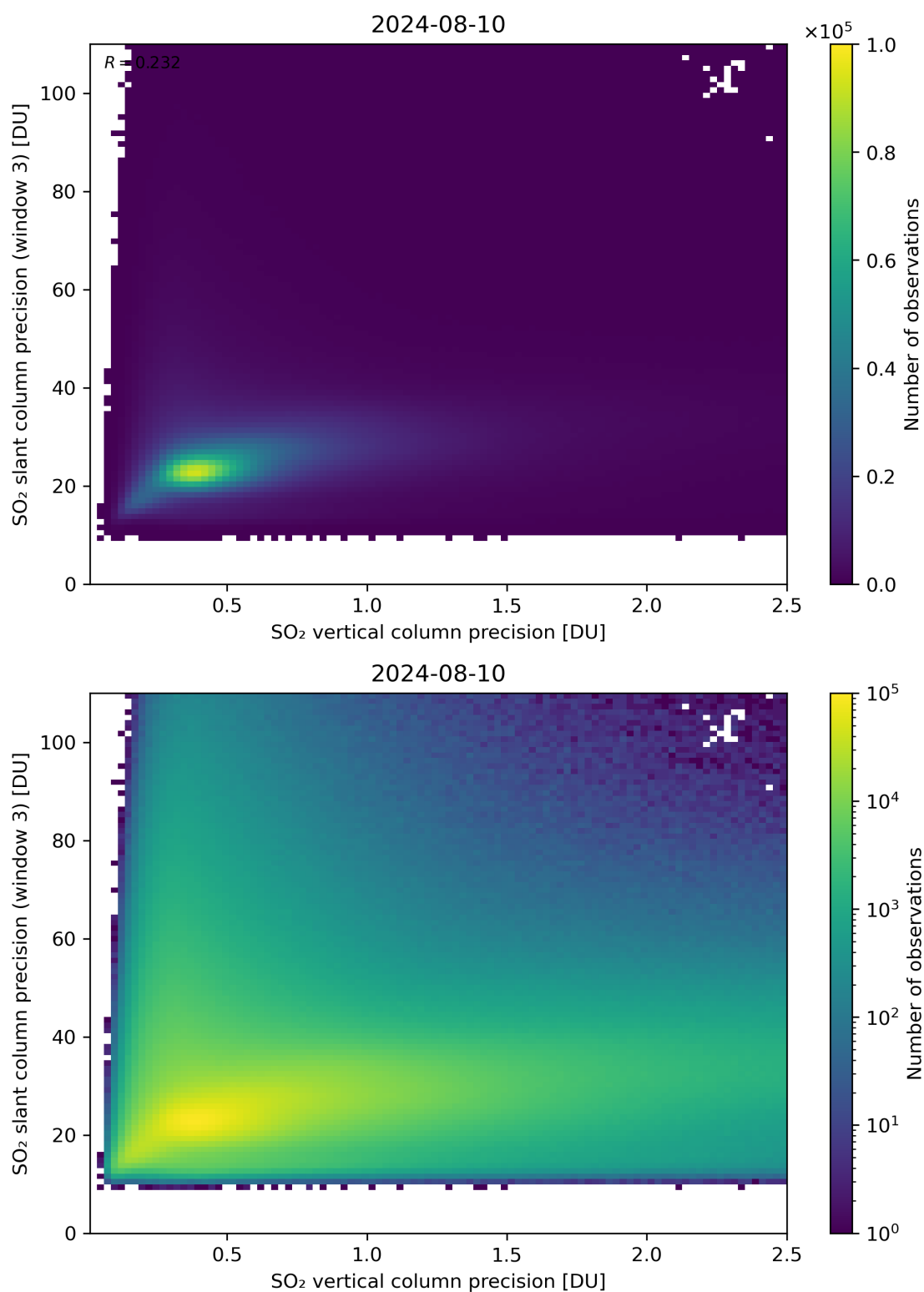
Figure 293: Scatter density plot of “SO 2 vertical column precision” against “SO 2 slant column precision (window 3)” for 2024-08-09 to 2024-08-11.
