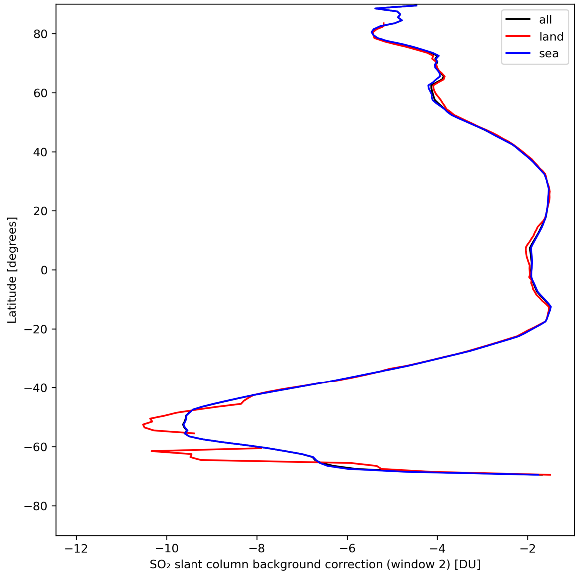
Figure 40: Zonal average of “SO 2 slant column background correction (window 2)” for 2024-08-09 to 2024-08-11.
