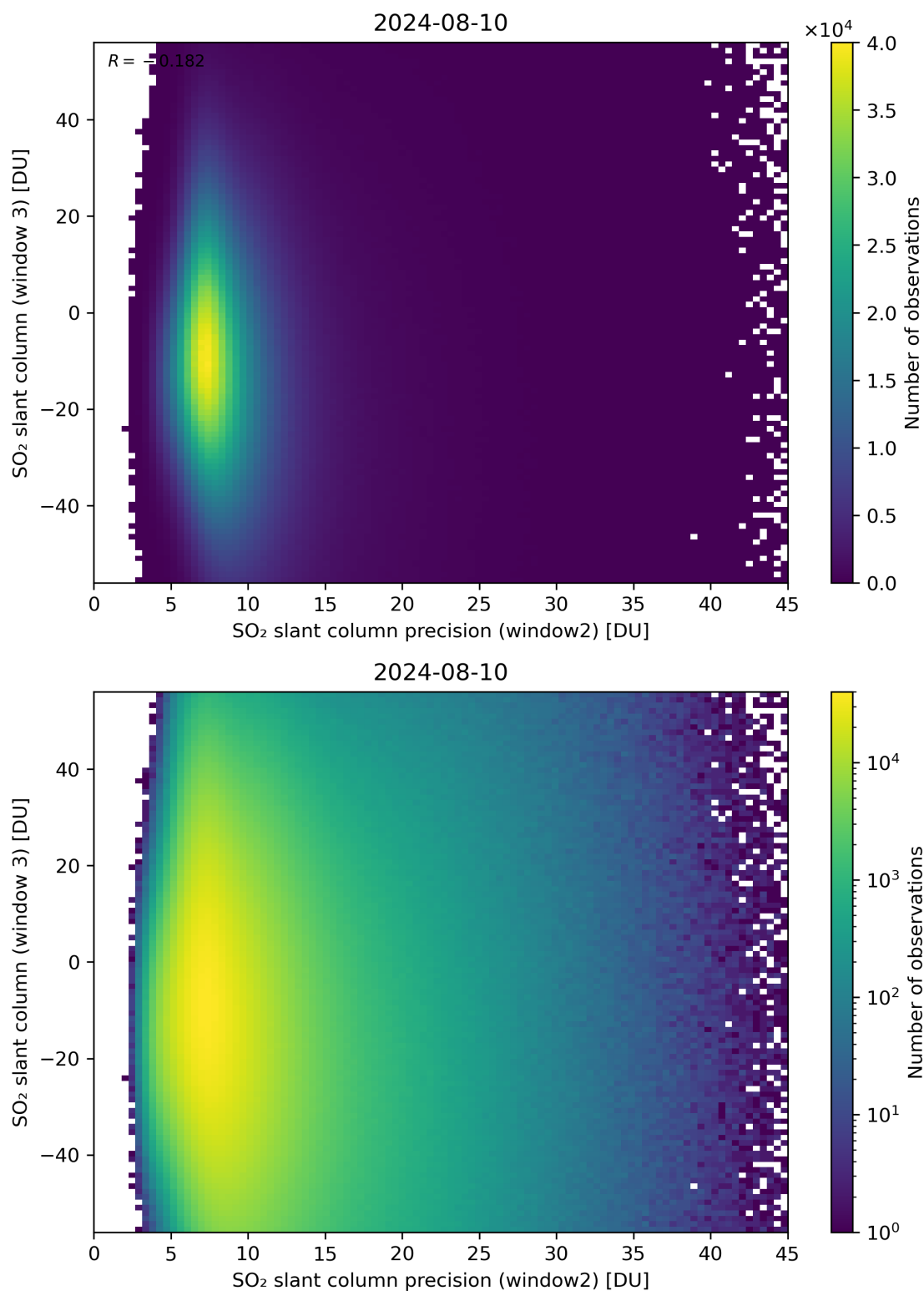
Figure 249: Scatter density plot of “SO 2 slant column precision (window2)” against “SO 2 slant column (window 3)” for 2024-08-09 to 2024-08-11.
