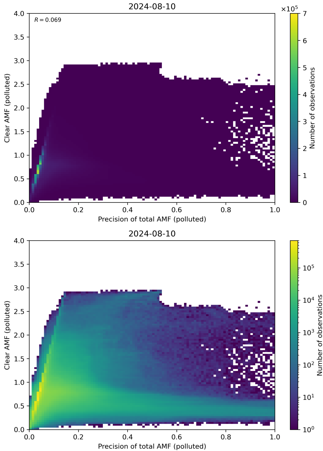
Figure 270: Scatter density plot of “Precision of total AMF (polluted)” against “Clear AMF (polluted)” for 2024-08-09 to 2024-08-11.
