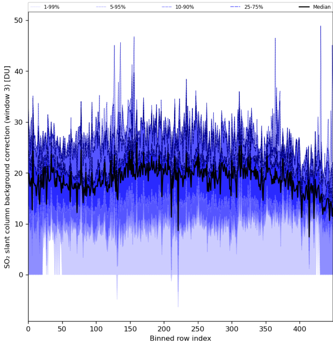
Figure 90: Along track statistics of “SO 2 slant column background correction (window 3)” for 2024-08-09 to 2024-08-11
