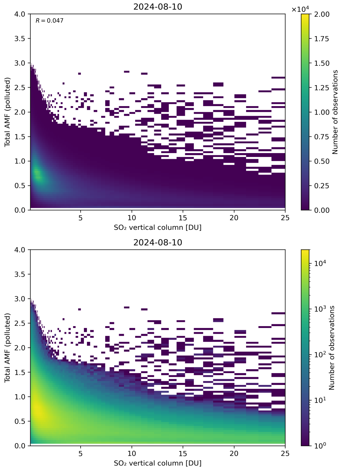
Figure 305: Scatter density plot of “SO 2 vertical column” against “Total AMF (polluted)” for 2024-08-09 to 2024-08-11.
