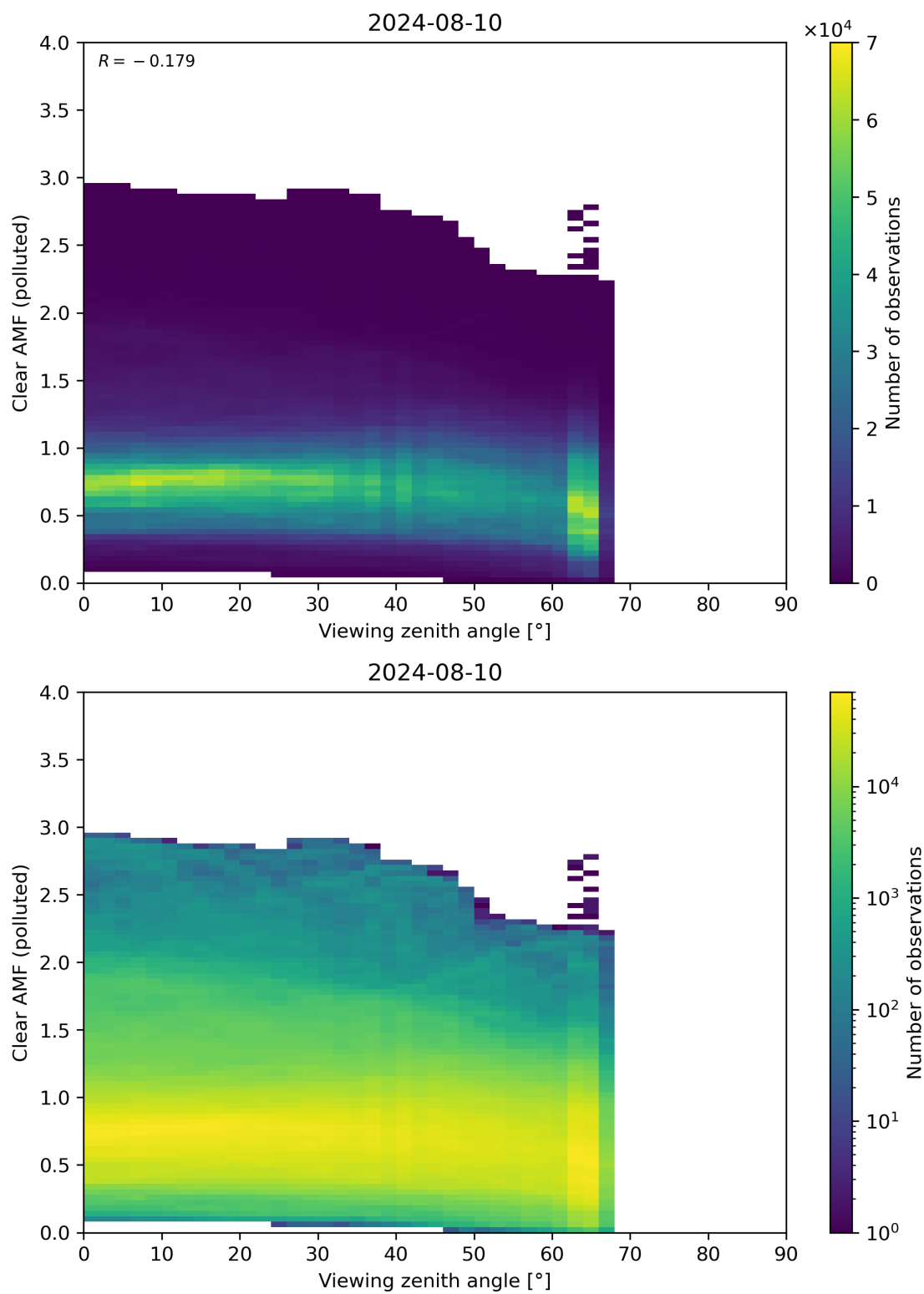
Figure 316: Scatter density plot of “Viewing zenith angle” against “Clear AMF (polluted)” for 2024-08-09 to 2024-08-11.
