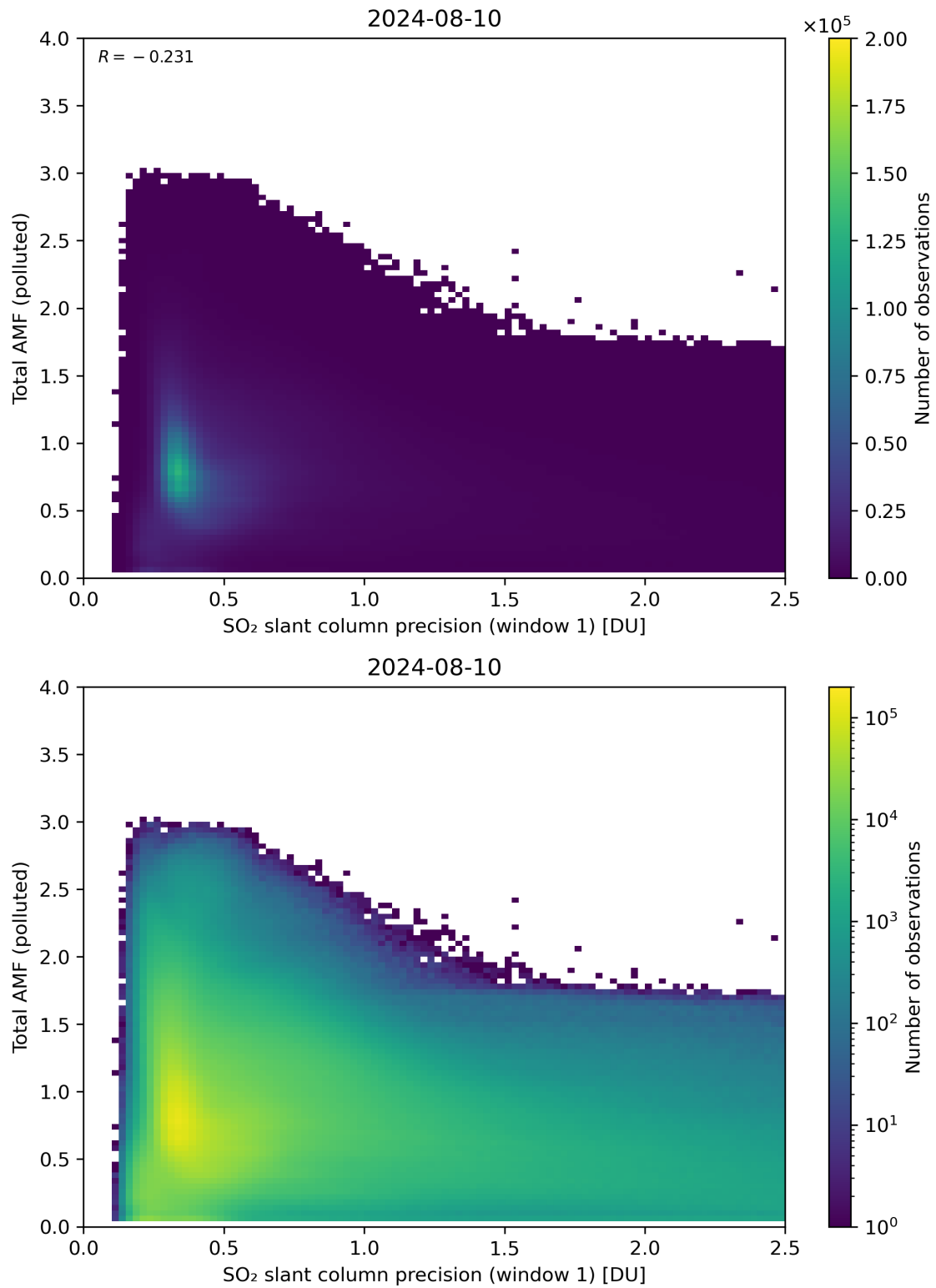
Figure 230: Scatter density plot of “SO 2 slant column precision (window 1)” against “Total AMF (polluted)” for 2024-08-09 to 2024-08-11.
