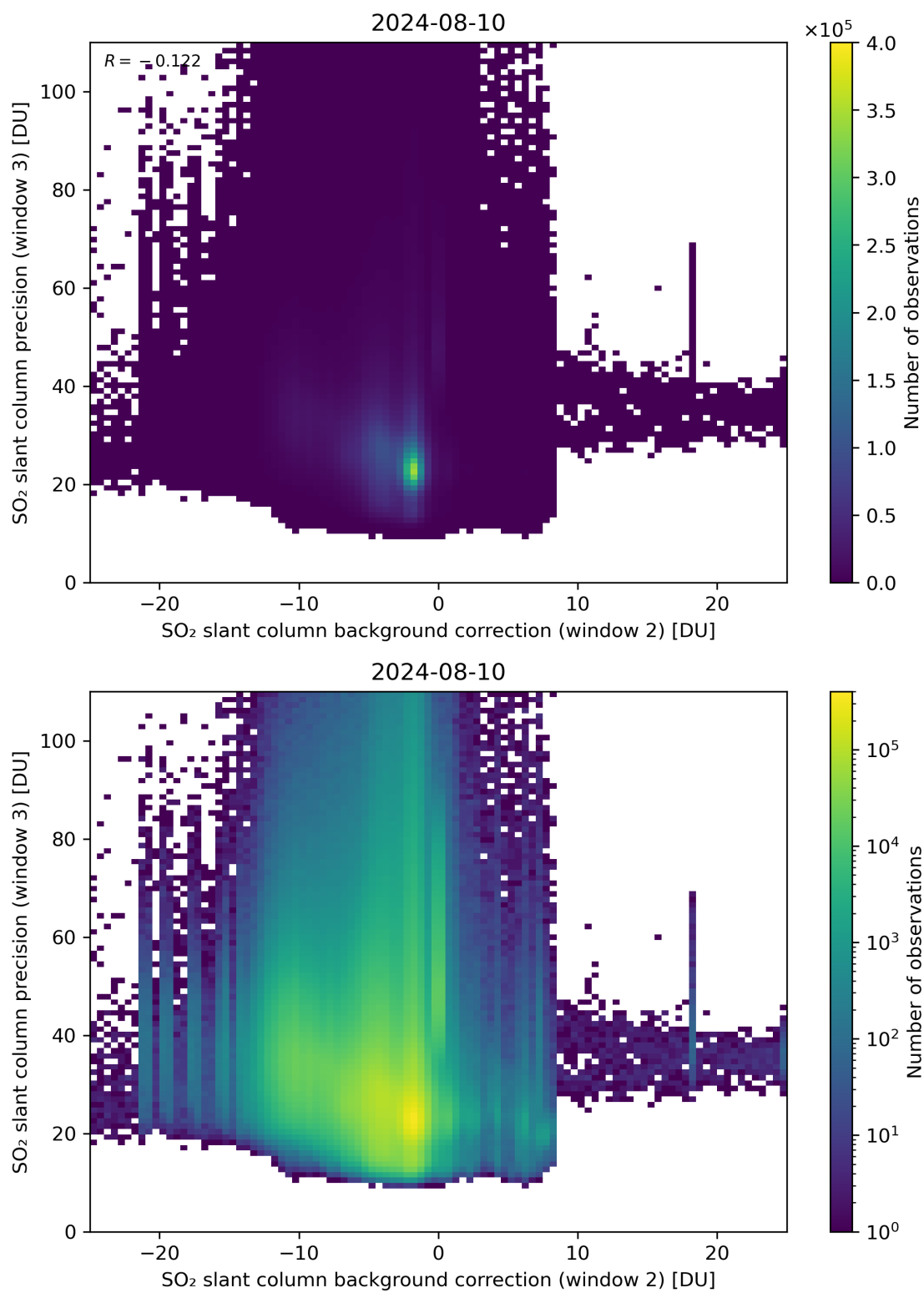
Figure 118: Scatter density plot of “SO 2 slant column background correction (window 2)” against “SO 2 slant column precision (window 3)” for 2024-08-09 to 2024-08-11.
