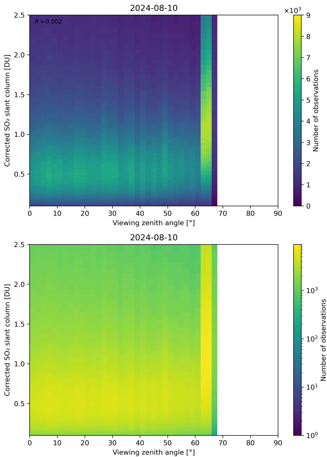
Figure 317: Scatter density plot of “Viewing zenith angle” against “Corrected SO 2 slant column” for 2024-08-09 to 2024-08-11.
