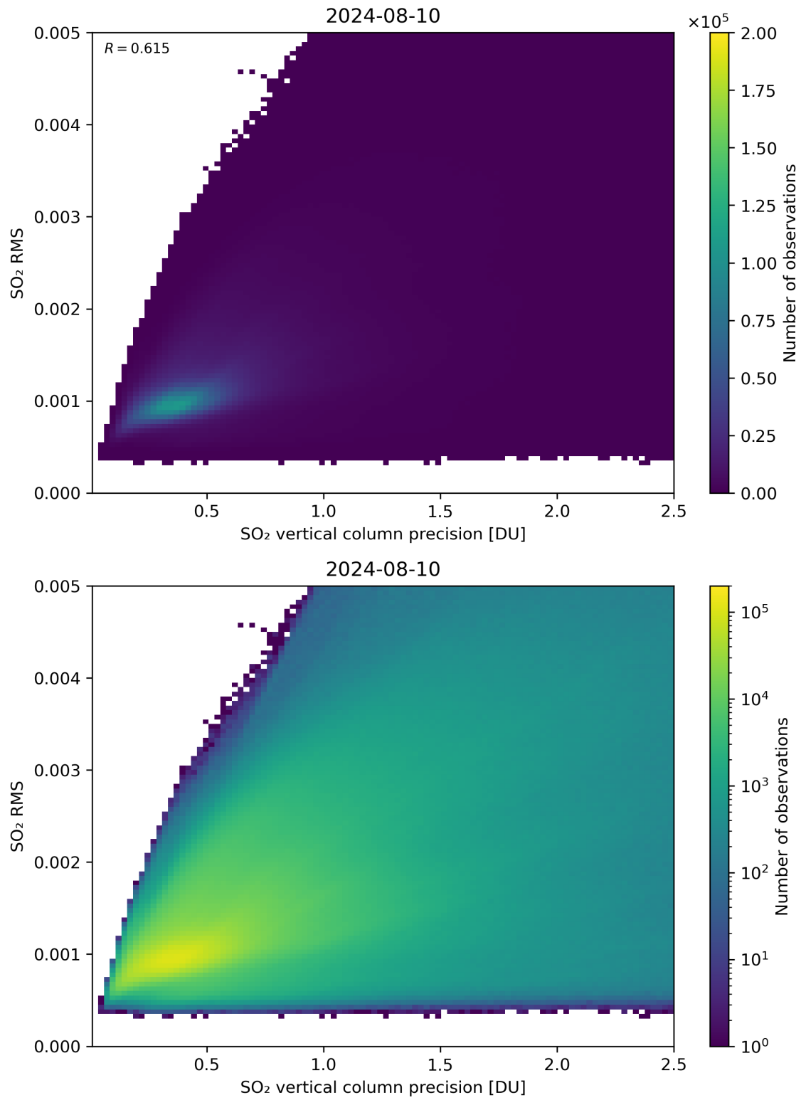
Figure 284: Scatter density plot of “SO 2 vertical column precision” against “SO 2 RMS” for 2024-08-09 to 2024-08-11.
