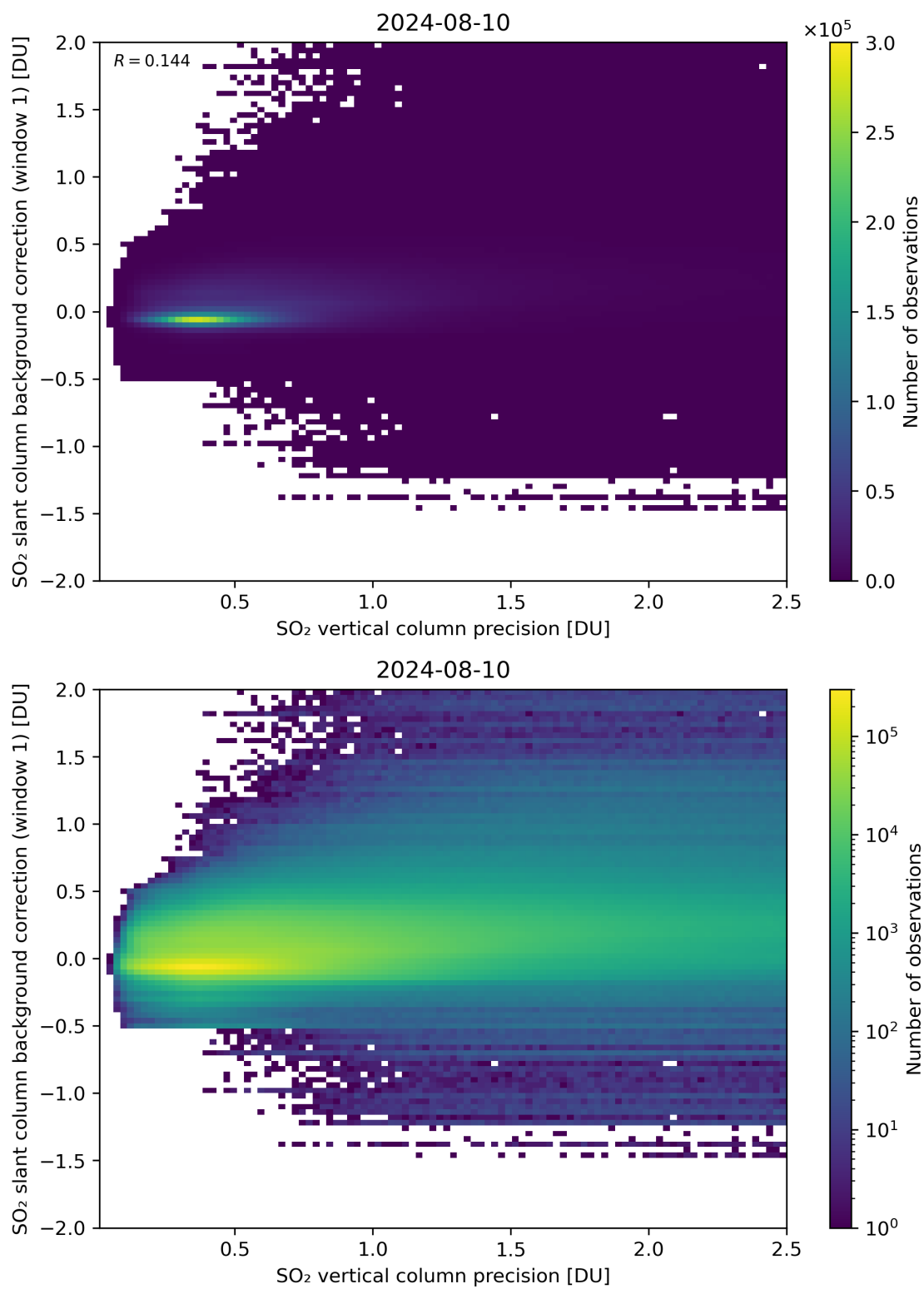
Figure 279: Scatter density plot of “SO 2 vertical column precision” against “SO 2 slant column background correction (window 1)” for 2024-08-09 to 2024-08-11.
