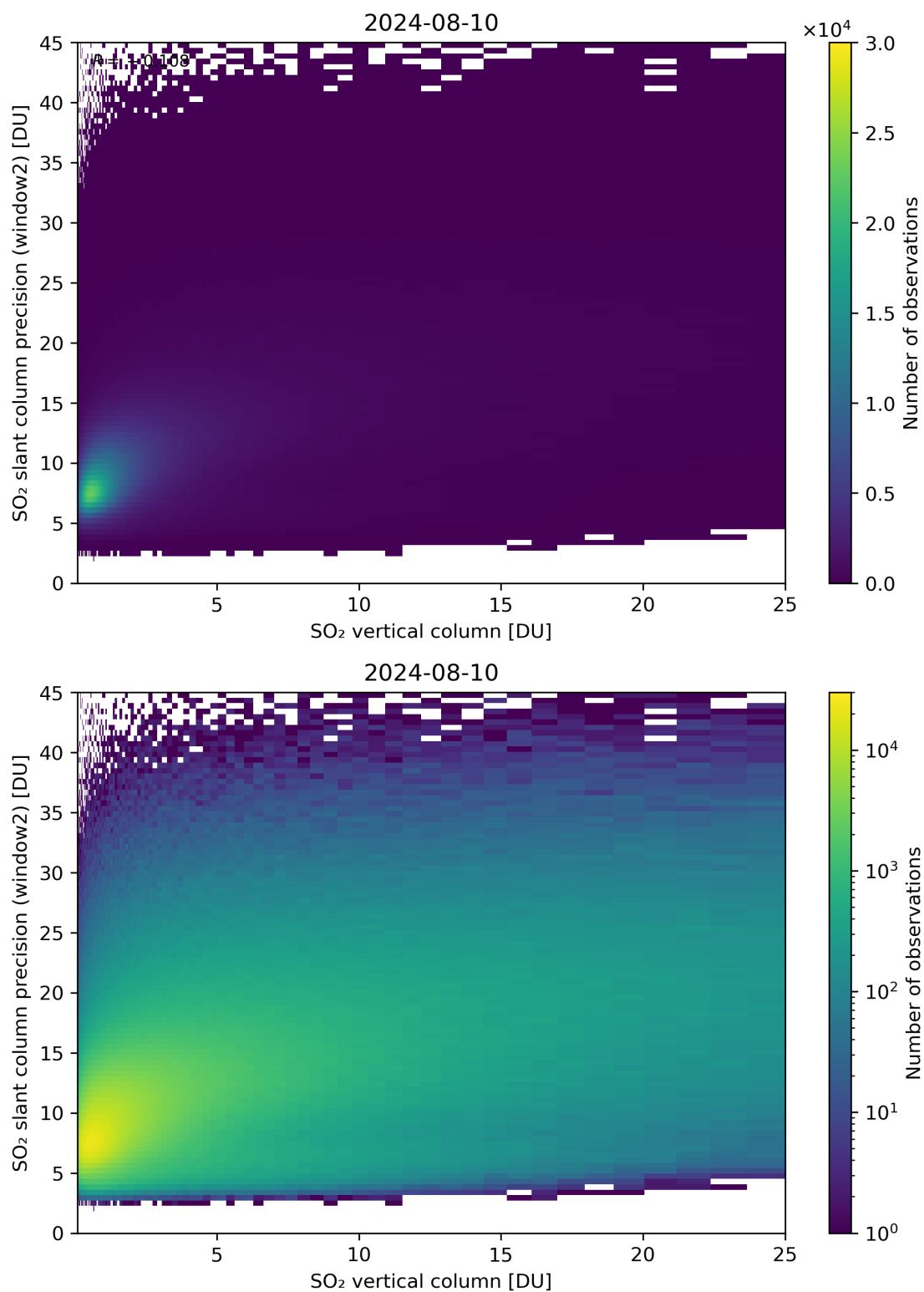
Figure 302: Scatter density plot of “SO 2 vertical column” against “SO 2 slant column precision (window2)” for 2024-08-09 to 2024-08-11.
