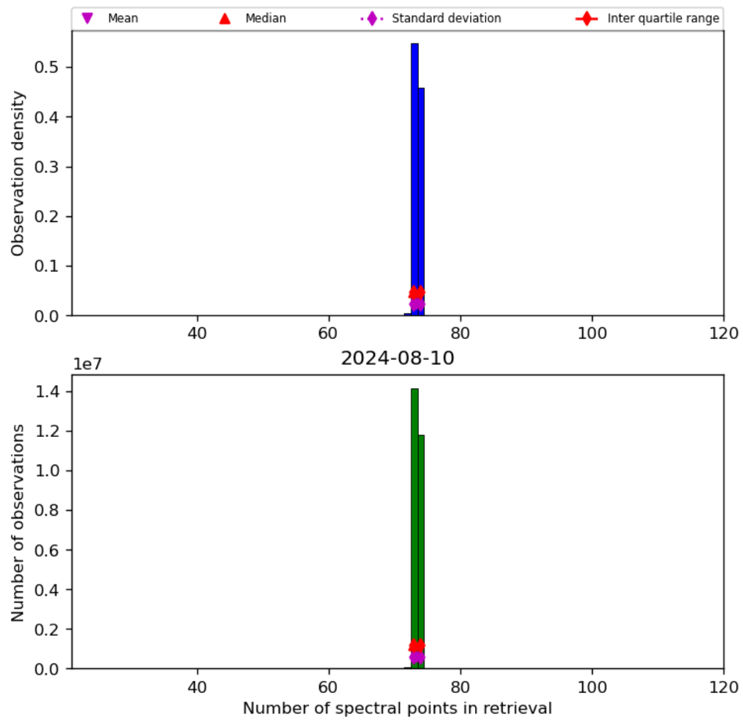
Figure 74: Histogram of “Number of spectral points in retrieval” for 2024-08-09 to 2024-08-11
