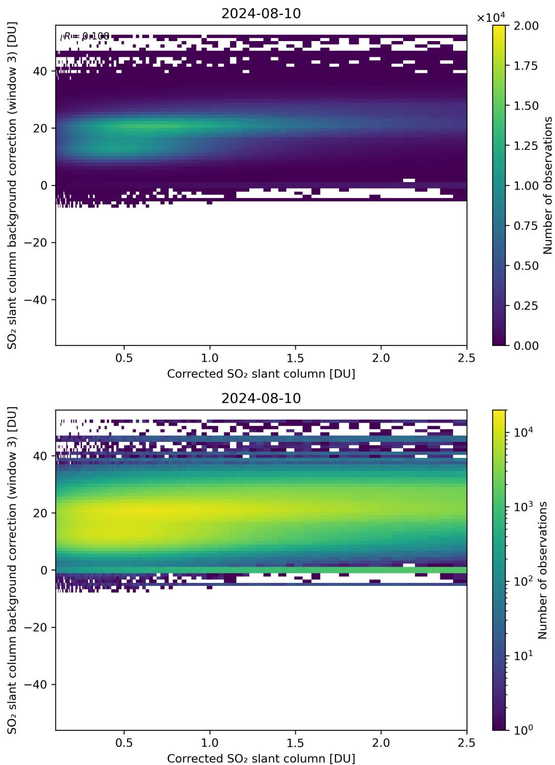
Figure 180: Scatter density plot of “Corrected SO 2 slant column” against “SO 2 slant column background correction (window 3)” for 2024-08-09 to 2024-08-11.
