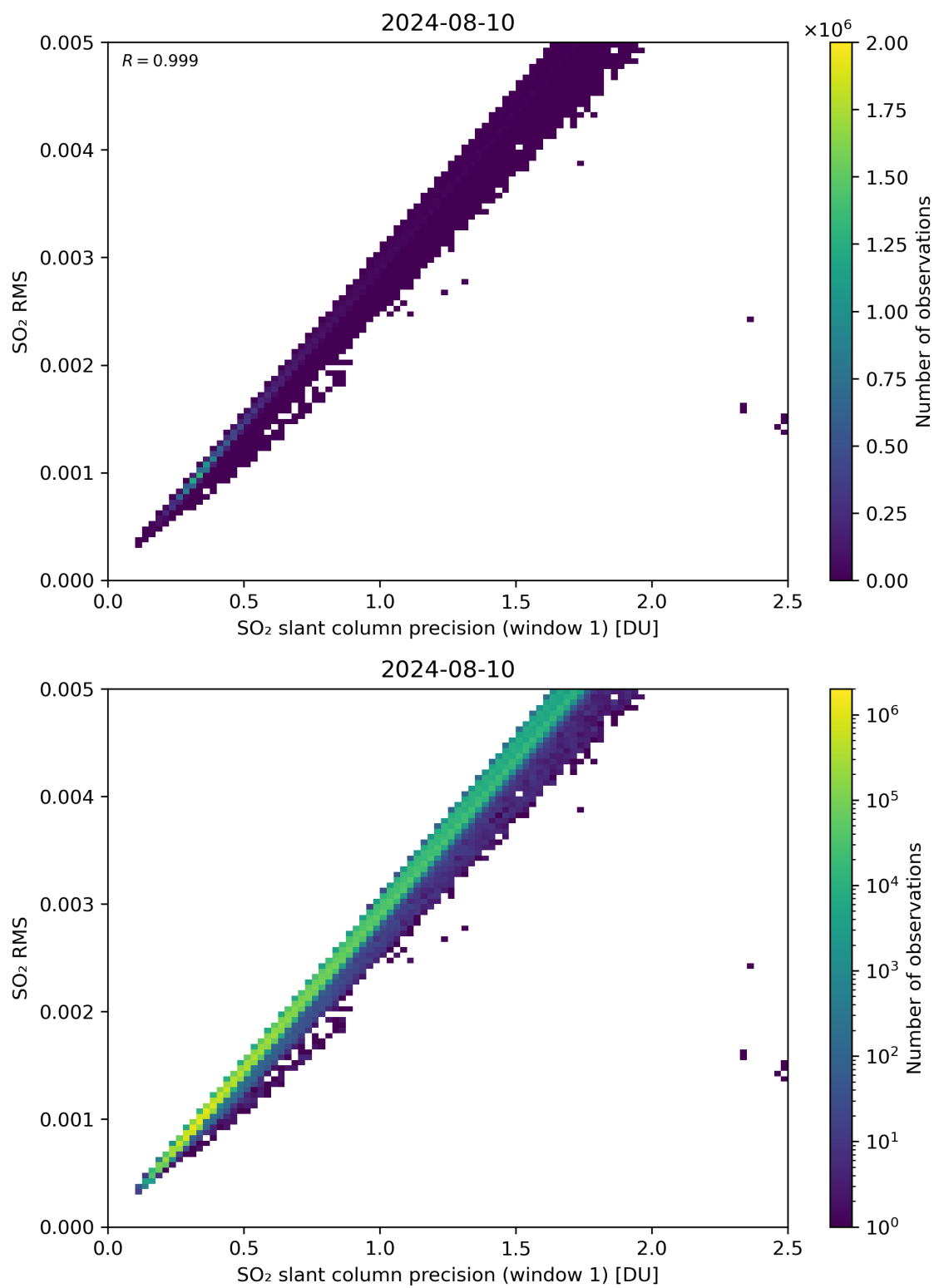
Figure 223: Scatter density plot of “SO 2 slant column precision (window 1)” against “SO 2 RMS” for 2024-08-09 to 2024-08-11.
