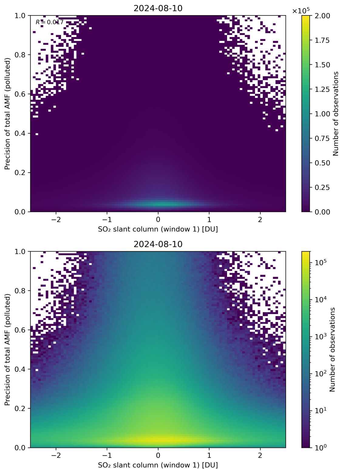
Figure 240: Scatter density plot of “SO 2 slant column (window 1)” against “Precision of total AMF (polluted)” for 2024-08-09 to 2024-08-11.
