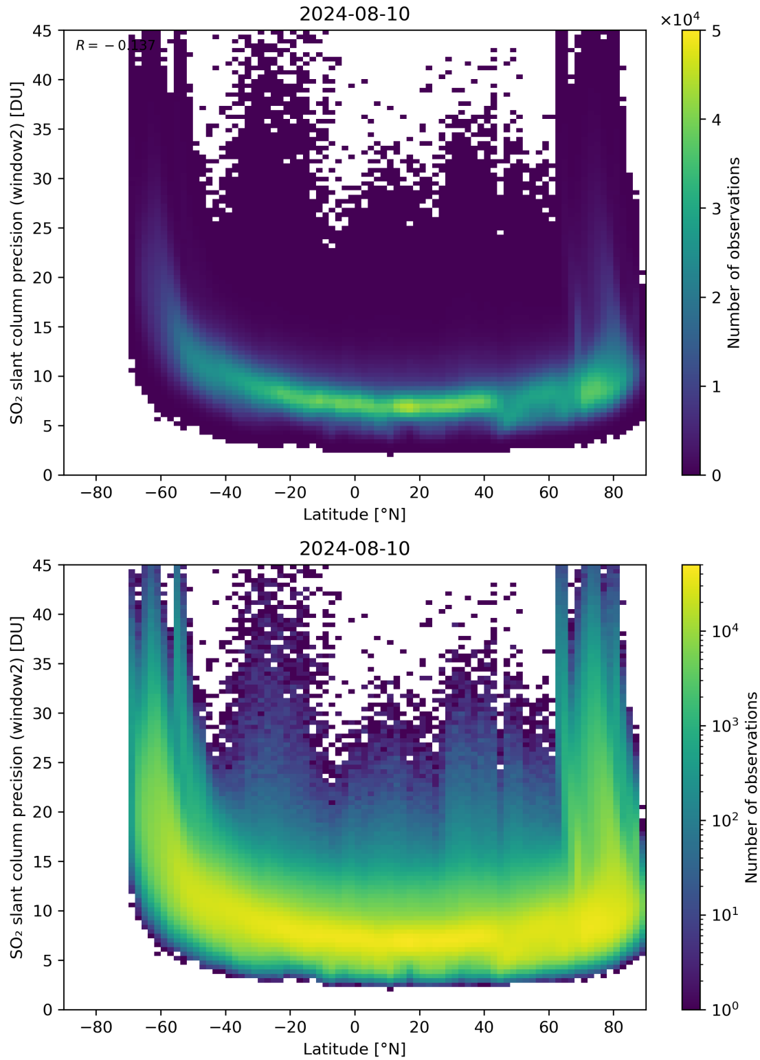
Figure 151: Scatter density plot of “Latitude” against “SO 2 slant column precision (window2)” for 2024-08-09 to 2024-08-11.
