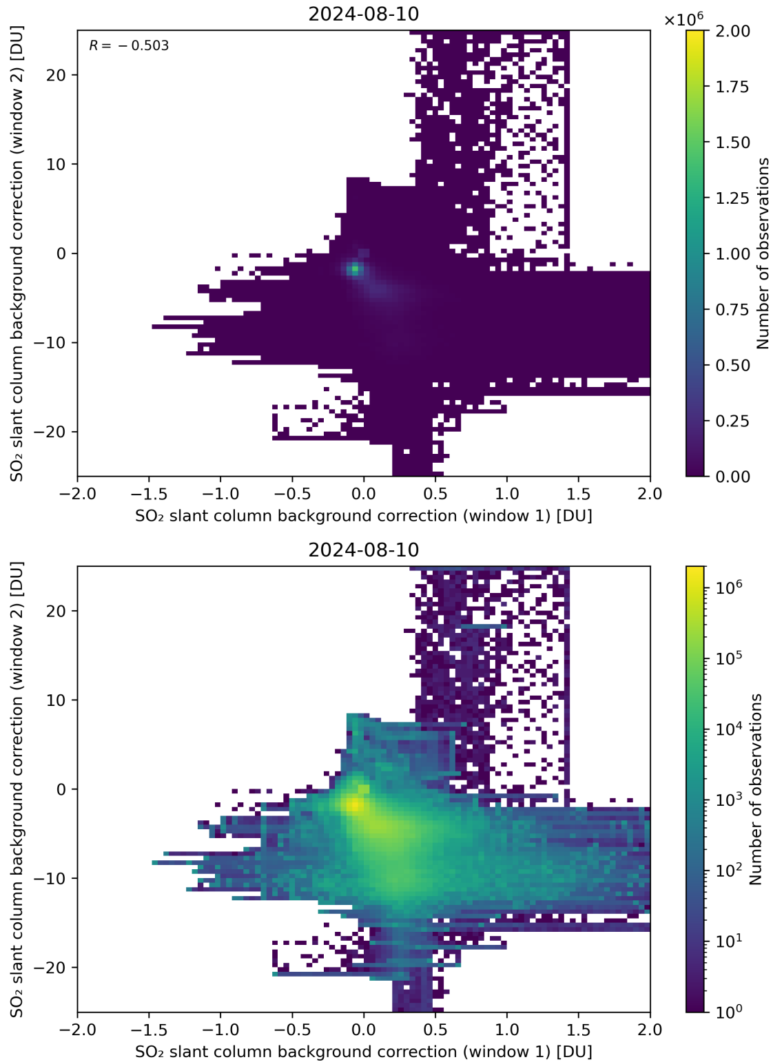
Figure 98: Scatter density plot of “SO 2 slant column background correction (window 1)” against “SO 2 slant column background correction (window 2)” for 2024-08-09 to 2024-08-11.
