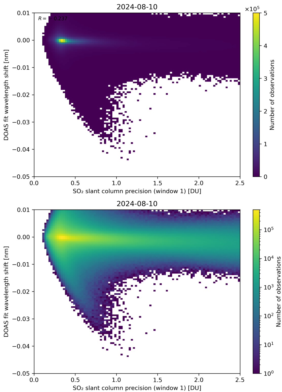
Figure 221: Scatter density plot of “SO 2 slant column precision (window 1)” against “DOAS fit wavelength shift” for 2024-08-09 to 2024-08-11.
