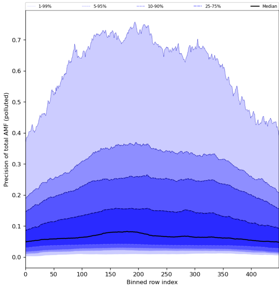
Figure 95: Along track statistics of “Precision of total AMF (polluted)” for 2024-08-09 to 2024-08-11
