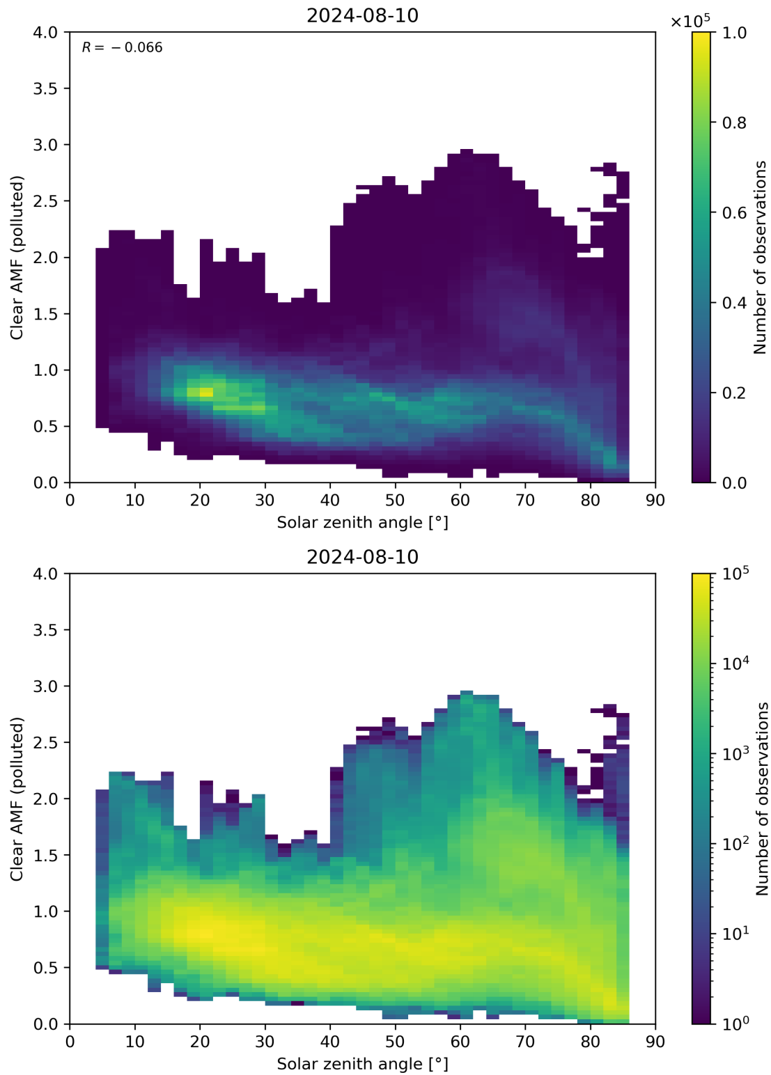
Figure 165: Scatter density plot of “Solar zenith angle” against “Clear AMF (polluted)” for 2024-08-09 to 2024-08-11.
