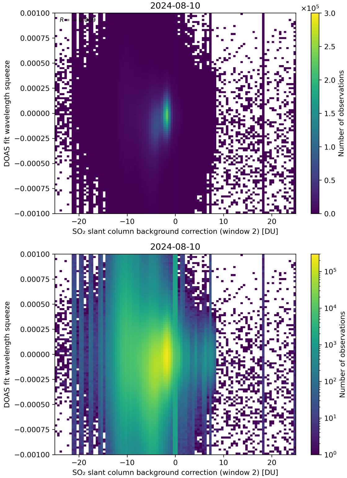
Figure 113: Scatter density plot of “SO 2 slant column background correction (window 2)” against “DOAS fit wavelength squeeze” for 2024-08-09 to 2024-08-11.
