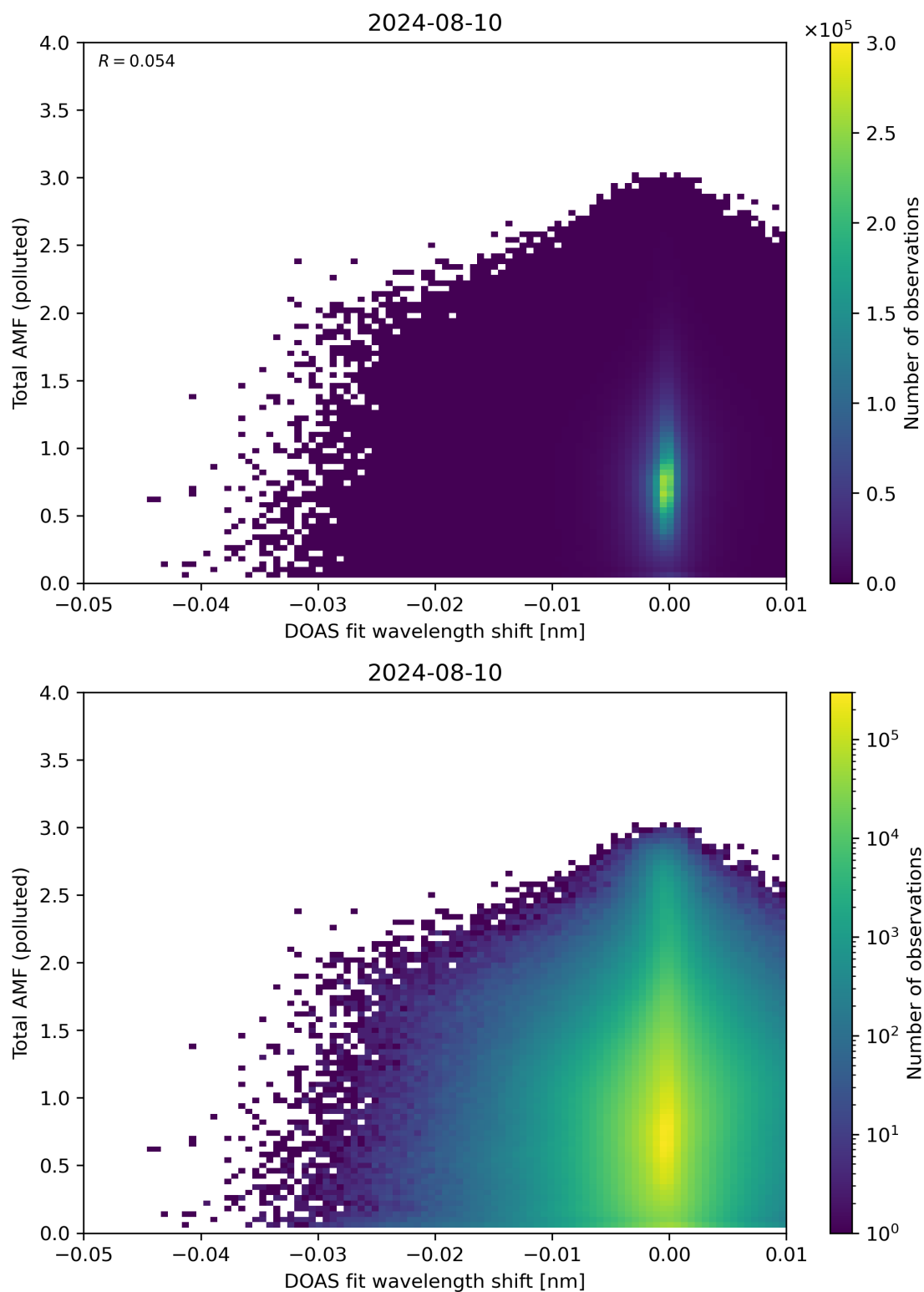
Figure 130: Scatter density plot of “DOAS fit wavelength shift” against “Total AMF (polluted)” for 2024-08-09 to 2024-08-11.
