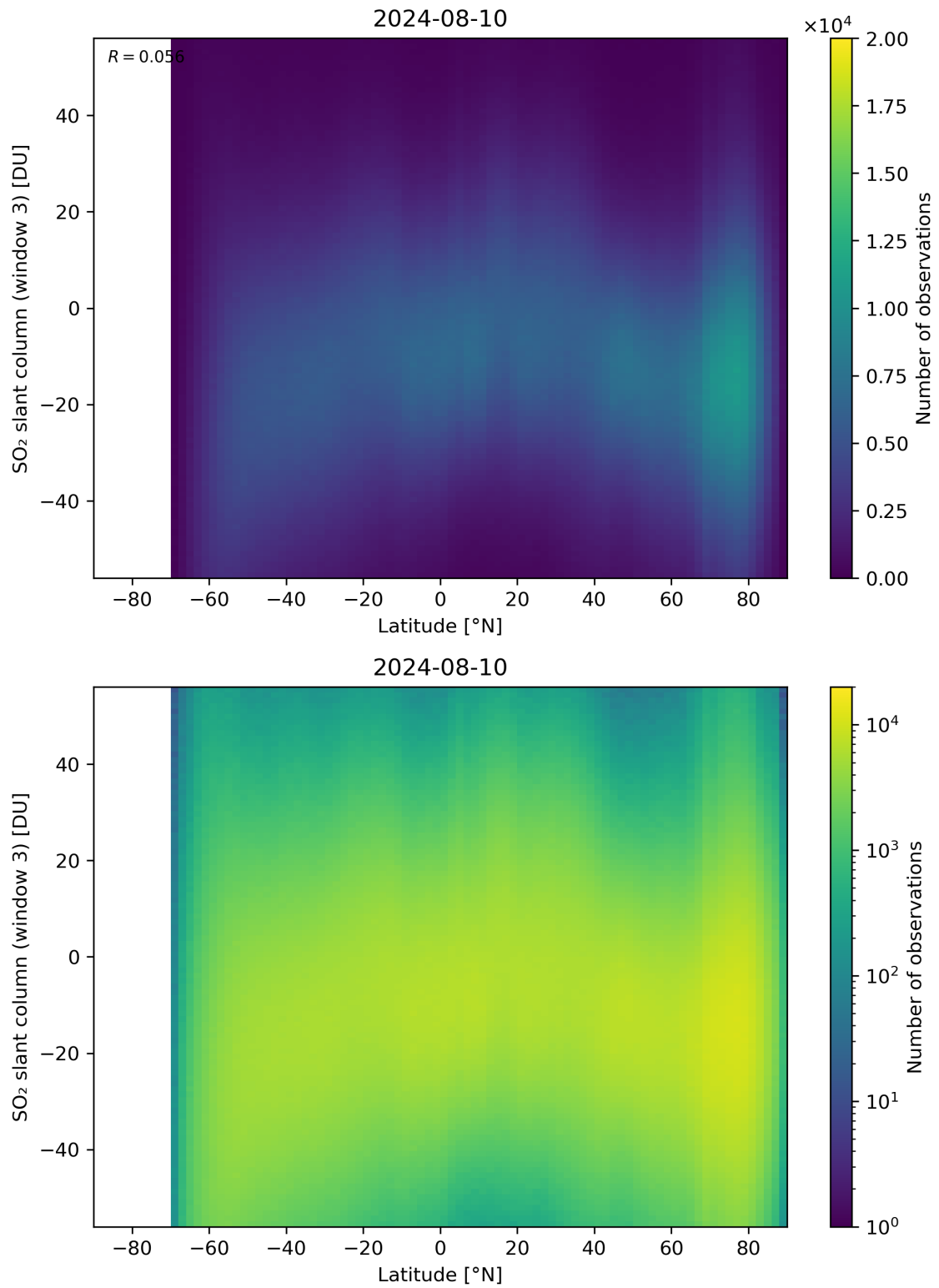
Figure 152: Scatter density plot of “Latitude” against “SO 2 slant column (window 3)” for 2024-08-09 to 2024-08-11.
