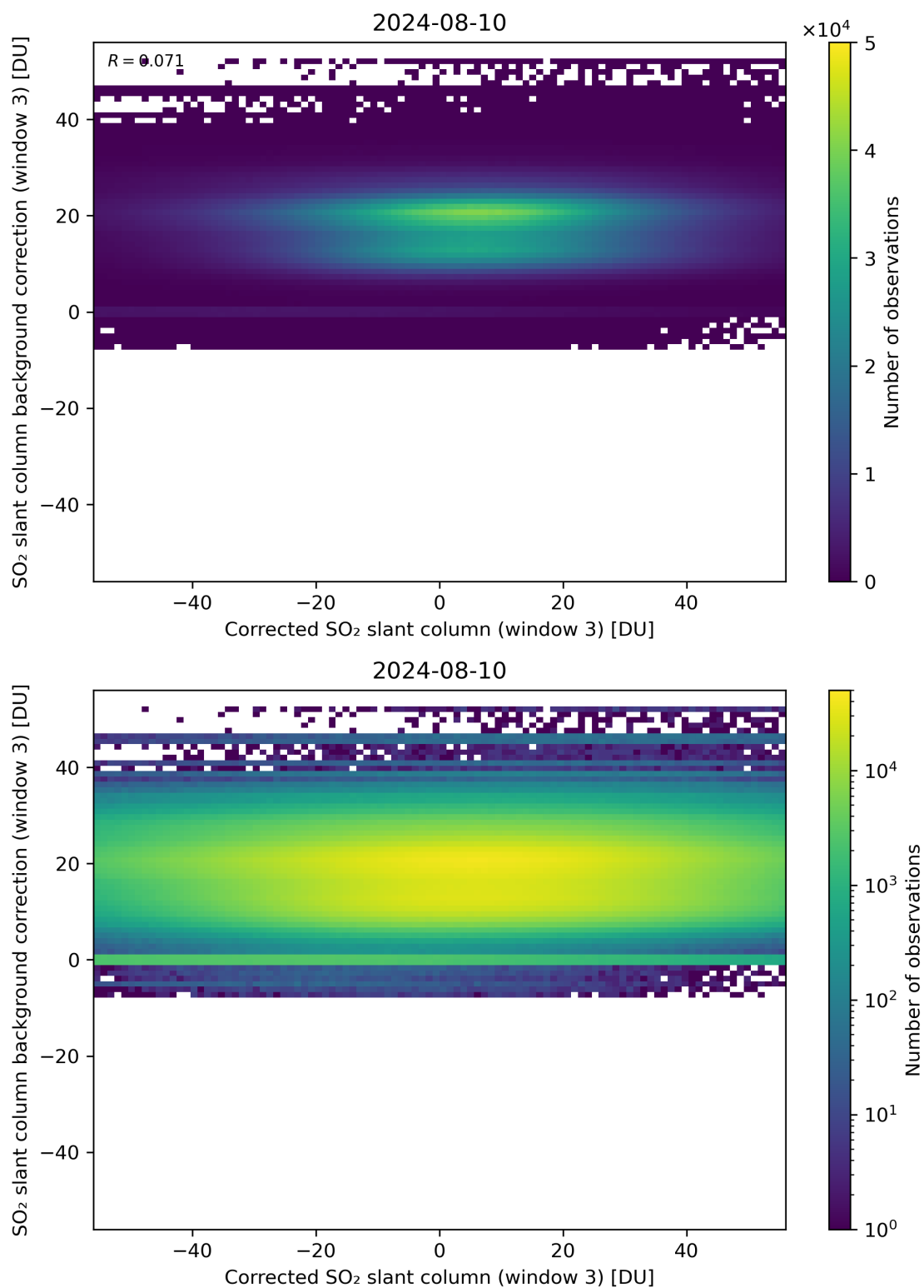
Figure 205: Scatter density plot of “Corrected SO 2 slant column (window 3)” against “SO 2 slant column background correction (window 3)” for 2024-08-09 to 2024-08-11.
