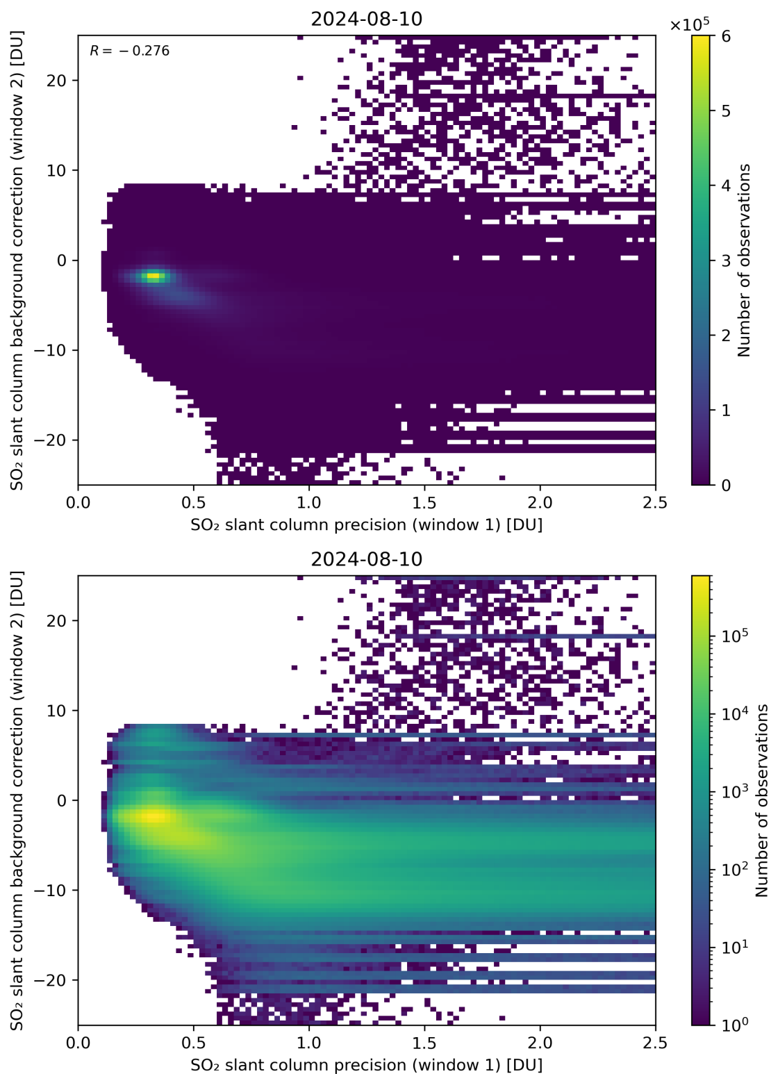
Figure 219: Scatter density plot of “SO 2 slant column precision (window 1)” against “SO 2 slant column background correction (window 2)” for 2024-08-09 to 2024-08-11.
