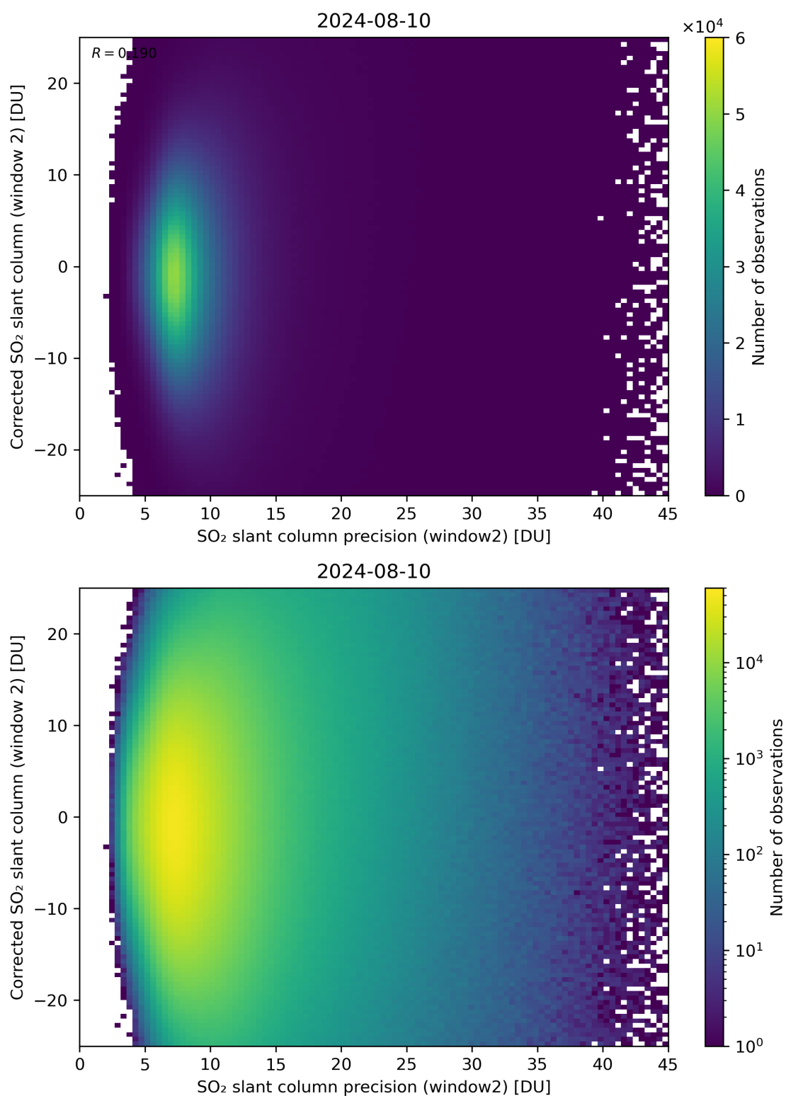
Figure 247: Scatter density plot of “SO 2 slant column precision (window2)” against “Corrected SO 2 slant column (window 2)” for 2024-08-09 to 2024-08-11.
