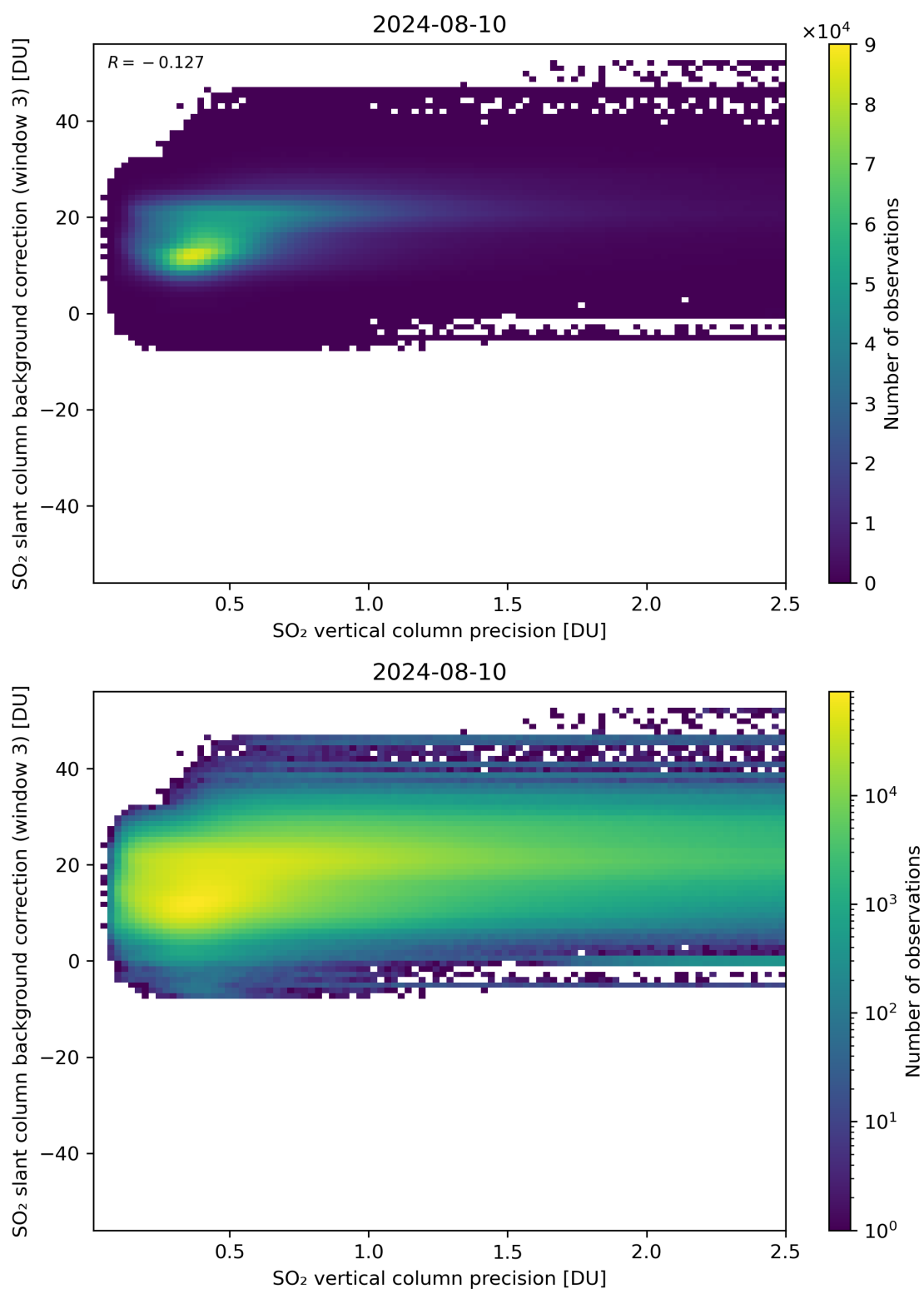
Figure 281: Scatter density plot of “SO 2 vertical column precision” against “SO 2 slant column background correction (window 3)” for 2024-08-09 to 2024-08-11.
