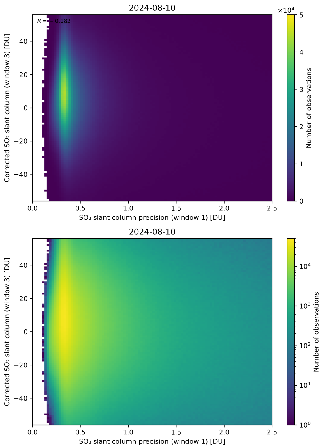
Figure 226: Scatter density plot of “SO 2 slant column precision (window 1)” against “Corrected SO 2 slant column (window 3)” for 2024-08-09 to 2024-08-11.
