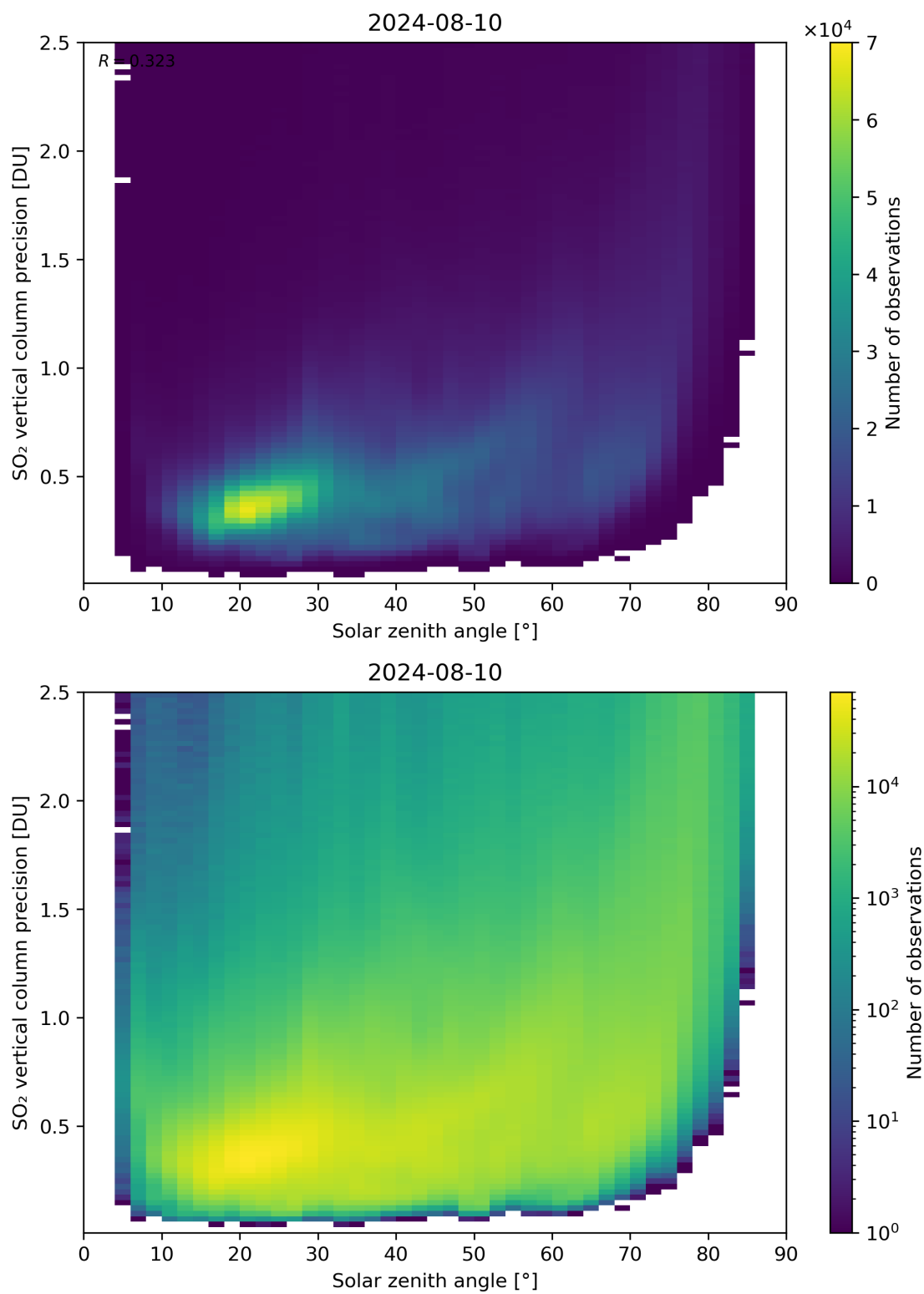
Figure 177: Scatter density plot of “Solar zenith angle” against “SO 2 vertical column precision” for 2024-08-09 to 2024-08-11.
