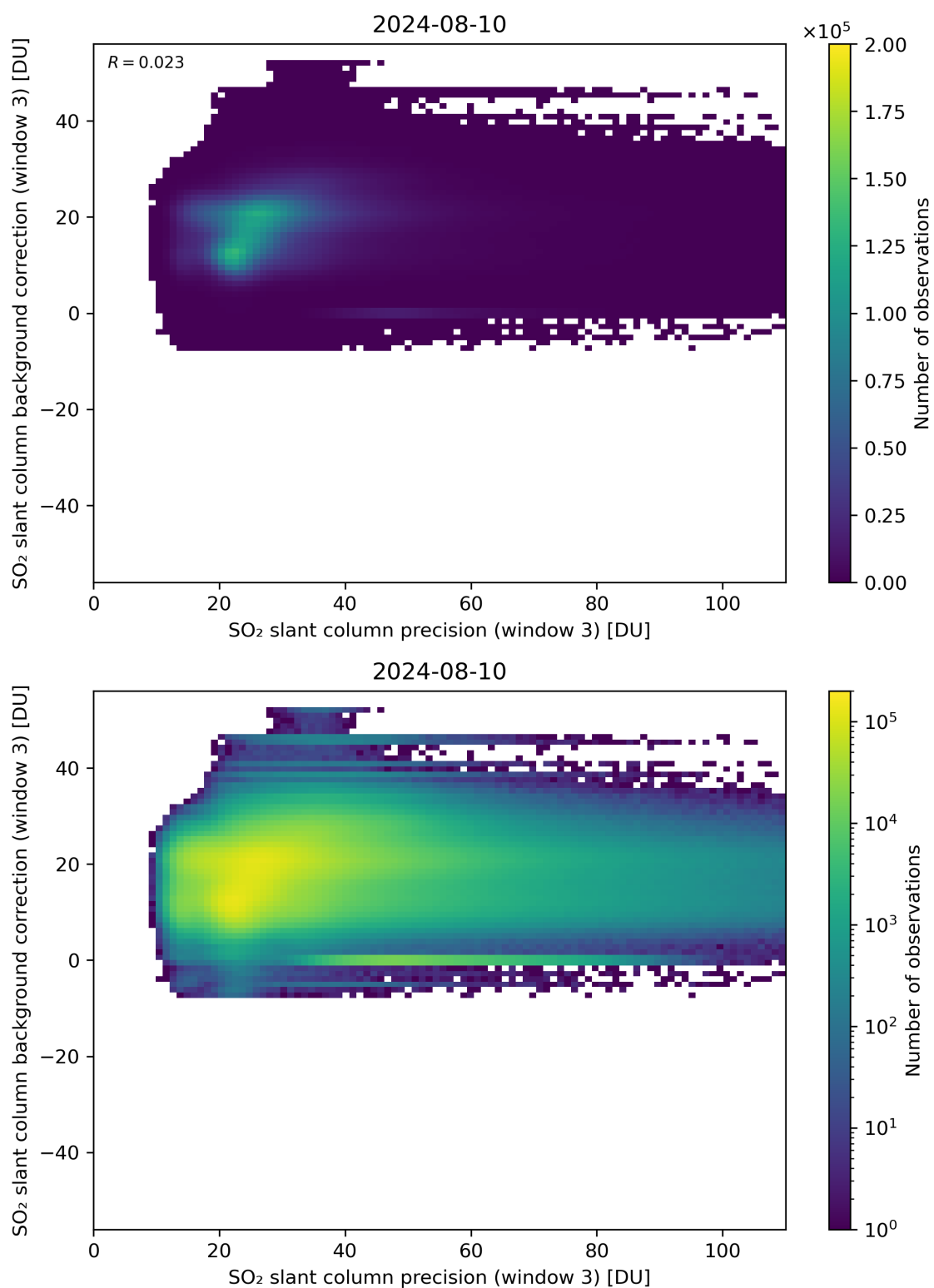
Figure 257: Scatter density plot of “SO 2 slant column precision (window 3)” against “SO 2 slant column background correction (window 3)” for 2024-08-09 to 2024-08-11.
