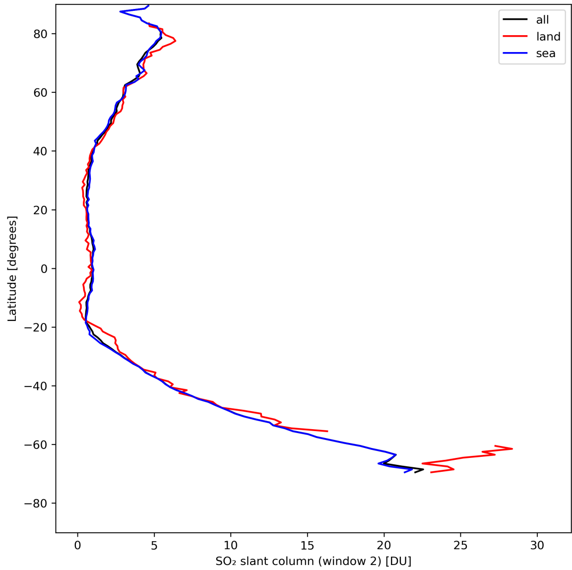
Figure 37: Zonal average of “SO 2 slant column (window 2)” for 2024-08-09 to 2024-08-11.
