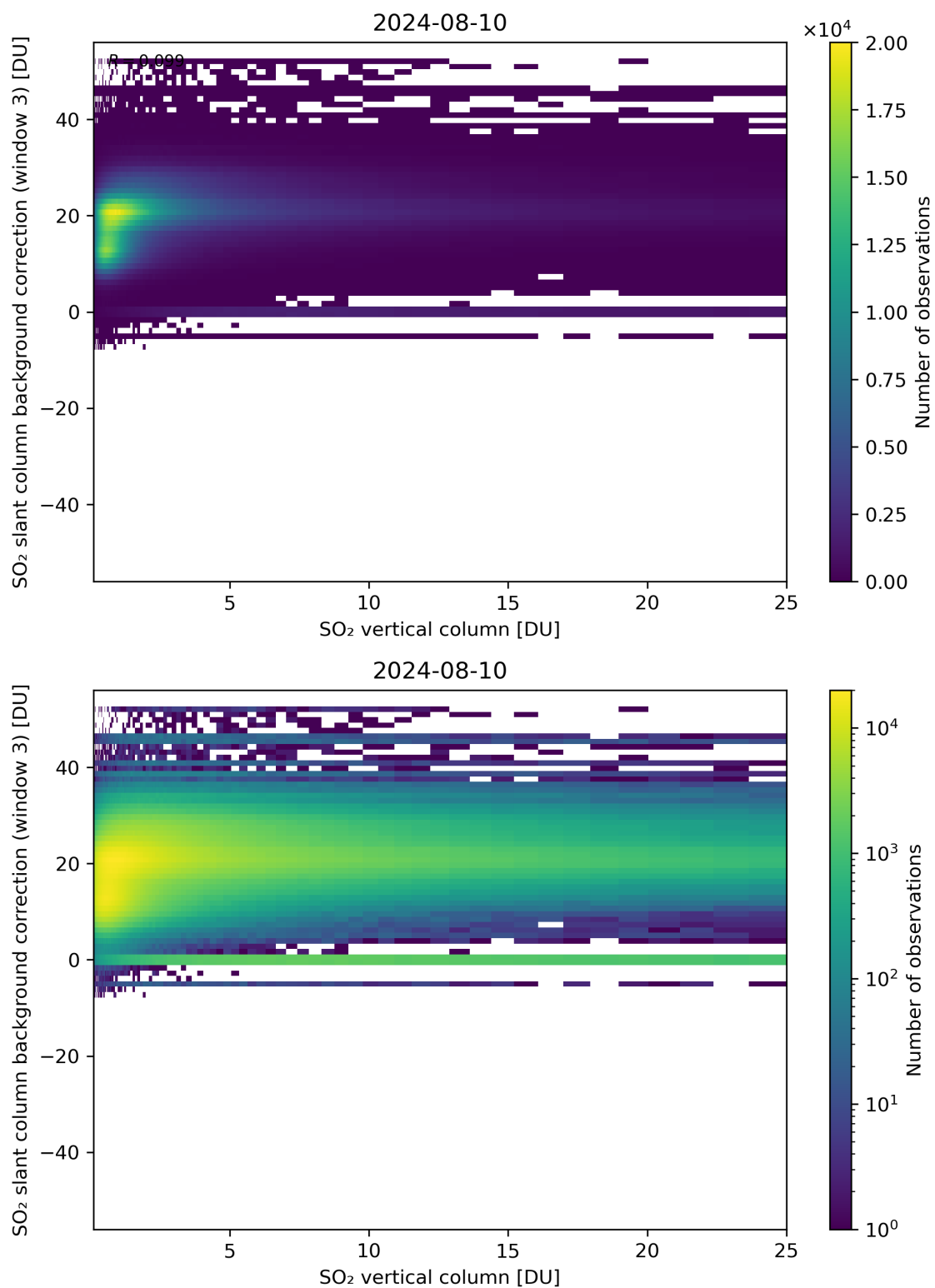
Figure 275: Scatter density plot of “SO 2 vertical column” against “SO 2 slant column background correction (window 3)” for 2024-08-09 to 2024-08-11.
