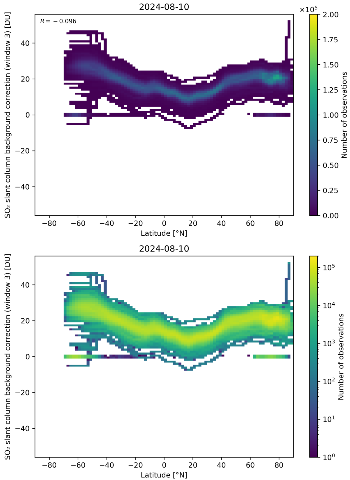
Figure 141: Scatter density plot of “Latitude” against “SO 2 slant column background correction (window 3)” for 2024-08-09 to 2024-08-11.
