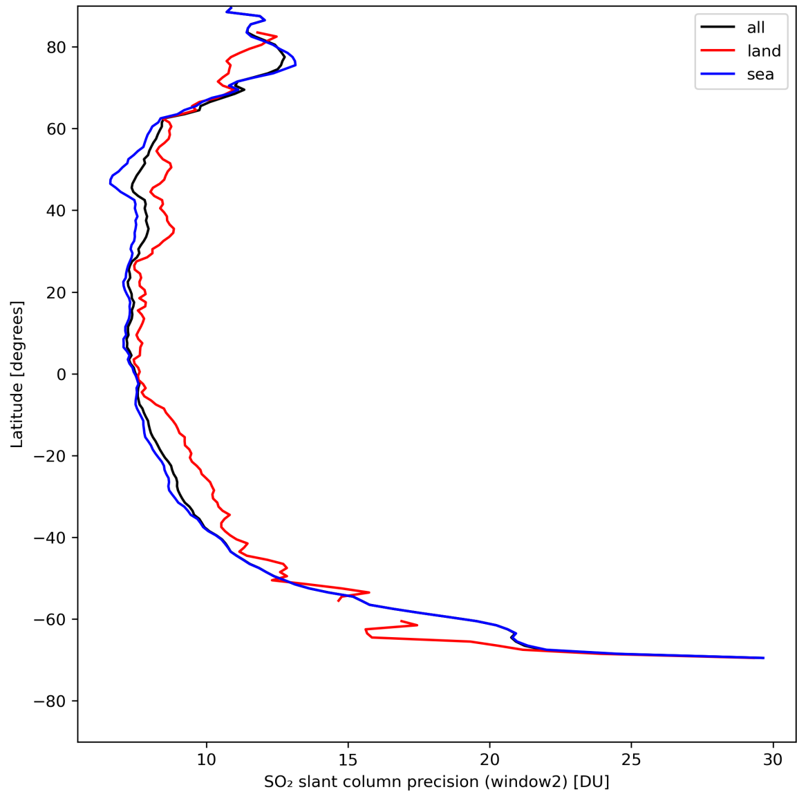
Figure 38: Zonal average of “SO 2 slant column precision (window2)” for 2024-08-09 to 2024-08-11.
