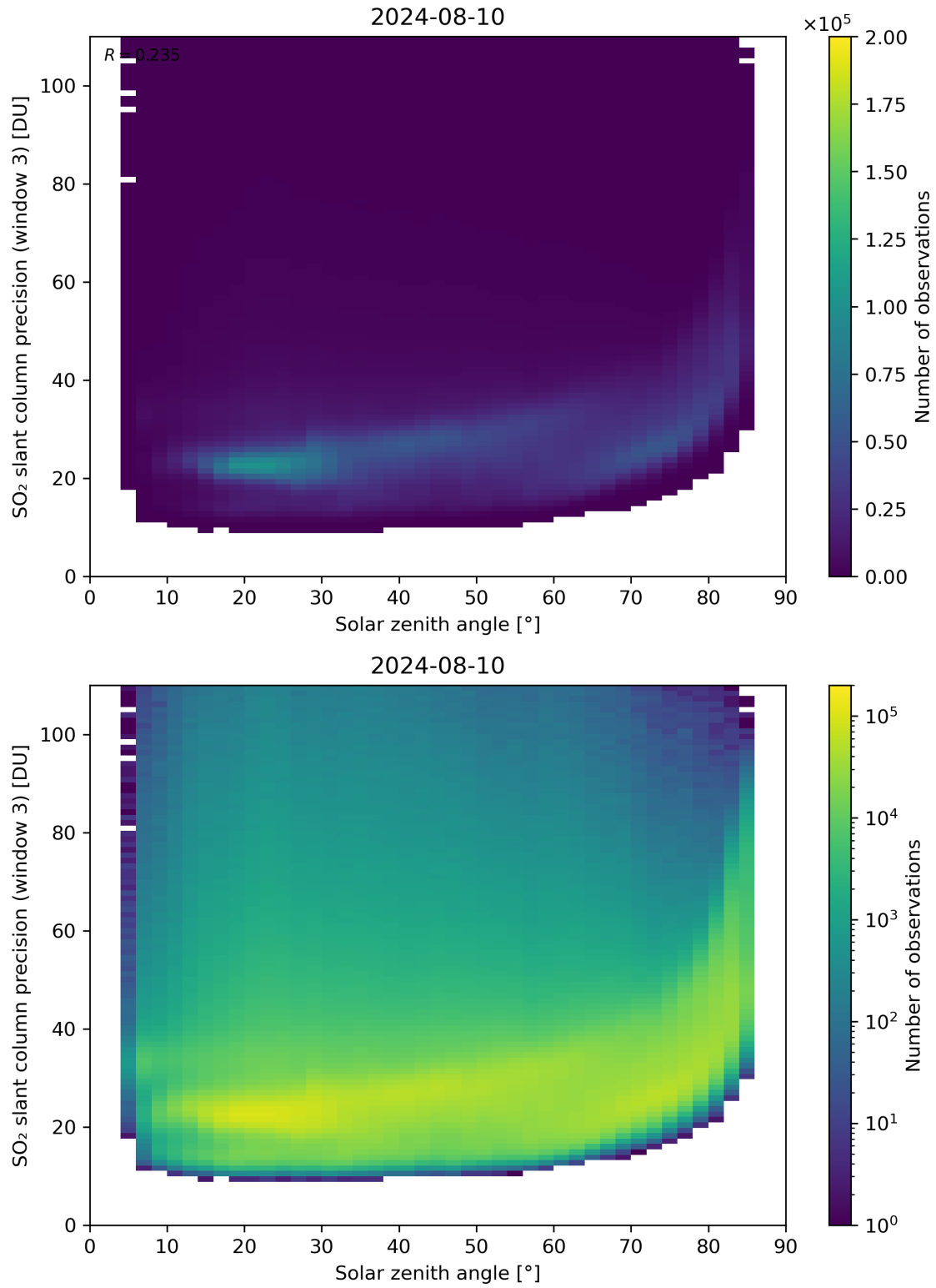
Figure 173: Scatter density plot of “Solar zenith angle” against “SO 2 slant column precision (window 3)” for 2024-08-09 to 2024-08-11.
