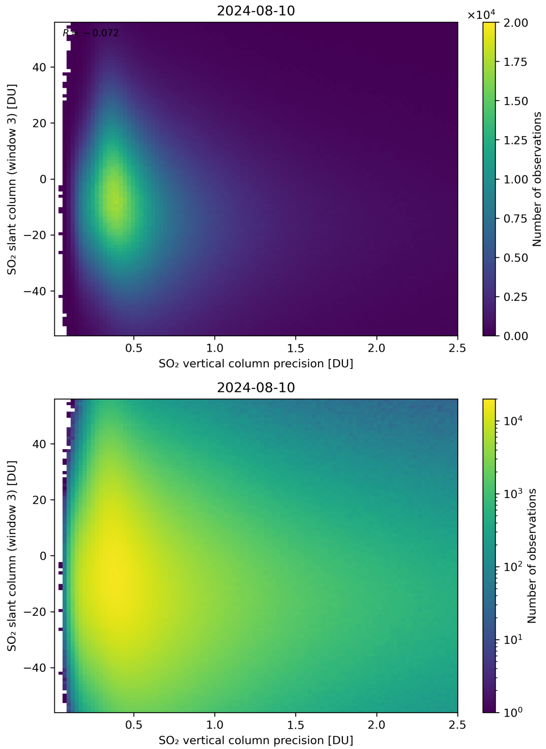
Figure 292: Scatter density plot of “SO 2 vertical column precision” against “SO 2 slant column (window 3)” for 2024-08-09 to 2024-08-11.
