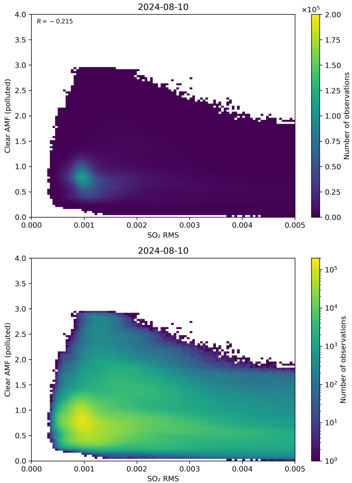
Figure 136: Scatter density plot of “SO 2 RMS” against “Clear AMF (polluted)” for 2024-08-09 to 2024-08-11.
