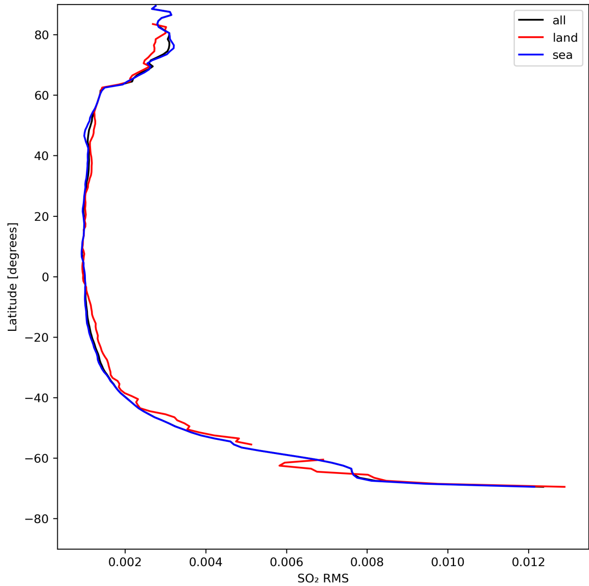
Figure 47: Zonal average of “SO 2 RMS” for 2024-08-09 to 2024-08-11.
