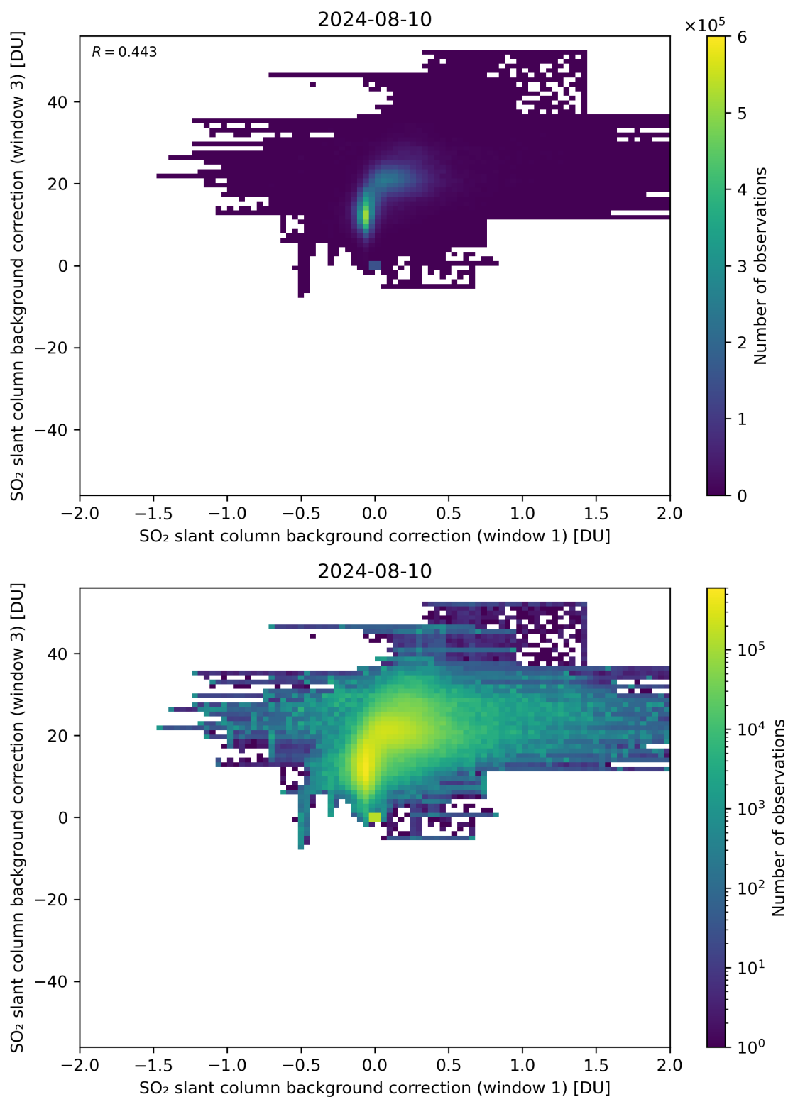
Figure 99: Scatter density plot of “SO 2 slant column background correction (window 1)” against “SO 2 slant column background correction (window 3)” for 2024-08-09 to 2024-08-11.
