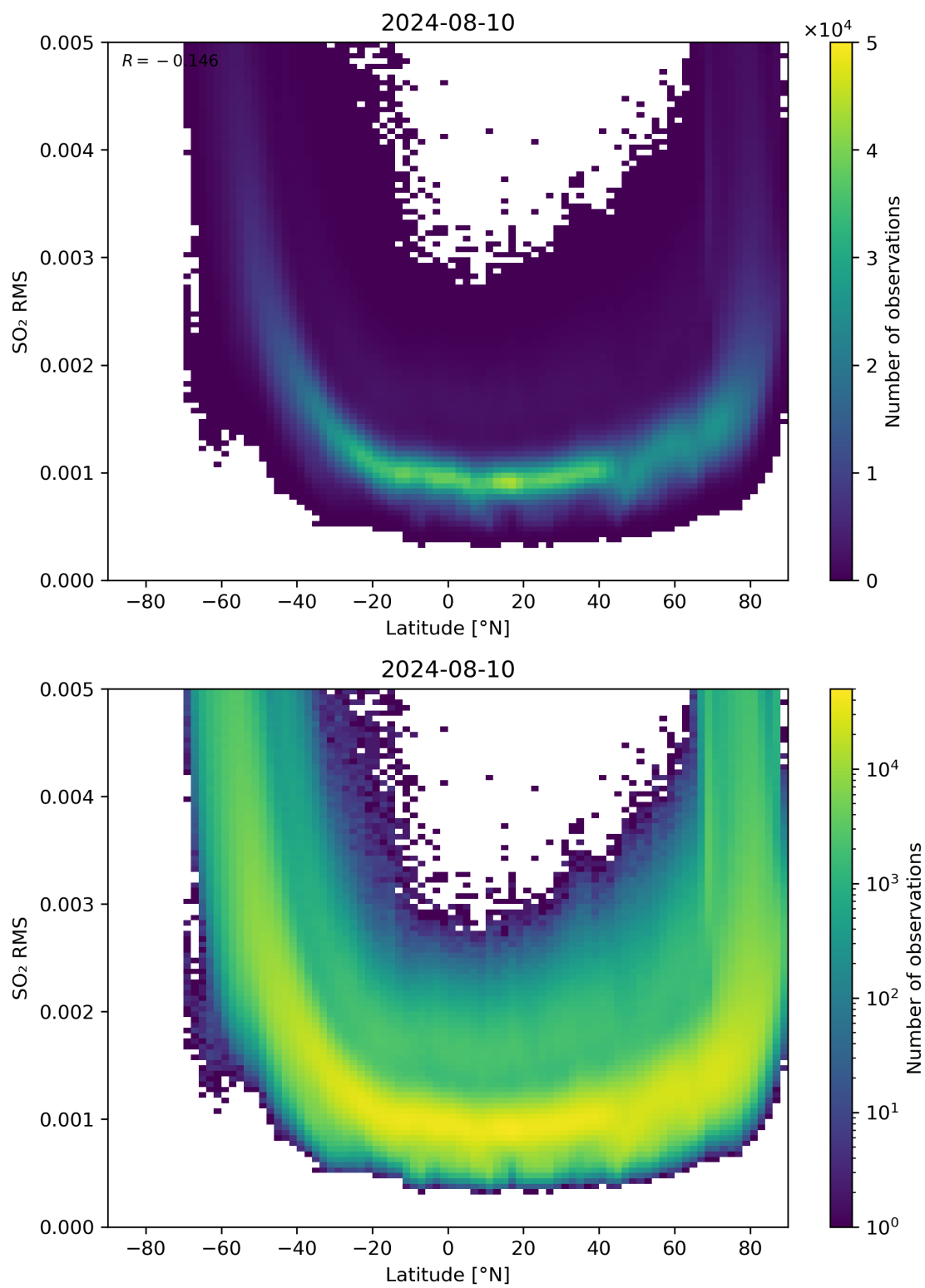
Figure 144: Scatter density plot of “Latitude” against “SO 2 RMS” for 2024-08-09 to 2024-08-11.
