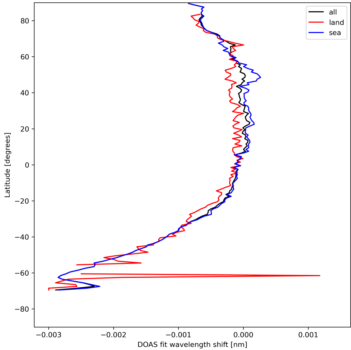
Figure 45: Zonal average of “DOAS fit wavelength shift” for 2024-08-09 to 2024-08-11.
