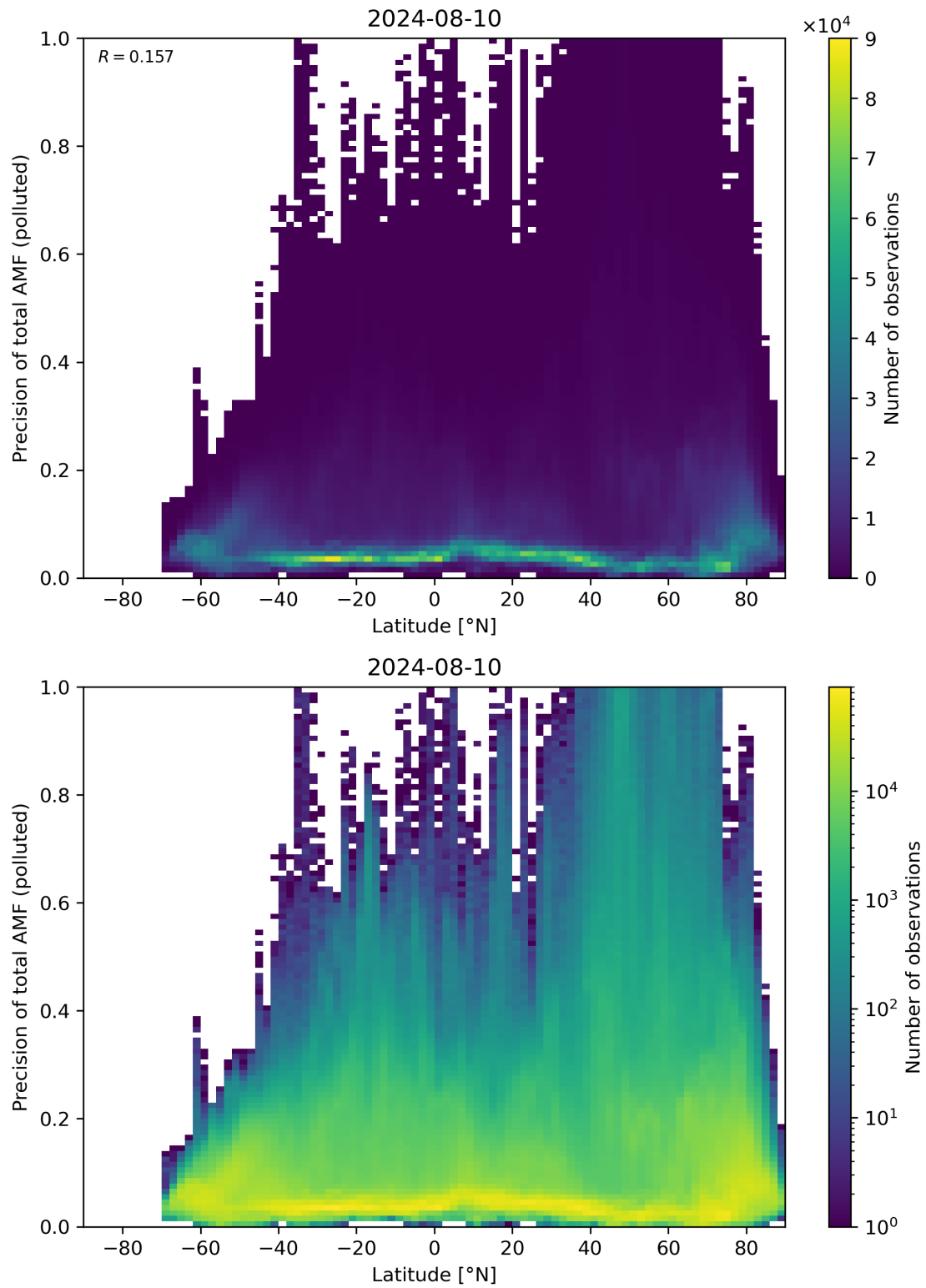
Figure 155: Scatter density plot of “Latitude” against “Precision of total AMF (polluted)” for 2024-08-09 to 2024-08-11.
