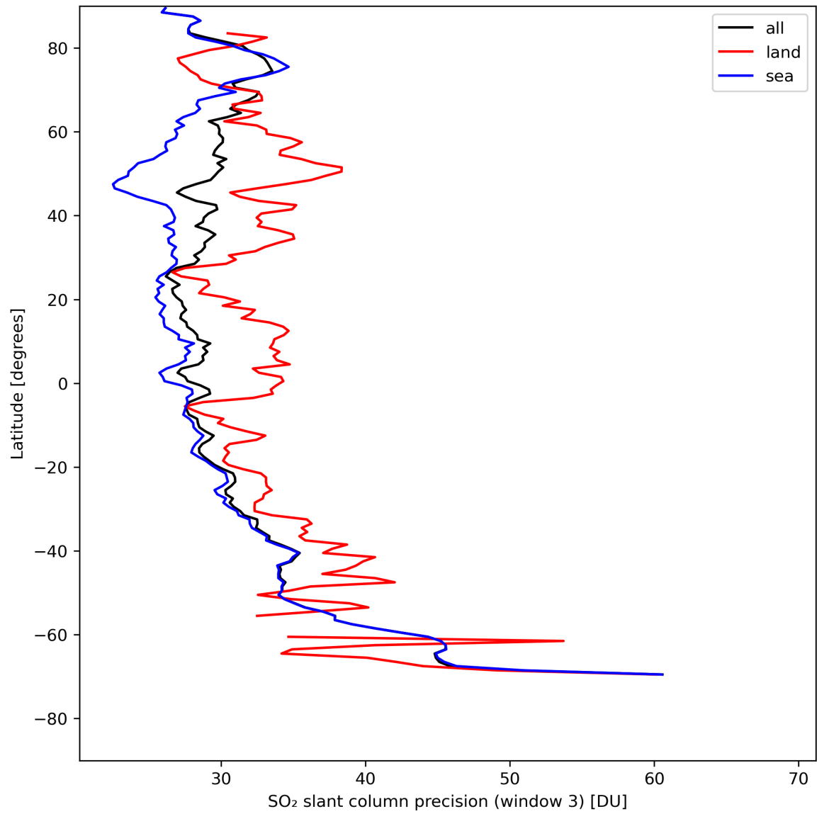
Figure 42: Zonal average of “SO 2 slant column precision (window 3)” for 2024-08-09 to 2024-08-11.
