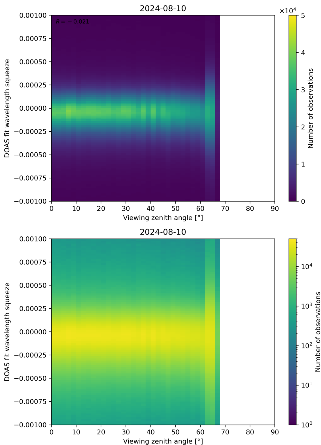
Figure 312: Scatter density plot of “Viewing zenith angle” against “DOAS fit wavelength squeeze” for 2024-08-09 to 2024-08-11.
