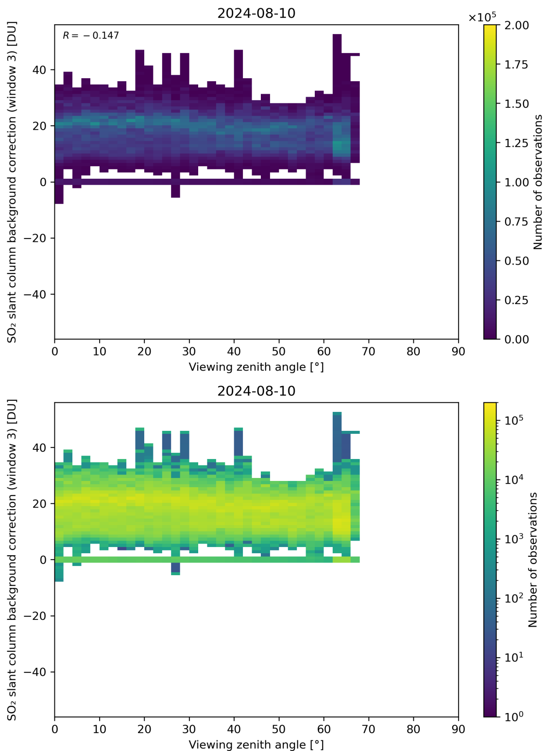
Figure 310: Scatter density plot of “Viewing zenith angle” against “SO 2 slant column background correction (window 3)” for 2024-08-09 to 2024-08-11.
