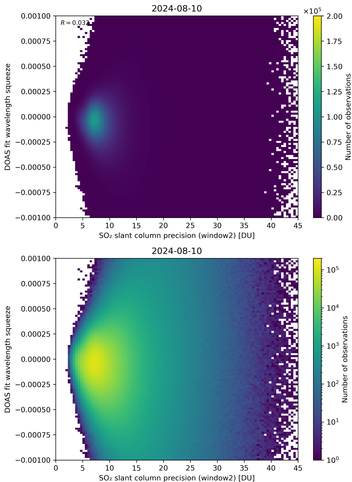
Figure 244: Scatter density plot of “SO 2 slant column precision (window2)” against “DOAS fit wavelength squeeze” for 2024-08-09 to 2024-08-11.
