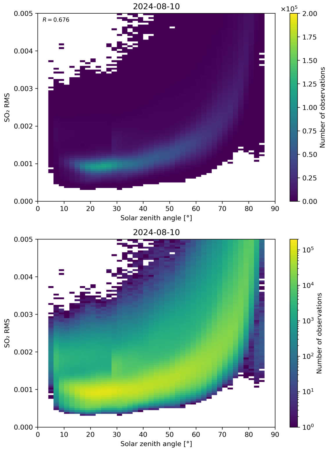
Figure 163: Scatter density plot of “Solar zenith angle” against “SO 2 RMS” for 2024-08-09 to 2024-08-11.
