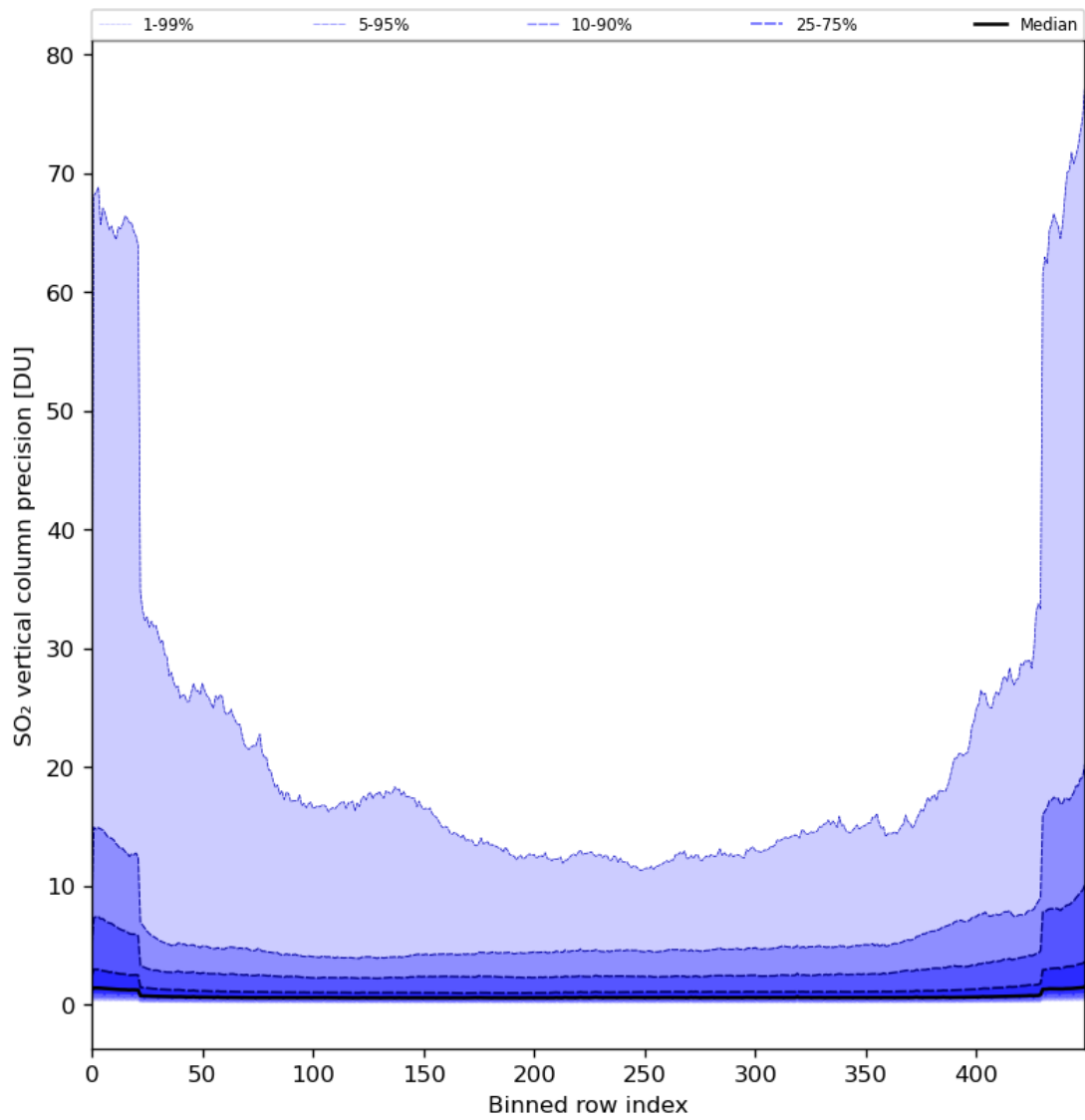
Figure 77: Along track statistics of “SO 2 vertical column precision” for 2024-08-09 to 2024-08-11
