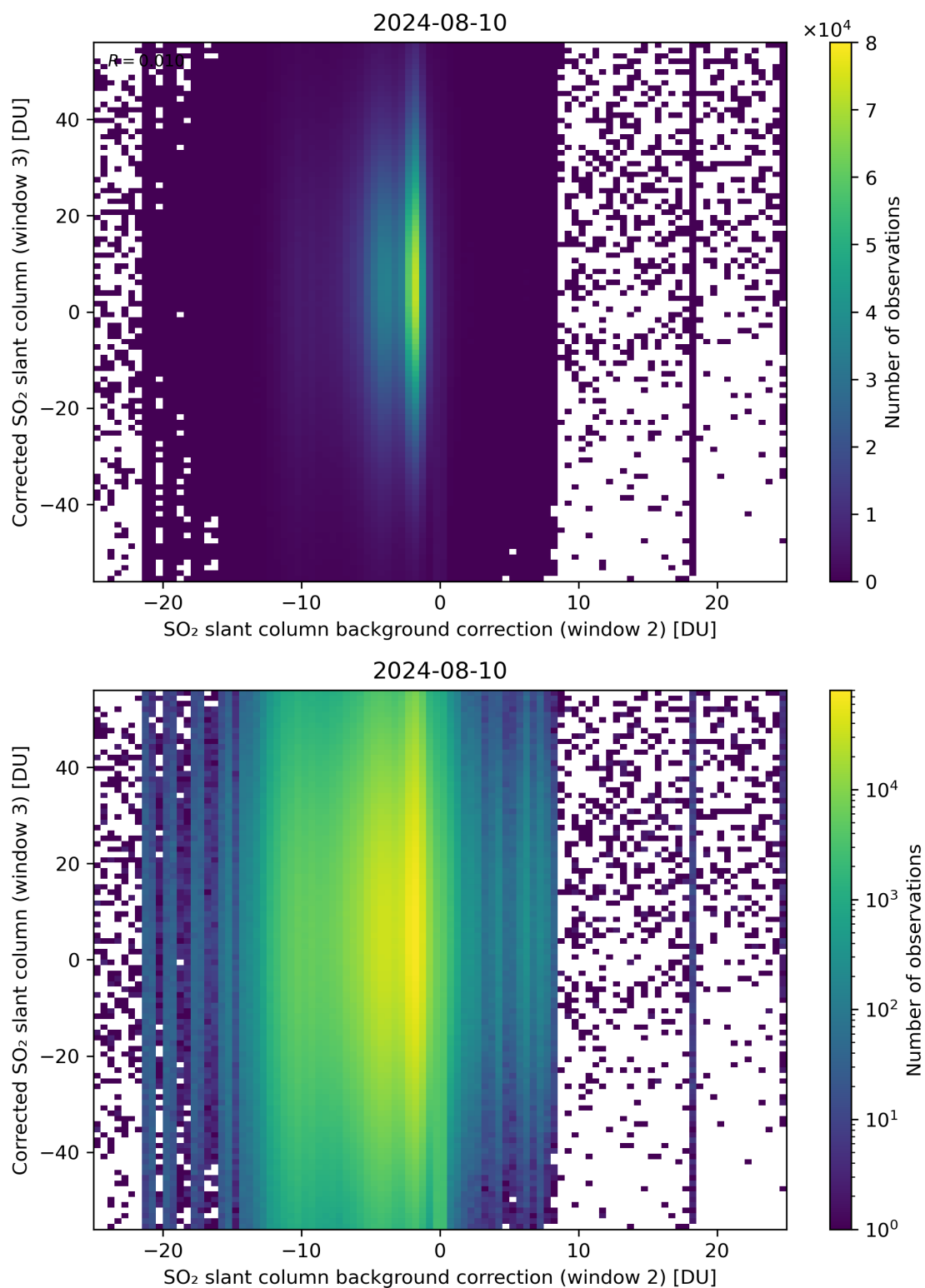
Figure 116: Scatter density plot of “SO 2 slant column background correction (window 2)” against “Corrected SO 2 slant column (window 3)” for 2024-08-09 to 2024-08-11.
