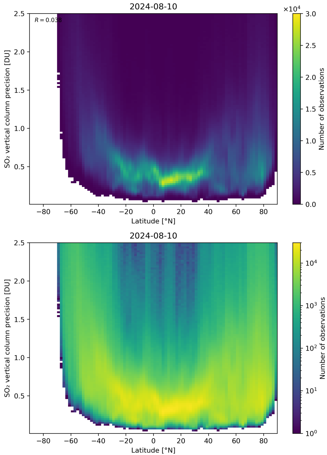
Figure 157: Scatter density plot of “Latitude” against “SO 2 vertical column precision” for 2024-08-09 to 2024-08-11.
