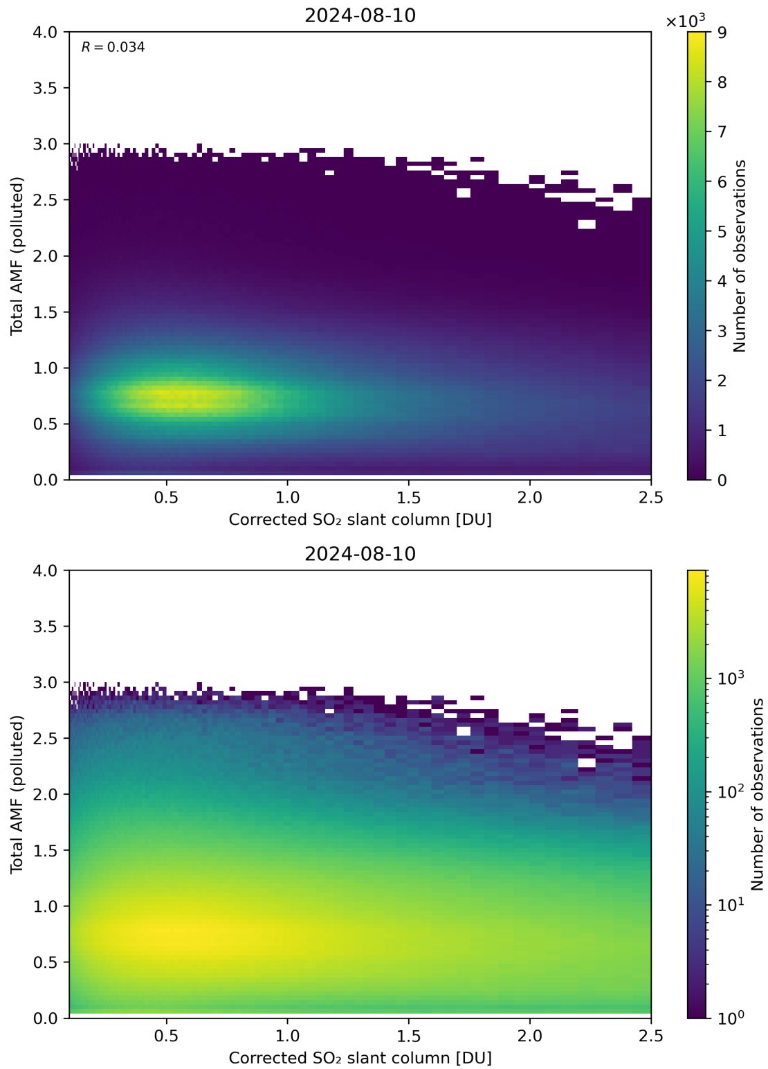
Figure 192: Scatter density plot of “Corrected SO 2 slant column” against “Total AMF (polluted)” for 2024-08-09 to 2024-08-11.
