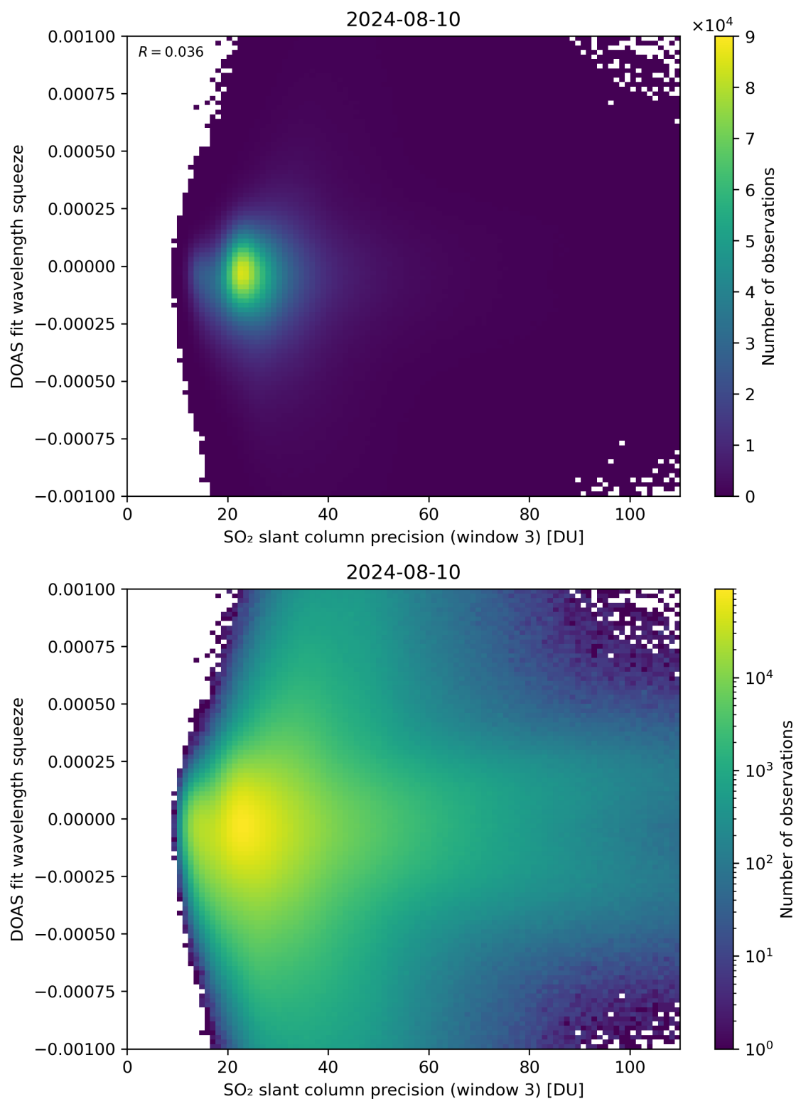
Figure 259: Scatter density plot of “SO 2 slant column precision (window 3)” against “DOAS fit wavelength squeeze” for 2024-08-09 to 2024-08-11.
