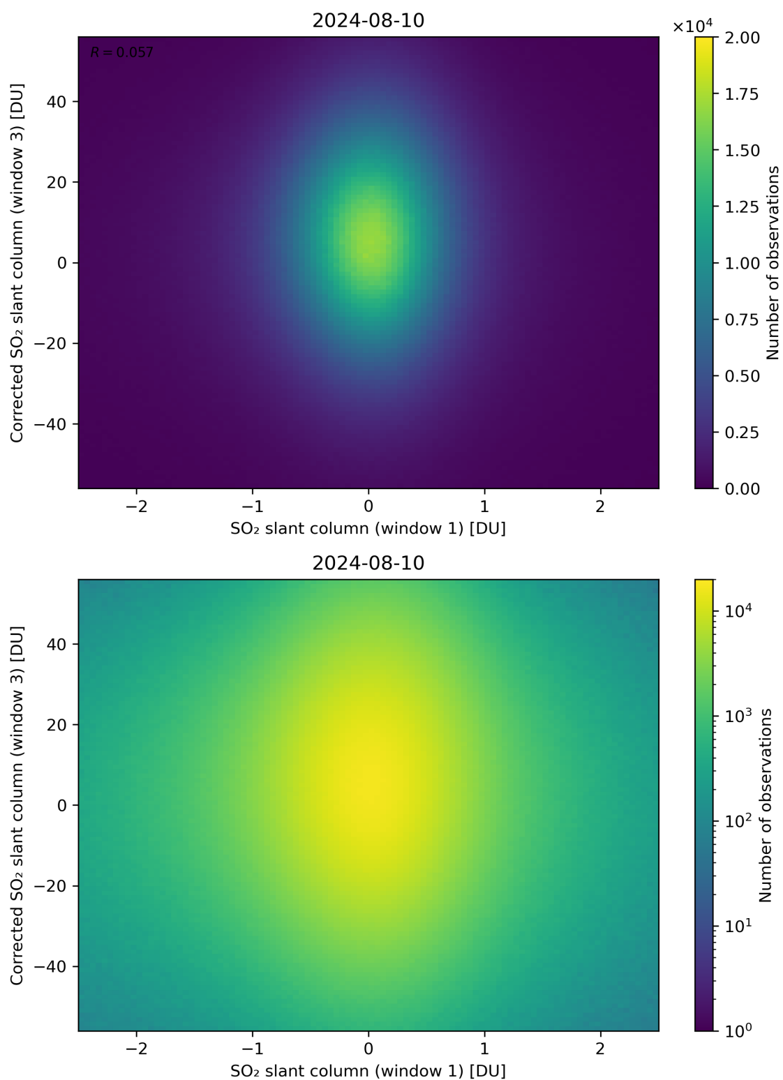
Figure 234: Scatter density plot of “SO 2 slant column (window 1)” against “Corrected SO 2 slant column (window 3)” for 2024-08-09 to 2024-08-11.
