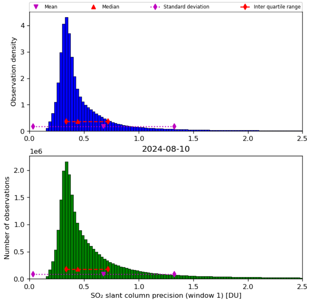
Figure 57: Histogram of “SO 2 slant column precision (window 1)” for 2024-08-09 to 2024-08-11
