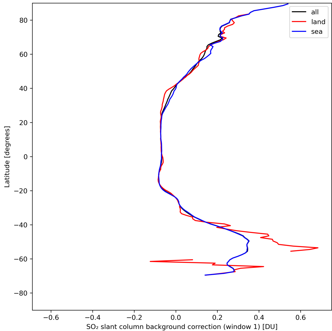
Figure 36: Zonal average of “SO 2 slant column background correction (window 1)” for 2024-08-09 to 2024-08-11.
