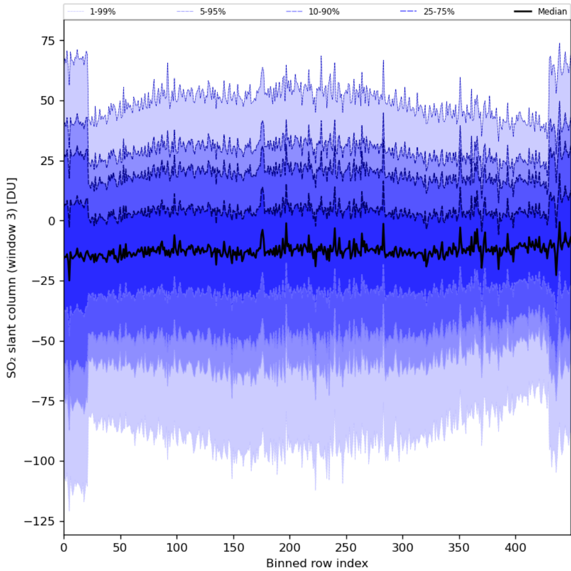
Figure 87: Along track statistics of “SO 2 slant column (window 3)” for 2024-08-09 to 2024-08-11
