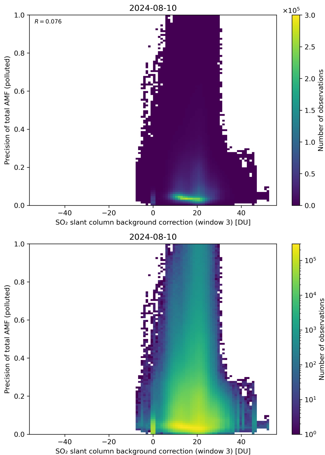
Figure 126: Scatter density plot of “SO 2 slant column background correction (window 3)” against “Precision of total AMF (polluted)” for 2024-08-09 to 2024-08-11.
