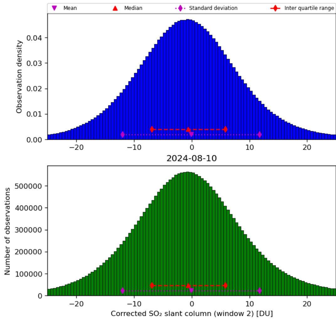
Figure 62: Histogram of “Corrected SO 2 slant column (window 2)” for 2024-08-09 to 2024-08-11
