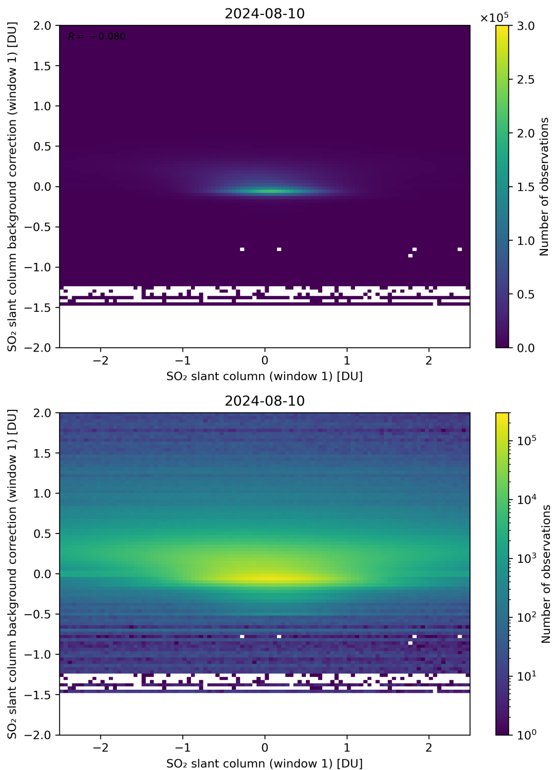
Figure 212: Scatter density plot of “SO 2 slant column (window 1)” against “SO 2 slant column background correction (window 1)” for 2024-08-09 to 2024-08-11.
