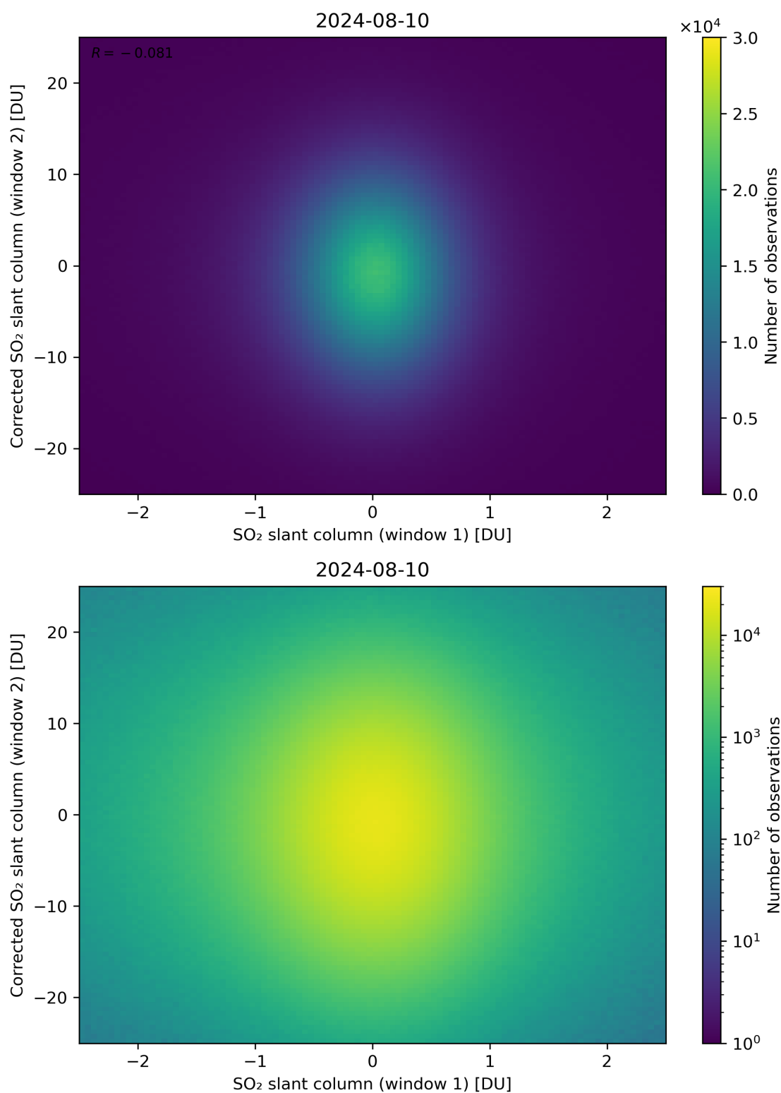
Figure 233: Scatter density plot of “SO 2 slant column (window 1)” against “Corrected SO 2 slant column (window 2)” for 2024-08-09 to 2024-08-11.
