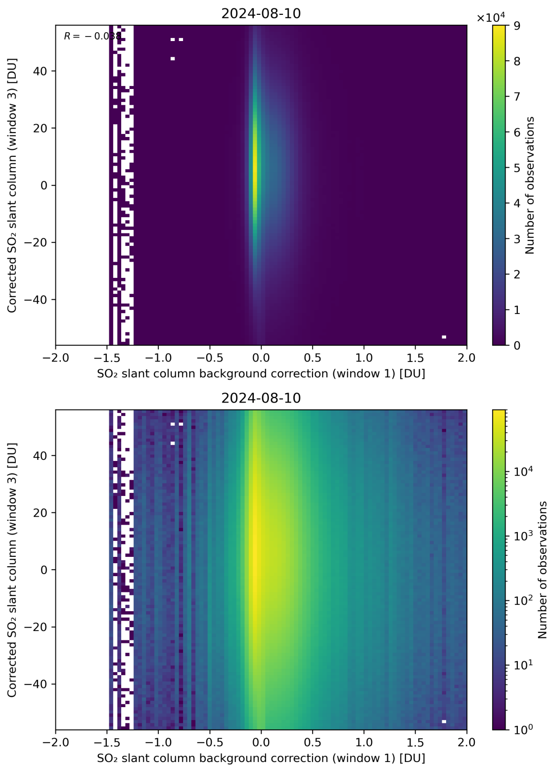
Figure 105: Scatter density plot of “SO 2 slant column background correction (window 1)” against “Corrected SO 2 slant column (window 3)” for 2024-08-09 to 2024-08-11.
