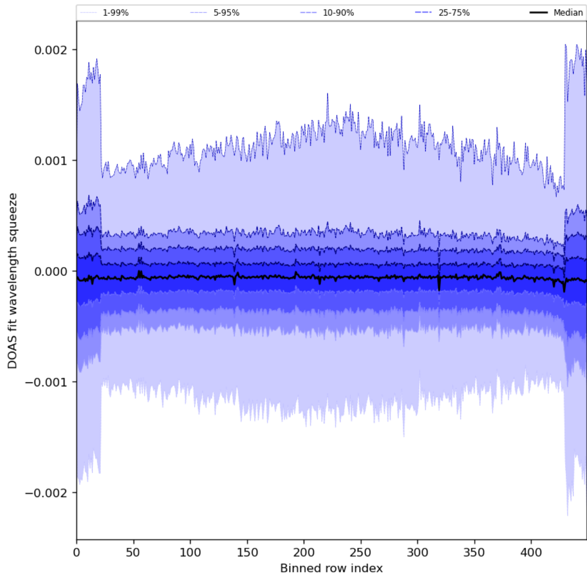
Figure 92: Along track statistics of “DOAS fit wavelength squeeze” for 2024-08-09 to 2024-08-11
