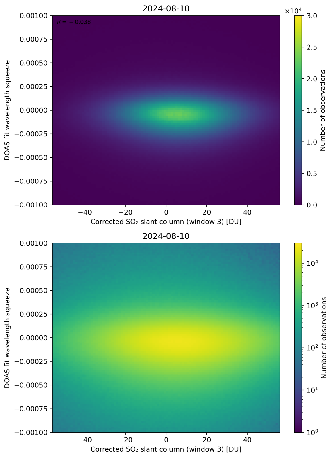
Figure 207: Scatter density plot of “Corrected SO 2 slant column (window 3)” against “DOAS fit wavelength squeeze” for 2024-08-09 to 2024-08-11.
