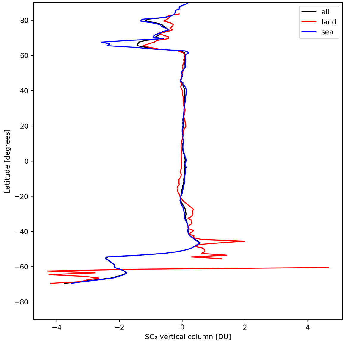
Figure 30: Zonal average of “SO 2 vertical column” for 2024-08-09 to 2024-08-11.
