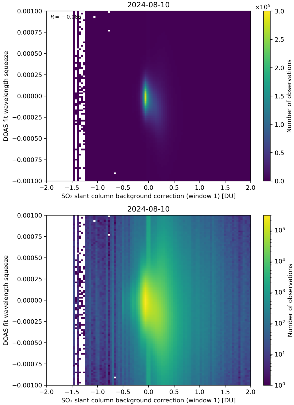
Figure 101: Scatter density plot of “SO 2 slant column background correction (window 1)” against “DOAS fit wavelength squeeze” for 2024-08-09 to 2024-08-11.
