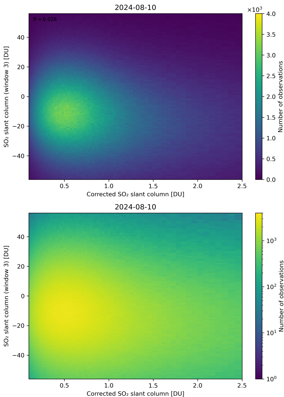
Figure 190: Scatter density plot of “Corrected SO 2 slant column” against “SO 2 slant column (window 3)” for 2024-08-09 to 2024-08-11.
