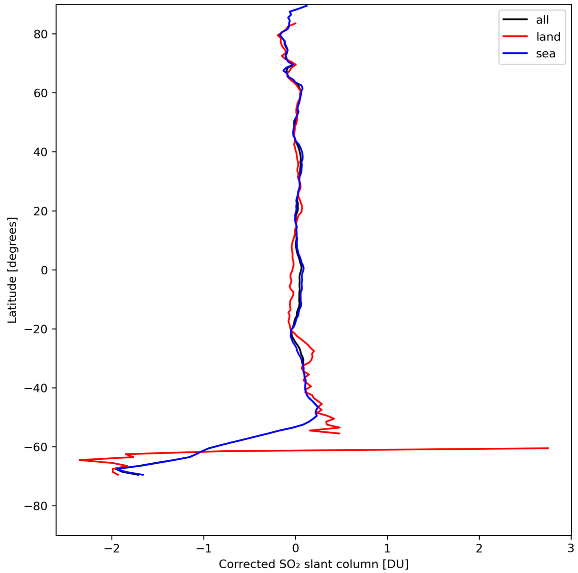
Figure 32: Zonal average of “Corrected SO 2 slant column” for 2024-08-09 to 2024-08-11.
