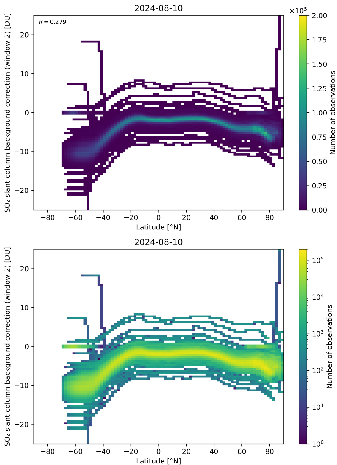
Figure 140: Scatter density plot of “Latitude” against “SO 2 slant column background correction (window 2)” for 2024-08-09 to 2024-08-11.
