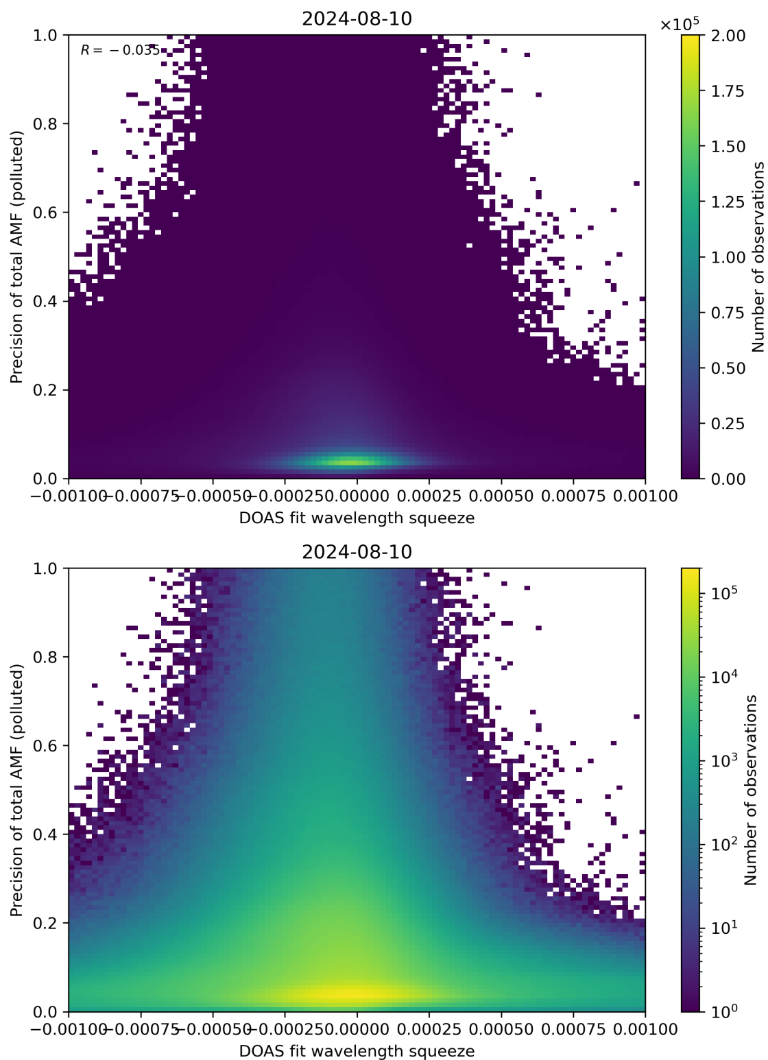
Figure 135: Scatter density plot of “DOAS fit wavelength squeeze” against “Precision of total AMF (polluted)” for 2024-08-09 to 2024-08-11.
