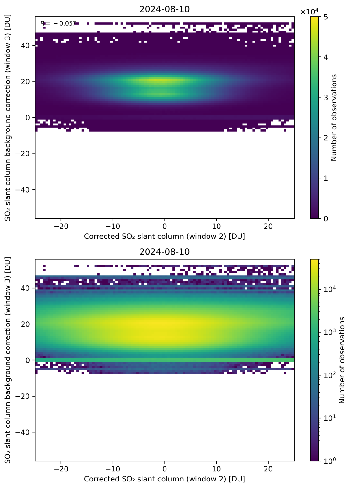
Figure 195: Scatter density plot of “Corrected SO 2 slant column (window 2)” against “SO 2 slant column background correction (window 3)” for 2024-08-09 to 2024-08-11.
