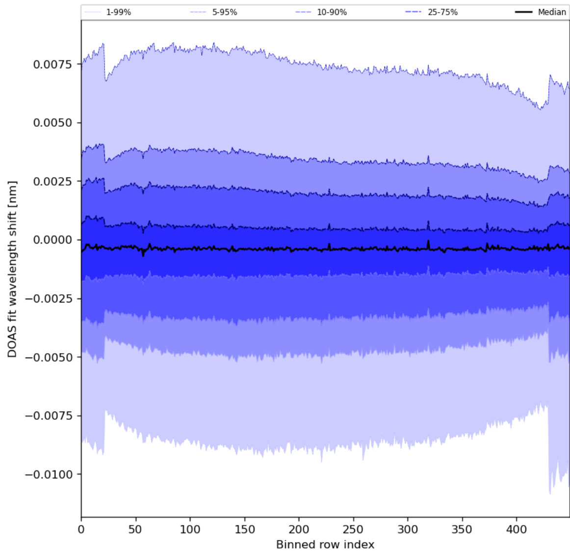
Figure 91: Along track statistics of “DOAS fit wavelength shift” for 2024-08-09 to 2024-08-11
