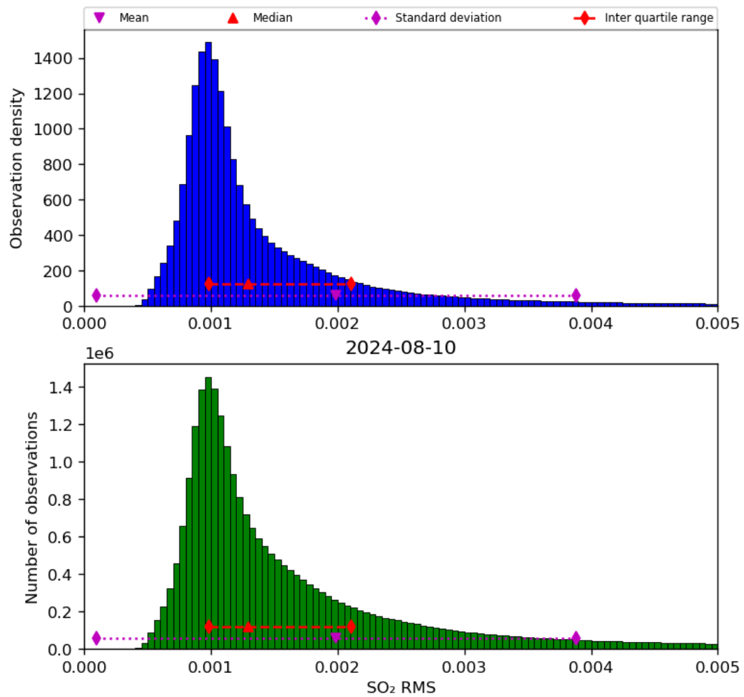
Figure 70: Histogram of “SO 2 RMS” for 2024-08-09 to 2024-08-11
