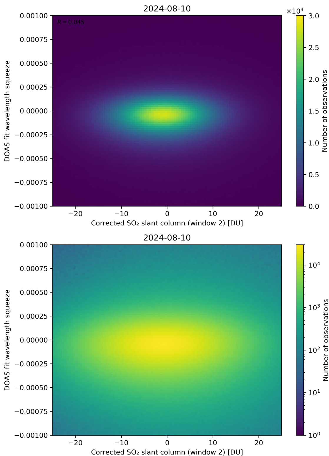
Figure 197: Scatter density plot of “Corrected SO 2 slant column (window 2)” against “DOAS fit wavelength squeeze” for 2024-08-09 to 2024-08-11.
