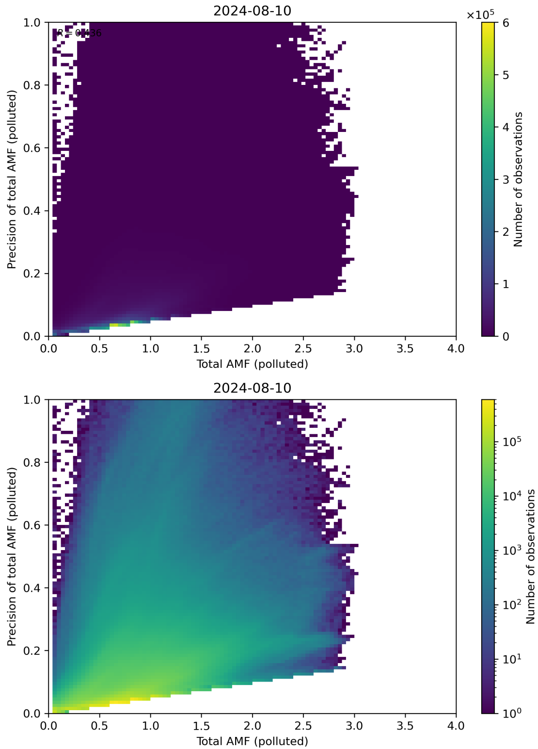
Figure 272: Scatter density plot of “Total AMF (polluted)” against “Precision of total AMF (polluted)” for 2024-08-09 to 2024-08-11.
