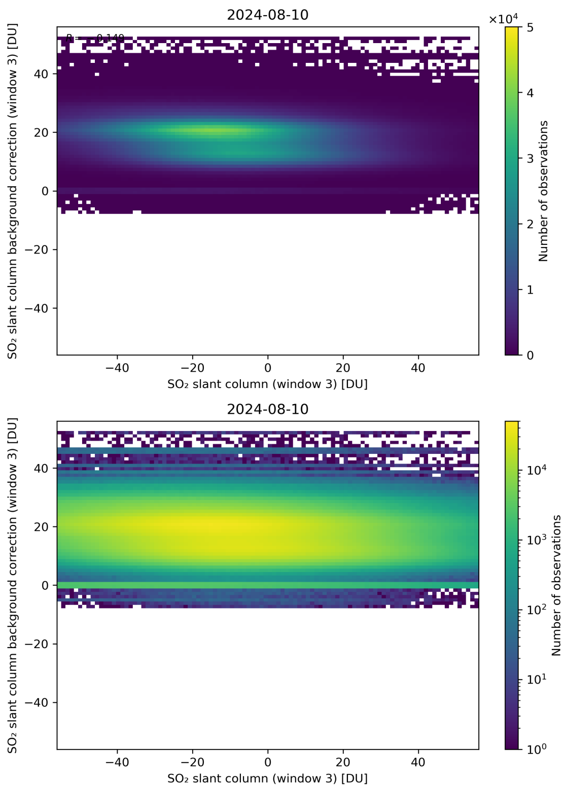
Figure 253: Scatter density plot of “SO 2 slant column (window 3)” against “SO 2 slant column background correction (window 3)” for 2024-08-09 to 2024-08-11.
