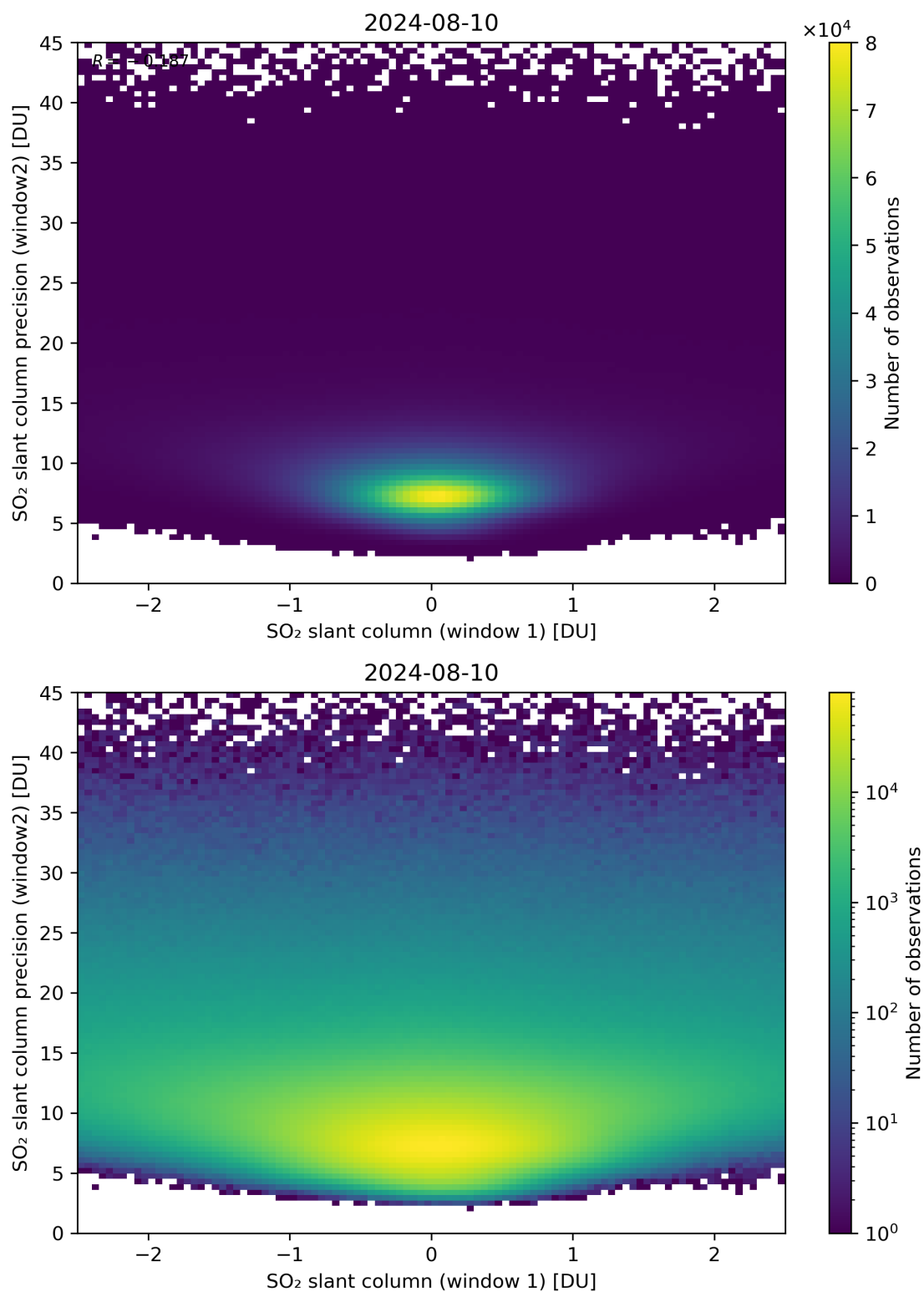
Figure 236: Scatter density plot of “SO 2 slant column (window 1)” against “SO 2 slant column precision (window2)” for 2024-08-09 to 2024-08-11.
