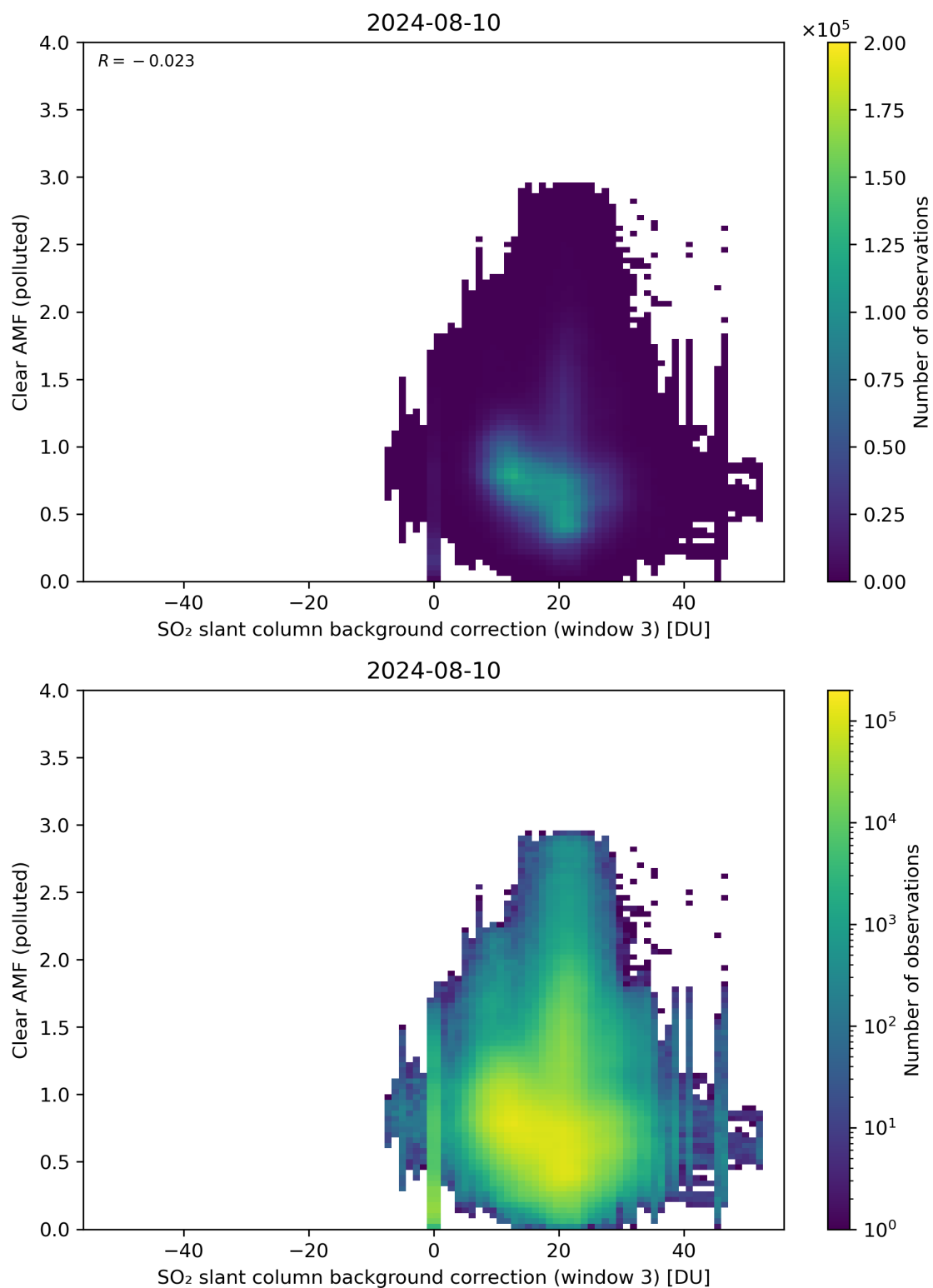
Figure 124: Scatter density plot of “SO 2 slant column background correction (window 3)” against “Clear AMF (polluted)” for 2024-08-09 to 2024-08-11.
