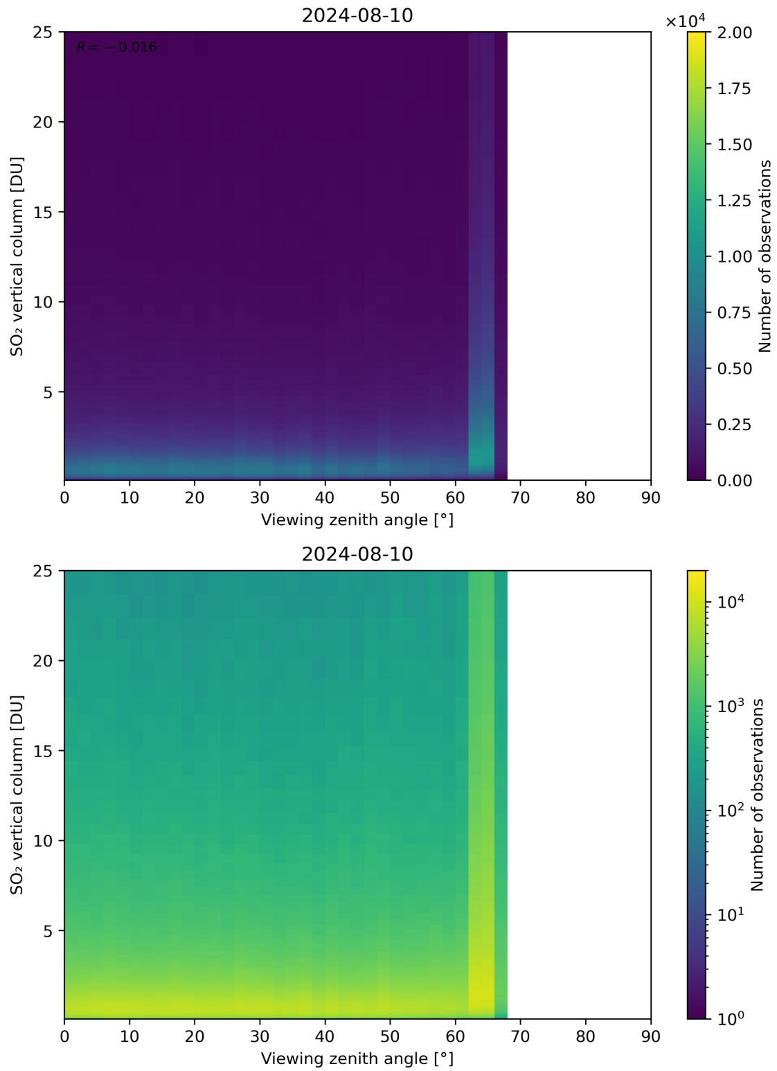
Figure 327: Scatter density plot of “Viewing zenith angle” against “SO 2 vertical column” for 2024-08-09 to 2024-08-11.
