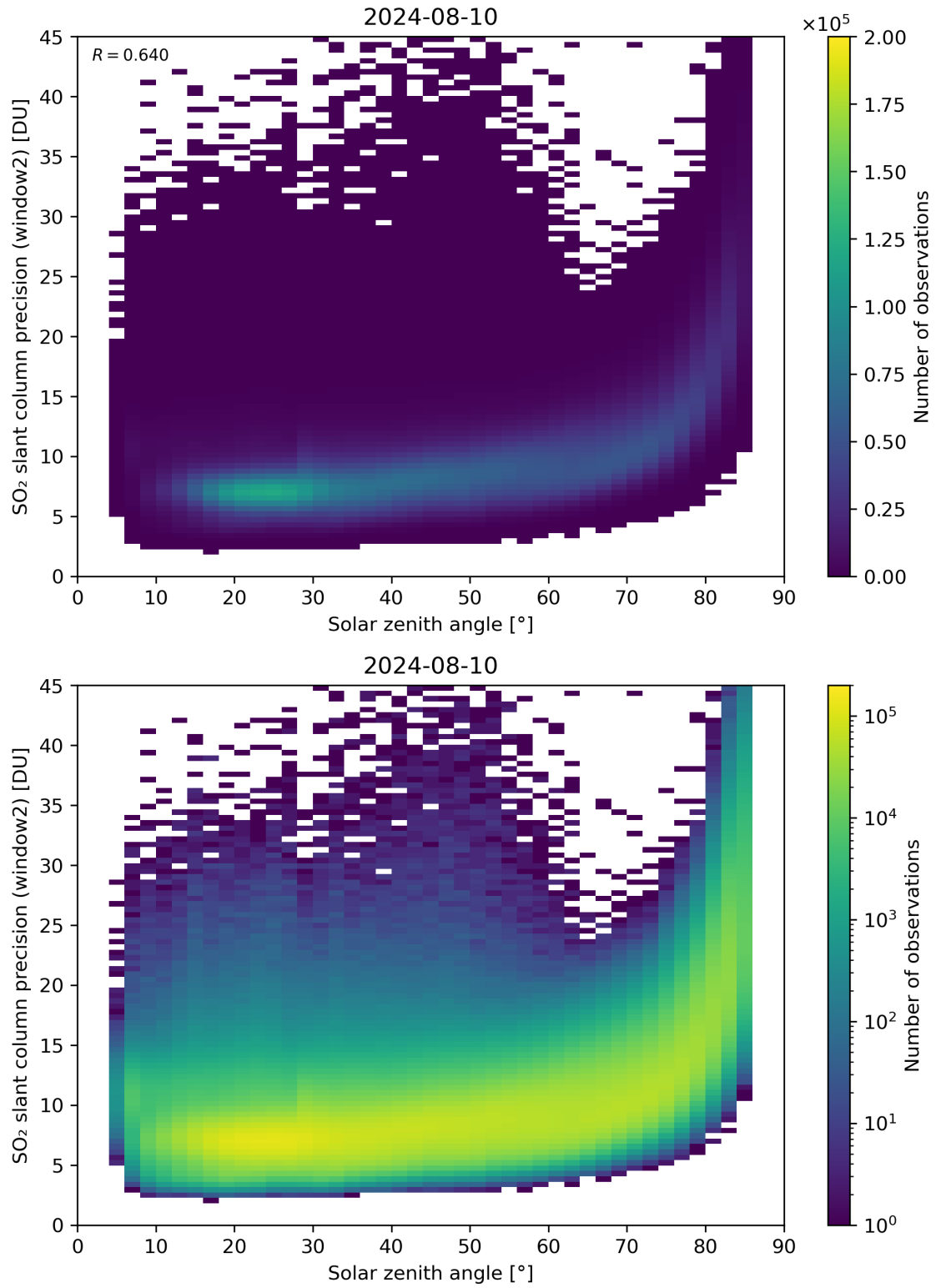
Figure 171: Scatter density plot of “Solar zenith angle” against “SO 2 slant column precision (window2)” for 2024-08-09 to 2024-08-11.
