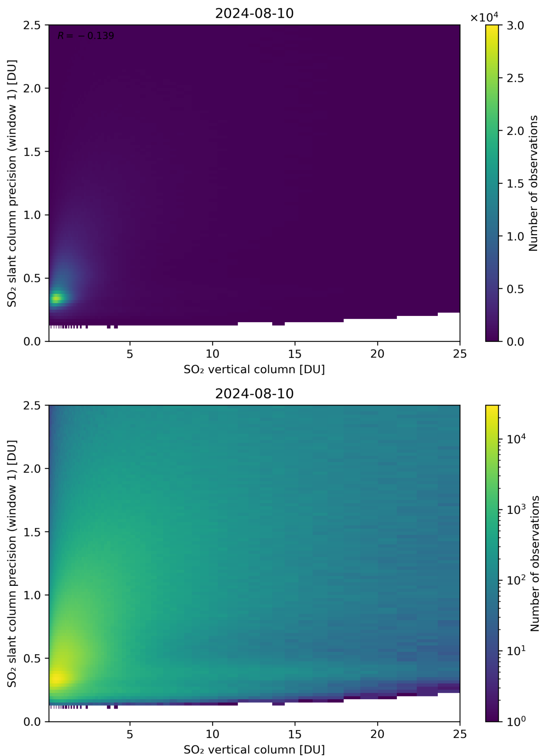
Figure 301: Scatter density plot of “SO 2 vertical column” against “SO 2 slant column precision (window 1)” for 2024-08-09 to 2024-08-11.
