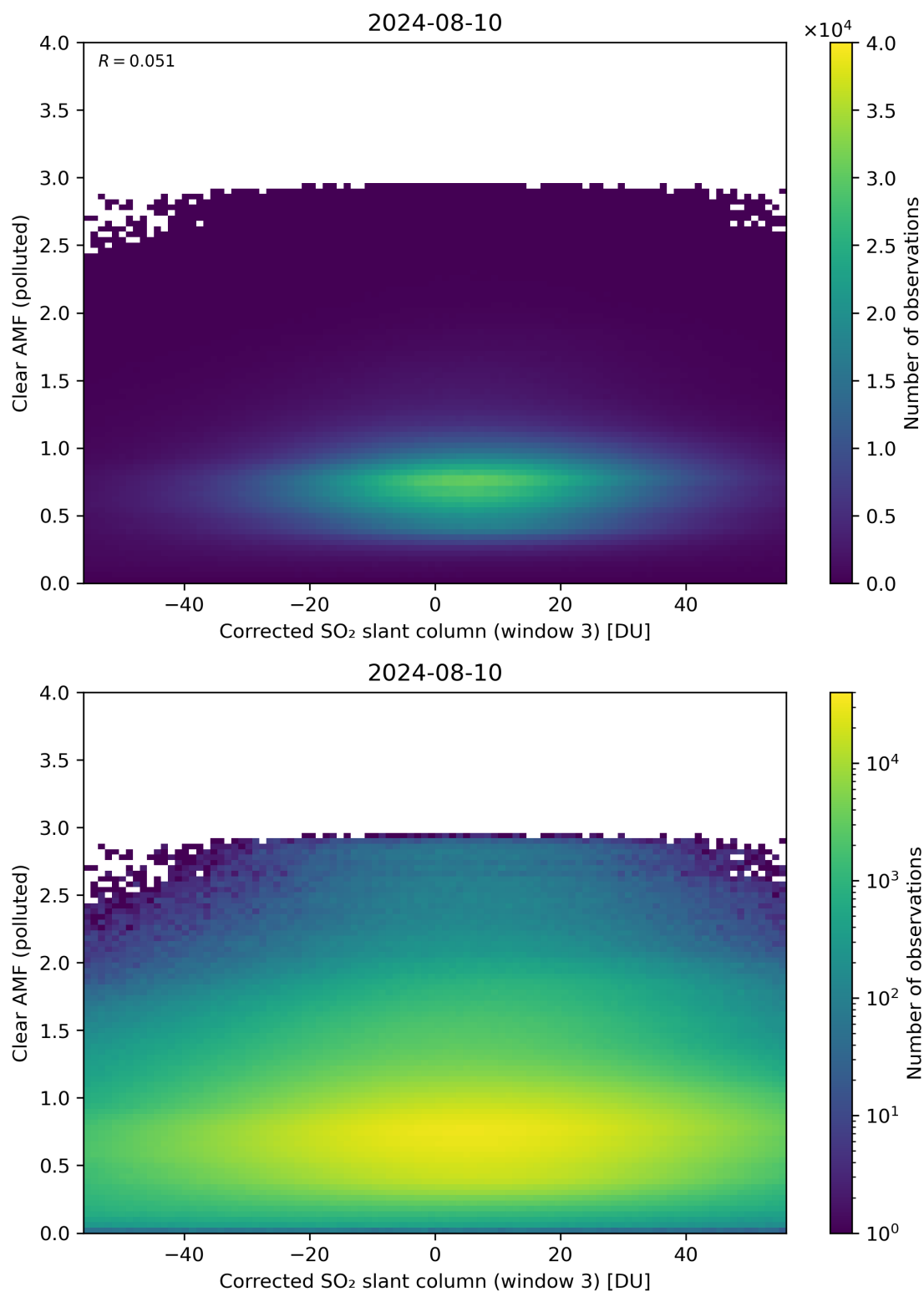
Figure 209: Scatter density plot of “Corrected SO 2 slant column (window 3)” against “Clear AMF (polluted)” for 2024-08-09 to 2024-08-11.
