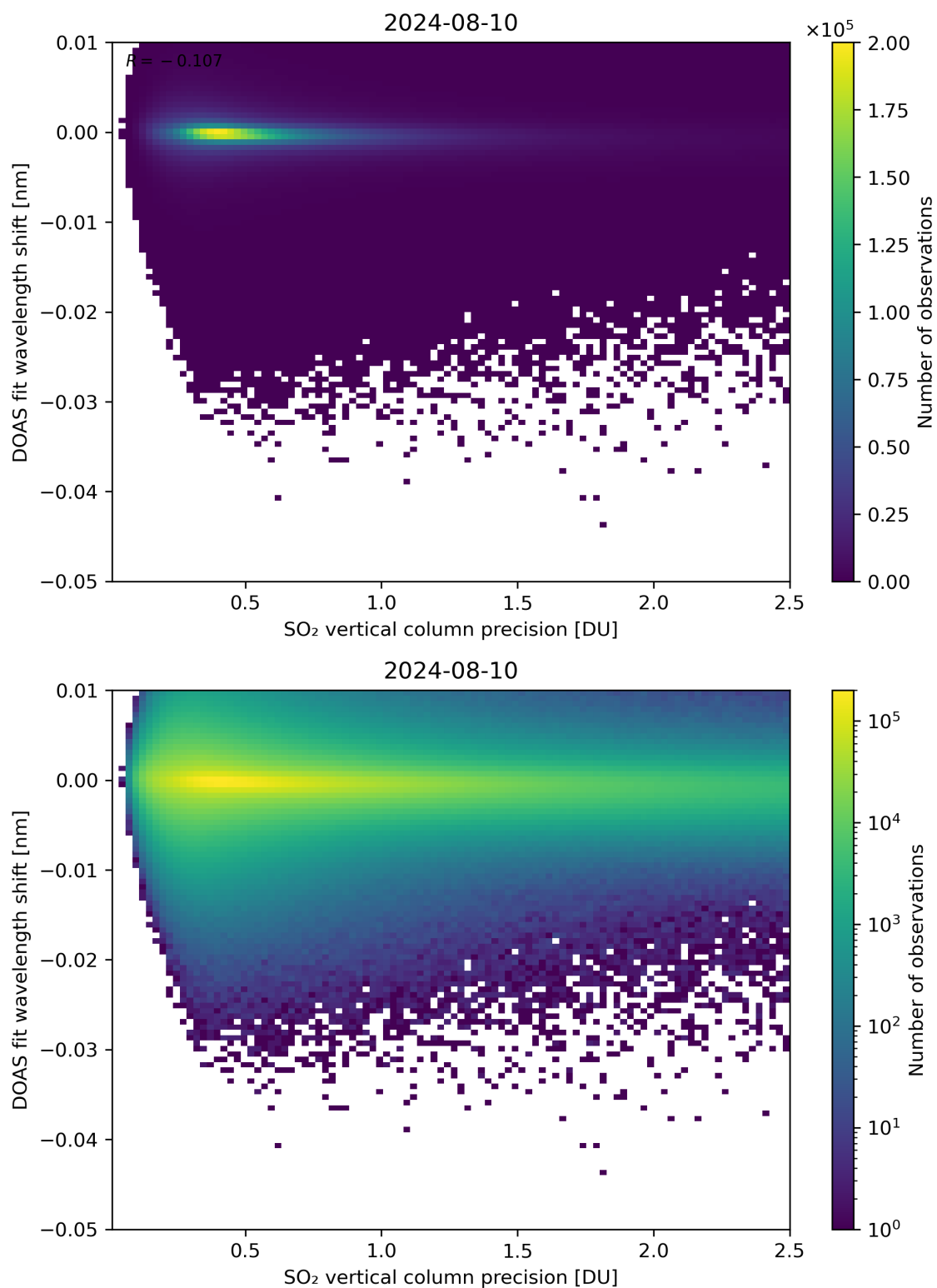
Figure 282: Scatter density plot of “SO 2 vertical column precision” against “DOAS fit wavelength shift” for 2024-08-09 to 2024-08-11.
