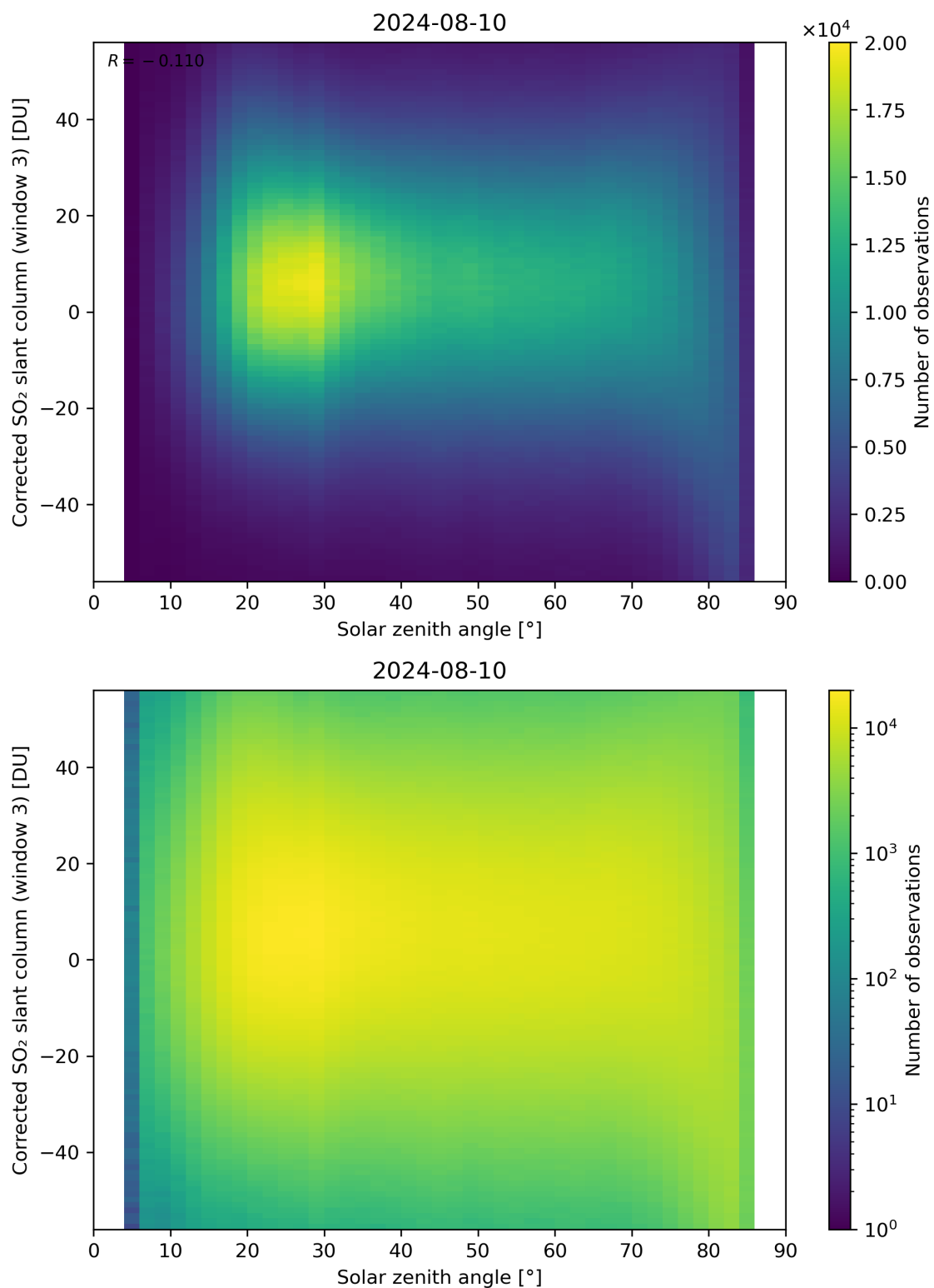
Figure 168: Scatter density plot of “Solar zenith angle” against “Corrected SO 2 slant column (window 3)” for 2024-08-09 to 2024-08-11.
