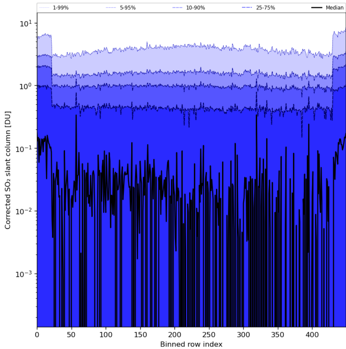
Figure 78: Along track statistics of “Corrected SO 2 slant column” for 2024-08-09 to 2024-08-11
