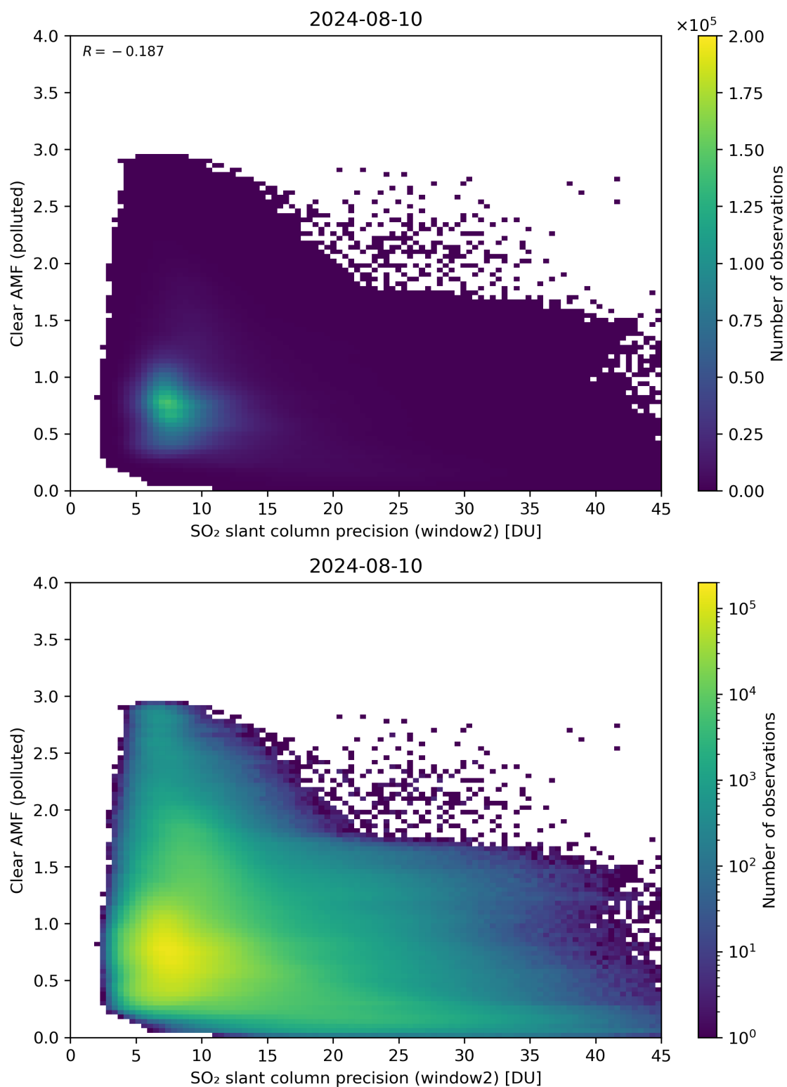
Figure 246: Scatter density plot of “SO 2 slant column precision (window2)” against “Clear AMF (polluted)” for 2024-08-09 to 2024-08-11.
