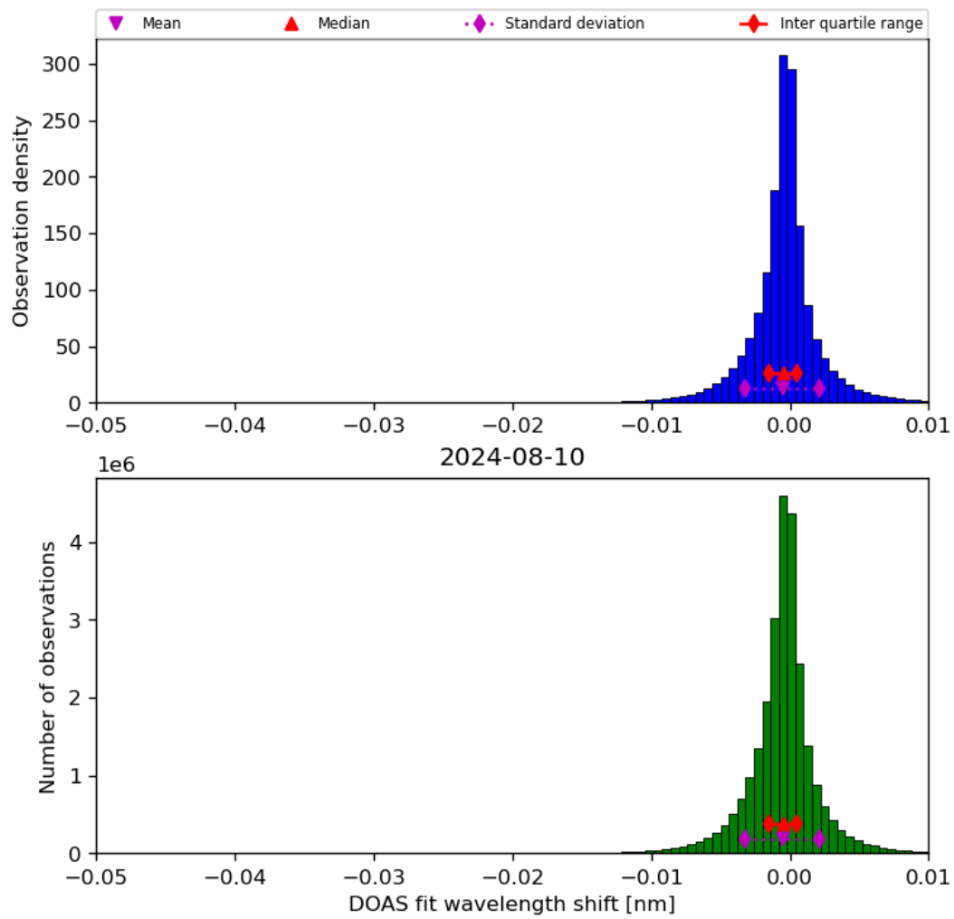
Figure 68: Histogram of “DOAS fit wavelength shift” for 2024-08-09 to 2024-08-11
