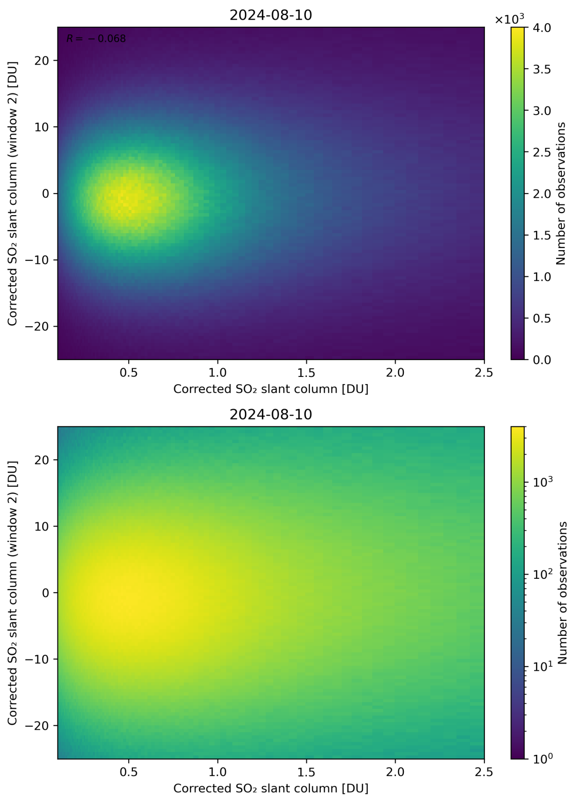
Figure 185: Scatter density plot of “Corrected SO 2 slant column” against “Corrected SO 2 slant column (window 2)” for 2024-08-09 to 2024-08-11.
