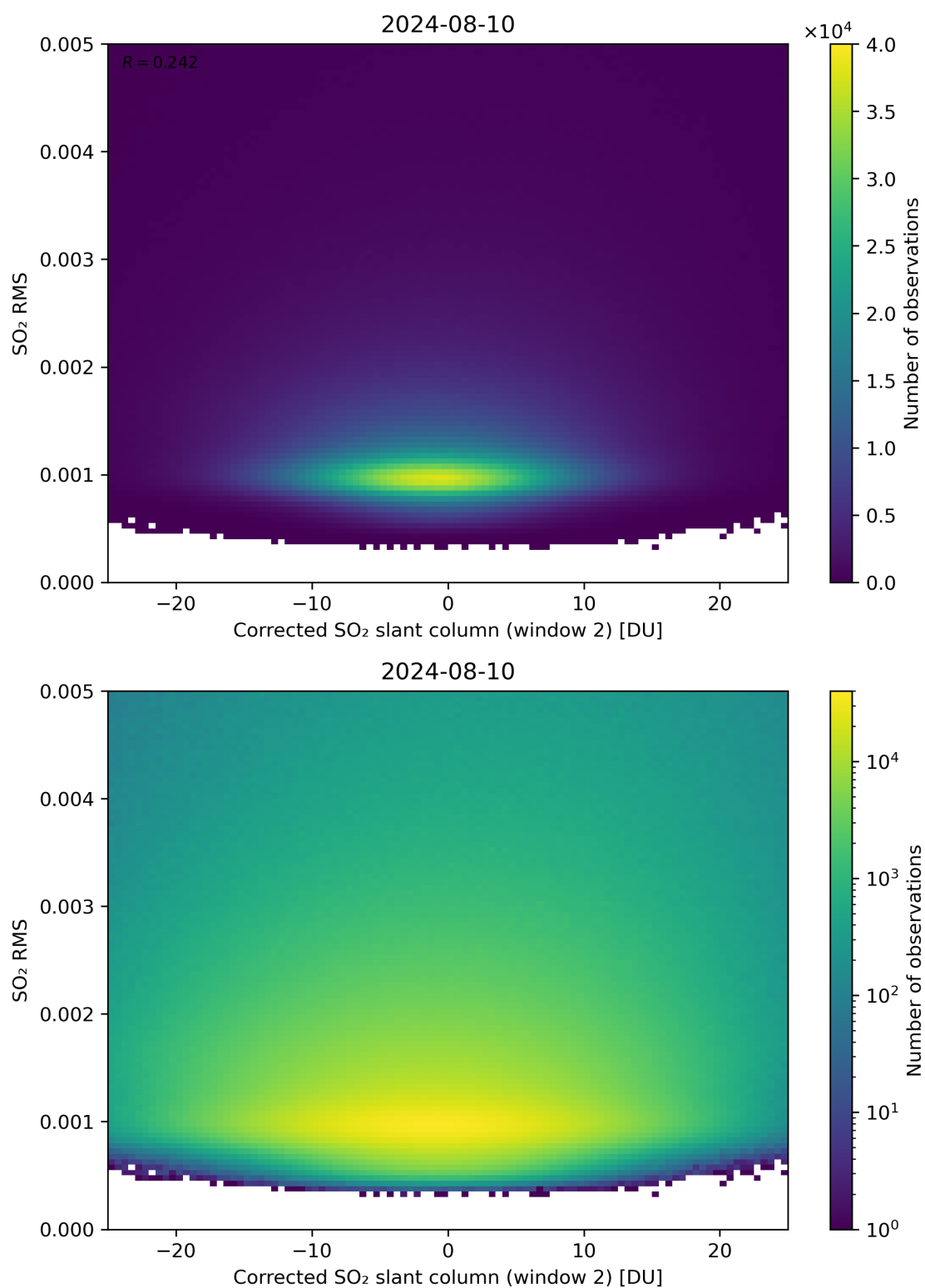
Figure 198: Scatter density plot of “Corrected SO 2 slant column (window 2)” against “SO 2 RMS” for 2024-08-09 to 2024-08-11.
