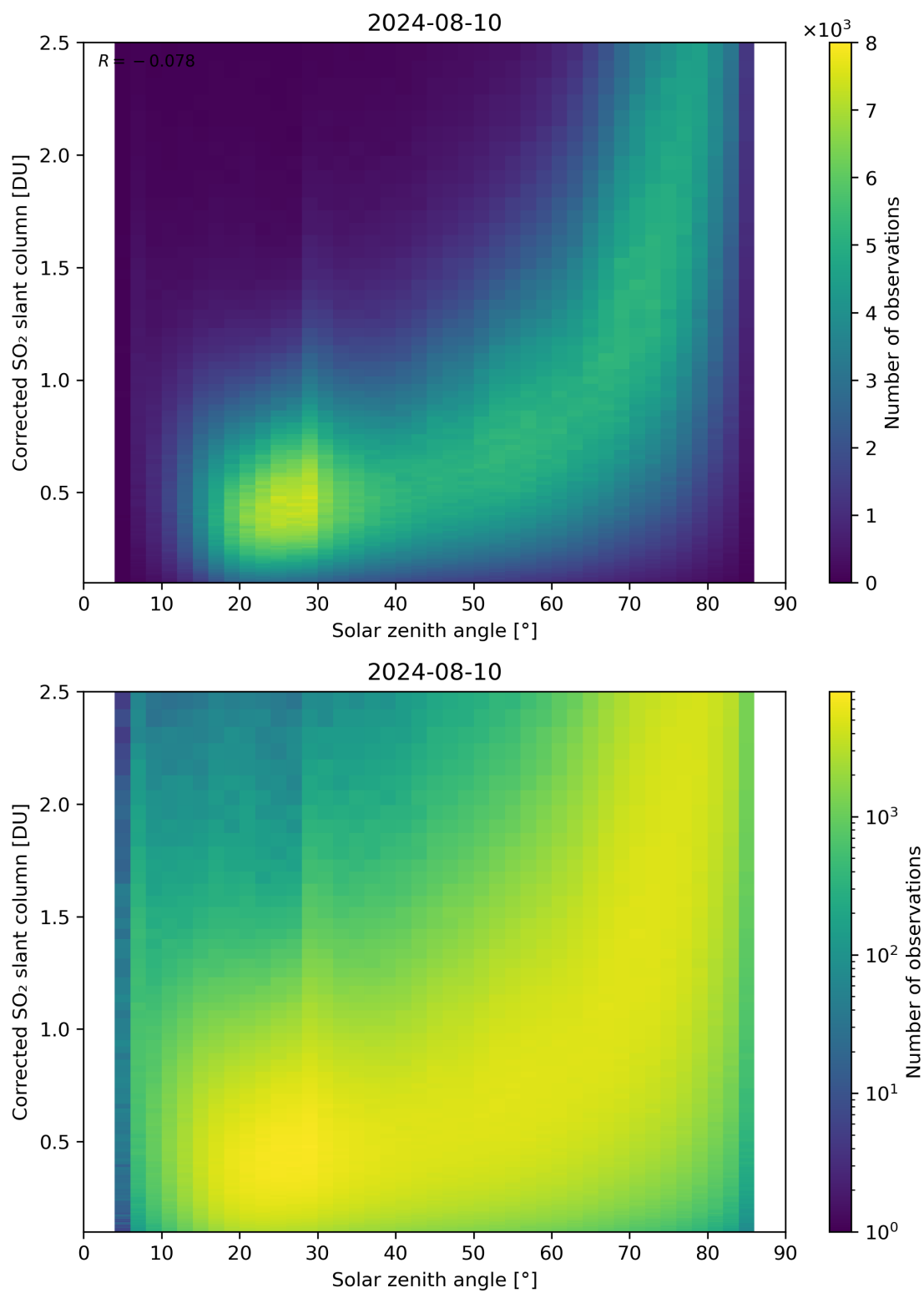
Figure 166: Scatter density plot of “Solar zenith angle” against “Corrected SO 2 slant column” for 2024-08-09 to 2024-08-11.
