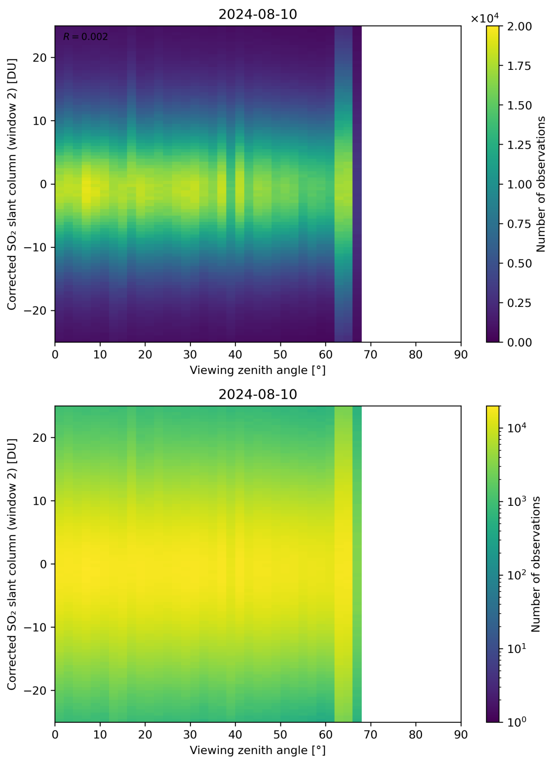
Figure 318: Scatter density plot of “Viewing zenith angle” against “Corrected SO 2 slant column (window 2)” for 2024-08-09 to 2024-08-11.
