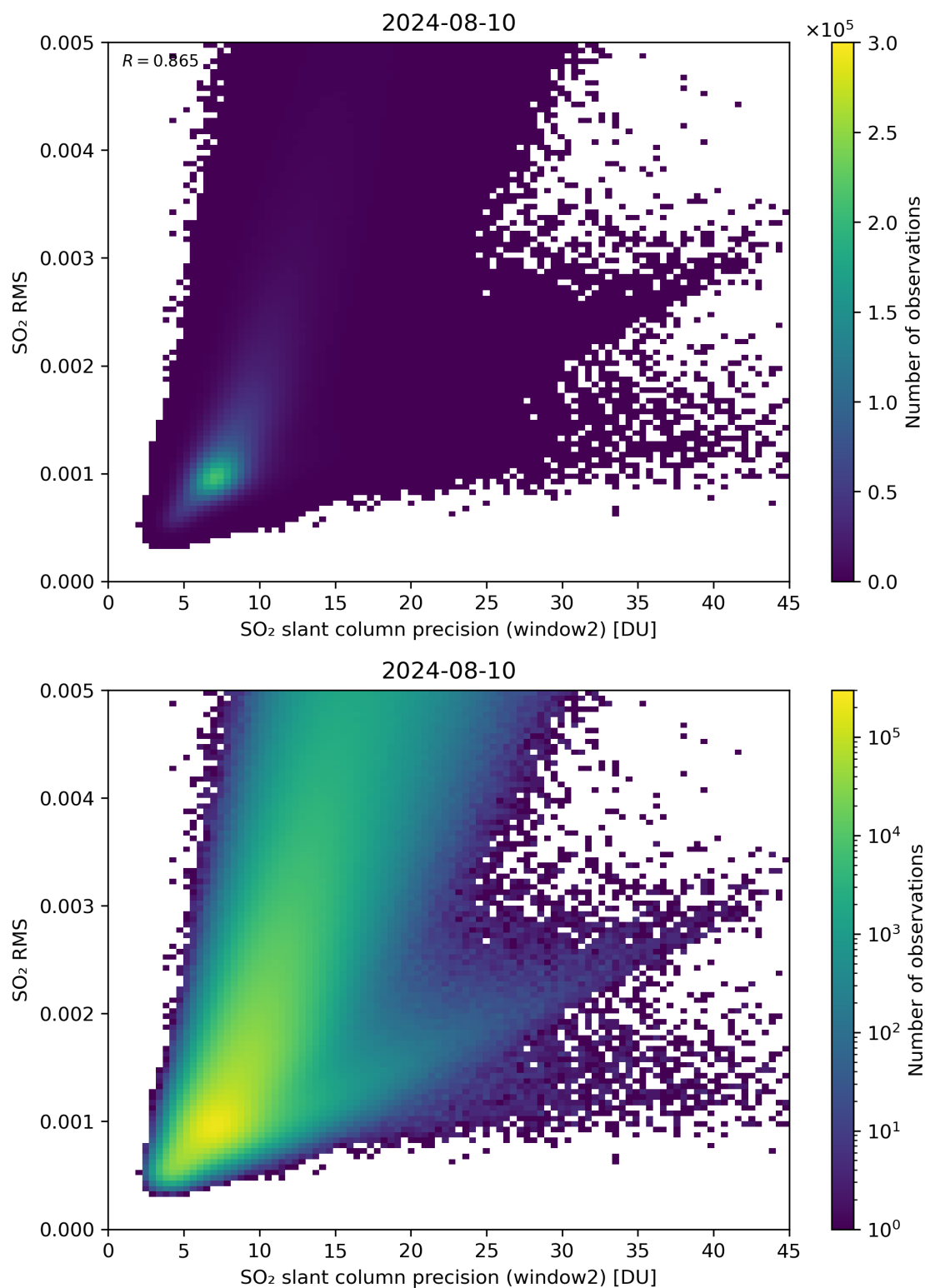
Figure 245: Scatter density plot of “SO 2 slant column precision (window2)” against “SO 2 RMS” for 2024-08-09 to 2024-08-11.
