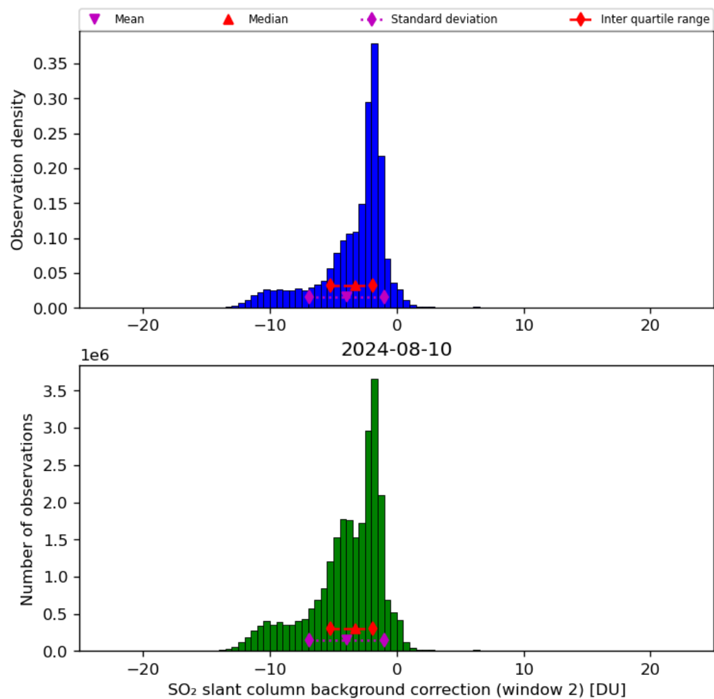
Figure 63: Histogram of “SO 2 slant column background correction (window 2)” for 2024-08-09 to 2024-08-11
