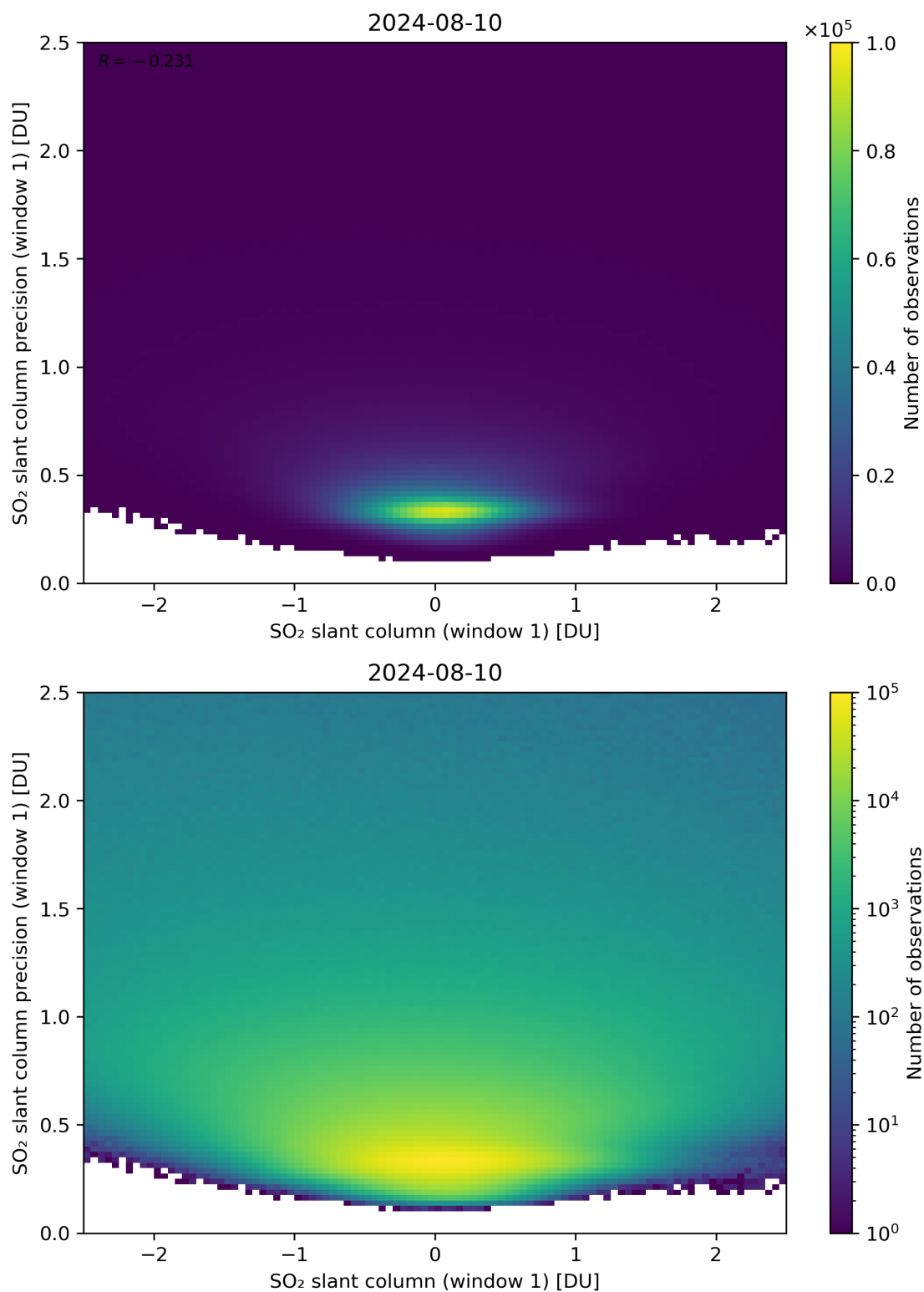
Figure 235: Scatter density plot of “SO 2 slant column (window 1)” against “SO 2 slant column precision (window 1)” for 2024-08-09 to 2024-08-11.
