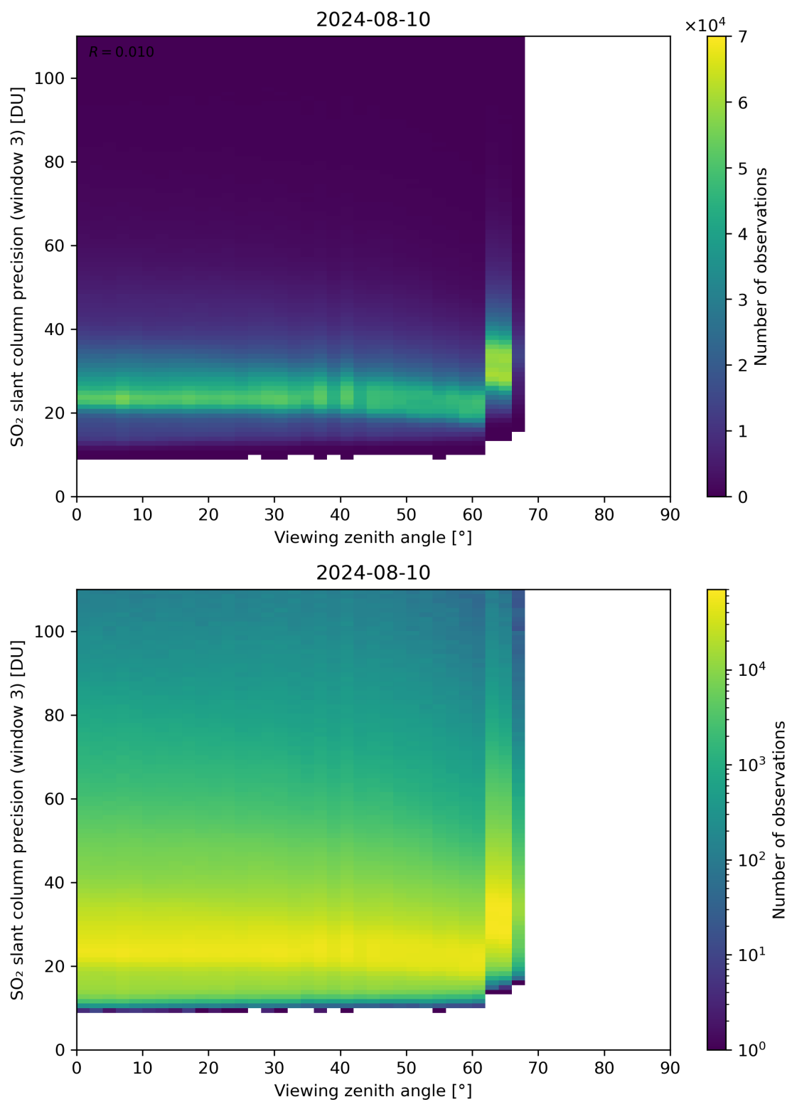
Figure 324: Scatter density plot of “Viewing zenith angle” against “SO 2 slant column precision (window 3)” for 2024-08-09 to 2024-08-11.
