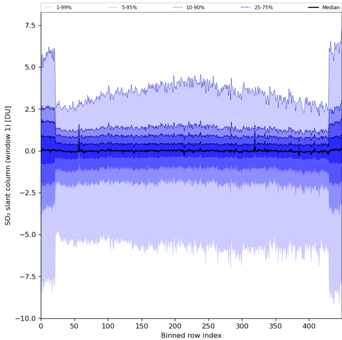
Figure 79: Along track statistics of “SO 2 slant column (window 1)” for 2024-08-09 to 2024-08-11
