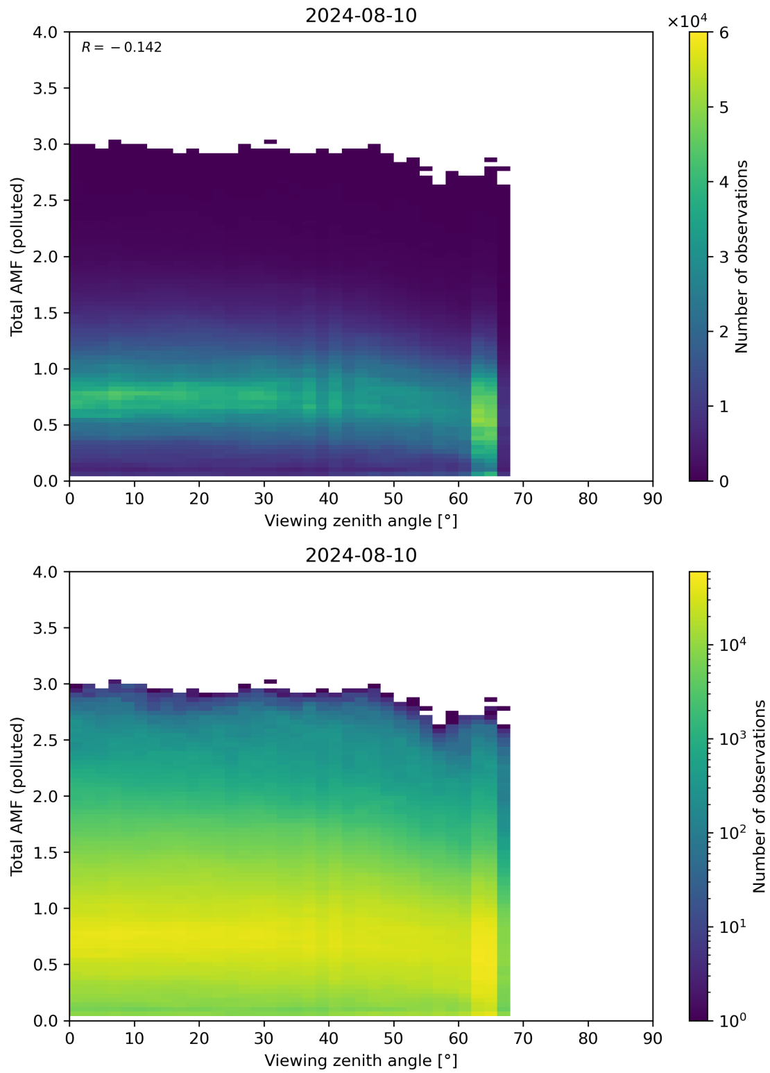
Figure 325: Scatter density plot of “Viewing zenith angle” against “Total AMF (polluted)” for 2024-08-09 to 2024-08-11.
