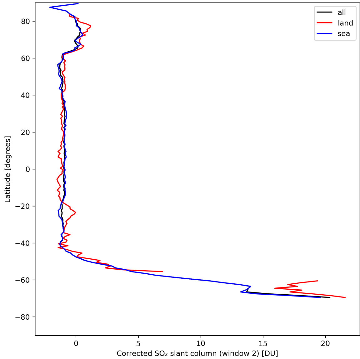
Figure 39: Zonal average of “Corrected SO 2 slant column (window 2)” for 2024-08-09 to 2024-08-11.
