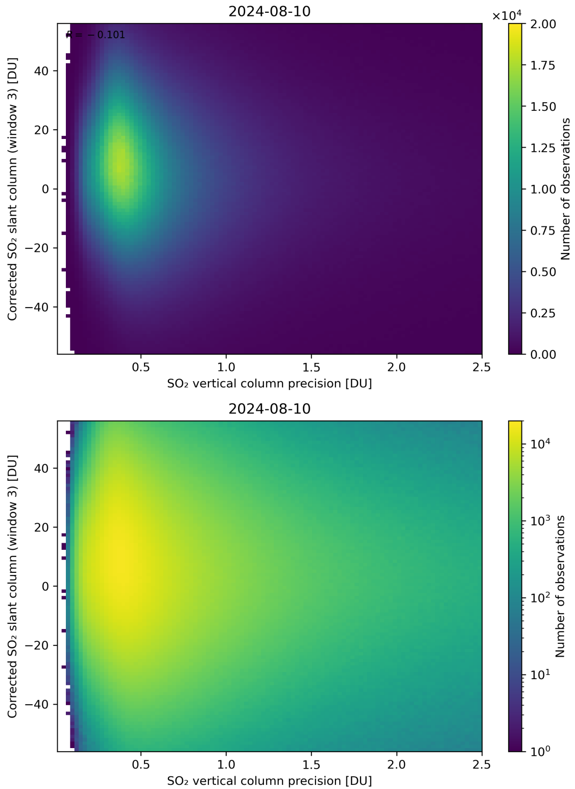
Figure 288: Scatter density plot of “SO 2 vertical column precision” against “Corrected SO 2 slant column (window 3)” for 2024-08-09 to 2024-08-11.
