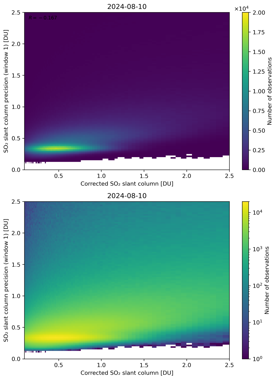
Figure 188: Scatter density plot of “Corrected SO 2 slant column” against “SO 2 slant column precision (window 1)” for 2024-08-09 to 2024-08-11.
