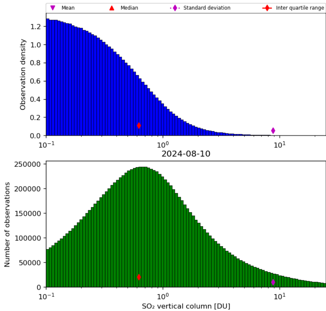
Figure 53: Histogram of “SO 2 vertical column” for 2024-08-09 to 2024-08-11
