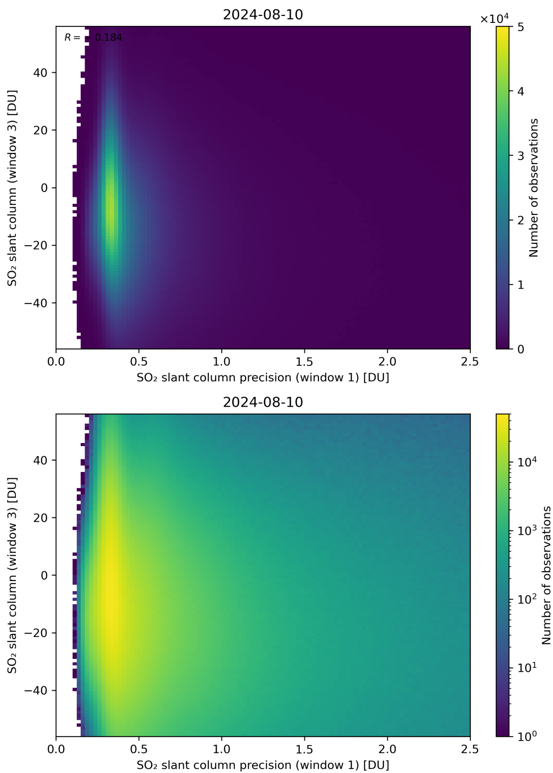
Figure 228: Scatter density plot of “SO 2 slant column precision (window 1)” against “SO 2 slant column (window 3)” for 2024-08-09 to 2024-08-11.
