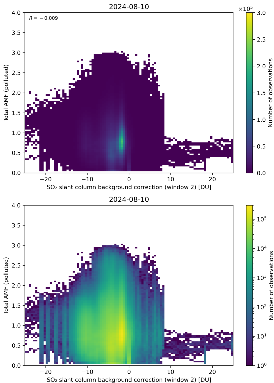
Figure 119: Scatter density plot of “SO 2 slant column background correction (window 2)” against “Total AMF (polluted)” for 2024-08-09 to 2024-08-11.
