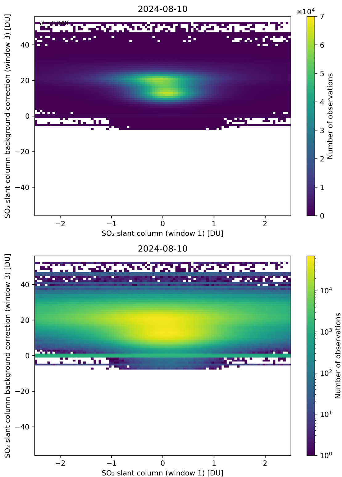
Figure 214: Scatter density plot of “SO 2 slant column (window 1)” against “SO 2 slant column background correction (window 3)” for 2024-08-09 to 2024-08-11.
