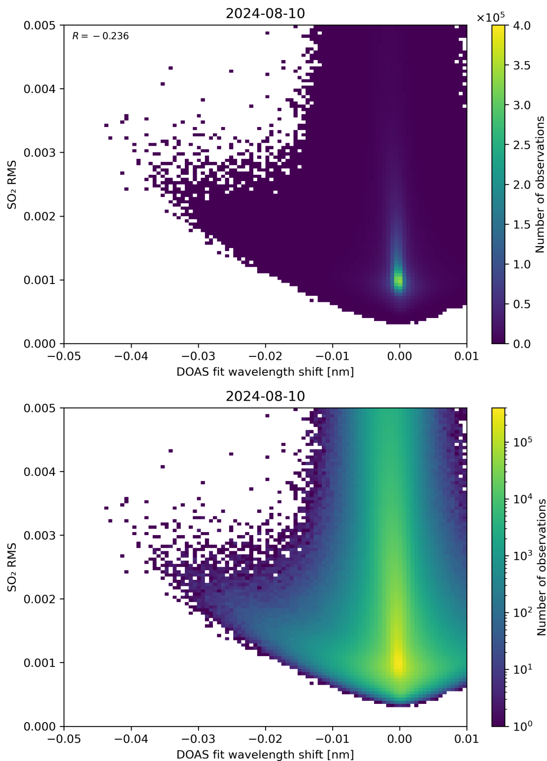
Figure 128: Scatter density plot of “DOAS fit wavelength shift” against “SO 2 RMS” for 2024-08-09 to 2024-08-11.
