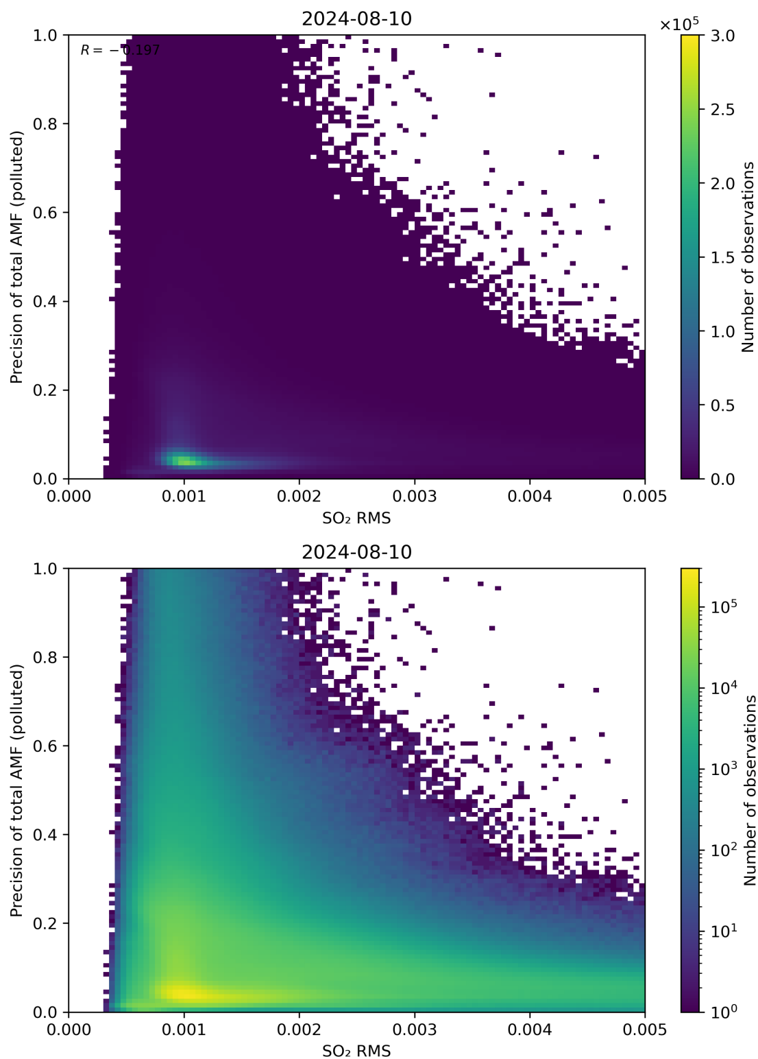
Figure 138: Scatter density plot of “SO 2 RMS” against “Precision of total AMF (polluted)” for 2024-08-09 to 2024-08-11.
