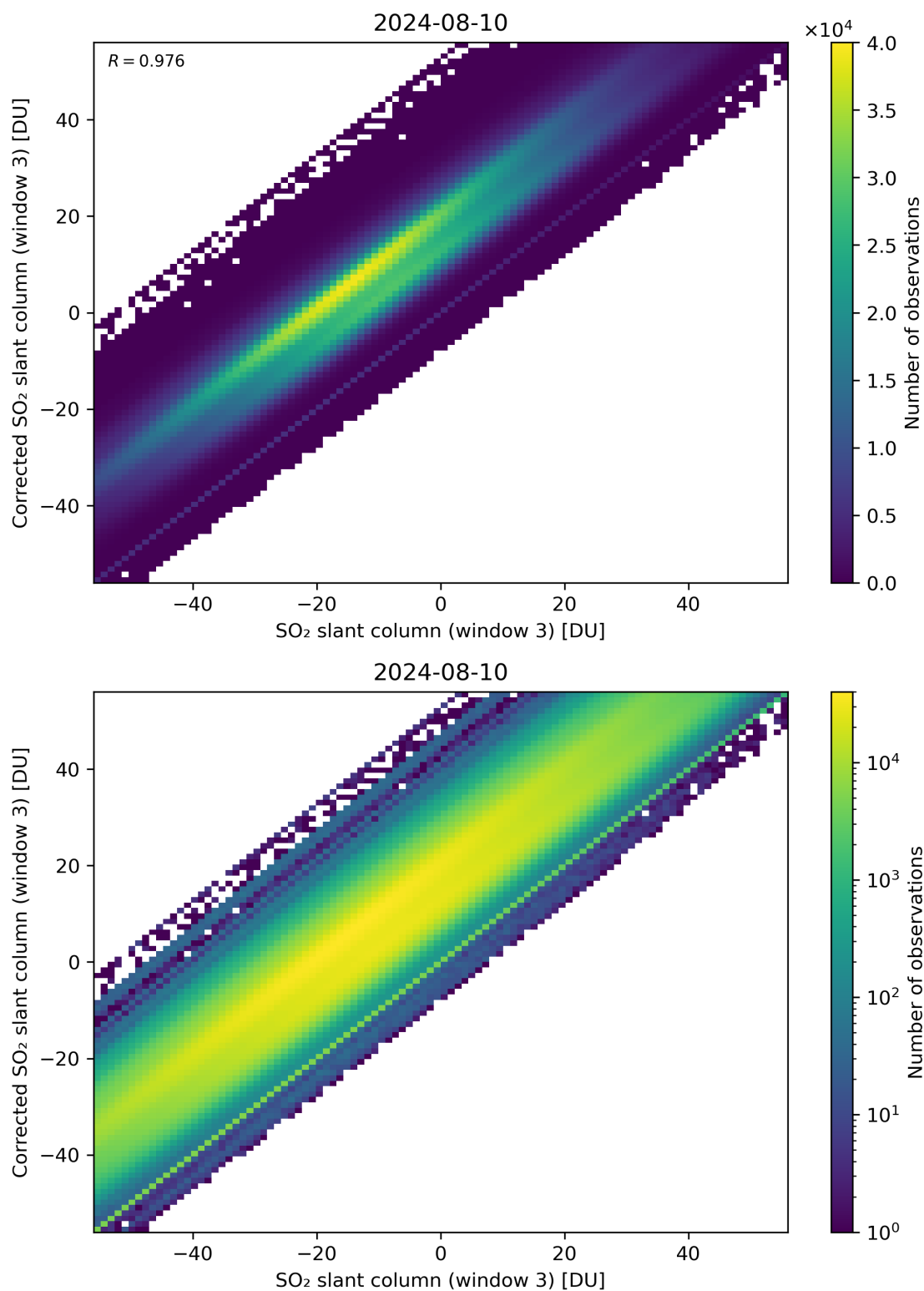
Figure 266: Scatter density plot of “SO 2 slant column (window 3)” against “Corrected SO 2 slant column (window 3)” for 2024-08-09 to 2024-08-11.
