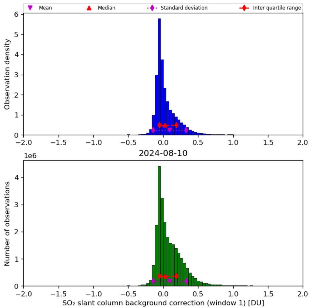
Figure 59: Histogram of “SO 2 slant column background correction (window 1)” for 2024-08-09 to 2024-08-11
