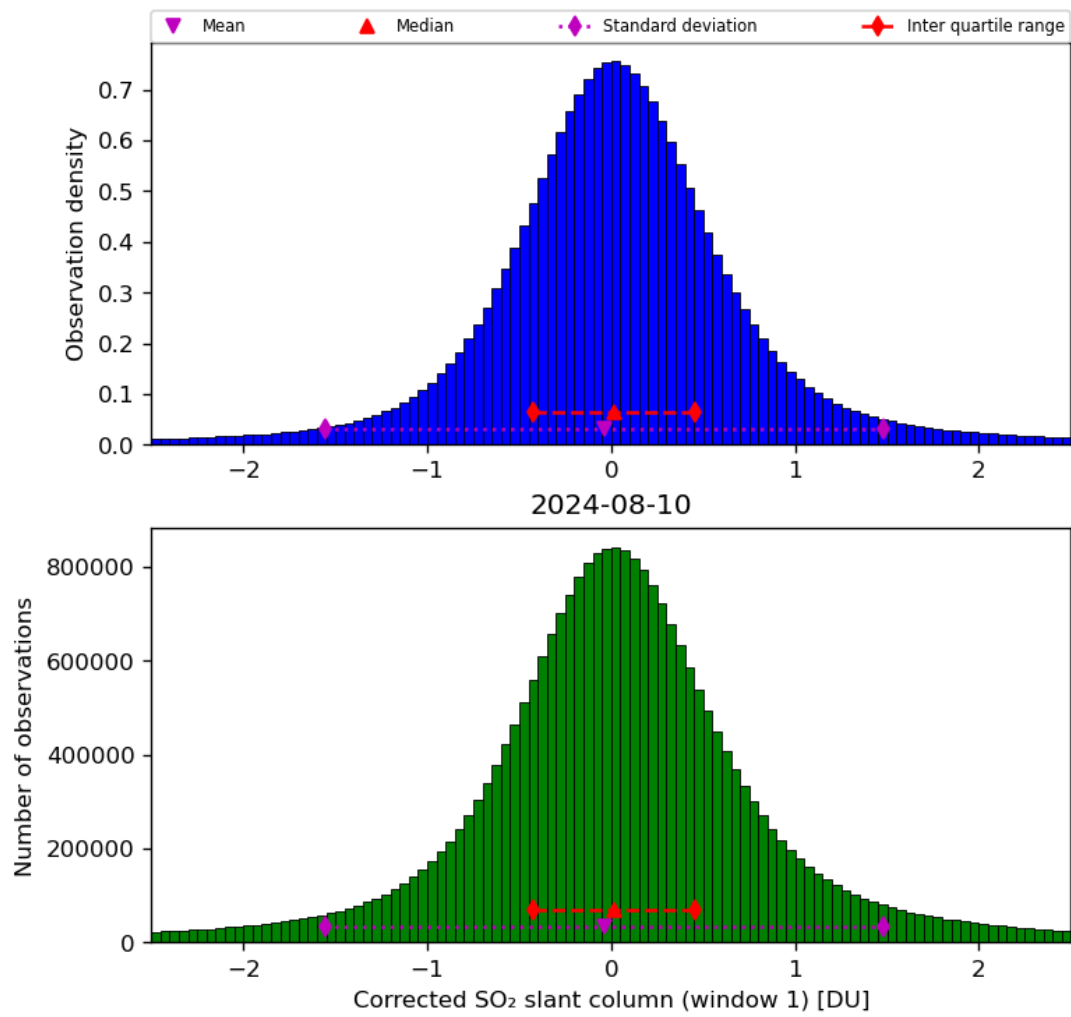
Figure 58: Histogram of “Corrected SO 2 slant column (window 1)” for 2024-08-09 to 2024-08-11
