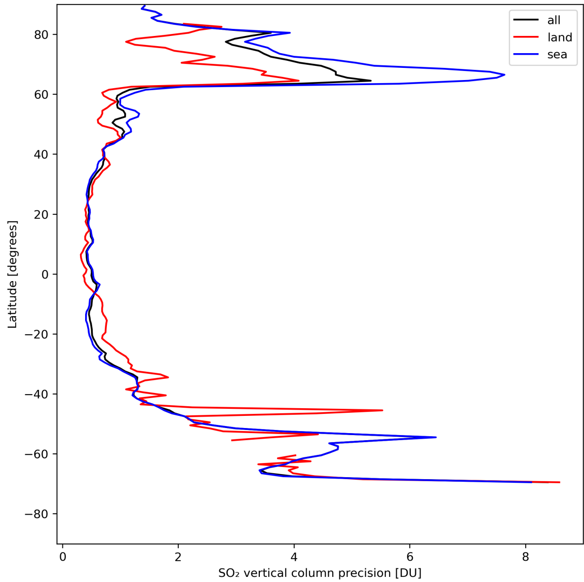
Figure 31: Zonal average of “SO 2 vertical column precision” for 2024-08-09 to 2024-08-11.
