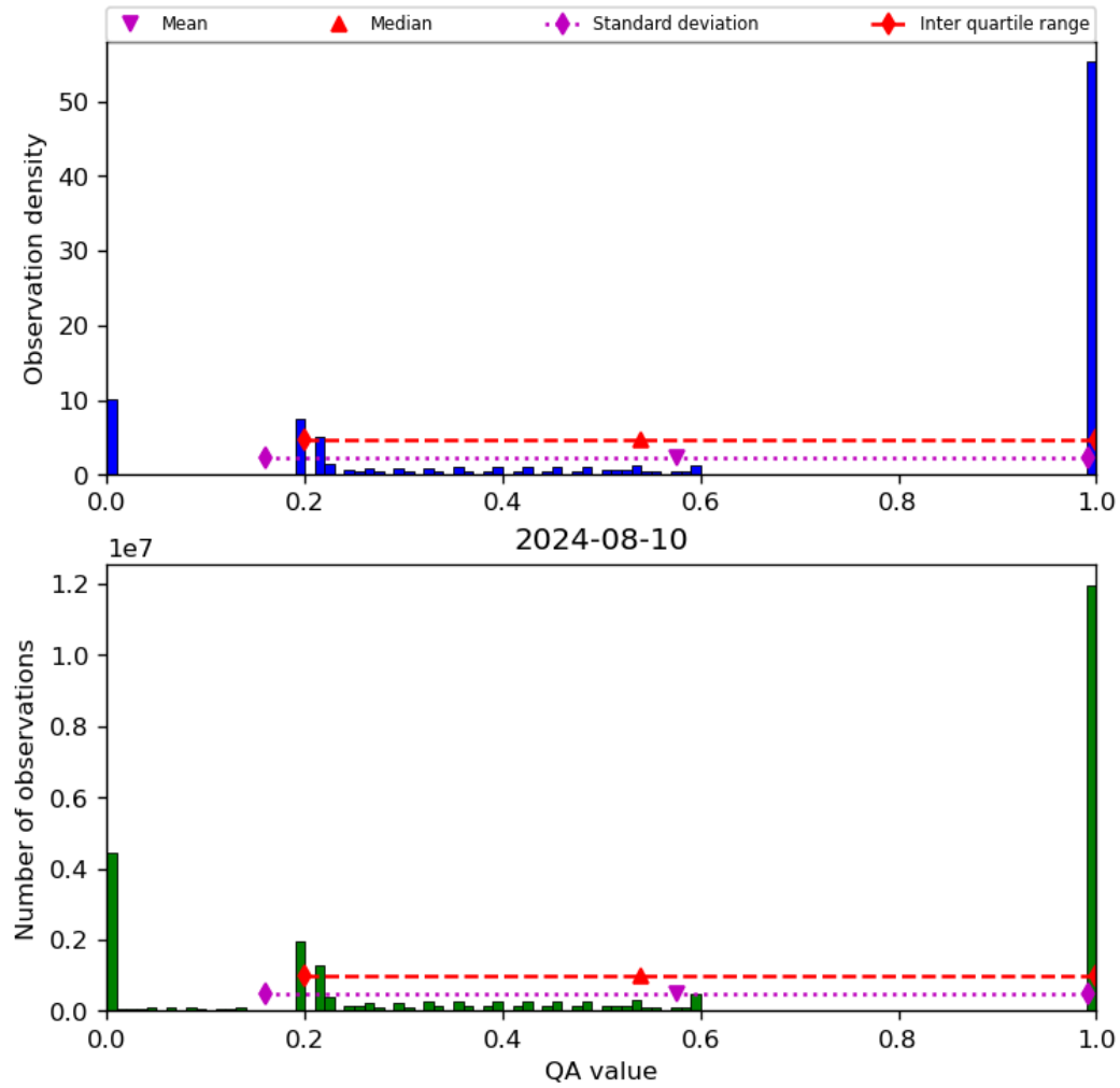
Figure 52: Histogram of “QA value” for 2024-08-09 to 2024-08-11
