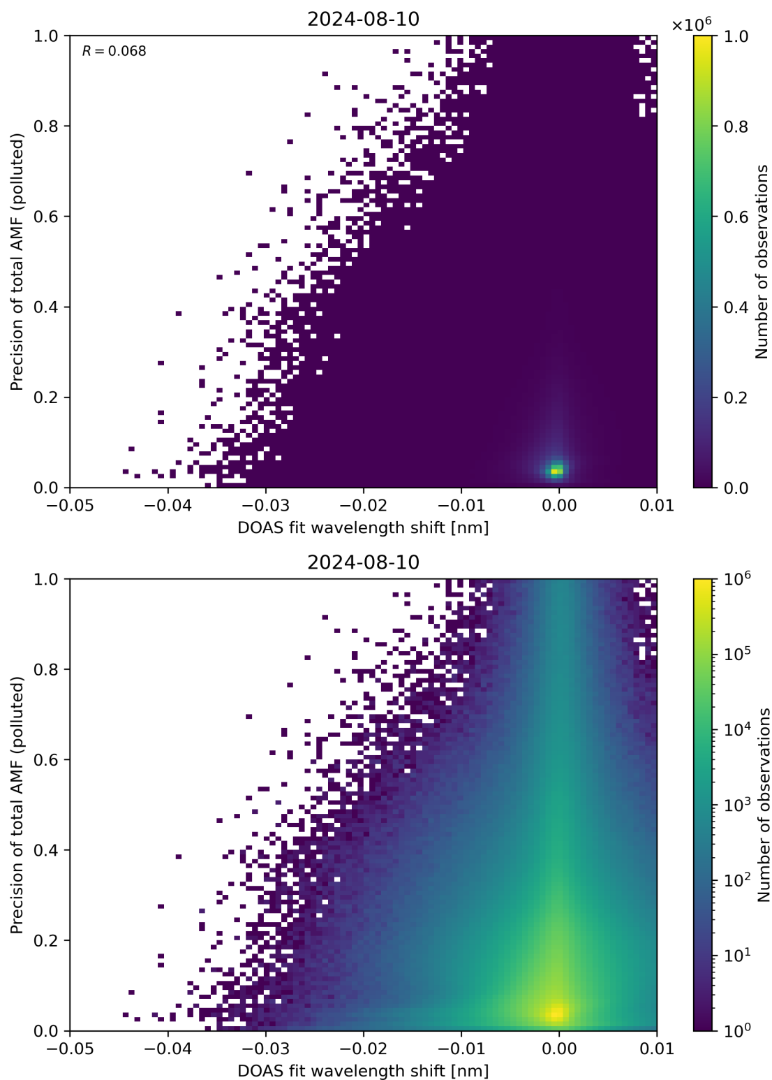
Figure 131: Scatter density plot of “DOAS fit wavelength shift” against “Precision of total AMF (polluted)” for 2024-08-09 to 2024-08-11.
