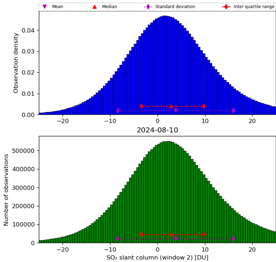
Figure 60: Histogram of “SO 2 slant column (window 2)” for 2024-08-09 to 2024-08-11
