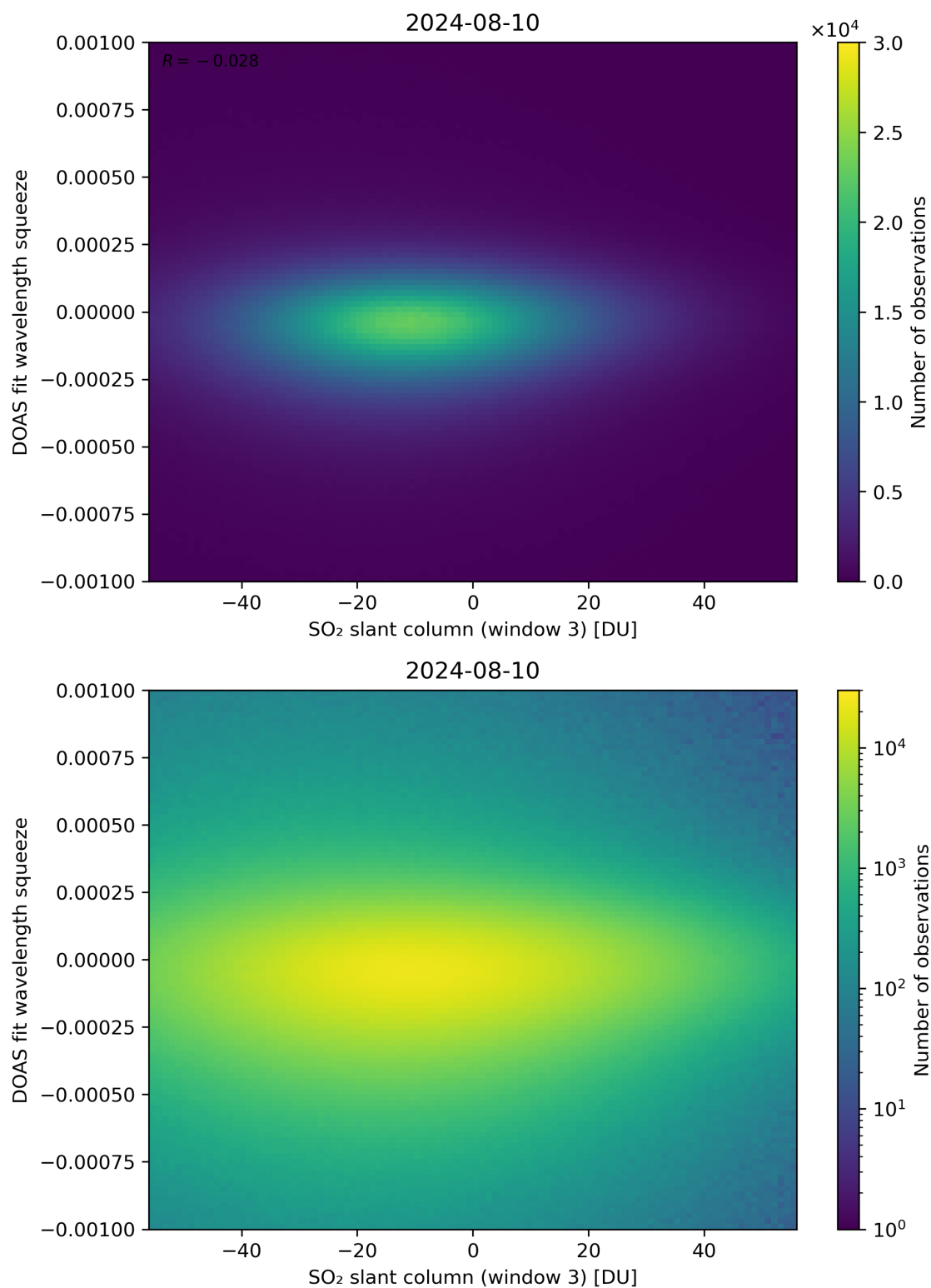
Figure 255: Scatter density plot of “SO 2 slant column (window 3)” against “DOAS fit wavelength squeeze” for 2024-08-09 to 2024-08-11.
