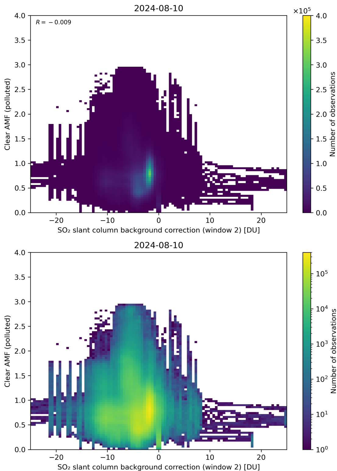
Figure 115: Scatter density plot of “SO 2 slant column background correction (window 2)” against “Clear AMF (polluted)” for 2024-08-09 to 2024-08-11.
