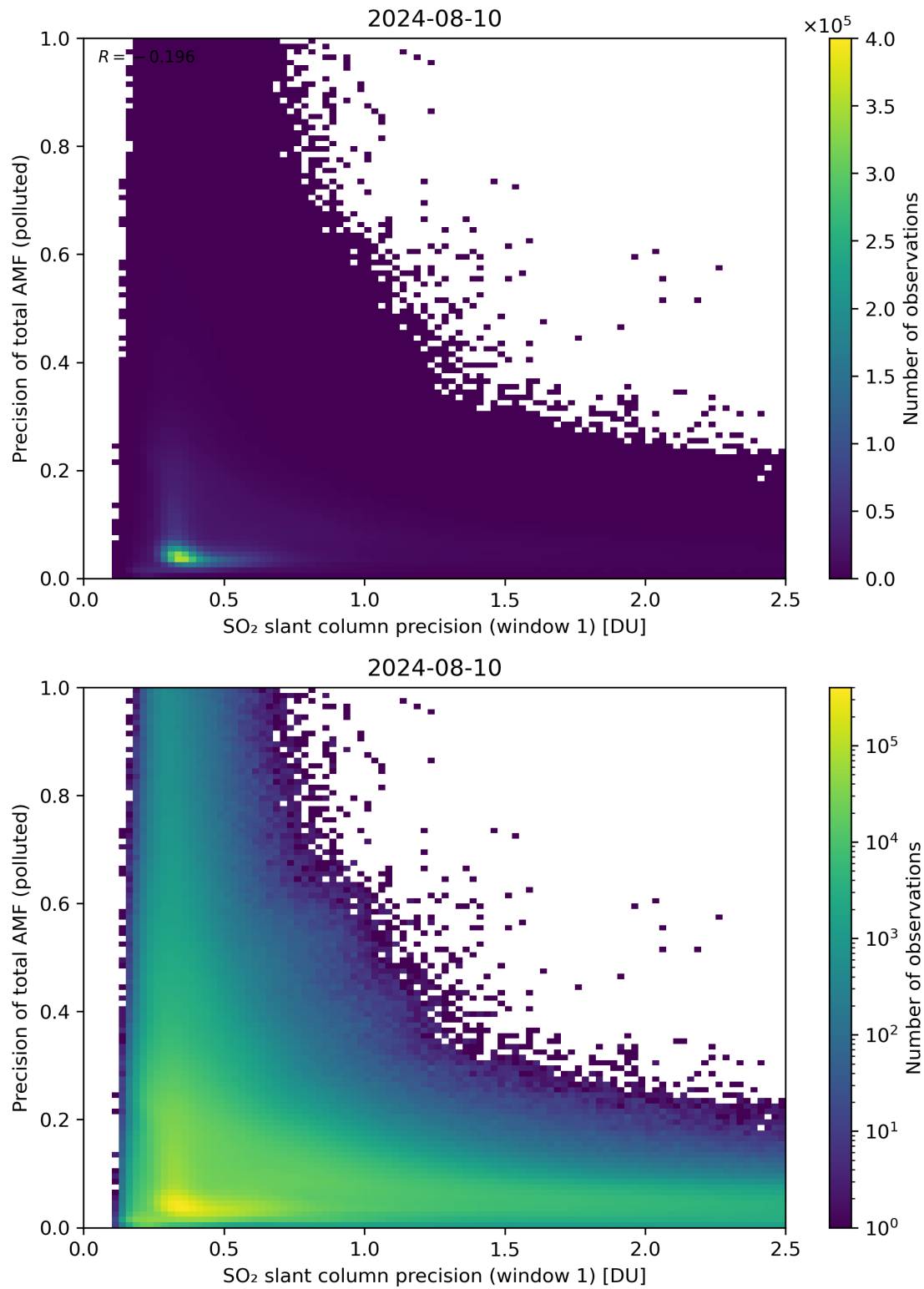
Figure 231: Scatter density plot of “SO 2 slant column precision (window 1)” against “Precision of total AMF (polluted)” for 2024-08-09 to 2024-08-11.
