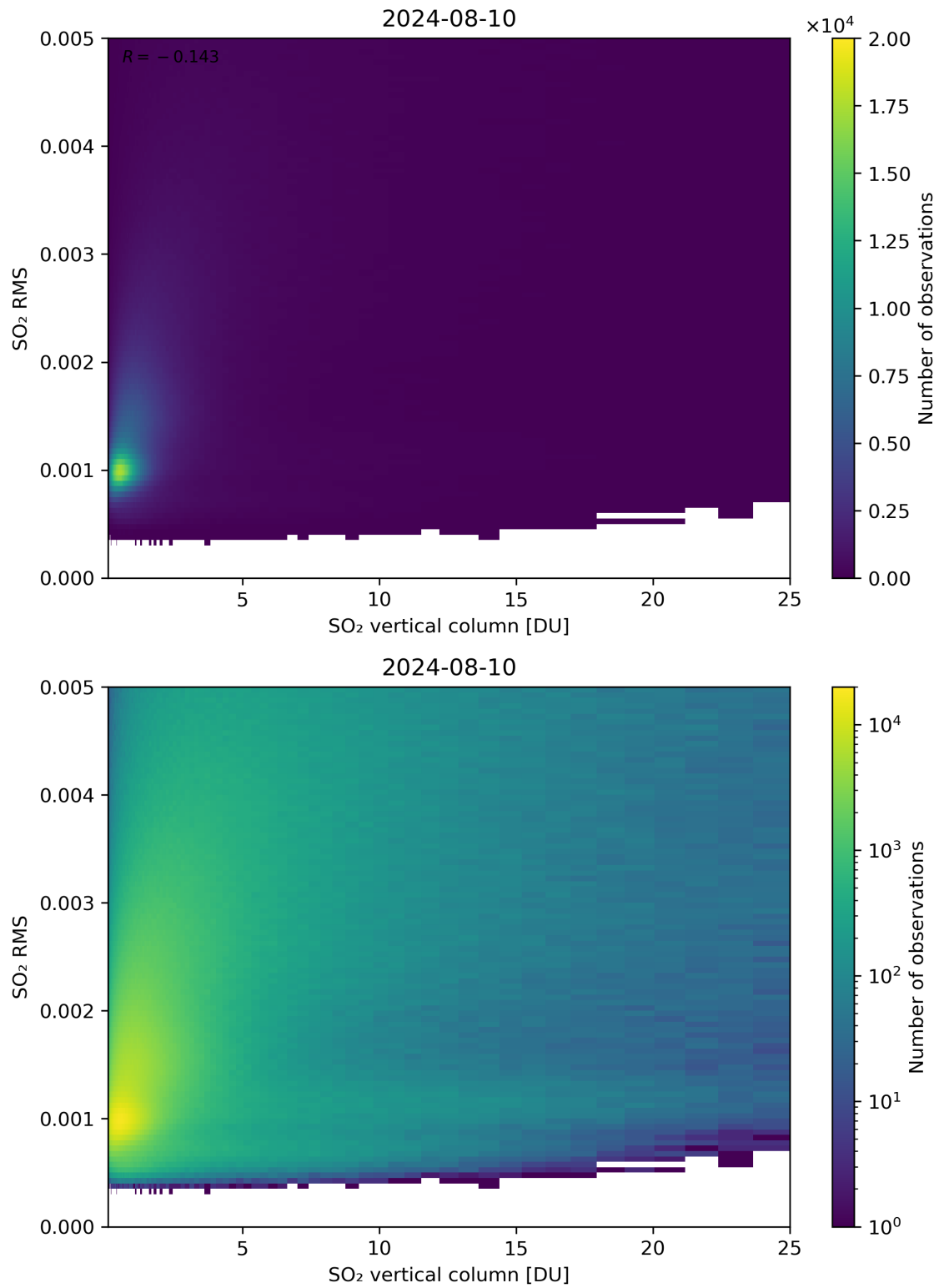
Figure 278: Scatter density plot of “SO 2 vertical column” against “SO 2 RMS” for 2024-08-09 to 2024-08-11.
