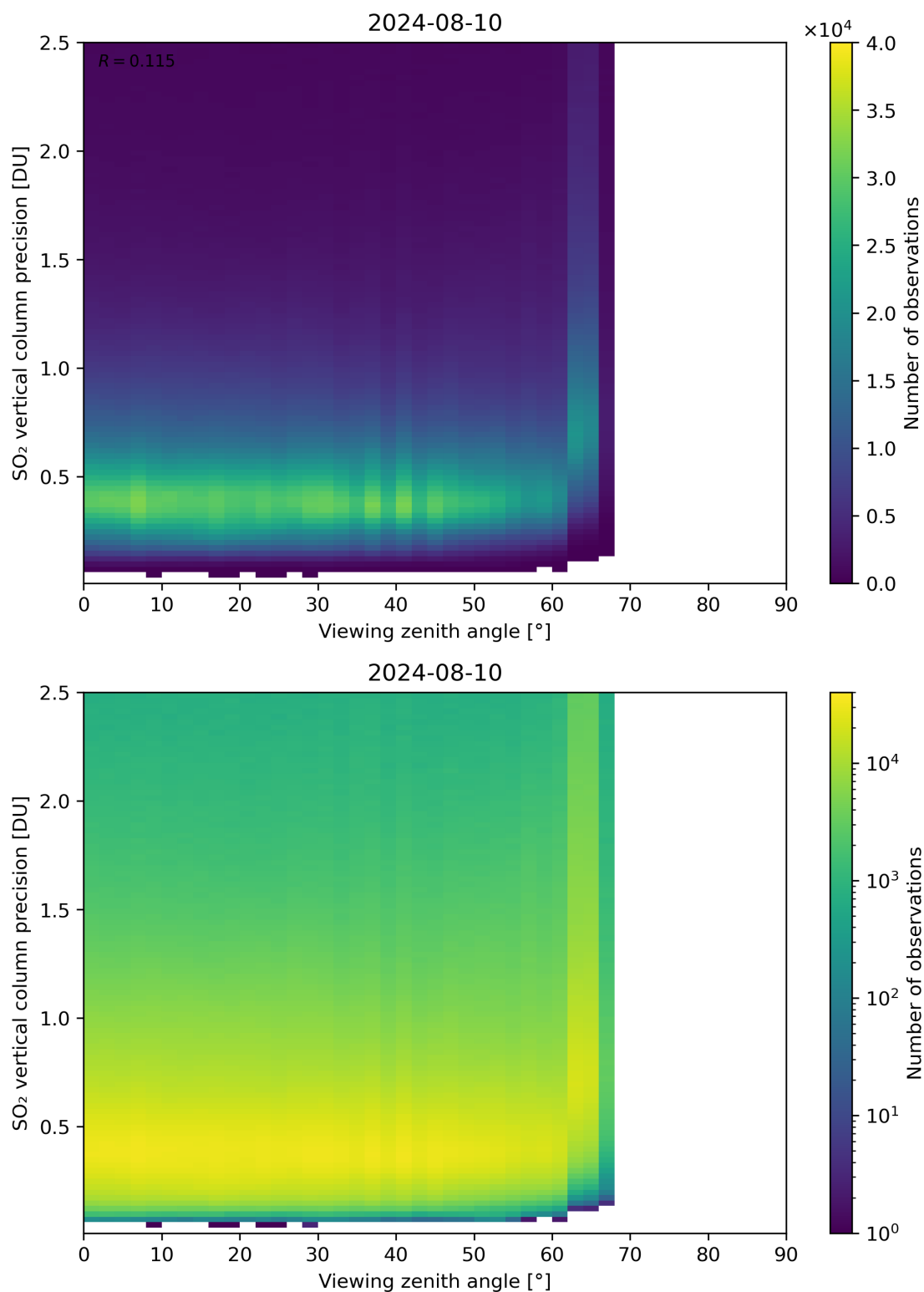
Figure 328: Scatter density plot of “Viewing zenith angle” against “SO 2 vertical column precision” for 2024-08-09 to 2024-08-11.
