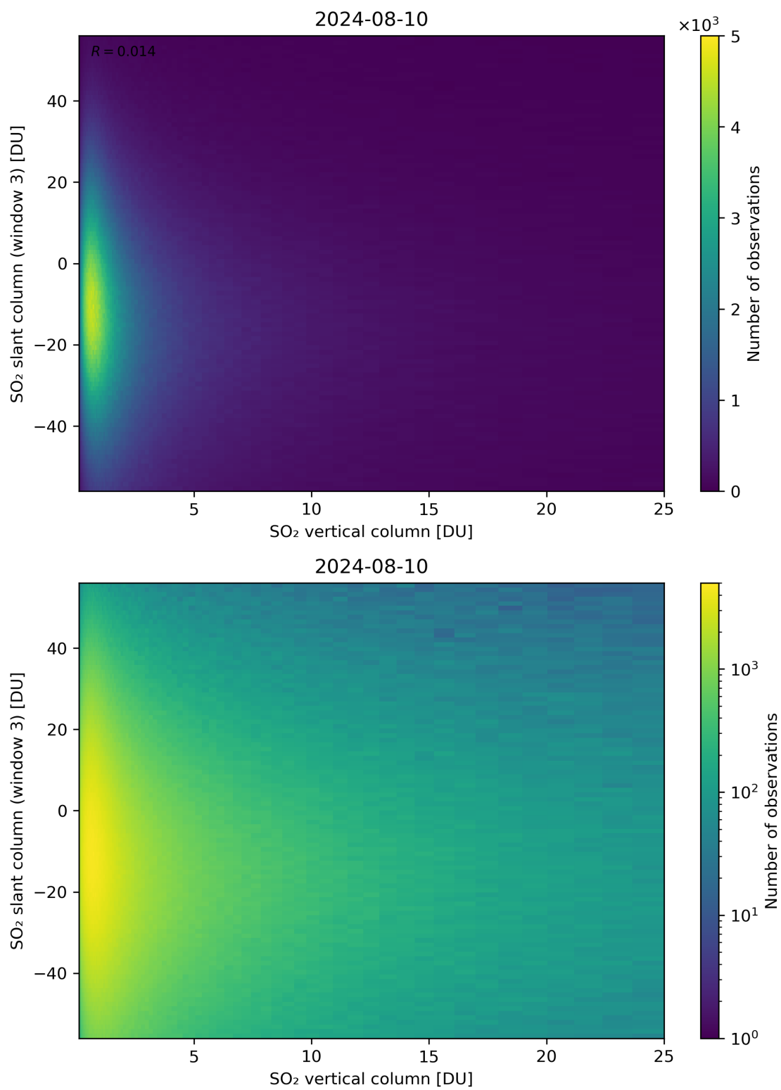
Figure 303: Scatter density plot of “SO 2 vertical column” against “SO 2 slant column (window 3)” for 2024-08-09 to 2024-08-11.
