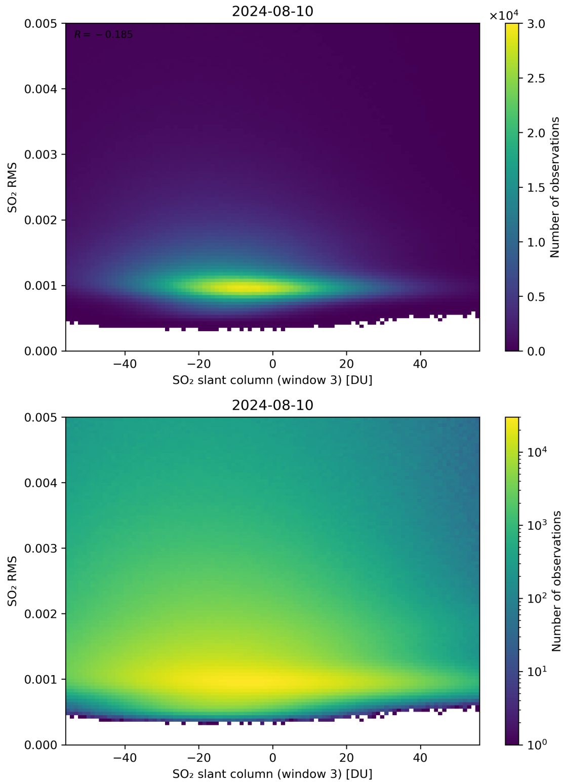
Figure 256: Scatter density plot of “SO 2 slant column (window 3)” against “SO 2 RMS” for 2024-08-09 to 2024-08-11.
