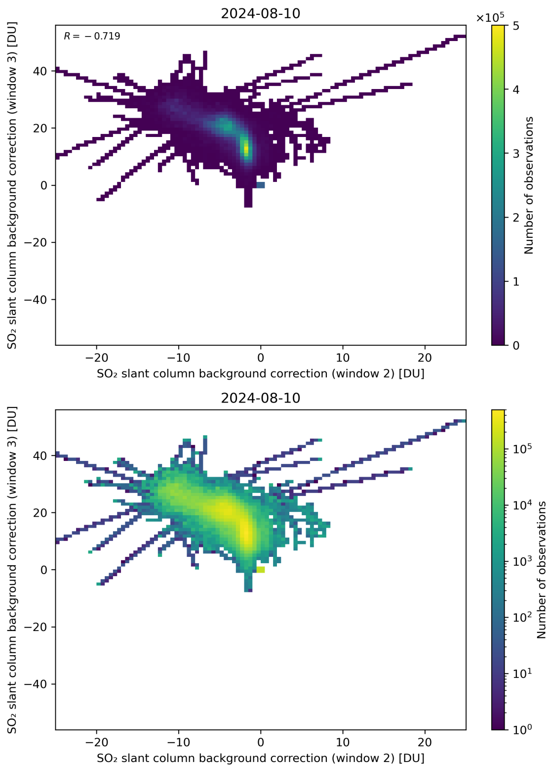
Figure 111: Scatter density plot of “SO 2 slant column background correction (window 2)” against “SO 2 slant column background correction (window 3)” for 2024-08-09 to 2024-08-11.
