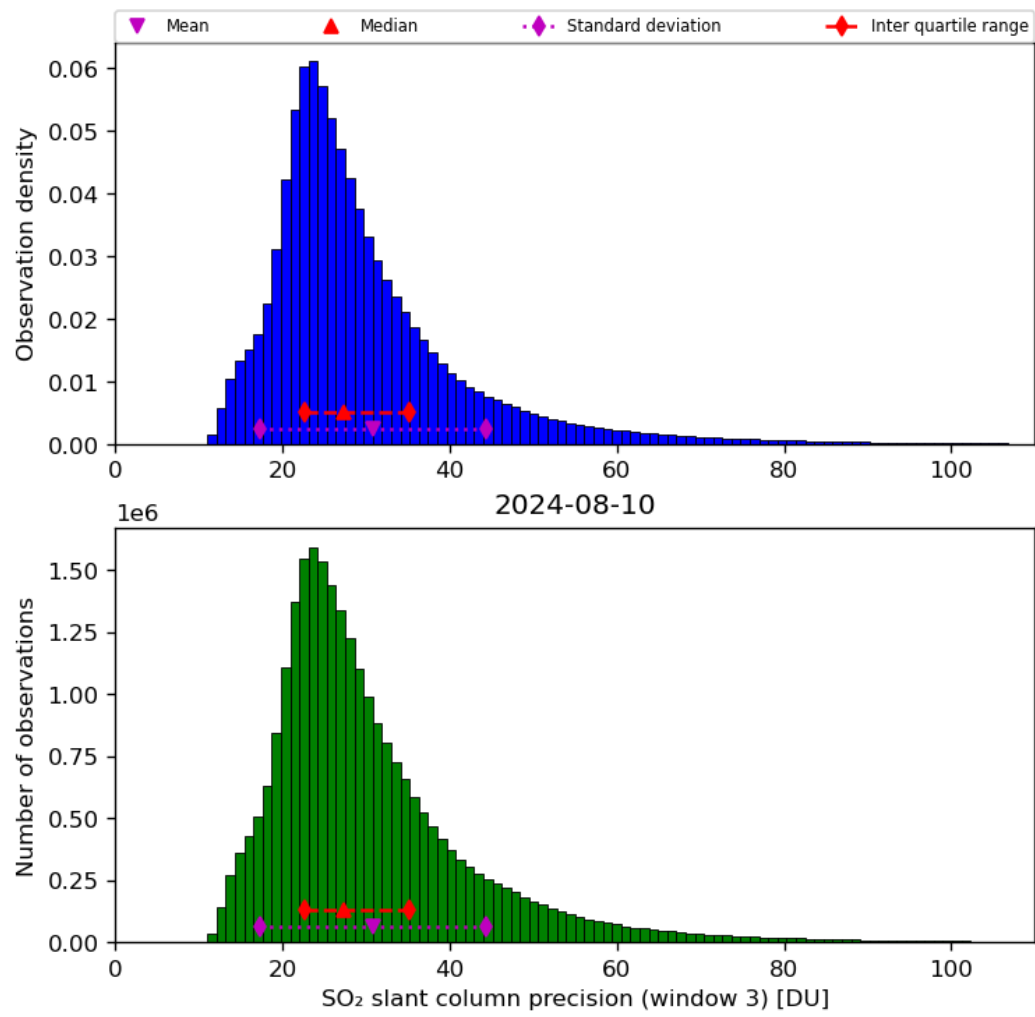
Figure 65: Histogram of “SO 2 slant column precision (window 3)” for 2024-08-09 to 2024-08-11
