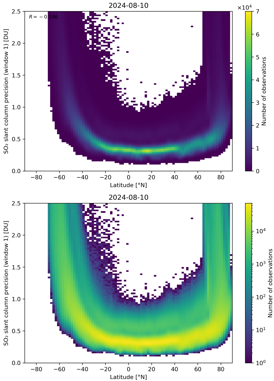
Figure 150: Scatter density plot of “Latitude” against “SO 2 slant column precision (window 1)” for 2024-08-09 to 2024-08-11.
