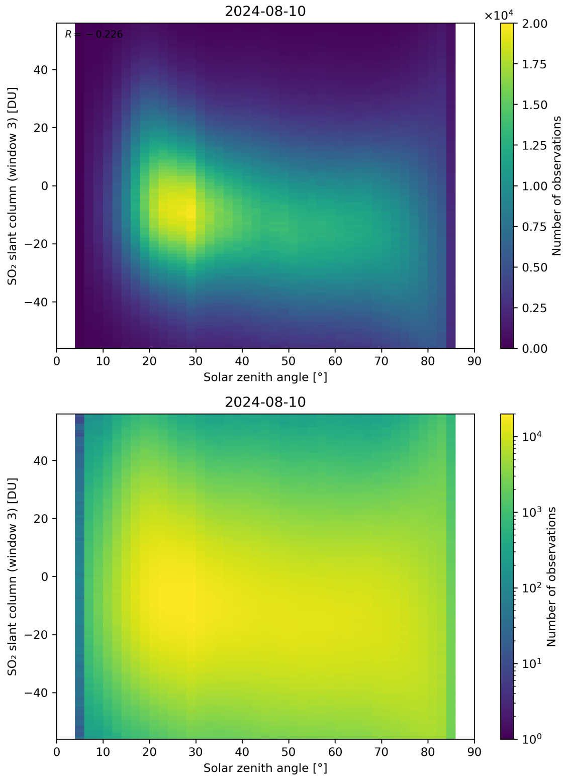
Figure 172: Scatter density plot of “Solar zenith angle” against “SO 2 slant column (window 3)” for 2024-08-09 to 2024-08-11.
