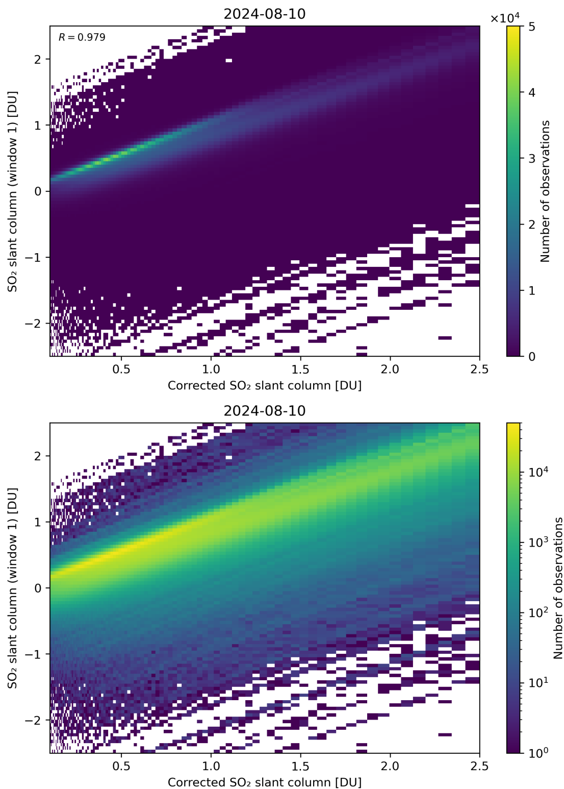
Figure 187: Scatter density plot of “Corrected SO 2 slant column” against “SO 2 slant column (window 1)” for 2024-08-09 to 2024-08-11.
