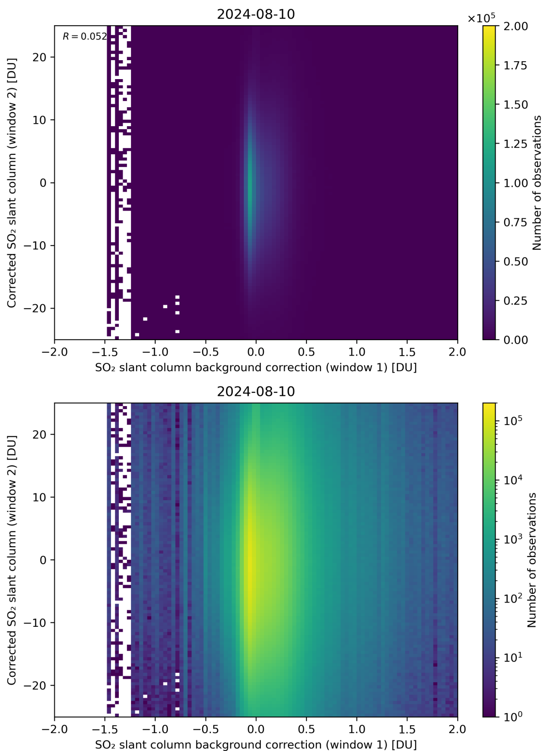
Figure 104: Scatter density plot of “SO 2 slant column background correction (window 1)” against “Corrected SO 2 slant column (window 2)” for 2024-08-09 to 2024-08-11.
