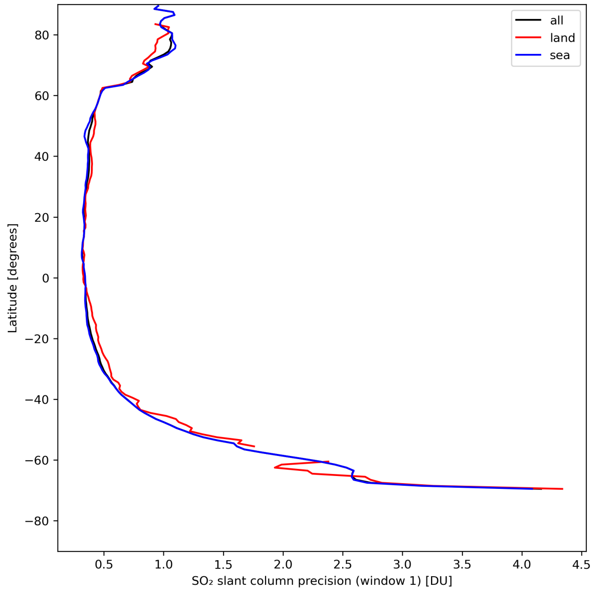
Figure 34: Zonal average of “SO 2 slant column precision (window 1)” for 2024-08-09 to 2024-08-11.
