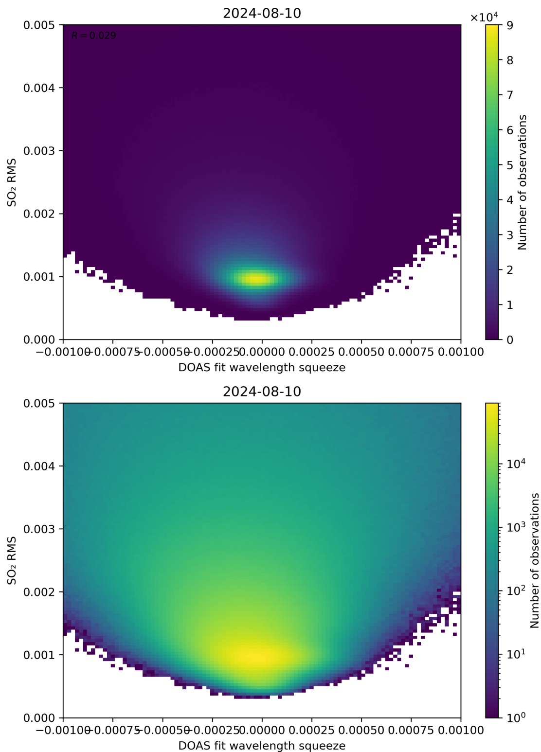
Figure 132: Scatter density plot of “DOAS fit wavelength squeeze” against “SO 2 RMS” for 2024-08-09 to 2024-08-11.
