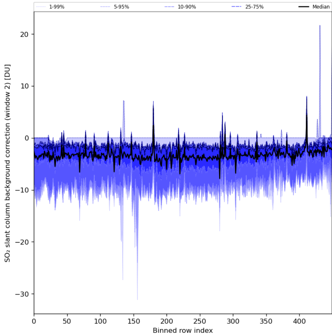
Figure 86: Along track statistics of “SO 2 slant column background correction (window 2)” for 2024-08-09 to 2024-08-11
