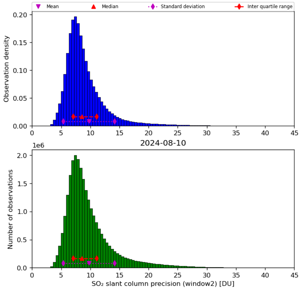
Figure 61: Histogram of “SO 2 slant column precision (window2)” for 2024-08-09 to 2024-08-11
