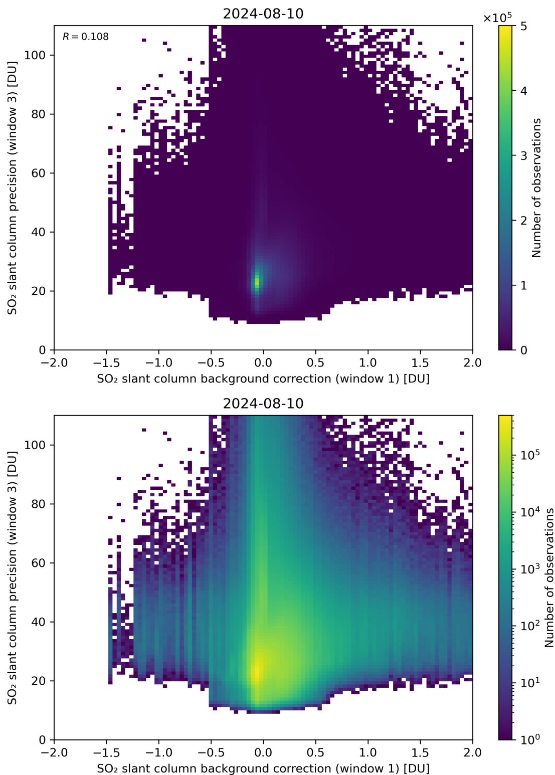
Figure 108: Scatter density plot of “SO 2 slant column background correction (window 1)” against “SO 2 slant column precision (window 3)” for 2024-08-09 to 2024-08-11.
