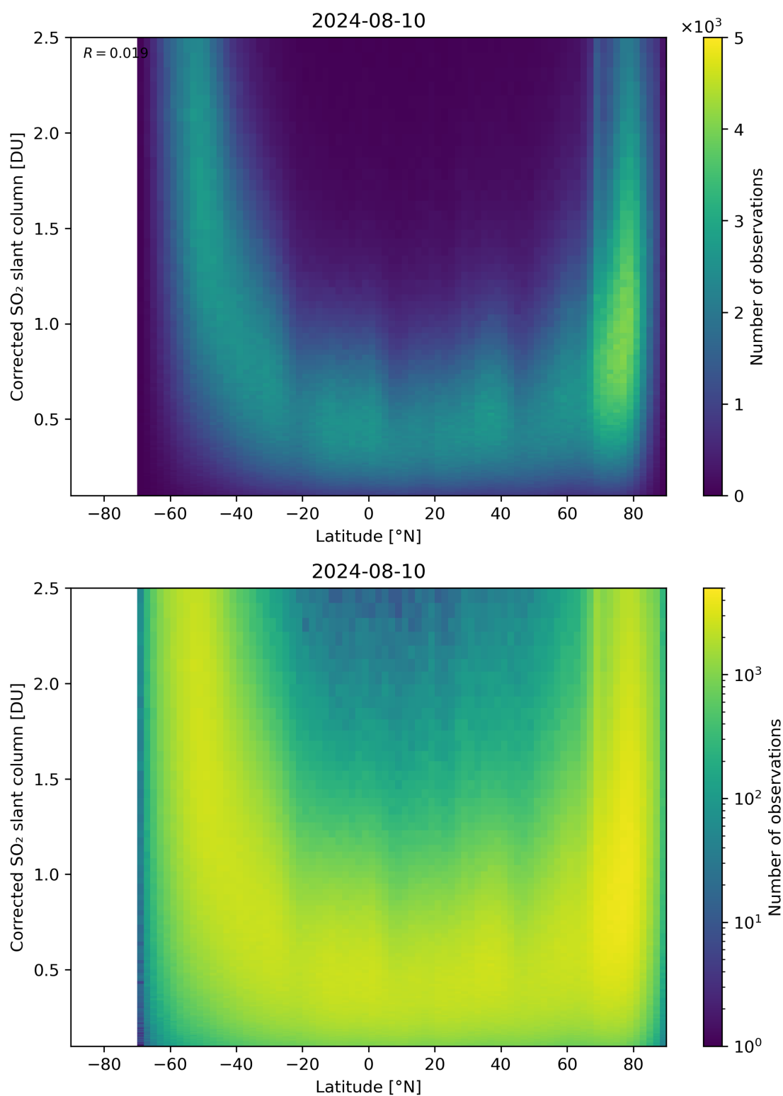
Figure 146: Scatter density plot of “Latitude” against “Corrected SO 2 slant column” for 2024-08-09 to 2024-08-11.
