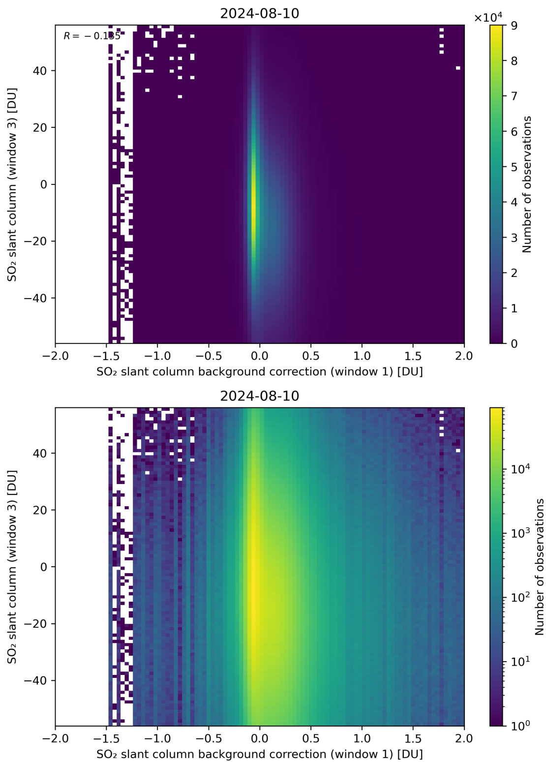
Figure 107: Scatter density plot of “SO 2 slant column background correction (window 1)” against “SO 2 slant column (window 3)” for 2024-08-09 to 2024-08-11.
