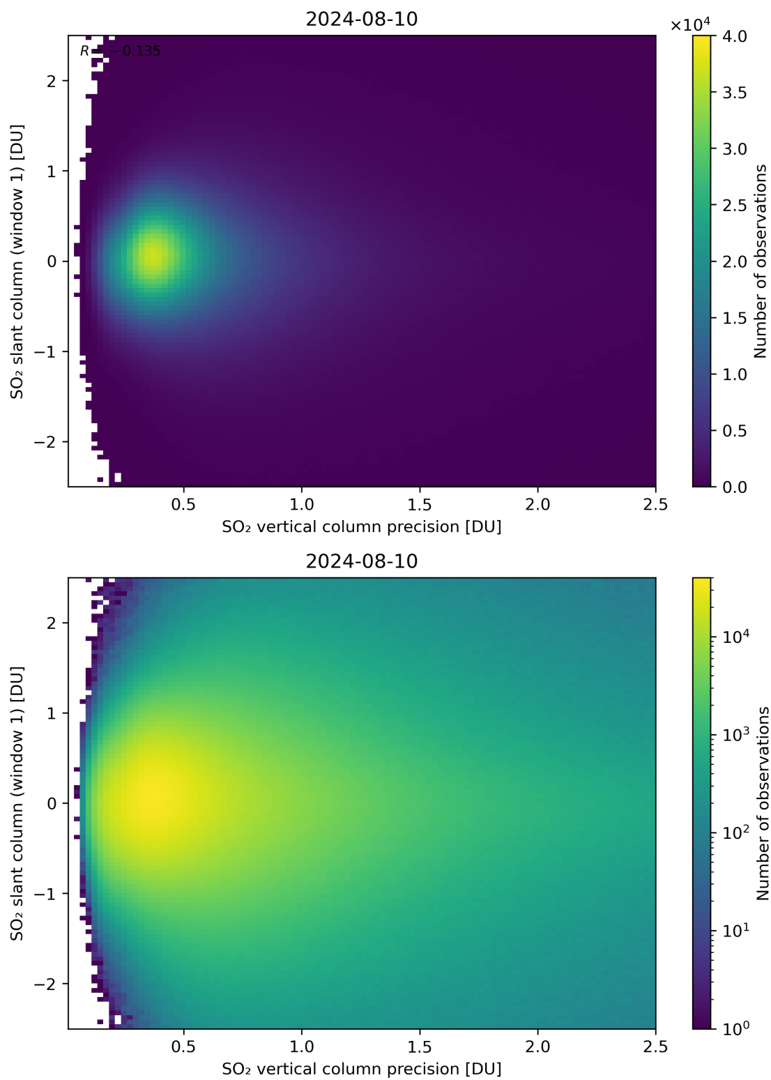
Figure 289: Scatter density plot of “SO 2 vertical column precision” against “SO 2 slant column (window 1)” for 2024-08-09 to 2024-08-11.
