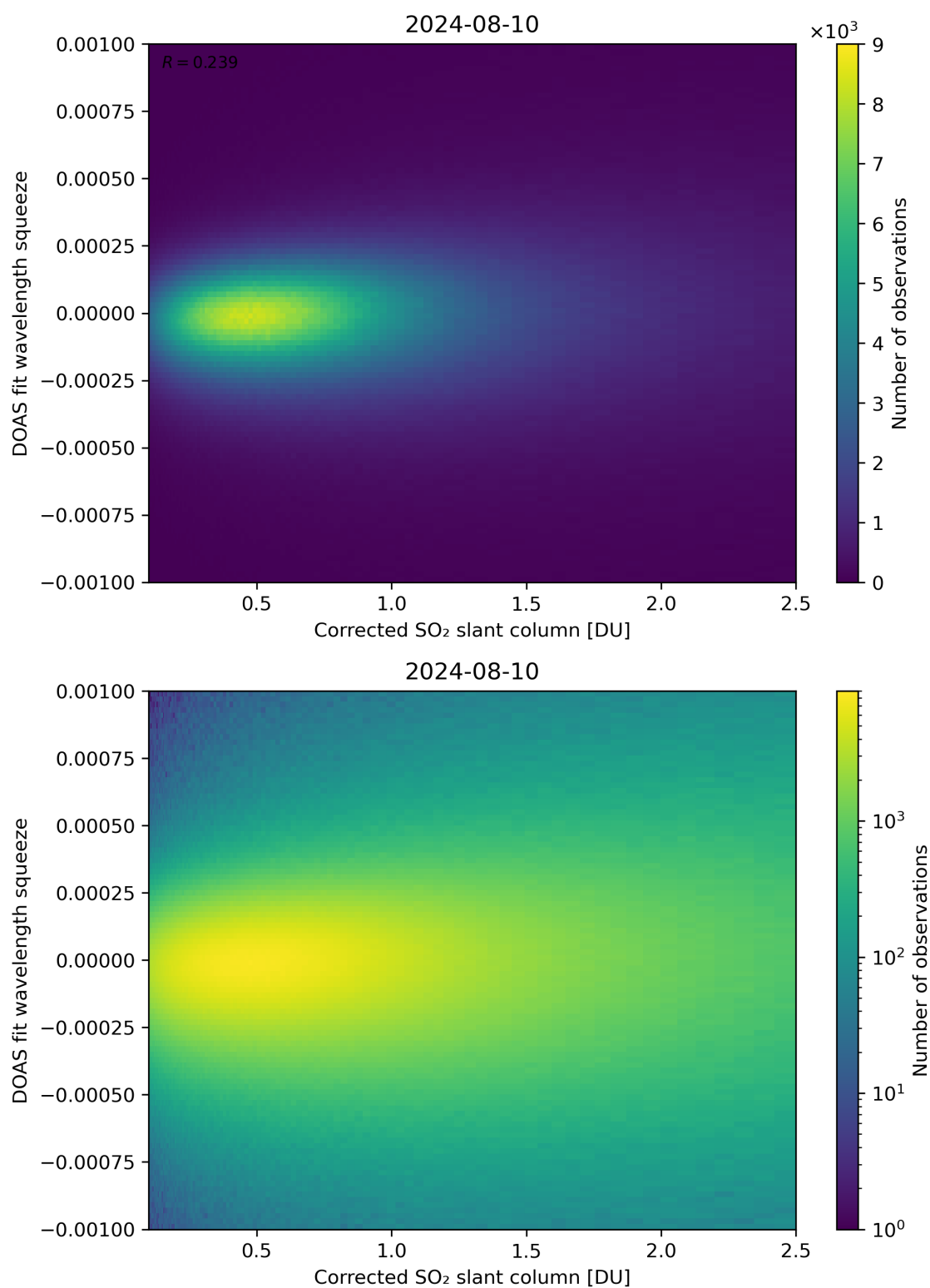
Figure 182: Scatter density plot of “Corrected SO 2 slant column” against “DOAS fit wavelength squeeze” for 2024-08-09 to 2024-08-11.
