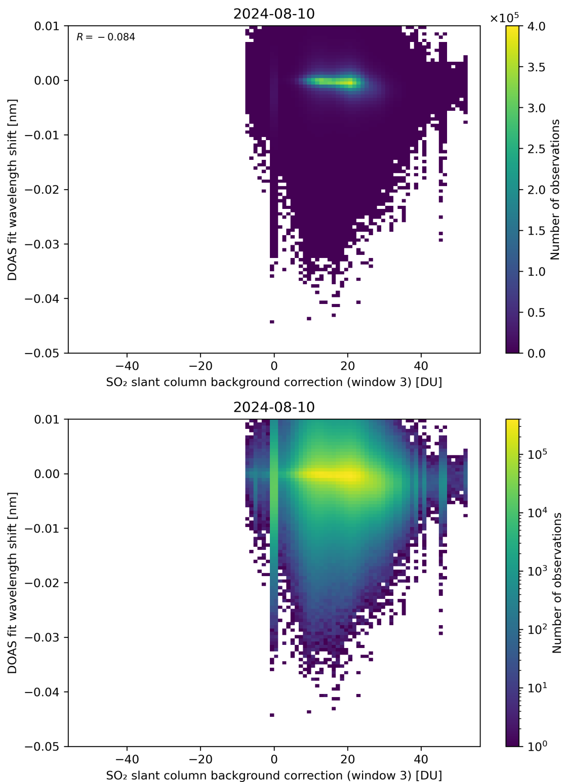
Figure 121: Scatter density plot of “SO 2 slant column background correction (window 3)” against “DOAS fit wavelength shift” for 2024-08-09 to 2024-08-11.
