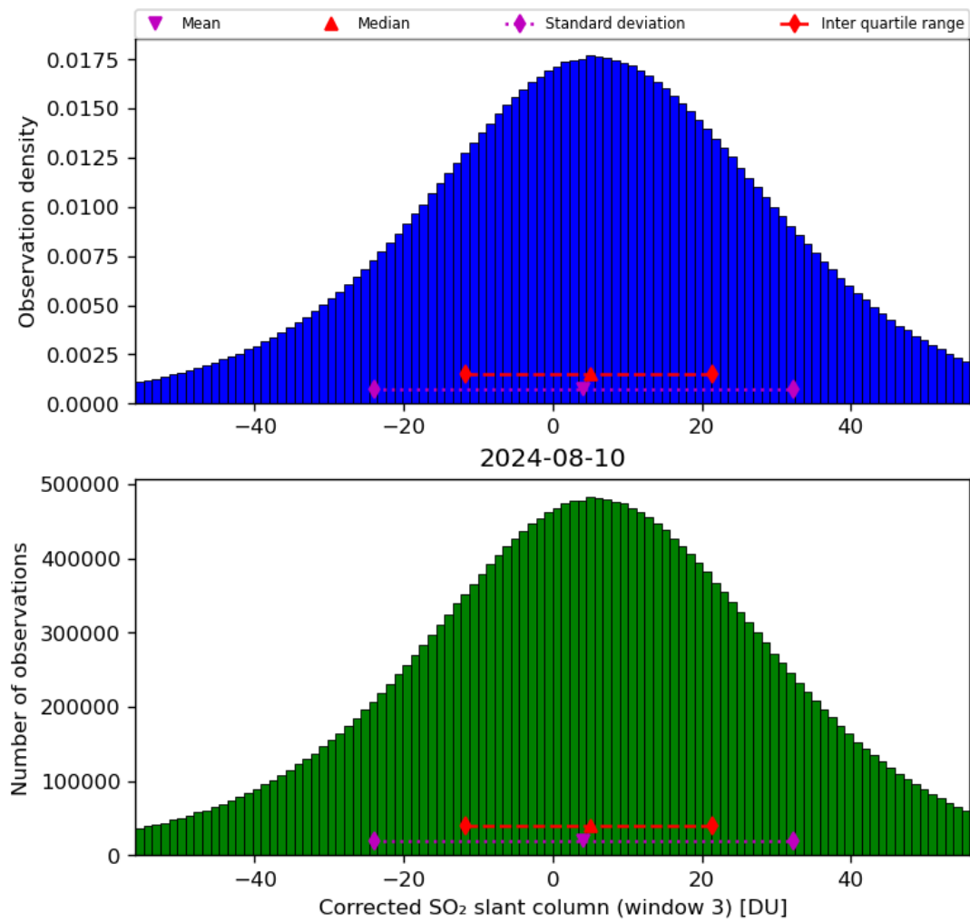
Figure 66: Histogram of “Corrected SO 2 slant column (window 3)” for 2024-08-09 to 2024-08-11
