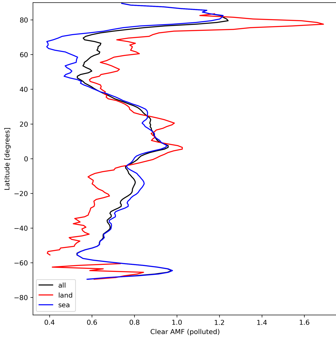
Figure 50: Zonal average of “Clear AMF (polluted)” for 2024-08-09 to 2024-08-11.
