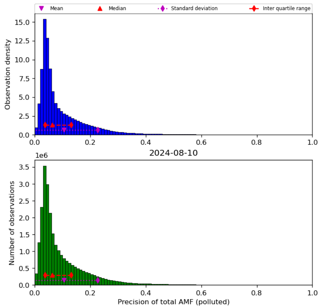
Figure 72: Histogram of “Precision of total AMF (polluted)” for 2024-08-09 to 2024-08-11
