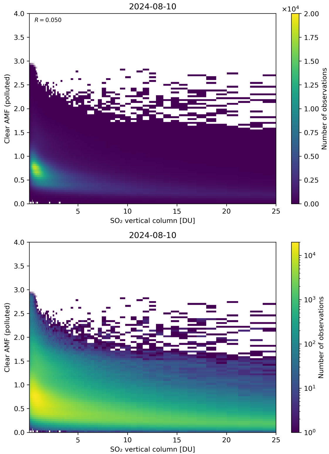
Figure 296: Scatter density plot of “SO 2 vertical column” against “Clear AMF (polluted)” for 2024-08-09 to 2024-08-11.
