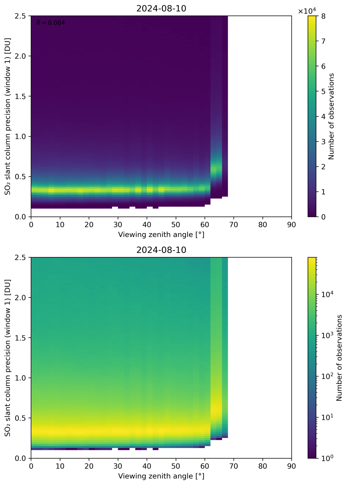
Figure 321: Scatter density plot of “Viewing zenith angle” against “SO 2 slant column precision (window 1)” for 2024-08-09 to 2024-08-11.
