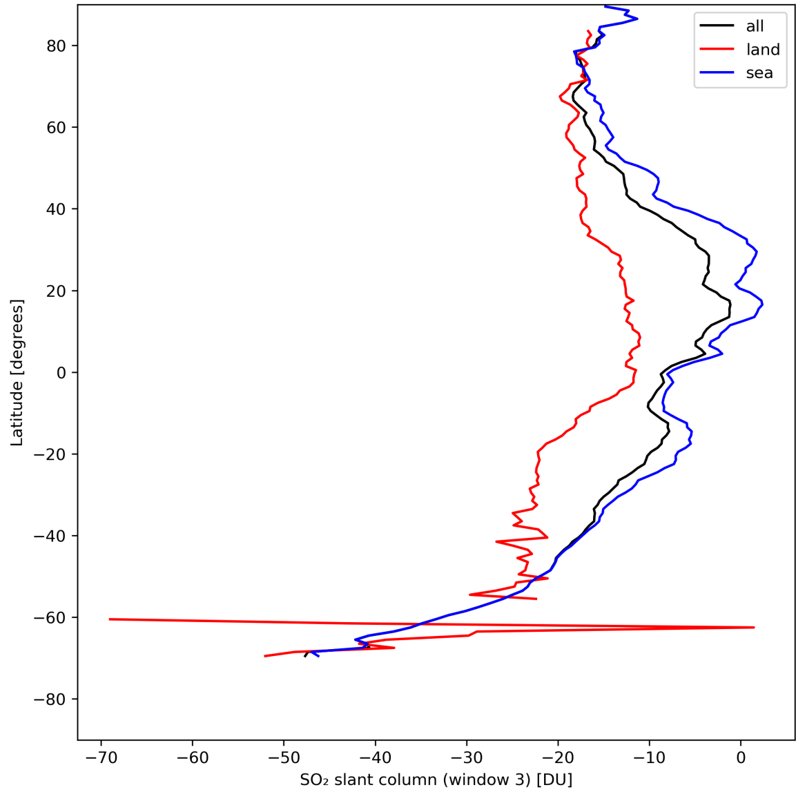
Figure 41: Zonal average of “SO 2 slant column (window 3)” for 2024-08-09 to 2024-08-11.
