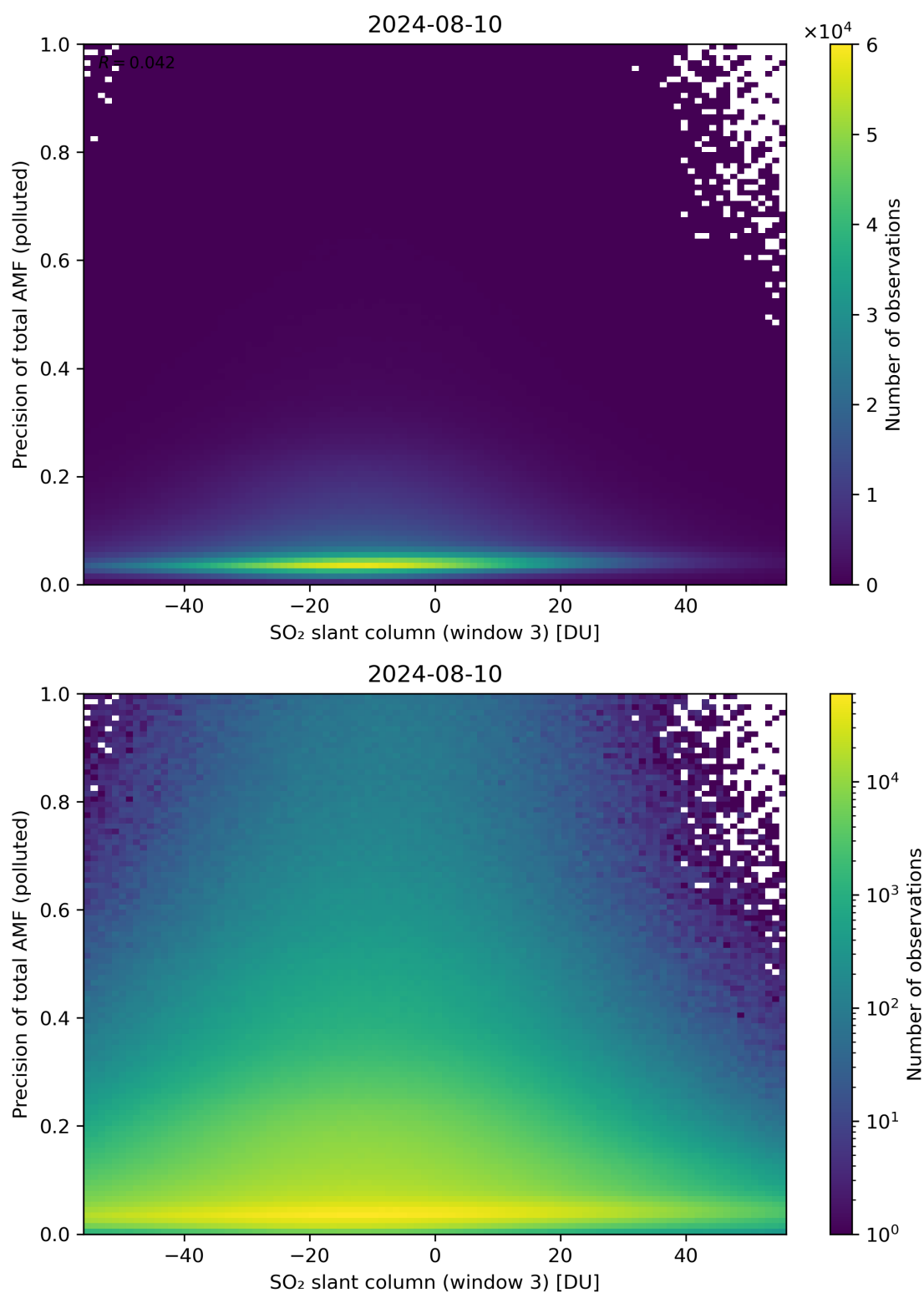
Figure 269: Scatter density plot of “SO 2 slant column (window 3)” against “Precision of total AMF (polluted)” for 2024-08-09 to 2024-08-11.
