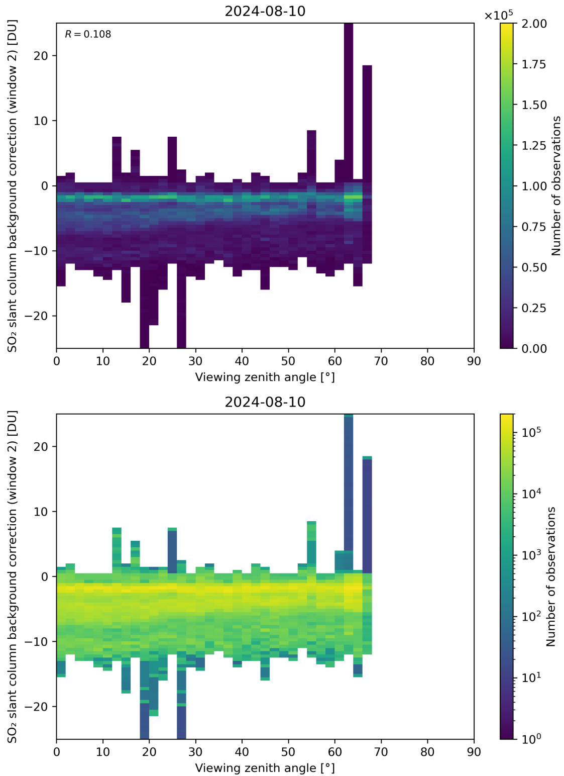
Figure 309: Scatter density plot of “Viewing zenith angle” against “SO 2 slant column background correction (window 2)” for 2024-08-09 to 2024-08-11.
