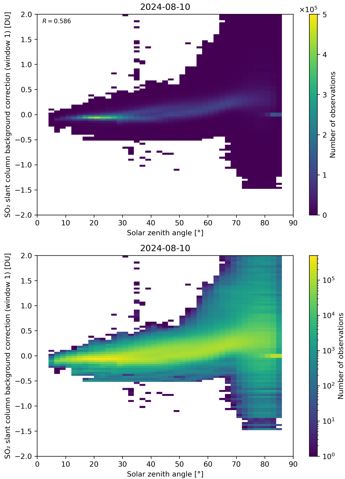
Figure 158: Scatter density plot of “Solar zenith angle” against “SO 2 slant column background correction (window 1)” for 2024-08-09 to 2024-08-11.
