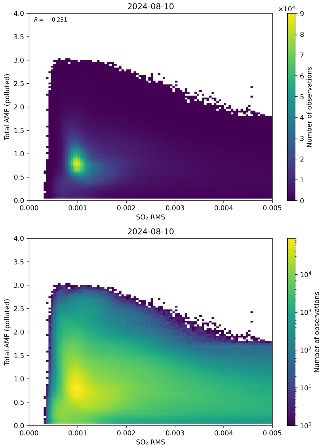
Figure 137: Scatter density plot of “SO 2 RMS” against “Total AMF (polluted)” for 2024-08-09 to 2024-08-11.
