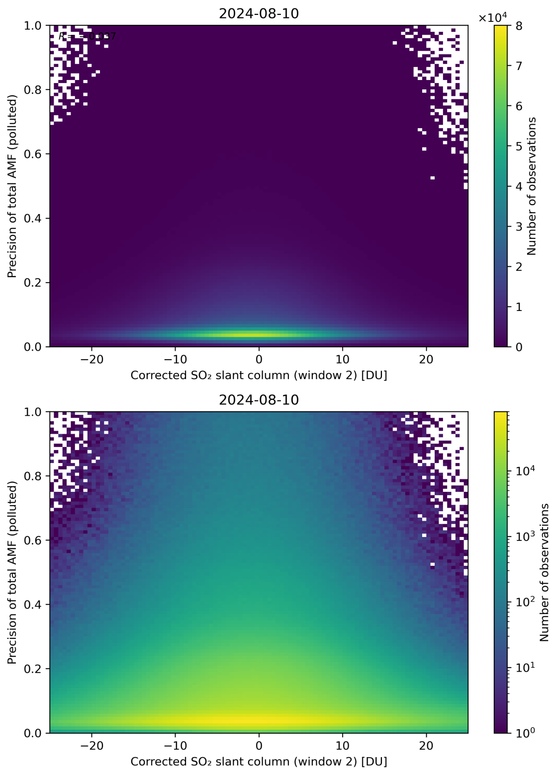
Figure 204: Scatter density plot of “Corrected SO 2 slant column (window 2)” against “Precision of total AMF (polluted)” for 2024-08-09 to 2024-08-11.
