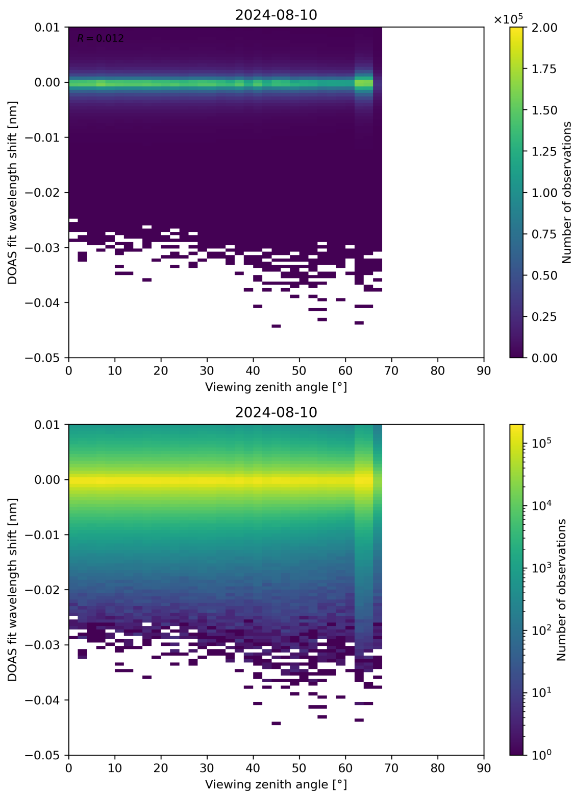
Figure 311: Scatter density plot of “Viewing zenith angle” against “DOAS fit wavelength shift” for 2024-08-09 to 2024-08-11.
