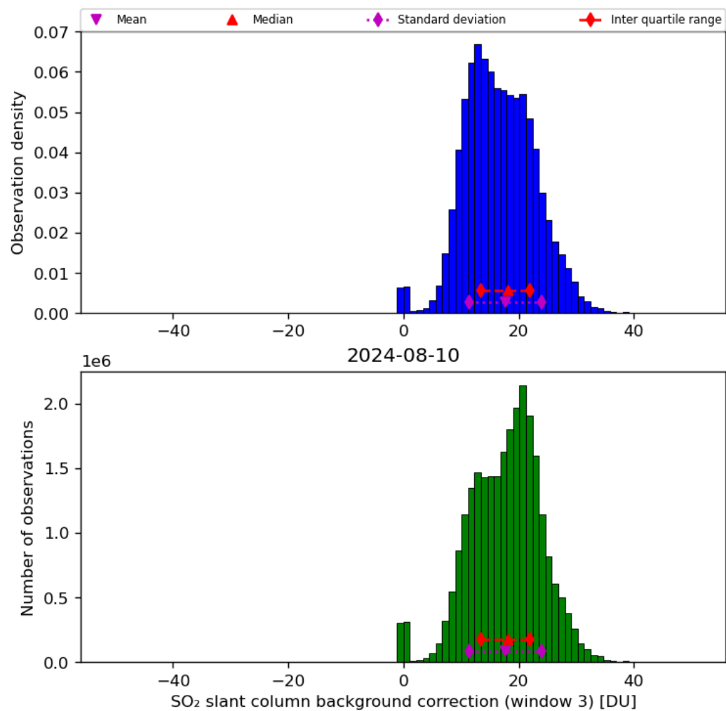
Figure 67: Histogram of “SO 2 slant column background correction (window 3)” for 2024-08-09 to 2024-08-11
