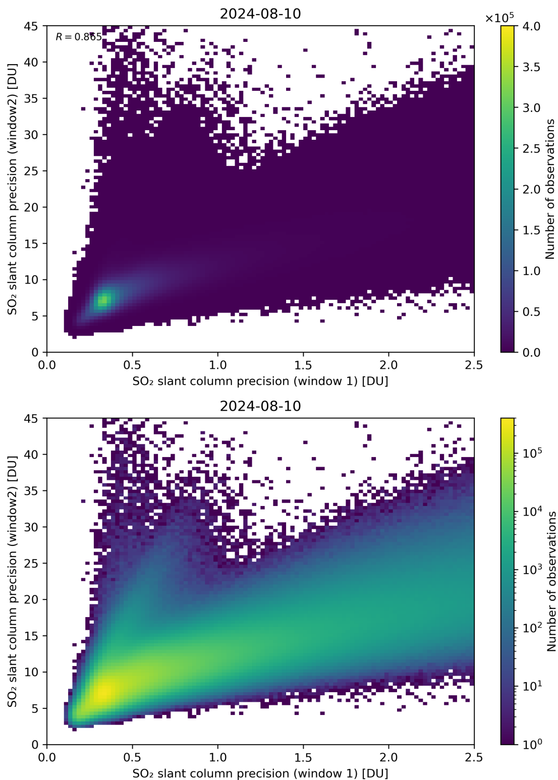
Figure 227: Scatter density plot of “SO 2 slant column precision (window 1)” against “SO 2 slant column precision (window2)” for 2024-08-09 to 2024-08-11.
