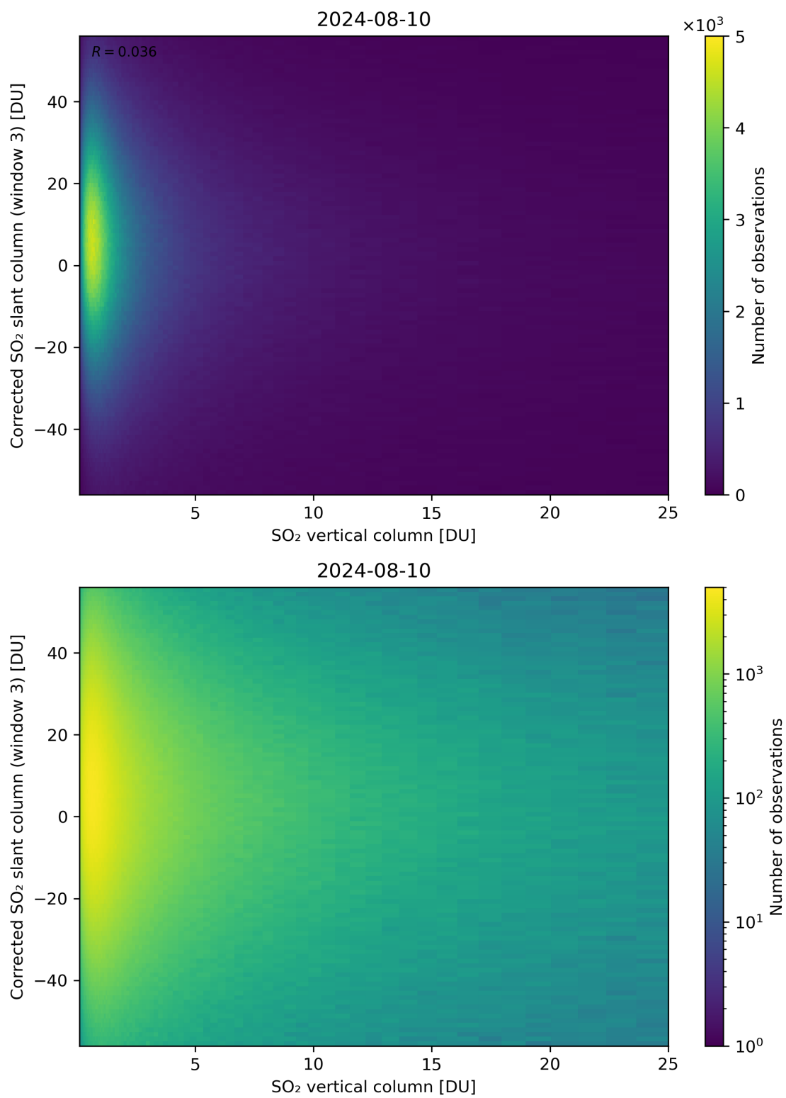
Figure 299: Scatter density plot of “SO 2 vertical column” against “Corrected SO 2 slant column (window 3)” for 2024-08-09 to 2024-08-11.
