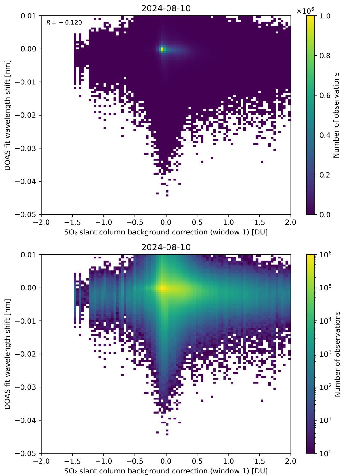
Figure 100: Scatter density plot of “SO 2 slant column background correction (window 1)” against “DOAS fit wavelength shift” for 2024-08-09 to 2024-08-11.
