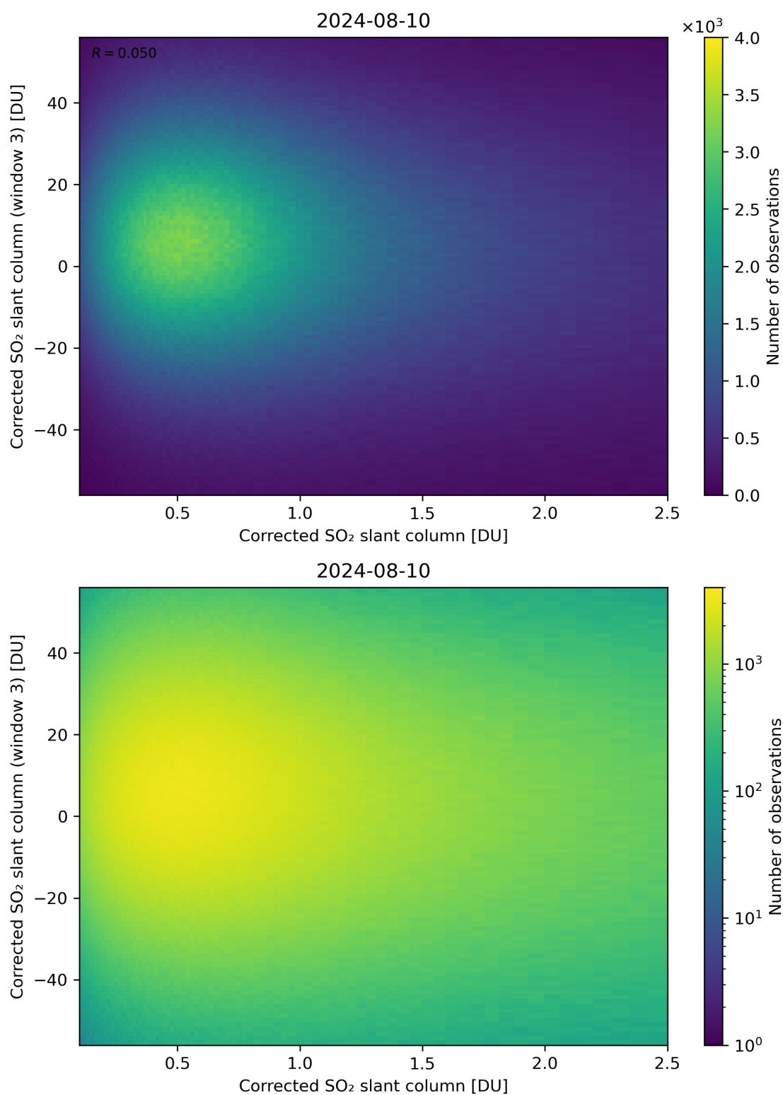
Figure 186: Scatter density plot of “Corrected SO 2 slant column” against “Corrected SO 2 slant column (window 3)” for 2024-08-09 to 2024-08-11.
