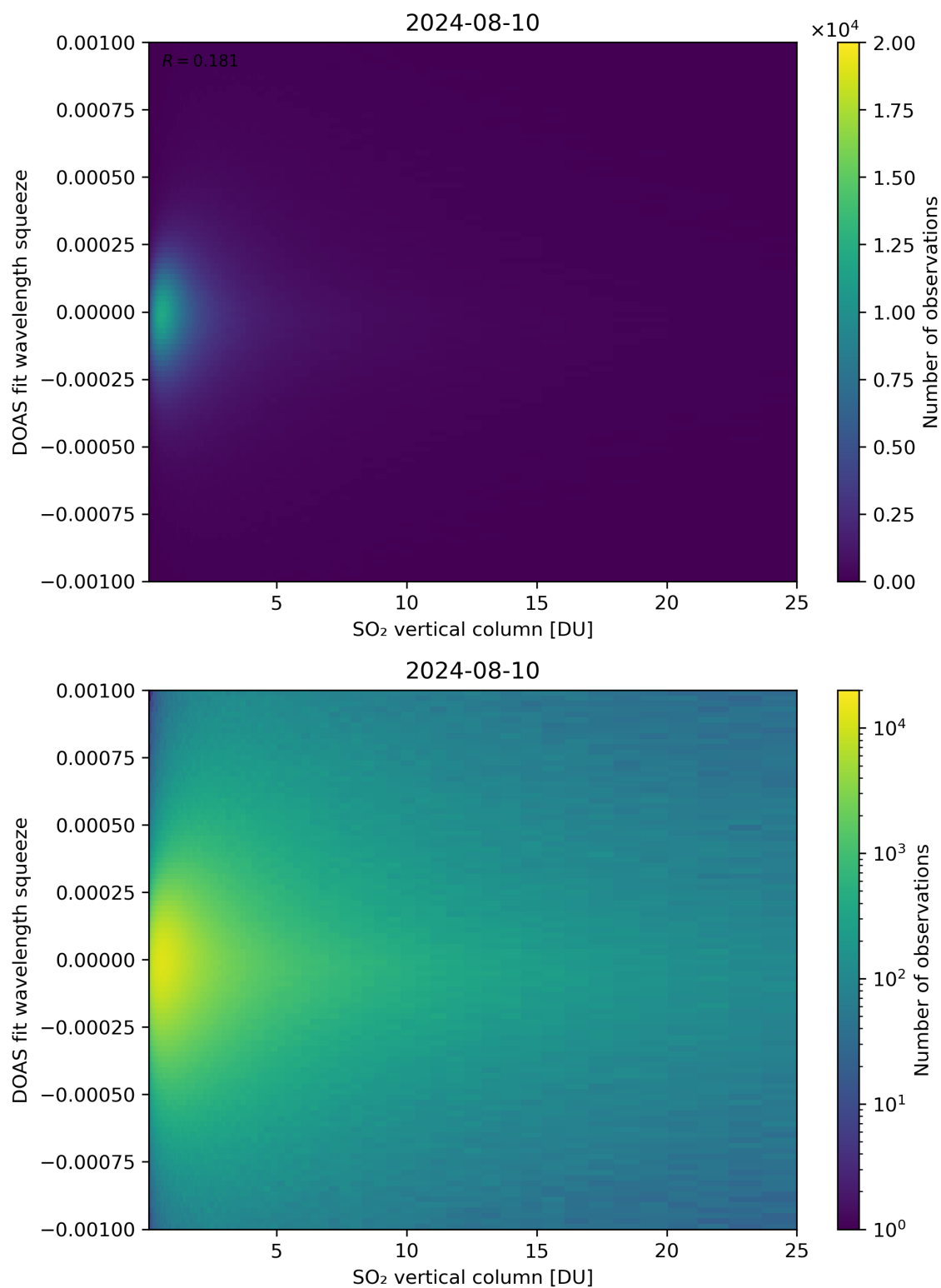
Figure 277: Scatter density plot of “SO 2 vertical column” against “DOAS fit wavelength squeeze” for 2024-08-09 to 2024-08-11.
