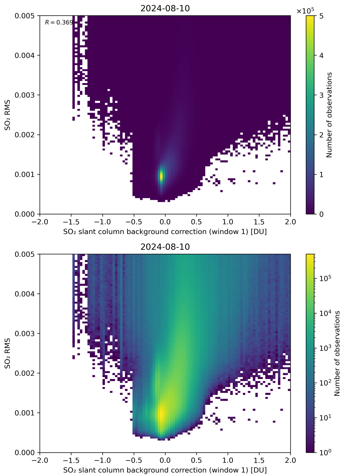
Figure 102: Scatter density plot of “SO 2 slant column background correction (window 1)” against “SO 2 RMS” for 2024-08-09 to 2024-08-11.
