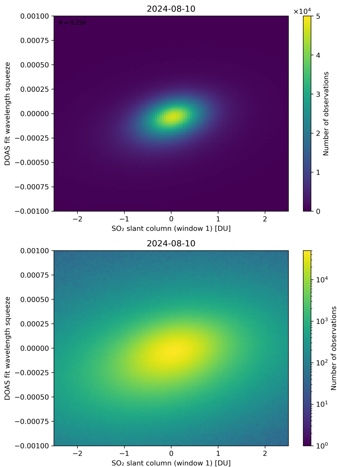
Figure 216: Scatter density plot of “SO 2 slant column (window 1)” against “DOAS fit wavelength squeeze” for 2024-08-09 to 2024-08-11.
