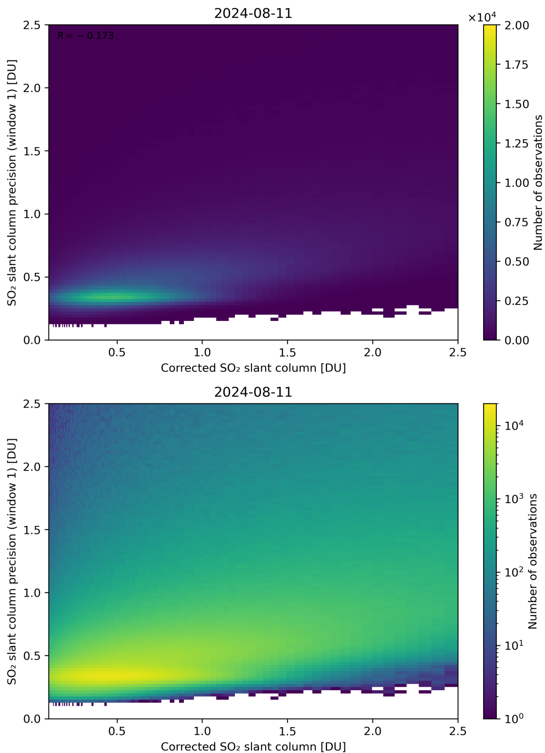
Figure 188: Scatter density plot of “Corrected SO 2 slant column” against “SO 2 slant column precision (window 1)” for 2024-08-11 to 2024-08-11.
