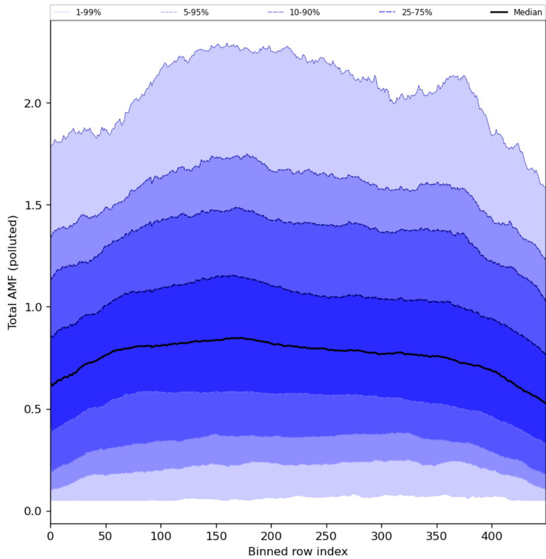
Figure 94: Along track statistics of “Total AMF (polluted)” for 2024-08-11 to 2024-08-11
