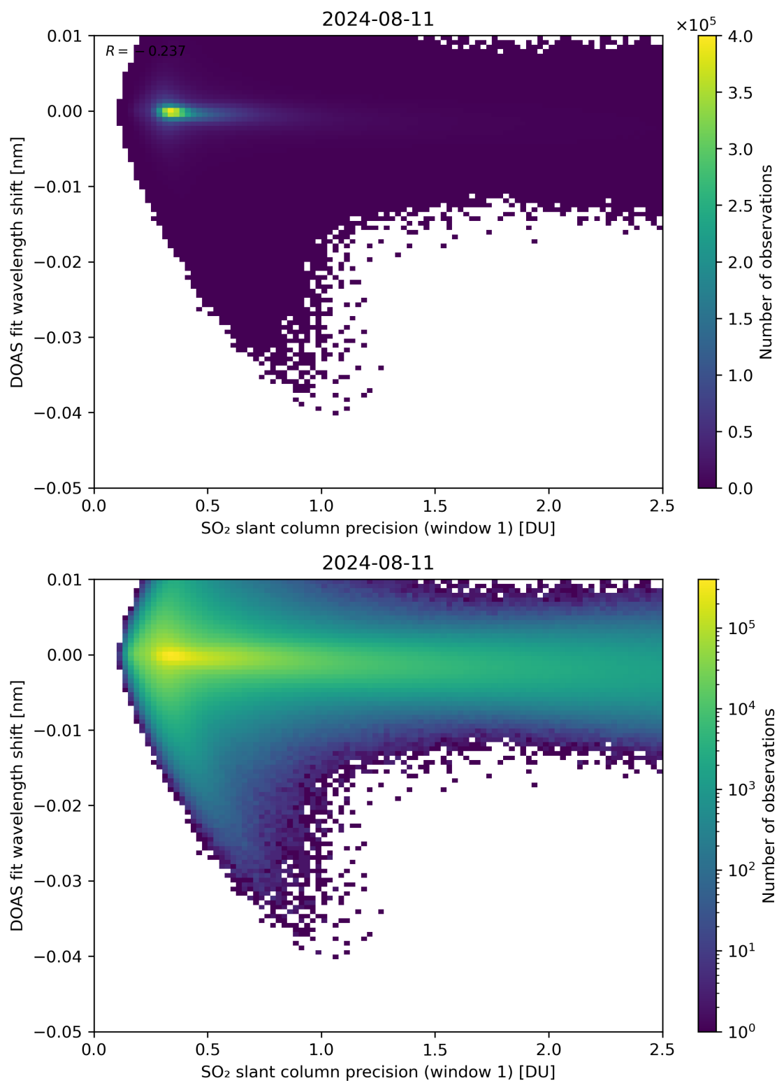
Figure 221: Scatter density plot of “SO 2 slant column precision (window 1)” against “DOAS fit wavelength shift” for 2024-08-11 to 2024-08-11.
