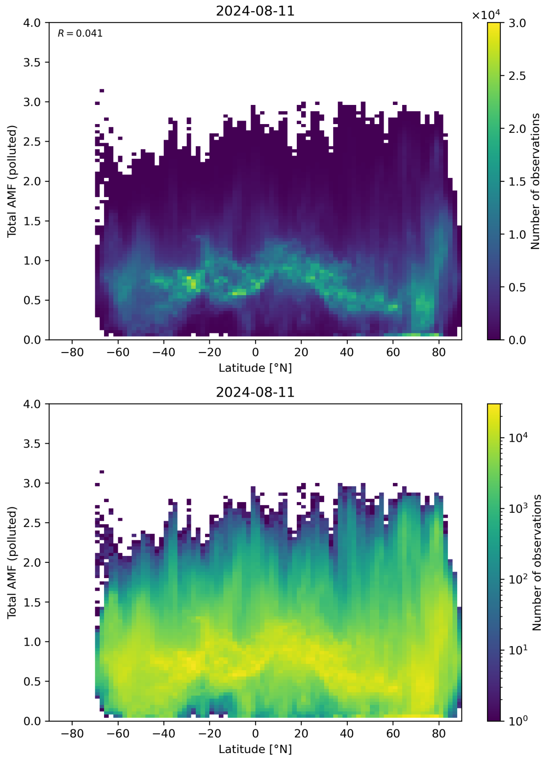
Figure 154: Scatter density plot of “Latitude” against “Total AMF (polluted)” for 2024-08-11 to 2024-08-11.
