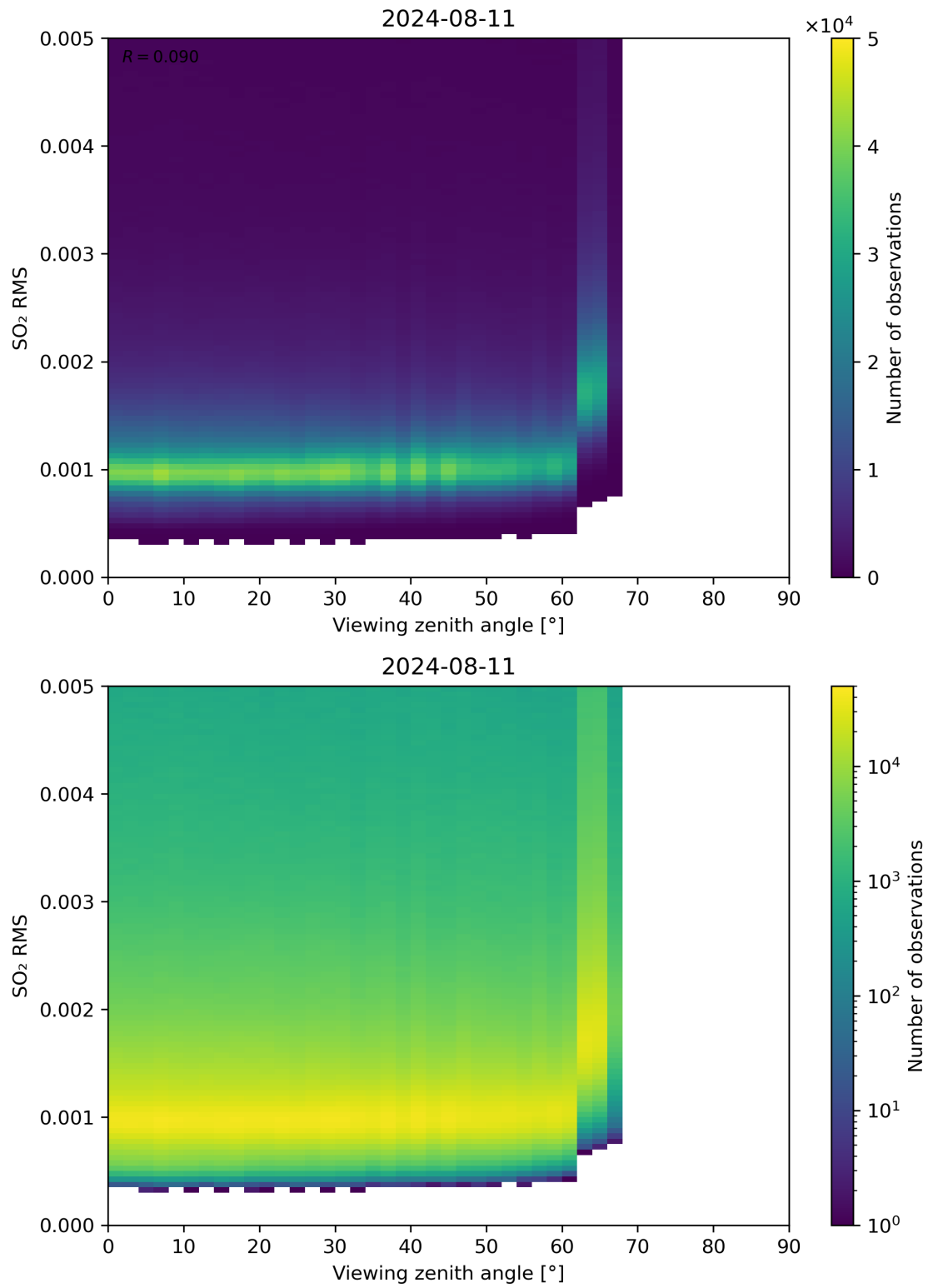
Figure 313: Scatter density plot of “Viewing zenith angle” against “SO 2 RMS” for 2024-08-11 to 2024-08-11.
