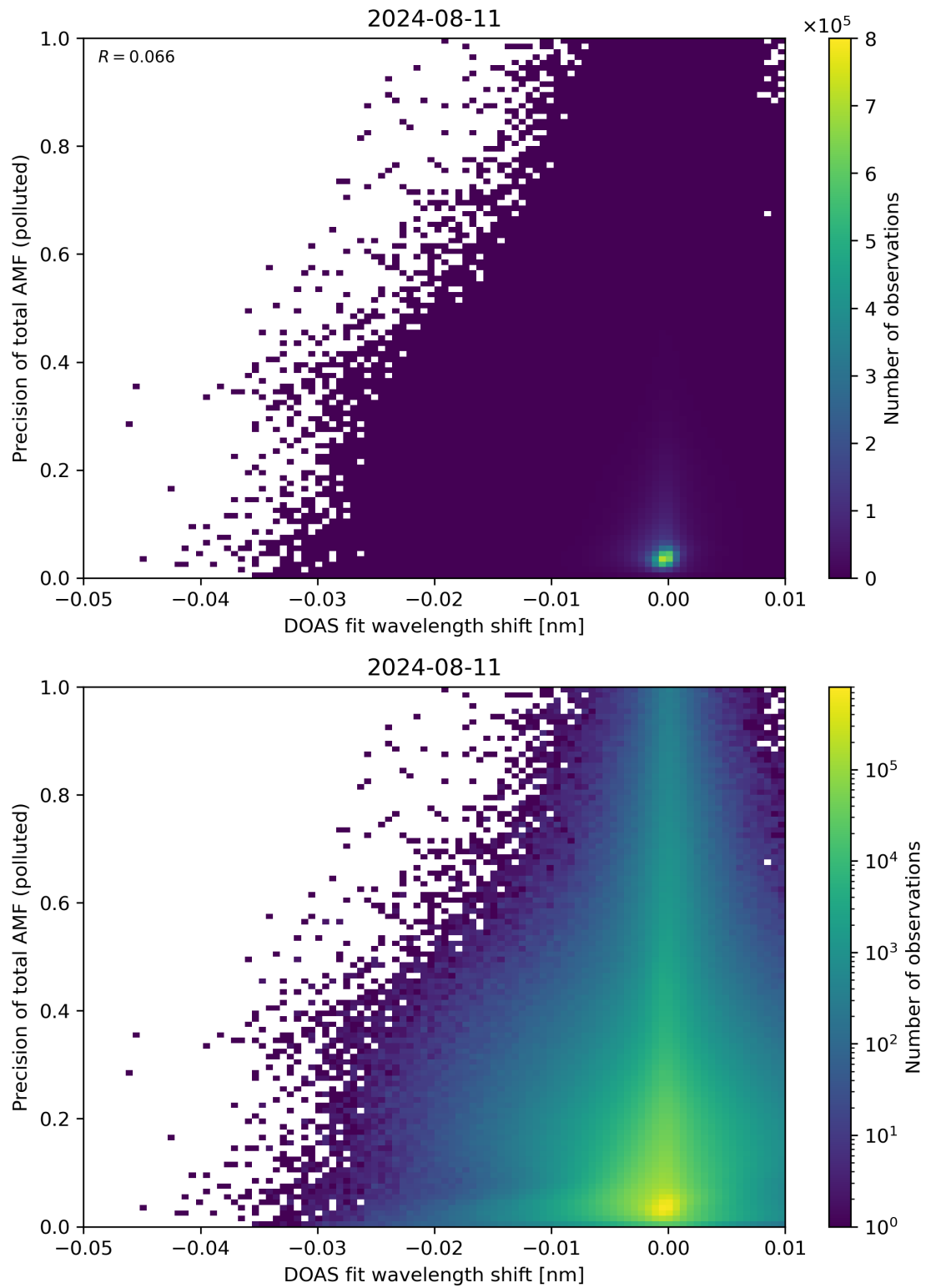
Figure 131: Scatter density plot of “DOAS fit wavelength shift” against “Precision of total AMF (polluted)” for 2024-08-11 to 2024-08-11.
