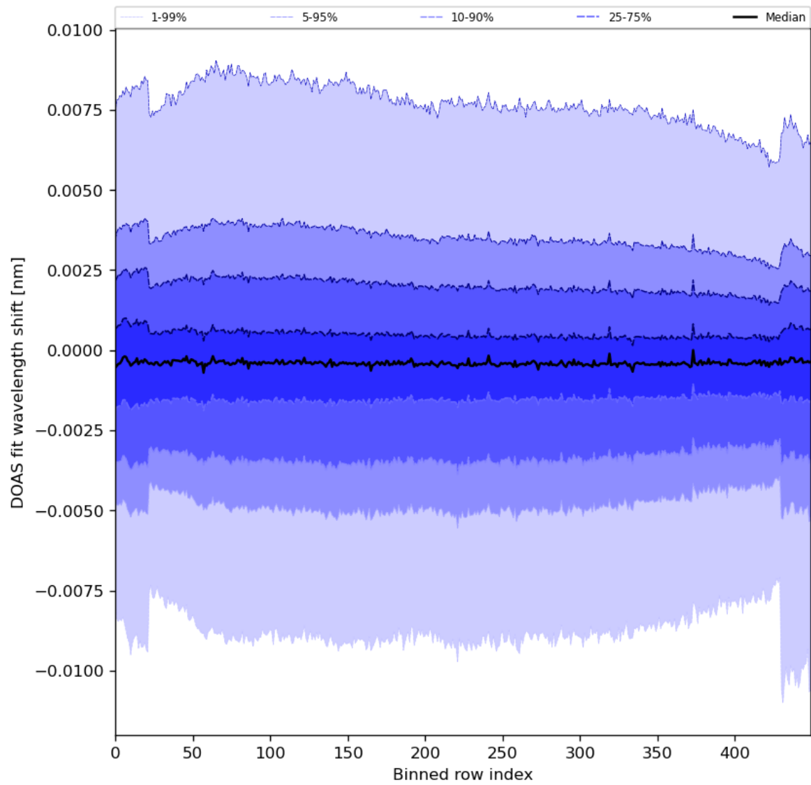
Figure 91: Along track statistics of “DOAS fit wavelength shift” for 2024-08-11 to 2024-08-11
