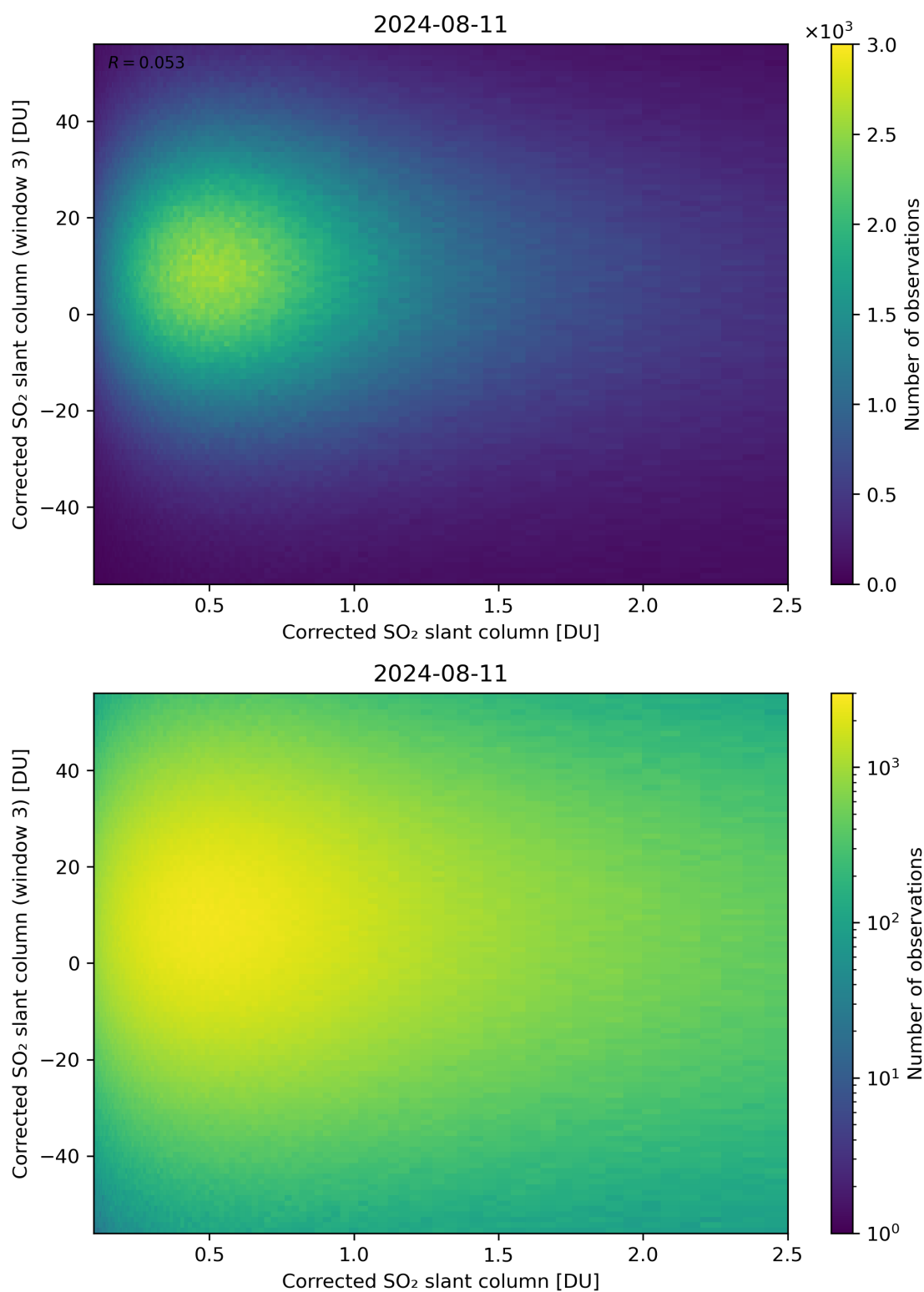
Figure 186: Scatter density plot of “Corrected SO 2 slant column” against “Corrected SO 2 slant column (window 3)” for 2024-08-11 to 2024-08-11.
