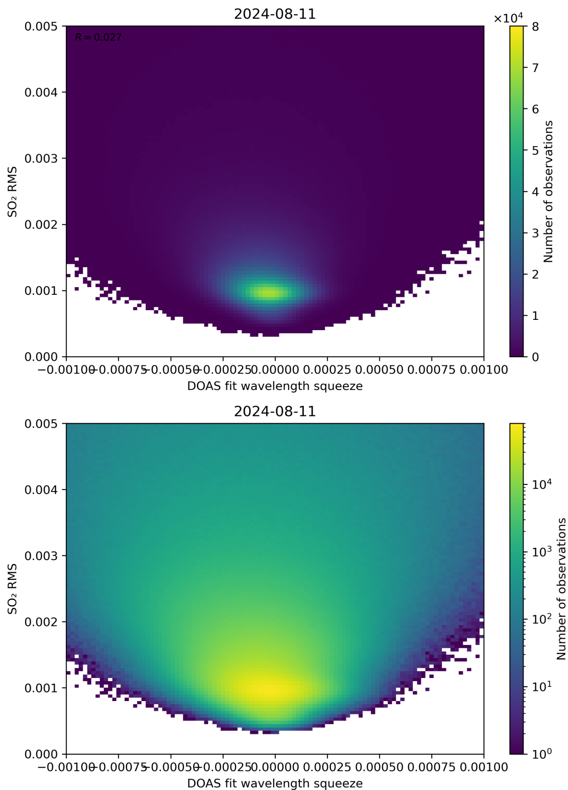
Figure 132: Scatter density plot of “DOAS fit wavelength squeeze” against “SO 2 RMS” for 2024-08-11 to 2024-08-11.
