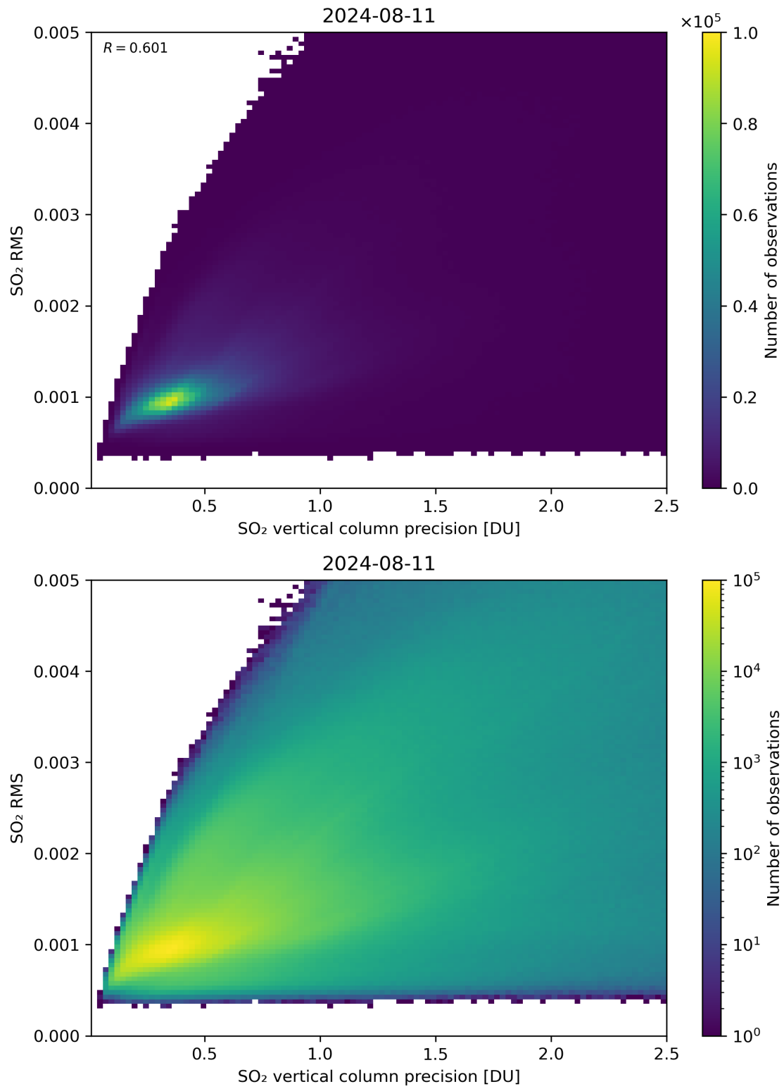
Figure 284: Scatter density plot of “SO 2 vertical column precision” against “SO 2 RMS” for 2024-08-11 to 2024-08-11.
