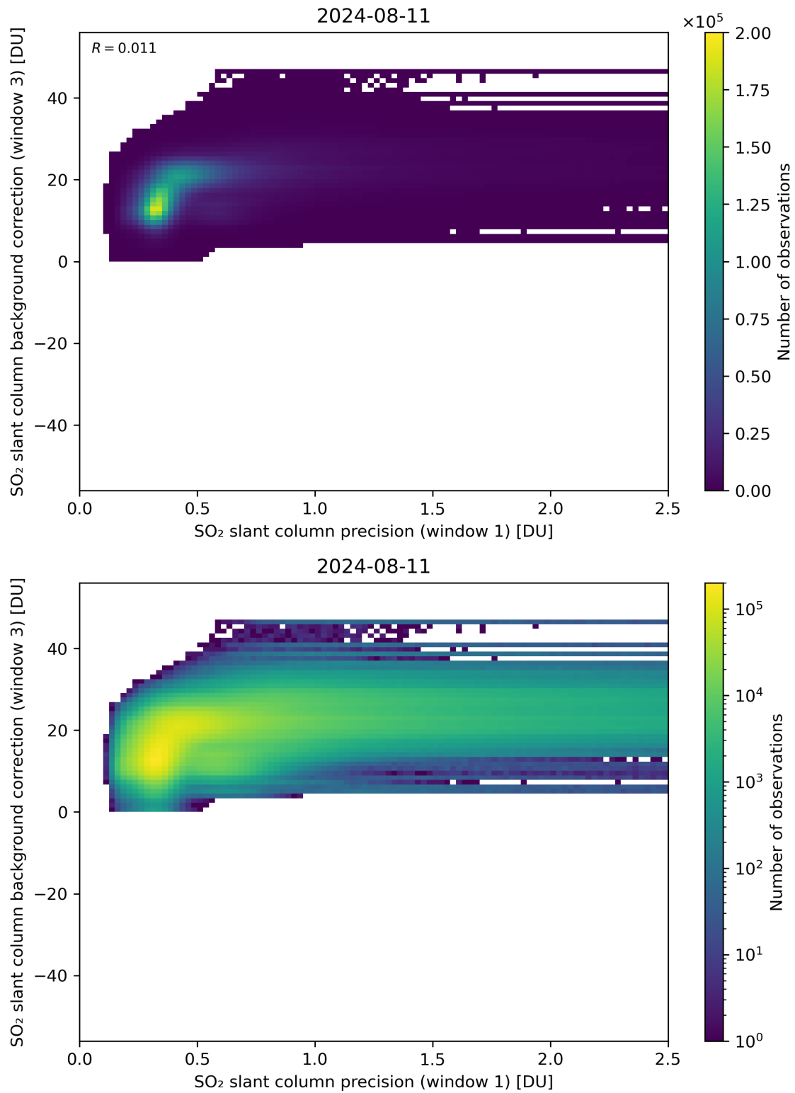
Figure 220: Scatter density plot of “SO 2 slant column precision (window 1)” against “SO 2 slant column background correction (window 3)” for 2024-08-11 to 2024-08-11.
