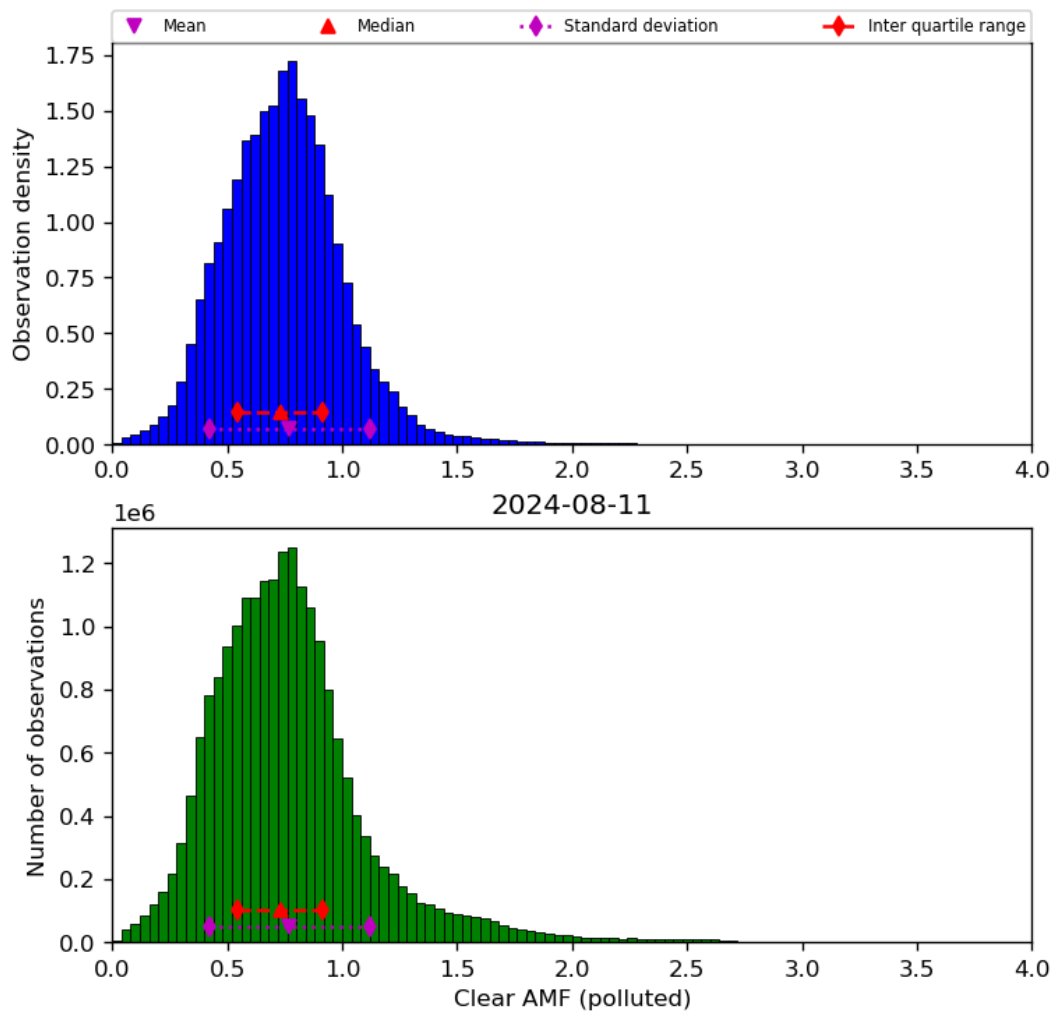
Figure 73: Histogram of “Clear AMF (polluted)” for 2024-08-11 to 2024-08-11
