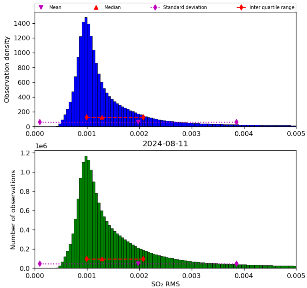
Figure 70: Histogram of “SO 2 RMS” for 2024-08-11 to 2024-08-11
