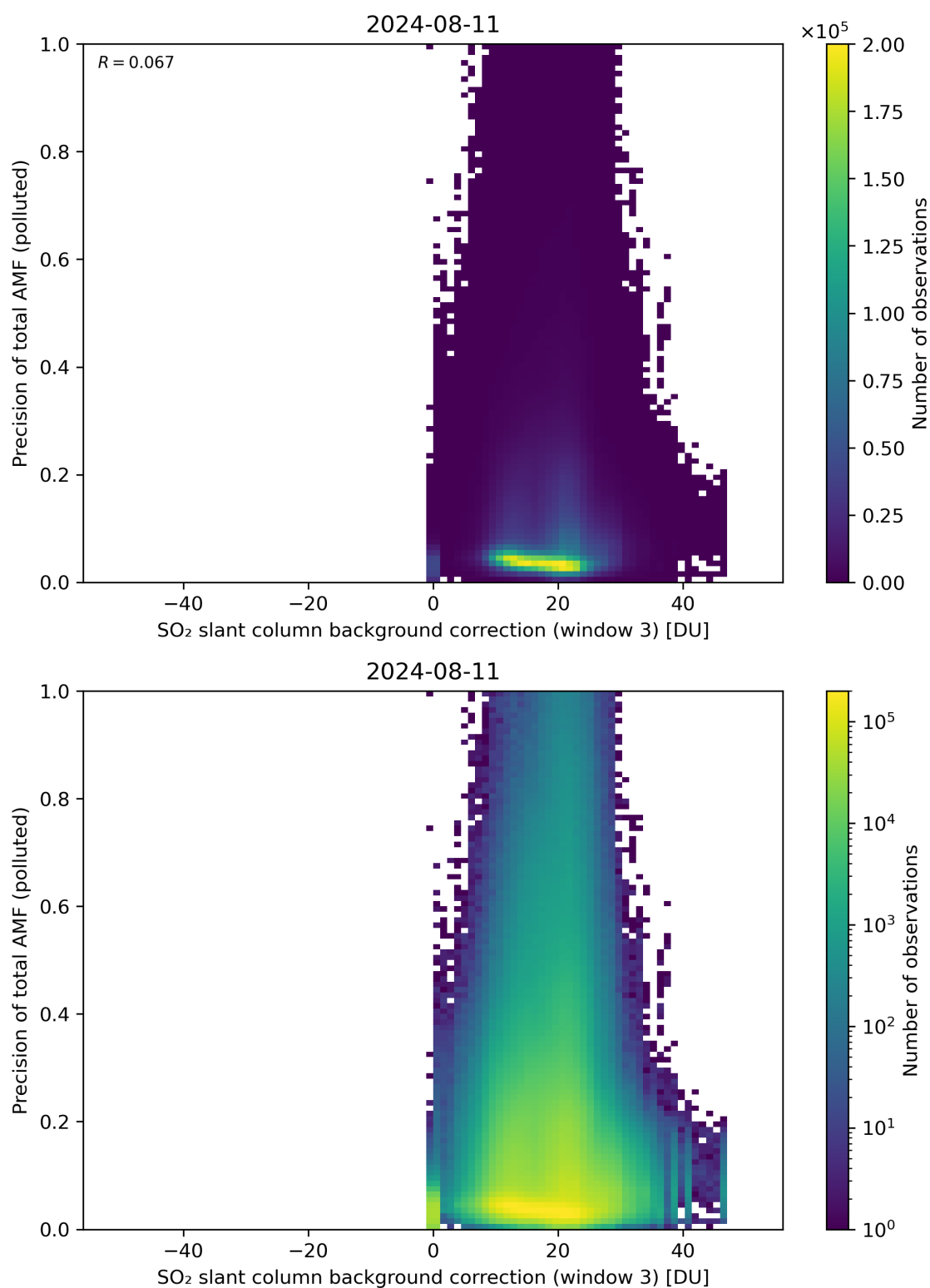
Figure 126: Scatter density plot of “SO 2 slant column background correction (window 3)” against “Precision of total AMF (polluted)” for 2024-08-11 to 2024-08-11.
