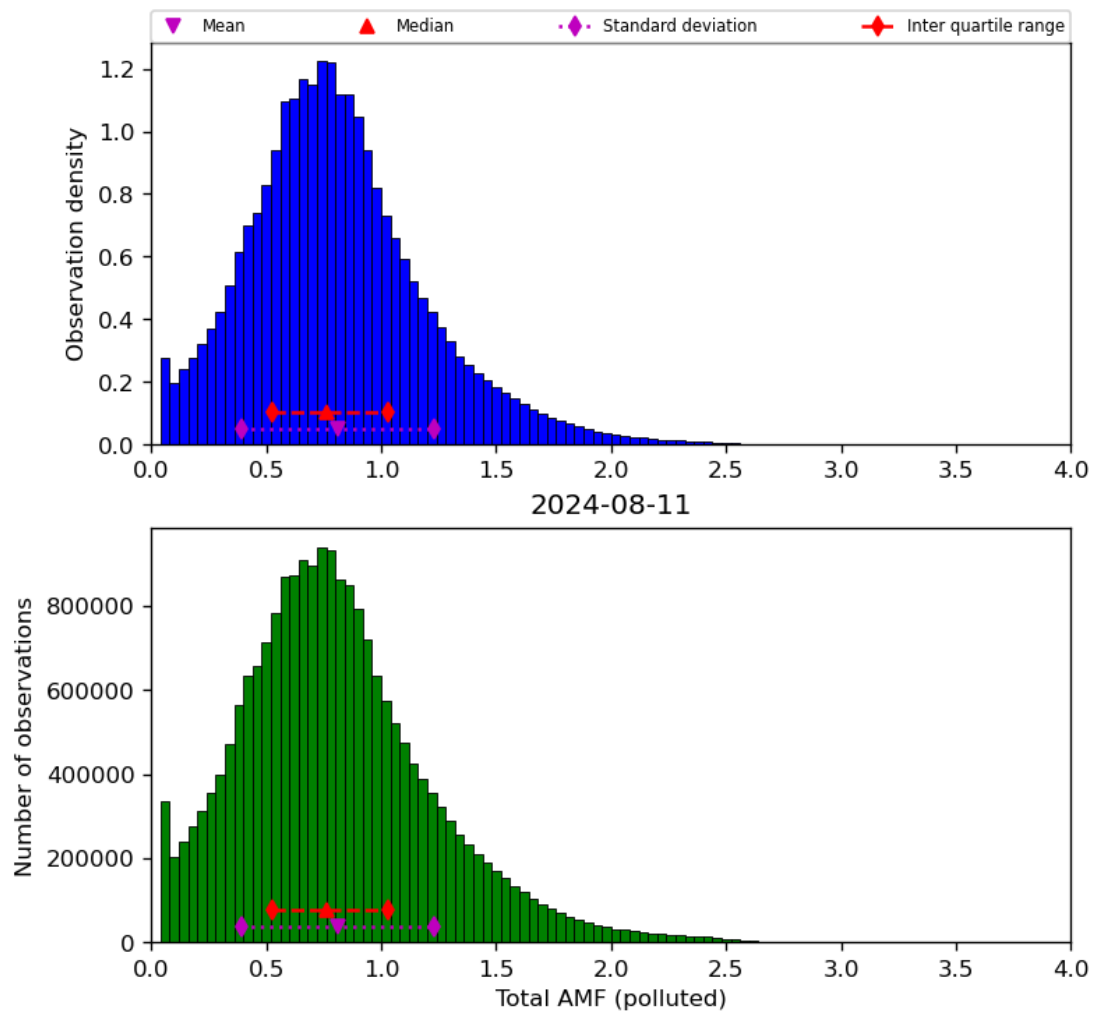
Figure 71: Histogram of “Total AMF (polluted)” for 2024-08-11 to 2024-08-11
