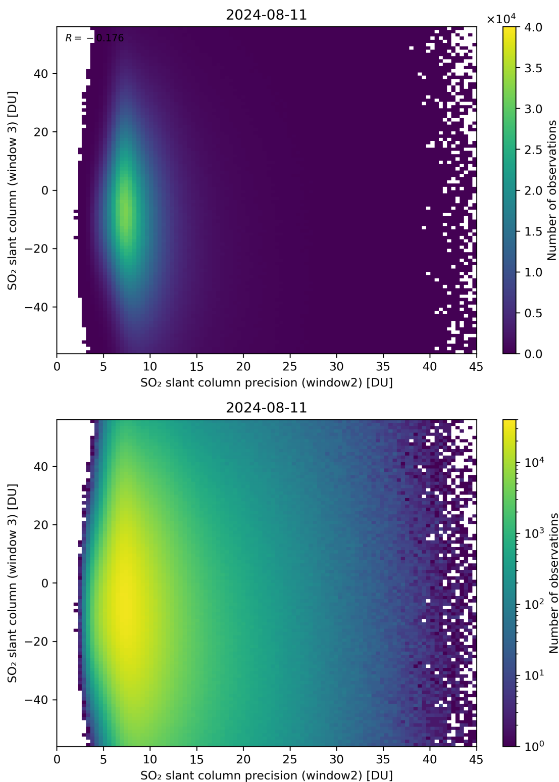
Figure 249: Scatter density plot of “SO 2 slant column precision (window2)” against “SO 2 slant column (window 3)” for 2024-08-11 to 2024-08-11.
