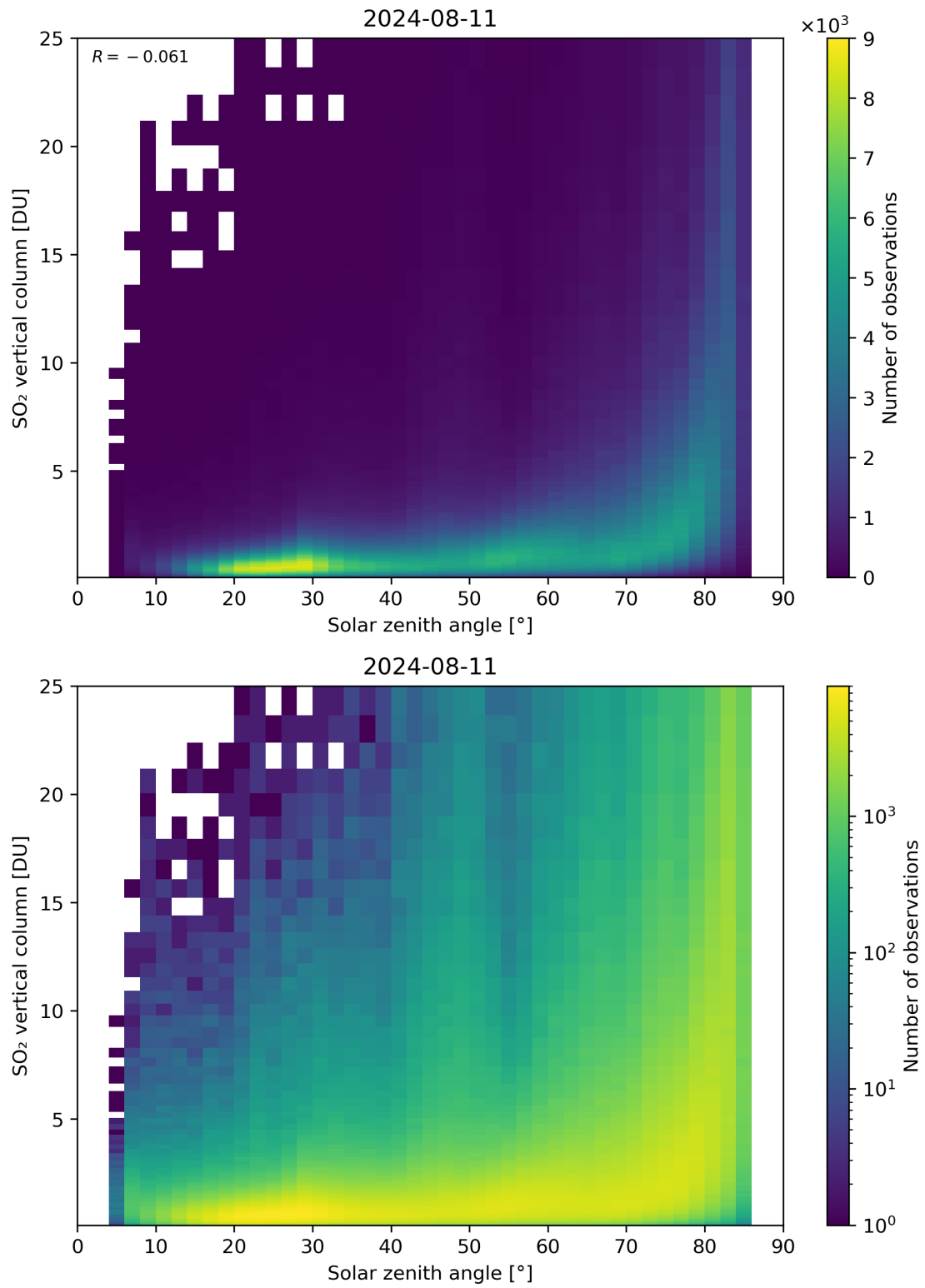
Figure 176: Scatter density plot of “Solar zenith angle” against “SO 2 vertical column” for 2024-08-11 to 2024-08-11.
