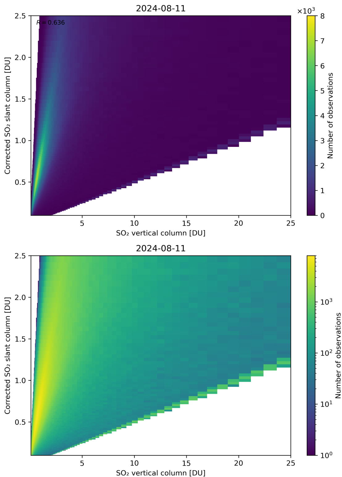
Figure 297: Scatter density plot of “SO 2 vertical column” against “Corrected SO 2 slant column” for 2024-08-11 to 2024-08-11.
