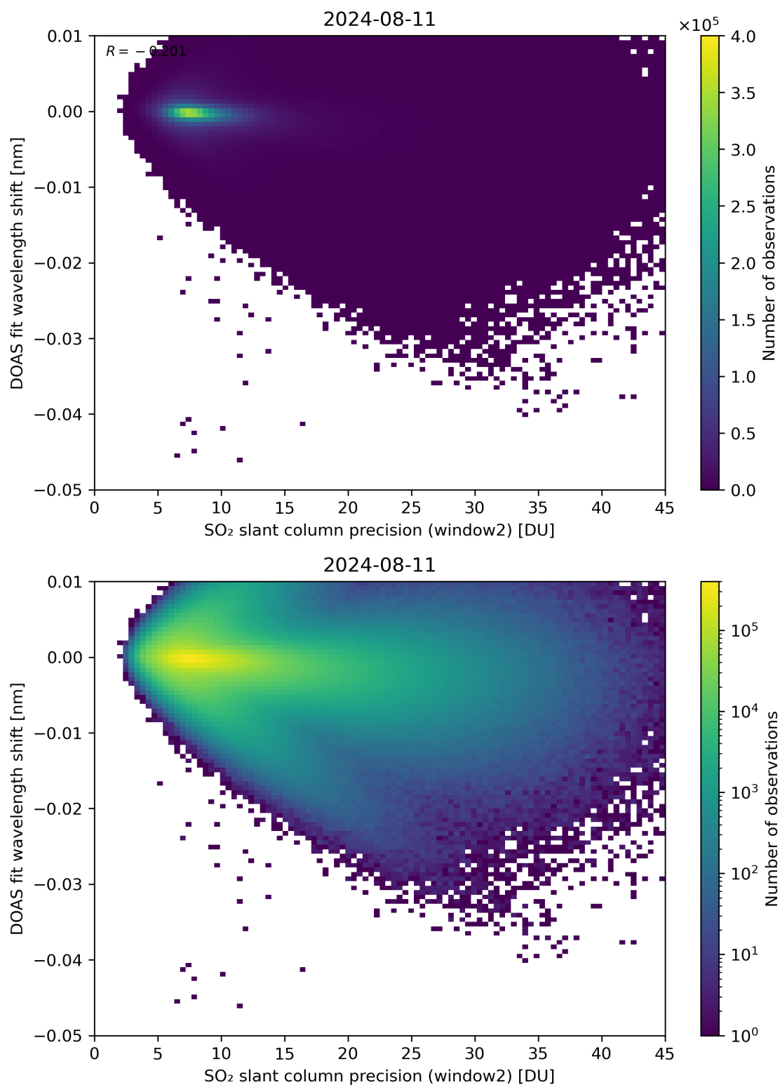
Figure 243: Scatter density plot of “SO 2 slant column precision (window2)” against “DOAS fit wavelength shift” for 2024-08-11 to 2024-08-11.
