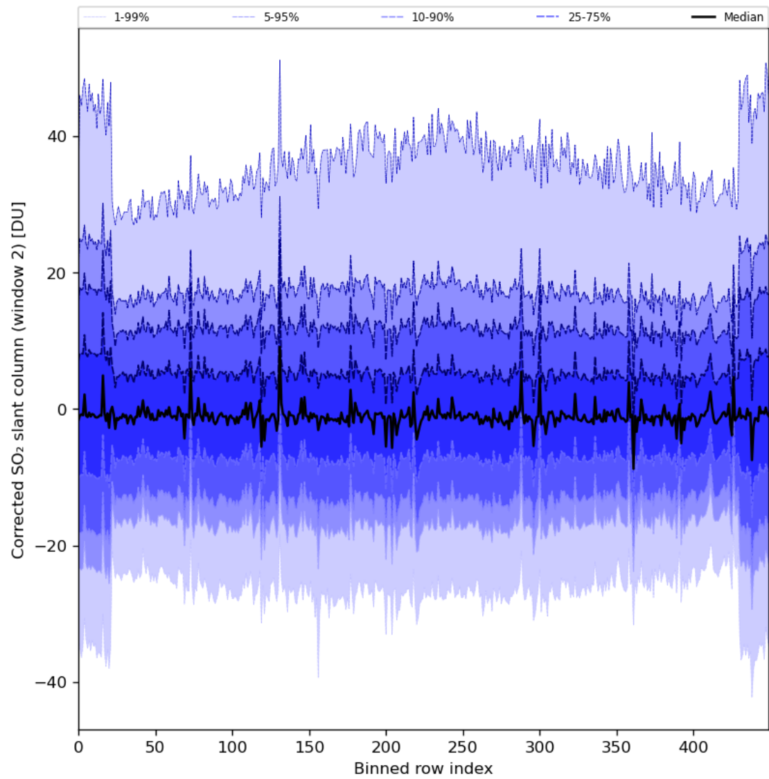
Figure 85: Along track statistics of “Corrected SO 2 slant column (window 2)” for 2024-08-11 to 2024-08-11
