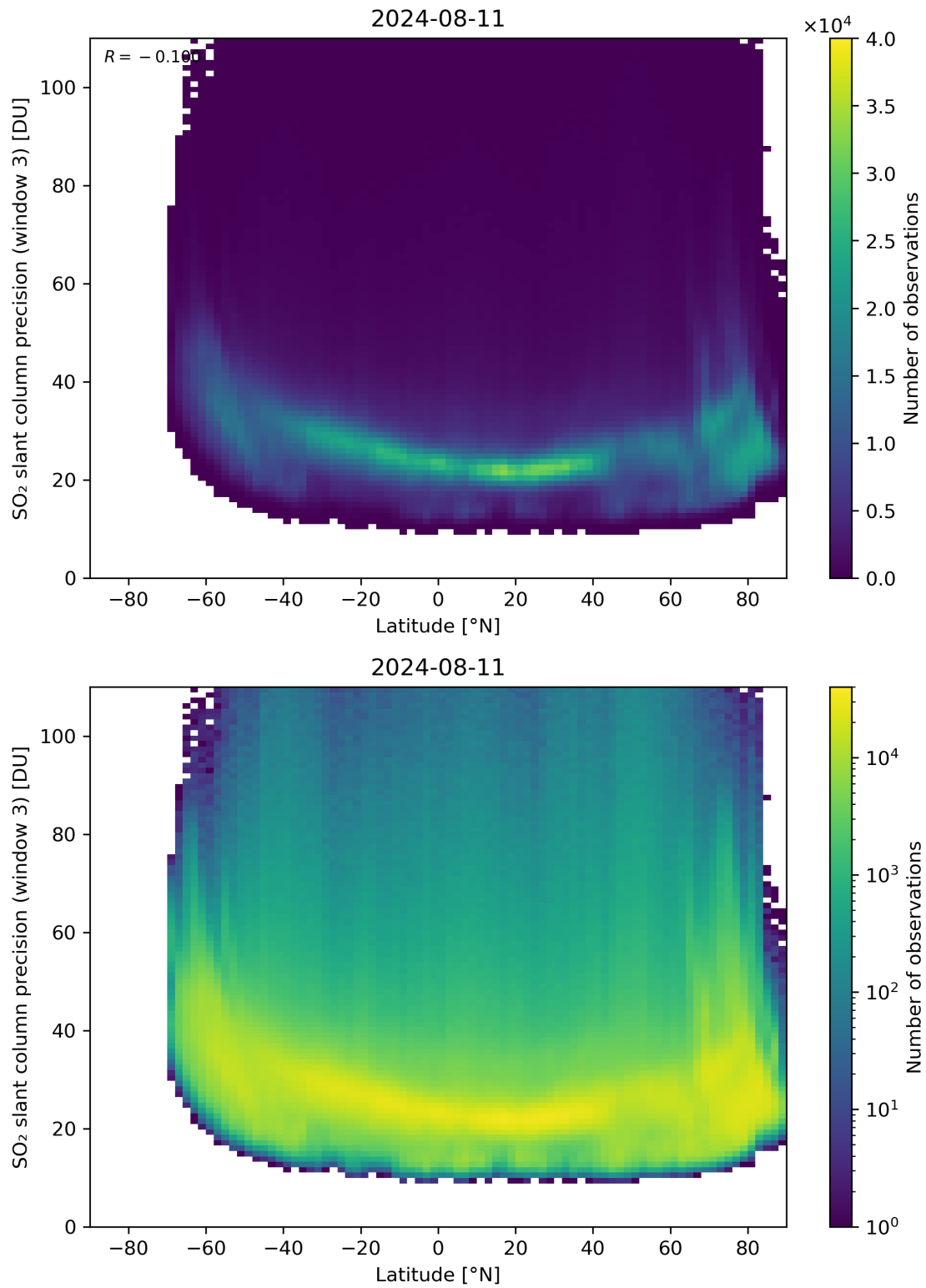
Figure 153: Scatter density plot of “Latitude” against “SO 2 slant column precision (window 3)” for 2024-08-11 to 2024-08-11.
