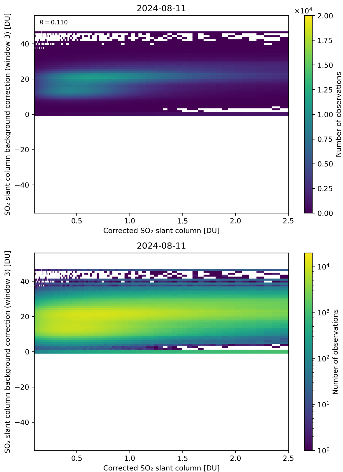
Figure 180: Scatter density plot of “Corrected SO 2 slant column” against “SO 2 slant column background correction (window 3)” for 2024-08-11 to 2024-08-11.
