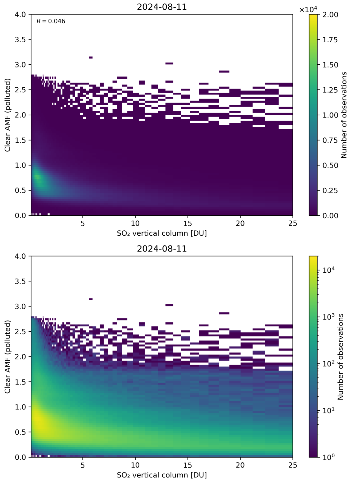
Figure 296: Scatter density plot of “SO 2 vertical column” against “Clear AMF (polluted)” for 2024-08-11 to 2024-08-11.
