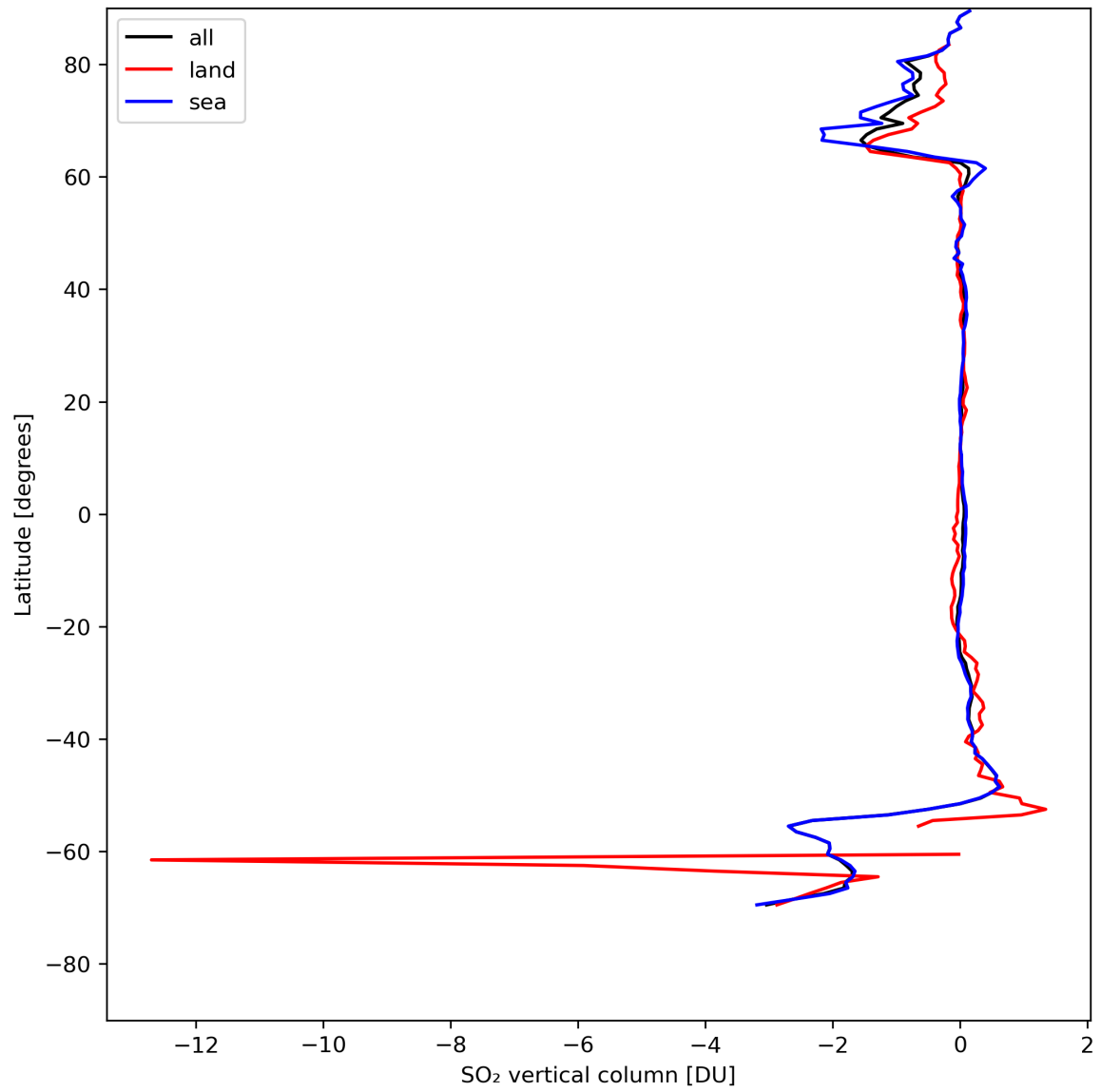
Figure 30: Zonal average of “SO 2 vertical column” for 2024-08-11 to 2024-08-11.
