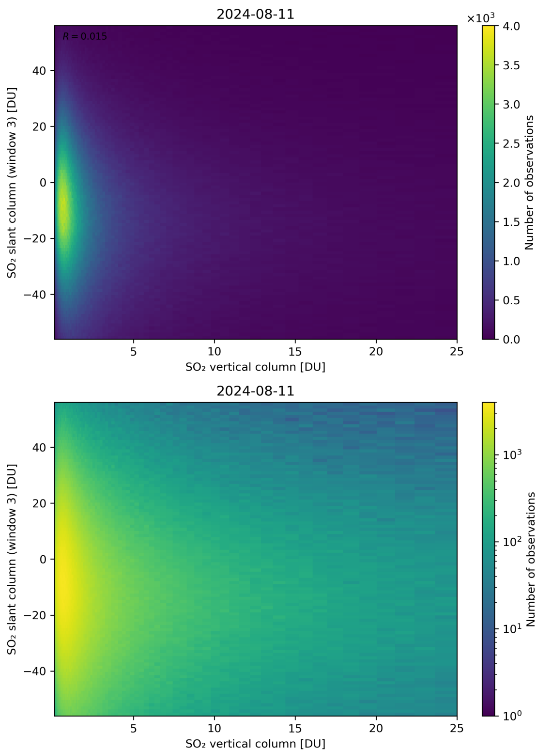
Figure 303: Scatter density plot of “SO 2 vertical column” against “SO 2 slant column (window 3)” for 2024-08-11 to 2024-08-11.
