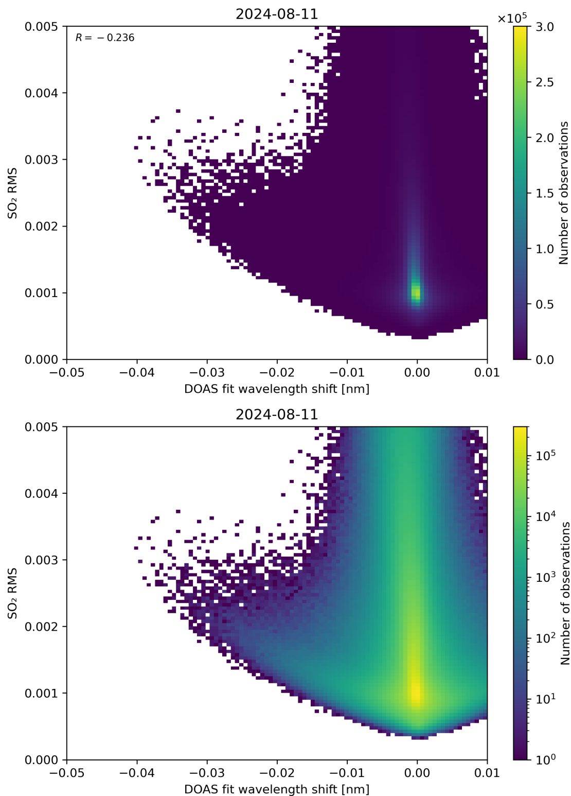
Figure 128: Scatter density plot of “DOAS fit wavelength shift” against “SO 2 RMS” for 2024-08-11 to 2024-08-11.
