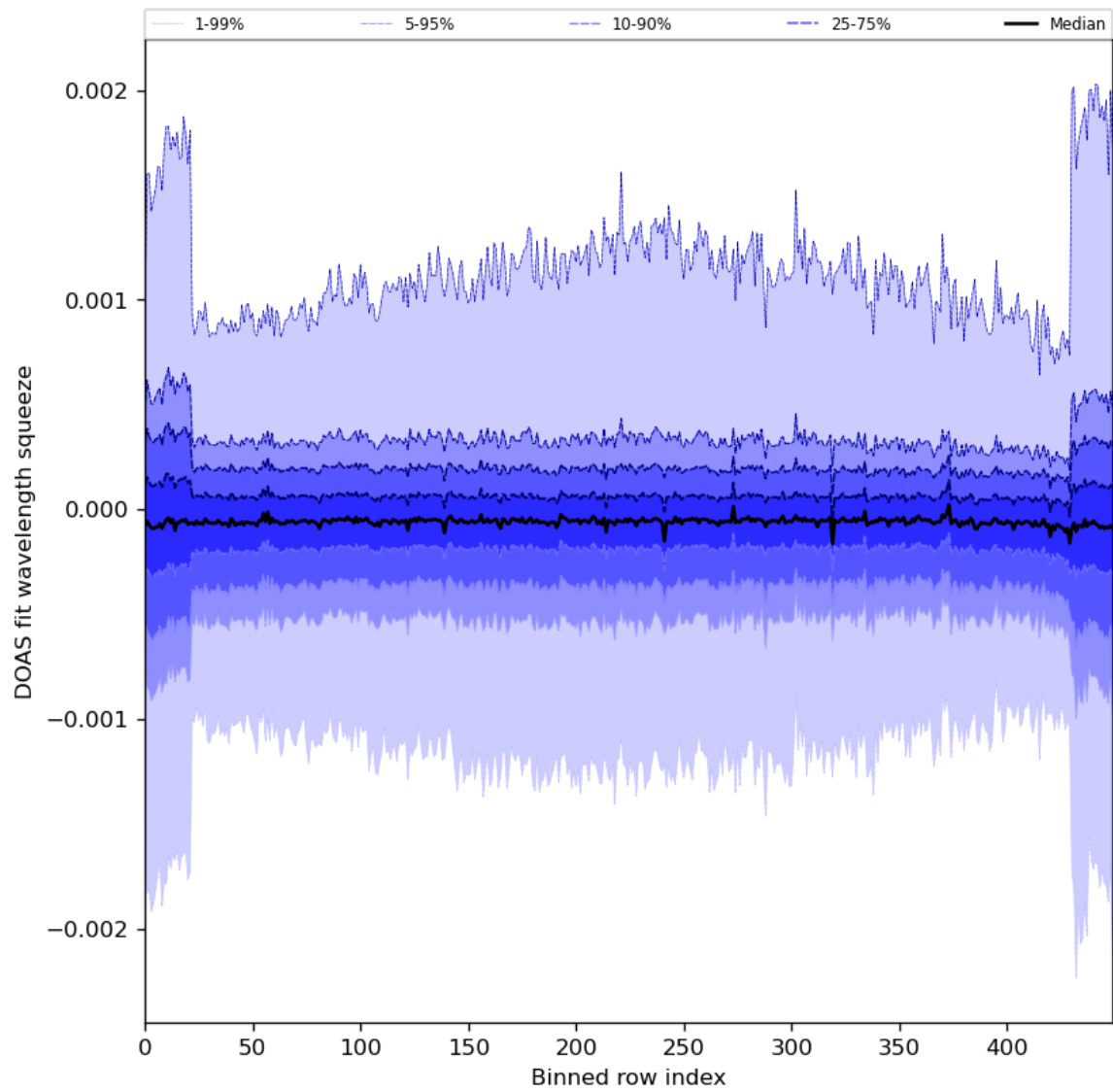
Figure 92: Along track statistics of “DOAS fit wavelength squeeze” for 2024-08-11 to 2024-08-11
