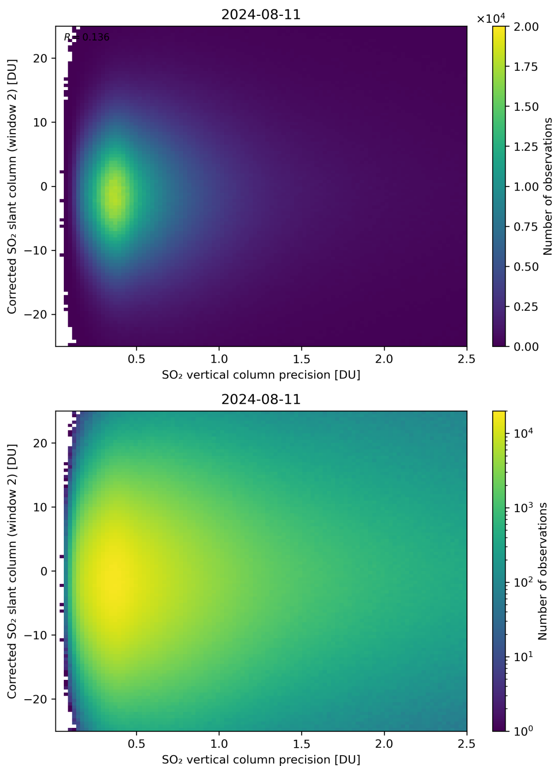
Figure 287: Scatter density plot of “SO 2 vertical column precision” against “Corrected SO 2 slant column (window 2)” for 2024-08-11 to 2024-08-11.
