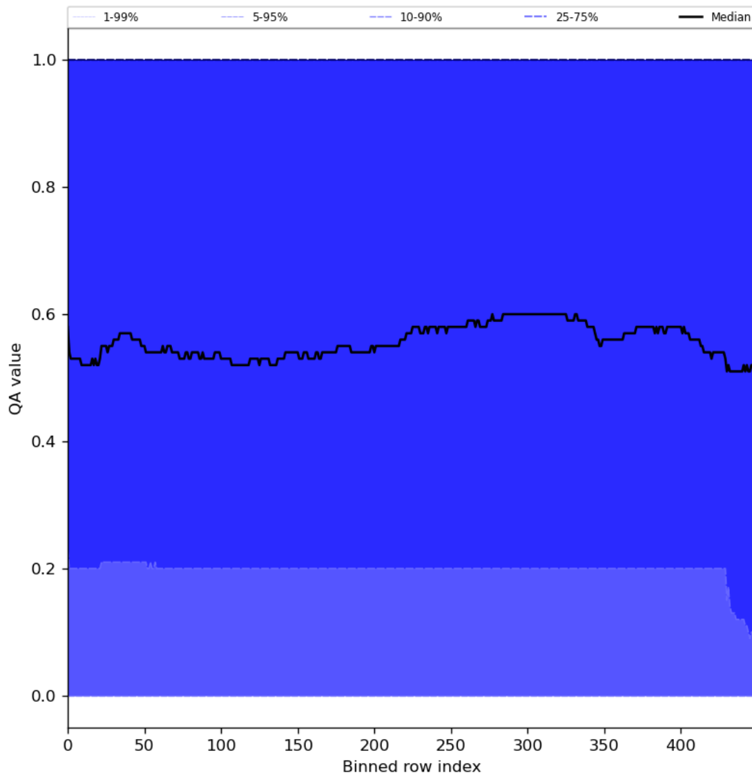
Figure 75: Along track statistics of “QA value” for 2024-08-11 to 2024-08-11
