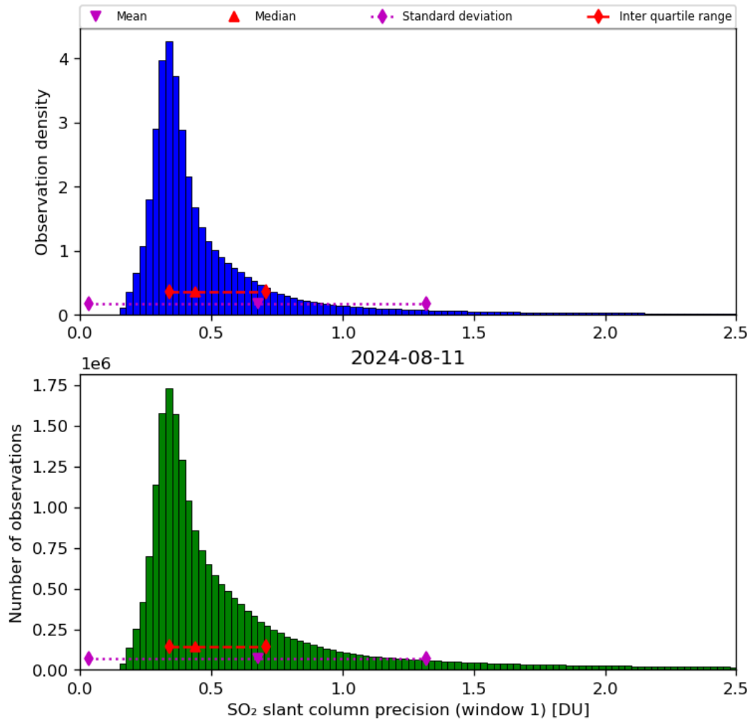
Figure 57: Histogram of “SO 2 slant column precision (window 1)” for 2024-08-11 to 2024-08-11
