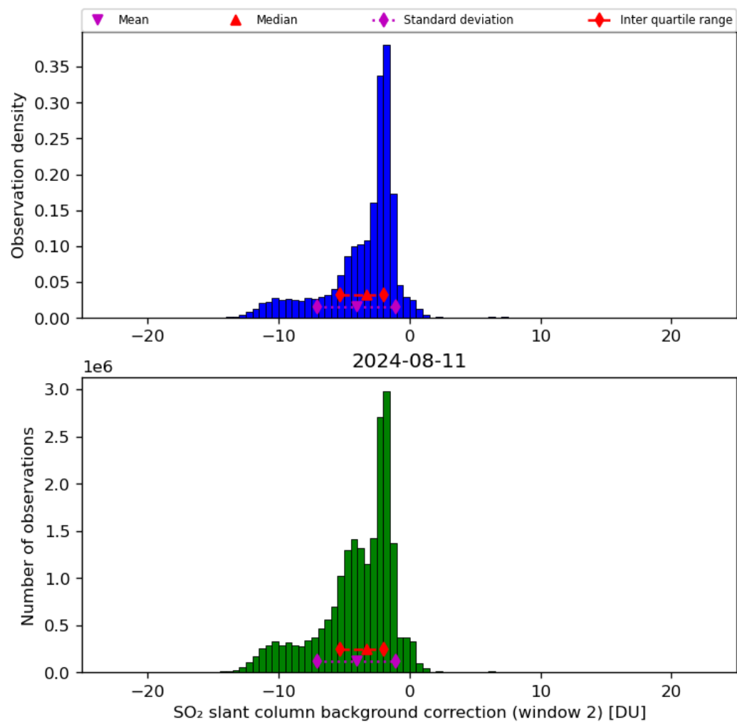
Figure 63: Histogram of “SO 2 slant column background correction (window 2)” for 2024-08-11 to 2024-08-11
