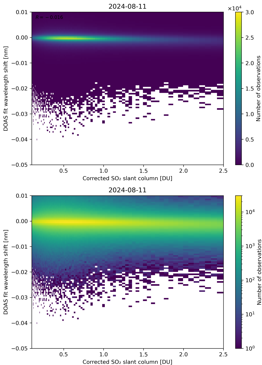
Figure 181: Scatter density plot of “Corrected SO 2 slant column” against “DOAS fit wavelength shift” for 2024-08-11 to 2024-08-11.
