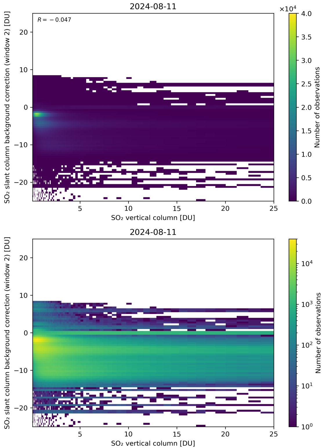
Figure 274: Scatter density plot of “SO 2 vertical column” against “SO 2 slant column background correction (window 2)” for 2024-08-11 to 2024-08-11.
