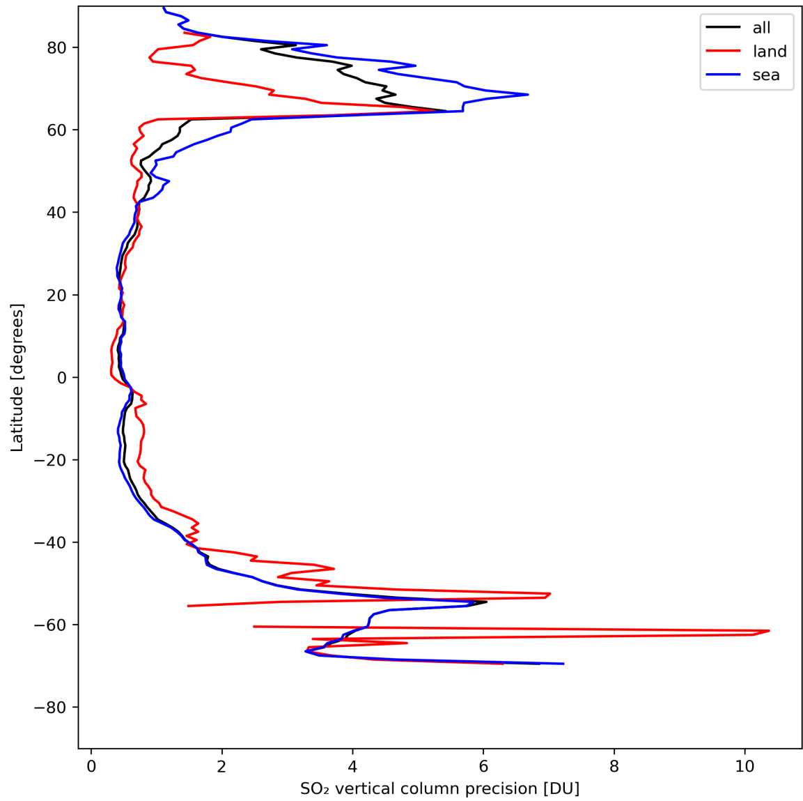
Figure 31: Zonal average of “SO 2 vertical column precision” for 2024-08-11 to 2024-08-11.
