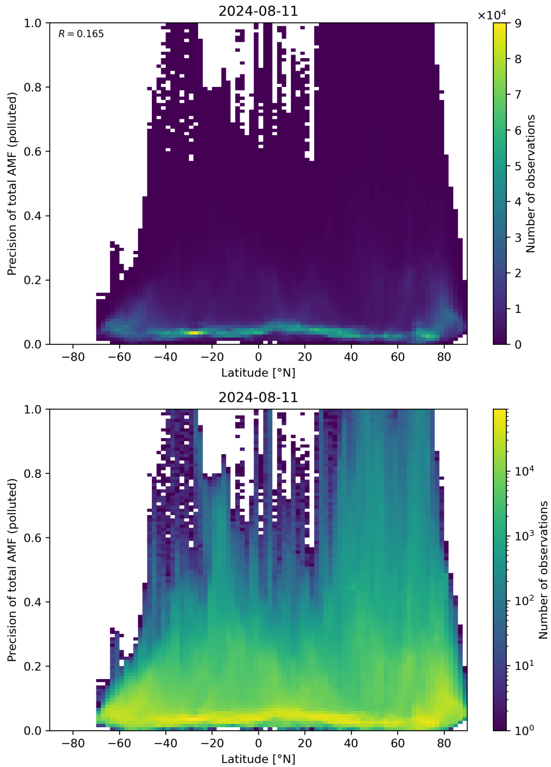
Figure 155: Scatter density plot of “Latitude” against “Precision of total AMF (polluted)” for 2024-08-11 to 2024-08-11.
