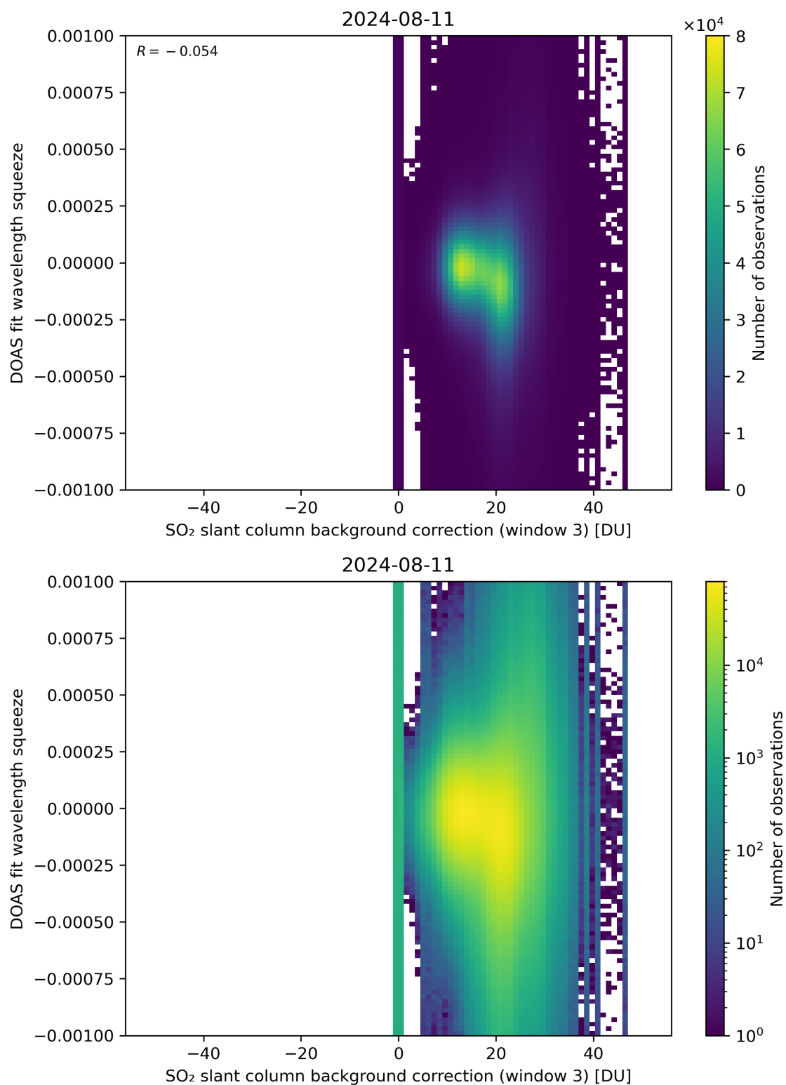
Figure 122: Scatter density plot of “SO 2 slant column background correction (window 3)” against “DOAS fit wavelength squeeze” for 2024-08-11 to 2024-08-11.
