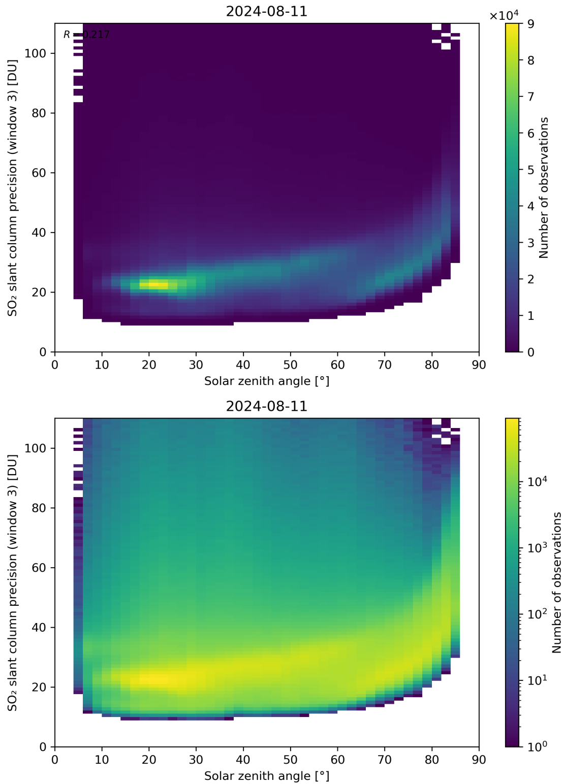
Figure 173: Scatter density plot of “Solar zenith angle” against “SO 2 slant column precision (window 3)” for 2024-08-11 to 2024-08-11.
