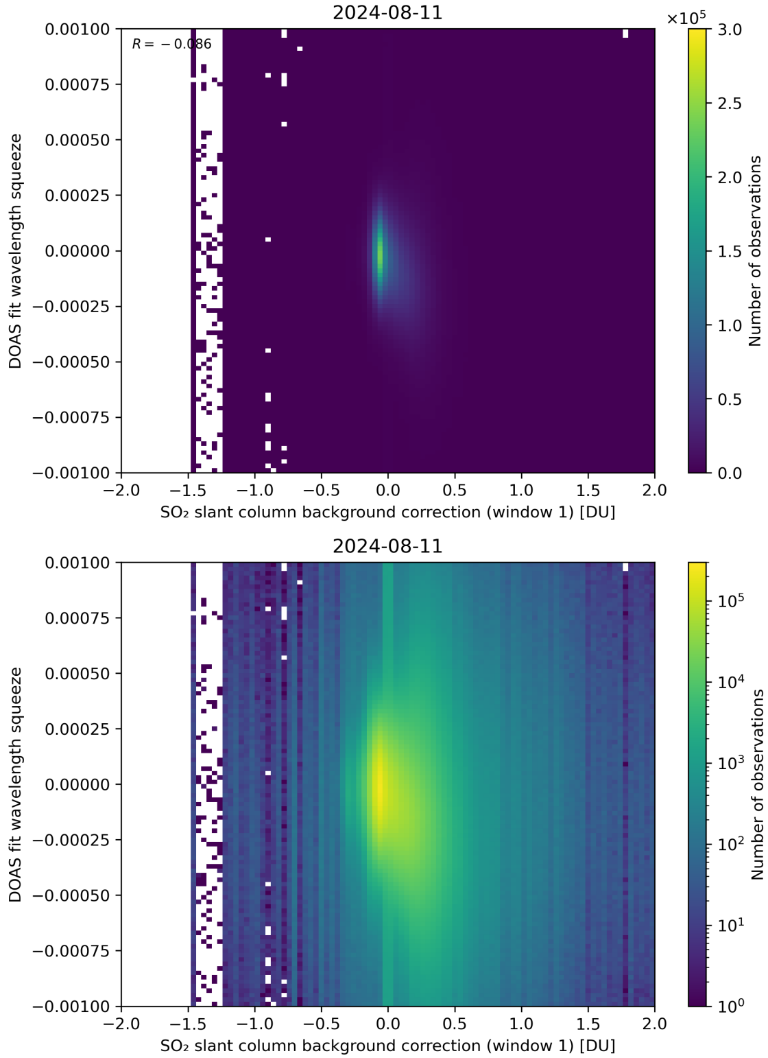
Figure 101: Scatter density plot of “SO 2 slant column background correction (window 1)” against “DOAS fit wavelength squeeze” for 2024-08-11 to 2024-08-11.
