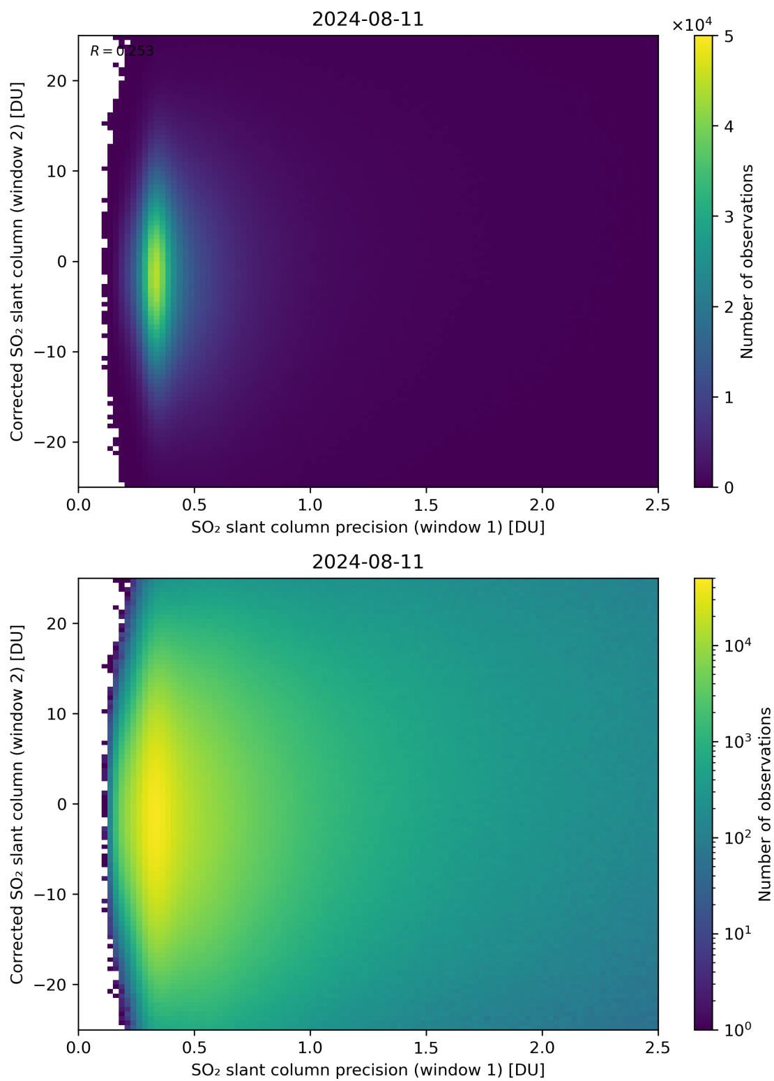
Figure 225: Scatter density plot of “SO 2 slant column precision (window 1)” against “Corrected SO 2 slant column (window 2)” for 2024-08-11 to 2024-08-11.
