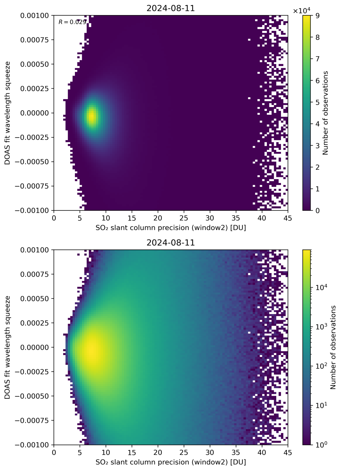
Figure 244: Scatter density plot of “SO 2 slant column precision (window2)” against “DOAS fit wavelength squeeze” for 2024-08-11 to 2024-08-11.
