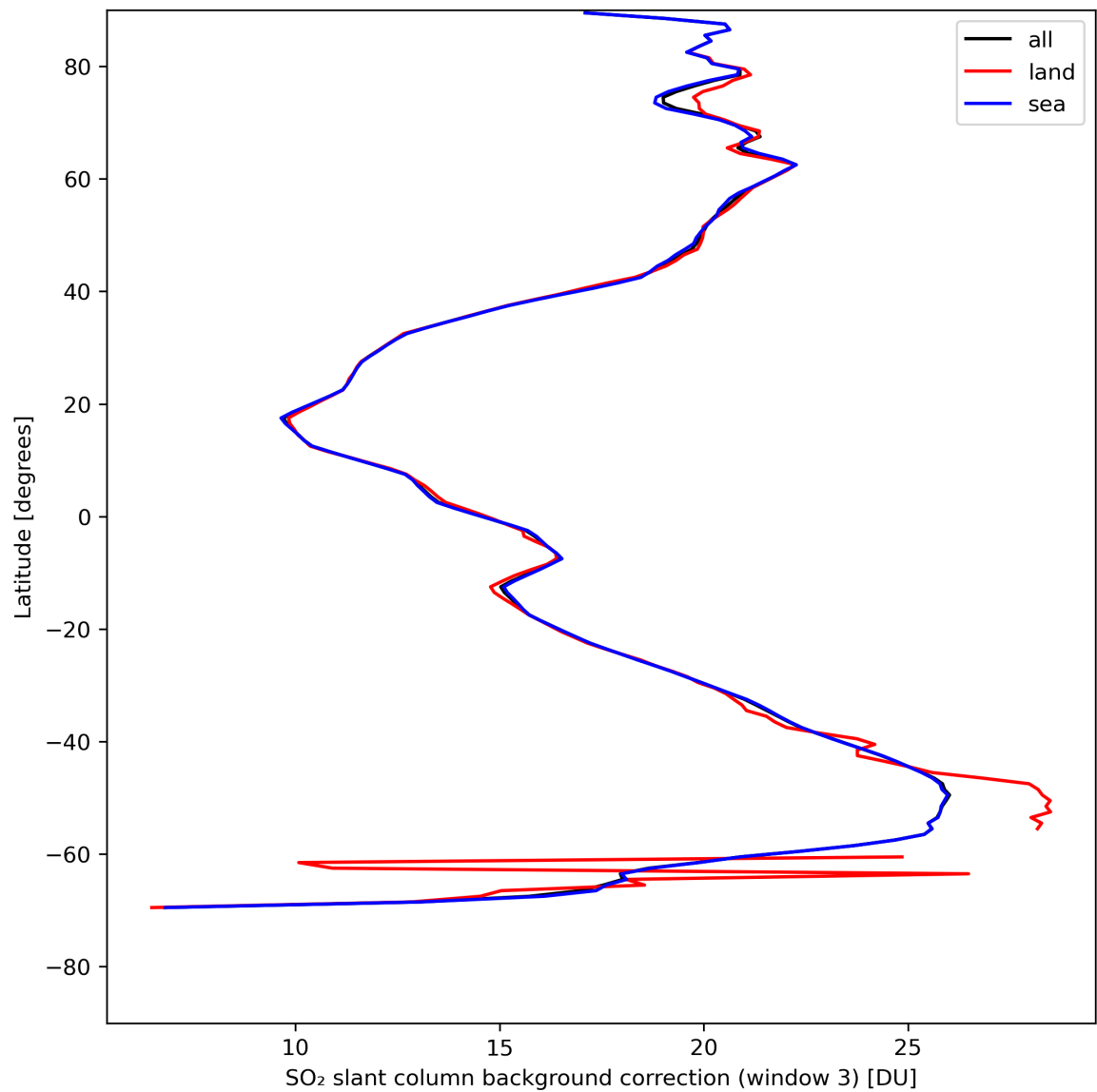
Figure 44: Zonal average of “SO 2 slant column background correction (window 3)” for 2024-08-11 to 2024-08-11.
