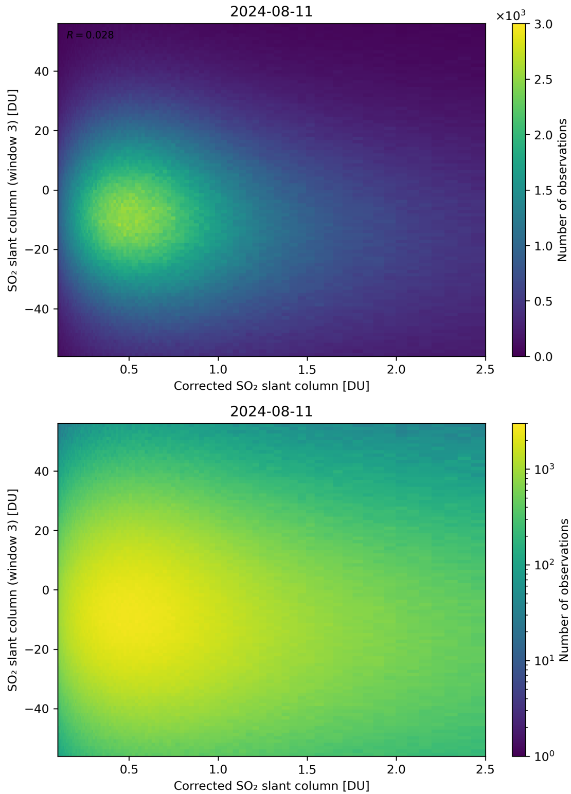
Figure 190: Scatter density plot of “Corrected SO 2 slant column” against “SO 2 slant column (window 3)” for 2024-08-11 to 2024-08-11.
