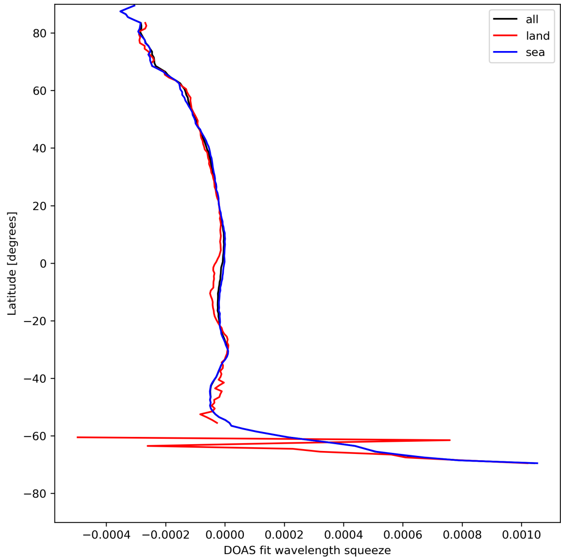
Figure 46: Zonal average of “DOAS fit wavelength squeeze” for 2024-08-11 to 2024-08-11.
