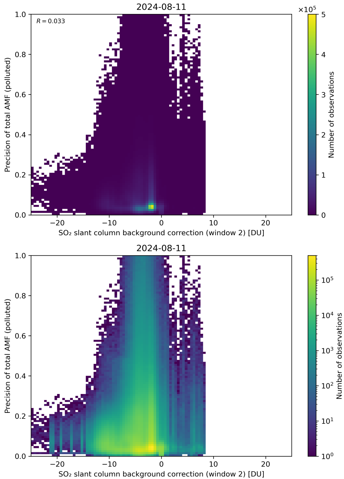
Figure 120: Scatter density plot of “SO 2 slant column background correction (window 2)” against “Precision of total AMF (polluted)” for 2024-08-11 to 2024-08-11.
