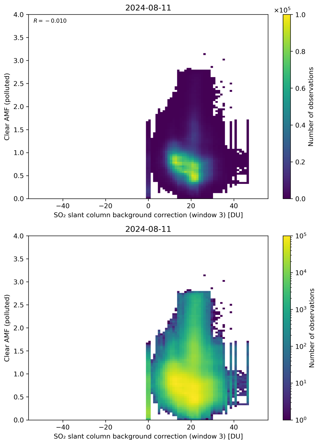
Figure 124: Scatter density plot of “SO 2 slant column background correction (window 3)” against “Clear AMF (polluted)” for 2024-08-11 to 2024-08-11.
