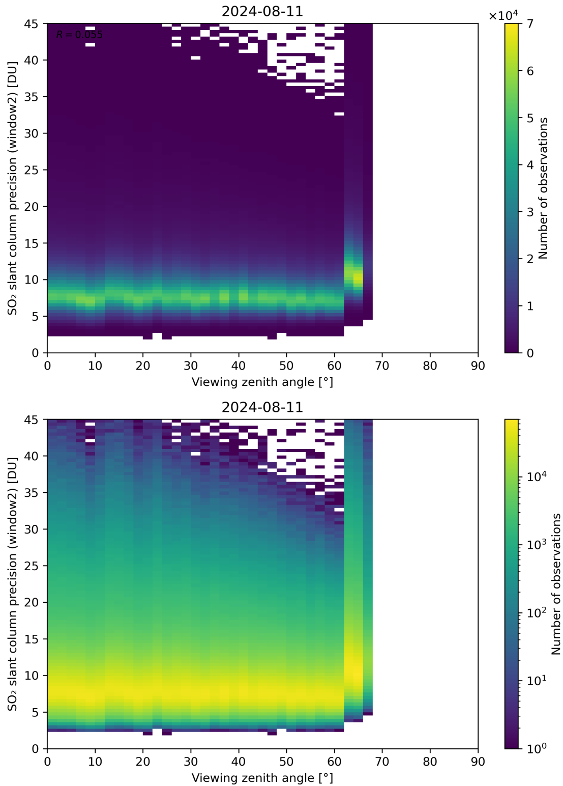
Figure 322: Scatter density plot of “Viewing zenith angle” against “SO 2 slant column precision (window2)” for 2024-08-11 to 2024-08-11.
