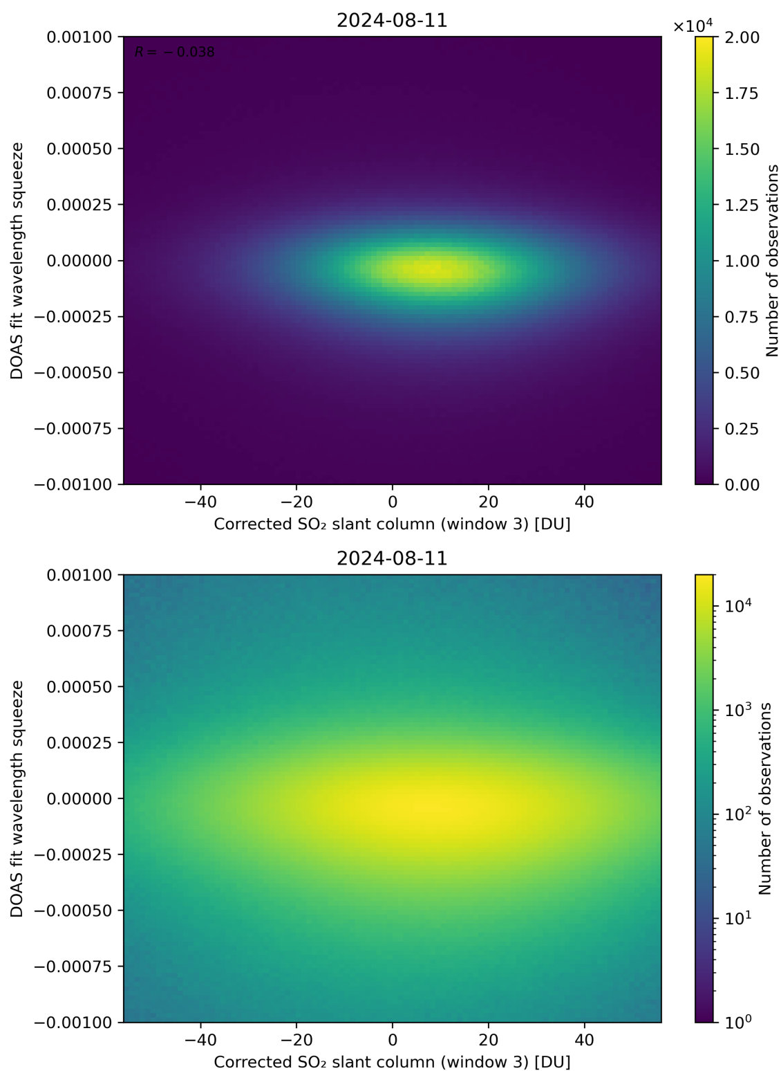
Figure 207: Scatter density plot of “Corrected SO 2 slant column (window 3)” against “DOAS fit wavelength squeeze” for 2024-08-11 to 2024-08-11.
