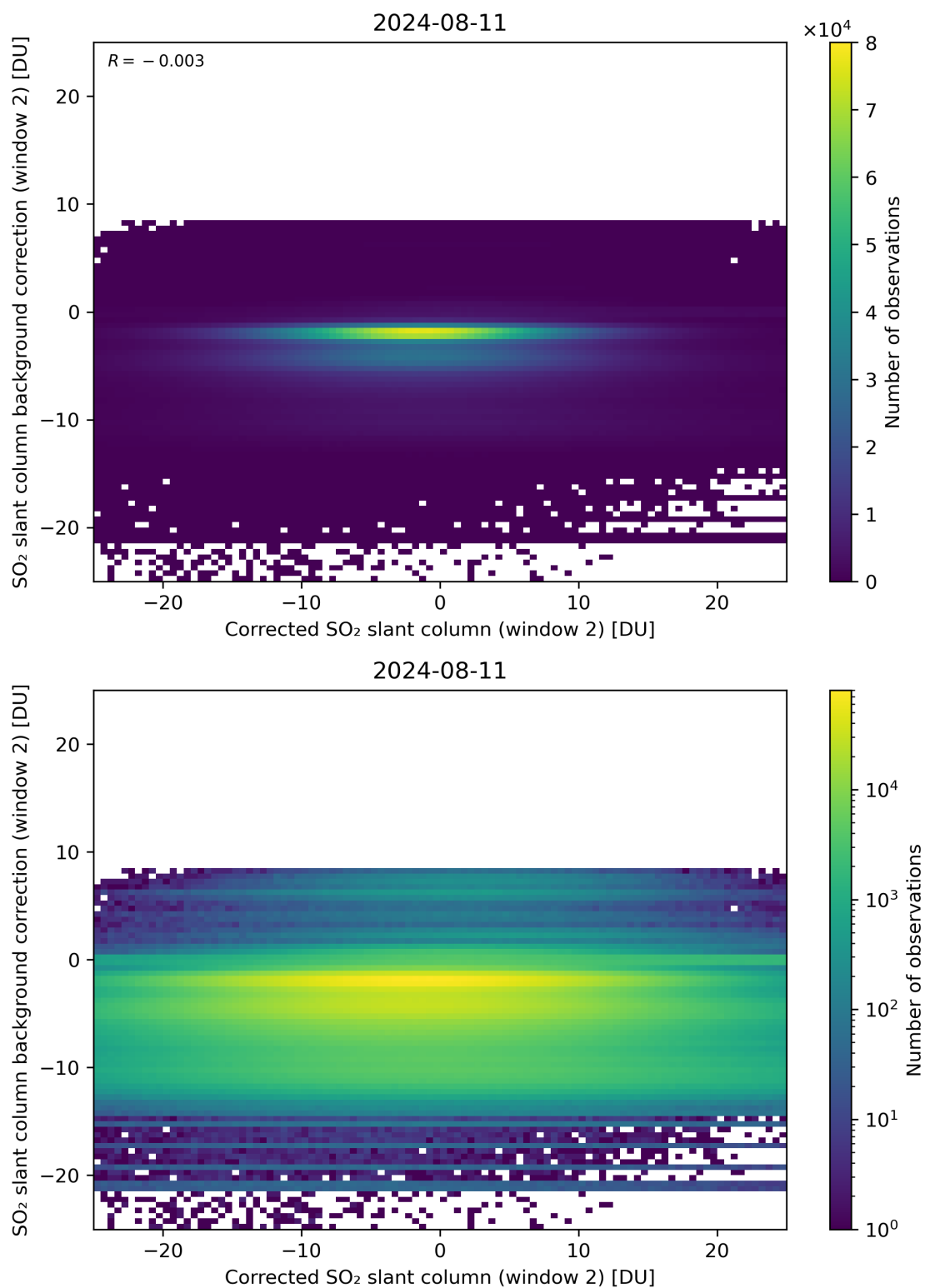
Figure 194: Scatter density plot of “Corrected SO 2 slant column (window 2)” against “SO 2 slant column background correction (window 2)” for 2024-08-11 to 2024-08-11.
