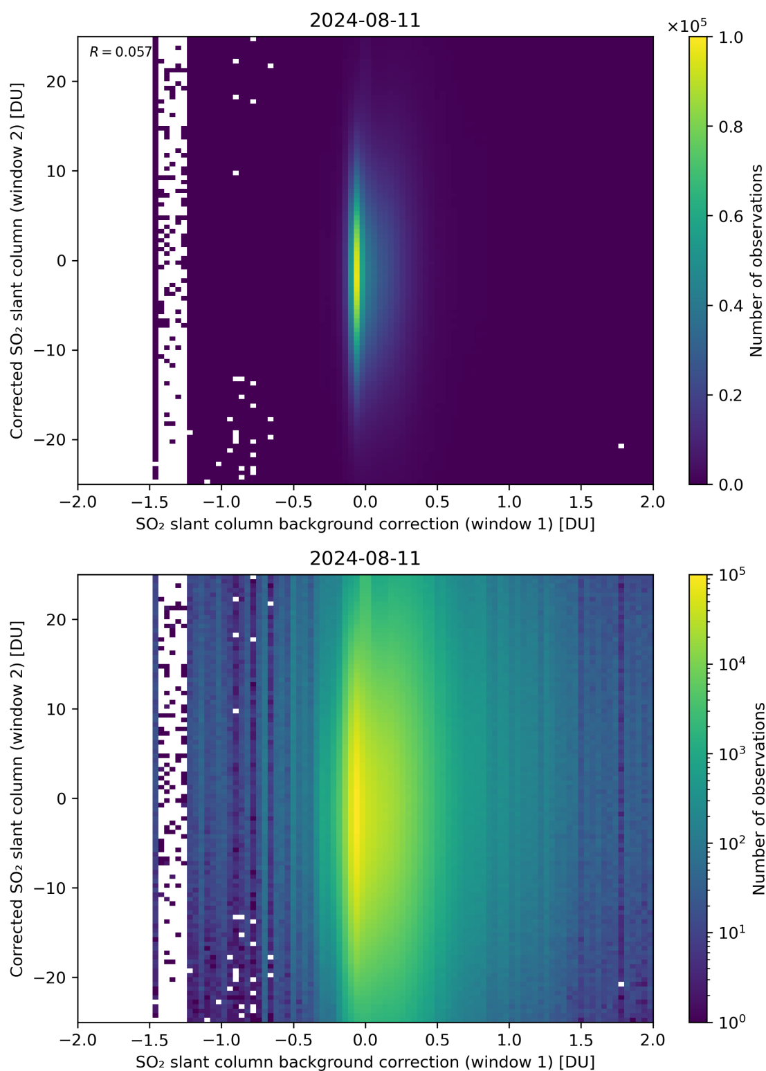
Figure 104: Scatter density plot of “SO 2 slant column background correction (window 1)” against “Corrected SO 2 slant column (window 2)” for 2024-08-11 to 2024-08-11.
