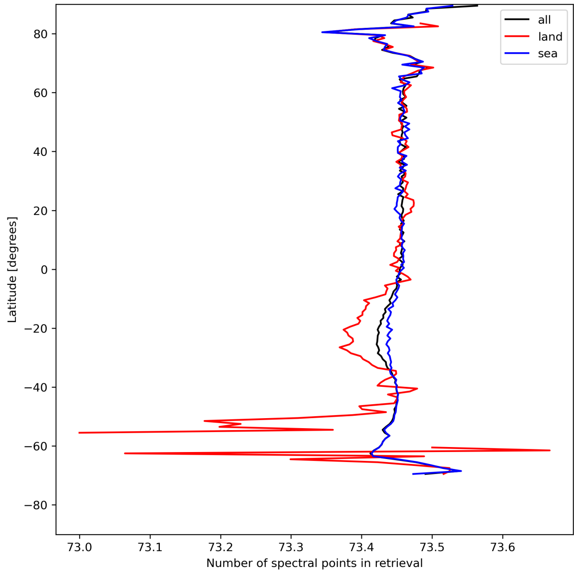
Figure 51: Zonal average of “Number of spectral points in retrieval” for 2024-08-11 to 2024-08-11.
