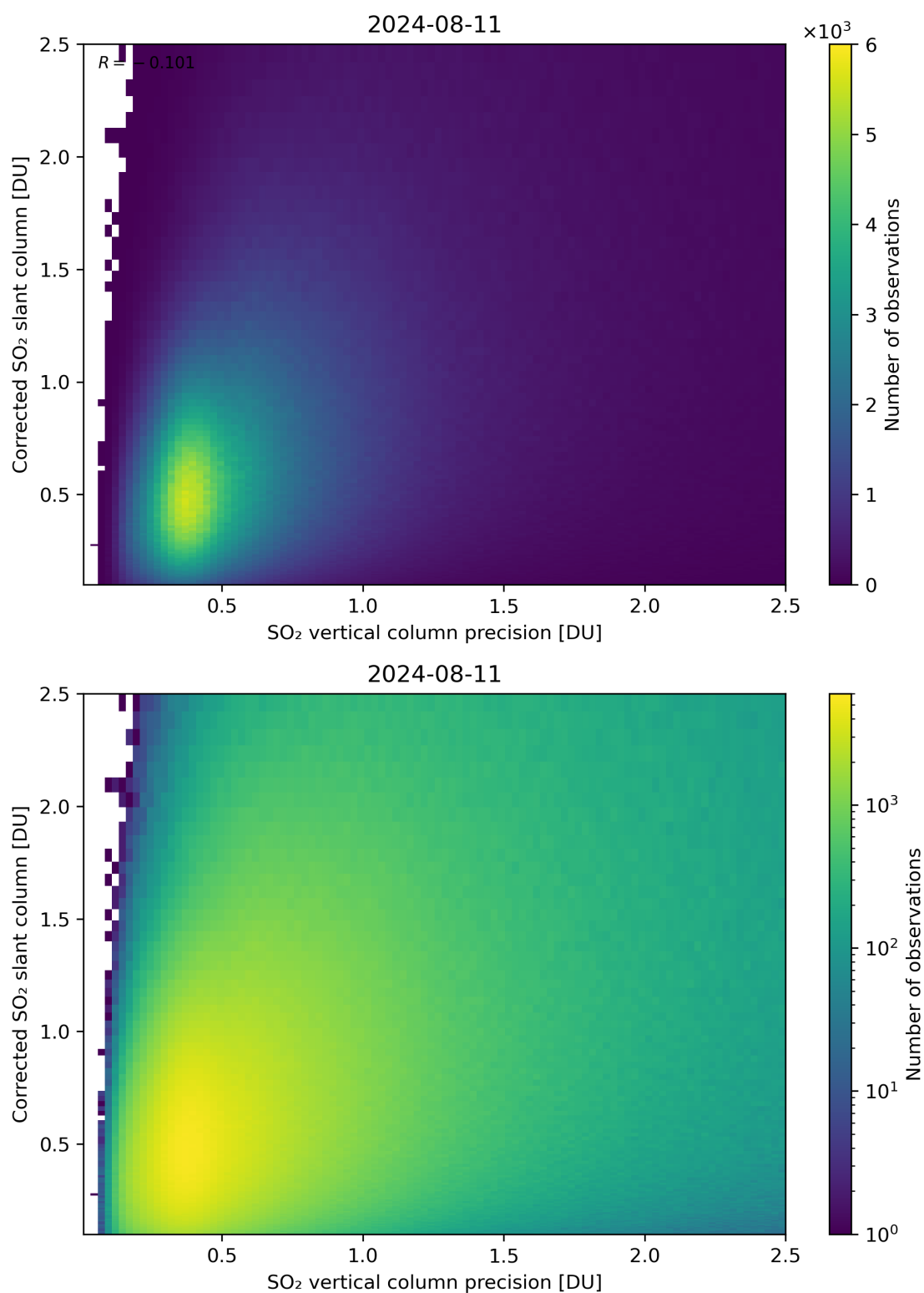
Figure 286: Scatter density plot of “SO 2 vertical column precision” against “Corrected SO 2 slant column” for 2024-08-11 to 2024-08-11.
