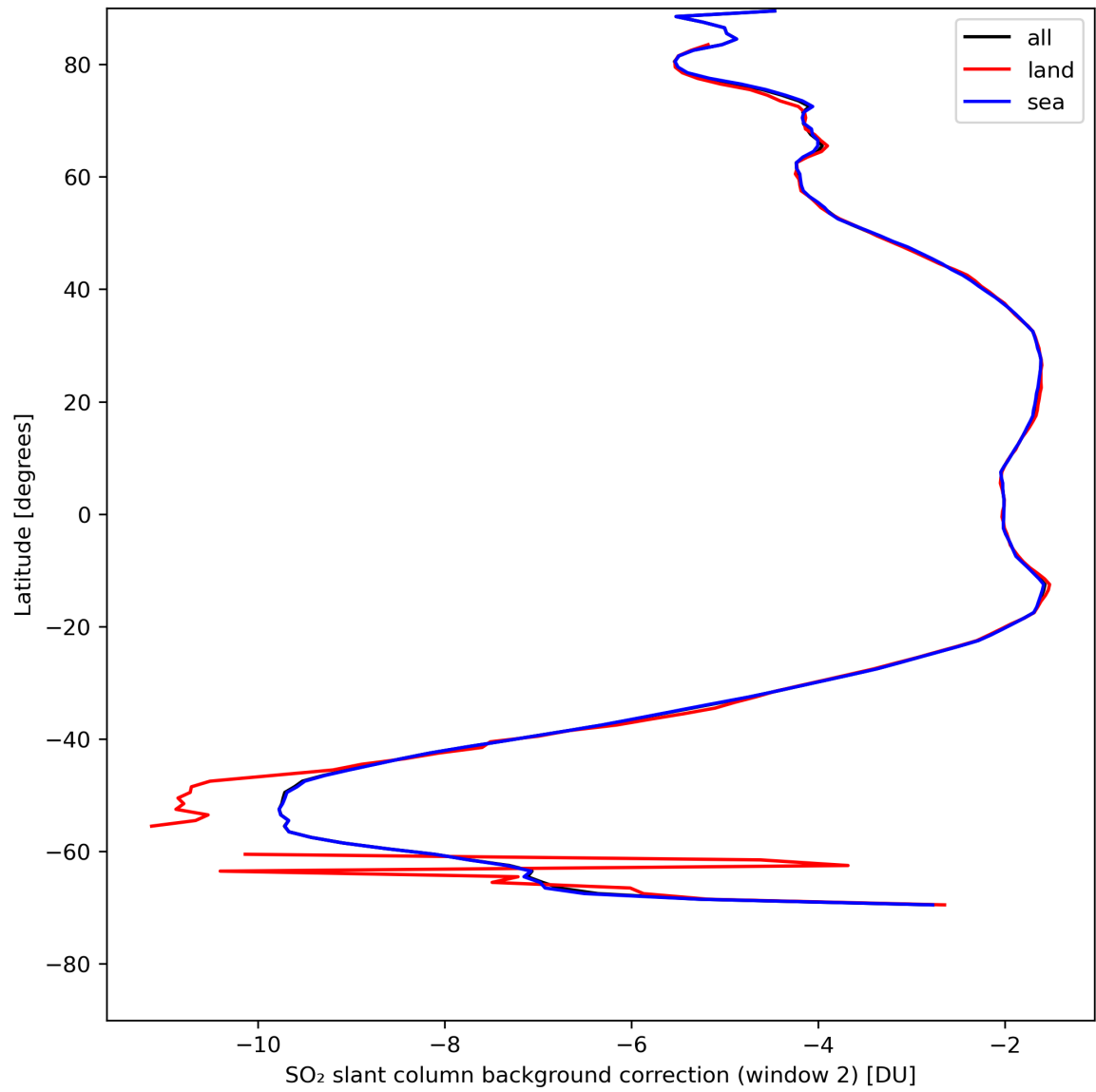
Figure 40: Zonal average of “SO 2 slant column background correction (window 2)” for 2024-08-11 to 2024-08-11.
