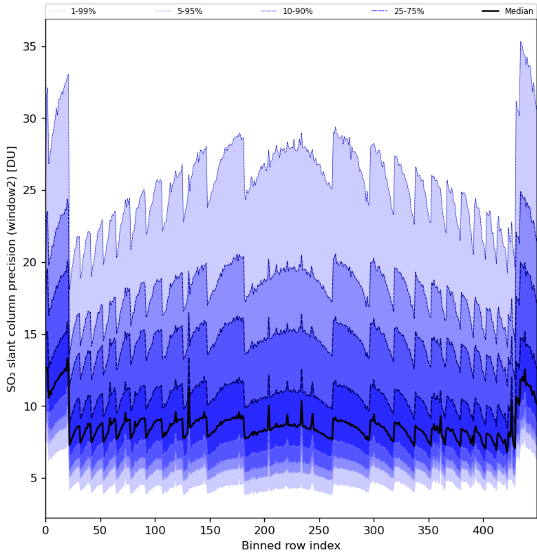
Figure 84: Along track statistics of “SO 2 slant column precision (window2)” for 2024-08-11 to 2024-08-11
