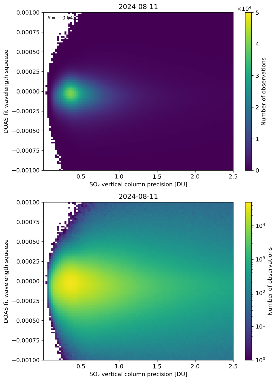
Figure 283: Scatter density plot of “SO 2 vertical column precision” against “DOAS fit wavelength squeeze” for 2024-08-11 to 2024-08-11.
