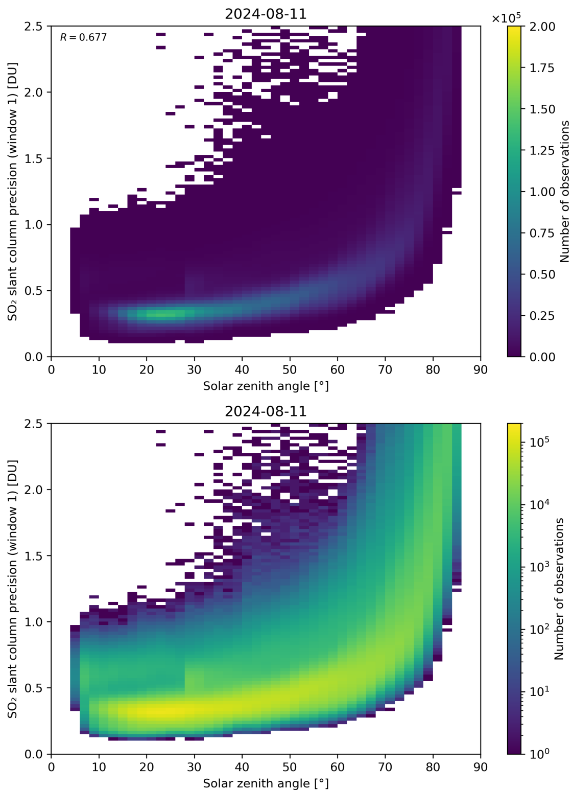
Figure 170: Scatter density plot of “Solar zenith angle” against “SO 2 slant column precision (window 1)” for 2024-08-11 to 2024-08-11.
