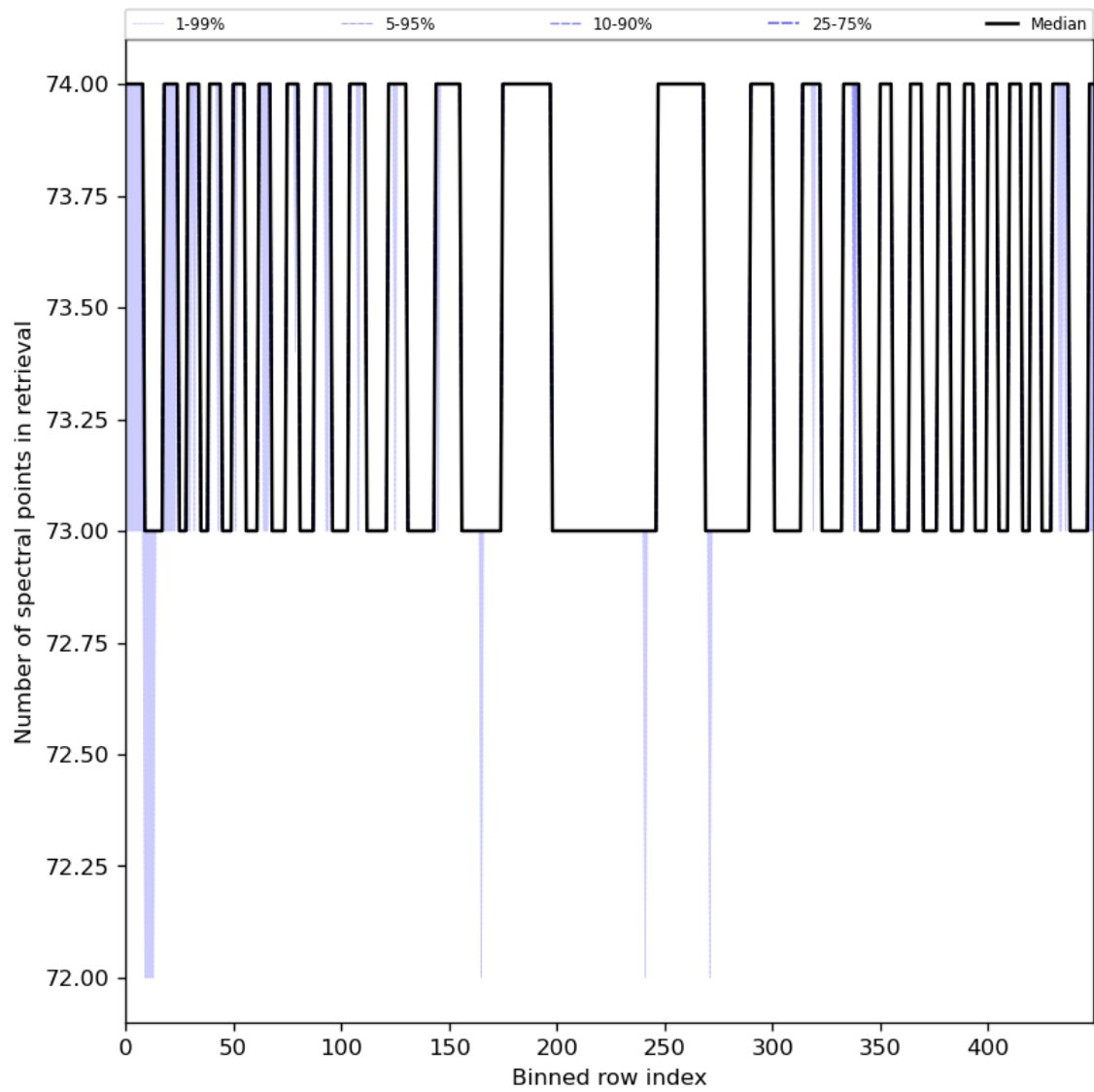
Figure 97: Along track statistics of “Number of spectral points in retrieval” for 2024-08-11 to 2024-08-11
