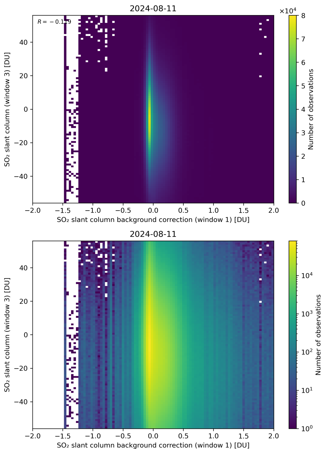
Figure 107: Scatter density plot of “SO 2 slant column background correction (window 1)” against “SO 2 slant column (window 3)” for 2024-08-11 to 2024-08-11.
