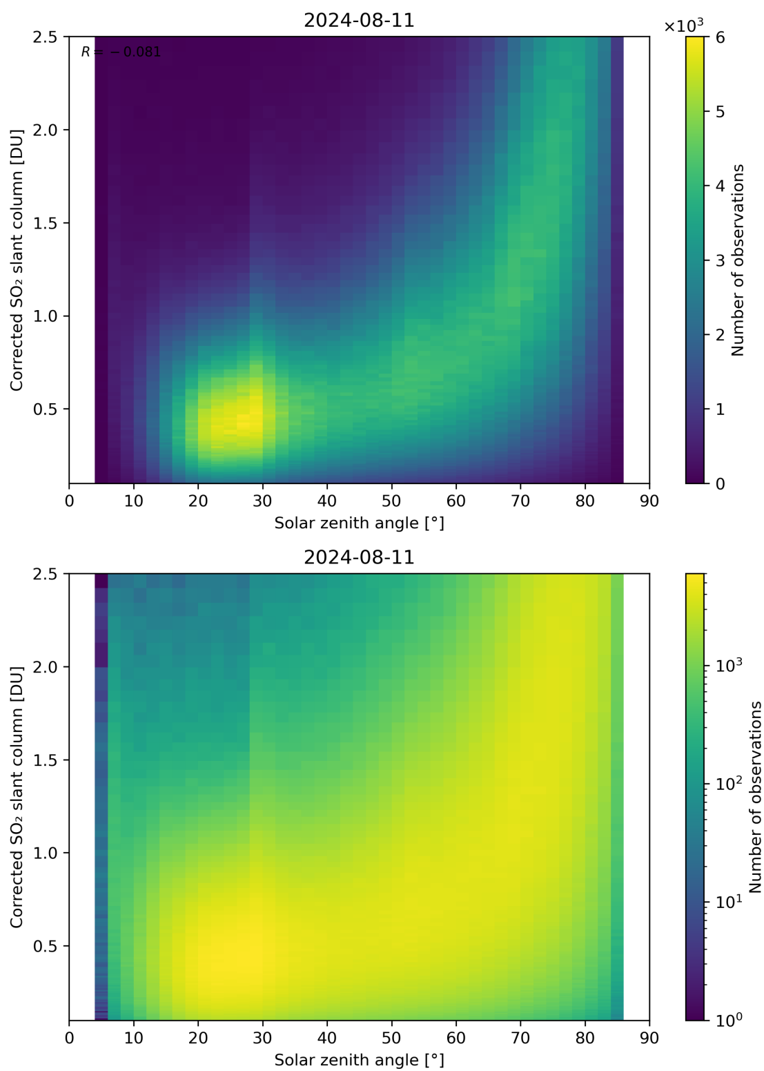
Figure 166: Scatter density plot of “Solar zenith angle” against “Corrected SO 2 slant column” for 2024-08-11 to 2024-08-11.
