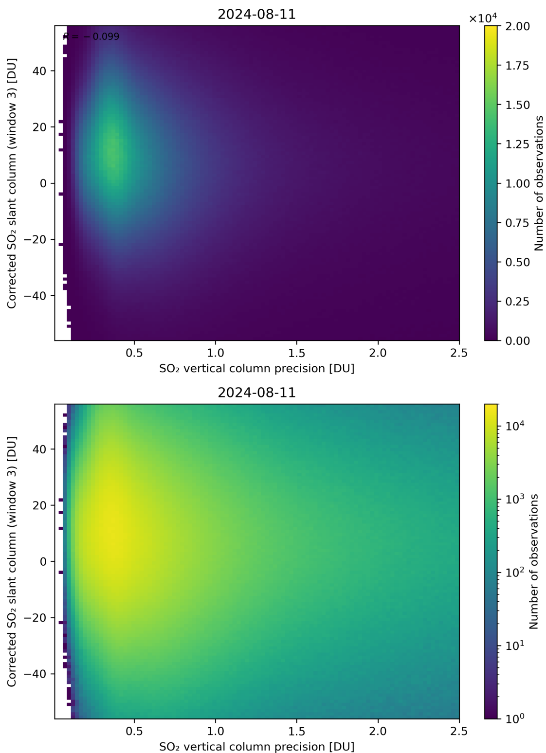
Figure 288: Scatter density plot of “SO 2 vertical column precision” against “Corrected SO 2 slant column (window 3)” for 2024-08-11 to 2024-08-11.
