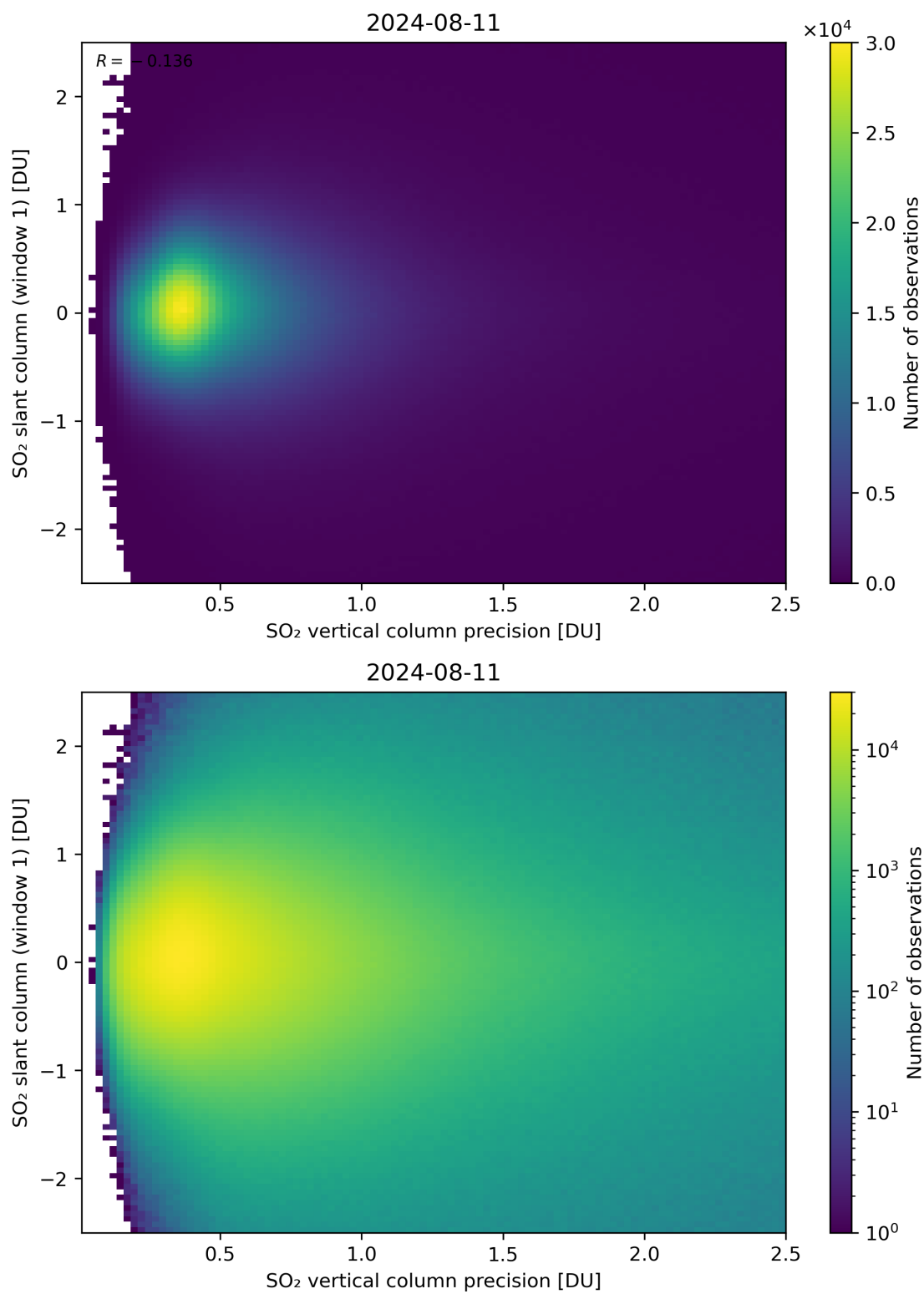
Figure 289: Scatter density plot of “SO 2 vertical column precision” against “SO 2 slant column (window 1)” for 2024-08-11 to 2024-08-11.
