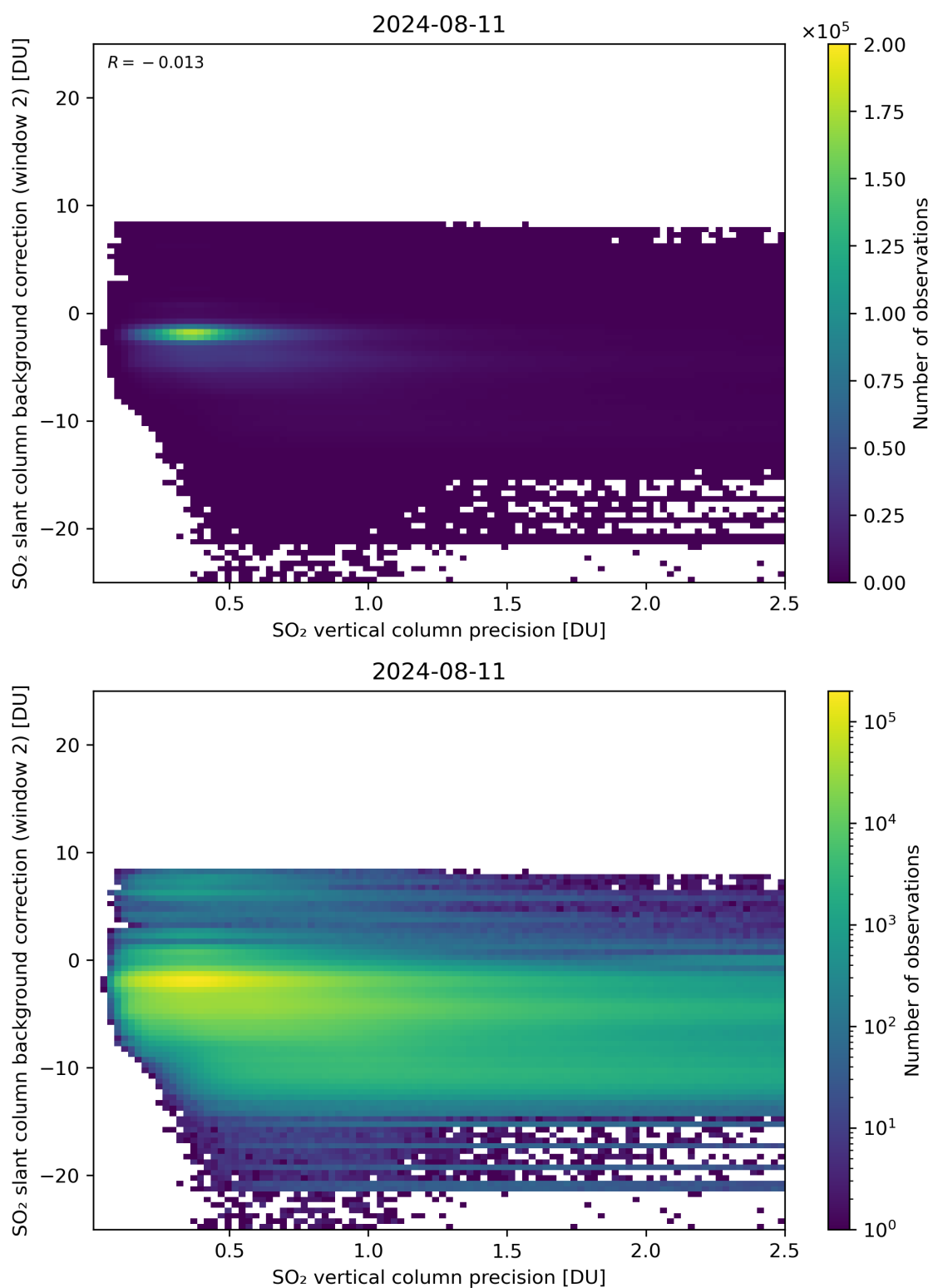
Figure 280: Scatter density plot of “SO 2 vertical column precision” against “SO 2 slant column background correction (window 2)” for 2024-08-11 to 2024-08-11.
