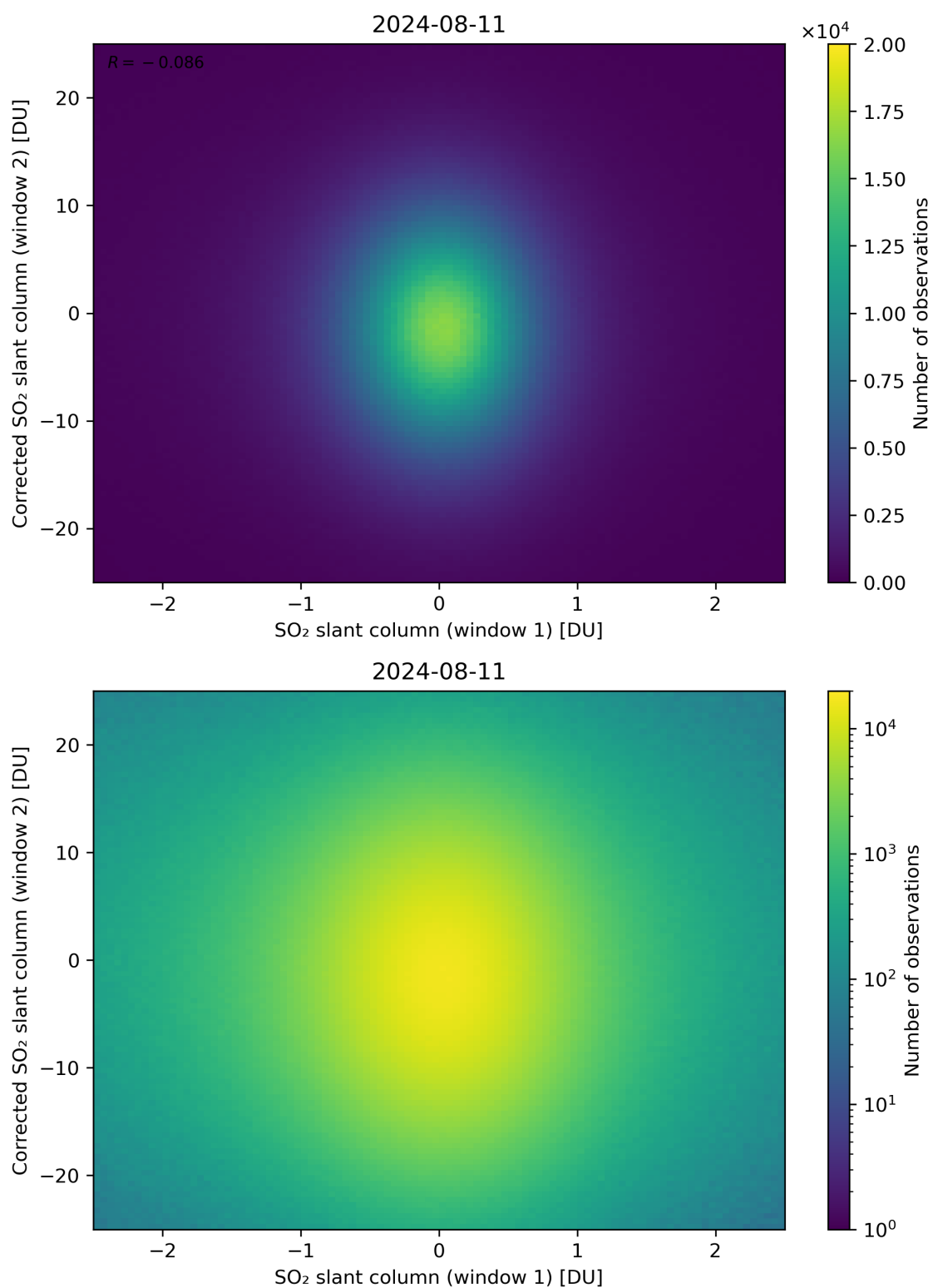
Figure 233: Scatter density plot of “SO 2 slant column (window 1)” against “Corrected SO 2 slant column (window 2)” for 2024-08-11 to 2024-08-11.
