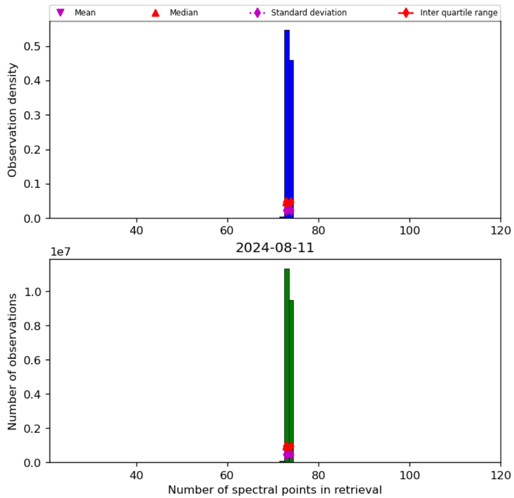
Figure 74: Histogram of "Number of spectral points in retrieval" for 2024-08-11 to 2024-08-11
