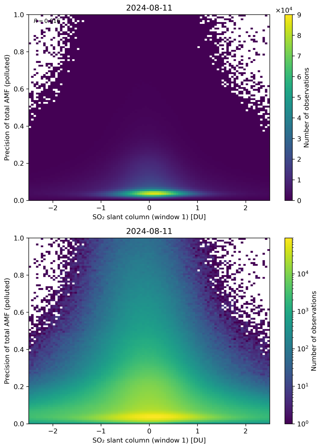
Figure 240: Scatter density plot of “SO 2 slant column (window 1)” against “Precision of total AMF (polluted)” for 2024-08-11 to 2024-08-11.
