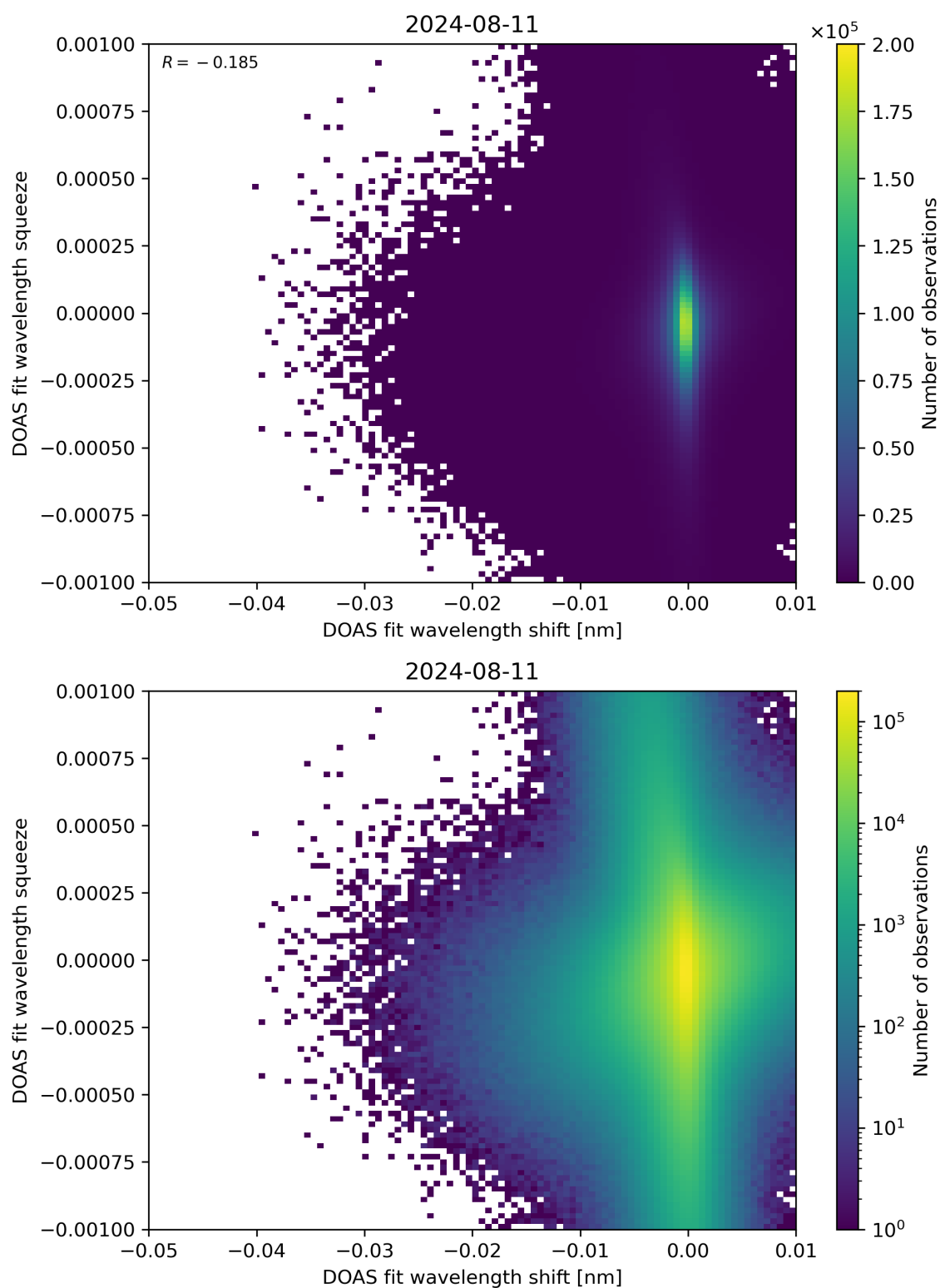
Figure 127: Scatter density plot of “DOAS fit wavelength shift” against “DOAS fit wavelength squeeze” for 2024-08-11 to 2024-08-11.
