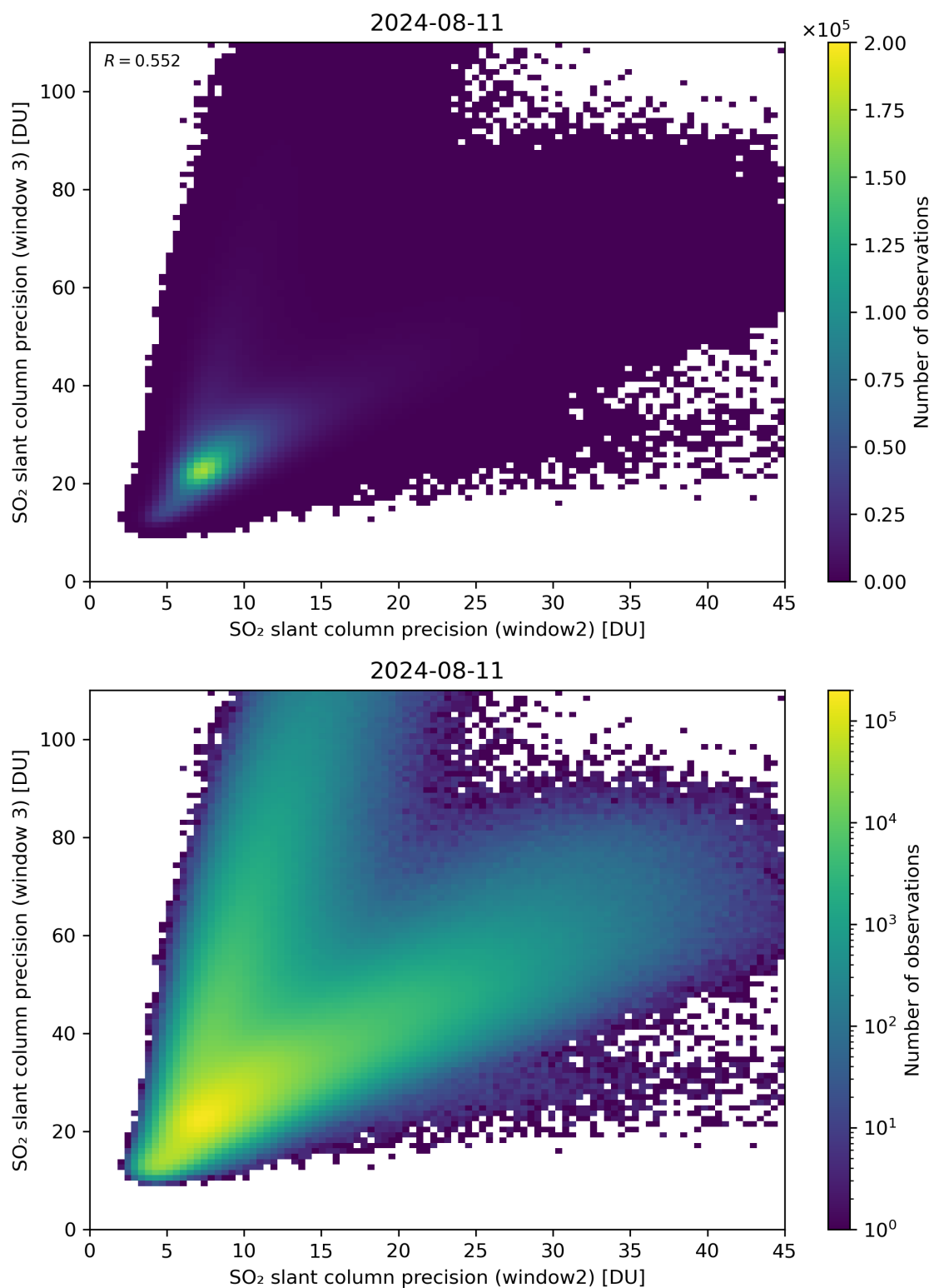
Figure 250: Scatter density plot of “SO 2 slant column precision (window2)” against “SO 2 slant column precision (window 3)” for 2024-08-11 to 2024-08-11.
