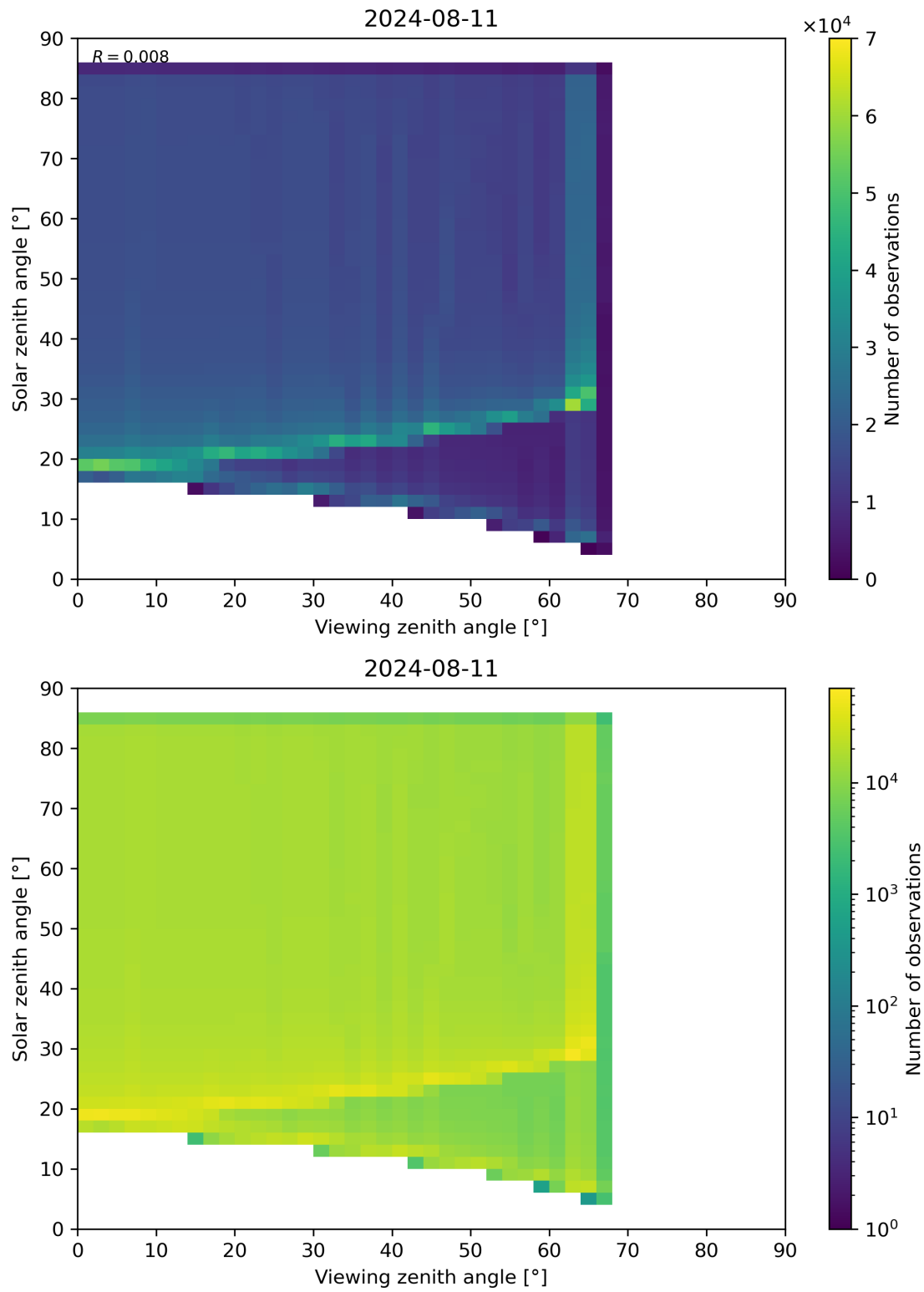
Figure 315: Scatter density plot of “Viewing zenith angle” against “Solar zenith angle” for 2024-08-11 to 2024-08-11.
