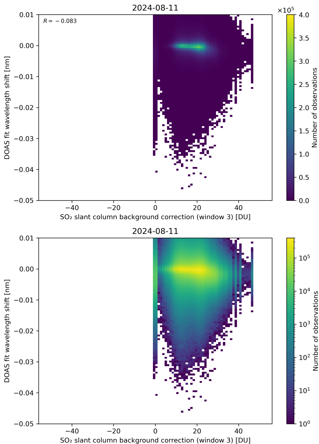
Figure 121: Scatter density plot of “SO 2 slant column background correction (window 3)” against “DOAS fit wavelength shift” for 2024-08-11 to 2024-08-11.
