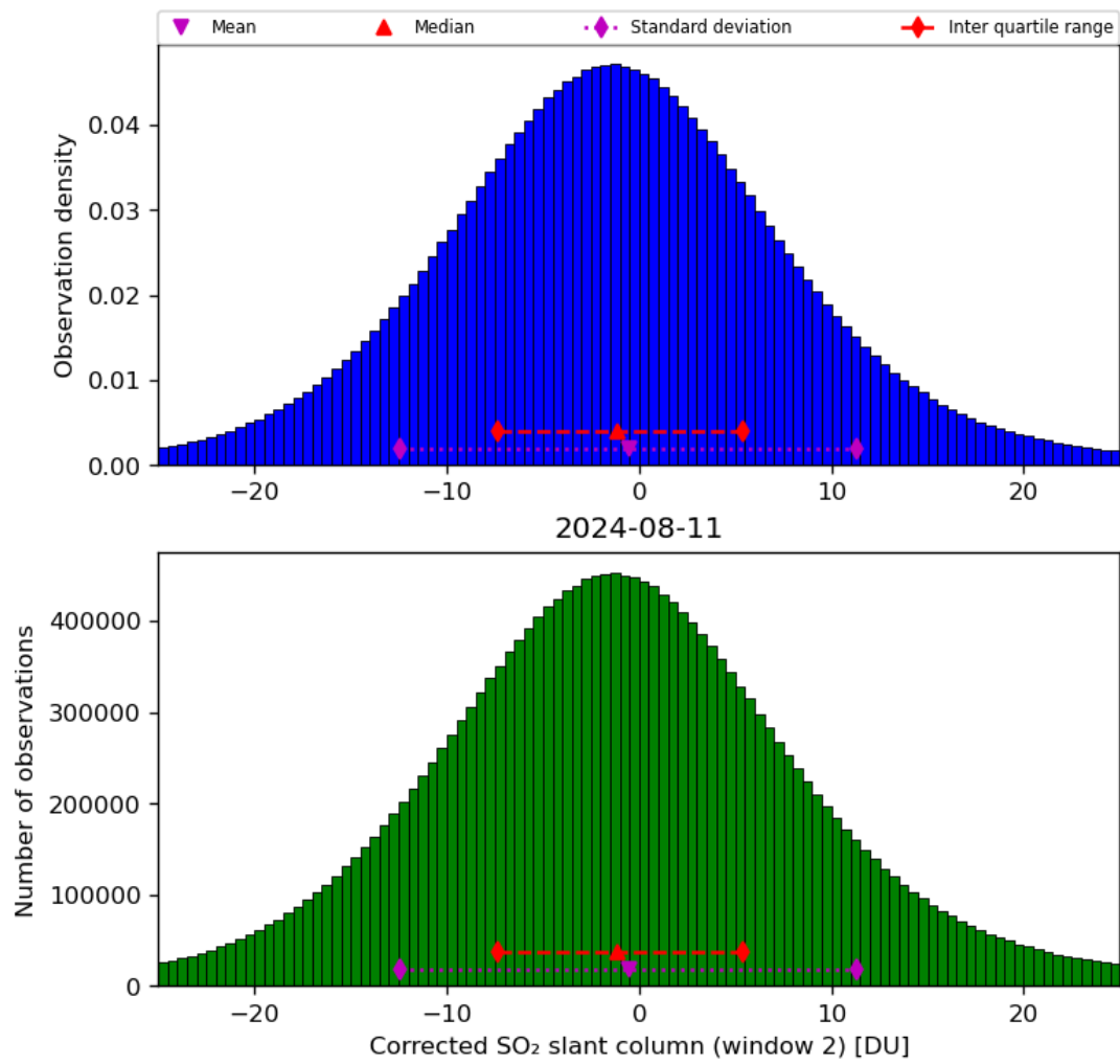
Figure 62: Histogram of “Corrected SO 2 slant column (window 2)” for 2024-08-11 to 2024-08-11
