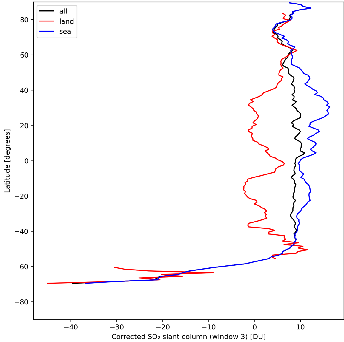
Figure 43: Zonal average of “Corrected SO 2 slant column (window 3)” for 2024-08-11 to 2024-08-11.
