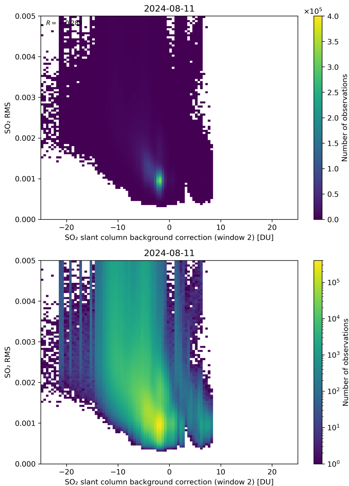
Figure 114: Scatter density plot of “SO 2 slant column background correction (window 2)” against “SO 2 RMS” for 2024-08-11 to 2024-08-11.
