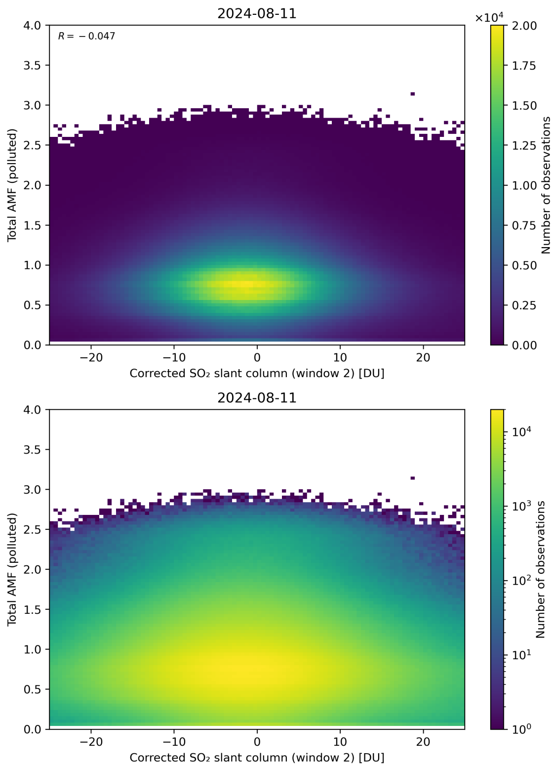
Figure 203: Scatter density plot of “Corrected SO 2 slant column (window 2)” against “Total AMF (polluted)” for 2024-08-11 to 2024-08-11.
