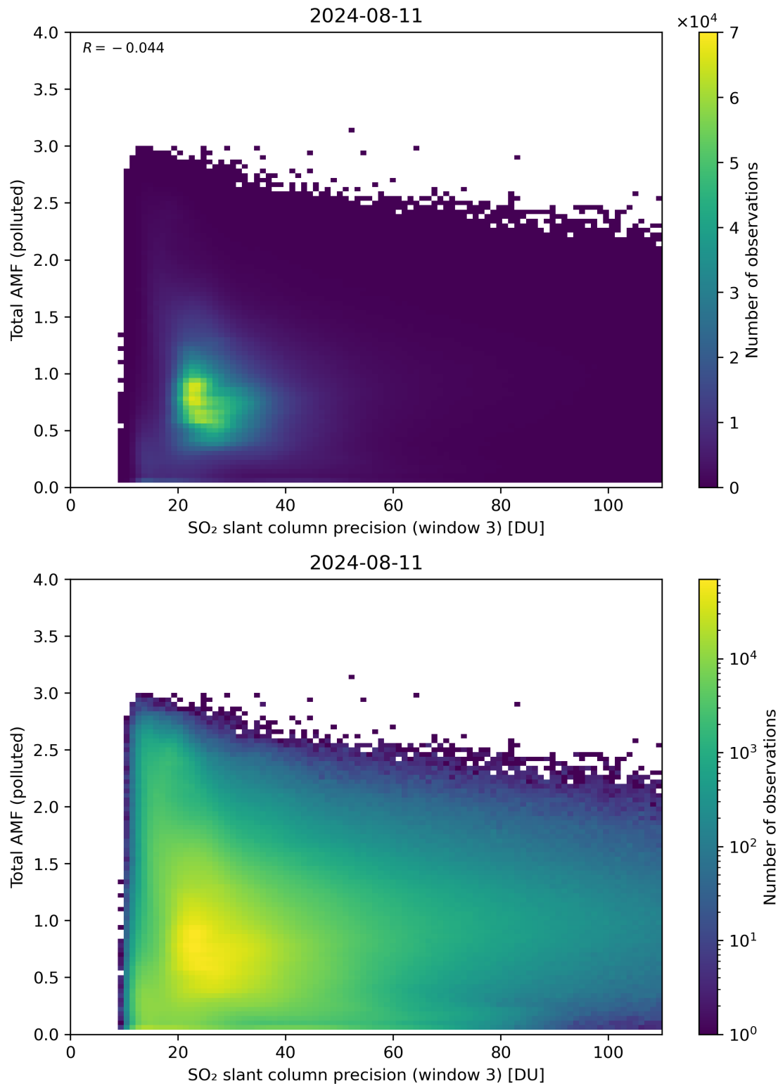
Figure 263: Scatter density plot of “SO 2 slant column precision (window 3)” against “Total AMF (polluted)” for 2024-08-11 to 2024-08-11.
