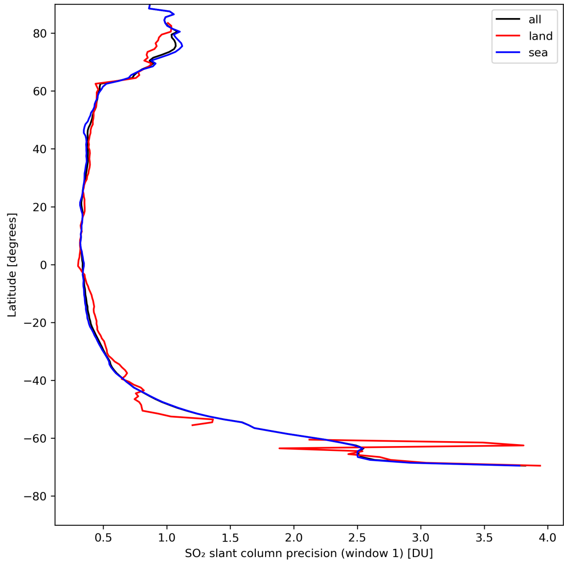
Figure 34: Zonal average of "SO 2 slant column precision (window 1)" for 2024-08-11 to 2024-08-11.
