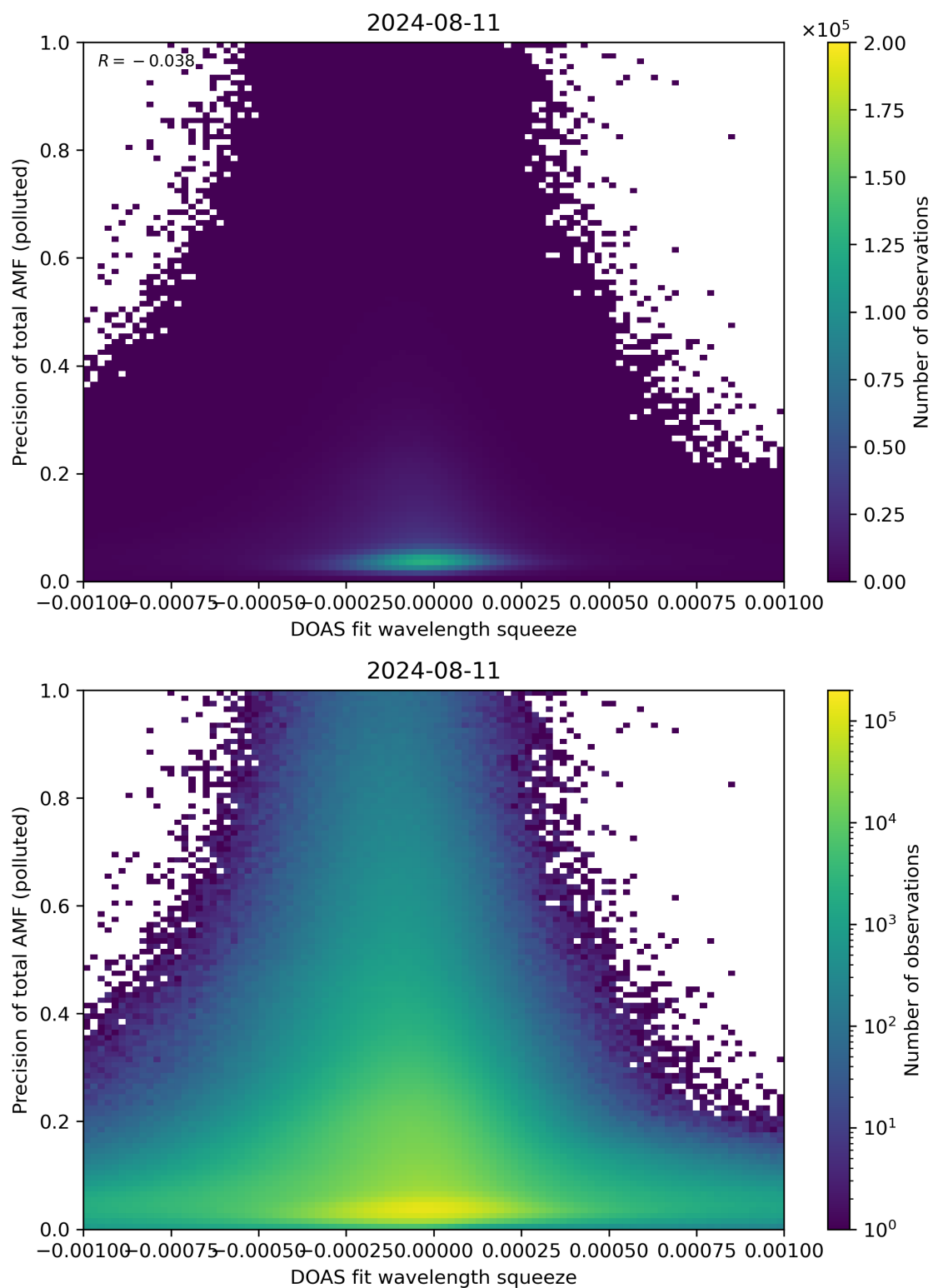
Figure 135: Scatter density plot of “DOAS fit wavelength squeeze” against “Precision of total AMF (polluted)” for 2024-08-11 to 2024-08-11.
