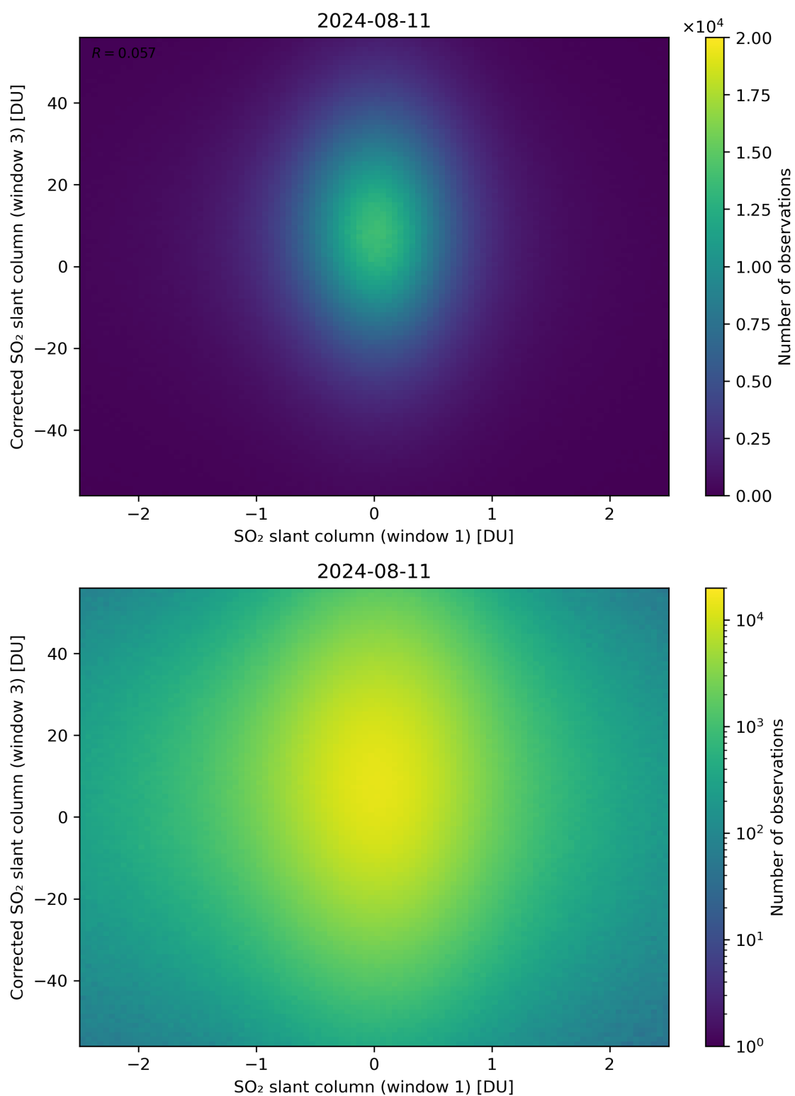
Figure 234: Scatter density plot of “SO 2 slant column (window 1)” against “Corrected SO 2 slant column (window 3)” for 2024-08-11 to 2024-08-11.
