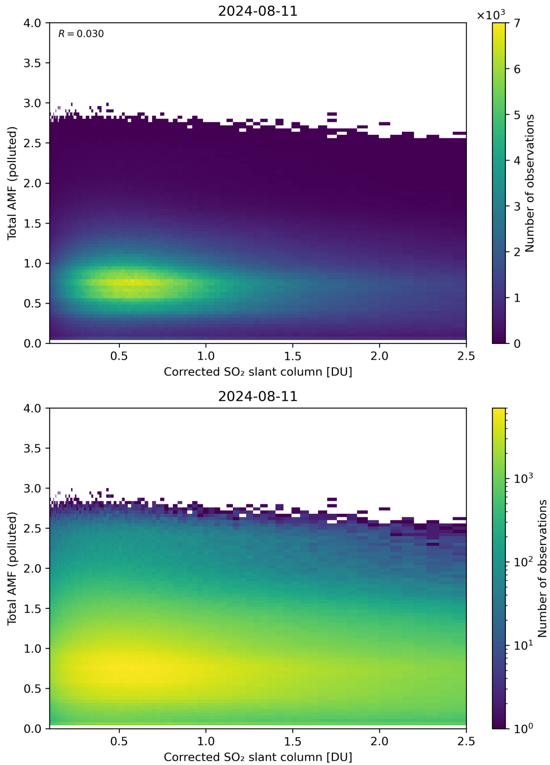
Figure 192: Scatter density plot of “Corrected SO 2 slant column” against “Total AMF (polluted)” for 2024-08-11 to 2024-08-11.
