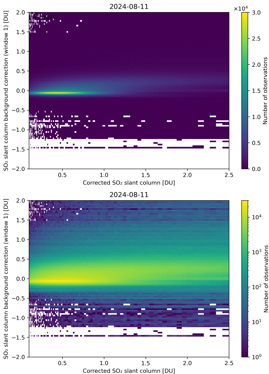
Figure 178: Scatter density plot of “Corrected SO 2 slant column” against “SO 2 slant column background correction (window 1)” for 2024-08-11 to 2024-08-11.
