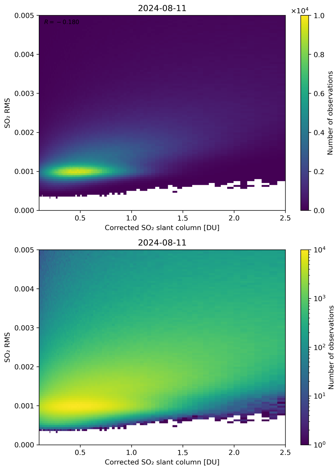
Figure 183: Scatter density plot of “Corrected SO 2 slant column” against “SO 2 RMS” for 2024-08-11 to 2024-08-11.
