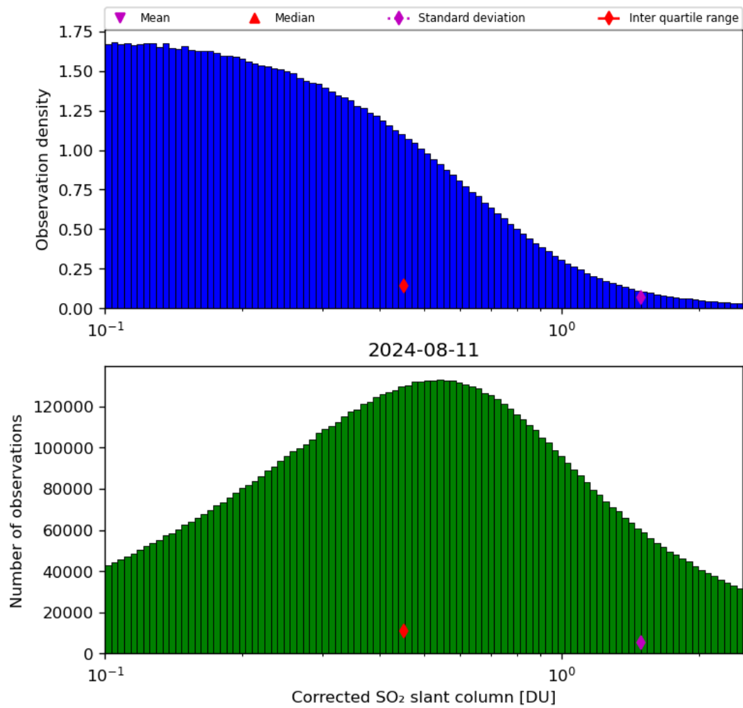
Figure 55: Histogram of “Corrected SO 2 slant column” for 2024-08-11 to 2024-08-11
