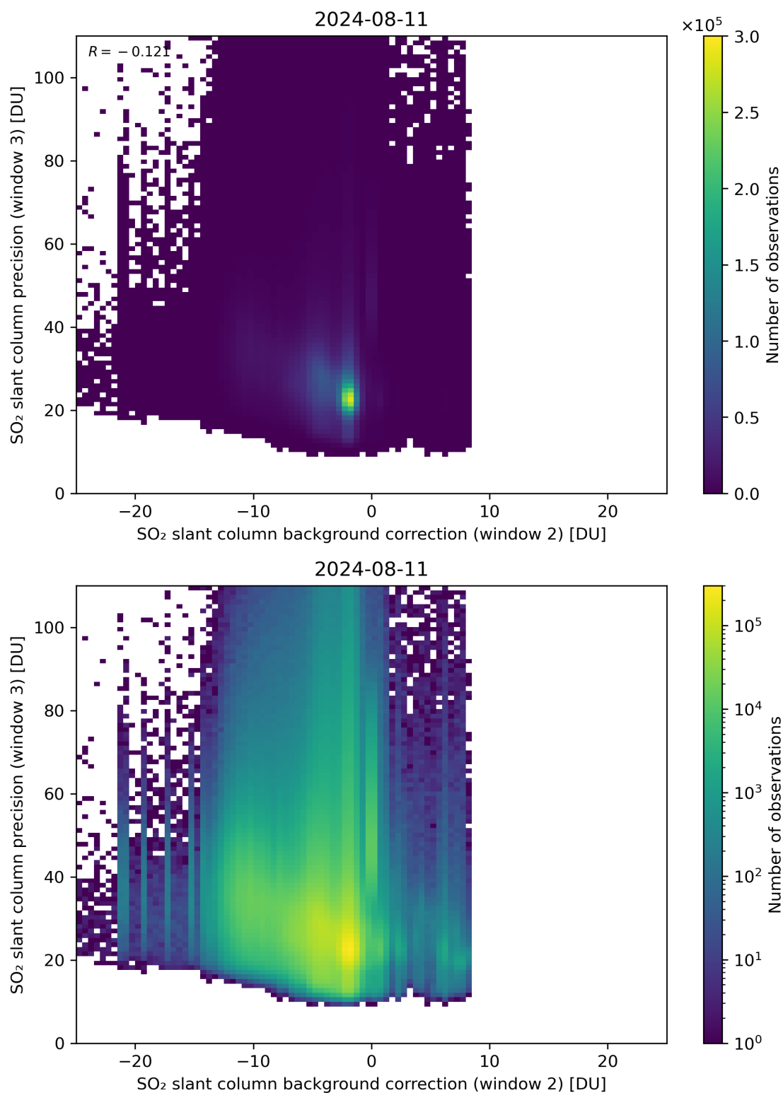
Figure 118: Scatter density plot of “SO 2 slant column background correction (window 2)” against “SO 2 slant column precision (window 3)” for 2024-08-11 to 2024-08-11.
