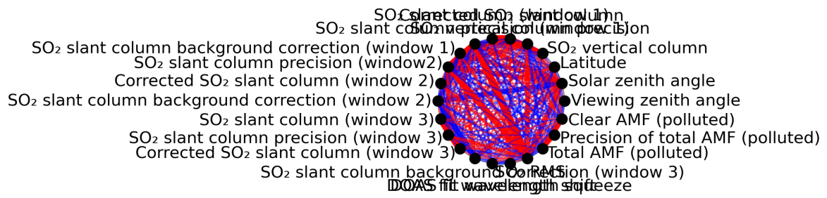
Figure 1: Map of correlation graph for 2024-08-11 to 2024-08-11.
