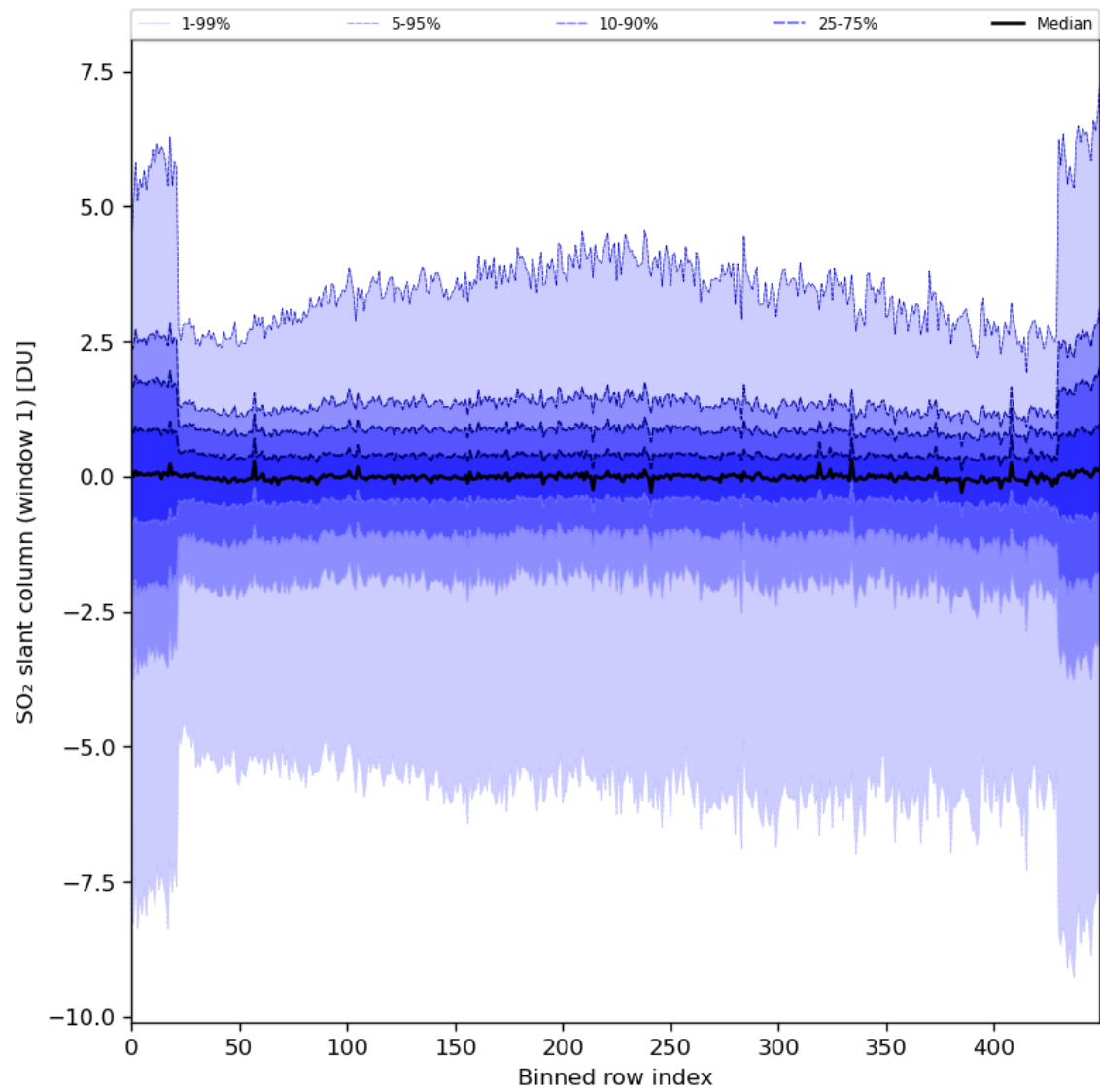
Figure 79: Along track statistics of “SO 2 slant column (window 1)” for 2024-08-11 to 2024-08-11
