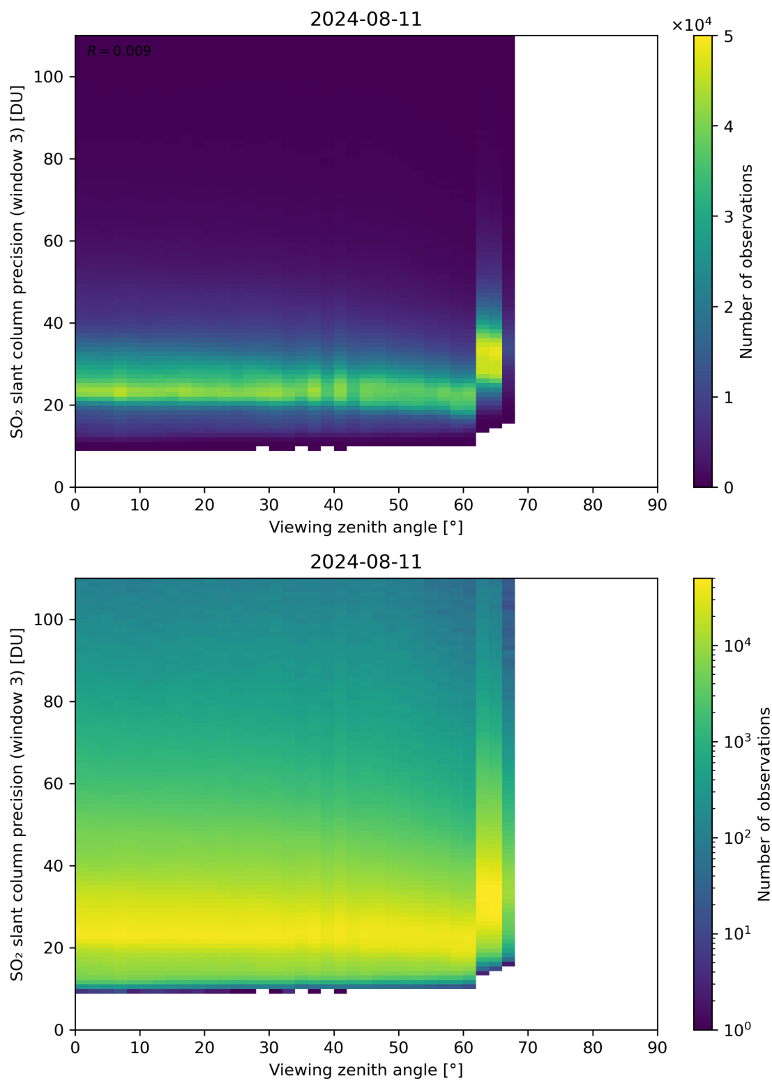
Figure 324: Scatter density plot of “Viewing zenith angle” against “SO 2 slant column precision (window 3)” for 2024-08-11 to 2024-08-11.
