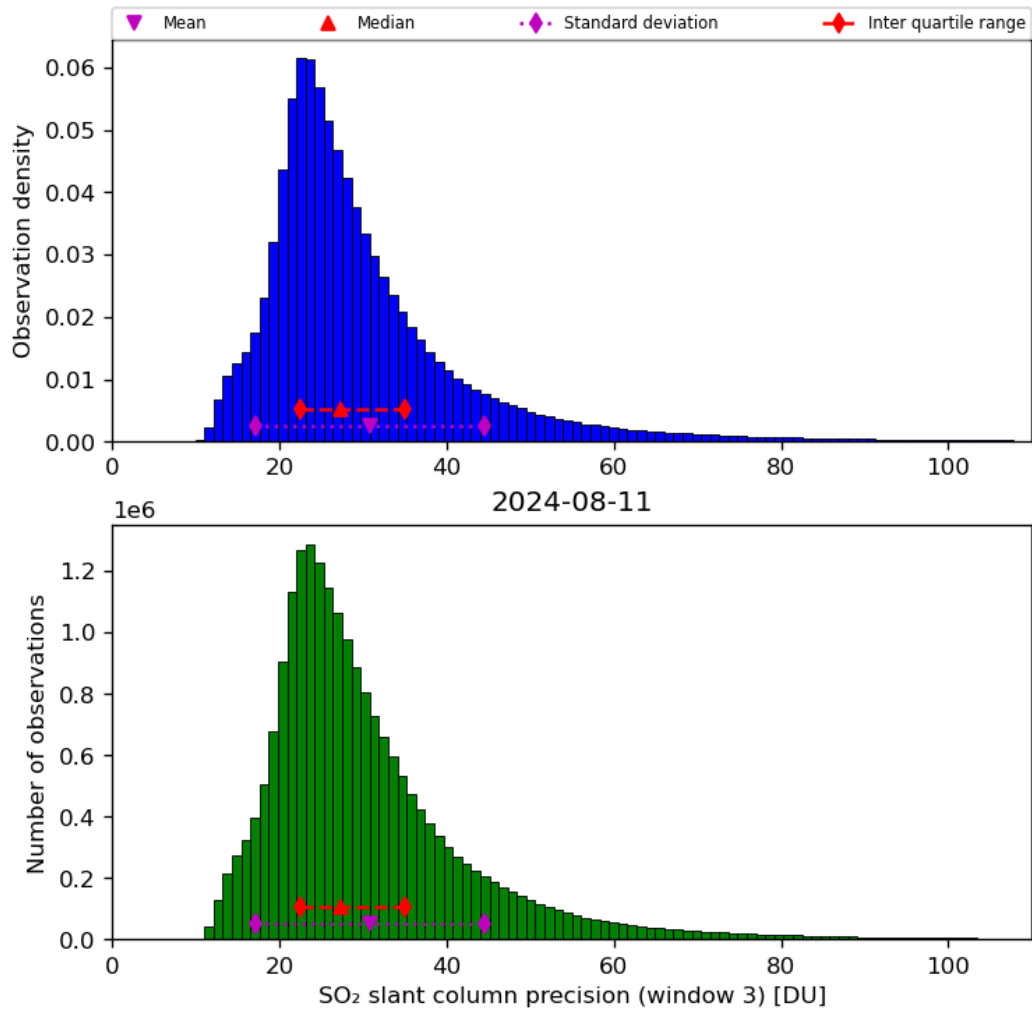
Figure 65: Histogram of “SO 2 slant column precision (window 3)” for 2024-08-11 to 2024-08-11
