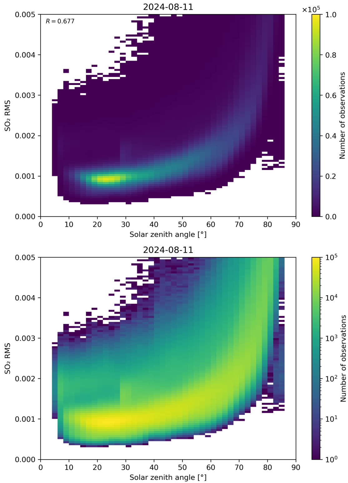
Figure 163: Scatter density plot of “Solar zenith angle” against “SO 2 RMS” for 2024-08-11 to 2024-08-11.
