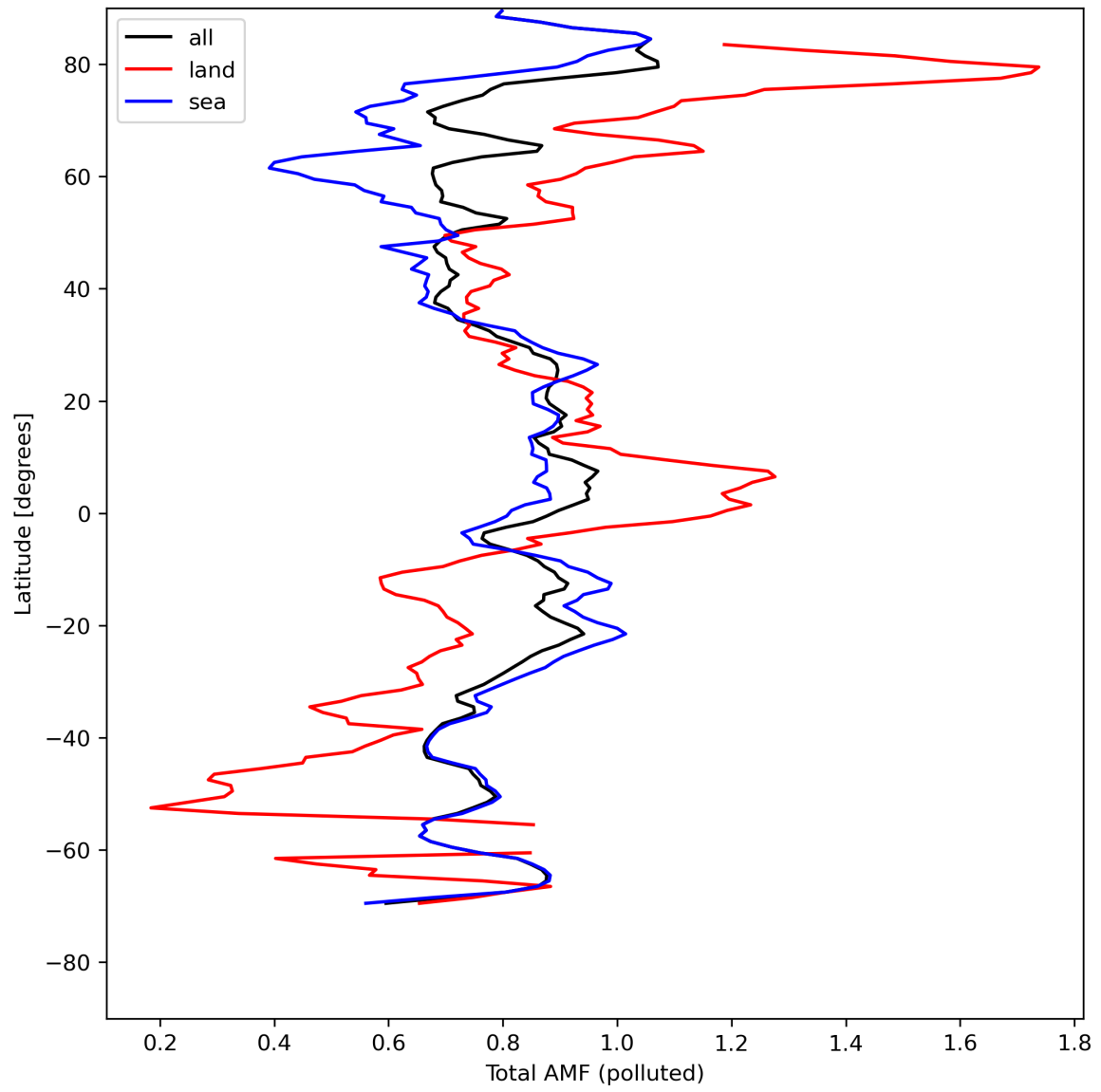
Figure 48: Zonal average of “Total AMF (polluted)” for 2024-08-11 to 2024-08-11.
