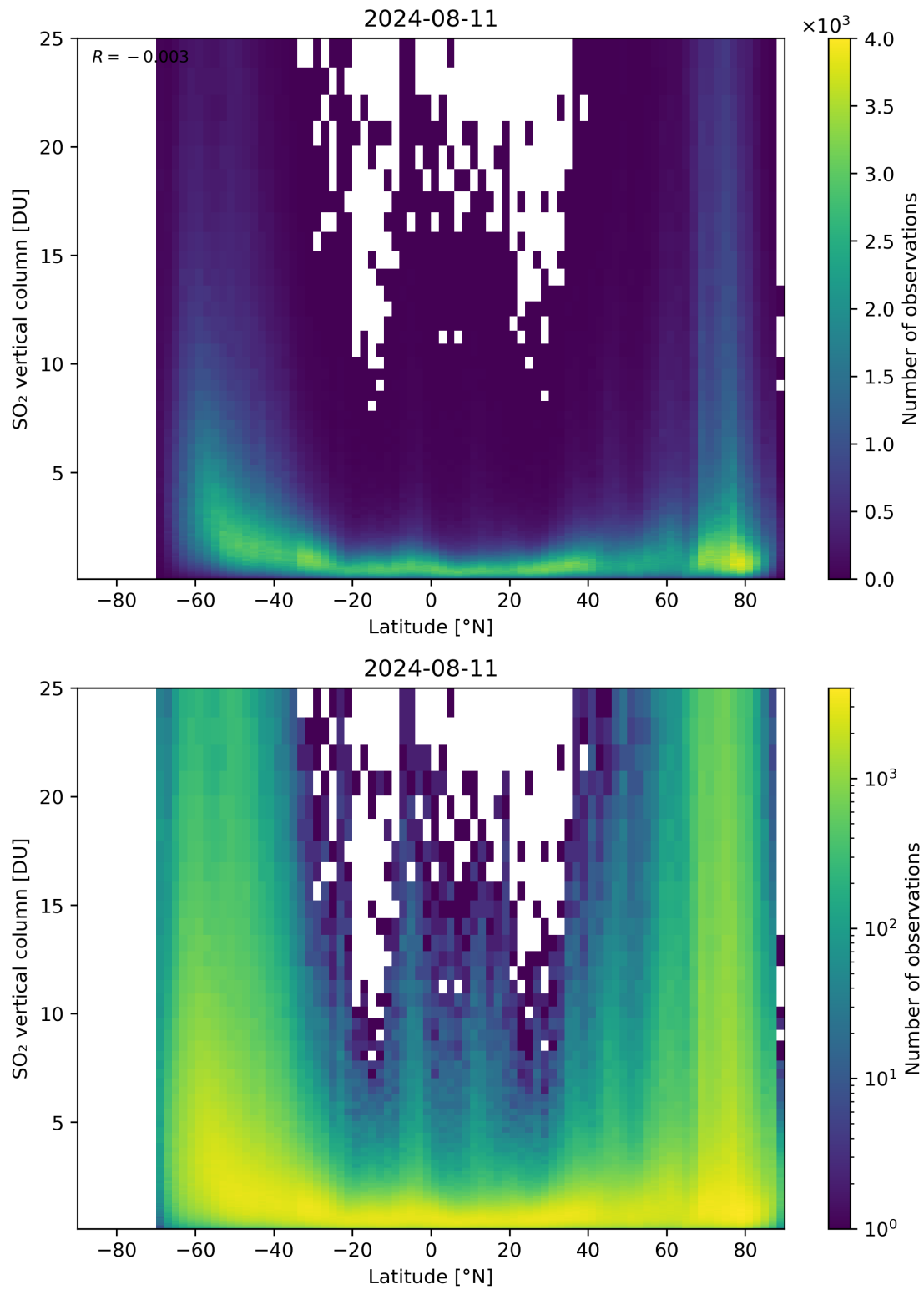
Figure 156: Scatter density plot of “Latitude” against “SO 2 vertical column” for 2024-08-11 to 2024-08-11.
