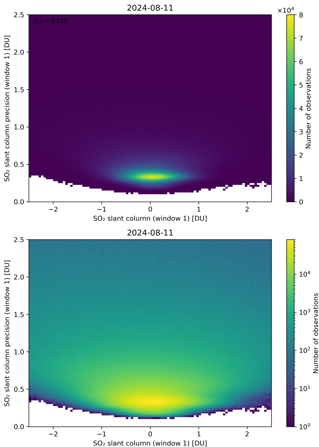
Figure 235: Scatter density plot of “SO 2 slant column (window 1)” against “SO 2 slant column precision (window 1)” for 2024-08-11 to 2024-08-11.
