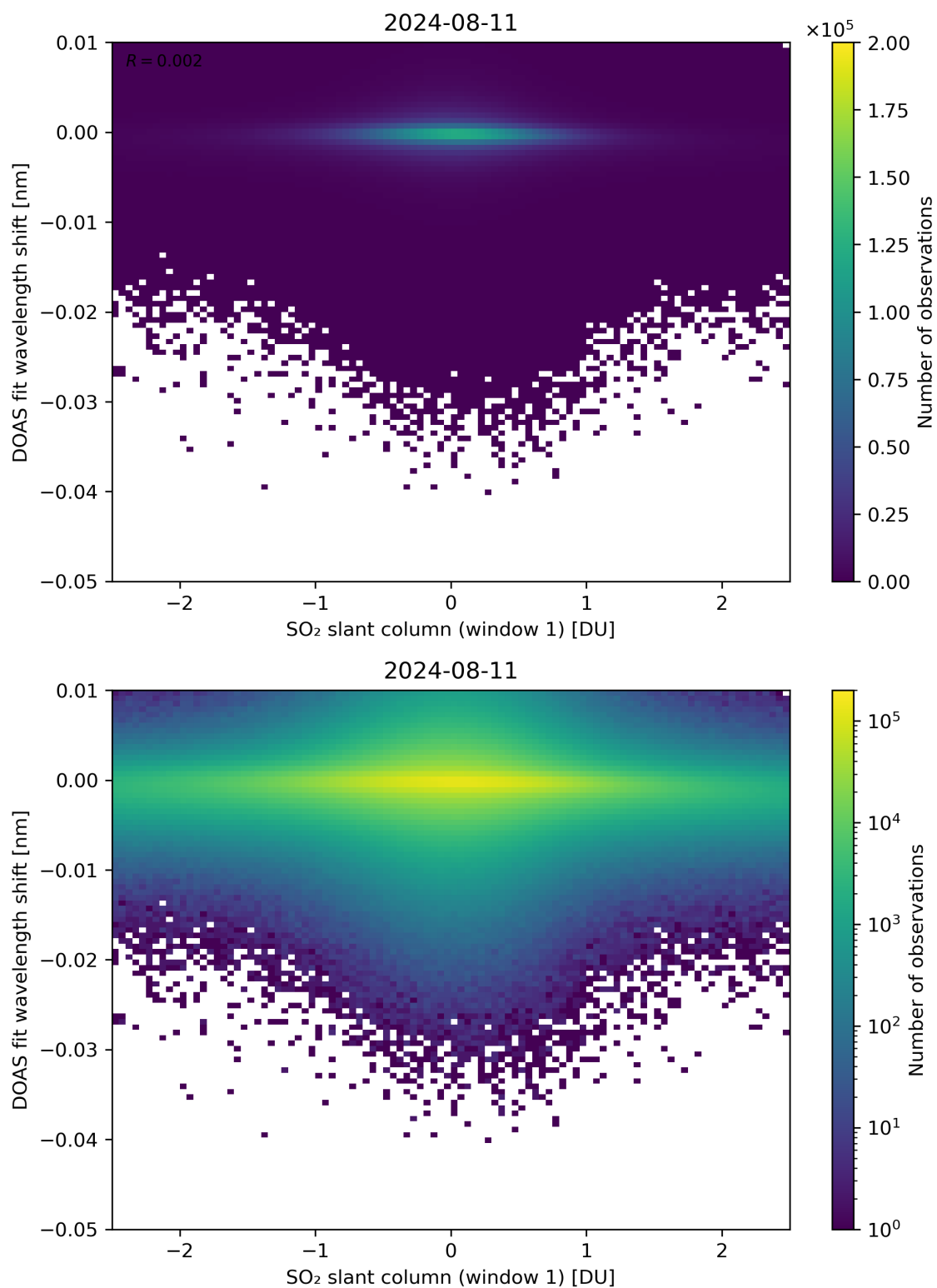
Figure 215: Scatter density plot of “SO 2 slant column (window 1)” against “DOAS fit wavelength shift” for 2024-08-11 to 2024-08-11.
