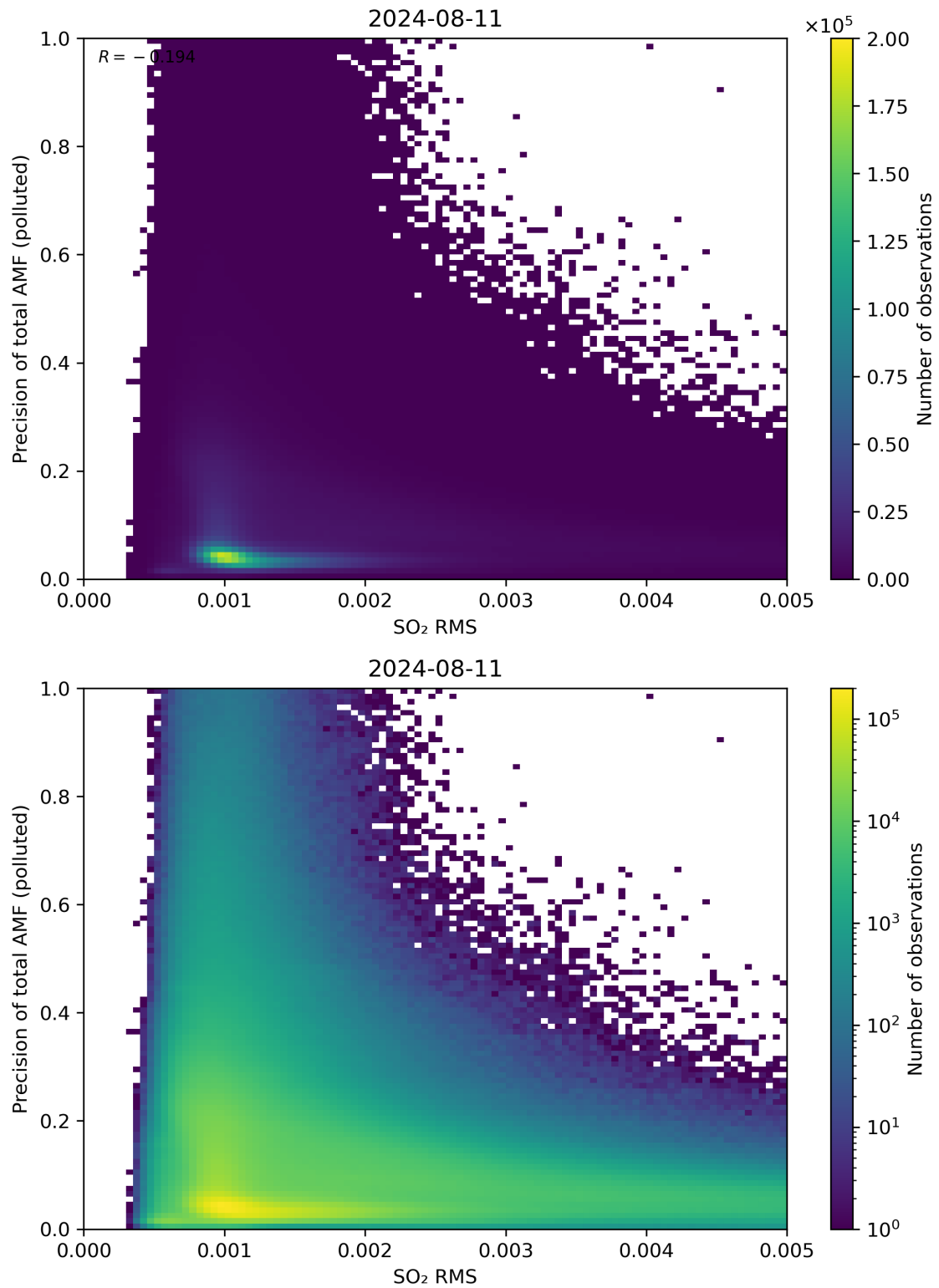
Figure 138: Scatter density plot of “SO 2 RMS” against “Precision of total AMF (polluted)” for 2024-08-11 to 2024-08-11.
