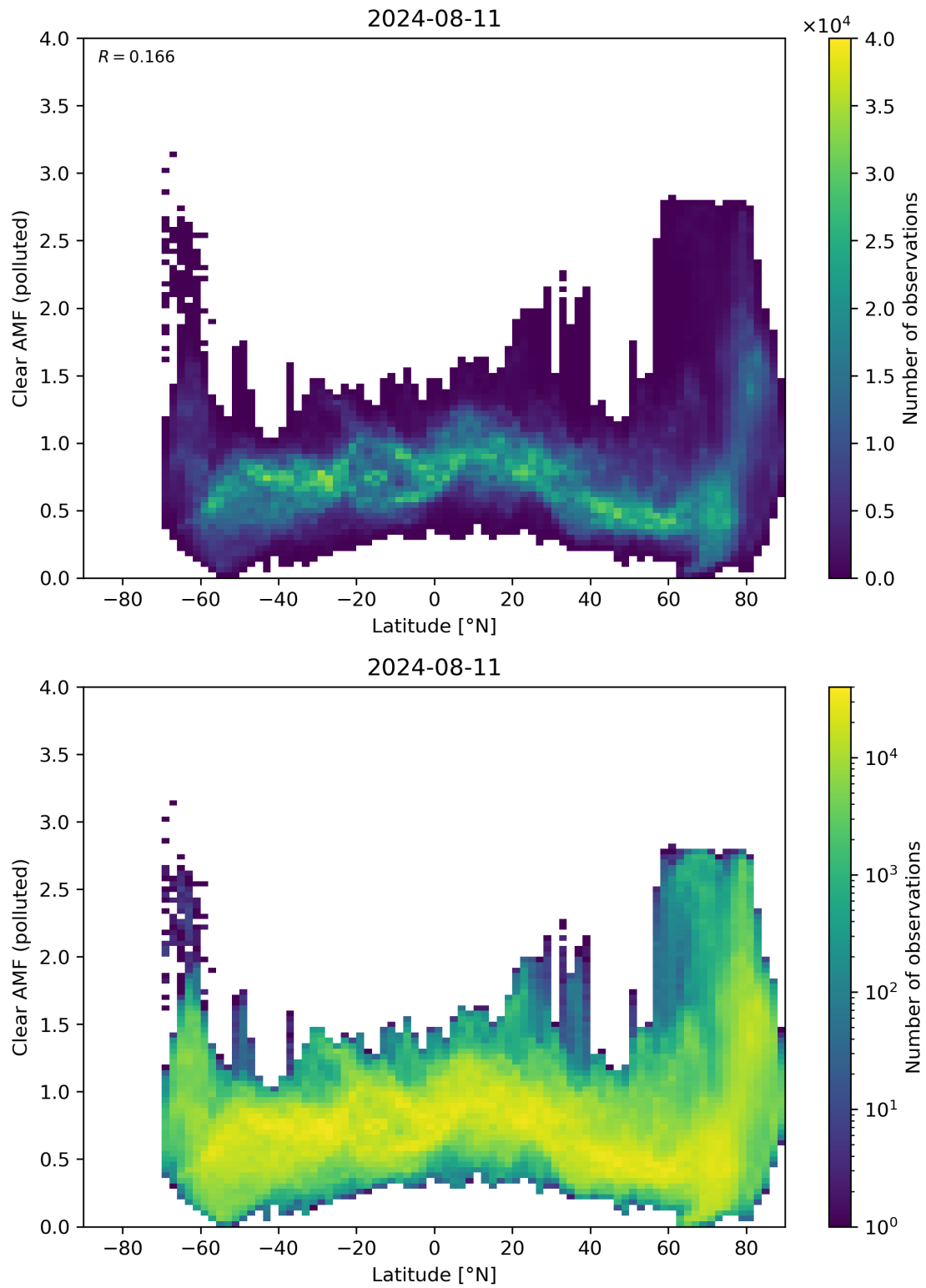
Figure 145: Scatter density plot of “Latitude” against “Clear AMF (polluted)” for 2024-08-11 to 2024-08-11.
