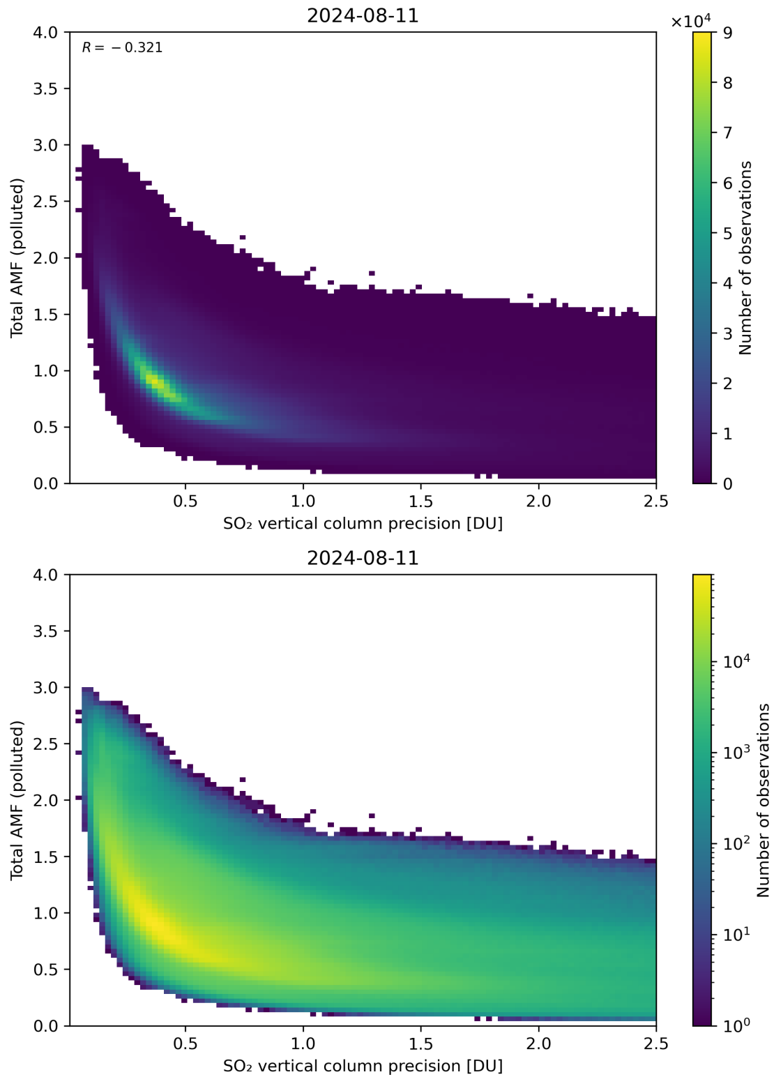
Figure 294: Scatter density plot of “SO 2 vertical column precision” against “Total AMF (polluted)” for 2024-08-11 to 2024-08-11.
