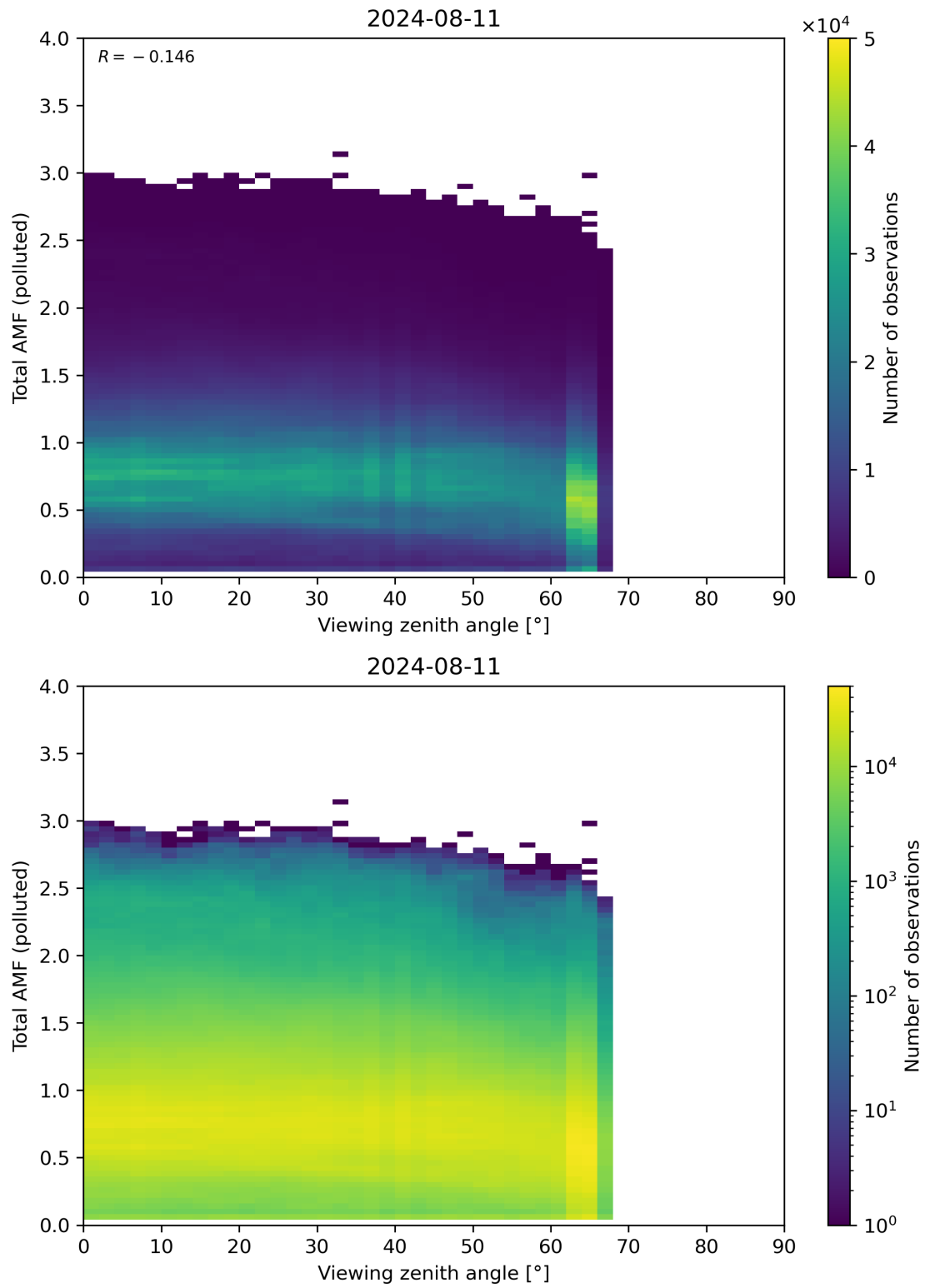
Figure 325: Scatter density plot of “Viewing zenith angle” against “Total AMF (polluted)” for 2024-08-11 to 2024-08-11.
