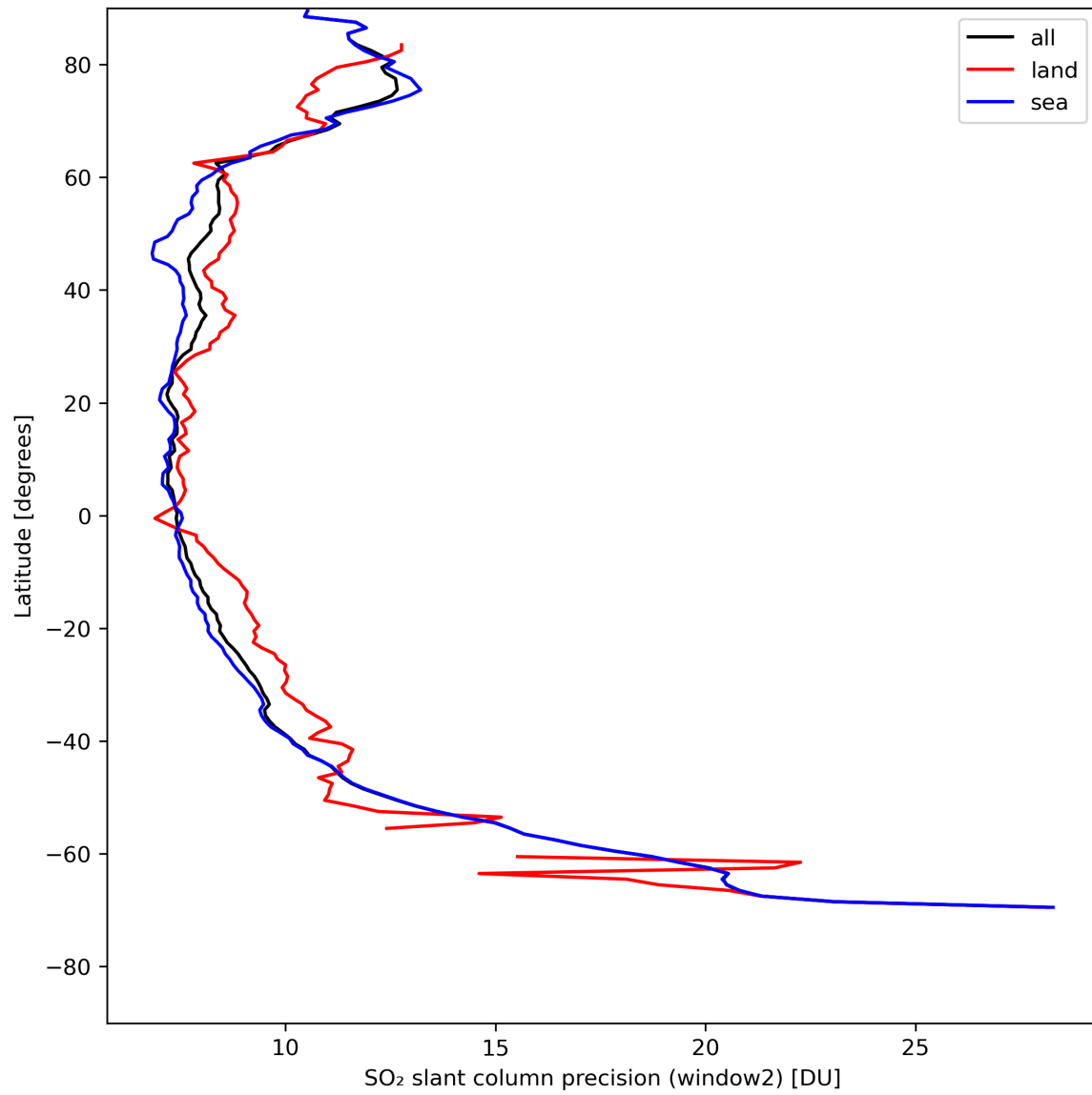
Figure 38: Zonal average of “SO 2 slant column precision (window2)” for 2024-08-11 to 2024-08-11.
