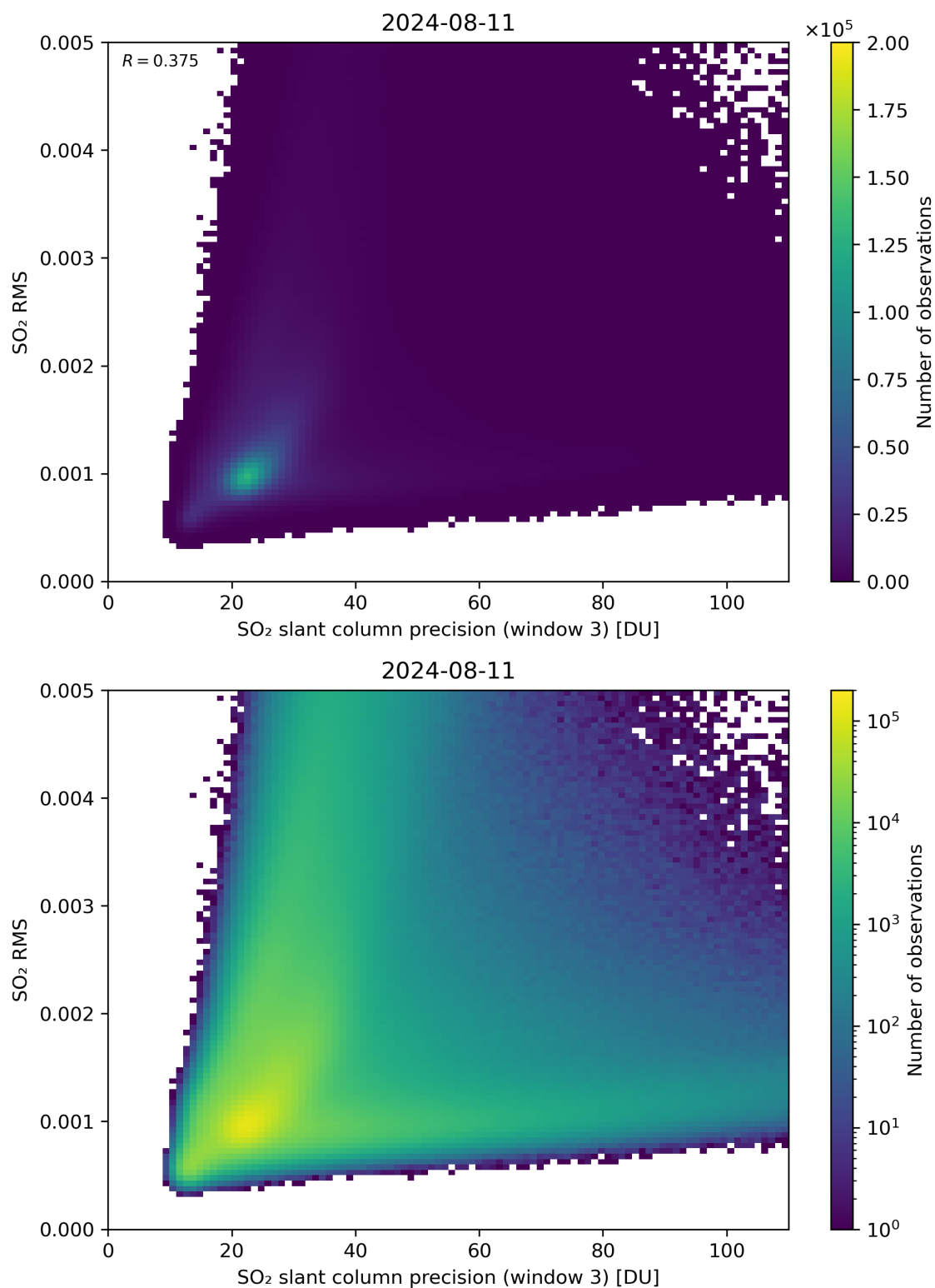
Figure 260: Scatter density plot of “SO 2 slant column precision (window 3)” against “SO 2 RMS” for 2024-08-11 to 2024-08-11.
