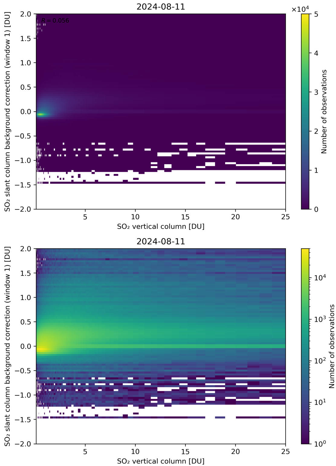
Figure 273: Scatter density plot of “SO 2 vertical column” against “SO 2 slant column background correction (window 1)” for 2024-08-11 to 2024-08-11.
