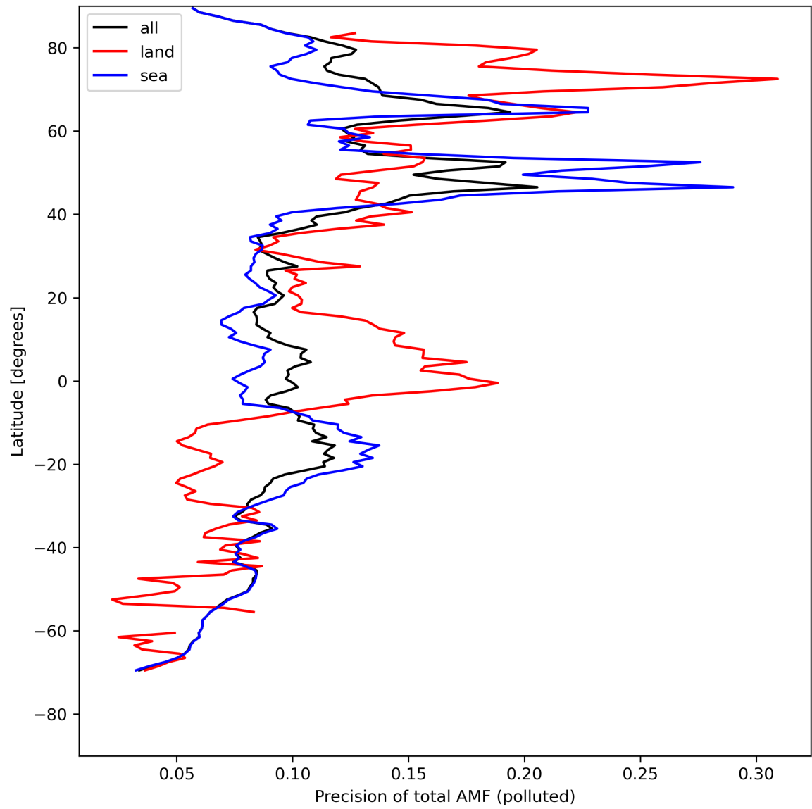
Figure 49: Zonal average of “Precision of total AMF (polluted)” for 2024-08-11 to 2024-08-11.
