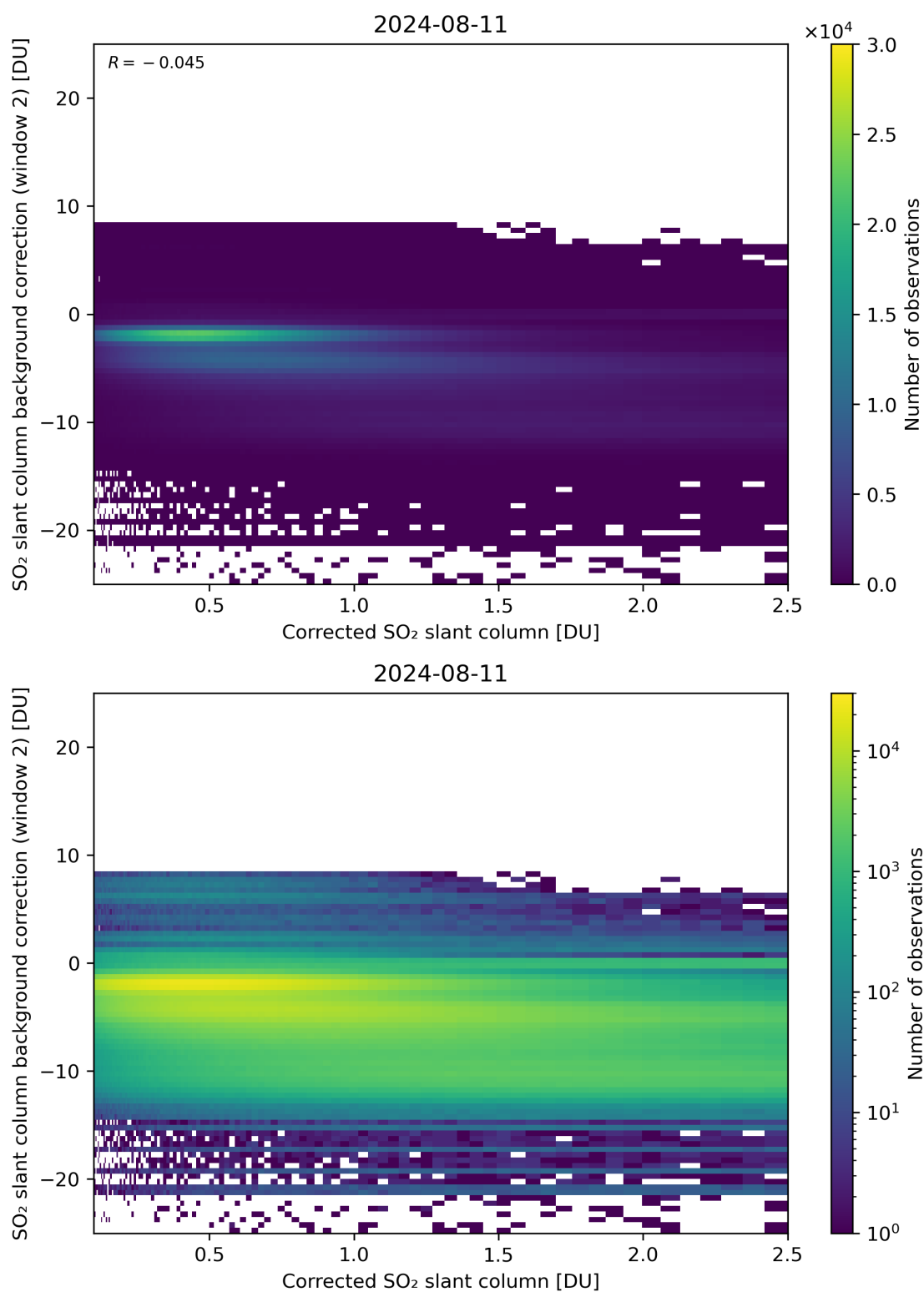
Figure 179: Scatter density plot of “Corrected SO 2 slant column” against “SO 2 slant column background correction (window 2)” for 2024-08-11 to 2024-08-11.
