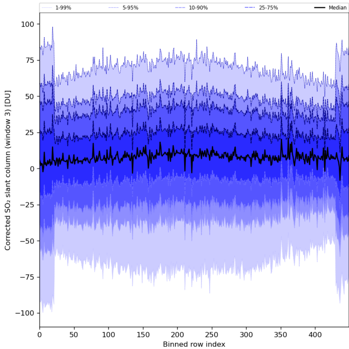
Figure 89: Along track statistics of “Corrected SO 2 slant column (window 3)” for 2024-08-11 to 2024-08-11
