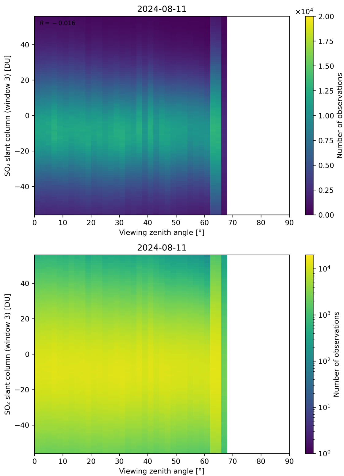
Figure 323: Scatter density plot of “Viewing zenith angle” against “SO 2 slant column (window 3)” for 2024-08-11 to 2024-08-11.
