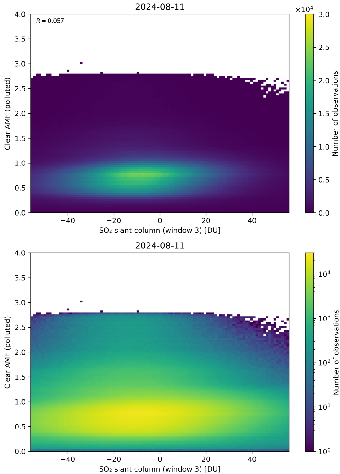
Figure 265: Scatter density plot of “SO 2 slant column (window 3)” against “Clear AMF (polluted)” for 2024-08-11 to 2024-08-11.
