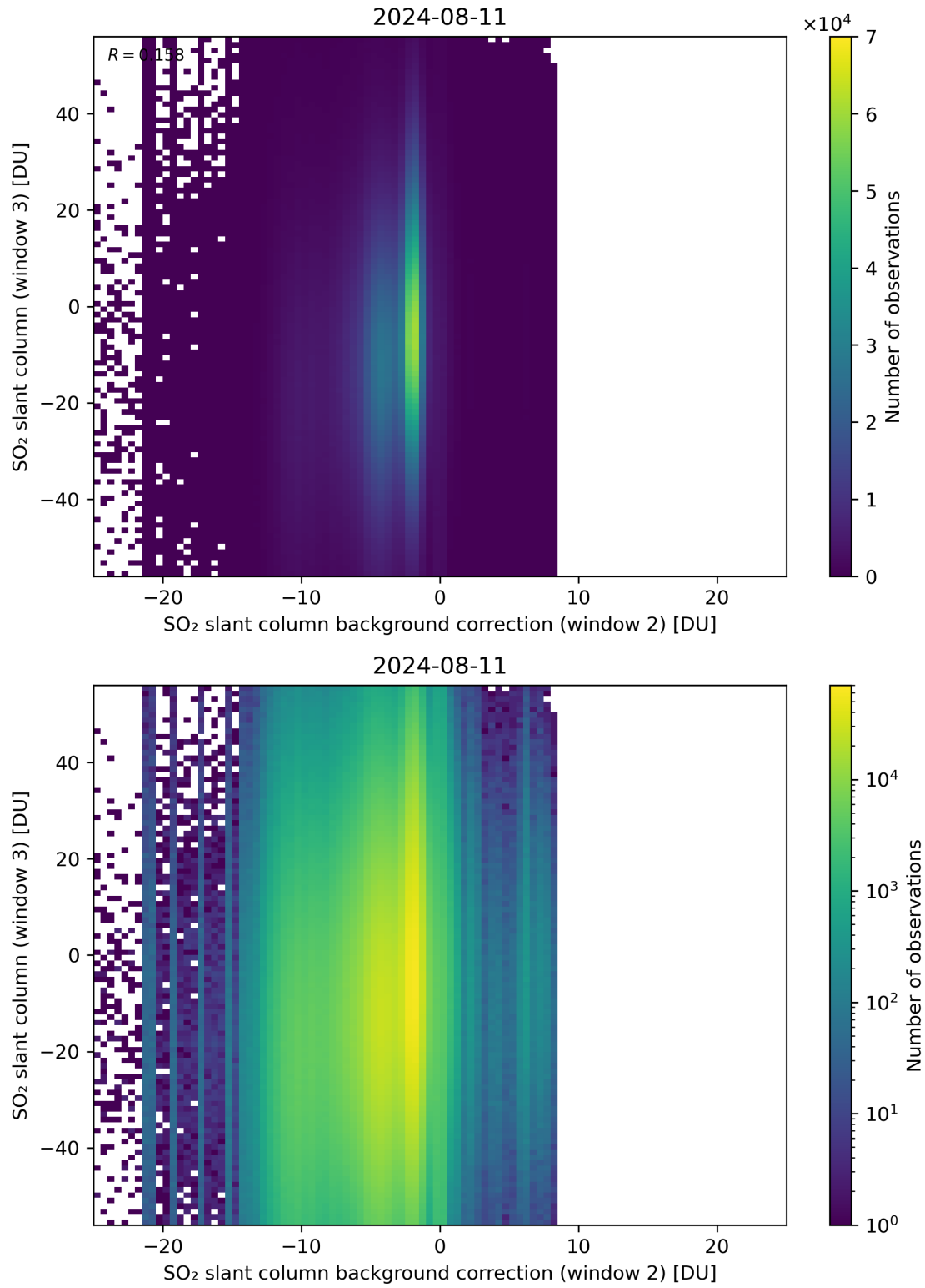
Figure 117: Scatter density plot of “SO 2 slant column background correction (window 2)” against “SO 2 slant column (window 3)” for 2024-08-11 to 2024-08-11.
