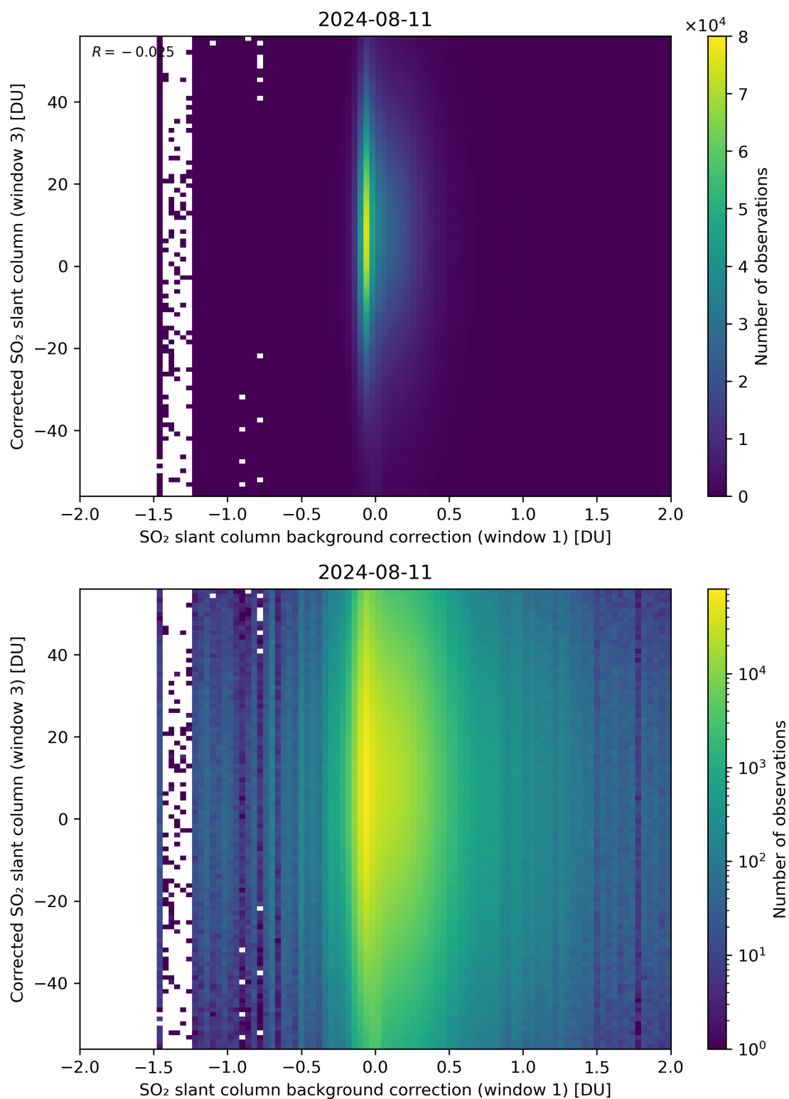
Figure 105: Scatter density plot of “SO 2 slant column background correction (window 1)” against “Corrected SO 2 slant column (window 3)” for 2024-08-11 to 2024-08-11.
