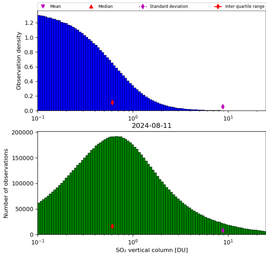
Figure 53: Histogram of “SO 2 vertical column” for 2024-08-11 to 2024-08-11
