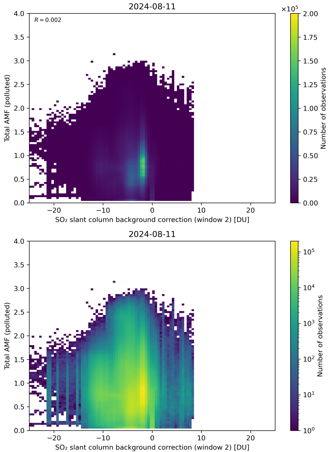
Figure 119: Scatter density plot of “SO 2 slant column background correction (window 2)” against “Total AMF (polluted)” for 2024-08-11 to 2024-08-11.
