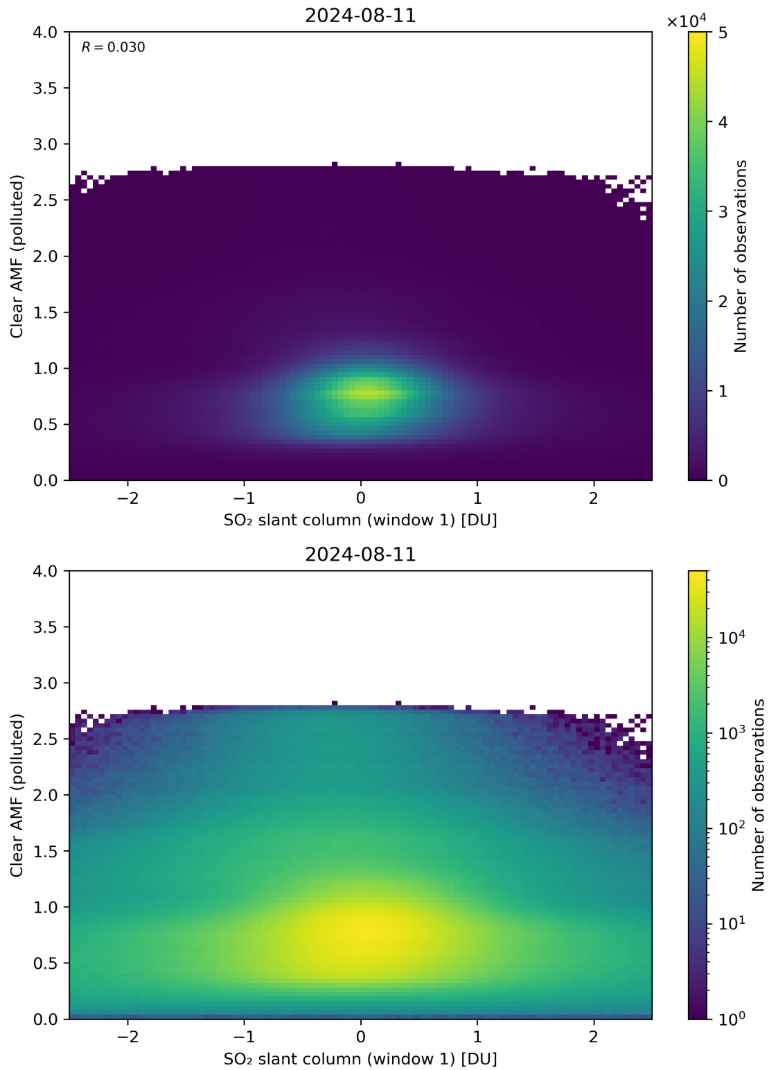
Figure 232: Scatter density plot of “SO 2 slant column (window 1)” against “Clear AMF (polluted)” for 2024-08-11 to 2024-08-11.
