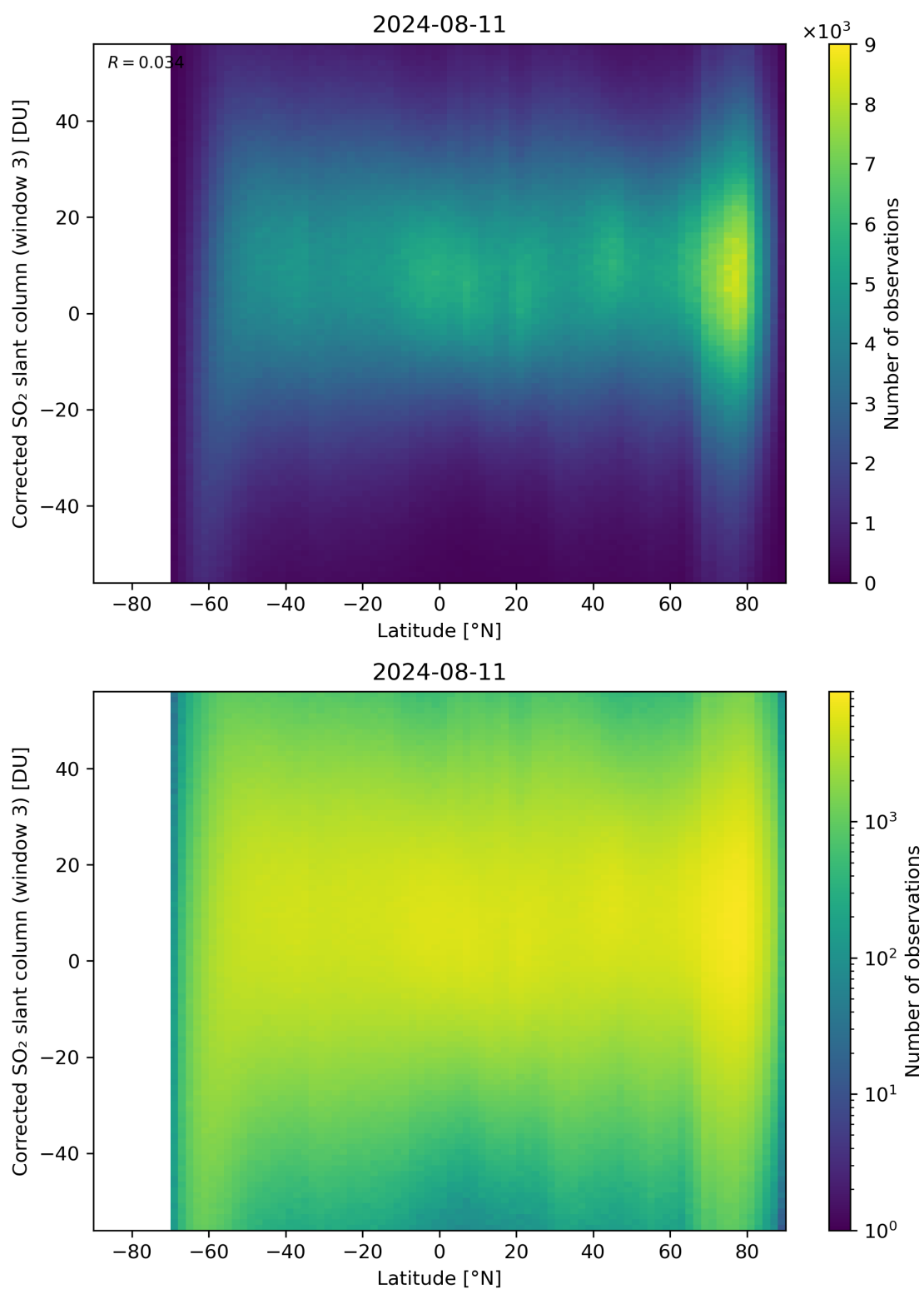
Figure 148: Scatter density plot of “Latitude” against “Corrected SO 2 slant column (window 3)” for 2024-08-11 to 2024-08-11.
