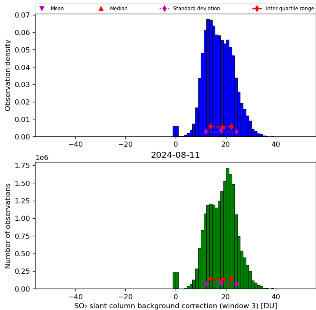
Figure 67: Histogram of “SO 2 slant column background correction (window 3)” for 2024-08-11 to 2024-08-11
