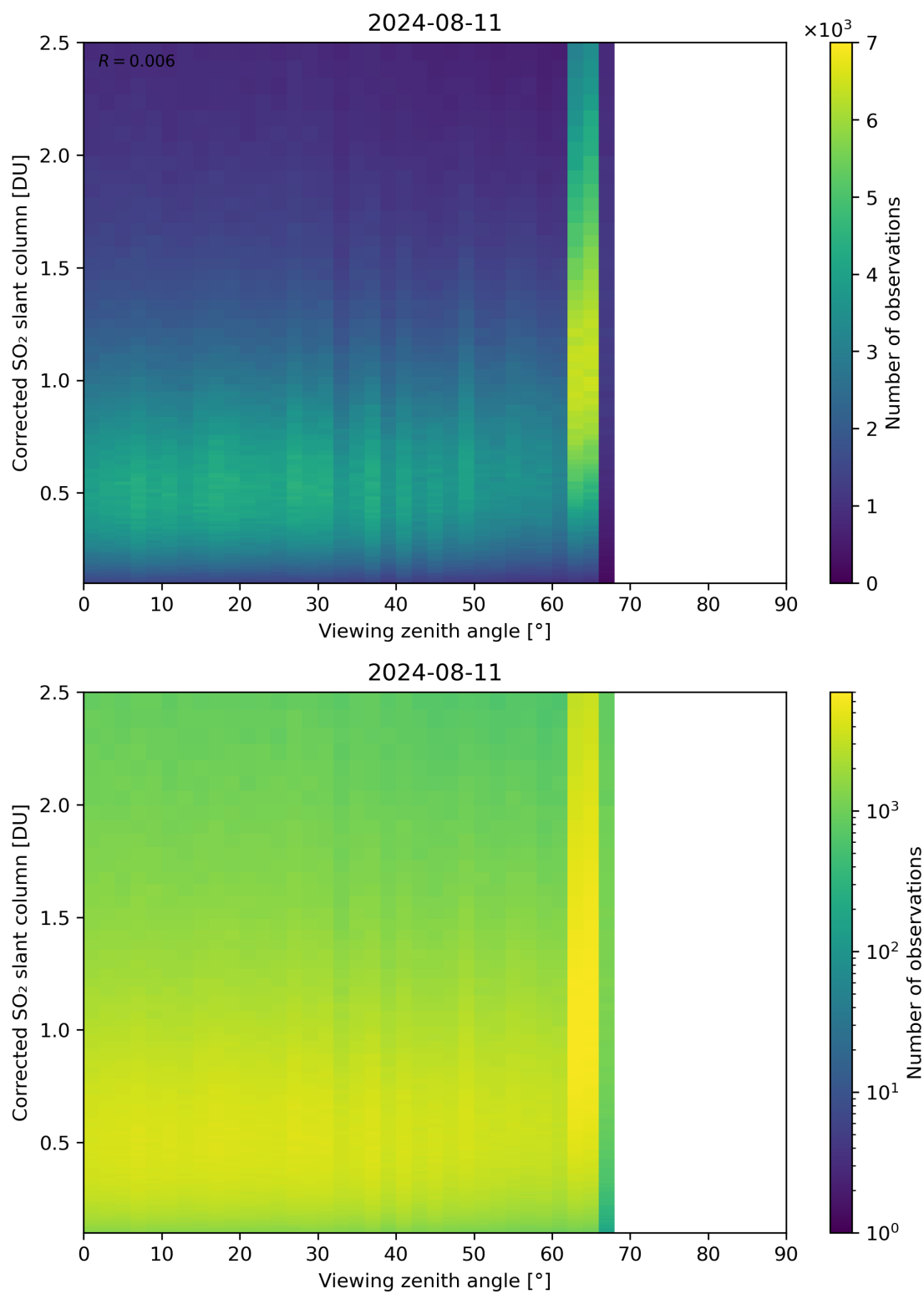
Figure 317: Scatter density plot of “Viewing zenith angle” against “Corrected SO 2 slant column” for 2024-08-11 to 2024-08-11.
