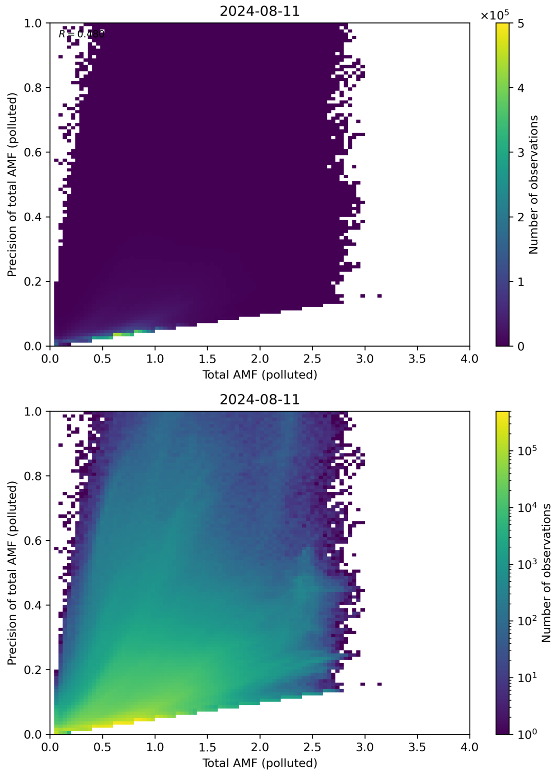
Figure 272: Scatter density plot of “Total AMF (polluted)” against “Precision of total AMF (polluted)” for 2024-08-11 to 2024-08-11.
