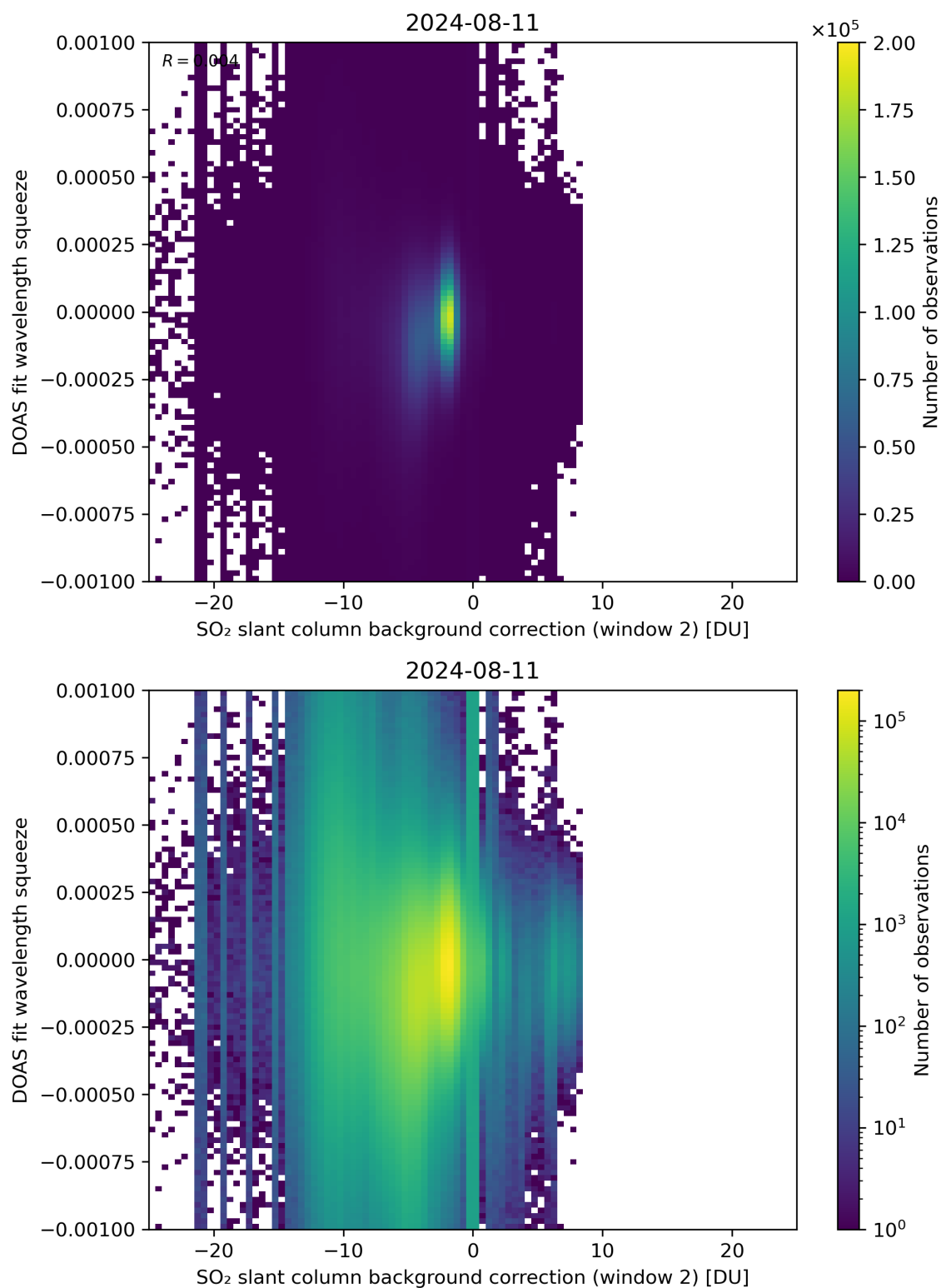
Figure 113: Scatter density plot of “SO 2 slant column background correction (window 2)” against “DOAS fit wavelength squeeze” for 2024-08-11 to 2024-08-11.
