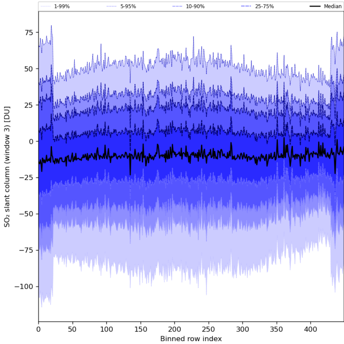
Figure 87: Along track statistics of “SO 2 slant column (window 3)” for 2024-08-11 to 2024-08-11
