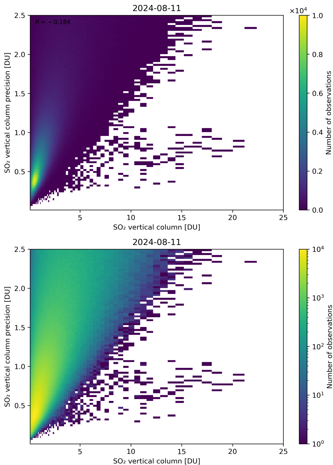
Figure 307: Scatter density plot of “SO 2 vertical column” against “SO 2 vertical column precision” for 2024-08-11 to 2024-08-11.
