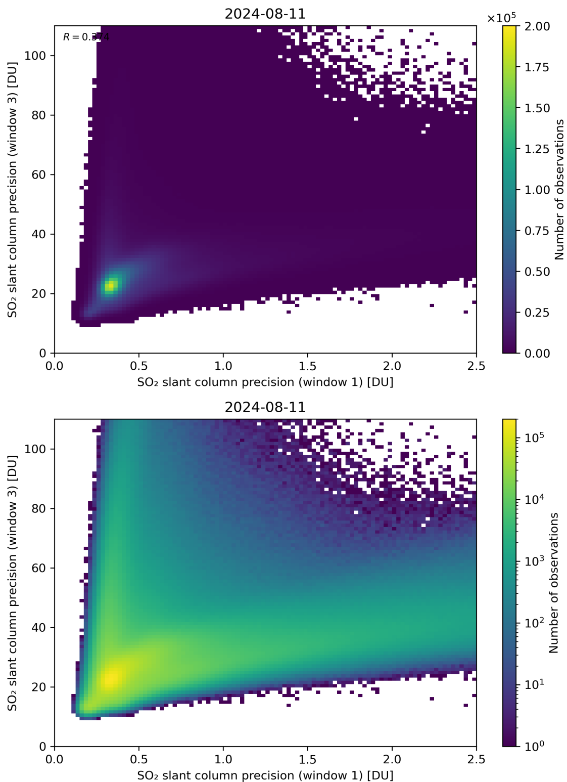
Figure 229: Scatter density plot of “SO 2 slant column precision (window 1)” against “SO 2 slant column precision (window 3)” for 2024-08-11 to 2024-08-11.
