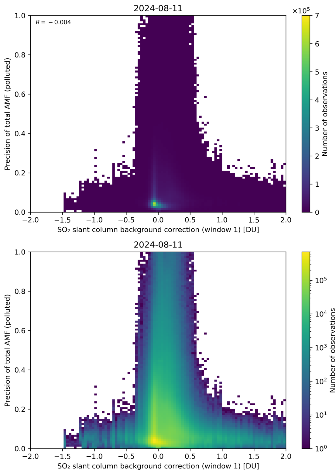
Figure 110: Scatter density plot of “SO 2 slant column background correction (window 1)” against “Precision of total AMF (polluted)” for 2024-08-11 to 2024-08-11.
