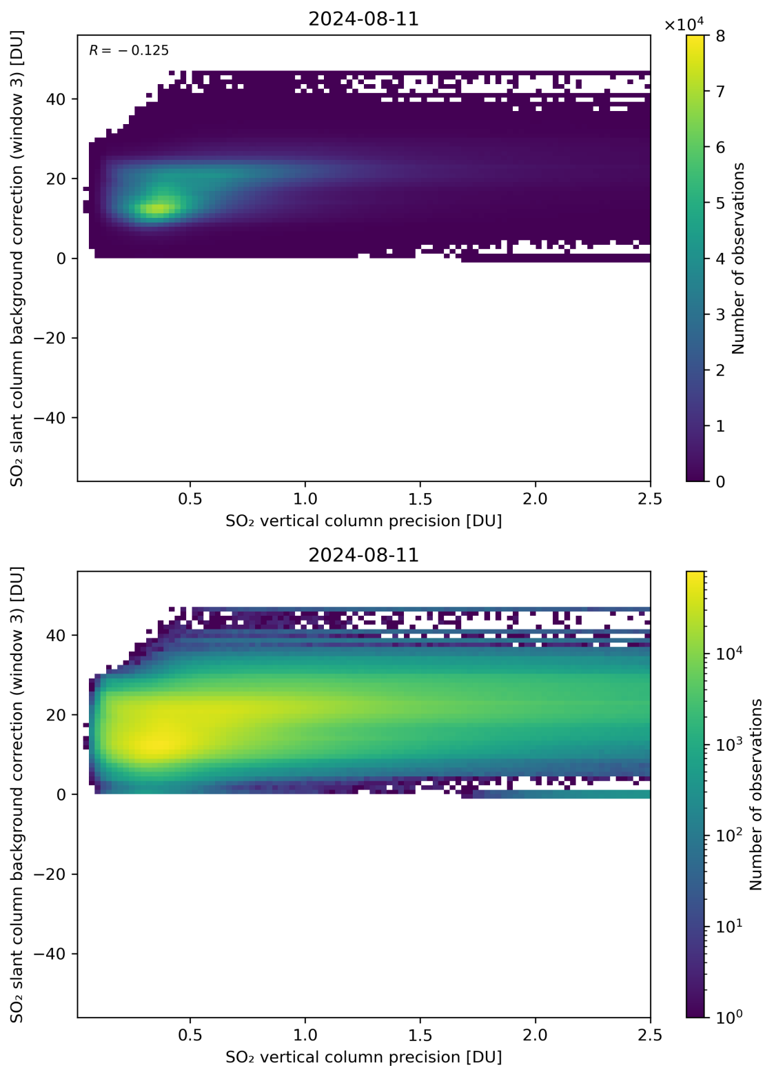
Figure 281: Scatter density plot of “SO 2 vertical column precision” against “SO 2 slant column background correction (window 3)” for 2024-08-11 to 2024-08-11.
