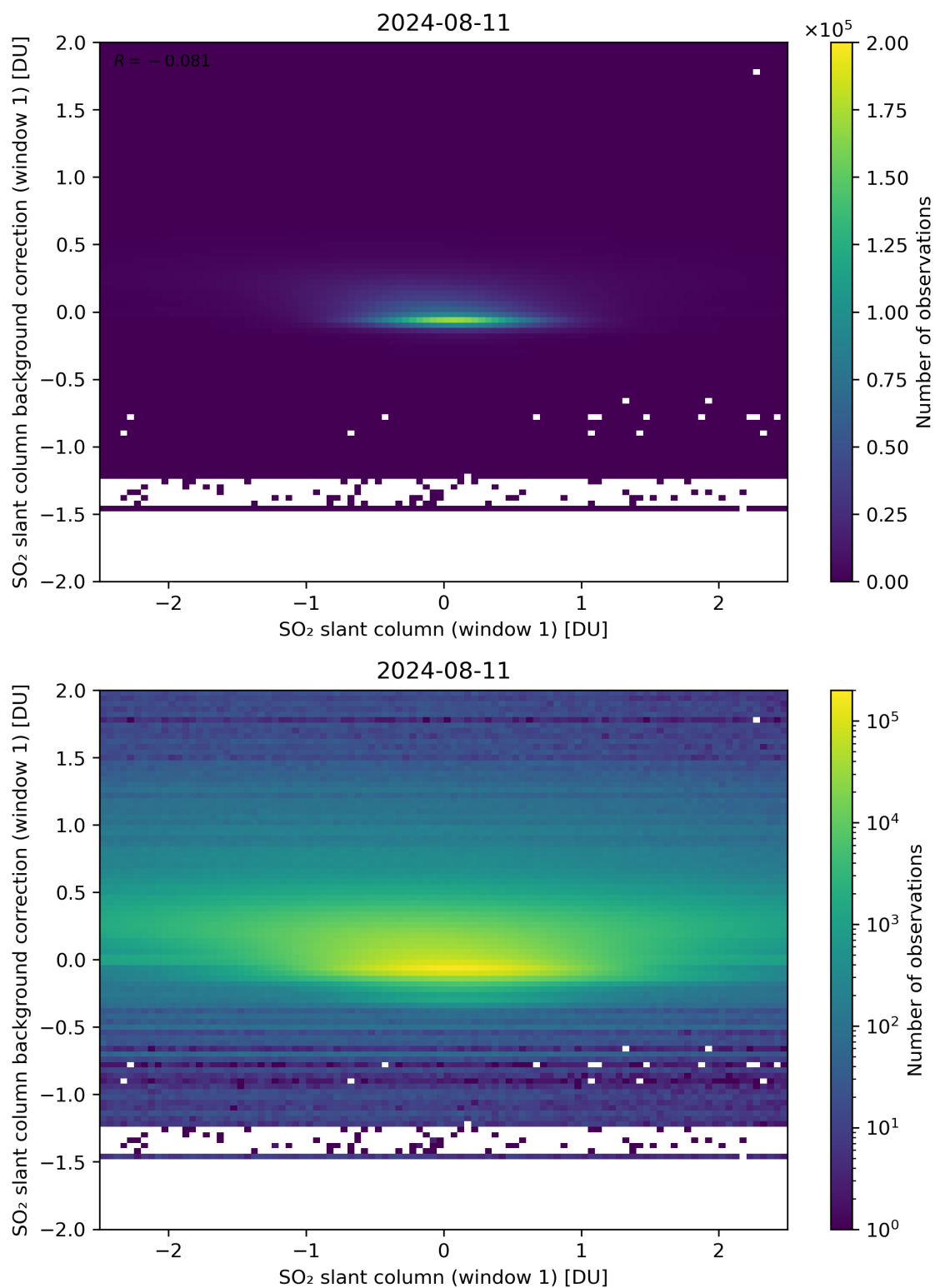
Figure 212: Scatter density plot of “SO 2 slant column (window 1)” against “SO 2 slant column background correction (window 1)” for 2024-08-11 to 2024-08-11.
