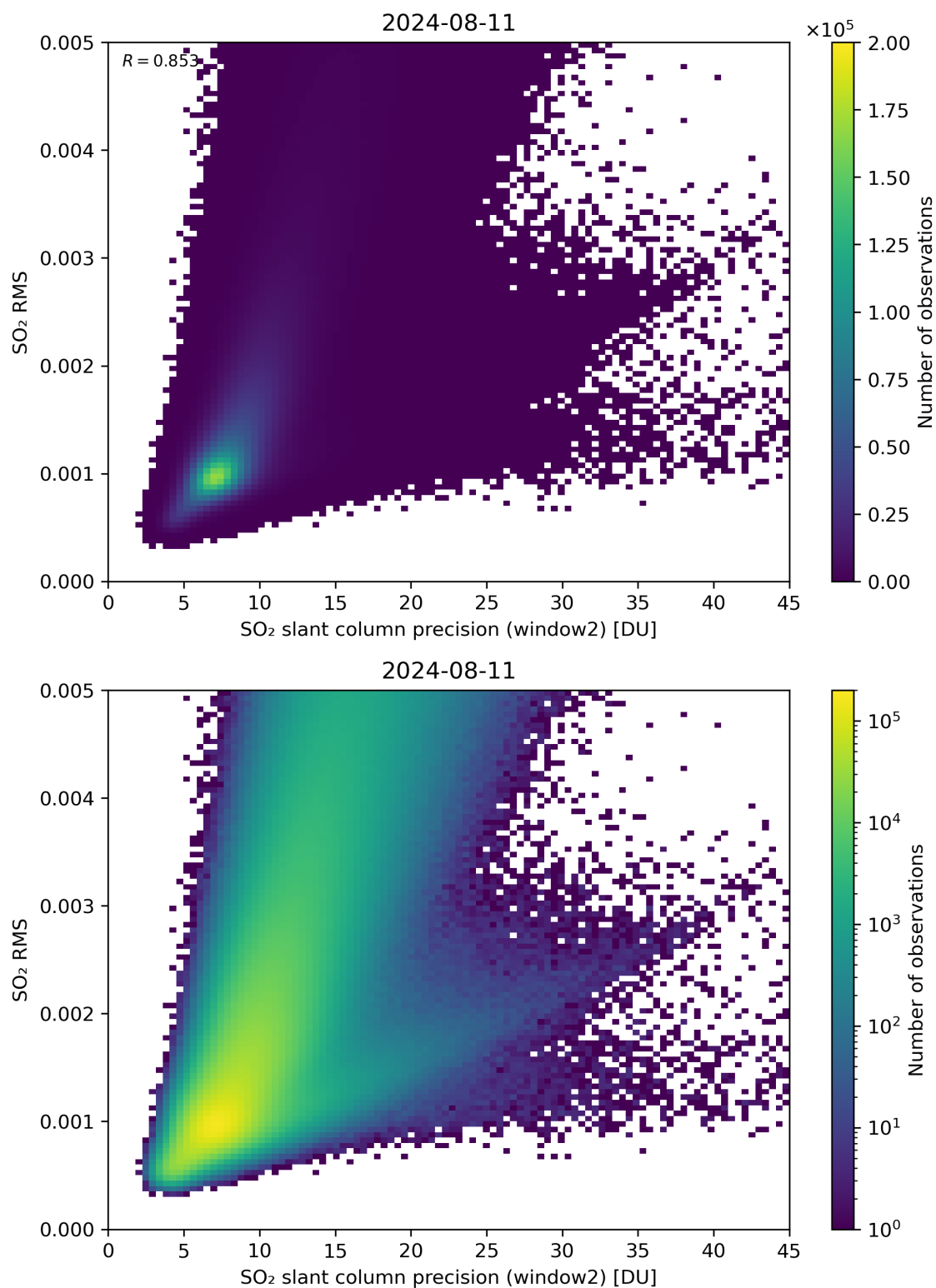
Figure 245: Scatter density plot of “SO 2 slant column precision (window2)” against “SO 2 RMS” for 2024-08-11 to 2024-08-11.
