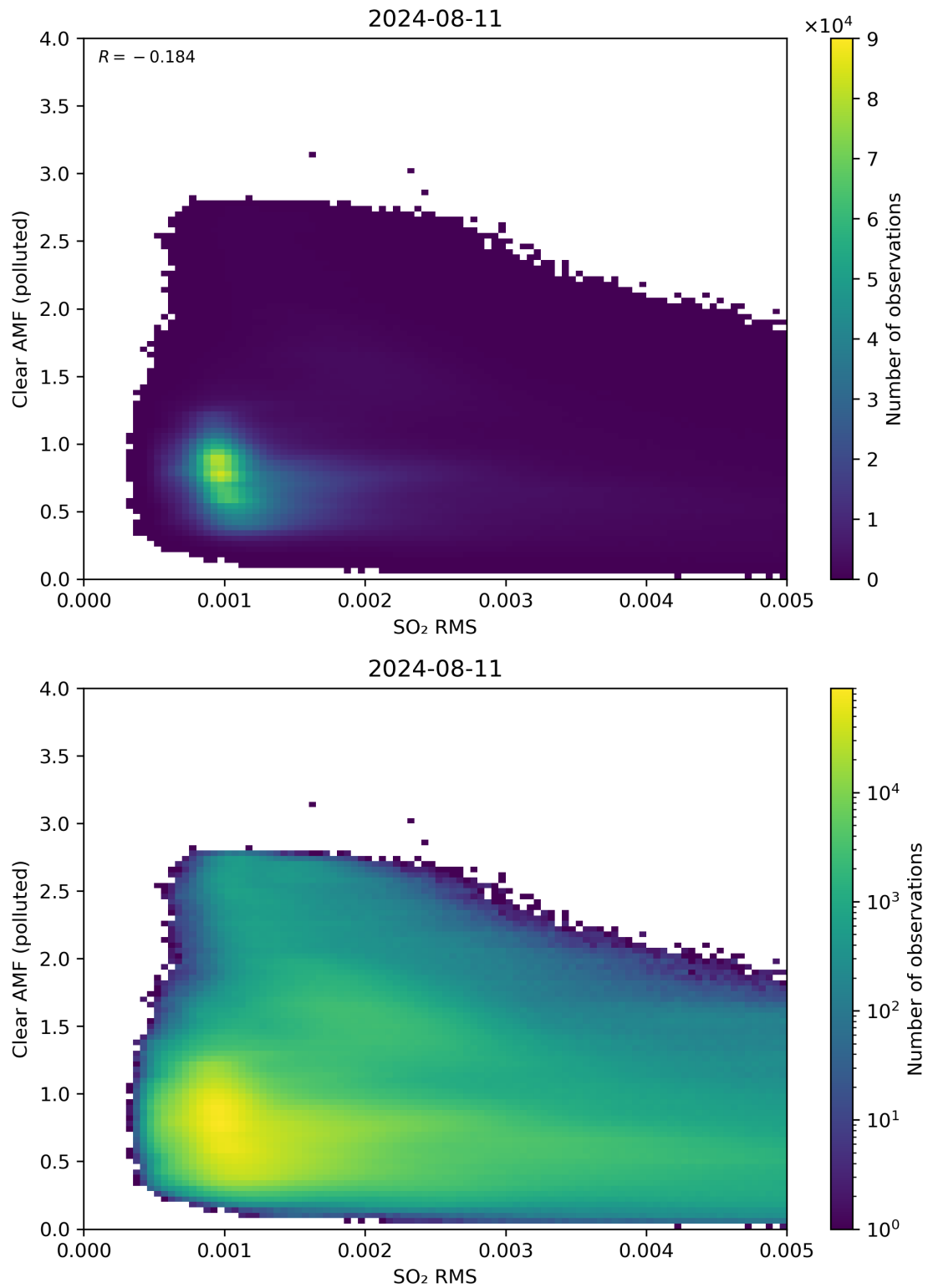
Figure 136: Scatter density plot of “SO 2 RMS” against “Clear AMF (polluted)” for 2024-08-11 to 2024-08-11.
