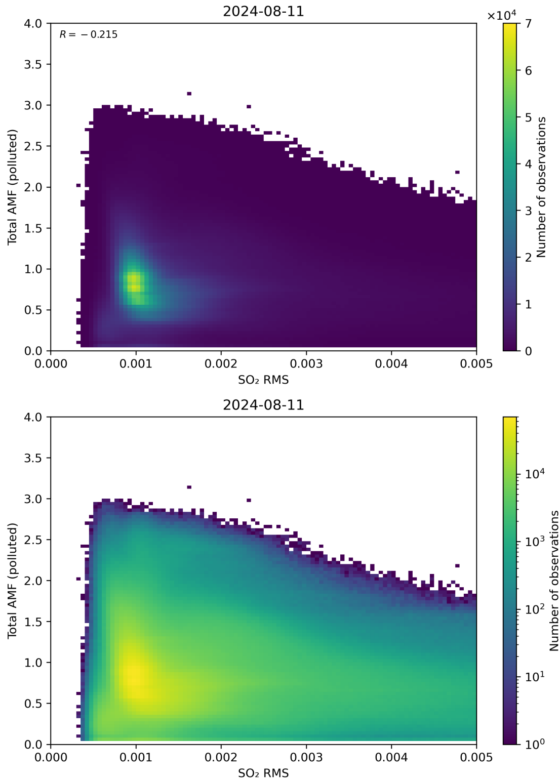
Figure 137: Scatter density plot of “SO 2 RMS” against “Total AMF (polluted)” for 2024-08-11 to 2024-08-11.
