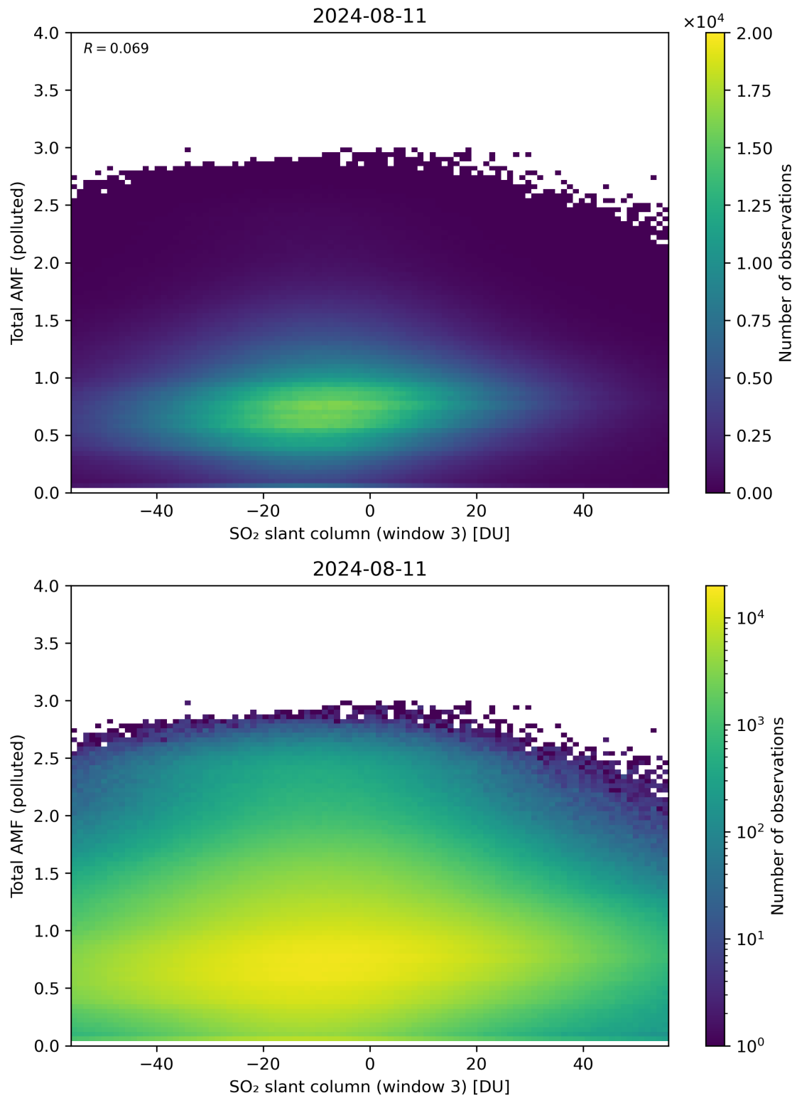
Figure 268: Scatter density plot of “SO 2 slant column (window 3)” against “Total AMF (polluted)” for 2024-08-11 to 2024-08-11.
