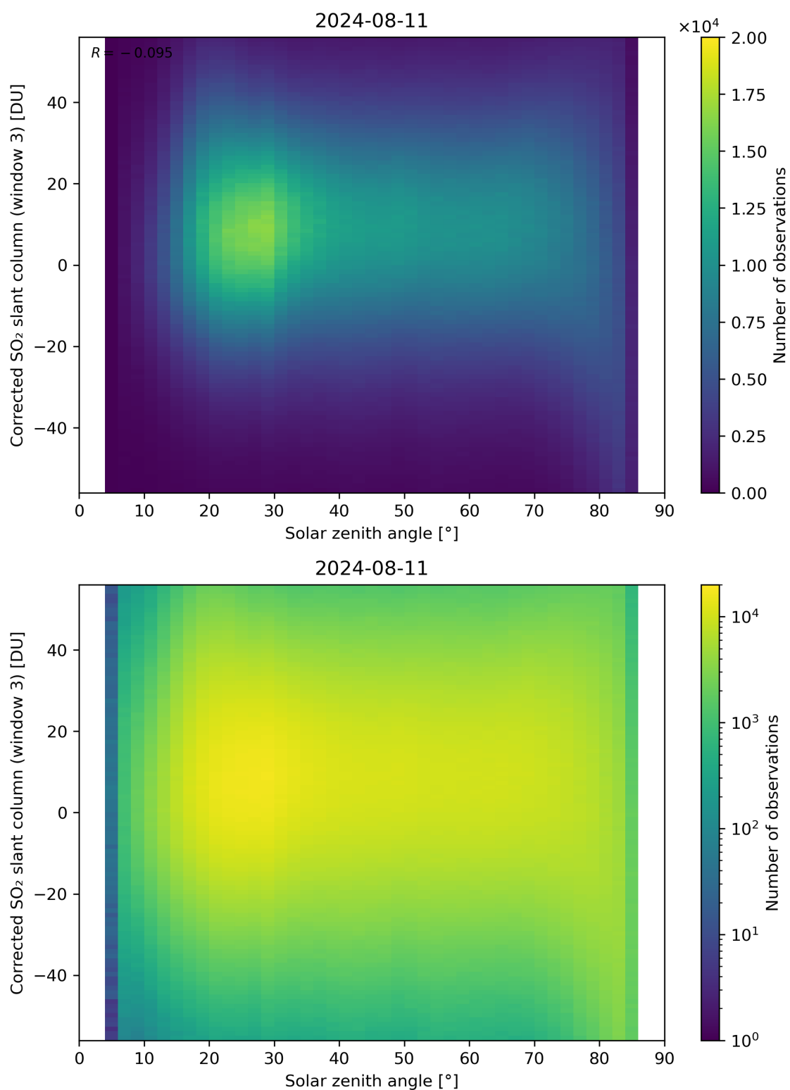
Figure 168: Scatter density plot of “Solar zenith angle” against “Corrected SO 2 slant column (window 3)” for 2024-08-11 to 2024-08-11.
