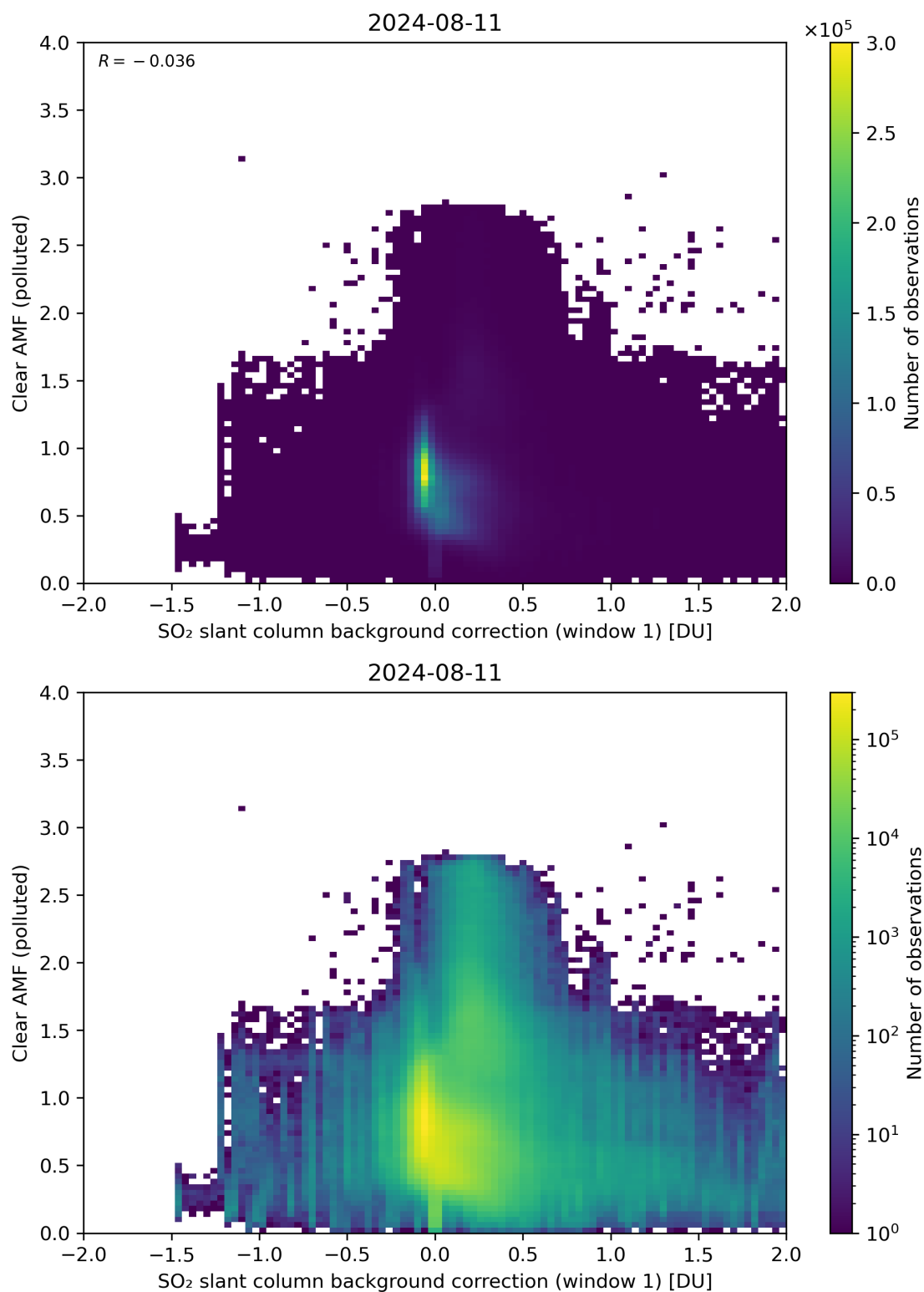
Figure 103: Scatter density plot of “SO 2 slant column background correction (window 1)” against “Clear AMF (polluted)” for 2024-08-11 to 2024-08-11.
