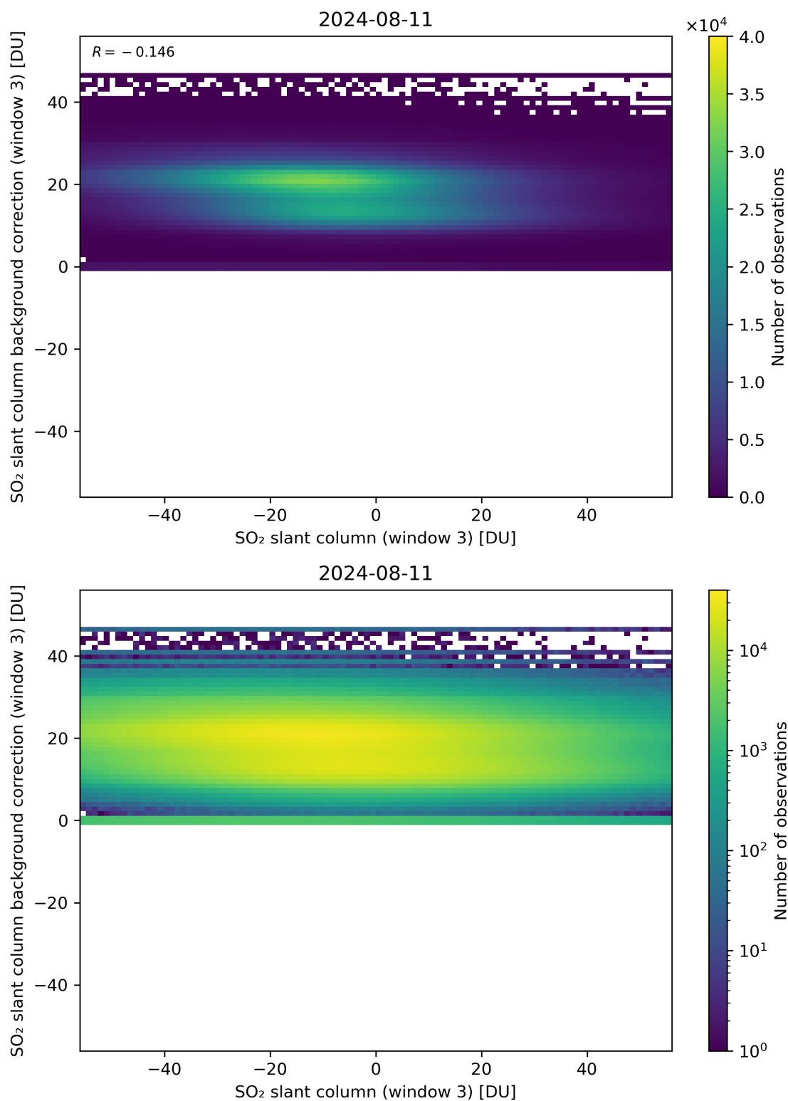
Figure 253: Scatter density plot of “SO 2 slant column (window 3)” against “SO 2 slant column background correction (window 3)” for 2024-08-11 to 2024-08-11.
