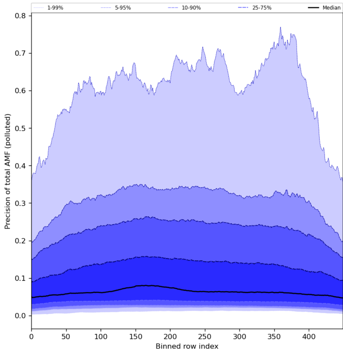
Figure 95: Along track statistics of “Precision of total AMF (polluted)” for 2024-08-11 to 2024-08-11
