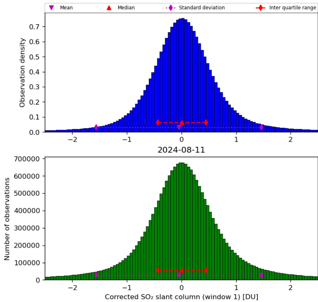
Figure 58: Histogram of “Corrected SO 2 slant column (window 1)” for 2024-08-11 to 2024-08-11
