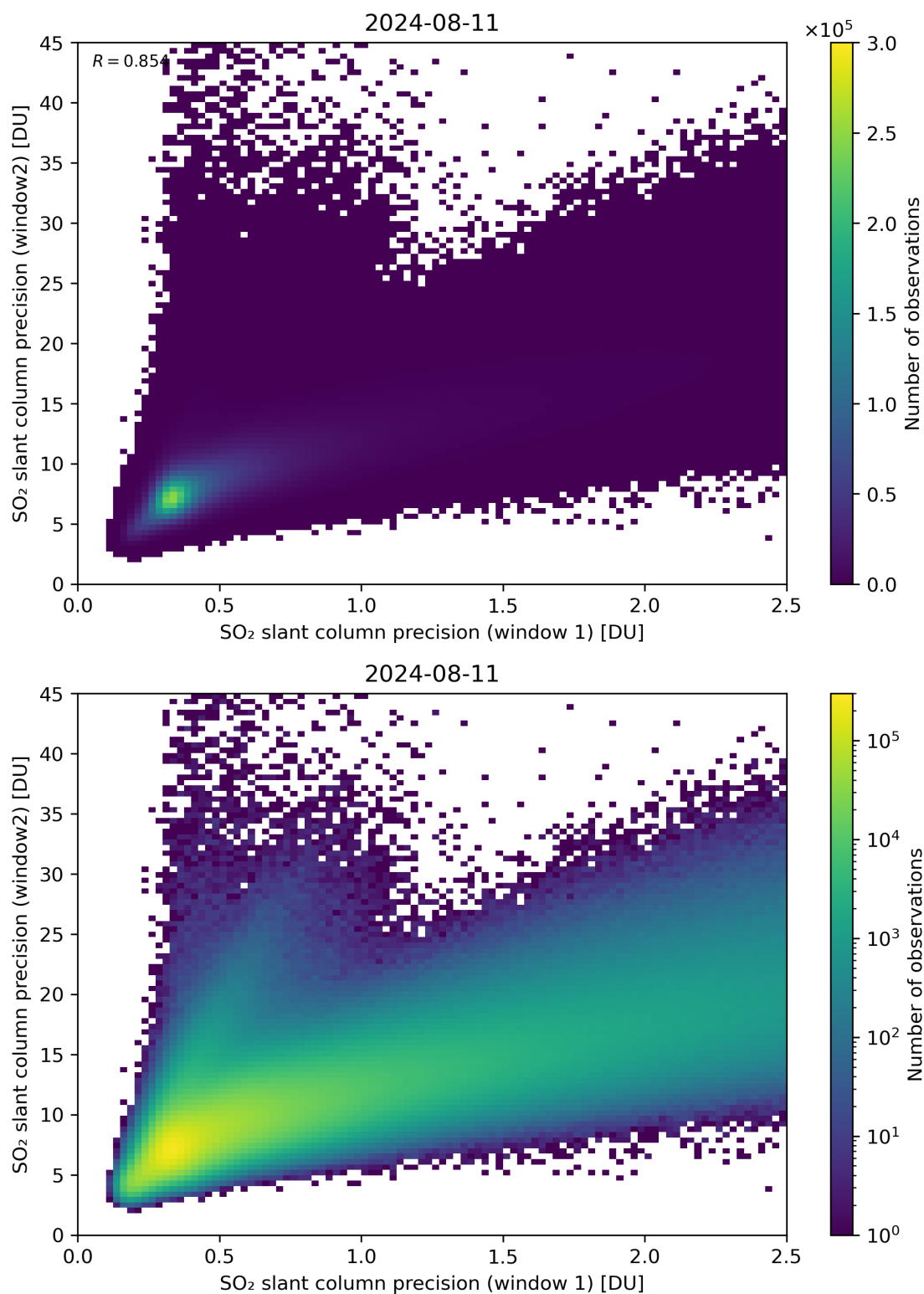
Figure 227: Scatter density plot of “SO 2 slant column precision (window 1)” against “SO 2 slant column precision (window2)” for 2024-08-11 to 2024-08-11.
