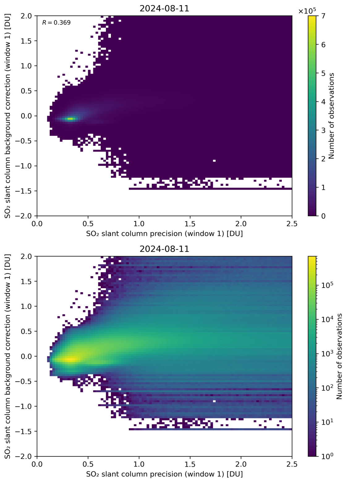
Figure 218: Scatter density plot of “SO 2 slant column precision (window 1)” against “SO 2 slant column background correction (window 1)” for 2024-08-11 to 2024-08-11.
