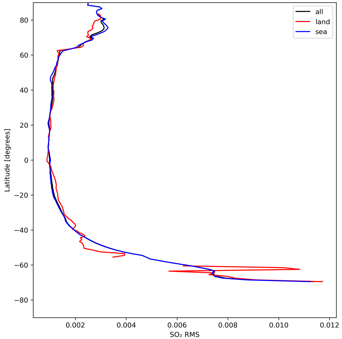
Figure 47: Zonal average of “SO 2 RMS” for 2024-08-11 to 2024-08-11.
