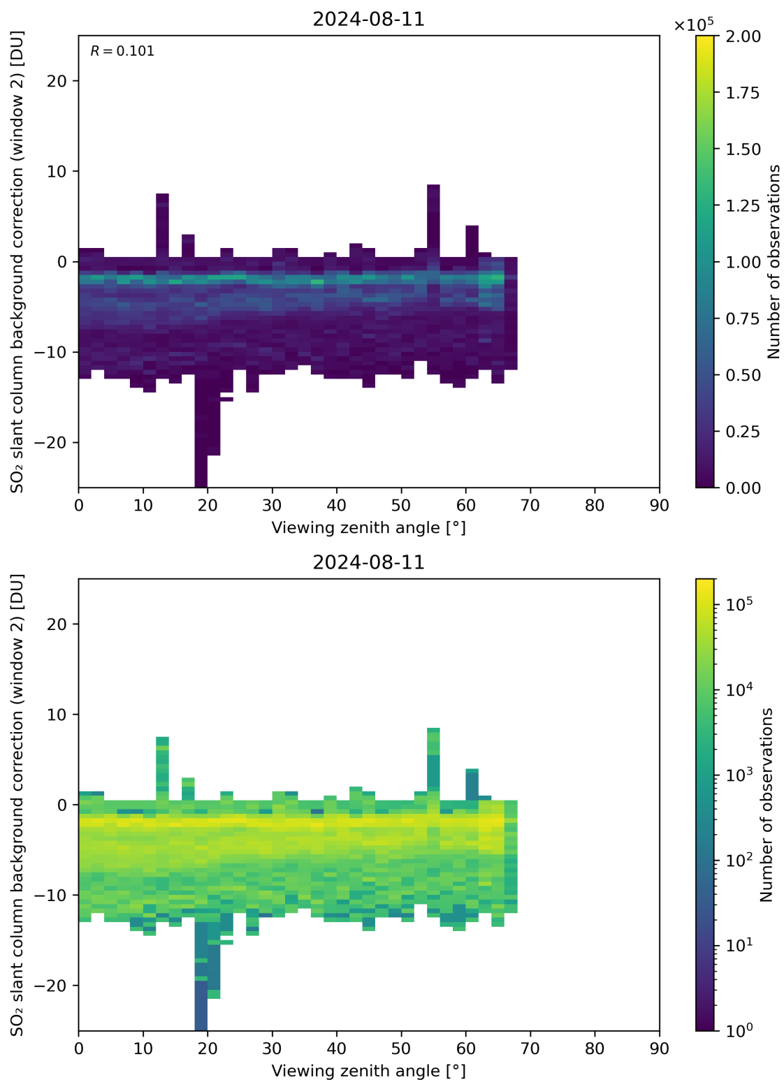
Figure 309: Scatter density plot of “Viewing zenith angle” against “SO 2 slant column background correction (window 2)” for 2024-08-11 to 2024-08-11.
