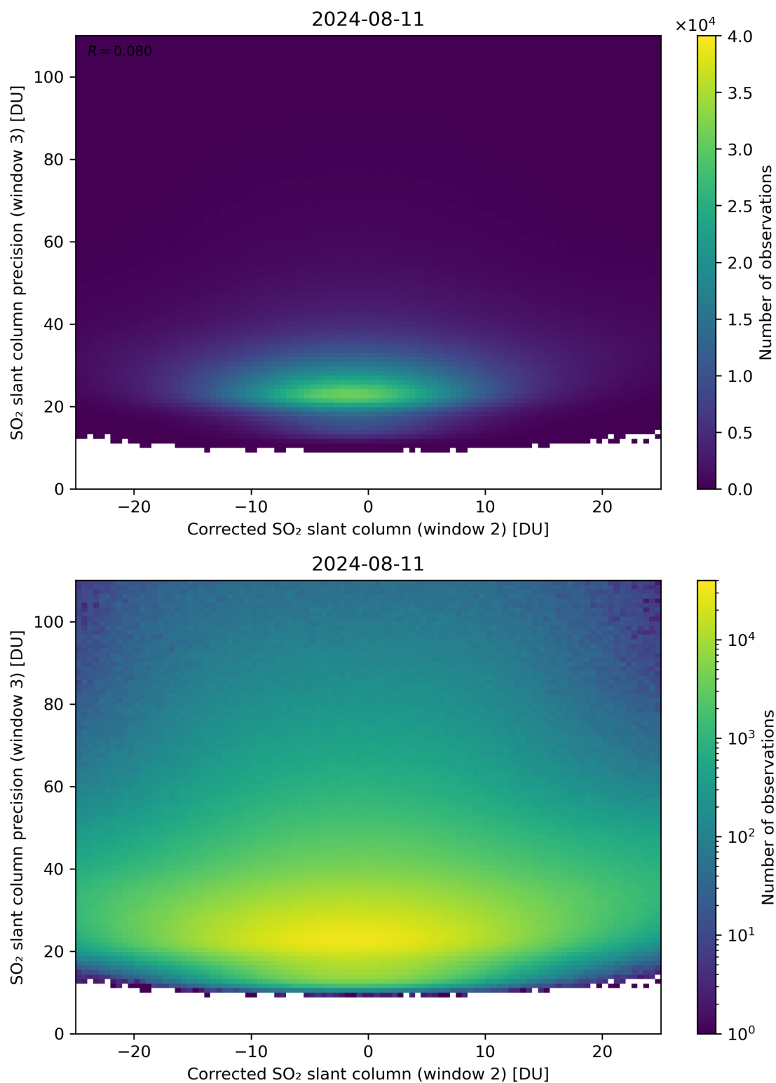
Figure 202: Scatter density plot of “Corrected SO 2 slant column (window 2)” against “SO 2 slant column precision (window 3)” for 2024-08-11 to 2024-08-11.
