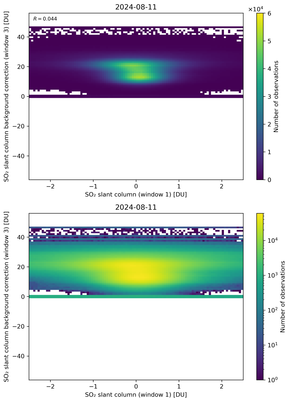
Figure 214: Scatter density plot of “SO 2 slant column (window 1)” against “SO 2 slant column background correction (window 3)” for 2024-08-11 to 2024-08-11.
