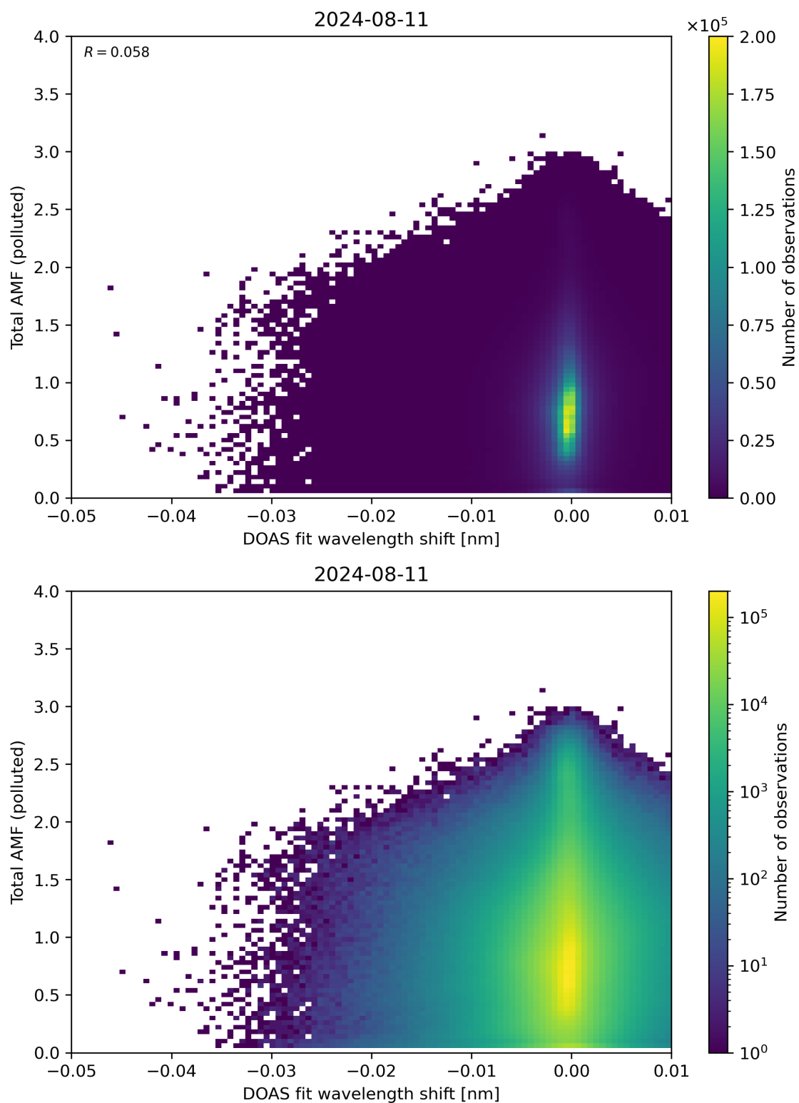
Figure 130: Scatter density plot of “DOAS fit wavelength shift” against “Total AMF (polluted)” for 2024-08-11 to 2024-08-11.
