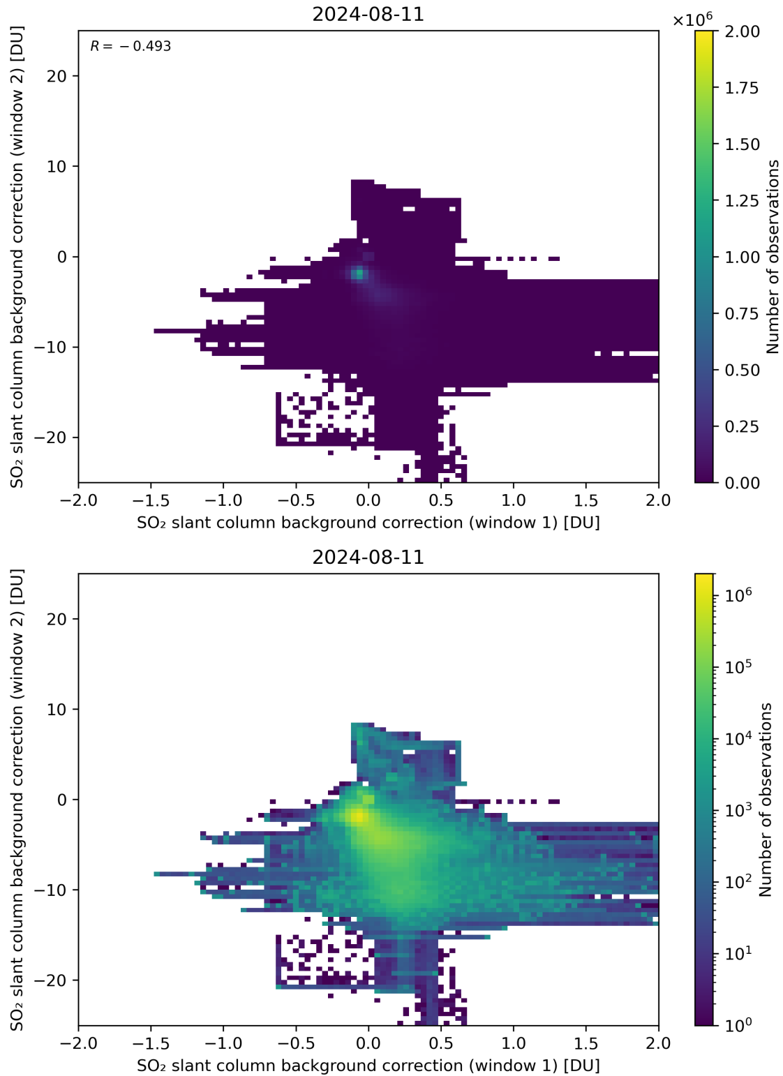
Figure 98: Scatter density plot of “SO 2 slant column background correction (window 1)” against “SO 2 slant column background correction (window 2)” for 2024-08-11 to 2024-08-11.
