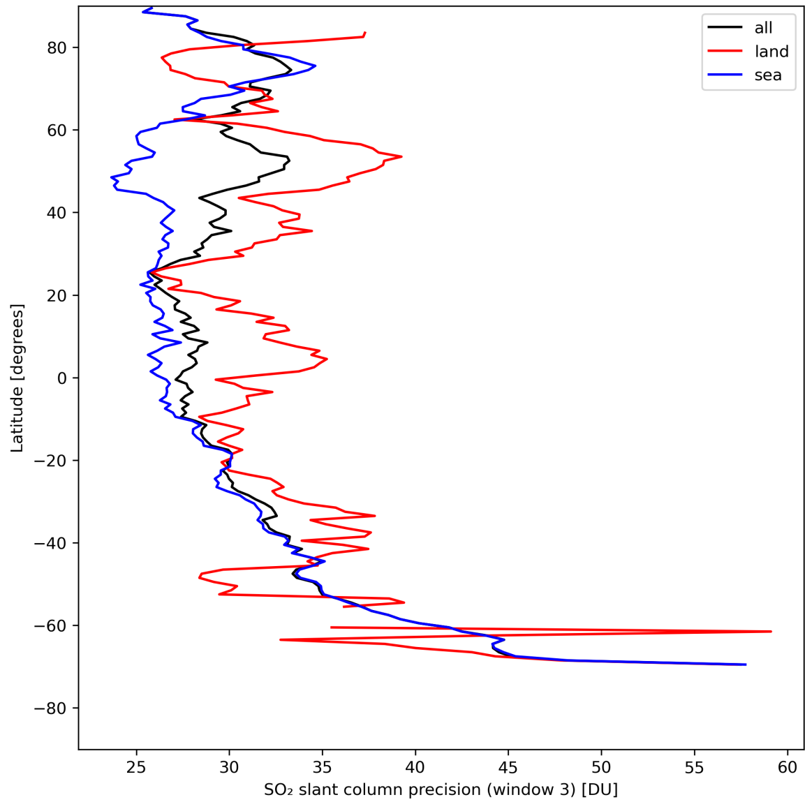
Figure 42: Zonal average of “SO 2 slant column precision (window 3)” for 2024-08-11 to 2024-08-11.
