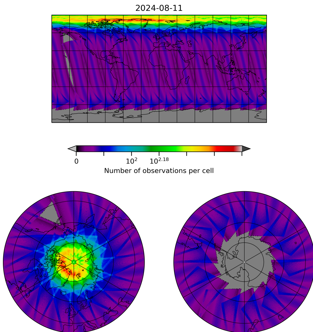
Figure 28: Map of the number of observations for 2024-08-11 to 2024-08-11
