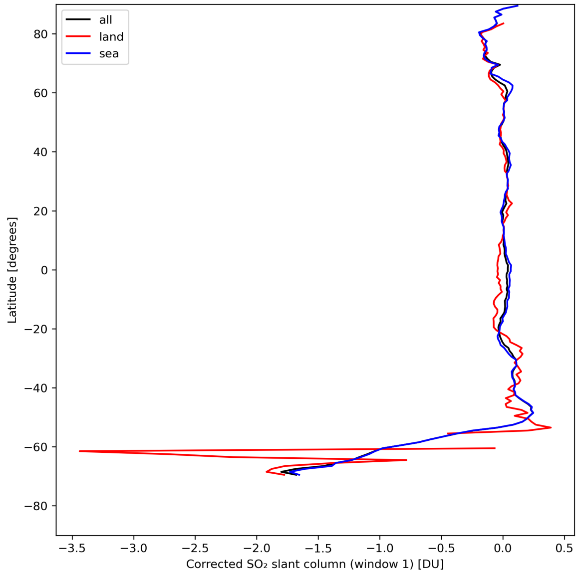
Figure 35: Zonal average of “Corrected SO 2 slant column (window 1)” for 2024-08-11 to 2024-08-11.
