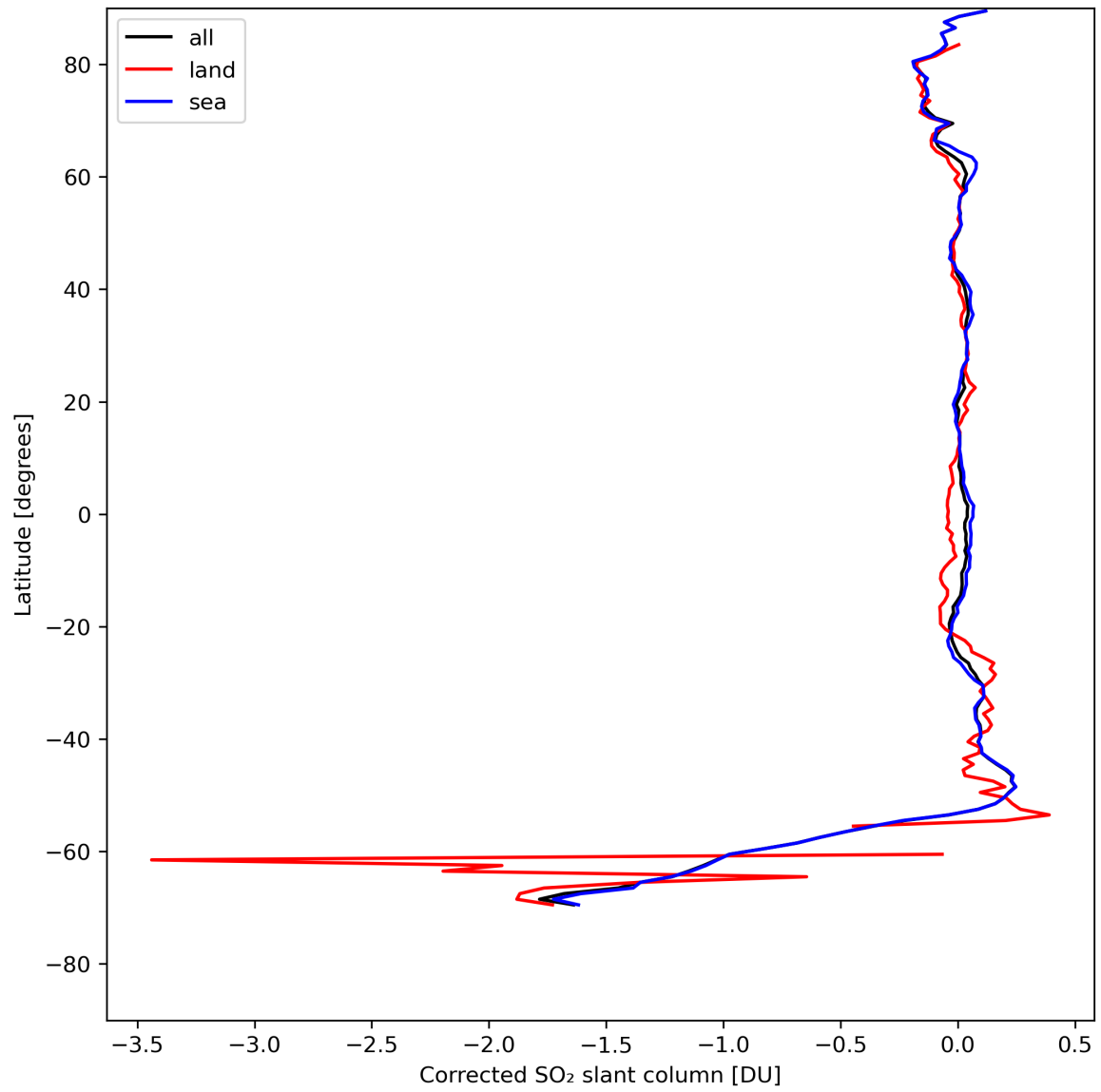
Figure 32: Zonal average of “Corrected SO 2 slant column” for 2024-08-11 to 2024-08-11.
