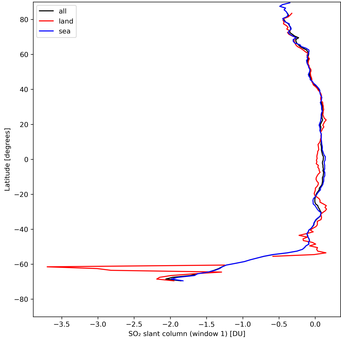
Figure 33: Zonal average of “SO 2 slant column (window 1)” for 2024-08-11 to 2024-08-11.
