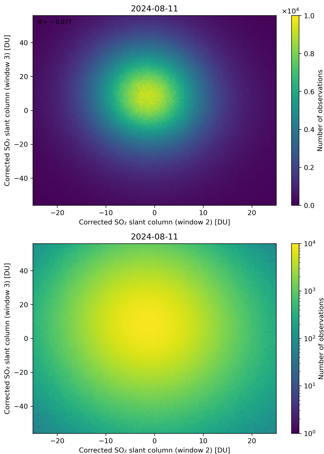
Figure 200: Scatter density plot of “Corrected SO 2 slant column (window 2)” against “Corrected SO 2 slant column (window 3)” for 2024-08-11 to 2024-08-11.
