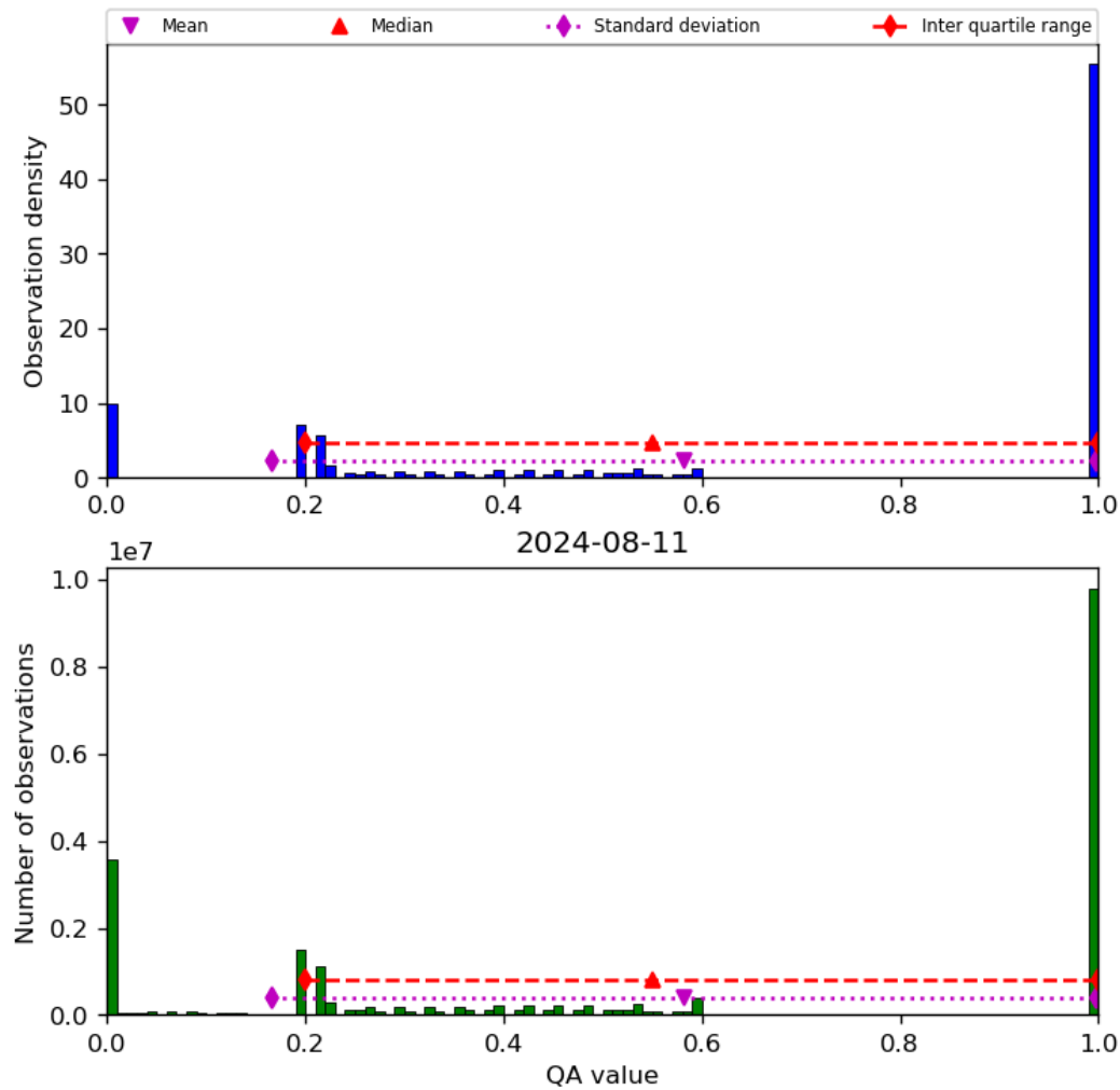
Figure 52: Histogram of “QA value” for 2024-08-11 to 2024-08-11
