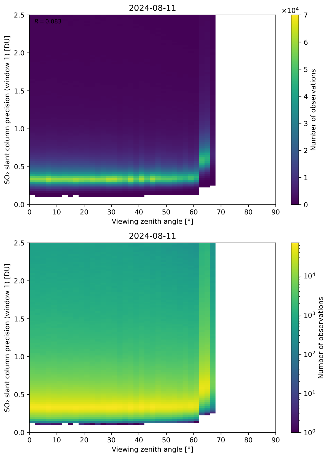
Figure 321: Scatter density plot of “Viewing zenith angle” against “SO 2 slant column precision (window 1)” for 2024-08-11 to 2024-08-11.
