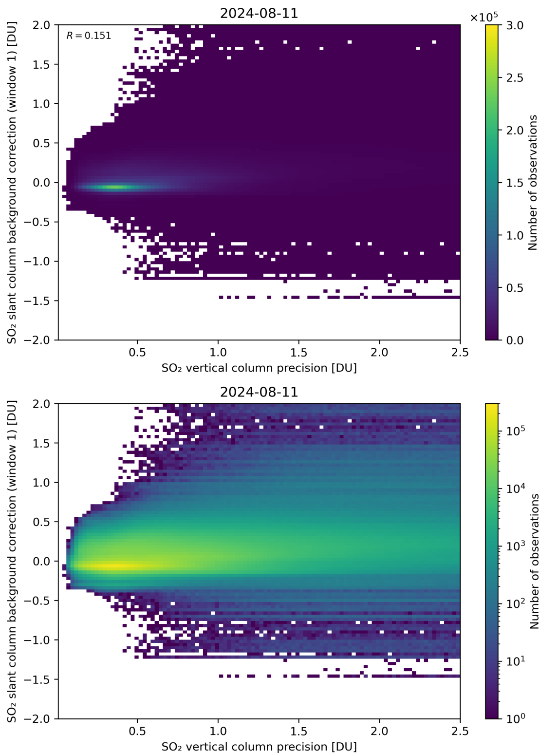
Figure 279: Scatter density plot of “SO 2 vertical column precision” against “SO 2 slant column background correction (window 1)” for 2024-08-11 to 2024-08-11.
