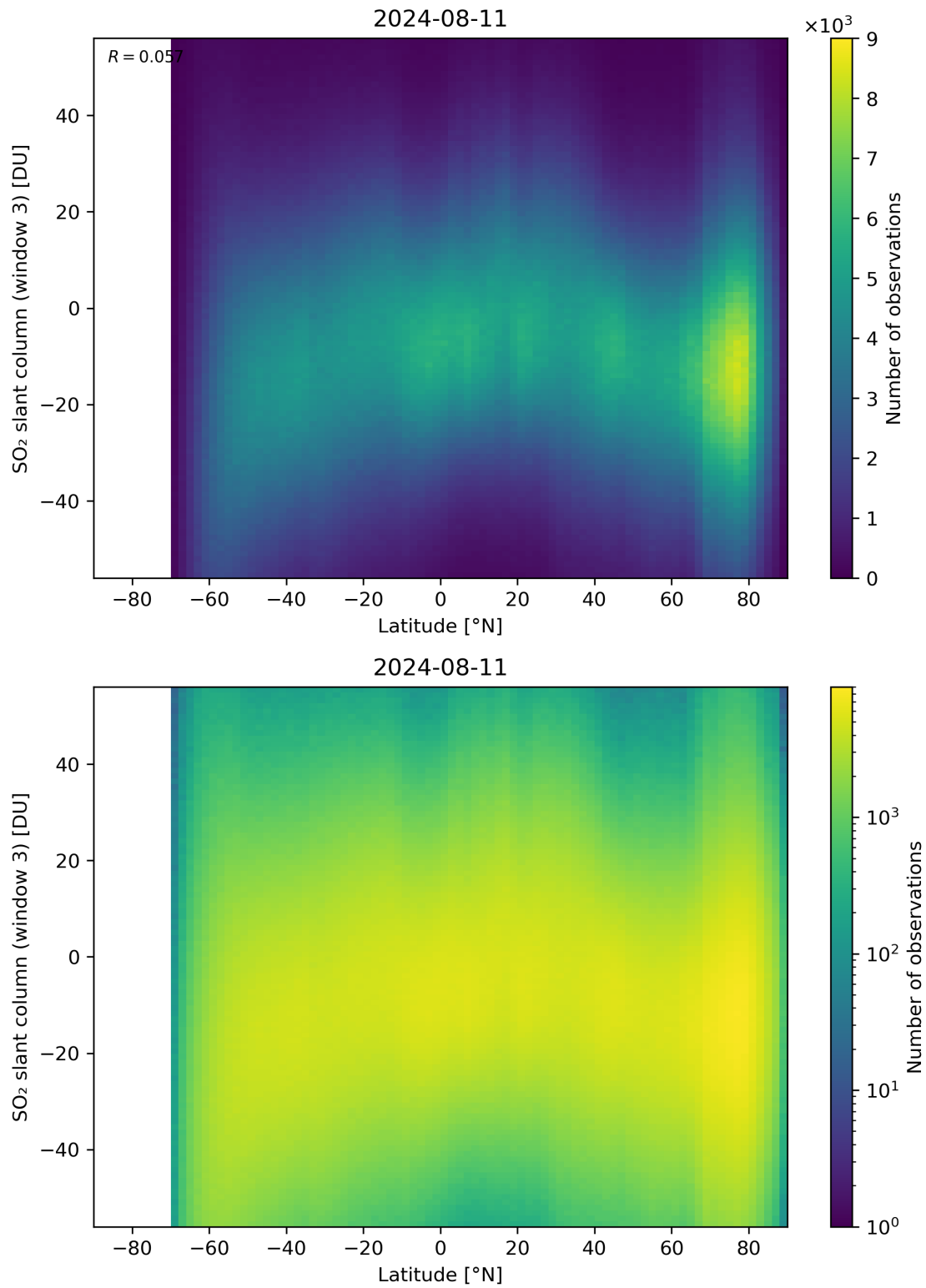
Figure 152: Scatter density plot of “Latitude” against “SO 2 slant column (window 3)” for 2024-08-11 to 2024-08-11.
