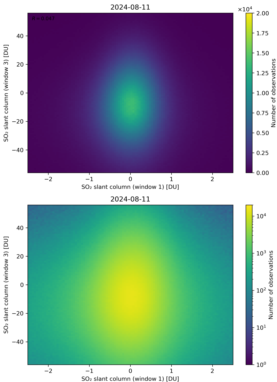
Figure 237: Scatter density plot of “SO 2 slant column (window 1)” against “SO 2 slant column (window 3)” for 2024-08-11 to 2024-08-11.
