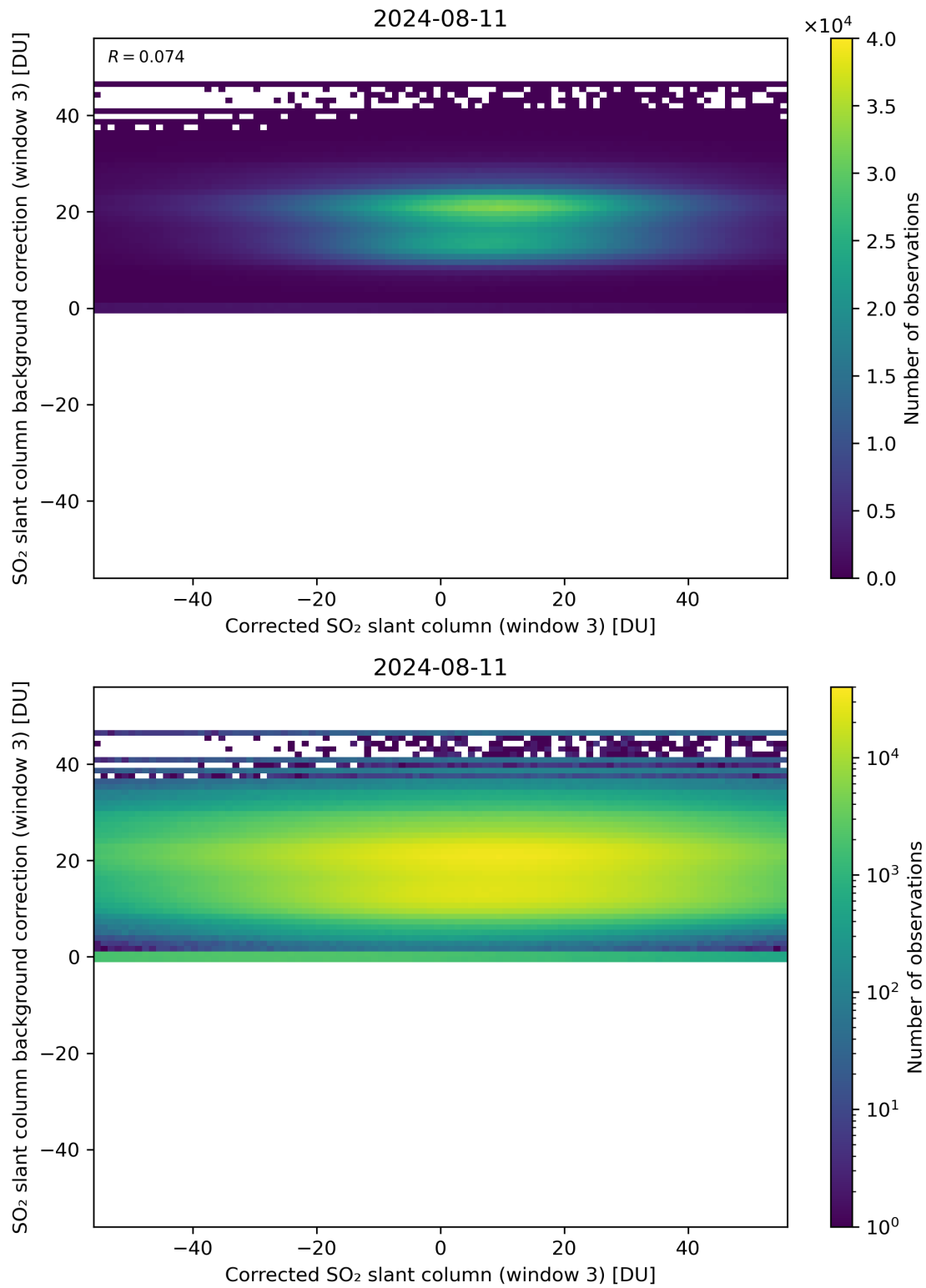
Figure 205: Scatter density plot of “Corrected SO 2 slant column (window 3)” against “SO 2 slant column background correction (window 3)” for 2024-08-11 to 2024-08-11.
