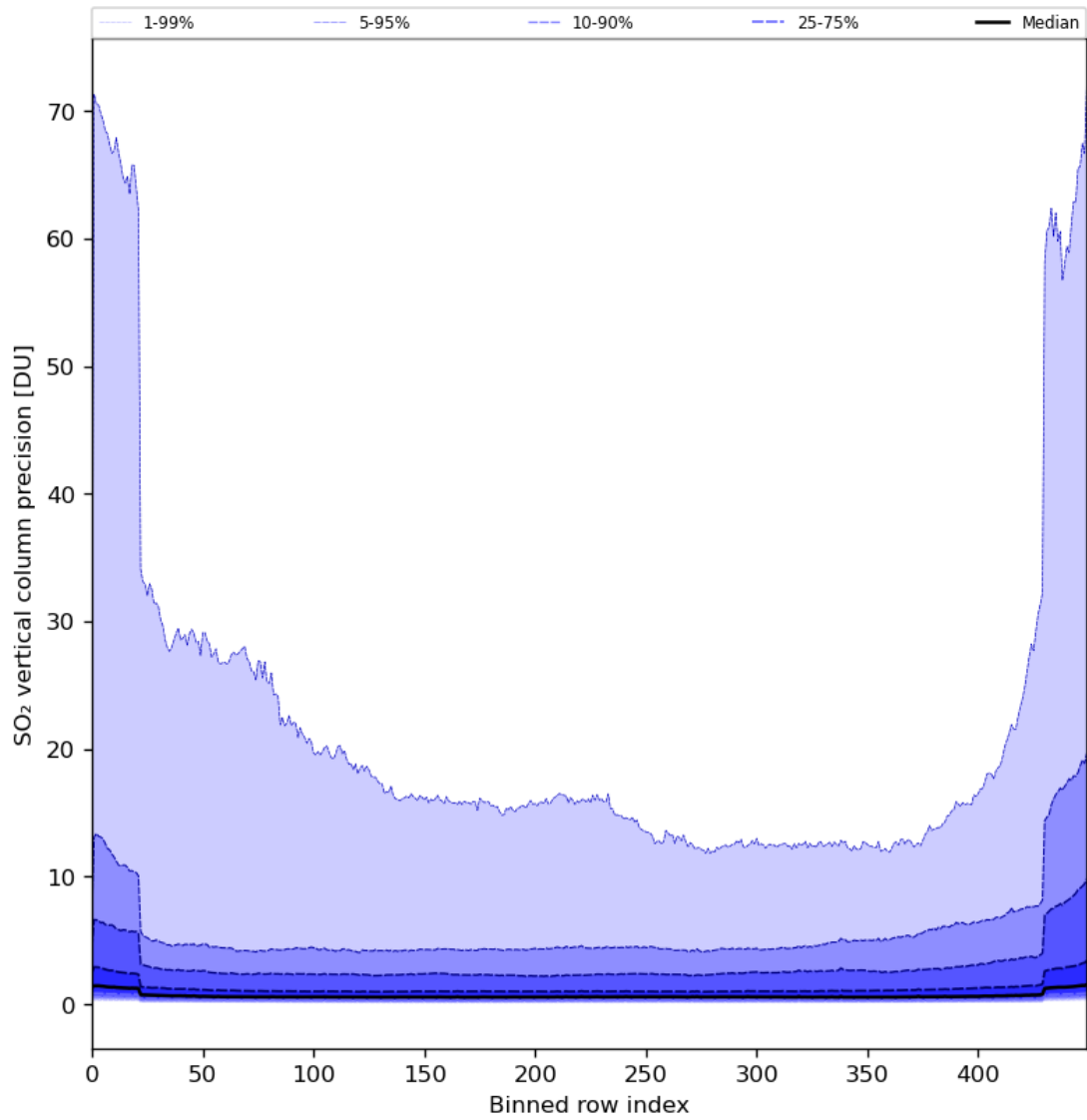
Figure 77: Along track statistics of “SO 2 vertical column precision” for 2024-08-11 to 2024-08-11
