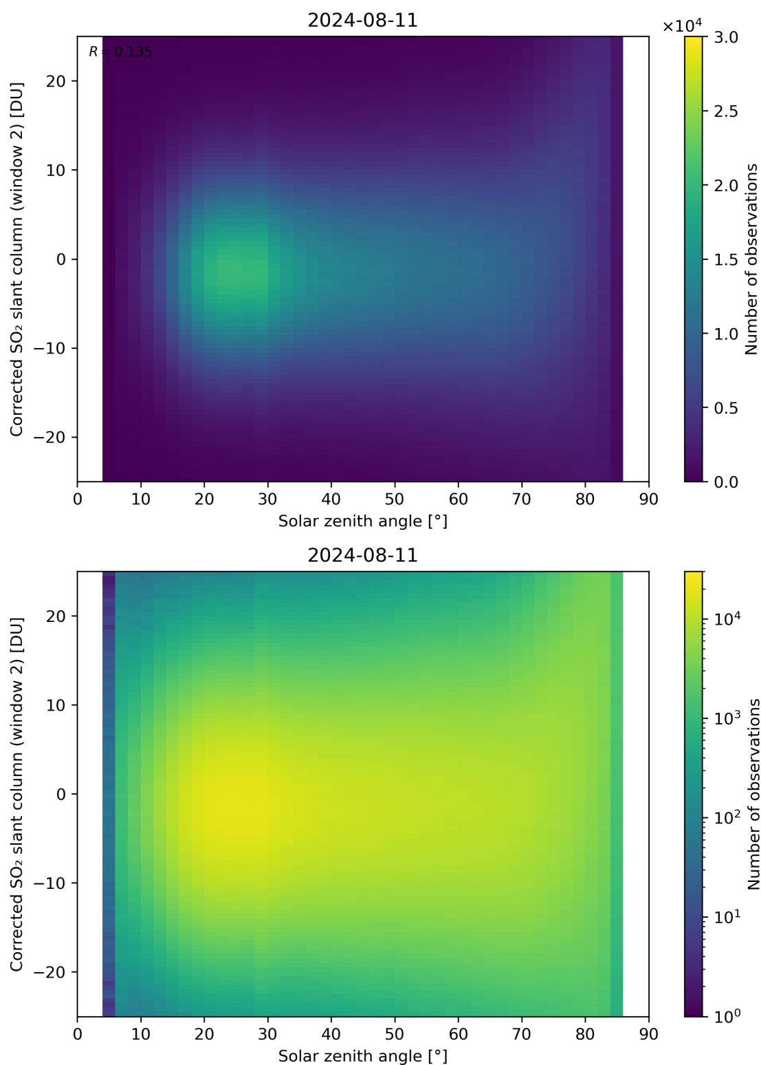
Figure 167: Scatter density plot of “Solar zenith angle” against “Corrected SO 2 slant column (window 2)” for 2024-08-11 to 2024-08-11.
