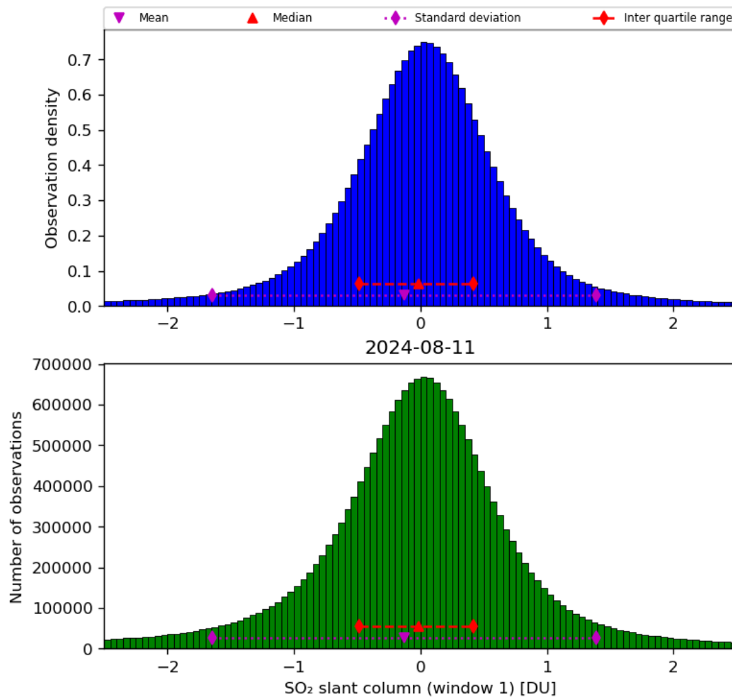
Figure 56: Histogram of “SO 2 slant column (window 1)” for 2024-08-11 to 2024-08-11
