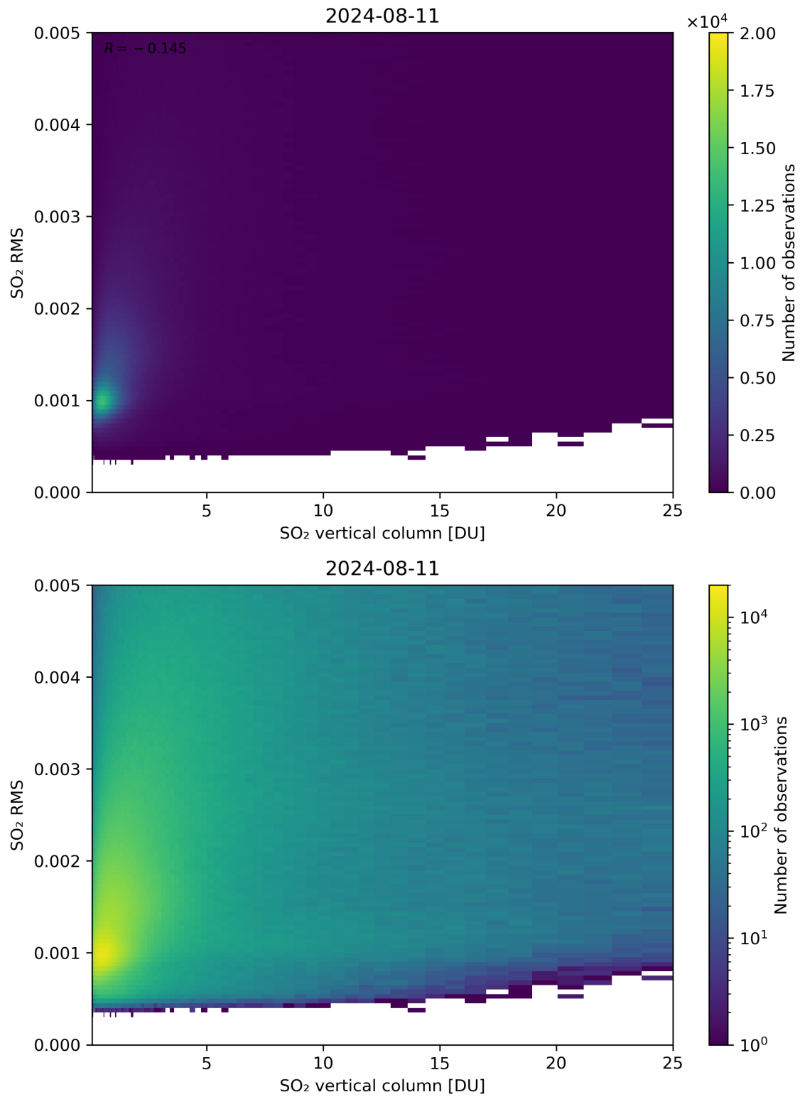
Figure 278: Scatter density plot of “SO 2 vertical column” against “SO 2 RMS” for 2024-08-11 to 2024-08-11.
