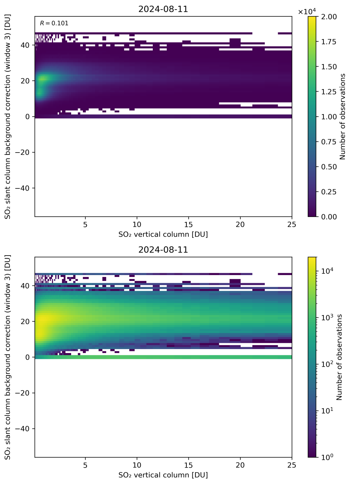
Figure 275: Scatter density plot of “SO 2 vertical column” against “SO 2 slant column background correction (window 3)” for 2024-08-11 to 2024-08-11.
