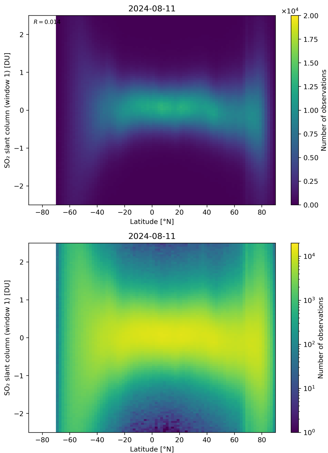
Figure 149: Scatter density plot of “Latitude” against “SO 2 slant column (window 1)” for 2024-08-11 to 2024-08-11.
