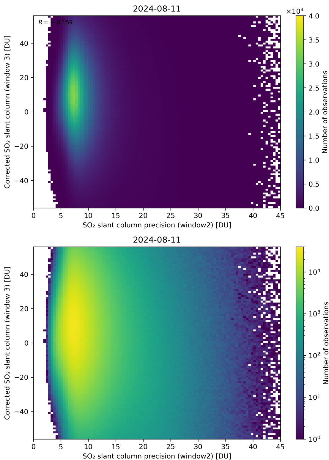
Figure 248: Scatter density plot of “SO 2 slant column precision (window2)” against “Corrected SO 2 slant column (window 3)” for 2024-08-11 to 2024-08-11.
