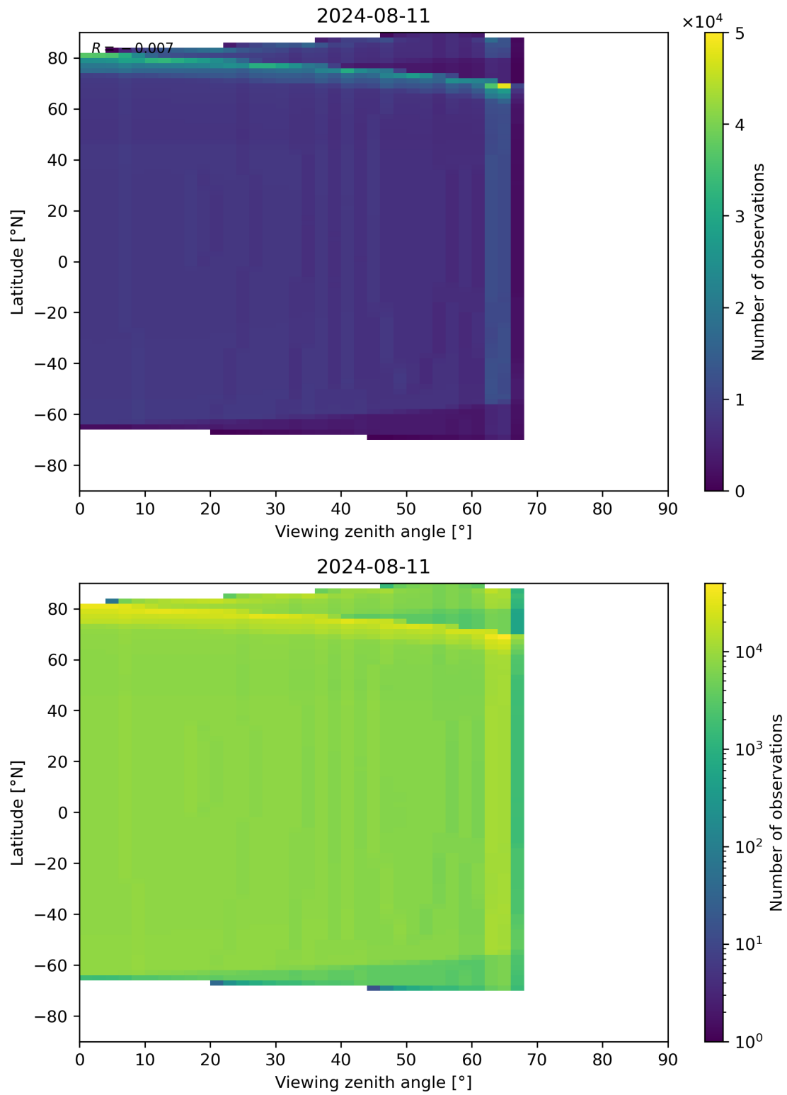
Figure 314: Scatter density plot of “Viewing zenith angle” against “Latitude” for 2024-08-11 to 2024-08-11.
