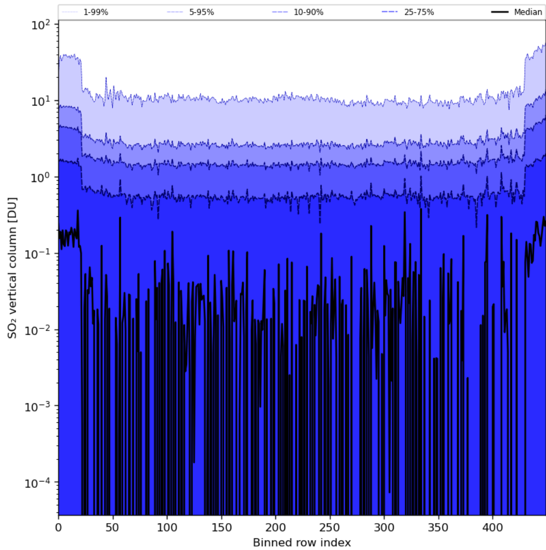
Figure 76: Along track statistics of “SO 2 vertical column” for 2024-08-11 to 2024-08-11
