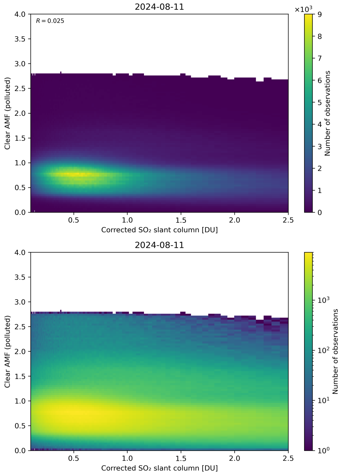
Figure 184: Scatter density plot of “Corrected SO 2 slant column” against “Clear AMF (polluted)” for 2024-08-11 to 2024-08-11.
