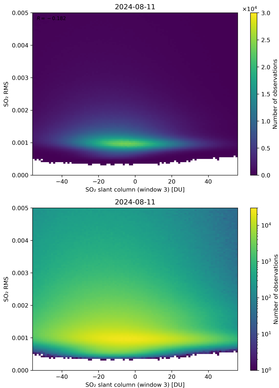
Figure 256: Scatter density plot of “SO 2 slant column (window 3)” against “SO 2 RMS” for 2024-08-11 to 2024-08-11.
