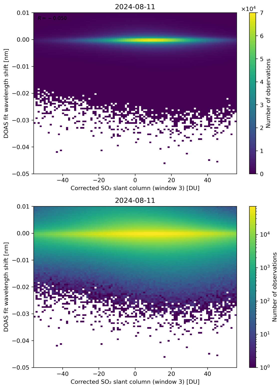
Figure 206: Scatter density plot of “Corrected SO 2 slant column (window 3)” against “DOAS fit wavelength shift” for 2024-08-11 to 2024-08-11.
