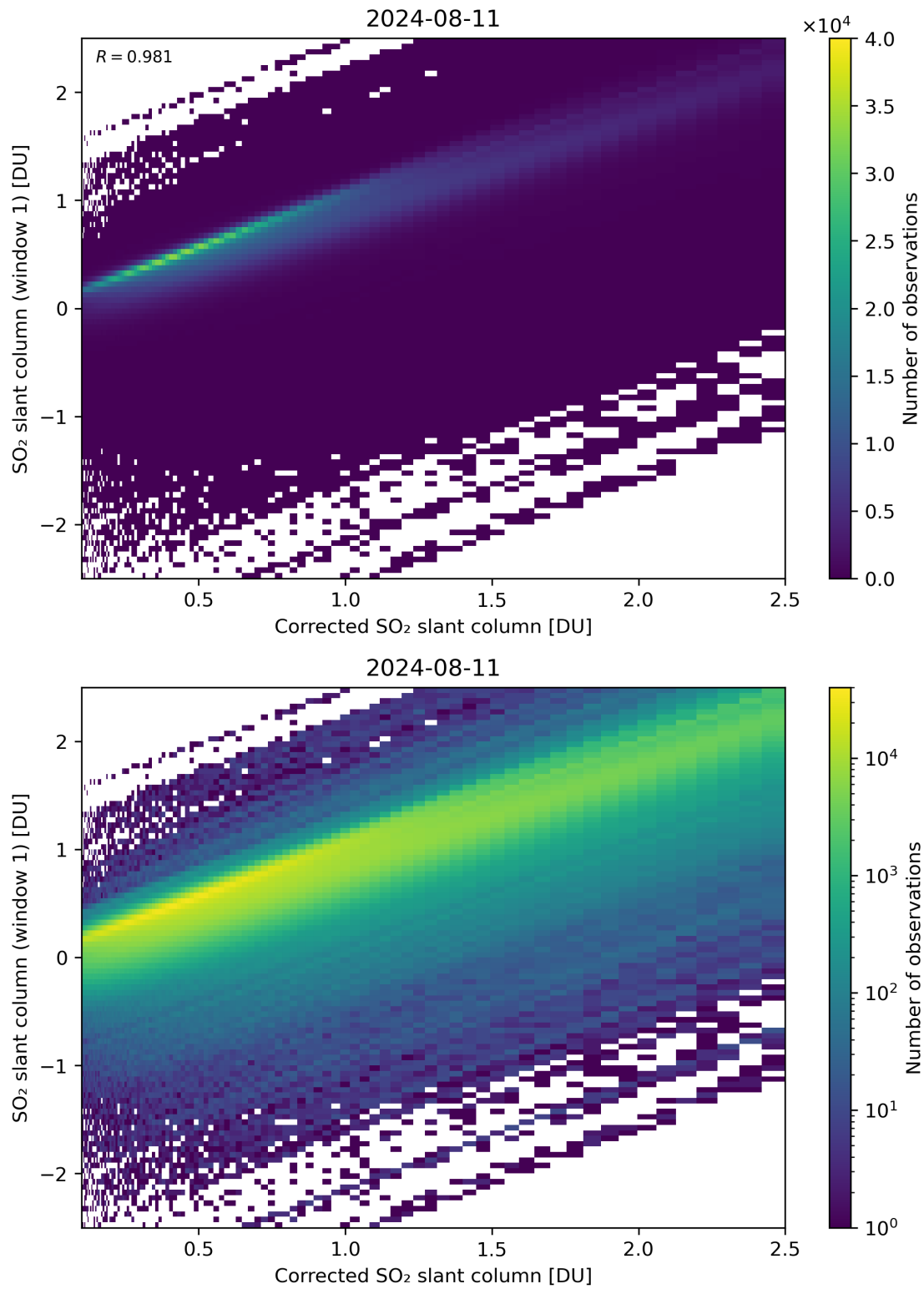
Figure 187: Scatter density plot of “Corrected SO 2 slant column” against “SO 2 slant column (window 1)” for 2024-08-11 to 2024-08-11.
