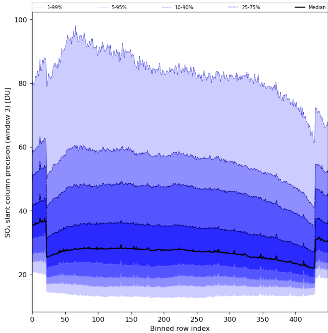
Figure 88: Along track statistics of “SO 2 slant column precision (window 3)” for 2024-08-11 to 2024-08-11
