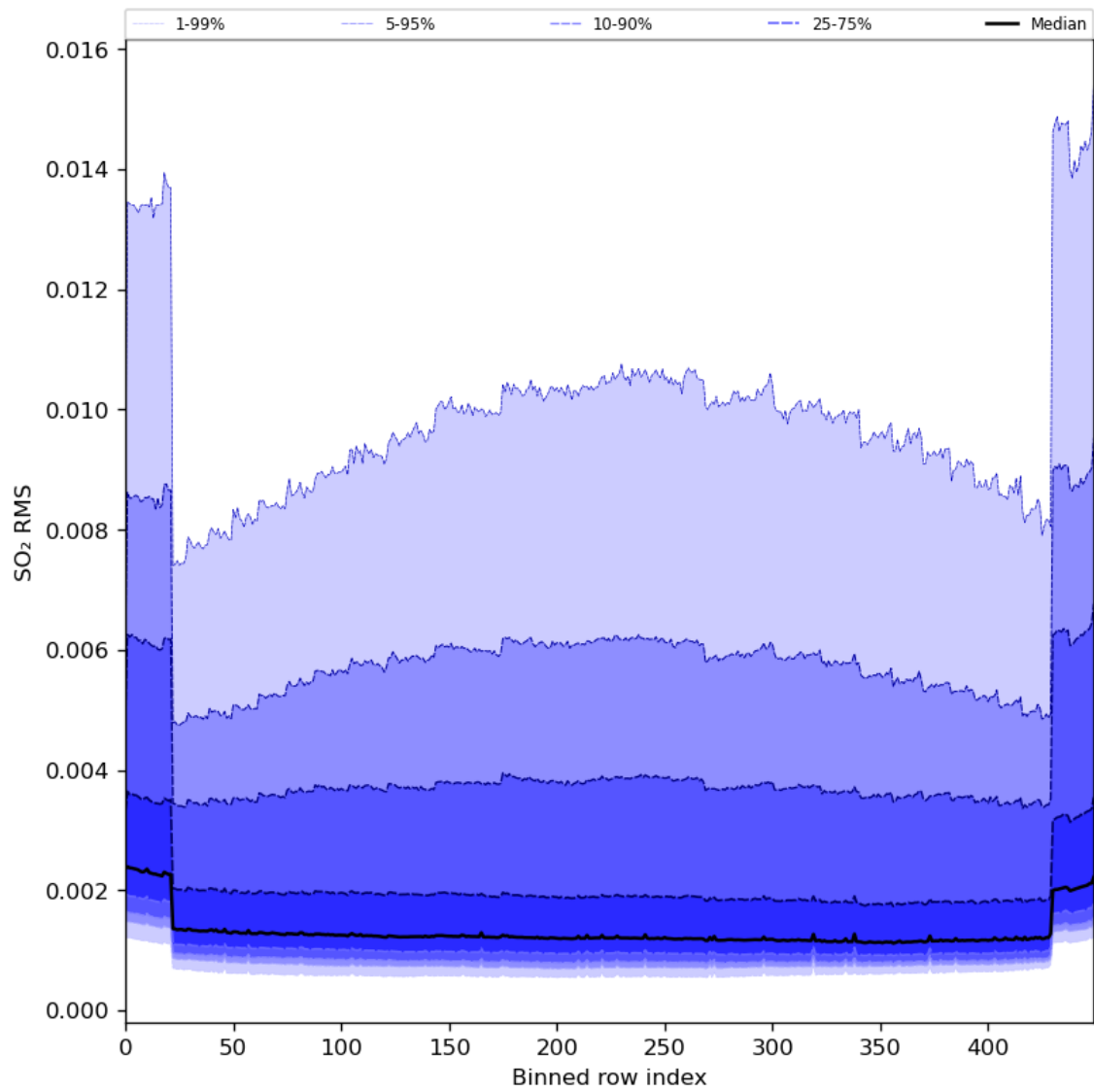
Figure 93: Along track statistics of “SO 2 RMS” for 2024-08-11 to 2024-08-11
