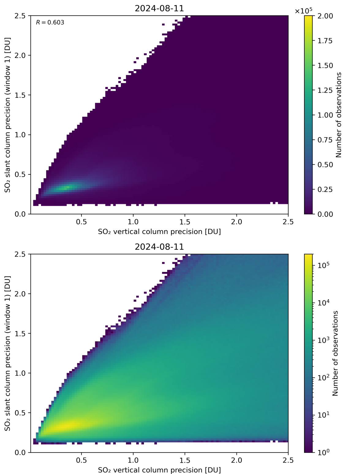
Figure 290: Scatter density plot of “SO 2 vertical column precision” against “SO 2 slant column precision (window 1)” for 2024-08-11 to 2024-08-11.
