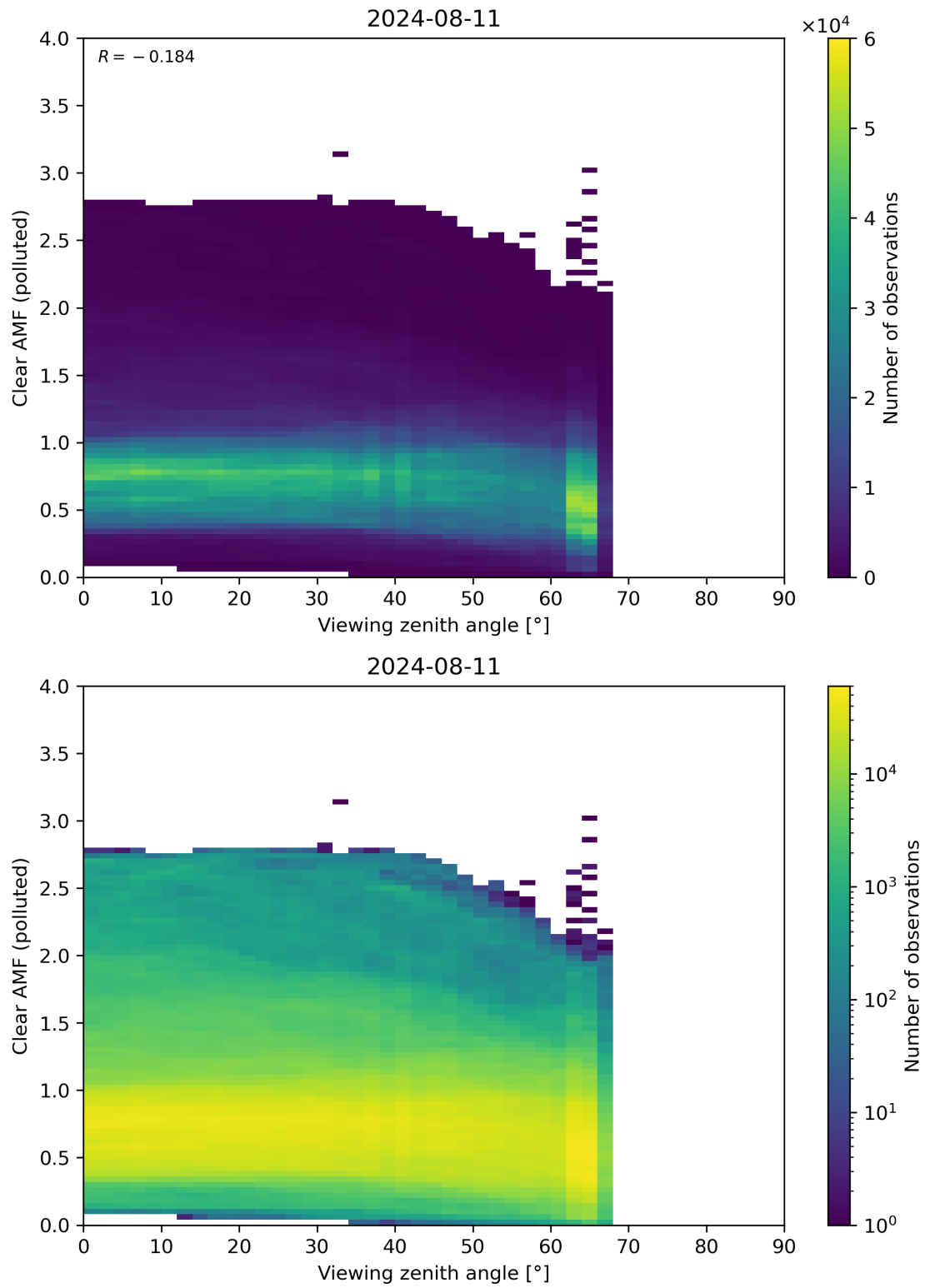
Figure 316: Scatter density plot of “Viewing zenith angle” against “Clear AMF (polluted)” for 2024-08-11 to 2024-08-11.
