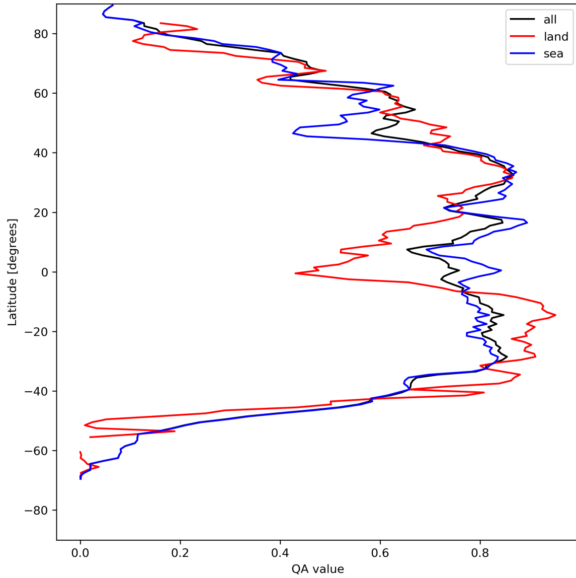
Figure 29: Zonal average of “QA value” for 2024-08-11 to 2024-08-11.
