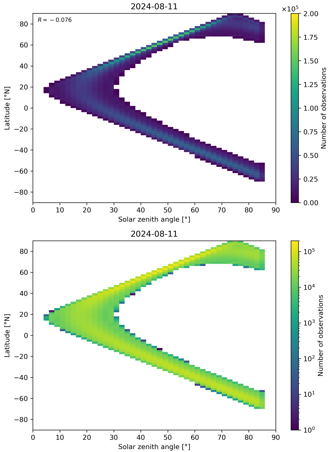
Figure 164: Scatter density plot of “Solar zenith angle” against “Latitude” for 2024-08-11 to 2024-08-11.
