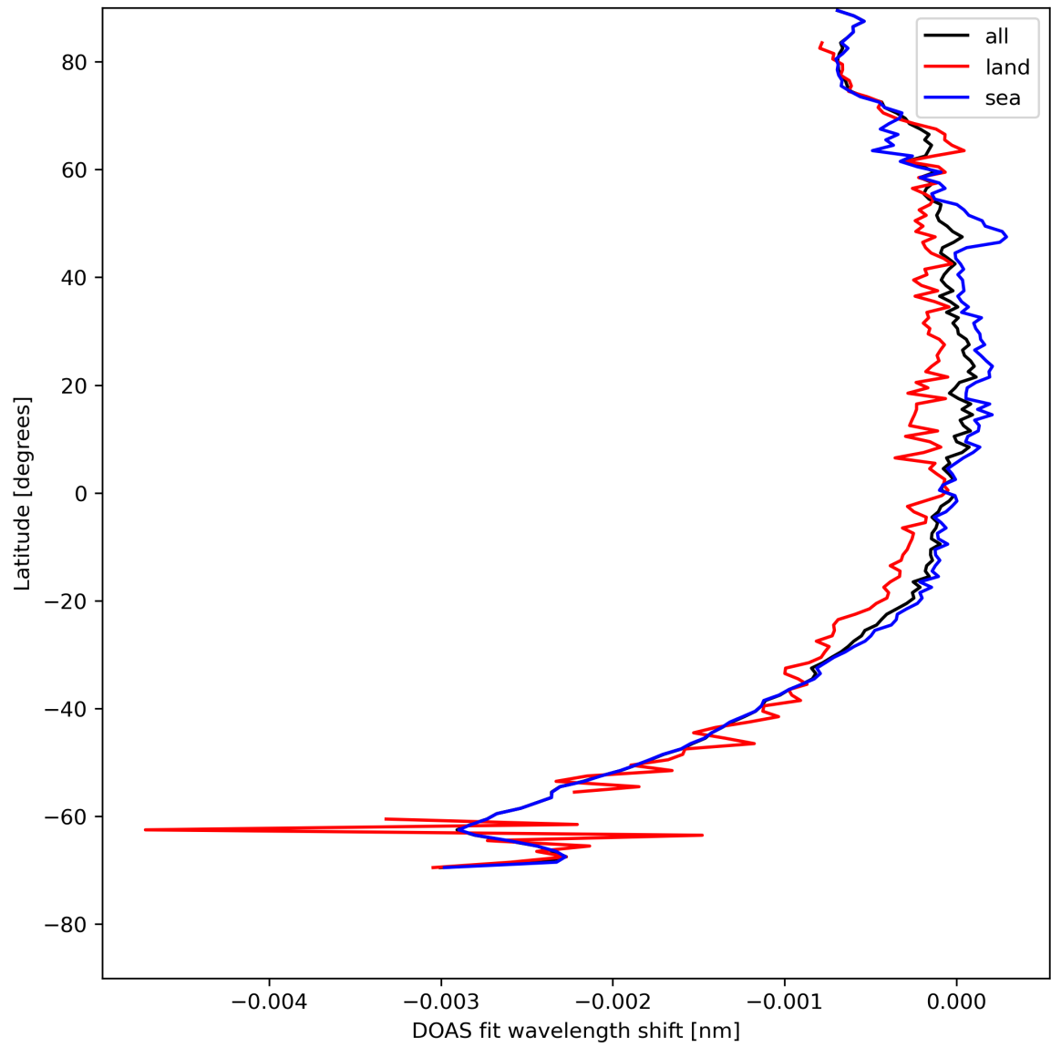
Figure 45: Zonal average of "DOAS fit wavelength shift" for 2024-08-11 to 2024-08-11.
