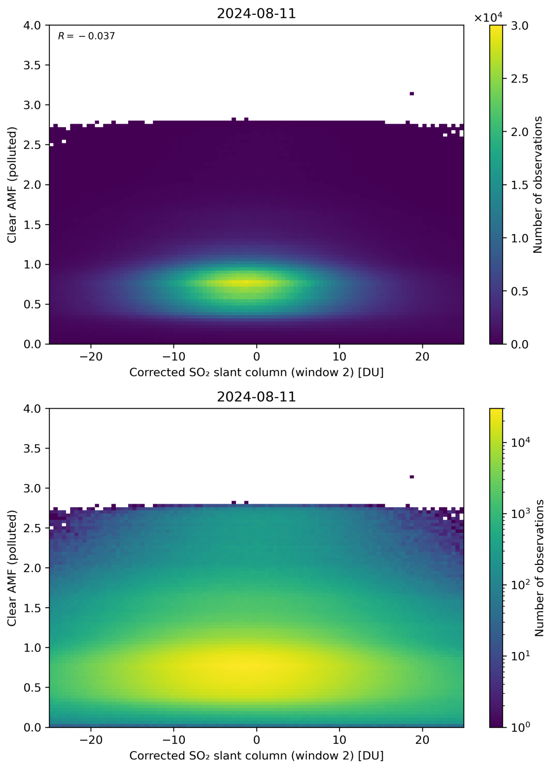
Figure 199: Scatter density plot of “Corrected SO 2 slant column (window 2)” against “Clear AMF (polluted)” for 2024-08-11 to 2024-08-11.
