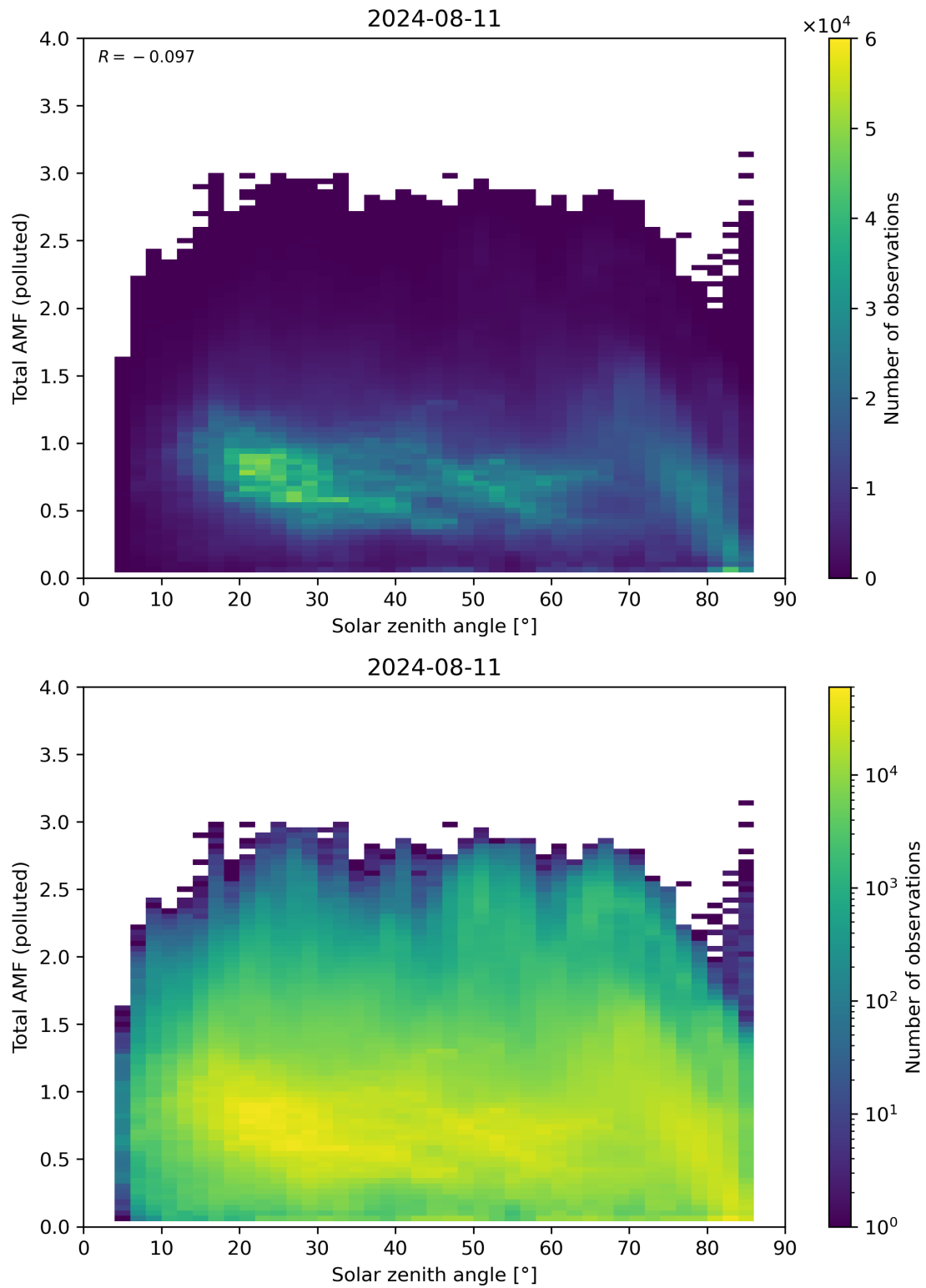
Figure 174: Scatter density plot of “Solar zenith angle” against “Total AMF (polluted)” for 2024-08-11 to 2024-08-11.
