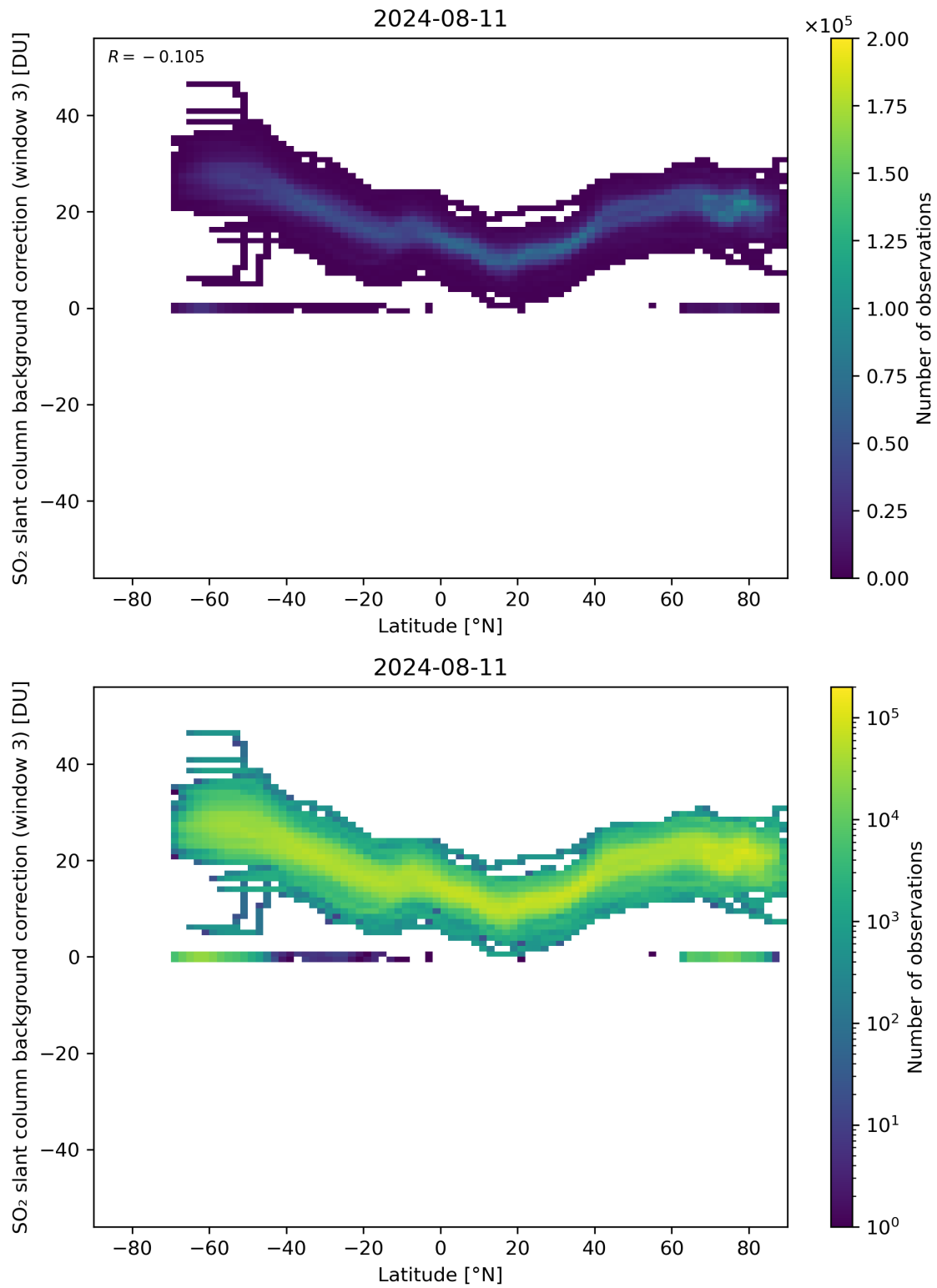
Figure 141: Scatter density plot of “Latitude” against “SO 2 slant column background correction (window 3)” for 2024-08-11 to 2024-08-11.
