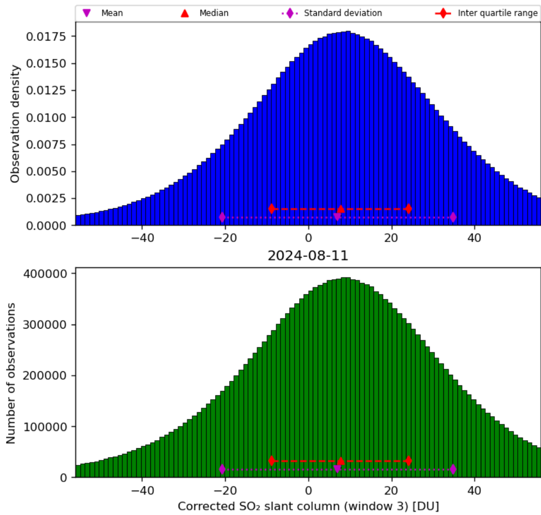
Figure 66: Histogram of “Corrected SO 2 slant column (window 3)” for 2024-08-11 to 2024-08-11
