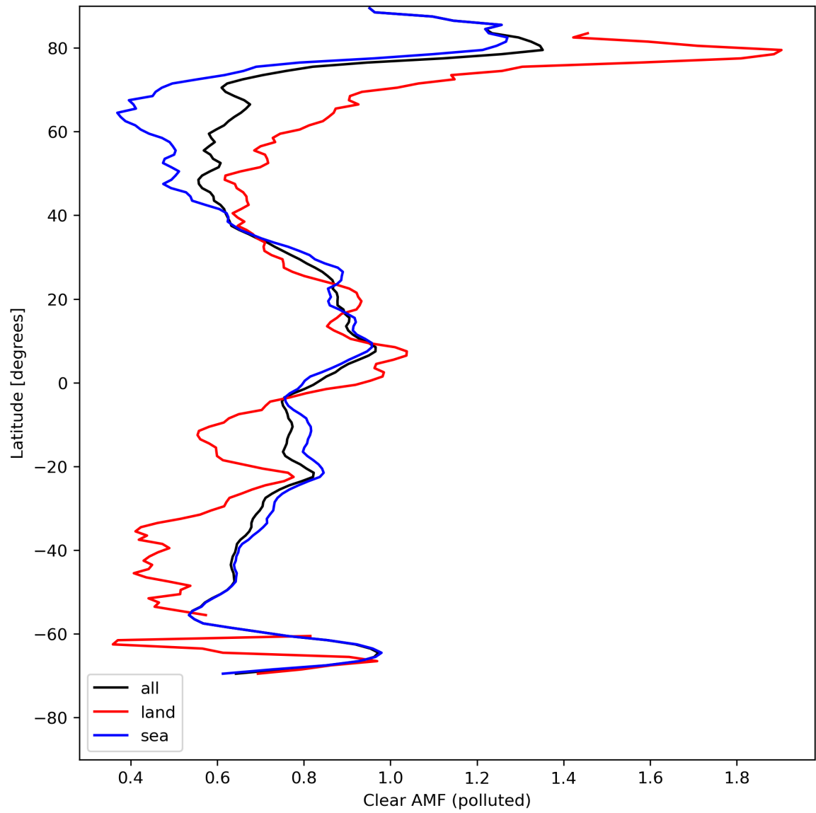
Figure 50: Zonal average of “Clear AMF (polluted)” for 2024-08-11 to 2024-08-11.
