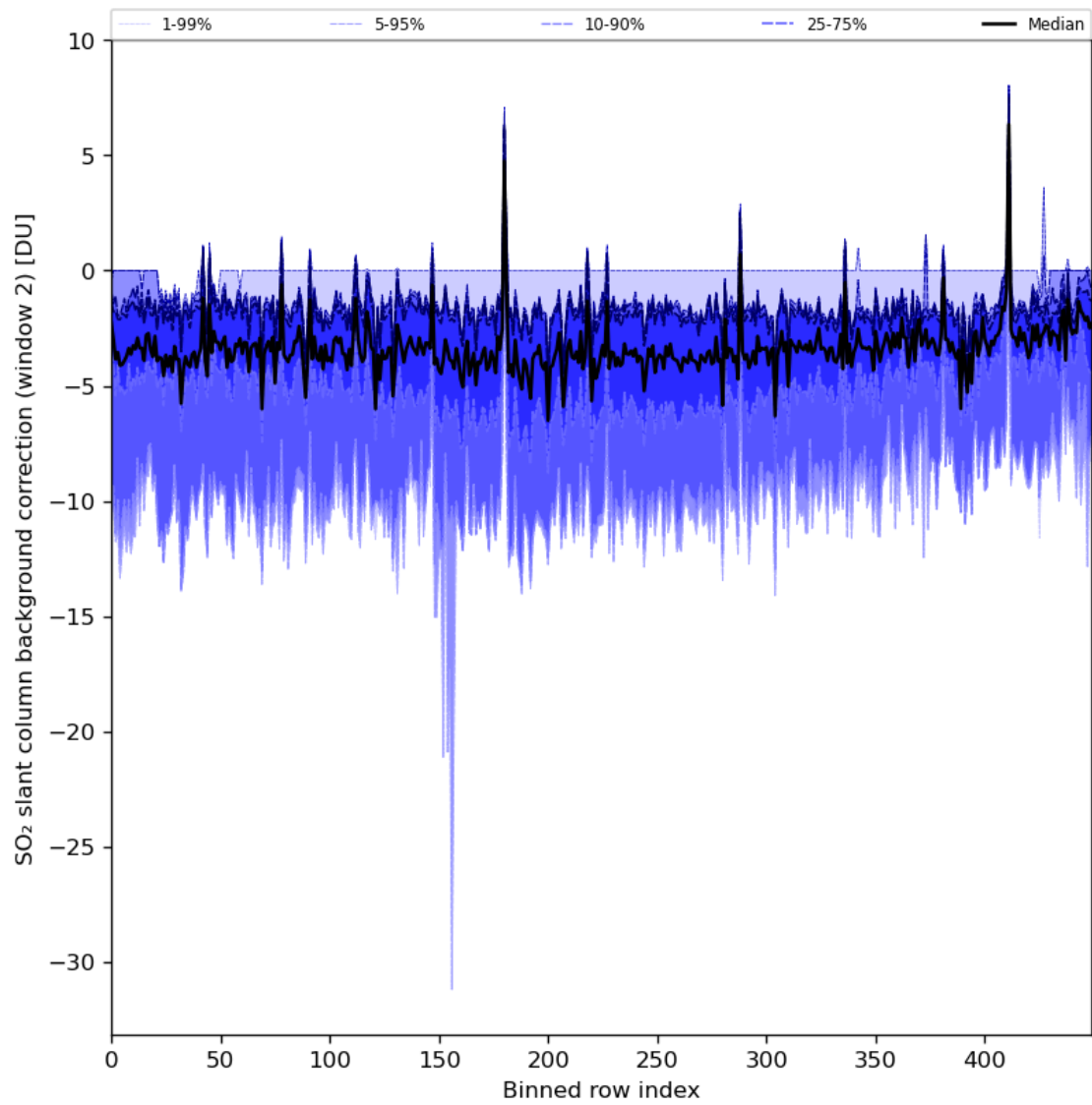
Figure 86: Along track statistics of “SO 2 slant column background correction (window 2)” for 2024-08-11 to 2024-08-11
