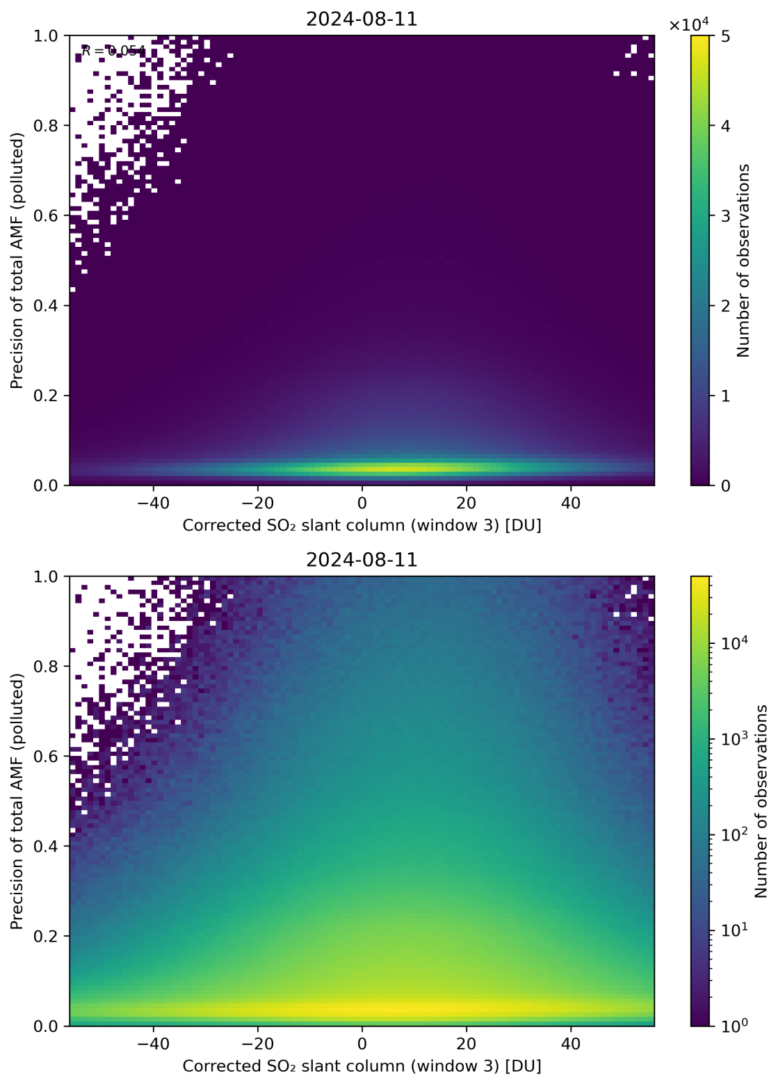
Figure 211: Scatter density plot of “Corrected SO 2 slant column (window 3)” against “Precision of total AMF (polluted)” for 2024-08-11 to 2024-08-11.
