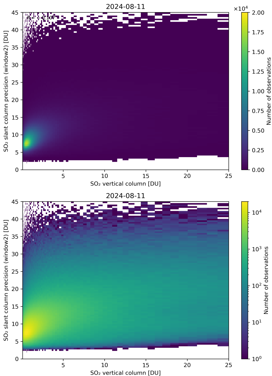
Figure 302: Scatter density plot of “SO 2 vertical column” against “SO 2 slant column precision (window2)” for 2024-08-11 to 2024-08-11.
