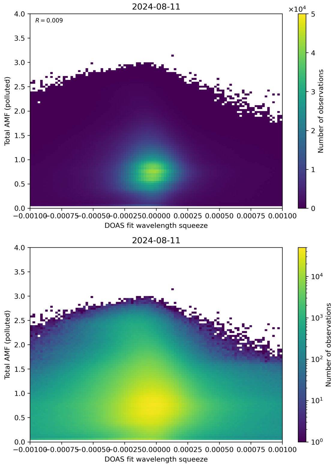
Figure 134: Scatter density plot of “DOAS fit wavelength squeeze” against “Total AMF (polluted)” for 2024-08-11 to 2024-08-11.
