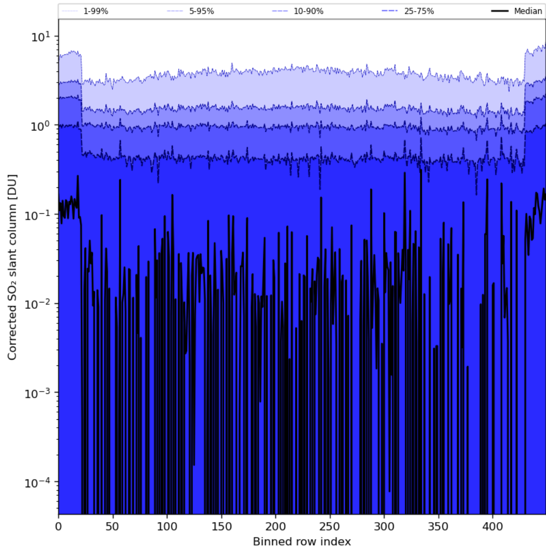
Figure 78: Along track statistics of “Corrected SO 2 slant column” for 2024-08-11 to 2024-08-11
