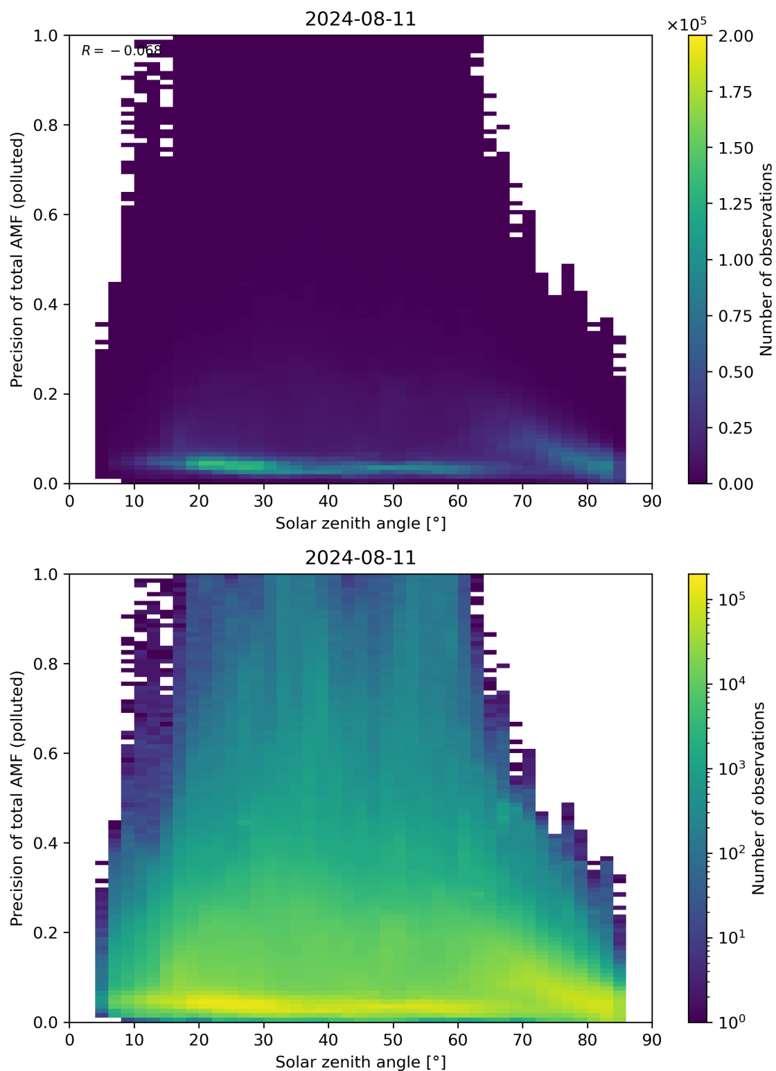
Figure 175: Scatter density plot of “Solar zenith angle” against “Precision of total AMF (polluted)” for 2024-08-11 to 2024-08-11.
