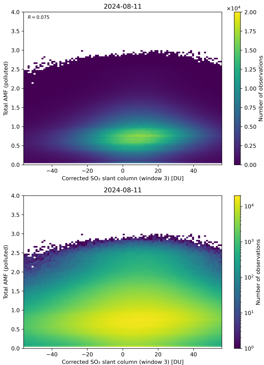
Figure 210: Scatter density plot of “Corrected SO 2 slant column (window 3)” against “Total AMF (polluted)” for 2024-08-11 to 2024-08-11.
