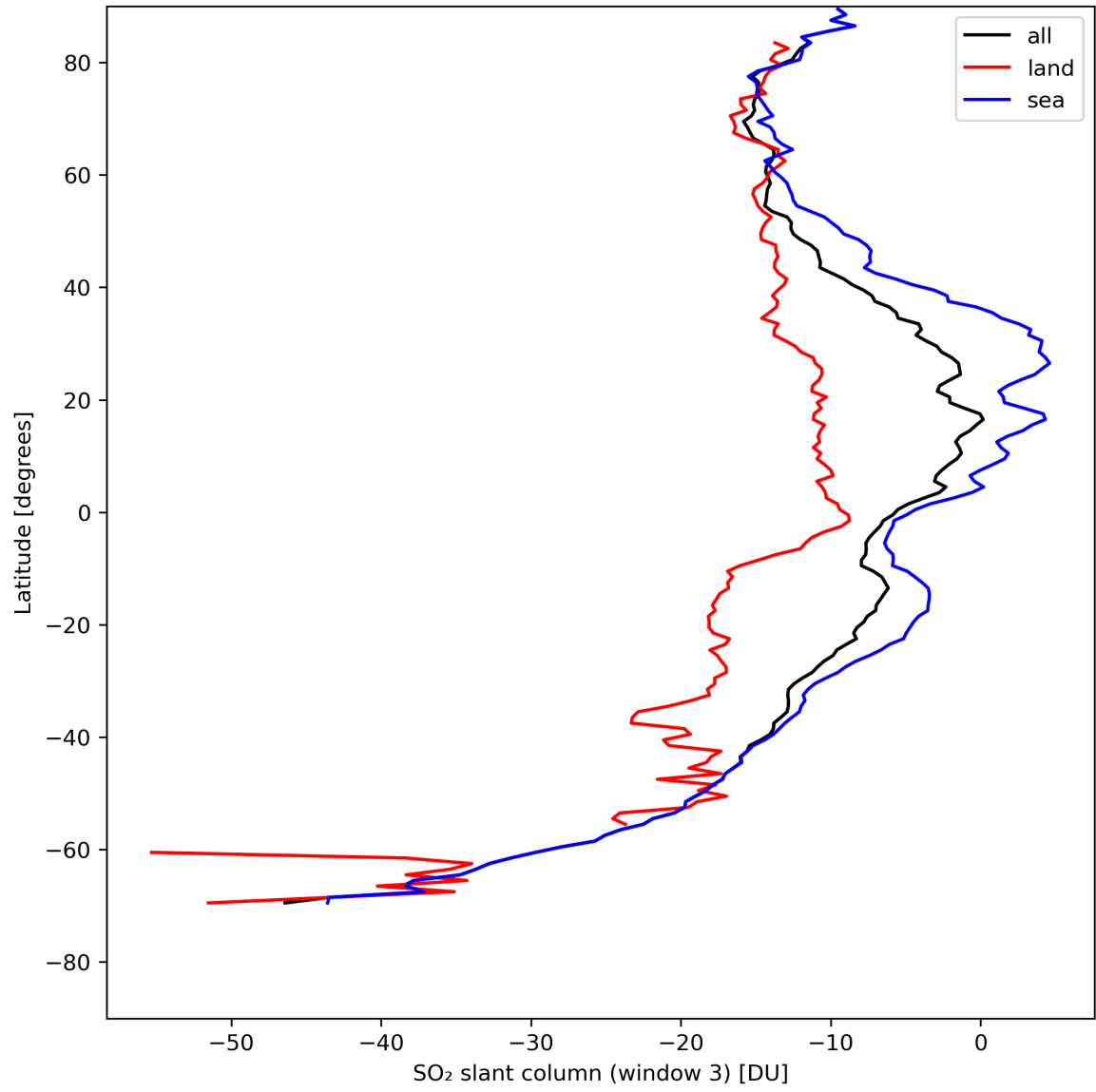
Figure 41: Zonal average of “SO 2 slant column (window 3)” for 2024-08-11 to 2024-08-11.
