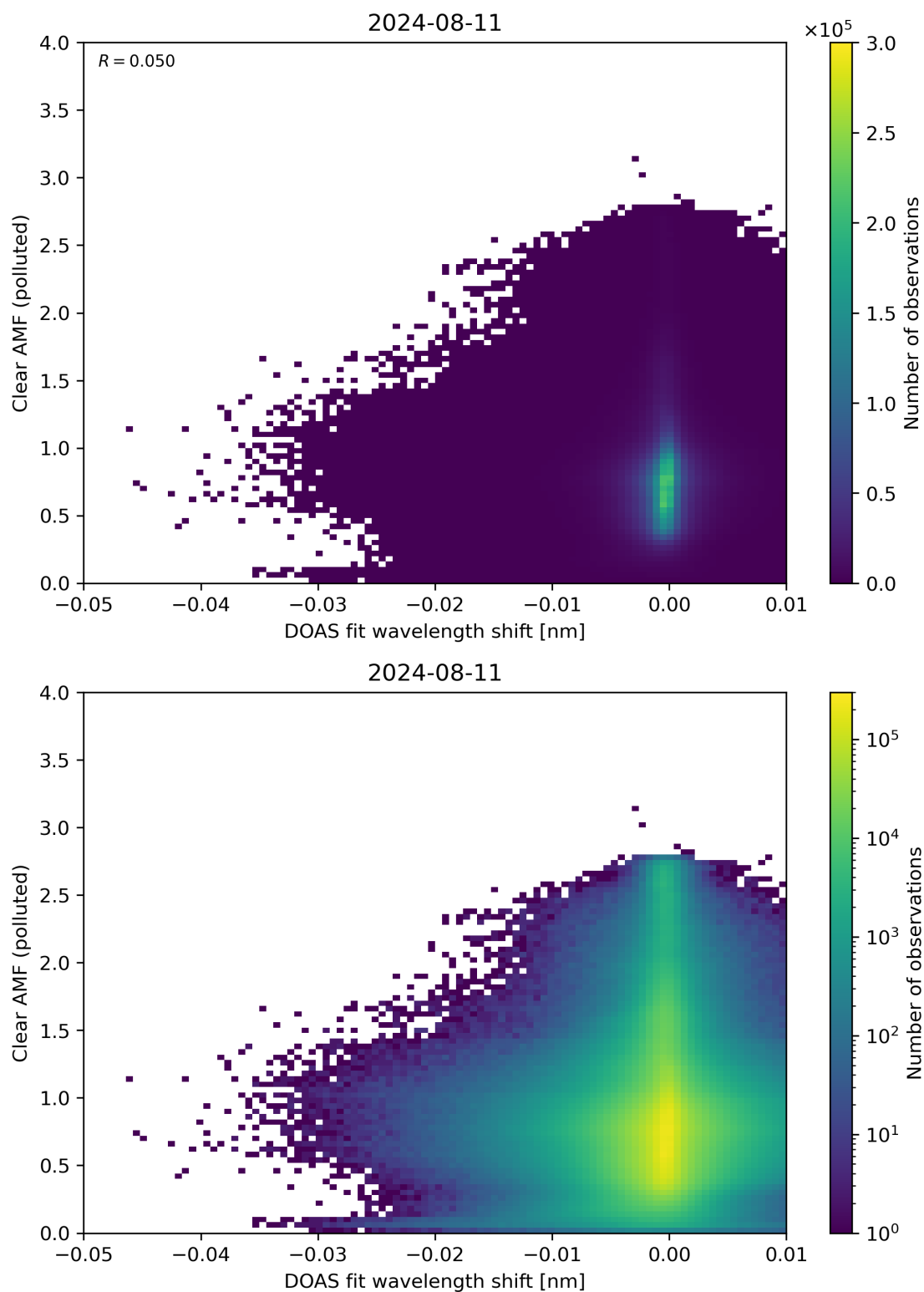
Figure 129: Scatter density plot of “DOAS fit wavelength shift” against “Clear AMF (polluted)” for 2024-08-11 to 2024-08-11.
