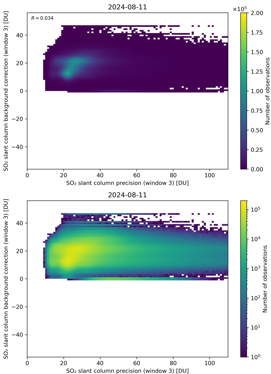
Figure 257: Scatter density plot of “SO 2 slant column precision (window 3)” against “SO 2 slant column background correction (window 3)” for 2024-08-11 to 2024-08-11.
