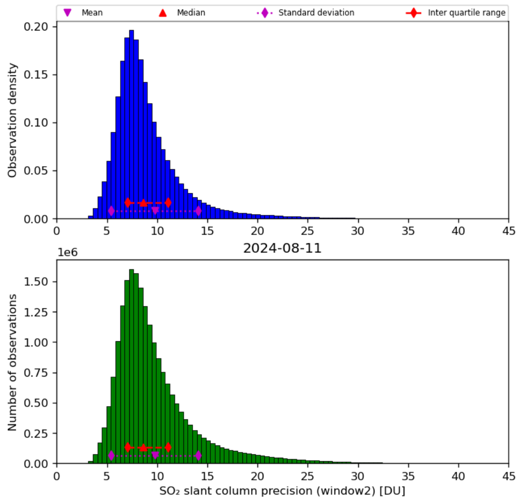
Figure 61: Histogram of “SO 2 slant column precision (window2)” for 2024-08-11 to 2024-08-11
