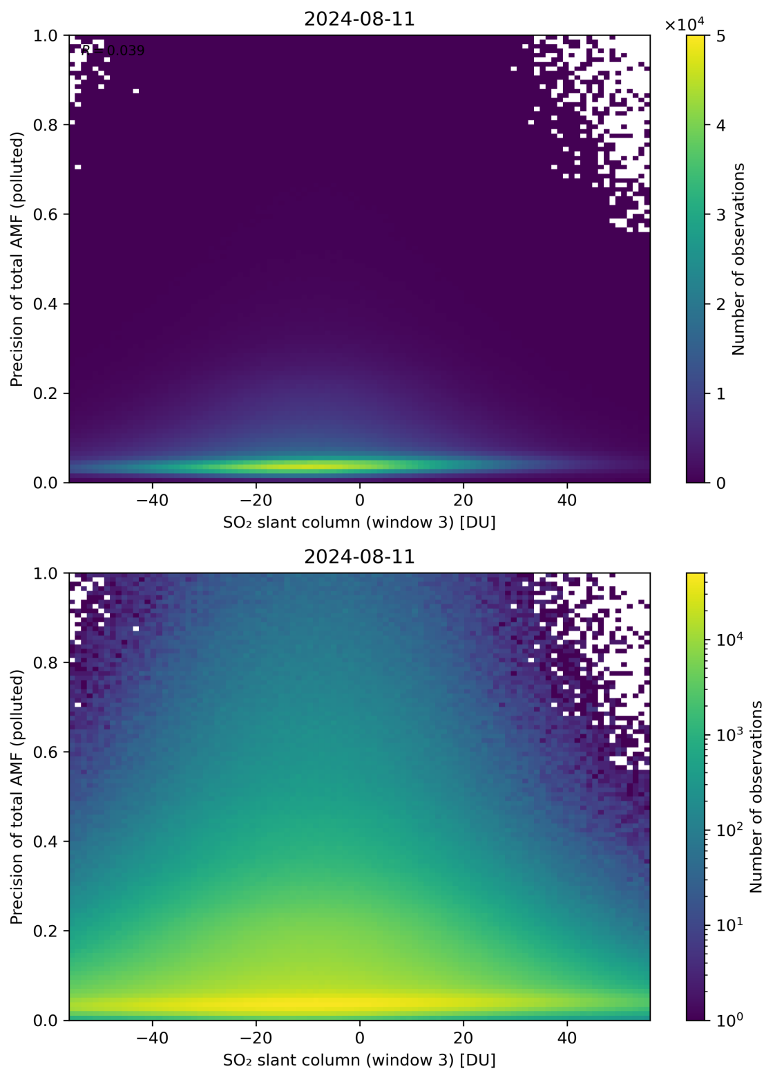
Figure 269: Scatter density plot of “SO 2 slant column (window 3)” against “Precision of total AMF (polluted)” for 2024-08-11 to 2024-08-11.
