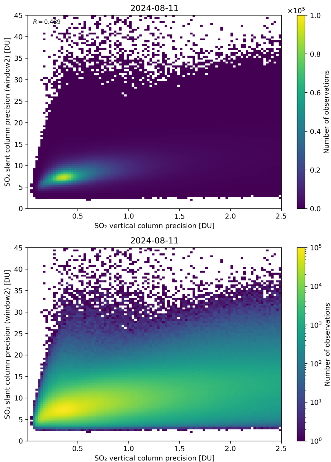
Figure 291: Scatter density plot of “SO 2 vertical column precision” against “SO 2 slant column precision (window2)” for 2024-08-11 to 2024-08-11.
