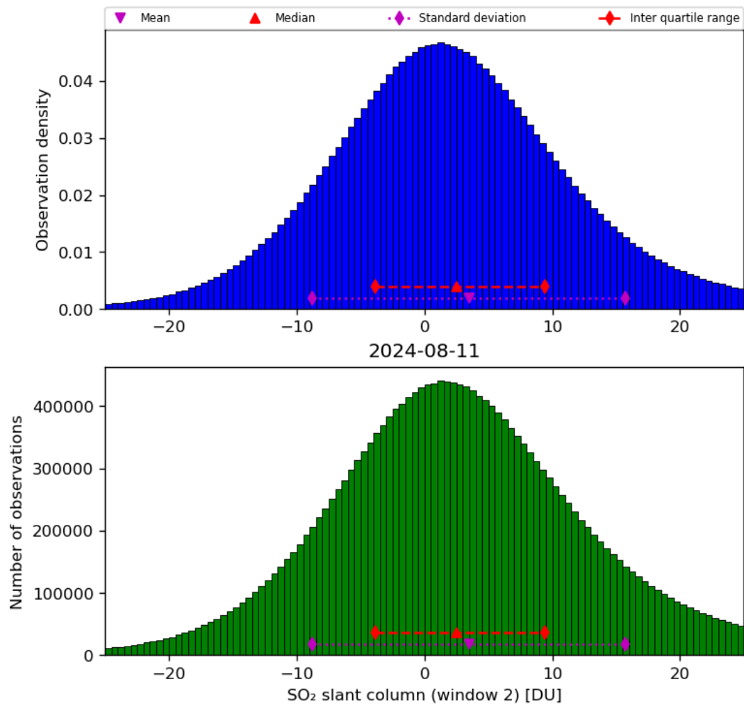
Figure 60: Histogram of “SO 2 slant column (window 2)” for 2024-08-11 to 2024-08-11
