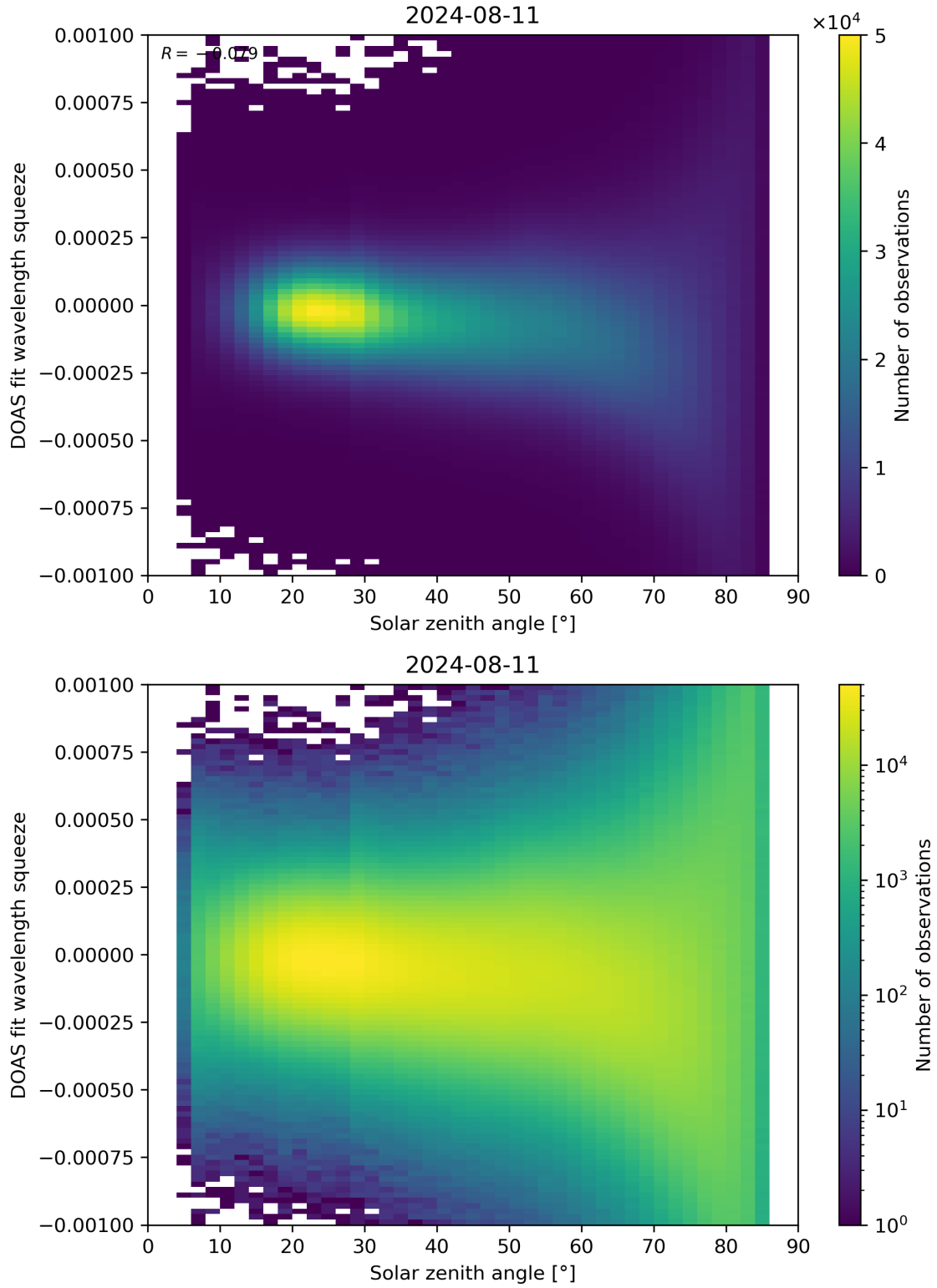
Figure 162: Scatter density plot of “Solar zenith angle” against “DOAS fit wavelength squeeze” for 2024-08-11 to 2024-08-11.
