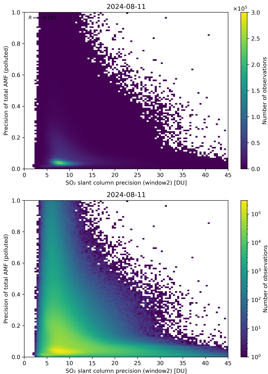
Figure 252: Scatter density plot of “SO 2 slant column precision (window2)” against “Precision of total AMF (polluted)” for 2024-08-11 to 2024-08-11.
