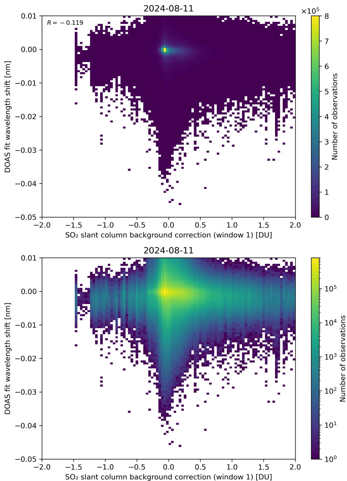
Figure 100: Scatter density plot of “SO 2 slant column background correction (window 1)” against “DOAS fit wavelength shift” for 2024-08-11 to 2024-08-11.
