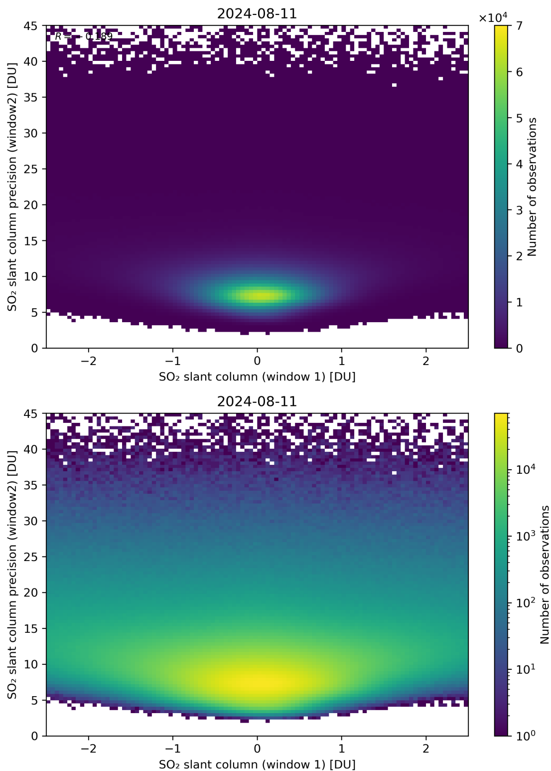
Figure 236: Scatter density plot of “SO 2 slant column (window 1)” against “SO 2 slant column precision (window2)” for 2024-08-11 to 2024-08-11.
