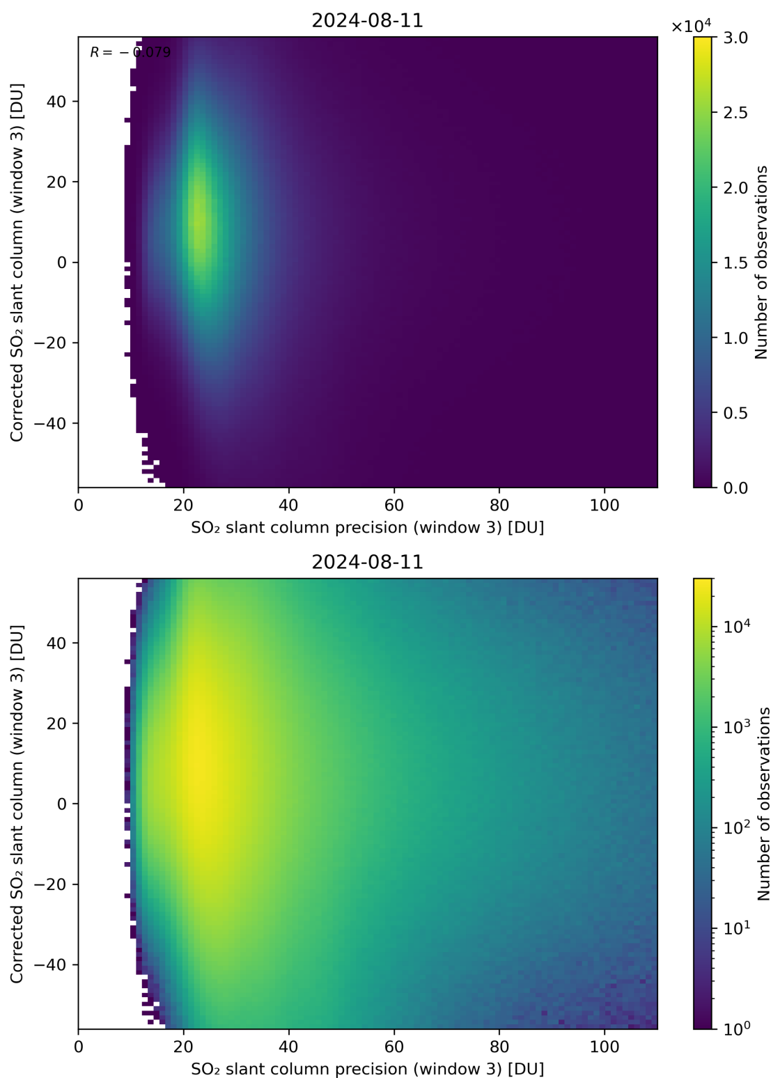
Figure 262: Scatter density plot of “SO 2 slant column precision (window 3)” against “Corrected SO 2 slant column (window 3)” for 2024-08-11 to 2024-08-11.
