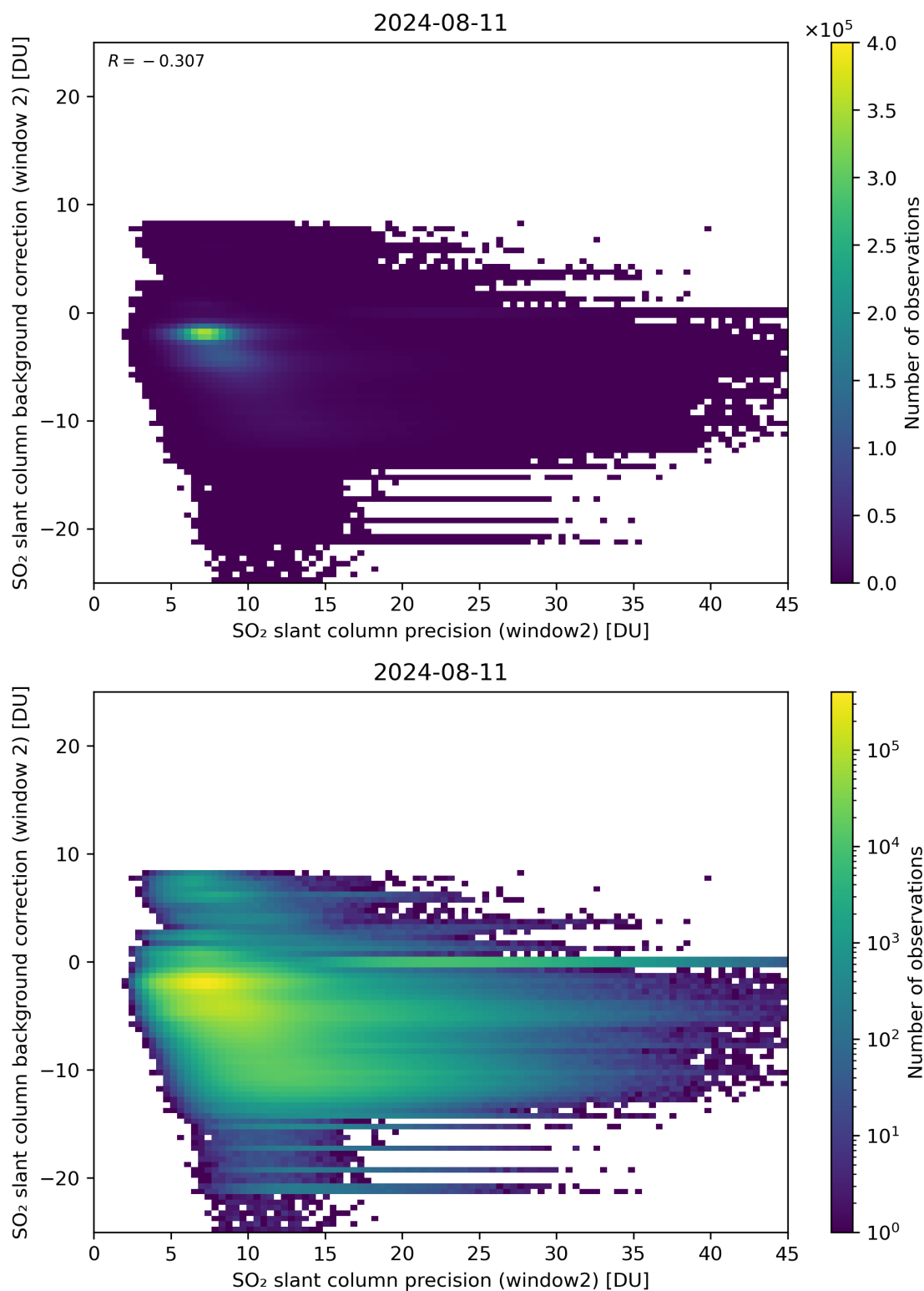
Figure 241: Scatter density plot of “SO 2 slant column precision (window2)” against “SO 2 slant column background correction (window 2)” for 2024-08-11 to 2024-08-11.
