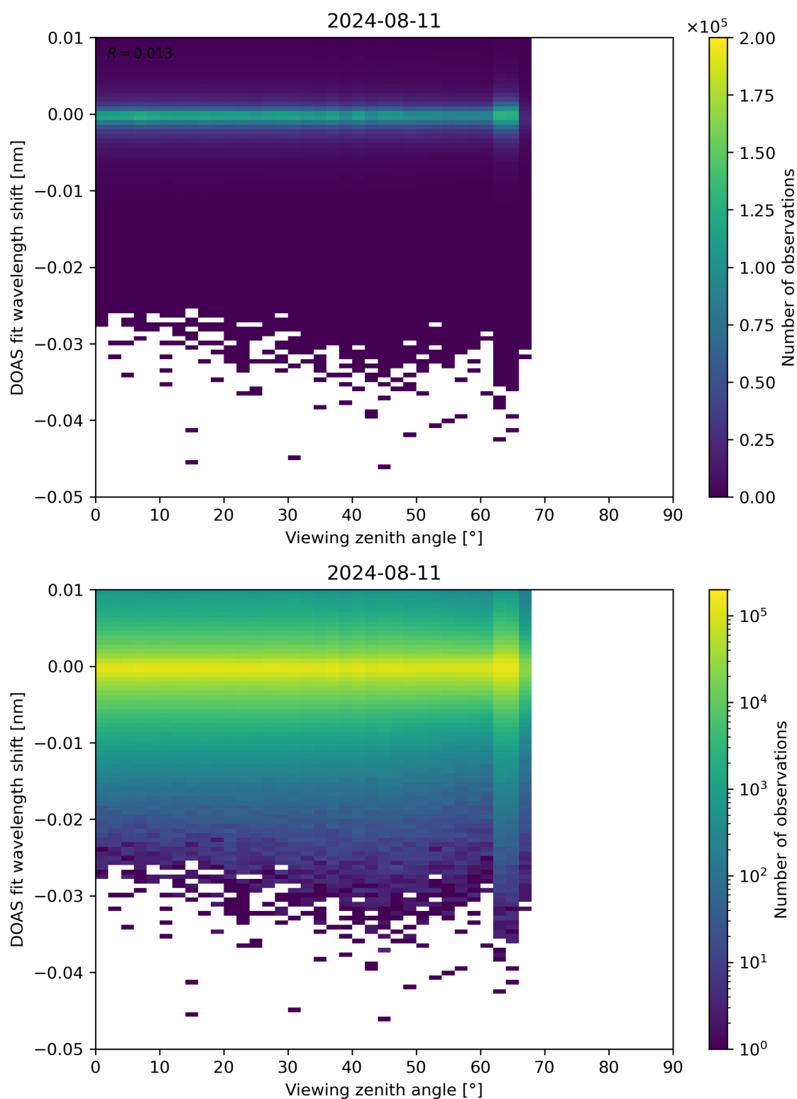
Figure 311: Scatter density plot of “Viewing zenith angle” against “DOAS fit wavelength shift” for 2024-08-11 to 2024-08-11.
