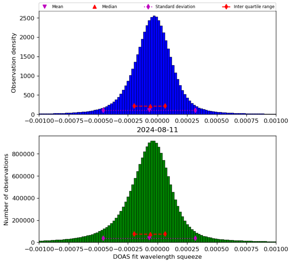
Figure 69: Histogram of “DOAS fit wavelength squeeze” for 2024-08-11 to 2024-08-11
