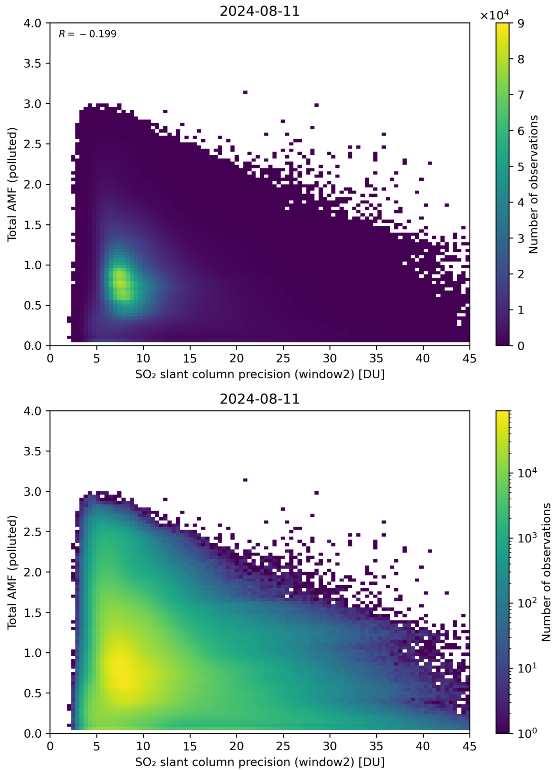
Figure 251: Scatter density plot of “SO 2 slant column precision (window2)” against “Total AMF (polluted)” for 2024-08-11 to 2024-08-11.
