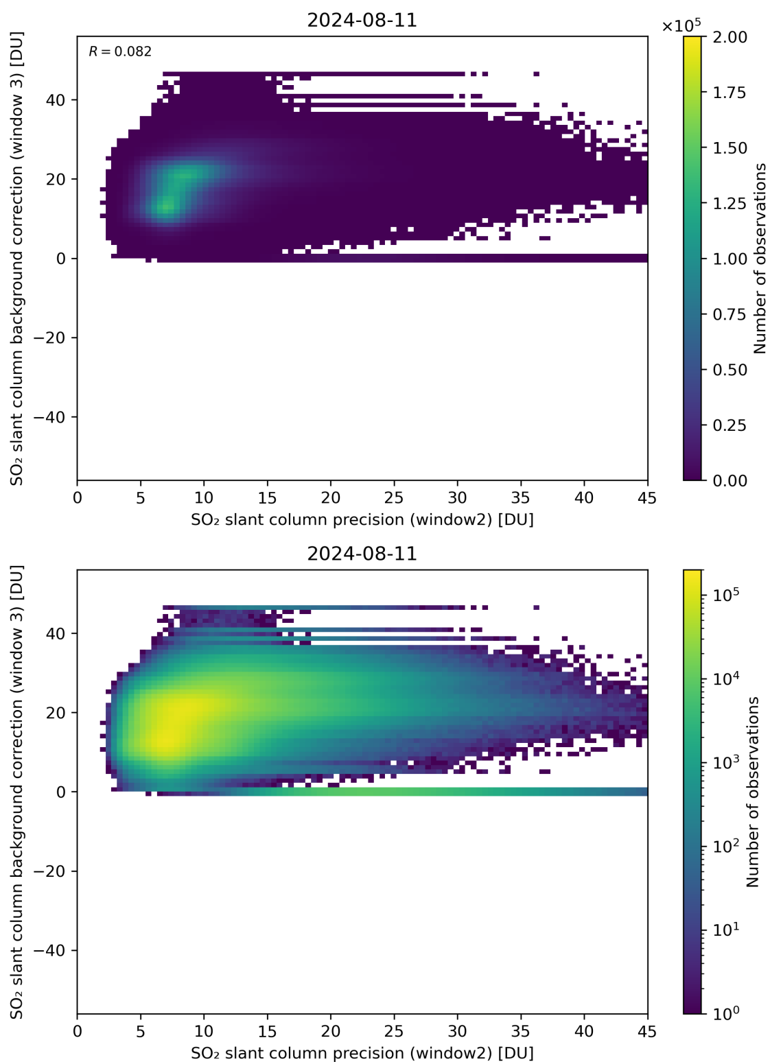
Figure 242: Scatter density plot of “SO 2 slant column precision (window2)” against “SO 2 slant column background correction (window 3)” for 2024-08-11 to 2024-08-11.
