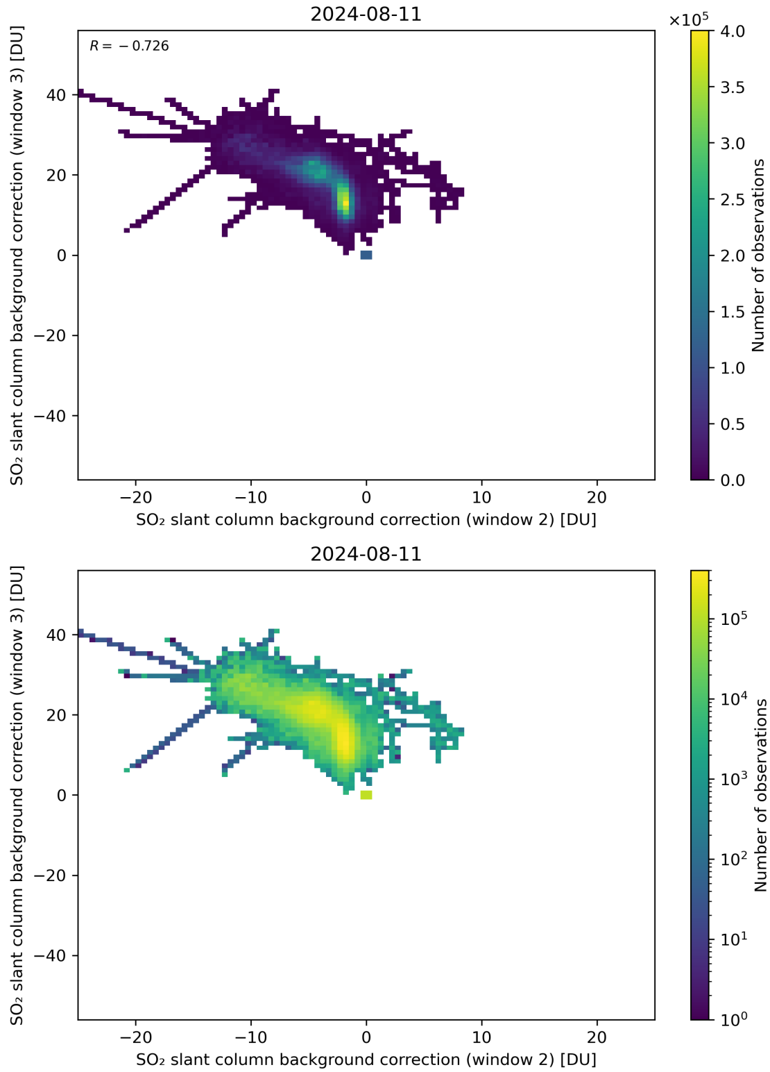
Figure 111: Scatter density plot of “SO 2 slant column background correction (window 2)” against “SO 2 slant column background correction (window 3)” for 2024-08-11 to 2024-08-11.
