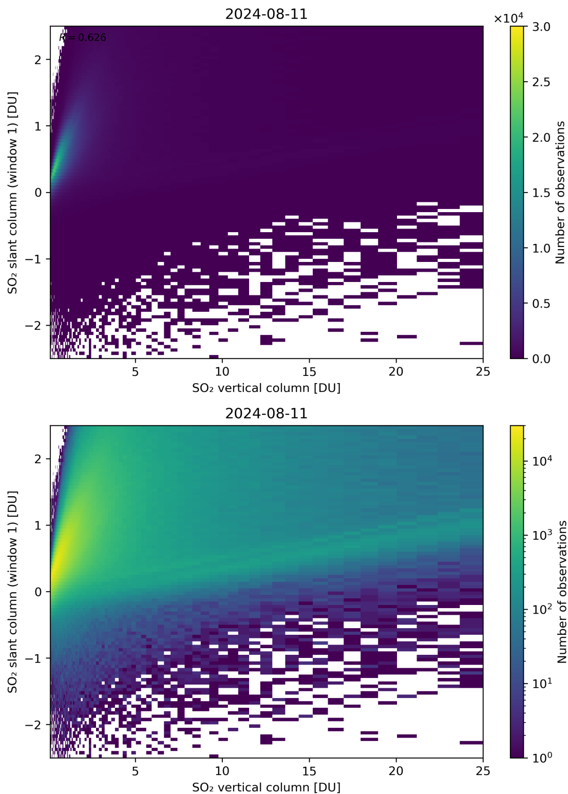
Figure 300: Scatter density plot of “SO 2 vertical column” against “SO 2 slant column (window 1)” for 2024-08-11 to 2024-08-11.
