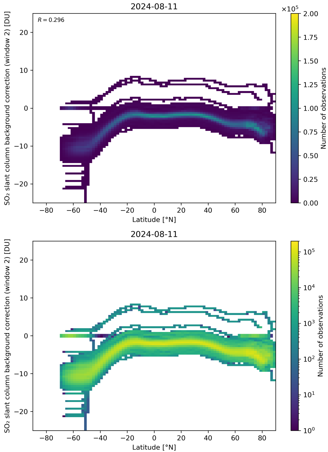
Figure 140: Scatter density plot of “Latitude” against “SO 2 slant column background correction (window 2)” for 2024-08-11 to 2024-08-11.
