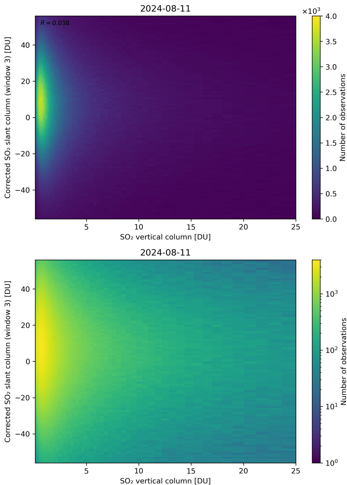
Figure 299: Scatter density plot of “SO 2 vertical column” against “Corrected SO 2 slant column (window 3)” for 2024-08-11 to 2024-08-11.
