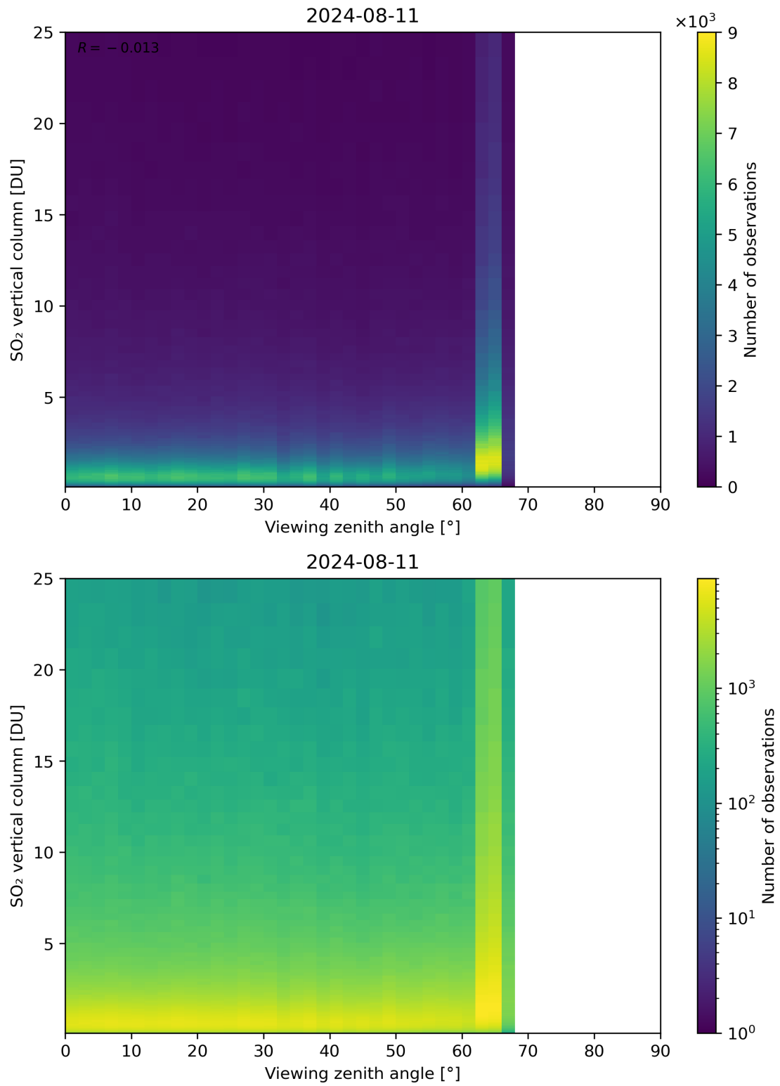
Figure 327: Scatter density plot of “Viewing zenith angle” against “SO 2 vertical column” for 2024-08-11 to 2024-08-11.
