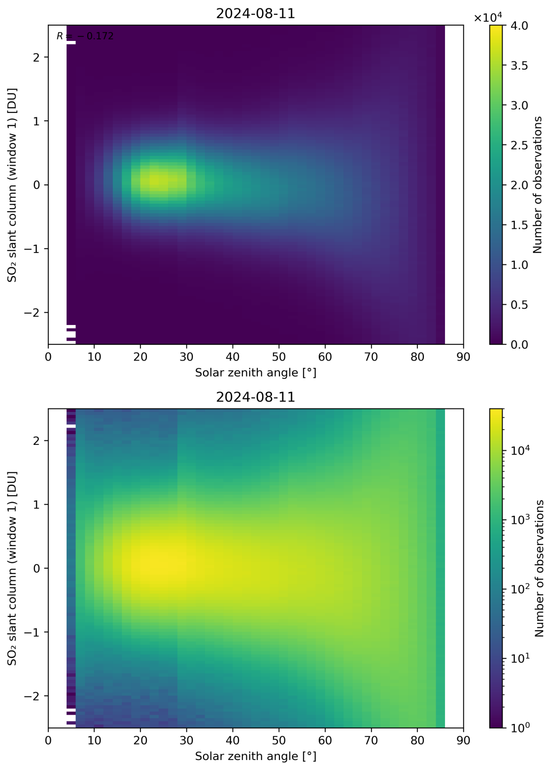
Figure 169: Scatter density plot of “Solar zenith angle” against “SO 2 slant column (window 1)” for 2024-08-11 to 2024-08-11.
