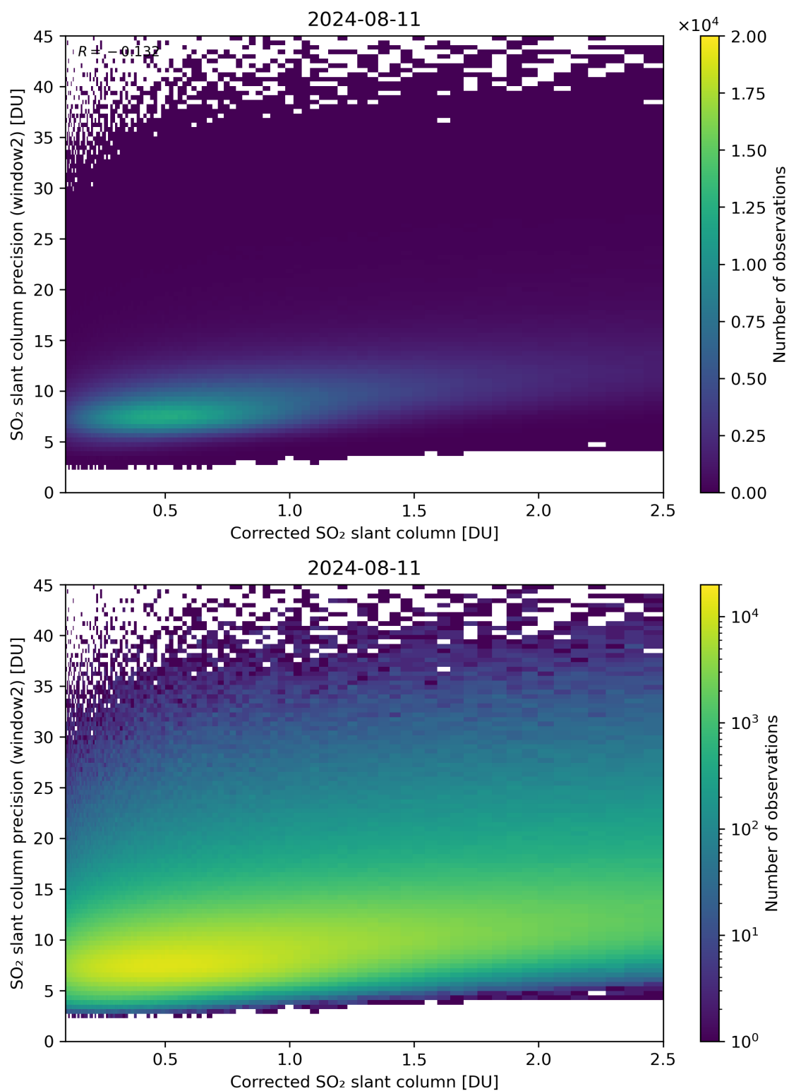
Figure 189: Scatter density plot of “Corrected SO 2 slant column” against “SO 2 slant column precision (window2)” for 2024-08-11 to 2024-08-11.
