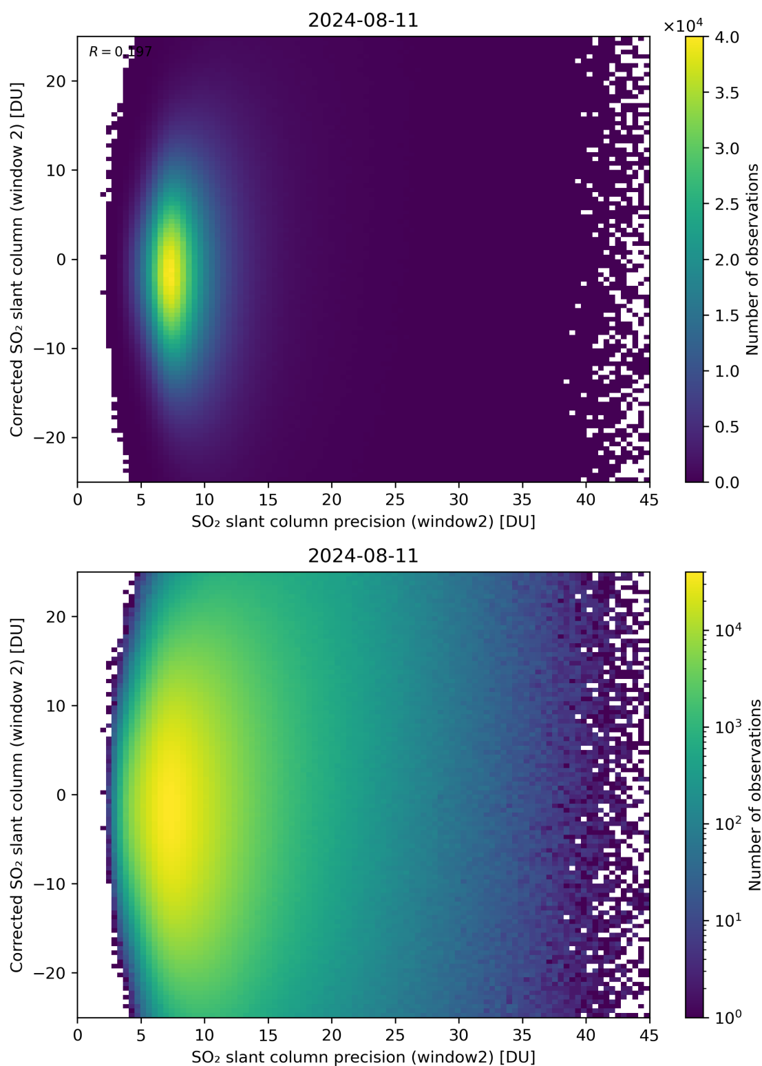
Figure 247: Scatter density plot of “SO 2 slant column precision (window2)” against “Corrected SO 2 slant column (window 2)” for 2024-08-11 to 2024-08-11.
