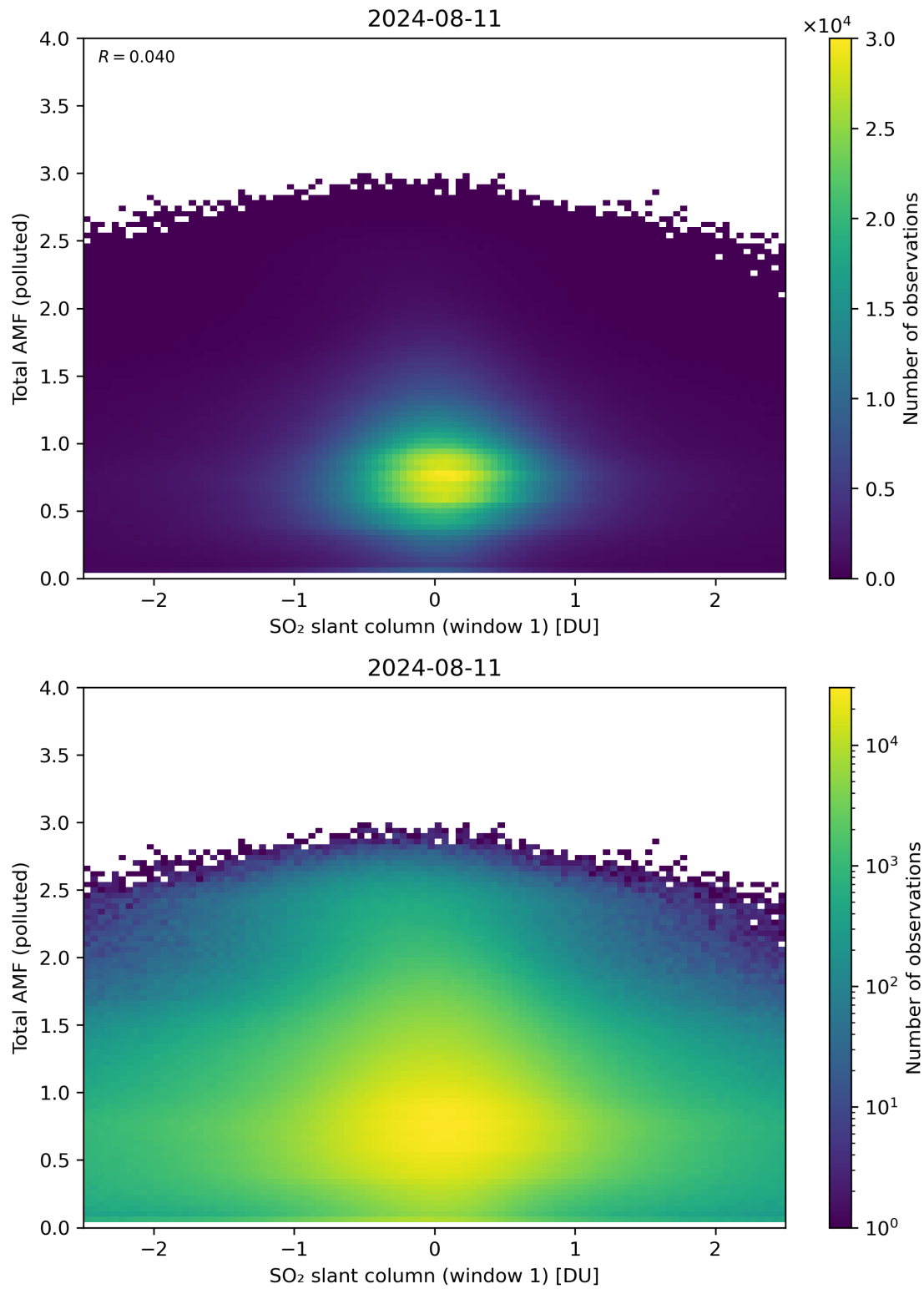
Figure 239: Scatter density plot of “SO 2 slant column (window 1)” against “Total AMF (polluted)” for 2024-08-11 to 2024-08-11.
