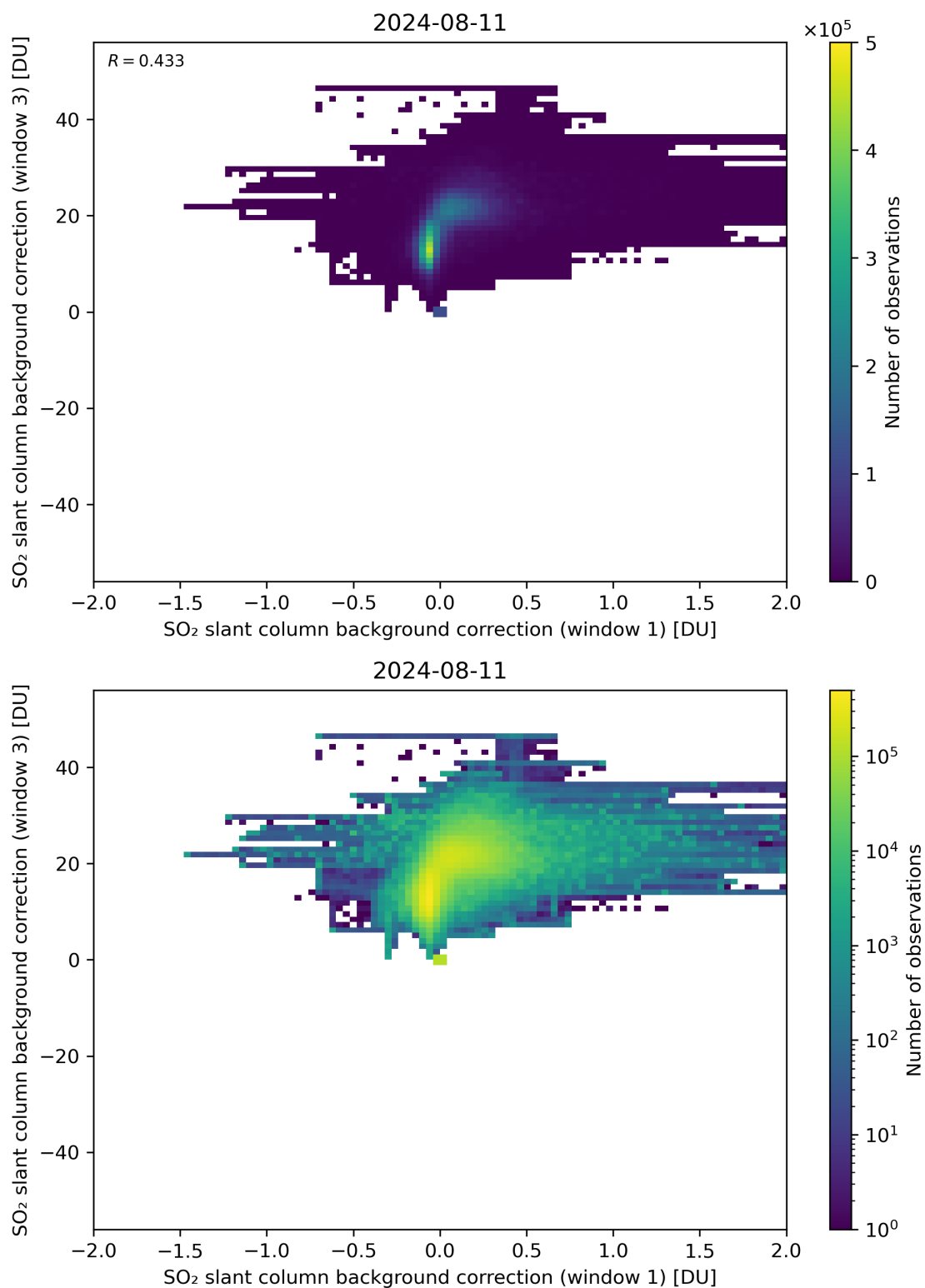
Figure 99: Scatter density plot of “SO 2 slant column background correction (window 1)” against “SO 2 slant column background correction (window 3)” for 2024-08-11 to 2024-08-11.
