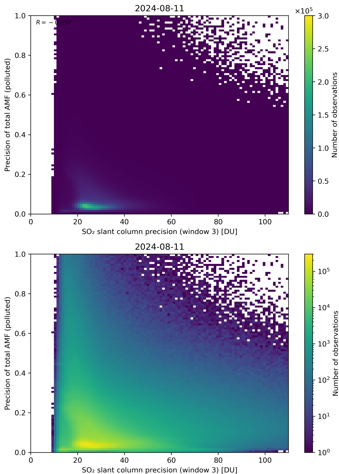
Figure 264: Scatter density plot of “SO 2 slant column precision (window 3)” against “Precision of total AMF (polluted)” for 2024-08-11 to 2024-08-11.
