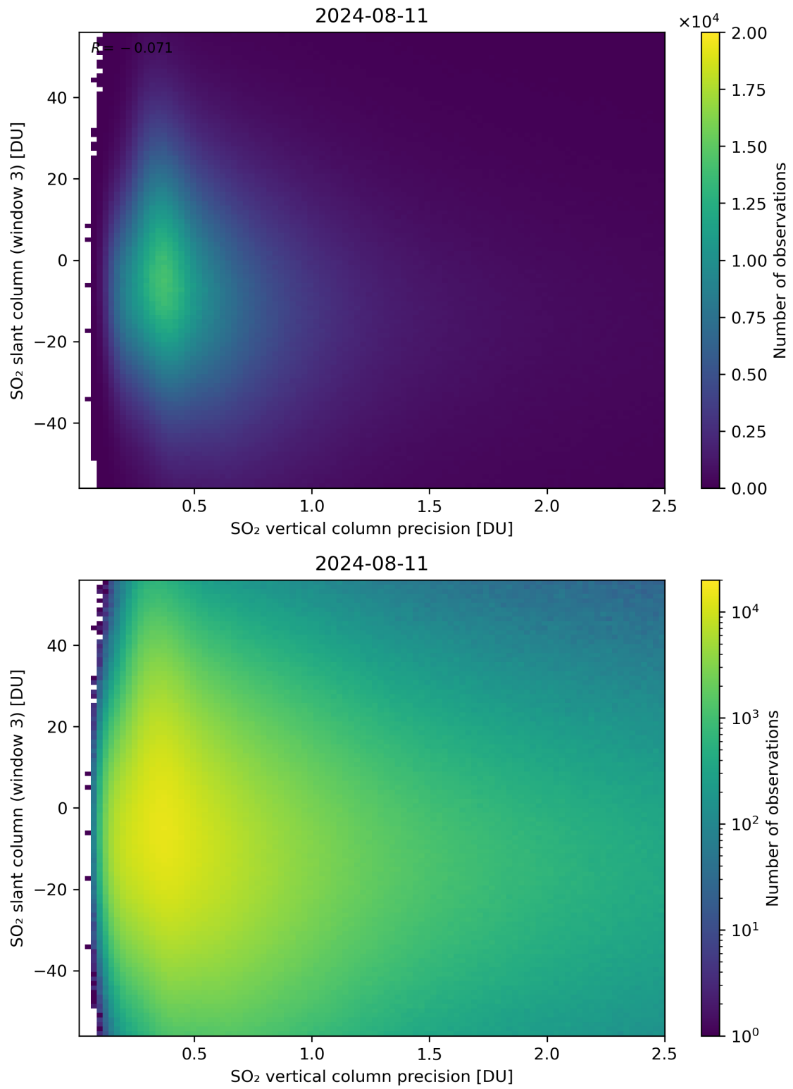
Figure 292: Scatter density plot of “SO 2 vertical column precision” against “SO 2 slant column (window 3)” for 2024-08-11 to 2024-08-11.
