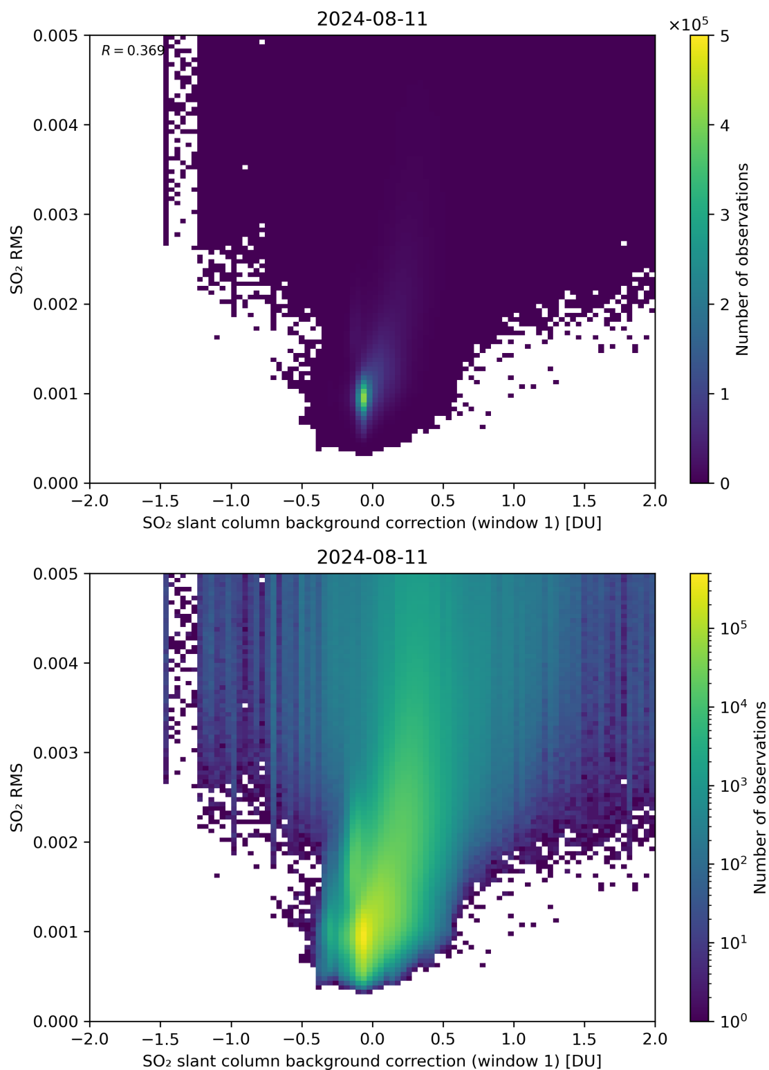
Figure 102: Scatter density plot of “SO 2 slant column background correction (window 1)” against “SO 2 RMS” for 2024-08-11 to 2024-08-11.
