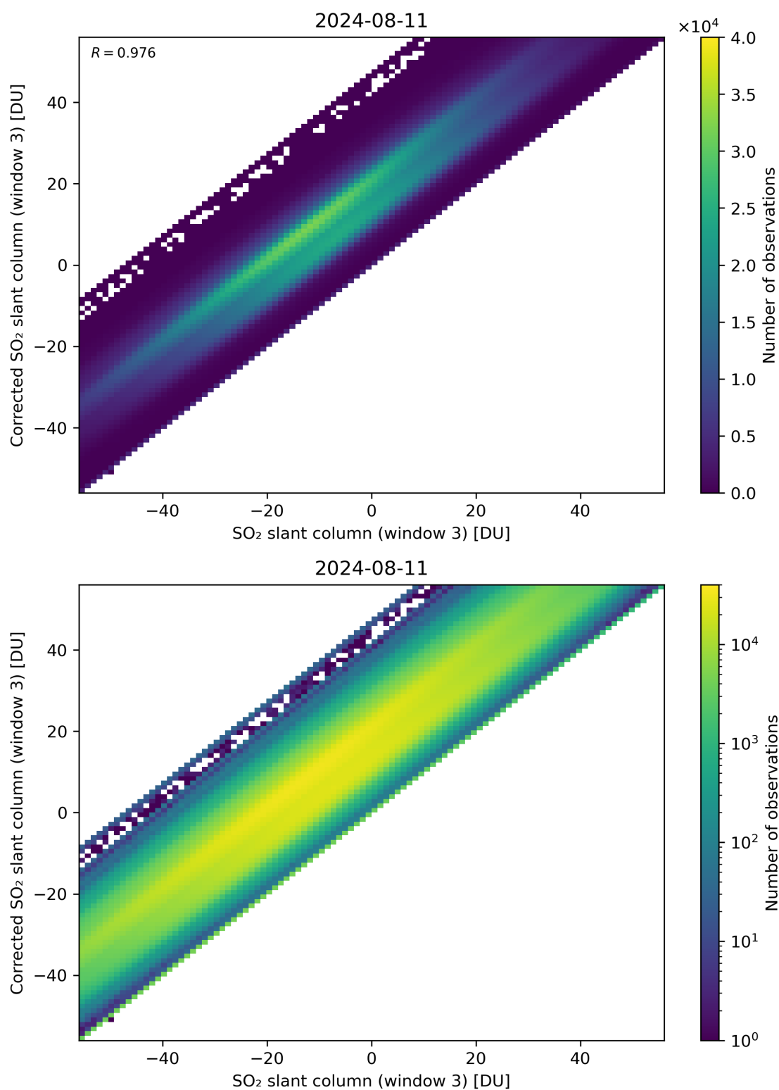
Figure 266: Scatter density plot of “SO 2 slant column (window 3)” against “Corrected SO 2 slant column (window 3)” for 2024-08-11 to 2024-08-11.
