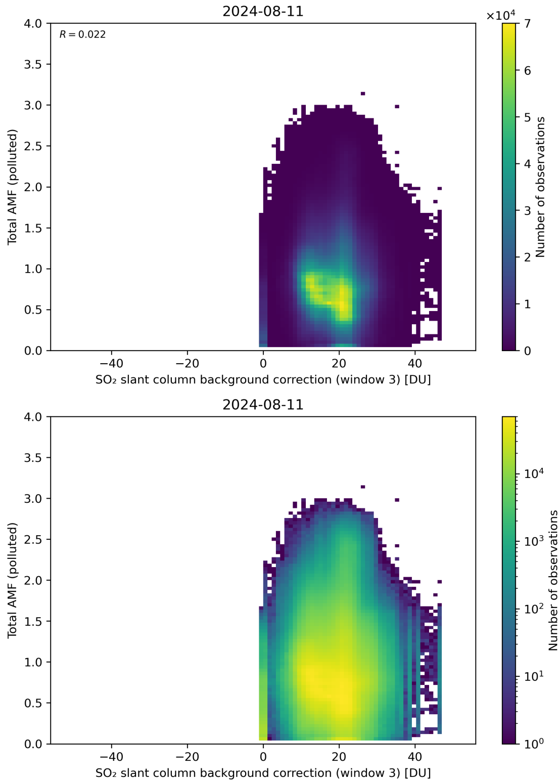
Figure 125: Scatter density plot of “SO 2 slant column background correction (window 3)” against “Total AMF (polluted)” for 2024-08-11 to 2024-08-11.
