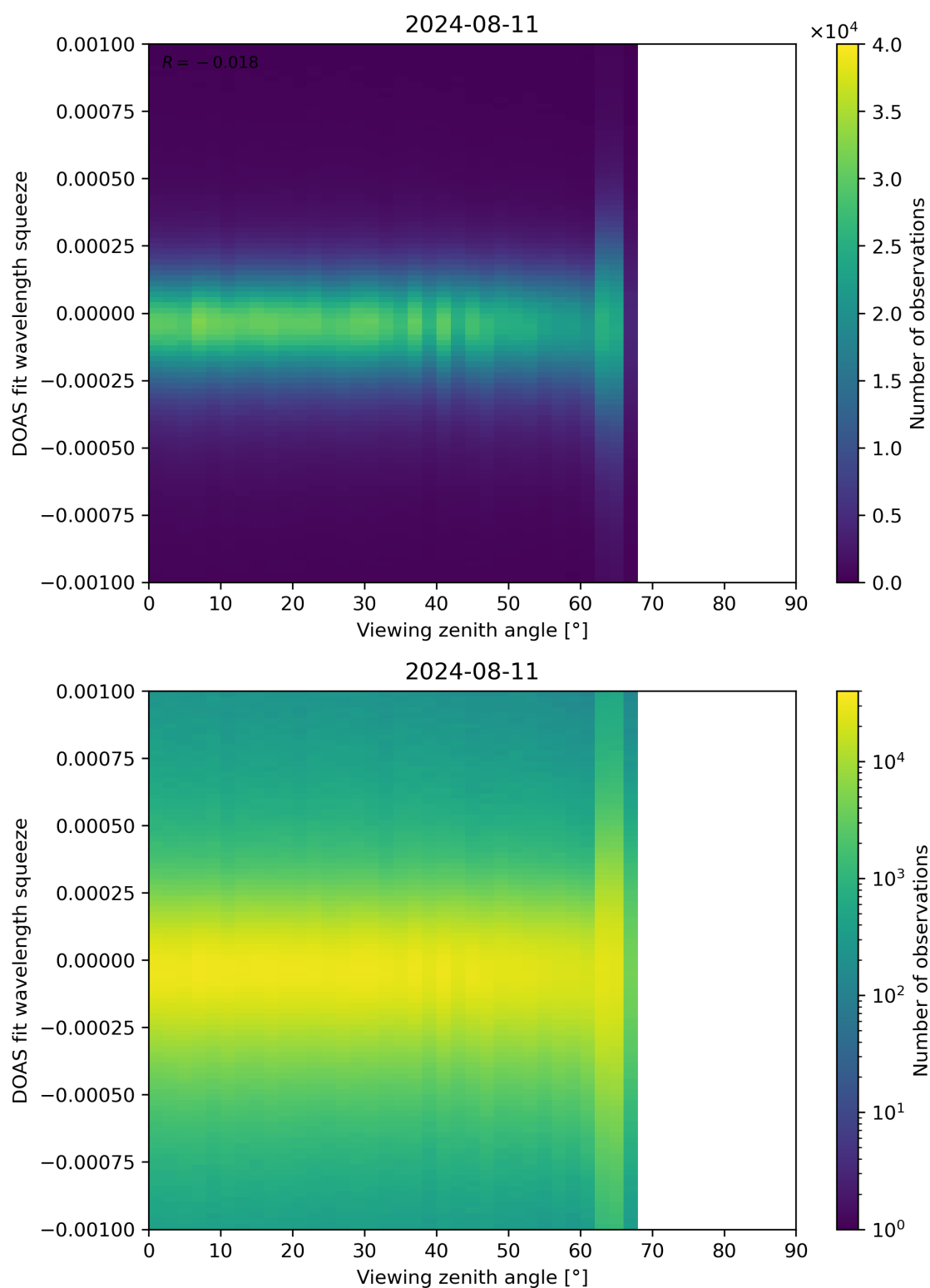
Figure 312: Scatter density plot of “Viewing zenith angle” against “DOAS fit wavelength squeeze” for 2024-08-11 to 2024-08-11.
