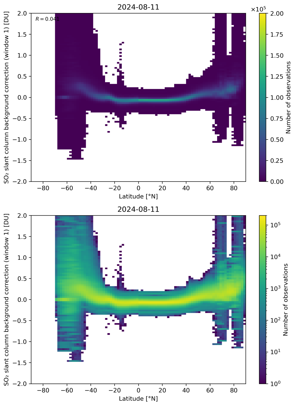
Figure 139: Scatter density plot of “Latitude” against “SO 2 slant column background correction (window 1)” for 2024-08-11 to 2024-08-11.
