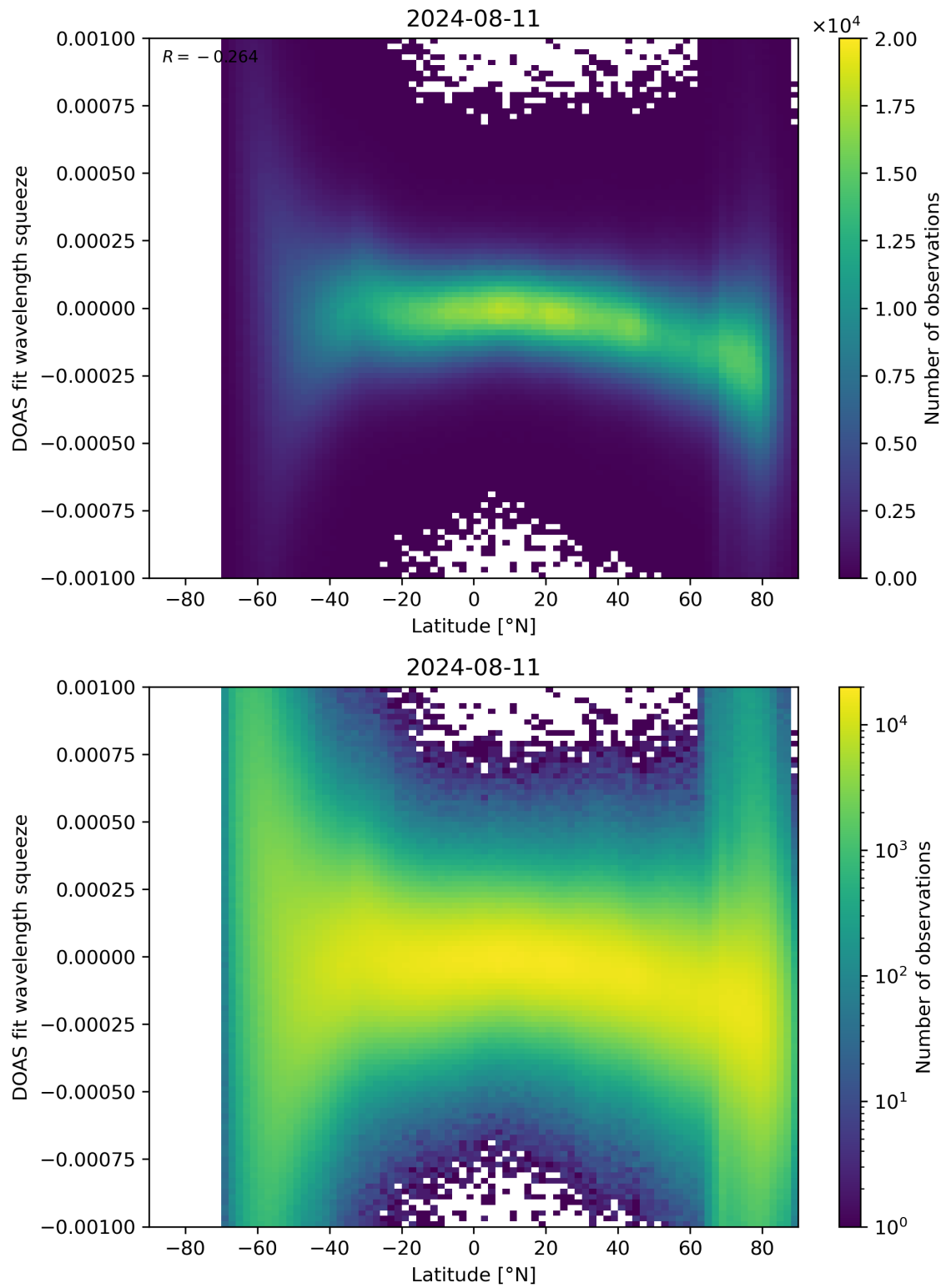
Figure 143: Scatter density plot of “Latitude” against “DOAS fit wavelength squeeze” for 2024-08-11 to 2024-08-11.
