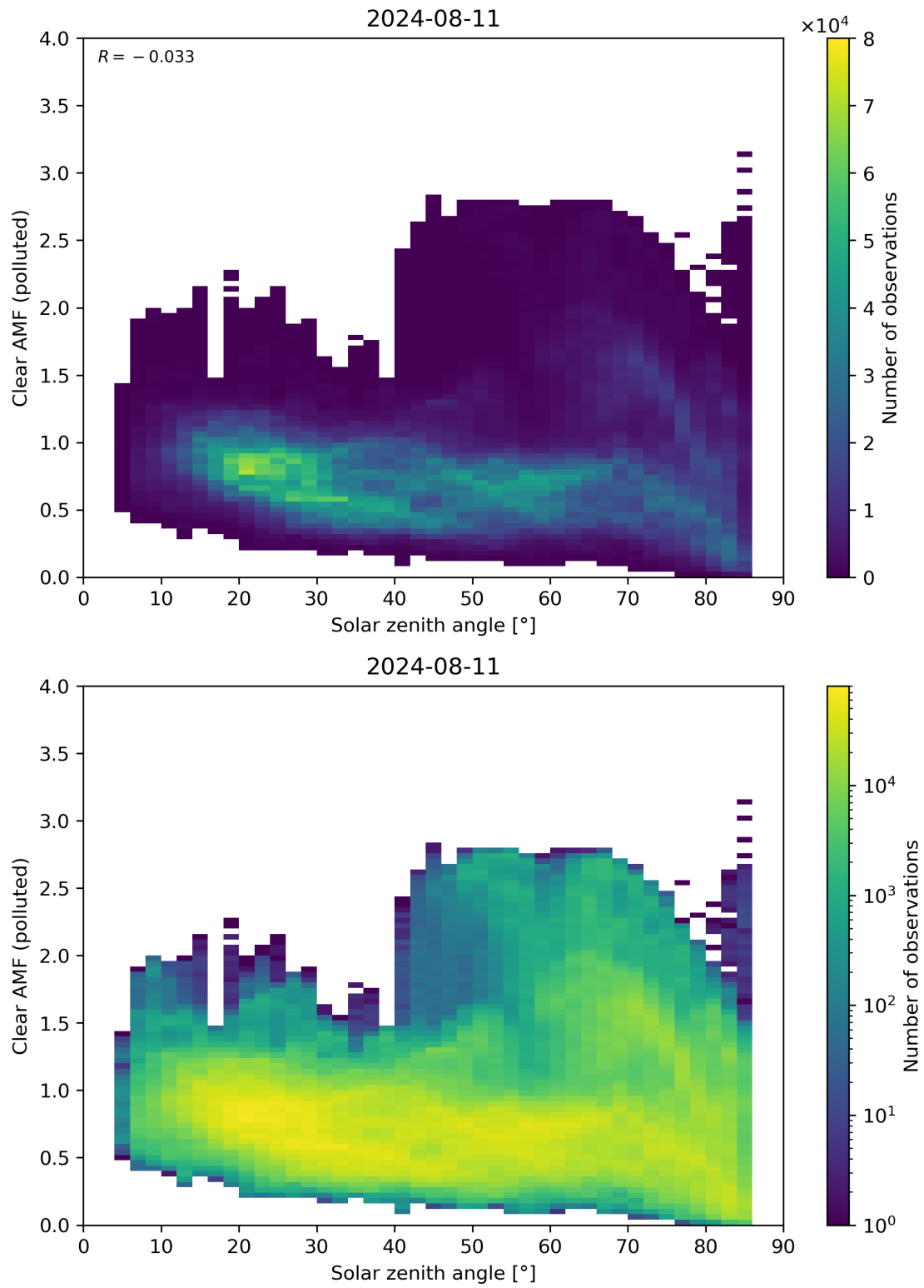
Figure 165: Scatter density plot of “Solar zenith angle” against “Clear AMF (polluted)” for 2024-08-11 to 2024-08-11.
