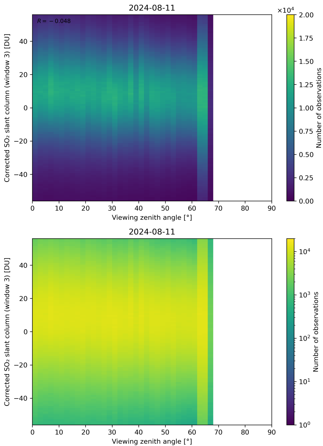
Figure 319: Scatter density plot of “Viewing zenith angle” against “Corrected SO 2 slant column (window 3)” for 2024-08-11 to 2024-08-11.
