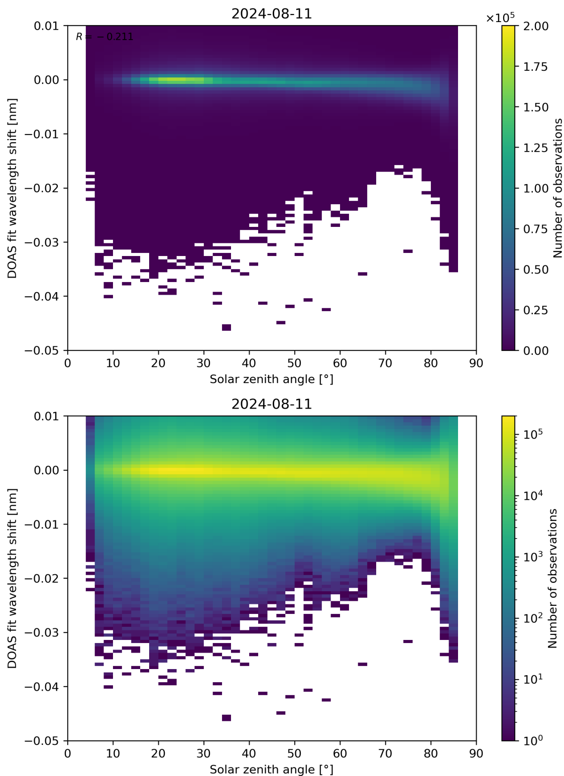
Figure 161: Scatter density plot of “Solar zenith angle” against “DOAS fit wavelength shift” for 2024-08-11 to 2024-08-11.
