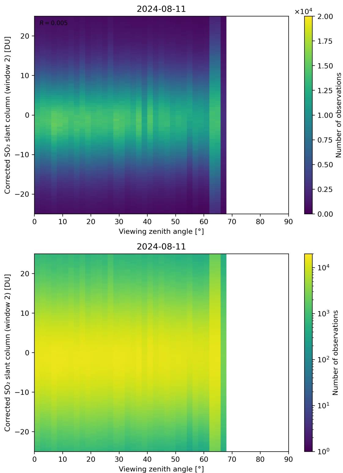
Figure 318: Scatter density plot of “Viewing zenith angle” against “Corrected SO 2 slant column (window 2)” for 2024-08-11 to 2024-08-11.
