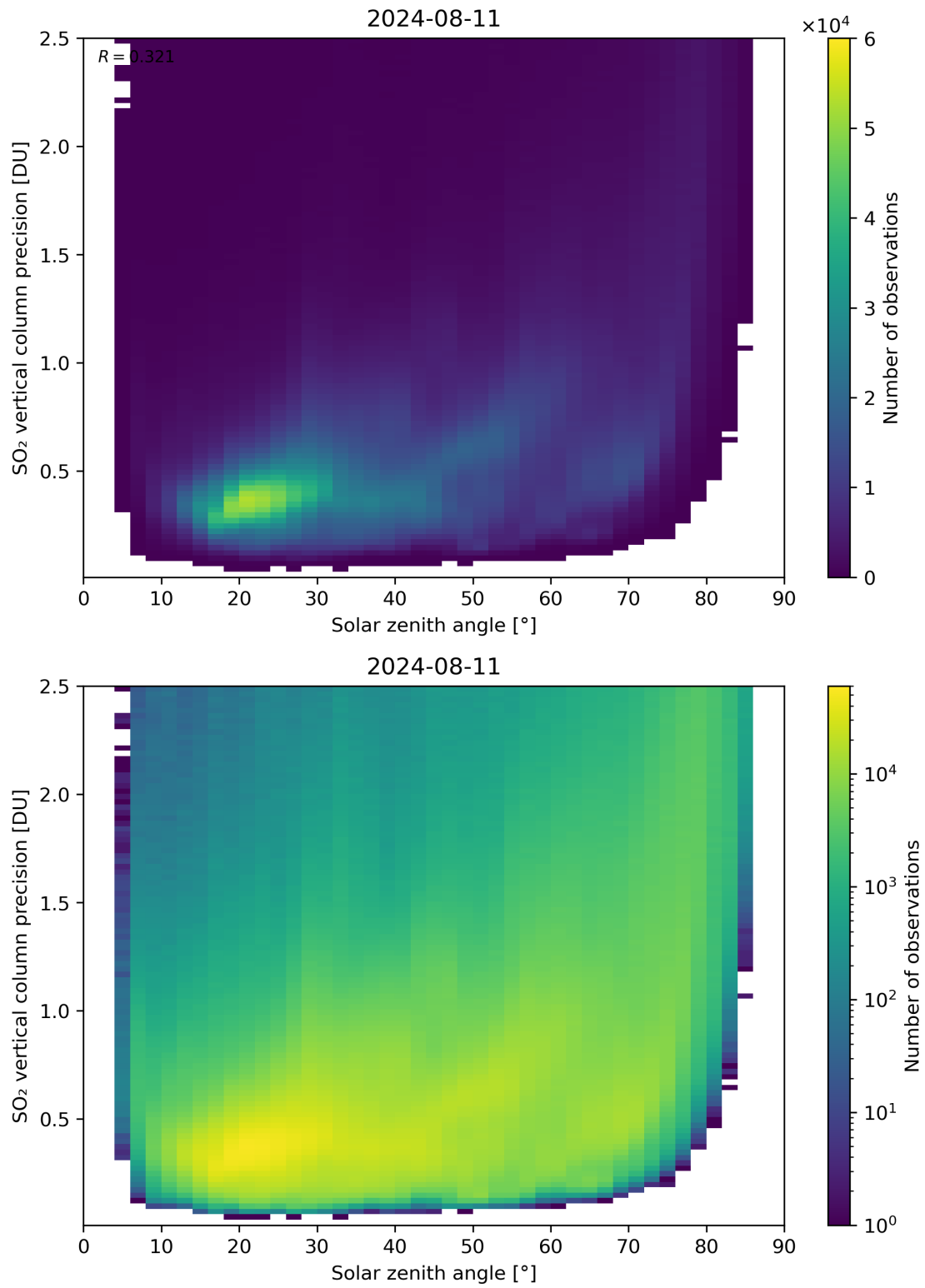
Figure 177: Scatter density plot of “Solar zenith angle” against “SO 2 vertical column precision” for 2024-08-11 to 2024-08-11.
