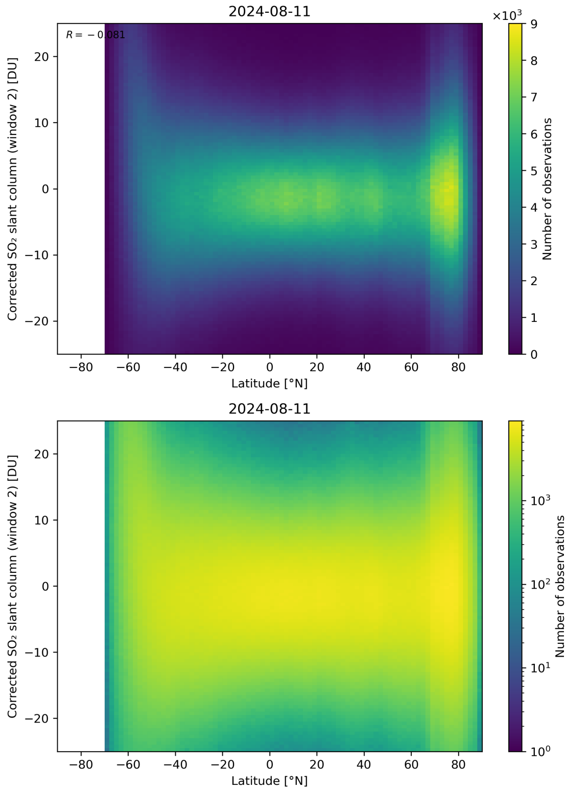
Figure 147: Scatter density plot of “Latitude” against “Corrected SO 2 slant column (window 2)” for 2024-08-11 to 2024-08-11.
