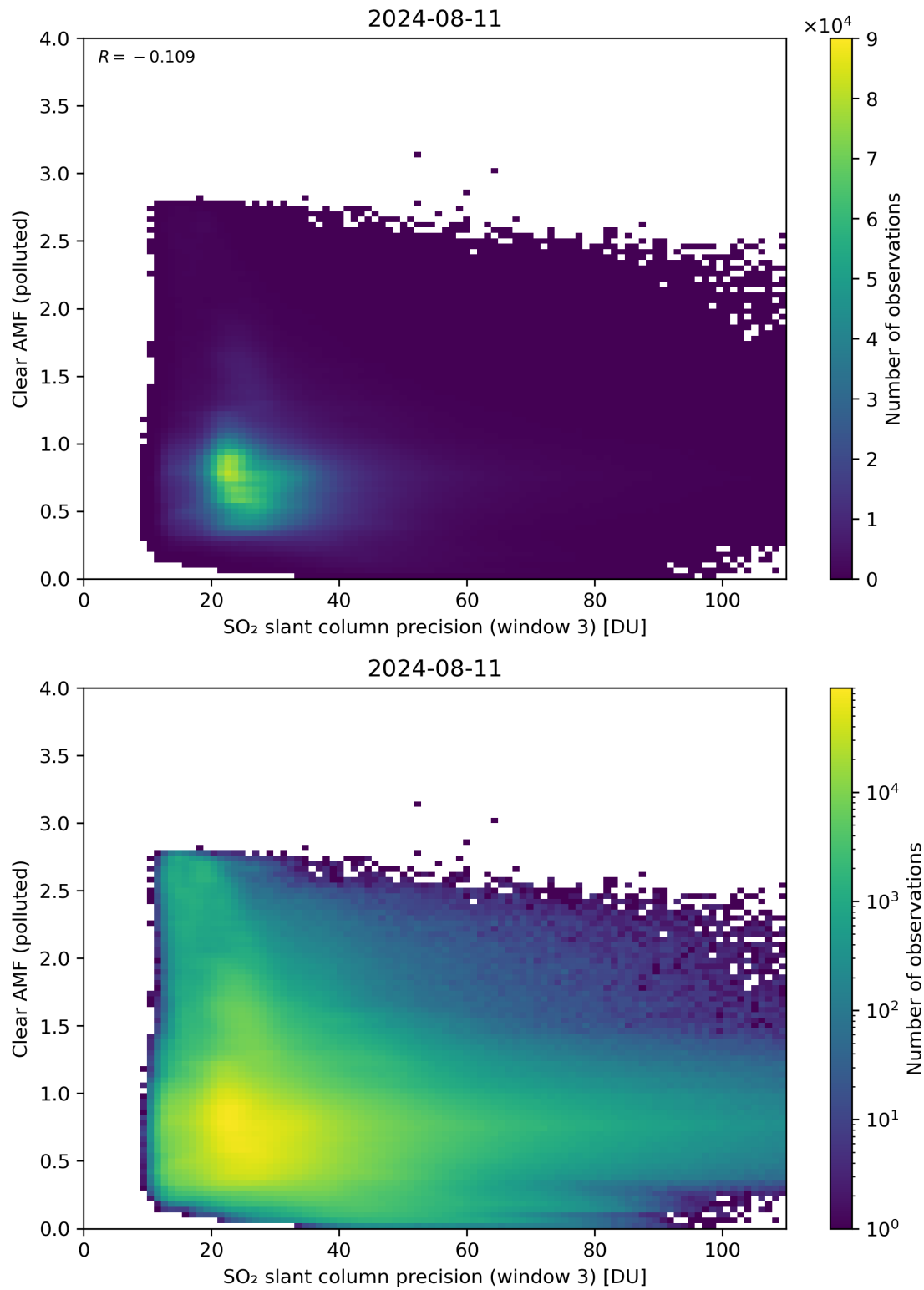
Figure 261: Scatter density plot of “SO 2 slant column precision (window 3)” against “Clear AMF (polluted)” for 2024-08-11 to 2024-08-11.
