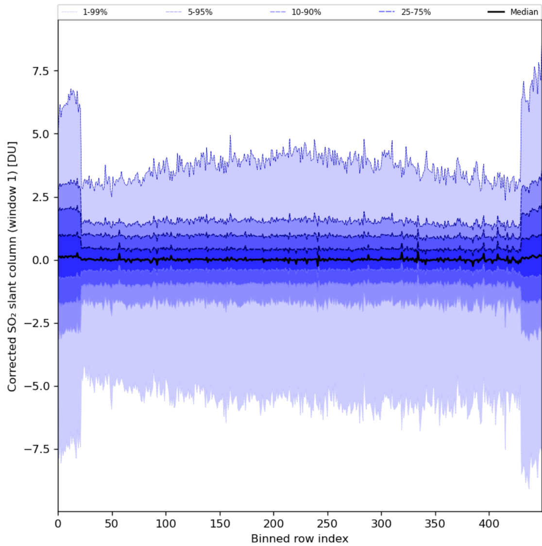
Figure 81: Along track statistics of “Corrected SO 2 slant column (window 1)” for 2024-08-11 to 2024-08-11
