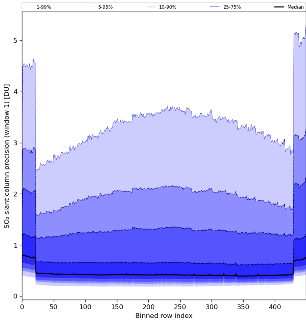
Figure 80: Along track statistics of “SO 2 slant column precision (window 1)” for 2024-08-11 to 2024-08-11
