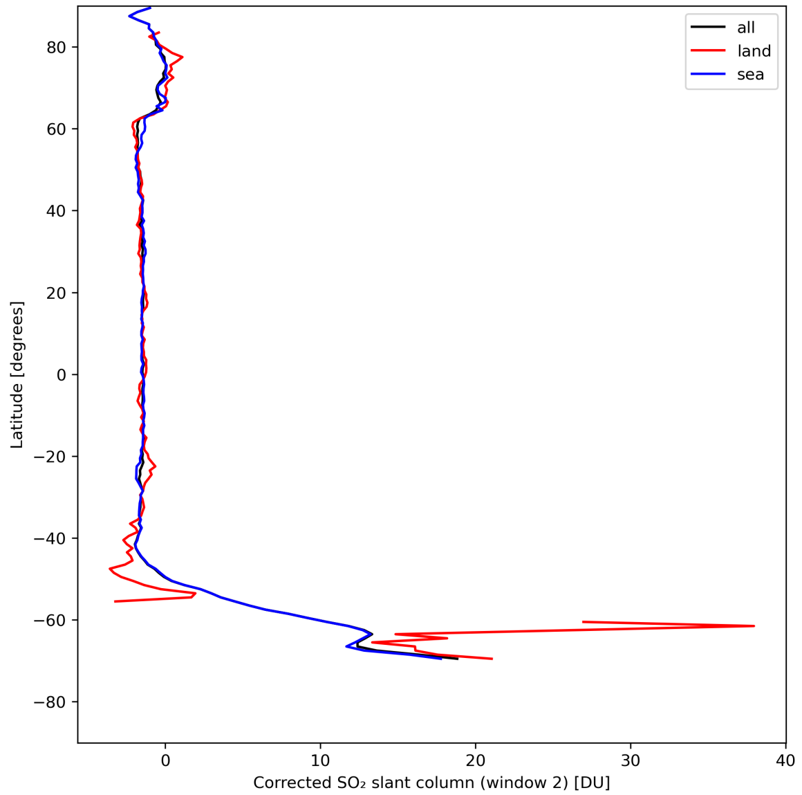
Figure 39: Zonal average of “Corrected SO 2 slant column (window 2)” for 2024-08-11 to 2024-08-11.
