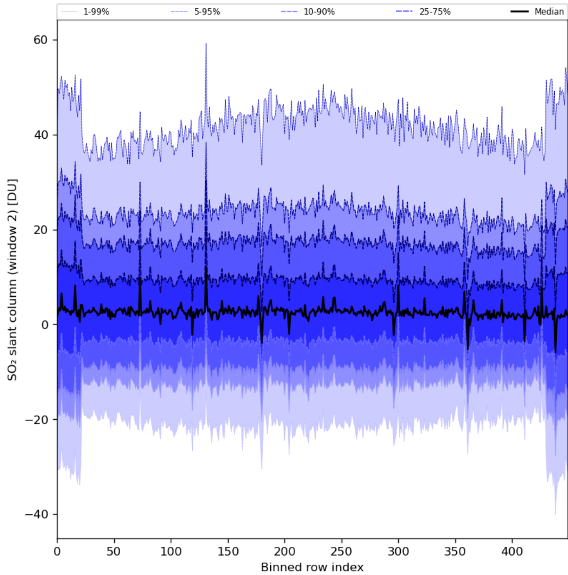
Figure 83: Along track statistics of “SO 2 slant column (window 2)” for 2024-08-11 to 2024-08-11
