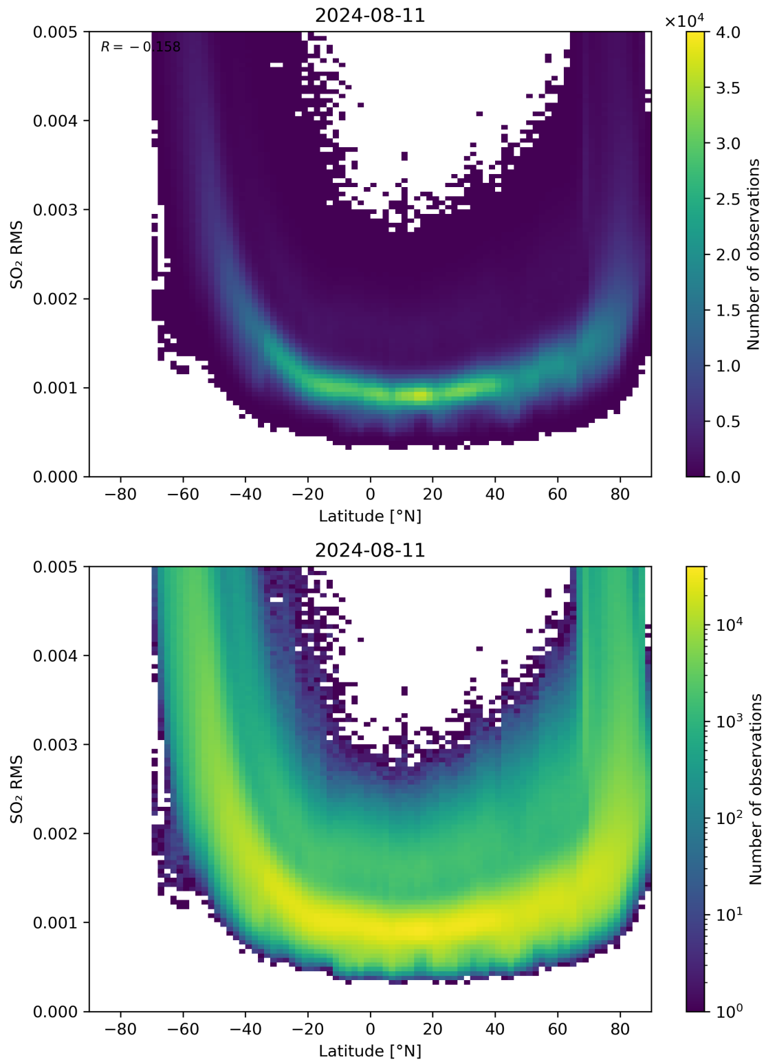
Figure 144: Scatter density plot of “Latitude” against “SO 2 RMS” for 2024-08-11 to 2024-08-11.
