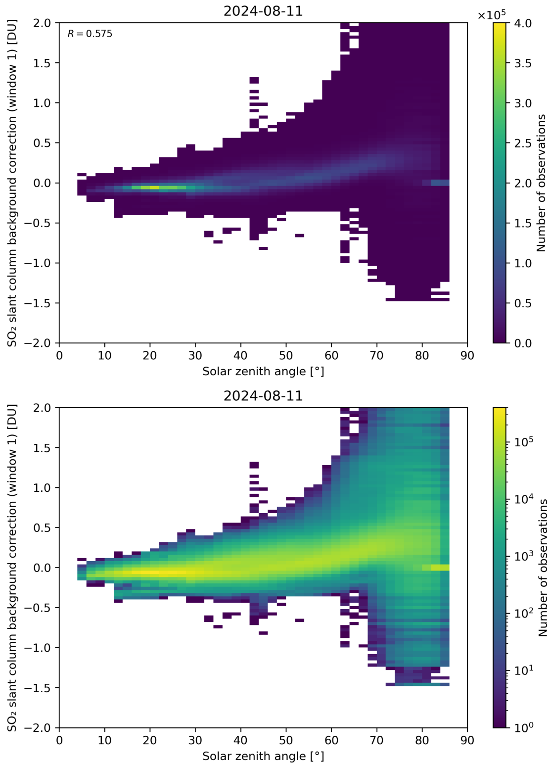
Figure 158: Scatter density plot of “Solar zenith angle” against “SO 2 slant column background correction (window 1)” for 2024-08-11 to 2024-08-11.
