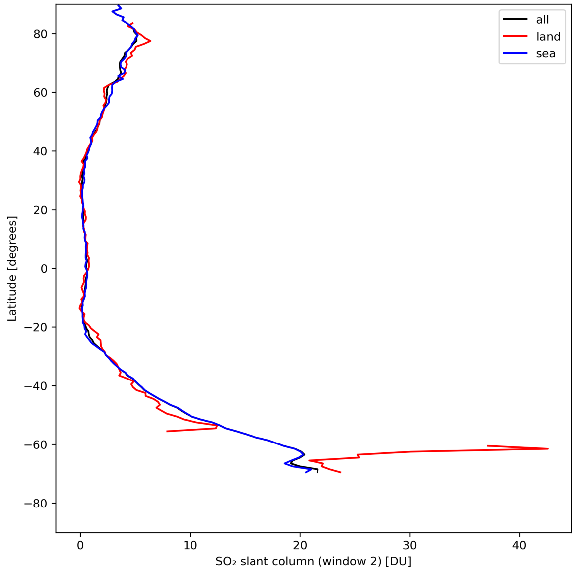
Figure 37: Zonal average of “SO 2 slant column (window 2)” for 2024-08-11 to 2024-08-11.
