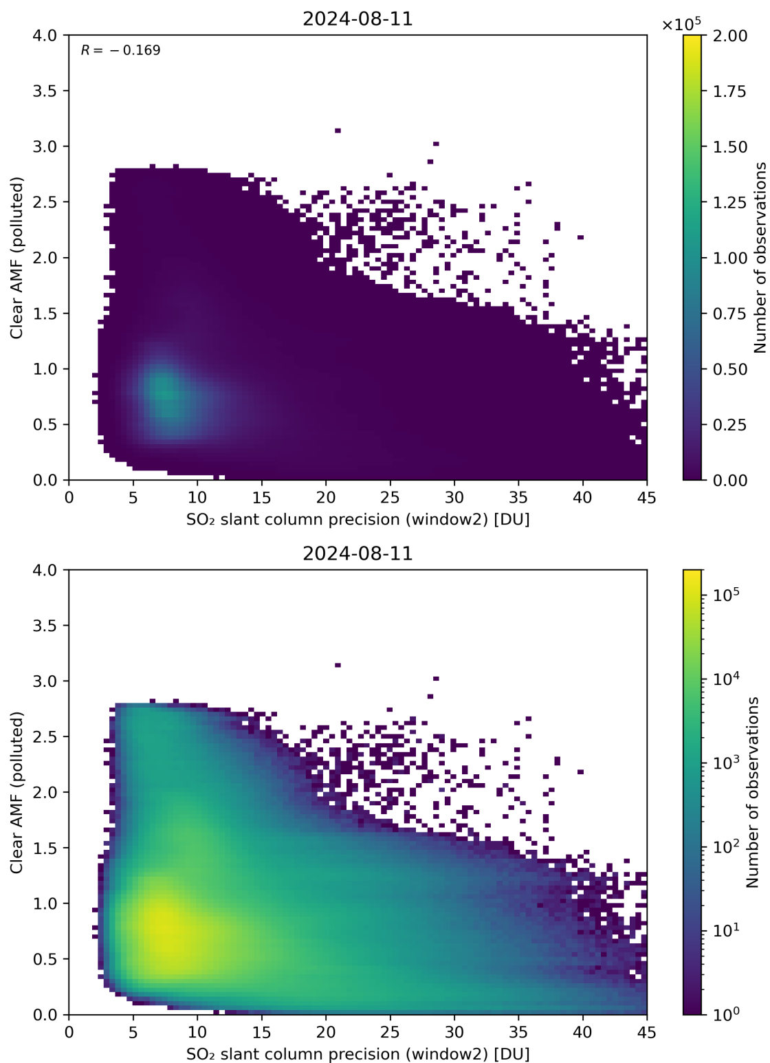
Figure 246: Scatter density plot of “SO 2 slant column precision (window2)” against “Clear AMF (polluted)” for 2024-08-11 to 2024-08-11.
