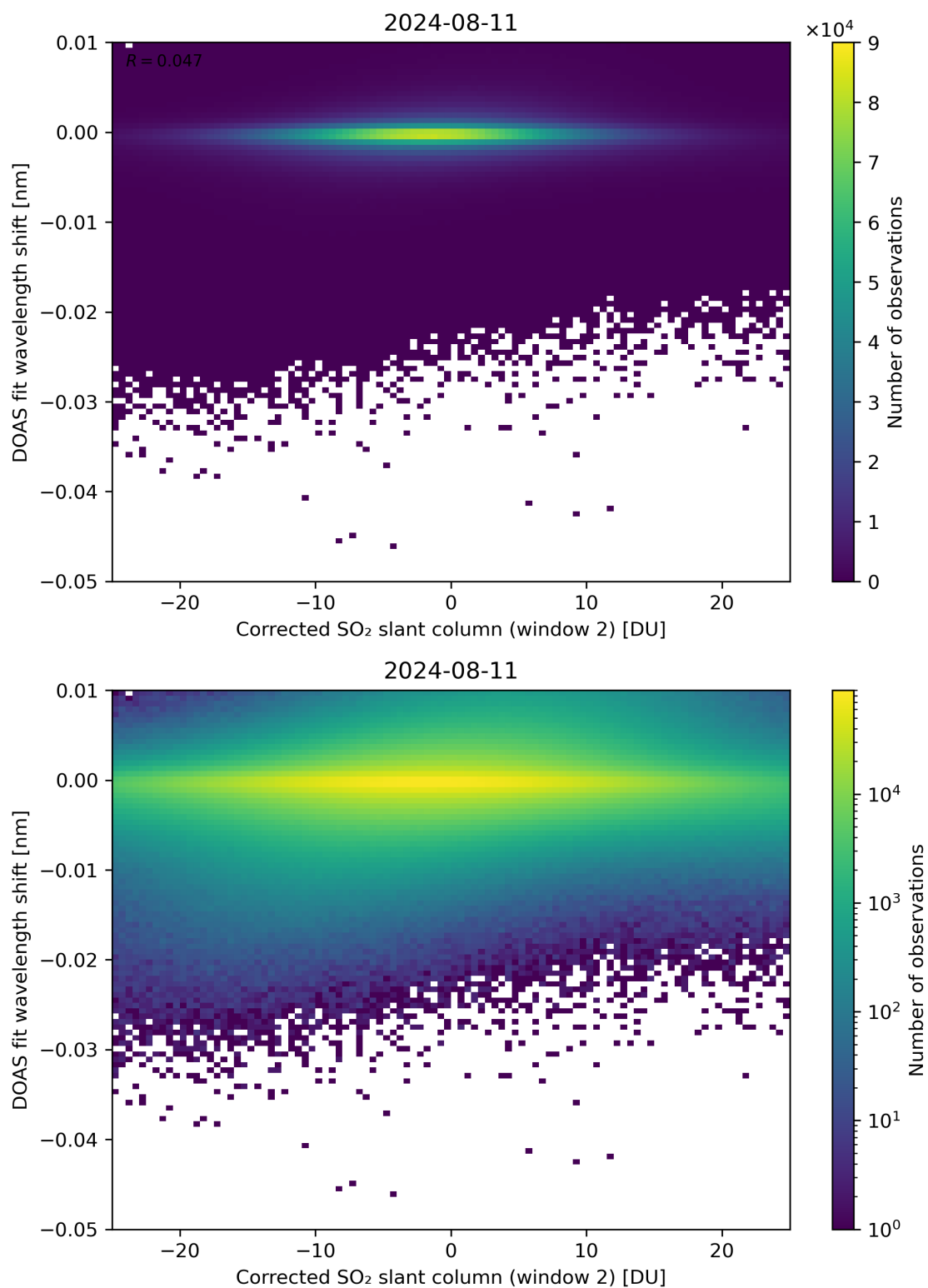
Figure 196: Scatter density plot of “Corrected SO 2 slant column (window 2)” against “DOAS fit wavelength shift” for 2024-08-11 to 2024-08-11.
