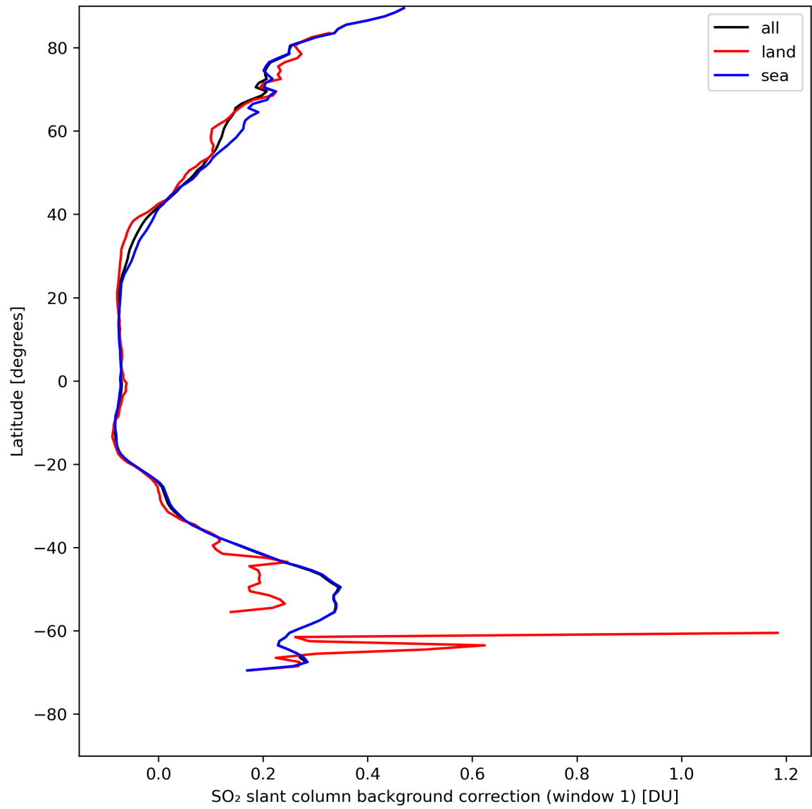
Figure 36: Zonal average of “SO 2 slant column background correction (window 1)” for 2024-08-11 to 2024-08-11.
