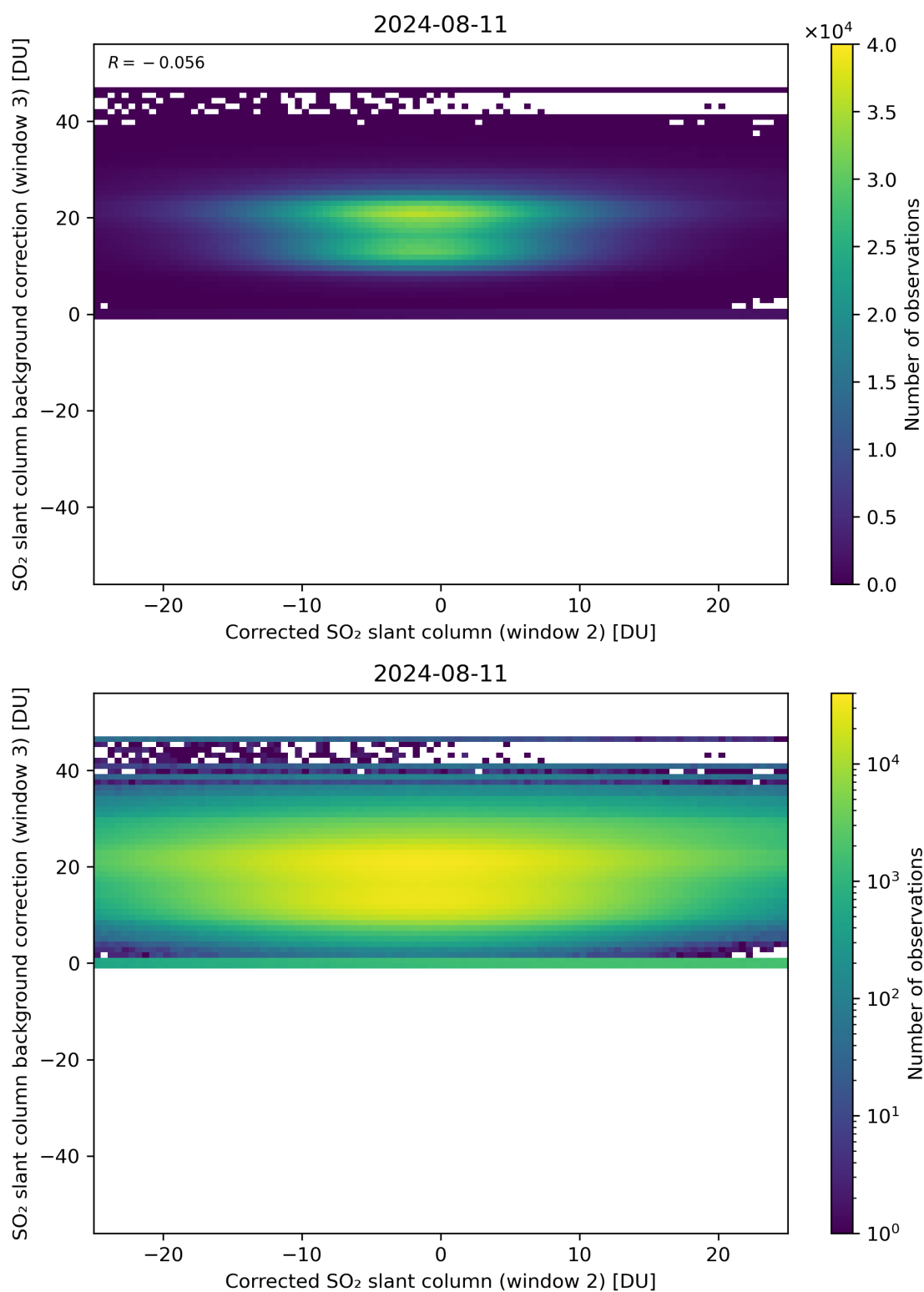
Figure 195: Scatter density plot of “Corrected SO 2 slant column (window 2)” against “SO 2 slant column background correction (window 3)” for 2024-08-11 to 2024-08-11.
