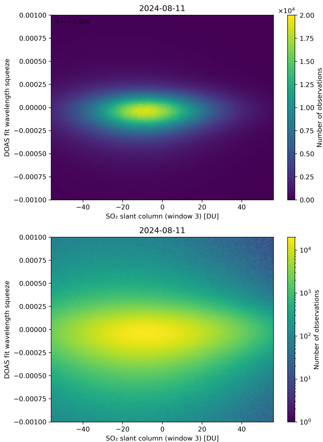
Figure 255: Scatter density plot of “SO 2 slant column (window 3)” against “DOAS fit wavelength squeeze” for 2024-08-11 to 2024-08-11.
