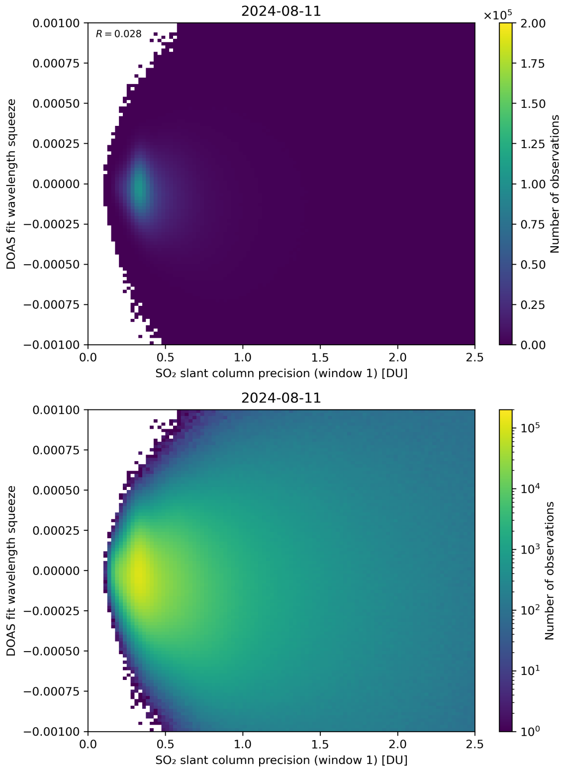
Figure 222: Scatter density plot of “SO 2 slant column precision (window 1)” against “DOAS fit wavelength squeeze” for 2024-08-11 to 2024-08-11.
