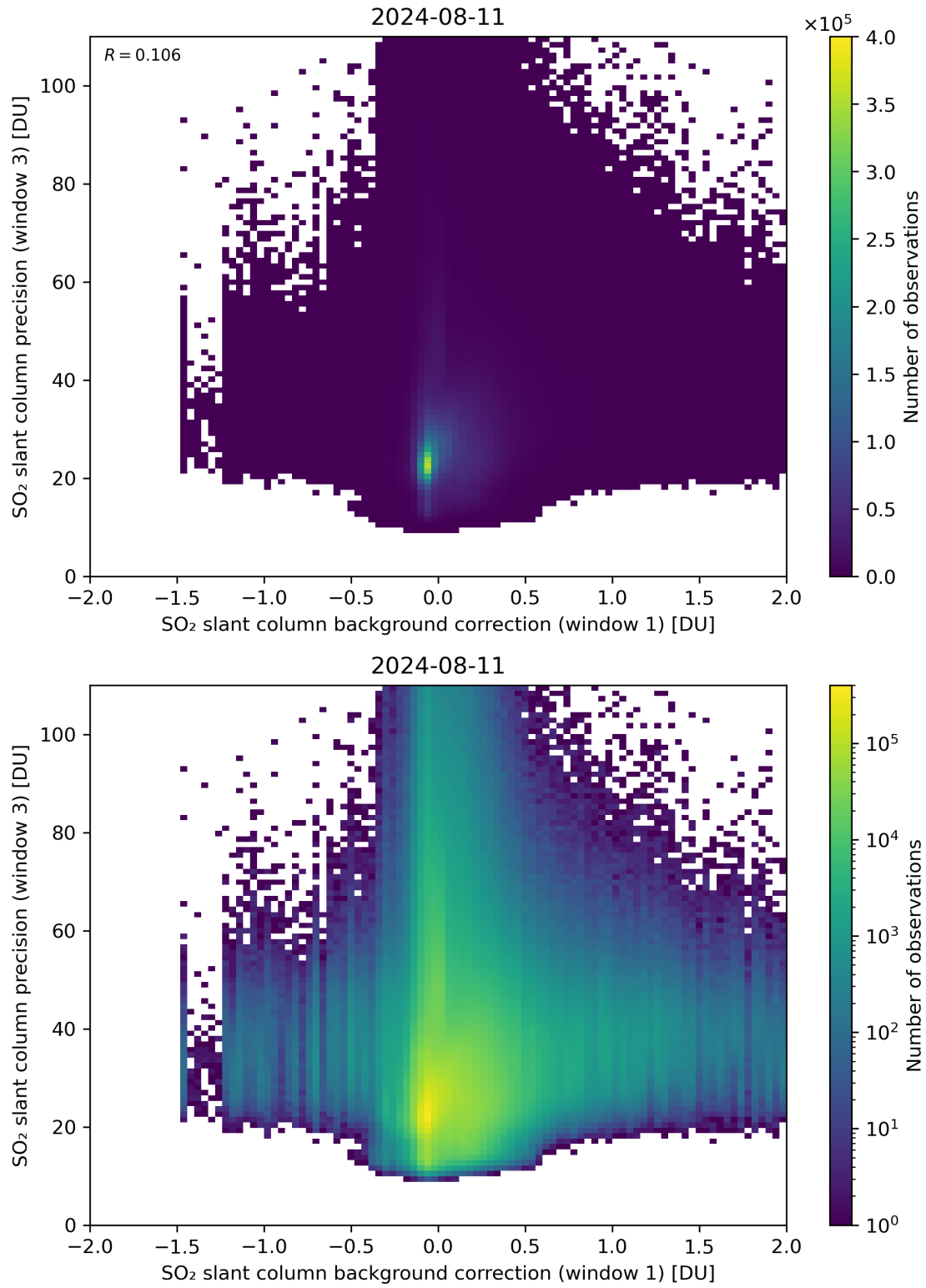
Figure 108: Scatter density plot of “SO 2 slant column background correction (window 1)” against “SO 2 slant column precision (window 3)” for 2024-08-11 to 2024-08-11.
