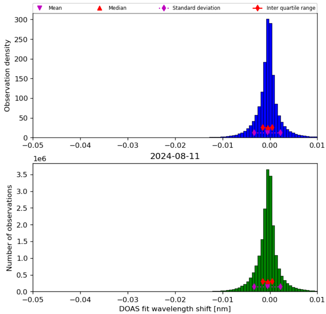
Figure 68: Histogram of “DOAS fit wavelength shift” for 2024-08-11 to 2024-08-11
