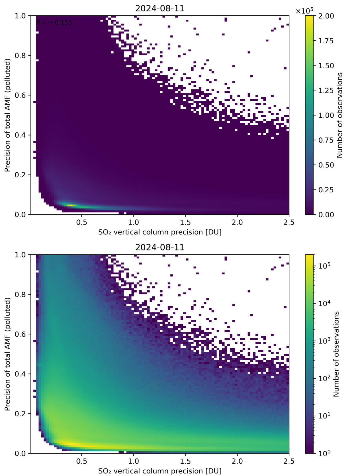
Figure 295: Scatter density plot of “SO 2 vertical column precision” against “Precision of total AMF (polluted)” for 2024-08-11 to 2024-08-11.
