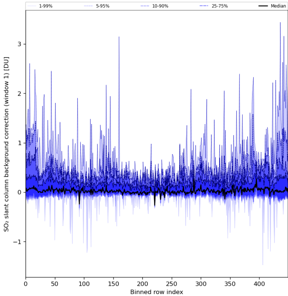
Figure 82: Along track statistics of “SO 2 slant column background correction (window 1)” for 2024-08-11 to 2024-08-11
