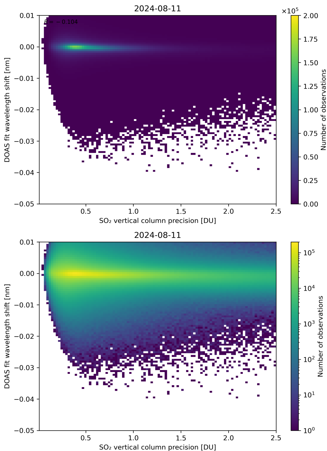
Figure 282: Scatter density plot of “SO 2 vertical column precision” against “DOAS fit wavelength shift” for 2024-08-11 to 2024-08-11.
