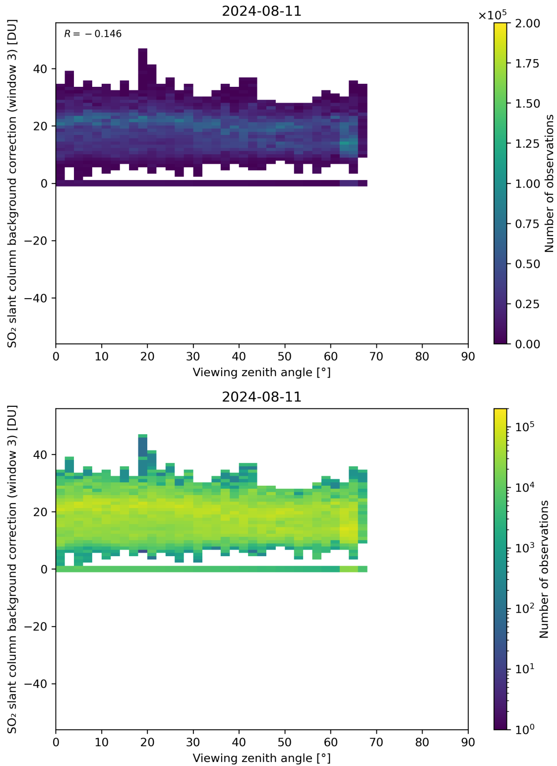
Figure 310: Scatter density plot of “Viewing zenith angle” against “SO 2 slant column background correction (window 3)” for 2024-08-11 to 2024-08-11.
