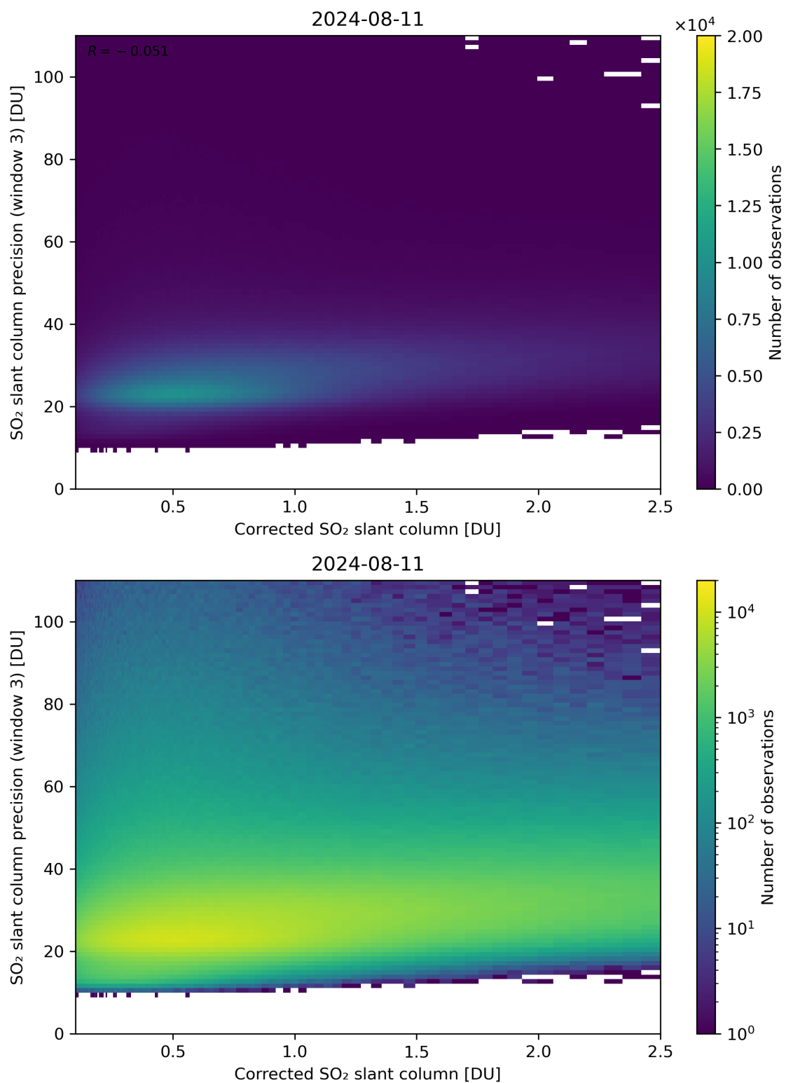
Figure 191: Scatter density plot of “Corrected SO 2 slant column” against “SO 2 slant column precision (window 3)” for 2024-08-11 to 2024-08-11.
