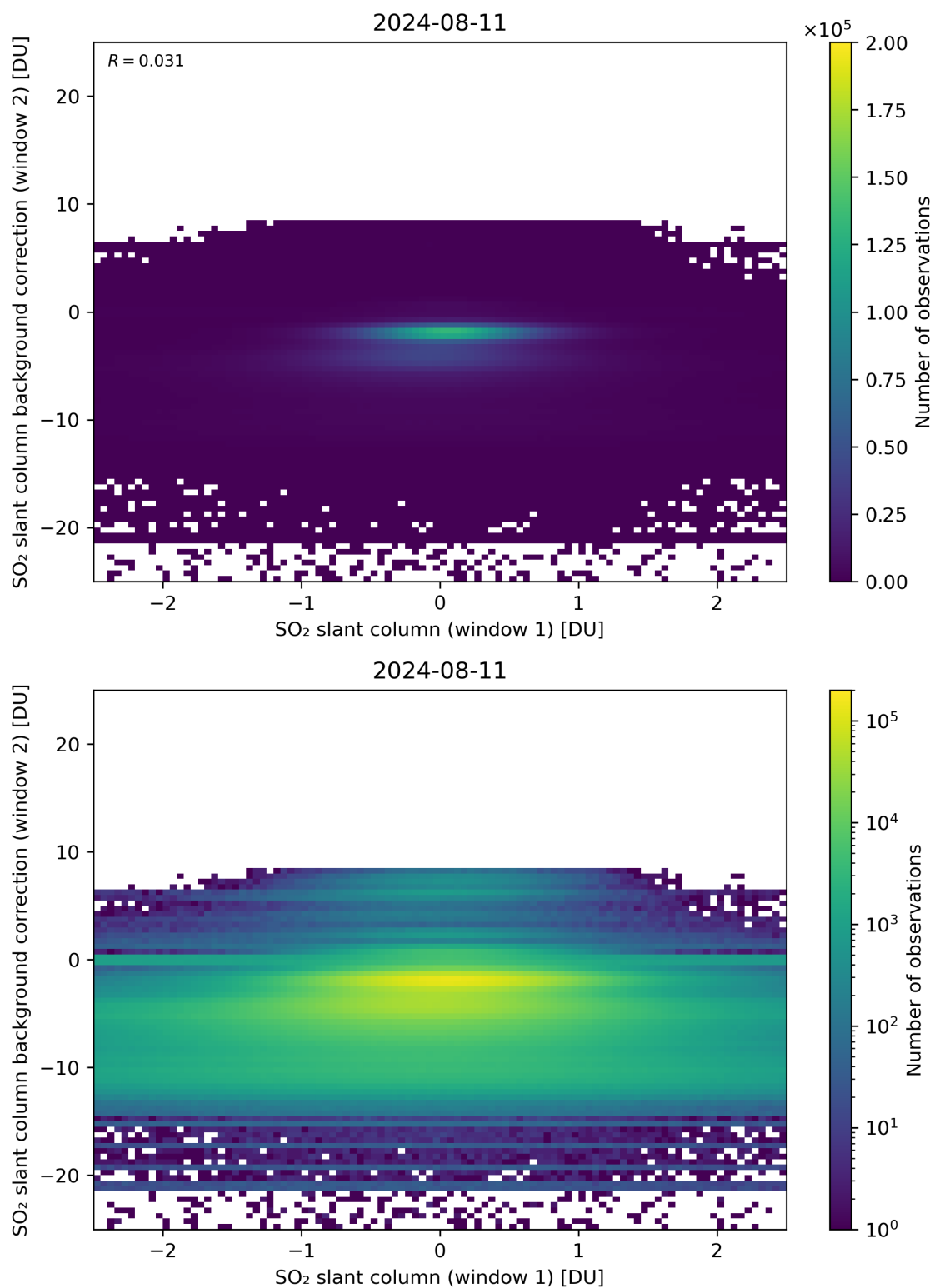
Figure 213: Scatter density plot of “SO 2 slant column (window 1)” against “SO 2 slant column background correction (window 2)” for 2024-08-11 to 2024-08-11.
