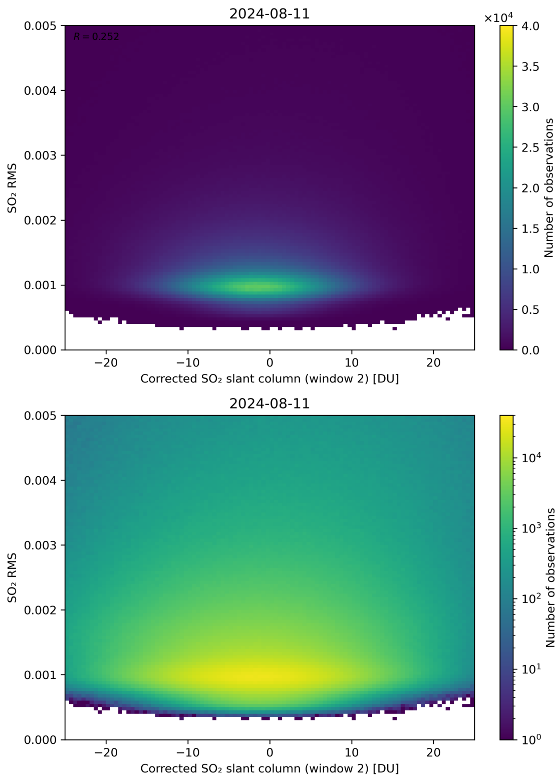
Figure 198: Scatter density plot of “Corrected SO 2 slant column (window 2)” against “SO 2 RMS” for 2024-08-11 to 2024-08-11.
