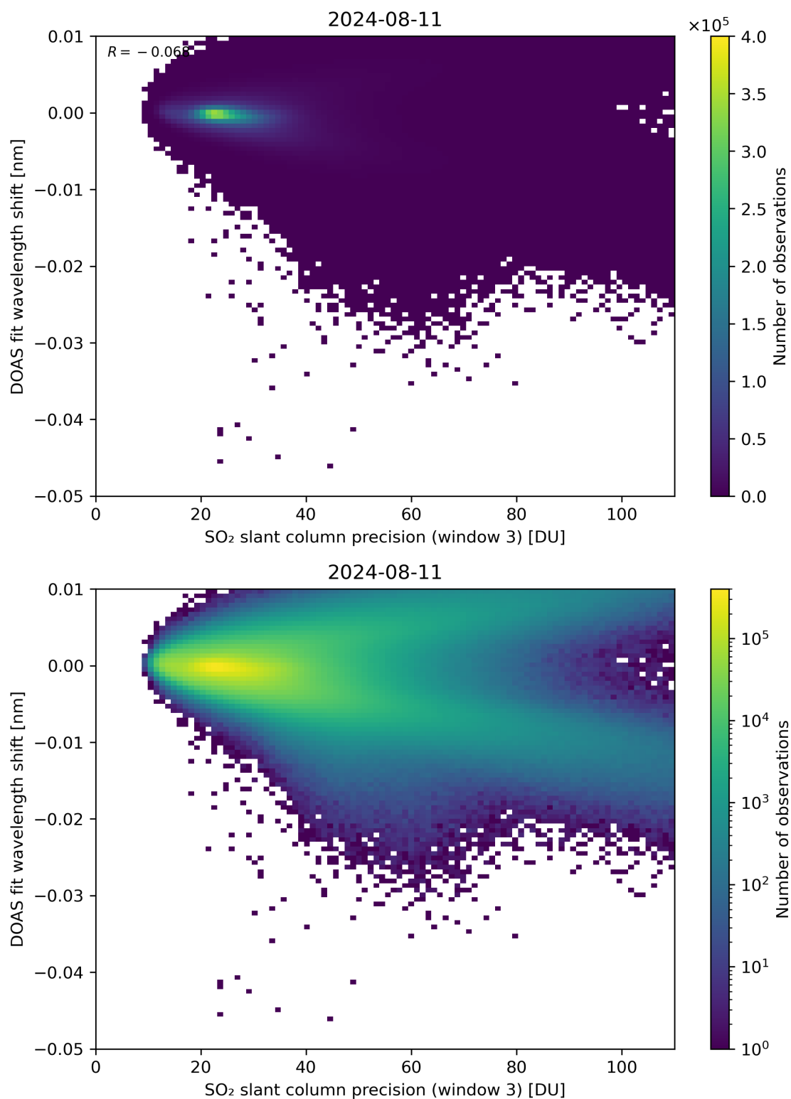
Figure 258: Scatter density plot of “SO 2 slant column precision (window 3)” against “DOAS fit wavelength shift” for 2024-08-11 to 2024-08-11.
