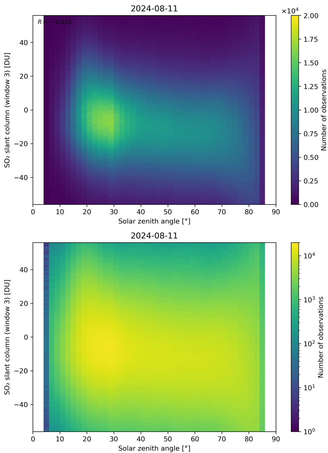
Figure 172: Scatter density plot of “Solar zenith angle” against “SO 2 slant column (window 3)” for 2024-08-11 to 2024-08-11.
