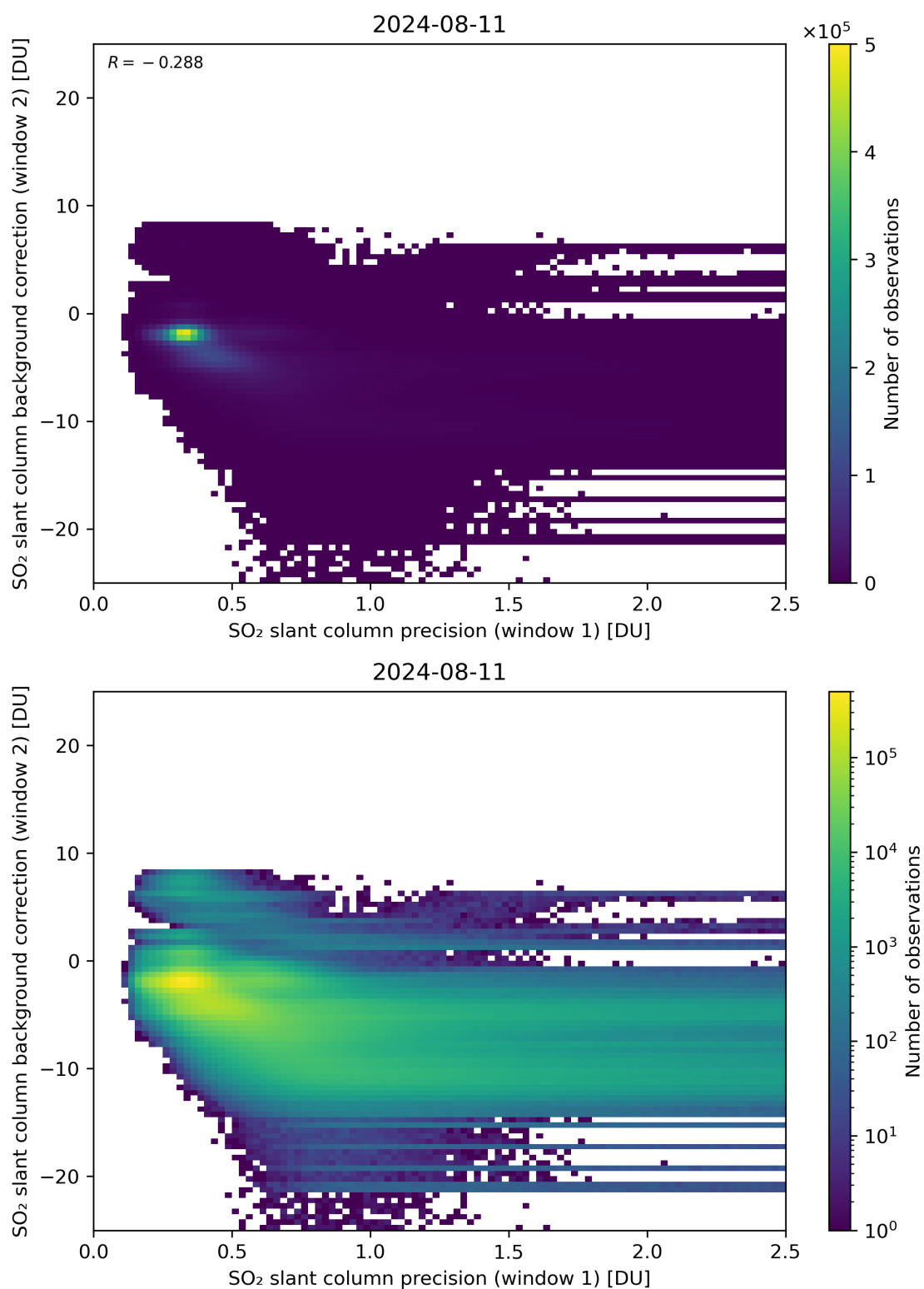
Figure 219: Scatter density plot of “SO 2 slant column precision (window 1)” against “SO 2 slant column background correction (window 2)” for 2024-08-11 to 2024-08-11.
