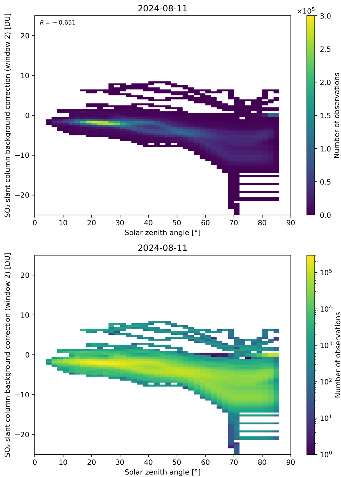
Figure 159: Scatter density plot of “Solar zenith angle” against “SO 2 slant column background correction (window 2)” for 2024-08-11 to 2024-08-11.
