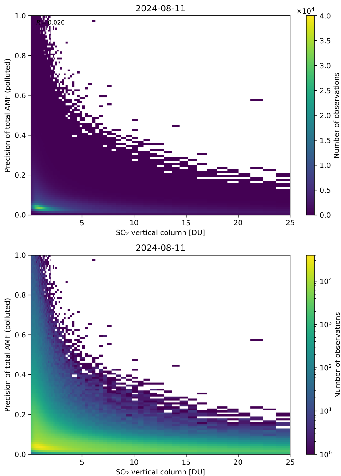
Figure 306: Scatter density plot of “SO 2 vertical column” against “Precision of total AMF (polluted)” for 2024-08-11 to 2024-08-11.
