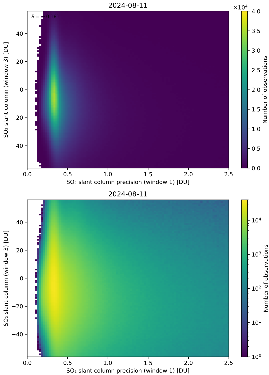
Figure 228: Scatter density plot of “SO 2 slant column precision (window 1)” against “SO 2 slant column (window 3)” for 2024-08-11 to 2024-08-11.
