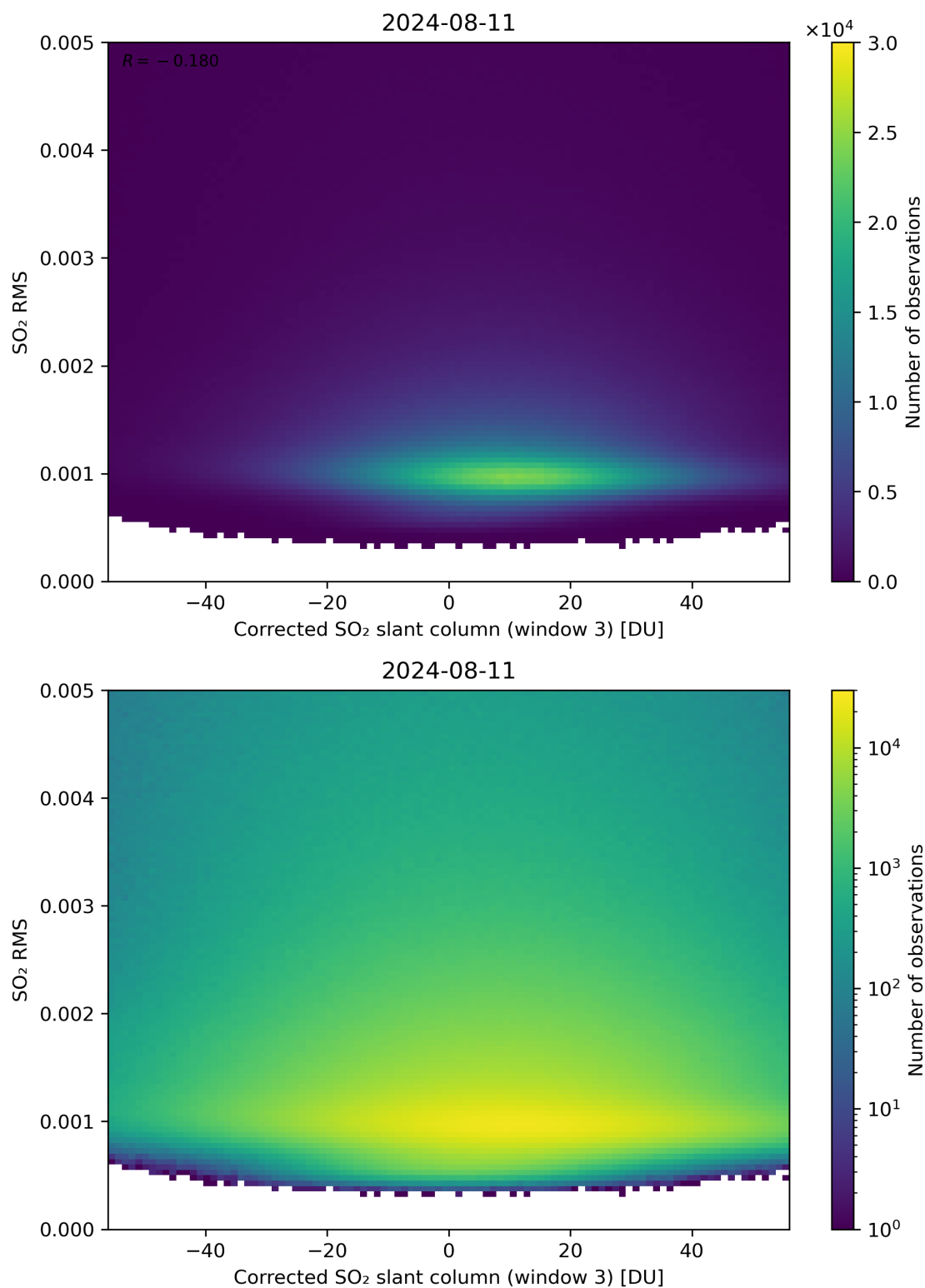
Figure 208: Scatter density plot of “Corrected SO 2 slant column (window 3)” against “SO 2 RMS” for 2024-08-11 to 2024-08-11.
