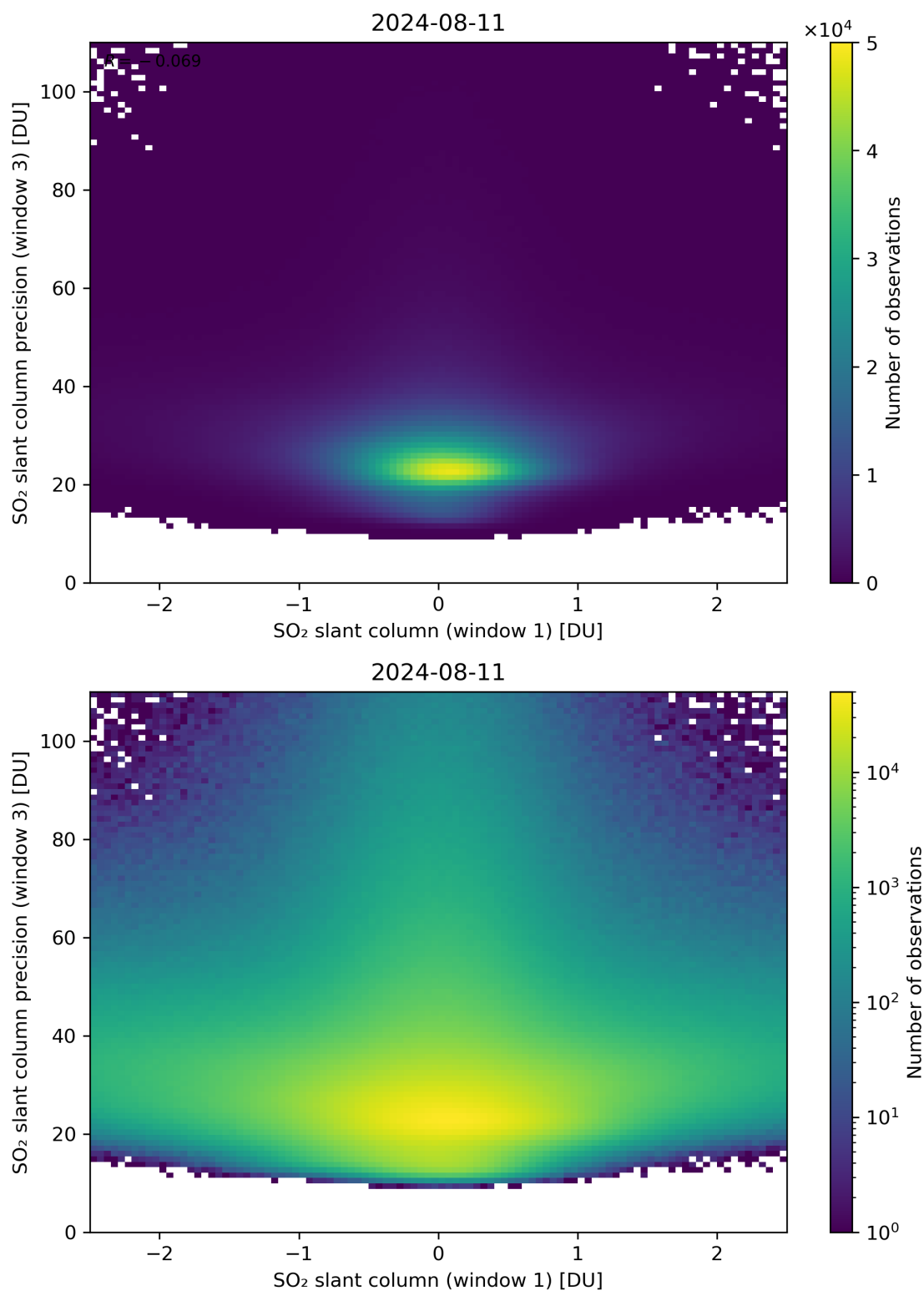
Figure 238: Scatter density plot of “SO 2 slant column (window 1)” against “SO 2 slant column precision (window 3)” for 2024-08-11 to 2024-08-11.
