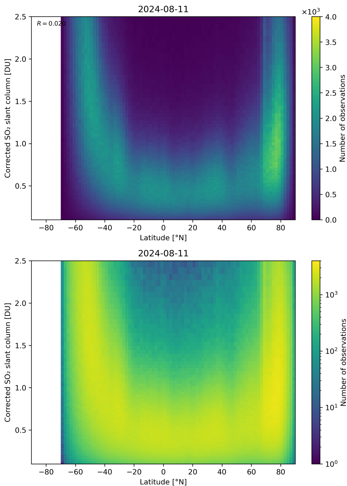
Figure 146: Scatter density plot of “Latitude” against “Corrected SO 2 slant column” for 2024-08-11 to 2024-08-11.
