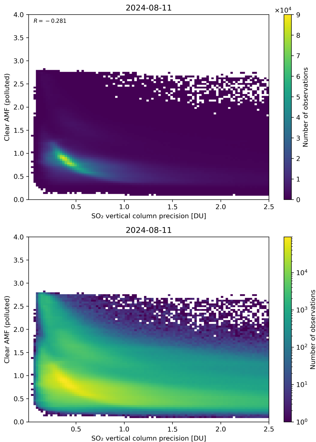
Figure 285: Scatter density plot of “SO 2 vertical column precision” against “Clear AMF (polluted)” for 2024-08-11 to 2024-08-11.
