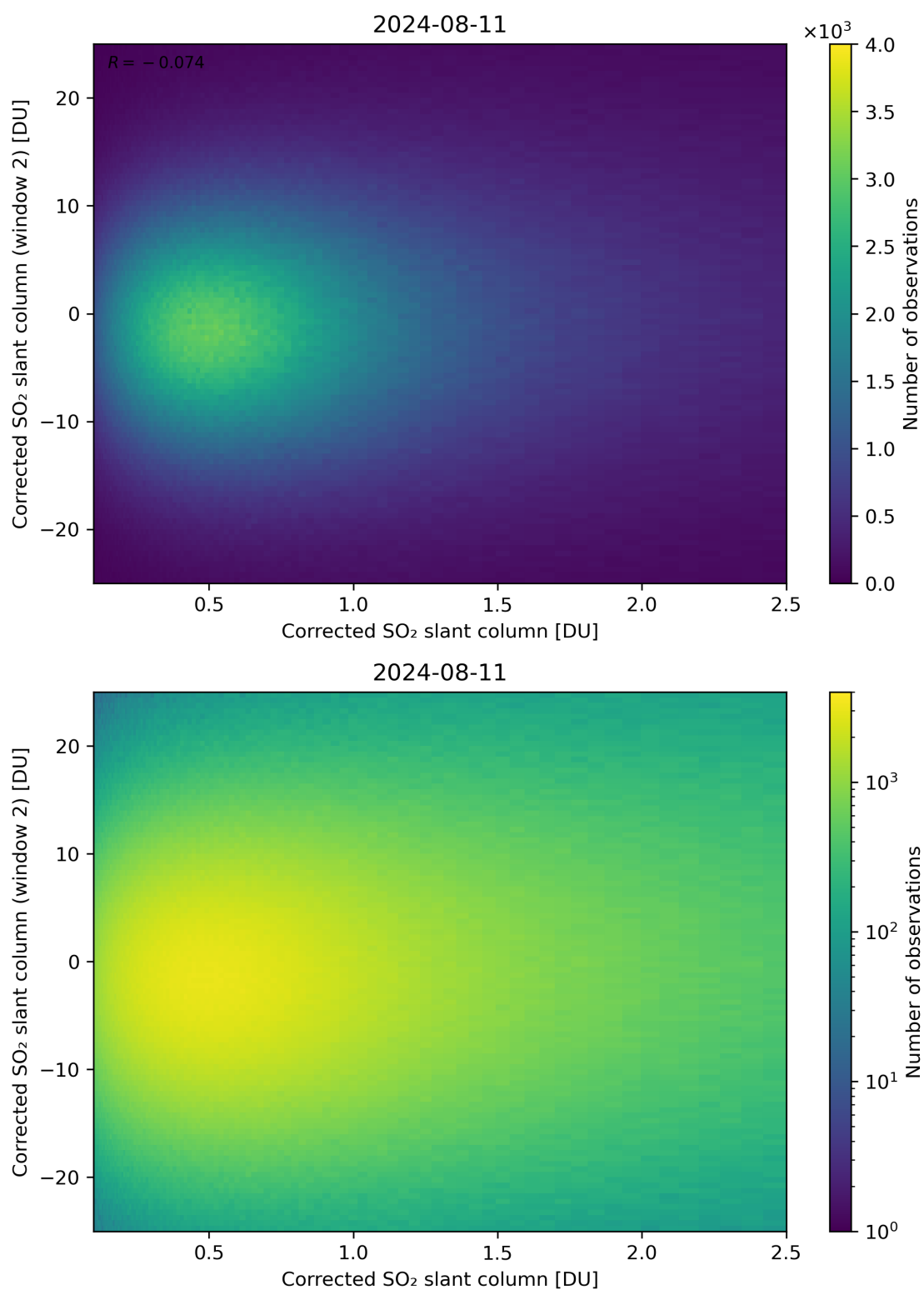
Figure 185: Scatter density plot of “Corrected SO 2 slant column” against “Corrected SO 2 slant column (window 2)” for 2024-08-11 to 2024-08-11.
