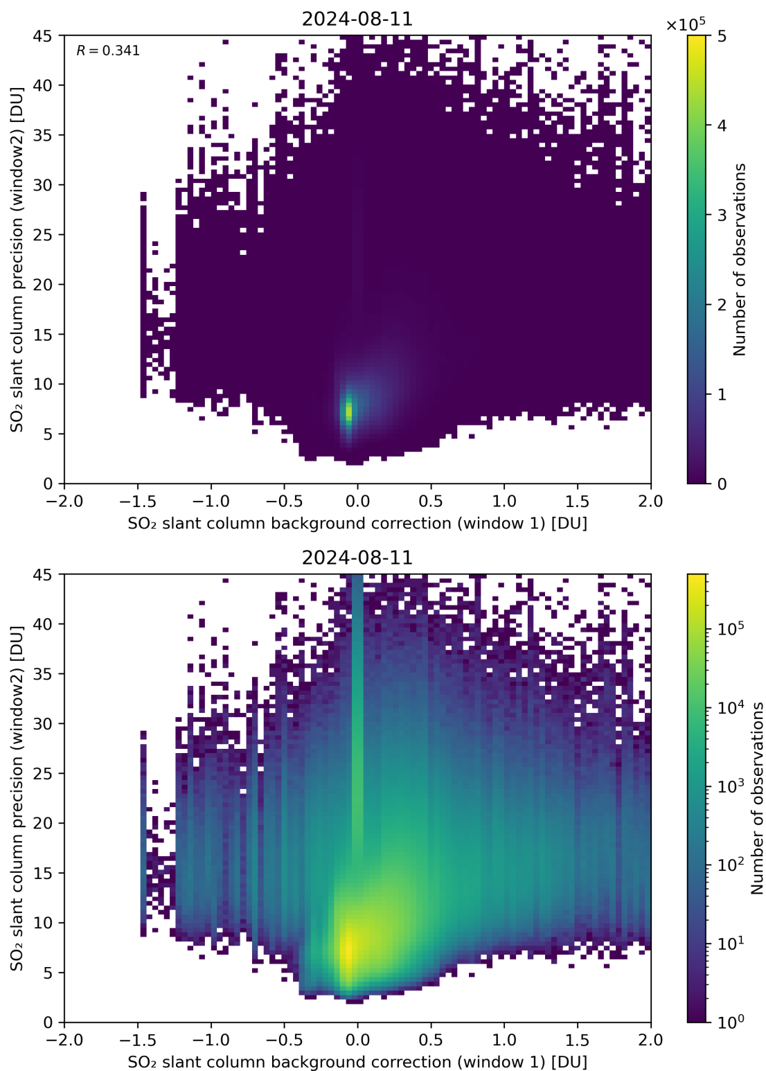
Figure 106: Scatter density plot of “SO 2 slant column background correction (window 1)” against “SO 2 slant column precision (window2)” for 2024-08-11 to 2024-08-11.
