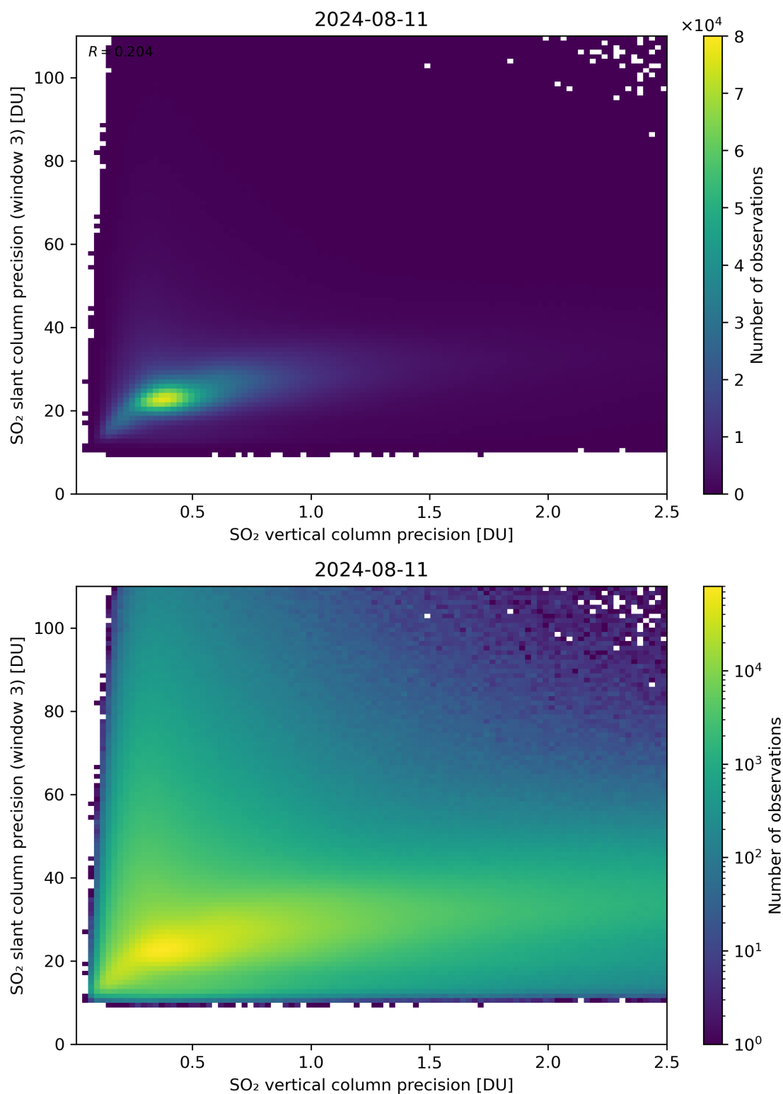
Figure 293: Scatter density plot of “SO 2 vertical column precision” against “SO 2 slant column precision (window 3)” for 2024-08-11 to 2024-08-11.
