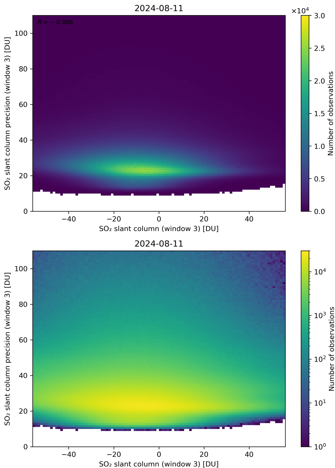
Figure 267: Scatter density plot of “SO 2 slant column (window 3)” against “SO 2 slant column precision (window 3)” for 2024-08-11 to 2024-08-11.
