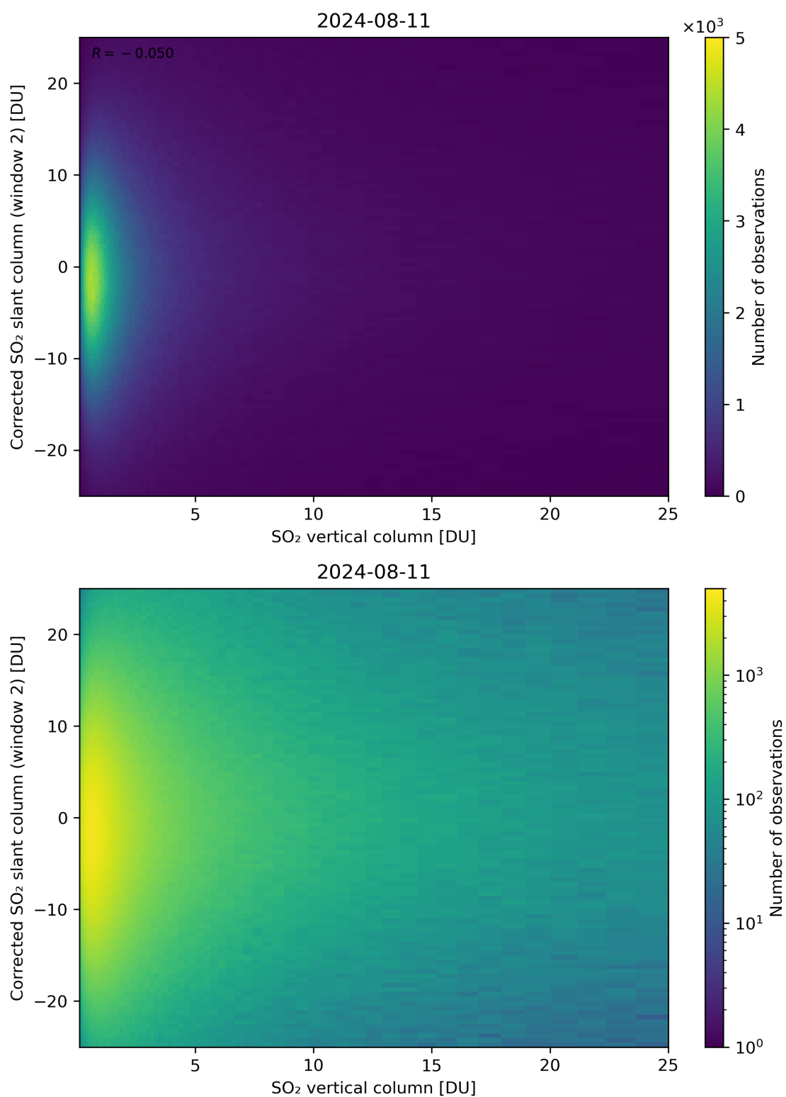
Figure 298: Scatter density plot of “SO 2 vertical column” against “Corrected SO 2 slant column (window 2)” for 2024-08-11 to 2024-08-11.
