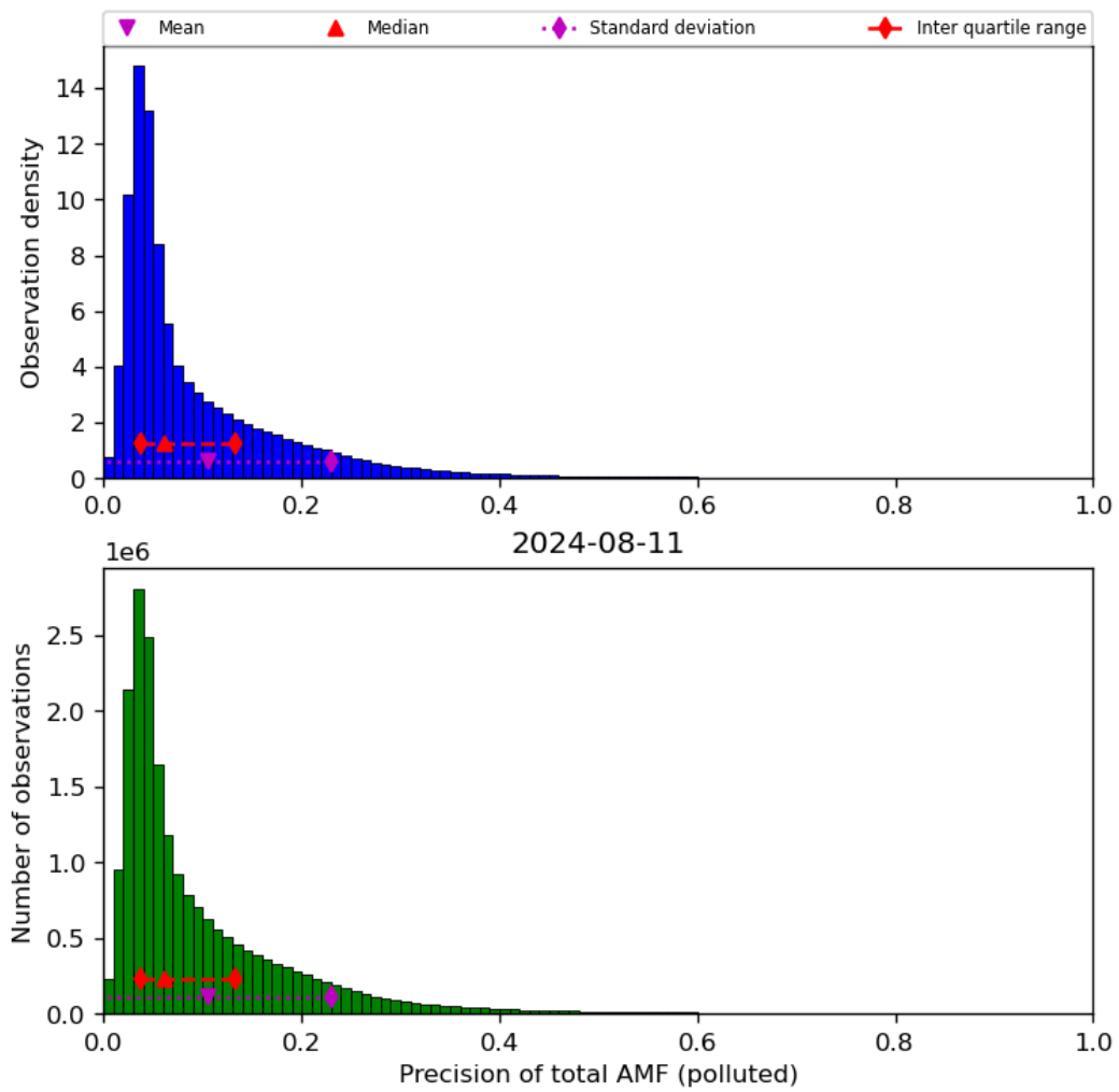
Figure 72: Histogram of “Precision of total AMF (polluted)” for 2024-08-11 to 2024-08-11
