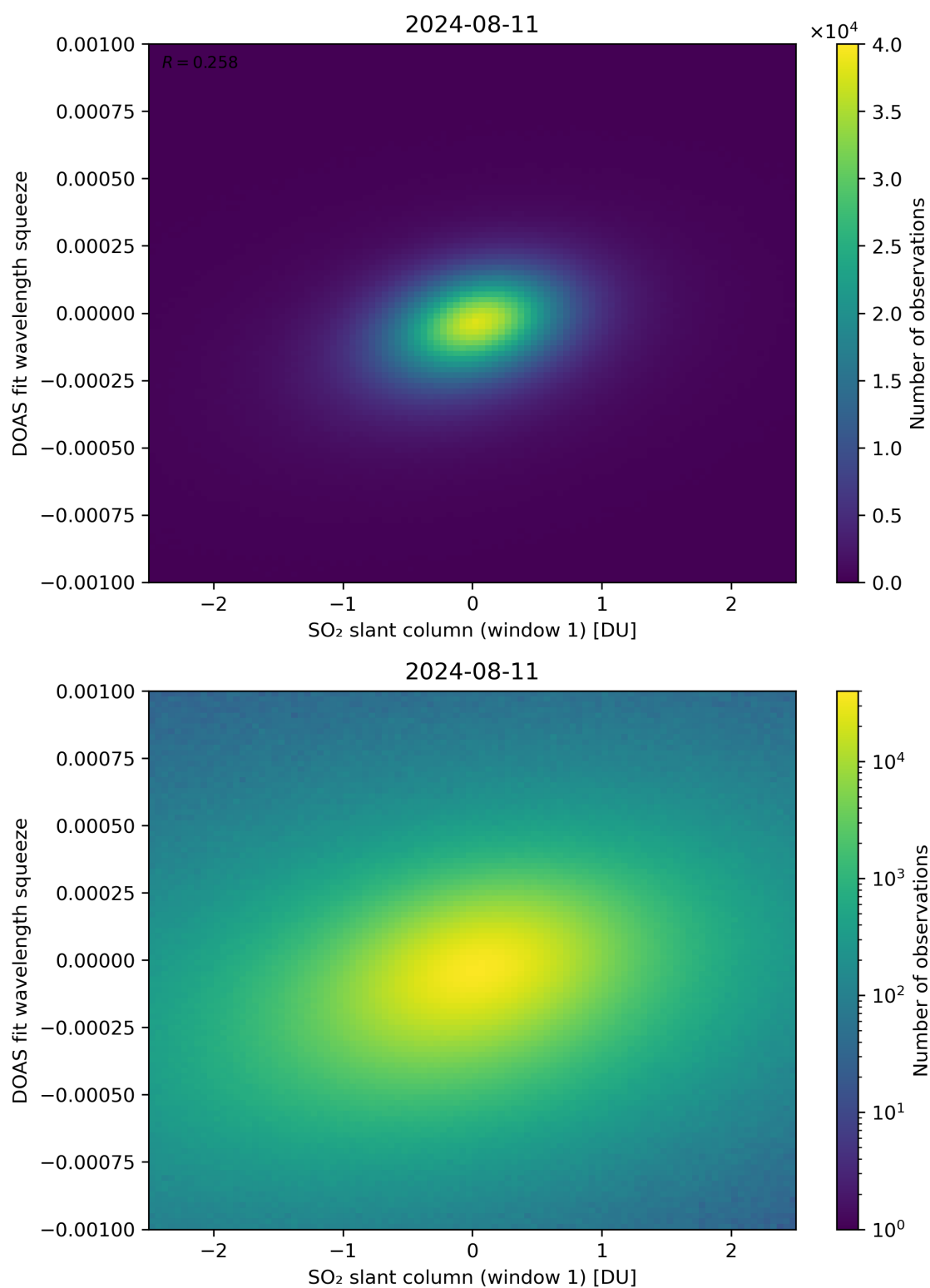
Figure 216: Scatter density plot of “SO 2 slant column (window 1)” against “DOAS fit wavelength squeeze” for 2024-08-11 to 2024-08-11.
