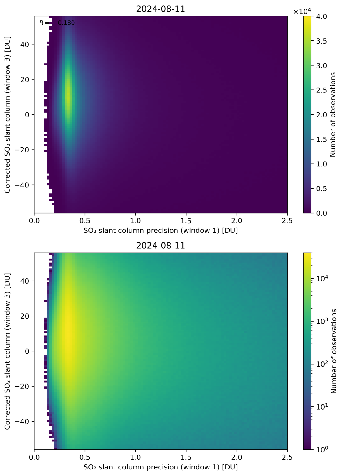
Figure 226: Scatter density plot of “SO 2 slant column precision (window 1)” against “Corrected SO 2 slant column (window 3)” for 2024-08-11 to 2024-08-11.
