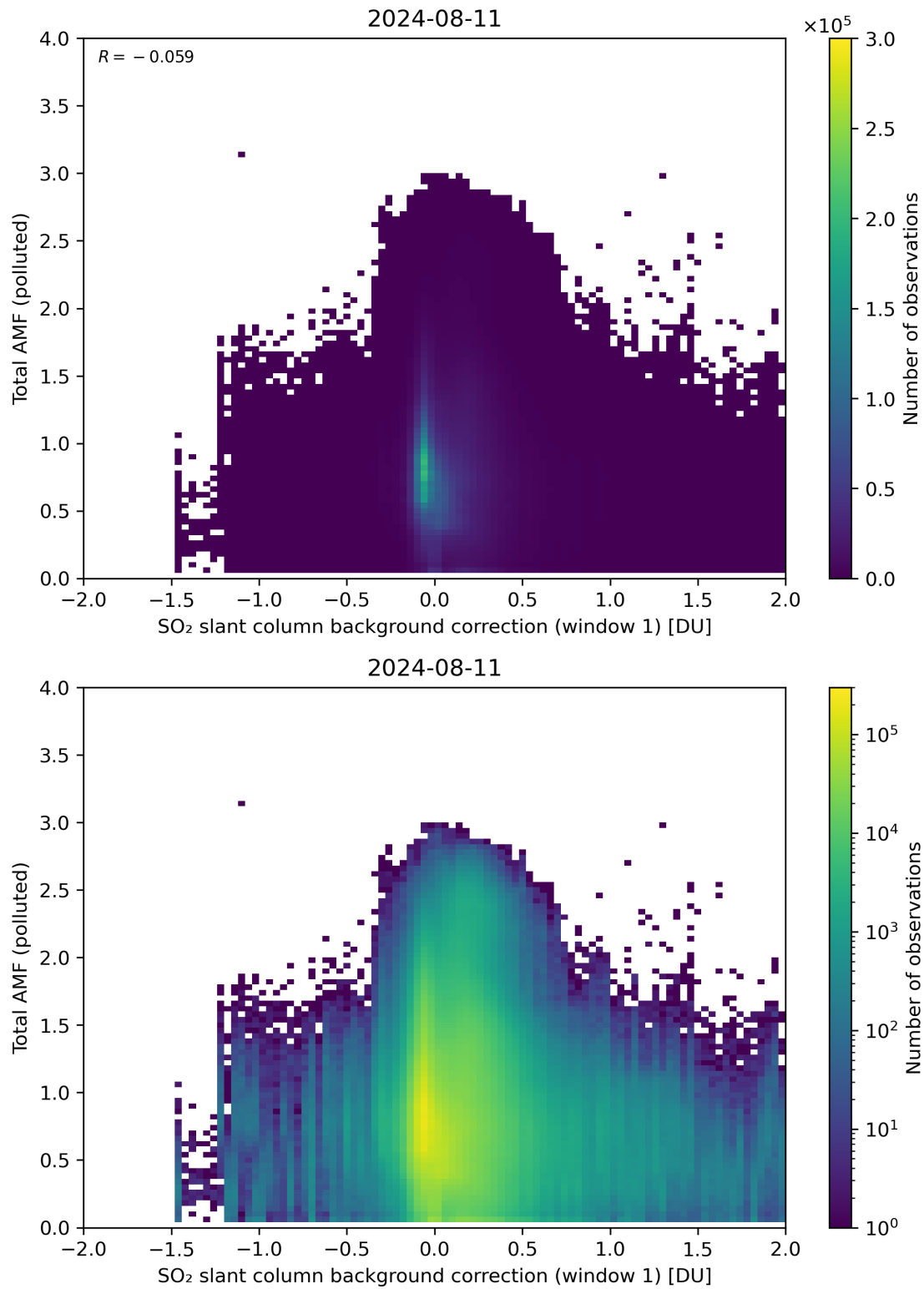
Figure 109: Scatter density plot of “SO 2 slant column background correction (window 1)” against “Total AMF (polluted)” for 2024-08-11 to 2024-08-11.
