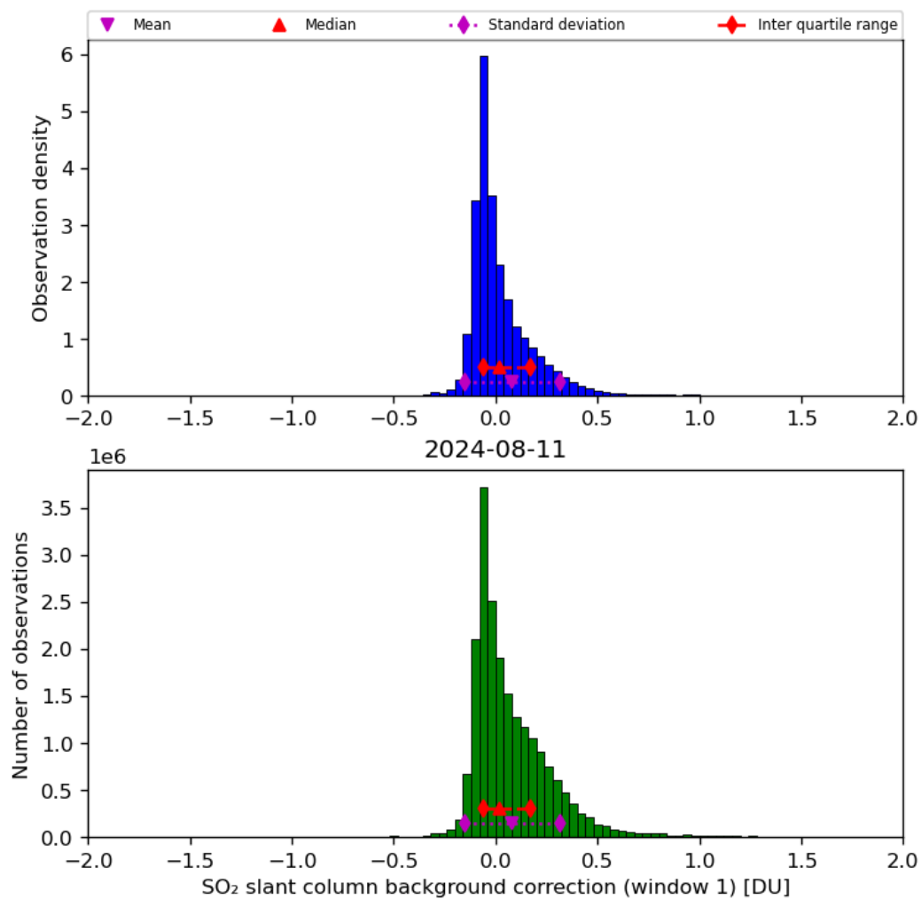
Figure 59: Histogram of “SO 2 slant column background correction (window 1)” for 2024-08-11 to 2024-08-11
