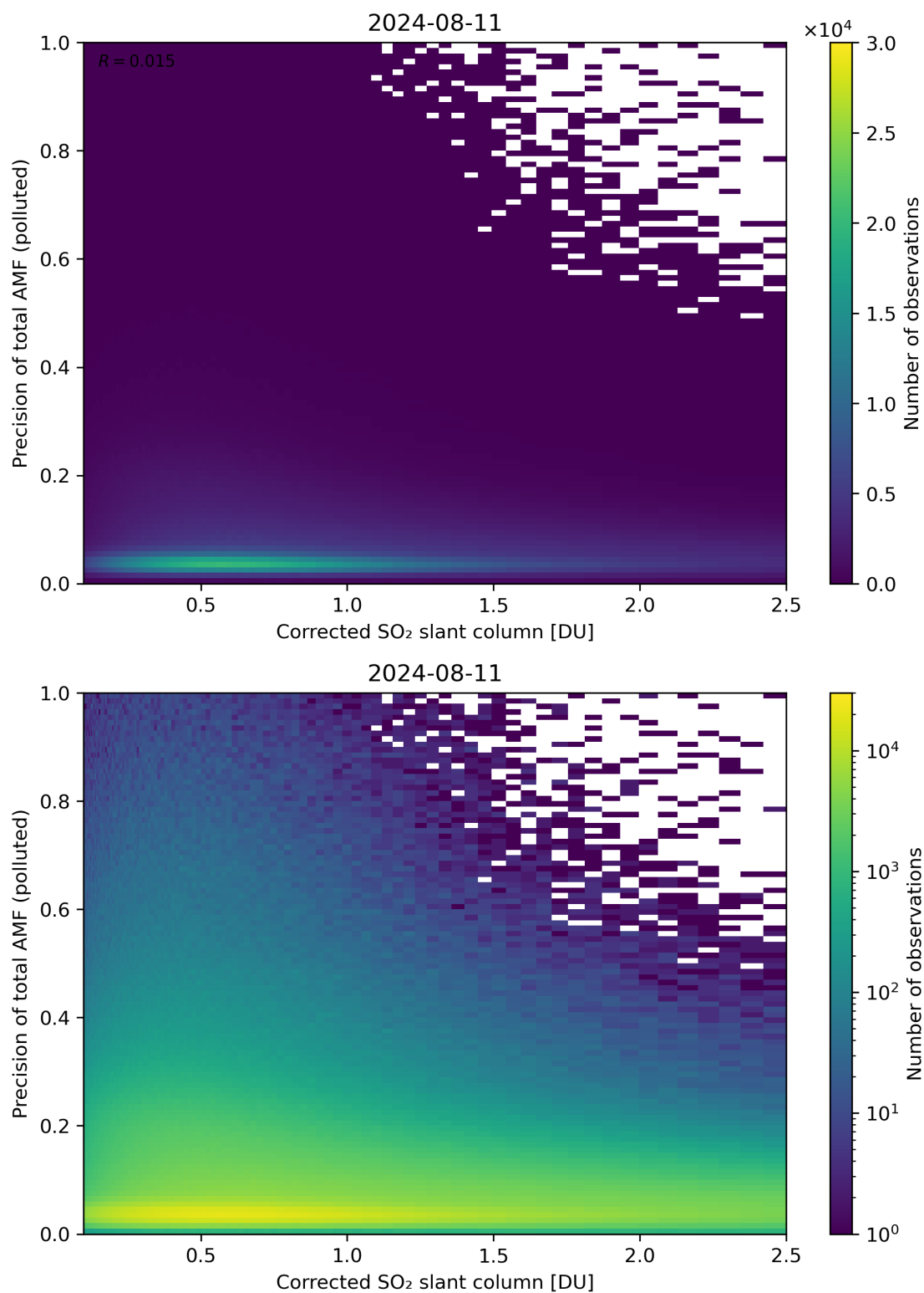
Figure 193: Scatter density plot of “Corrected SO 2 slant column” against “Precision of total AMF (polluted)” for 2024-08-11 to 2024-08-11.
