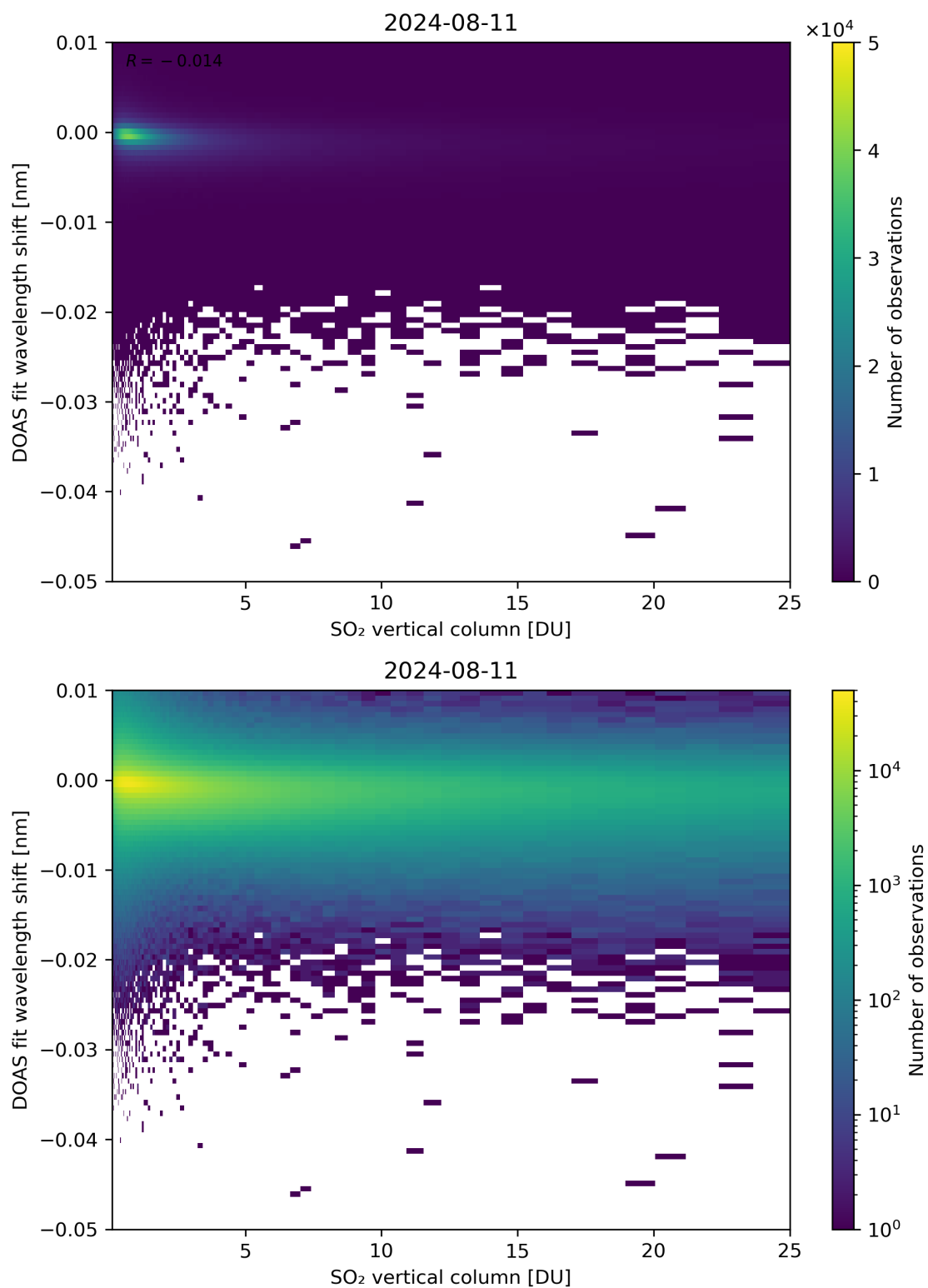
Figure 276: Scatter density plot of “SO 2 vertical column” against “DOAS fit wavelength shift” for 2024-08-11 to 2024-08-11.
