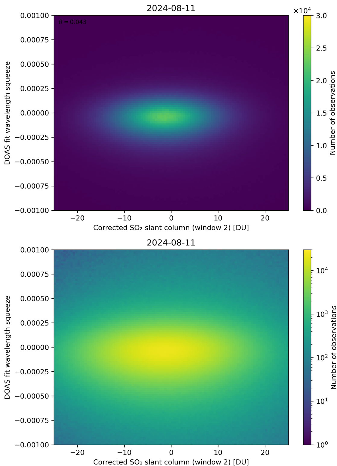
Figure 197: Scatter density plot of “Corrected SO 2 slant column (window 2)” against “DOAS fit wavelength squeeze” for 2024-08-11 to 2024-08-11.
