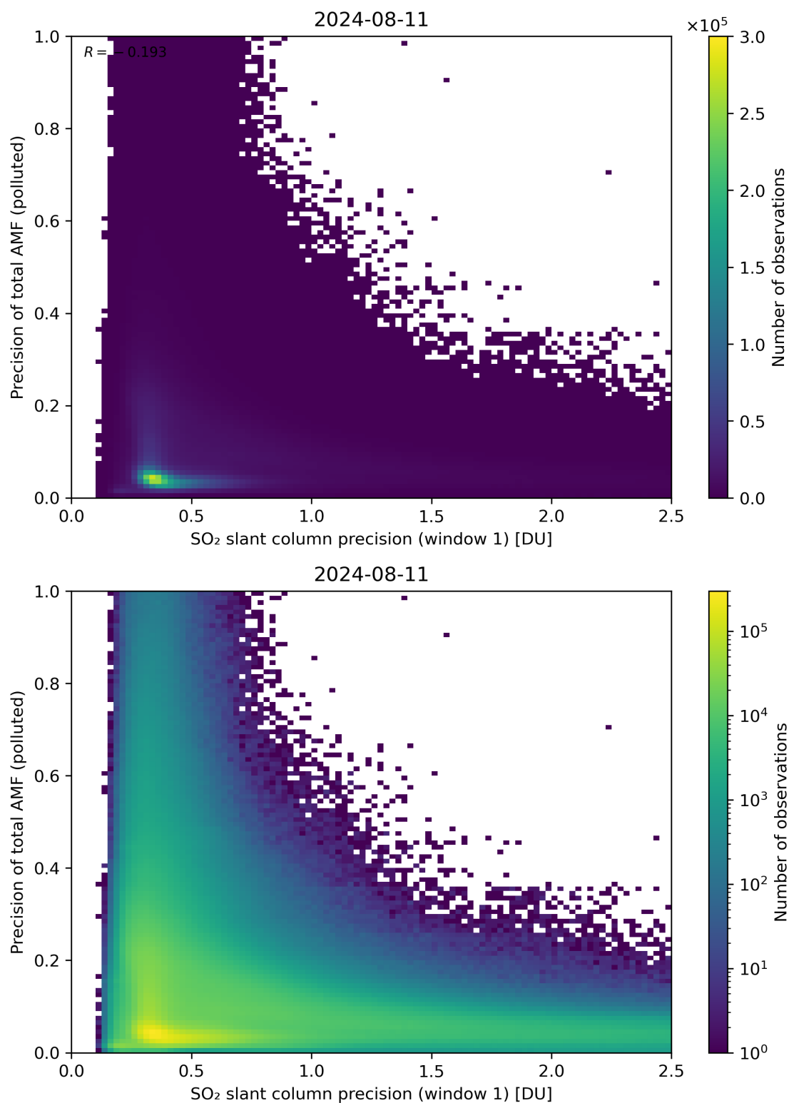
Figure 231: Scatter density plot of “SO 2 slant column precision (window 1)” against “Precision of total AMF (polluted)” for 2024-08-11 to 2024-08-11.
