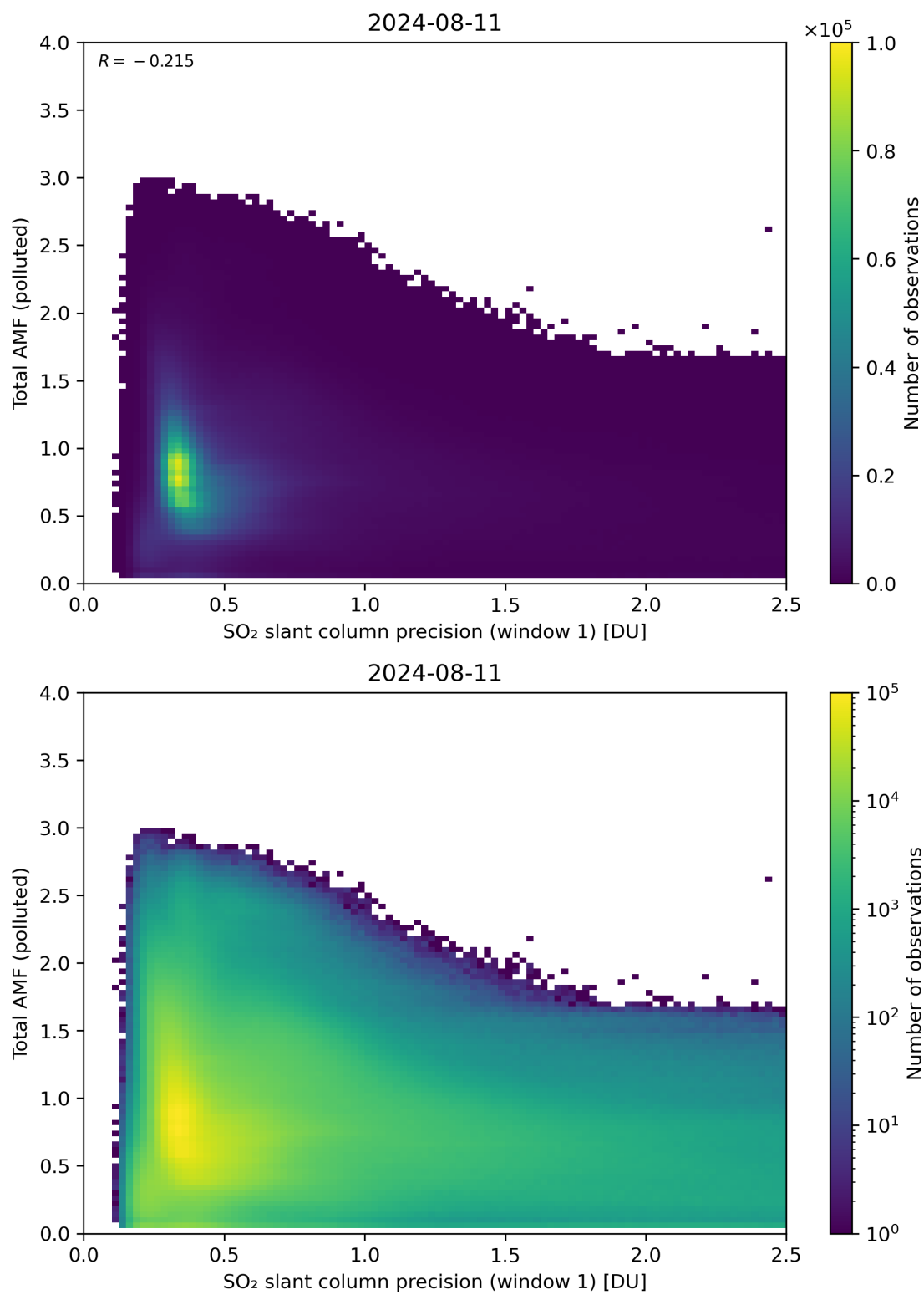
Figure 230: Scatter density plot of “SO 2 slant column precision (window 1)” against “Total AMF (polluted)” for 2024-08-11 to 2024-08-11.
