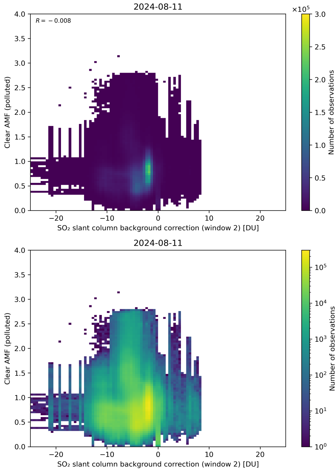
Figure 115: Scatter density plot of “SO 2 slant column background correction (window 2)” against “Clear AMF (polluted)” for 2024-08-11 to 2024-08-11.
