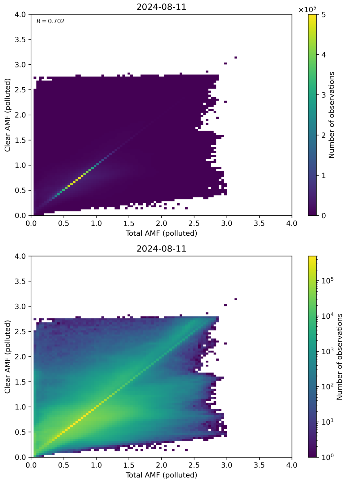
Figure 271: Scatter density plot of “Total AMF (polluted)” against “Clear AMF (polluted)” for 2024-08-11 to 2024-08-11.
