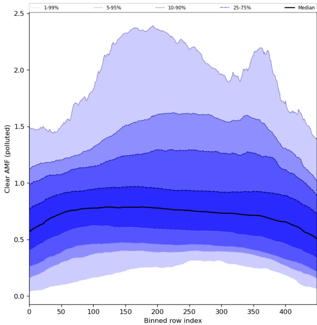
Figure 96: Along track statistics of “Clear AMF (polluted)” for 2024-08-11 to 2024-08-11
