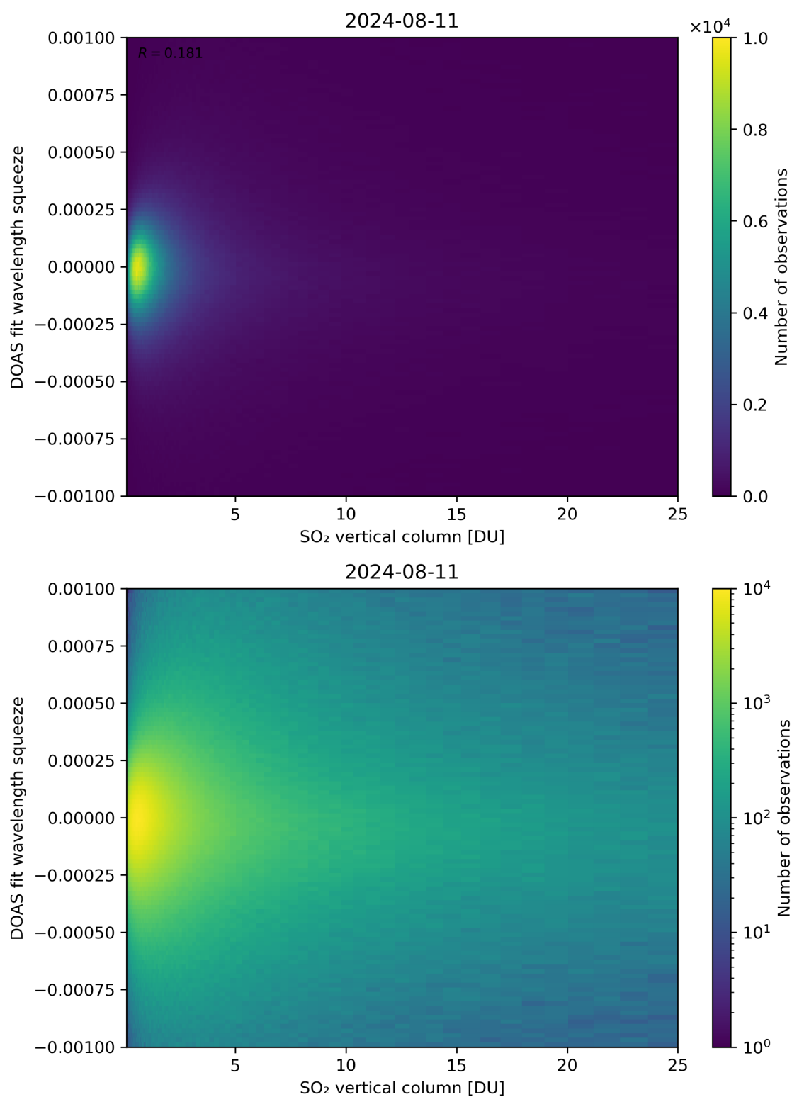
Figure 277: Scatter density plot of “SO 2 vertical column” against “DOAS fit wavelength squeeze” for 2024-08-11 to 2024-08-11.
