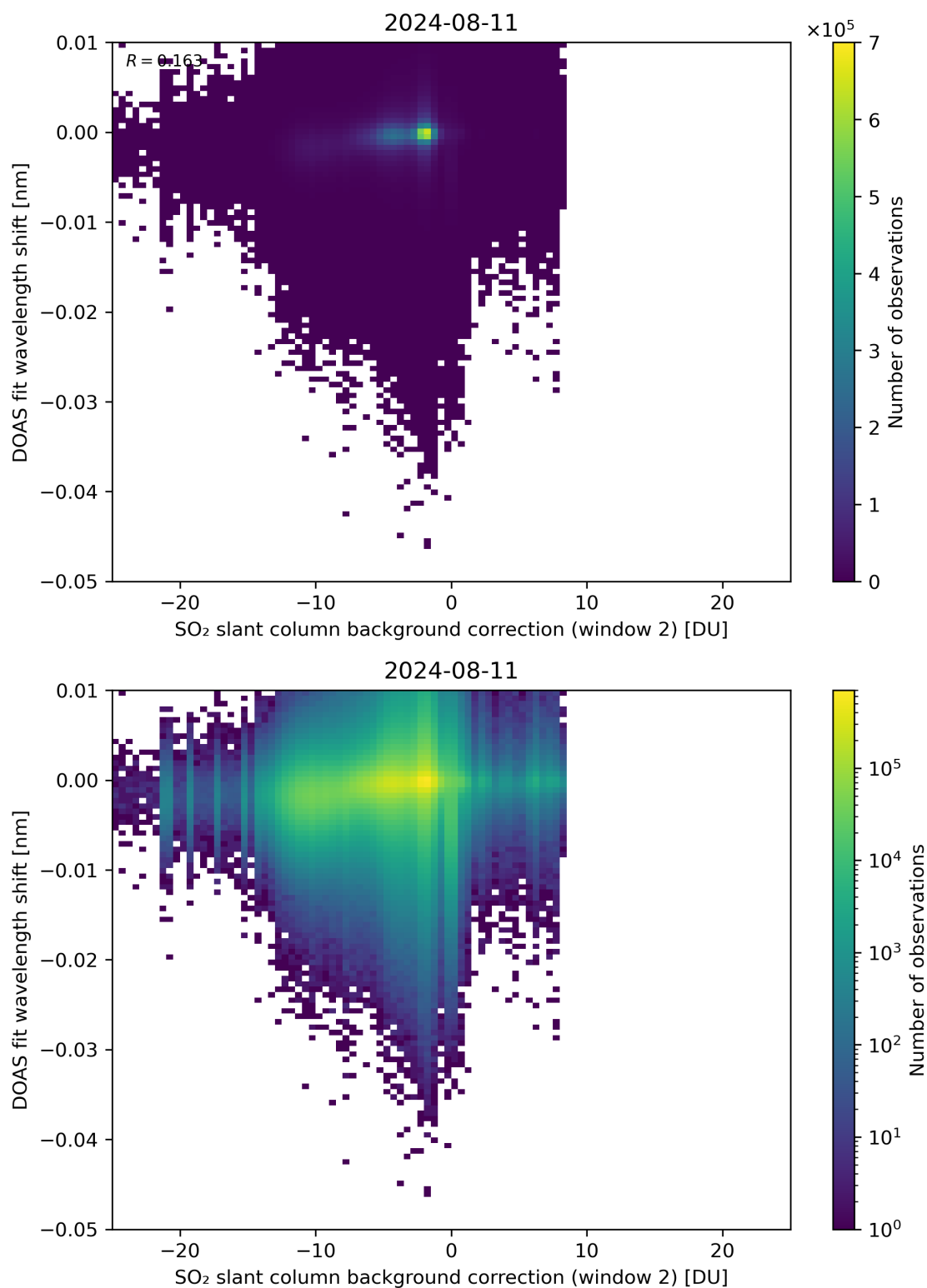
Figure 112: Scatter density plot of “SO 2 slant column background correction (window 2)” against “DOAS fit wavelength shift” for 2024-08-11 to 2024-08-11.
