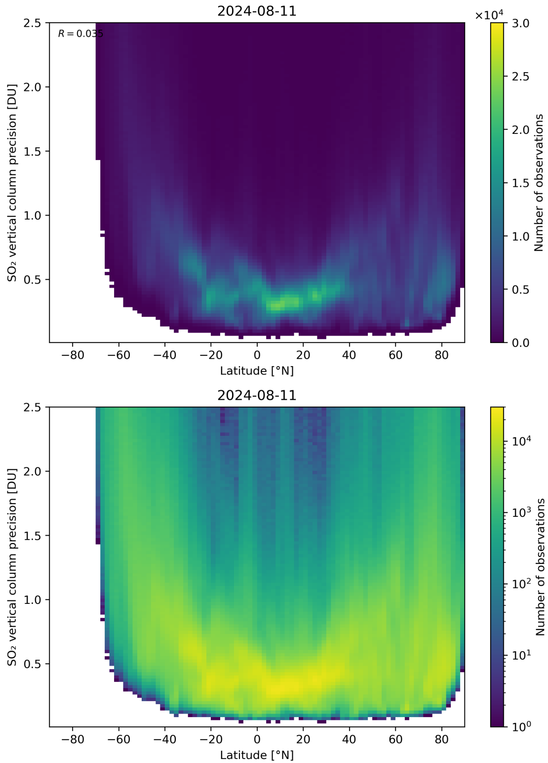
Figure 157: Scatter density plot of “Latitude” against “SO 2 vertical column precision” for 2024-08-11 to 2024-08-11.
