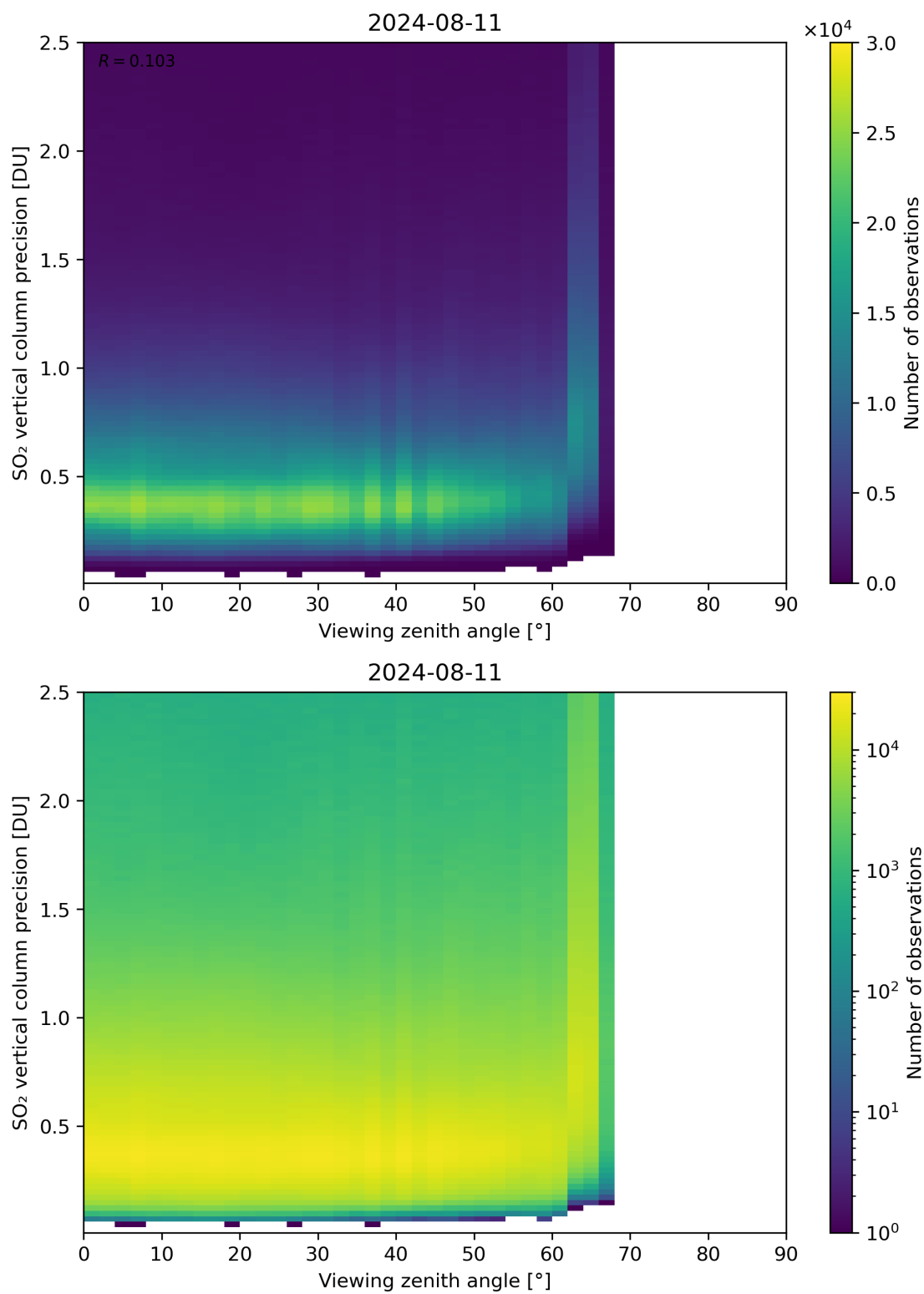
Figure 328: Scatter density plot of “Viewing zenith angle” against “SO 2 vertical column precision” for 2024-08-11 to 2024-08-11.
