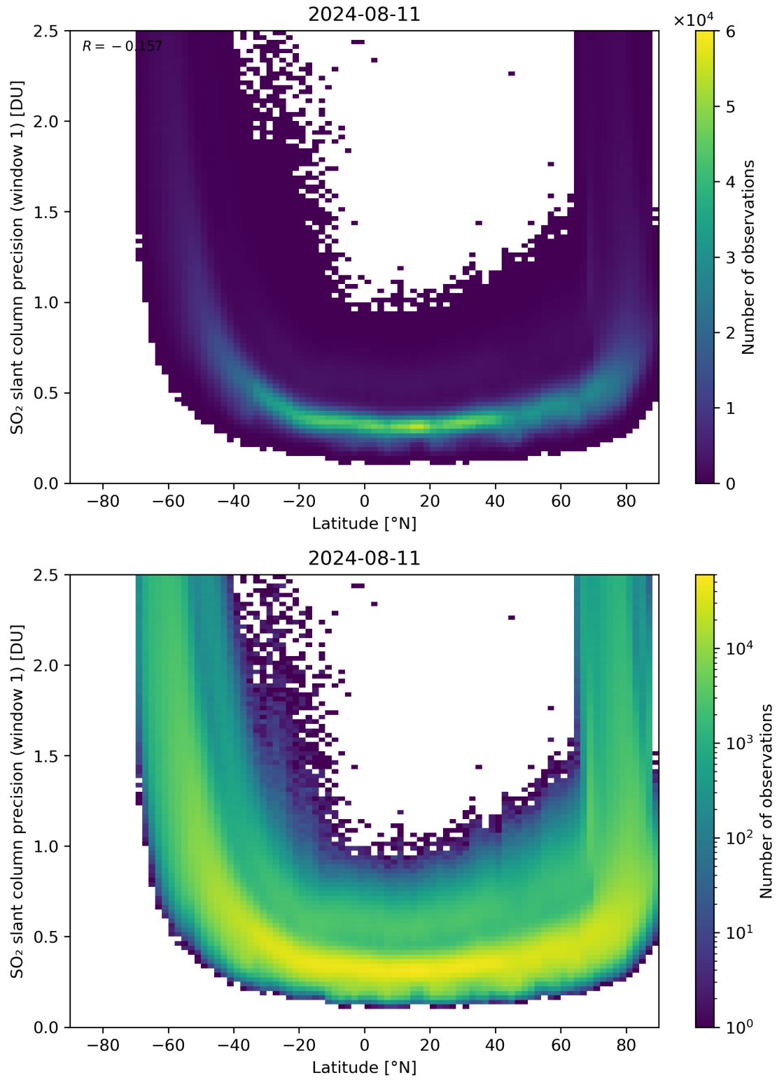
Figure 150: Scatter density plot of “Latitude” against “SO 2 slant column precision (window 1)” for 2024-08-11 to 2024-08-11.
