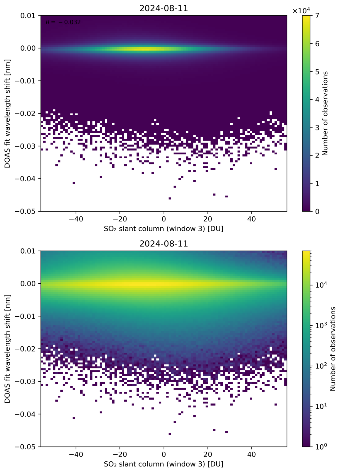
Figure 254: Scatter density plot of “SO 2 slant column (window 3)” against “DOAS fit wavelength shift” for 2024-08-11 to 2024-08-11.
