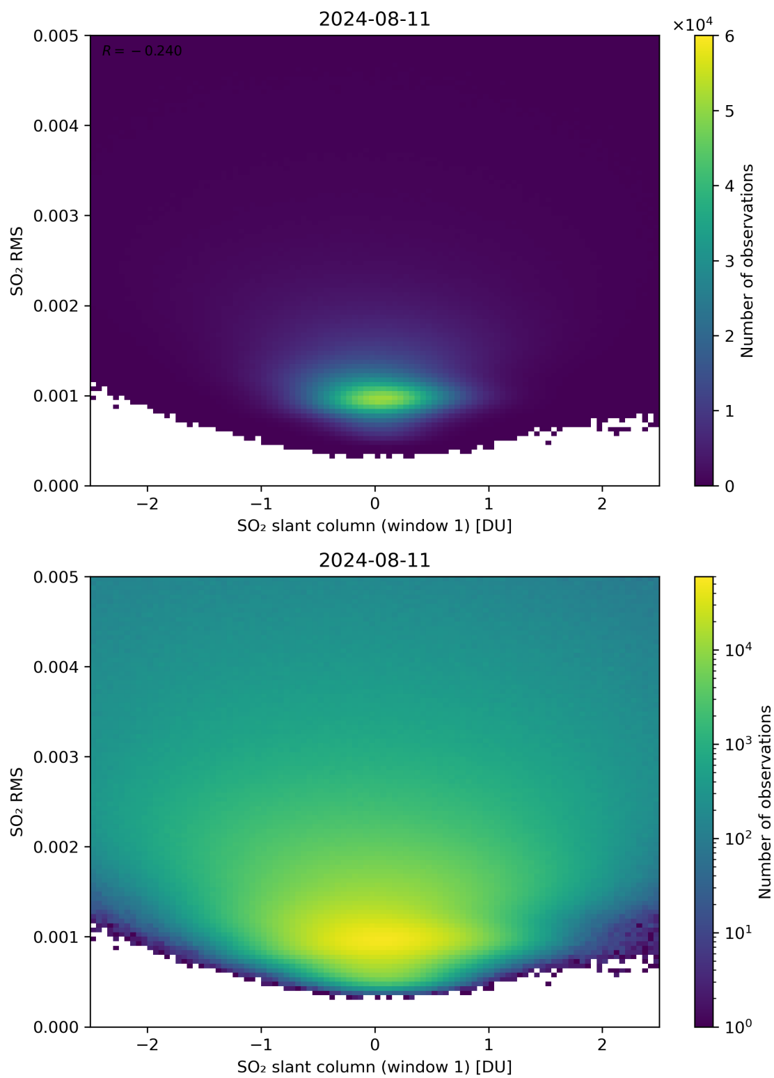
Figure 217: Scatter density plot of “SO 2 slant column (window 1)” against “SO 2 RMS” for 2024-08-11 to 2024-08-11.
