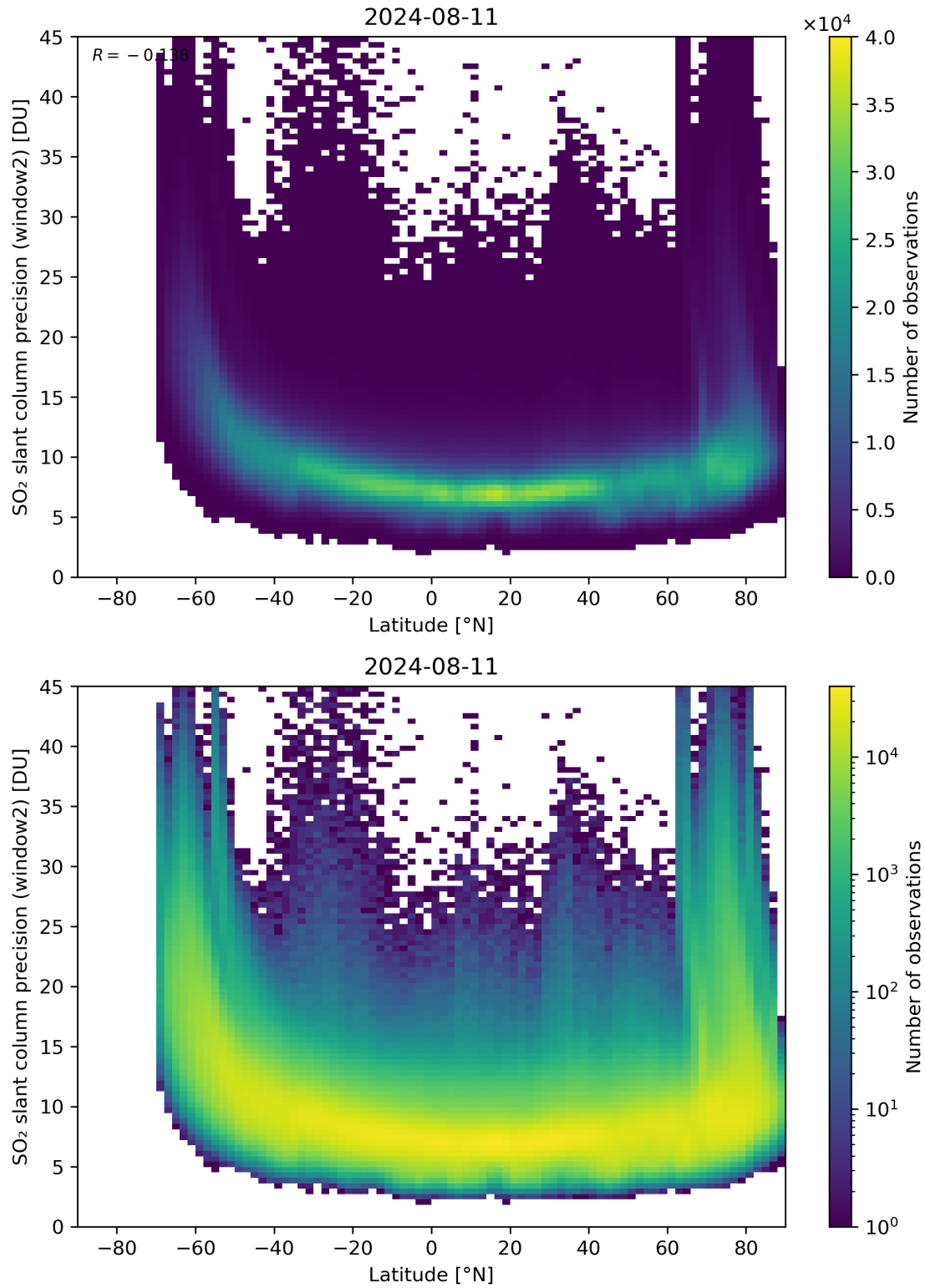
Figure 151: Scatter density plot of “Latitude” against “SO 2 slant column precision (window2)” for 2024-08-11 to 2024-08-11.
