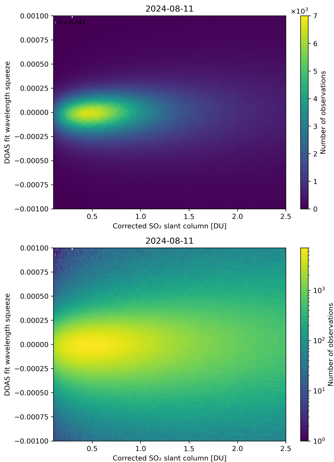
Figure 182: Scatter density plot of “Corrected SO 2 slant column” against “DOAS fit wavelength squeeze” for 2024-08-11 to 2024-08-11.
