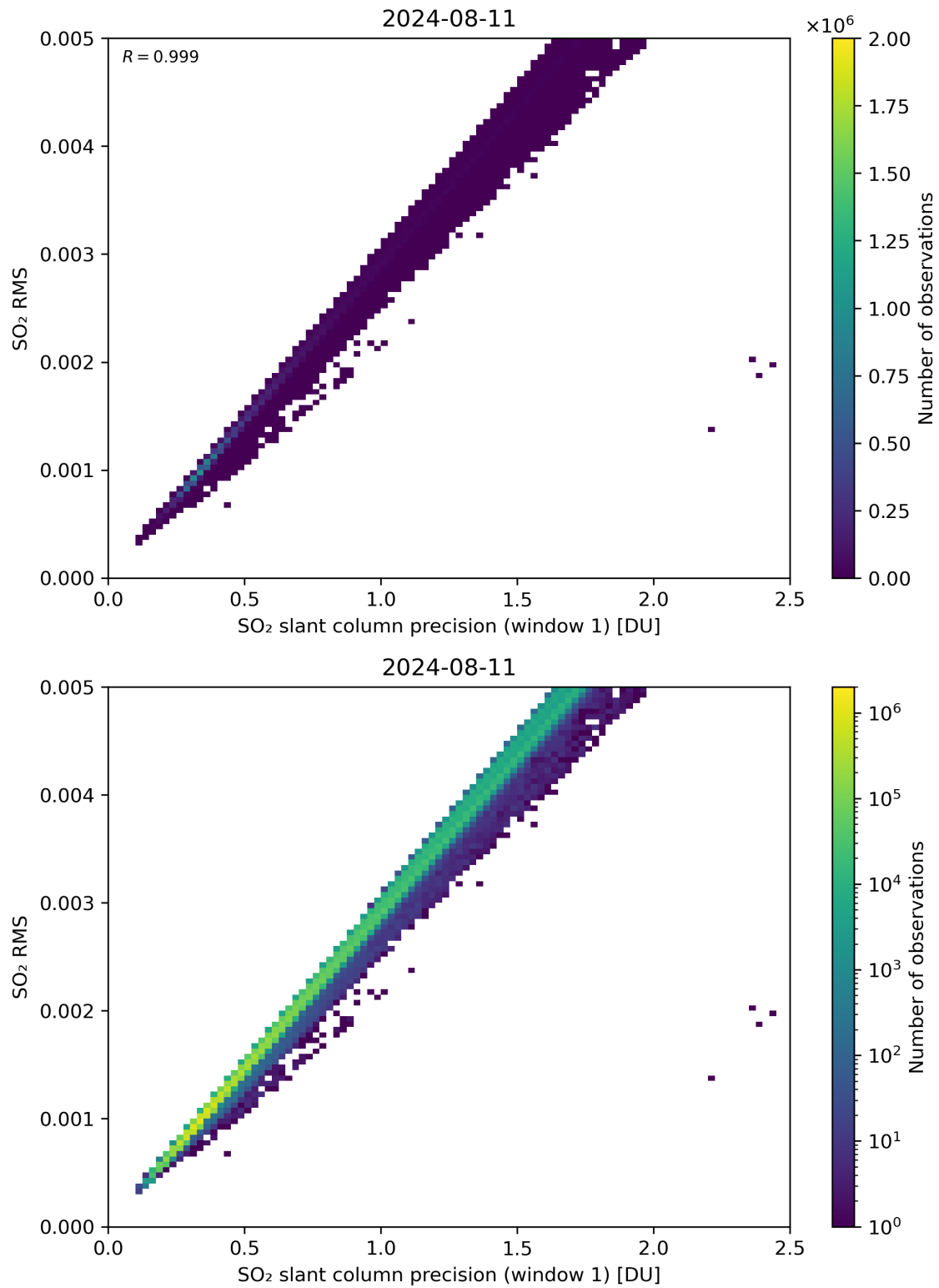
Figure 223: Scatter density plot of “SO 2 slant column precision (window 1)” against “SO 2 RMS” for 2024-08-11 to 2024-08-11.
