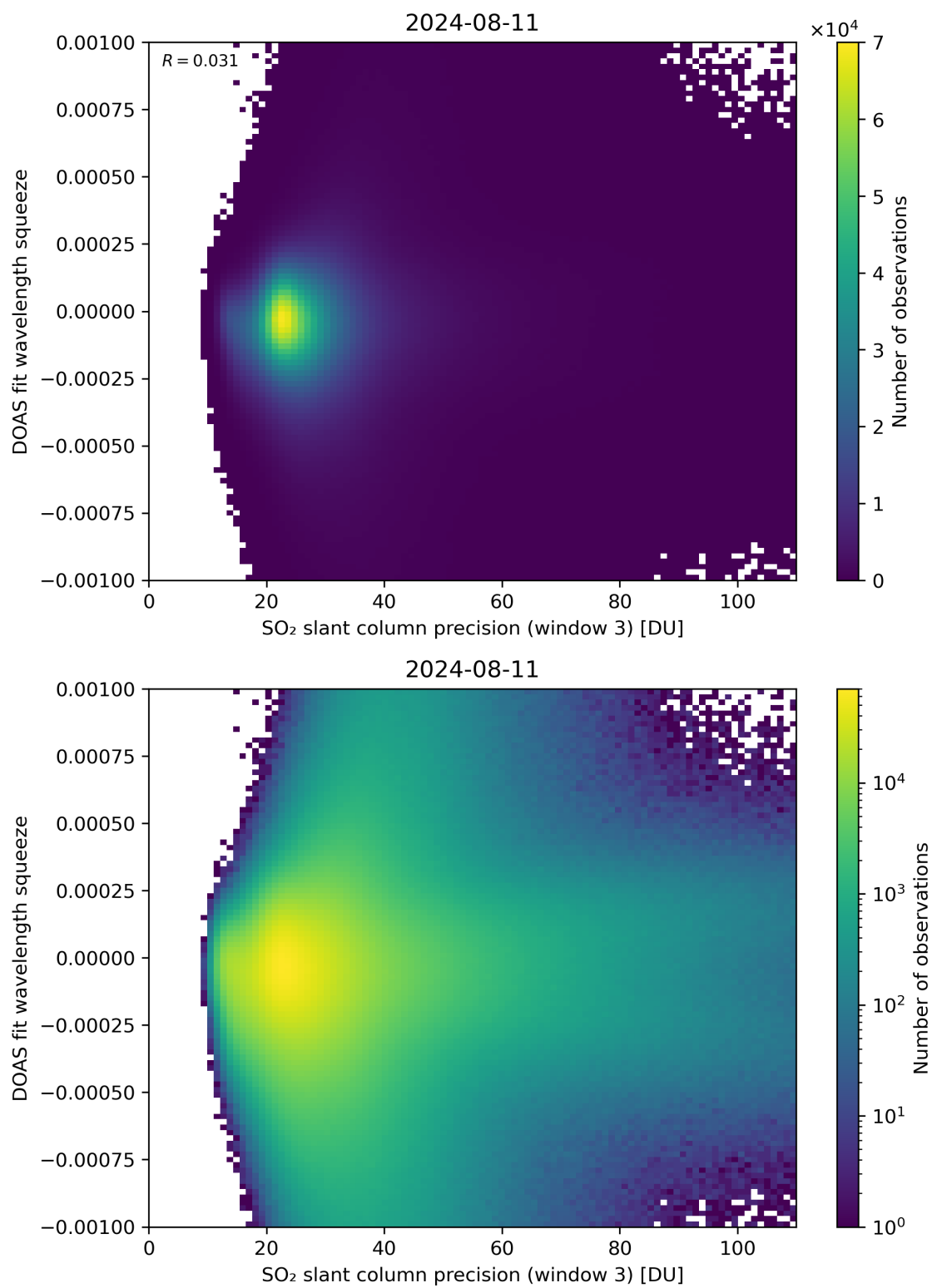
Figure 259: Scatter density plot of “SO 2 slant column precision (window 3)” against “DOAS fit wavelength squeeze” for 2024-08-11 to 2024-08-11.
