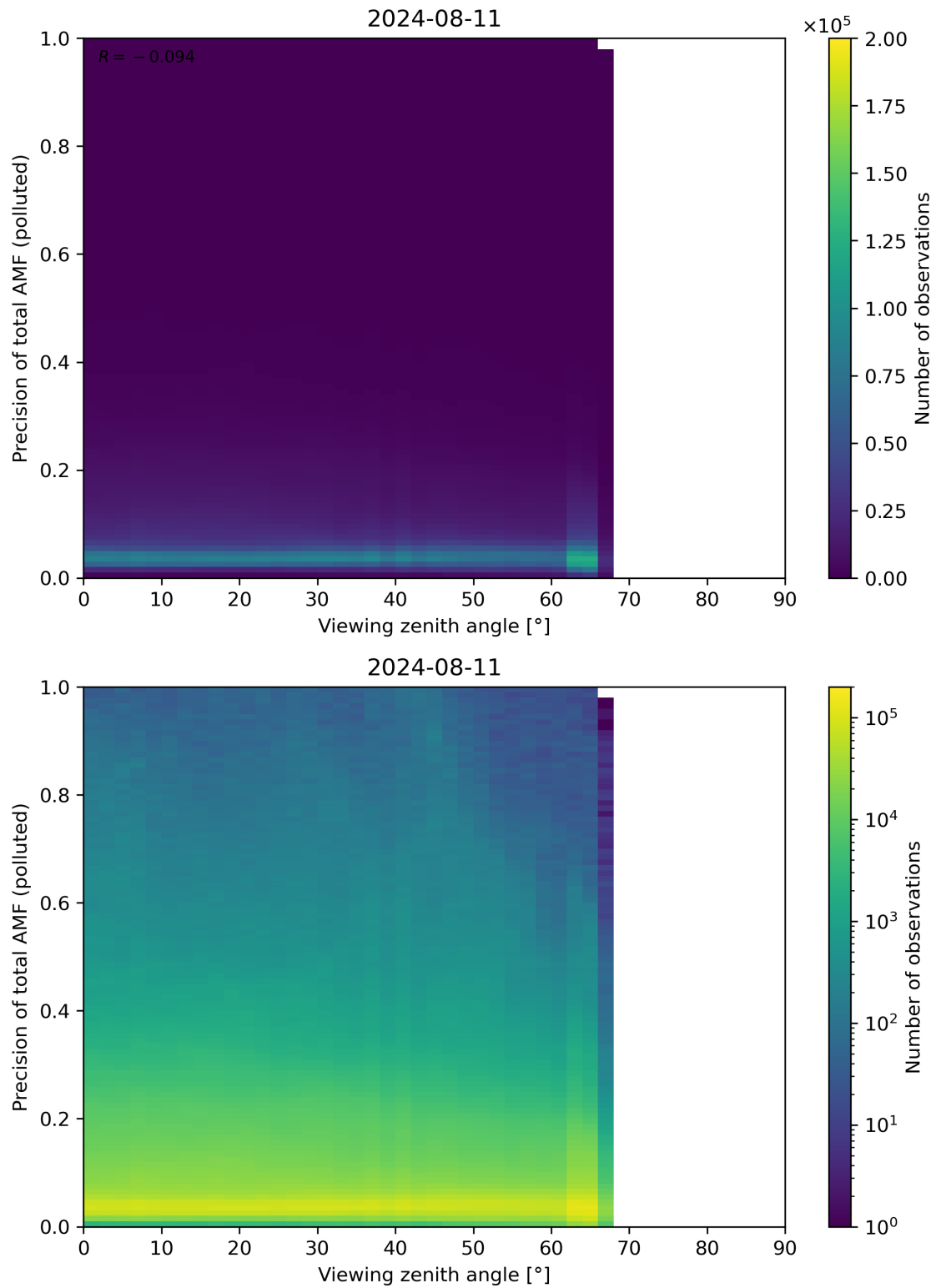
Figure 326: Scatter density plot of “Viewing zenith angle” against “Precision of total AMF (polluted)” for 2024-08-11 to 2024-08-11.
