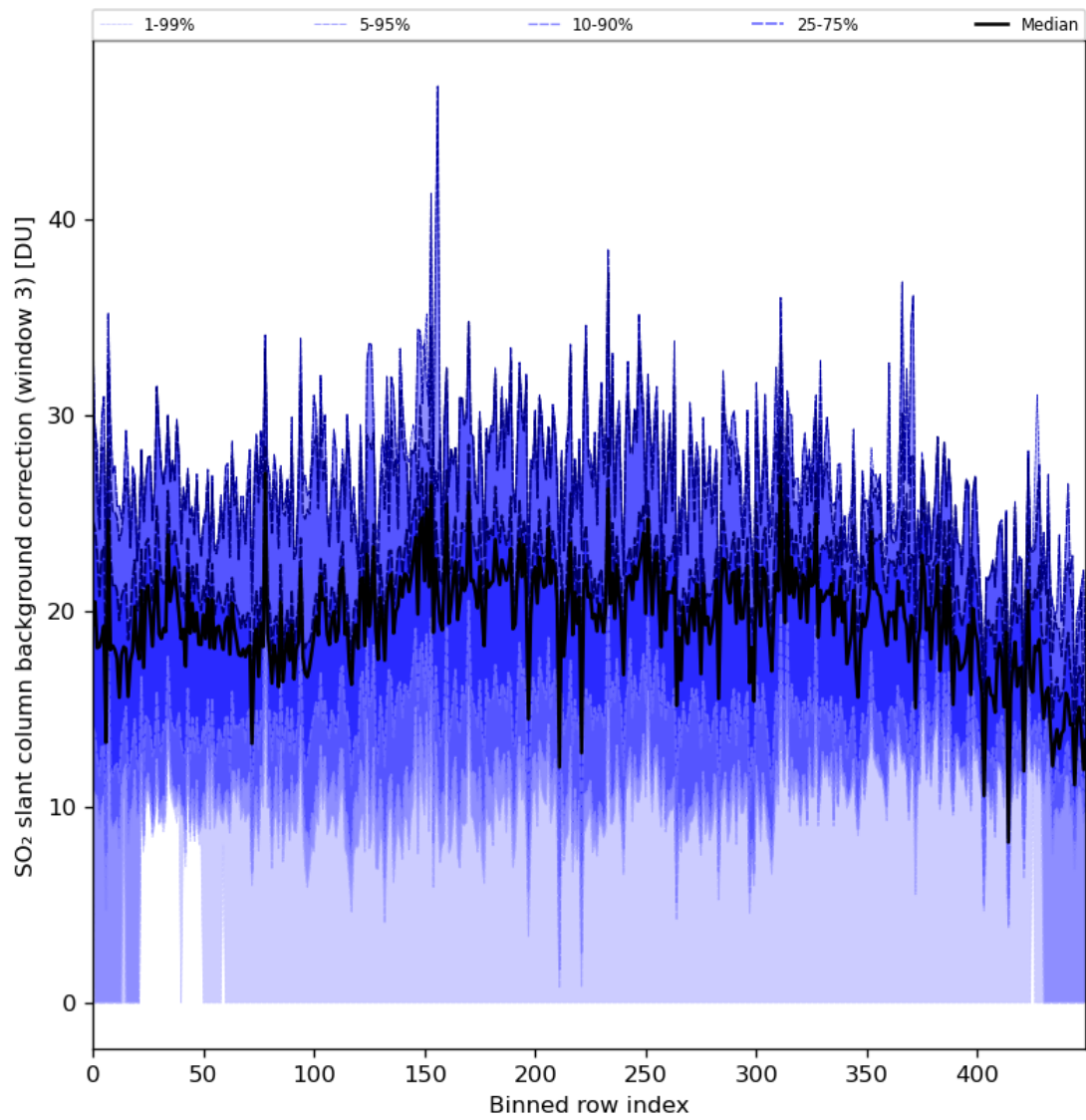
Figure 90: Along track statistics of “SO 2 slant column background correction (window 3)” for 2024-08-11 to 2024-08-11
