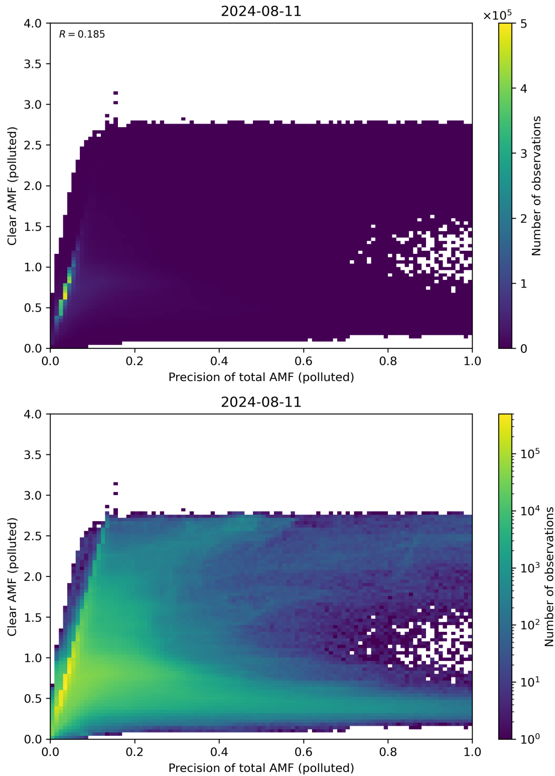
Figure 270: Scatter density plot of “Precision of total AMF (polluted)” against “Clear AMF (polluted)” for 2024-08-11 to 2024-08-11.
