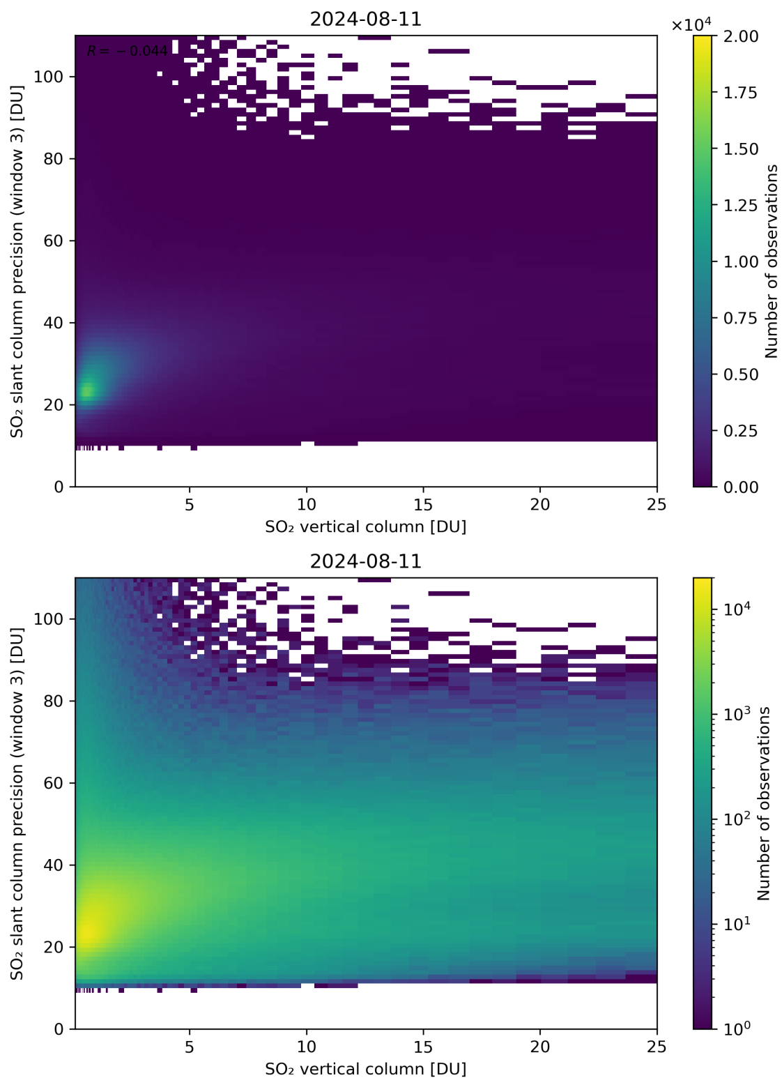
Figure 304: Scatter density plot of “SO 2 vertical column” against “SO 2 slant column precision (window 3)” for 2024-08-11 to 2024-08-11.
