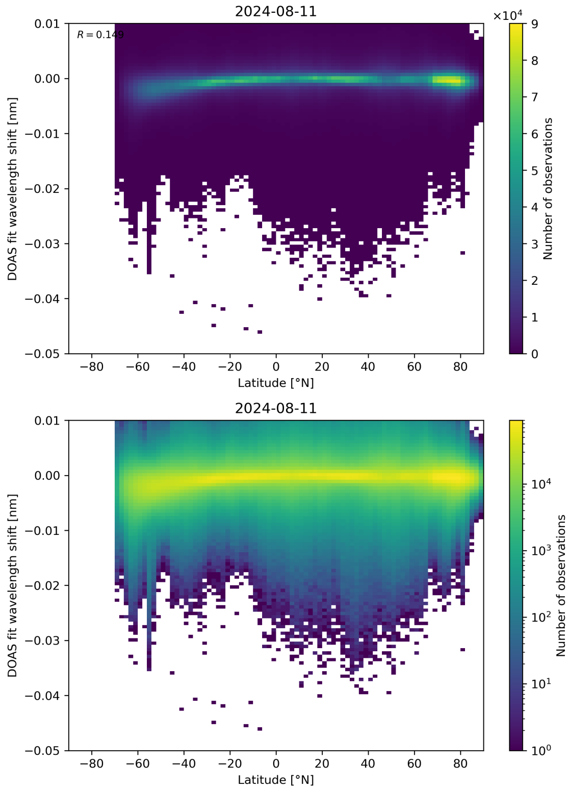
Figure 142: Scatter density plot of “Latitude” against “DOAS fit wavelength shift” for 2024-08-11 to 2024-08-11.
