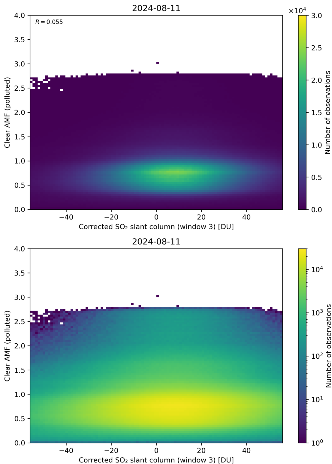
Figure 209: Scatter density plot of “Corrected SO 2 slant column (window 3)” against “Clear AMF (polluted)” for 2024-08-11 to 2024-08-11.
