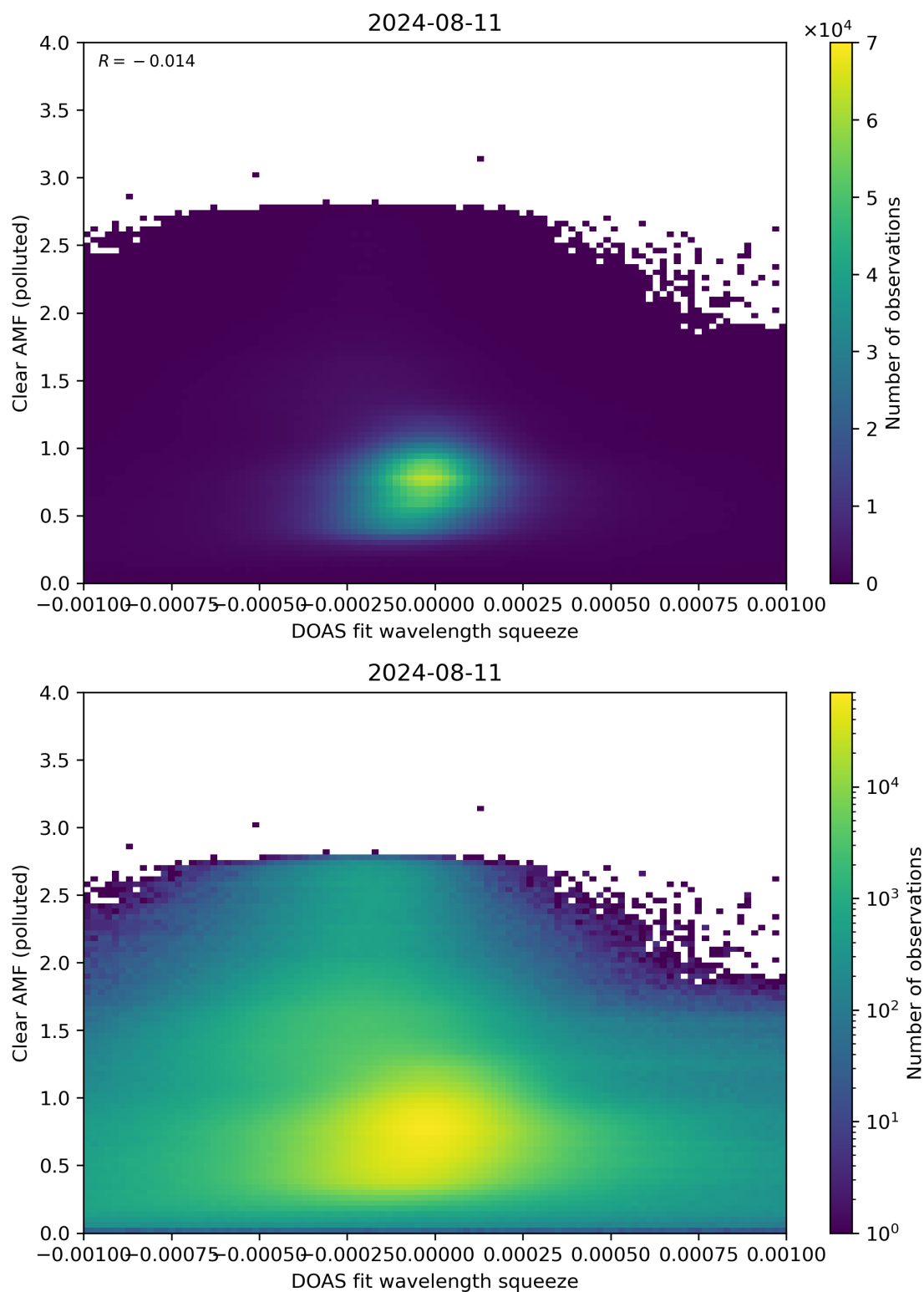
Figure 133: Scatter density plot of “DOAS fit wavelength squeeze” against “Clear AMF (polluted)” for 2024-08-11 to 2024-08-11.
