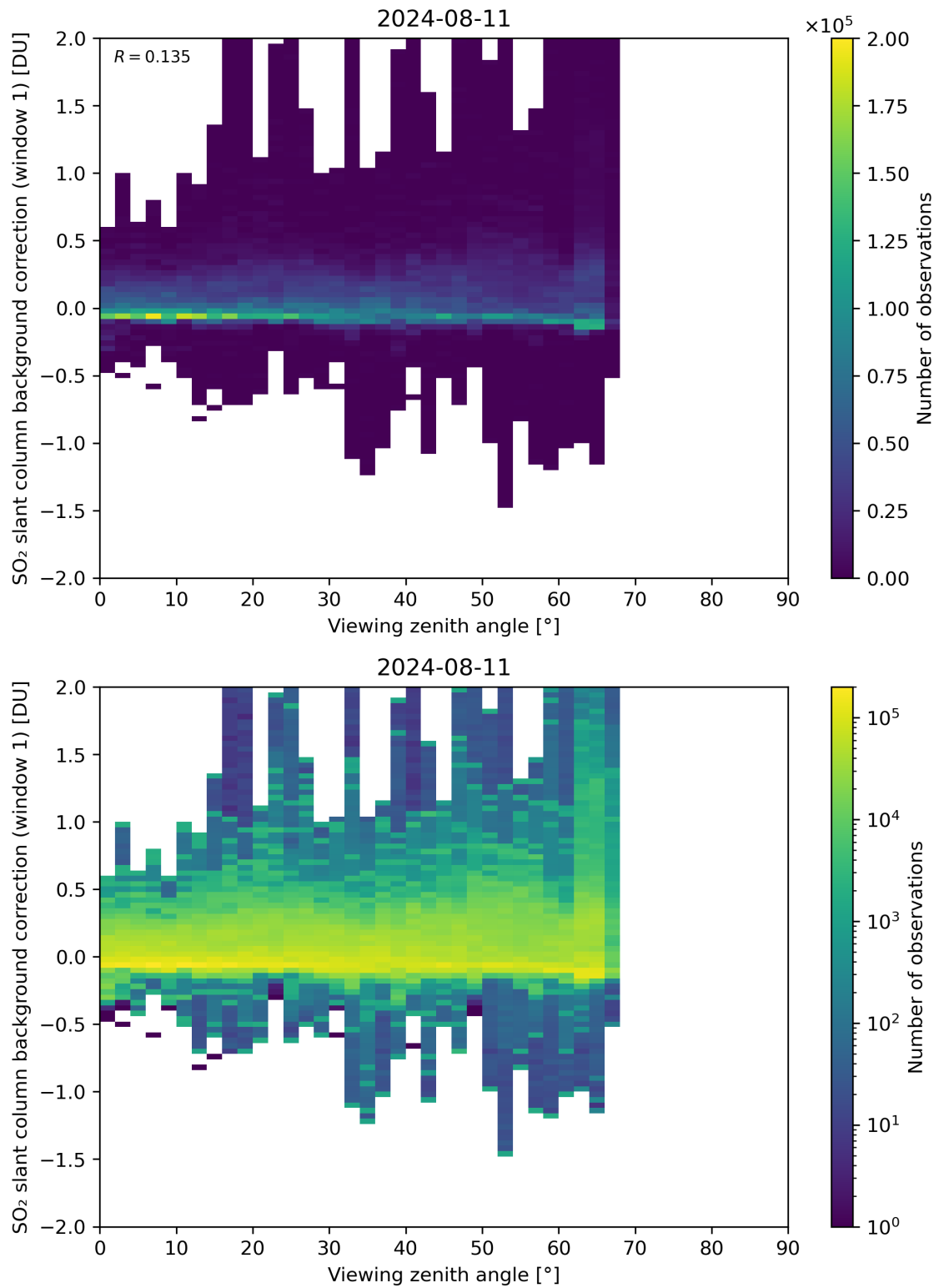
Figure 308: Scatter density plot of “Viewing zenith angle” against “SO 2 slant column background correction (window 1)” for 2024-08-11 to 2024-08-11.
