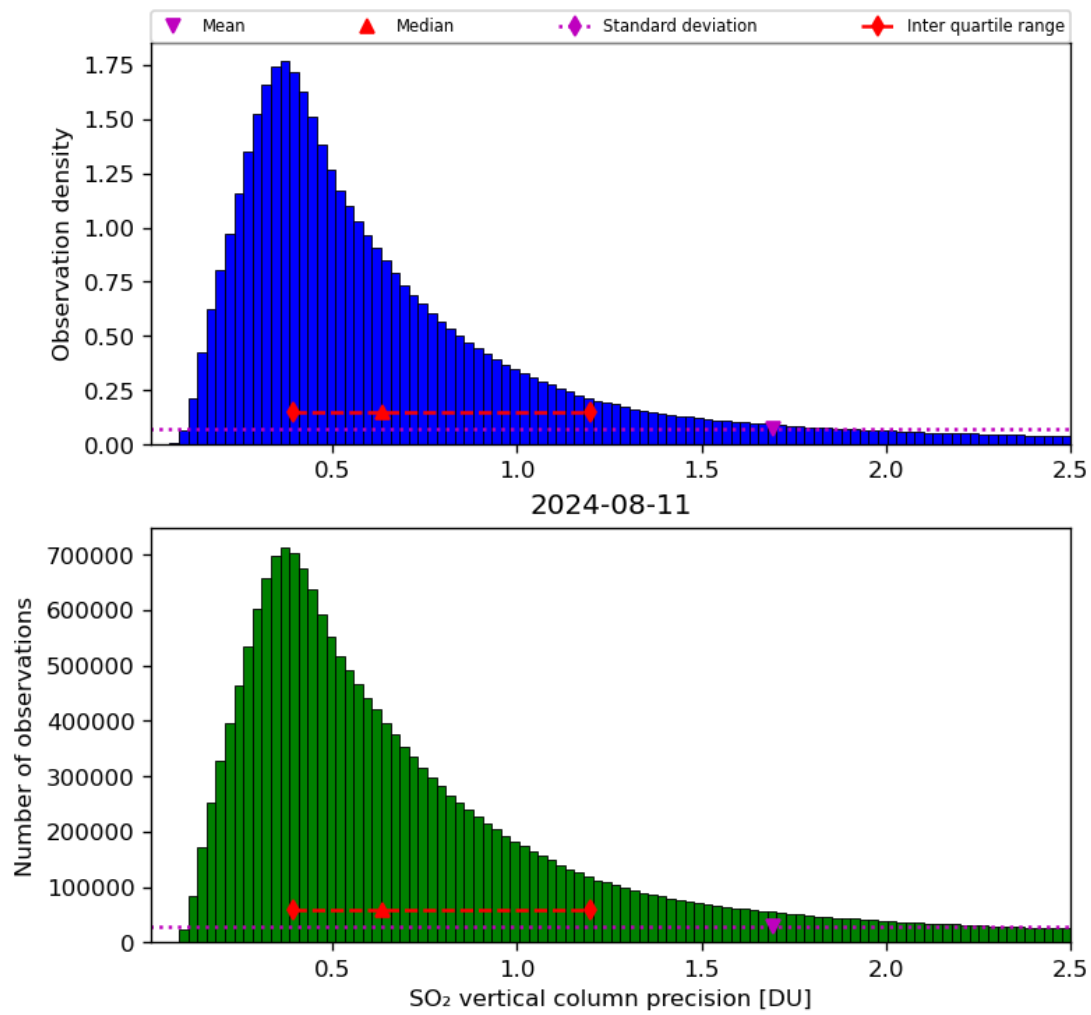
Figure 54: Histogram of “SO 2 vertical column precision” for 2024-08-11 to 2024-08-11
