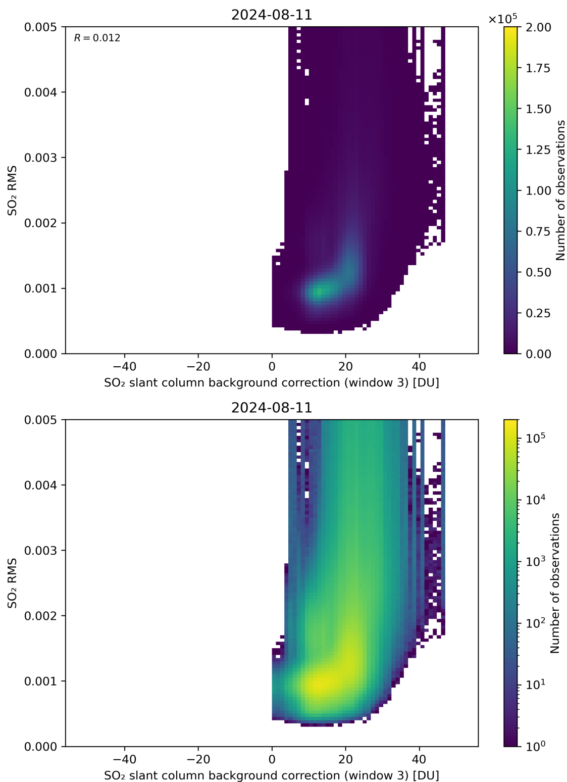
Figure 123: Scatter density plot of “SO 2 slant column background correction (window 3)” against “SO 2 RMS” for 2024-08-11 to 2024-08-11.
