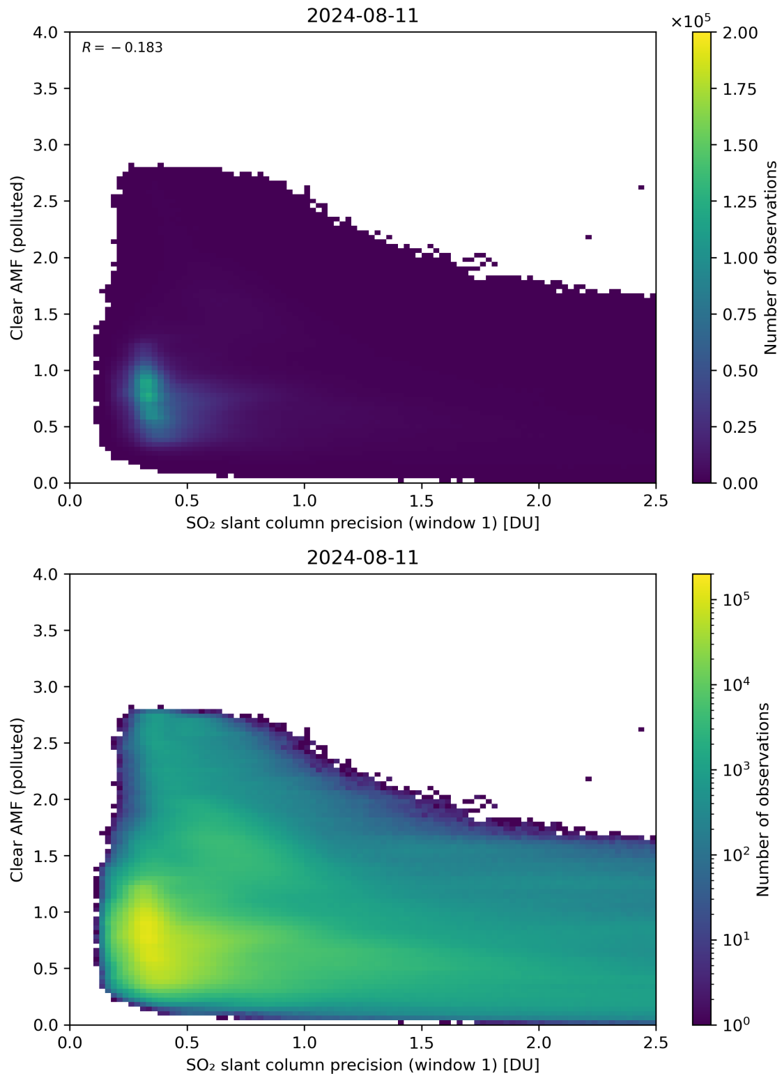
Figure 224: Scatter density plot of “SO 2 slant column precision (window 1)” against “Clear AMF (polluted)” for 2024-08-11 to 2024-08-11.
