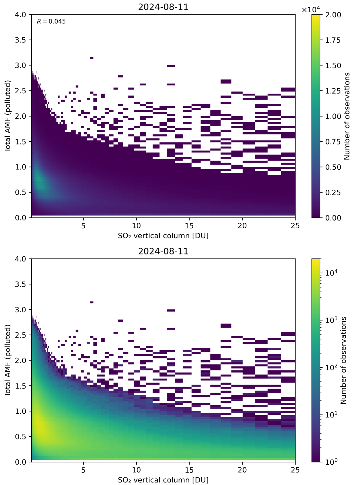
Figure 305: Scatter density plot of “SO 2 vertical column” against “Total AMF (polluted)” for 2024-08-11 to 2024-08-11.
