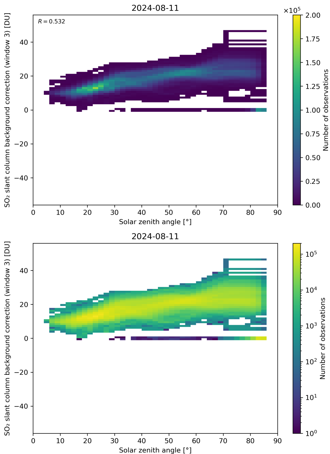
Figure 160: Scatter density plot of “Solar zenith angle” against “SO 2 slant column background correction (window 3)” for 2024-08-11 to 2024-08-11.
