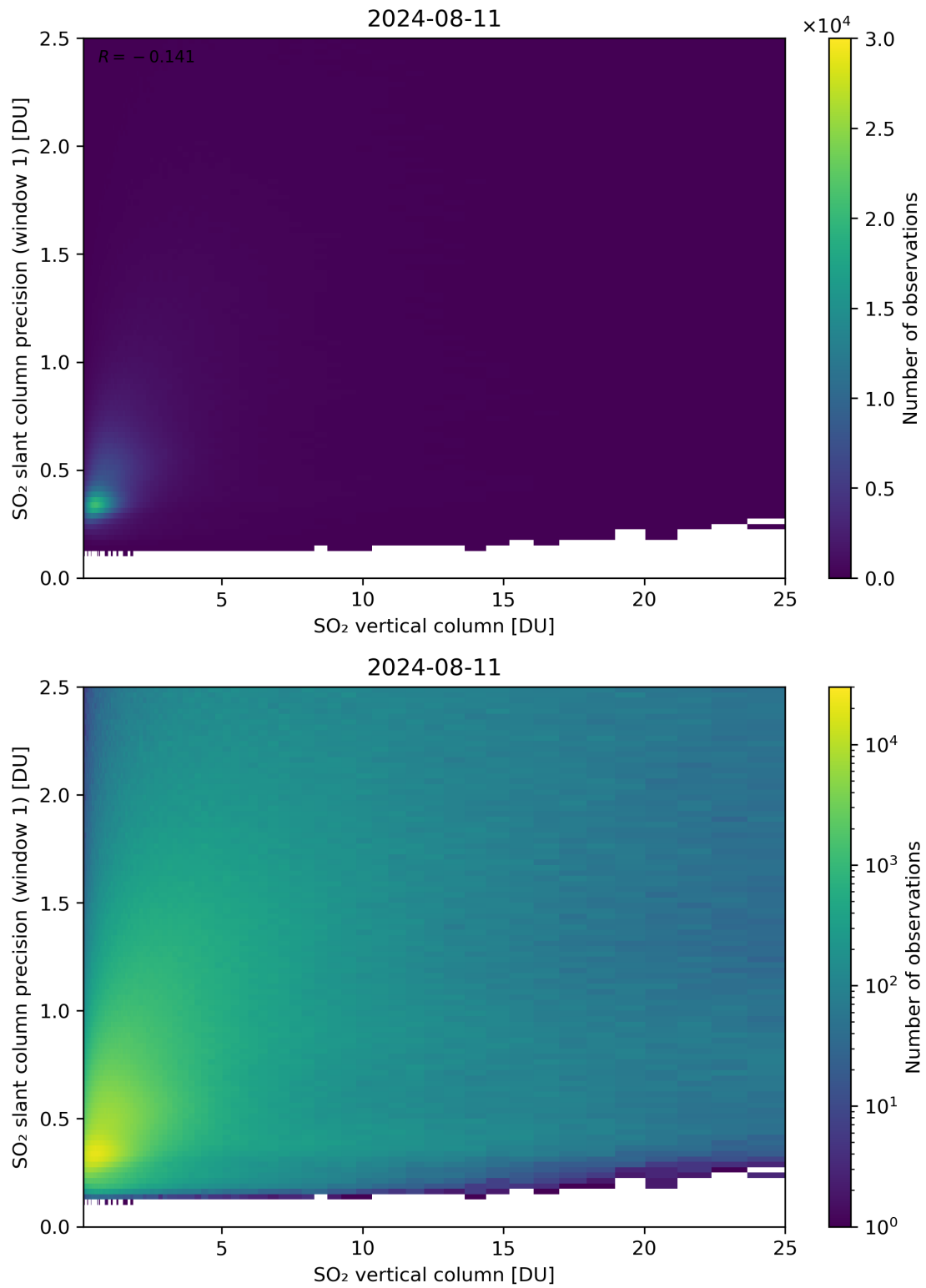
Figure 301: Scatter density plot of “SO 2 vertical column” against “SO 2 slant column precision (window 1)” for 2024-08-11 to 2024-08-11.
