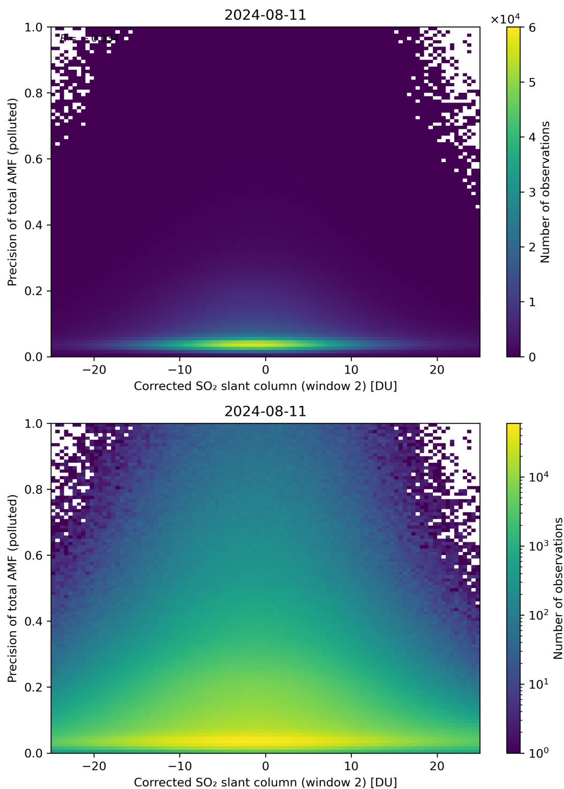
Figure 204: Scatter density plot of “Corrected SO 2 slant column (window 2)” against “Precision of total AMF (polluted)” for 2024-08-11 to 2024-08-11.
