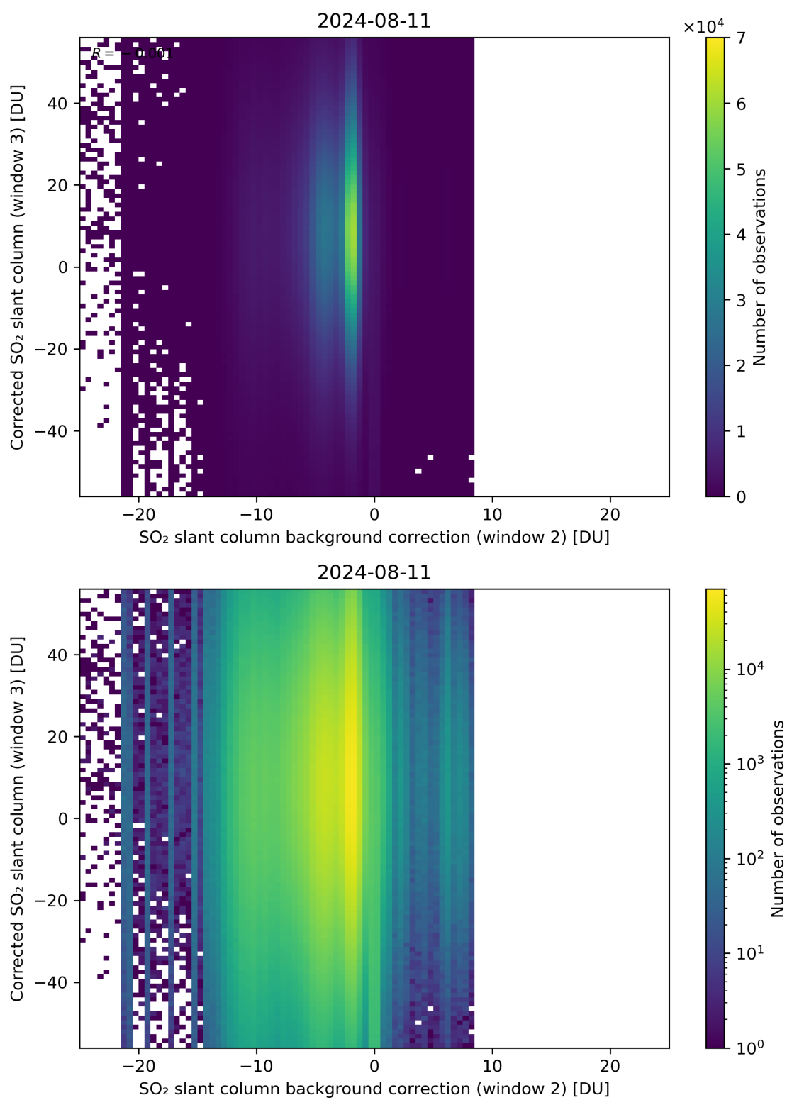
Figure 116: Scatter density plot of “SO 2 slant column background correction (window 2)” against “Corrected SO 2 slant column (window 3)” for 2024-08-11 to 2024-08-11.
