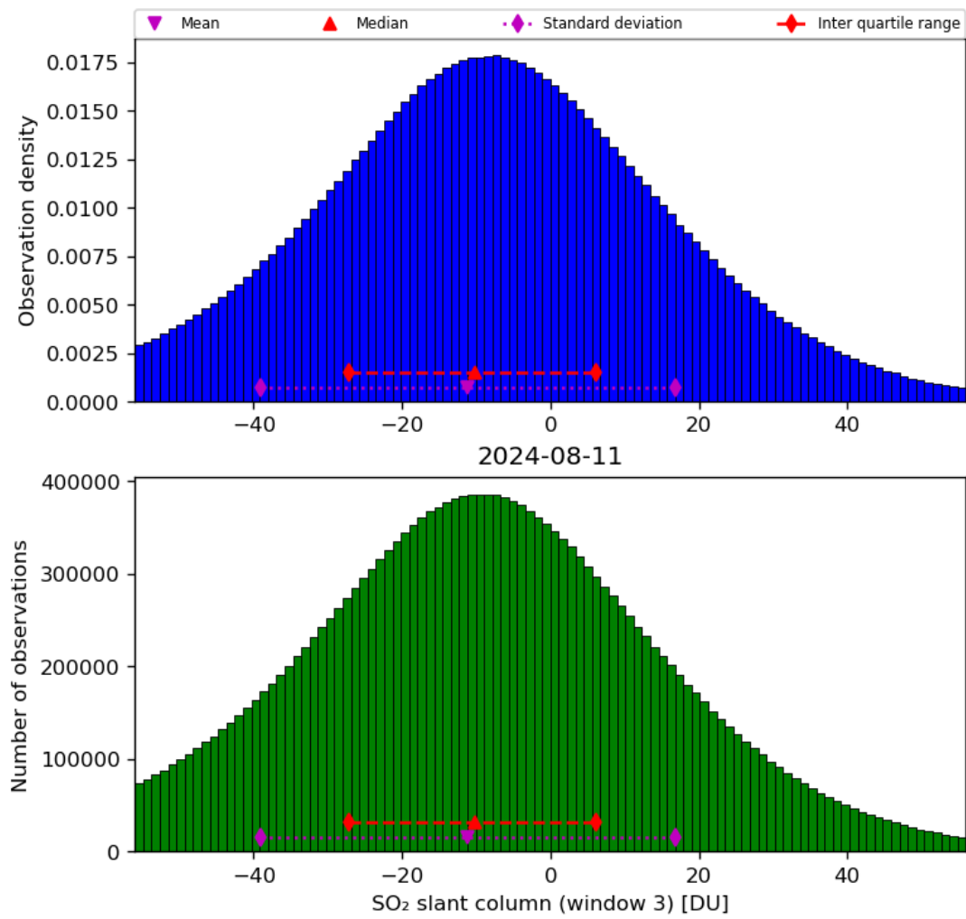
Figure 64: Histogram of “SO 2 slant column (window 3)” for 2024-08-11 to 2024-08-11
