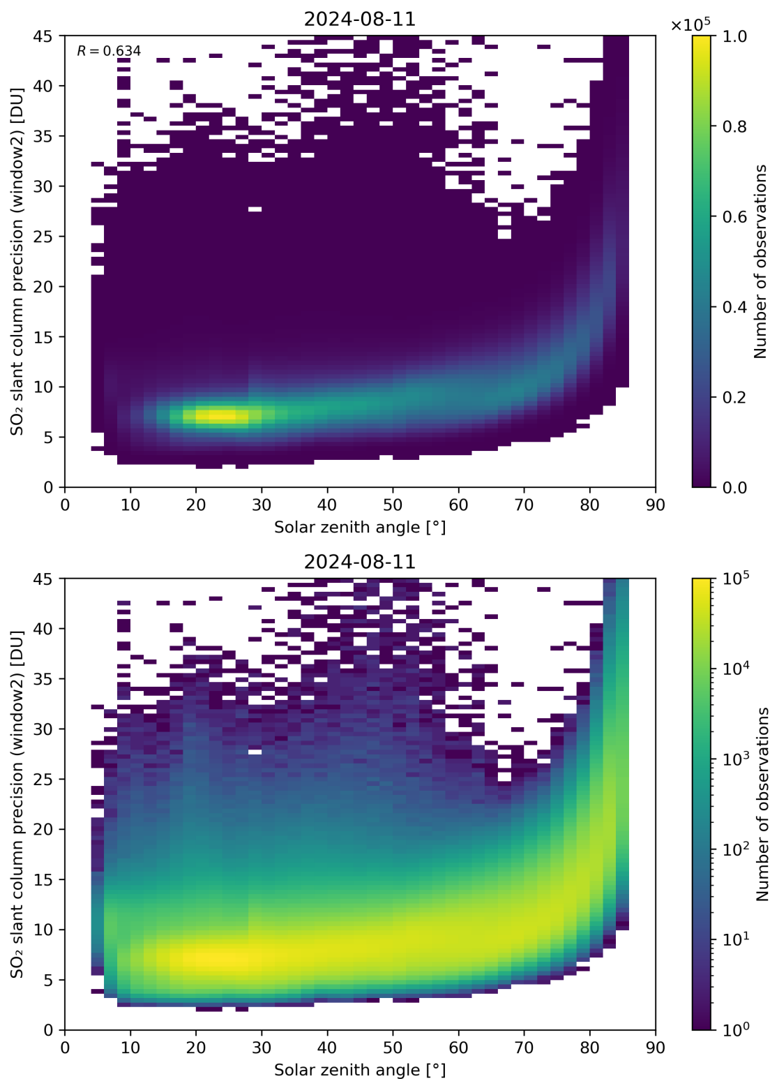
Figure 171: Scatter density plot of “Solar zenith angle” against “SO 2 slant column precision (window2)” for 2024-08-11 to 2024-08-11.
