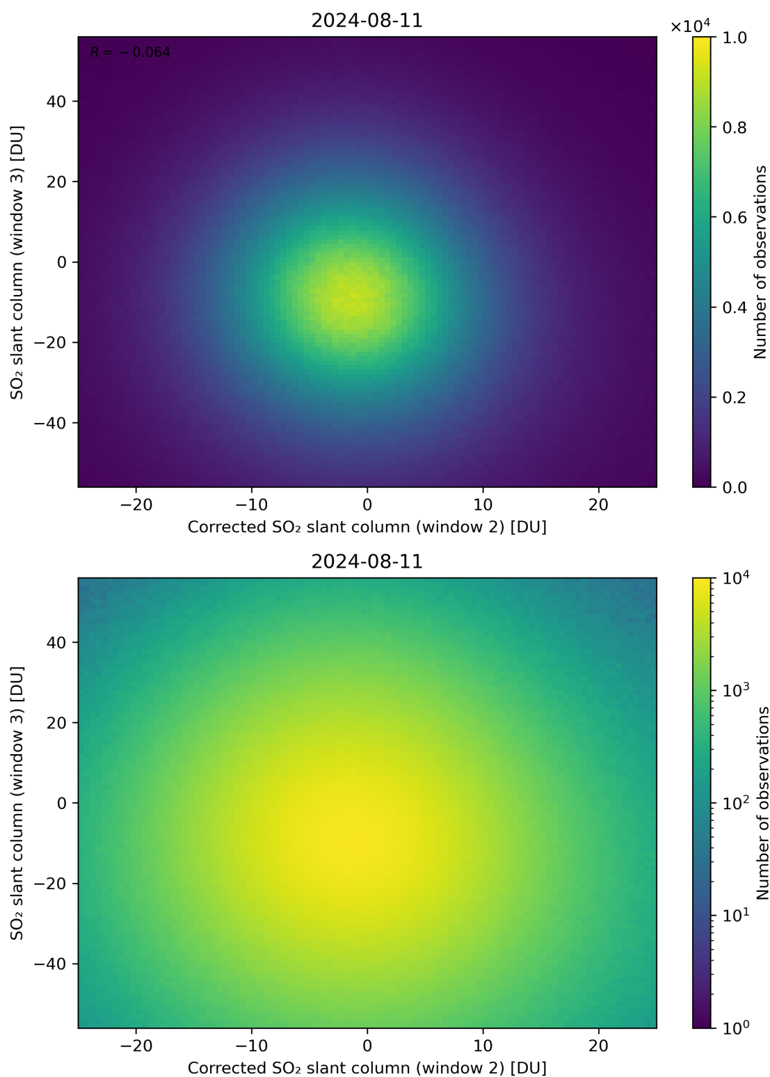
Figure 201: Scatter density plot of “Corrected SO 2 slant column (window 2)” against “SO 2 slant column (window 3)” for 2024-08-11 to 2024-08-11.
