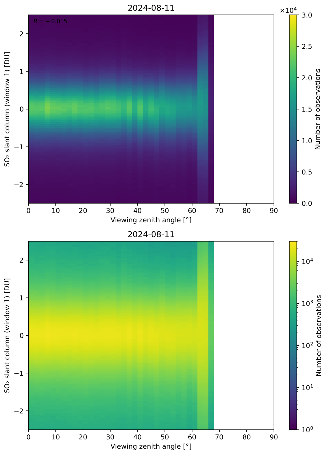
Figure 320: Scatter density plot of “Viewing zenith angle” against “SO 2 slant column (window 1)” for 2024-08-11 to 2024-08-11.
