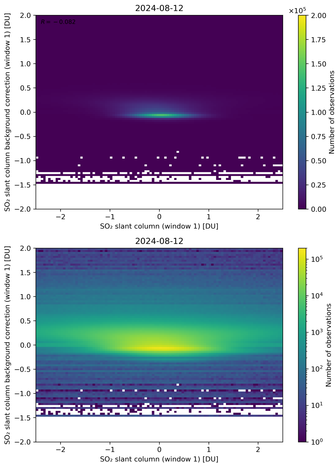
Figure 212: Scatter density plot of “SO 2 slant column (window 1)” against “SO 2 slant column background correction (window 1)” for 2024-08-12 to 2024-08-13.
