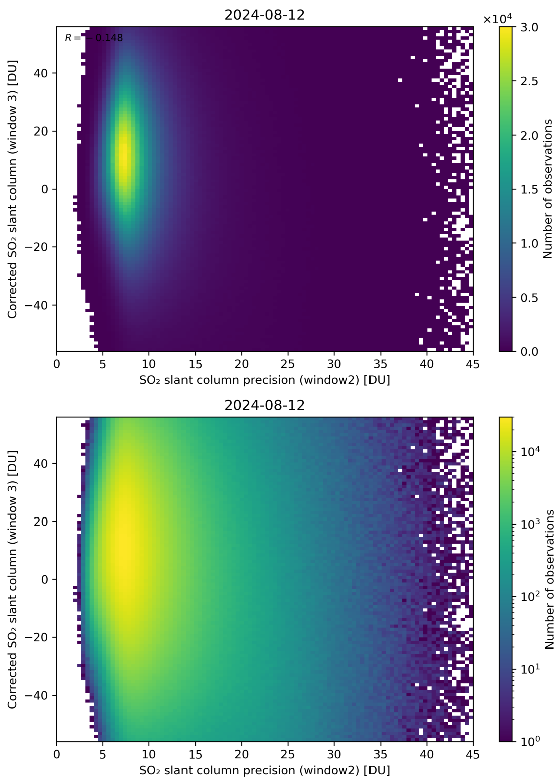
Figure 248: Scatter density plot of “SO 2 slant column precision (window2)” against “Corrected SO 2 slant column (window 3)” for 2024-08-12 to 2024-08-13.
