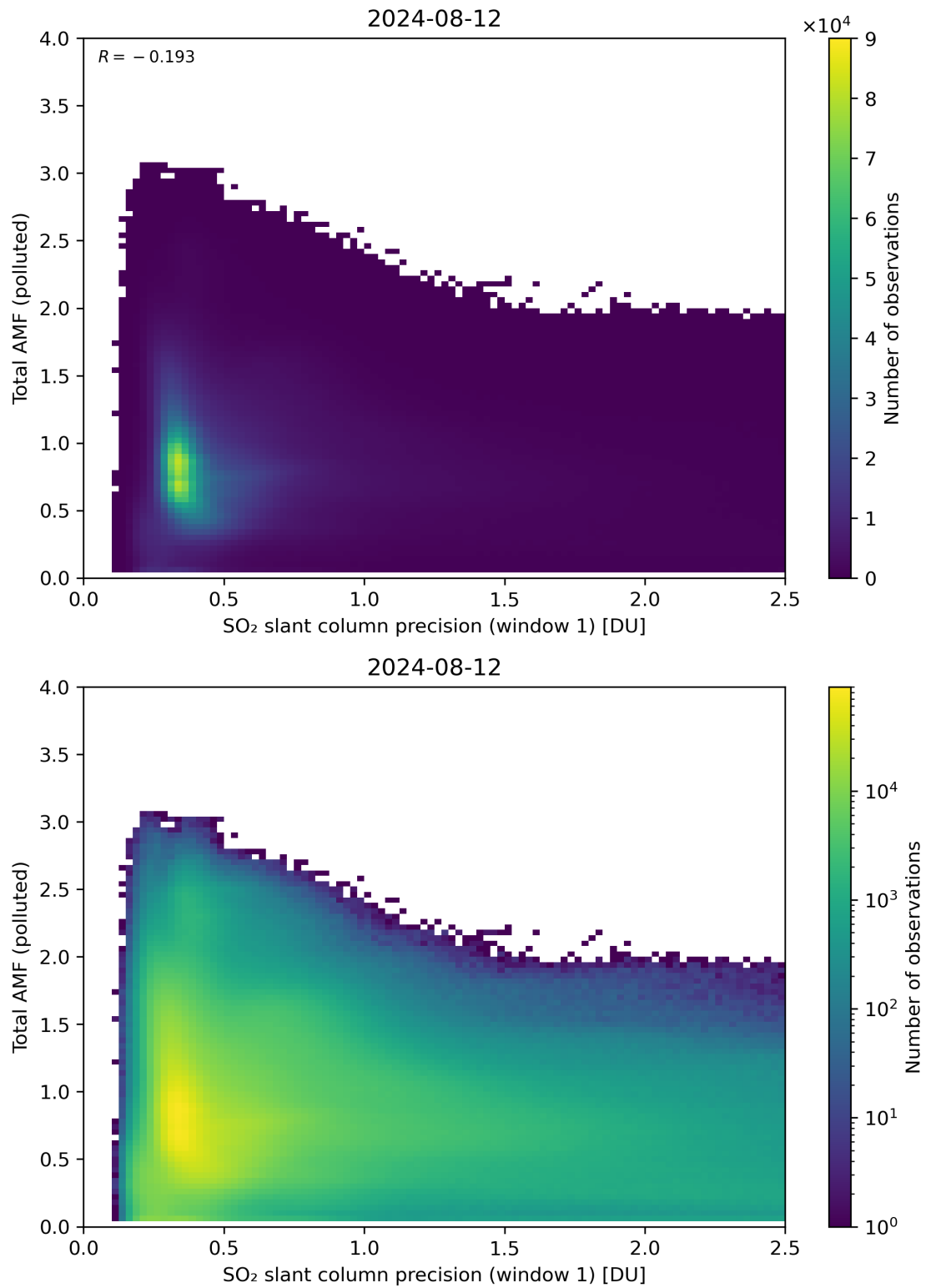
Figure 230: Scatter density plot of “SO 2 slant column precision (window 1)” against “Total AMF (polluted)” for 2024-08-12 to 2024-08-13.
