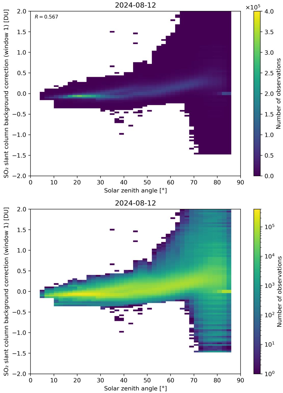
Figure 158: Scatter density plot of “Solar zenith angle” against “SO 2 slant column background correction (window 1)” for 2024-08-12 to 2024-08-13.
