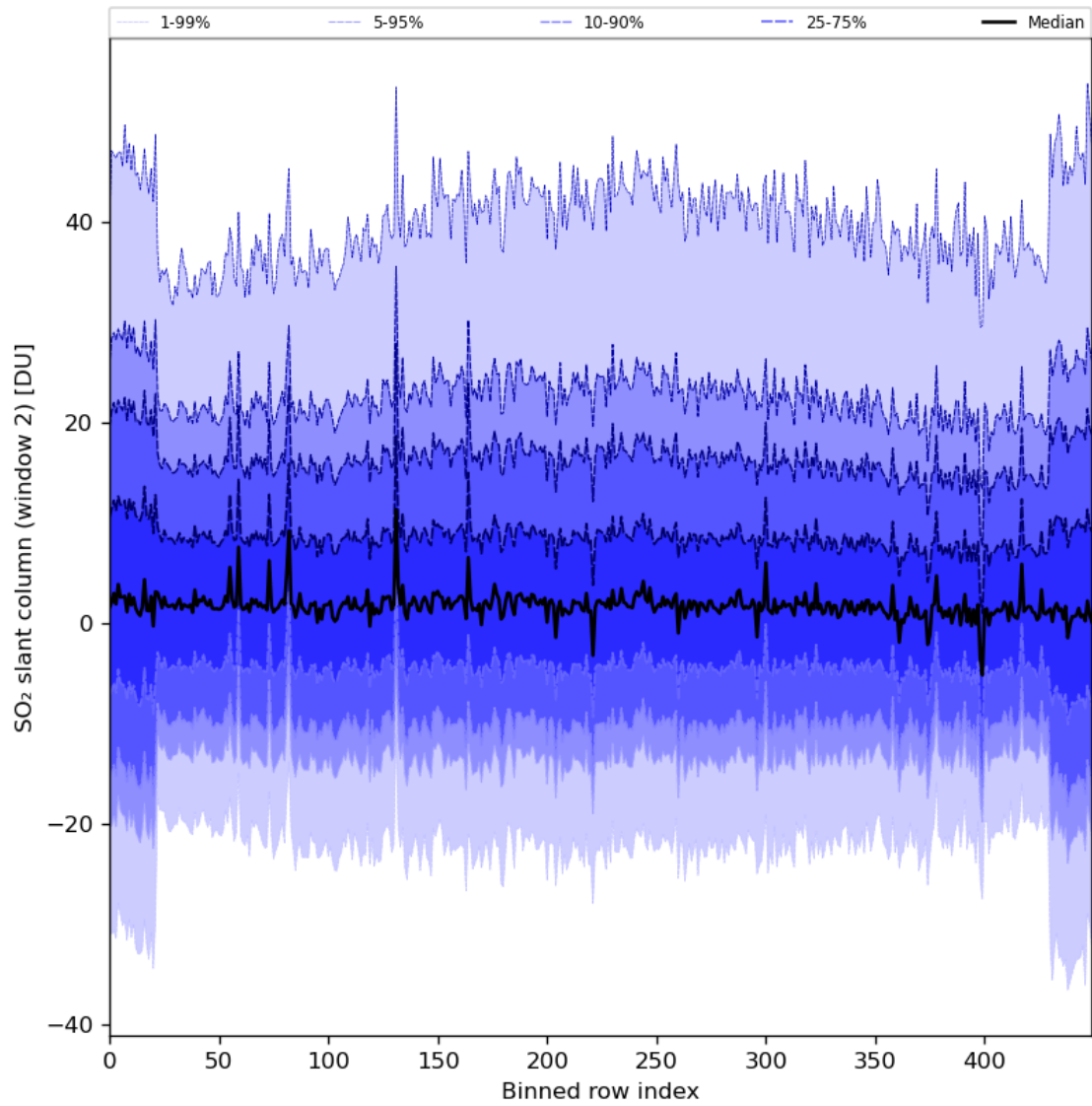
Figure 83: Along track statistics of “SO 2 slant column (window 2)” for 2024-08-12 to 2024-08-13
