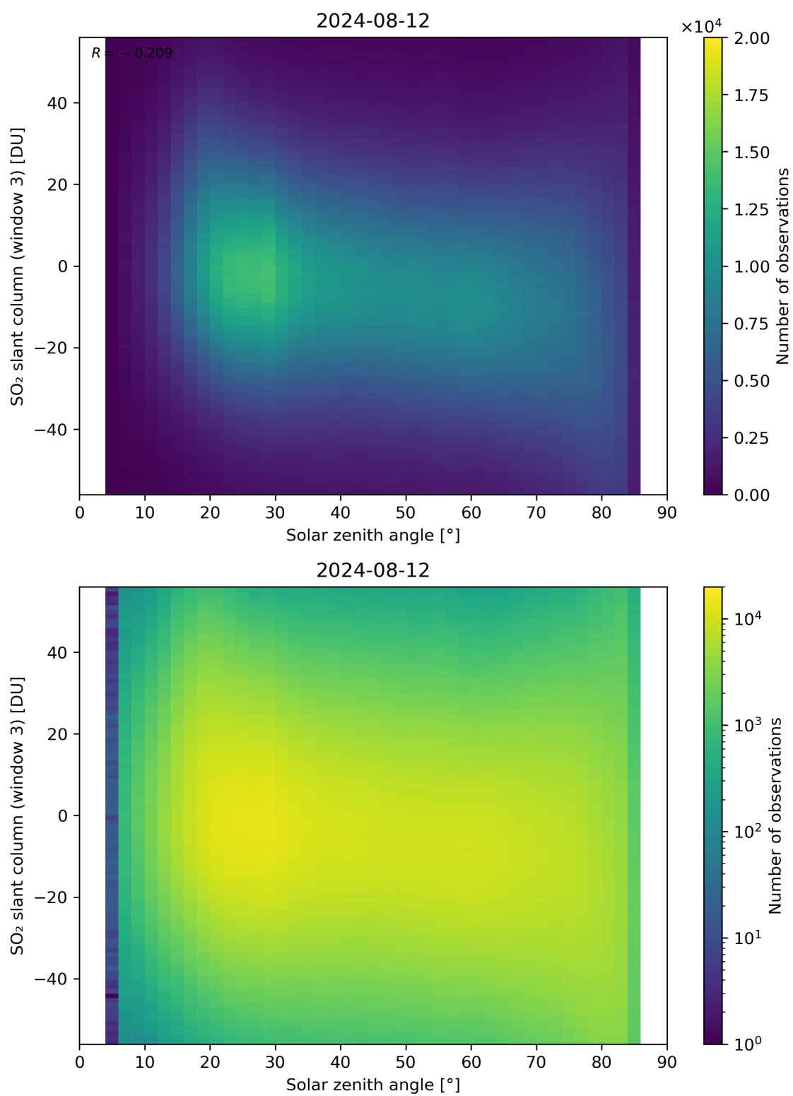
Figure 172: Scatter density plot of “Solar zenith angle” against “SO 2 slant column (window 3)” for 2024-08-12 to 2024-08-13.
