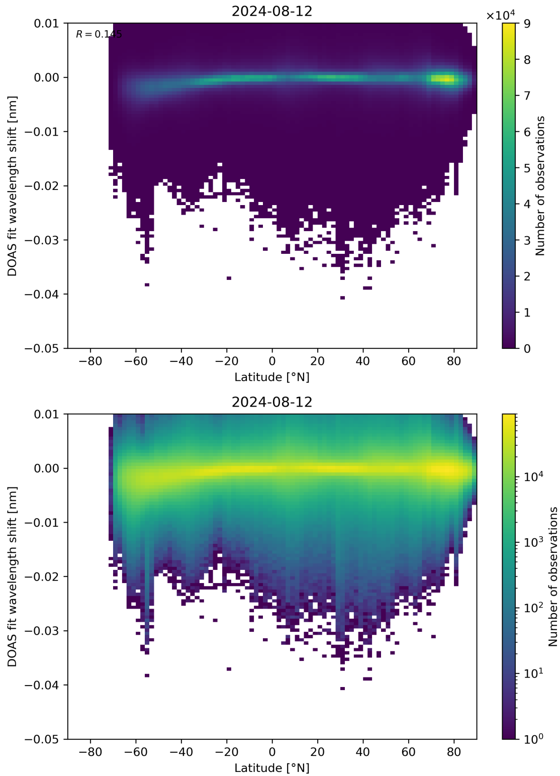
Figure 142: Scatter density plot of “Latitude” against “DOAS fit wavelength shift” for 2024-08-12 to 2024-08-13.
