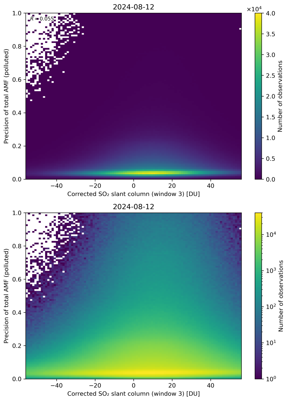
Figure 211: Scatter density plot of “Corrected SO 2 slant column (window 3)” against “Precision of total AMF (polluted)” for 2024-08-12 to 2024-08-13.
