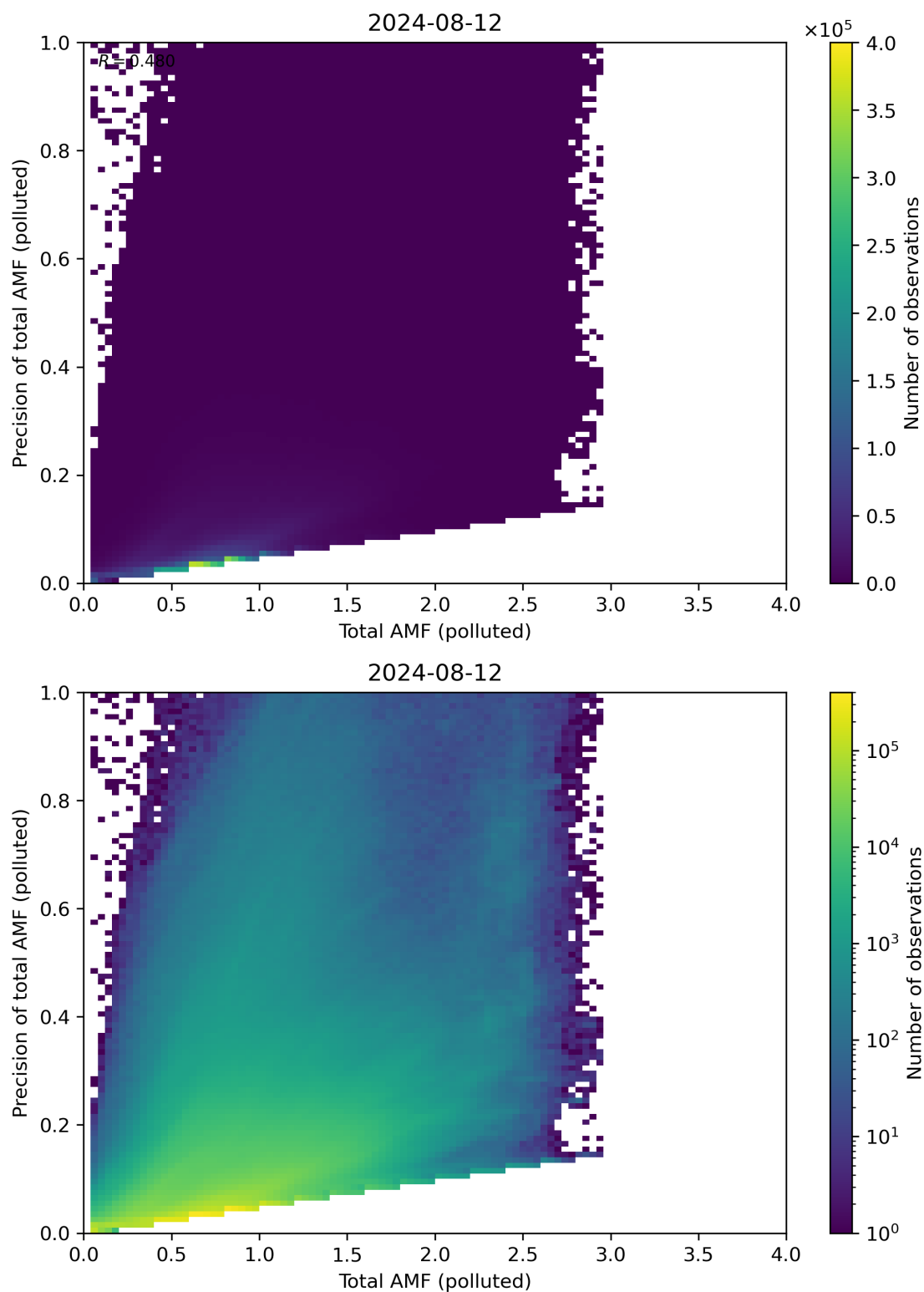
Figure 272: Scatter density plot of “Total AMF (polluted)” against “Precision of total AMF (polluted)” for 2024-08-12 to 2024-08-13.
