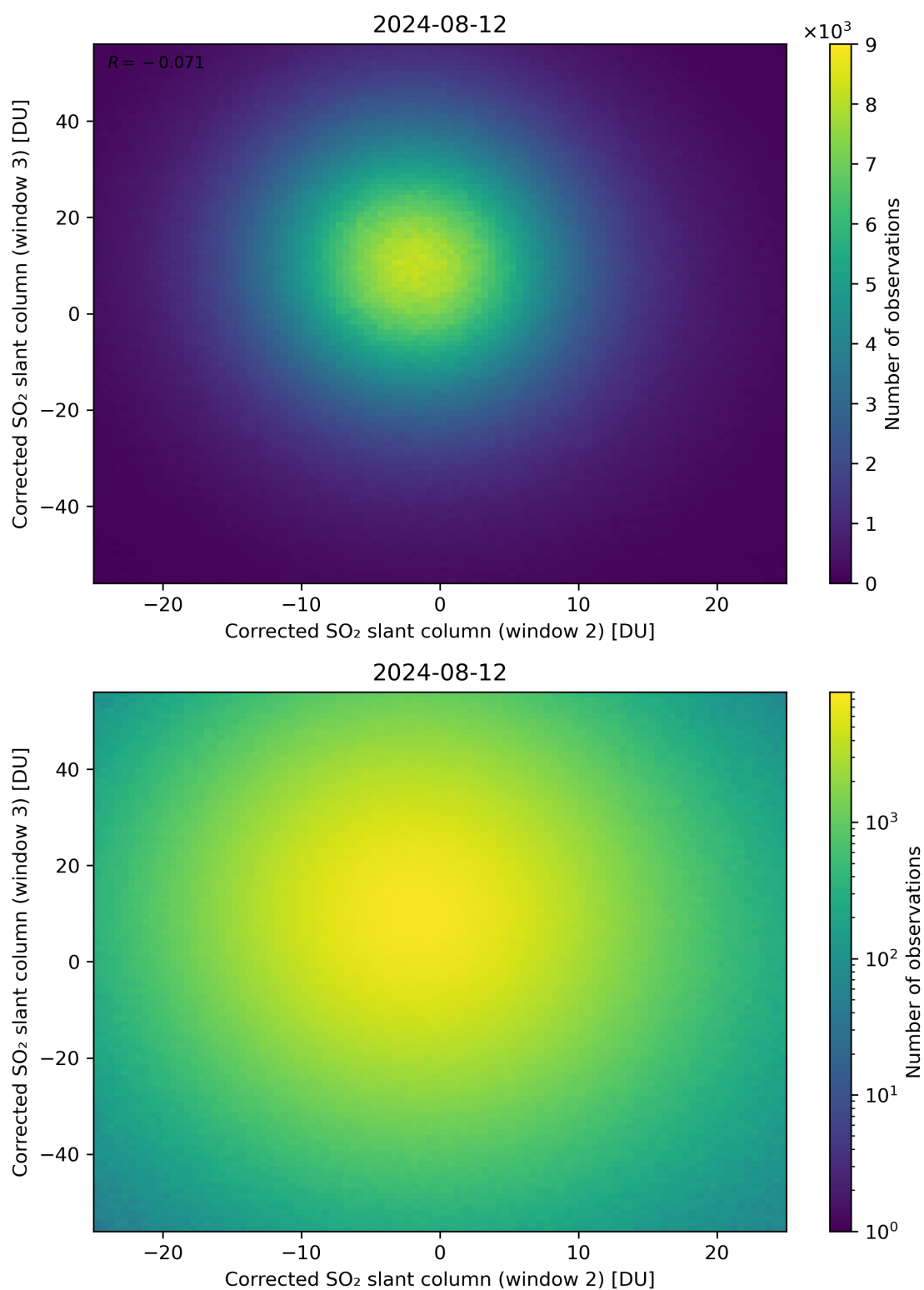
Figure 200: Scatter density plot of “Corrected SO 2 slant column (window 2)” against “Corrected SO 2 slant column (window 3)” for 2024-08-12 to 2024-08-13.
