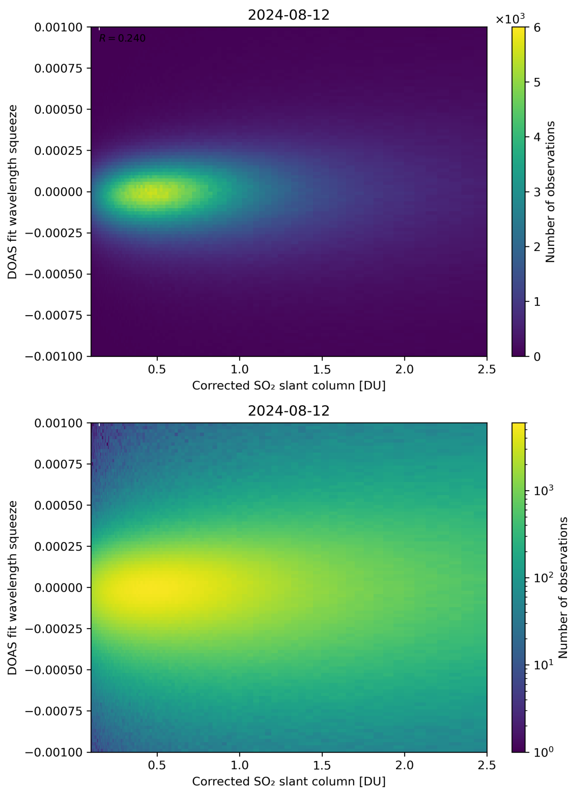
Figure 182: Scatter density plot of “Corrected SO 2 slant column” against “DOAS fit wavelength squeeze” for 2024-08-12 to 2024-08-13.
