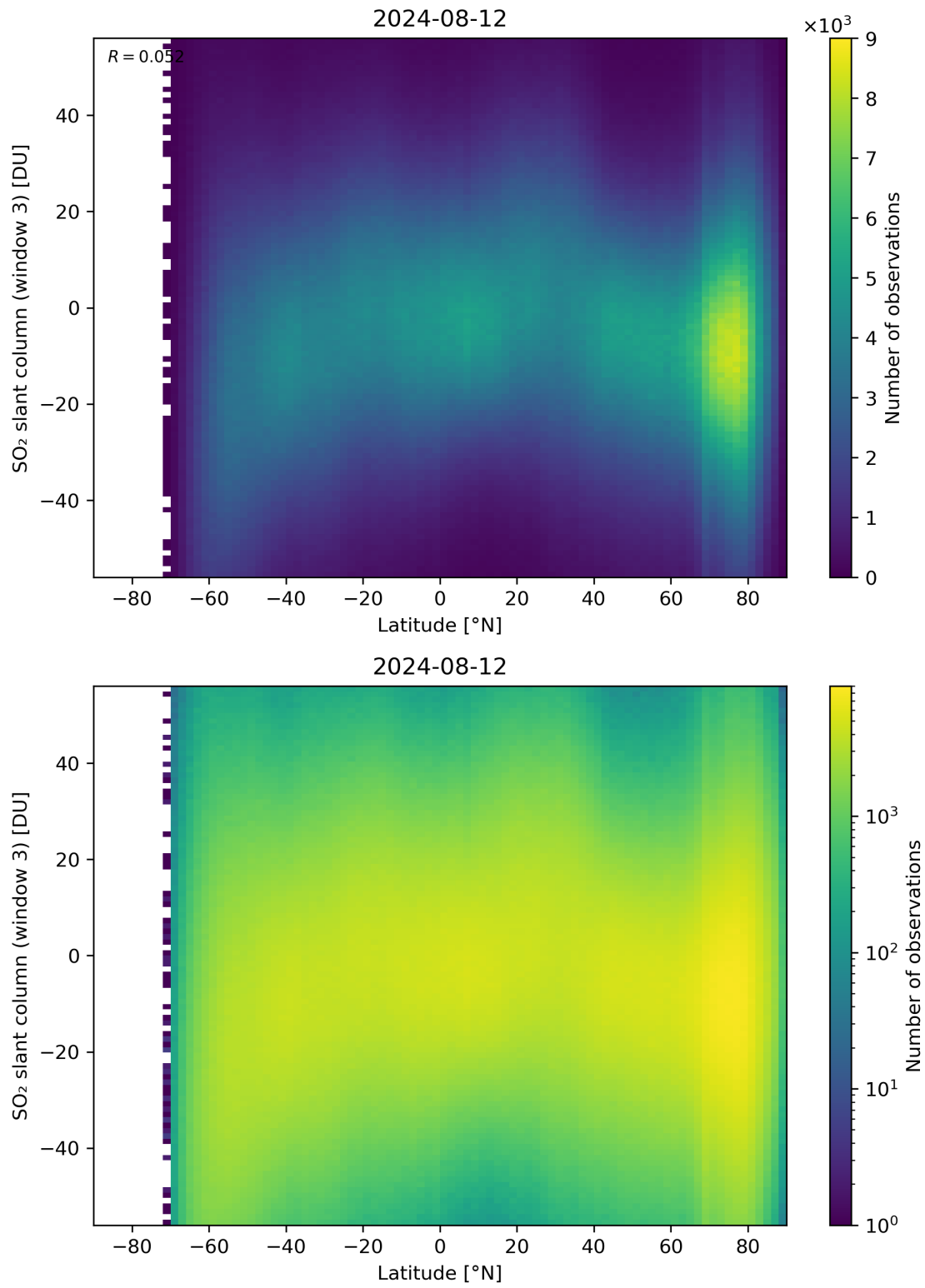
Figure 152: Scatter density plot of “Latitude” against “SO 2 slant column (window 3)” for 2024-08-12 to 2024-08-13.
