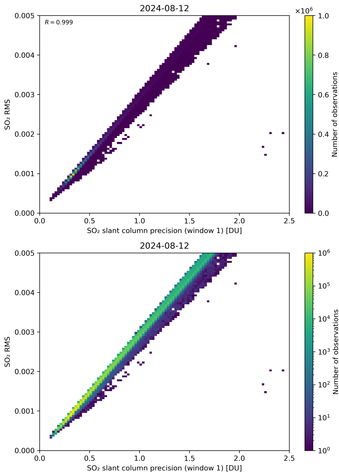
Figure 223: Scatter density plot of “SO 2 slant column precision (window 1)” against “SO 2 RMS” for 2024-08-12 to 2024-08-13.
