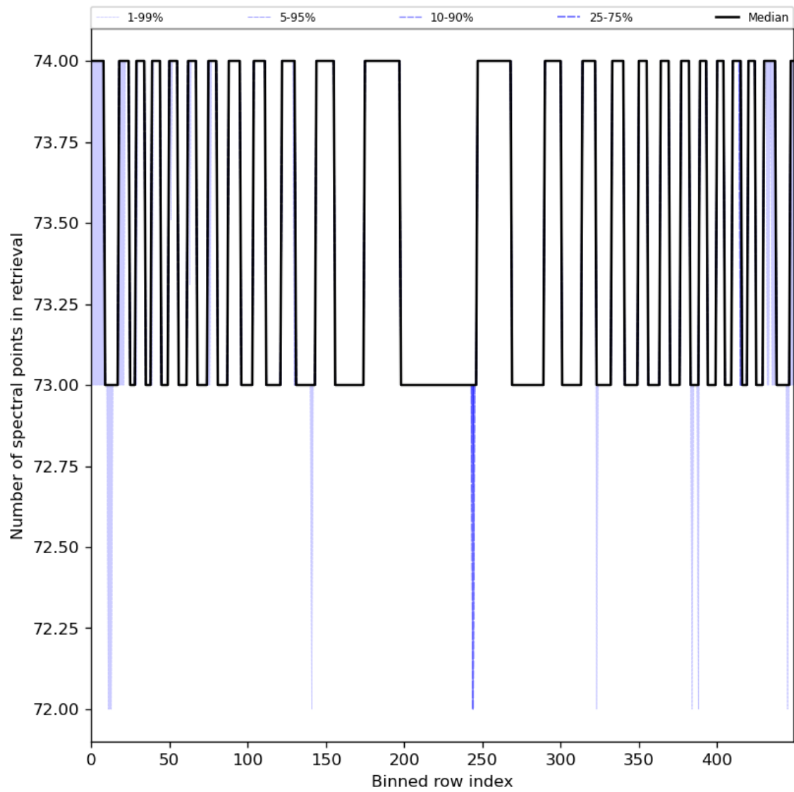
Figure 97: Along track statistics of “Number of spectral points in retrieval” for 2024-08-12 to 2024-08-13
