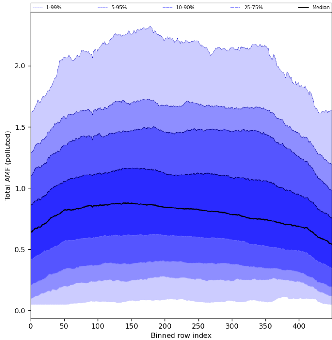
Figure 94: Along track statistics of “Total AMF (polluted)” for 2024-08-12 to 2024-08-13
