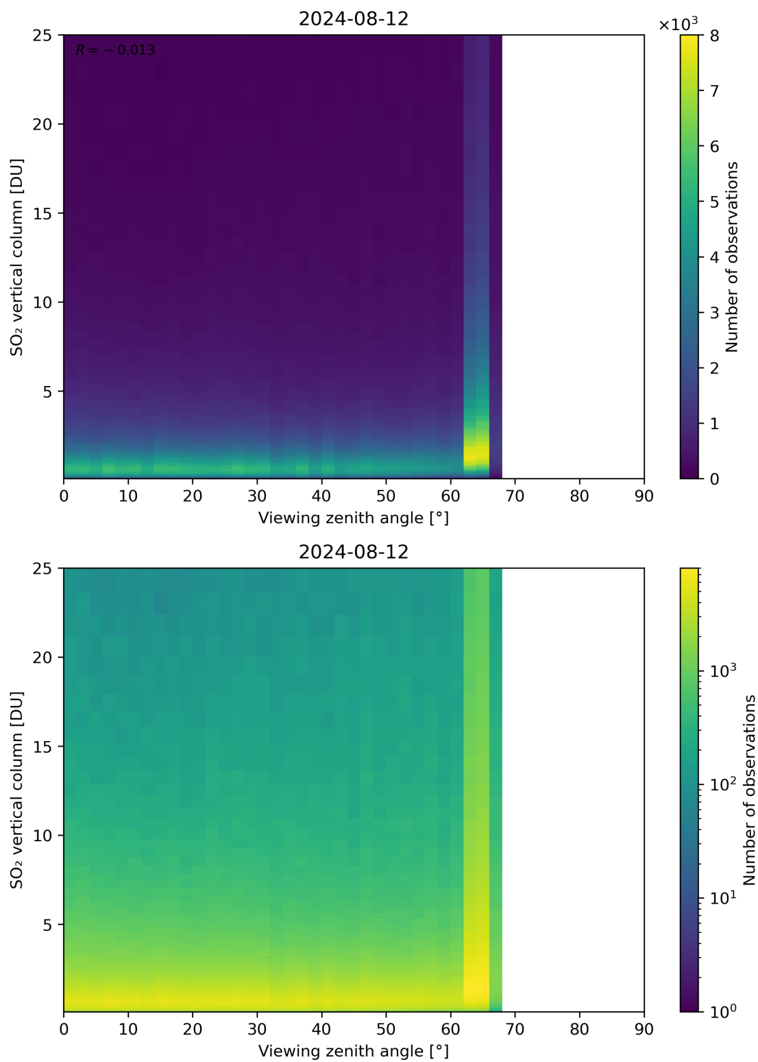
Figure 327: Scatter density plot of “Viewing zenith angle” against “SO 2 vertical column” for 2024-08-12 to 2024-08-13.
