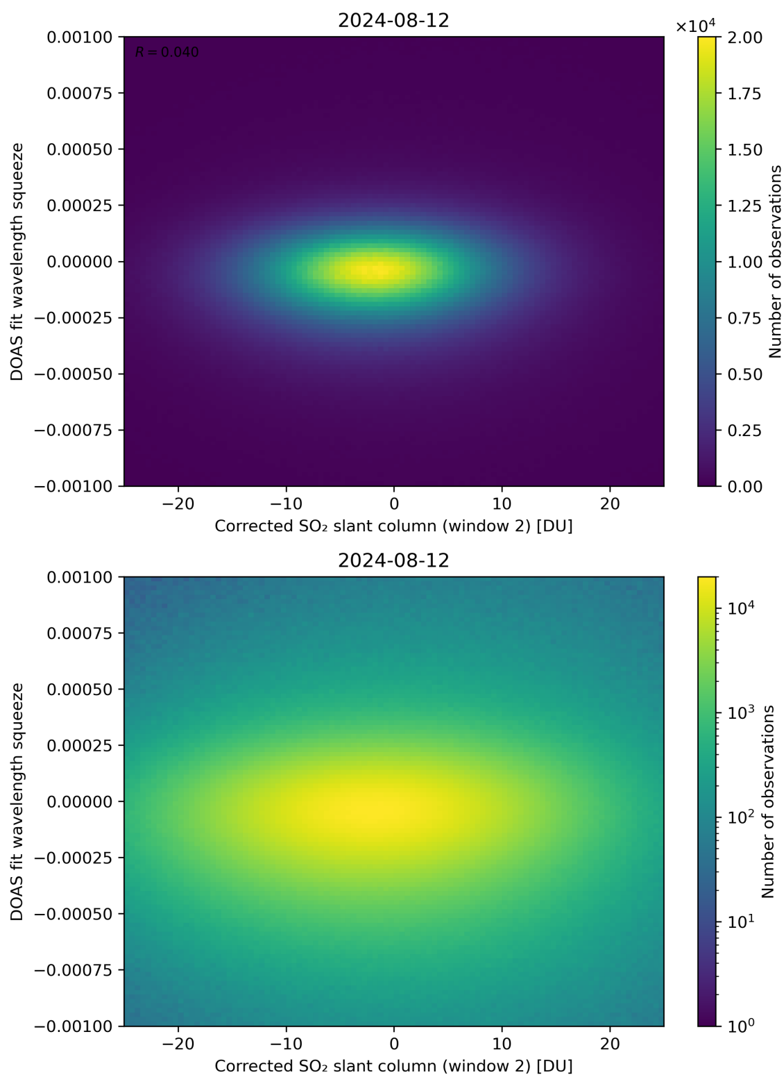
Figure 197: Scatter density plot of “Corrected SO 2 slant column (window 2)” against “DOAS fit wavelength squeeze” for 2024-08-12 to 2024-08-13.
