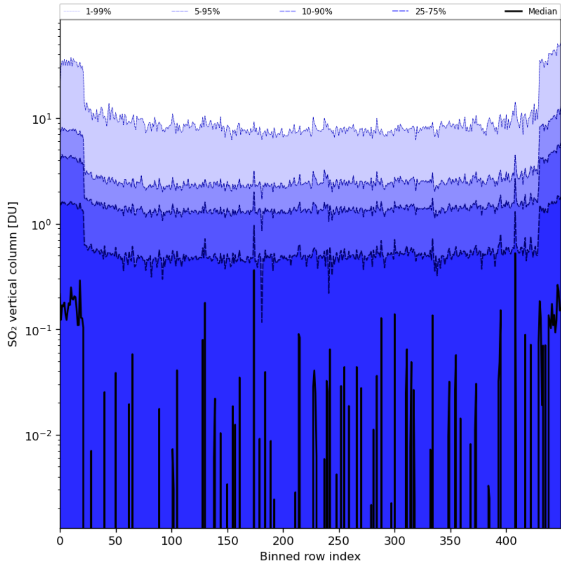
Figure 76: Along track statistics of “SO 2 vertical column” for 2024-08-12 to 2024-08-13
