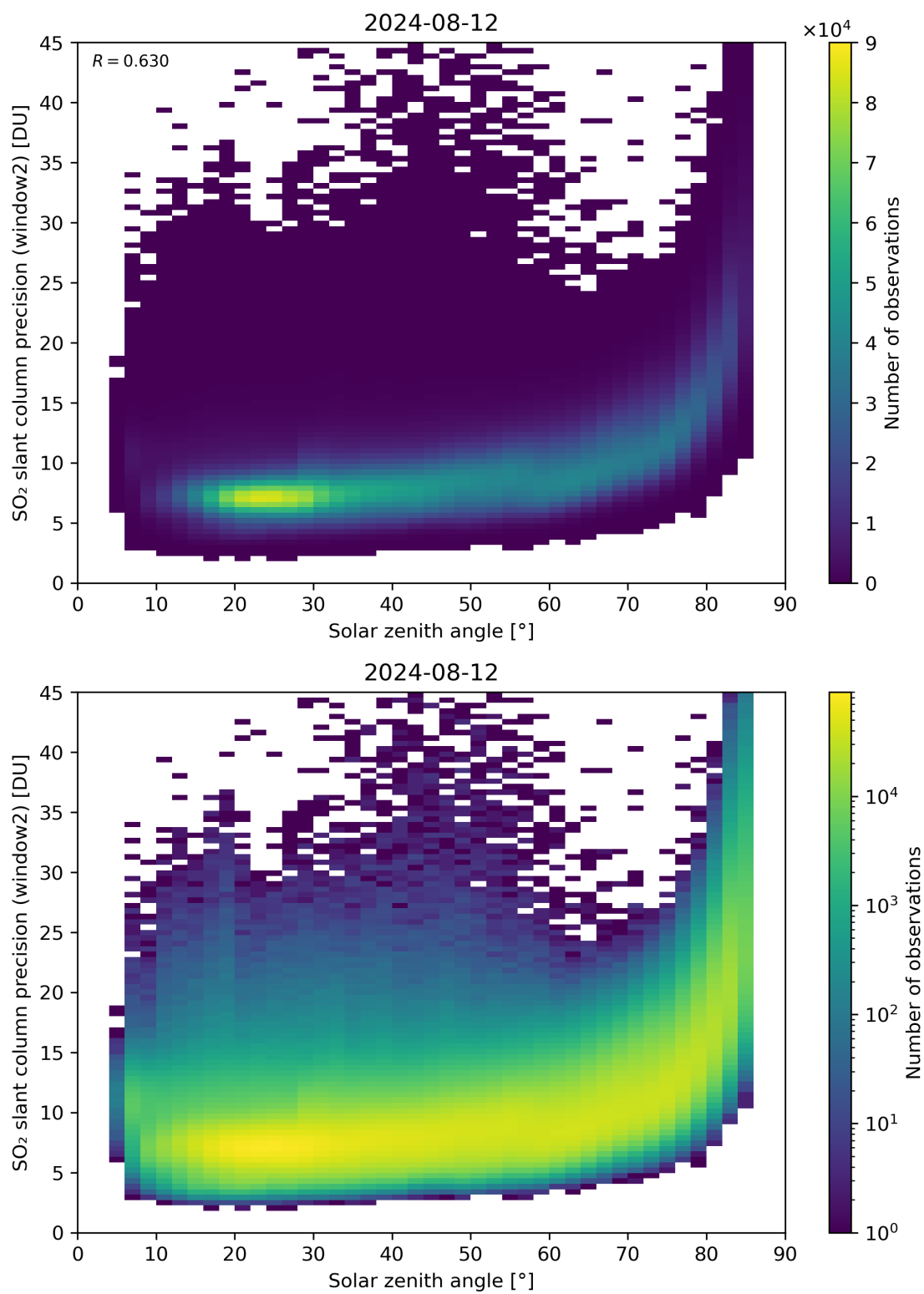
Figure 171: Scatter density plot of “Solar zenith angle” against “SO 2 slant column precision (window2)” for 2024-08-12 to 2024-08-13.
