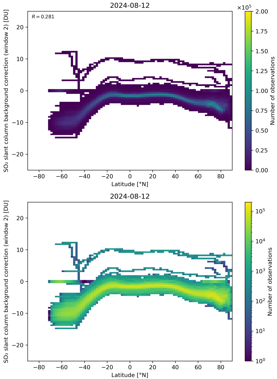
Figure 140: Scatter density plot of “Latitude” against “SO 2 slant column background correction (window 2)” for 2024-08-12 to 2024-08-13.
