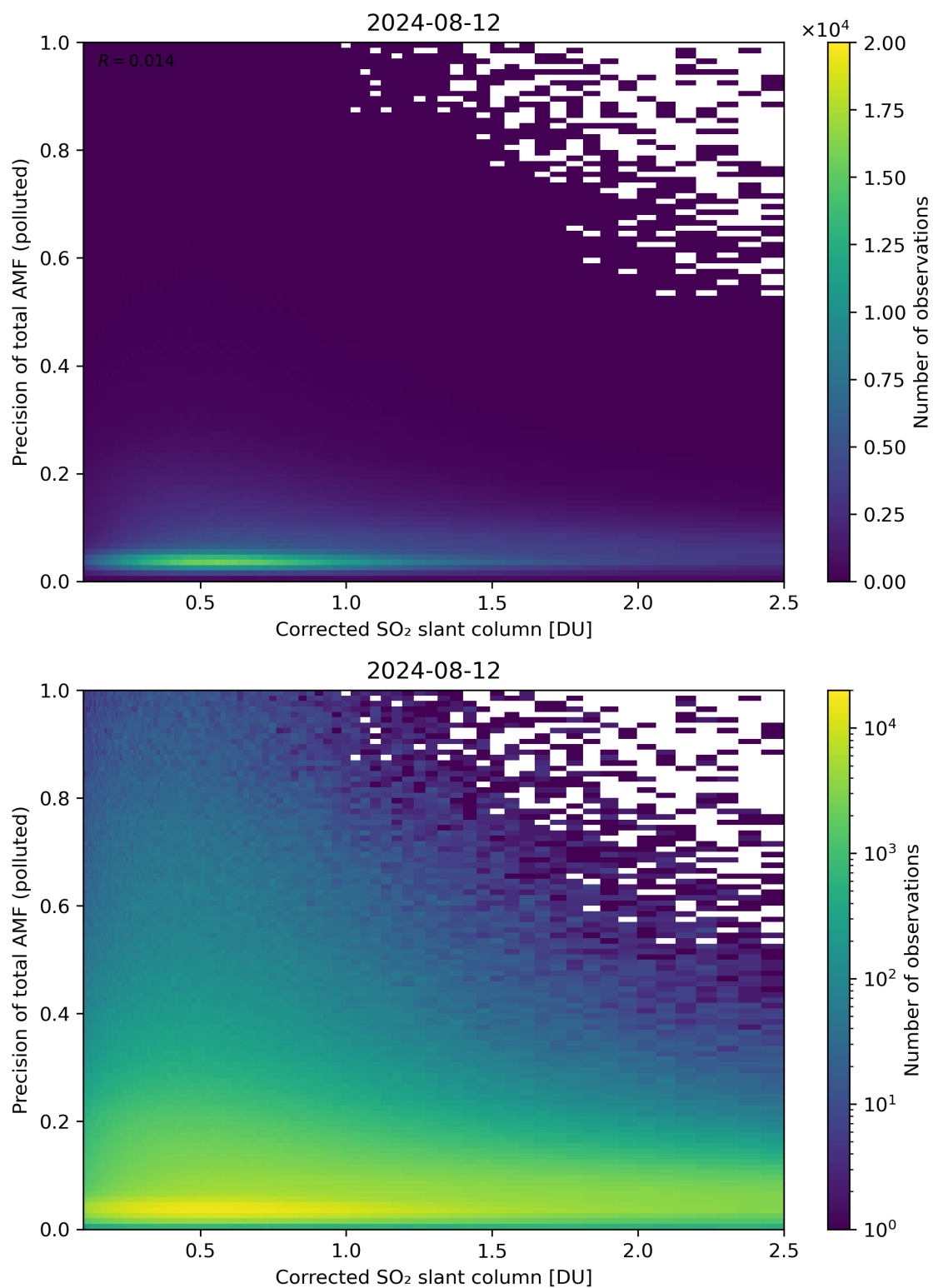
Figure 193: Scatter density plot of “Corrected SO 2 slant column” against “Precision of total AMF (polluted)” for 2024-08-12 to 2024-08-13.
