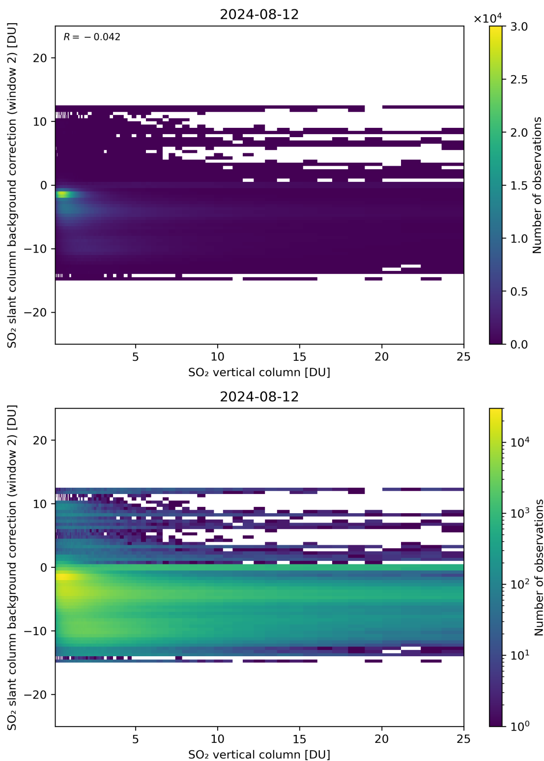
Figure 274: Scatter density plot of “SO 2 vertical column” against “SO 2 slant column background correction (window 2)” for 2024-08-12 to 2024-08-13.
