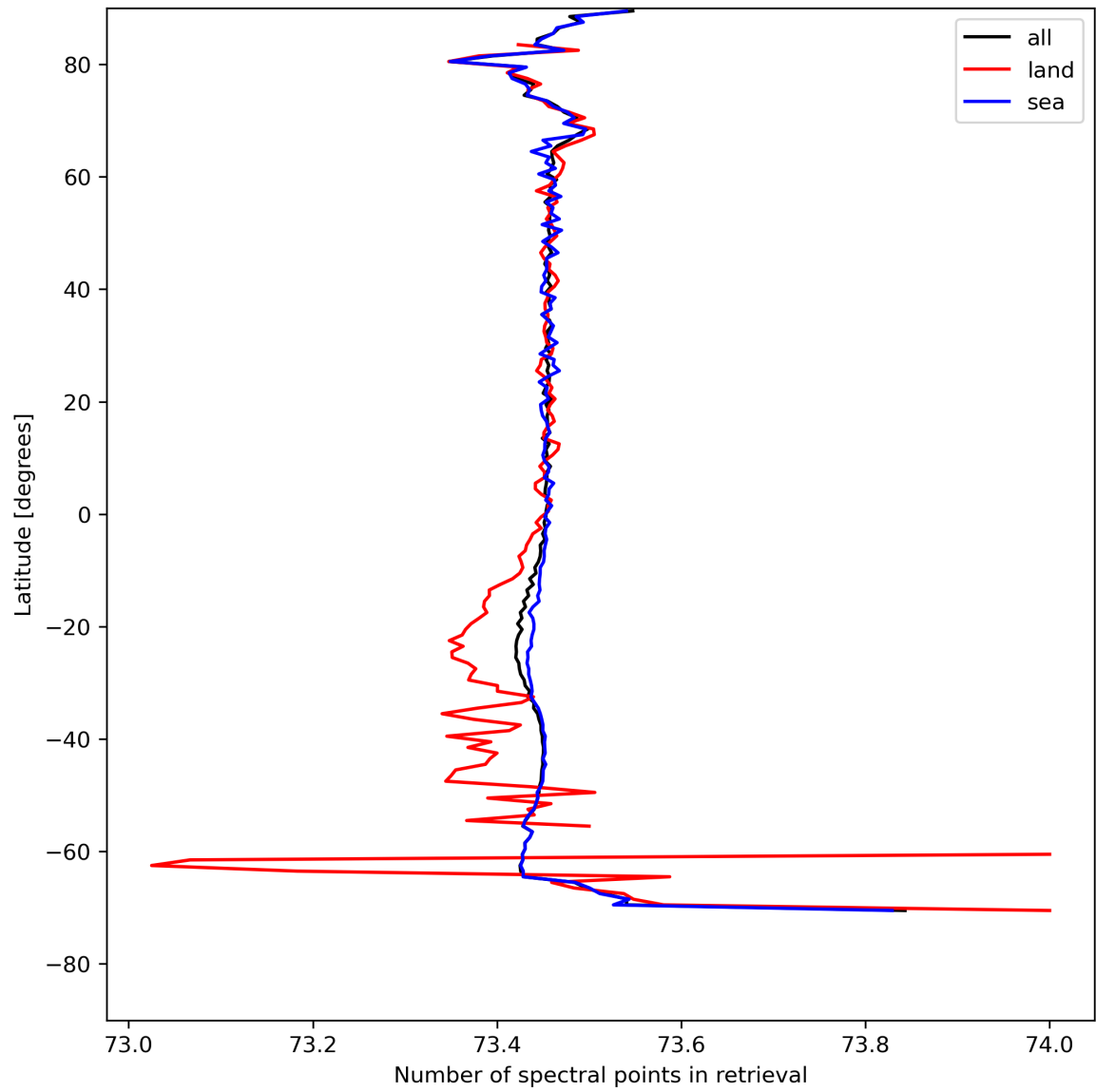
Figure 51: Zonal average of “Number of spectral points in retrieval” for 2024-08-12 to 2024-08-13.
