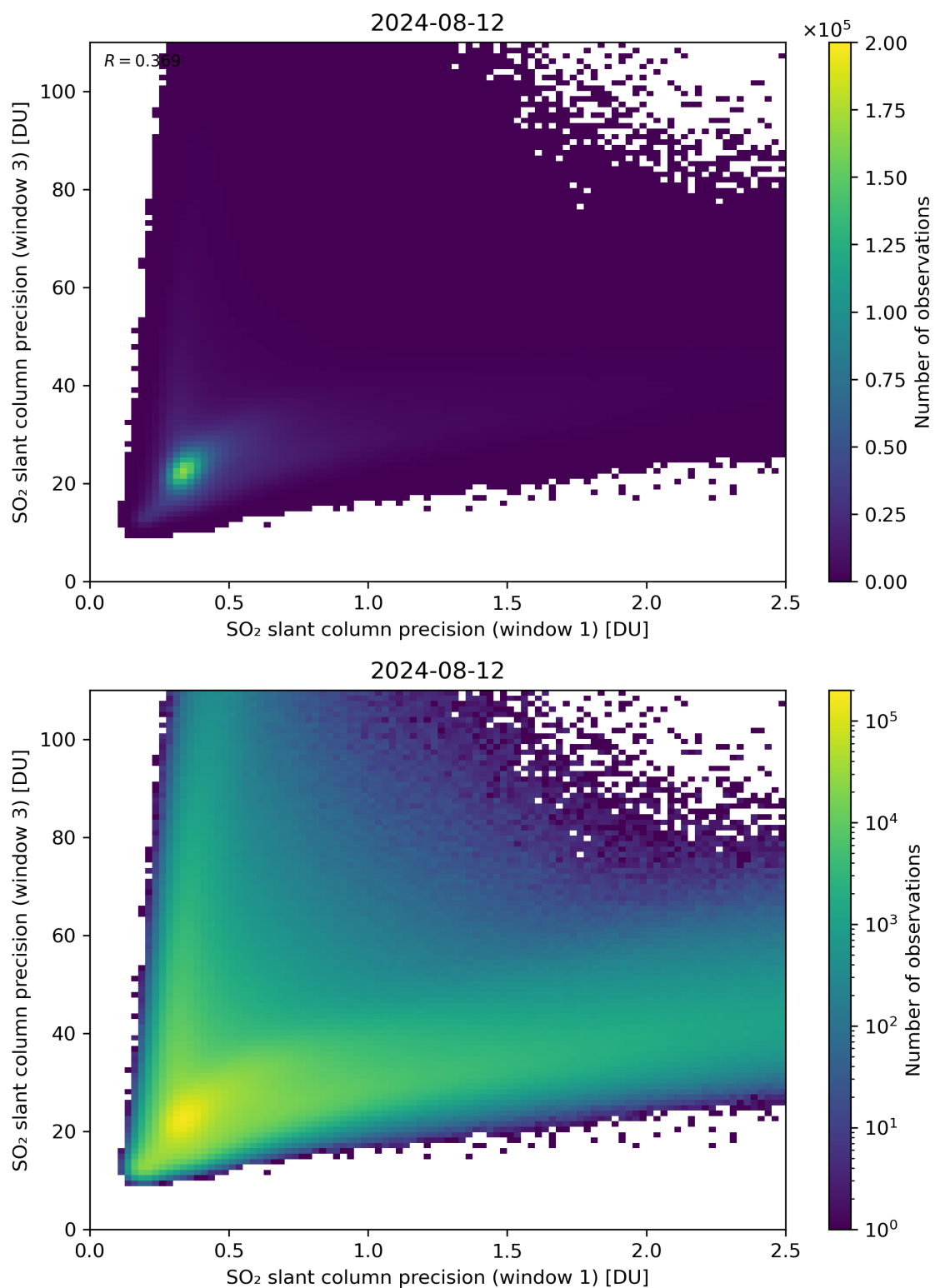
Figure 229: Scatter density plot of “SO 2 slant column precision (window 1)” against “SO 2 slant column precision (window 3)” for 2024-08-12 to 2024-08-13.
