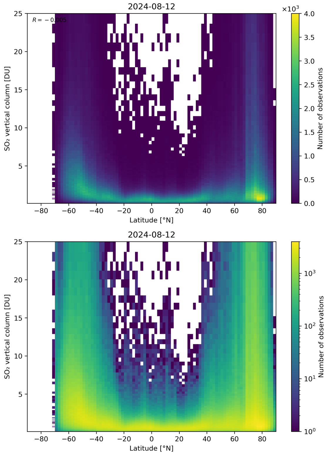
Figure 156: Scatter density plot of “Latitude” against “SO 2 vertical column” for 2024-08-12 to 2024-08-13.
