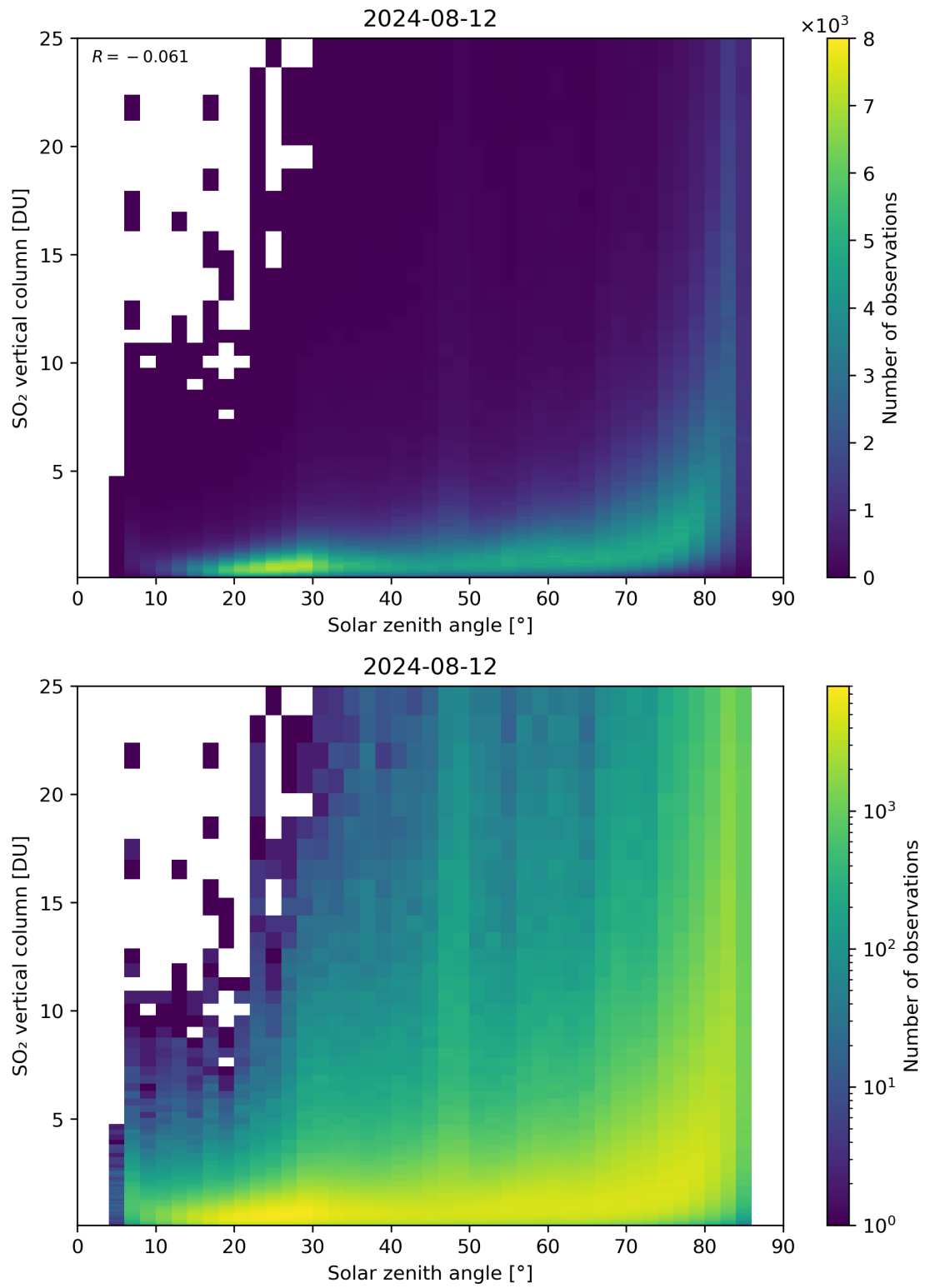
Figure 176: Scatter density plot of “Solar zenith angle” against “SO 2 vertical column” for 2024-08-12 to 2024-08-13.
