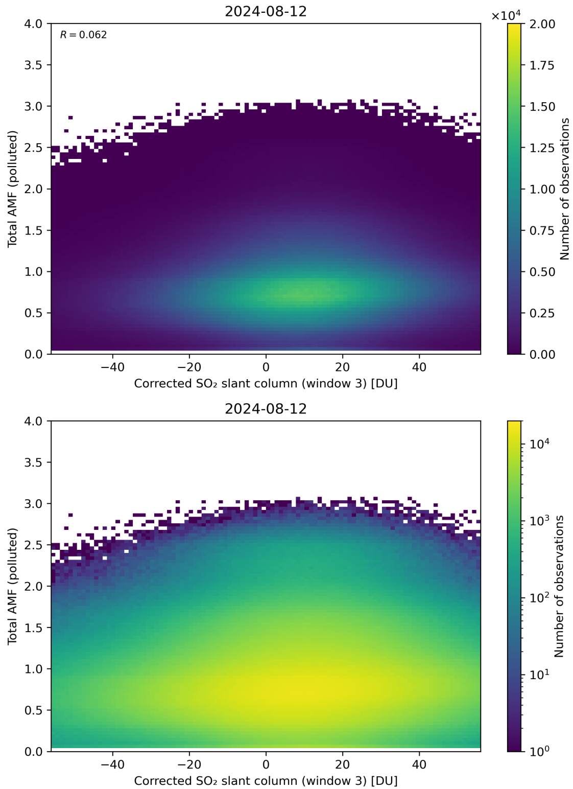
Figure 210: Scatter density plot of “Corrected SO 2 slant column (window 3)” against “Total AMF (polluted)” for 2024-08-12 to 2024-08-13.
