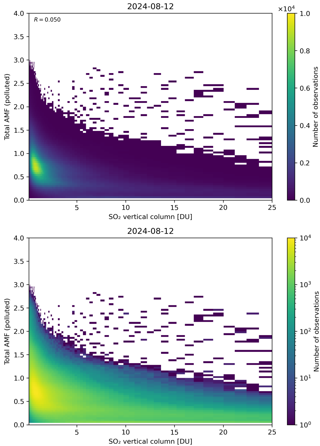
Figure 305: Scatter density plot of “SO 2 vertical column” against “Total AMF (polluted)” for 2024-08-12 to 2024-08-13.
