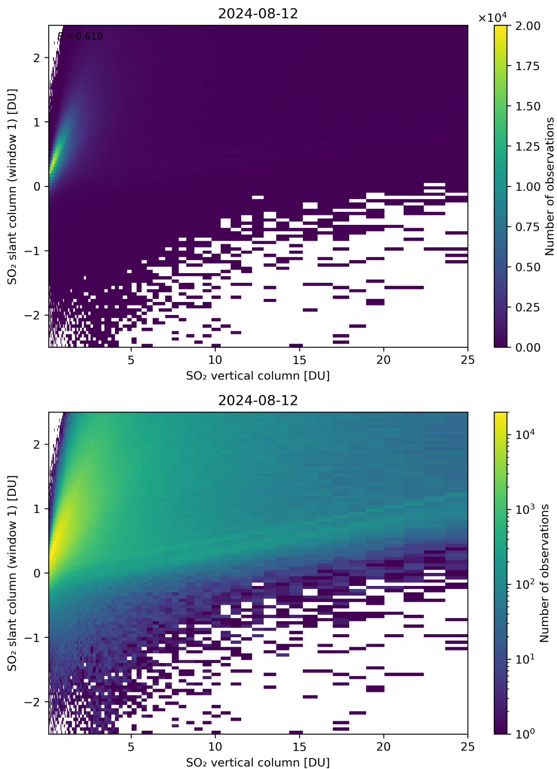
Figure 300: Scatter density plot of “SO 2 vertical column” against “SO 2 slant column (window 1)” for 2024-08-12 to 2024-08-13.
