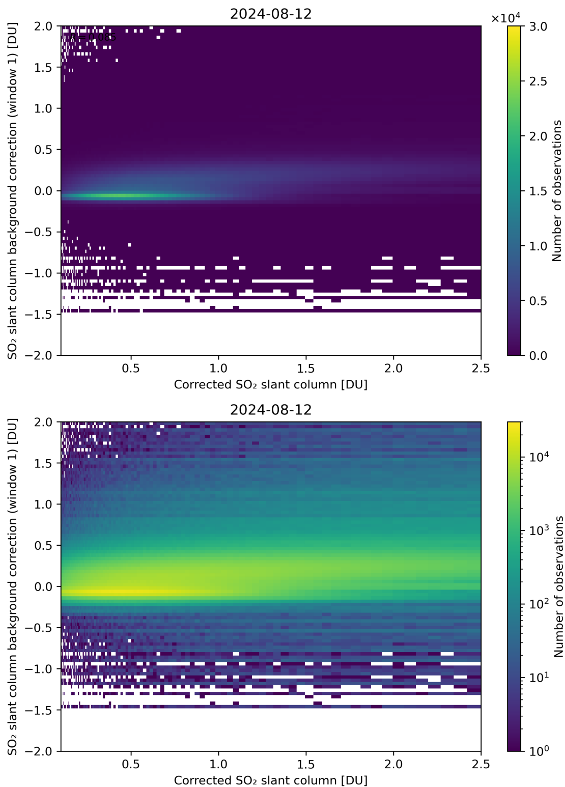
Figure 178: Scatter density plot of “Corrected SO 2 slant column” against “SO 2 slant column background correction (window 1)” for 2024-08-12 to 2024-08-13.
