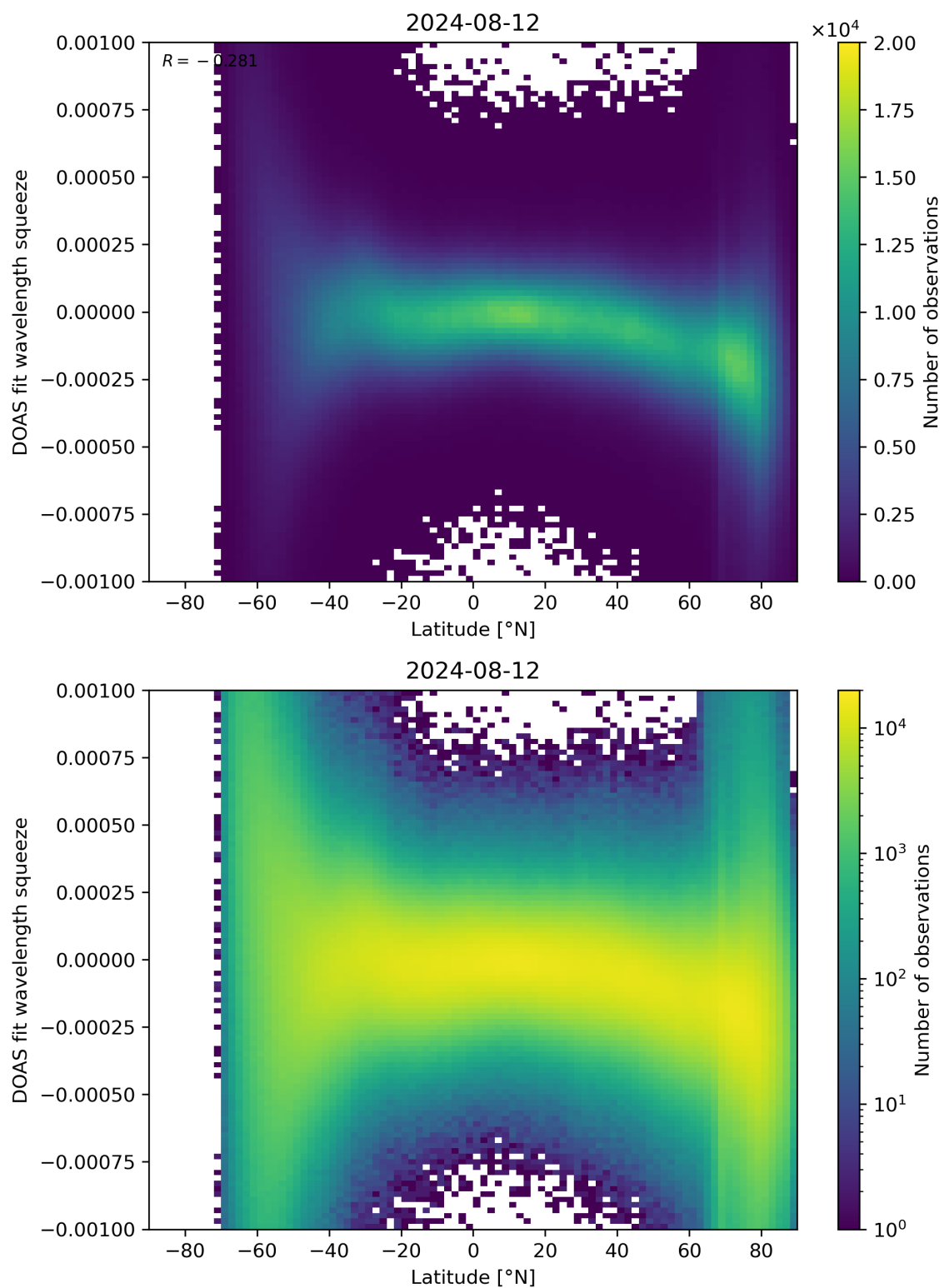
Figure 143: Scatter density plot of “Latitude” against “DOAS fit wavelength squeeze” for 2024-08-12 to 2024-08-13.
