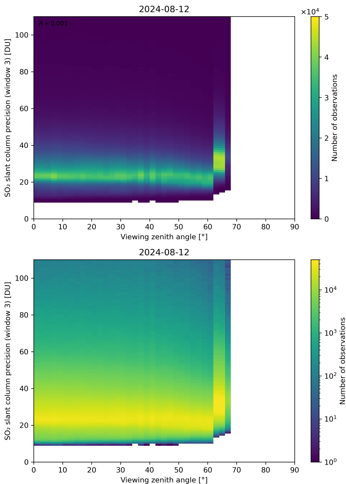
Figure 324: Scatter density plot of “Viewing zenith angle” against “SO 2 slant column precision (window 3)” for 2024-08-12 to 2024-08-13.
