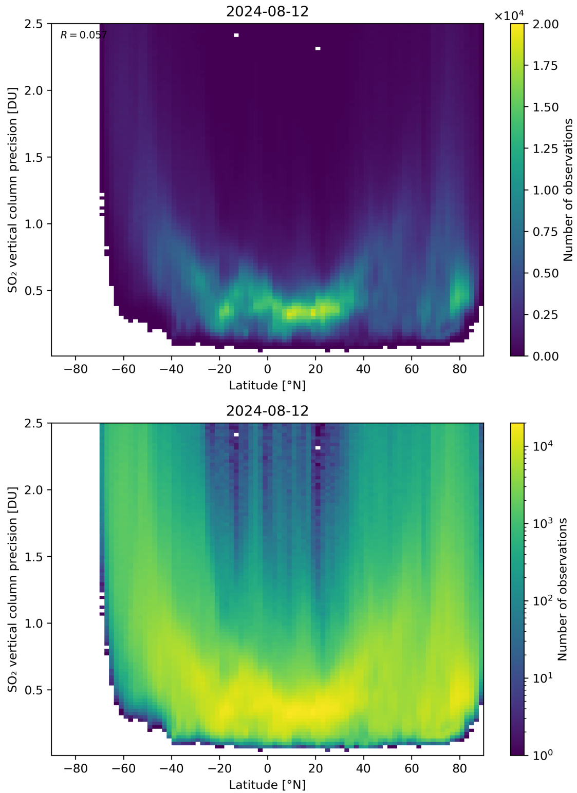
Figure 157: Scatter density plot of “Latitude” against “SO 2 vertical column precision” for 2024-08-12 to 2024-08-13.
