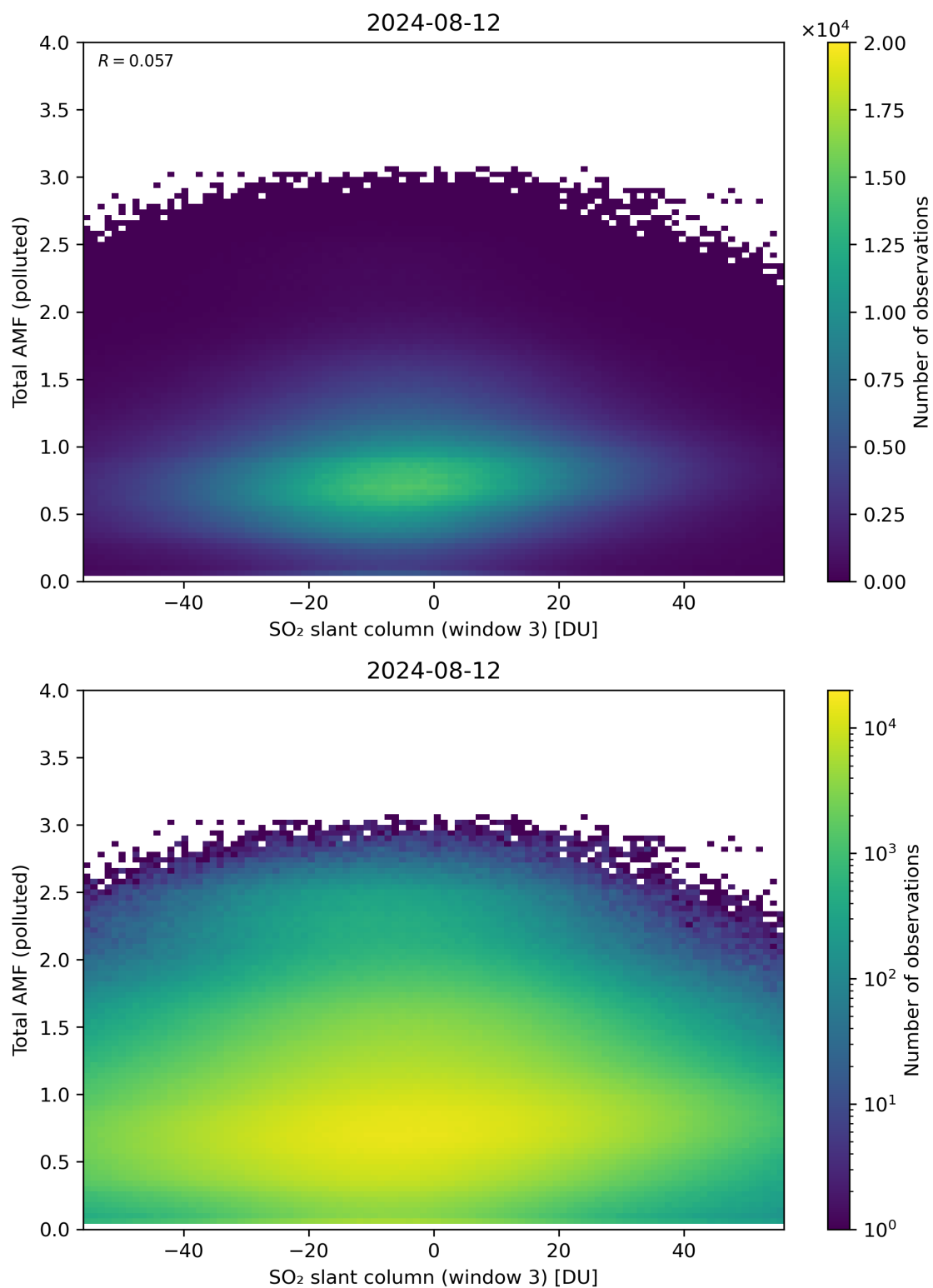
Figure 268: Scatter density plot of “SO 2 slant column (window 3)” against “Total AMF (polluted)” for 2024-08-12 to 2024-08-13.
