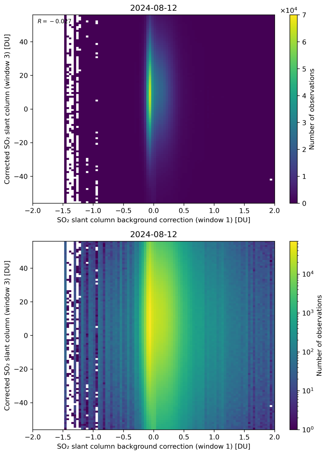
Figure 105: Scatter density plot of “SO 2 slant column background correction (window 1)” against “Corrected SO 2 slant column (window 3)” for 2024-08-12 to 2024-08-13.
