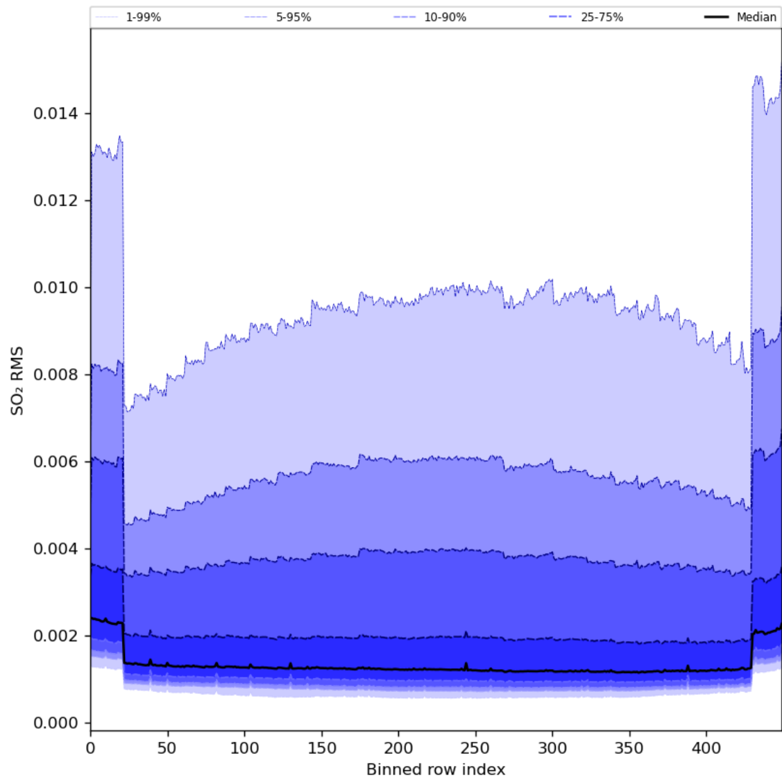
Figure 93: Along track statistics of “SO 2 RMS” for 2024-08-12 to 2024-08-13
