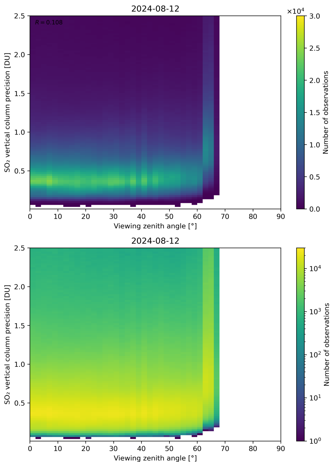
Figure 328: Scatter density plot of “Viewing zenith angle” against “SO 2 vertical column precision” for 2024-08-12 to 2024-08-13.
