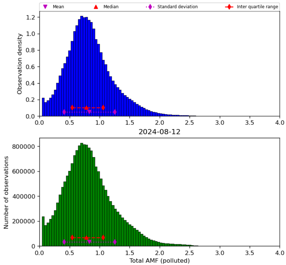
Figure 71: Histogram of “Total AMF (polluted)” for 2024-08-12 to 2024-08-13
