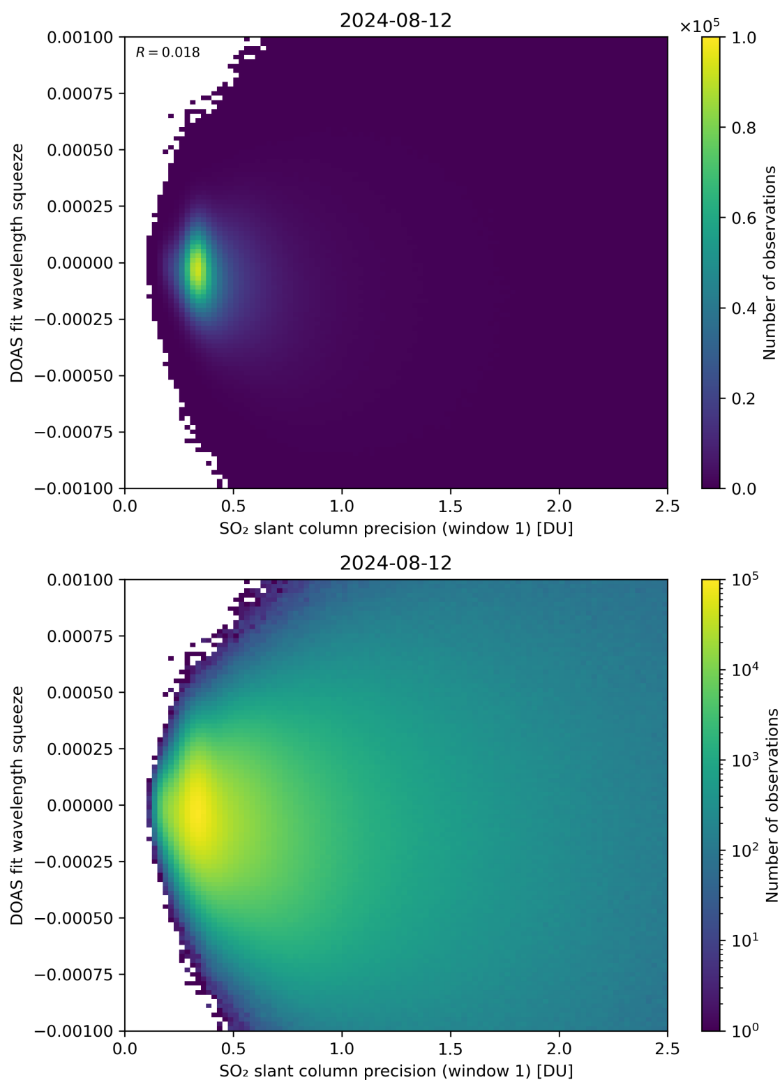
Figure 222: Scatter density plot of “SO 2 slant column precision (window 1)” against “DOAS fit wavelength squeeze” for 2024-08-12 to 2024-08-13.
