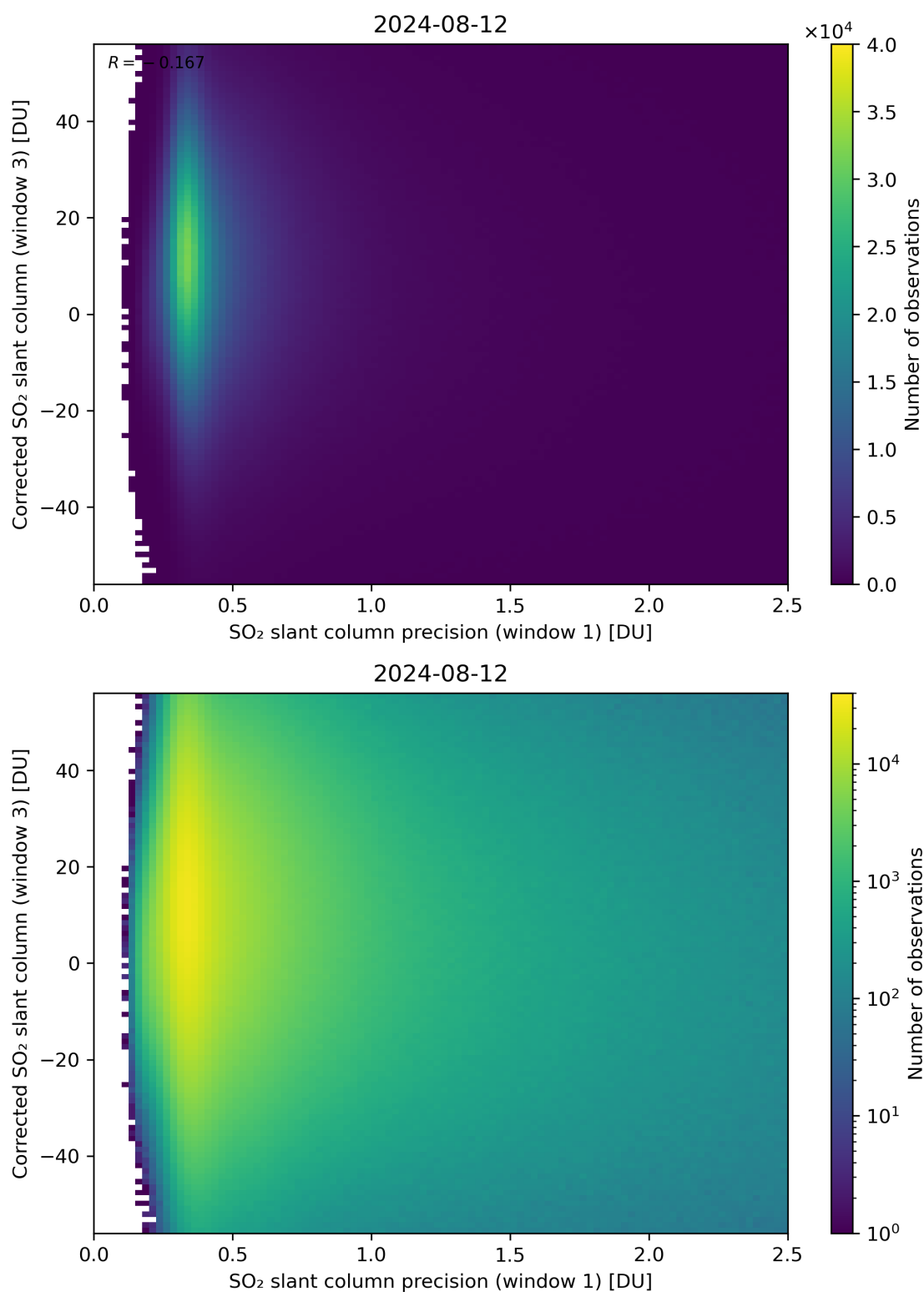
Figure 226: Scatter density plot of “SO 2 slant column precision (window 1)” against “Corrected SO 2 slant column (window 3)” for 2024-08-12 to 2024-08-13.
