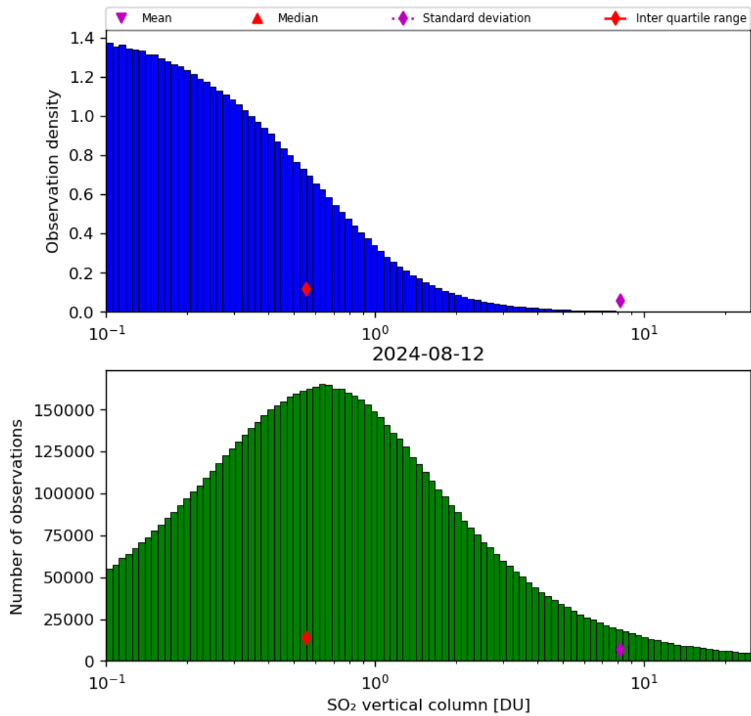
Figure 53: Histogram of “SO 2 vertical column” for 2024-08-12 to 2024-08-13
