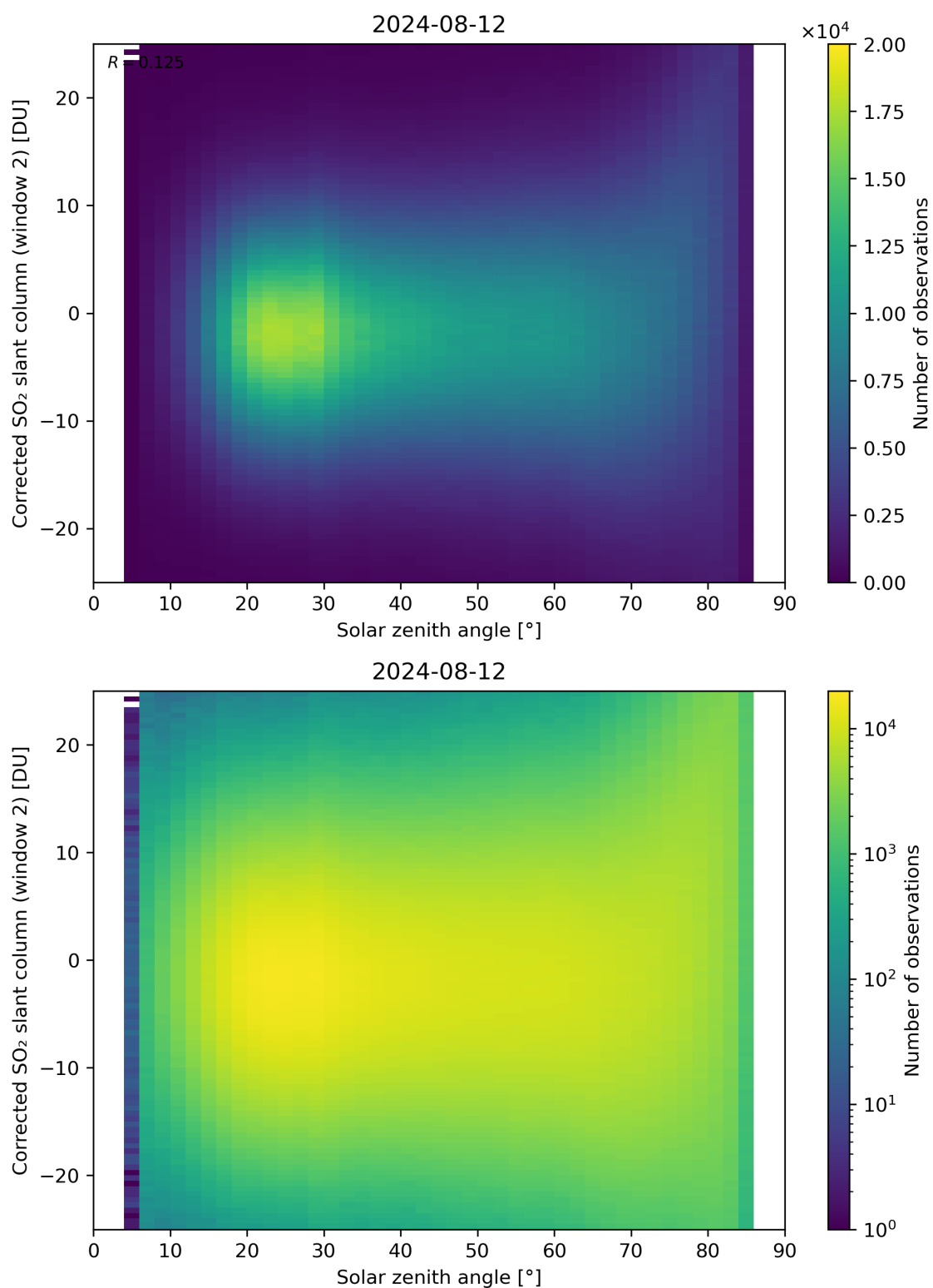
Figure 167: Scatter density plot of “Solar zenith angle” against “Corrected SO 2 slant column (window 2)” for 2024-08-12 to 2024-08-13.
