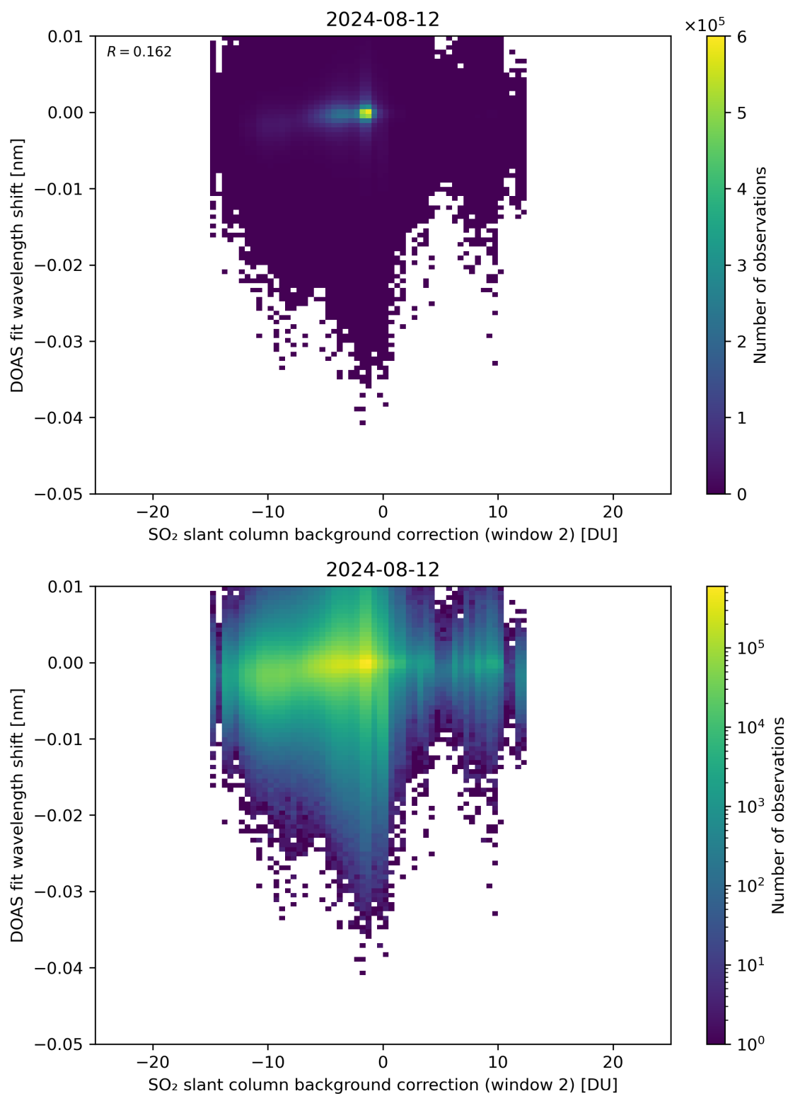
Figure 112: Scatter density plot of “SO 2 slant column background correction (window 2)” against “DOAS fit wavelength shift” for 2024-08-12 to 2024-08-13.
