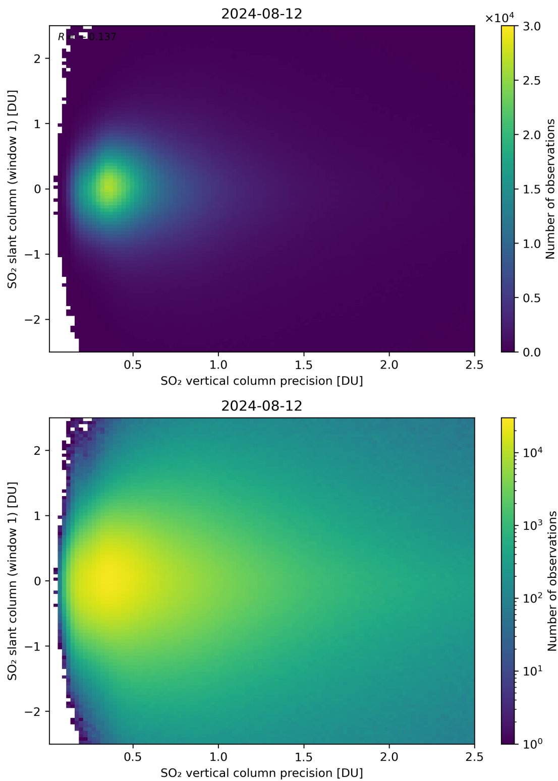
Figure 289: Scatter density plot of “SO 2 vertical column precision” against “SO 2 slant column (window 1)” for 2024-08-12 to 2024-08-13.
