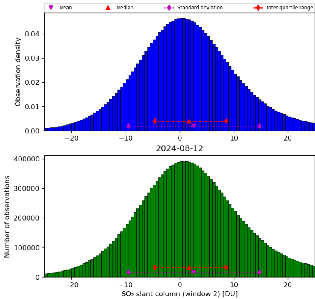
Figure 60: Histogram of “SO 2 slant column (window 2)” for 2024-08-12 to 2024-08-13
