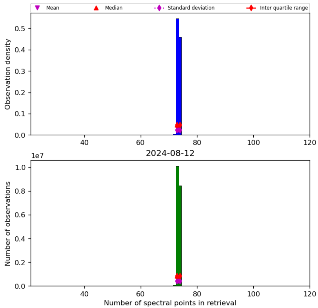
Figure 74: Histogram of “Number of spectral points in retrieval” for 2024-08-12 to 2024-08-13
