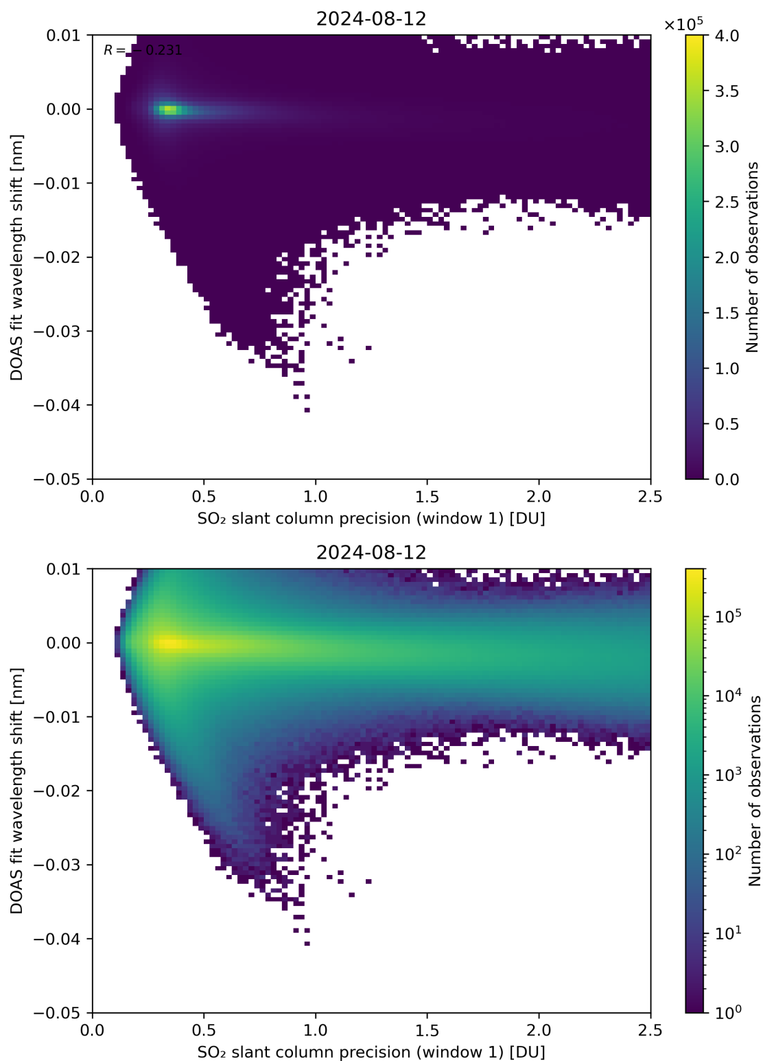
Figure 221: Scatter density plot of “SO 2 slant column precision (window 1)” against “DOAS fit wavelength shift” for 2024-08-12 to 2024-08-13.
