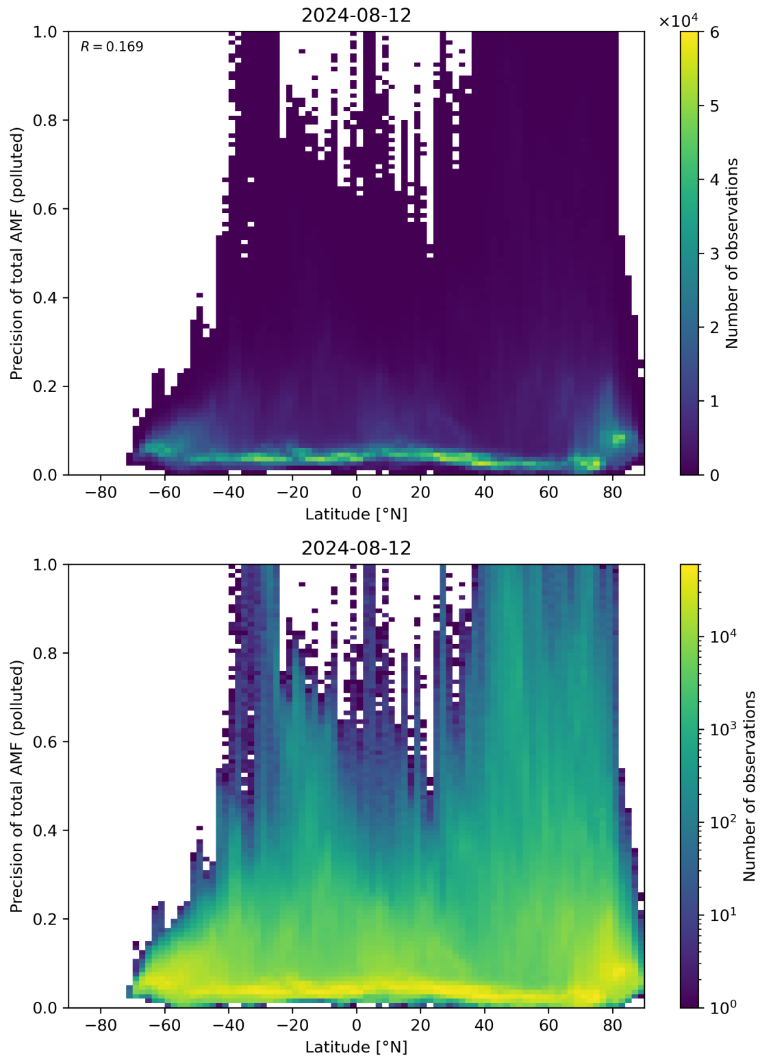
Figure 155: Scatter density plot of “Latitude” against “Precision of total AMF (polluted)” for 2024-08-12 to 2024-08-13.
