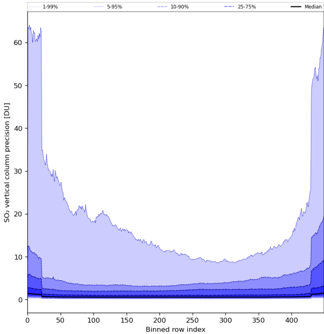
Figure 77: Along track statistics of “SO 2 vertical column precision” for 2024-08-12 to 2024-08-13
