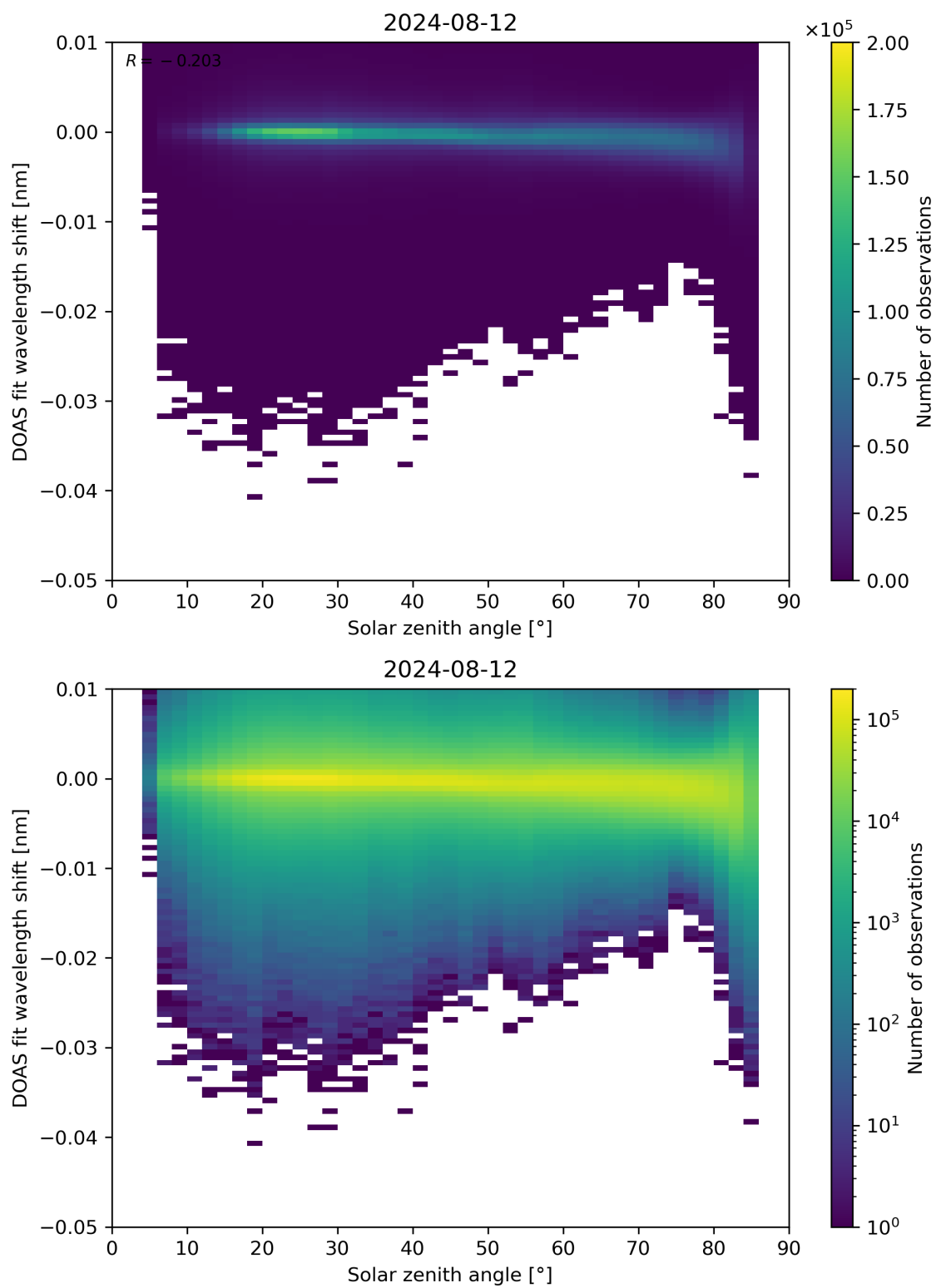
Figure 161: Scatter density plot of “Solar zenith angle” against “DOAS fit wavelength shift” for 2024-08-12 to 2024-08-13.
