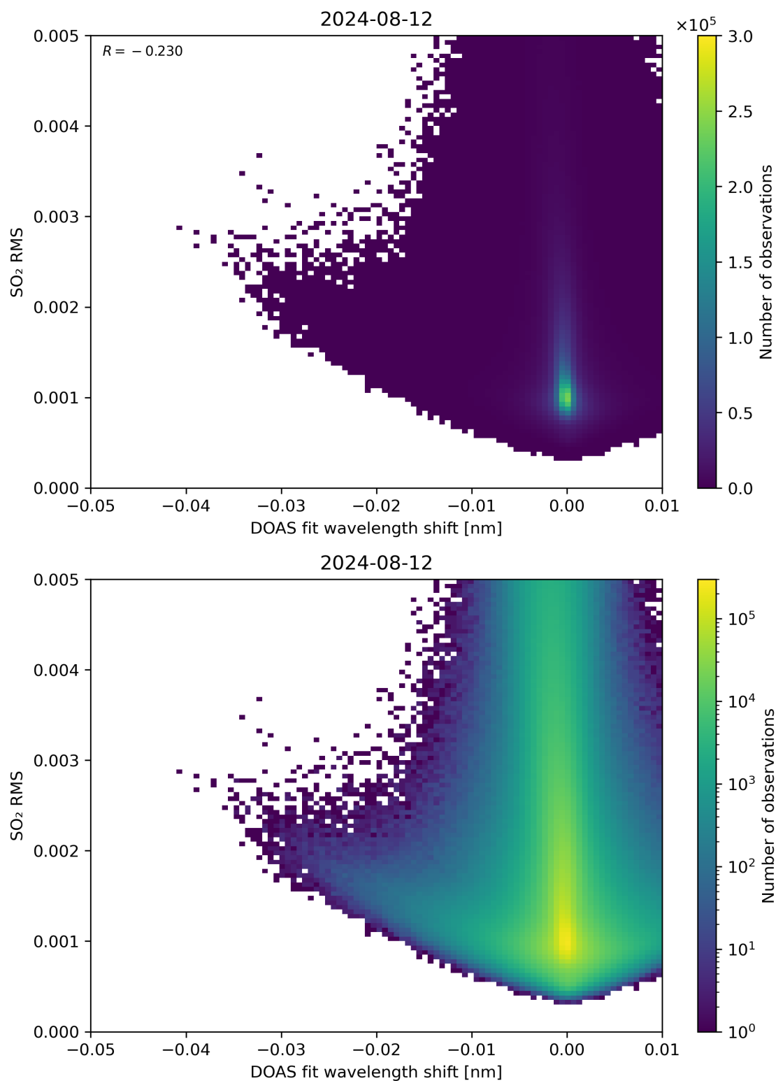
Figure 128: Scatter density plot of “DOAS fit wavelength shift” against “SO 2 RMS” for 2024-08-12 to 2024-08-13.
