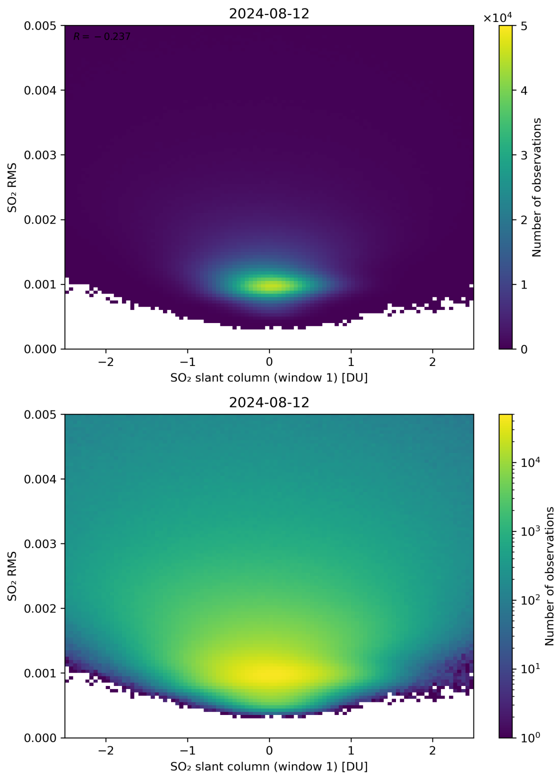
Figure 217: Scatter density plot of “SO 2 slant column (window 1)” against “SO 2 RMS” for 2024-08-12 to 2024-08-13.
