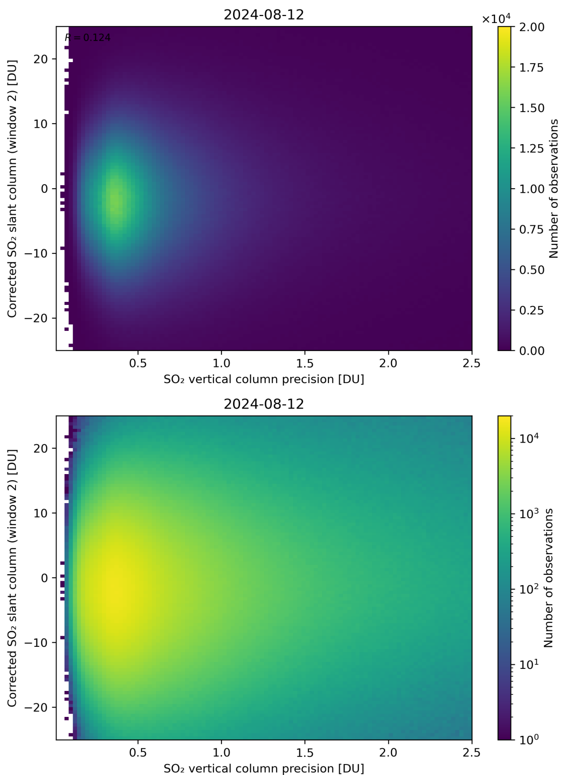
Figure 287: Scatter density plot of “SO 2 vertical column precision” against “Corrected SO 2 slant column (window 2)” for 2024-08-12 to 2024-08-13.
