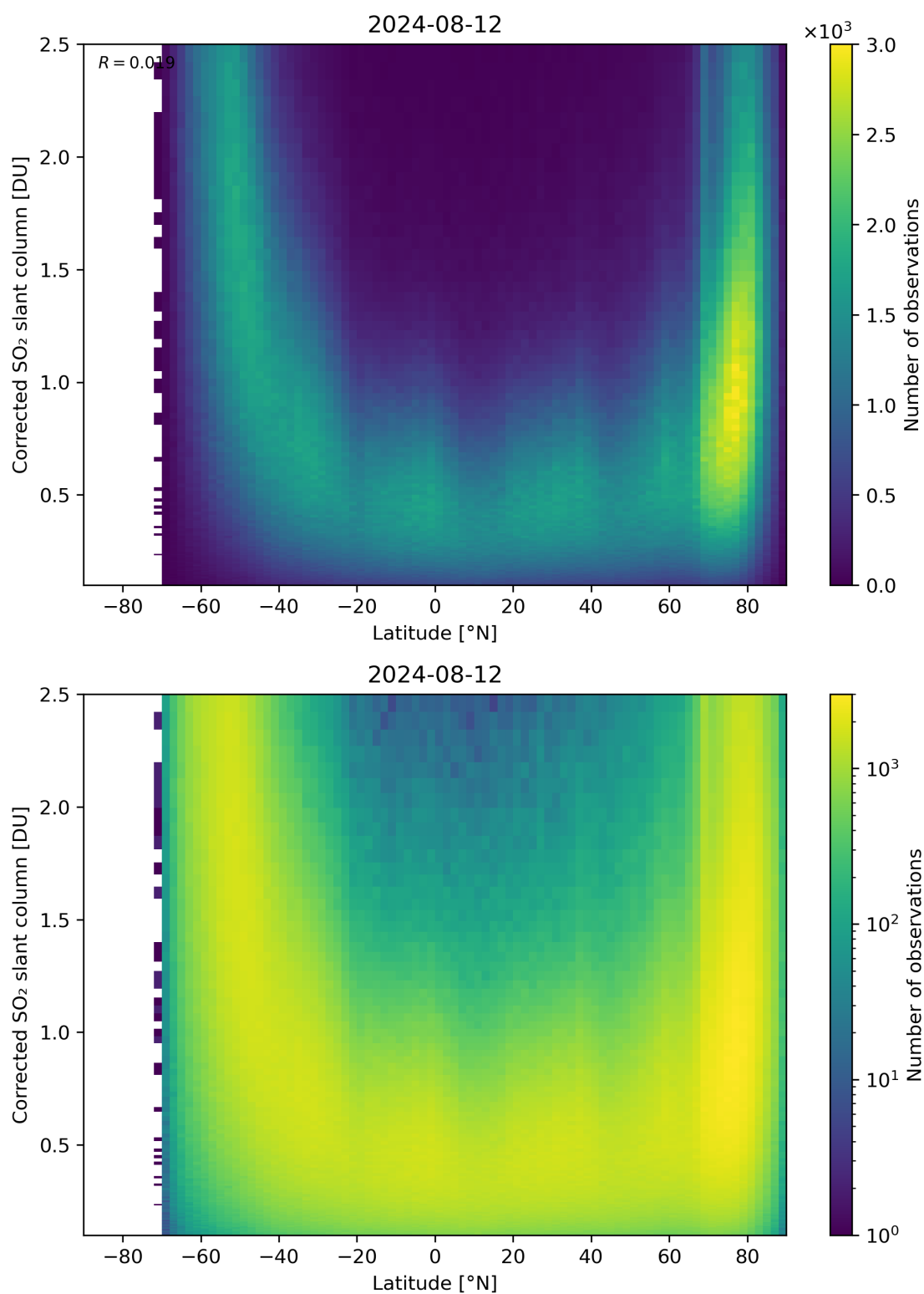
Figure 146: Scatter density plot of “Latitude” against “Corrected SO 2 slant column” for 2024-08-12 to 2024-08-13.
