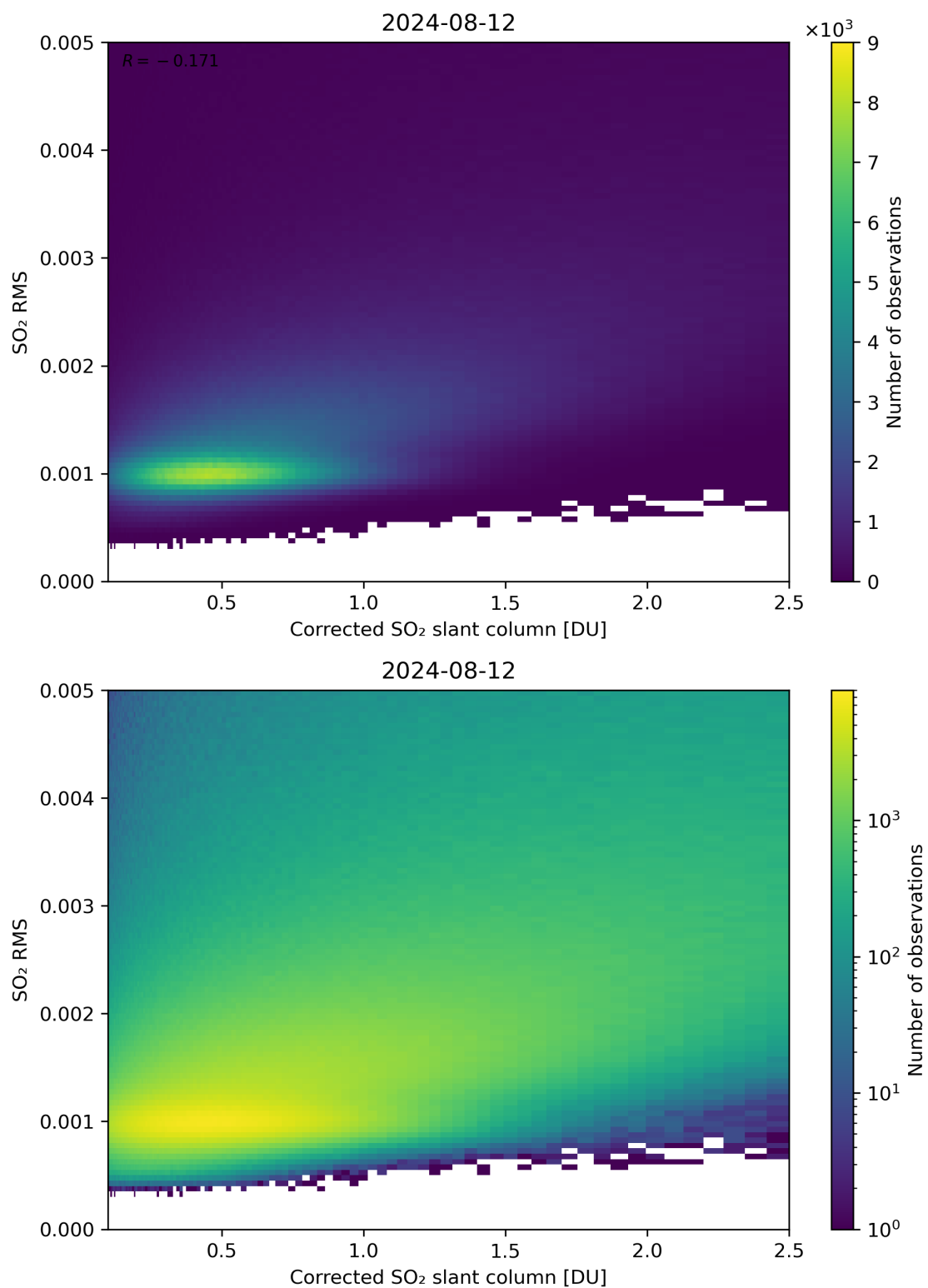
Figure 183: Scatter density plot of “Corrected SO 2 slant column” against “SO 2 RMS” for 2024-08-12 to 2024-08-13.
