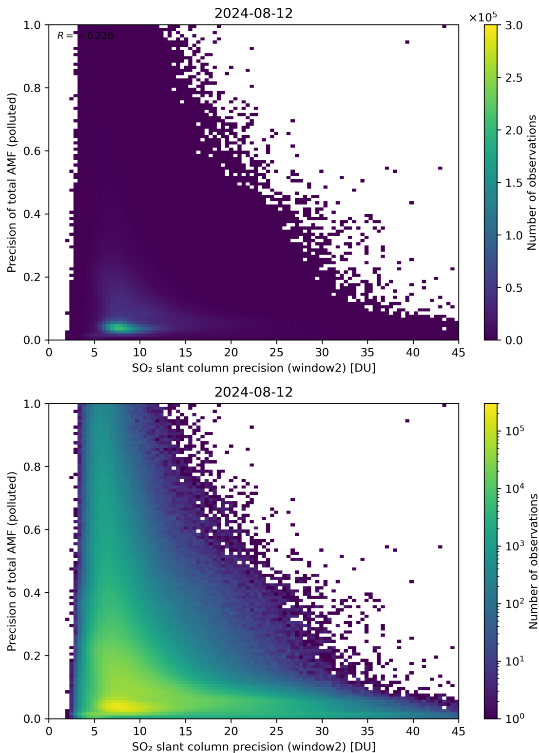
Figure 252: Scatter density plot of “SO 2 slant column precision (window2)” against “Precision of total AMF (polluted)” for 2024-08-12 to 2024-08-13.
