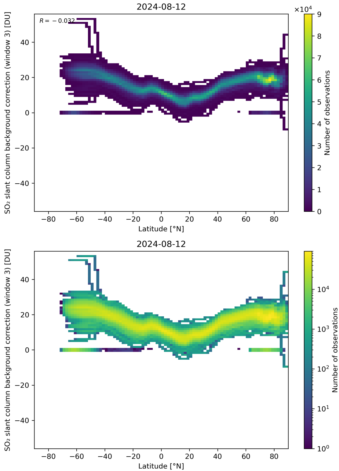
Figure 141: Scatter density plot of “Latitude” against “SO 2 slant column background correction (window 3)” for 2024-08-12 to 2024-08-13.
