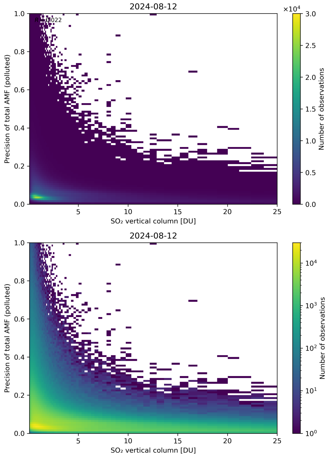
Figure 306: Scatter density plot of “SO 2 vertical column” against “Precision of total AMF (polluted)” for 2024-08-12 to 2024-08-13.
