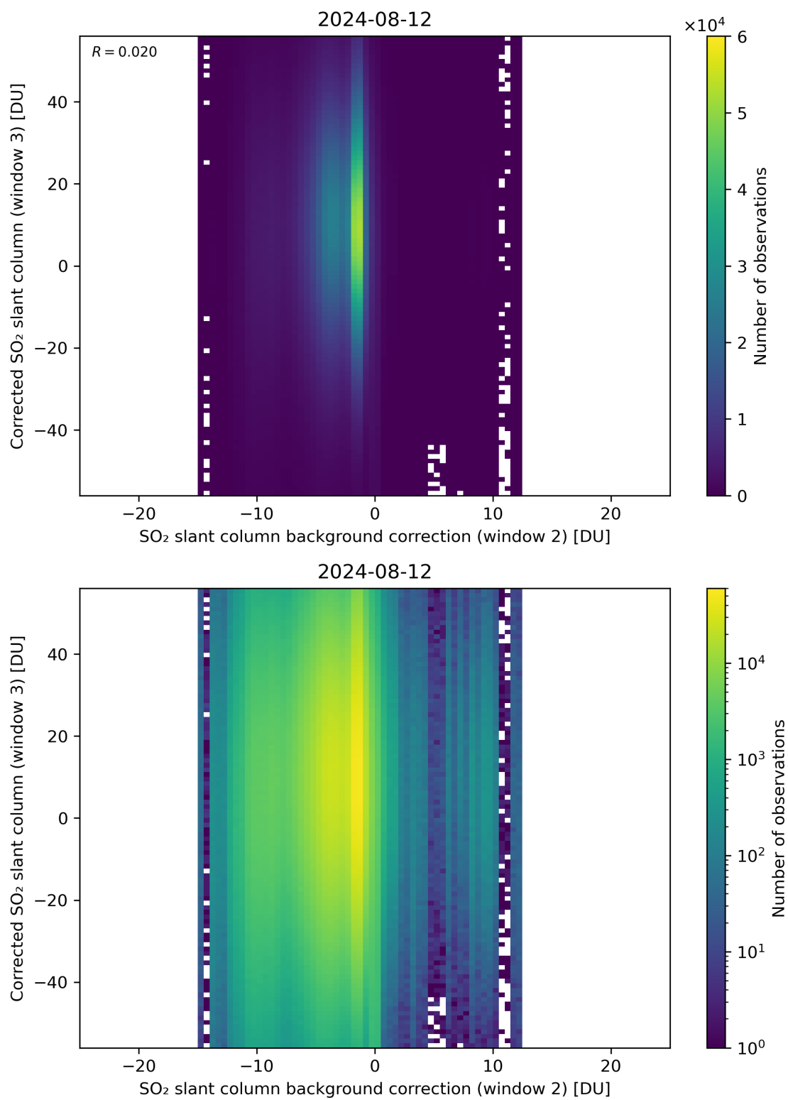
Figure 116: Scatter density plot of “SO 2 slant column background correction (window 2)” against “Corrected SO 2 slant column (window 3)” for 2024-08-12 to 2024-08-13.
