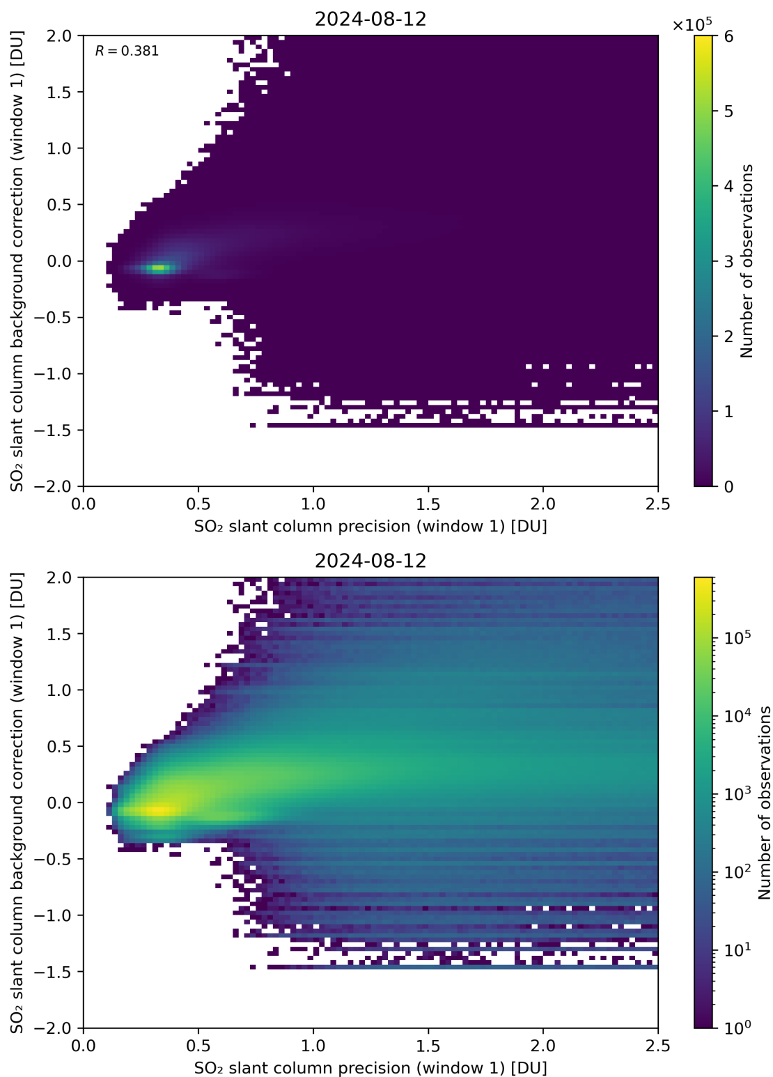
Figure 218: Scatter density plot of “SO 2 slant column precision (window 1)” against “SO 2 slant column background correction (window 1)” for 2024-08-12 to 2024-08-13.
