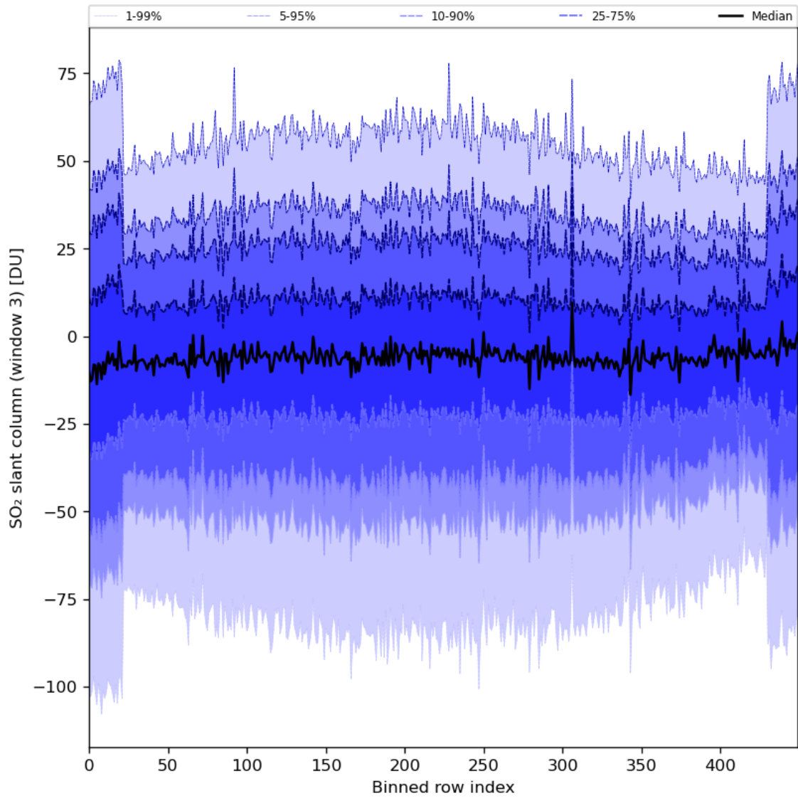
Figure 87: Along track statistics of “SO 2 slant column (window 3)” for 2024-08-12 to 2024-08-13
