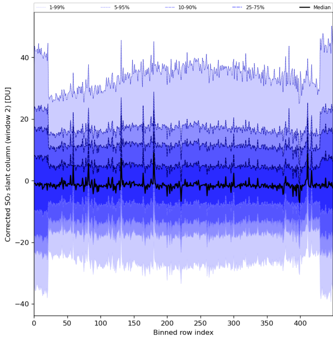
Figure 85: Along track statistics of “Corrected SO 2 slant column (window 2)” for 2024-08-12 to 2024-08-13
