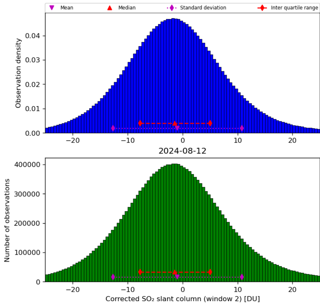
Figure 62: Histogram of “Corrected SO 2 slant column (window 2)” for 2024-08-12 to 2024-08-13
