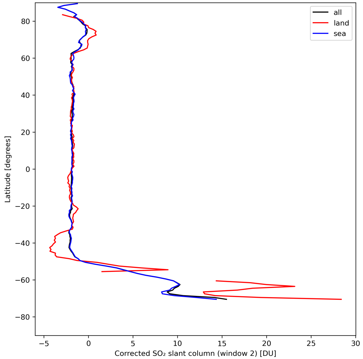
Figure 39: Zonal average of “Corrected SO 2 slant column (window 2)” for 2024-08-12 to 2024-08-13.
