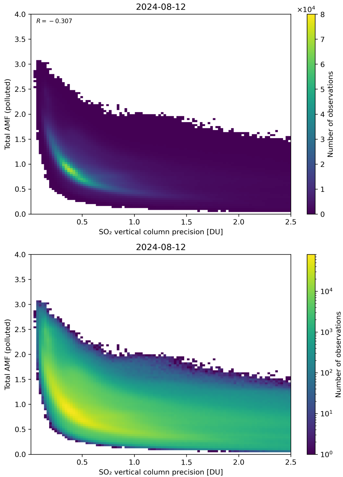
Figure 294: Scatter density plot of “SO 2 vertical column precision” against “Total AMF (polluted)” for 2024-08-12 to 2024-08-13.
