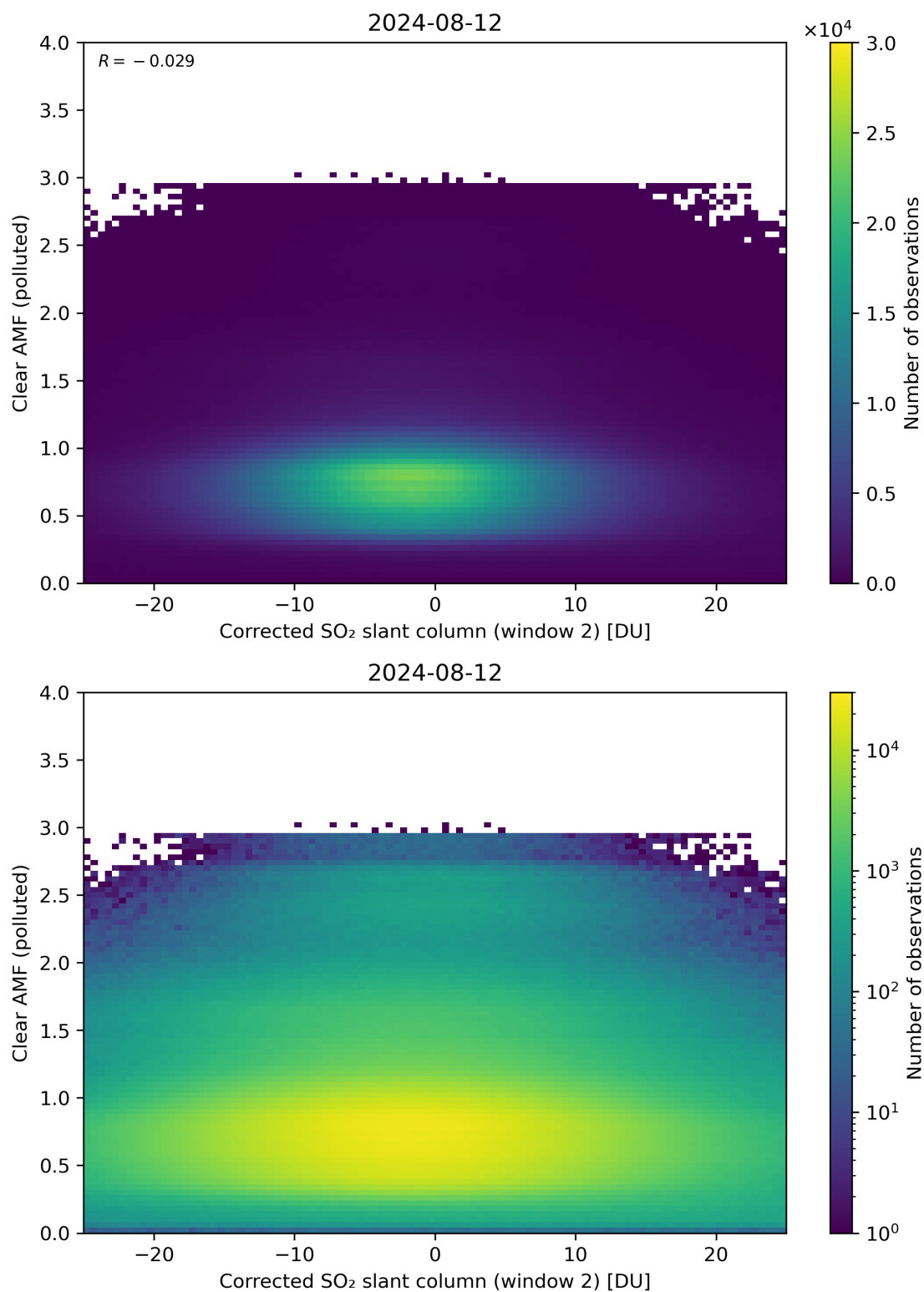
Figure 199: Scatter density plot of “Corrected SO 2 slant column (window 2)” against “Clear AMF (polluted)” for 2024-08-12 to 2024-08-13.
