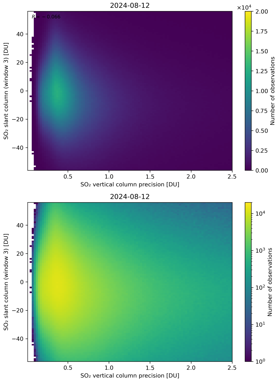
Figure 292: Scatter density plot of “SO 2 vertical column precision” against “SO 2 slant column (window 3)” for 2024-08-12 to 2024-08-13.
