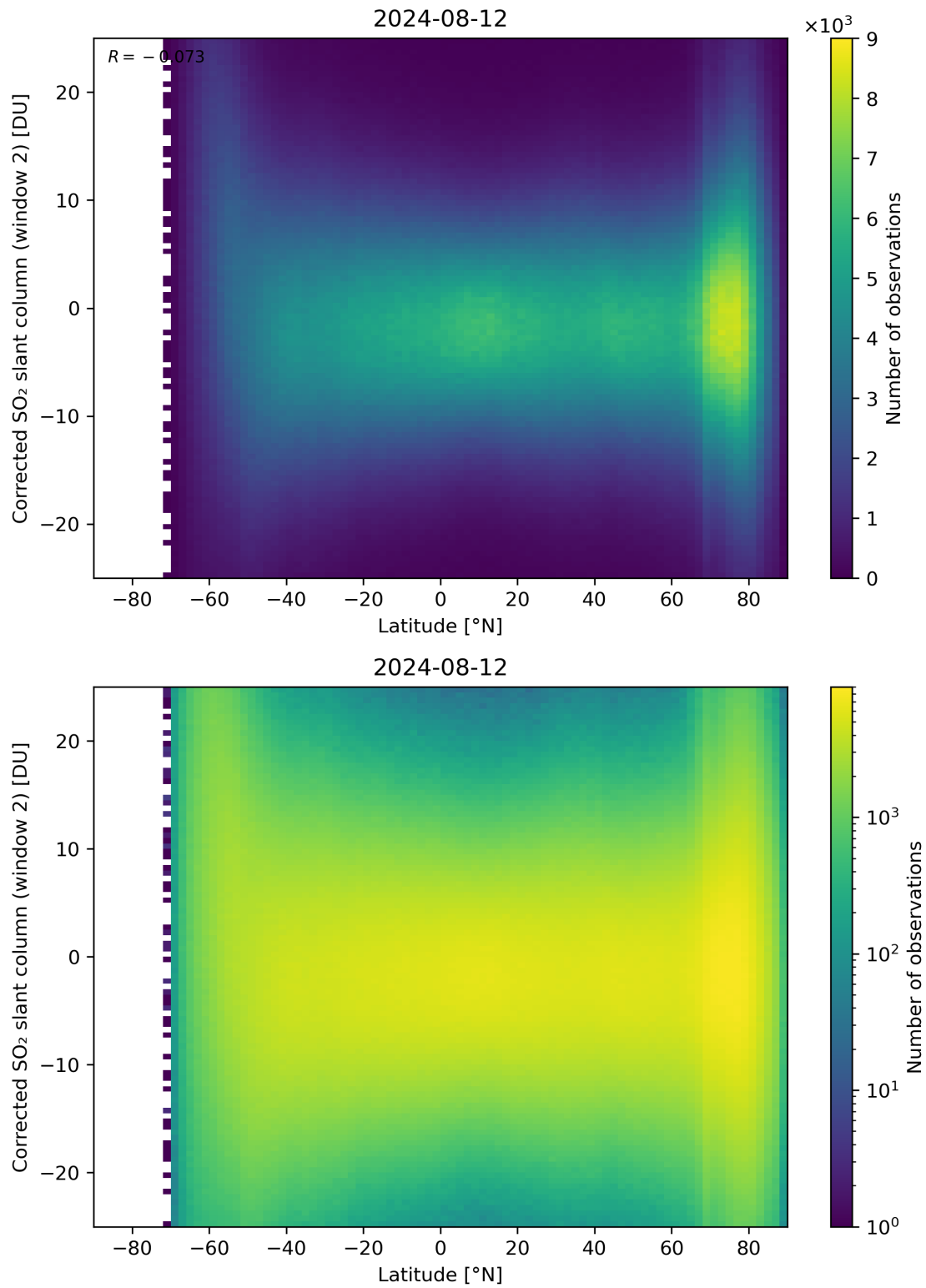
Figure 147: Scatter density plot of “Latitude” against “Corrected SO 2 slant column (window 2)” for 2024-08-12 to 2024-08-13.
