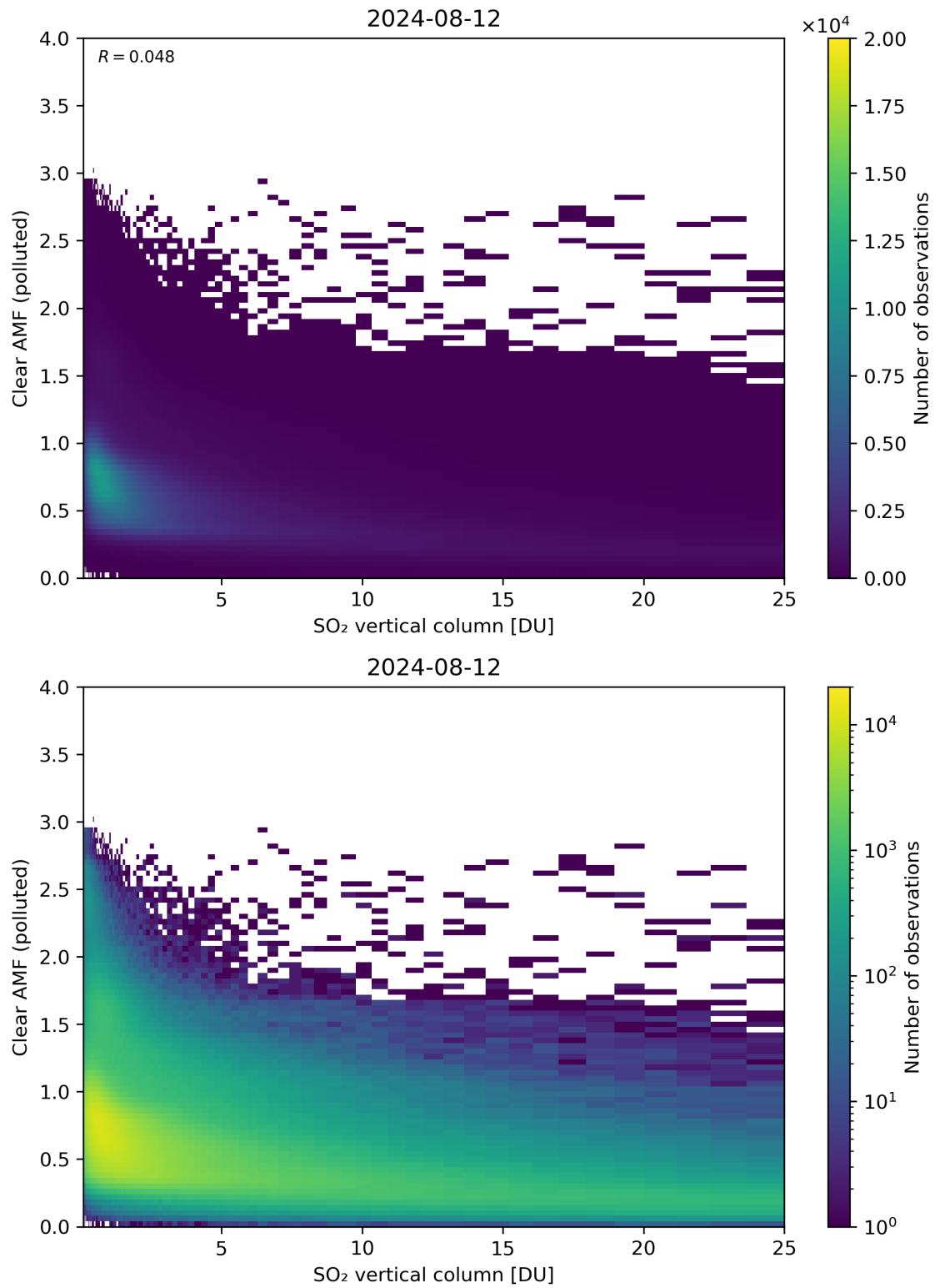
Figure 296: Scatter density plot of “SO 2 vertical column” against “Clear AMF (polluted)” for 2024-08-12 to 2024-08-13.
