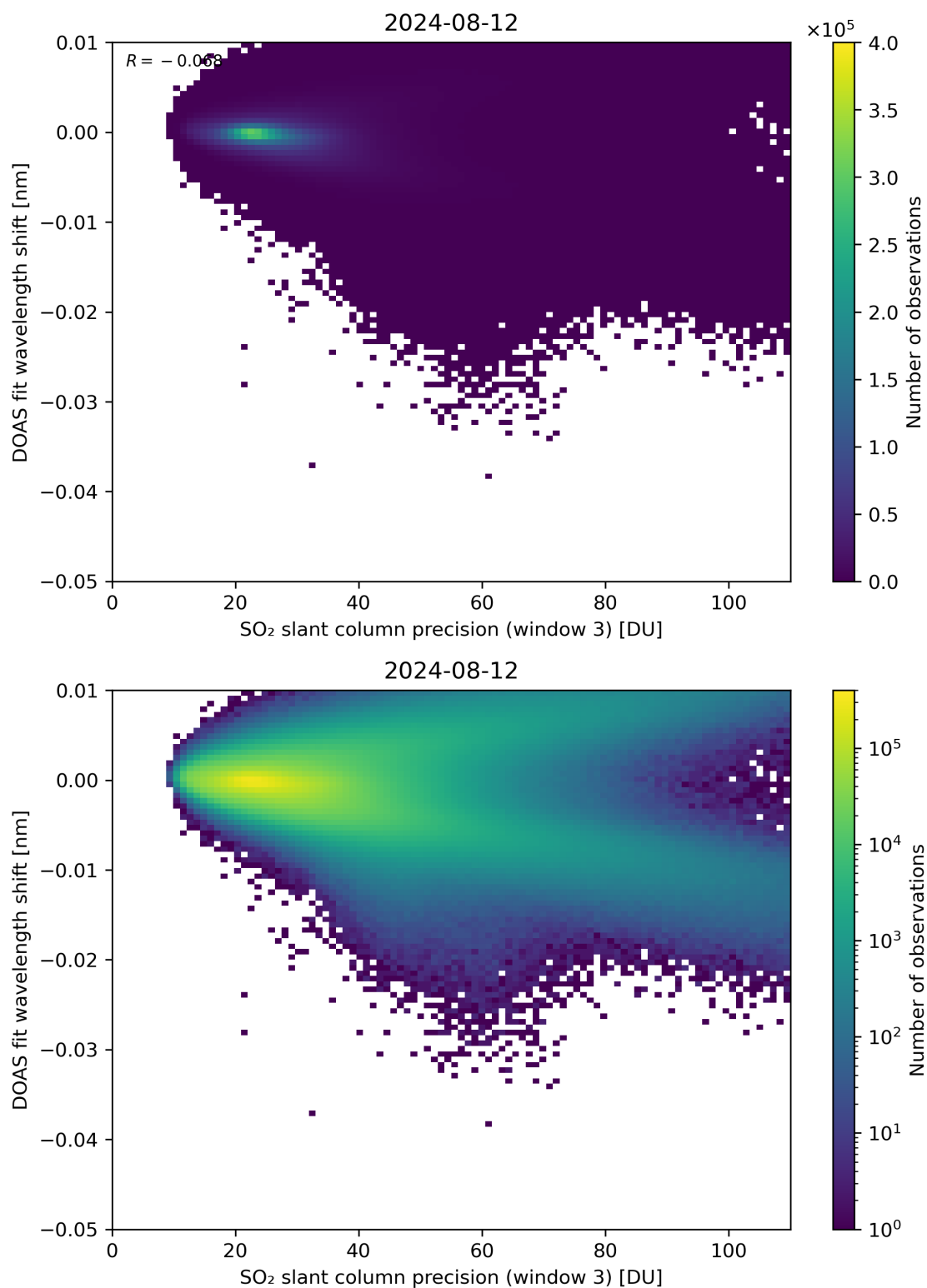
Figure 258: Scatter density plot of “SO 2 slant column precision (window 3)” against “DOAS fit wavelength shift” for 2024-08-12 to 2024-08-13.
