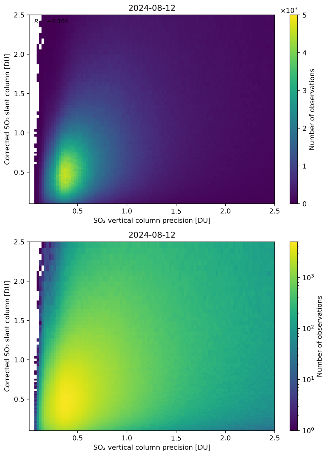
Figure 286: Scatter density plot of “SO 2 vertical column precision” against “Corrected SO 2 slant column” for 2024-08-12 to 2024-08-13.
