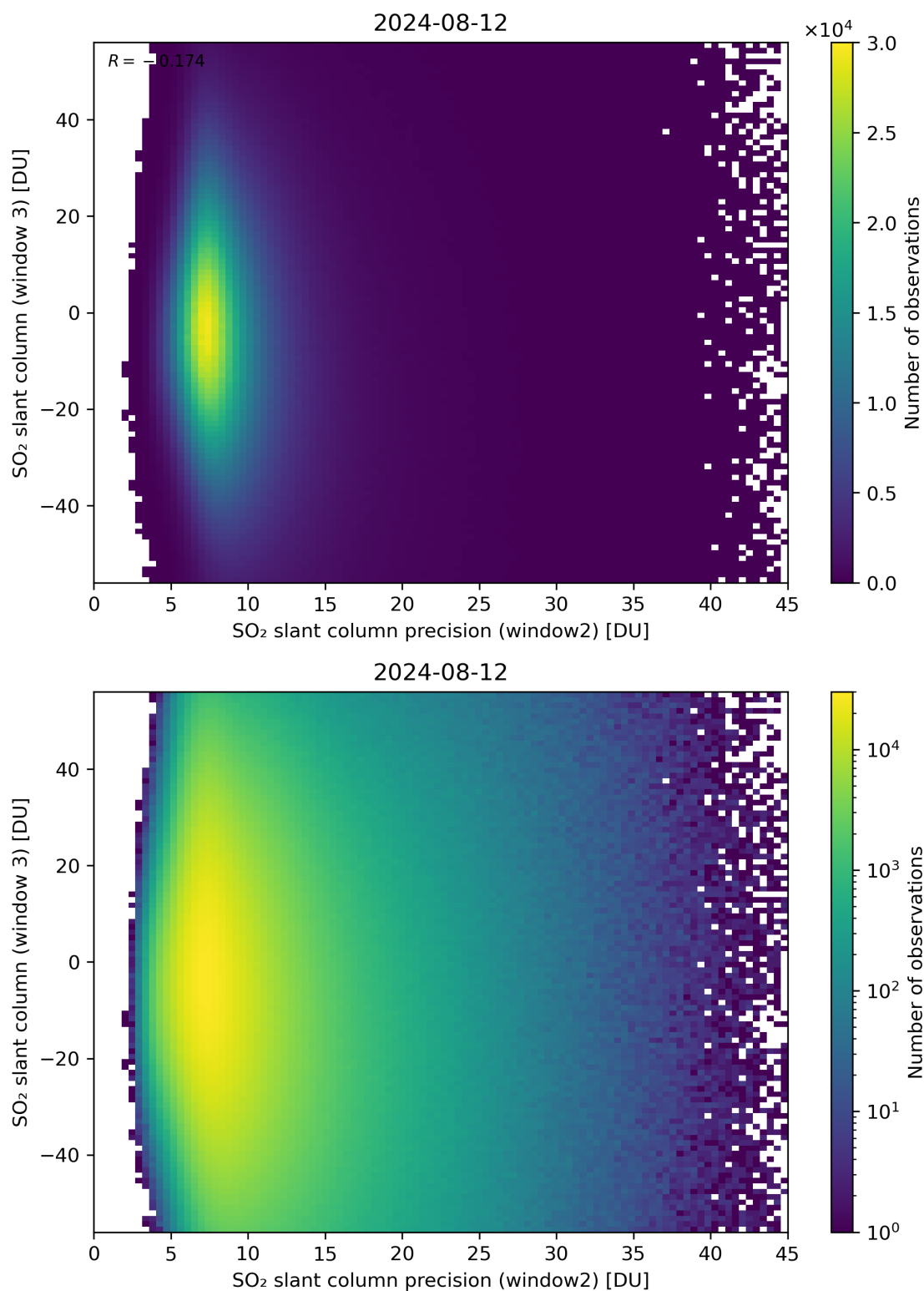
Figure 249: Scatter density plot of “SO 2 slant column precision (window2)” against “SO 2 slant column (window 3)” for 2024-08-12 to 2024-08-13.
