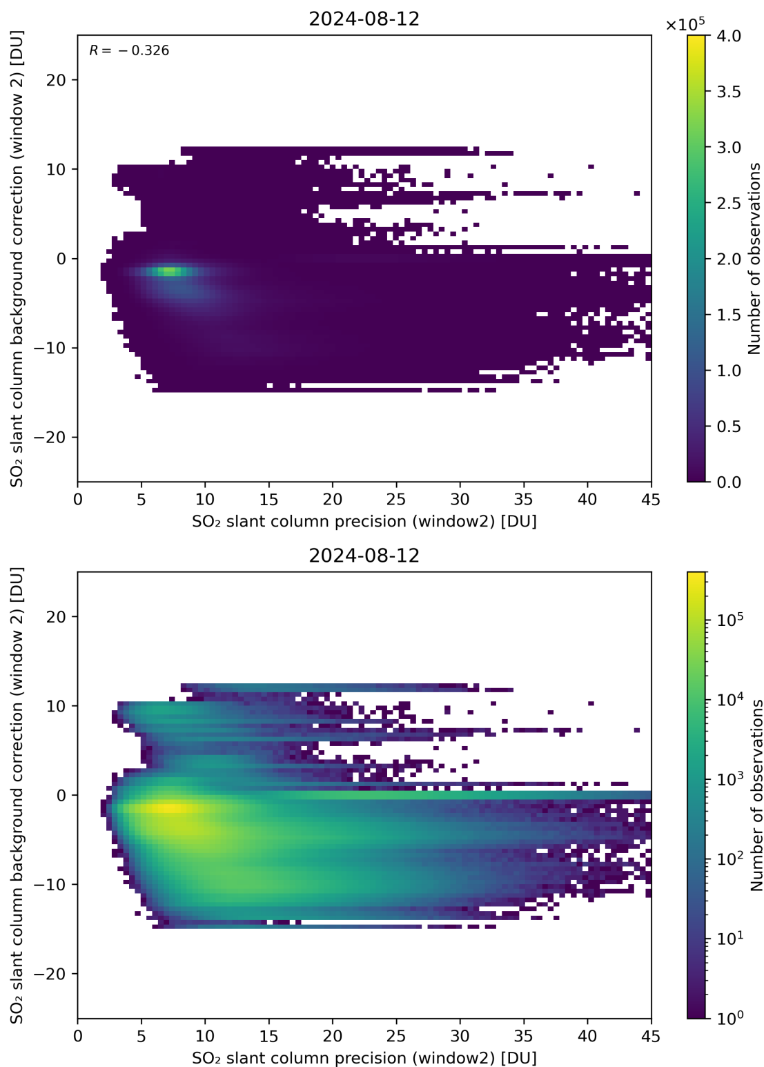
Figure 241: Scatter density plot of “SO 2 slant column precision (window2)” against “SO 2 slant column background correction (window 2)” for 2024-08-12 to 2024-08-13.
