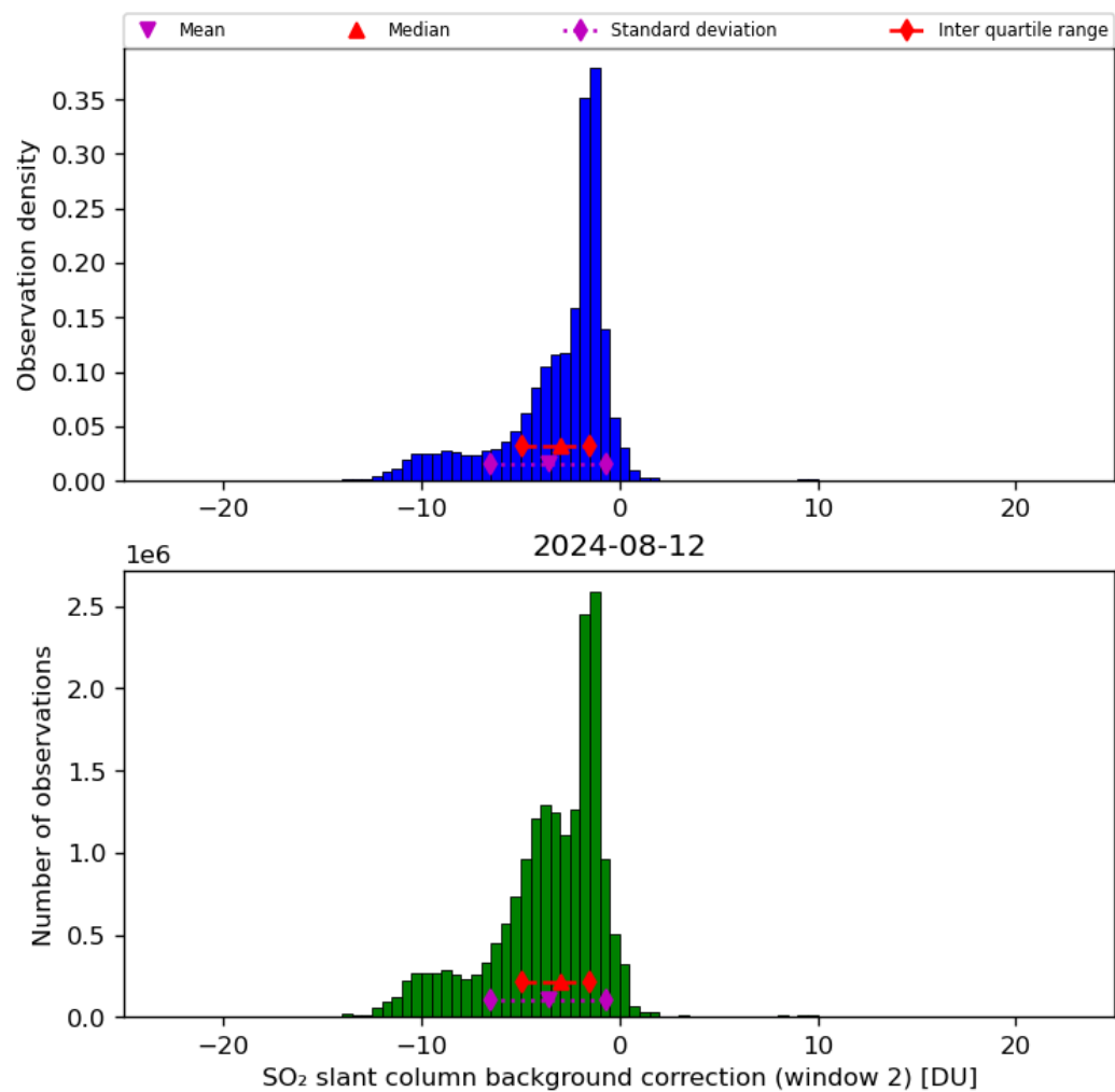
Figure 63: Histogram of “SO 2 slant column background correction (window 2)” for 2024-08-12 to 2024-08-13
