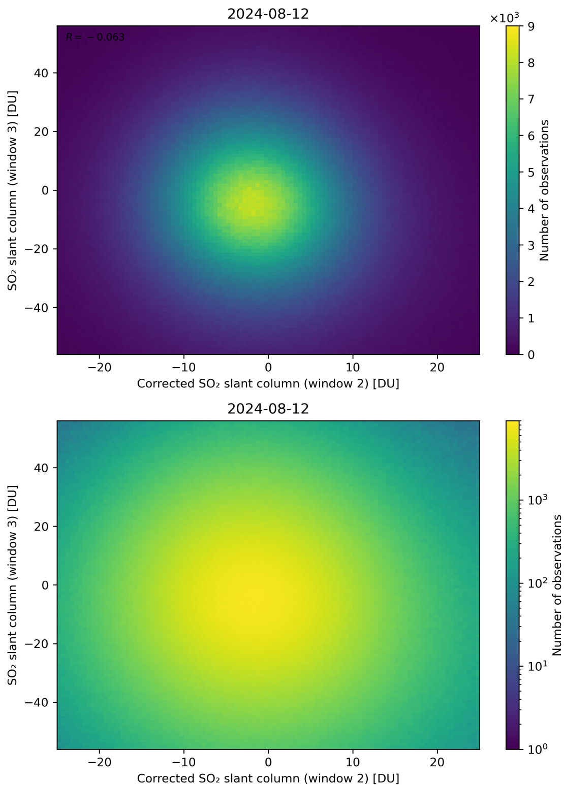
Figure 201: Scatter density plot of “Corrected SO 2 slant column (window 2)” against “SO 2 slant column (window 3)” for 2024-08-12 to 2024-08-13.
