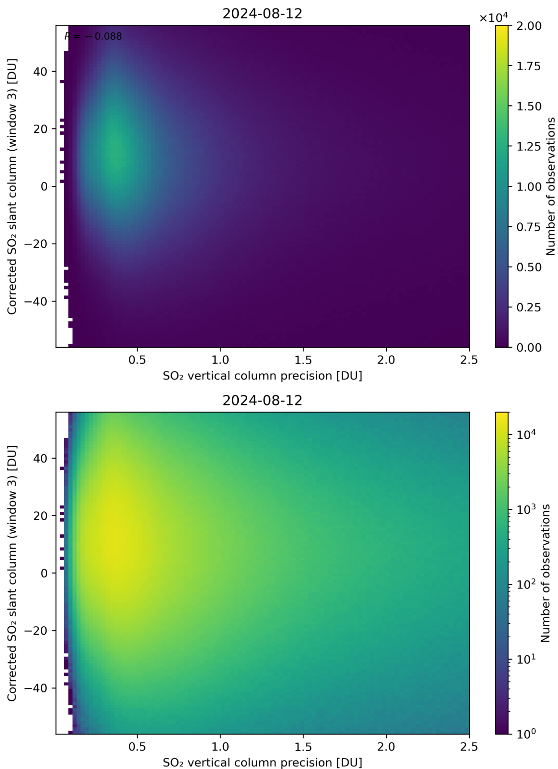
Figure 288: Scatter density plot of “SO 2 vertical column precision” against “Corrected SO 2 slant column (window 3)” for 2024-08-12 to 2024-08-13.
