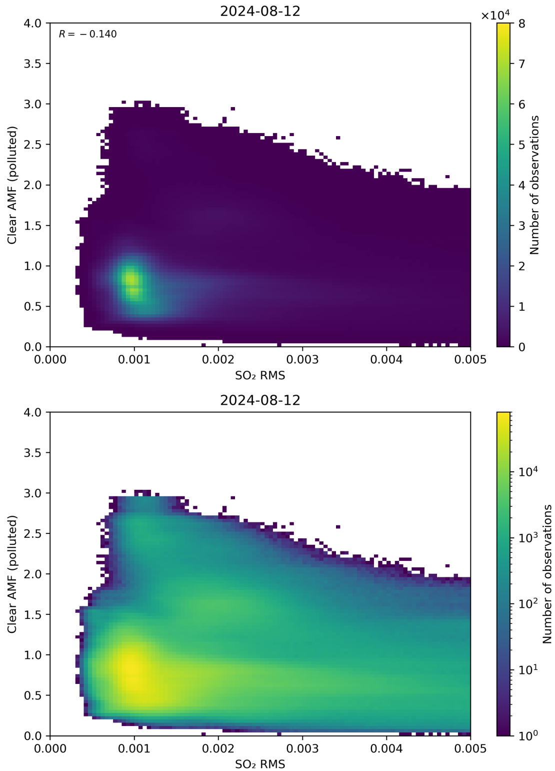
Figure 136: Scatter density plot of “SO 2 RMS” against “Clear AMF (polluted)” for 2024-08-12 to 2024-08-13.
