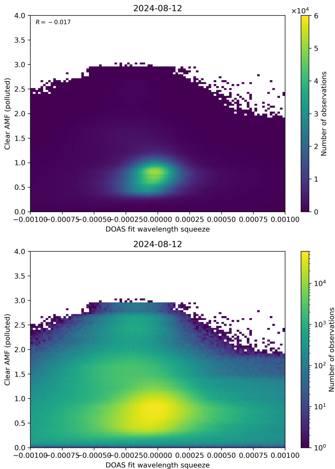
Figure 133: Scatter density plot of “DOAS fit wavelength squeeze” against “Clear AMF (polluted)” for 2024-08-12 to 2024-08-13.
