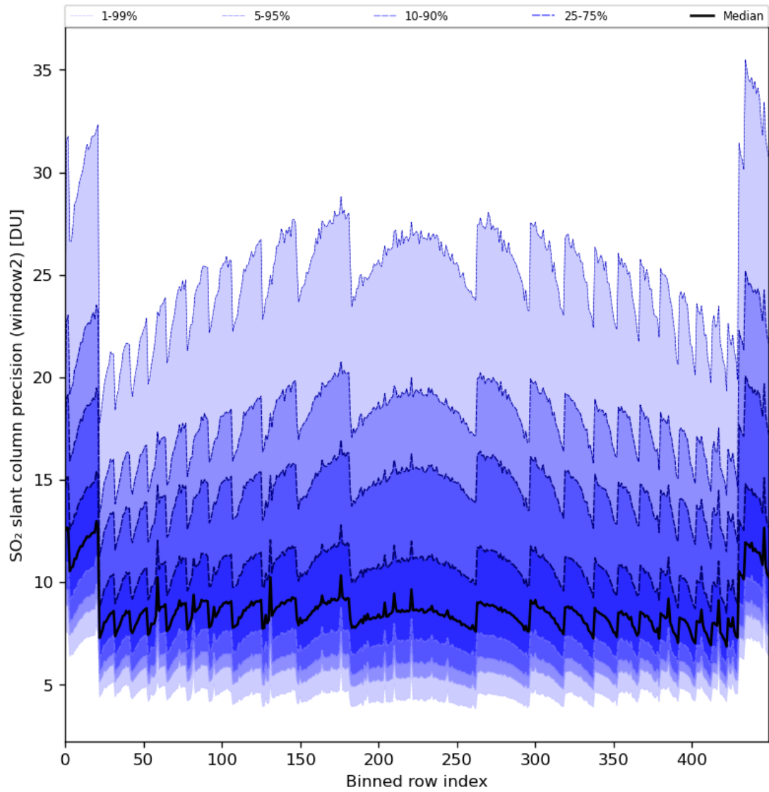
Figure 84: Along track statistics of “SO 2 slant column precision (window2)” for 2024-08-12 to 2024-08-13
