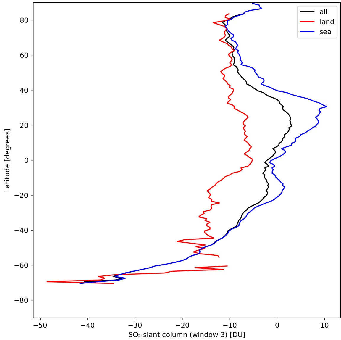
Figure 41: Zonal average of “SO 2 slant column (window 3)” for 2024-08-12 to 2024-08-13.
