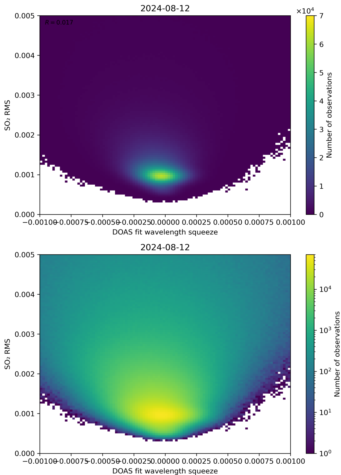
Figure 132: Scatter density plot of “DOAS fit wavelength squeeze” against “SO 2 RMS” for 2024-08-12 to 2024-08-13.
