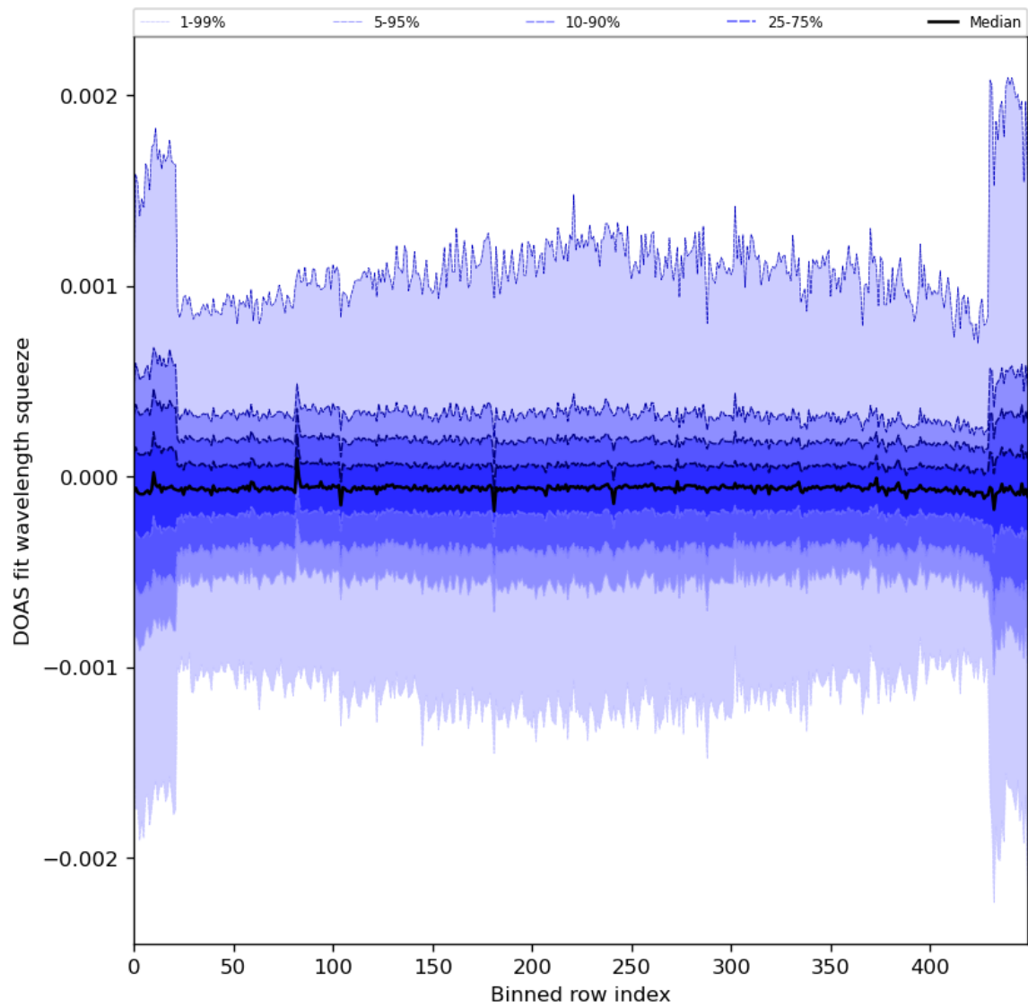
Figure 92: Along track statistics of “DOAS fit wavelength squeeze” for 2024-08-12 to 2024-08-13
