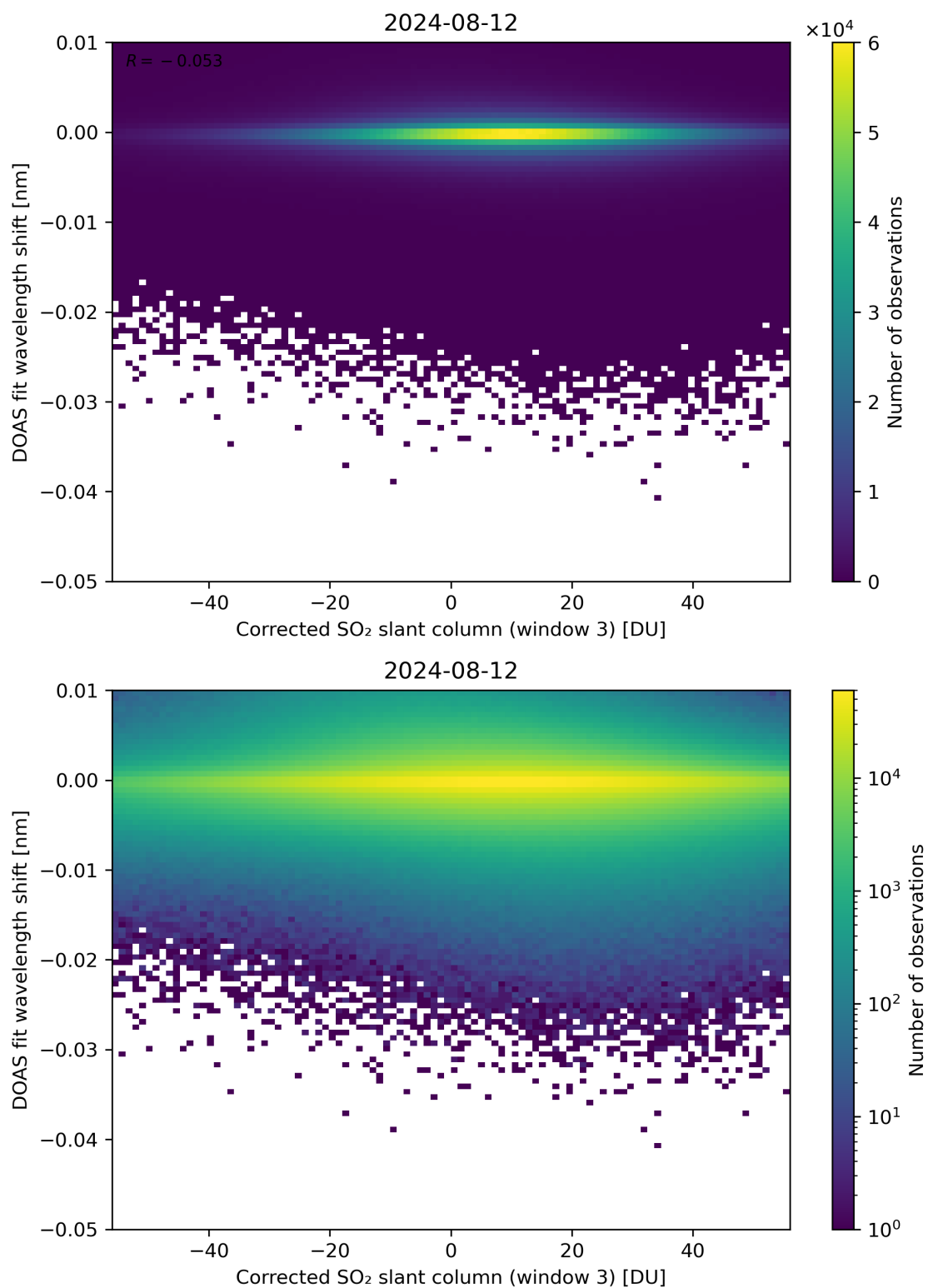
Figure 206: Scatter density plot of “Corrected SO 2 slant column (window 3)” against “DOAS fit wavelength shift” for 2024-08-12 to 2024-08-13.
