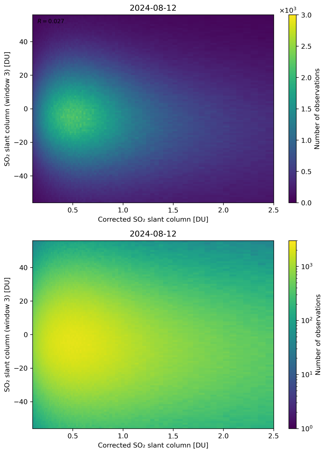
Figure 190: Scatter density plot of “Corrected SO 2 slant column” against “SO 2 slant column (window 3)” for 2024-08-12 to 2024-08-13.
