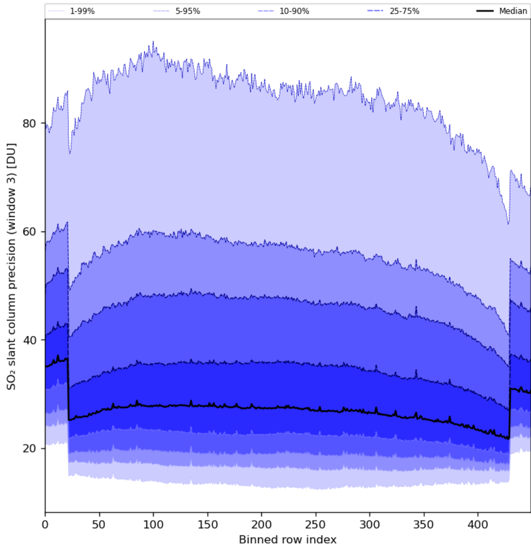
Figure 88: Along track statistics of “SO 2 slant column precision (window 3)” for 2024-08-12 to 2024-08-13
