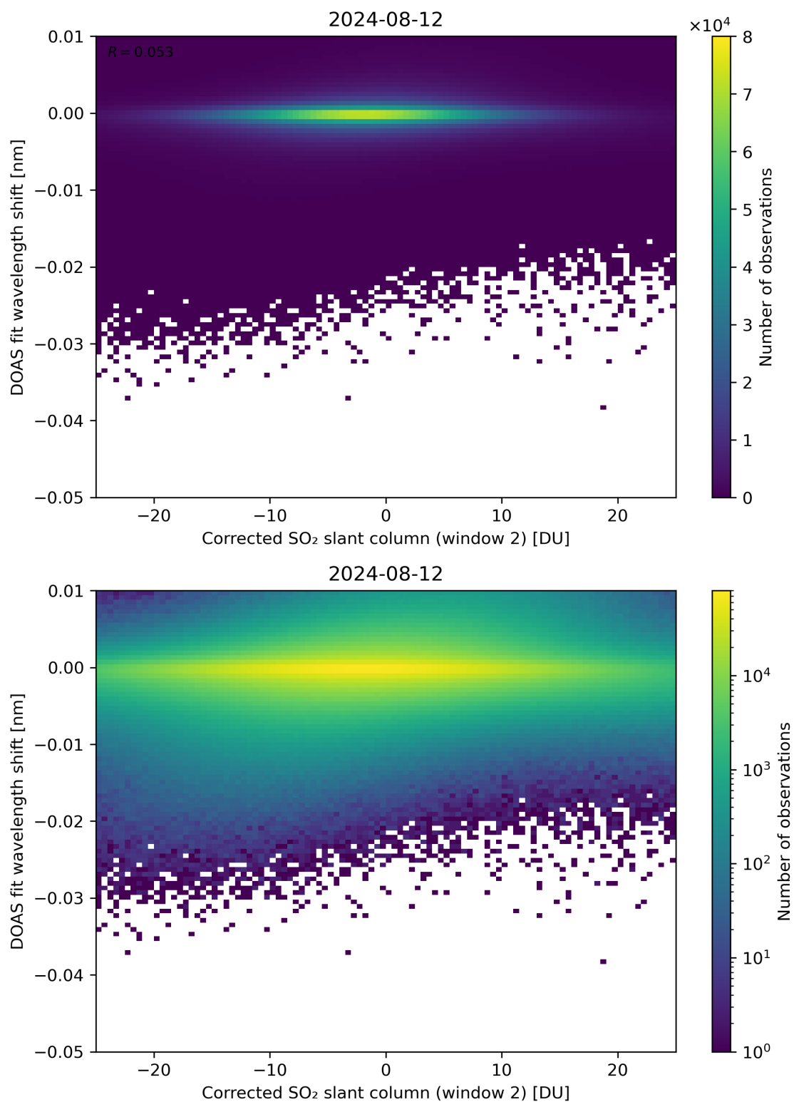
Figure 196: Scatter density plot of “Corrected SO 2 slant column (window 2)” against “DOAS fit wavelength shift” for 2024-08-12 to 2024-08-13.
