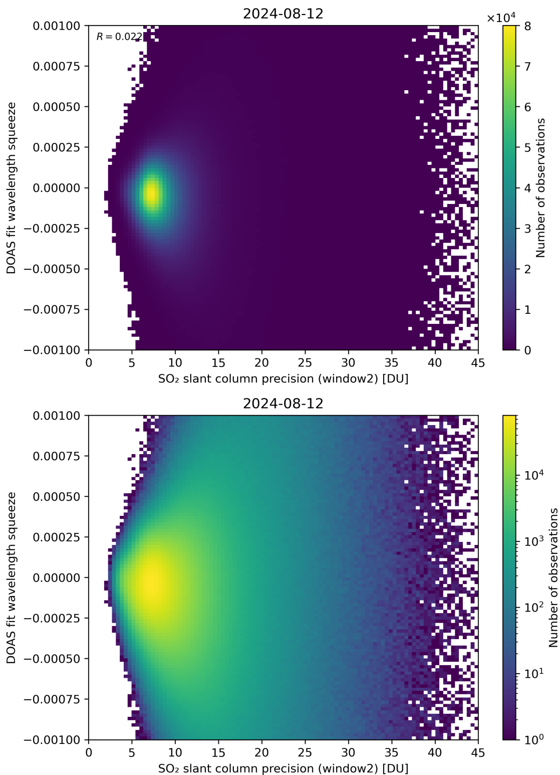
Figure 244: Scatter density plot of “SO 2 slant column precision (window2)” against “DOAS fit wavelength squeeze” for 2024-08-12 to 2024-08-13.
