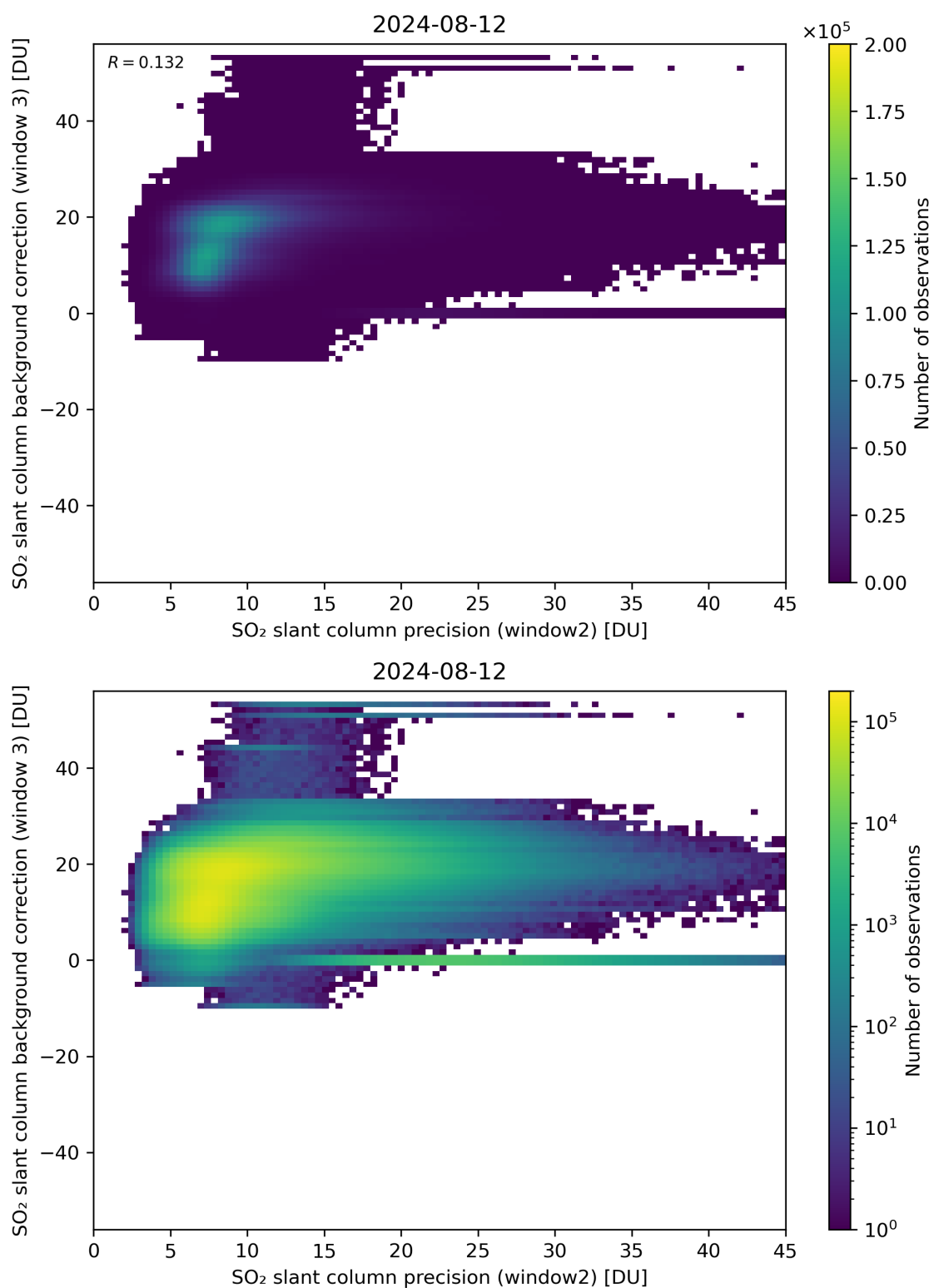
Figure 242: Scatter density plot of “SO 2 slant column precision (window2)” against “SO 2 slant column background correction (window 3)” for 2024-08-12 to 2024-08-13.
