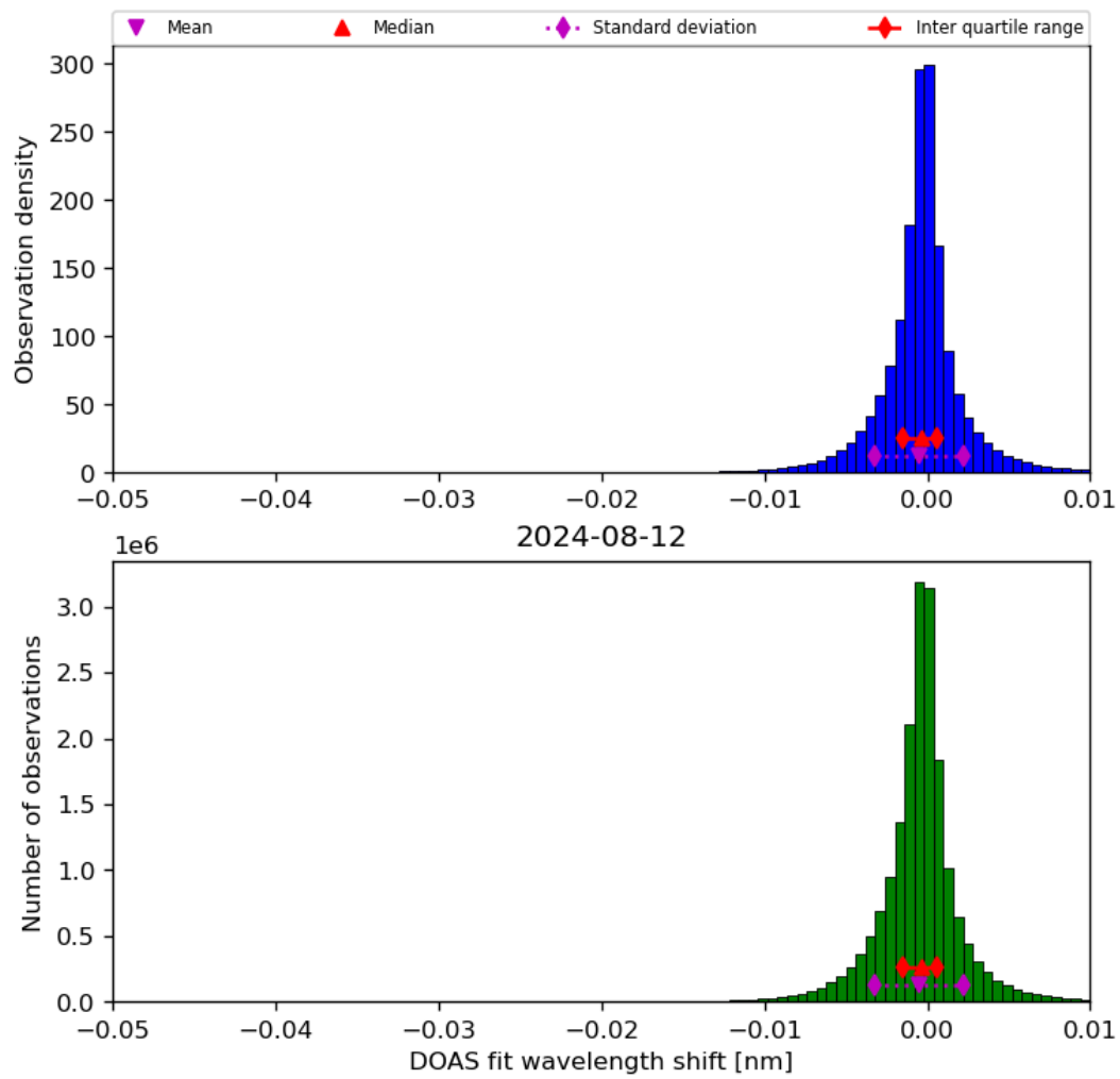
Figure 68: Histogram of “DOAS fit wavelength shift” for 2024-08-12 to 2024-08-13
