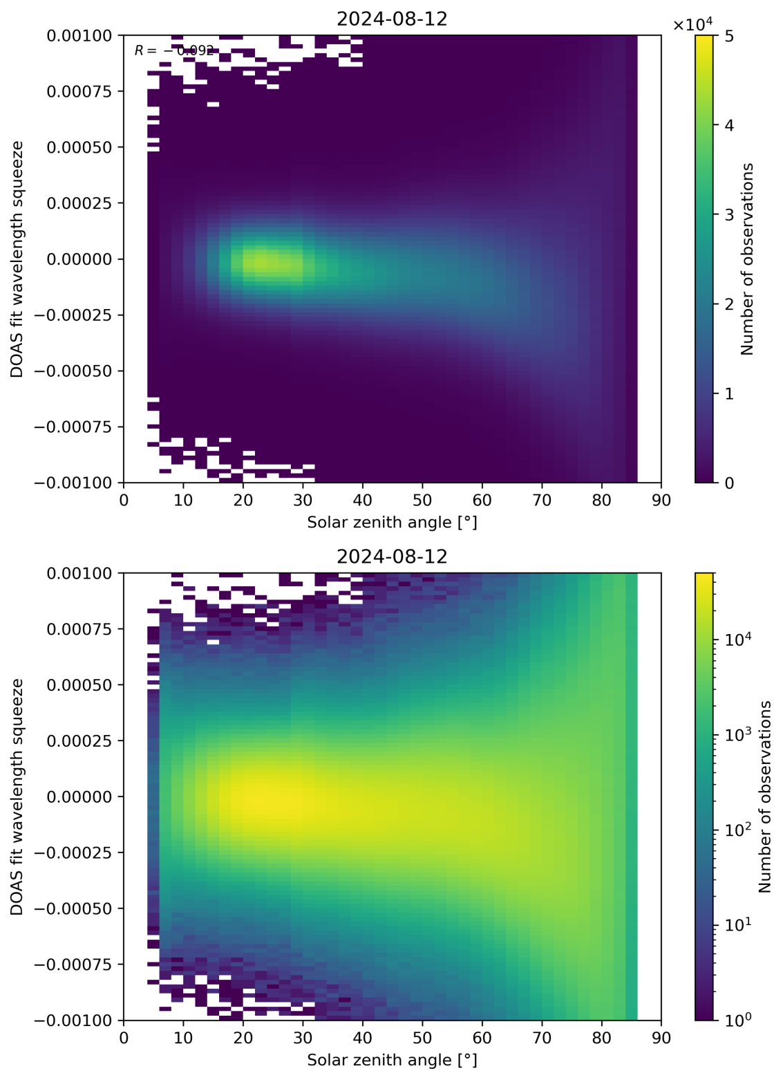
Figure 162: Scatter density plot of “Solar zenith angle” against “DOAS fit wavelength squeeze” for 2024-08-12 to 2024-08-13.
