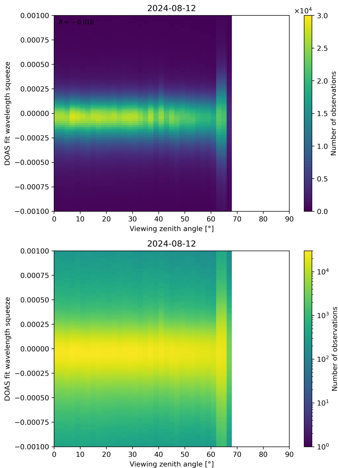
Figure 312: Scatter density plot of “Viewing zenith angle” against “DOAS fit wavelength squeeze” for 2024-08-12 to 2024-08-13.
