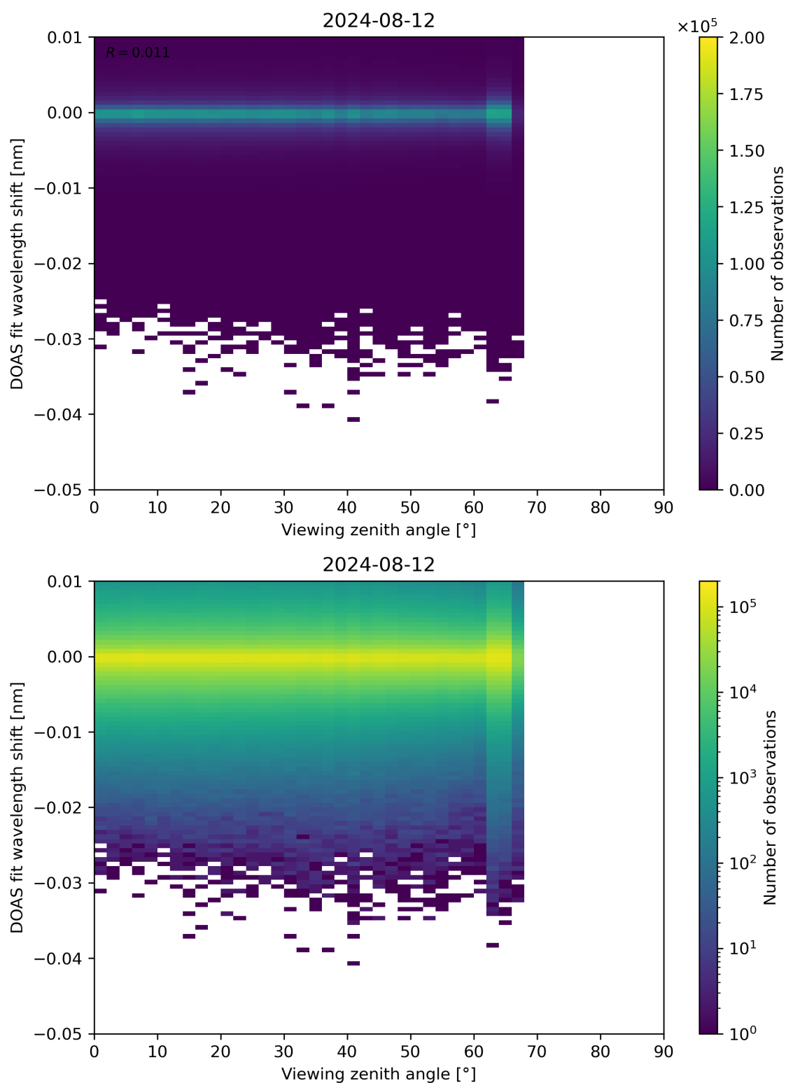
Figure 311: Scatter density plot of “Viewing zenith angle” against “DOAS fit wavelength shift” for 2024-08-12 to 2024-08-13.
