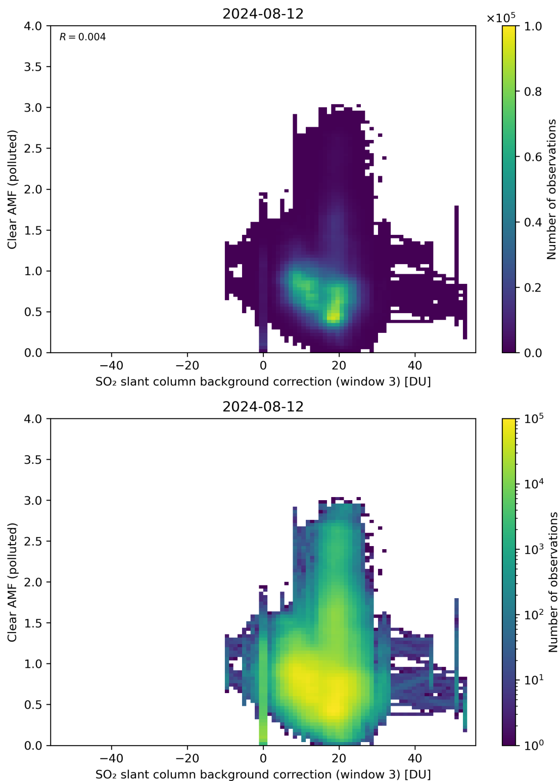
Figure 124: Scatter density plot of “SO 2 slant column background correction (window 3)” against “Clear AMF (polluted)” for 2024-08-12 to 2024-08-13.
