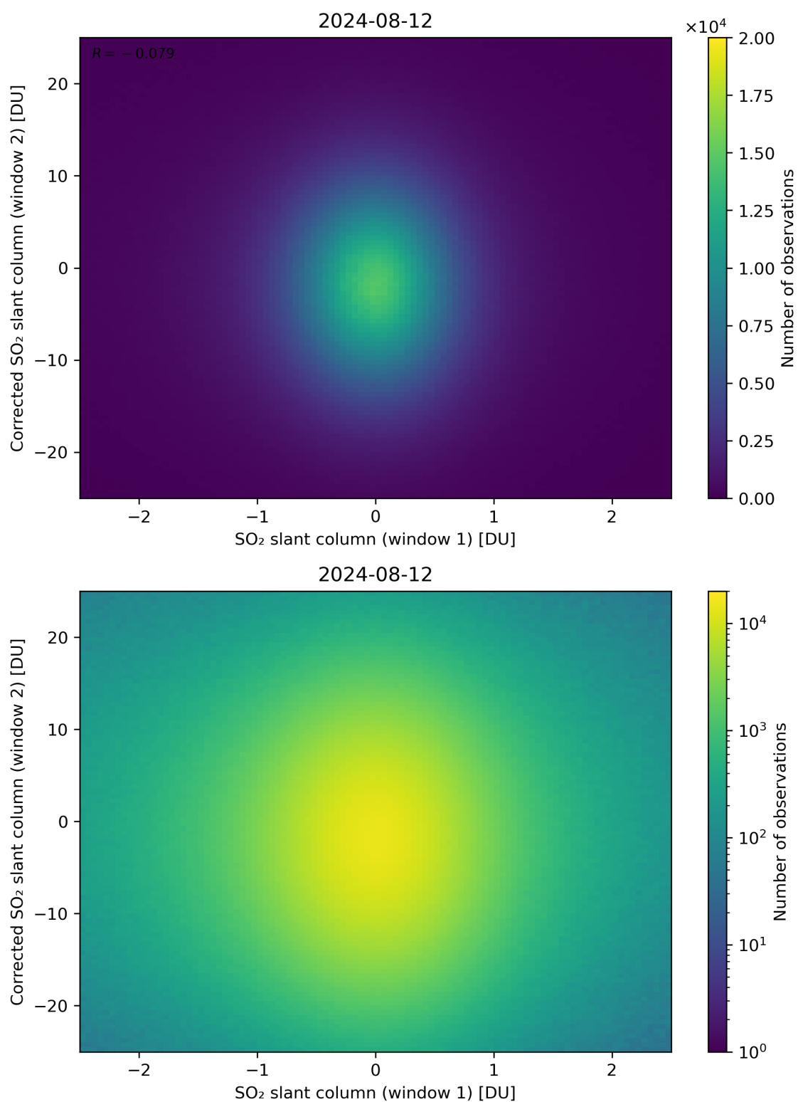
Figure 233: Scatter density plot of “SO 2 slant column (window 1)” against “Corrected SO 2 slant column (window 2)” for 2024-08-12 to 2024-08-13.
