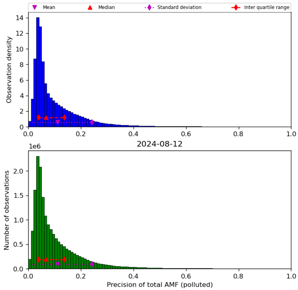
Figure 72: Histogram of “Precision of total AMF (polluted)” for 2024-08-12 to 2024-08-13
