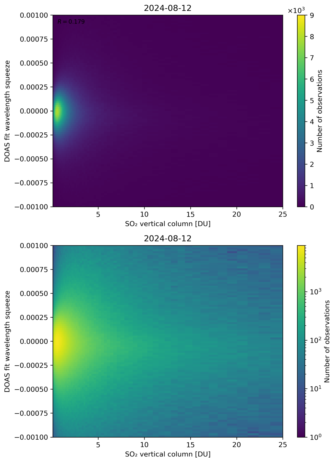
Figure 277: Scatter density plot of “SO 2 vertical column” against “DOAS fit wavelength squeeze” for 2024-08-12 to 2024-08-13.
