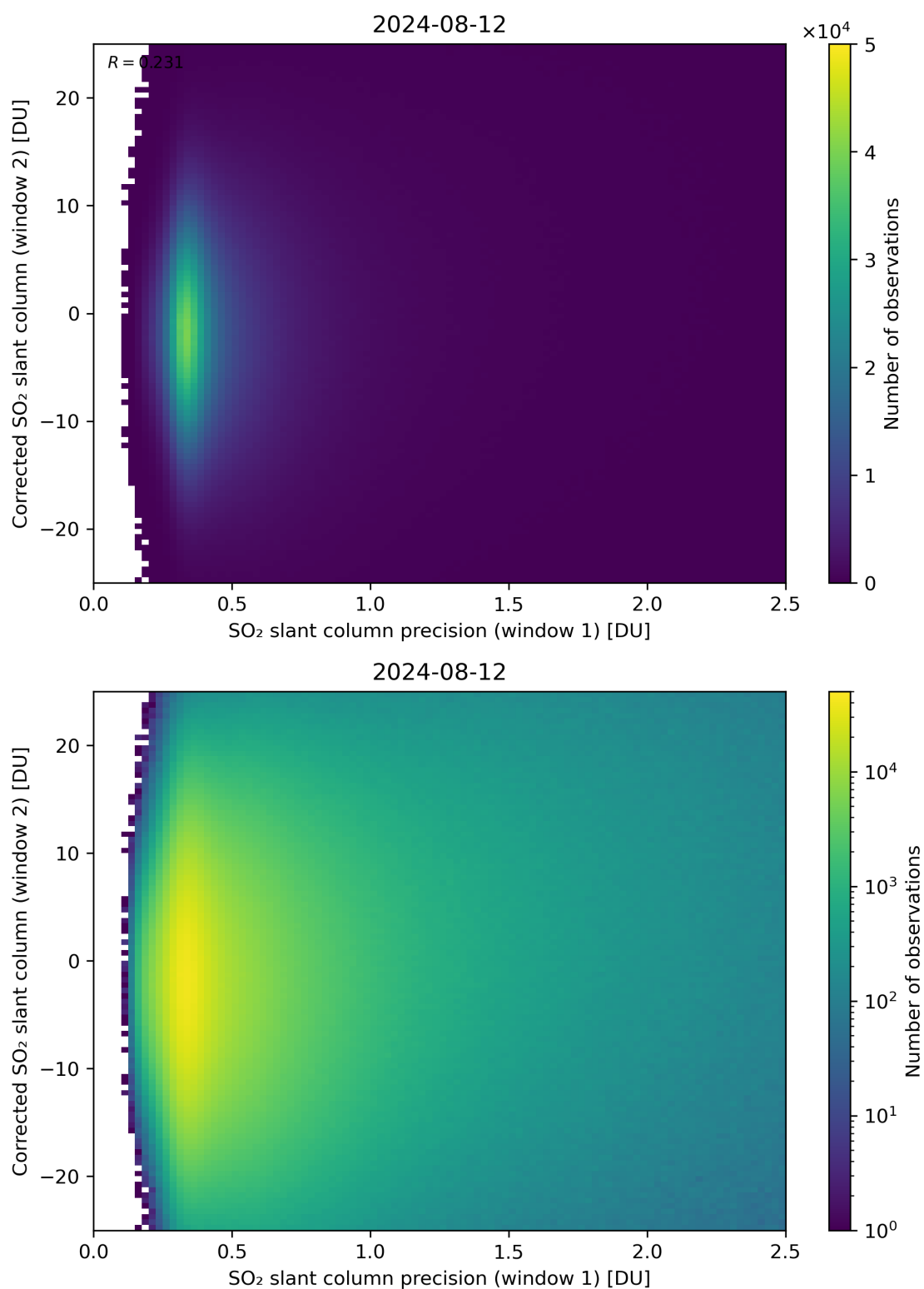
Figure 225: Scatter density plot of “SO 2 slant column precision (window 1)” against “Corrected SO 2 slant column (window 2)” for 2024-08-12 to 2024-08-13.
