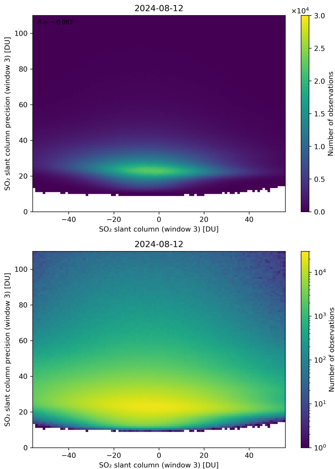
Figure 267: Scatter density plot of “SO 2 slant column (window 3)” against “SO 2 slant column precision (window 3)” for 2024-08-12 to 2024-08-13.
