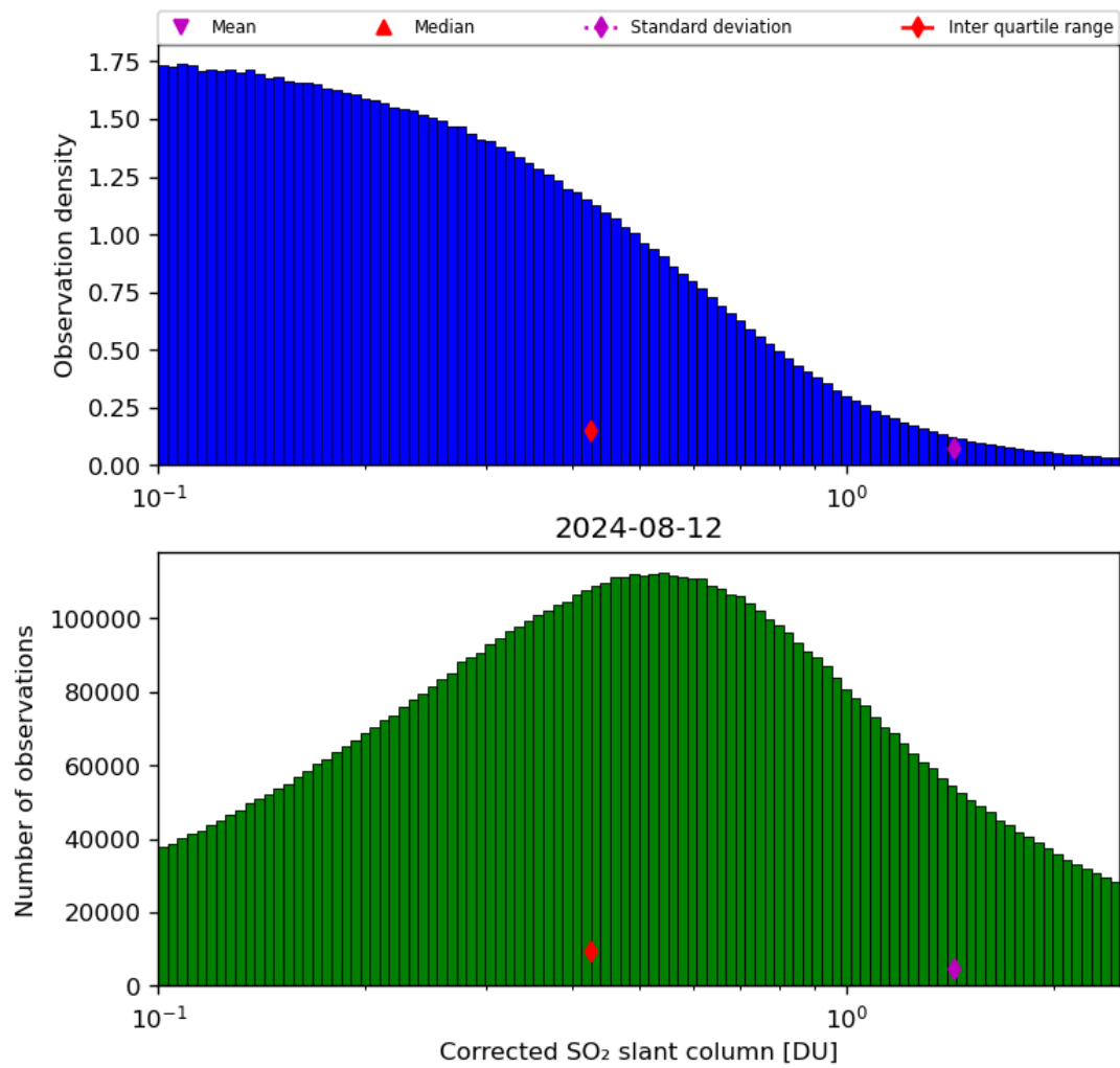
Figure 55: Histogram of “Corrected SO 2 slant column” for 2024-08-12 to 2024-08-13
