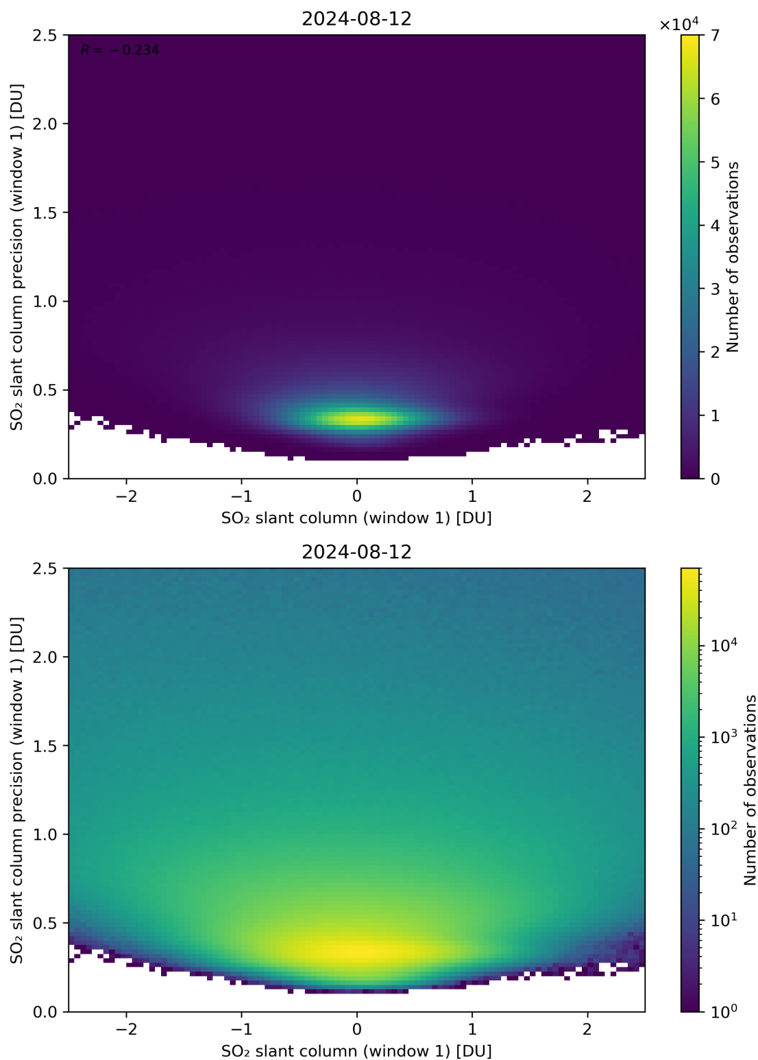
Figure 235: Scatter density plot of “SO 2 slant column (window 1)” against “SO 2 slant column precision (window 1)” for 2024-08-12 to 2024-08-13.
