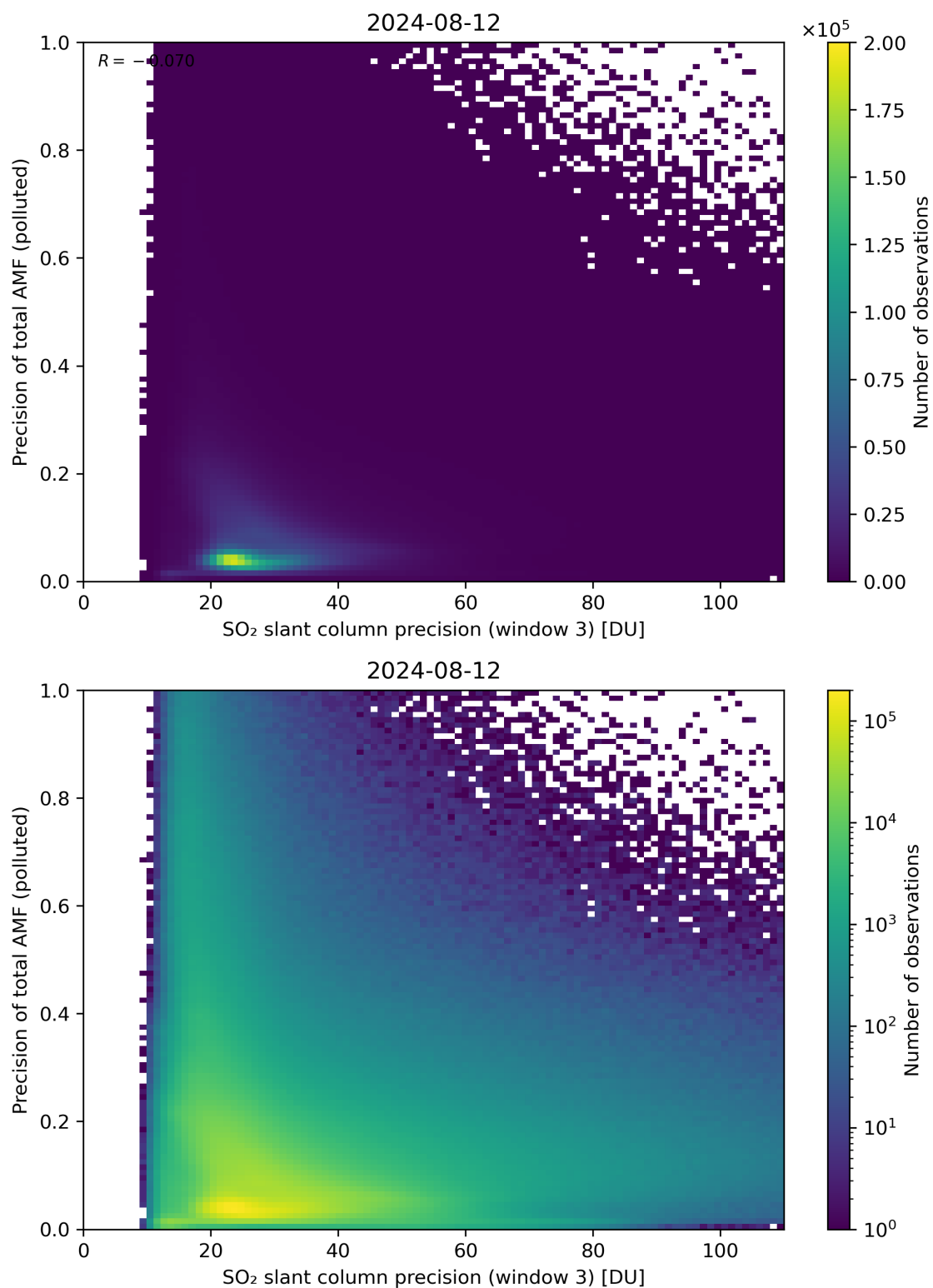
Figure 264: Scatter density plot of “SO 2 slant column precision (window 3)” against “Precision of total AMF (polluted)” for 2024-08-12 to 2024-08-13.
