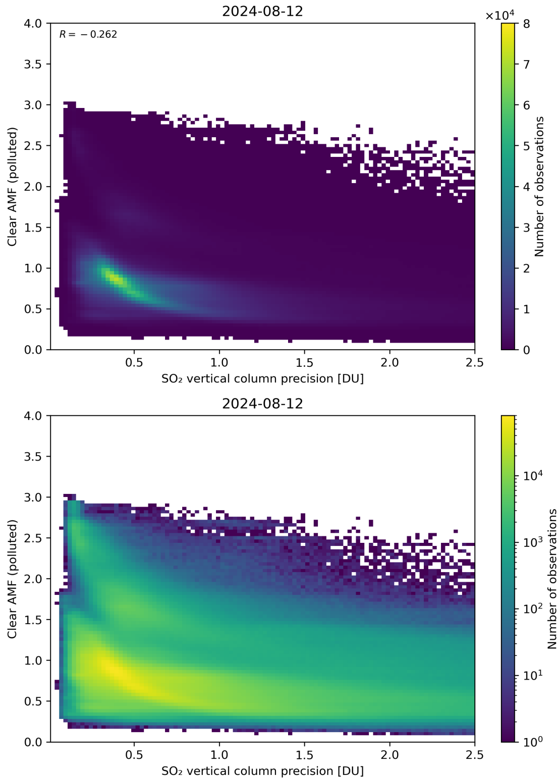
Figure 285: Scatter density plot of “SO 2 vertical column precision” against “Clear AMF (polluted)” for 2024-08-12 to 2024-08-13.
