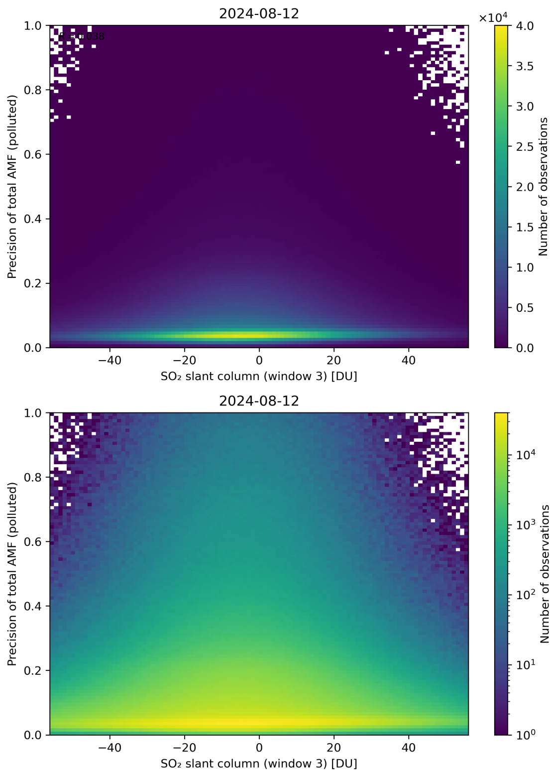
Figure 269: Scatter density plot of “SO 2 slant column (window 3)” against “Precision of total AMF (polluted)” for 2024-08-12 to 2024-08-13.
