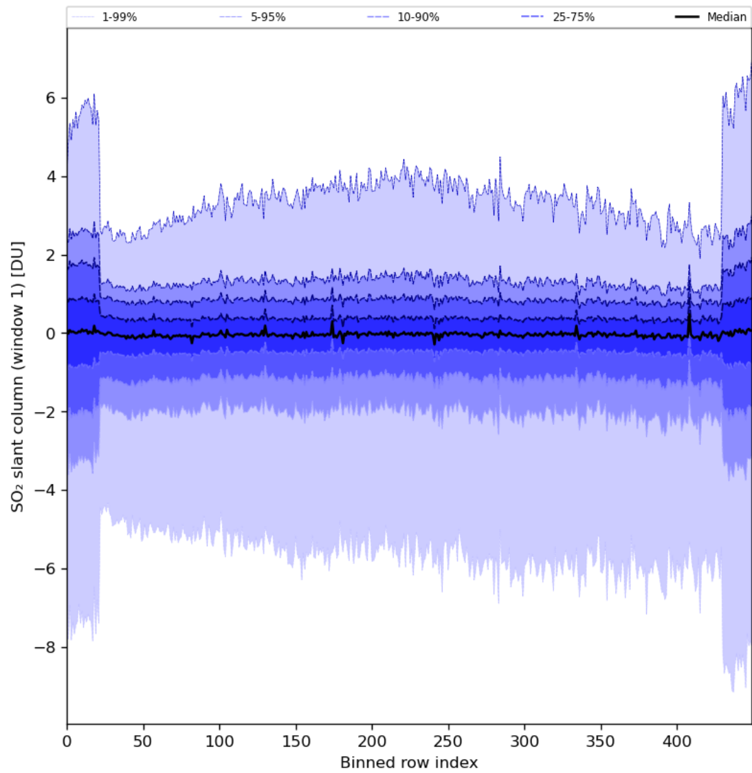
Figure 79: Along track statistics of “SO 2 slant column (window 1)” for 2024-08-12 to 2024-08-13
