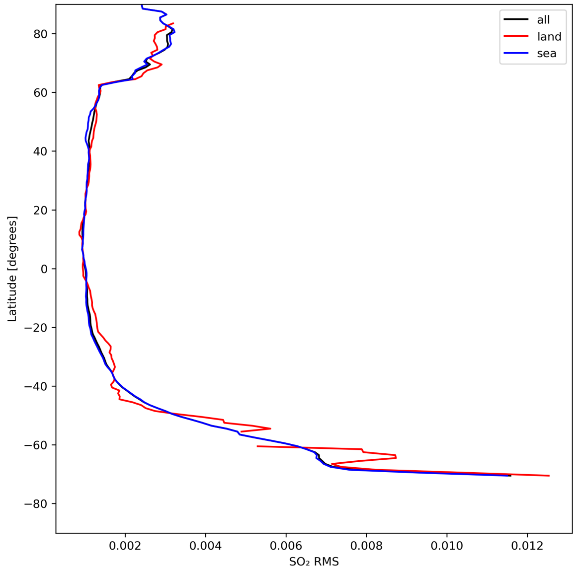
Figure 47: Zonal average of “SO 2 RMS” for 2024-08-12 to 2024-08-13.
