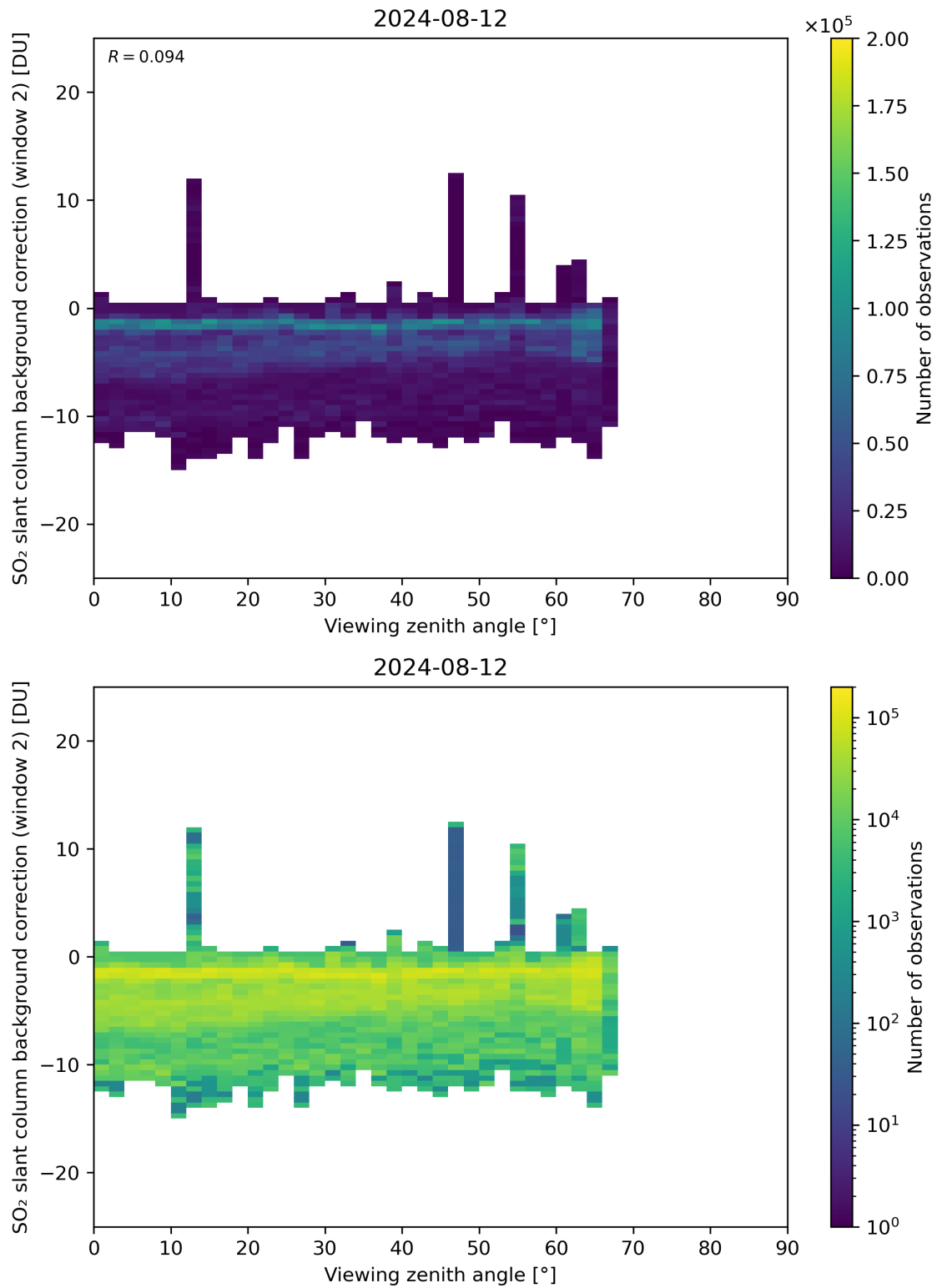
Figure 309: Scatter density plot of “Viewing zenith angle” against “SO 2 slant column background correction (window 2)” for 2024-08-12 to 2024-08-13.
