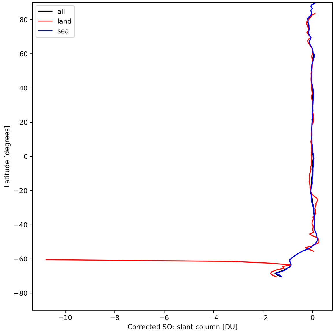
Figure 32: Zonal average of “Corrected SO 2 slant column” for 2024-08-12 to 2024-08-13.
