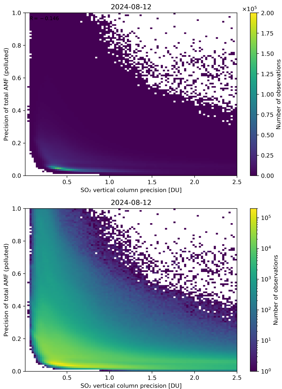
Figure 295: Scatter density plot of “SO 2 vertical column precision” against “Precision of total AMF (polluted)” for 2024-08-12 to 2024-08-13.
