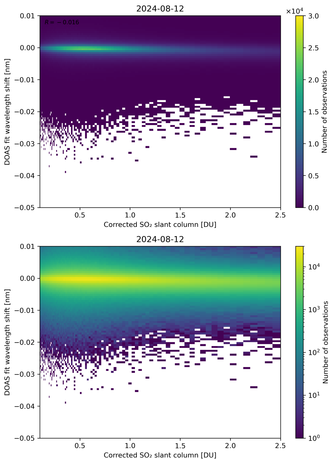
Figure 181: Scatter density plot of “Corrected SO 2 slant column” against “DOAS fit wavelength shift” for 2024-08-12 to 2024-08-13.
