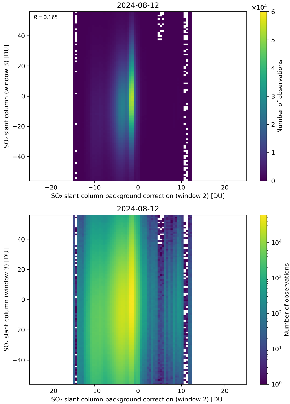
Figure 117: Scatter density plot of “SO 2 slant column background correction (window 2)” against “SO 2 slant column (window 3)” for 2024-08-12 to 2024-08-13.
