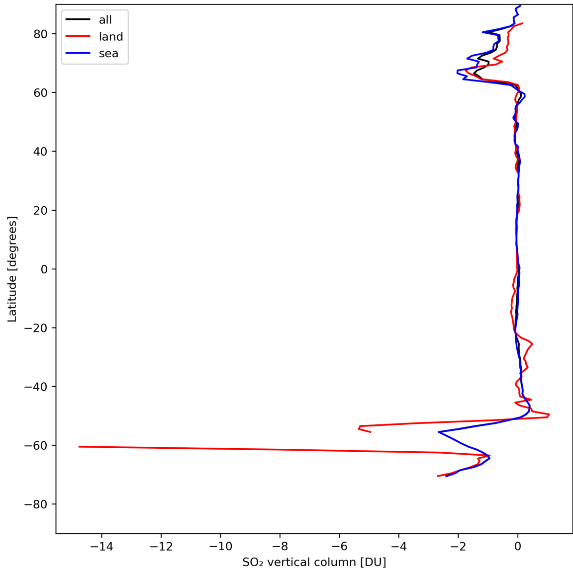
Figure 30: Zonal average of “SO 2 vertical column” for 2024-08-12 to 2024-08-13.
