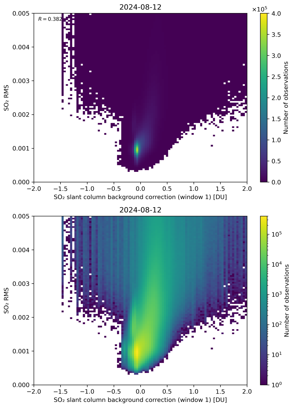
Figure 102: Scatter density plot of “SO 2 slant column background correction (window 1)” against “SO 2 RMS” for 2024-08-12 to 2024-08-13.
