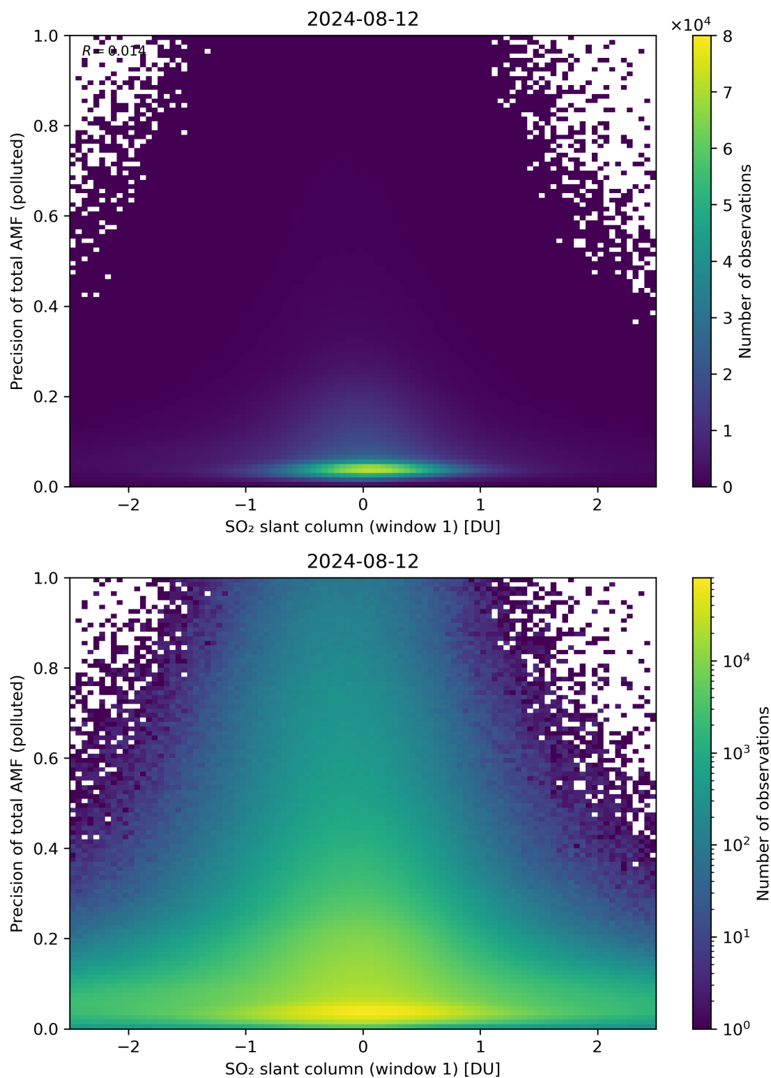
Figure 240: Scatter density plot of “SO 2 slant column (window 1)” against “Precision of total AMF (polluted)” for 2024-08-12 to 2024-08-13.
