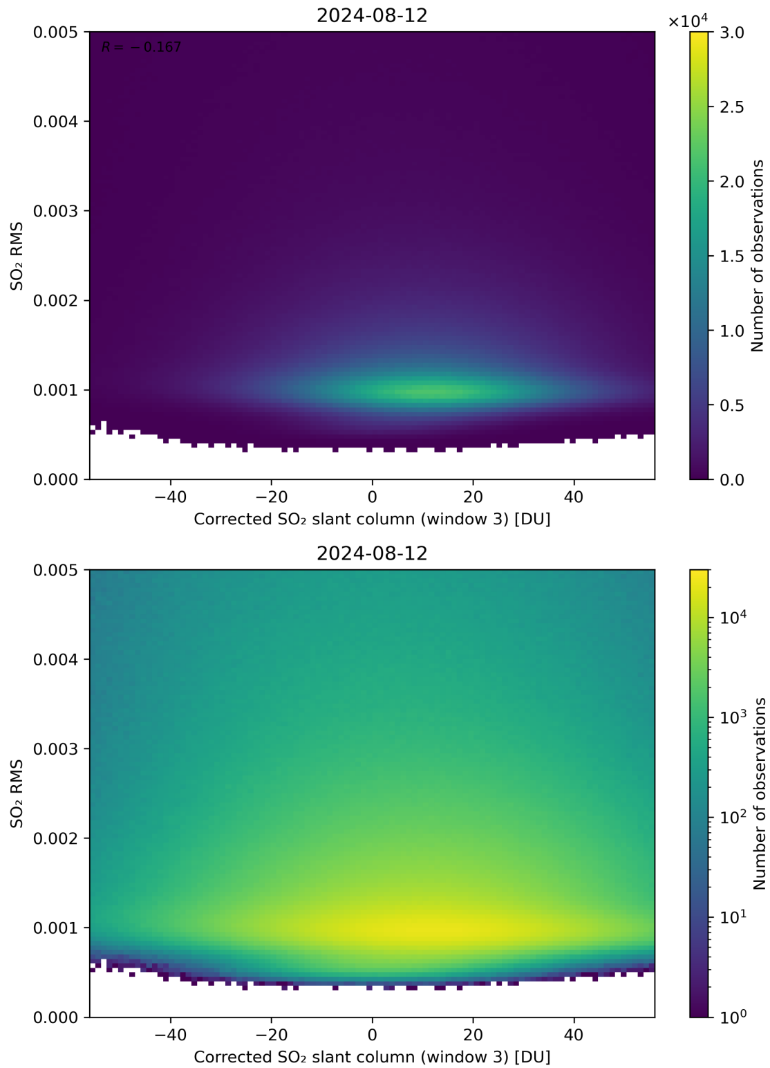
Figure 208: Scatter density plot of “Corrected SO 2 slant column (window 3)” against “SO 2 RMS” for 2024-08-12 to 2024-08-13.
