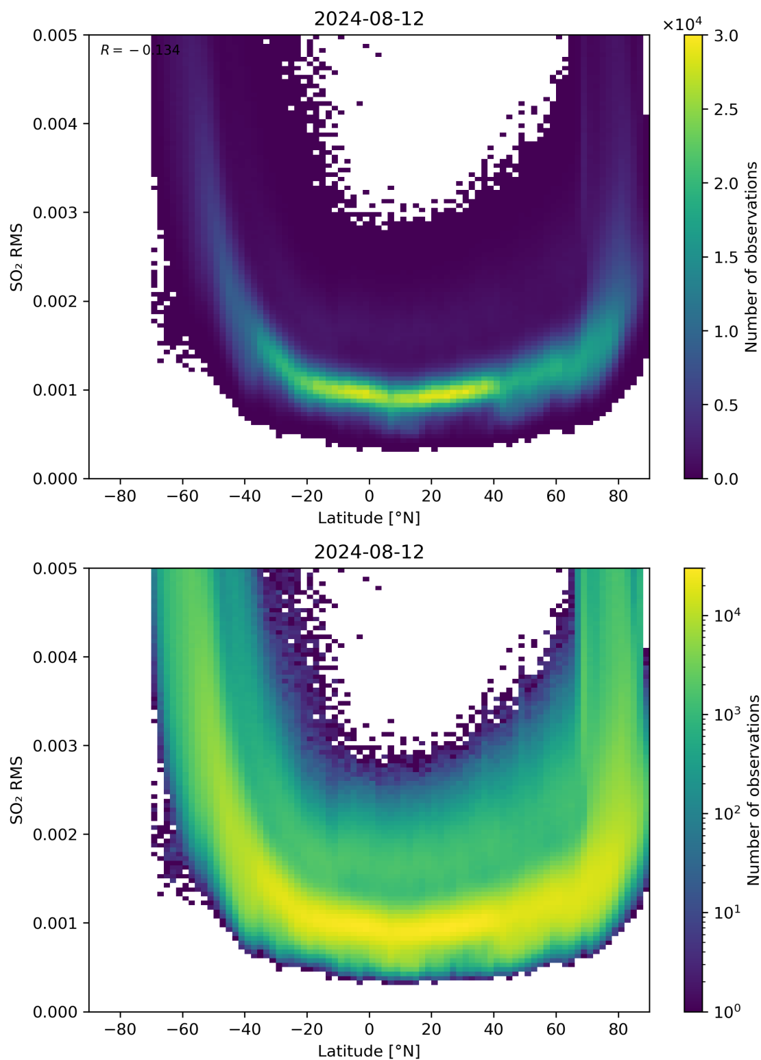
Figure 144: Scatter density plot of “Latitude” against “SO 2 RMS” for 2024-08-12 to 2024-08-13.
