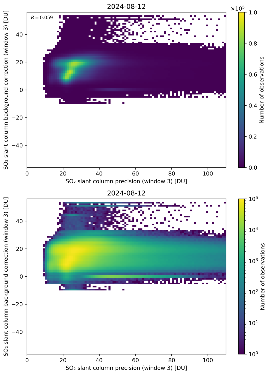
Figure 257: Scatter density plot of “SO 2 slant column precision (window 3)” against “SO 2 slant column background correction (window 3)” for 2024-08-12 to 2024-08-13.
