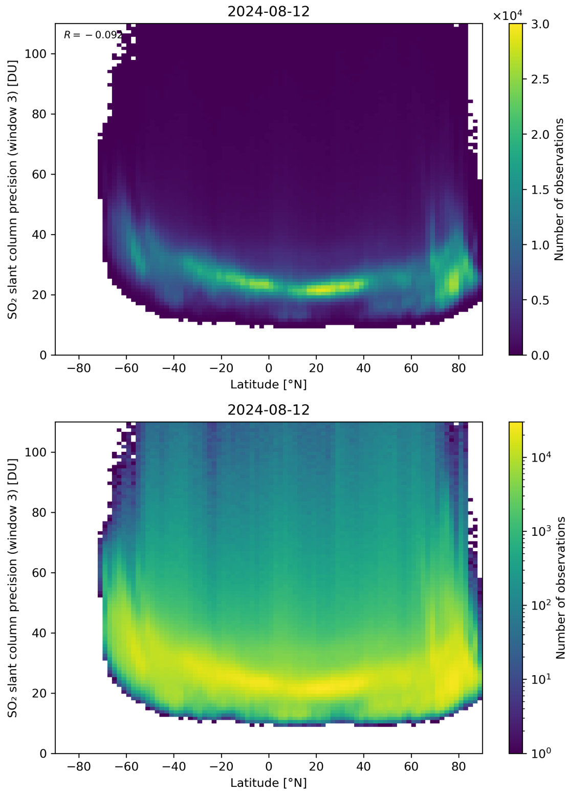
Figure 153: Scatter density plot of “Latitude” against “SO 2 slant column precision (window 3)” for 2024-08-12 to 2024-08-13.
