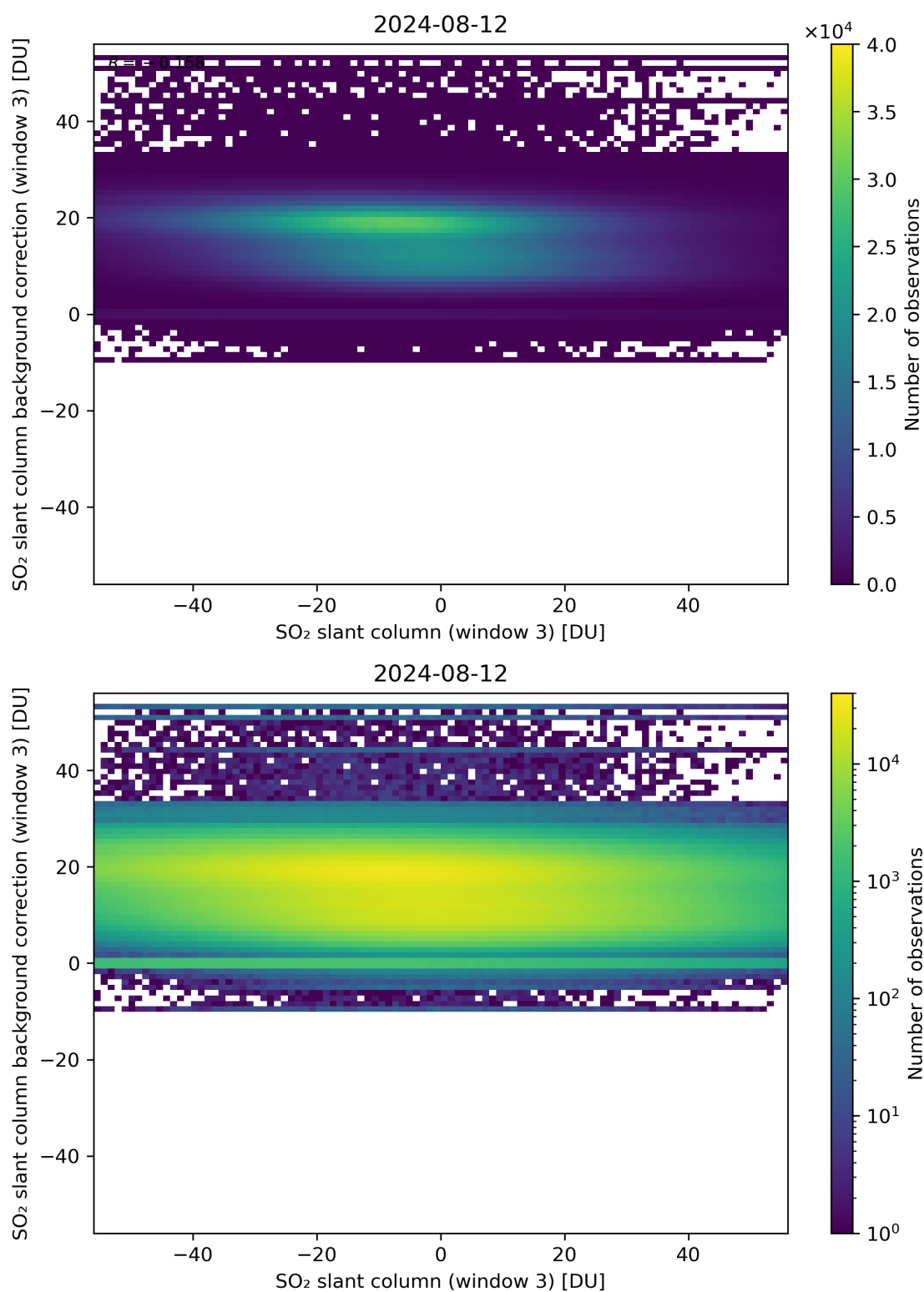
Figure 253: Scatter density plot of “SO 2 slant column (window 3)” against “SO 2 slant column background correction (window 3)” for 2024-08-12 to 2024-08-13.
