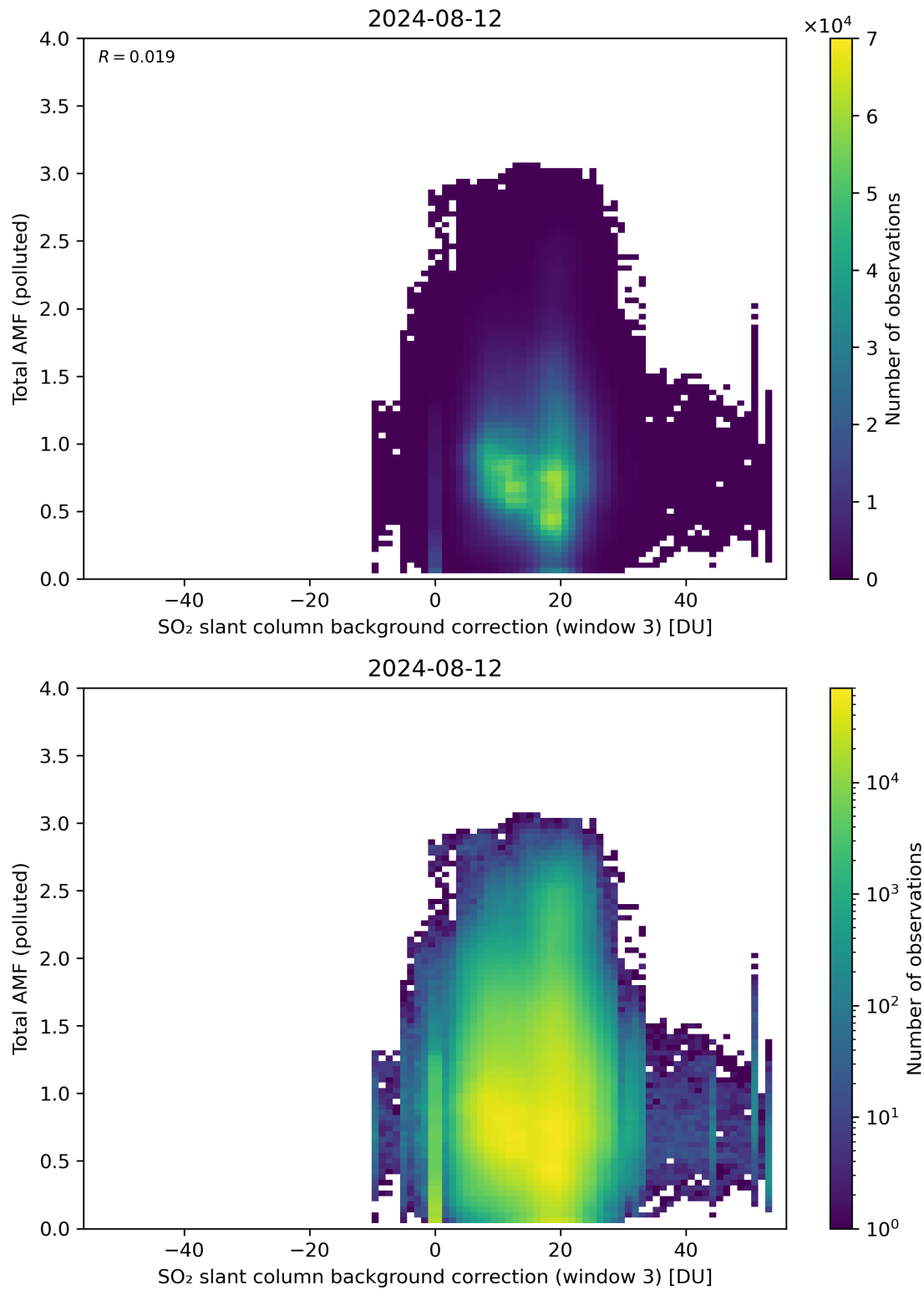
Figure 125: Scatter density plot of “SO 2 slant column background correction (window 3)” against “Total AMF (polluted)” for 2024-08-12 to 2024-08-13.
