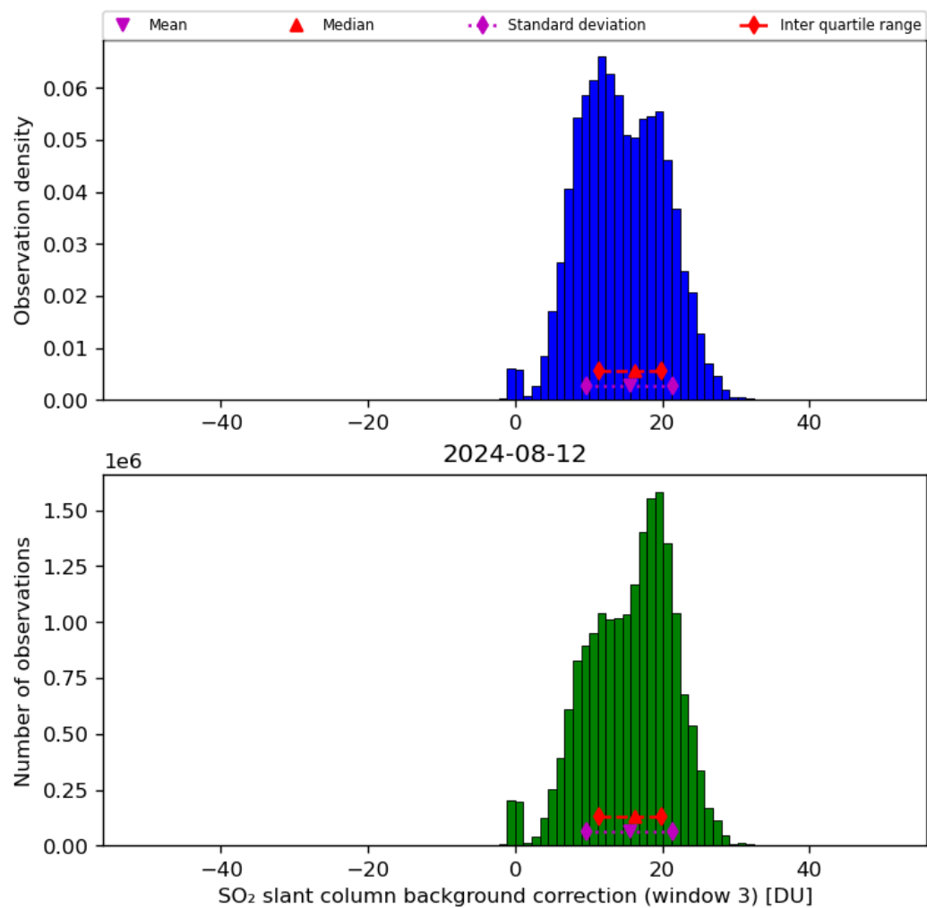
Figure 67: Histogram of “SO 2 slant column background correction (window 3)” for 2024-08-12 to 2024-08-13
