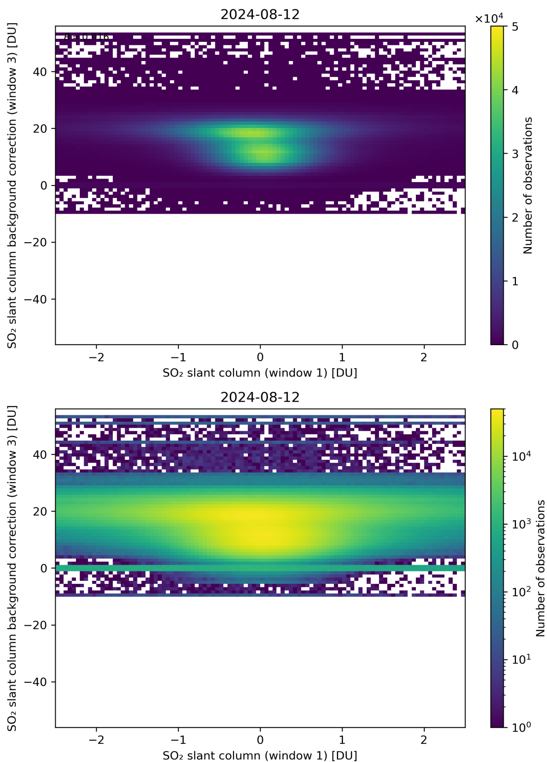
Figure 214: Scatter density plot of “SO 2 slant column (window 1)” against “SO 2 slant column background correction (window 3)” for 2024-08-12 to 2024-08-13.
