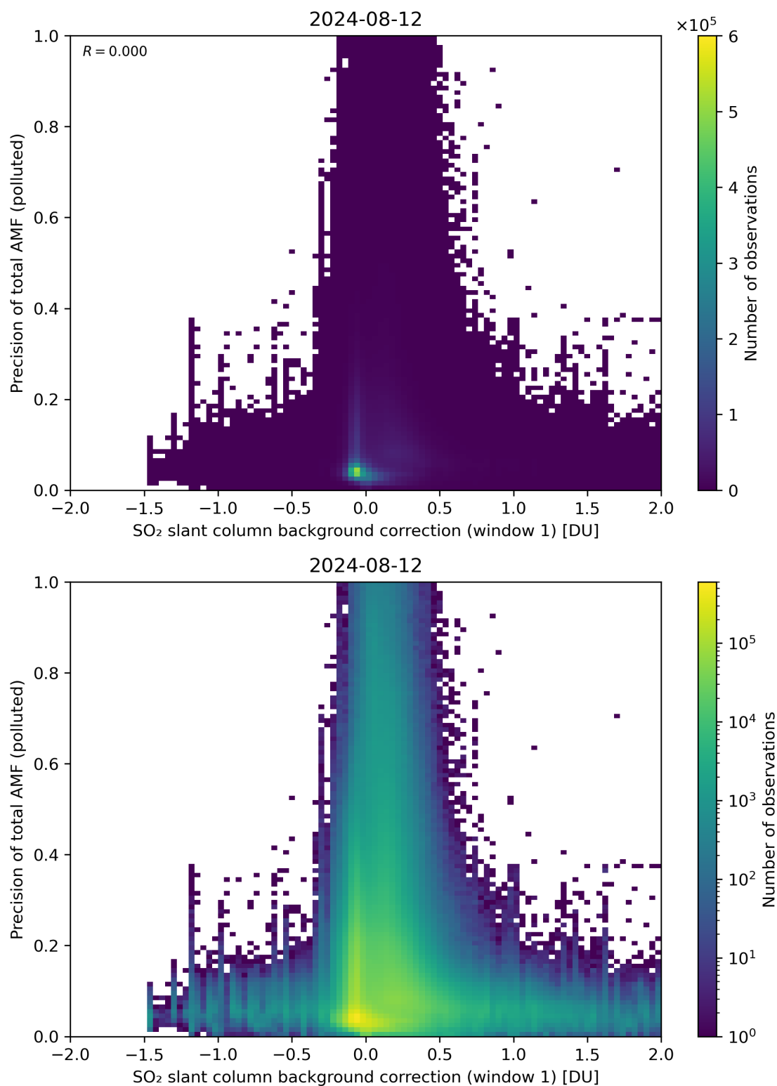
Figure 110: Scatter density plot of “SO 2 slant column background correction (window 1)” against “Precision of total AMF (polluted)” for 2024-08-12 to 2024-08-13.
