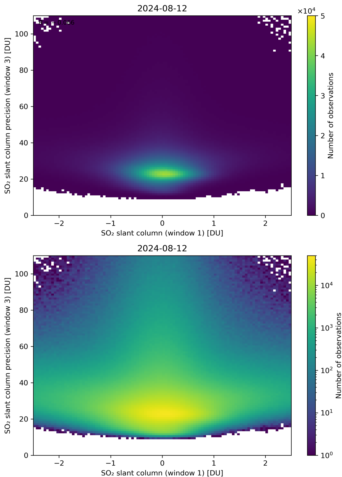
Figure 238: Scatter density plot of “SO 2 slant column (window 1)” against “SO 2 slant column precision (window 3)” for 2024-08-12 to 2024-08-13.
