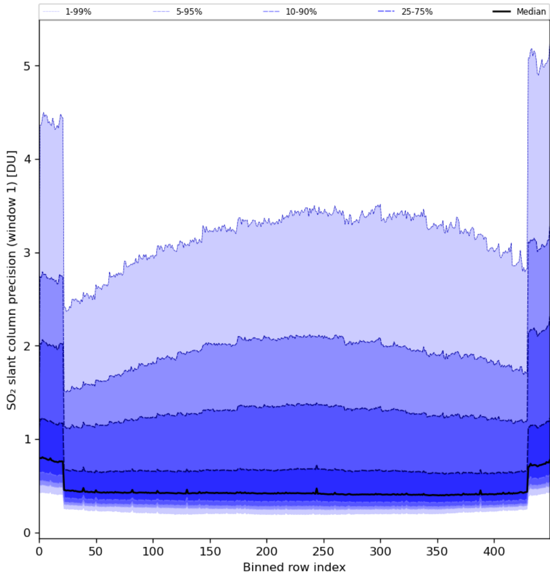
Figure 80: Along track statistics of “SO 2 slant column precision (window 1)” for 2024-08-12 to 2024-08-13
