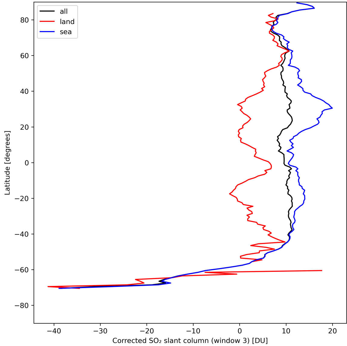
Figure 43: Zonal average of “Corrected SO 2 slant column (window 3)” for 2024-08-12 to 2024-08-13.
