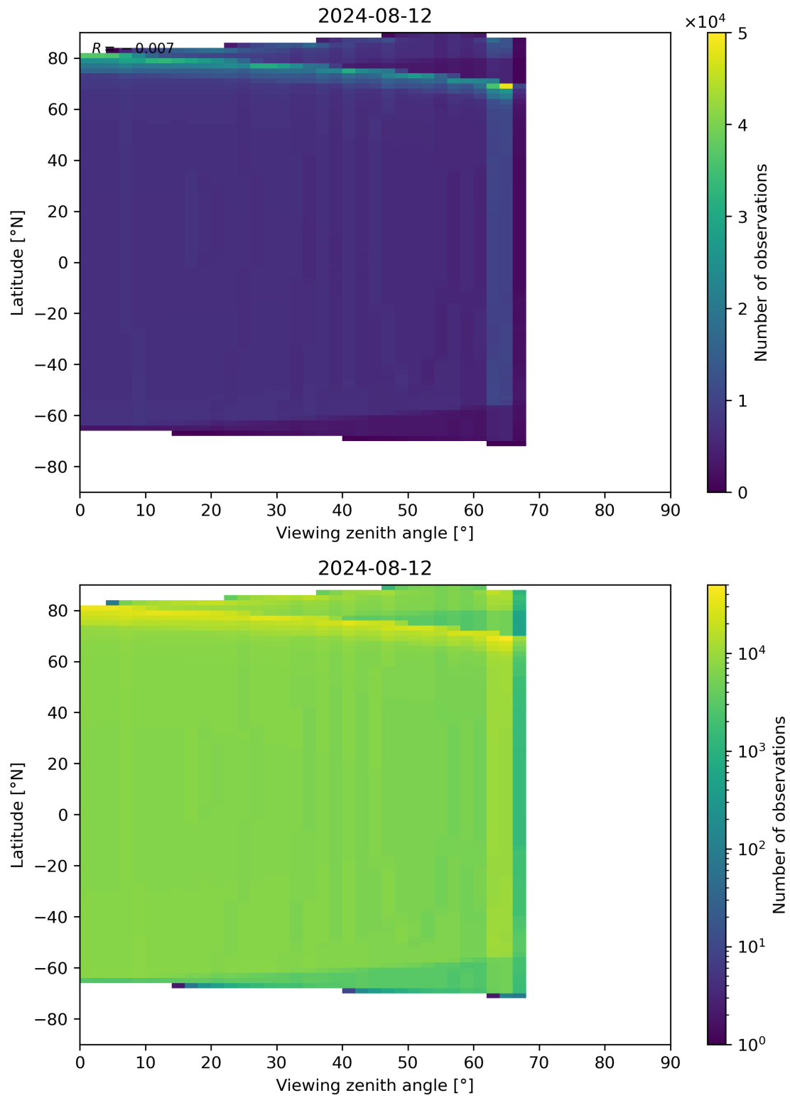
Figure 314: Scatter density plot of “Viewing zenith angle” against “Latitude” for 2024-08-12 to 2024-08-13.
