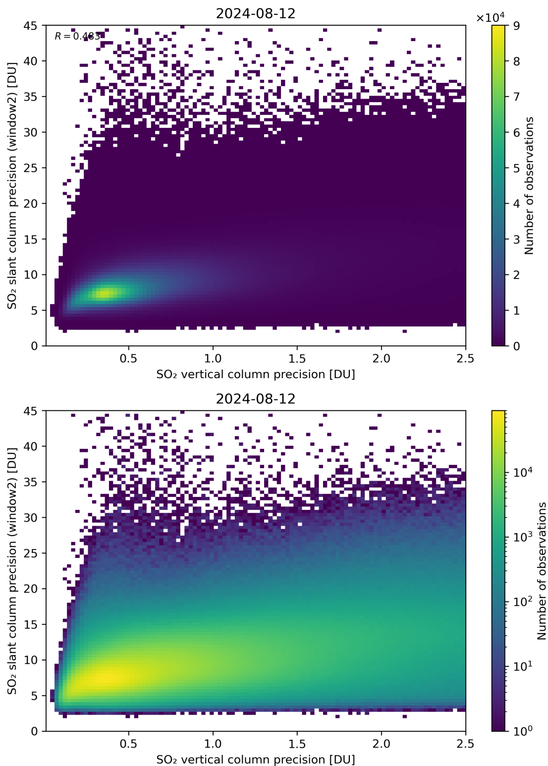
Figure 291: Scatter density plot of “SO 2 vertical column precision” against “SO 2 slant column precision (window2)” for 2024-08-12 to 2024-08-13.
