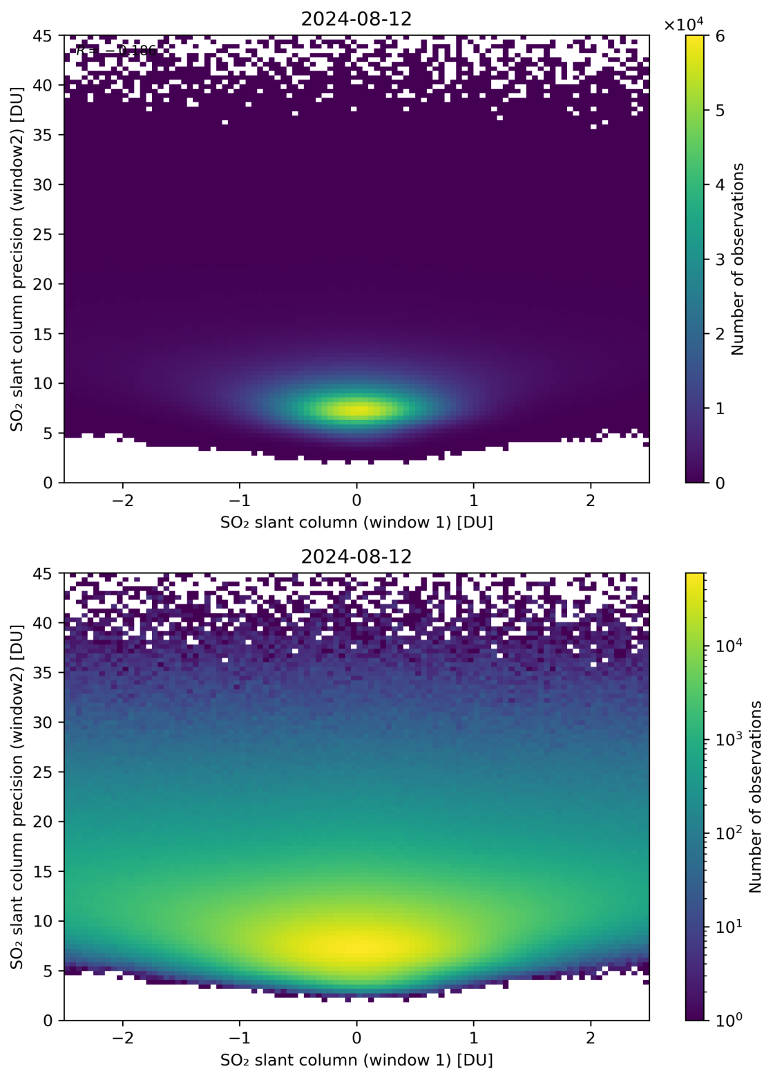
Figure 236: Scatter density plot of “SO 2 slant column (window 1)” against “SO 2 slant column precision (window2)” for 2024-08-12 to 2024-08-13.
