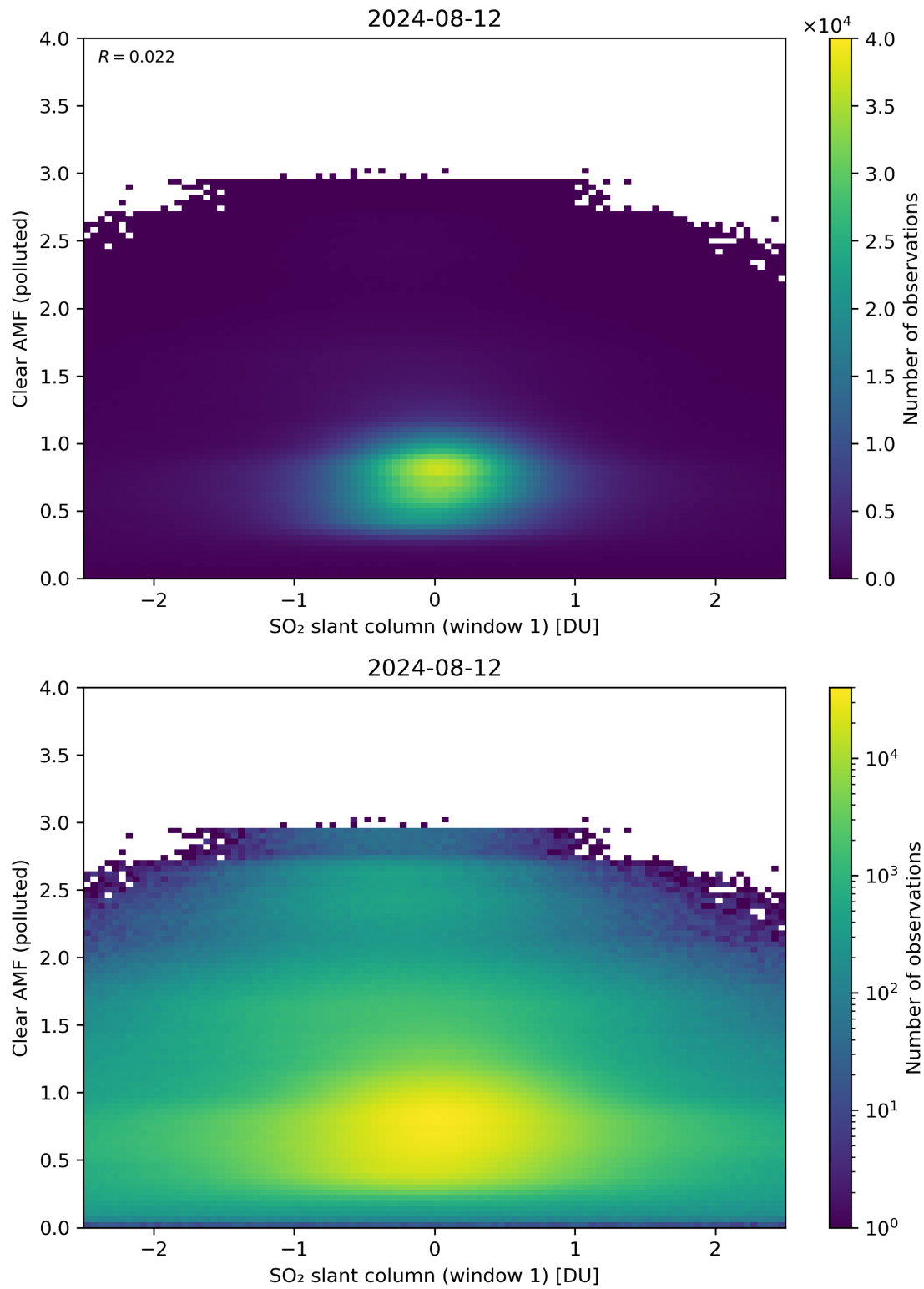
Figure 232: Scatter density plot of “SO 2 slant column (window 1)” against “Clear AMF (polluted)” for 2024-08-12 to 2024-08-13.
