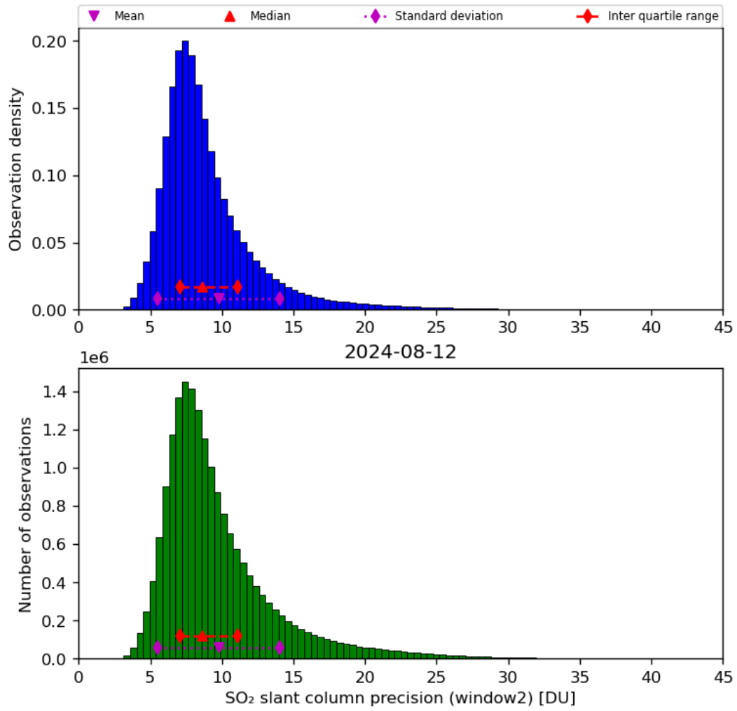
Figure 61: Histogram of “SO 2 slant column precision (window2)” for 2024-08-12 to 2024-08-13
