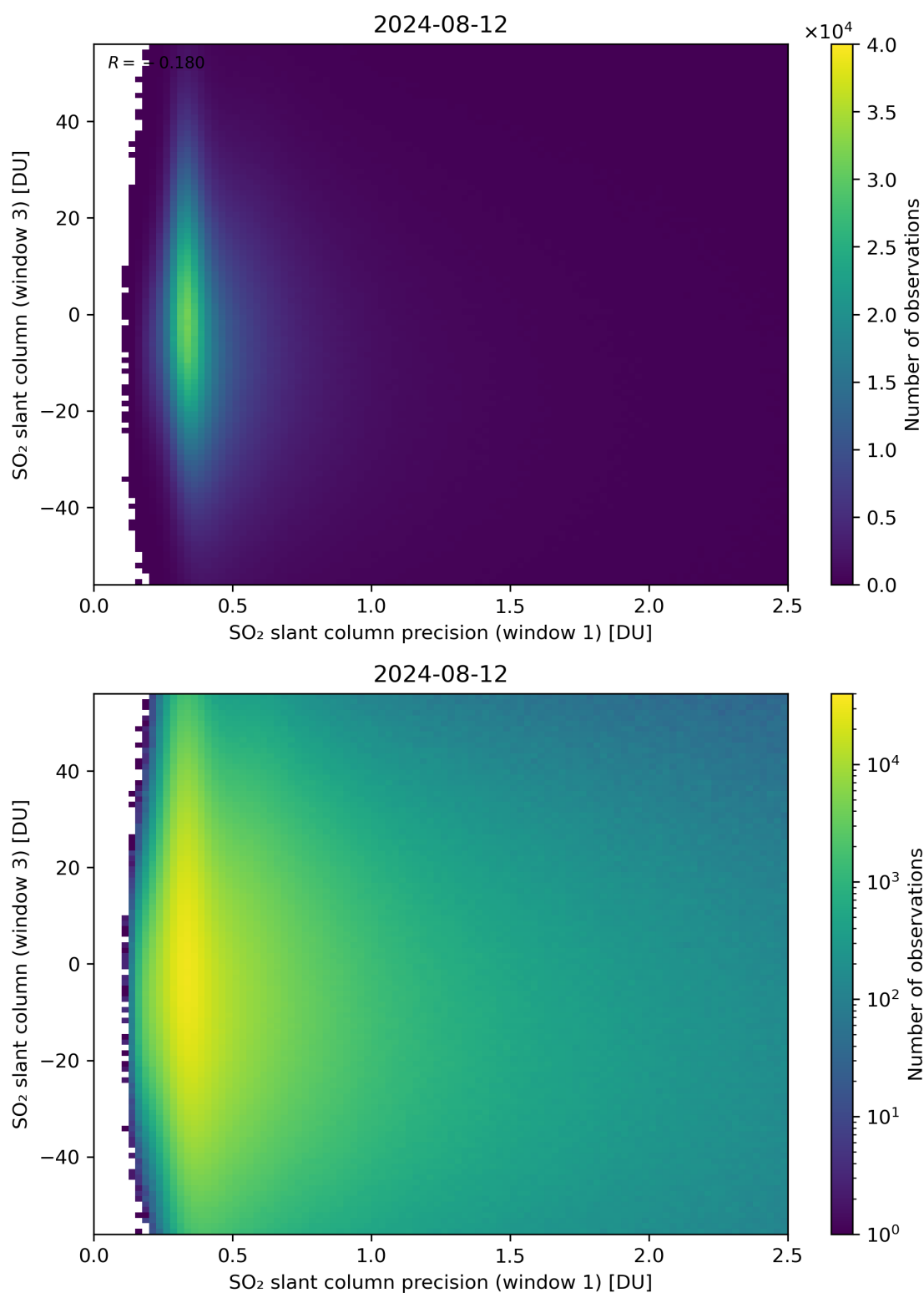
Figure 228: Scatter density plot of “SO 2 slant column precision (window 1)” against “SO 2 slant column (window 3)” for 2024-08-12 to 2024-08-13.
