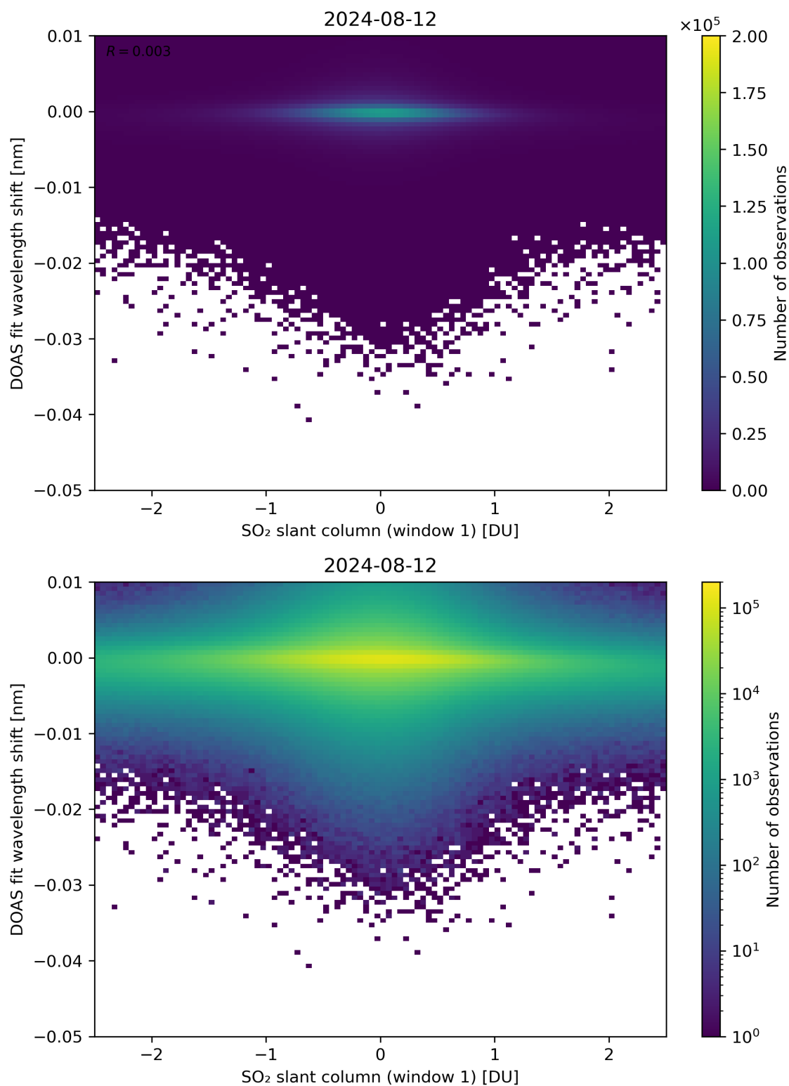
Figure 215: Scatter density plot of “SO 2 slant column (window 1)” against “DOAS fit wavelength shift” for 2024-08-12 to 2024-08-13.
