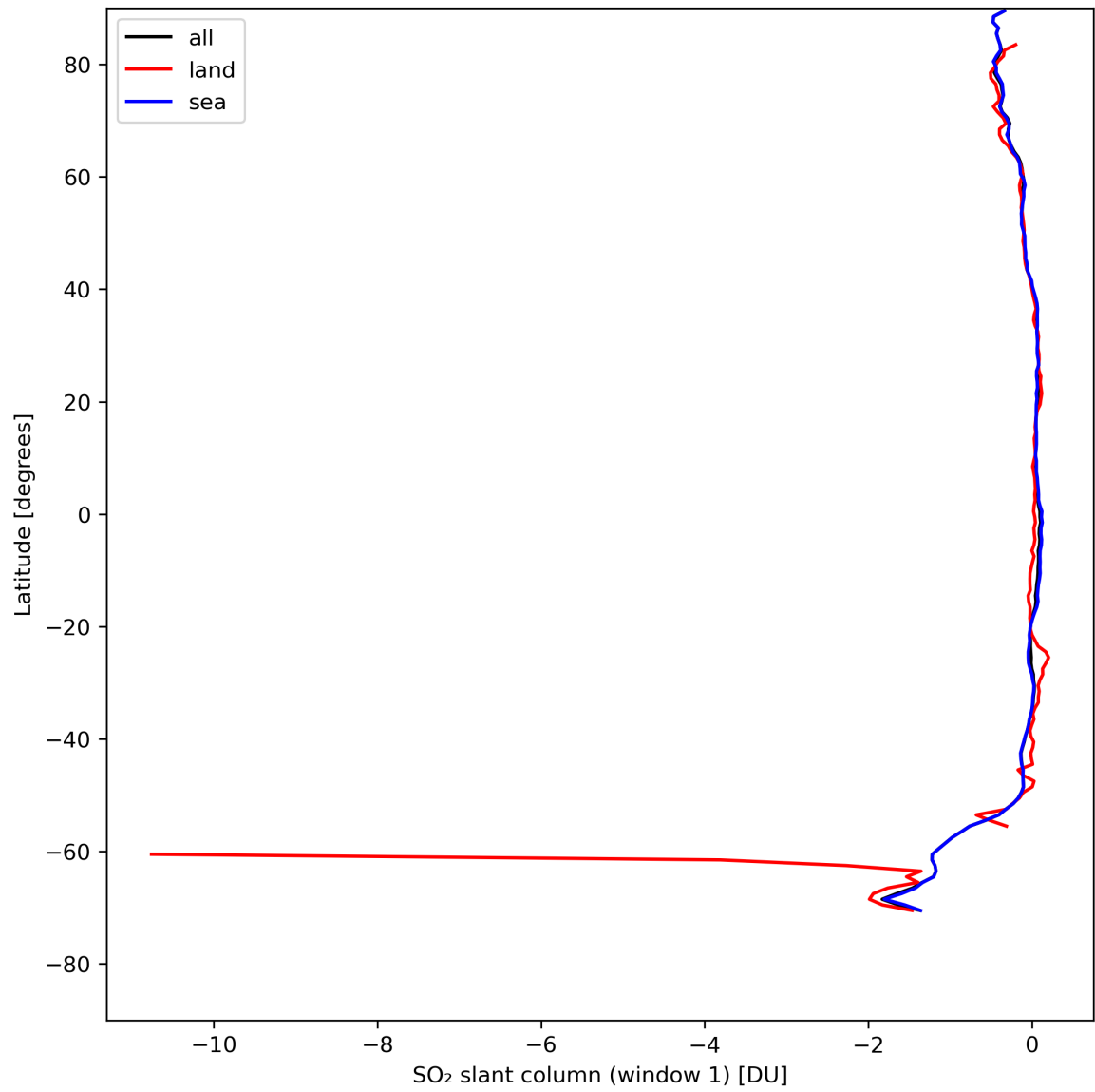
Figure 33: Zonal average of “SO 2 slant column (window 1)” for 2024-08-12 to 2024-08-13.
