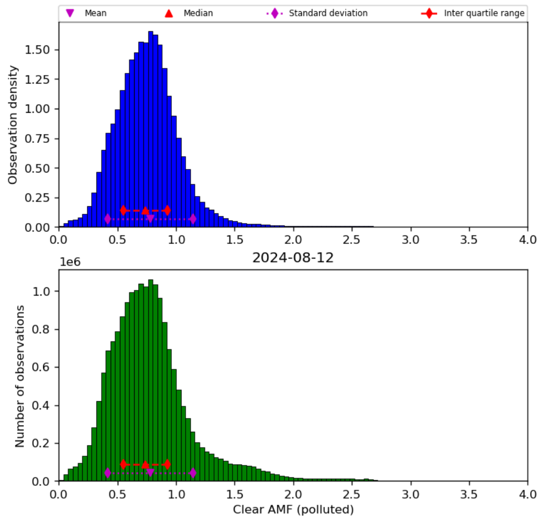
Figure 73: Histogram of “Clear AMF (polluted)” for 2024-08-12 to 2024-08-13
