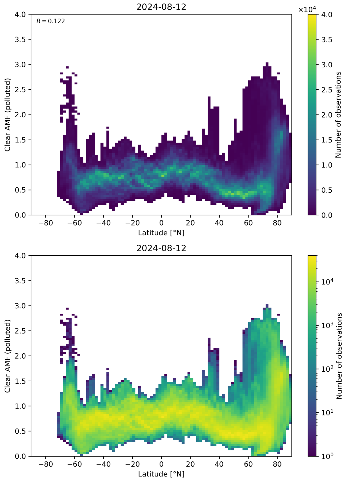
Figure 145: Scatter density plot of “Latitude” against “Clear AMF (polluted)” for 2024-08-12 to 2024-08-13.
