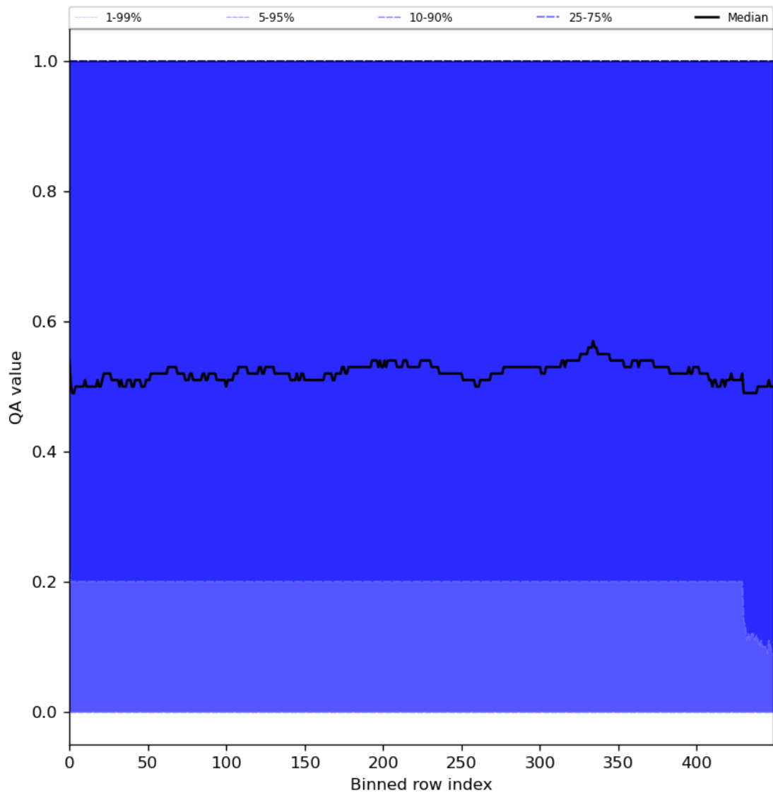
Figure 75: Along track statistics of “QA value” for 2024-08-12 to 2024-08-13
