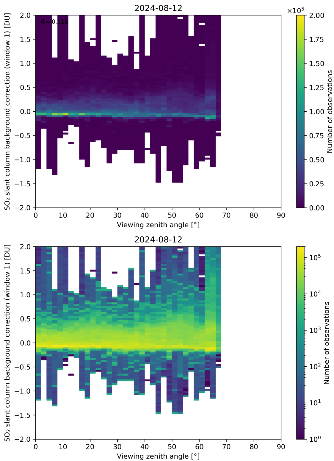
Figure 308: Scatter density plot of “Viewing zenith angle” against “SO 2 slant column background correction (window 1)” for 2024-08-12 to 2024-08-13.
