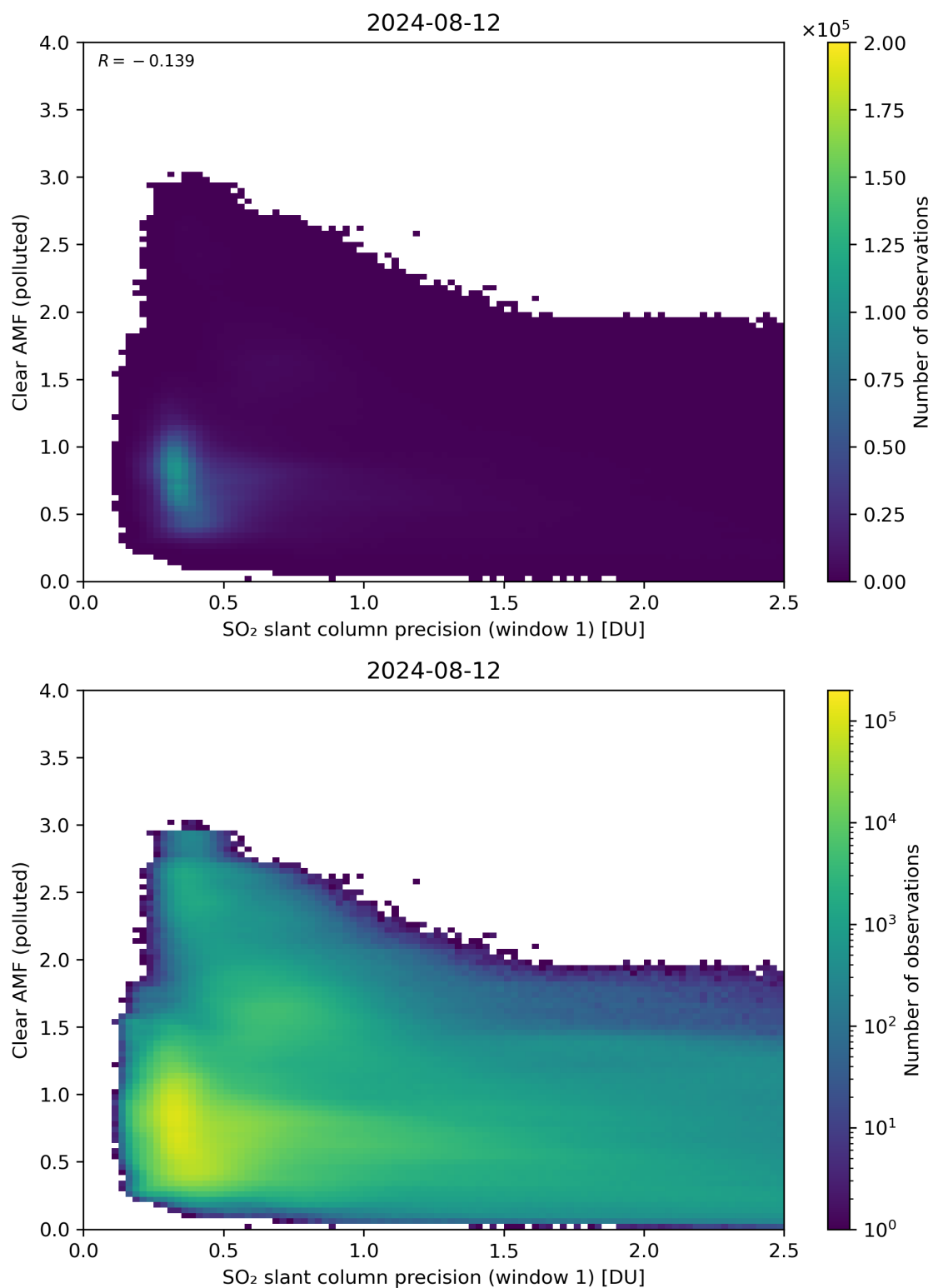
Figure 224: Scatter density plot of “SO 2 slant column precision (window 1)” against “Clear AMF (polluted)” for 2024-08-12 to 2024-08-13.
