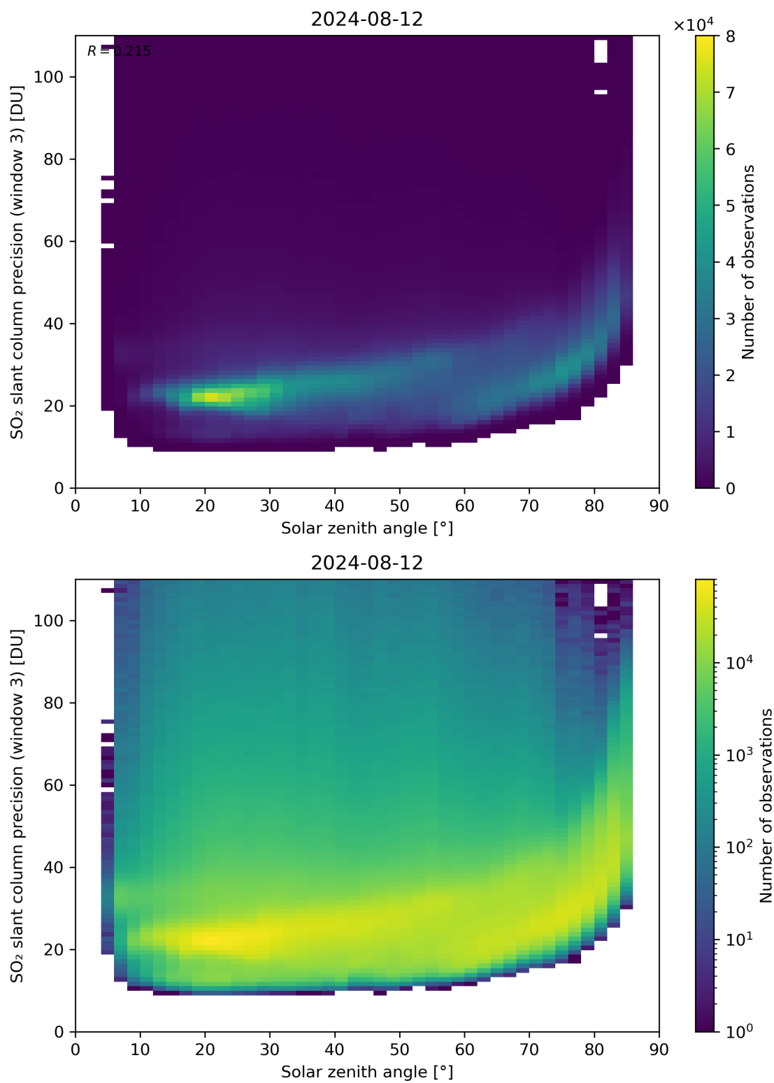
Figure 173: Scatter density plot of “Solar zenith angle” against “SO 2 slant column precision (window 3)” for 2024-08-12 to 2024-08-13.
