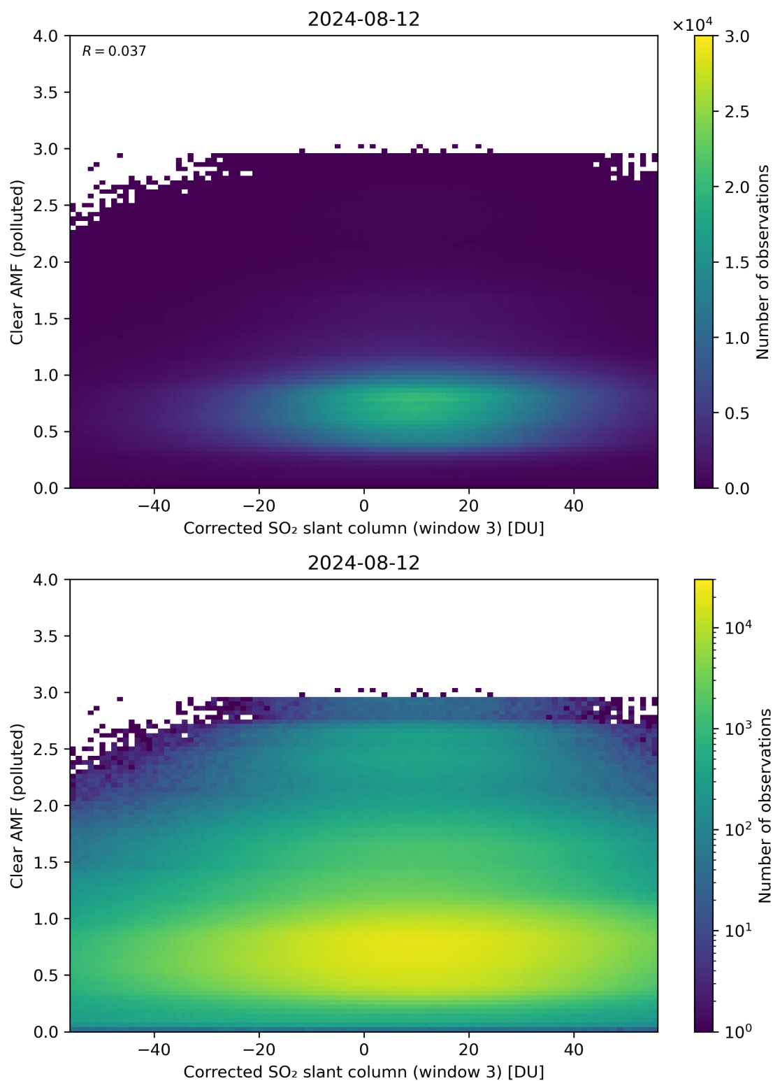
Figure 209: Scatter density plot of “Corrected SO 2 slant column (window 3)” against “Clear AMF (polluted)” for 2024-08-12 to 2024-08-13.
