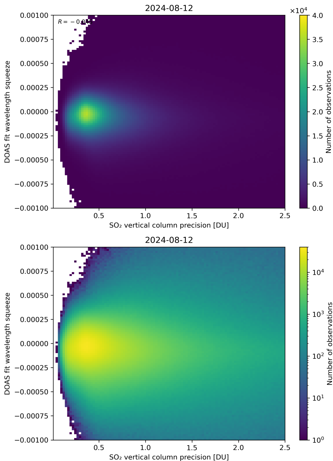
Figure 283: Scatter density plot of “SO 2 vertical column precision” against “DOAS fit wavelength squeeze” for 2024-08-12 to 2024-08-13.
