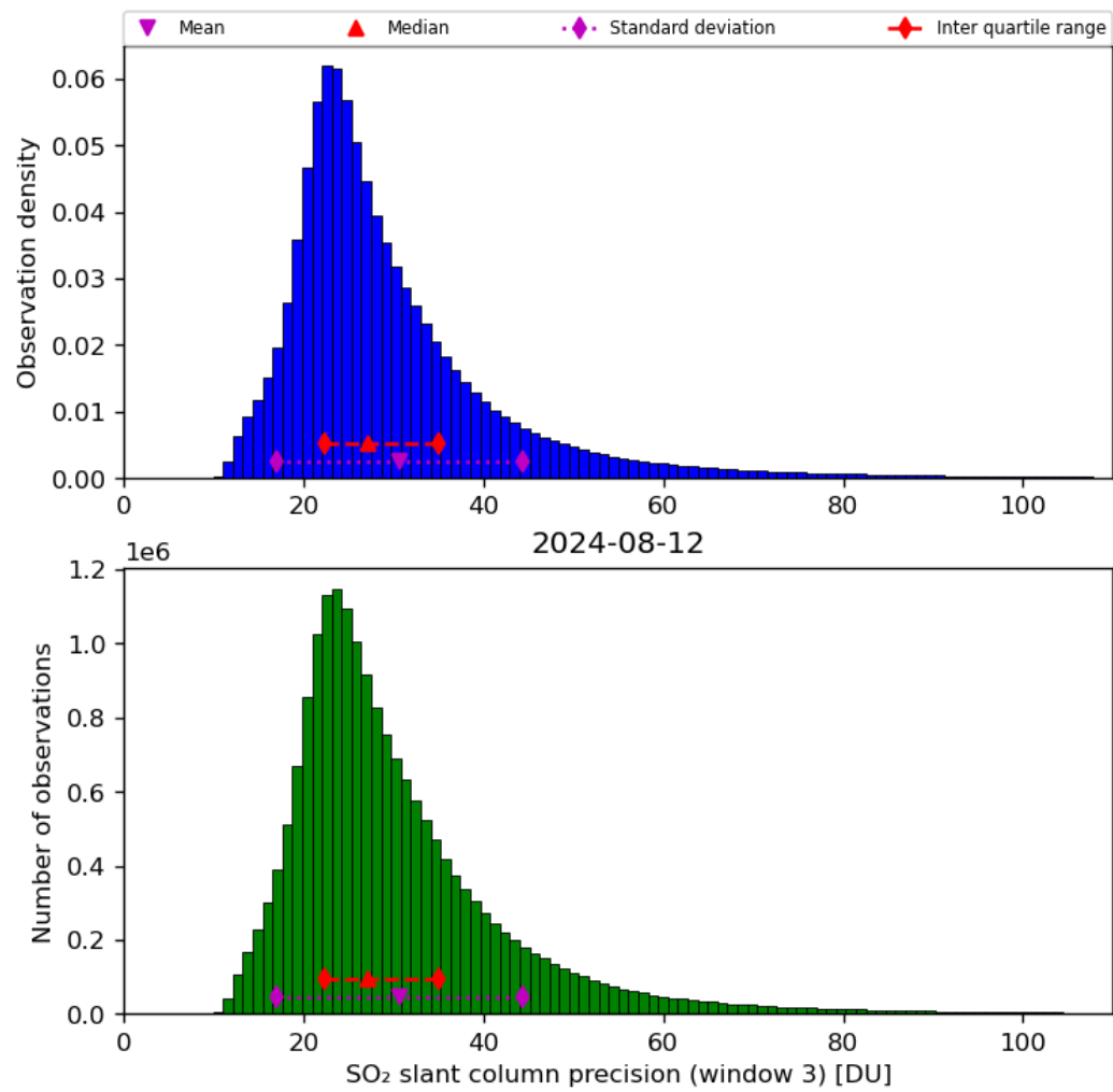
Figure 65: Histogram of “SO 2 slant column precision (window 3)” for 2024-08-12 to 2024-08-13
