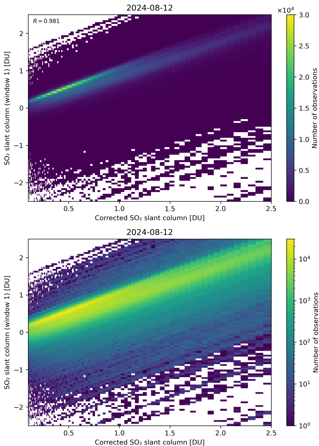
Figure 187: Scatter density plot of “Corrected SO 2 slant column” against “SO 2 slant column (window 1)” for 2024-08-12 to 2024-08-13.
