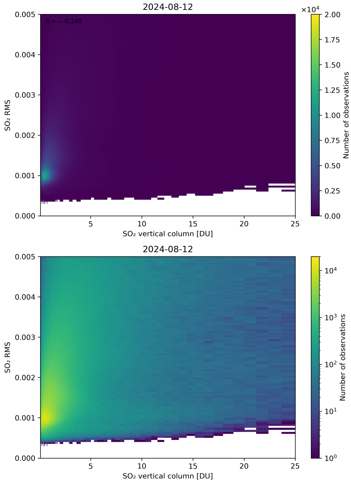
Figure 278: Scatter density plot of “SO 2 vertical column” against “SO 2 RMS” for 2024-08-12 to 2024-08-13.
