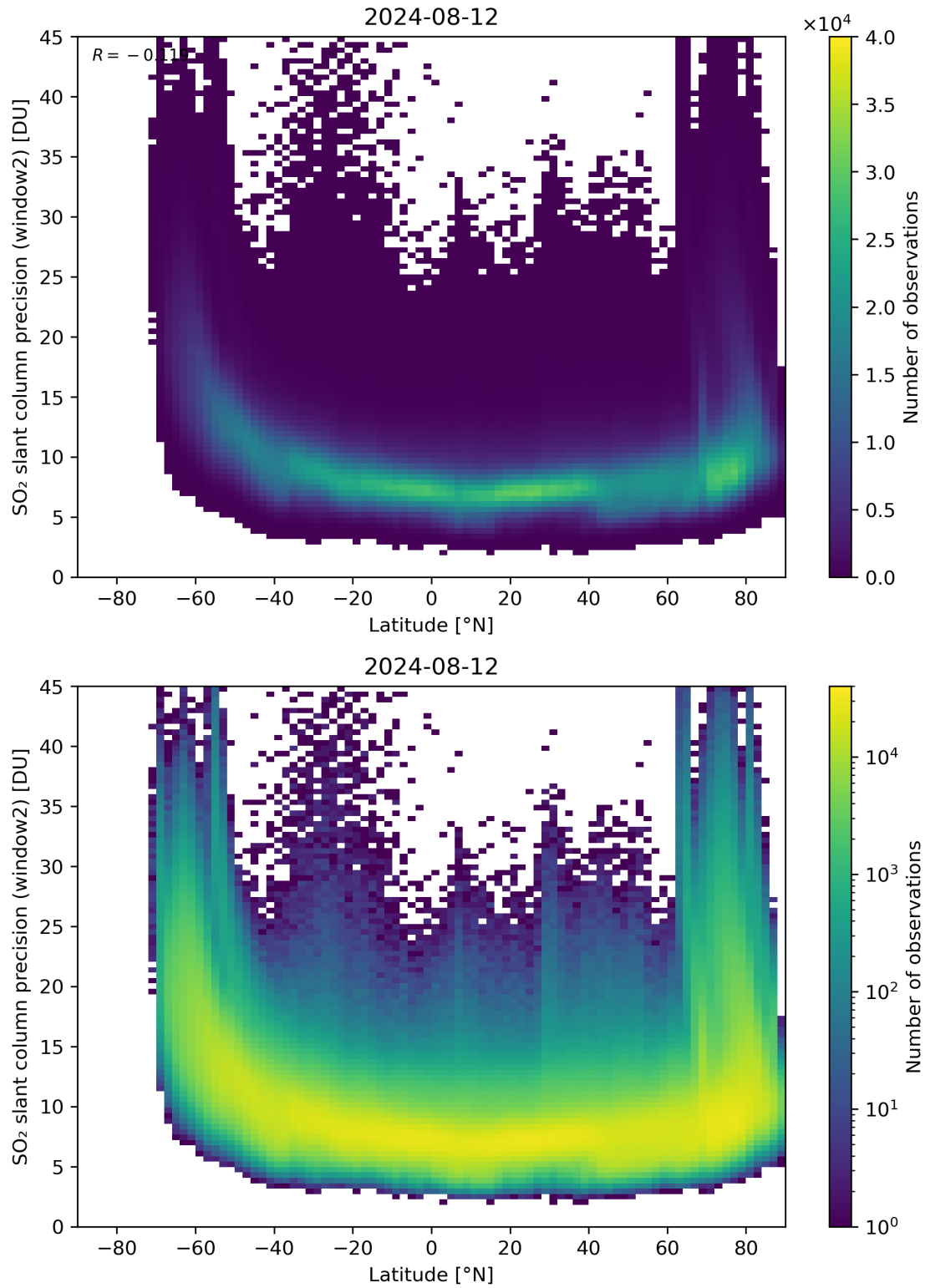
Figure 151: Scatter density plot of “Latitude” against “SO 2 slant column precision (window2)” for 2024-08-12 to 2024-08-13.
