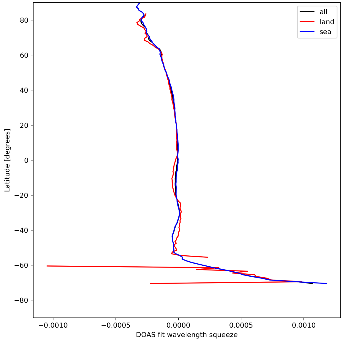
Figure 46: Zonal average of "DOAS fit wavelength squeeze" for 2024-08-12 to 2024-08-13.
