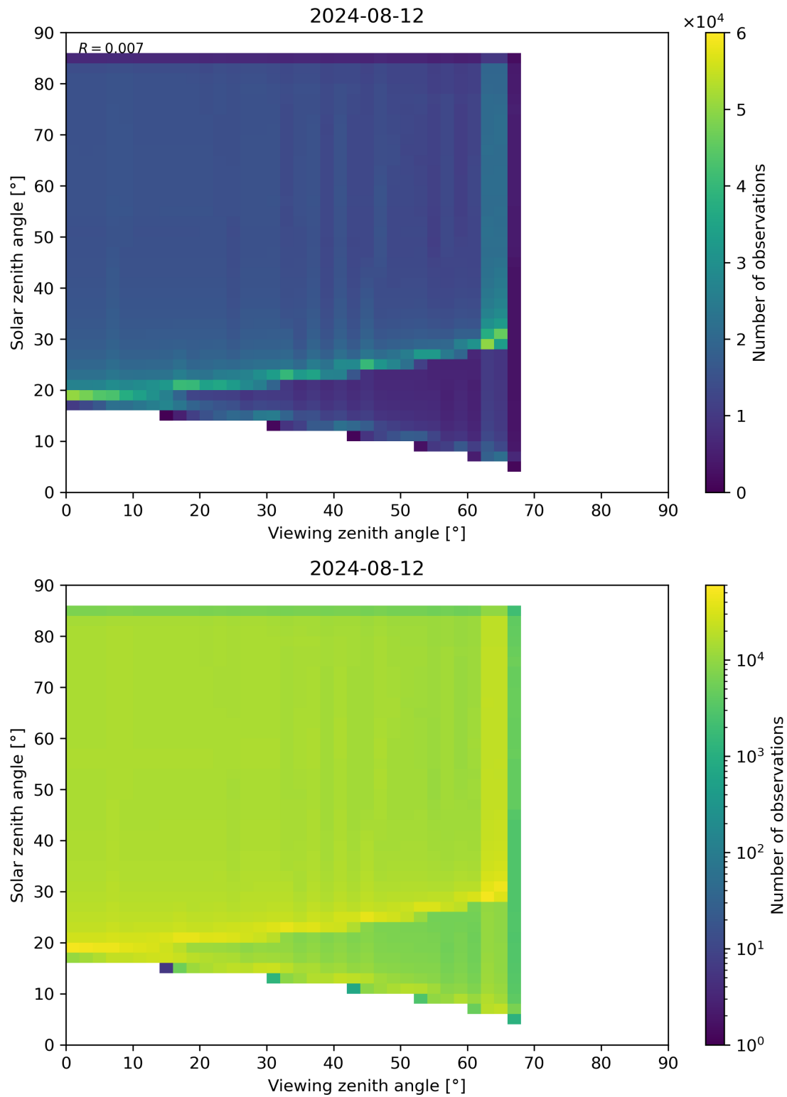
Figure 315: Scatter density plot of “Viewing zenith angle” against “Solar zenith angle” for 2024-08-12 to 2024-08-13.
