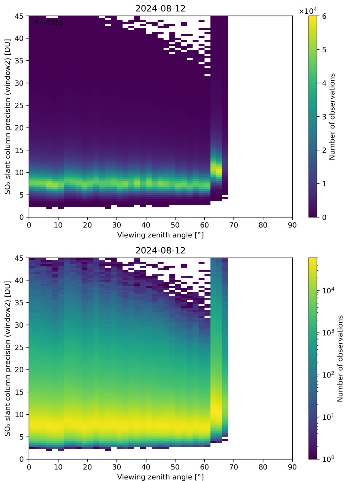
Figure 322: Scatter density plot of “Viewing zenith angle” against “SO 2 slant column precision (window2)” for 2024-08-12 to 2024-08-13.
