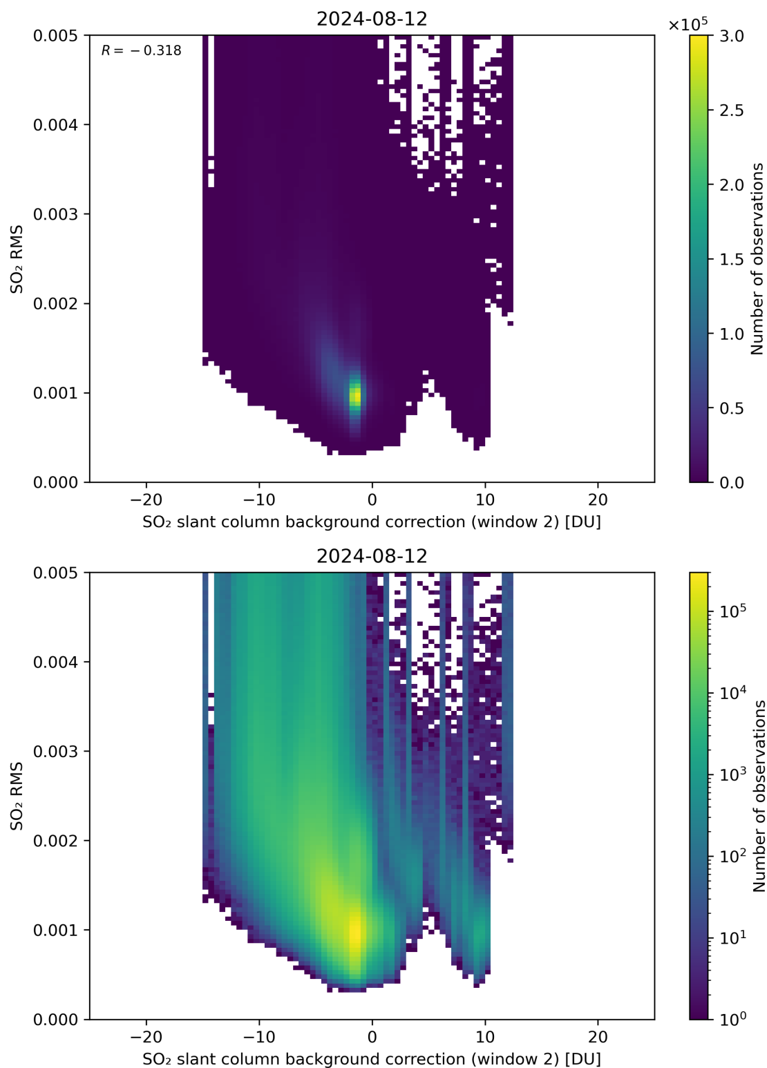
Figure 114: Scatter density plot of “SO 2 slant column background correction (window 2)” against “SO 2 RMS” for 2024-08-12 to 2024-08-13.
