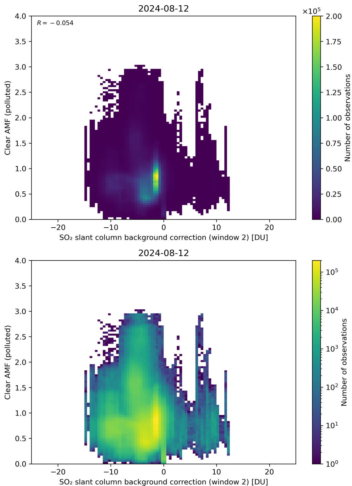
Figure 115: Scatter density plot of “SO 2 slant column background correction (window 2)” against “Clear AMF (polluted)” for 2024-08-12 to 2024-08-13.
