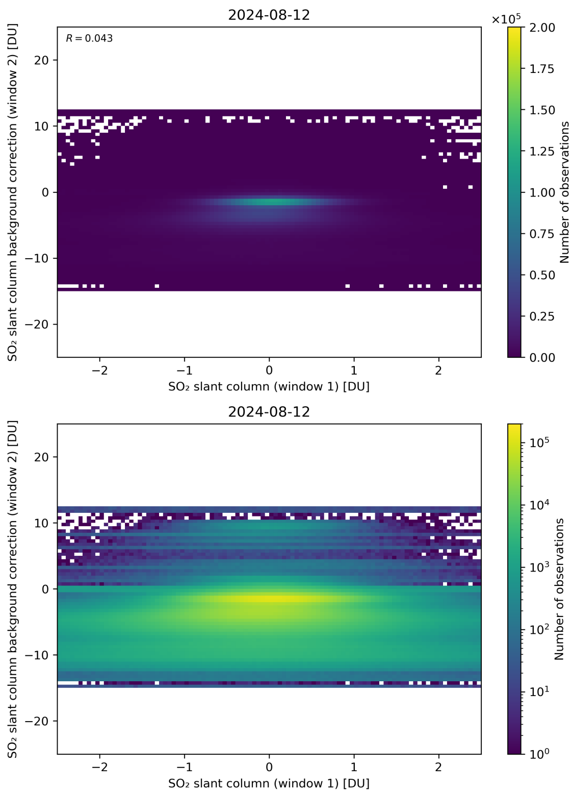
Figure 213: Scatter density plot of “SO 2 slant column (window 1)” against “SO 2 slant column background correction (window 2)” for 2024-08-12 to 2024-08-13.
