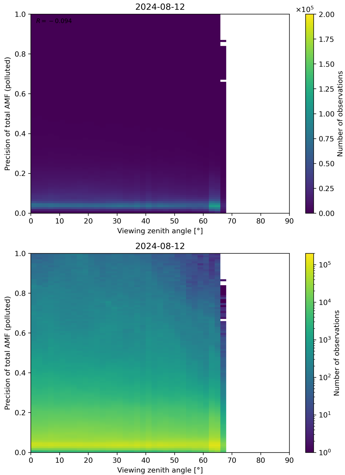
Figure 326: Scatter density plot of “Viewing zenith angle” against “Precision of total AMF (polluted)” for 2024-08-12 to 2024-08-13.
