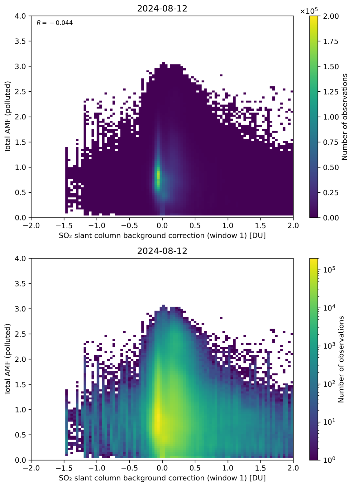
Figure 109: Scatter density plot of “SO 2 slant column background correction (window 1)” against “Total AMF (polluted)” for 2024-08-12 to 2024-08-13.
