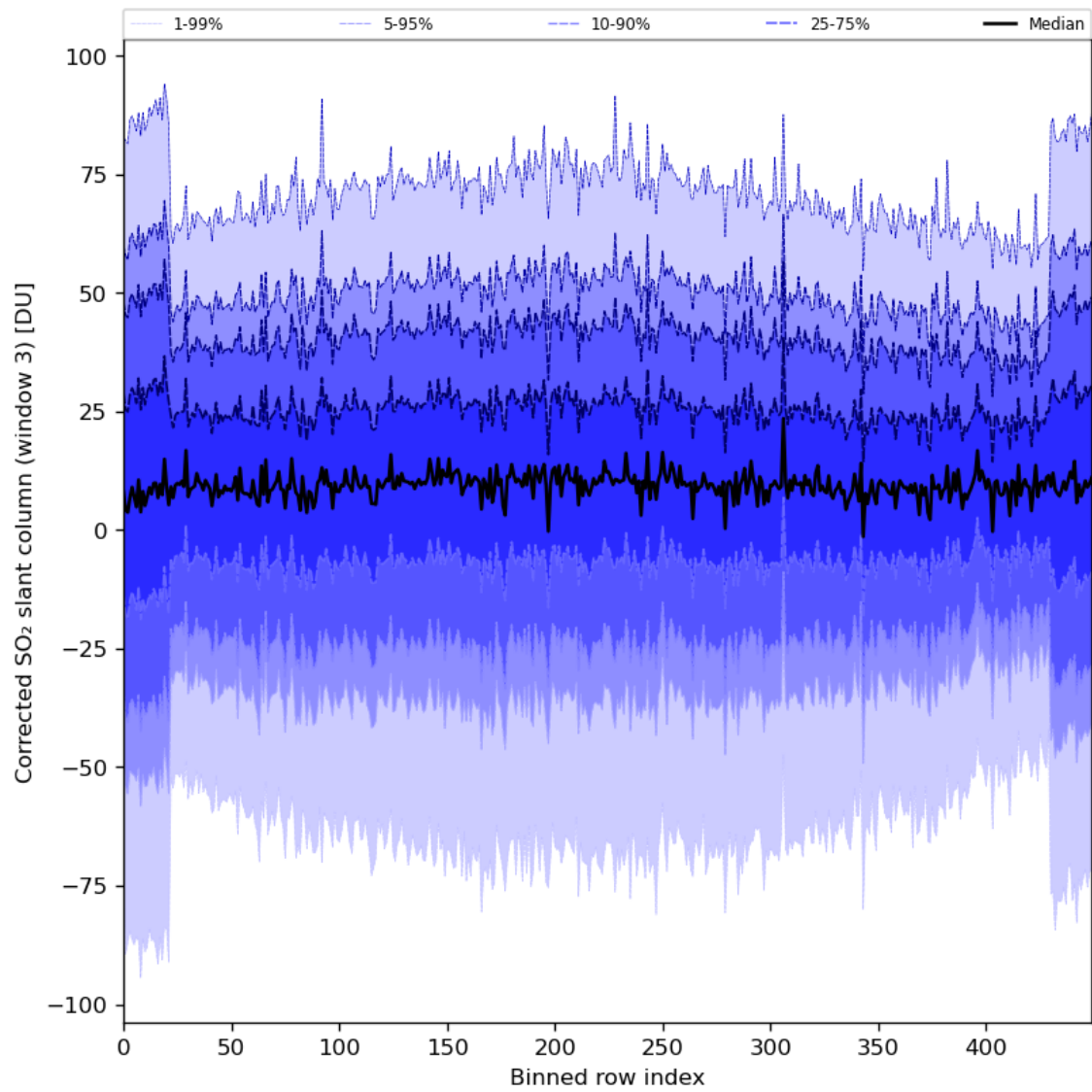
Figure 89: Along track statistics of “Corrected SO 2 slant column (window 3)” for 2024-08-12 to 2024-08-13
