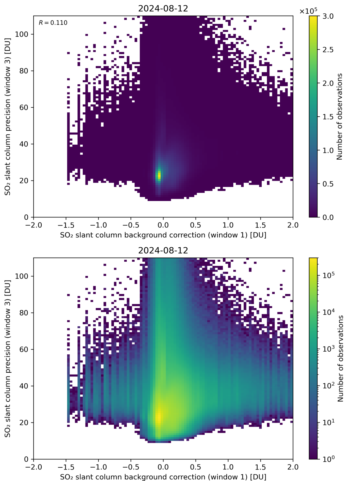
Figure 108: Scatter density plot of “SO 2 slant column background correction (window 1)” against “SO 2 slant column precision (window 3)” for 2024-08-12 to 2024-08-13.
