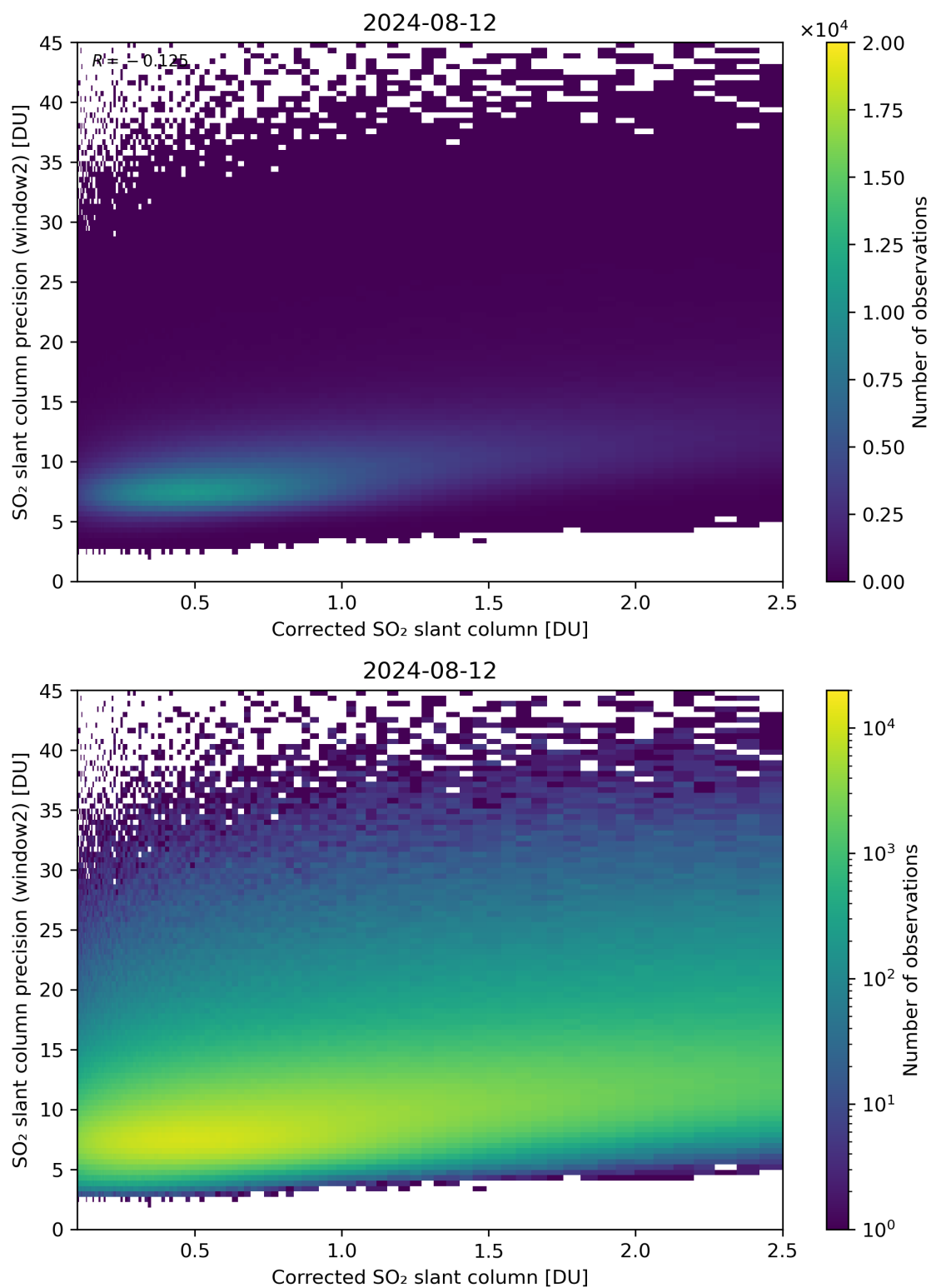
Figure 189: Scatter density plot of “Corrected SO 2 slant column” against “SO 2 slant column precision (window2)” for 2024-08-12 to 2024-08-13.
