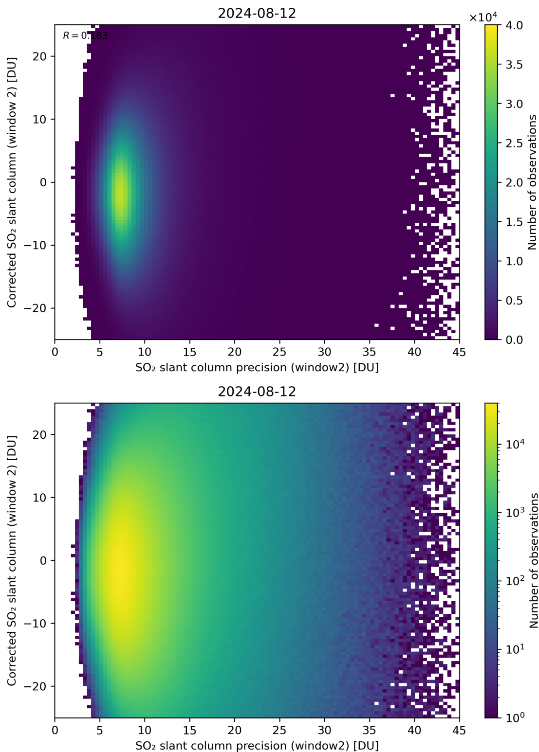
Figure 247: Scatter density plot of “SO 2 slant column precision (window2)” against “Corrected SO 2 slant column (window 2)” for 2024-08-12 to 2024-08-13.
