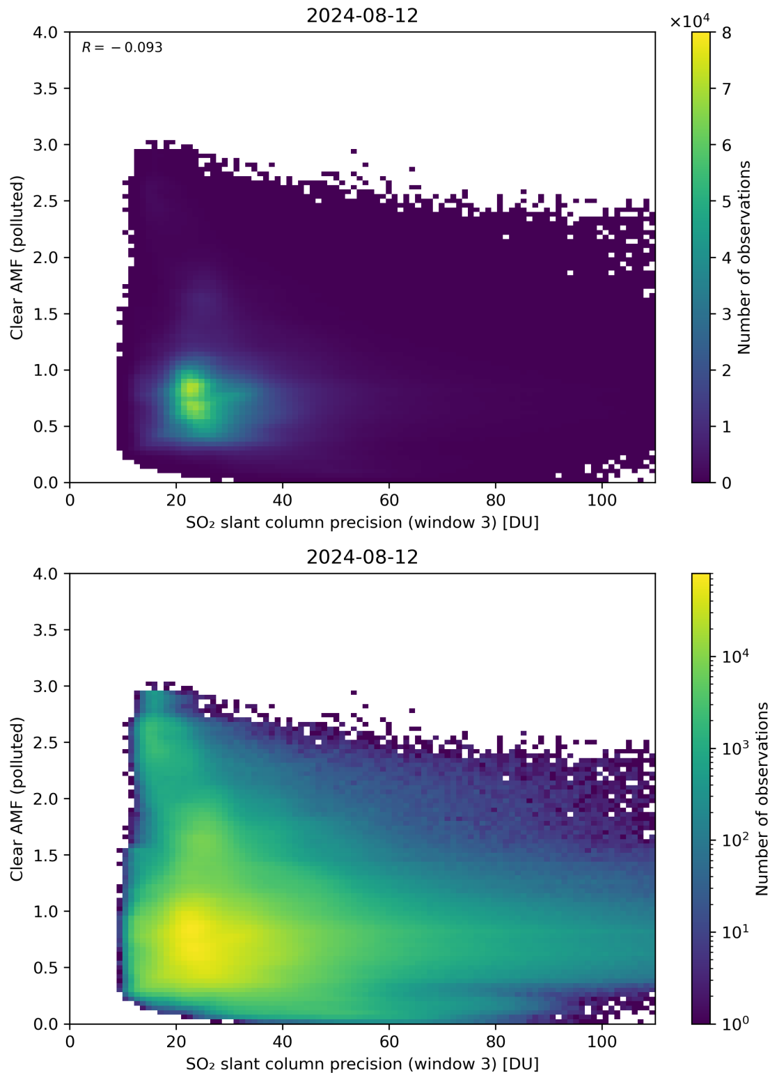
Figure 261: Scatter density plot of “SO 2 slant column precision (window 3)” against “Clear AMF (polluted)” for 2024-08-12 to 2024-08-13.
