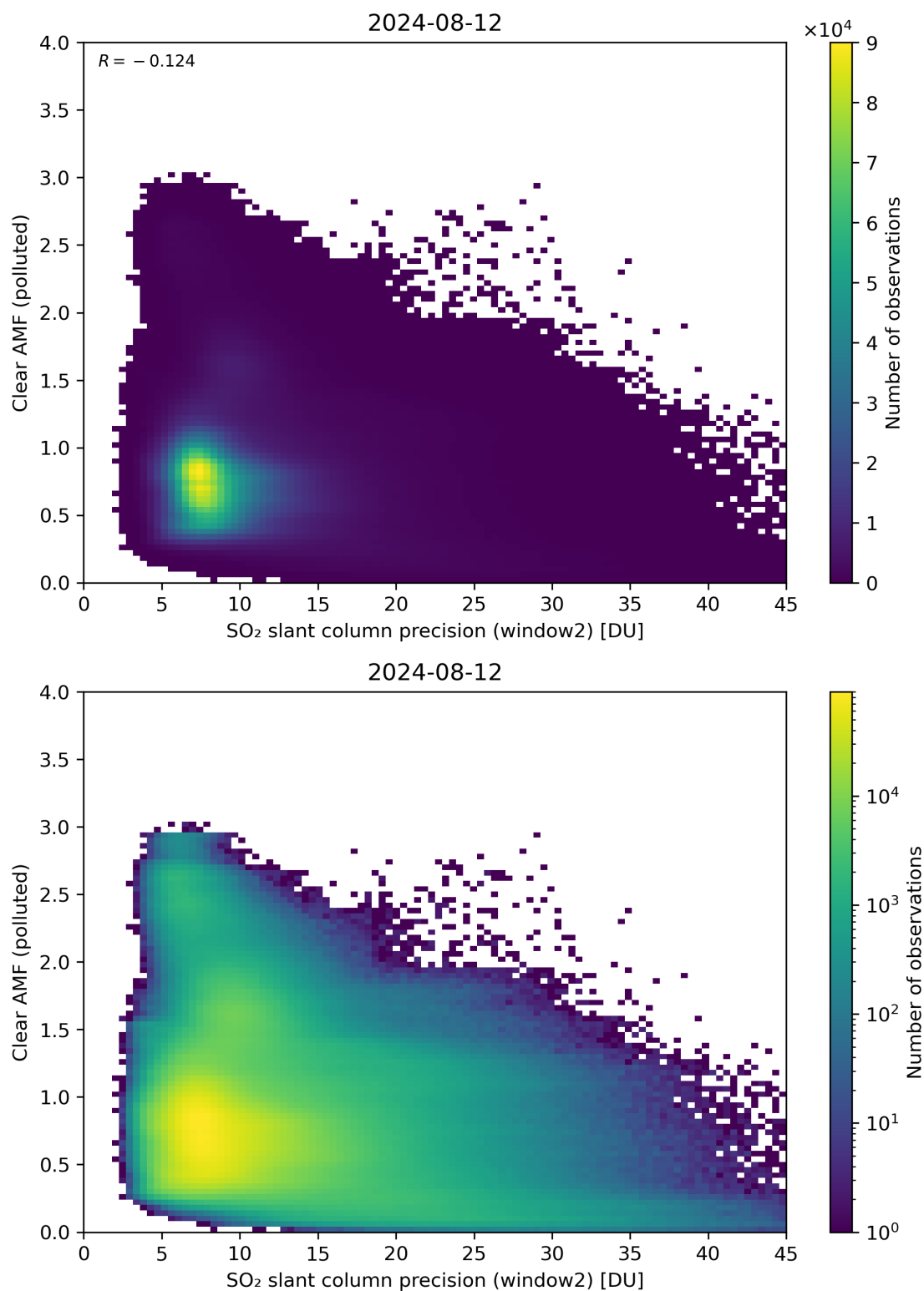
Figure 246: Scatter density plot of “SO 2 slant column precision (window2)” against “Clear AMF (polluted)” for 2024-08-12 to 2024-08-13.
