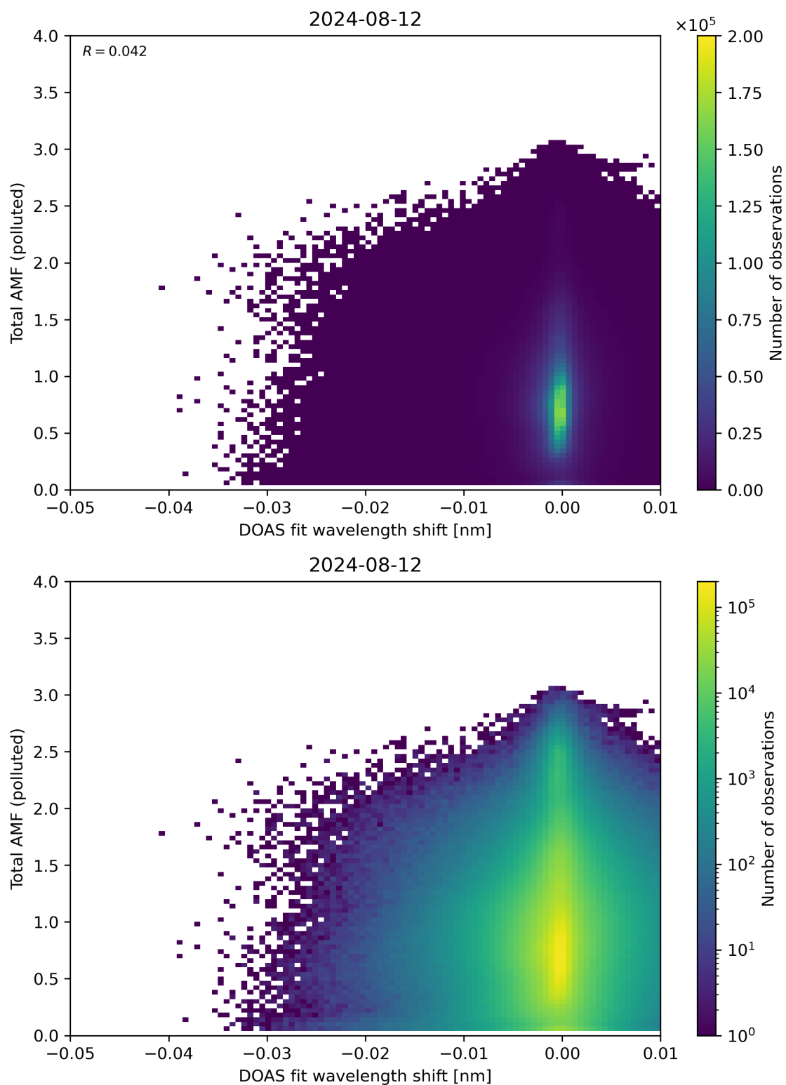
Figure 130: Scatter density plot of “DOAS fit wavelength shift” against “Total AMF (polluted)” for 2024-08-12 to 2024-08-13.
