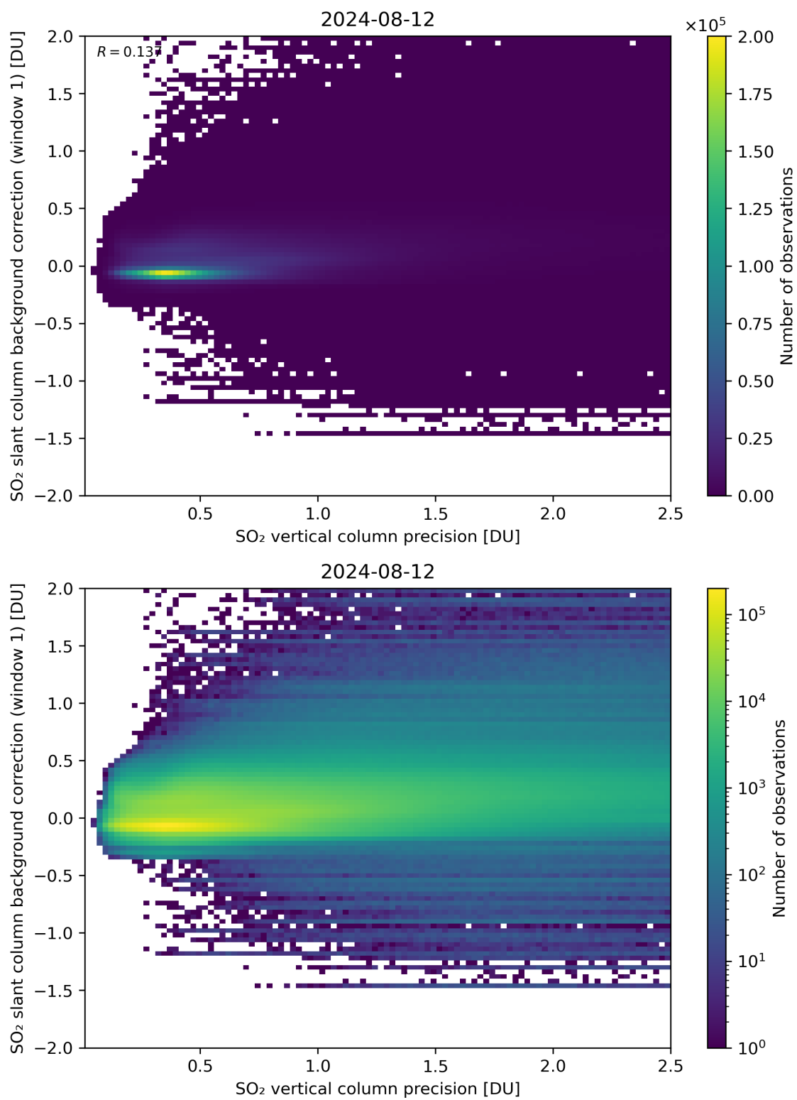
Figure 279: Scatter density plot of “SO 2 vertical column precision” against “SO 2 slant column background correction (window 1)” for 2024-08-12 to 2024-08-13.
