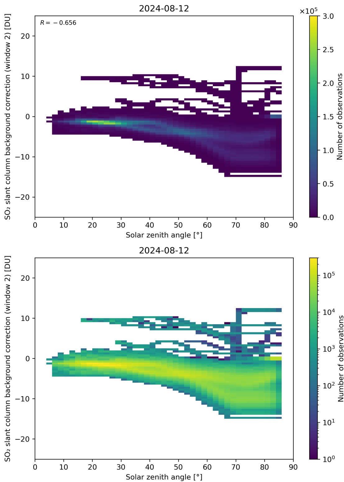
Figure 159: Scatter density plot of “Solar zenith angle” against “SO 2 slant column background correction (window 2)” for 2024-08-12 to 2024-08-13.
