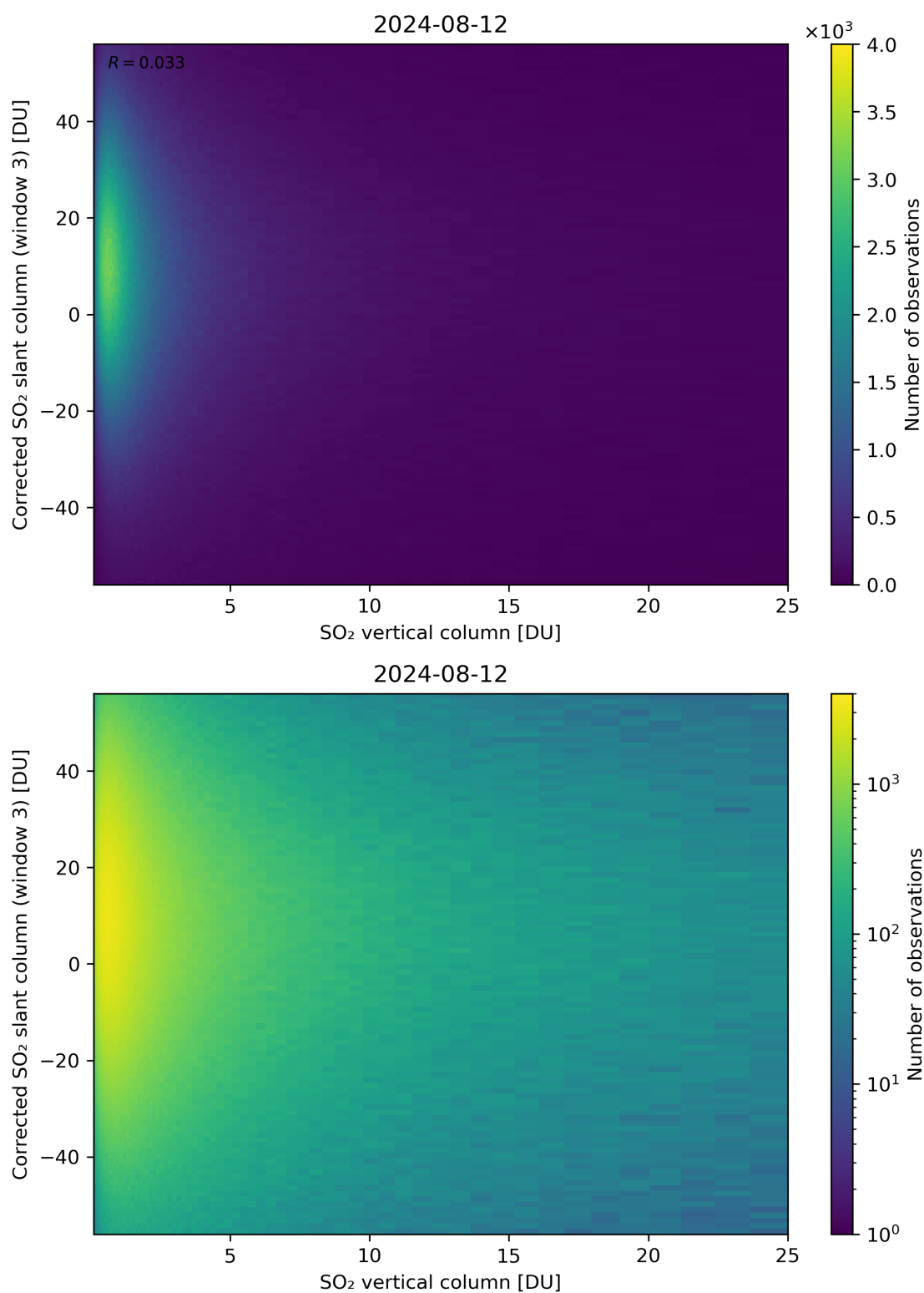
Figure 299: Scatter density plot of “SO 2 vertical column” against “Corrected SO 2 slant column (window 3)” for 2024-08-12 to 2024-08-13.
