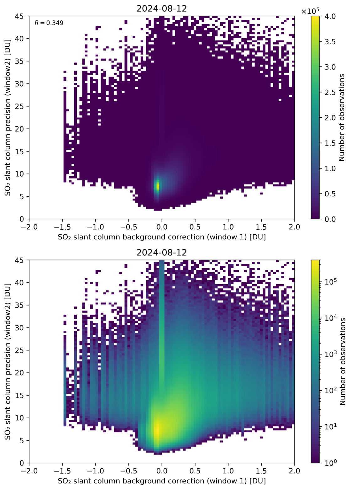
Figure 106: Scatter density plot of “SO 2 slant column background correction (window 1)” against “SO 2 slant column precision (window2)” for 2024-08-12 to 2024-08-13.
