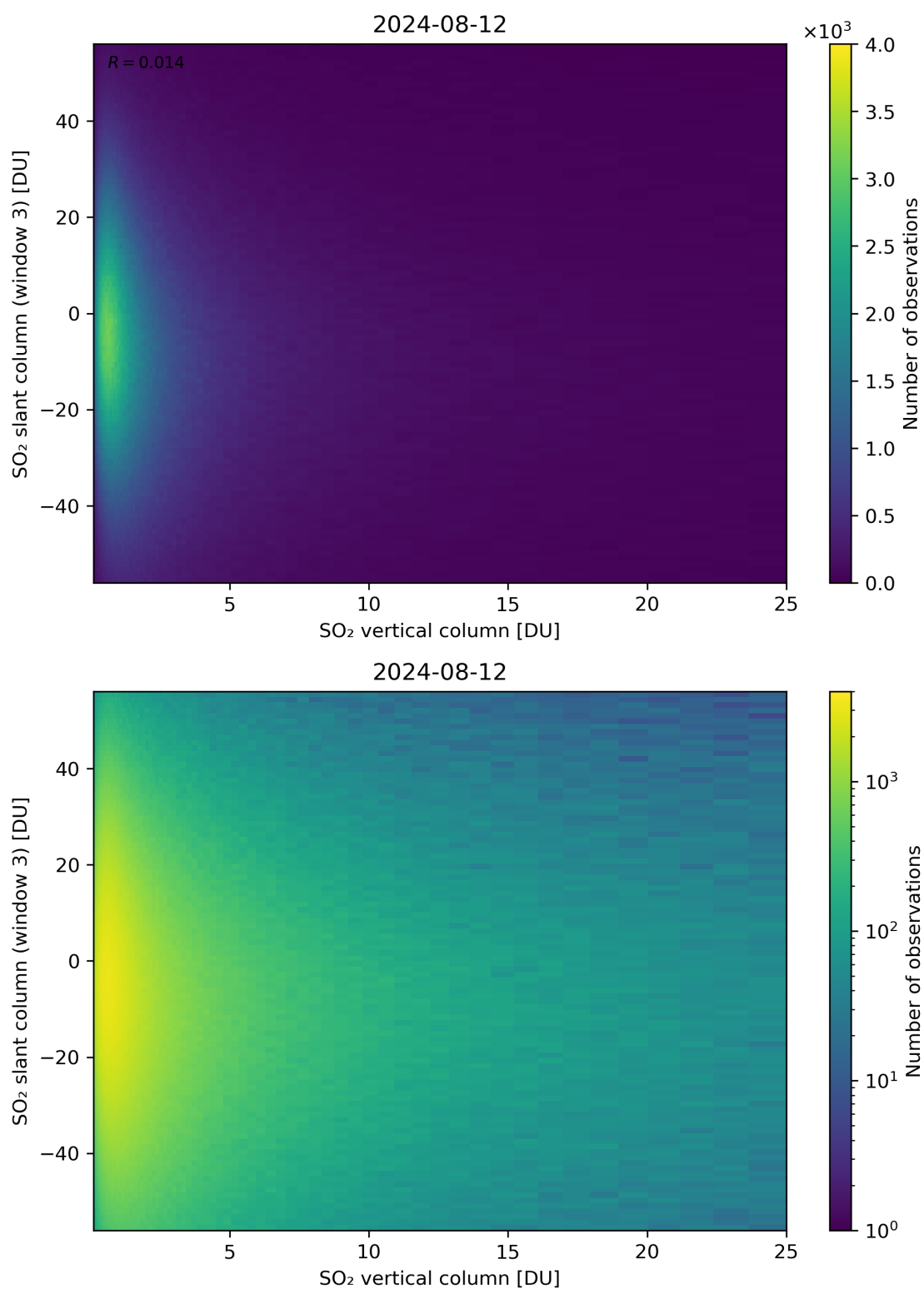
Figure 303: Scatter density plot of “SO 2 vertical column” against “SO 2 slant column (window 3)” for 2024-08-12 to 2024-08-13.
