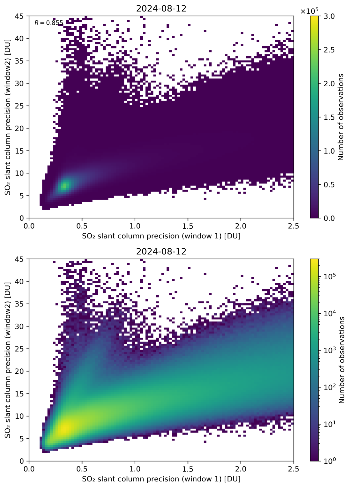
Figure 227: Scatter density plot of “SO 2 slant column precision (window 1)” against “SO 2 slant column precision (window2)” for 2024-08-12 to 2024-08-13.
