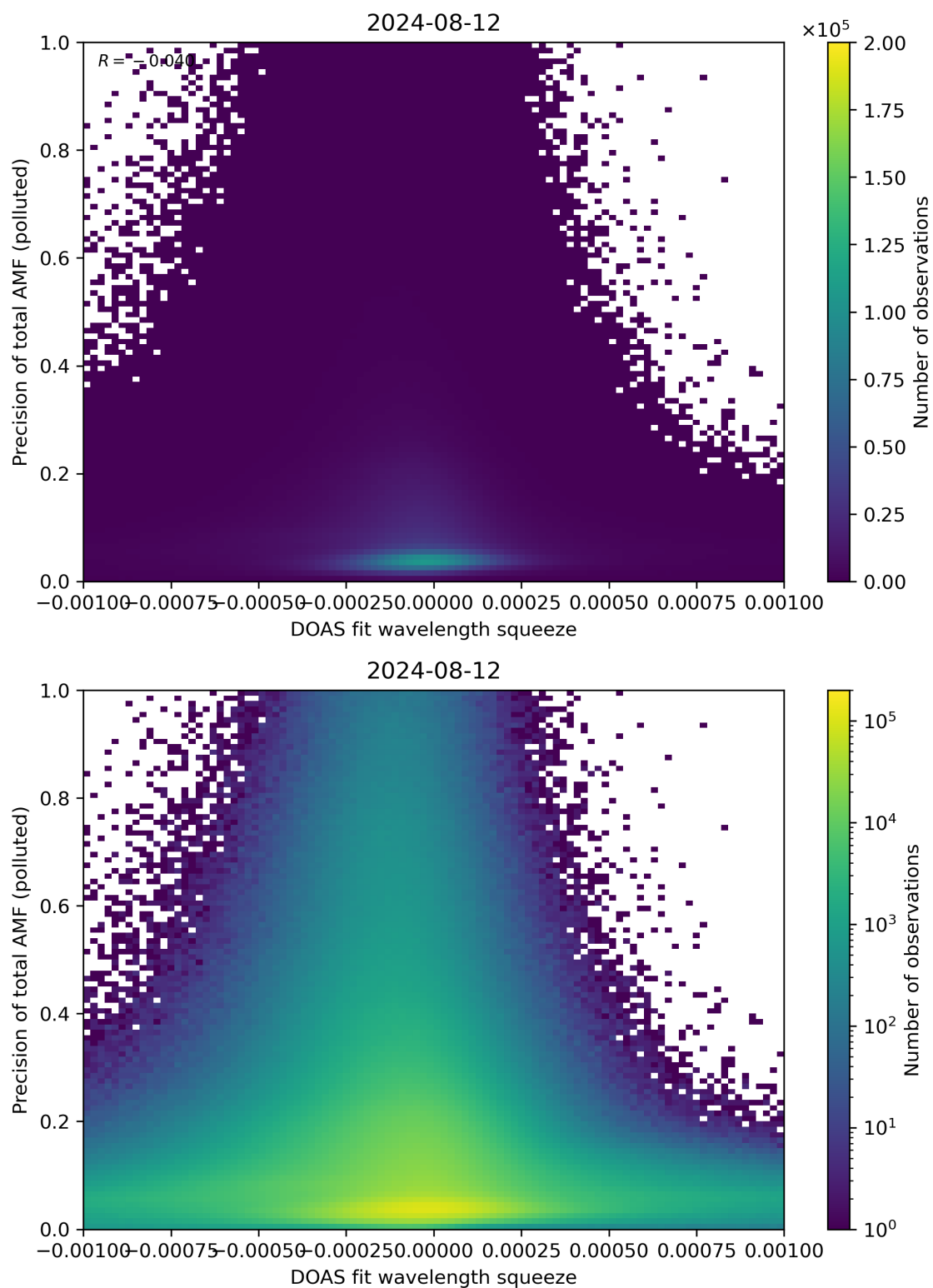
Figure 135: Scatter density plot of “DOAS fit wavelength squeeze” against “Precision of total AMF (polluted)” for 2024-08-12 to 2024-08-13.
