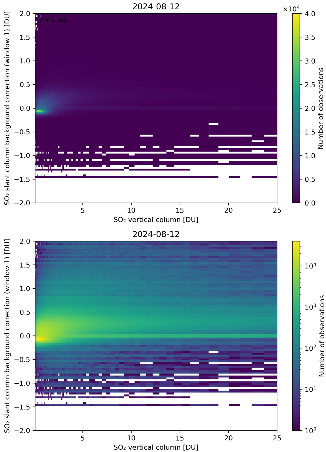
Figure 273: Scatter density plot of “SO 2 vertical column” against “SO 2 slant column background correction (window 1)” for 2024-08-12 to 2024-08-13.
