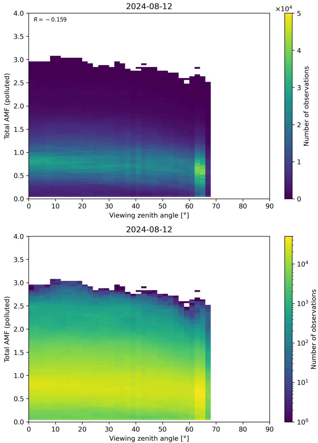
Figure 325: Scatter density plot of “Viewing zenith angle” against “Total AMF (polluted)” for 2024-08-12 to 2024-08-13.
