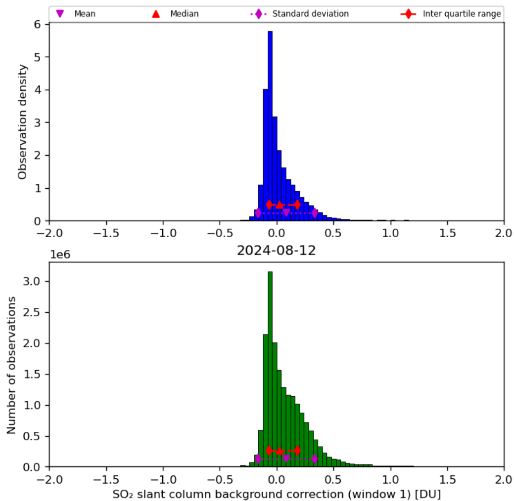
Figure 59: Histogram of “SO 2 slant column background correction (window 1)” for 2024-08-12 to 2024-08-13
