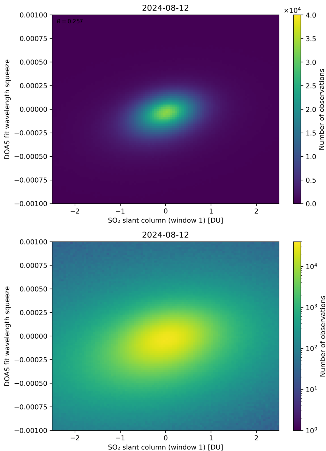
Figure 216: Scatter density plot of “SO 2 slant column (window 1)” against “DOAS fit wavelength squeeze” for 2024-08-12 to 2024-08-13.
