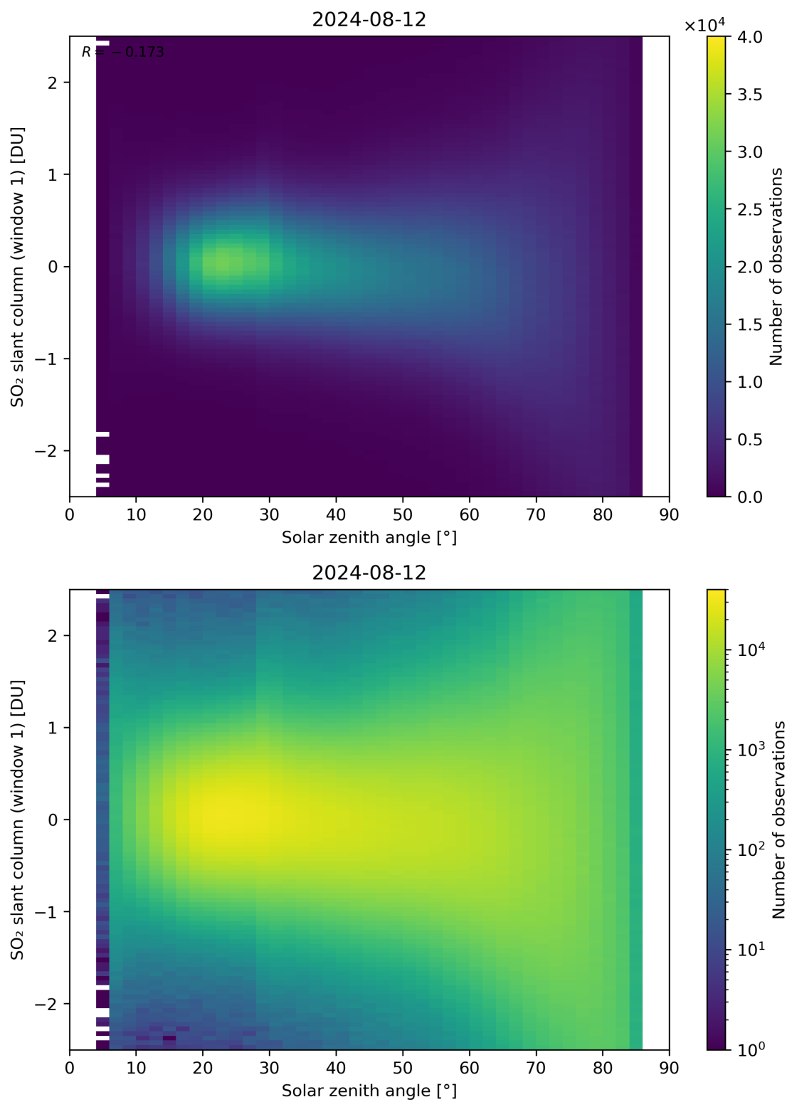
Figure 169: Scatter density plot of “Solar zenith angle” against “SO 2 slant column (window 1)” for 2024-08-12 to 2024-08-13.
