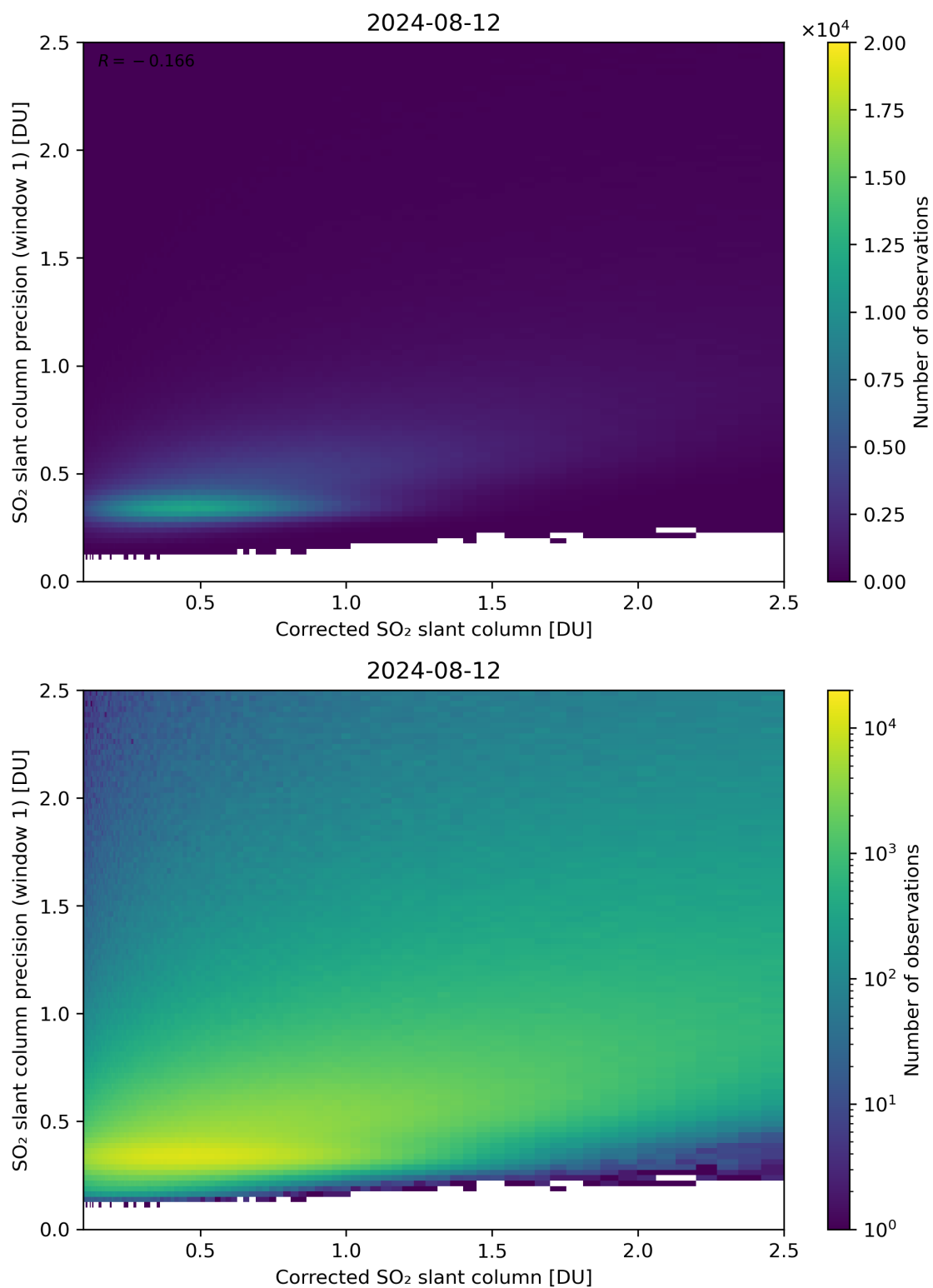
Figure 188: Scatter density plot of “Corrected SO 2 slant column” against “SO 2 slant column precision (window 1)” for 2024-08-12 to 2024-08-13.
