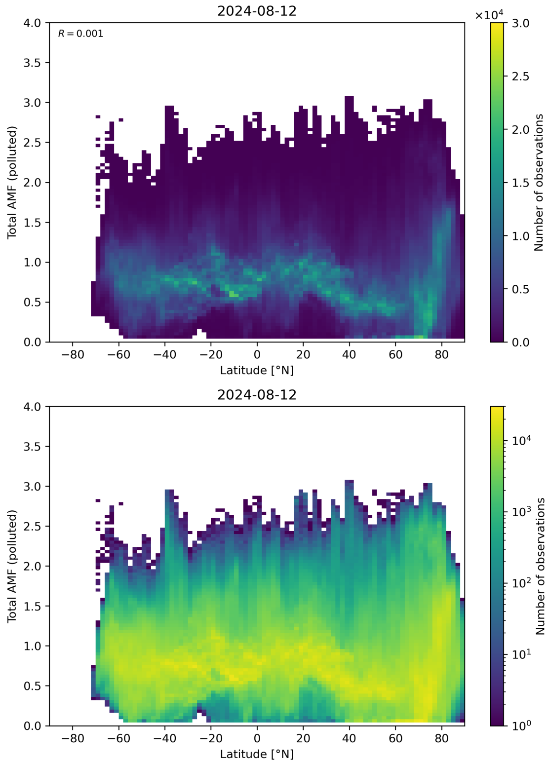
Figure 154: Scatter density plot of “Latitude” against “Total AMF (polluted)” for 2024-08-12 to 2024-08-13.
