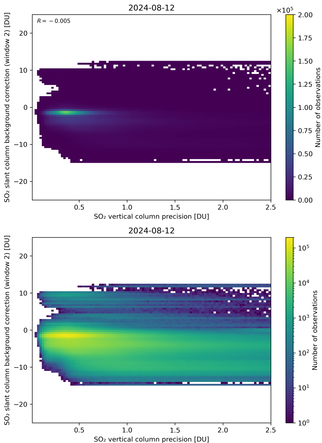
Figure 280: Scatter density plot of “SO 2 vertical column precision” against “SO 2 slant column background correction (window 2)” for 2024-08-12 to 2024-08-13.
