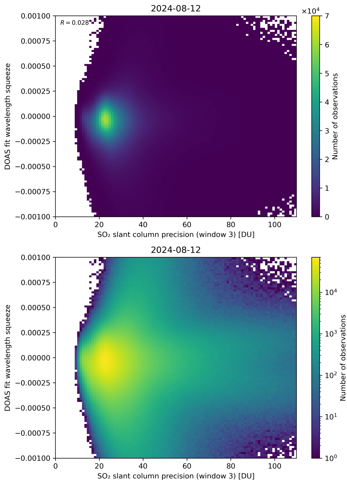
Figure 259: Scatter density plot of “SO 2 slant column precision (window 3)” against “DOAS fit wavelength squeeze” for 2024-08-12 to 2024-08-13.
