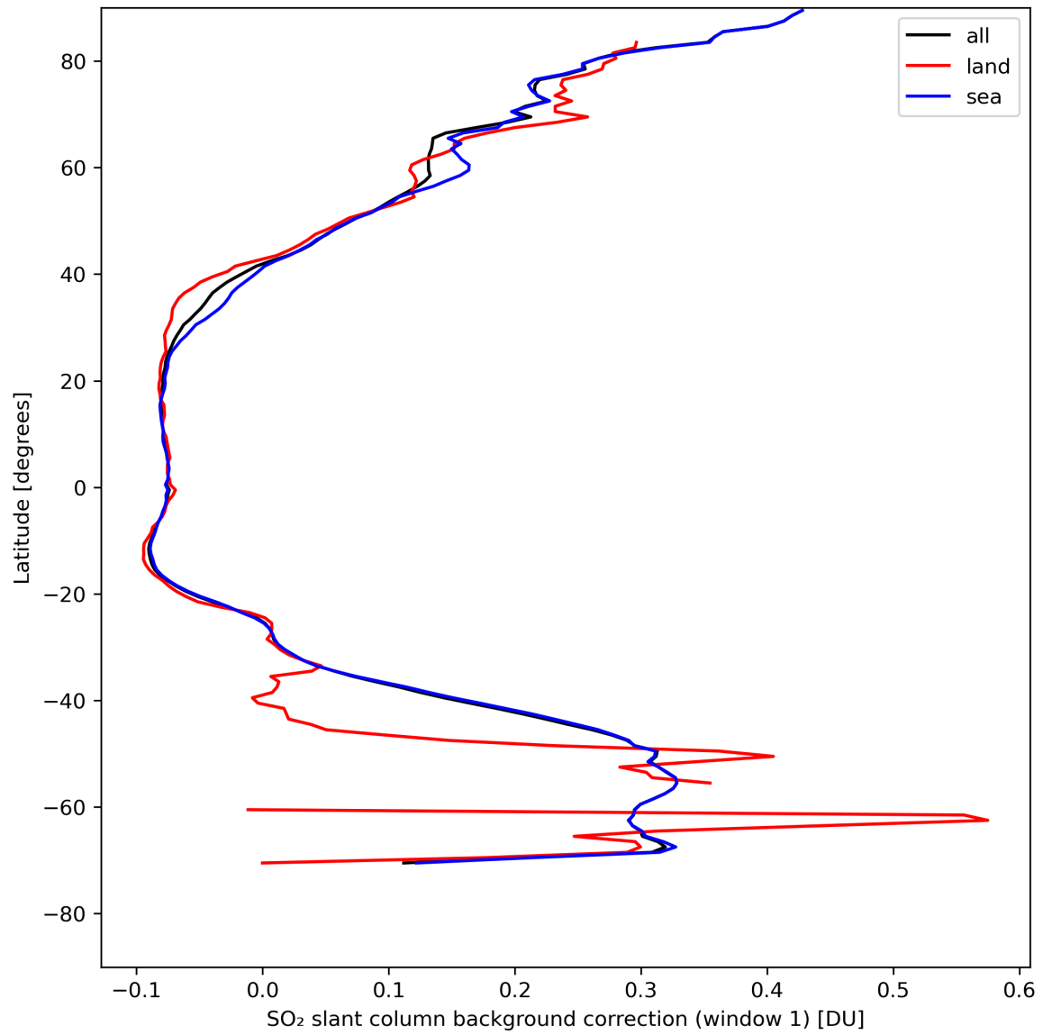
Figure 36: Zonal average of “SO 2 slant column background correction (window 1)” for 2024-08-12 to 2024-08-13.
