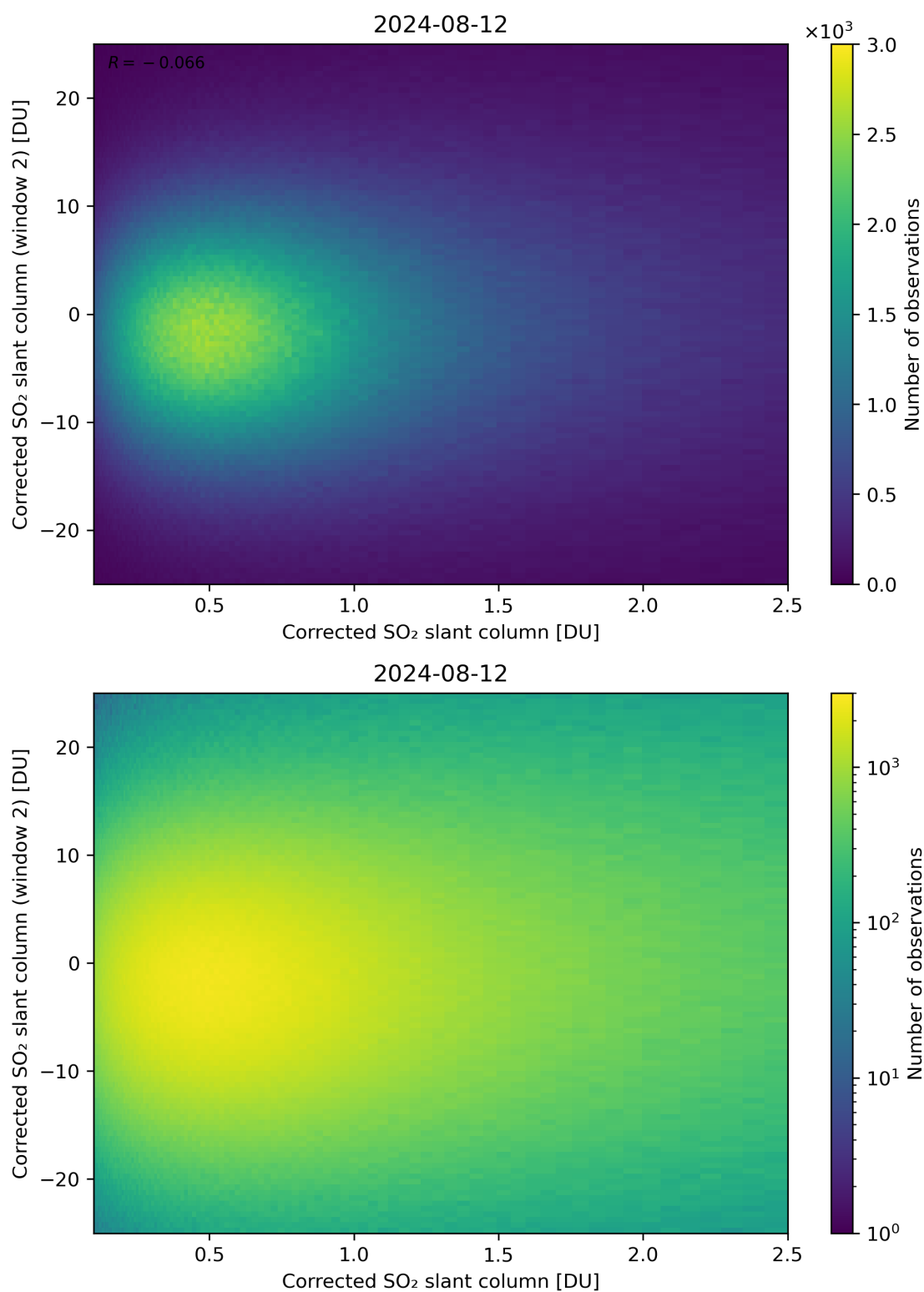
Figure 185: Scatter density plot of “Corrected SO 2 slant column” against “Corrected SO 2 slant column (window 2)” for 2024-08-12 to 2024-08-13.
