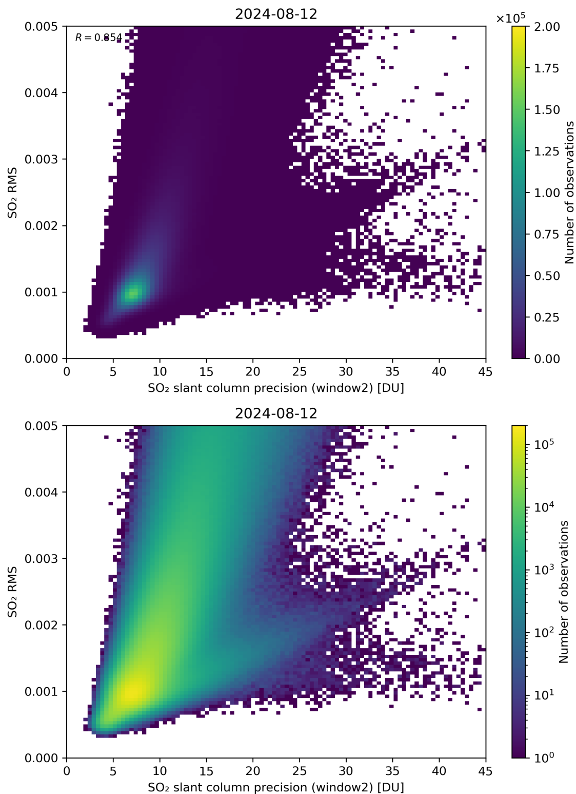
Figure 245: Scatter density plot of “SO 2 slant column precision (window2)” against “SO 2 RMS” for 2024-08-12 to 2024-08-13.
