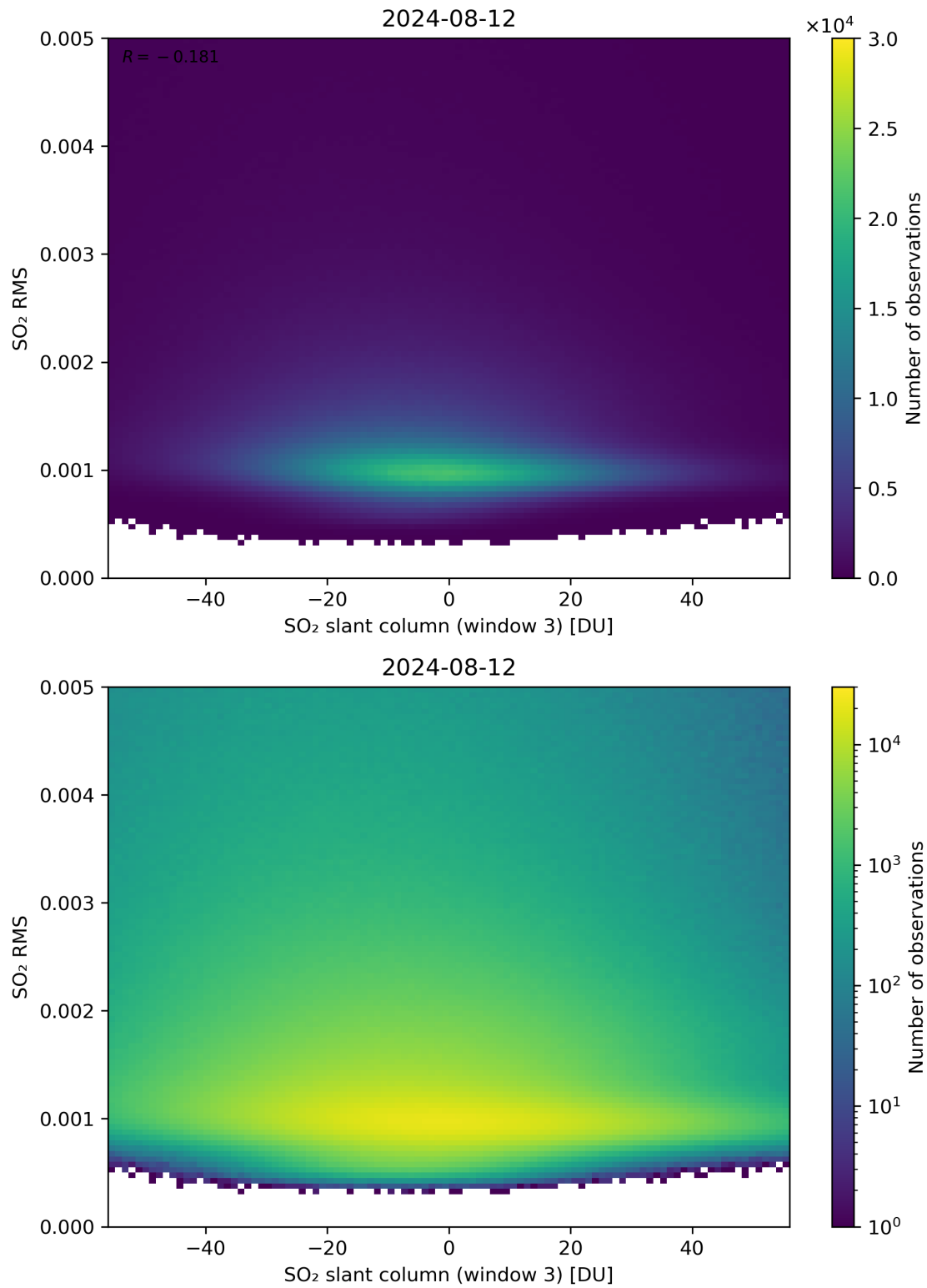
Figure 256: Scatter density plot of “SO 2 slant column (window 3)” against “SO 2 RMS” for 2024-08-12 to 2024-08-13.
