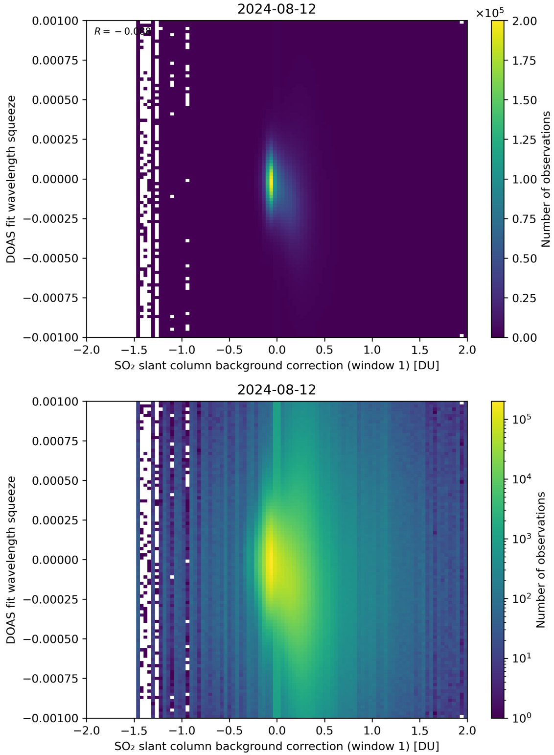
Figure 101: Scatter density plot of “SO 2 slant column background correction (window 1)” against “DOAS fit wavelength squeeze” for 2024-08-12 to 2024-08-13.
