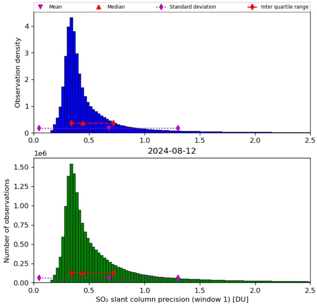
Figure 57: Histogram of “SO 2 slant column precision (window 1)” for 2024-08-12 to 2024-08-13
