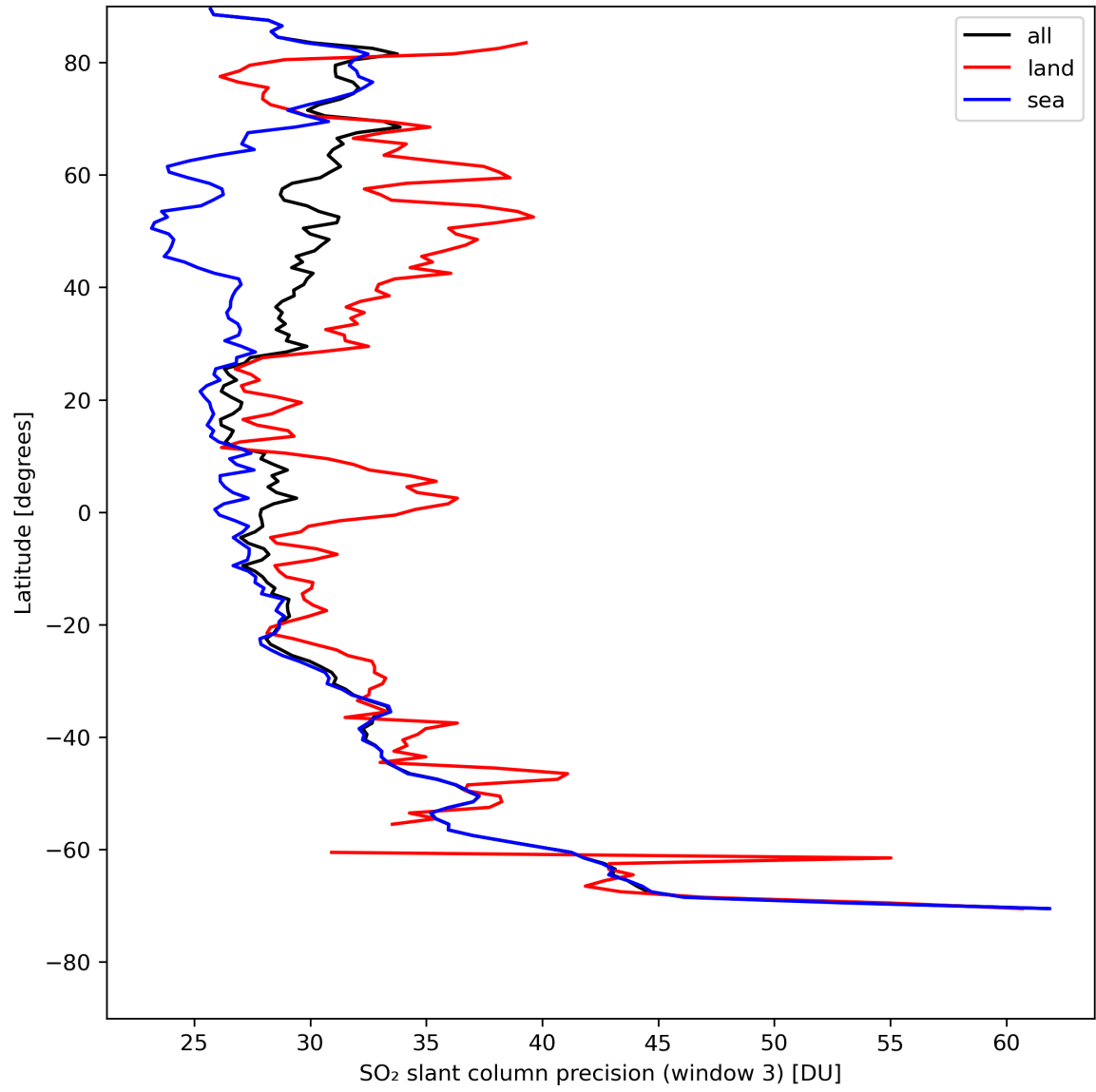
Figure 42: Zonal average of “SO 2 slant column precision (window 3)” for 2024-08-12 to 2024-08-13.
