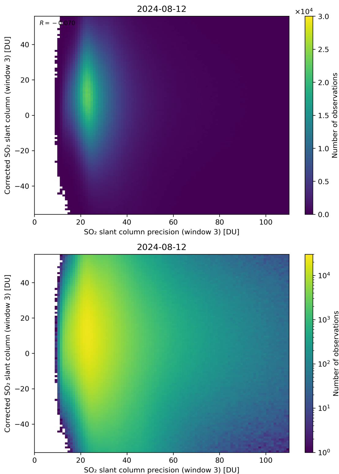
Figure 262: Scatter density plot of “SO 2 slant column precision (window 3)” against “Corrected SO 2 slant column (window 3)” for 2024-08-12 to 2024-08-13.
