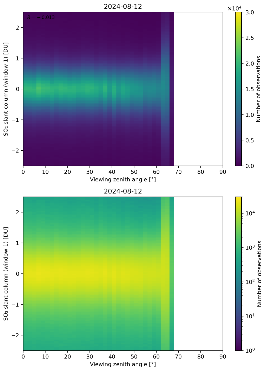
Figure 320: Scatter density plot of “Viewing zenith angle” against “SO 2 slant column (window 1)” for 2024-08-12 to 2024-08-13.
