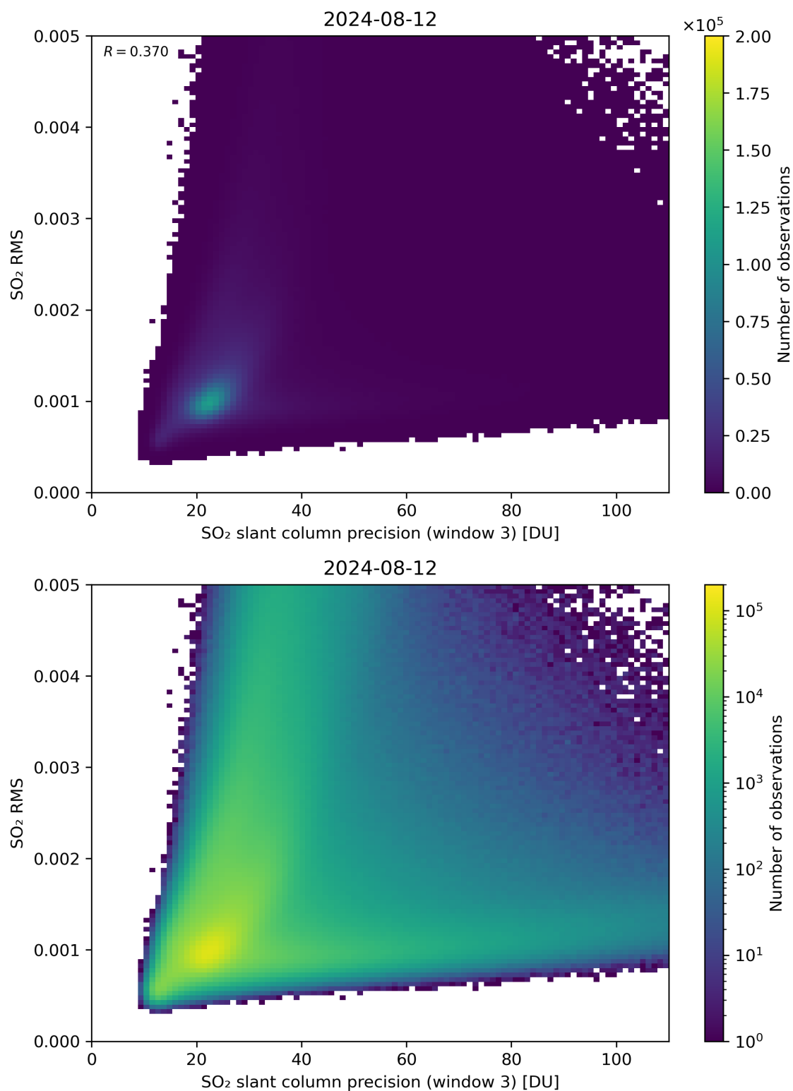
Figure 260: Scatter density plot of “SO 2 slant column precision (window 3)” against “SO 2 RMS” for 2024-08-12 to 2024-08-13.
