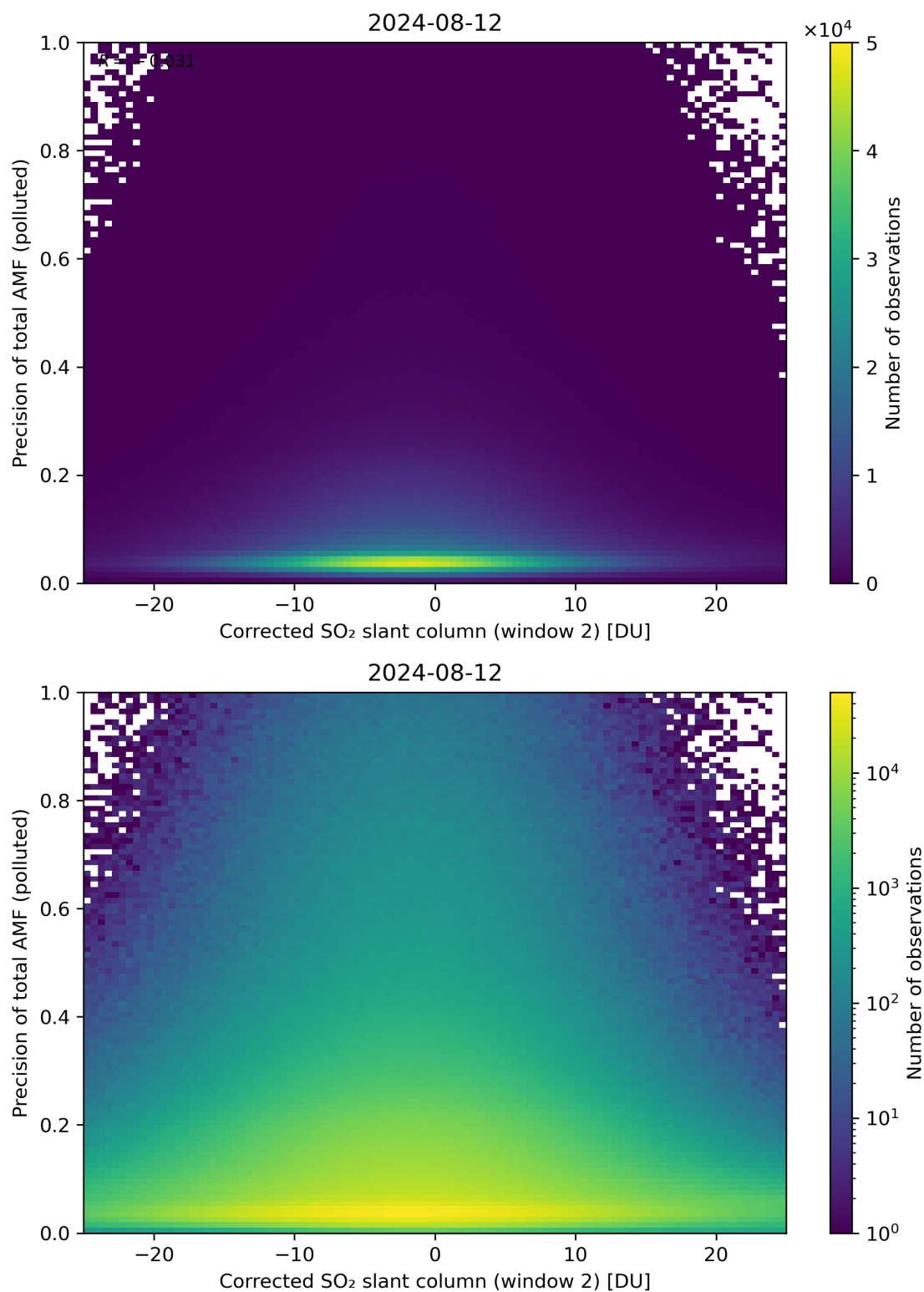
Figure 204: Scatter density plot of “Corrected SO 2 slant column (window 2)” against “Precision of total AMF (polluted)” for 2024-08-12 to 2024-08-13.
