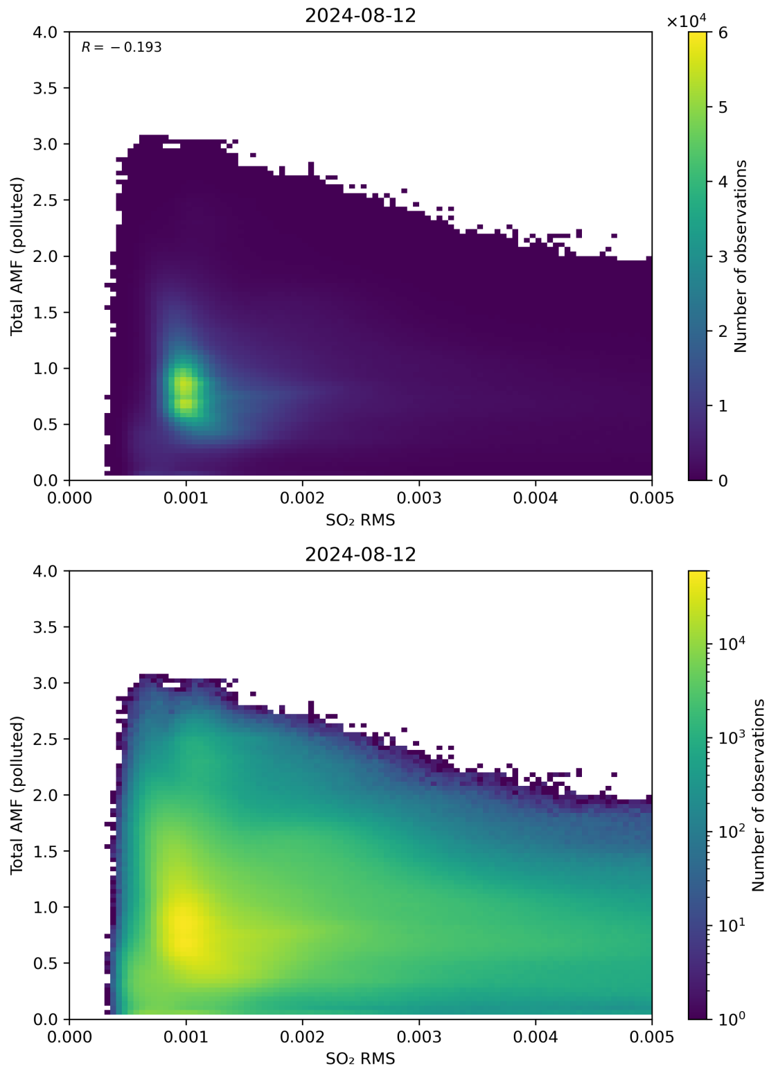
Figure 137: Scatter density plot of “SO 2 RMS” against “Total AMF (polluted)” for 2024-08-12 to 2024-08-13.
