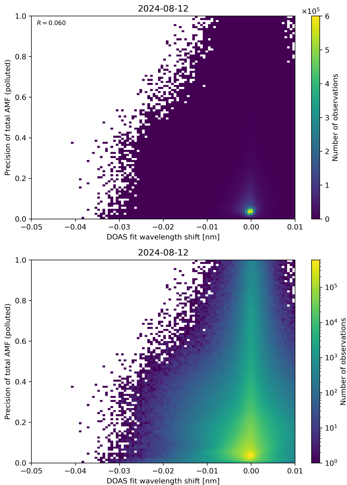
Figure 131: Scatter density plot of “DOAS fit wavelength shift” against “Precision of total AMF (polluted)” for 2024-08-12 to 2024-08-13.
