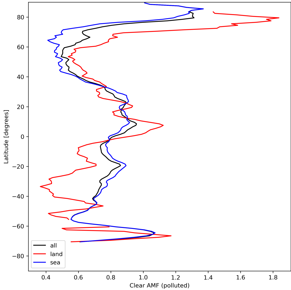
Figure 50: Zonal average of “Clear AMF (polluted)” for 2024-08-12 to 2024-08-13.
