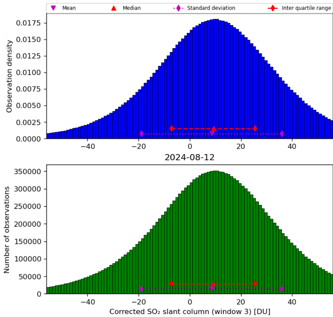
Figure 66: Histogram of “Corrected SO 2 slant column (window 3)” for 2024-08-12 to 2024-08-13
