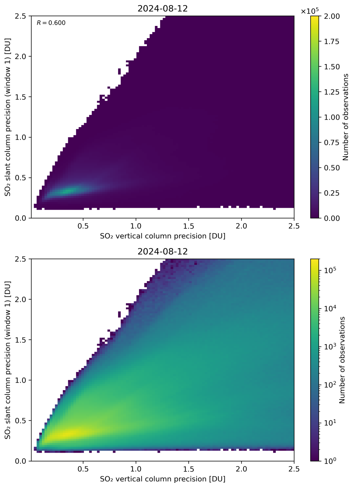
Figure 290: Scatter density plot of “SO 2 vertical column precision” against “SO 2 slant column precision (window 1)” for 2024-08-12 to 2024-08-13.
