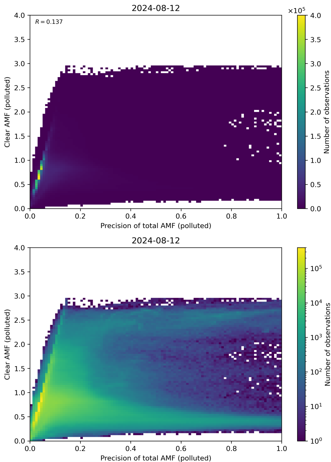
Figure 270: Scatter density plot of “Precision of total AMF (polluted)” against “Clear AMF (polluted)” for 2024-08-12 to 2024-08-13.
