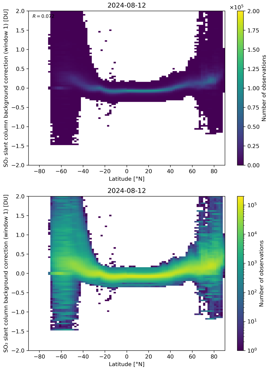
Figure 139: Scatter density plot of “Latitude” against “SO 2 slant column background correction (window 1)” for 2024-08-12 to 2024-08-13.
