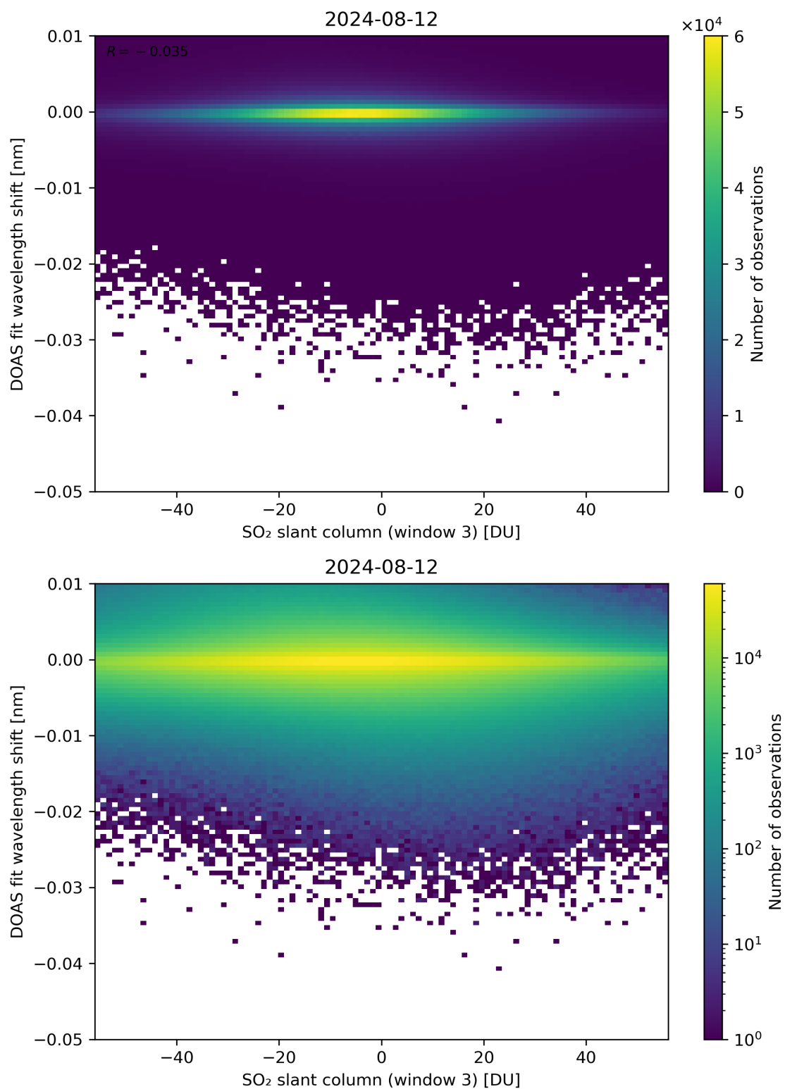
Figure 254: Scatter density plot of “SO 2 slant column (window 3)” against “DOAS fit wavelength shift” for 2024-08-12 to 2024-08-13.
