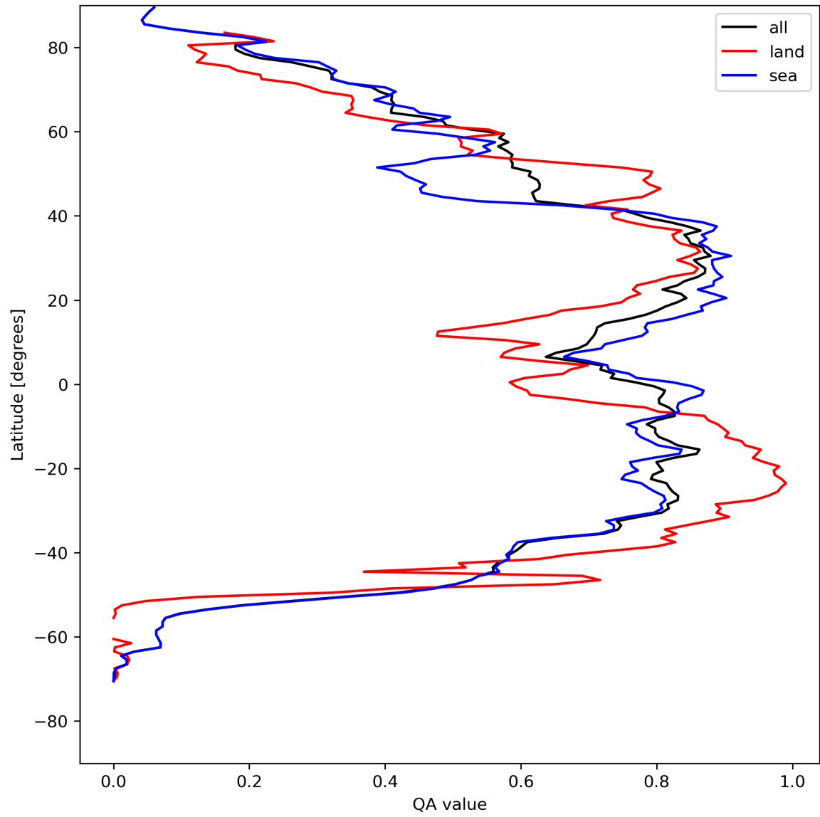
Figure 29: Zonal average of “QA value” for 2024-08-12 to 2024-08-13.
