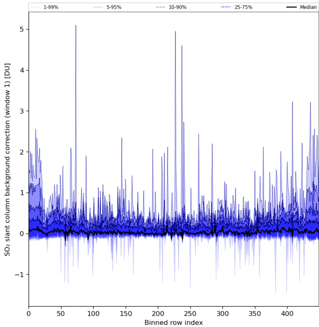
Figure 82: Along track statistics of “SO 2 slant column background correction (window 1)” for 2024-08-12 to 2024-08-13
