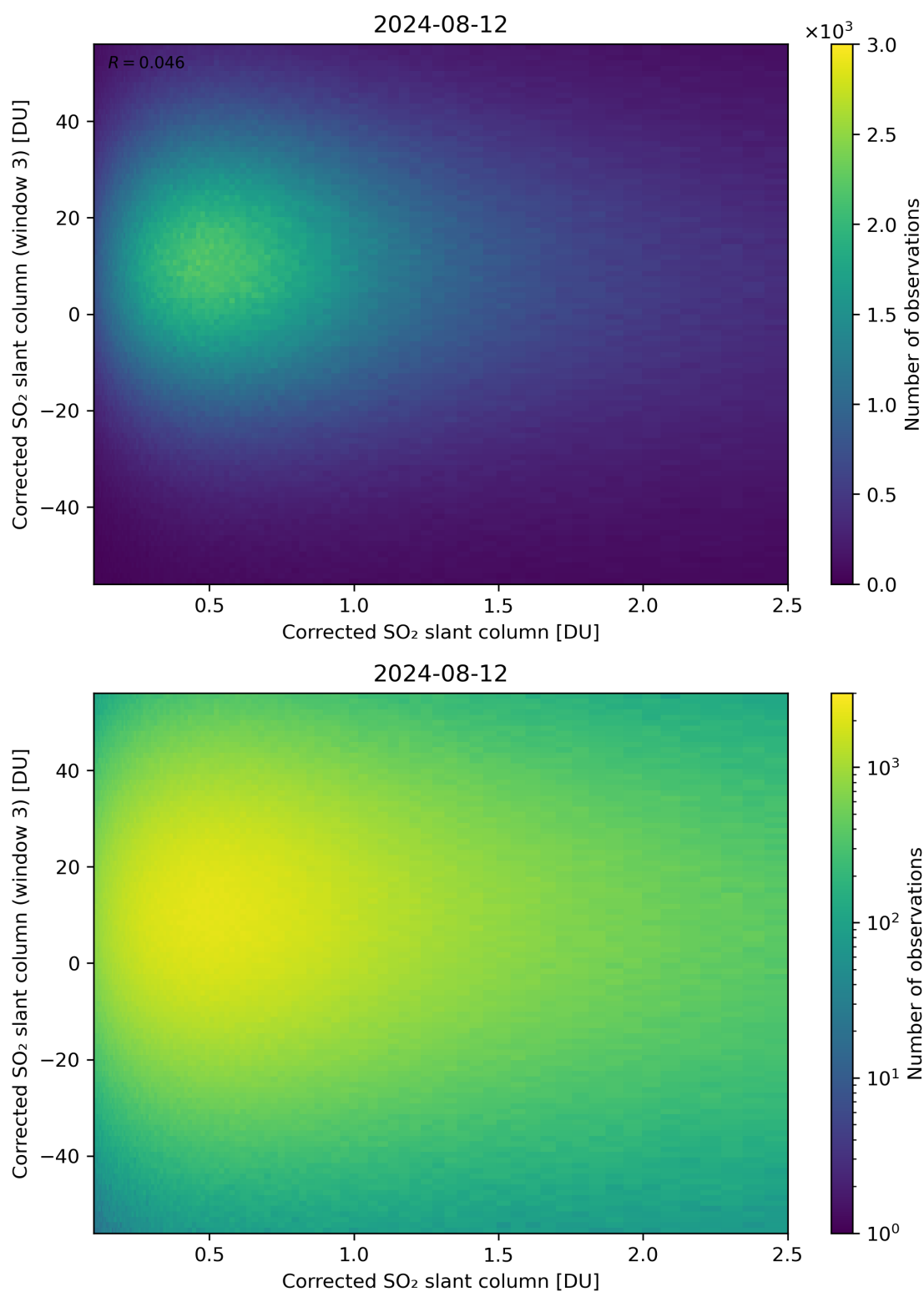
Figure 186: Scatter density plot of “Corrected SO 2 slant column” against “Corrected SO 2 slant column (window 3)” for 2024-08-12 to 2024-08-13.
