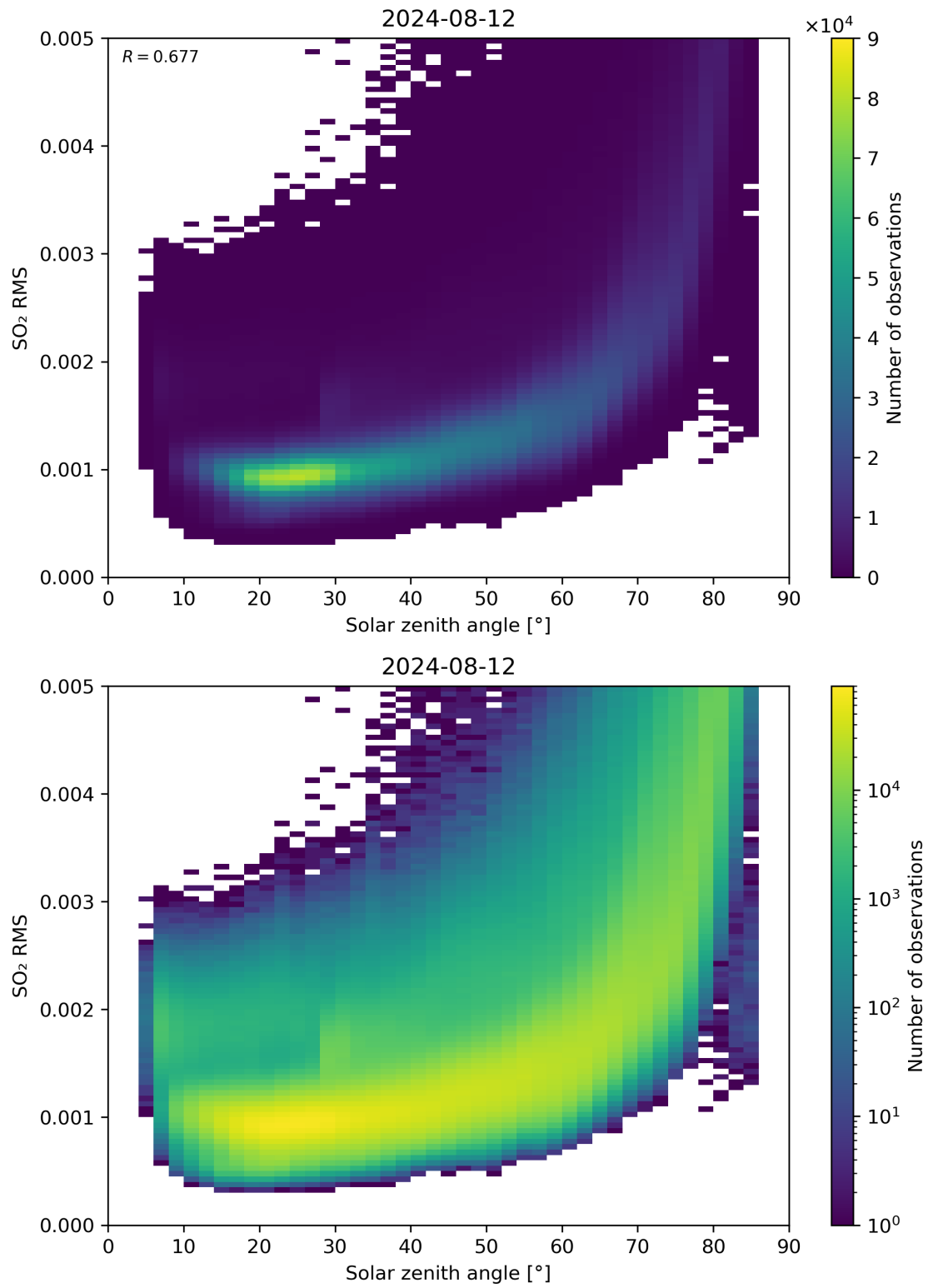
Figure 163: Scatter density plot of “Solar zenith angle” against “SO 2 RMS” for 2024-08-12 to 2024-08-13.
