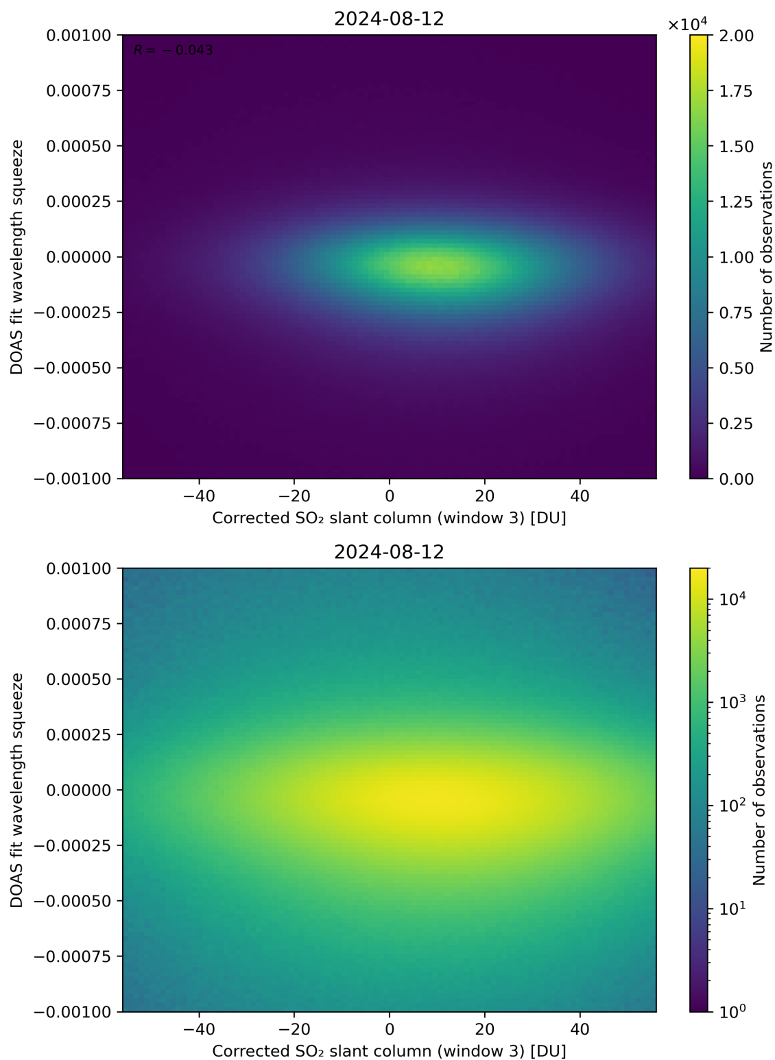
Figure 207: Scatter density plot of “Corrected SO 2 slant column (window 3)” against “DOAS fit wavelength squeeze” for 2024-08-12 to 2024-08-13.
