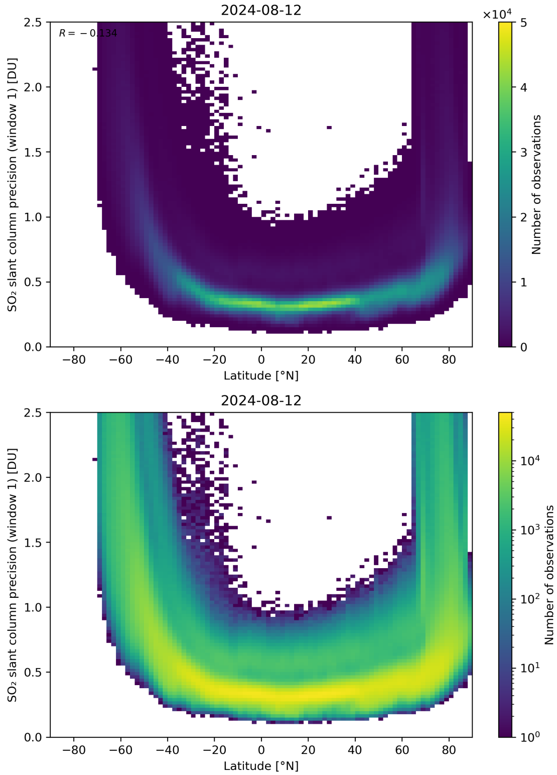
Figure 150: Scatter density plot of “Latitude” against “SO 2 slant column precision (window 1)” for 2024-08-12 to 2024-08-13.
