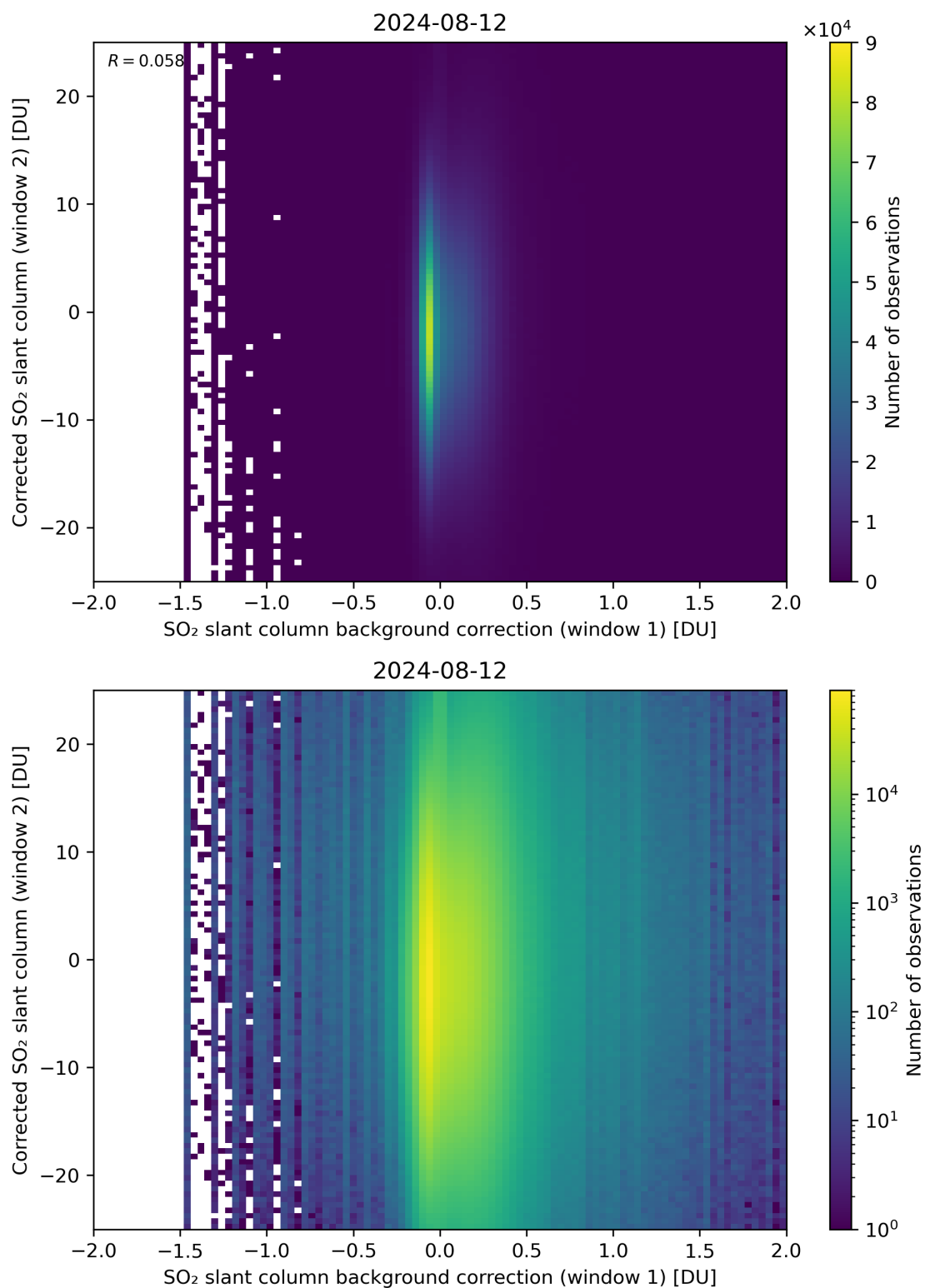
Figure 104: Scatter density plot of “SO 2 slant column background correction (window 1)” against “Corrected SO 2 slant column (window 2)” for 2024-08-12 to 2024-08-13.
