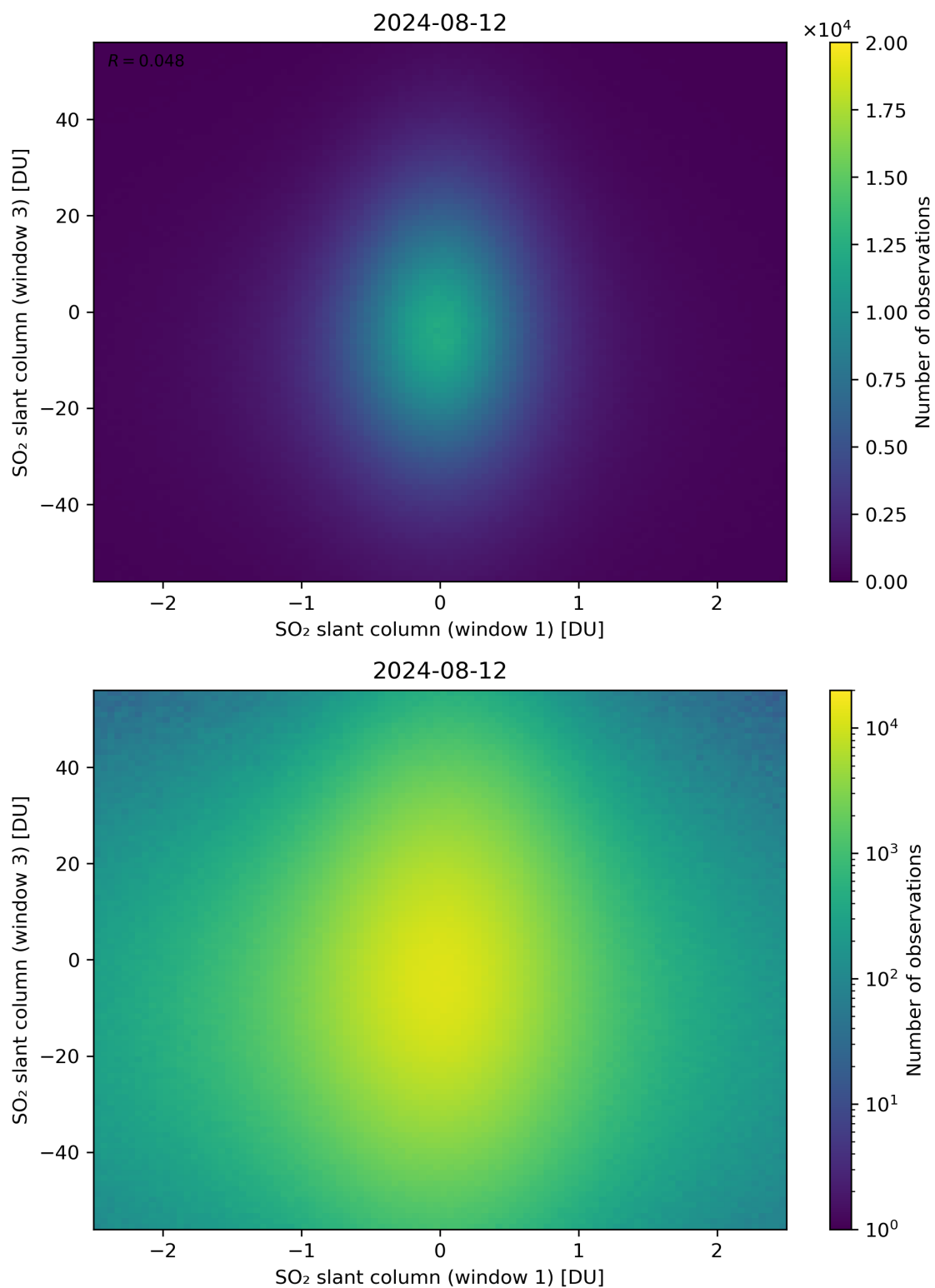
Figure 237: Scatter density plot of “SO 2 slant column (window 1)” against “SO 2 slant column (window 3)” for 2024-08-12 to 2024-08-13.
