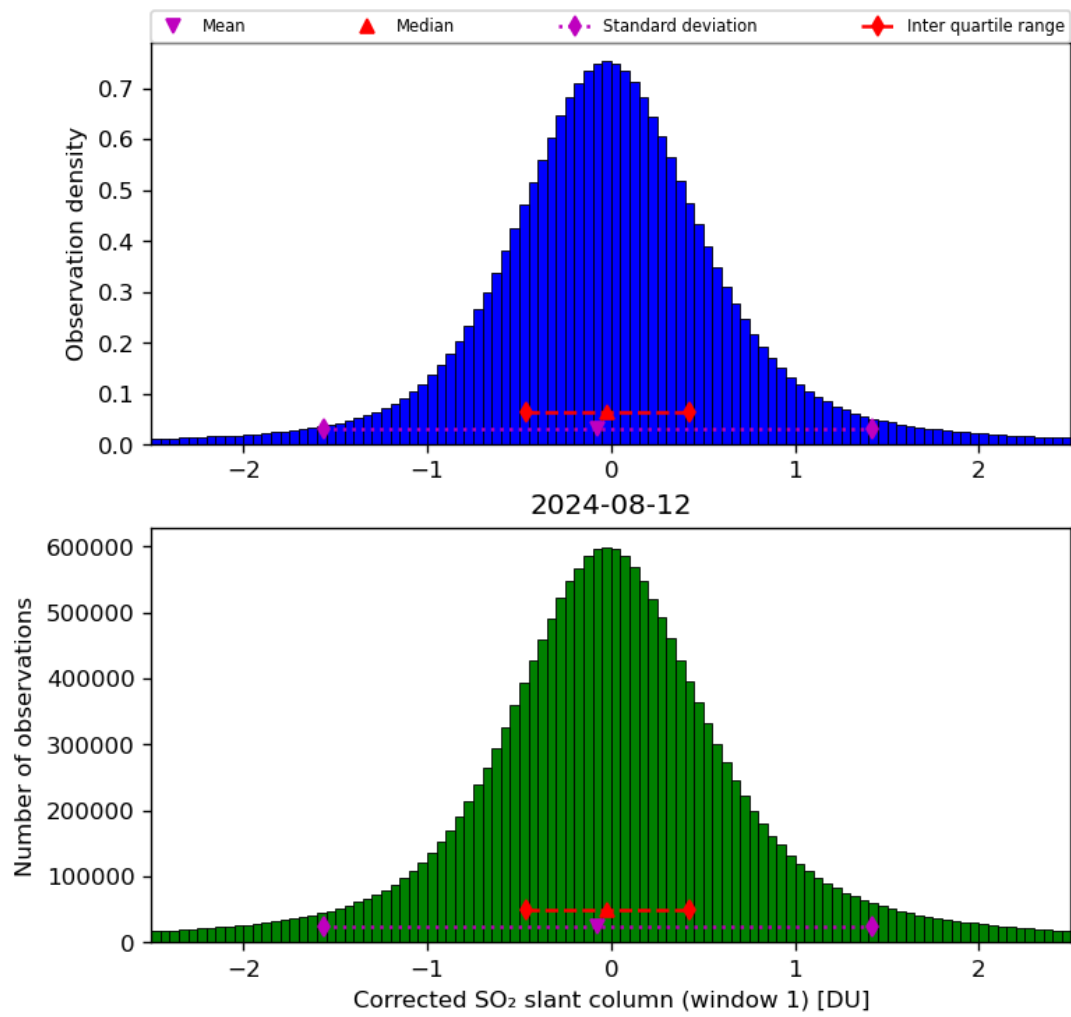
Figure 58: Histogram of “Corrected SO 2 slant column (window 1)” for 2024-08-12 to 2024-08-13
