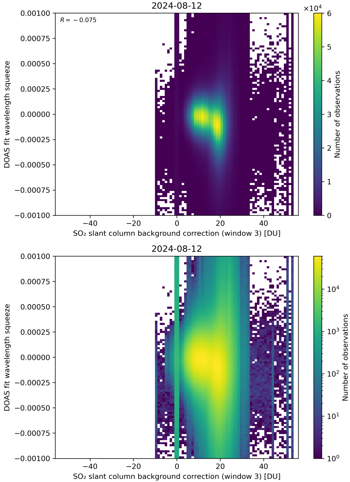
Figure 122: Scatter density plot of “SO 2 slant column background correction (window 3)” against “DOAS fit wavelength squeeze” for 2024-08-12 to 2024-08-13.
