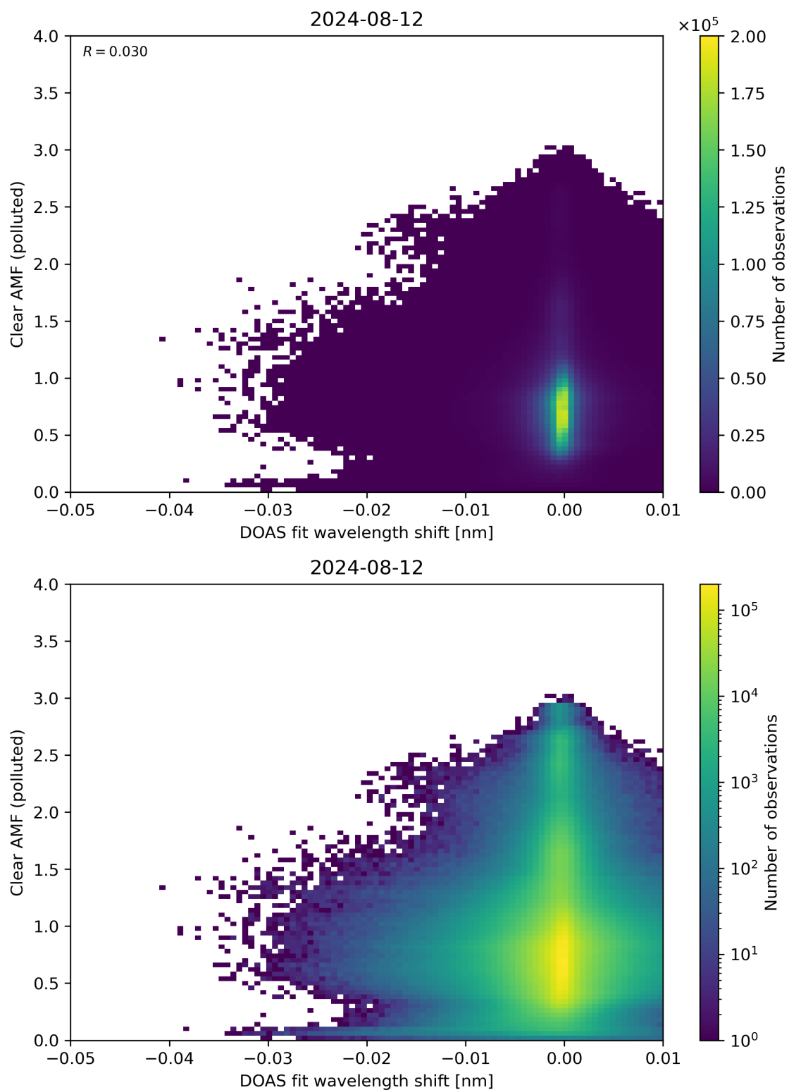
Figure 129: Scatter density plot of “DOAS fit wavelength shift” against “Clear AMF (polluted)” for 2024-08-12 to 2024-08-13.
