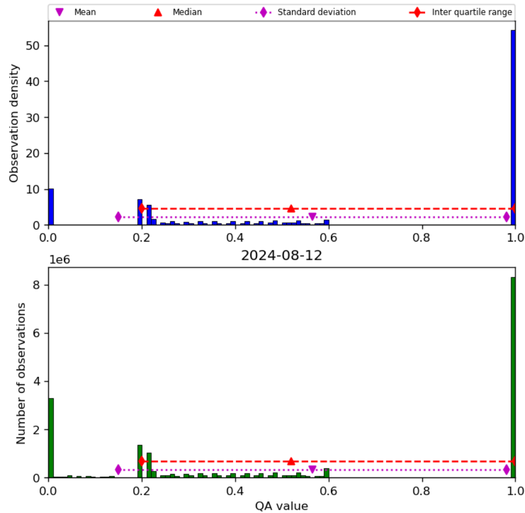
Figure 52: Histogram of “QA value” for 2024-08-12 to 2024-08-13
