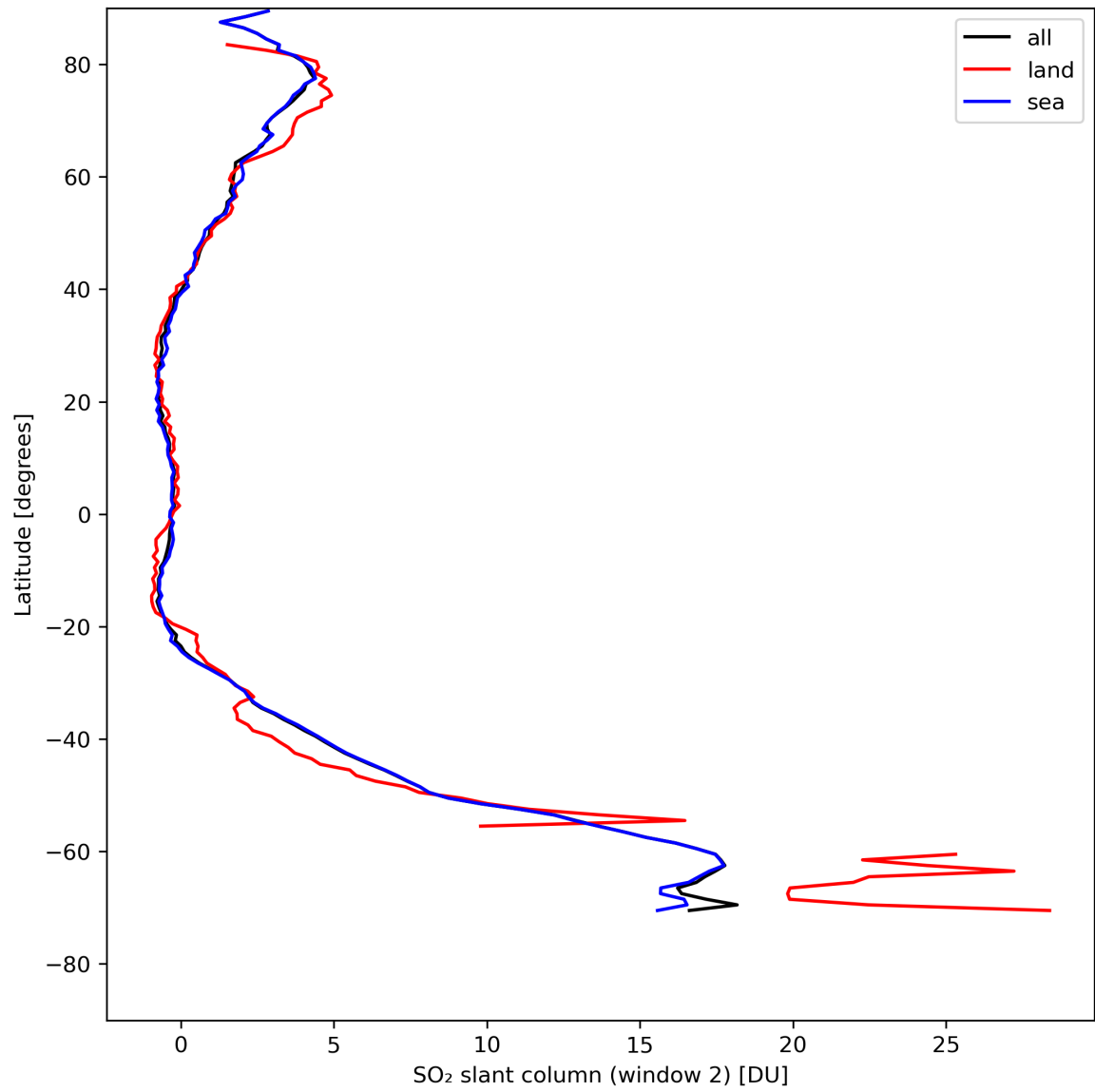
Figure 37: Zonal average of “SO 2 slant column (window 2)” for 2024-08-12 to 2024-08-13.
