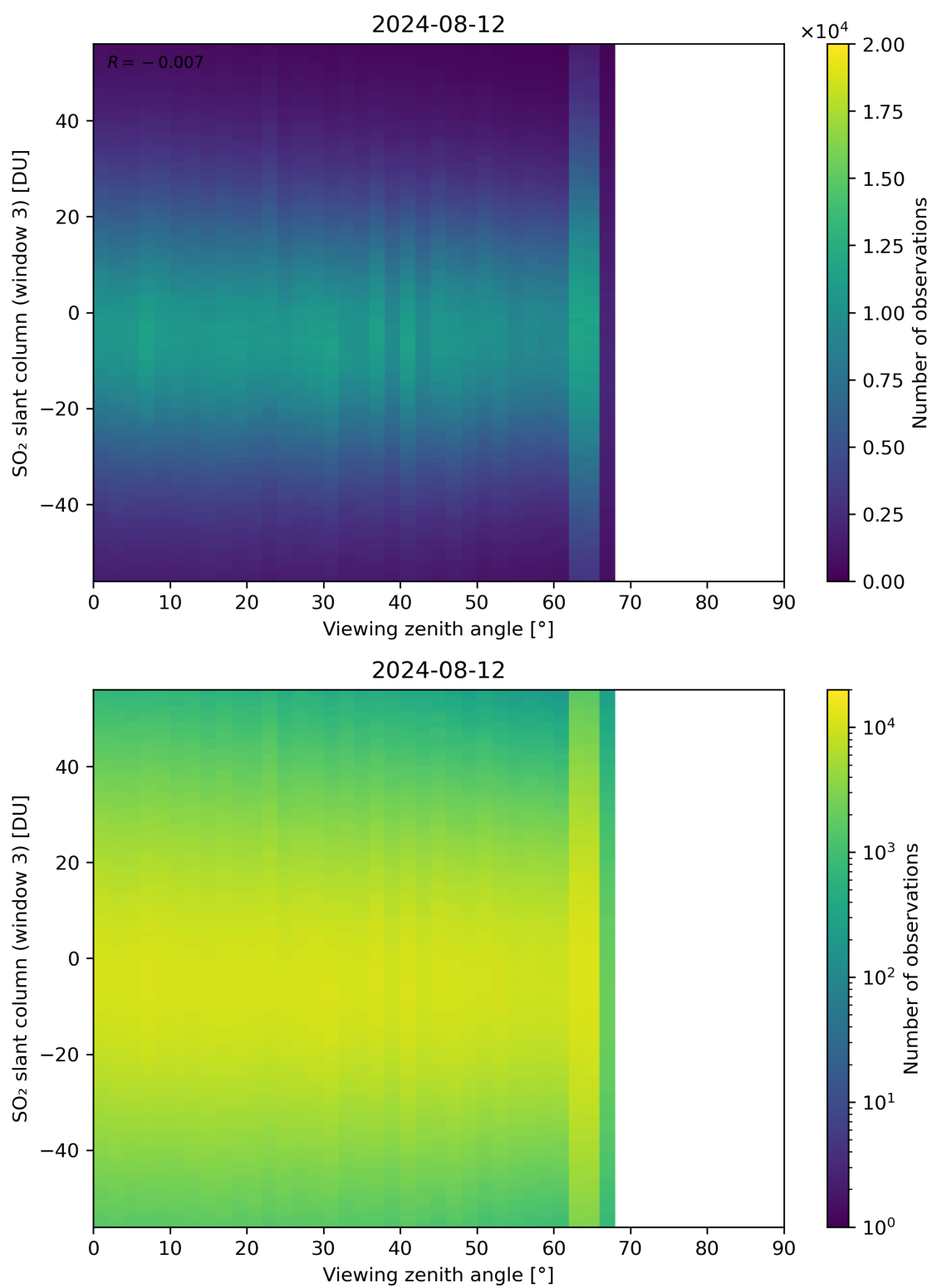
Figure 323: Scatter density plot of “Viewing zenith angle” against “SO 2 slant column (window 3)” for 2024-08-12 to 2024-08-13.
