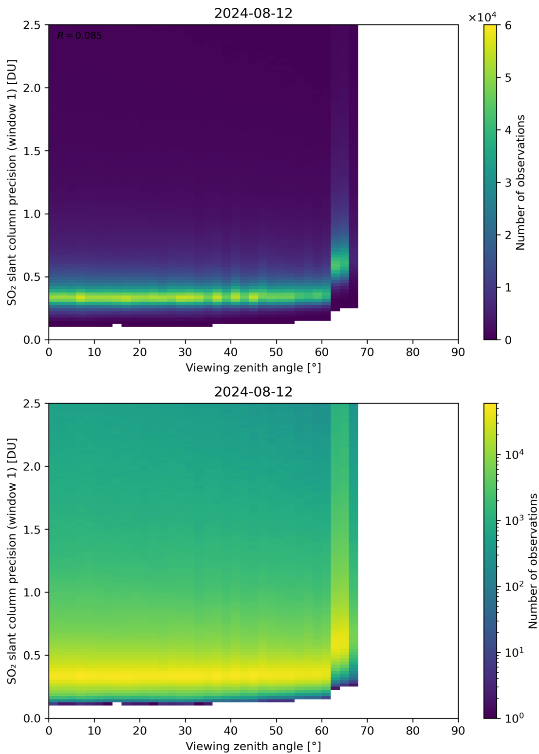
Figure 321: Scatter density plot of “Viewing zenith angle” against “SO 2 slant column precision (window 1)” for 2024-08-12 to 2024-08-13.
