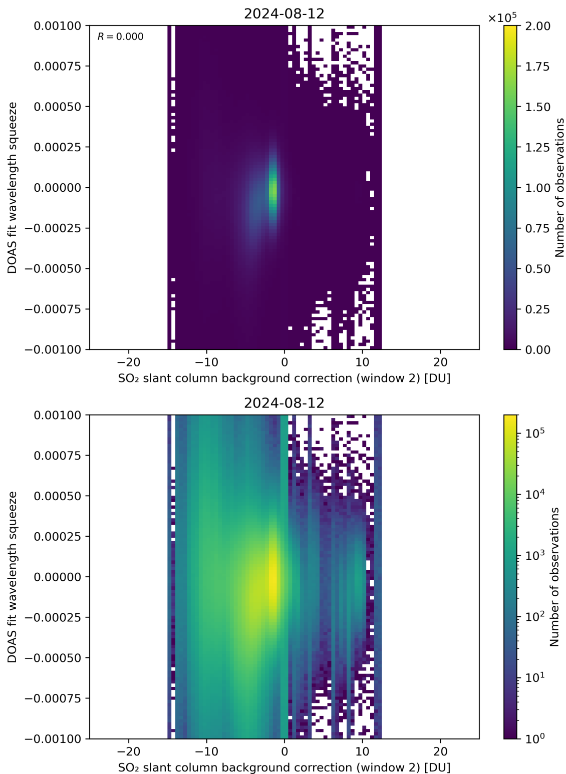
Figure 113: Scatter density plot of “SO 2 slant column background correction (window 2)” against “DOAS fit wavelength squeeze” for 2024-08-12 to 2024-08-13.
