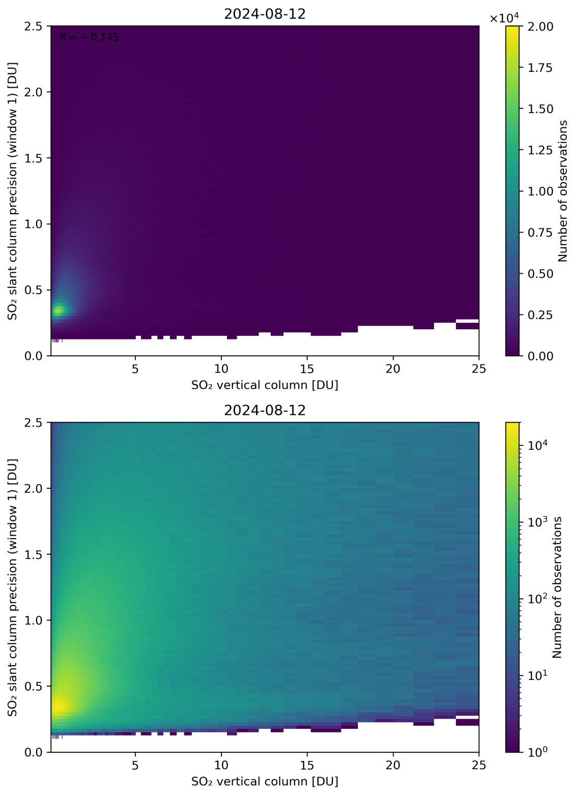
Figure 301: Scatter density plot of “SO 2 vertical column” against “SO 2 slant column precision (window 1)” for 2024-08-12 to 2024-08-13.
