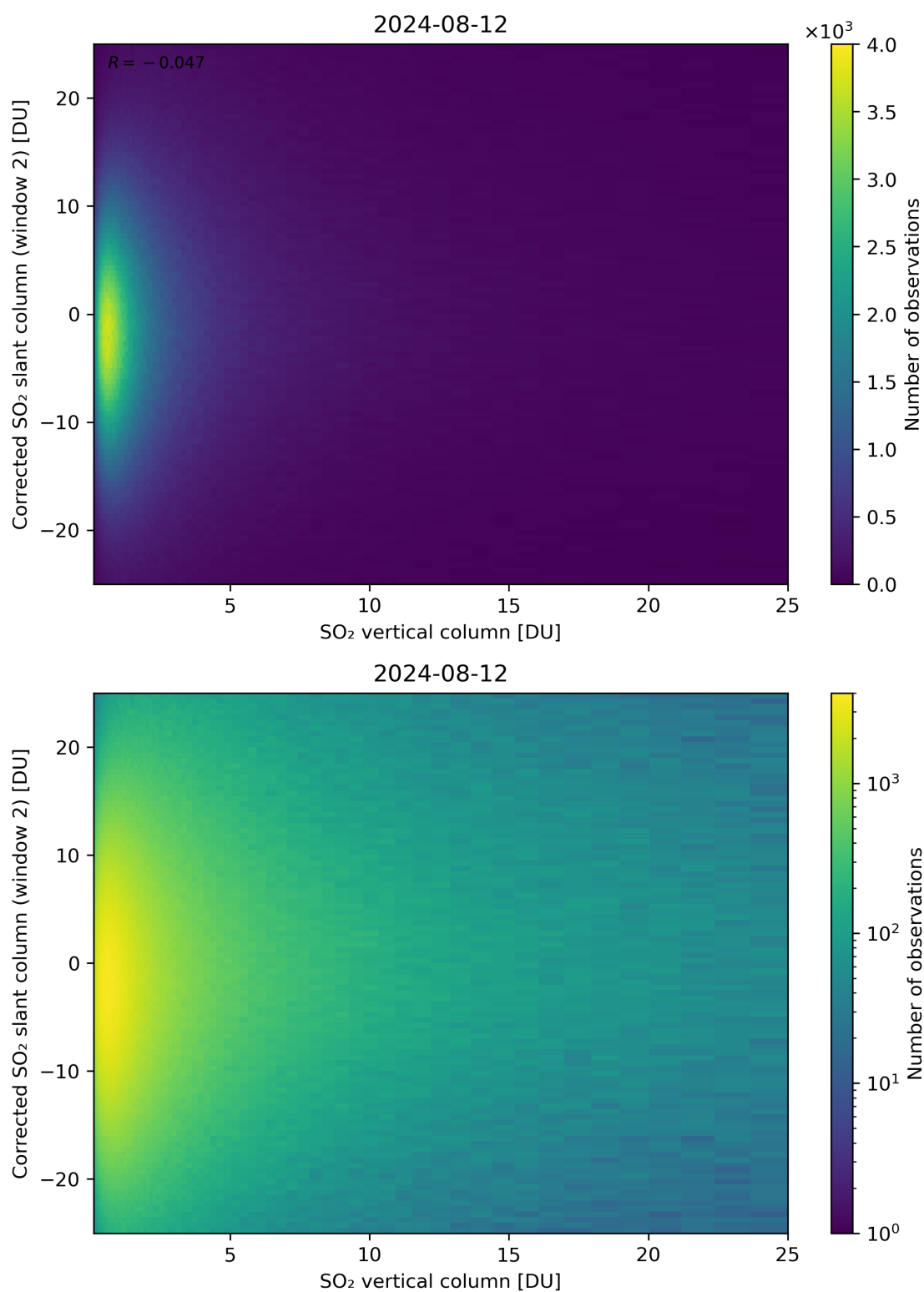
Figure 298: Scatter density plot of “SO 2 vertical column” against “Corrected SO 2 slant column (window 2)” for 2024-08-12 to 2024-08-13.
