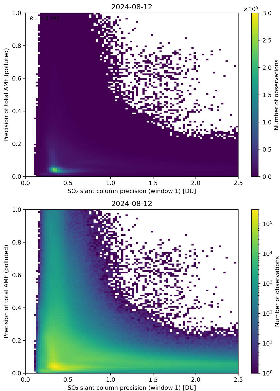
Figure 231: Scatter density plot of “SO 2 slant column precision (window 1)” against “Precision of total AMF (polluted)” for 2024-08-12 to 2024-08-13.
