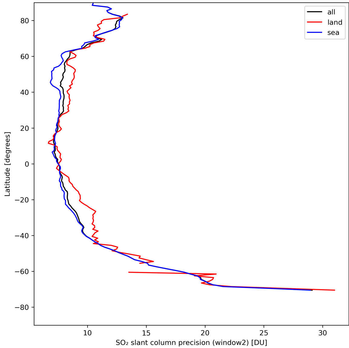
Figure 38: Zonal average of “SO 2 slant column precision (window2)” for 2024-08-12 to 2024-08-13.
