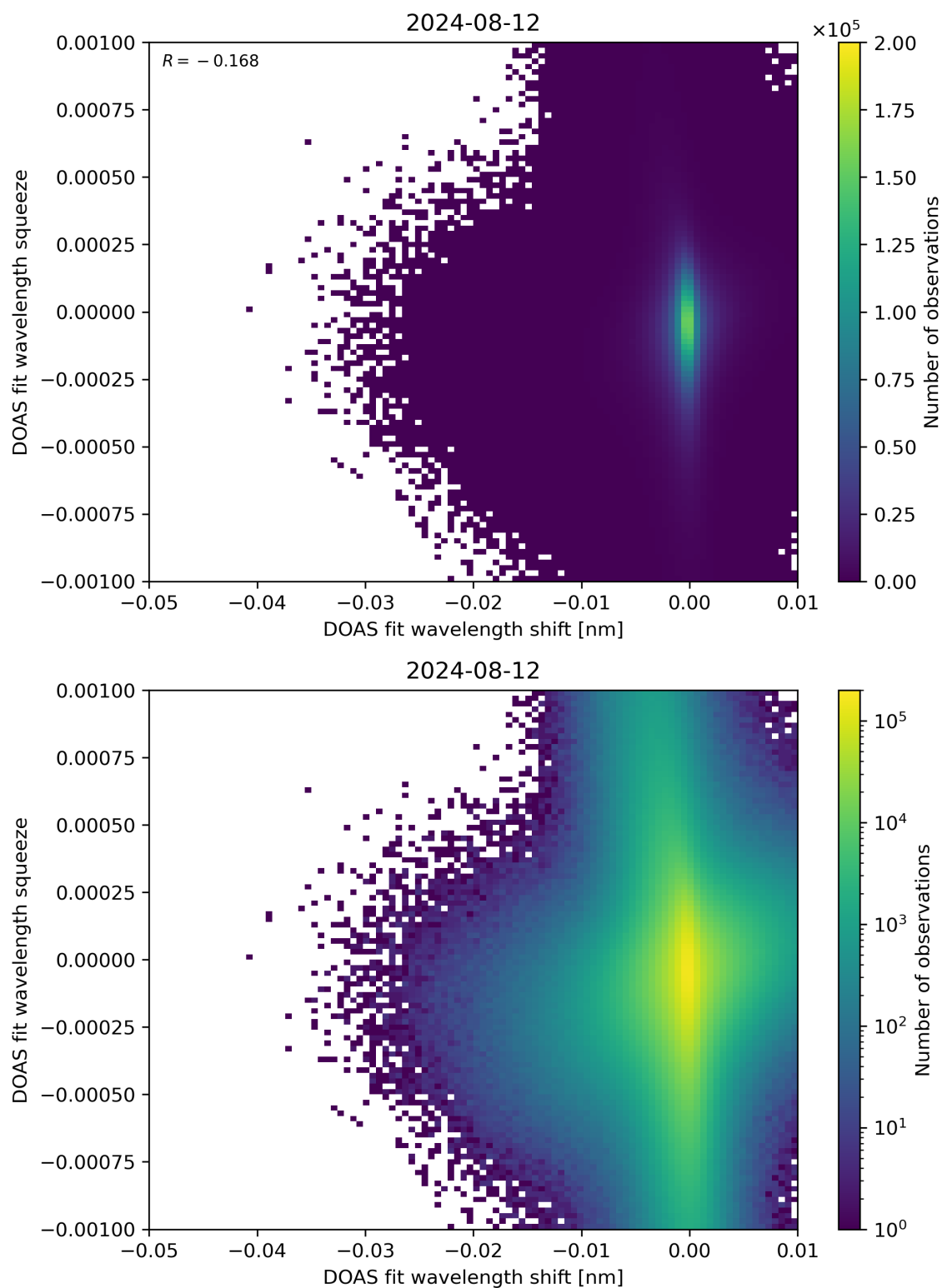
Figure 127: Scatter density plot of “DOAS fit wavelength shift” against “DOAS fit wavelength squeeze” for 2024-08-12 to 2024-08-13.
