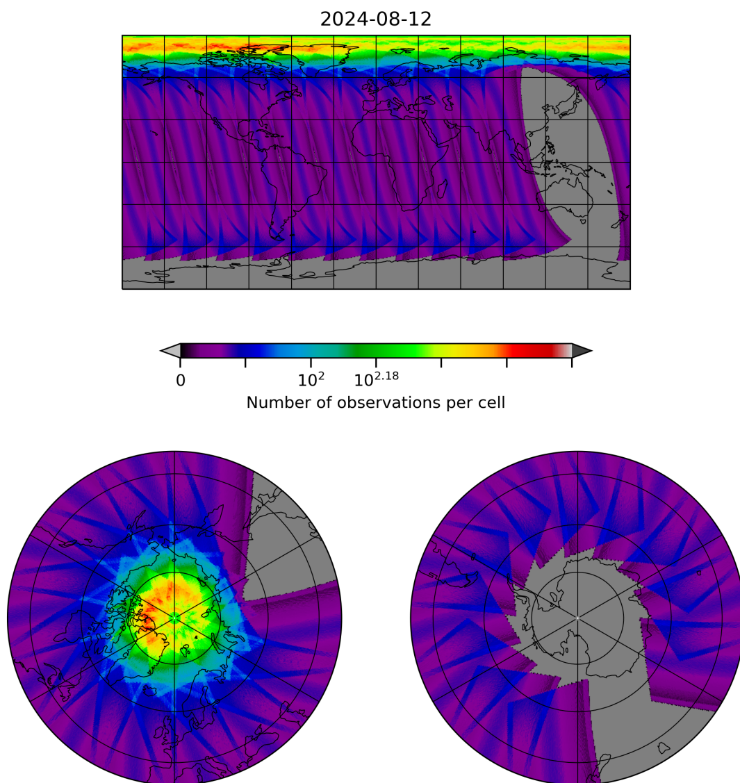
Figure 28: Map of the number of observations for 2024-08-12 to 2024-08-13
