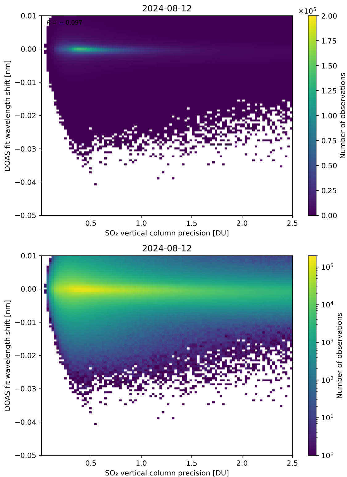
Figure 282: Scatter density plot of “SO 2 vertical column precision” against “DOAS fit wavelength shift” for 2024-08-12 to 2024-08-13.
