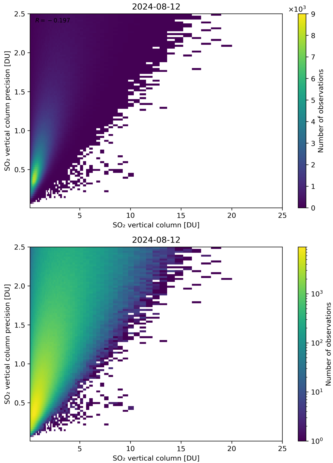
Figure 307: Scatter density plot of “SO 2 vertical column” against “SO 2 vertical column precision” for 2024-08-12 to 2024-08-13.
