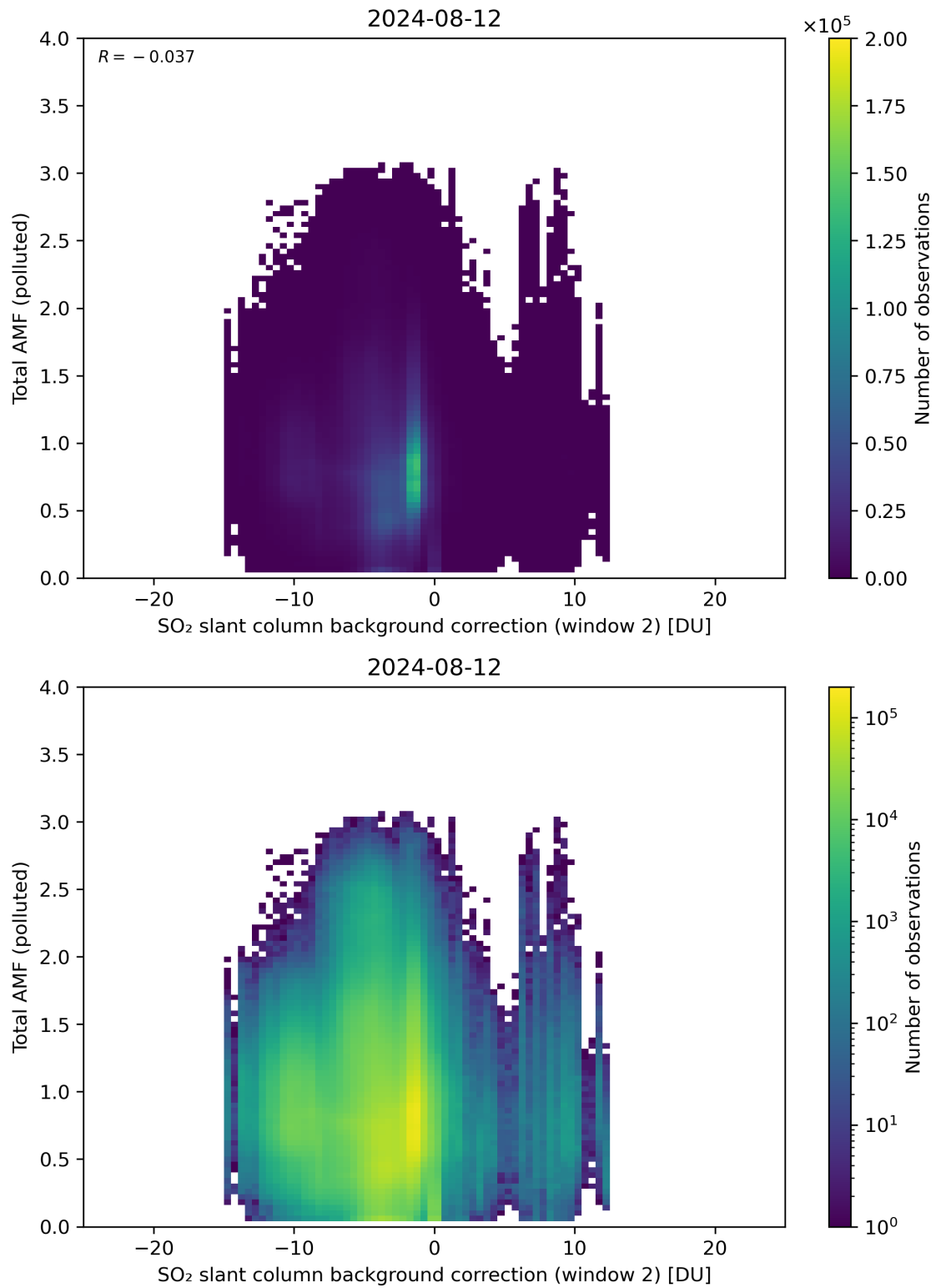
Figure 119: Scatter density plot of “SO 2 slant column background correction (window 2)” against “Total AMF (polluted)” for 2024-08-12 to 2024-08-13.
