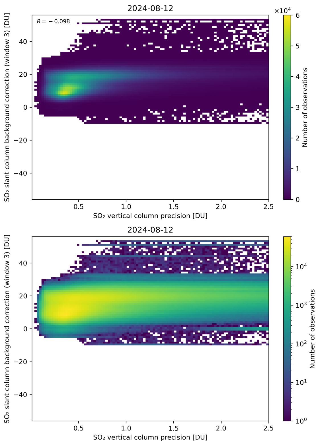
Figure 281: Scatter density plot of “SO 2 vertical column precision” against “SO 2 slant column background correction (window 3)” for 2024-08-12 to 2024-08-13.
