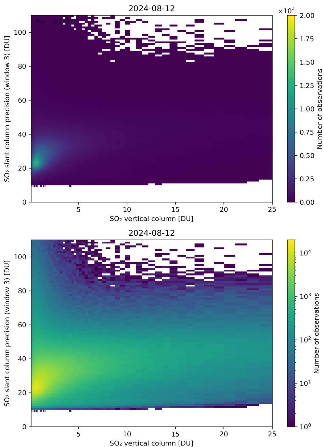
Figure 304: Scatter density plot of “SO 2 vertical column” against “SO 2 slant column precision (window 3)” for 2024-08-12 to 2024-08-13.
