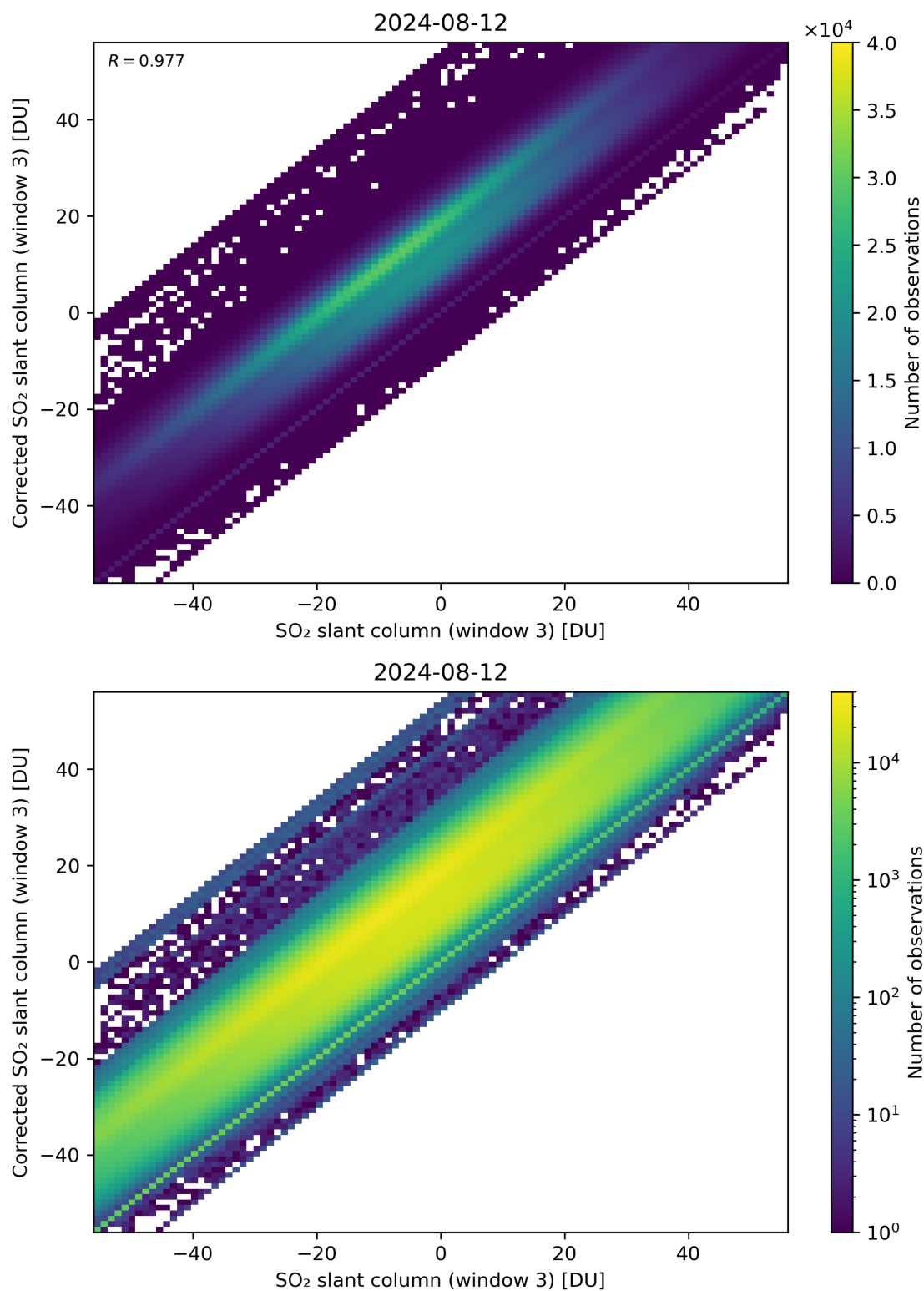
Figure 266: Scatter density plot of “SO 2 slant column (window 3)” against “Corrected SO 2 slant column (window 3)” for 2024-08-12 to 2024-08-13.
