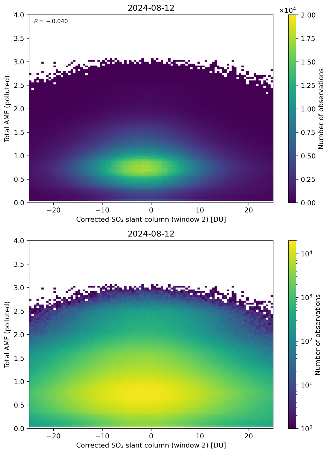
Figure 203: Scatter density plot of “Corrected SO 2 slant column (window 2)” against “Total AMF (polluted)” for 2024-08-12 to 2024-08-13.
