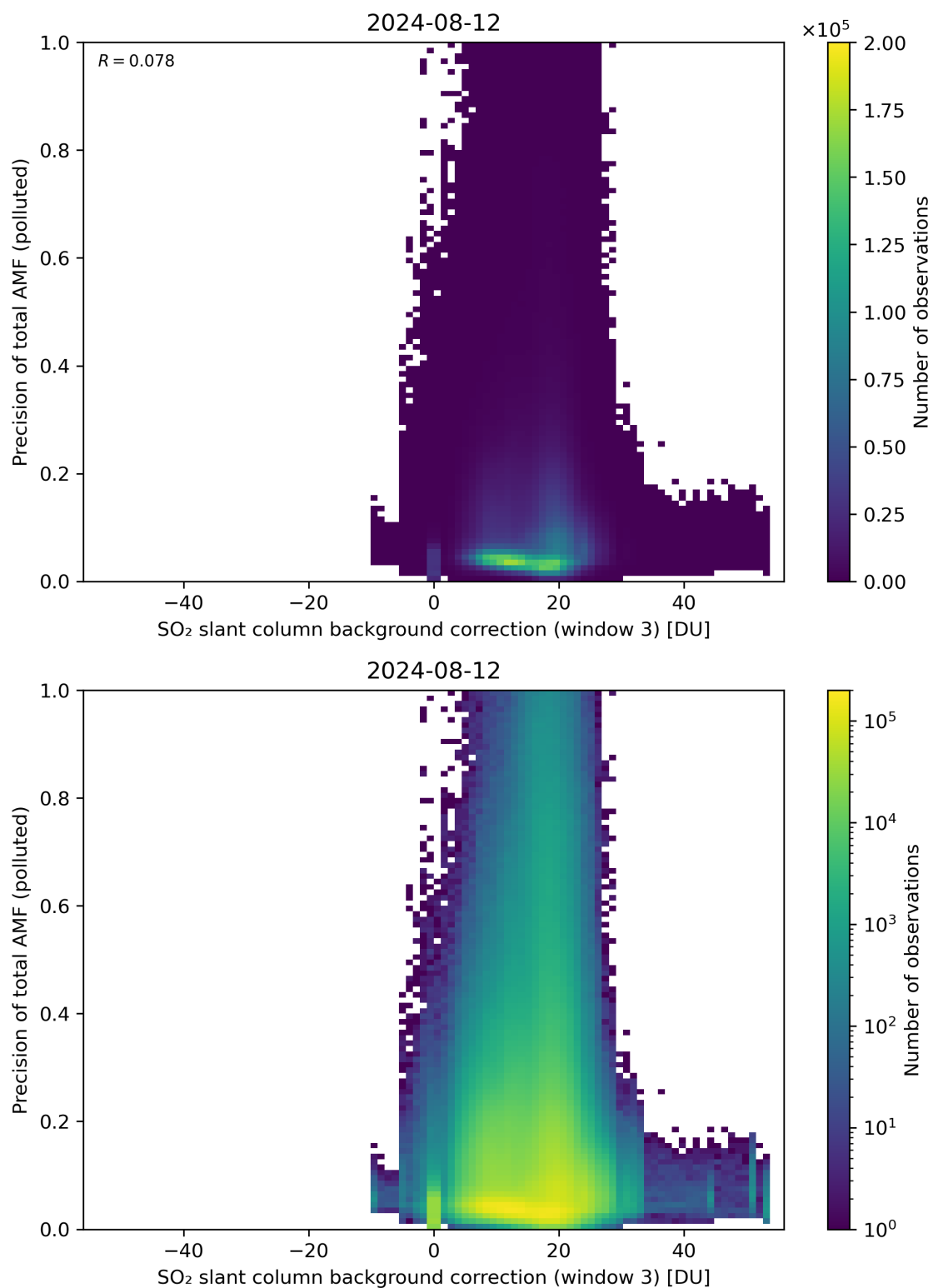
Figure 126: Scatter density plot of “SO 2 slant column background correction (window 3)” against “Precision of total AMF (polluted)” for 2024-08-12 to 2024-08-13.
