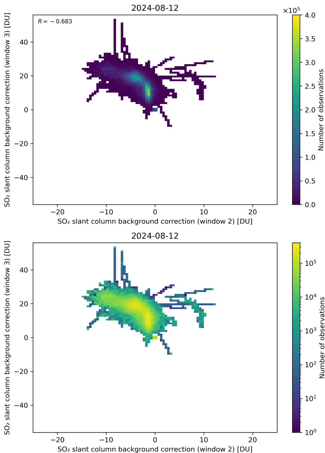
Figure 111: Scatter density plot of “SO 2 slant column background correction (window 2)” against “SO 2 slant column background correction (window 3)” for 2024-08-12 to 2024-08-13.
