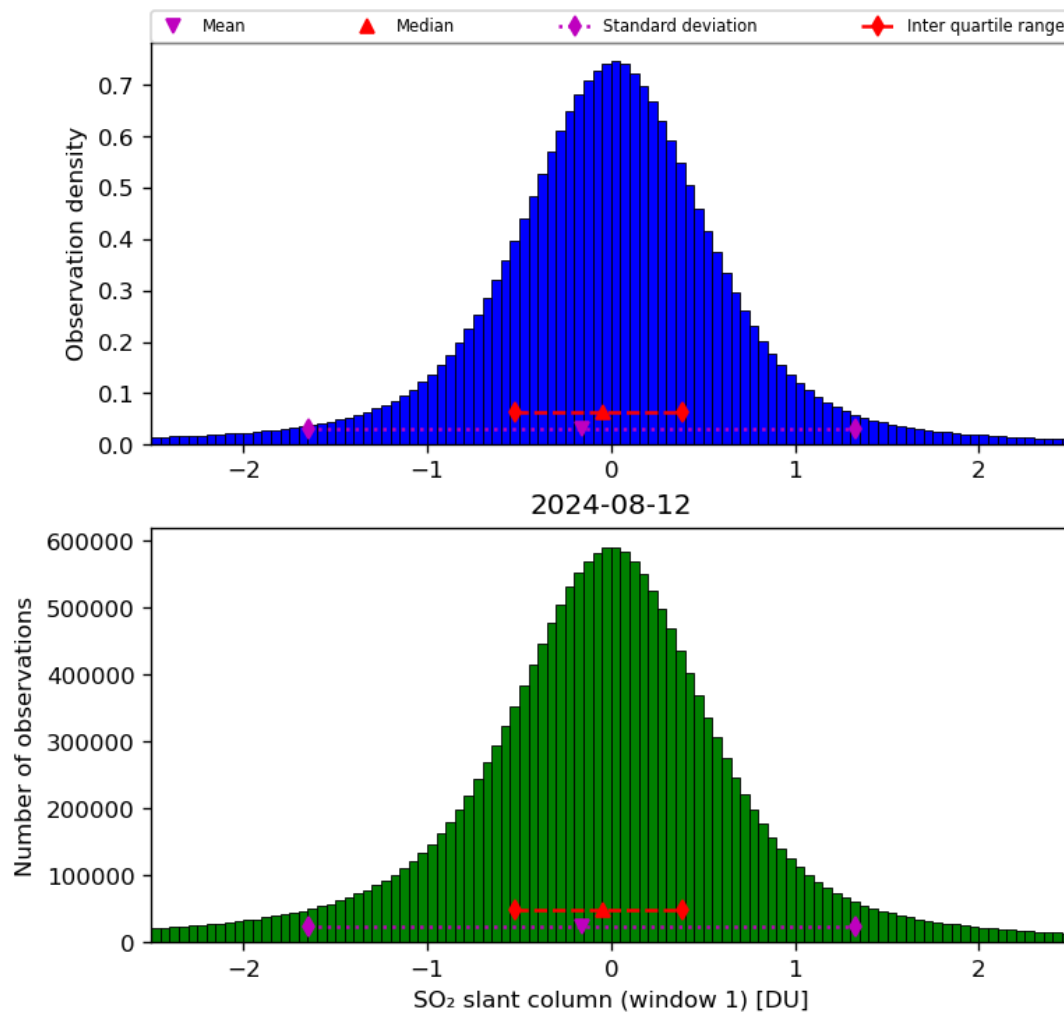
Figure 56: Histogram of “SO 2 slant column (window 1)” for 2024-08-12 to 2024-08-13
