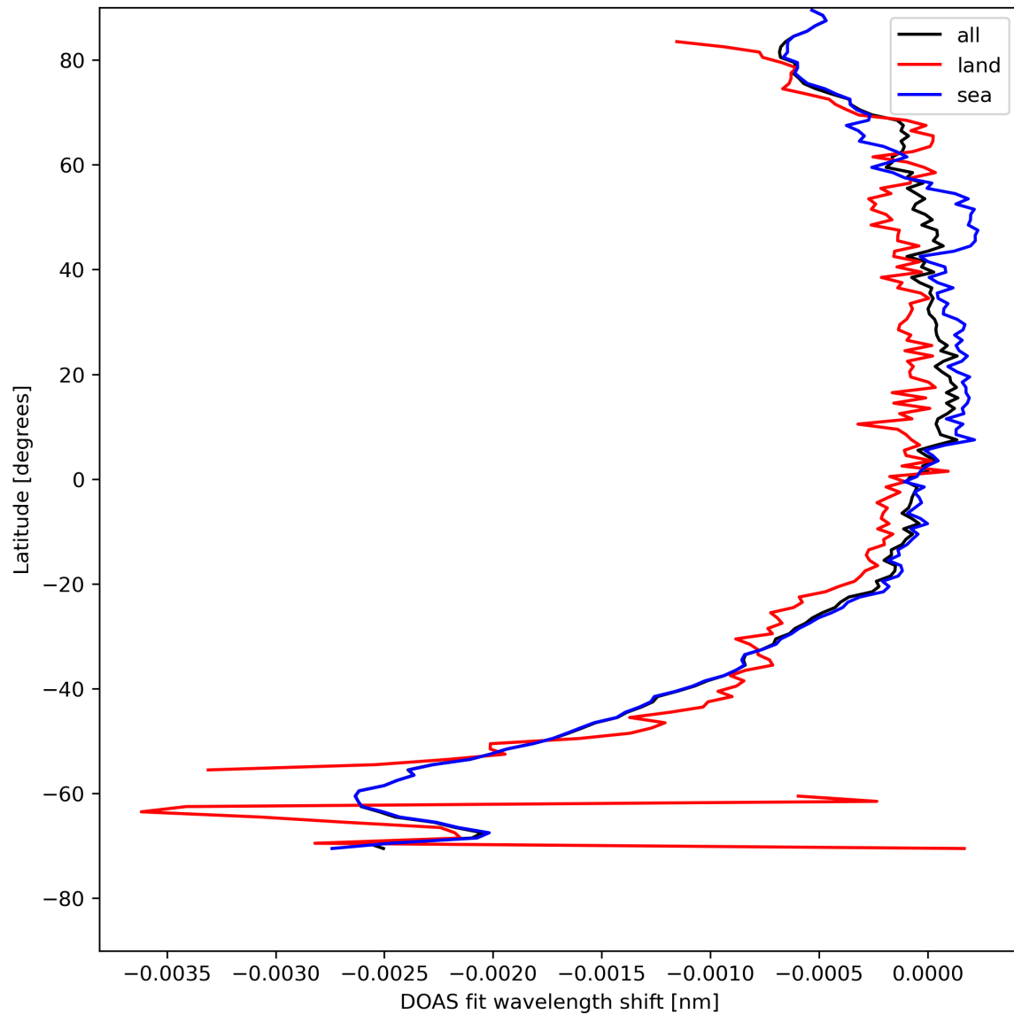
Figure 45: Zonal average of “DOAS fit wavelength shift” for 2024-08-12 to 2024-08-13.
