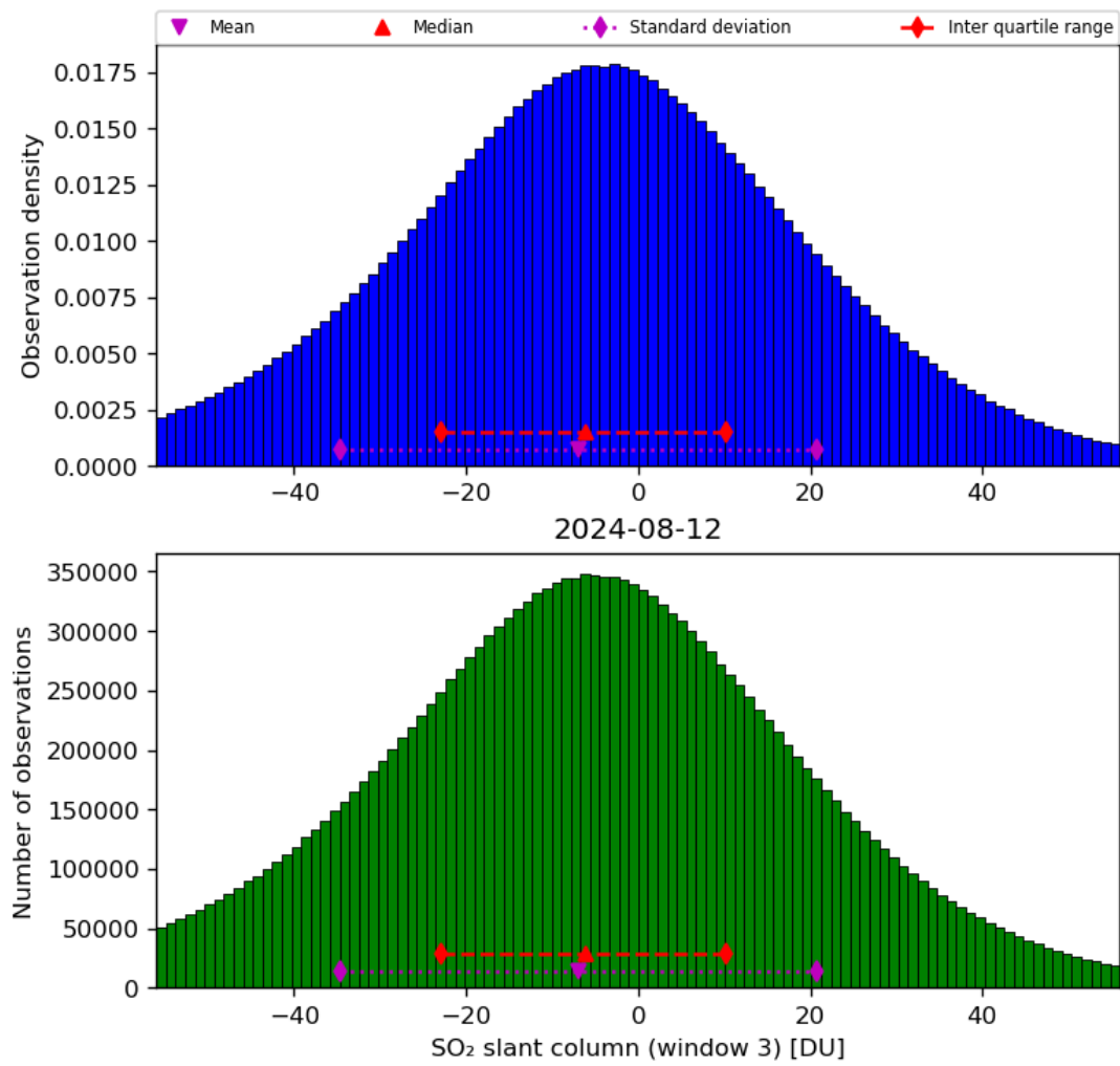
Figure 64: Histogram of “SO 2 slant column (window 3)” for 2024-08-12 to 2024-08-13
