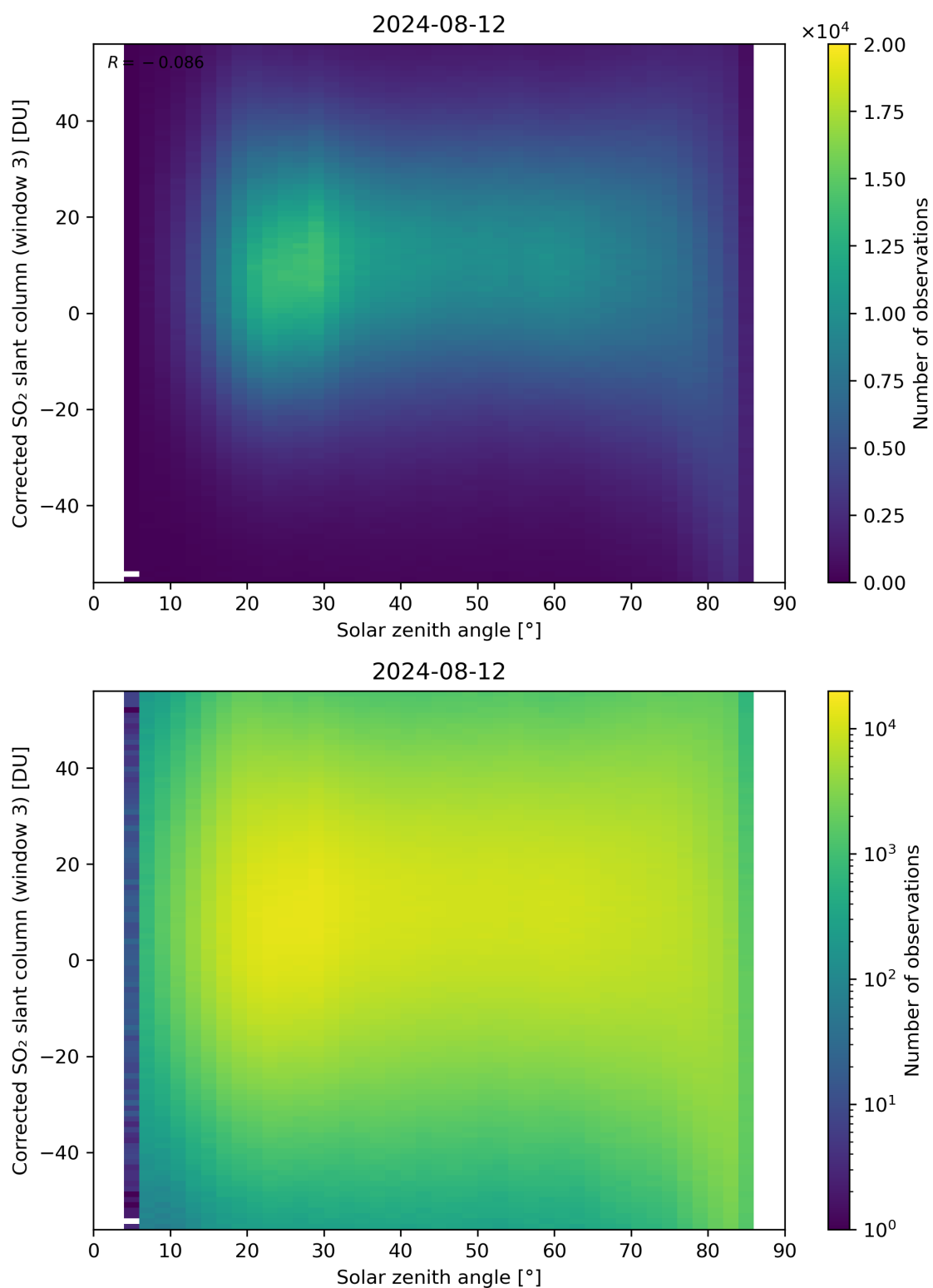
Figure 168: Scatter density plot of “Solar zenith angle” against “Corrected SO 2 slant column (window 3)” for 2024-08-12 to 2024-08-13.
