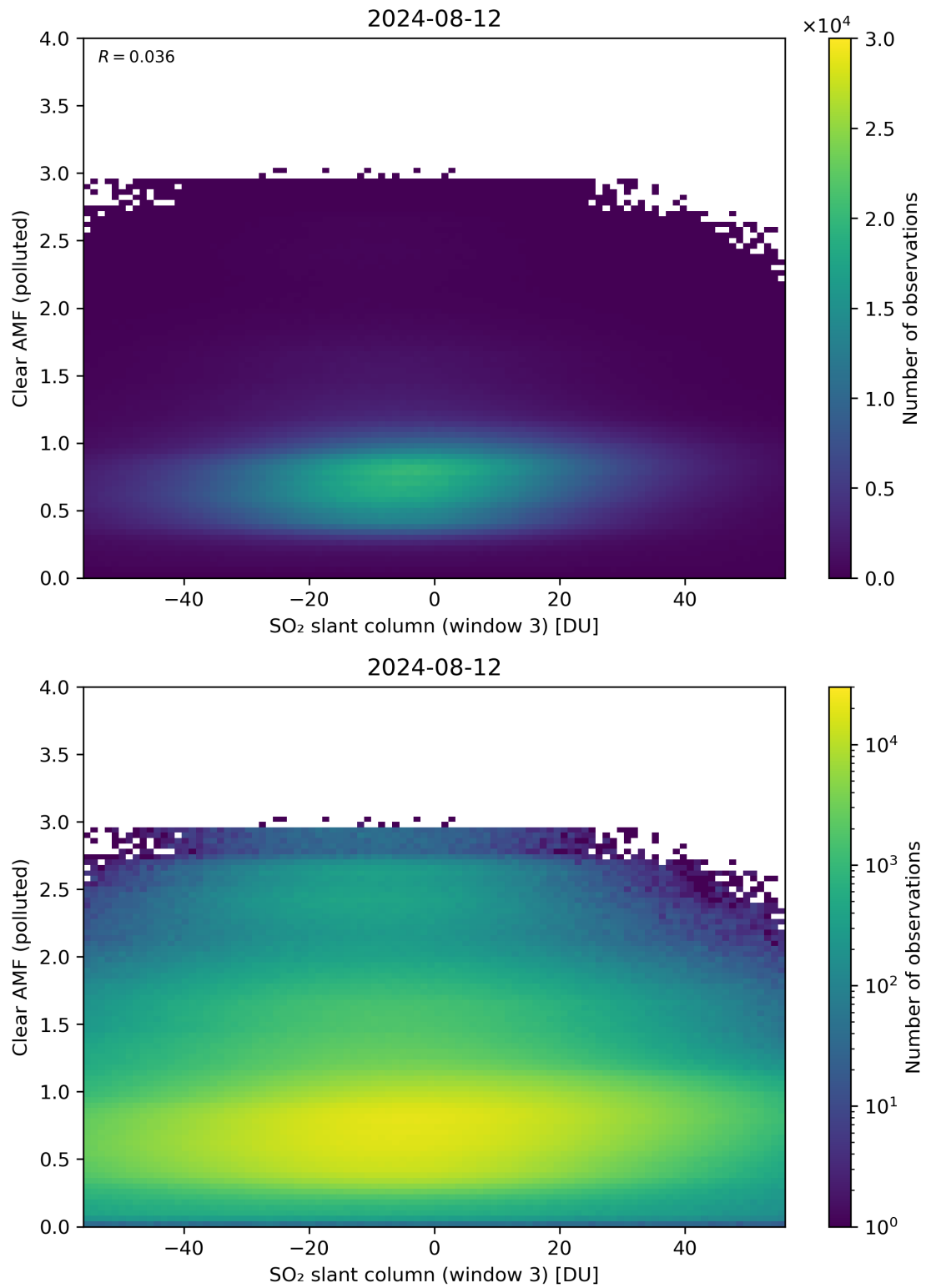
Figure 265: Scatter density plot of “SO 2 slant column (window 3)” against “Clear AMF (polluted)” for 2024-08-12 to 2024-08-13.
