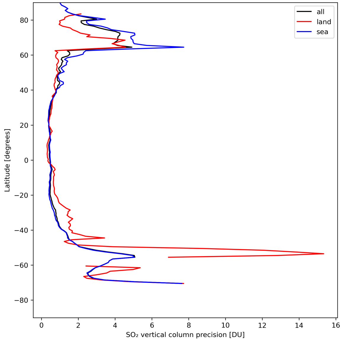
Figure 31: Zonal average of “SO 2 vertical column precision” for 2024-08-12 to 2024-08-13.
