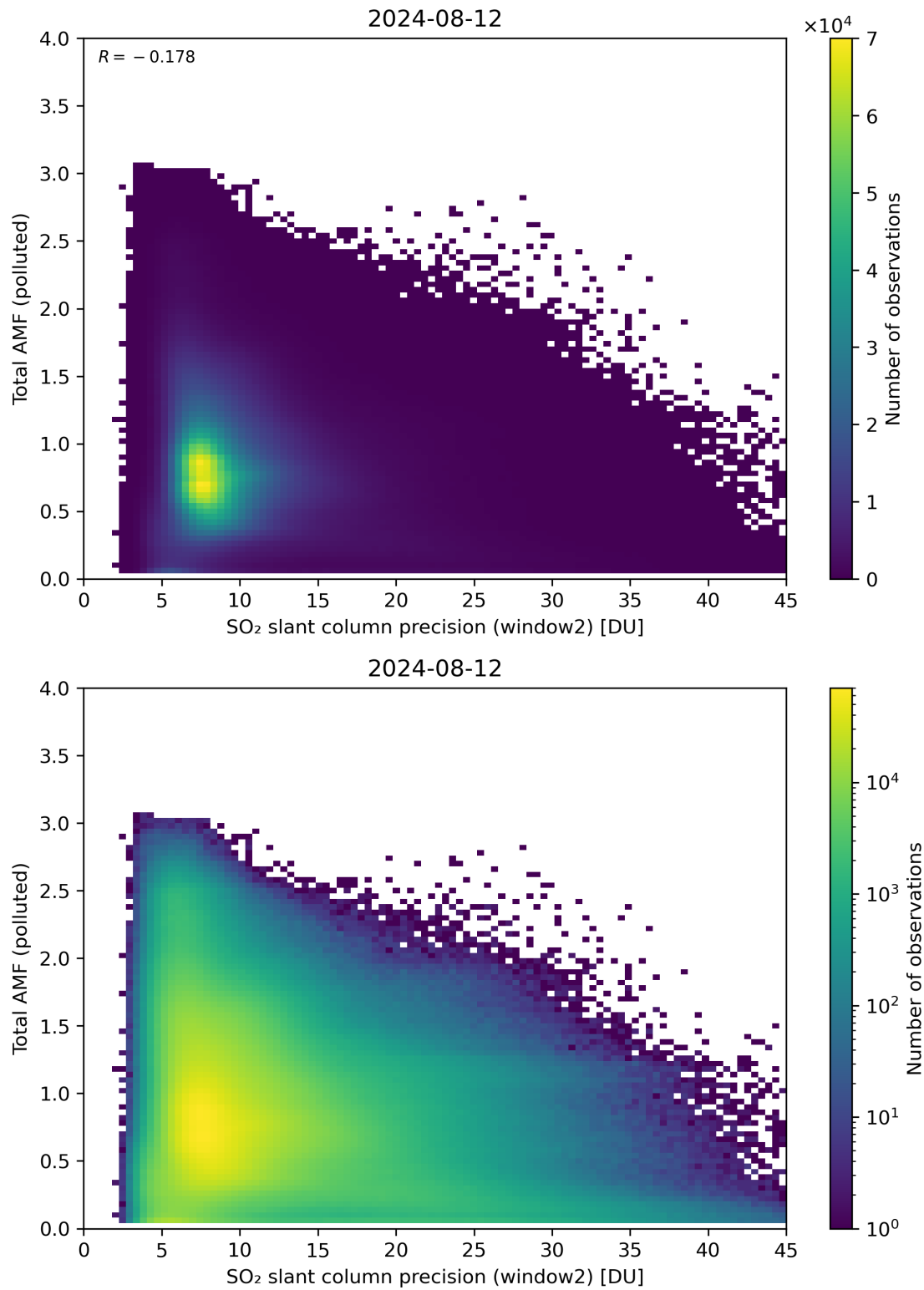
Figure 251: Scatter density plot of “SO 2 slant column precision (window2)” against “Total AMF (polluted)” for 2024-08-12 to 2024-08-13.
