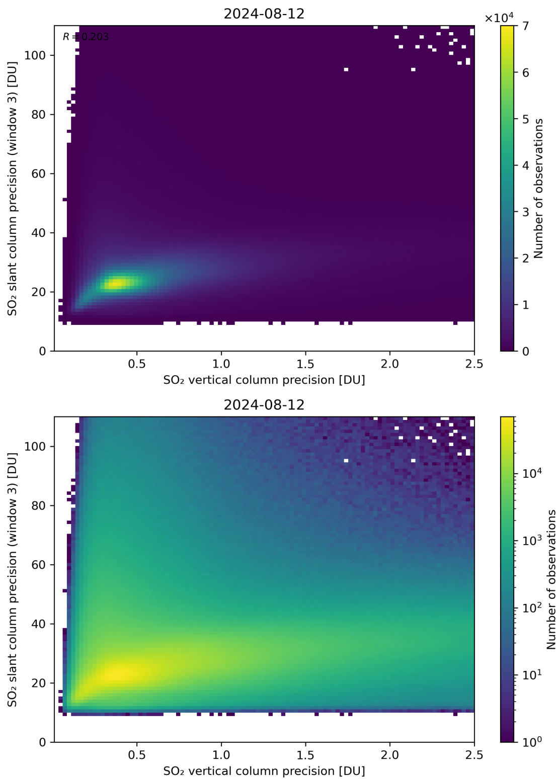
Figure 293: Scatter density plot of “SO 2 vertical column precision” against “SO 2 slant column precision (window 3)” for 2024-08-12 to 2024-08-13.
