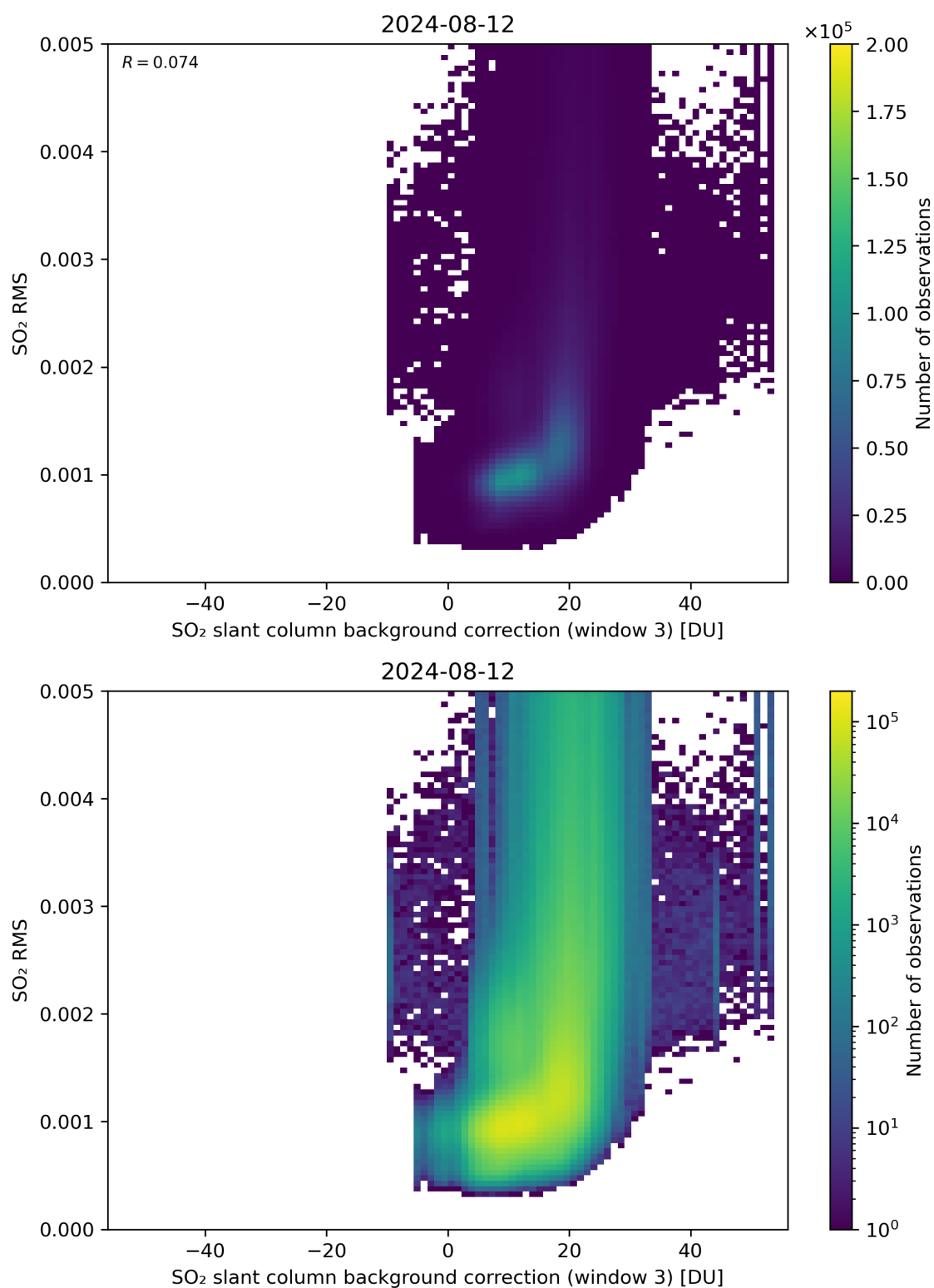
Figure 123: Scatter density plot of “SO 2 slant column background correction (window 3)” against “SO 2 RMS” for 2024-08-12 to 2024-08-13.
