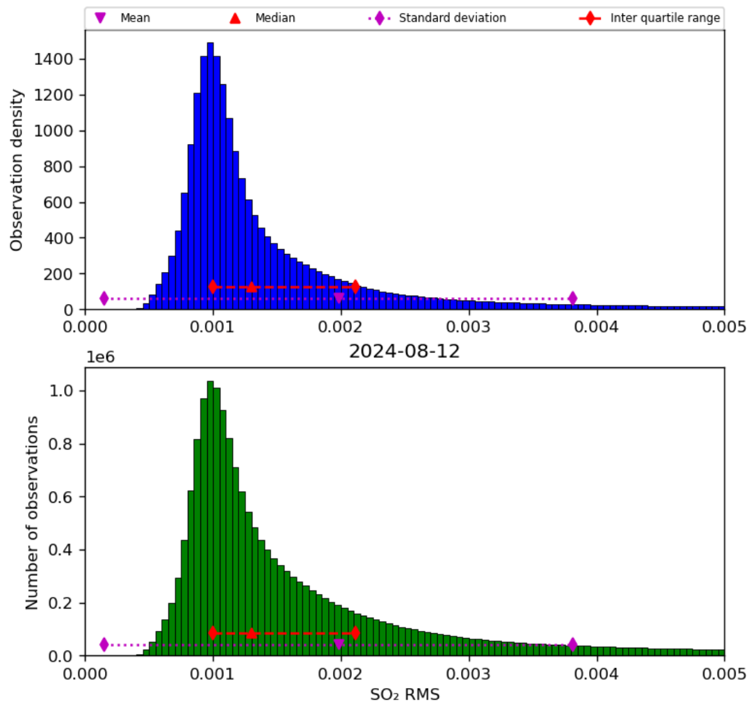
Figure 70: Histogram of “SO 2 RMS” for 2024-08-12 to 2024-08-13
