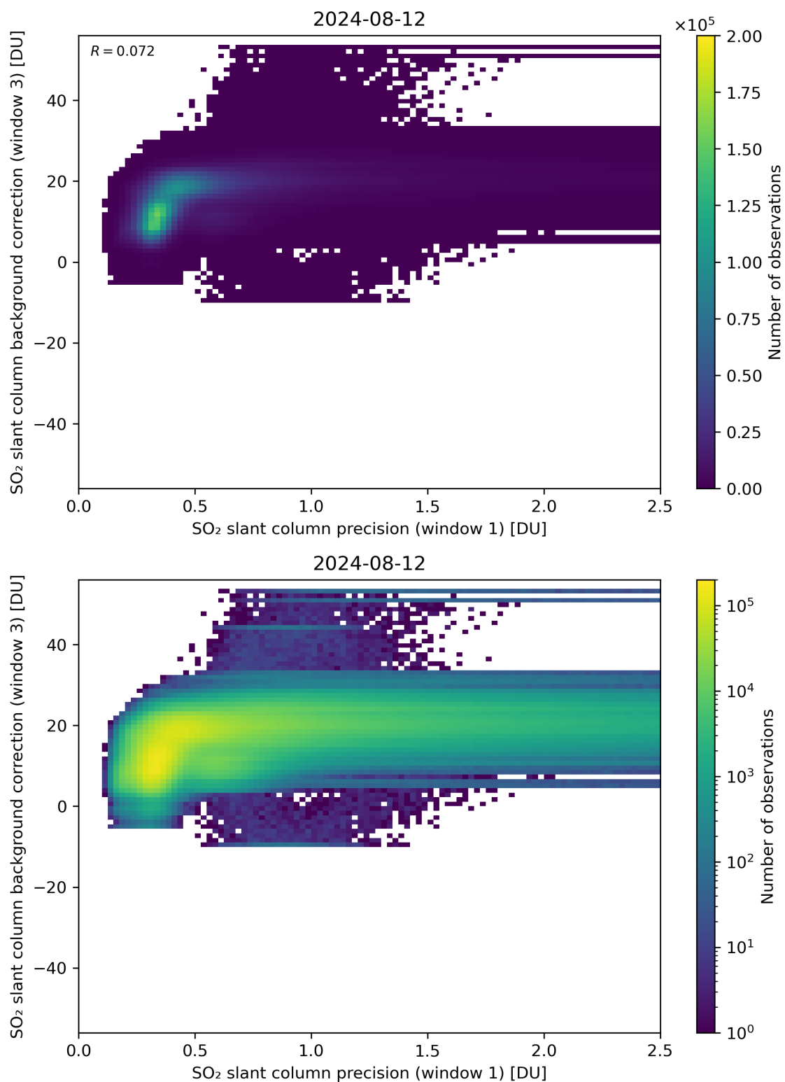
Figure 220: Scatter density plot of “SO 2 slant column precision (window 1)” against “SO 2 slant column background correction (window 3)” for 2024-08-12 to 2024-08-13.
