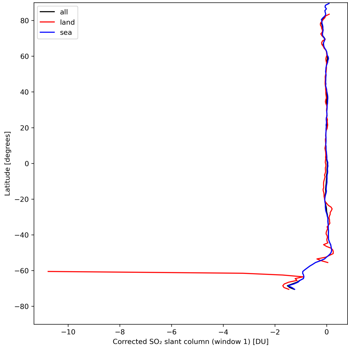
Figure 35: Zonal average of “Corrected SO 2 slant column (window 1)” for 2024-08-12 to 2024-08-13.
