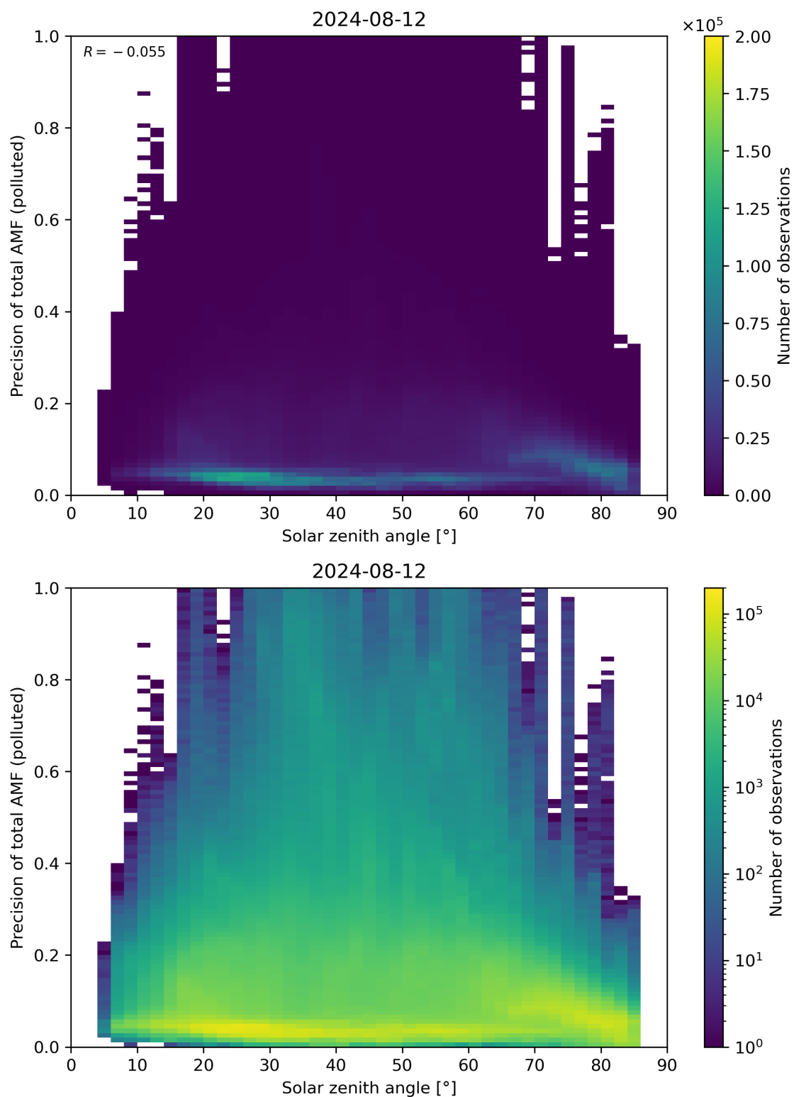
Figure 175: Scatter density plot of “Solar zenith angle” against “Precision of total AMF (polluted)” for 2024-08-12 to 2024-08-13.
