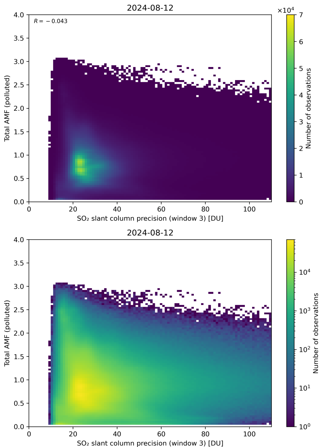
Figure 263: Scatter density plot of “SO 2 slant column precision (window 3)” against “Total AMF (polluted)” for 2024-08-12 to 2024-08-13.
