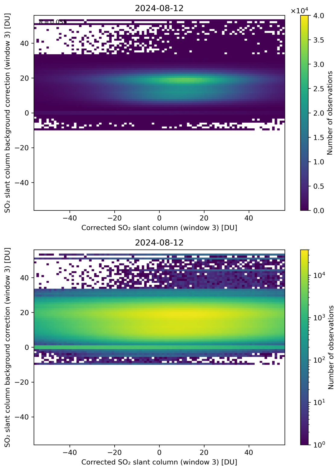
Figure 205: Scatter density plot of “Corrected SO 2 slant column (window 3)” against “SO 2 slant column background correction (window 3)” for 2024-08-12 to 2024-08-13.
