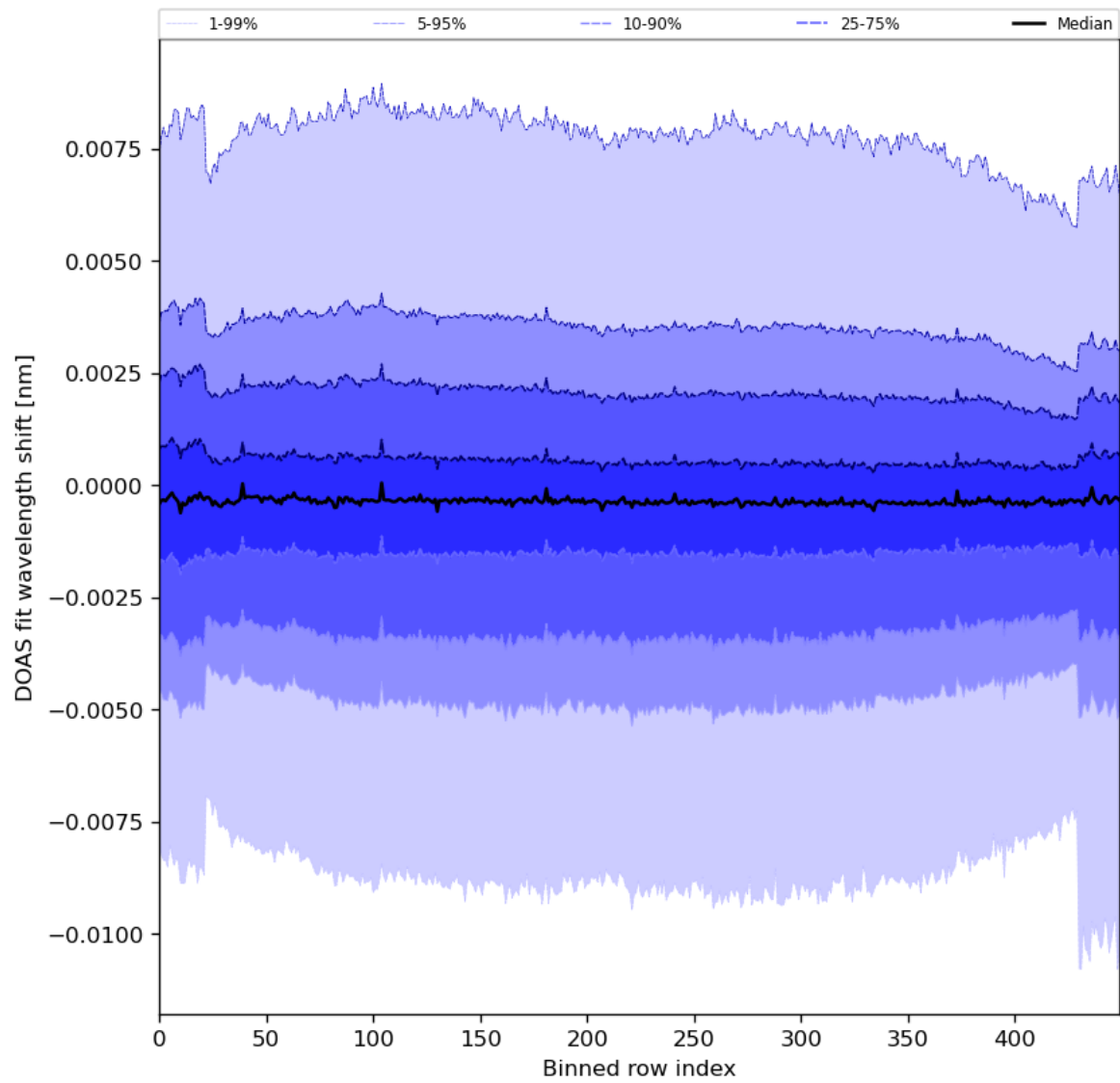
Figure 91: Along track statistics of “DOAS fit wavelength shift” for 2024-08-12 to 2024-08-13
