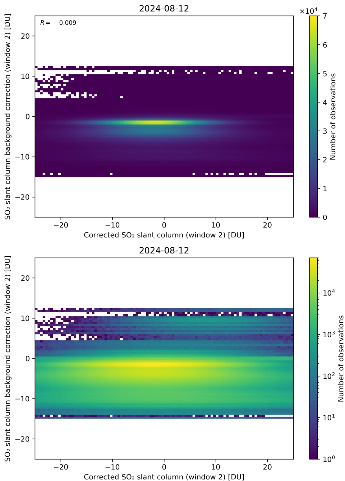
Figure 194: Scatter density plot of “Corrected SO 2 slant column (window 2)” against “SO 2 slant column background correction (window 2)” for 2024-08-12 to 2024-08-13.
