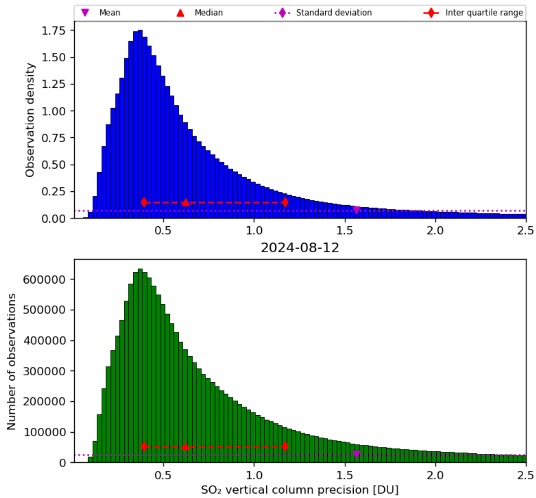
Figure 54: Histogram of “SO 2 vertical column precision” for 2024-08-12 to 2024-08-13
