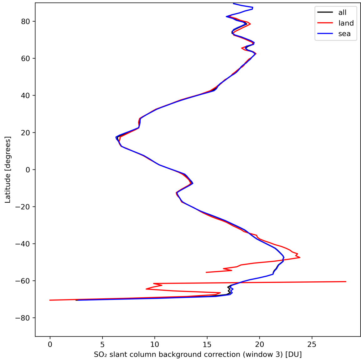
Figure 44: Zonal average of “SO 2 slant column background correction (window 3)” for 2024-08-12 to 2024-08-13.
