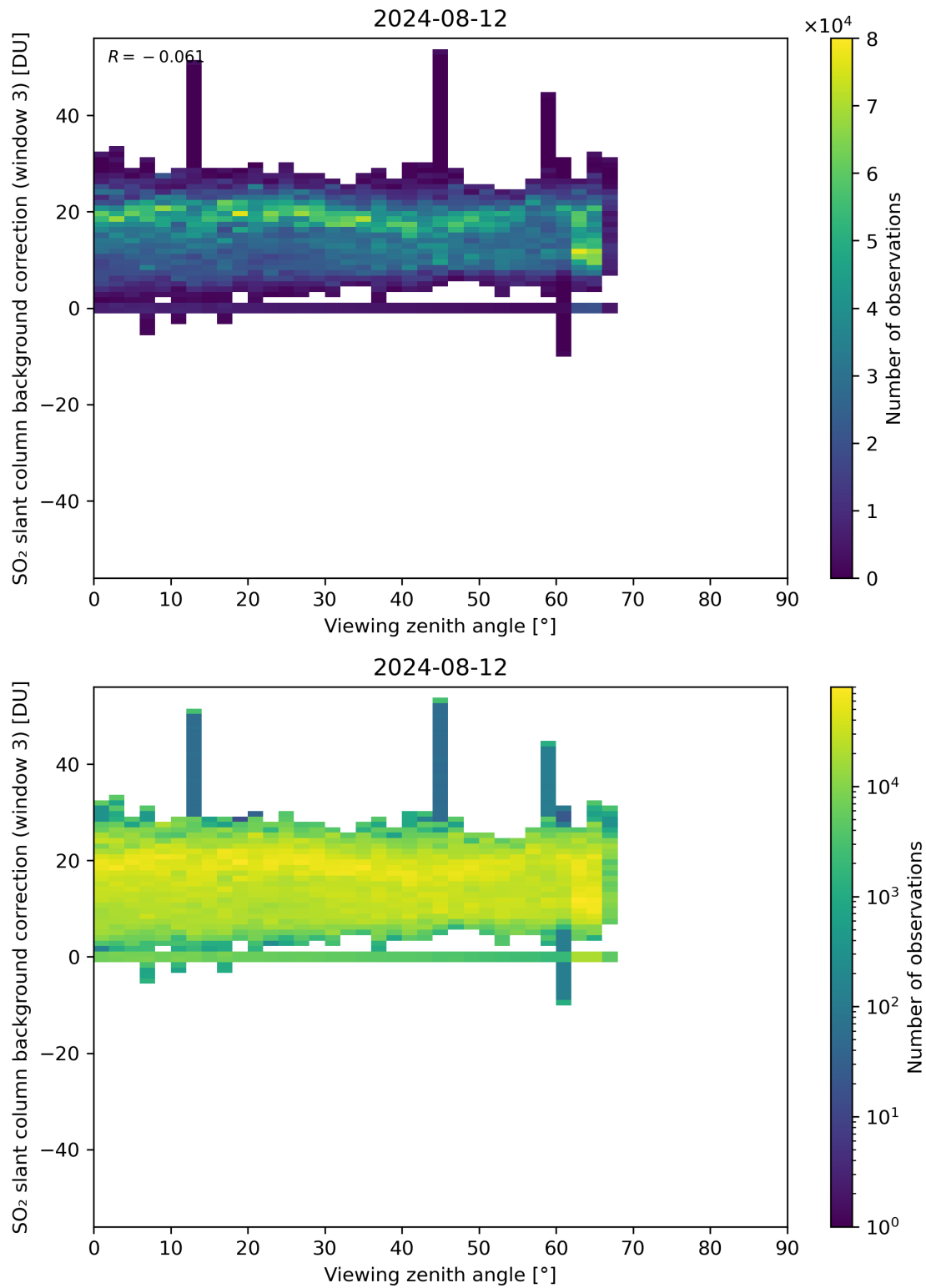
Figure 310: Scatter density plot of “Viewing zenith angle” against “SO 2 slant column background correction (window 3)” for 2024-08-12 to 2024-08-13.
