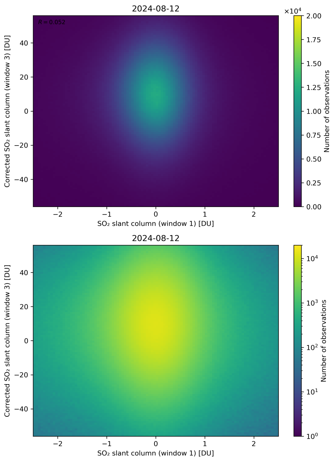
Figure 234: Scatter density plot of “SO 2 slant column (window 1)” against “Corrected SO 2 slant column (window 3)” for 2024-08-12 to 2024-08-13.
