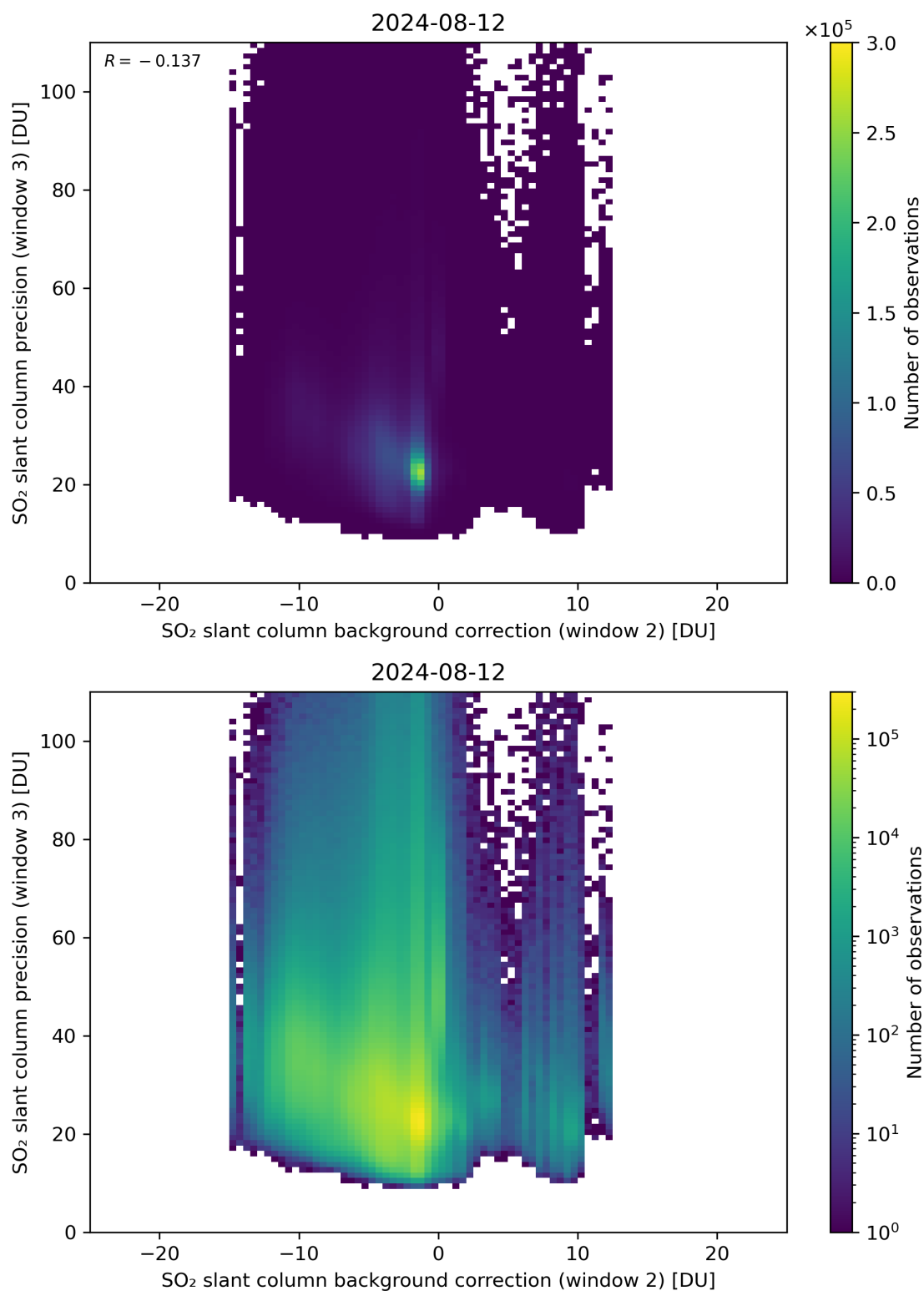
Figure 118: Scatter density plot of “SO 2 slant column background correction (window 2)” against “SO 2 slant column precision (window 3)” for 2024-08-12 to 2024-08-13.
