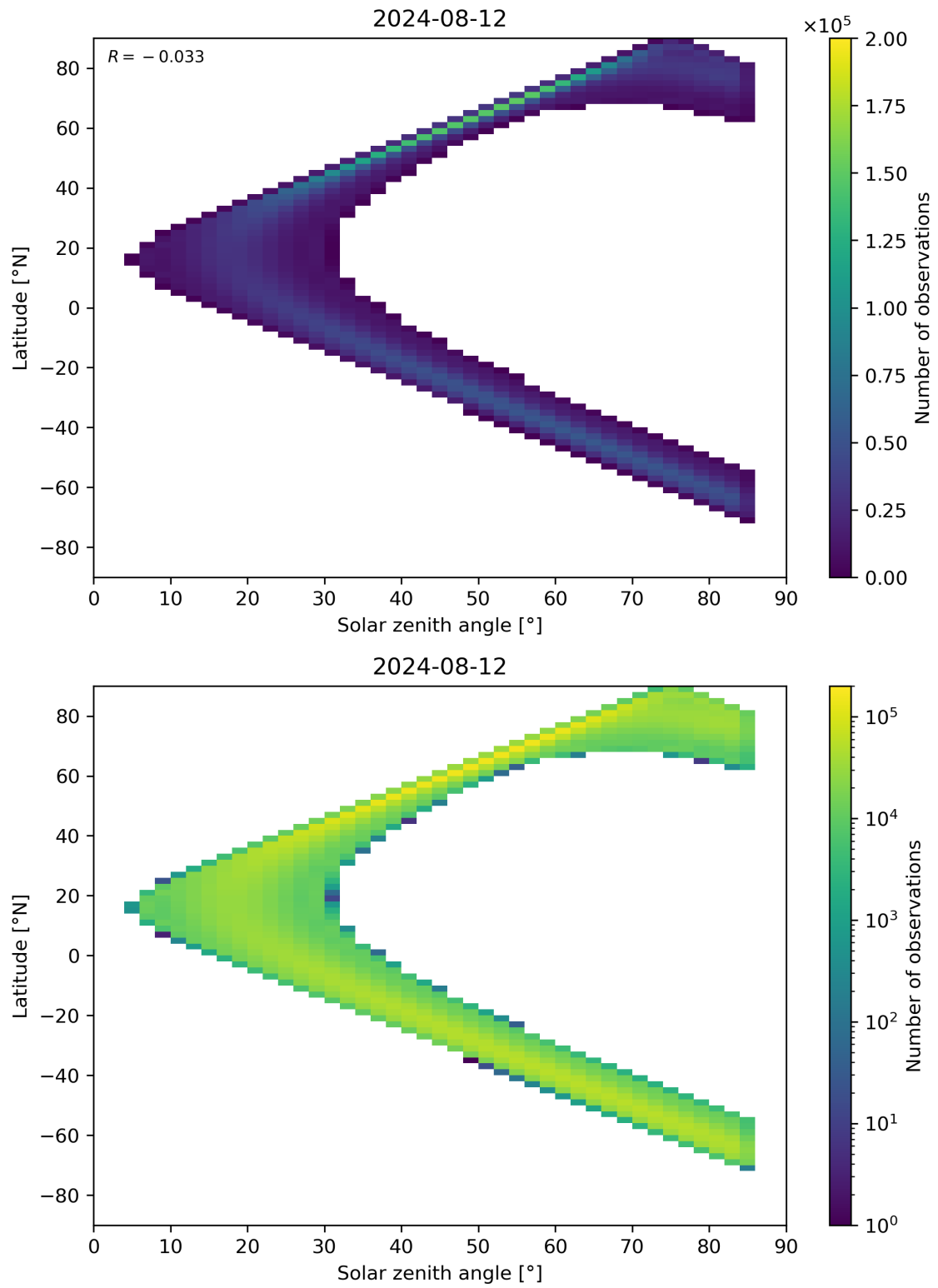
Figure 164: Scatter density plot of “Solar zenith angle” against “Latitude” for 2024-08-12 to 2024-08-13.
