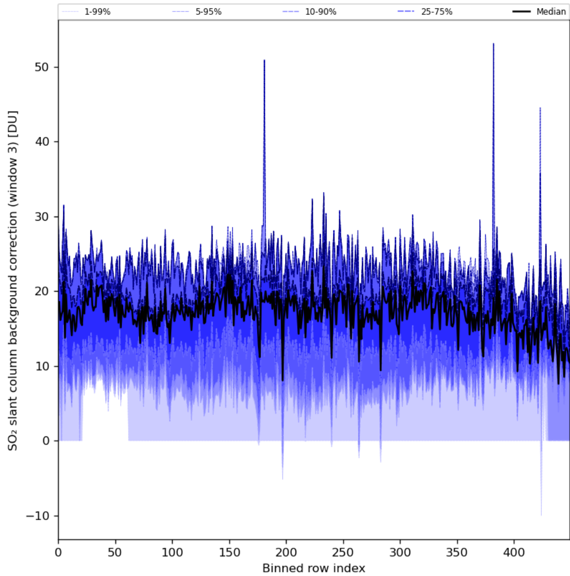
Figure 90: Along track statistics of “SO 2 slant column background correction (window 3)” for 2024-08-12 to 2024-08-13
