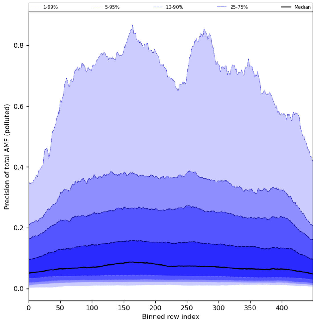
Figure 95: Along track statistics of “Precision of total AMF (polluted)” for 2024-08-12 to 2024-08-13
