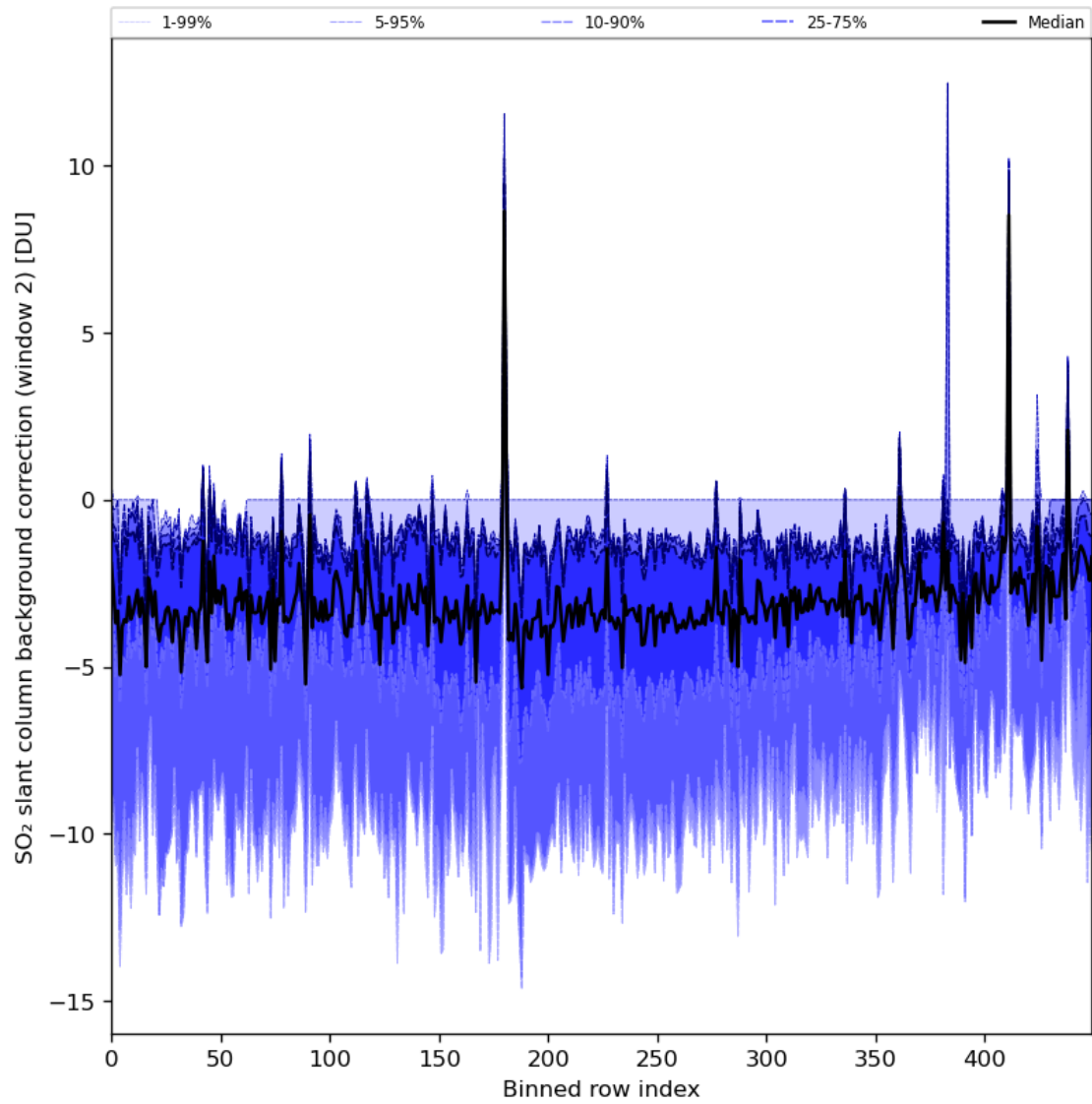
Figure 86: Along track statistics of “SO 2 slant column background correction (window 2)” for 2024-08-12 to 2024-08-13
