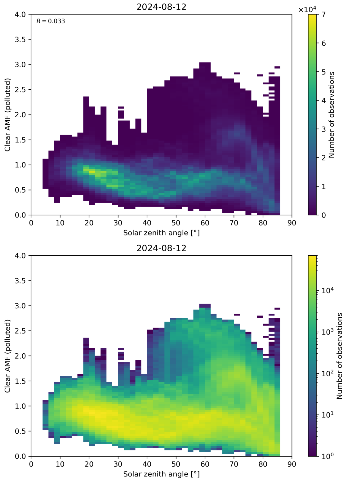
Figure 165: Scatter density plot of “Solar zenith angle” against “Clear AMF (polluted)” for 2024-08-12 to 2024-08-13.
