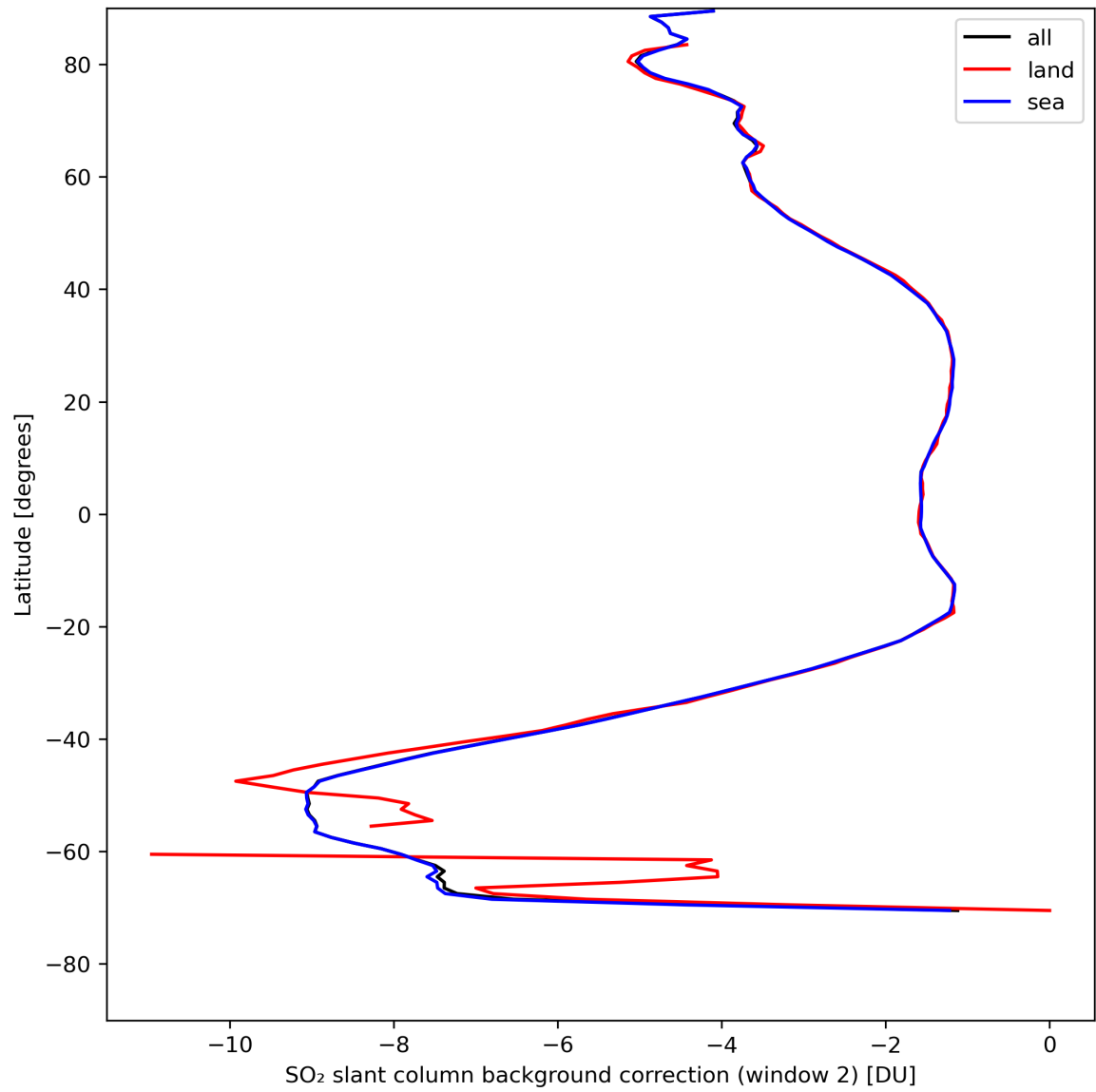
Figure 40: Zonal average of “SO 2 slant column background correction (window 2)” for 2024-08-12 to 2024-08-13.
