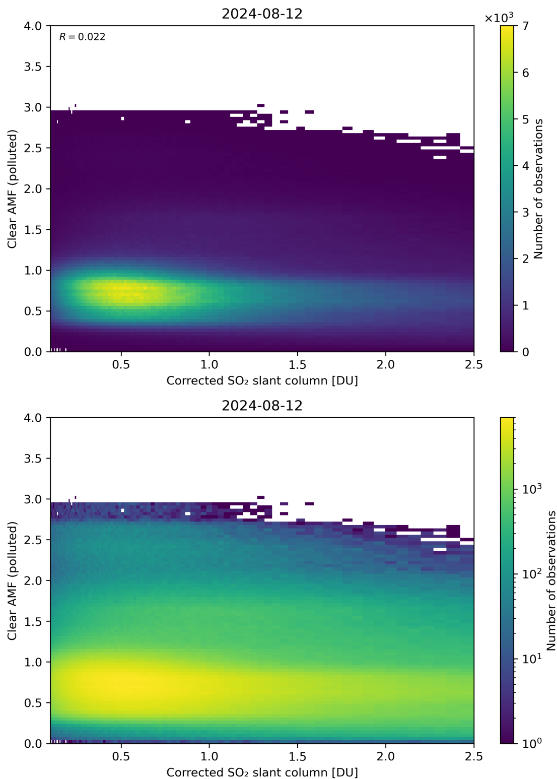
Figure 184: Scatter density plot of “Corrected SO 2 slant column” against “Clear AMF (polluted)” for 2024-08-12 to 2024-08-13.
