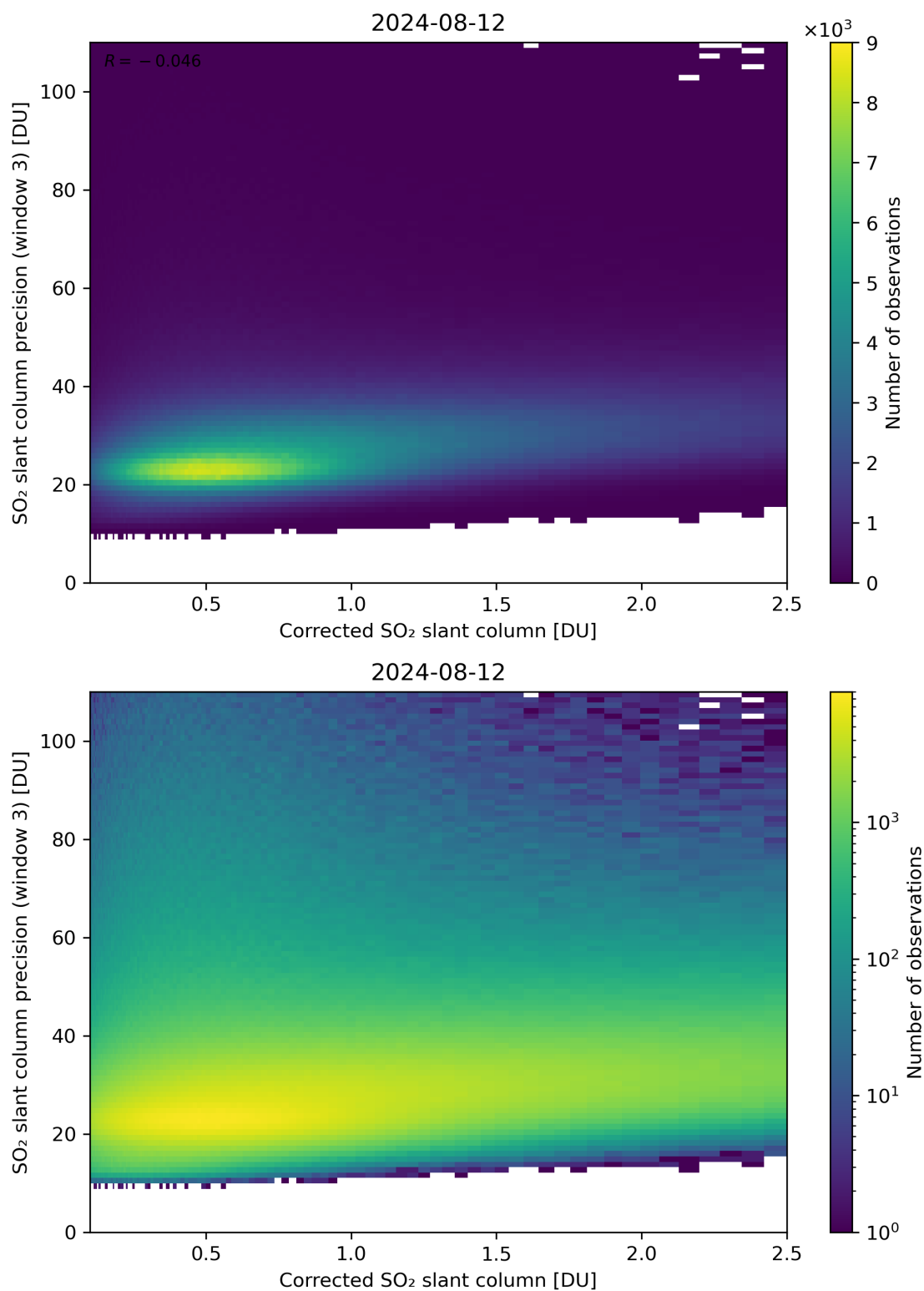
Figure 191: Scatter density plot of “Corrected SO 2 slant column” against “SO 2 slant column precision (window 3)” for 2024-08-12 to 2024-08-13.
