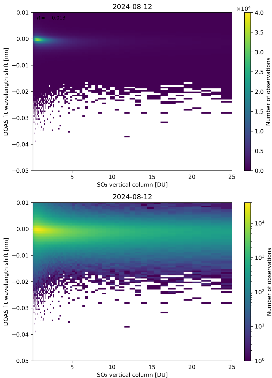
Figure 276: Scatter density plot of “SO 2 vertical column” against “DOAS fit wavelength shift” for 2024-08-12 to 2024-08-13.
