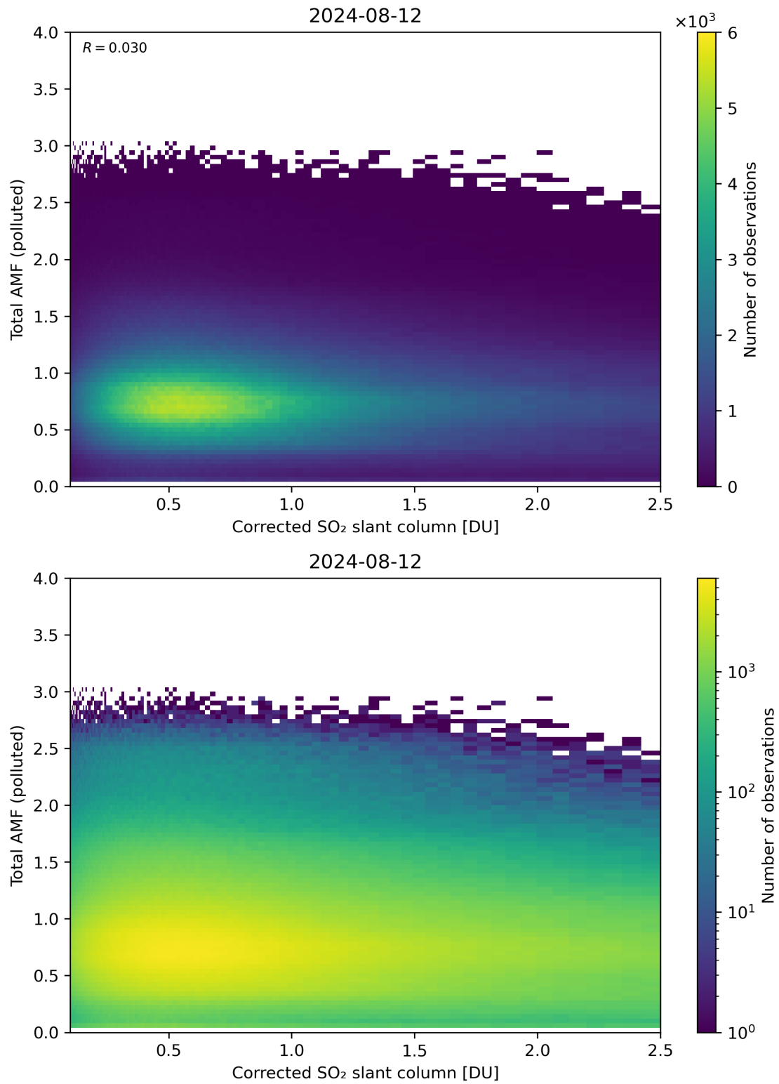
Figure 192: Scatter density plot of “Corrected SO 2 slant column” against “Total AMF (polluted)” for 2024-08-12 to 2024-08-13.
