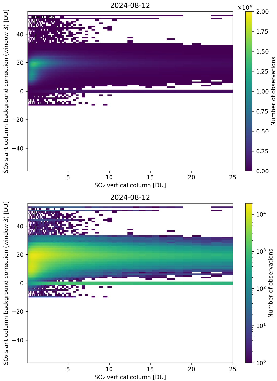
Figure 275: Scatter density plot of “SO 2 vertical column” against “SO 2 slant column background correction (window 3)” for 2024-08-12 to 2024-08-13.
