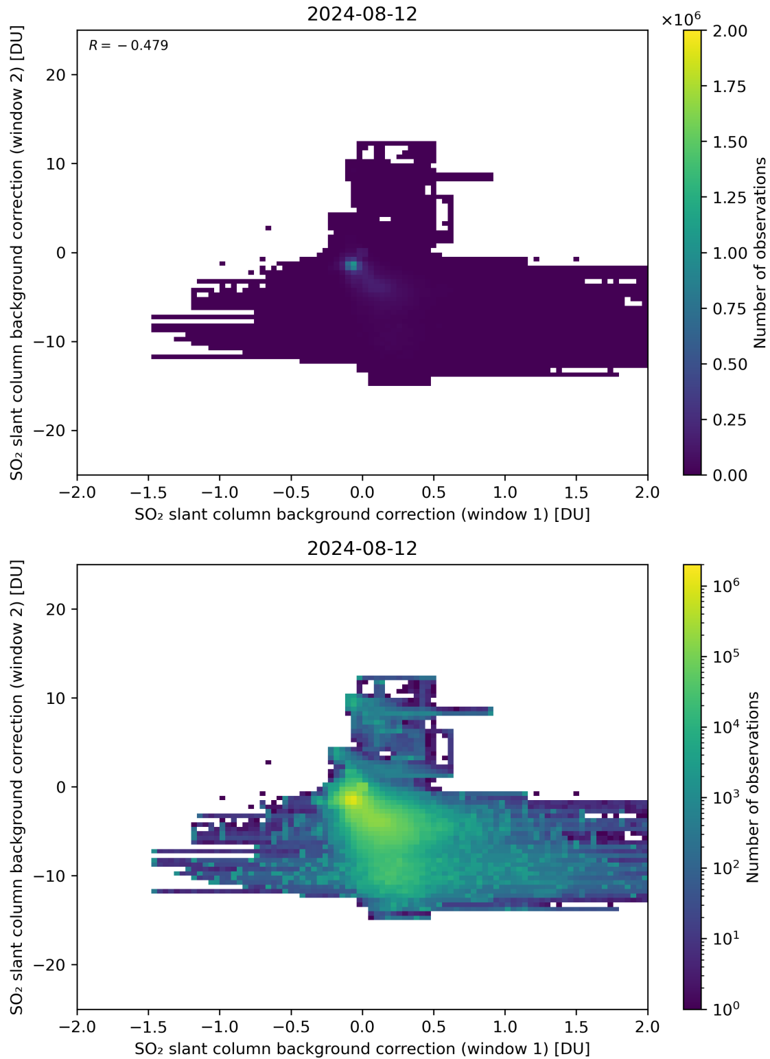
Figure 98: Scatter density plot of “SO 2 slant column background correction (window 1)” against “SO 2 slant column background correction (window 2)” for 2024-08-12 to 2024-08-13.
