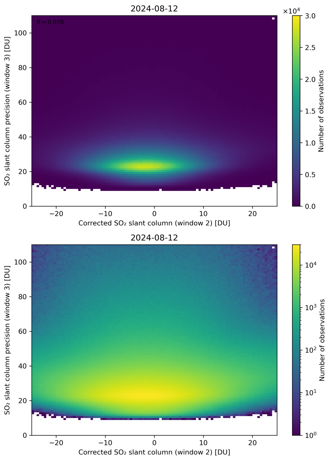
Figure 202: Scatter density plot of “Corrected SO 2 slant column (window 2)” against “SO 2 slant column precision (window 3)” for 2024-08-12 to 2024-08-13.
