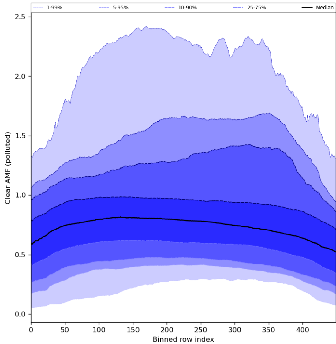
Figure 96: Along track statistics of “Clear AMF (polluted)” for 2024-08-12 to 2024-08-13
