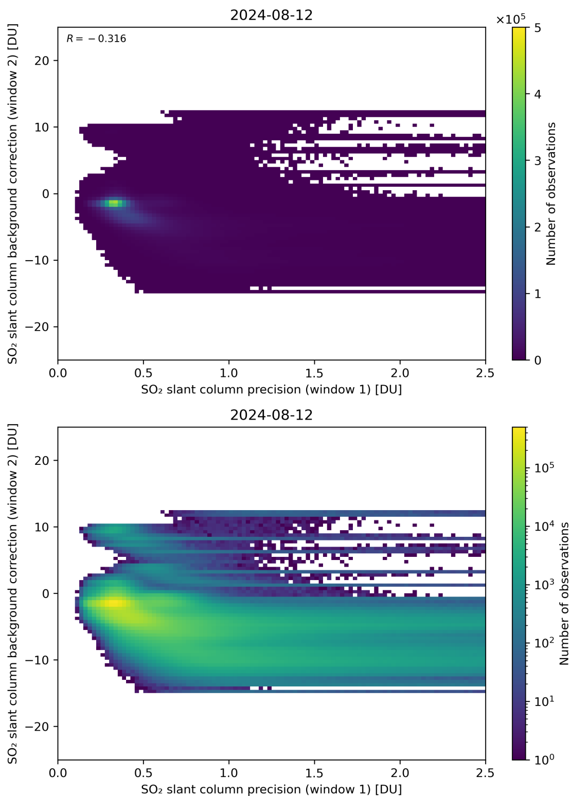
Figure 219: Scatter density plot of “SO 2 slant column precision (window 1)” against “SO 2 slant column background correction (window 2)” for 2024-08-12 to 2024-08-13.
