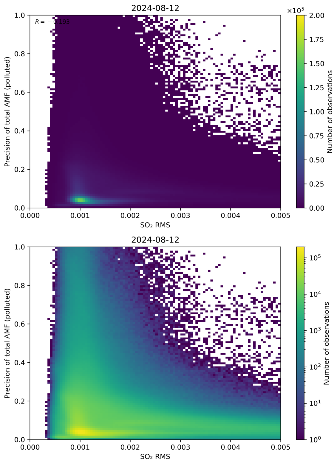
Figure 138: Scatter density plot of “SO 2 RMS” against “Precision of total AMF (polluted)” for 2024-08-12 to 2024-08-13.
