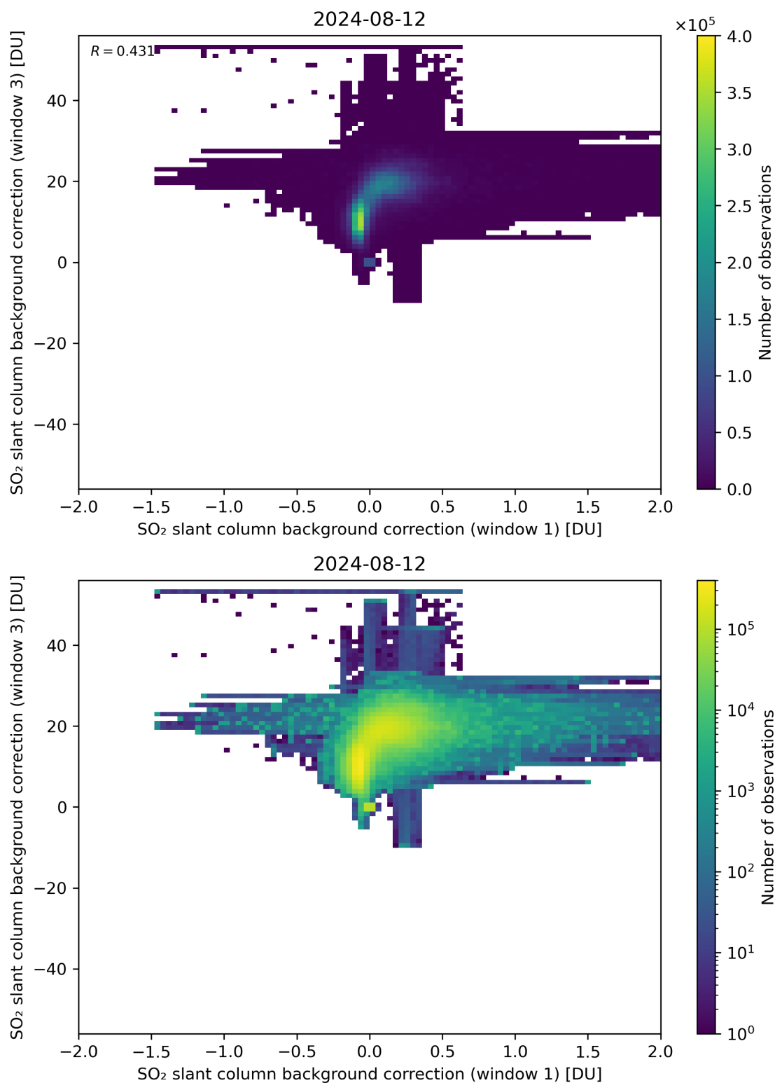
Figure 99: Scatter density plot of “SO 2 slant column background correction (window 1)” against “SO 2 slant column background correction (window 3)” for 2024-08-12 to 2024-08-13.
