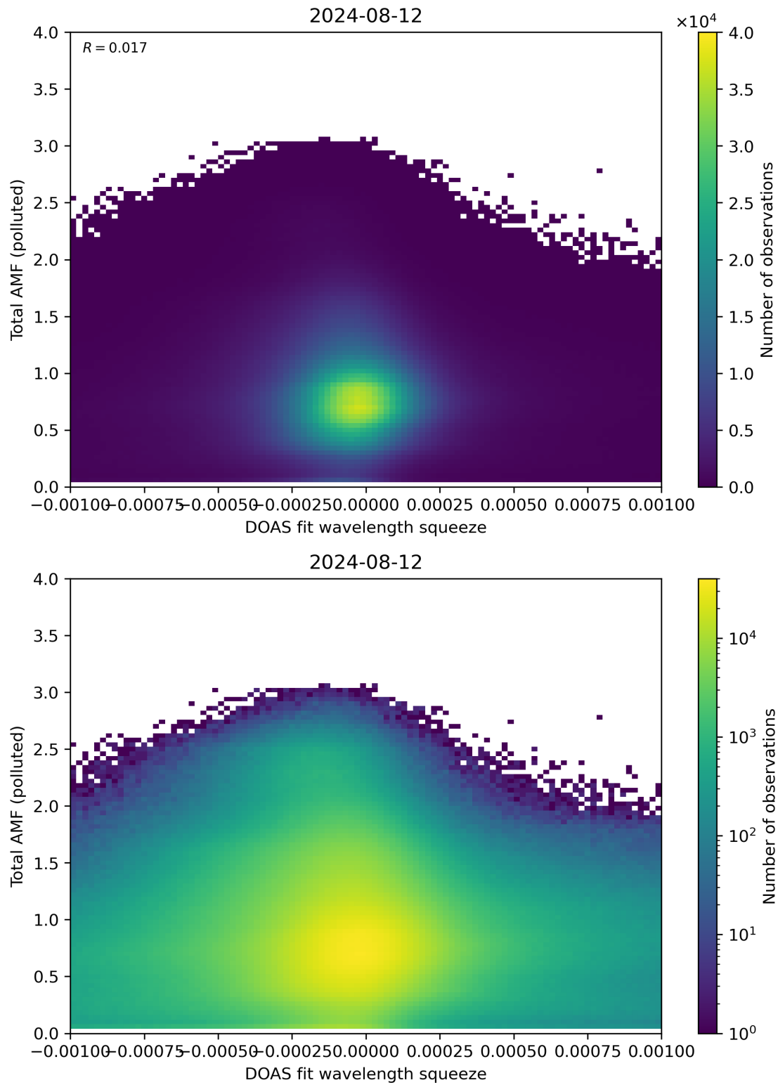
Figure 134: Scatter density plot of “DOAS fit wavelength squeeze” against “Total AMF (polluted)” for 2024-08-12 to 2024-08-13.
