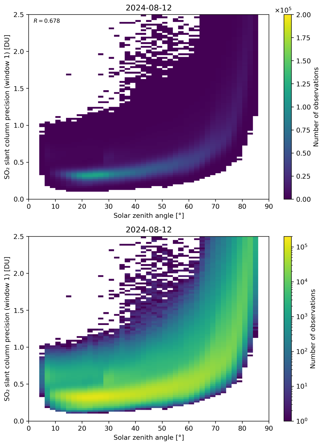
Figure 170: Scatter density plot of “Solar zenith angle” against “SO 2 slant column precision (window 1)” for 2024-08-12 to 2024-08-13.
