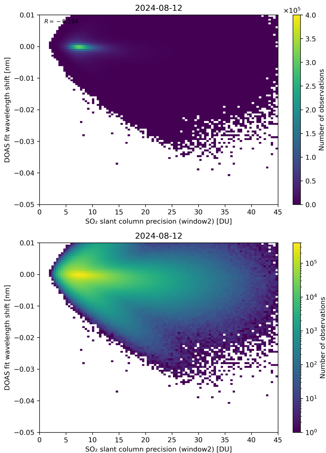
Figure 243: Scatter density plot of “SO 2 slant column precision (window2)” against “DOAS fit wavelength shift” for 2024-08-12 to 2024-08-13.
