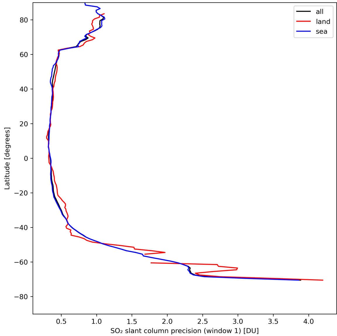
Figure 34: Zonal average of “SO 2 slant column precision (window 1)” for 2024-08-12 to 2024-08-13.
