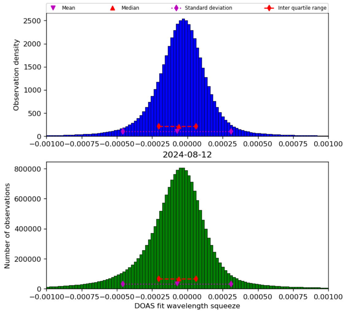
Figure 69: Histogram of “DOAS fit wavelength squeeze” for 2024-08-12 to 2024-08-13
