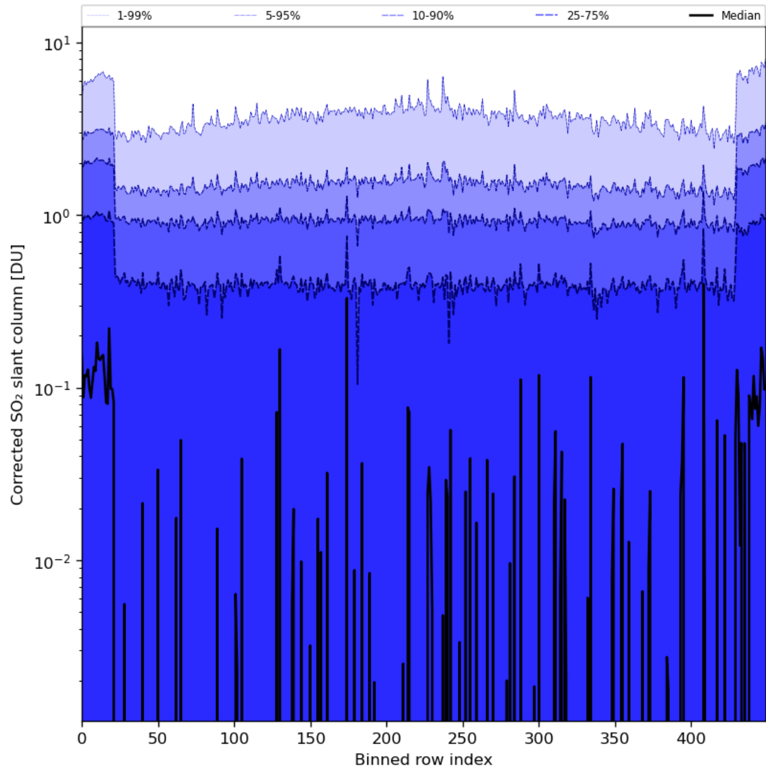
Figure 78: Along track statistics of “Corrected SO 2 slant column” for 2024-08-12 to 2024-08-13
