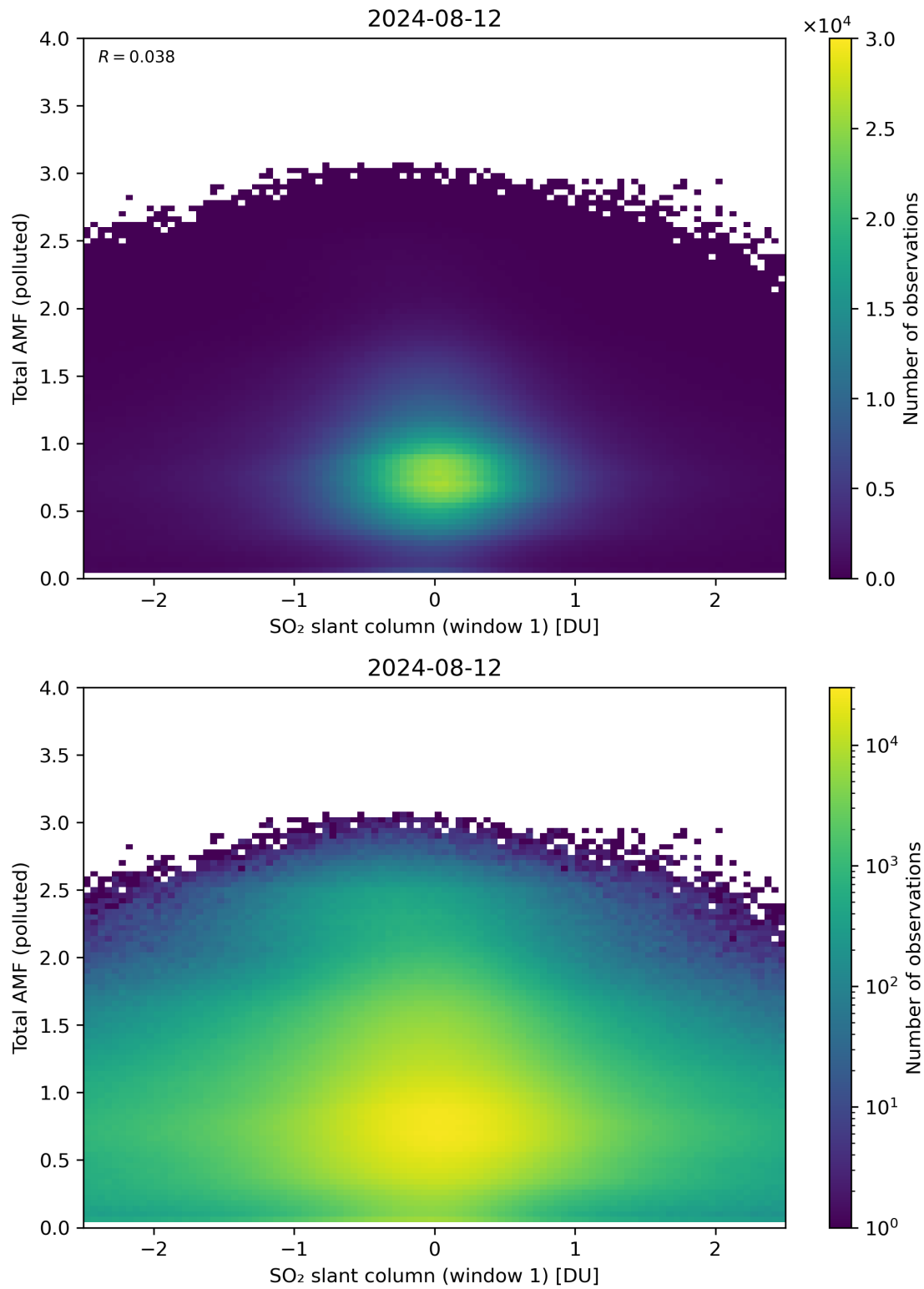
Figure 239: Scatter density plot of “SO 2 slant column (window 1)” against “Total AMF (polluted)” for 2024-08-12 to 2024-08-13.
