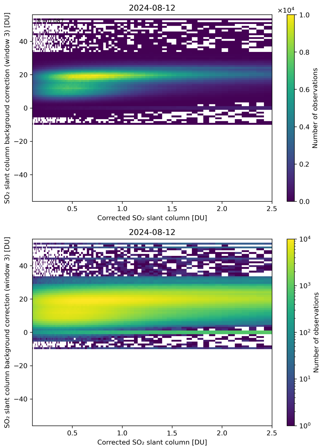
Figure 180: Scatter density plot of “Corrected SO 2 slant column” against “SO 2 slant column background correction (window 3)” for 2024-08-12 to 2024-08-13.
