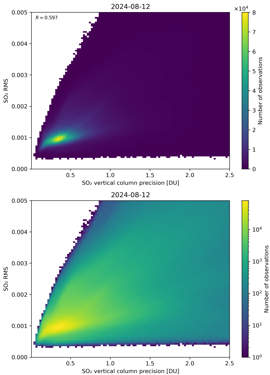
Figure 284: Scatter density plot of “SO 2 vertical column precision” against “SO 2 RMS” for 2024-08-12 to 2024-08-13.
