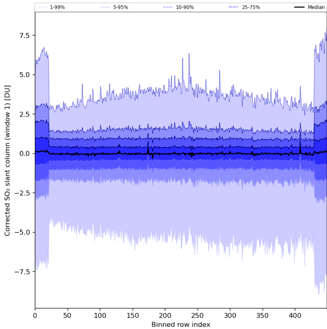
Figure 81: Along track statistics of "Corrected SO 2 slant column (window 1)" for 2024-08-12 to 2024-08-13
