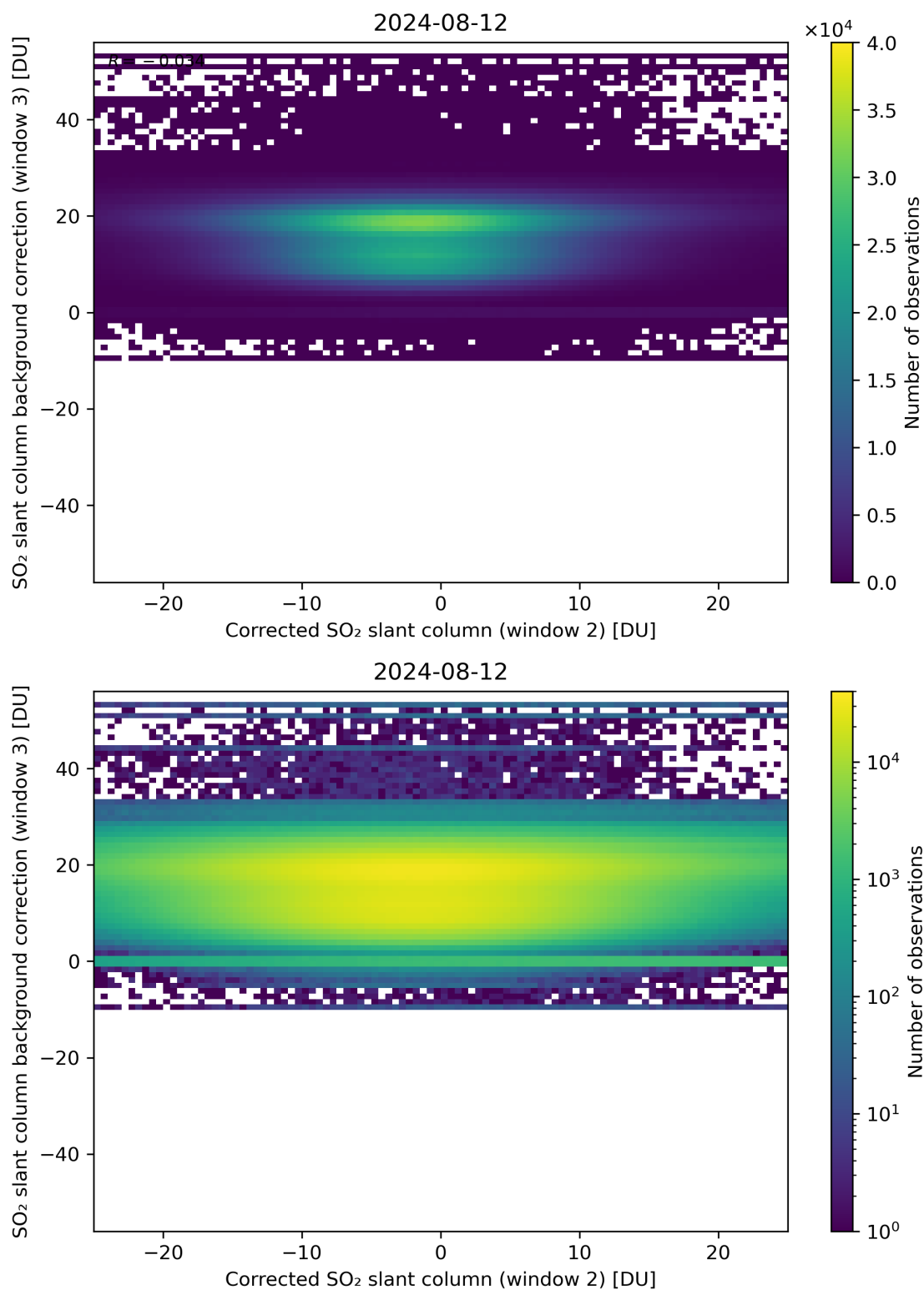
Figure 195: Scatter density plot of “Corrected SO 2 slant column (window 2)” against “SO 2 slant column background correction (window 3)” for 2024-08-12 to 2024-08-13.
