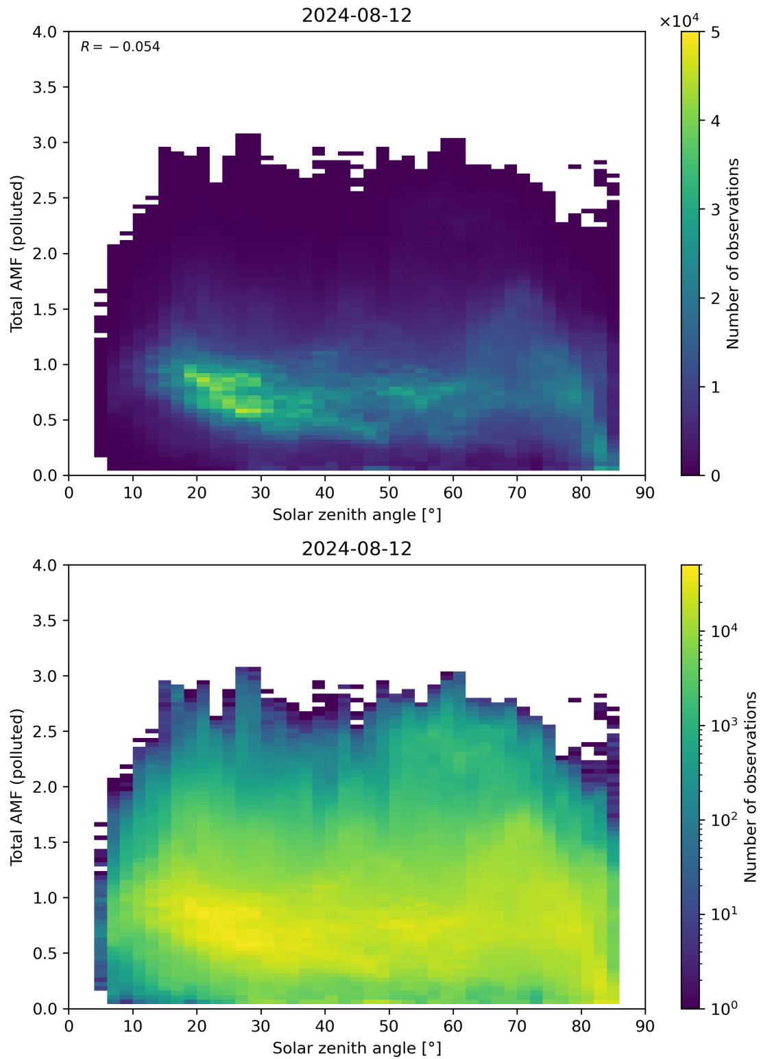
Figure 174: Scatter density plot of “Solar zenith angle” against “Total AMF (polluted)” for 2024-08-12 to 2024-08-13.
