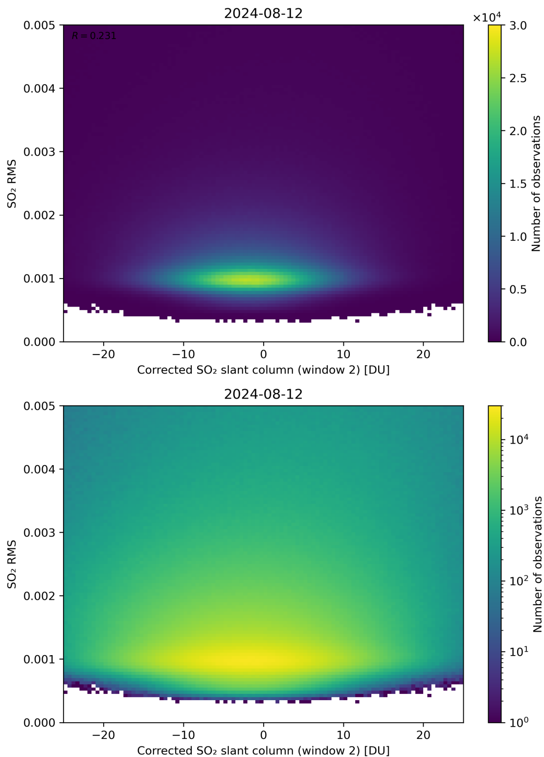
Figure 198: Scatter density plot of “Corrected SO 2 slant column (window 2)” against “SO 2 RMS” for 2024-08-12 to 2024-08-13.
