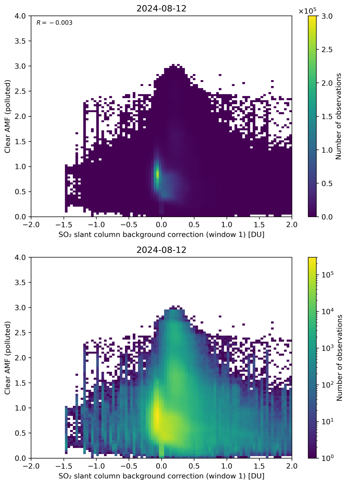
Figure 103: Scatter density plot of “SO 2 slant column background correction (window 1)” against “Clear AMF (polluted)” for 2024-08-12 to 2024-08-13.
