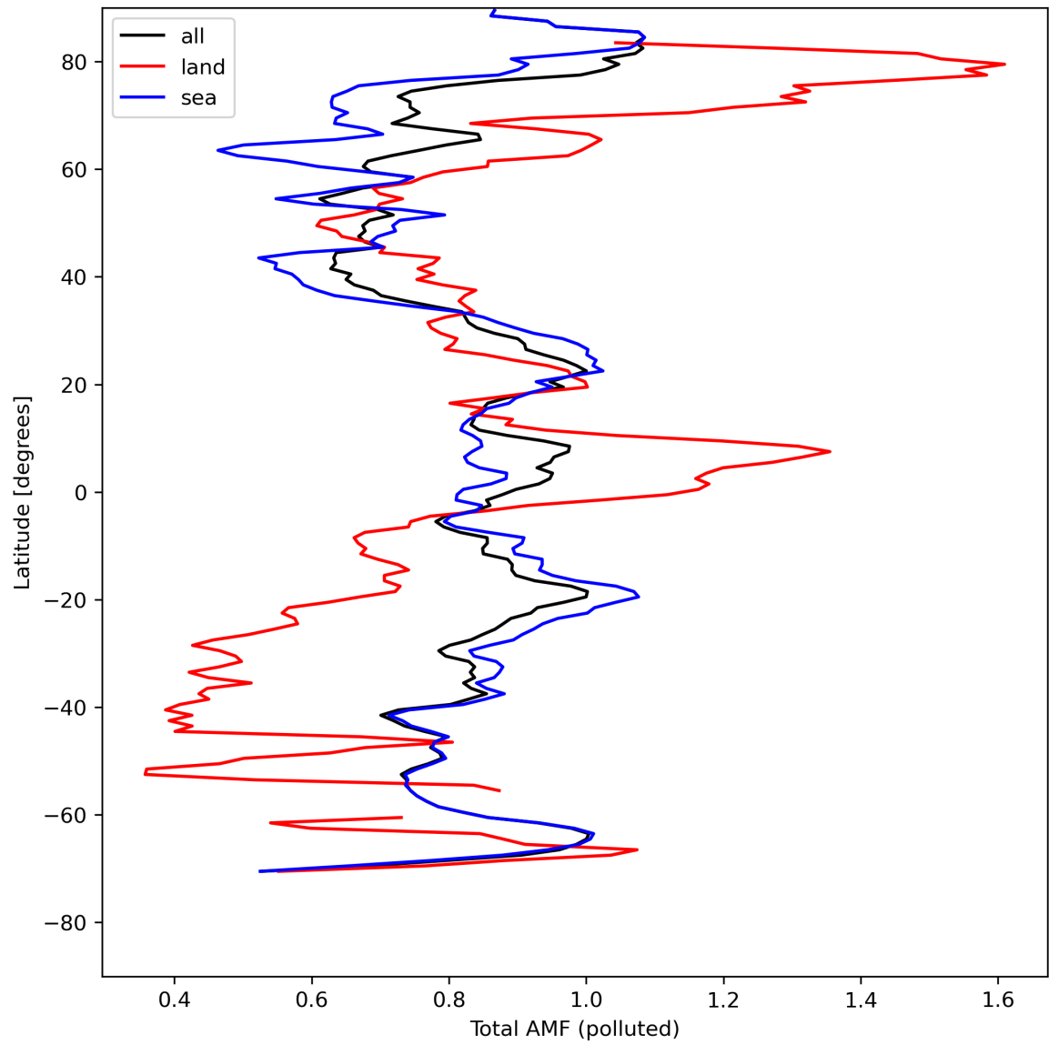
Figure 48: Zonal average of “Total AMF (polluted)” for 2024-08-12 to 2024-08-13.
