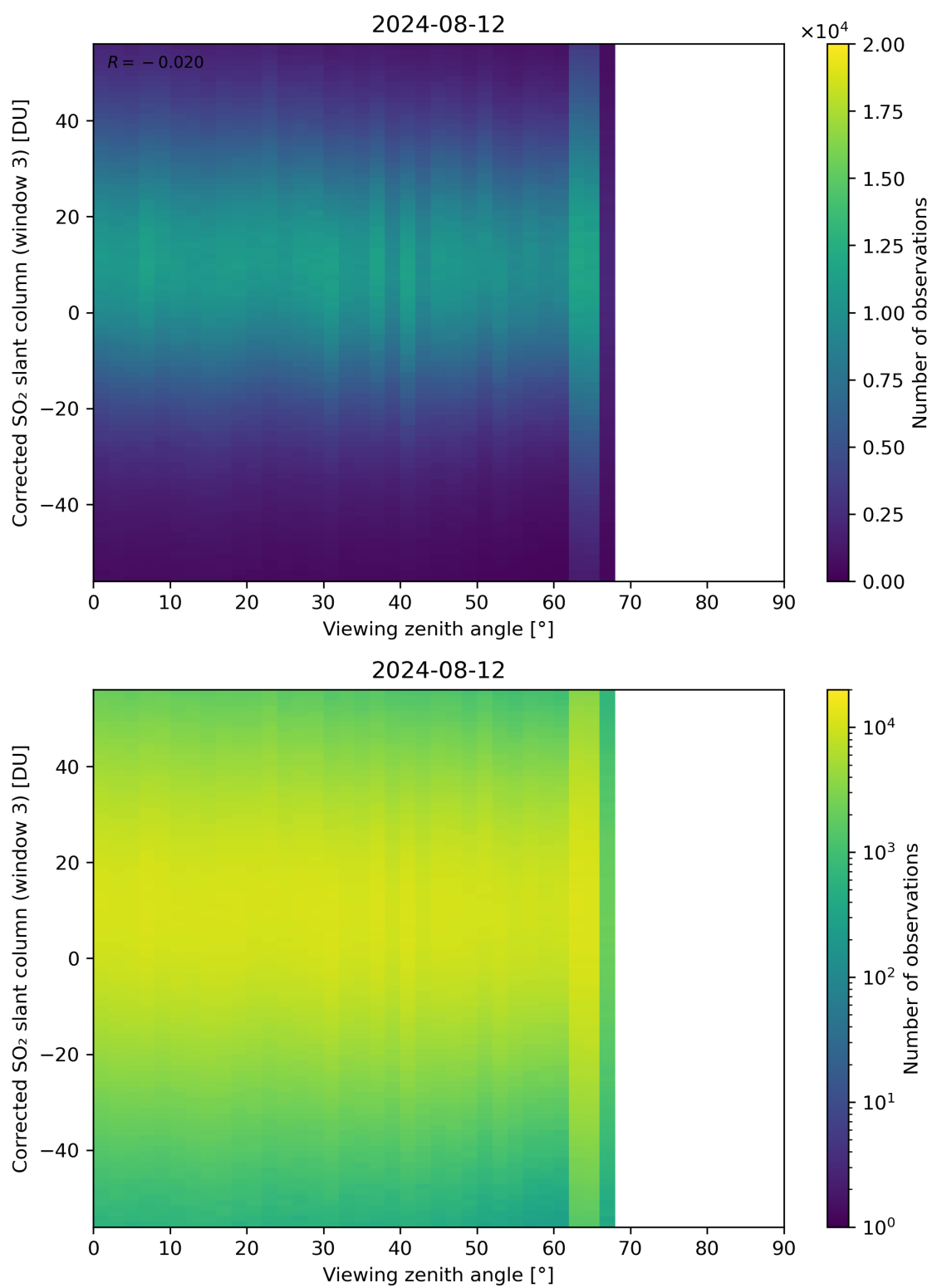
Figure 319: Scatter density plot of “Viewing zenith angle” against “Corrected SO 2 slant column (window 3)” for 2024-08-12 to 2024-08-13.
