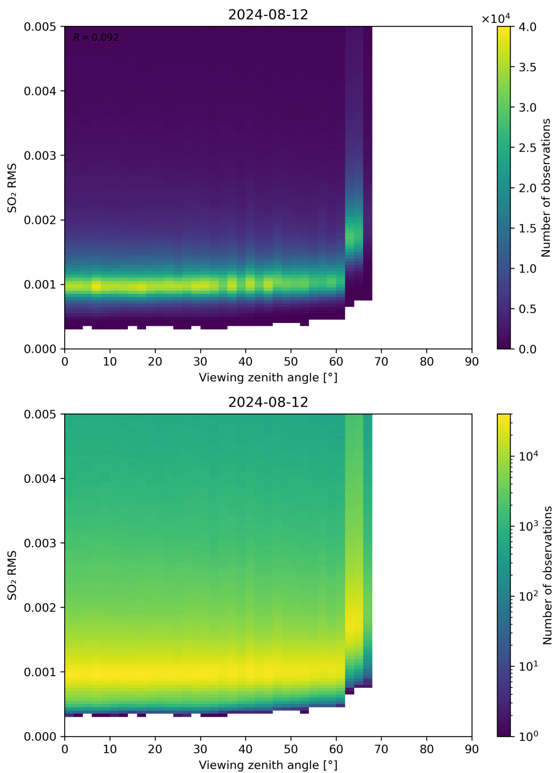
Figure 313: Scatter density plot of “Viewing zenith angle” against “SO 2 RMS” for 2024-08-12 to 2024-08-13.
