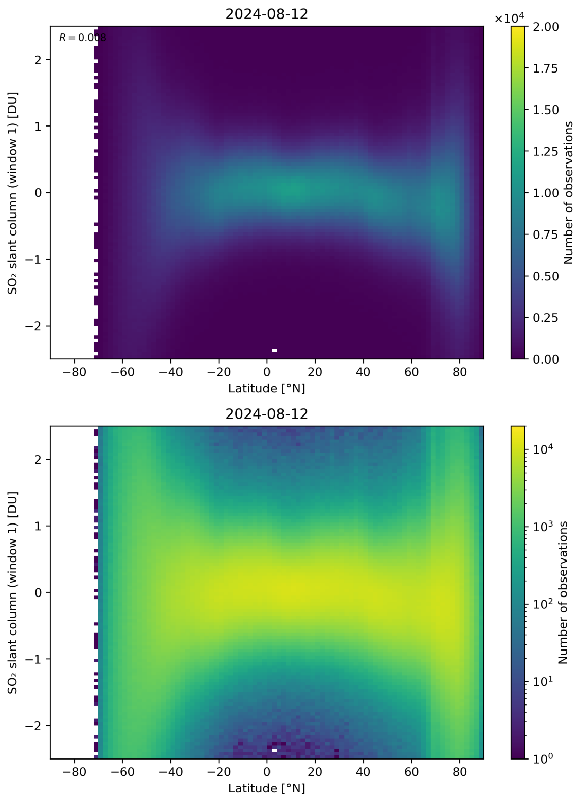
Figure 149: Scatter density plot of “Latitude” against “SO 2 slant column (window 1)” for 2024-08-12 to 2024-08-13.
