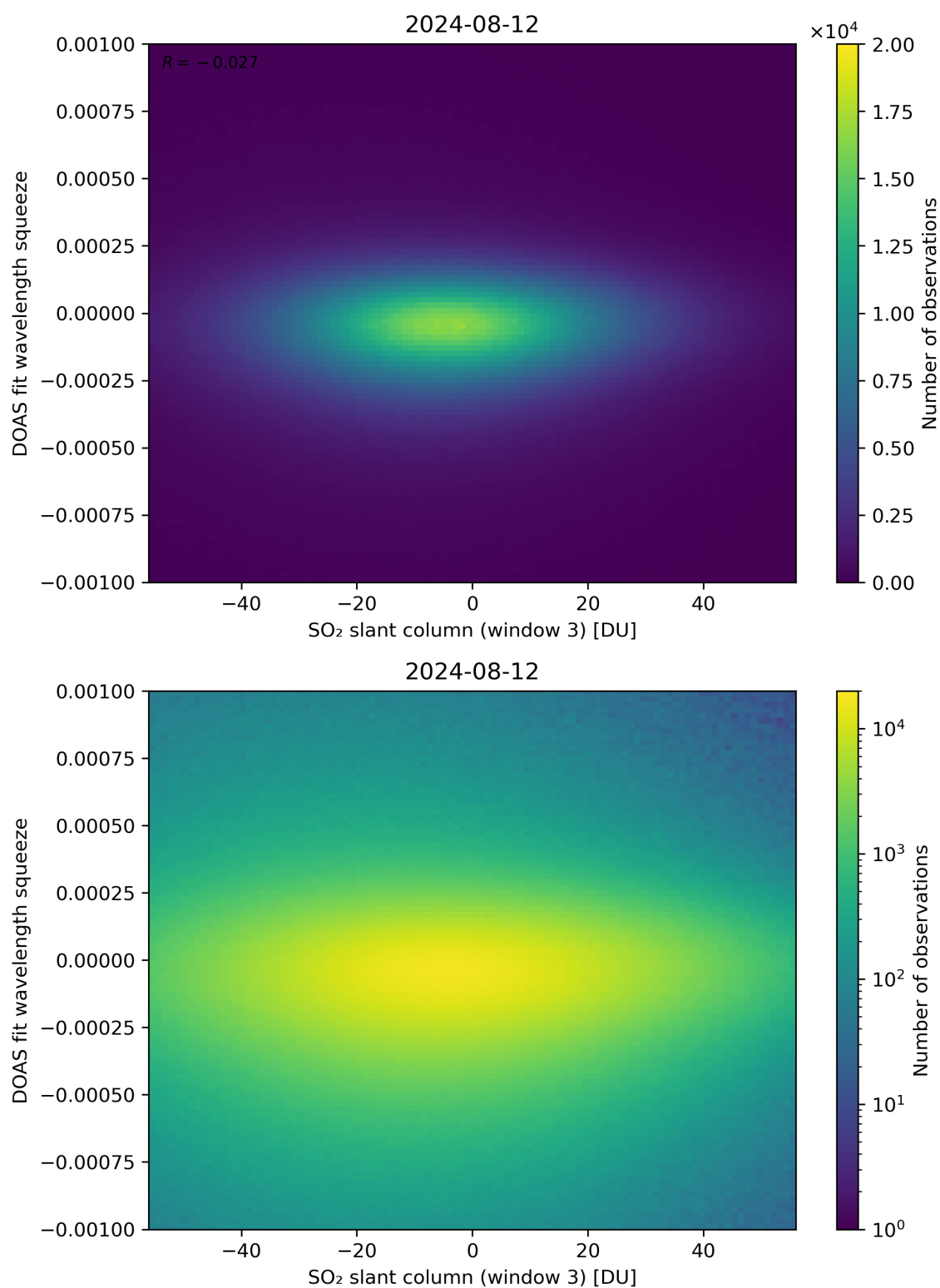
Figure 255: Scatter density plot of “SO 2 slant column (window 3)” against “DOAS fit wavelength squeeze” for 2024-08-12 to 2024-08-13.
