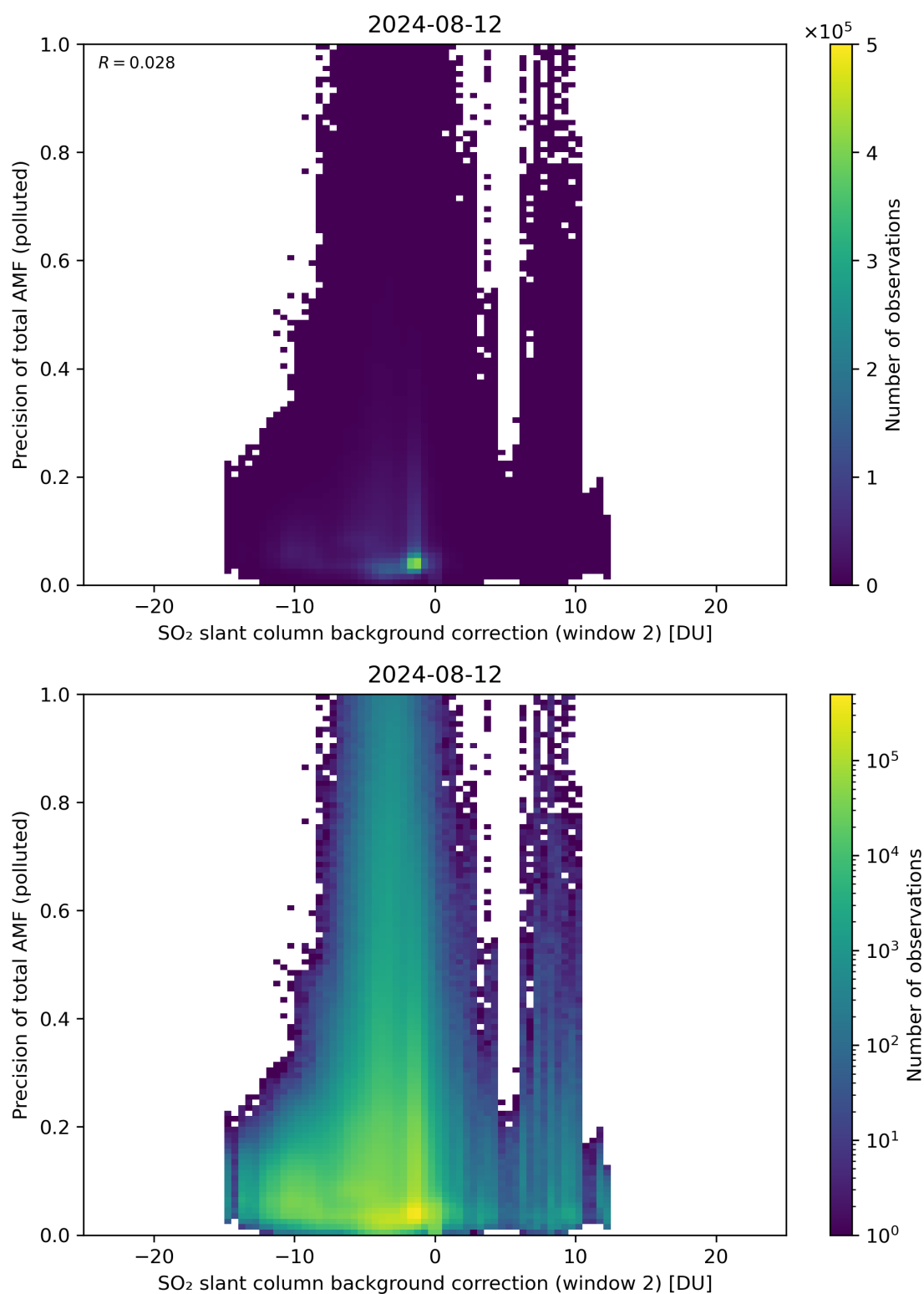
Figure 120: Scatter density plot of “SO 2 slant column background correction (window 2)” against “Precision of total AMF (polluted)” for 2024-08-12 to 2024-08-13.
