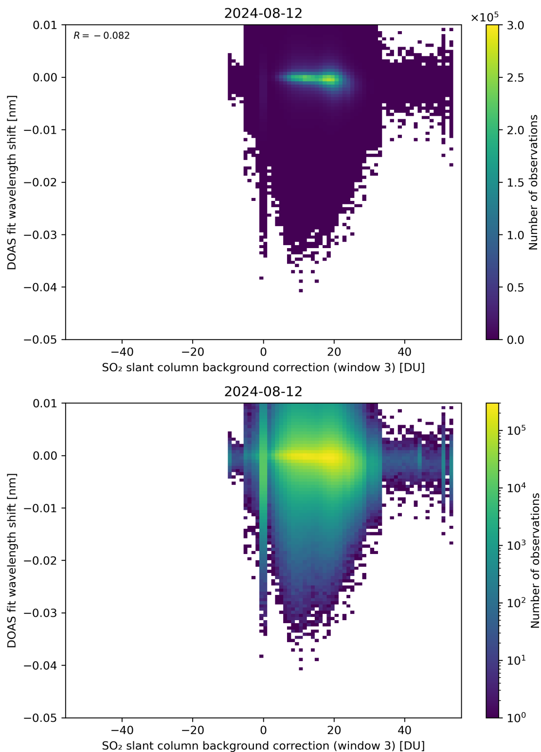
Figure 121: Scatter density plot of “SO 2 slant column background correction (window 3)” against “DOAS fit wavelength shift” for 2024-08-12 to 2024-08-13.
