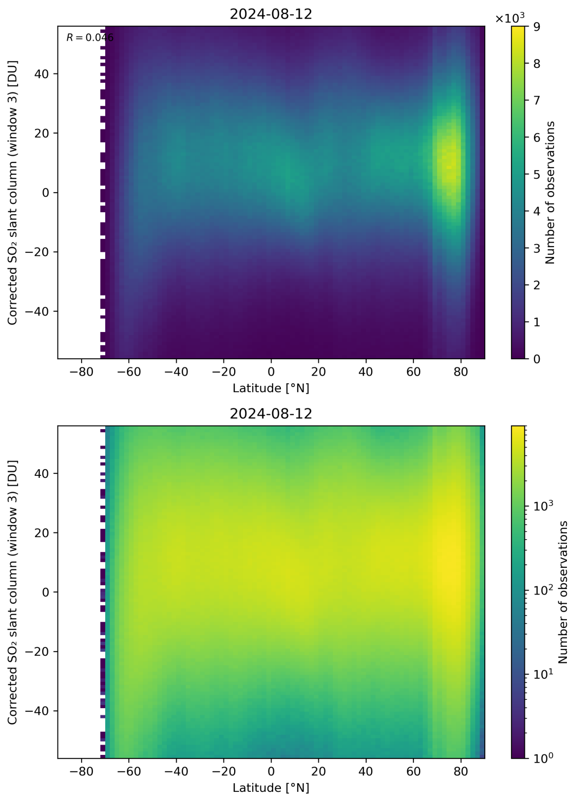
Figure 148: Scatter density plot of “Latitude” against “Corrected SO 2 slant column (window 3)” for 2024-08-12 to 2024-08-13.
