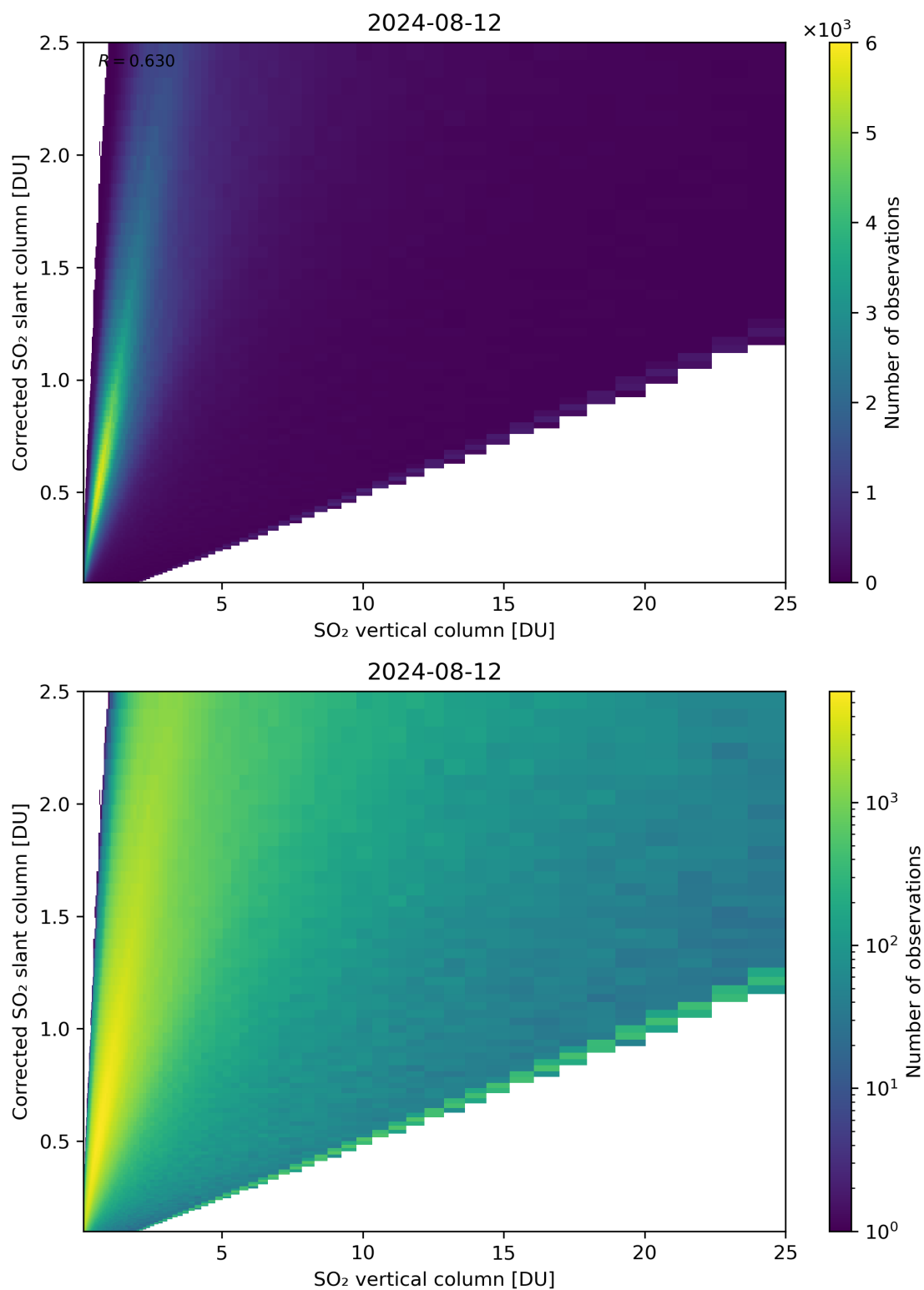
Figure 297: Scatter density plot of “SO 2 vertical column” against “Corrected SO 2 slant column” for 2024-08-12 to 2024-08-13.
