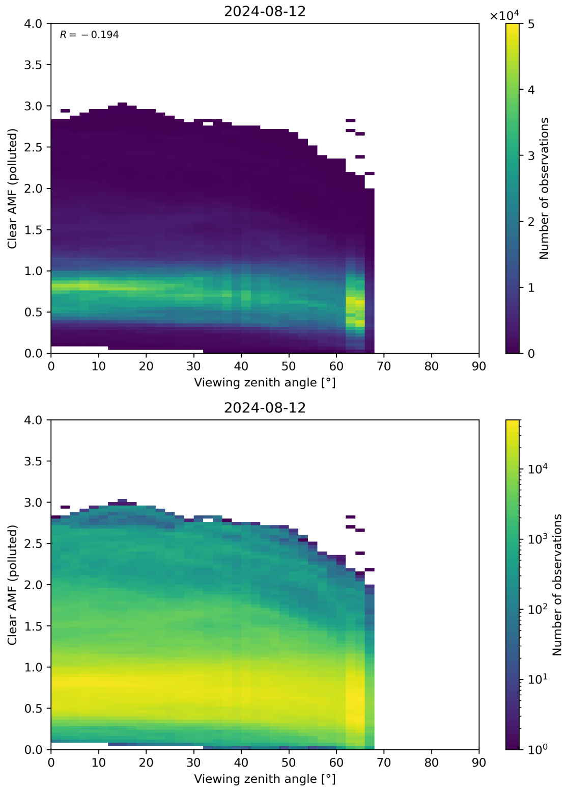
Figure 316: Scatter density plot of “Viewing zenith angle” against “Clear AMF (polluted)” for 2024-08-12 to 2024-08-13.
