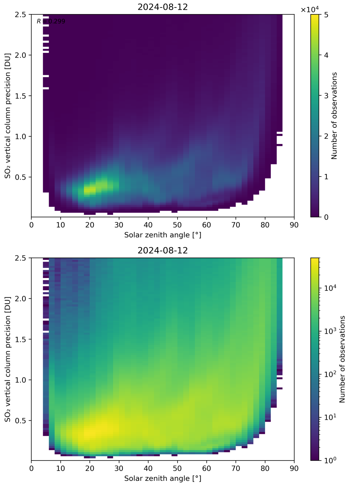
Figure 177: Scatter density plot of “Solar zenith angle” against “SO 2 vertical column precision” for 2024-08-12 to 2024-08-13.
