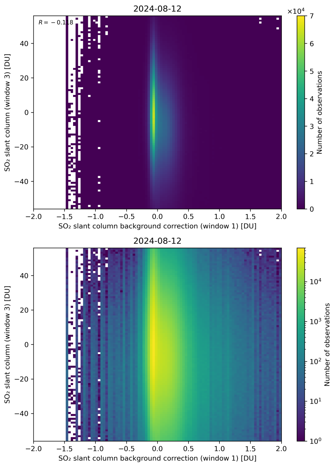
Figure 107: Scatter density plot of “SO 2 slant column background correction (window 1)” against “SO 2 slant column (window 3)” for 2024-08-12 to 2024-08-13.
