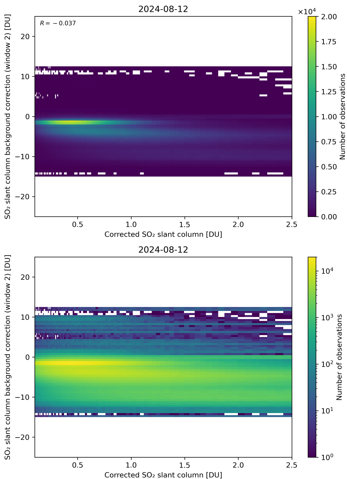
Figure 179: Scatter density plot of “Corrected SO 2 slant column” against “SO 2 slant column background correction (window 2)” for 2024-08-12 to 2024-08-13.
