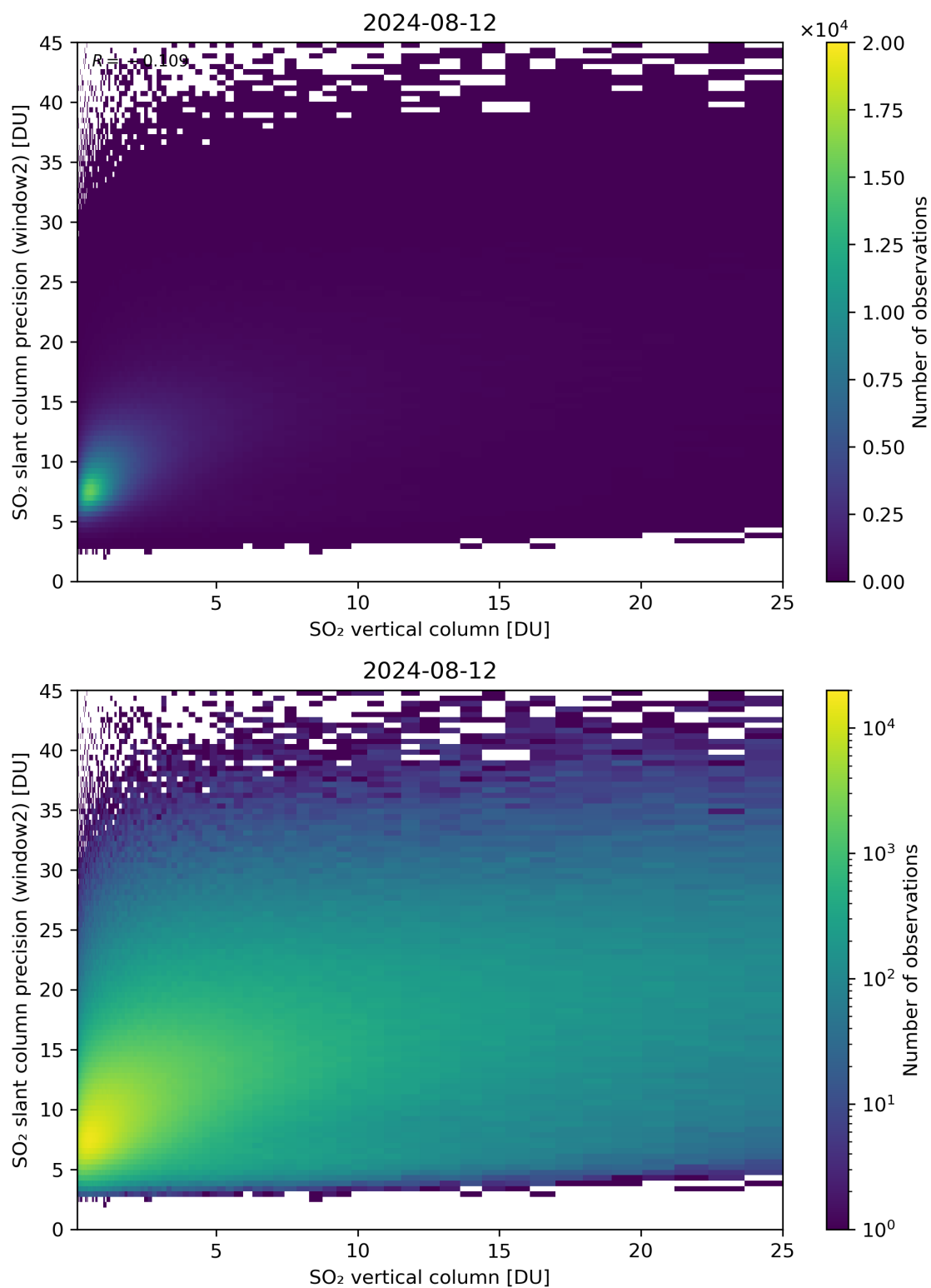
Figure 302: Scatter density plot of “SO 2 vertical column” against “SO 2 slant column precision (window2)” for 2024-08-12 to 2024-08-13.
