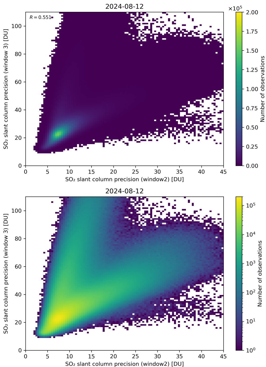
Figure 250: Scatter density plot of “SO 2 slant column precision (window2)” against “SO 2 slant column precision (window 3)” for 2024-08-12 to 2024-08-13.
