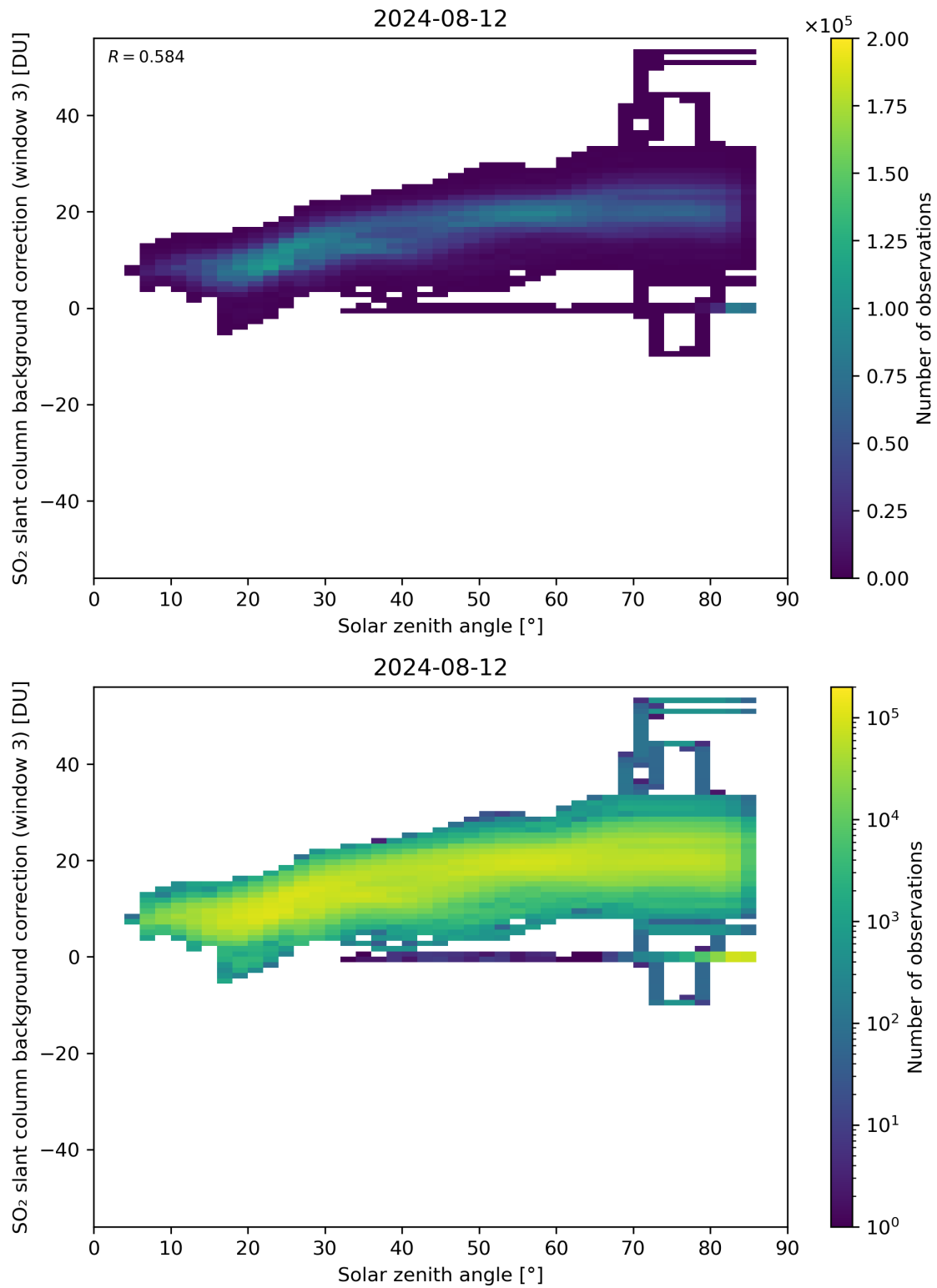
Figure 160: Scatter density plot of “Solar zenith angle” against “SO 2 slant column background correction (window 3)” for 2024-08-12 to 2024-08-13.
