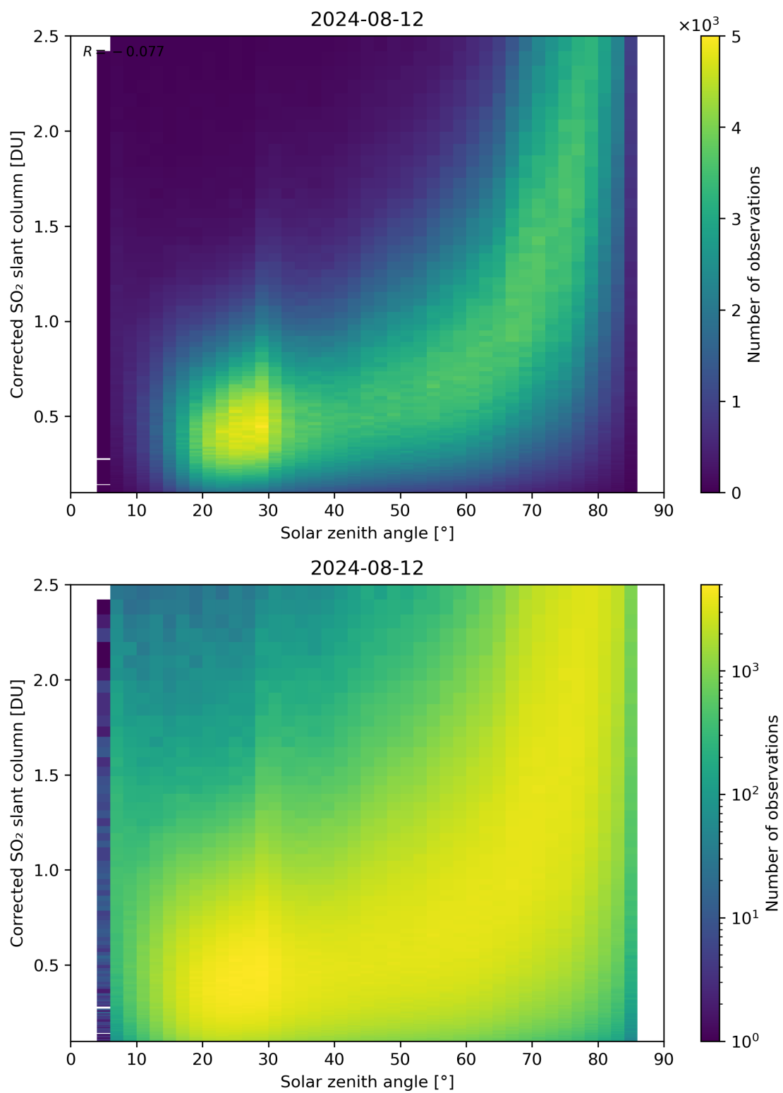
Figure 166: Scatter density plot of “Solar zenith angle” against “Corrected SO 2 slant column” for 2024-08-12 to 2024-08-13.
