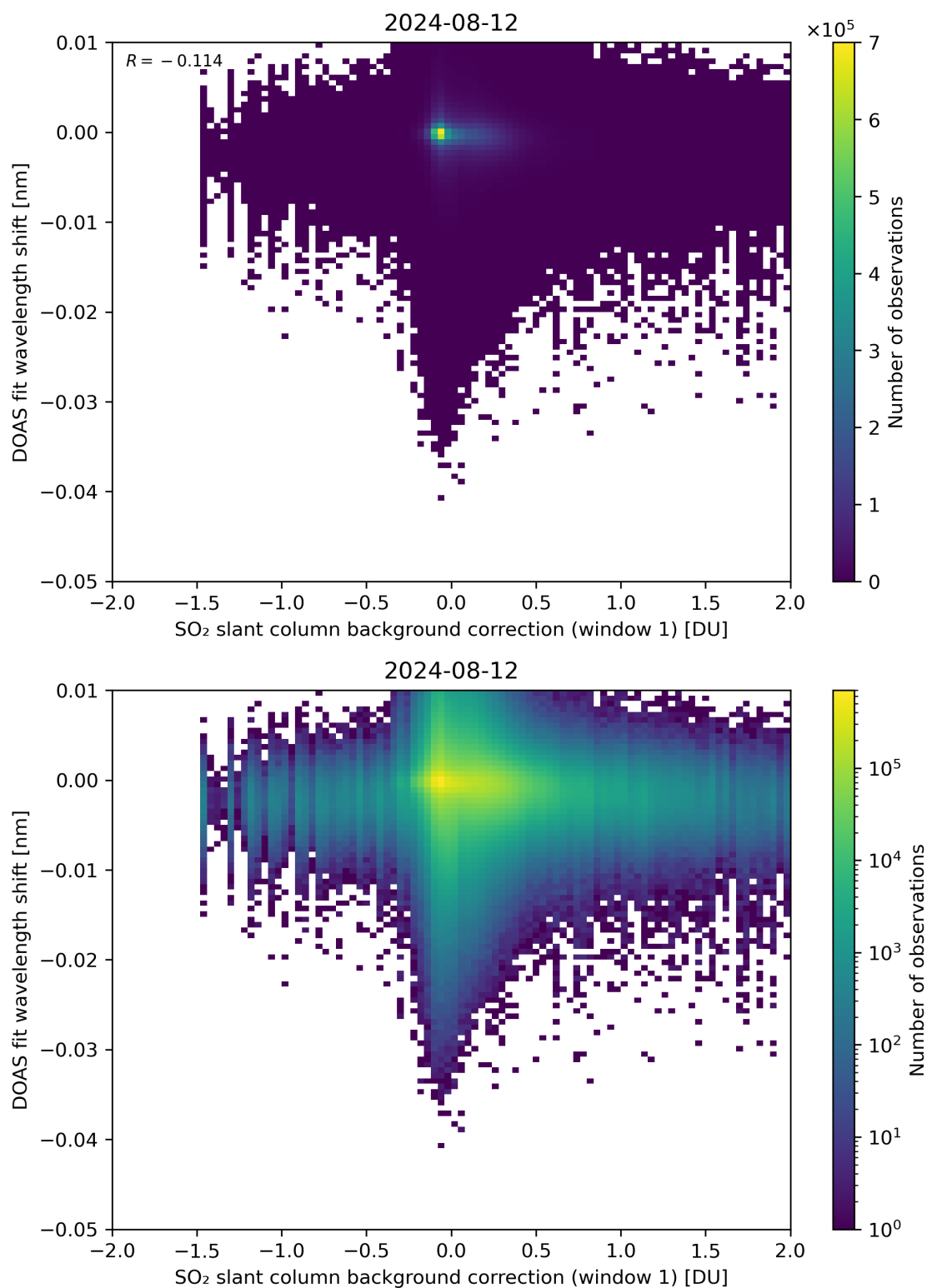
Figure 100: Scatter density plot of “SO 2 slant column background correction (window 1)” against “DOAS fit wavelength shift” for 2024-08-12 to 2024-08-13.
