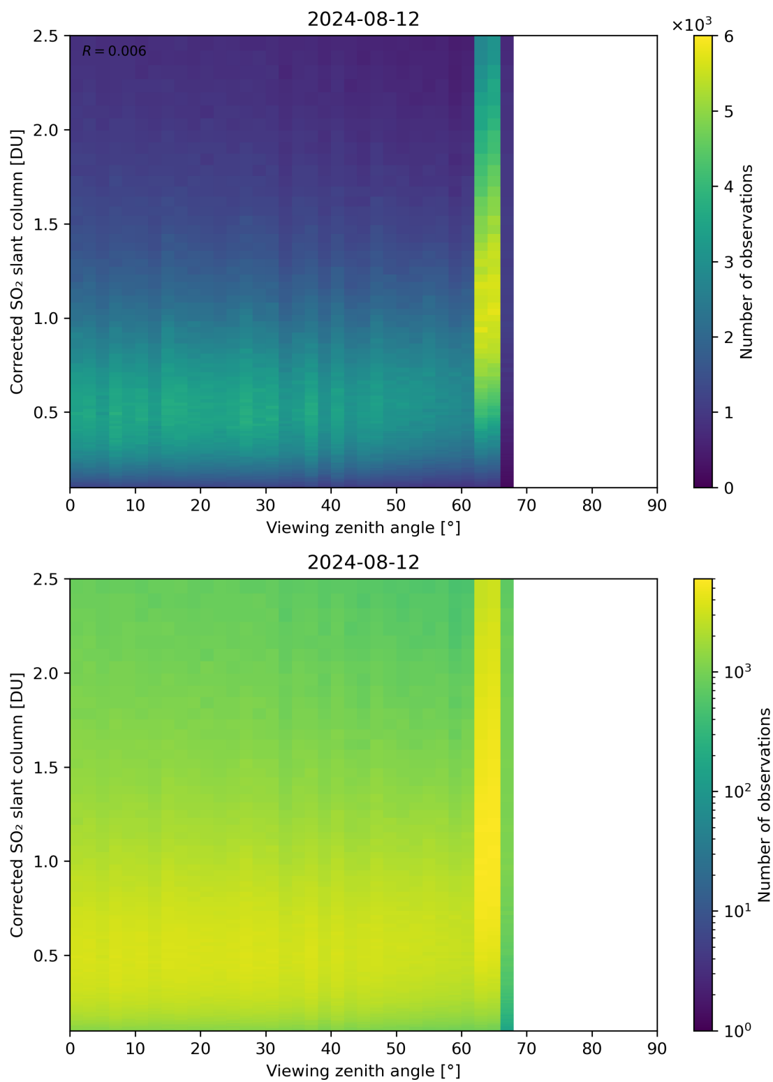
Figure 317: Scatter density plot of “Viewing zenith angle” against “Corrected SO 2 slant column” for 2024-08-12 to 2024-08-13.
