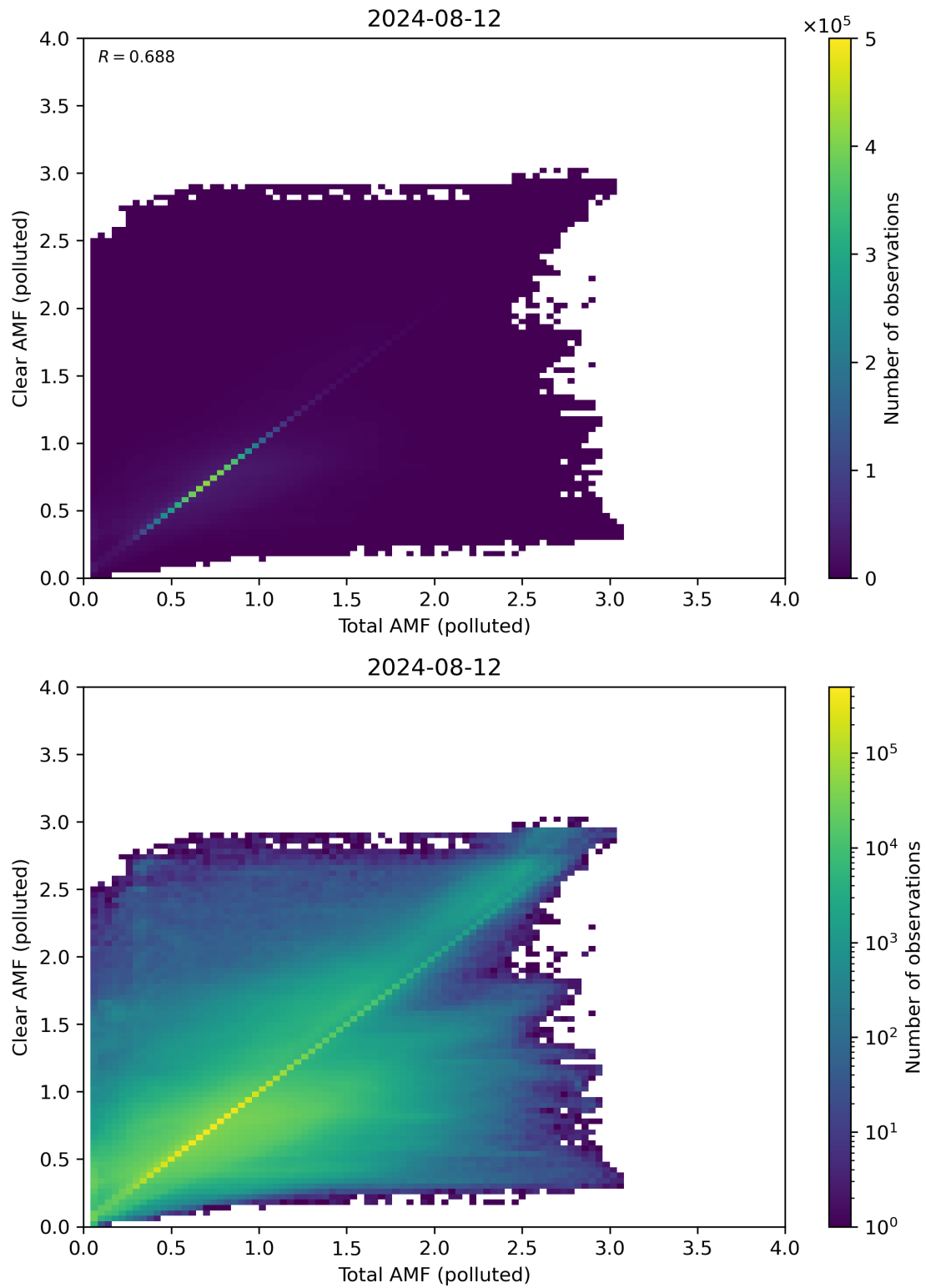
Figure 271: Scatter density plot of “Total AMF (polluted)” against “Clear AMF (polluted)” for 2024-08-12 to 2024-08-13.
