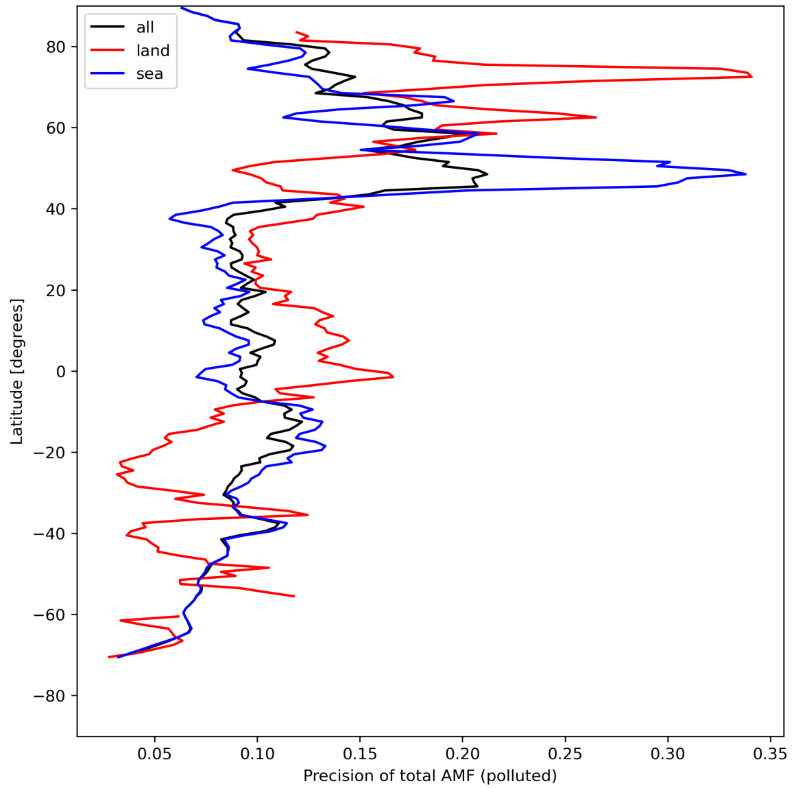
Figure 49: Zonal average of “Precision of total AMF (polluted)” for 2024-08-12 to 2024-08-13.
