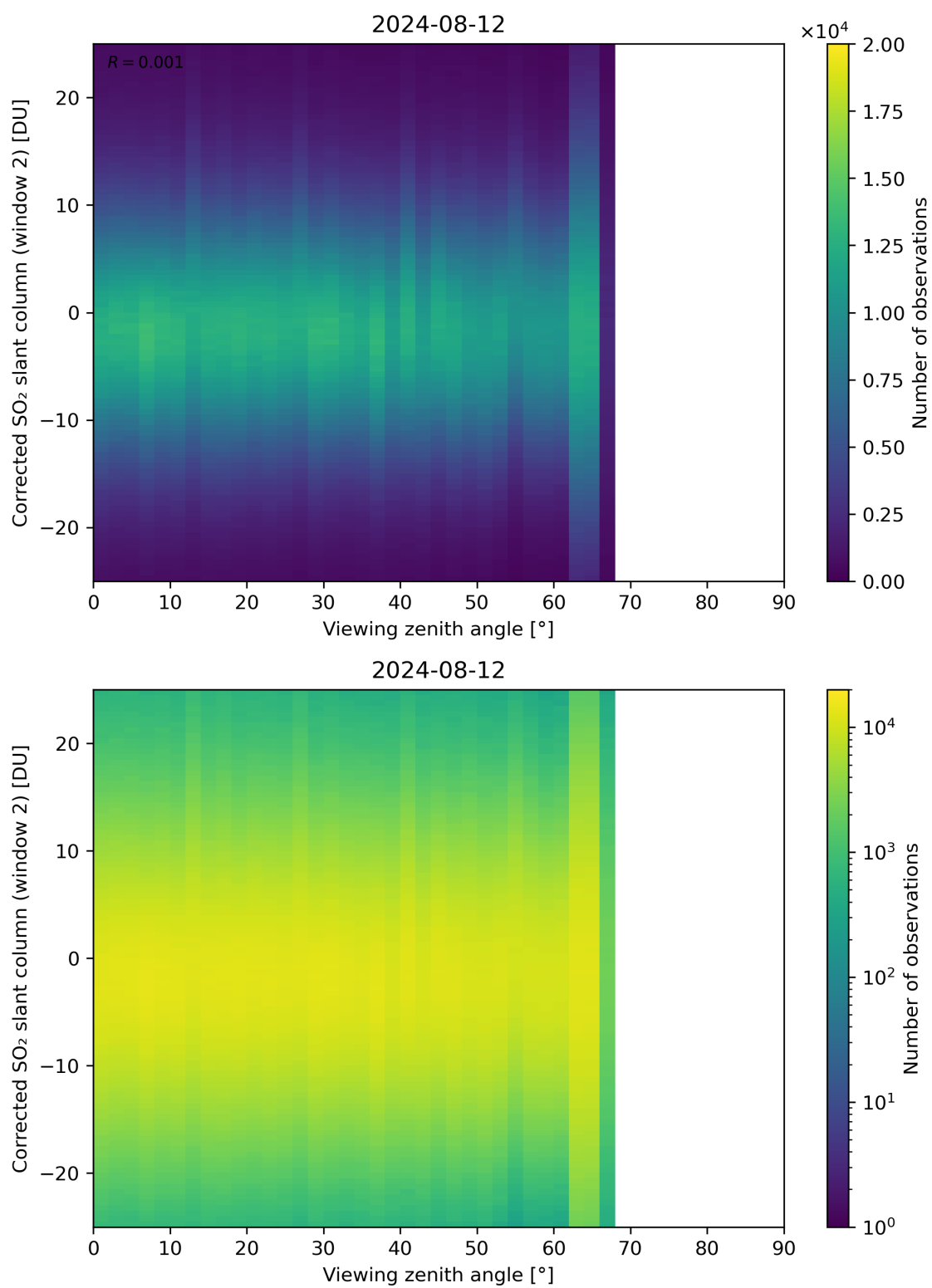
Figure 318: Scatter density plot of “Viewing zenith angle” against “Corrected SO 2 slant column (window 2)” for 2024-08-12 to 2024-08-13.
