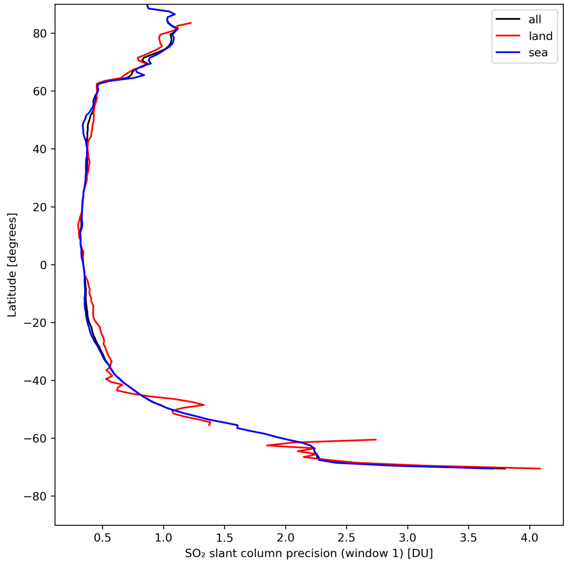
Figure 34: Zonal average of “SO 2 slant column precision (window 1)” for 2024-08-12 to 2024-08-14.
