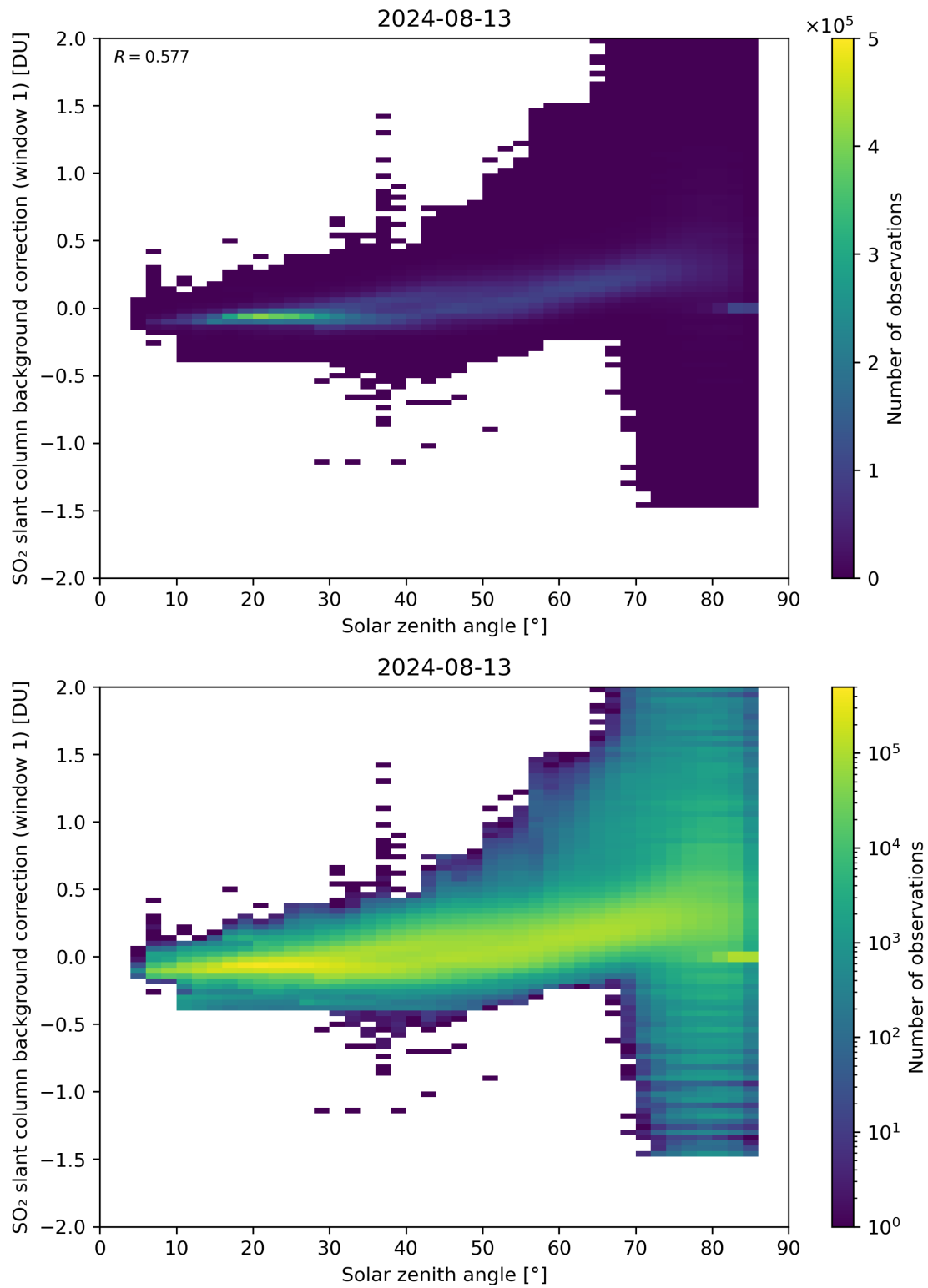
Figure 158: Scatter density plot of “Solar zenith angle” against “SO 2 slant column background correction (window 1)” for 2024-08-12 to 2024-08-14.
