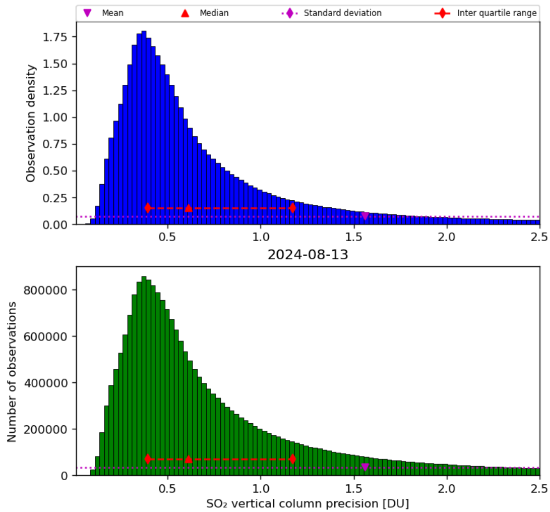
Figure 54: Histogram of “SO 2 vertical column precision” for 2024-08-12 to 2024-08-14
