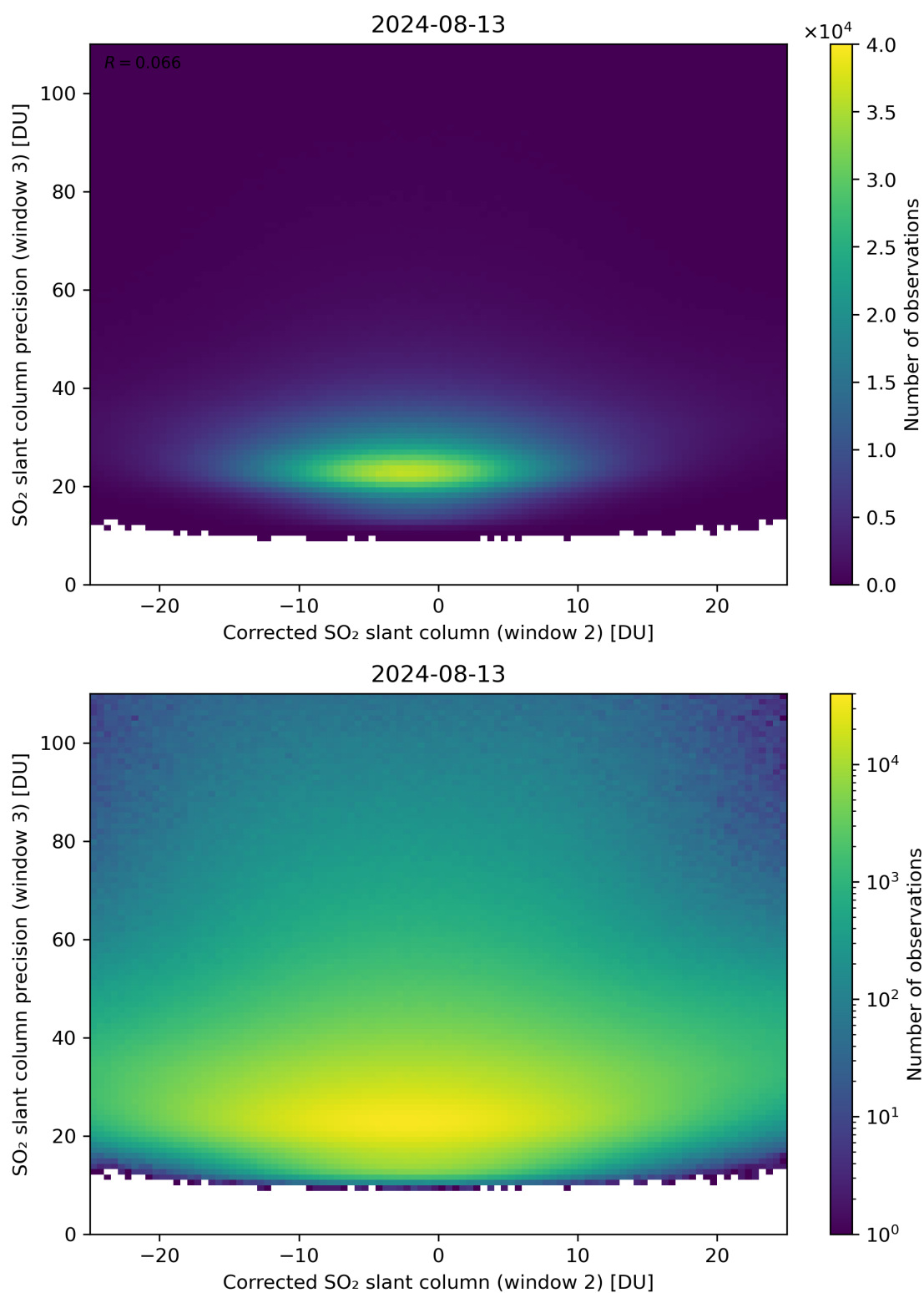
Figure 202: Scatter density plot of “Corrected SO 2 slant column (window 2)” against “SO 2 slant column precision (window 3)” for 2024-08-12 to 2024-08-14.
