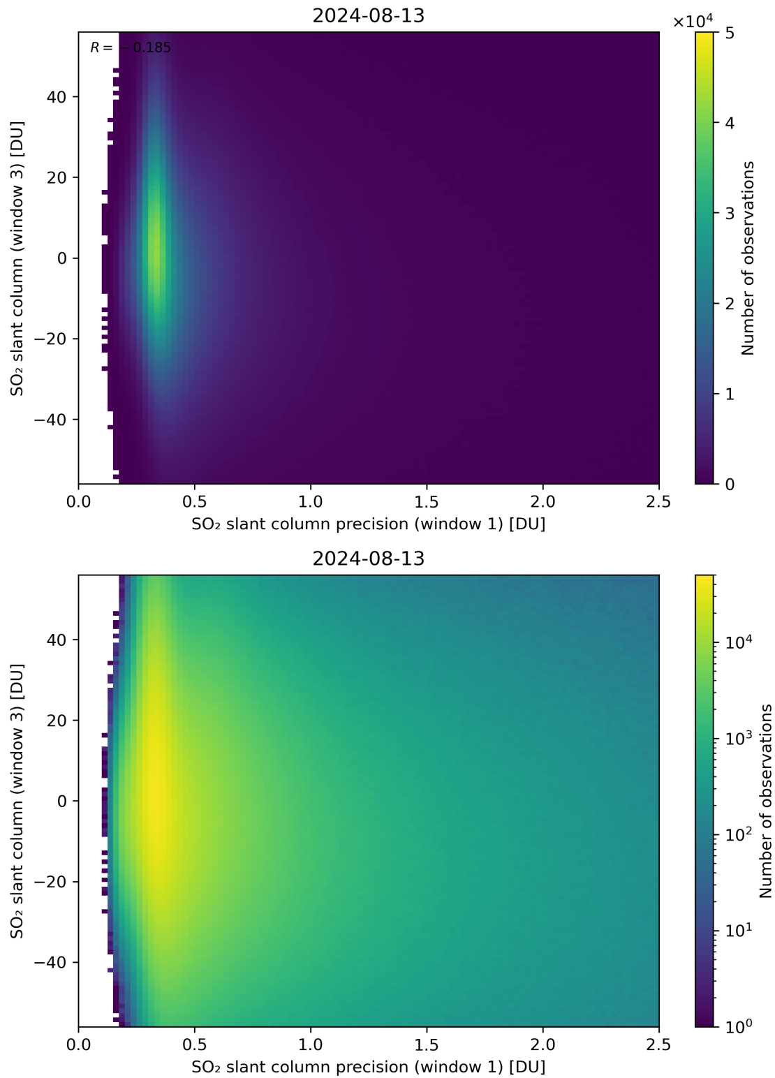
Figure 228: Scatter density plot of “SO 2 slant column precision (window 1)” against “SO 2 slant column (window 3)” for 2024-08-12 to 2024-08-14.
