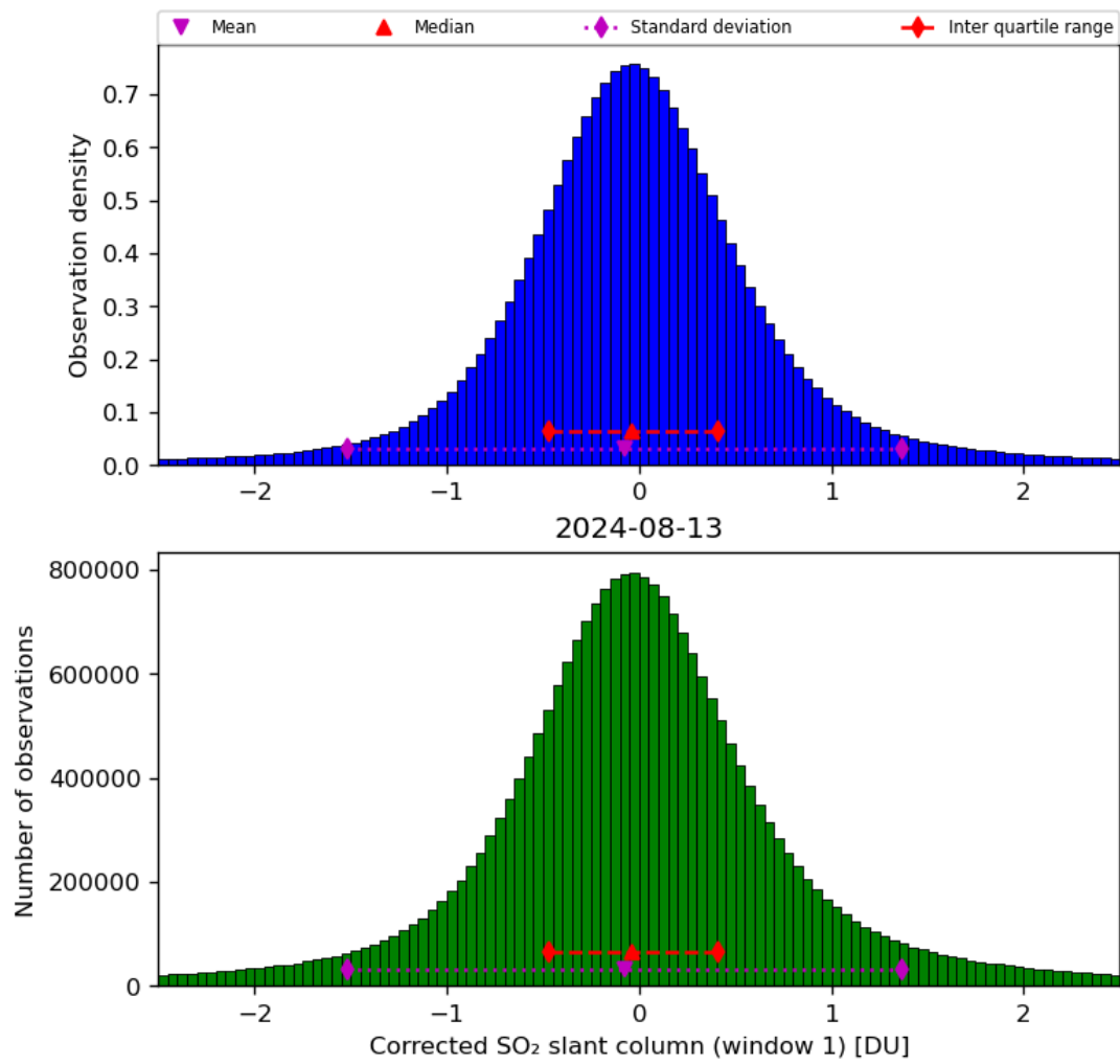
Figure 58: Histogram of “Corrected SO 2 slant column (window 1)” for 2024-08-12 to 2024-08-14
