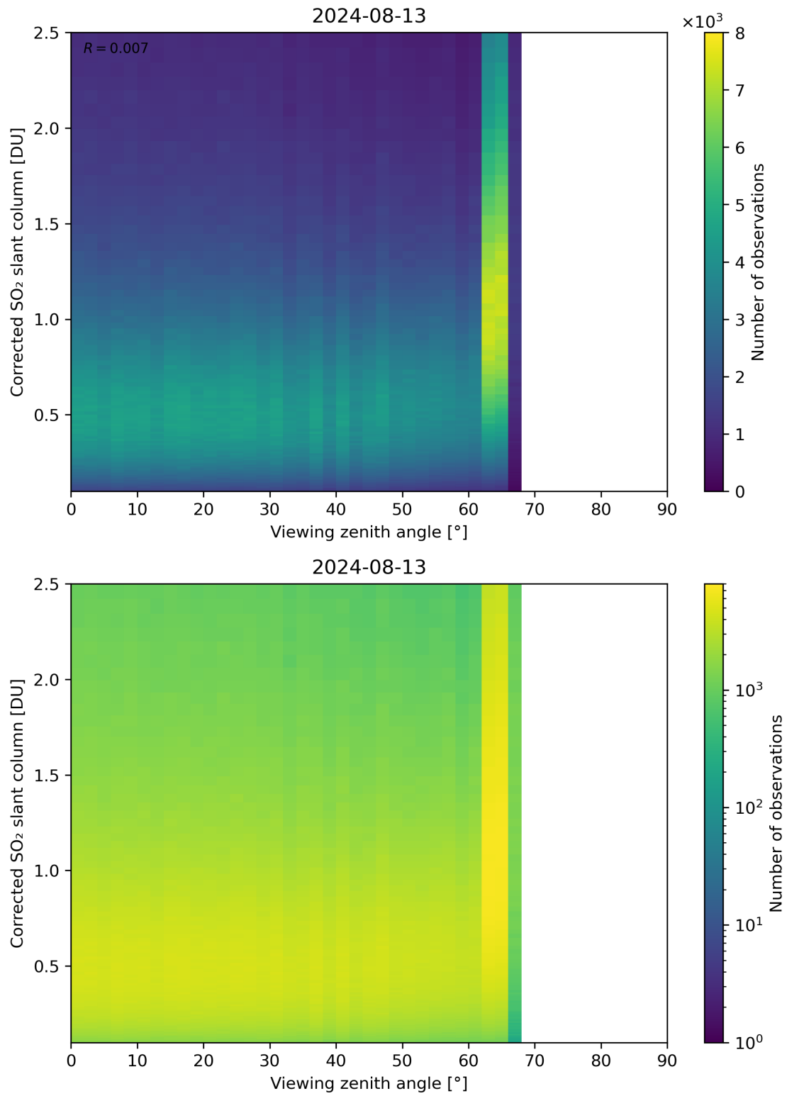
Figure 317: Scatter density plot of “Viewing zenith angle” against “Corrected SO 2 slant column” for 2024-08-12 to 2024-08-14.
