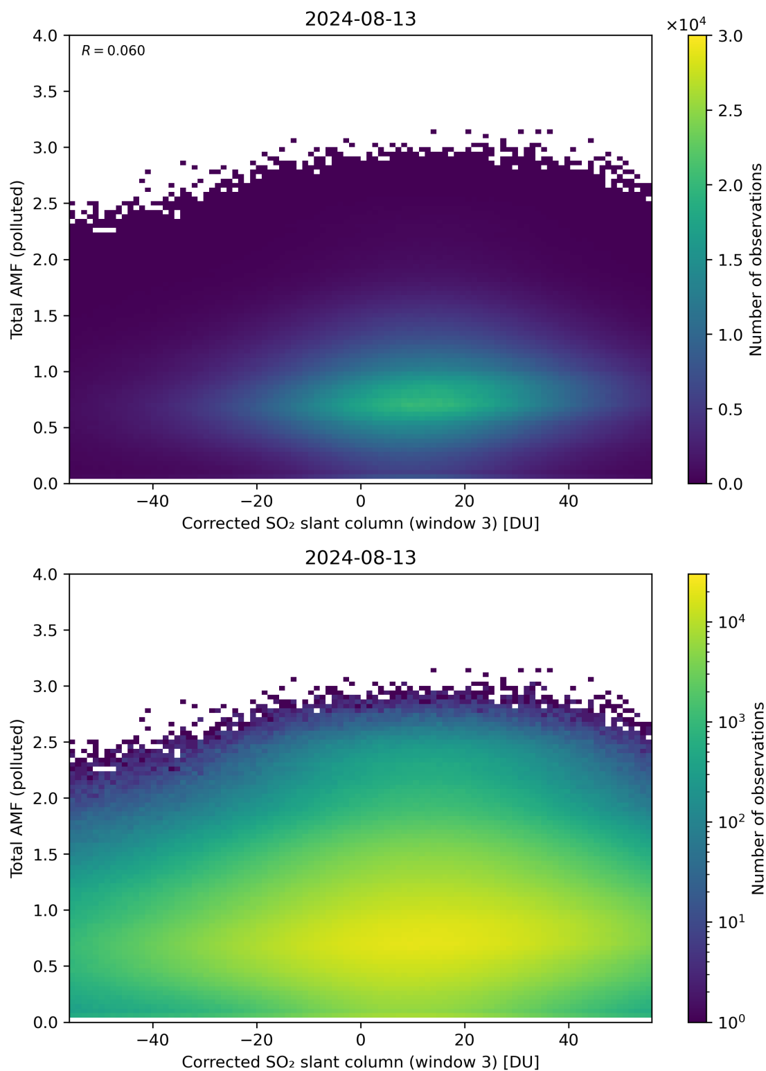
Figure 210: Scatter density plot of “Corrected SO 2 slant column (window 3)” against “Total AMF (polluted)” for 2024-08-12 to 2024-08-14.
