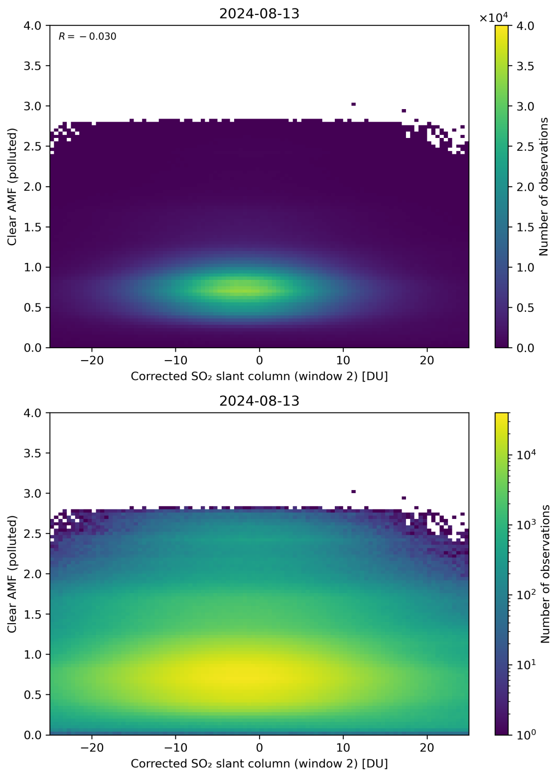
Figure 199: Scatter density plot of “Corrected SO 2 slant column (window 2)” against “Clear AMF (polluted)” for 2024-08-12 to 2024-08-14.
