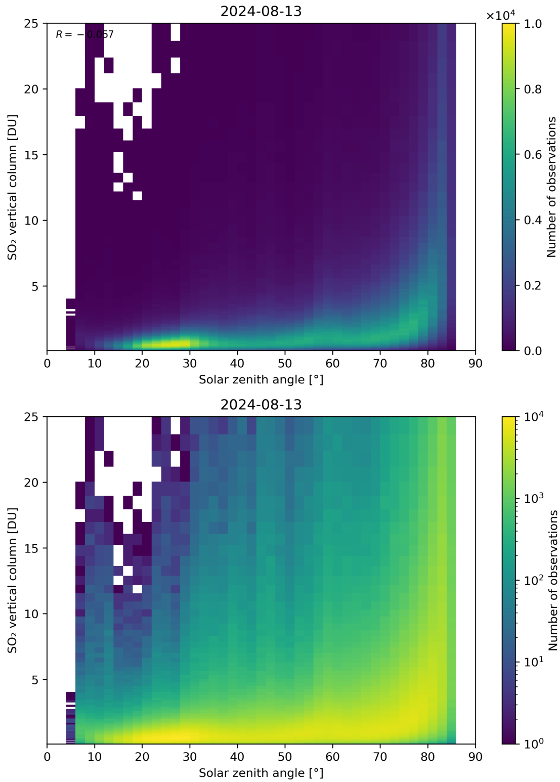
Figure 176: Scatter density plot of “Solar zenith angle” against “SO 2 vertical column” for 2024-08-12 to 2024-08-14.
