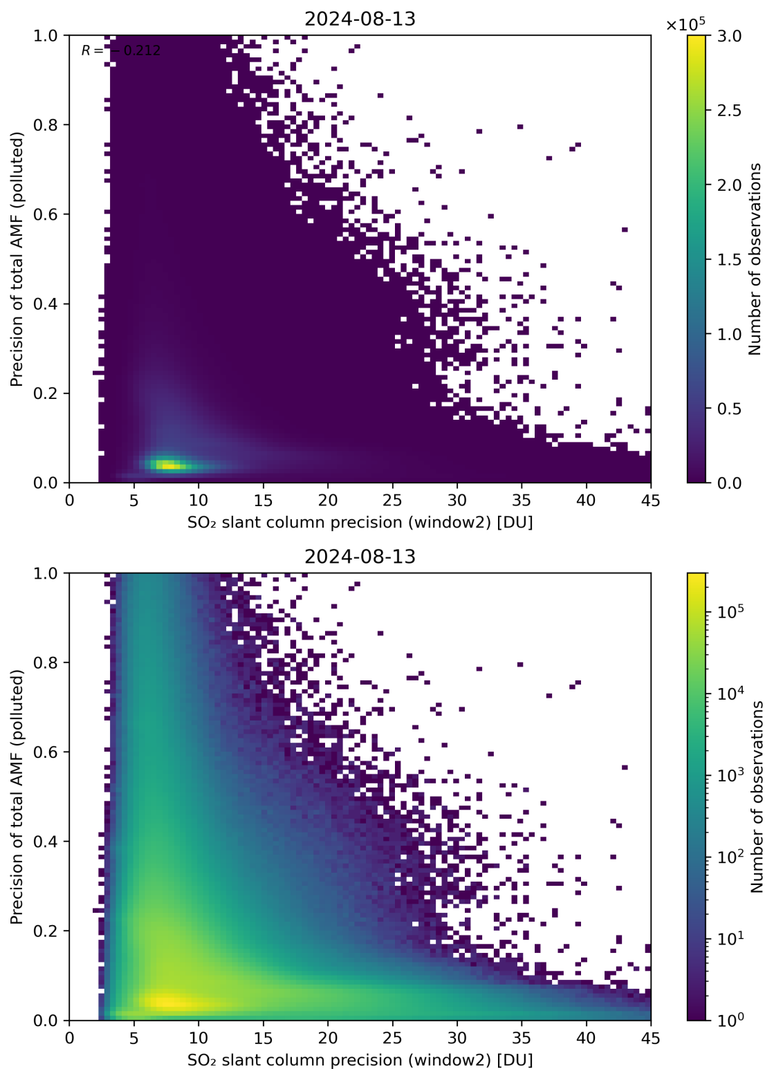
Figure 252: Scatter density plot of “SO 2 slant column precision (window2)” against “Precision of total AMF (polluted)” for 2024-08-12 to 2024-08-14.
