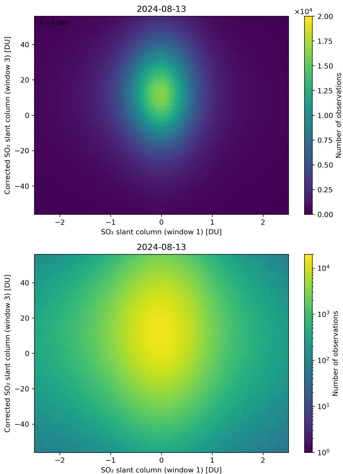
Figure 234: Scatter density plot of “SO 2 slant column (window 1)” against “Corrected SO 2 slant column (window 3)” for 2024-08-12 to 2024-08-14.
