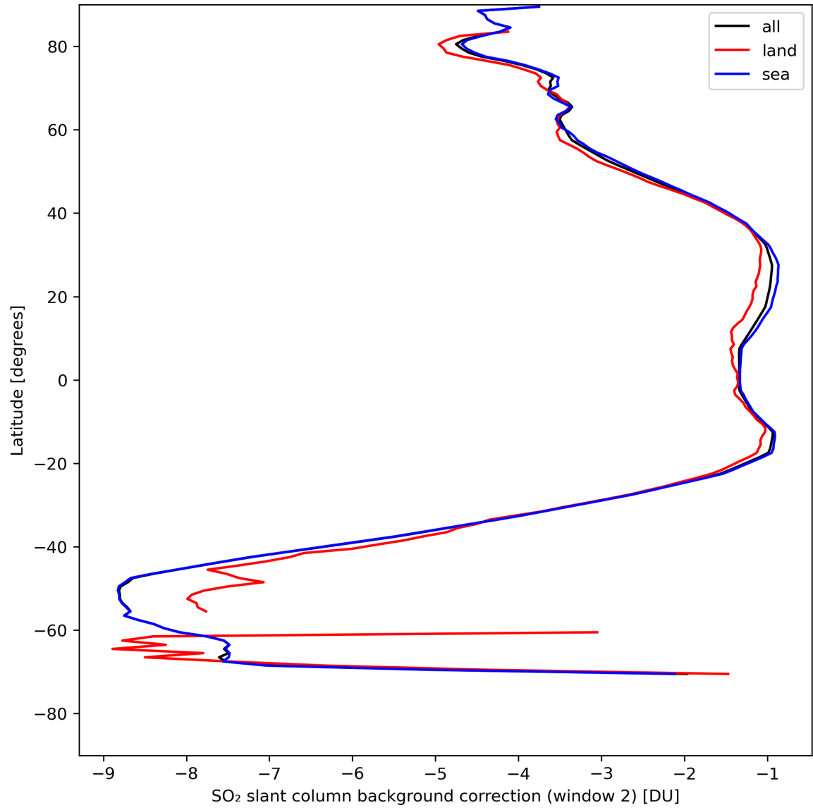
Figure 40: Zonal average of “SO 2 slant column background correction (window 2)” for 2024-08-12 to 2024-08-14.
