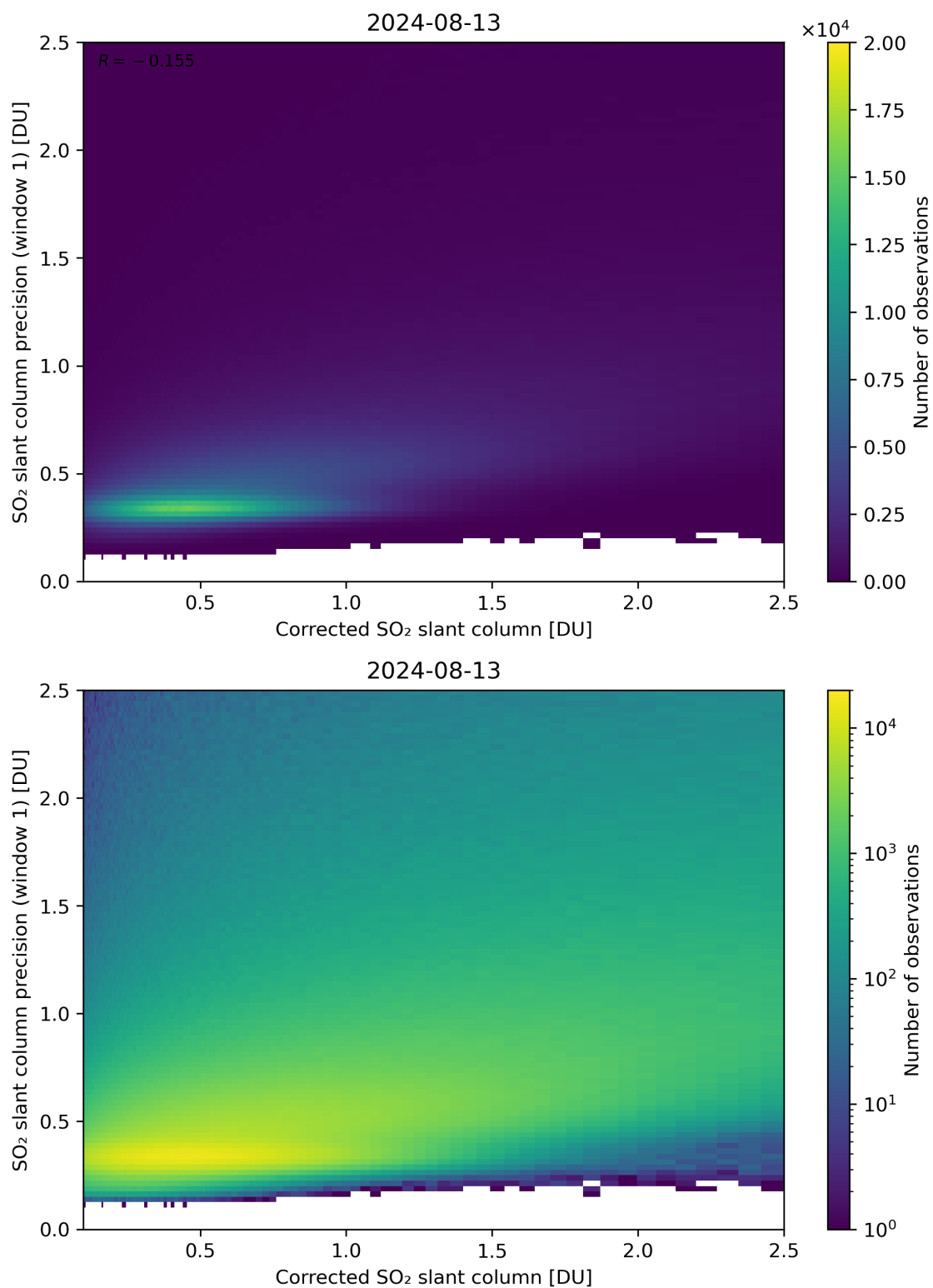
Figure 188: Scatter density plot of “Corrected SO 2 slant column” against “SO 2 slant column precision (window 1)” for 2024-08-12 to 2024-08-14.
