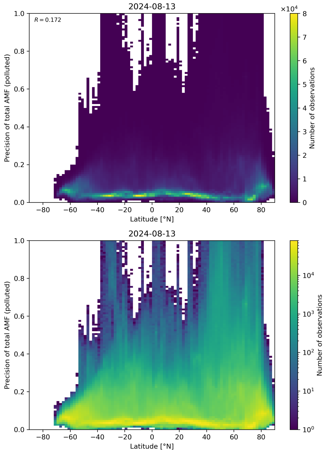
Figure 155: Scatter density plot of “Latitude” against “Precision of total AMF (polluted)” for 2024-08-12 to 2024-08-14.
