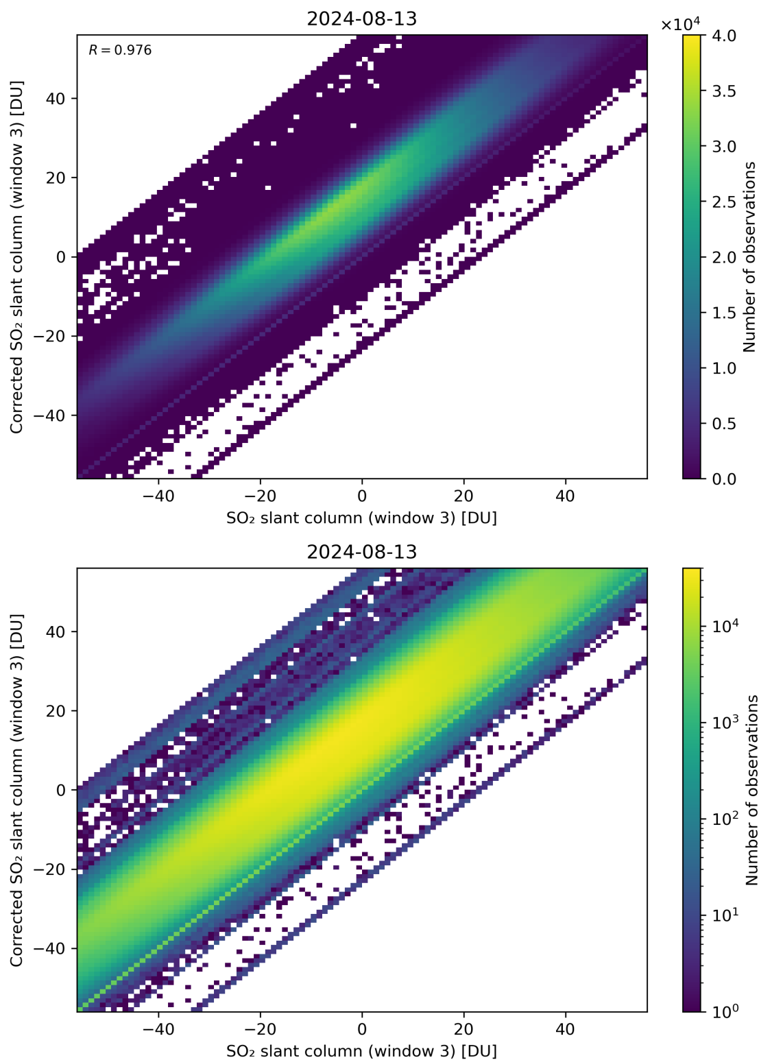
Figure 266: Scatter density plot of “SO 2 slant column (window 3)” against “Corrected SO 2 slant column (window 3)” for 2024-08-12 to 2024-08-14.
