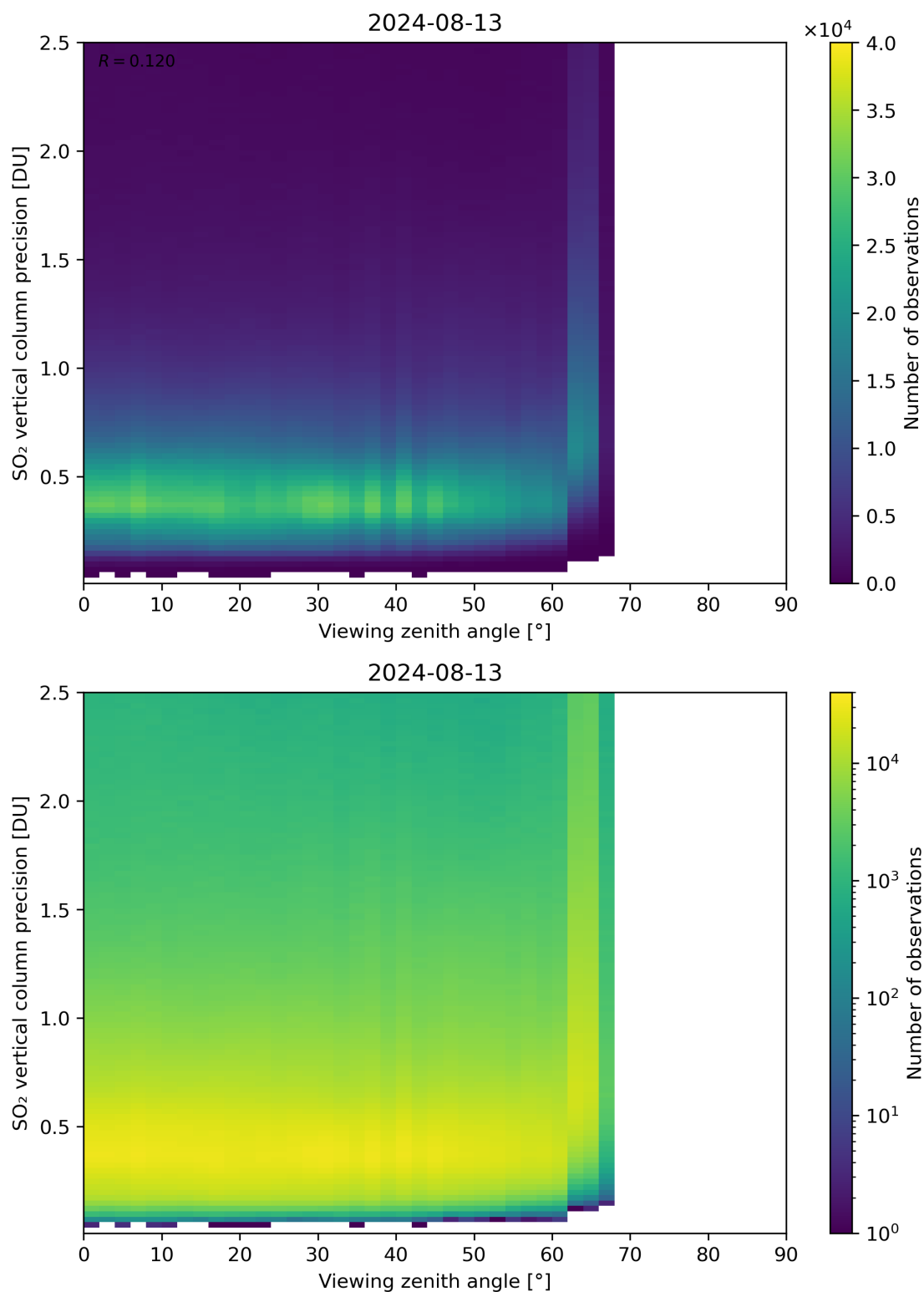
Figure 328: Scatter density plot of “Viewing zenith angle” against “SO 2 vertical column precision” for 2024-08-12 to 2024-08-14.
