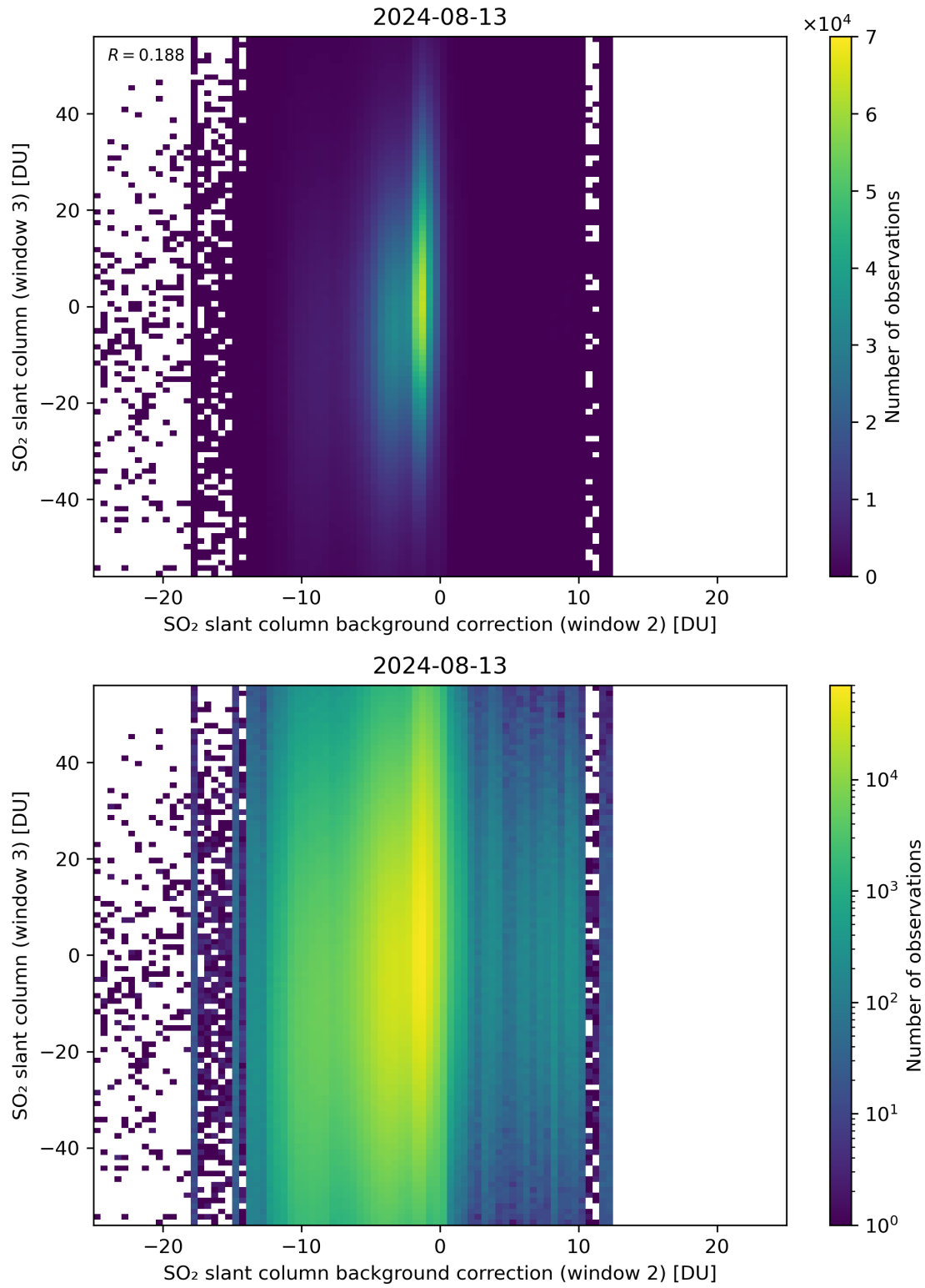
Figure 117: Scatter density plot of “SO 2 slant column background correction (window 2)” against “SO 2 slant column (window 3)” for 2024-08-12 to 2024-08-14.
