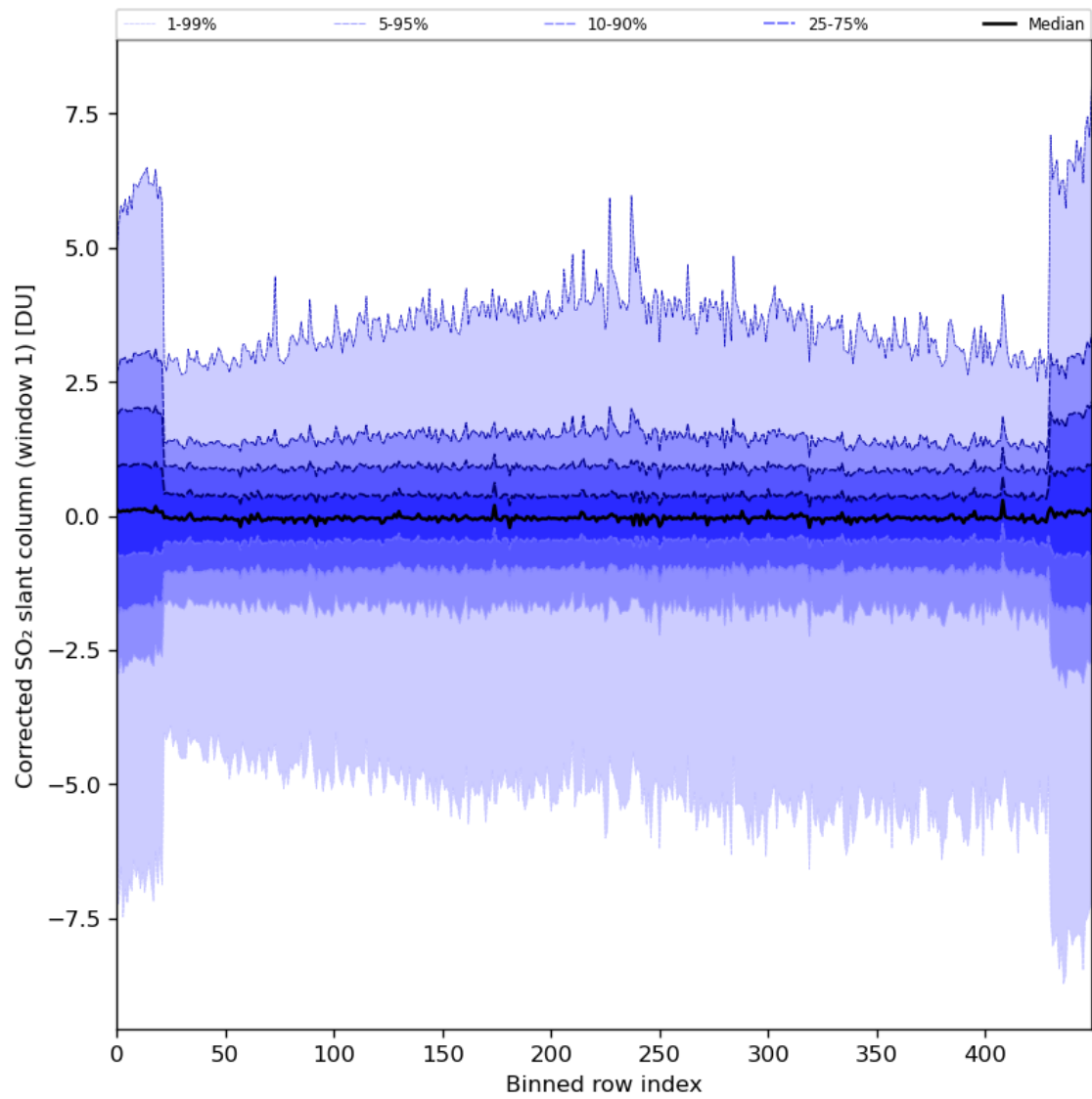
Figure 81: Along track statistics of “Corrected SO 2 slant column (window 1)” for 2024-08-12 to 2024-08-14
