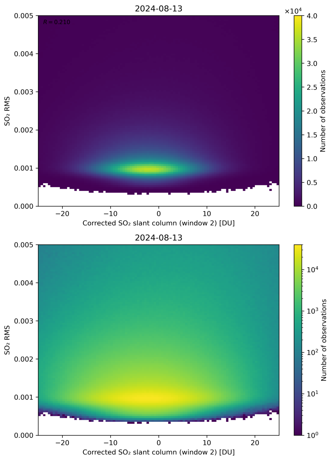
Figure 198: Scatter density plot of “Corrected SO 2 slant column (window 2)” against “SO 2 RMS” for 2024-08-12 to 2024-08-14.
