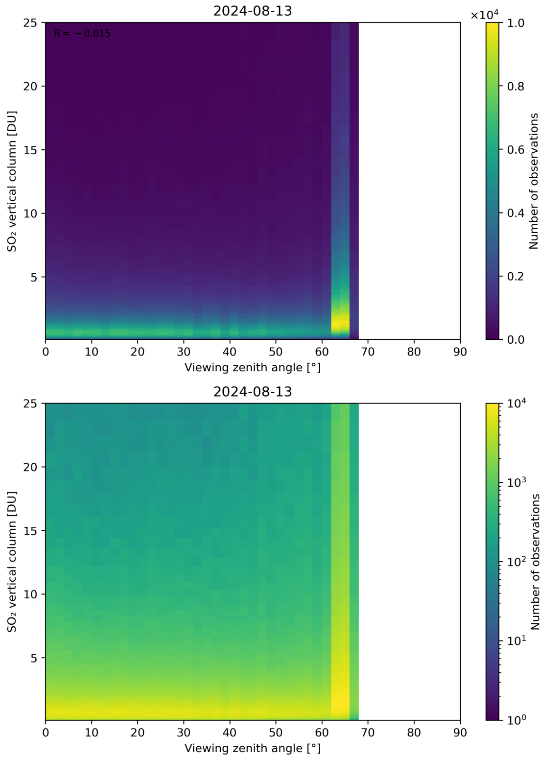
Figure 327: Scatter density plot of “Viewing zenith angle” against “SO 2 vertical column” for 2024-08-12 to 2024-08-14.
