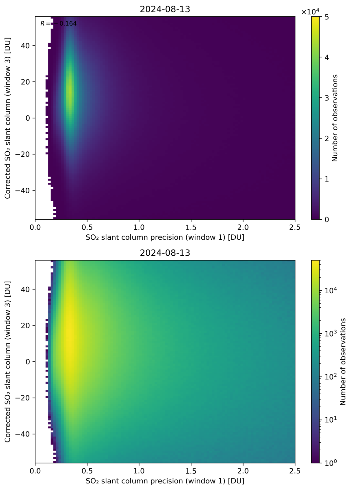
Figure 226: Scatter density plot of “SO 2 slant column precision (window 1)” against “Corrected SO 2 slant column (window 3)” for 2024-08-12 to 2024-08-14.
