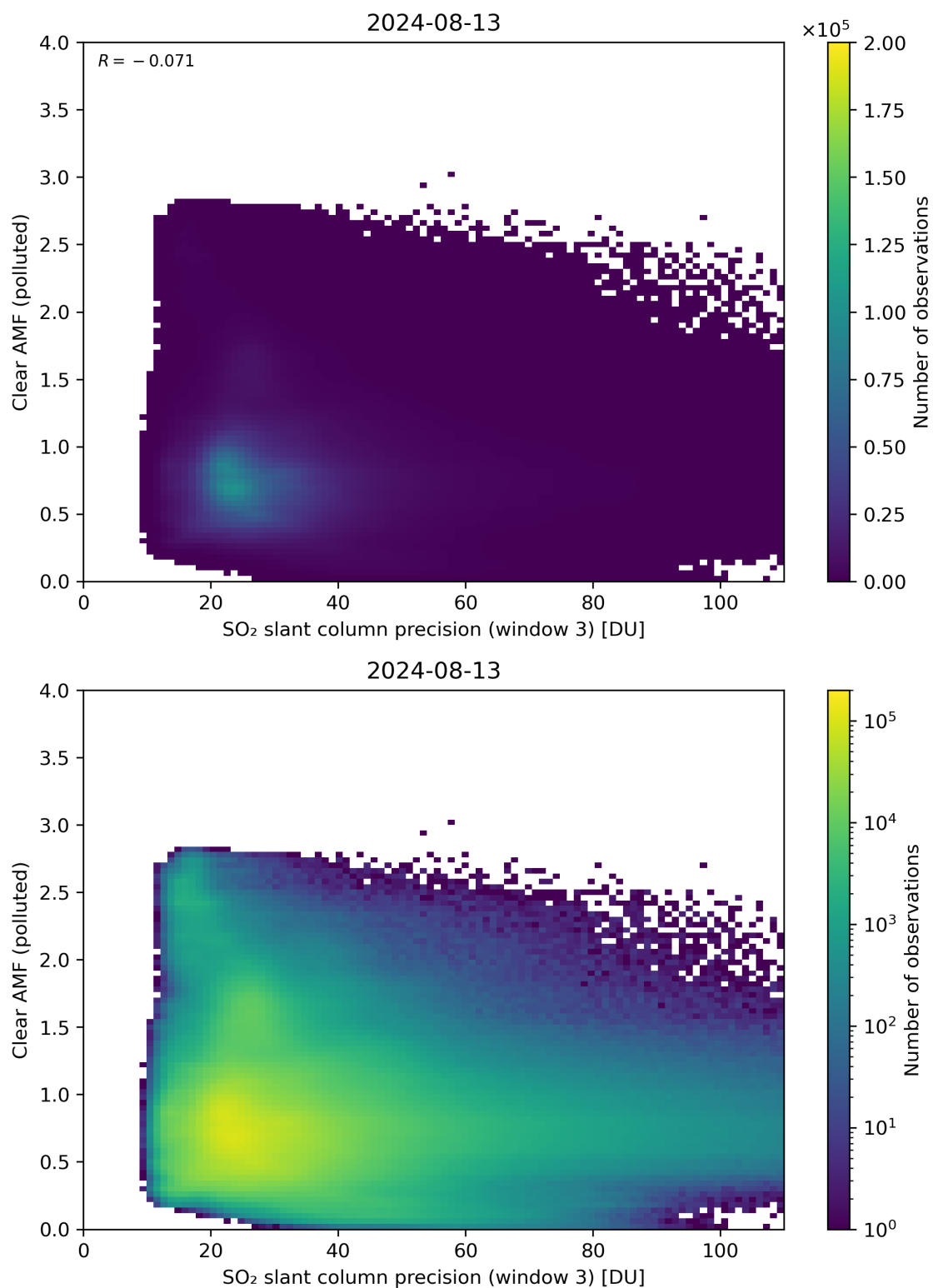
Figure 261: Scatter density plot of “SO 2 slant column precision (window 3)” against “Clear AMF (polluted)” for 2024-08-12 to 2024-08-14.
