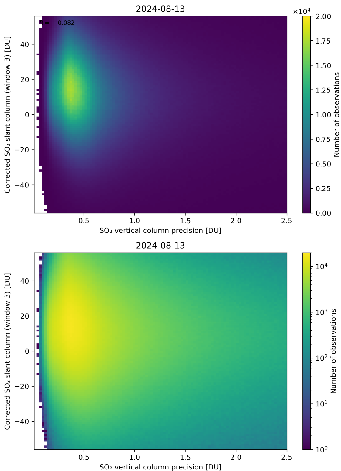
Figure 288: Scatter density plot of “SO 2 vertical column precision” against “Corrected SO 2 slant column (window 3)” for 2024-08-12 to 2024-08-14.
