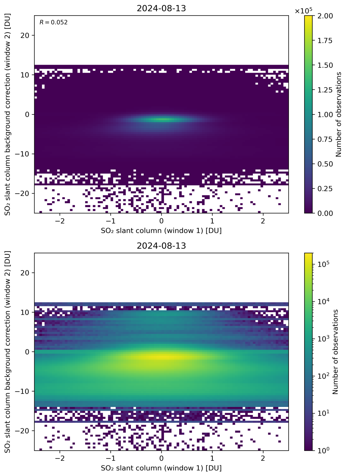
Figure 213: Scatter density plot of “SO 2 slant column (window 1)” against “SO 2 slant column background correction (window 2)” for 2024-08-12 to 2024-08-14.
