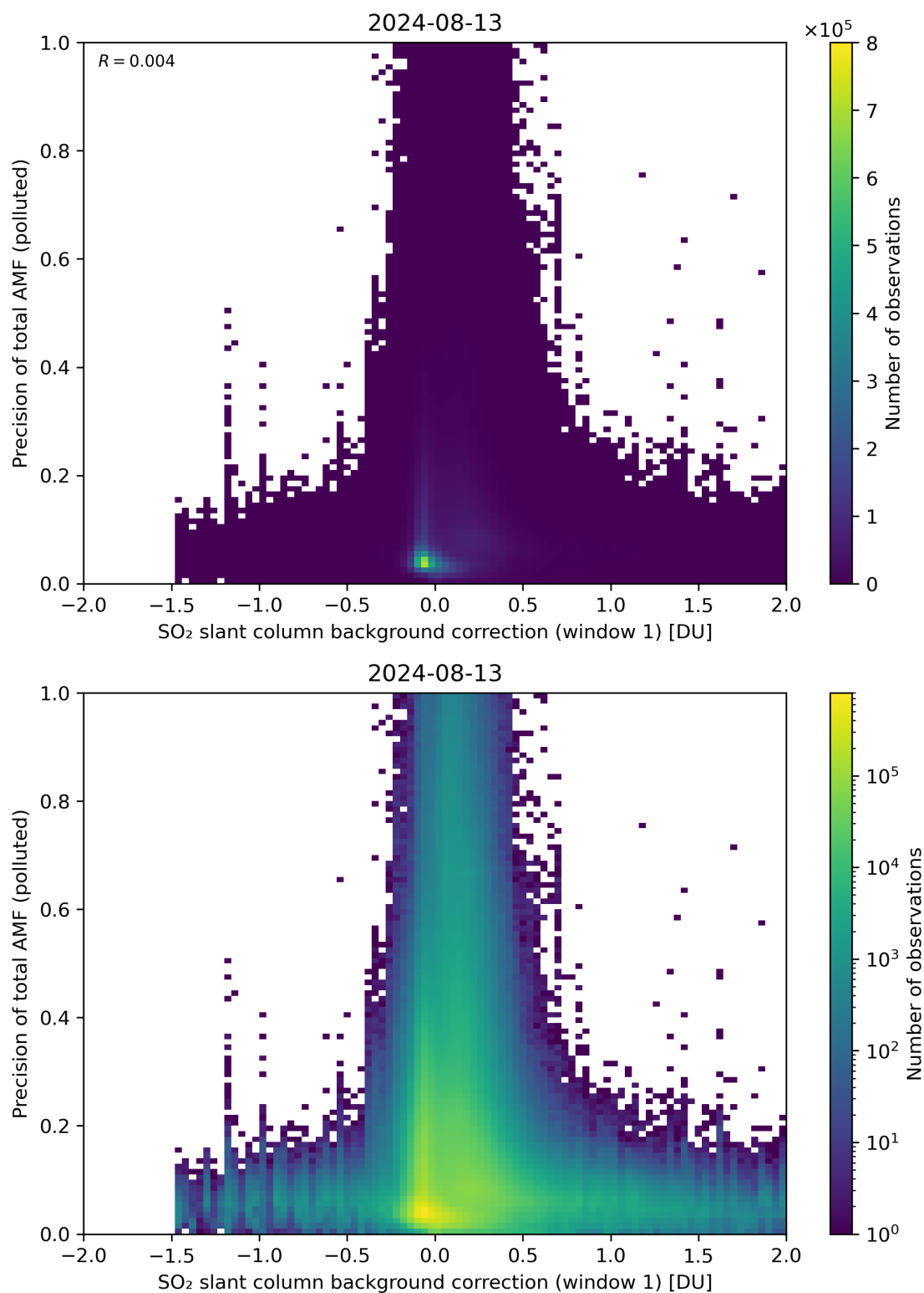
Figure 110: Scatter density plot of “SO 2 slant column background correction (window 1)” against “Precision of total AMF (polluted)” for 2024-08-12 to 2024-08-14.
