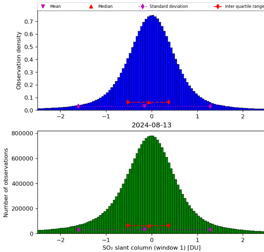
Figure 56: Histogram of “SO 2 slant column (window 1)” for 2024-08-12 to 2024-08-14
