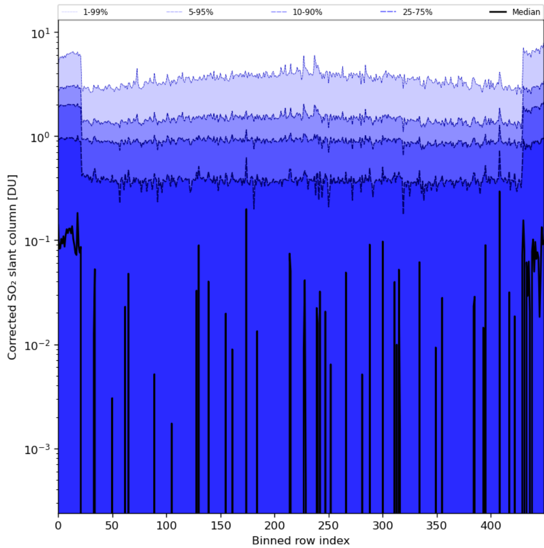
Figure 78: Along track statistics of “Corrected SO 2 slant column” for 2024-08-12 to 2024-08-14
