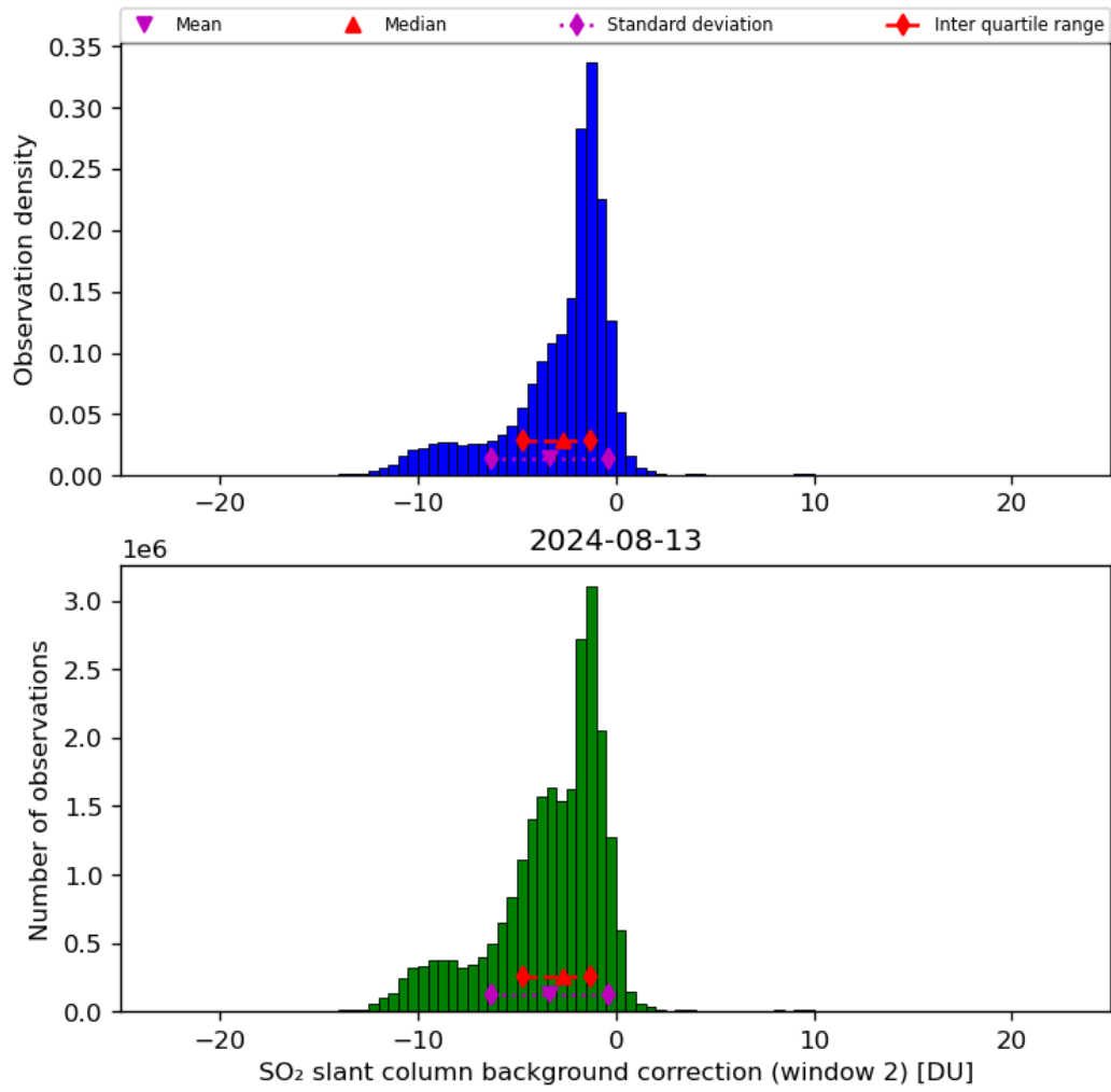
Figure 63: Histogram of “SO 2 slant column background correction (window 2)” for 2024-08-12 to 2024-08-14
