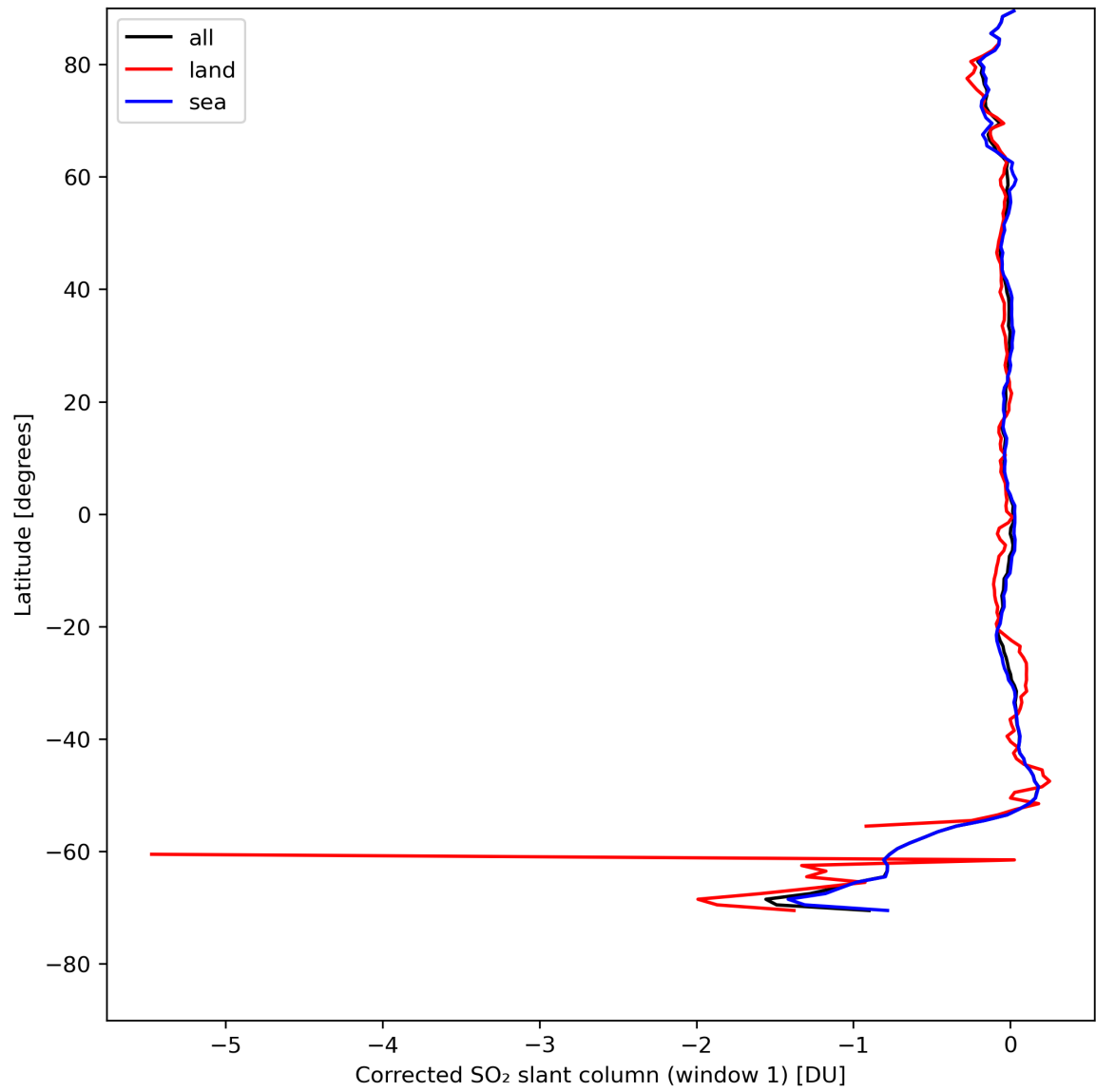
Figure 35: Zonal average of “Corrected SO 2 slant column (window 1)” for 2024-08-12 to 2024-08-14.
