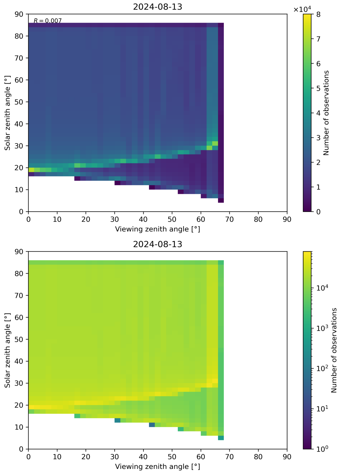
Figure 315: Scatter density plot of “Viewing zenith angle” against “Solar zenith angle” for 2024-08-12 to 2024-08-14.
