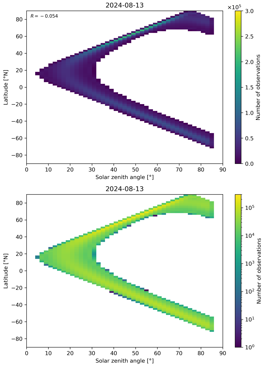
Figure 164: Scatter density plot of “Solar zenith angle” against “Latitude” for 2024-08-12 to 2024-08-14.
