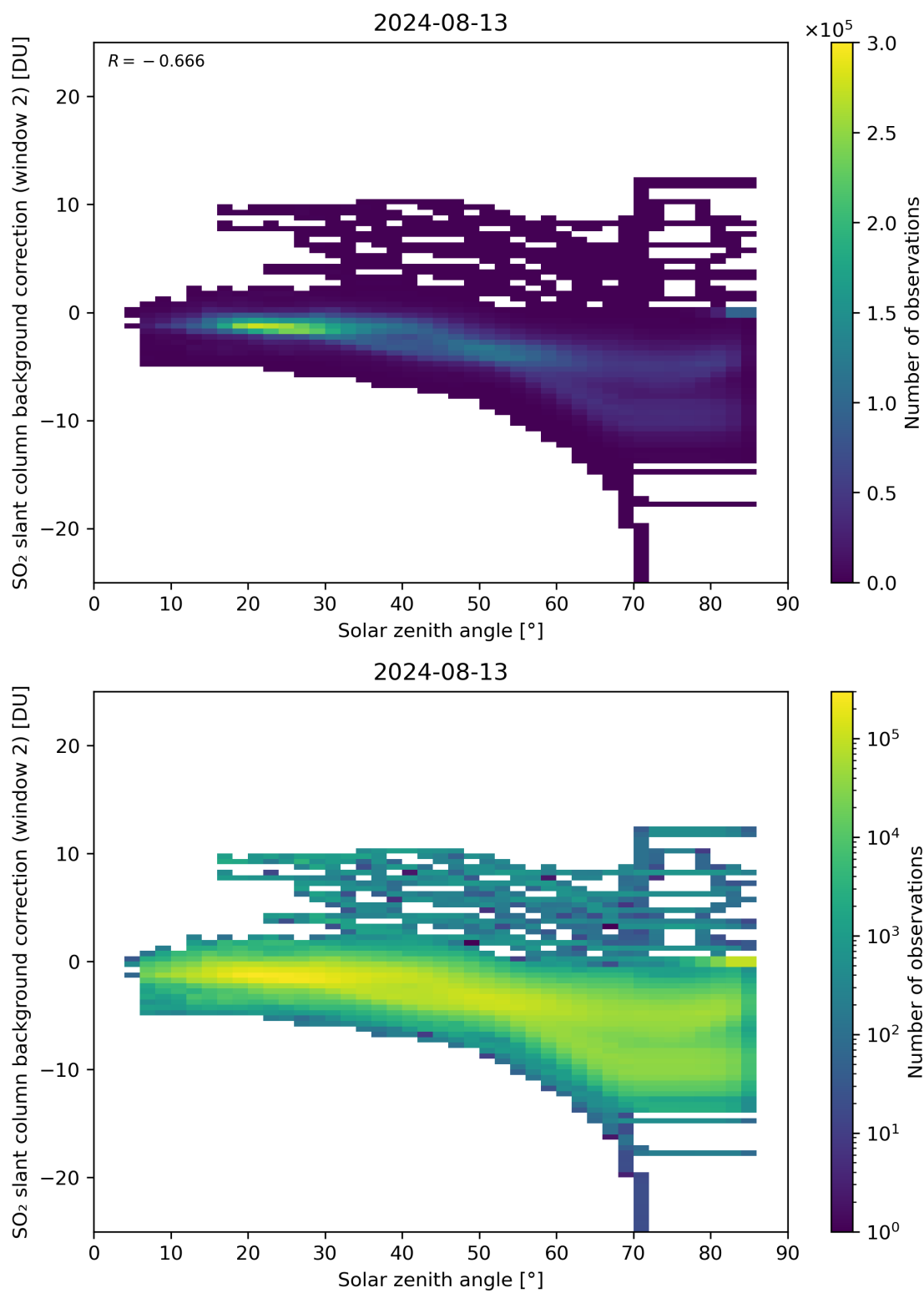
Figure 159: Scatter density plot of “Solar zenith angle” against “SO 2 slant column background correction (window 2)” for 2024-08-12 to 2024-08-14.
