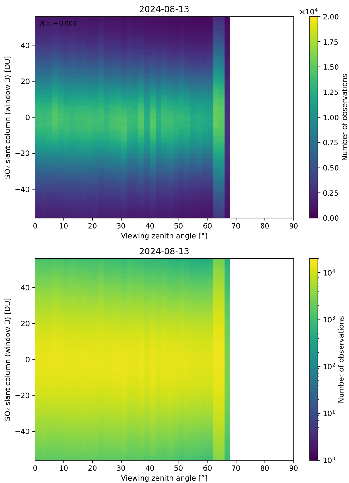
Figure 323: Scatter density plot of “Viewing zenith angle” against “SO 2 slant column (window 3)” for 2024-08-12 to 2024-08-14.
