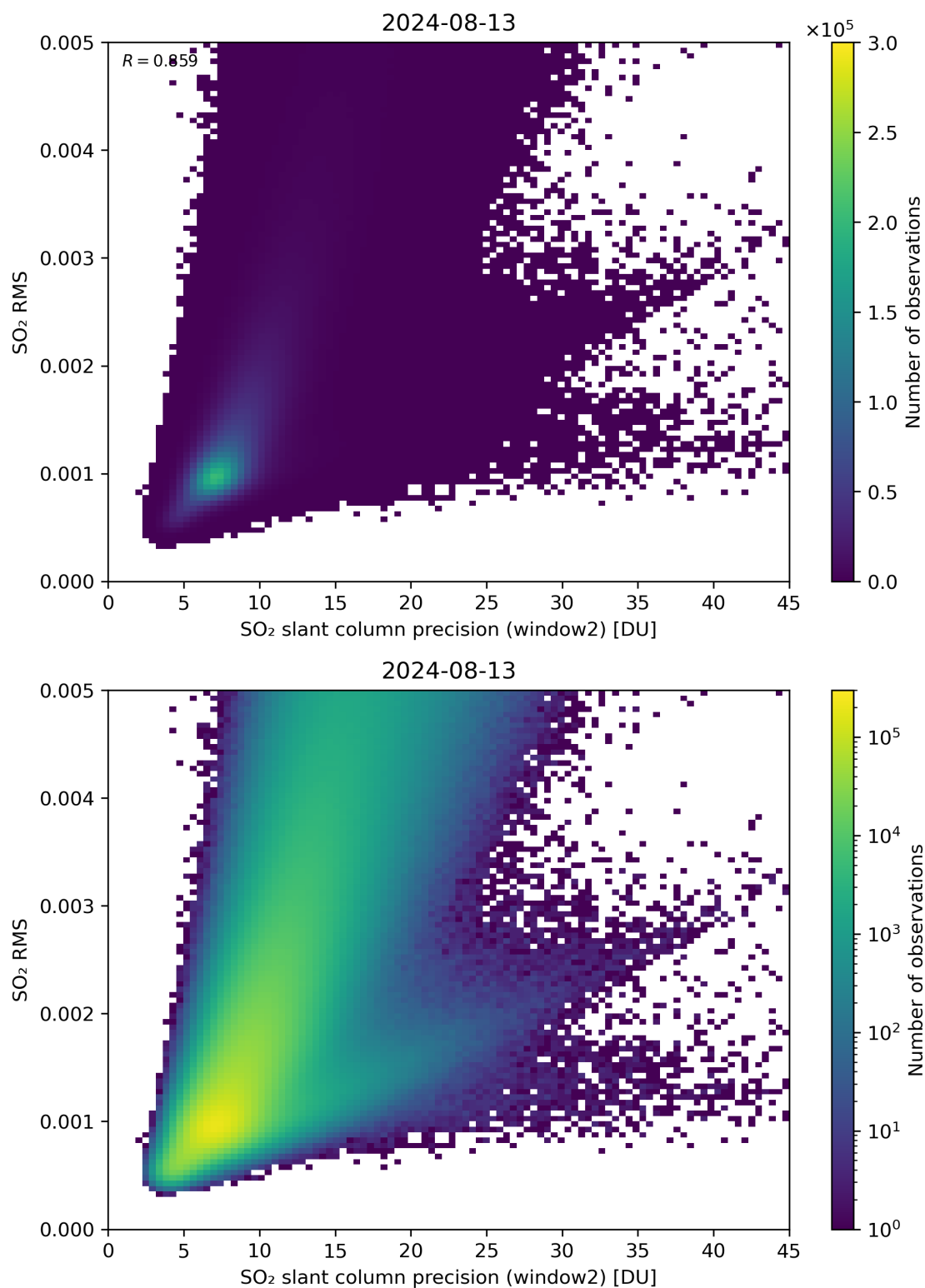
Figure 245: Scatter density plot of “SO 2 slant column precision (window2)” against “SO 2 RMS” for 2024-08-12 to 2024-08-14.
