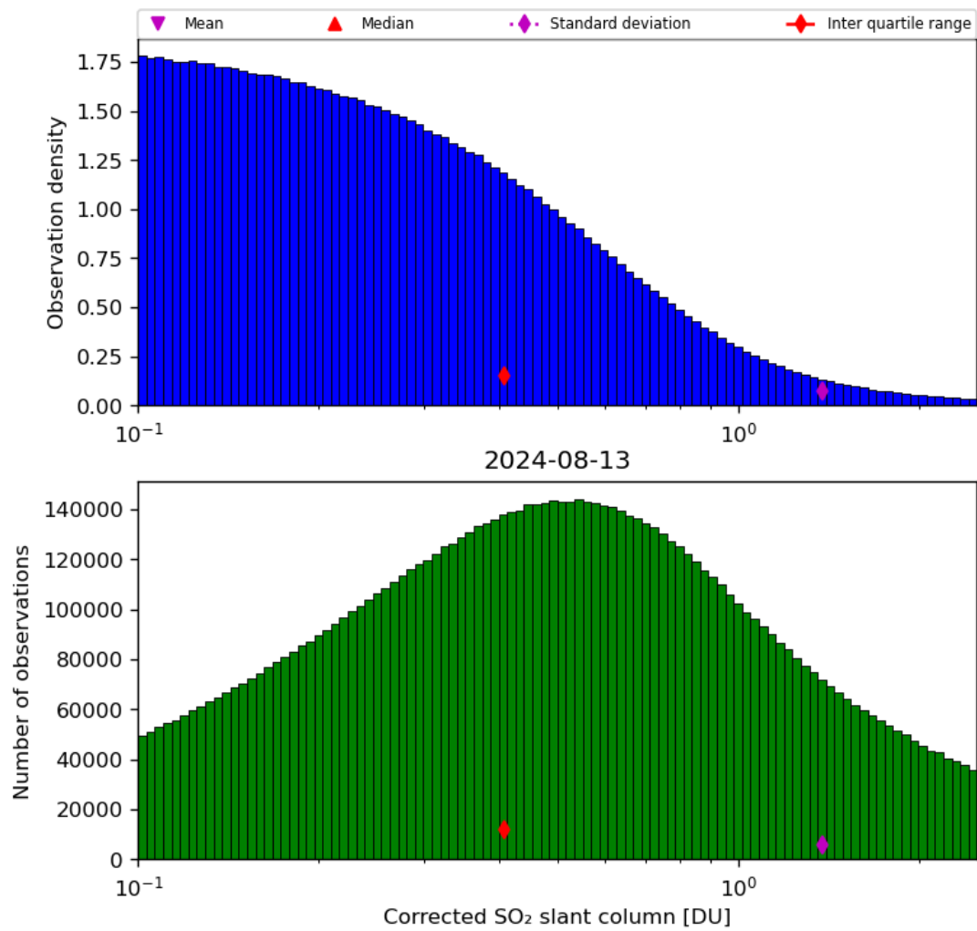
Figure 55: Histogram of “Corrected SO 2 slant column” for 2024-08-12 to 2024-08-14
