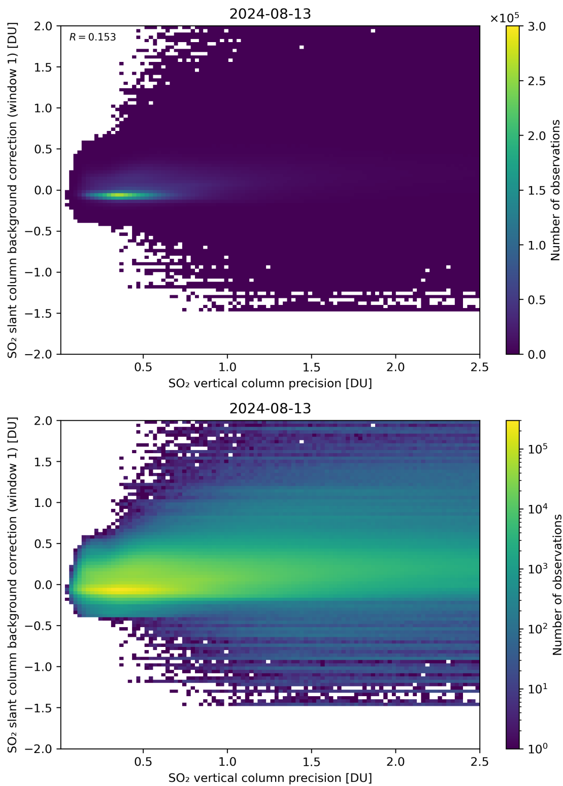
Figure 279: Scatter density plot of “SO 2 vertical column precision” against “SO 2 slant column background correction (window 1)” for 2024-08-12 to 2024-08-14.
