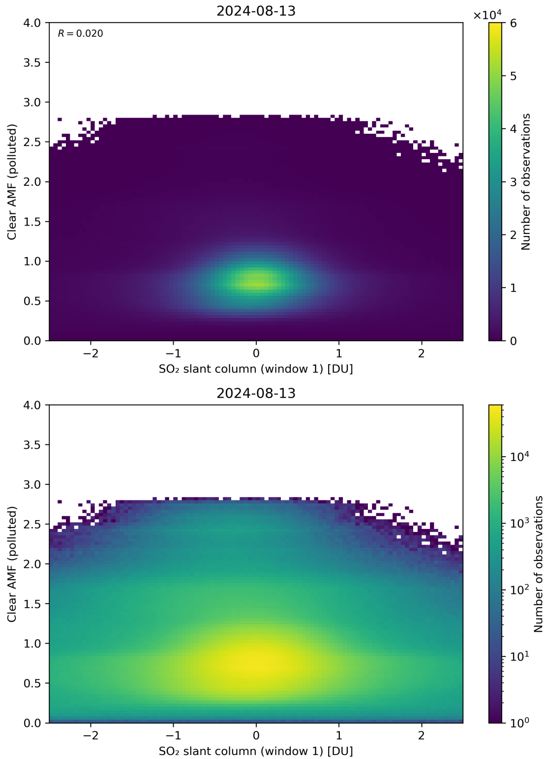
Figure 232: Scatter density plot of “SO 2 slant column (window 1)” against “Clear AMF (polluted)” for 2024-08-12 to 2024-08-14.
