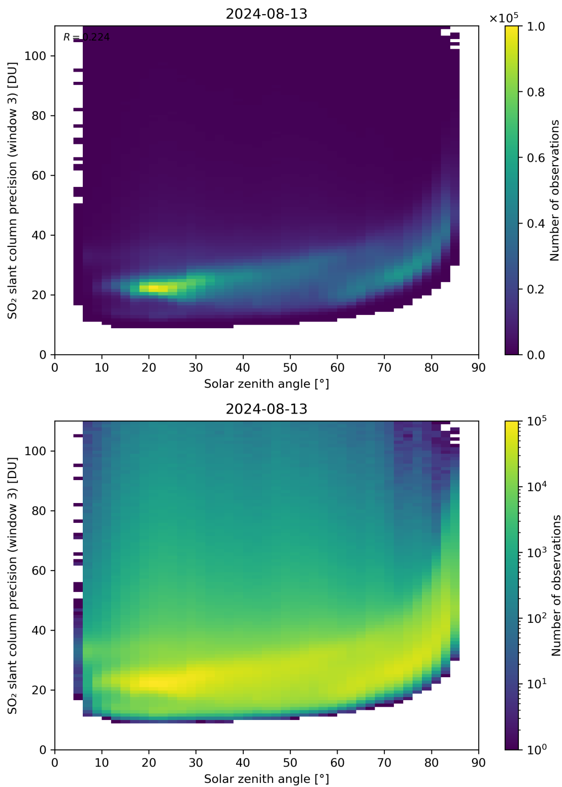
Figure 173: Scatter density plot of “Solar zenith angle” against “SO 2 slant column precision (window 3)” for 2024-08-12 to 2024-08-14.
