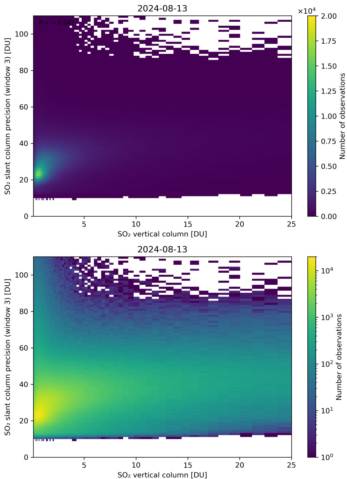
Figure 304: Scatter density plot of “SO 2 vertical column” against “SO 2 slant column precision (window 3)” for 2024-08-12 to 2024-08-14.
