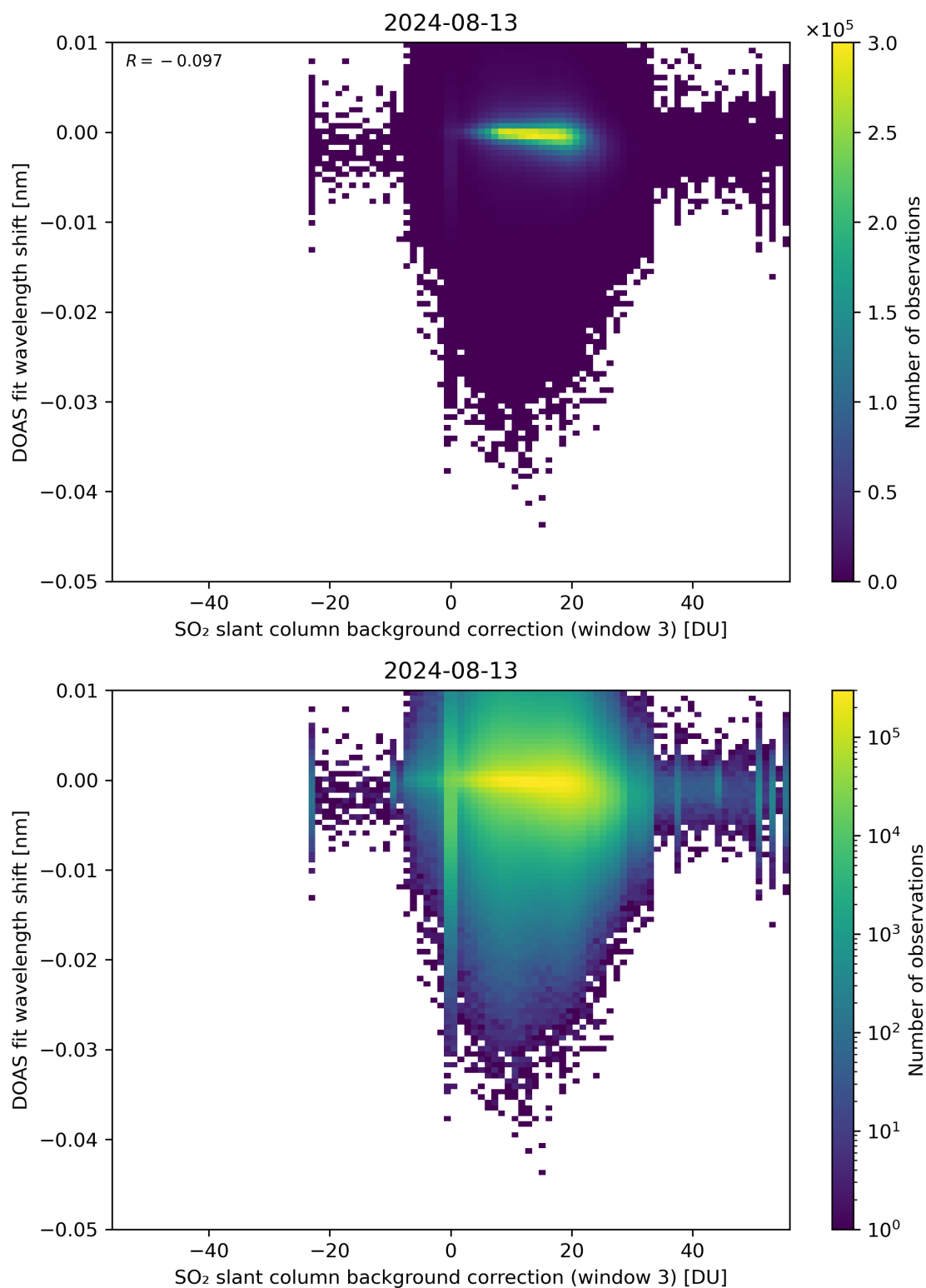
Figure 121: Scatter density plot of “SO 2 slant column background correction (window 3)” against “DOAS fit wavelength shift” for 2024-08-12 to 2024-08-14.
