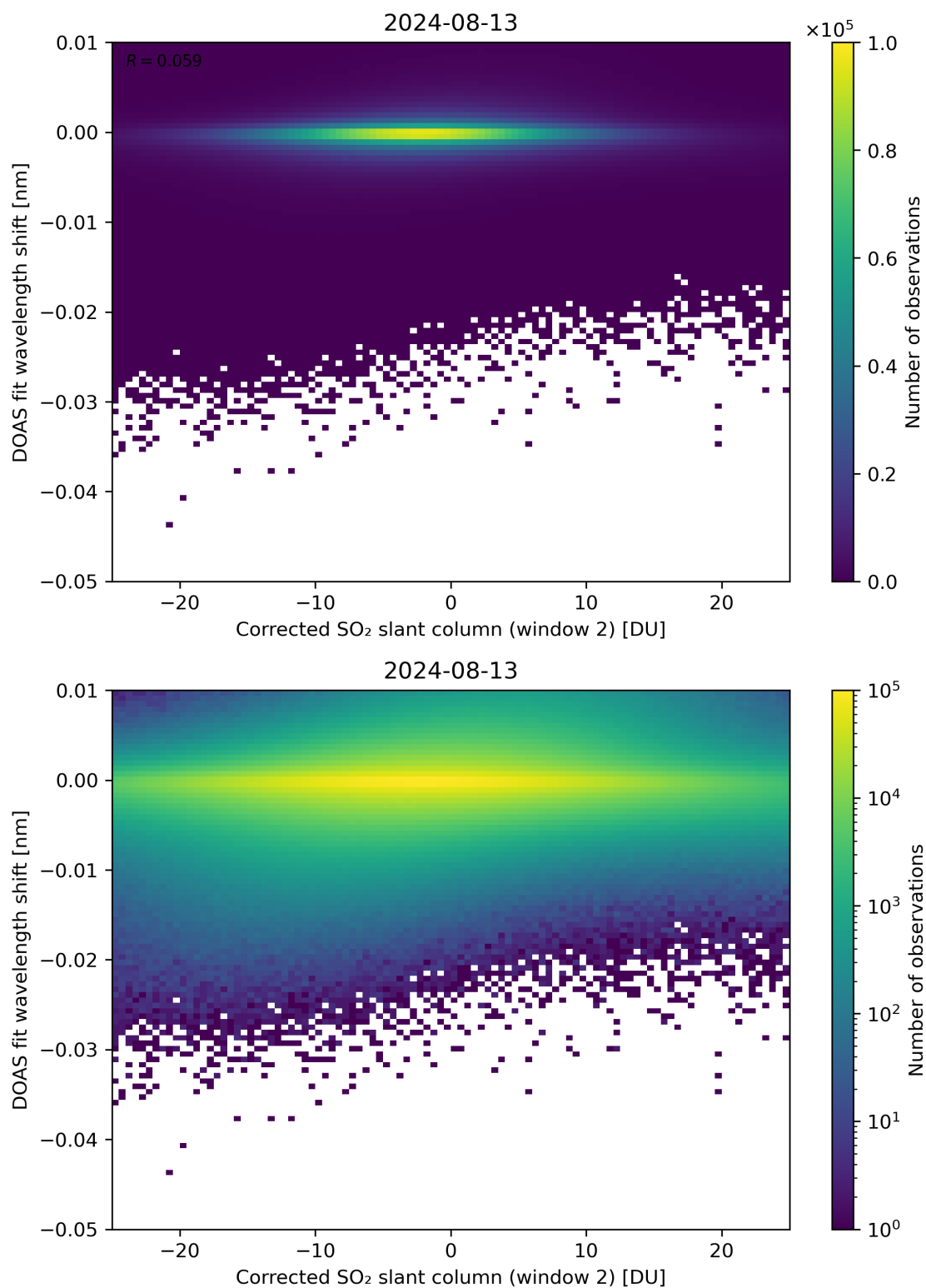
Figure 196: Scatter density plot of “Corrected SO 2 slant column (window 2)” against “DOAS fit wavelength shift” for 2024-08-12 to 2024-08-14.
