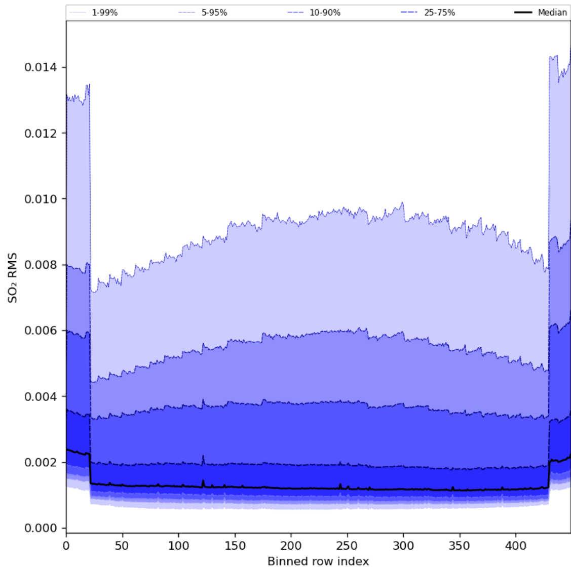
Figure 93: Along track statistics of “SO 2 RMS” for 2024-08-12 to 2024-08-14
