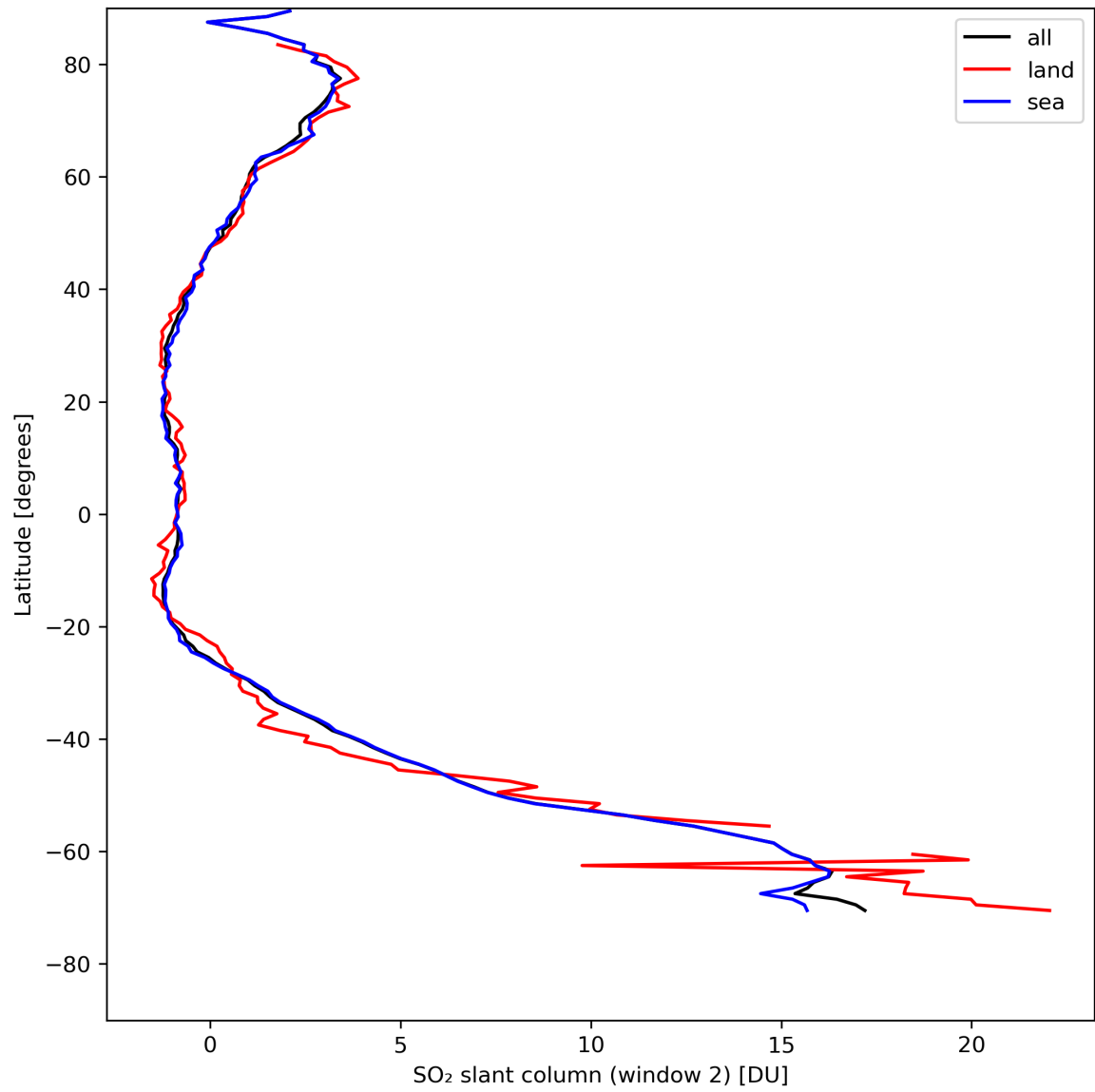
Figure 37: Zonal average of “SO 2 slant column (window 2)” for 2024-08-12 to 2024-08-14.
