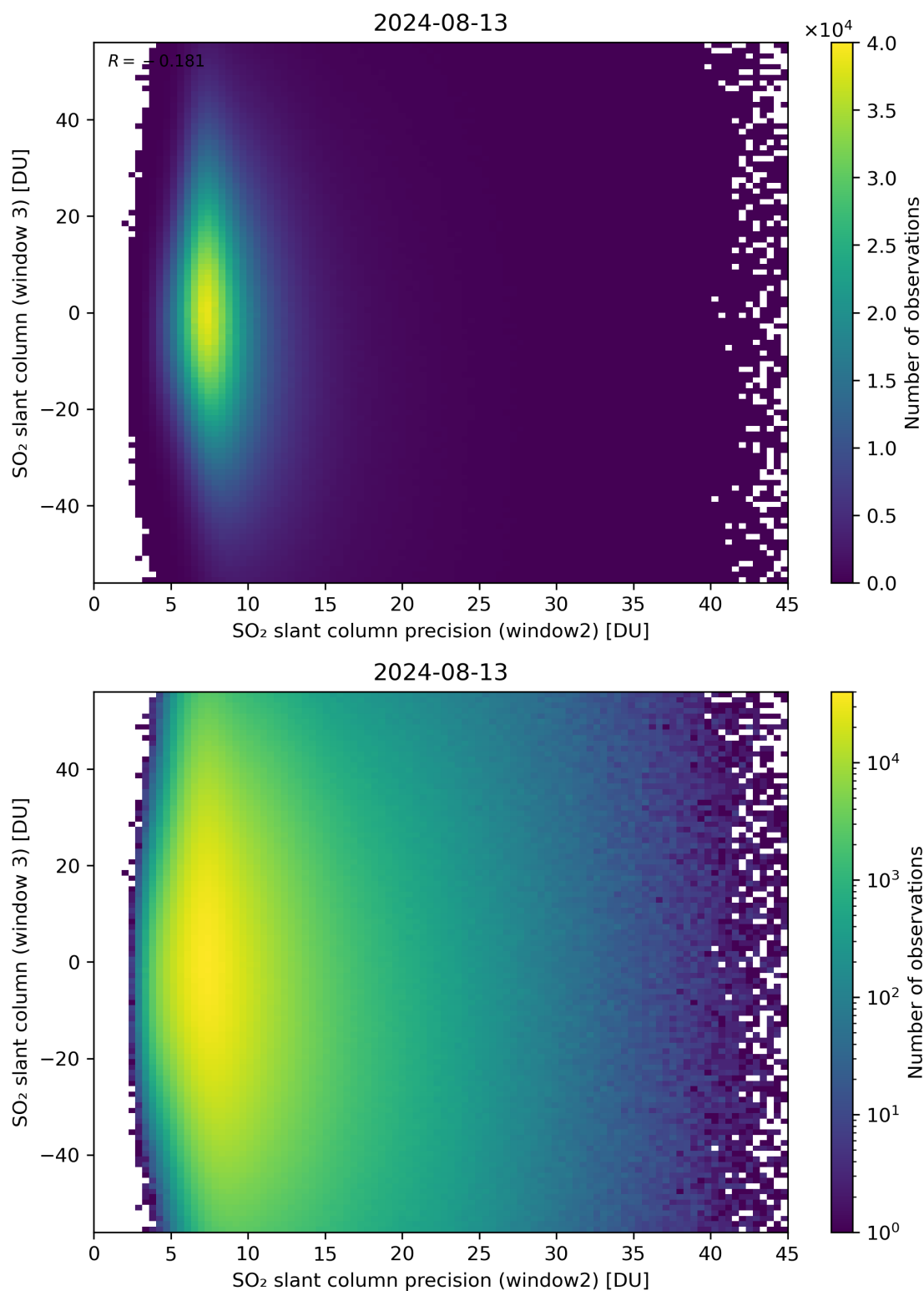
Figure 249: Scatter density plot of “SO 2 slant column precision (window2)” against “SO 2 slant column (window 3)” for 2024-08-12 to 2024-08-14.
