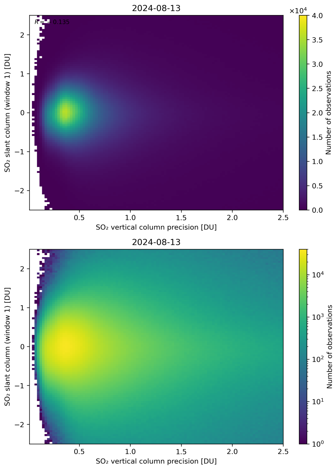
Figure 289: Scatter density plot of “SO 2 vertical column precision” against “SO 2 slant column (window 1)” for 2024-08-12 to 2024-08-14.
