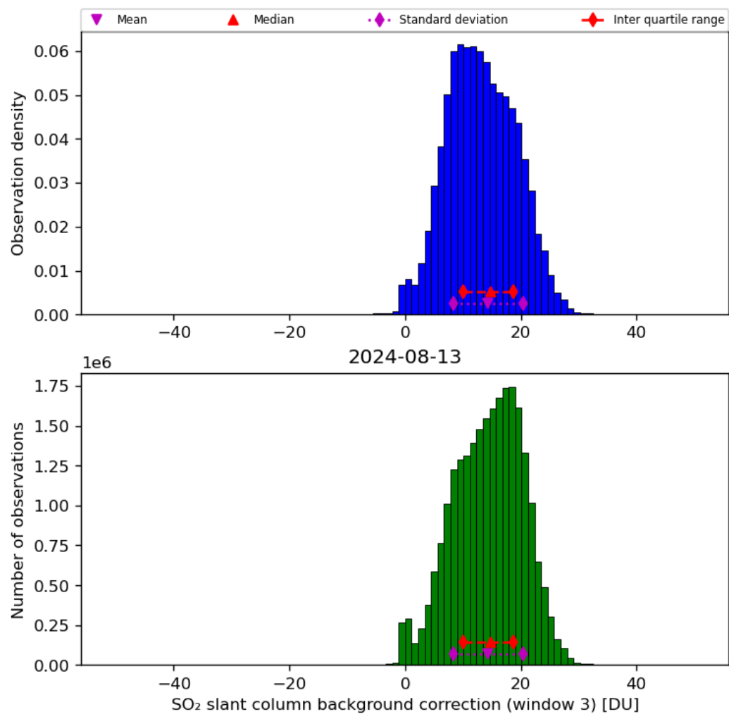
Figure 67: Histogram of “SO 2 slant column background correction (window 3)” for 2024-08-12 to 2024-08-14
