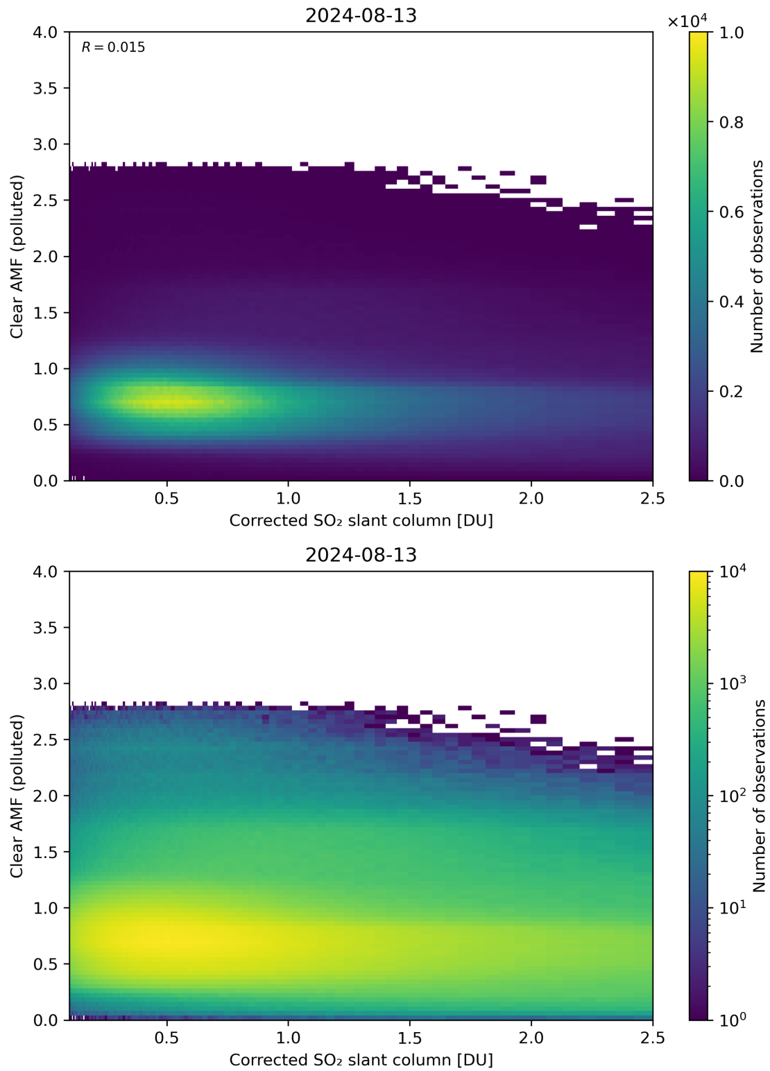
Figure 184: Scatter density plot of “Corrected SO 2 slant column” against “Clear AMF (polluted)” for 2024-08-12 to 2024-08-14.
