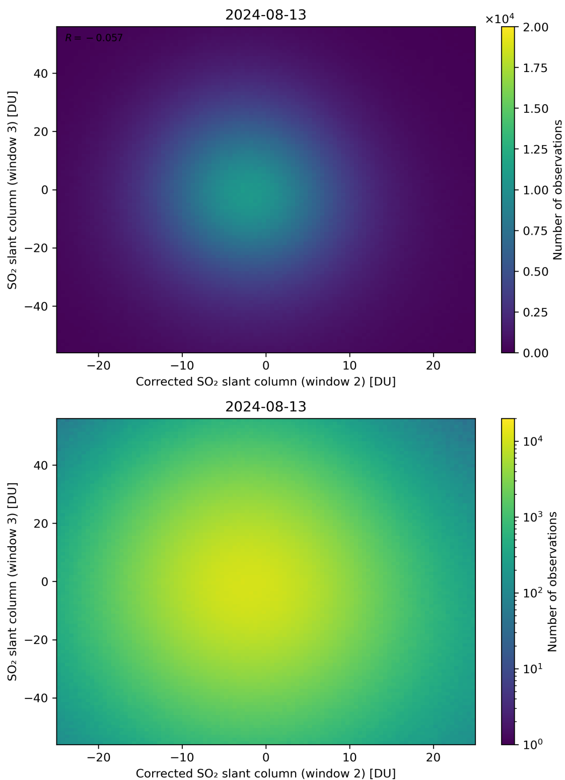
Figure 201: Scatter density plot of “Corrected SO 2 slant column (window 2)” against “SO 2 slant column (window 3)” for 2024-08-12 to 2024-08-14.
