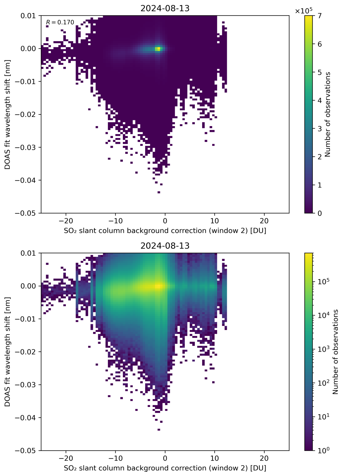
Figure 112: Scatter density plot of “SO 2 slant column background correction (window 2)” against “DOAS fit wavelength shift” for 2024-08-12 to 2024-08-14.
