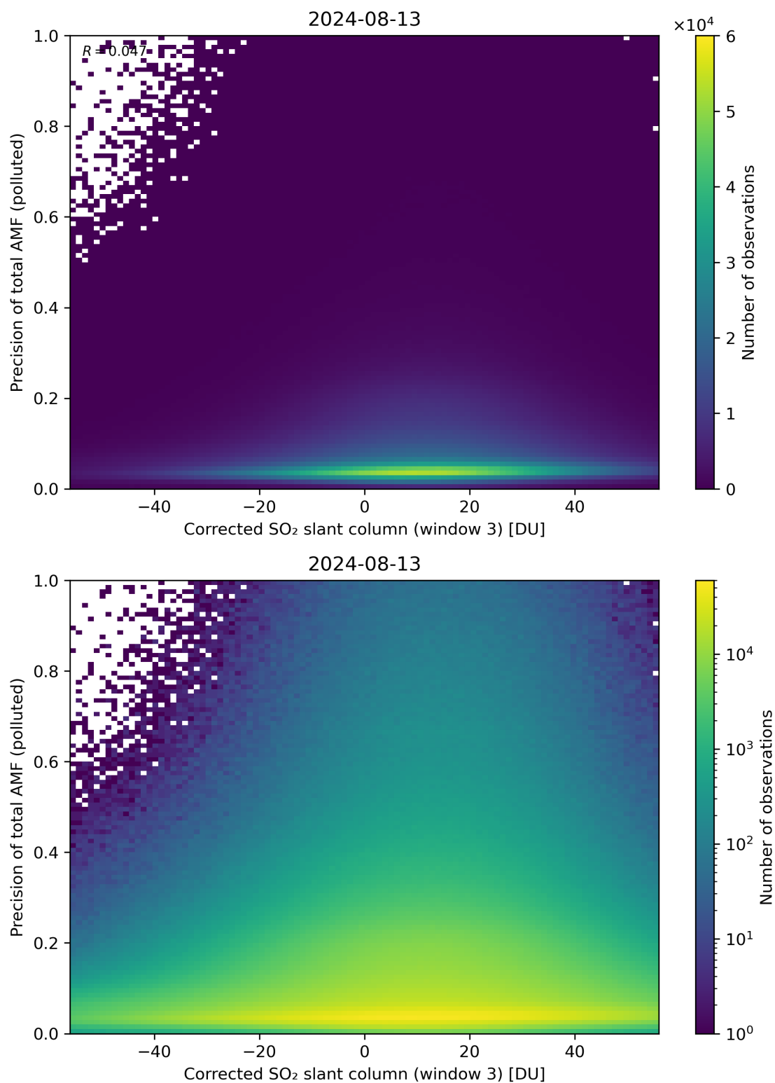
Figure 211: Scatter density plot of “Corrected SO 2 slant column (window 3)” against “Precision of total AMF (polluted)” for 2024-08-12 to 2024-08-14.
