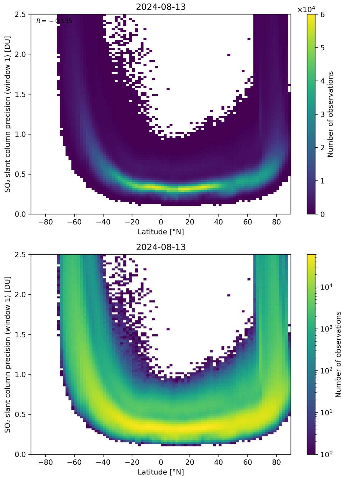
Figure 150: Scatter density plot of “Latitude” against “SO 2 slant column precision (window 1)” for 2024-08-12 to 2024-08-14.
