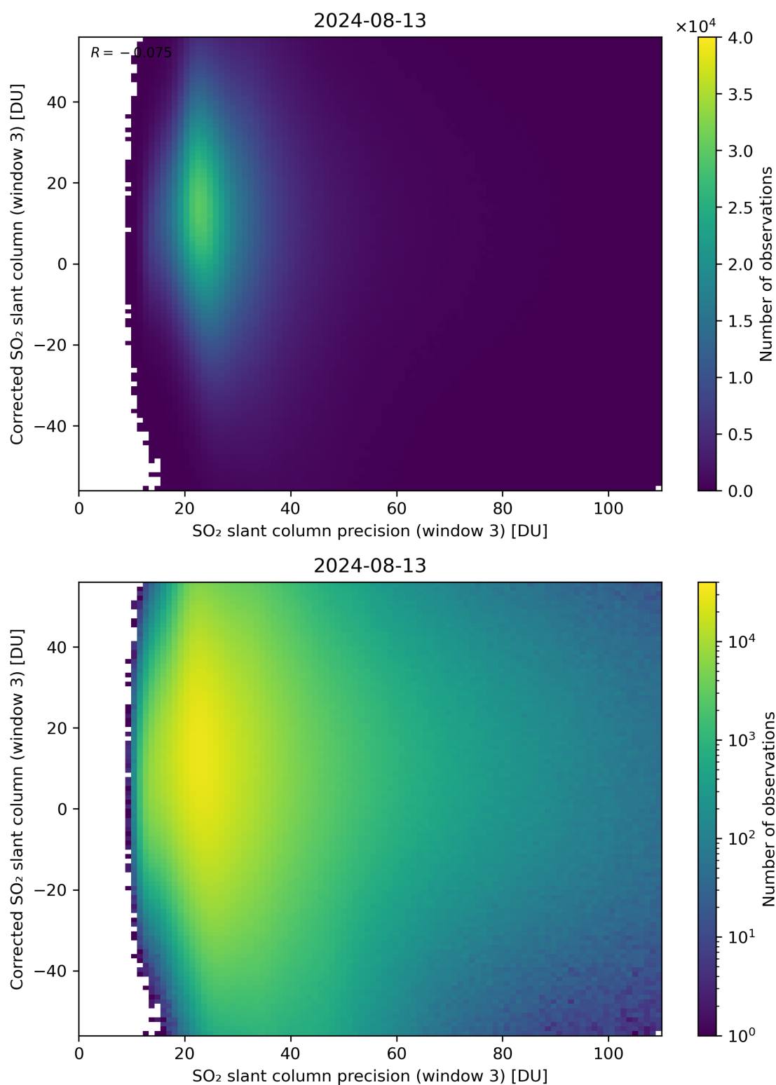
Figure 262: Scatter density plot of “SO 2 slant column precision (window 3)” against “Corrected SO 2 slant column (window 3)” for 2024-08-12 to 2024-08-14.
