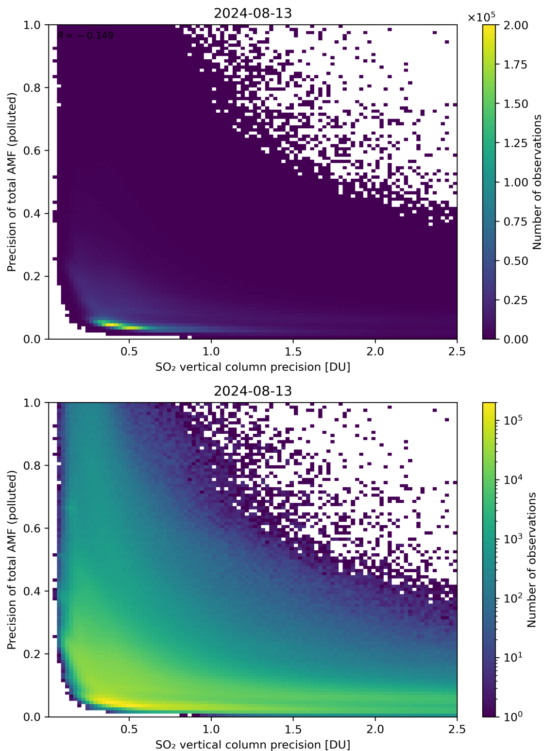
Figure 295: Scatter density plot of “SO 2 vertical column precision” against “Precision of total AMF (polluted)” for 2024-08-12 to 2024-08-14.
