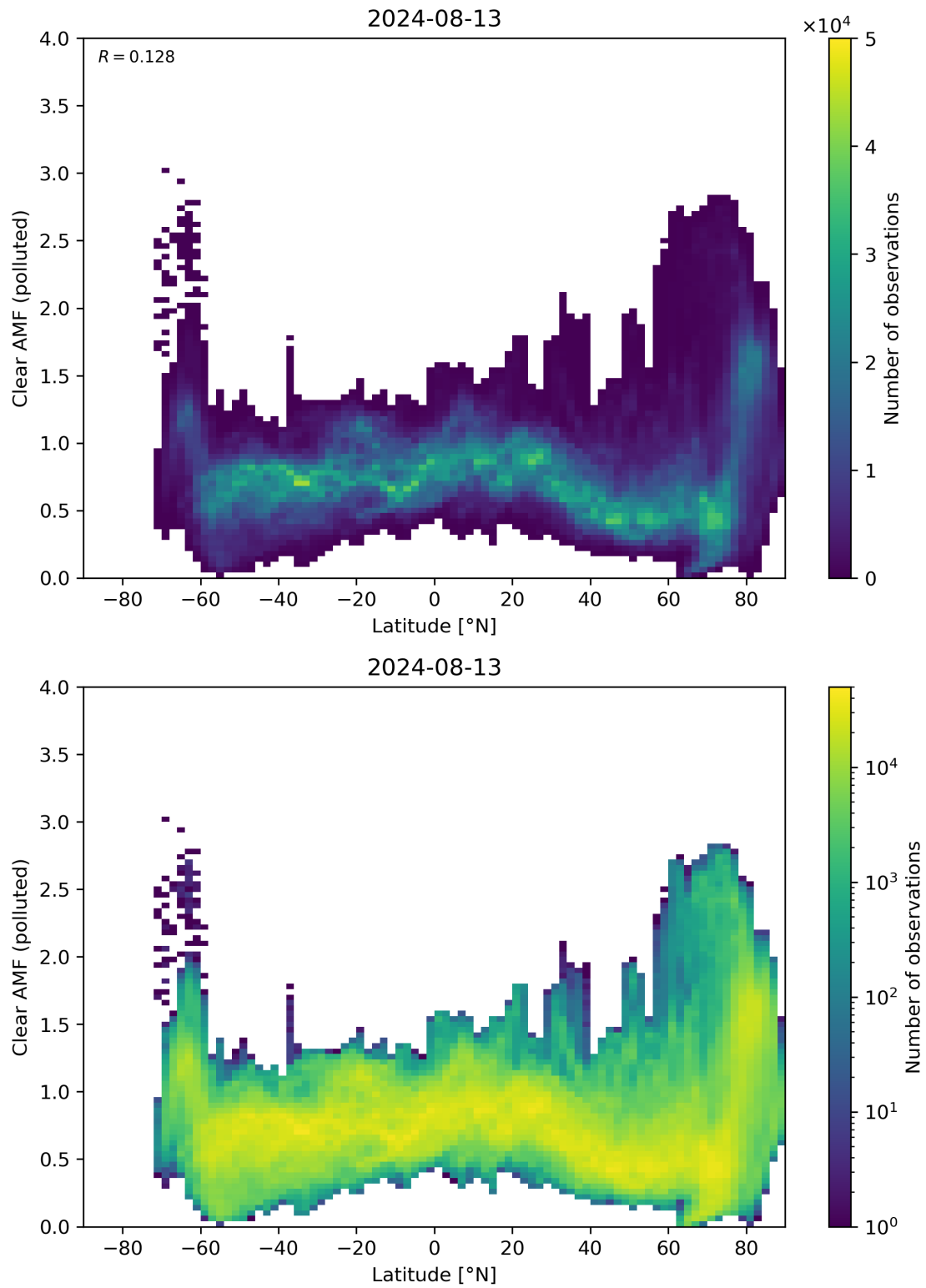
Figure 145: Scatter density plot of “Latitude” against “Clear AMF (polluted)” for 2024-08-12 to 2024-08-14.
