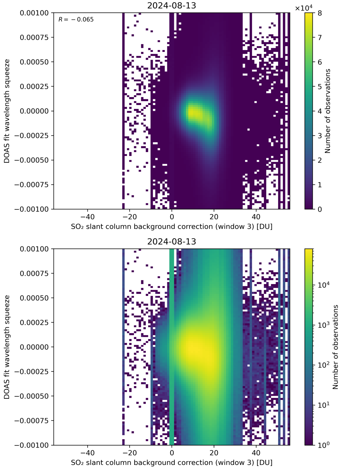
Figure 122: Scatter density plot of “SO 2 slant column background correction (window 3)” against “DOAS fit wavelength squeeze” for 2024-08-12 to 2024-08-14.
