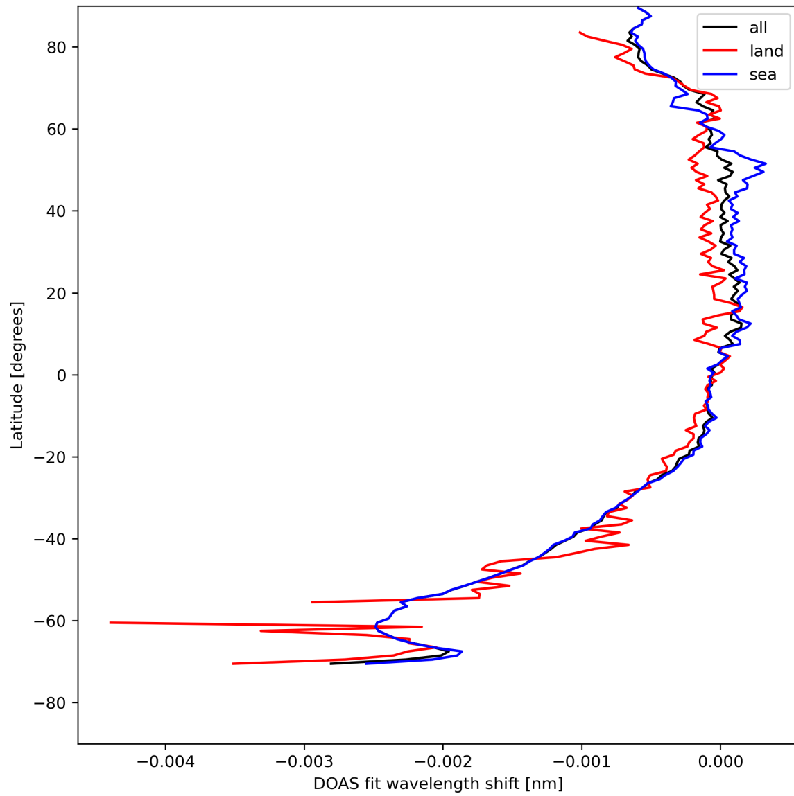
Figure 45: Zonal average of "DOAS fit wavelength shift" for 2024-08-12 to 2024-08-14.
