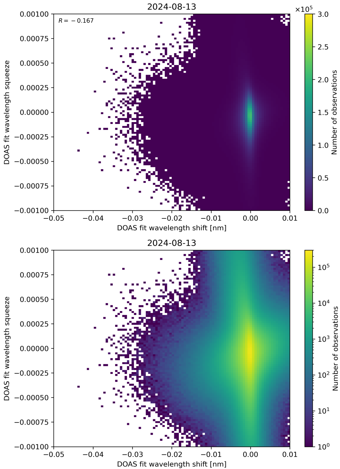
Figure 127: Scatter density plot of “DOAS fit wavelength shift” against “DOAS fit wavelength squeeze” for 2024-08-12 to 2024-08-14.
