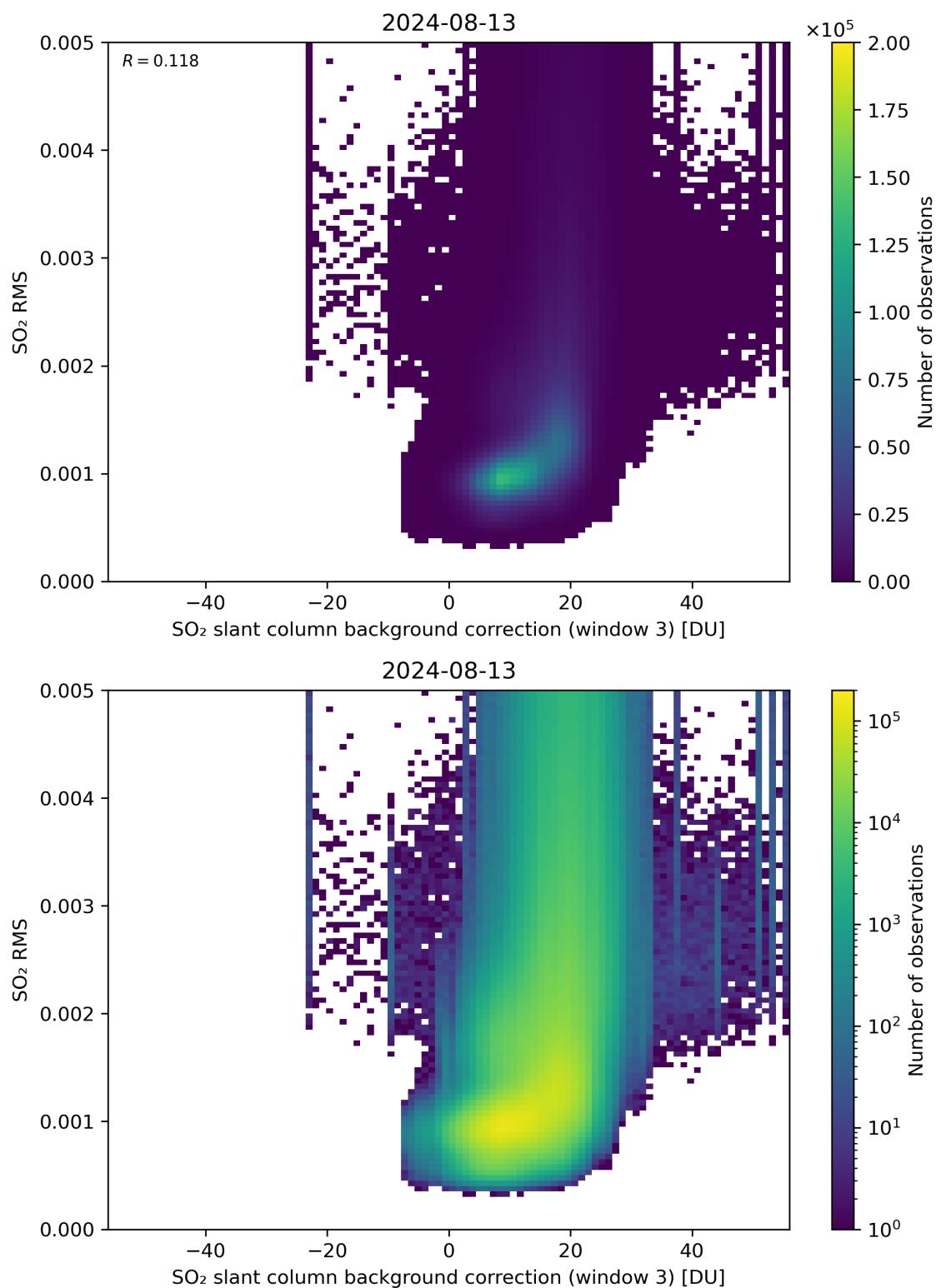
Figure 123: Scatter density plot of “SO 2 slant column background correction (window 3)” against “SO 2 RMS” for 2024-08-12 to 2024-08-14.
