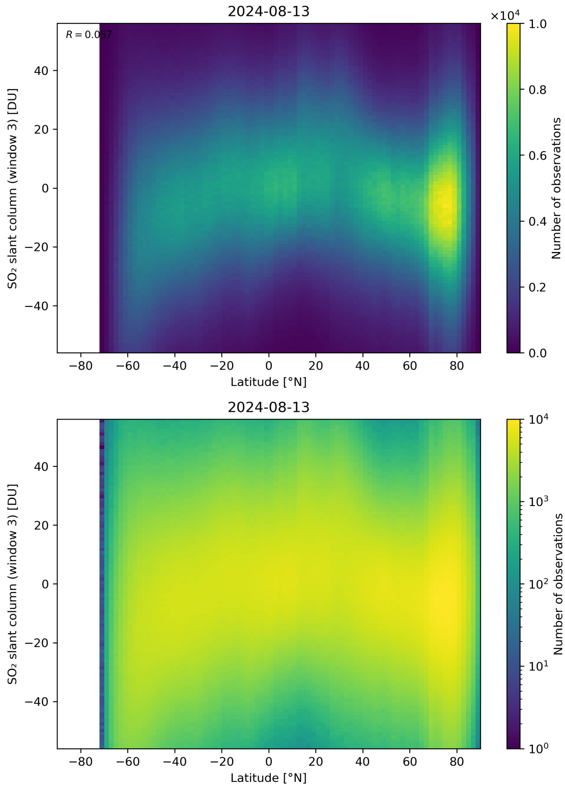
Figure 152: Scatter density plot of “Latitude” against “SO 2 slant column (window 3)” for 2024-08-12 to 2024-08-14.
