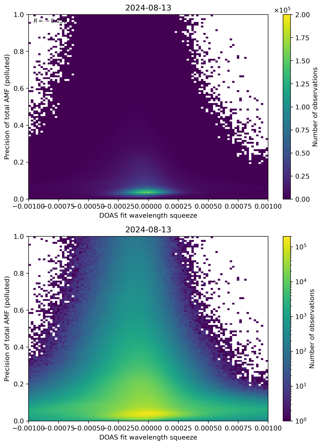
Figure 135: Scatter density plot of “DOAS fit wavelength squeeze” against “Precision of total AMF (polluted)” for 2024-08-12 to 2024-08-14.
