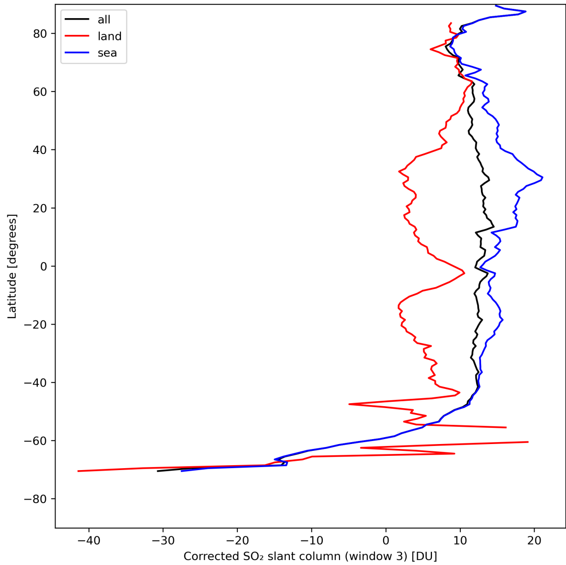
Figure 43: Zonal average of “Corrected SO 2 slant column (window 3)” for 2024-08-12 to 2024-08-14.
