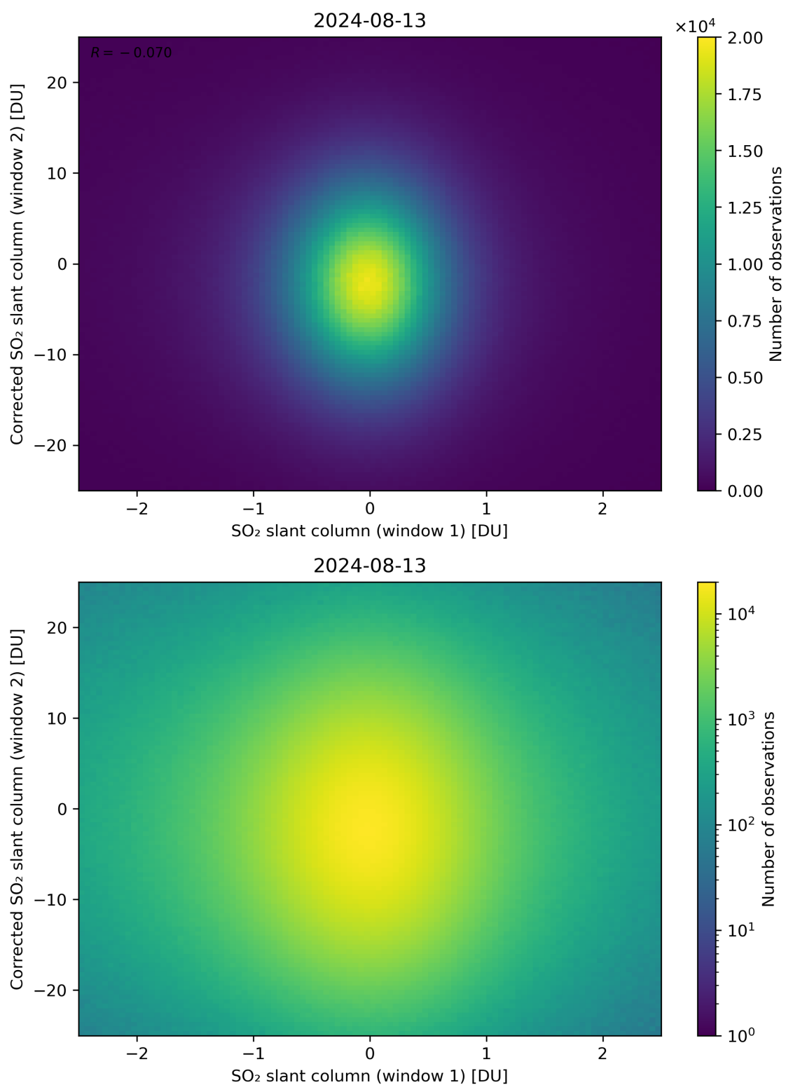
Figure 233: Scatter density plot of “SO 2 slant column (window 1)” against “Corrected SO 2 slant column (window 2)” for 2024-08-12 to 2024-08-14.
