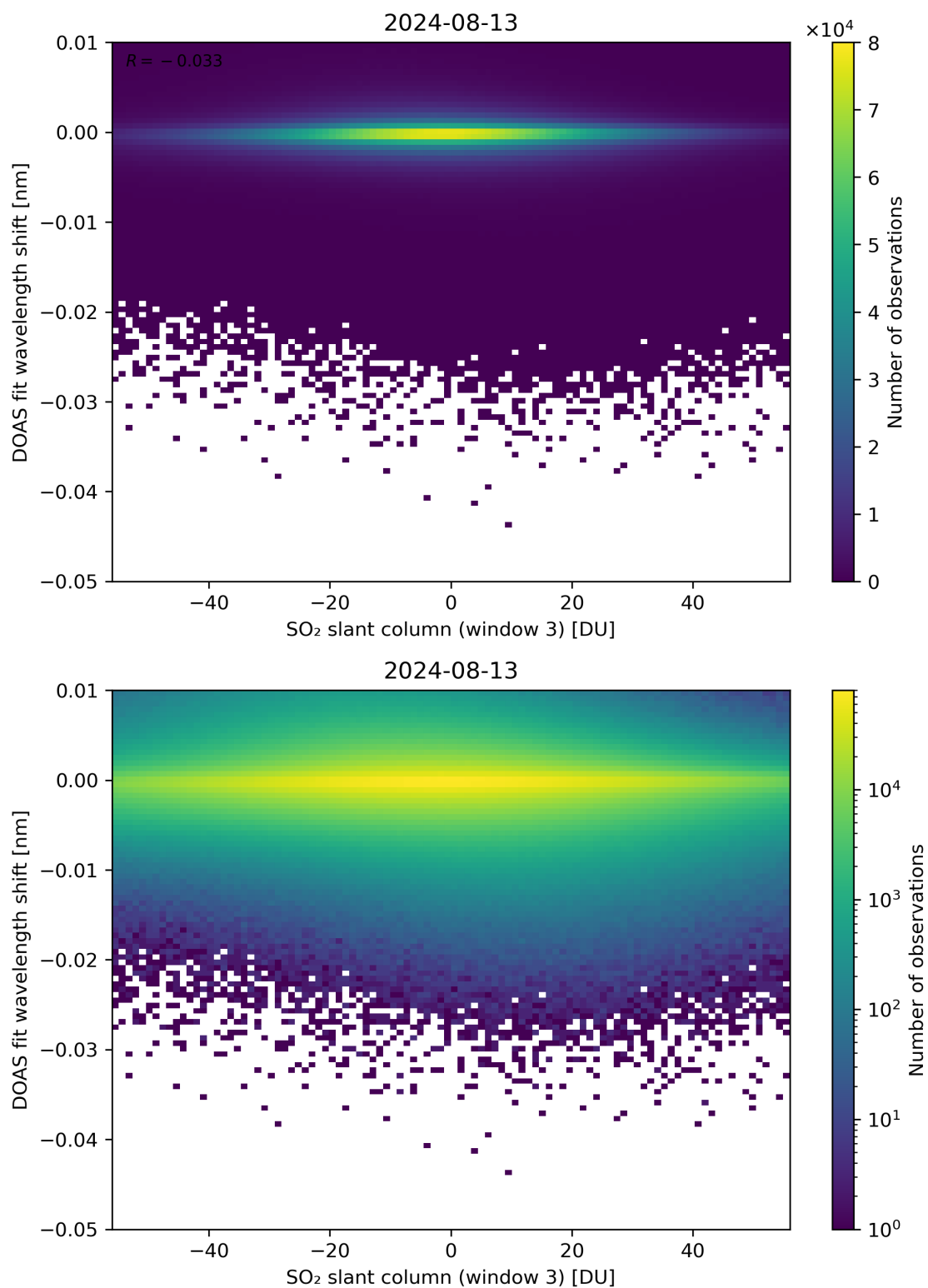
Figure 254: Scatter density plot of “SO 2 slant column (window 3)” against “DOAS fit wavelength shift” for 2024-08-12 to 2024-08-14.
