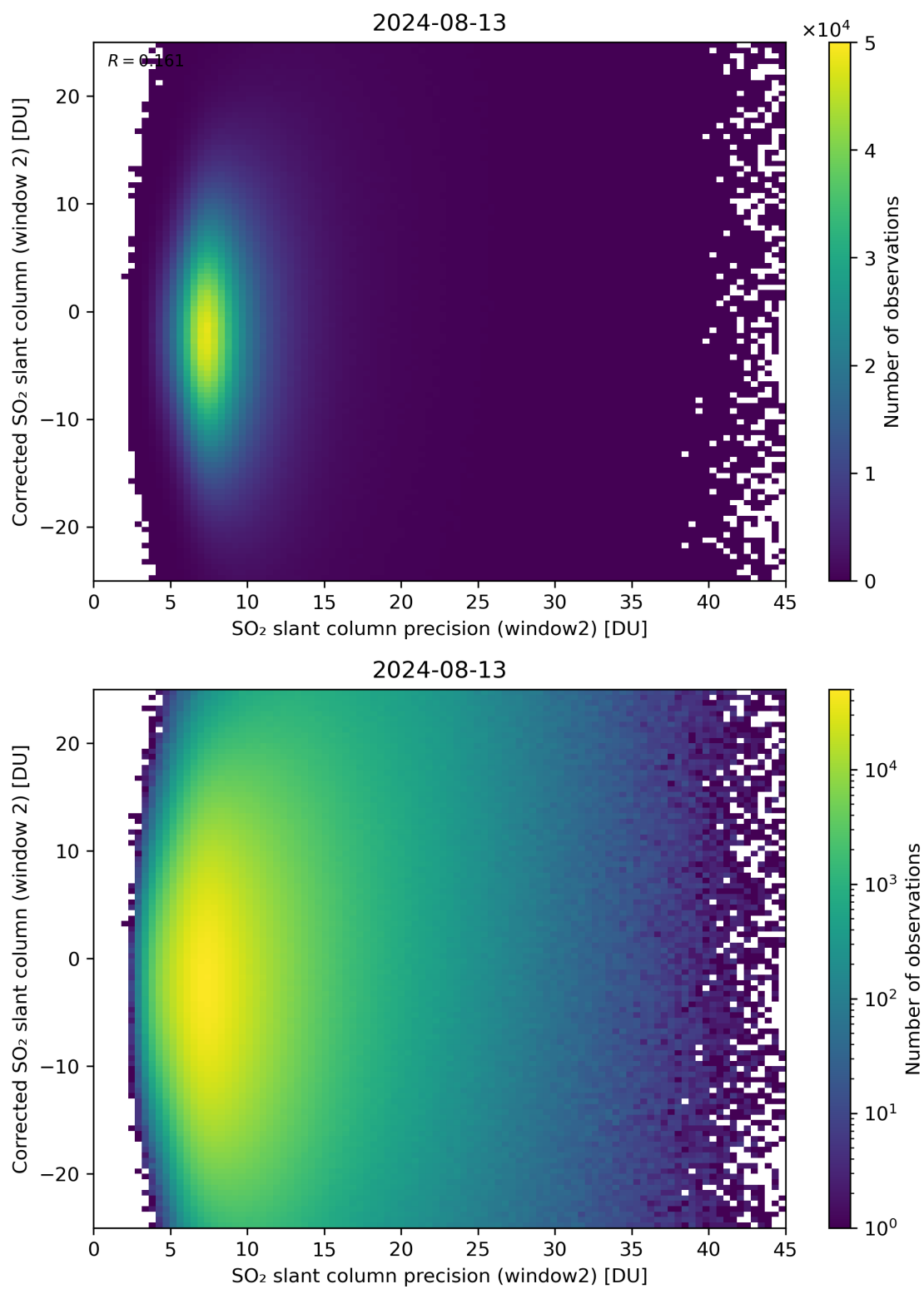
Figure 247: Scatter density plot of “SO 2 slant column precision (window2)” against “Corrected SO 2 slant column (window 2)” for 2024-08-12 to 2024-08-14.
