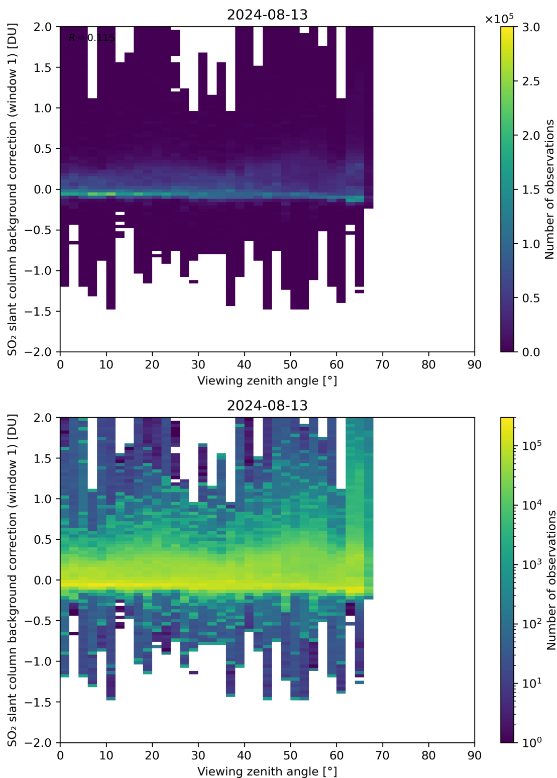
Figure 308: Scatter density plot of “Viewing zenith angle” against “SO 2 slant column background correction (window 1)” for 2024-08-12 to 2024-08-14.
