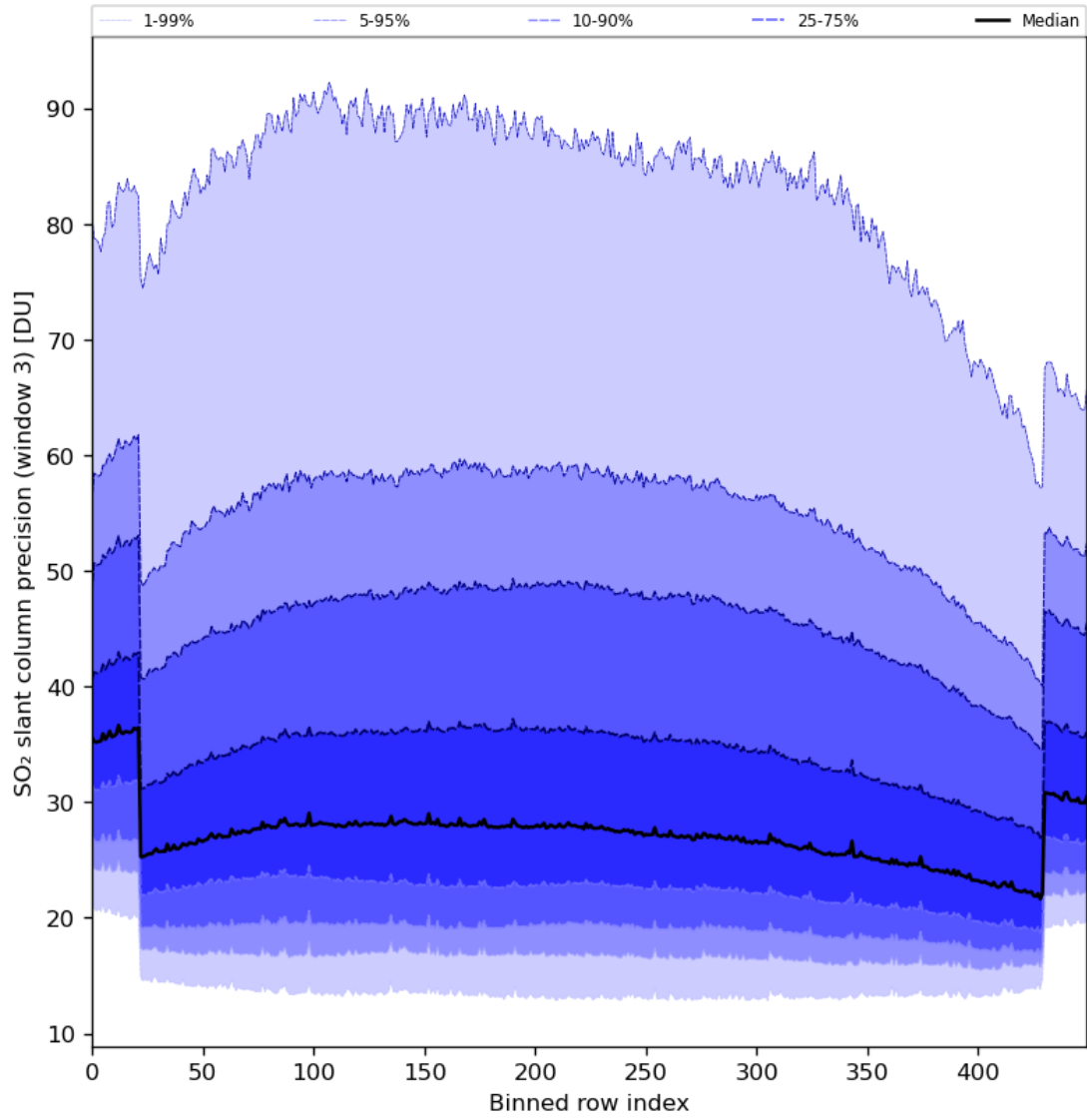
Figure 88: Along track statistics of “SO 2 slant column precision (window 3)” for 2024-08-12 to 2024-08-14
