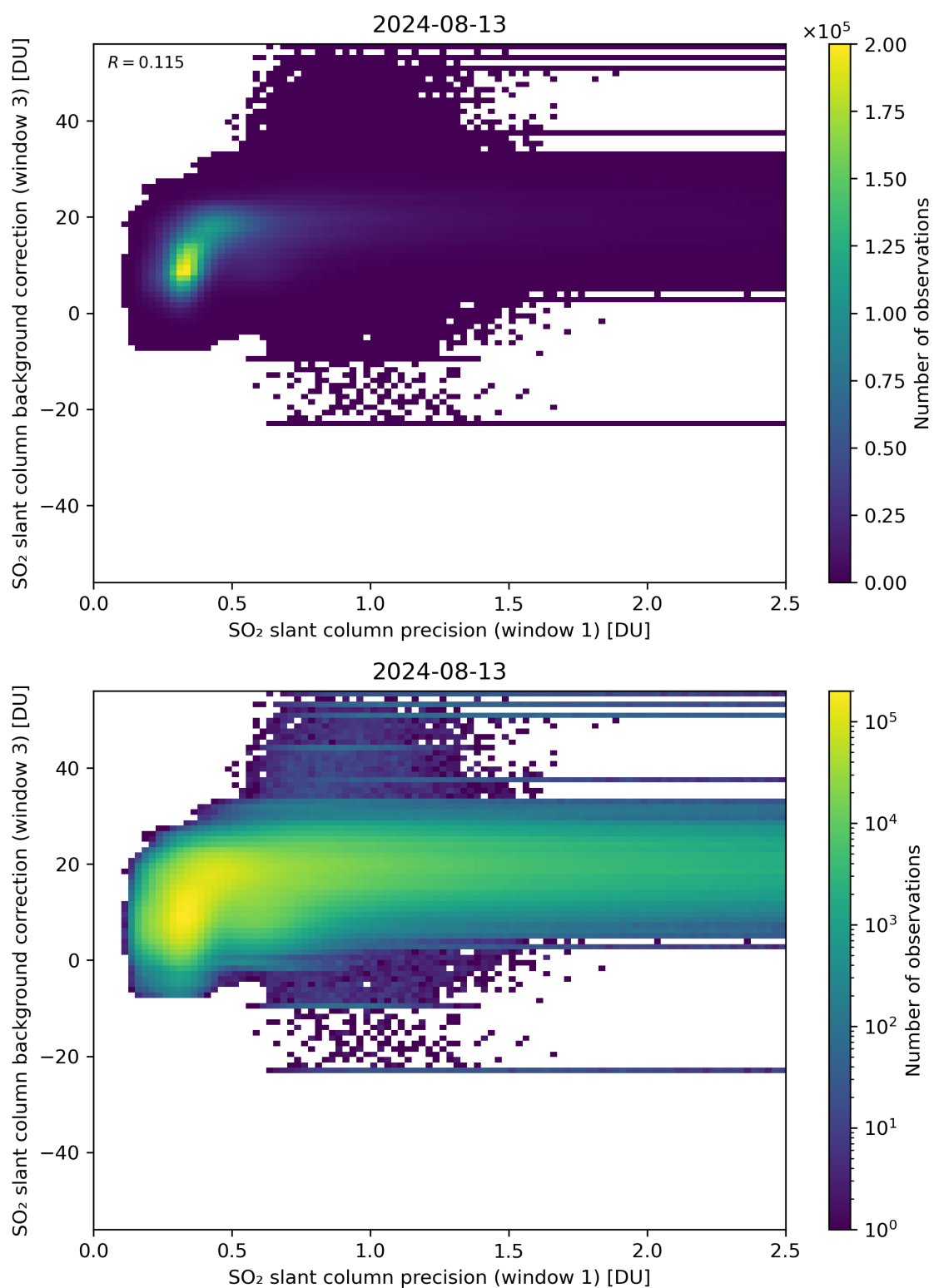
Figure 220: Scatter density plot of “SO 2 slant column precision (window 1)” against “SO 2 slant column background correction (window 3)” for 2024-08-12 to 2024-08-14.
