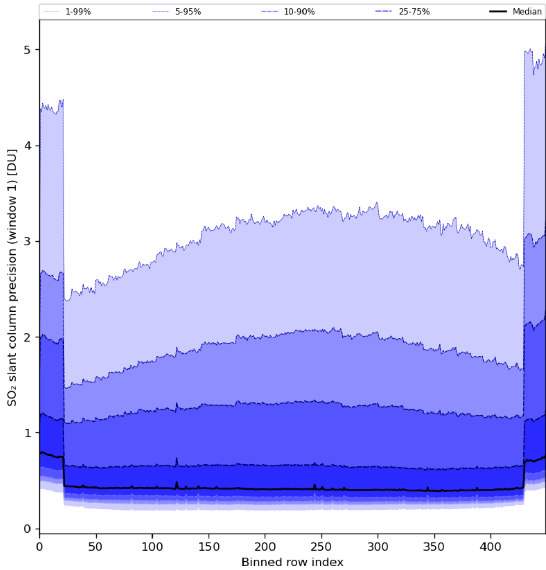
Figure 80: Along track statistics of “SO 2 slant column precision (window 1)” for 2024-08-12 to 2024-08-14
