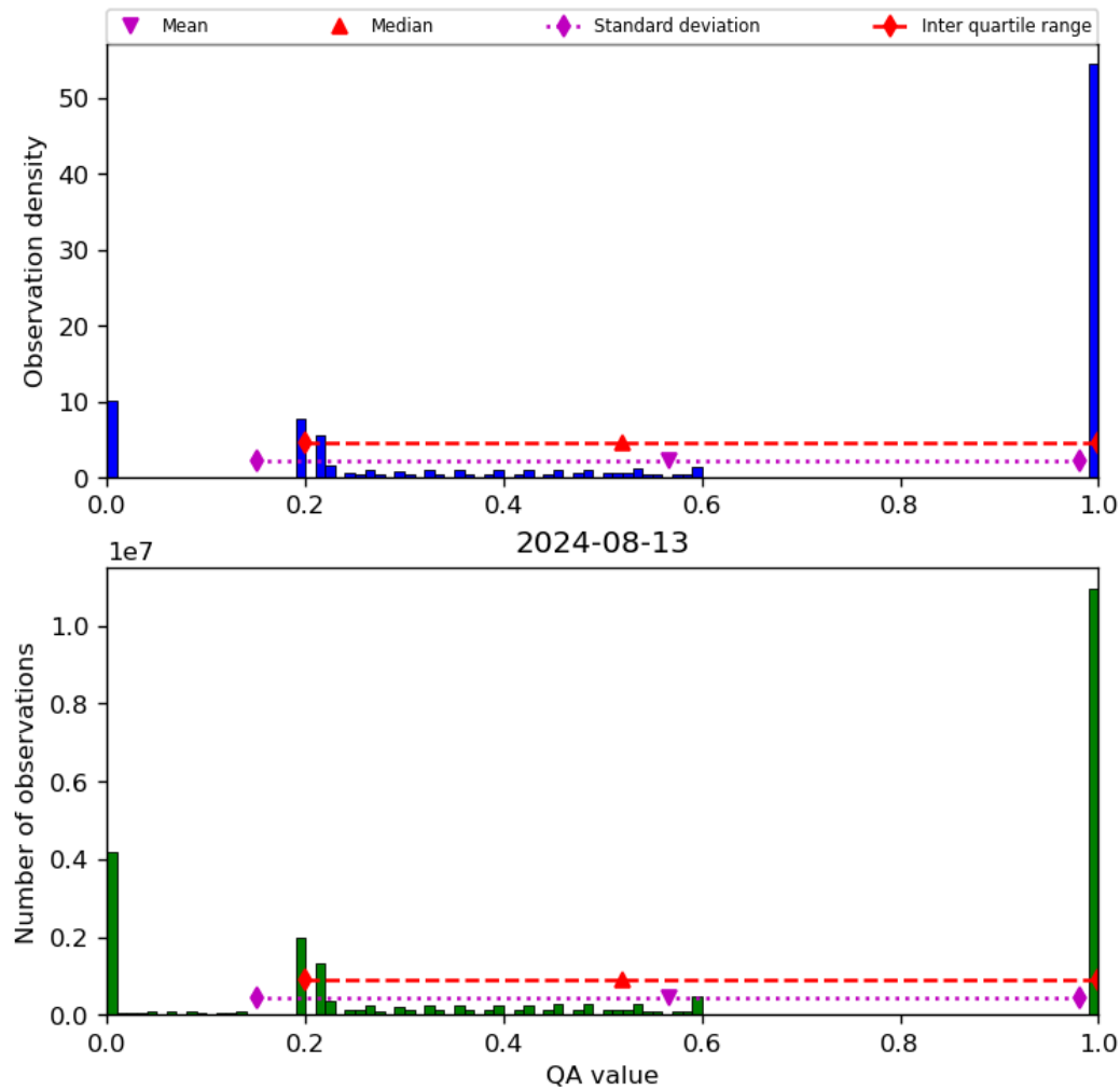
Figure 52: Histogram of “QA value” for 2024-08-12 to 2024-08-14
