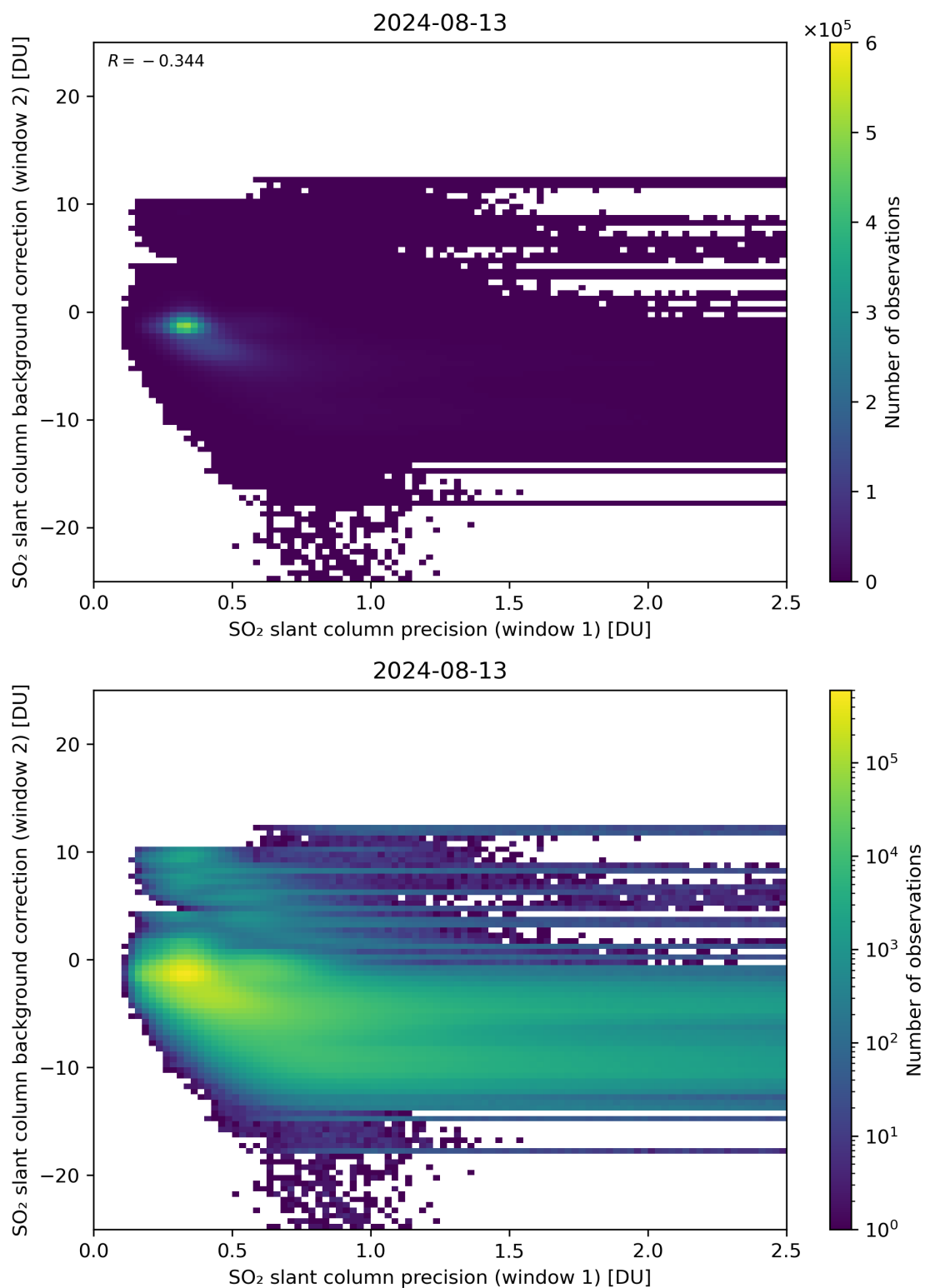
Figure 219: Scatter density plot of “SO 2 slant column precision (window 1)” against “SO 2 slant column background correction (window 2)” for 2024-08-12 to 2024-08-14.
