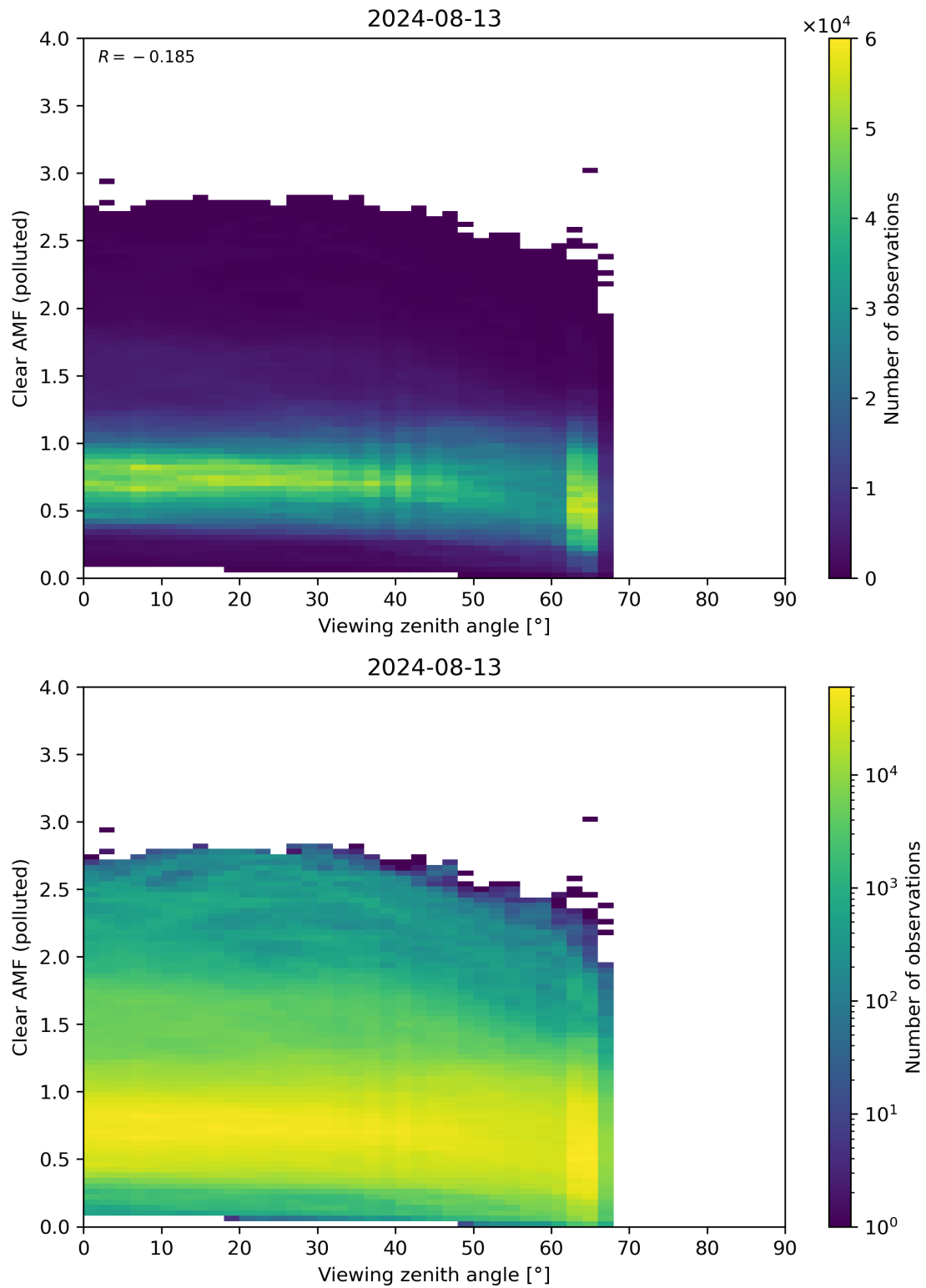
Figure 316: Scatter density plot of “Viewing zenith angle” against “Clear AMF (polluted)” for 2024-08-12 to 2024-08-14.
