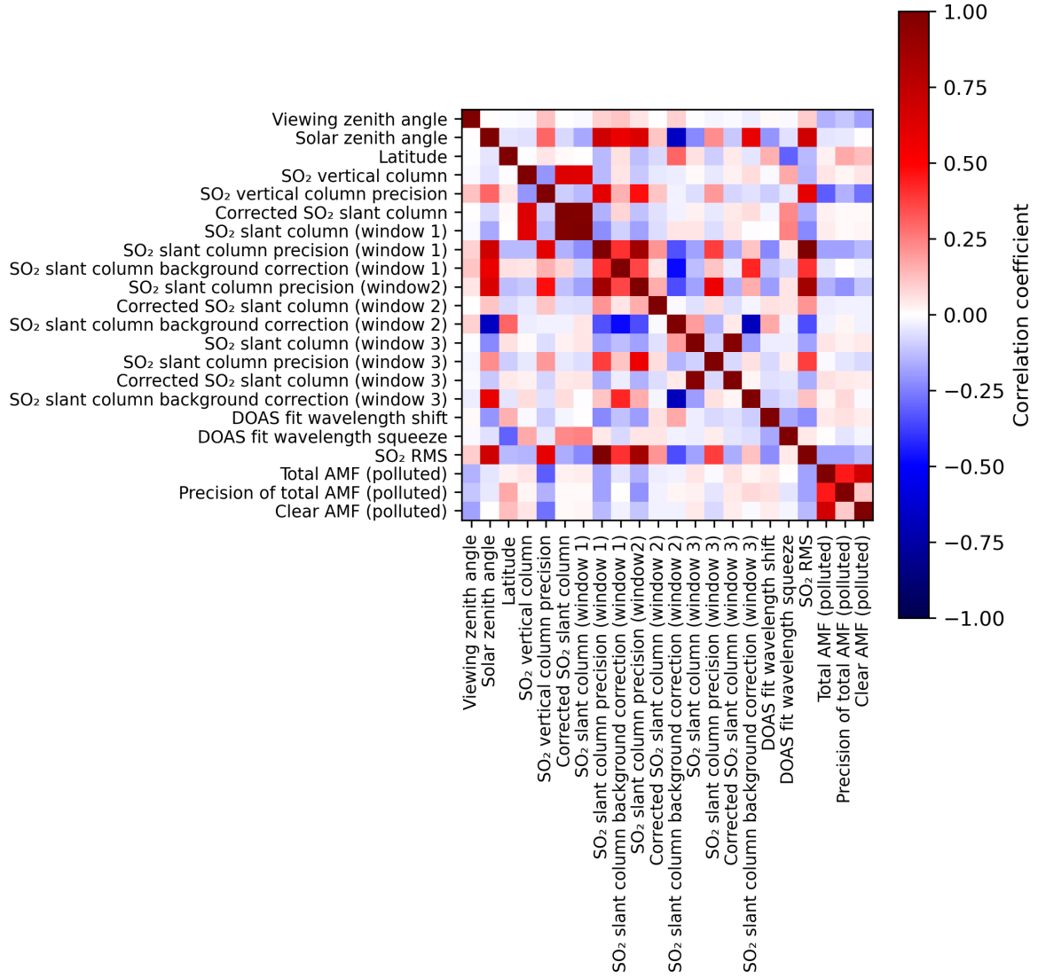
Figure 2: Map of correlation matrix for 2024-08-12 to 2024-08-14.
