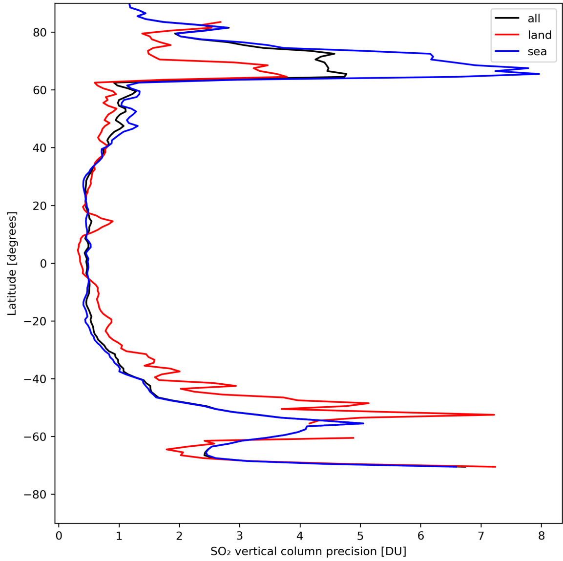
Figure 31: Zonal average of “SO 2 vertical column precision” for 2024-08-12 to 2024-08-14.
