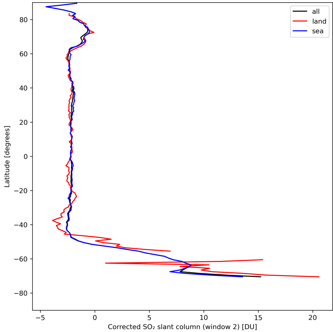
Figure 39: Zonal average of “Corrected SO 2 slant column (window 2)” for 2024-08-12 to 2024-08-14.
