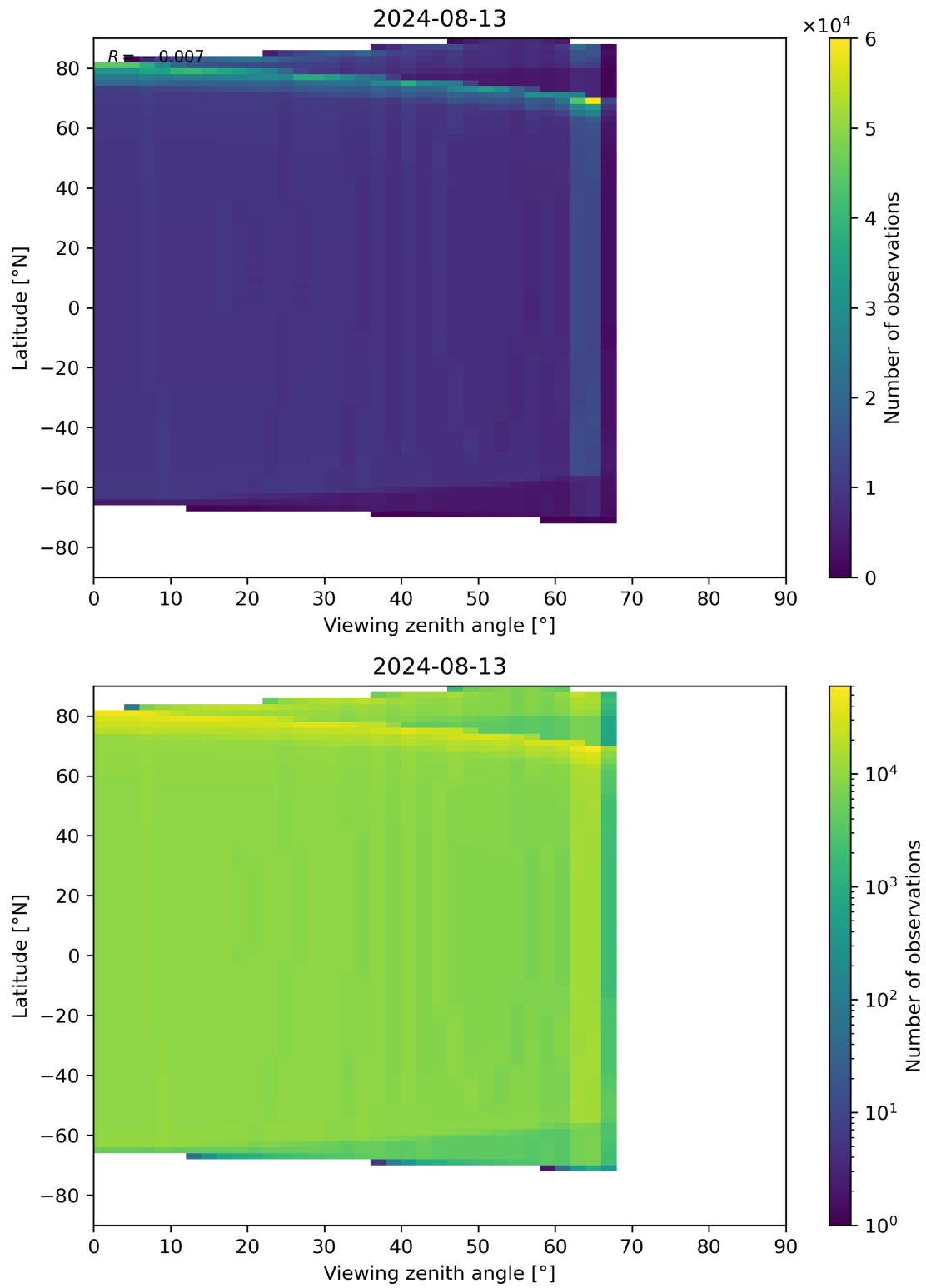
Figure 314: Scatter density plot of “Viewing zenith angle” against “Latitude” for 2024-08-12 to 2024-08-14.
