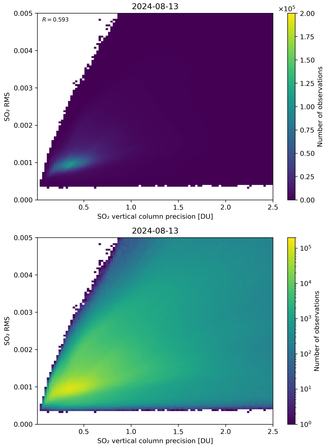
Figure 284: Scatter density plot of “SO 2 vertical column precision” against “SO 2 RMS” for 2024-08-12 to 2024-08-14.
