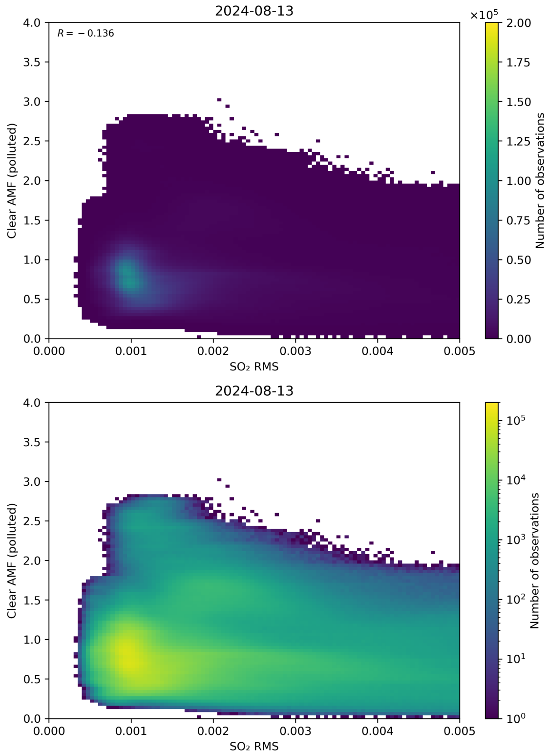
Figure 136: Scatter density plot of “SO 2 RMS” against “Clear AMF (polluted)” for 2024-08-12 to 2024-08-14.
