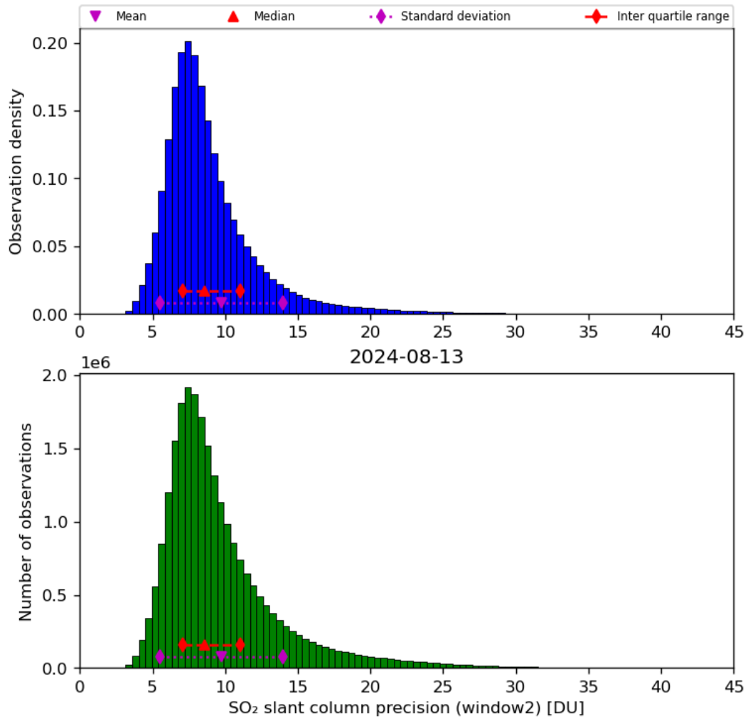
Figure 61: Histogram of “SO 2 slant column precision (window2)” for 2024-08-12 to 2024-08-14
