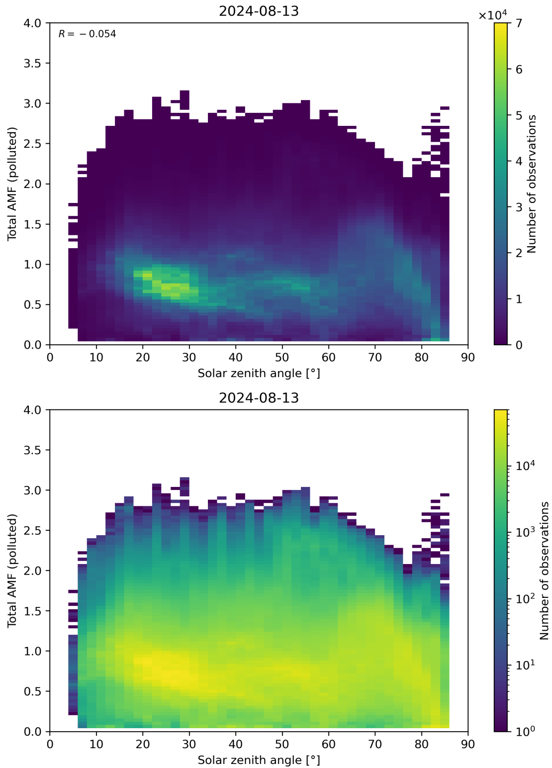
Figure 174: Scatter density plot of “Solar zenith angle” against “Total AMF (polluted)” for 2024-08-12 to 2024-08-14.
