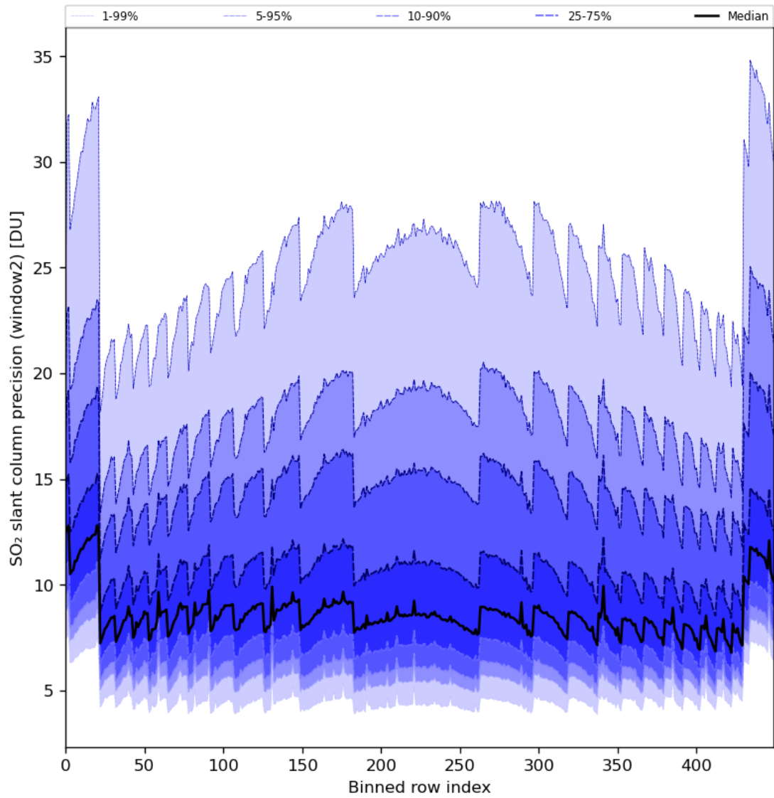
Figure 84: Along track statistics of “SO 2 slant column precision (window2)” for 2024-08-12 to 2024-08-14
