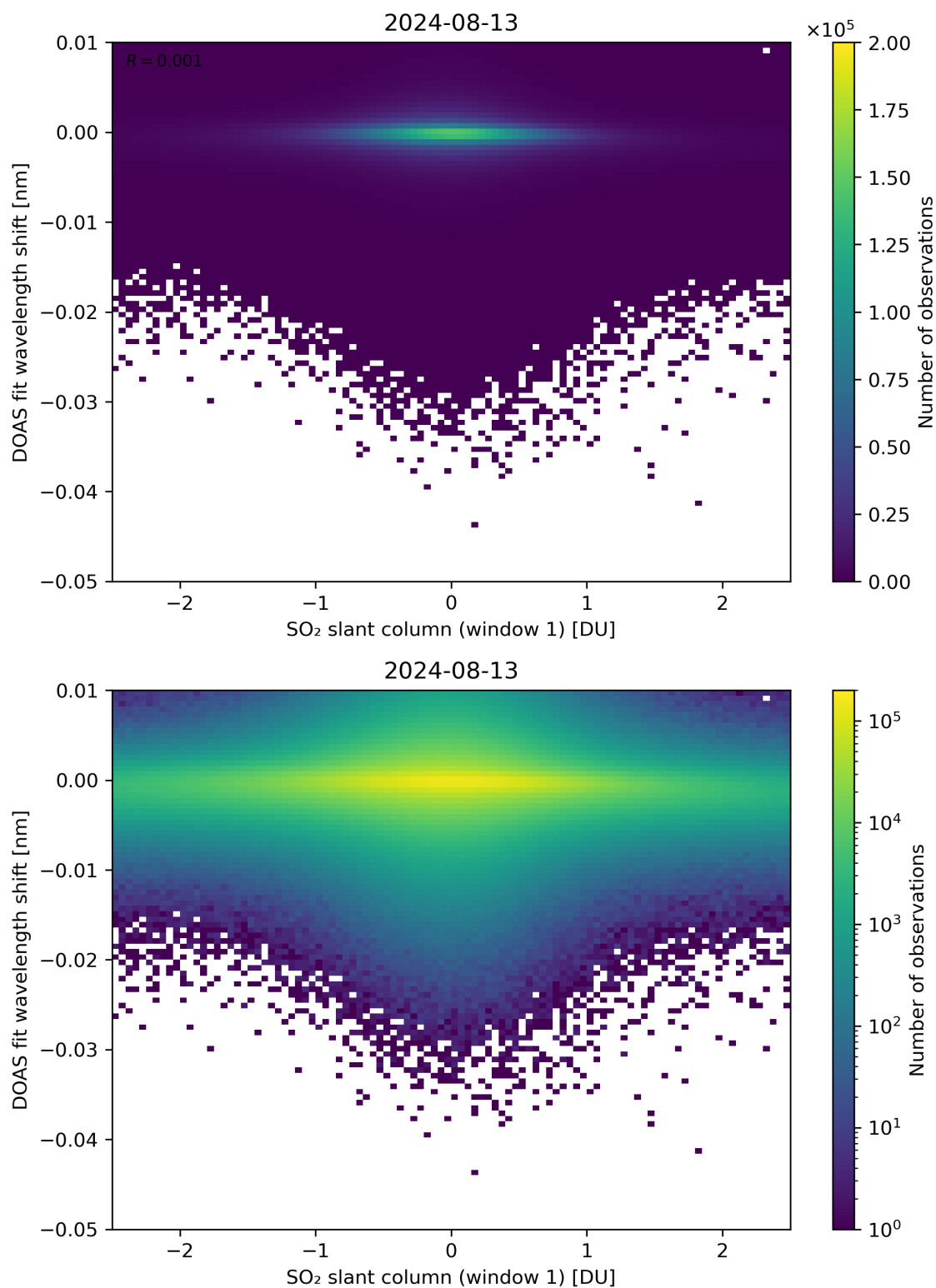
Figure 215: Scatter density plot of “SO 2 slant column (window 1)” against “DOAS fit wavelength shift” for 2024-08-12 to 2024-08-14.
