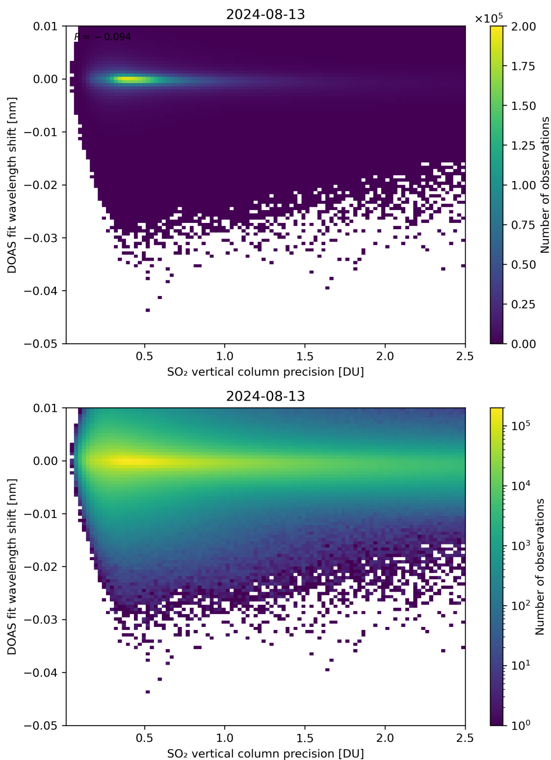
Figure 282: Scatter density plot of “SO 2 vertical column precision” against “DOAS fit wavelength shift” for 2024-08-12 to 2024-08-14.
