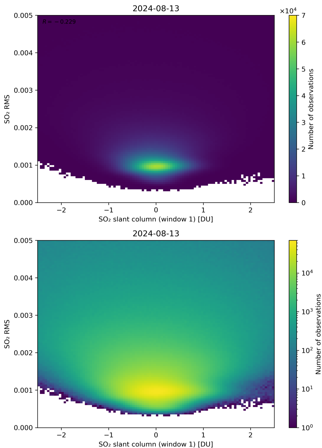
Figure 217: Scatter density plot of “SO 2 slant column (window 1)” against “SO 2 RMS” for 2024-08-12 to 2024-08-14.
