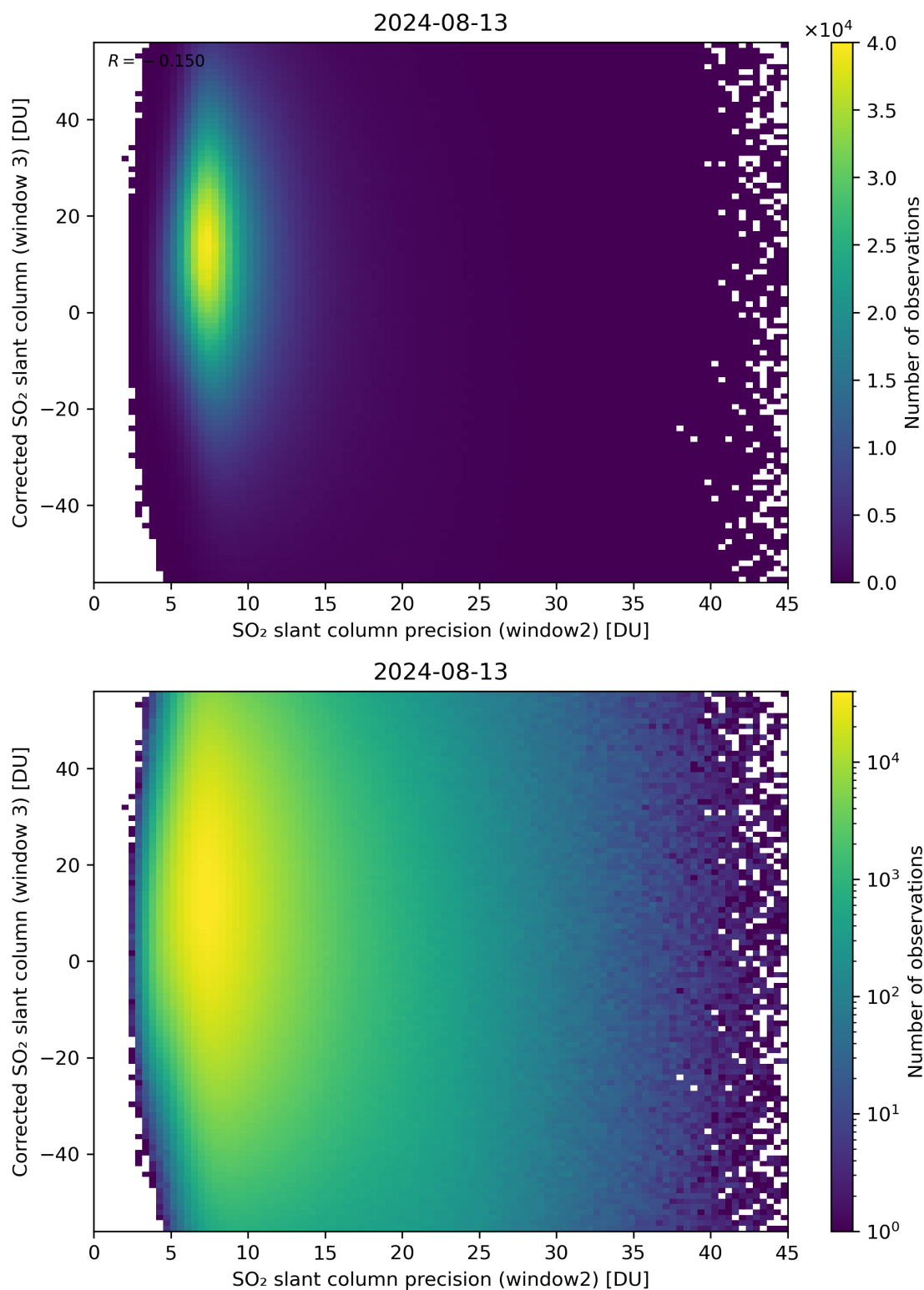
Figure 248: Scatter density plot of “SO 2 slant column precision (window2)” against “Corrected SO 2 slant column (window 3)” for 2024-08-12 to 2024-08-14.
