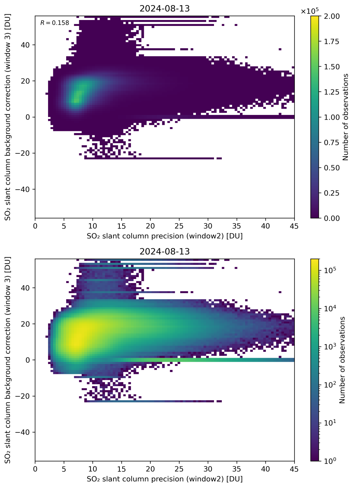
Figure 242: Scatter density plot of “SO 2 slant column precision (window2)” against “SO 2 slant column background correction (window 3)” for 2024-08-12 to 2024-08-14.
