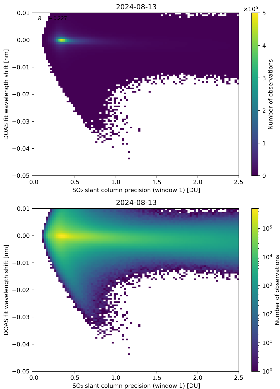
Figure 221: Scatter density plot of “SO 2 slant column precision (window 1)” against “DOAS fit wavelength shift” for 2024-08-12 to 2024-08-14.
