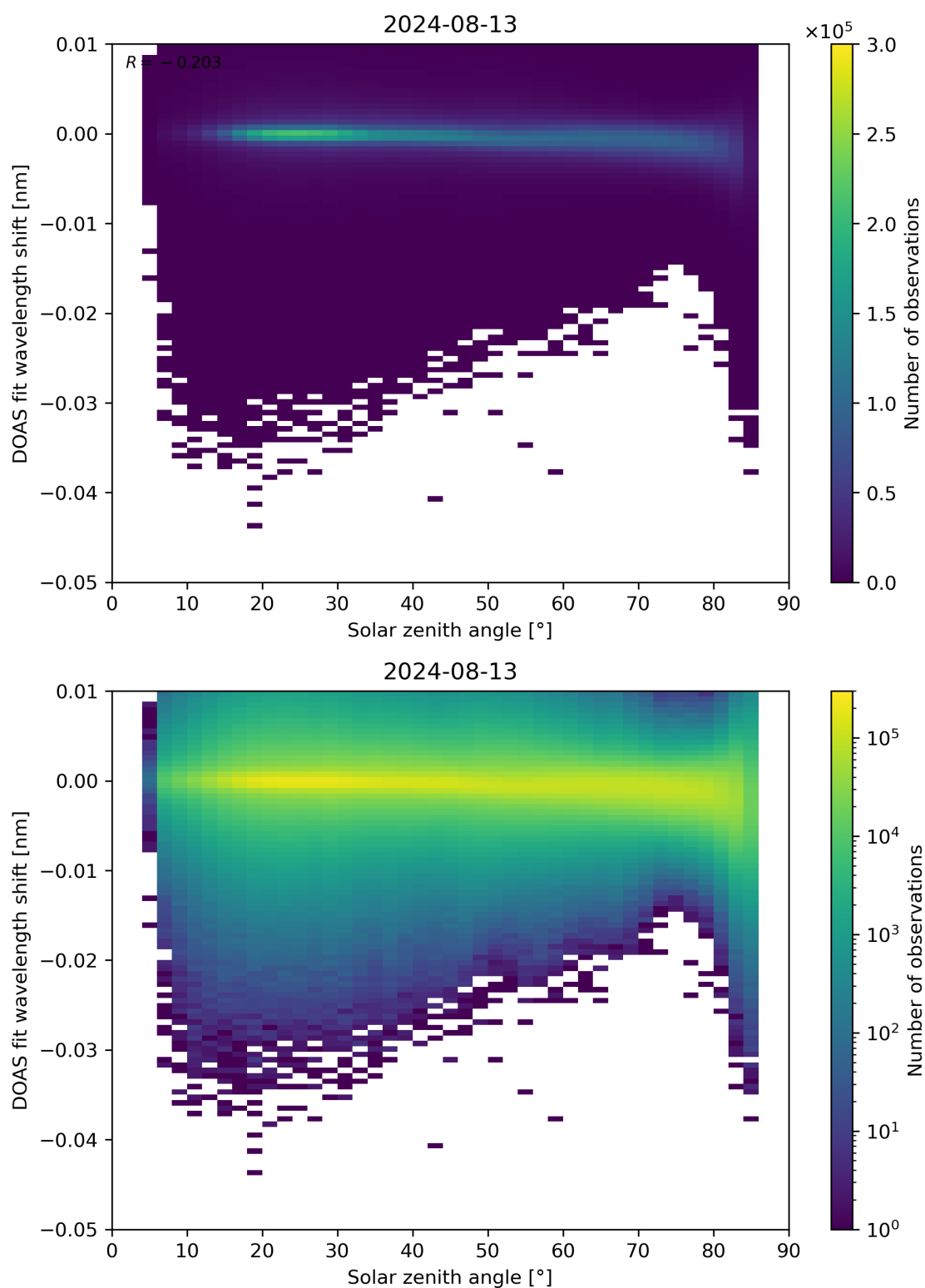
Figure 161: Scatter density plot of “Solar zenith angle” against “DOAS fit wavelength shift” for 2024-08-12 to 2024-08-14.
