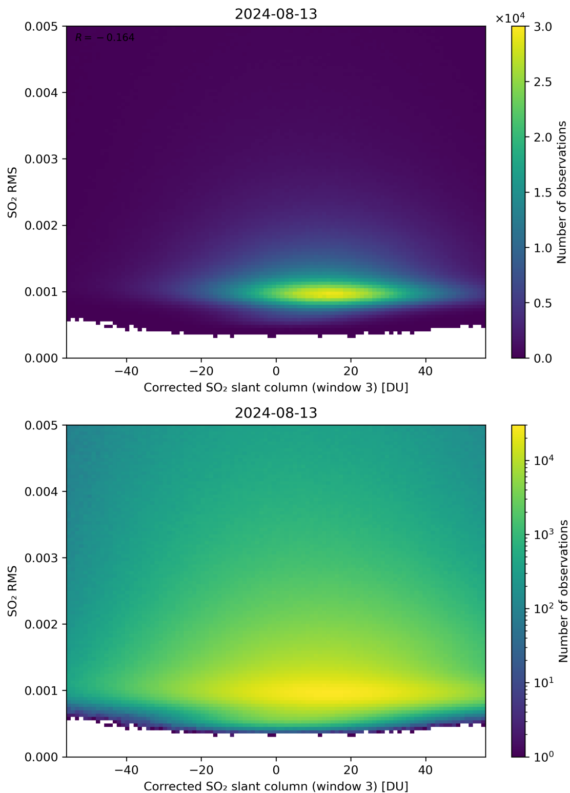
Figure 208: Scatter density plot of “Corrected SO 2 slant column (window 3)” against “SO 2 RMS” for 2024-08-12 to 2024-08-14.
