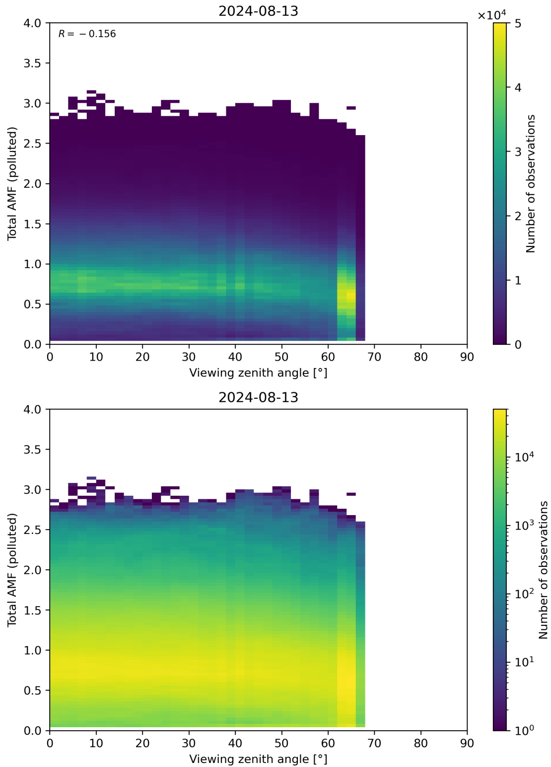
Figure 325: Scatter density plot of “Viewing zenith angle” against “Total AMF (polluted)” for 2024-08-12 to 2024-08-14.
