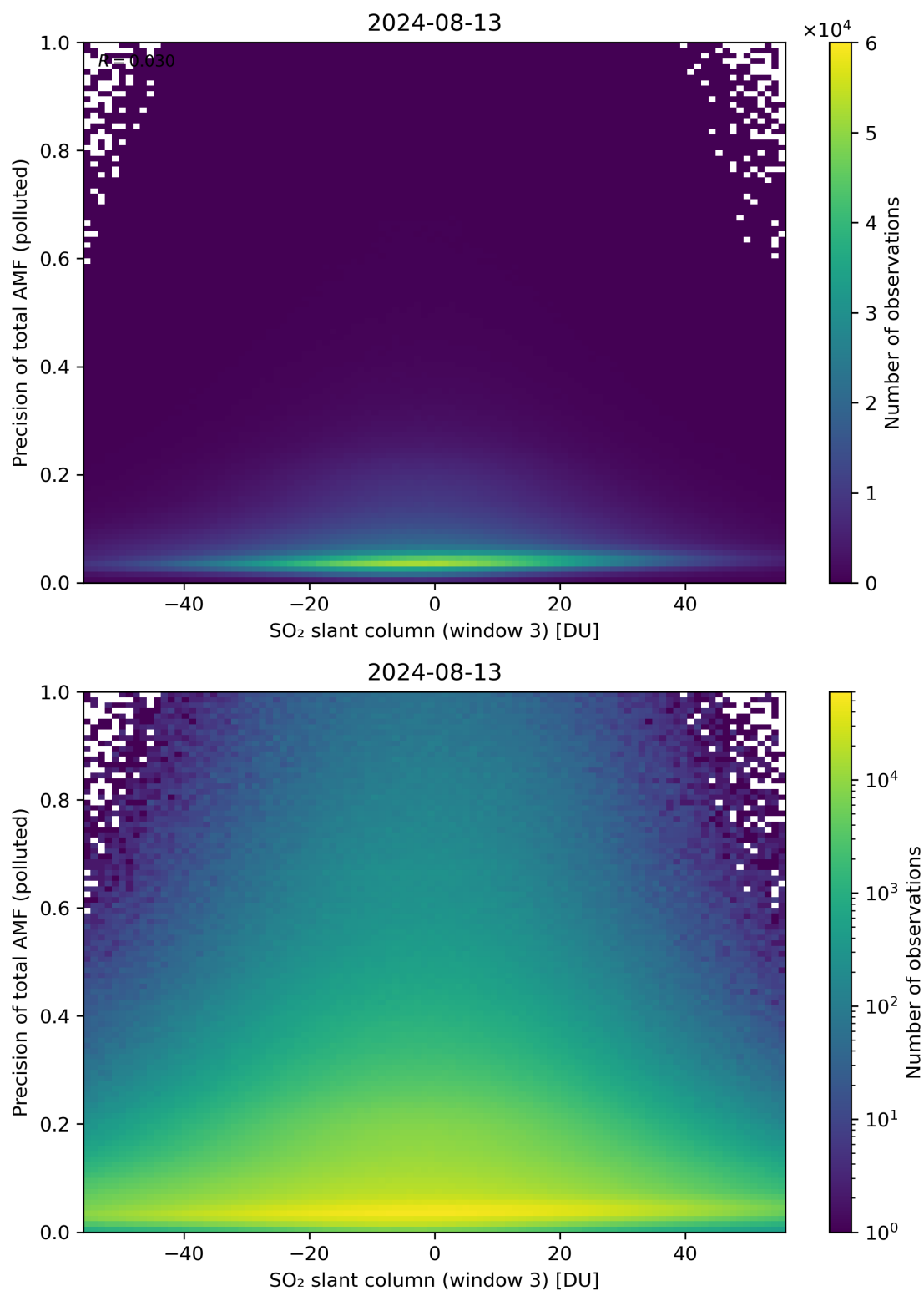
Figure 269: Scatter density plot of “SO 2 slant column (window 3)” against “Precision of total AMF (polluted)” for 2024-08-12 to 2024-08-14.
