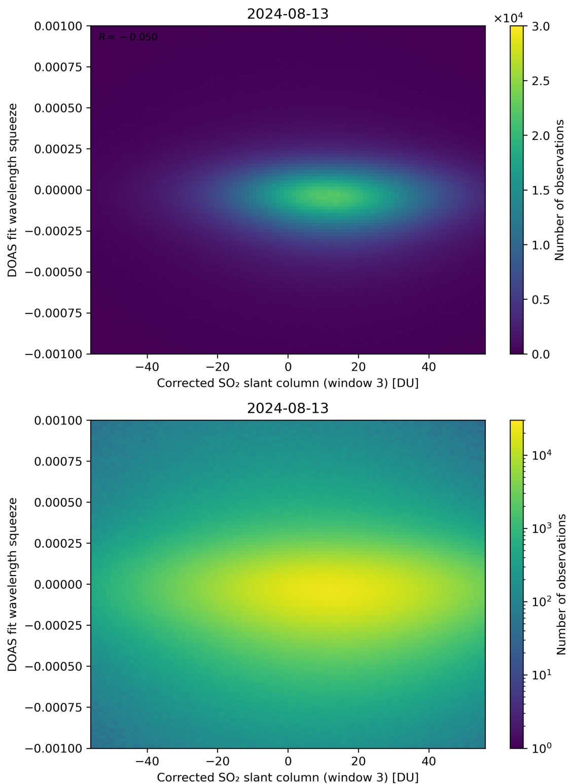
Figure 207: Scatter density plot of “Corrected SO 2 slant column (window 3)” against “DOAS fit wavelength squeeze” for 2024-08-12 to 2024-08-14.
