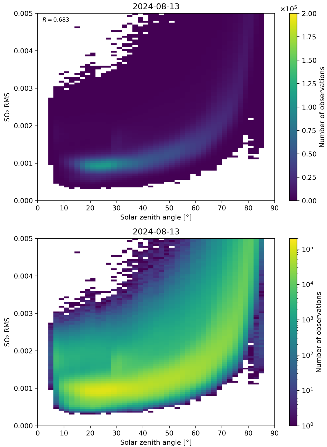
Figure 163: Scatter density plot of “Solar zenith angle” against “SO 2 RMS” for 2024-08-12 to 2024-08-14.
