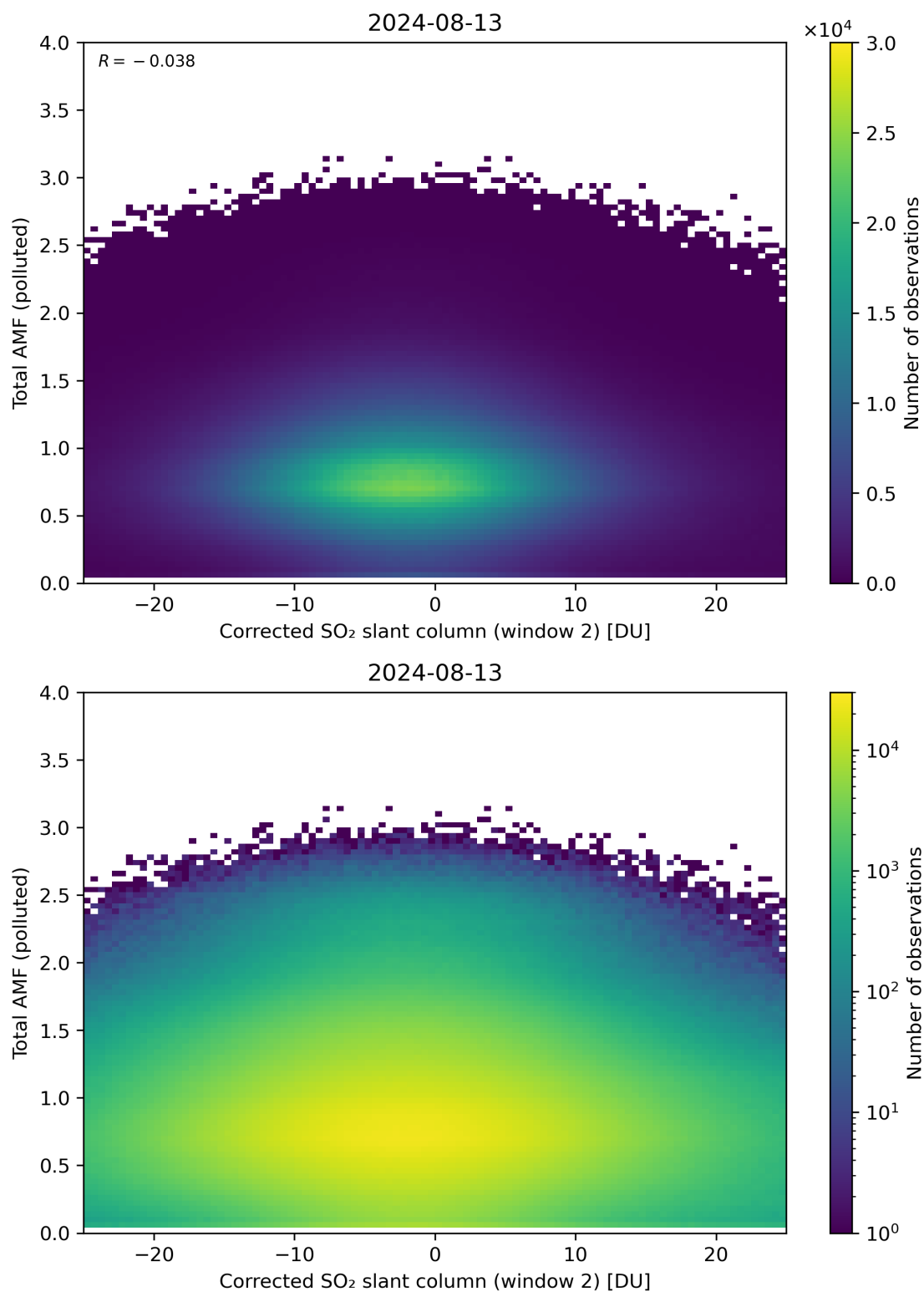
Figure 203: Scatter density plot of “Corrected SO 2 slant column (window 2)” against “Total AMF (polluted)” for 2024-08-12 to 2024-08-14.
