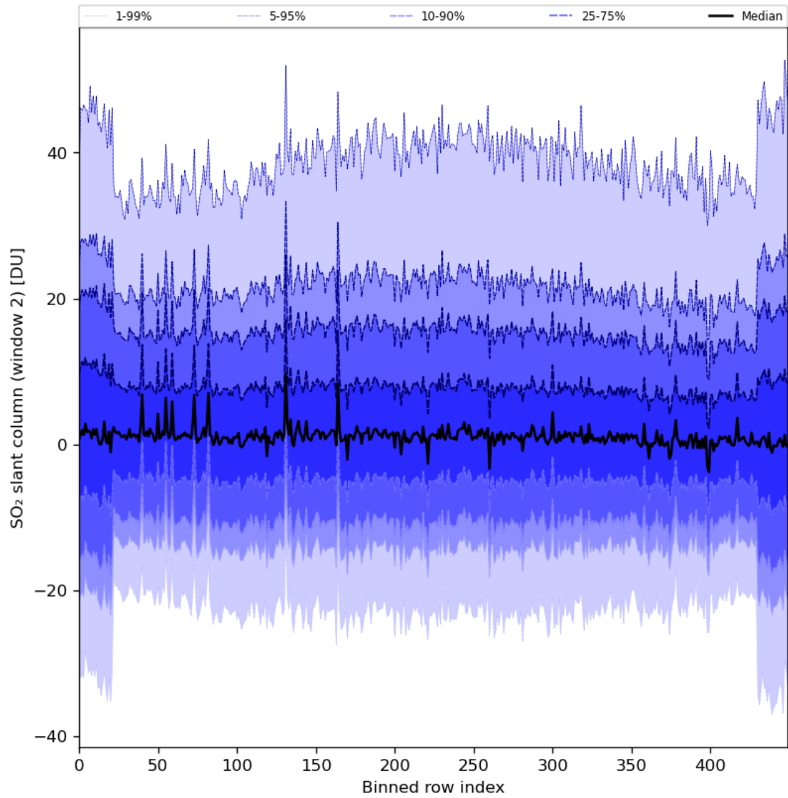
Figure 83: Along track statistics of “SO 2 slant column (window 2)” for 2024-08-12 to 2024-08-14
