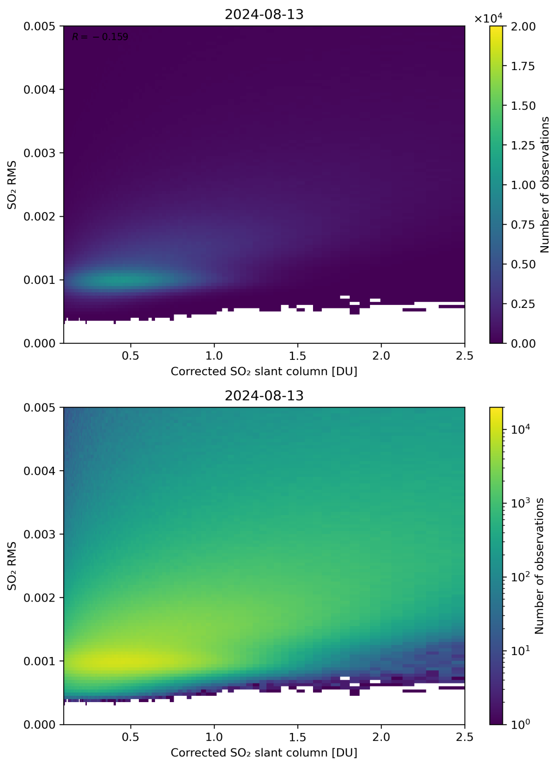
Figure 183: Scatter density plot of “Corrected SO 2 slant column” against “SO 2 RMS” for 2024-08-12 to 2024-08-14.
