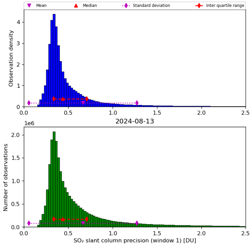
Figure 57: Histogram of “SO 2 slant column precision (window 1)” for 2024-08-12 to 2024-08-14
