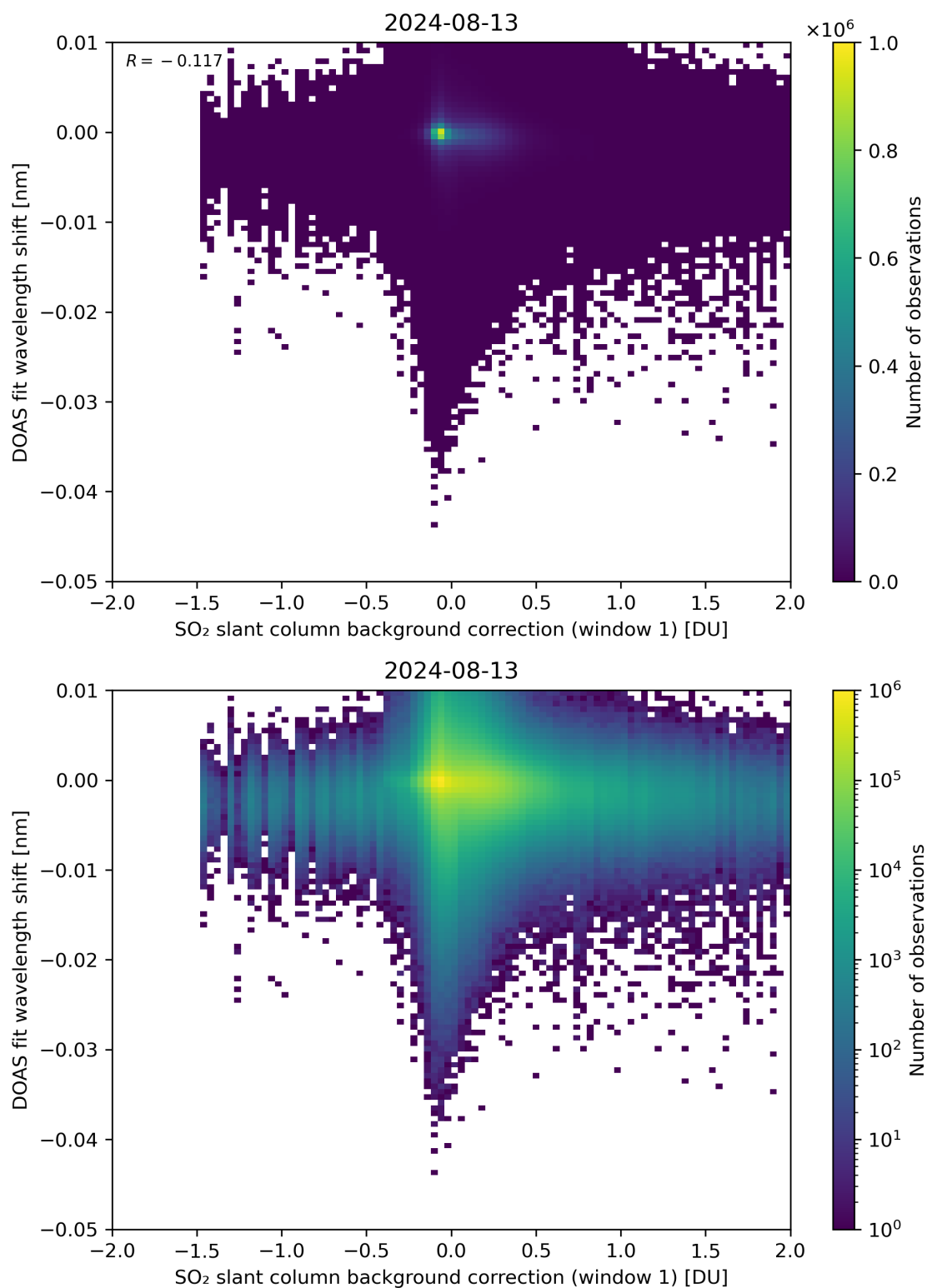
Figure 100: Scatter density plot of “SO 2 slant column background correction (window 1)” against “DOAS fit wavelength shift” for 2024-08-12 to 2024-08-14.
