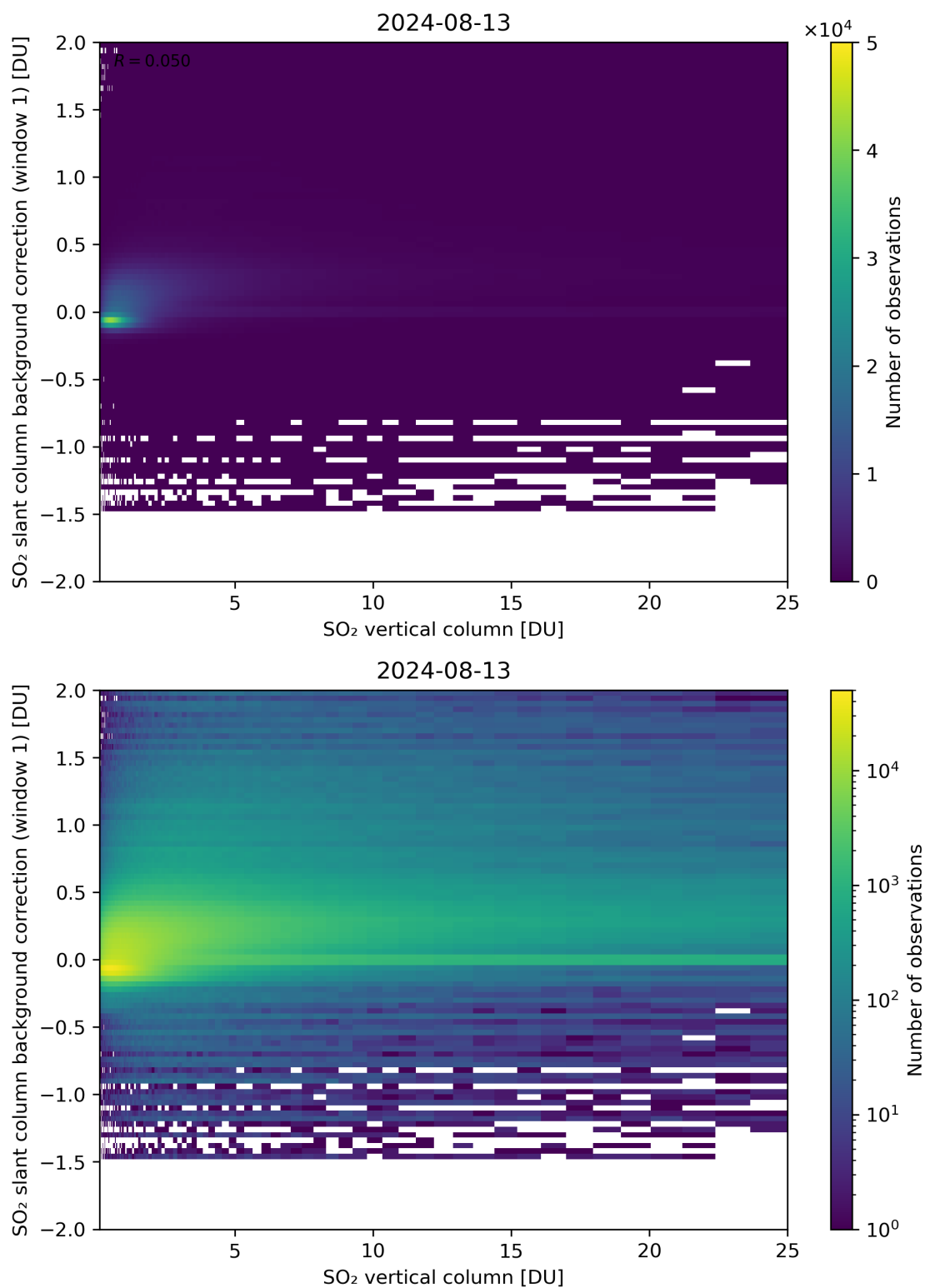
Figure 273: Scatter density plot of “SO 2 vertical column” against “SO 2 slant column background correction (window 1)” for 2024-08-12 to 2024-08-14.
