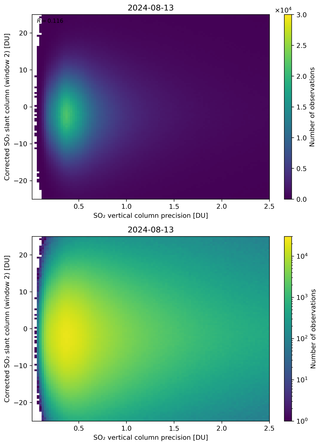
Figure 287: Scatter density plot of “SO 2 vertical column precision” against “Corrected SO 2 slant column (window 2)” for 2024-08-12 to 2024-08-14.
