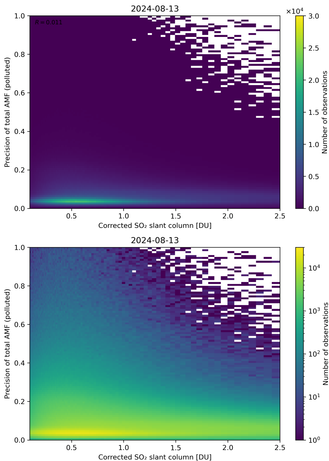
Figure 193: Scatter density plot of “Corrected SO 2 slant column” against “Precision of total AMF (polluted)” for 2024-08-12 to 2024-08-14.
