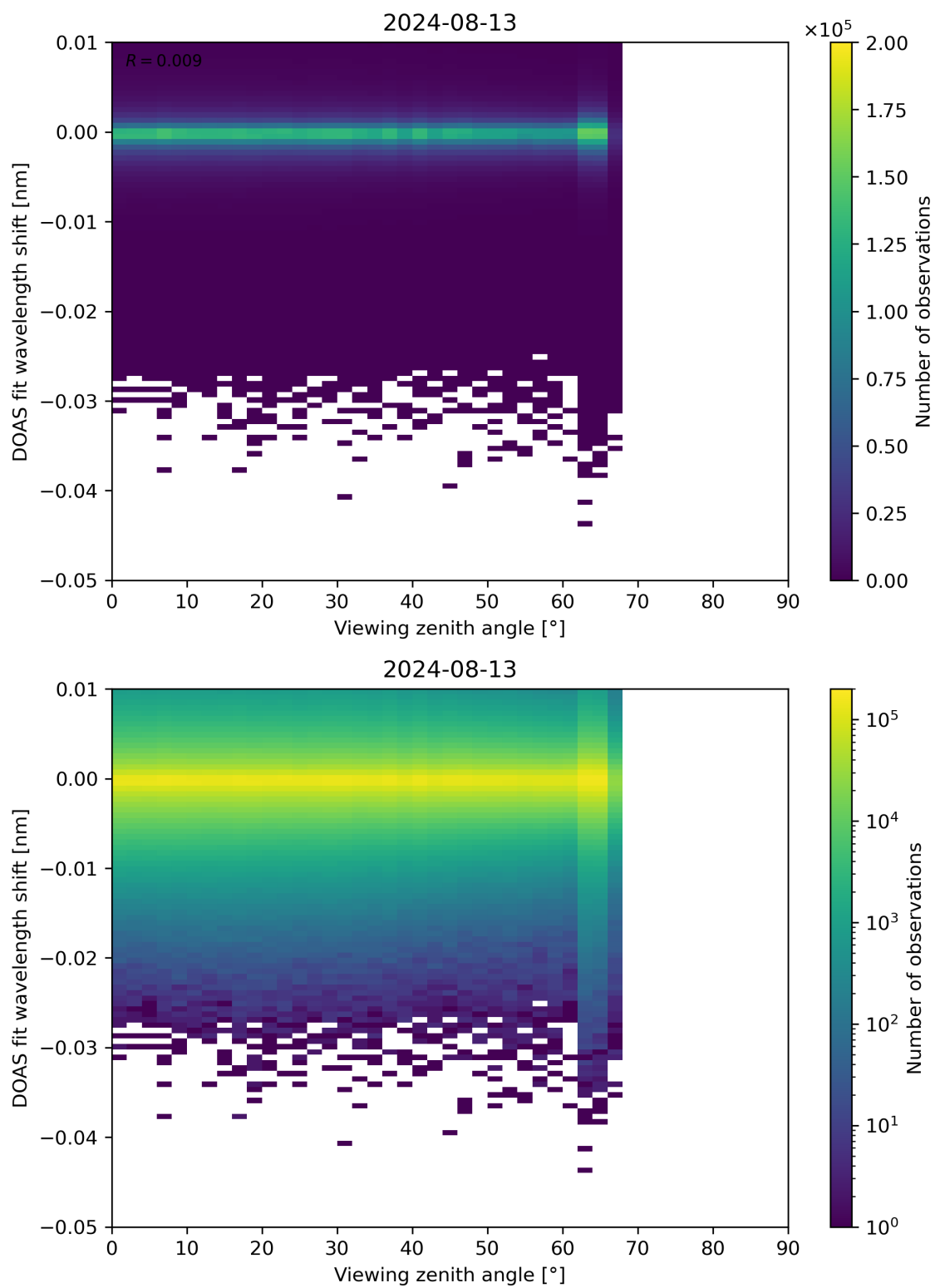
Figure 311: Scatter density plot of “Viewing zenith angle” against “DOAS fit wavelength shift” for 2024-08-12 to 2024-08-14.
