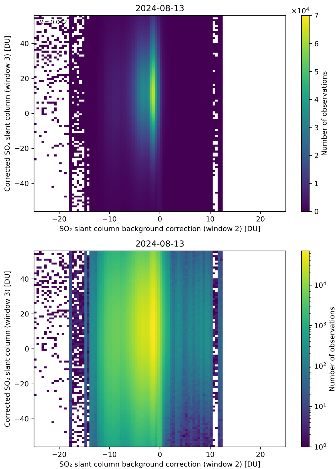
Figure 116: Scatter density plot of “SO 2 slant column background correction (window 2)” against “Corrected SO 2 slant column (window 3)” for 2024-08-12 to 2024-08-14.
