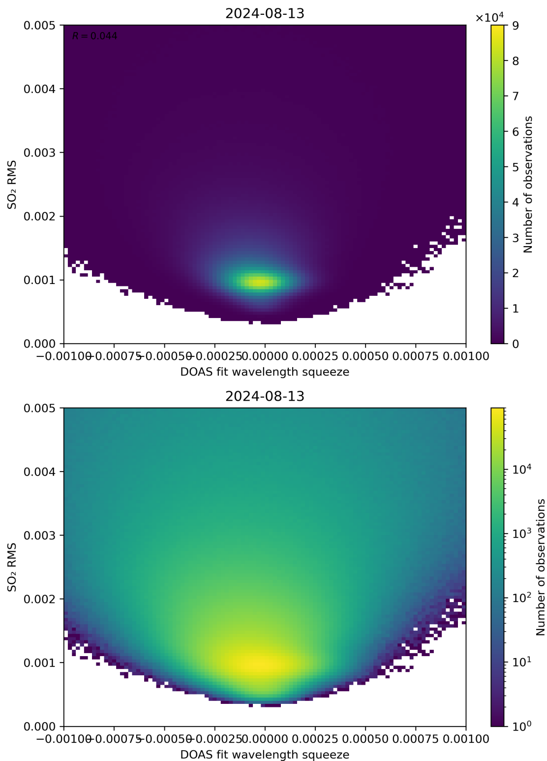
Figure 132: Scatter density plot of “DOAS fit wavelength squeeze” against “SO 2 RMS” for 2024-08-12 to 2024-08-14.
