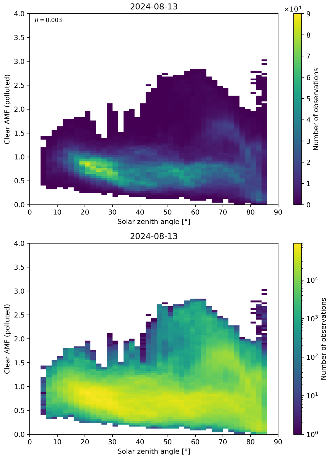
Figure 165: Scatter density plot of “Solar zenith angle” against “Clear AMF (polluted)” for 2024-08-12 to 2024-08-14.
