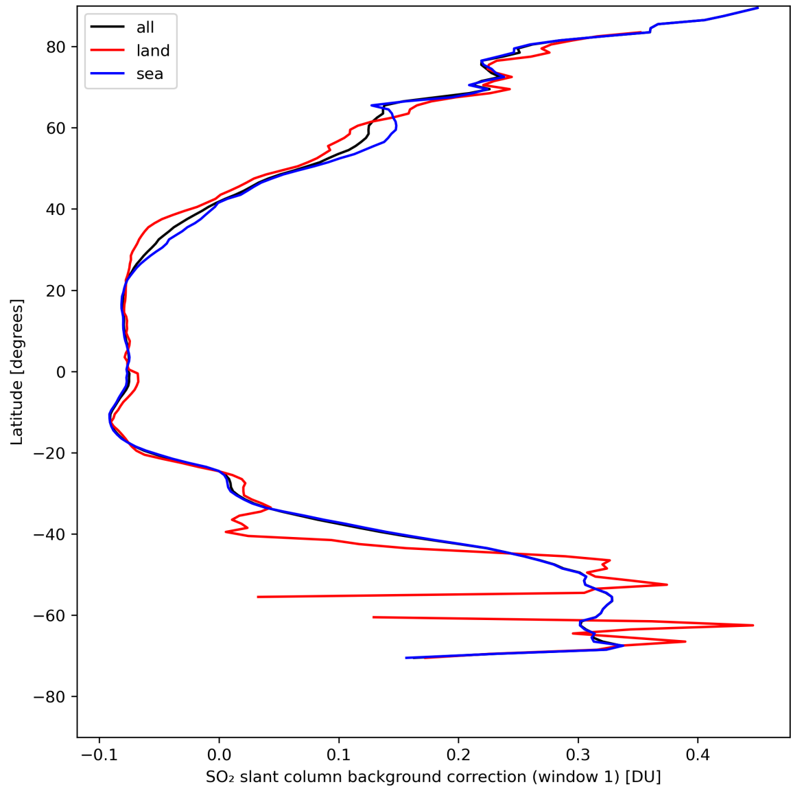
Figure 36: Zonal average of “SO 2 slant column background correction (window 1)” for 2024-08-12 to 2024-08-14.
