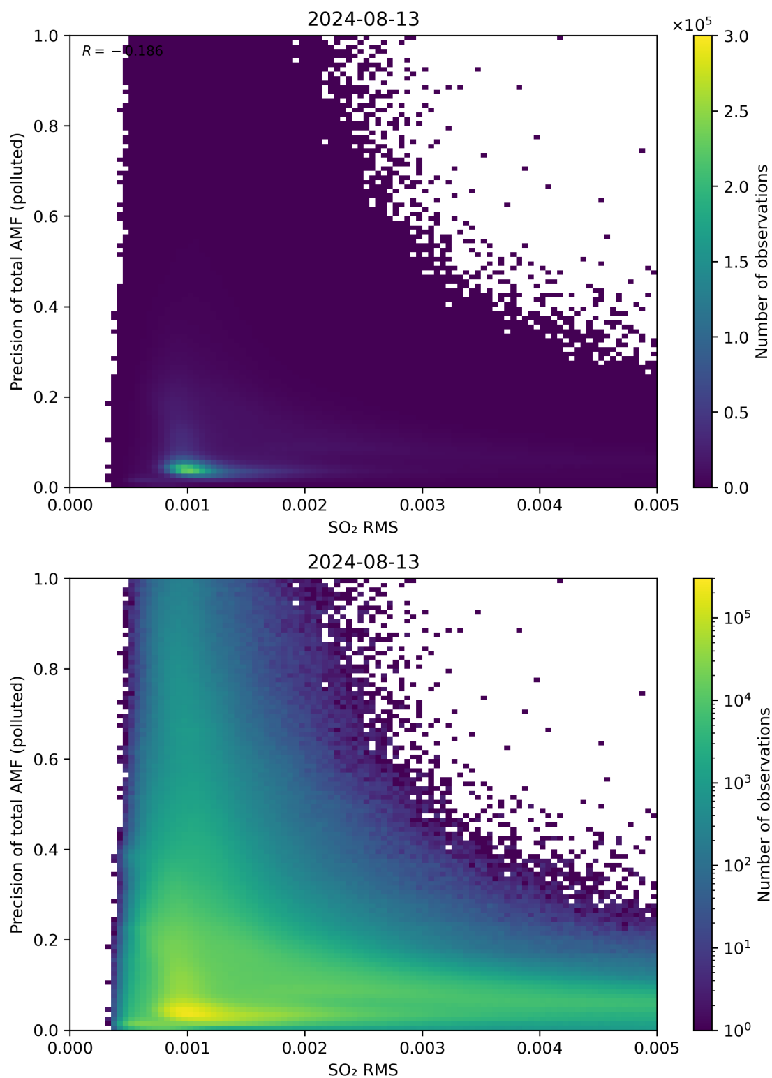
Figure 138: Scatter density plot of “SO 2 RMS” against “Precision of total AMF (polluted)” for 2024-08-12 to 2024-08-14.
