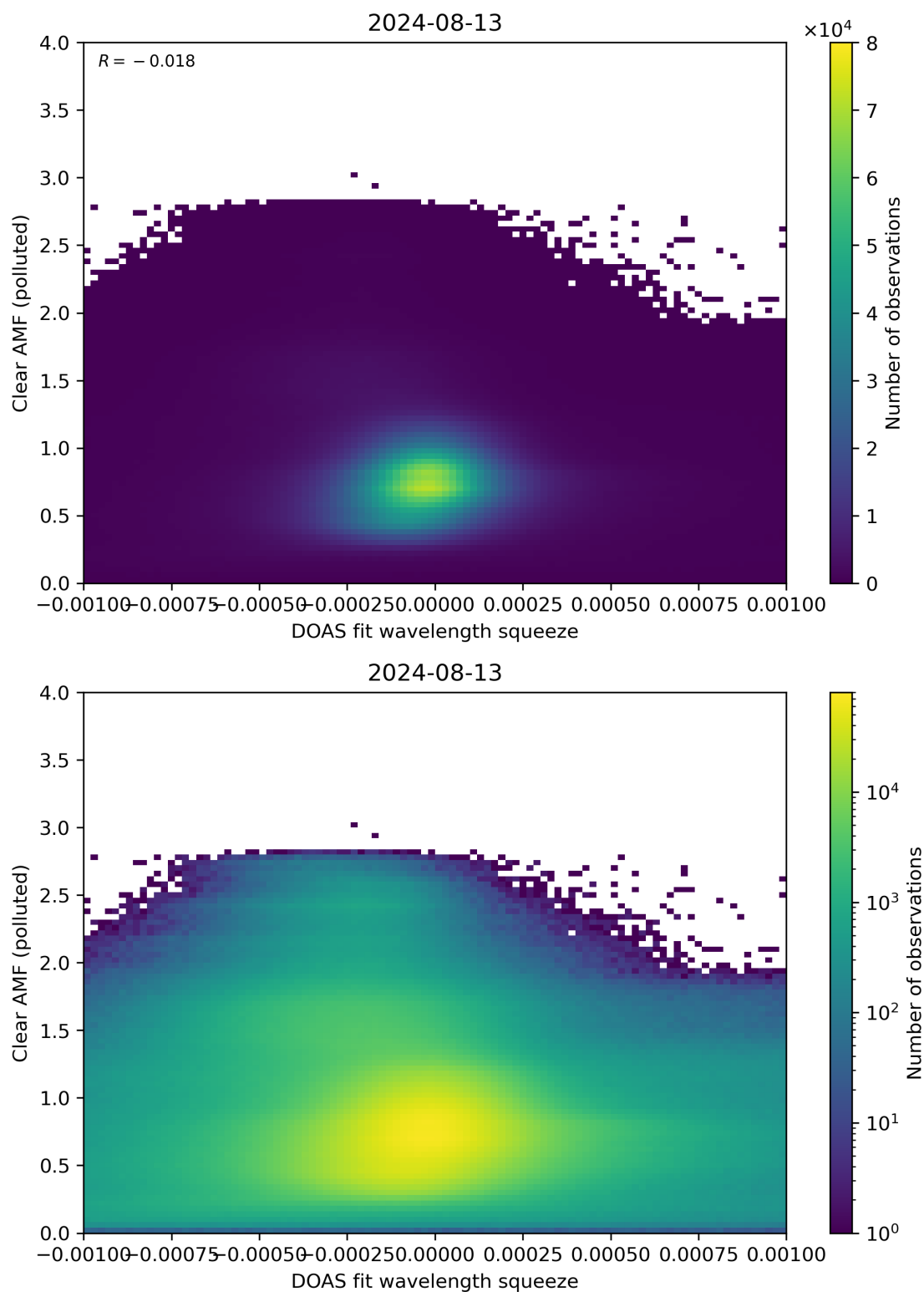
Figure 133: Scatter density plot of “DOAS fit wavelength squeeze” against “Clear AMF (polluted)” for 2024-08-12 to 2024-08-14.
