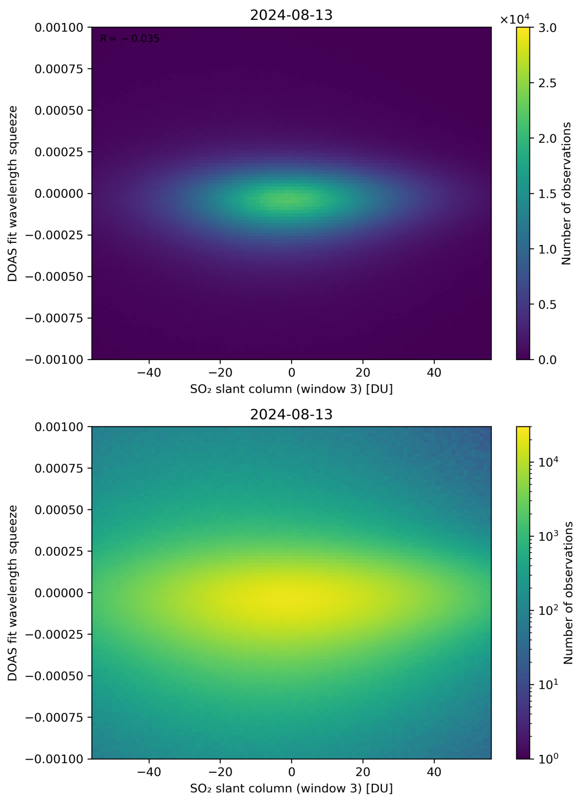
Figure 255: Scatter density plot of “SO 2 slant column (window 3)” against “DOAS fit wavelength squeeze” for 2024-08-12 to 2024-08-14.
