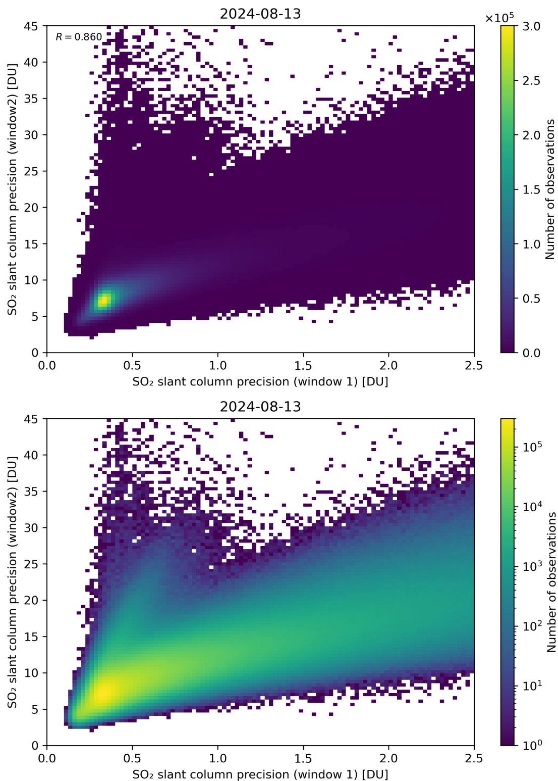
Figure 227: Scatter density plot of “SO 2 slant column precision (window 1)” against “SO 2 slant column precision (window2)” for 2024-08-12 to 2024-08-14.
