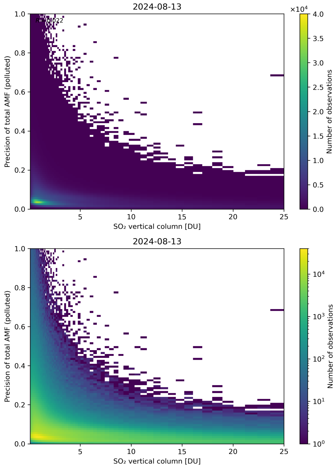
Figure 306: Scatter density plot of “SO 2 vertical column” against “Precision of total AMF (polluted)” for 2024-08-12 to 2024-08-14.
