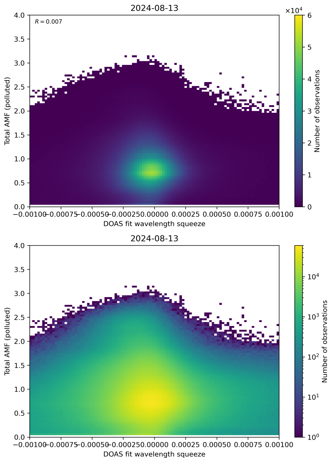
Figure 134: Scatter density plot of “DOAS fit wavelength squeeze” against “Total AMF (polluted)” for 2024-08-12 to 2024-08-14.
