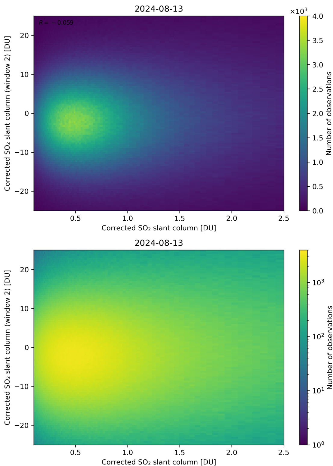
Figure 185: Scatter density plot of “Corrected SO 2 slant column” against “Corrected SO 2 slant column (window 2)” for 2024-08-12 to 2024-08-14.
