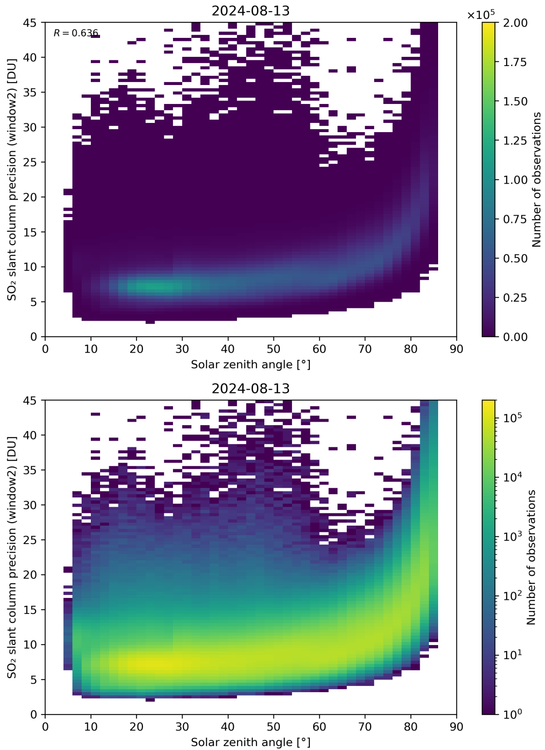
Figure 171: Scatter density plot of “Solar zenith angle” against “SO 2 slant column precision (window2)” for 2024-08-12 to 2024-08-14.
