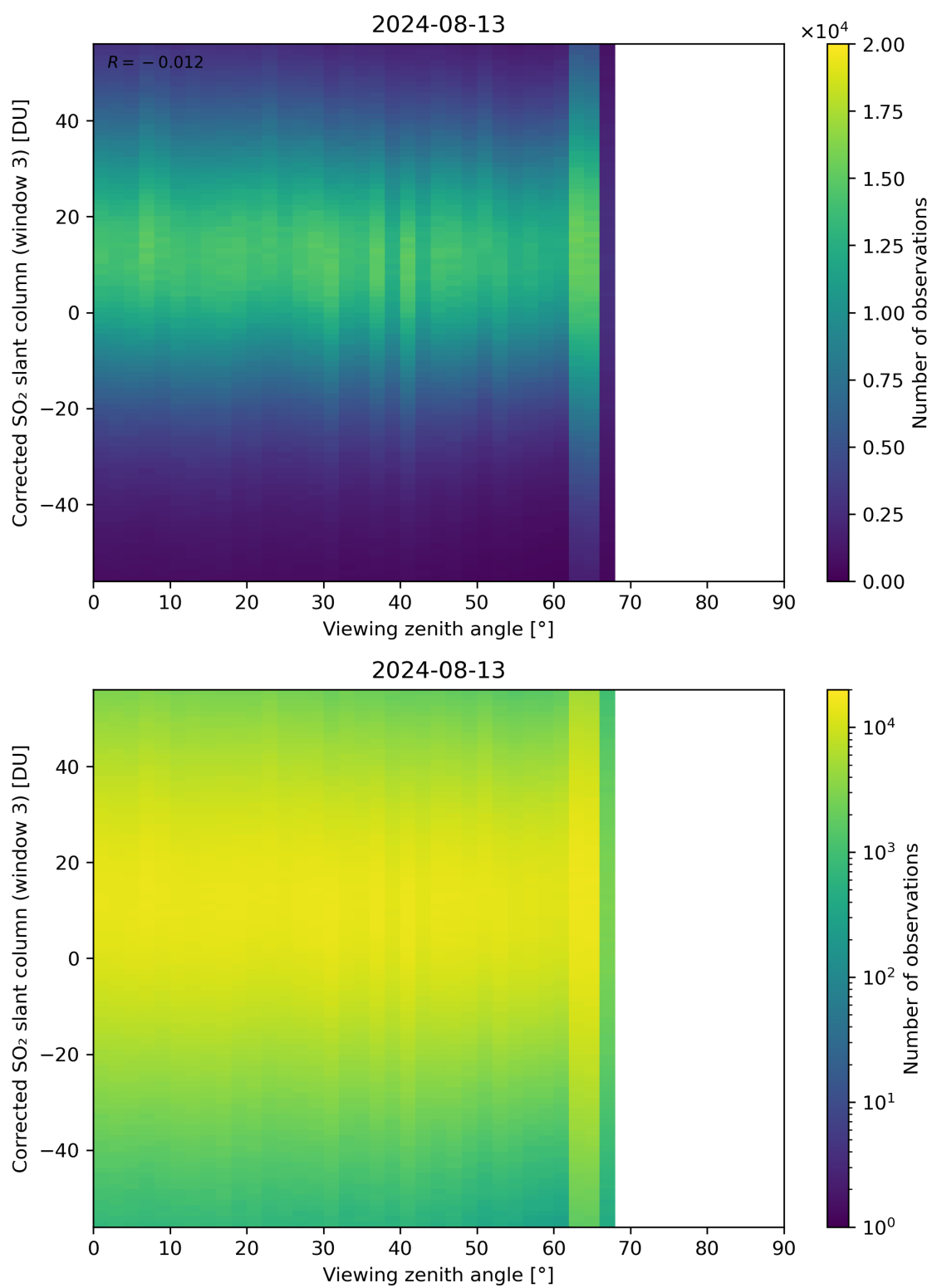
Figure 319: Scatter density plot of “Viewing zenith angle” against “Corrected SO 2 slant column (window 3)” for 2024-08-12 to 2024-08-14.
