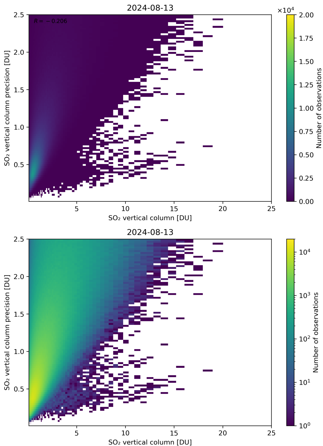
Figure 307: Scatter density plot of “SO 2 vertical column” against “SO 2 vertical column precision” for 2024-08-12 to 2024-08-14.
