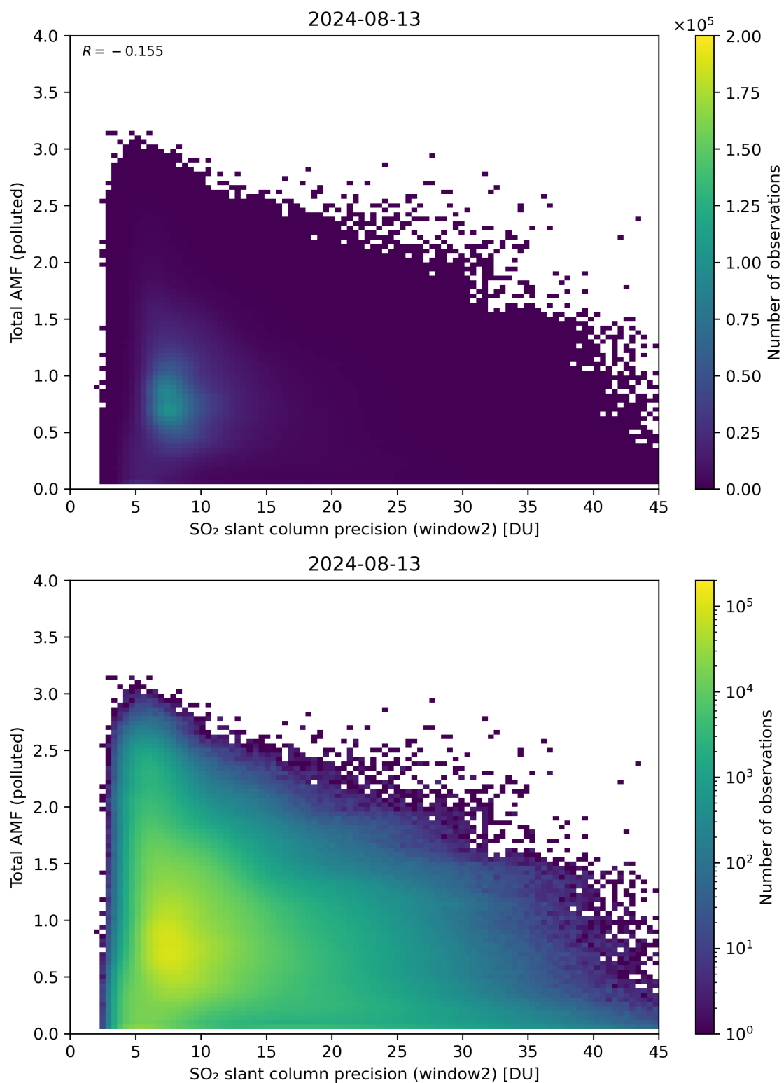
Figure 251: Scatter density plot of “SO 2 slant column precision (window2)” against “Total AMF (polluted)” for 2024-08-12 to 2024-08-14.
