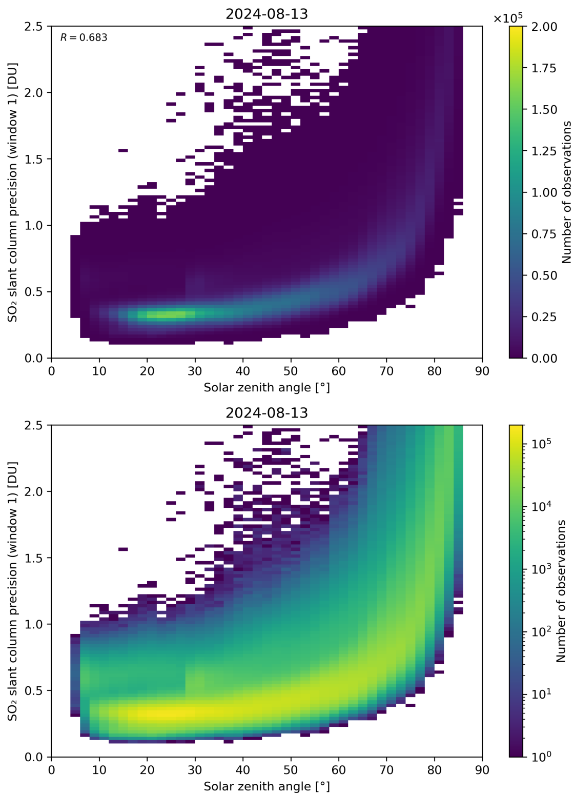
Figure 170: Scatter density plot of “Solar zenith angle” against “SO 2 slant column precision (window 1)” for 2024-08-12 to 2024-08-14.
