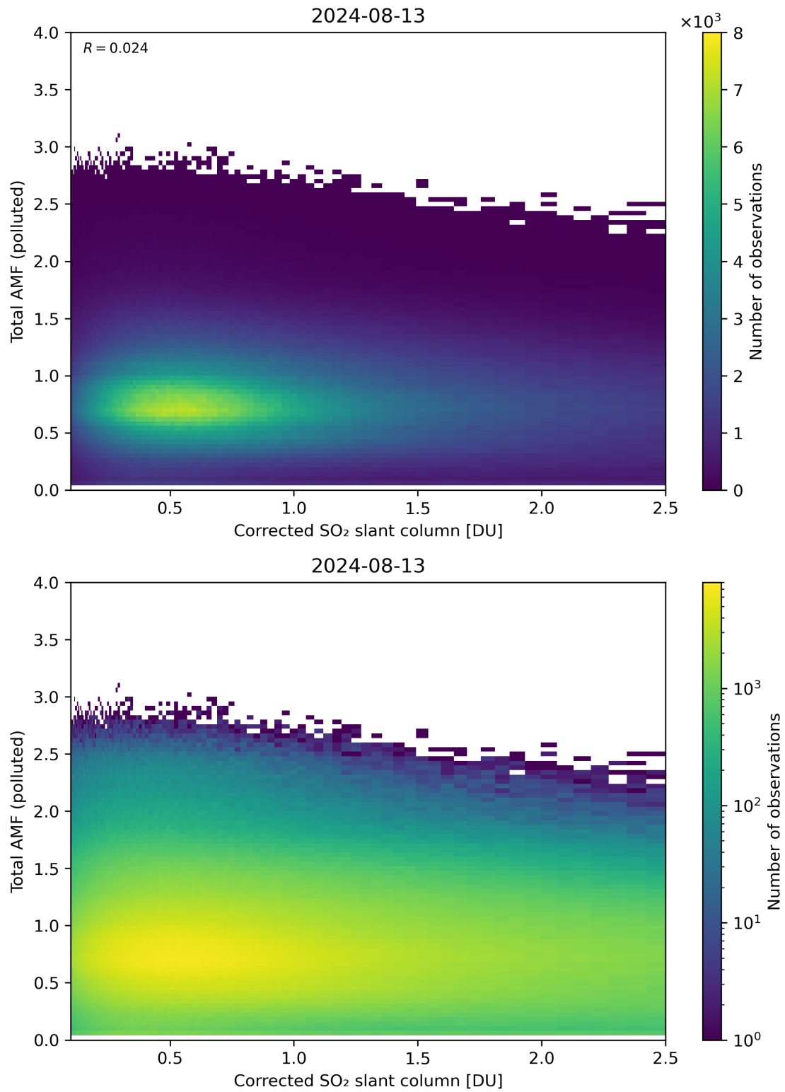
Figure 192: Scatter density plot of “Corrected SO 2 slant column” against “Total AMF (polluted)” for 2024-08-12 to 2024-08-14.
