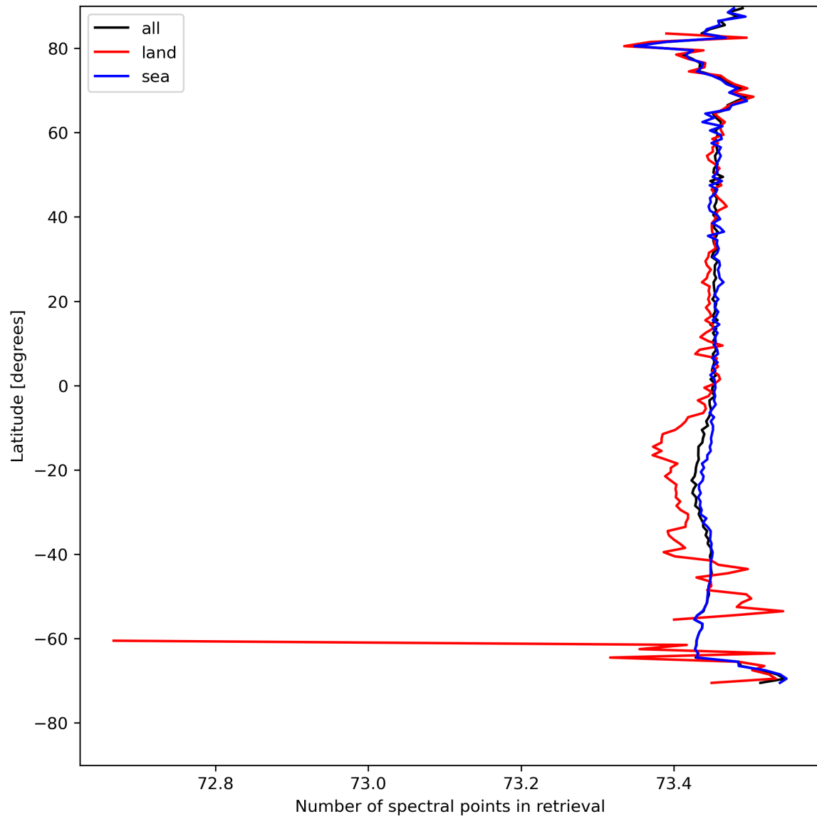
Figure 51: Zonal average of “Number of spectral points in retrieval” for 2024-08-12 to 2024-08-14.
