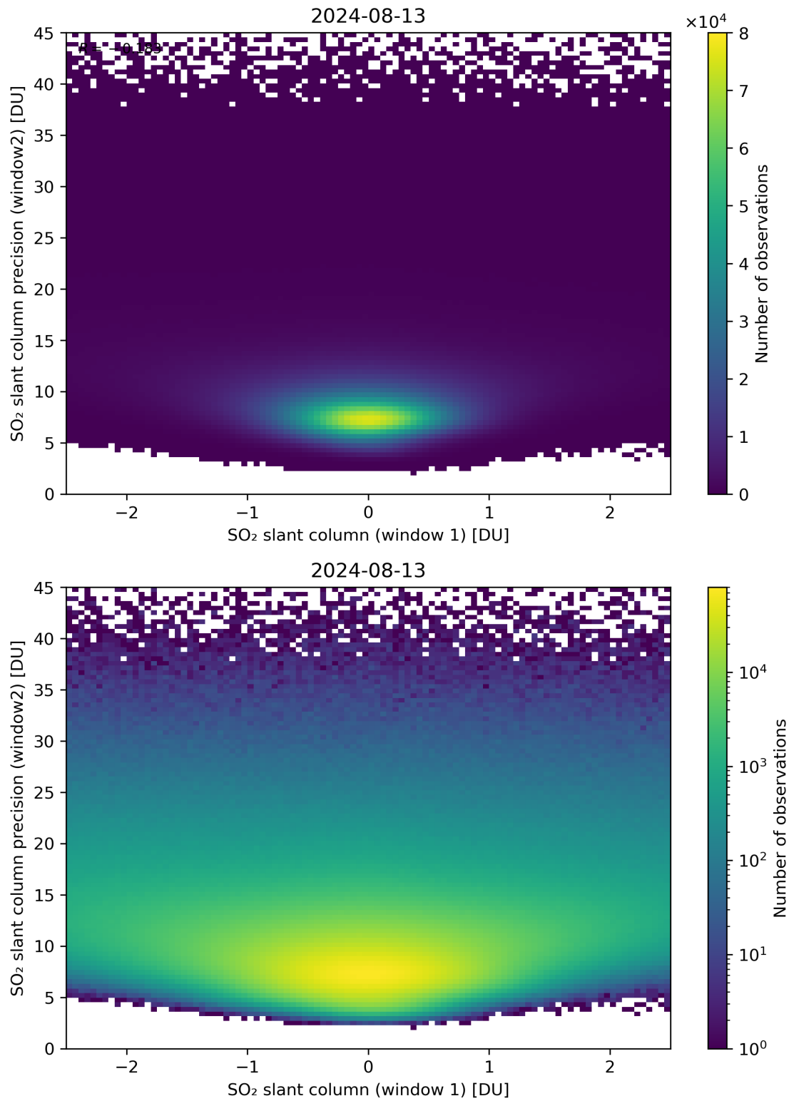
Figure 236: Scatter density plot of “SO 2 slant column (window 1)” against “SO 2 slant column precision (window2)” for 2024-08-12 to 2024-08-14.
