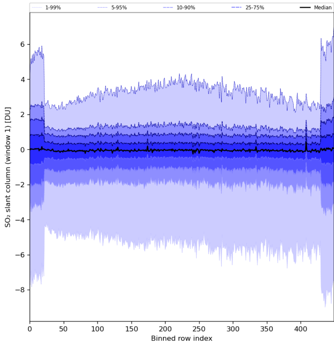
Figure 79: Along track statistics of “SO 2 slant column (window 1)” for 2024-08-12 to 2024-08-14
