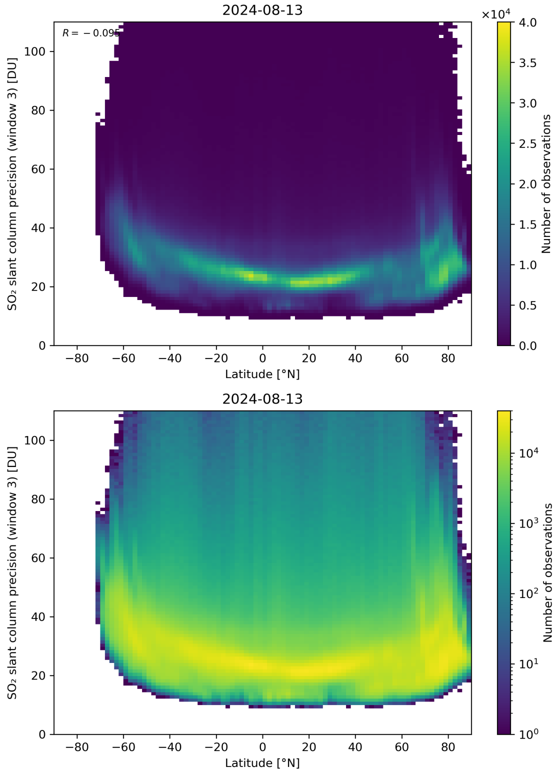
Figure 153: Scatter density plot of “Latitude” against “SO 2 slant column precision (window 3)” for 2024-08-12 to 2024-08-14.
