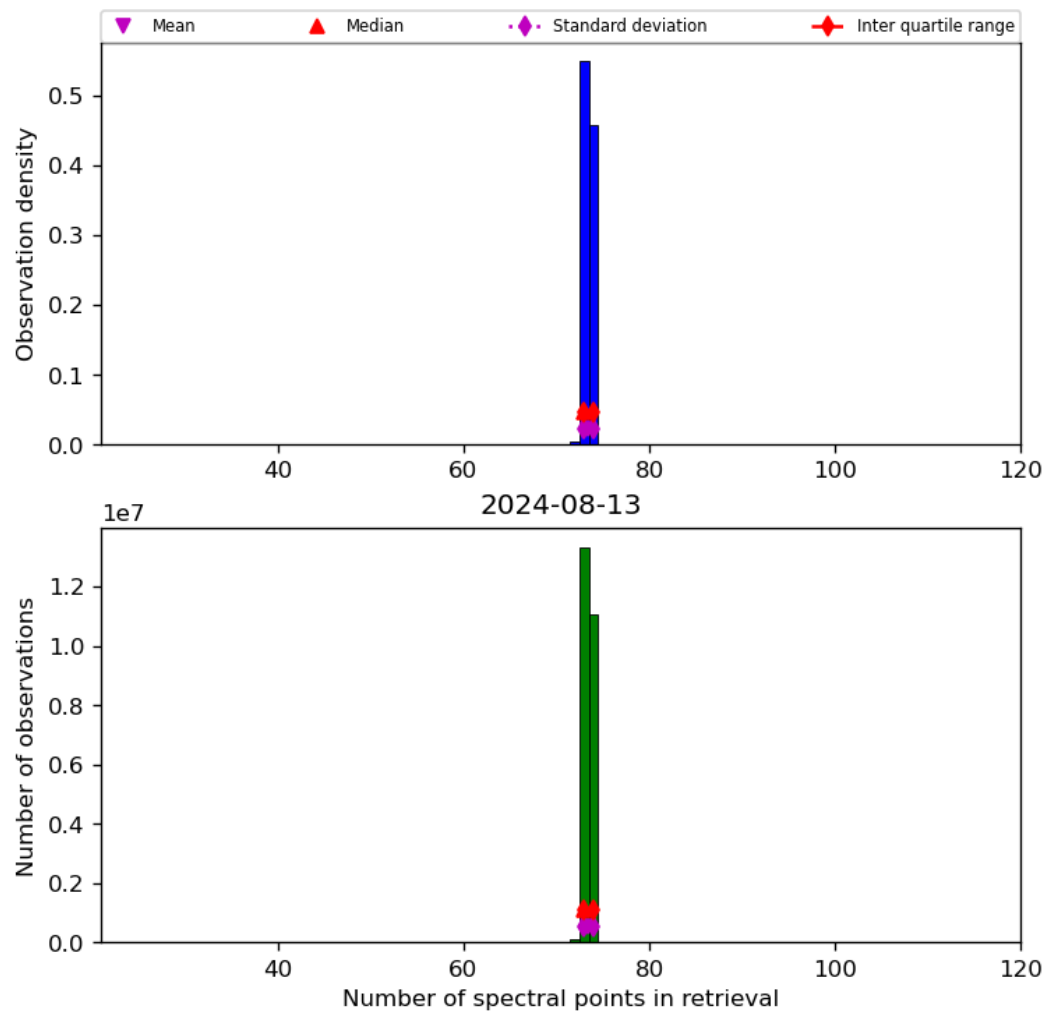
Figure 74: Histogram of “Number of spectral points in retrieval” for 2024-08-12 to 2024-08-14
