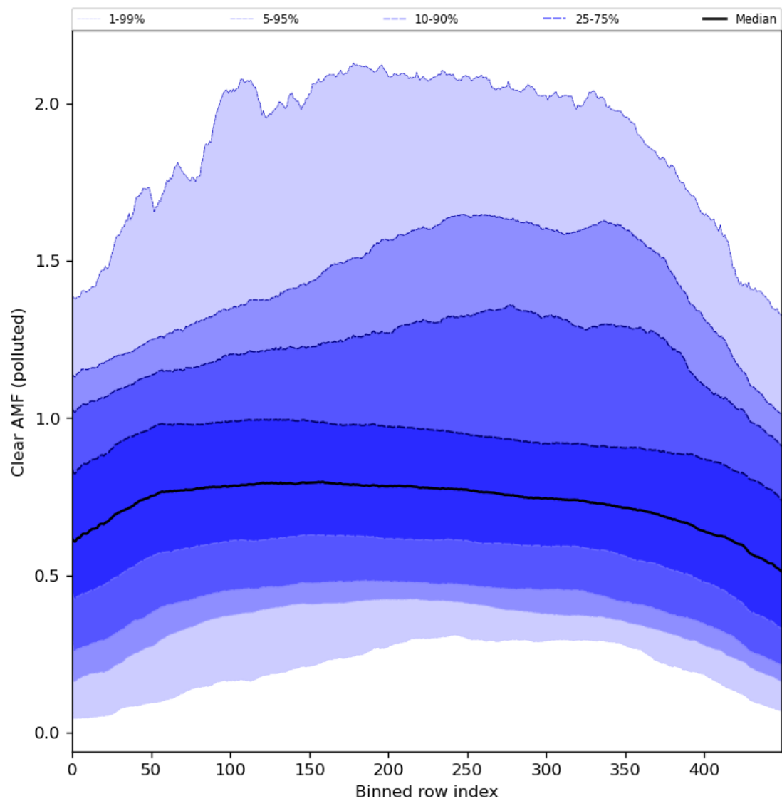
Figure 96: Along track statistics of “Clear AMF (polluted)” for 2024-08-12 to 2024-08-14
