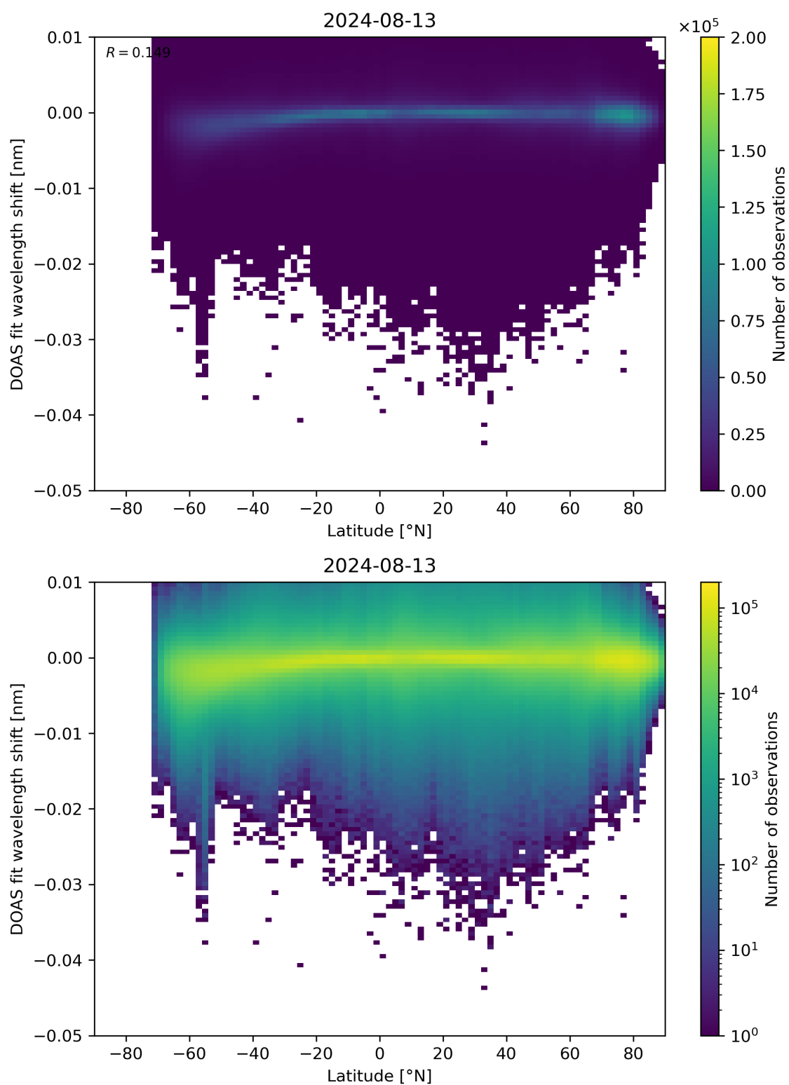
Figure 142: Scatter density plot of “Latitude” against “DOAS fit wavelength shift” for 2024-08-12 to 2024-08-14.
