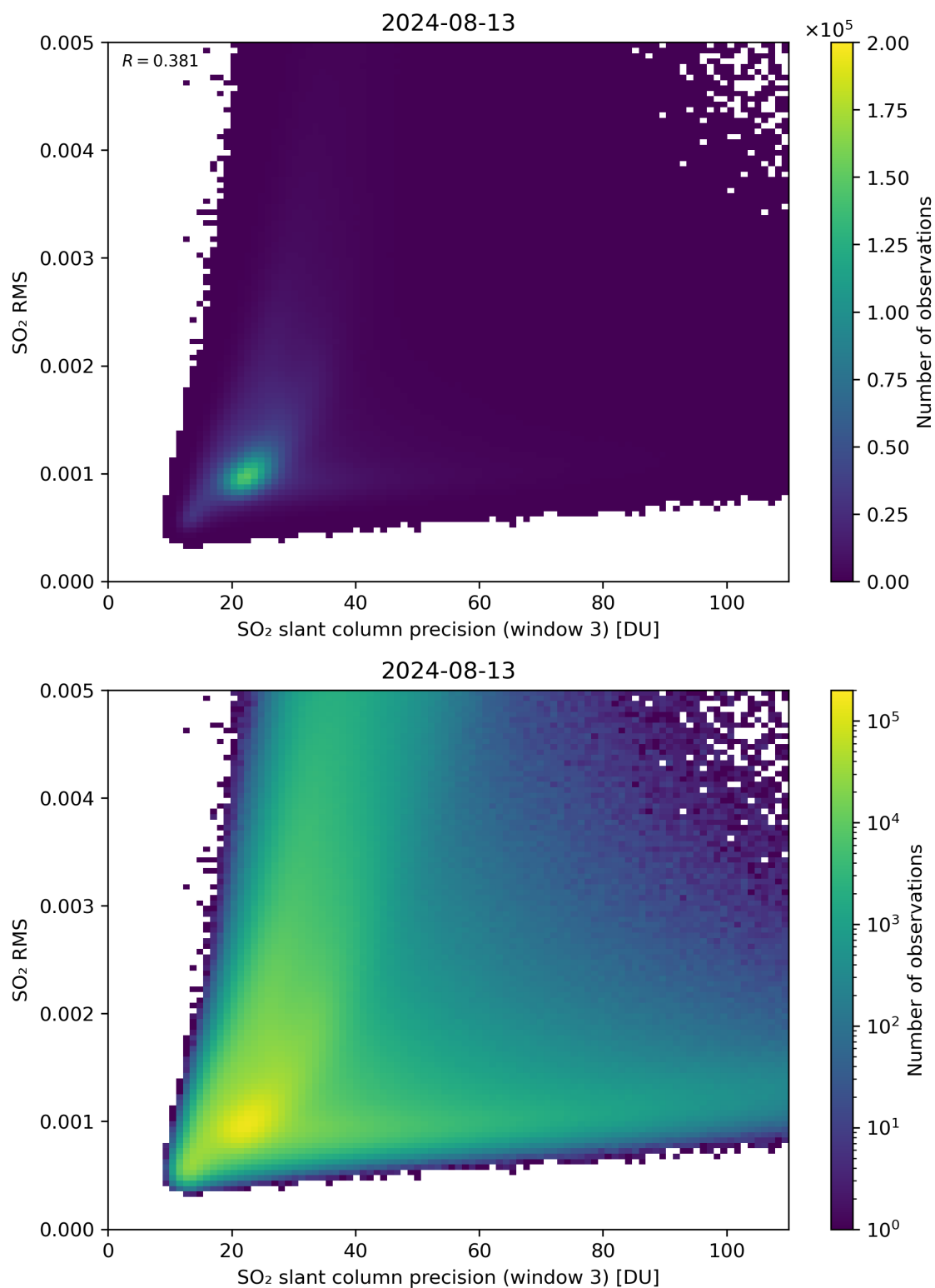
Figure 260: Scatter density plot of “SO 2 slant column precision (window 3)” against “SO 2 RMS” for 2024-08-12 to 2024-08-14.
