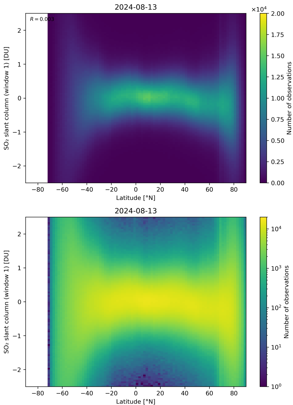
Figure 149: Scatter density plot of “Latitude” against “SO 2 slant column (window 1)” for 2024-08-12 to 2024-08-14.
