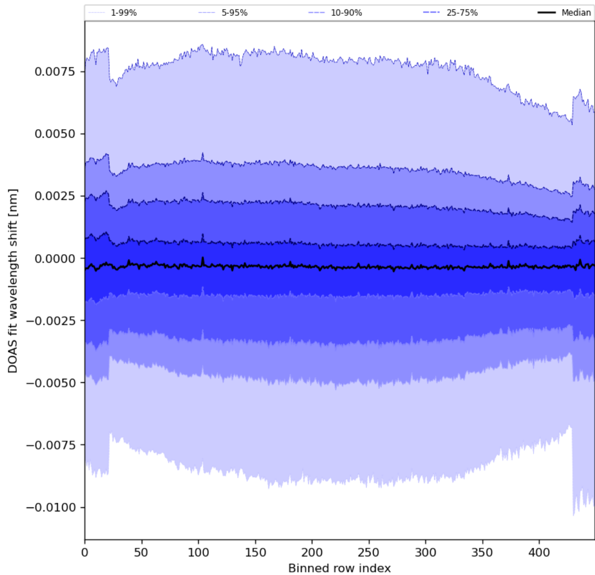
Figure 91: Along track statistics of “DOAS fit wavelength shift” for 2024-08-12 to 2024-08-14
