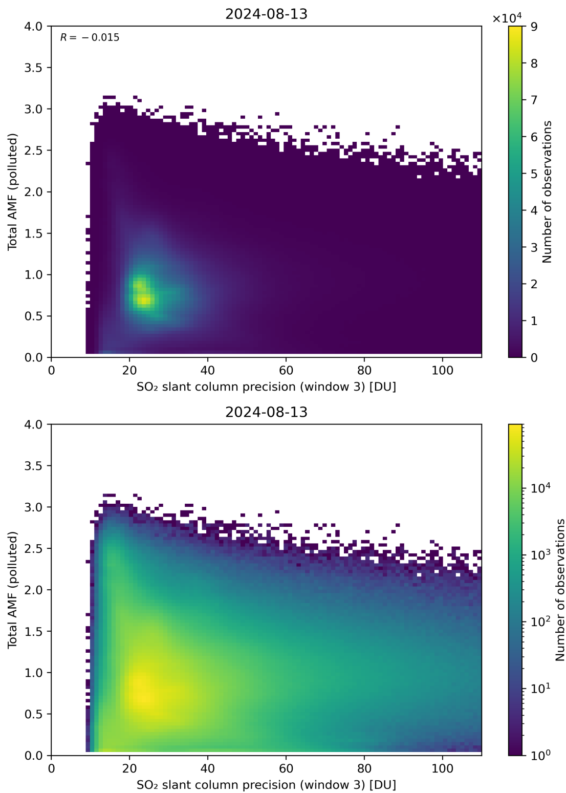
Figure 263: Scatter density plot of “SO 2 slant column precision (window 3)” against “Total AMF (polluted)” for 2024-08-12 to 2024-08-14.
