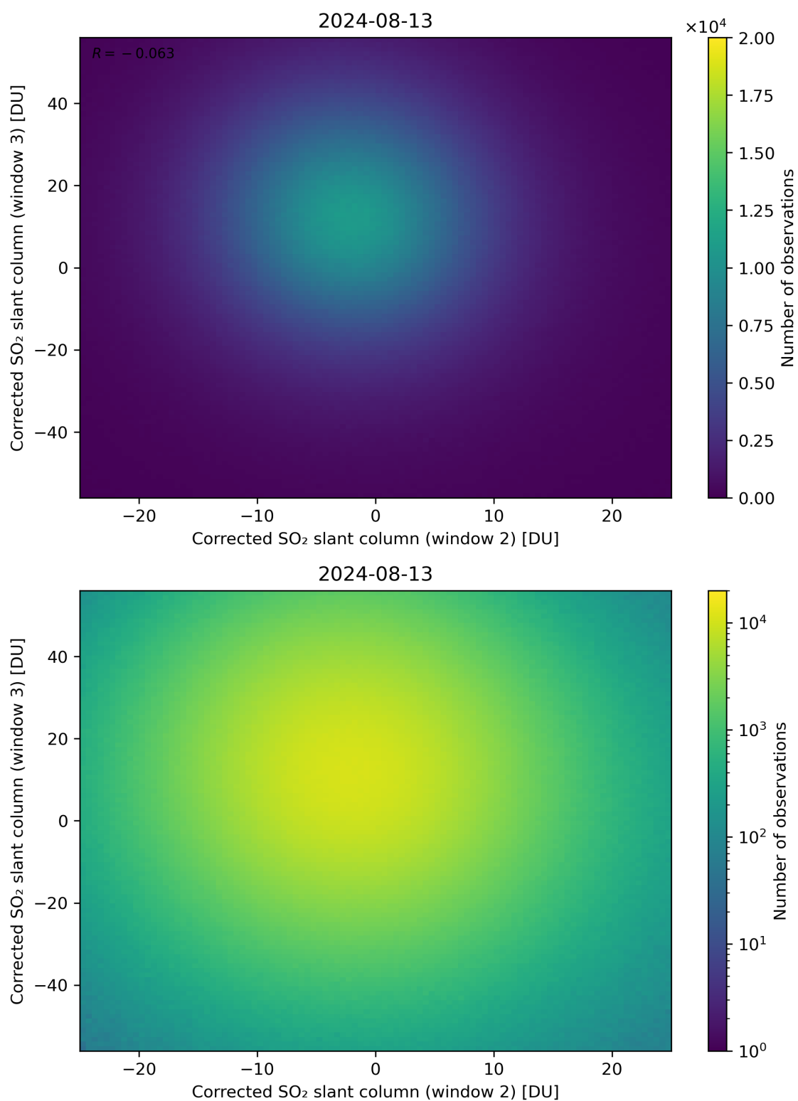
Figure 200: Scatter density plot of “Corrected SO 2 slant column (window 2)” against “Corrected SO 2 slant column (window 3)” for 2024-08-12 to 2024-08-14.
