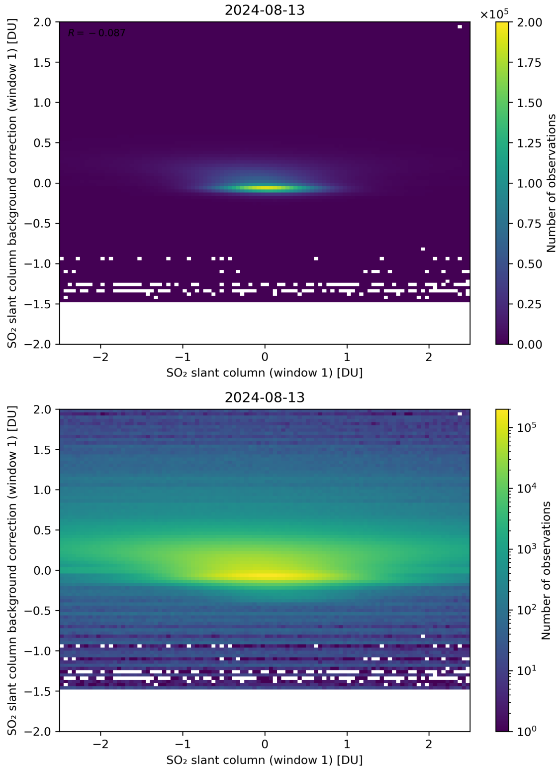
Figure 212: Scatter density plot of “SO 2 slant column (window 1)” against “SO 2 slant column background correction (window 1)” for 2024-08-12 to 2024-08-14.
