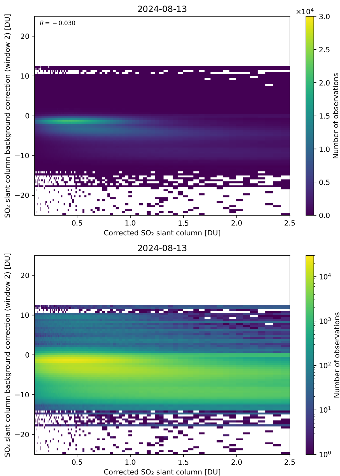
Figure 179: Scatter density plot of “Corrected SO 2 slant column” against “SO 2 slant column background correction (window 2)” for 2024-08-12 to 2024-08-14.
