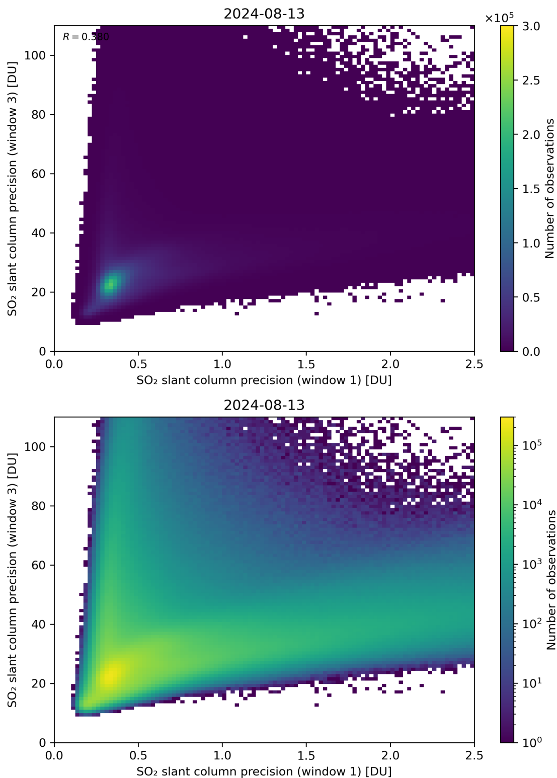
Figure 229: Scatter density plot of “SO 2 slant column precision (window 1)” against “SO 2 slant column precision (window 3)” for 2024-08-12 to 2024-08-14.
