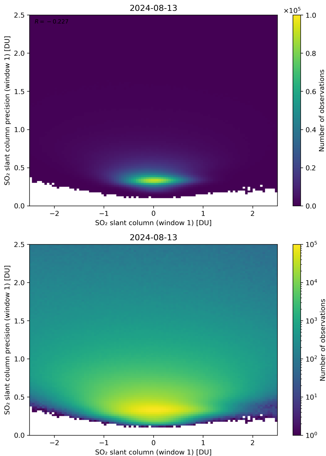
Figure 235: Scatter density plot of “SO 2 slant column (window 1)” against “SO 2 slant column precision (window 1)” for 2024-08-12 to 2024-08-14.
