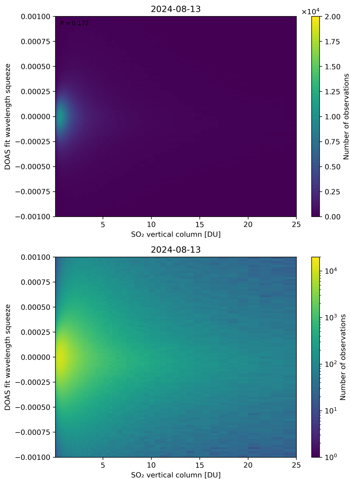
Figure 277: Scatter density plot of “SO 2 vertical column” against “DOAS fit wavelength squeeze” for 2024-08-12 to 2024-08-14.
