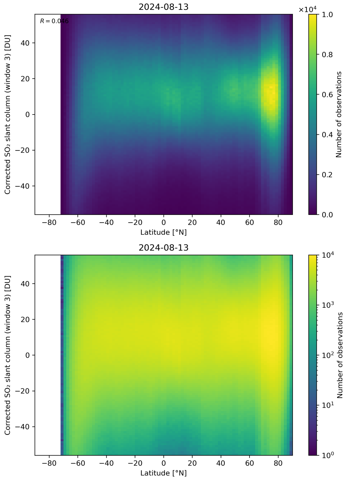
Figure 148: Scatter density plot of “Latitude” against “Corrected SO 2 slant column (window 3)” for 2024-08-12 to 2024-08-14.
