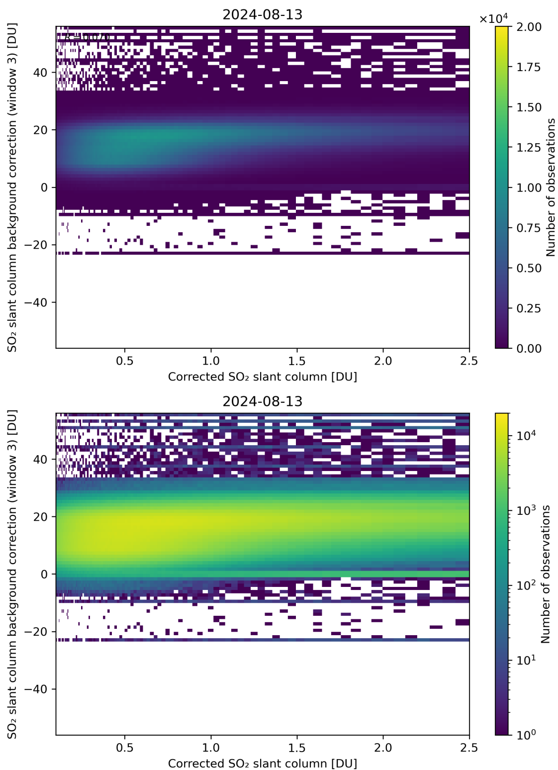
Figure 180: Scatter density plot of “Corrected SO 2 slant column” against “SO 2 slant column background correction (window 3)” for 2024-08-12 to 2024-08-14.
