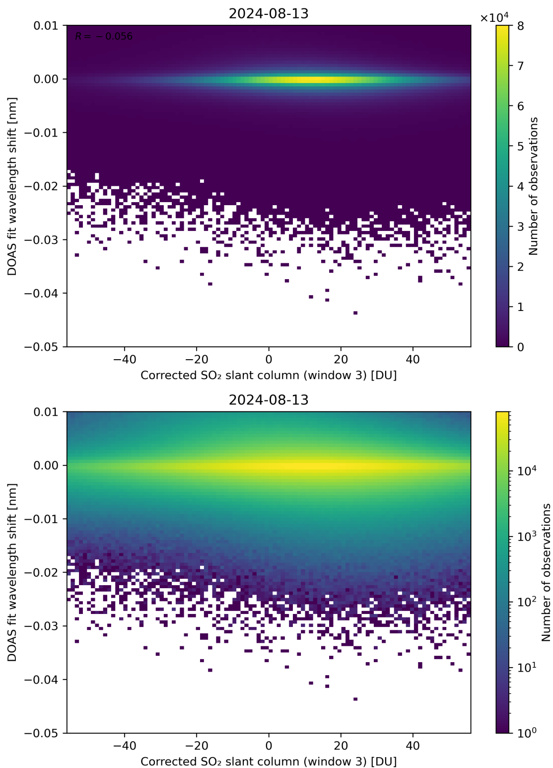
Figure 206: Scatter density plot of “Corrected SO 2 slant column (window 3)” against “DOAS fit wavelength shift” for 2024-08-12 to 2024-08-14.
