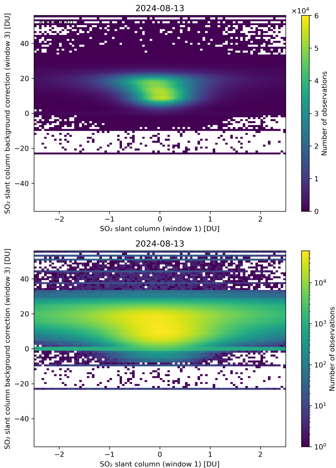
Figure 214: Scatter density plot of “SO 2 slant column (window 1)” against “SO 2 slant column background correction (window 3)” for 2024-08-12 to 2024-08-14.
