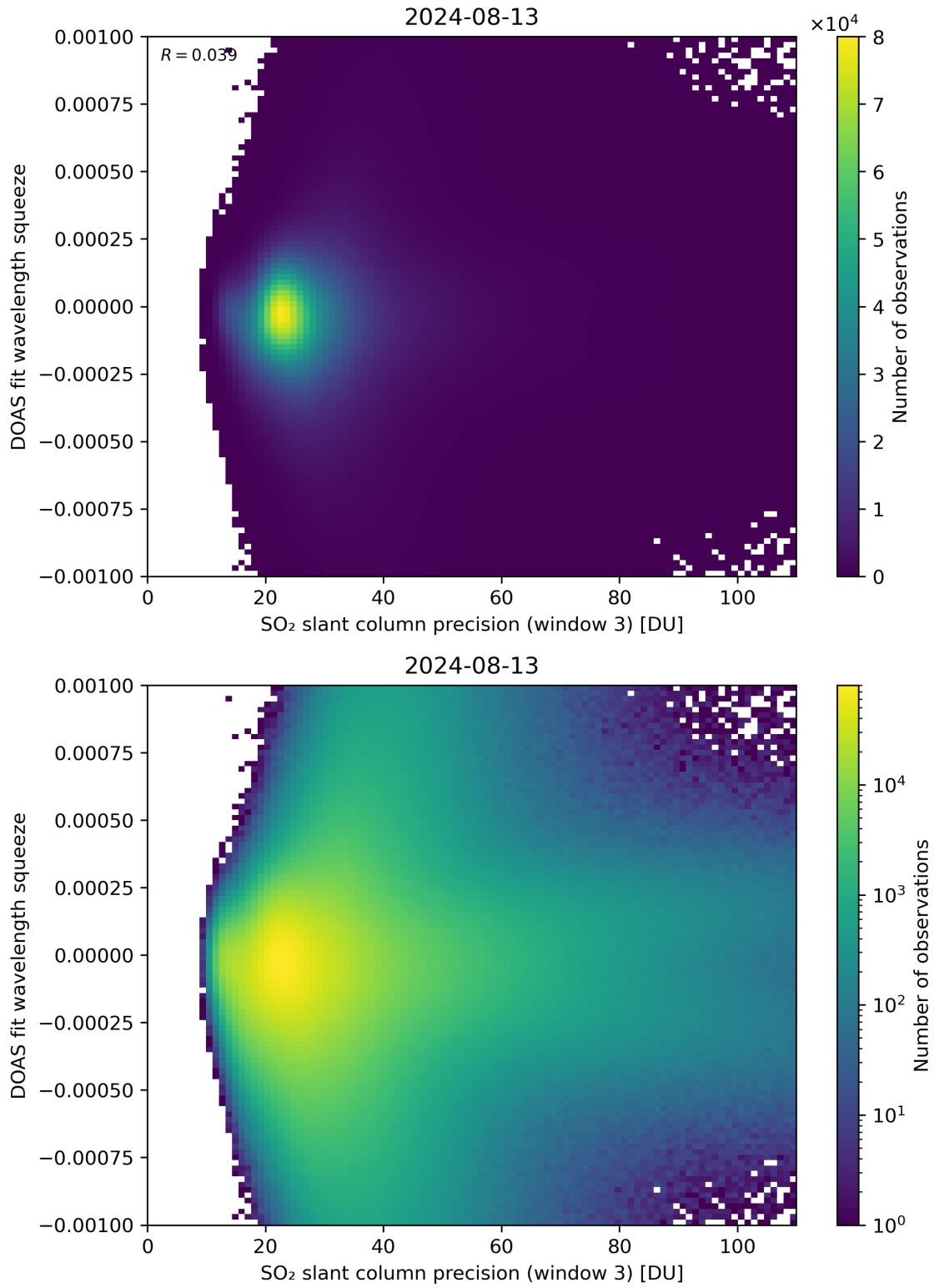
Figure 259: Scatter density plot of “SO 2 slant column precision (window 3)” against “DOAS fit wavelength squeeze” for 2024-08-12 to 2024-08-14.
