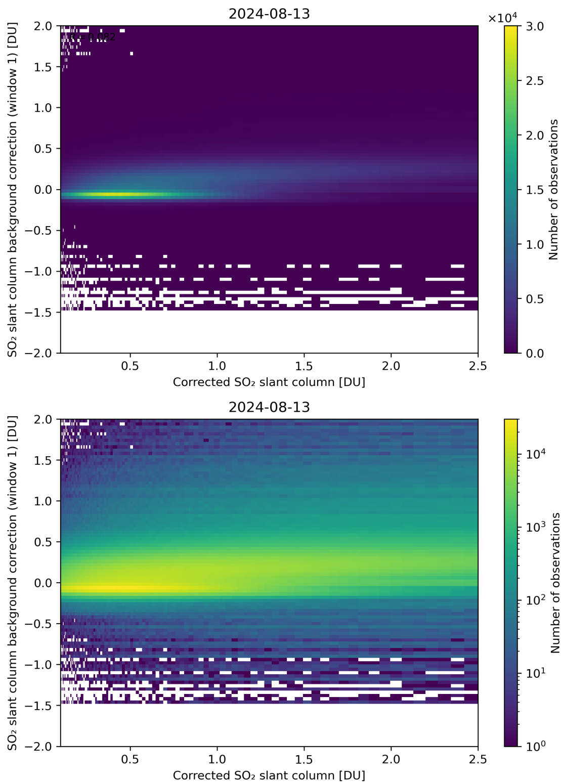
Figure 178: Scatter density plot of “Corrected SO 2 slant column” against “SO 2 slant column background correction (window 1)” for 2024-08-12 to 2024-08-14.
