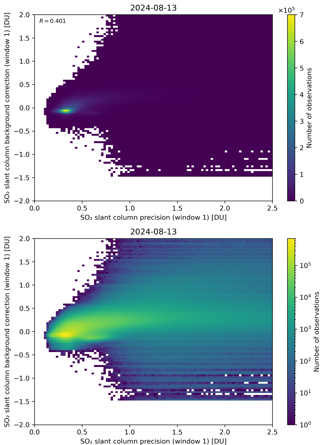
Figure 218: Scatter density plot of “SO 2 slant column precision (window 1)” against “SO 2 slant column background correction (window 1)” for 2024-08-12 to 2024-08-14.
