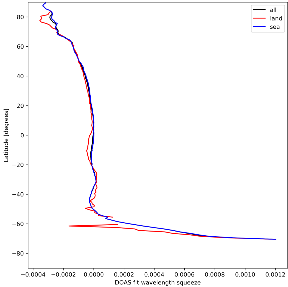
Figure 46: Zonal average of “DOAS fit wavelength squeeze” for 2024-08-12 to 2024-08-14.
