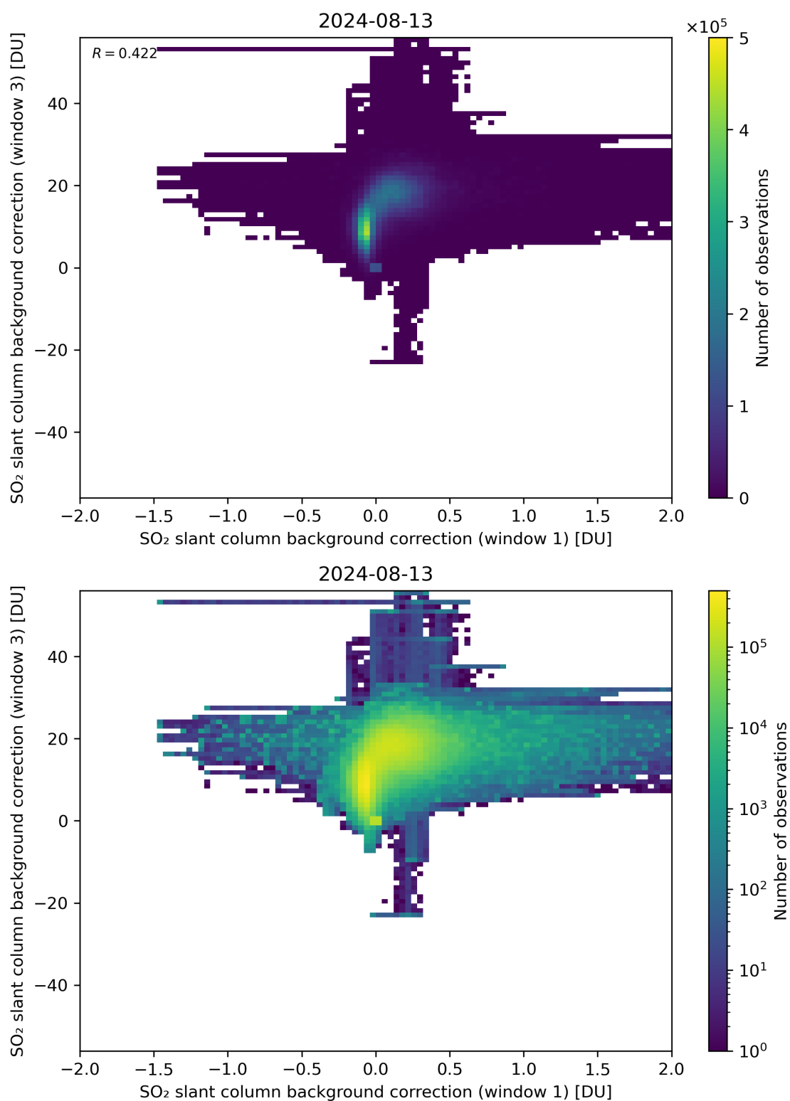
Figure 99: Scatter density plot of “SO 2 slant column background correction (window 1)” against “SO 2 slant column background correction (window 3)” for 2024-08-12 to 2024-08-14.
