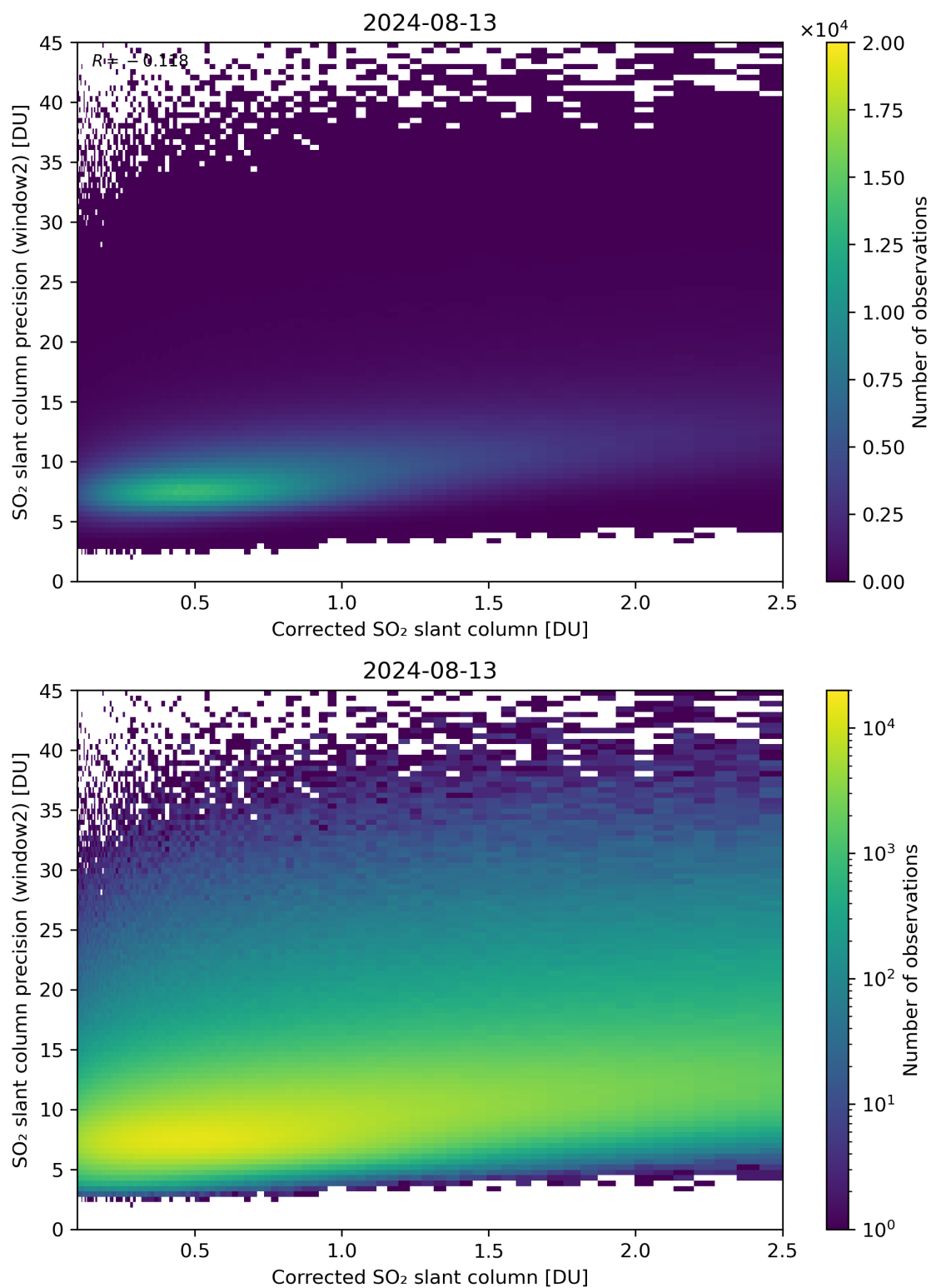
Figure 189: Scatter density plot of “Corrected SO 2 slant column” against “SO 2 slant column precision (window2)” for 2024-08-12 to 2024-08-14.
