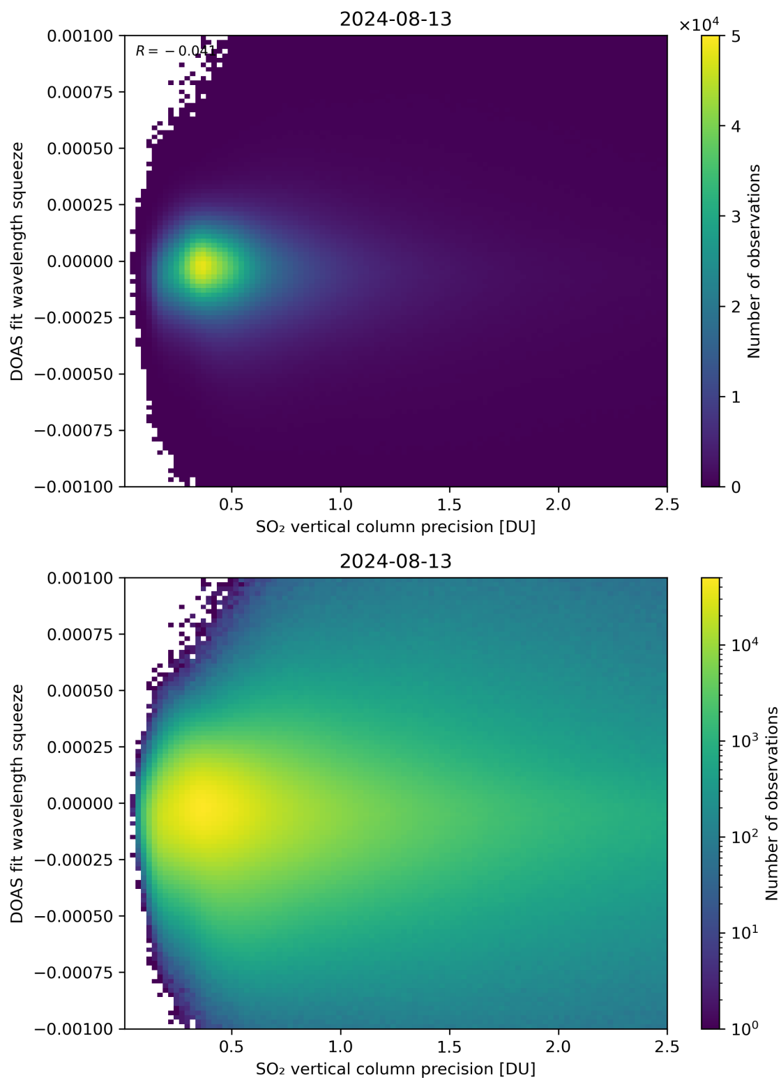
Figure 283: Scatter density plot of “SO 2 vertical column precision” against “DOAS fit wavelength squeeze” for 2024-08-12 to 2024-08-14.
