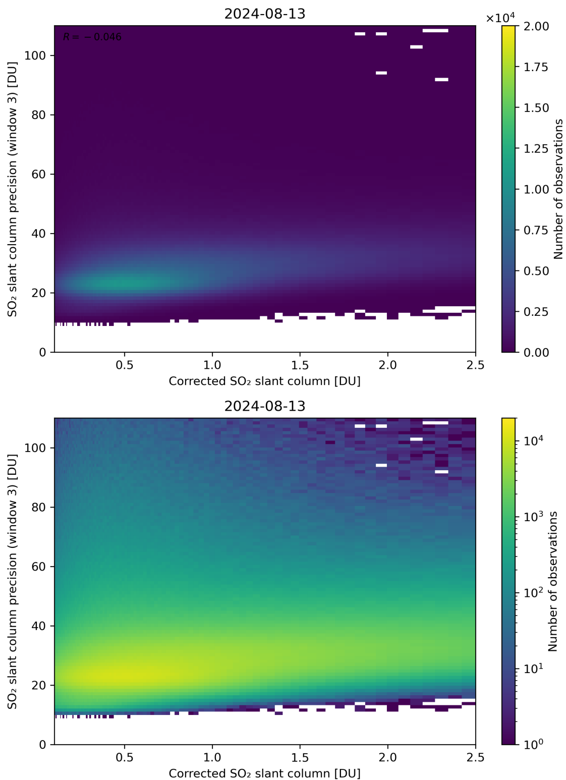
Figure 191: Scatter density plot of “Corrected SO 2 slant column” against “SO 2 slant column precision (window 3)” for 2024-08-12 to 2024-08-14.
