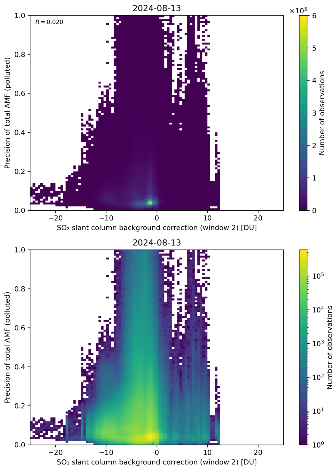
Figure 120: Scatter density plot of “SO 2 slant column background correction (window 2)” against “Precision of total AMF (polluted)” for 2024-08-12 to 2024-08-14.
