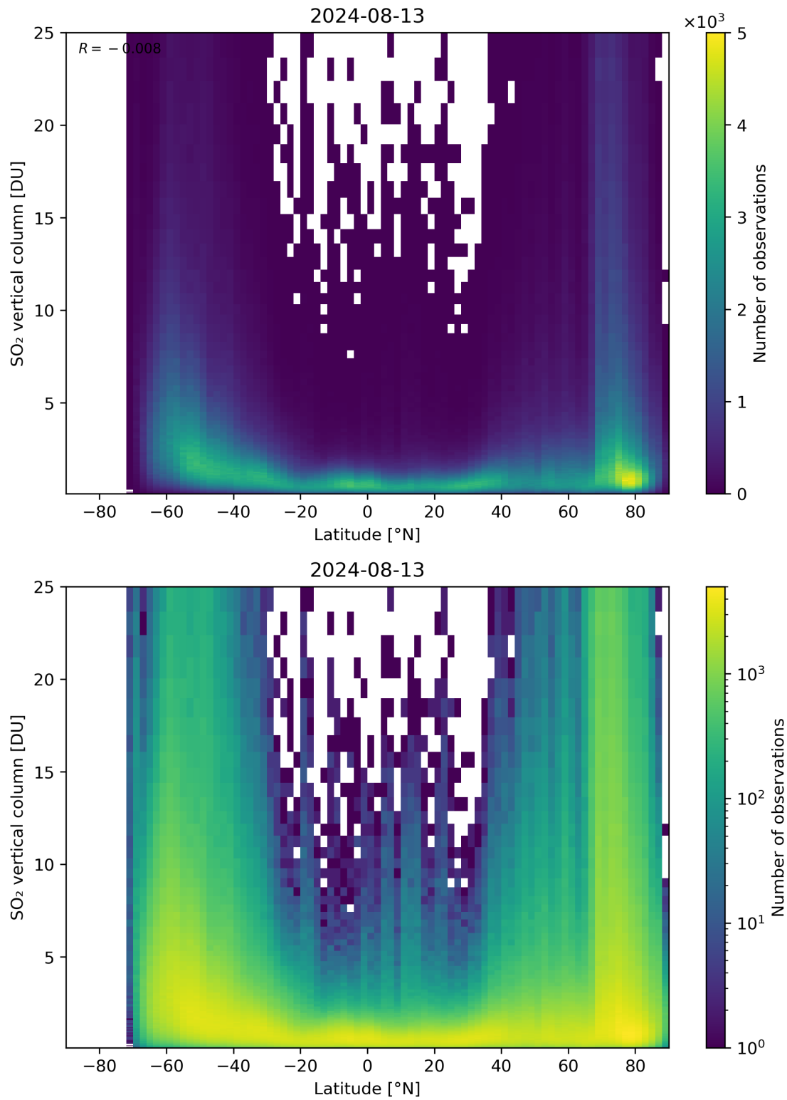
Figure 156: Scatter density plot of “Latitude” against “SO 2 vertical column” for 2024-08-12 to 2024-08-14.
