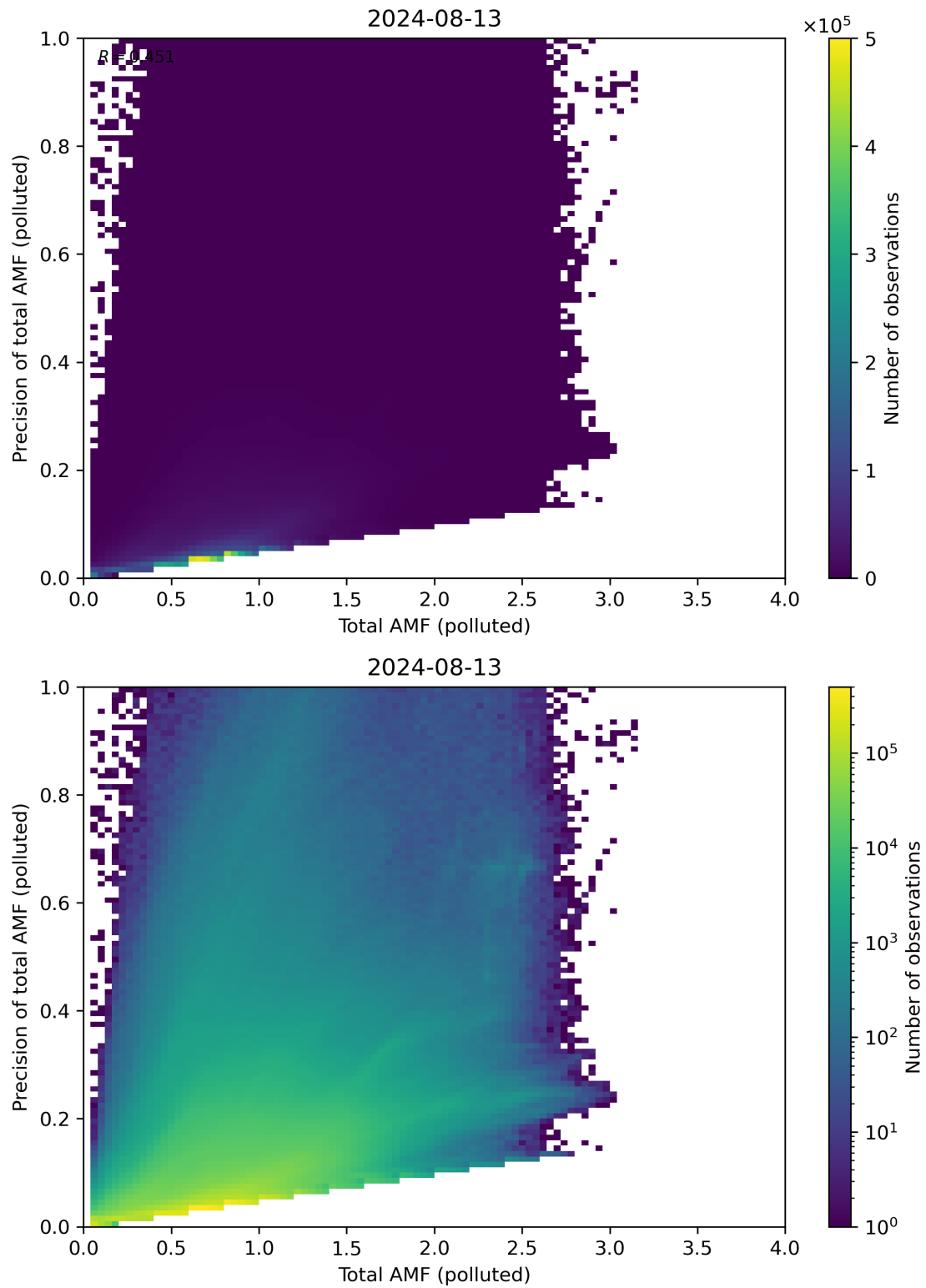
Figure 272: Scatter density plot of “Total AMF (polluted)” against “Precision of total AMF (polluted)” for 2024-08-12 to 2024-08-14.
