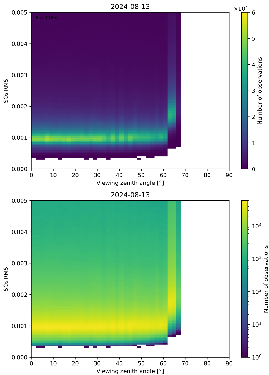
Figure 313: Scatter density plot of “Viewing zenith angle” against “SO 2 RMS” for 2024-08-12 to 2024-08-14.
