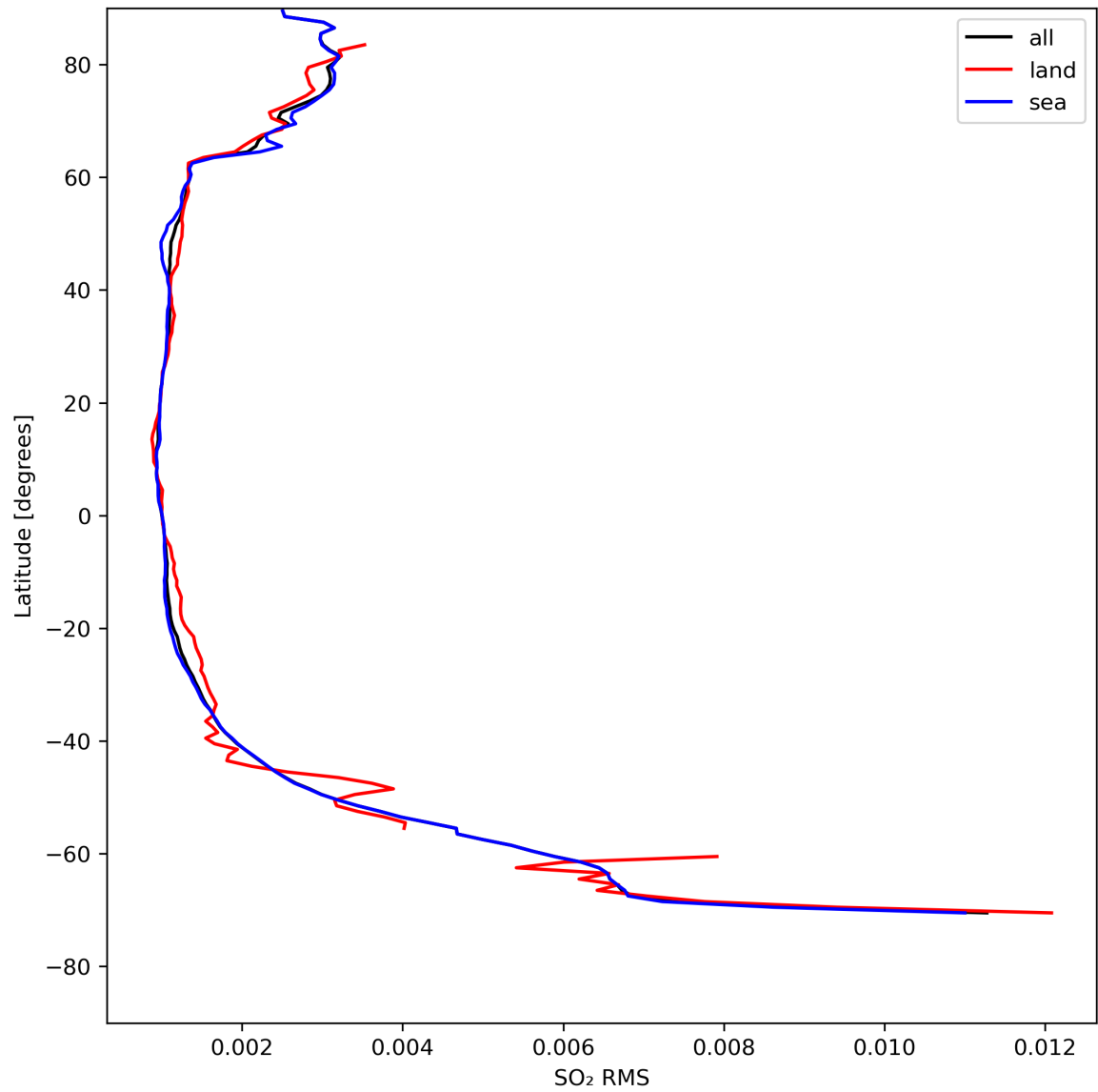
Figure 47: Zonal average of “SO 2 RMS” for 2024-08-12 to 2024-08-14.
