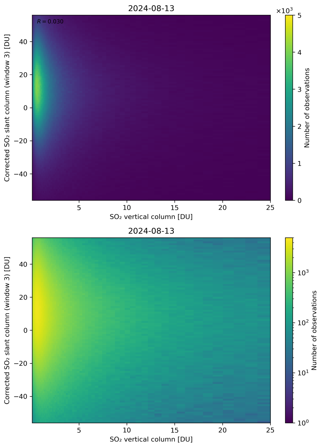
Figure 299: Scatter density plot of “SO 2 vertical column” against “Corrected SO 2 slant column (window 3)” for 2024-08-12 to 2024-08-14.
