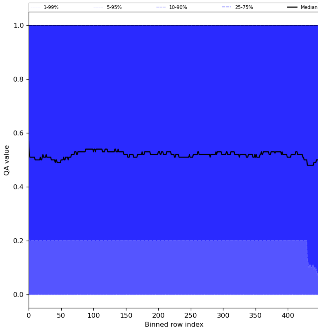
Figure 75: Along track statistics of “QA value” for 2024-08-12 to 2024-08-14
