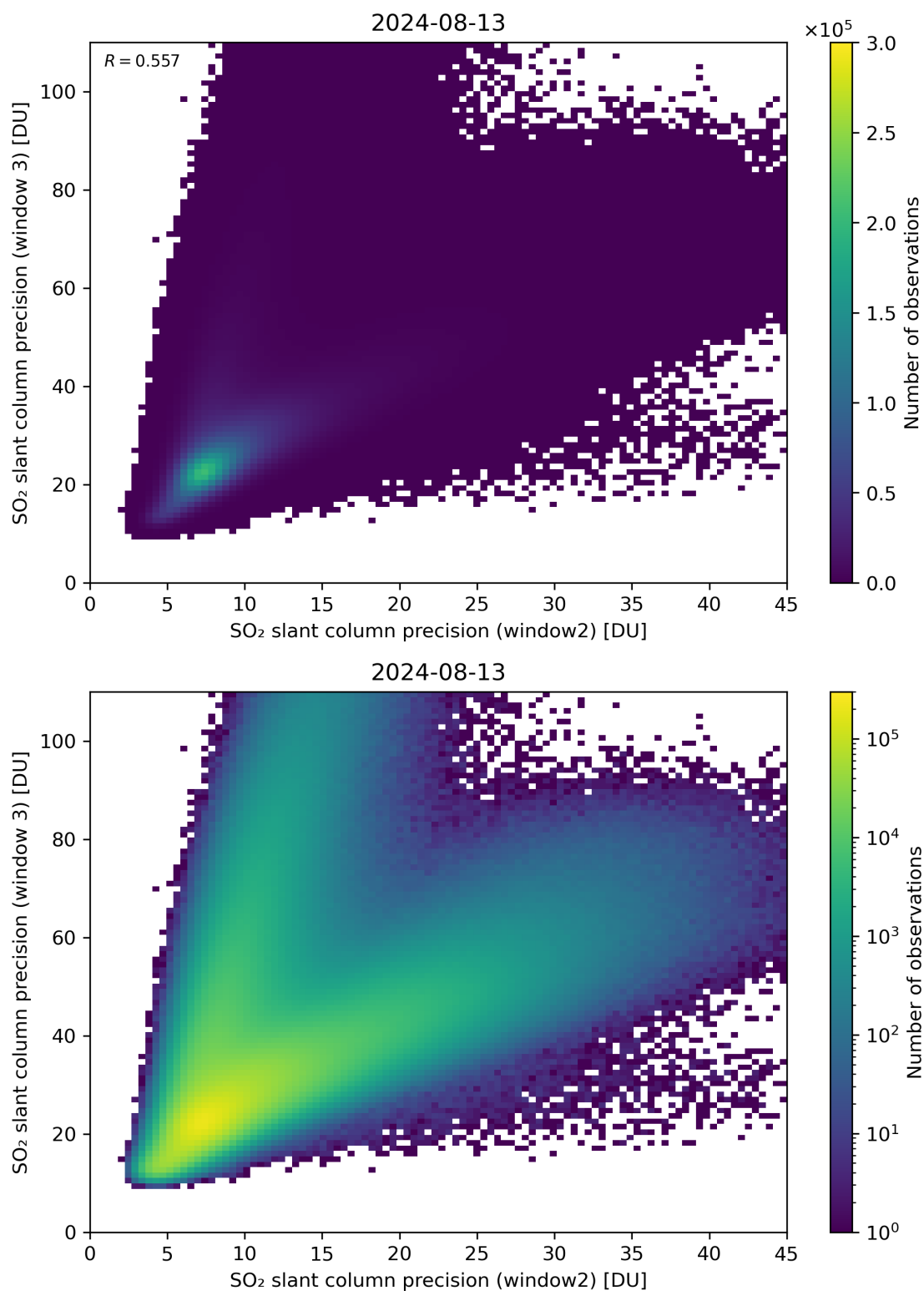
Figure 250: Scatter density plot of “SO 2 slant column precision (window2)” against “SO 2 slant column precision (window 3)” for 2024-08-12 to 2024-08-14.
