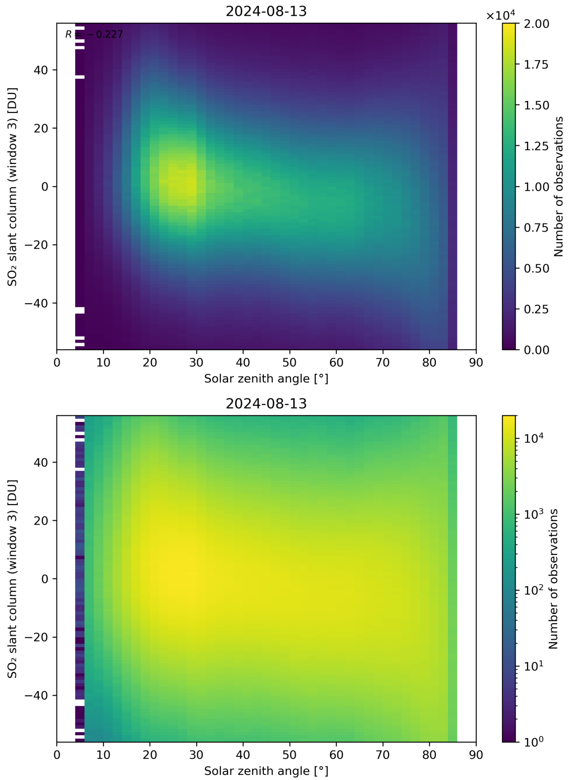
Figure 172: Scatter density plot of “Solar zenith angle” against “SO 2 slant column (window 3)” for 2024-08-12 to 2024-08-14.
