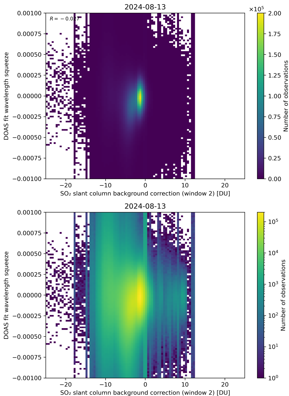
Figure 113: Scatter density plot of “SO 2 slant column background correction (window 2)” against “DOAS fit wavelength squeeze” for 2024-08-12 to 2024-08-14.
