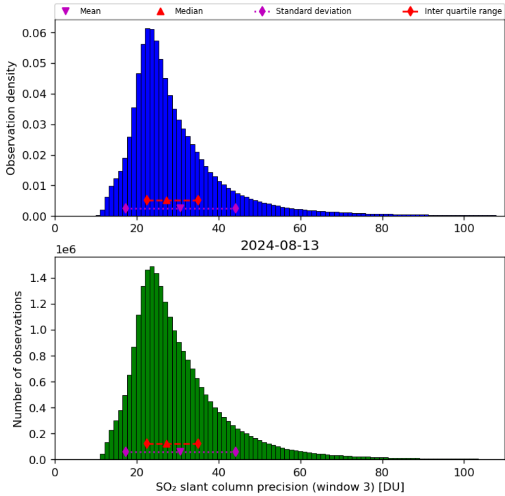
Figure 65: Histogram of “SO 2 slant column precision (window 3)” for 2024-08-12 to 2024-08-14
