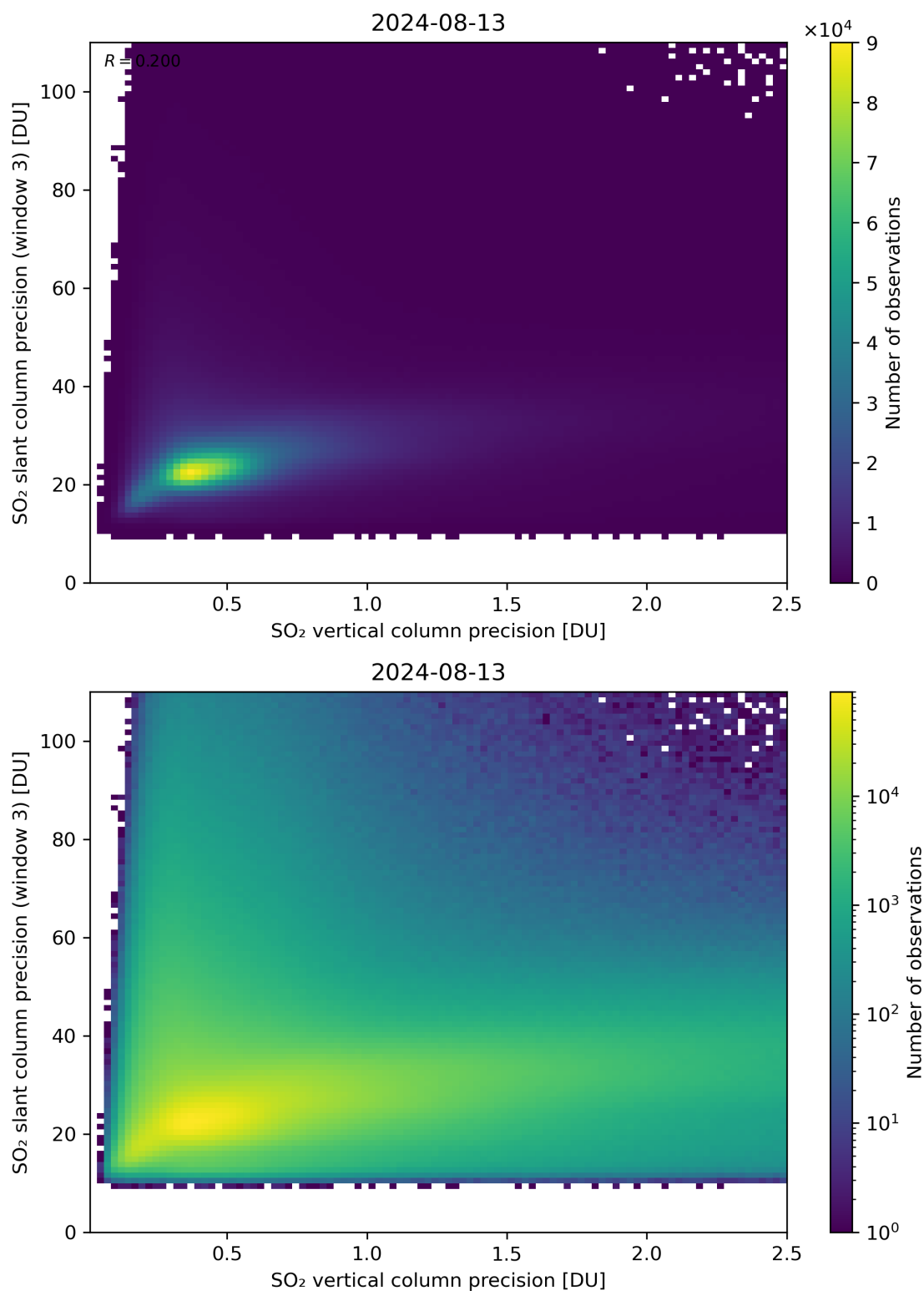
Figure 293: Scatter density plot of “SO 2 vertical column precision” against “SO 2 slant column precision (window 3)” for 2024-08-12 to 2024-08-14.
