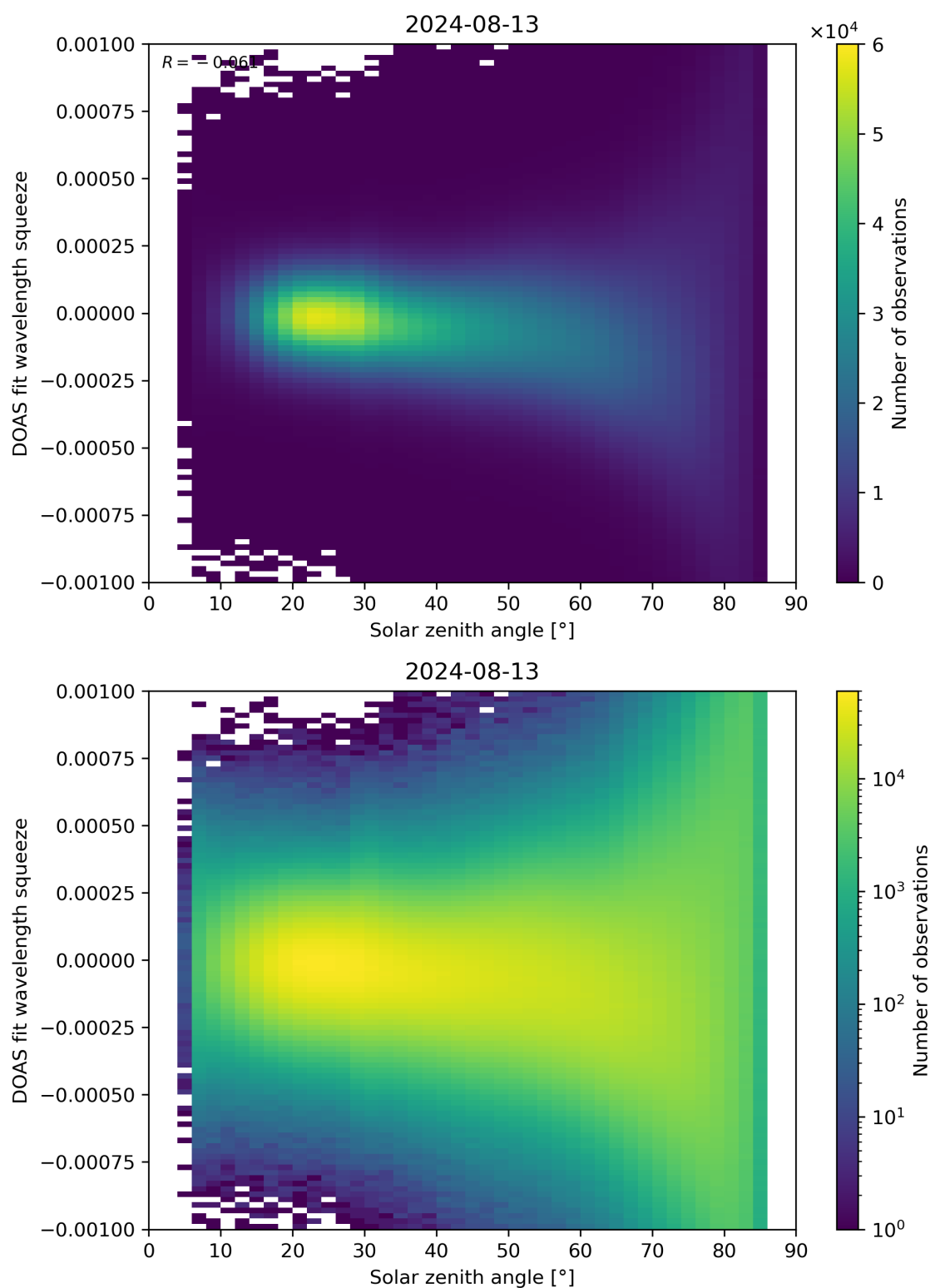
Figure 162: Scatter density plot of “Solar zenith angle” against “DOAS fit wavelength squeeze” for 2024-08-12 to 2024-08-14.
