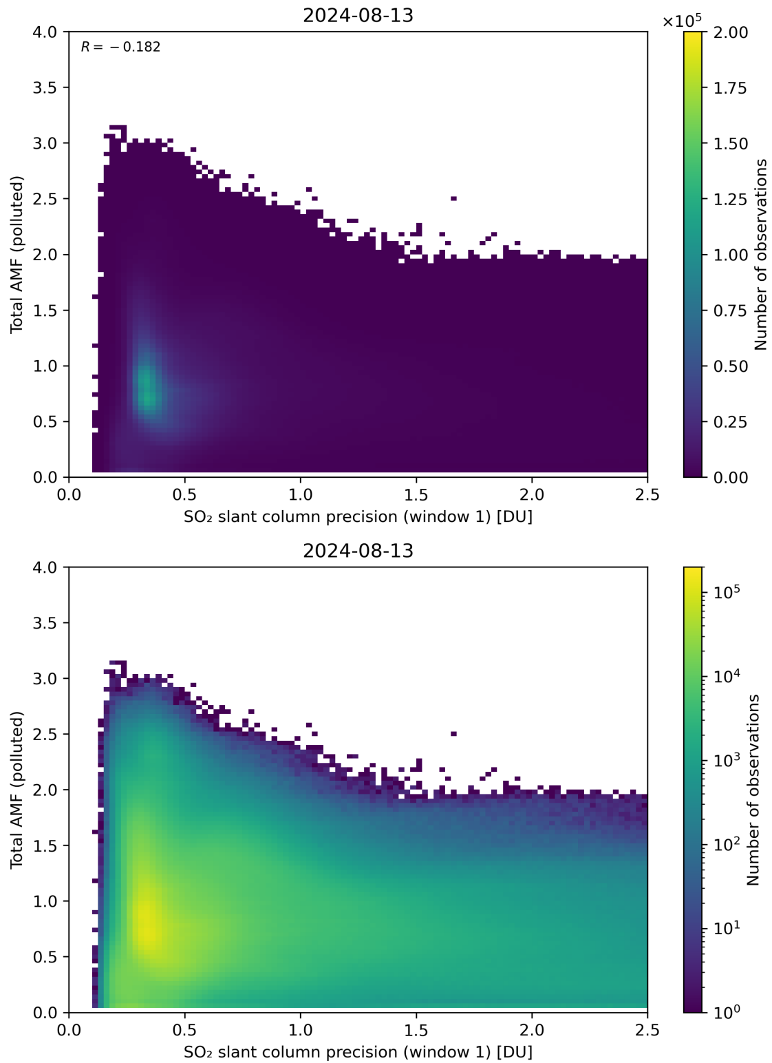
Figure 230: Scatter density plot of “SO 2 slant column precision (window 1)” against “Total AMF (polluted)” for 2024-08-12 to 2024-08-14.
