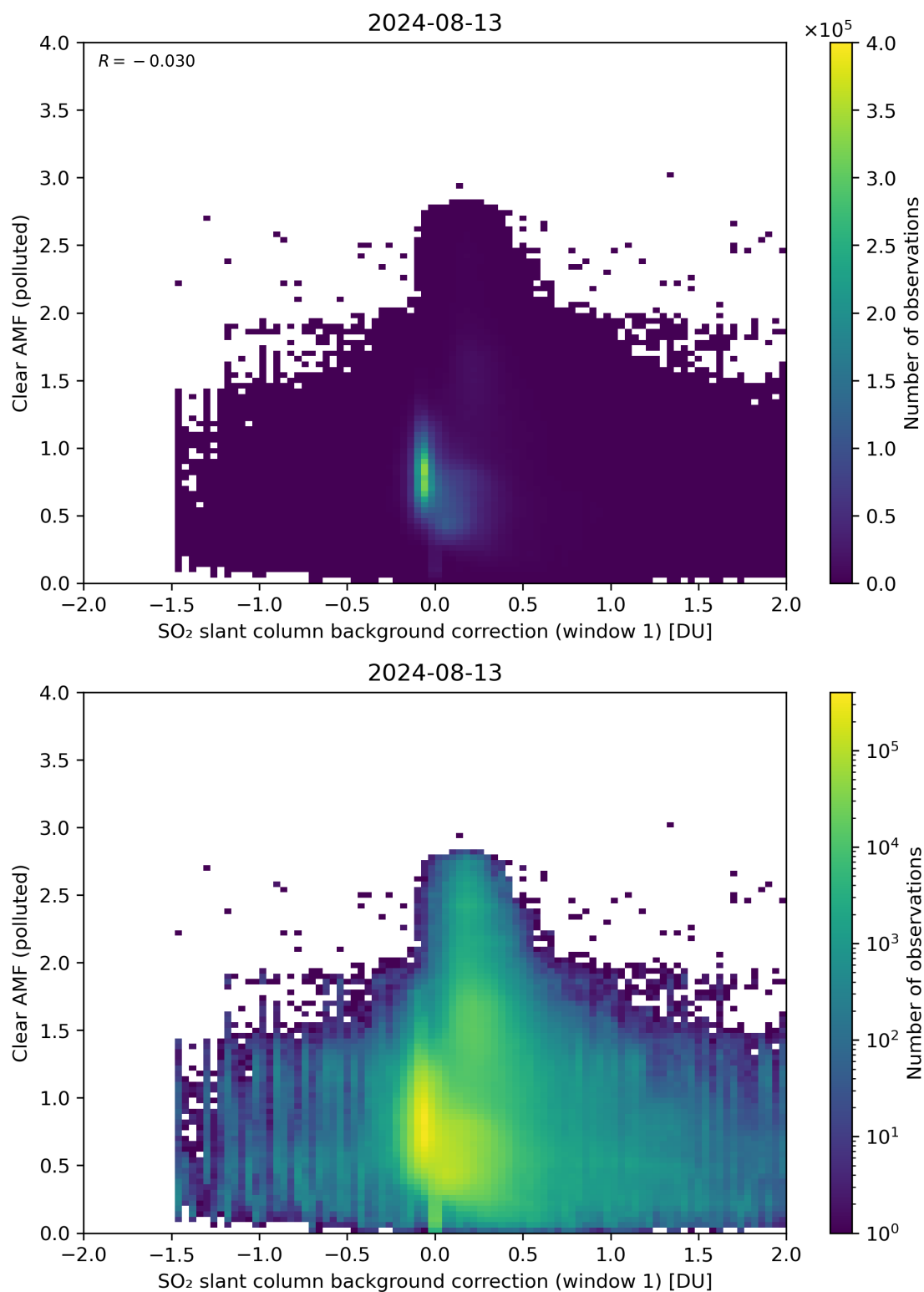
Figure 103: Scatter density plot of “SO 2 slant column background correction (window 1)” against “Clear AMF (polluted)” for 2024-08-12 to 2024-08-14.
