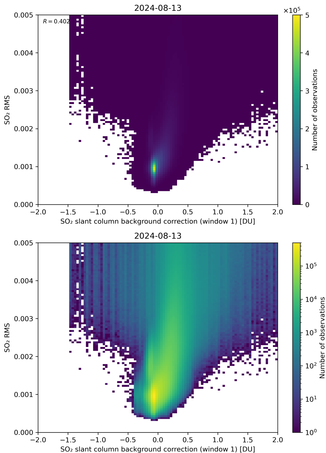
Figure 102: Scatter density plot of “SO 2 slant column background correction (window 1)” against “SO 2 RMS” for 2024-08-12 to 2024-08-14.
