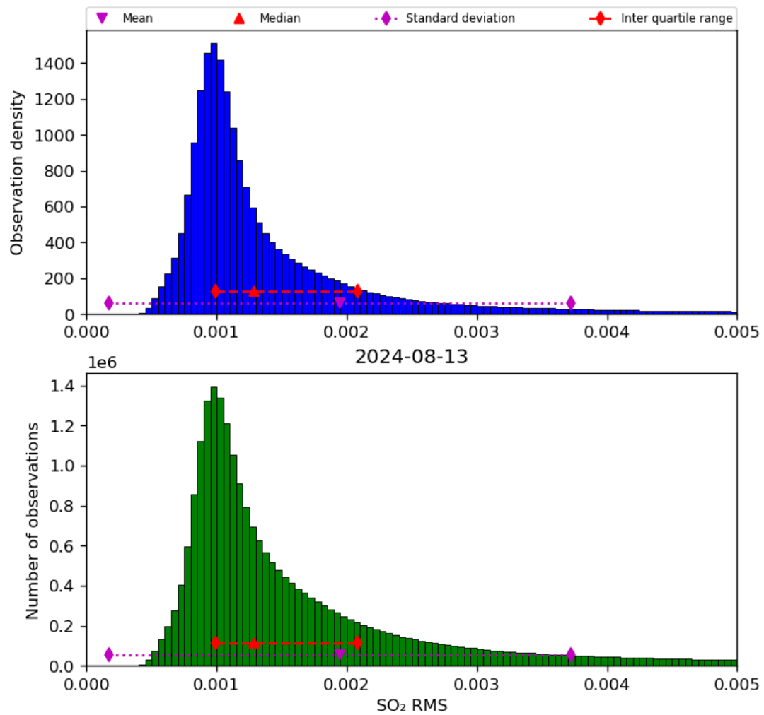
Figure 70: Histogram of “SO 2 RMS” for 2024-08-12 to 2024-08-14
