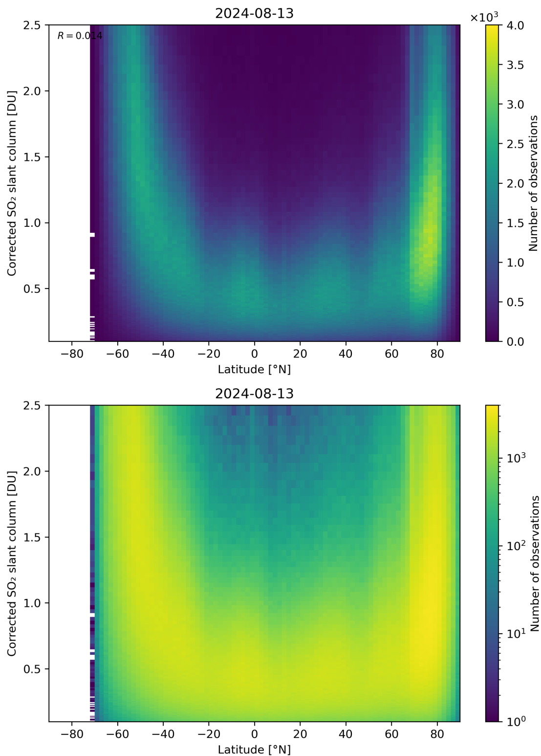
Figure 146: Scatter density plot of “Latitude” against “Corrected SO 2 slant column” for 2024-08-12 to 2024-08-14.
