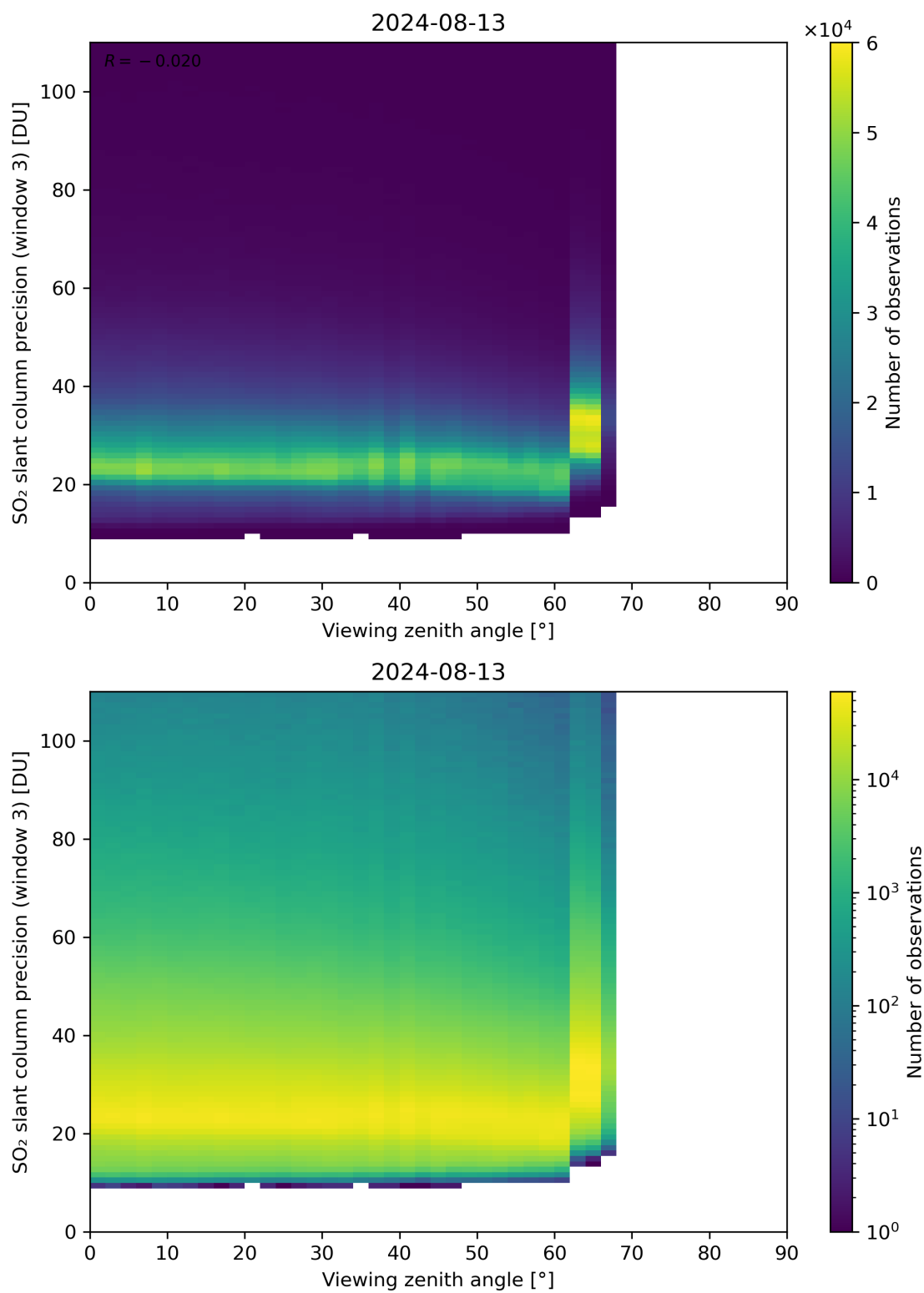
Figure 324: Scatter density plot of “Viewing zenith angle” against “SO 2 slant column precision (window 3)” for 2024-08-12 to 2024-08-14.
