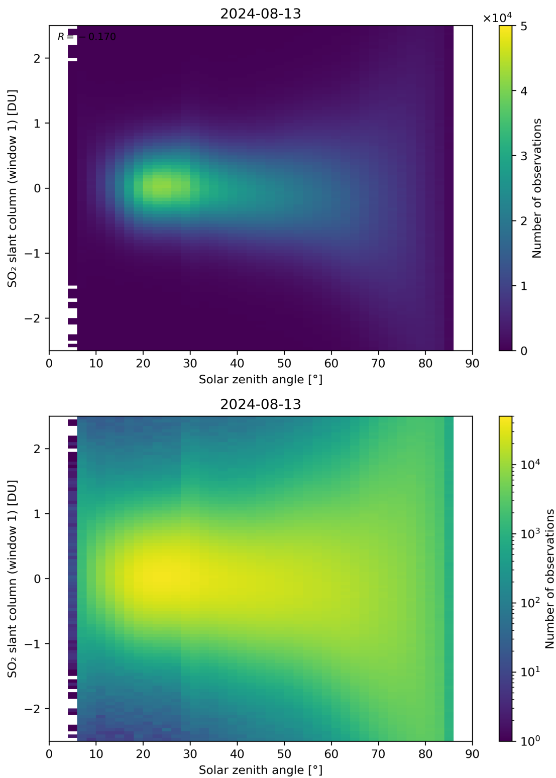
Figure 169: Scatter density plot of “Solar zenith angle” against “SO 2 slant column (window 1)” for 2024-08-12 to 2024-08-14.
