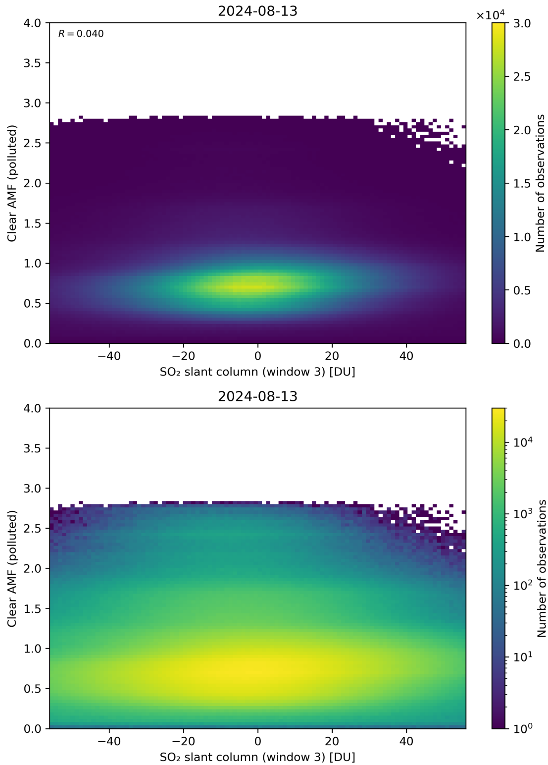
Figure 265: Scatter density plot of “SO 2 slant column (window 3)” against “Clear AMF (polluted)” for 2024-08-12 to 2024-08-14.
