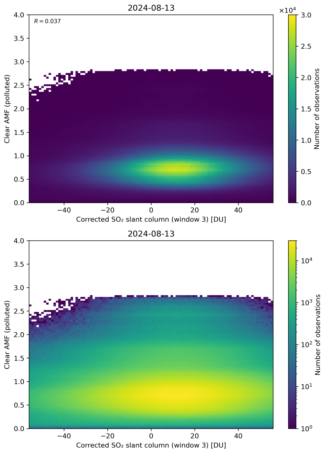
Figure 209: Scatter density plot of “Corrected SO 2 slant column (window 3)” against “Clear AMF (polluted)” for 2024-08-12 to 2024-08-14.
