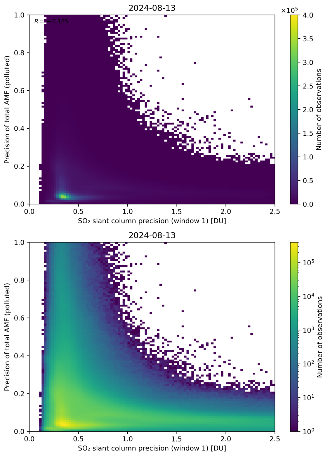
Figure 231: Scatter density plot of “SO 2 slant column precision (window 1)” against “Precision of total AMF (polluted)” for 2024-08-12 to 2024-08-14.
