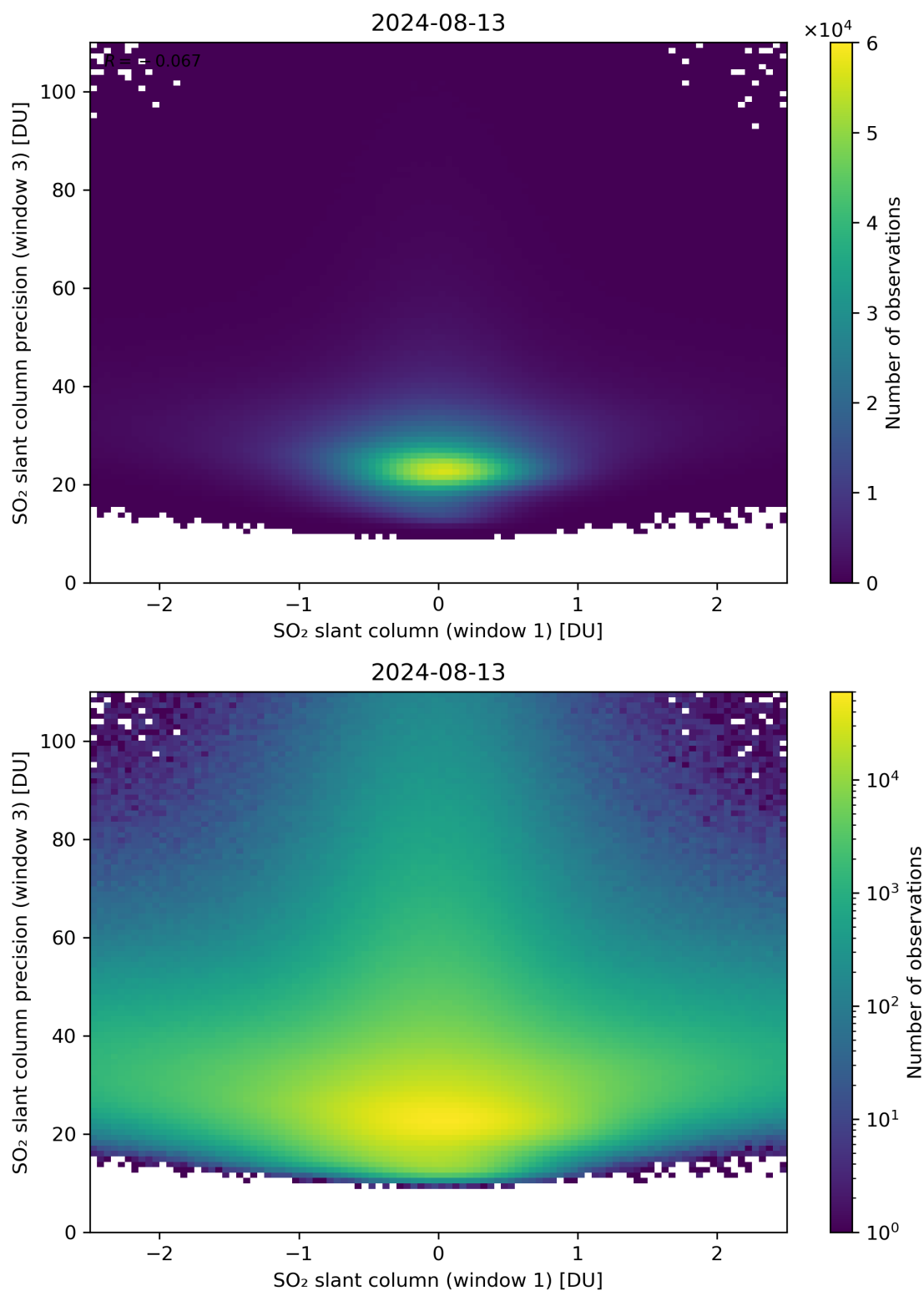
Figure 238: Scatter density plot of “SO 2 slant column (window 1)” against “SO 2 slant column precision (window 3)” for 2024-08-12 to 2024-08-14.
