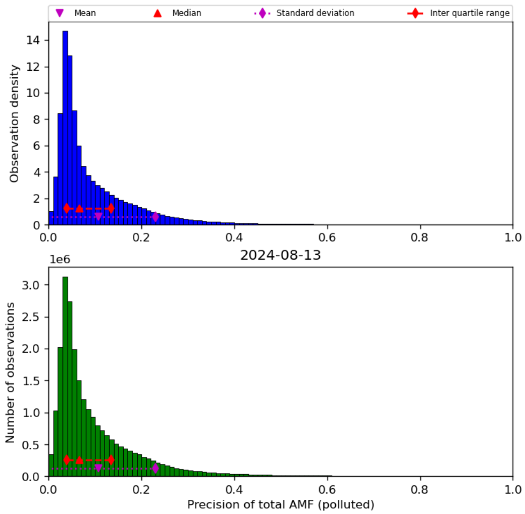
Figure 72: Histogram of “Precision of total AMF (polluted)” for 2024-08-12 to 2024-08-14
