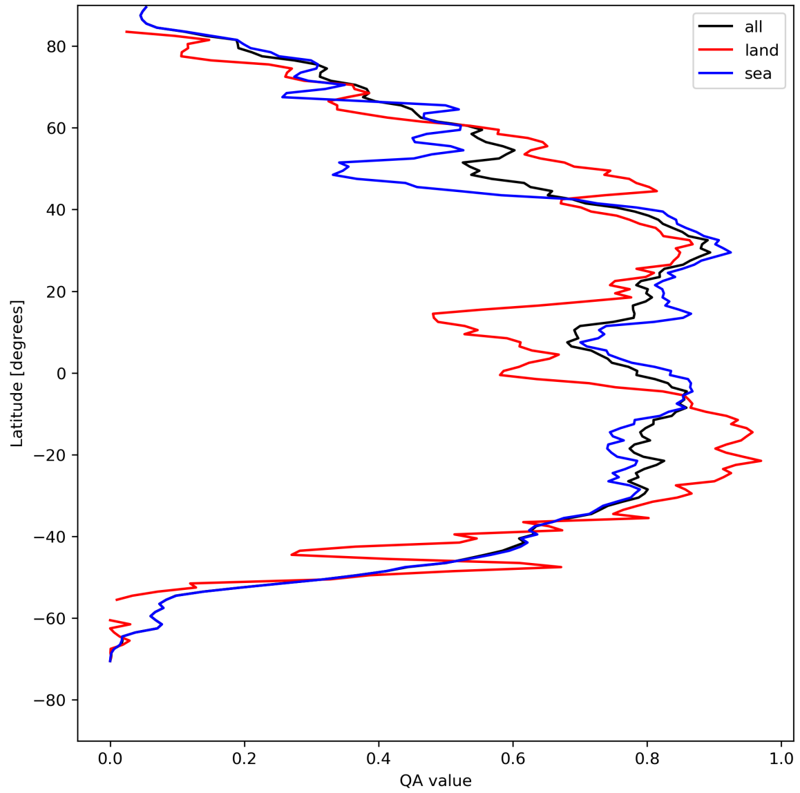
Figure 29: Zonal average of “QA value” for 2024-08-12 to 2024-08-14.
