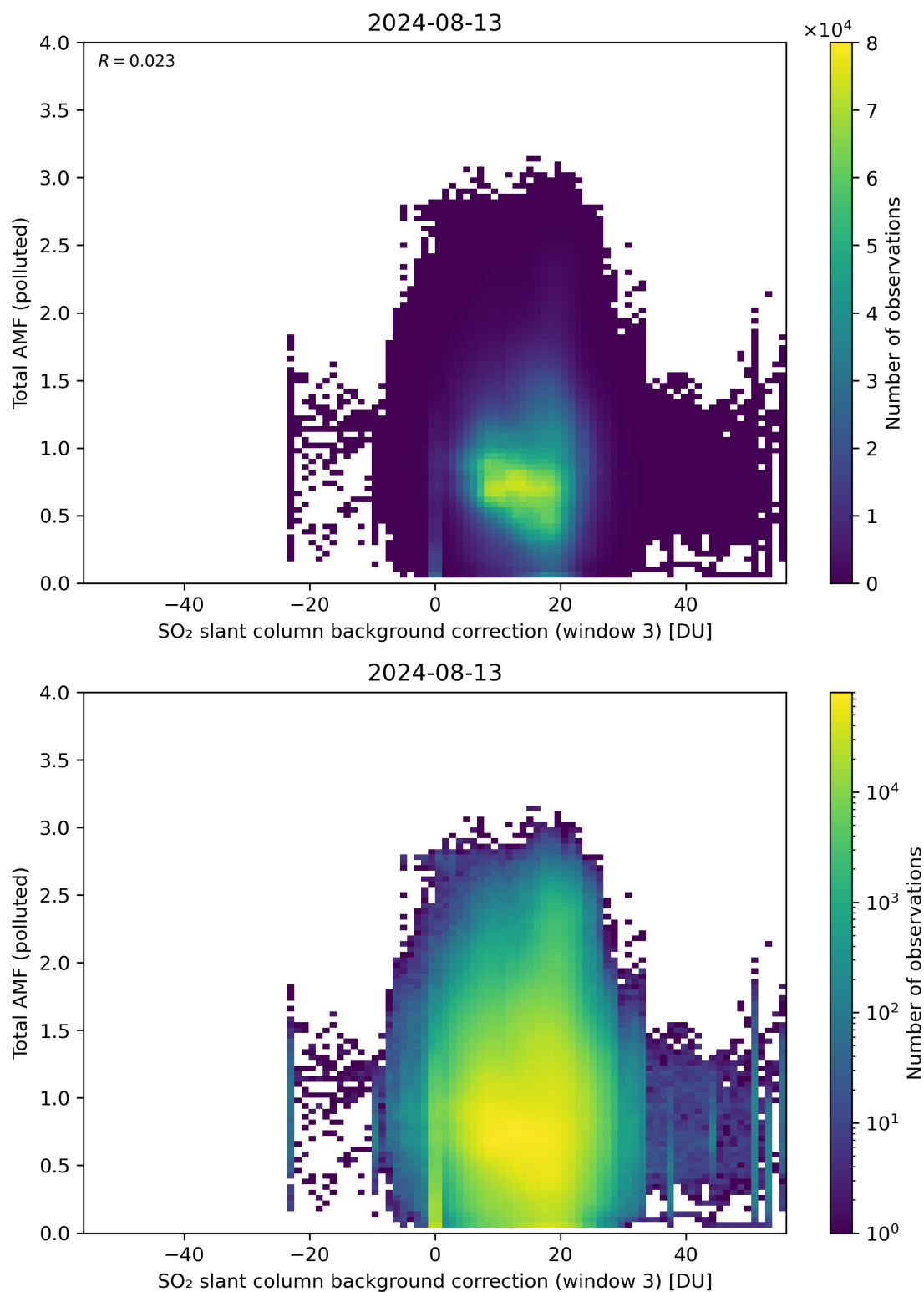
Figure 125: Scatter density plot of “SO 2 slant column background correction (window 3)” against “Total AMF (polluted)” for 2024-08-12 to 2024-08-14.
