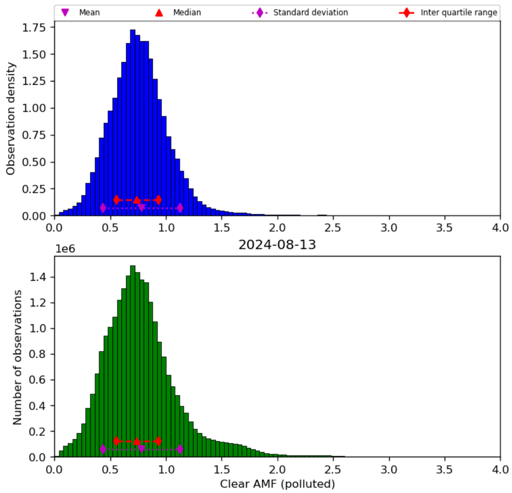
Figure 73: Histogram of “Clear AMF (polluted)” for 2024-08-12 to 2024-08-14
