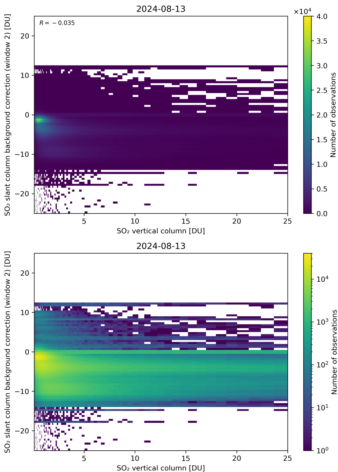
Figure 274: Scatter density plot of “SO 2 vertical column” against “SO 2 slant column background correction (window 2)” for 2024-08-12 to 2024-08-14.
