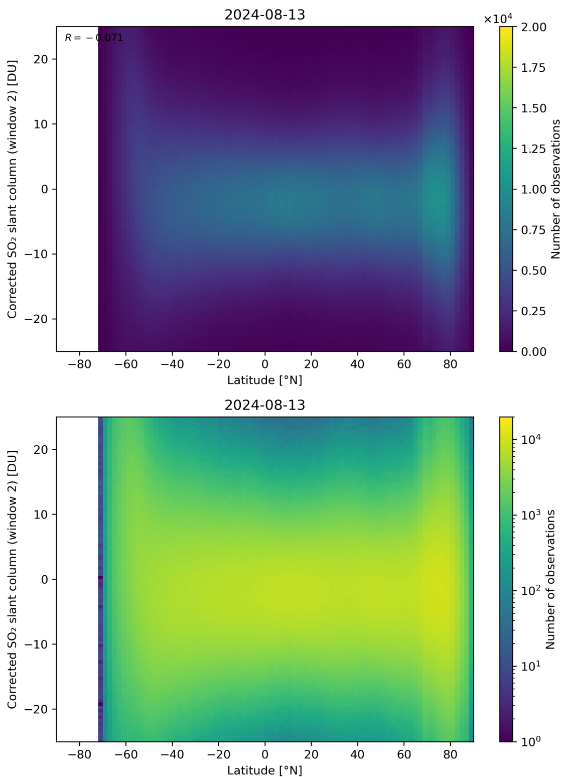
Figure 147: Scatter density plot of “Latitude” against “Corrected SO 2 slant column (window 2)” for 2024-08-12 to 2024-08-14.
