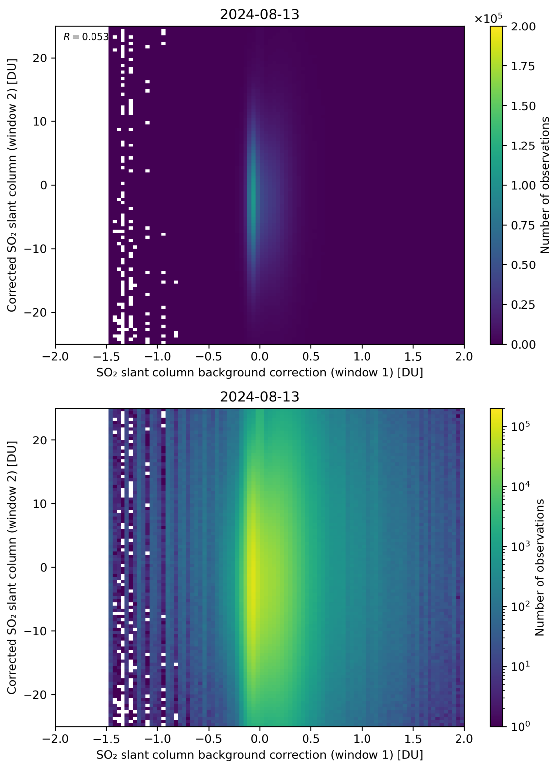
Figure 104: Scatter density plot of “SO 2 slant column background correction (window 1)” against “Corrected SO 2 slant column (window 2)” for 2024-08-12 to 2024-08-14.
