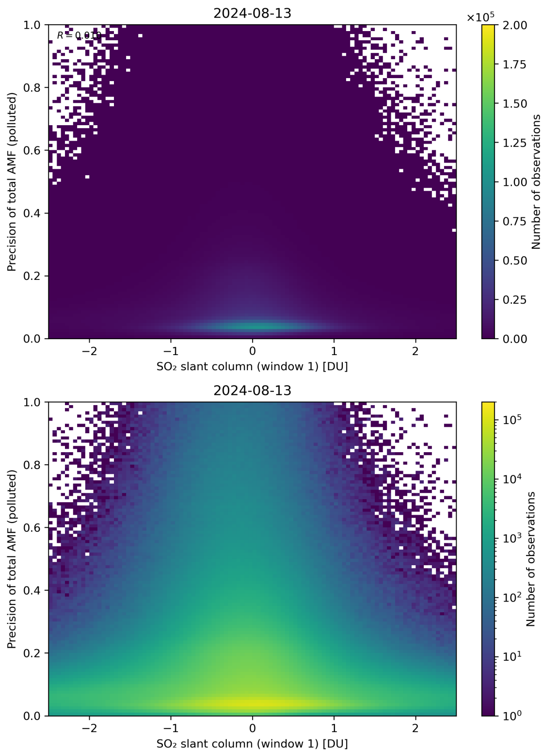
Figure 240: Scatter density plot of “SO 2 slant column (window 1)” against “Precision of total AMF (polluted)” for 2024-08-12 to 2024-08-14.
