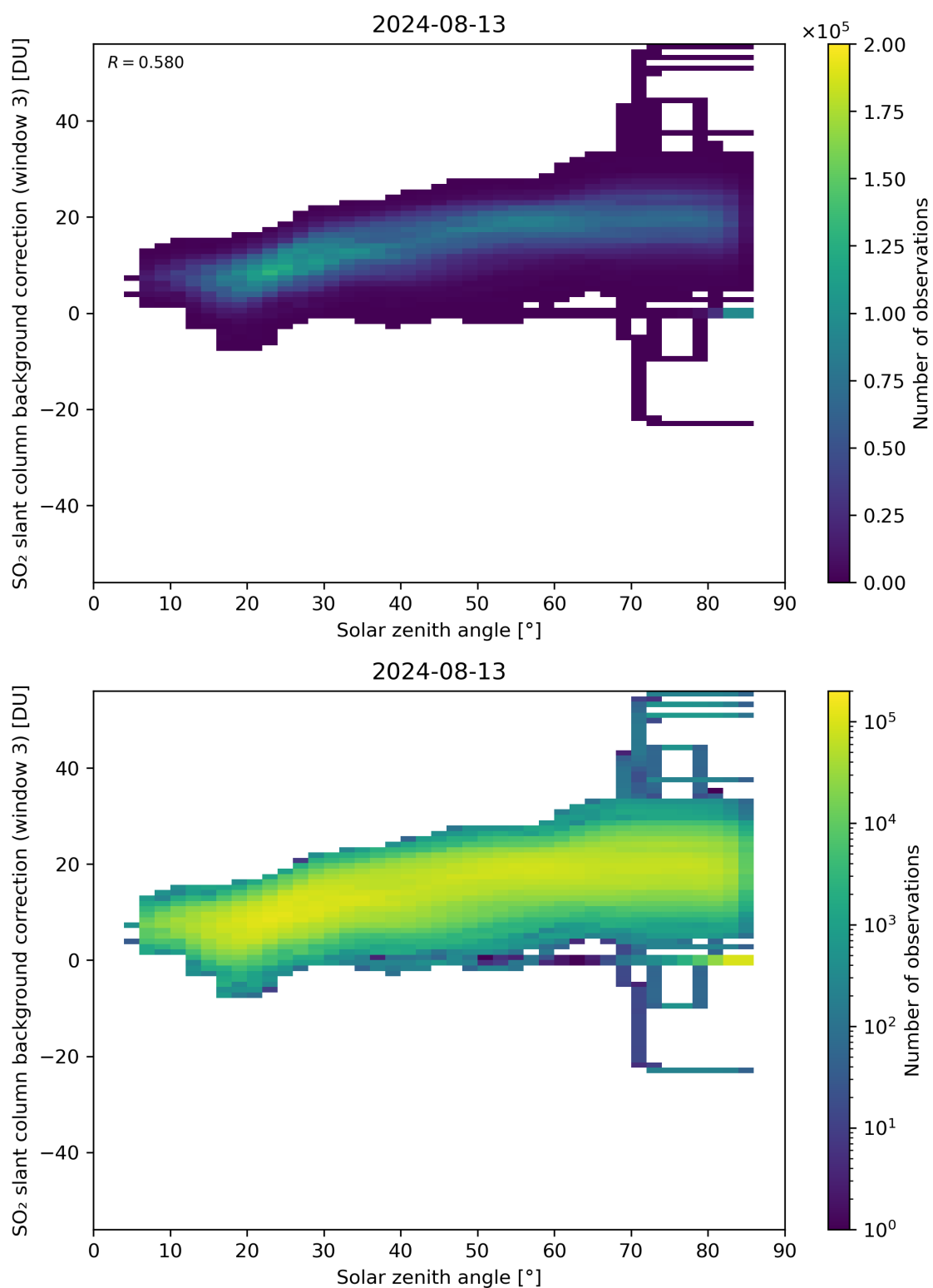
Figure 160: Scatter density plot of “Solar zenith angle” against “SO 2 slant column background correction (window 3)” for 2024-08-12 to 2024-08-14.
