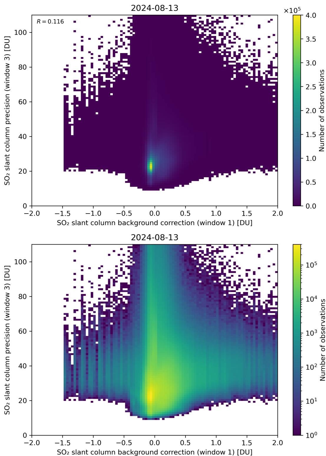
Figure 108: Scatter density plot of “SO 2 slant column background correction (window 1)” against “SO 2 slant column precision (window 3)” for 2024-08-12 to 2024-08-14.
