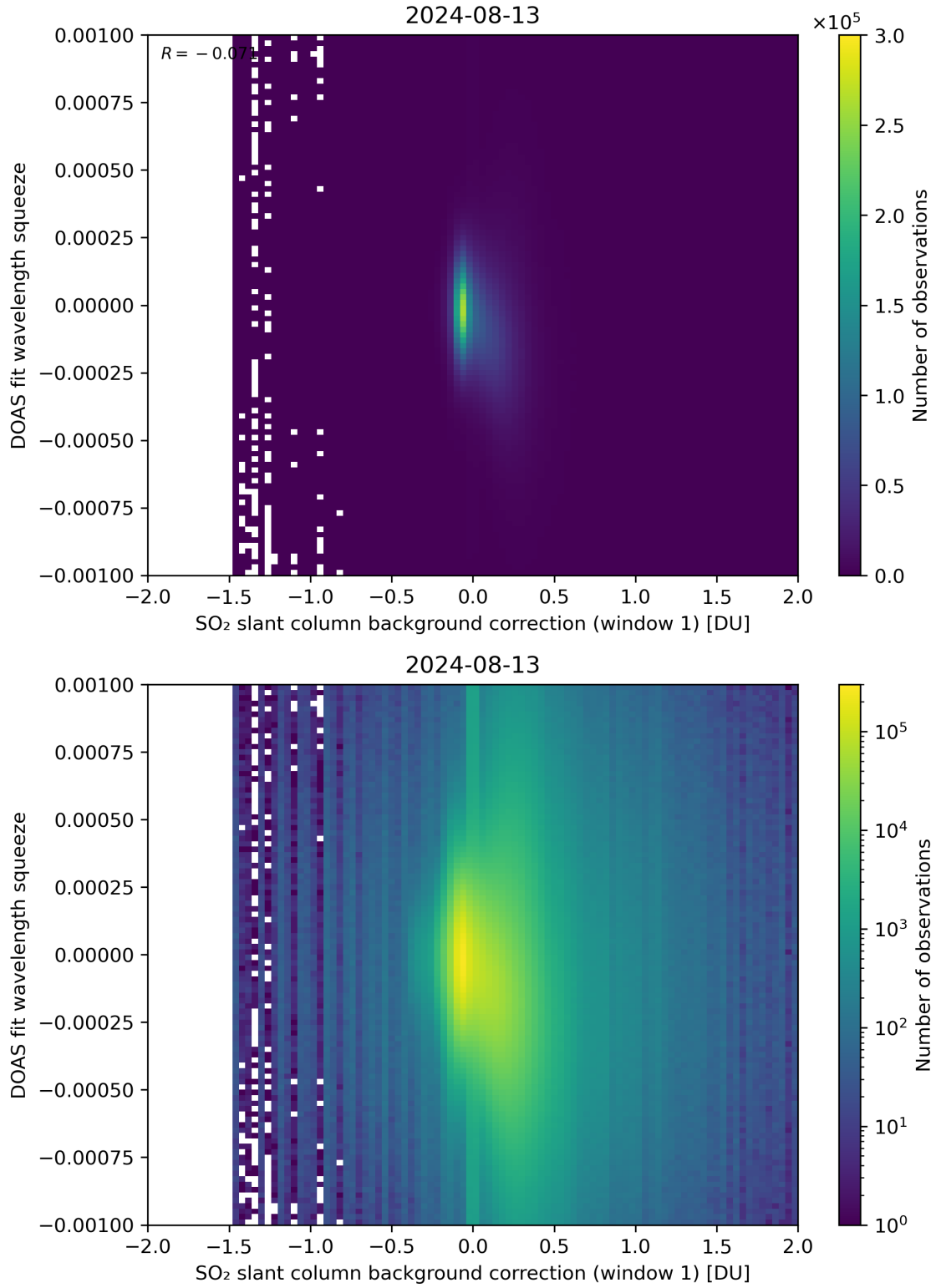
Figure 101: Scatter density plot of “SO 2 slant column background correction (window 1)” against “DOAS fit wavelength squeeze” for 2024-08-12 to 2024-08-14.
