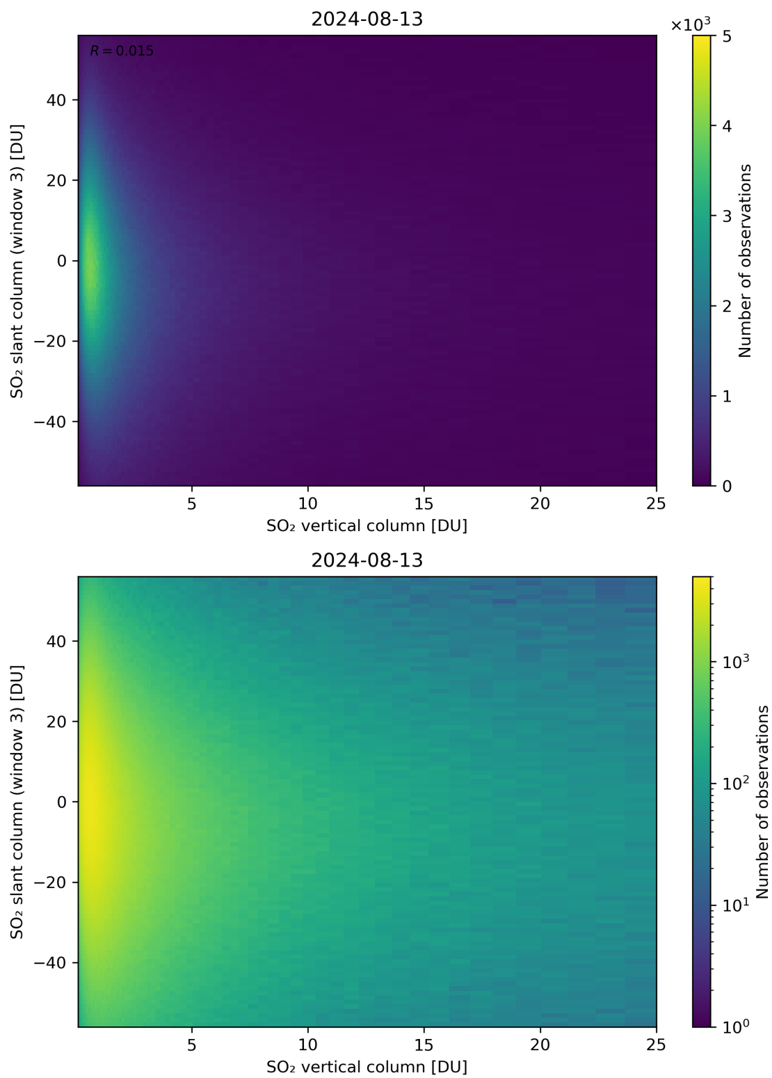
Figure 303: Scatter density plot of “SO 2 vertical column” against “SO 2 slant column (window 3)” for 2024-08-12 to 2024-08-14.
