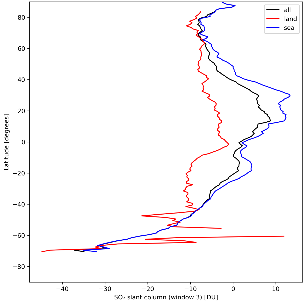
Figure 41: Zonal average of “SO 2 slant column (window 3)” for 2024-08-12 to 2024-08-14.
