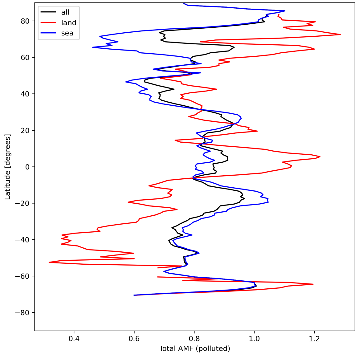
Figure 48: Zonal average of “Total AMF (polluted)” for 2024-08-12 to 2024-08-14.
