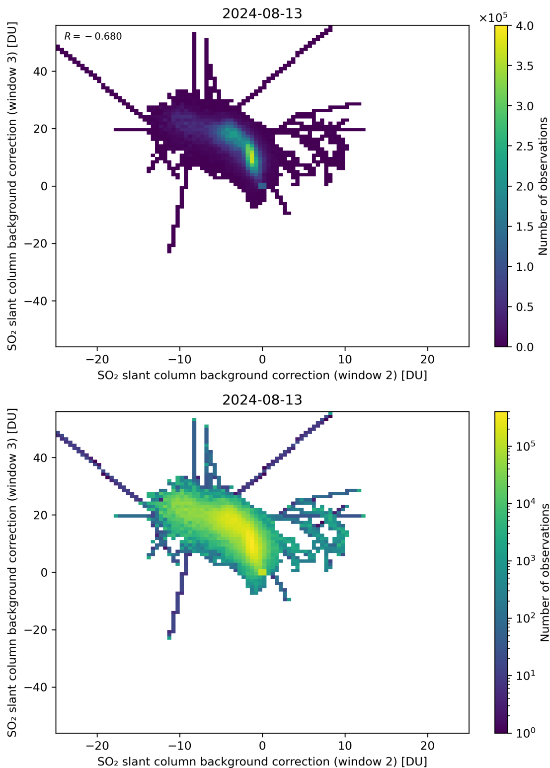
Figure 111: Scatter density plot of “SO 2 slant column background correction (window 2)” against “SO 2 slant column background correction (window 3)” for 2024-08-12 to 2024-08-14.
