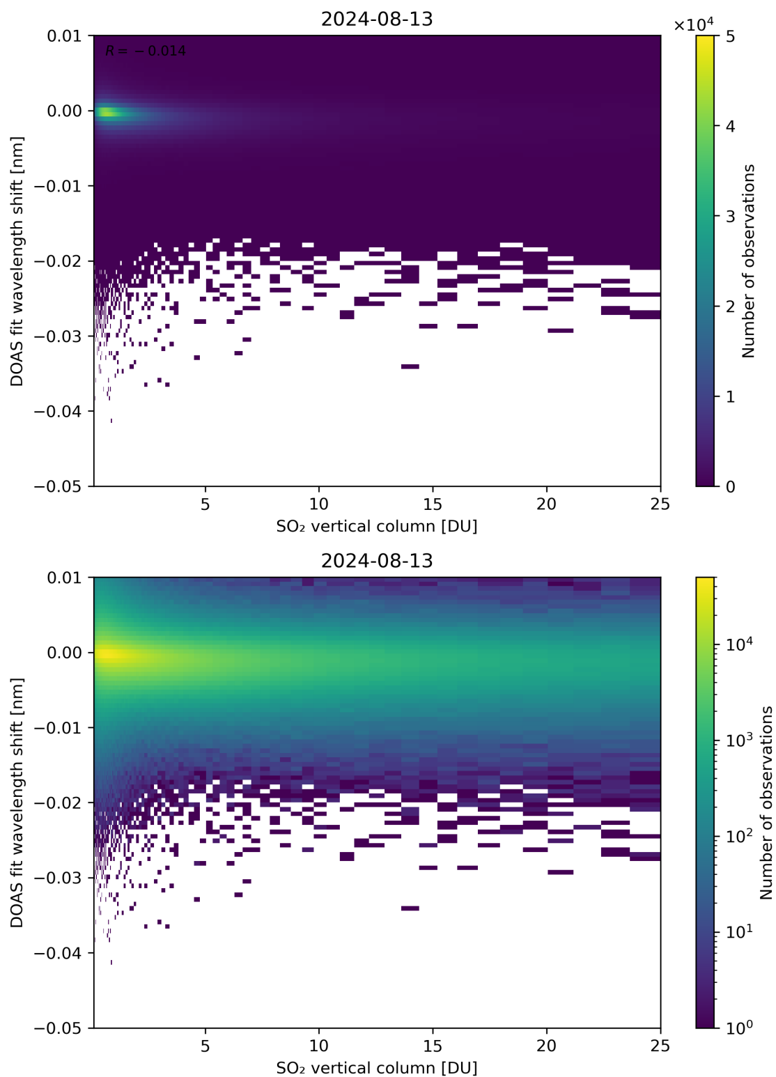
Figure 276: Scatter density plot of “SO 2 vertical column” against “DOAS fit wavelength shift” for 2024-08-12 to 2024-08-14.
