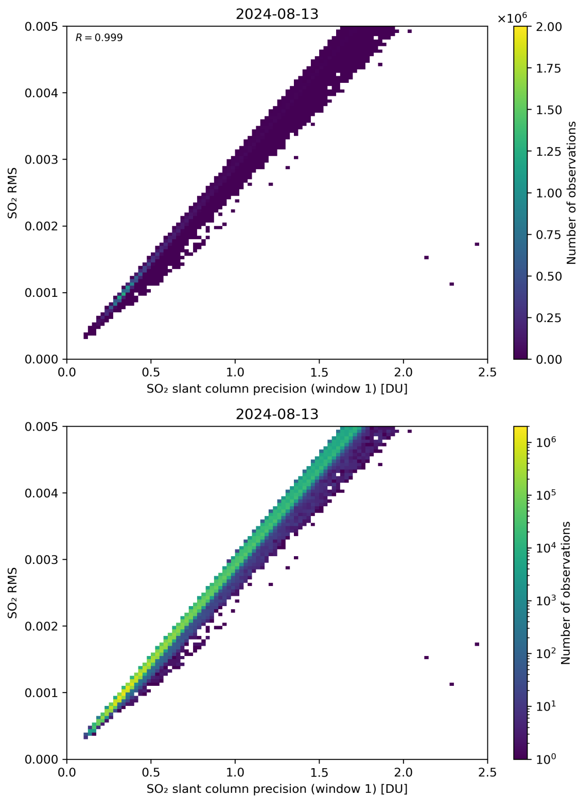
Figure 223: Scatter density plot of “SO 2 slant column precision (window 1)” against “SO 2 RMS” for 2024-08-12 to 2024-08-14.
