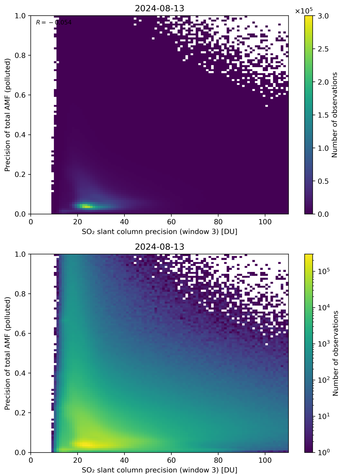
Figure 264: Scatter density plot of “SO 2 slant column precision (window 3)” against “Precision of total AMF (polluted)” for 2024-08-12 to 2024-08-14.
