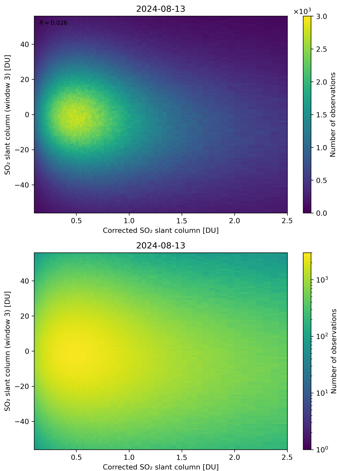
Figure 190: Scatter density plot of “Corrected SO 2 slant column” against “SO 2 slant column (window 3)” for 2024-08-12 to 2024-08-14.
