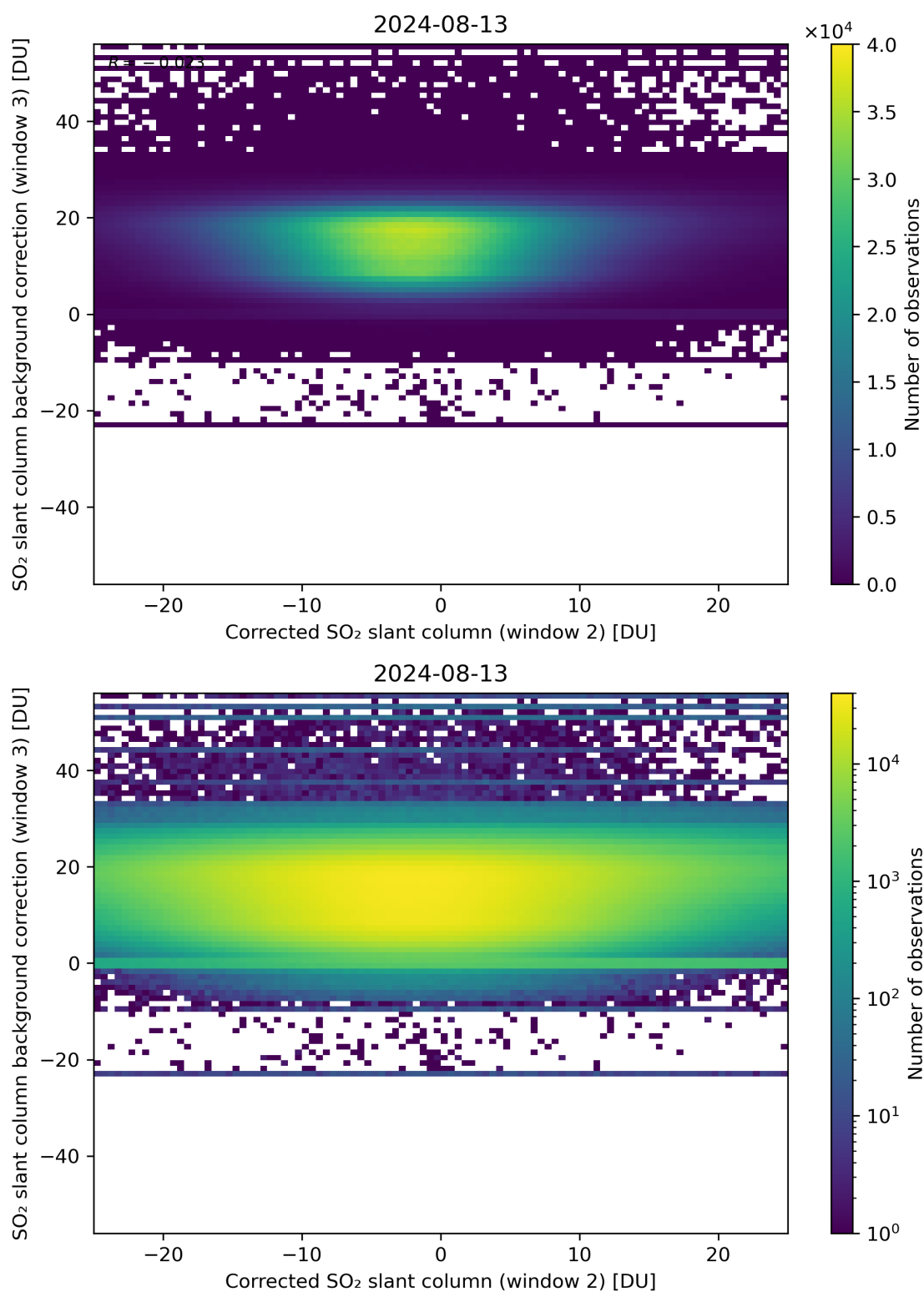
Figure 195: Scatter density plot of “Corrected SO 2 slant column (window 2)” against “SO 2 slant column background correction (window 3)” for 2024-08-12 to 2024-08-14.
