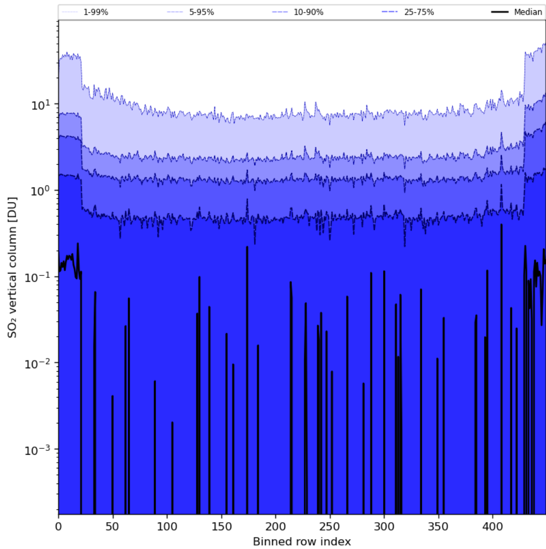
Figure 76: Along track statistics of “SO 2 vertical column” for 2024-08-12 to 2024-08-14
