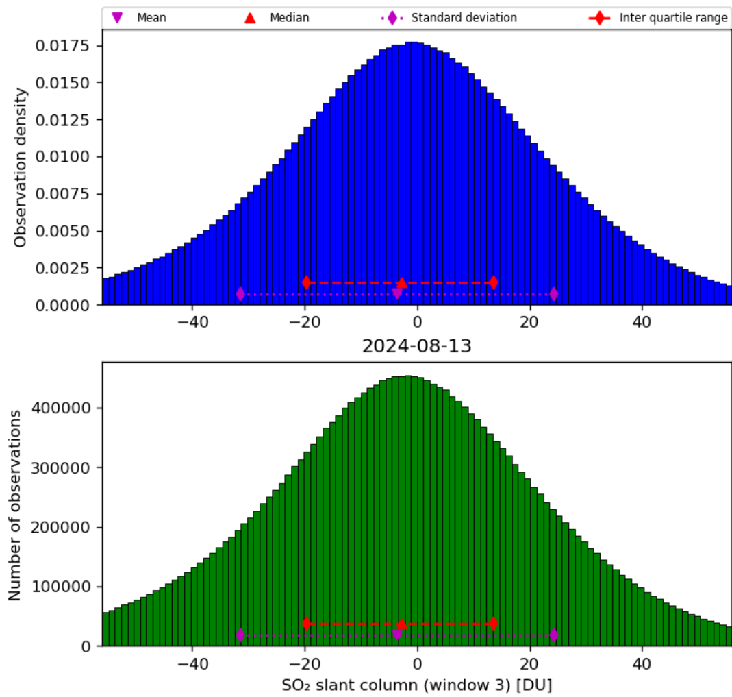
Figure 64: Histogram of “SO 2 slant column (window 3)” for 2024-08-12 to 2024-08-14
