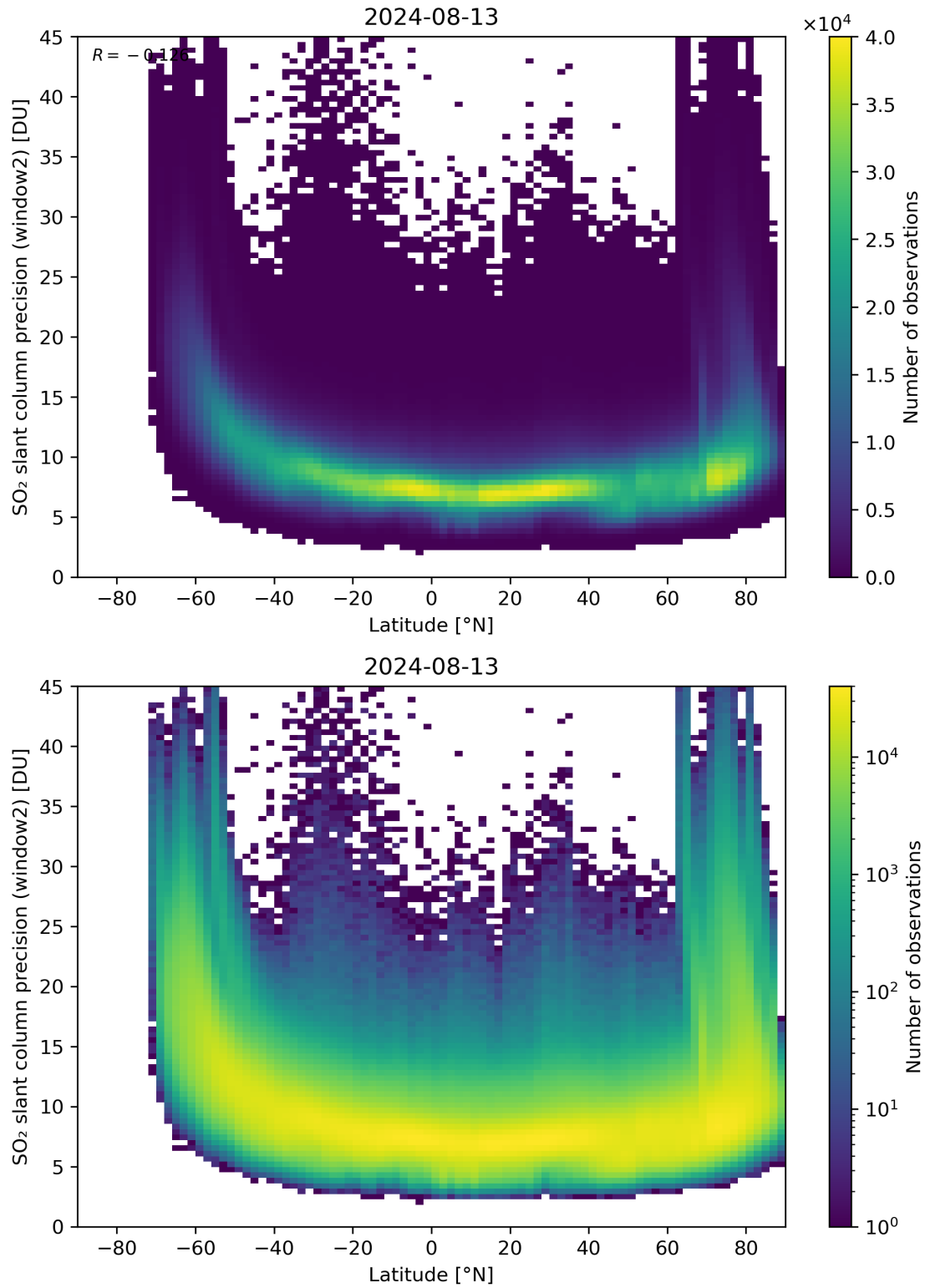
Figure 151: Scatter density plot of “Latitude” against “SO 2 slant column precision (window2)” for 2024-08-12 to 2024-08-14.
