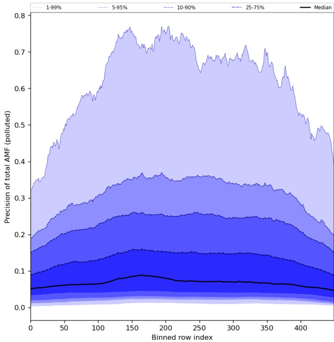
Figure 95: Along track statistics of “Precision of total AMF (polluted)” for 2024-08-12 to 2024-08-14
