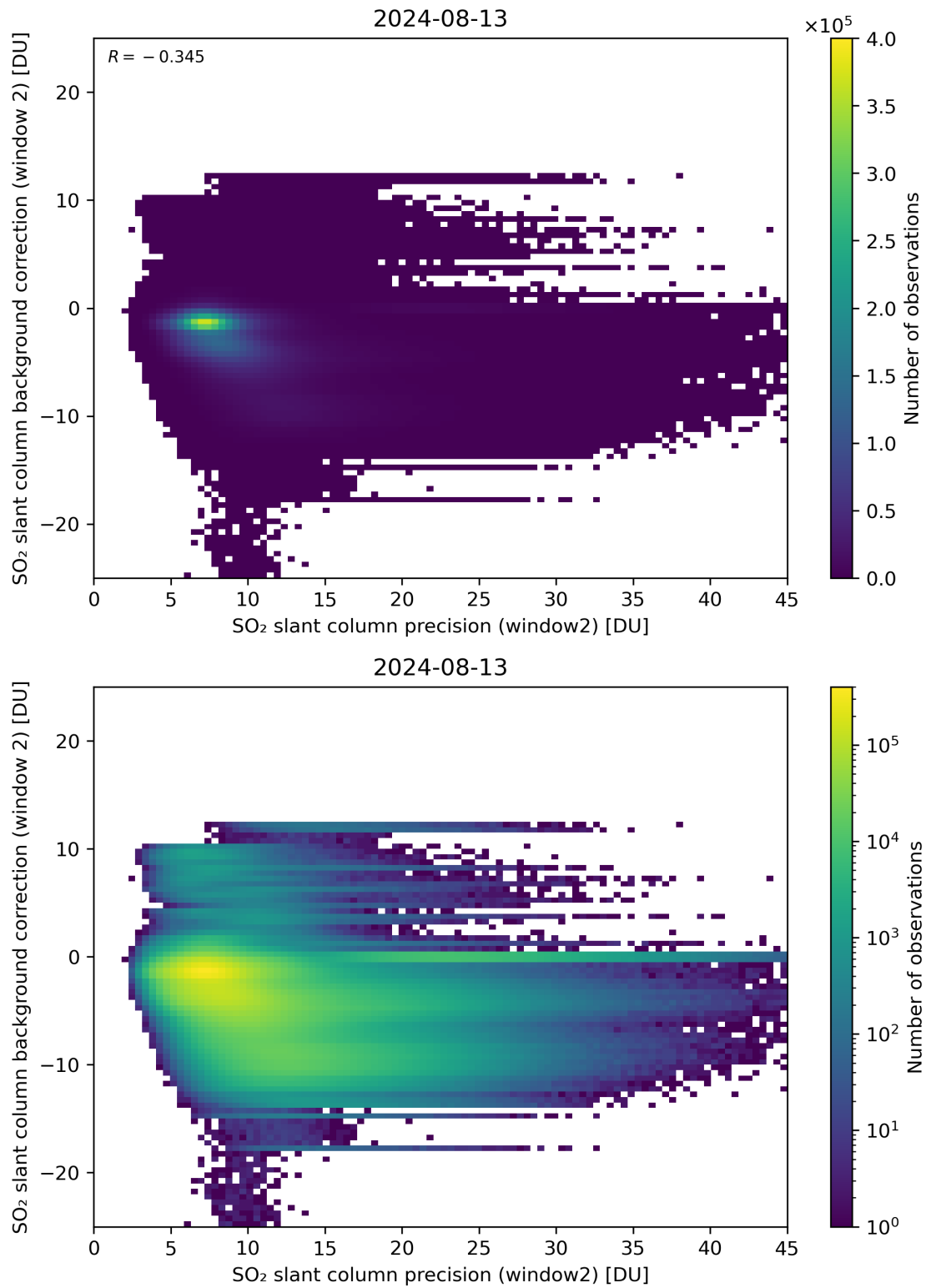
Figure 241: Scatter density plot of “SO 2 slant column precision (window2)” against “SO 2 slant column background correction (window 2)” for 2024-08-12 to 2024-08-14.
