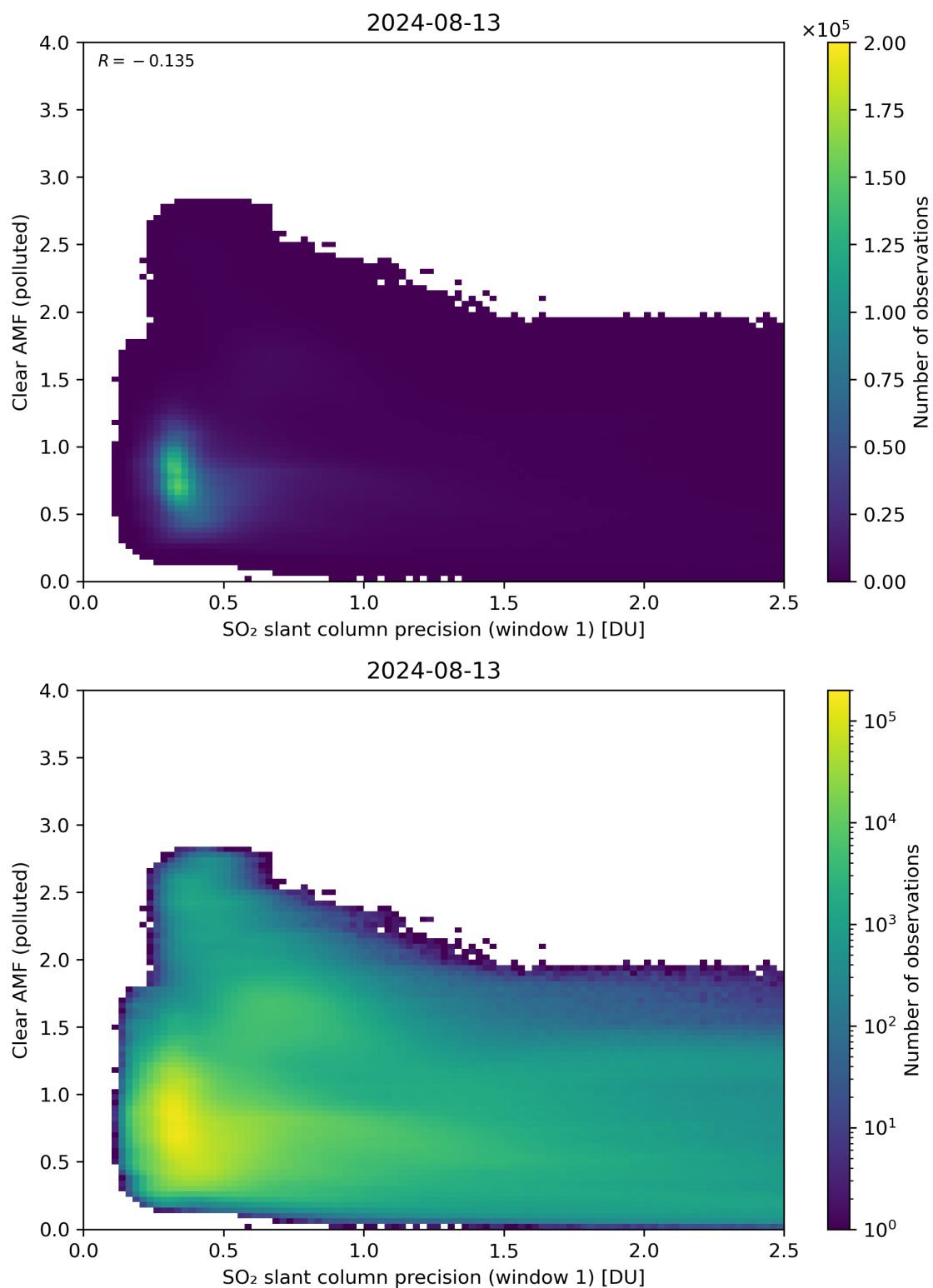
Figure 224: Scatter density plot of “SO 2 slant column precision (window 1)” against “Clear AMF (polluted)” for 2024-08-12 to 2024-08-14.
