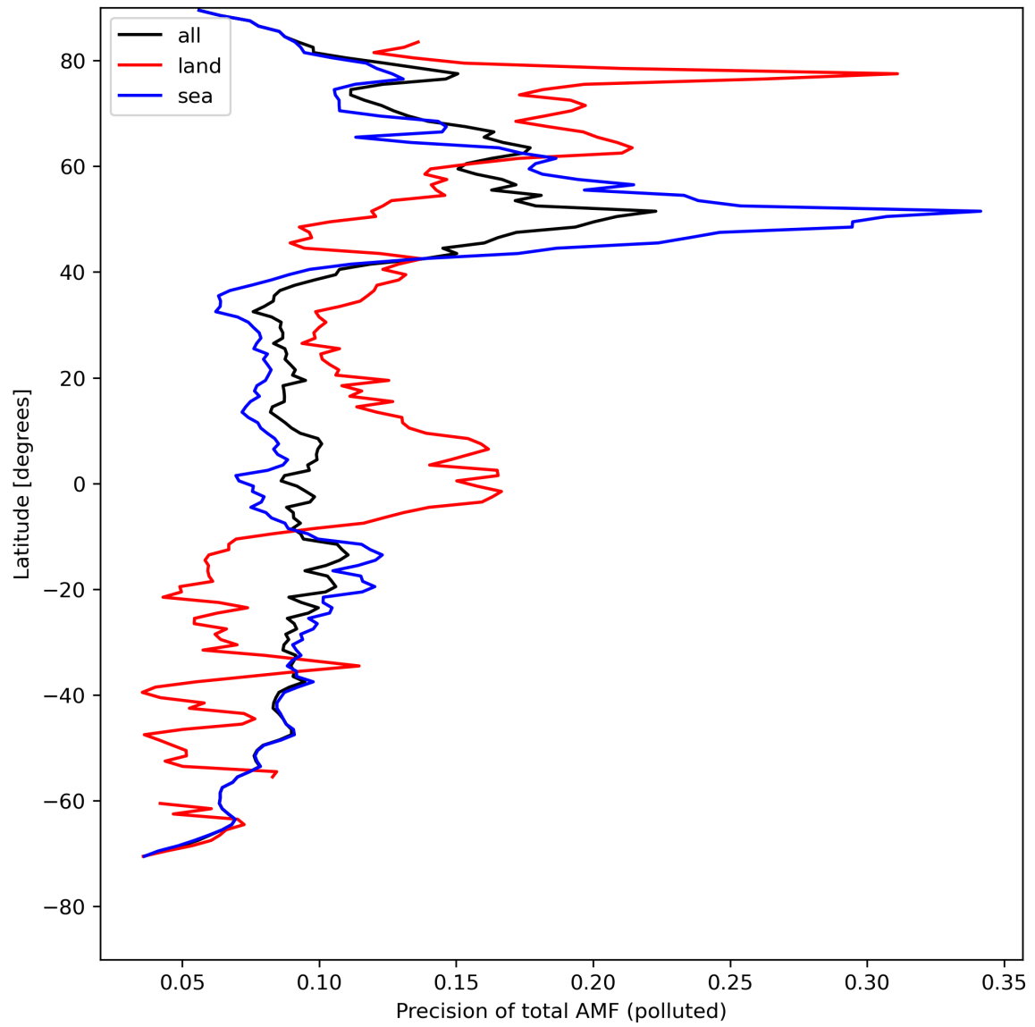
Figure 49: Zonal average of “Precision of total AMF (polluted)” for 2024-08-12 to 2024-08-14.
