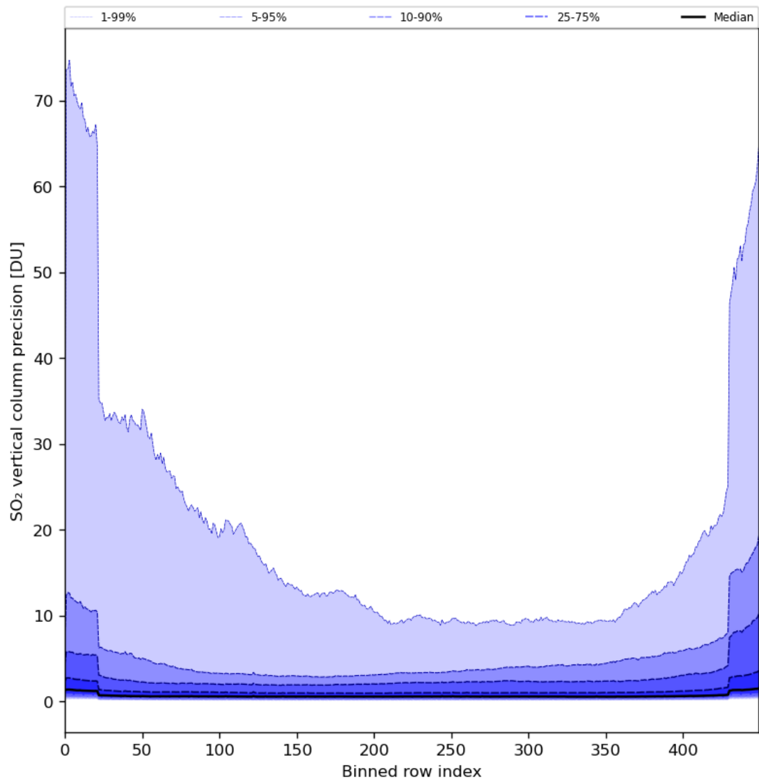
Figure 77: Along track statistics of “SO 2 vertical column precision” for 2024-08-12 to 2024-08-14
