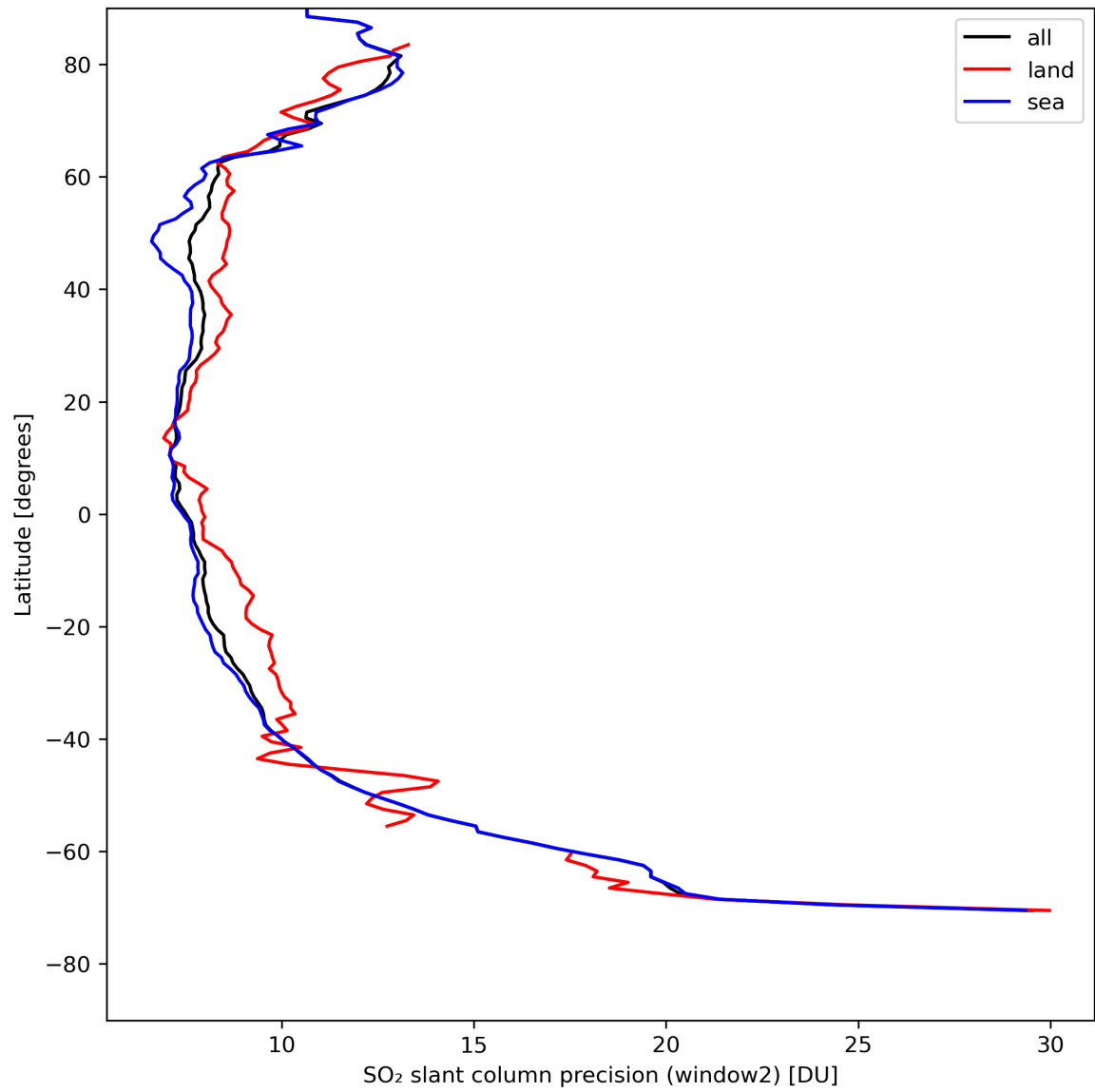
Figure 38: Zonal average of “SO 2 slant column precision (window2)” for 2024-08-12 to 2024-08-14.
