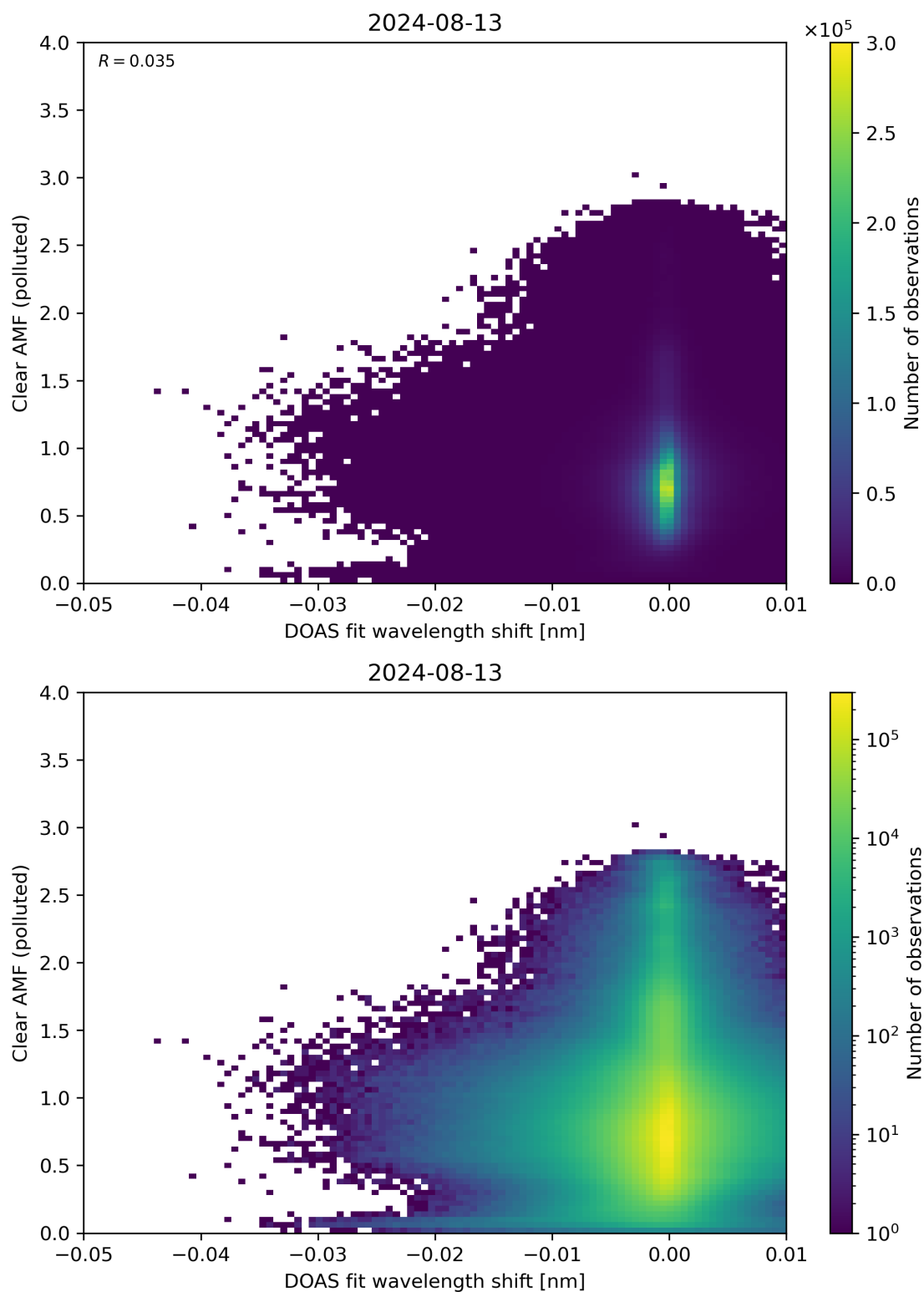
Figure 129: Scatter density plot of “DOAS fit wavelength shift” against “Clear AMF (polluted)” for 2024-08-12 to 2024-08-14.
