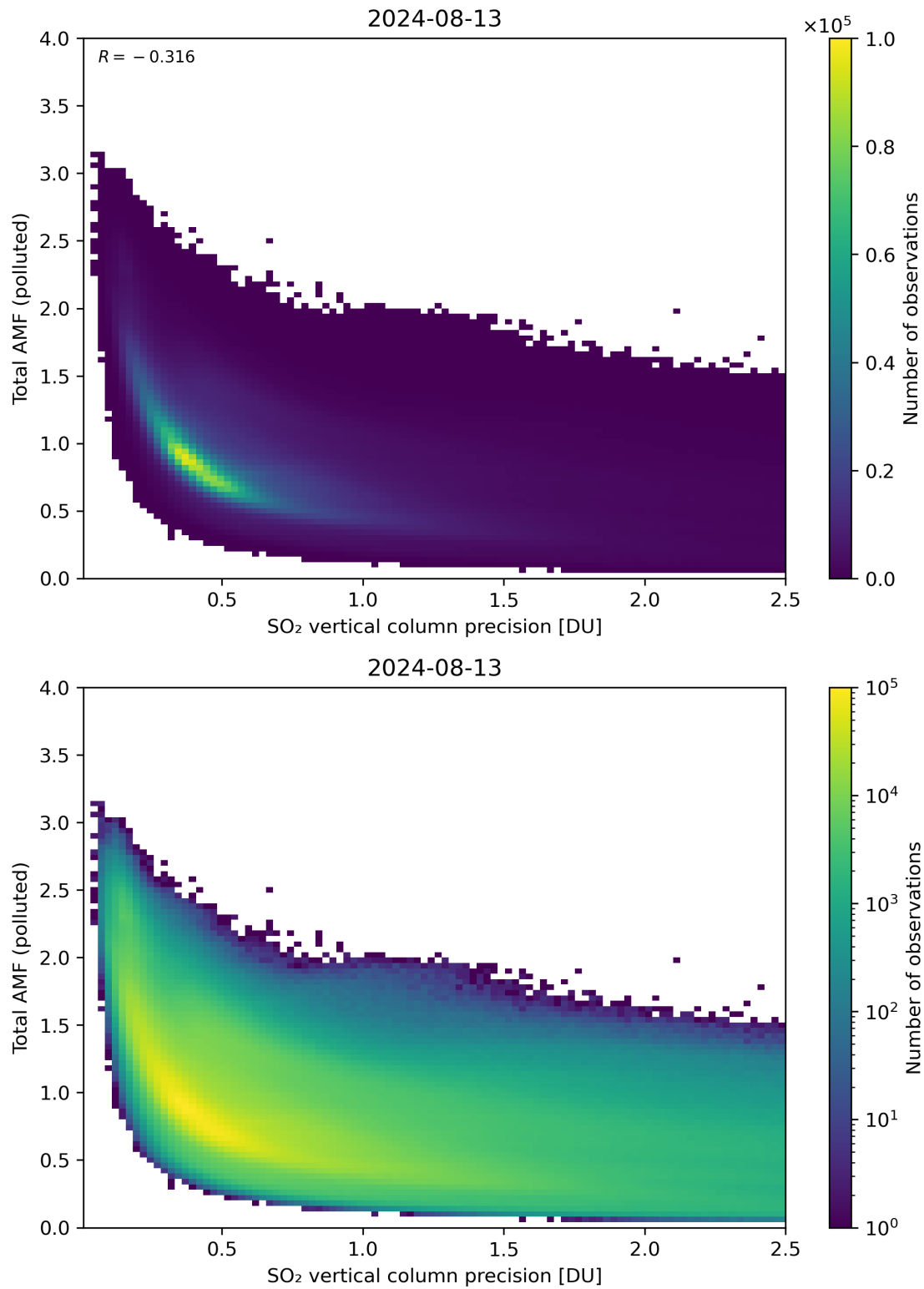
Figure 294: Scatter density plot of “SO 2 vertical column precision” against “Total AMF (polluted)” for 2024-08-12 to 2024-08-14.
