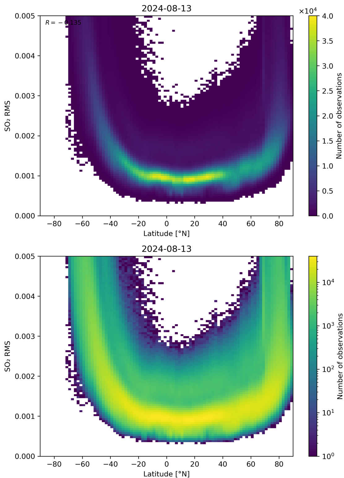
Figure 144: Scatter density plot of “Latitude” against “SO 2 RMS” for 2024-08-12 to 2024-08-14.
