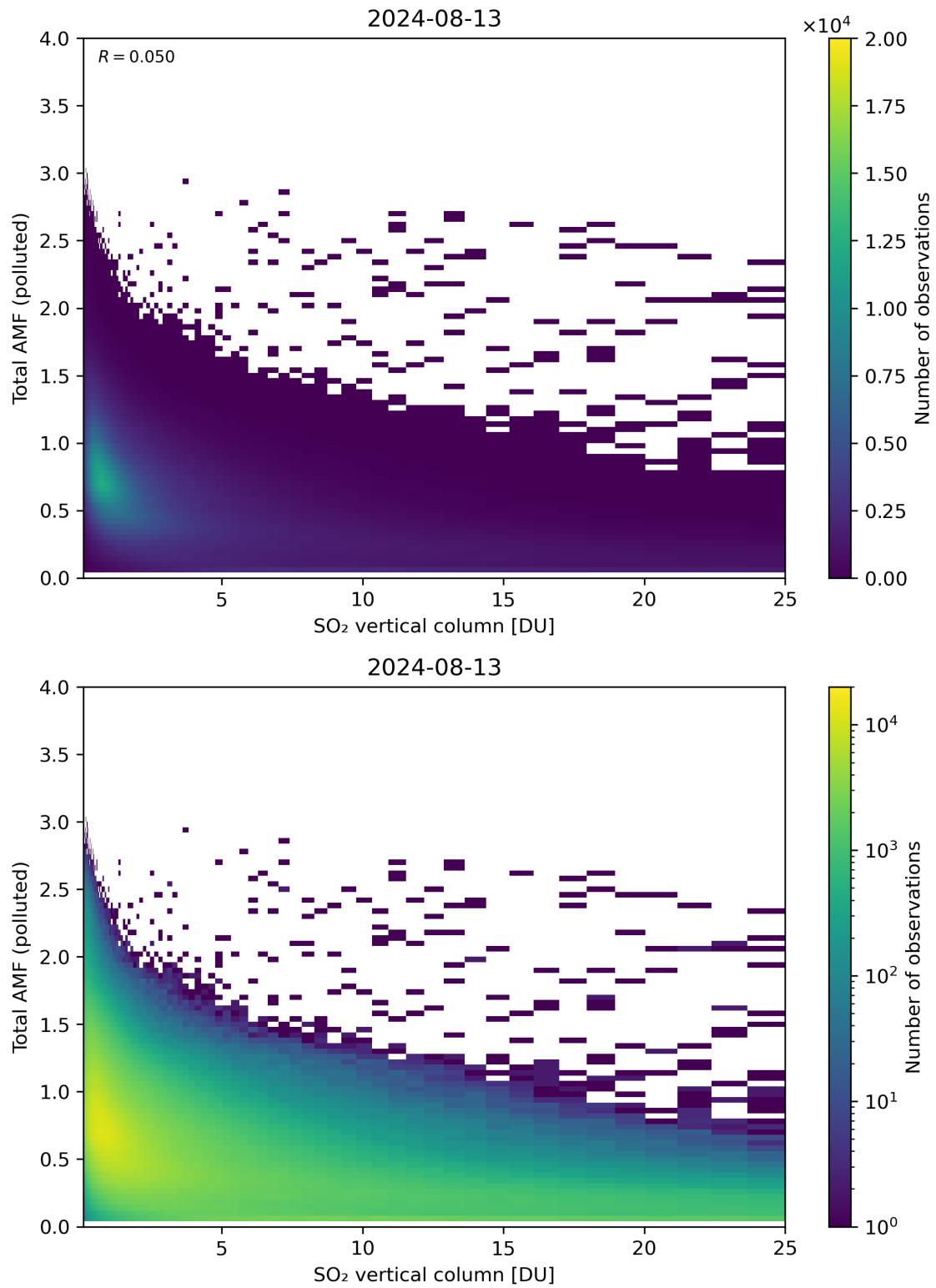
Figure 305: Scatter density plot of “SO 2 vertical column” against “Total AMF (polluted)” for 2024-08-12 to 2024-08-14.
