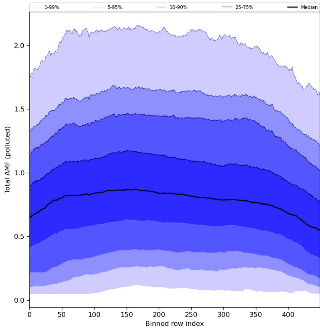
Figure 94: Along track statistics of “Total AMF (polluted)” for 2024-08-12 to 2024-08-14
