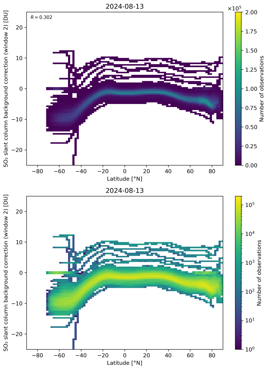
Figure 140: Scatter density plot of “Latitude” against “SO 2 slant column background correction (window 2)” for 2024-08-12 to 2024-08-14.
