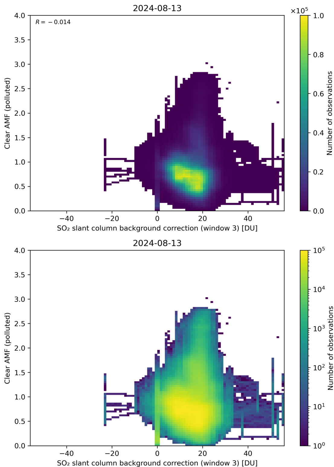
Figure 124: Scatter density plot of “SO 2 slant column background correction (window 3)” against “Clear AMF (polluted)” for 2024-08-12 to 2024-08-14.
