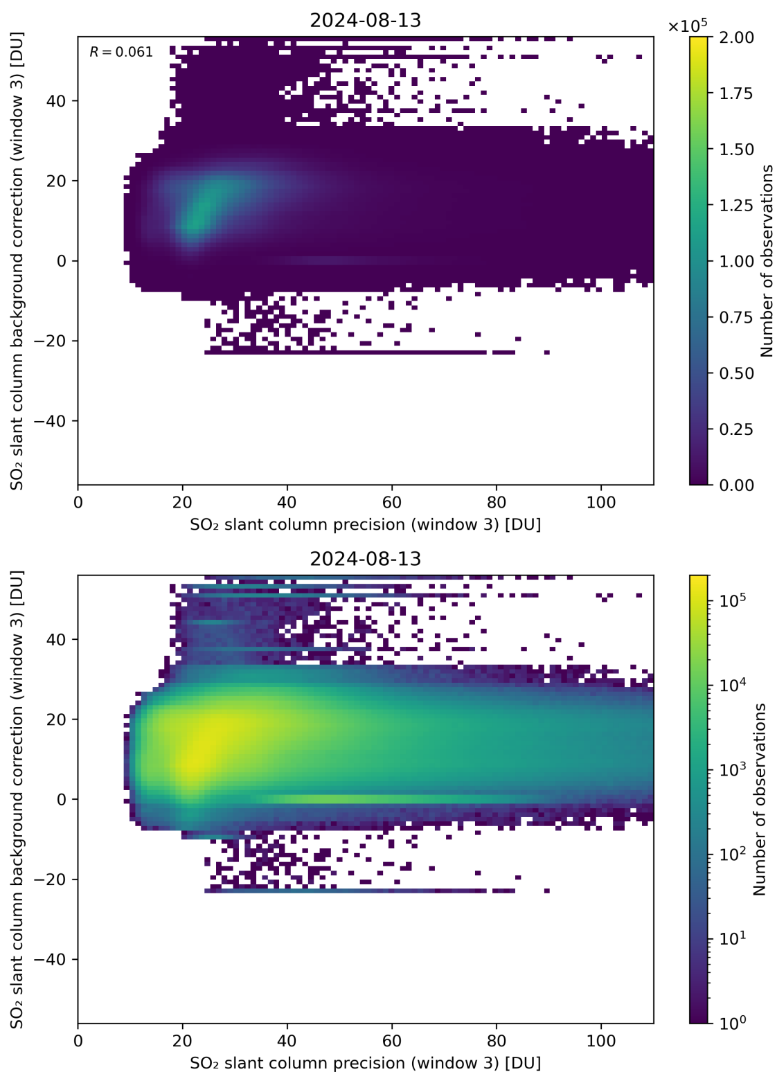
Figure 257: Scatter density plot of “SO 2 slant column precision (window 3)” against “SO 2 slant column background correction (window 3)” for 2024-08-12 to 2024-08-14.
