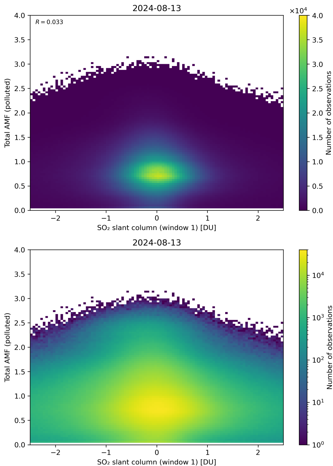
Figure 239: Scatter density plot of “SO 2 slant column (window 1)” against “Total AMF (polluted)” for 2024-08-12 to 2024-08-14.
