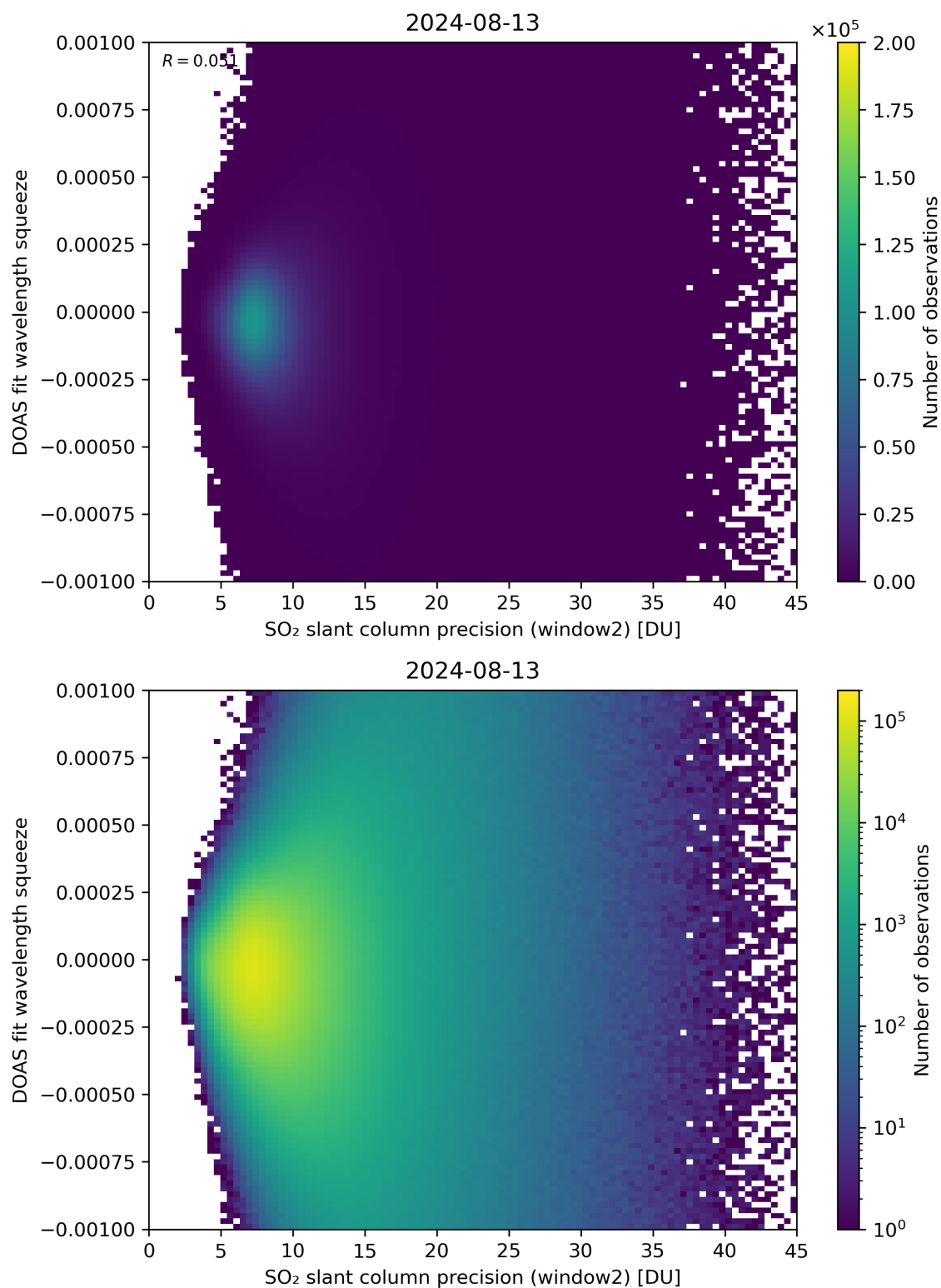
Figure 244: Scatter density plot of “SO 2 slant column precision (window2)” against “DOAS fit wavelength squeeze” for 2024-08-12 to 2024-08-14.
