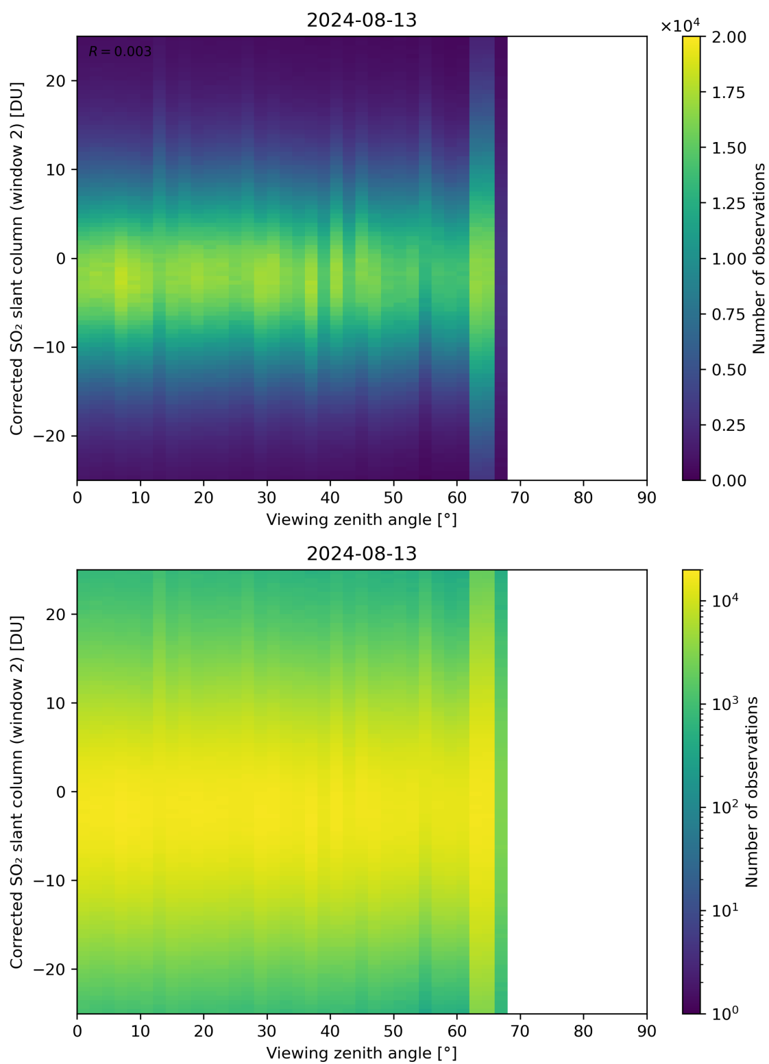
Figure 318: Scatter density plot of “Viewing zenith angle” against “Corrected SO 2 slant column (window 2)” for 2024-08-12 to 2024-08-14.
