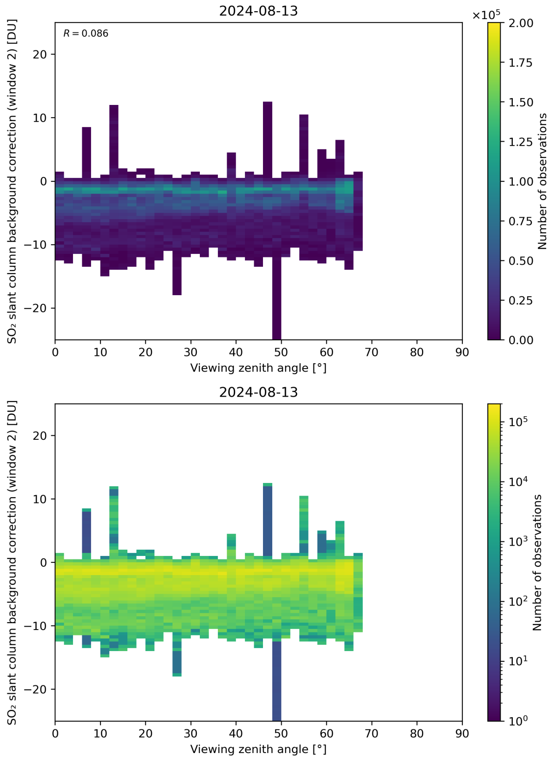
Figure 309: Scatter density plot of “Viewing zenith angle” against “SO 2 slant column background correction (window 2)” for 2024-08-12 to 2024-08-14.
