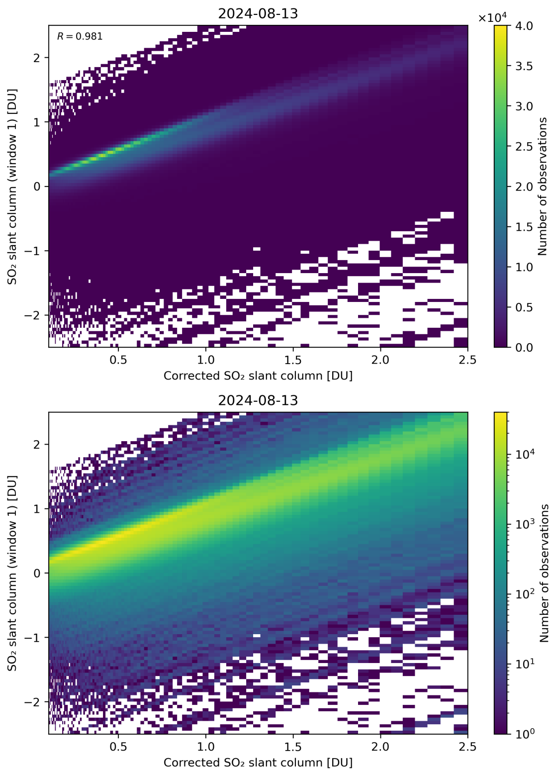
Figure 187: Scatter density plot of “Corrected SO 2 slant column” against “SO 2 slant column (window 1)” for 2024-08-12 to 2024-08-14.
