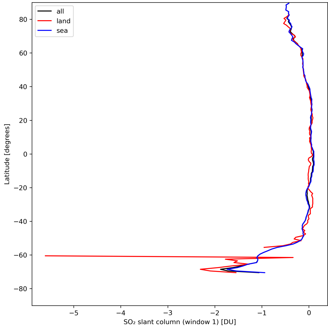
Figure 33: Zonal average of “SO 2 slant column (window 1)” for 2024-08-12 to 2024-08-14.
