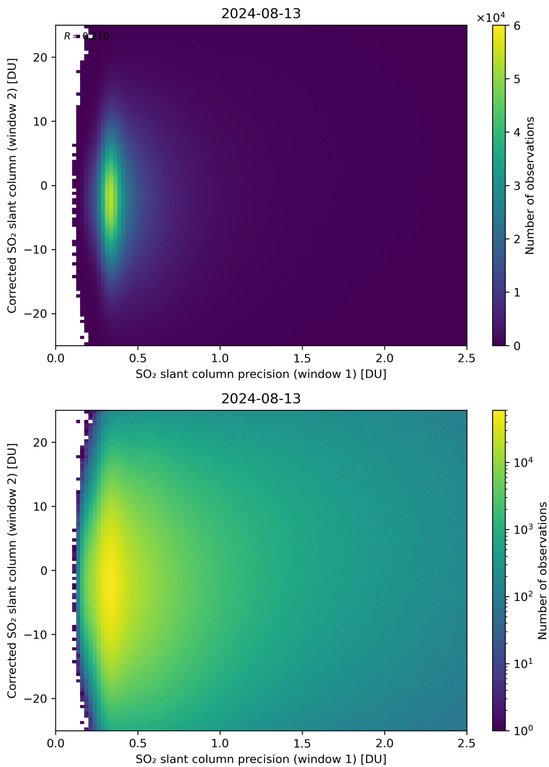
Figure 225: Scatter density plot of “SO 2 slant column precision (window 1)” against “Corrected SO 2 slant column (window 2)” for 2024-08-12 to 2024-08-14.
