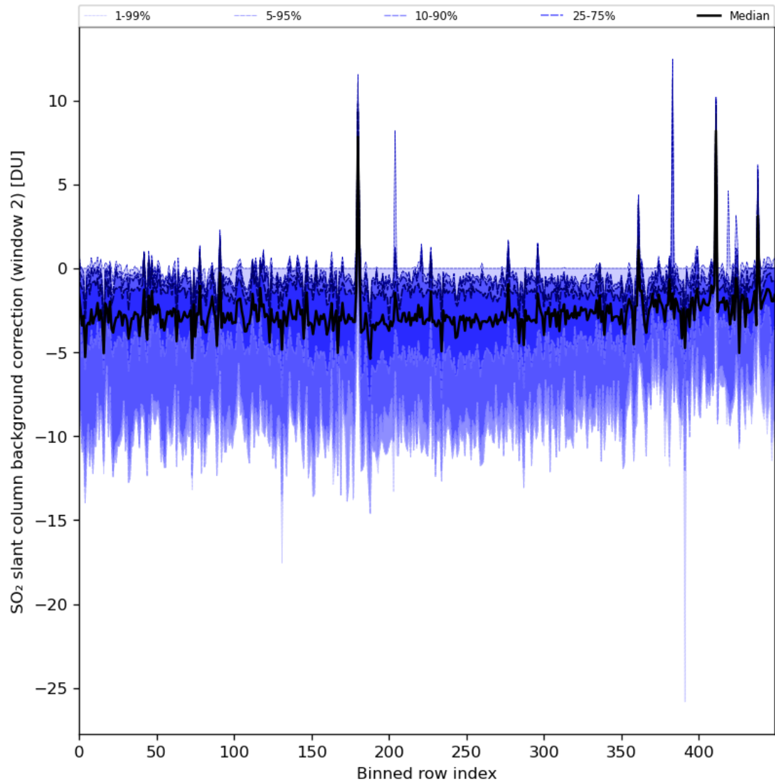
Figure 86: Along track statistics of “SO 2 slant column background correction (window 2)” for 2024-08-12 to 2024-08-14
