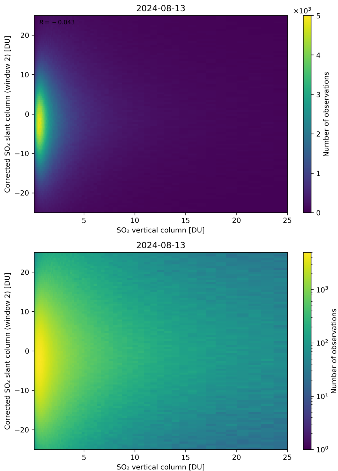
Figure 298: Scatter density plot of “SO 2 vertical column” against “Corrected SO 2 slant column (window 2)” for 2024-08-12 to 2024-08-14.
