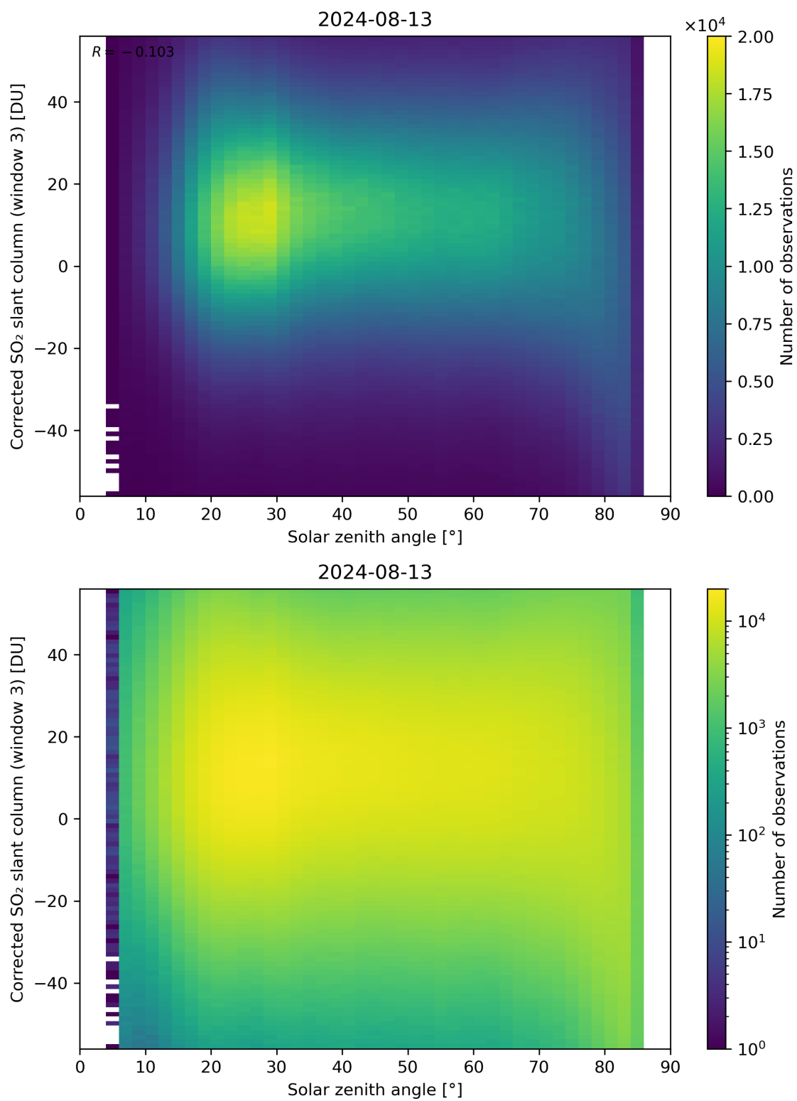
Figure 168: Scatter density plot of “Solar zenith angle” against “Corrected SO 2 slant column (window 3)” for 2024-08-12 to 2024-08-14.
