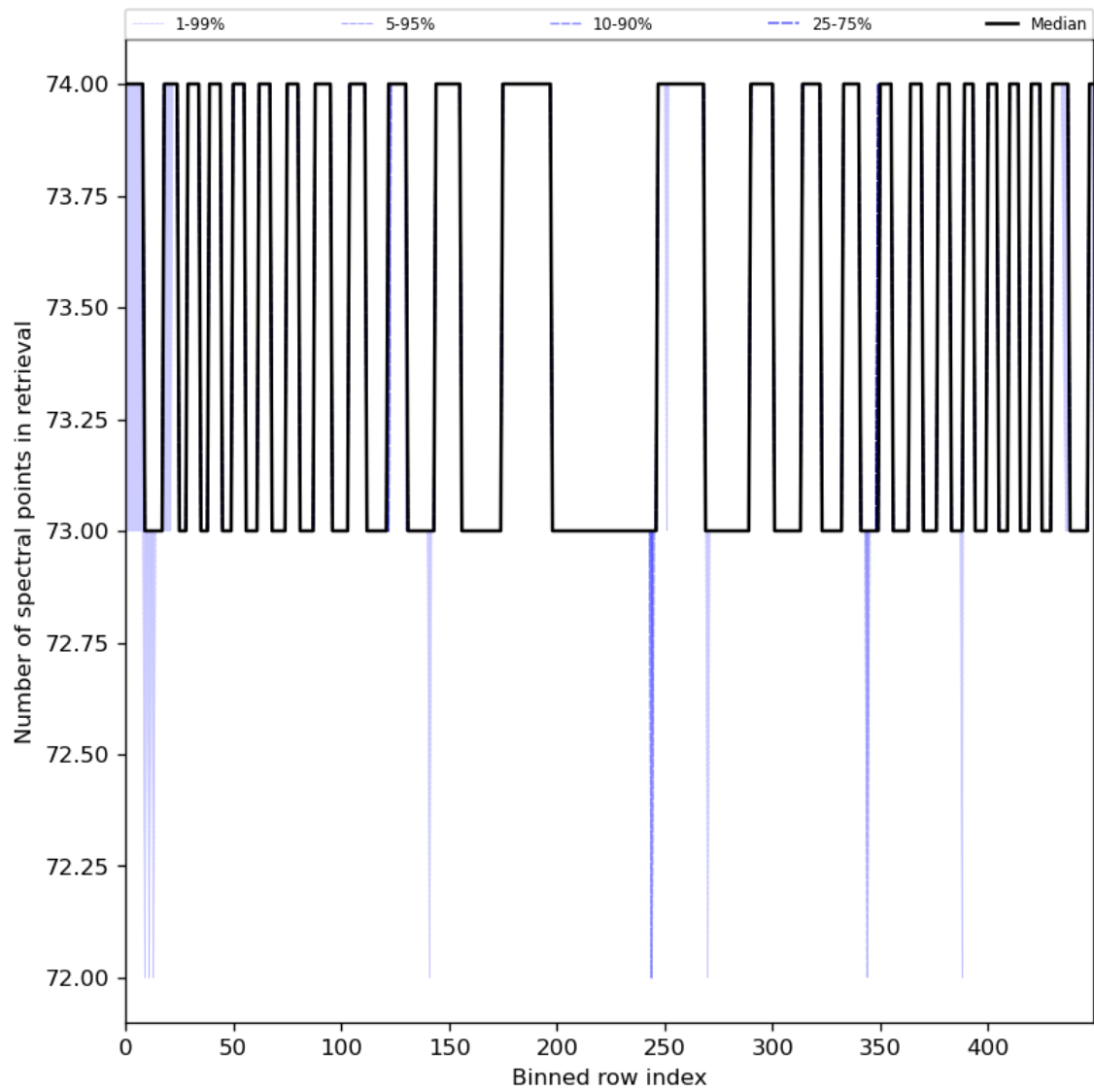
Figure 97: Along track statistics of “Number of spectral points in retrieval” for 2024-08-12 to 2024-08-14
