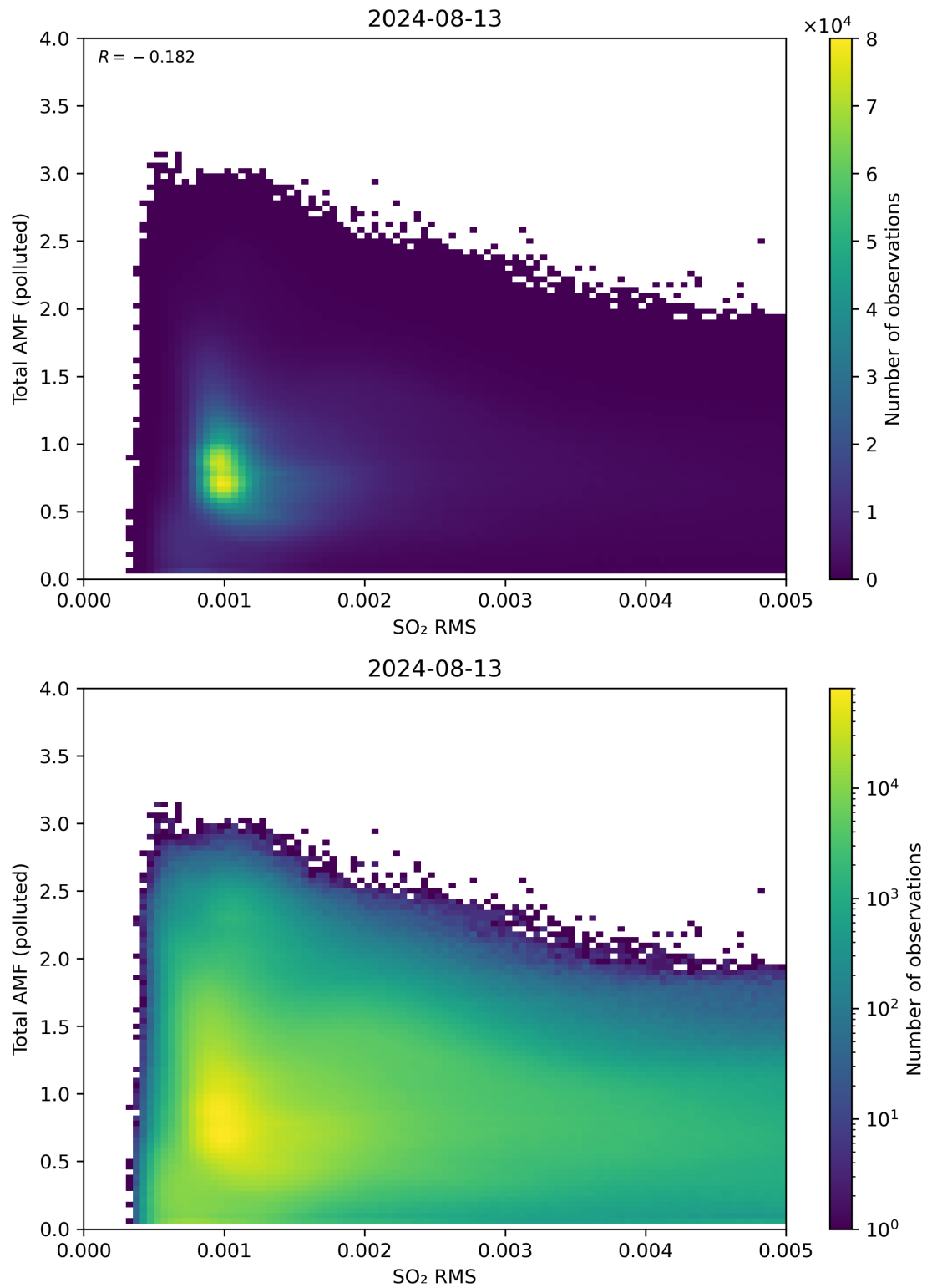
Figure 137: Scatter density plot of “SO 2 RMS” against “Total AMF (polluted)” for 2024-08-12 to 2024-08-14.
