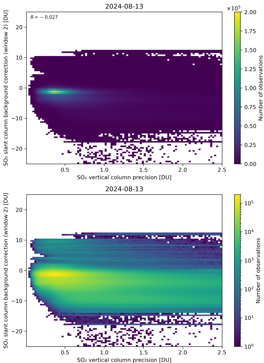
Figure 280: Scatter density plot of “SO 2 vertical column precision” against “SO 2 slant column background correction (window 2)” for 2024-08-12 to 2024-08-14.
