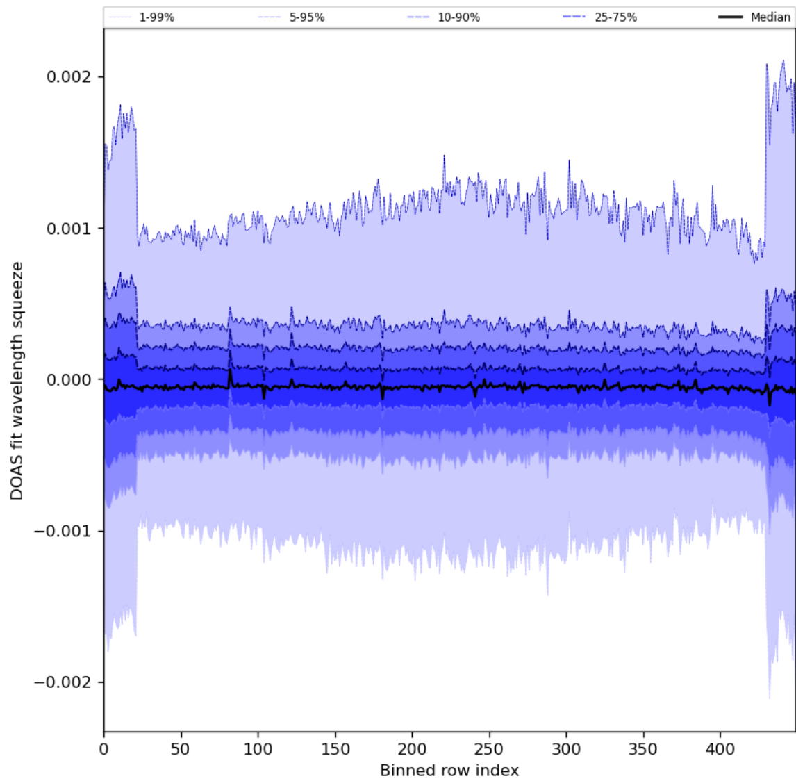
Figure 92: Along track statistics of “DOAS fit wavelength squeeze” for 2024-08-12 to 2024-08-14
