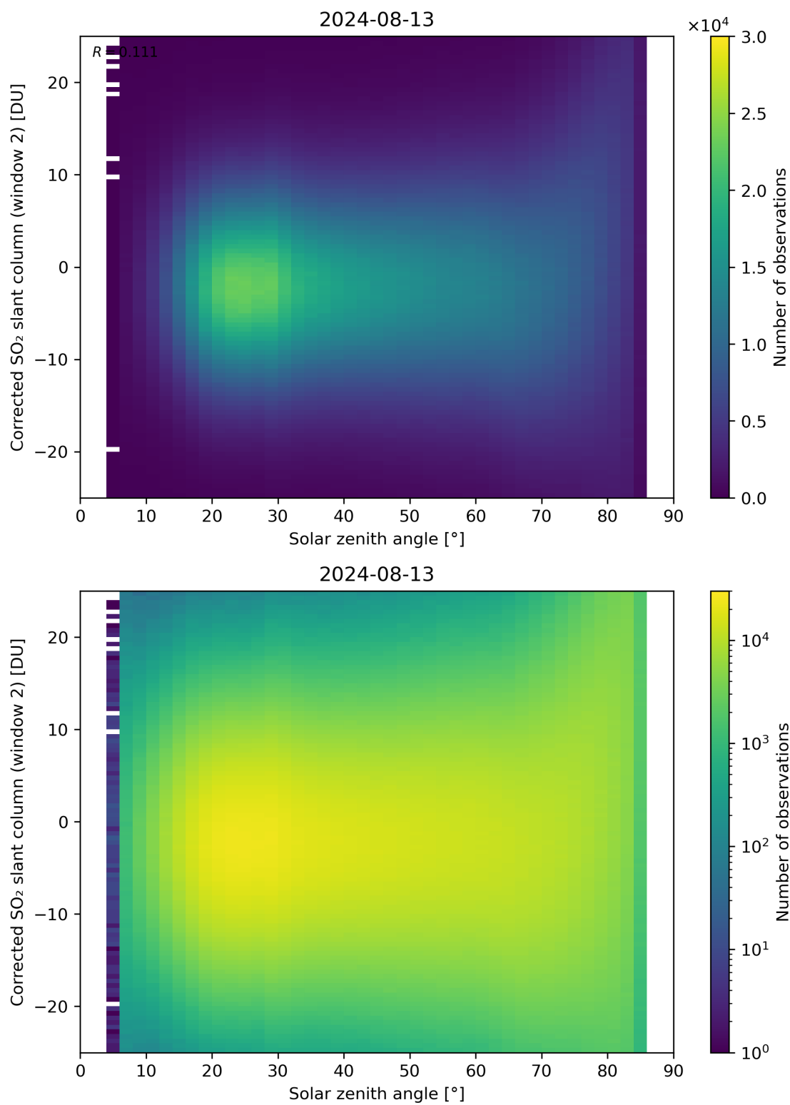
Figure 167: Scatter density plot of “Solar zenith angle” against “Corrected SO 2 slant column (window 2)” for 2024-08-12 to 2024-08-14.
