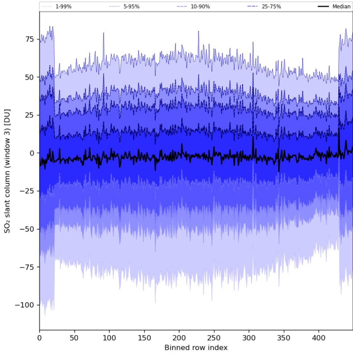
Figure 87: Along track statistics of “SO 2 slant column (window 3)” for 2024-08-12 to 2024-08-14
