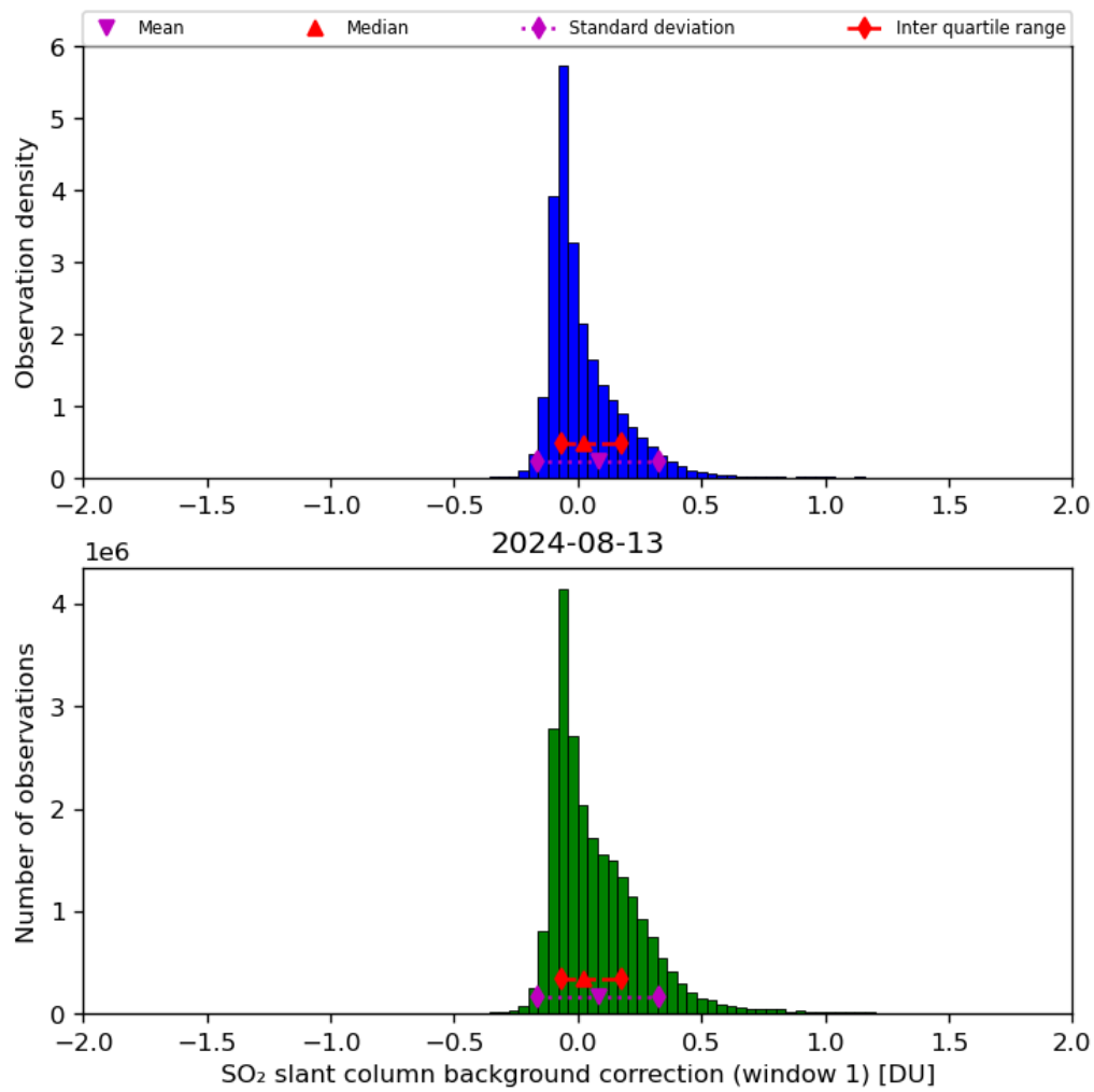
Figure 59: Histogram of “SO 2 slant column background correction (window 1)” for 2024-08-12 to 2024-08-14
