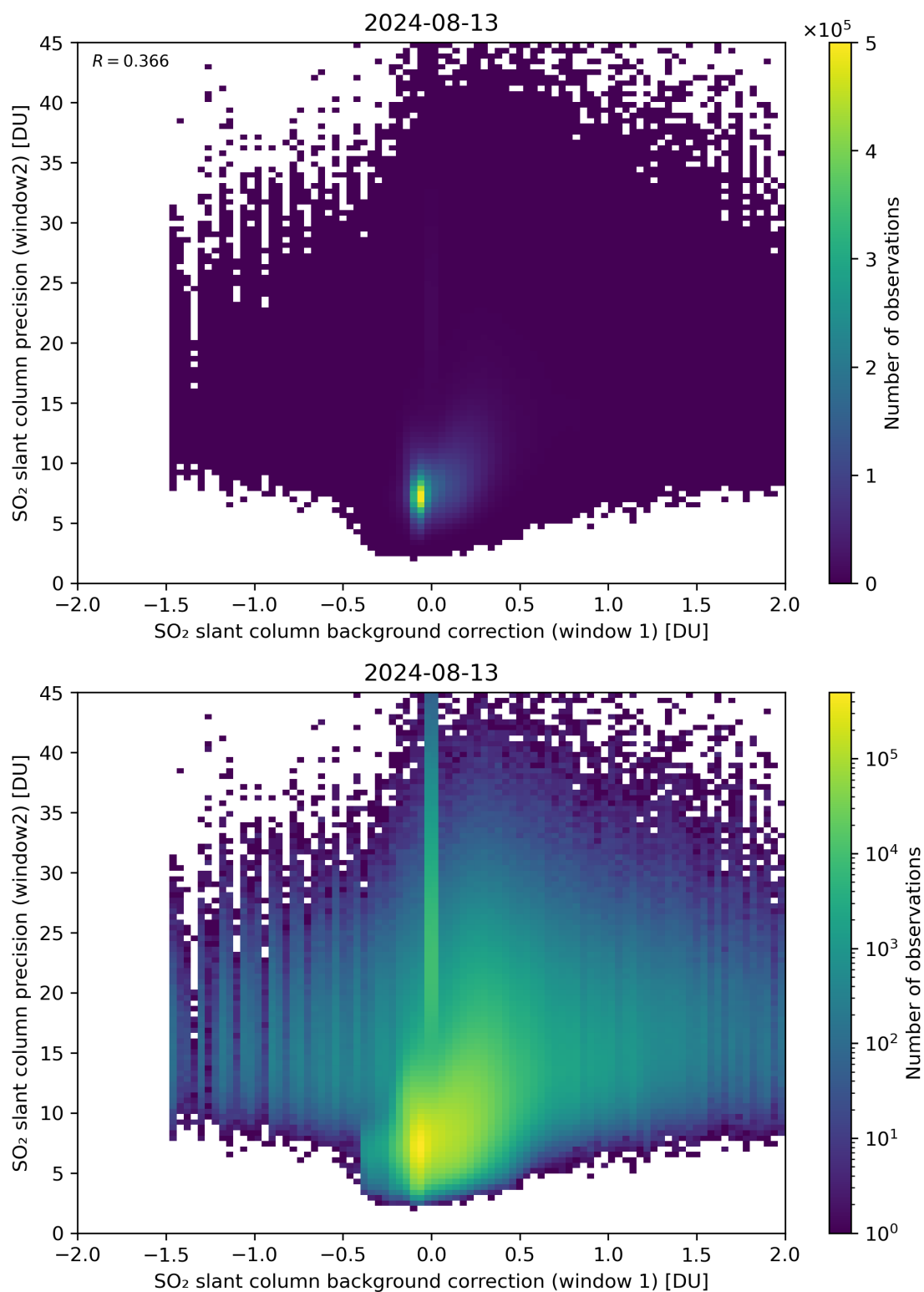
Figure 106: Scatter density plot of “SO 2 slant column background correction (window 1)” against “SO 2 slant column precision (window2)” for 2024-08-12 to 2024-08-14.
