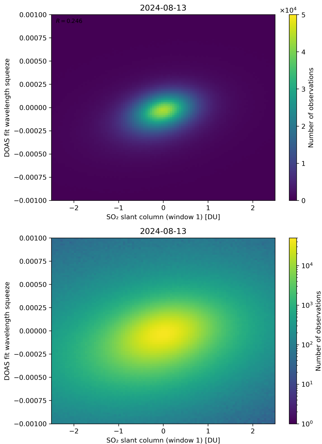
Figure 216: Scatter density plot of “SO 2 slant column (window 1)” against “DOAS fit wavelength squeeze” for 2024-08-12 to 2024-08-14.
