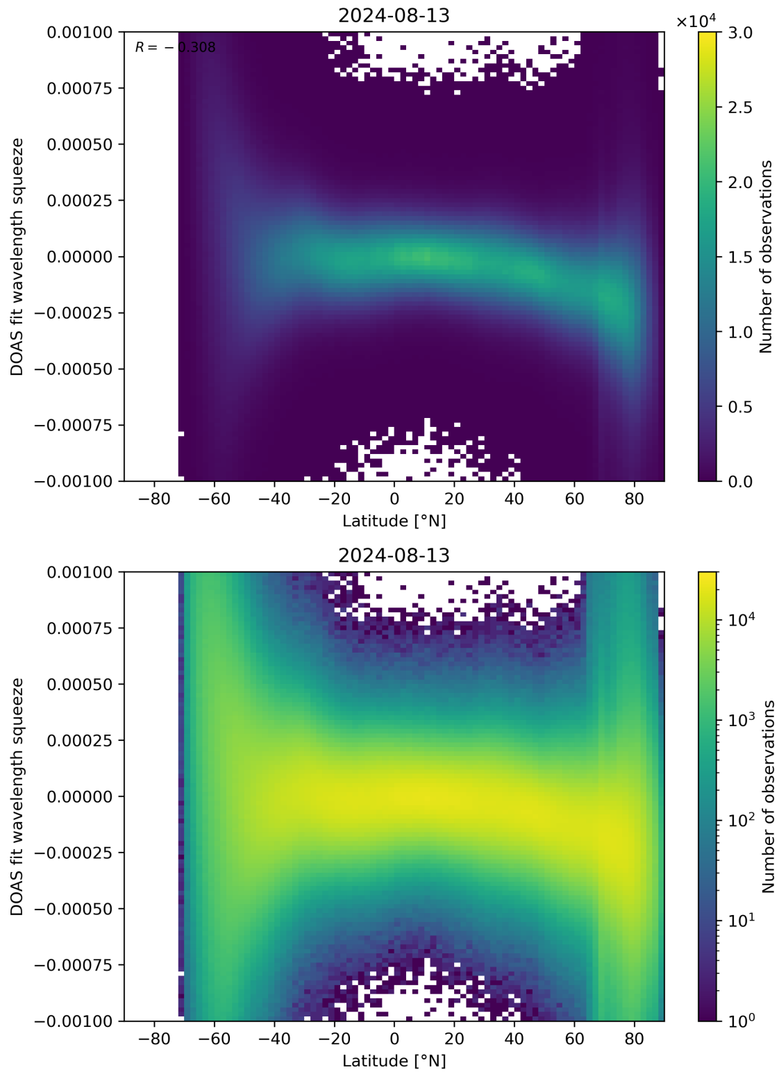
Figure 143: Scatter density plot of “Latitude” against “DOAS fit wavelength squeeze” for 2024-08-12 to 2024-08-14.
