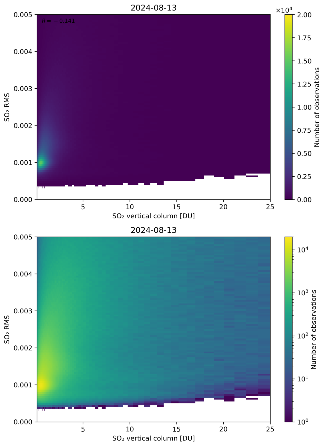
Figure 278: Scatter density plot of “SO 2 vertical column” against “SO 2 RMS” for 2024-08-12 to 2024-08-14.
