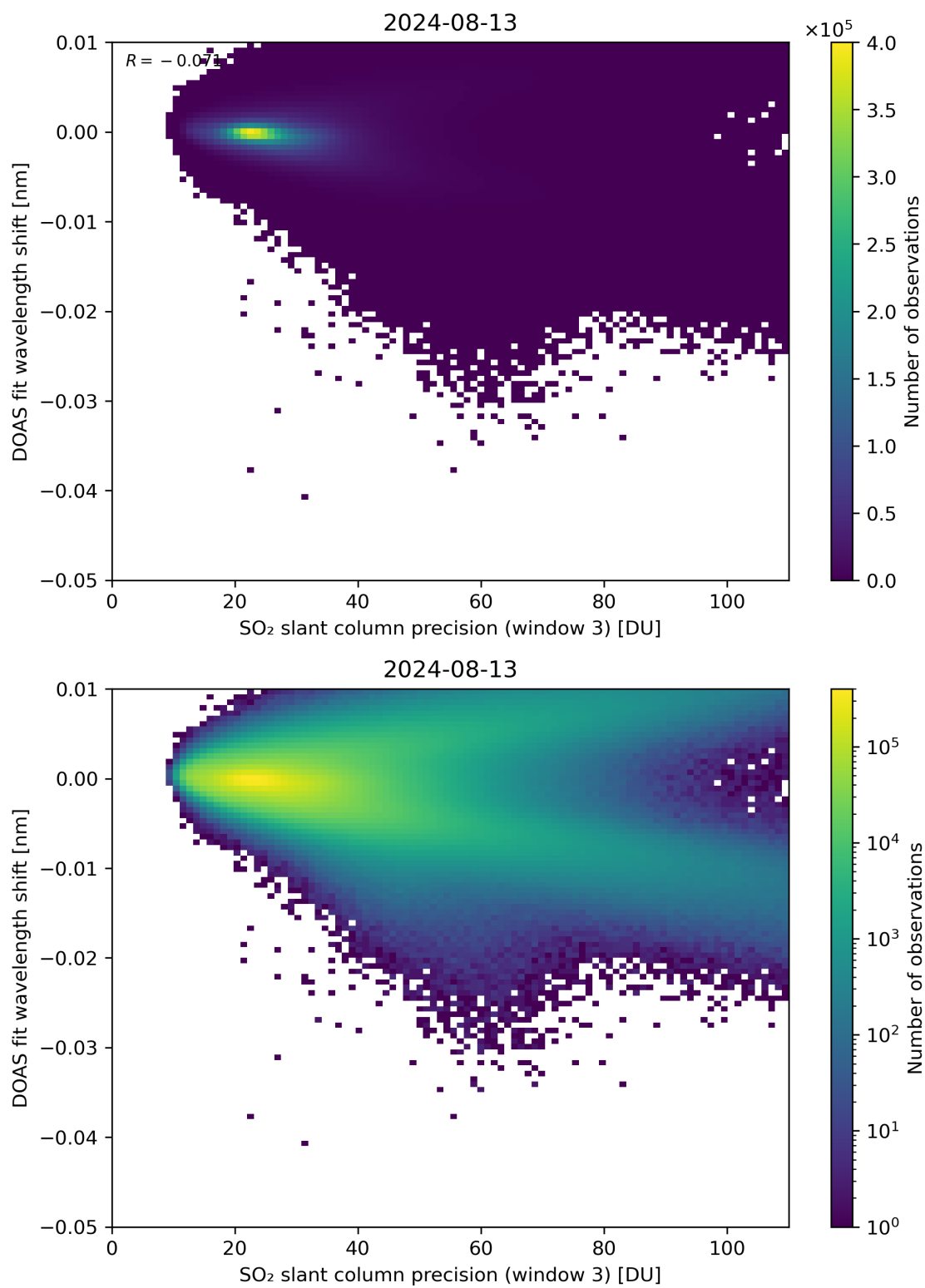
Figure 258: Scatter density plot of “SO 2 slant column precision (window 3)” against “DOAS fit wavelength shift” for 2024-08-12 to 2024-08-14.
