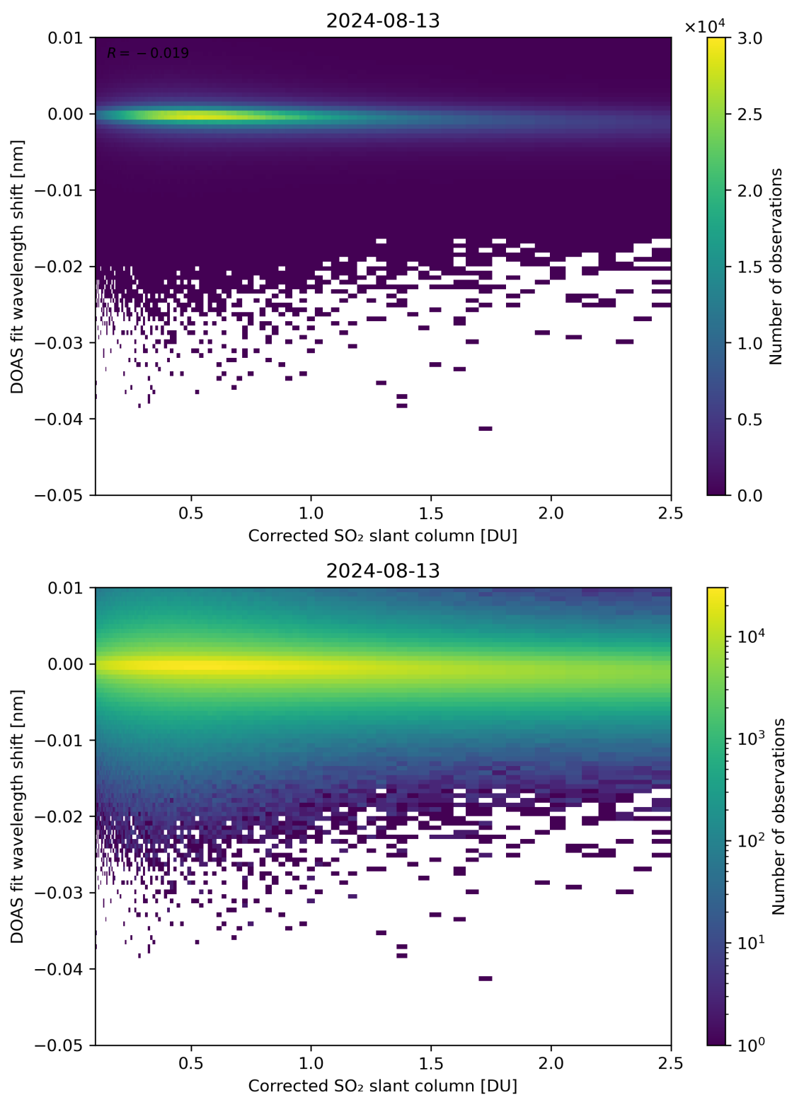
Figure 181: Scatter density plot of “Corrected SO 2 slant column” against “DOAS fit wavelength shift” for 2024-08-12 to 2024-08-14.
