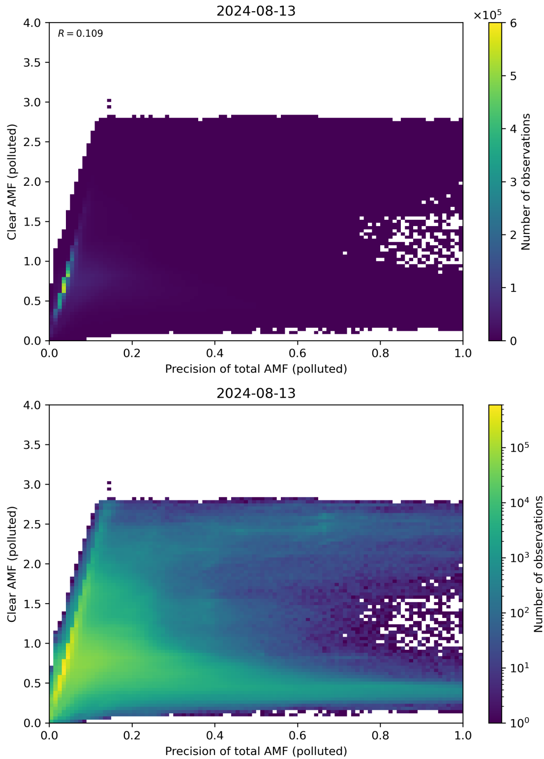
Figure 270: Scatter density plot of “Precision of total AMF (polluted)” against “Clear AMF (polluted)” for 2024-08-12 to 2024-08-14.
