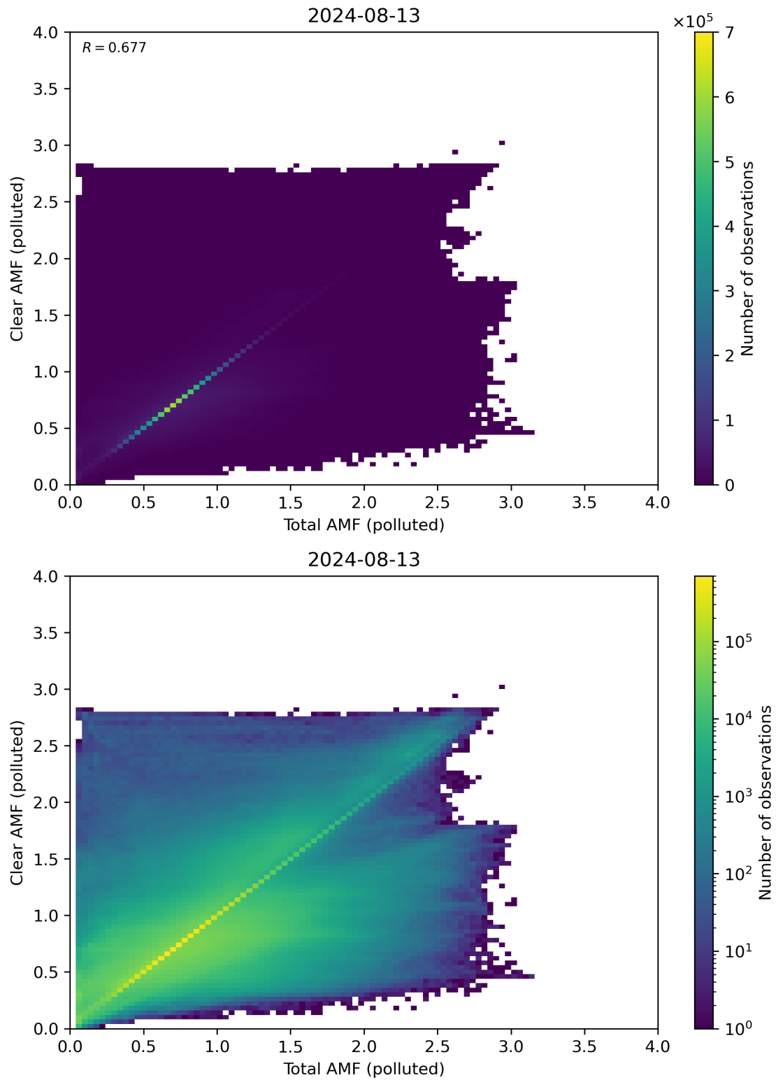
Figure 271: Scatter density plot of “Total AMF (polluted)” against “Clear AMF (polluted)” for 2024-08-12 to 2024-08-14.
