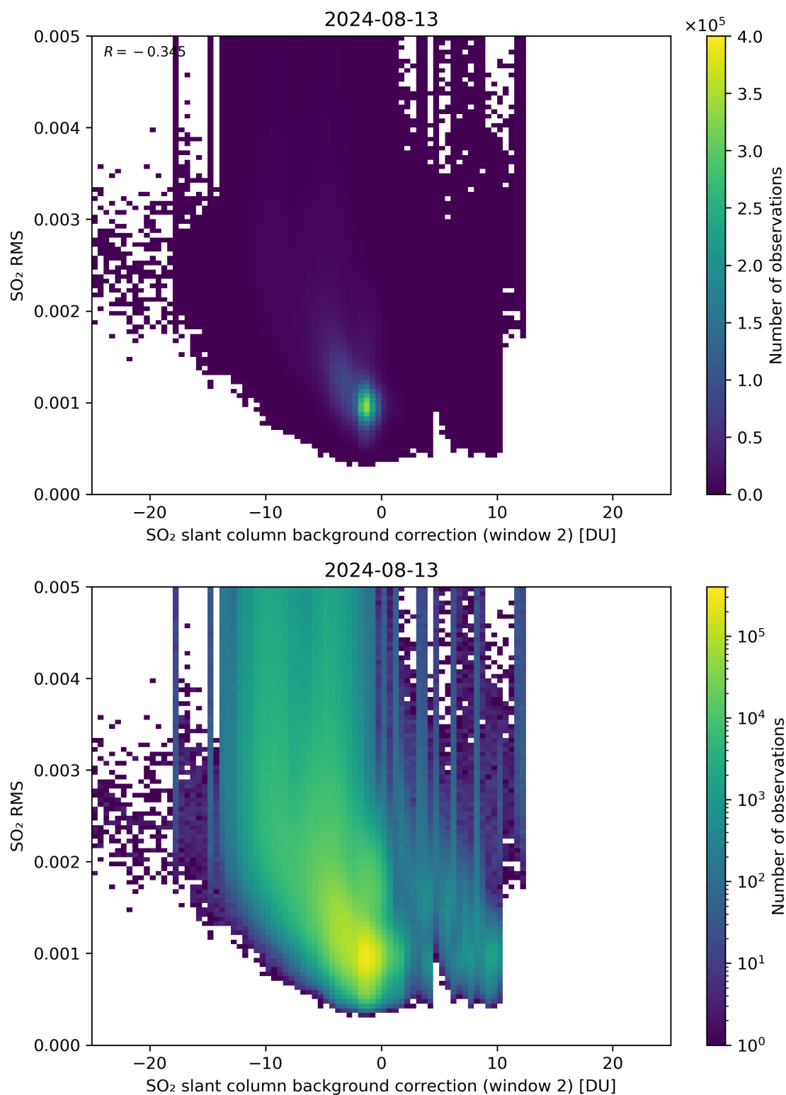
Figure 114: Scatter density plot of “SO 2 slant column background correction (window 2)” against “SO 2 RMS” for 2024-08-12 to 2024-08-14.
