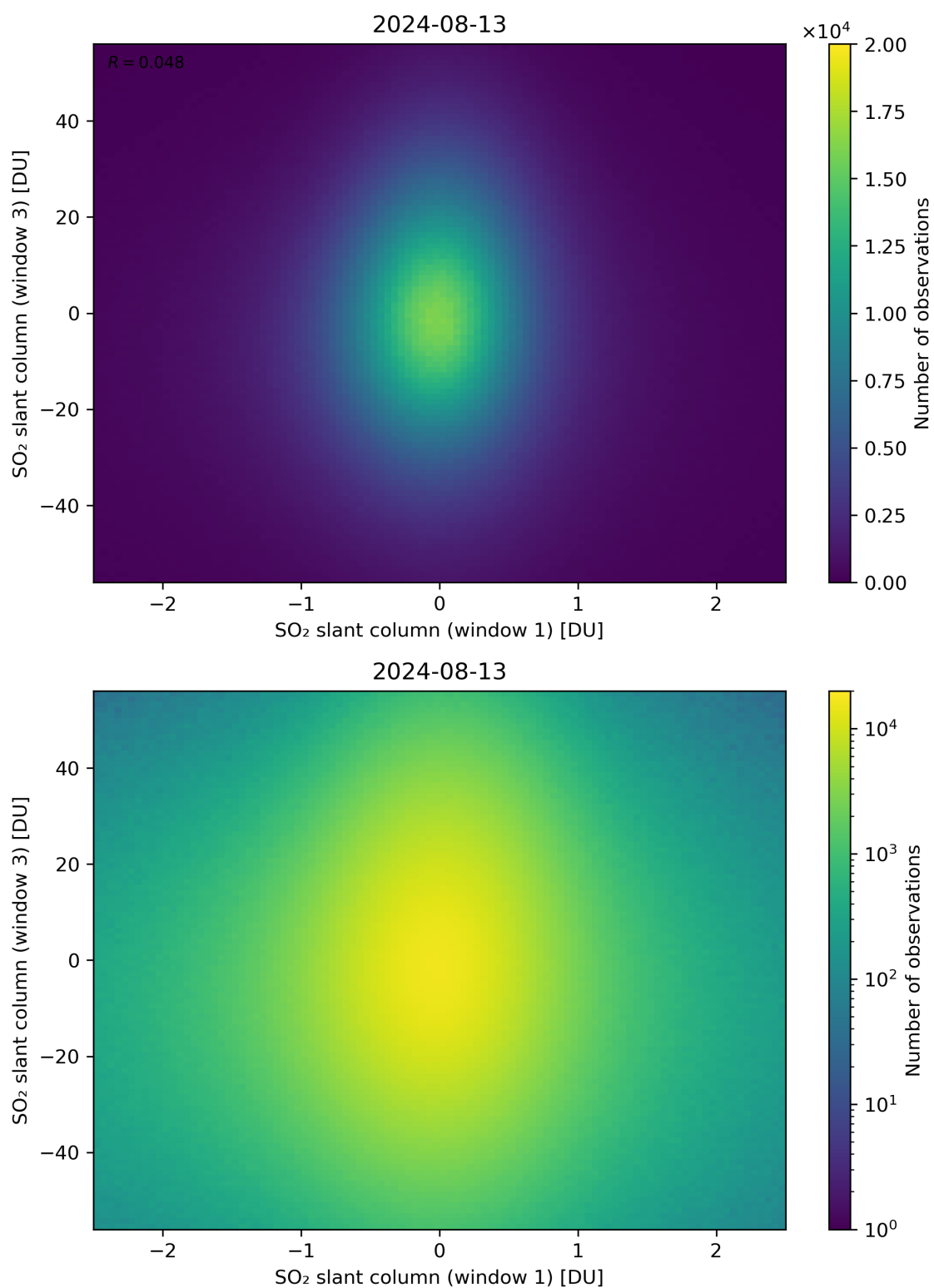
Figure 237: Scatter density plot of “SO 2 slant column (window 1)” against “SO 2 slant column (window 3)” for 2024-08-12 to 2024-08-14.
