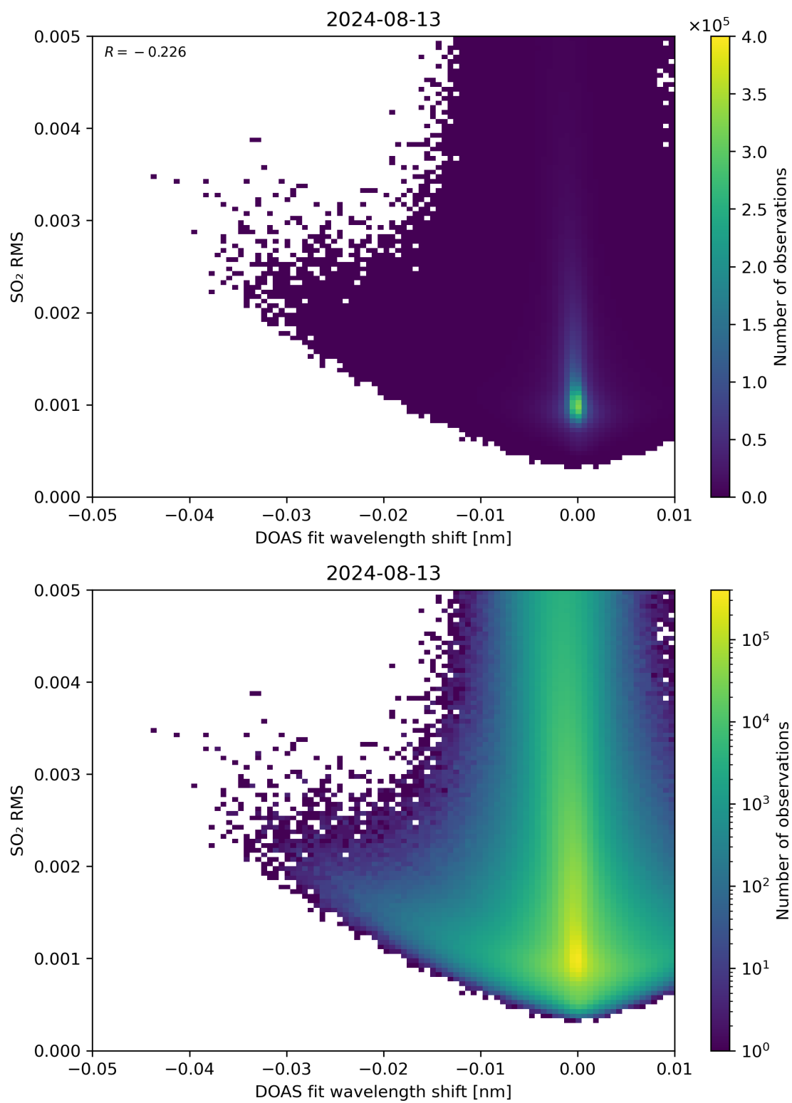
Figure 128: Scatter density plot of “DOAS fit wavelength shift” against “SO 2 RMS” for 2024-08-12 to 2024-08-14.
