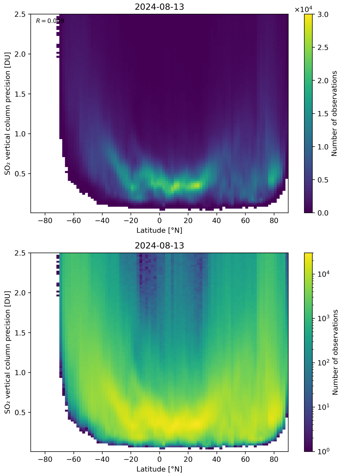
Figure 157: Scatter density plot of “Latitude” against “SO 2 vertical column precision” for 2024-08-12 to 2024-08-14.
