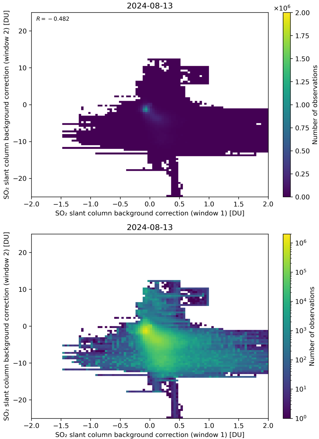
Figure 98: Scatter density plot of “SO 2 slant column background correction (window 1)” against “SO 2 slant column background correction (window 2)” for 2024-08-12 to 2024-08-14.
