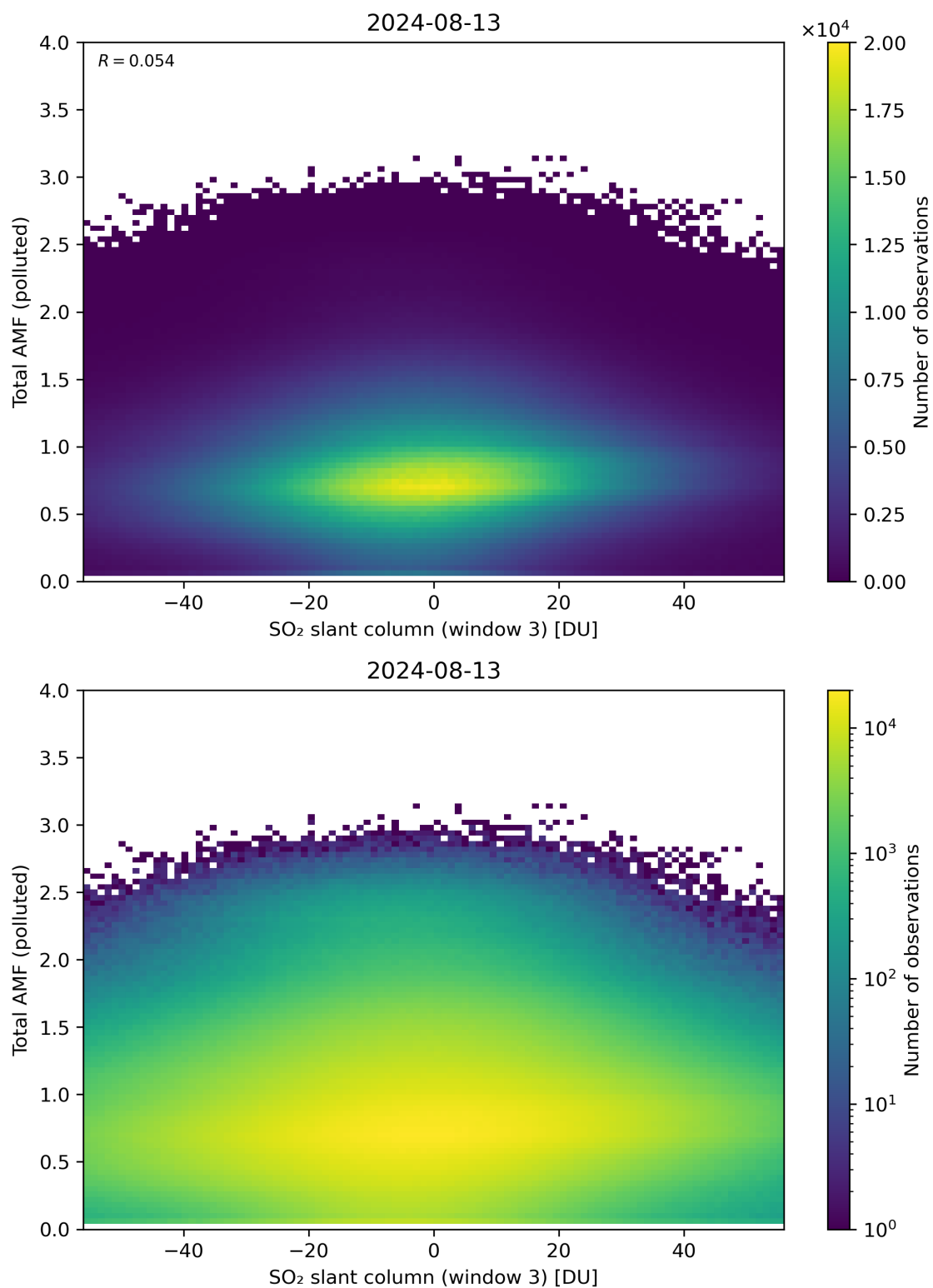
Figure 268: Scatter density plot of “SO 2 slant column (window 3)” against “Total AMF (polluted)” for 2024-08-12 to 2024-08-14.
