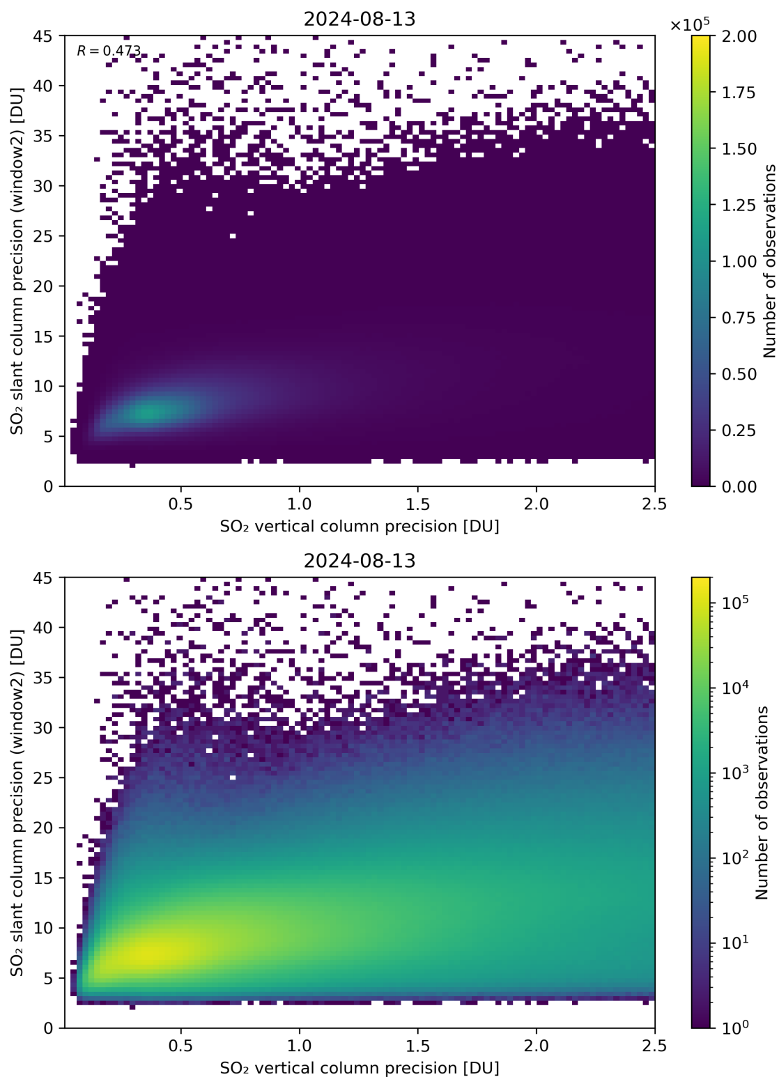
Figure 291: Scatter density plot of “SO 2 vertical column precision” against “SO 2 slant column precision (window2)” for 2024-08-12 to 2024-08-14.
