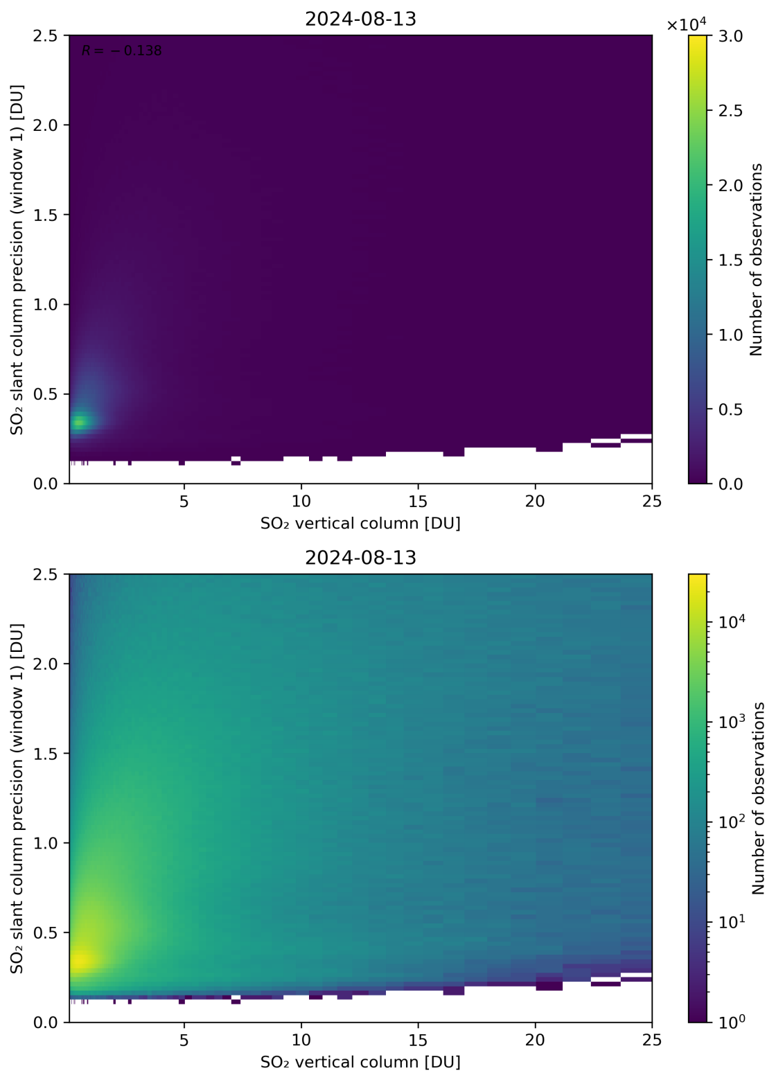
Figure 301: Scatter density plot of “SO 2 vertical column” against “SO 2 slant column precision (window 1)” for 2024-08-12 to 2024-08-14.
