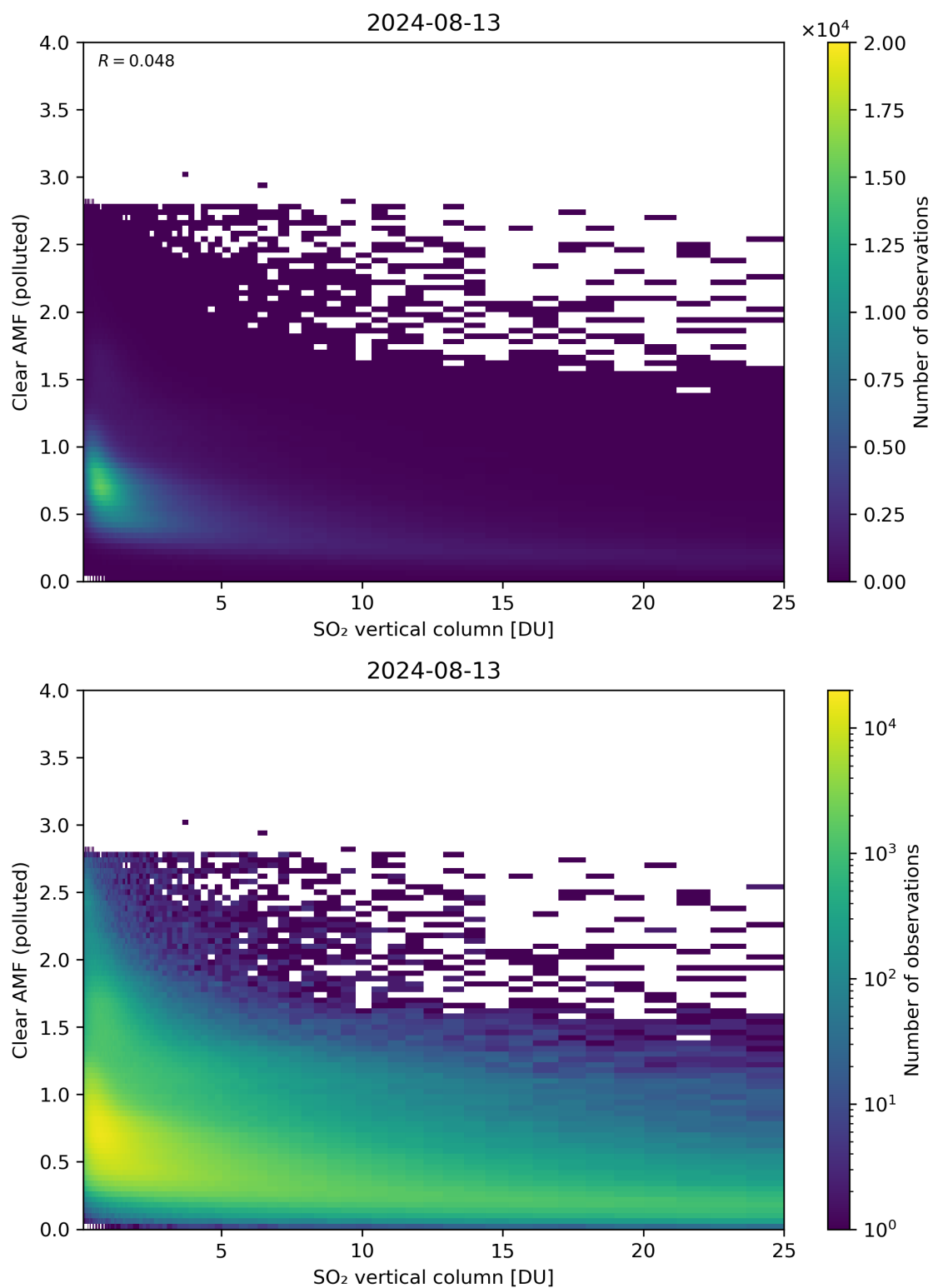
Figure 296: Scatter density plot of “SO 2 vertical column” against “Clear AMF (polluted)” for 2024-08-12 to 2024-08-14.
