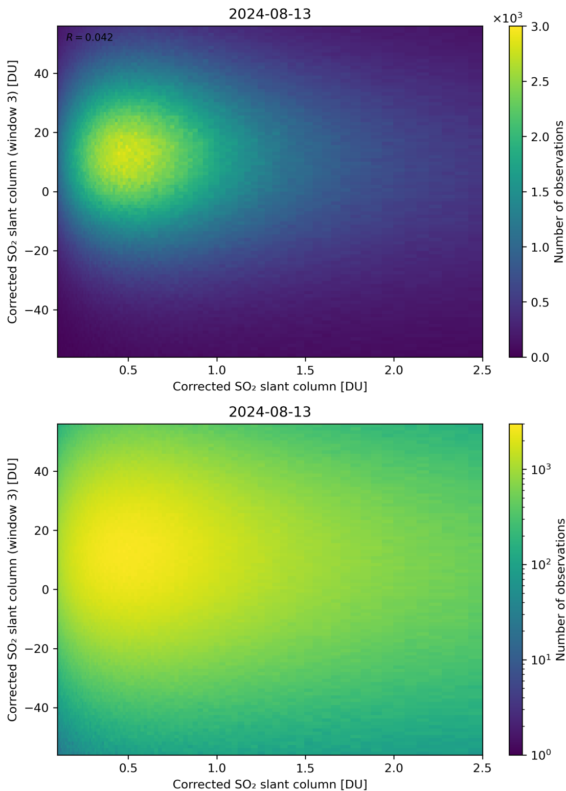
Figure 186: Scatter density plot of “Corrected SO 2 slant column” against “Corrected SO 2 slant column (window 3)” for 2024-08-12 to 2024-08-14.
