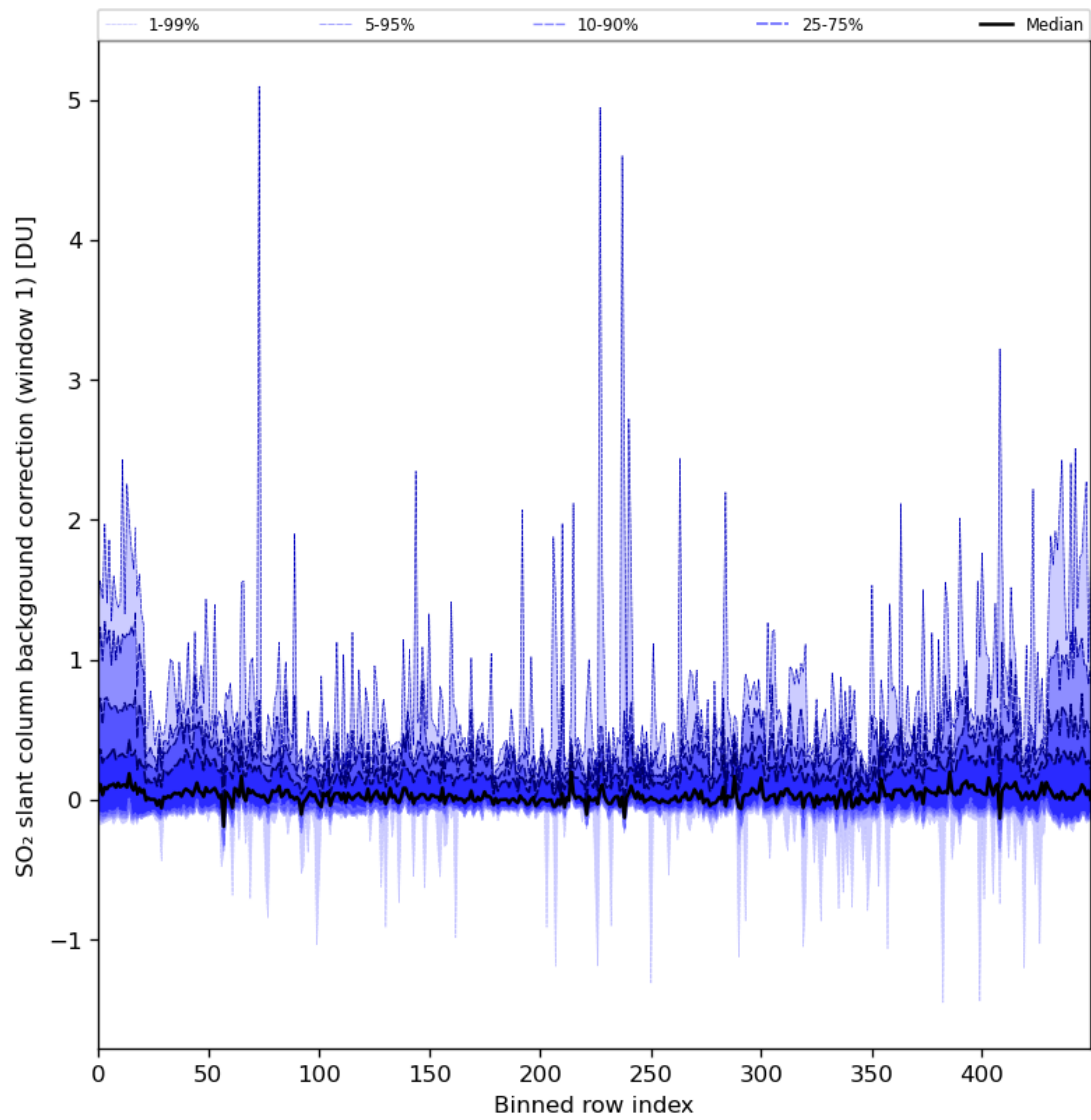
Figure 82: Along track statistics of “SO 2 slant column background correction (window 1)” for 2024-08-12 to 2024-08-14
