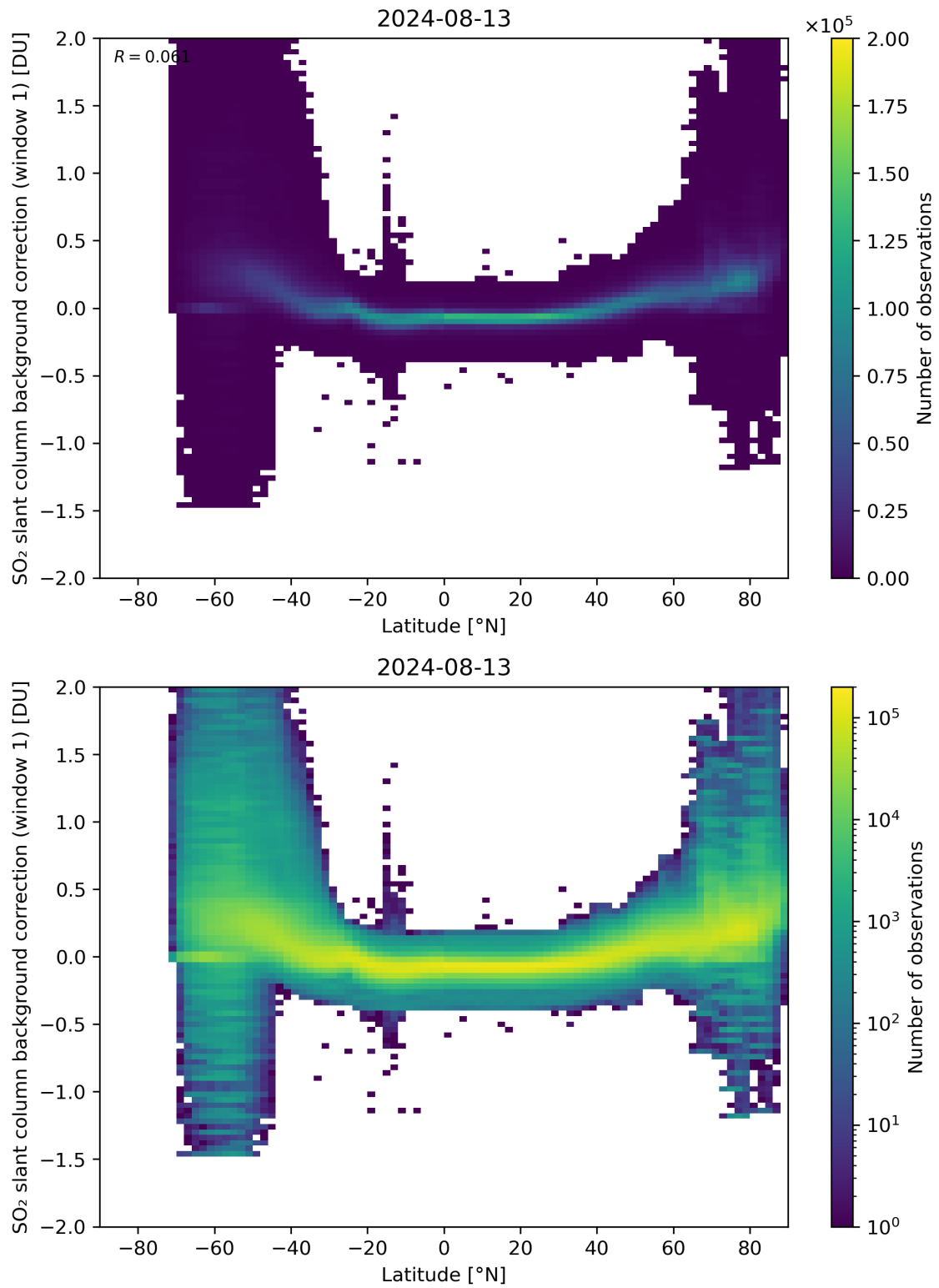
Figure 139: Scatter density plot of “Latitude” against “SO 2 slant column background correction (window 1)” for 2024-08-12 to 2024-08-14.
