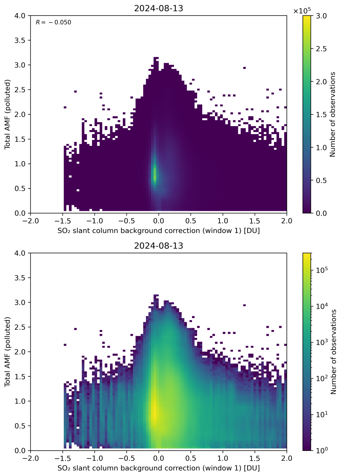
Figure 109: Scatter density plot of “SO 2 slant column background correction (window 1)” against “Total AMF (polluted)” for 2024-08-12 to 2024-08-14.
