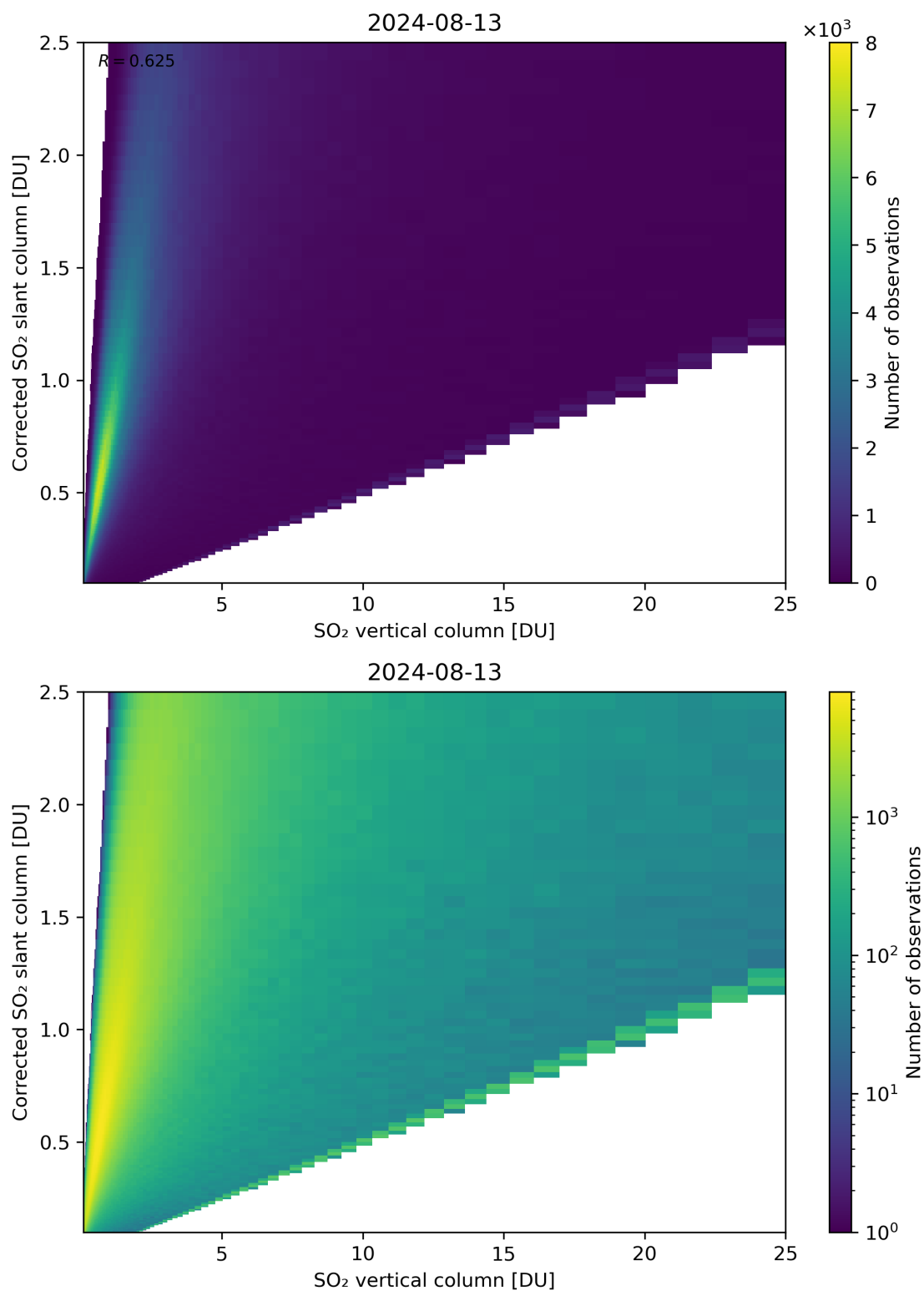
Figure 297: Scatter density plot of “SO 2 vertical column” against “Corrected SO 2 slant column” for 2024-08-12 to 2024-08-14.
