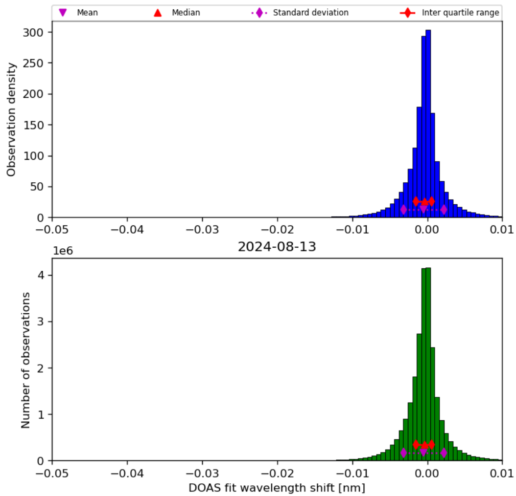
Figure 68: Histogram of “DOAS fit wavelength shift” for 2024-08-12 to 2024-08-14
