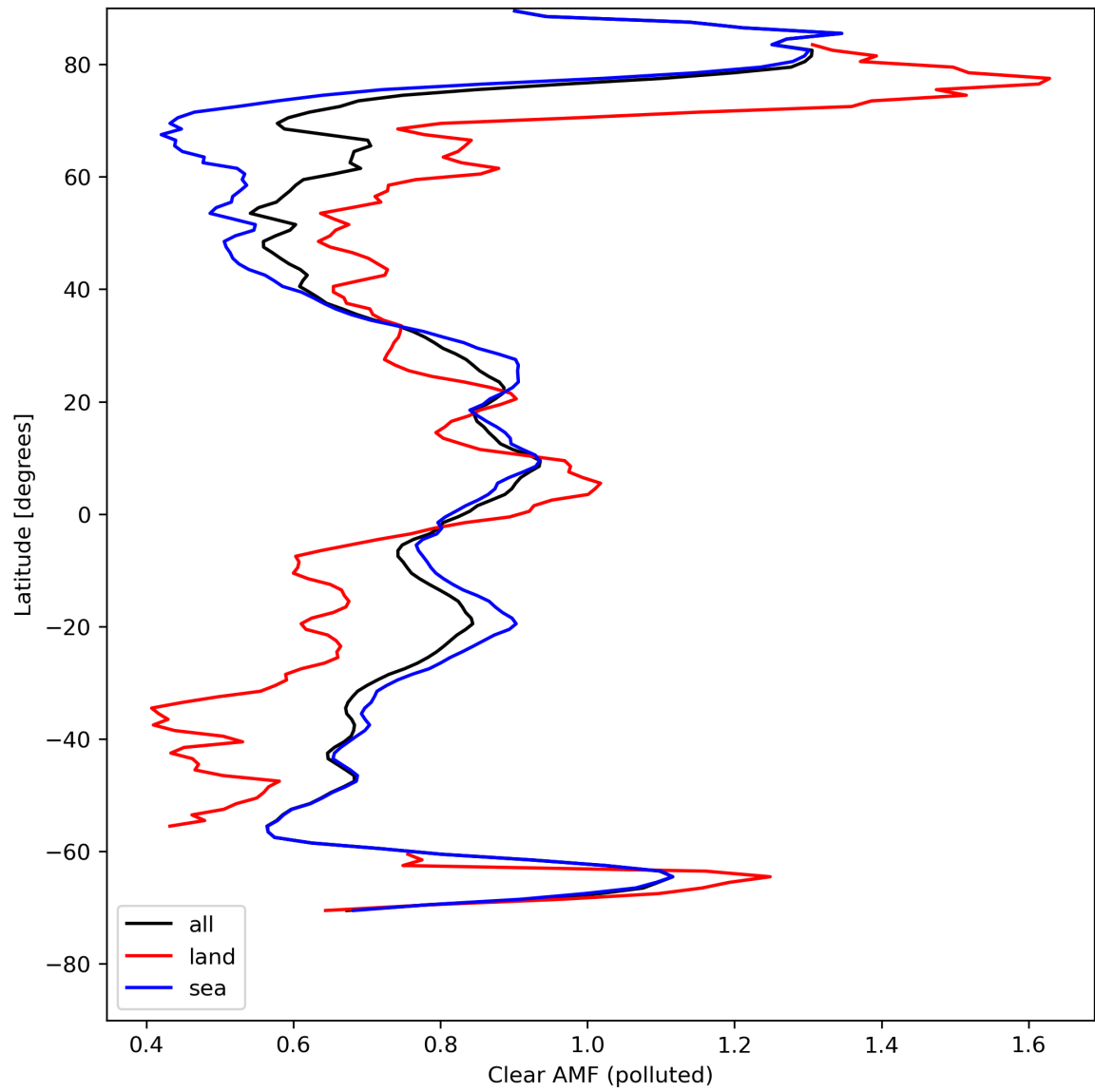
Figure 50: Zonal average of “Clear AMF (polluted)” for 2024-08-12 to 2024-08-14.
