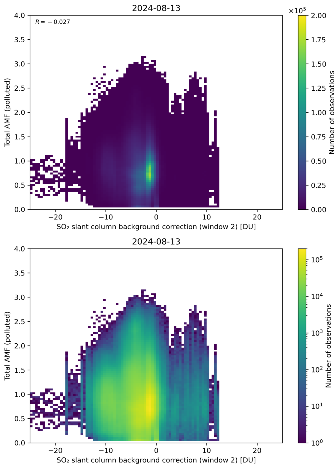
Figure 119: Scatter density plot of “SO 2 slant column background correction (window 2)” against “Total AMF (polluted)” for 2024-08-12 to 2024-08-14.
