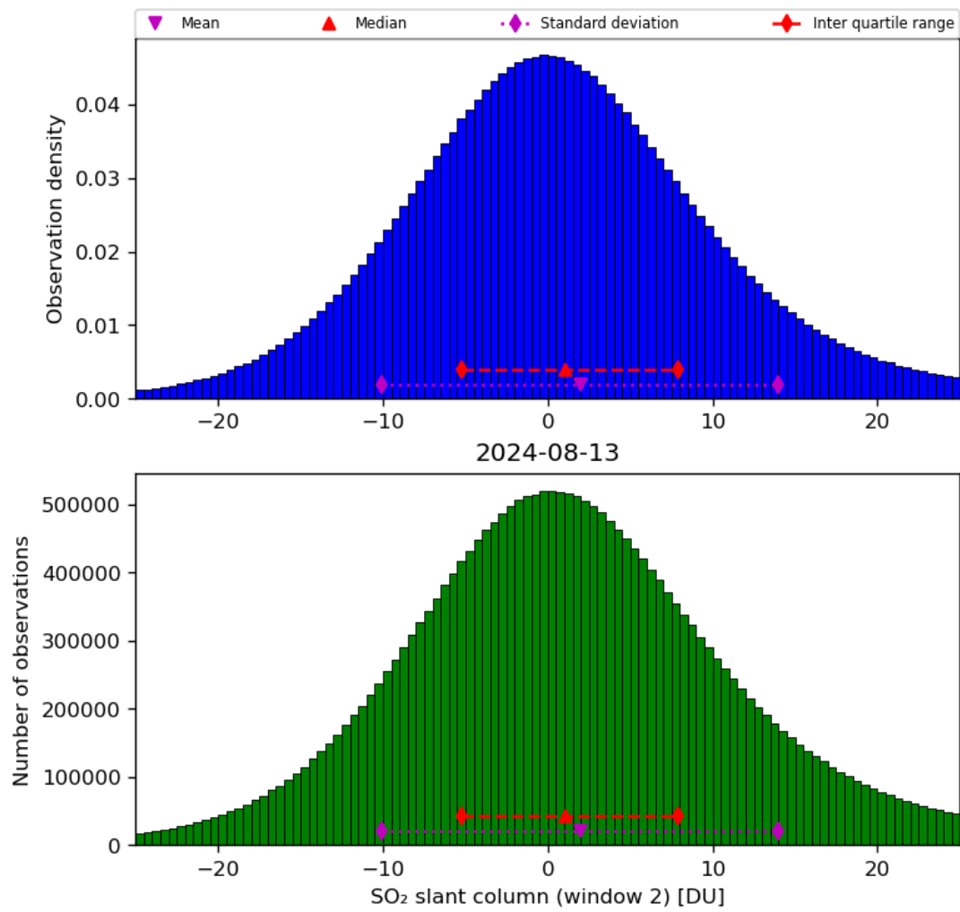
Figure 60: Histogram of “SO 2 slant column (window 2)” for 2024-08-12 to 2024-08-14
