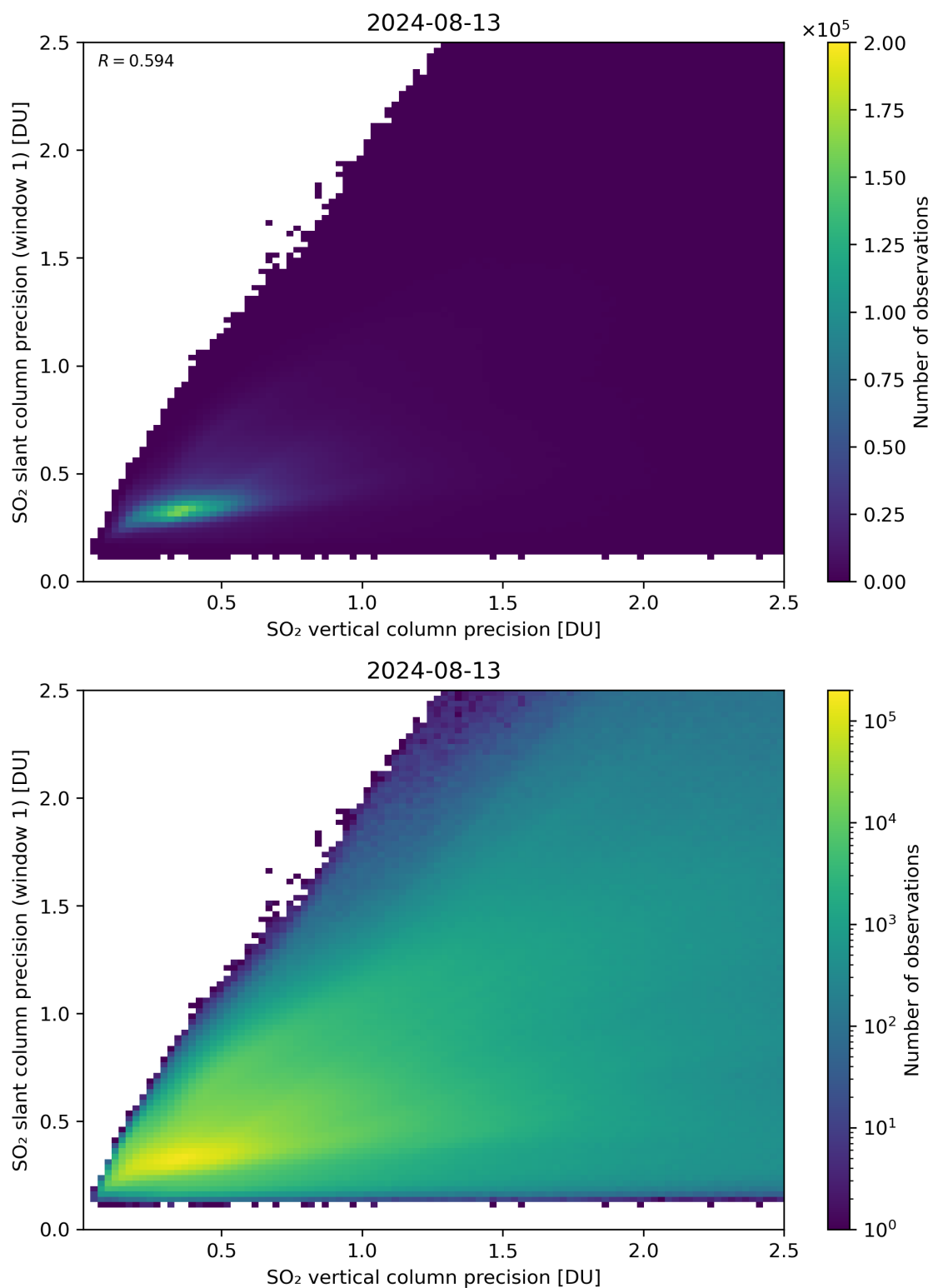
Figure 290: Scatter density plot of “SO 2 vertical column precision” against “SO 2 slant column precision (window 1)” for 2024-08-12 to 2024-08-14.
