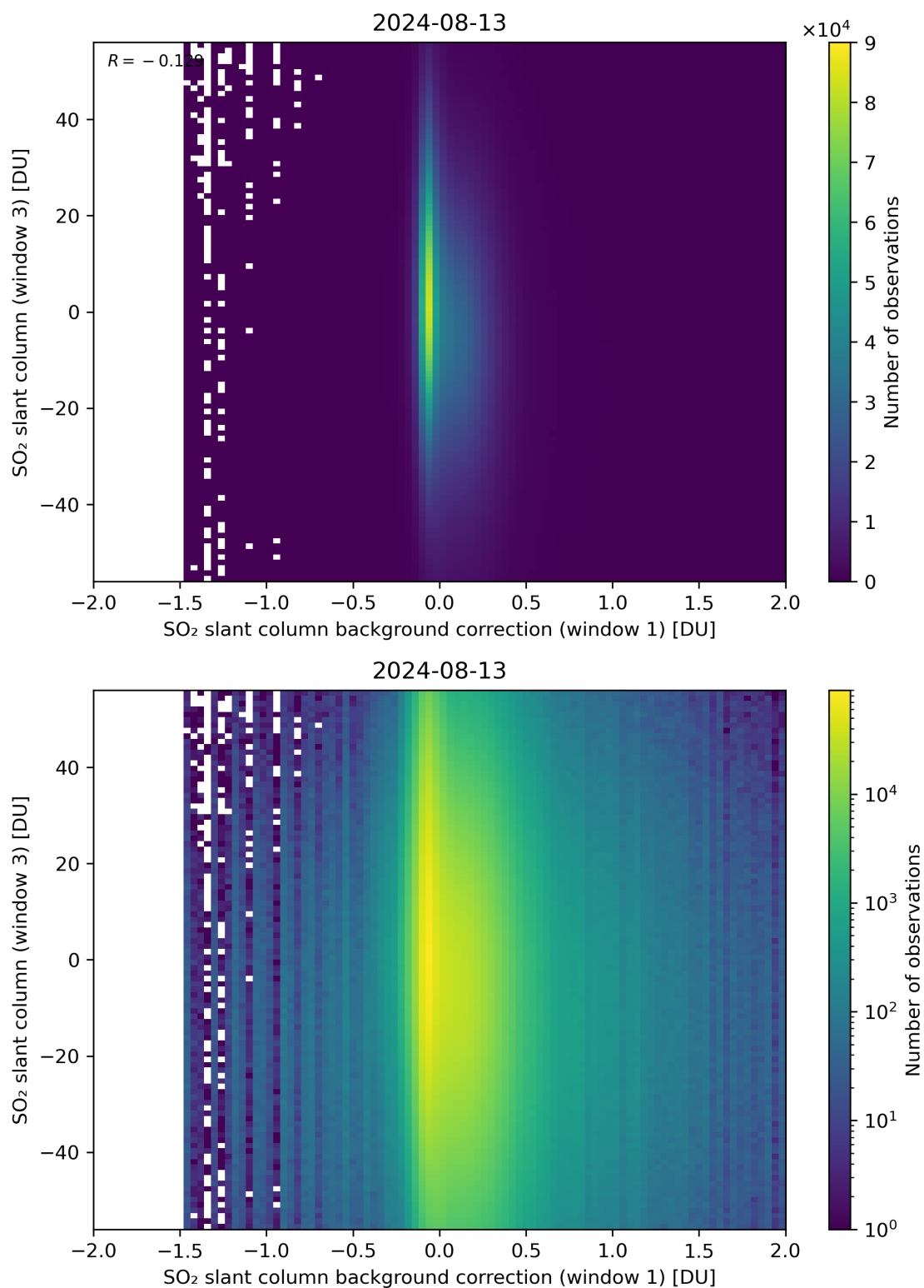
Figure 107: Scatter density plot of “SO 2 slant column background correction (window 1)” against “SO 2 slant column (window 3)” for 2024-08-12 to 2024-08-14.
