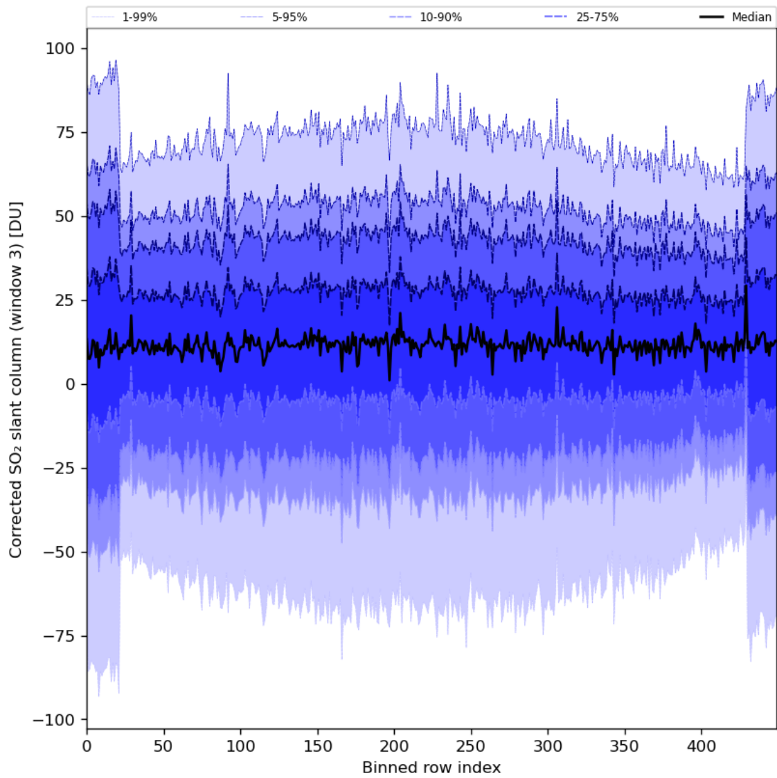
Figure 89: Along track statistics of “Corrected SO 2 slant column (window 3)” for 2024-08-12 to 2024-08-14
