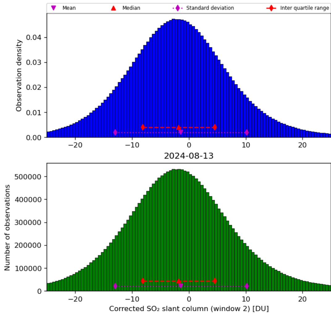
Figure 62: Histogram of “Corrected SO 2 slant column (window 2)” for 2024-08-12 to 2024-08-14
