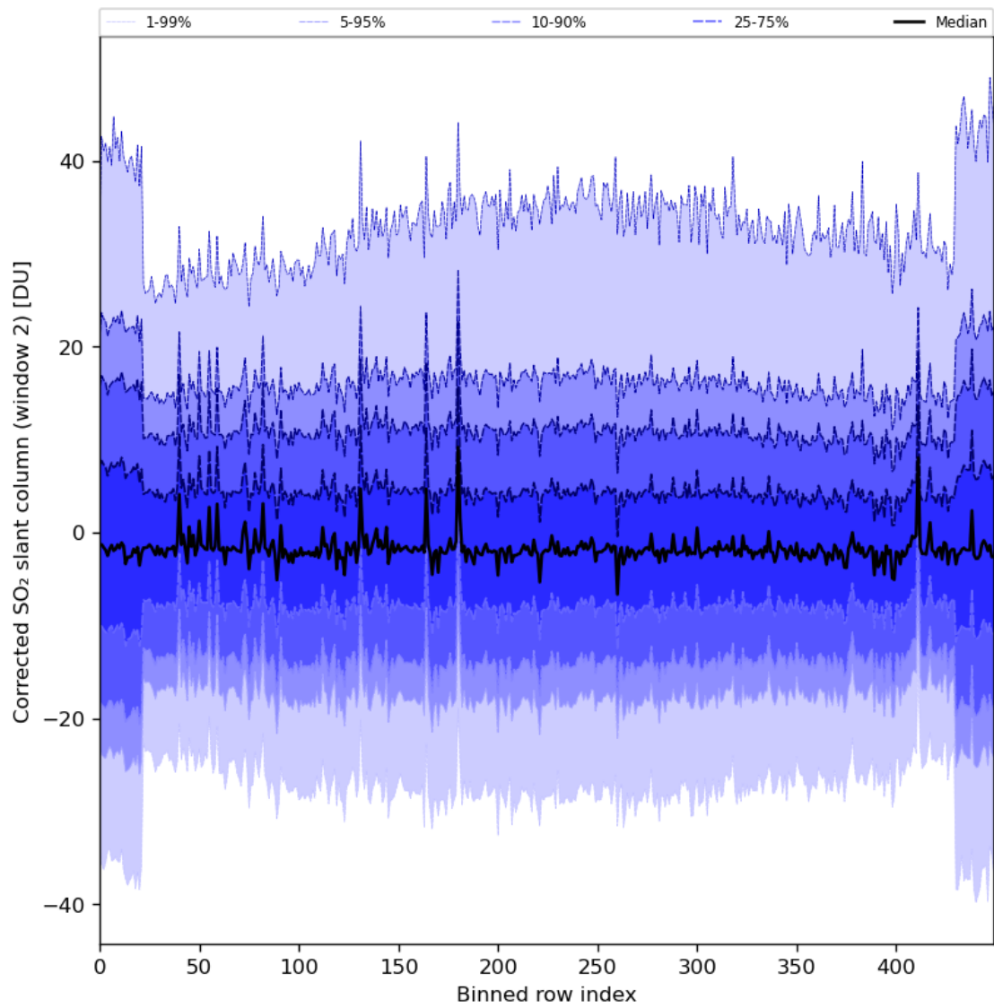
Figure 85: Along track statistics of “Corrected SO 2 slant column (window 2)” for 2024-08-12 to 2024-08-14
