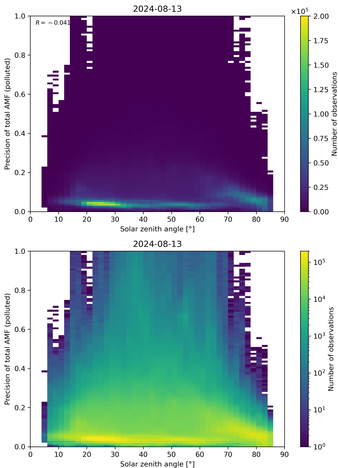
Figure 175: Scatter density plot of “Solar zenith angle” against “Precision of total AMF (polluted)” for 2024-08-12 to 2024-08-14.
