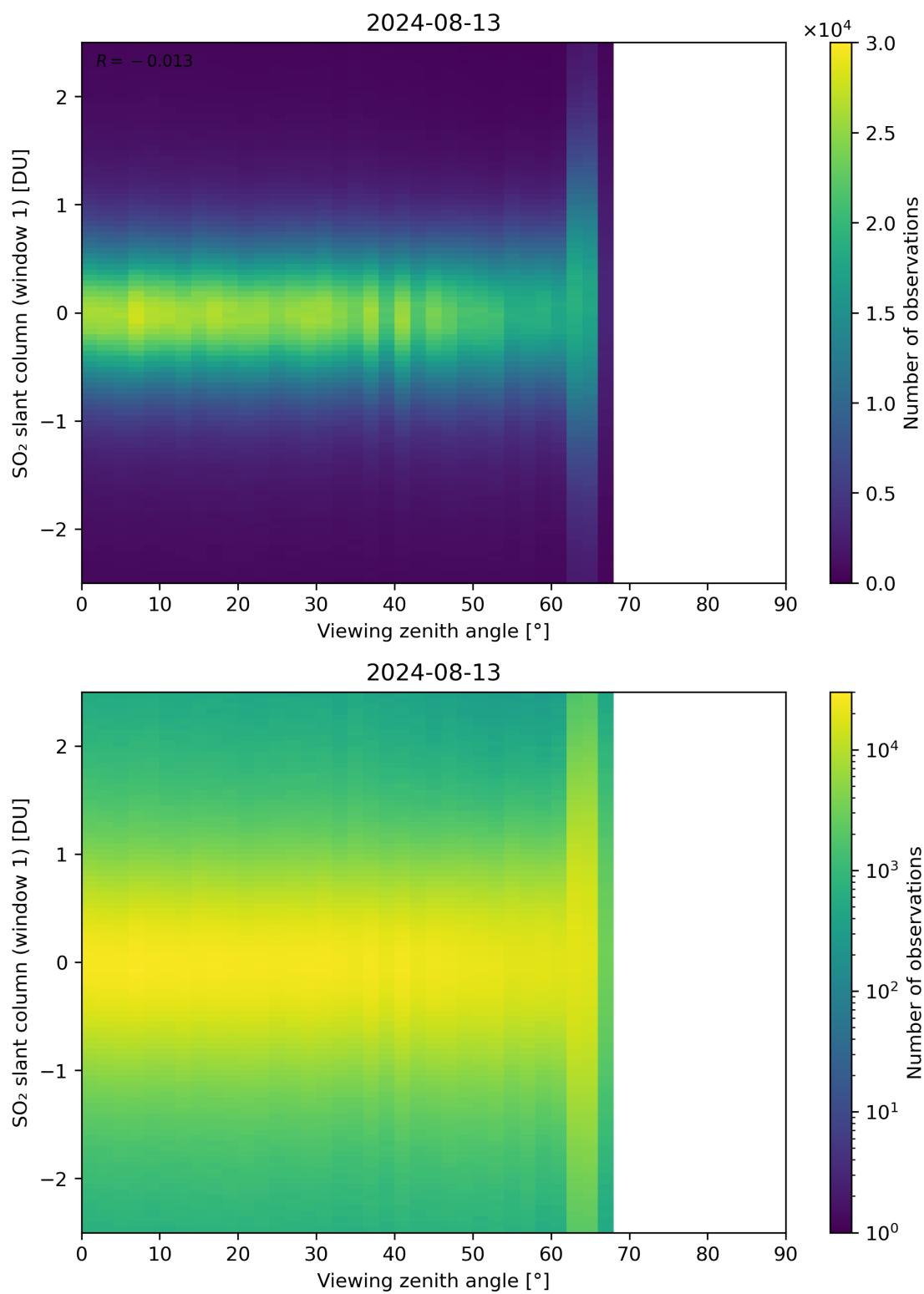
Figure 320: Scatter density plot of “Viewing zenith angle” against “SO 2 slant column (window 1)” for 2024-08-12 to 2024-08-14.
