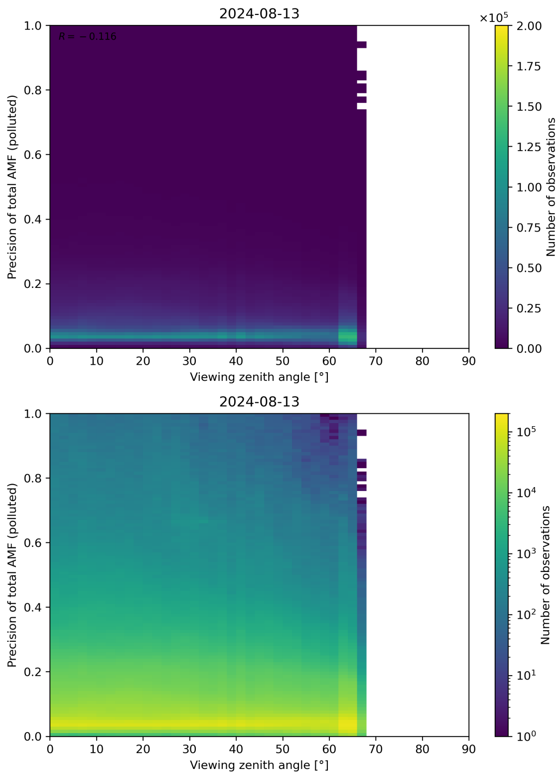
Figure 326: Scatter density plot of “Viewing zenith angle” against “Precision of total AMF (polluted)” for 2024-08-12 to 2024-08-14.
