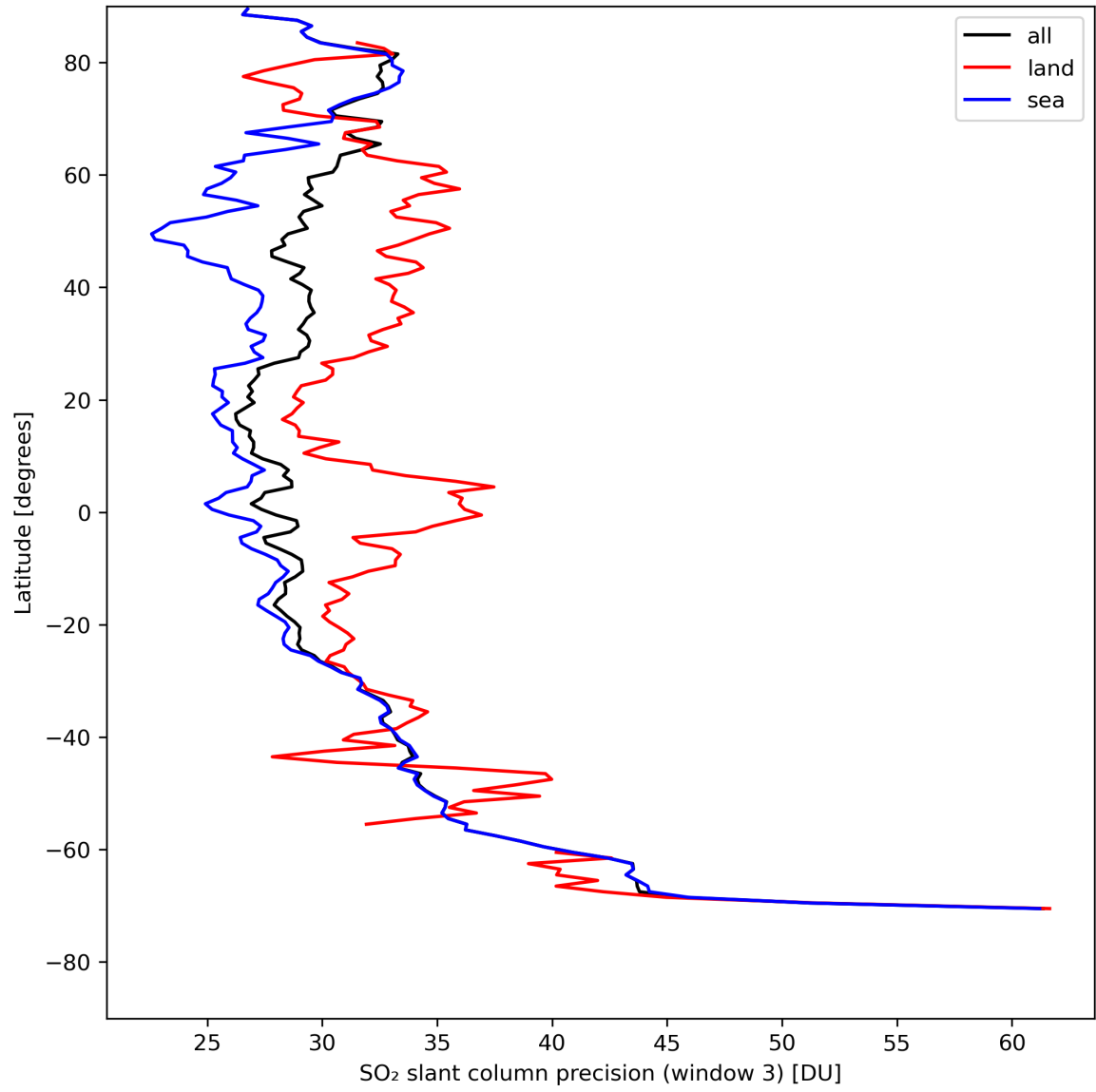
Figure 42: Zonal average of “SO 2 slant column precision (window 3)” for 2024-08-12 to 2024-08-14.
