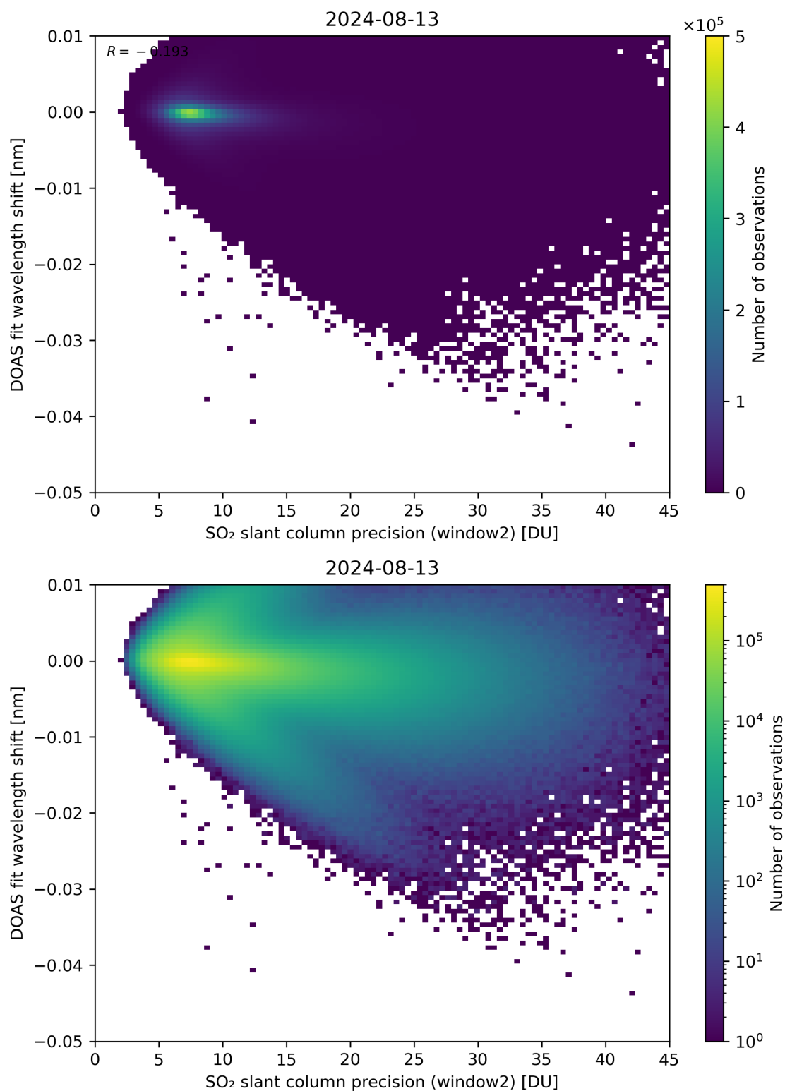
Figure 243: Scatter density plot of “SO 2 slant column precision (window2)” against “DOAS fit wavelength shift” for 2024-08-12 to 2024-08-14.
