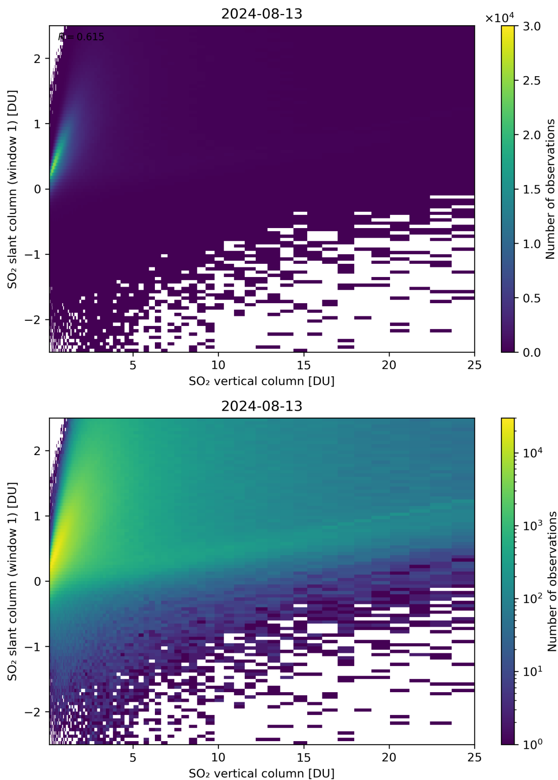
Figure 300: Scatter density plot of “SO 2 vertical column” against “SO 2 slant column (window 1)” for 2024-08-12 to 2024-08-14.
