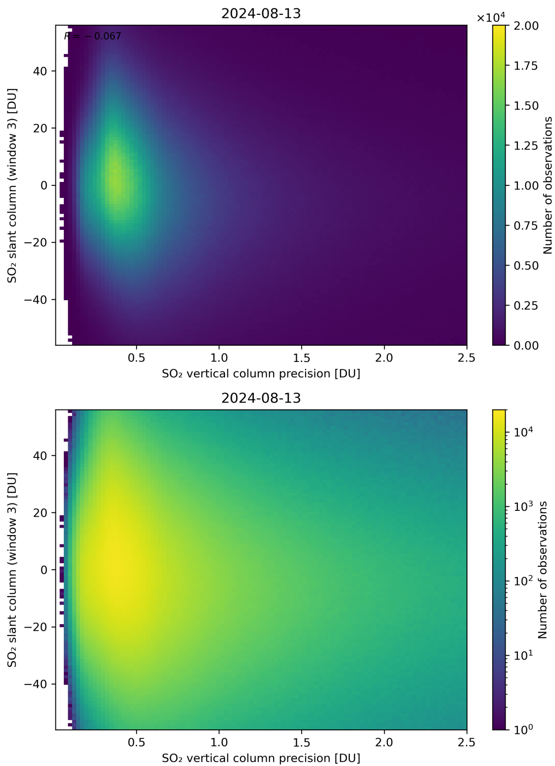
Figure 292: Scatter density plot of “SO 2 vertical column precision” against “SO 2 slant column (window 3)” for 2024-08-12 to 2024-08-14.
