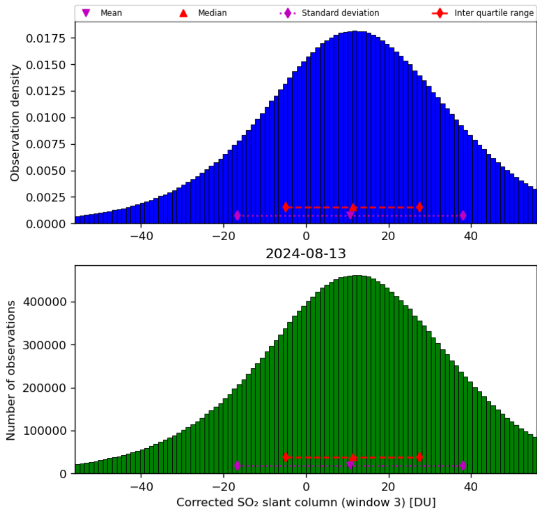
Figure 66: Histogram of “Corrected SO 2 slant column (window 3)” for 2024-08-12 to 2024-08-14
