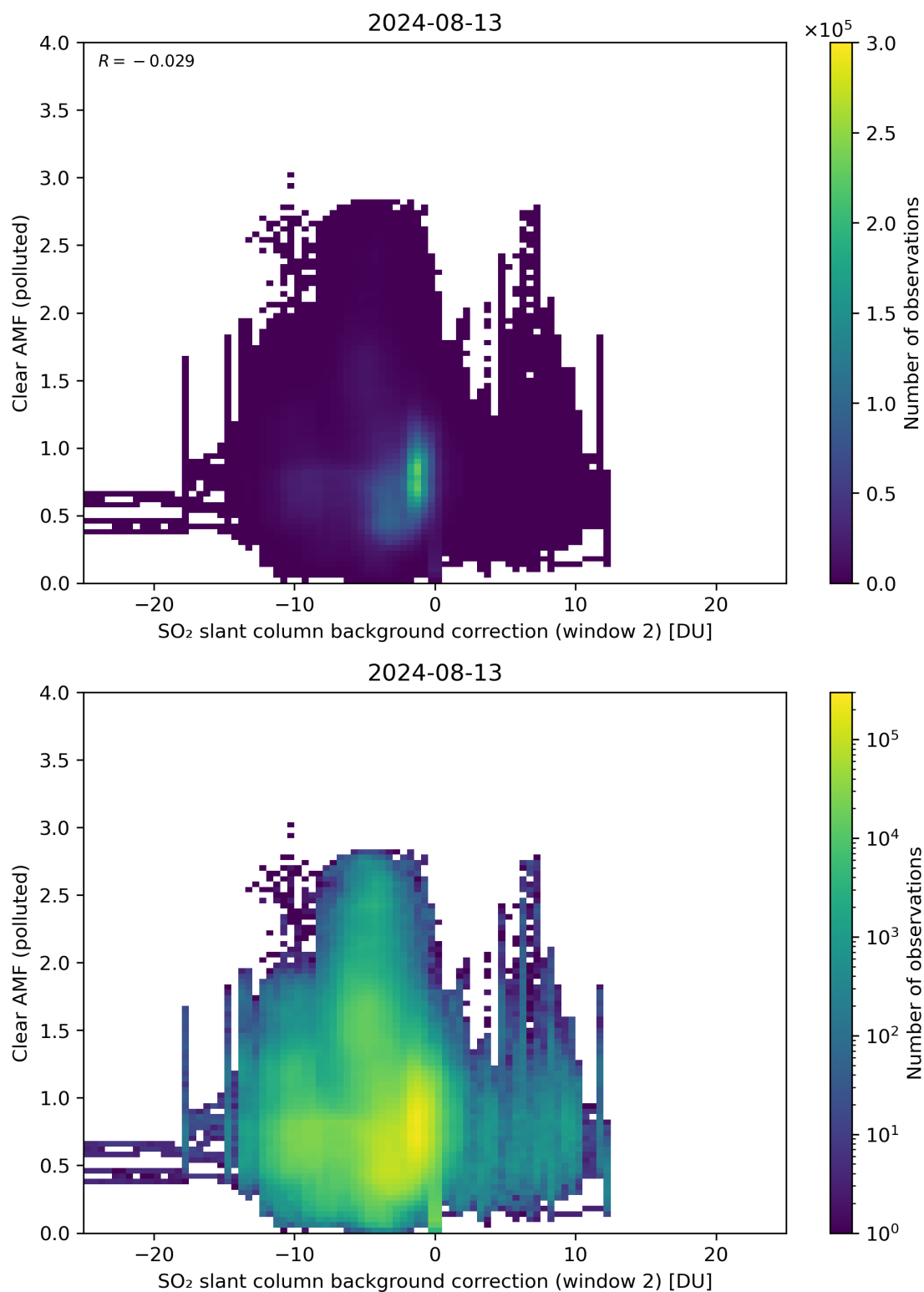
Figure 115: Scatter density plot of “SO 2 slant column background correction (window 2)” against “Clear AMF (polluted)” for 2024-08-12 to 2024-08-14.
