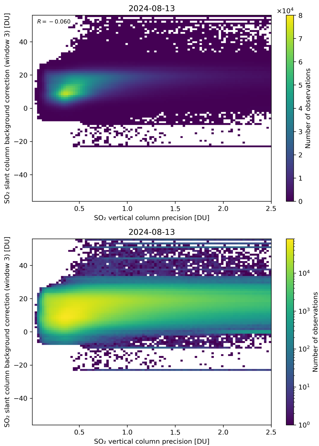
Figure 281: Scatter density plot of “SO 2 vertical column precision” against “SO 2 slant column background correction (window 3)” for 2024-08-12 to 2024-08-14.
