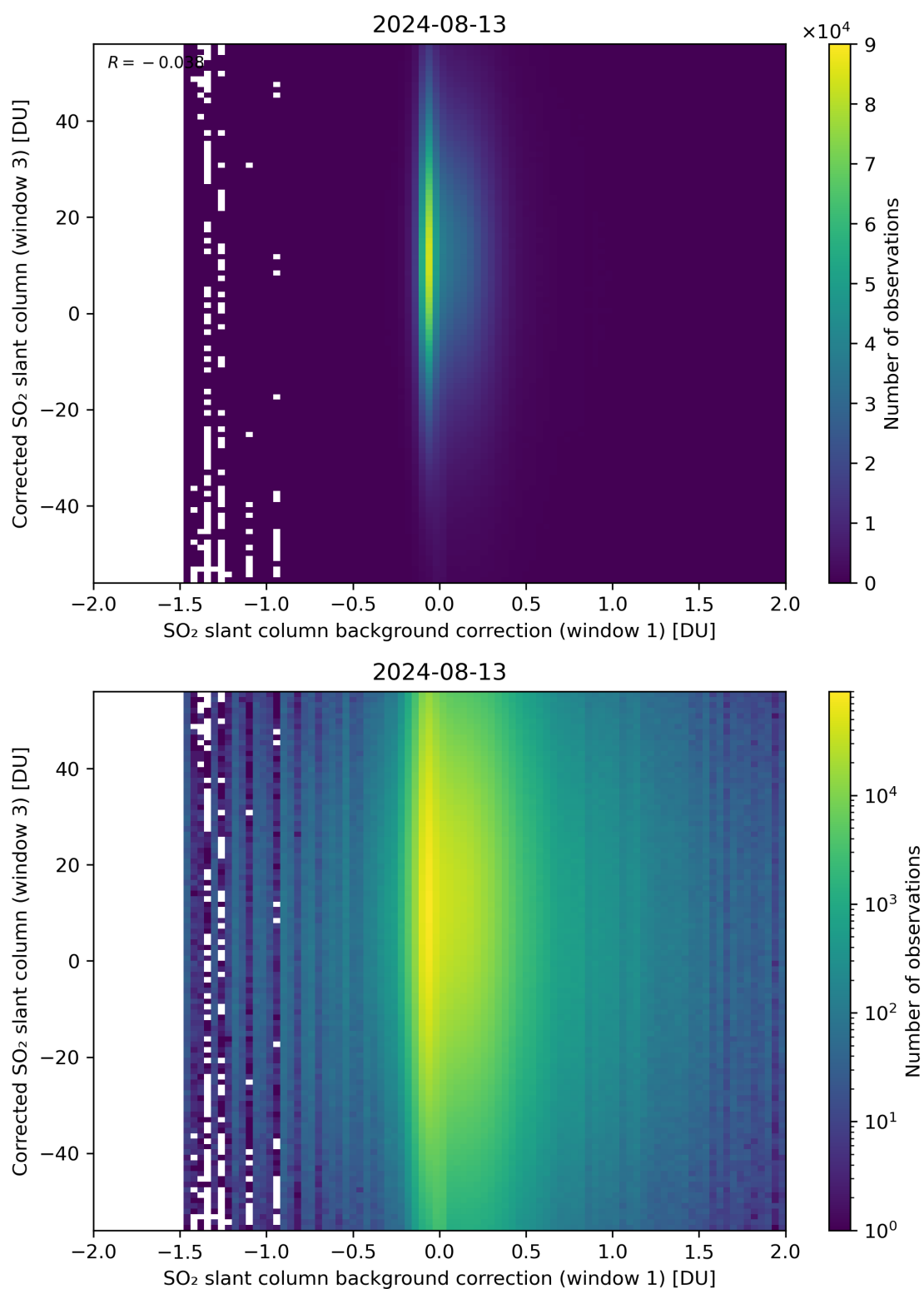
Figure 105: Scatter density plot of “SO 2 slant column background correction (window 1)” against “Corrected SO 2 slant column (window 3)” for 2024-08-12 to 2024-08-14.
