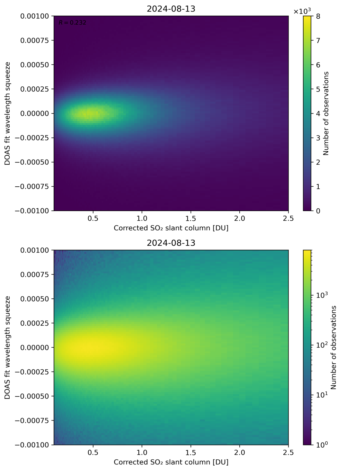
Figure 182: Scatter density plot of “Corrected SO 2 slant column” against “DOAS fit wavelength squeeze” for 2024-08-12 to 2024-08-14.
