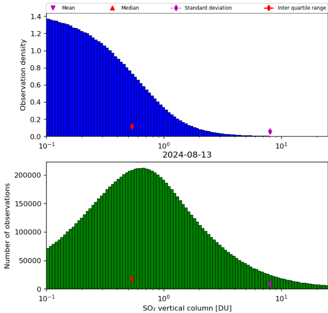
Figure 53: Histogram of “SO 2 vertical column” for 2024-08-12 to 2024-08-14
