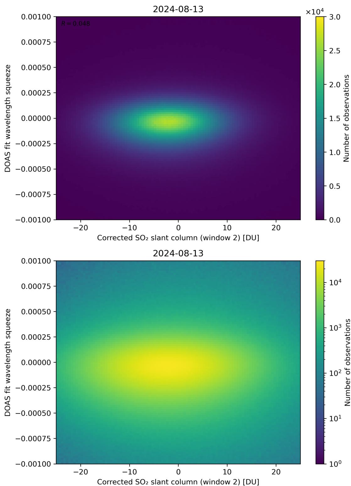
Figure 197: Scatter density plot of “Corrected SO 2 slant column (window 2)” against “DOAS fit wavelength squeeze” for 2024-08-12 to 2024-08-14.
