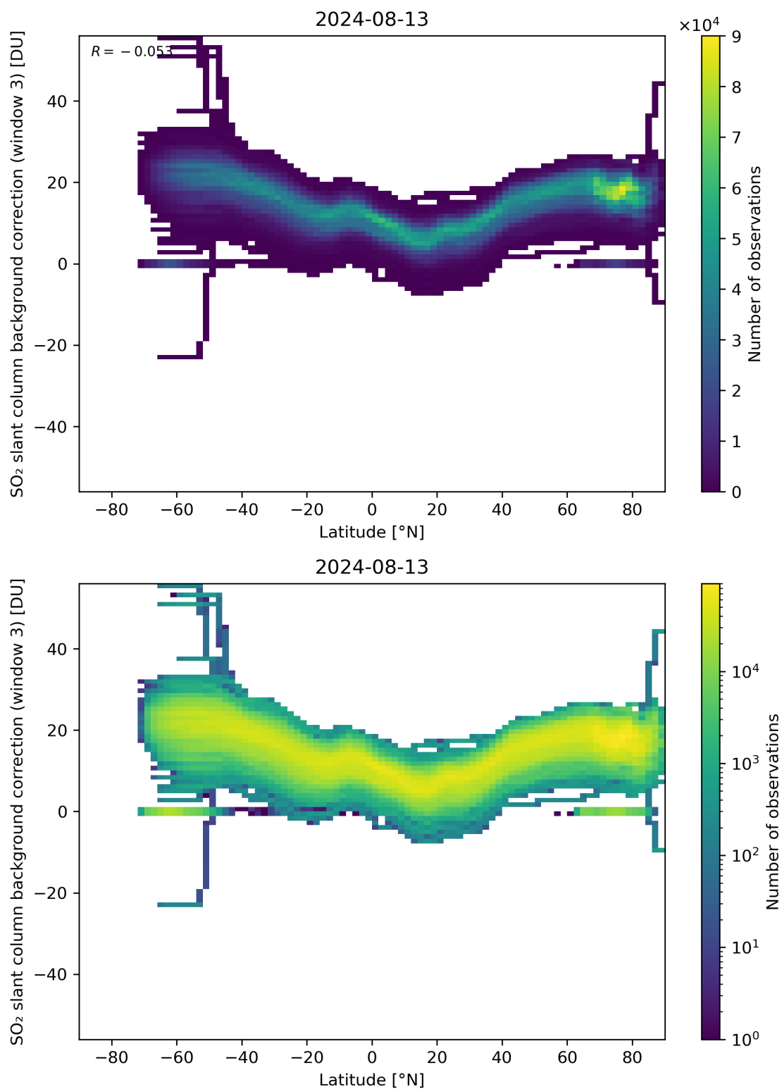
Figure 141: Scatter density plot of “Latitude” against “SO 2 slant column background correction (window 3)” for 2024-08-12 to 2024-08-14.
