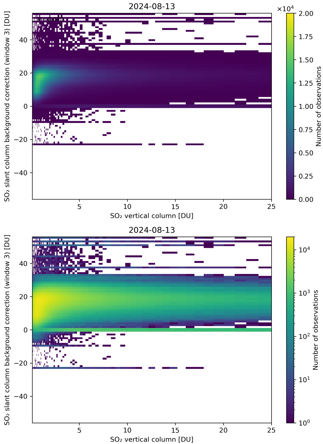
Figure 275: Scatter density plot of “SO 2 vertical column” against “SO 2 slant column background correction (window 3)” for 2024-08-12 to 2024-08-14.
