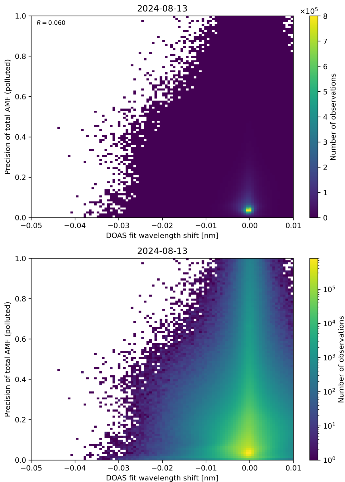
Figure 131: Scatter density plot of “DOAS fit wavelength shift” against “Precision of total AMF (polluted)” for 2024-08-12 to 2024-08-14.
