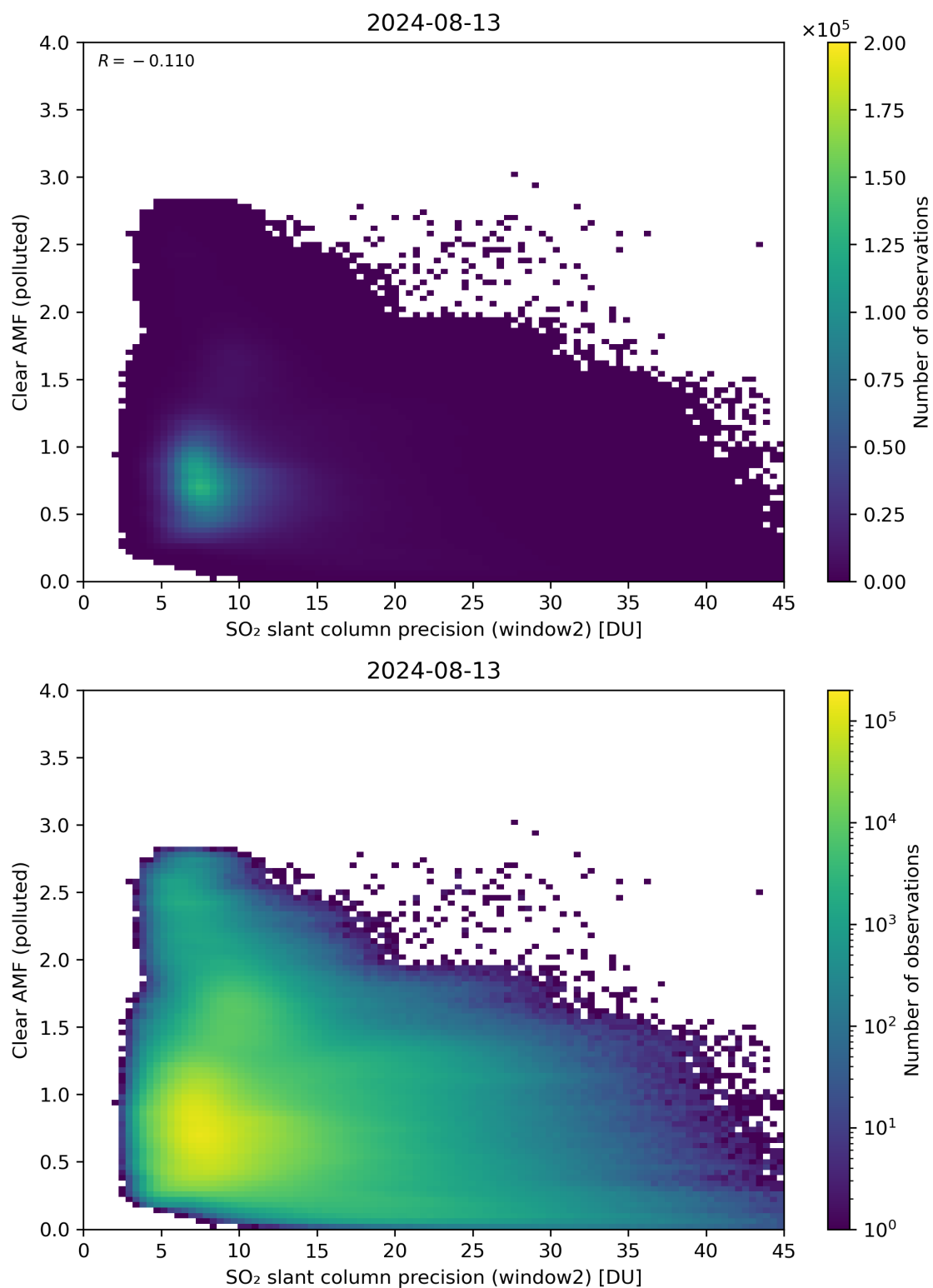
Figure 246: Scatter density plot of “SO 2 slant column precision (window2)” against “Clear AMF (polluted)” for 2024-08-12 to 2024-08-14.
