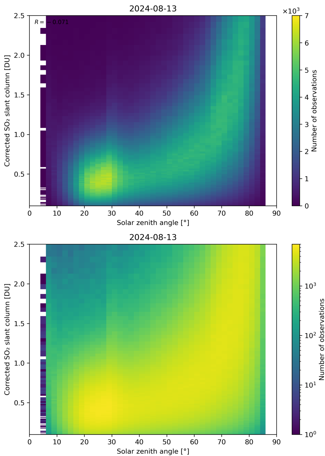
Figure 166: Scatter density plot of “Solar zenith angle” against “Corrected SO 2 slant column” for 2024-08-12 to 2024-08-14.
