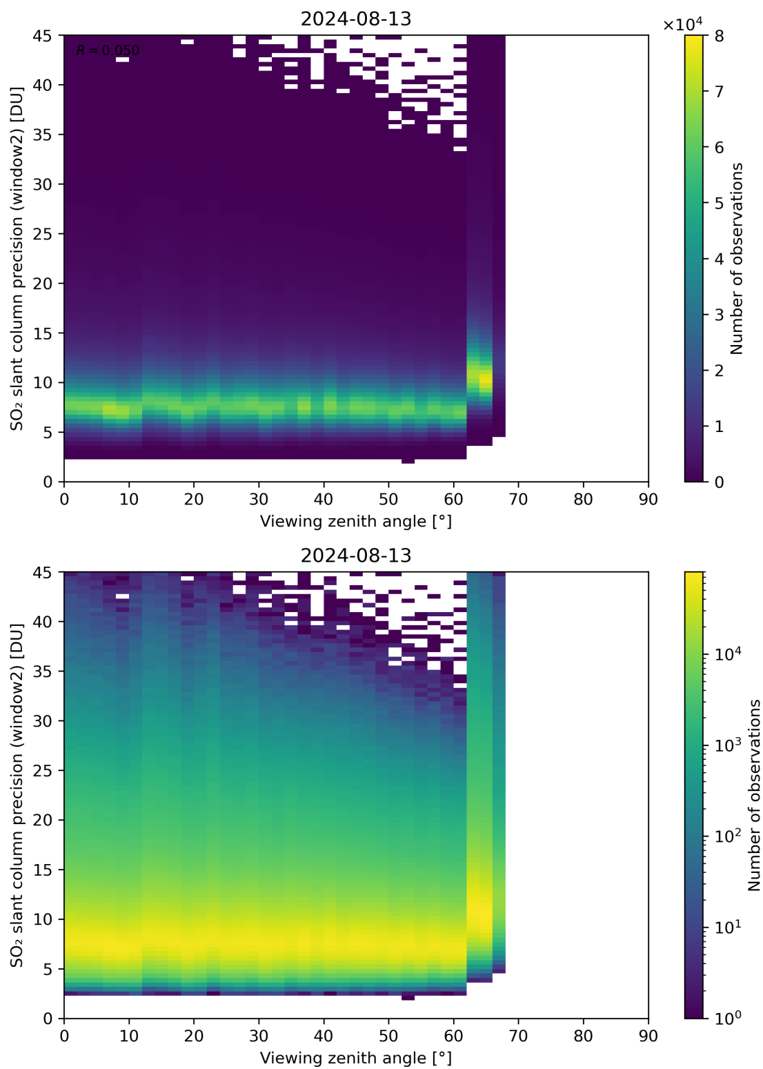
Figure 322: Scatter density plot of “Viewing zenith angle” against “SO 2 slant column precision (window2)” for 2024-08-12 to 2024-08-14.
