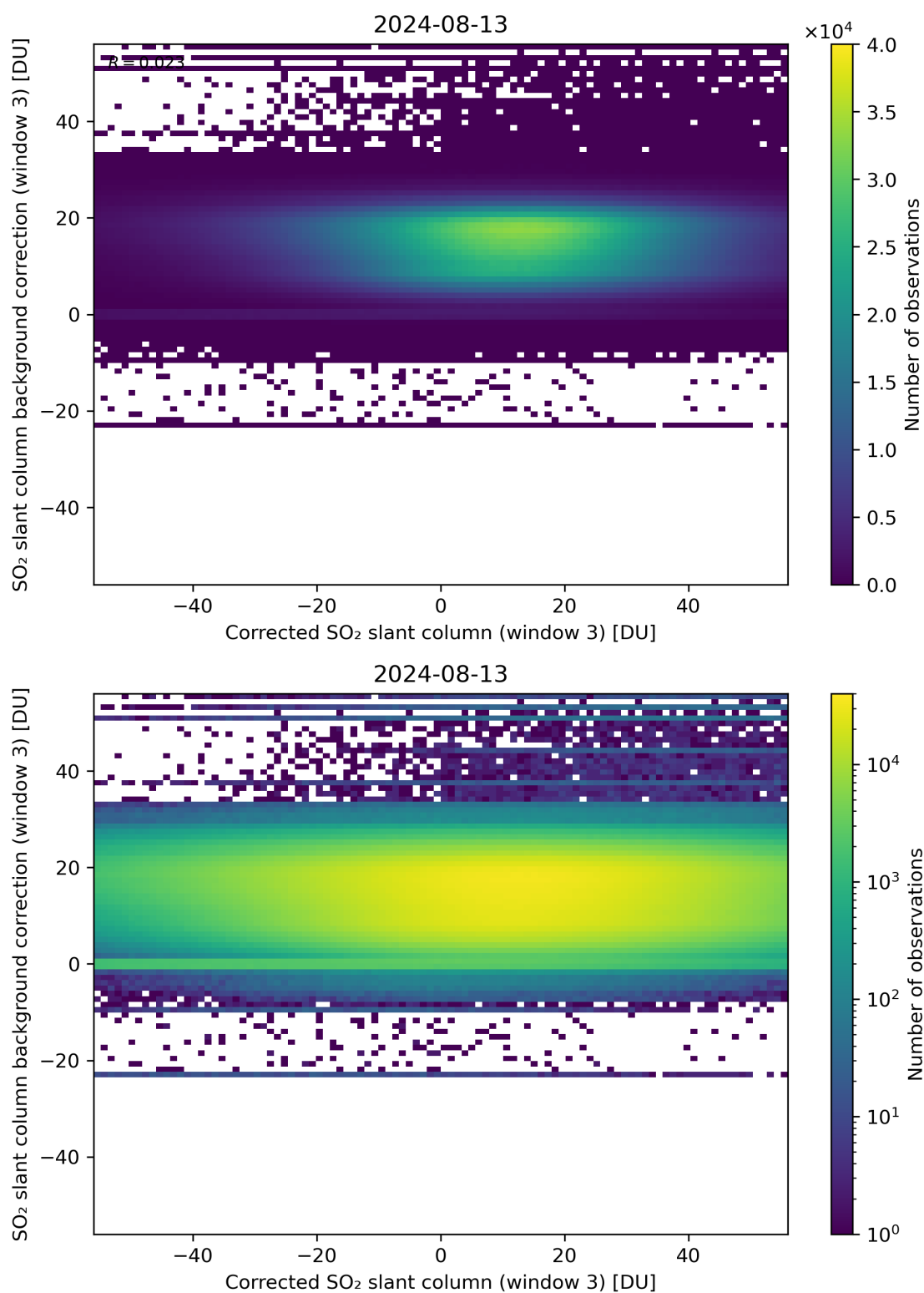
Figure 205: Scatter density plot of “Corrected SO 2 slant column (window 3)” against “SO 2 slant column background correction (window 3)” for 2024-08-12 to 2024-08-14.
