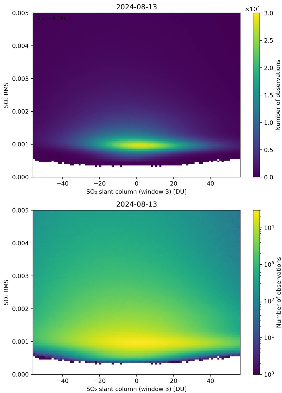
Figure 256: Scatter density plot of “SO 2 slant column (window 3)” against “SO 2 RMS” for 2024-08-12 to 2024-08-14.
