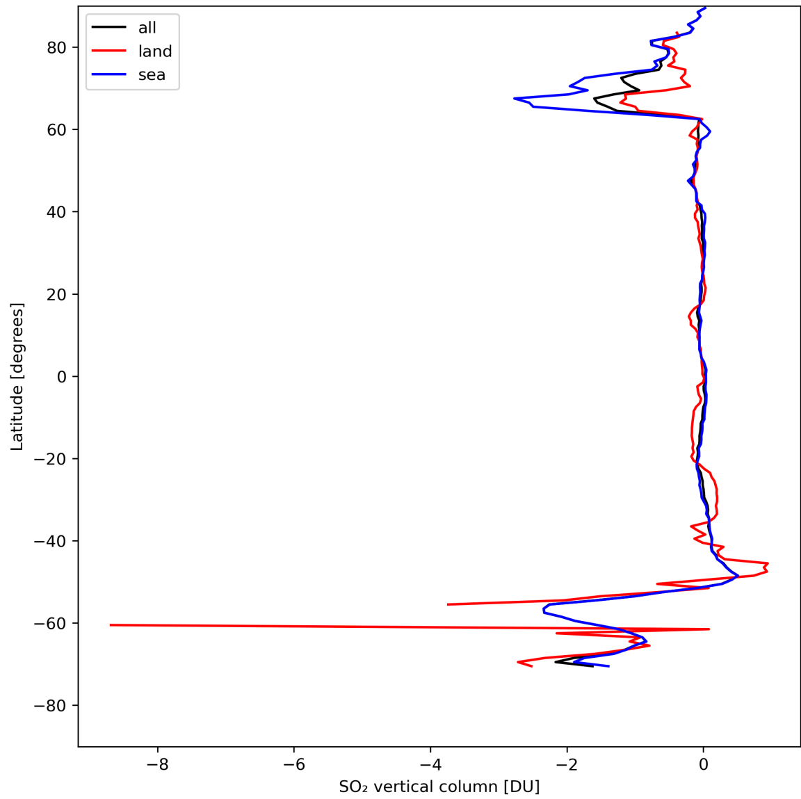
Figure 30: Zonal average of “SO 2 vertical column” for 2024-08-12 to 2024-08-14.
