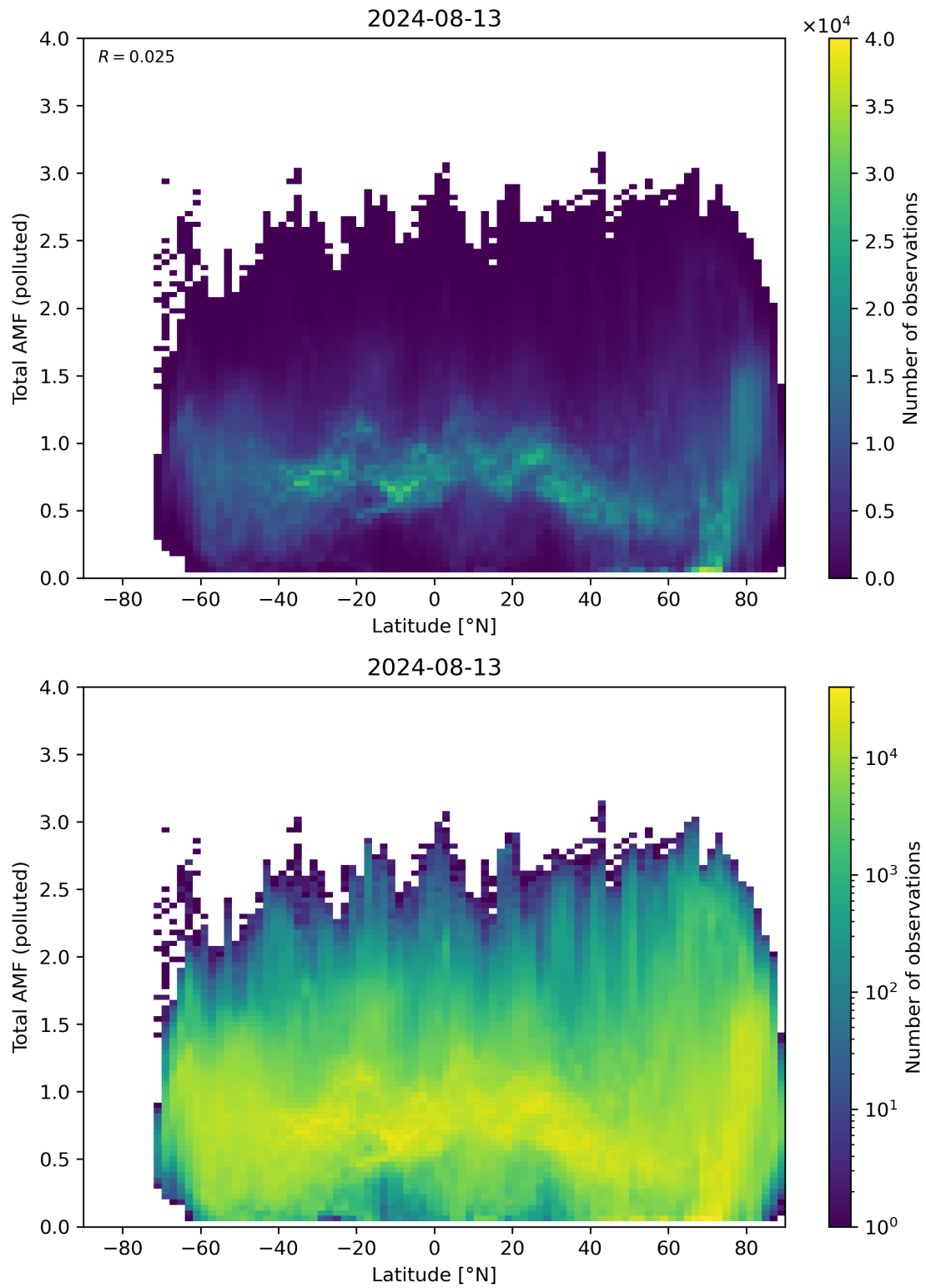
Figure 154: Scatter density plot of “Latitude” against “Total AMF (polluted)” for 2024-08-12 to 2024-08-14.
