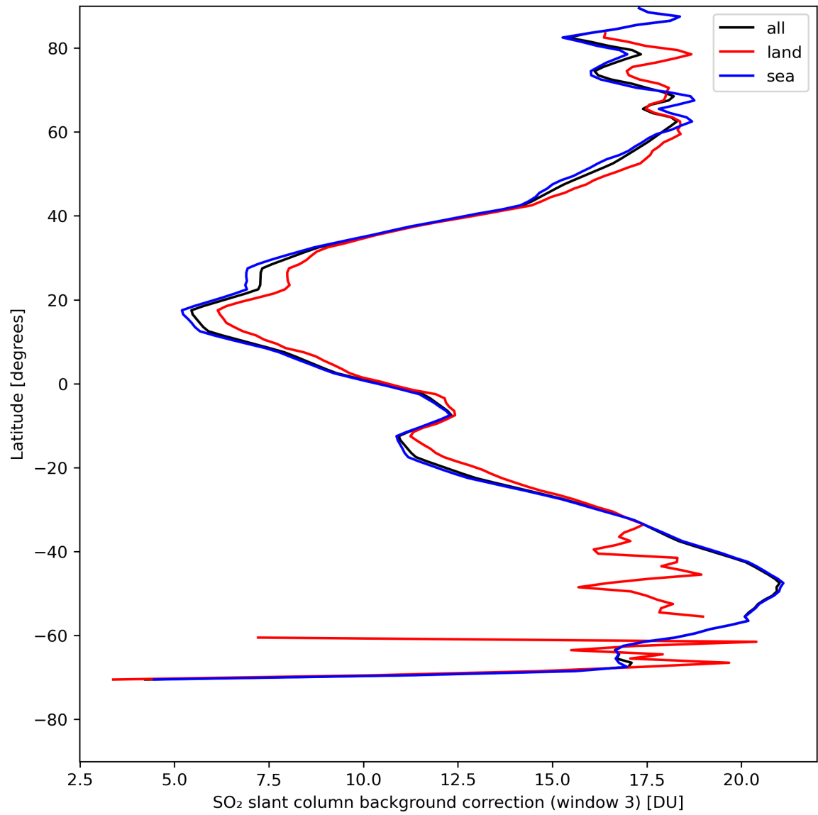
Figure 44: Zonal average of “SO 2 slant column background correction (window 3)” for 2024-08-12 to 2024-08-14.
