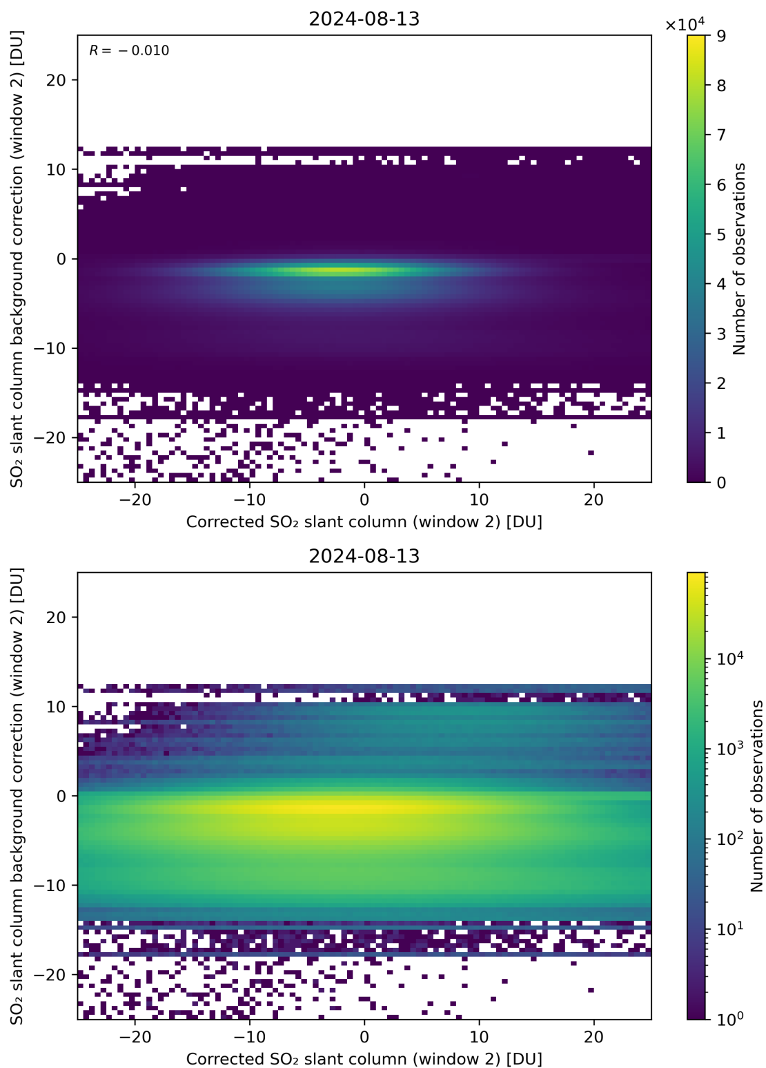
Figure 194: Scatter density plot of “Corrected SO 2 slant column (window 2)” against “SO 2 slant column background correction (window 2)” for 2024-08-12 to 2024-08-14.
