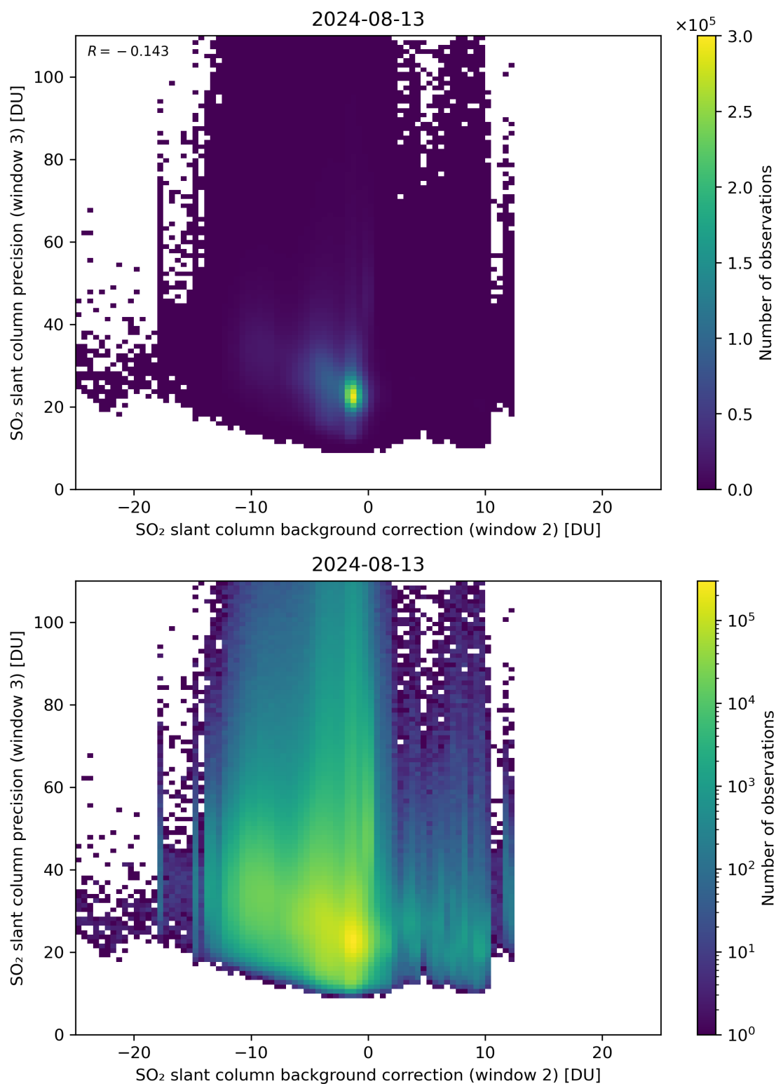
Figure 118: Scatter density plot of “SO 2 slant column background correction (window 2)” against “SO 2 slant column precision (window 3)” for 2024-08-12 to 2024-08-14.
