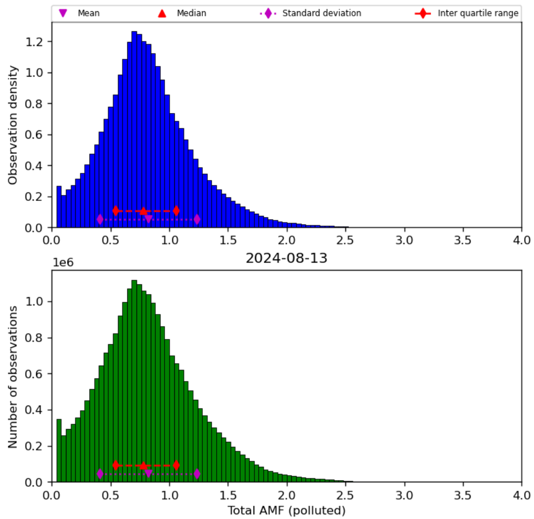
Figure 71: Histogram of “Total AMF (polluted)” for 2024-08-12 to 2024-08-14
