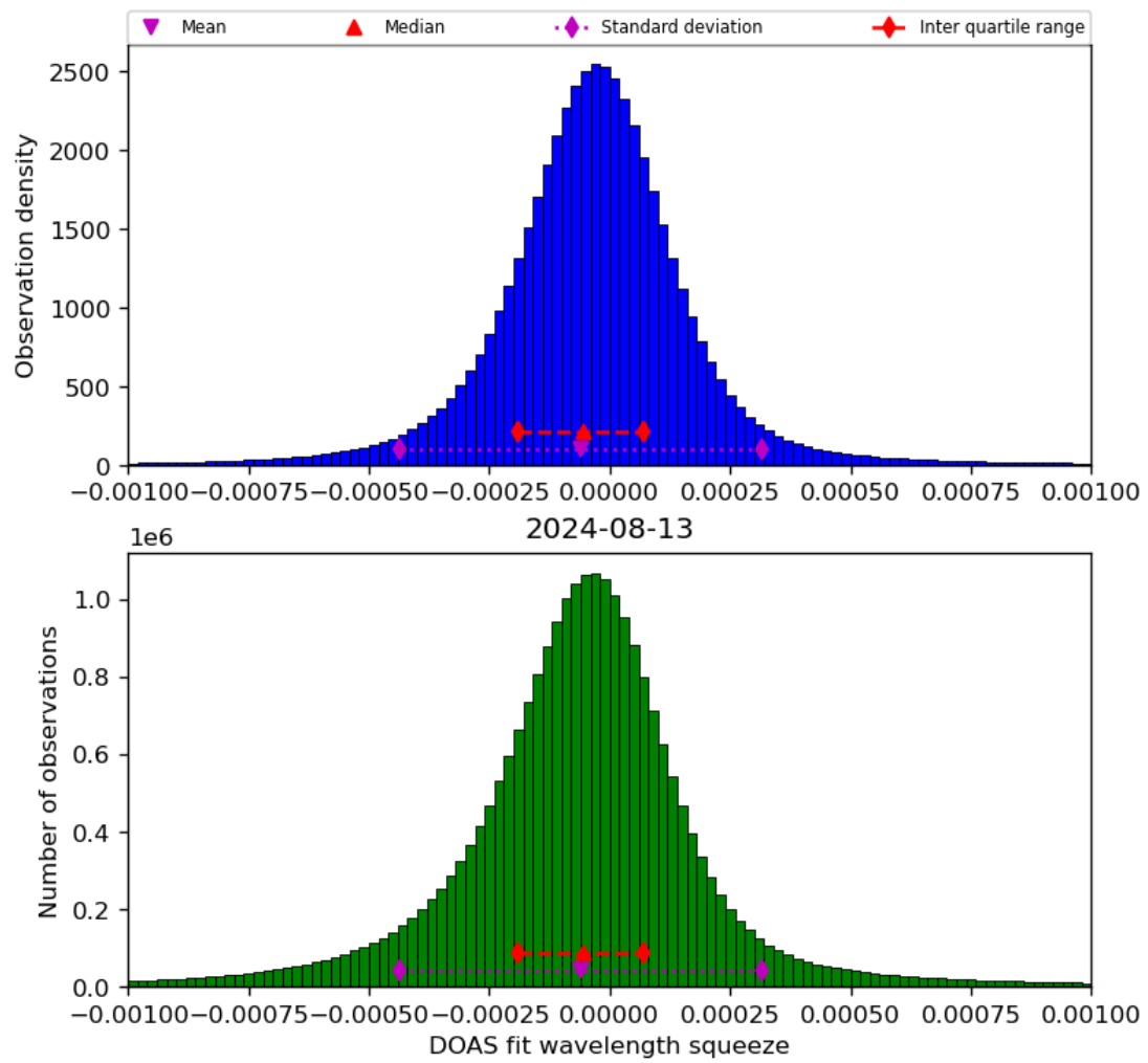
Figure 69: Histogram of “DOAS fit wavelength squeeze” for 2024-08-12 to 2024-08-14
