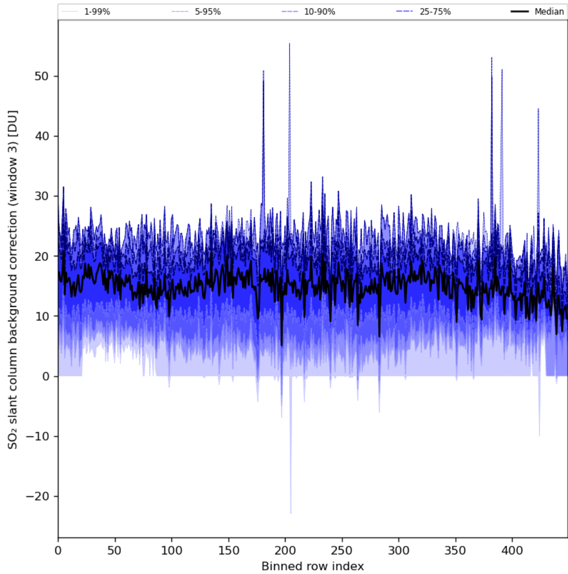
Figure 90: Along track statistics of “SO 2 slant column background correction (window 3)” for 2024-08-12 to 2024-08-14
