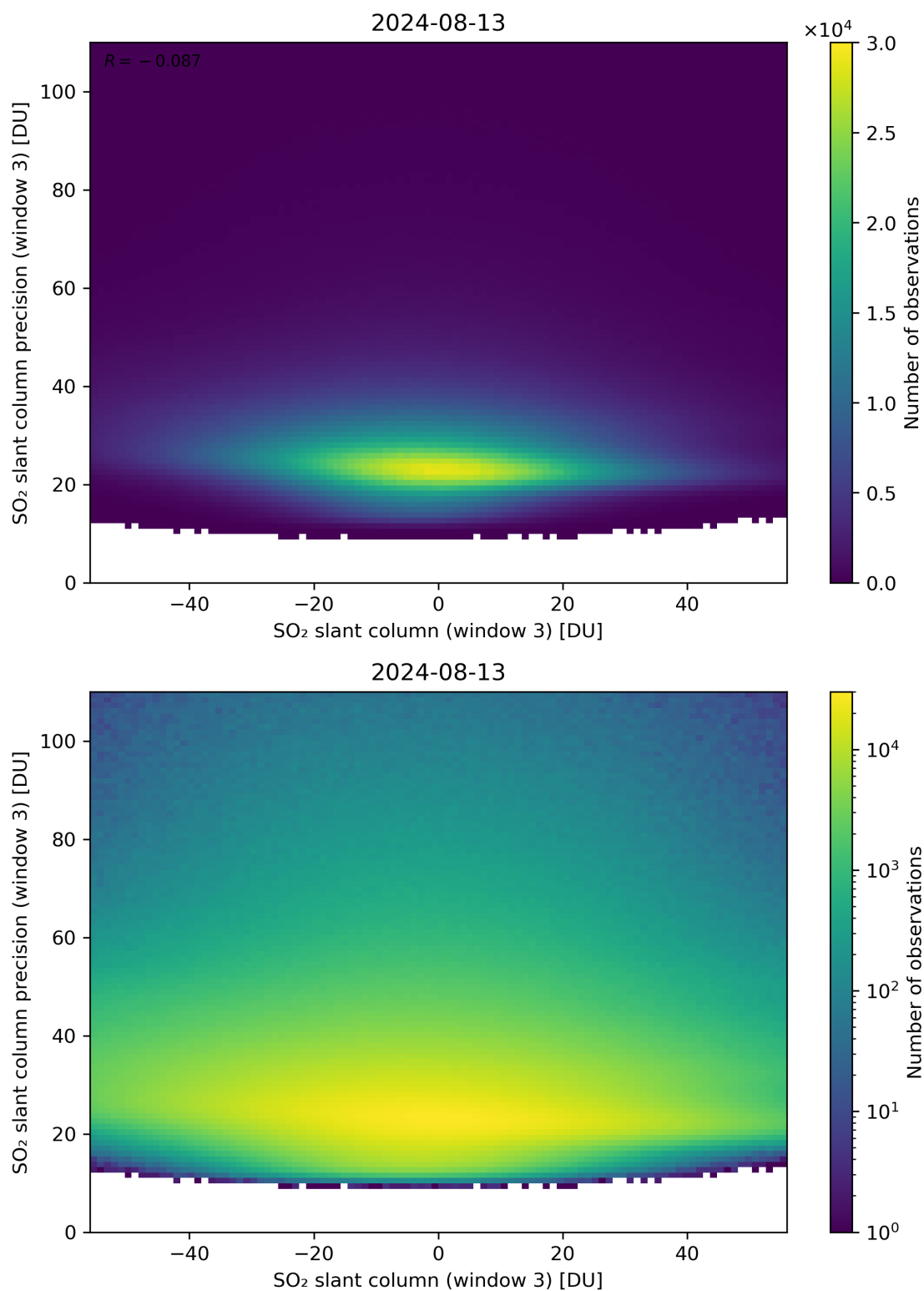
Figure 267: Scatter density plot of “SO 2 slant column (window 3)” against “SO 2 slant column precision (window 3)” for 2024-08-12 to 2024-08-14.
