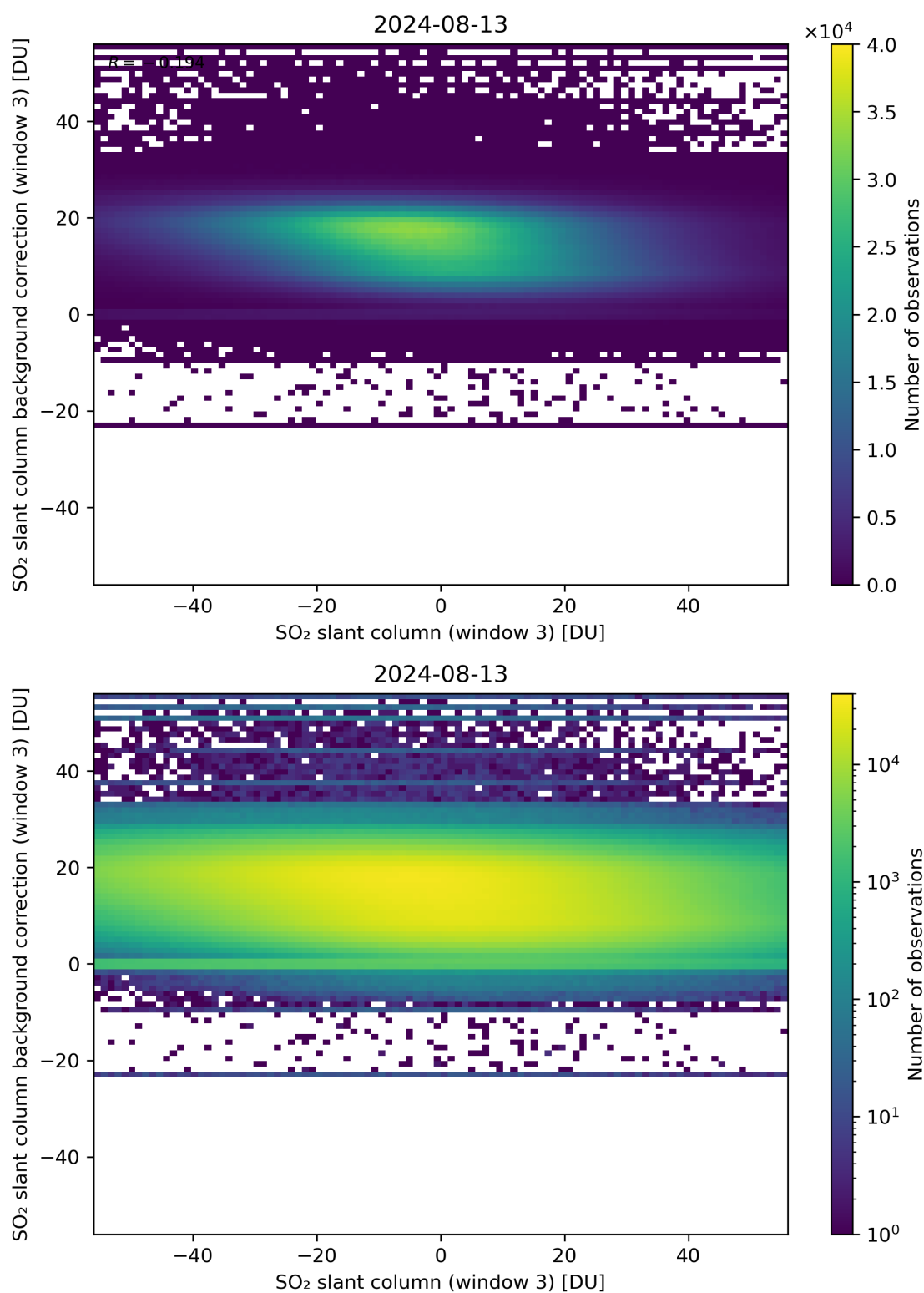
Figure 253: Scatter density plot of “SO 2 slant column (window 3)” against “SO 2 slant column background correction (window 3)” for 2024-08-12 to 2024-08-14.
