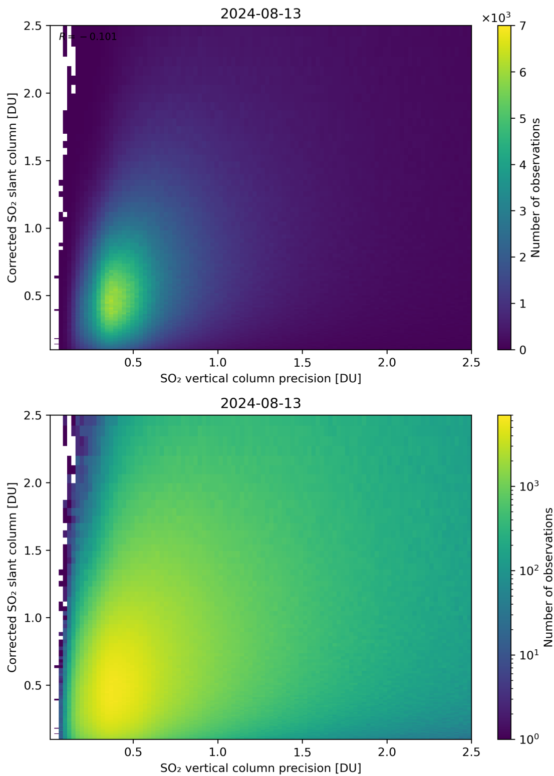
Figure 286: Scatter density plot of “SO 2 vertical column precision” against “Corrected SO 2 slant column” for 2024-08-12 to 2024-08-14.
