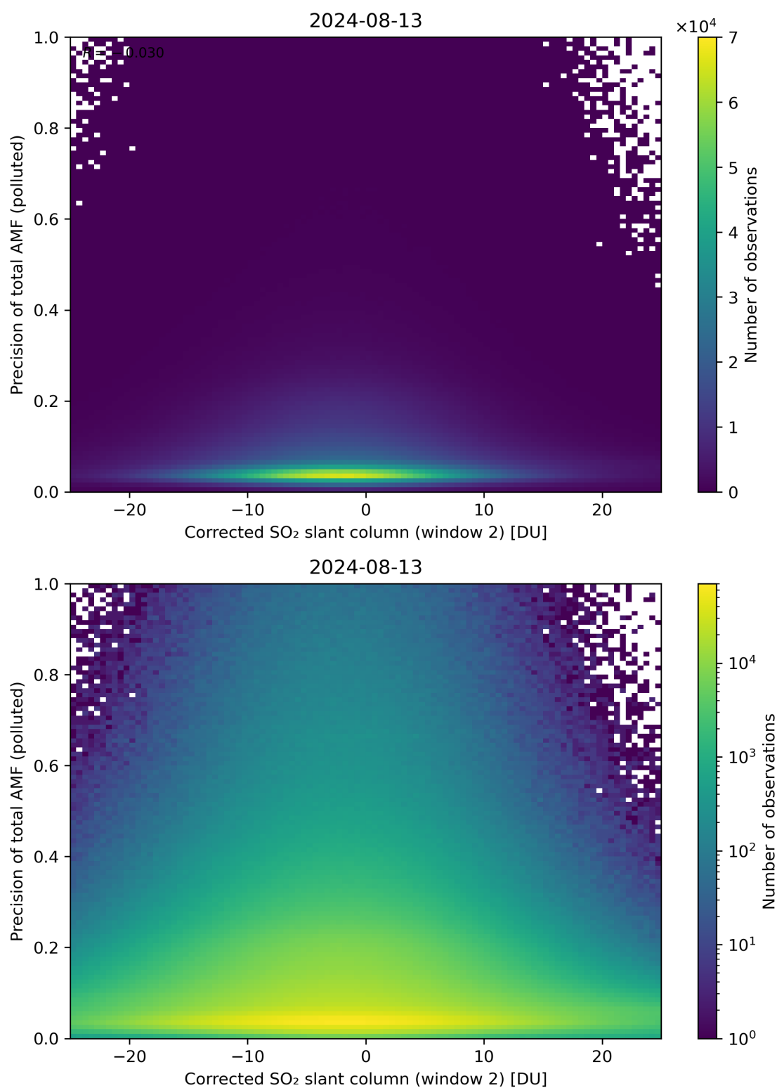
Figure 204: Scatter density plot of “Corrected SO 2 slant column (window 2)” against “Precision of total AMF (polluted)” for 2024-08-12 to 2024-08-14.
