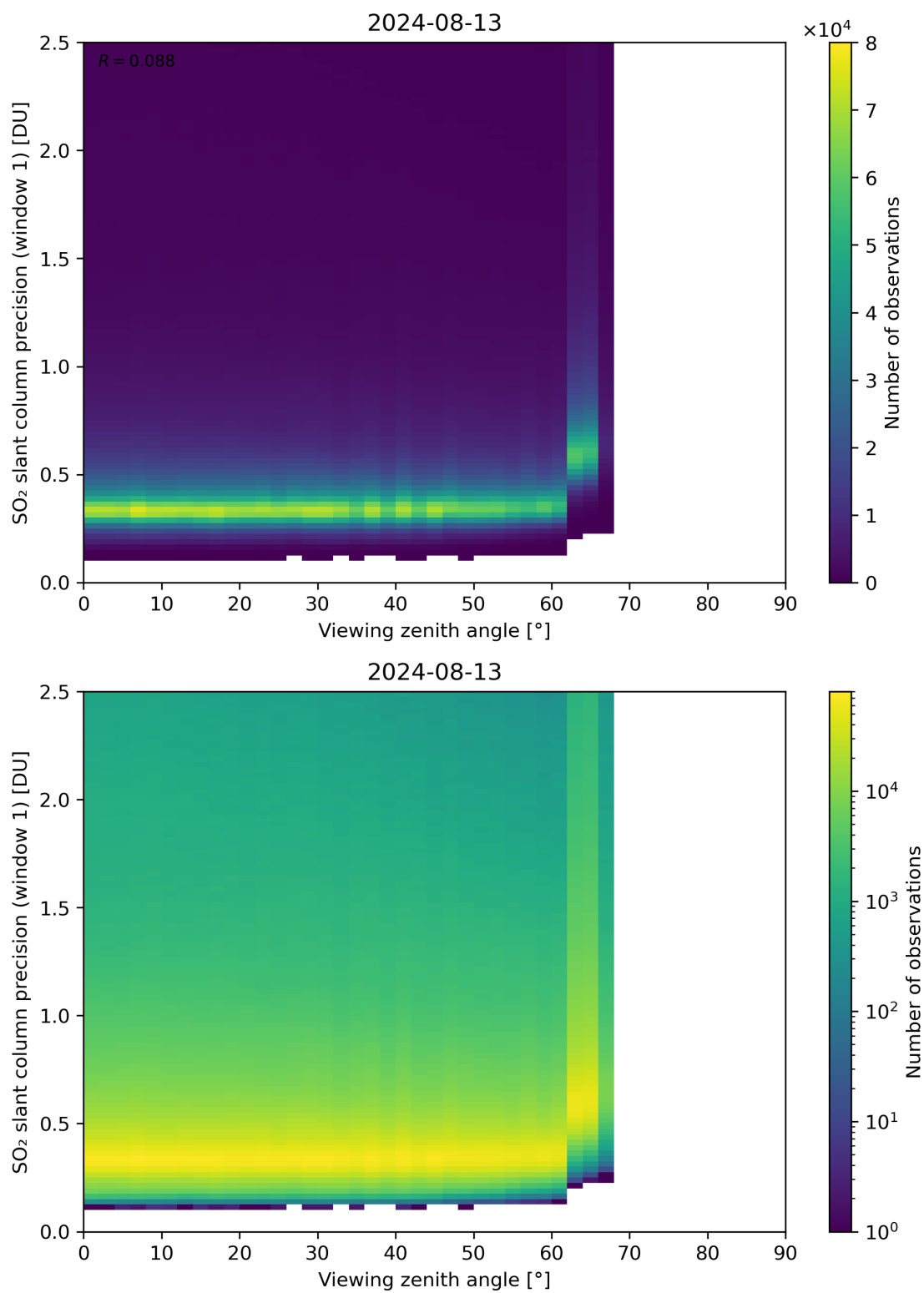
Figure 321: Scatter density plot of “Viewing zenith angle” against “SO 2 slant column precision (window 1)” for 2024-08-12 to 2024-08-14.
