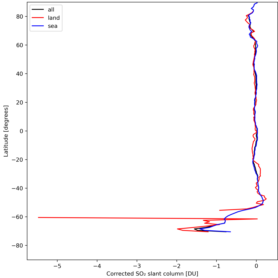
Figure 32: Zonal average of “Corrected SO 2 slant column” for 2024-08-12 to 2024-08-14.
