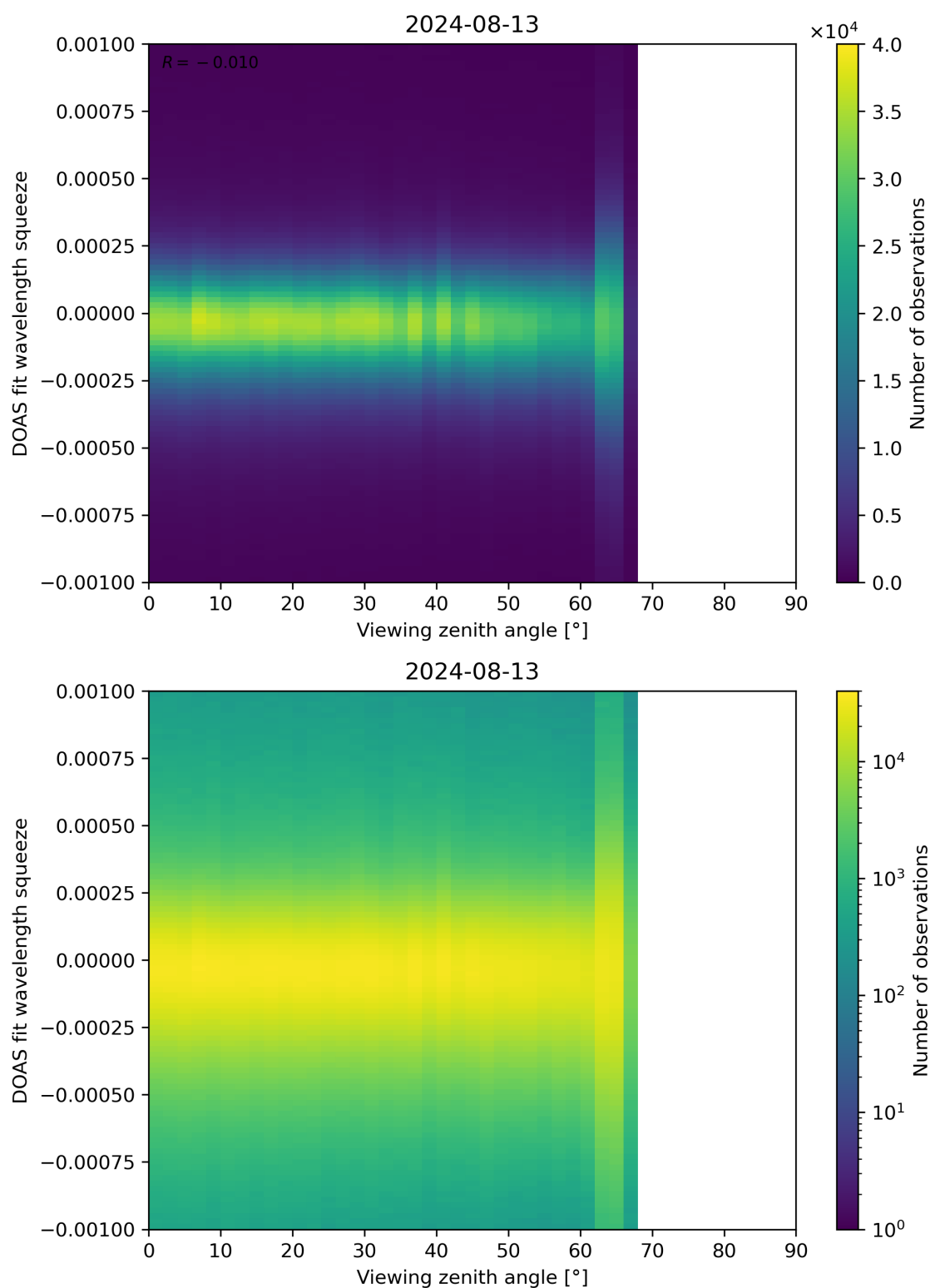
Figure 312: Scatter density plot of “Viewing zenith angle” against “DOAS fit wavelength squeeze” for 2024-08-12 to 2024-08-14.
