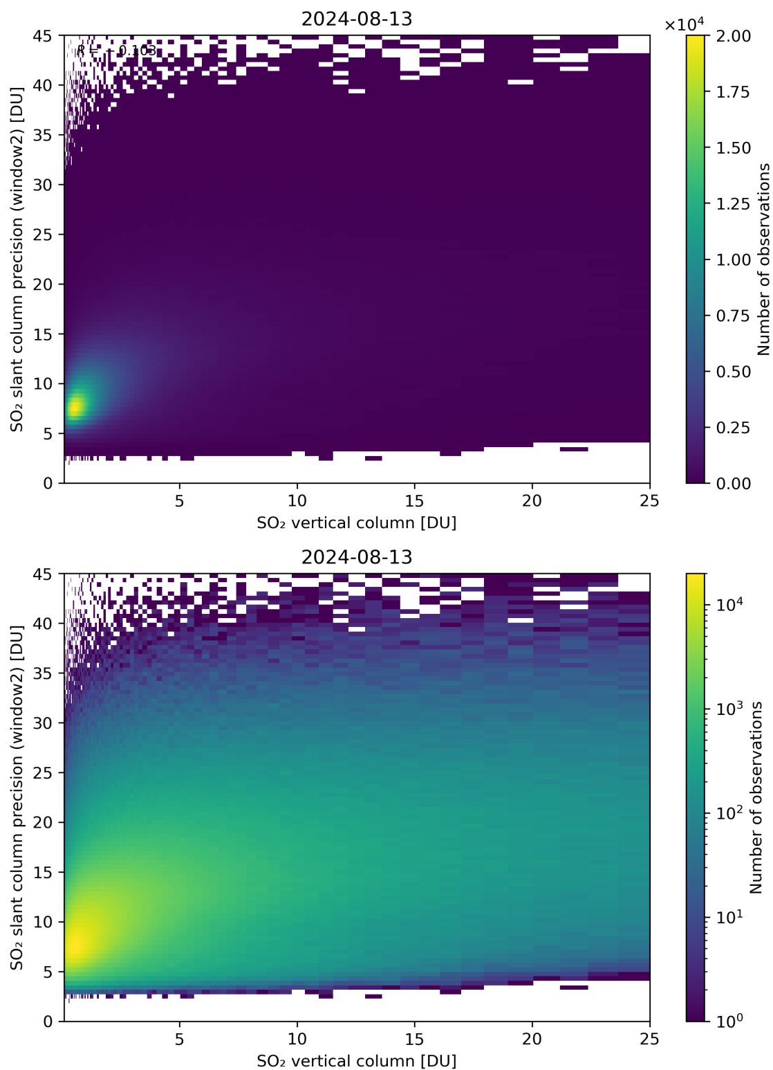
Figure 302: Scatter density plot of “SO 2 vertical column” against “SO 2 slant column precision (window2)” for 2024-08-12 to 2024-08-14.
