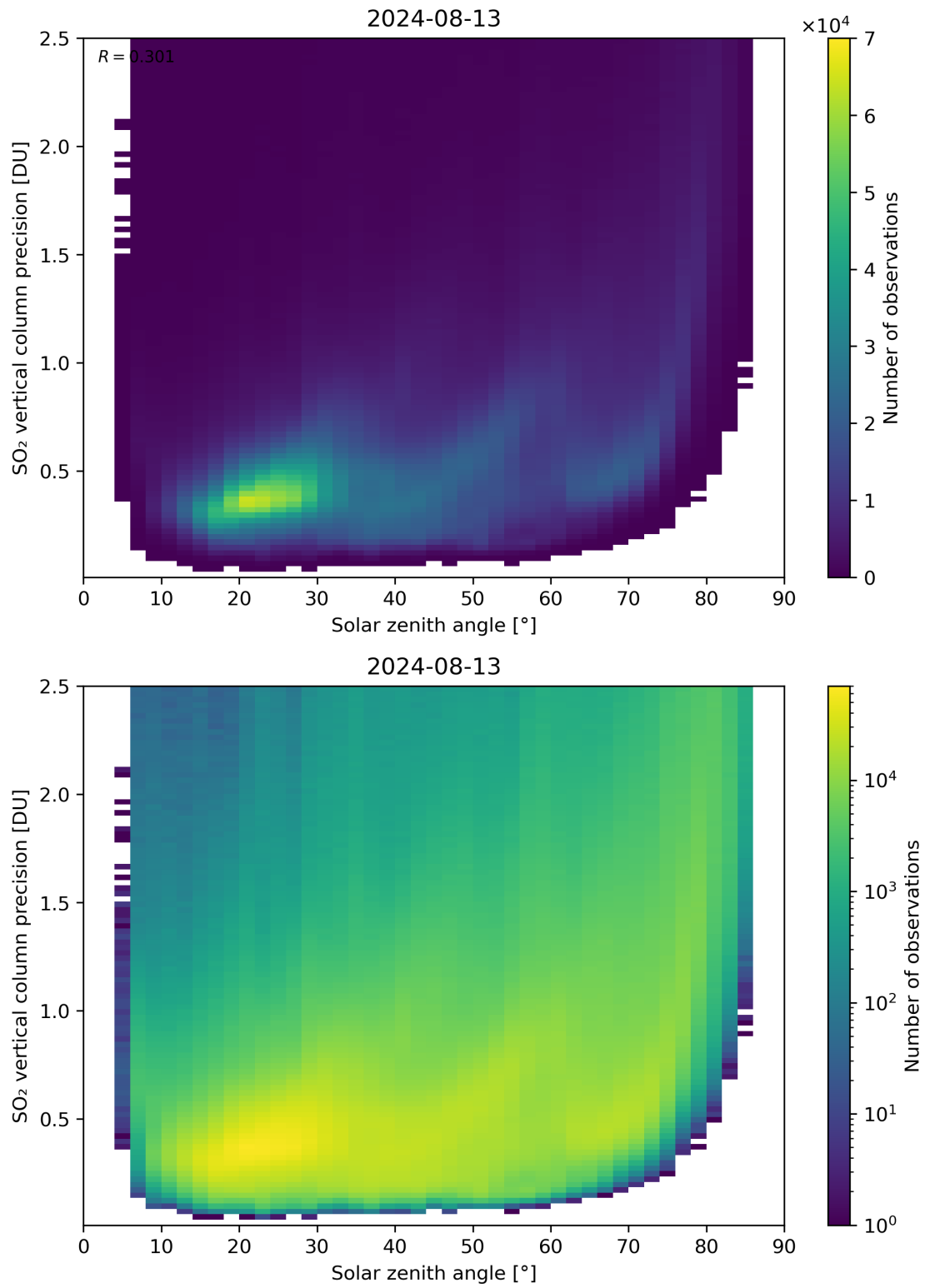
Figure 177: Scatter density plot of “Solar zenith angle” against “SO 2 vertical column precision” for 2024-08-12 to 2024-08-14.
