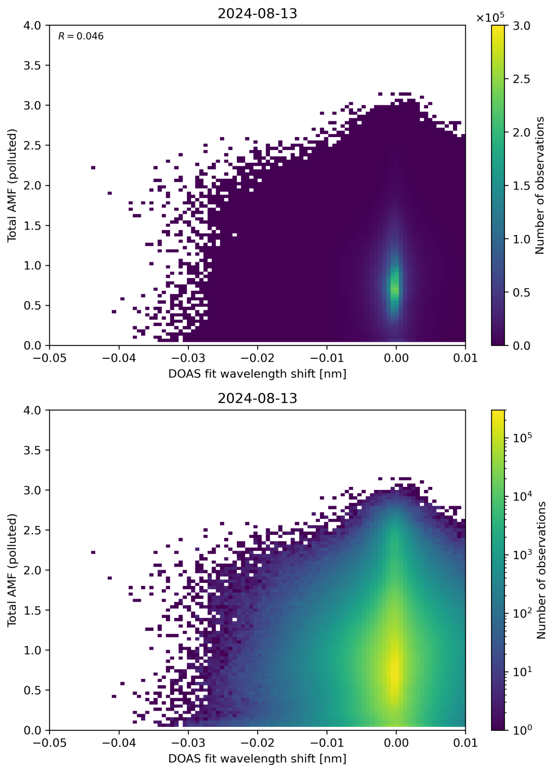
Figure 130: Scatter density plot of “DOAS fit wavelength shift” against “Total AMF (polluted)” for 2024-08-12 to 2024-08-14.
