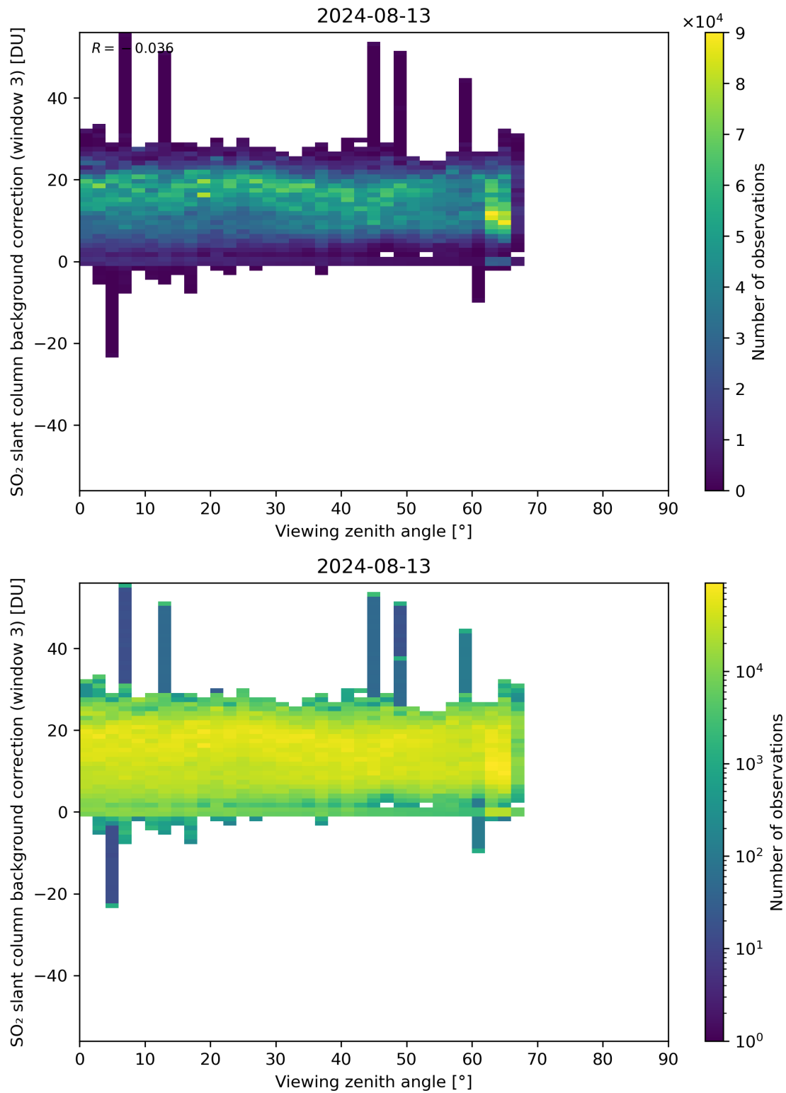
Figure 310: Scatter density plot of “Viewing zenith angle” against “SO 2 slant column background correction (window 3)” for 2024-08-12 to 2024-08-14.
