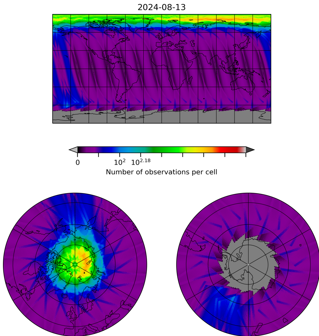
Figure 28: Map of the number of observations for 2024-08-12 to 2024-08-14
