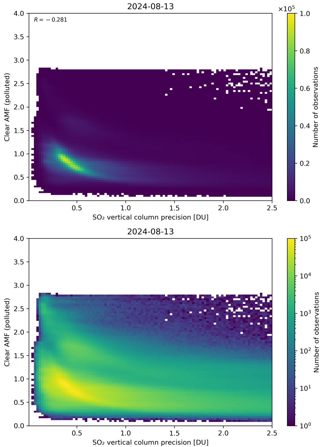
Figure 285: Scatter density plot of “SO 2 vertical column precision” against “Clear AMF (polluted)” for 2024-08-12 to 2024-08-14.
