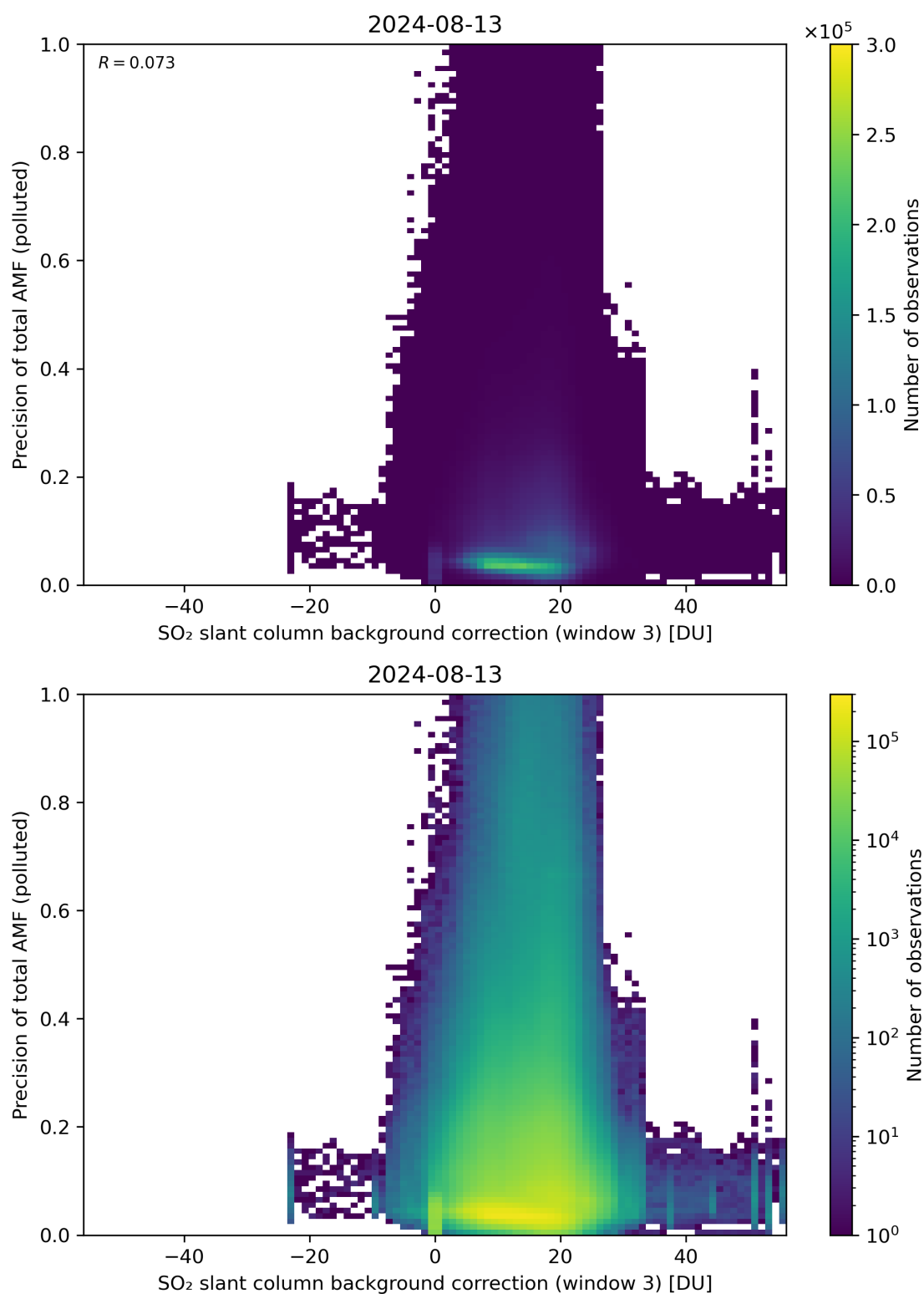
Figure 126: Scatter density plot of “SO 2 slant column background correction (window 3)” against “Precision of total AMF (polluted)” for 2024-08-12 to 2024-08-14.
