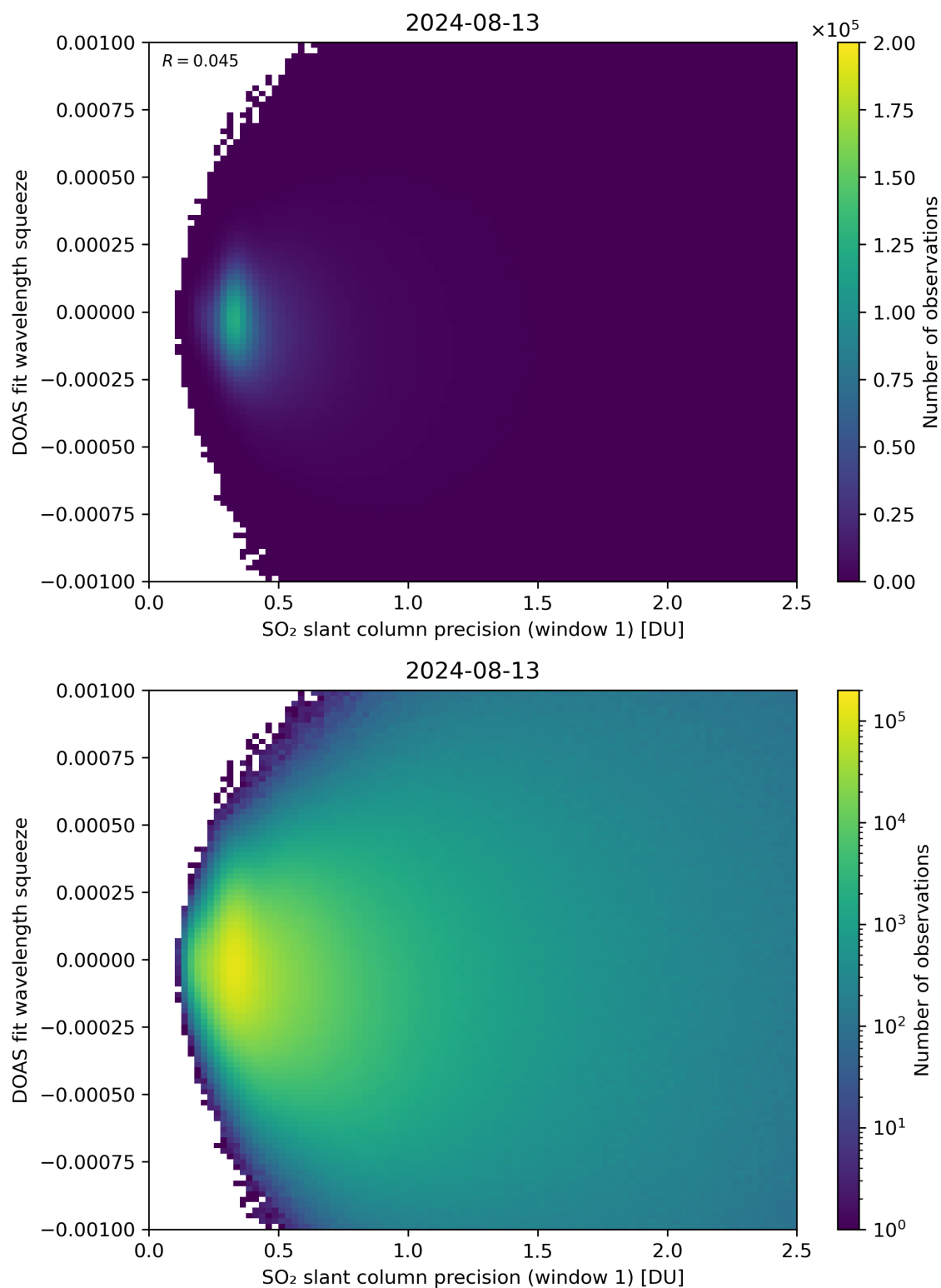
Figure 222: Scatter density plot of “SO 2 slant column precision (window 1)” against “DOAS fit wavelength squeeze” for 2024-08-12 to 2024-08-14.
