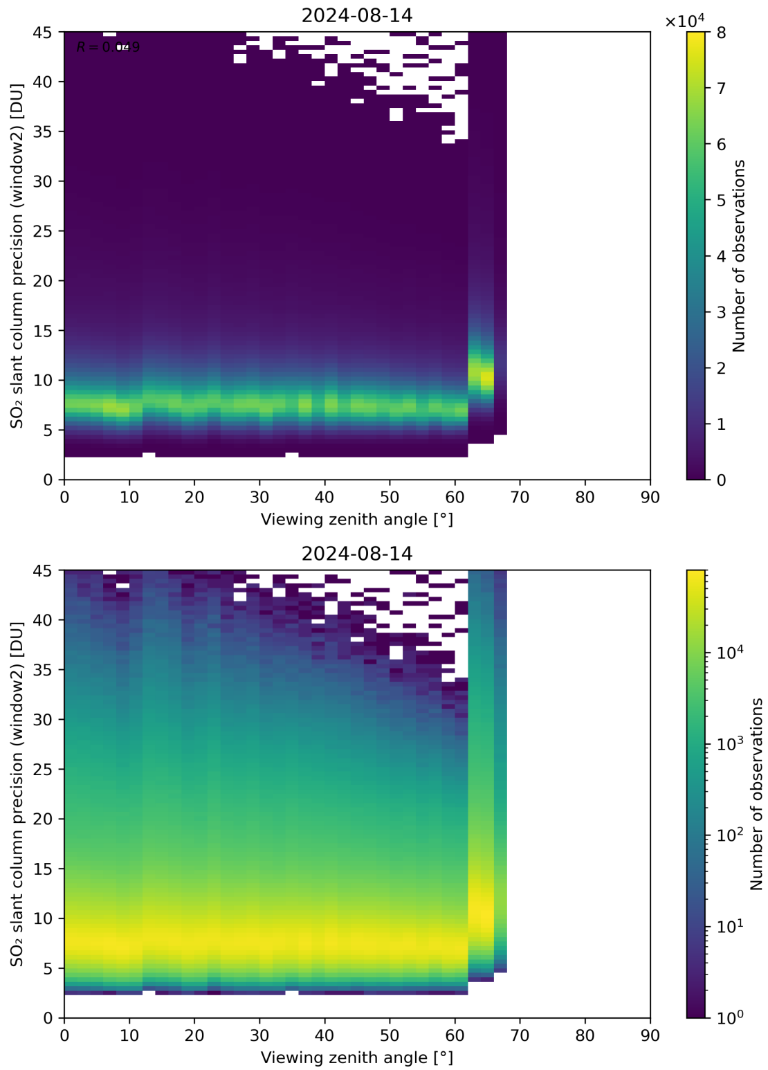
Figure 322: Scatter density plot of “Viewing zenith angle” against “SO 2 slant column precision (window2)” for 2024-08-13 to 2024-08-15.
