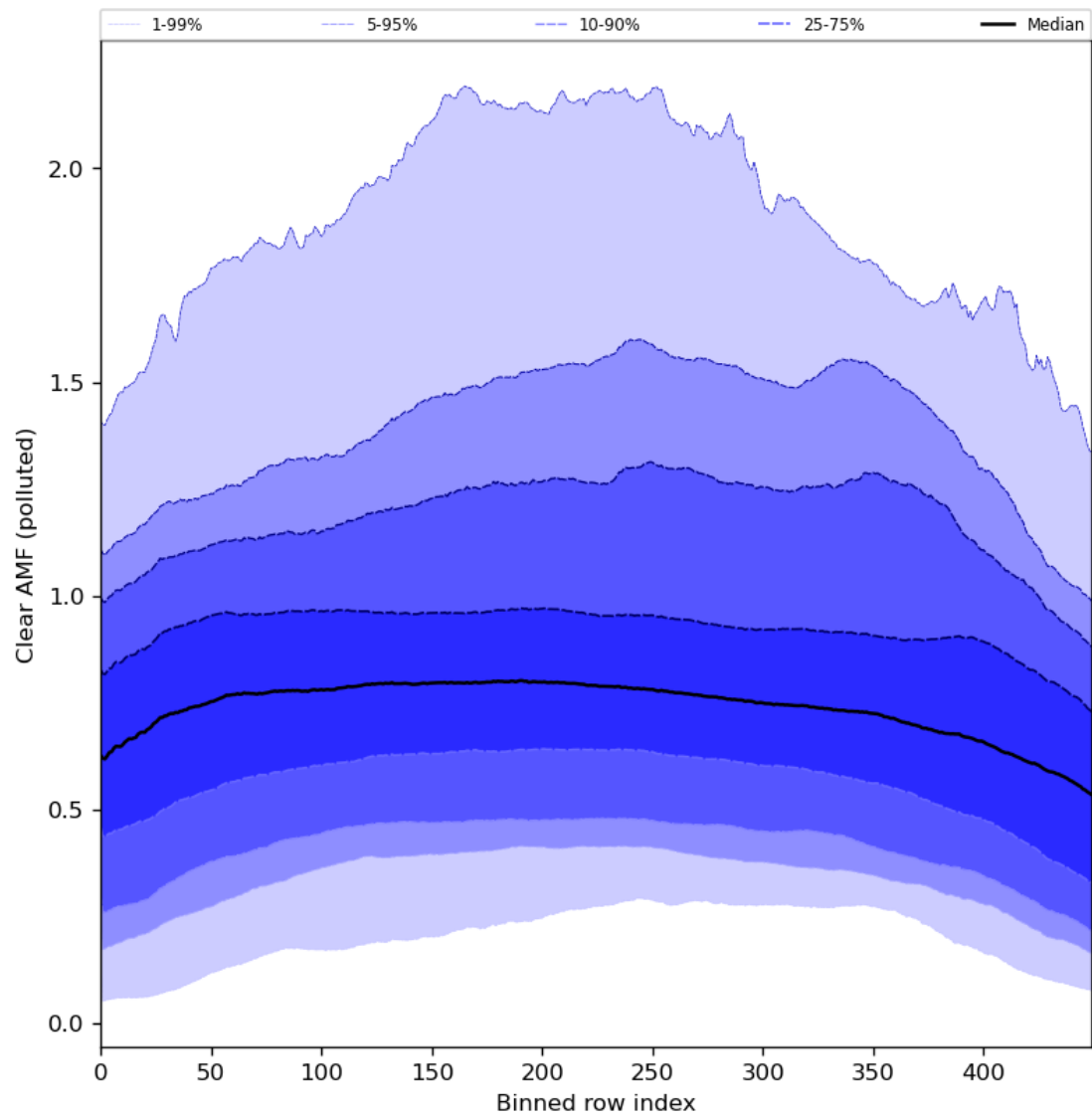
Figure 96: Along track statistics of “Clear AMF (polluted)” for 2024-08-13 to 2024-08-15
