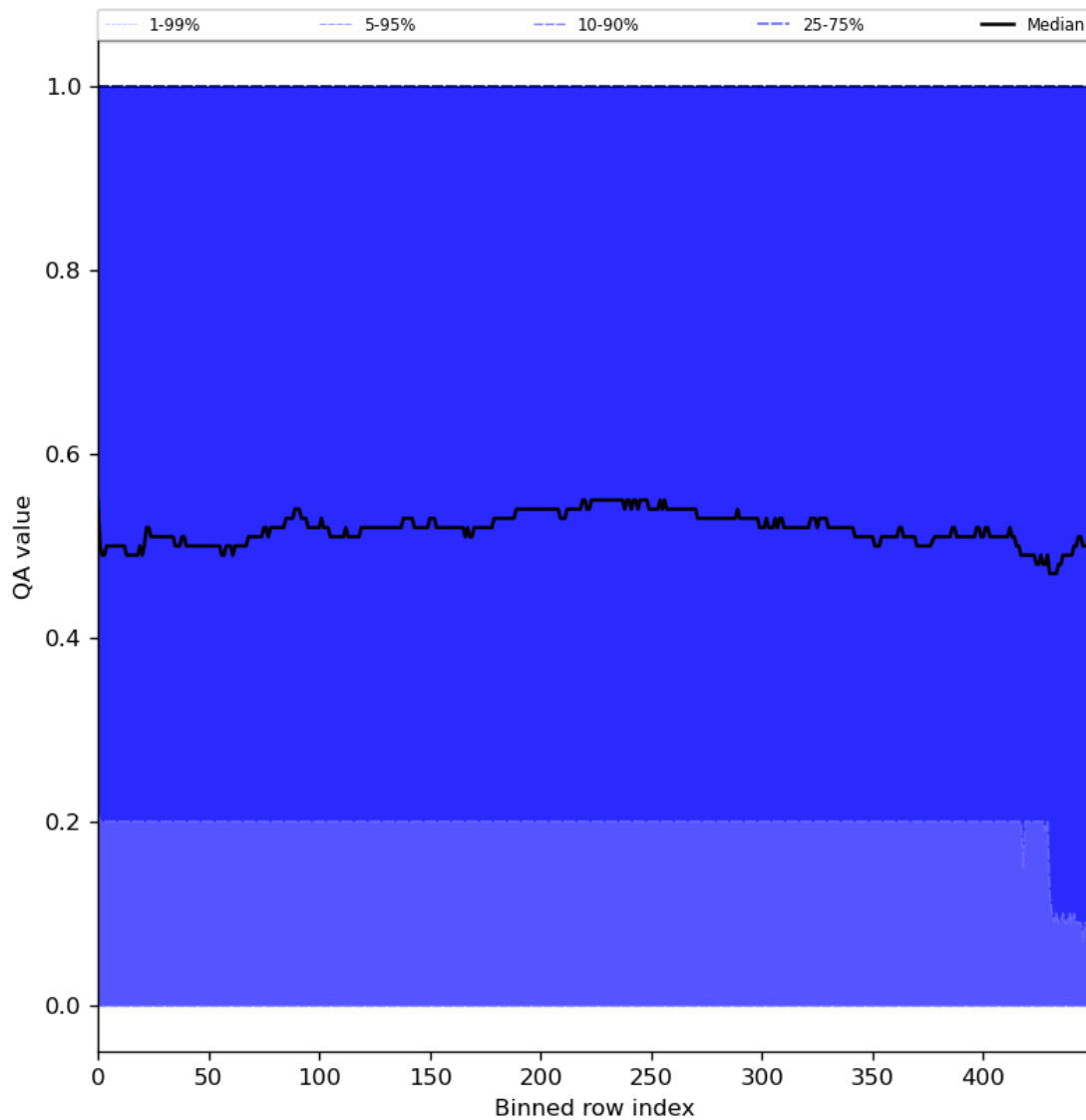
Figure 75: Along track statistics of “QA value” for 2024-08-13 to 2024-08-15
