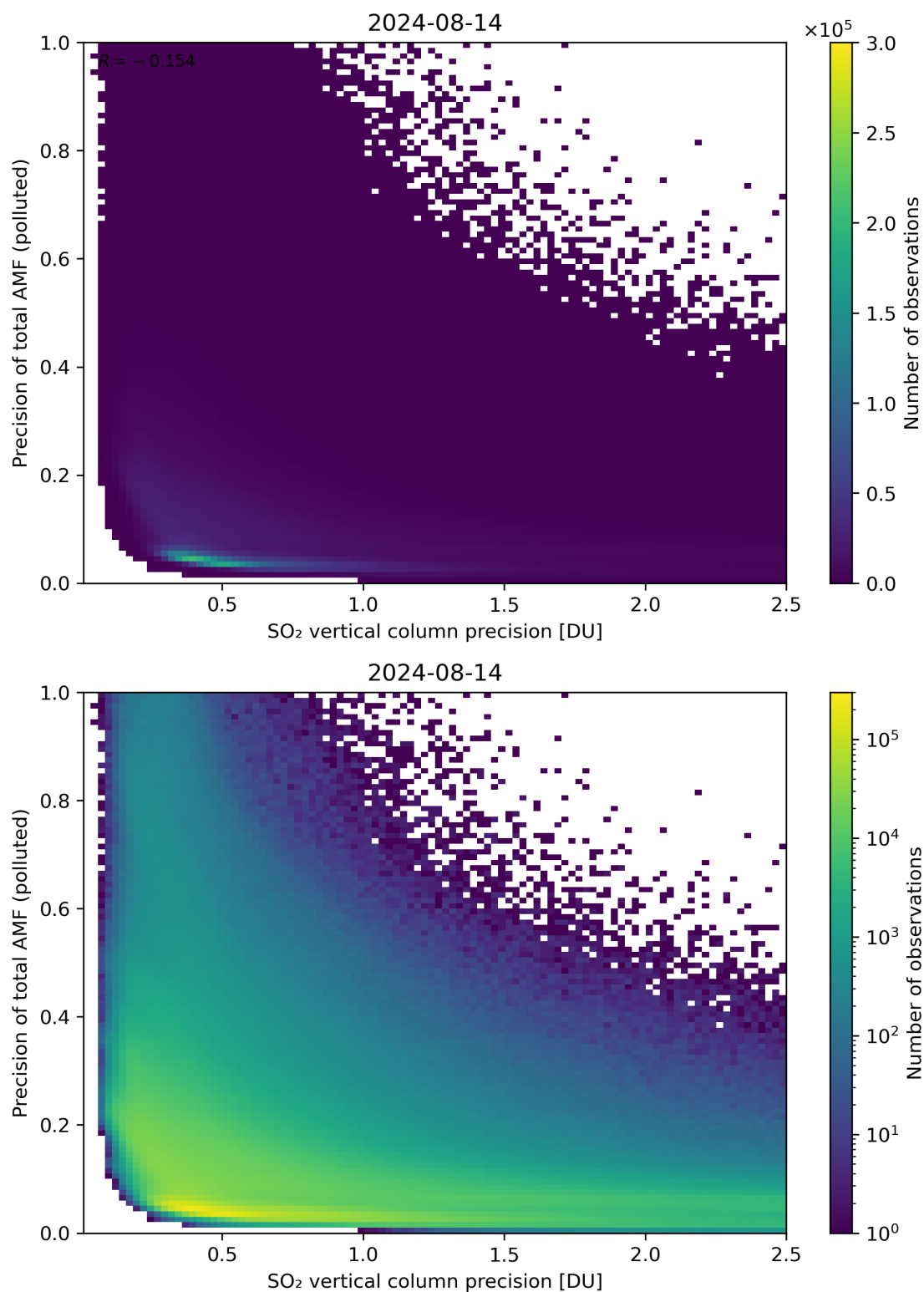
Figure 295: Scatter density plot of “SO 2 vertical column precision” against “Precision of total AMF (polluted)” for 2024-08-13 to 2024-08-15.
