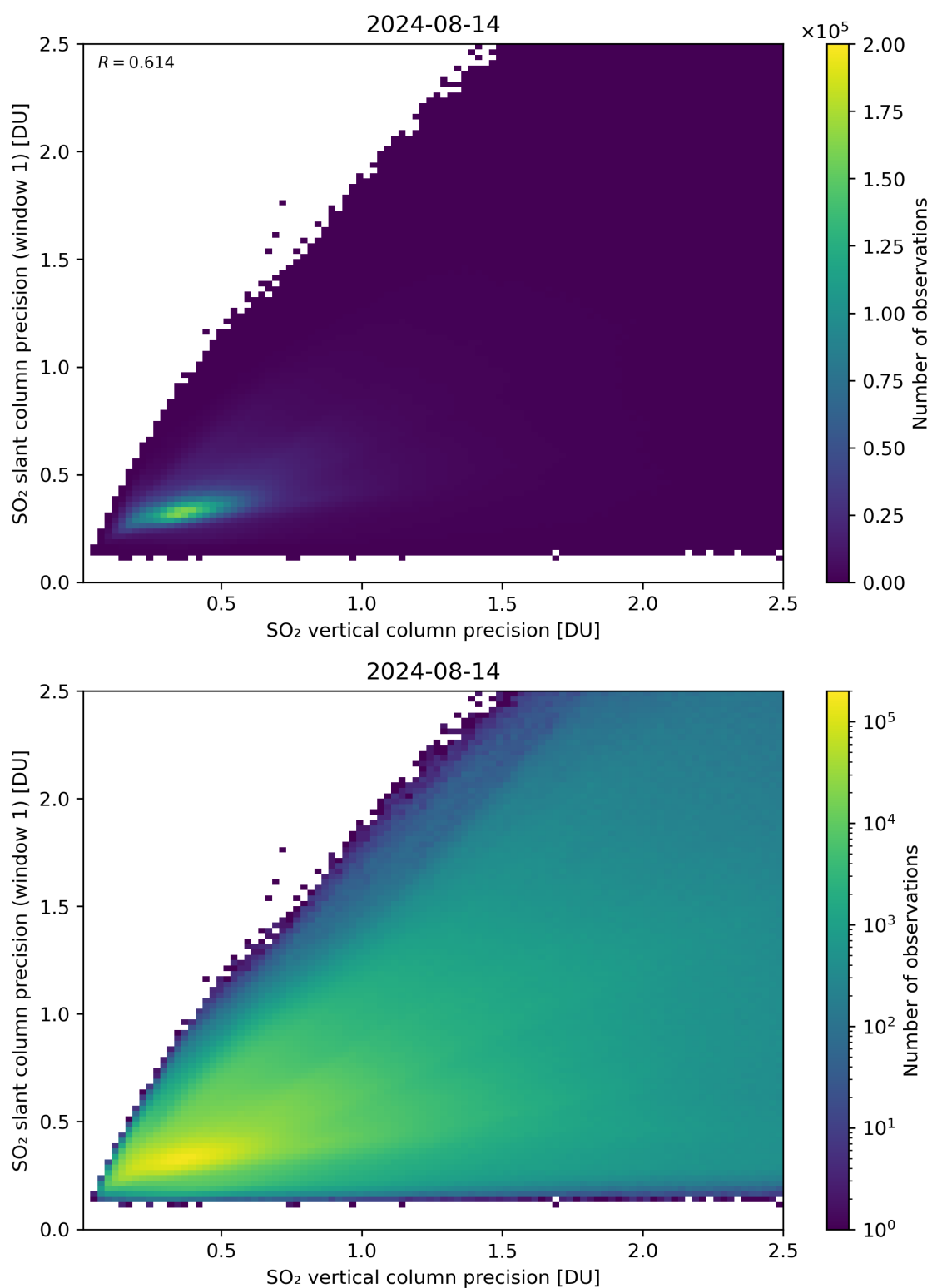
Figure 290: Scatter density plot of “SO 2 vertical column precision” against “SO 2 slant column precision (window 1)” for 2024-08-13 to 2024-08-15.
