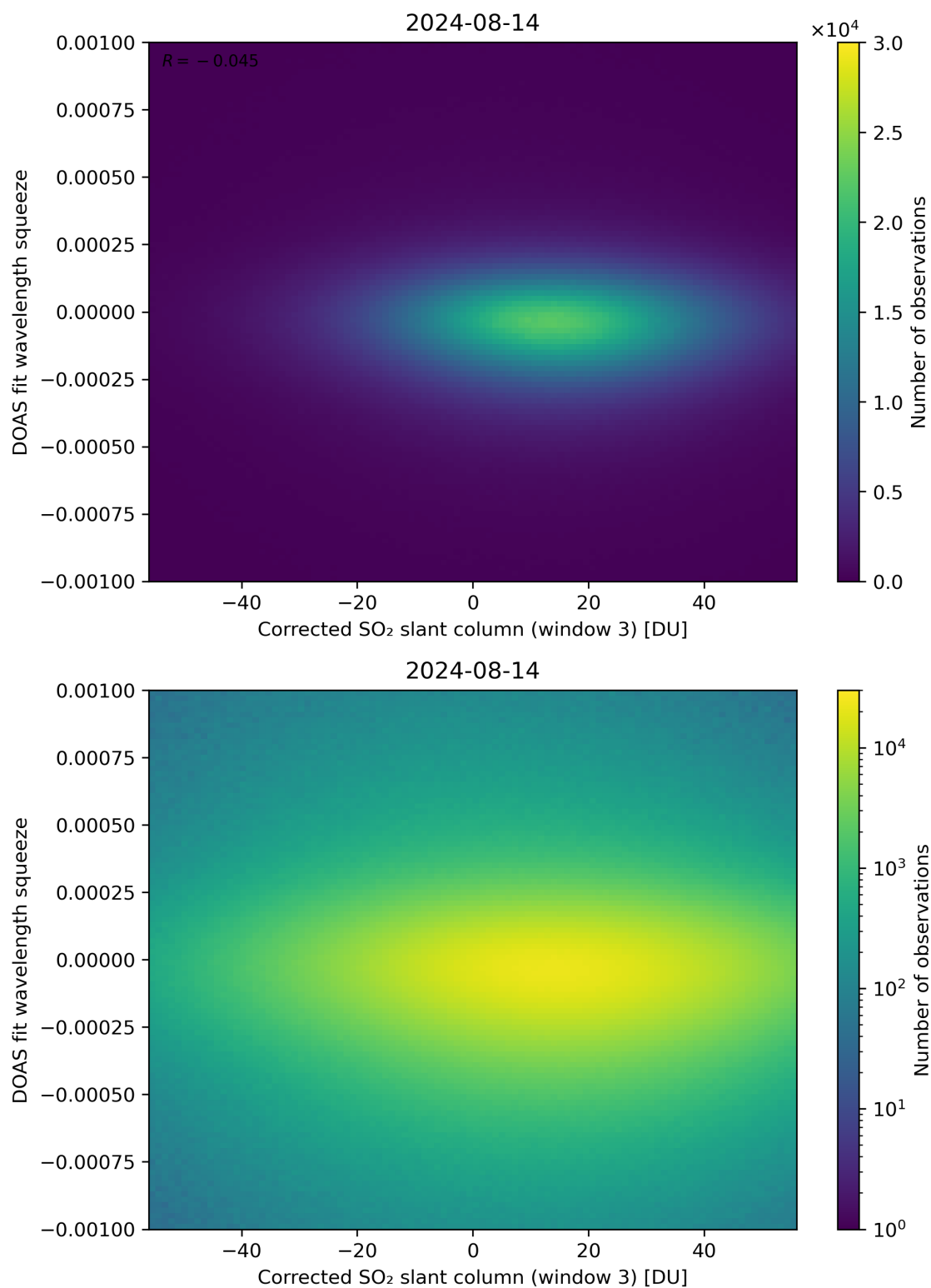
Figure 207: Scatter density plot of “Corrected SO 2 slant column (window 3)” against “DOAS fit wavelength squeeze” for 2024-08-13 to 2024-08-15.
