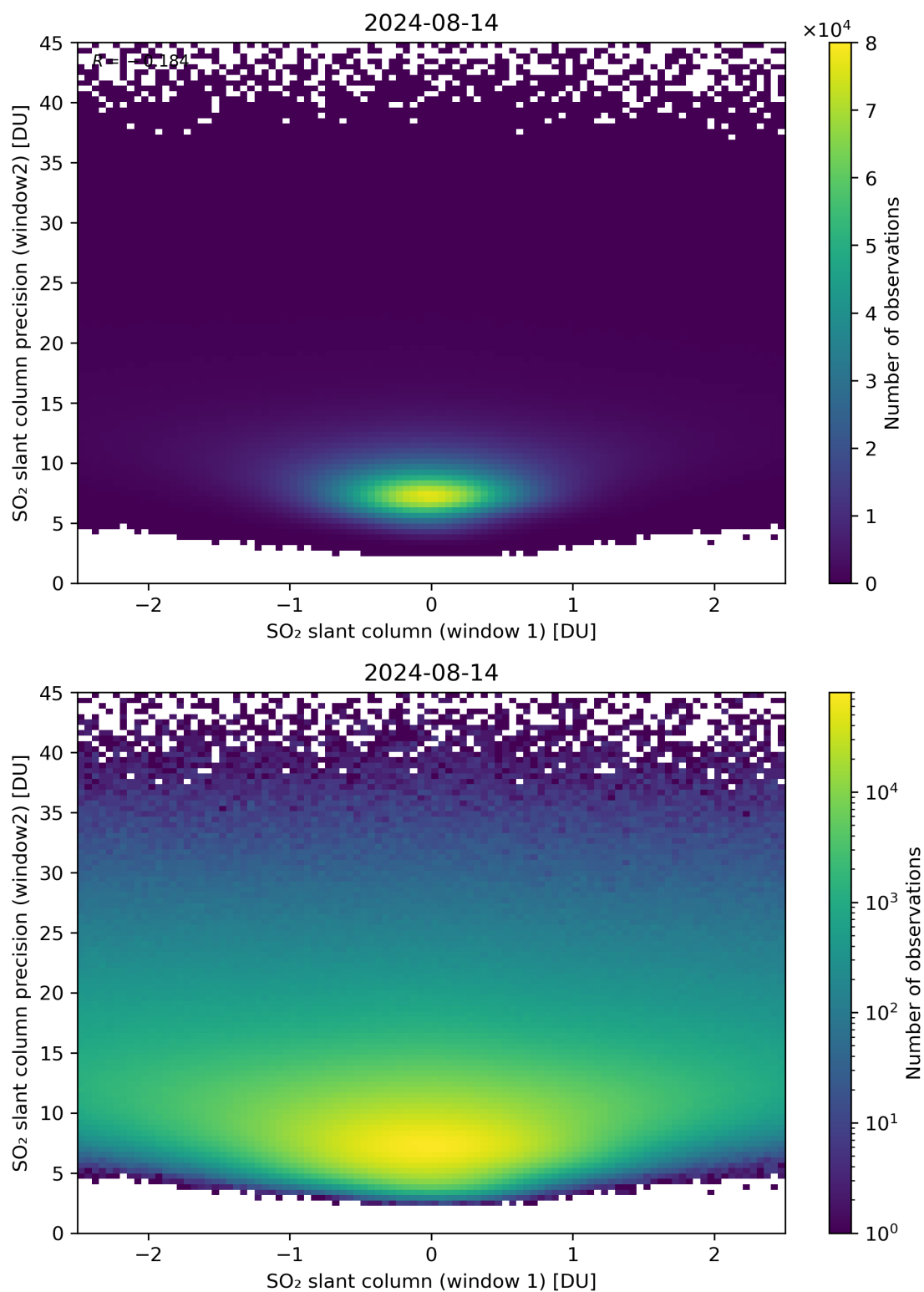
Figure 236: Scatter density plot of “SO 2 slant column (window 1)” against “SO 2 slant column precision (window2)” for 2024-08-13 to 2024-08-15.
