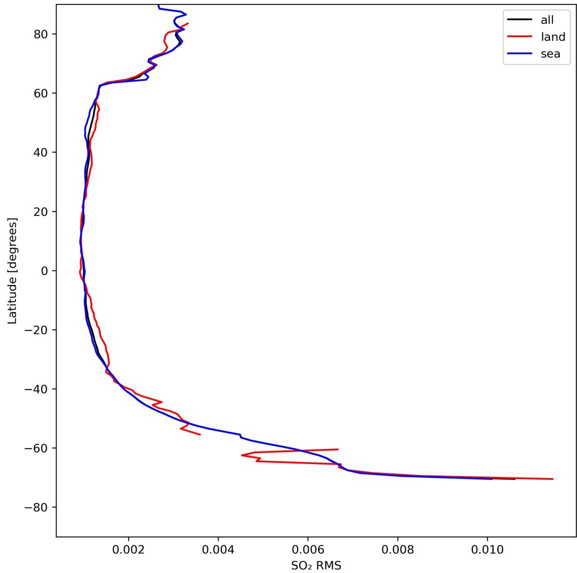
Figure 47: Zonal average of “SO 2 RMS” for 2024-08-13 to 2024-08-15.
