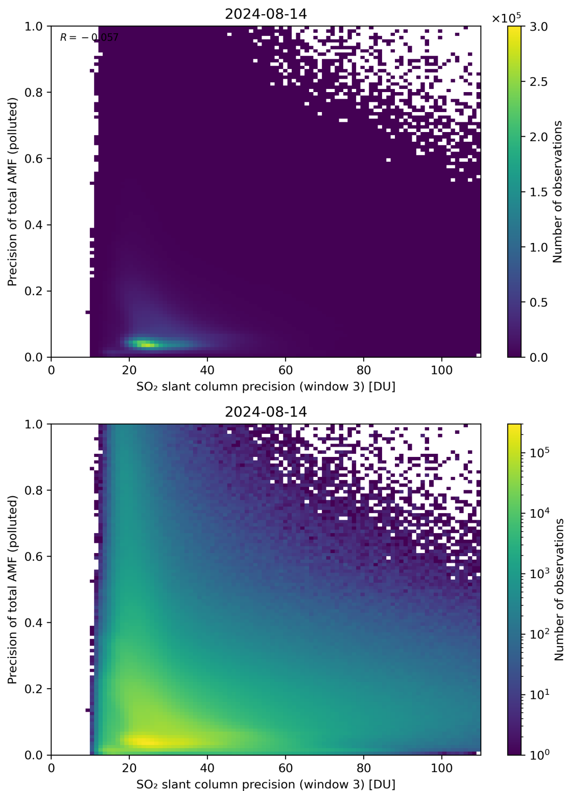
Figure 264: Scatter density plot of “SO 2 slant column precision (window 3)” against “Precision of total AMF (polluted)” for 2024-08-13 to 2024-08-15.
