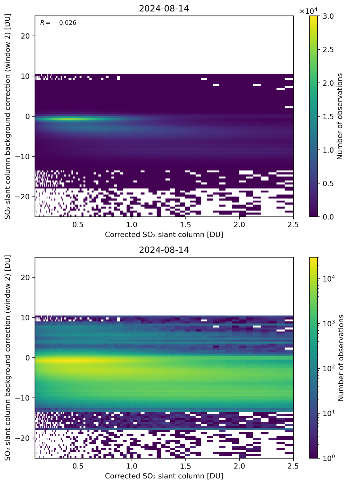
Figure 179: Scatter density plot of “Corrected SO 2 slant column” against “SO 2 slant column background correction (window 2)” for 2024-08-13 to 2024-08-15.
