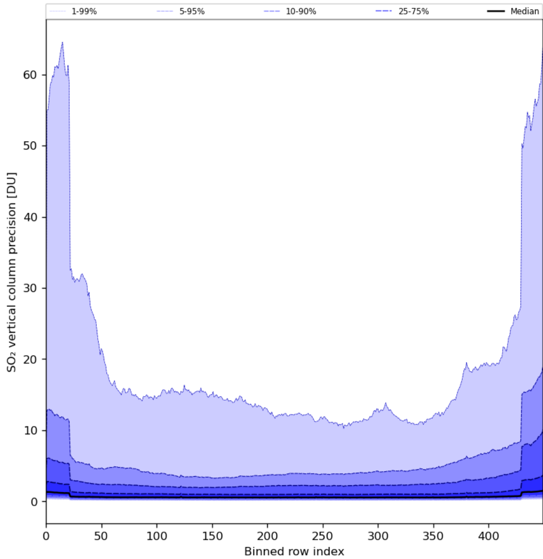
Figure 77: Along track statistics of “SO 2 vertical column precision” for 2024-08-13 to 2024-08-15
