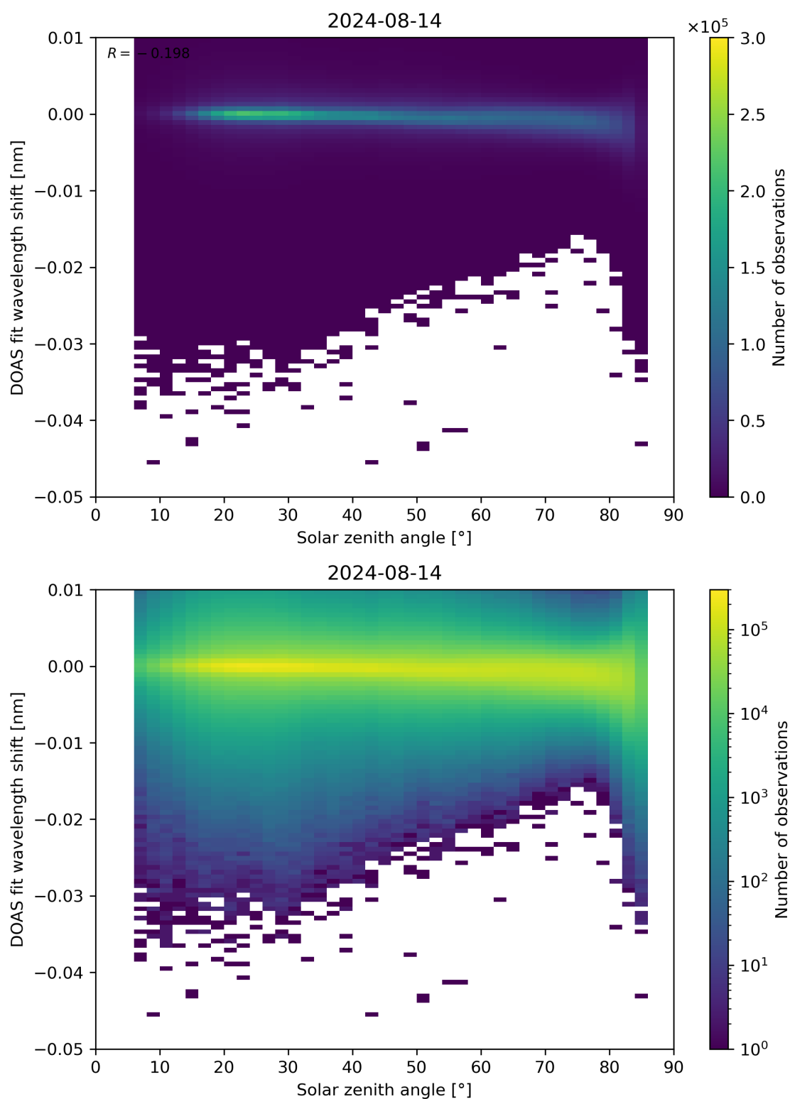
Figure 161: Scatter density plot of “Solar zenith angle” against “DOAS fit wavelength shift” for 2024-08-13 to 2024-08-15.
