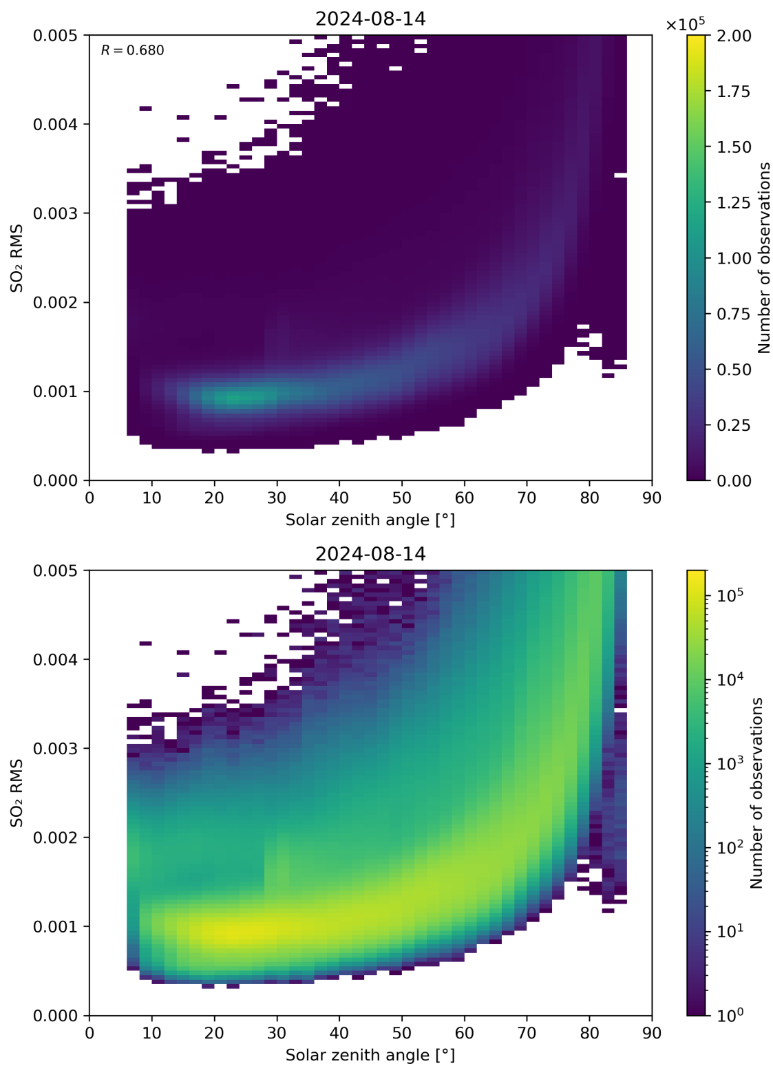
Figure 163: Scatter density plot of “Solar zenith angle” against “SO 2 RMS” for 2024-08-13 to 2024-08-15.
