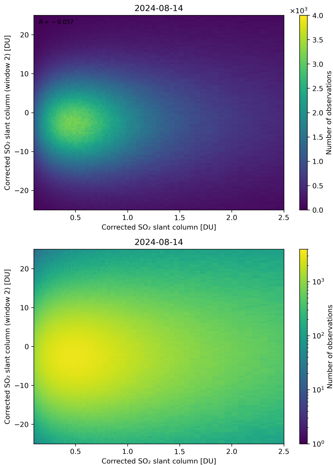
Figure 185: Scatter density plot of “Corrected SO 2 slant column” against “Corrected SO 2 slant column (window 2)” for 2024-08-13 to 2024-08-15.
