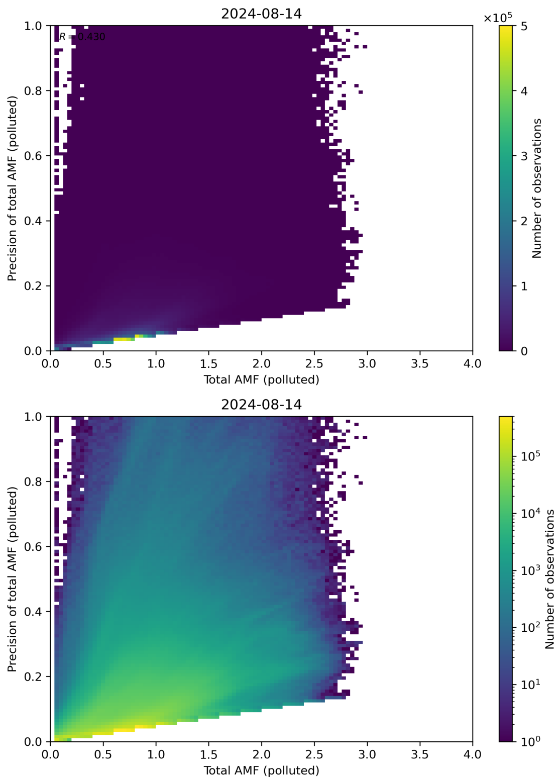
Figure 272: Scatter density plot of “Total AMF (polluted)” against “Precision of total AMF (polluted)” for 2024-08-13 to 2024-08-15.
