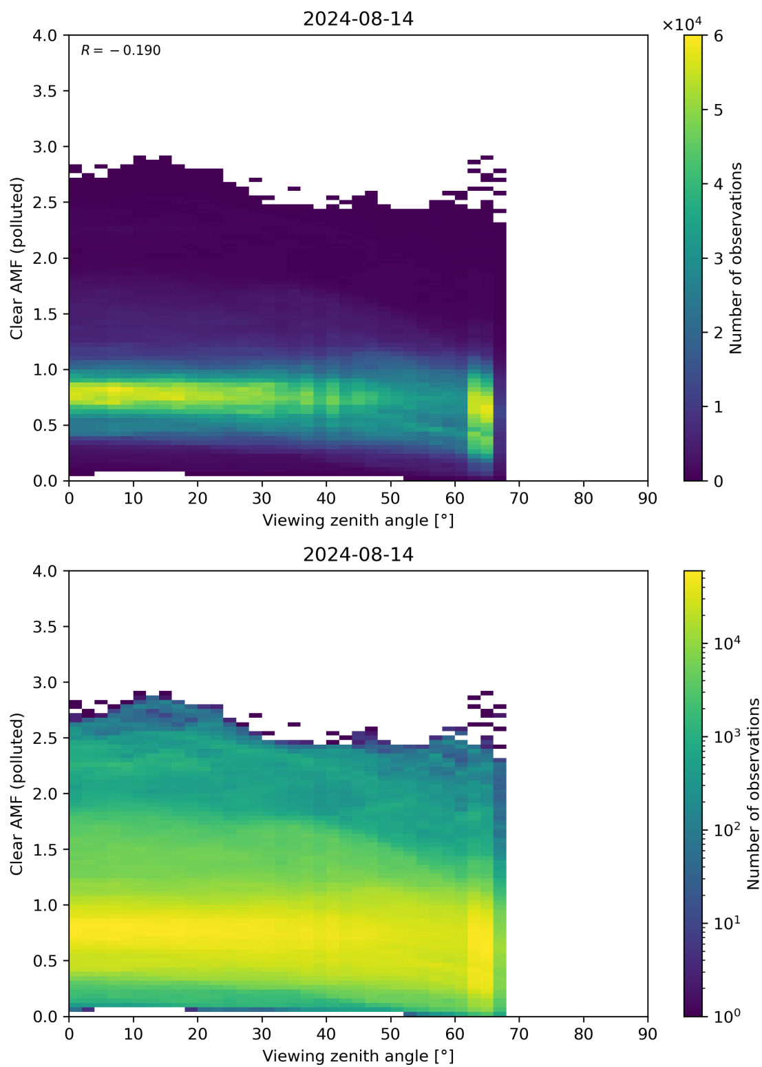
Figure 316: Scatter density plot of “Viewing zenith angle” against “Clear AMF (polluted)” for 2024-08-13 to 2024-08-15.
