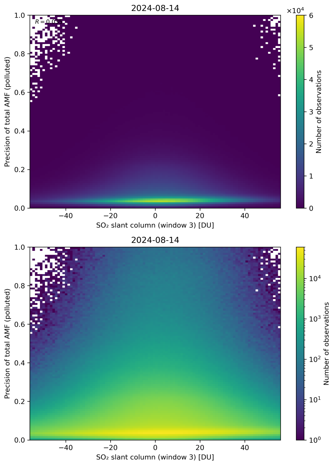
Figure 269: Scatter density plot of “SO 2 slant column (window 3)” against “Precision of total AMF (polluted)” for 2024-08-13 to 2024-08-15.
