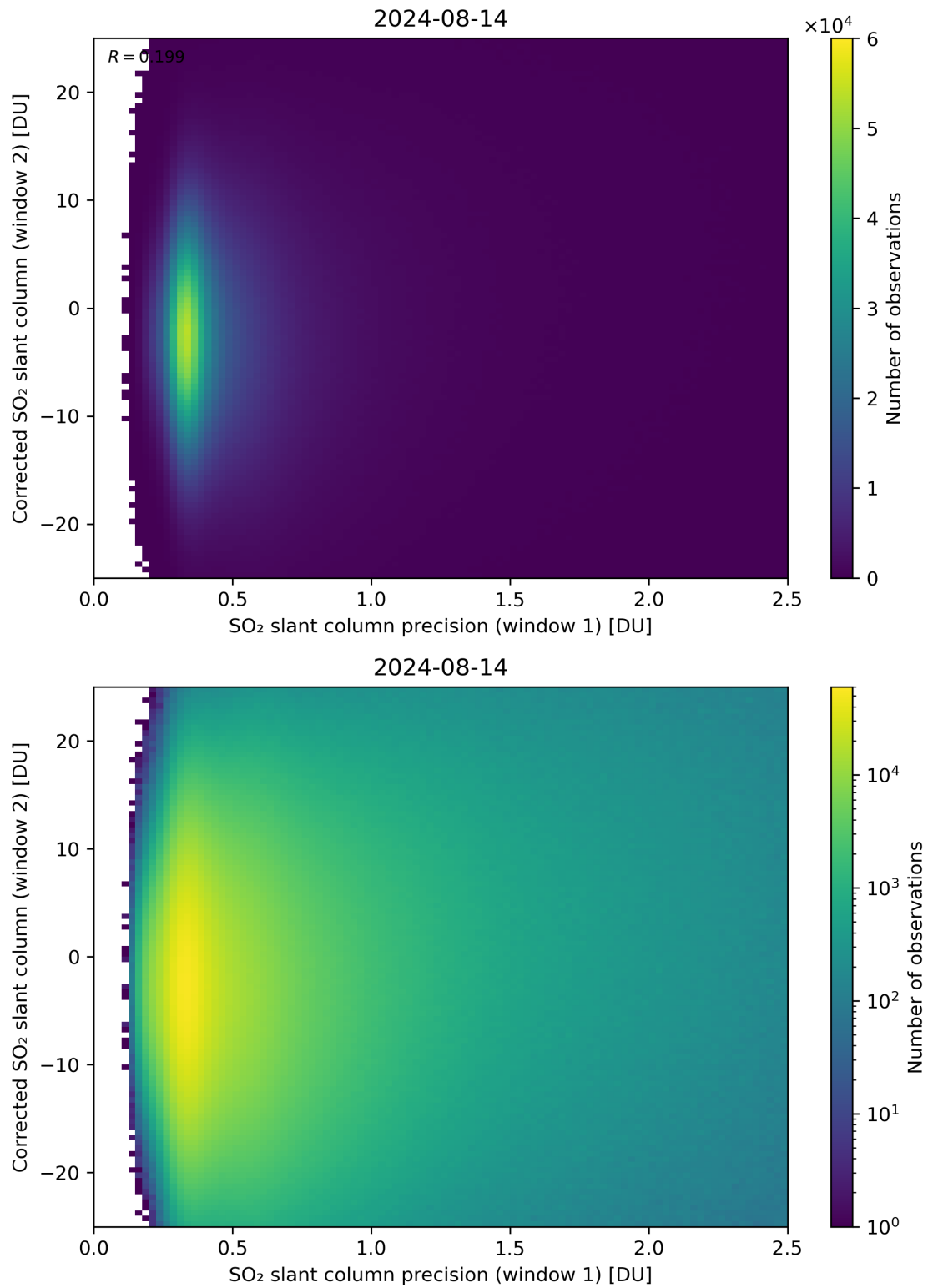
Figure 225: Scatter density plot of “SO 2 slant column precision (window 1)” against “Corrected SO 2 slant column (window 2)” for 2024-08-13 to 2024-08-15.
