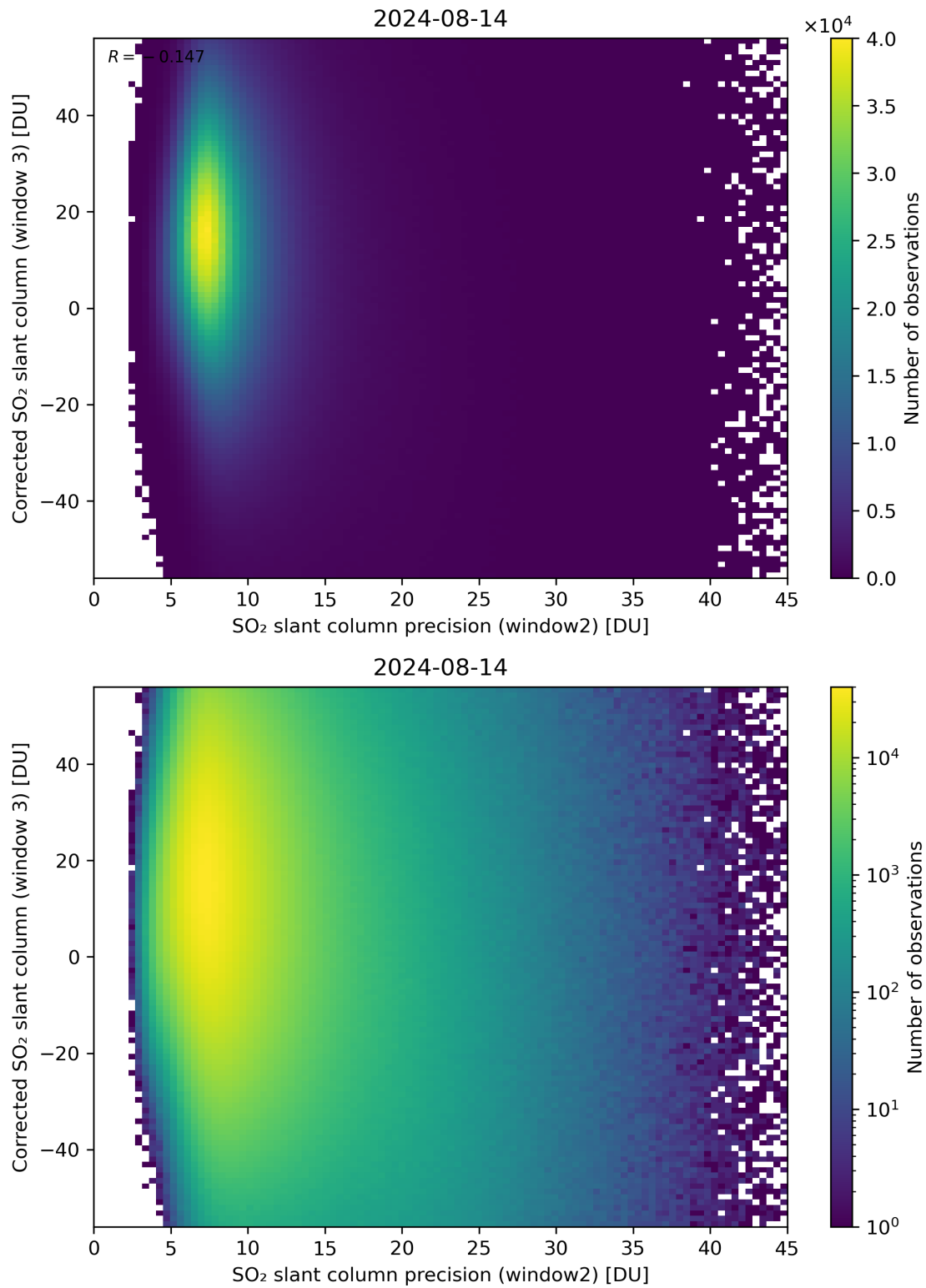
Figure 248: Scatter density plot of “SO 2 slant column precision (window2)” against “Corrected SO 2 slant column (window 3)” for 2024-08-13 to 2024-08-15.
