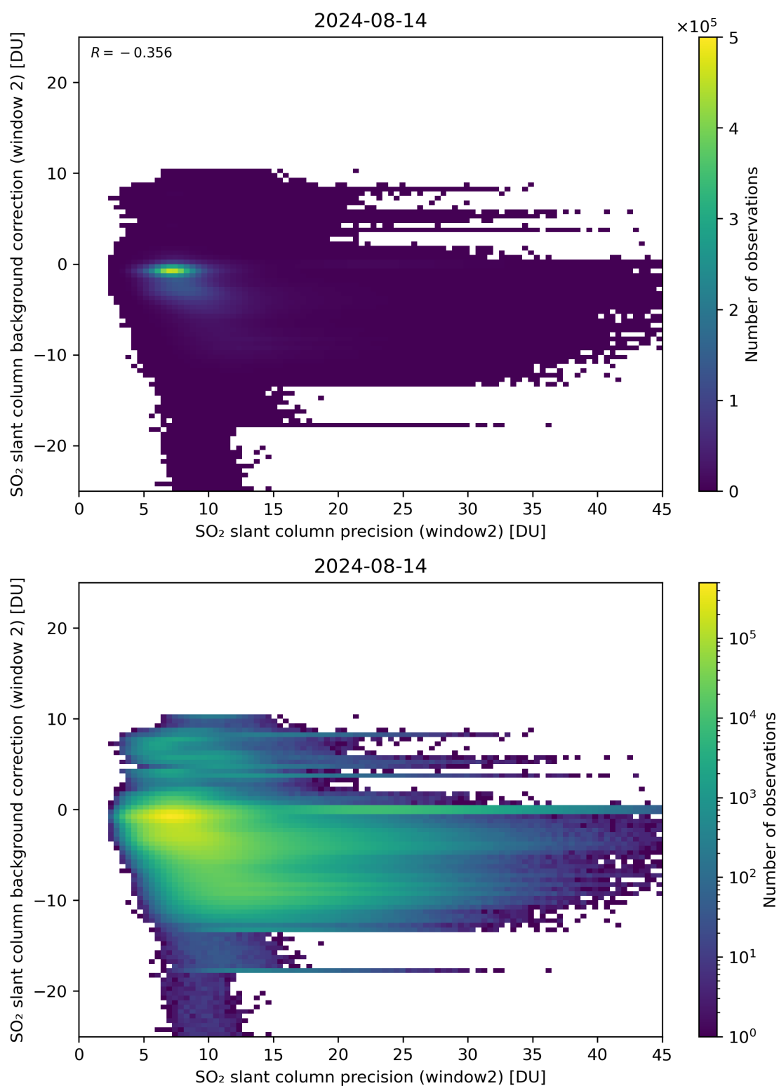
Figure 241: Scatter density plot of “SO 2 slant column precision (window2)” against “SO 2 slant column background correction (window 2)” for 2024-08-13 to 2024-08-15.
