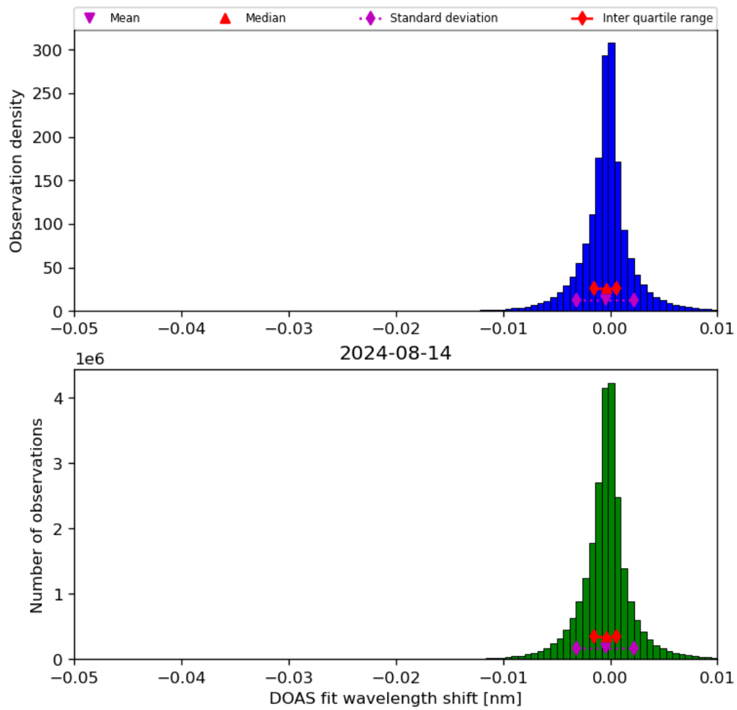
Figure 68: Histogram of “DOAS fit wavelength shift” for 2024-08-13 to 2024-08-15
