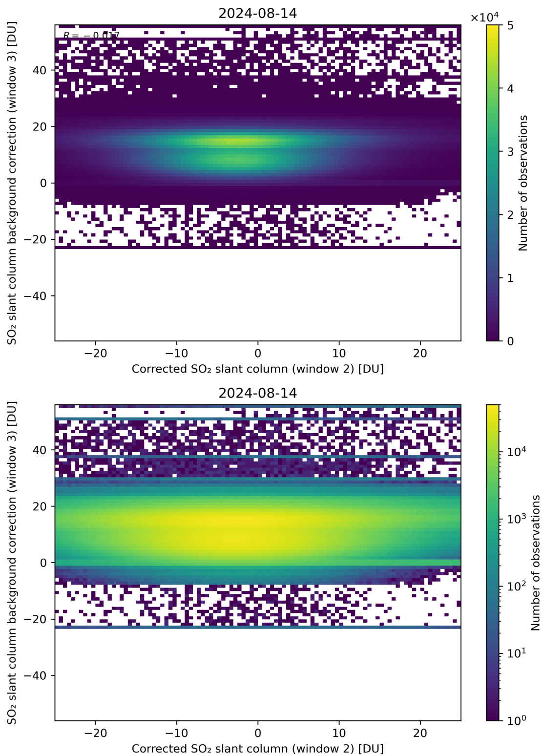
Figure 195: Scatter density plot of “Corrected SO 2 slant column (window 2)” against “SO 2 slant column background correction (window 3)” for 2024-08-13 to 2024-08-15.
