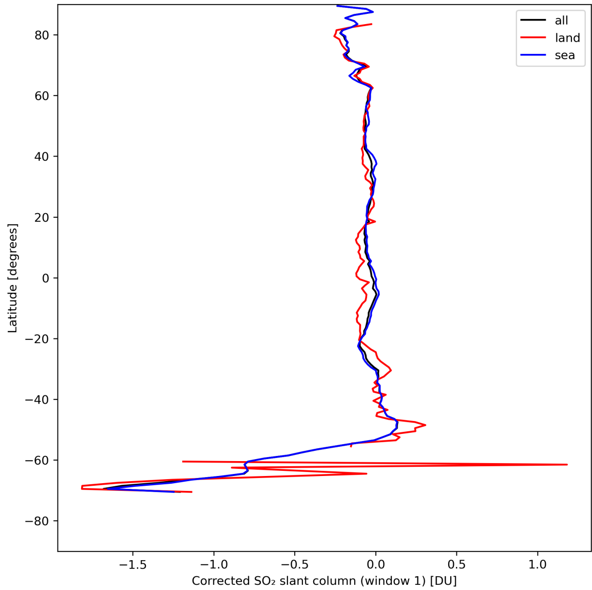
Figure 35: Zonal average of “Corrected SO 2 slant column (window 1)” for 2024-08-13 to 2024-08-15.
