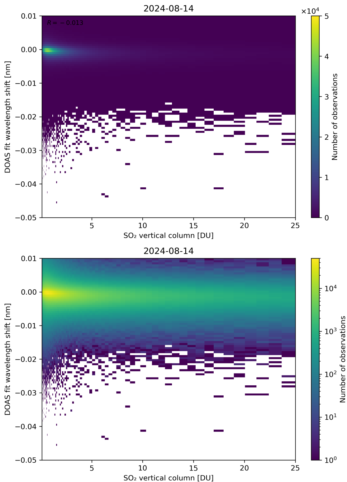
Figure 276: Scatter density plot of “SO 2 vertical column” against “DOAS fit wavelength shift” for 2024-08-13 to 2024-08-15.
