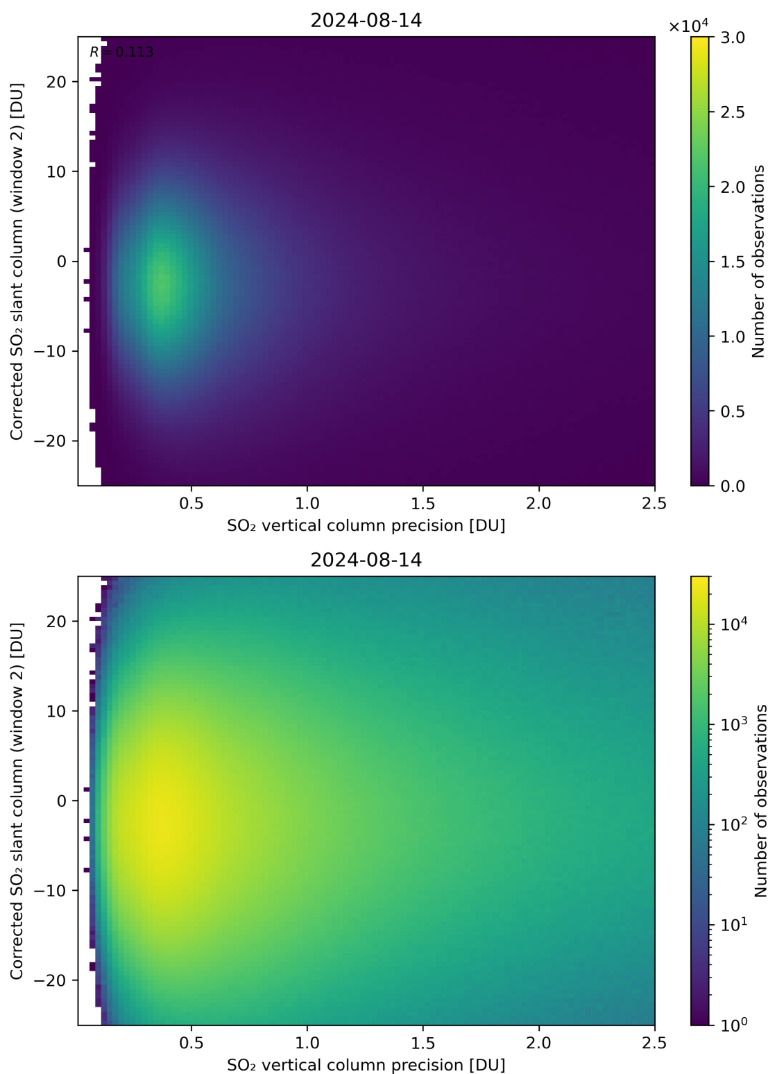
Figure 287: Scatter density plot of “SO 2 vertical column precision” against “Corrected SO 2 slant column (window 2)” for 2024-08-13 to 2024-08-15.
