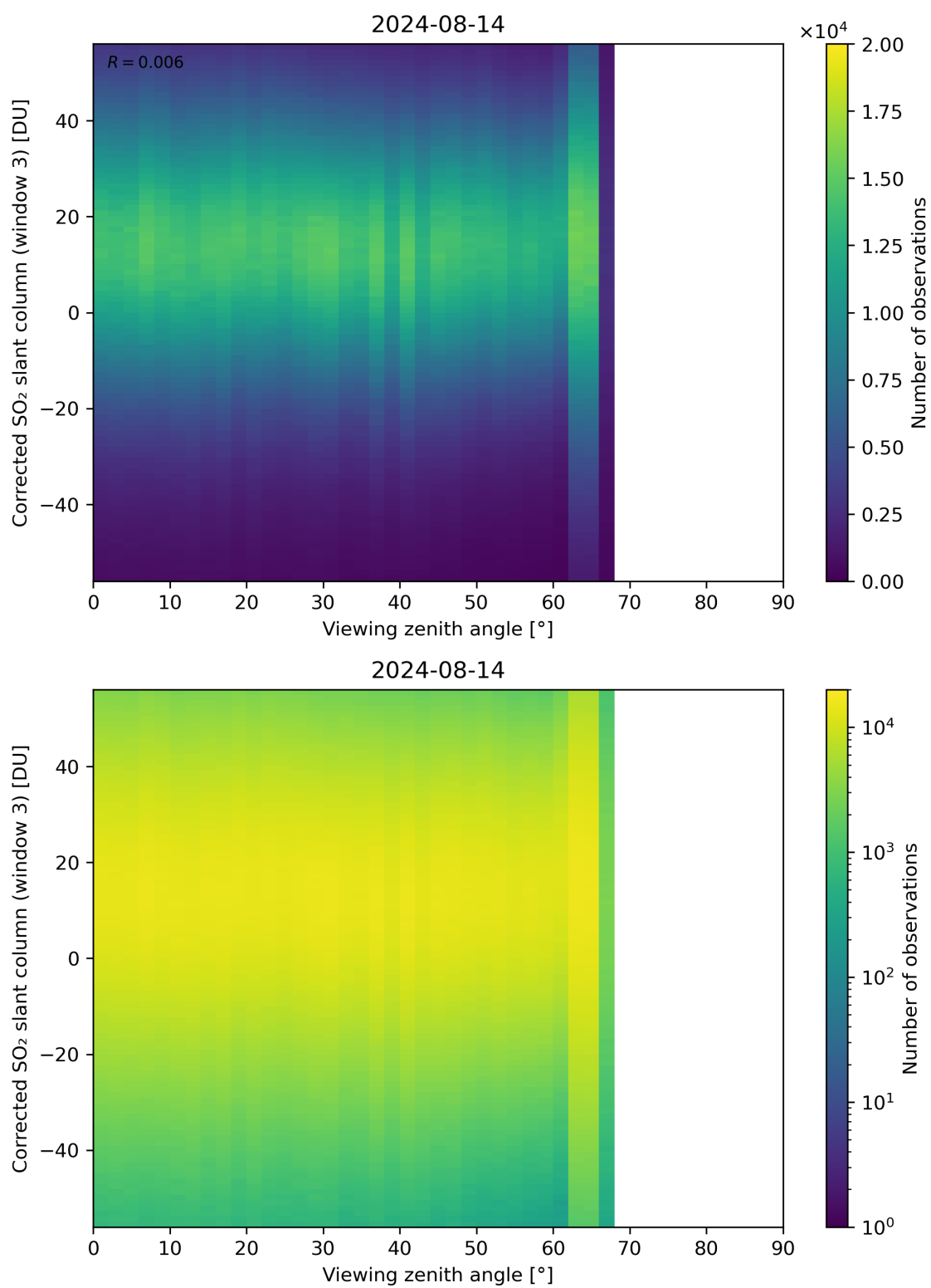
Figure 319: Scatter density plot of “Viewing zenith angle” against “Corrected SO 2 slant column (window 3)” for 2024-08-13 to 2024-08-15.
