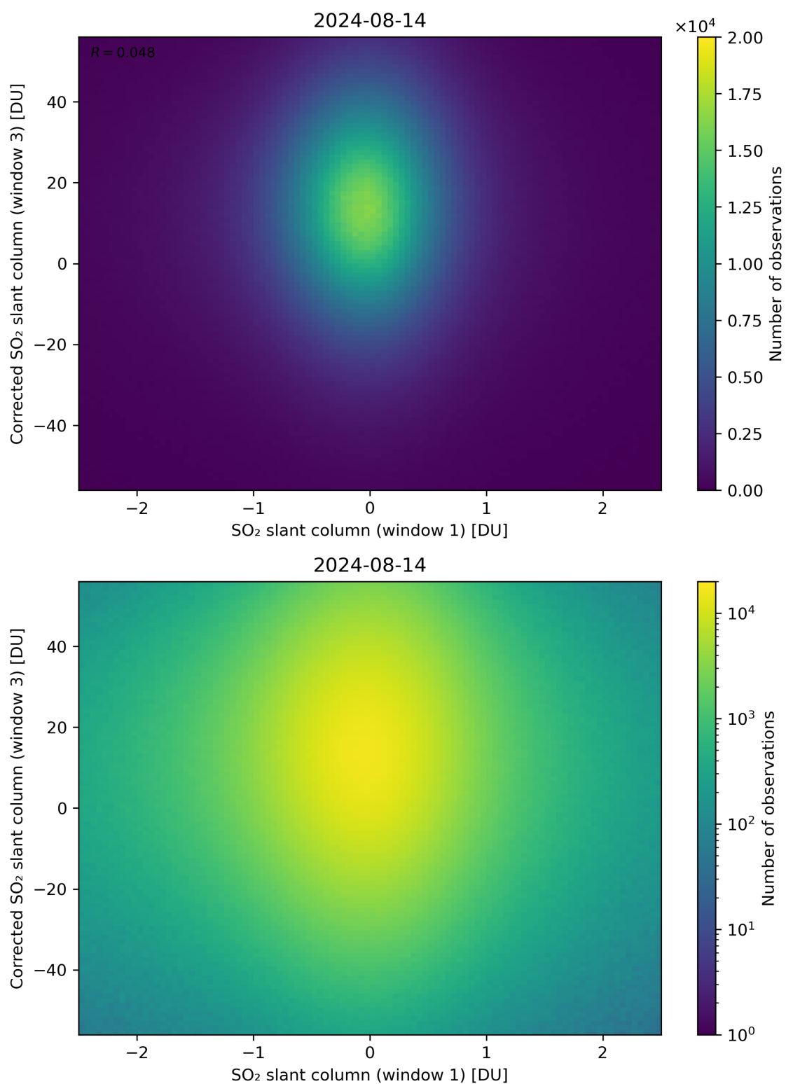
Figure 234: Scatter density plot of “SO 2 slant column (window 1)” against “Corrected SO 2 slant column (window 3)” for 2024-08-13 to 2024-08-15.
