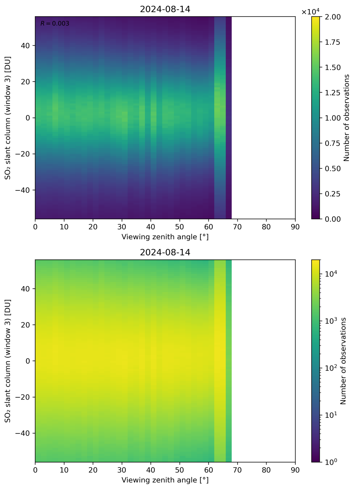
Figure 323: Scatter density plot of “Viewing zenith angle” against “SO 2 slant column (window 3)” for 2024-08-13 to 2024-08-15.
