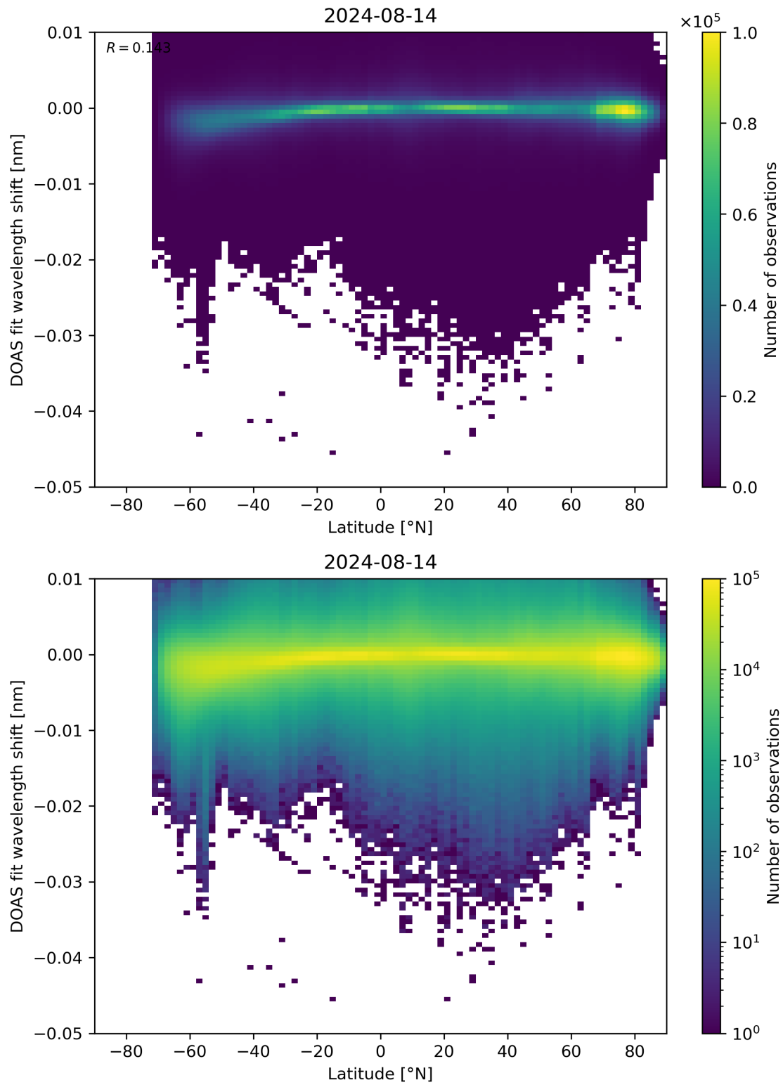
Figure 142: Scatter density plot of “Latitude” against “DOAS fit wavelength shift” for 2024-08-13 to 2024-08-15.
