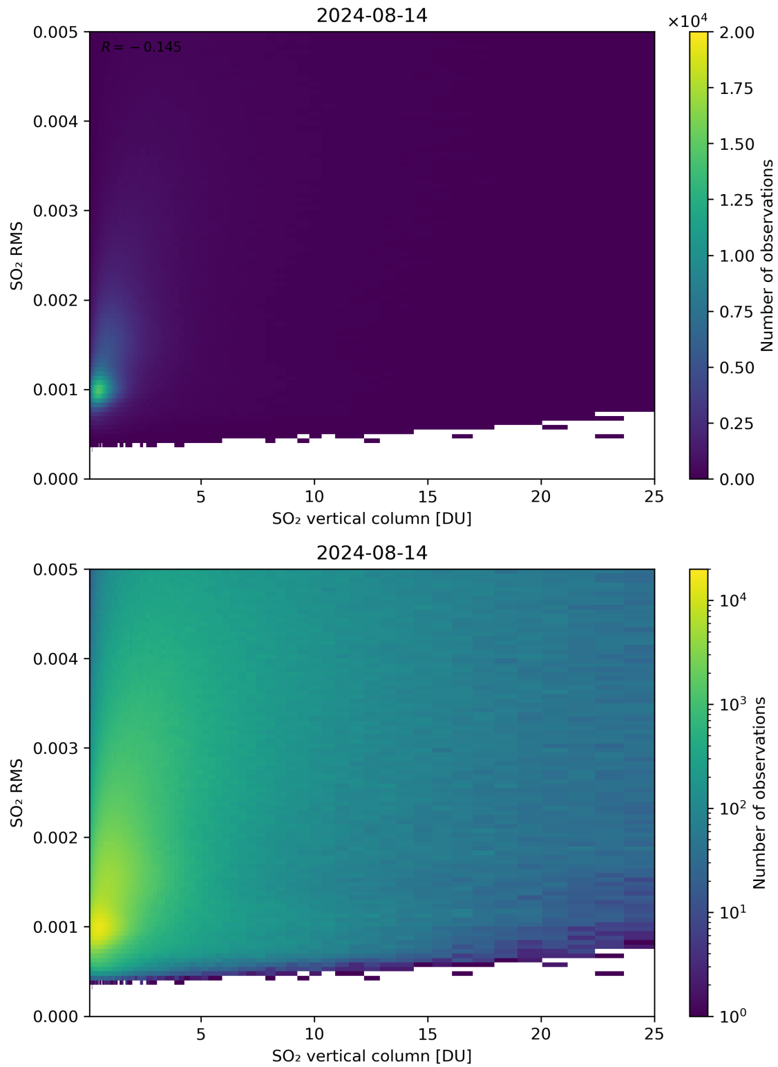
Figure 278: Scatter density plot of “SO 2 vertical column” against “SO 2 RMS” for 2024-08-13 to 2024-08-15.
