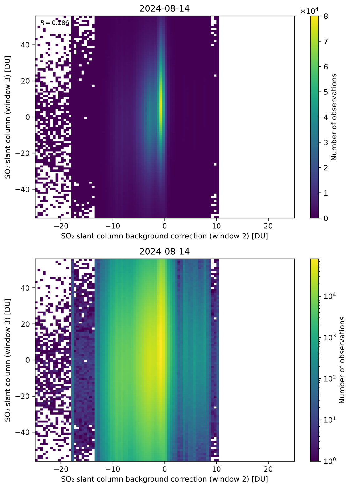
Figure 117: Scatter density plot of “SO 2 slant column background correction (window 2)” against “SO 2 slant column (window 3)” for 2024-08-13 to 2024-08-15.
