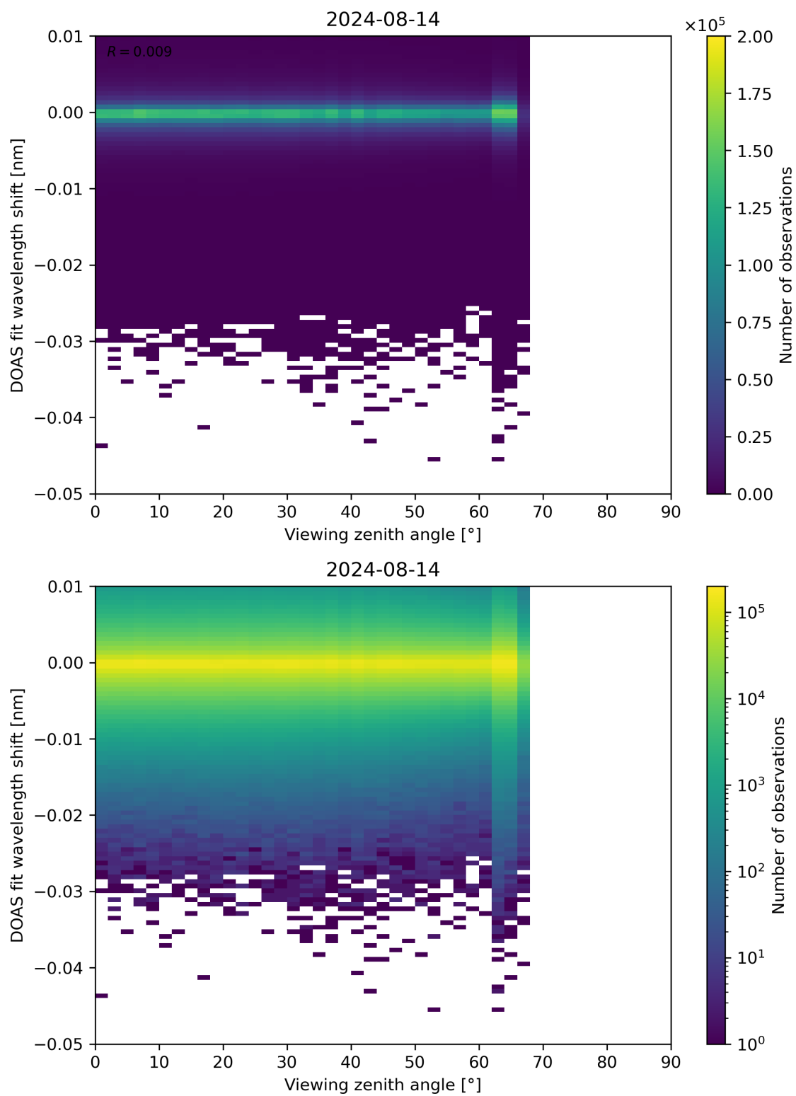
Figure 311: Scatter density plot of “Viewing zenith angle” against “DOAS fit wavelength shift” for 2024-08-13 to 2024-08-15.
