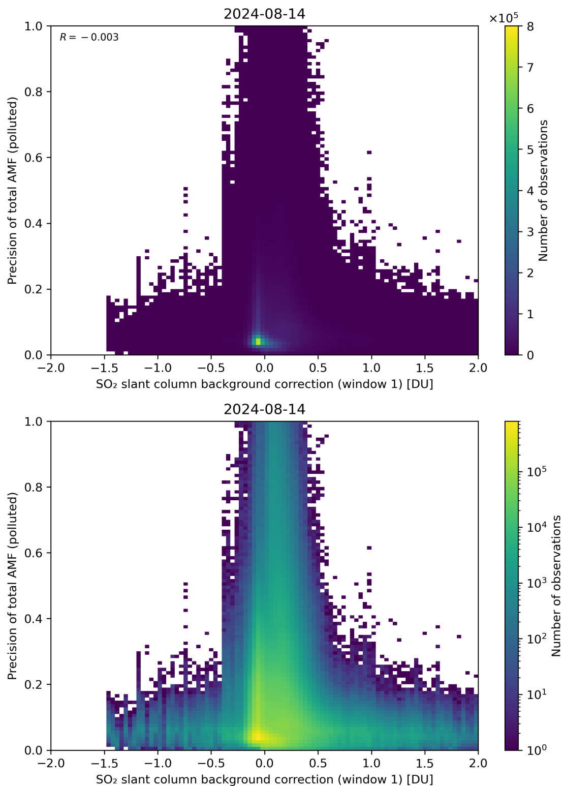
Figure 110: Scatter density plot of “SO 2 slant column background correction (window 1)” against “Precision of total AMF (polluted)” for 2024-08-13 to 2024-08-15.
