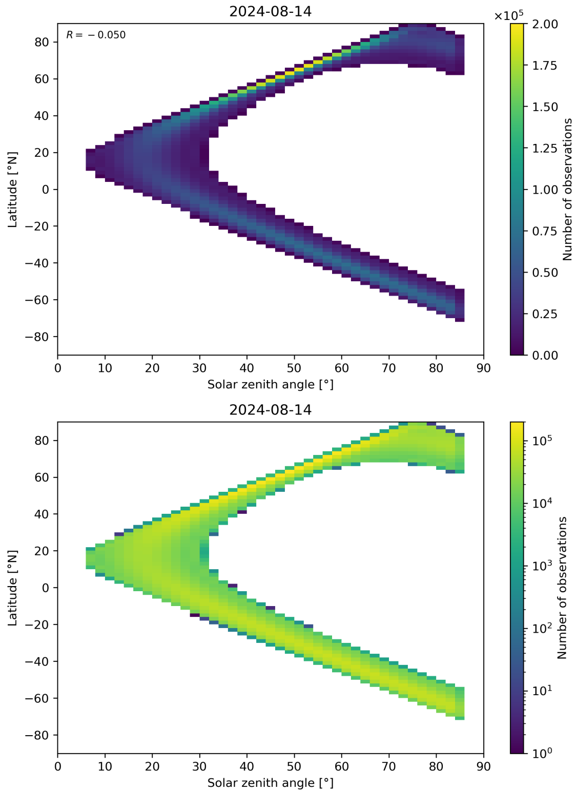
Figure 164: Scatter density plot of “Solar zenith angle” against “Latitude” for 2024-08-13 to 2024-08-15.
