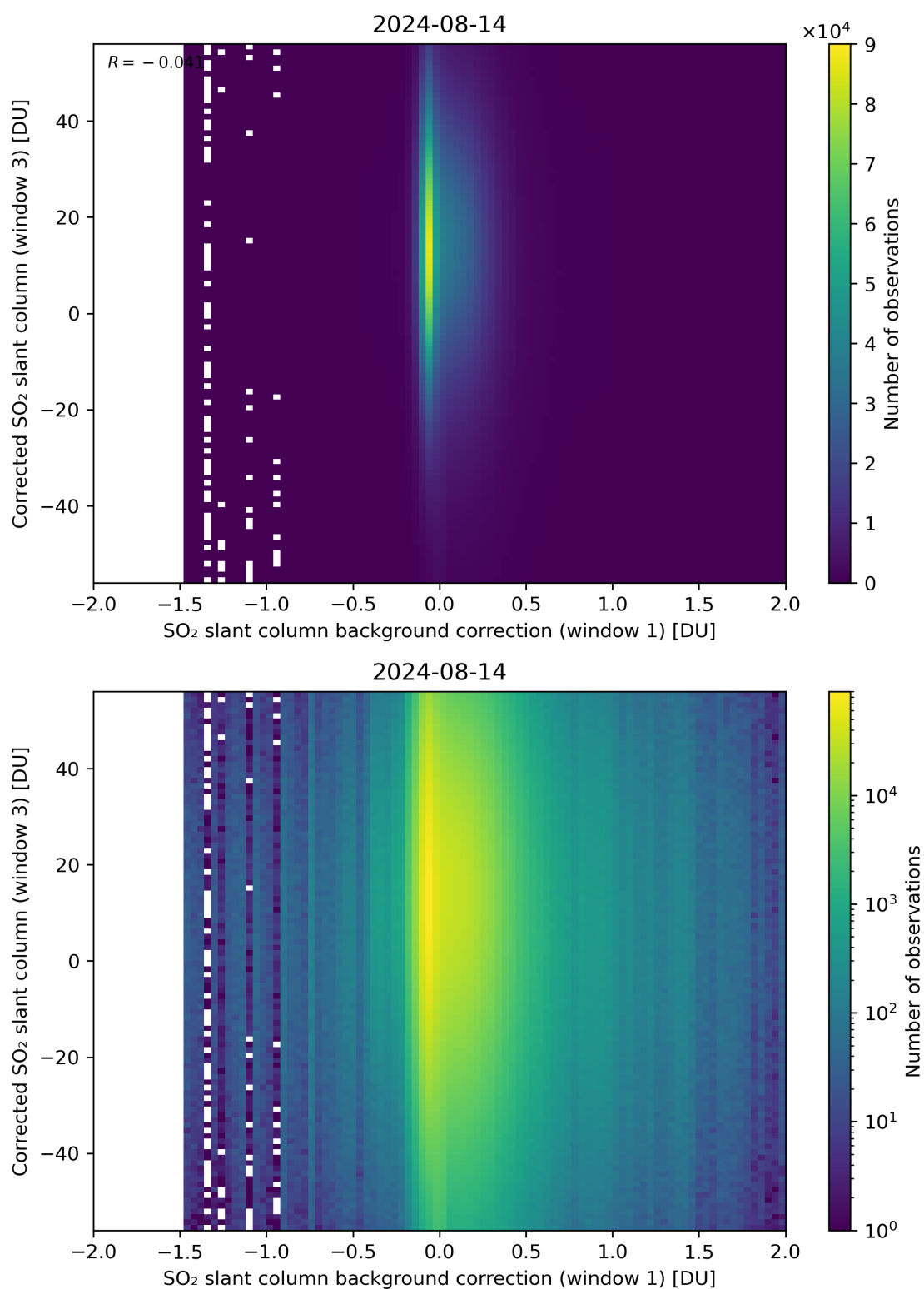
Figure 105: Scatter density plot of “SO 2 slant column background correction (window 1)” against “Corrected SO 2 slant column (window 3)” for 2024-08-13 to 2024-08-15.
