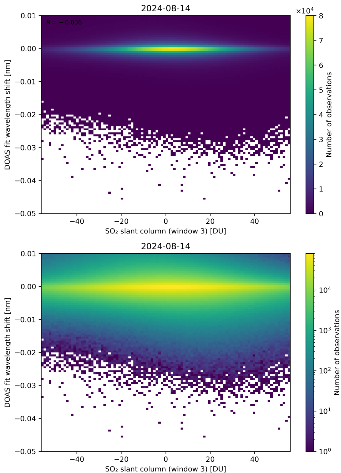
Figure 254: Scatter density plot of “SO 2 slant column (window 3)” against “DOAS fit wavelength shift” for 2024-08-13 to 2024-08-15.
