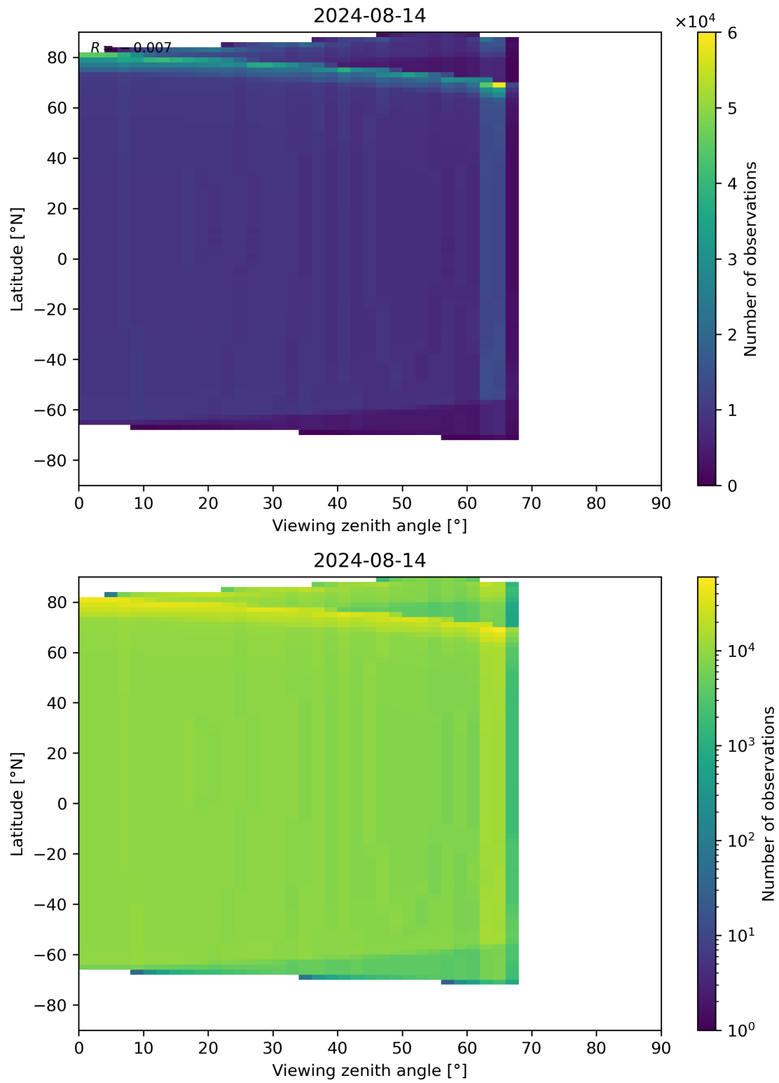
Figure 314: Scatter density plot of “Viewing zenith angle” against “Latitude” for 2024-08-13 to 2024-08-15.
