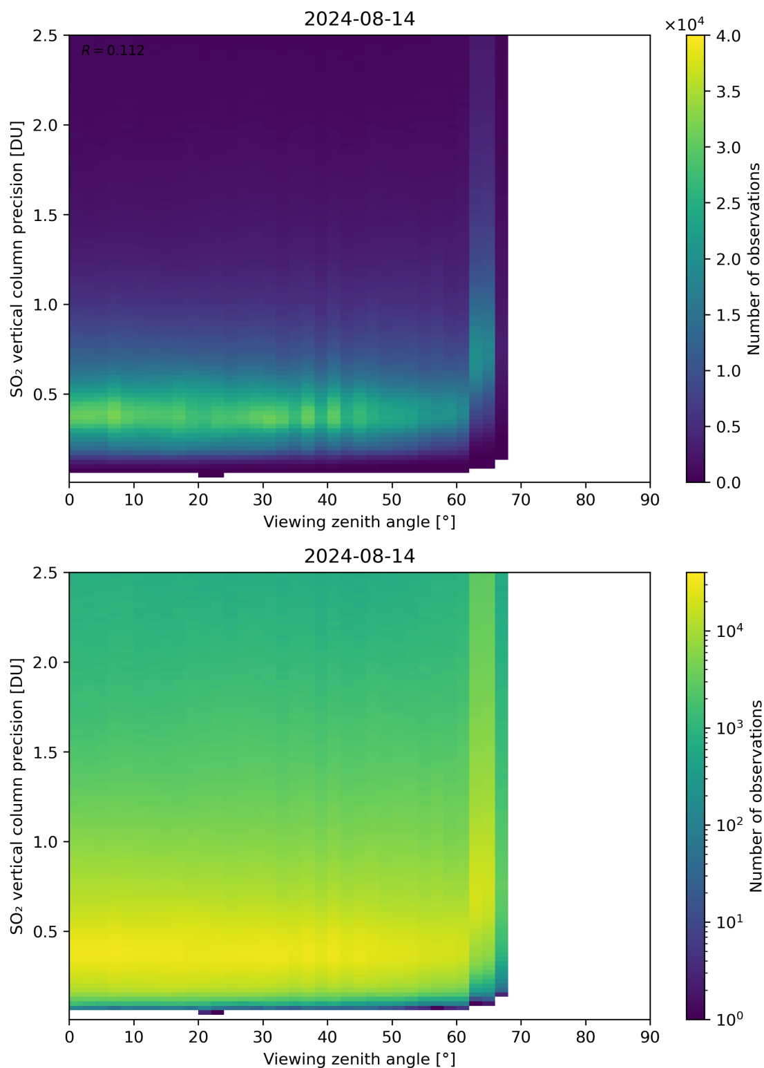
Figure 328: Scatter density plot of “Viewing zenith angle” against “SO 2 vertical column precision” for 2024-08-13 to 2024-08-15.
