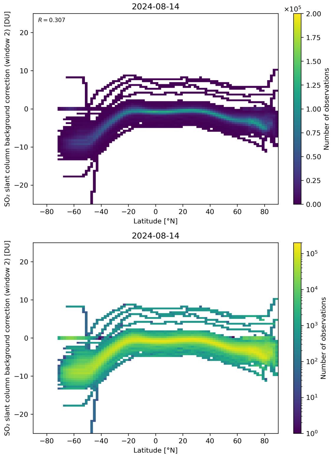
Figure 140: Scatter density plot of “Latitude” against “SO 2 slant column background correction (window 2)” for 2024-08-13 to 2024-08-15.
