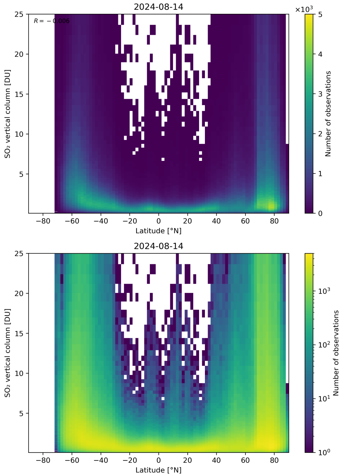
Figure 156: Scatter density plot of “Latitude” against “SO 2 vertical column” for 2024-08-13 to 2024-08-15.
