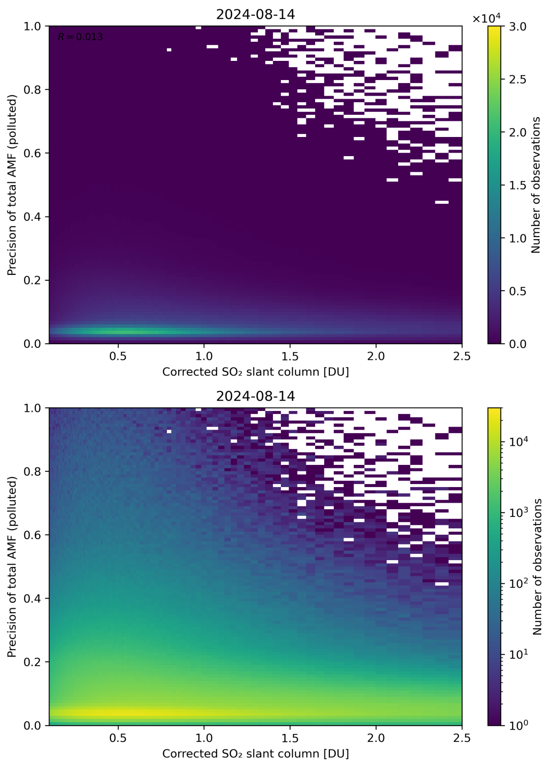
Figure 193: Scatter density plot of “Corrected SO 2 slant column” against “Precision of total AMF (polluted)” for 2024-08-13 to 2024-08-15.
