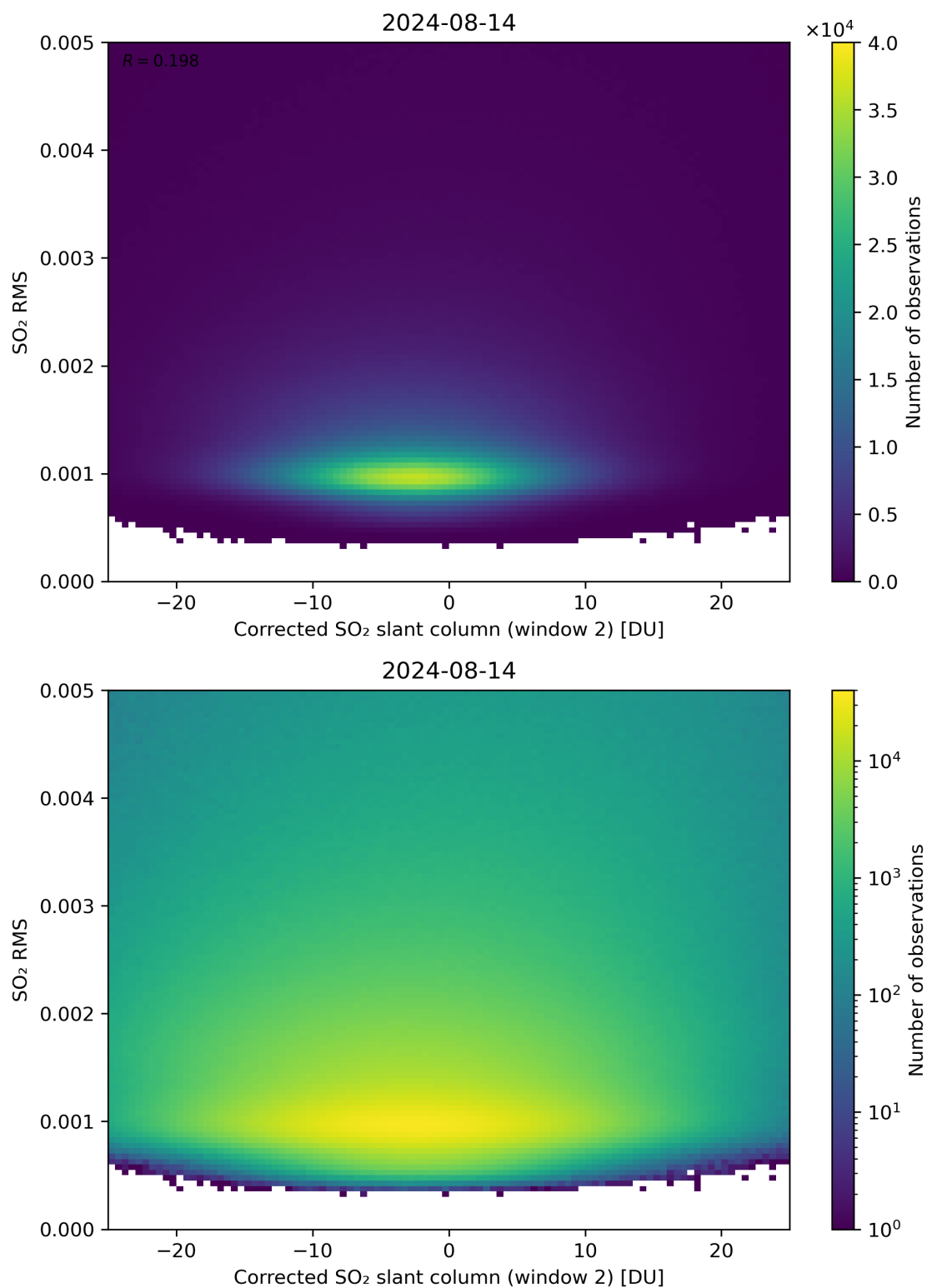
Figure 198: Scatter density plot of “Corrected SO 2 slant column (window 2)” against “SO 2 RMS” for 2024-08-13 to 2024-08-15.
