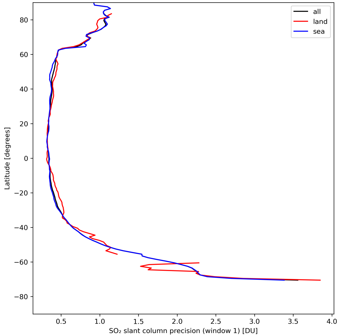
Figure 34: Zonal average of “SO 2 slant column precision (window 1)” for 2024-08-13 to 2024-08-15.
