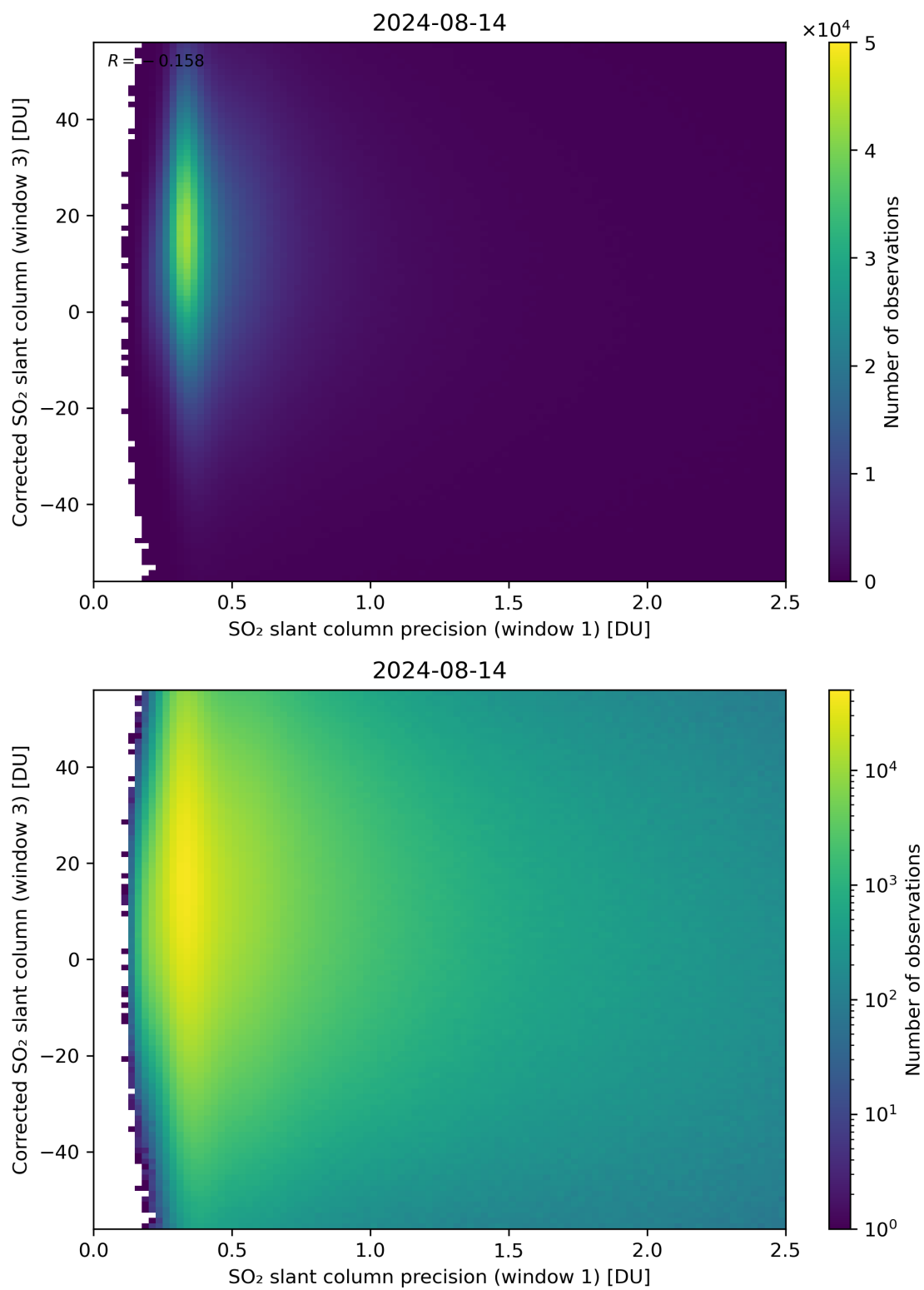
Figure 226: Scatter density plot of “SO 2 slant column precision (window 1)” against “Corrected SO 2 slant column (window 3)” for 2024-08-13 to 2024-08-15.
