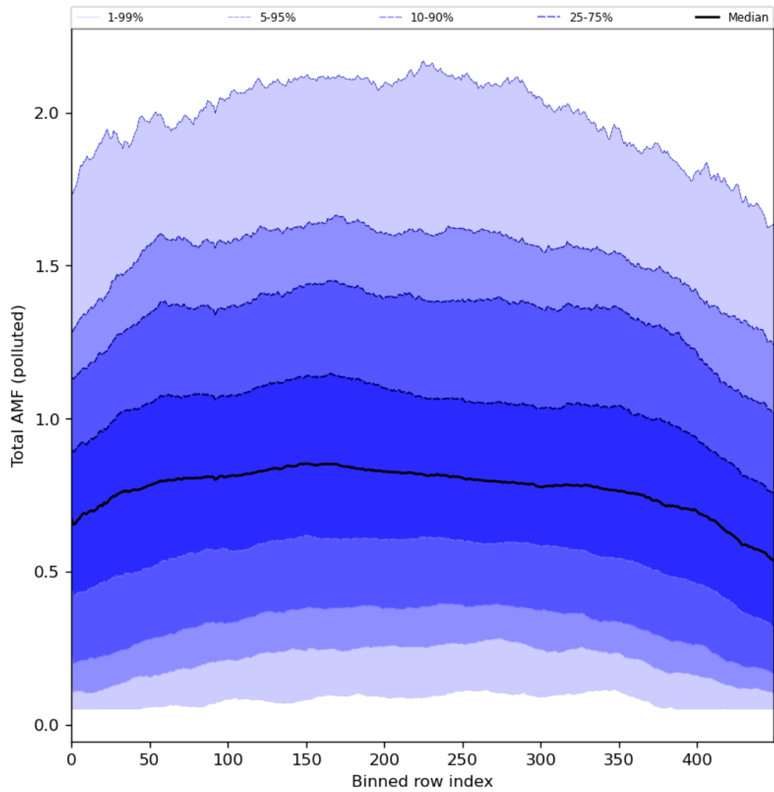
Figure 94: Along track statistics of “Total AMF (polluted)” for 2024-08-13 to 2024-08-15
