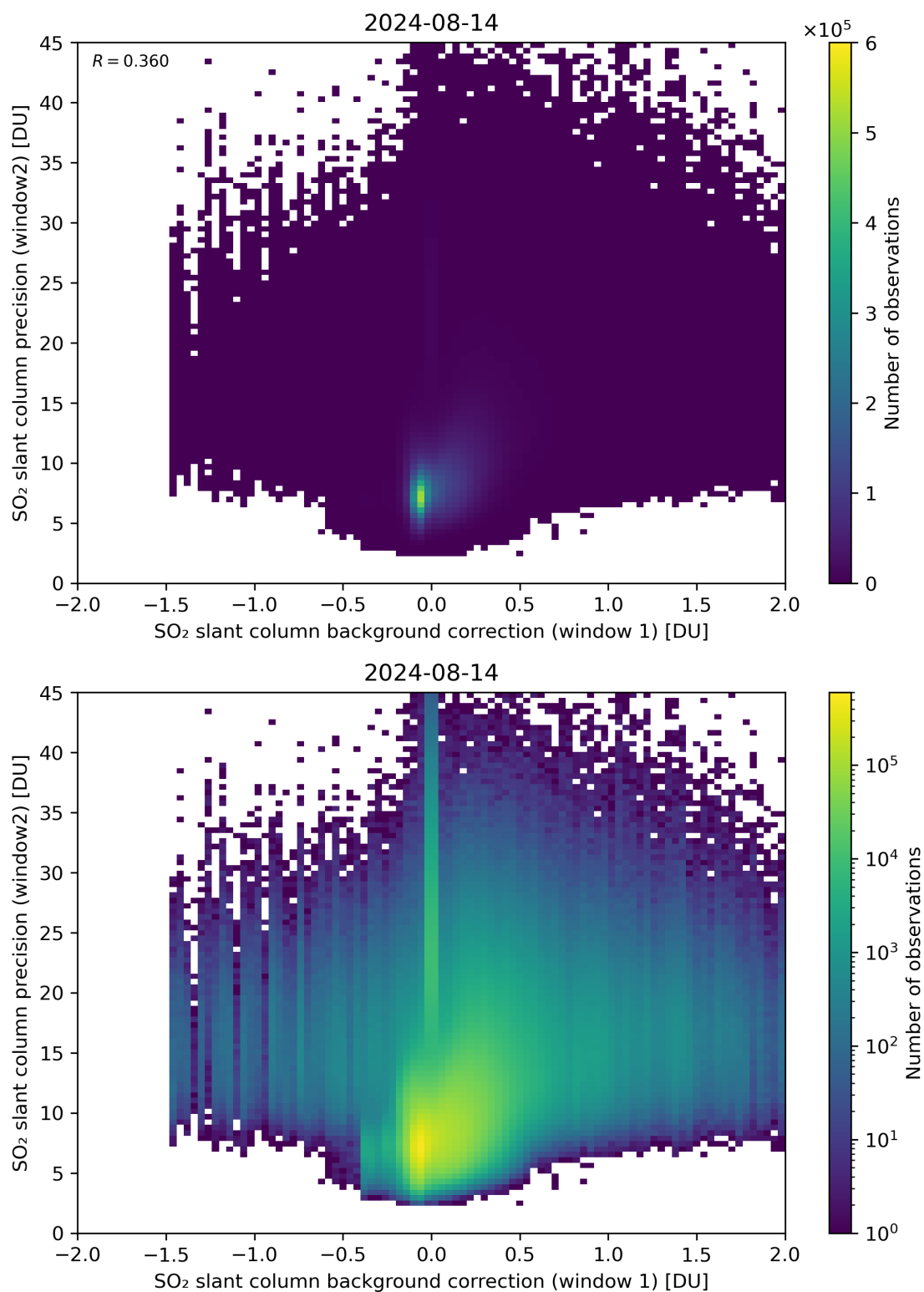
Figure 106: Scatter density plot of “SO 2 slant column background correction (window 1)” against “SO 2 slant column precision (window2)” for 2024-08-13 to 2024-08-15.
