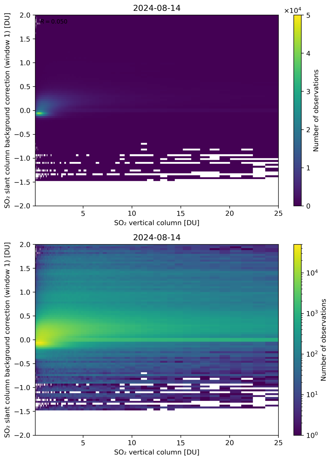
Figure 273: Scatter density plot of “SO 2 vertical column” against “SO 2 slant column background correction (window 1)” for 2024-08-13 to 2024-08-15.
