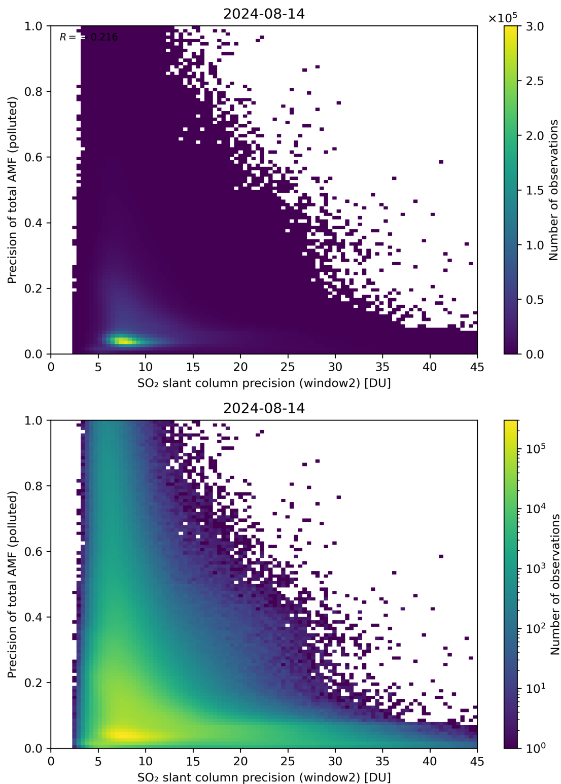
Figure 252: Scatter density plot of “SO 2 slant column precision (window2)” against “Precision of total AMF (polluted)” for 2024-08-13 to 2024-08-15.
