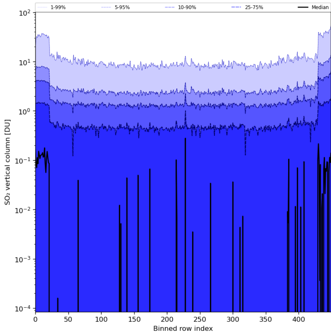
Figure 76: Along track statistics of “SO 2 vertical column” for 2024-08-13 to 2024-08-15
