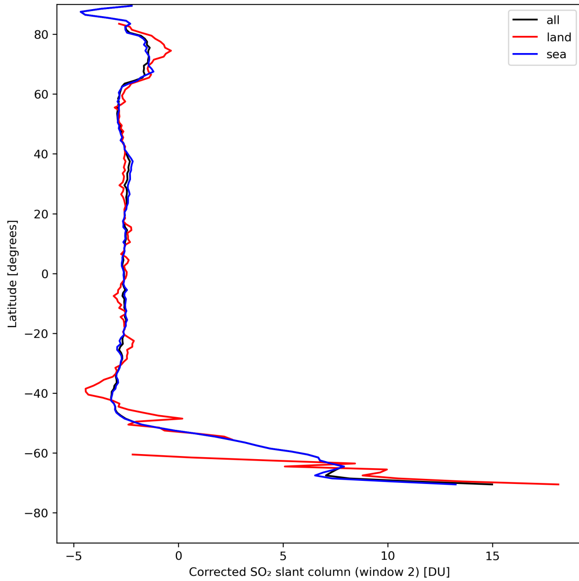
Figure 39: Zonal average of “Corrected SO 2 slant column (window 2)” for 2024-08-13 to 2024-08-15.
