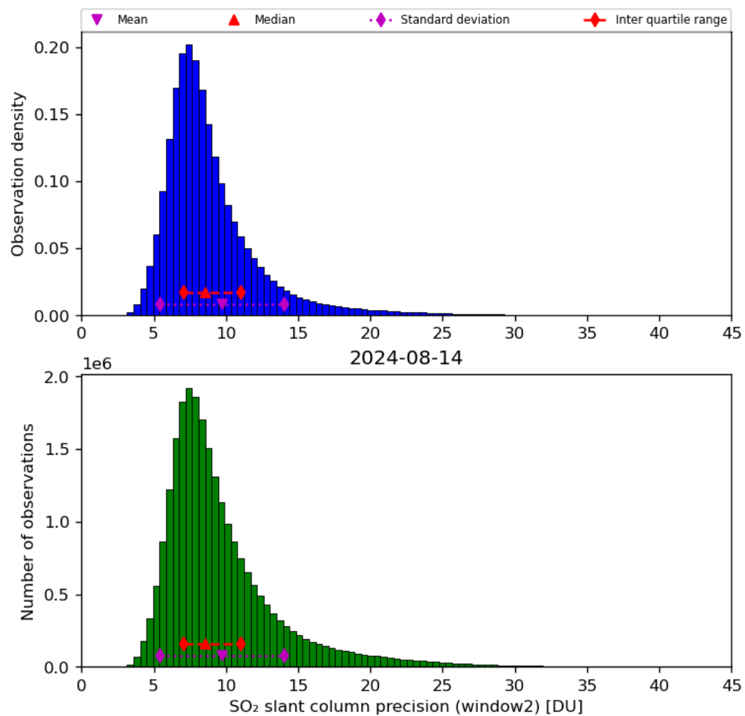
Figure 61: Histogram of “SO 2 slant column precision (window2)” for 2024-08-13 to 2024-08-15
