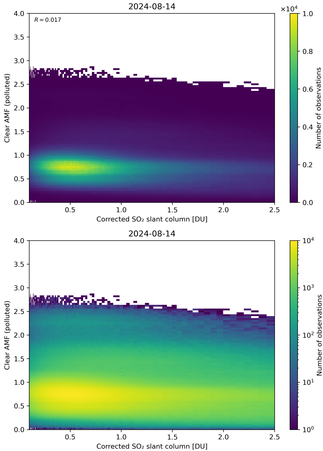
Figure 184: Scatter density plot of “Corrected SO 2 slant column” against “Clear AMF (polluted)” for 2024-08-13 to 2024-08-15.
