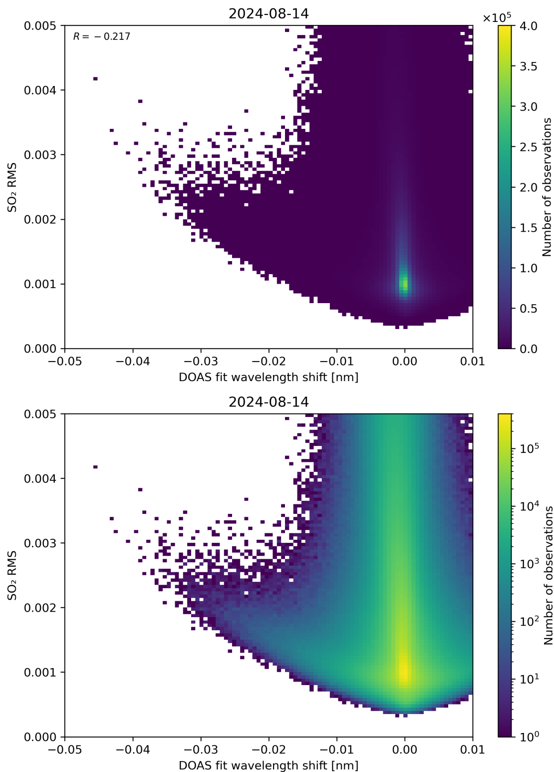
Figure 128: Scatter density plot of “DOAS fit wavelength shift” against “SO 2 RMS” for 2024-08-13 to 2024-08-15.
