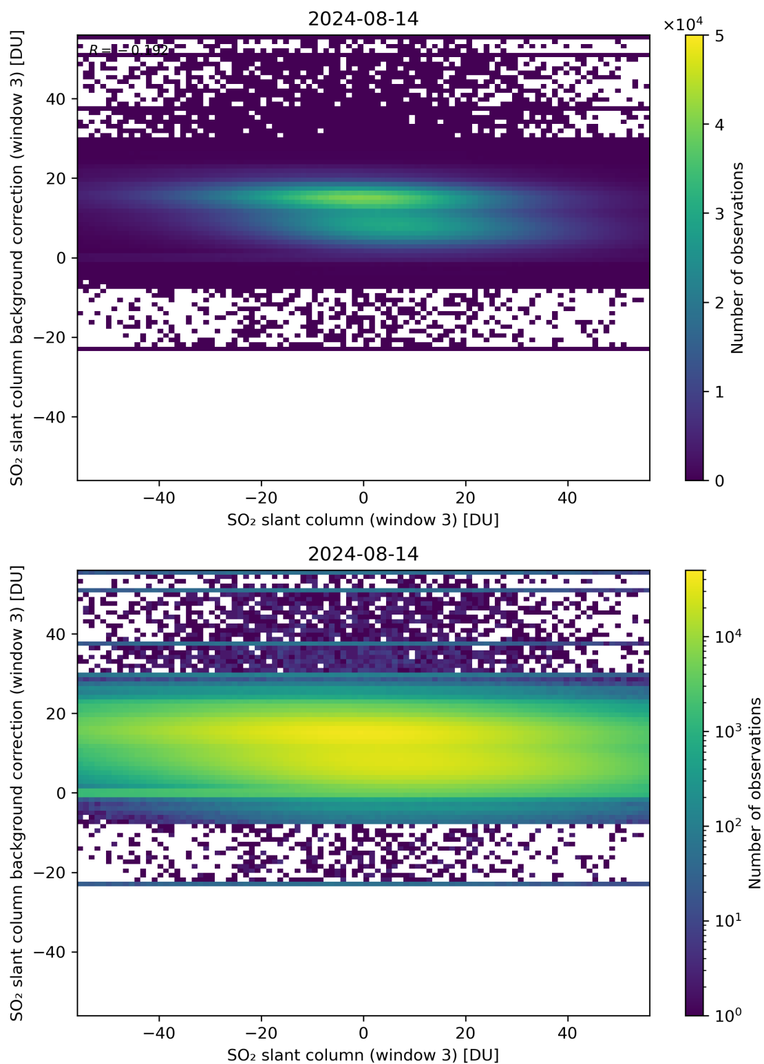
Figure 253: Scatter density plot of “SO 2 slant column (window 3)” against “SO 2 slant column background correction (window 3)” for 2024-08-13 to 2024-08-15.
