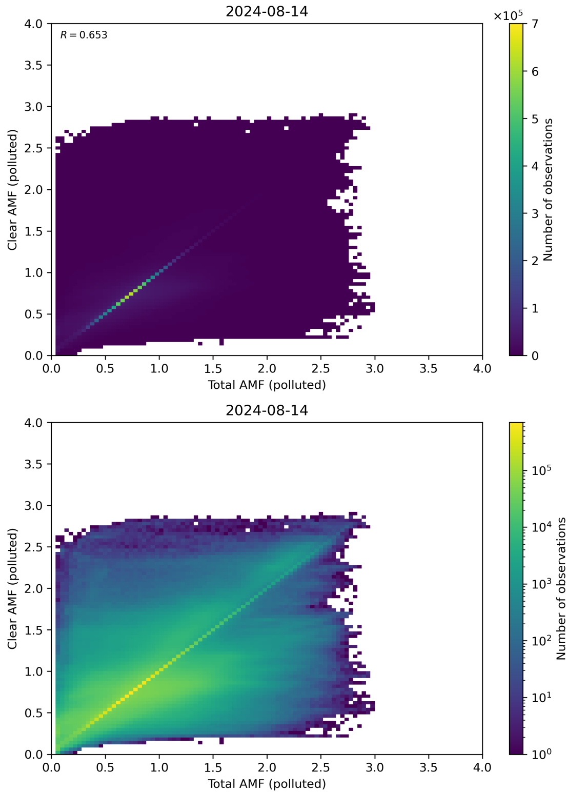
Figure 271: Scatter density plot of “Total AMF (polluted)” against “Clear AMF (polluted)” for 2024-08-13 to 2024-08-15.
