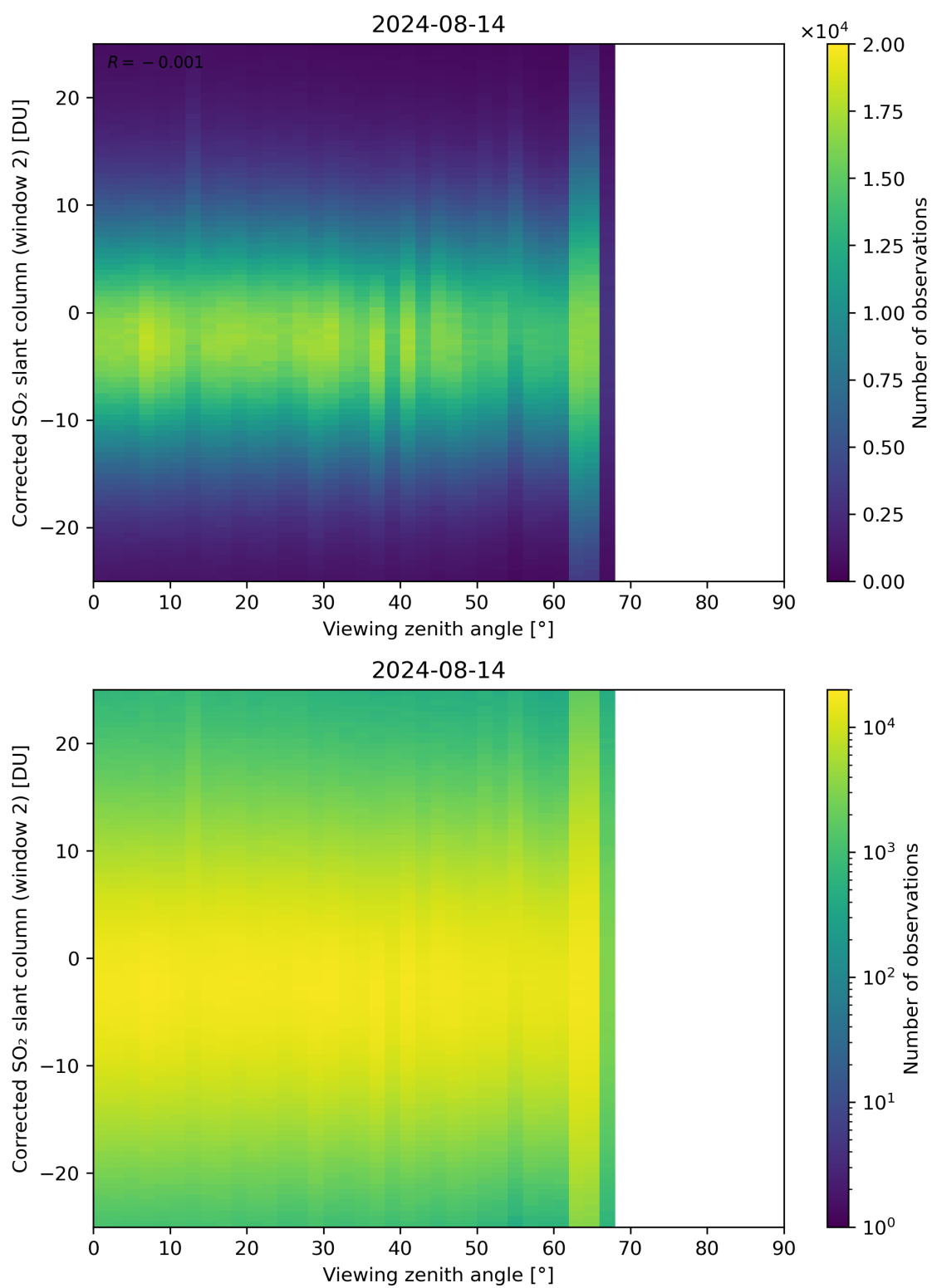
Figure 318: Scatter density plot of “Viewing zenith angle” against “Corrected SO 2 slant column (window 2)” for 2024-08-13 to 2024-08-15.
