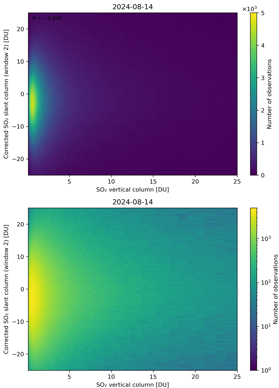
Figure 298: Scatter density plot of “SO 2 vertical column” against “Corrected SO 2 slant column (window 2)” for 2024-08-13 to 2024-08-15.
