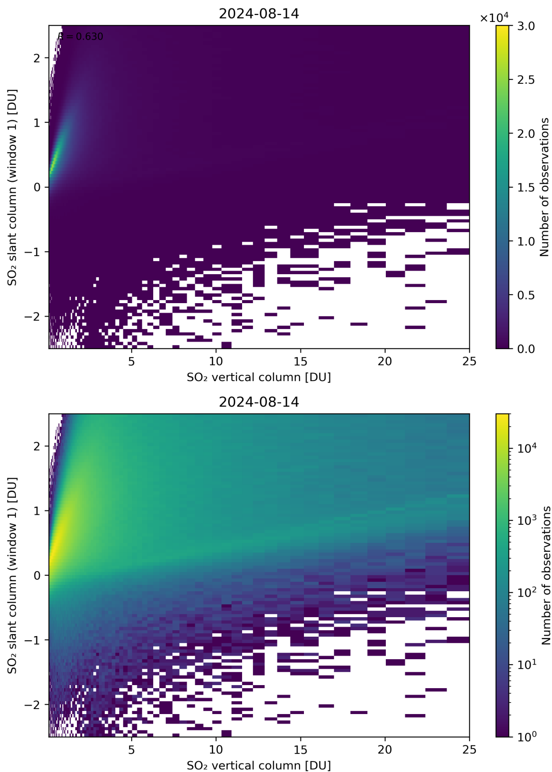
Figure 300: Scatter density plot of “SO 2 vertical column” against “SO 2 slant column (window 1)” for 2024-08-13 to 2024-08-15.
