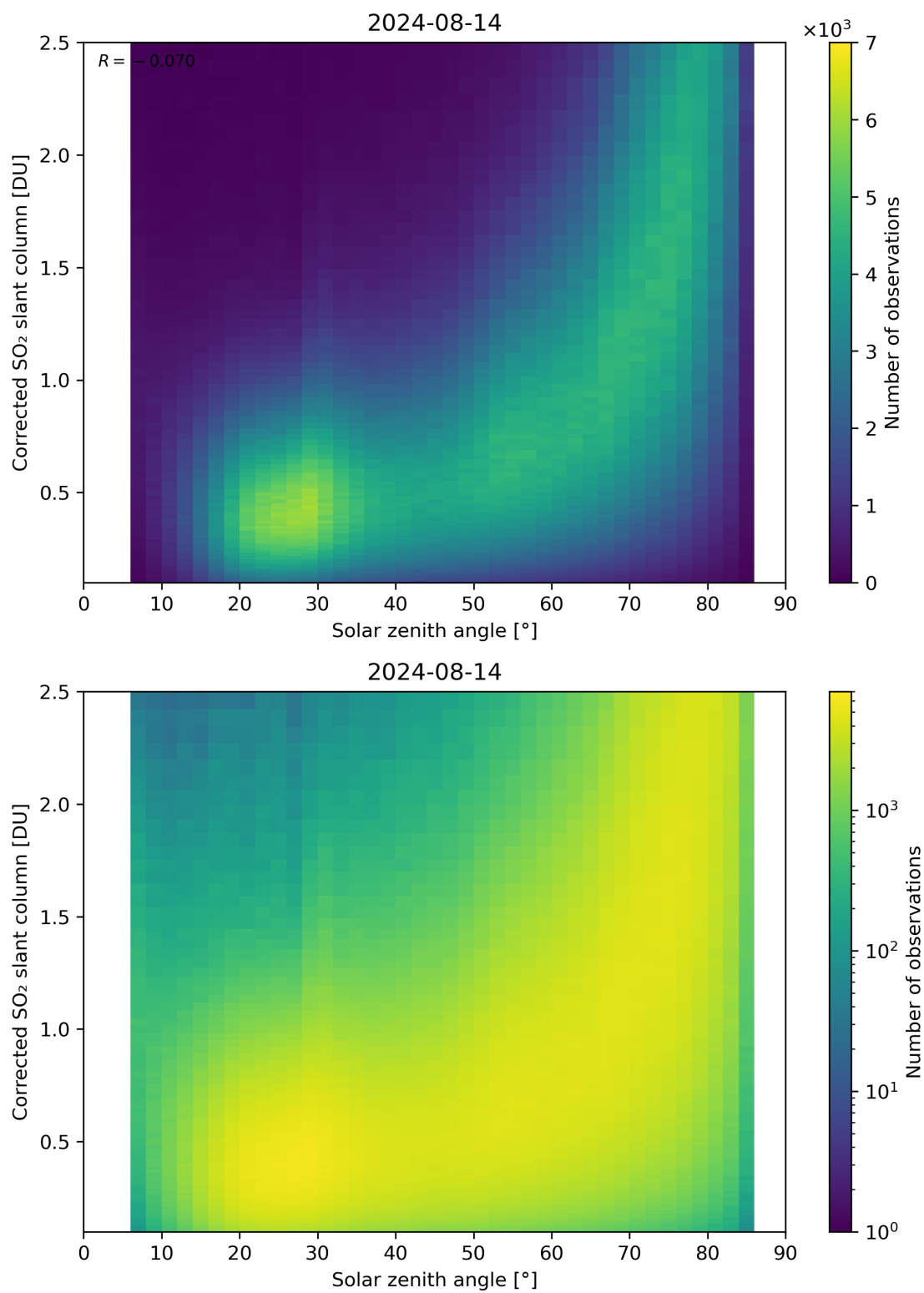
Figure 166: Scatter density plot of “Solar zenith angle” against “Corrected SO 2 slant column” for 2024-08-13 to 2024-08-15.
