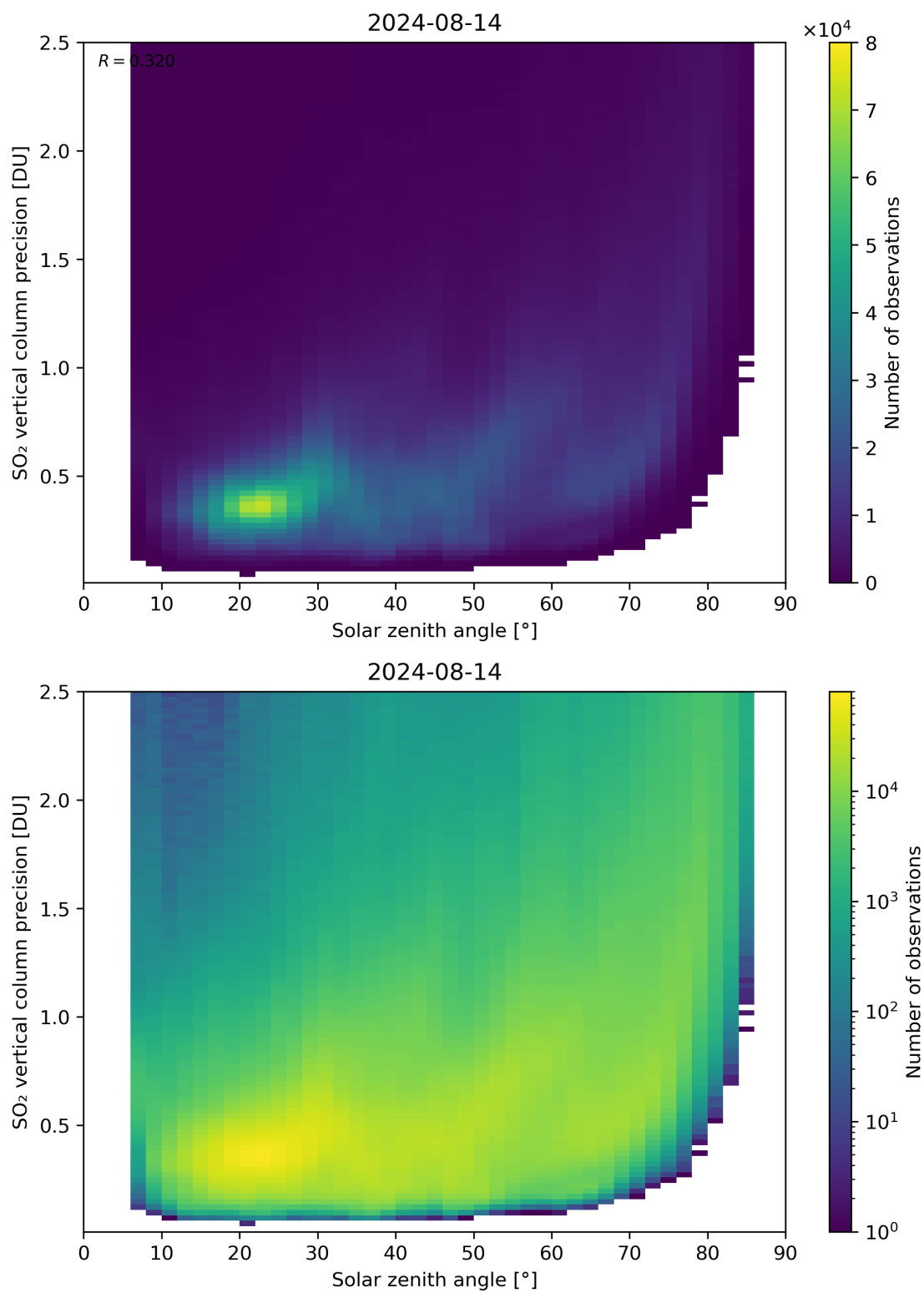
Figure 177: Scatter density plot of “Solar zenith angle” against “SO 2 vertical column precision” for 2024-08-13 to 2024-08-15.
