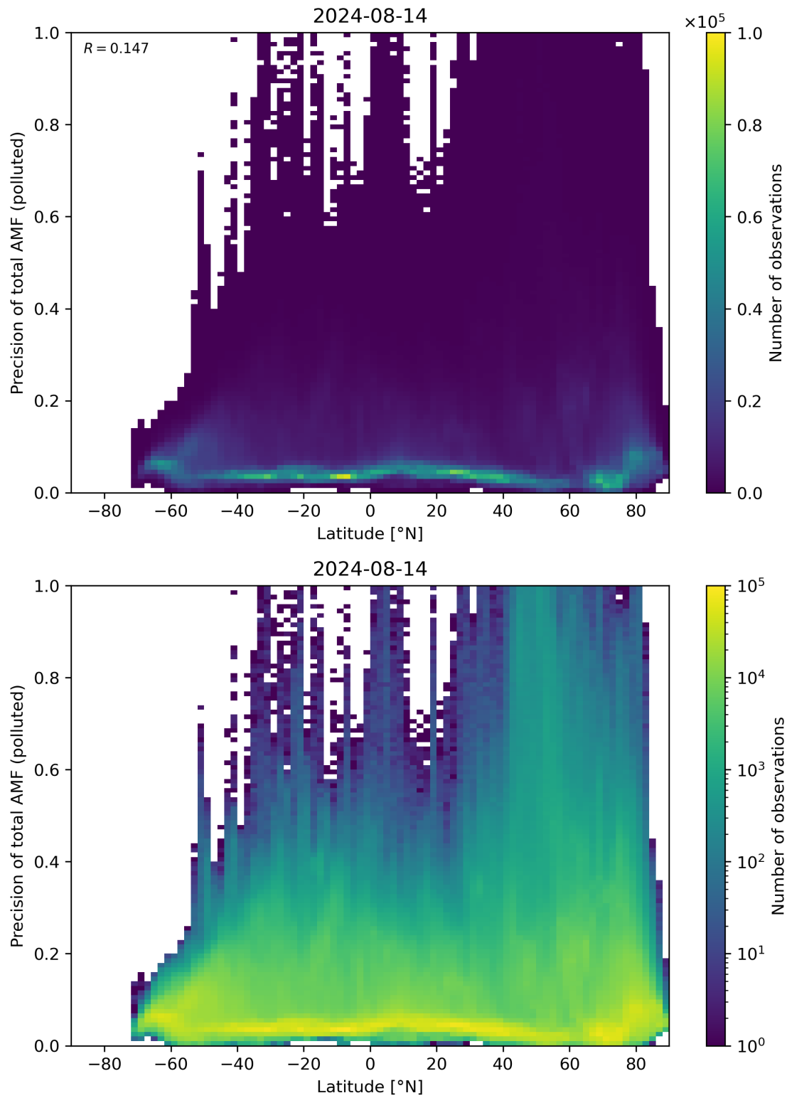
Figure 155: Scatter density plot of “Latitude” against “Precision of total AMF (polluted)” for 2024-08-13 to 2024-08-15.
