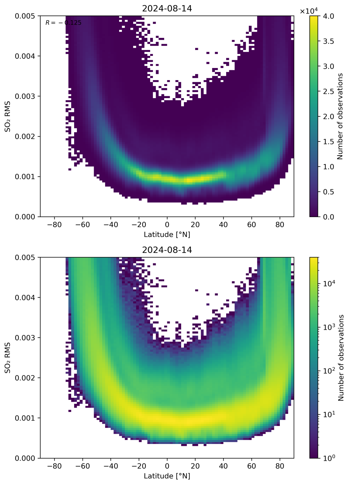
Figure 144: Scatter density plot of “Latitude” against “SO 2 RMS” for 2024-08-13 to 2024-08-15.
