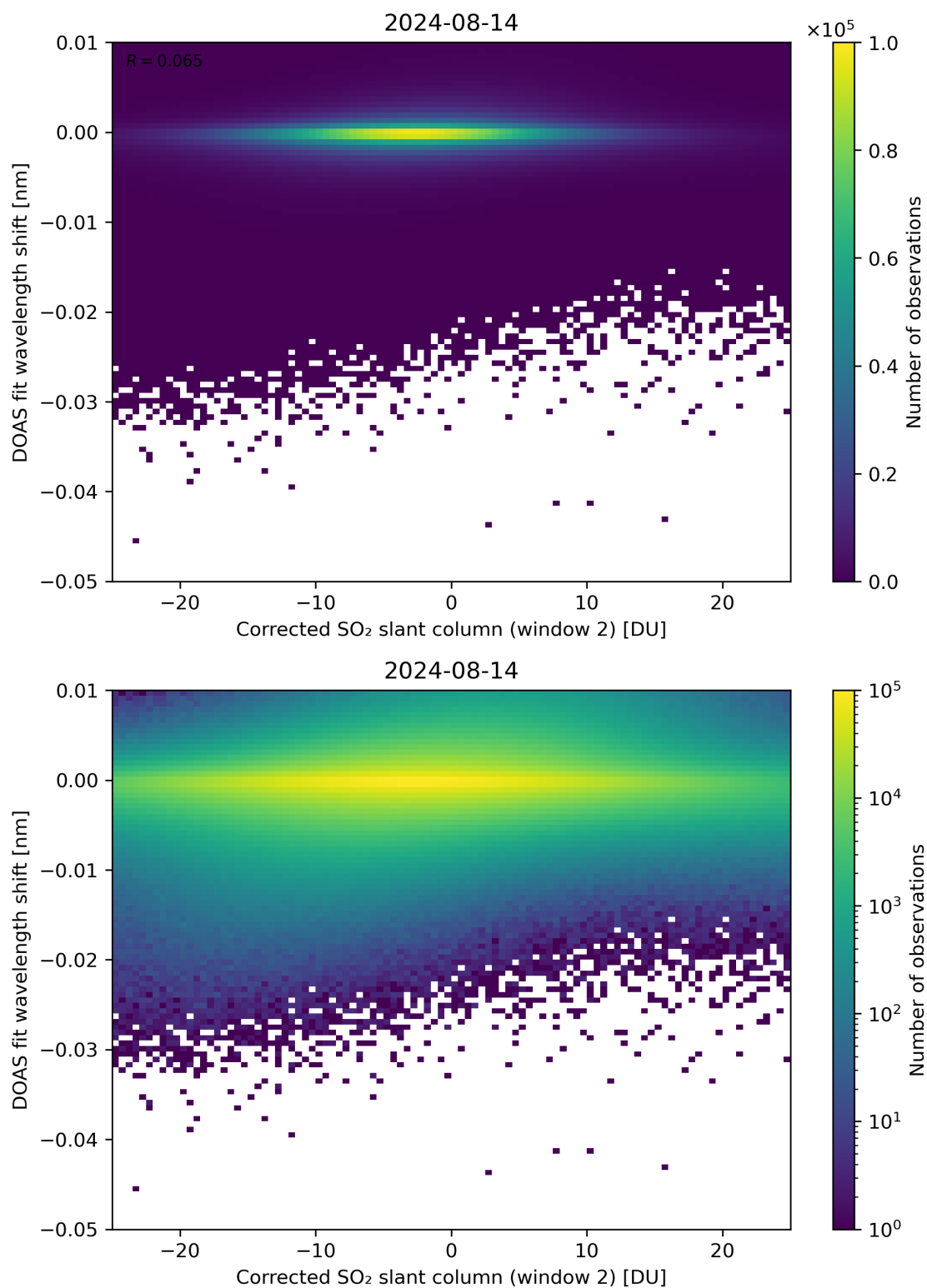
Figure 196: Scatter density plot of “Corrected SO 2 slant column (window 2)” against “DOAS fit wavelength shift” for 2024-08-13 to 2024-08-15.
