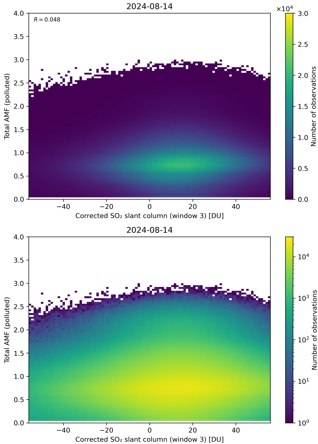
Figure 210: Scatter density plot of “Corrected SO 2 slant column (window 3)” against “Total AMF (polluted)” for 2024-08-13 to 2024-08-15.
