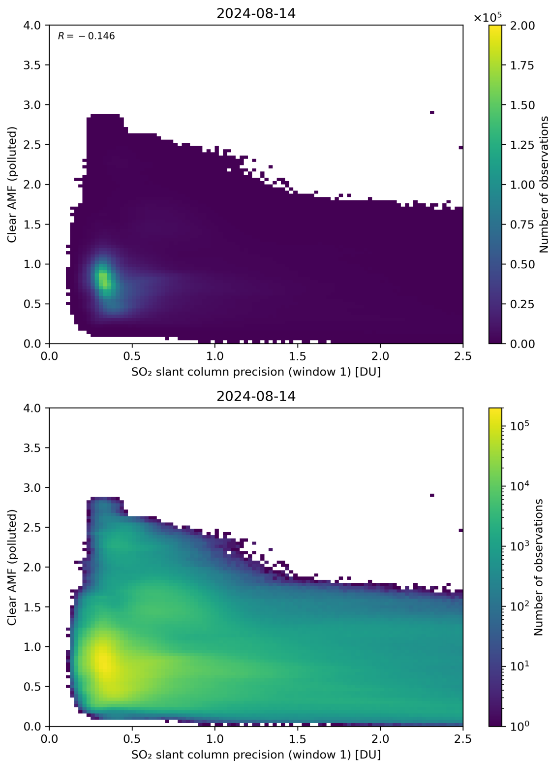
Figure 224: Scatter density plot of “SO 2 slant column precision (window 1)” against “Clear AMF (polluted)” for 2024-08-13 to 2024-08-15.
