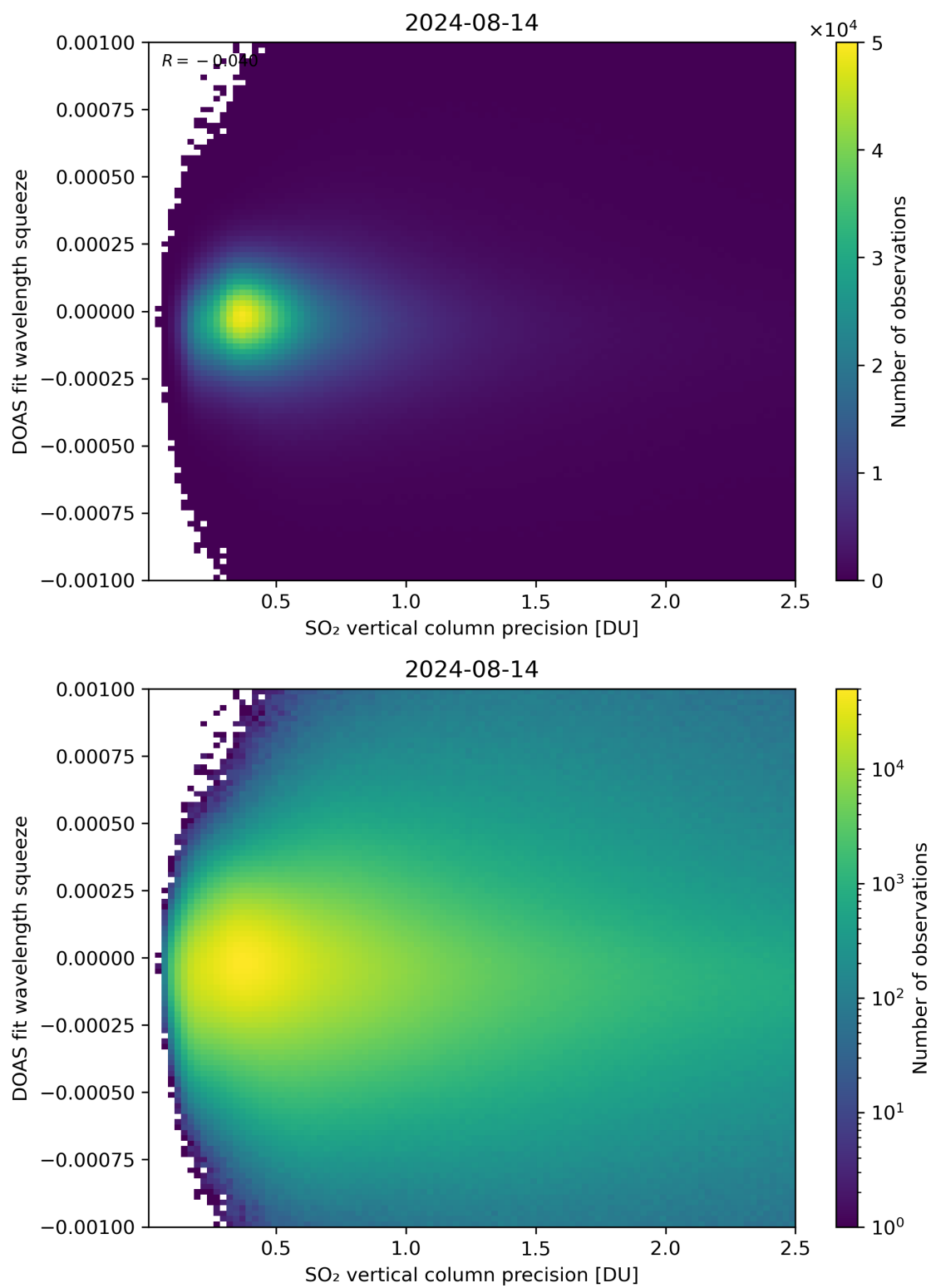
Figure 283: Scatter density plot of “SO 2 vertical column precision” against “DOAS fit wavelength squeeze” for 2024-08-13 to 2024-08-15.
