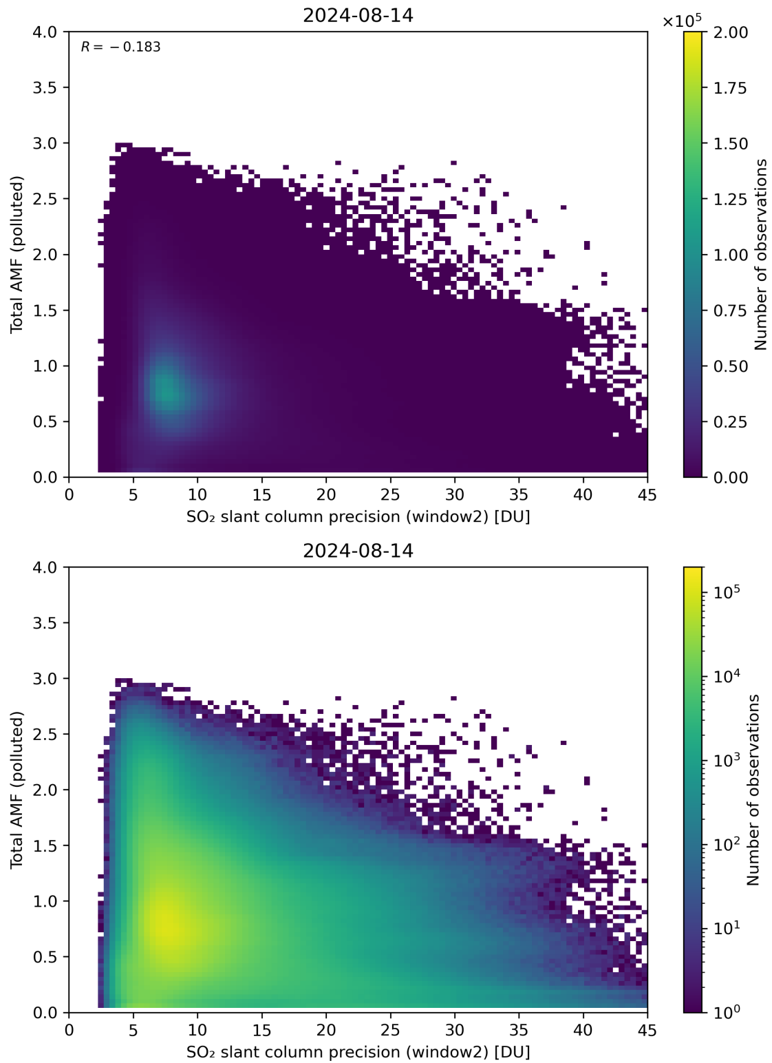
Figure 251: Scatter density plot of “SO 2 slant column precision (window2)” against “Total AMF (polluted)” for 2024-08-13 to 2024-08-15.
