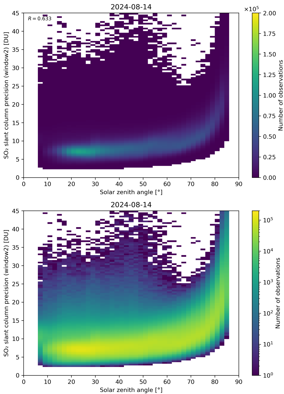
Figure 171: Scatter density plot of “Solar zenith angle” against “SO 2 slant column precision (window2)” for 2024-08-13 to 2024-08-15.
