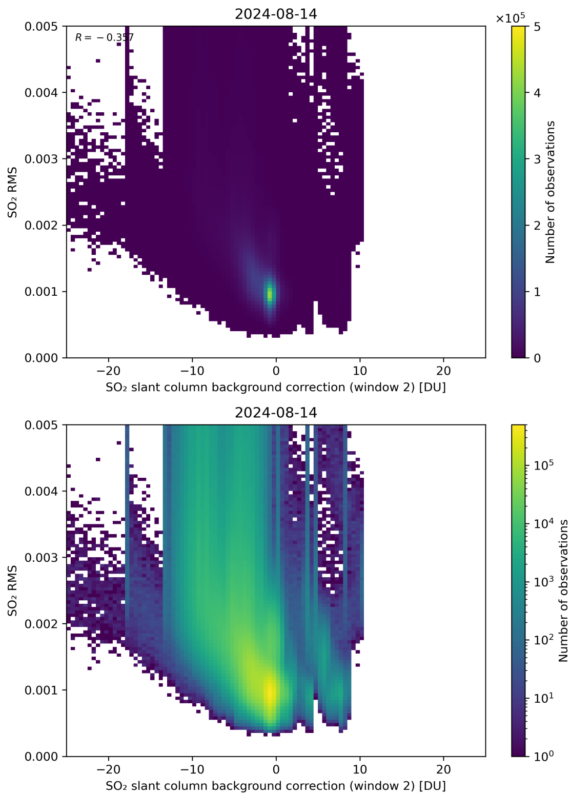
Figure 114: Scatter density plot of “SO 2 slant column background correction (window 2)” against “SO 2 RMS” for 2024-08-13 to 2024-08-15.
