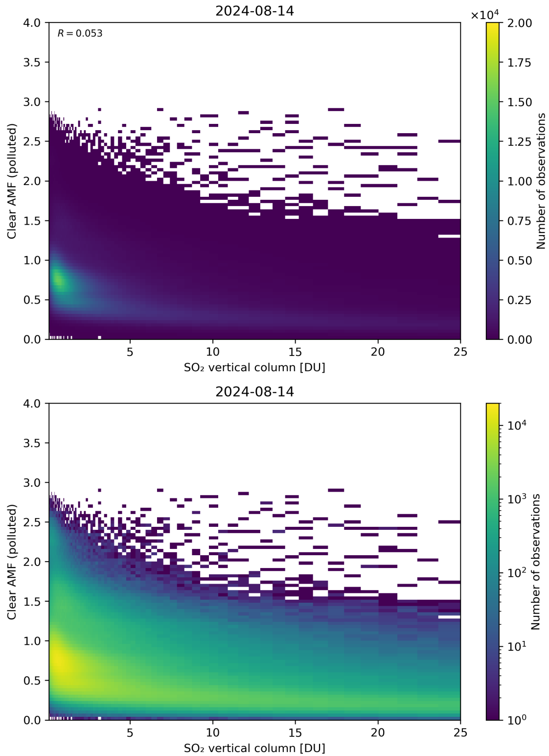
Figure 296: Scatter density plot of “SO 2 vertical column” against “Clear AMF (polluted)” for 2024-08-13 to 2024-08-15.
