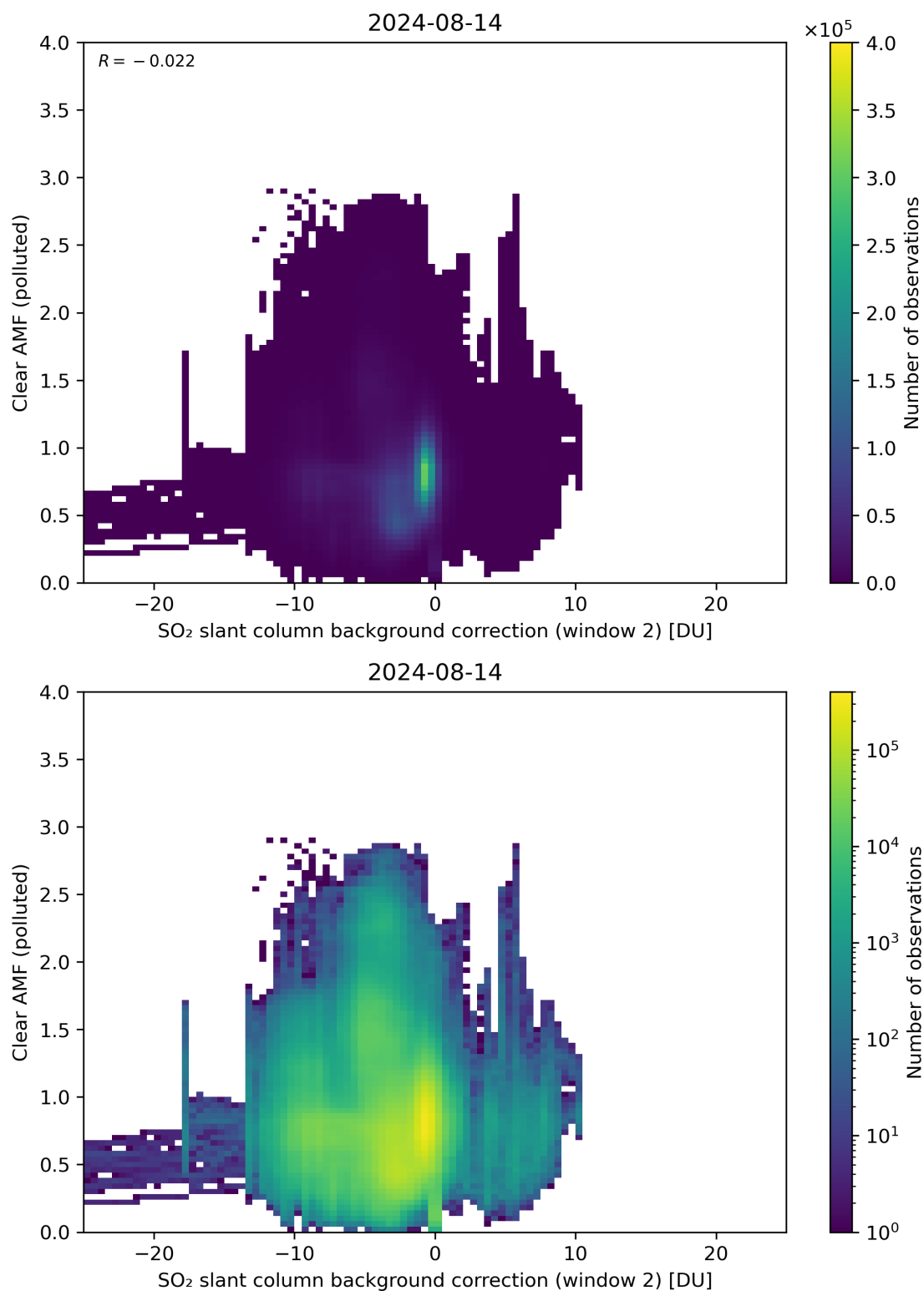
Figure 115: Scatter density plot of “SO 2 slant column background correction (window 2)” against “Clear AMF (polluted)” for 2024-08-13 to 2024-08-15.
