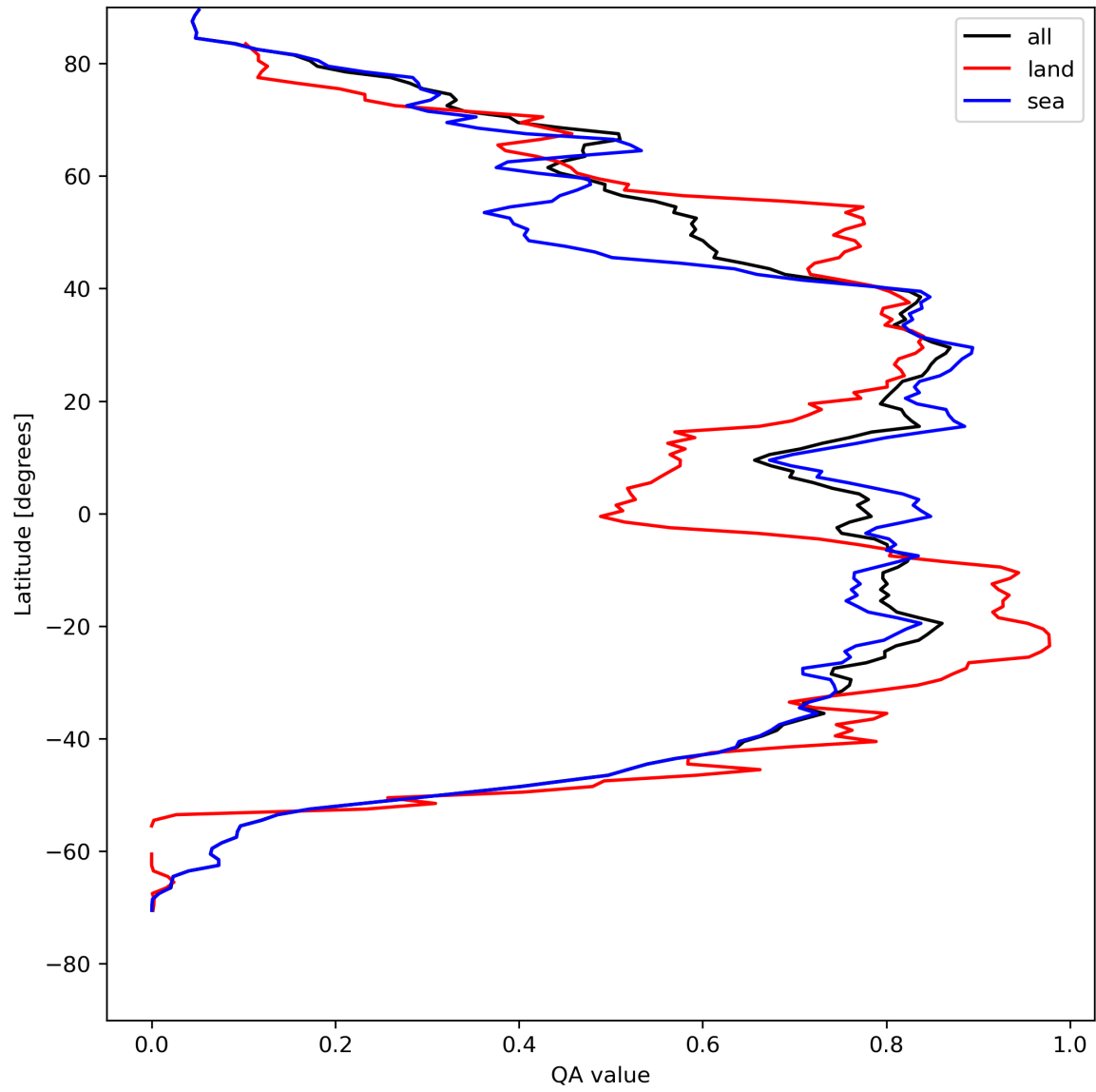
Figure 29: Zonal average of “QA value” for 2024-08-13 to 2024-08-15.
