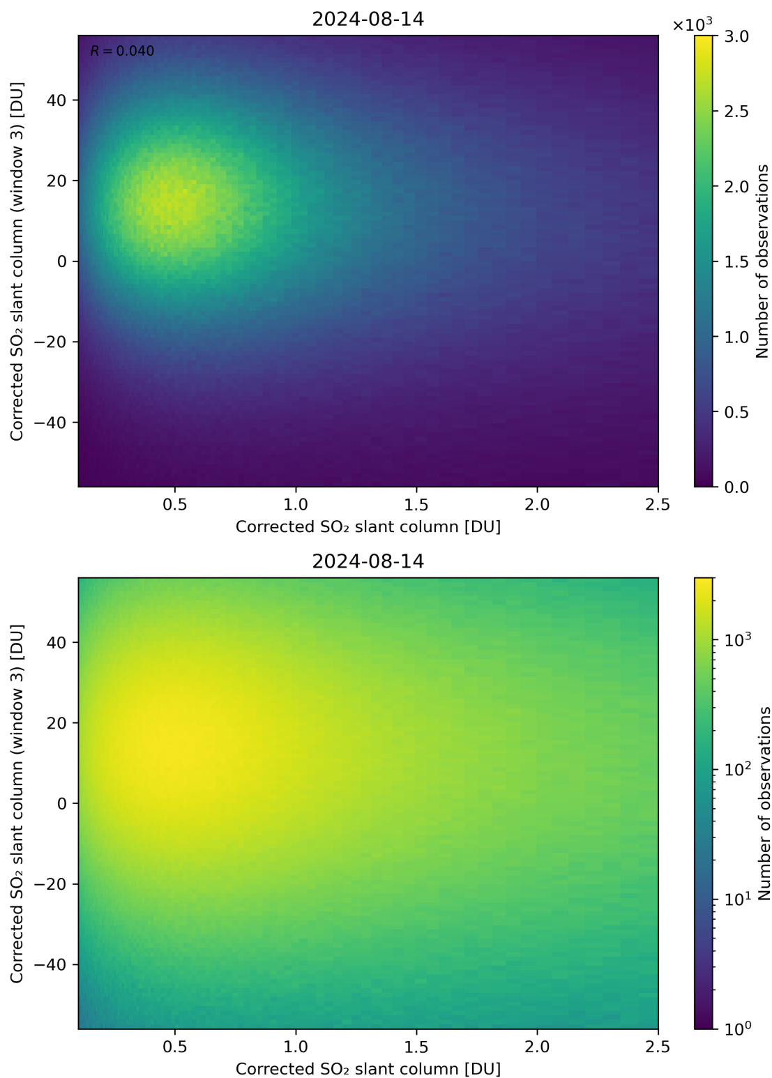
Figure 186: Scatter density plot of “Corrected SO 2 slant column” against “Corrected SO 2 slant column (window 3)” for 2024-08-13 to 2024-08-15.
