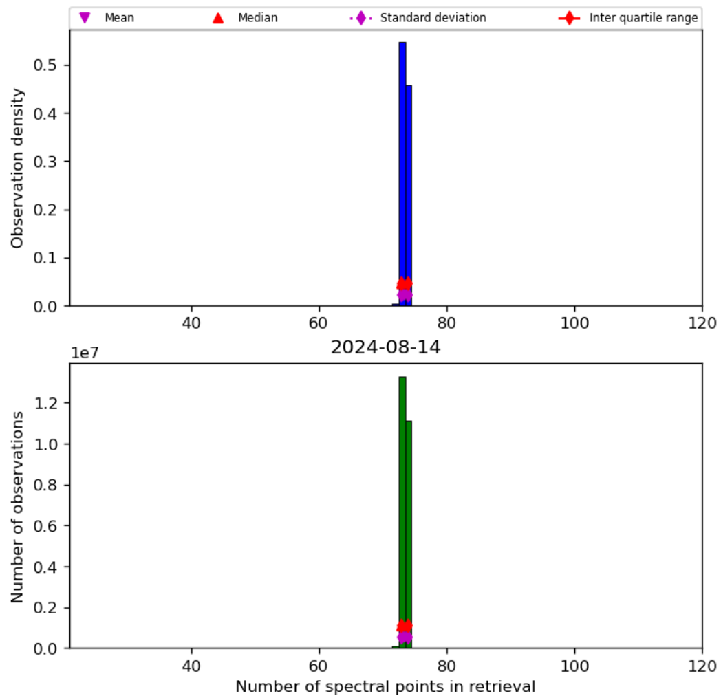
Figure 74: Histogram of “Number of spectral points in retrieval” for 2024-08-13 to 2024-08-15
