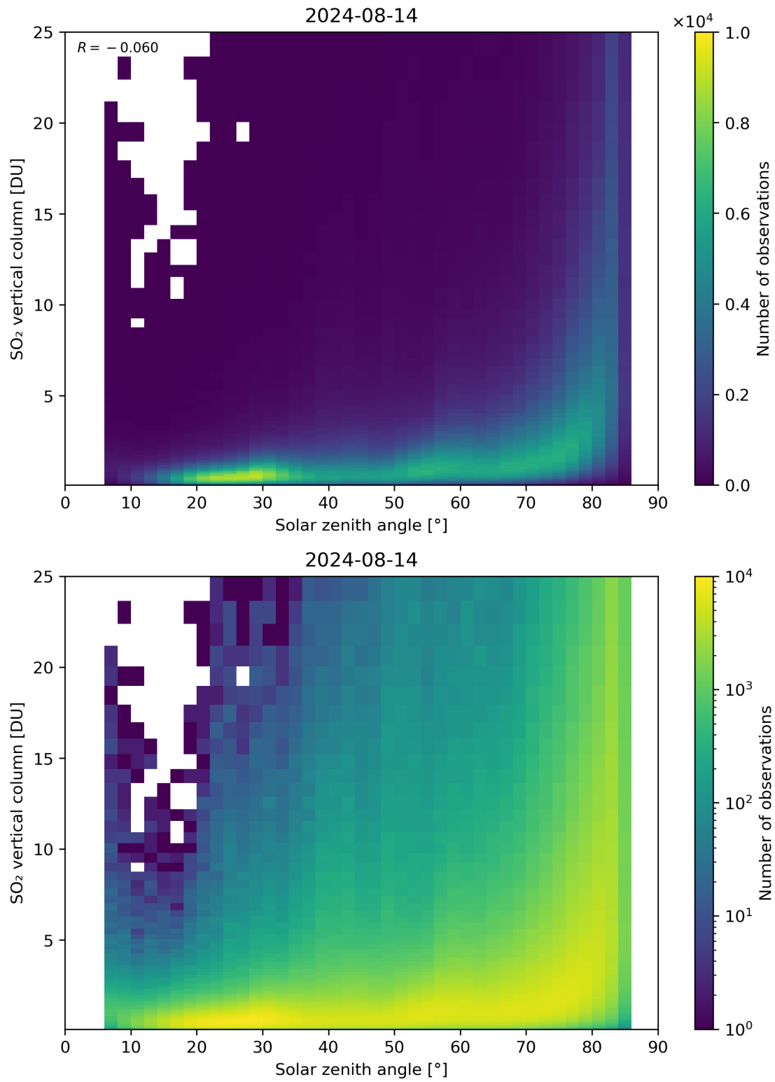
Figure 176: Scatter density plot of “Solar zenith angle” against “SO 2 vertical column” for 2024-08-13 to 2024-08-15.
