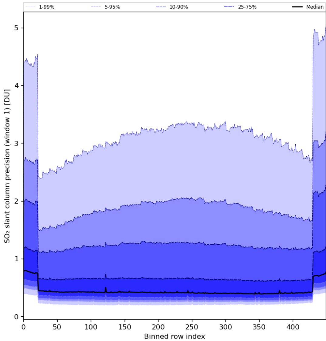
Figure 80: Along track statistics of “SO 2 slant column precision (window 1)” for 2024-08-13 to 2024-08-15
