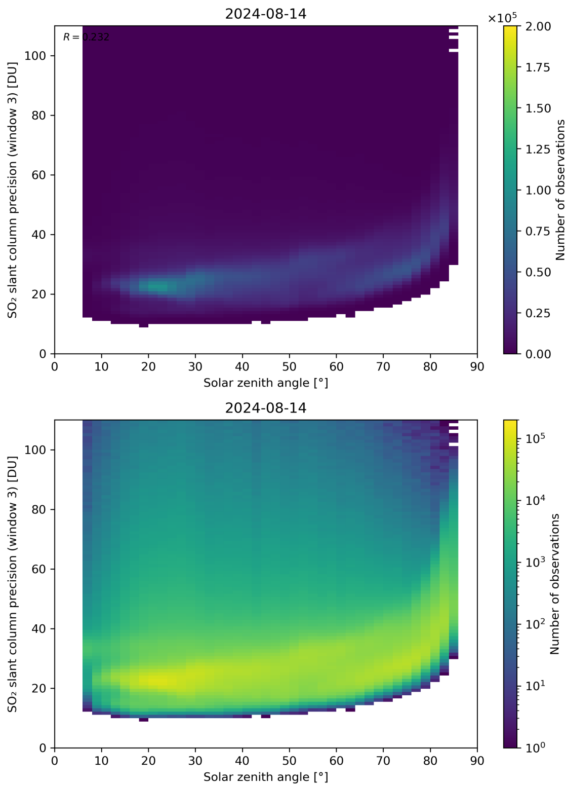
Figure 173: Scatter density plot of “Solar zenith angle” against “SO 2 slant column precision (window 3)” for 2024-08-13 to 2024-08-15.
