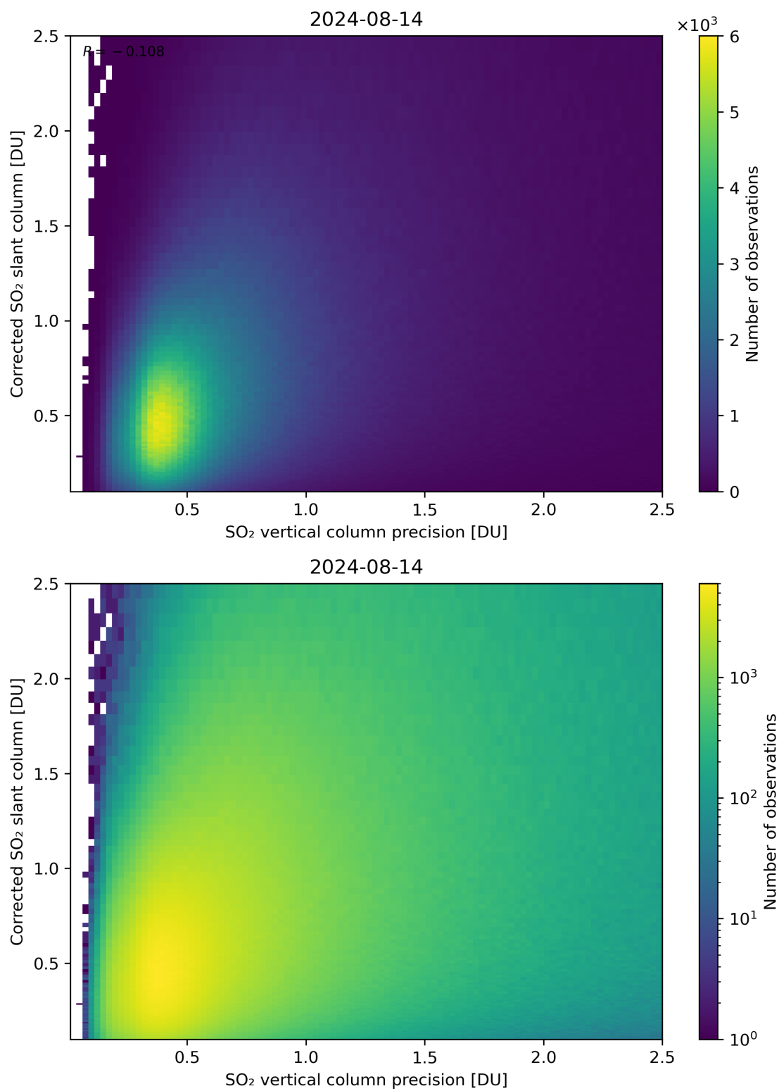
Figure 286: Scatter density plot of “SO 2 vertical column precision” against “Corrected SO 2 slant column” for 2024-08-13 to 2024-08-15.
