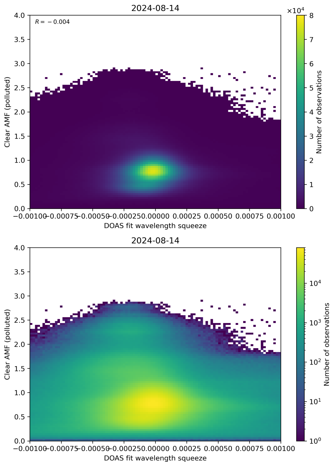
Figure 133: Scatter density plot of “DOAS fit wavelength squeeze” against “Clear AMF (polluted)” for 2024-08-13 to 2024-08-15.
