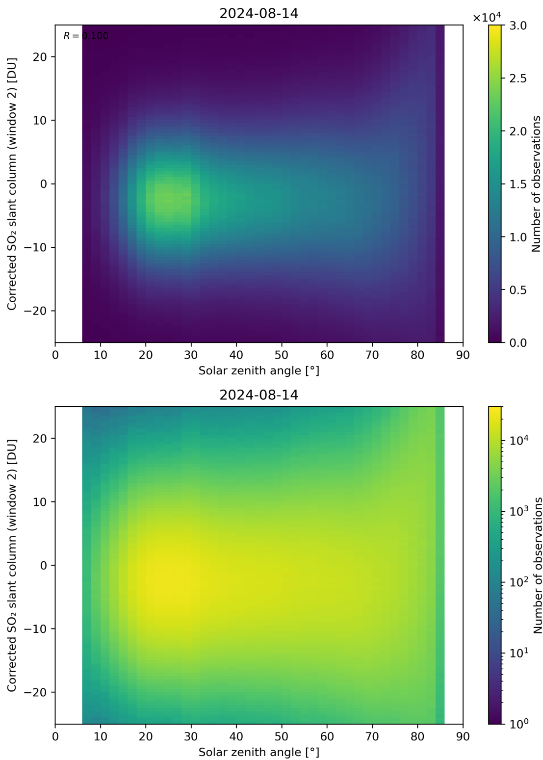
Figure 167: Scatter density plot of “Solar zenith angle” against “Corrected SO 2 slant column (window 2)” for 2024-08-13 to 2024-08-15.
