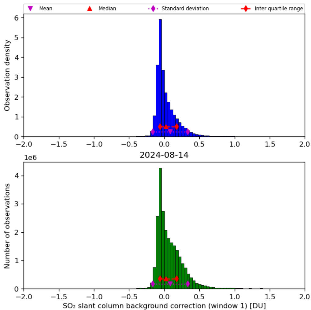
Figure 59: Histogram of “SO 2 slant column background correction (window 1)” for 2024-08-13 to 2024-08-15
