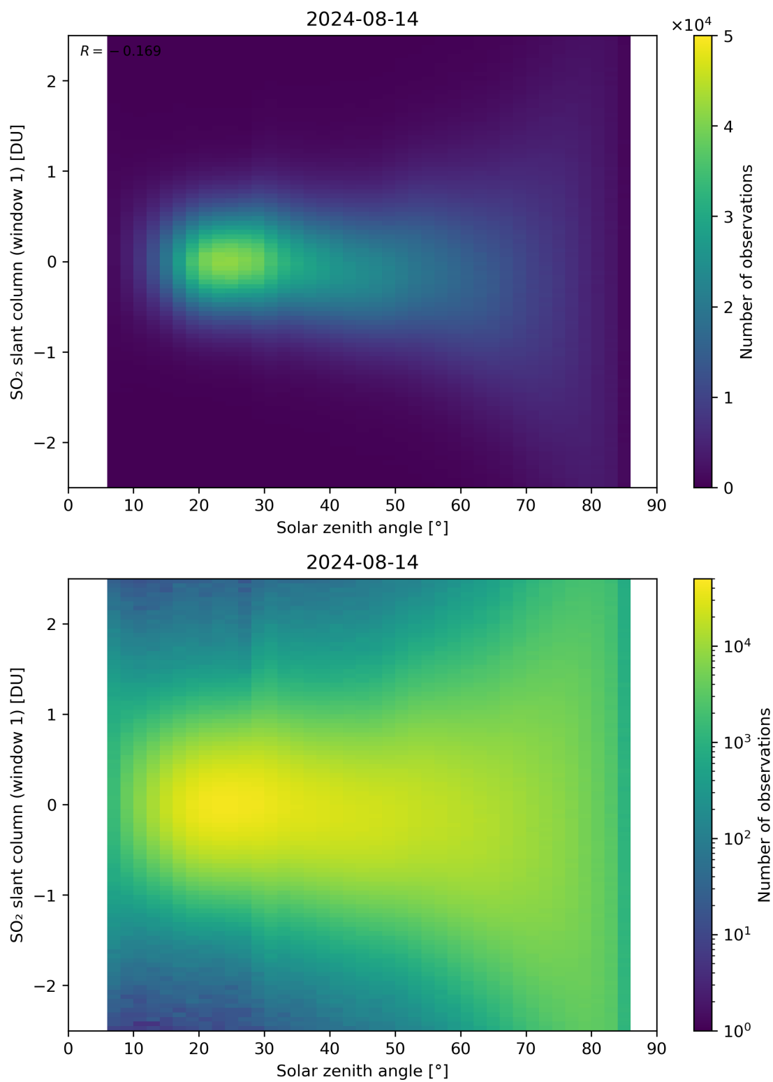
Figure 169: Scatter density plot of “Solar zenith angle” against “SO 2 slant column (window 1)” for 2024-08-13 to 2024-08-15.
