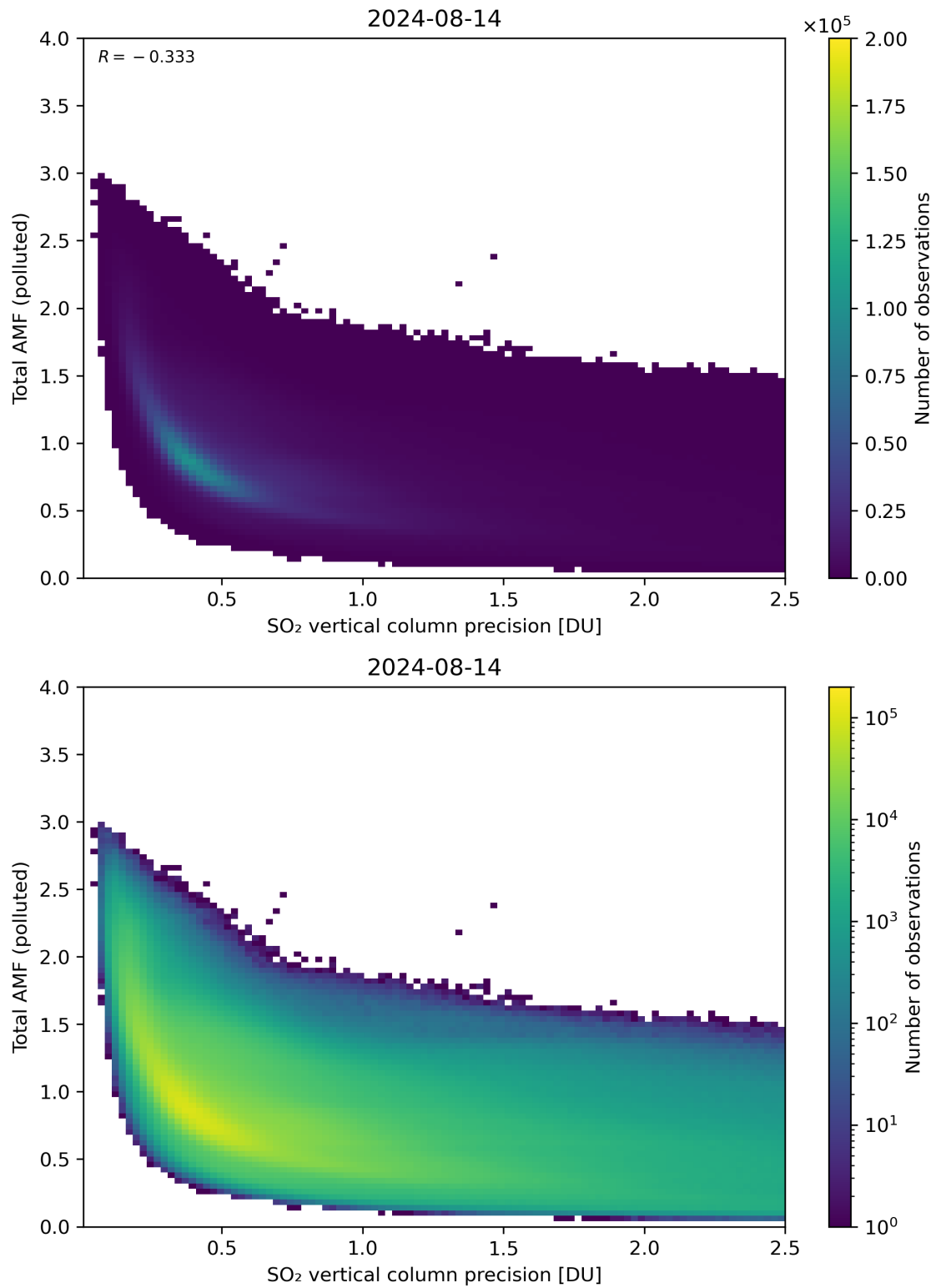
Figure 294: Scatter density plot of “SO 2 vertical column precision” against “Total AMF (polluted)” for 2024-08-13 to 2024-08-15.
