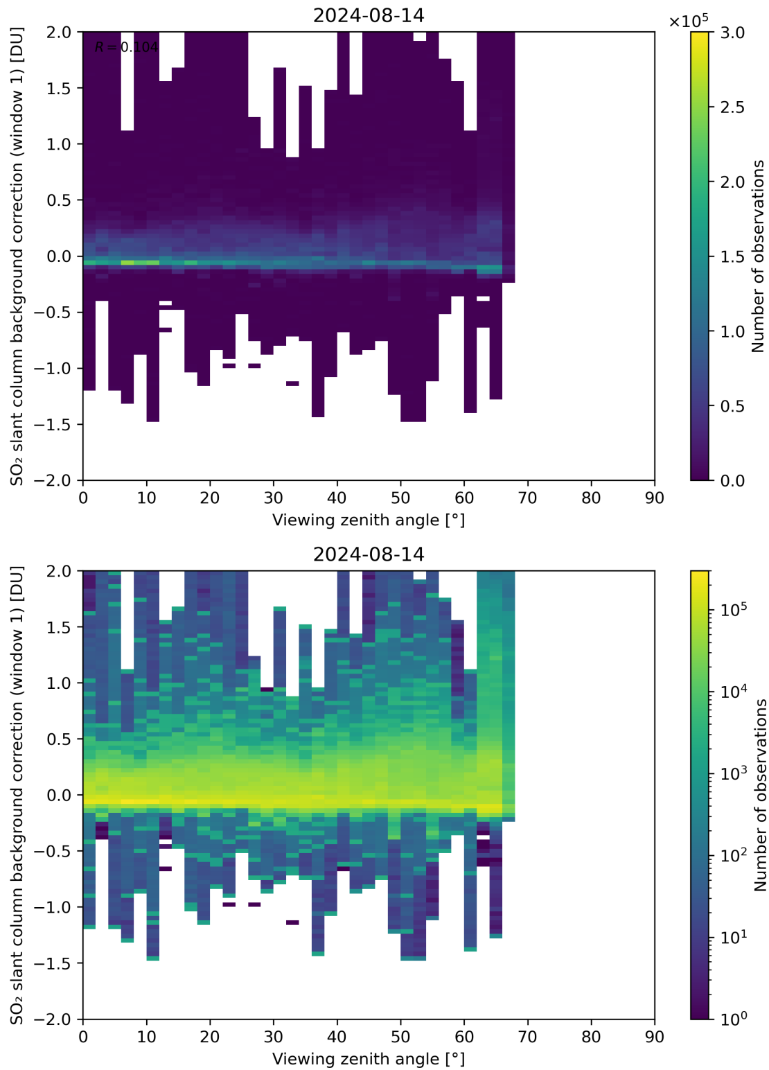
Figure 308: Scatter density plot of “Viewing zenith angle” against “SO 2 slant column background correction (window 1)” for 2024-08-13 to 2024-08-15.
