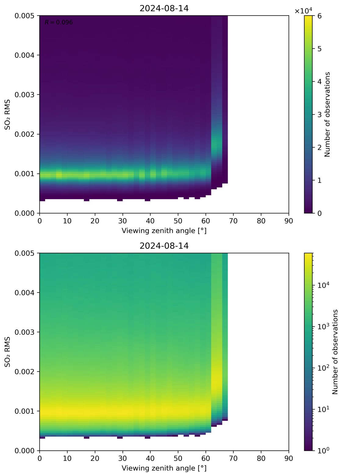
Figure 313: Scatter density plot of “Viewing zenith angle” against “SO 2 RMS” for 2024-08-13 to 2024-08-15.
