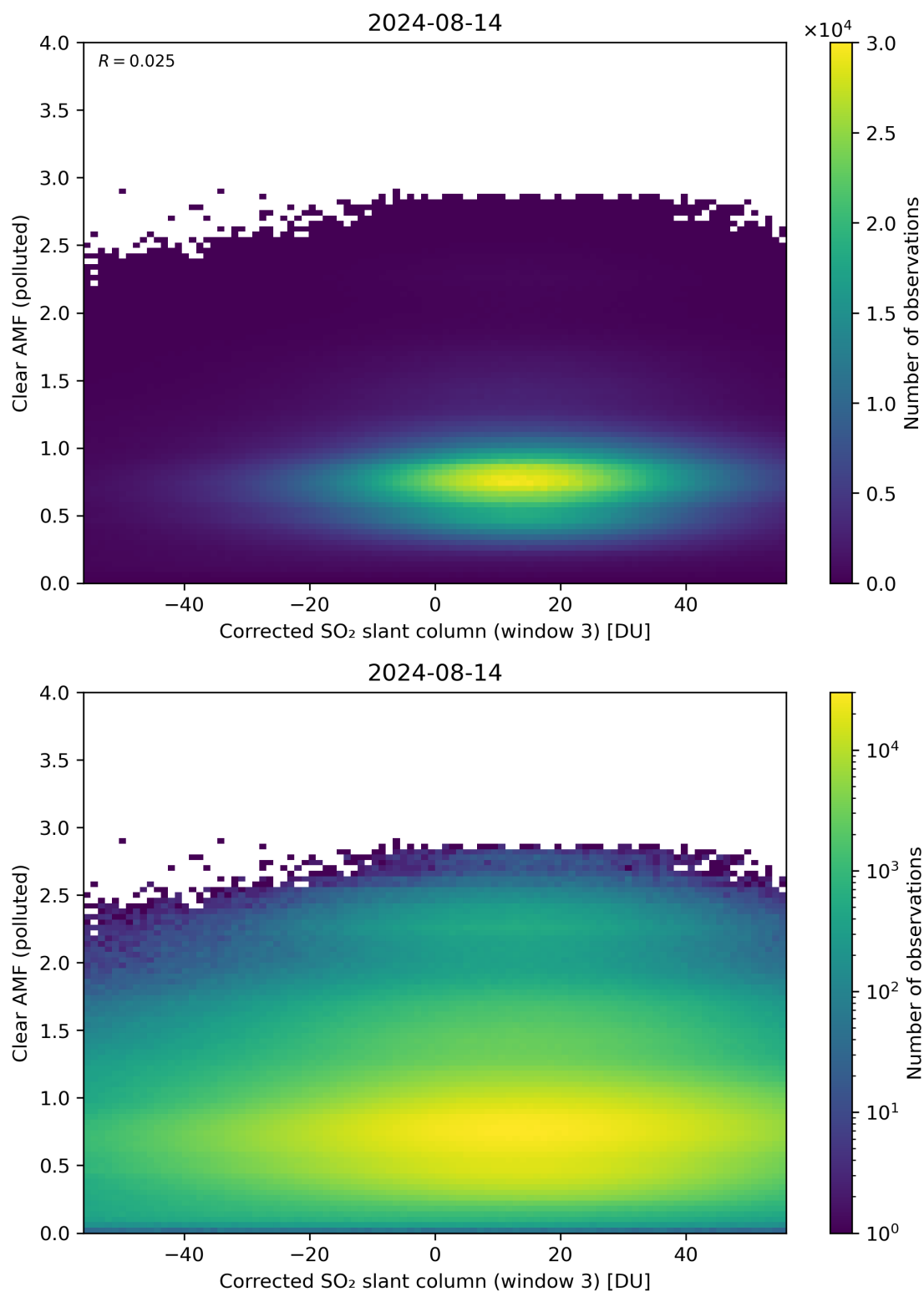
Figure 209: Scatter density plot of “Corrected SO 2 slant column (window 3)” against “Clear AMF (polluted)” for 2024-08-13 to 2024-08-15.
