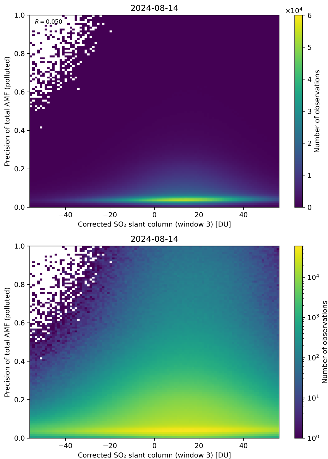
Figure 211: Scatter density plot of “Corrected SO 2 slant column (window 3)” against “Precision of total AMF (polluted)” for 2024-08-13 to 2024-08-15.
