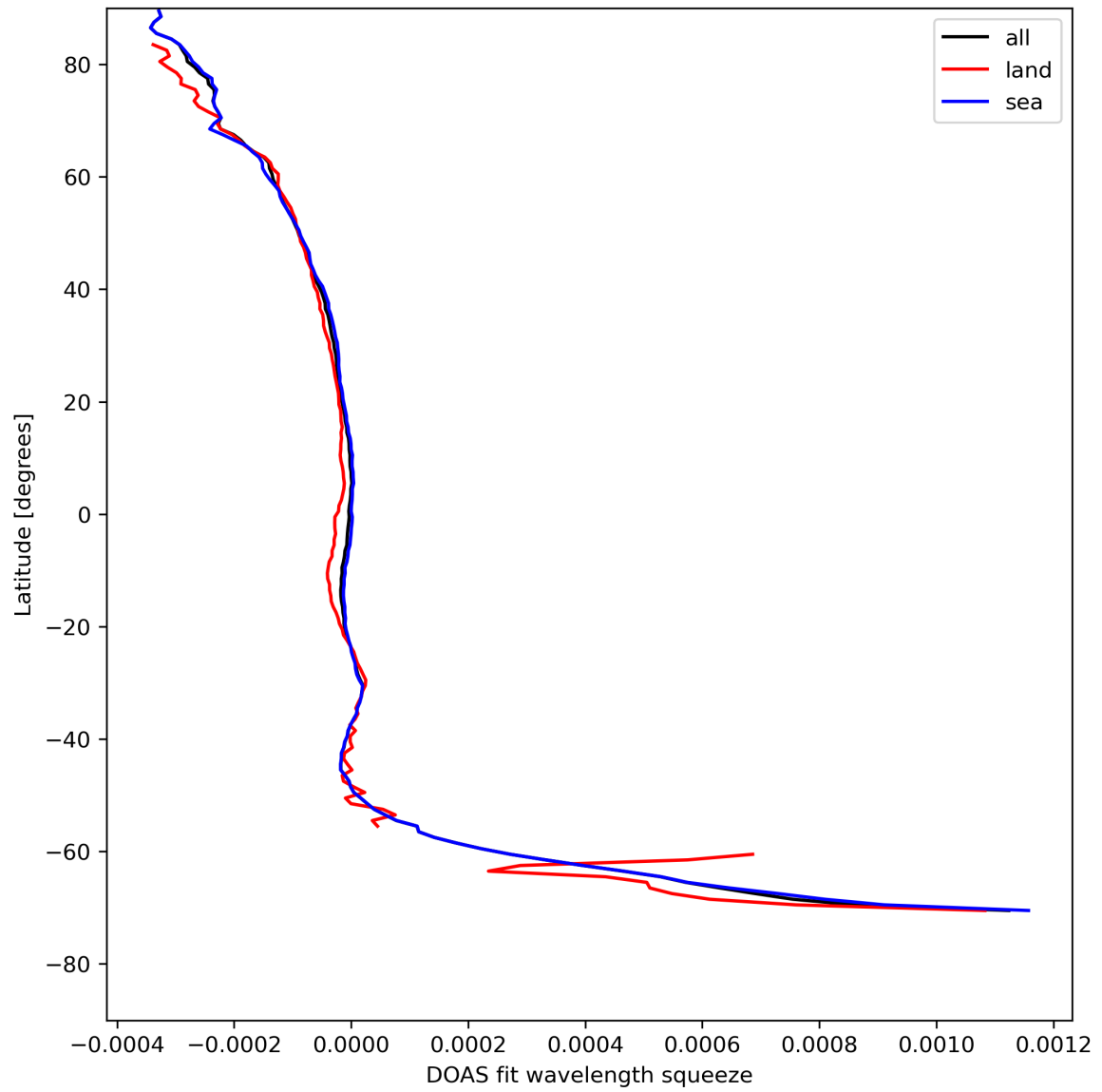
Figure 46: Zonal average of “DOAS fit wavelength squeeze” for 2024-08-13 to 2024-08-15.
