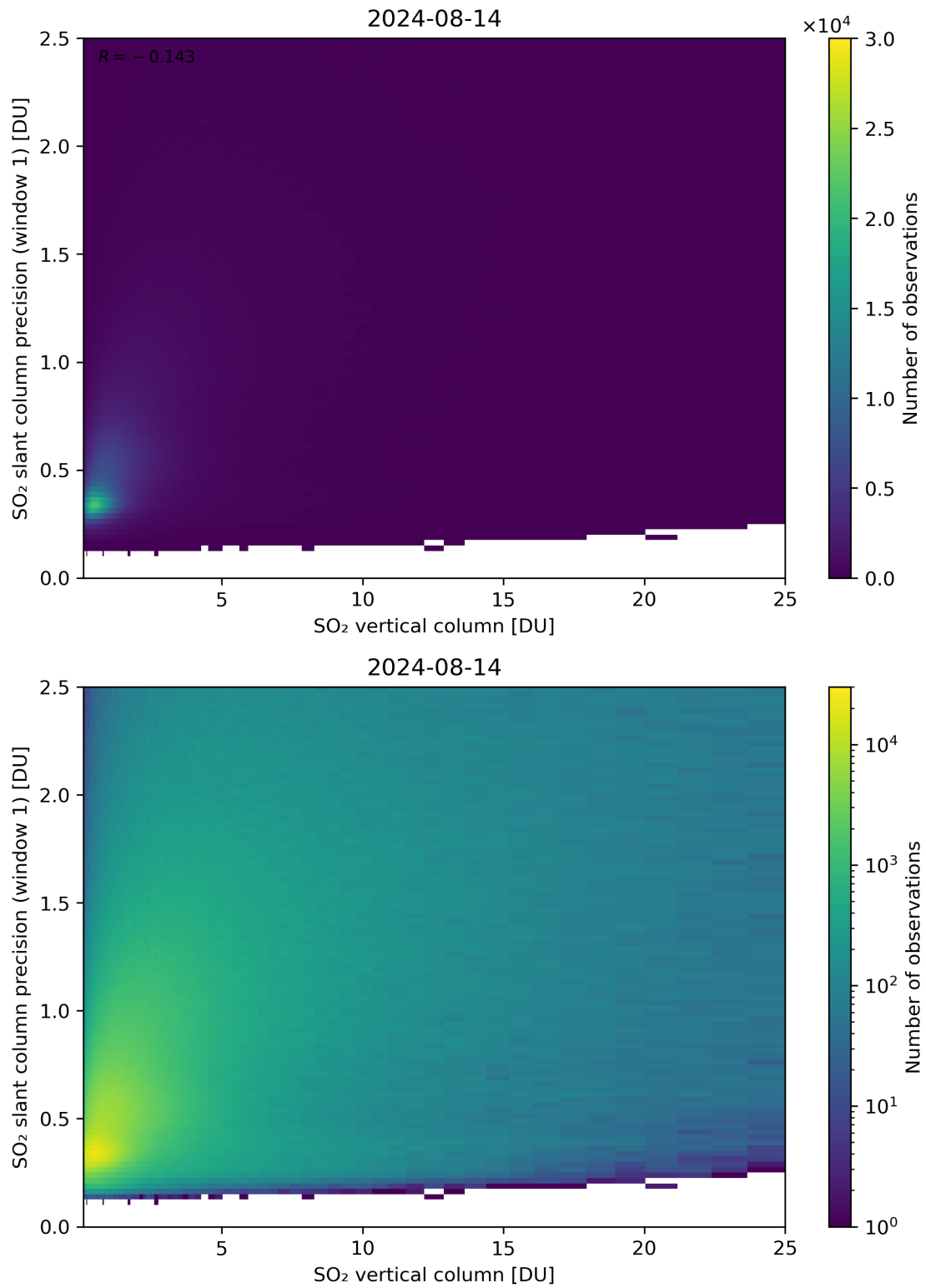
Figure 301: Scatter density plot of “SO 2 vertical column” against “SO 2 slant column precision (window 1)” for 2024-08-13 to 2024-08-15.
