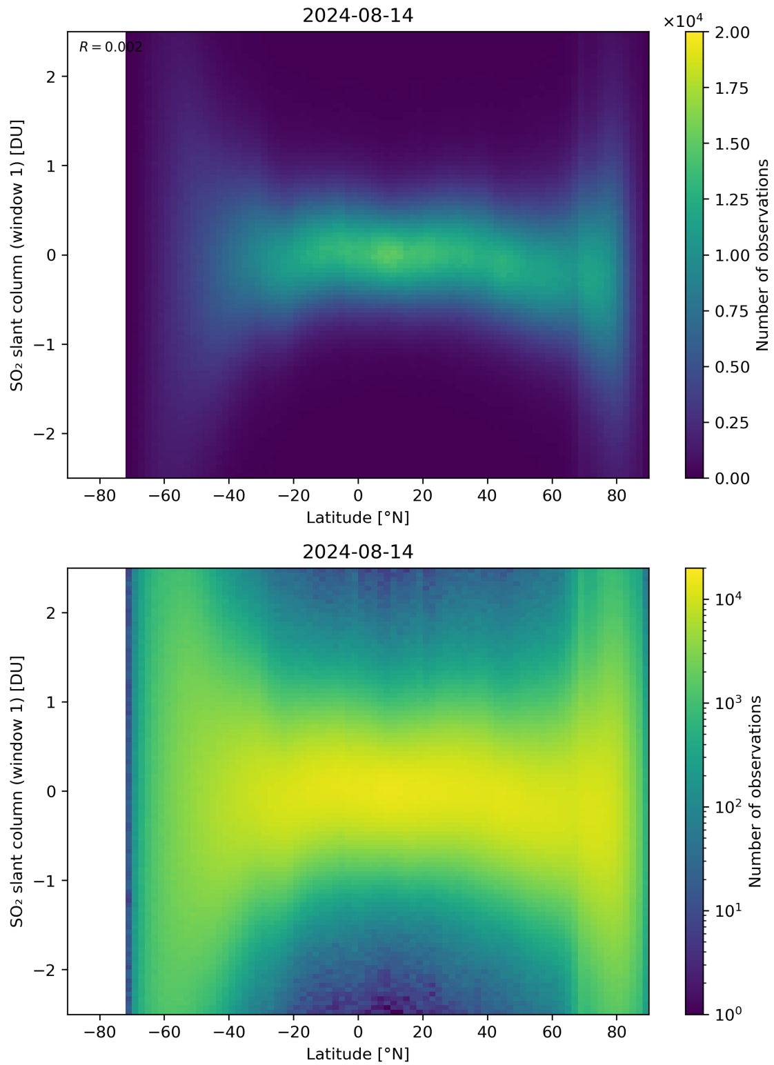
Figure 149: Scatter density plot of “Latitude” against “SO 2 slant column (window 1)” for 2024-08-13 to 2024-08-15.
