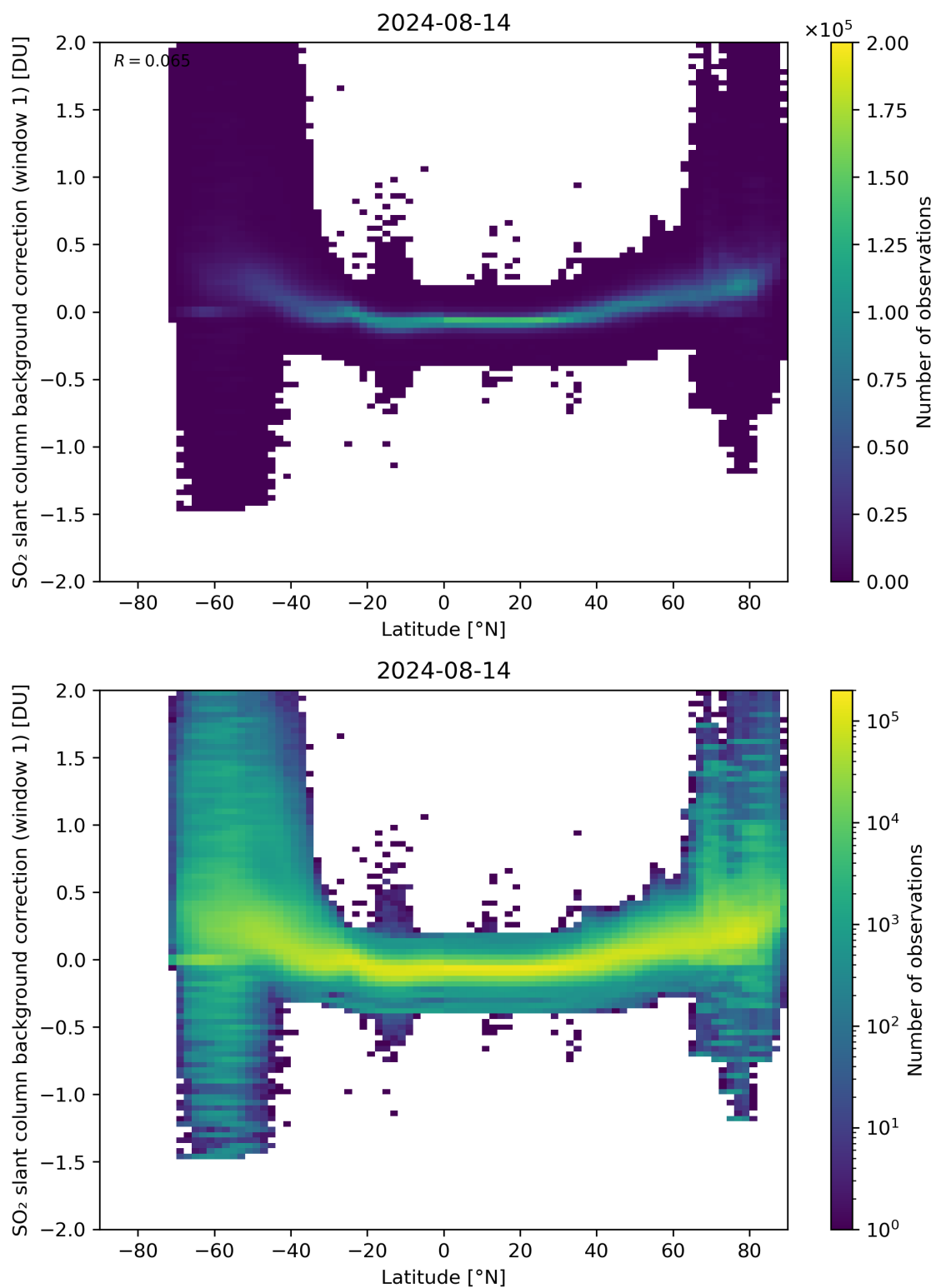
Figure 139: Scatter density plot of “Latitude” against “SO 2 slant column background correction (window 1)” for 2024-08-13 to 2024-08-15.
