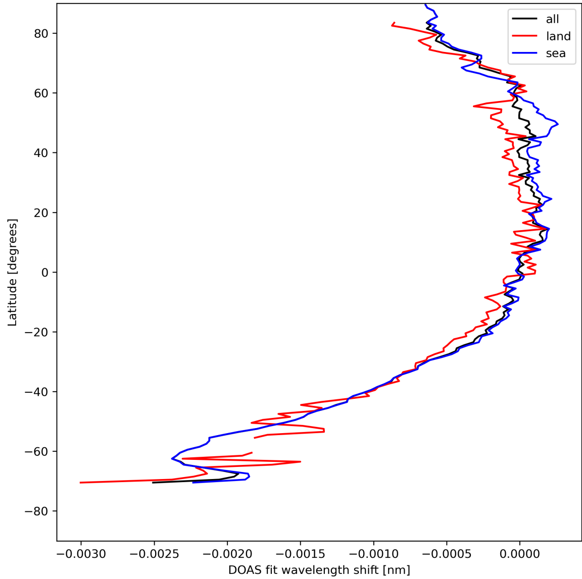
Figure 45: Zonal average of "DOAS fit wavelength shift" for 2024-08-13 to 2024-08-15.
