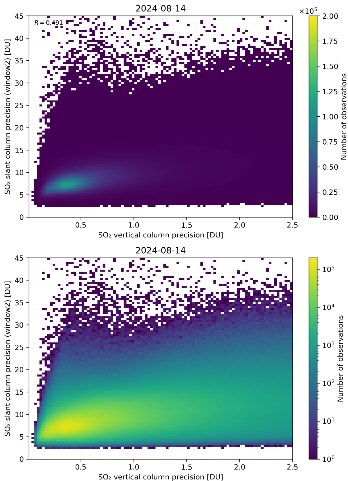
Figure 291: Scatter density plot of “SO 2 vertical column precision” against “SO 2 slant column precision (window2)” for 2024-08-13 to 2024-08-15.
