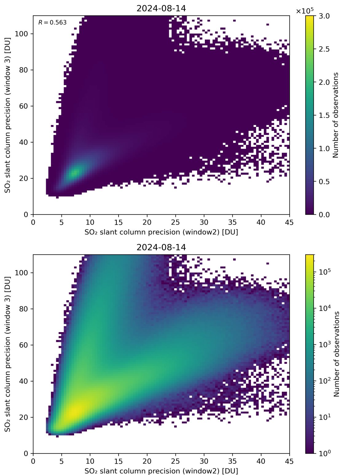
Figure 250: Scatter density plot of “SO 2 slant column precision (window2)” against “SO 2 slant column precision (window 3)” for 2024-08-13 to 2024-08-15.
