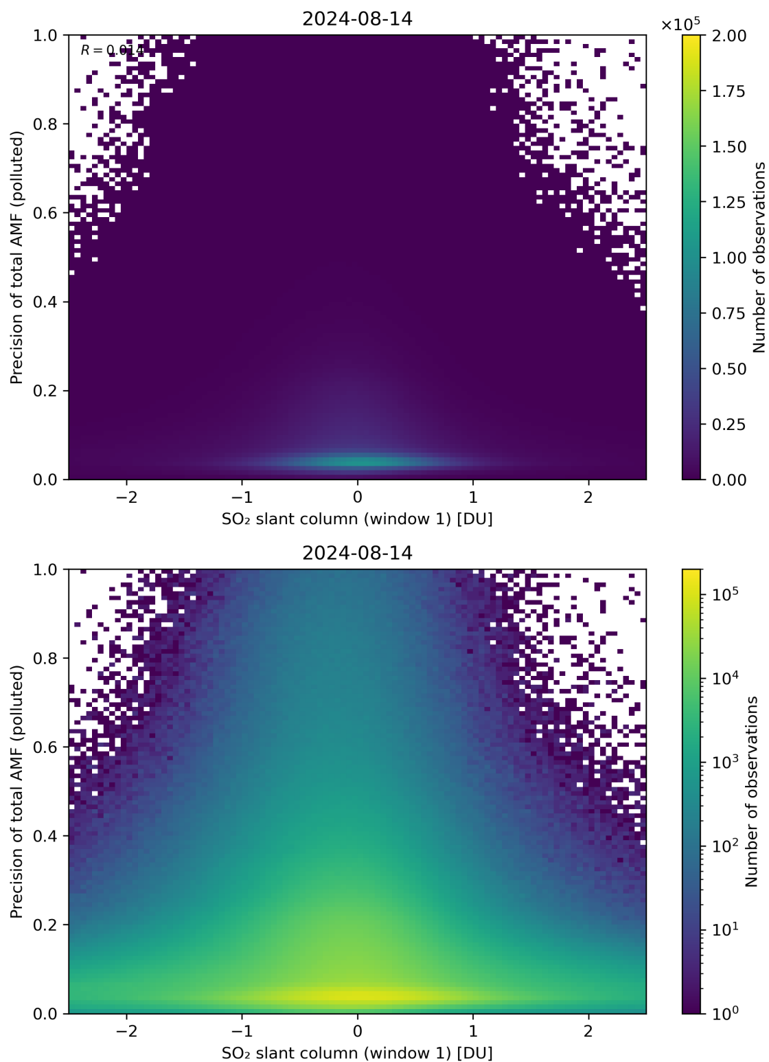
Figure 240: Scatter density plot of “SO 2 slant column (window 1)” against “Precision of total AMF (polluted)” for 2024-08-13 to 2024-08-15.
