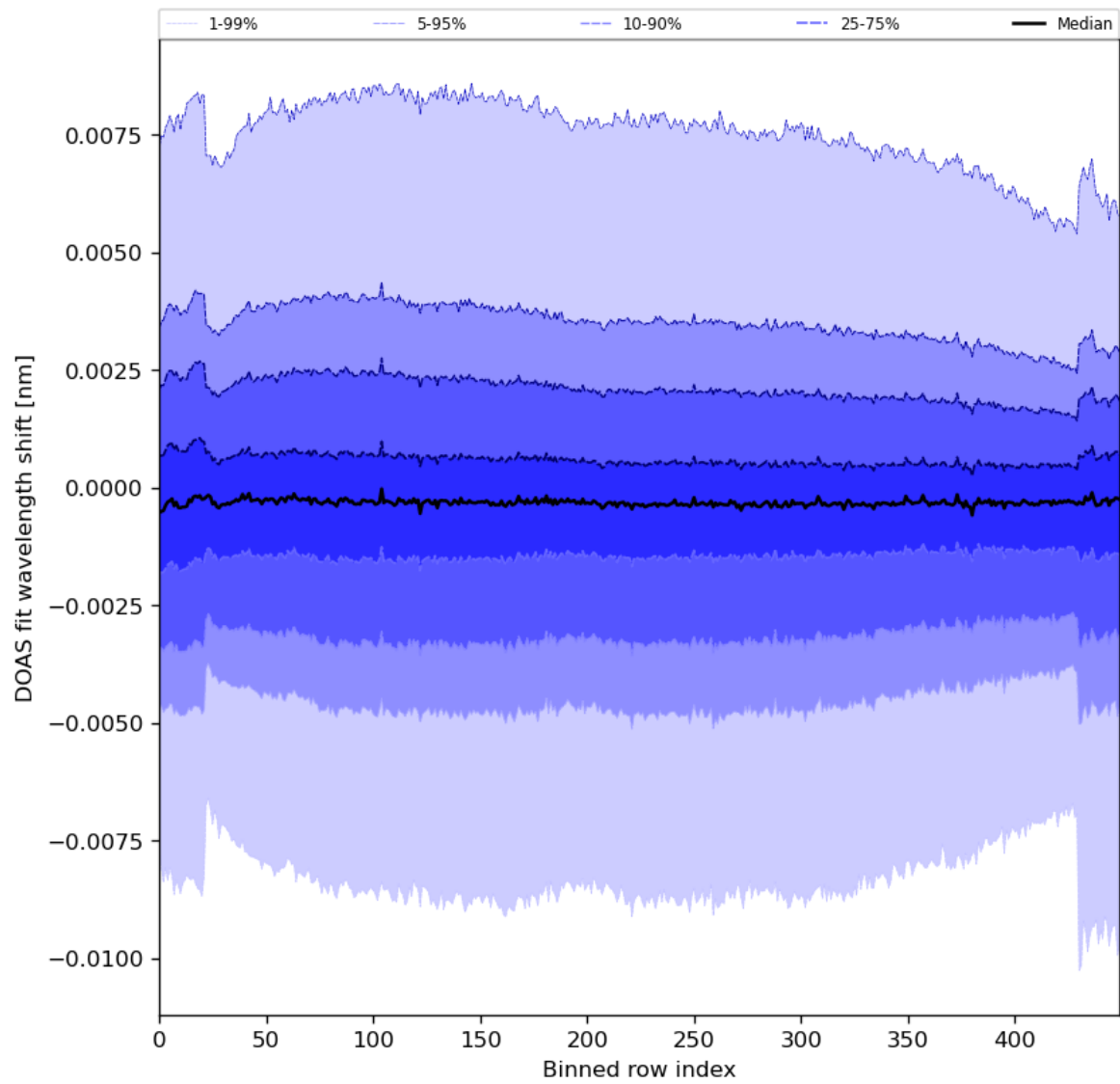
Figure 91: Along track statistics of “DOAS fit wavelength shift” for 2024-08-13 to 2024-08-15
