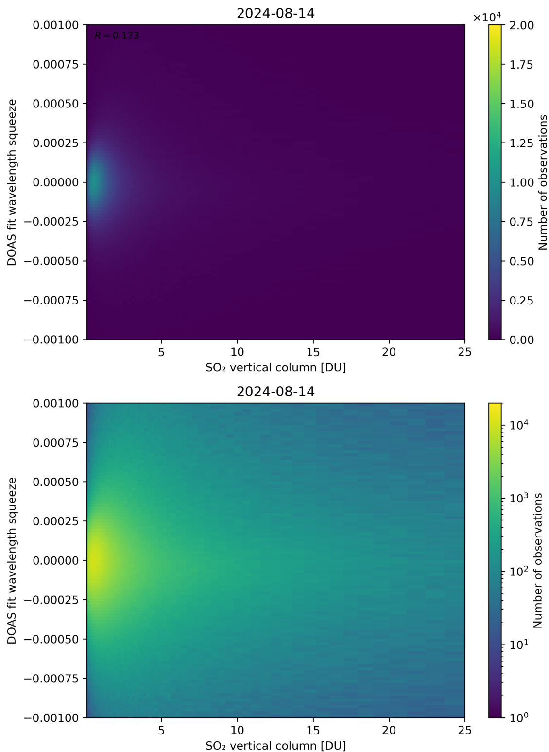
Figure 277: Scatter density plot of “SO 2 vertical column” against “DOAS fit wavelength squeeze” for 2024-08-13 to 2024-08-15.
