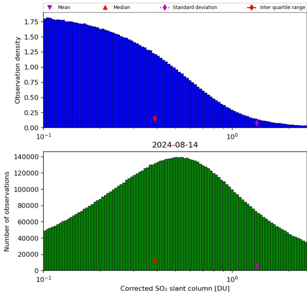
Figure 55: Histogram of “Corrected SO 2 slant column” for 2024-08-13 to 2024-08-15
