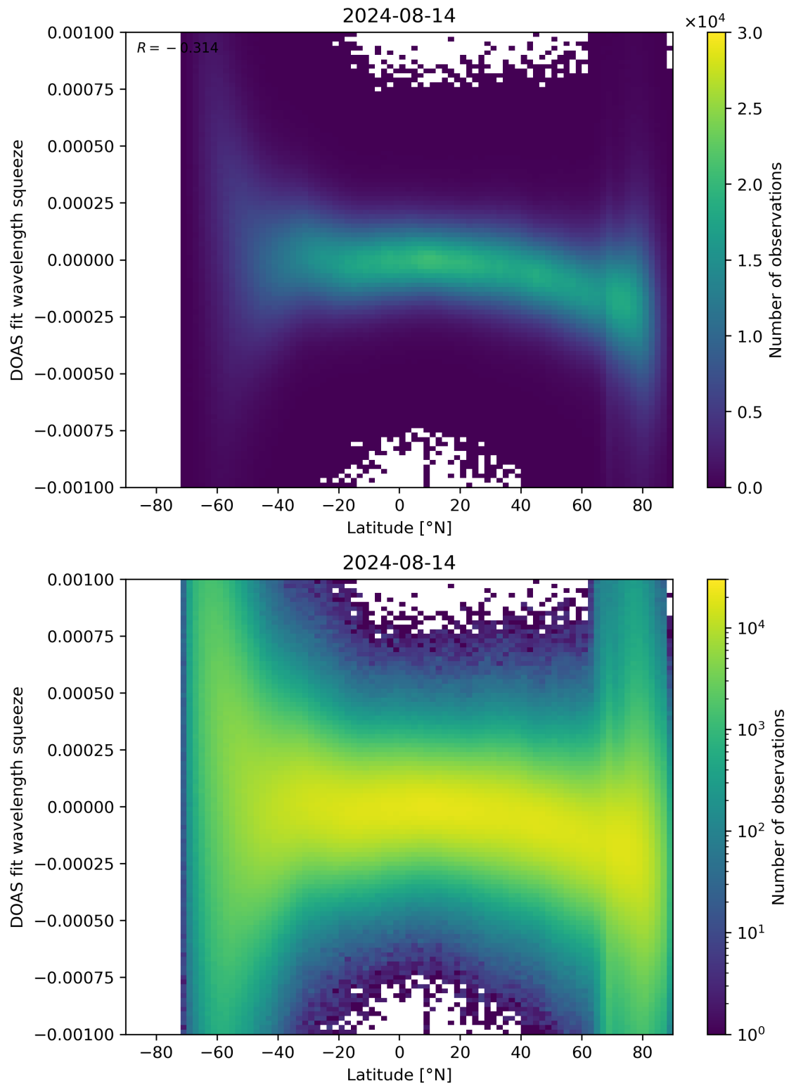
Figure 143: Scatter density plot of “Latitude” against “DOAS fit wavelength squeeze” for 2024-08-13 to 2024-08-15.
