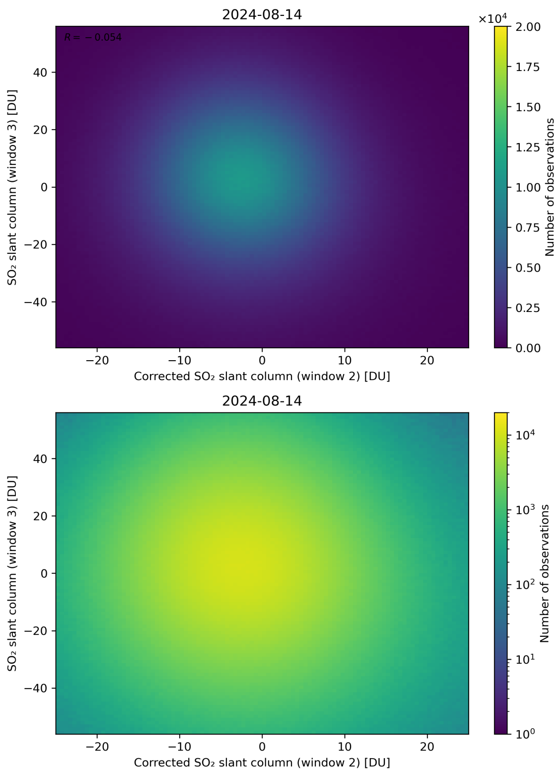
Figure 201: Scatter density plot of “Corrected SO 2 slant column (window 2)” against “SO 2 slant column (window 3)” for 2024-08-13 to 2024-08-15.
