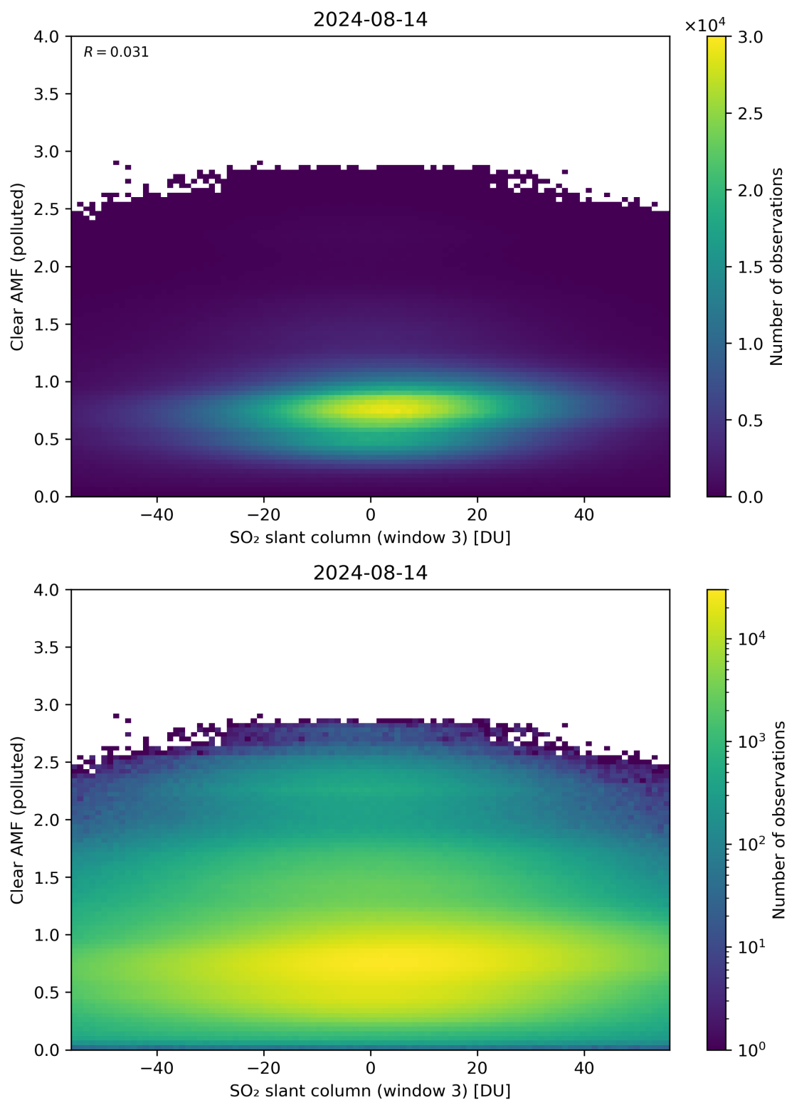
Figure 265: Scatter density plot of “SO 2 slant column (window 3)” against “Clear AMF (polluted)” for 2024-08-13 to 2024-08-15.
