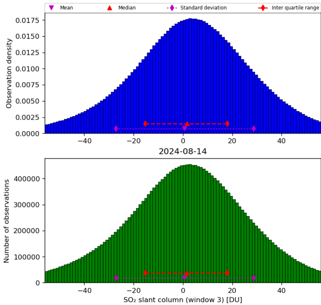
Figure 64: Histogram of “SO 2 slant column (window 3)” for 2024-08-13 to 2024-08-15
