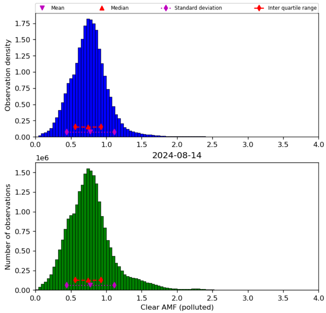
Figure 73: Histogram of “Clear AMF (polluted)” for 2024-08-13 to 2024-08-15
