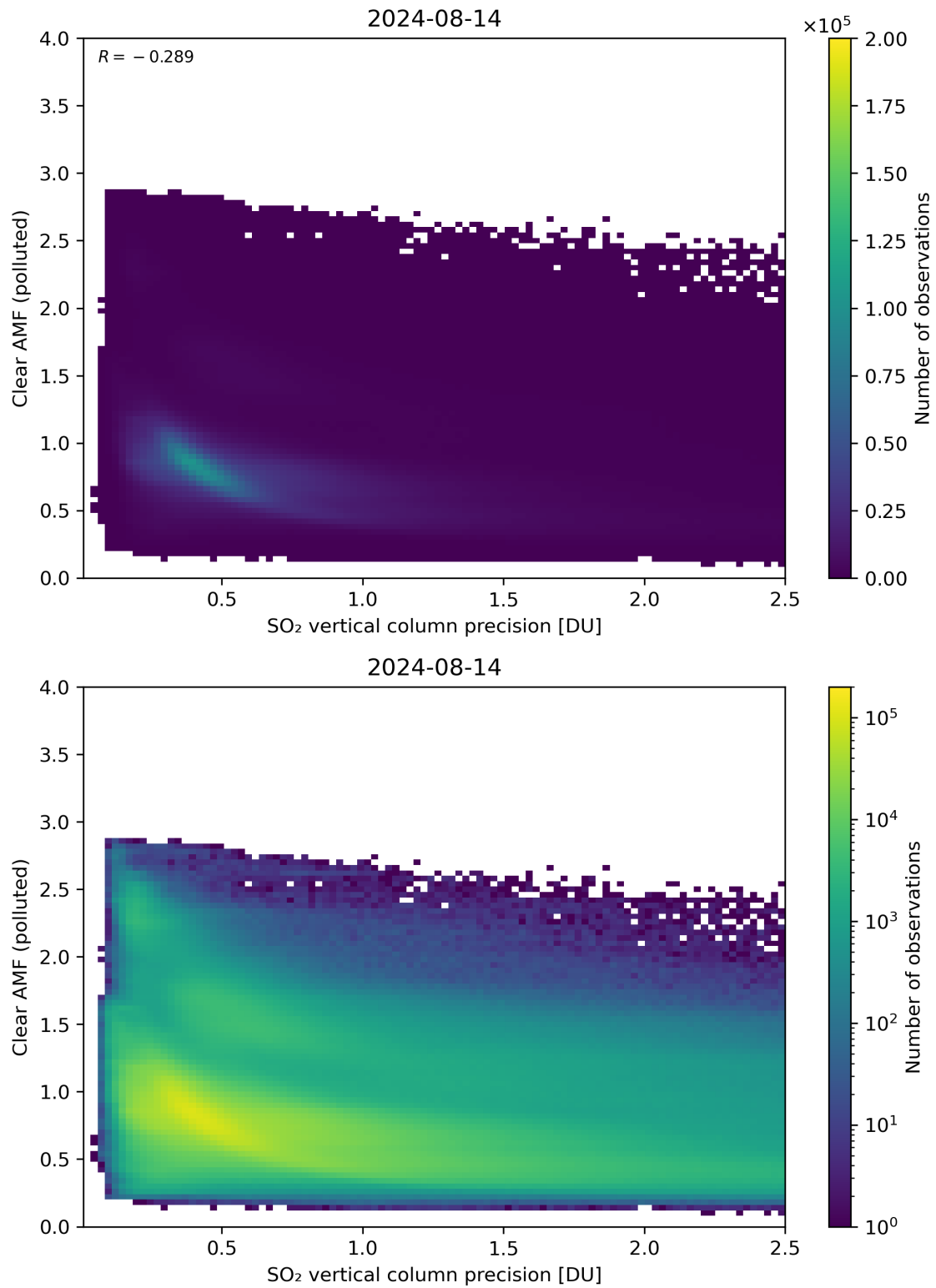
Figure 285: Scatter density plot of “SO 2 vertical column precision” against “Clear AMF (polluted)” for 2024-08-13 to 2024-08-15.
