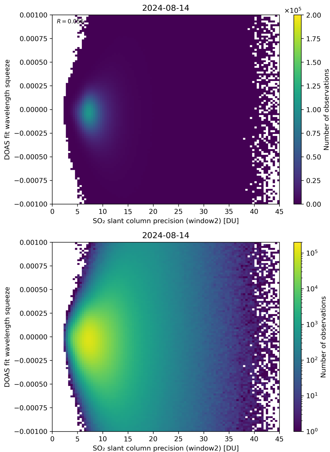
Figure 244: Scatter density plot of “SO 2 slant column precision (window2)” against “DOAS fit wavelength squeeze” for 2024-08-13 to 2024-08-15.
