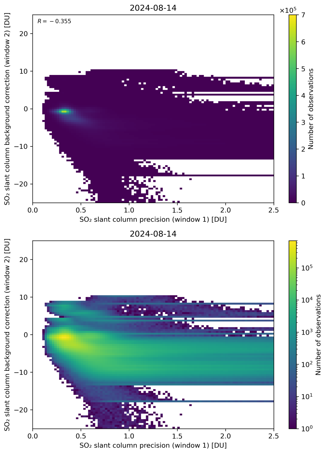
Figure 219: Scatter density plot of “SO 2 slant column precision (window 1)” against “SO 2 slant column background correction (window 2)” for 2024-08-13 to 2024-08-15.
