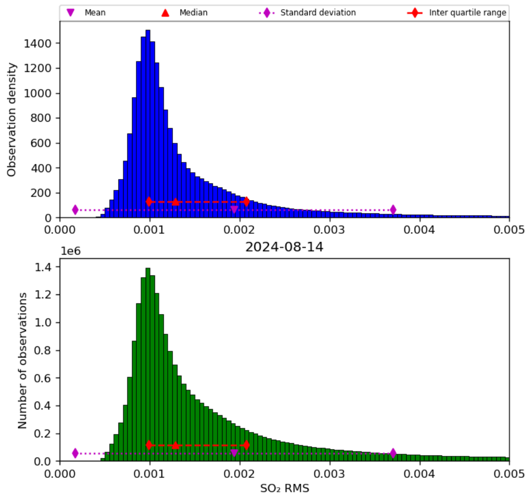
Figure 70: Histogram of “SO 2 RMS” for 2024-08-13 to 2024-08-15
