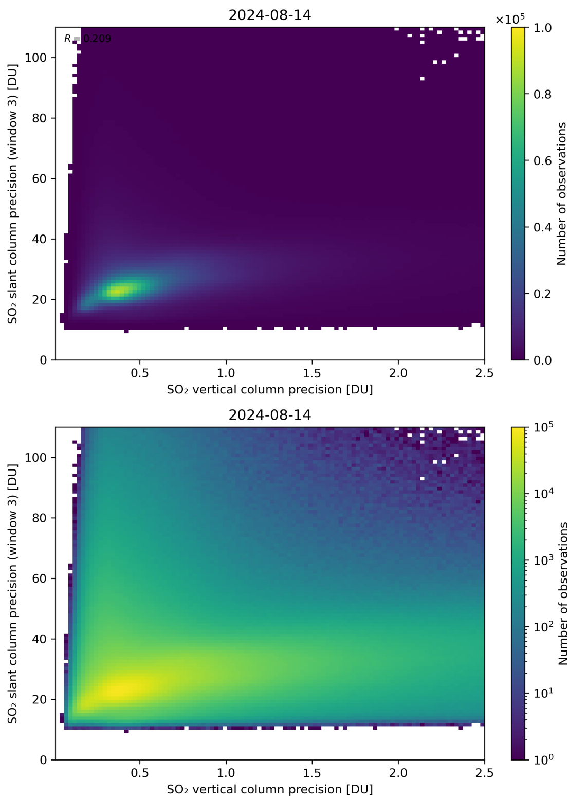
Figure 293: Scatter density plot of “SO 2 vertical column precision” against “SO 2 slant column precision (window 3)” for 2024-08-13 to 2024-08-15.
