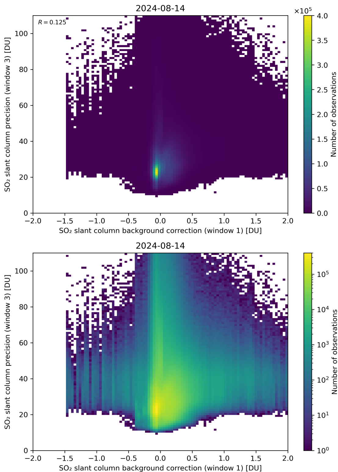
Figure 108: Scatter density plot of “SO 2 slant column background correction (window 1)” against “SO 2 slant column precision (window 3)” for 2024-08-13 to 2024-08-15.
