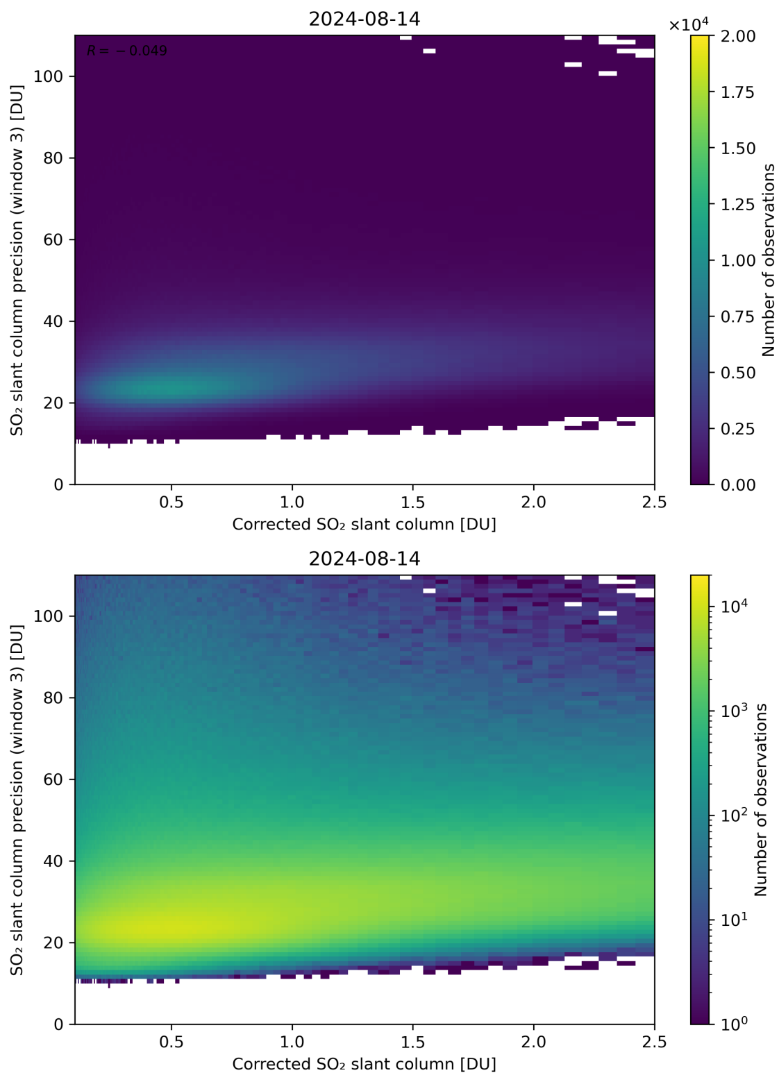
Figure 191: Scatter density plot of “Corrected SO 2 slant column” against “SO 2 slant column precision (window 3)” for 2024-08-13 to 2024-08-15.
