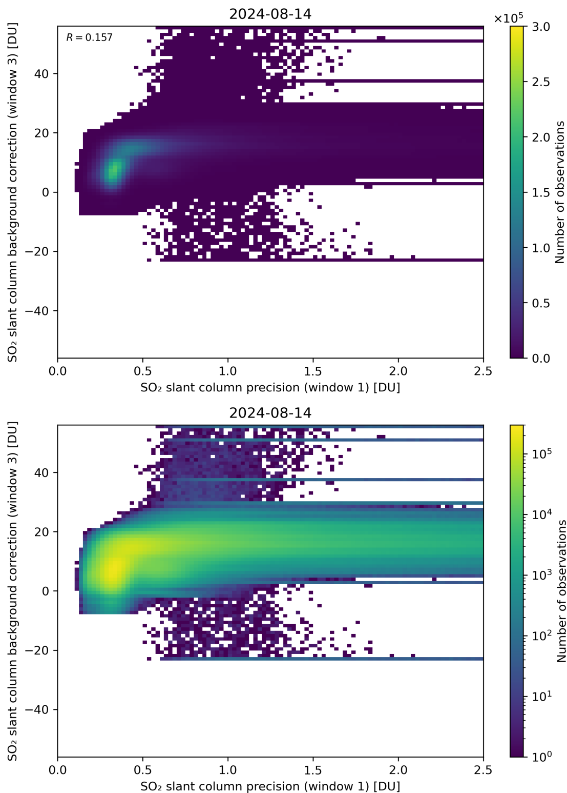
Figure 220: Scatter density plot of “SO 2 slant column precision (window 1)” against “SO 2 slant column background correction (window 3)” for 2024-08-13 to 2024-08-15.
