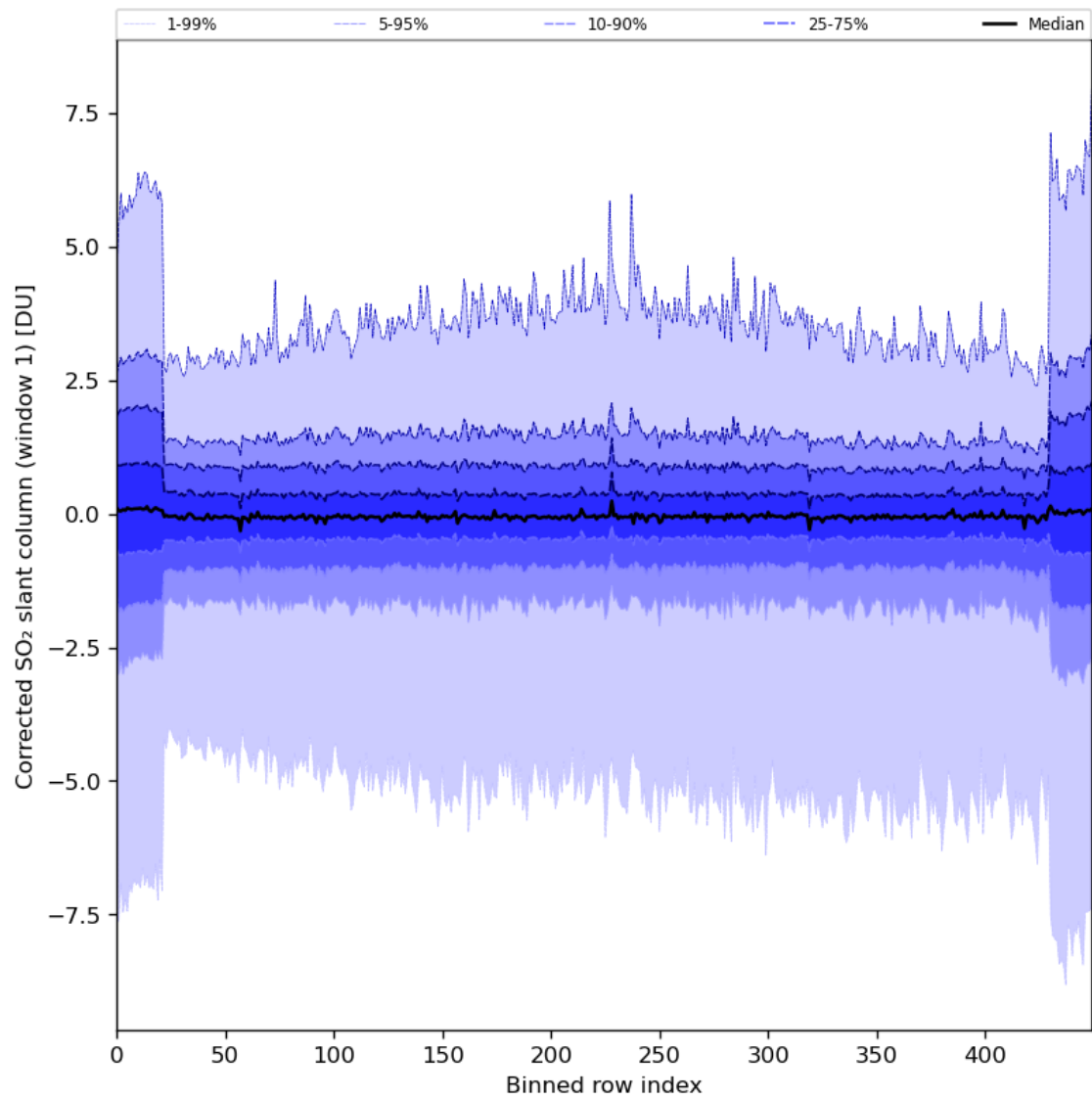
Figure 81: Along track statistics of “Corrected SO 2 slant column (window 1)” for 2024-08-13 to 2024-08-15
