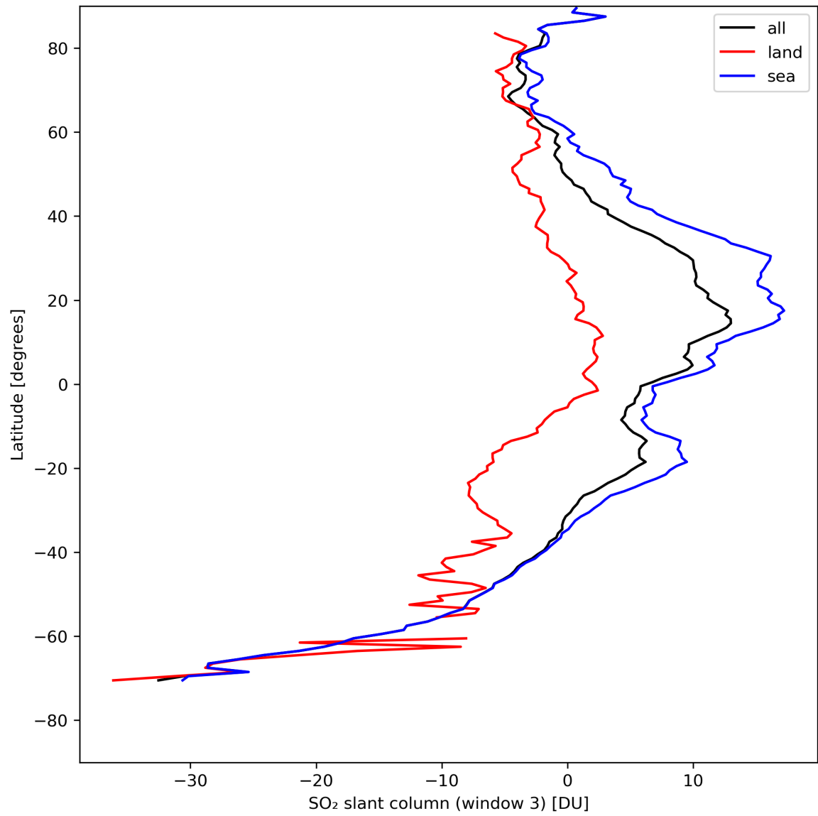
Figure 41: Zonal average of “SO 2 slant column (window 3)” for 2024-08-13 to 2024-08-15.
