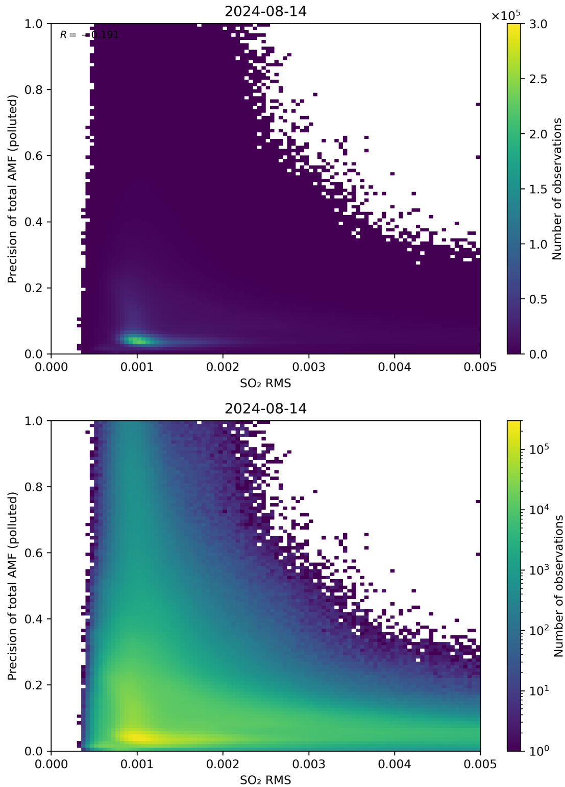
Figure 138: Scatter density plot of “SO 2 RMS” against “Precision of total AMF (polluted)” for 2024-08-13 to 2024-08-15.
