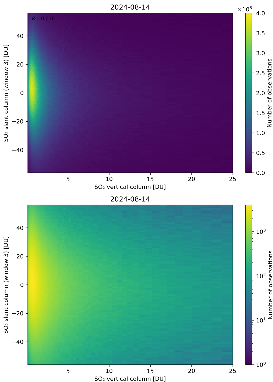
Figure 303: Scatter density plot of “SO 2 vertical column” against “SO 2 slant column (window 3)” for 2024-08-13 to 2024-08-15.
