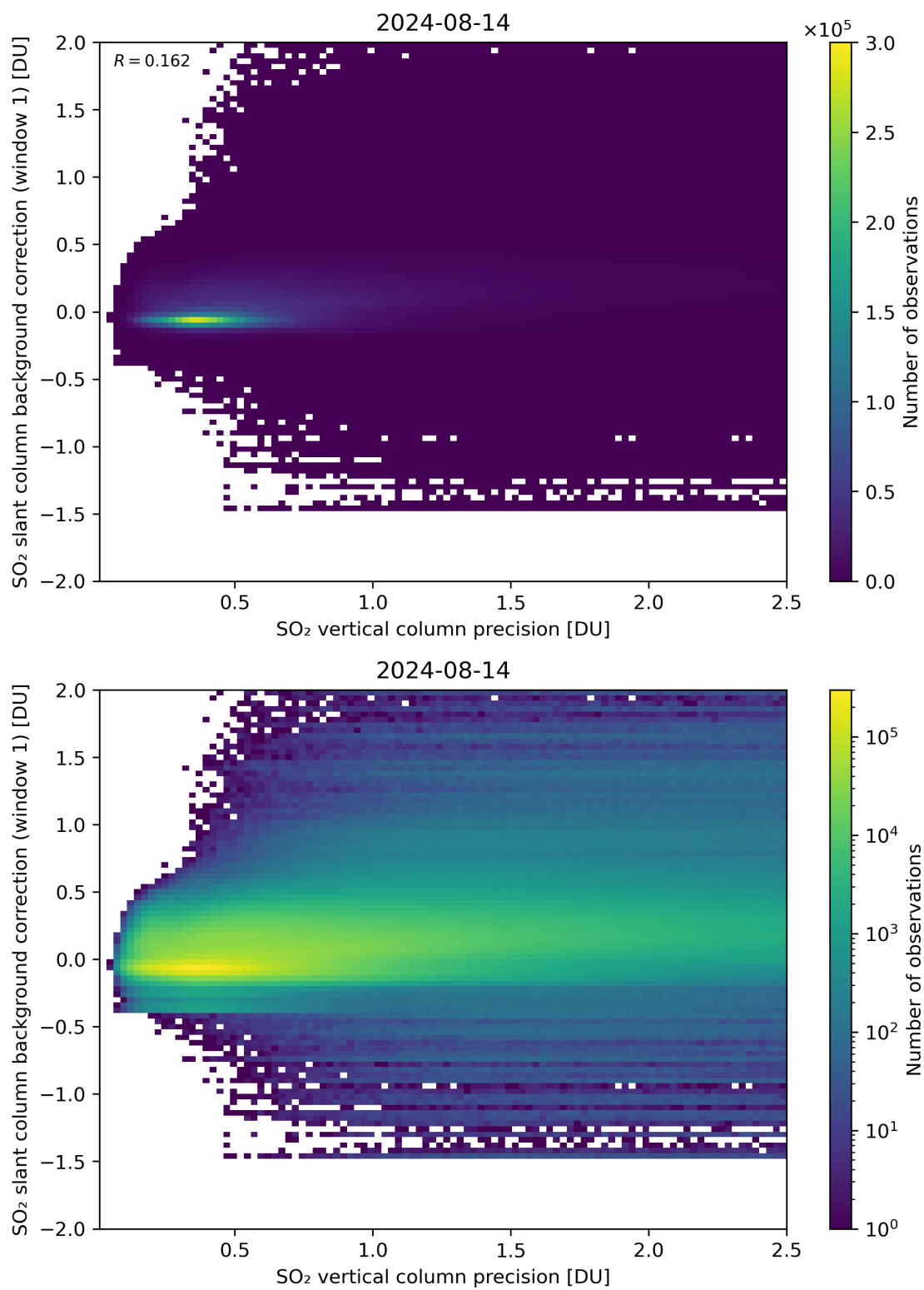
Figure 279: Scatter density plot of “SO 2 vertical column precision” against “SO 2 slant column background correction (window 1)” for 2024-08-13 to 2024-08-15.
