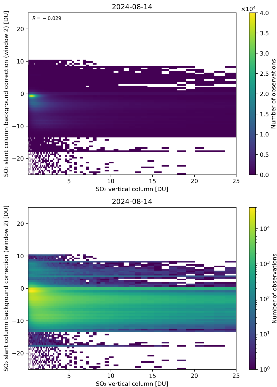
Figure 274: Scatter density plot of “SO 2 vertical column” against “SO 2 slant column background correction (window 2)” for 2024-08-13 to 2024-08-15.
