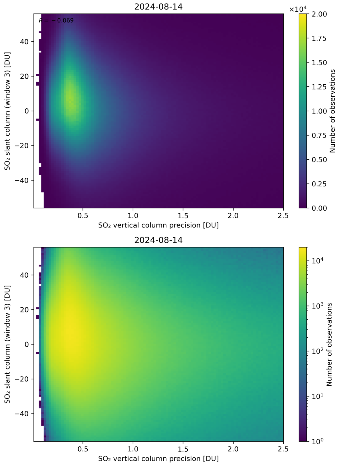
Figure 292: Scatter density plot of “SO 2 vertical column precision” against “SO 2 slant column (window 3)” for 2024-08-13 to 2024-08-15.
