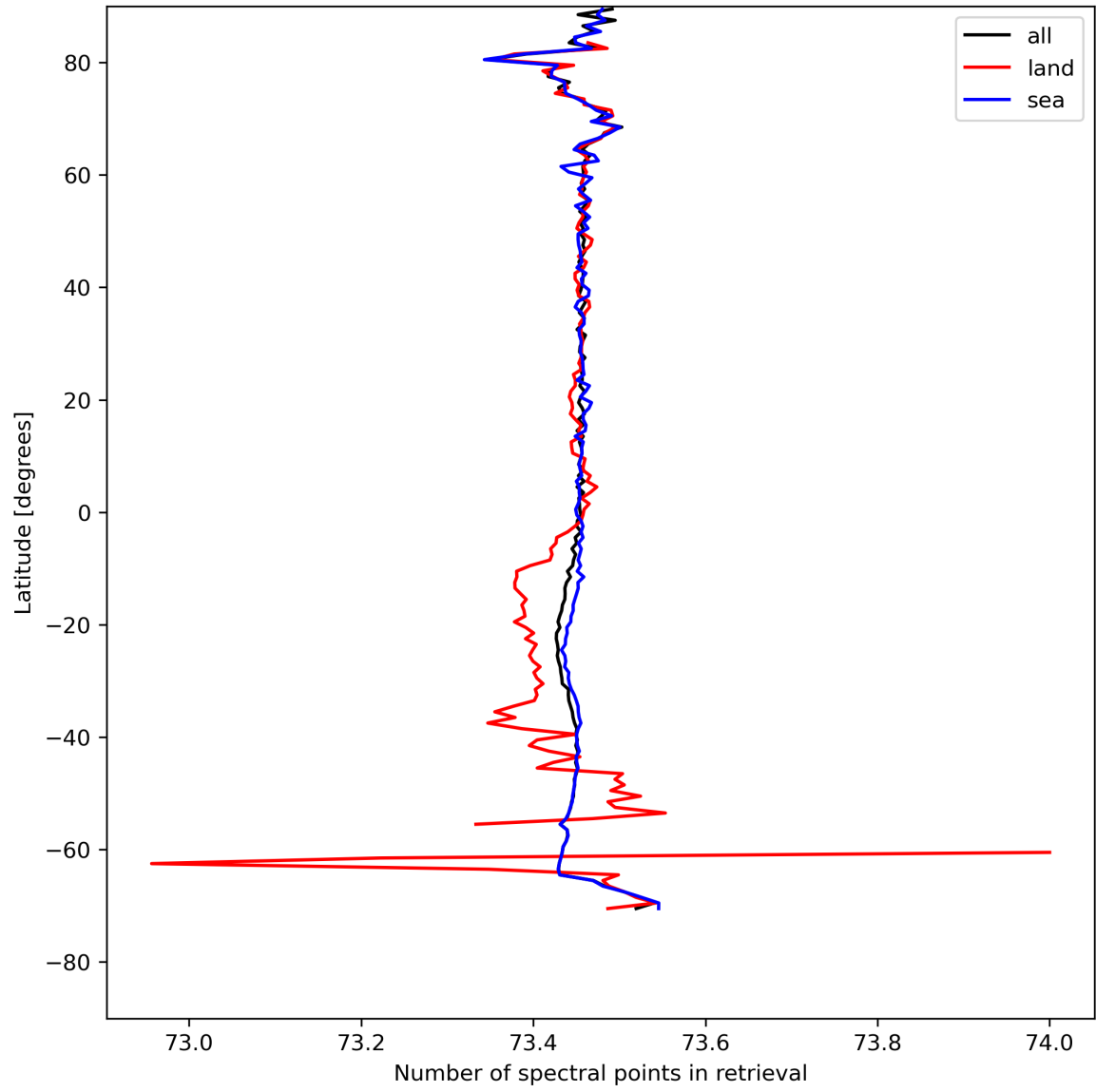
Figure 51: Zonal average of “Number of spectral points in retrieval” for 2024-08-13 to 2024-08-15.
