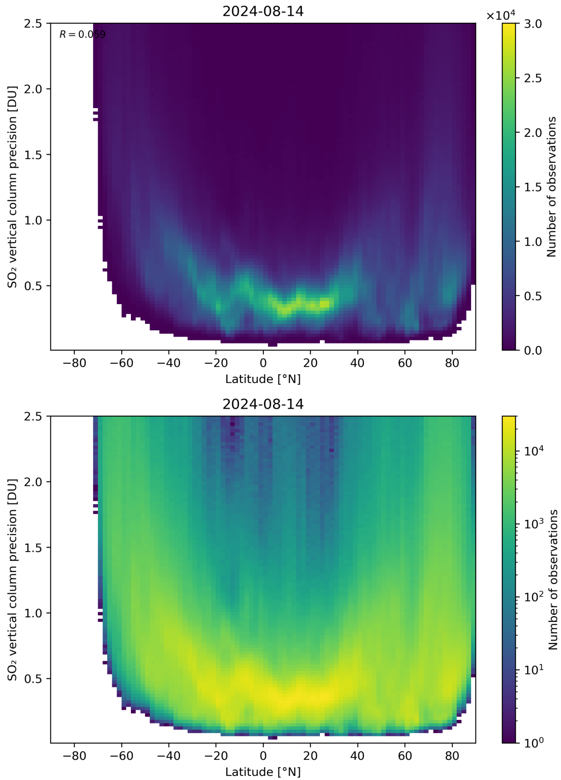
Figure 157: Scatter density plot of “Latitude” against “SO 2 vertical column precision” for 2024-08-13 to 2024-08-15.
