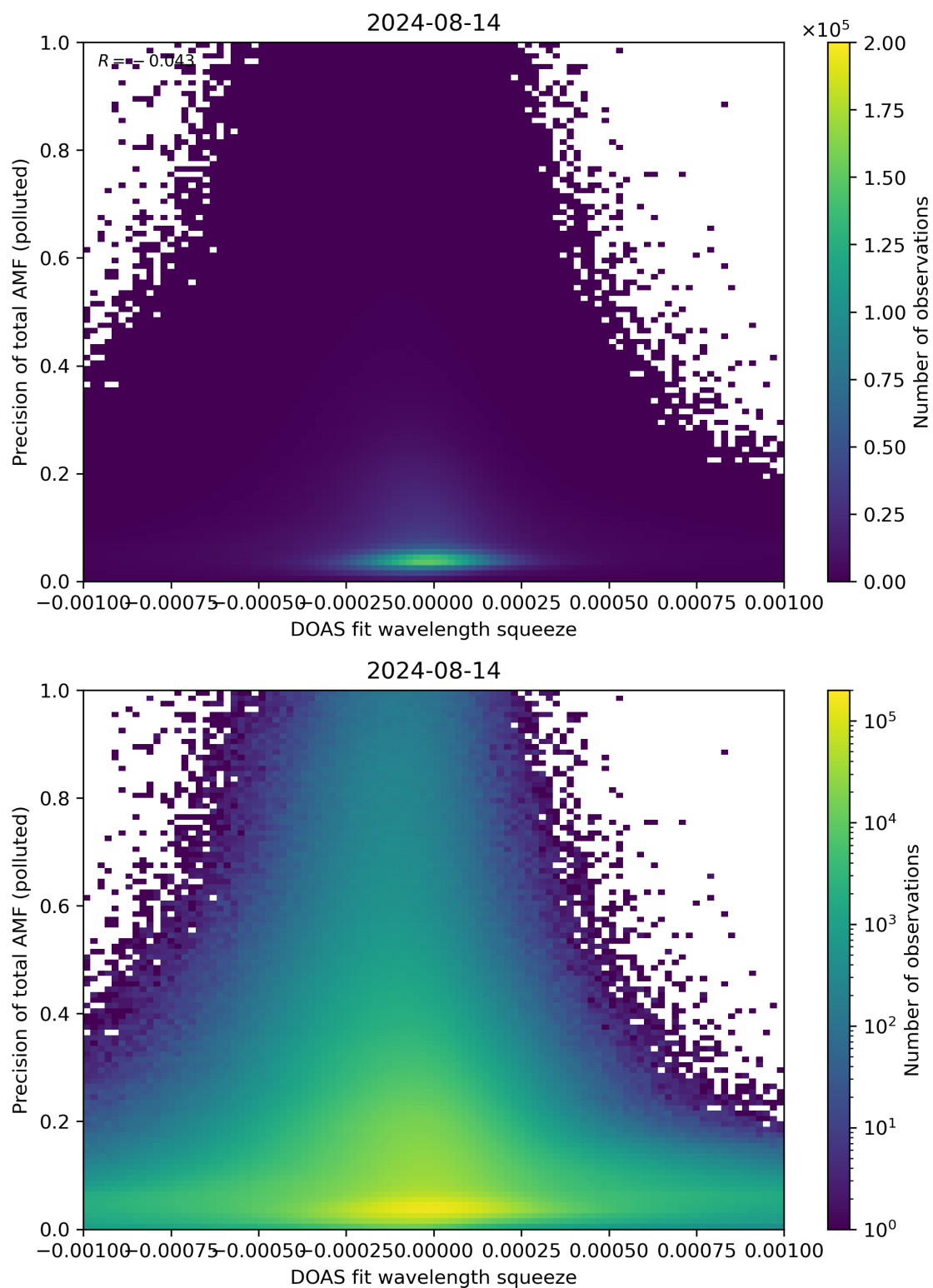
Figure 135: Scatter density plot of “DOAS fit wavelength squeeze” against “Precision of total AMF (polluted)” for 2024-08-13 to 2024-08-15.
