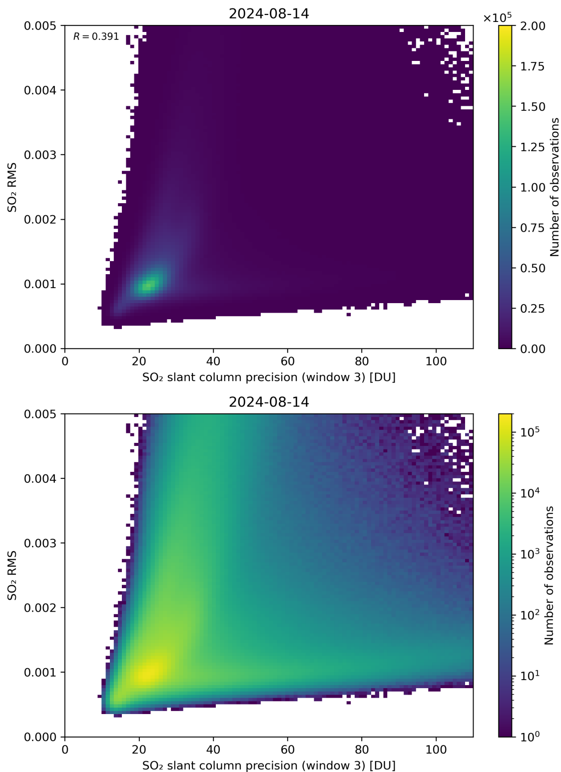
Figure 260: Scatter density plot of “SO 2 slant column precision (window 3)” against “SO 2 RMS” for 2024-08-13 to 2024-08-15.
