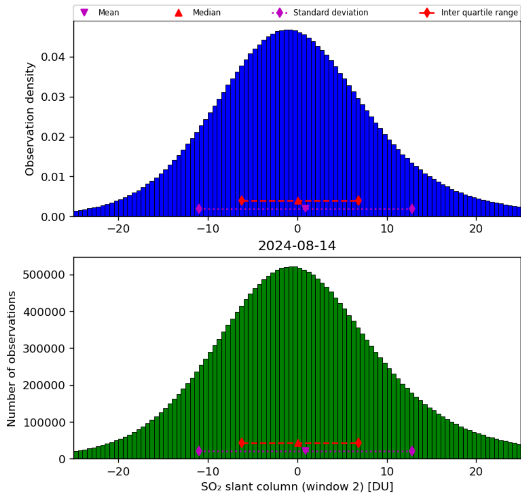
Figure 60: Histogram of “SO 2 slant column (window 2)” for 2024-08-13 to 2024-08-15
