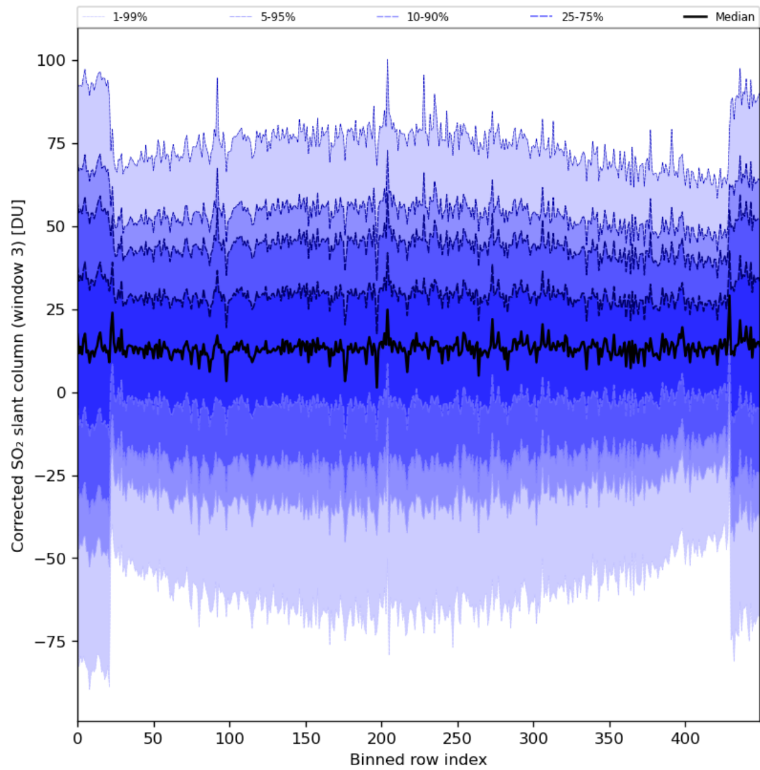
Figure 89: Along track statistics of “Corrected SO 2 slant column (window 3)” for 2024-08-13 to 2024-08-15
