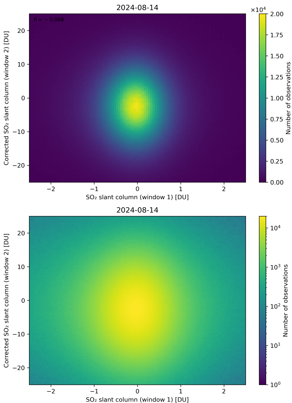
Figure 233: Scatter density plot of “SO 2 slant column (window 1)” against “Corrected SO 2 slant column (window 2)” for 2024-08-13 to 2024-08-15.
