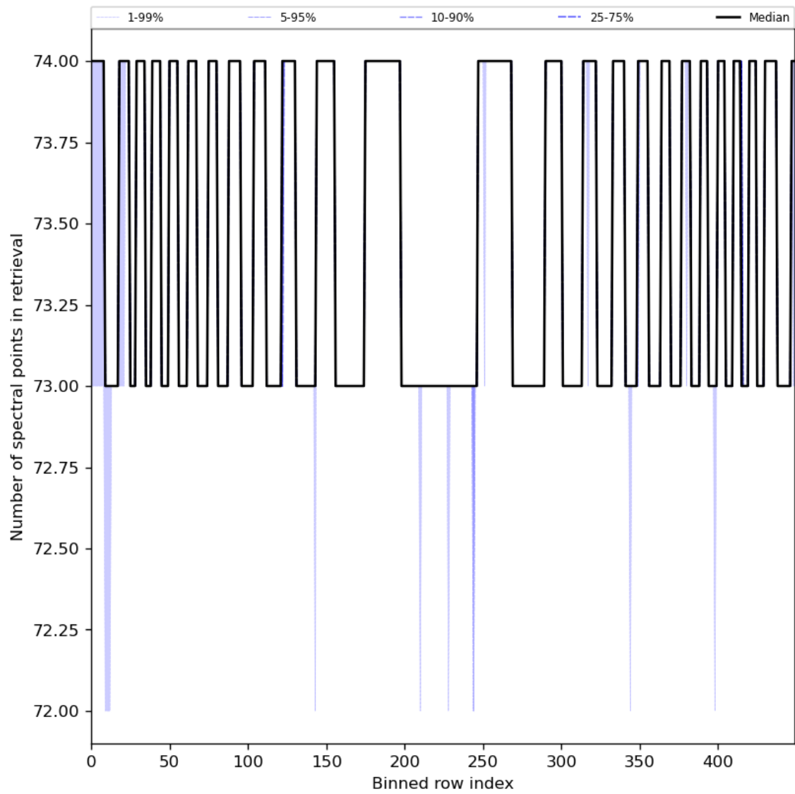
Figure 97: Along track statistics of “Number of spectral points in retrieval” for 2024-08-13 to 2024-08-15
