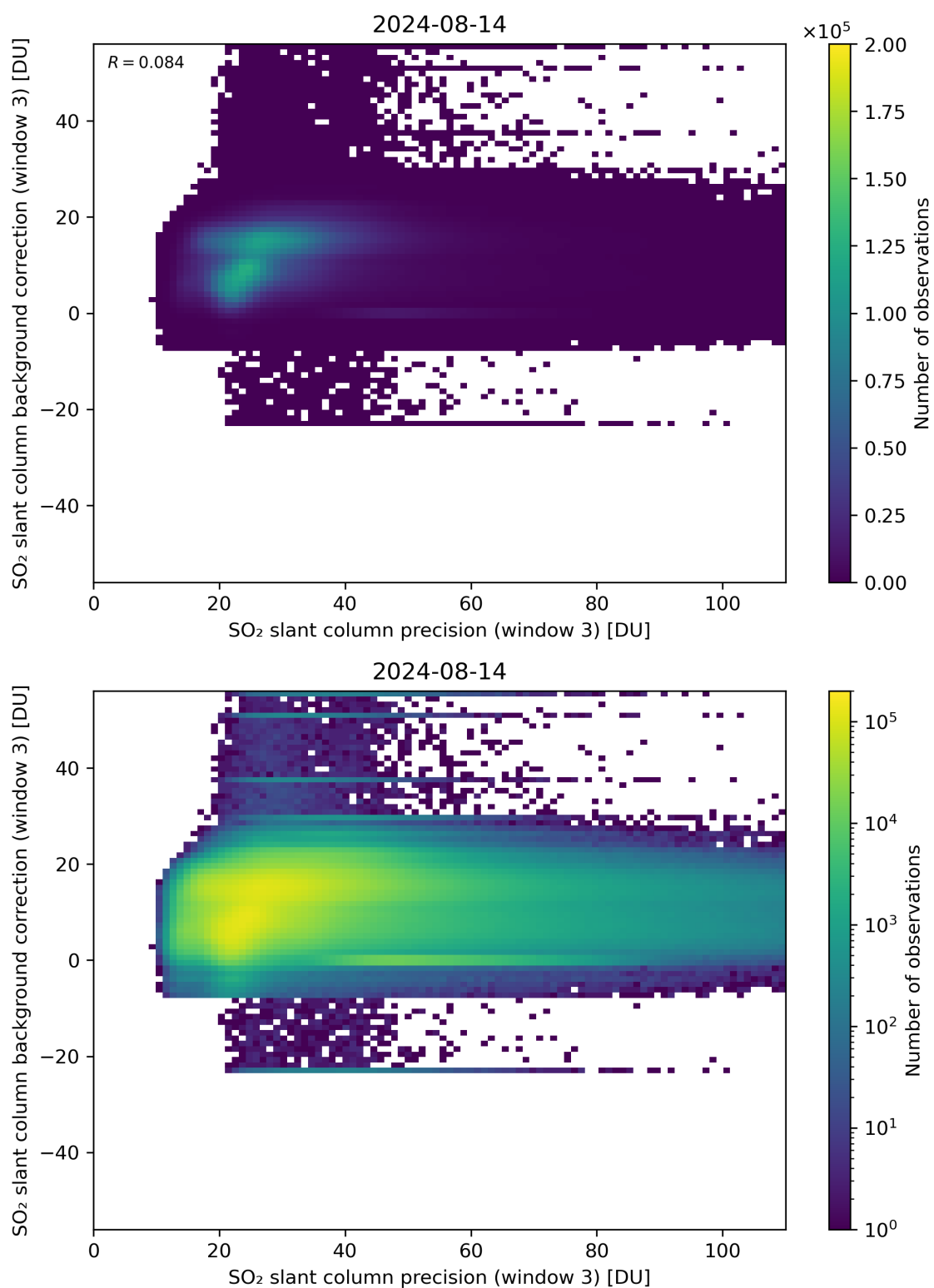
Figure 257: Scatter density plot of “SO 2 slant column precision (window 3)” against “SO 2 slant column background correction (window 3)” for 2024-08-13 to 2024-08-15.
