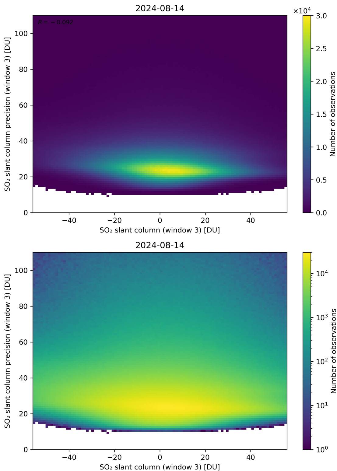
Figure 267: Scatter density plot of “SO 2 slant column (window 3)” against “SO 2 slant column precision (window 3)” for 2024-08-13 to 2024-08-15.
