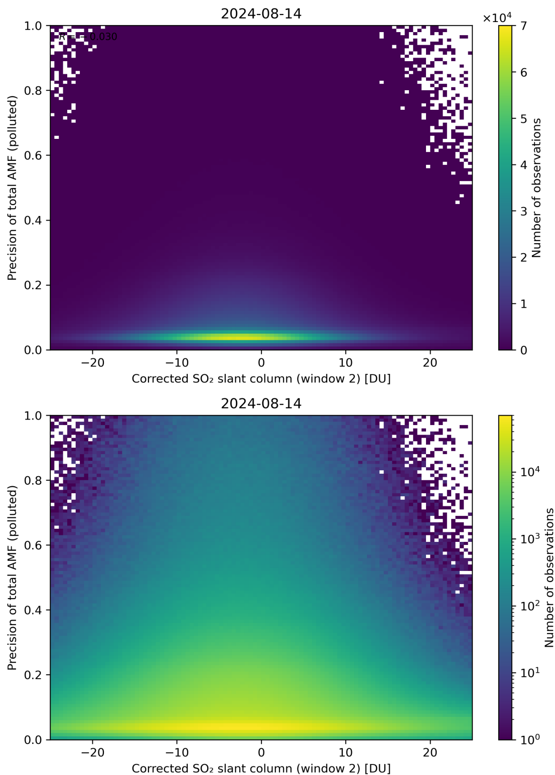
Figure 204: Scatter density plot of “Corrected SO 2 slant column (window 2)” against “Precision of total AMF (polluted)” for 2024-08-13 to 2024-08-15.
