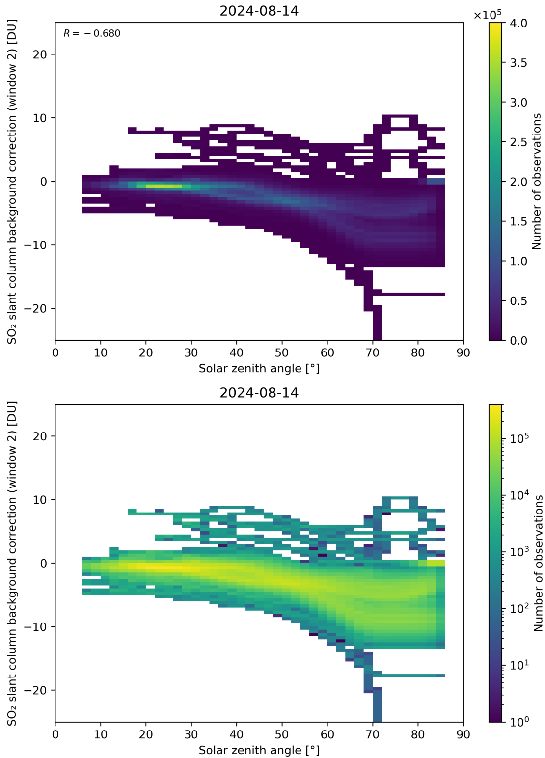
Figure 159: Scatter density plot of “Solar zenith angle” against “SO 2 slant column background correction (window 2)” for 2024-08-13 to 2024-08-15.
