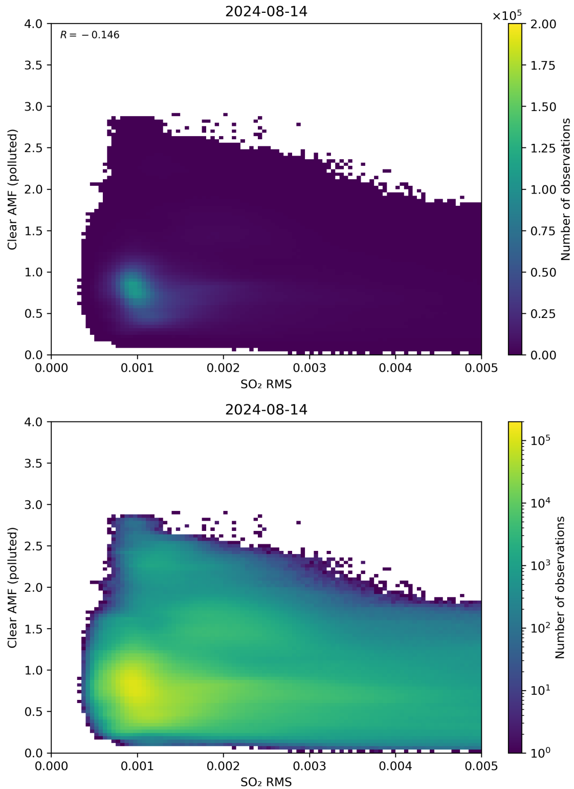
Figure 136: Scatter density plot of “SO 2 RMS” against “Clear AMF (polluted)” for 2024-08-13 to 2024-08-15.
