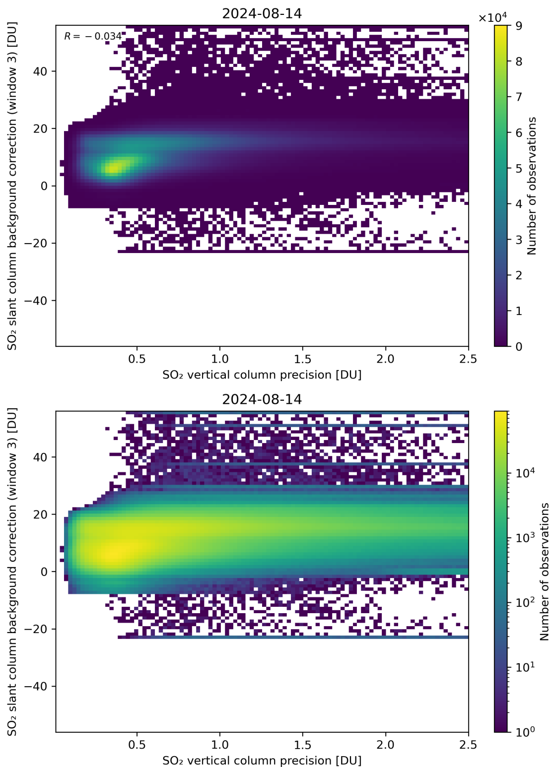
Figure 281: Scatter density plot of “SO 2 vertical column precision” against “SO 2 slant column background correction (window 3)” for 2024-08-13 to 2024-08-15.
