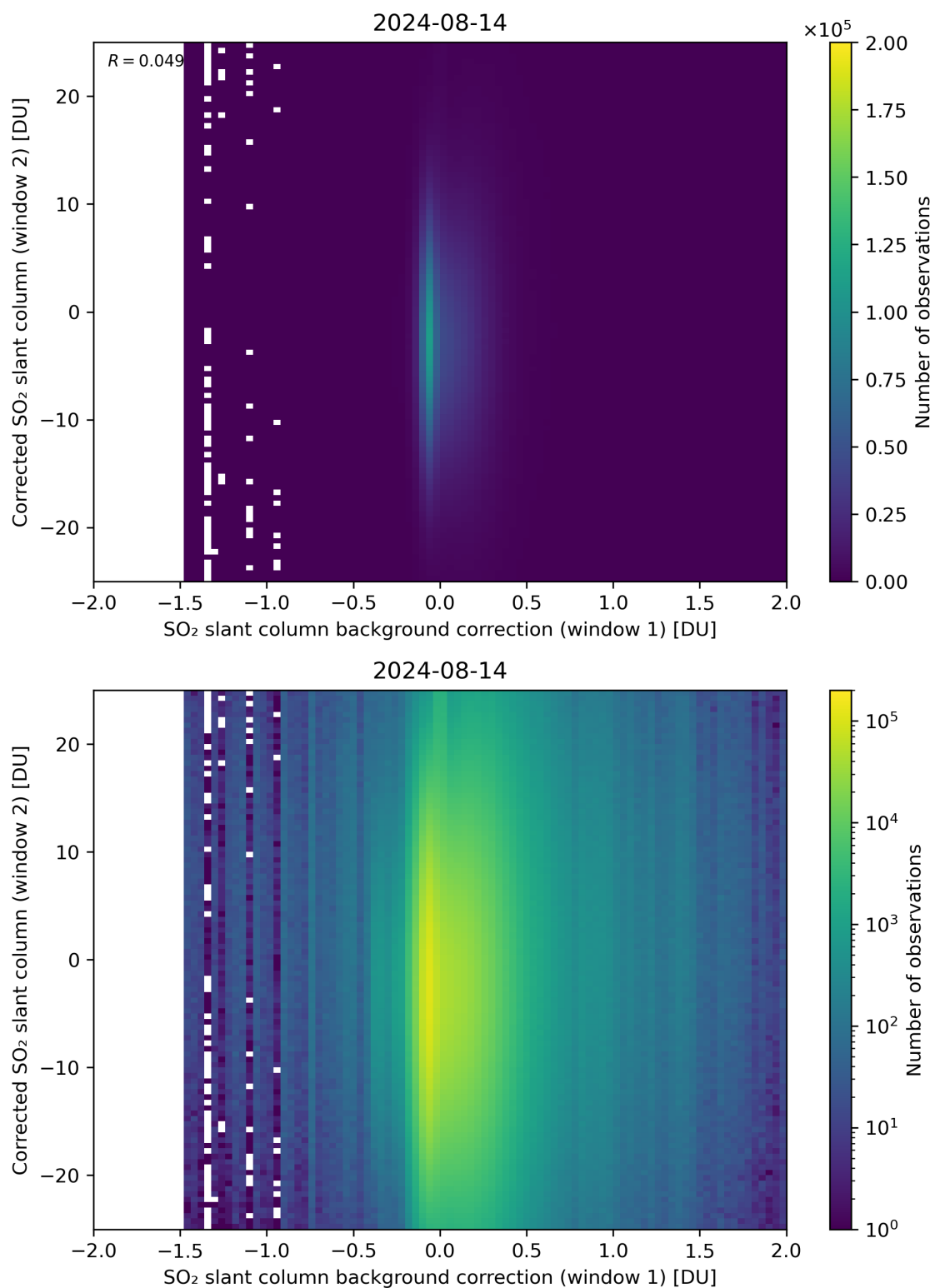
Figure 104: Scatter density plot of “SO 2 slant column background correction (window 1)” against “Corrected SO 2 slant column (window 2)” for 2024-08-13 to 2024-08-15.
