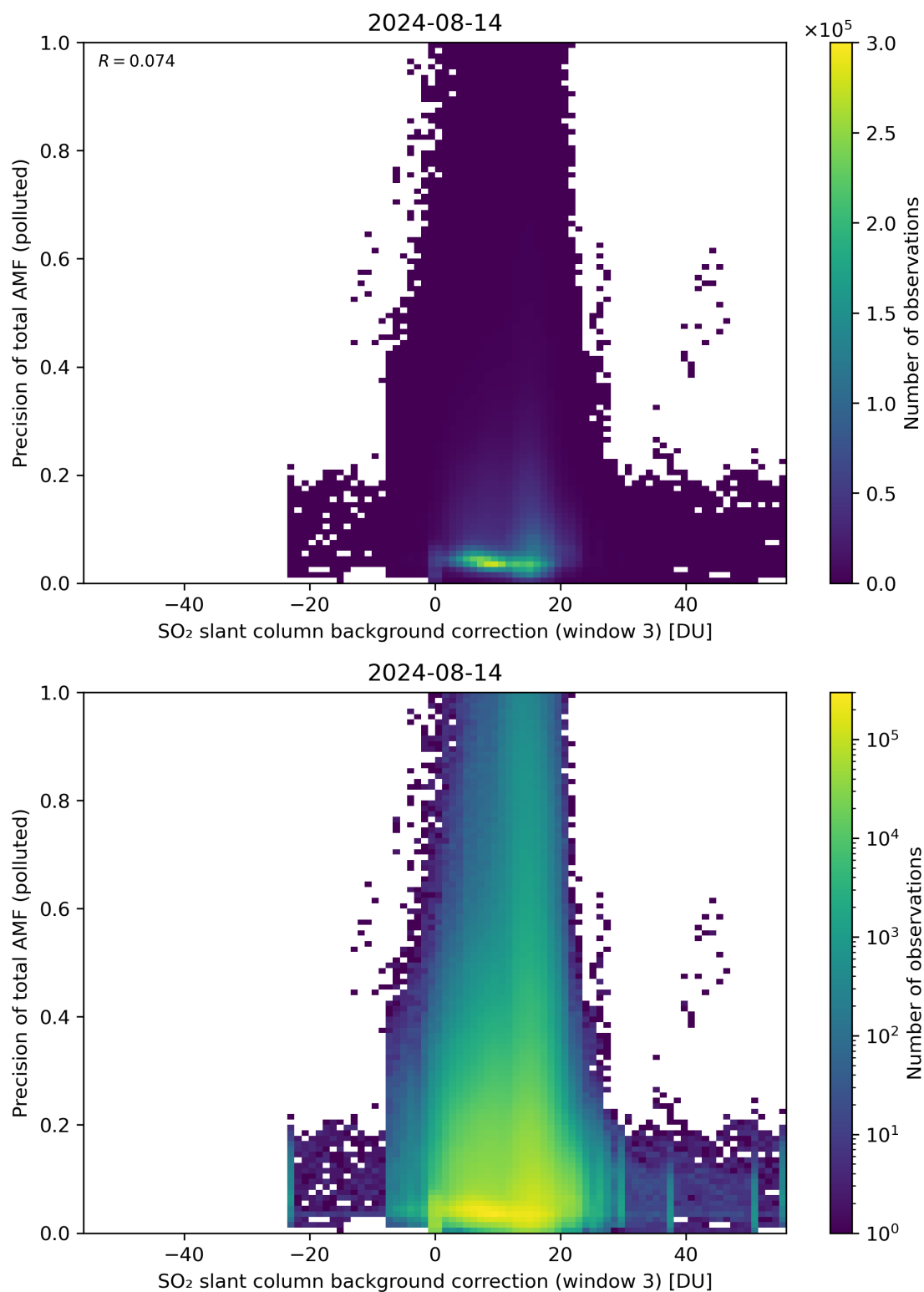
Figure 126: Scatter density plot of “SO 2 slant column background correction (window 3)” against “Precision of total AMF (polluted)” for 2024-08-13 to 2024-08-15.
