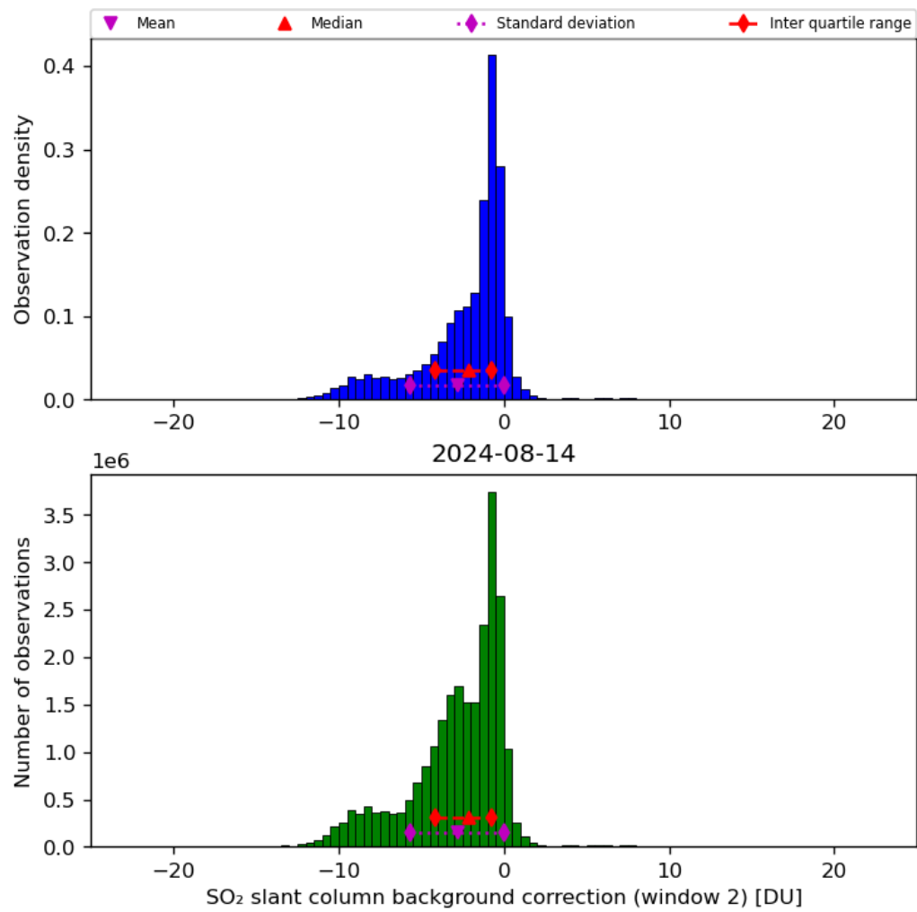
Figure 63: Histogram of “SO 2 slant column background correction (window 2)” for 2024-08-13 to 2024-08-15
