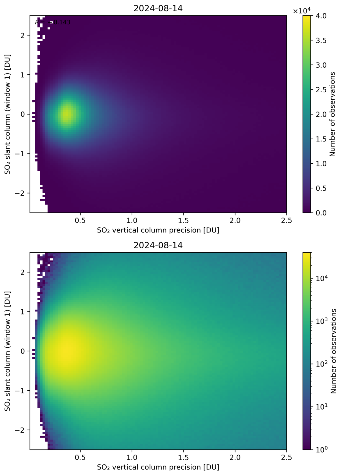
Figure 289: Scatter density plot of “SO 2 vertical column precision” against “SO 2 slant column (window 1)” for 2024-08-13 to 2024-08-15.
