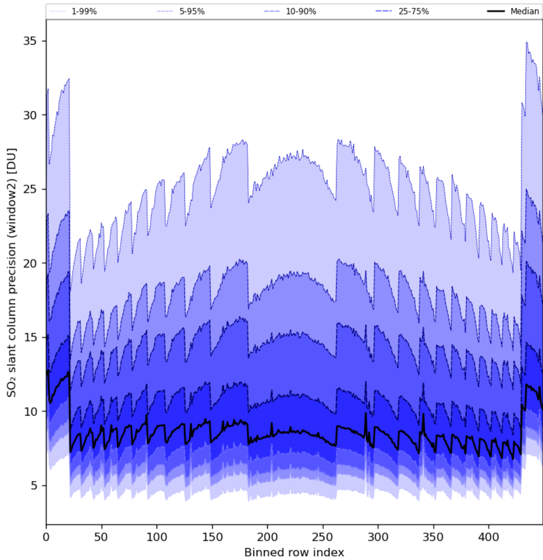
Figure 84: Along track statistics of “SO 2 slant column precision (window2)” for 2024-08-13 to 2024-08-15
