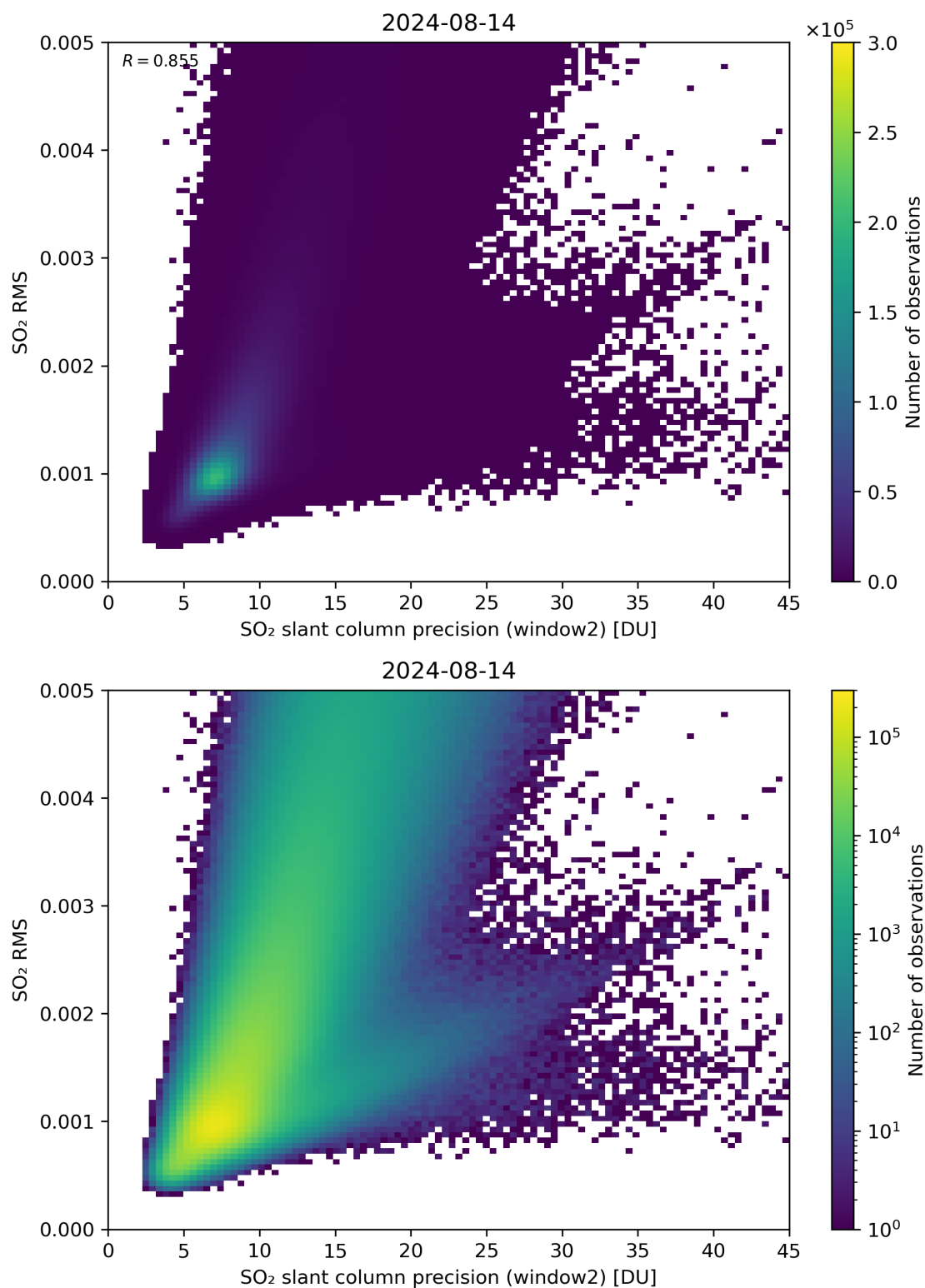
Figure 245: Scatter density plot of “SO 2 slant column precision (window2)” against “SO 2 RMS” for 2024-08-13 to 2024-08-15.
