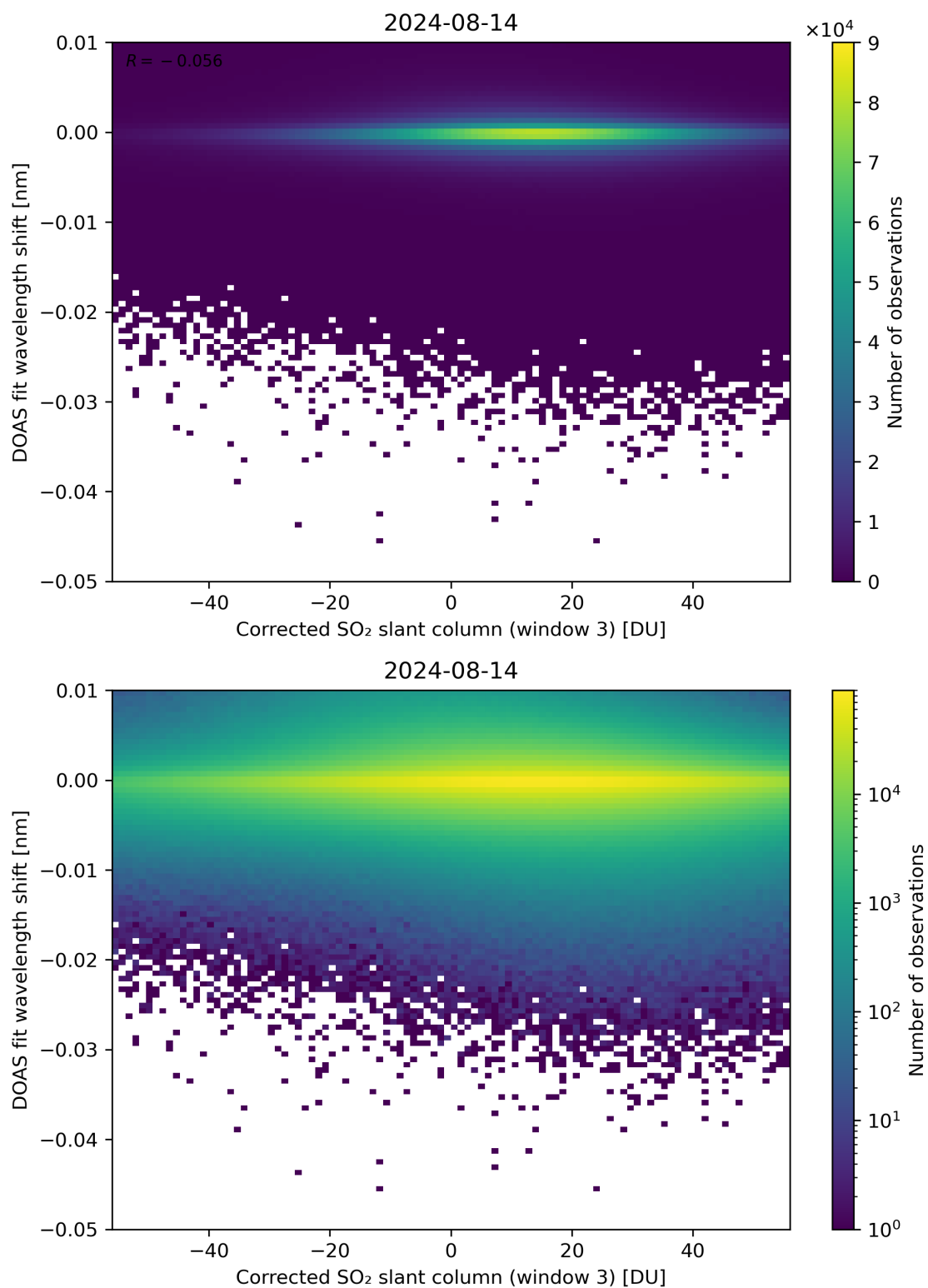
Figure 206: Scatter density plot of “Corrected SO 2 slant column (window 3)” against “DOAS fit wavelength shift” for 2024-08-13 to 2024-08-15.
