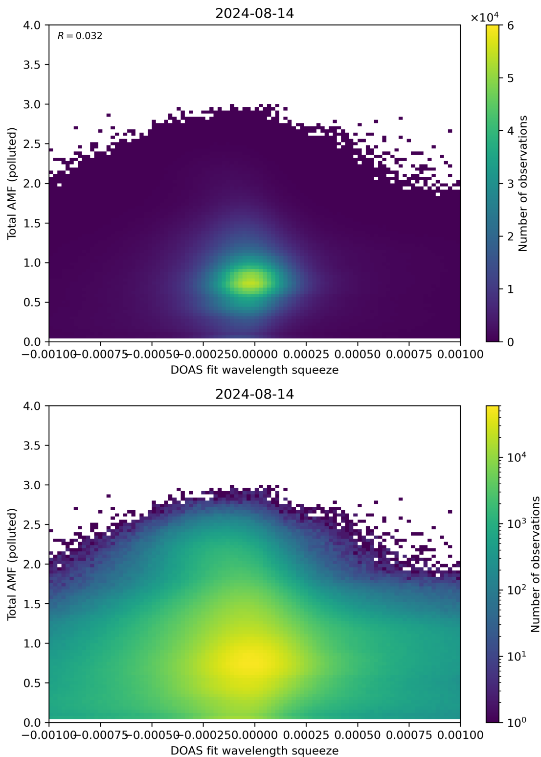
Figure 134: Scatter density plot of “DOAS fit wavelength squeeze” against “Total AMF (polluted)” for 2024-08-13 to 2024-08-15.
