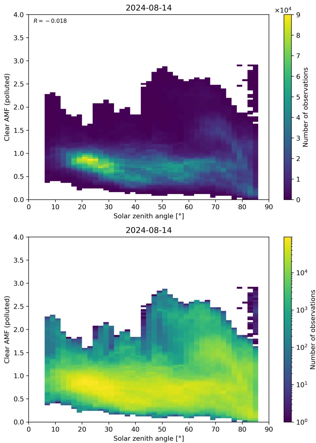
Figure 165: Scatter density plot of “Solar zenith angle” against “Clear AMF (polluted)” for 2024-08-13 to 2024-08-15.
