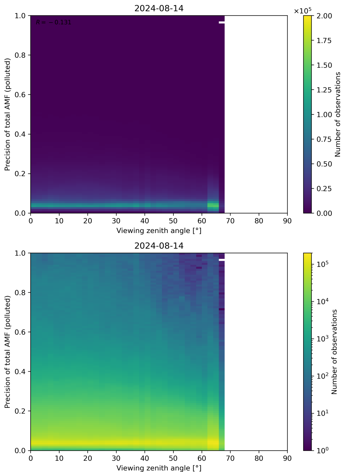
Figure 326: Scatter density plot of “Viewing zenith angle” against “Precision of total AMF (polluted)” for 2024-08-13 to 2024-08-15.
