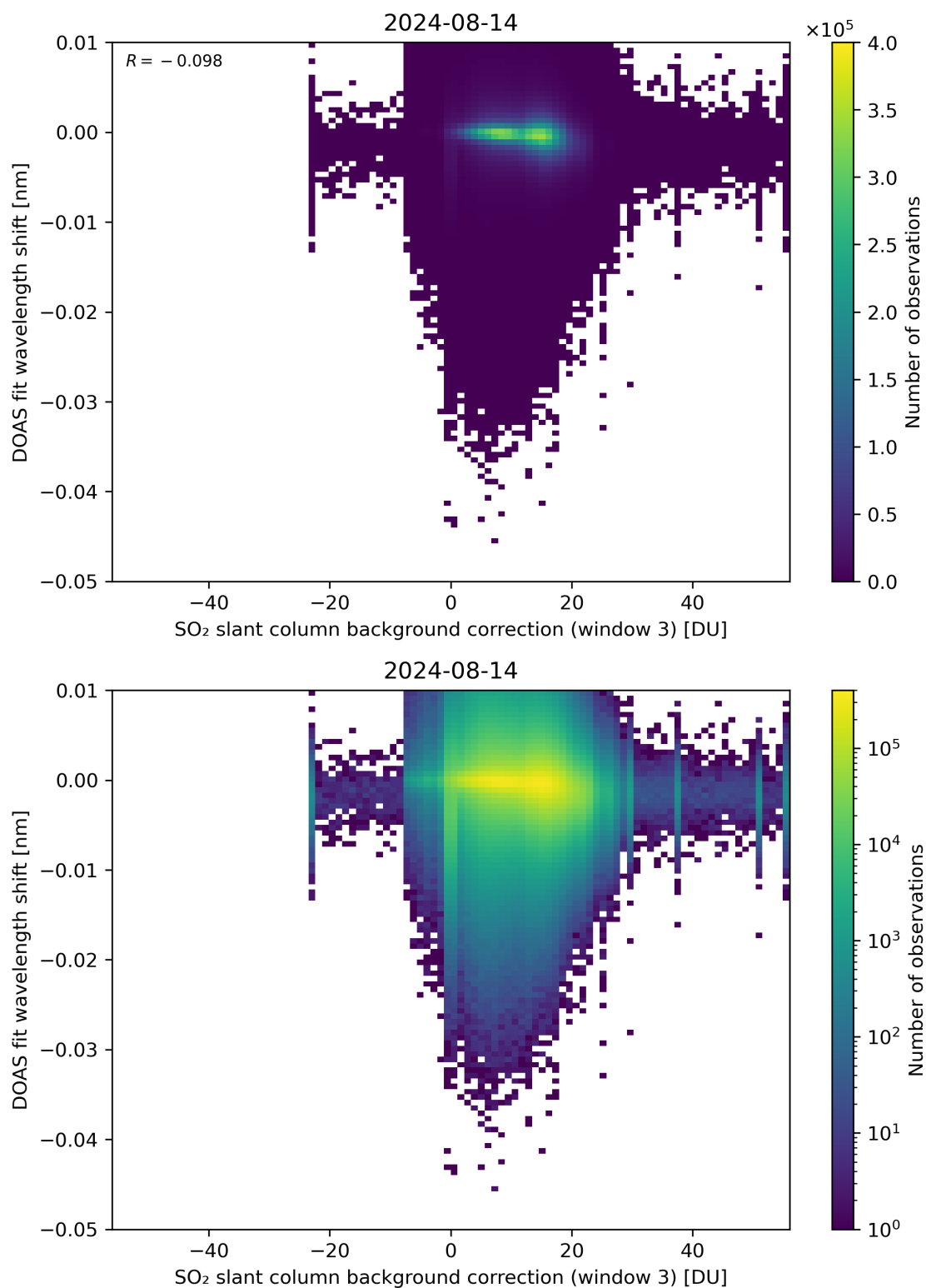
Figure 121: Scatter density plot of “SO 2 slant column background correction (window 3)” against “DOAS fit wavelength shift” for 2024-08-13 to 2024-08-15.
