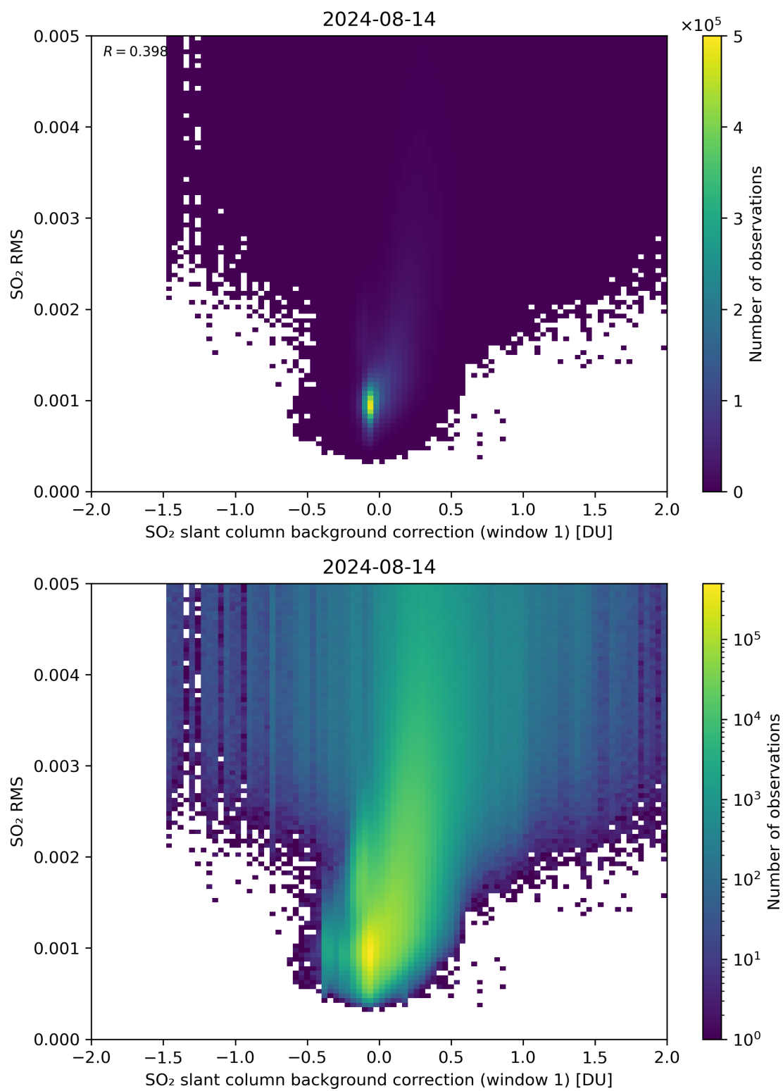
Figure 102: Scatter density plot of “SO 2 slant column background correction (window 1)” against “SO 2 RMS” for 2024-08-13 to 2024-08-15.
