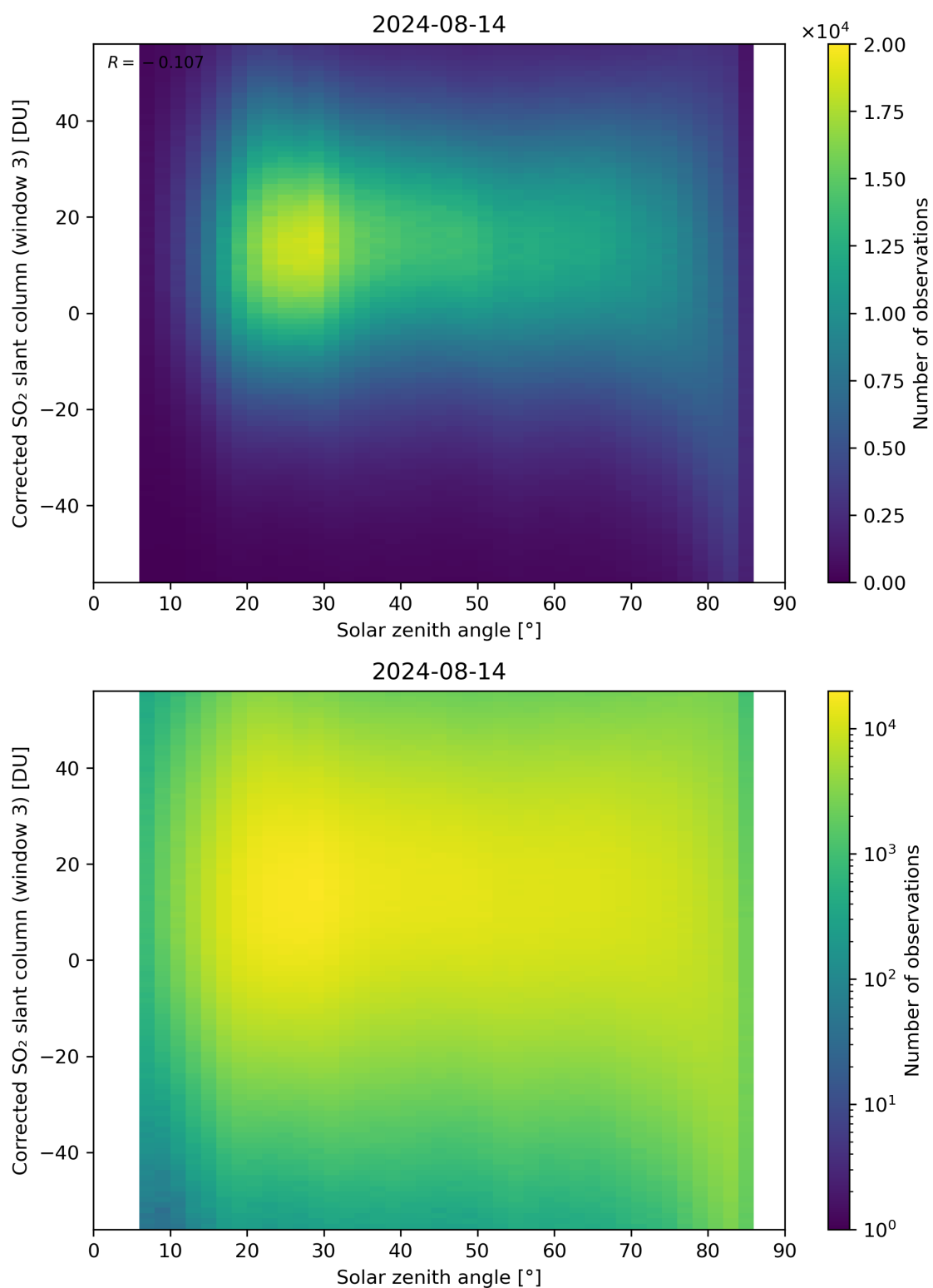
Figure 168: Scatter density plot of “Solar zenith angle” against “Corrected SO 2 slant column (window 3)” for 2024-08-13 to 2024-08-15.
