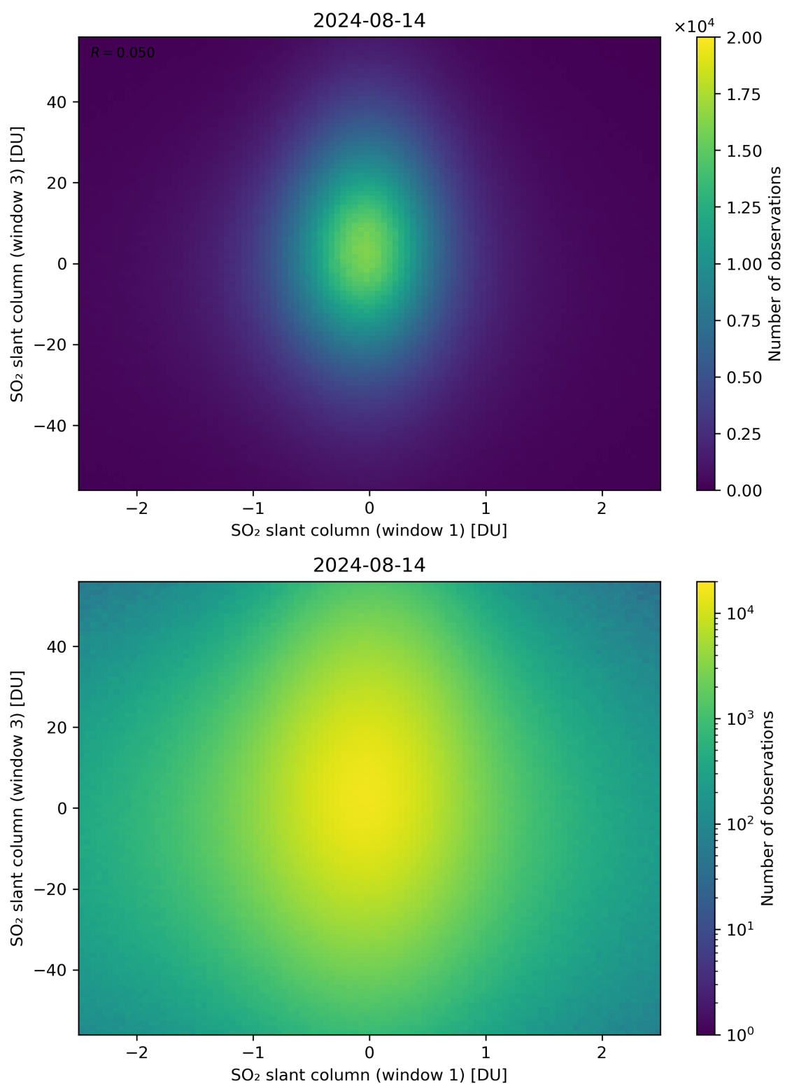
Figure 237: Scatter density plot of “SO 2 slant column (window 1)” against “SO 2 slant column (window 3)” for 2024-08-13 to 2024-08-15.
