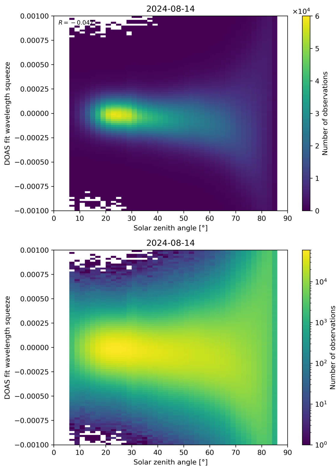
Figure 162: Scatter density plot of “Solar zenith angle” against “DOAS fit wavelength squeeze” for 2024-08-13 to 2024-08-15.
