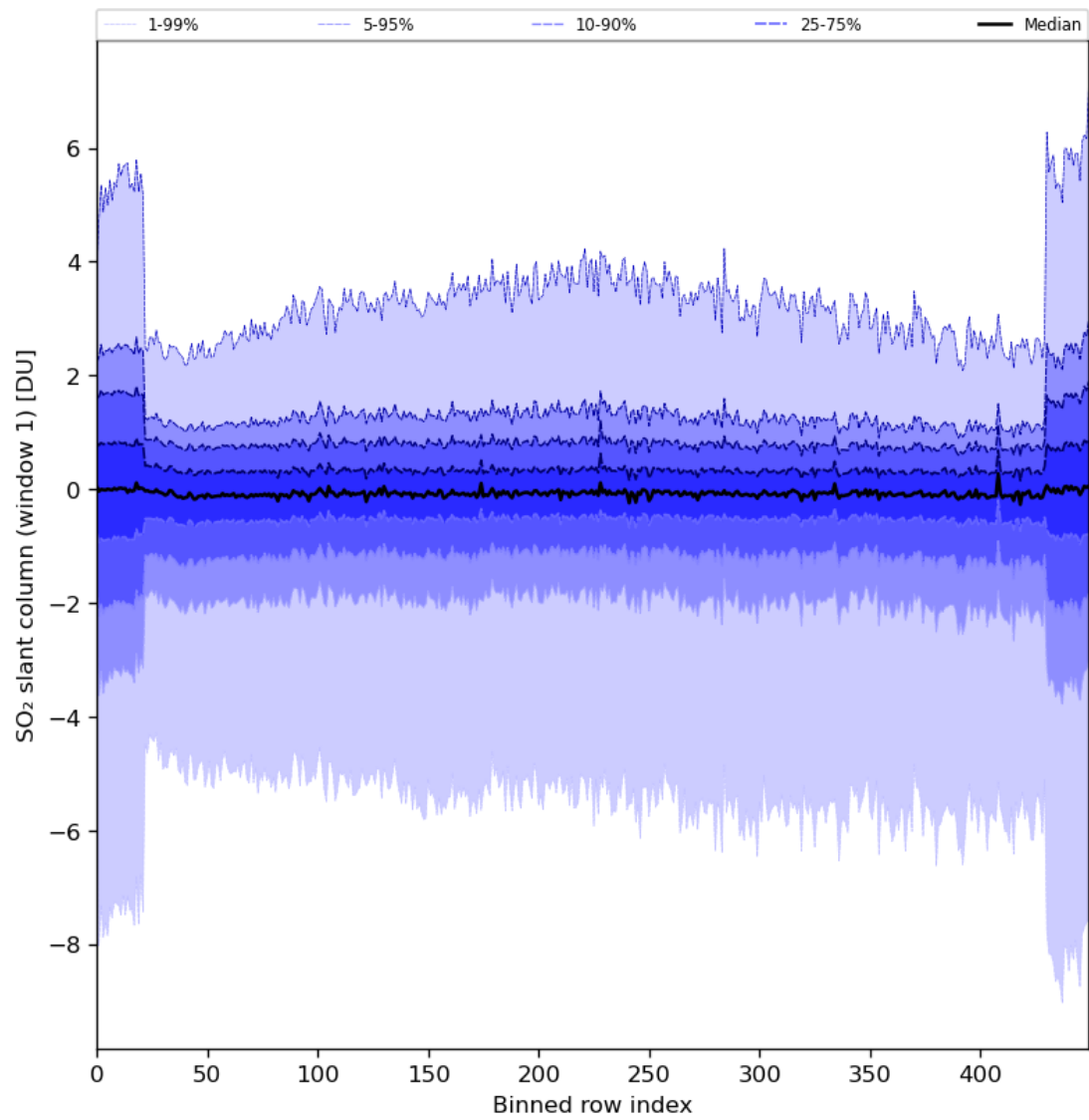
Figure 79: Along track statistics of “SO 2 slant column (window 1)” for 2024-08-13 to 2024-08-15
