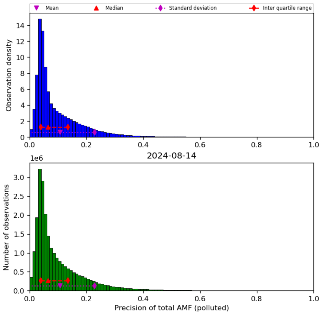
Figure 72: Histogram of “Precision of total AMF (polluted)” for 2024-08-13 to 2024-08-15
