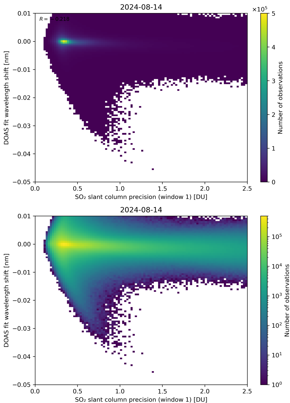
Figure 221: Scatter density plot of “SO 2 slant column precision (window 1)” against “DOAS fit wavelength shift” for 2024-08-13 to 2024-08-15.
