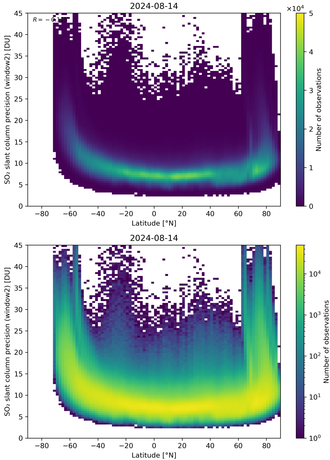
Figure 151: Scatter density plot of “Latitude” against “SO 2 slant column precision (window2)” for 2024-08-13 to 2024-08-15.
