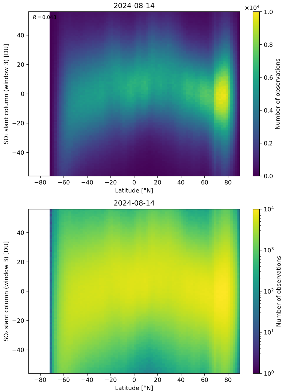
Figure 152: Scatter density plot of “Latitude” against “SO 2 slant column (window 3)” for 2024-08-13 to 2024-08-15.
