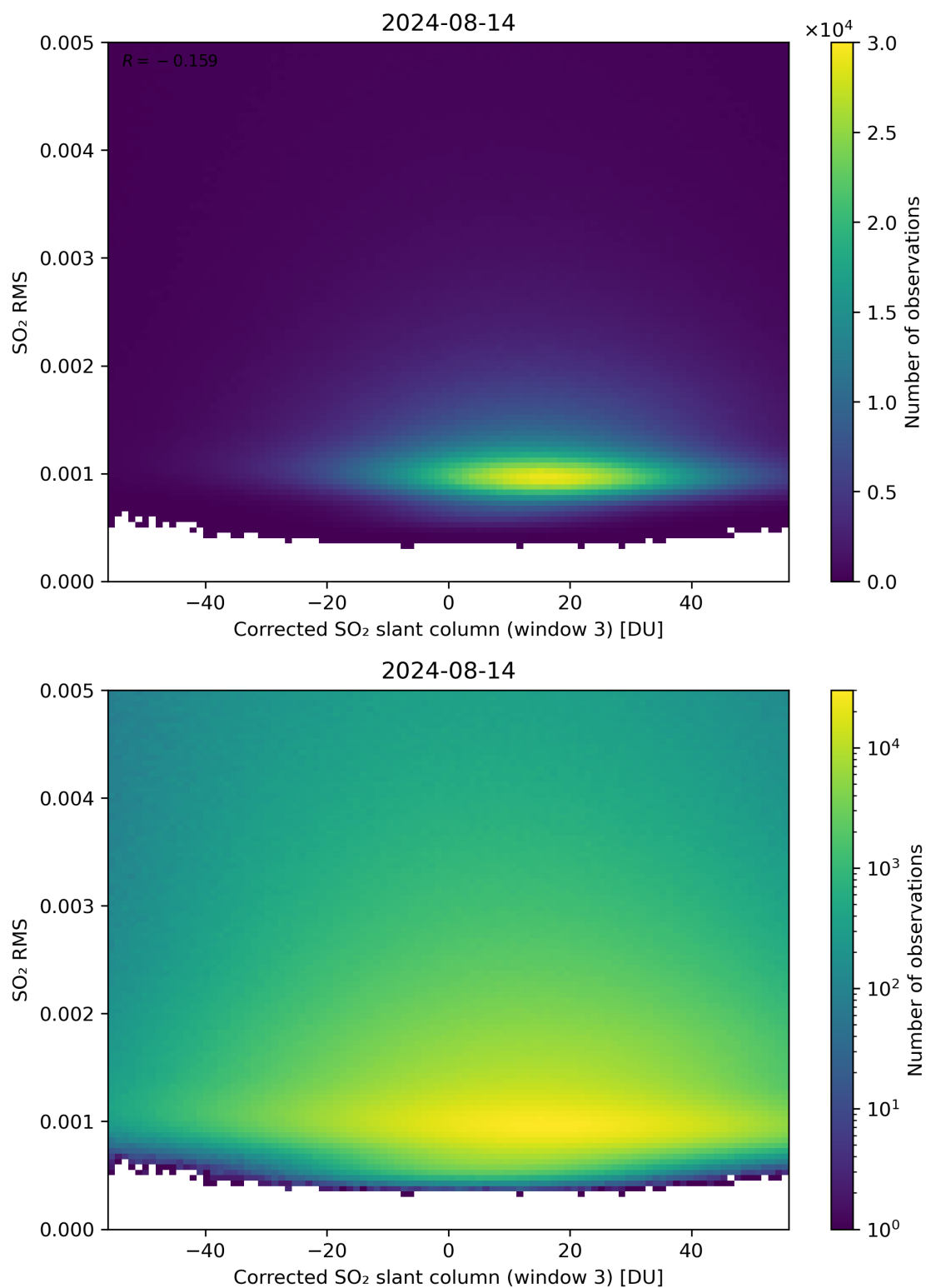
Figure 208: Scatter density plot of “Corrected SO 2 slant column (window 3)” against “SO 2 RMS” for 2024-08-13 to 2024-08-15.
