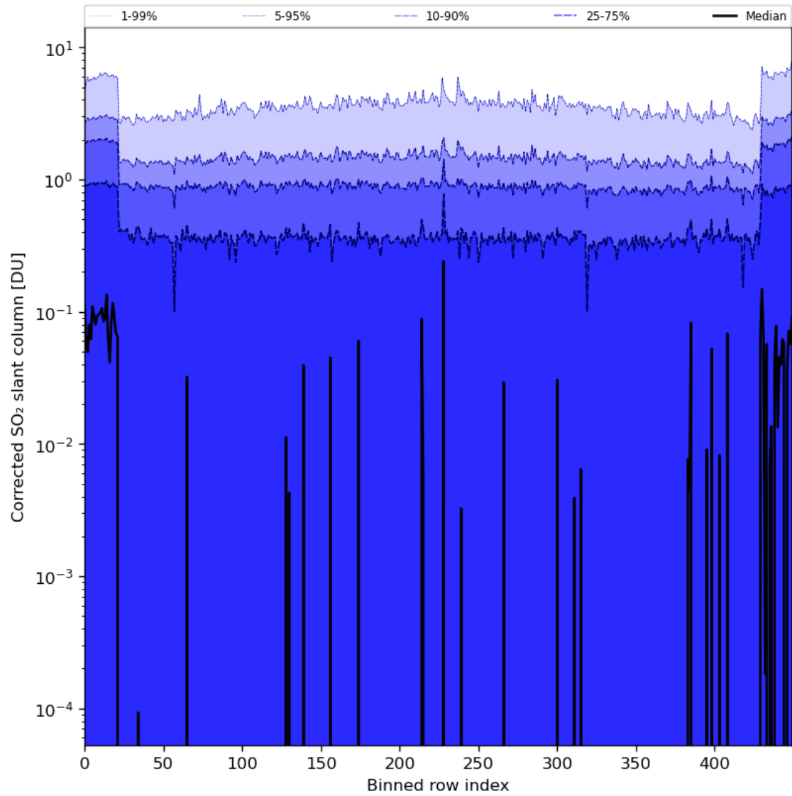
Figure 78: Along track statistics of “Corrected SO 2 slant column” for 2024-08-13 to 2024-08-15
