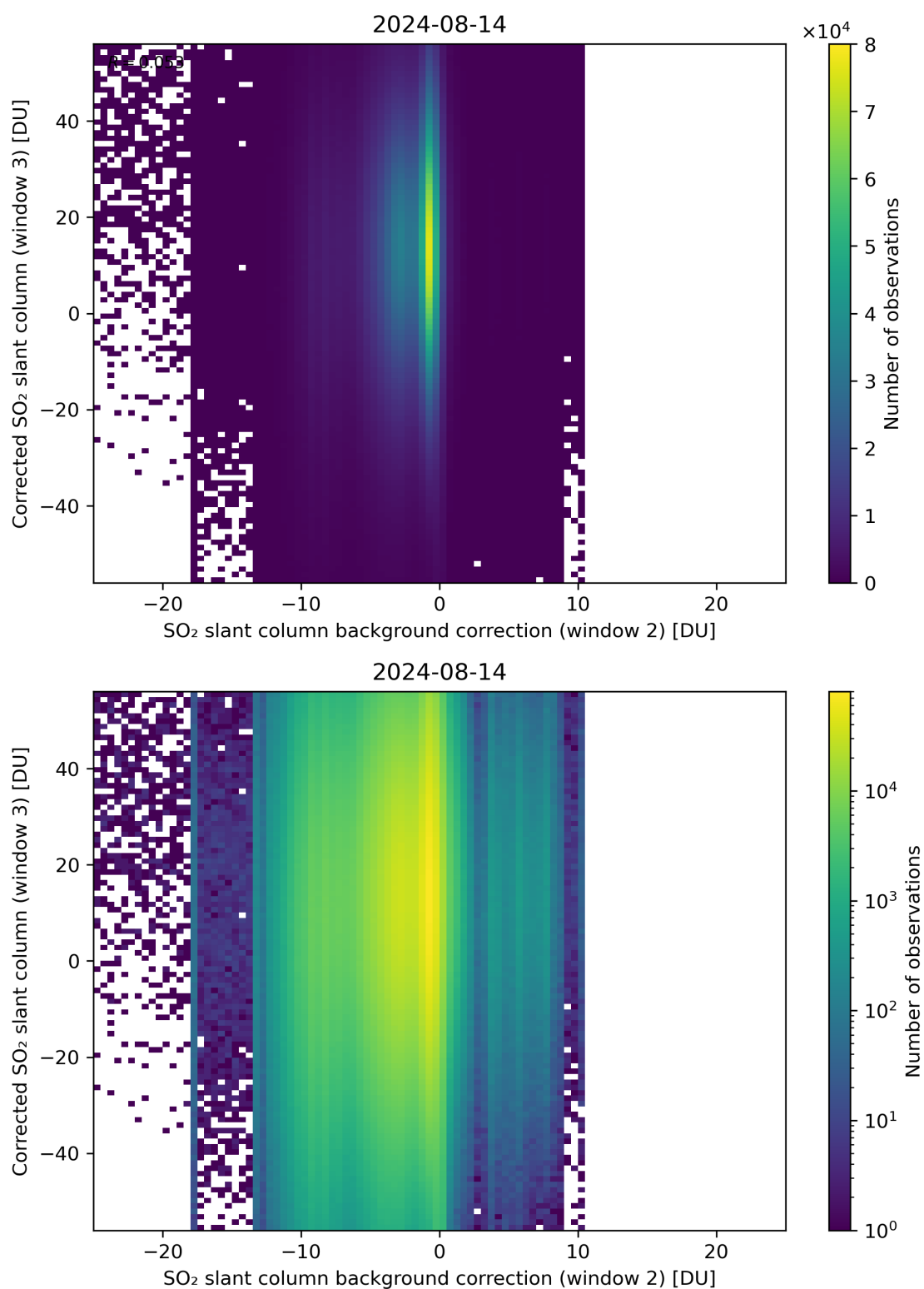
Figure 116: Scatter density plot of “SO 2 slant column background correction (window 2)” against “Corrected SO 2 slant column (window 3)” for 2024-08-13 to 2024-08-15.
