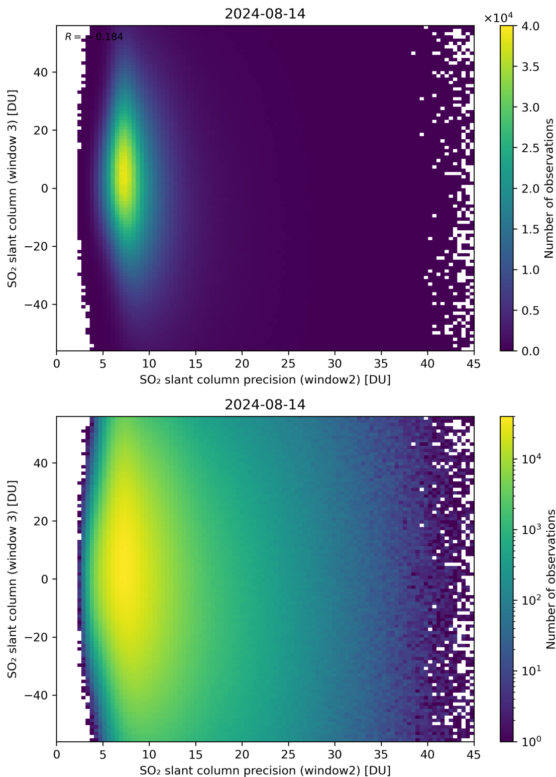
Figure 249: Scatter density plot of “SO 2 slant column precision (window2)” against “SO 2 slant column (window 3)” for 2024-08-13 to 2024-08-15.
