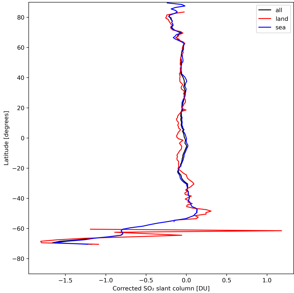
Figure 32: Zonal average of “Corrected SO 2 slant column” for 2024-08-13 to 2024-08-15.
