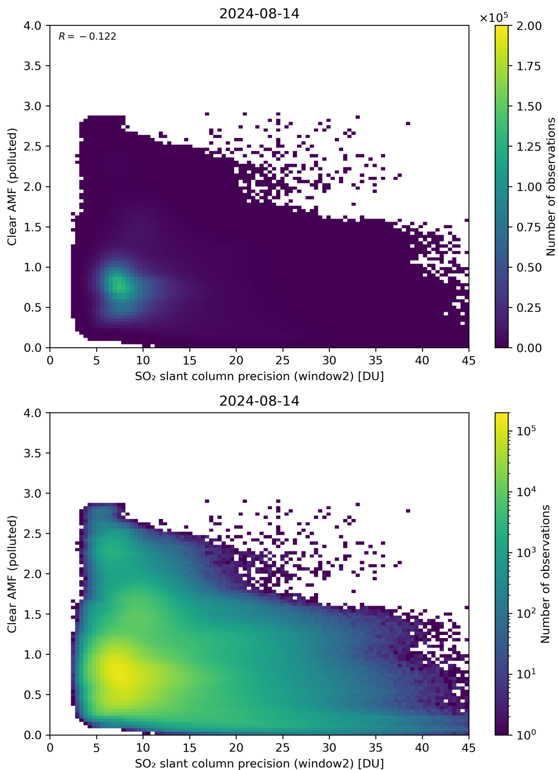
Figure 246: Scatter density plot of “SO 2 slant column precision (window2)” against “Clear AMF (polluted)” for 2024-08-13 to 2024-08-15.
