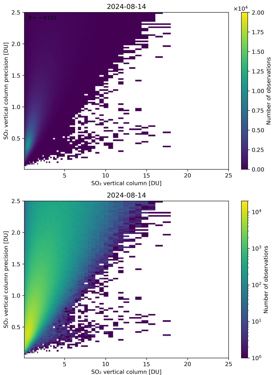
Figure 307: Scatter density plot of “SO 2 vertical column” against “SO 2 vertical column precision” for 2024-08-13 to 2024-08-15.
