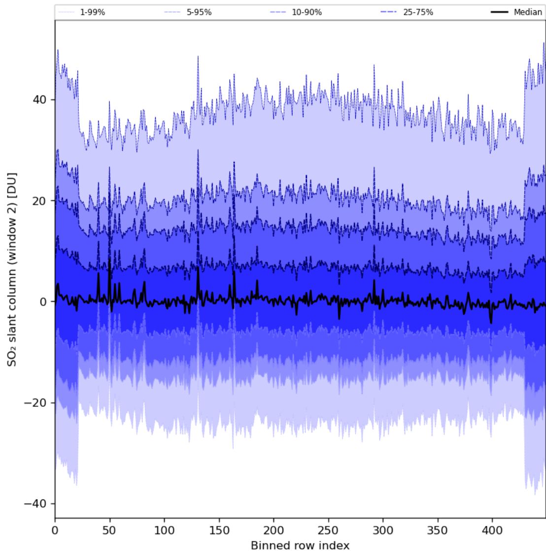
Figure 83: Along track statistics of “SO 2 slant column (window 2)” for 2024-08-13 to 2024-08-15
