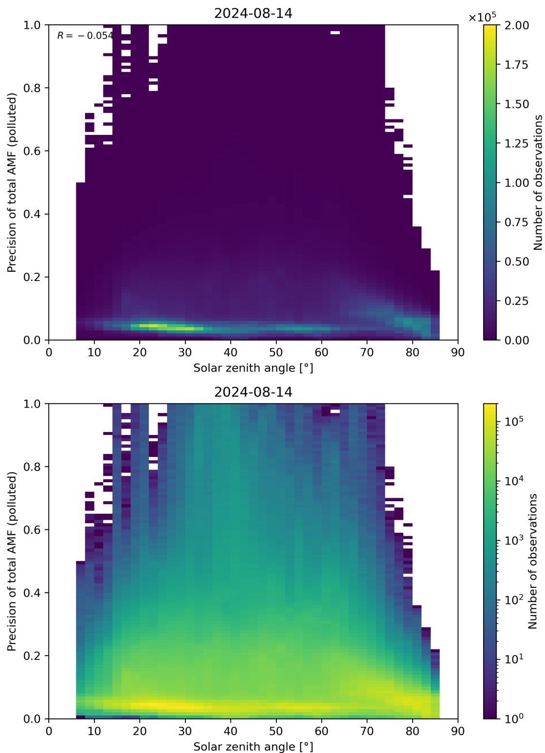
Figure 175: Scatter density plot of “Solar zenith angle” against “Precision of total AMF (polluted)” for 2024-08-13 to 2024-08-15.
