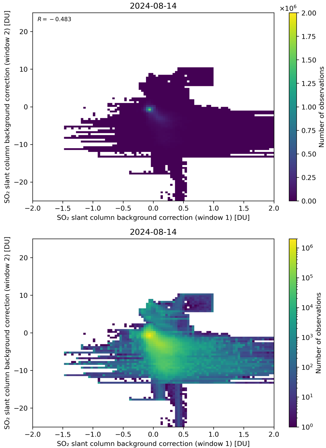
Figure 98: Scatter density plot of “SO 2 slant column background correction (window 1)” against “SO 2 slant column background correction (window 2)” for 2024-08-13 to 2024-08-15.
