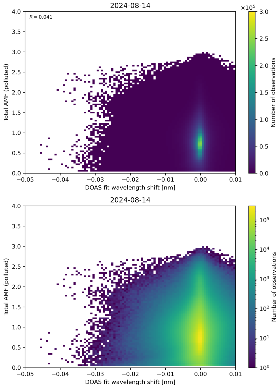
Figure 130: Scatter density plot of “DOAS fit wavelength shift” against “Total AMF (polluted)” for 2024-08-13 to 2024-08-15.
