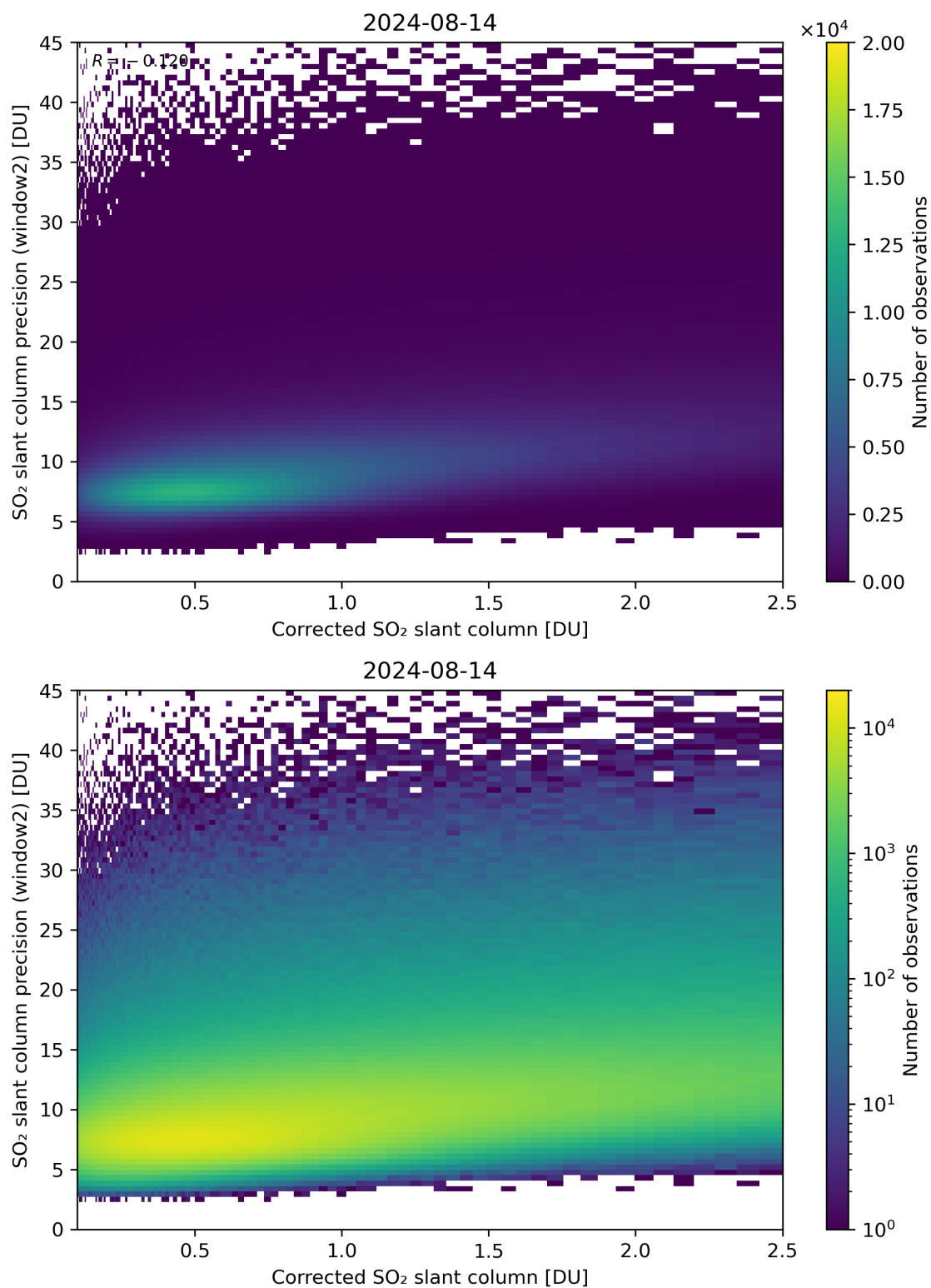
Figure 189: Scatter density plot of “Corrected SO 2 slant column” against “SO 2 slant column precision (window2)” for 2024-08-13 to 2024-08-15.
