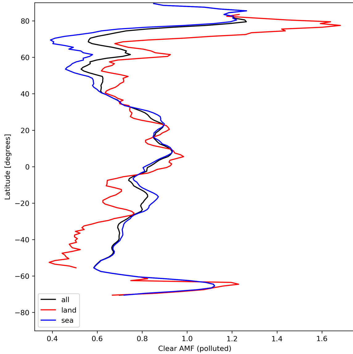
Figure 50: Zonal average of “Clear AMF (polluted)” for 2024-08-13 to 2024-08-15.
