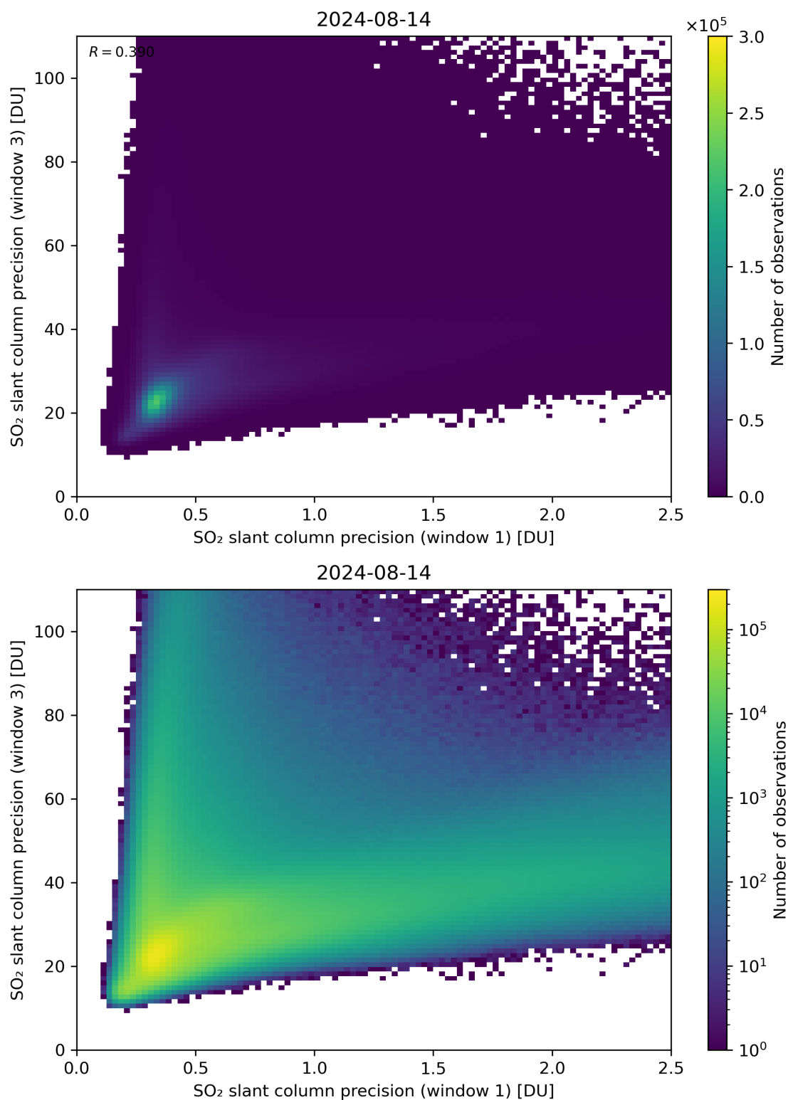
Figure 229: Scatter density plot of “SO 2 slant column precision (window 1)” against “SO 2 slant column precision (window 3)” for 2024-08-13 to 2024-08-15.
