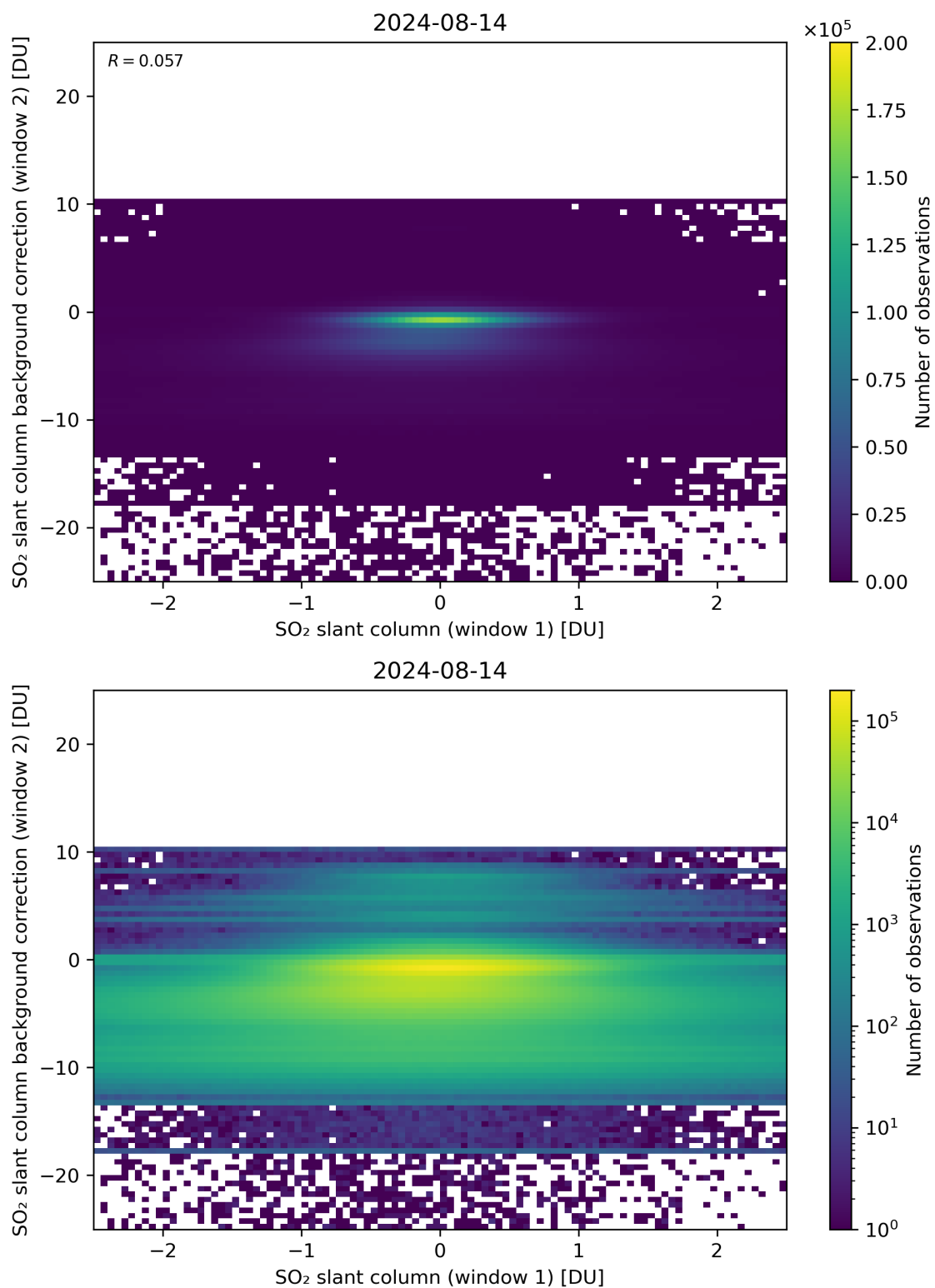
Figure 213: Scatter density plot of “SO 2 slant column (window 1)” against “SO 2 slant column background correction (window 2)” for 2024-08-13 to 2024-08-15.
