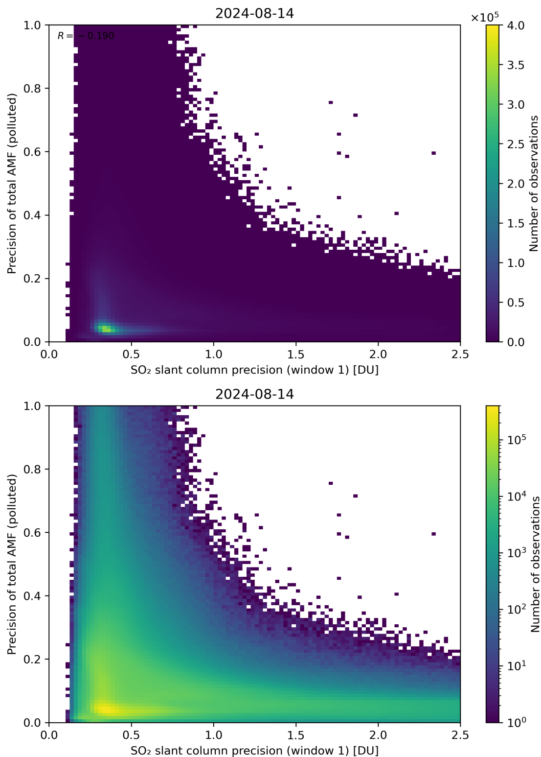
Figure 231: Scatter density plot of “SO 2 slant column precision (window 1)” against “Precision of total AMF (polluted)” for 2024-08-13 to 2024-08-15.
