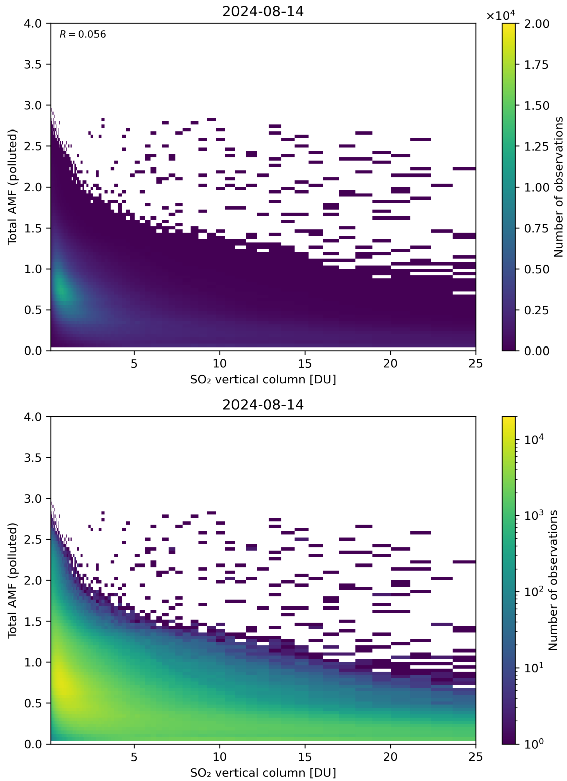
Figure 305: Scatter density plot of “SO 2 vertical column” against “Total AMF (polluted)” for 2024-08-13 to 2024-08-15.
