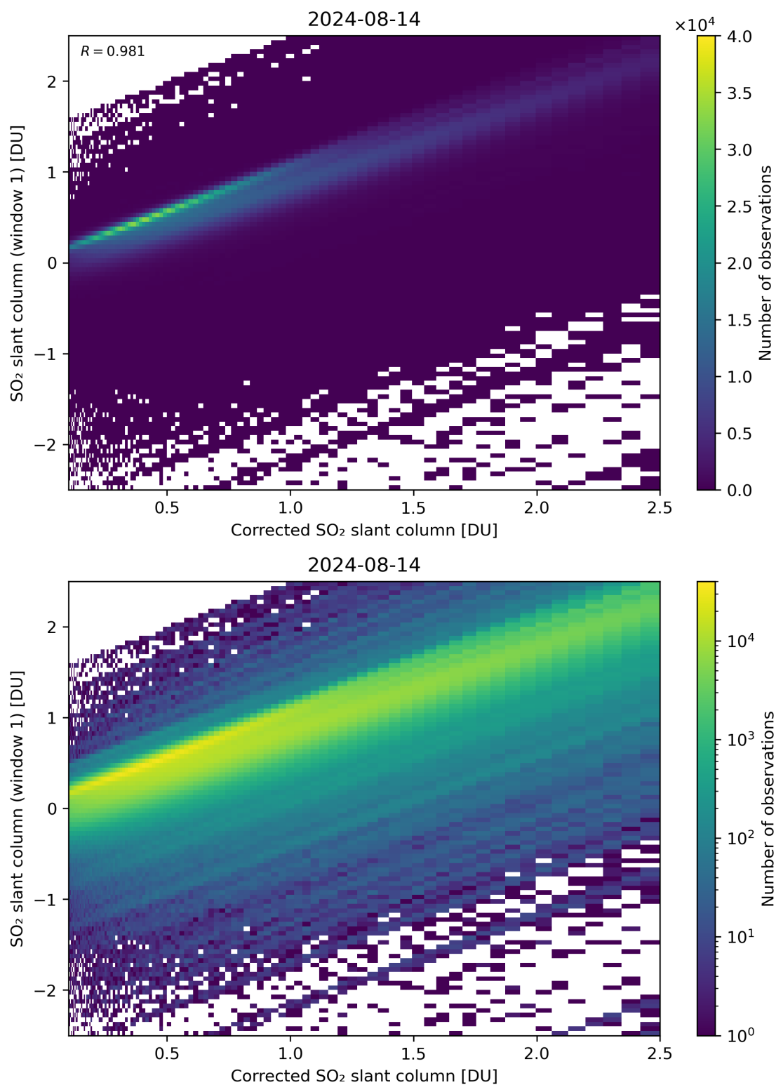
Figure 187: Scatter density plot of “Corrected SO 2 slant column” against “SO 2 slant column (window 1)” for 2024-08-13 to 2024-08-15.
