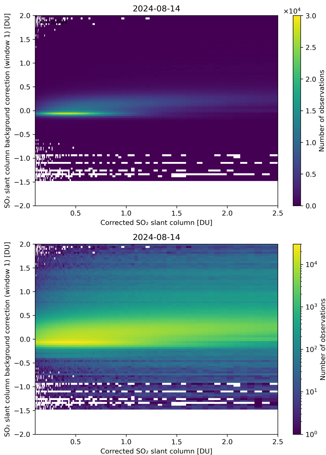
Figure 178: Scatter density plot of “Corrected SO 2 slant column” against “SO 2 slant column background correction (window 1)” for 2024-08-13 to 2024-08-15.
