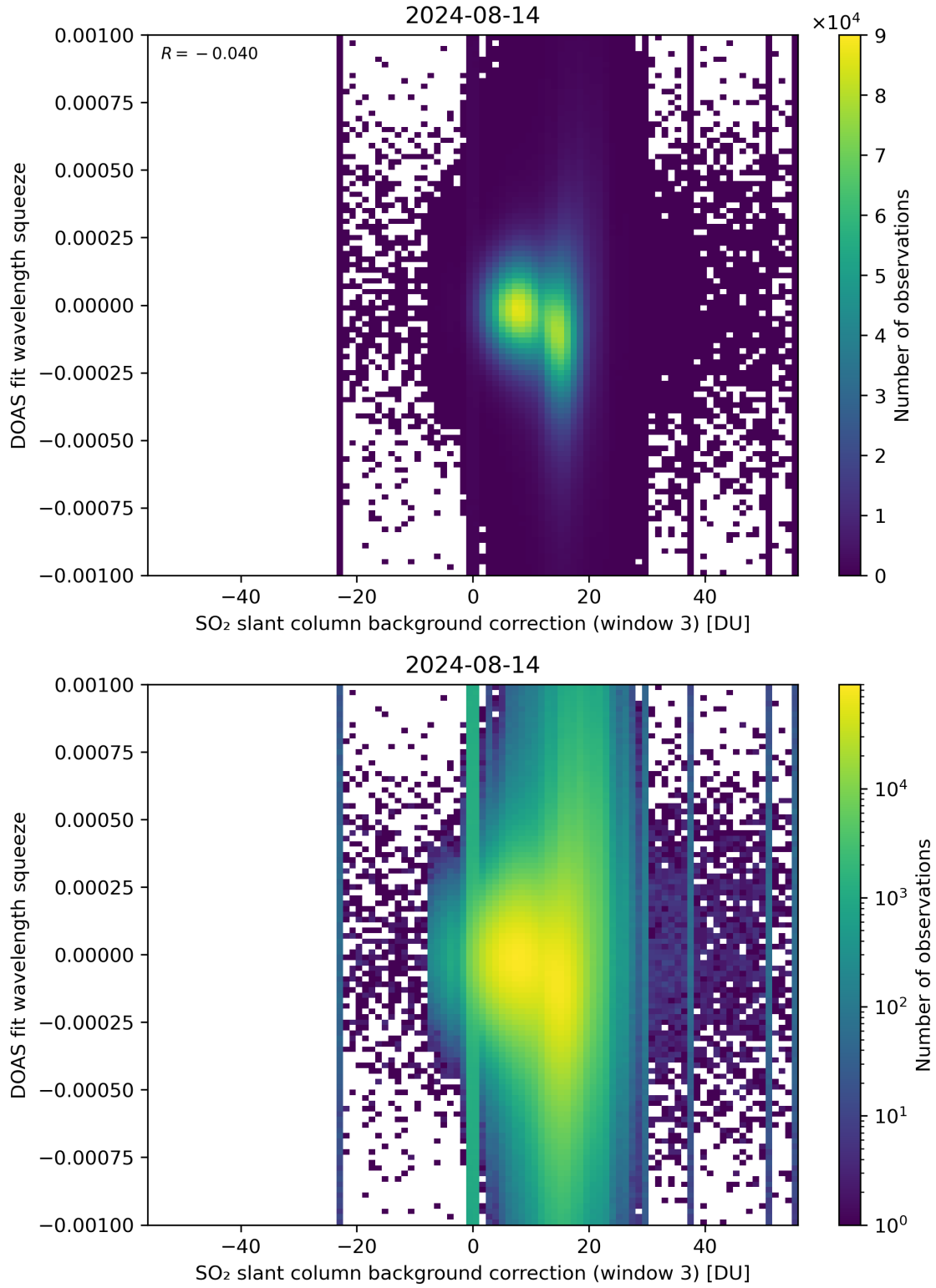
Figure 122: Scatter density plot of “SO 2 slant column background correction (window 3)” against “DOAS fit wavelength squeeze” for 2024-08-13 to 2024-08-15.
