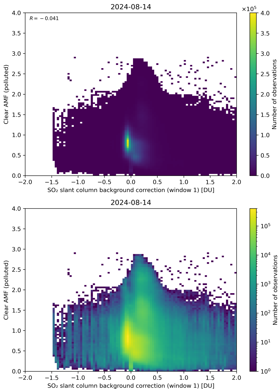
Figure 103: Scatter density plot of “SO 2 slant column background correction (window 1)” against “Clear AMF (polluted)” for 2024-08-13 to 2024-08-15.
