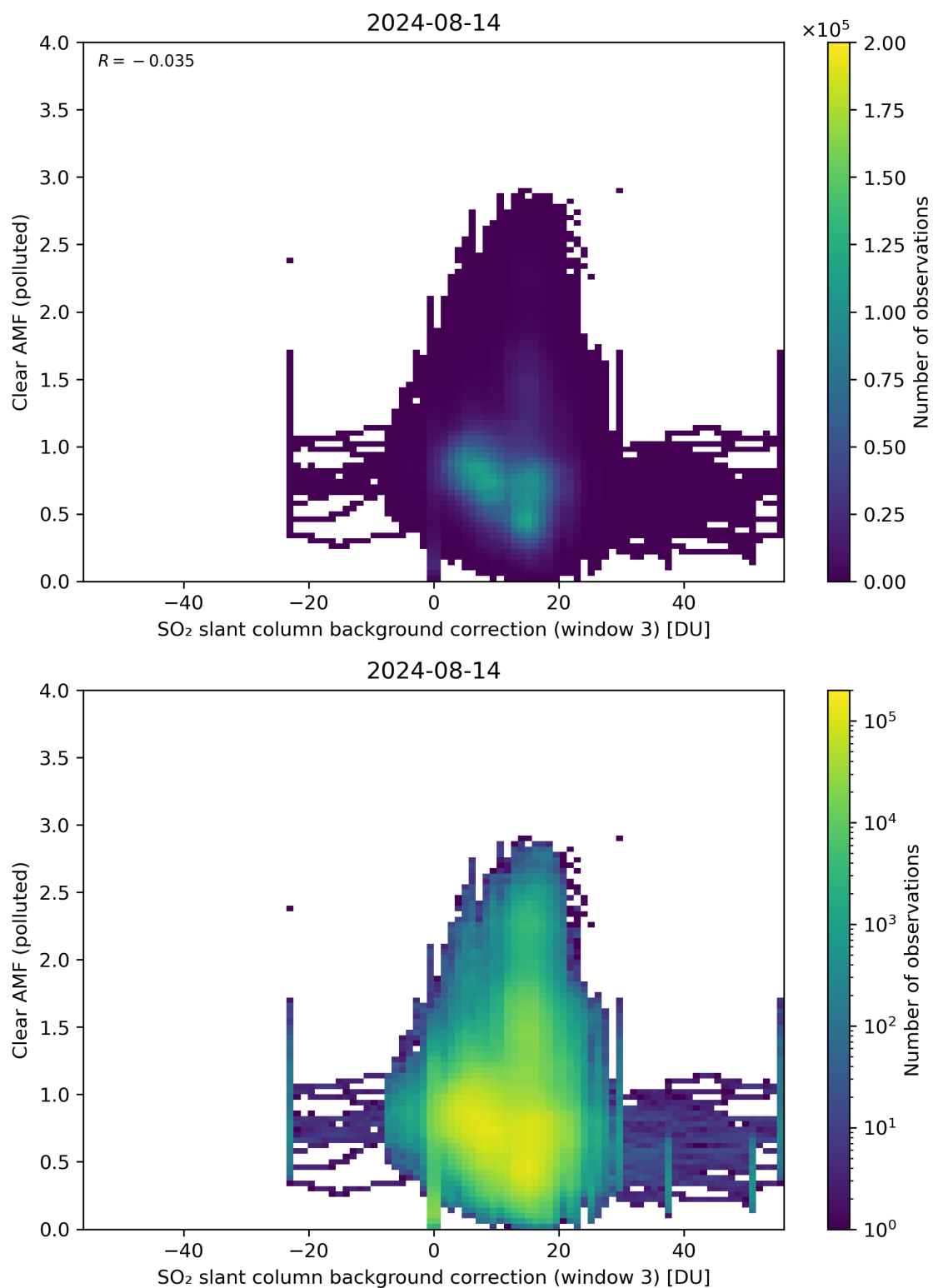
Figure 124: Scatter density plot of “SO 2 slant column background correction (window 3)” against “Clear AMF (polluted)” for 2024-08-13 to 2024-08-15.
