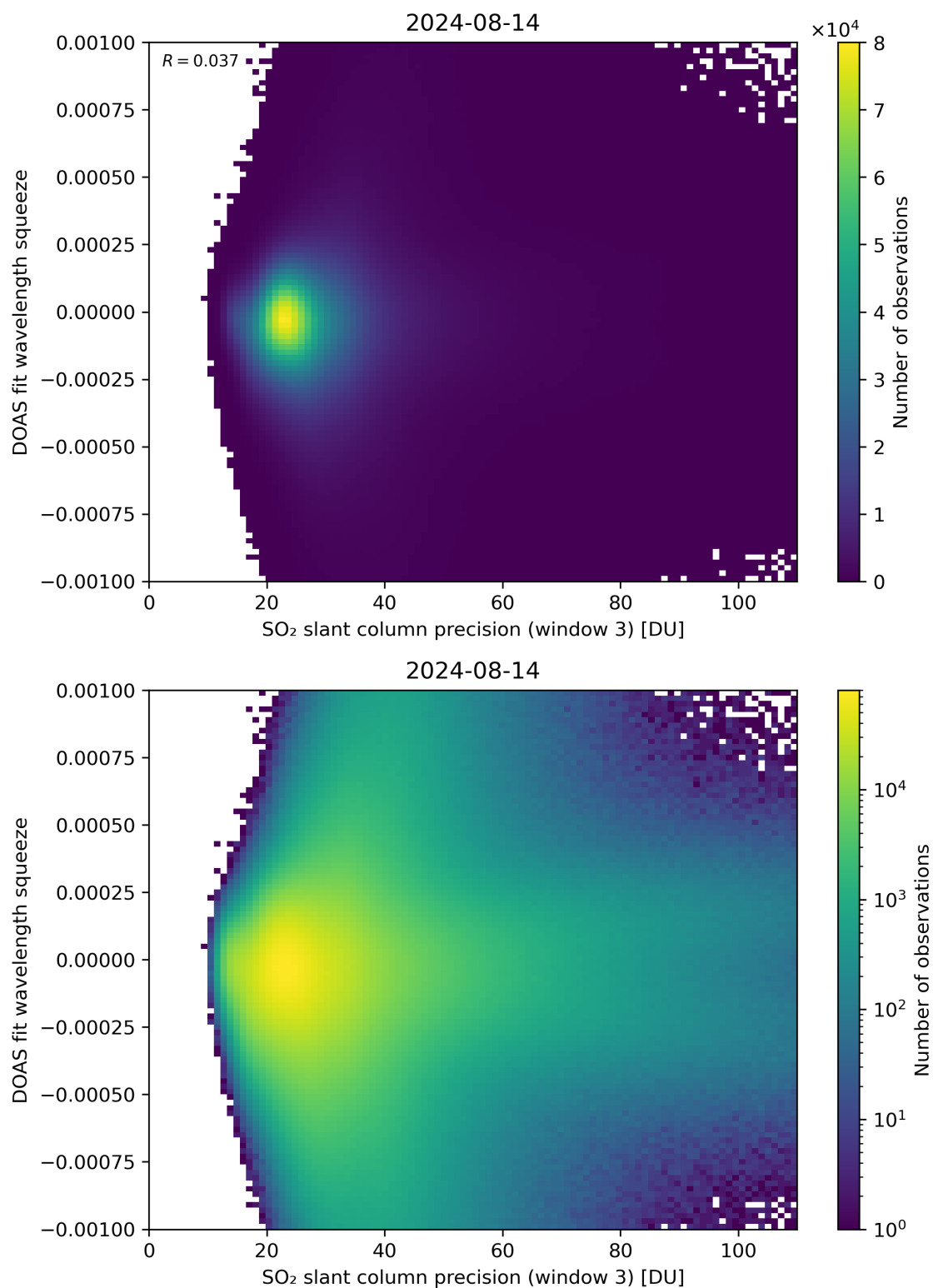
Figure 259: Scatter density plot of “SO 2 slant column precision (window 3)” against “DOAS fit wavelength squeeze” for 2024-08-13 to 2024-08-15.
