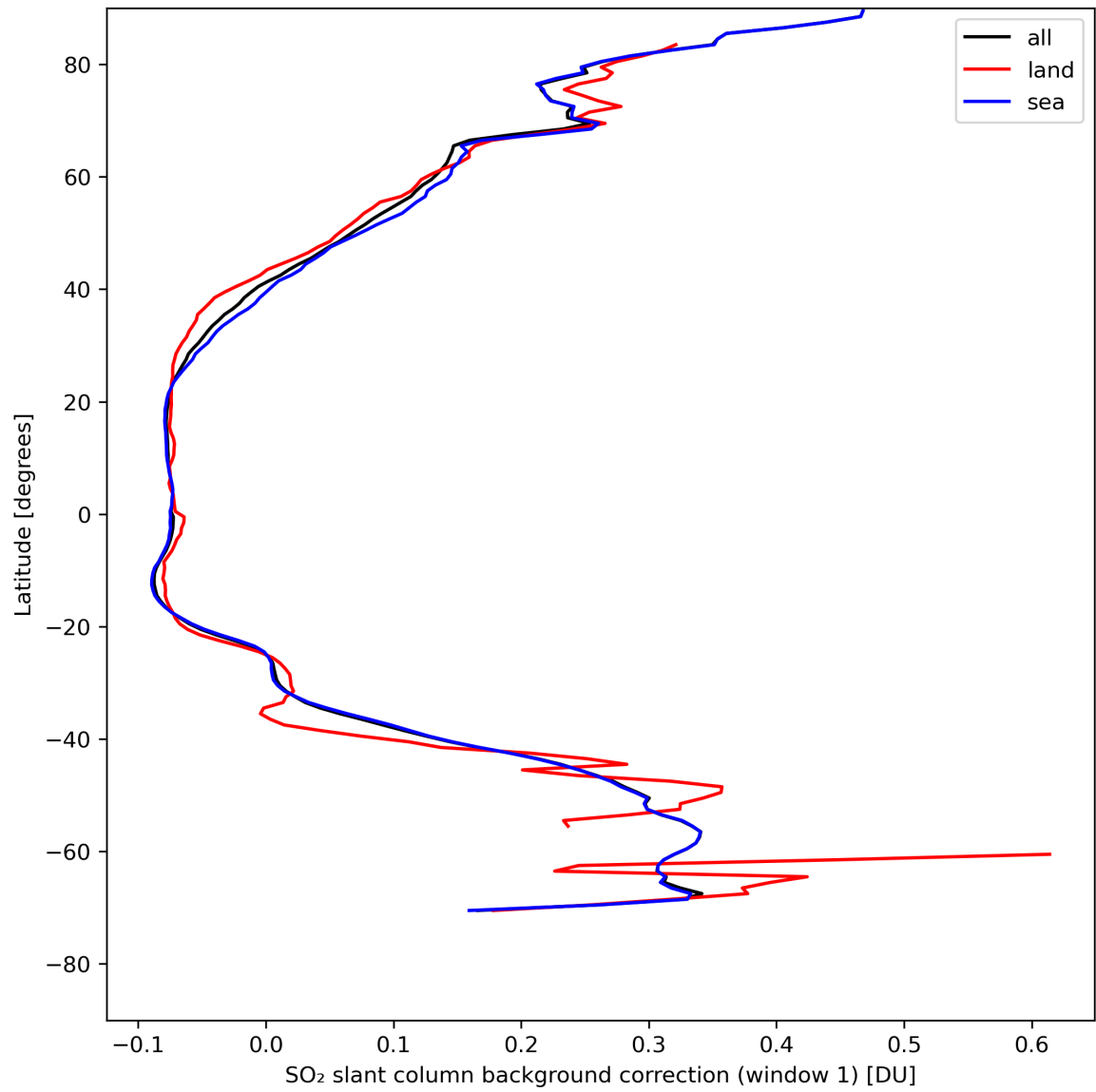
Figure 36: Zonal average of “SO 2 slant column background correction (window 1)” for 2024-08-13 to 2024-08-15.
