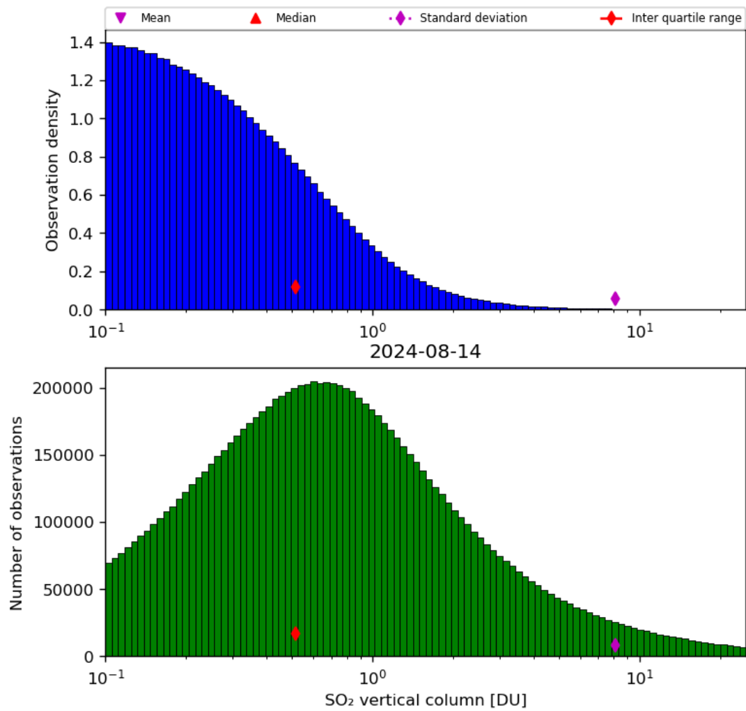
Figure 53: Histogram of “SO 2 vertical column” for 2024-08-13 to 2024-08-15
