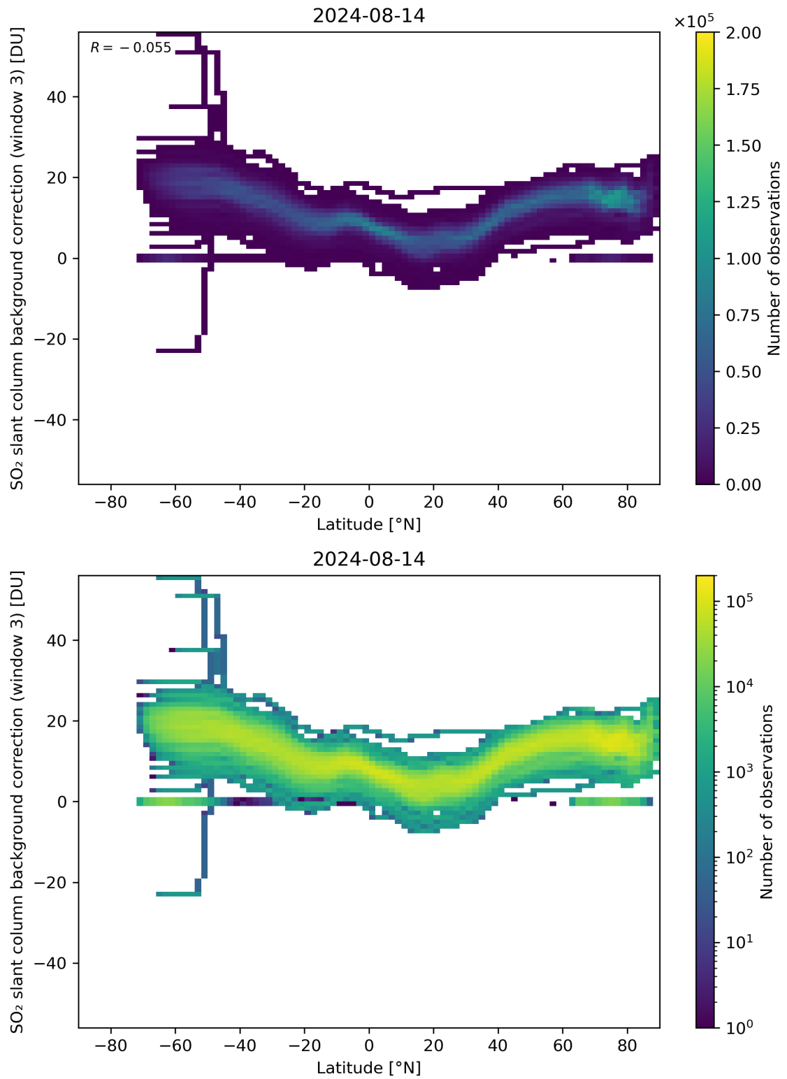
Figure 141: Scatter density plot of “Latitude” against “SO 2 slant column background correction (window 3)” for 2024-08-13 to 2024-08-15.
