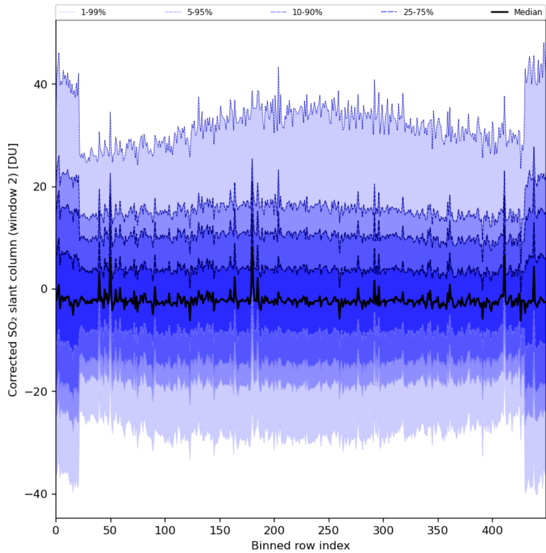
Figure 85: Along track statistics of “Corrected SO 2 slant column (window 2)” for 2024-08-13 to 2024-08-15
