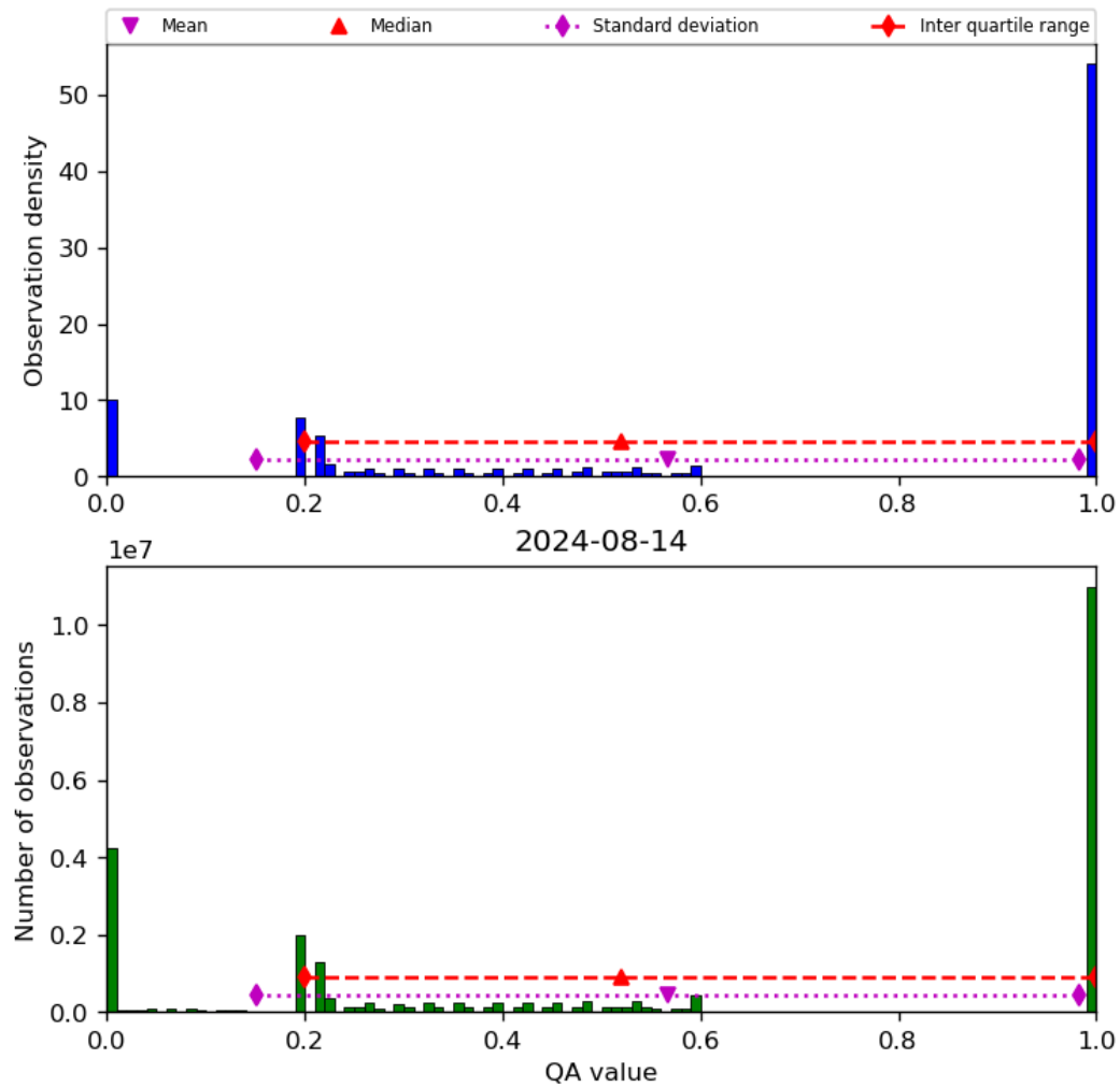
Figure 52: Histogram of “QA value” for 2024-08-13 to 2024-08-15
