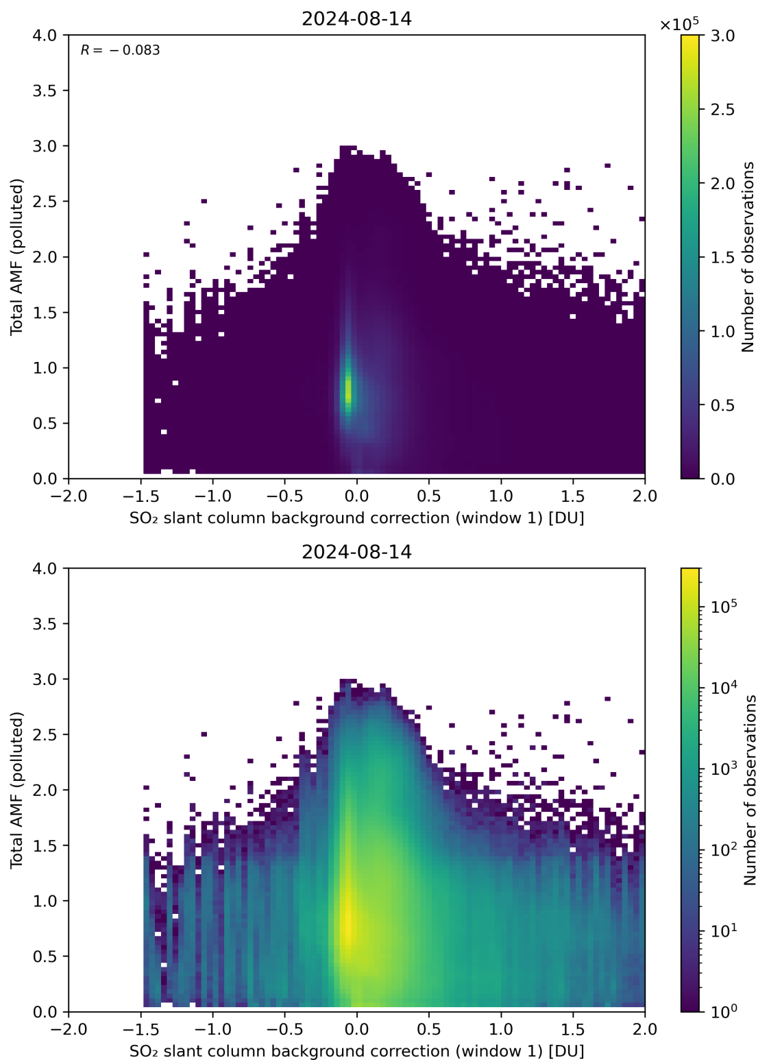
Figure 109: Scatter density plot of “SO 2 slant column background correction (window 1)” against “Total AMF (polluted)” for 2024-08-13 to 2024-08-15.
