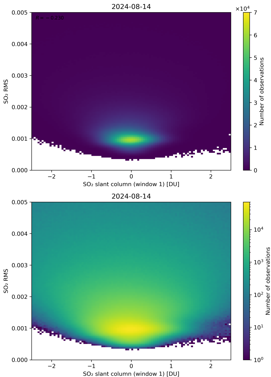
Figure 217: Scatter density plot of “SO 2 slant column (window 1)” against “SO 2 RMS” for 2024-08-13 to 2024-08-15.
