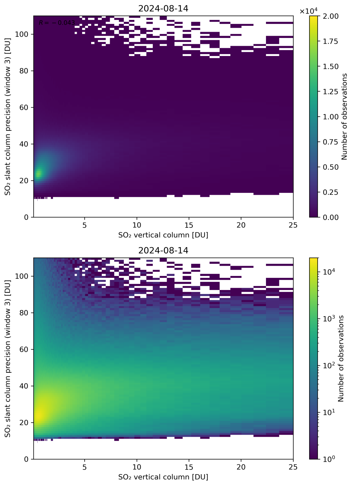
Figure 304: Scatter density plot of “SO 2 vertical column” against “SO 2 slant column precision (window 3)” for 2024-08-13 to 2024-08-15.
