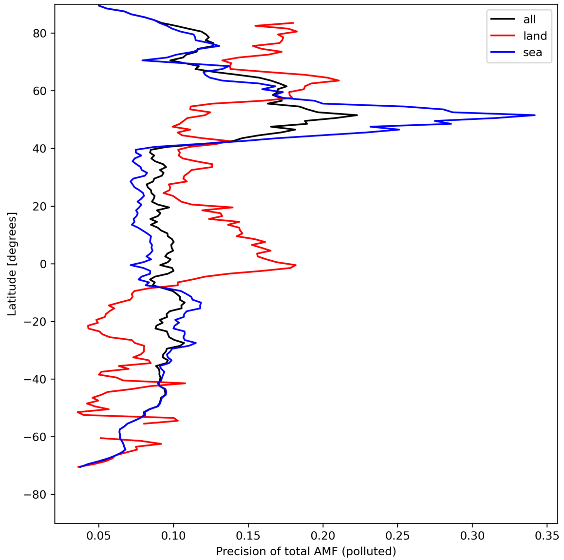
Figure 49: Zonal average of “Precision of total AMF (polluted)” for 2024-08-13 to 2024-08-15.
