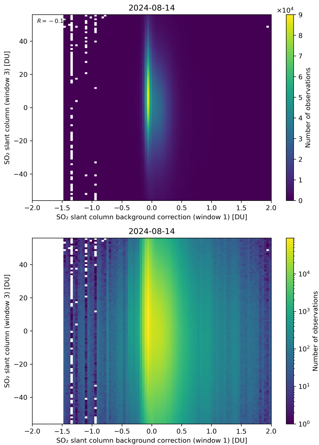
Figure 107: Scatter density plot of “SO 2 slant column background correction (window 1)” against “SO 2 slant column (window 3)” for 2024-08-13 to 2024-08-15.
