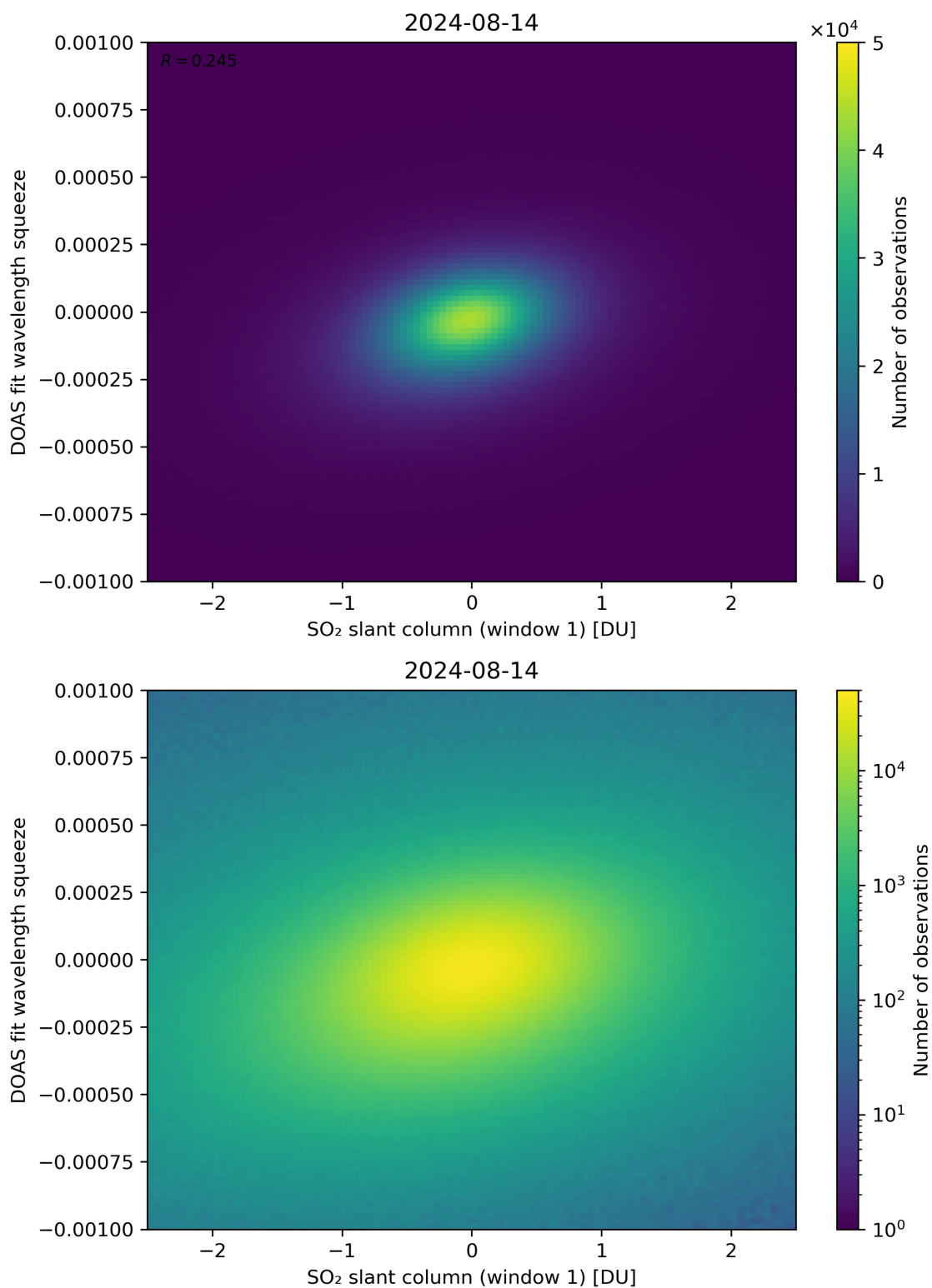
Figure 216: Scatter density plot of “SO 2 slant column (window 1)” against “DOAS fit wavelength squeeze” for 2024-08-13 to 2024-08-15.
