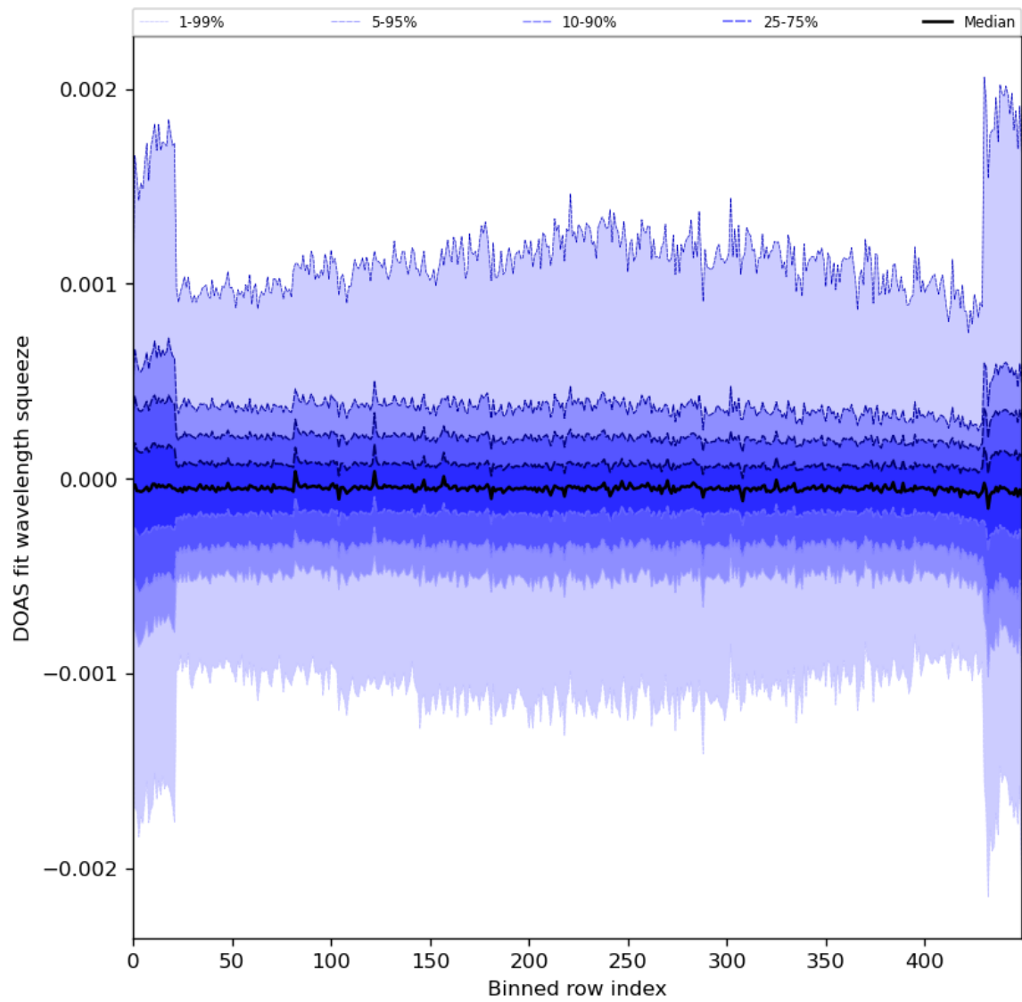
Figure 92: Along track statistics of “DOAS fit wavelength squeeze” for 2024-08-13 to 2024-08-15
