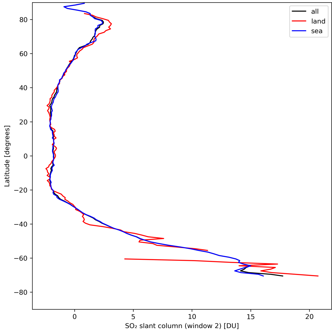
Figure 37: Zonal average of “SO 2 slant column (window 2)” for 2024-08-13 to 2024-08-15.
