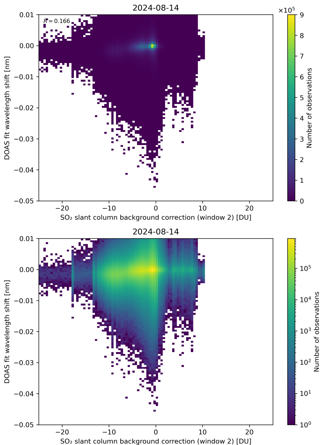
Figure 112: Scatter density plot of “SO 2 slant column background correction (window 2)” against “DOAS fit wavelength shift” for 2024-08-13 to 2024-08-15.
