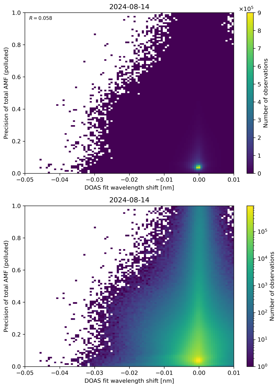
Figure 131: Scatter density plot of “DOAS fit wavelength shift” against “Precision of total AMF (polluted)” for 2024-08-13 to 2024-08-15.
