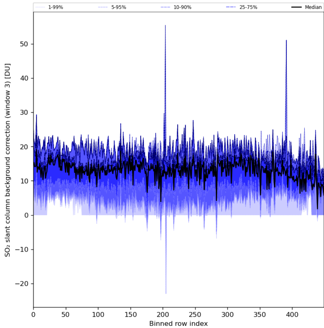
Figure 90: Along track statistics of “SO 2 slant column background correction (window 3)” for 2024-08-13 to 2024-08-15
