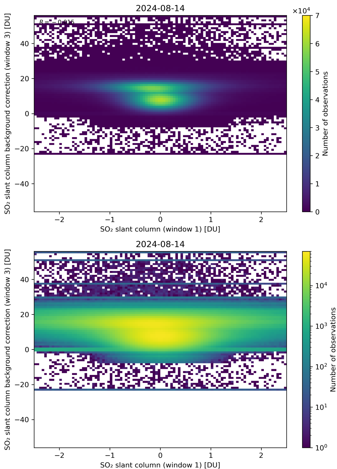
Figure 214: Scatter density plot of “SO 2 slant column (window 1)” against “SO 2 slant column background correction (window 3)” for 2024-08-13 to 2024-08-15.
