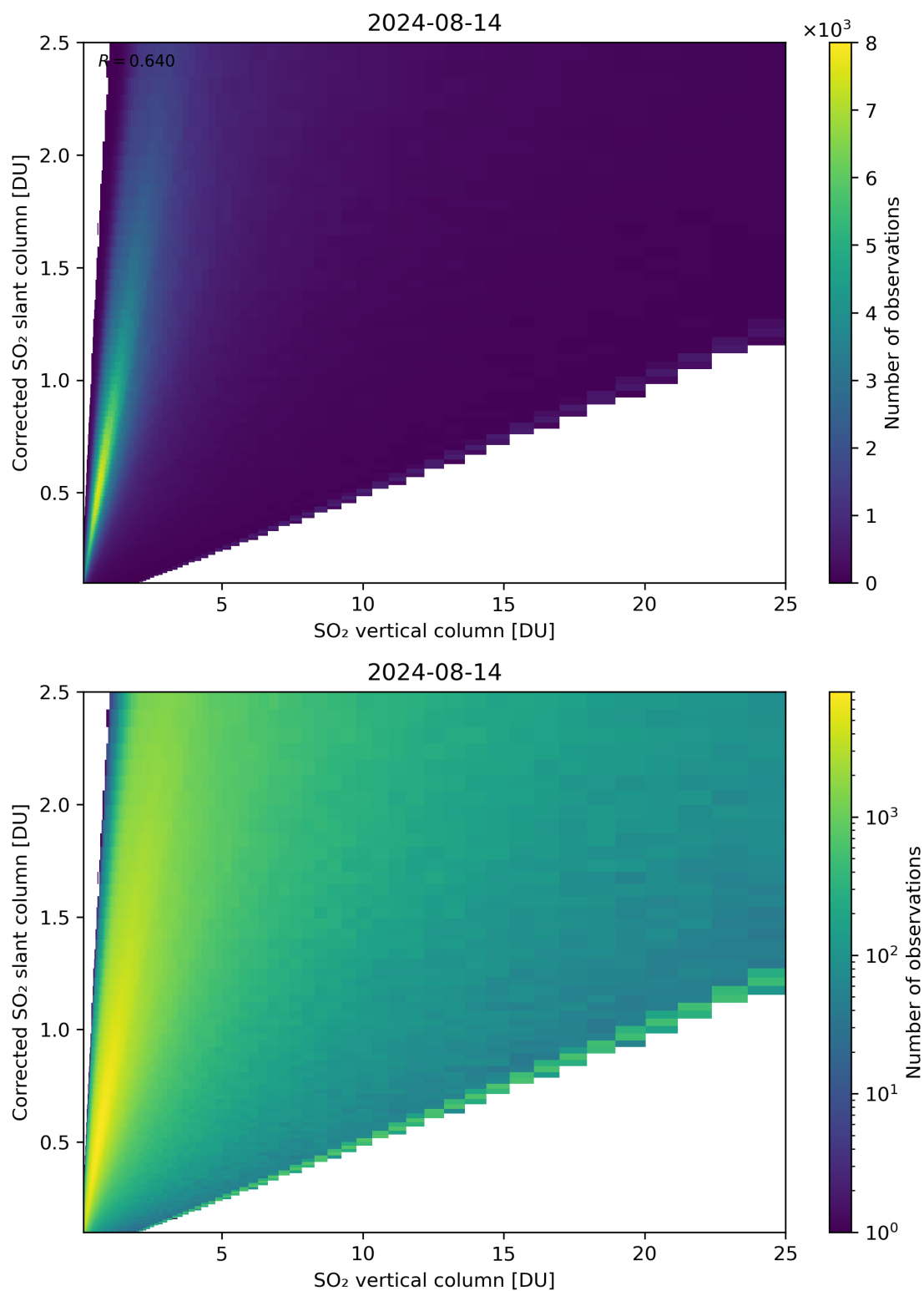
Figure 297: Scatter density plot of “SO 2 vertical column” against “Corrected SO 2 slant column” for 2024-08-13 to 2024-08-15.
