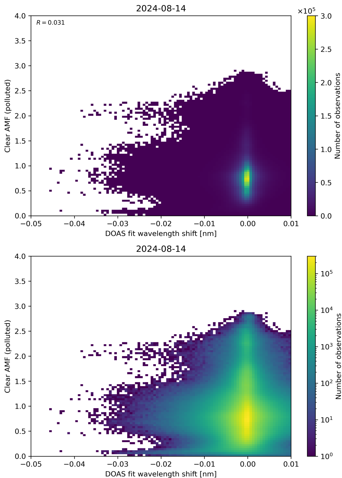
Figure 129: Scatter density plot of “DOAS fit wavelength shift” against “Clear AMF (polluted)” for 2024-08-13 to 2024-08-15.
