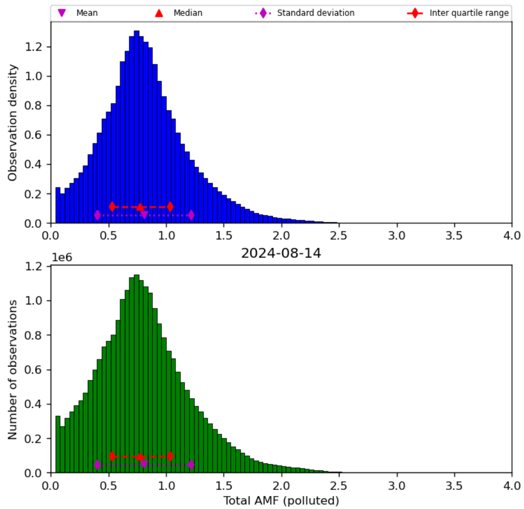
Figure 71: Histogram of “Total AMF (polluted)” for 2024-08-13 to 2024-08-15
