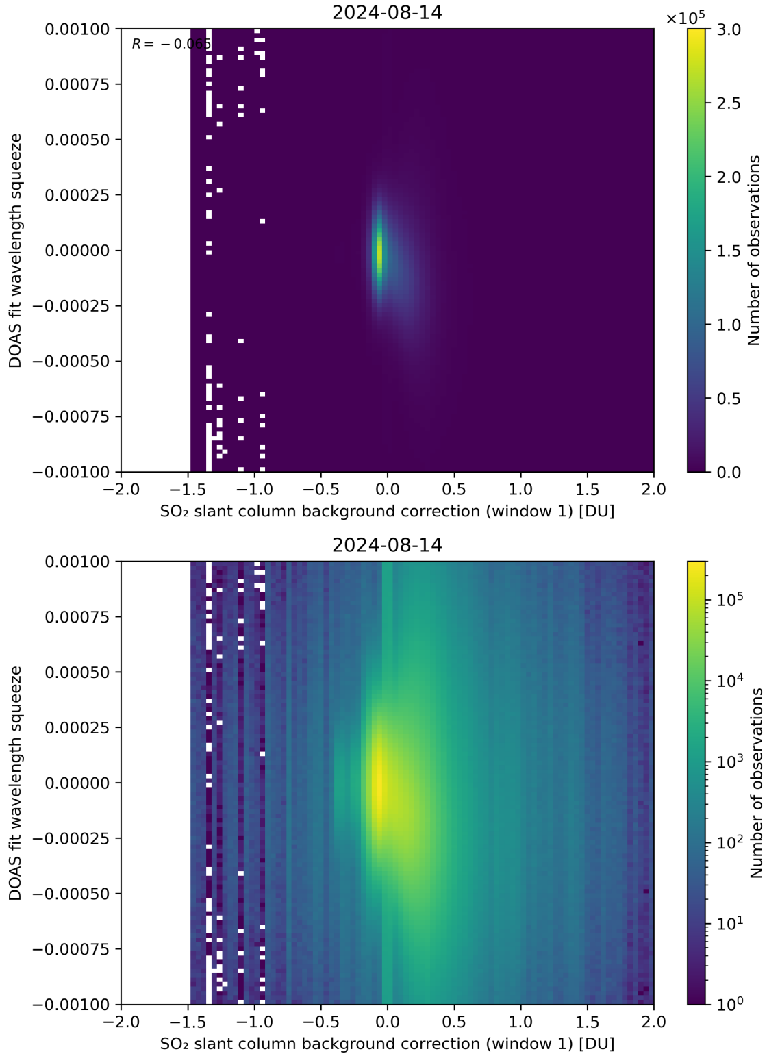
Figure 101: Scatter density plot of “SO 2 slant column background correction (window 1)” against “DOAS fit wavelength squeeze” for 2024-08-13 to 2024-08-15.
