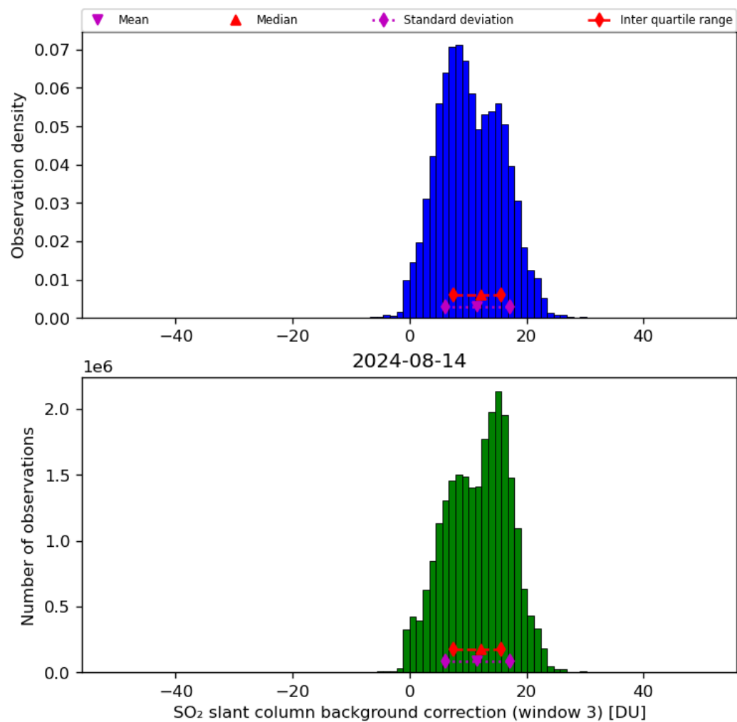
Figure 67: Histogram of “SO 2 slant column background correction (window 3)” for 2024-08-13 to 2024-08-15
