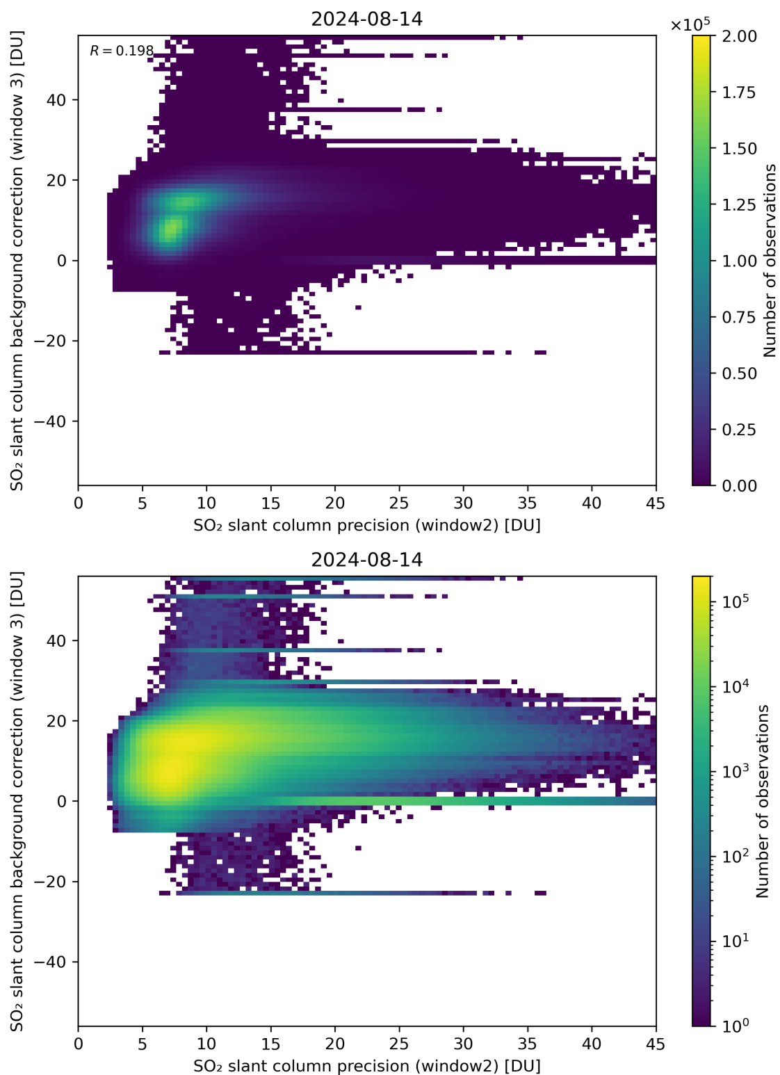
Figure 242: Scatter density plot of “SO 2 slant column precision (window2)” against “SO 2 slant column background correction (window 3)” for 2024-08-13 to 2024-08-15.
