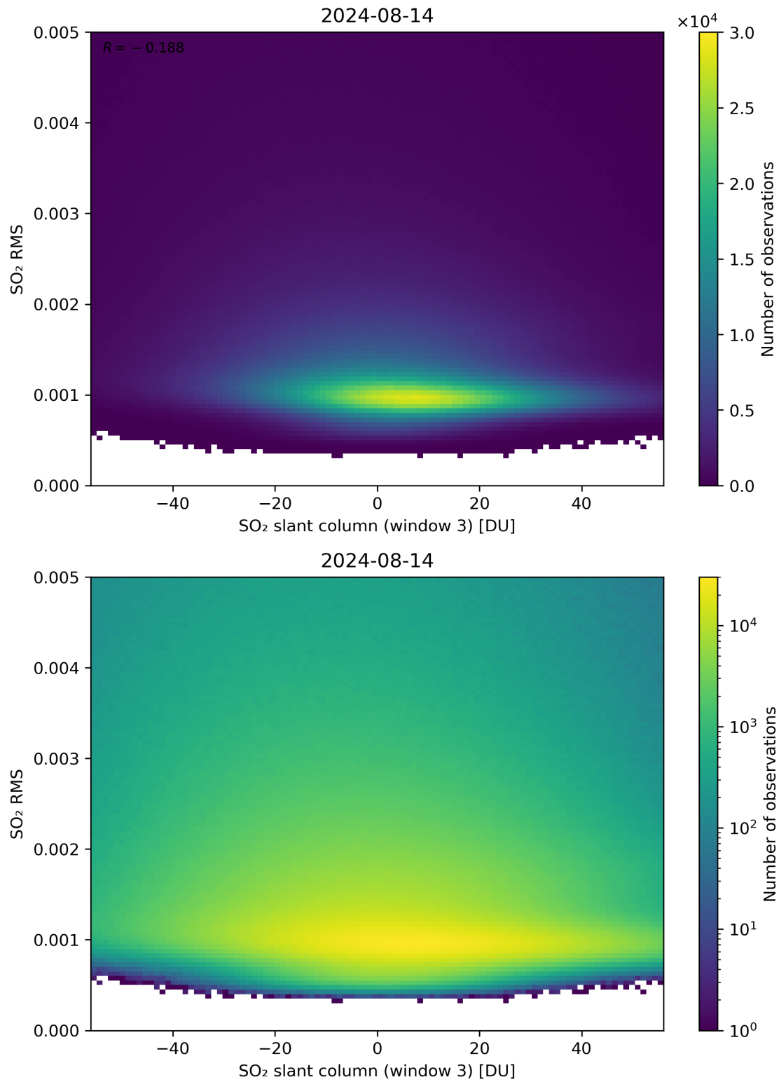
Figure 256: Scatter density plot of “SO 2 slant column (window 3)” against “SO 2 RMS” for 2024-08-13 to 2024-08-15.
