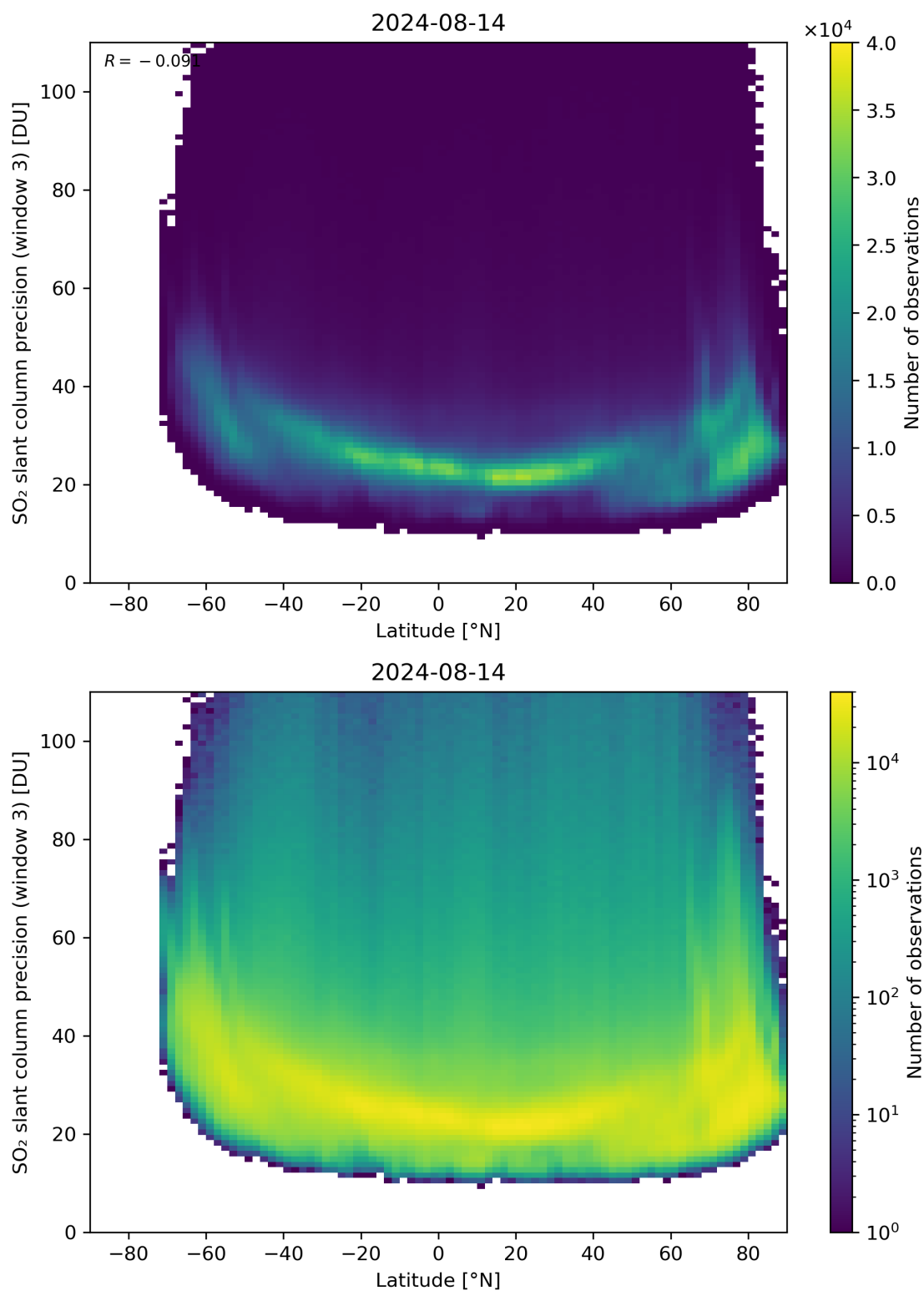
Figure 153: Scatter density plot of “Latitude” against “SO 2 slant column precision (window 3)” for 2024-08-13 to 2024-08-15.
