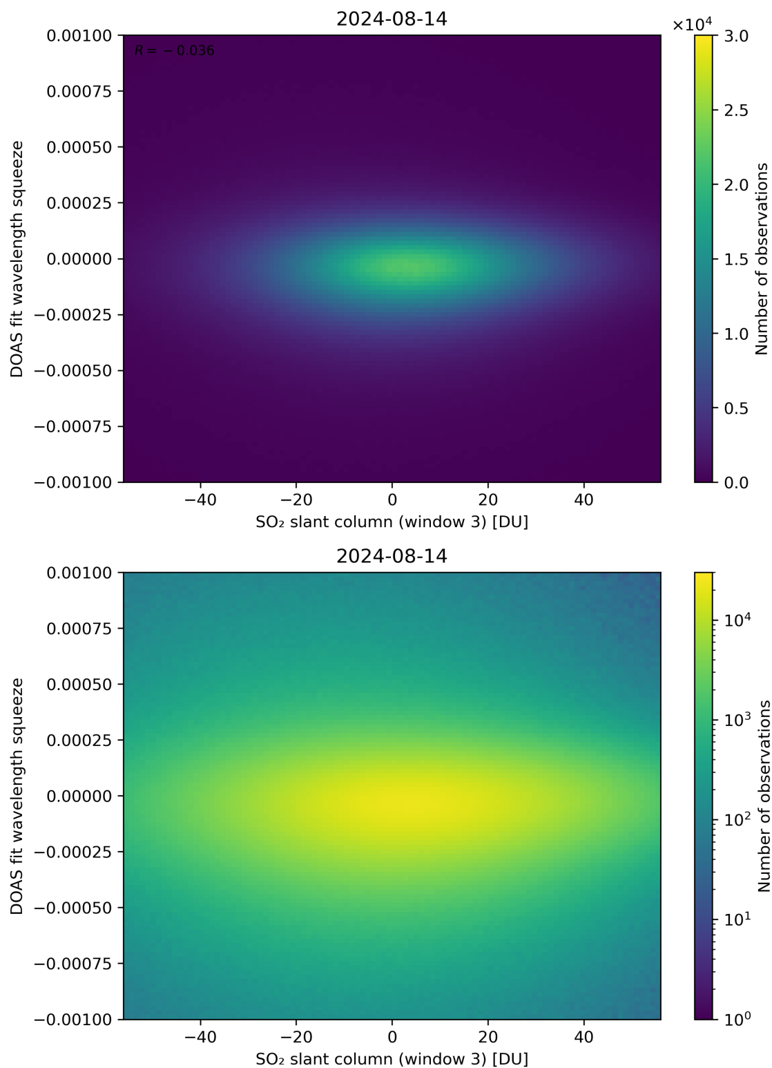
Figure 255: Scatter density plot of “SO 2 slant column (window 3)” against “DOAS fit wavelength squeeze” for 2024-08-13 to 2024-08-15.
