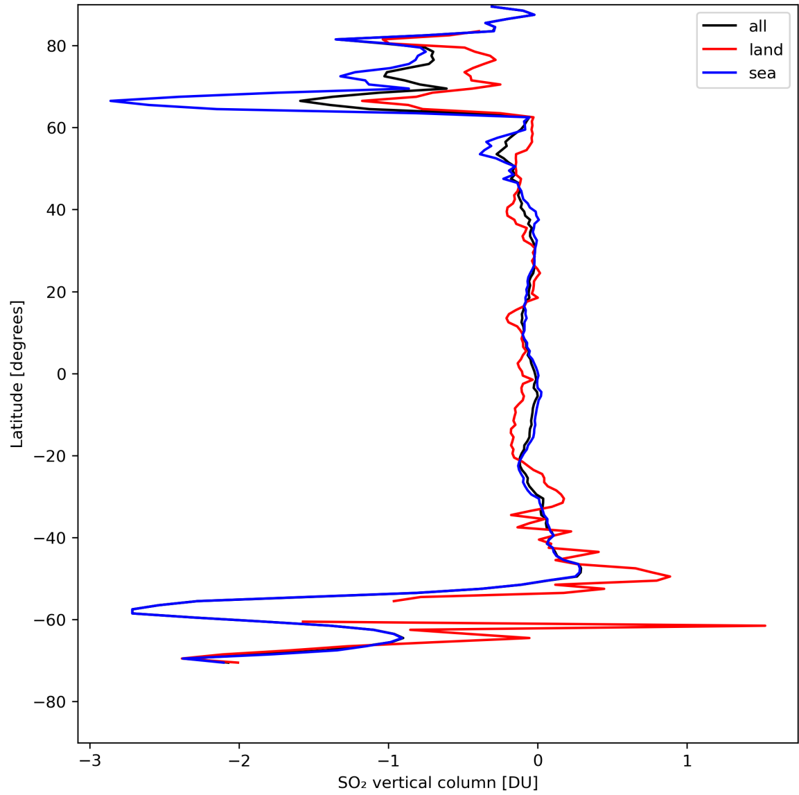
Figure 30: Zonal average of “SO 2 vertical column” for 2024-08-13 to 2024-08-15.
