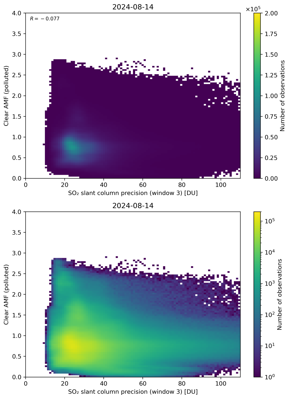
Figure 261: Scatter density plot of “SO 2 slant column precision (window 3)” against “Clear AMF (polluted)” for 2024-08-13 to 2024-08-15.
