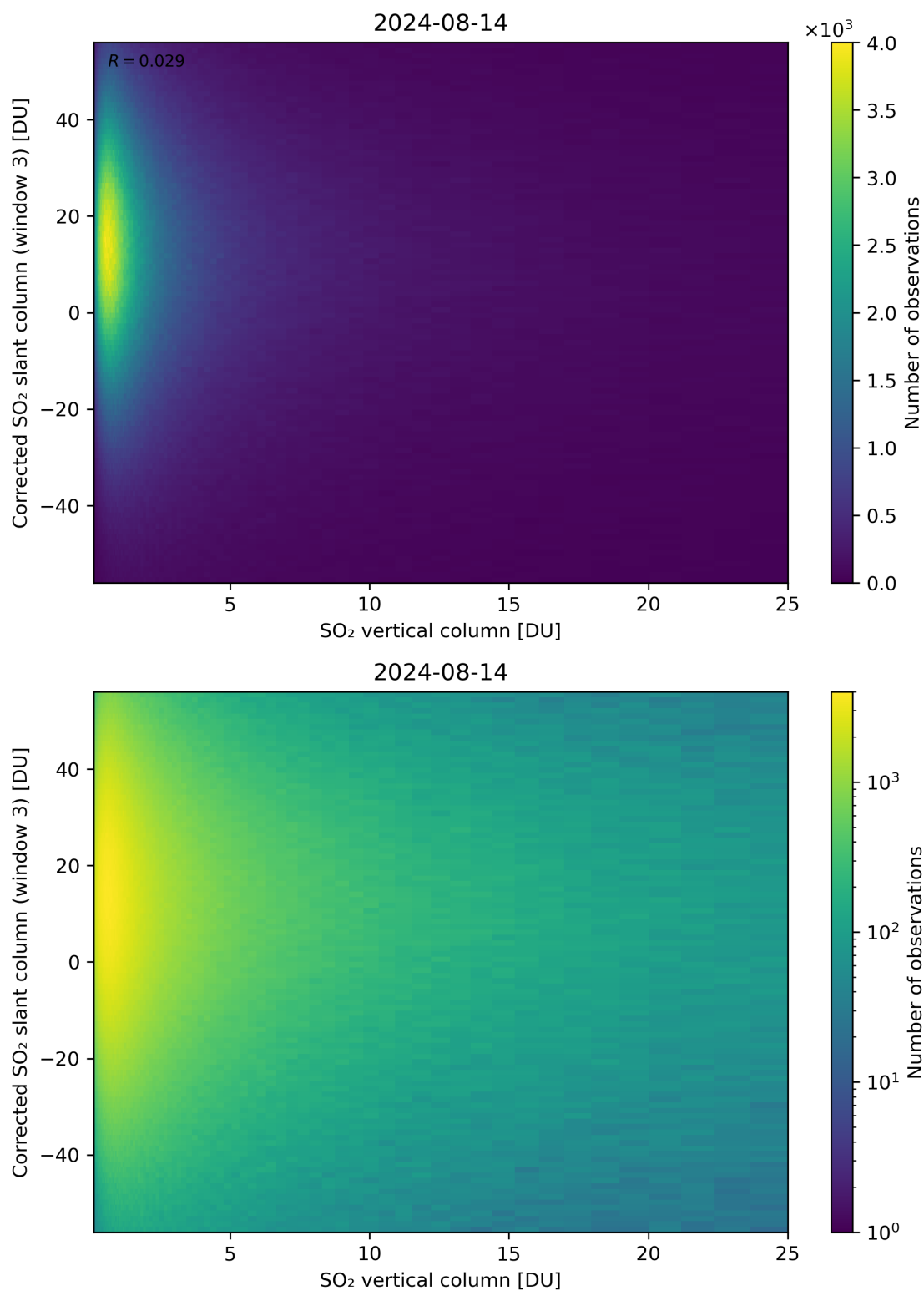
Figure 299: Scatter density plot of “SO 2 vertical column” against “Corrected SO 2 slant column (window 3)” for 2024-08-13 to 2024-08-15.
