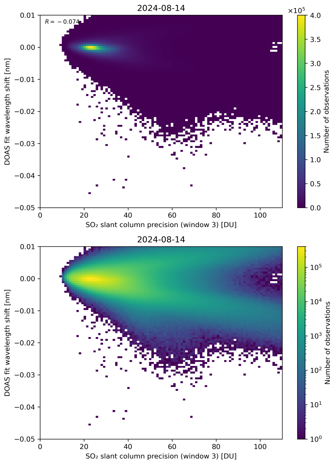
Figure 258: Scatter density plot of “SO 2 slant column precision (window 3)” against “DOAS fit wavelength shift” for 2024-08-13 to 2024-08-15.
