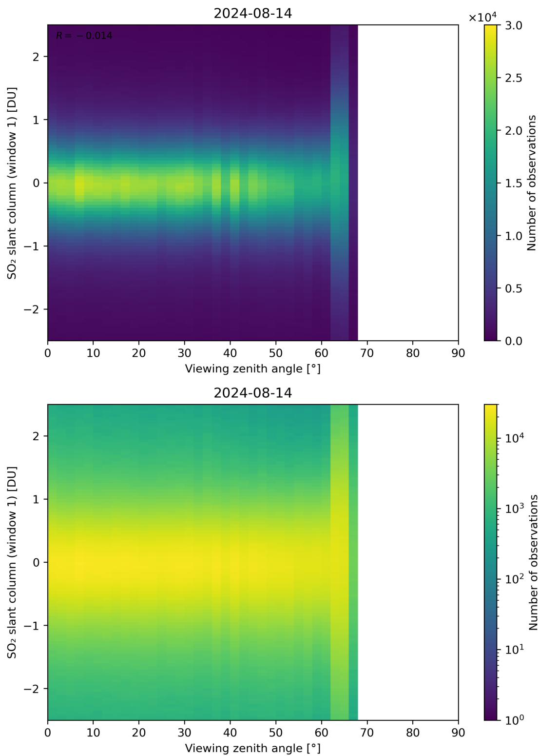
Figure 320: Scatter density plot of “Viewing zenith angle” against “SO 2 slant column (window 1)” for 2024-08-13 to 2024-08-15.
