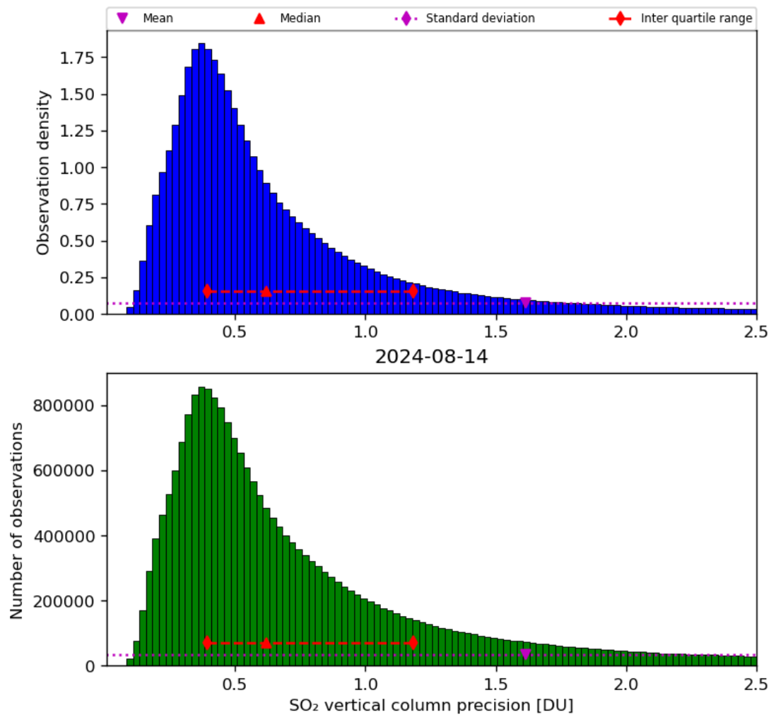
Figure 54: Histogram of “SO 2 vertical column precision” for 2024-08-13 to 2024-08-15
