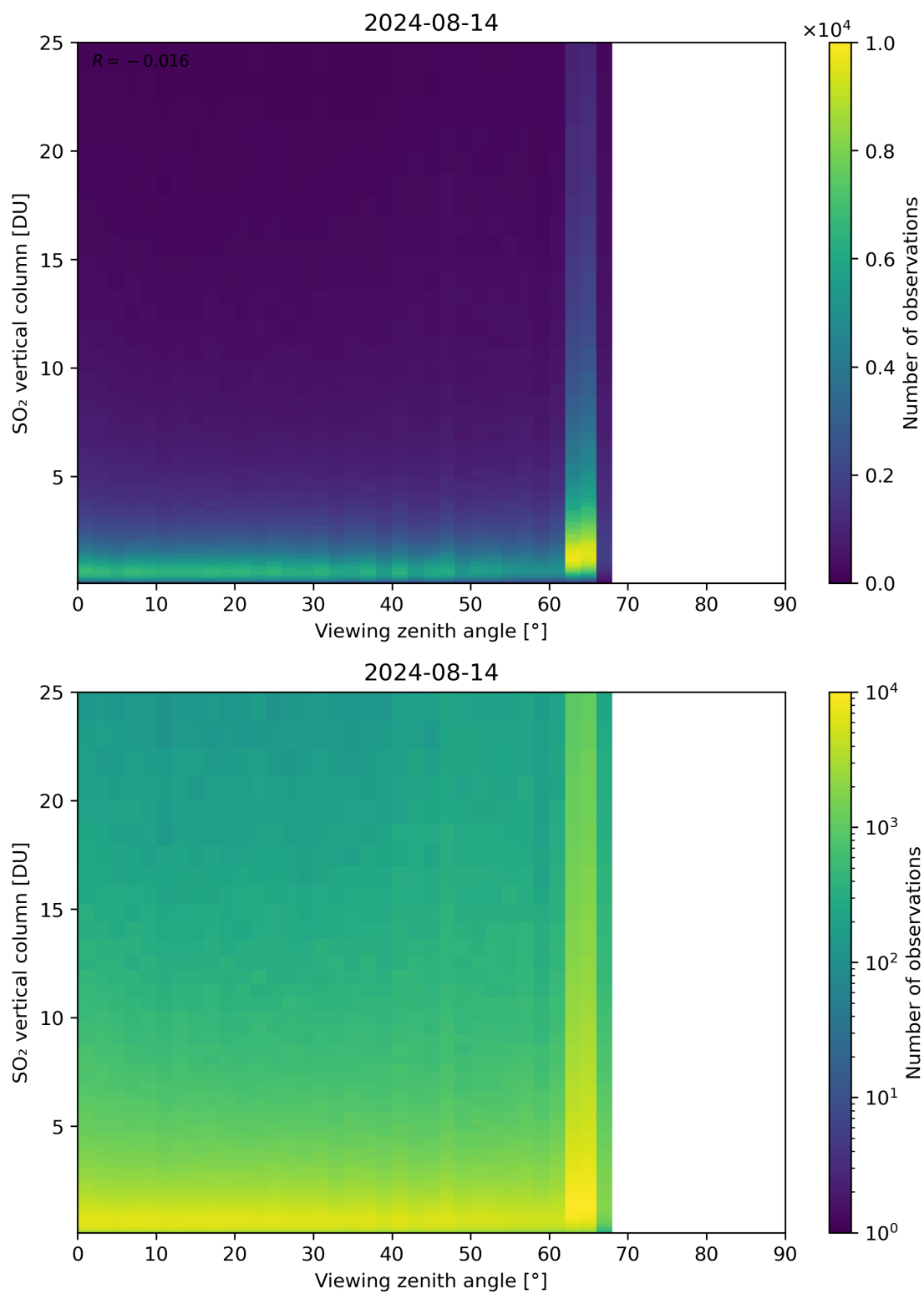
Figure 327: Scatter density plot of “Viewing zenith angle” against “SO 2 vertical column” for 2024-08-13 to 2024-08-15.
