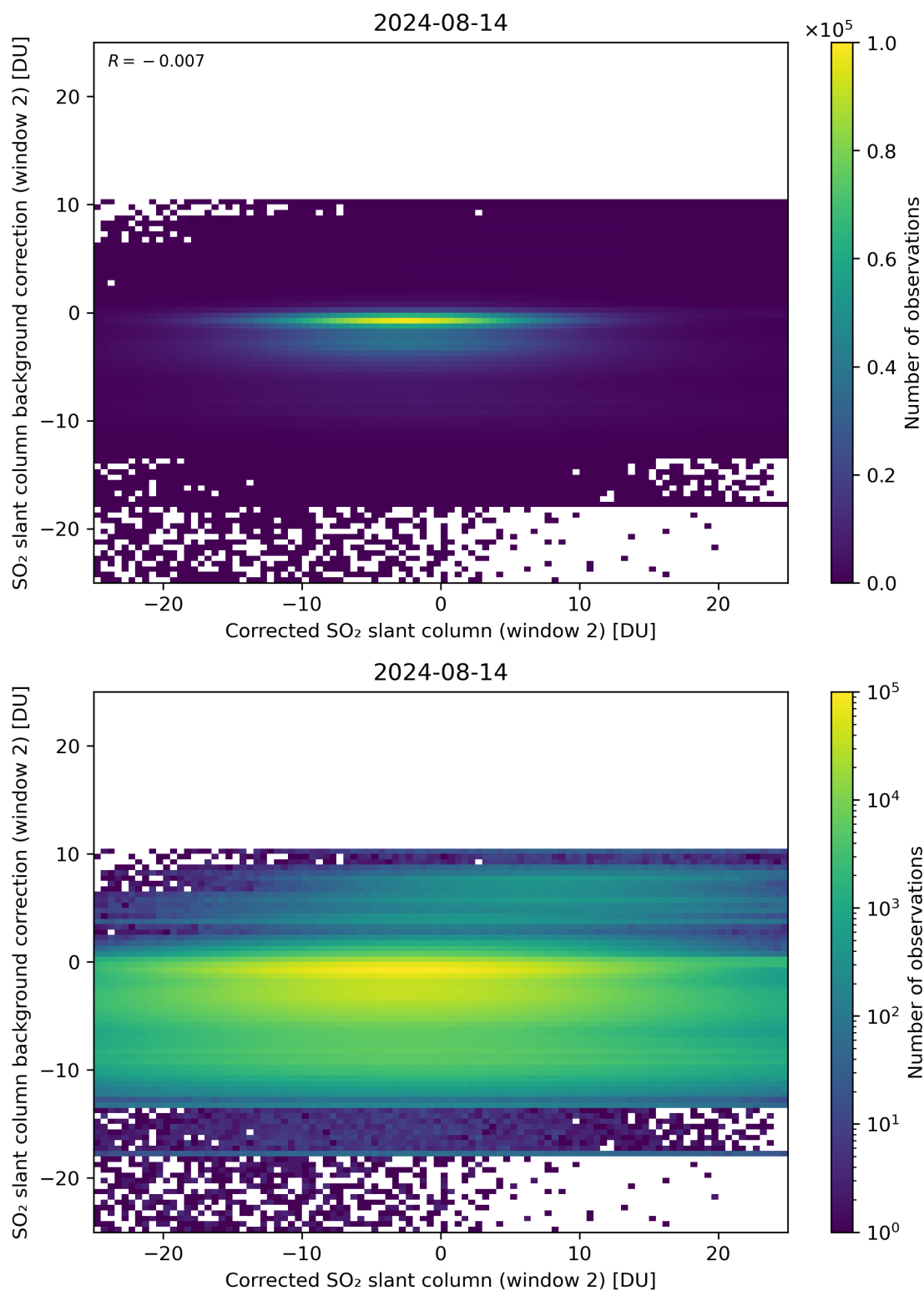
Figure 194: Scatter density plot of “Corrected SO 2 slant column (window 2)” against “SO 2 slant column background correction (window 2)” for 2024-08-13 to 2024-08-15.
