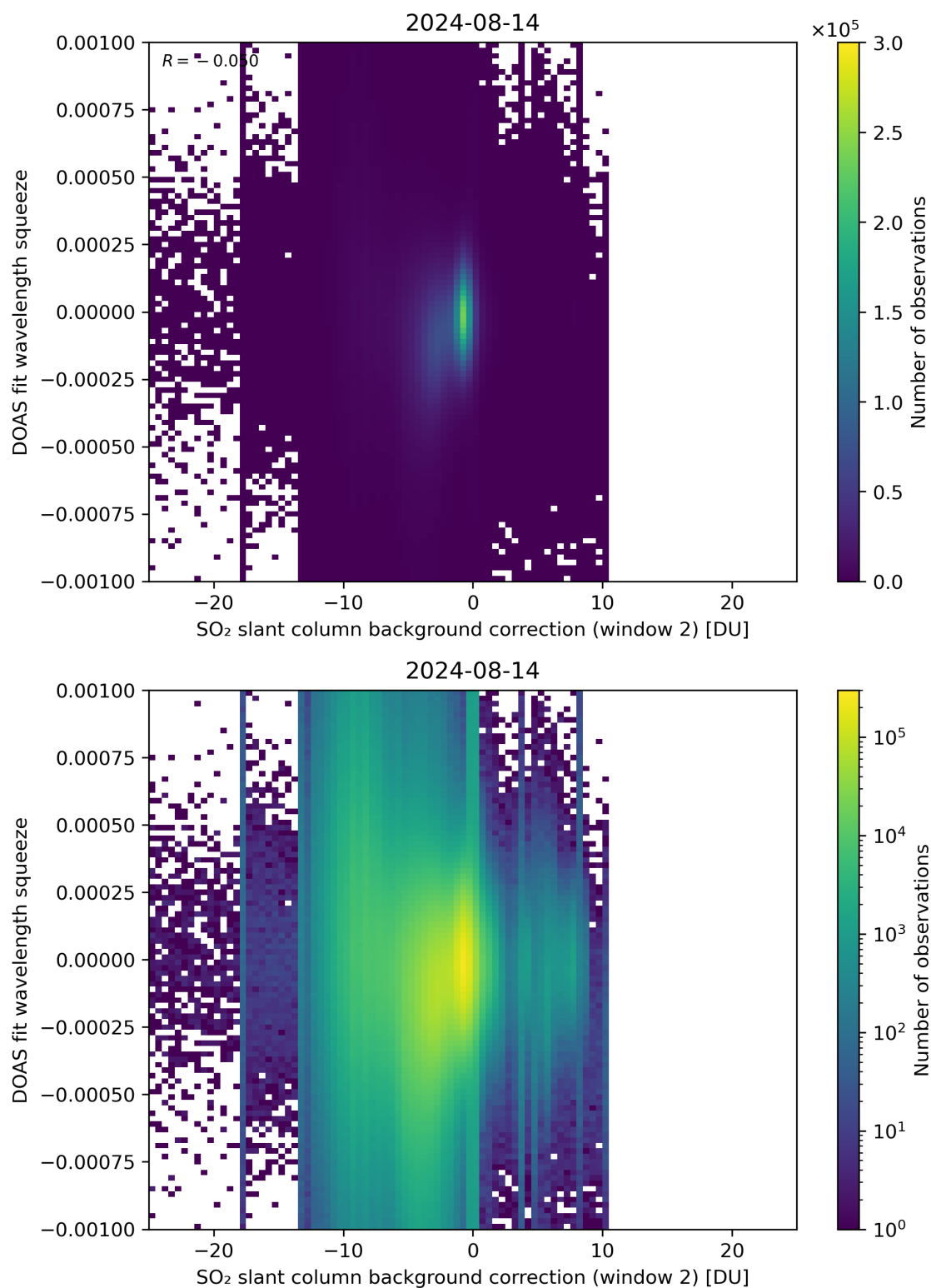
Figure 113: Scatter density plot of “SO 2 slant column background correction (window 2)” against “DOAS fit wavelength squeeze” for 2024-08-13 to 2024-08-15.
