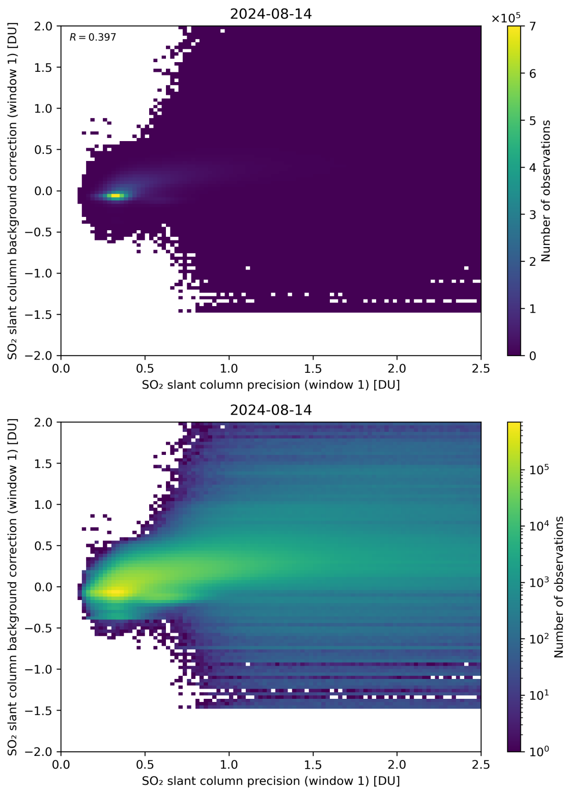
Figure 218: Scatter density plot of “SO 2 slant column precision (window 1)” against “SO 2 slant column background correction (window 1)” for 2024-08-13 to 2024-08-15.
