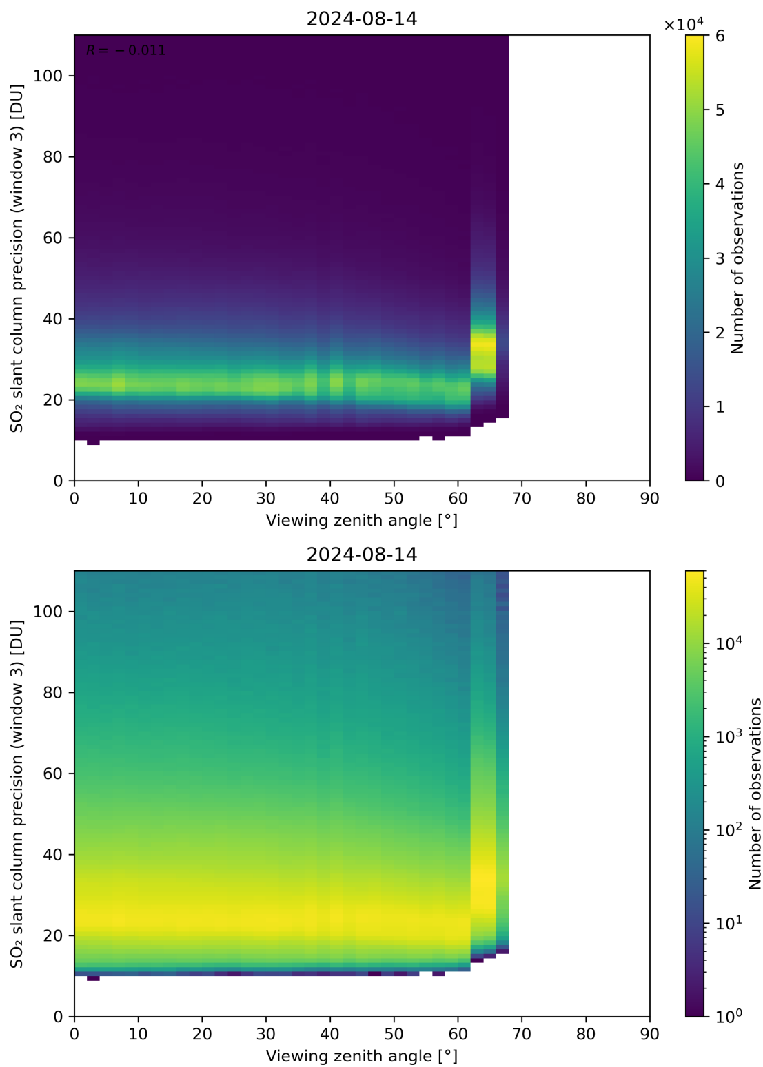
Figure 324: Scatter density plot of “Viewing zenith angle” against “SO 2 slant column precision (window 3)” for 2024-08-13 to 2024-08-15.
