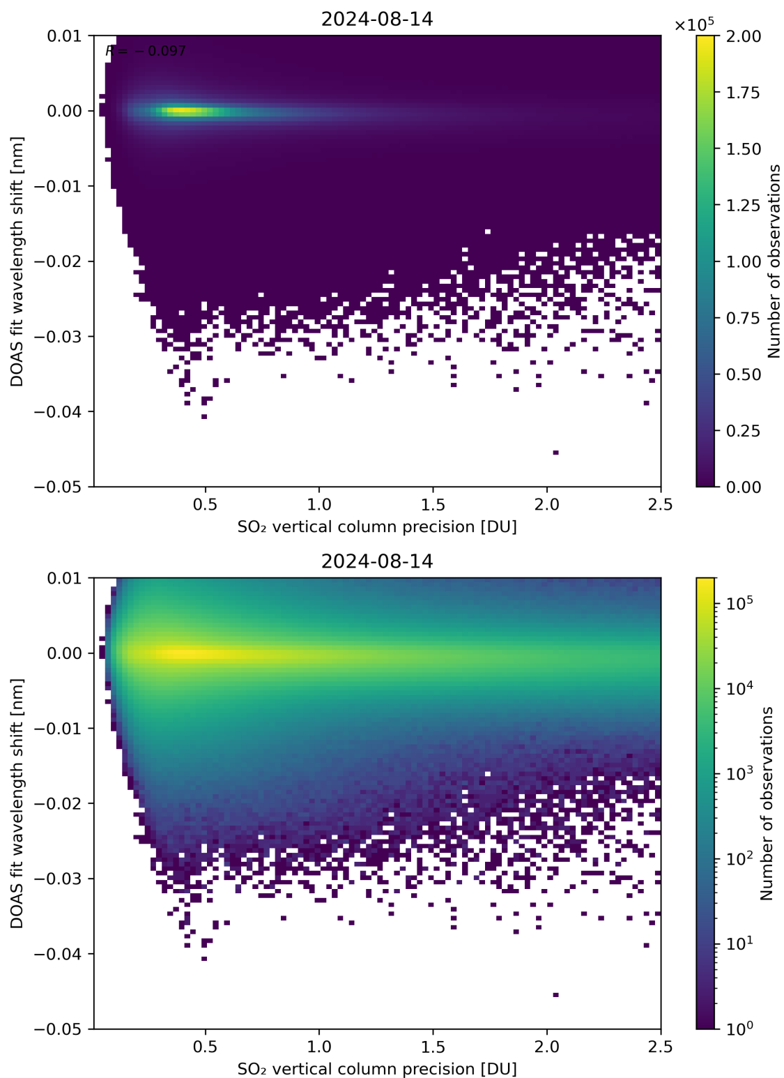
Figure 282: Scatter density plot of “SO 2 vertical column precision” against “DOAS fit wavelength shift” for 2024-08-13 to 2024-08-15.
