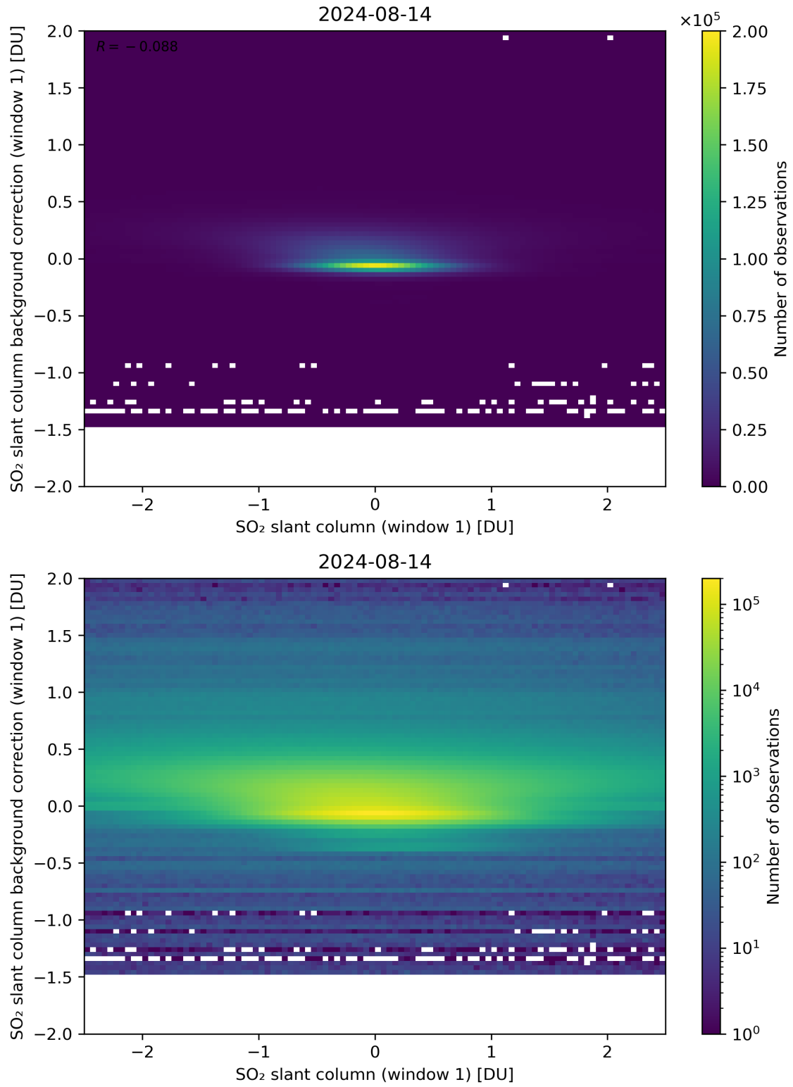
Figure 212: Scatter density plot of “SO 2 slant column (window 1)” against “SO 2 slant column background correction (window 1)” for 2024-08-13 to 2024-08-15.
