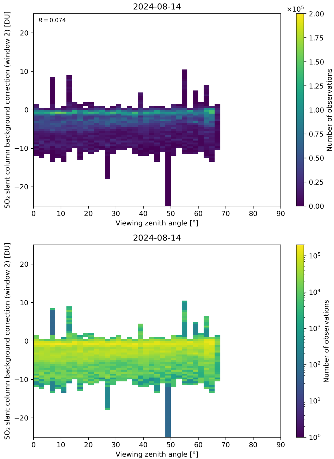
Figure 309: Scatter density plot of “Viewing zenith angle” against “SO 2 slant column background correction (window 2)” for 2024-08-13 to 2024-08-15.
