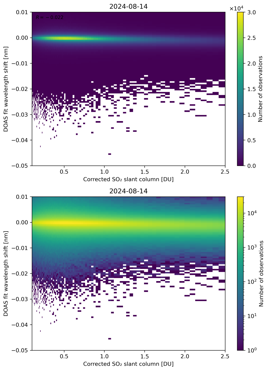
Figure 181: Scatter density plot of “Corrected SO 2 slant column” against “DOAS fit wavelength shift” for 2024-08-13 to 2024-08-15.
