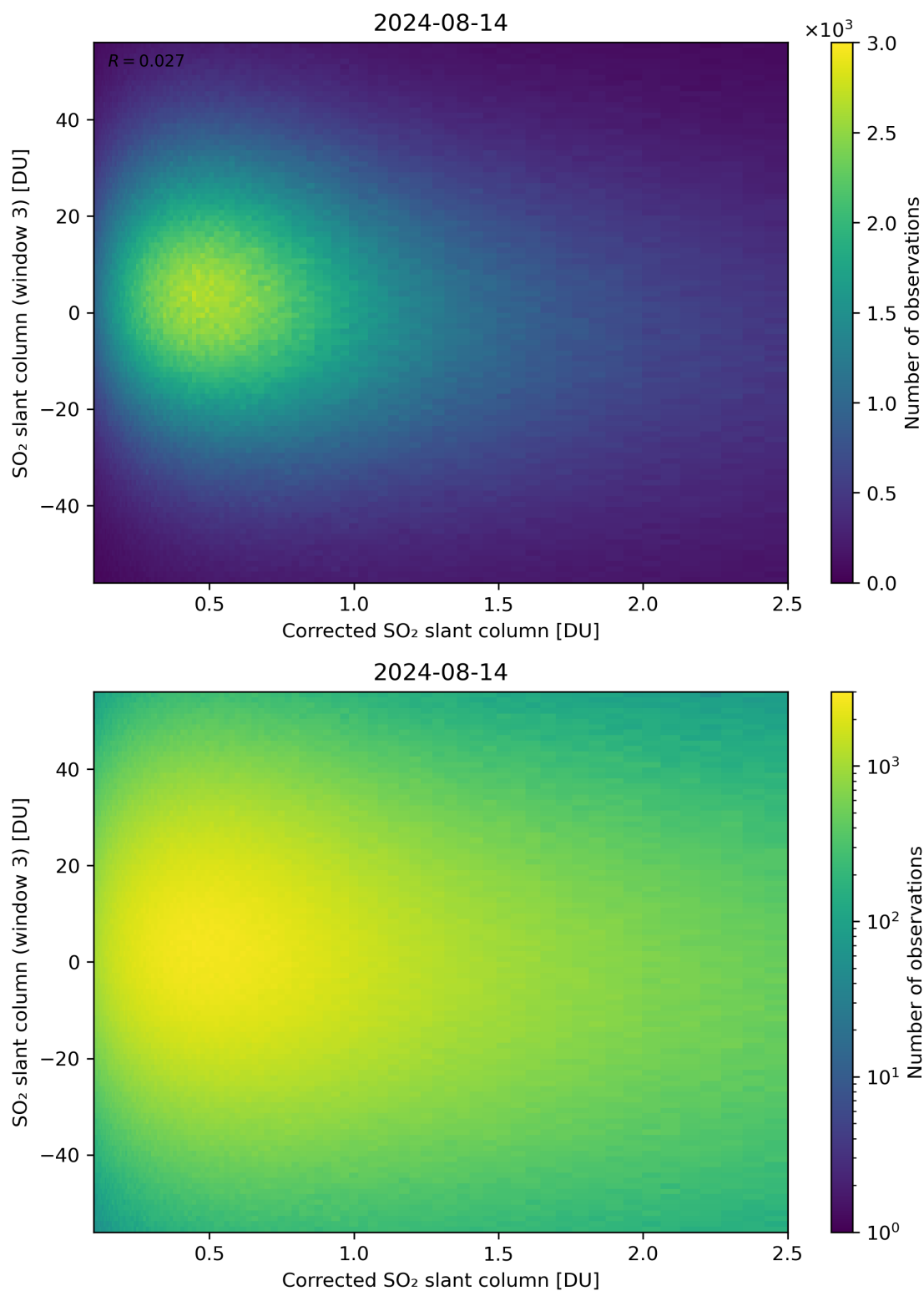
Figure 190: Scatter density plot of “Corrected SO 2 slant column” against “SO 2 slant column (window 3)” for 2024-08-13 to 2024-08-15.
