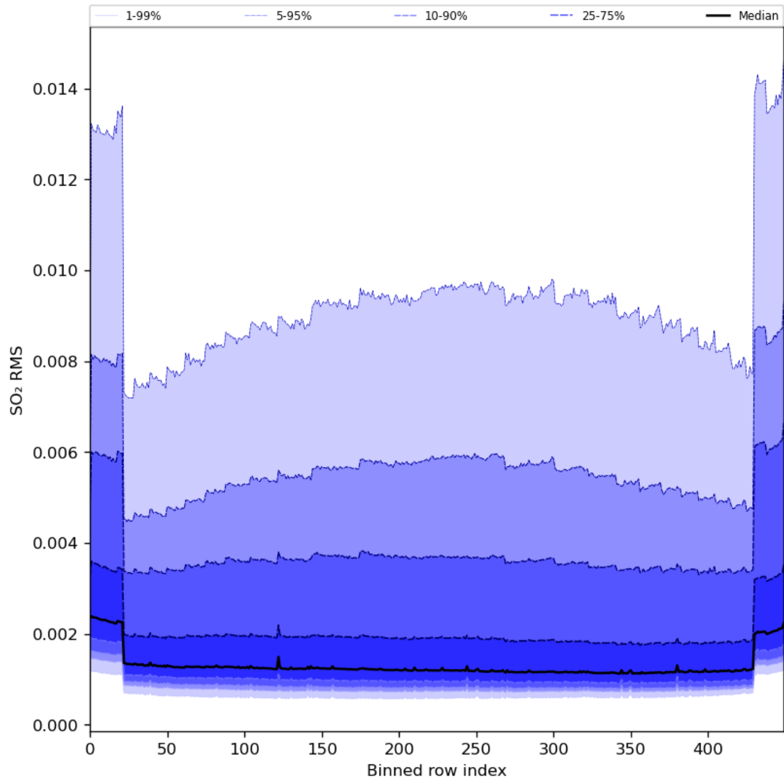
Figure 93: Along track statistics of “SO 2 RMS” for 2024-08-13 to 2024-08-15
