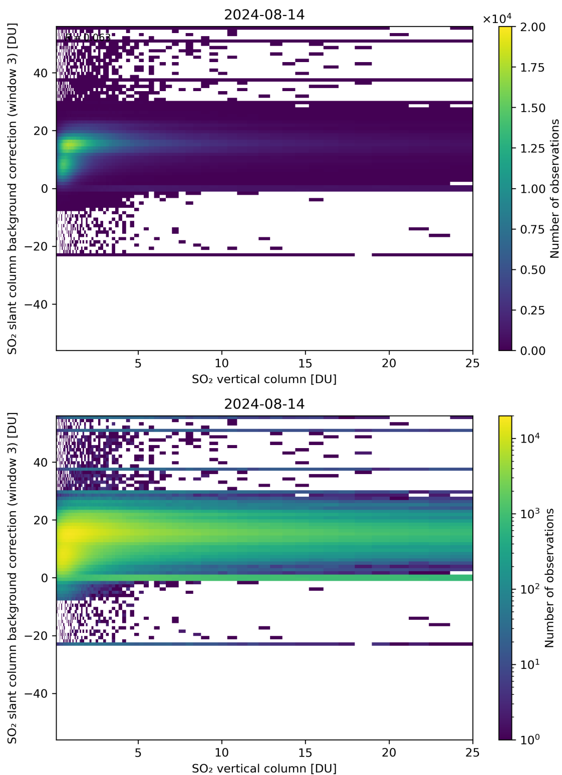
Figure 275: Scatter density plot of “SO 2 vertical column” against “SO 2 slant column background correction (window 3)” for 2024-08-13 to 2024-08-15.
