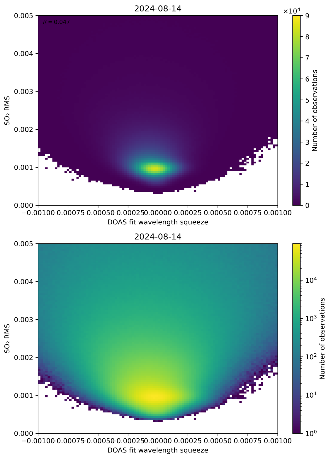
Figure 132: Scatter density plot of “DOAS fit wavelength squeeze” against “SO 2 RMS” for 2024-08-13 to 2024-08-15.
