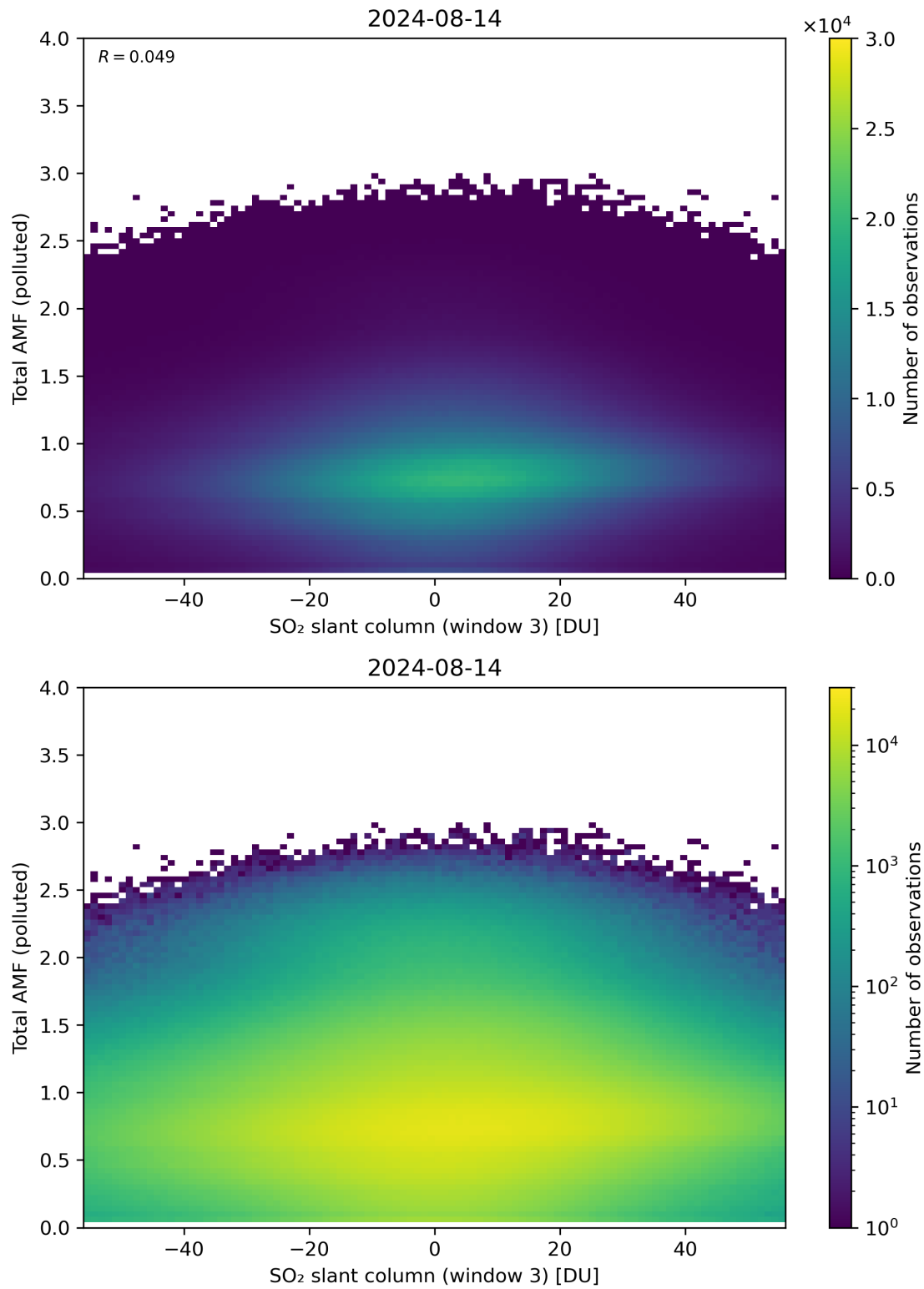
Figure 268: Scatter density plot of “SO 2 slant column (window 3)” against “Total AMF (polluted)” for 2024-08-13 to 2024-08-15.
