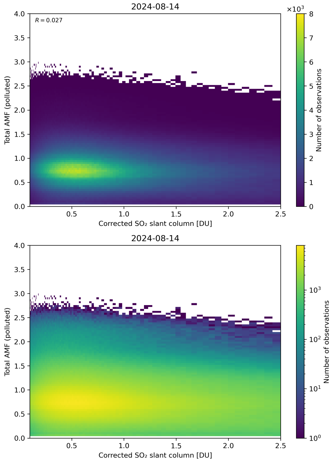
Figure 192: Scatter density plot of “Corrected SO 2 slant column” against “Total AMF (polluted)” for 2024-08-13 to 2024-08-15.
