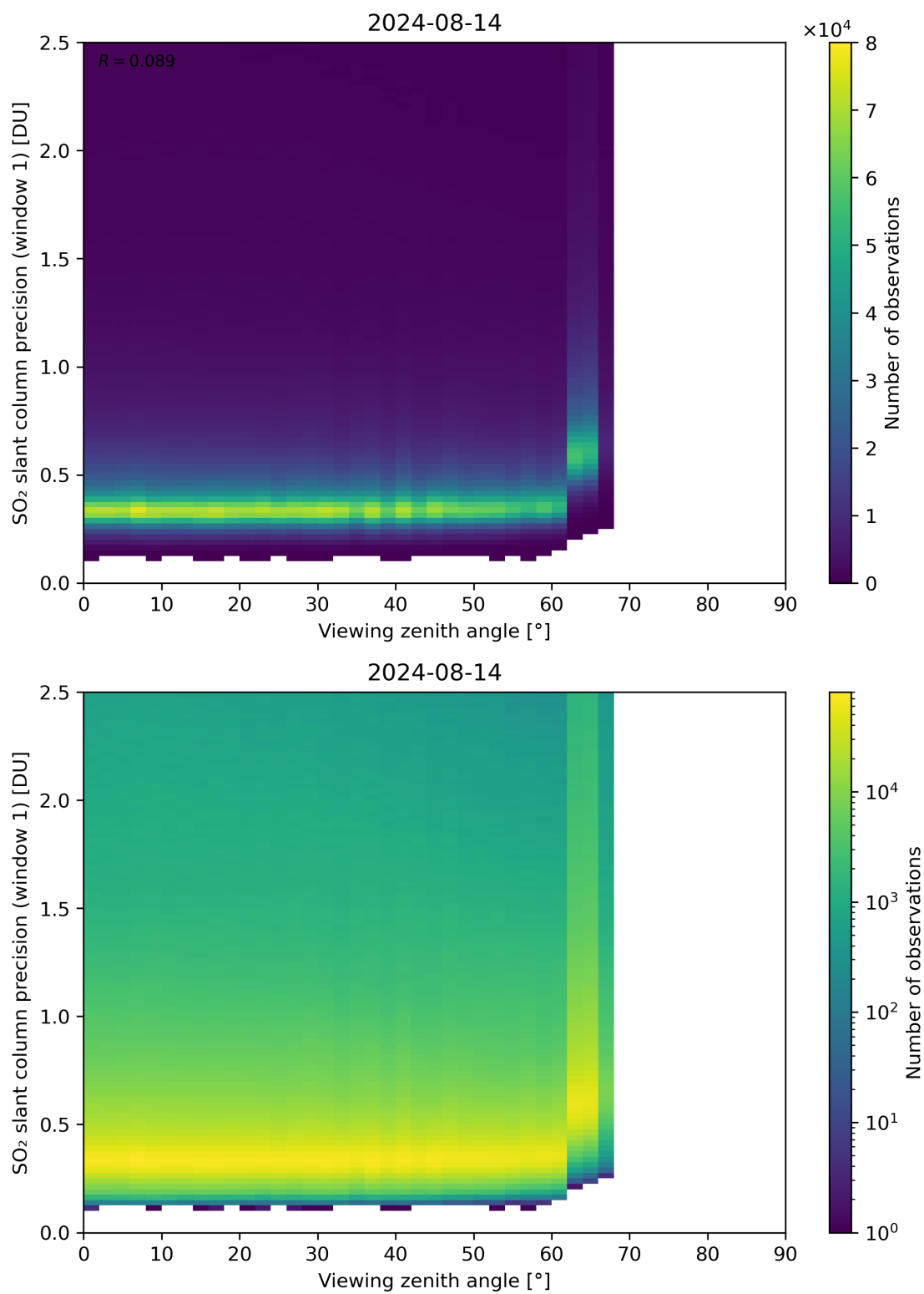
Figure 321: Scatter density plot of “Viewing zenith angle” against “SO 2 slant column precision (window 1)” for 2024-08-13 to 2024-08-15.
