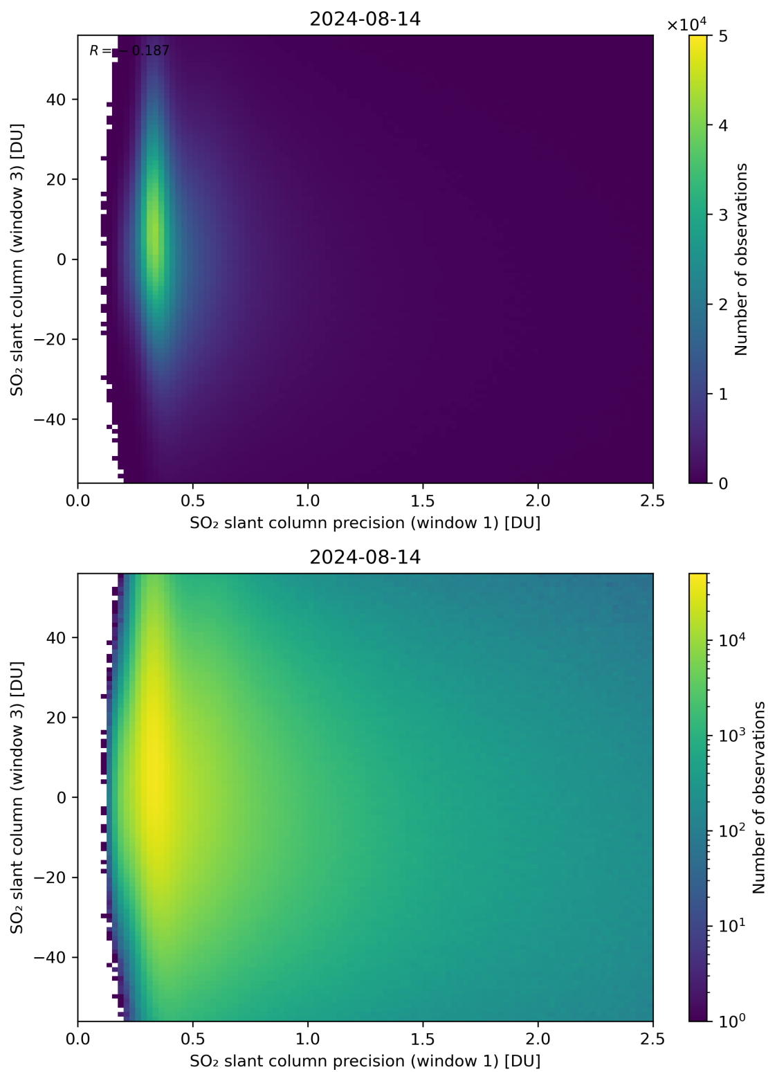
Figure 228: Scatter density plot of “SO 2 slant column precision (window 1)” against “SO 2 slant column (window 3)” for 2024-08-13 to 2024-08-15.
