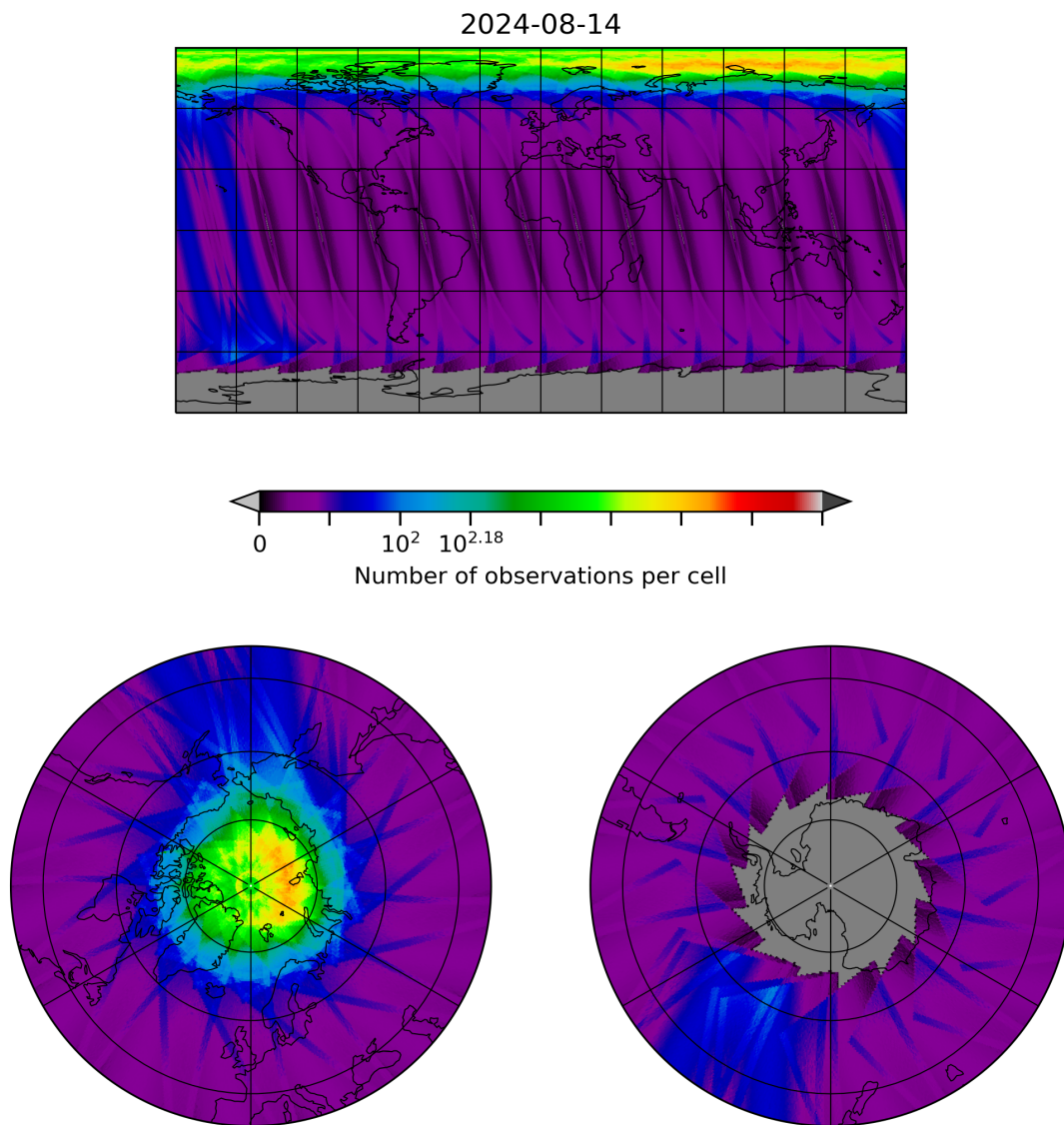
Figure 28: Map of the number of observations for 2024-08-13 to 2024-08-15
