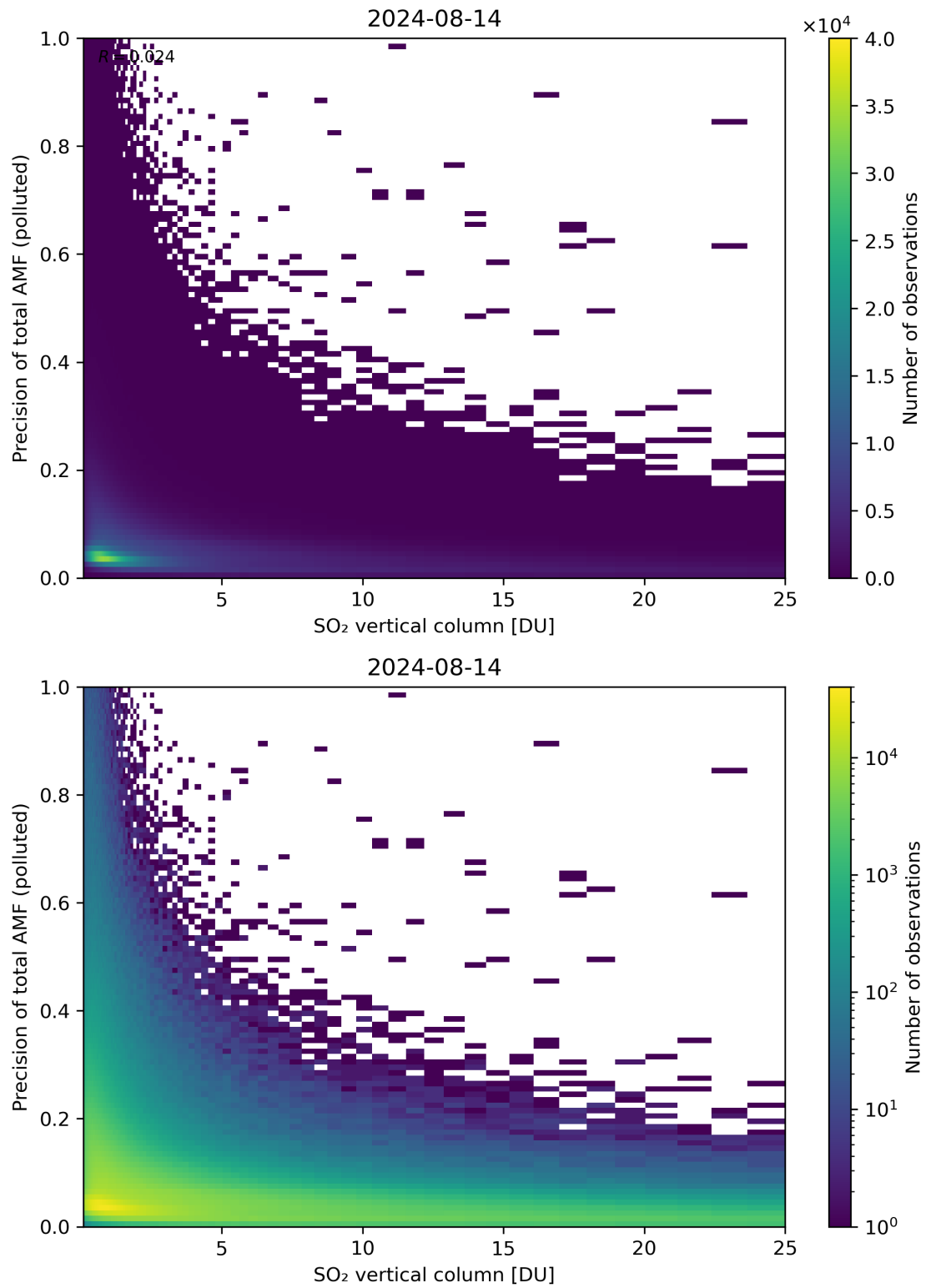
Figure 306: Scatter density plot of “SO 2 vertical column” against “Precision of total AMF (polluted)” for 2024-08-13 to 2024-08-15.
