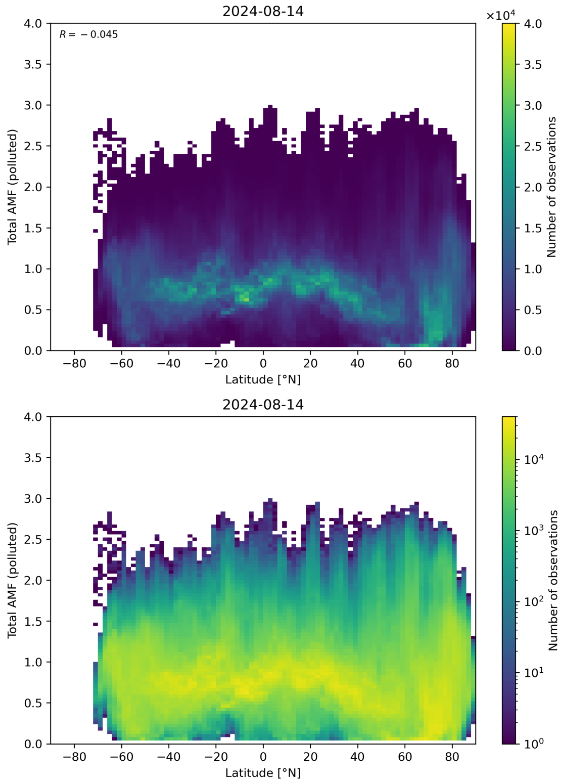
Figure 154: Scatter density plot of “Latitude” against “Total AMF (polluted)” for 2024-08-13 to 2024-08-15.
