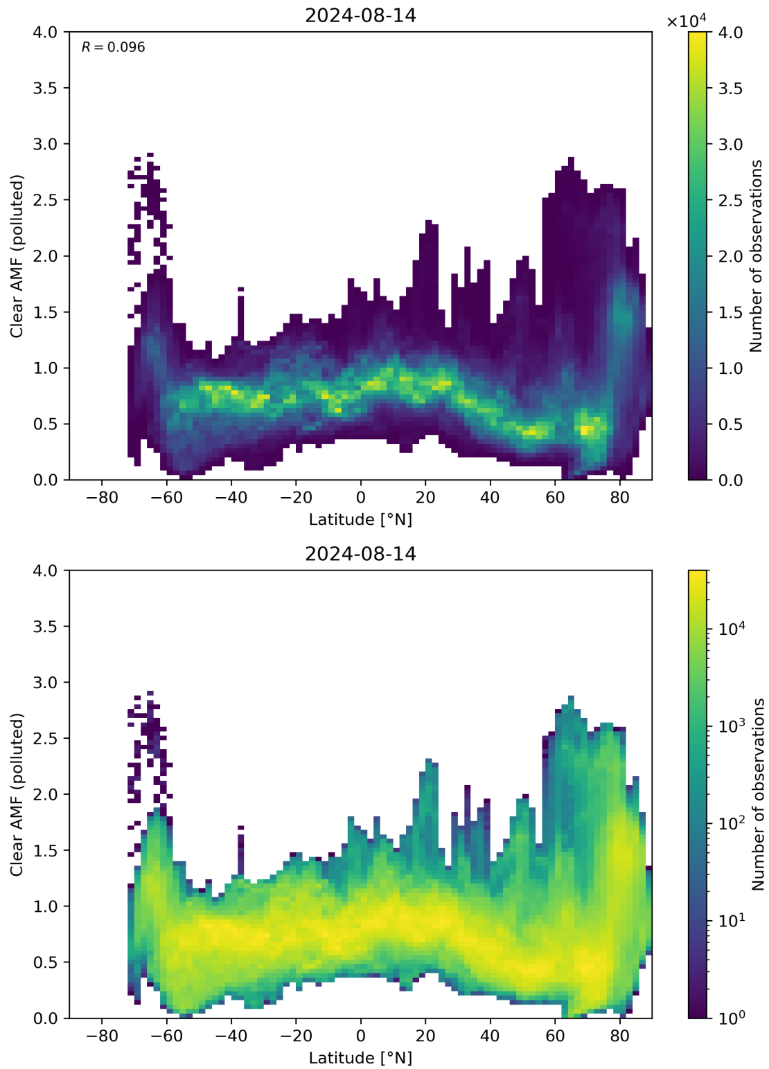
Figure 145: Scatter density plot of “Latitude” against “Clear AMF (polluted)” for 2024-08-13 to 2024-08-15.
