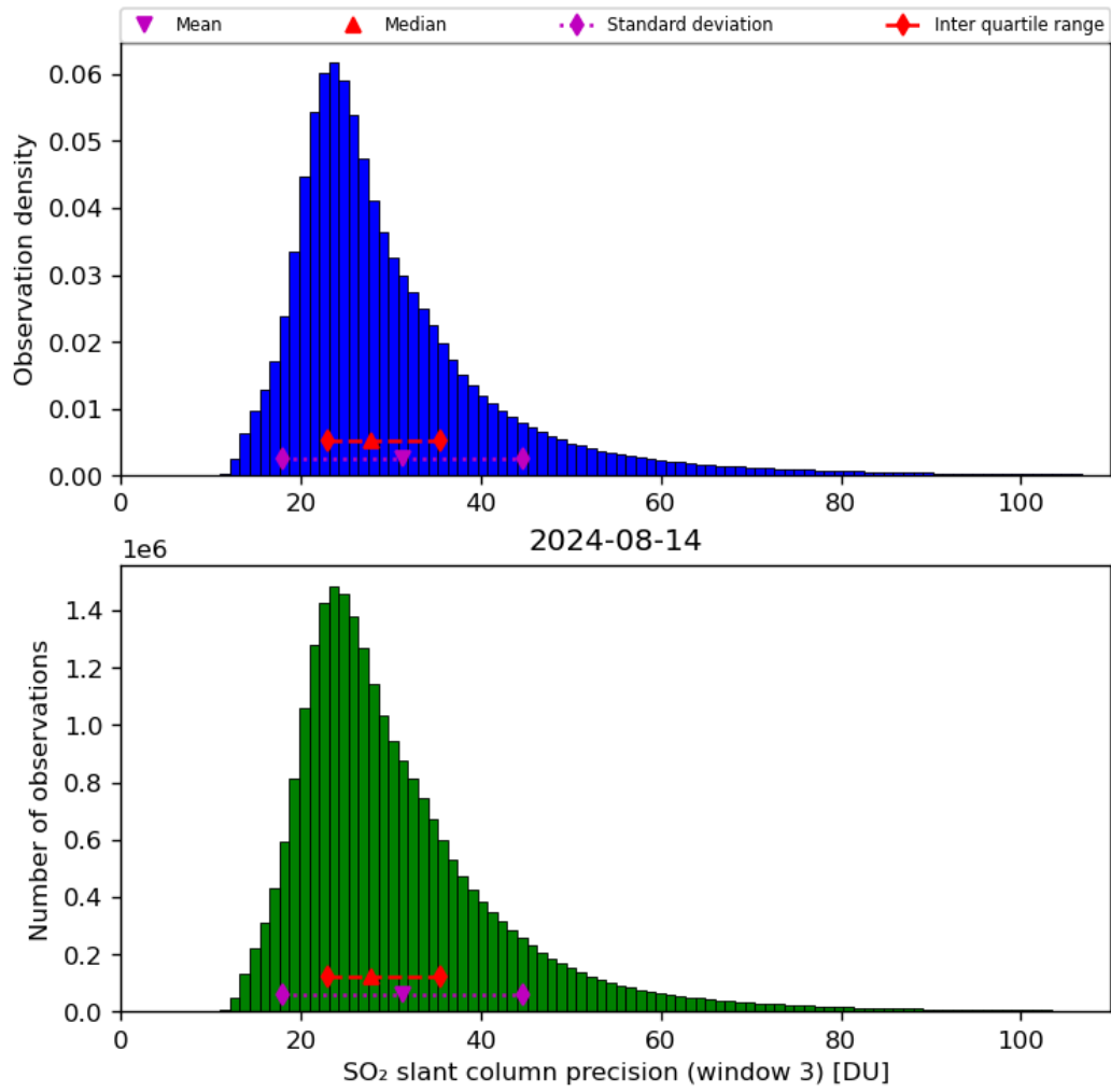
Figure 65: Histogram of “SO 2 slant column precision (window 3)” for 2024-08-13 to 2024-08-15
