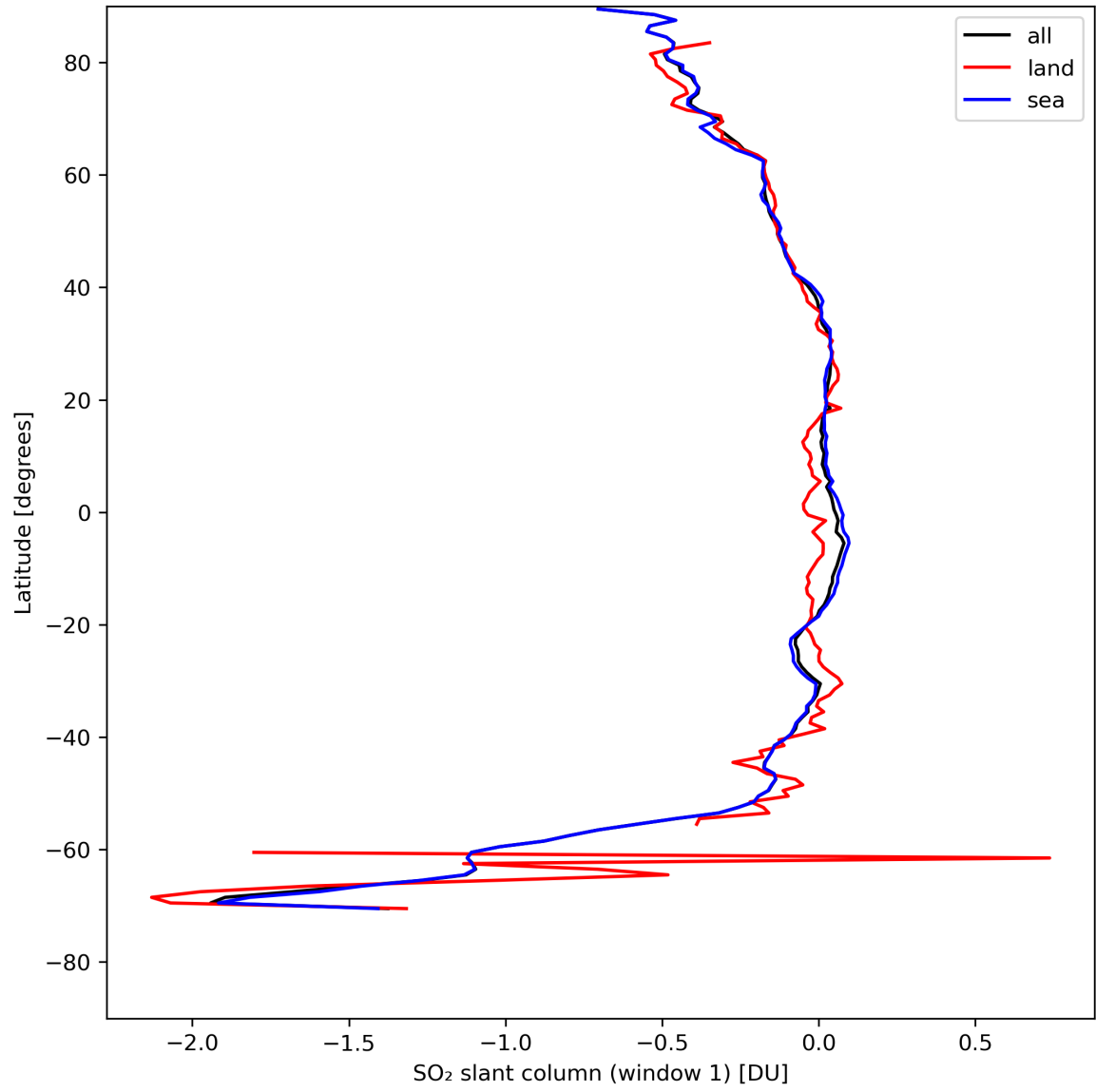
Figure 33: Zonal average of “SO 2 slant column (window 1)” for 2024-08-13 to 2024-08-15.
