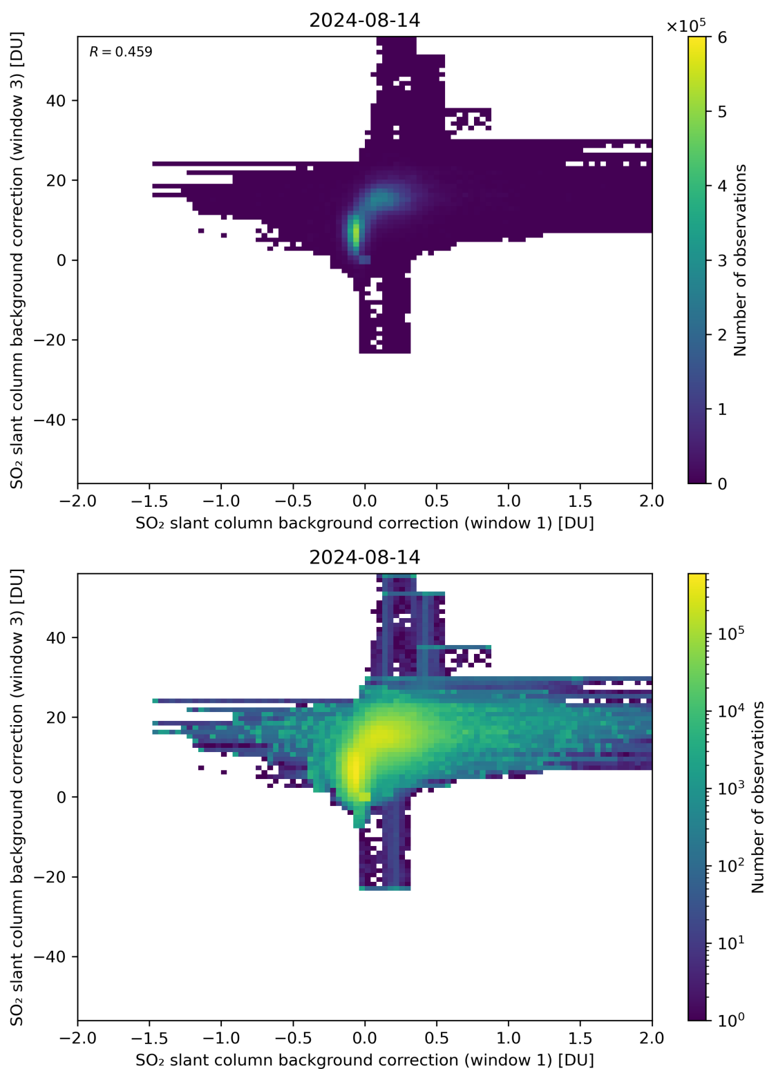
Figure 99: Scatter density plot of “SO 2 slant column background correction (window 1)” against “SO 2 slant column background correction (window 3)” for 2024-08-13 to 2024-08-15.
