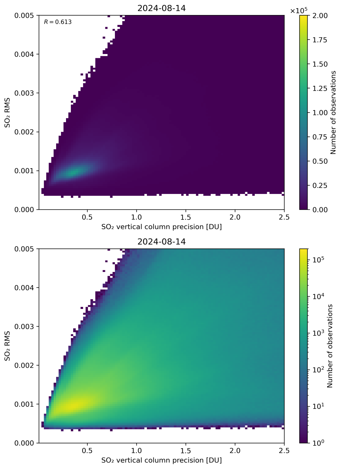
Figure 284: Scatter density plot of “SO 2 vertical column precision” against “SO 2 RMS” for 2024-08-13 to 2024-08-15.
