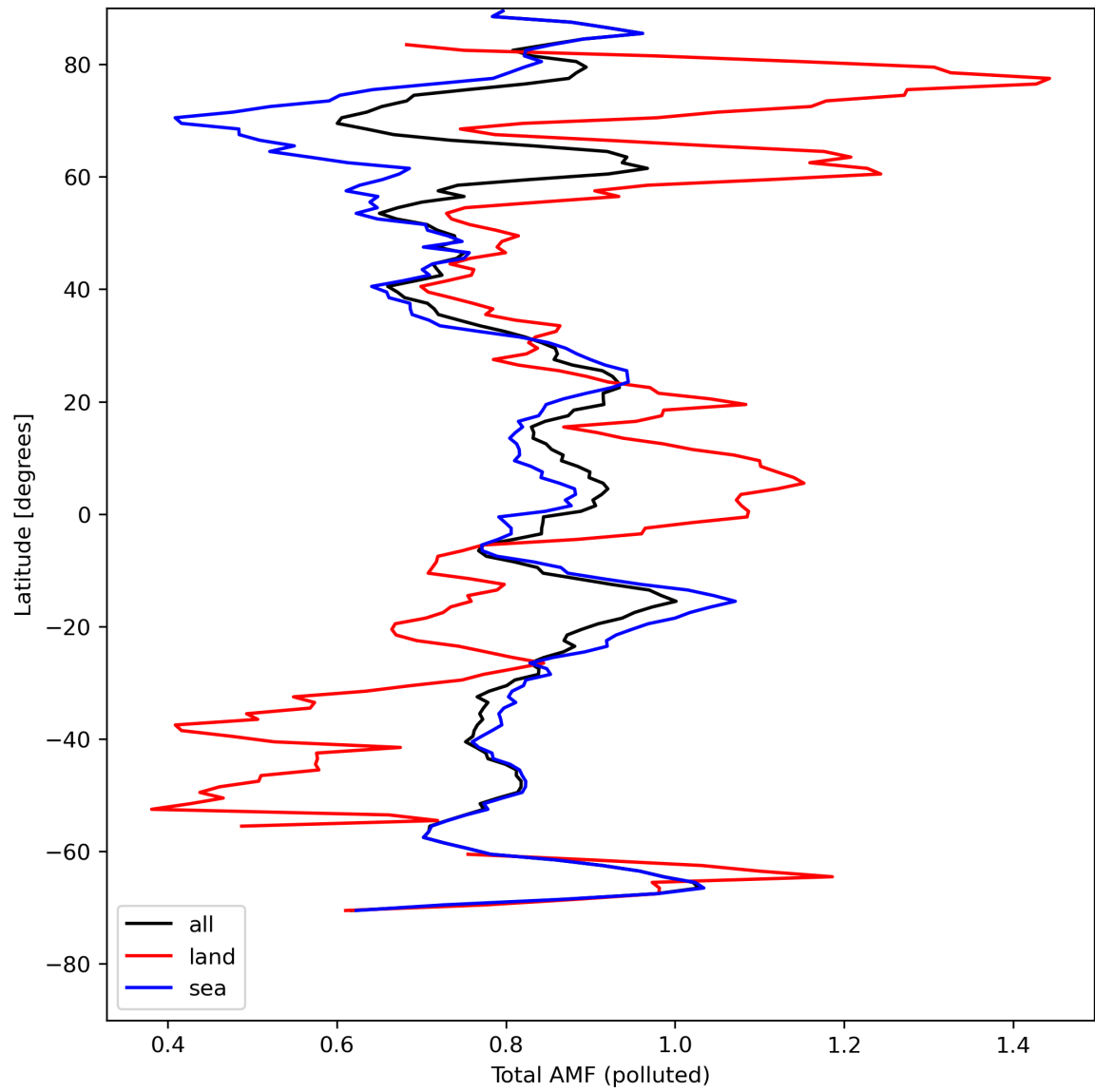
Figure 48: Zonal average of “Total AMF (polluted)” for 2024-08-13 to 2024-08-15.
