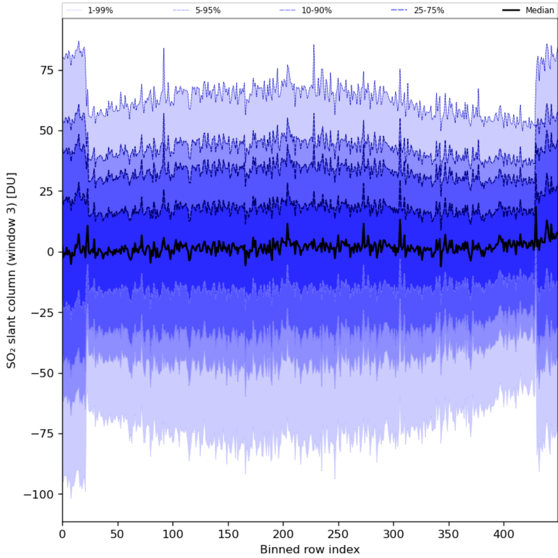
Figure 87: Along track statistics of “SO 2 slant column (window 3)” for 2024-08-13 to 2024-08-15
