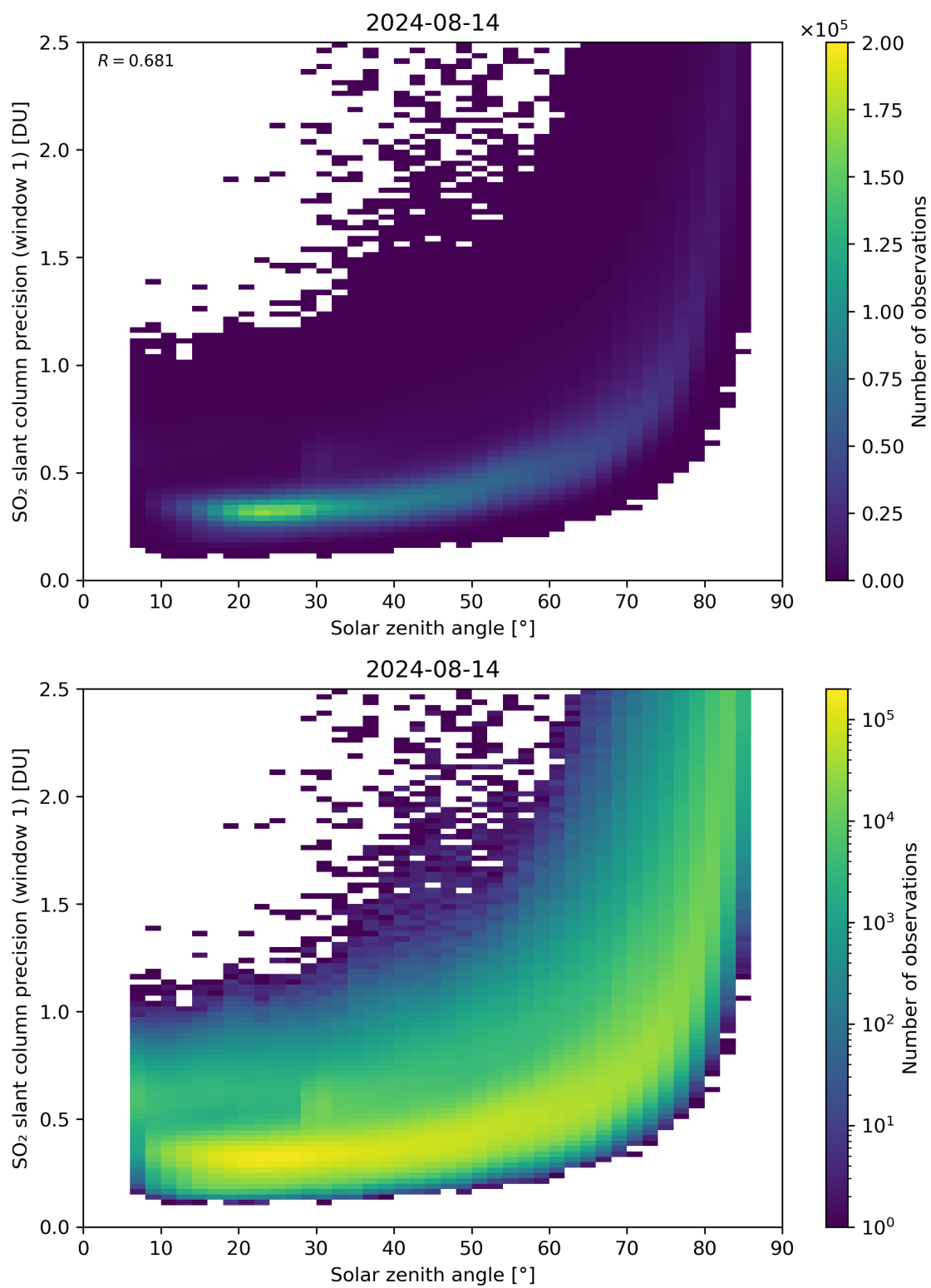
Figure 170: Scatter density plot of “Solar zenith angle” against “SO 2 slant column precision (window 1)” for 2024-08-13 to 2024-08-15.
