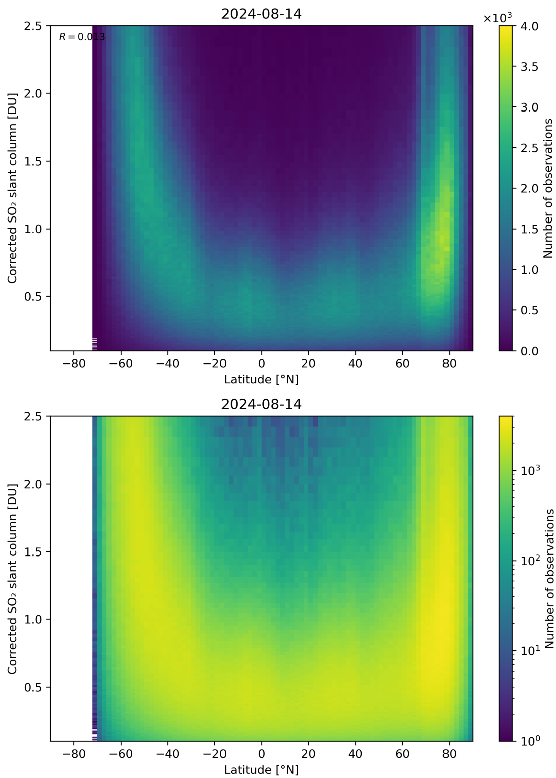
Figure 146: Scatter density plot of “Latitude” against “Corrected SO 2 slant column” for 2024-08-13 to 2024-08-15.
