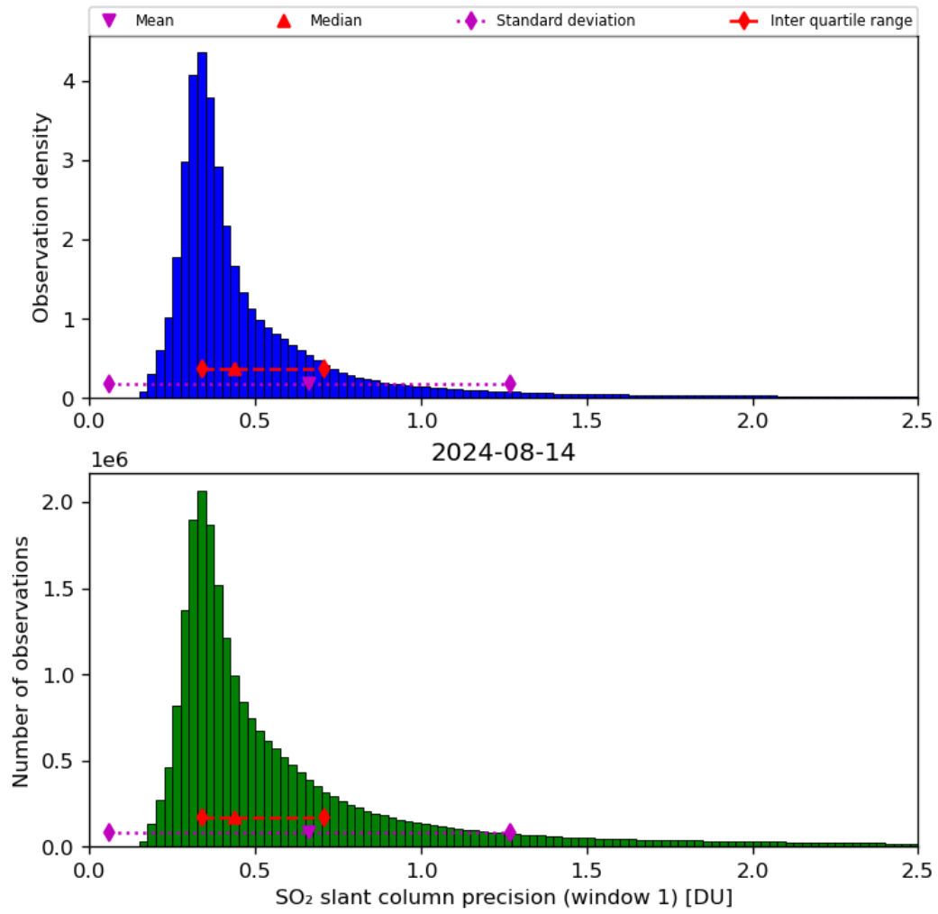
Figure 57: Histogram of “SO 2 slant column precision (window 1)” for 2024-08-13 to 2024-08-15
