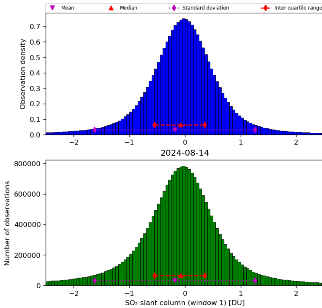
Figure 56: Histogram of “SO 2 slant column (window 1)” for 2024-08-13 to 2024-08-15
