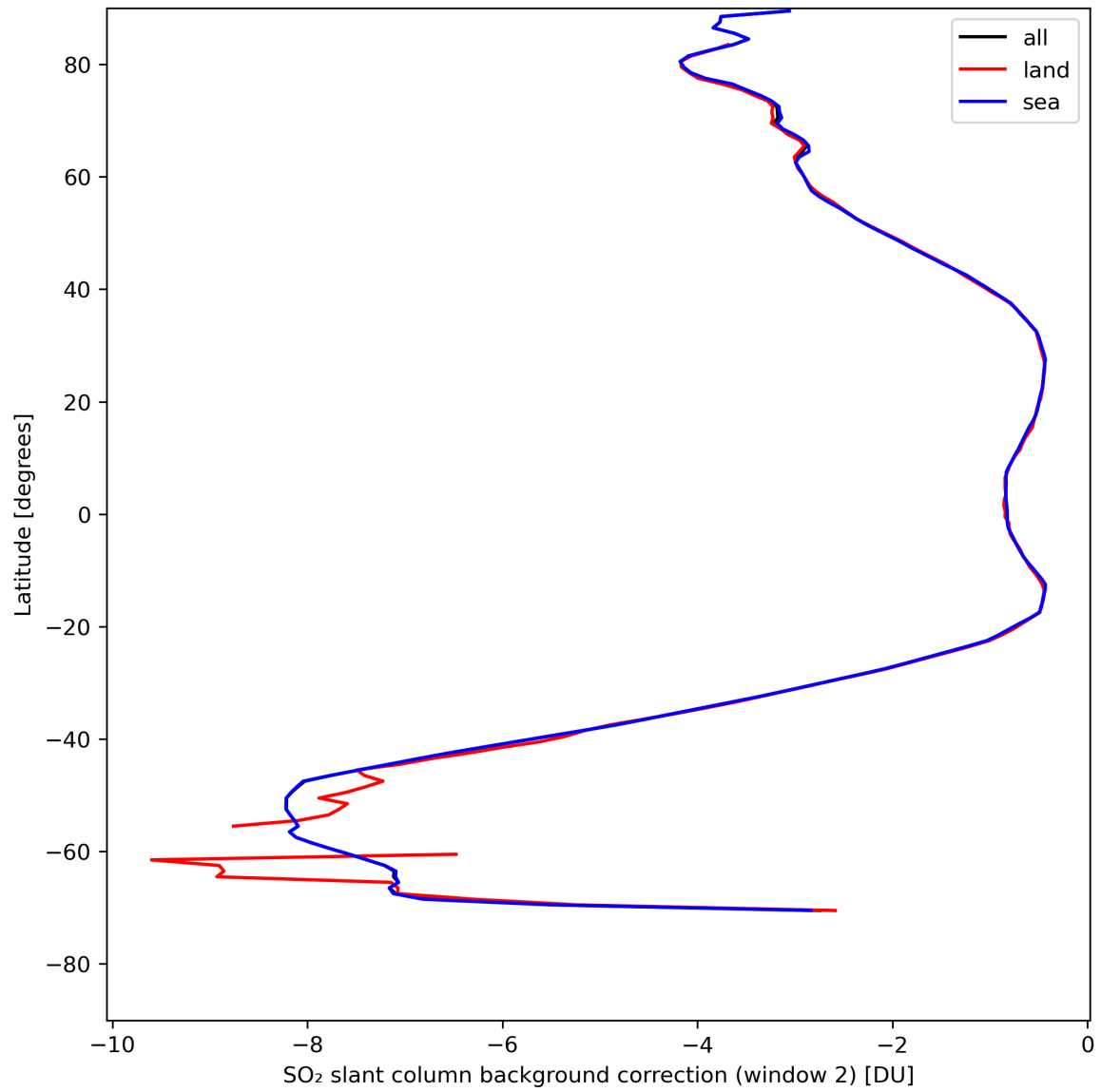
Figure 40: Zonal average of “SO 2 slant column background correction (window 2)” for 2024-08-13 to 2024-08-15.
