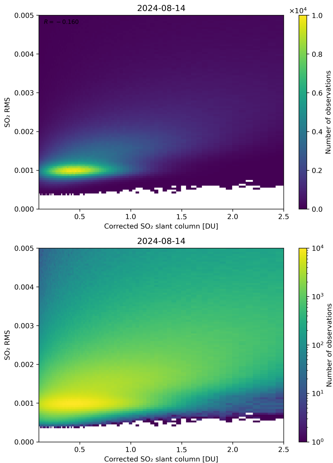
Figure 183: Scatter density plot of “Corrected SO 2 slant column” against “SO 2 RMS” for 2024-08-13 to 2024-08-15.
