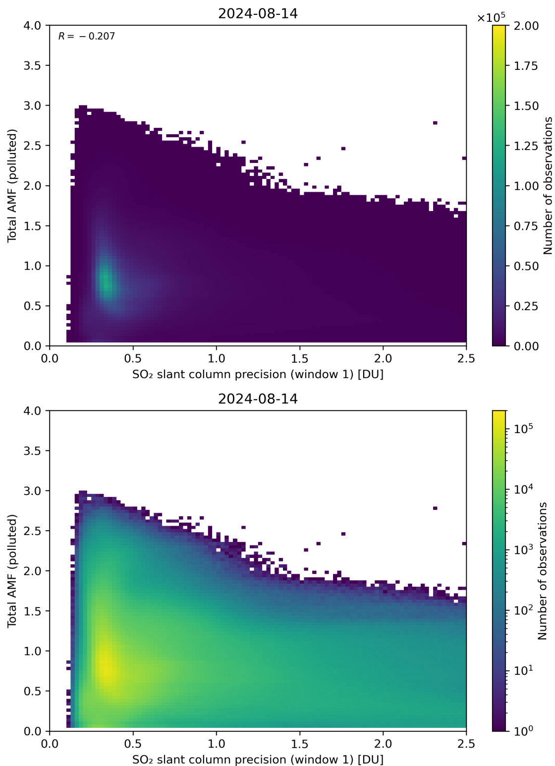
Figure 230: Scatter density plot of “SO 2 slant column precision (window 1)” against “Total AMF (polluted)” for 2024-08-13 to 2024-08-15.
