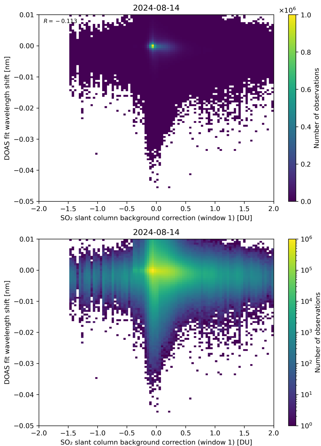
Figure 100: Scatter density plot of “SO 2 slant column background correction (window 1)” against “DOAS fit wavelength shift” for 2024-08-13 to 2024-08-15.
