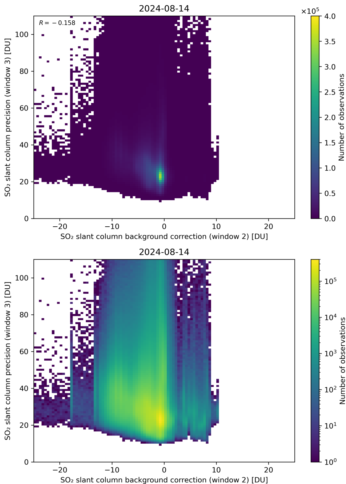
Figure 118: Scatter density plot of “SO 2 slant column background correction (window 2)” against “SO 2 slant column precision (window 3)” for 2024-08-13 to 2024-08-15.
