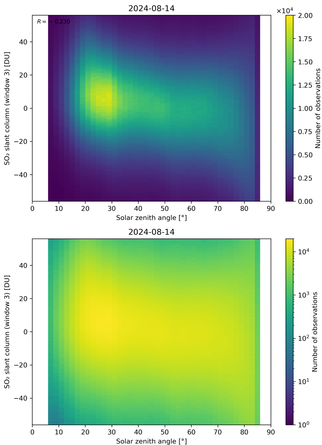
Figure 172: Scatter density plot of “Solar zenith angle” against “SO 2 slant column (window 3)” for 2024-08-13 to 2024-08-15.
