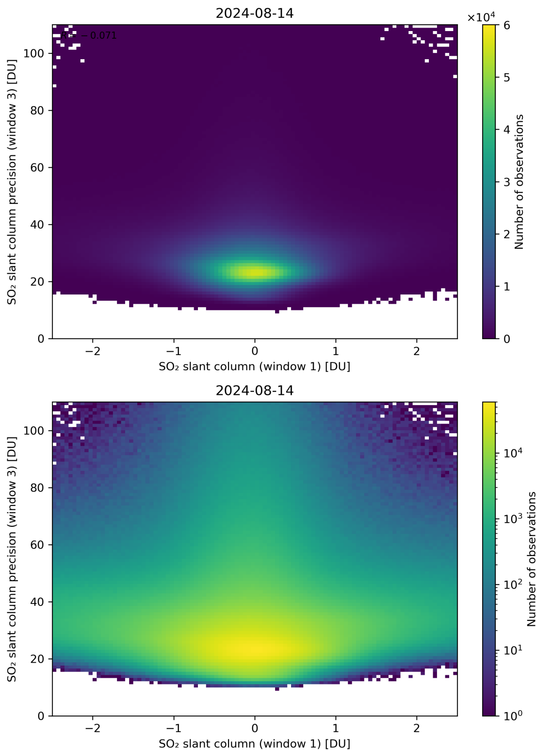
Figure 238: Scatter density plot of “SO 2 slant column (window 1)” against “SO 2 slant column precision (window 3)” for 2024-08-13 to 2024-08-15.
