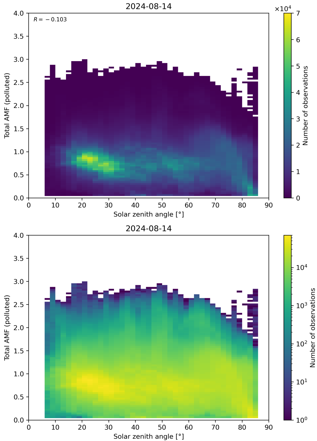
Figure 174: Scatter density plot of “Solar zenith angle” against “Total AMF (polluted)” for 2024-08-13 to 2024-08-15.
