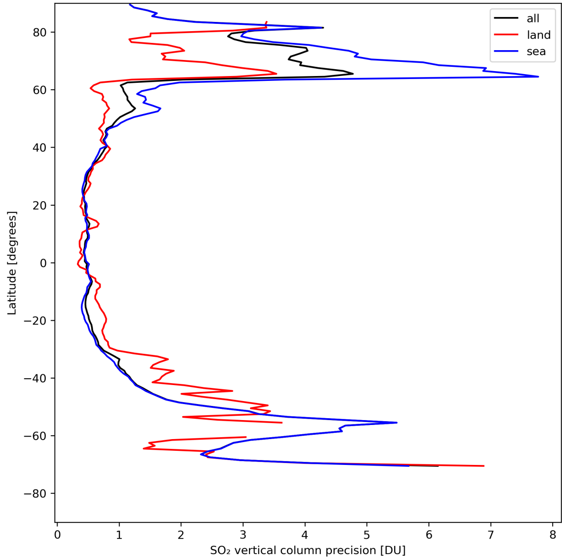
Figure 31: Zonal average of “SO 2 vertical column precision” for 2024-08-13 to 2024-08-15.
