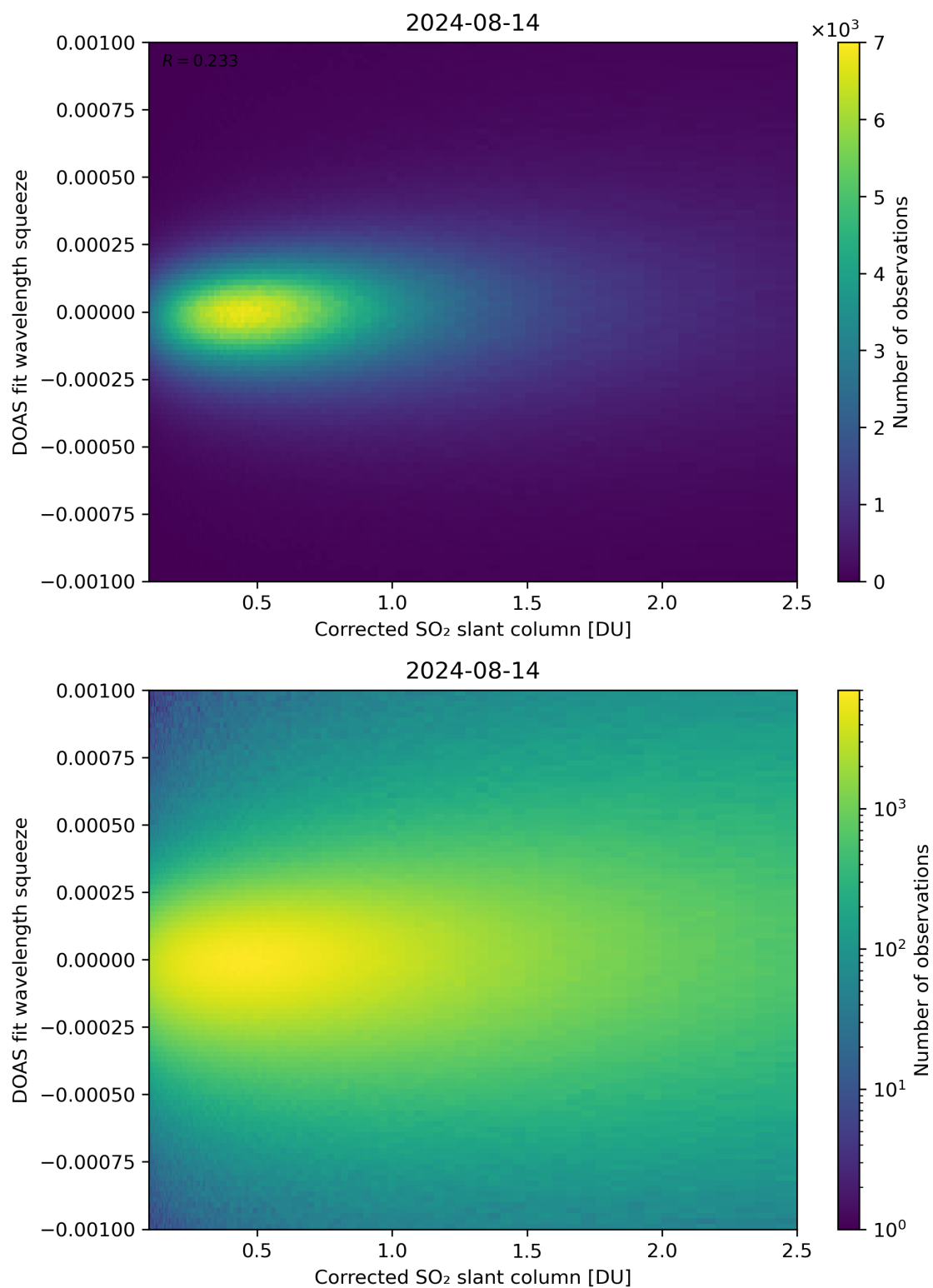
Figure 182: Scatter density plot of “Corrected SO 2 slant column” against “DOAS fit wavelength squeeze” for 2024-08-13 to 2024-08-15.
