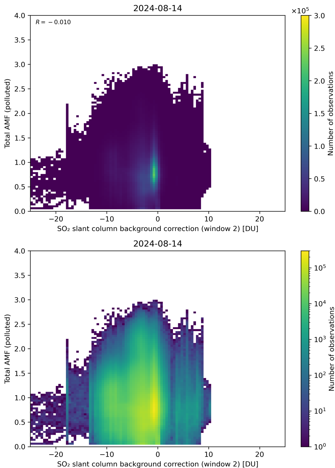
Figure 119: Scatter density plot of “SO 2 slant column background correction (window 2)” against “Total AMF (polluted)” for 2024-08-13 to 2024-08-15.
