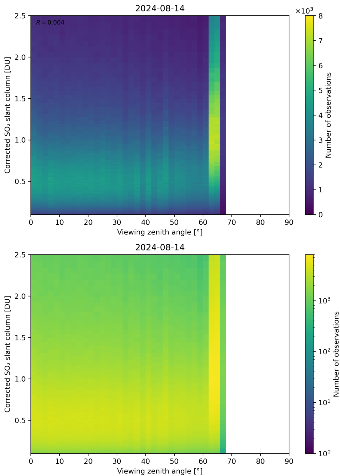
Figure 317: Scatter density plot of “Viewing zenith angle” against “Corrected SO 2 slant column” for 2024-08-13 to 2024-08-15.
