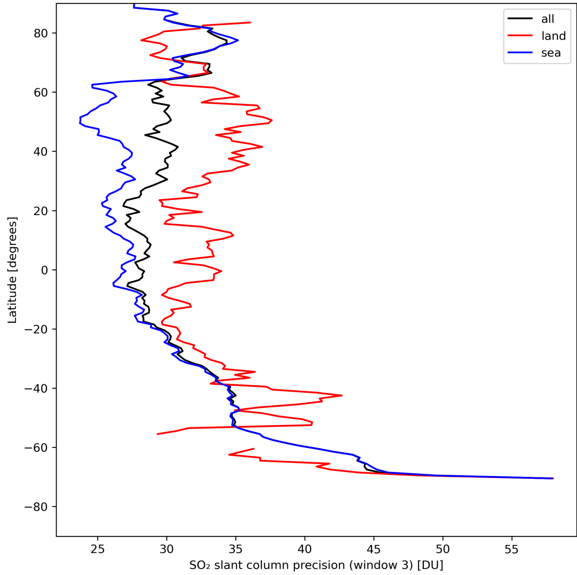
Figure 42: Zonal average of “SO 2 slant column precision (window 3)” for 2024-08-13 to 2024-08-15.
