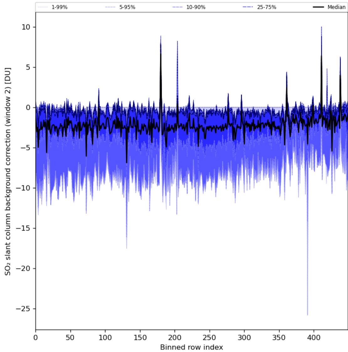
Figure 86: Along track statistics of “SO 2 slant column background correction (window 2)” for 2024-08-13 to 2024-08-15
