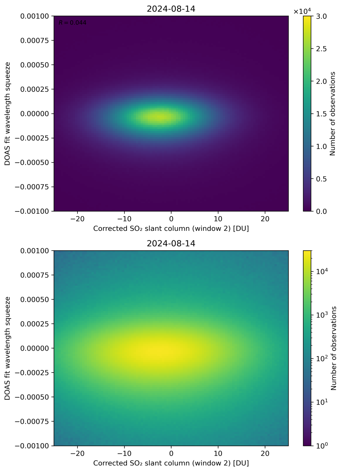
Figure 197: Scatter density plot of “Corrected SO 2 slant column (window 2)” against “DOAS fit wavelength squeeze” for 2024-08-13 to 2024-08-15.
