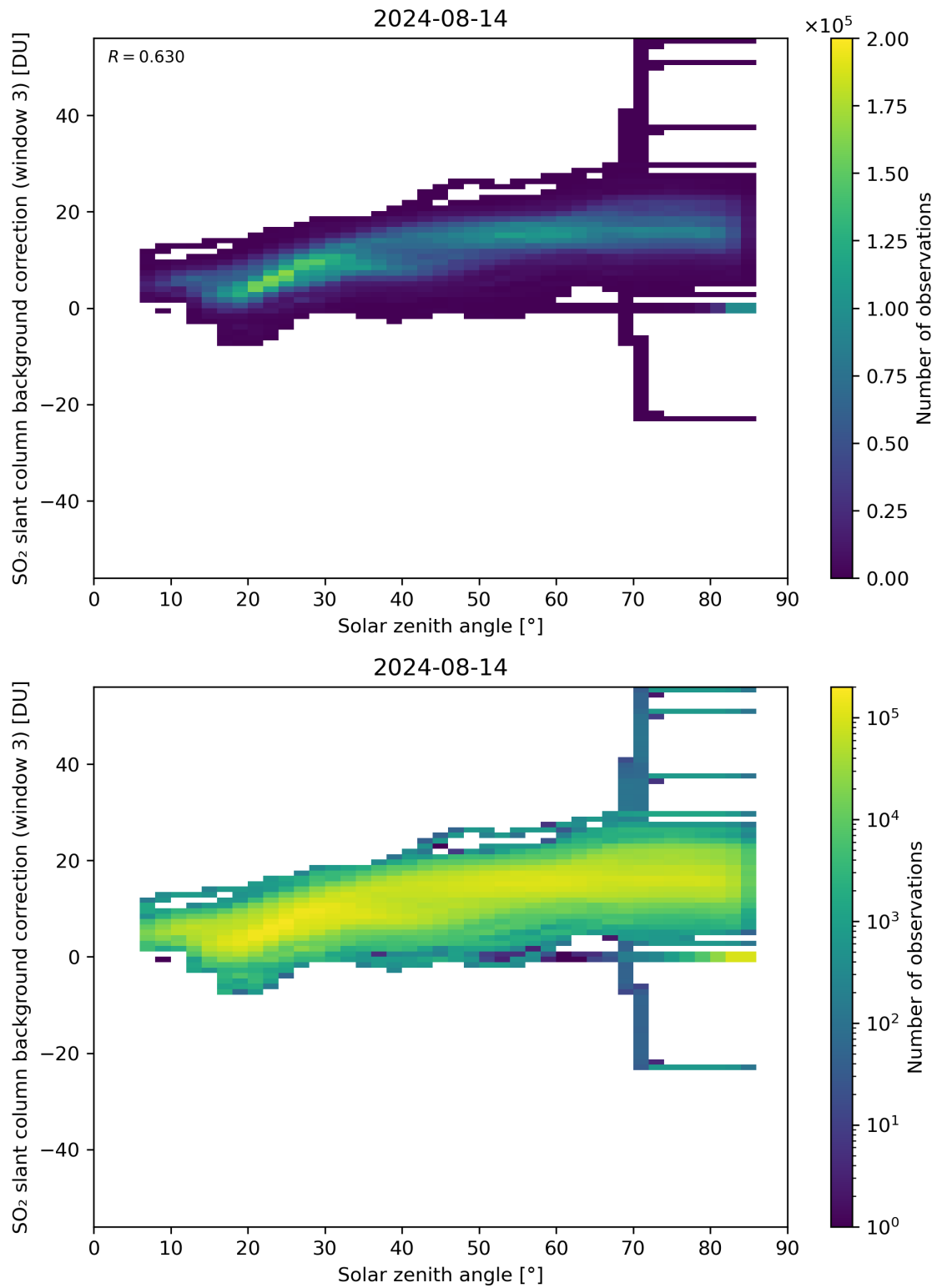
Figure 160: Scatter density plot of “Solar zenith angle” against “SO 2 slant column background correction (window 3)” for 2024-08-13 to 2024-08-15.
