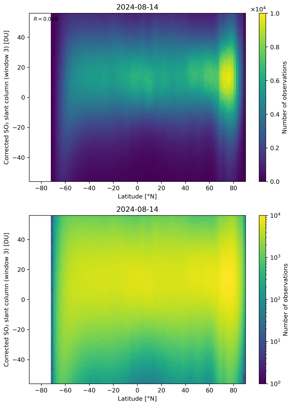
Figure 148: Scatter density plot of “Latitude” against “Corrected SO 2 slant column (window 3)” for 2024-08-13 to 2024-08-15.
