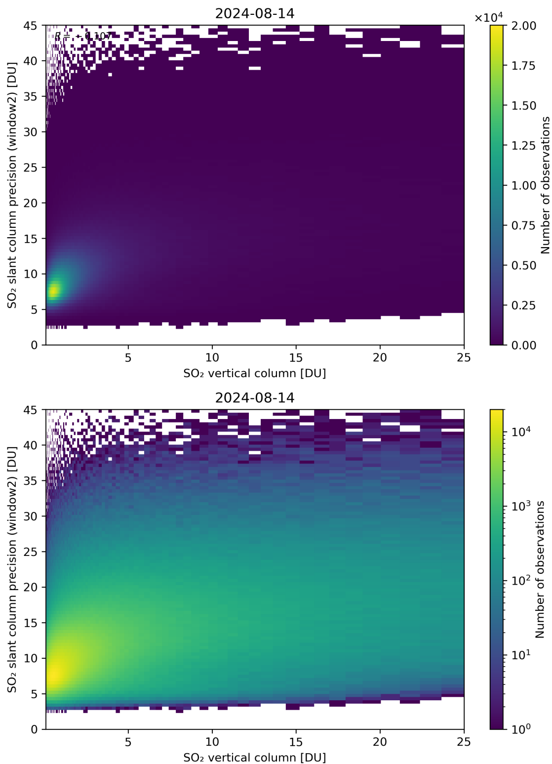
Figure 302: Scatter density plot of “SO 2 vertical column” against “SO 2 slant column precision (window2)” for 2024-08-13 to 2024-08-15.
