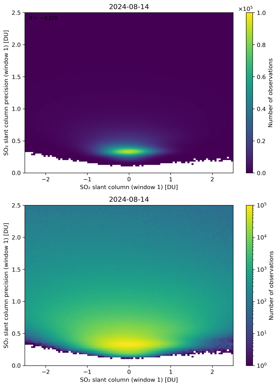
Figure 235: Scatter density plot of “SO 2 slant column (window 1)” against “SO 2 slant column precision (window 1)” for 2024-08-13 to 2024-08-15.
