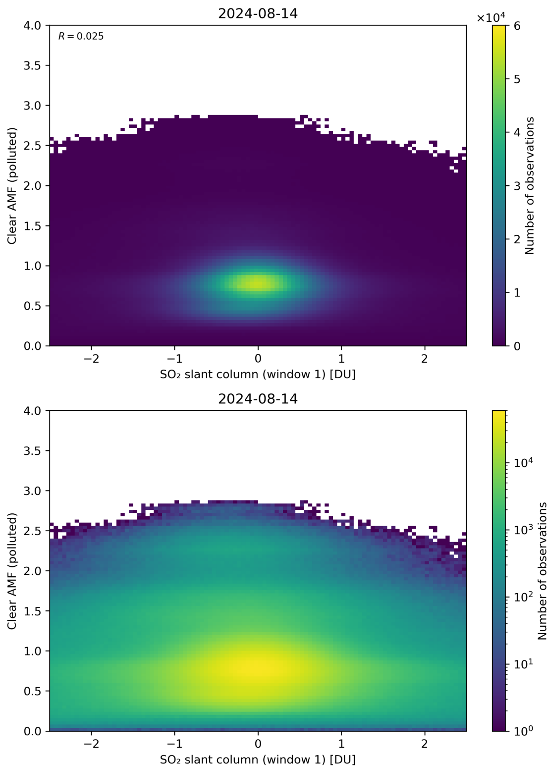
Figure 232: Scatter density plot of “SO 2 slant column (window 1)” against “Clear AMF (polluted)” for 2024-08-13 to 2024-08-15.
