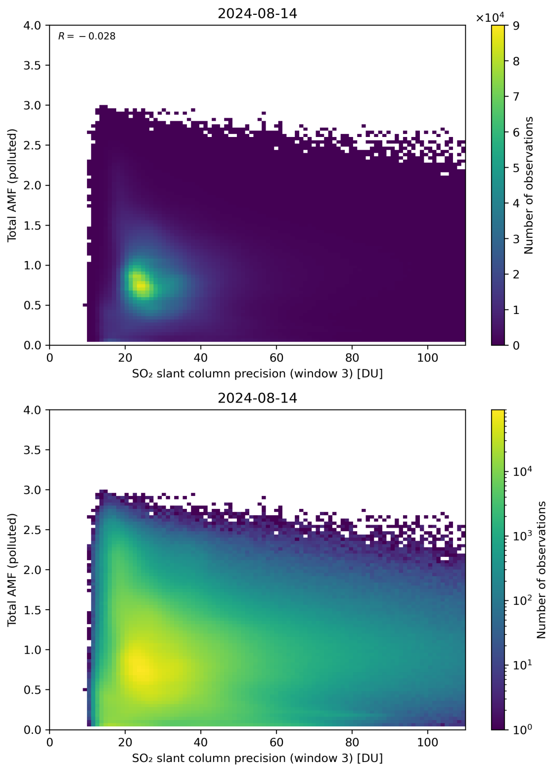
Figure 263: Scatter density plot of “SO 2 slant column precision (window 3)” against “Total AMF (polluted)” for 2024-08-13 to 2024-08-15.
