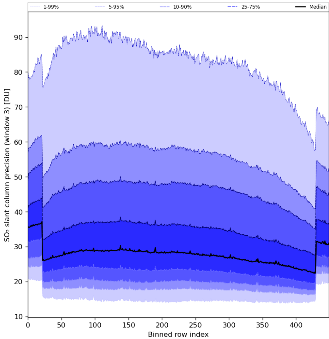
Figure 88: Along track statistics of “SO 2 slant column precision (window 3)” for 2024-08-13 to 2024-08-15
