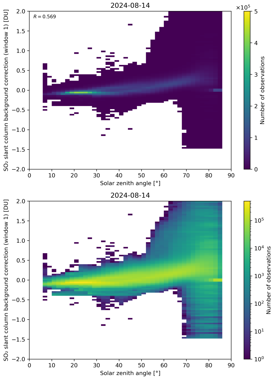
Figure 158: Scatter density plot of “Solar zenith angle” against “SO 2 slant column background correction (window 1)” for 2024-08-13 to 2024-08-15.
