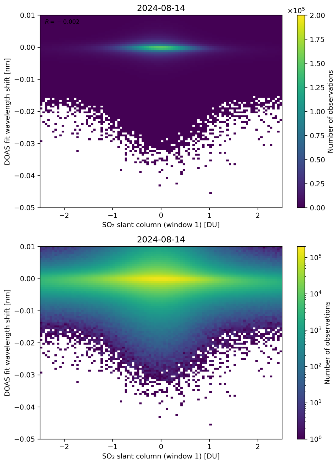
Figure 215: Scatter density plot of “SO 2 slant column (window 1)” against “DOAS fit wavelength shift” for 2024-08-13 to 2024-08-15.
