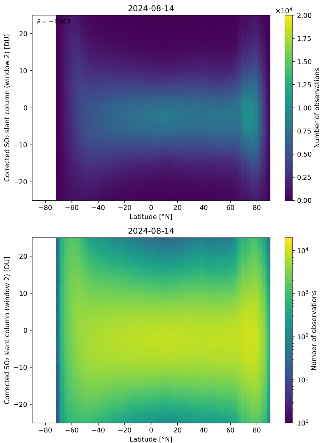
Figure 147: Scatter density plot of “Latitude” against “Corrected SO 2 slant column (window 2)” for 2024-08-13 to 2024-08-15.
