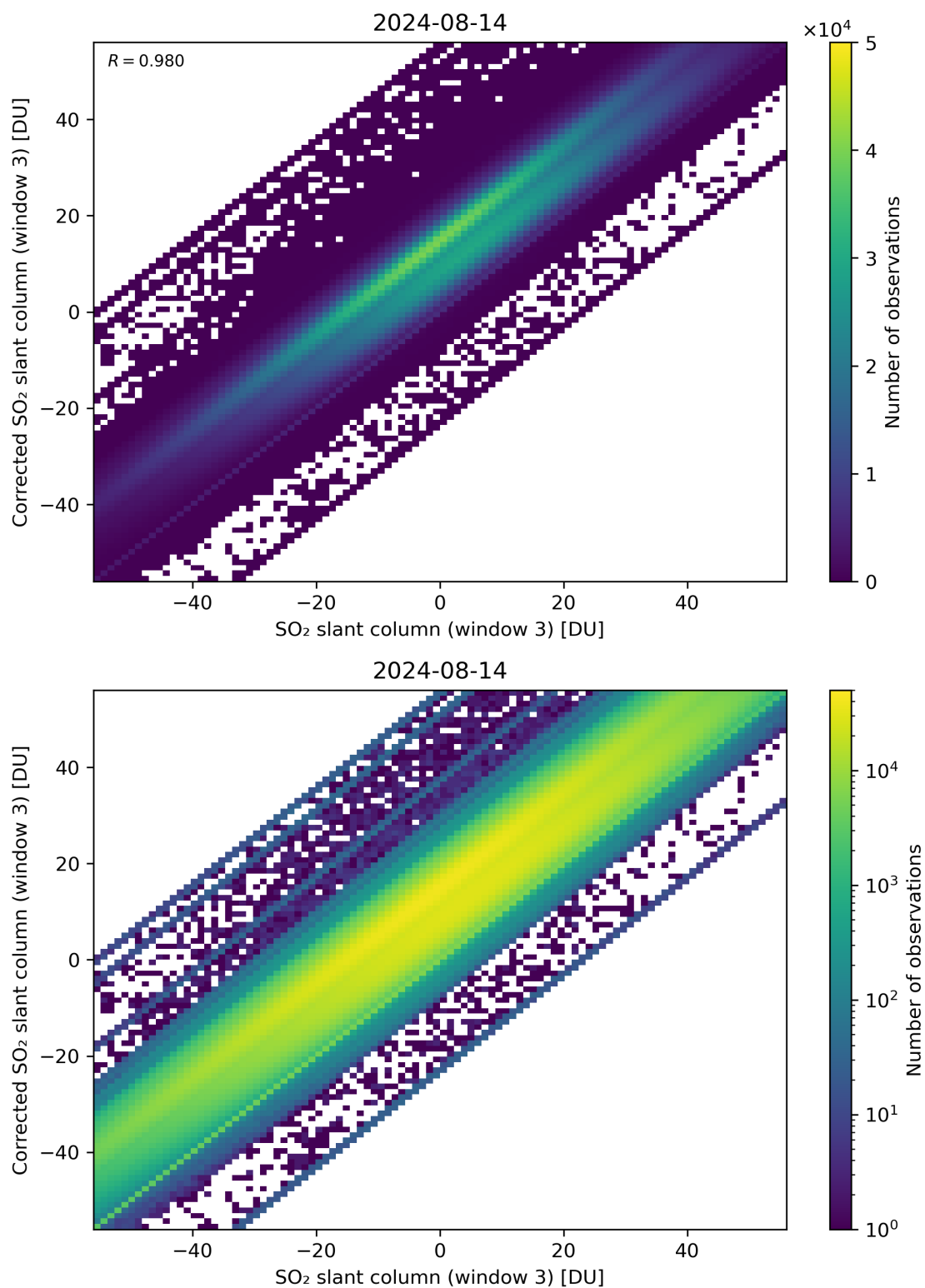
Figure 266: Scatter density plot of “SO 2 slant column (window 3)” against “Corrected SO 2 slant column (window 3)” for 2024-08-13 to 2024-08-15.
