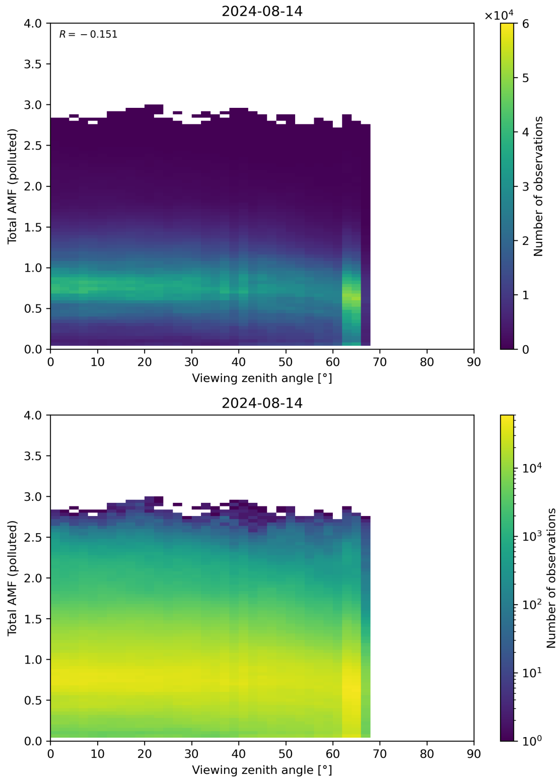
Figure 325: Scatter density plot of “Viewing zenith angle” against “Total AMF (polluted)” for 2024-08-13 to 2024-08-15.
