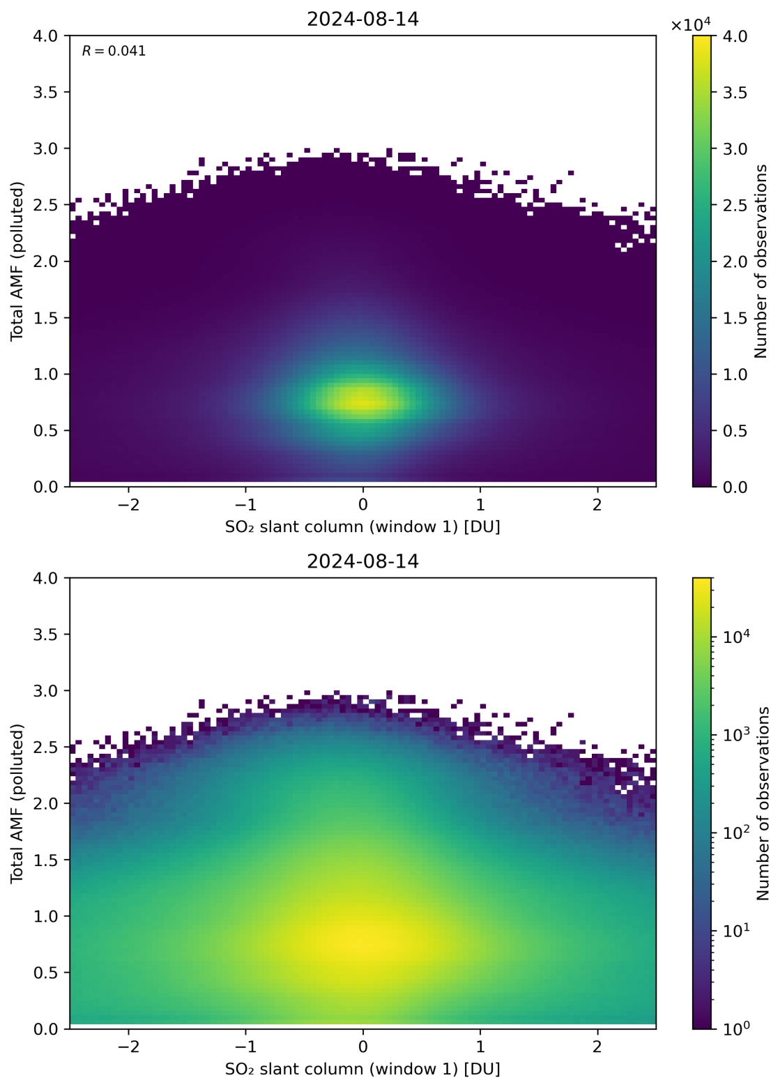
Figure 239: Scatter density plot of “SO 2 slant column (window 1)” against “Total AMF (polluted)” for 2024-08-13 to 2024-08-15.
