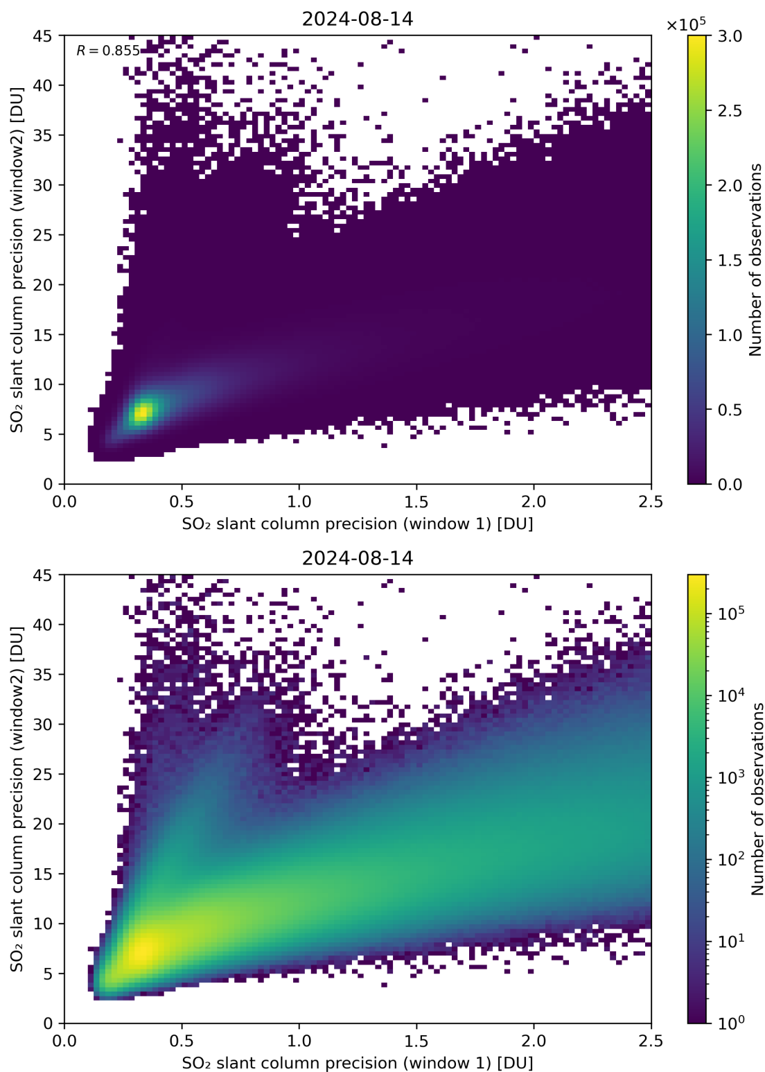
Figure 227: Scatter density plot of “SO 2 slant column precision (window 1)” against “SO 2 slant column precision (window2)” for 2024-08-13 to 2024-08-15.
