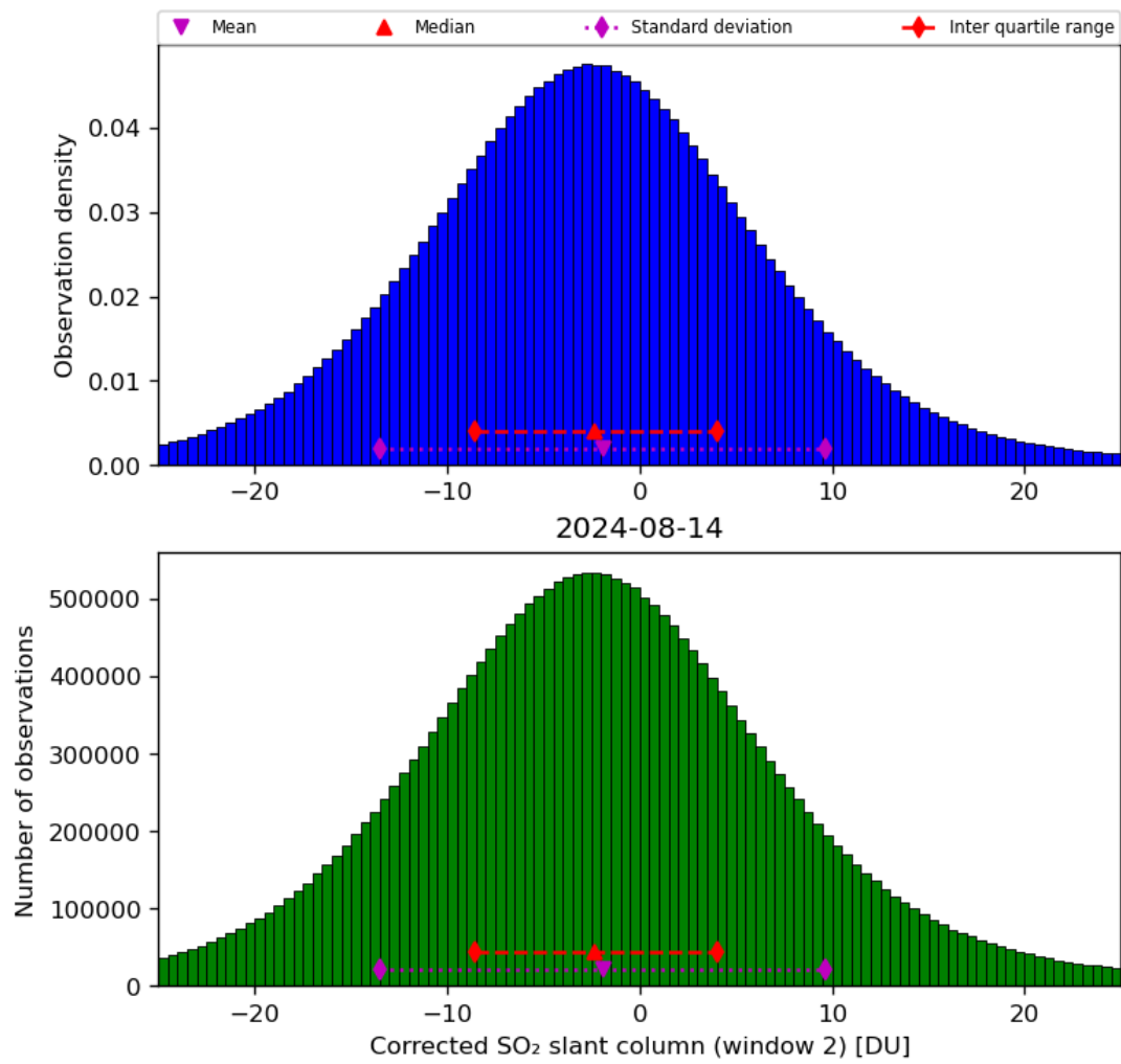
Figure 62: Histogram of “Corrected SO 2 slant column (window 2)” for 2024-08-13 to 2024-08-15
