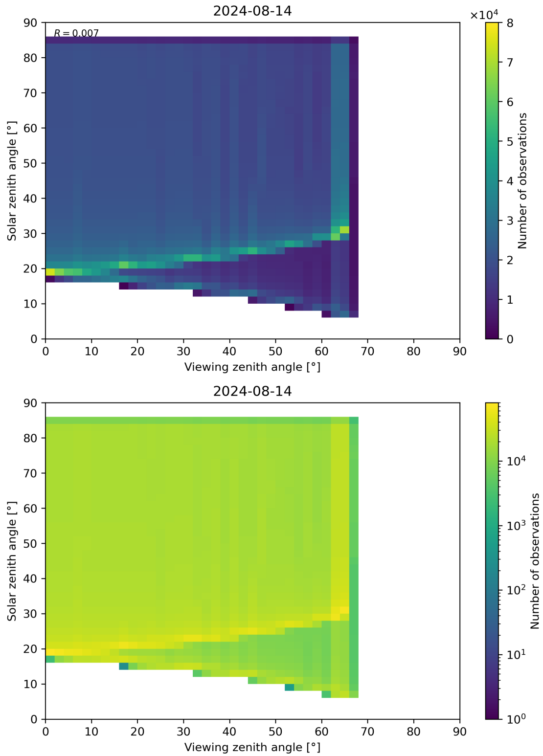
Figure 315: Scatter density plot of “Viewing zenith angle” against “Solar zenith angle” for 2024-08-13 to 2024-08-15.
