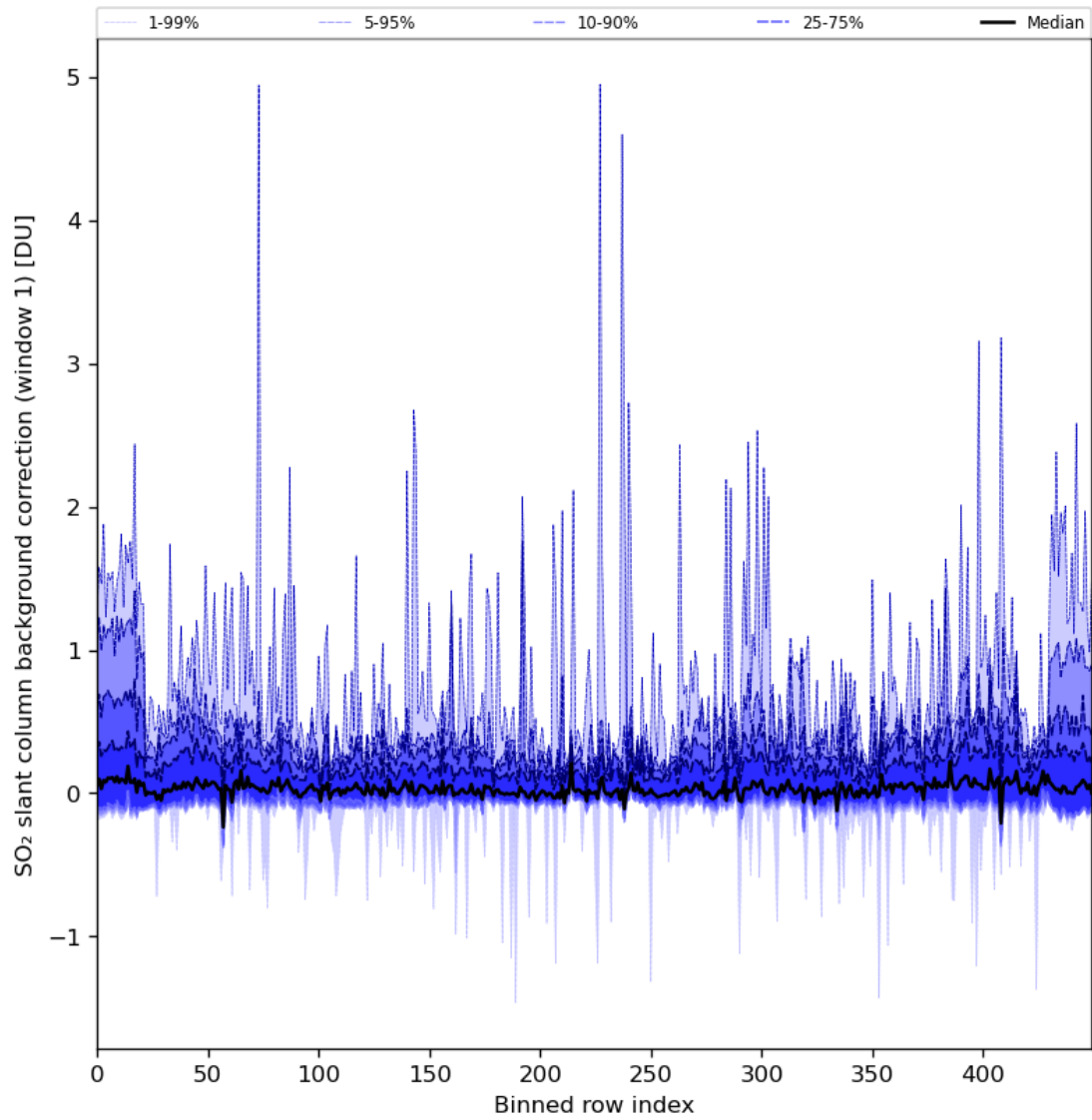
Figure 82: Along track statistics of “SO 2 slant column background correction (window 1)” for 2024-08-13 to 2024-08-15
