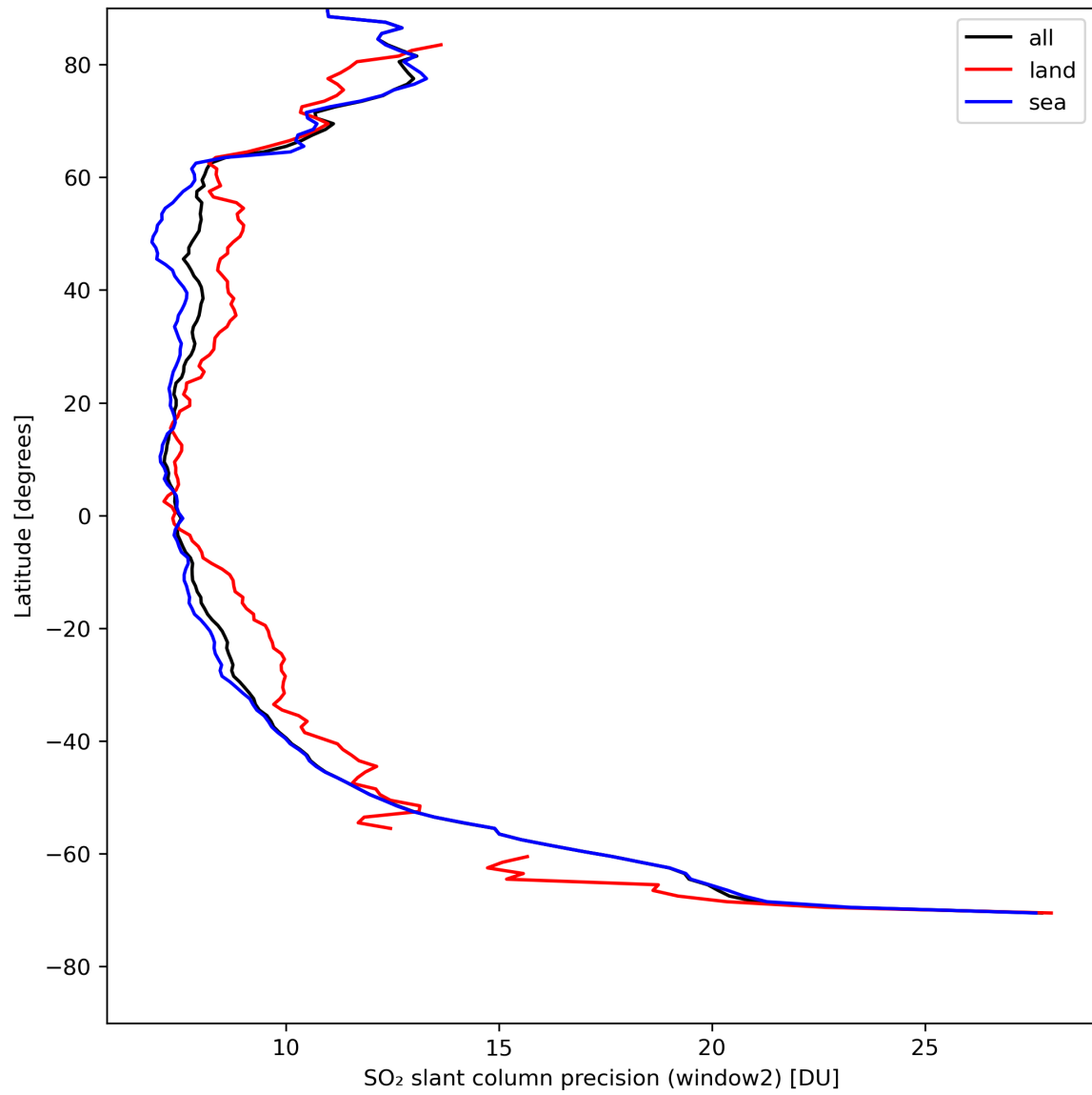
Figure 38: Zonal average of “SO 2 slant column precision (window2)” for 2024-08-13 to 2024-08-15.
