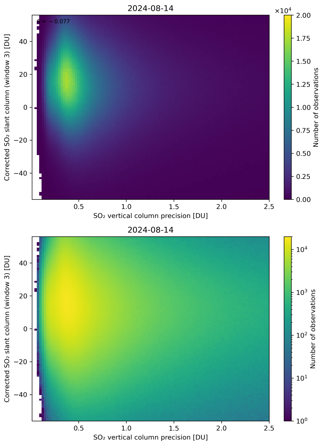
Figure 288: Scatter density plot of “SO 2 vertical column precision” against “Corrected SO 2 slant column (window 3)” for 2024-08-13 to 2024-08-15.
