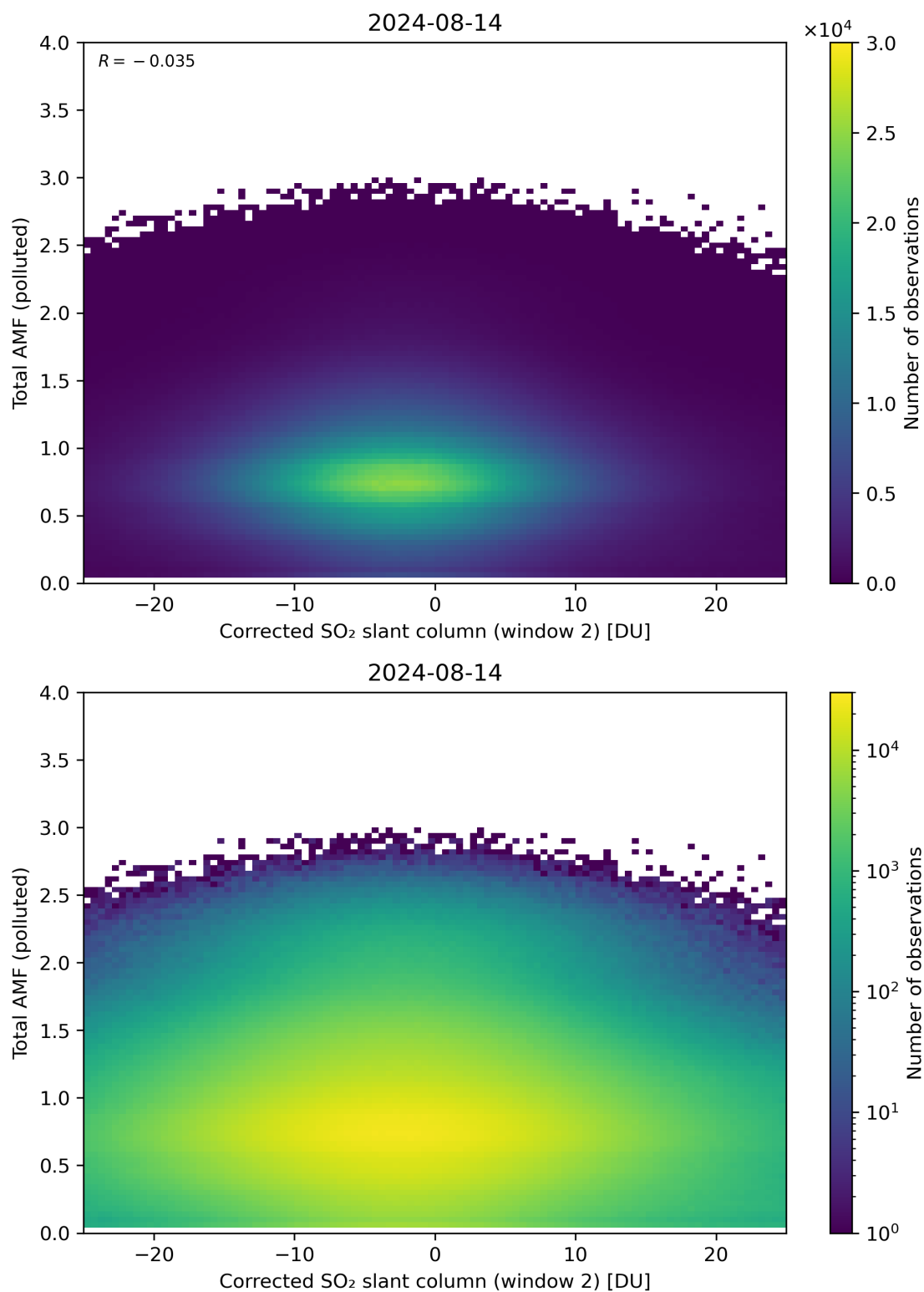
Figure 203: Scatter density plot of “Corrected SO 2 slant column (window 2)” against “Total AMF (polluted)” for 2024-08-13 to 2024-08-15.
