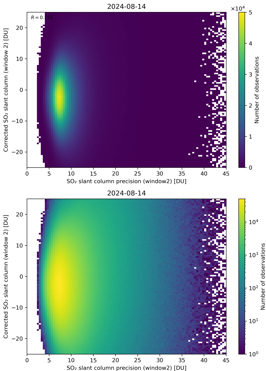
Figure 247: Scatter density plot of “SO 2 slant column precision (window2)” against “Corrected SO 2 slant column (window 2)” for 2024-08-13 to 2024-08-15.
