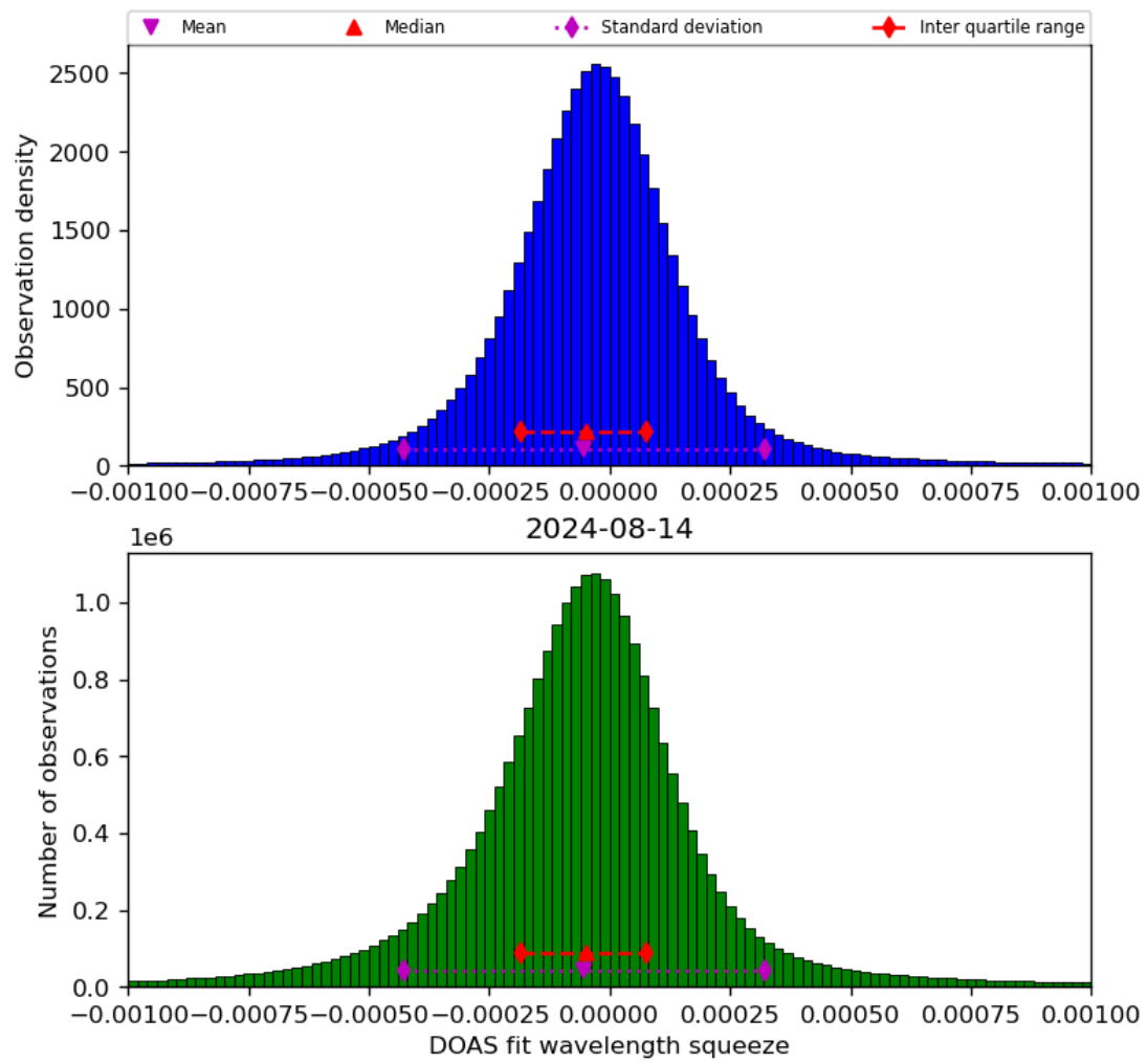
Figure 69: Histogram of “DOAS fit wavelength squeeze” for 2024-08-13 to 2024-08-15
