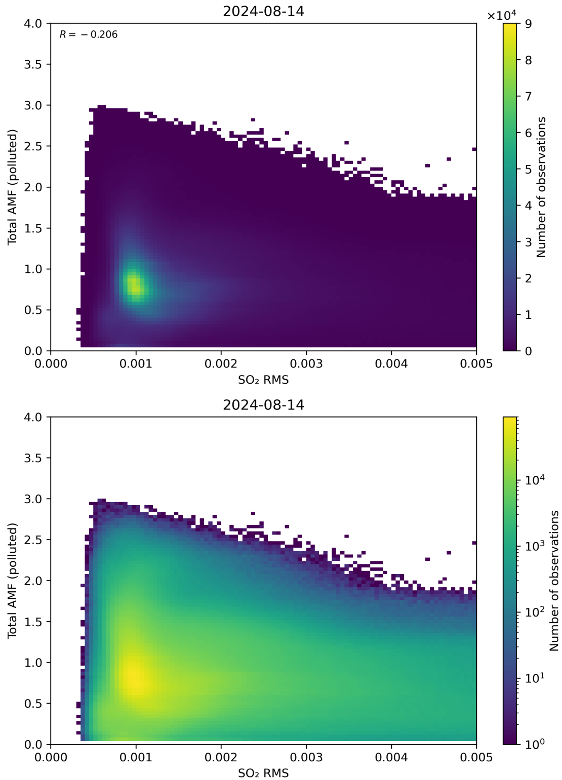
Figure 137: Scatter density plot of “SO 2 RMS” against “Total AMF (polluted)” for 2024-08-13 to 2024-08-15.
