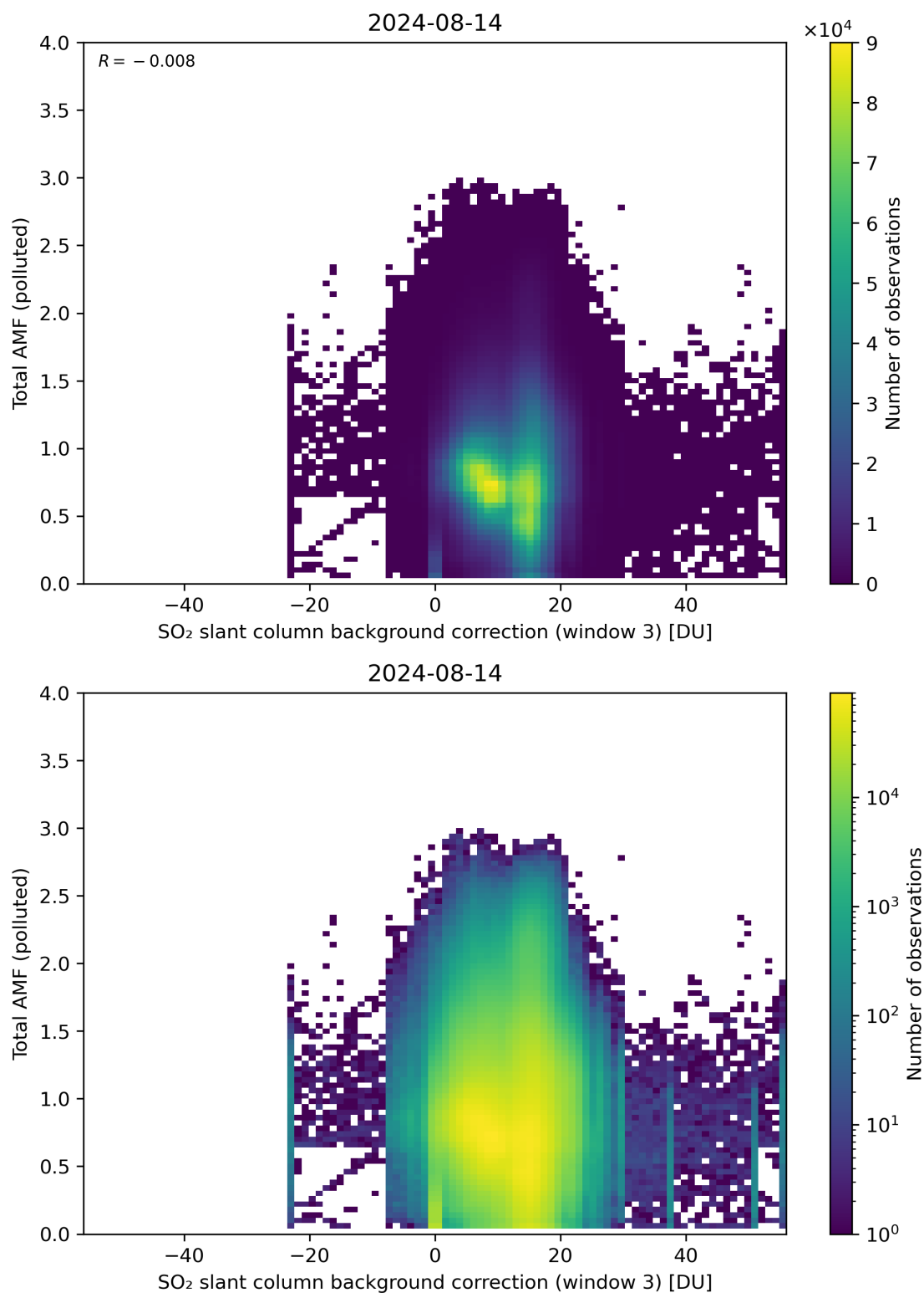
Figure 125: Scatter density plot of “SO 2 slant column background correction (window 3)” against “Total AMF (polluted)” for 2024-08-13 to 2024-08-15.
