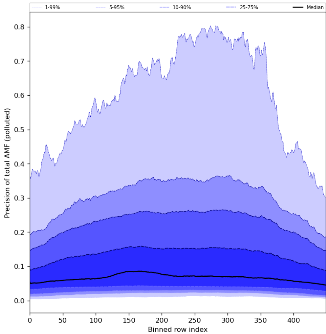
Figure 95: Along track statistics of “Precision of total AMF (polluted)” for 2024-08-13 to 2024-08-15
