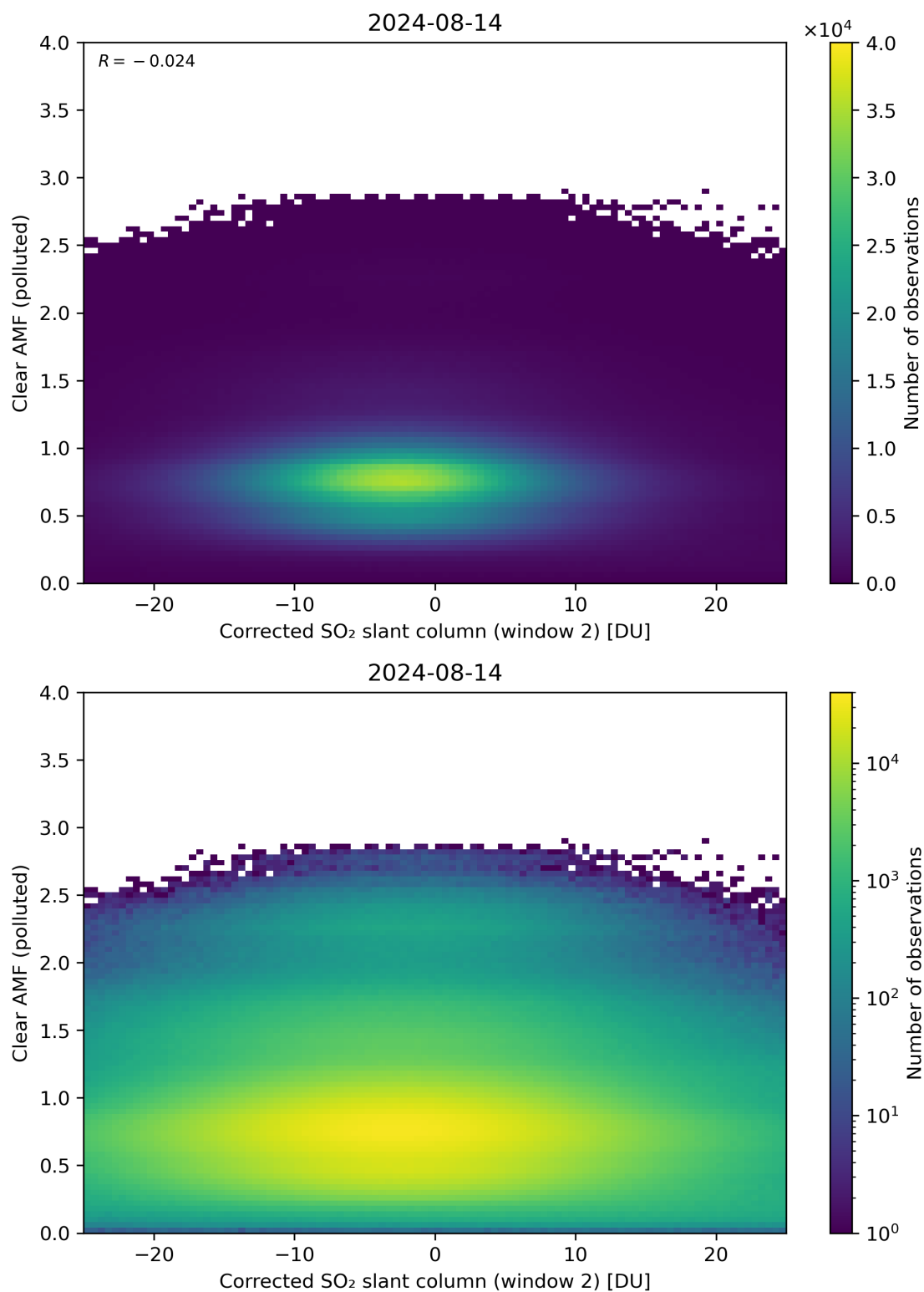
Figure 199: Scatter density plot of “Corrected SO 2 slant column (window 2)” against “Clear AMF (polluted)” for 2024-08-13 to 2024-08-15.
