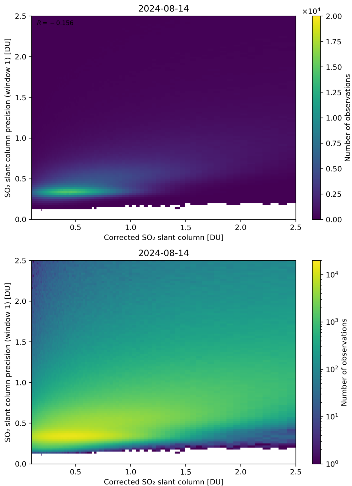
Figure 188: Scatter density plot of “Corrected SO 2 slant column” against “SO 2 slant column precision (window 1)” for 2024-08-13 to 2024-08-15.
