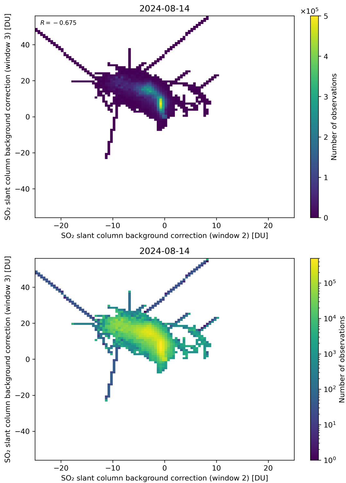
Figure 111: Scatter density plot of “SO 2 slant column background correction (window 2)” against “SO 2 slant column background correction (window 3)” for 2024-08-13 to 2024-08-15.
