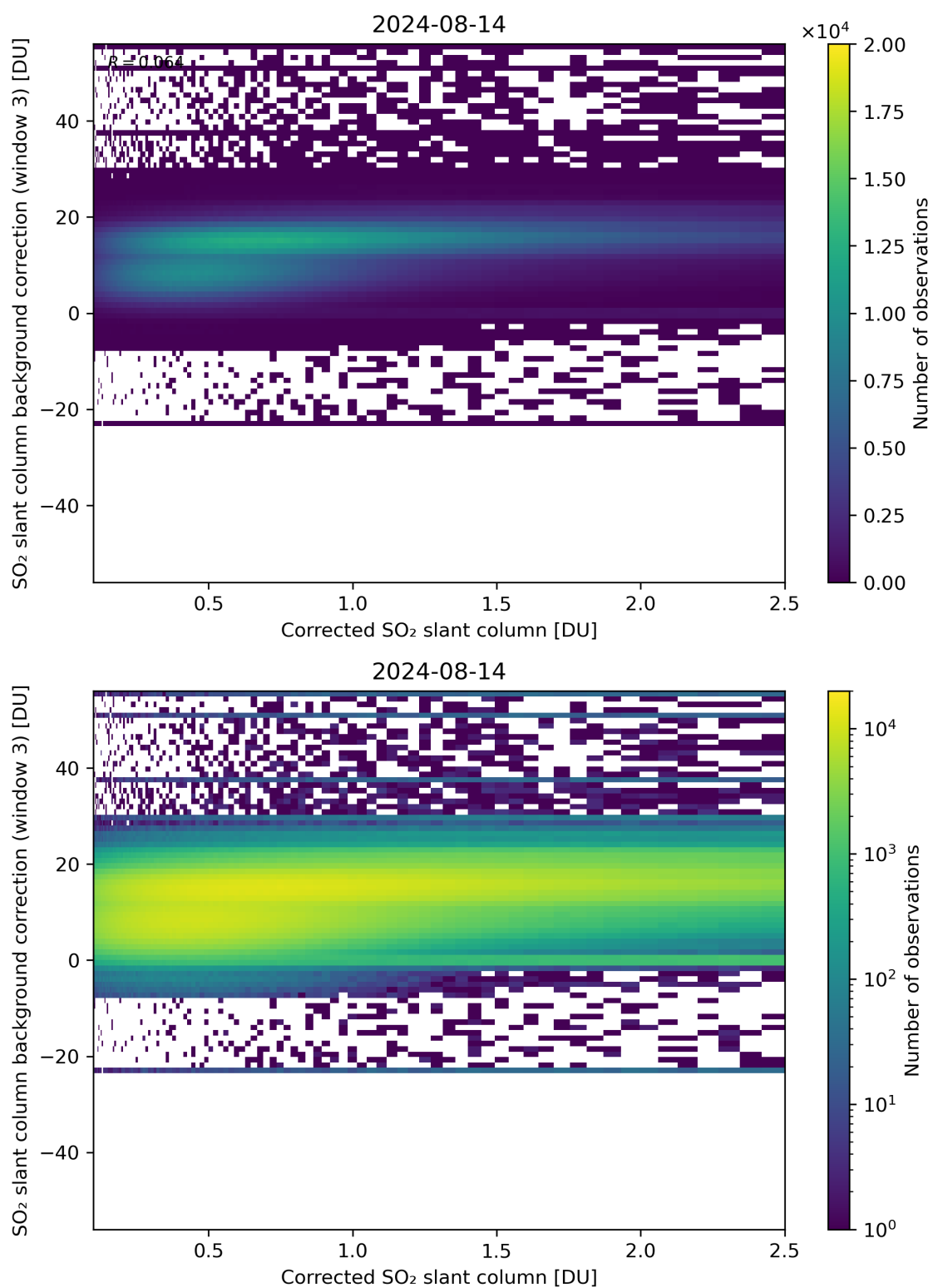
Figure 180: Scatter density plot of “Corrected SO 2 slant column” against “SO 2 slant column background correction (window 3)” for 2024-08-13 to 2024-08-15.
