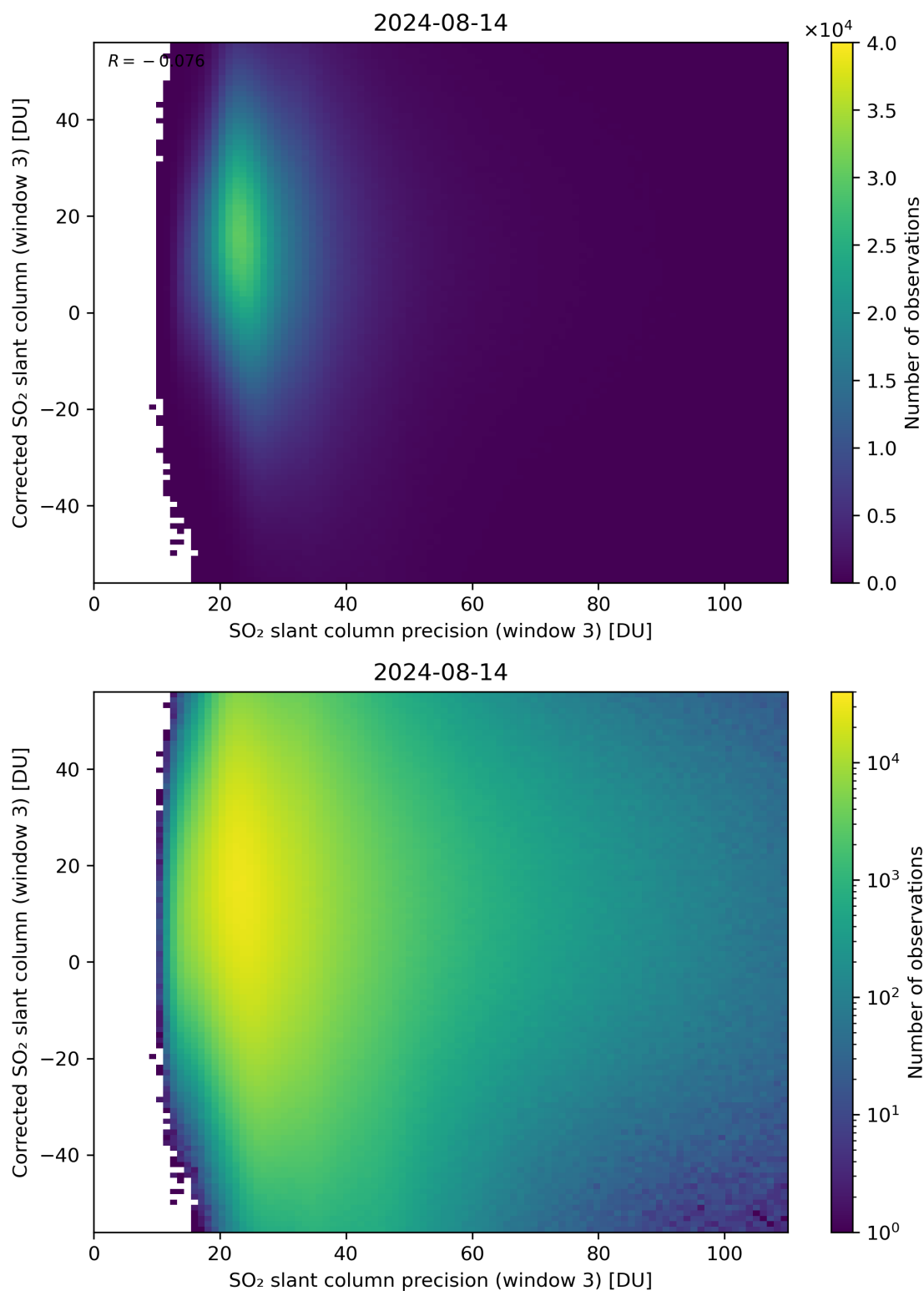
Figure 262: Scatter density plot of “SO 2 slant column precision (window 3)” against “Corrected SO 2 slant column (window 3)” for 2024-08-13 to 2024-08-15.
