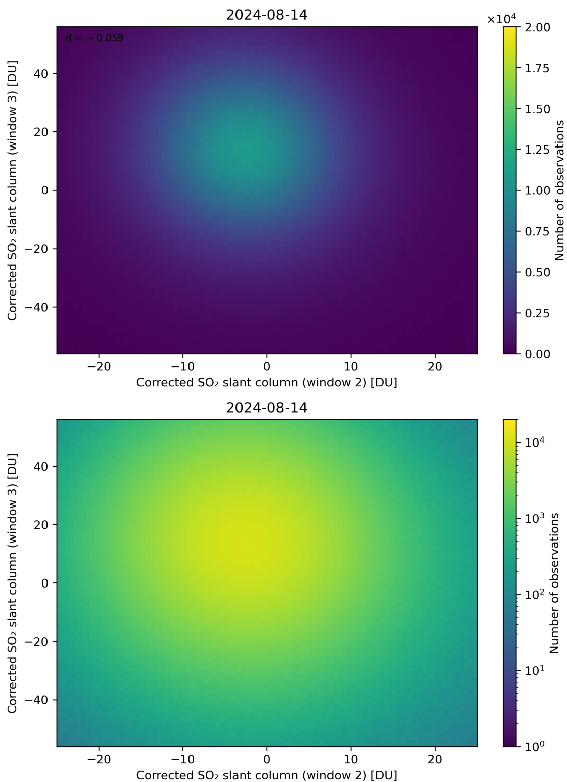
Figure 200: Scatter density plot of “Corrected SO 2 slant column (window 2)” against “Corrected SO 2 slant column (window 3)” for 2024-08-13 to 2024-08-15.
