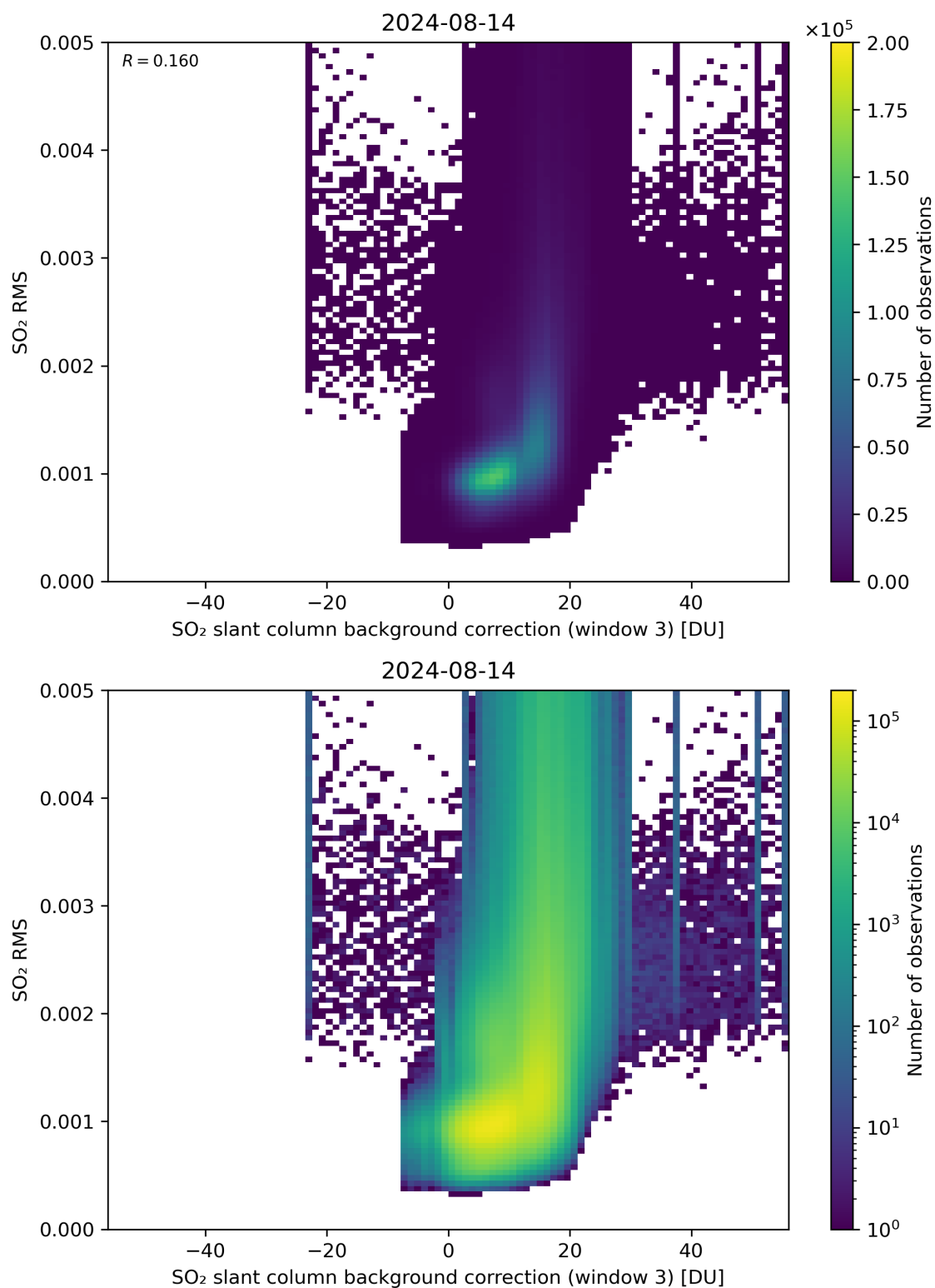
Figure 123: Scatter density plot of “SO 2 slant column background correction (window 3)” against “SO 2 RMS” for 2024-08-13 to 2024-08-15.
