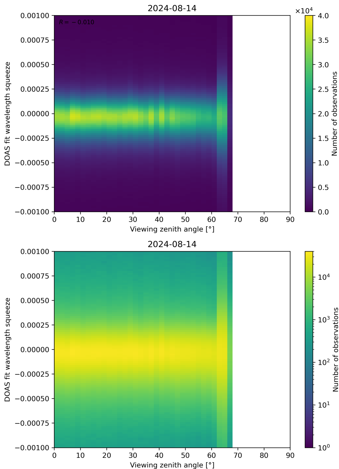
Figure 312: Scatter density plot of “Viewing zenith angle” against “DOAS fit wavelength squeeze” for 2024-08-13 to 2024-08-15.
