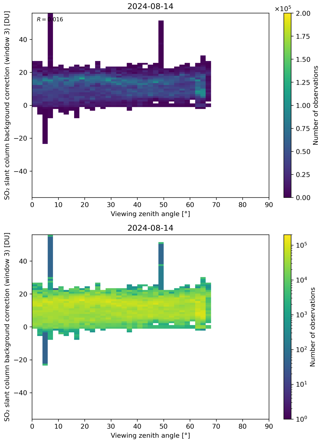
Figure 310: Scatter density plot of “Viewing zenith angle” against “SO 2 slant column background correction (window 3)” for 2024-08-13 to 2024-08-15.
