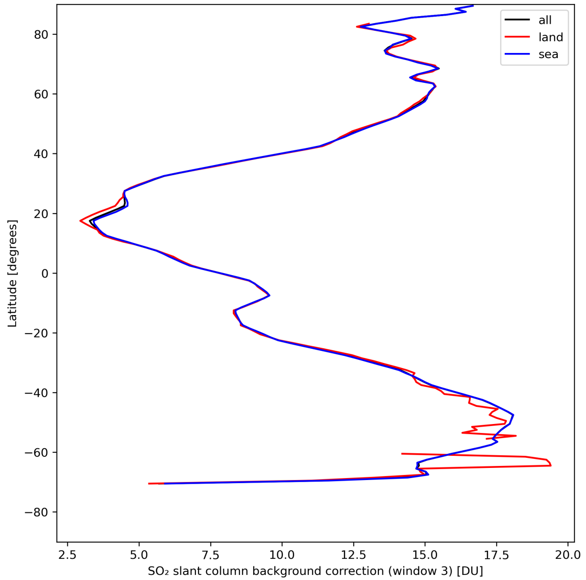
Figure 44: Zonal average of “SO 2 slant column background correction (window 3)” for 2024-08-13 to 2024-08-15.
