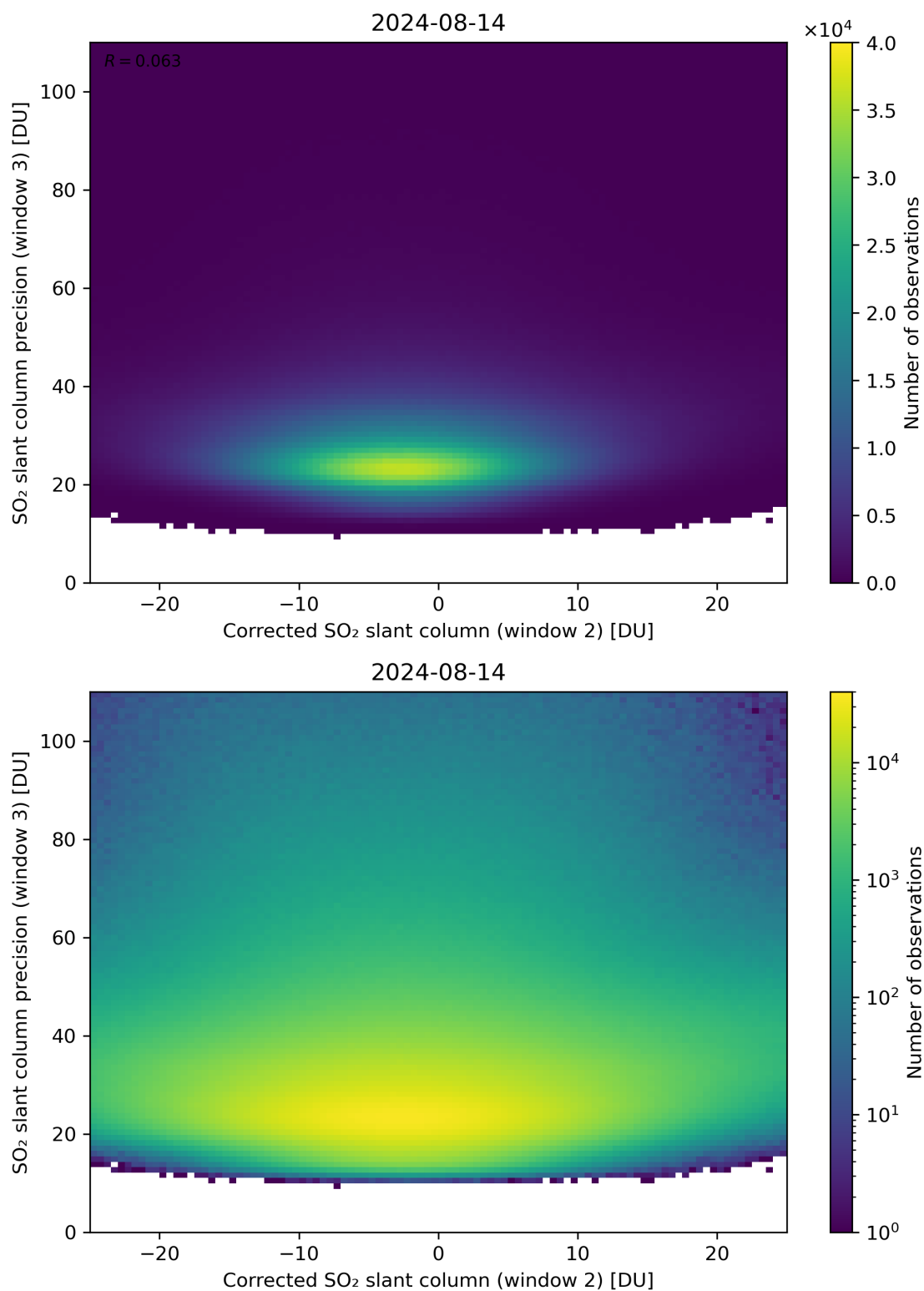
Figure 202: Scatter density plot of “Corrected SO 2 slant column (window 2)” against “SO 2 slant column precision (window 3)” for 2024-08-13 to 2024-08-15.
