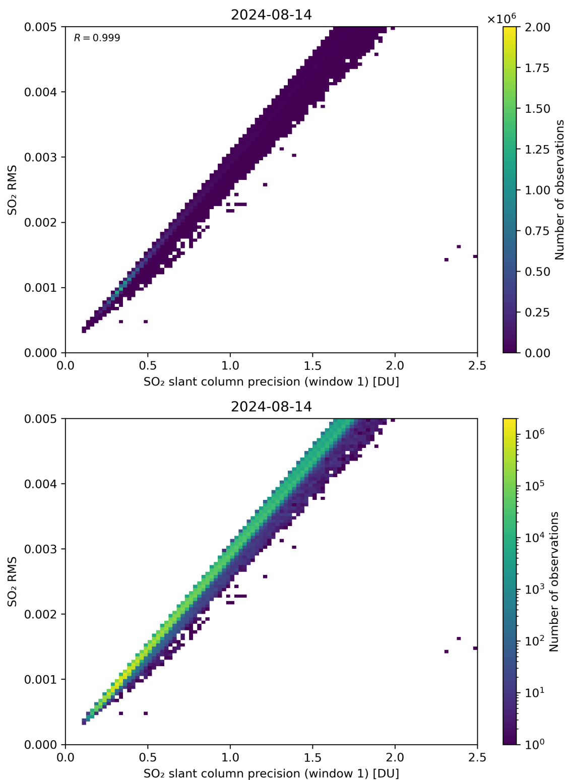
Figure 223: Scatter density plot of “SO 2 slant column precision (window 1)” against “SO 2 RMS” for 2024-08-13 to 2024-08-15.
