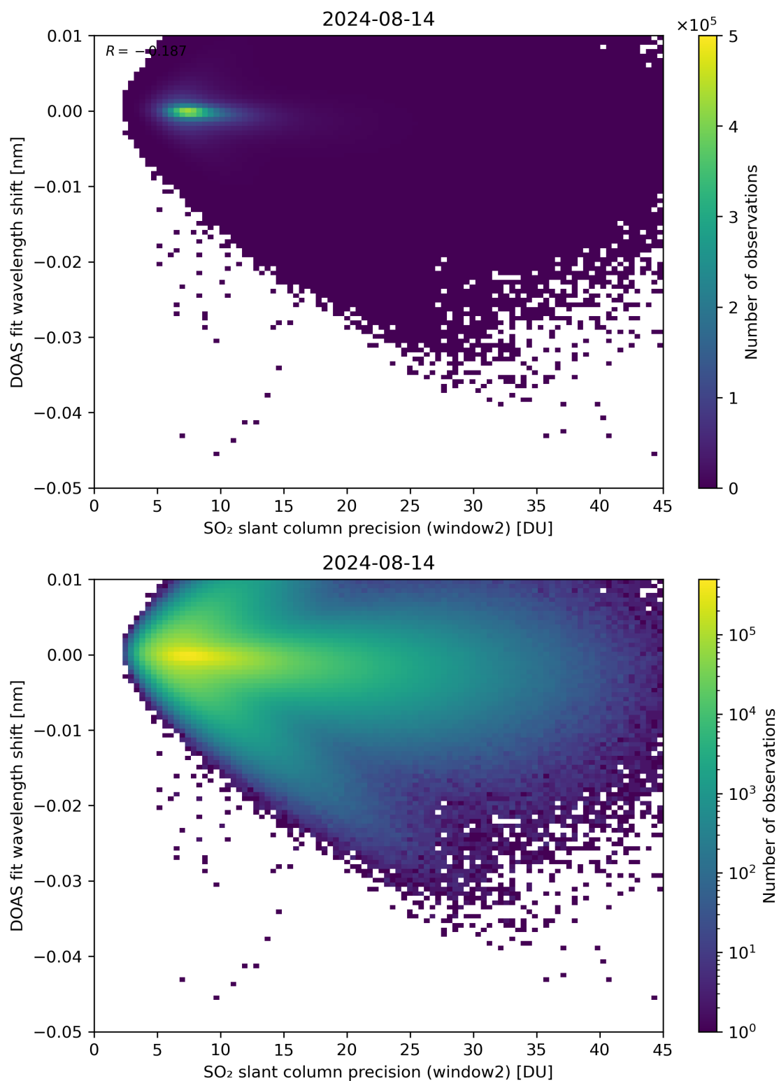
Figure 243: Scatter density plot of “SO 2 slant column precision (window2)” against “DOAS fit wavelength shift” for 2024-08-13 to 2024-08-15.
