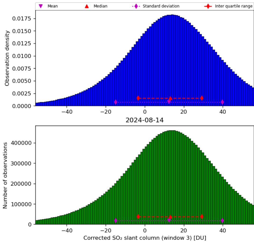
Figure 66: Histogram of “Corrected SO 2 slant column (window 3)” for 2024-08-13 to 2024-08-15
