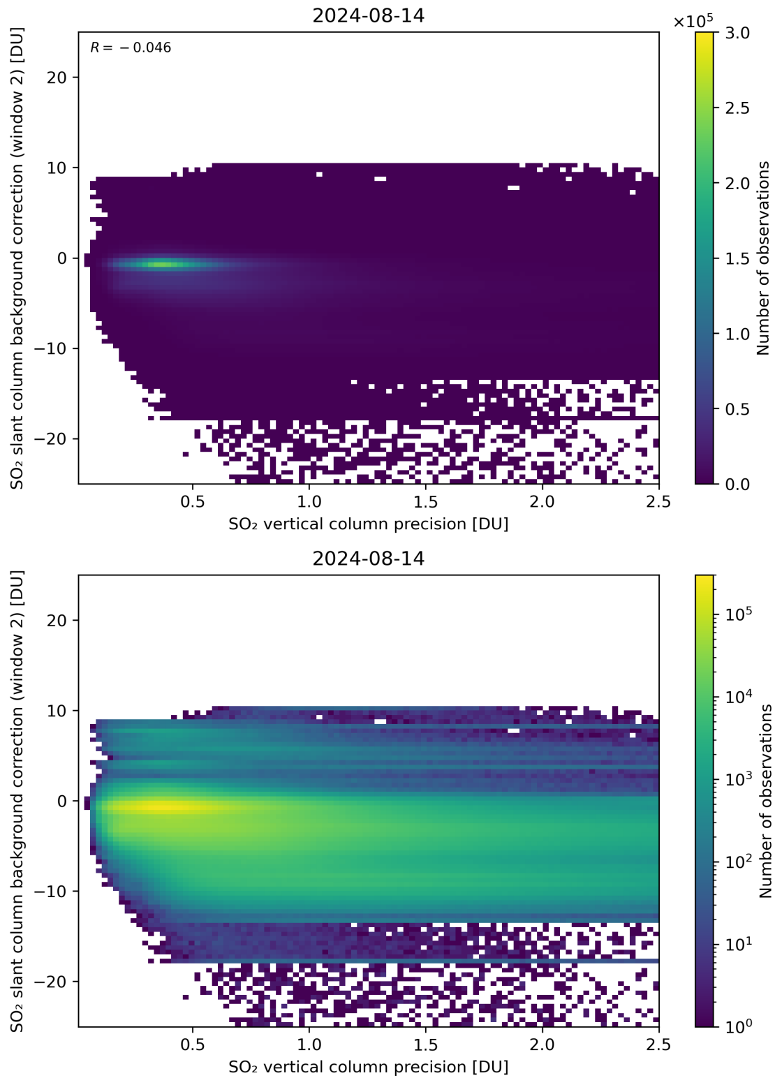
Figure 280: Scatter density plot of “SO 2 vertical column precision” against “SO 2 slant column background correction (window 2)” for 2024-08-13 to 2024-08-15.
