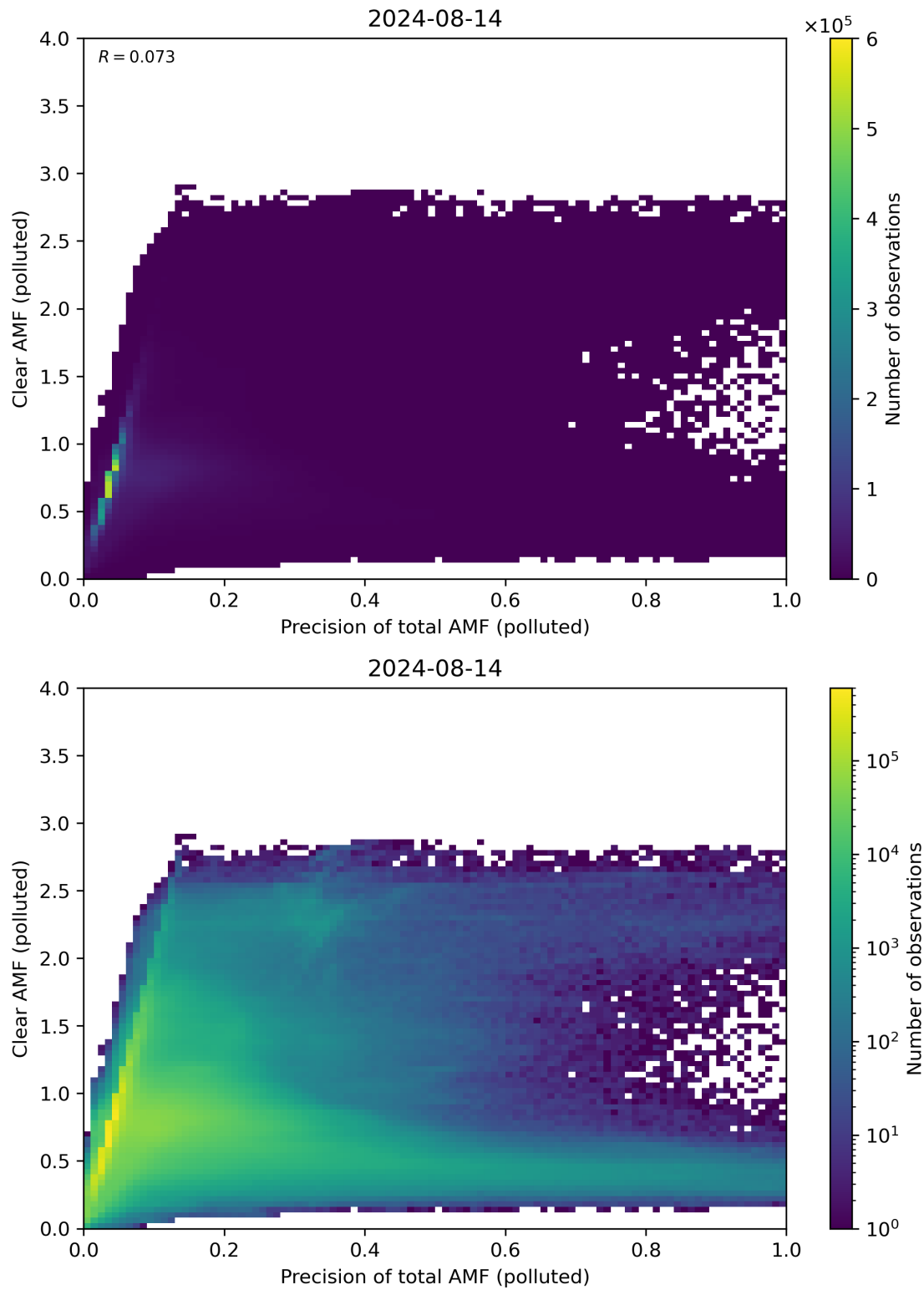
Figure 270: Scatter density plot of “Precision of total AMF (polluted)” against “Clear AMF (polluted)” for 2024-08-13 to 2024-08-15.
