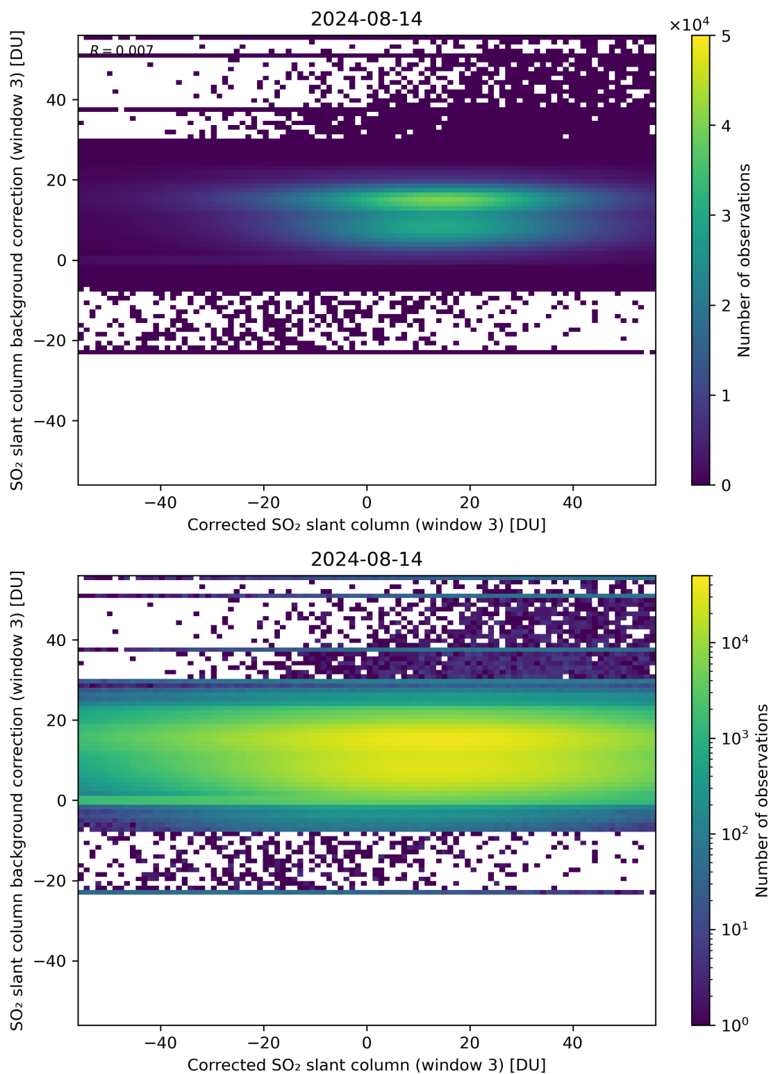
Figure 205: Scatter density plot of “Corrected SO 2 slant column (window 3)” against “SO 2 slant column background correction (window 3)” for 2024-08-13 to 2024-08-15.
