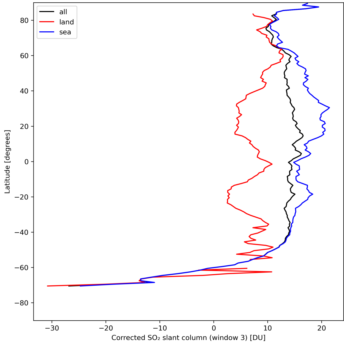
Figure 43: Zonal average of “Corrected SO 2 slant column (window 3)” for 2024-08-13 to 2024-08-15.
