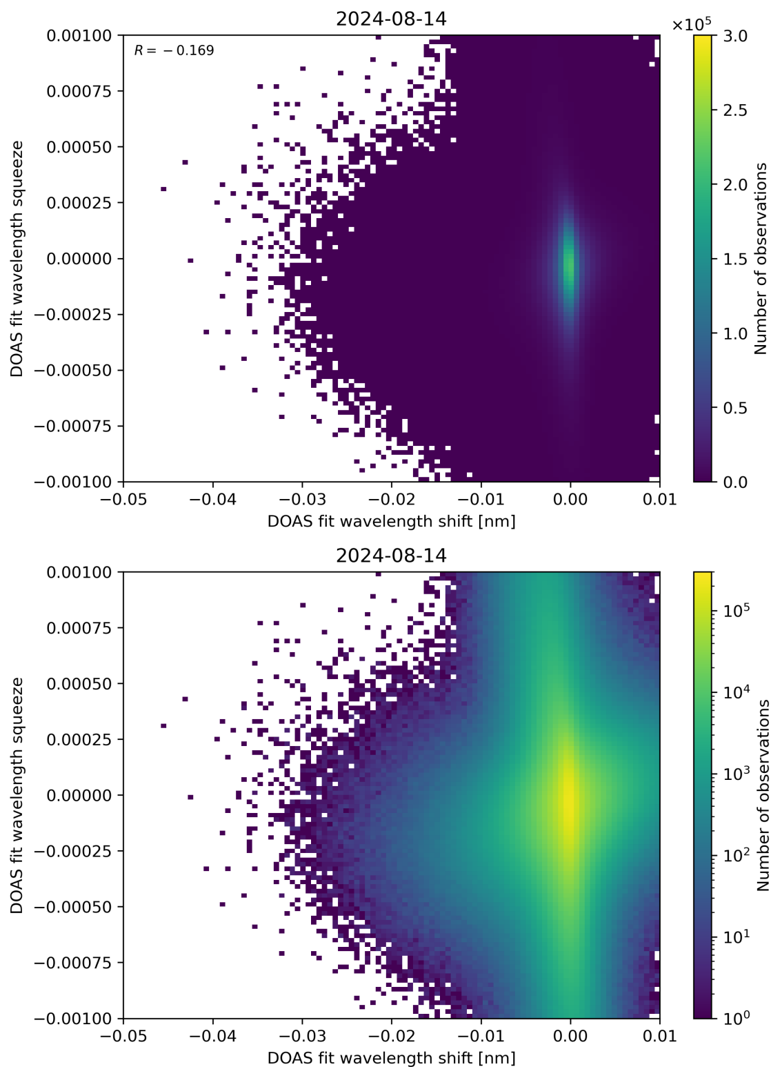
Figure 127: Scatter density plot of “DOAS fit wavelength shift” against “DOAS fit wavelength squeeze” for 2024-08-13 to 2024-08-15.
