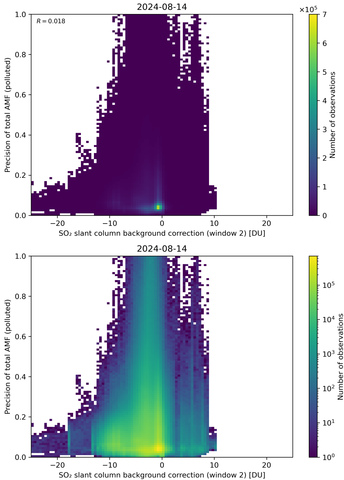
Figure 120: Scatter density plot of “SO 2 slant column background correction (window 2)” against “Precision of total AMF (polluted)” for 2024-08-13 to 2024-08-15.
