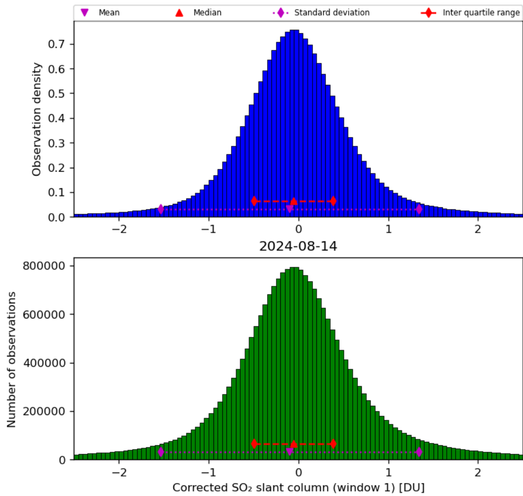
Figure 58: Histogram of “Corrected SO 2 slant column (window 1)” for 2024-08-13 to 2024-08-15
