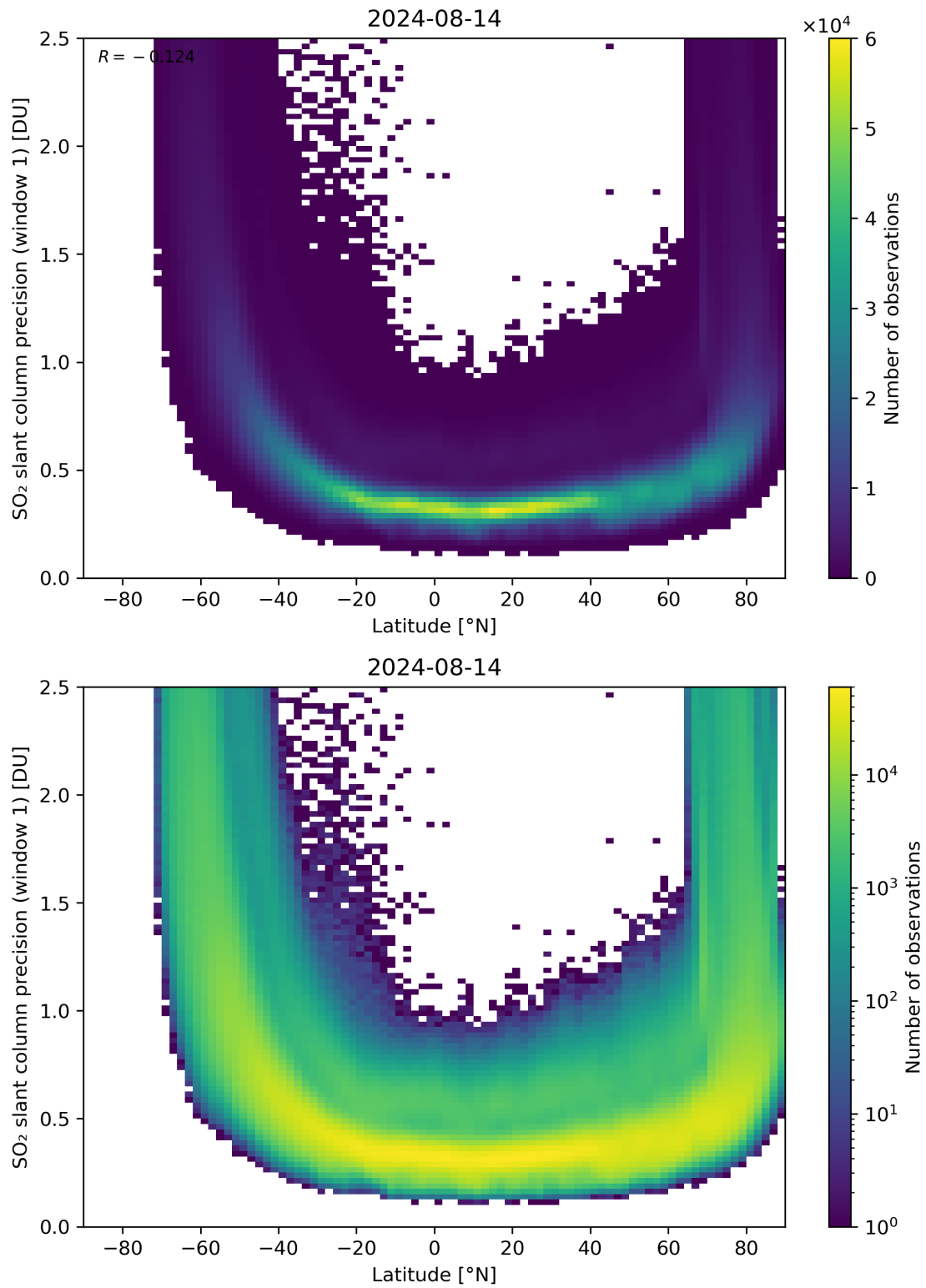
Figure 150: Scatter density plot of “Latitude” against “SO 2 slant column precision (window 1)” for 2024-08-13 to 2024-08-15.
