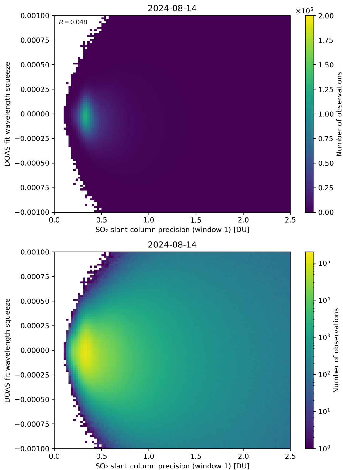
Figure 222: Scatter density plot of “SO 2 slant column precision (window 1)” against “DOAS fit wavelength squeeze” for 2024-08-13 to 2024-08-15.
