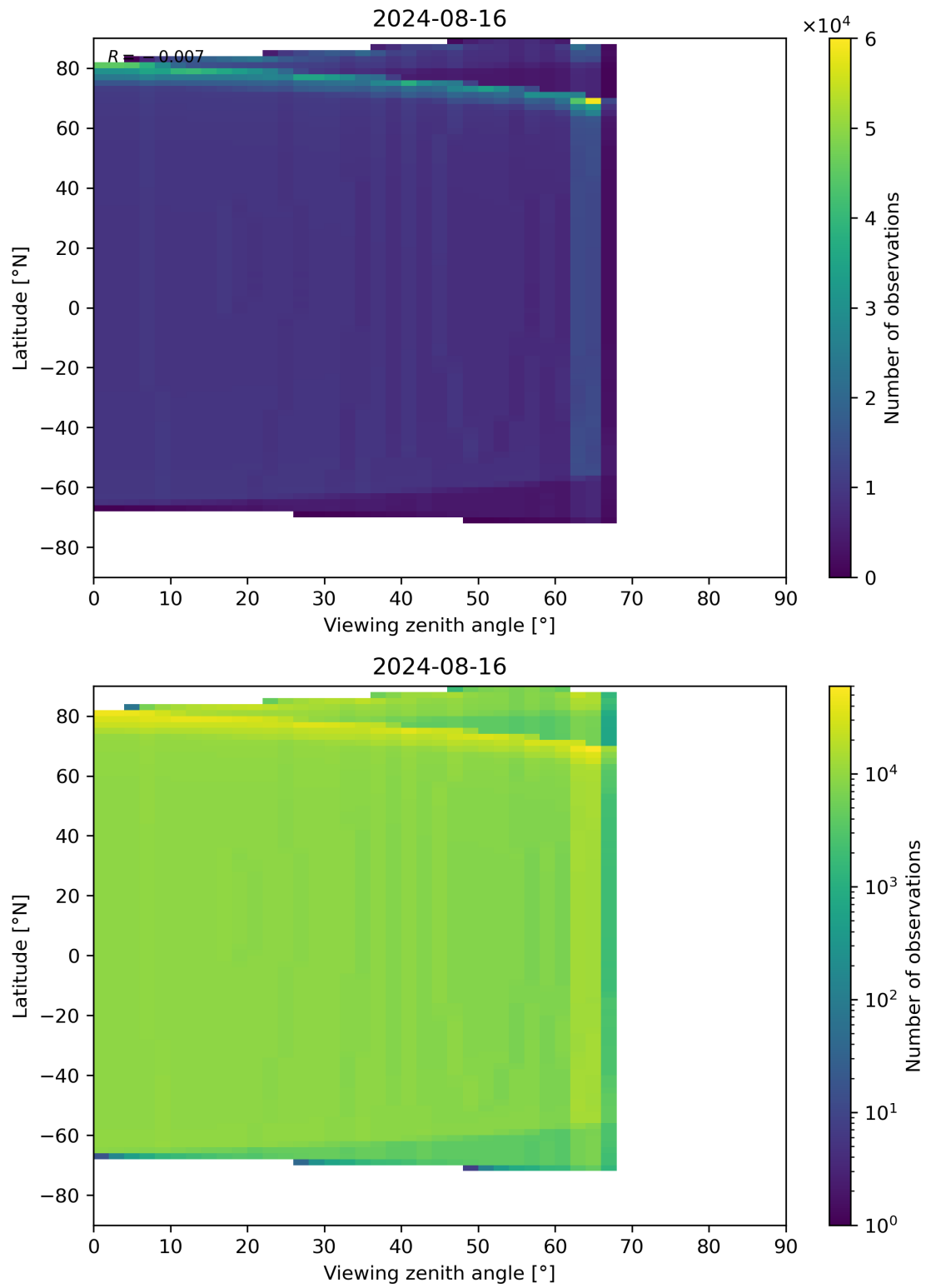
Figure 314: Scatter density plot of “Viewing zenith angle” against “Latitude” for 2024-08-16 to 2024-08-17.
