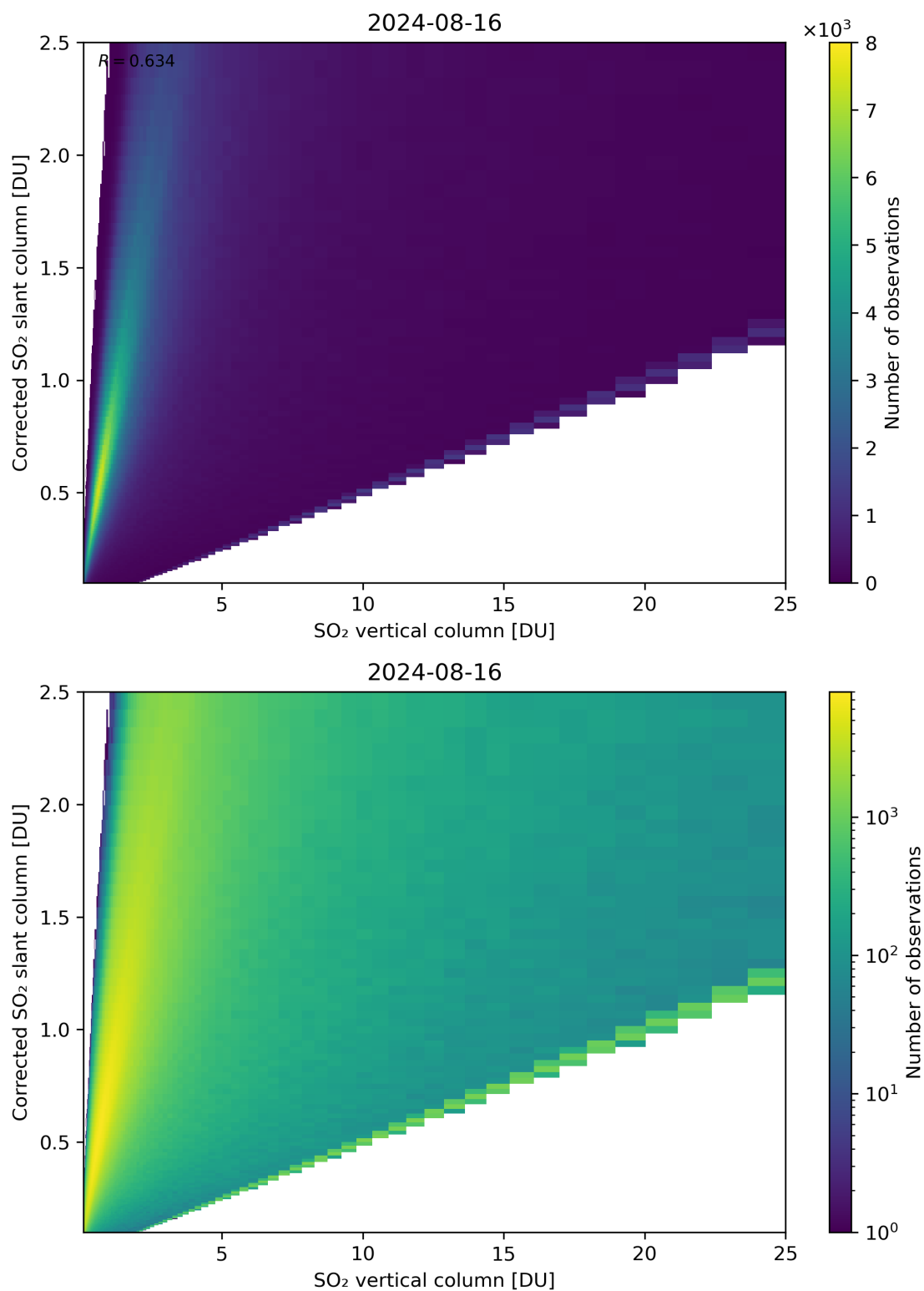
Figure 297: Scatter density plot of “SO 2 vertical column” against “Corrected SO 2 slant column” for 2024-08-16 to 2024-08-17.
