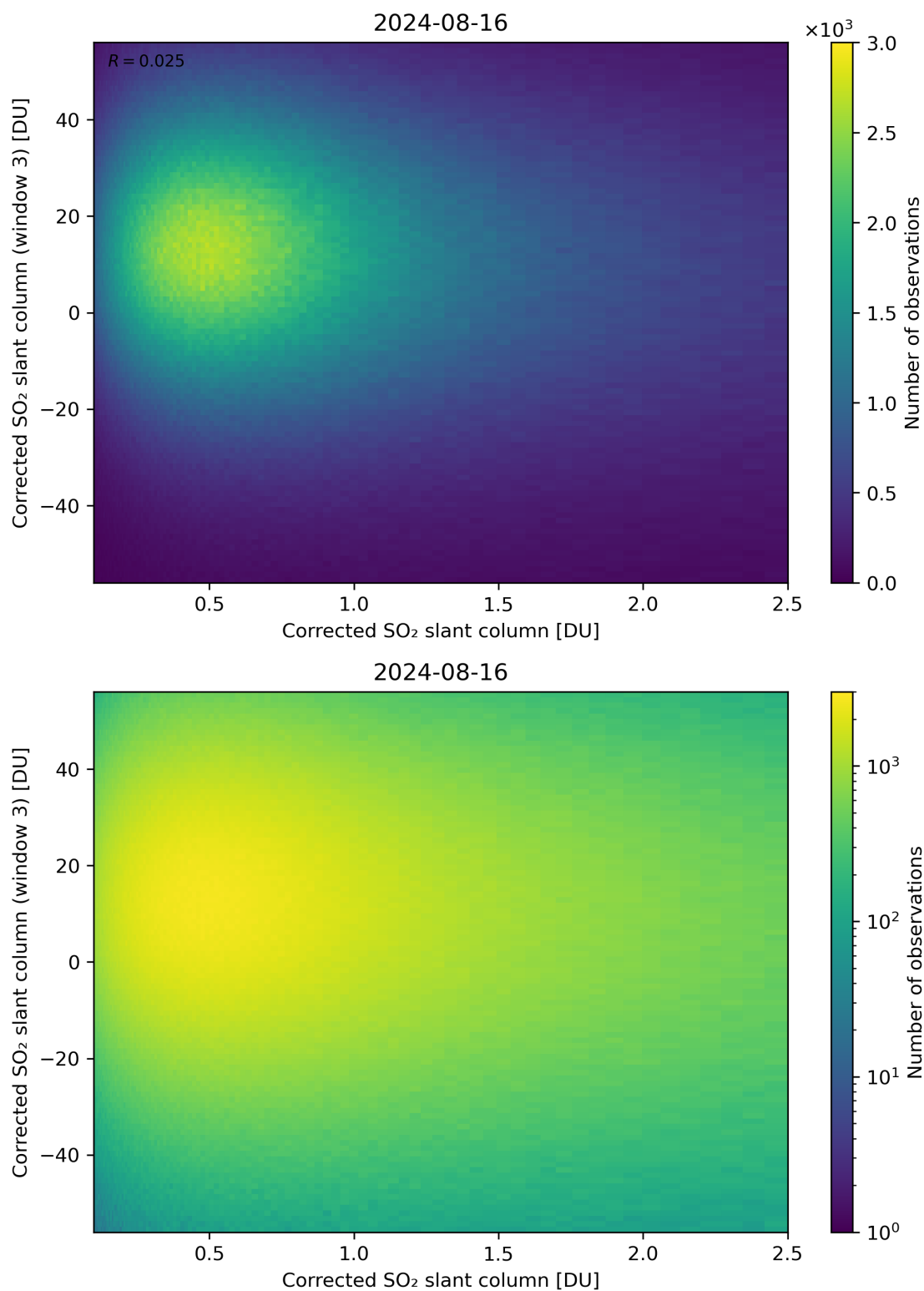
Figure 186: Scatter density plot of “Corrected SO 2 slant column” against “Corrected SO 2 slant column (window 3)” for 2024-08-16 to 2024-08-17.
