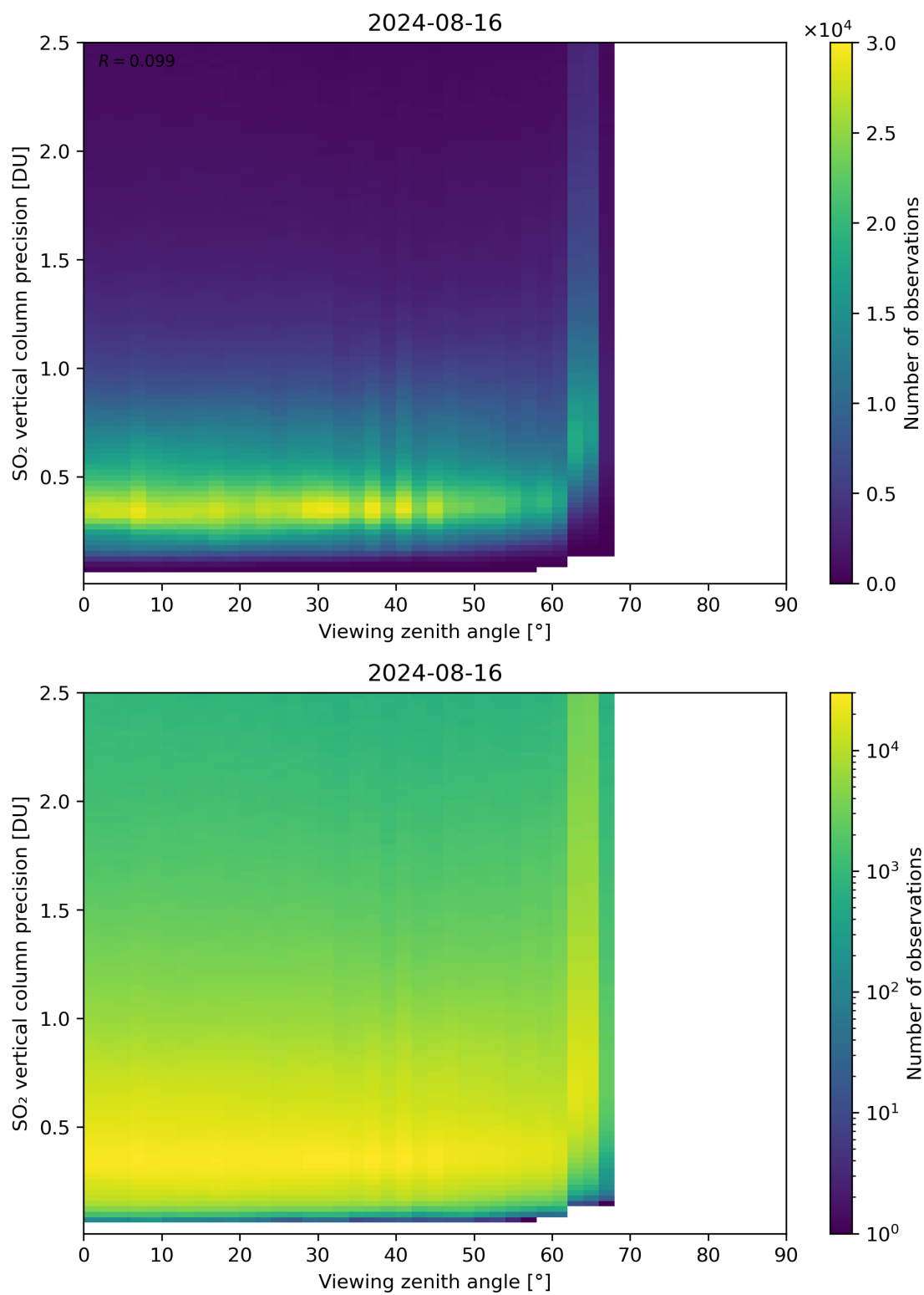
Figure 328: Scatter density plot of “Viewing zenith angle” against “SO 2 vertical column precision” for 2024-08-16 to 2024-08-17.
