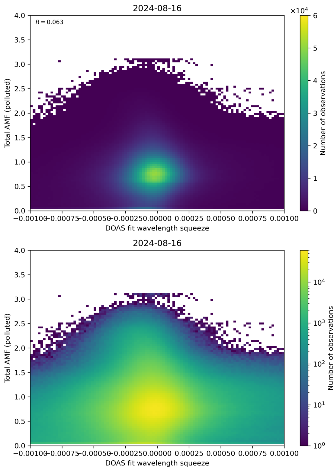
Figure 134: Scatter density plot of “DOAS fit wavelength squeeze” against “Total AMF (polluted)” for 2024-08-16 to 2024-08-17.
