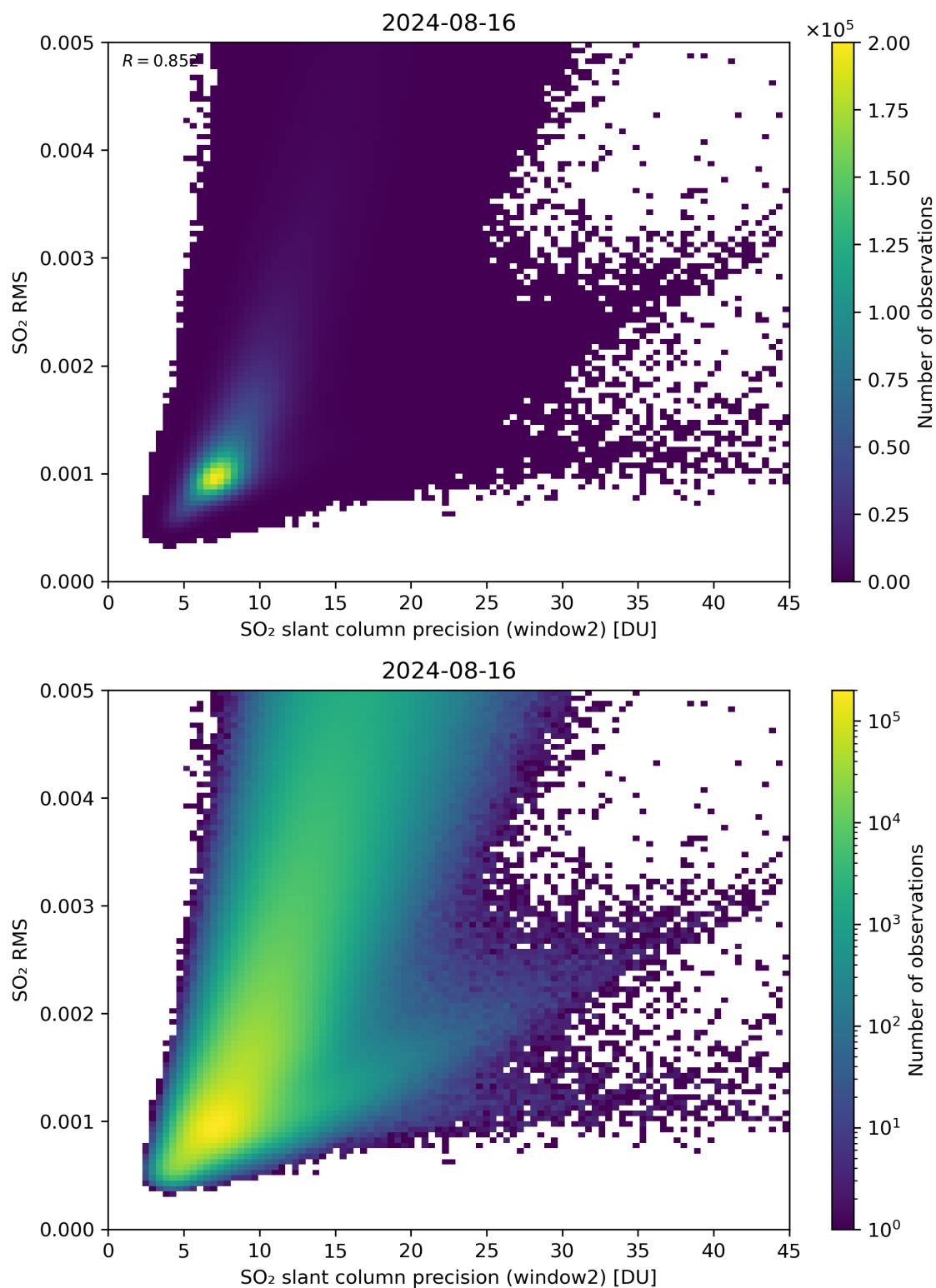
Figure 245: Scatter density plot of “SO 2 slant column precision (window2)” against “SO 2 RMS” for 2024-08-16 to 2024-08-17.
