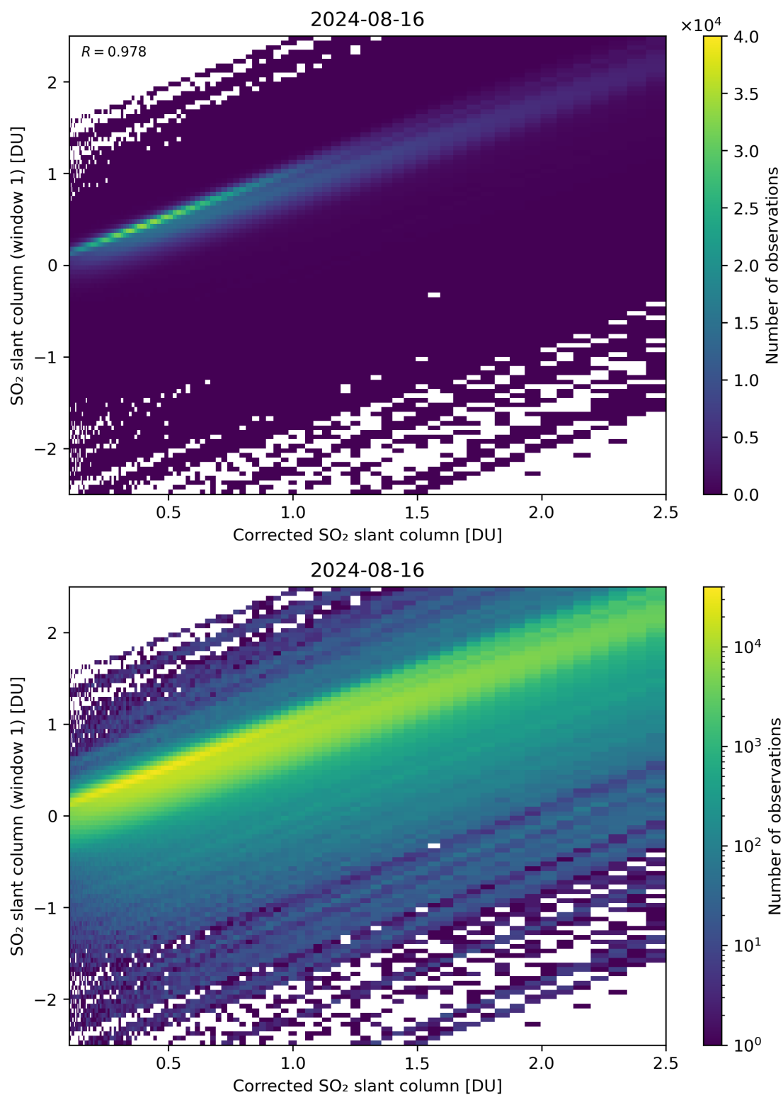
Figure 187: Scatter density plot of “Corrected SO 2 slant column” against “SO 2 slant column (window 1)” for 2024-08-16 to 2024-08-17.
