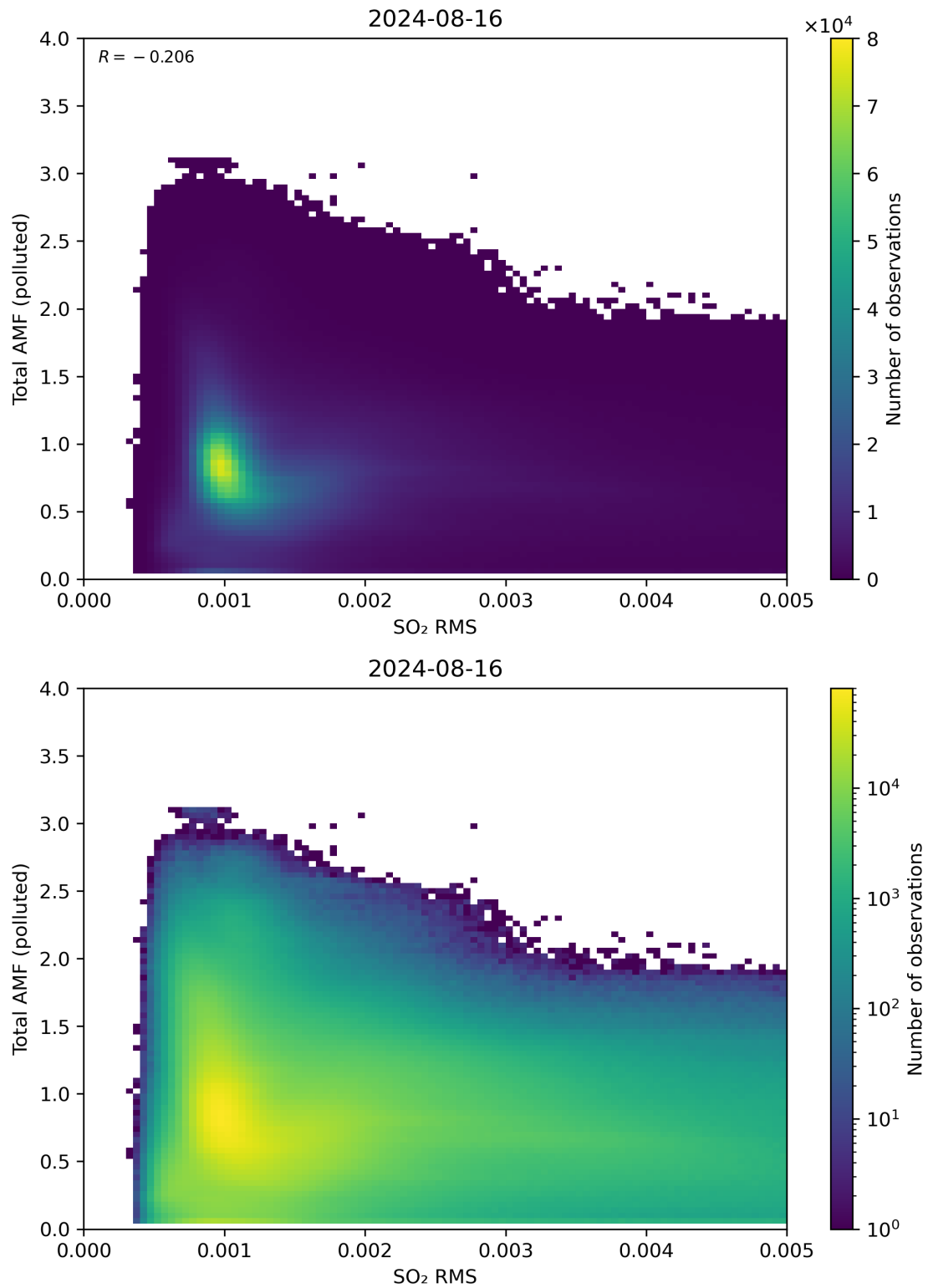
Figure 137: Scatter density plot of “SO 2 RMS” against “Total AMF (polluted)” for 2024-08-16 to 2024-08-17.
