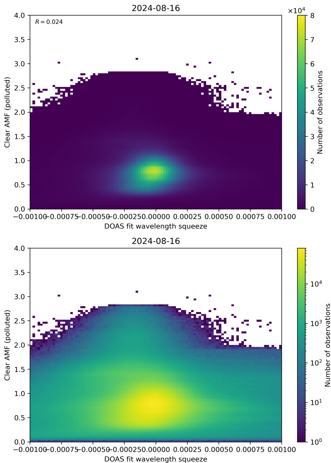
Figure 133: Scatter density plot of “DOAS fit wavelength squeeze” against “Clear AMF (polluted)” for 2024-08-16 to 2024-08-17.
