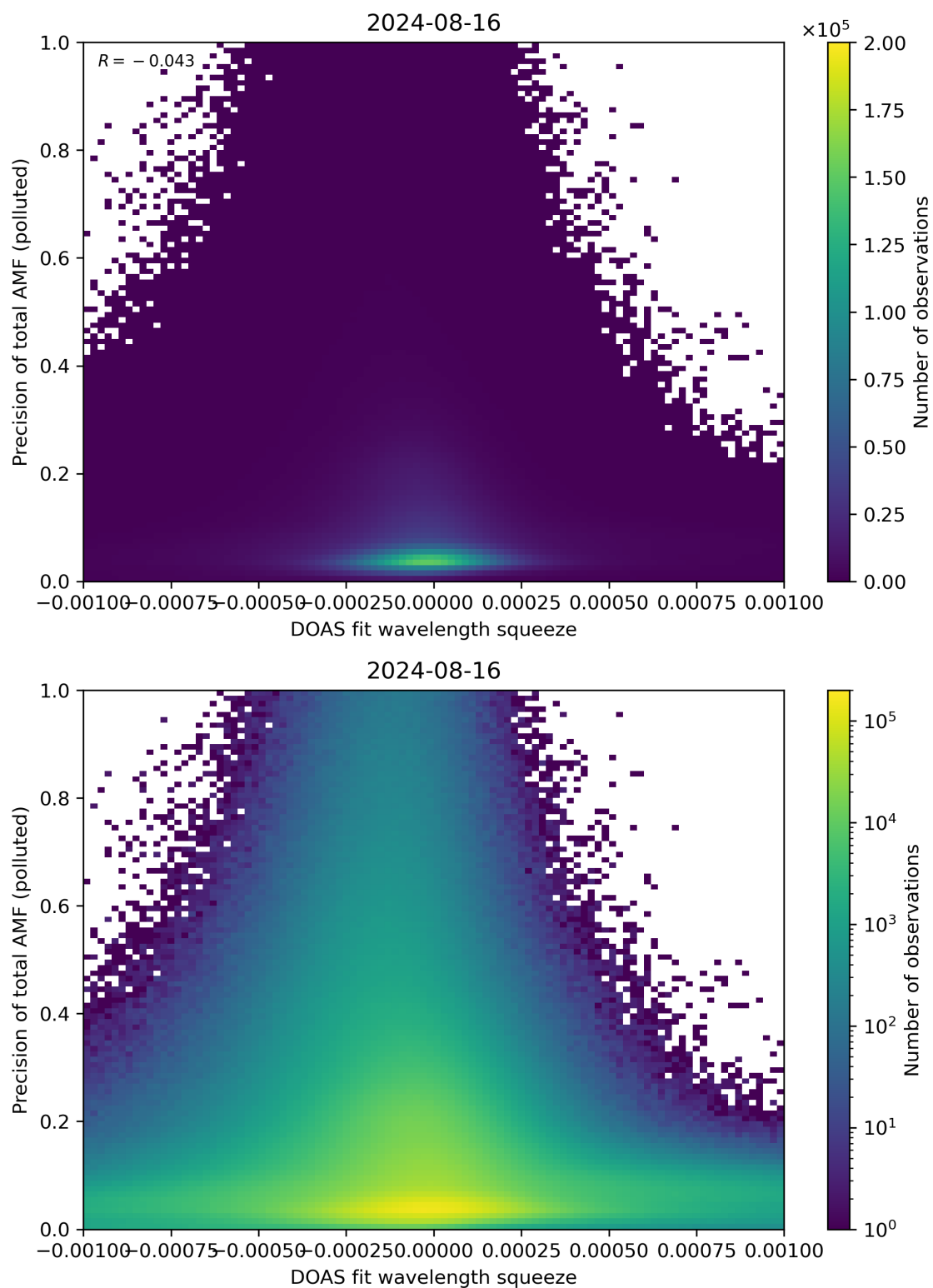
Figure 135: Scatter density plot of “DOAS fit wavelength squeeze” against “Precision of total AMF (polluted)” for 2024-08-16 to 2024-08-17.
