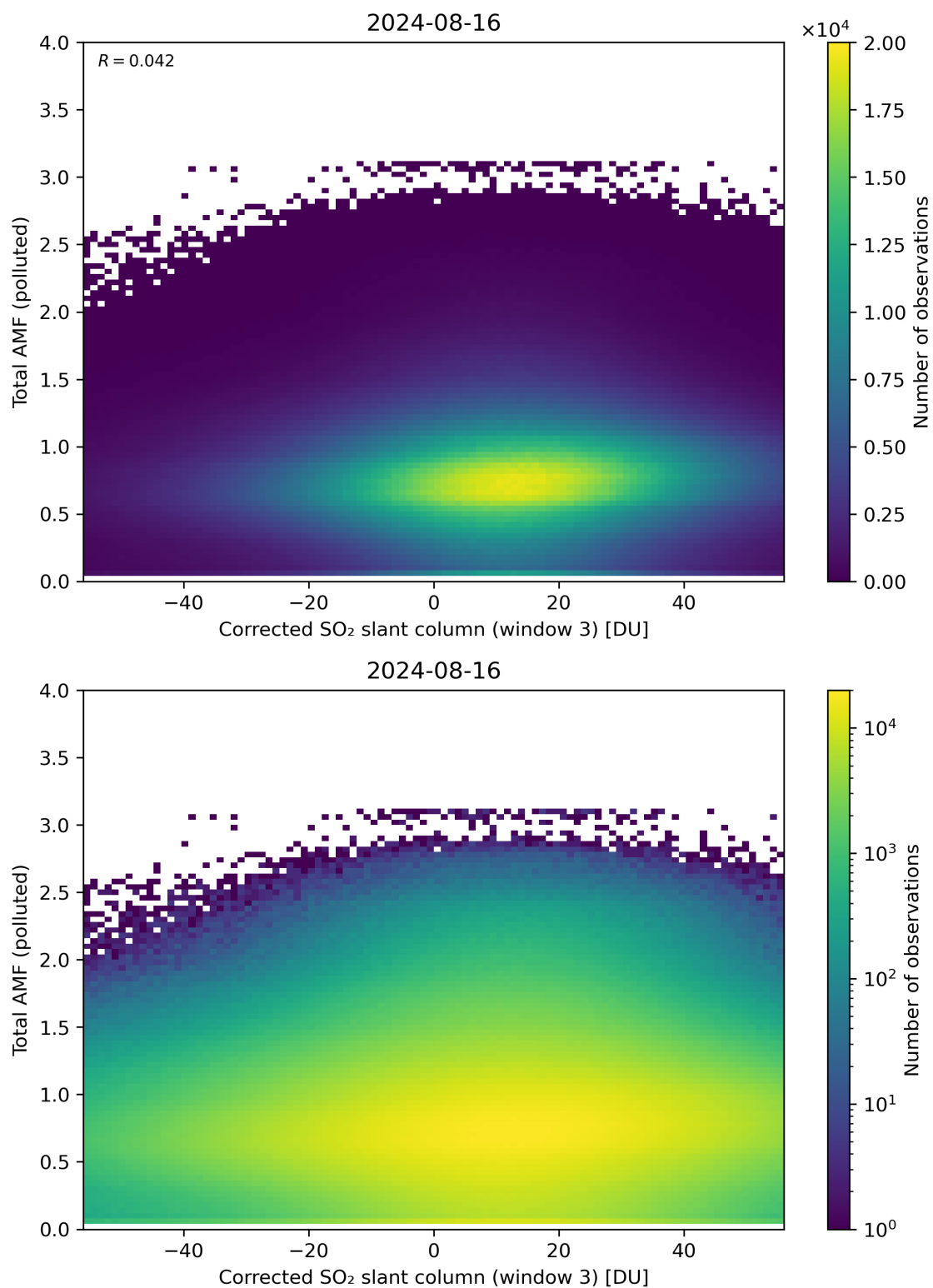
Figure 210: Scatter density plot of “Corrected SO 2 slant column (window 3)” against “Total AMF (polluted)” for 2024-08-16 to 2024-08-17.
