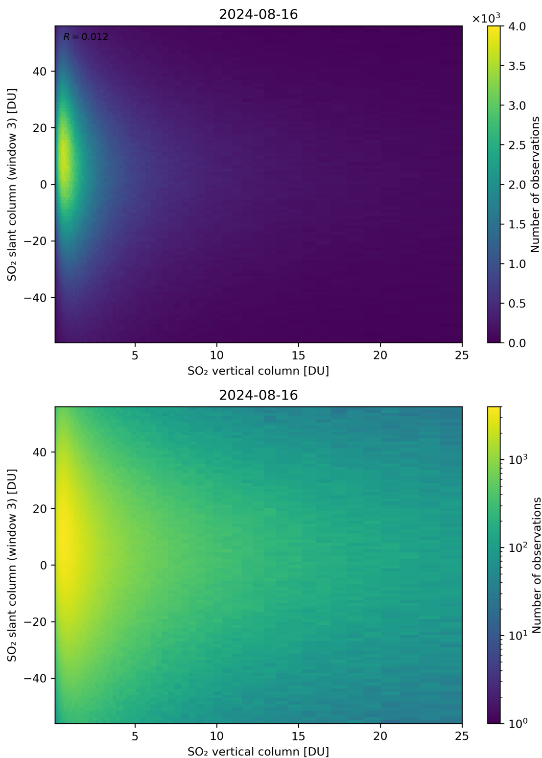
Figure 303: Scatter density plot of “SO 2 vertical column” against “SO 2 slant column (window 3)” for 2024-08-16 to 2024-08-17.
