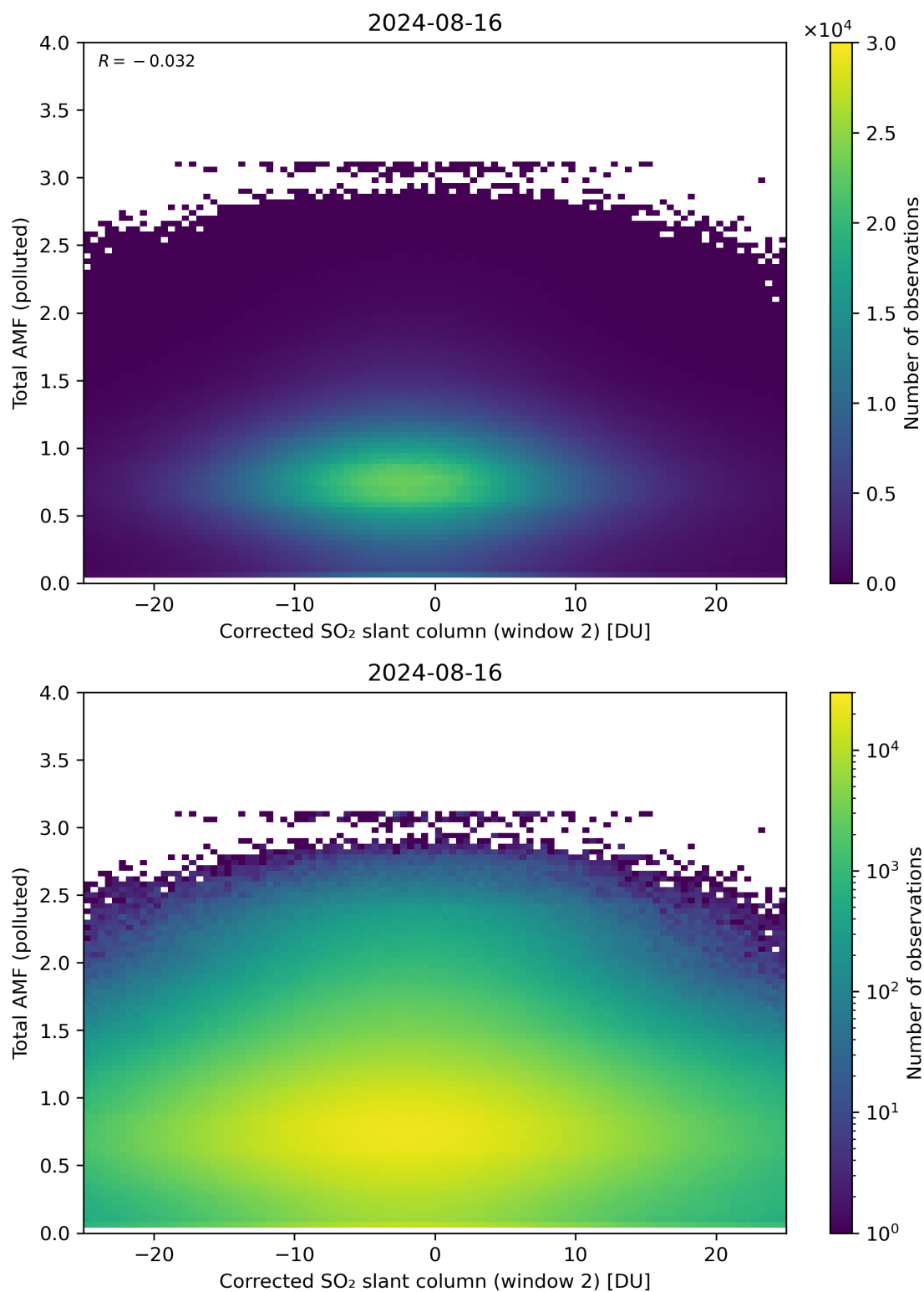
Figure 203: Scatter density plot of “Corrected SO 2 slant column (window 2)” against “Total AMF (polluted)” for 2024-08-16 to 2024-08-17.
