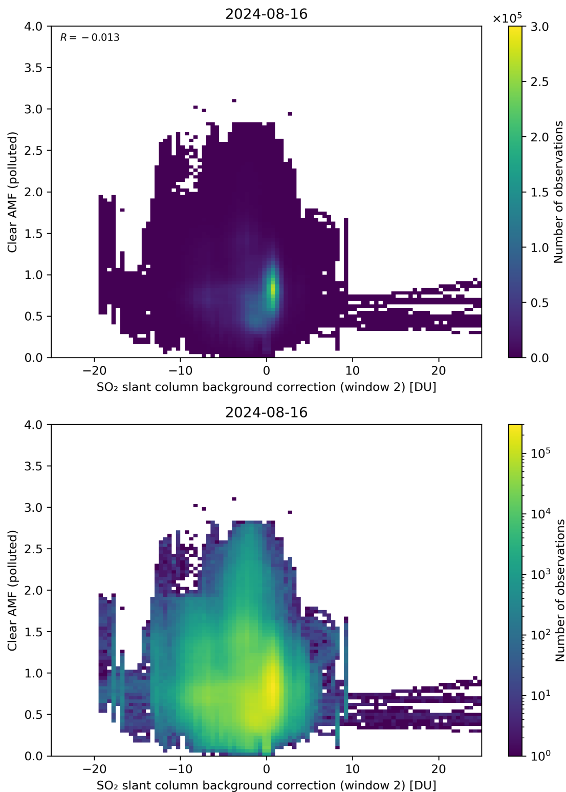
Figure 115: Scatter density plot of “SO 2 slant column background correction (window 2)” against “Clear AMF (polluted)” for 2024-08-16 to 2024-08-17.
