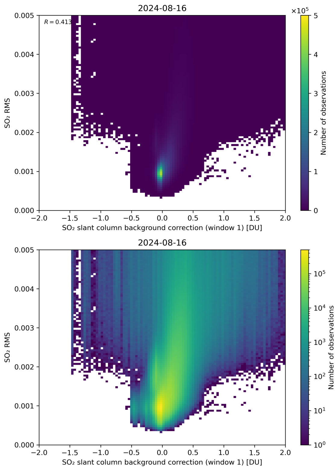
Figure 102: Scatter density plot of “SO 2 slant column background correction (window 1)” against “SO 2 RMS” for 2024-08-16 to 2024-08-17.
