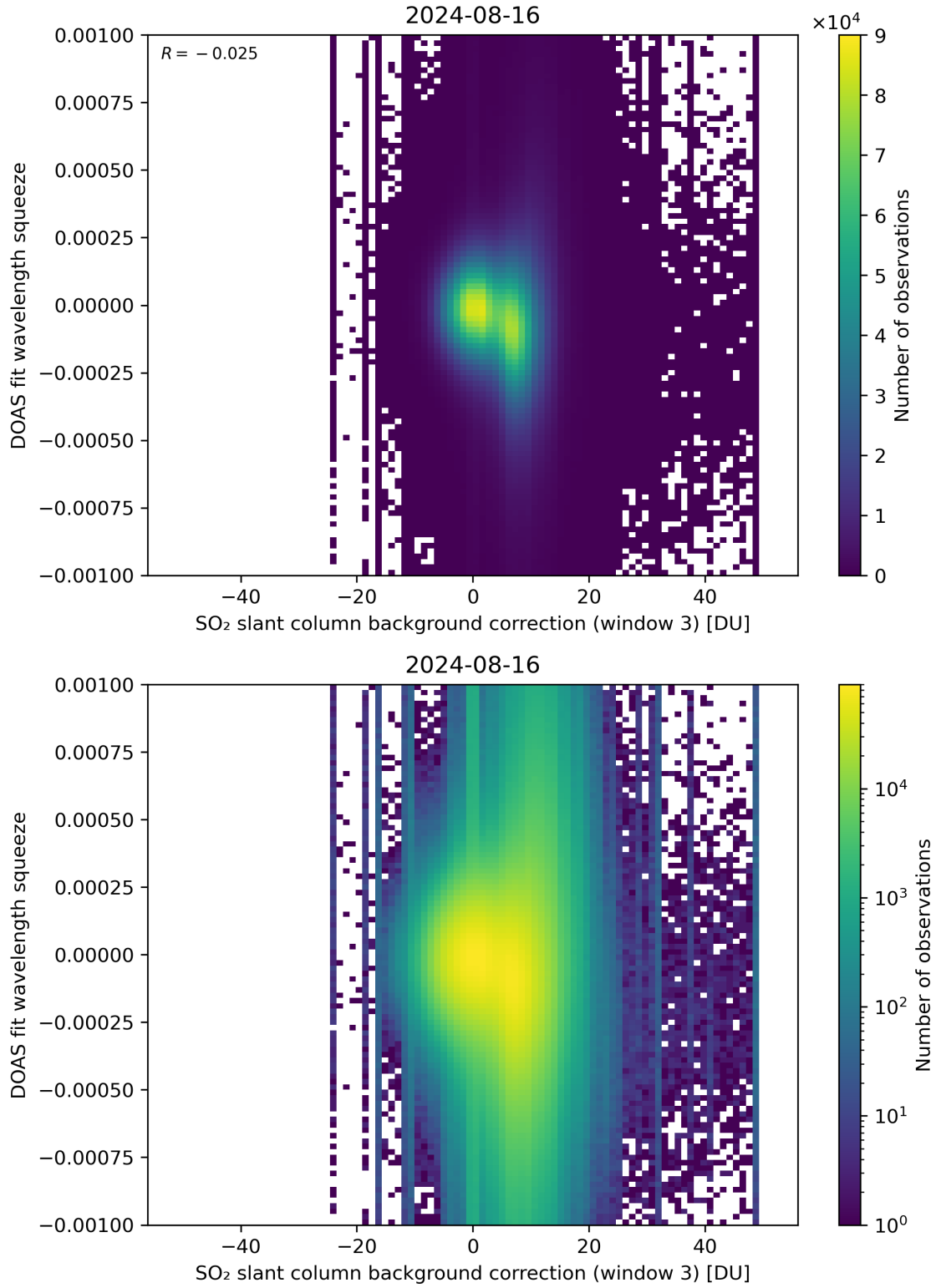
Figure 122: Scatter density plot of “SO 2 slant column background correction (window 3)” against “DOAS fit wavelength squeeze” for 2024-08-16 to 2024-08-17.
