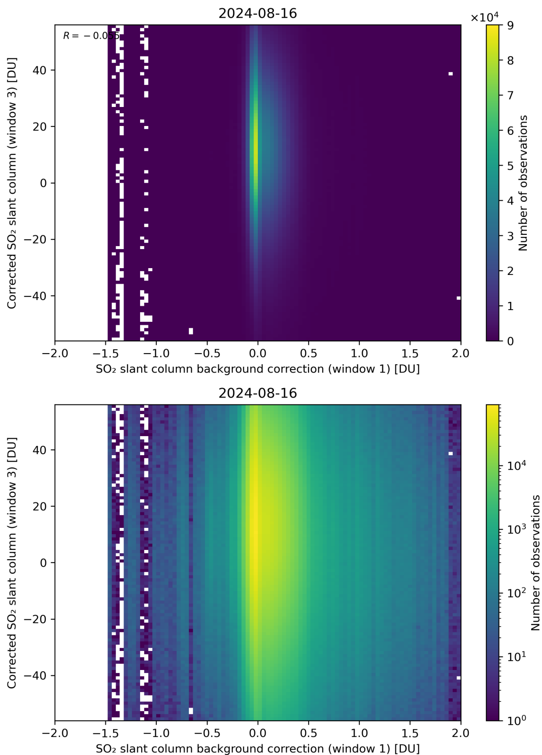
Figure 105: Scatter density plot of “SO 2 slant column background correction (window 1)” against “Corrected SO 2 slant column (window 3)” for 2024-08-16 to 2024-08-17.
