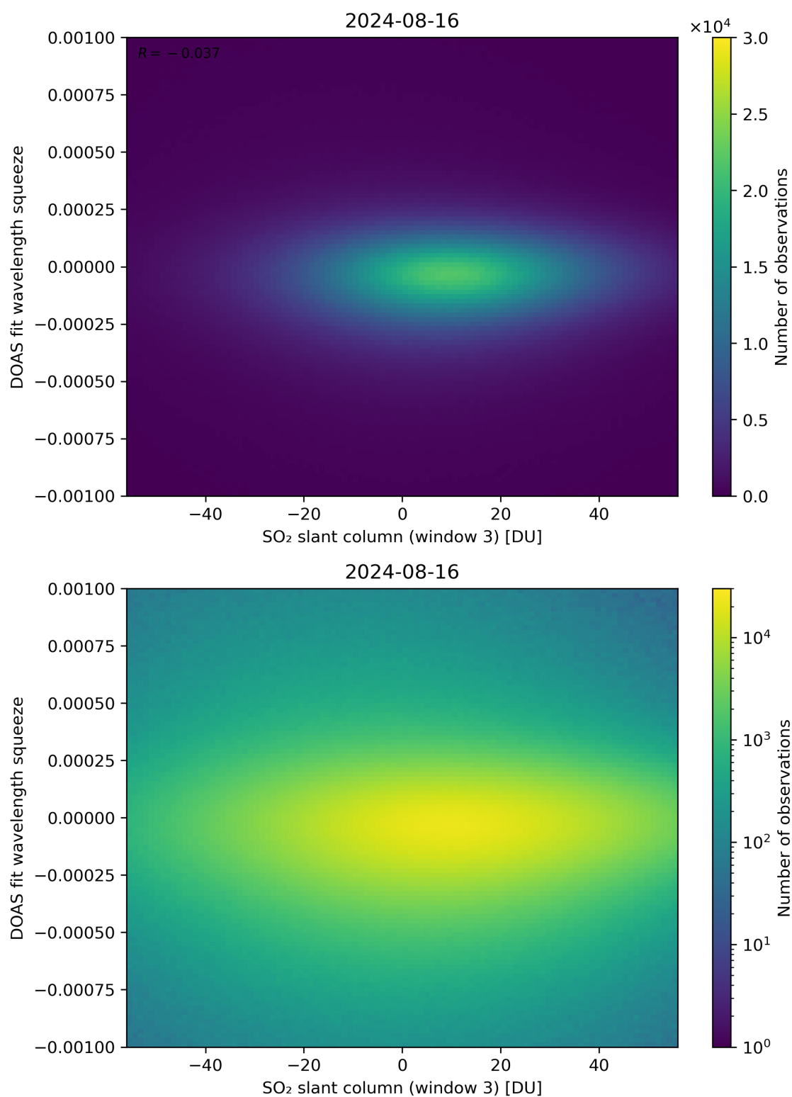
Figure 255: Scatter density plot of “SO 2 slant column (window 3)” against “DOAS fit wavelength squeeze” for 2024-08-16 to 2024-08-17.
