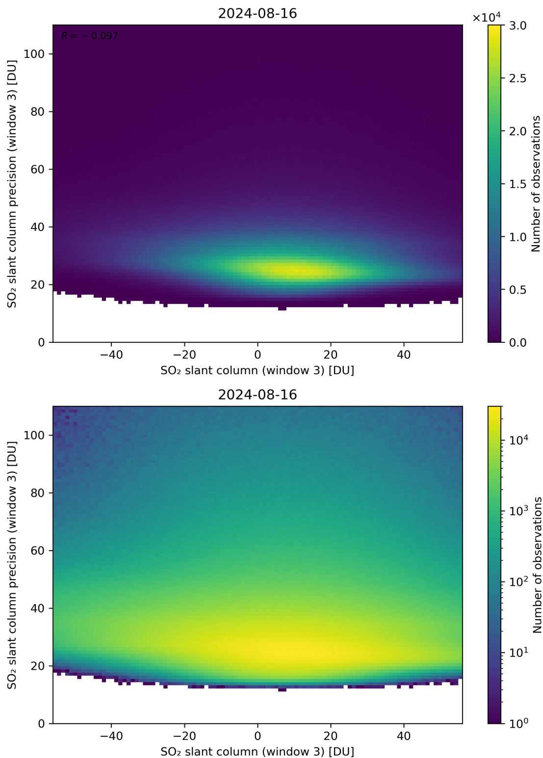
Figure 267: Scatter density plot of “SO 2 slant column (window 3)” against “SO 2 slant column precision (window 3)” for 2024-08-16 to 2024-08-17.
