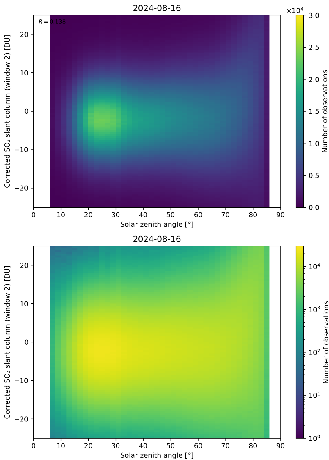
Figure 167: Scatter density plot of “Solar zenith angle” against “Corrected SO 2 slant column (window 2)” for 2024-08-16 to 2024-08-17.
