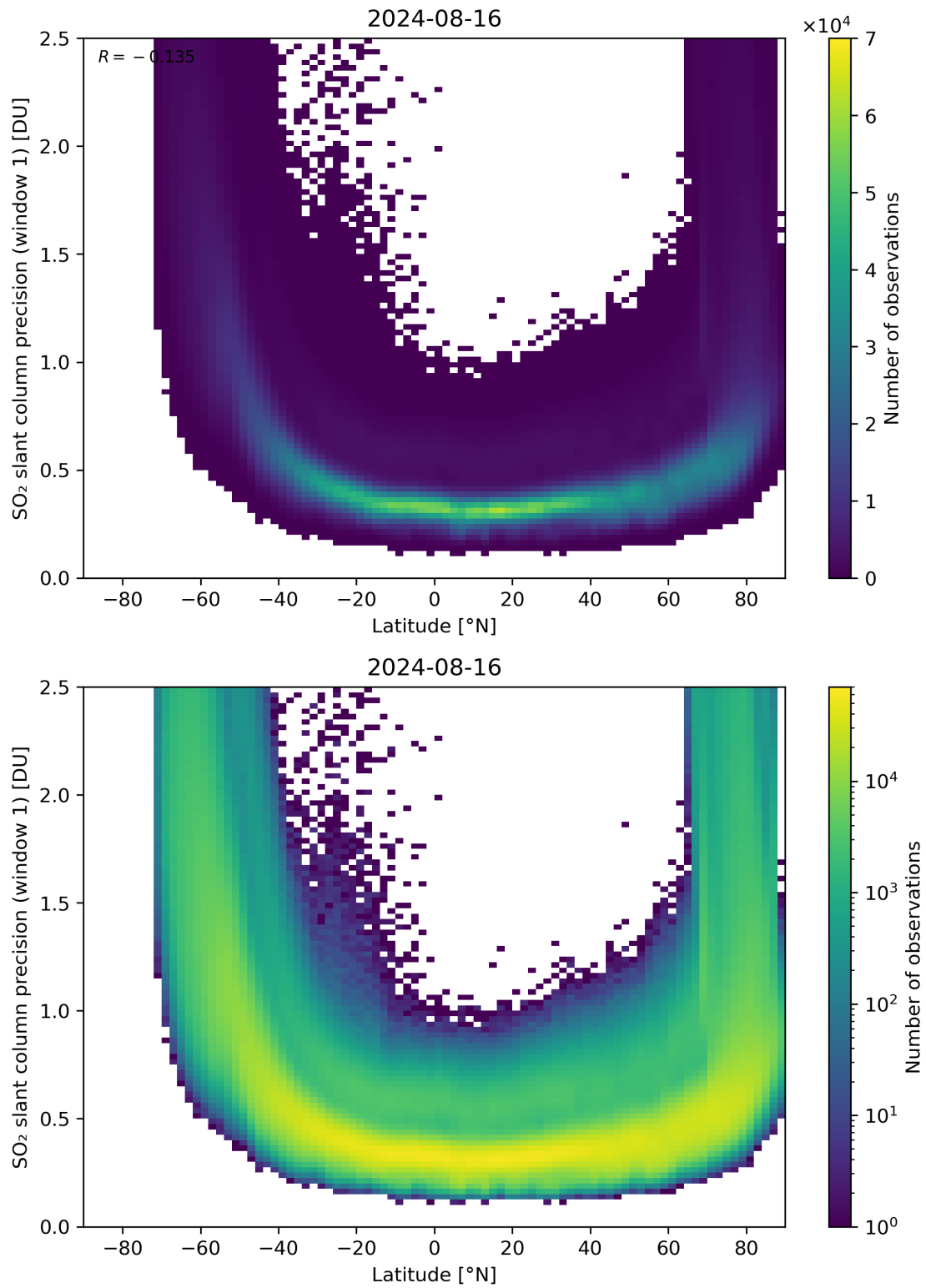
Figure 150: Scatter density plot of “Latitude” against “SO 2 slant column precision (window 1)” for 2024-08-16 to 2024-08-17.
