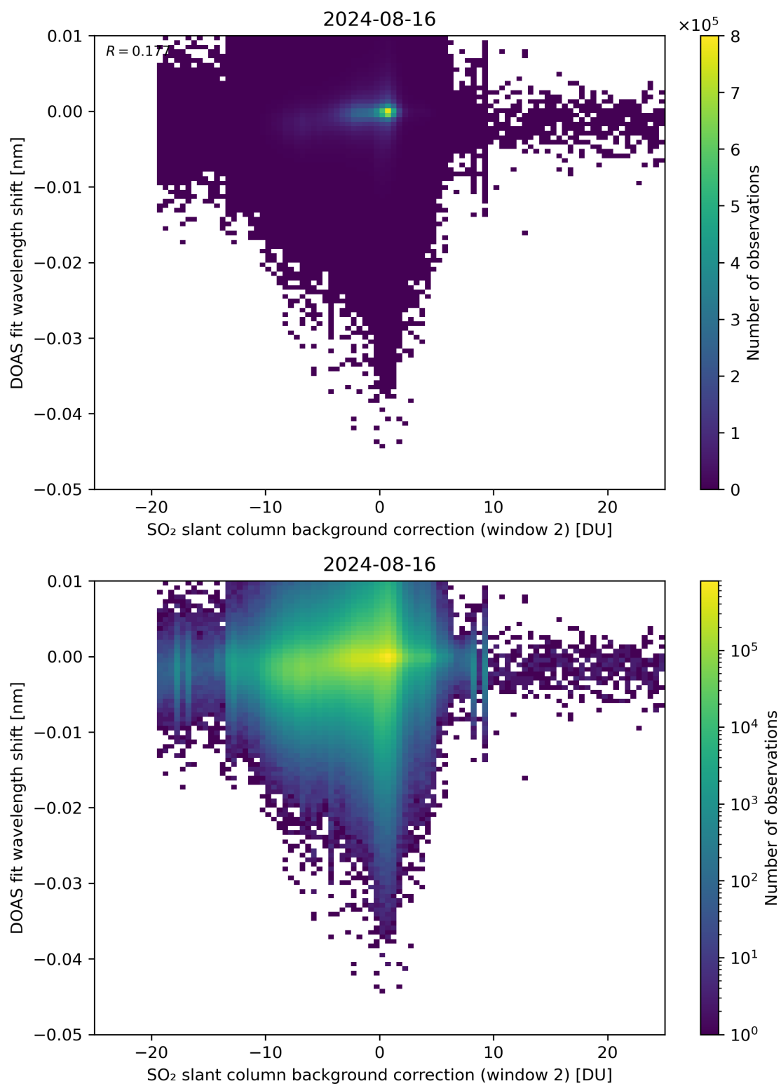
Figure 112: Scatter density plot of “SO 2 slant column background correction (window 2)” against “DOAS fit wavelength shift” for 2024-08-16 to 2024-08-17.
