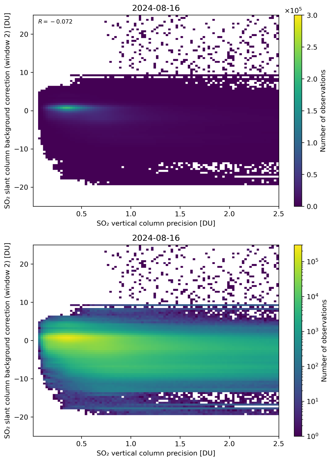
Figure 280: Scatter density plot of “SO 2 vertical column precision” against “SO 2 slant column background correction (window 2)” for 2024-08-16 to 2024-08-17.
