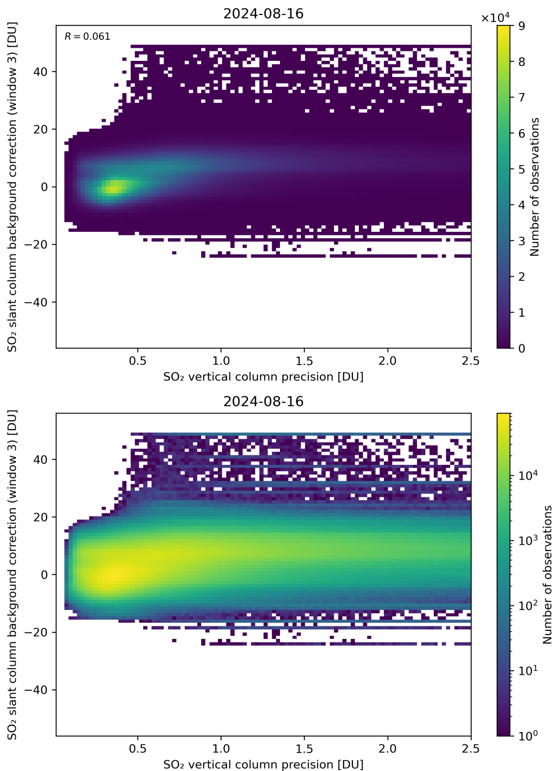
Figure 281: Scatter density plot of “SO 2 vertical column precision” against “SO 2 slant column background correction (window 3)” for 2024-08-16 to 2024-08-17.
