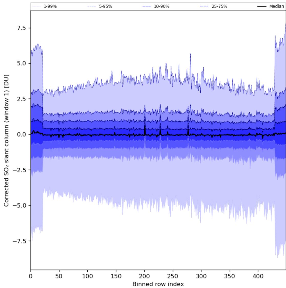
Figure 81: Along track statistics of “Corrected SO 2 slant column (window 1)” for 2024-08-16 to 2024-08-17
