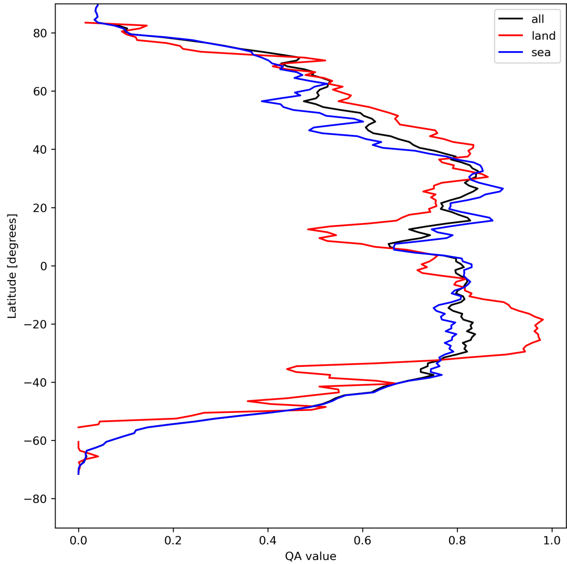
Figure 29: Zonal average of “QA value” for 2024-08-16 to 2024-08-17.
