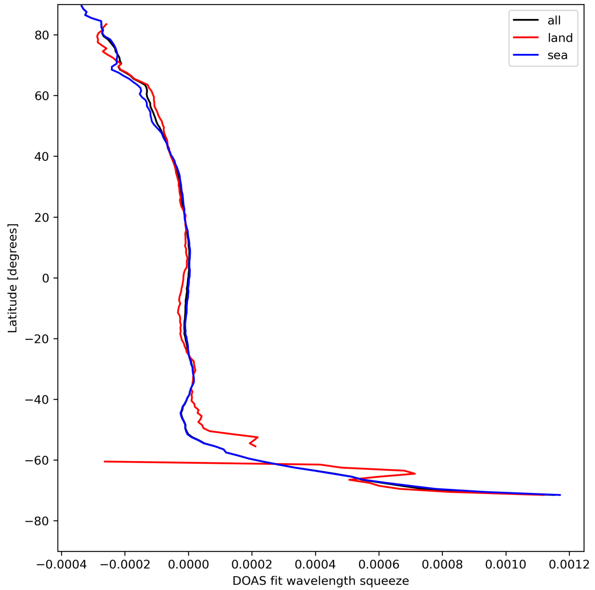
Figure 46: Zonal average of “DOAS fit wavelength squeeze” for 2024-08-16 to 2024-08-17.
