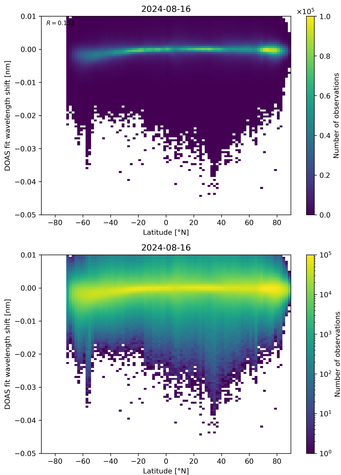
Figure 142: Scatter density plot of “Latitude” against “DOAS fit wavelength shift” for 2024-08-16 to 2024-08-17.
