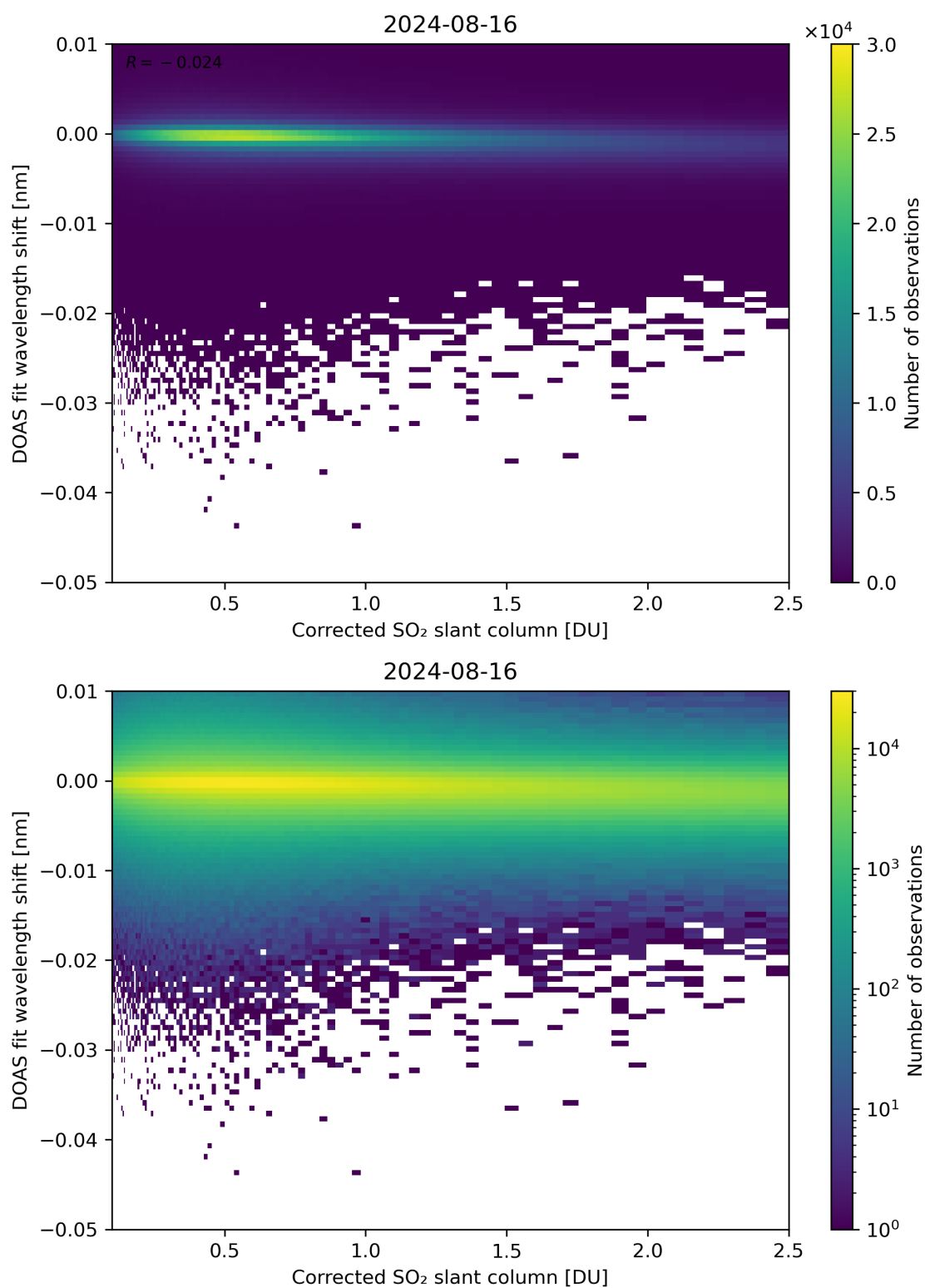
Figure 181: Scatter density plot of “Corrected SO 2 slant column” against “DOAS fit wavelength shift” for 2024-08-16 to 2024-08-17.
