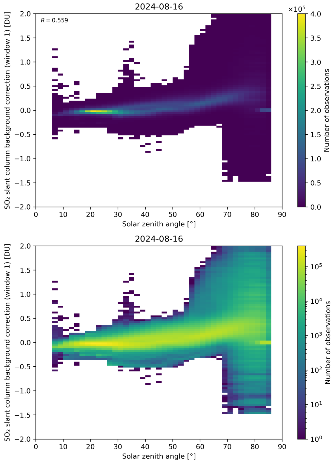
Figure 158: Scatter density plot of “Solar zenith angle” against “SO 2 slant column background correction (window 1)” for 2024-08-16 to 2024-08-17.
