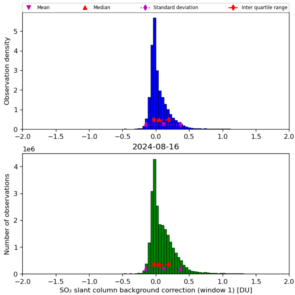
Figure 59: Histogram of “SO 2 slant column background correction (window 1)” for 2024-08-16 to 2024-08-17
