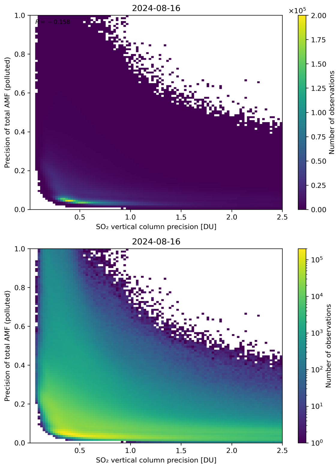
Figure 295: Scatter density plot of “SO 2 vertical column precision” against “Precision of total AMF (polluted)” for 2024-08-16 to 2024-08-17.
