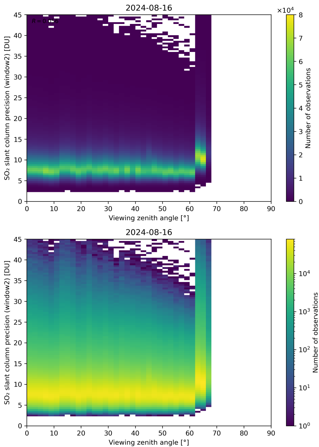
Figure 322: Scatter density plot of “Viewing zenith angle” against “SO 2 slant column precision (window2)” for 2024-08-16 to 2024-08-17.
