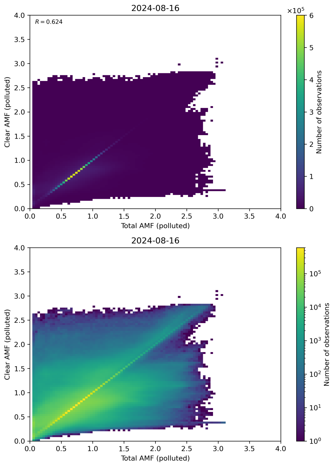
Figure 271: Scatter density plot of “Total AMF (polluted)” against “Clear AMF (polluted)” for 2024-08-16 to 2024-08-17.
