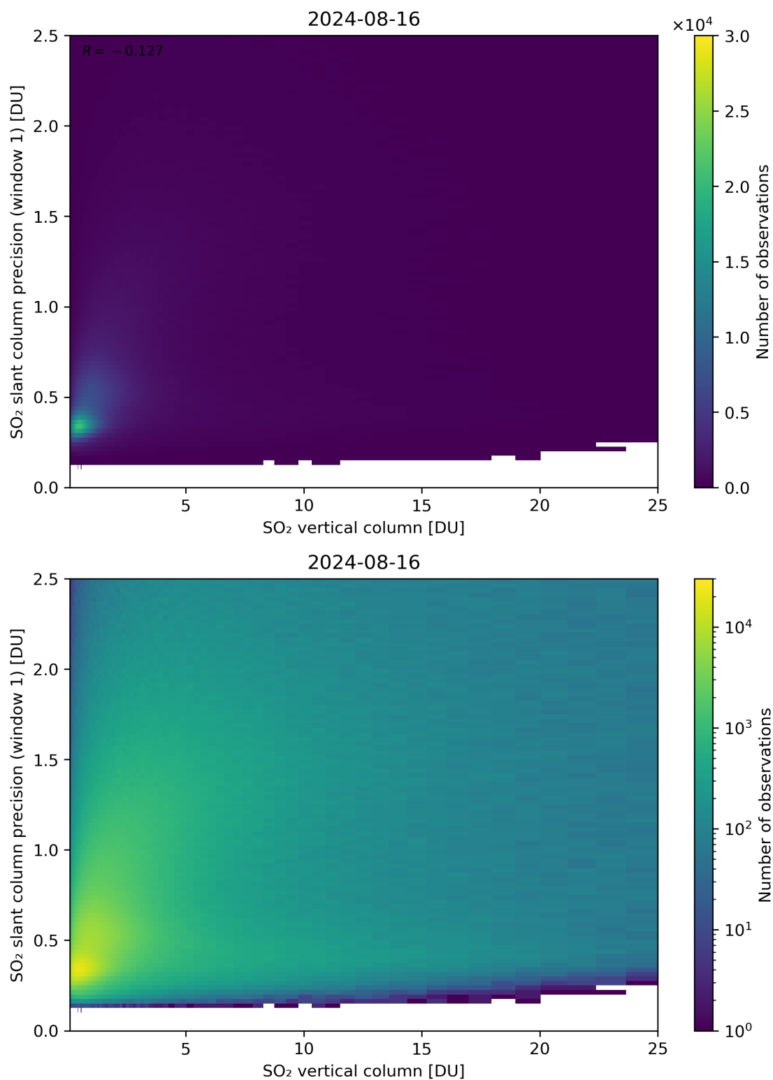
Figure 301: Scatter density plot of “SO 2 vertical column” against “SO 2 slant column precision (window 1)” for 2024-08-16 to 2024-08-17.
