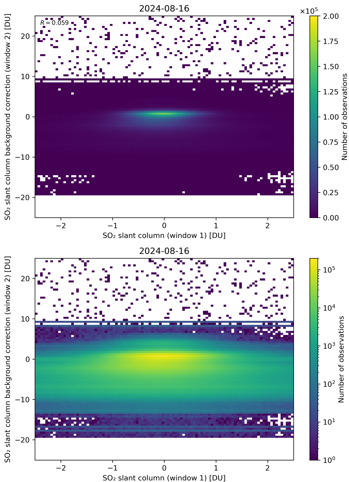
Figure 213: Scatter density plot of “SO 2 slant column (window 1)” against “SO 2 slant column background correction (window 2)” for 2024-08-16 to 2024-08-17.
