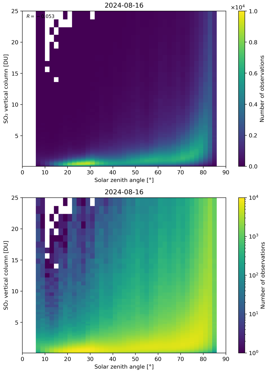
Figure 176: Scatter density plot of “Solar zenith angle” against “SO 2 vertical column” for 2024-08-16 to 2024-08-17.
