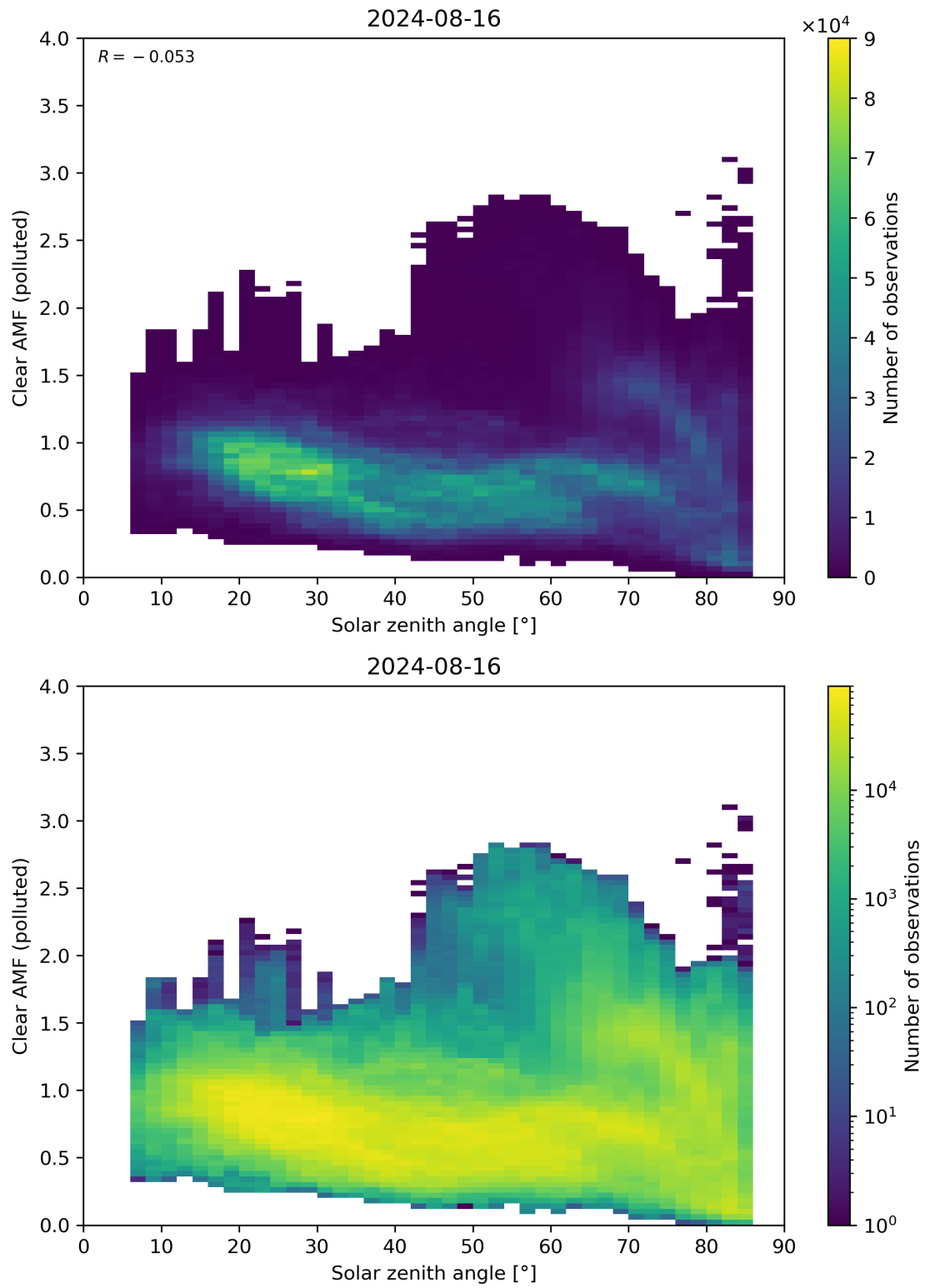
Figure 165: Scatter density plot of “Solar zenith angle” against “Clear AMF (polluted)” for 2024-08-16 to 2024-08-17.
