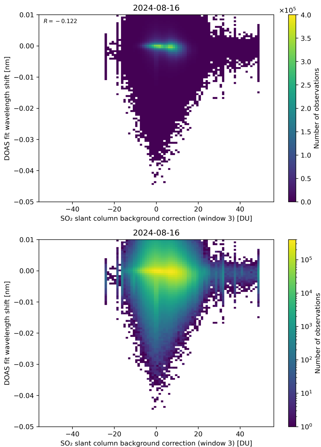
Figure 121: Scatter density plot of “SO 2 slant column background correction (window 3)” against “DOAS fit wavelength shift” for 2024-08-16 to 2024-08-17.
