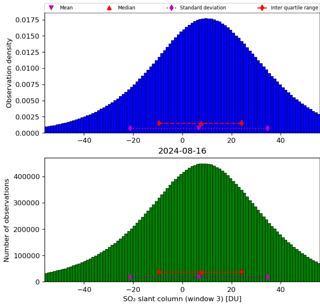
Figure 64: Histogram of “SO 2 slant column (window 3)” for 2024-08-16 to 2024-08-17
