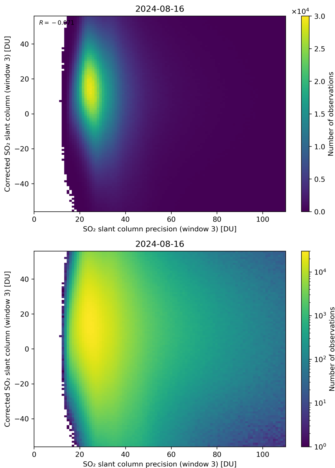
Figure 262: Scatter density plot of “SO 2 slant column precision (window 3)” against “Corrected SO 2 slant column (window 3)” for 2024-08-16 to 2024-08-17.
