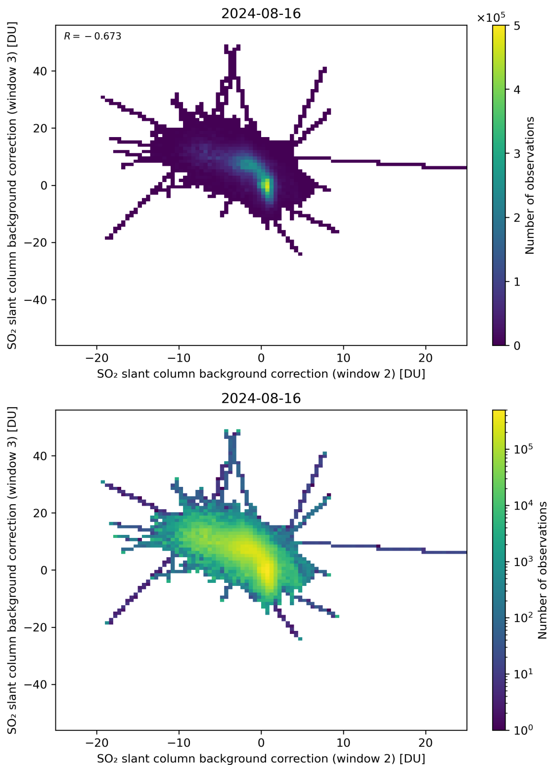
Figure 111: Scatter density plot of “SO 2 slant column background correction (window 2)” against “SO 2 slant column background correction (window 3)” for 2024-08-16 to 2024-08-17.
