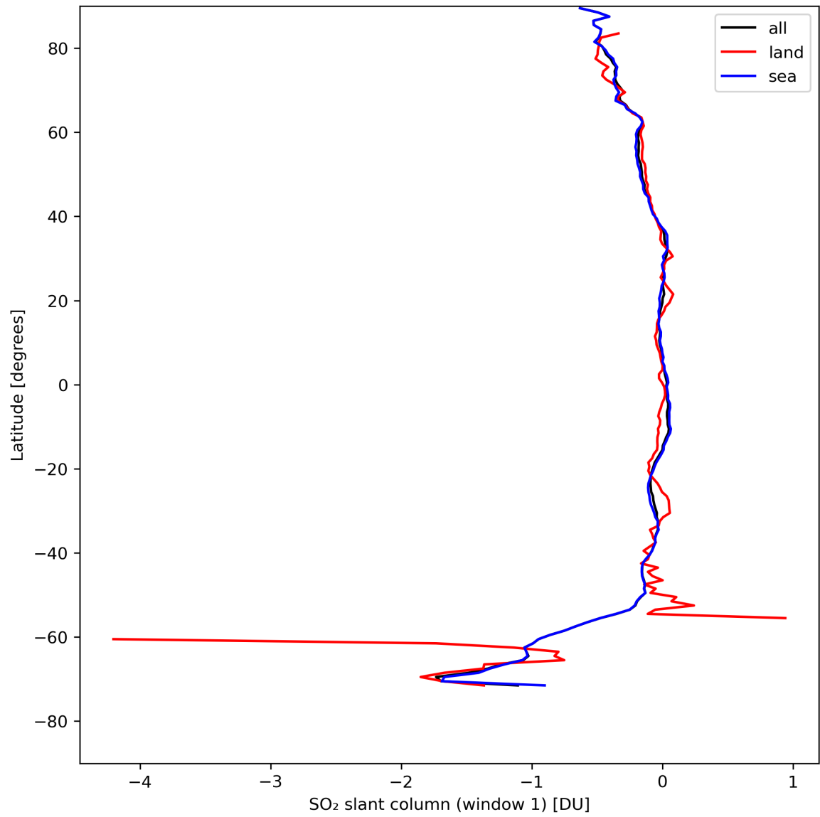
Figure 33: Zonal average of “SO 2 slant column (window 1)” for 2024-08-16 to 2024-08-17.
