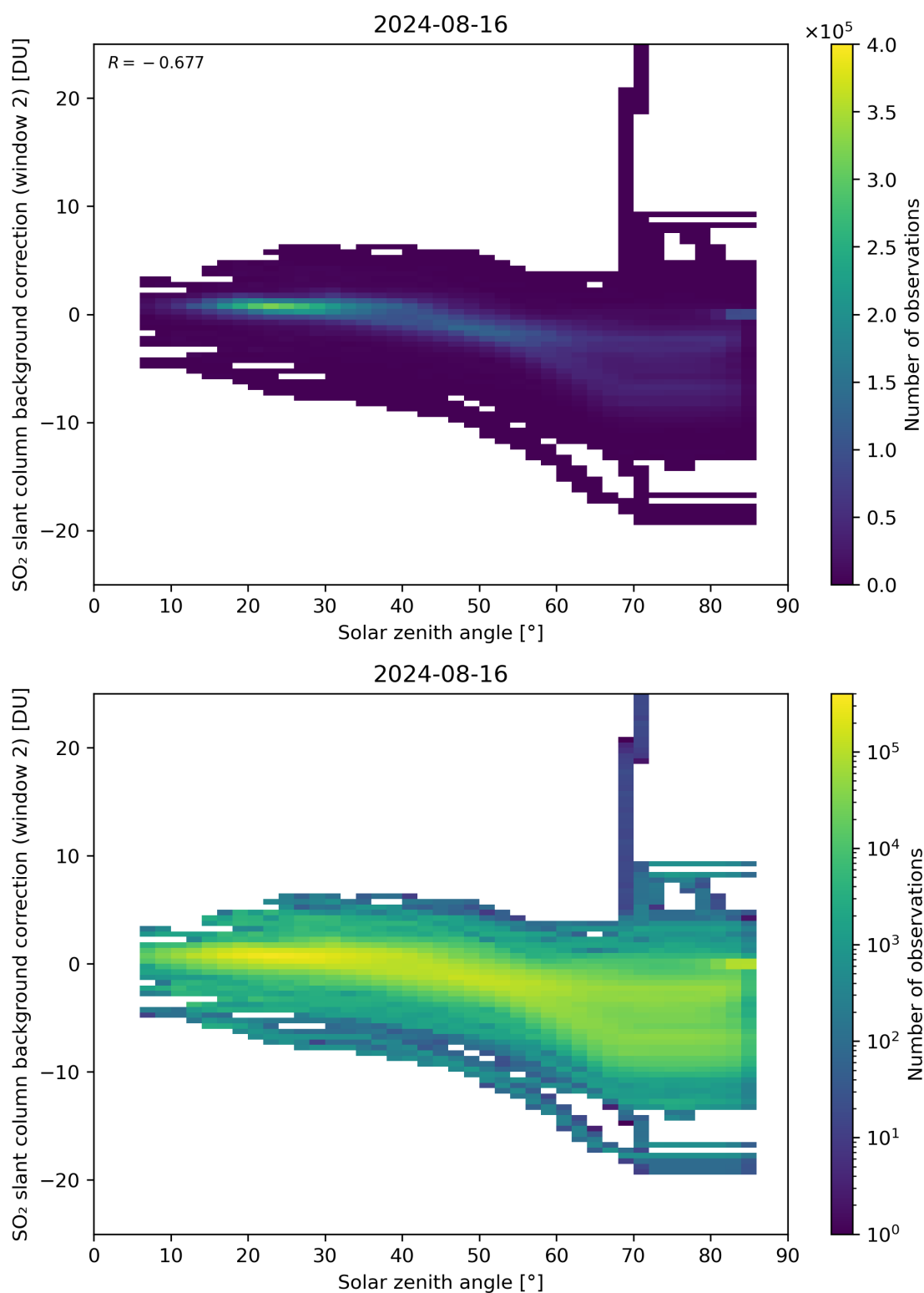
Figure 159: Scatter density plot of “Solar zenith angle” against “SO 2 slant column background correction (window 2)” for 2024-08-16 to 2024-08-17.
