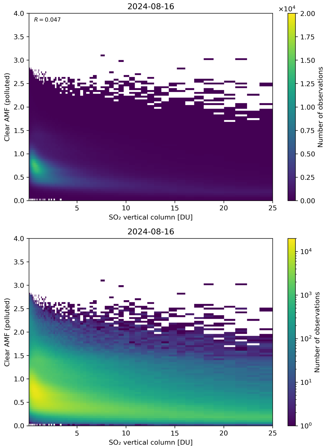
Figure 296: Scatter density plot of “SO 2 vertical column” against “Clear AMF (polluted)” for 2024-08-16 to 2024-08-17.
