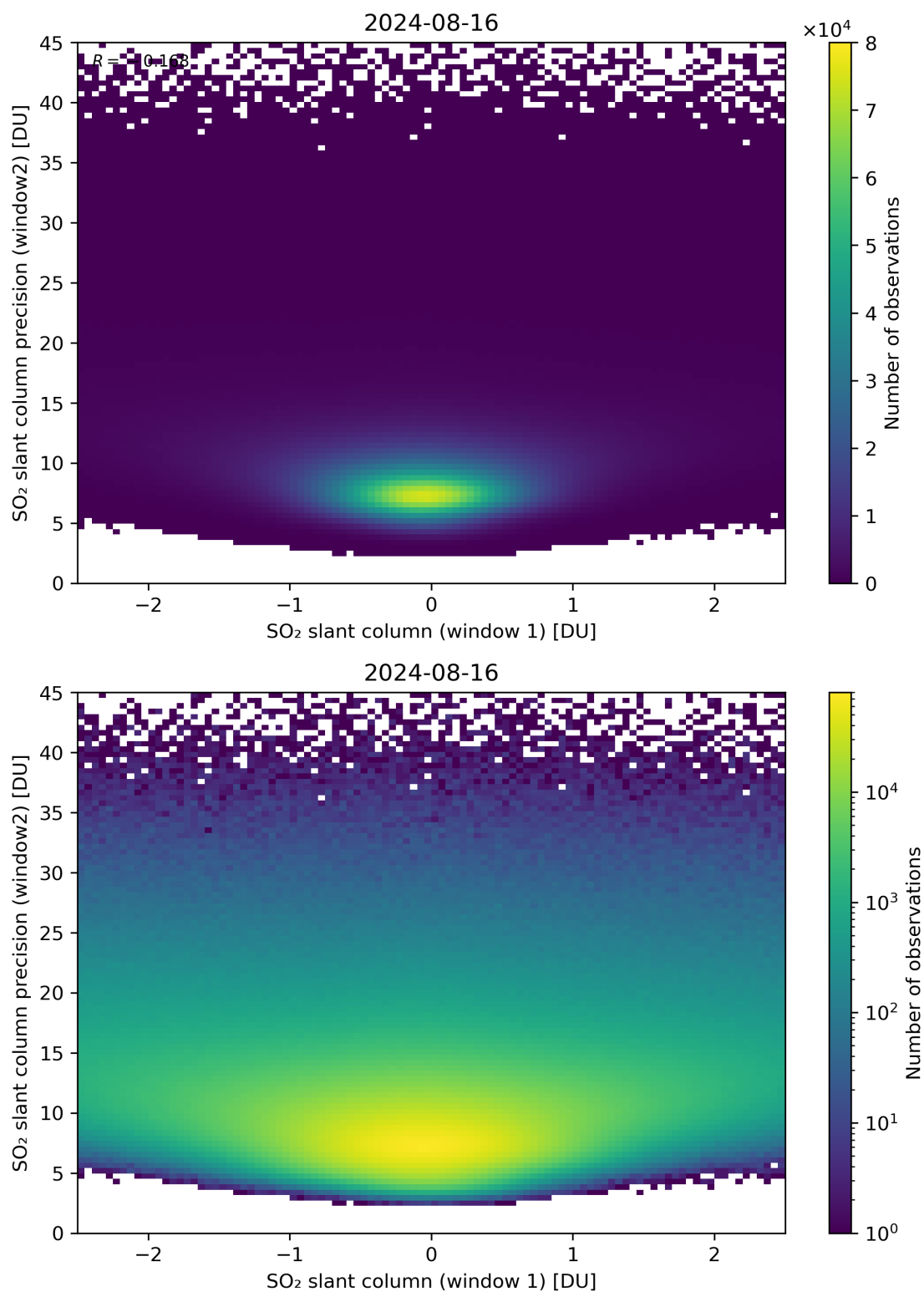
Figure 236: Scatter density plot of “SO 2 slant column (window 1)” against “SO 2 slant column precision (window2)” for 2024-08-16 to 2024-08-17.
