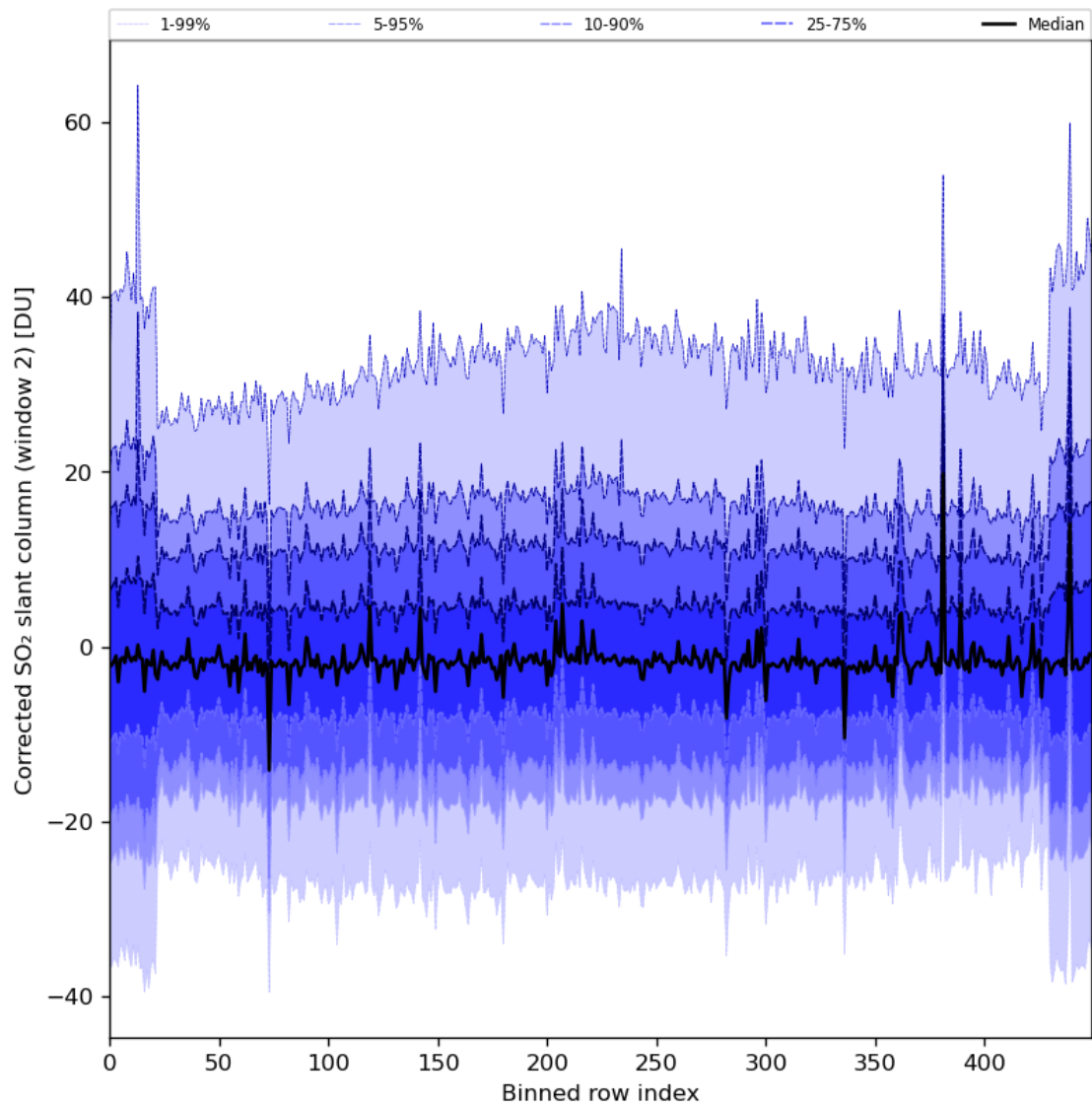
Figure 85: Along track statistics of “Corrected SO 2 slant column (window 2)” for 2024-08-16 to 2024-08-17
