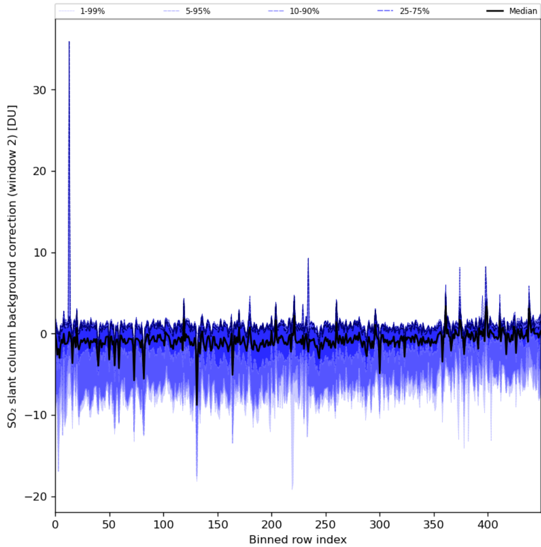
Figure 86: Along track statistics of “SO 2 slant column background correction (window 2)” for 2024-08-16 to 2024-08-17
