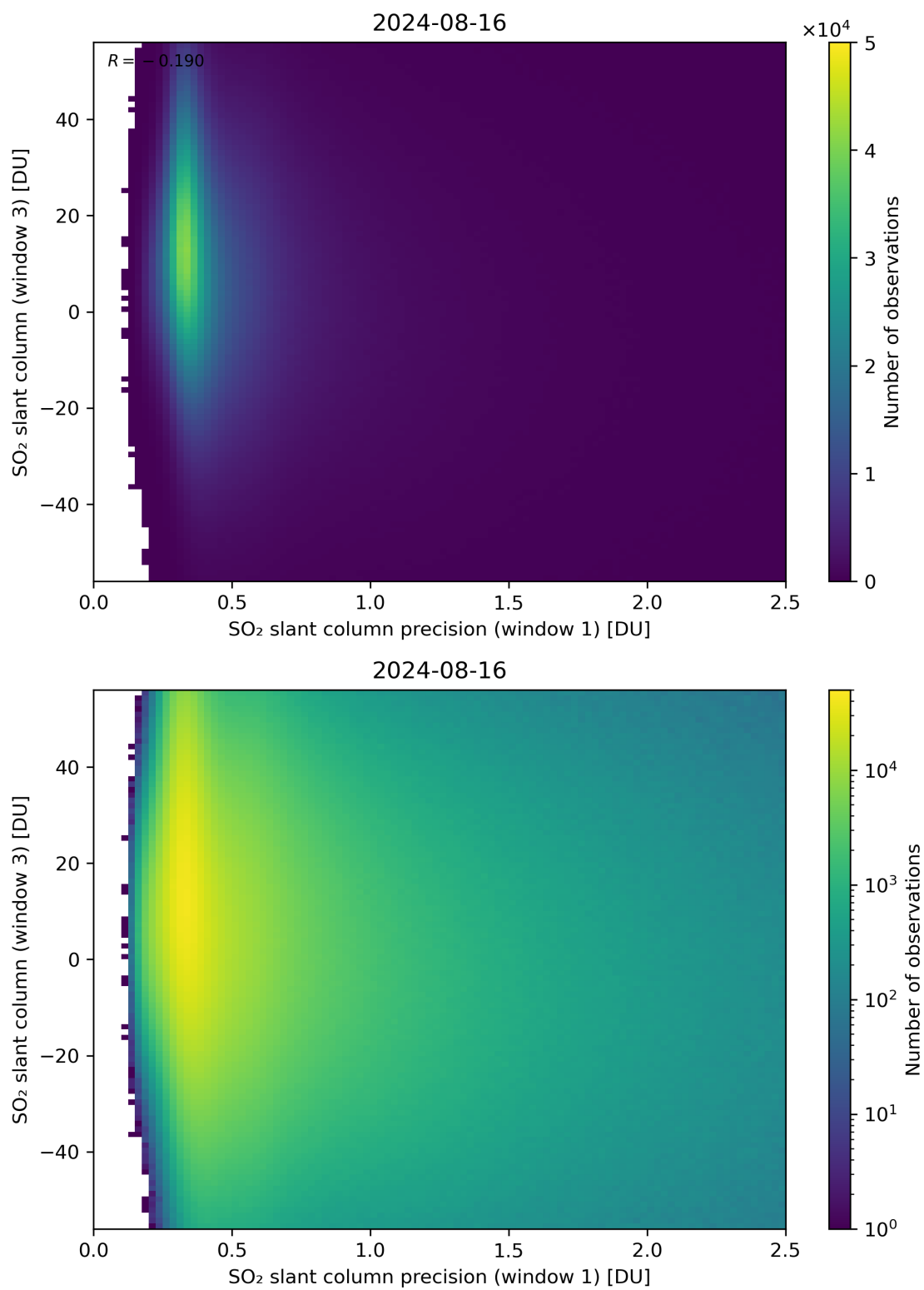
Figure 228: Scatter density plot of “SO 2 slant column precision (window 1)” against “SO 2 slant column (window 3)” for 2024-08-16 to 2024-08-17.
