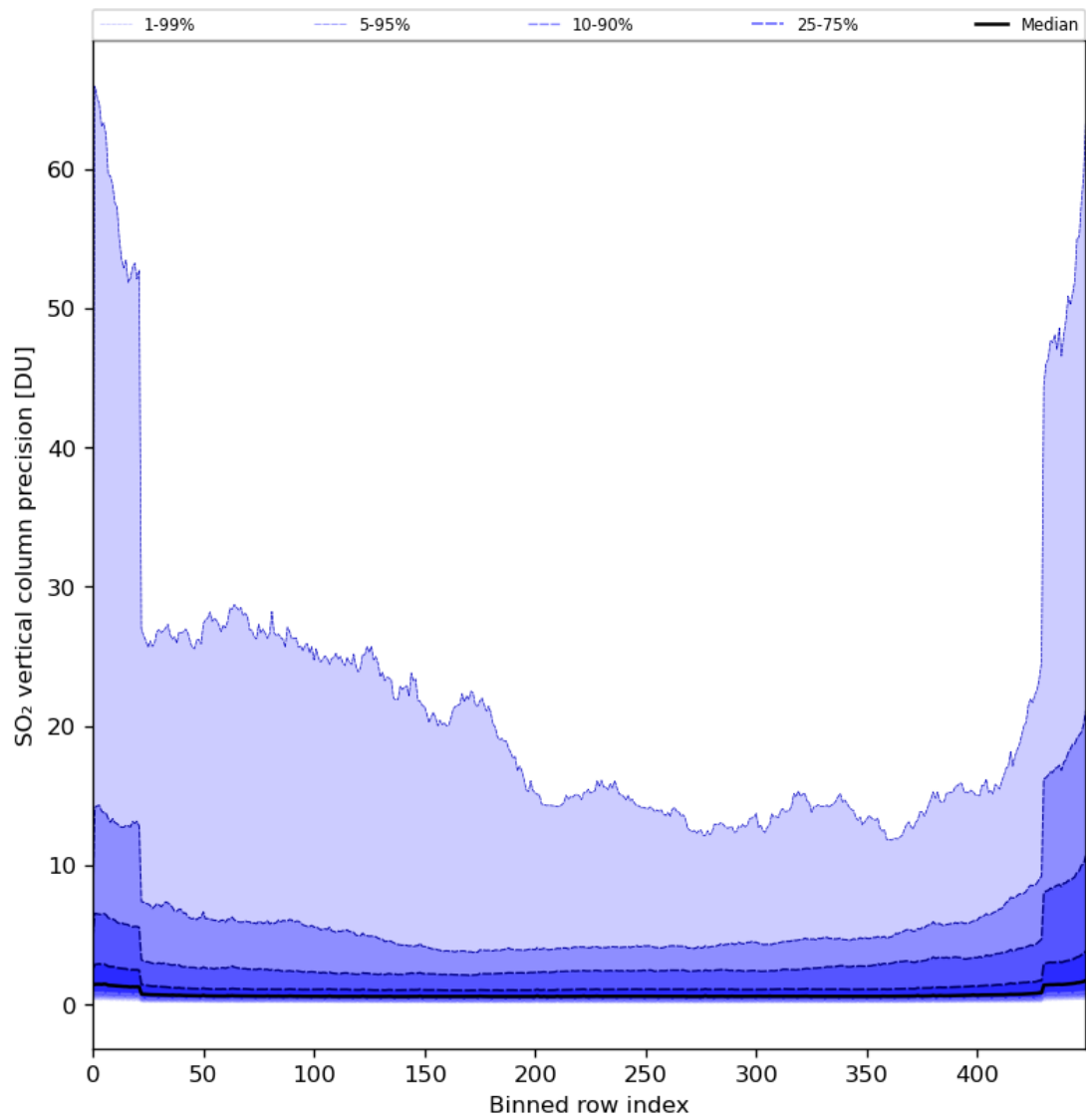
Figure 77: Along track statistics of “SO 2 vertical column precision” for 2024-08-16 to 2024-08-17
