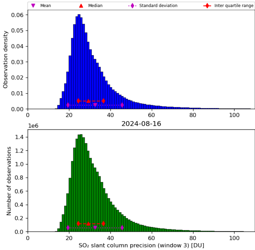
Figure 65: Histogram of “SO 2 slant column precision (window 3)” for 2024-08-16 to 2024-08-17
