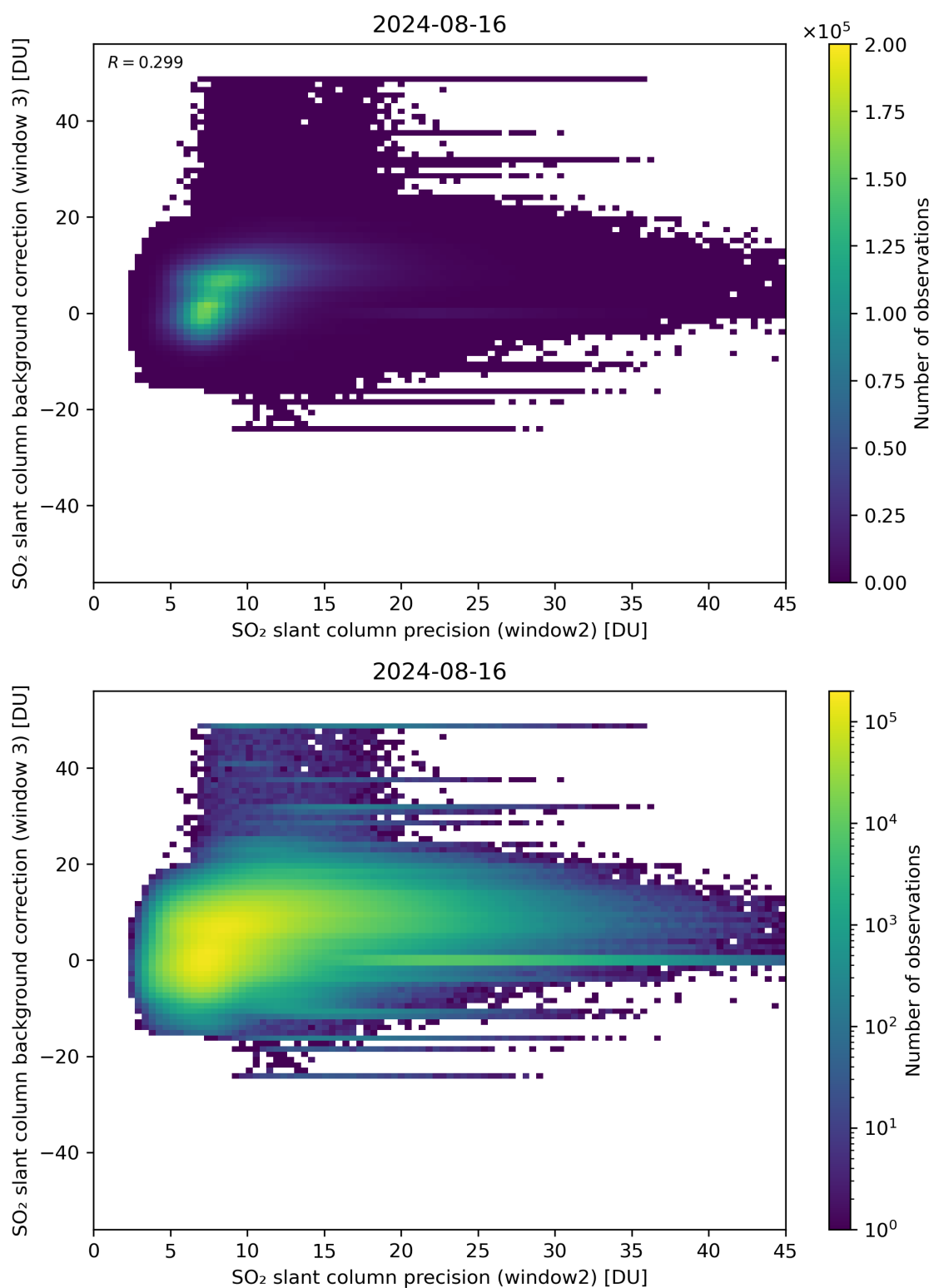
Figure 242: Scatter density plot of “SO 2 slant column precision (window2)” against “SO 2 slant column background correction (window 3)” for 2024-08-16 to 2024-08-17.
