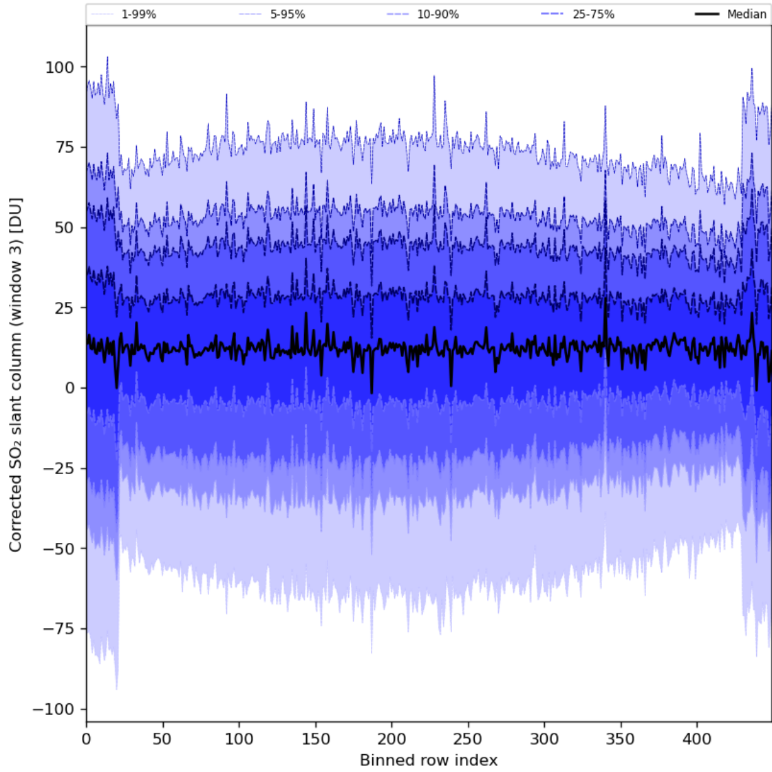
Figure 89: Along track statistics of “Corrected SO 2 slant column (window 3)” for 2024-08-16 to 2024-08-17
