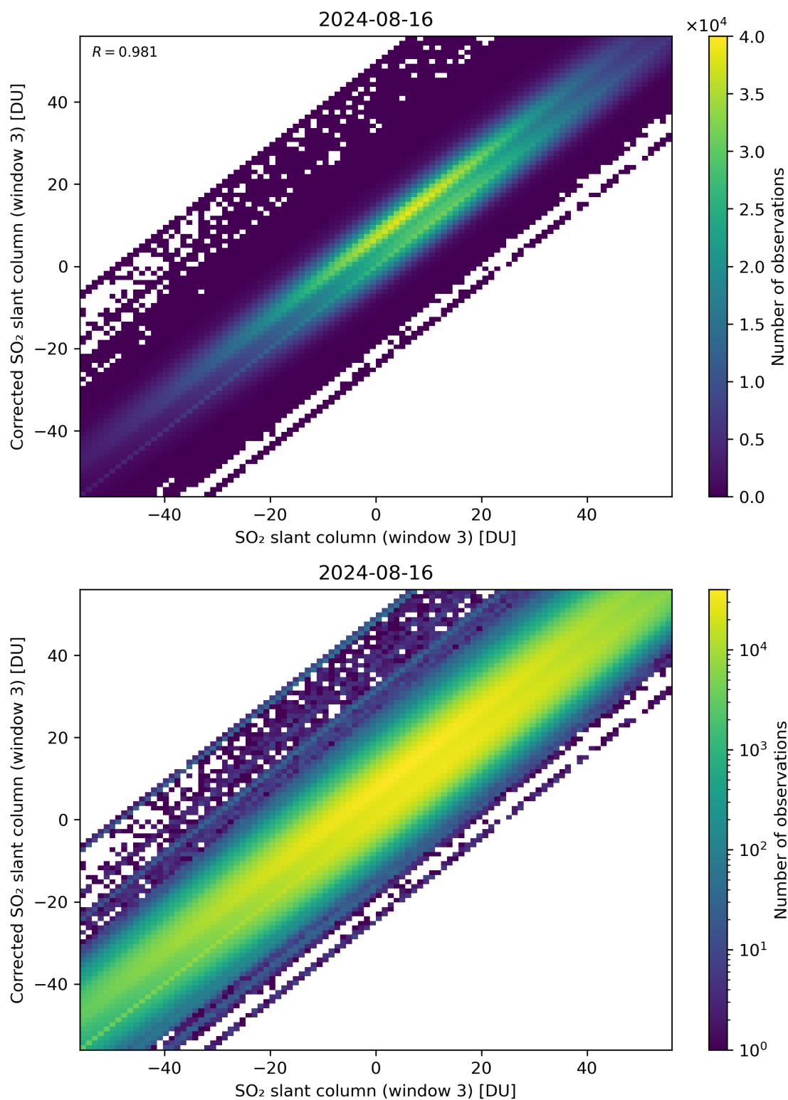
Figure 266: Scatter density plot of “SO 2 slant column (window 3)” against “Corrected SO 2 slant column (window 3)” for 2024-08-16 to 2024-08-17.
