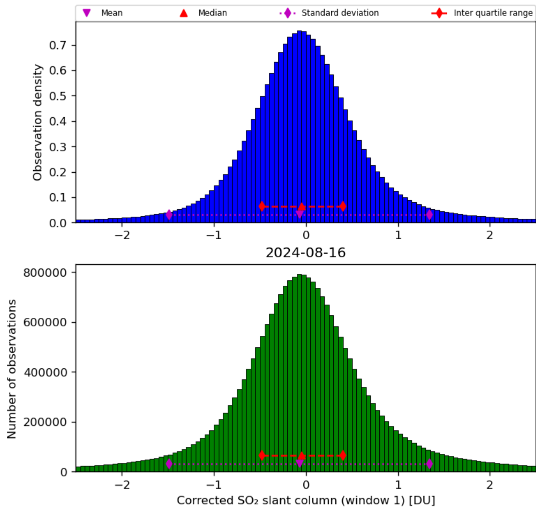
Figure 58: Histogram of “Corrected SO 2 slant column (window 1)” for 2024-08-16 to 2024-08-17
