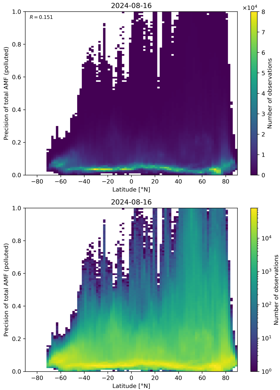
Figure 155: Scatter density plot of “Latitude” against “Precision of total AMF (polluted)” for 2024-08-16 to 2024-08-17.
