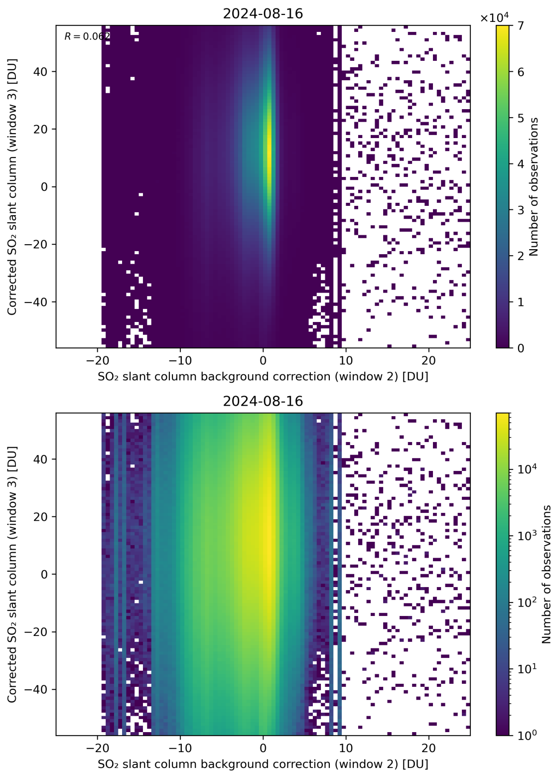
Figure 116: Scatter density plot of “SO 2 slant column background correction (window 2)” against “Corrected SO 2 slant column (window 3)” for 2024-08-16 to 2024-08-17.
