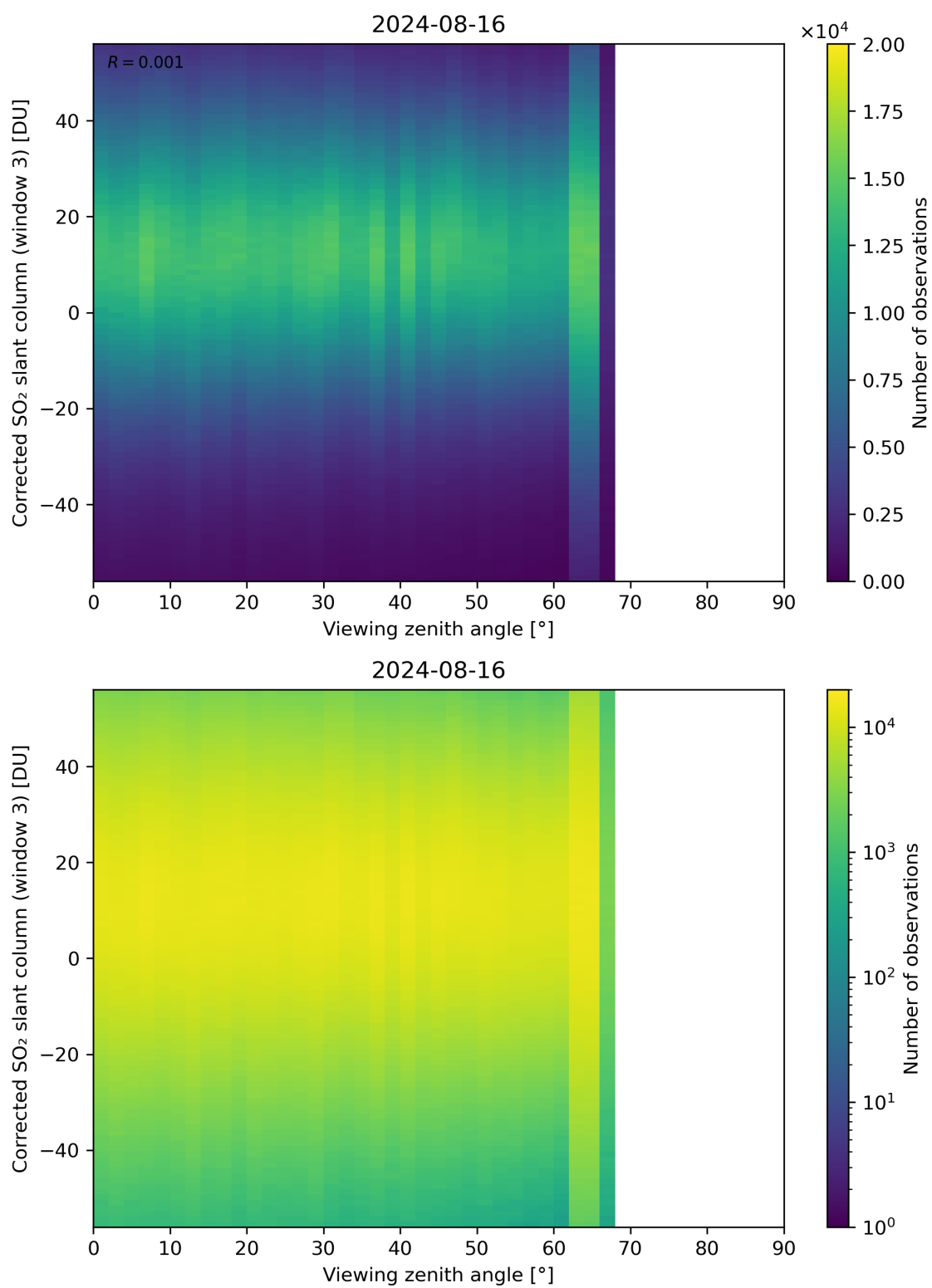
Figure 319: Scatter density plot of “Viewing zenith angle” against “Corrected SO 2 slant column (window 3)” for 2024-08-16 to 2024-08-17.
