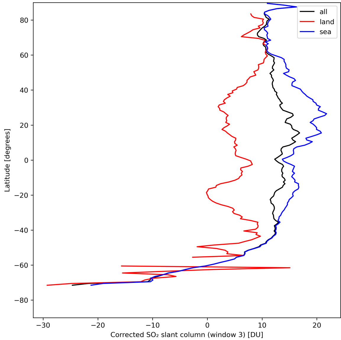
Figure 43: Zonal average of “Corrected SO 2 slant column (window 3)” for 2024-08-16 to 2024-08-17.
