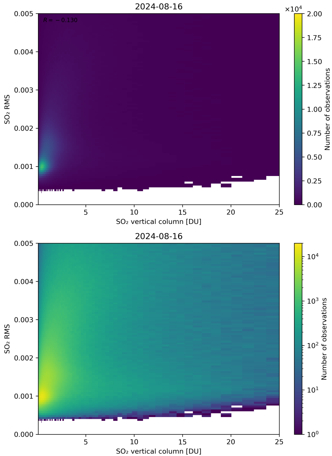
Figure 278: Scatter density plot of “SO 2 vertical column” against “SO 2 RMS” for 2024-08-16 to 2024-08-17.
