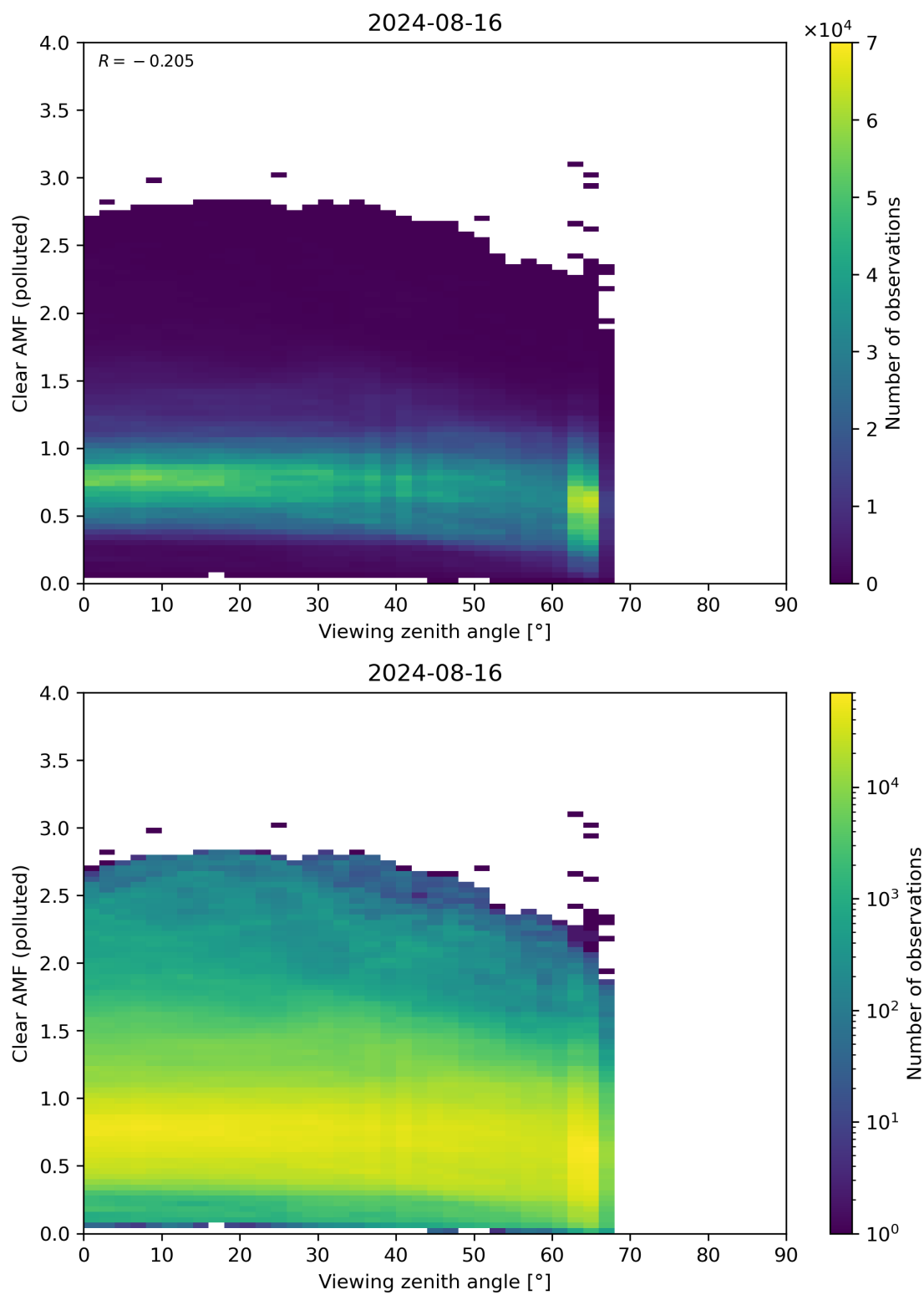
Figure 316: Scatter density plot of “Viewing zenith angle” against “Clear AMF (polluted)” for 2024-08-16 to 2024-08-17.
