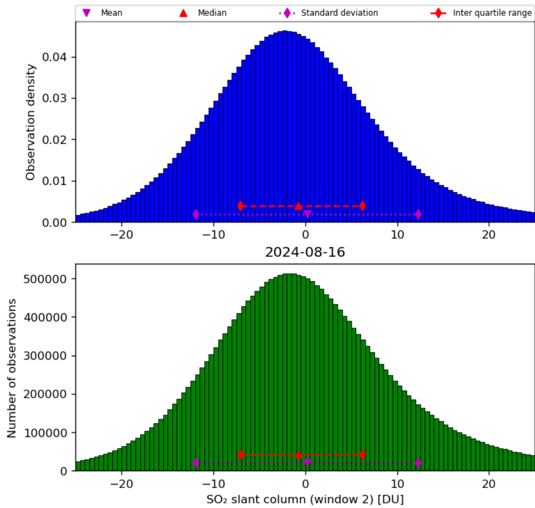
Figure 60: Histogram of “SO 2 slant column (window 2)” for 2024-08-16 to 2024-08-17
