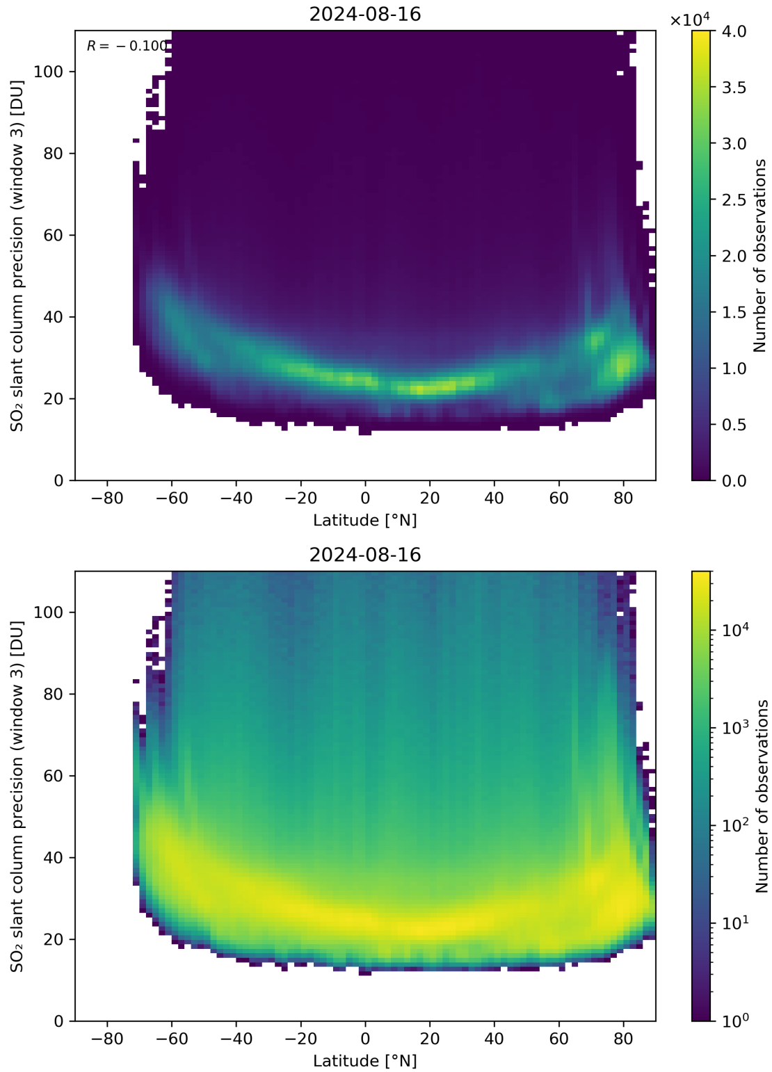
Figure 153: Scatter density plot of “Latitude” against “SO 2 slant column precision (window 3)” for 2024-08-16 to 2024-08-17.
