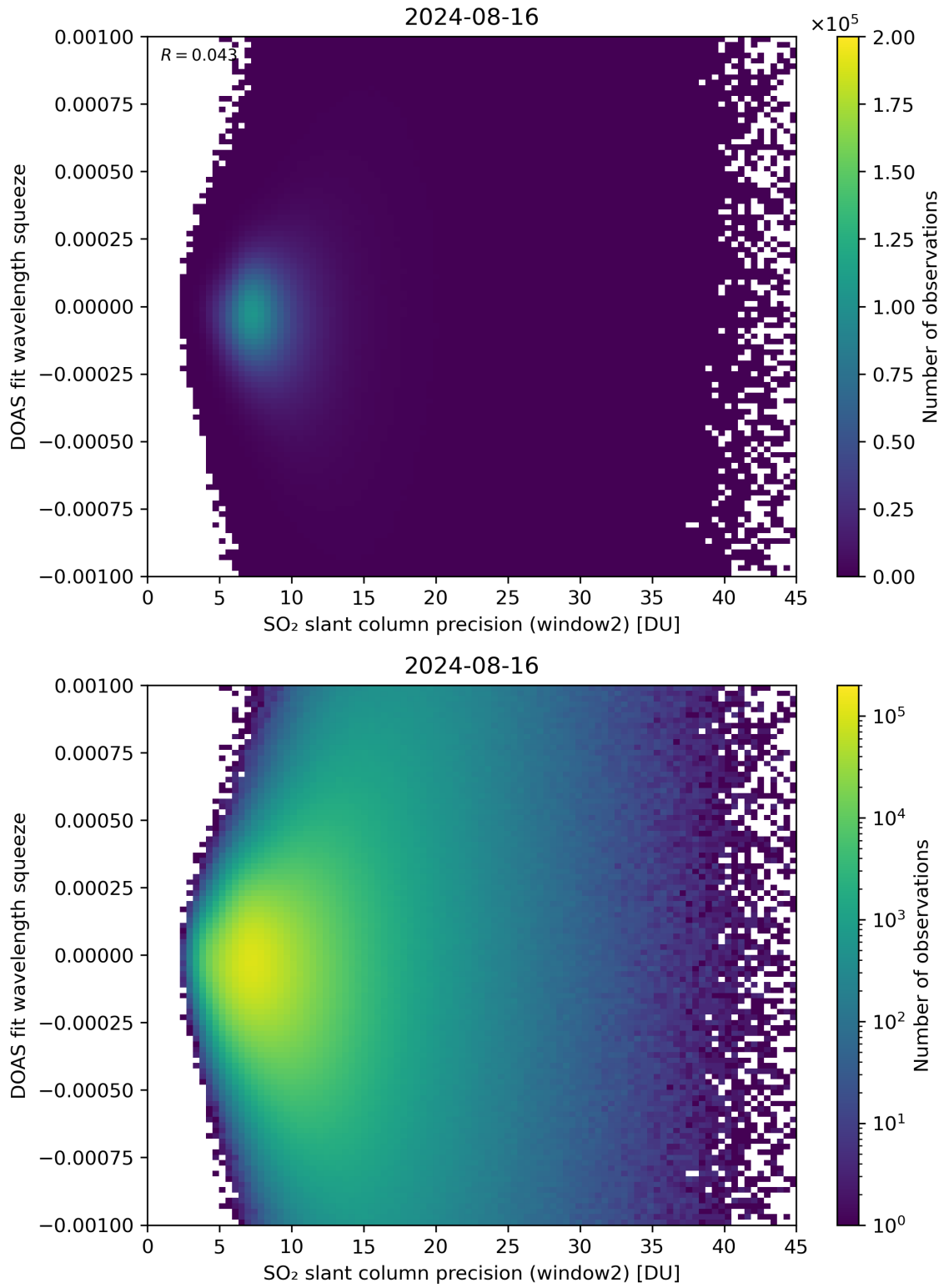
Figure 244: Scatter density plot of “SO 2 slant column precision (window2)” against “DOAS fit wavelength squeeze” for 2024-08-16 to 2024-08-17.
