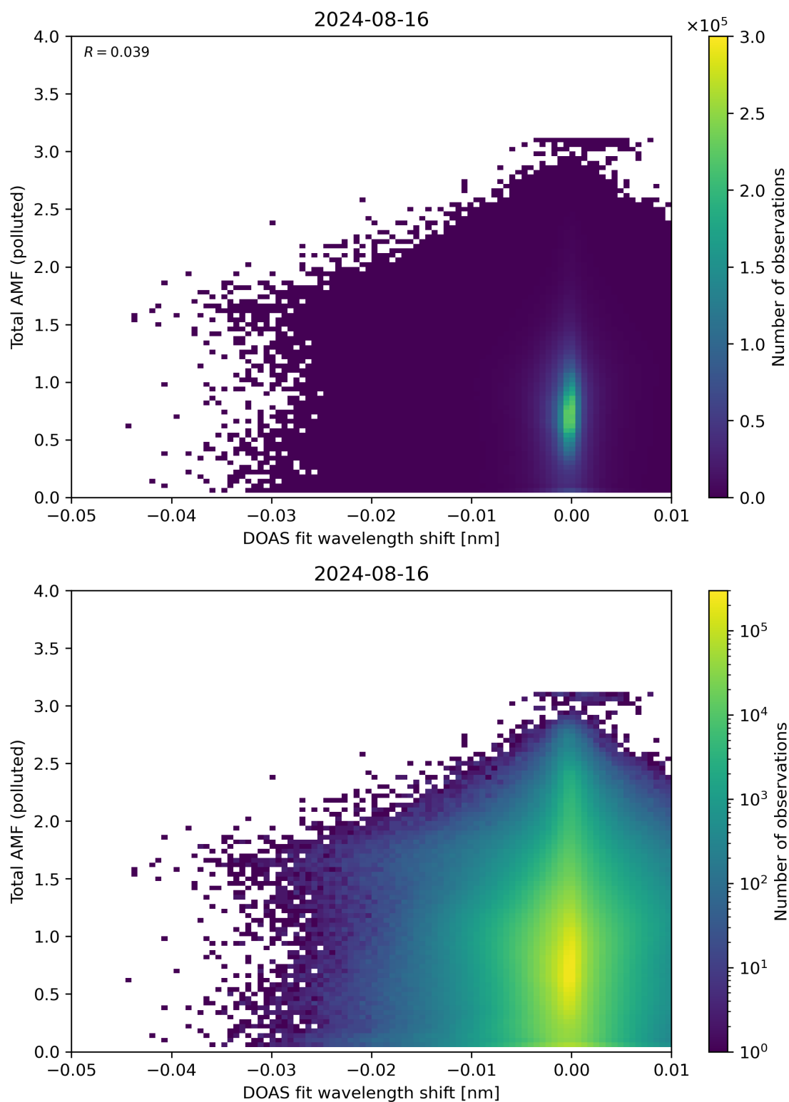
Figure 130: Scatter density plot of “DOAS fit wavelength shift” against “Total AMF (polluted)” for 2024-08-16 to 2024-08-17.
