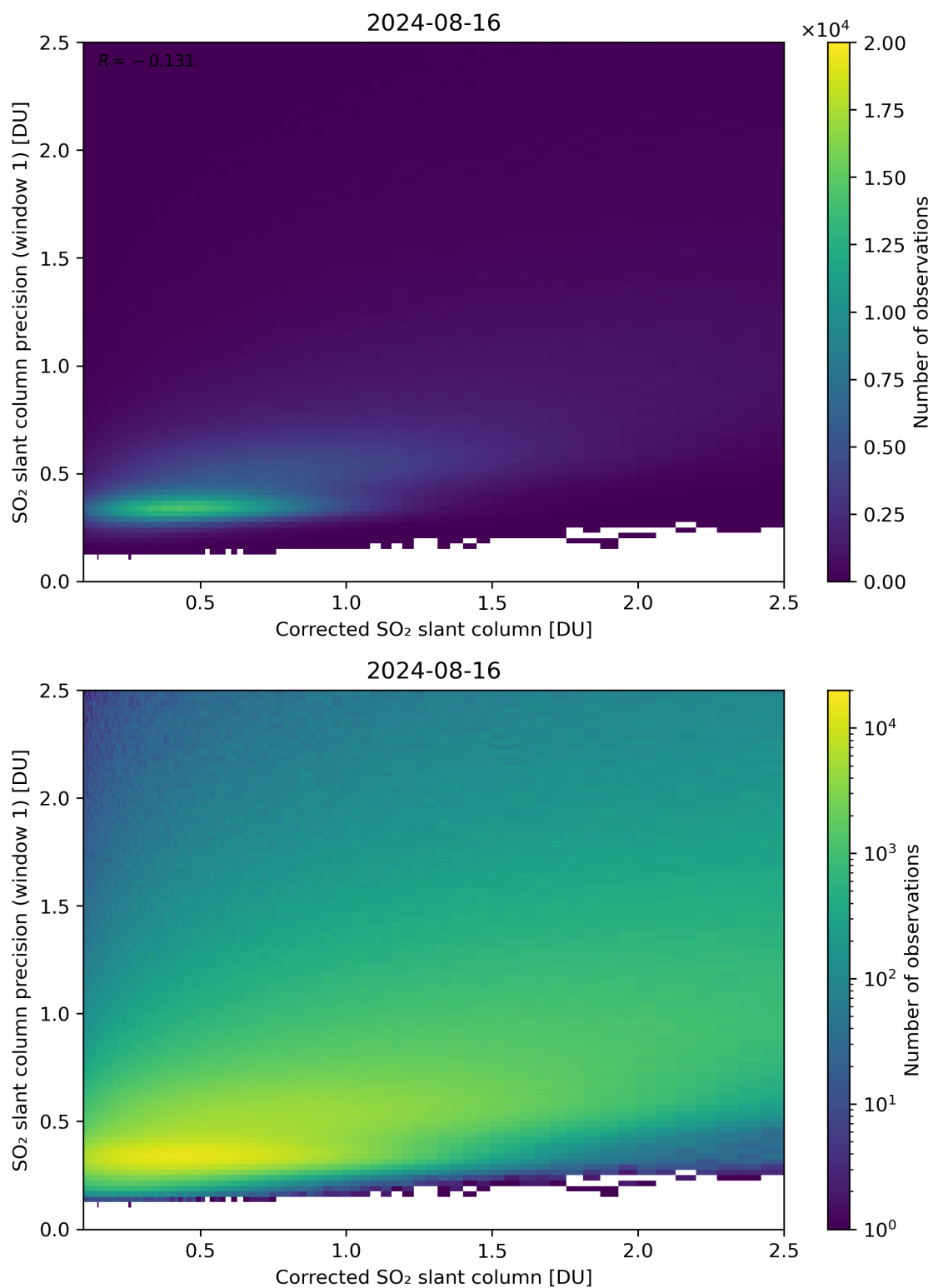
Figure 188: Scatter density plot of “Corrected SO 2 slant column” against “SO 2 slant column precision (window 1)” for 2024-08-16 to 2024-08-17.
