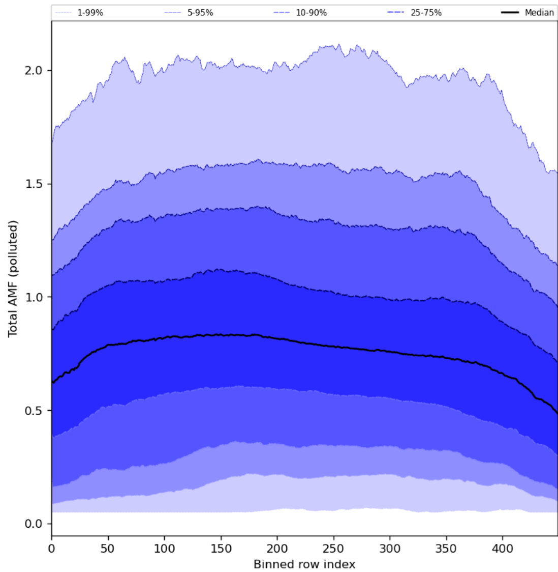
Figure 94: Along track statistics of “Total AMF (polluted)” for 2024-08-16 to 2024-08-17
