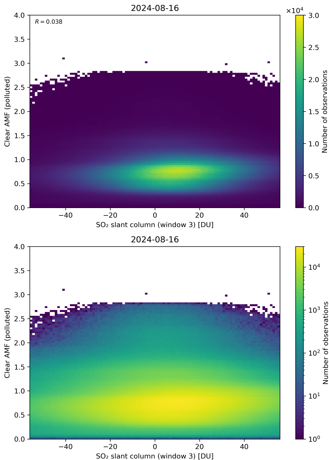
Figure 265: Scatter density plot of “SO 2 slant column (window 3)” against “Clear AMF (polluted)” for 2024-08-16 to 2024-08-17.
