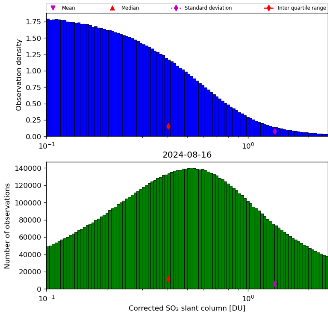
Figure 55: Histogram of “Corrected SO 2 slant column” for 2024-08-16 to 2024-08-17
