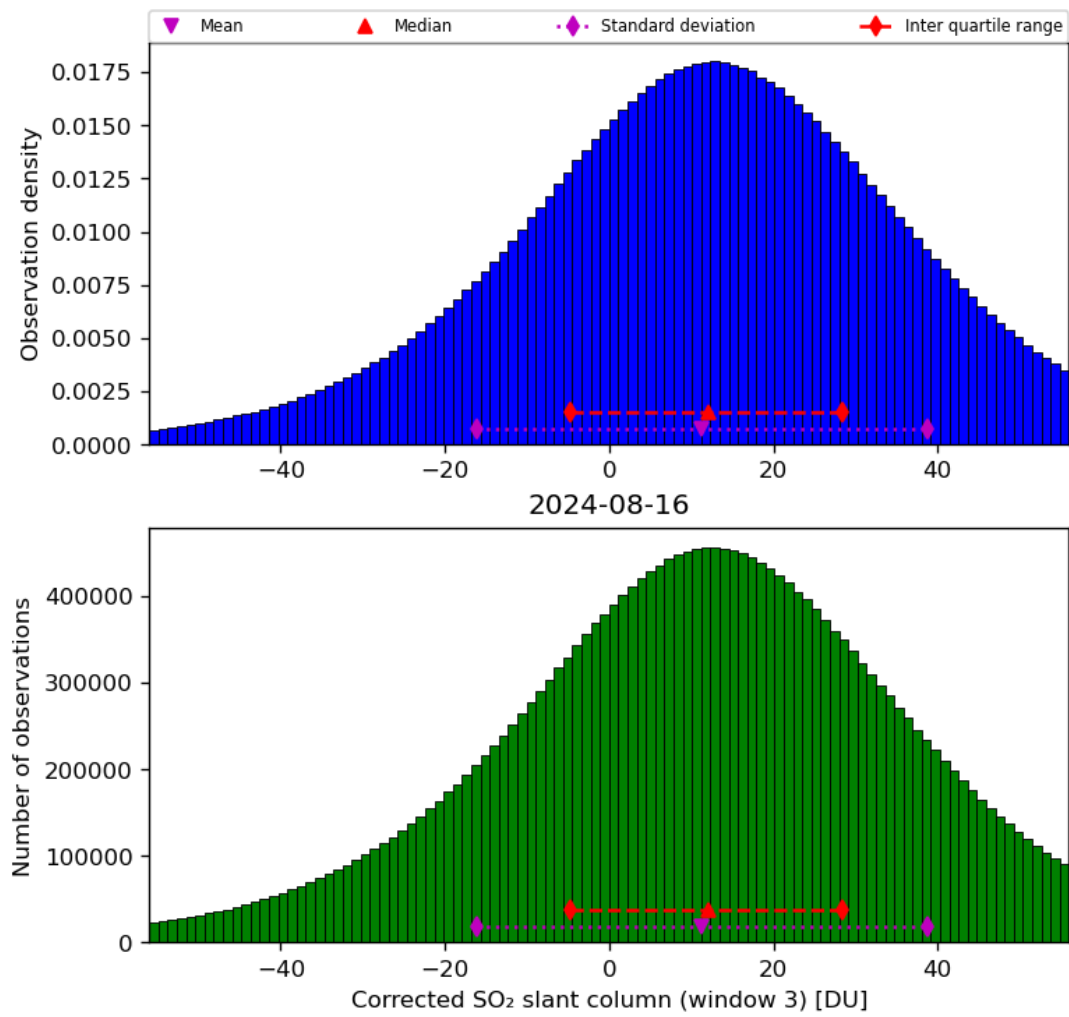
Figure 66: Histogram of “Corrected SO 2 slant column (window 3)” for 2024-08-16 to 2024-08-17
