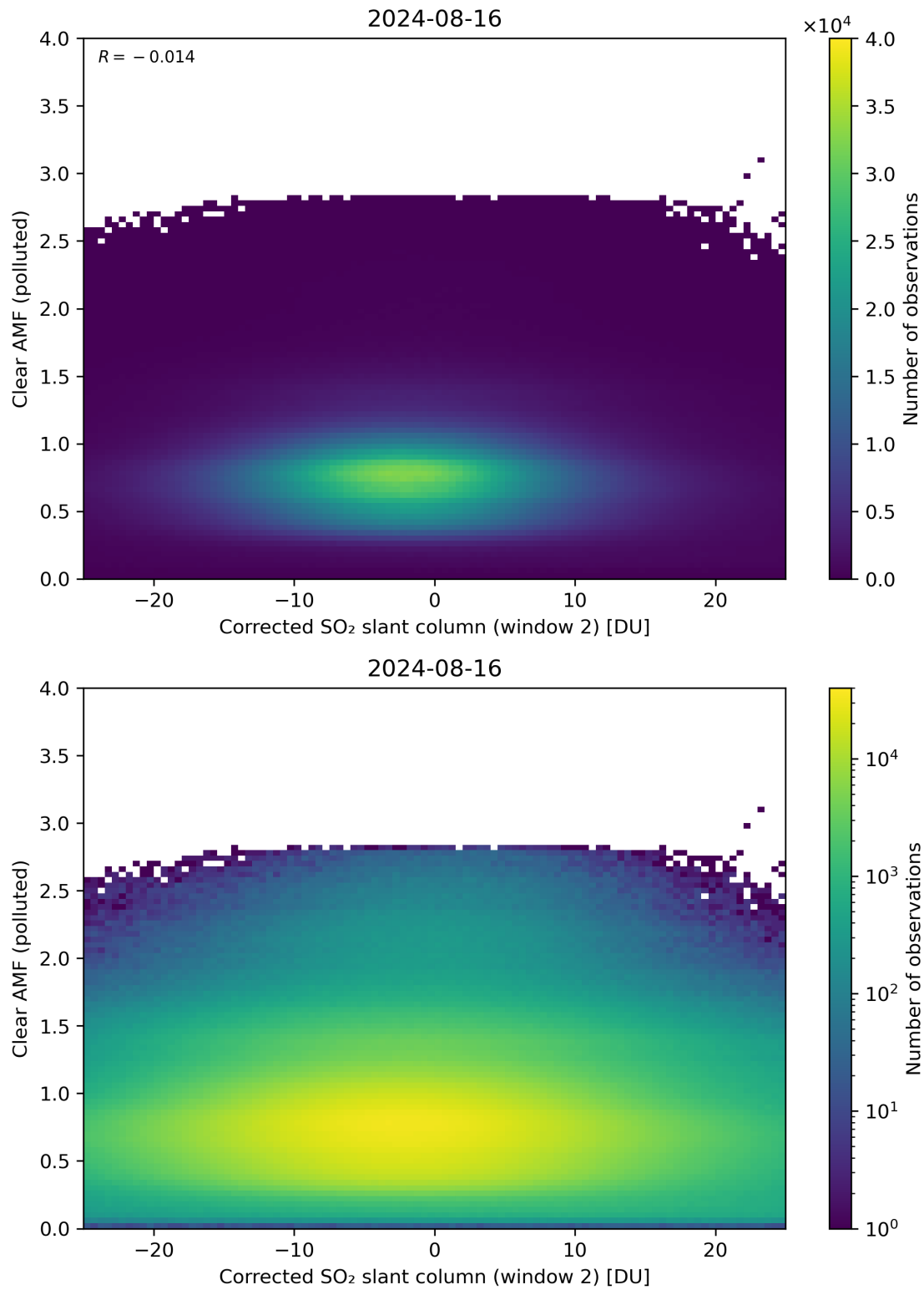
Figure 199: Scatter density plot of “Corrected SO 2 slant column (window 2)” against “Clear AMF (polluted)” for 2024-08-16 to 2024-08-17.
