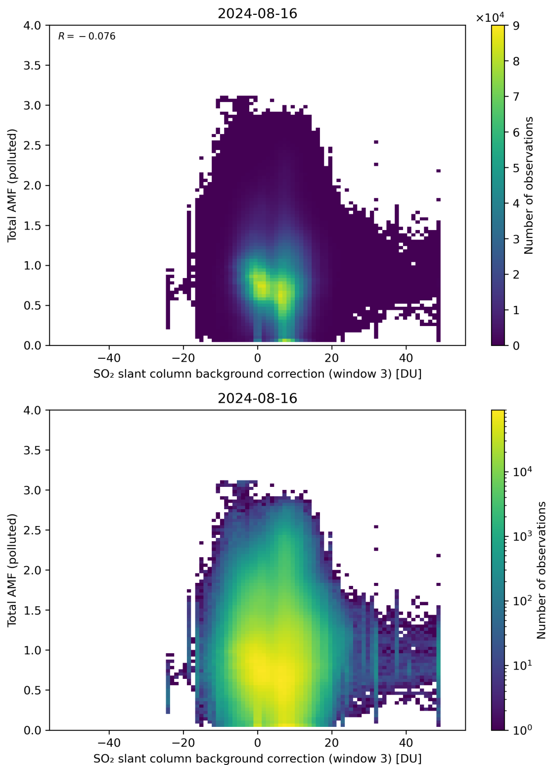
Figure 125: Scatter density plot of “SO 2 slant column background correction (window 3)” against “Total AMF (polluted)” for 2024-08-16 to 2024-08-17.
