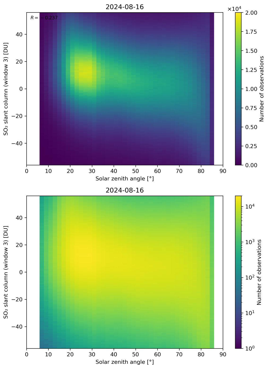
Figure 172: Scatter density plot of “Solar zenith angle” against “SO 2 slant column (window 3)” for 2024-08-16 to 2024-08-17.
