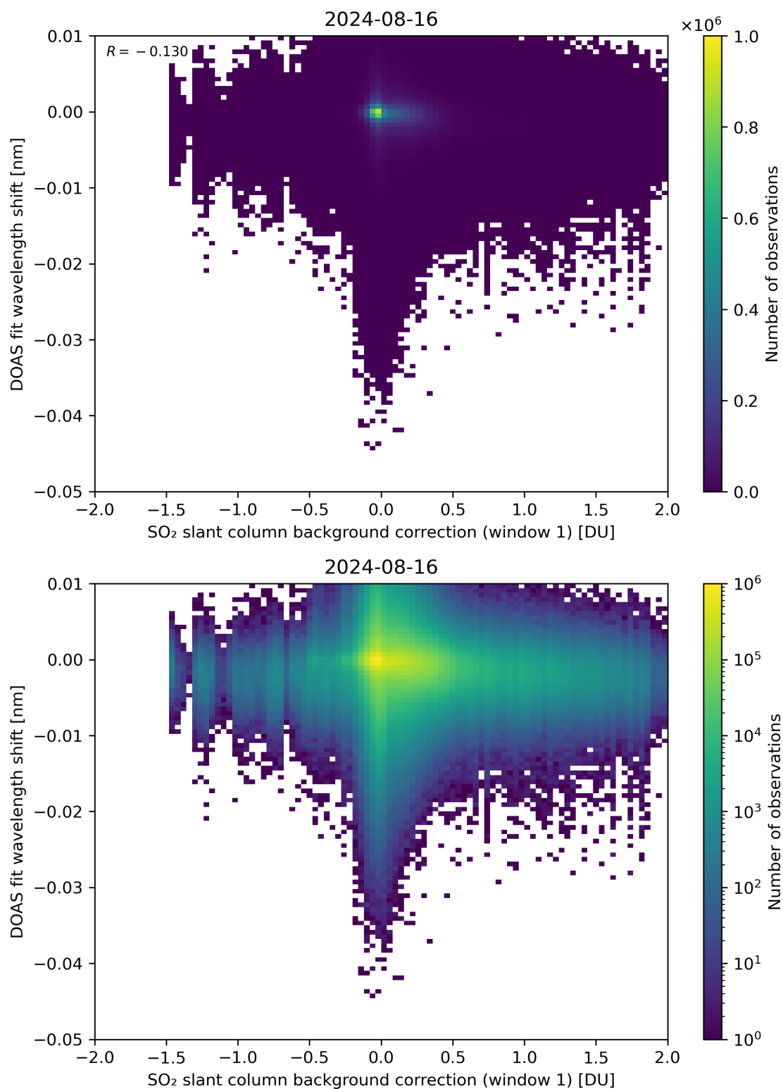
Figure 100: Scatter density plot of “SO 2 slant column background correction (window 1)” against “DOAS fit wavelength shift” for 2024-08-16 to 2024-08-17.
