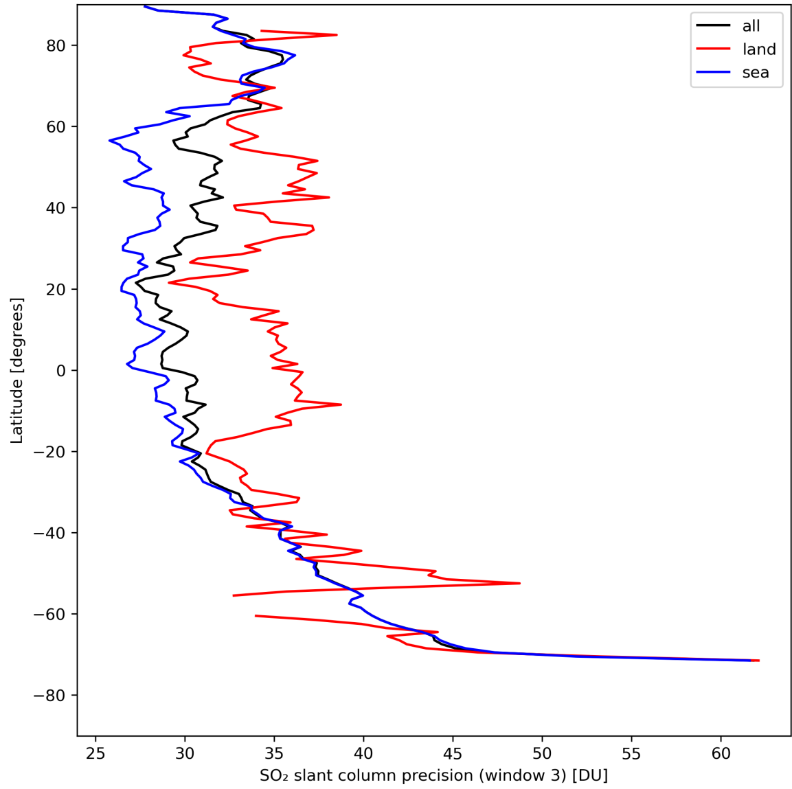
Figure 42: Zonal average of “SO 2 slant column precision (window 3)” for 2024-08-16 to 2024-08-17.
