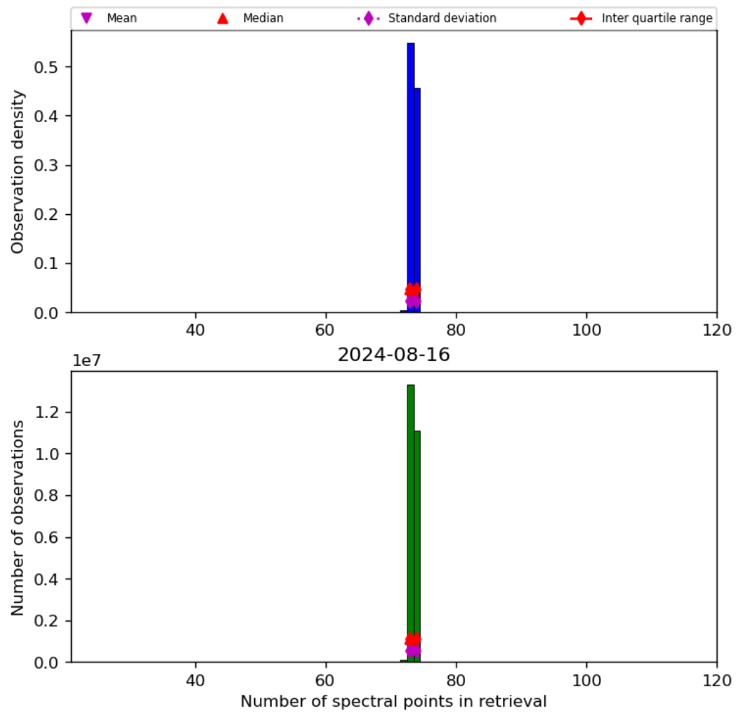
Figure 74: Histogram of “Number of spectral points in retrieval” for 2024-08-16 to 2024-08-17
