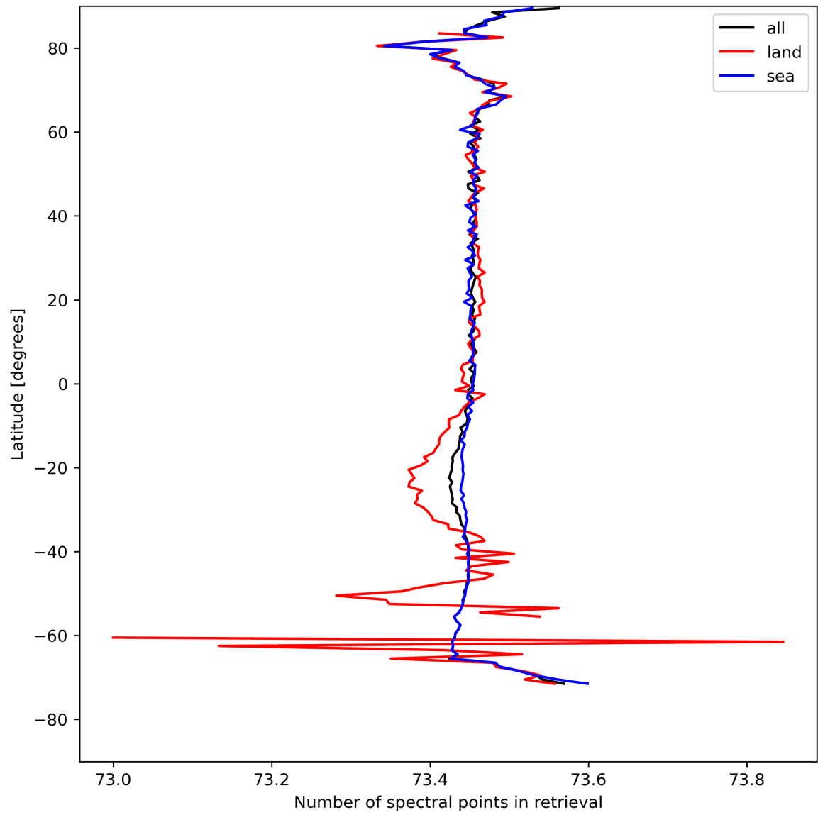
Figure 51: Zonal average of “Number of spectral points in retrieval” for 2024-08-16 to 2024-08-17.
