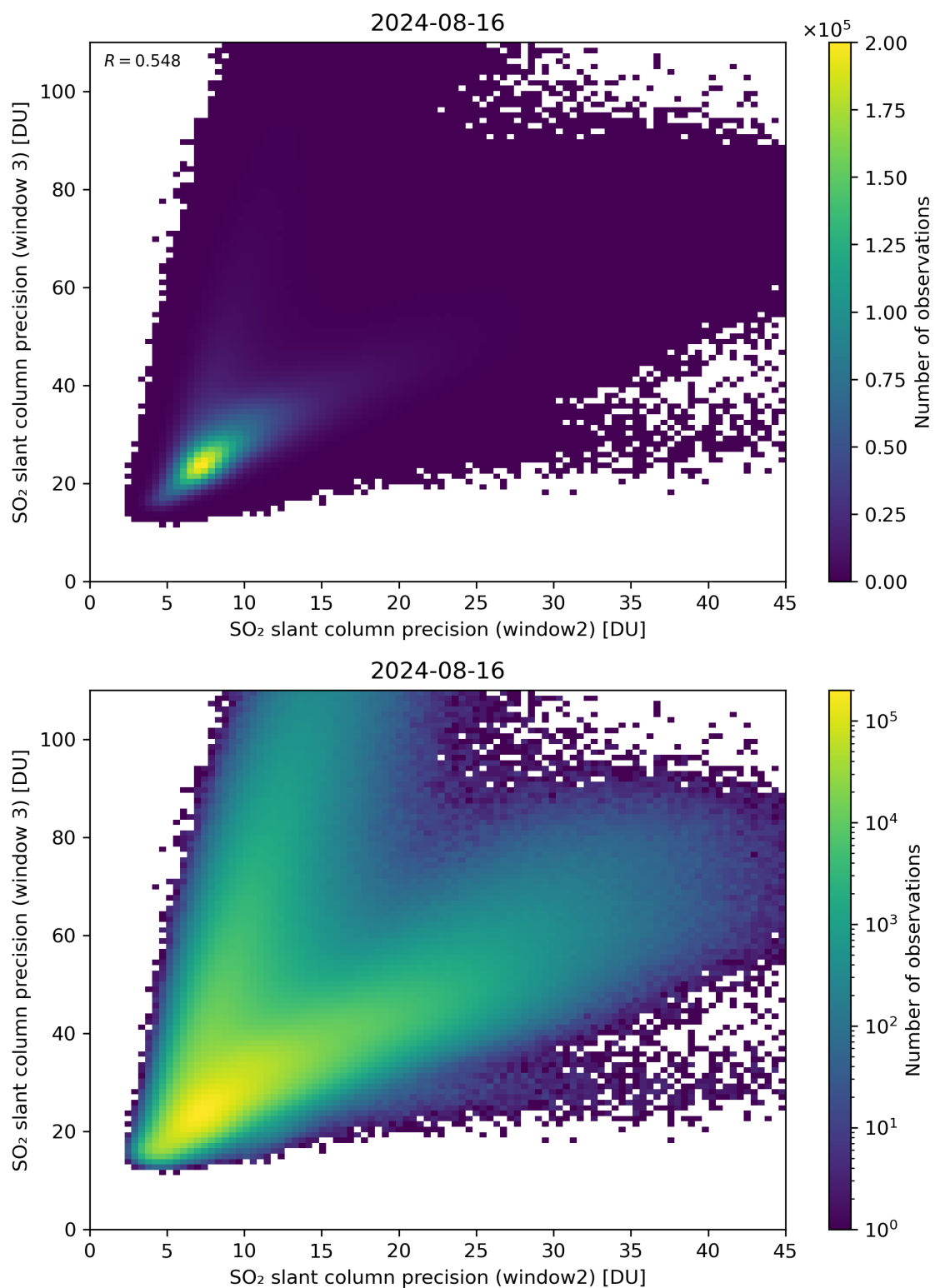
Figure 250: Scatter density plot of “SO 2 slant column precision (window2)” against “SO 2 slant column precision (window 3)” for 2024-08-16 to 2024-08-17.
