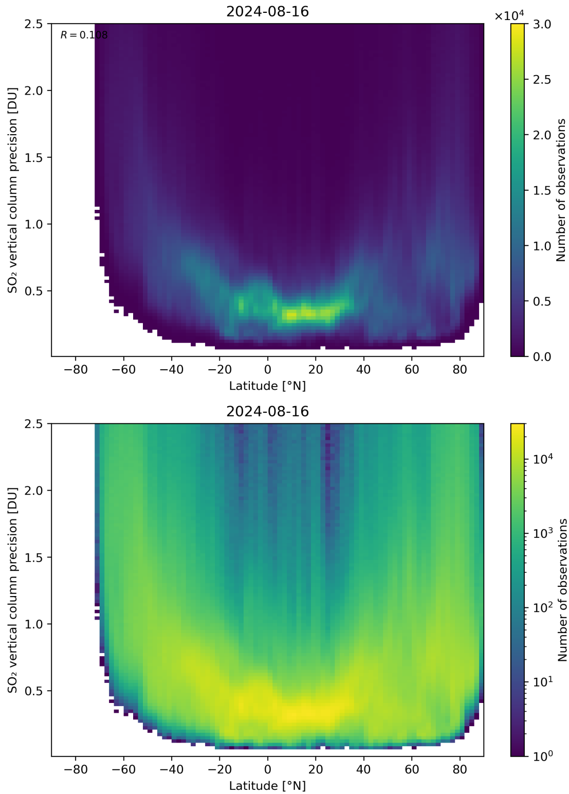
Figure 157: Scatter density plot of “Latitude” against “SO 2 vertical column precision” for 2024-08-16 to 2024-08-17.
