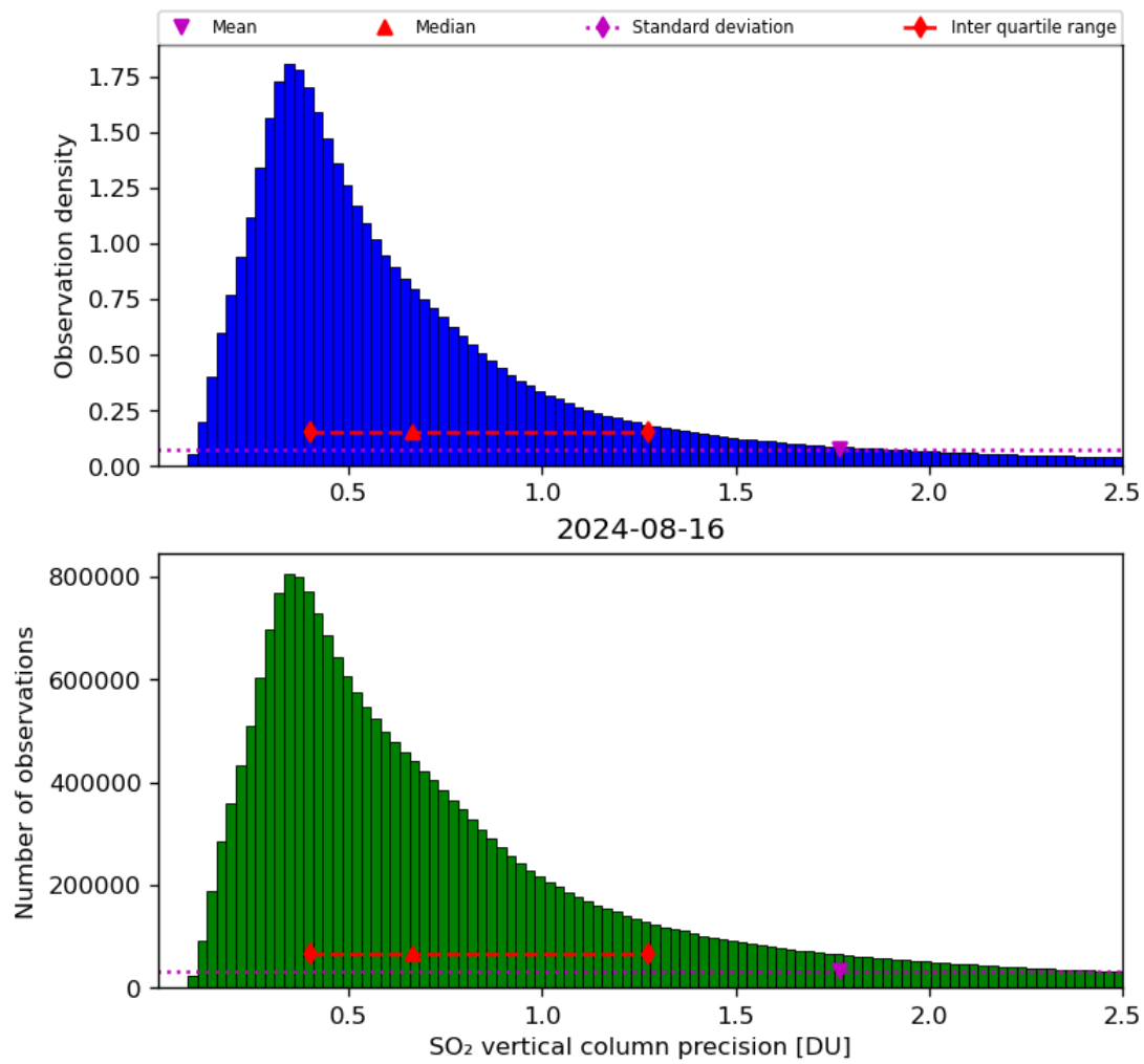
Figure 54: Histogram of “SO 2 vertical column precision” for 2024-08-16 to 2024-08-17
