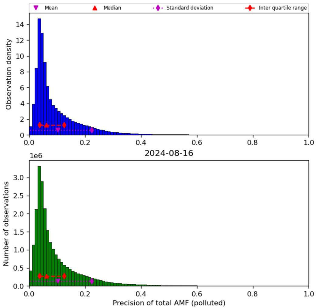
Figure 72: Histogram of “Precision of total AMF (polluted)” for 2024-08-16 to 2024-08-17
