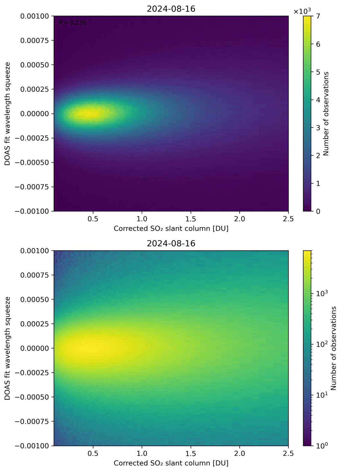
Figure 182: Scatter density plot of “Corrected SO 2 slant column” against “DOAS fit wavelength squeeze” for 2024-08-16 to 2024-08-17.
