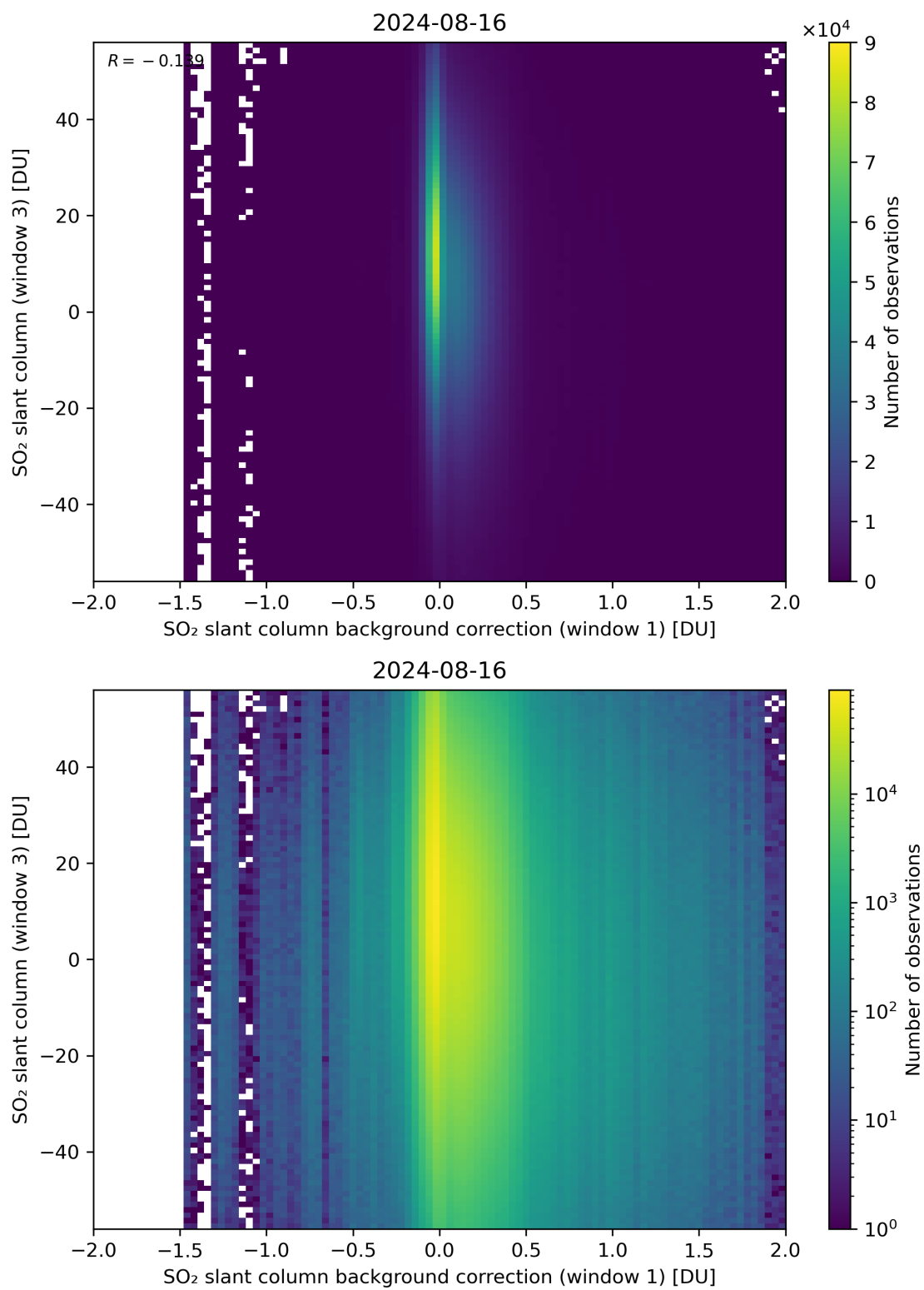
Figure 107: Scatter density plot of “SO 2 slant column background correction (window 1)” against “SO 2 slant column (window 3)” for 2024-08-16 to 2024-08-17.
