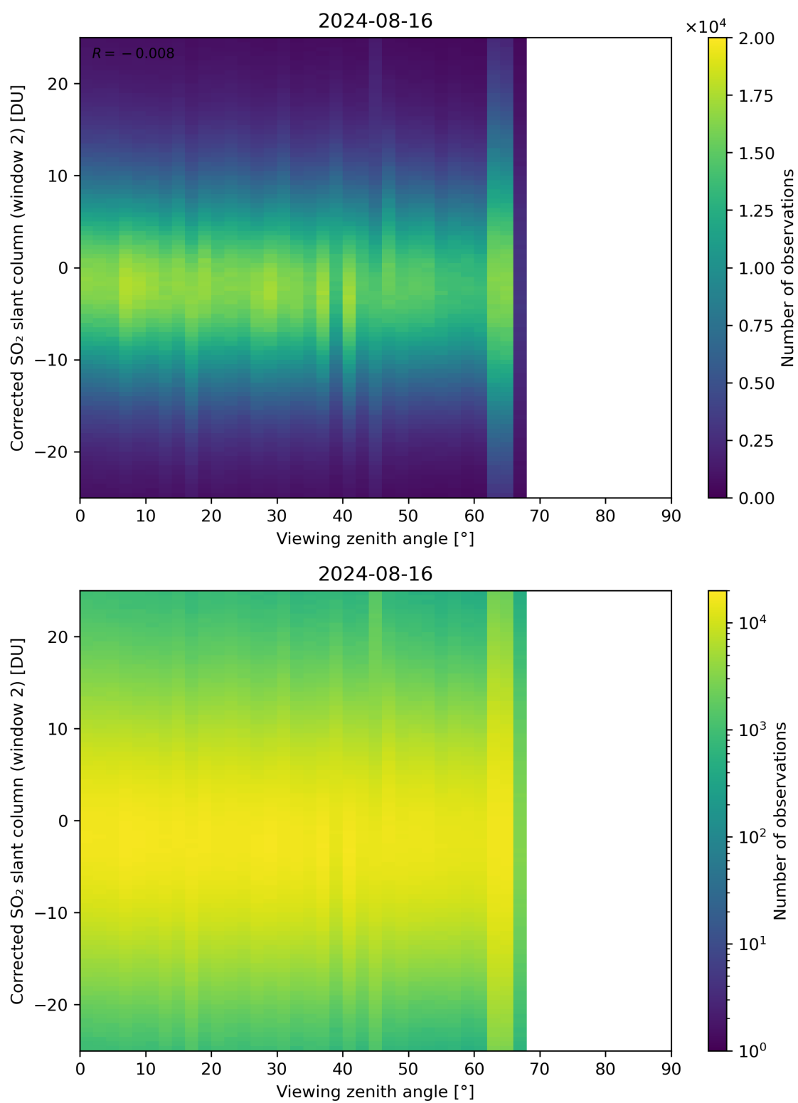
Figure 318: Scatter density plot of “Viewing zenith angle” against “Corrected SO 2 slant column (window 2)” for 2024-08-16 to 2024-08-17.
