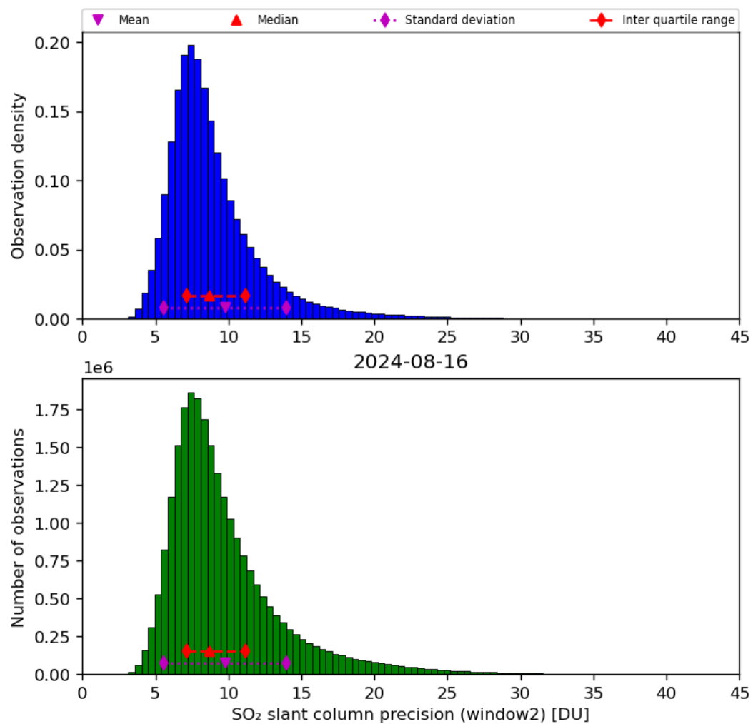
Figure 61: Histogram of “SO 2 slant column precision (window2)” for 2024-08-16 to 2024-08-17
