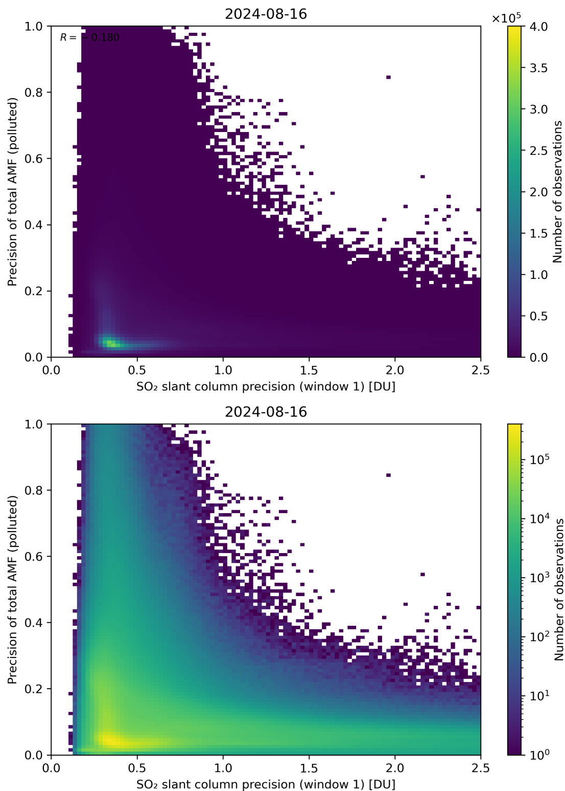
Figure 231: Scatter density plot of “SO 2 slant column precision (window 1)” against “Precision of total AMF (polluted)” for 2024-08-16 to 2024-08-17.
