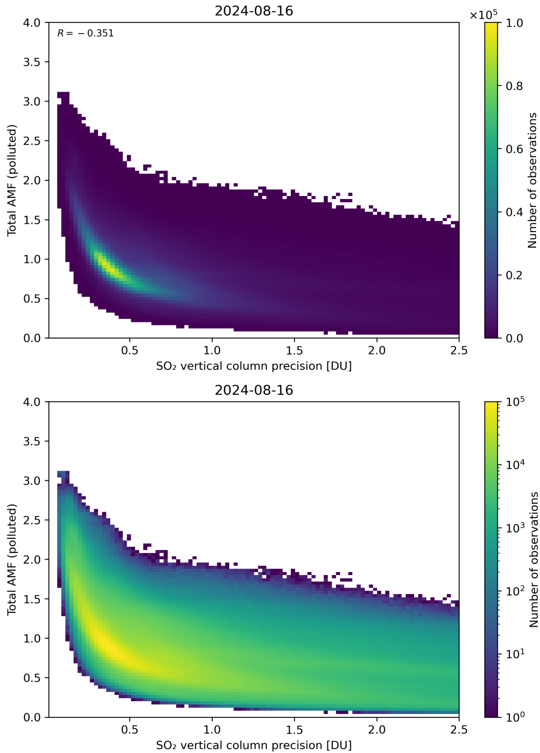
Figure 294: Scatter density plot of “SO 2 vertical column precision” against “Total AMF (polluted)” for 2024-08-16 to 2024-08-17.
