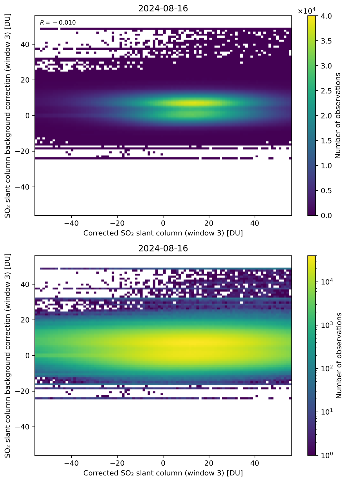
Figure 205: Scatter density plot of “Corrected SO 2 slant column (window 3)” against “SO 2 slant column background correction (window 3)” for 2024-08-16 to 2024-08-17.
