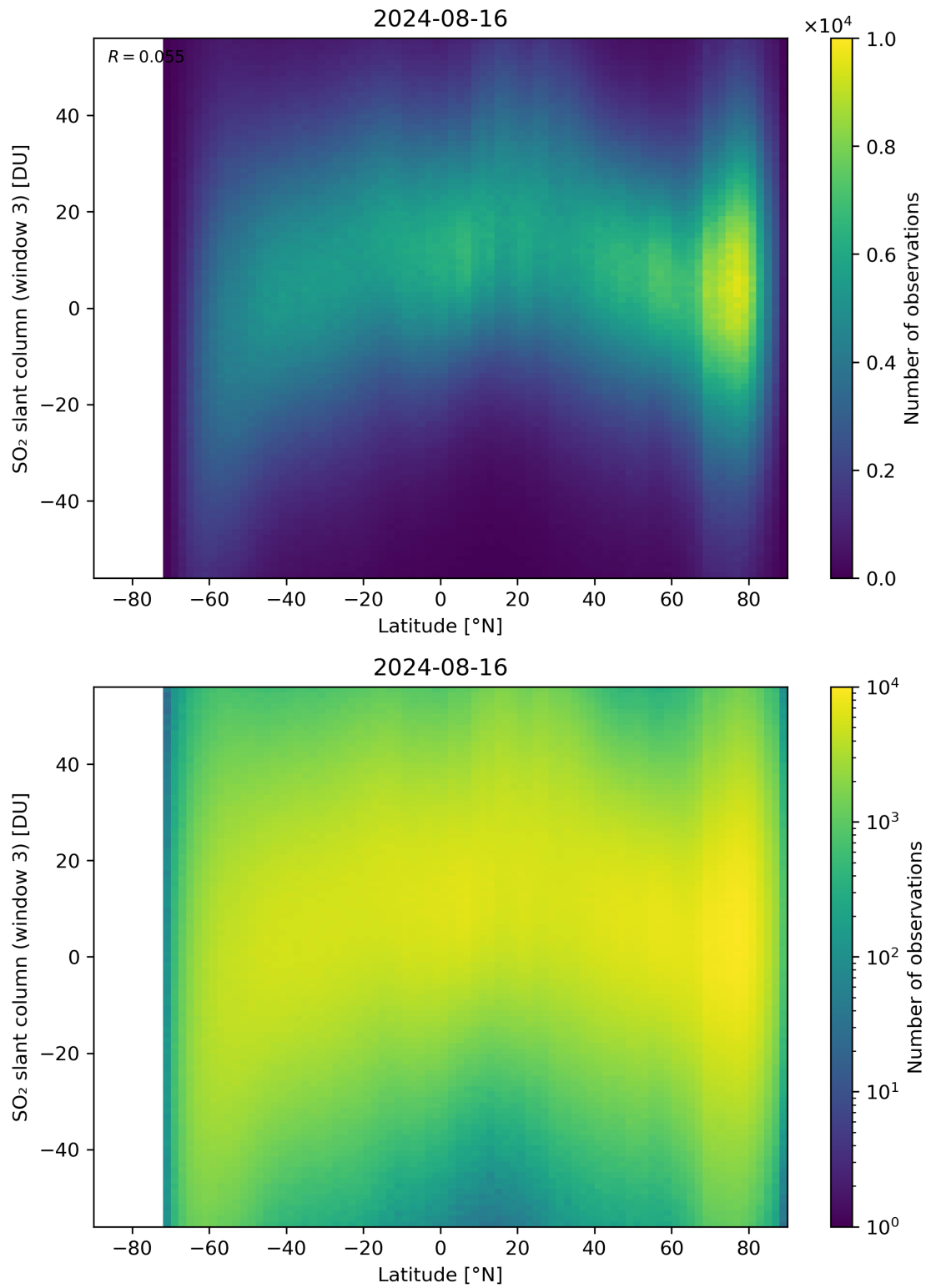
Figure 152: Scatter density plot of “Latitude” against “SO 2 slant column (window 3)” for 2024-08-16 to 2024-08-17.
