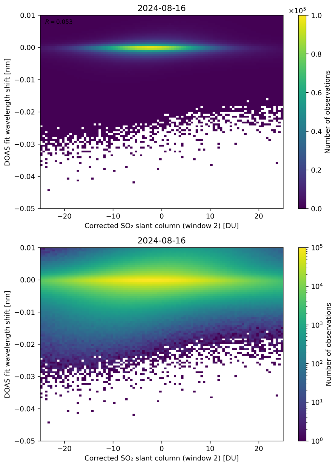
Figure 196: Scatter density plot of “Corrected SO 2 slant column (window 2)” against “DOAS fit wavelength shift” for 2024-08-16 to 2024-08-17.
