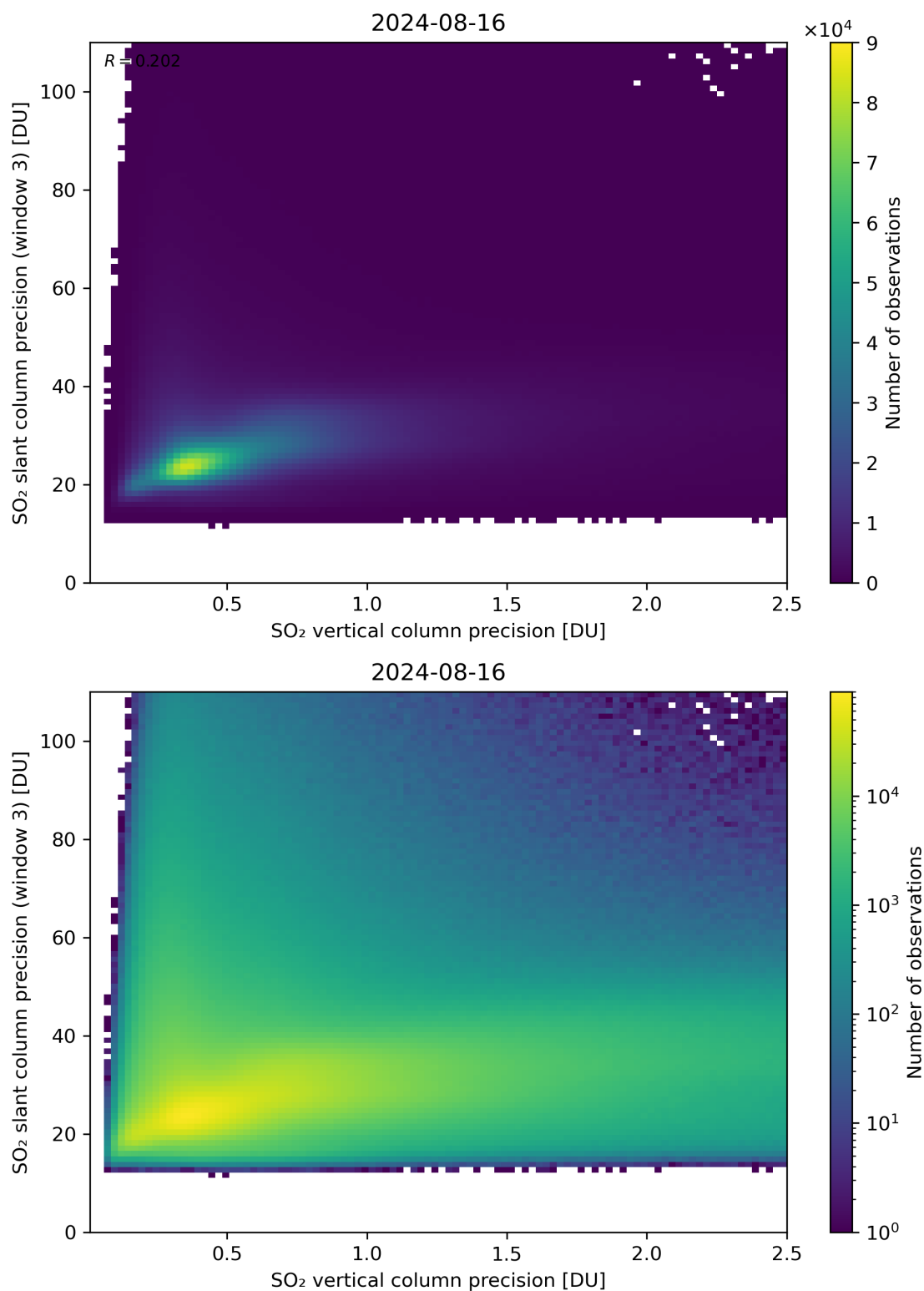
Figure 293: Scatter density plot of “SO 2 vertical column precision” against “SO 2 slant column precision (window 3)” for 2024-08-16 to 2024-08-17.
