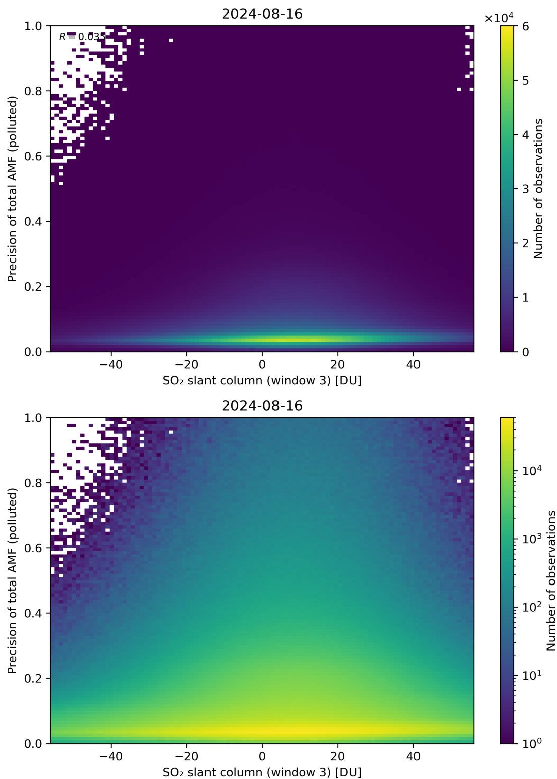
Figure 269: Scatter density plot of “SO 2 slant column (window 3)” against “Precision of total AMF (polluted)” for 2024-08-16 to 2024-08-17.
