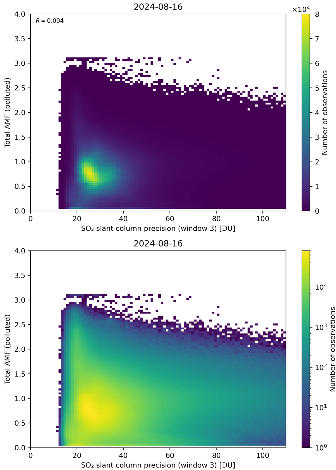
Figure 263: Scatter density plot of “SO 2 slant column precision (window 3)” against “Total AMF (polluted)” for 2024-08-16 to 2024-08-17.
