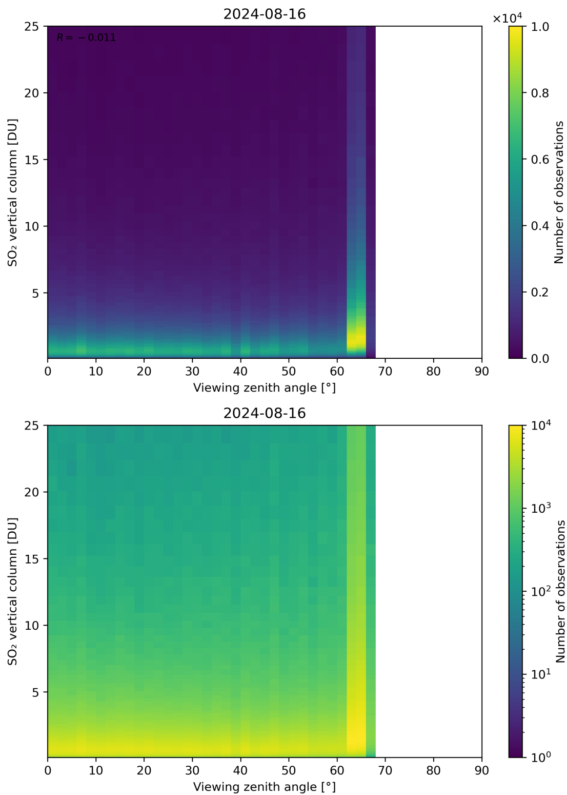
Figure 327: Scatter density plot of “Viewing zenith angle” against “SO 2 vertical column” for 2024-08-16 to 2024-08-17.
