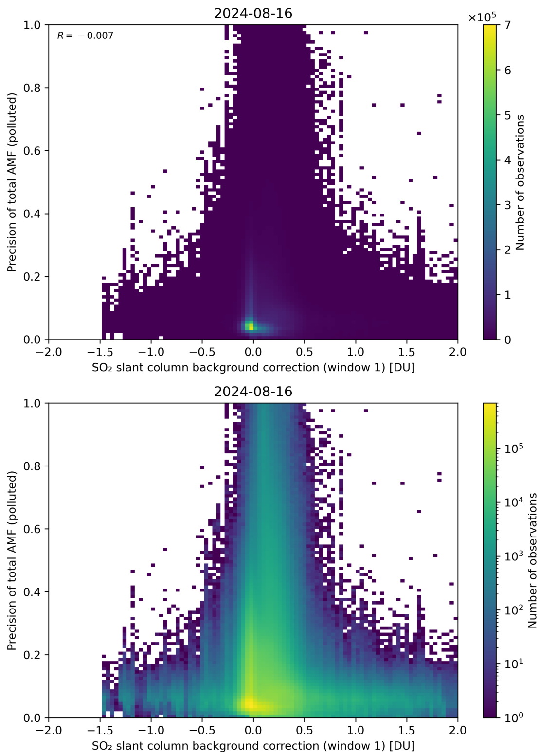
Figure 110: Scatter density plot of “SO 2 slant column background correction (window 1)” against “Precision of total AMF (polluted)” for 2024-08-16 to 2024-08-17.
