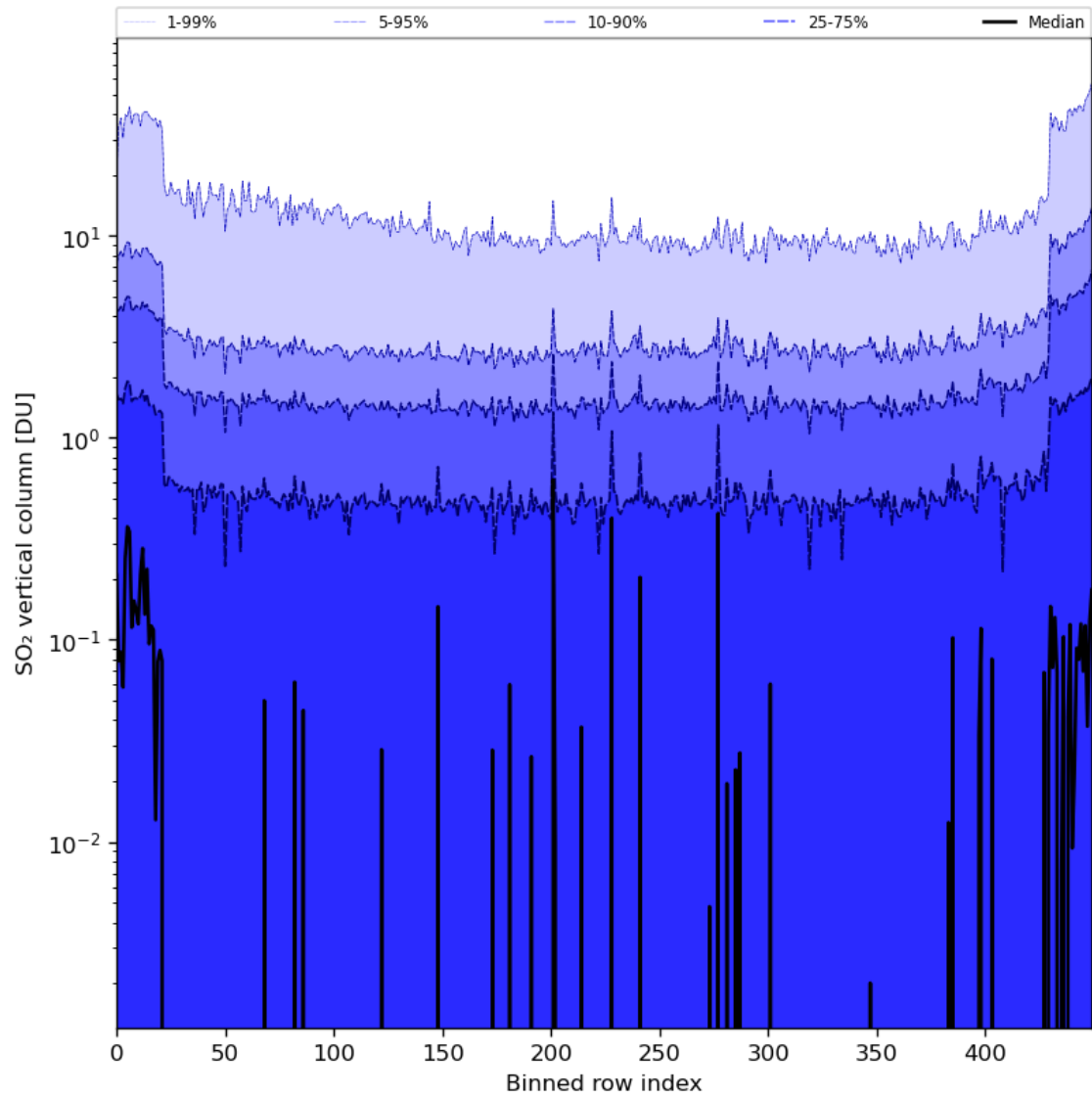
Figure 76: Along track statistics of “SO 2 vertical column” for 2024-08-16 to 2024-08-17
