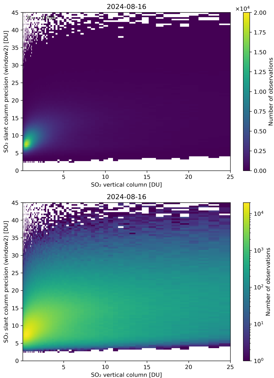
Figure 302: Scatter density plot of “SO 2 vertical column” against “SO 2 slant column precision (window2)” for 2024-08-16 to 2024-08-17.
