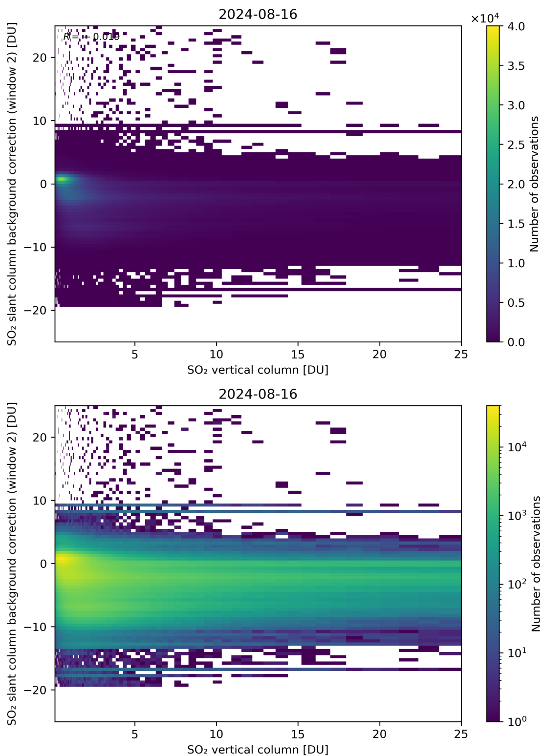
Figure 274: Scatter density plot of “SO 2 vertical column” against “SO 2 slant column background correction (window 2)” for 2024-08-16 to 2024-08-17.
