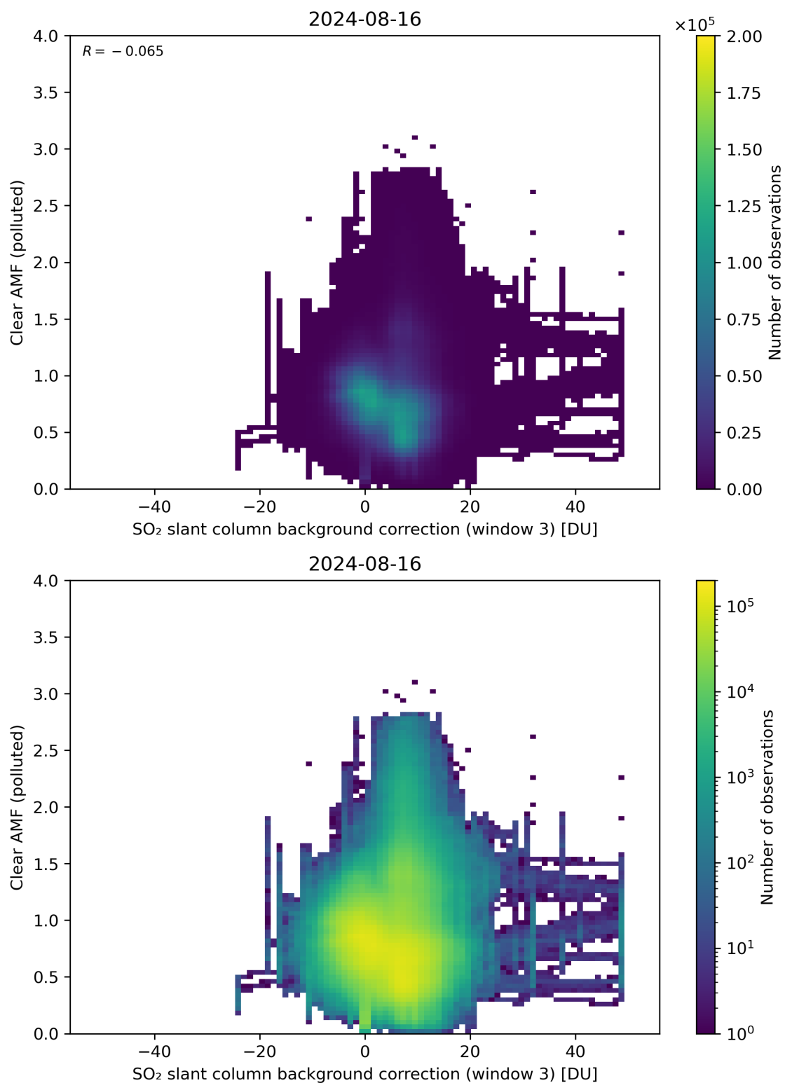
Figure 124: Scatter density plot of “SO 2 slant column background correction (window 3)” against “Clear AMF (polluted)” for 2024-08-16 to 2024-08-17.
