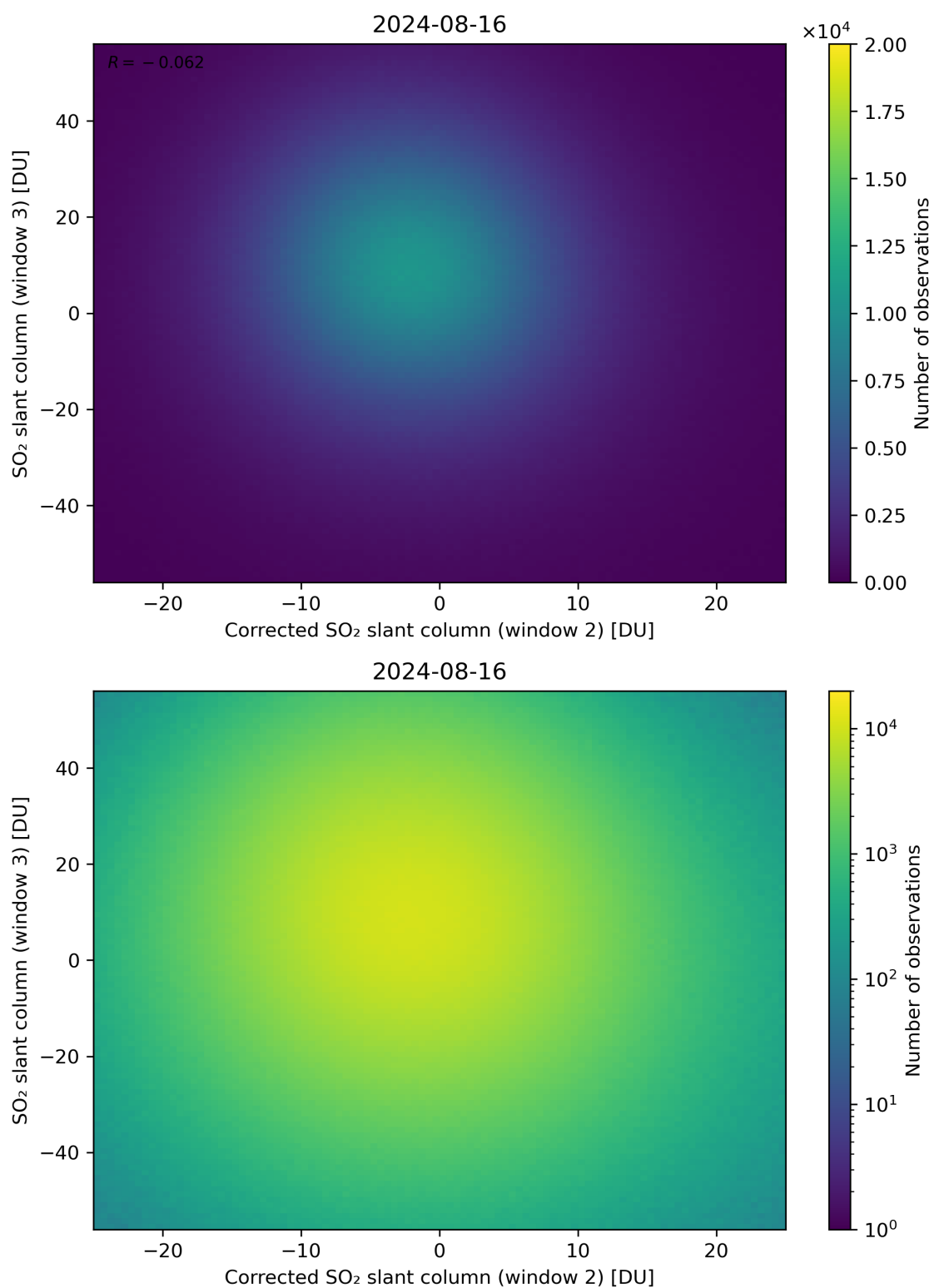
Figure 201: Scatter density plot of “Corrected SO 2 slant column (window 2)” against “SO 2 slant column (window 3)” for 2024-08-16 to 2024-08-17.
