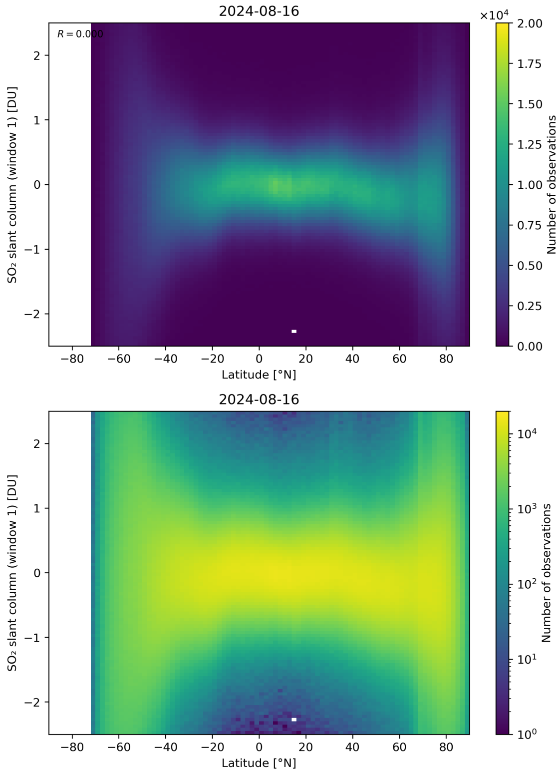
Figure 149: Scatter density plot of “Latitude” against “SO 2 slant column (window 1)” for 2024-08-16 to 2024-08-17.
