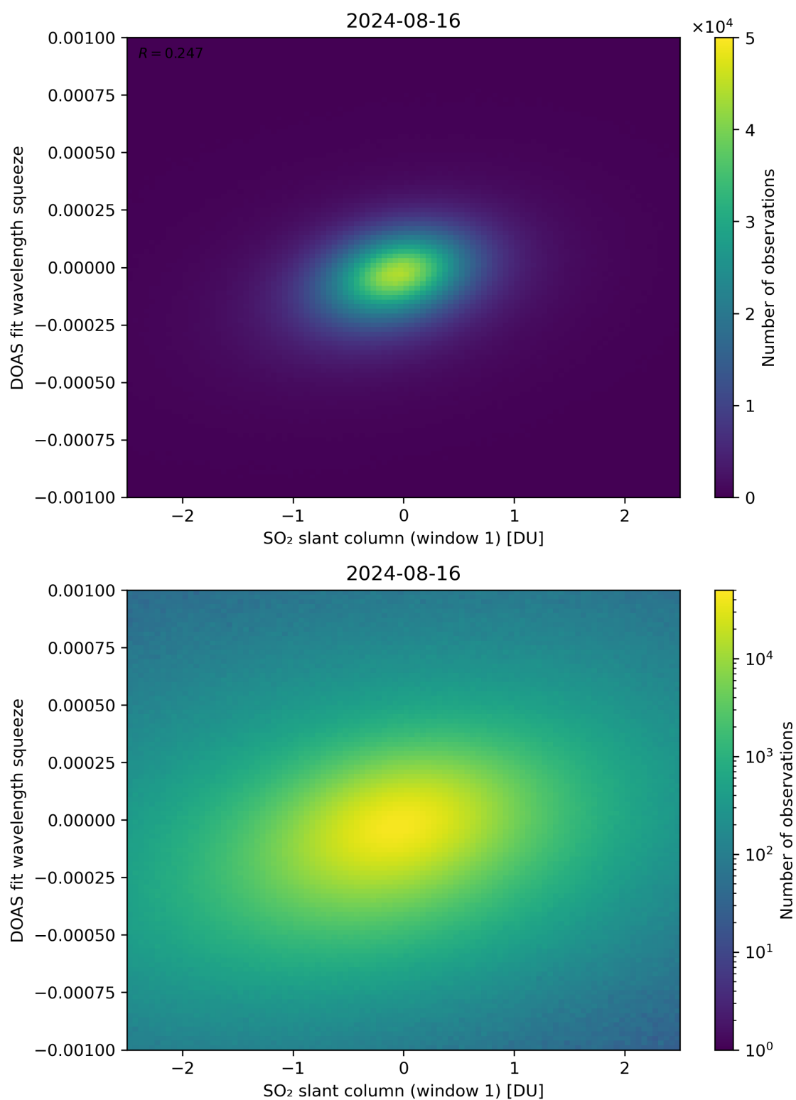
Figure 216: Scatter density plot of “SO 2 slant column (window 1)” against “DOAS fit wavelength squeeze” for 2024-08-16 to 2024-08-17.
