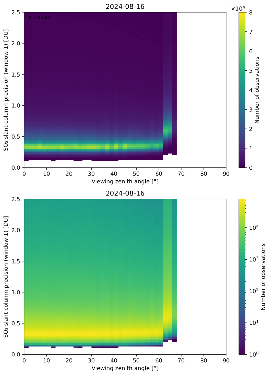
Figure 321: Scatter density plot of “Viewing zenith angle” against “SO 2 slant column precision (window 1)” for 2024-08-16 to 2024-08-17.
