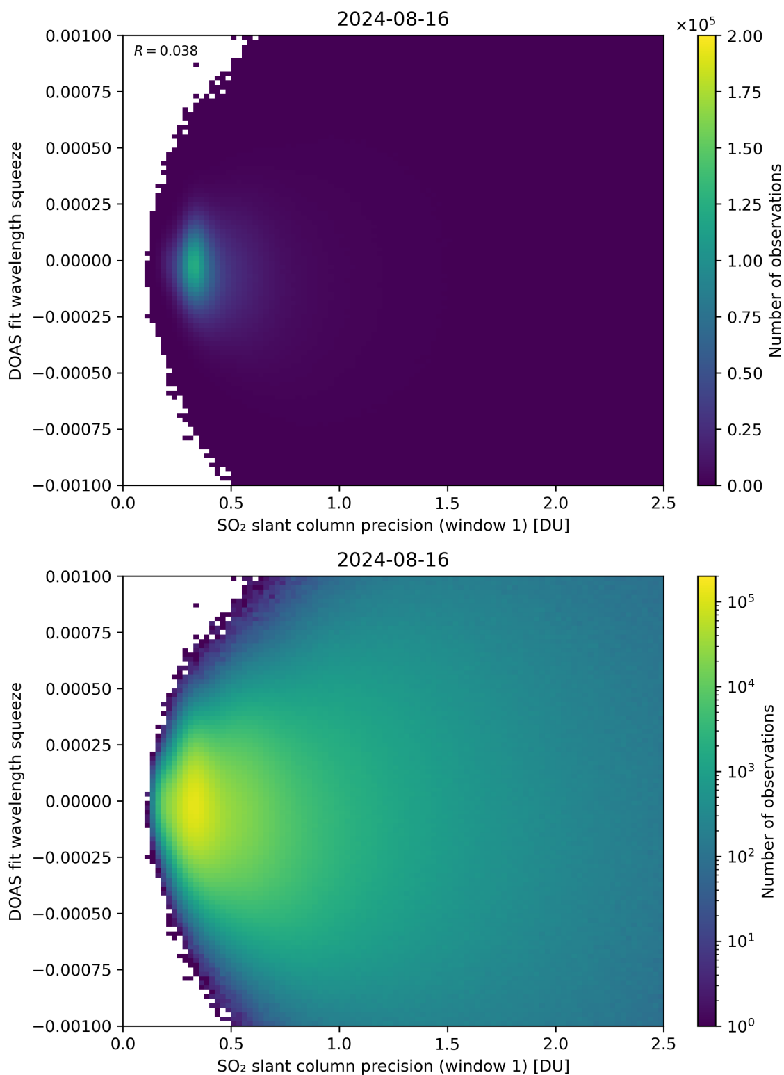
Figure 222: Scatter density plot of “SO 2 slant column precision (window 1)” against “DOAS fit wavelength squeeze” for 2024-08-16 to 2024-08-17.
