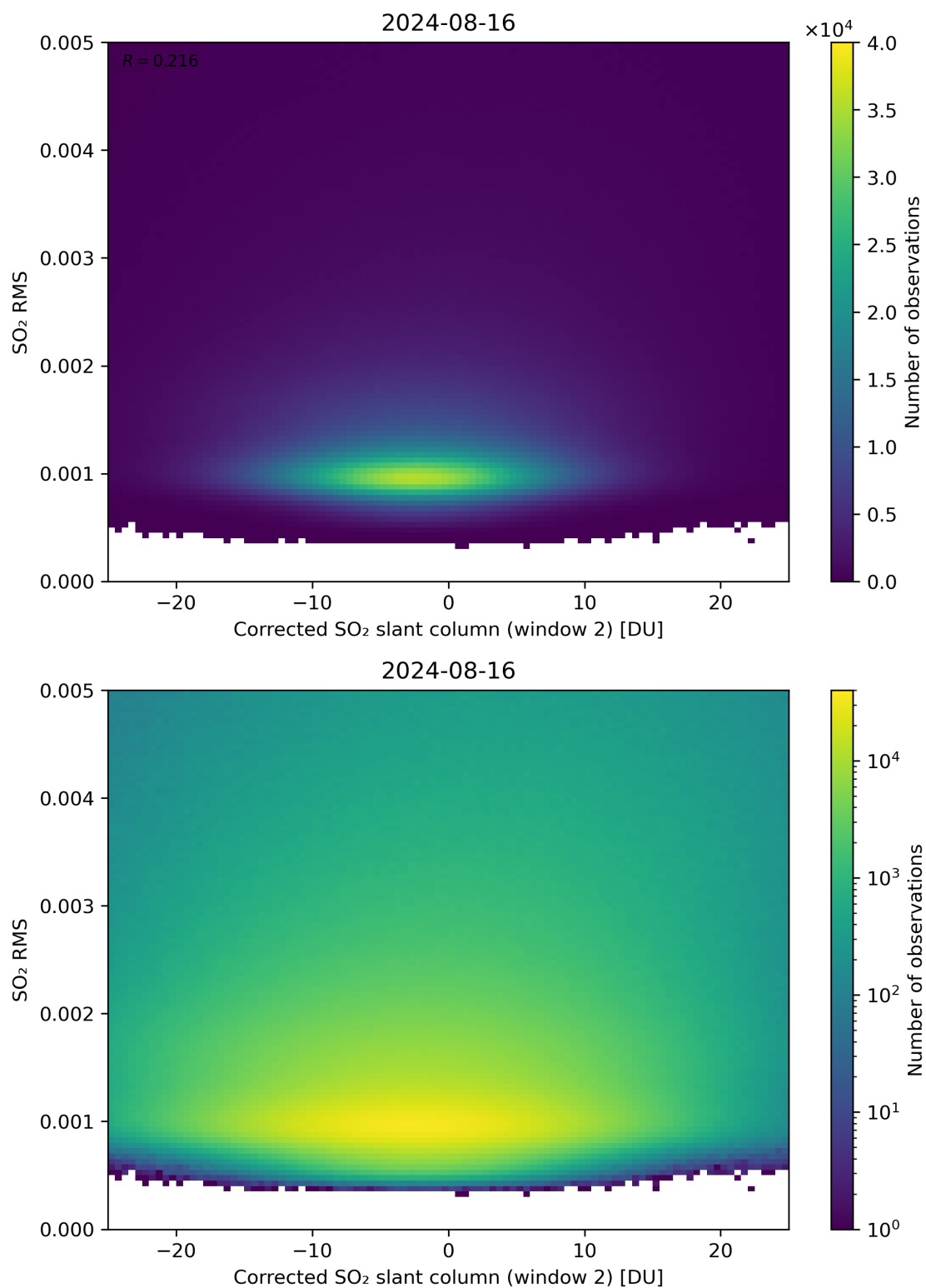
Figure 198: Scatter density plot of “Corrected SO 2 slant column (window 2)” against “SO 2 RMS” for 2024-08-16 to 2024-08-17.
