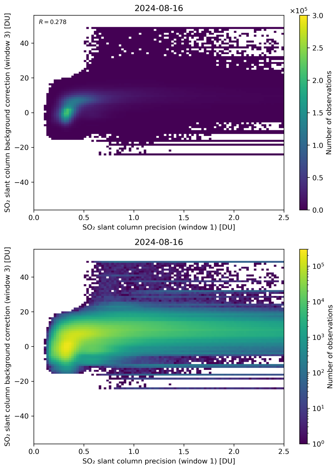
Figure 220: Scatter density plot of “SO 2 slant column precision (window 1)” against “SO 2 slant column background correction (window 3)” for 2024-08-16 to 2024-08-17.
