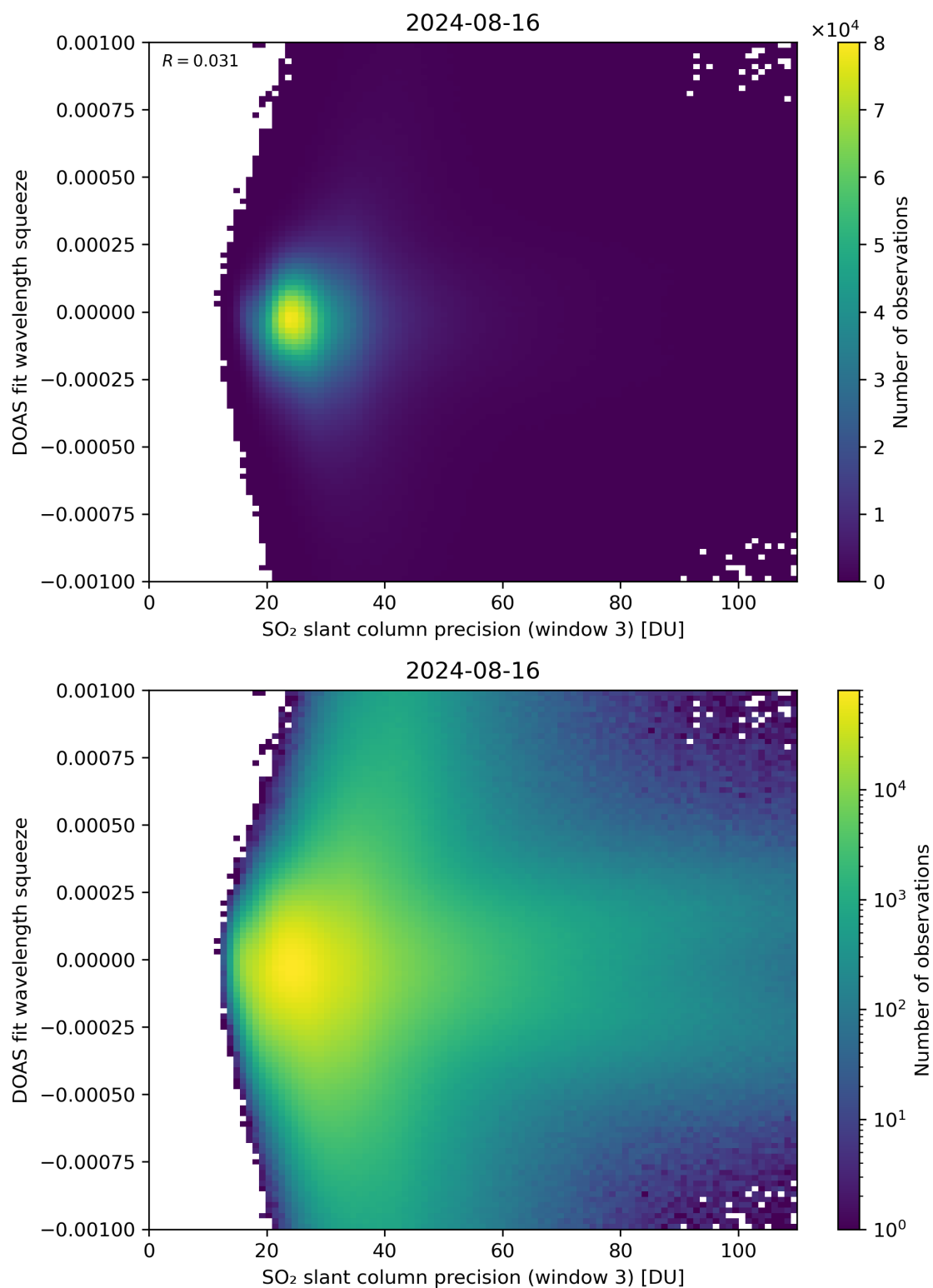
Figure 259: Scatter density plot of “SO 2 slant column precision (window 3)” against “DOAS fit wavelength squeeze” for 2024-08-16 to 2024-08-17.
