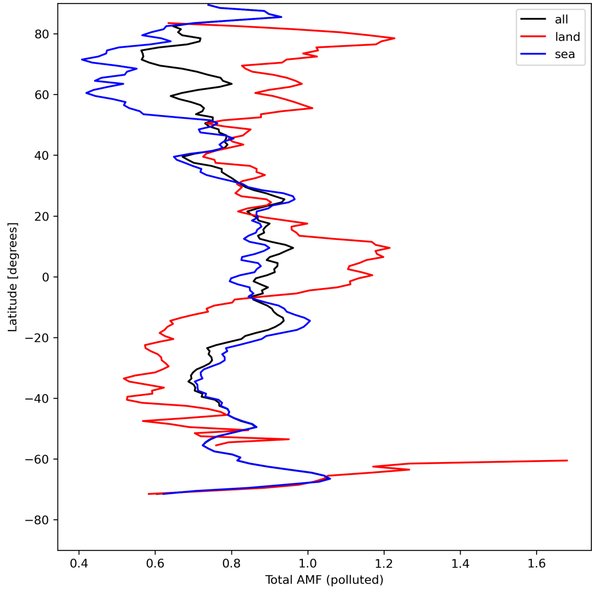
Figure 48: Zonal average of “Total AMF (polluted)” for 2024-08-16 to 2024-08-17.
