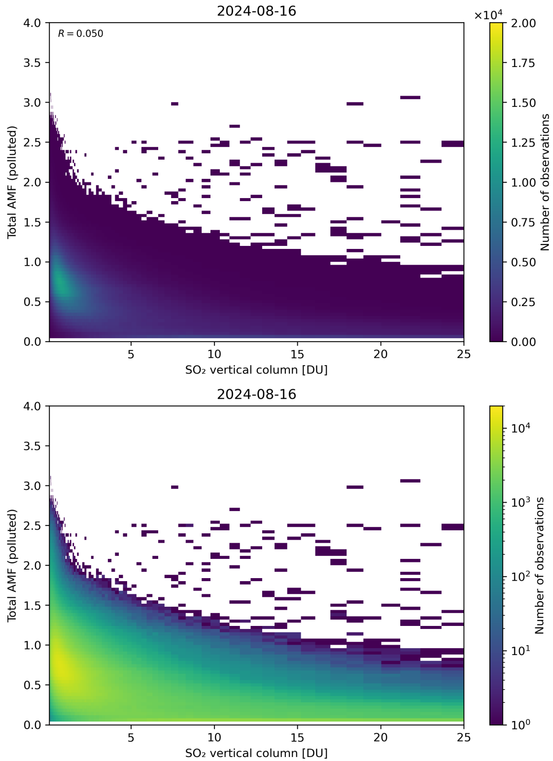
Figure 305: Scatter density plot of “SO 2 vertical column” against “Total AMF (polluted)” for 2024-08-16 to 2024-08-17.
