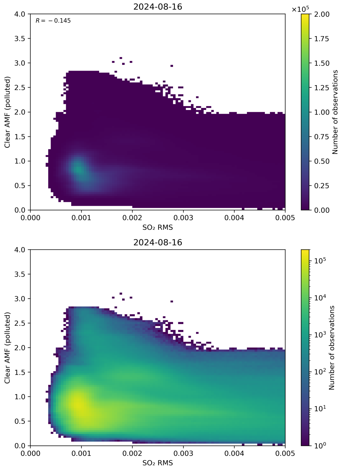
Figure 136: Scatter density plot of “SO 2 RMS” against “Clear AMF (polluted)” for 2024-08-16 to 2024-08-17.
