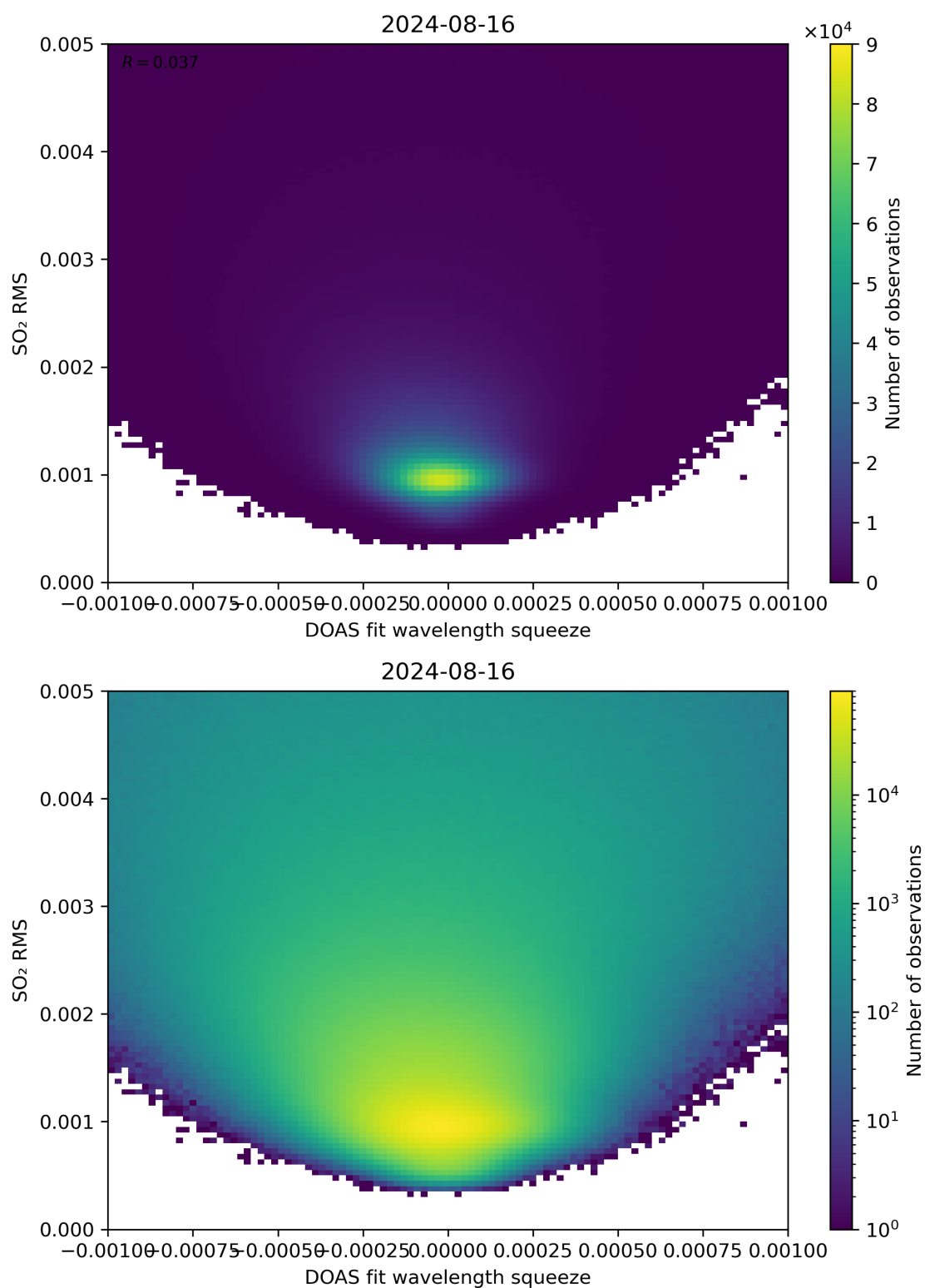
Figure 132: Scatter density plot of “DOAS fit wavelength squeeze” against “SO 2 RMS” for 2024-08-16 to 2024-08-17.
