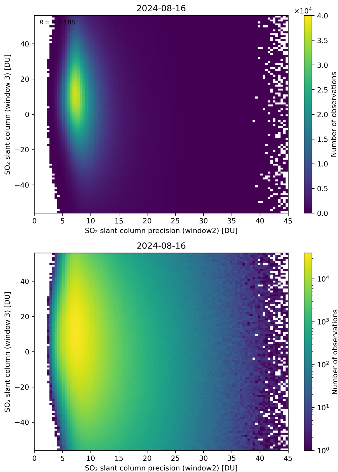
Figure 249: Scatter density plot of “SO 2 slant column precision (window2)” against “SO 2 slant column (window 3)” for 2024-08-16 to 2024-08-17.
