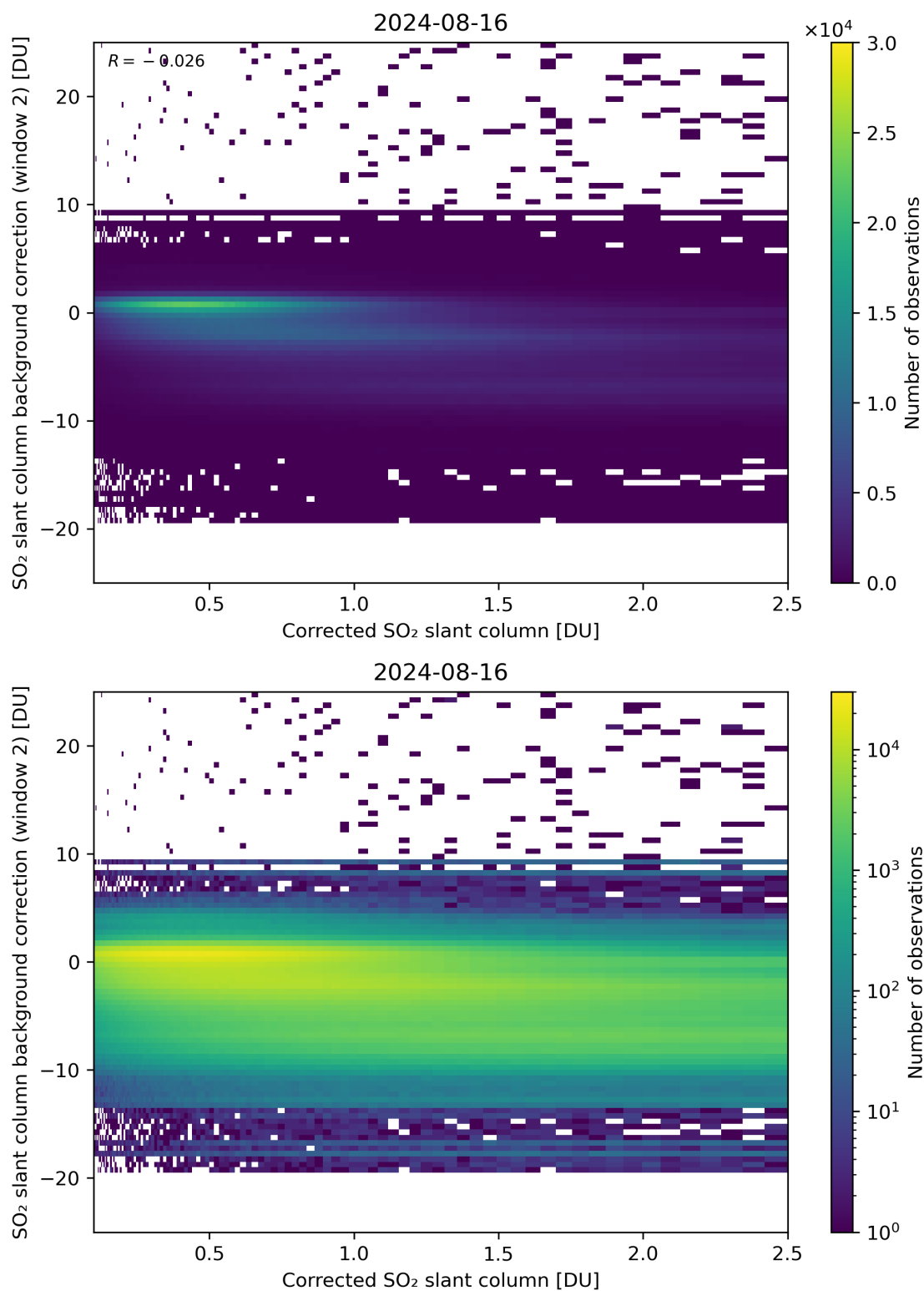
Figure 179: Scatter density plot of “Corrected SO 2 slant column” against “SO 2 slant column background correction (window 2)” for 2024-08-16 to 2024-08-17.
