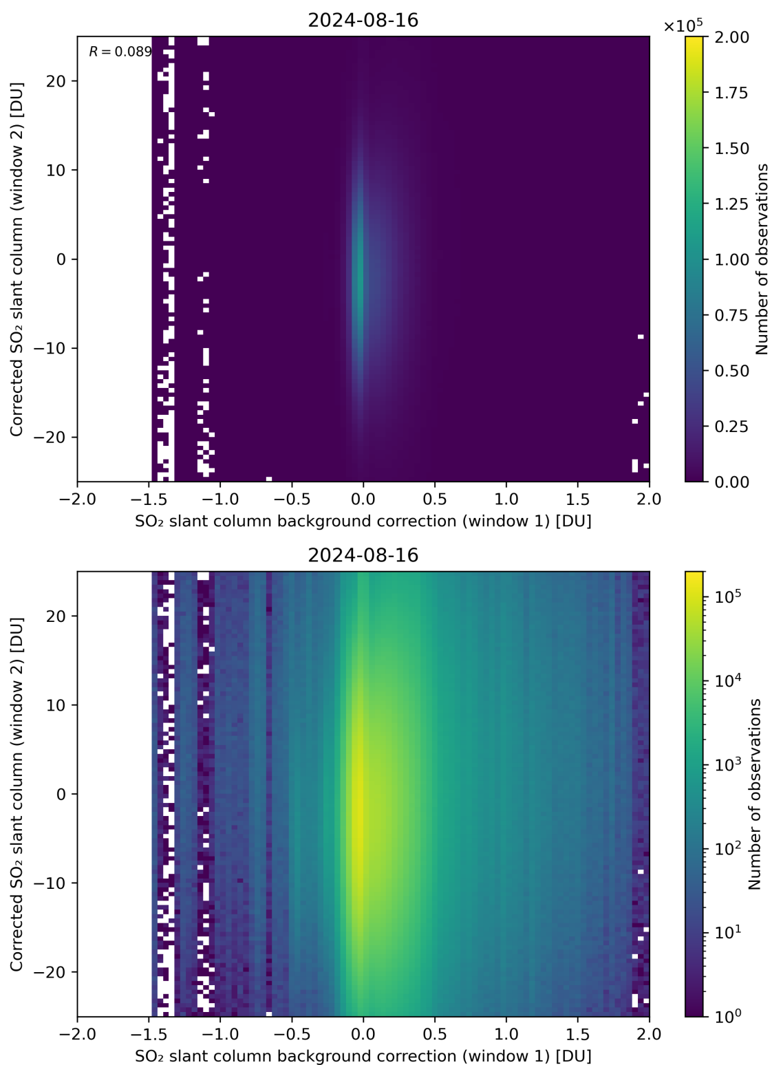
Figure 104: Scatter density plot of “SO 2 slant column background correction (window 1)” against “Corrected SO 2 slant column (window 2)” for 2024-08-16 to 2024-08-17.
