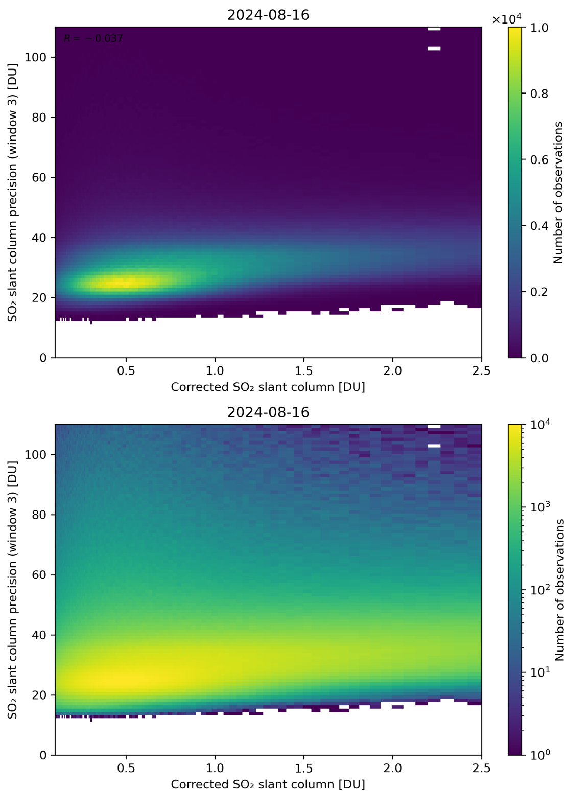
Figure 191: Scatter density plot of “Corrected SO 2 slant column” against “SO 2 slant column precision (window 3)” for 2024-08-16 to 2024-08-17.
