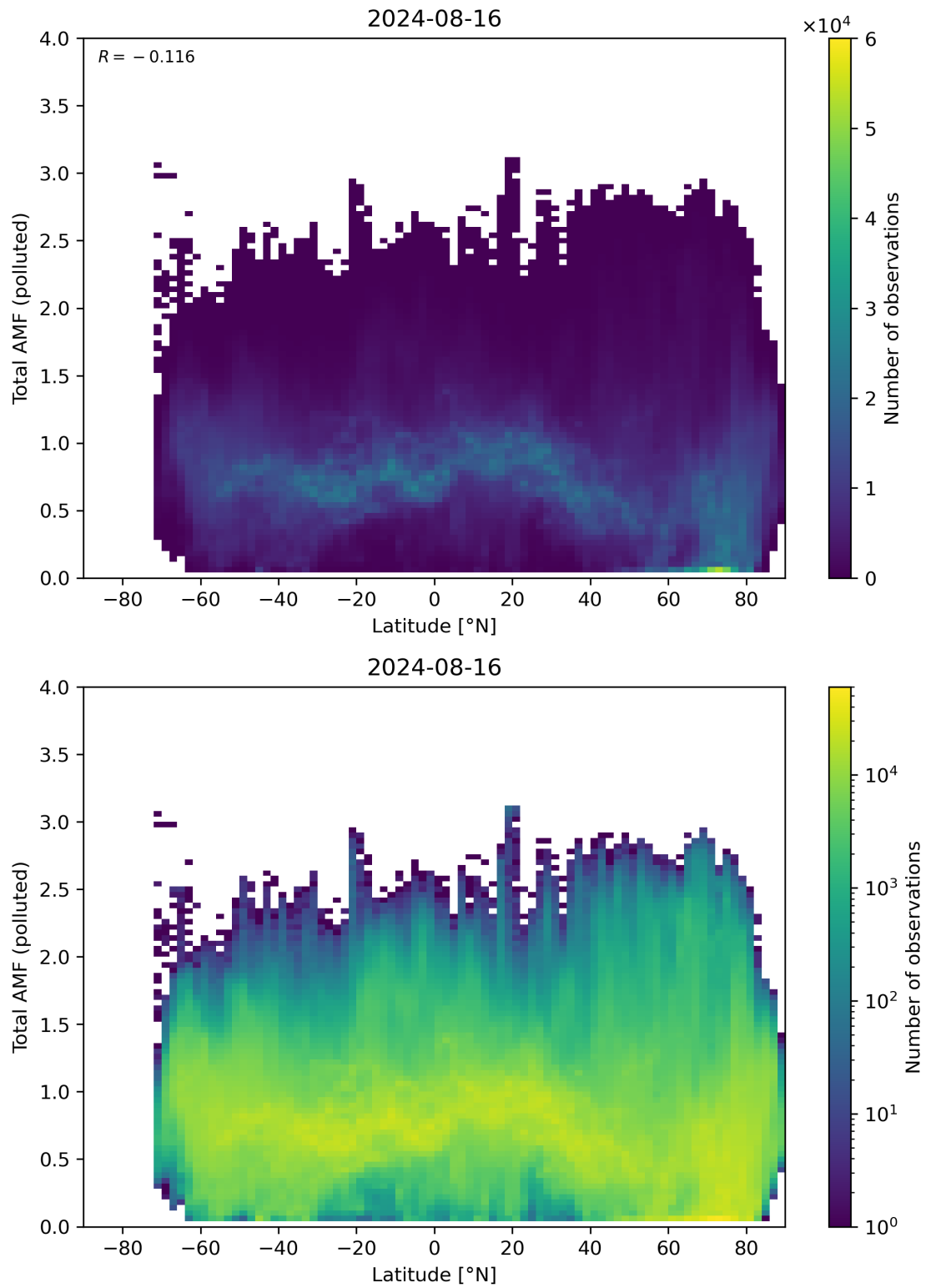
Figure 154: Scatter density plot of “Latitude” against “Total AMF (polluted)” for 2024-08-16 to 2024-08-17.
