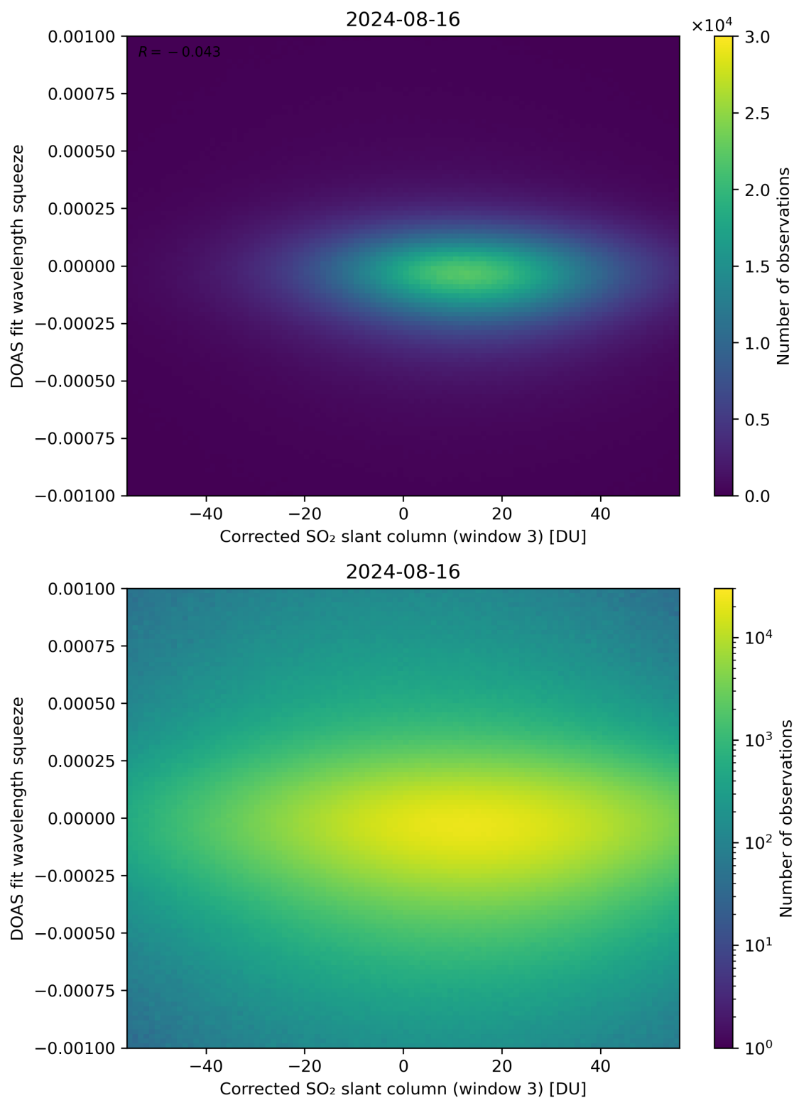
Figure 207: Scatter density plot of “Corrected SO 2 slant column (window 3)” against “DOAS fit wavelength squeeze” for 2024-08-16 to 2024-08-17.
