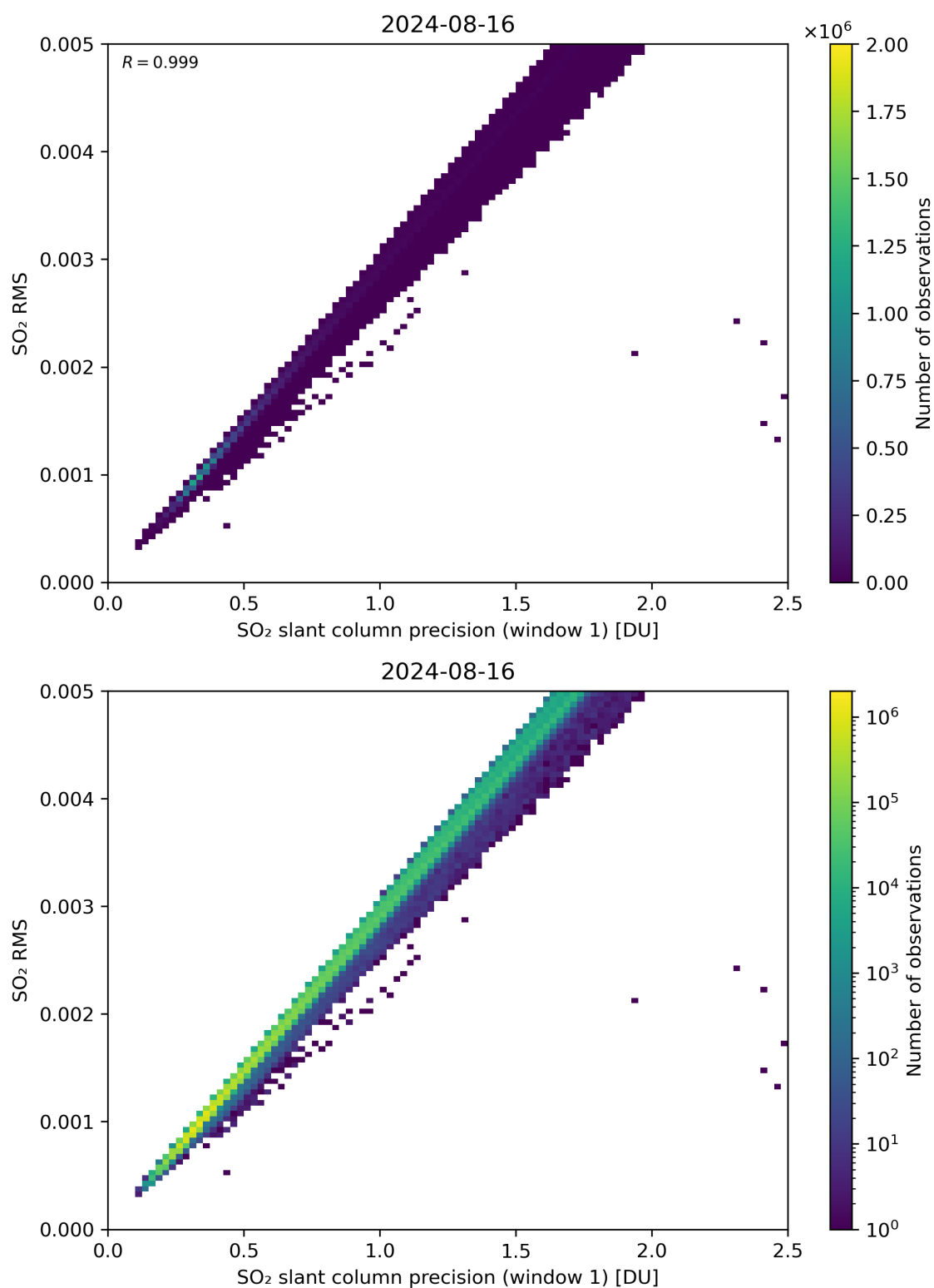
Figure 223: Scatter density plot of “SO 2 slant column precision (window 1)” against “SO 2 RMS” for 2024-08-16 to 2024-08-17.
