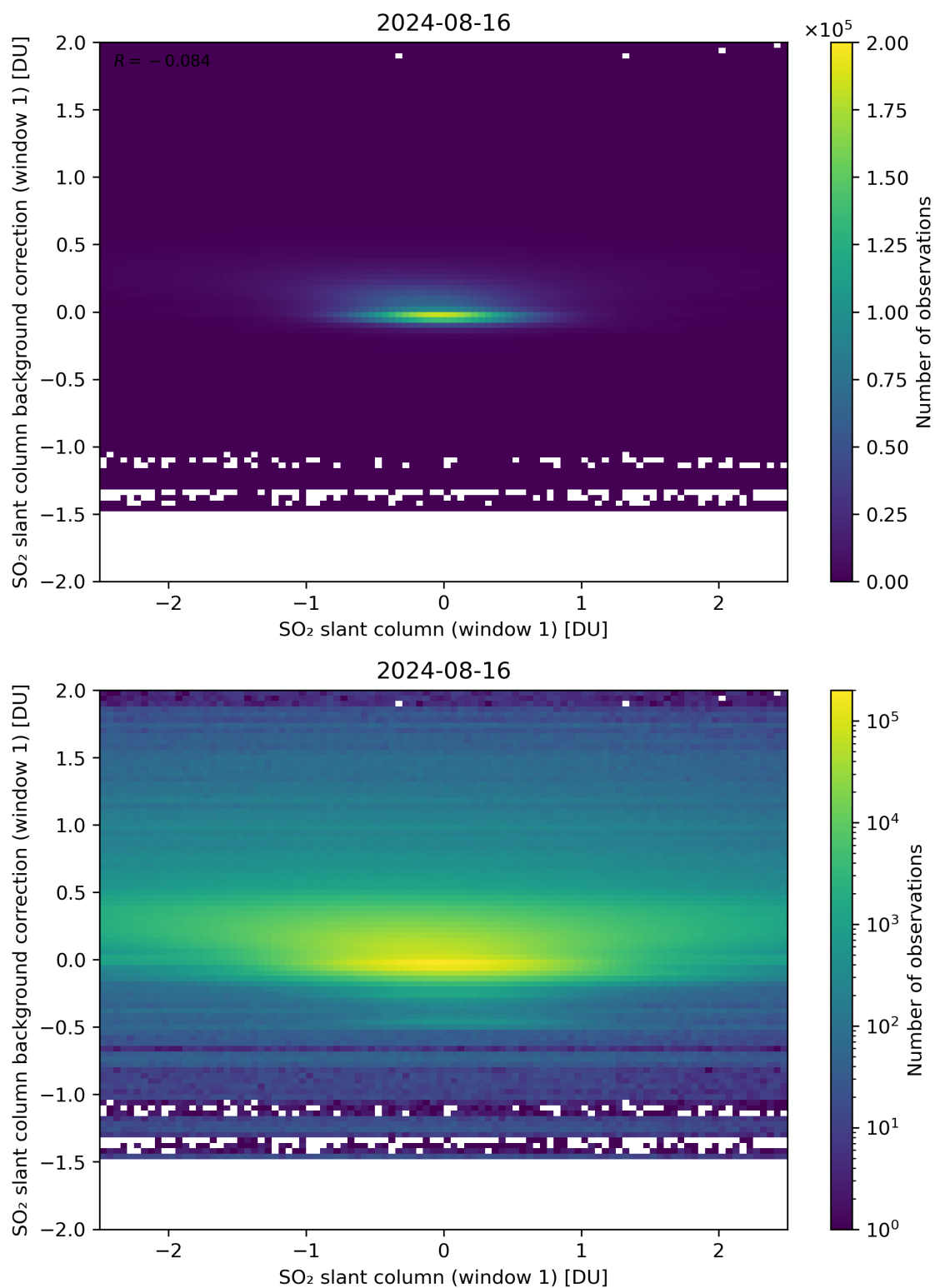
Figure 212: Scatter density plot of “SO 2 slant column (window 1)” against “SO 2 slant column background correction (window 1)” for 2024-08-16 to 2024-08-17.
