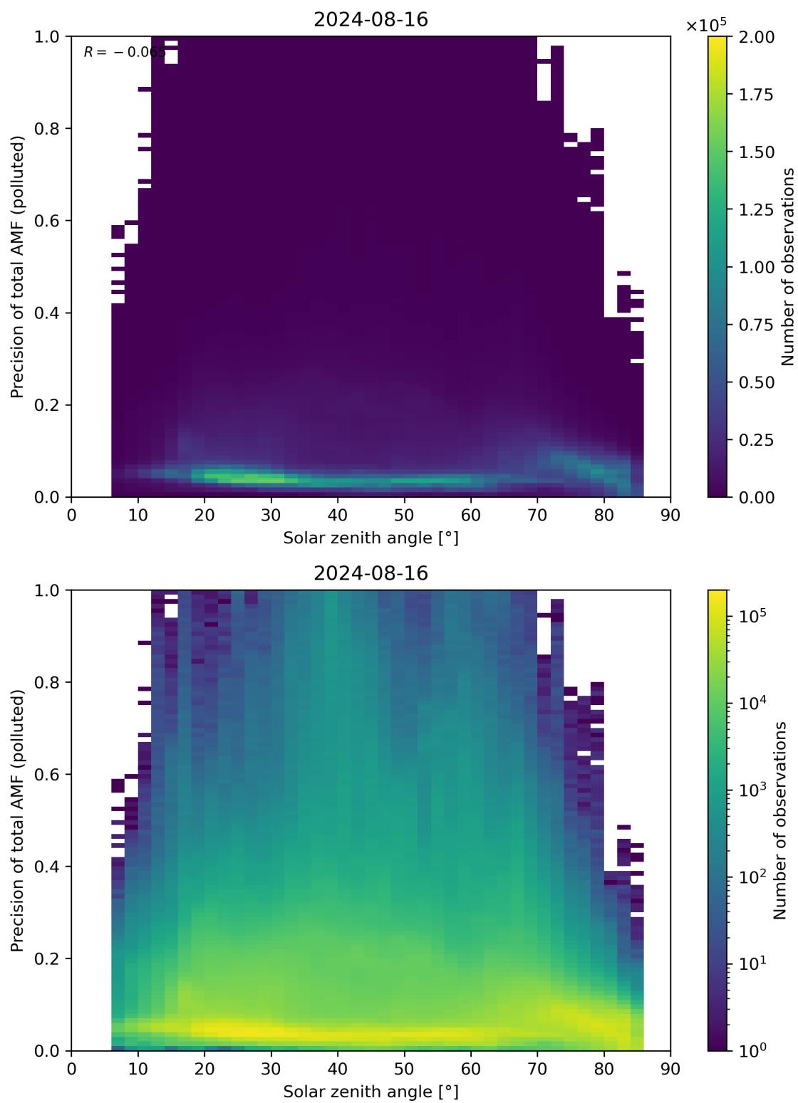
Figure 175: Scatter density plot of “Solar zenith angle” against “Precision of total AMF (polluted)” for 2024-08-16 to 2024-08-17.
