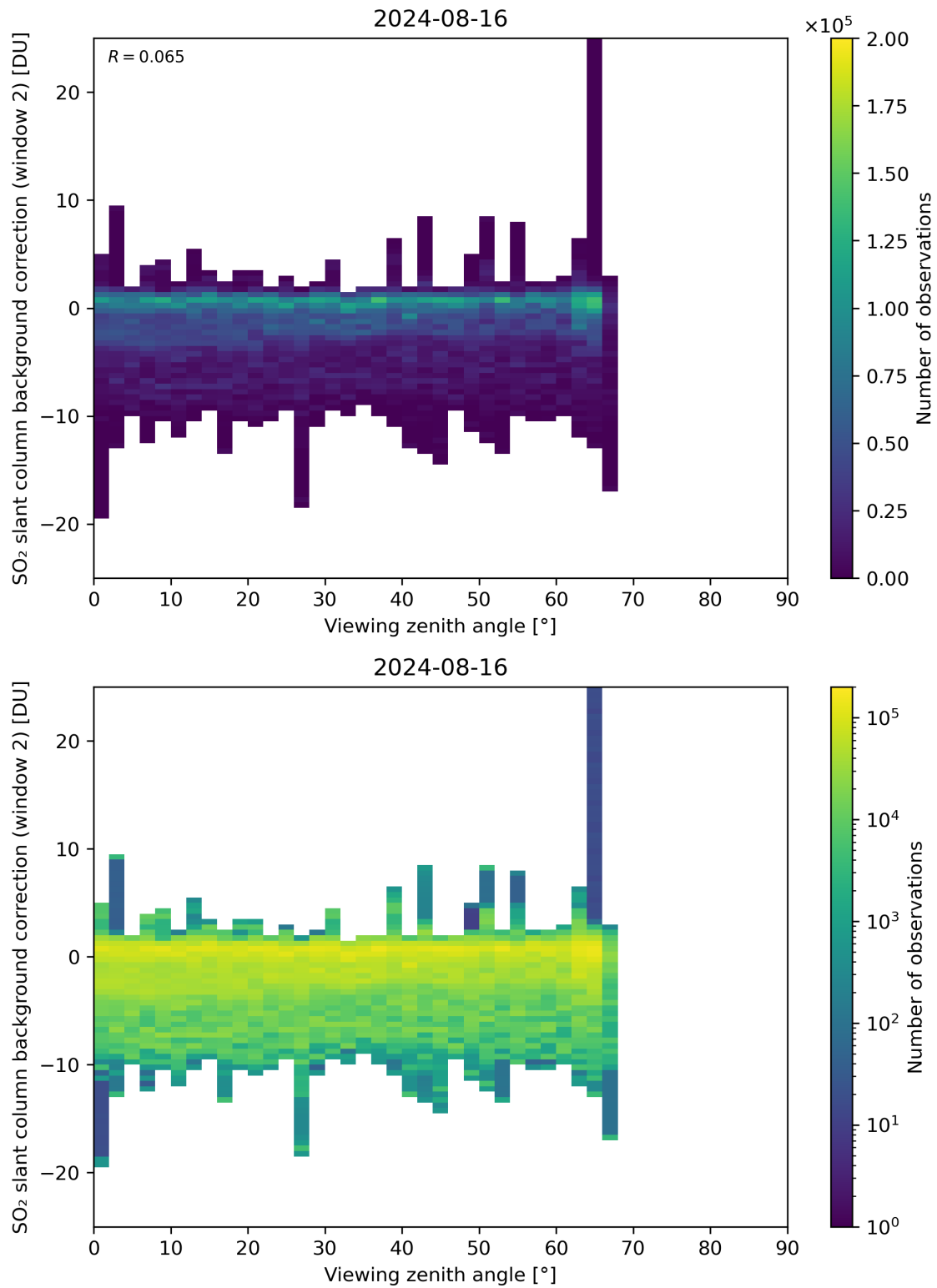
Figure 309: Scatter density plot of “Viewing zenith angle” against “SO 2 slant column background correction (window 2)” for 2024-08-16 to 2024-08-17.
