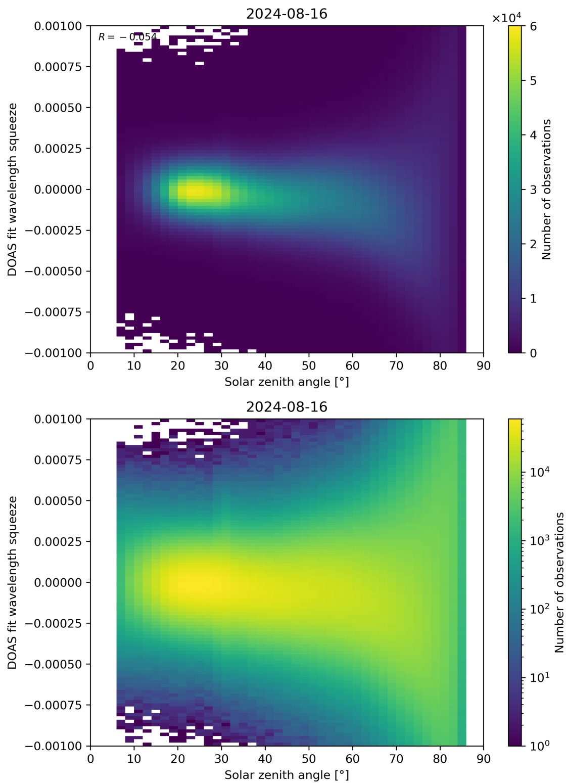
Figure 162: Scatter density plot of “Solar zenith angle” against “DOAS fit wavelength squeeze” for 2024-08-16 to 2024-08-17.
