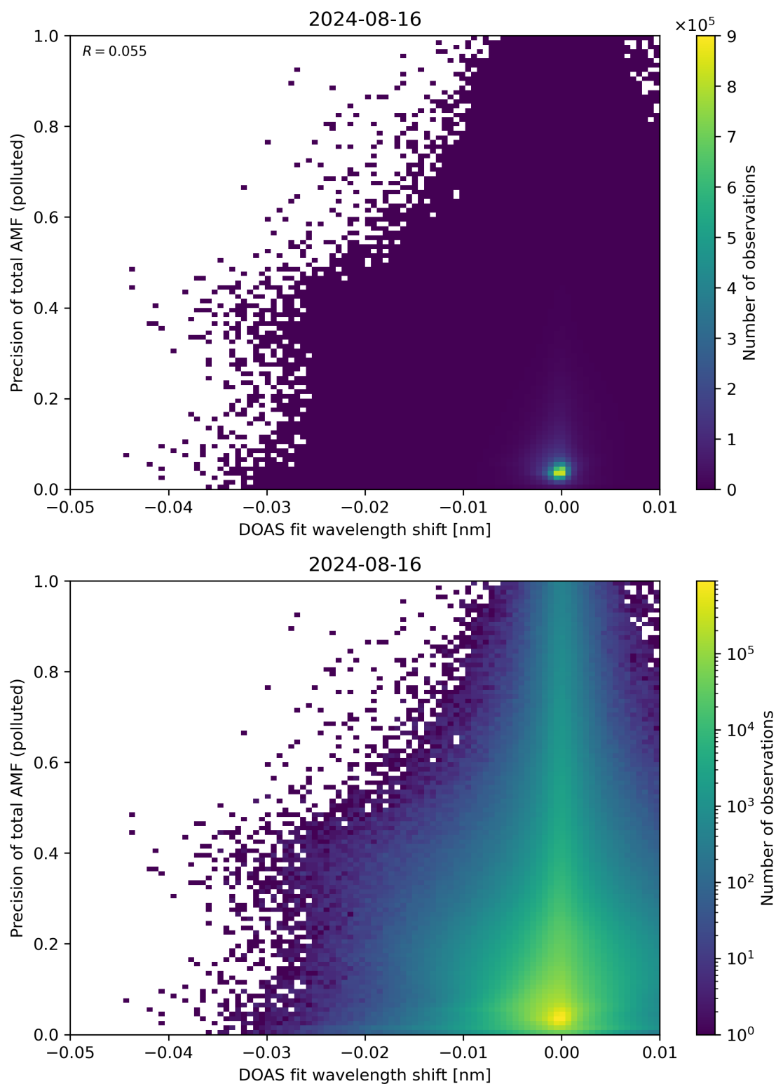
Figure 131: Scatter density plot of “DOAS fit wavelength shift” against “Precision of total AMF (polluted)” for 2024-08-16 to 2024-08-17.
