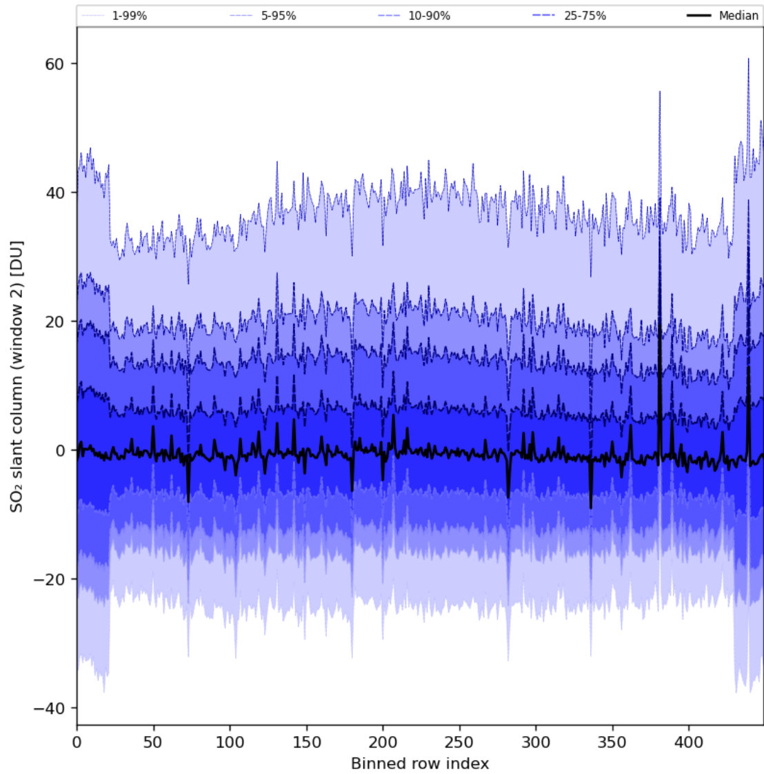
Figure 83: Along track statistics of “SO 2 slant column (window 2)” for 2024-08-16 to 2024-08-17
