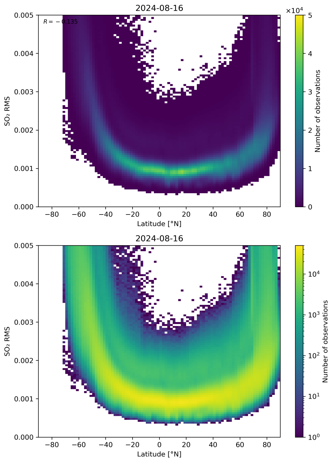
Figure 144: Scatter density plot of “Latitude” against “SO 2 RMS” for 2024-08-16 to 2024-08-17.
