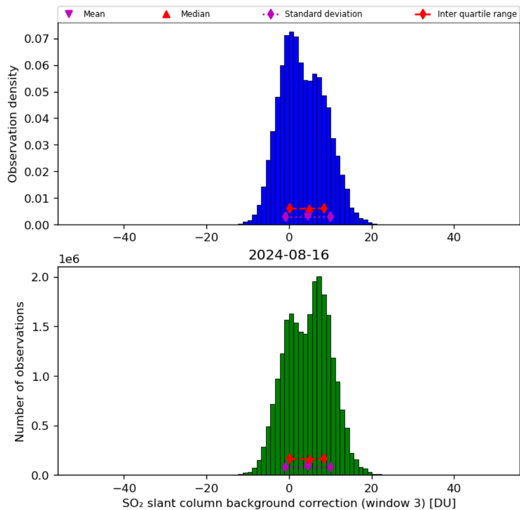
Figure 67: Histogram of “SO 2 slant column background correction (window 3)” for 2024-08-16 to 2024-08-17
