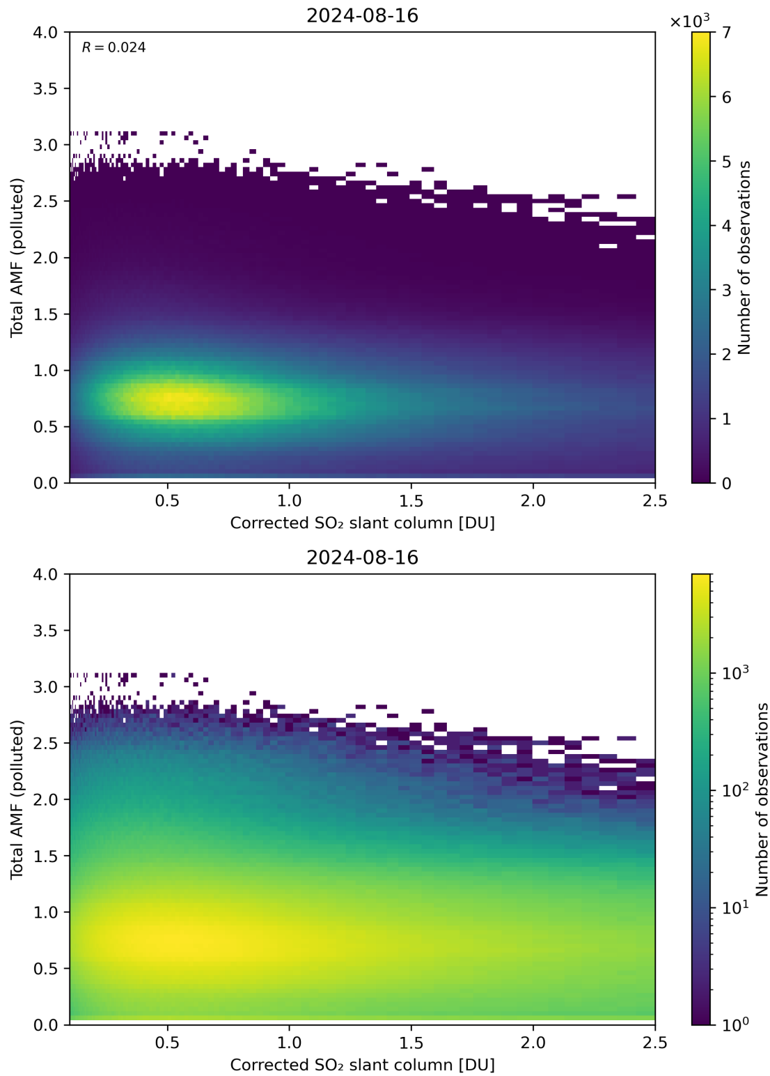
Figure 192: Scatter density plot of “Corrected SO 2 slant column” against “Total AMF (polluted)” for 2024-08-16 to 2024-08-17.
