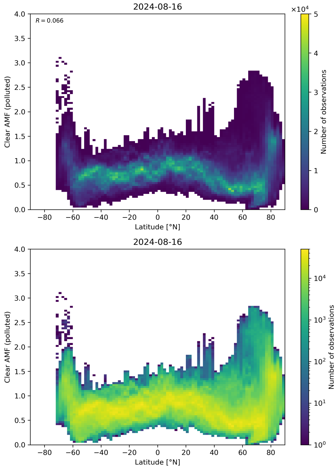
Figure 145: Scatter density plot of “Latitude” against “Clear AMF (polluted)” for 2024-08-16 to 2024-08-17.
