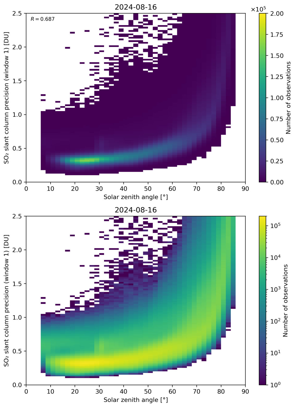
Figure 170: Scatter density plot of “Solar zenith angle” against “SO 2 slant column precision (window 1)” for 2024-08-16 to 2024-08-17.
