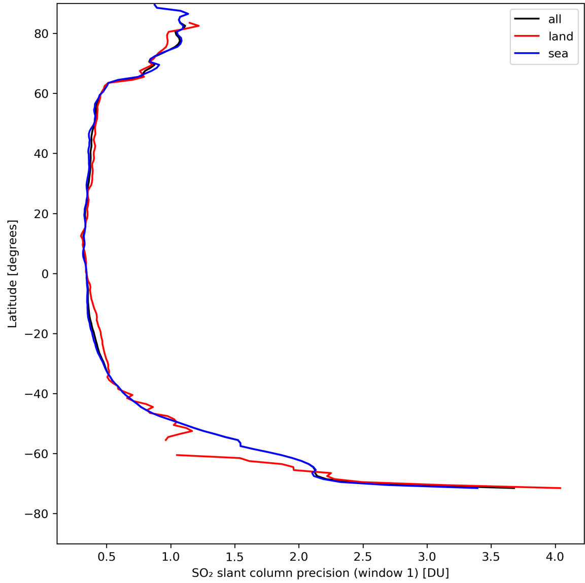
Figure 34: Zonal average of “SO 2 slant column precision (window 1)” for 2024-08-16 to 2024-08-17.
