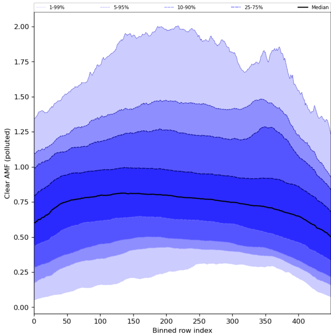
Figure 96: Along track statistics of “Clear AMF (polluted)” for 2024-08-16 to 2024-08-17
