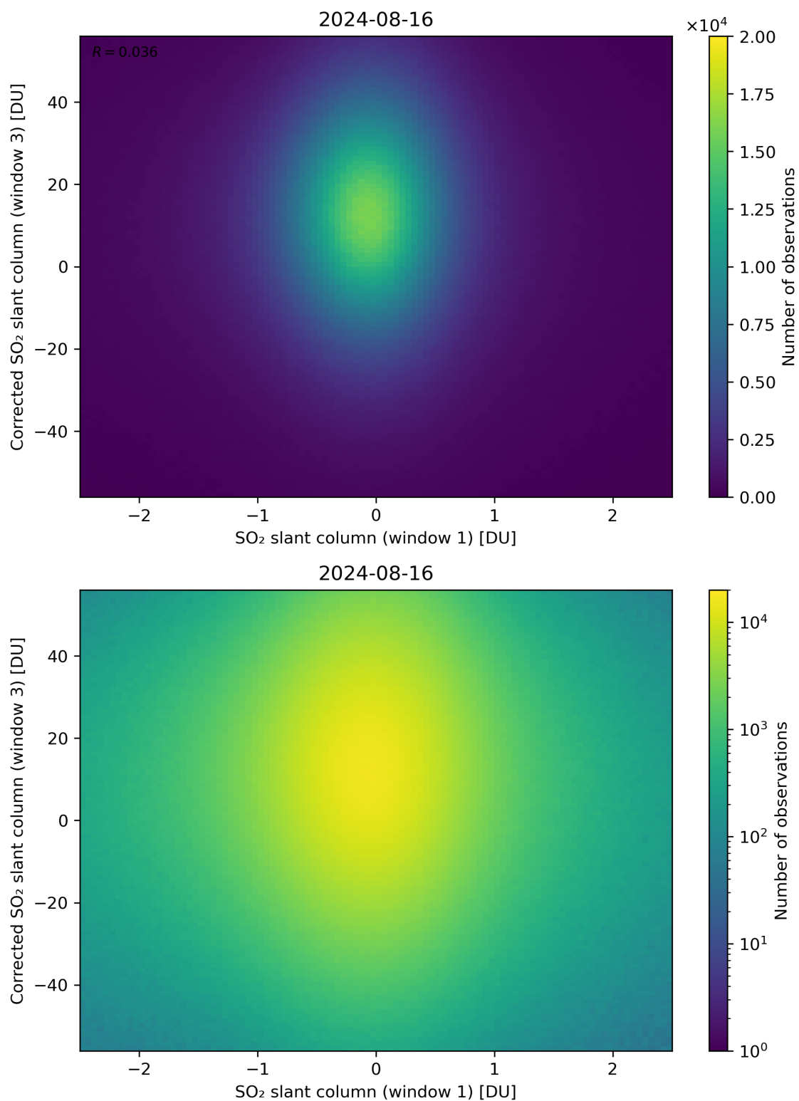
Figure 234: Scatter density plot of “SO 2 slant column (window 1)” against “Corrected SO 2 slant column (window 3)” for 2024-08-16 to 2024-08-17.
