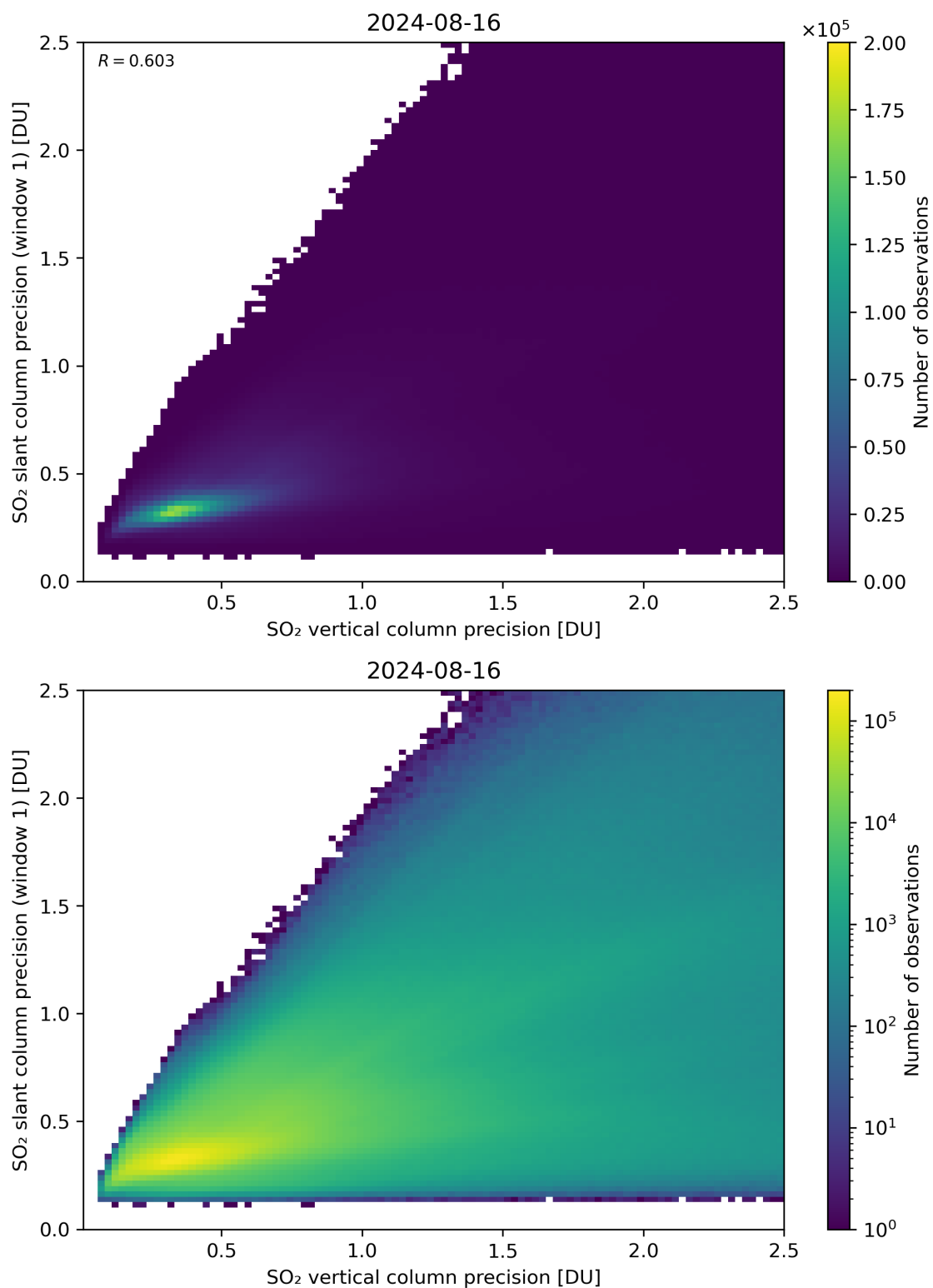
Figure 290: Scatter density plot of “SO 2 vertical column precision” against “SO 2 slant column precision (window 1)” for 2024-08-16 to 2024-08-17.
