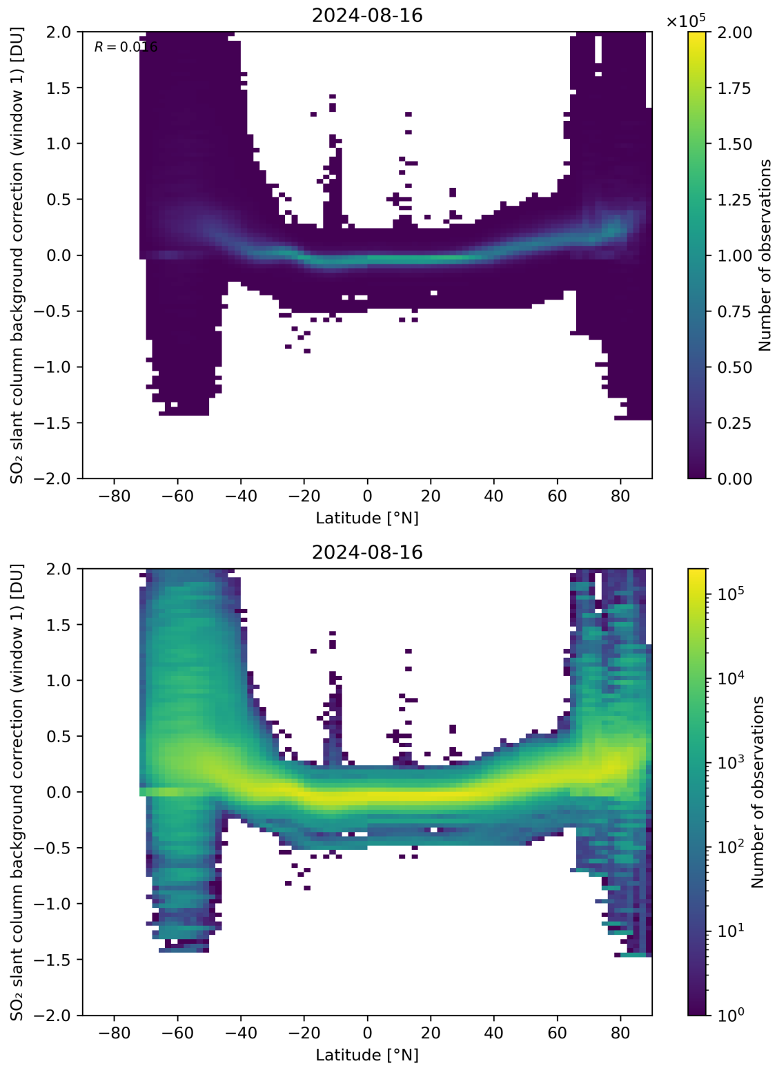
Figure 139: Scatter density plot of “Latitude” against “SO 2 slant column background correction (window 1)” for 2024-08-16 to 2024-08-17.
