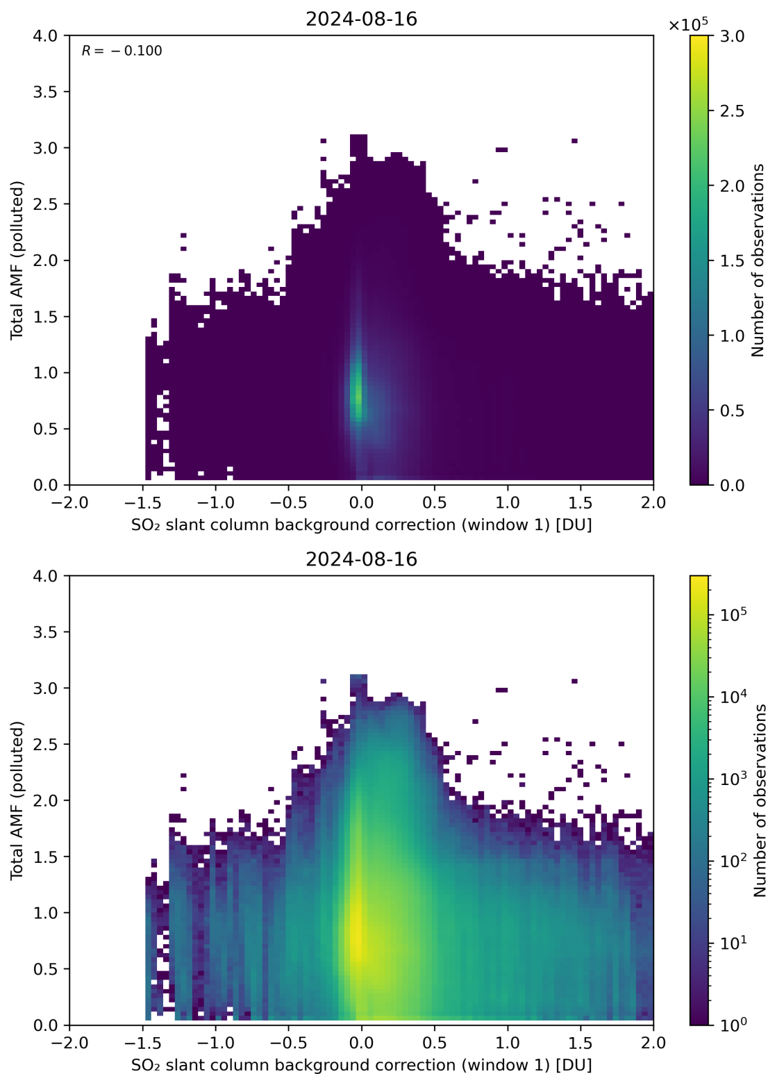
Figure 109: Scatter density plot of “SO 2 slant column background correction (window 1)” against “Total AMF (polluted)” for 2024-08-16 to 2024-08-17.
