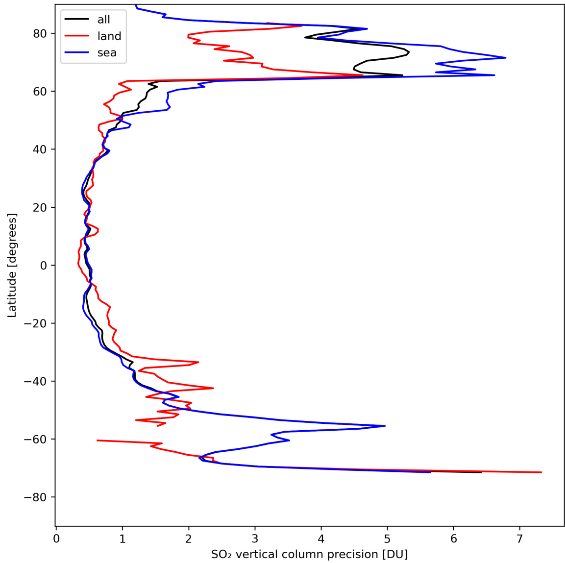
Figure 31: Zonal average of “SO 2 vertical column precision” for 2024-08-16 to 2024-08-17.
