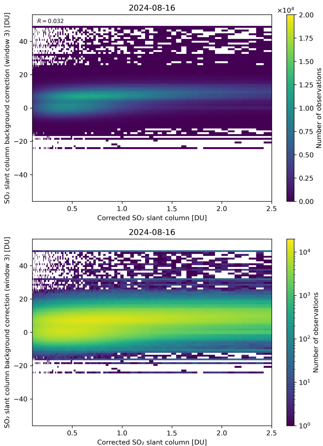
Figure 180: Scatter density plot of “Corrected SO 2 slant column” against “SO 2 slant column background correction (window 3)” for 2024-08-16 to 2024-08-17.
