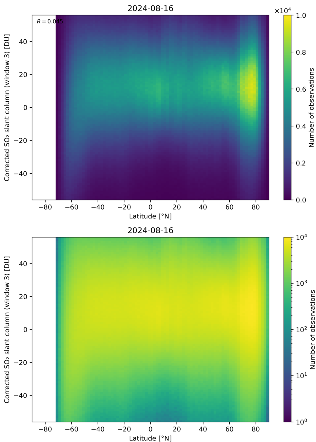
Figure 148: Scatter density plot of “Latitude” against “Corrected SO 2 slant column (window 3)” for 2024-08-16 to 2024-08-17.
