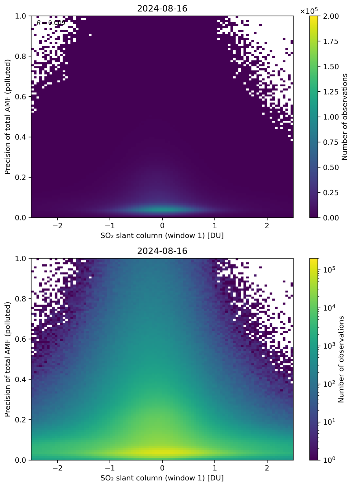
Figure 240: Scatter density plot of “SO 2 slant column (window 1)” against “Precision of total AMF (polluted)” for 2024-08-16 to 2024-08-17.
