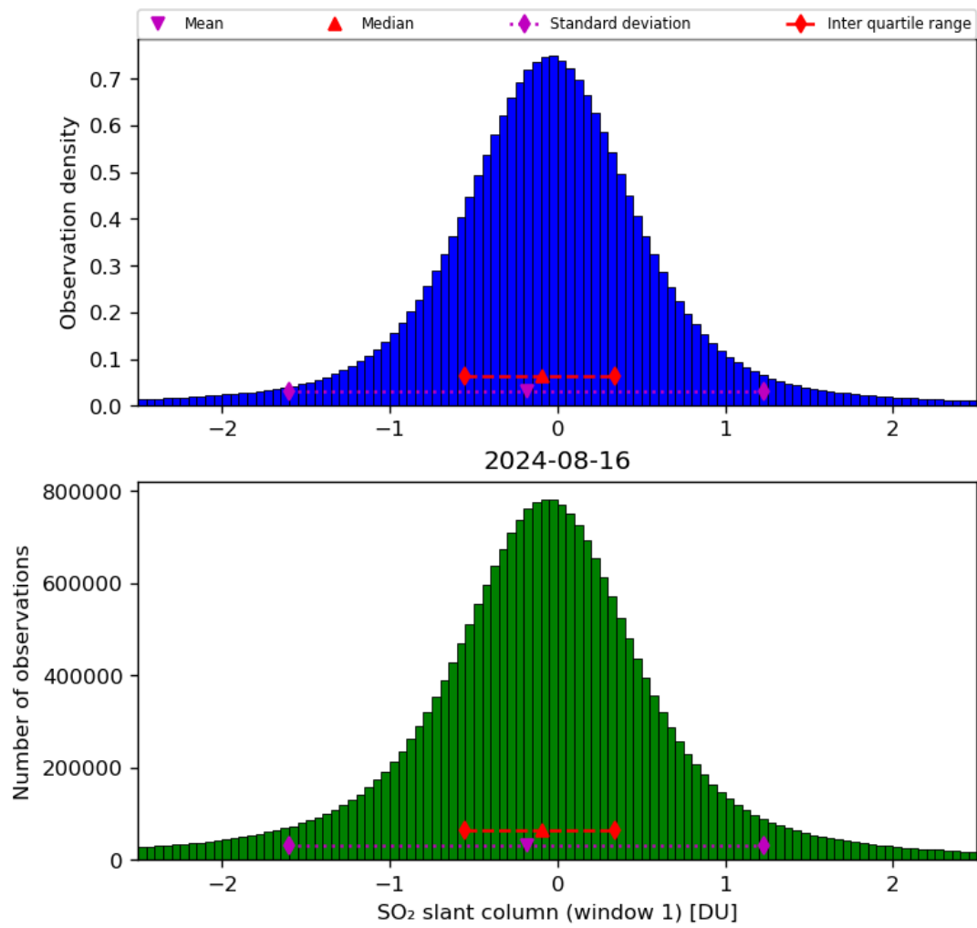
Figure 56: Histogram of “SO 2 slant column (window 1)” for 2024-08-16 to 2024-08-17
