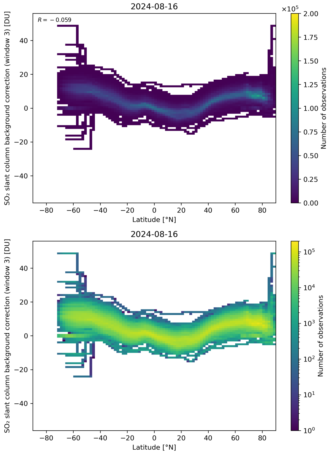
Figure 141: Scatter density plot of “Latitude” against “SO 2 slant column background correction (window 3)” for 2024-08-16 to 2024-08-17.
