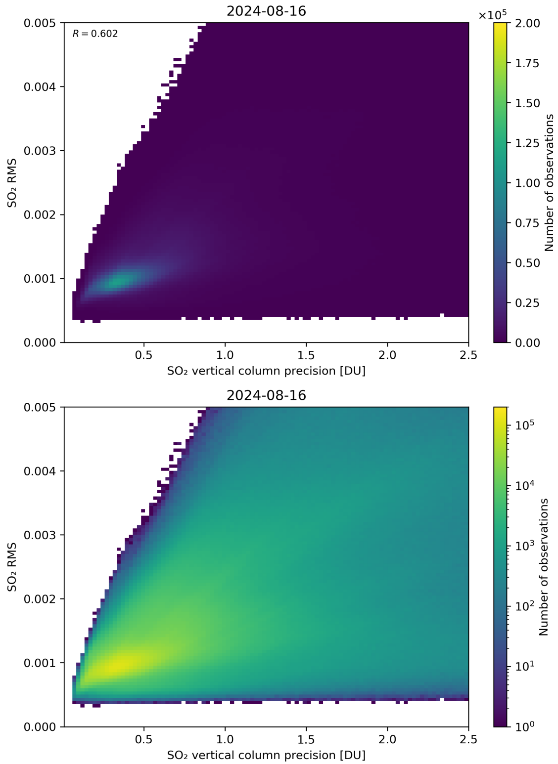
Figure 284: Scatter density plot of “SO 2 vertical column precision” against “SO 2 RMS” for 2024-08-16 to 2024-08-17.
