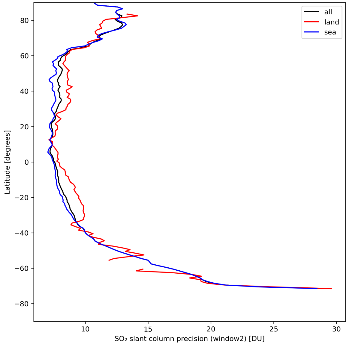
Figure 38: Zonal average of “SO 2 slant column precision (window2)” for 2024-08-16 to 2024-08-17.
