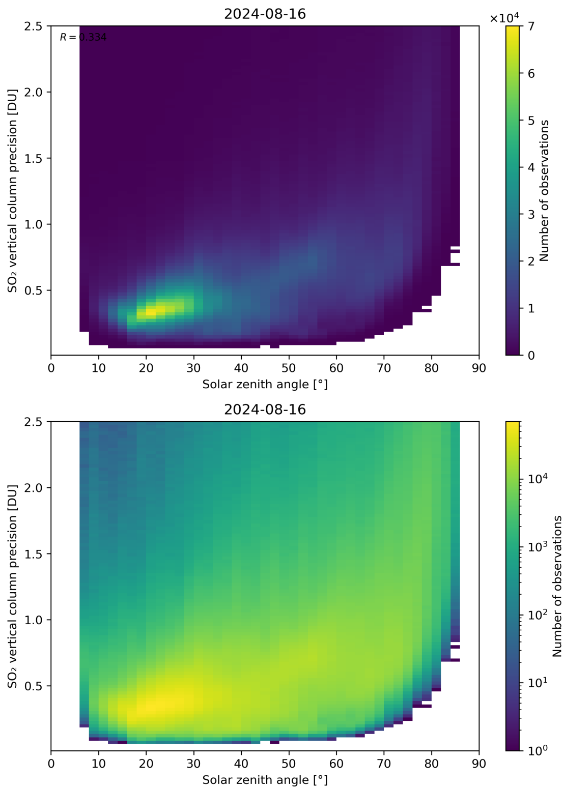
Figure 177: Scatter density plot of “Solar zenith angle” against “SO 2 vertical column precision” for 2024-08-16 to 2024-08-17.
