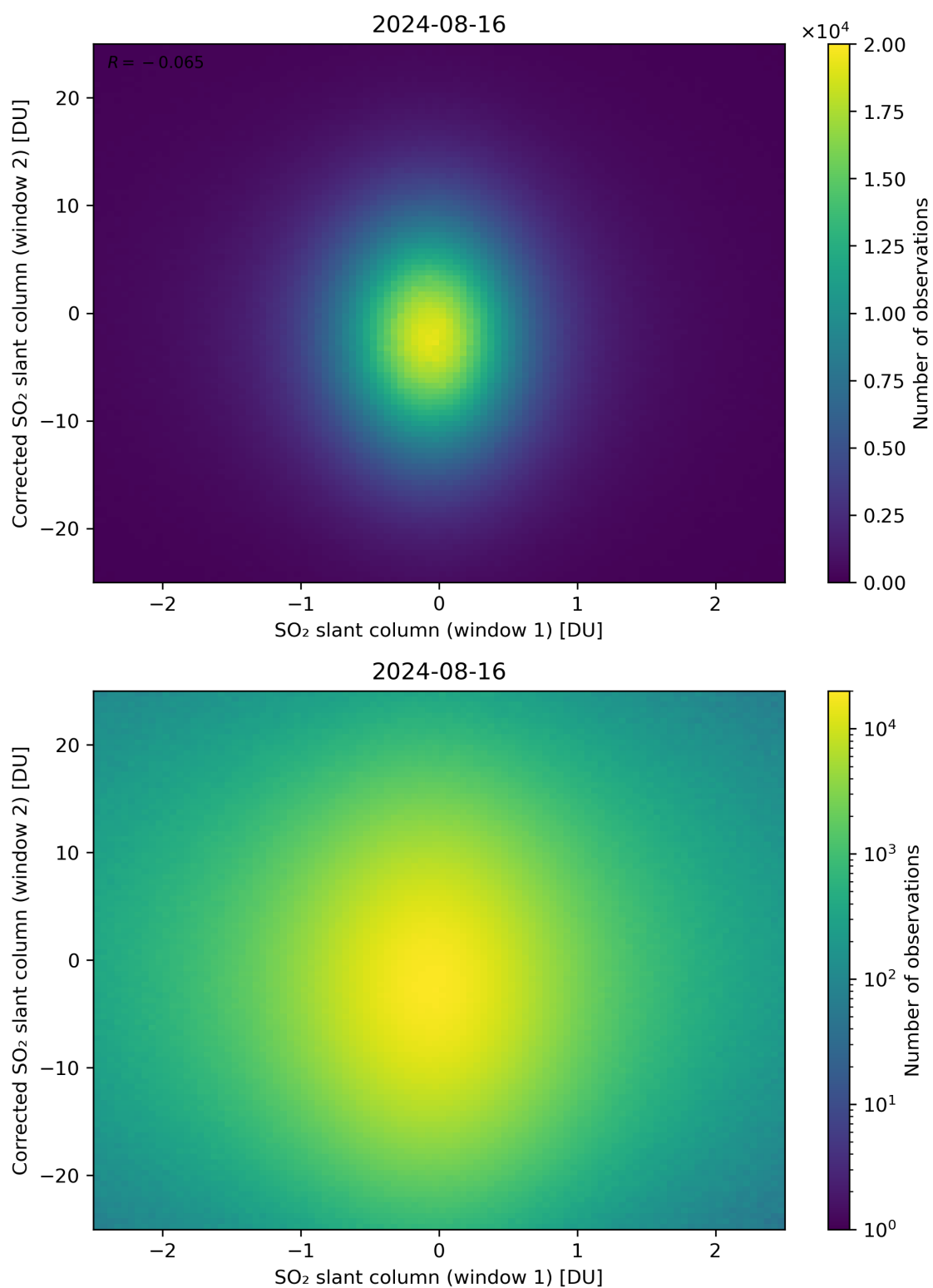
Figure 233: Scatter density plot of “SO 2 slant column (window 1)” against “Corrected SO 2 slant column (window 2)” for 2024-08-16 to 2024-08-17.
