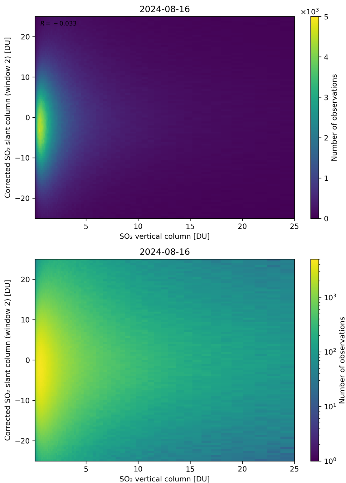
Figure 298: Scatter density plot of “SO 2 vertical column” against “Corrected SO 2 slant column (window 2)” for 2024-08-16 to 2024-08-17.
