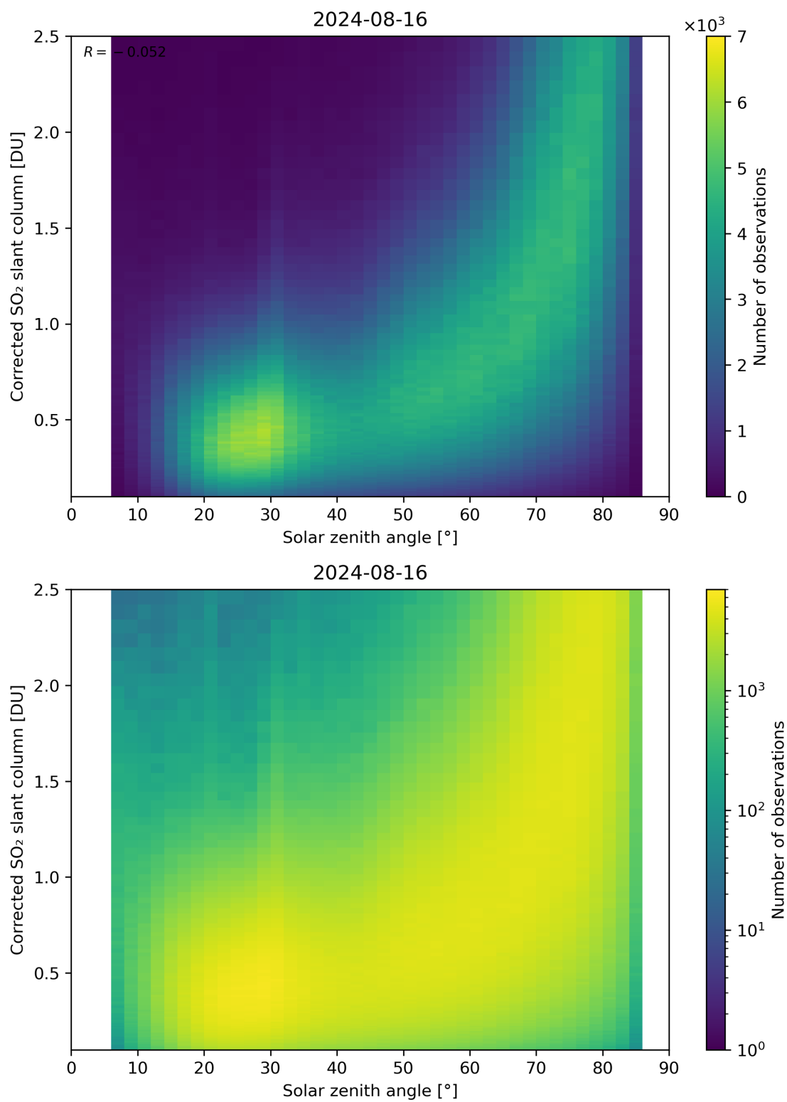
Figure 166: Scatter density plot of “Solar zenith angle” against “Corrected SO 2 slant column” for 2024-08-16 to 2024-08-17.
