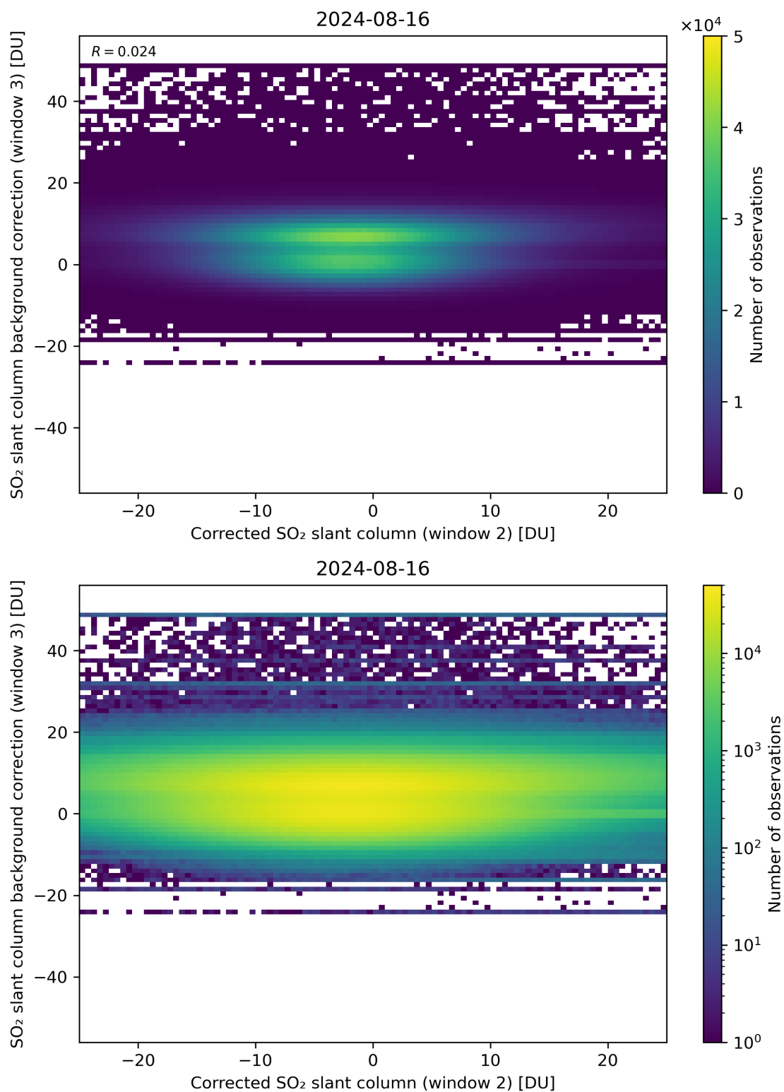
Figure 195: Scatter density plot of “Corrected SO 2 slant column (window 2)” against “SO 2 slant column background correction (window 3)” for 2024-08-16 to 2024-08-17.
