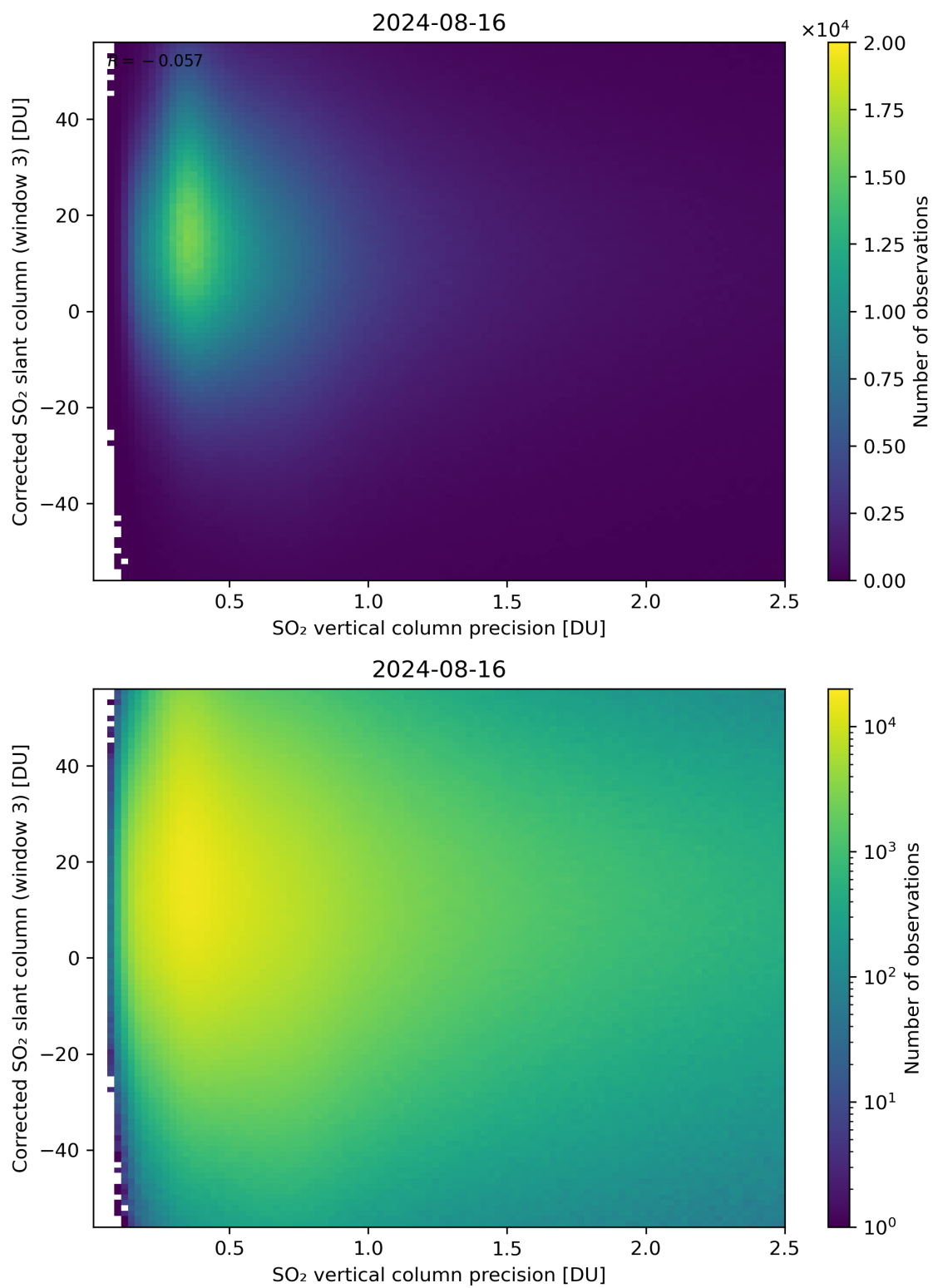
Figure 288: Scatter density plot of “SO 2 vertical column precision” against “Corrected SO 2 slant column (window 3)” for 2024-08-16 to 2024-08-17.
