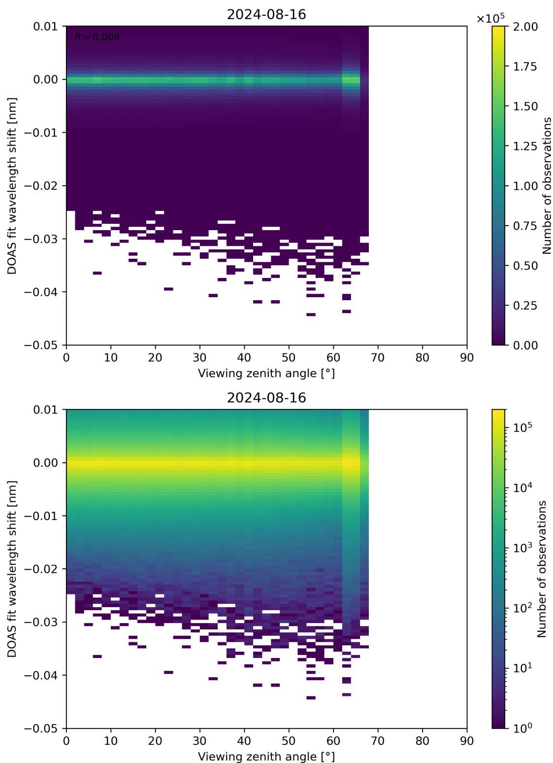
Figure 311: Scatter density plot of “Viewing zenith angle” against “DOAS fit wavelength shift” for 2024-08-16 to 2024-08-17.
