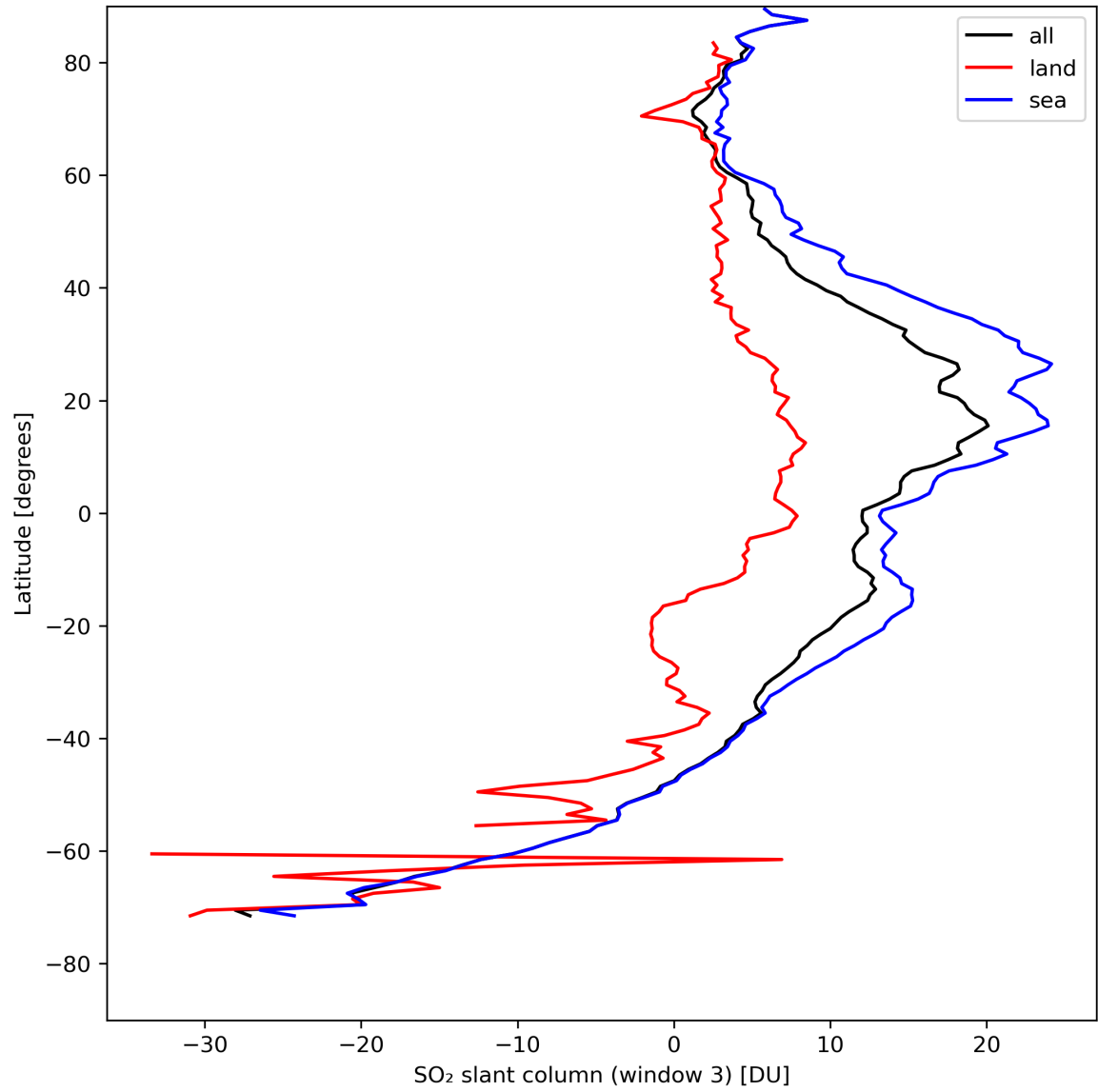
Figure 41: Zonal average of “SO 2 slant column (window 3)” for 2024-08-16 to 2024-08-17.
