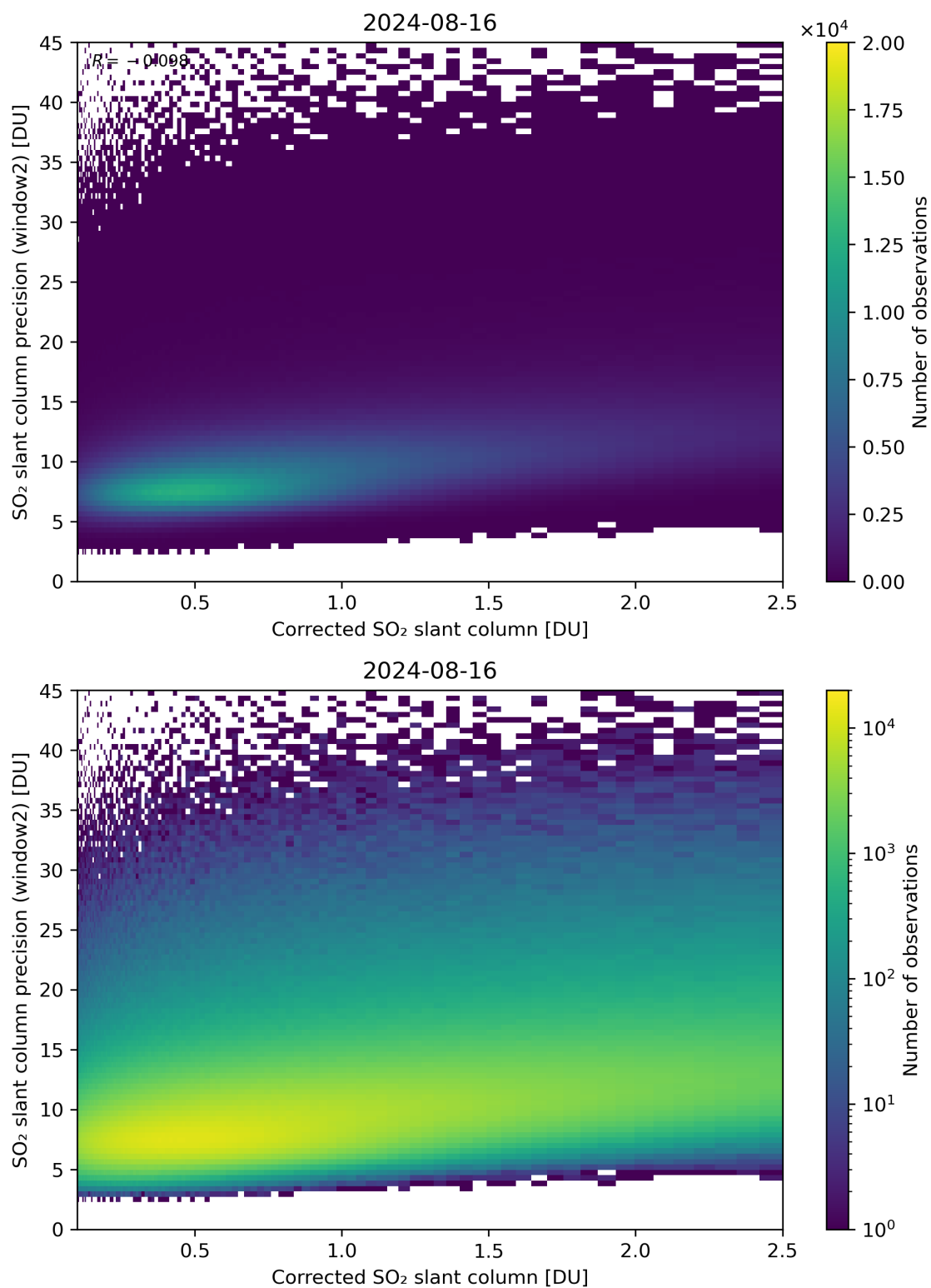
Figure 189: Scatter density plot of “Corrected SO 2 slant column” against “SO 2 slant column precision (window2)” for 2024-08-16 to 2024-08-17.
