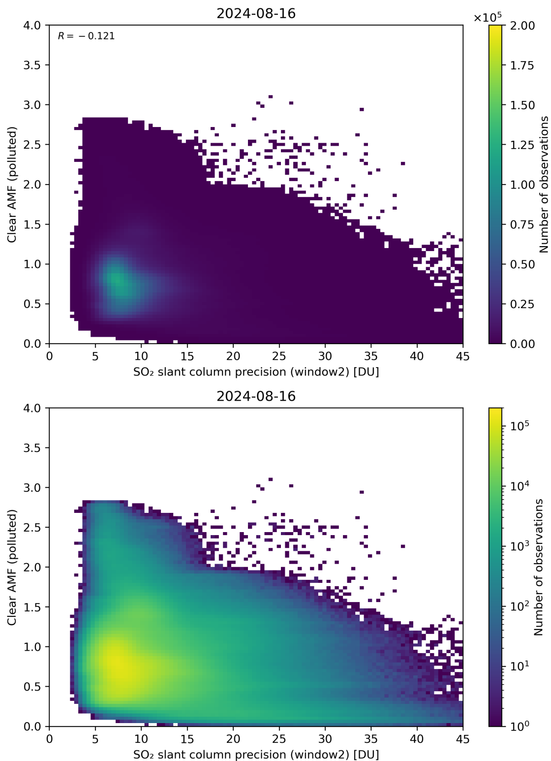
Figure 246: Scatter density plot of “SO 2 slant column precision (window2)” against “Clear AMF (polluted)” for 2024-08-16 to 2024-08-17.
