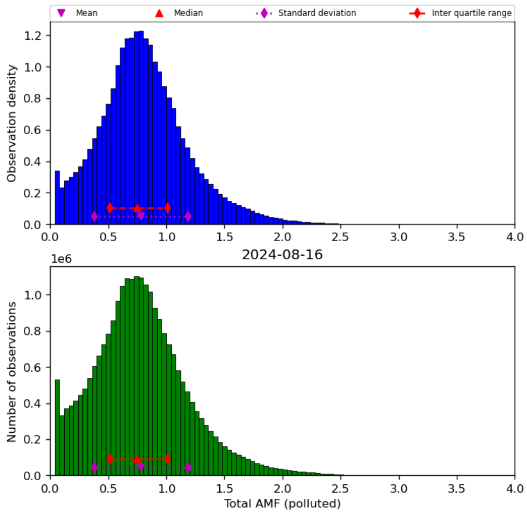
Figure 71: Histogram of “Total AMF (polluted)” for 2024-08-16 to 2024-08-17
