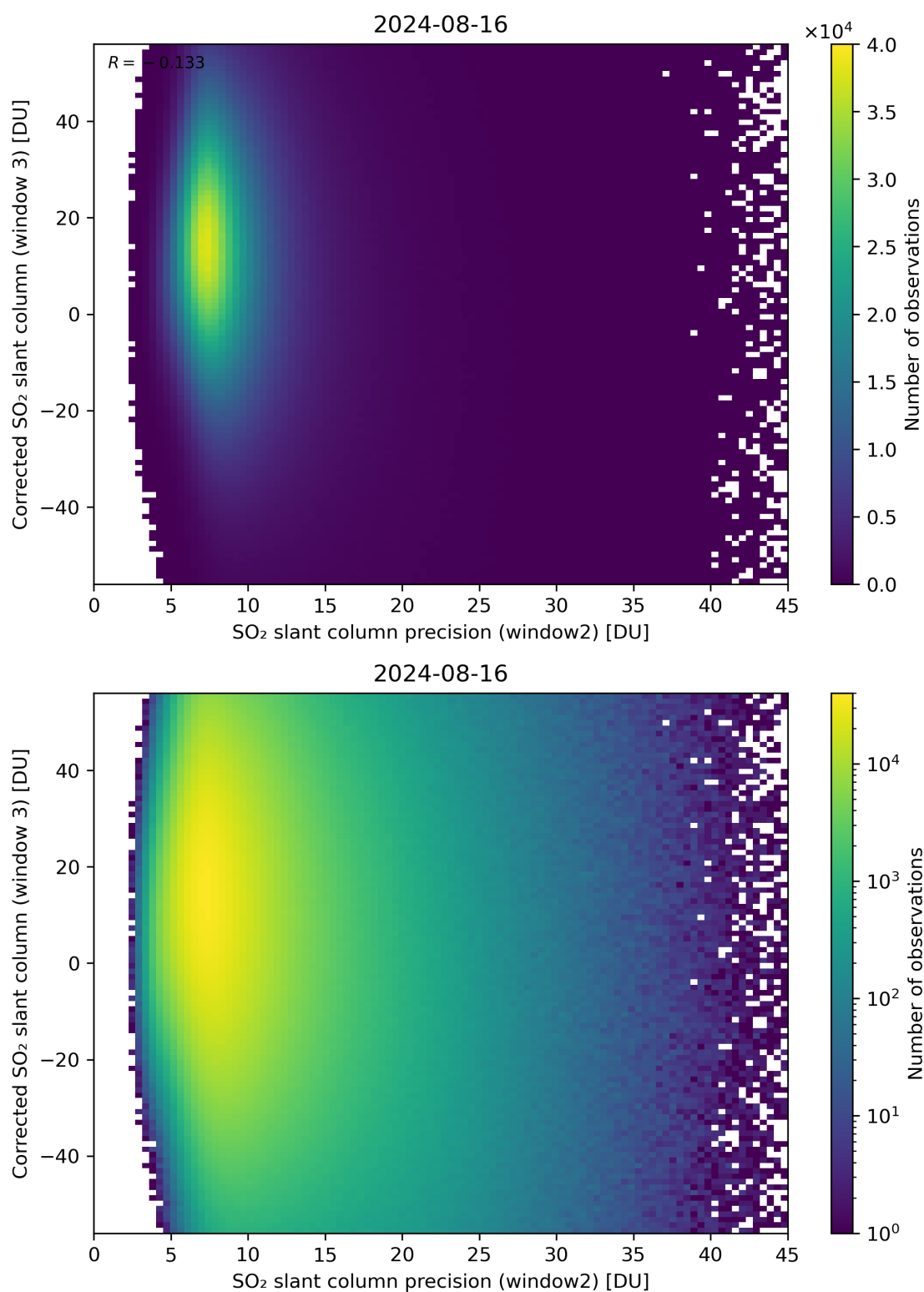
Figure 248: Scatter density plot of “SO 2 slant column precision (window2)” against “Corrected SO 2 slant column (window 3)” for 2024-08-16 to 2024-08-17.
