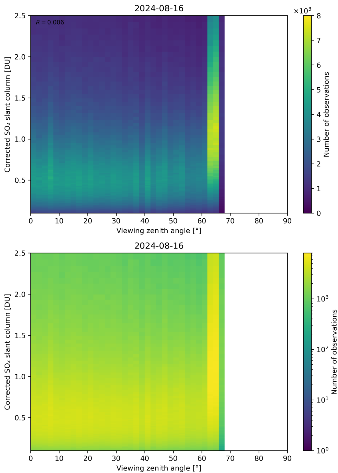
Figure 317: Scatter density plot of “Viewing zenith angle” against “Corrected SO 2 slant column” for 2024-08-16 to 2024-08-17.
