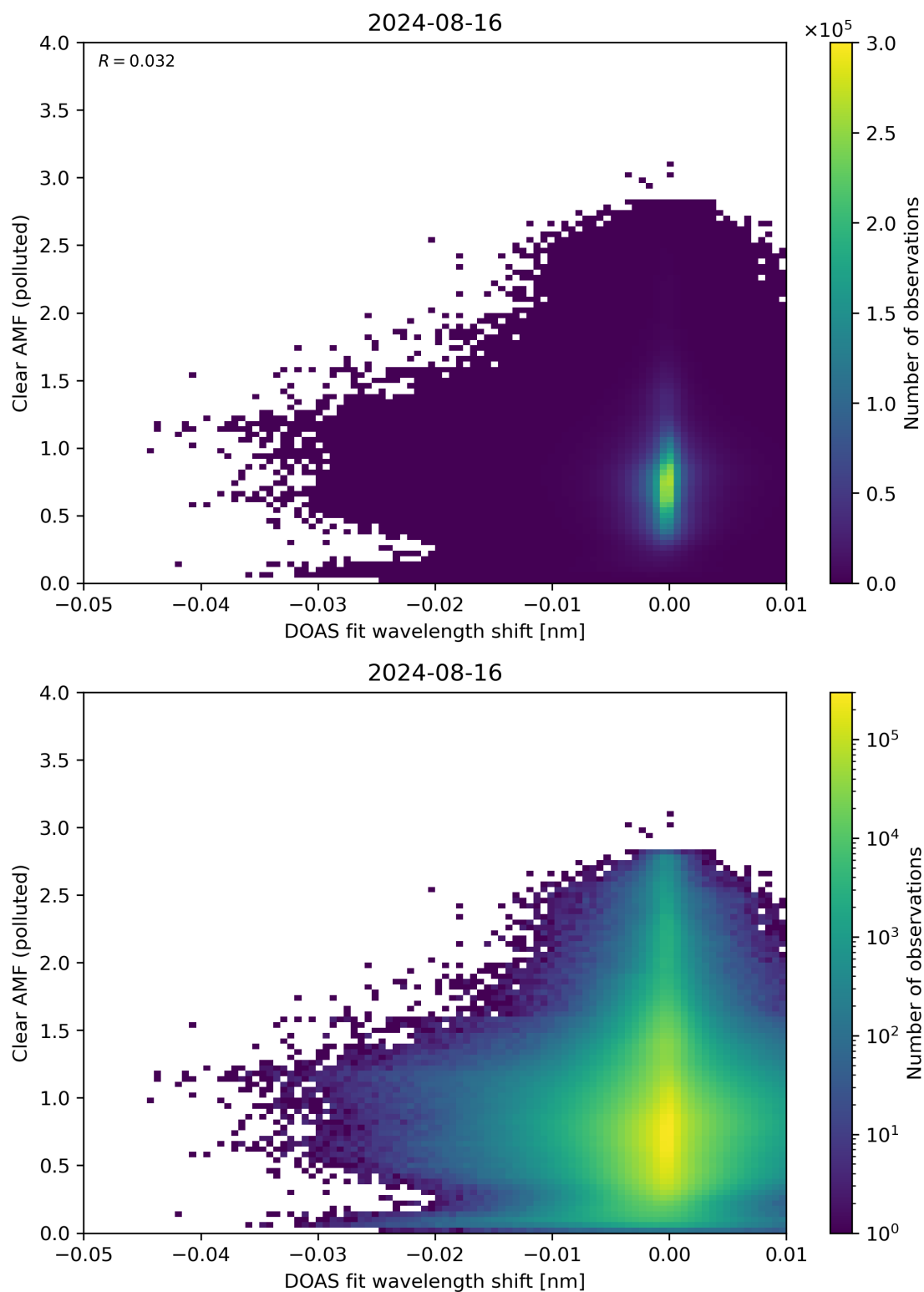
Figure 129: Scatter density plot of “DOAS fit wavelength shift” against “Clear AMF (polluted)” for 2024-08-16 to 2024-08-17.
