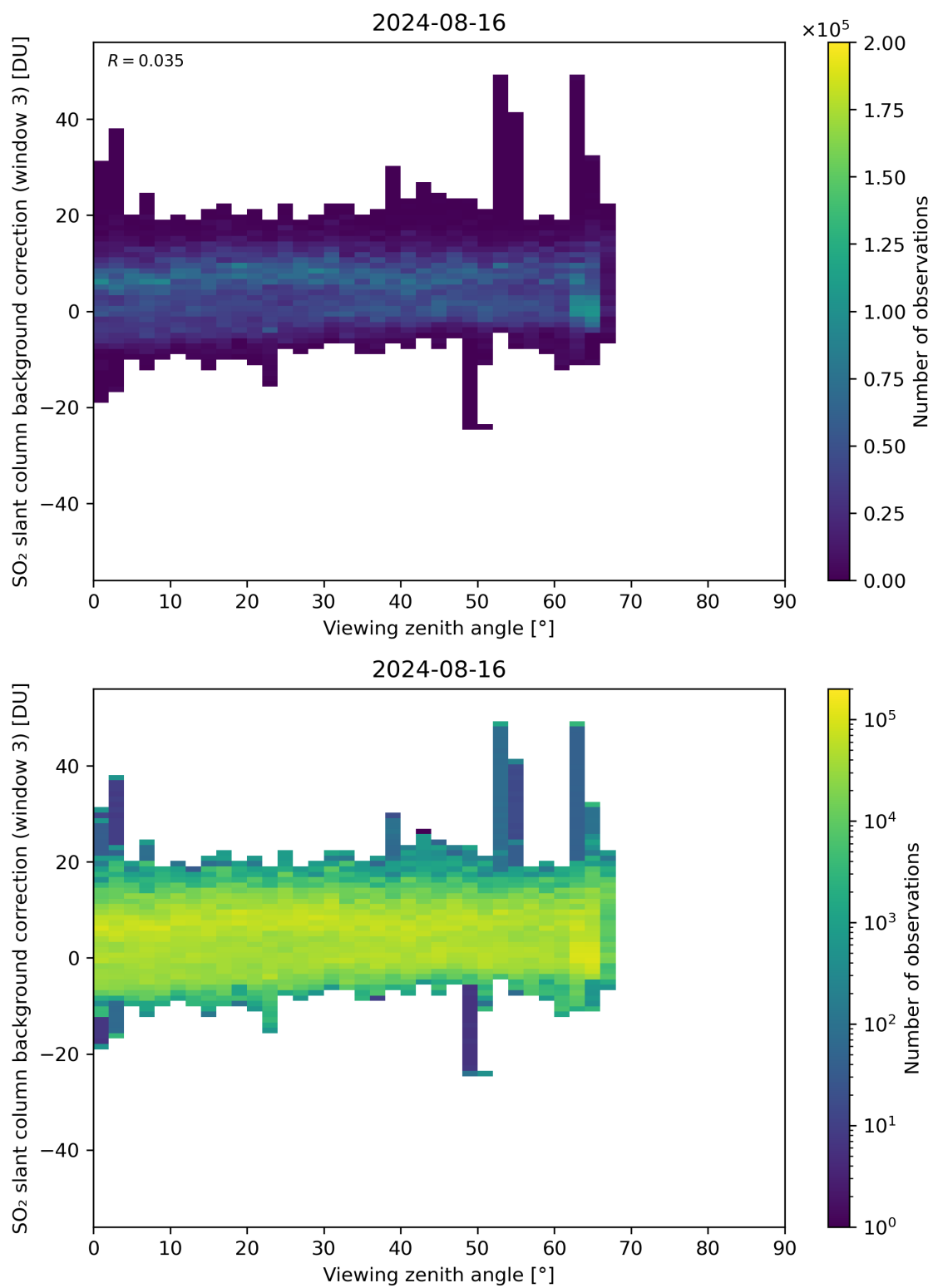
Figure 310: Scatter density plot of “Viewing zenith angle” against “SO 2 slant column background correction (window 3)” for 2024-08-16 to 2024-08-17.
