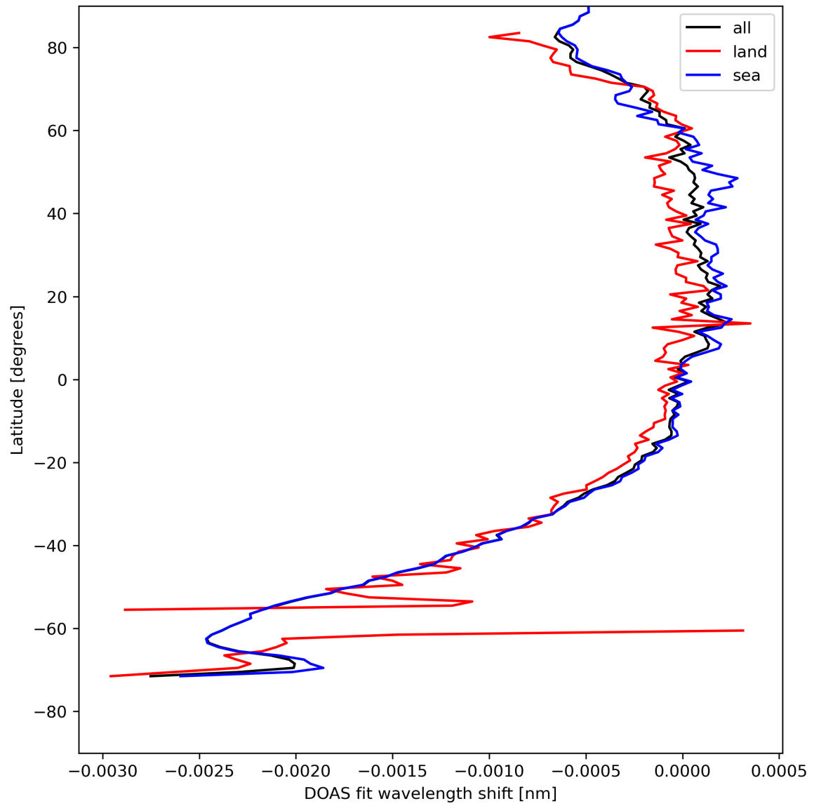
Figure 45: Zonal average of “DOAS fit wavelength shift” for 2024-08-16 to 2024-08-17.
