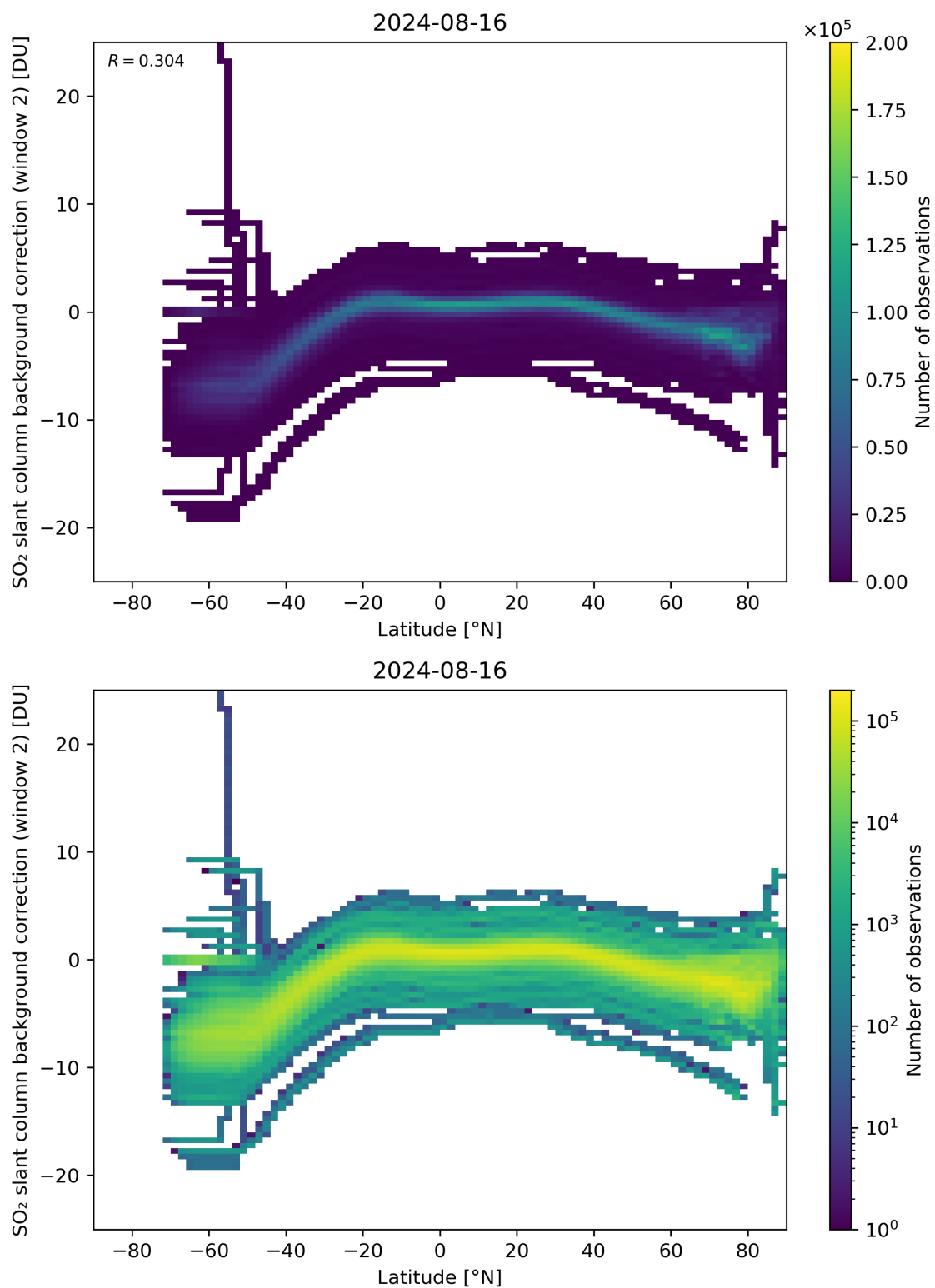
Figure 140: Scatter density plot of “Latitude” against “SO 2 slant column background correction (window 2)” for 2024-08-16 to 2024-08-17.
