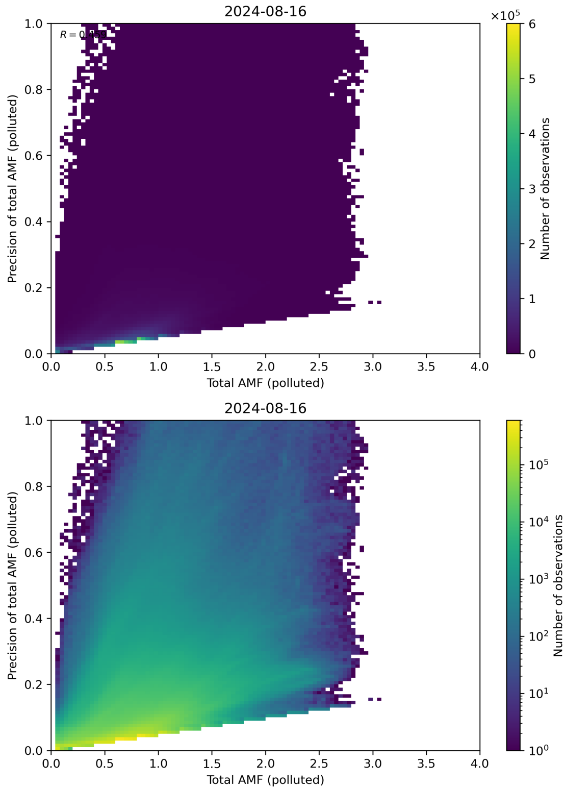
Figure 272: Scatter density plot of “Total AMF (polluted)” against “Precision of total AMF (polluted)” for 2024-08-16 to 2024-08-17.
