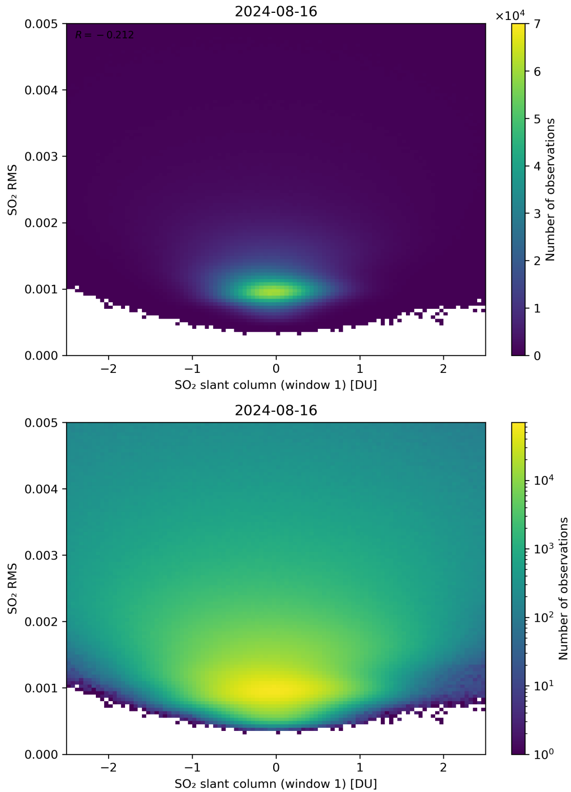
Figure 217: Scatter density plot of “SO 2 slant column (window 1)” against “SO 2 RMS” for 2024-08-16 to 2024-08-17.
