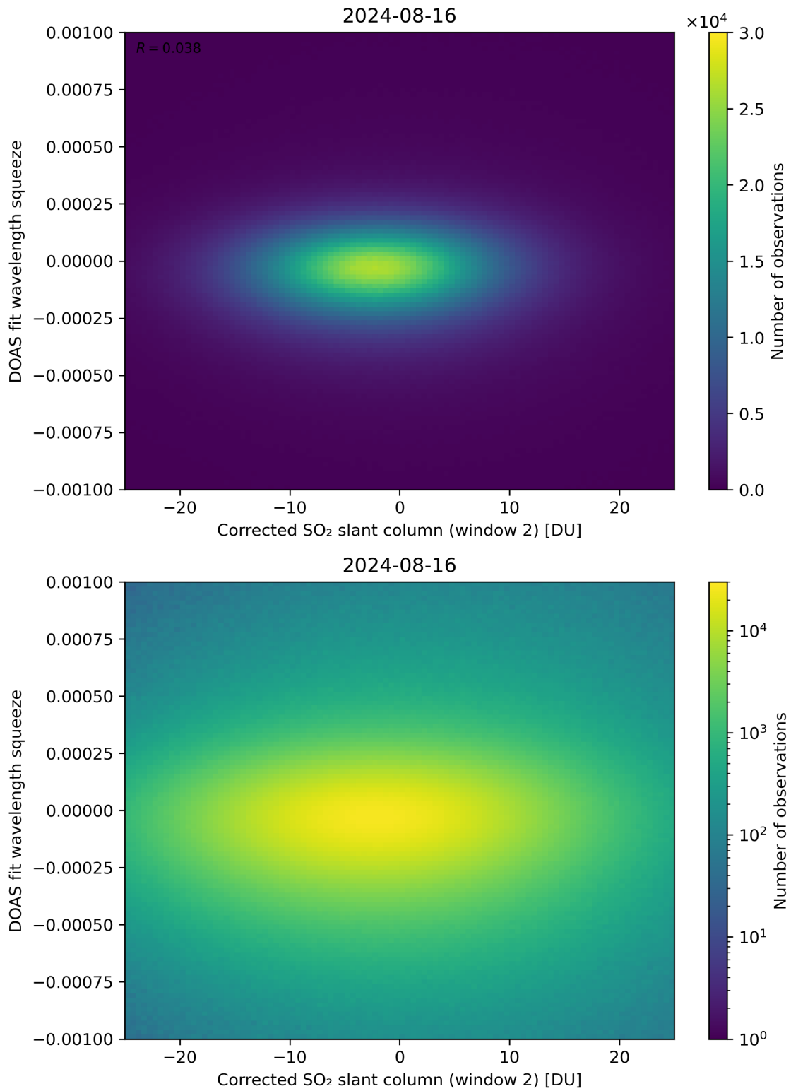
Figure 197: Scatter density plot of “Corrected SO 2 slant column (window 2)” against “DOAS fit wavelength squeeze” for 2024-08-16 to 2024-08-17.
