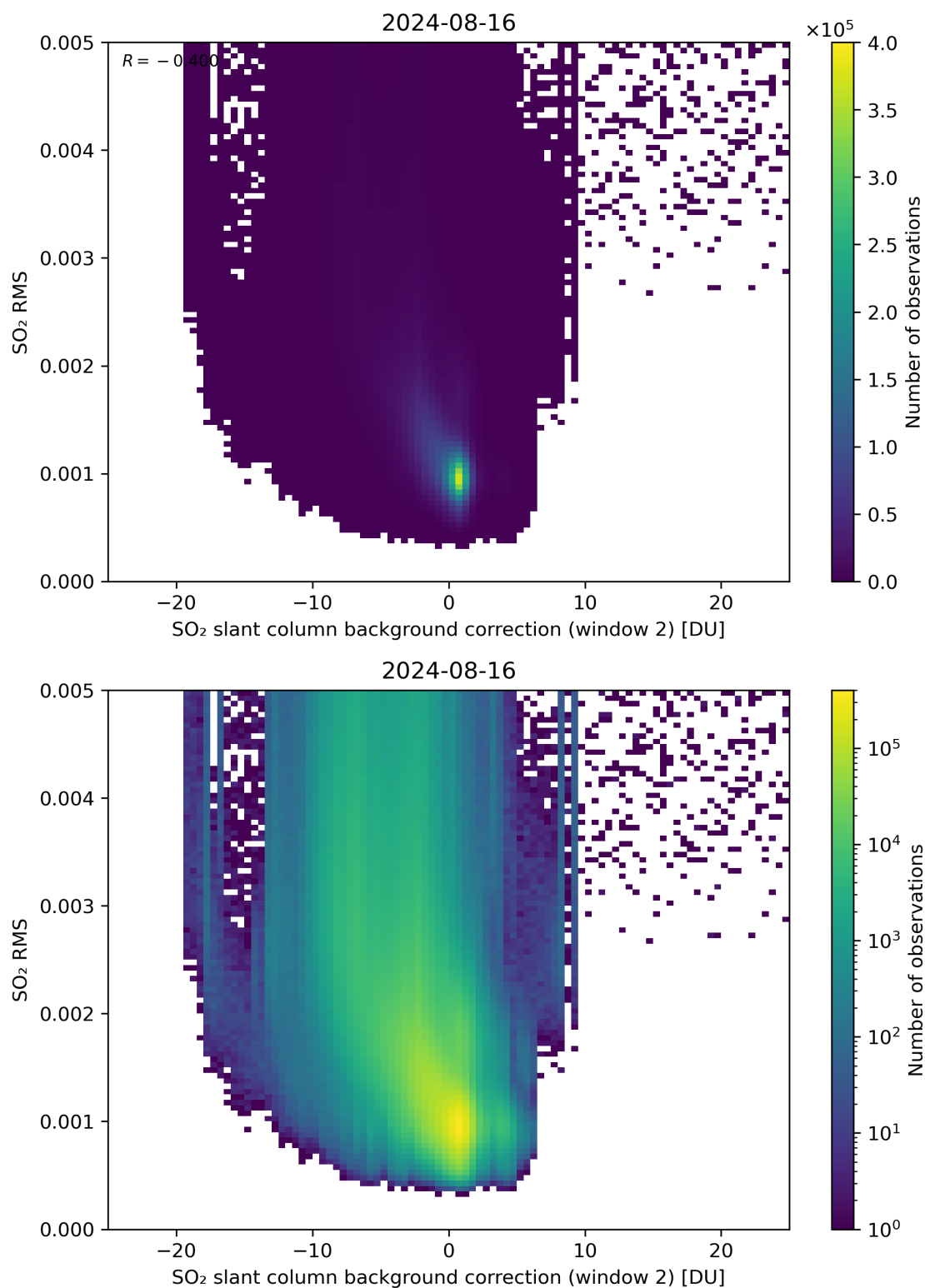
Figure 114: Scatter density plot of “SO 2 slant column background correction (window 2)” against “SO 2 RMS” for 2024-08-16 to 2024-08-17.
