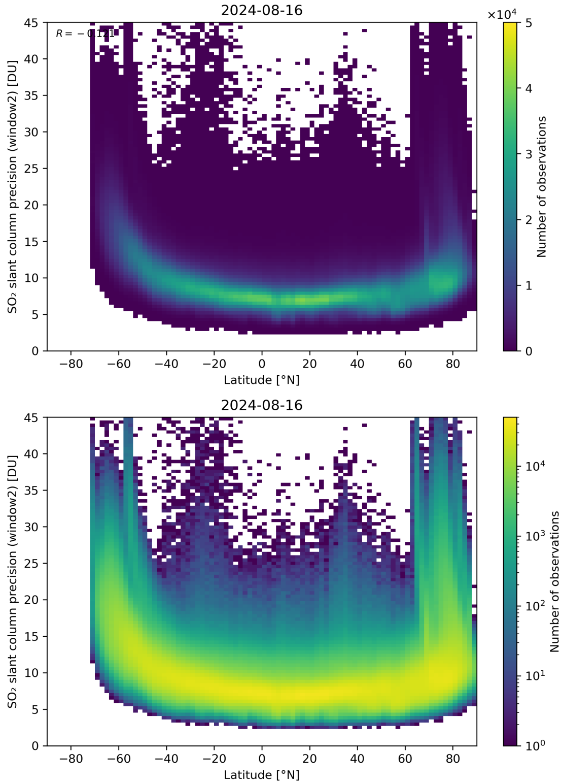
Figure 151: Scatter density plot of “Latitude” against “SO 2 slant column precision (window2)” for 2024-08-16 to 2024-08-17.
