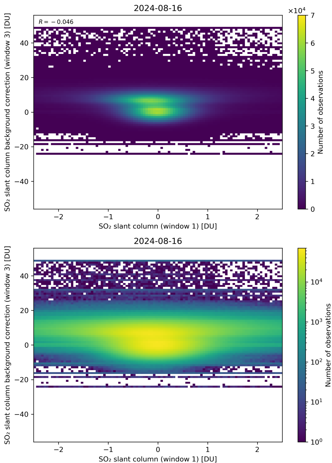
Figure 214: Scatter density plot of “SO 2 slant column (window 1)” against “SO 2 slant column background correction (window 3)” for 2024-08-16 to 2024-08-17.
