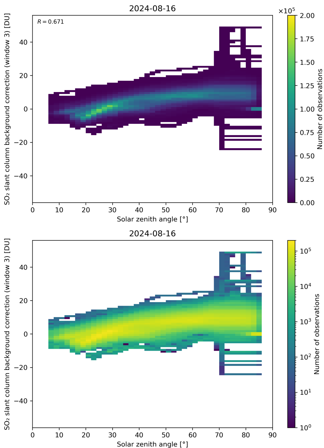
Figure 160: Scatter density plot of “Solar zenith angle” against “SO 2 slant column background correction (window 3)” for 2024-08-16 to 2024-08-17.
