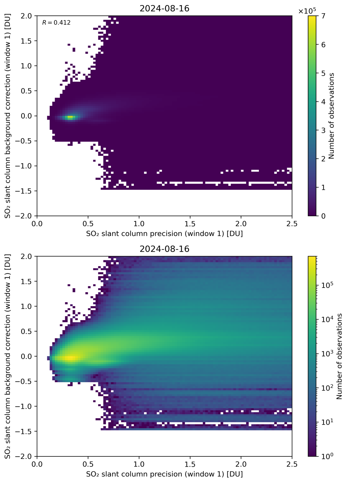
Figure 218: Scatter density plot of “SO 2 slant column precision (window 1)” against “SO 2 slant column background correction (window 1)” for 2024-08-16 to 2024-08-17.
