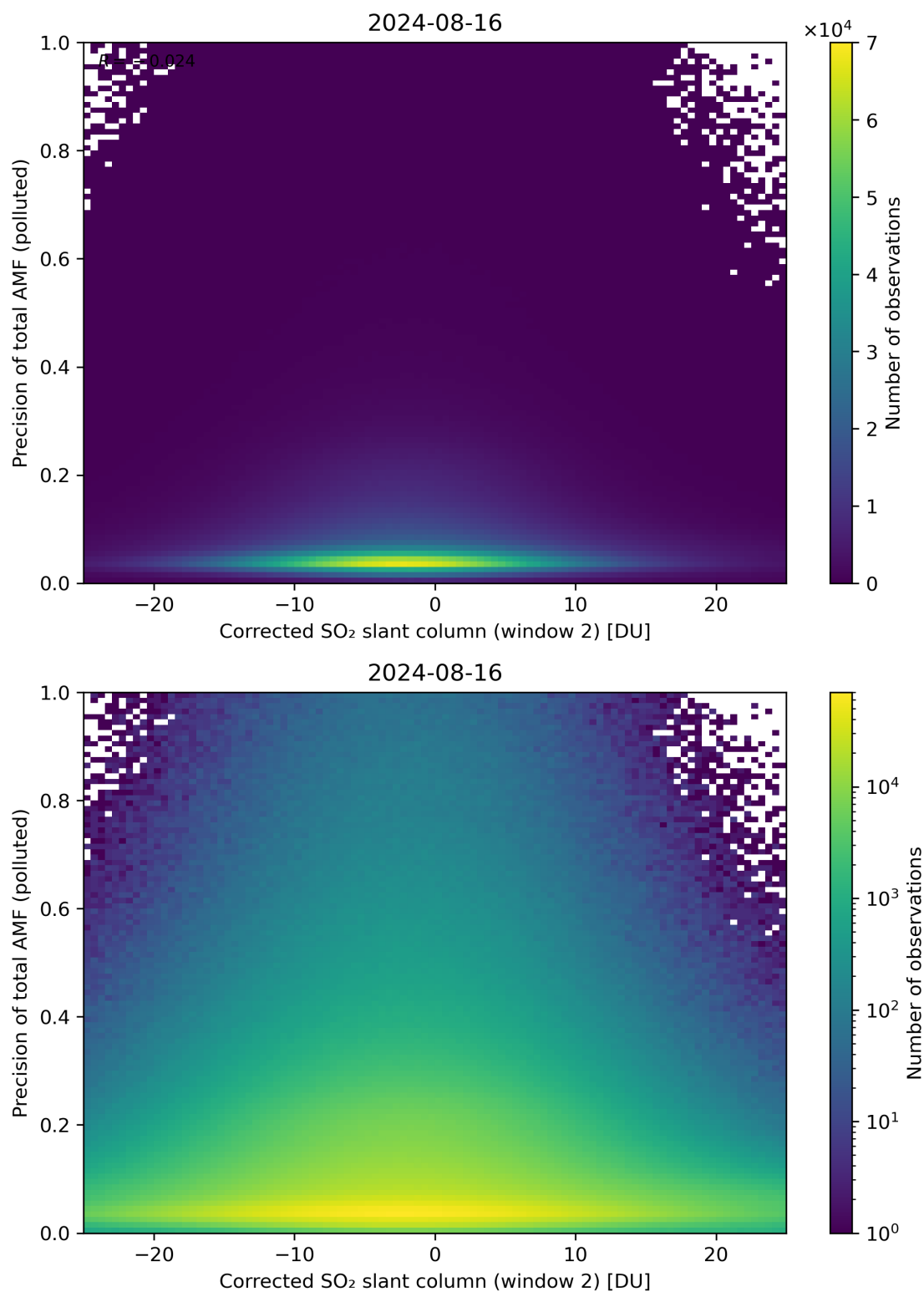
Figure 204: Scatter density plot of “Corrected SO 2 slant column (window 2)” against “Precision of total AMF (polluted)” for 2024-08-16 to 2024-08-17.
