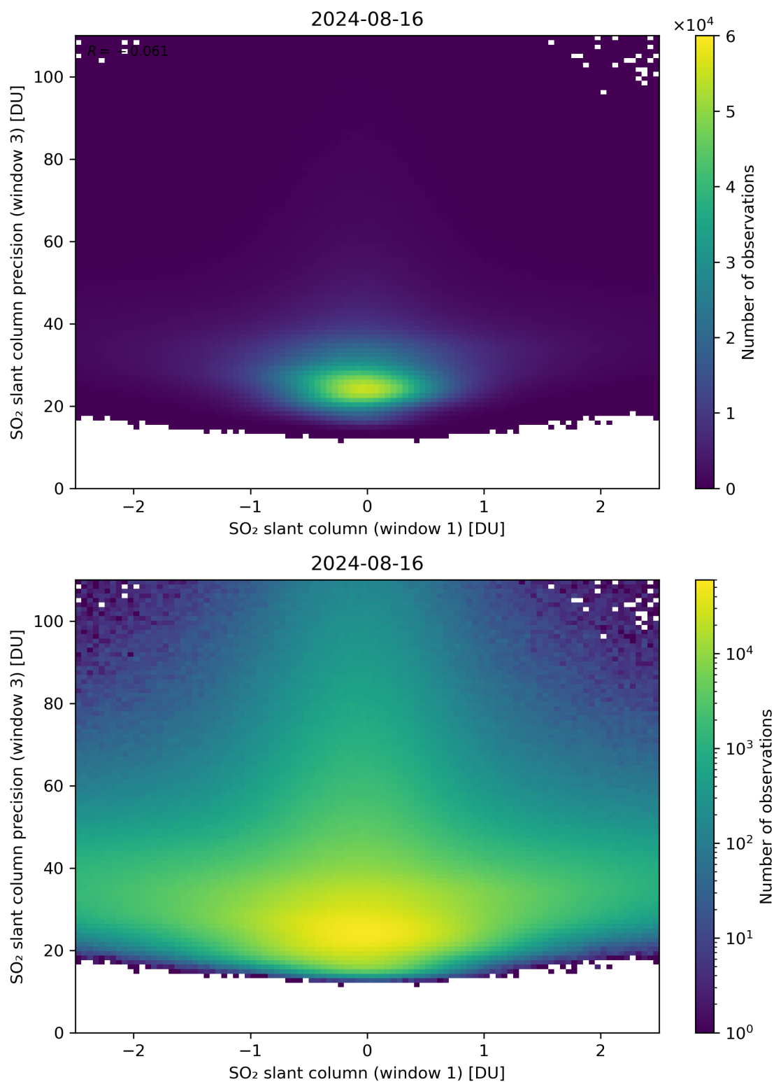
Figure 238: Scatter density plot of “SO 2 slant column (window 1)” against “SO 2 slant column precision (window 3)” for 2024-08-16 to 2024-08-17.
