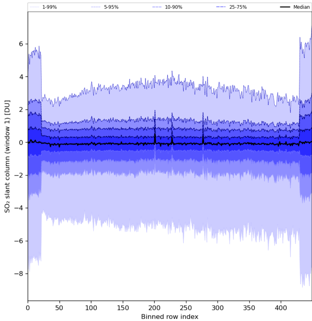
Figure 79: Along track statistics of “SO 2 slant column (window 1)” for 2024-08-16 to 2024-08-17
