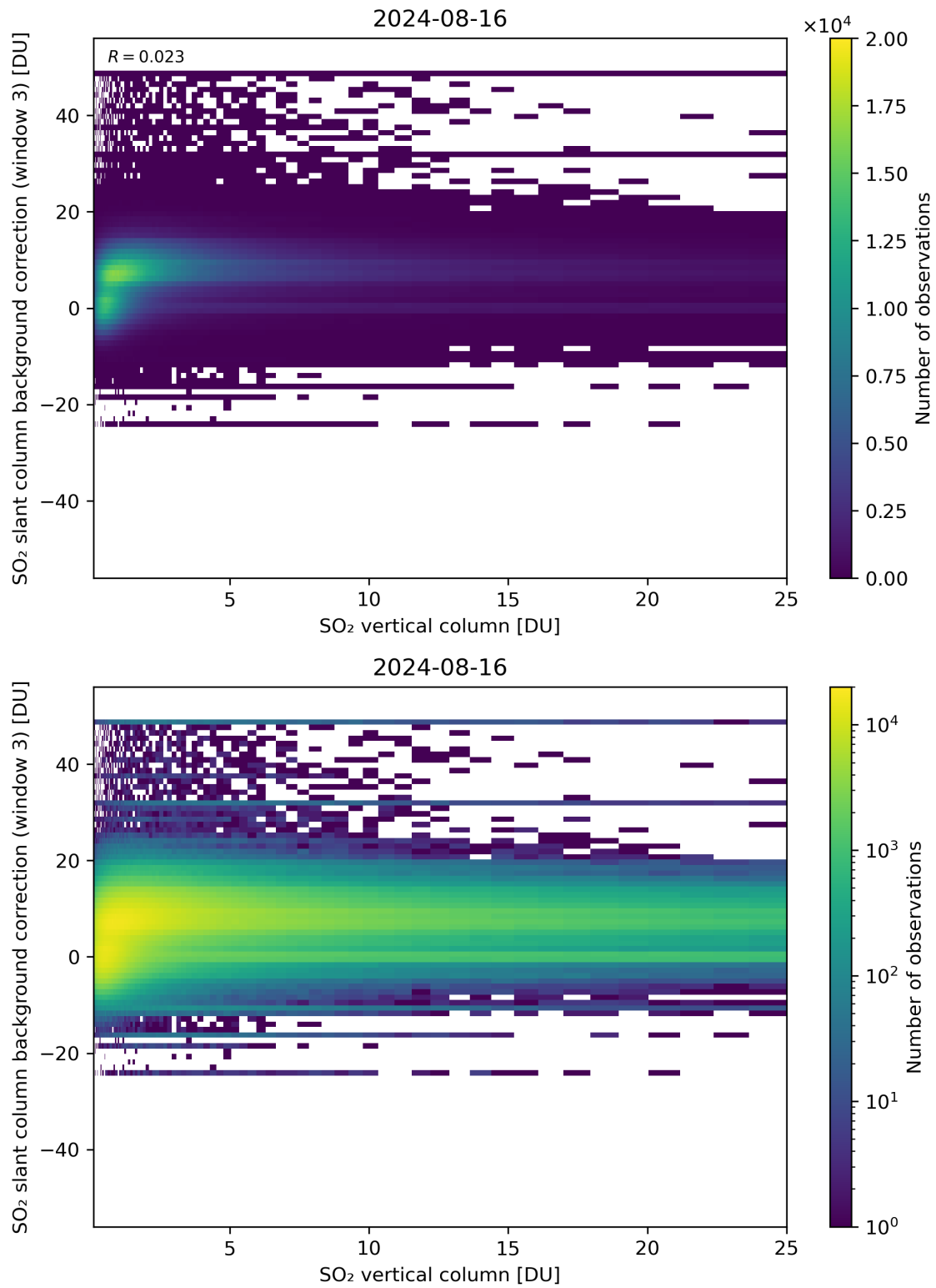
Figure 275: Scatter density plot of “SO 2 vertical column” against “SO 2 slant column background correction (window 3)” for 2024-08-16 to 2024-08-17.
