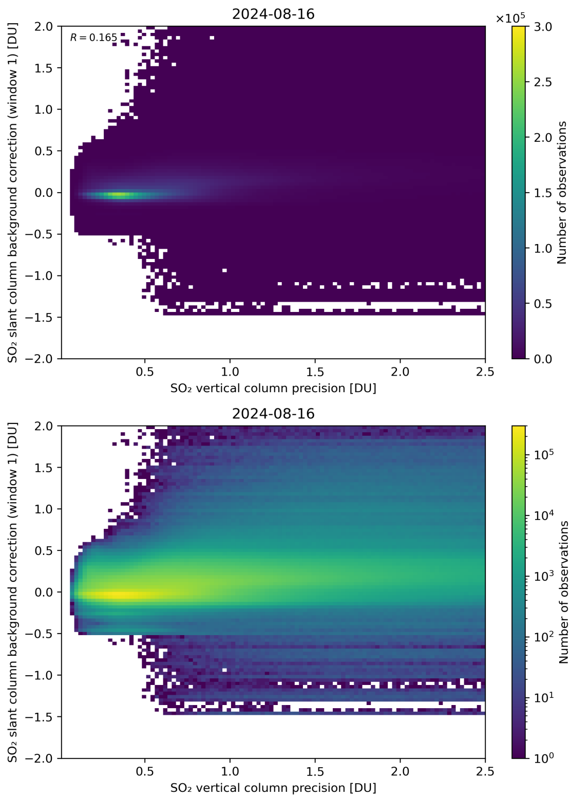
Figure 279: Scatter density plot of “SO 2 vertical column precision” against “SO 2 slant column background correction (window 1)” for 2024-08-16 to 2024-08-17.
