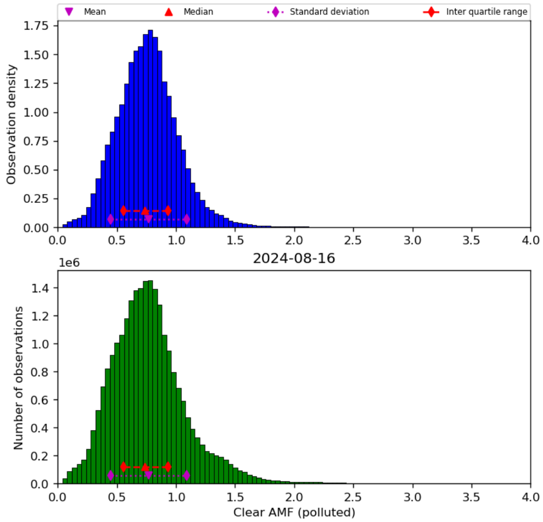
Figure 73: Histogram of “Clear AMF (polluted)” for 2024-08-16 to 2024-08-17
