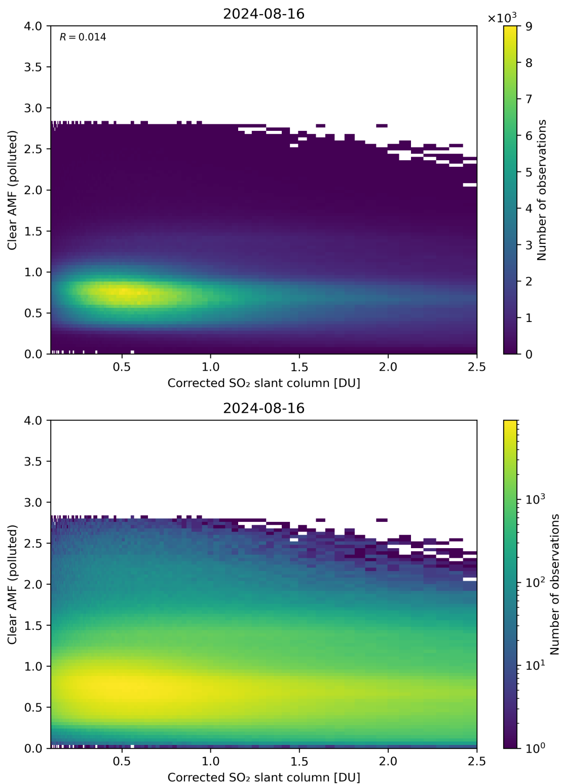
Figure 184: Scatter density plot of “Corrected SO 2 slant column” against “Clear AMF (polluted)” for 2024-08-16 to 2024-08-17.
