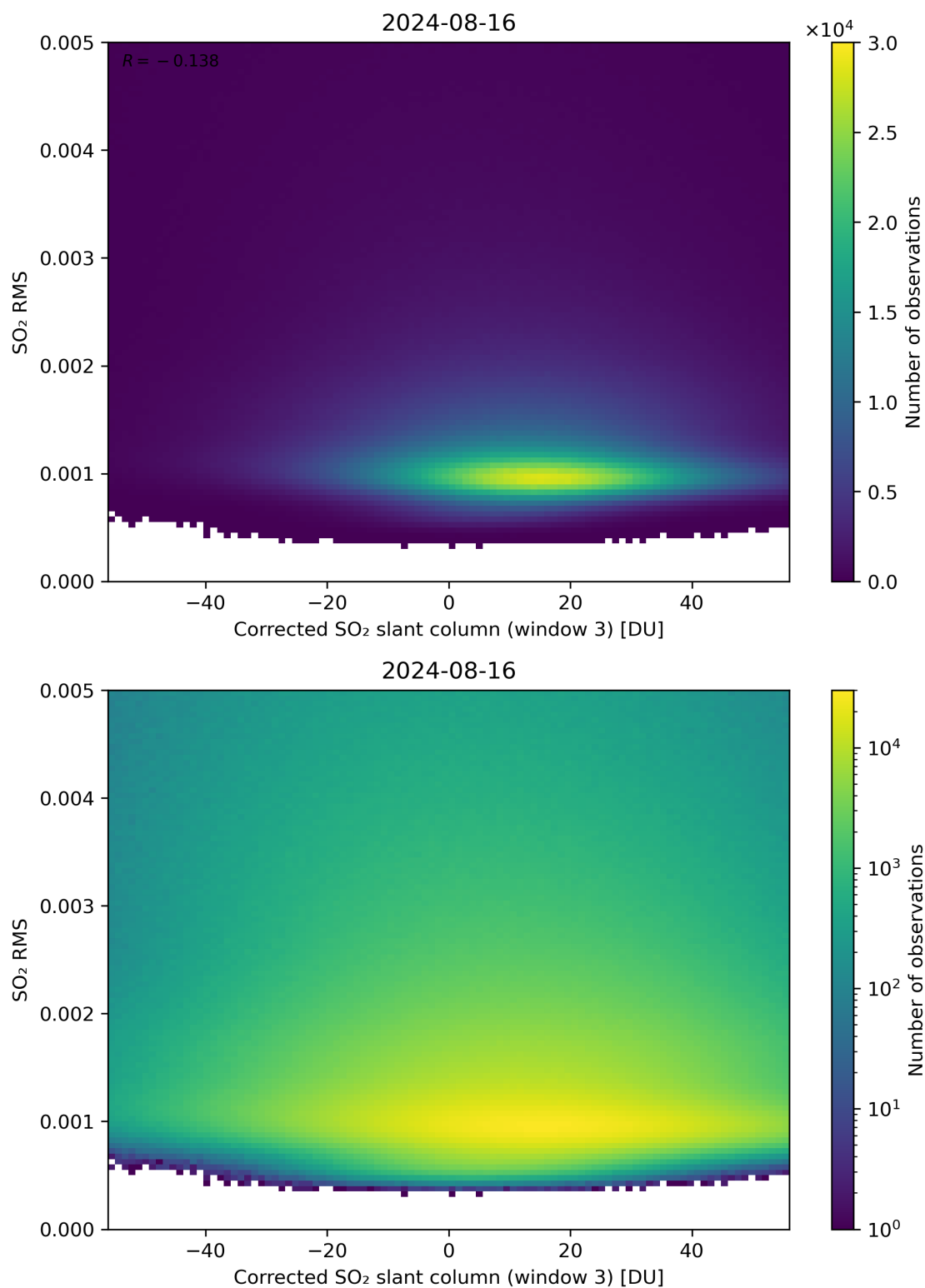
Figure 208: Scatter density plot of “Corrected SO 2 slant column (window 3)” against “SO 2 RMS” for 2024-08-16 to 2024-08-17.
