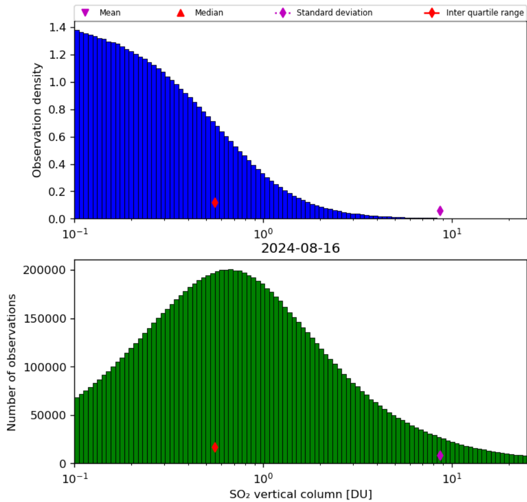
Figure 53: Histogram of “SO 2 vertical column” for 2024-08-16 to 2024-08-17
