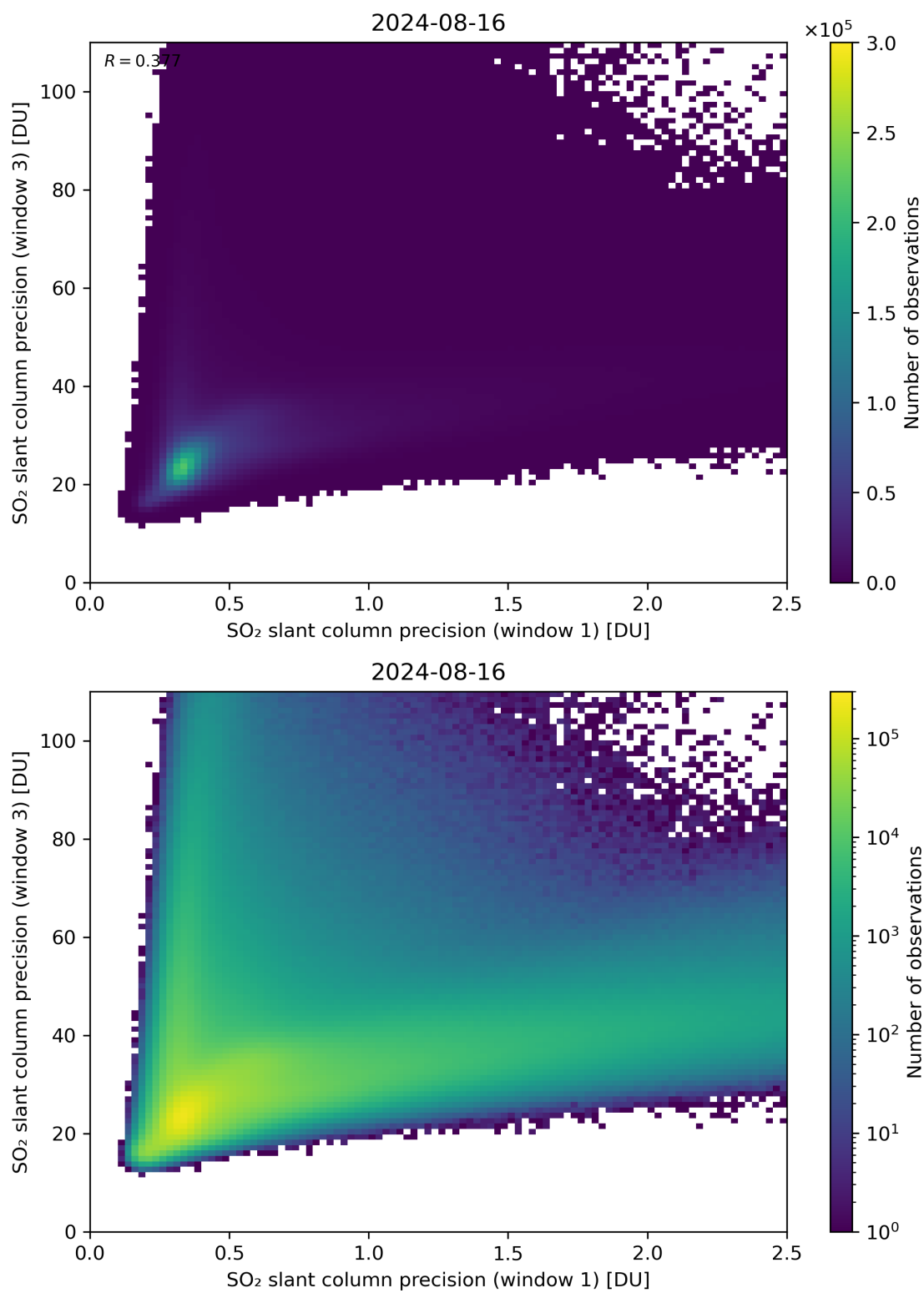
Figure 229: Scatter density plot of “SO 2 slant column precision (window 1)” against “SO 2 slant column precision (window 3)” for 2024-08-16 to 2024-08-17.
