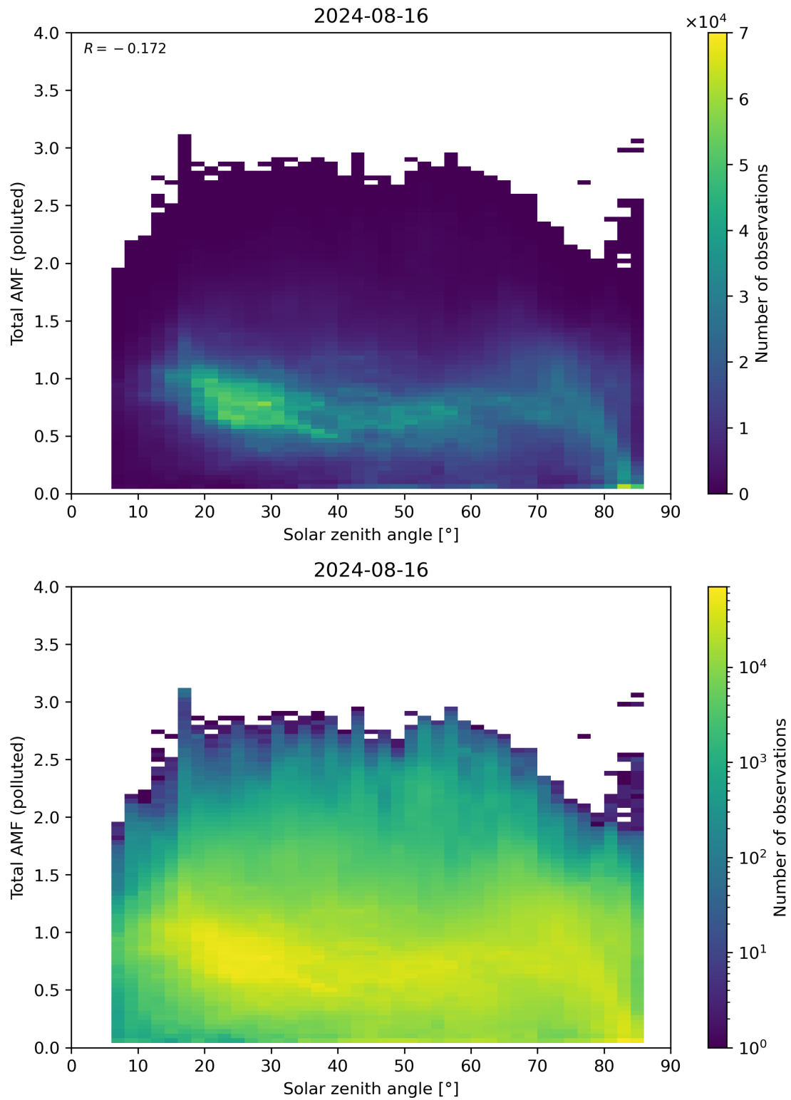
Figure 174: Scatter density plot of “Solar zenith angle” against “Total AMF (polluted)” for 2024-08-16 to 2024-08-17.
