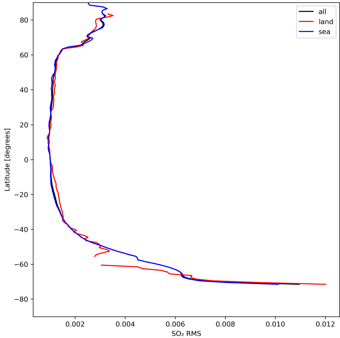
Figure 47: Zonal average of “SO 2 RMS” for 2024-08-16 to 2024-08-17.
