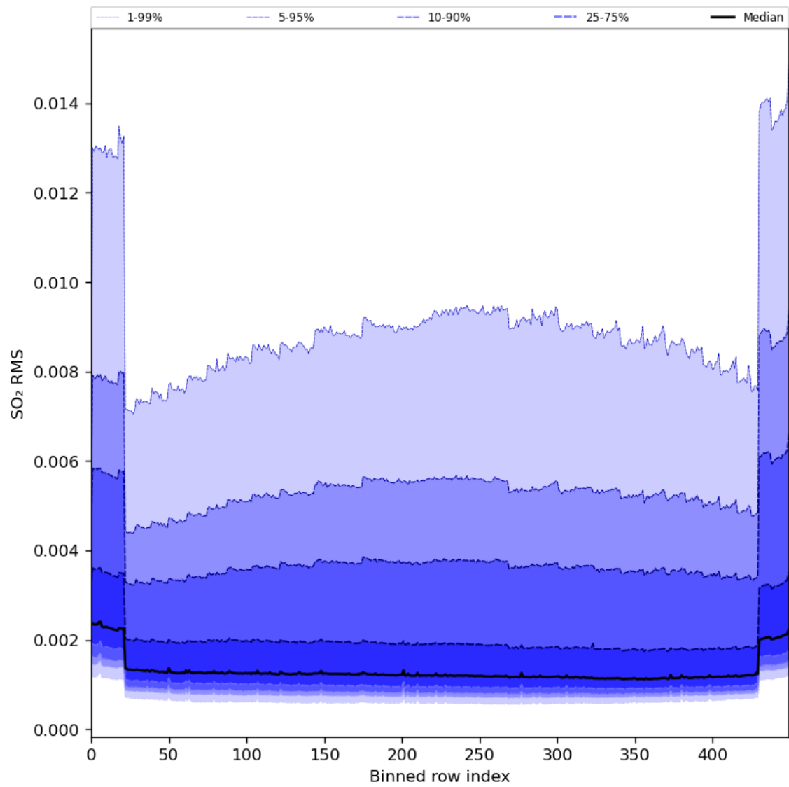
Figure 93: Along track statistics of “SO 2 RMS” for 2024-08-16 to 2024-08-17
