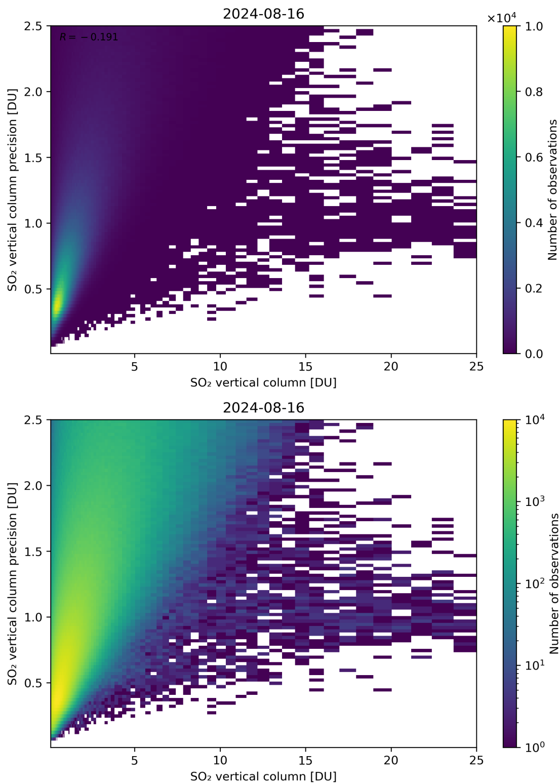
Figure 307: Scatter density plot of “SO 2 vertical column” against “SO 2 vertical column precision” for 2024-08-16 to 2024-08-17.
