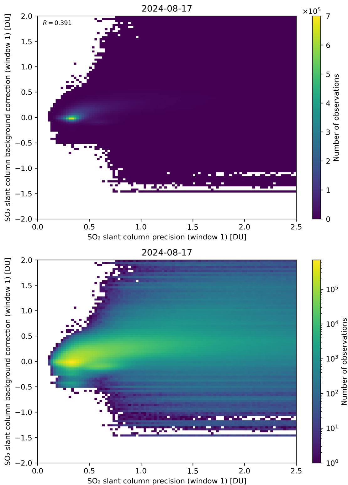
Figure 218: Scatter density plot of “SO 2 slant column precision (window 1)” against “SO 2 slant column background correction (window 1)” for 2024-08-16 to 2024-08-18.
