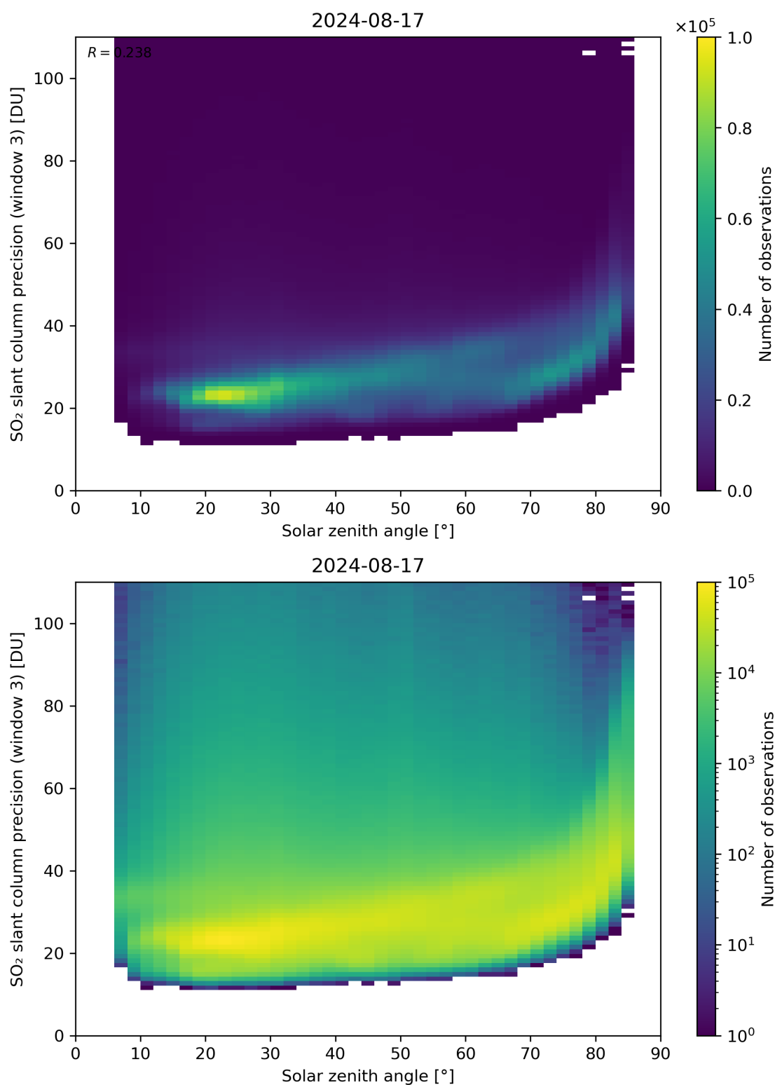
Figure 173: Scatter density plot of “Solar zenith angle” against “SO 2 slant column precision (window 3)” for 2024-08-16 to 2024-08-18.
