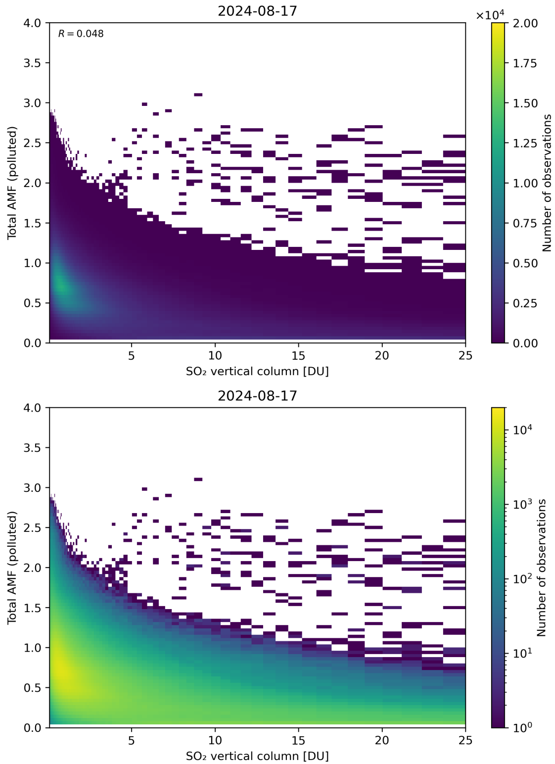
Figure 305: Scatter density plot of “SO 2 vertical column” against “Total AMF (polluted)” for 2024-08-16 to 2024-08-18.
