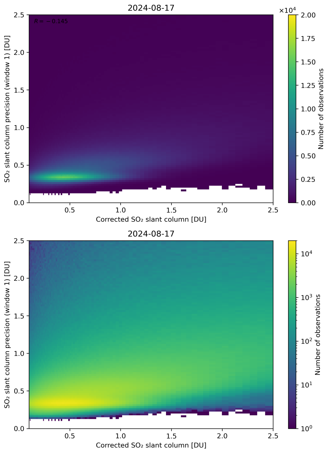
Figure 188: Scatter density plot of “Corrected SO 2 slant column” against “SO 2 slant column precision (window 1)” for 2024-08-16 to 2024-08-18.
