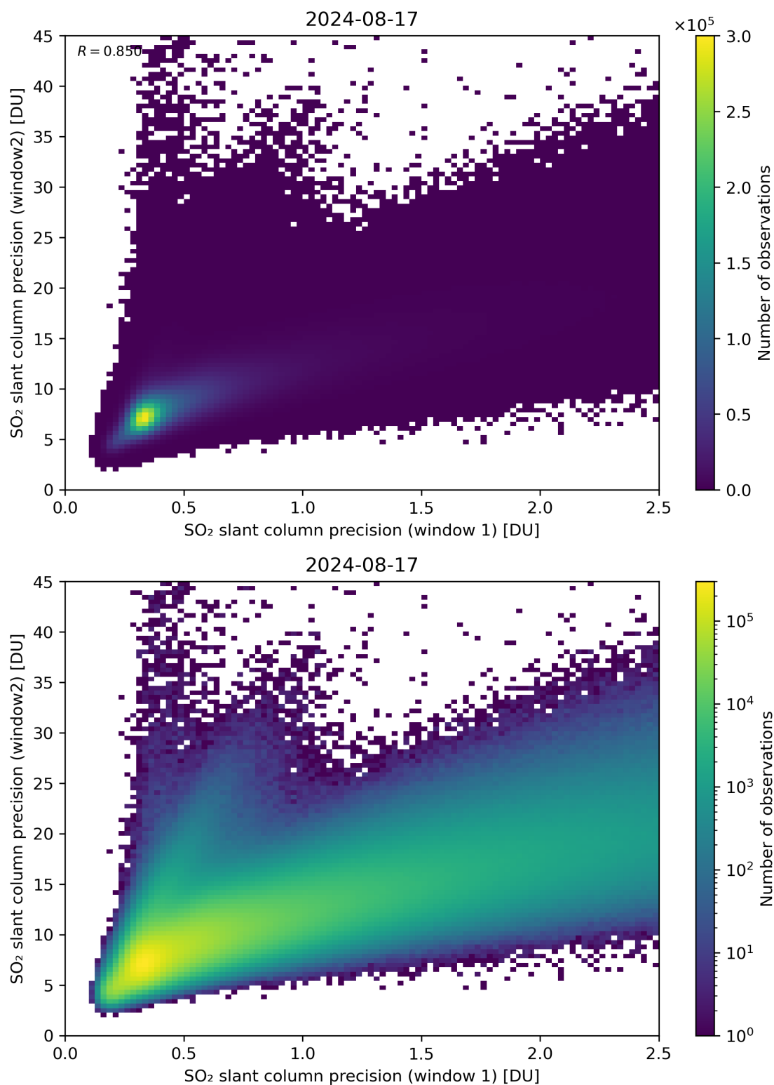
Figure 227: Scatter density plot of “SO 2 slant column precision (window 1)” against “SO 2 slant column precision (window2)” for 2024-08-16 to 2024-08-18.
