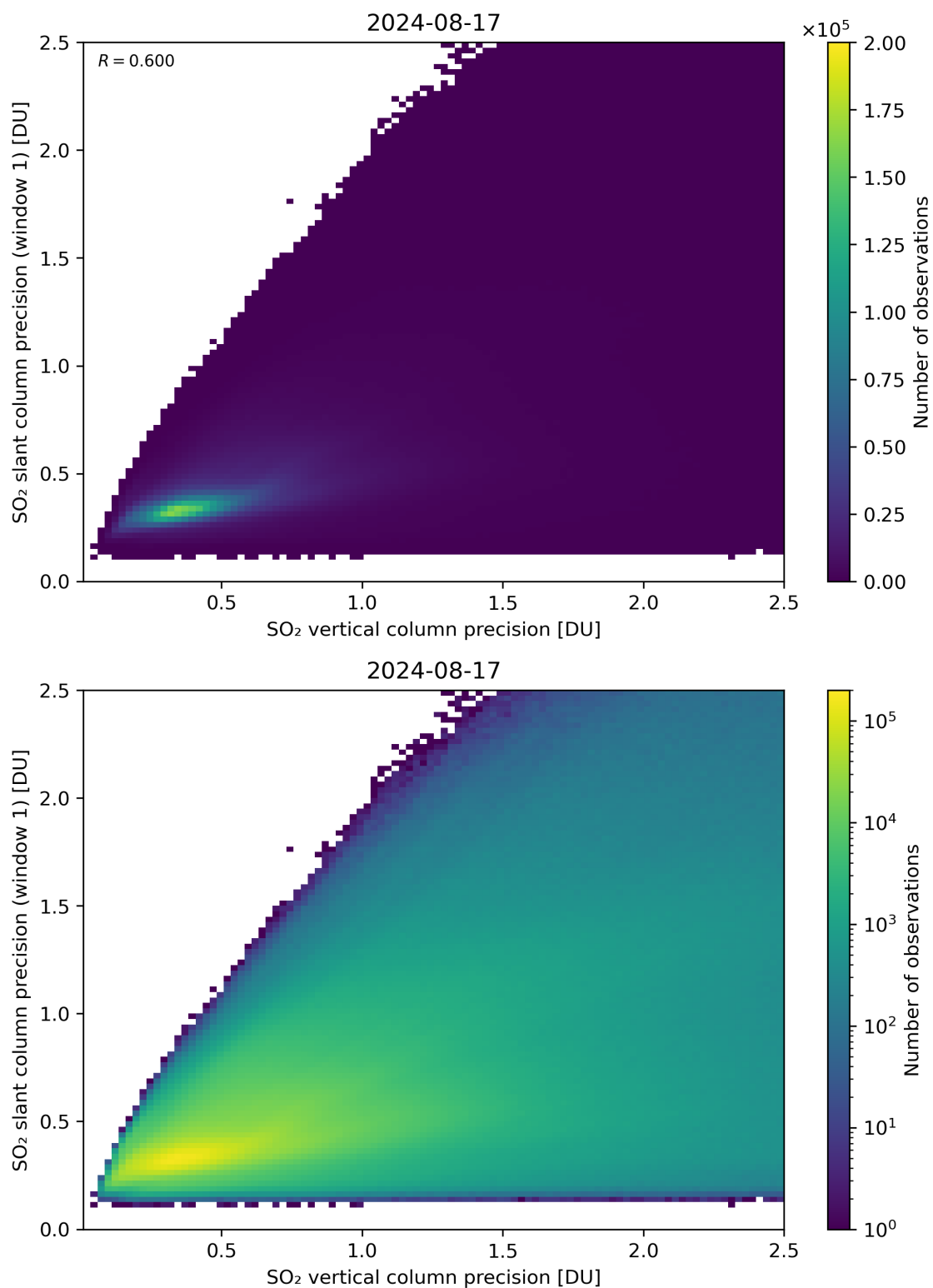
Figure 290: Scatter density plot of “SO 2 vertical column precision” against “SO 2 slant column precision (window 1)” for 2024-08-16 to 2024-08-18.
