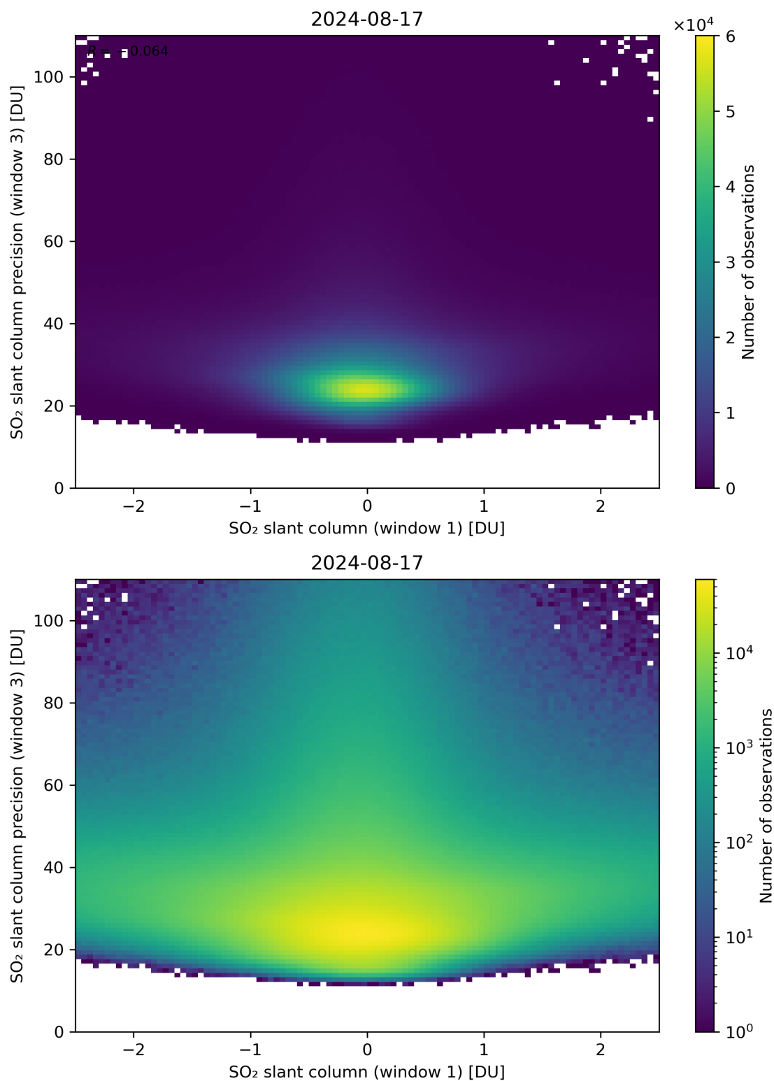
Figure 238: Scatter density plot of “SO 2 slant column (window 1)” against “SO 2 slant column precision (window 3)” for 2024-08-16 to 2024-08-18.
