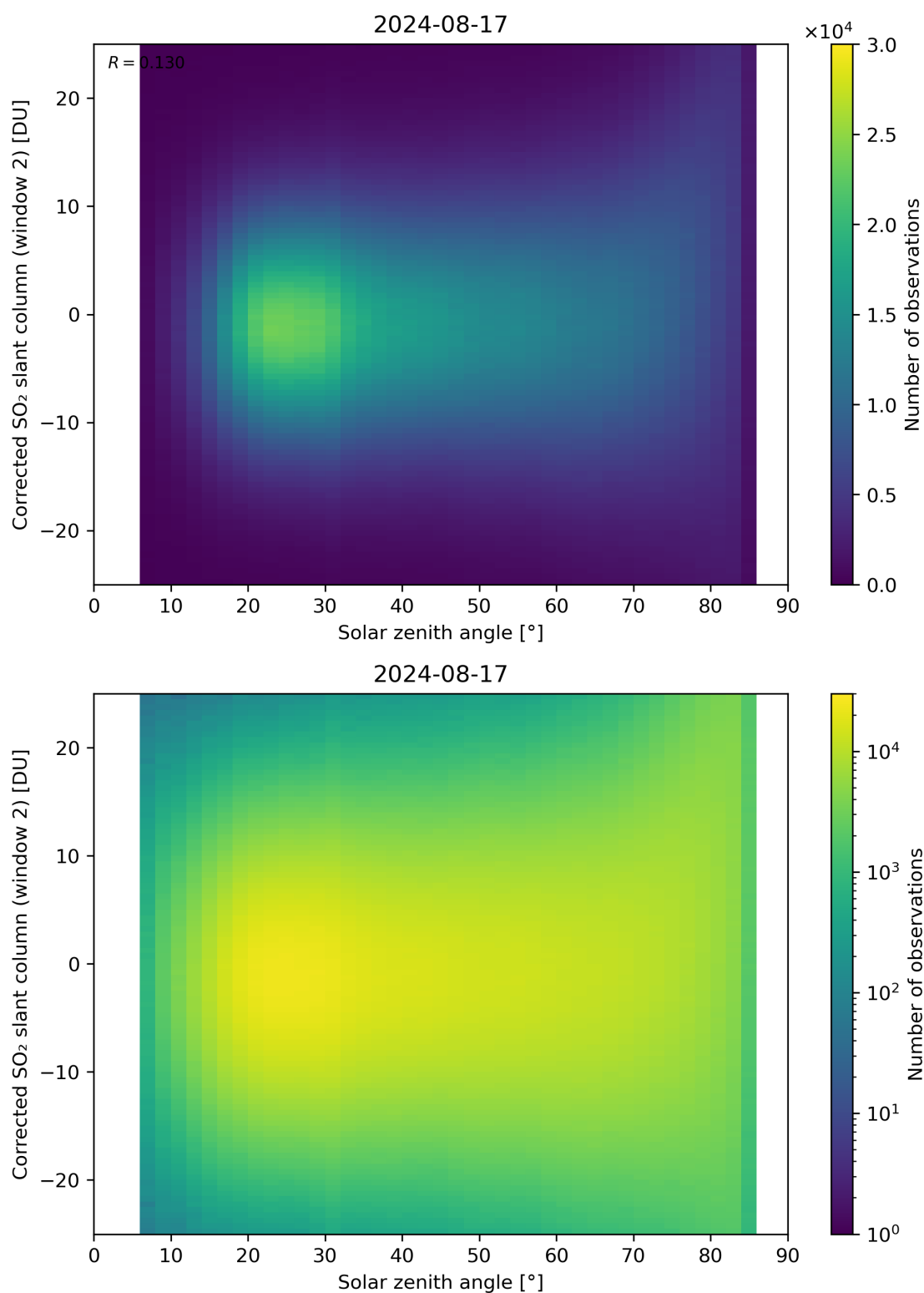
Figure 167: Scatter density plot of “Solar zenith angle” against “Corrected SO 2 slant column (window 2)” for 2024-08-16 to 2024-08-18.
