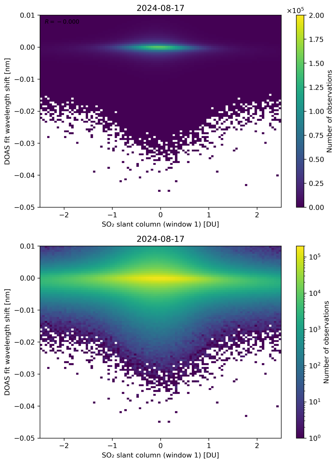
Figure 215: Scatter density plot of “SO 2 slant column (window 1)” against “DOAS fit wavelength shift” for 2024-08-16 to 2024-08-18.
