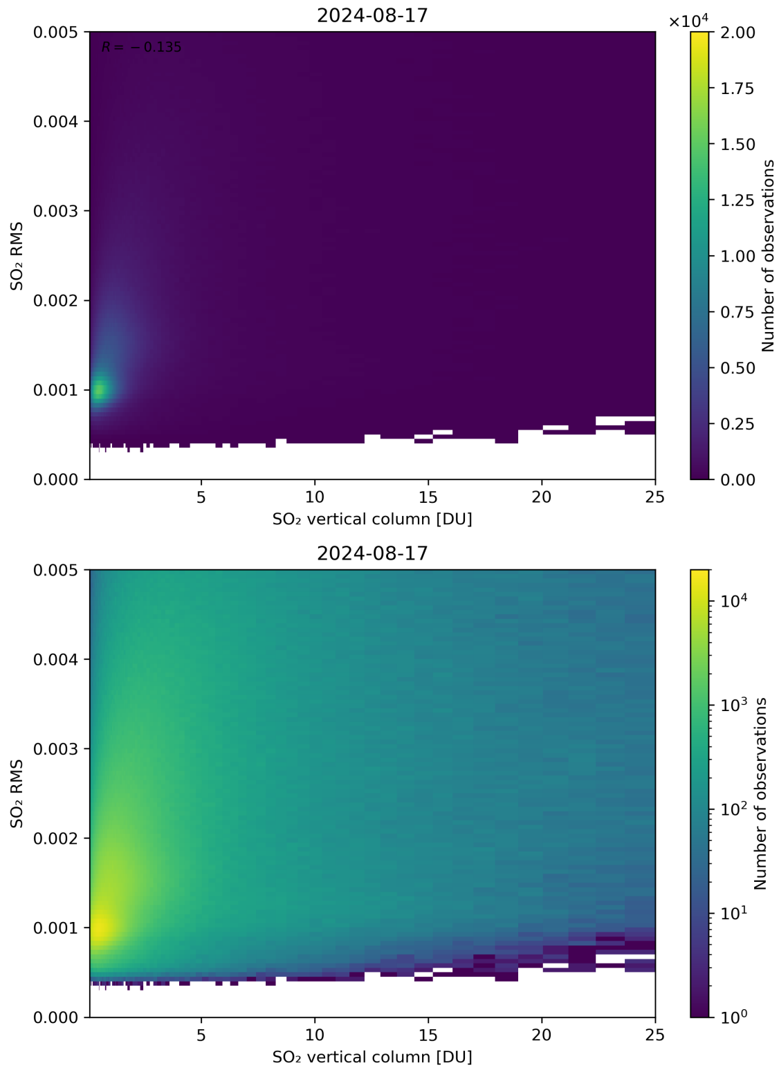
Figure 278: Scatter density plot of “SO 2 vertical column” against “SO 2 RMS” for 2024-08-16 to 2024-08-18.
