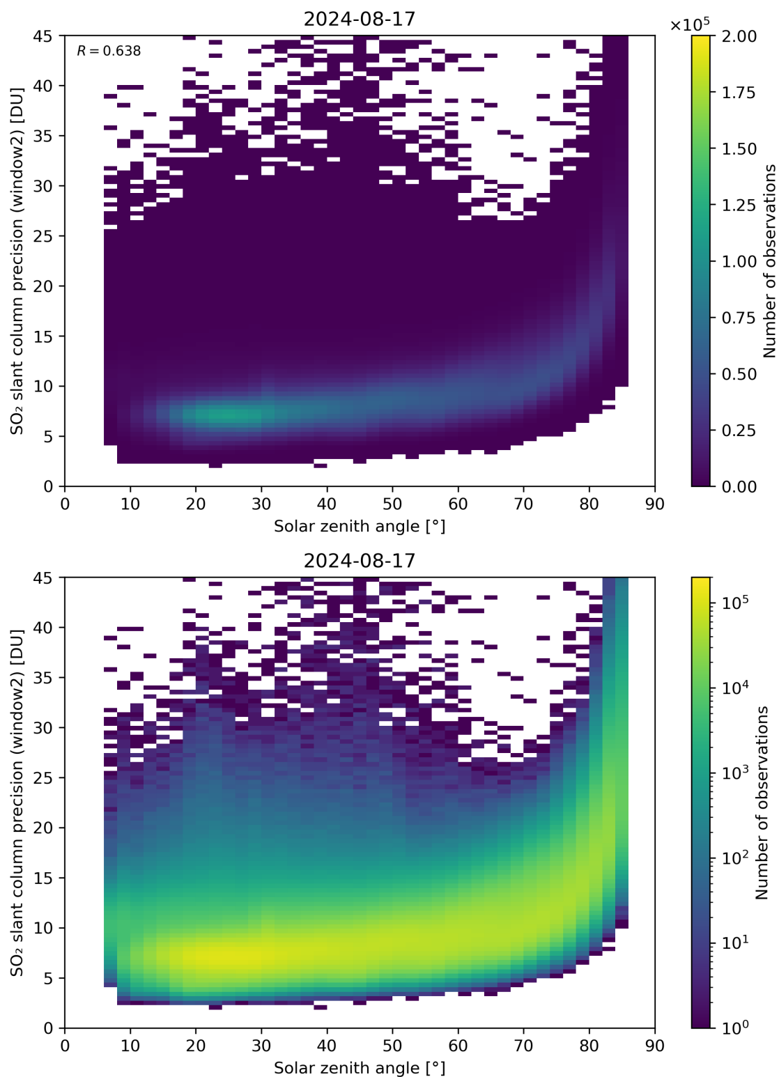
Figure 171: Scatter density plot of “Solar zenith angle” against “SO 2 slant column precision (window2)” for 2024-08-16 to 2024-08-18.
