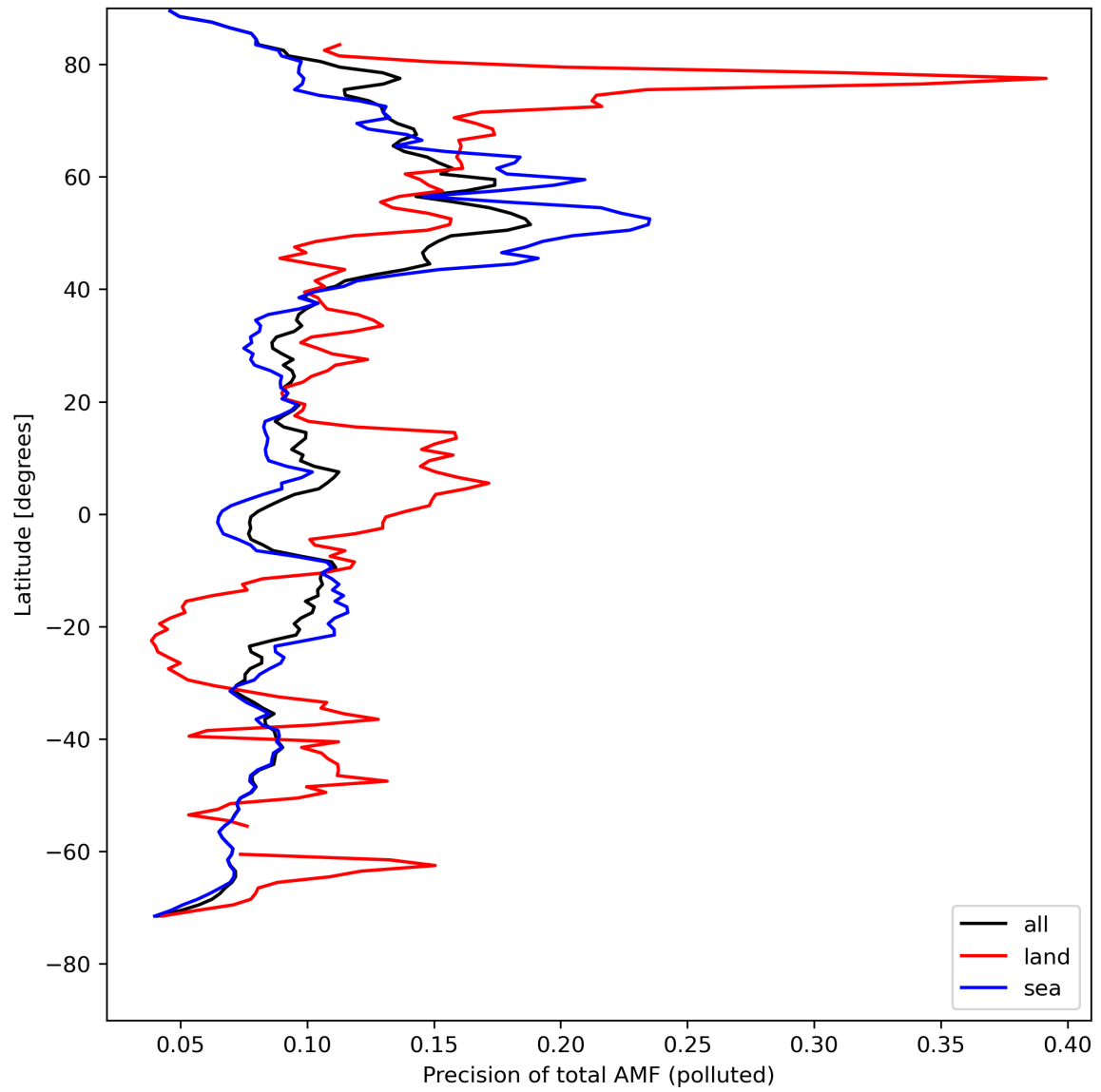
Figure 49: Zonal average of “Precision of total AMF (polluted)” for 2024-08-16 to 2024-08-18.
