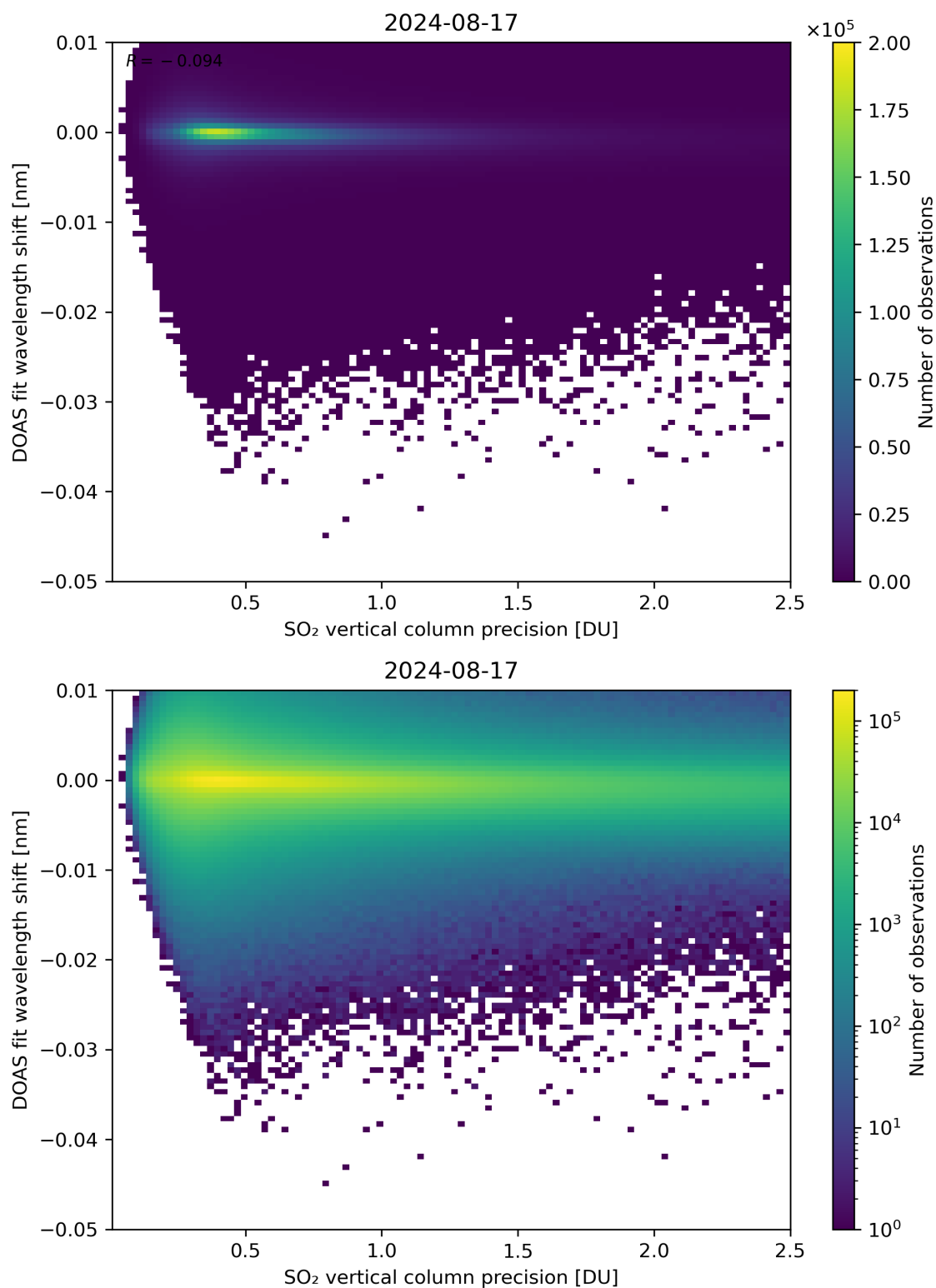
Figure 282: Scatter density plot of “SO 2 vertical column precision” against “DOAS fit wavelength shift” for 2024-08-16 to 2024-08-18.
