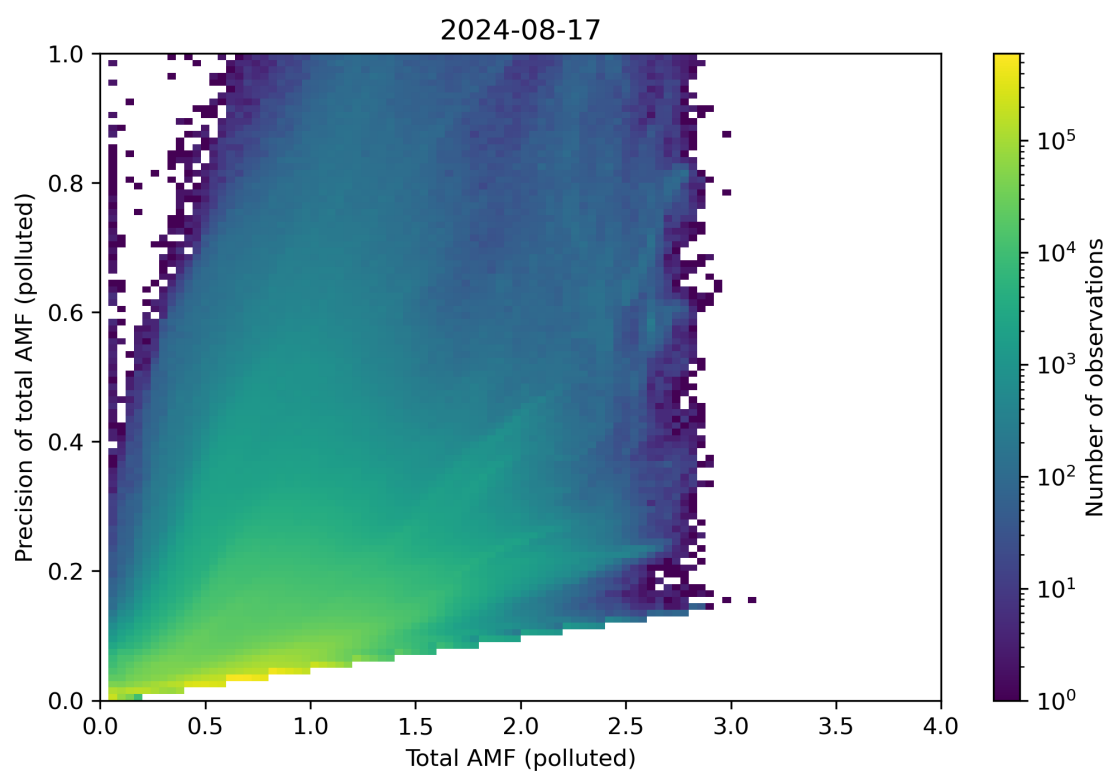
Figure 272: Scatter density plot of “Total AMF (polluted)” against “Precision of total AMF (polluted)” for 2024-08-16 to 2024-08-18.
