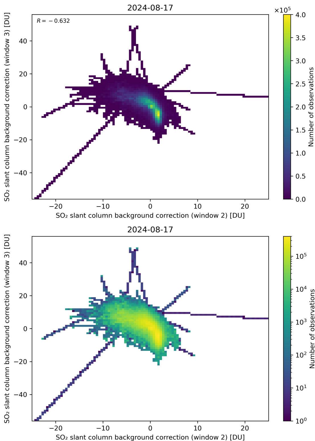
Figure 111: Scatter density plot of “SO 2 slant column background correction (window 2)” against “SO 2 slant column background correction (window 3)” for 2024-08-16 to 2024-08-18.
