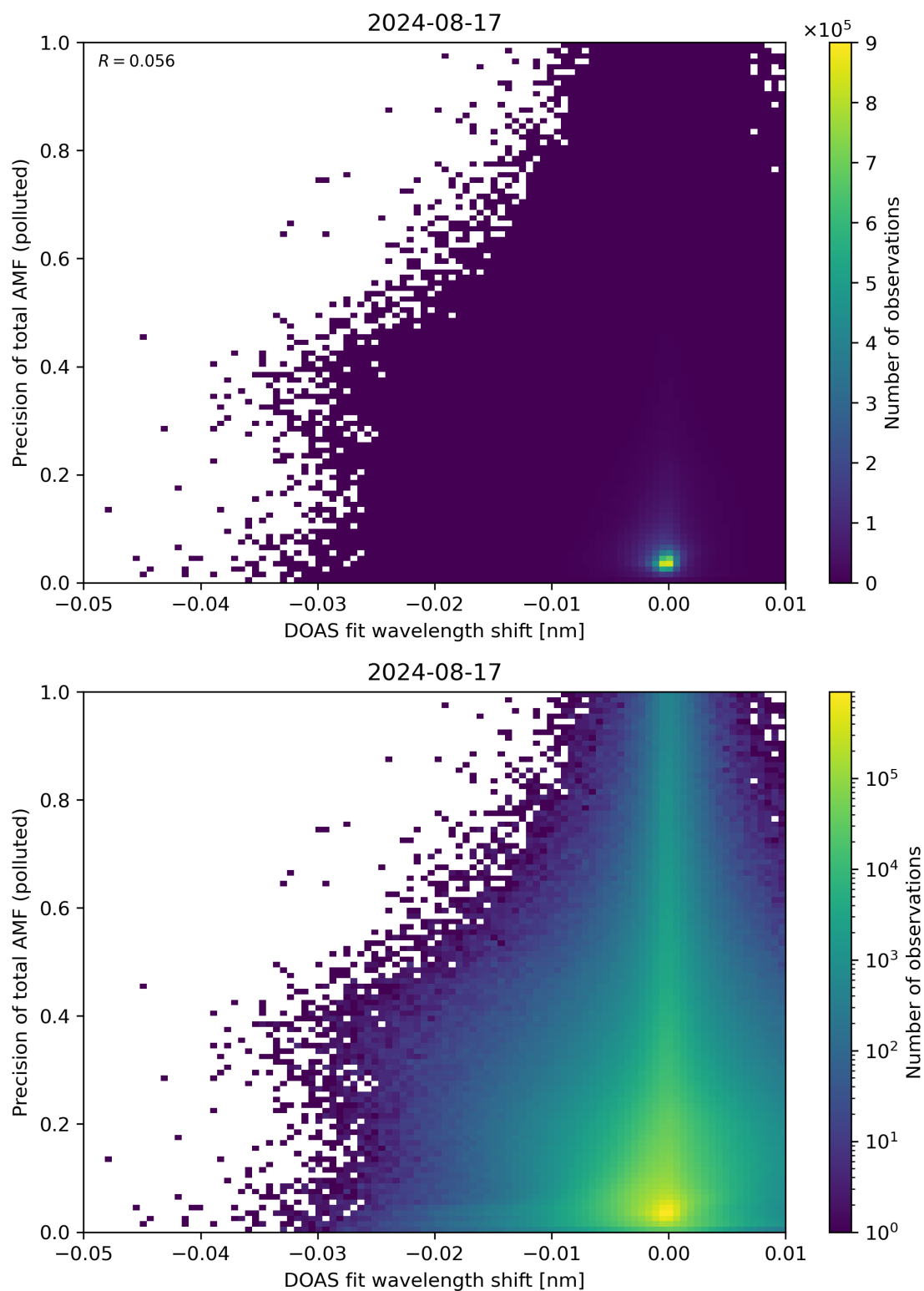
Figure 131: Scatter density plot of “DOAS fit wavelength shift” against “Precision of total AMF (polluted)” for 2024-08-16 to 2024-08-18.
