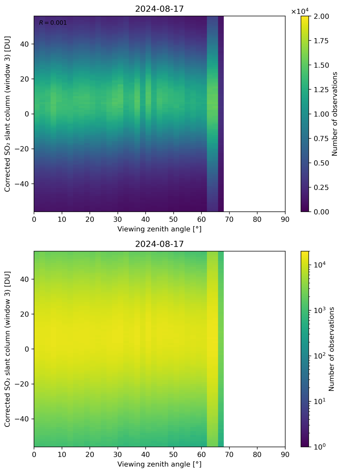
Figure 319: Scatter density plot of “Viewing zenith angle” against “Corrected SO 2 slant column (window 3)” for 2024-08-16 to 2024-08-18.
