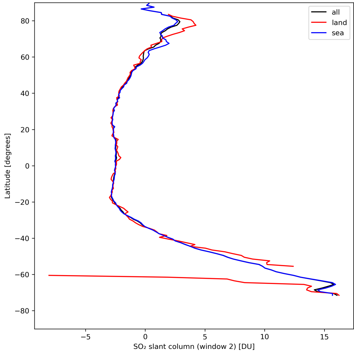
Figure 37: Zonal average of “SO 2 slant column (window 2)” for 2024-08-16 to 2024-08-18.
