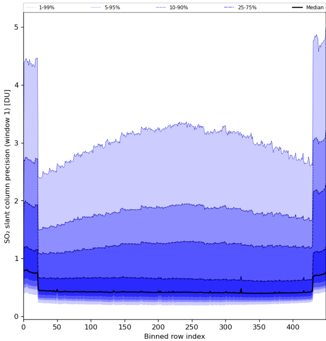
Figure 80: Along track statistics of “SO 2 slant column precision (window 1)” for 2024-08-16 to 2024-08-18
