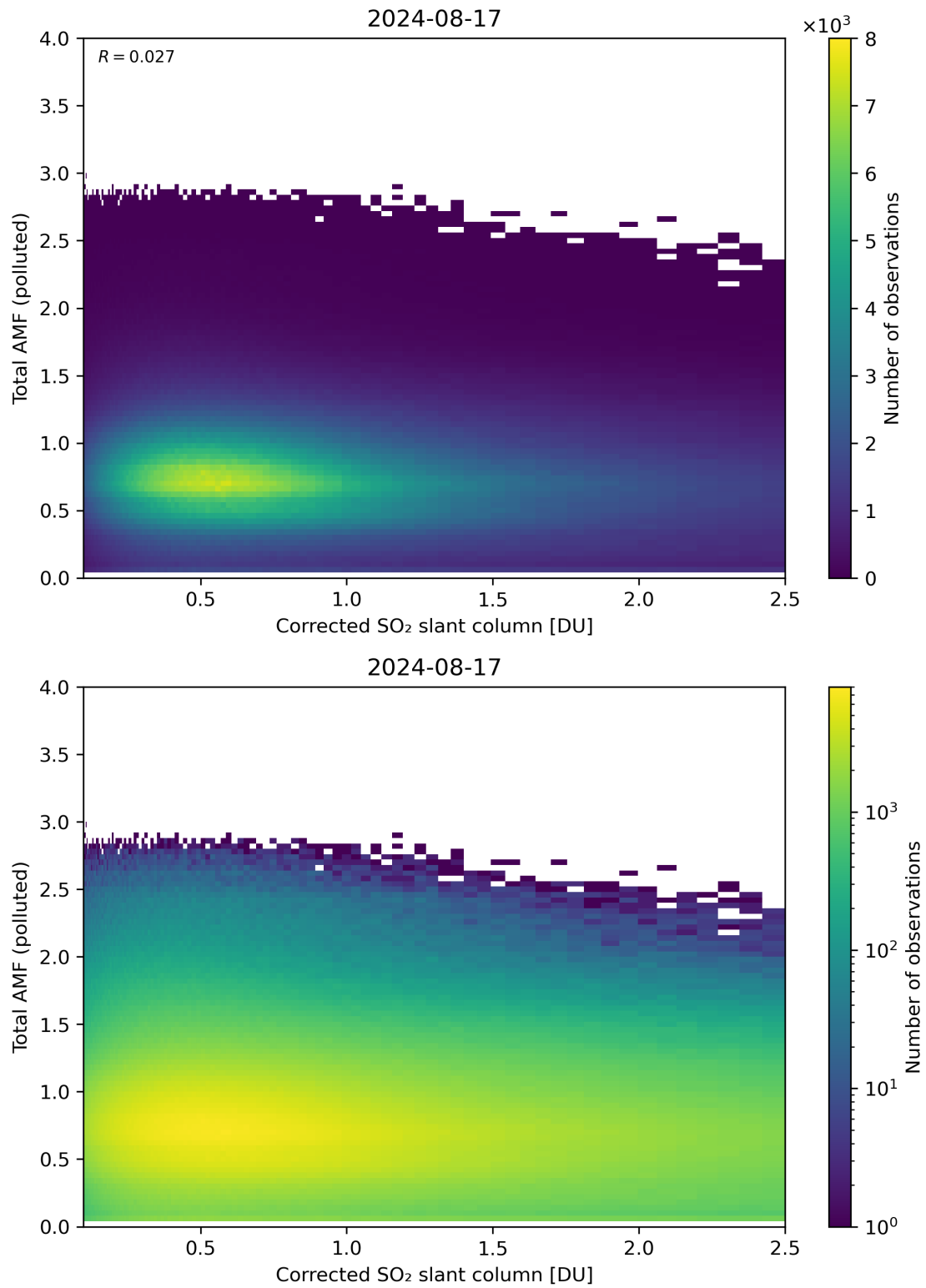
Figure 192: Scatter density plot of “Corrected SO 2 slant column” against “Total AMF (polluted)” for 2024-08-16 to 2024-08-18.
