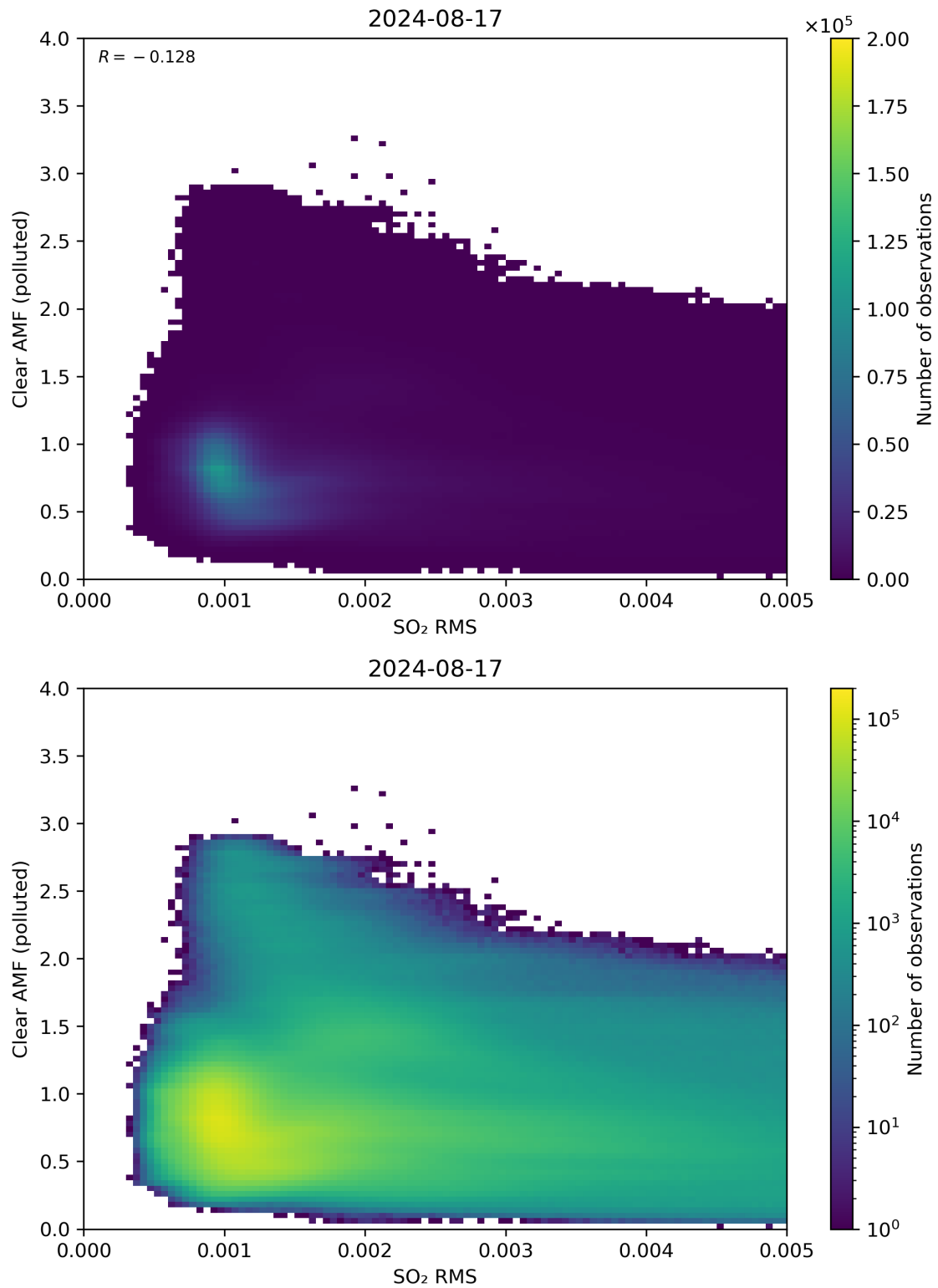
Figure 136: Scatter density plot of “SO 2 RMS” against “Clear AMF (polluted)” for 2024-08-16 to 2024-08-18.
