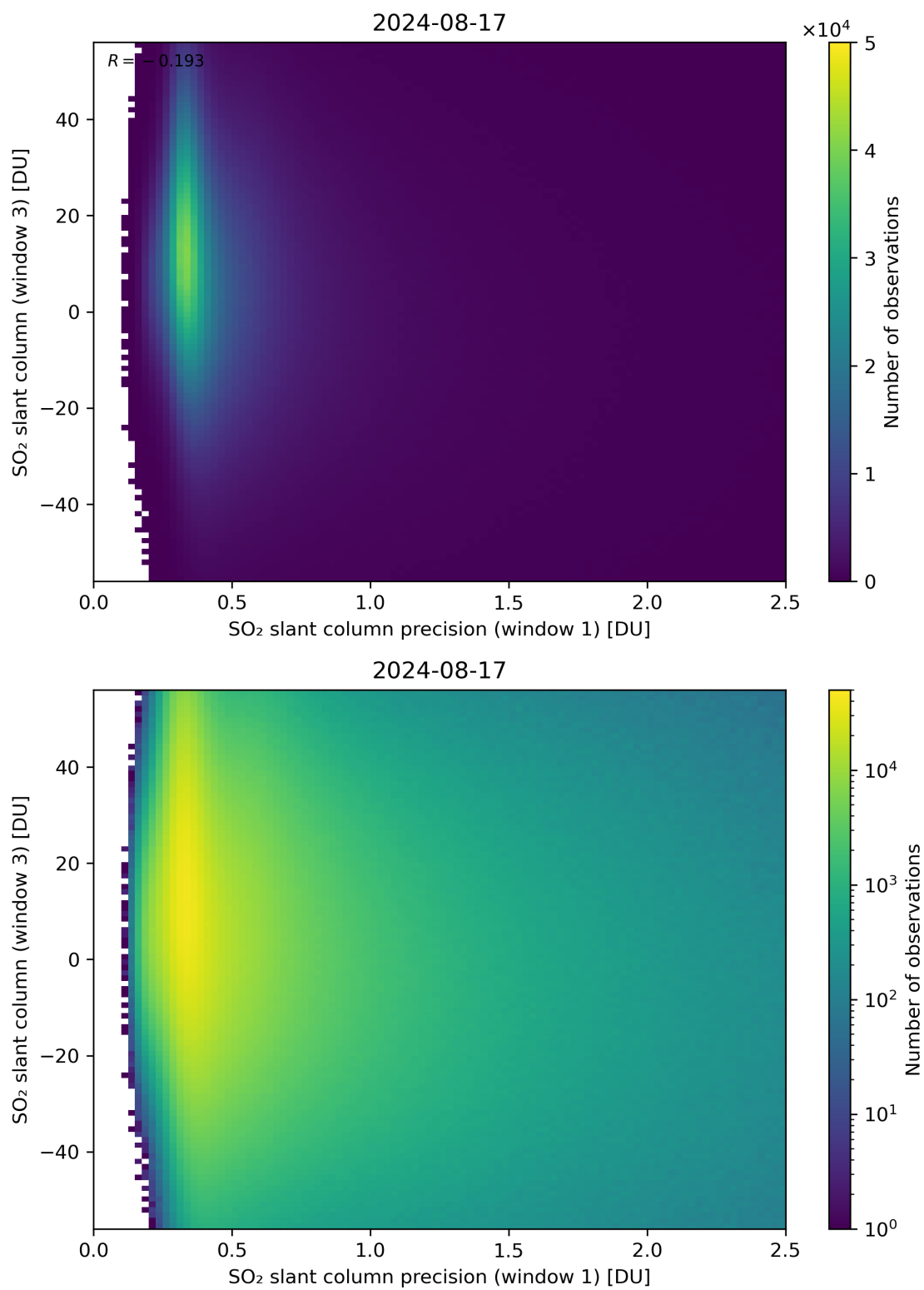
Figure 228: Scatter density plot of “SO 2 slant column precision (window 1)” against “SO 2 slant column (window 3)” for 2024-08-16 to 2024-08-18.
