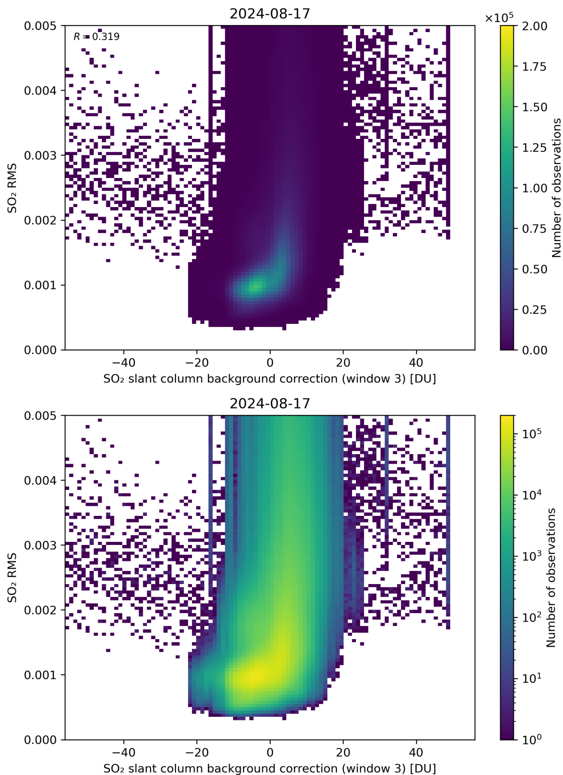
Figure 123: Scatter density plot of “SO 2 slant column background correction (window 3)” against “SO 2 RMS” for 2024-08-16 to 2024-08-18.
