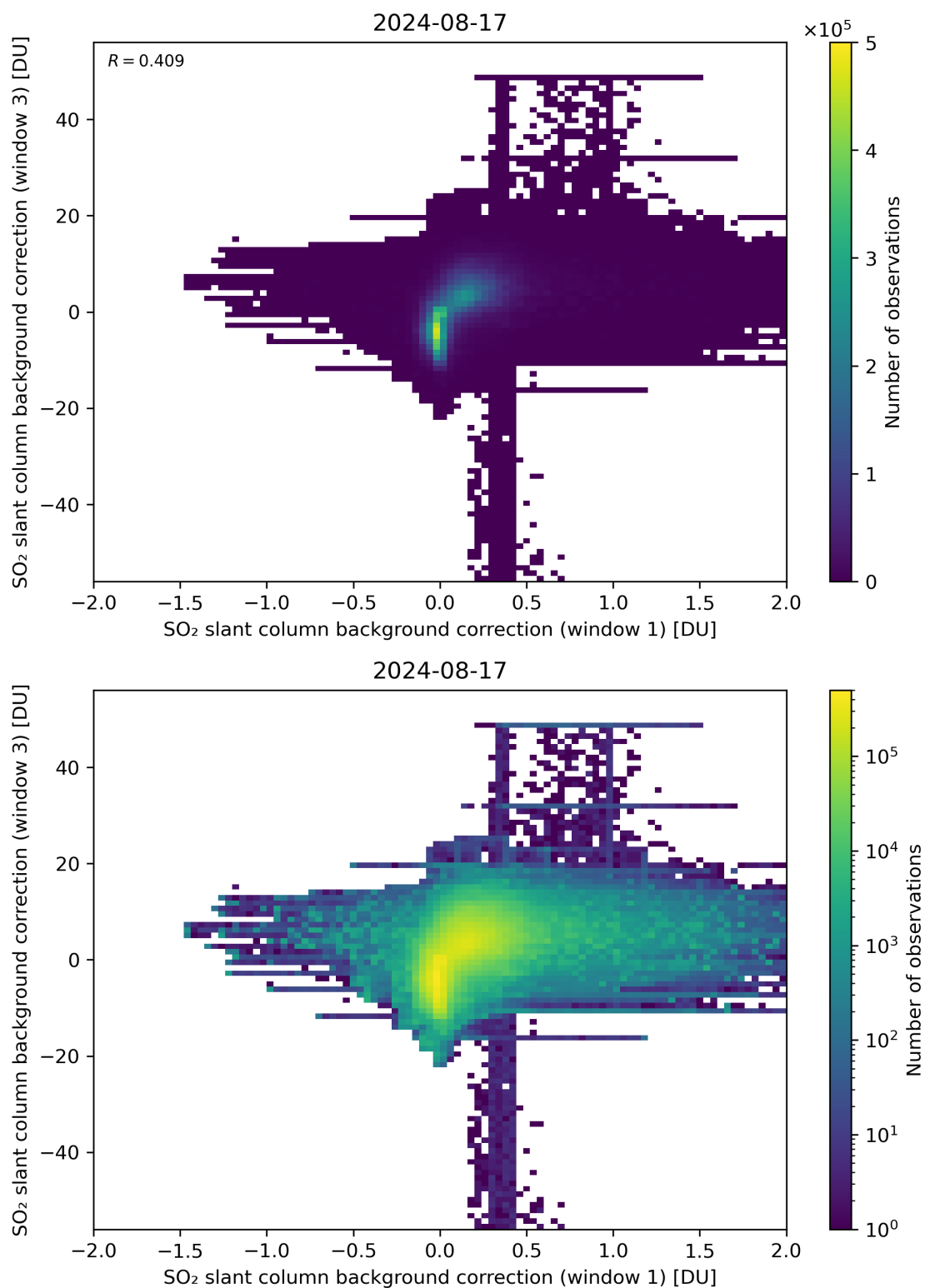
Figure 99: Scatter density plot of “SO 2 slant column background correction (window 1)” against “SO 2 slant column background correction (window 3)” for 2024-08-16 to 2024-08-18.
