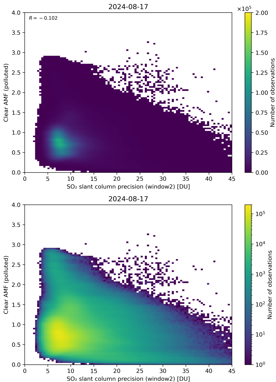
Figure 246: Scatter density plot of “SO 2 slant column precision (window2)” against “Clear AMF (polluted)” for 2024-08-16 to 2024-08-18.
