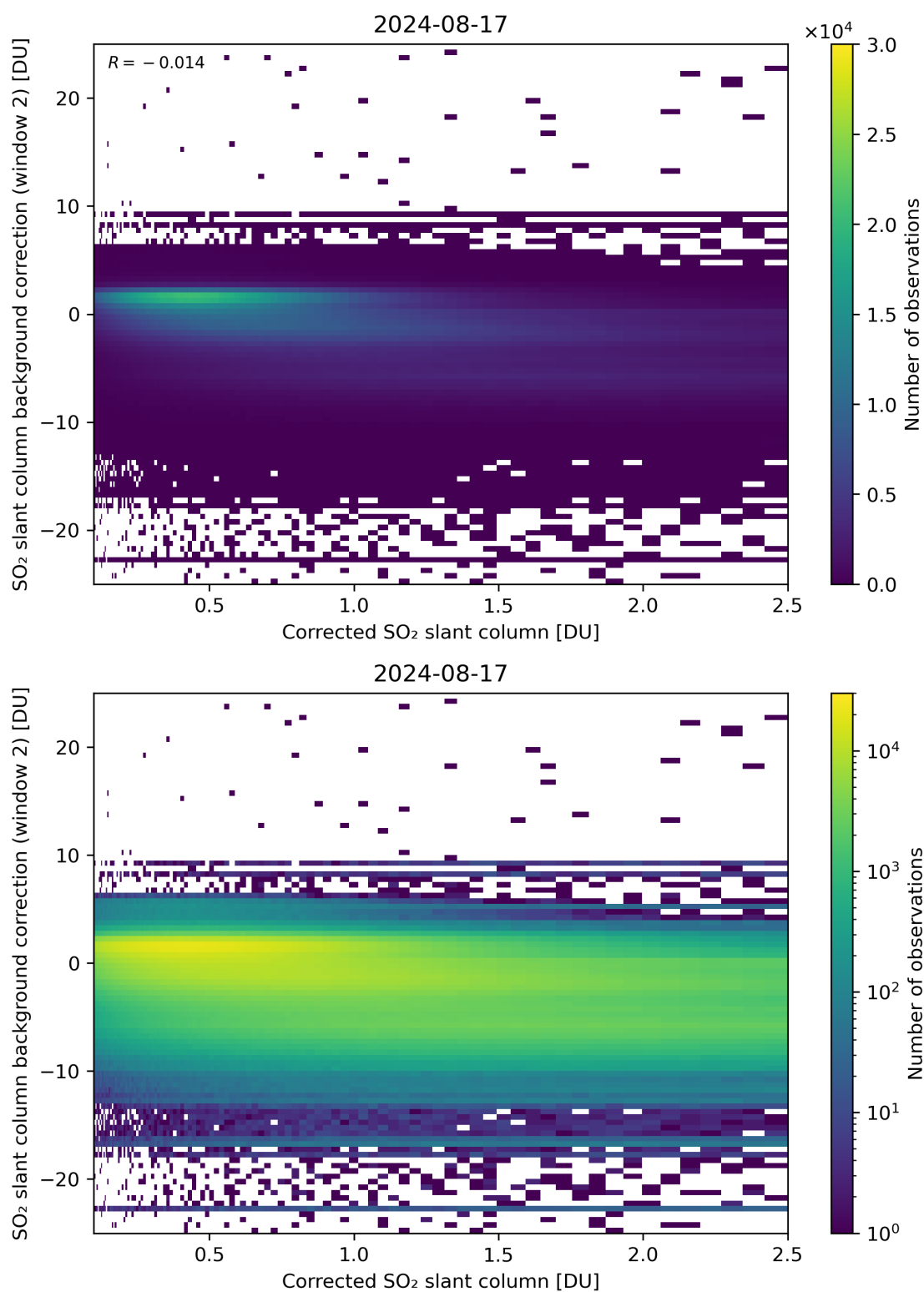
Figure 179: Scatter density plot of “Corrected SO 2 slant column” against “SO 2 slant column background correction (window 2)” for 2024-08-16 to 2024-08-18.
