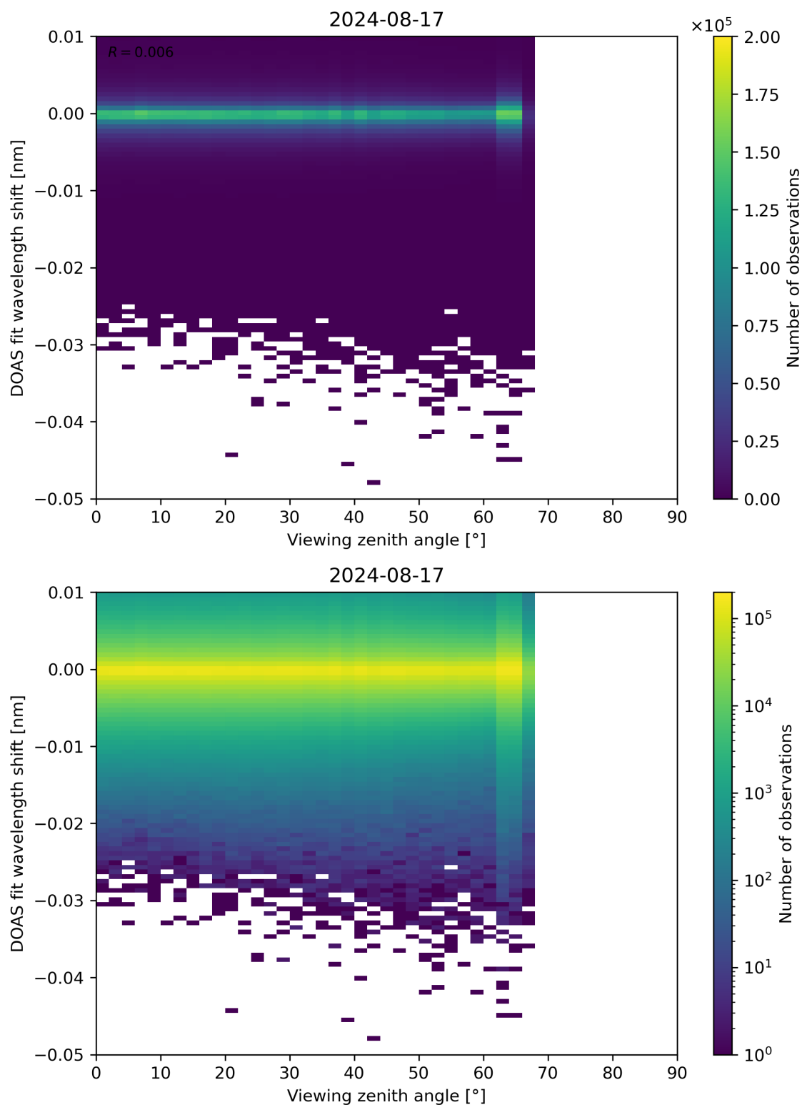
Figure 311: Scatter density plot of “Viewing zenith angle” against “DOAS fit wavelength shift” for 2024-08-16 to 2024-08-18.
