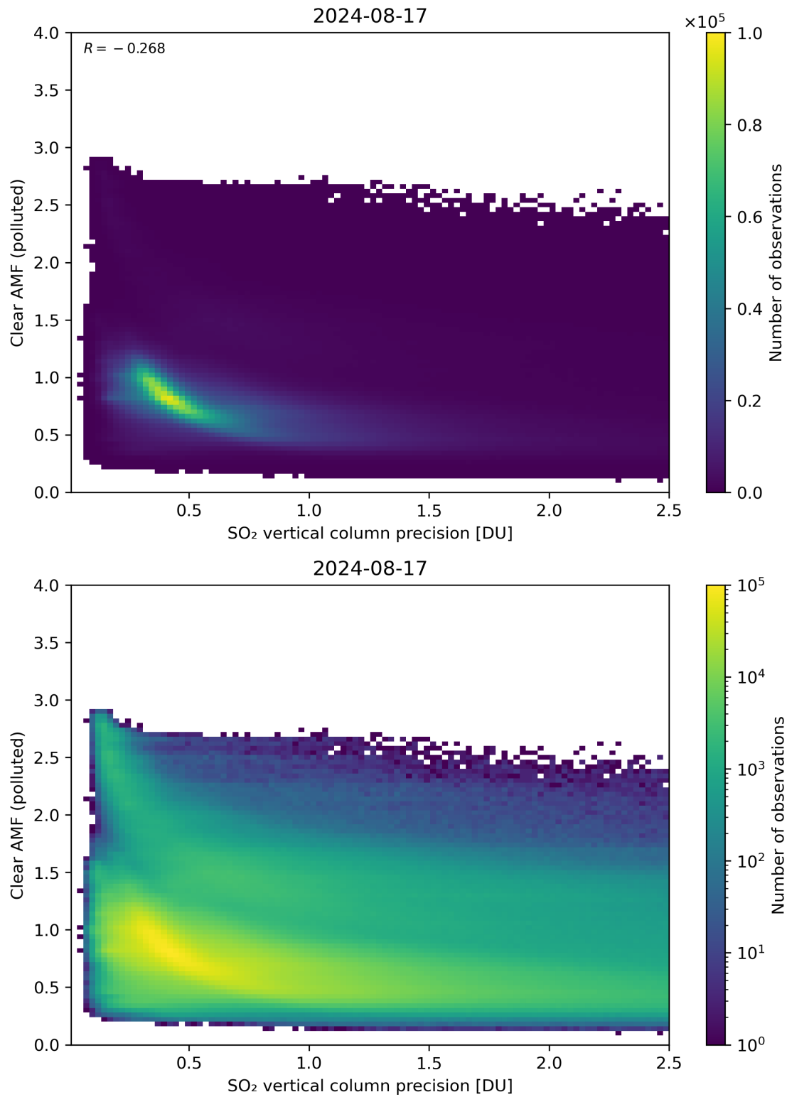
Figure 285: Scatter density plot of “SO 2 vertical column precision” against “Clear AMF (polluted)” for 2024-08-16 to 2024-08-18.
