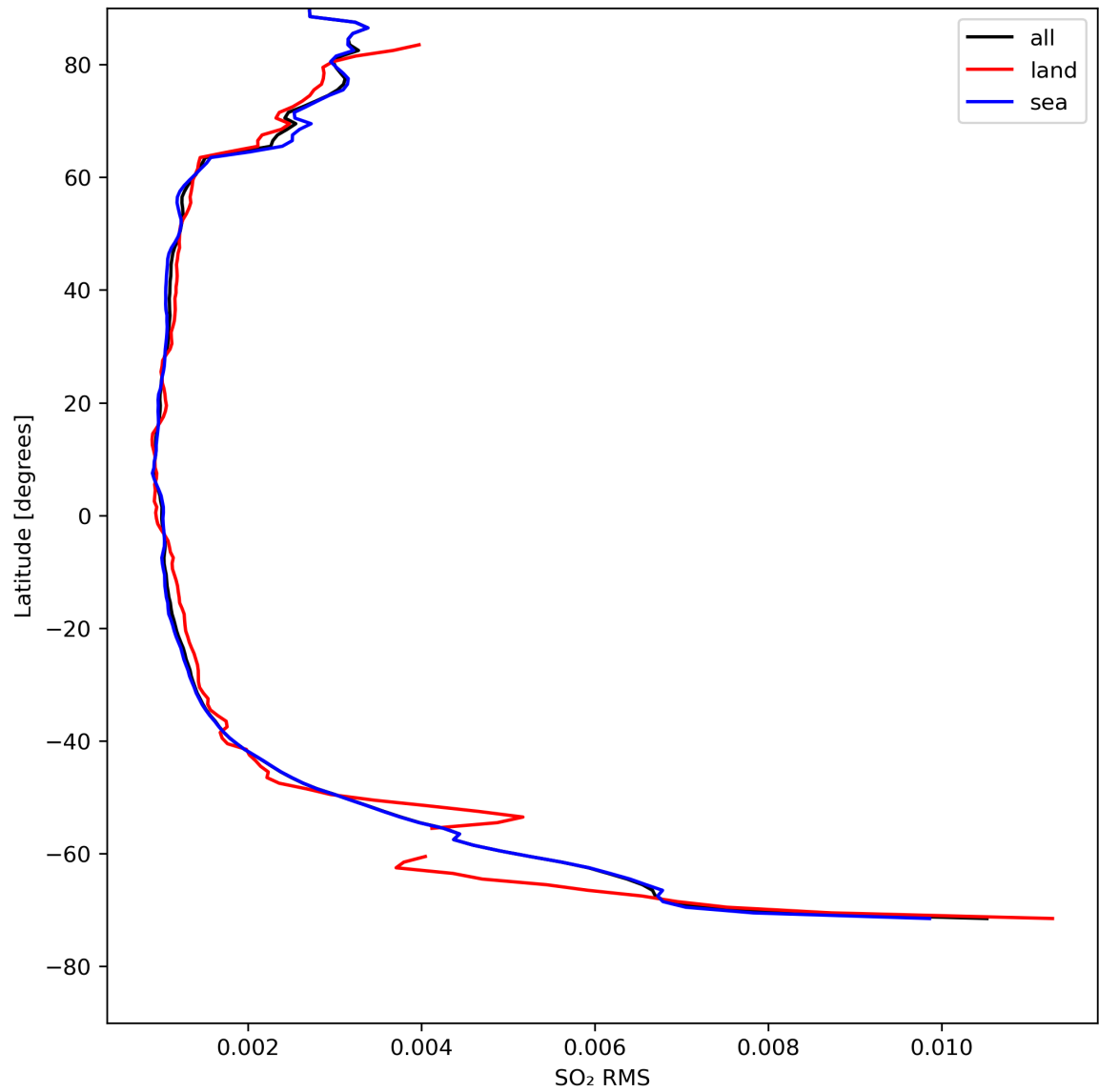
Figure 47: Zonal average of “SO 2 RMS” for 2024-08-16 to 2024-08-18.
