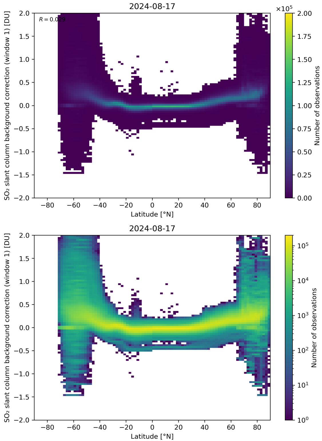
Figure 139: Scatter density plot of “Latitude” against “SO 2 slant column background correction (window 1)” for 2024-08-16 to 2024-08-18.
