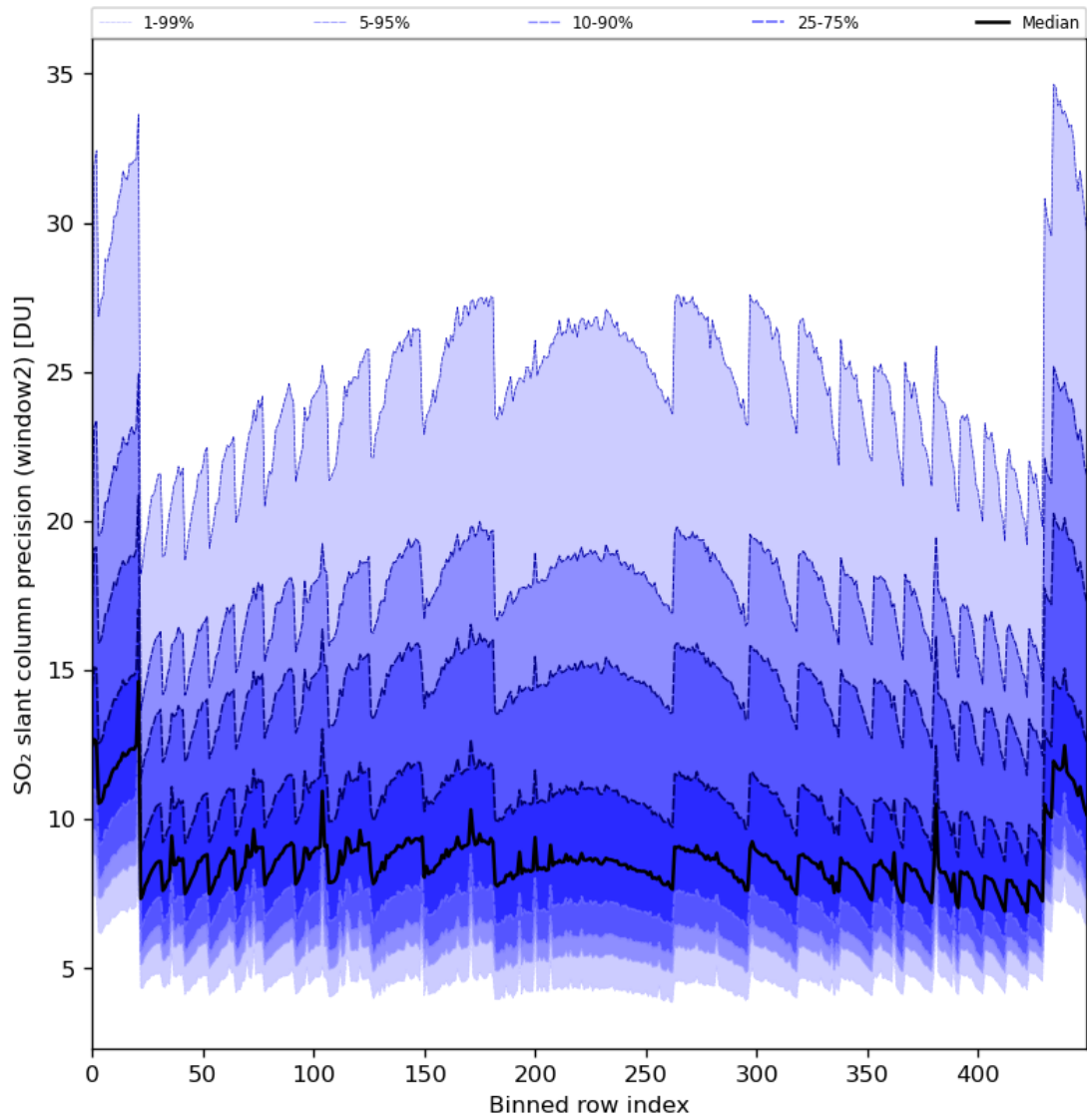
Figure 84: Along track statistics of “SO 2 slant column precision (window2)” for 2024-08-16 to 2024-08-18
