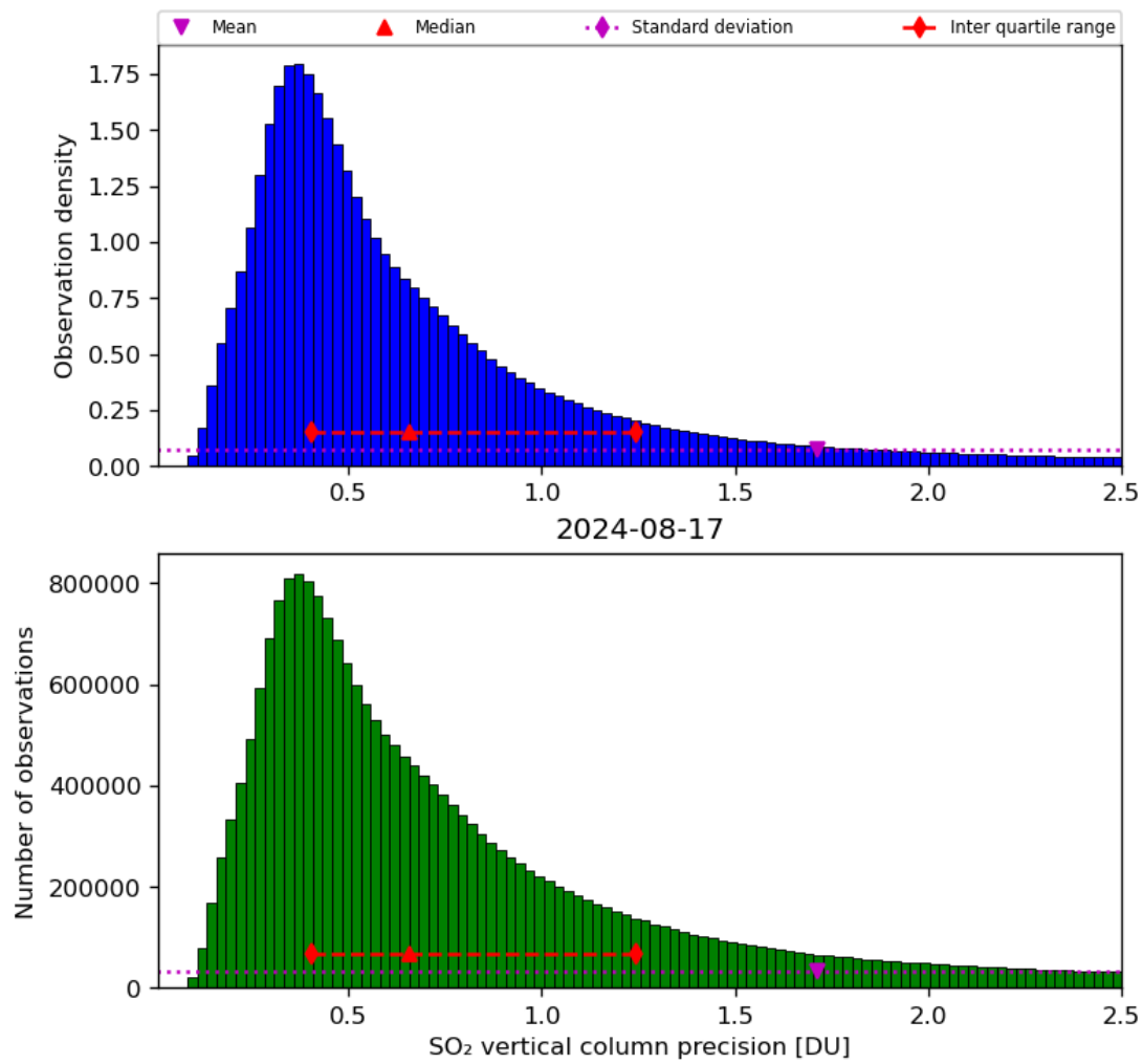
Figure 54: Histogram of “SO 2 vertical column precision” for 2024-08-16 to 2024-08-18
