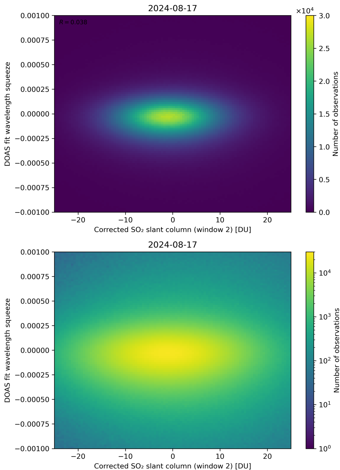
Figure 197: Scatter density plot of “Corrected SO 2 slant column (window 2)” against “DOAS fit wavelength squeeze” for 2024-08-16 to 2024-08-18.
