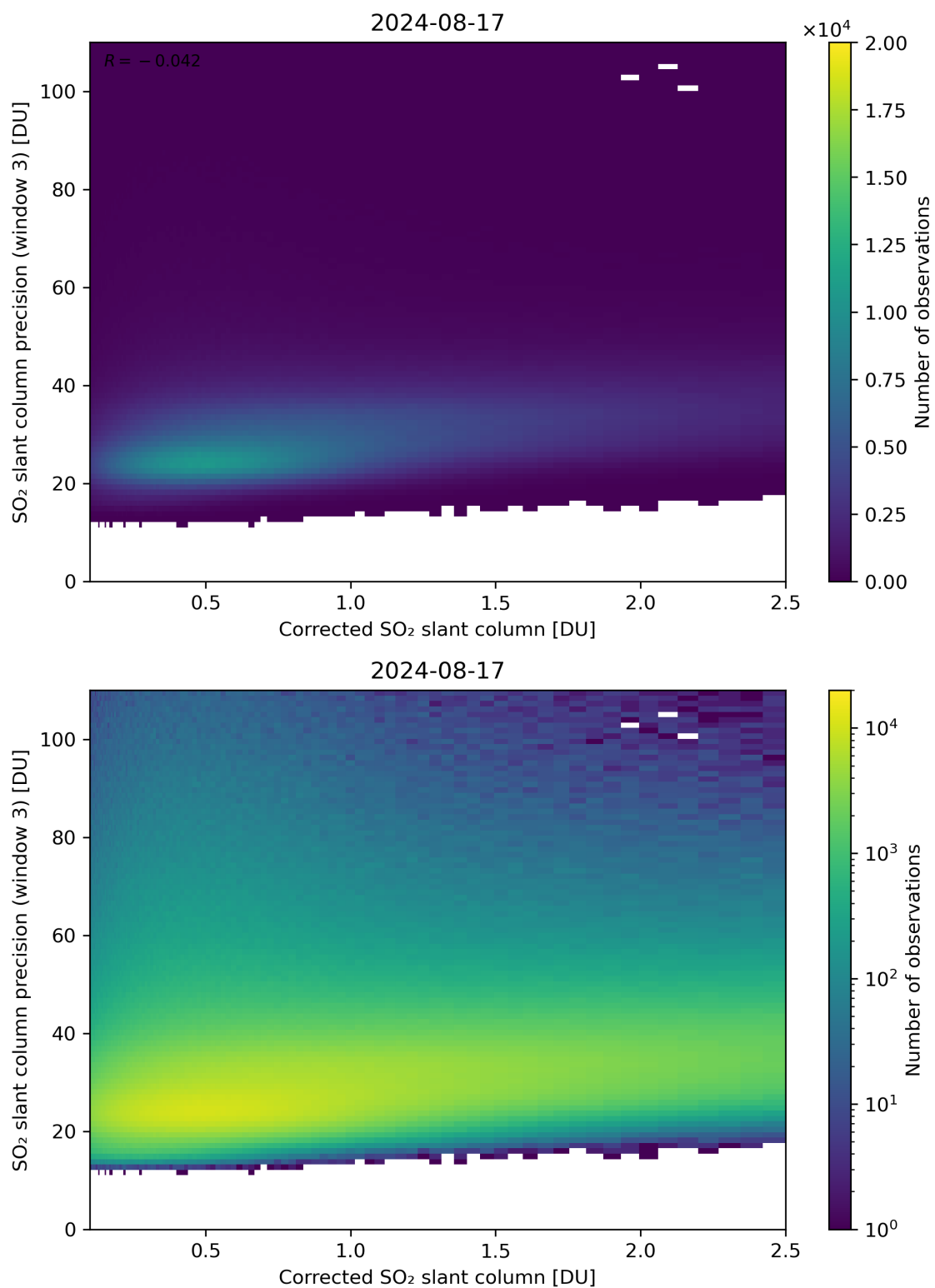
Figure 191: Scatter density plot of “Corrected SO 2 slant column” against “SO 2 slant column precision (window 3)” for 2024-08-16 to 2024-08-18.
