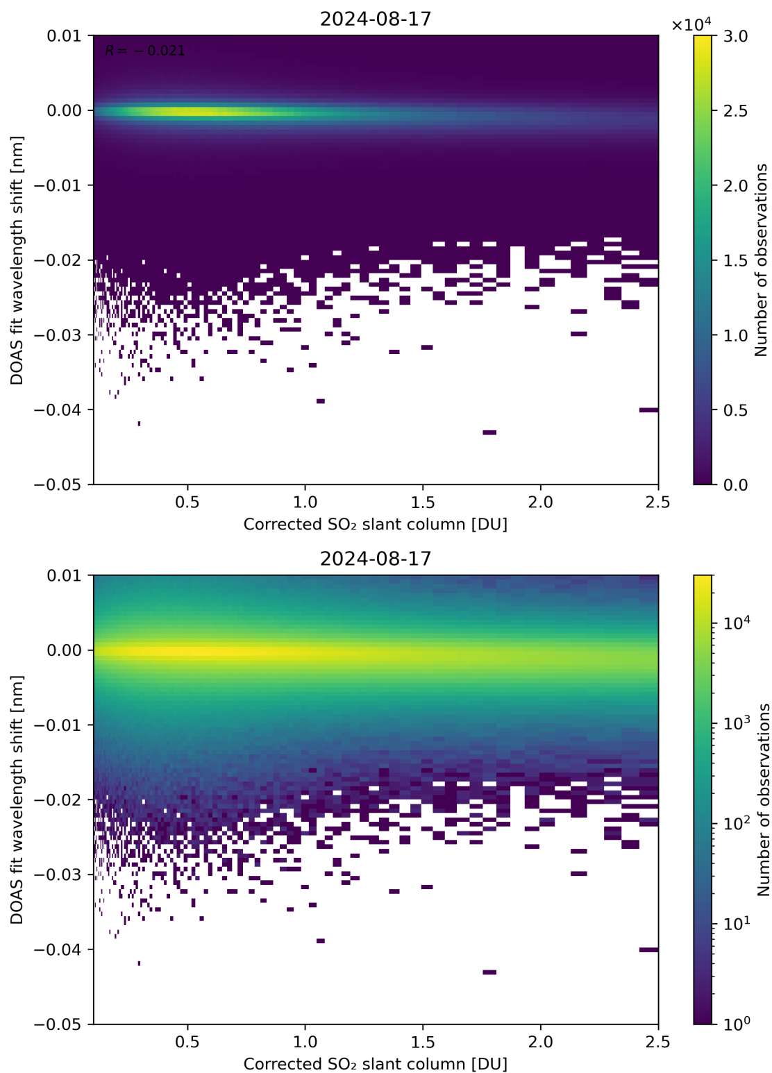
Figure 181: Scatter density plot of “Corrected SO 2 slant column” against “DOAS fit wavelength shift” for 2024-08-16 to 2024-08-18.
