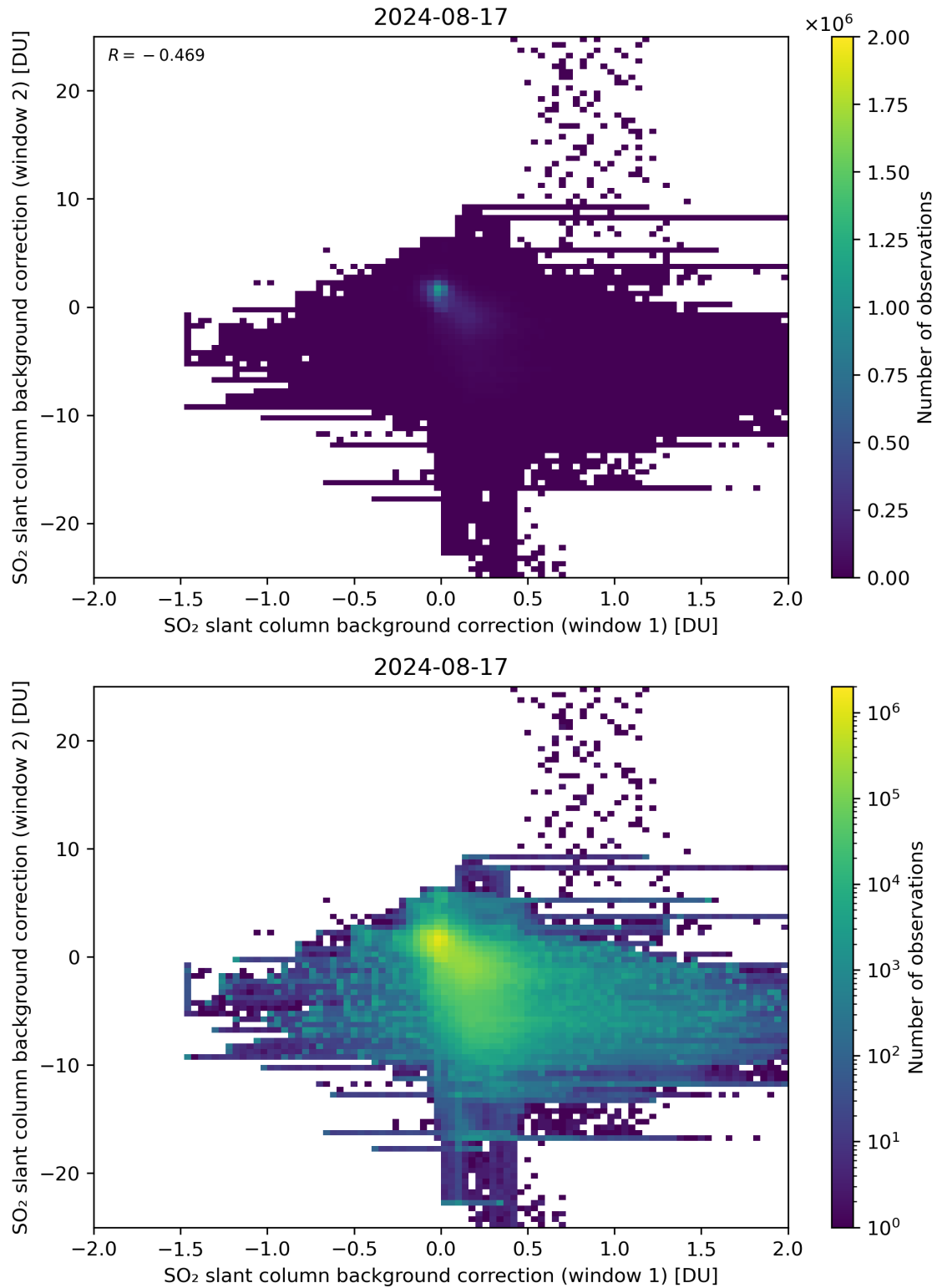
Figure 98: Scatter density plot of “SO 2 slant column background correction (window 1)” against “SO 2 slant column background correction (window 2)” for 2024-08-16 to 2024-08-18.
