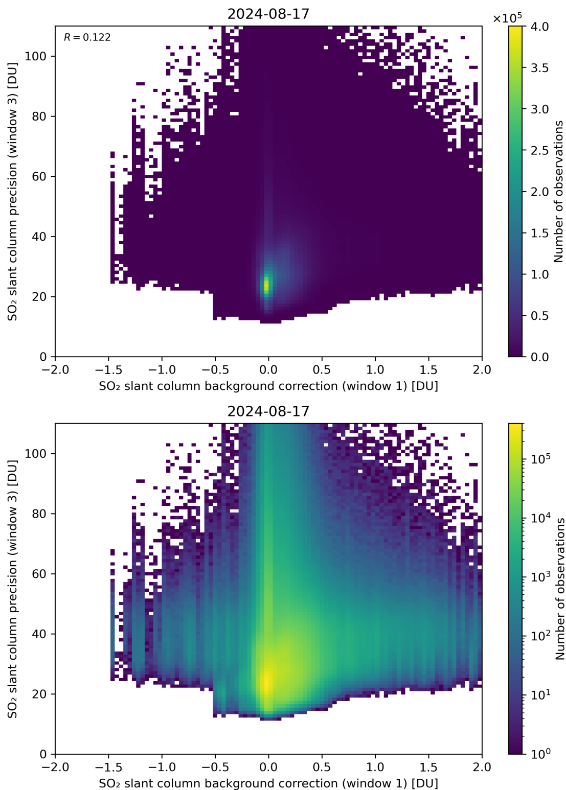
Figure 108: Scatter density plot of “SO 2 slant column background correction (window 1)” against “SO 2 slant column precision (window 3)” for 2024-08-16 to 2024-08-18.
