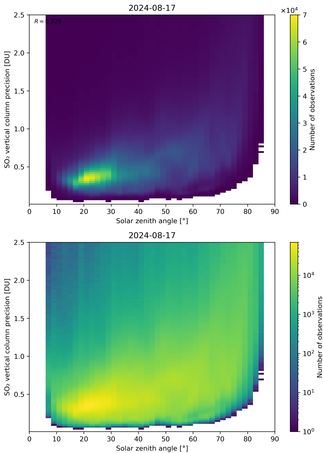
Figure 177: Scatter density plot of “Solar zenith angle” against “SO 2 vertical column precision” for 2024-08-16 to 2024-08-18.
