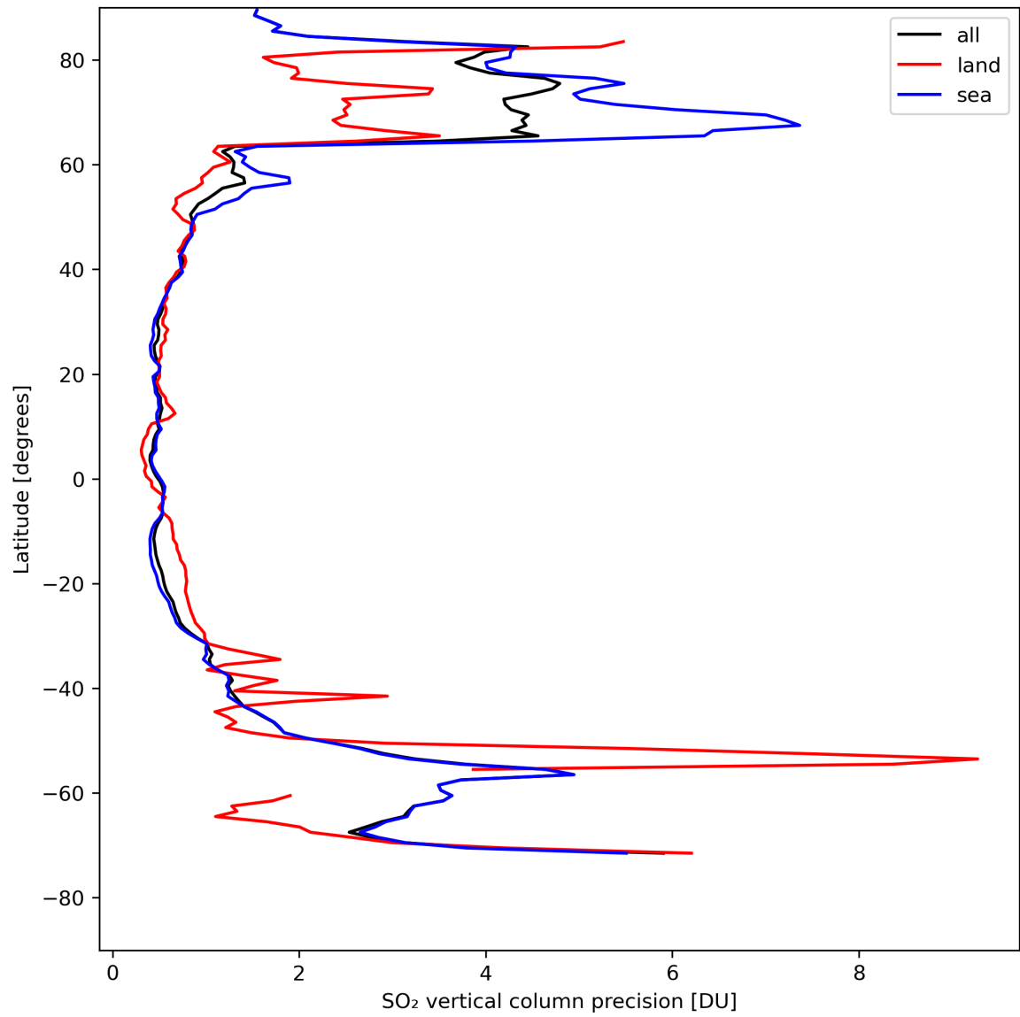
Figure 31: Zonal average of “SO 2 vertical column precision” for 2024-08-16 to 2024-08-18.
