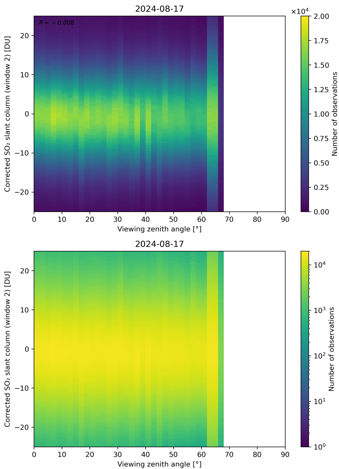
Figure 318: Scatter density plot of “Viewing zenith angle” against “Corrected SO 2 slant column (window 2)” for 2024-08-16 to 2024-08-18.
