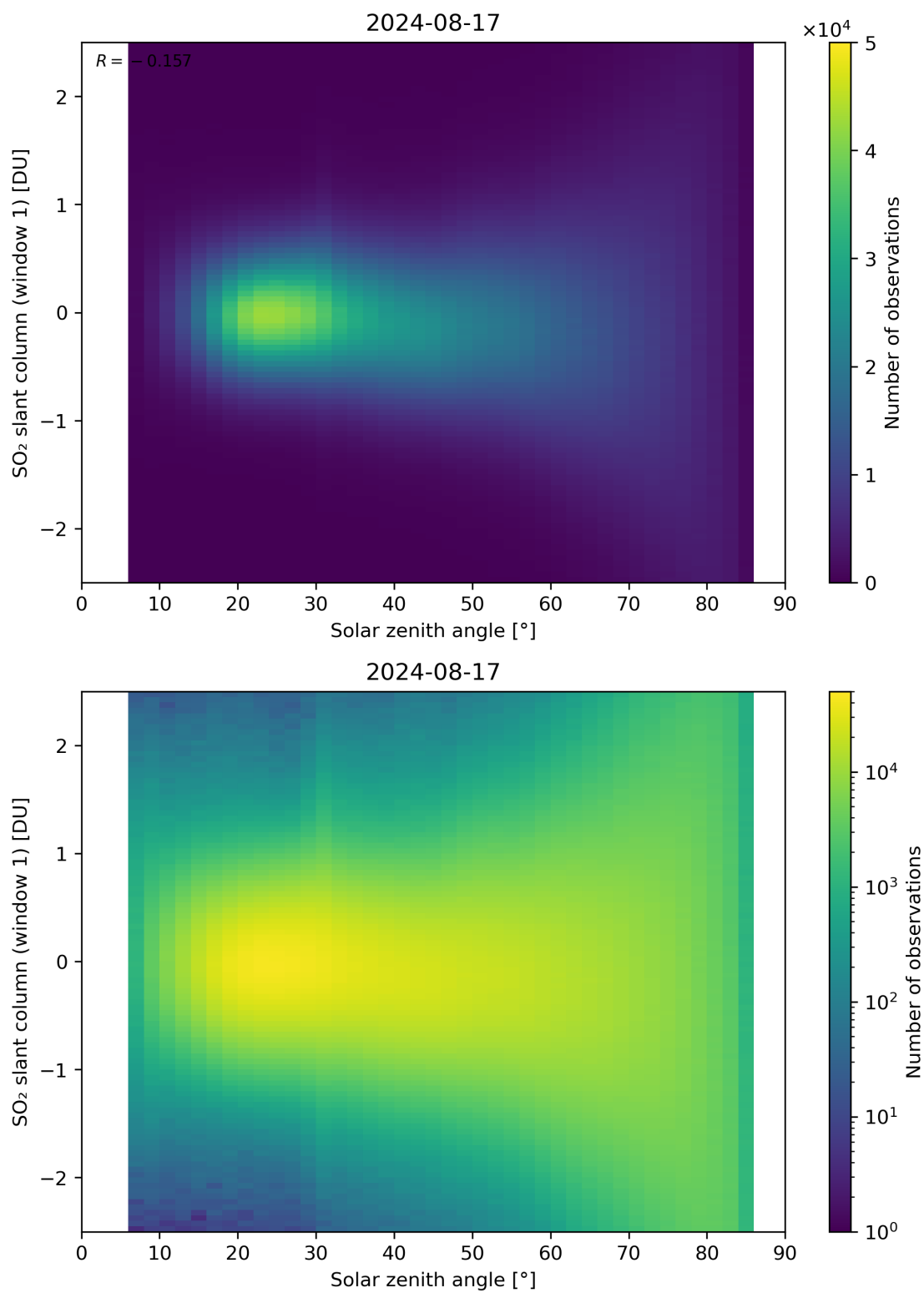
Figure 169: Scatter density plot of “Solar zenith angle” against “SO 2 slant column (window 1)” for 2024-08-16 to 2024-08-18.
