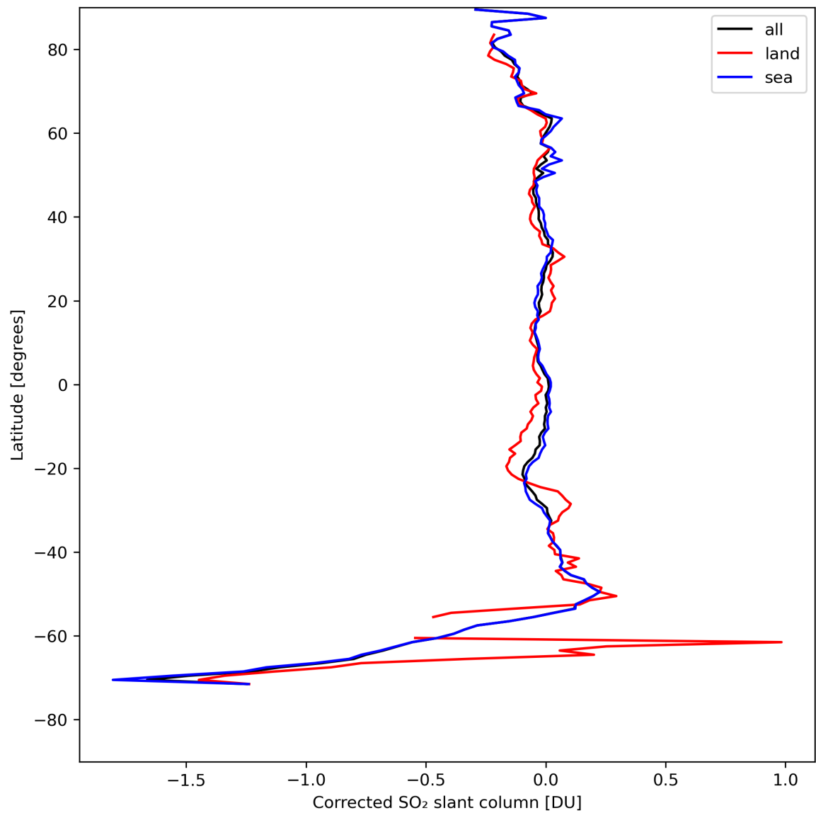
Figure 32: Zonal average of “Corrected SO 2 slant column” for 2024-08-16 to 2024-08-18.
