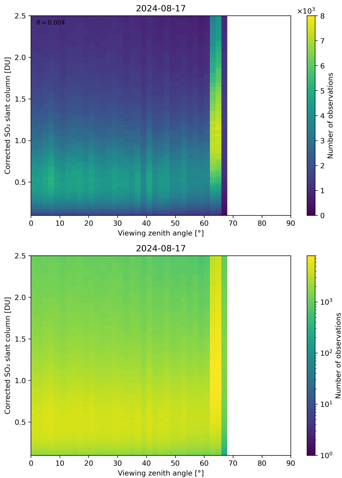
Figure 317: Scatter density plot of “Viewing zenith angle” against “Corrected SO 2 slant column” for 2024-08-16 to 2024-08-18.
