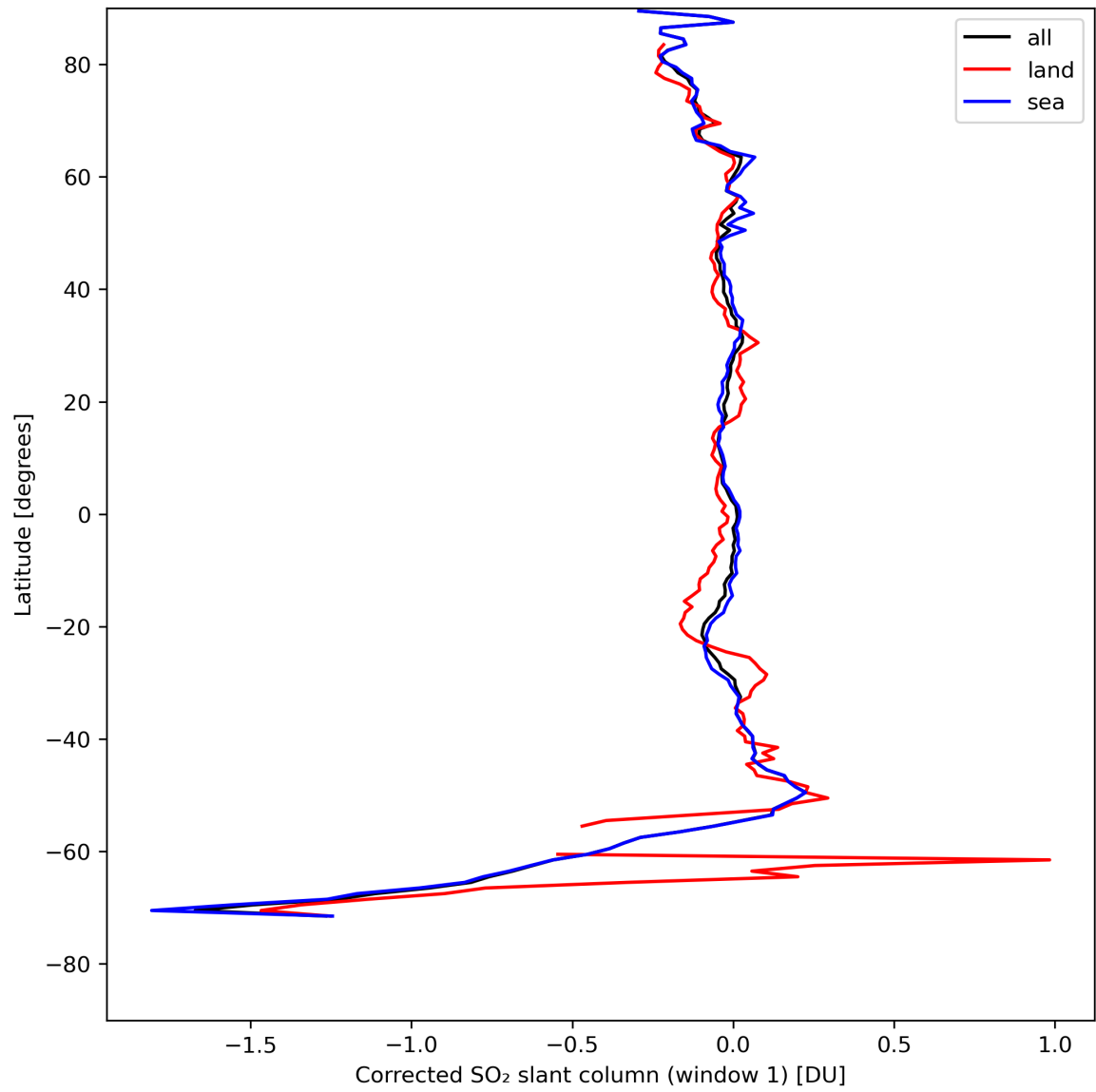
Figure 35: Zonal average of “Corrected SO 2 slant column (window 1)” for 2024-08-16 to 2024-08-18.
