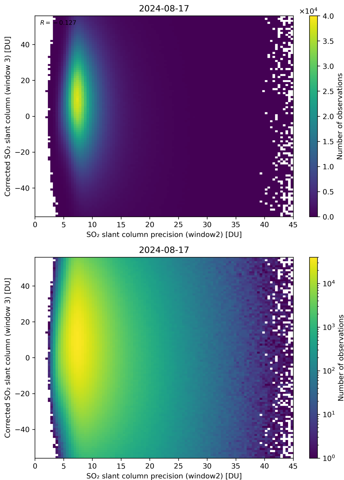
Figure 248: Scatter density plot of “SO 2 slant column precision (window2)” against “Corrected SO 2 slant column (window 3)” for 2024-08-16 to 2024-08-18.
