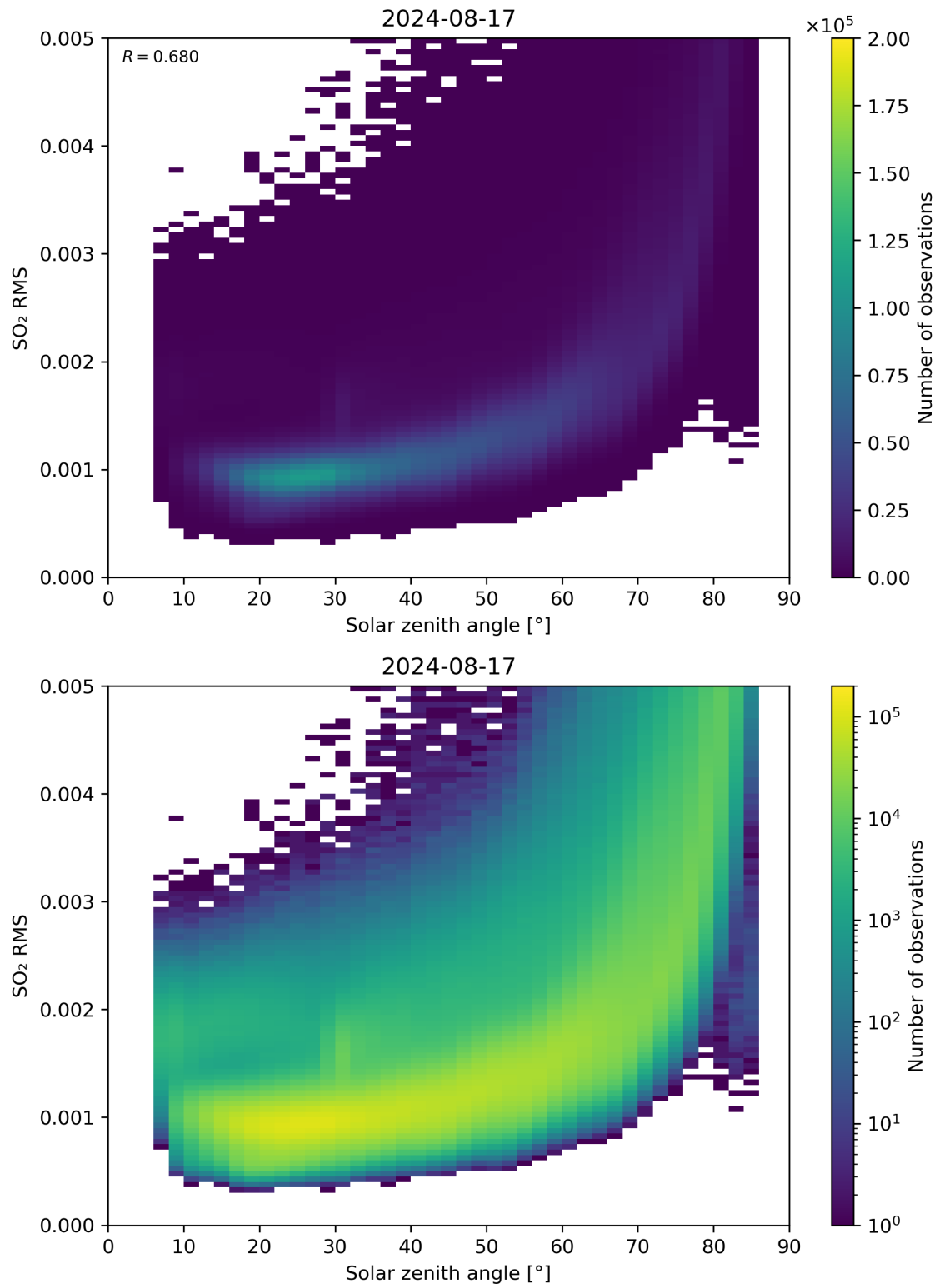
Figure 163: Scatter density plot of “Solar zenith angle” against “SO 2 RMS” for 2024-08-16 to 2024-08-18.
