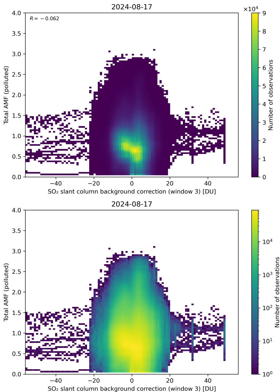
Figure 125: Scatter density plot of “SO 2 slant column background correction (window 3)” against “Total AMF (polluted)” for 2024-08-16 to 2024-08-18.
