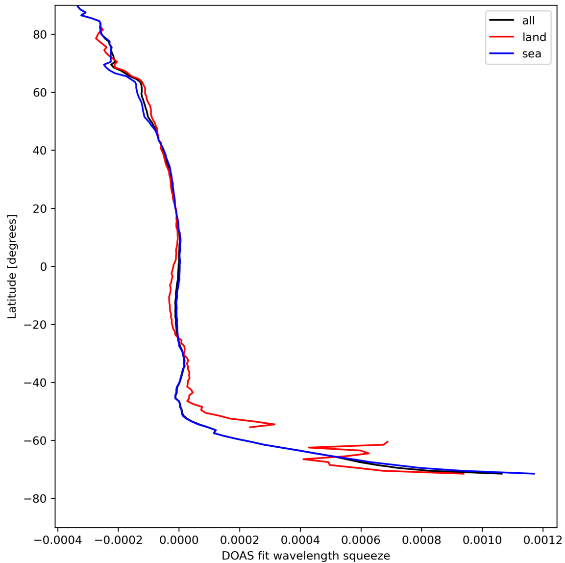
Figure 46: Zonal average of “DOAS fit wavelength squeeze” for 2024-08-16 to 2024-08-18.
