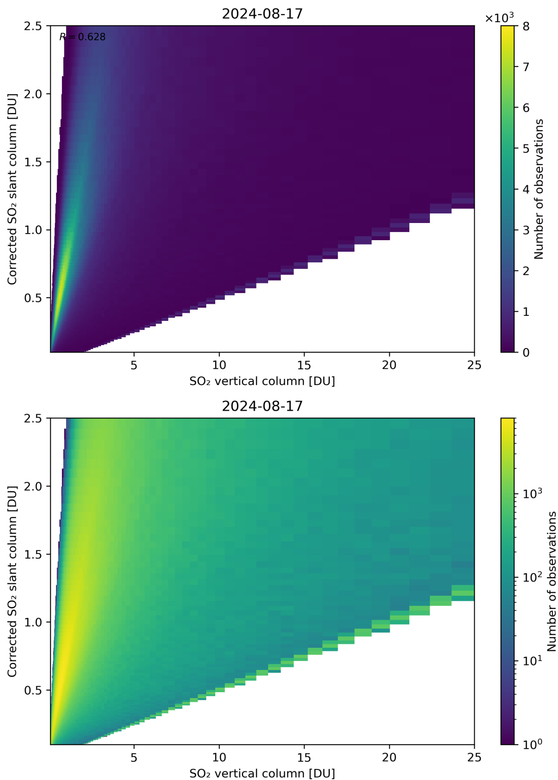
Figure 297: Scatter density plot of “SO 2 vertical column” against “Corrected SO 2 slant column” for 2024-08-16 to 2024-08-18.
