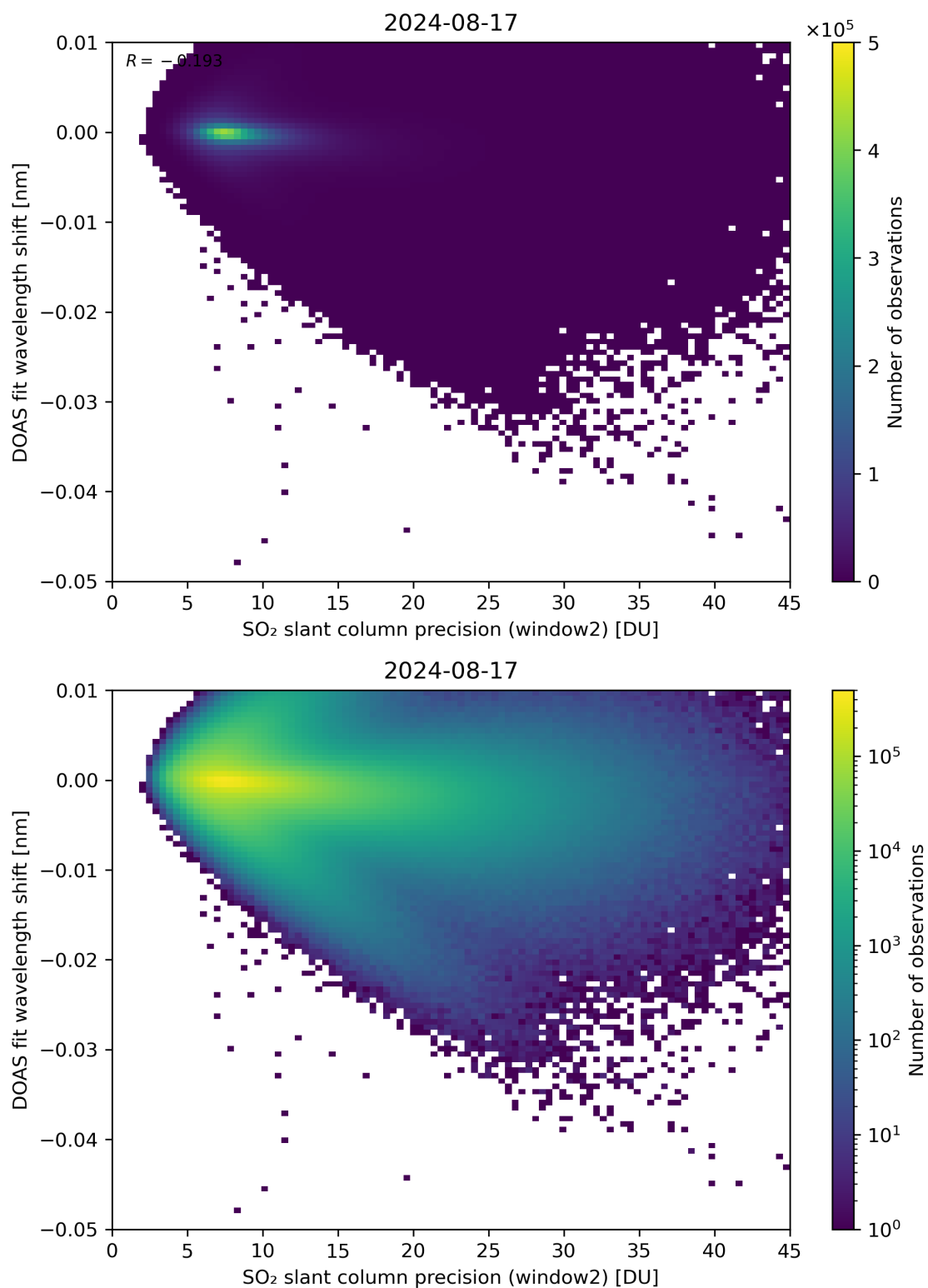
Figure 243: Scatter density plot of “SO 2 slant column precision (window2)” against “DOAS fit wavelength shift” for 2024-08-16 to 2024-08-18.
