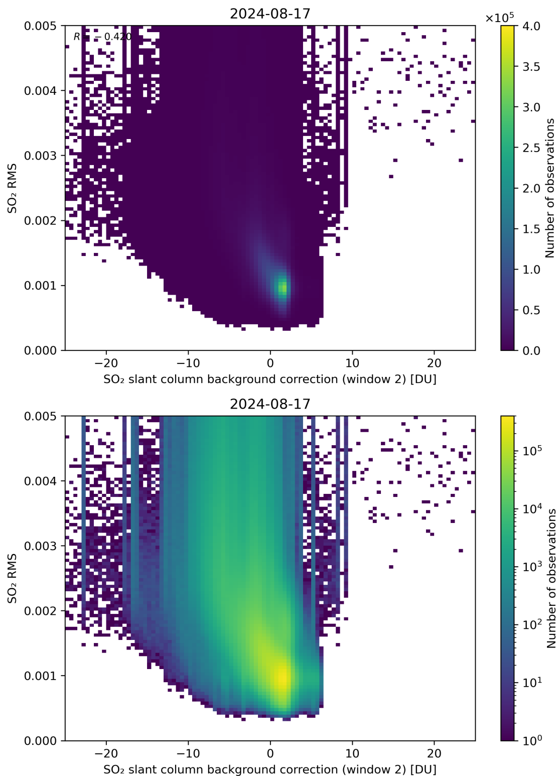
Figure 114: Scatter density plot of “SO 2 slant column background correction (window 2)” against “SO 2 RMS” for 2024-08-16 to 2024-08-18.
