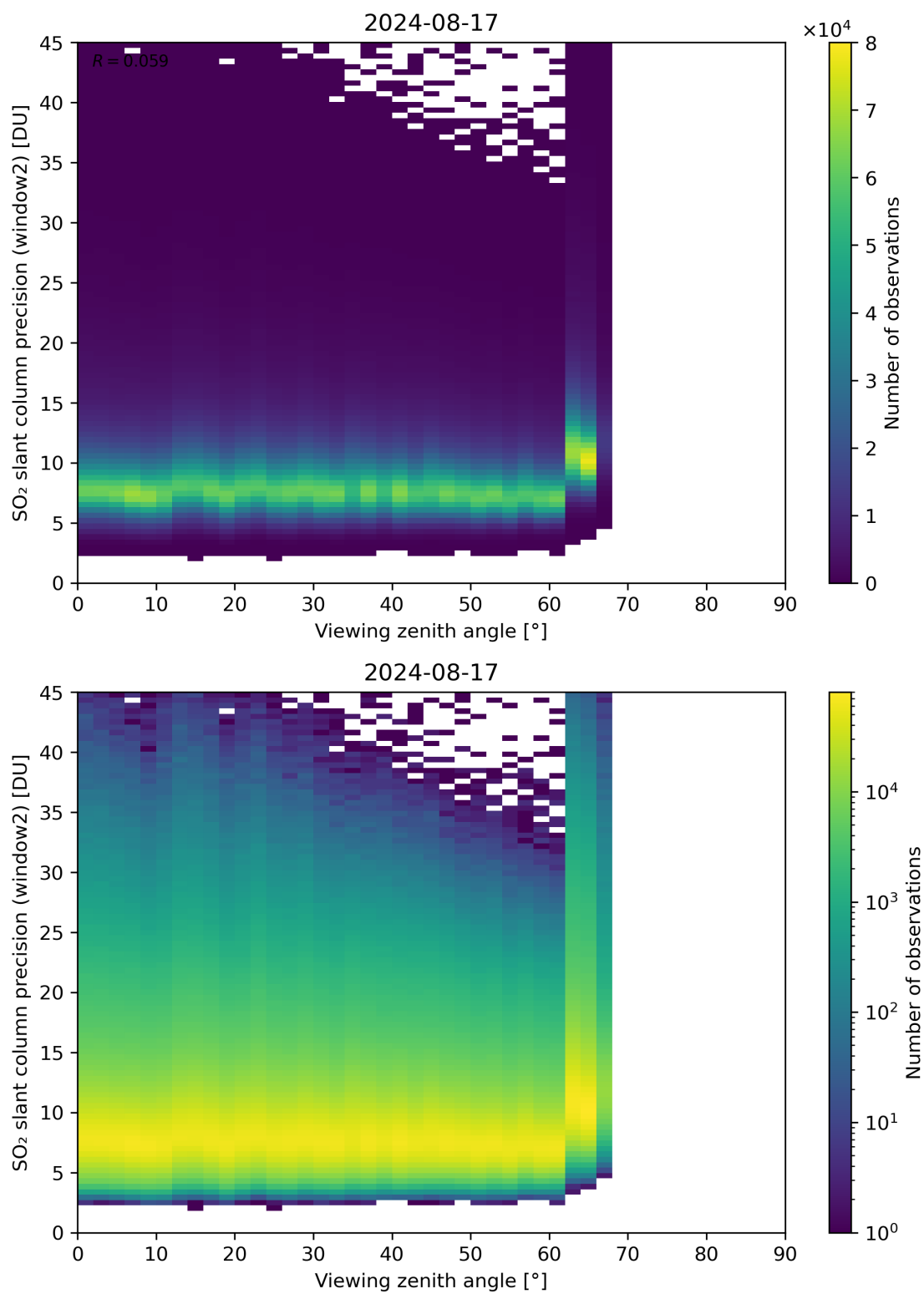
Figure 322: Scatter density plot of “Viewing zenith angle” against “SO 2 slant column precision (window2)” for 2024-08-16 to 2024-08-18.
