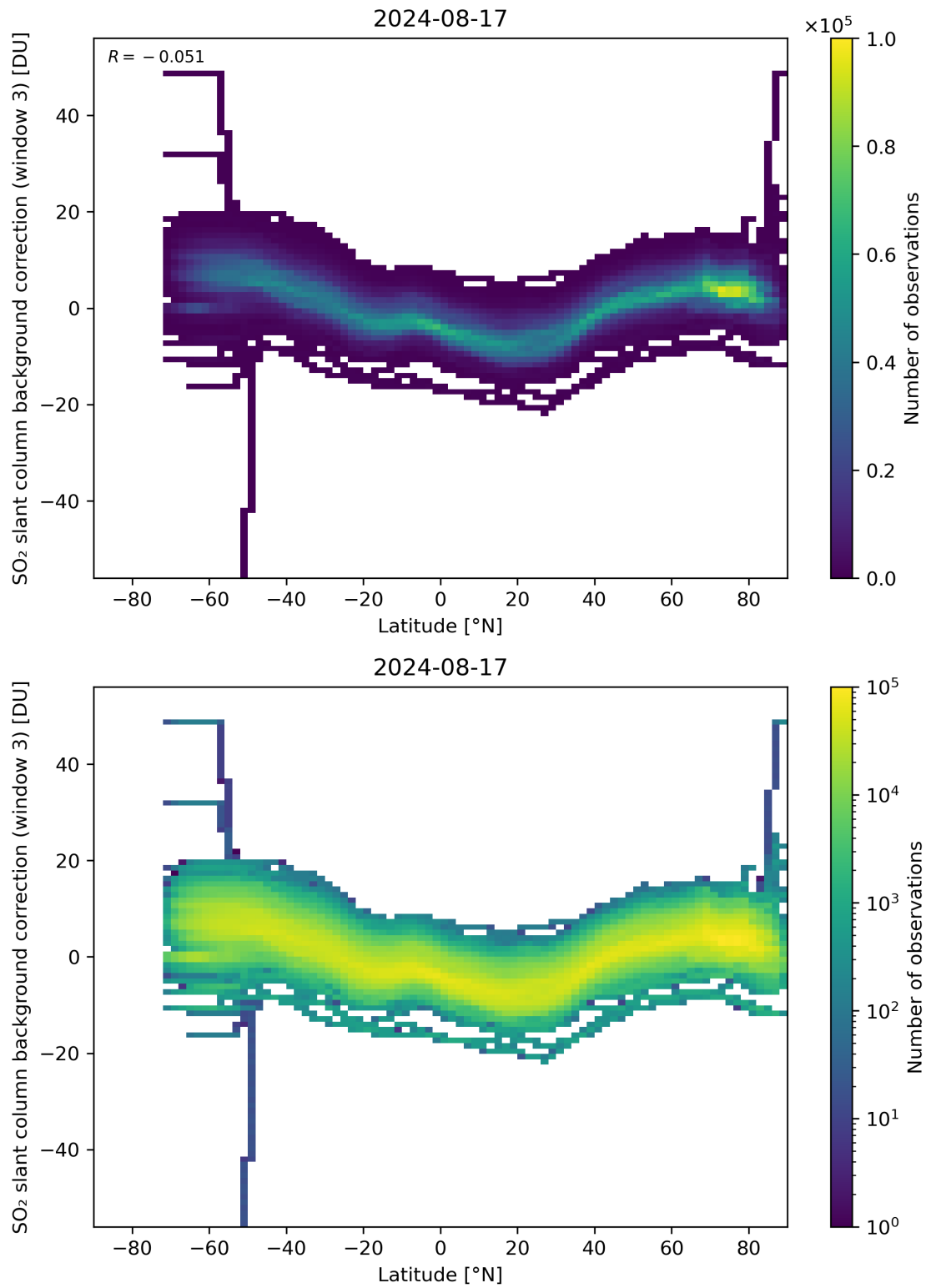
Figure 141: Scatter density plot of “Latitude” against “SO 2 slant column background correction (window 3)” for 2024-08-16 to 2024-08-18.
