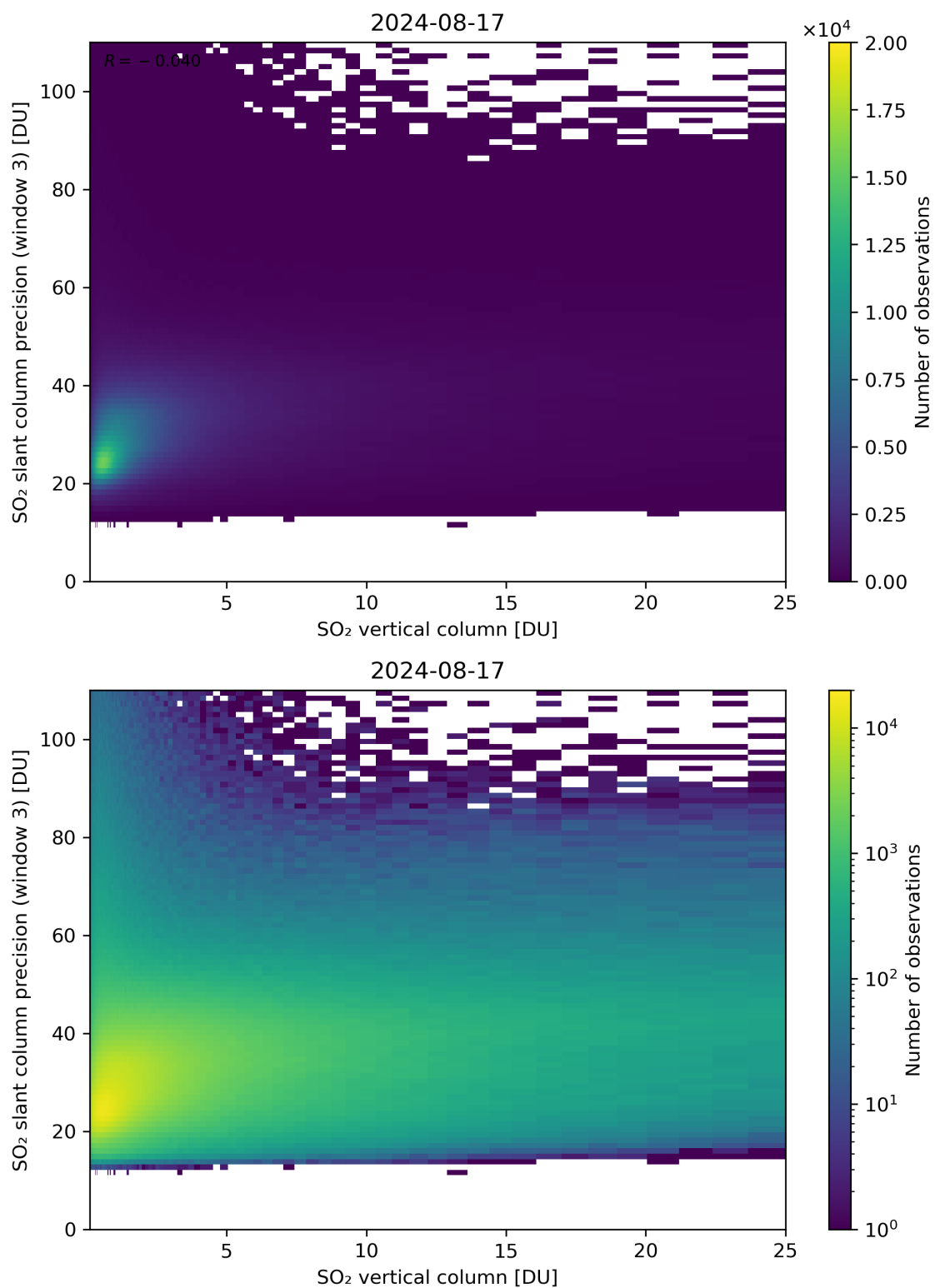
Figure 304: Scatter density plot of “SO 2 vertical column” against “SO 2 slant column precision (window 3)” for 2024-08-16 to 2024-08-18.
