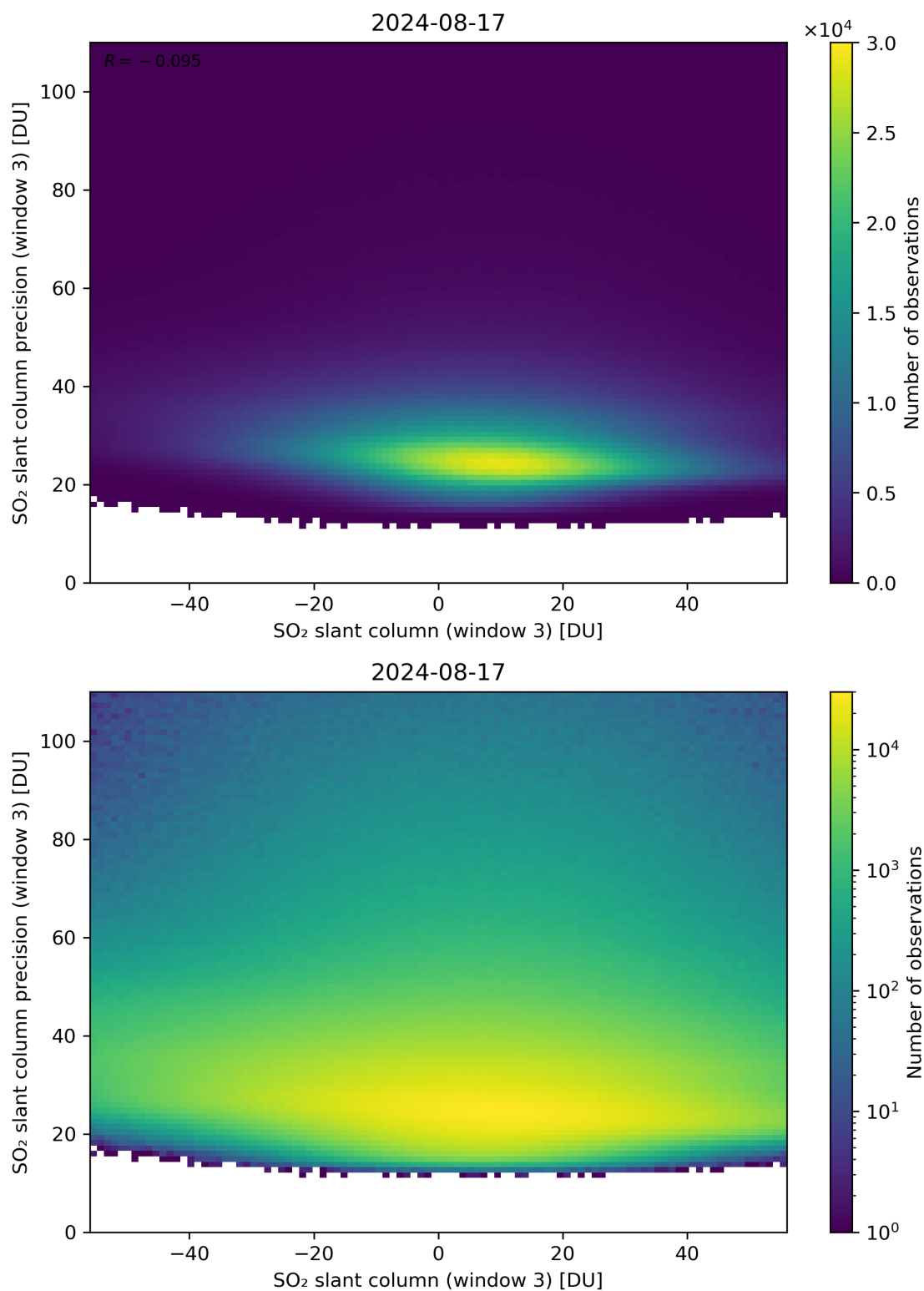
Figure 267: Scatter density plot of “SO 2 slant column (window 3)” against “SO 2 slant column precision (window 3)” for 2024-08-16 to 2024-08-18.
