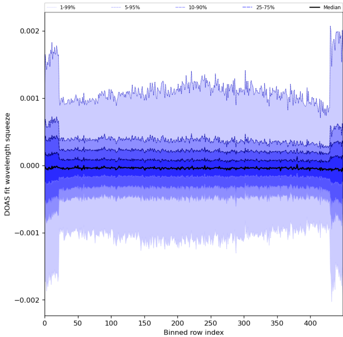
Figure 92: Along track statistics of “DOAS fit wavelength squeeze” for 2024-08-16 to 2024-08-18
