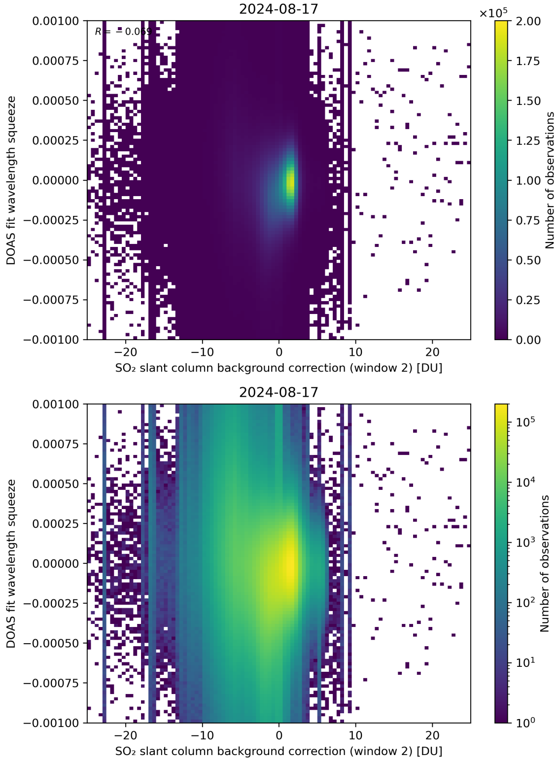
Figure 113: Scatter density plot of “SO 2 slant column background correction (window 2)” against “DOAS fit wavelength squeeze” for 2024-08-16 to 2024-08-18.
