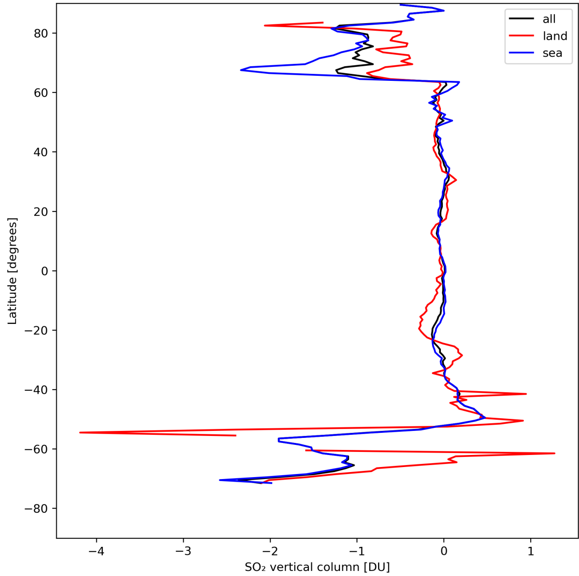
Figure 30: Zonal average of “SO 2 vertical column” for 2024-08-16 to 2024-08-18.
