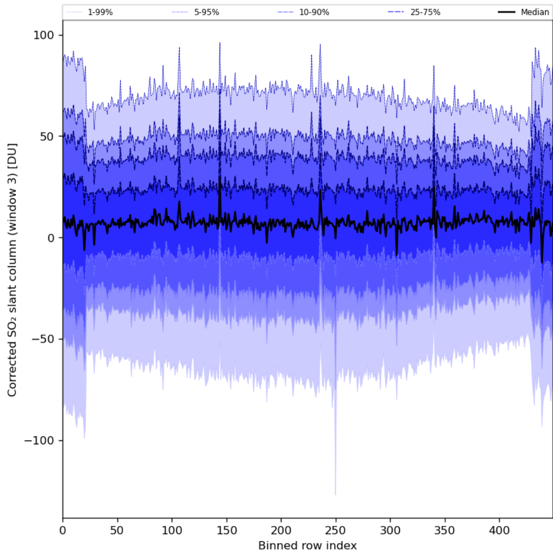
Figure 89: Along track statistics of “Corrected SO 2 slant column (window 3)” for 2024-08-16 to 2024-08-18
