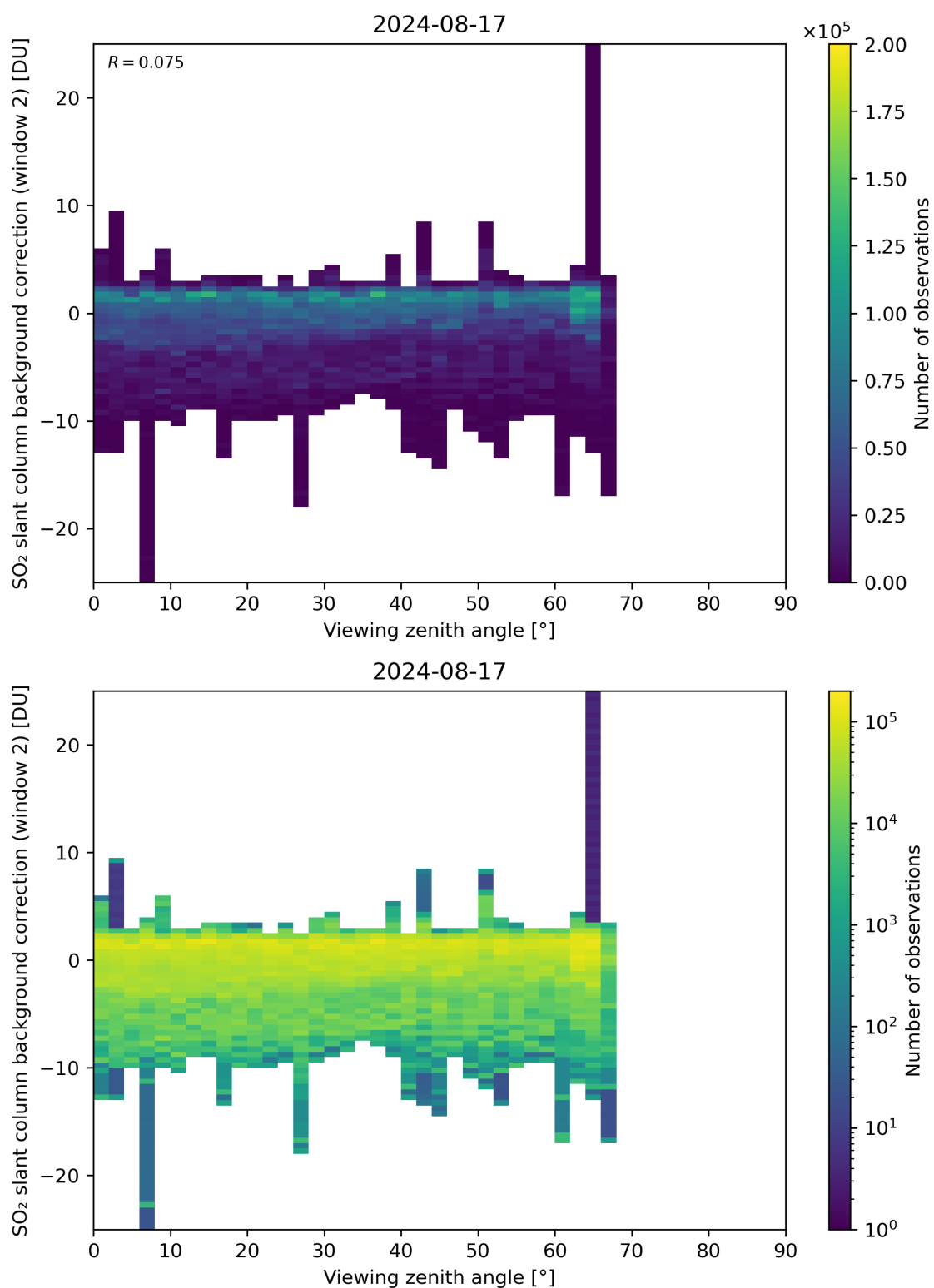
Figure 309: Scatter density plot of “Viewing zenith angle” against “SO 2 slant column background correction (window 2)” for 2024-08-16 to 2024-08-18.
