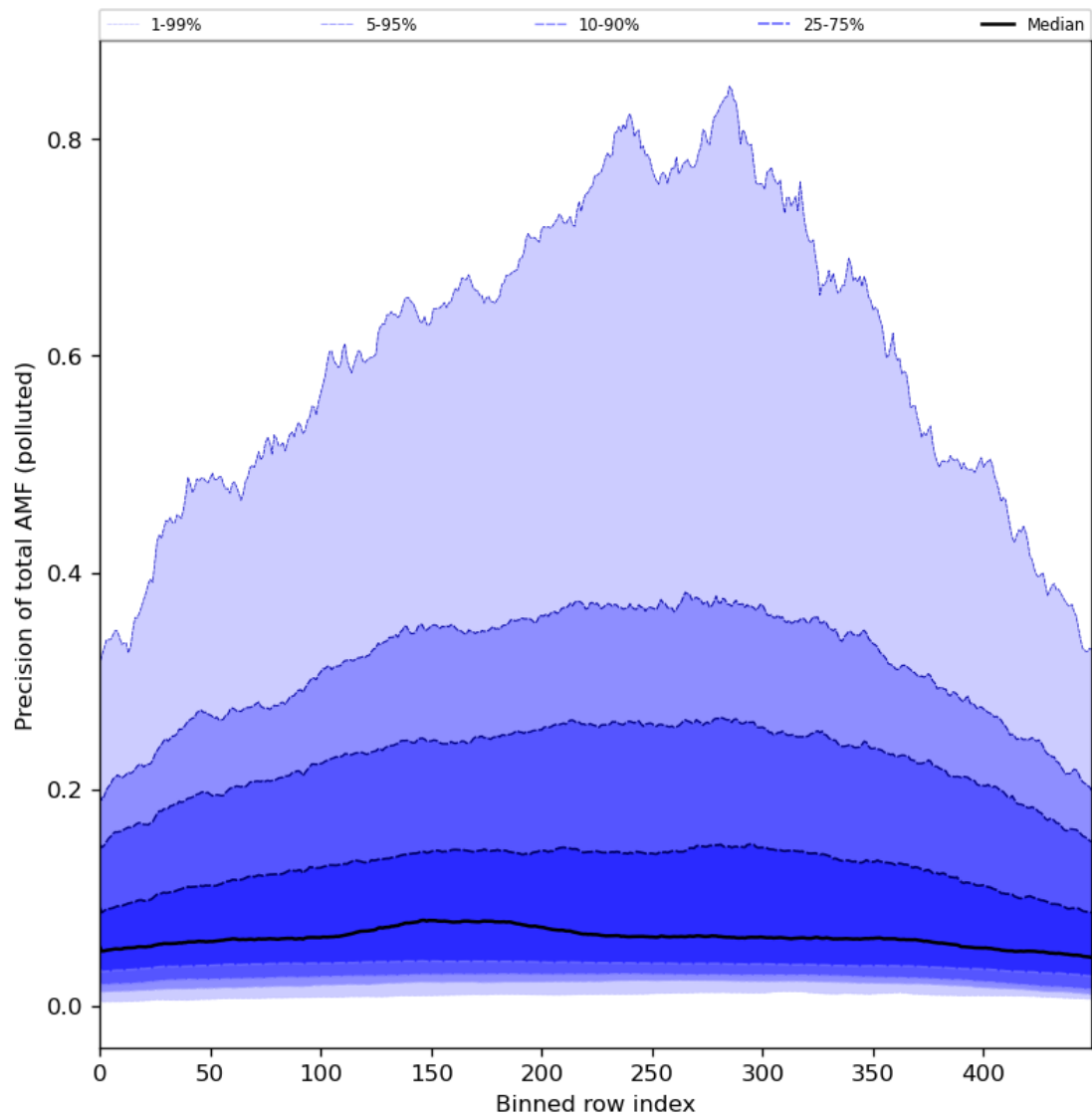
Figure 95: Along track statistics of “Precision of total AMF (polluted)” for 2024-08-16 to 2024-08-18
