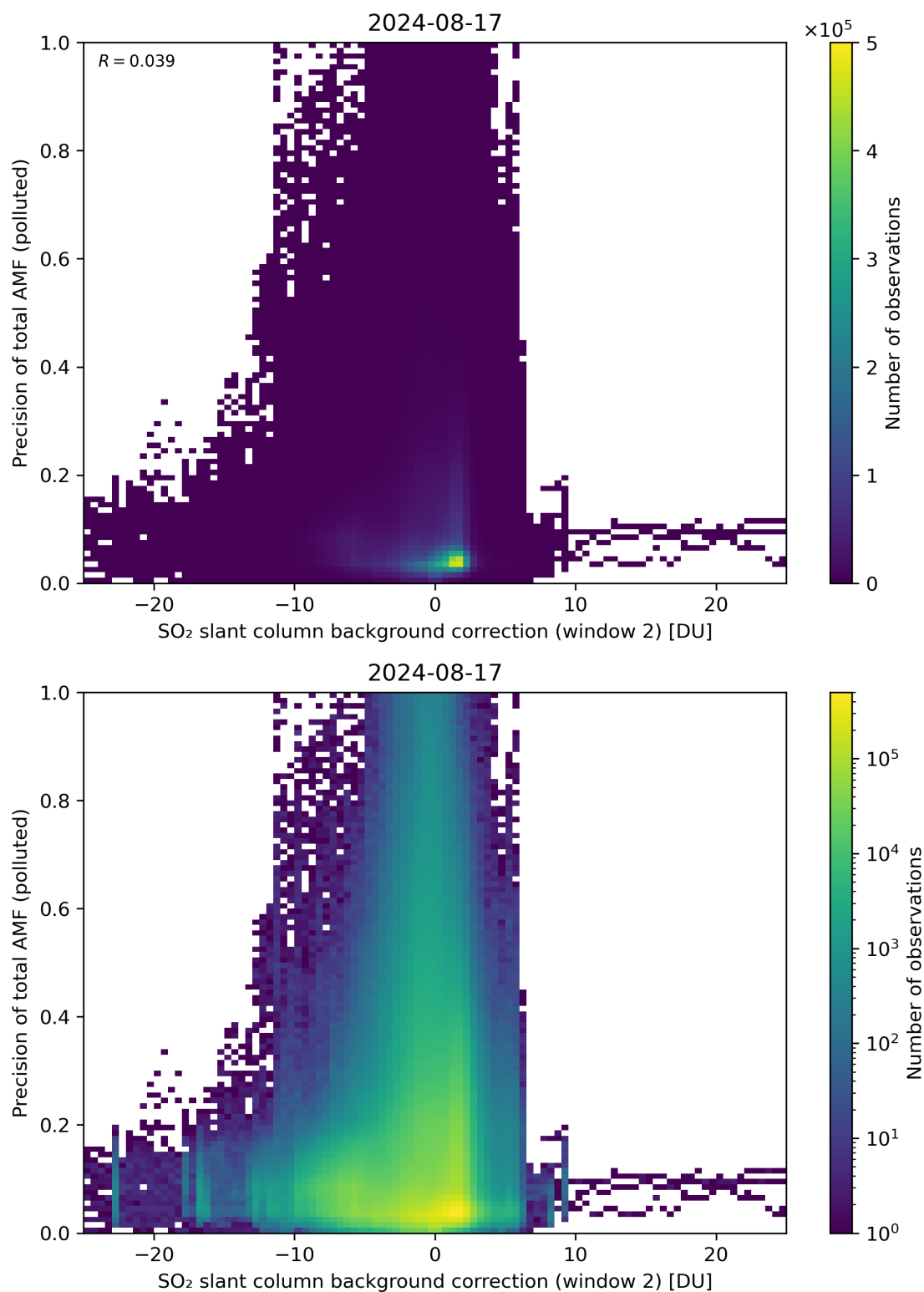
Figure 120: Scatter density plot of “SO 2 slant column background correction (window 2)” against “Precision of total AMF (polluted)” for 2024-08-16 to 2024-08-18.
