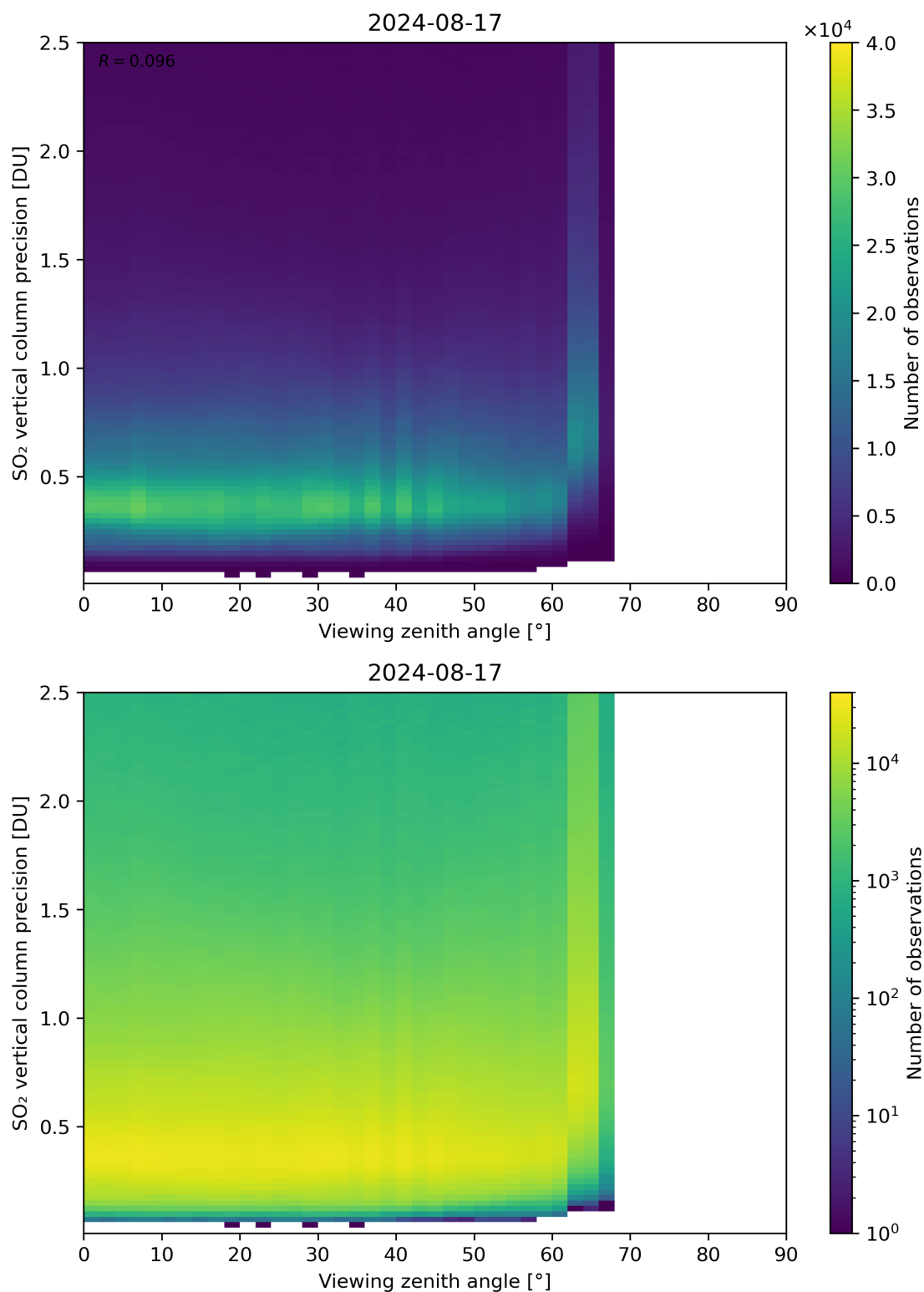
Figure 328: Scatter density plot of “Viewing zenith angle” against “SO 2 vertical column precision” for 2024-08-16 to 2024-08-18.
