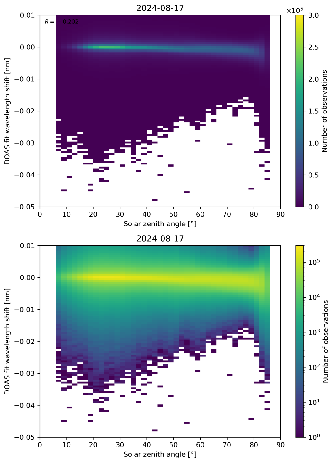
Figure 161: Scatter density plot of “Solar zenith angle” against “DOAS fit wavelength shift” for 2024-08-16 to 2024-08-18.
