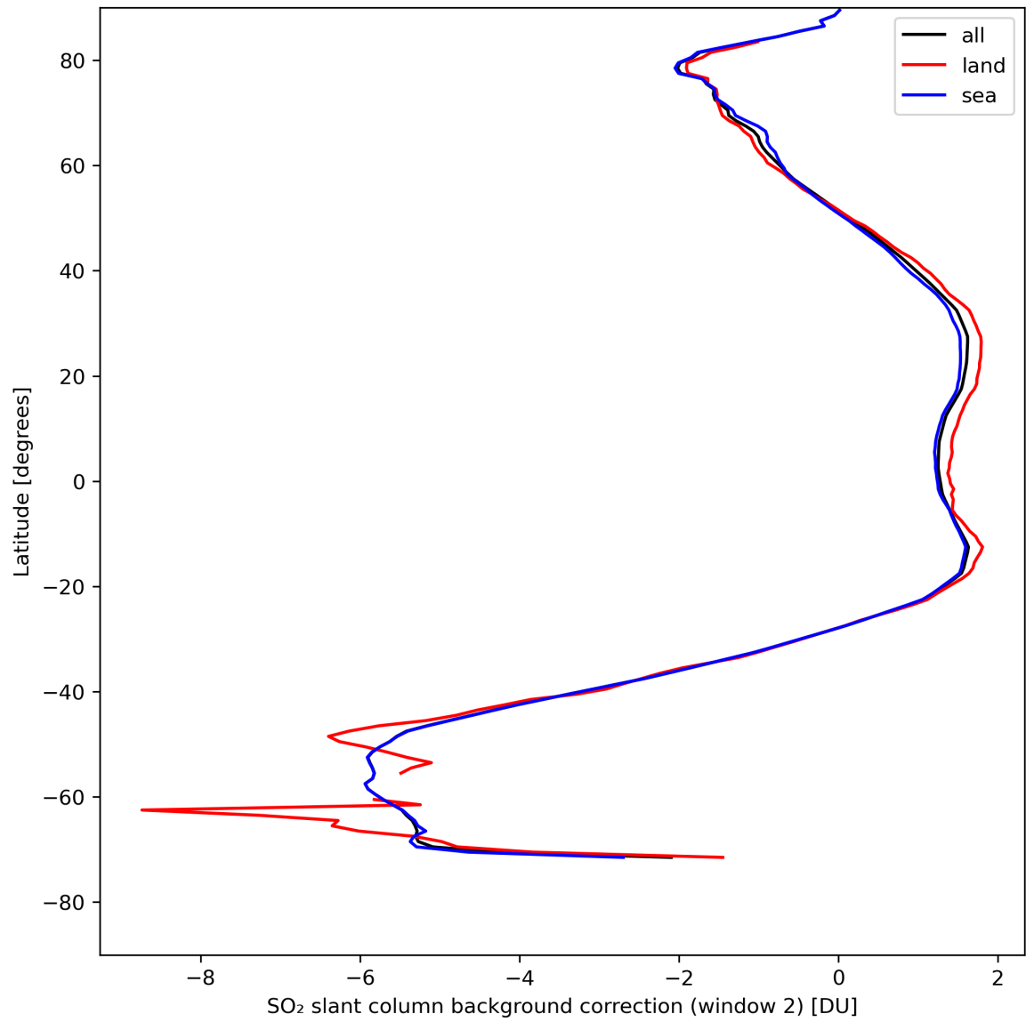
Figure 40: Zonal average of “SO 2 slant column background correction (window 2)” for 2024-08-16 to 2024-08-18.
