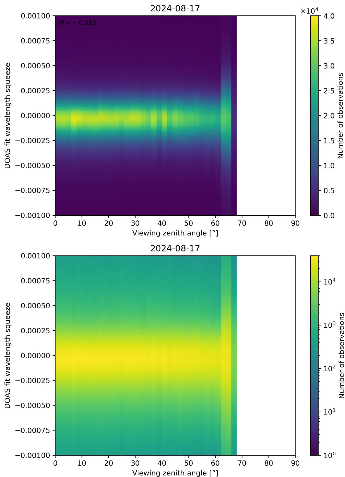
Figure 312: Scatter density plot of “Viewing zenith angle” against “DOAS fit wavelength squeeze” for 2024-08-16 to 2024-08-18.
