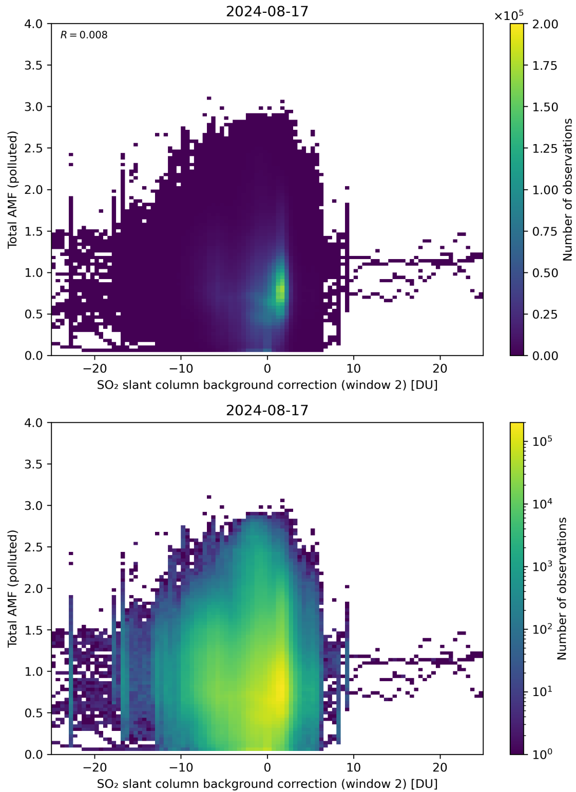
Figure 119: Scatter density plot of “SO 2 slant column background correction (window 2)” against “Total AMF (polluted)” for 2024-08-16 to 2024-08-18.
