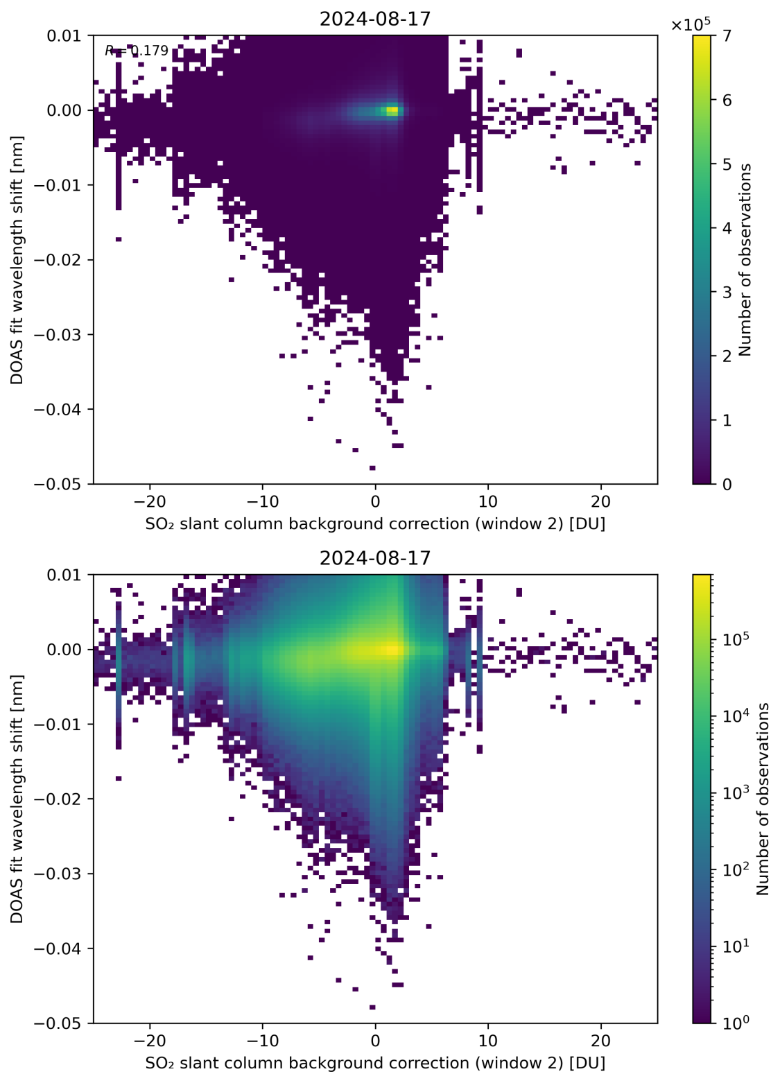
Figure 112: Scatter density plot of “SO 2 slant column background correction (window 2)” against “DOAS fit wavelength shift” for 2024-08-16 to 2024-08-18.
