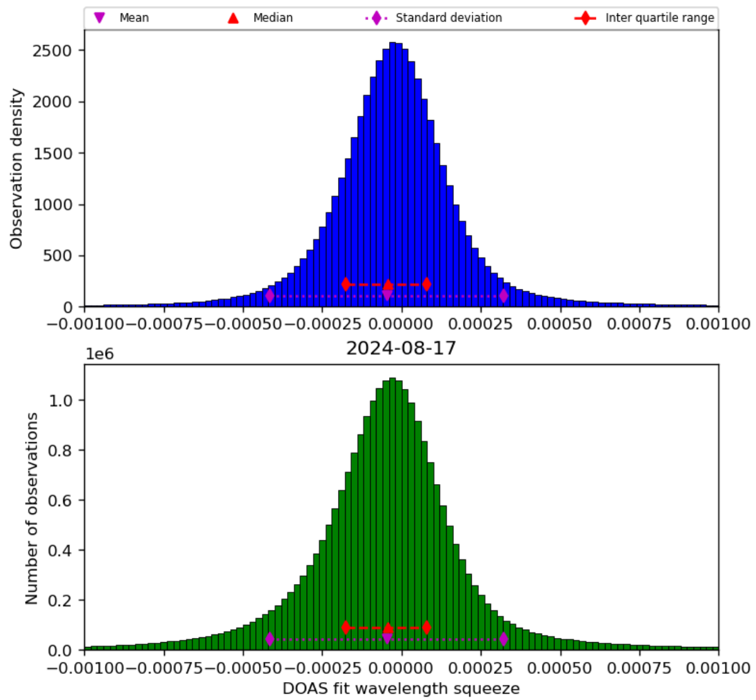
Figure 69: Histogram of “DOAS fit wavelength squeeze” for 2024-08-16 to 2024-08-18
