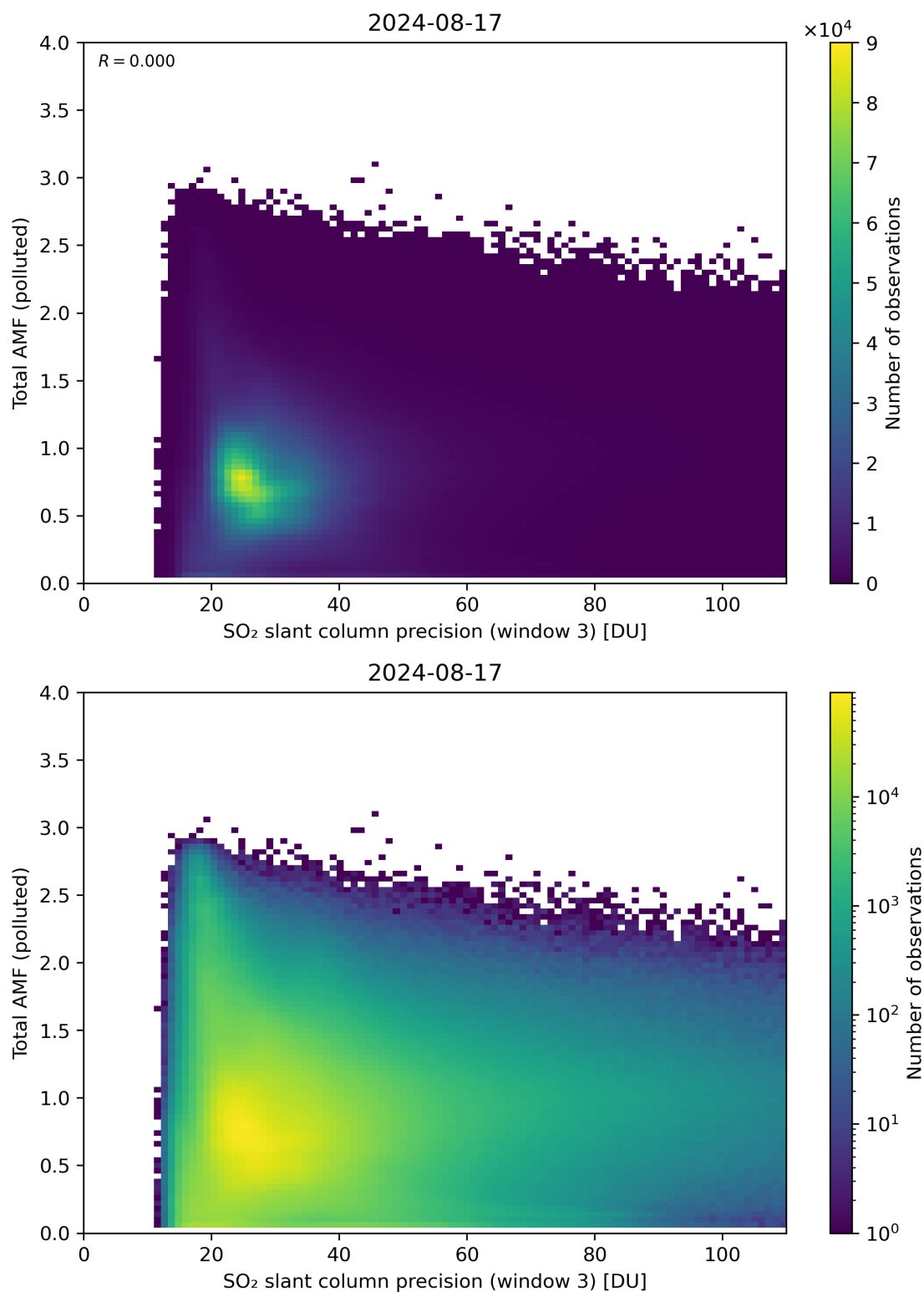
Figure 263: Scatter density plot of “SO 2 slant column precision (window 3)” against “Total AMF (polluted)” for 2024-08-16 to 2024-08-18.
