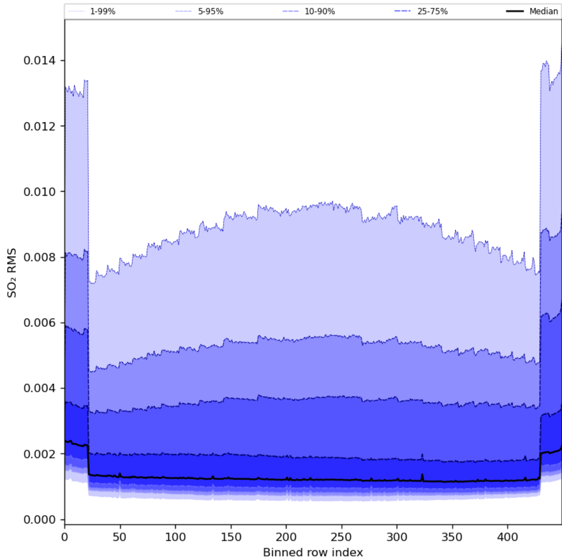
Figure 93: Along track statistics of “SO 2 RMS” for 2024-08-16 to 2024-08-18
