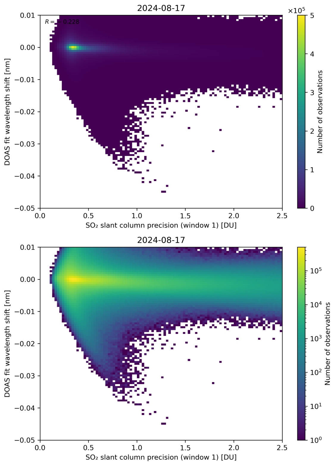
Figure 221: Scatter density plot of “SO 2 slant column precision (window 1)” against “DOAS fit wavelength shift” for 2024-08-16 to 2024-08-18.
