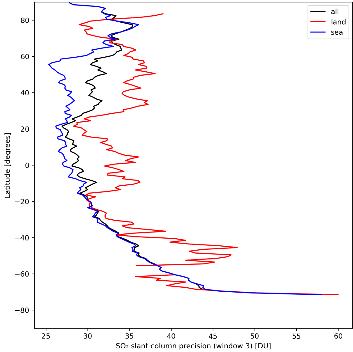
Figure 42: Zonal average of “SO 2 slant column precision (window 3)” for 2024-08-16 to 2024-08-18.
