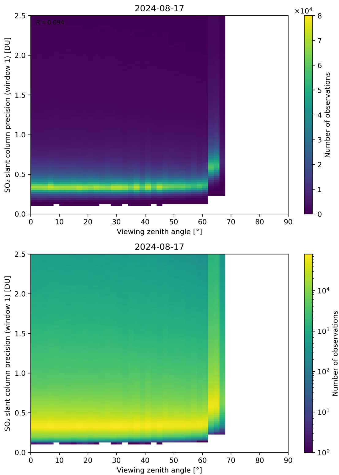
Figure 321: Scatter density plot of “Viewing zenith angle” against “SO 2 slant column precision (window 1)” for 2024-08-16 to 2024-08-18.
