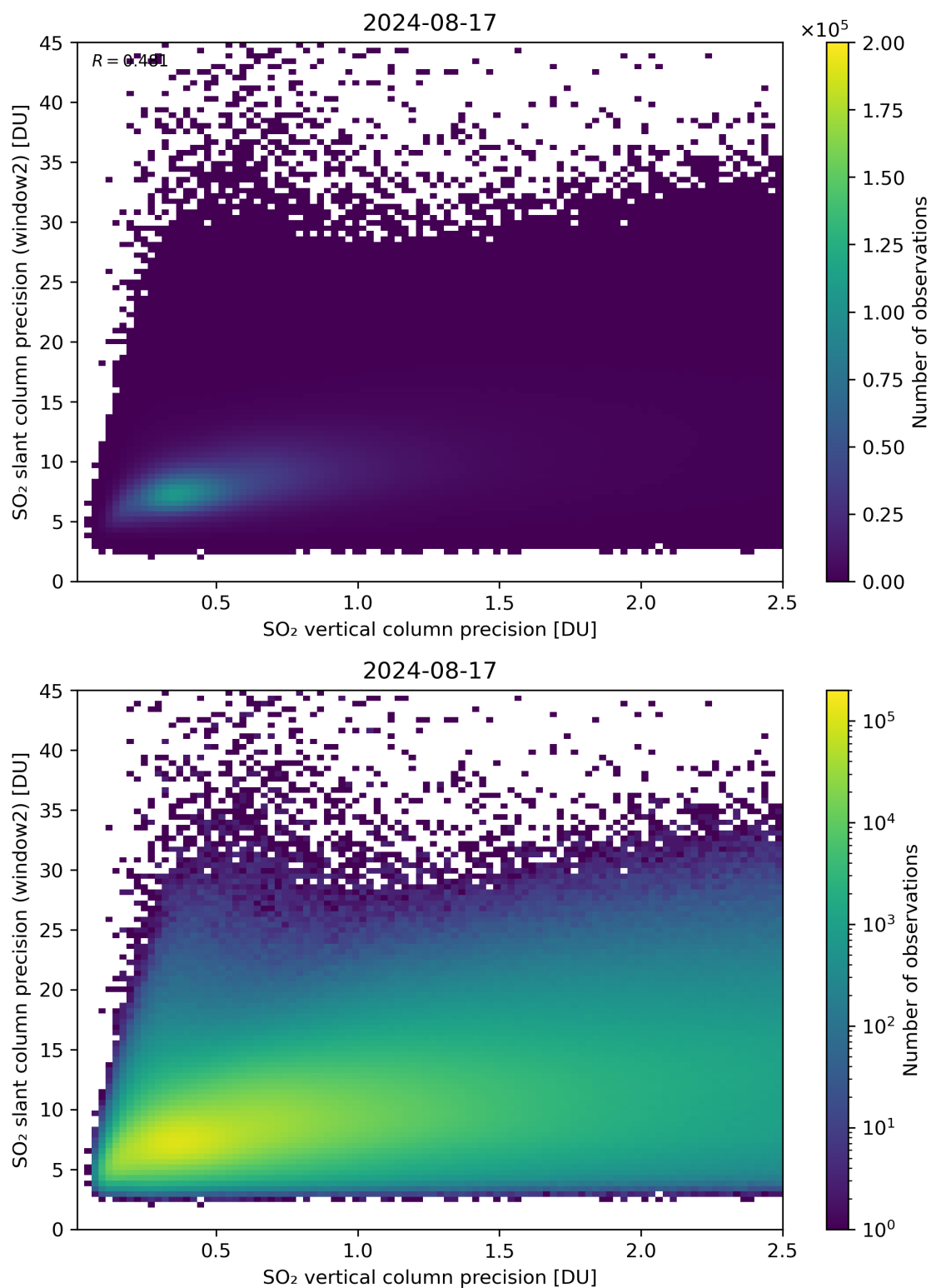
Figure 291: Scatter density plot of “SO 2 vertical column precision” against “SO 2 slant column precision (window2)” for 2024-08-16 to 2024-08-18.
