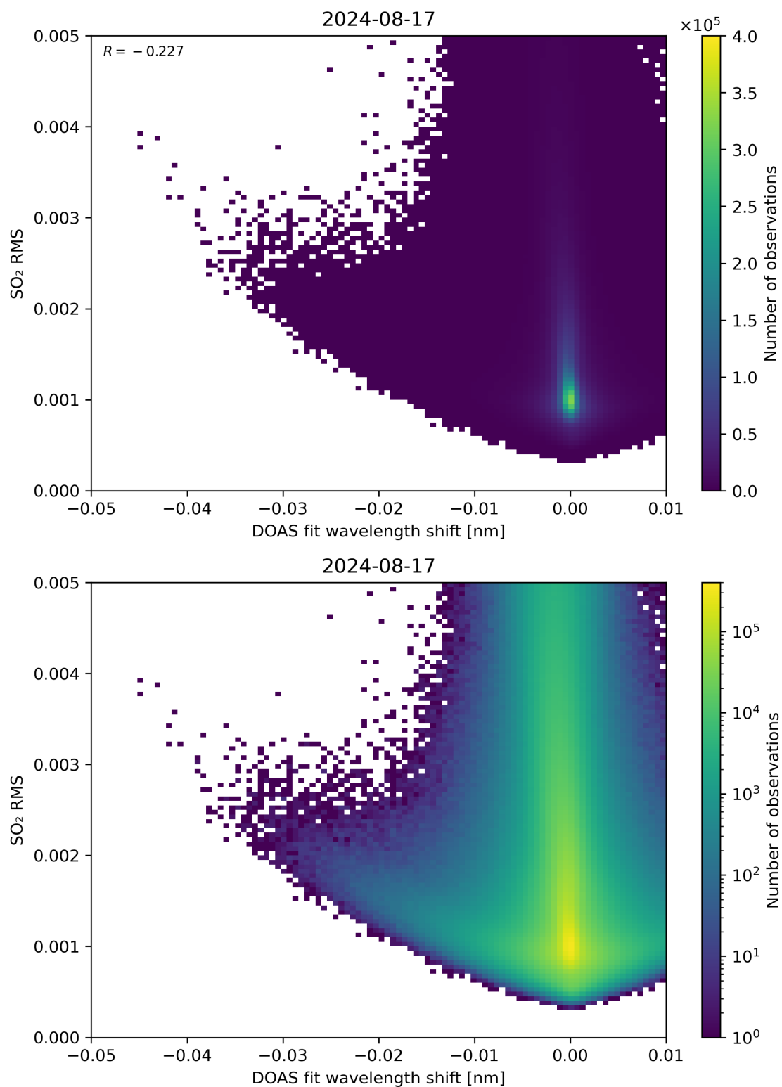
Figure 128: Scatter density plot of “DOAS fit wavelength shift” against “SO 2 RMS” for 2024-08-16 to 2024-08-18.
