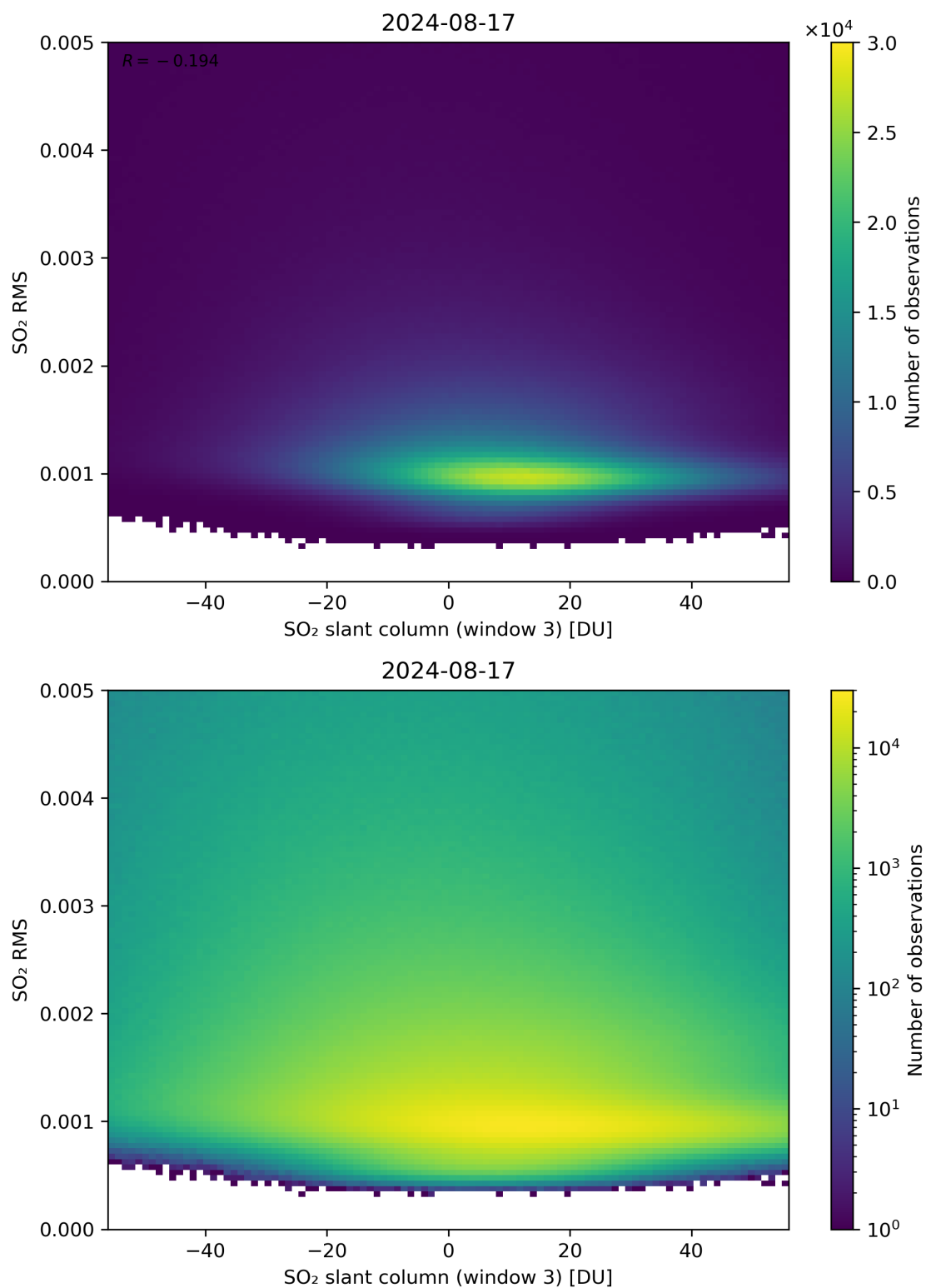
Figure 256: Scatter density plot of “SO 2 slant column (window 3)” against “SO 2 RMS” for 2024-08-16 to 2024-08-18.
