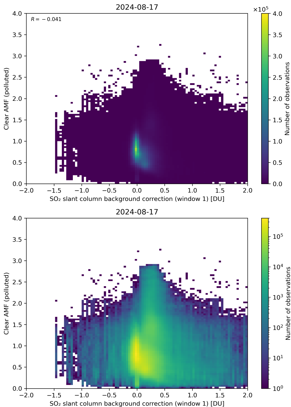
Figure 103: Scatter density plot of “SO 2 slant column background correction (window 1)” against “Clear AMF (polluted)” for 2024-08-16 to 2024-08-18.
