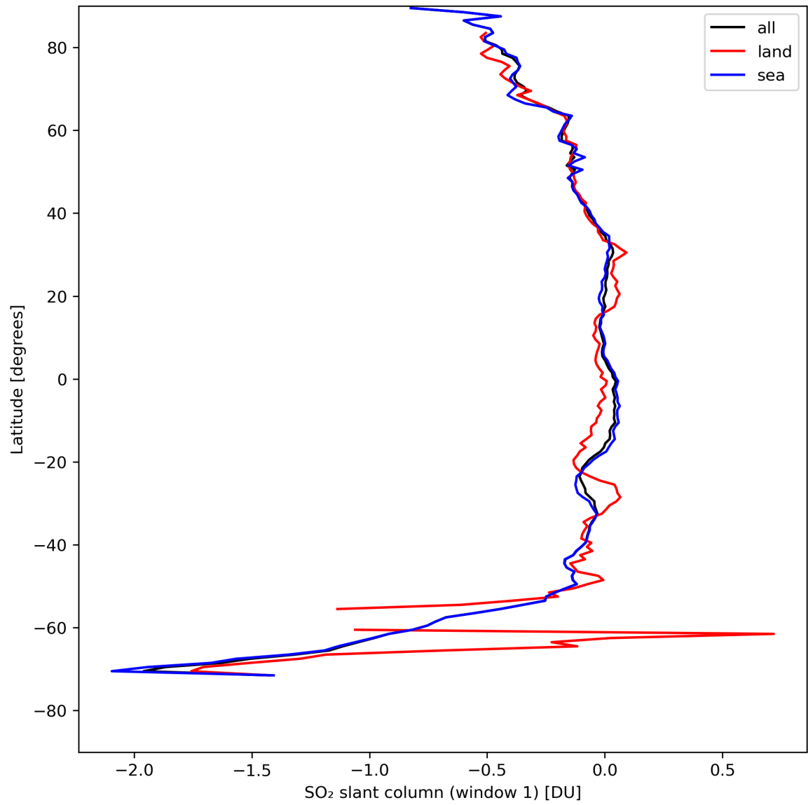
Figure 33: Zonal average of “SO 2 slant column (window 1)” for 2024-08-16 to 2024-08-18.
