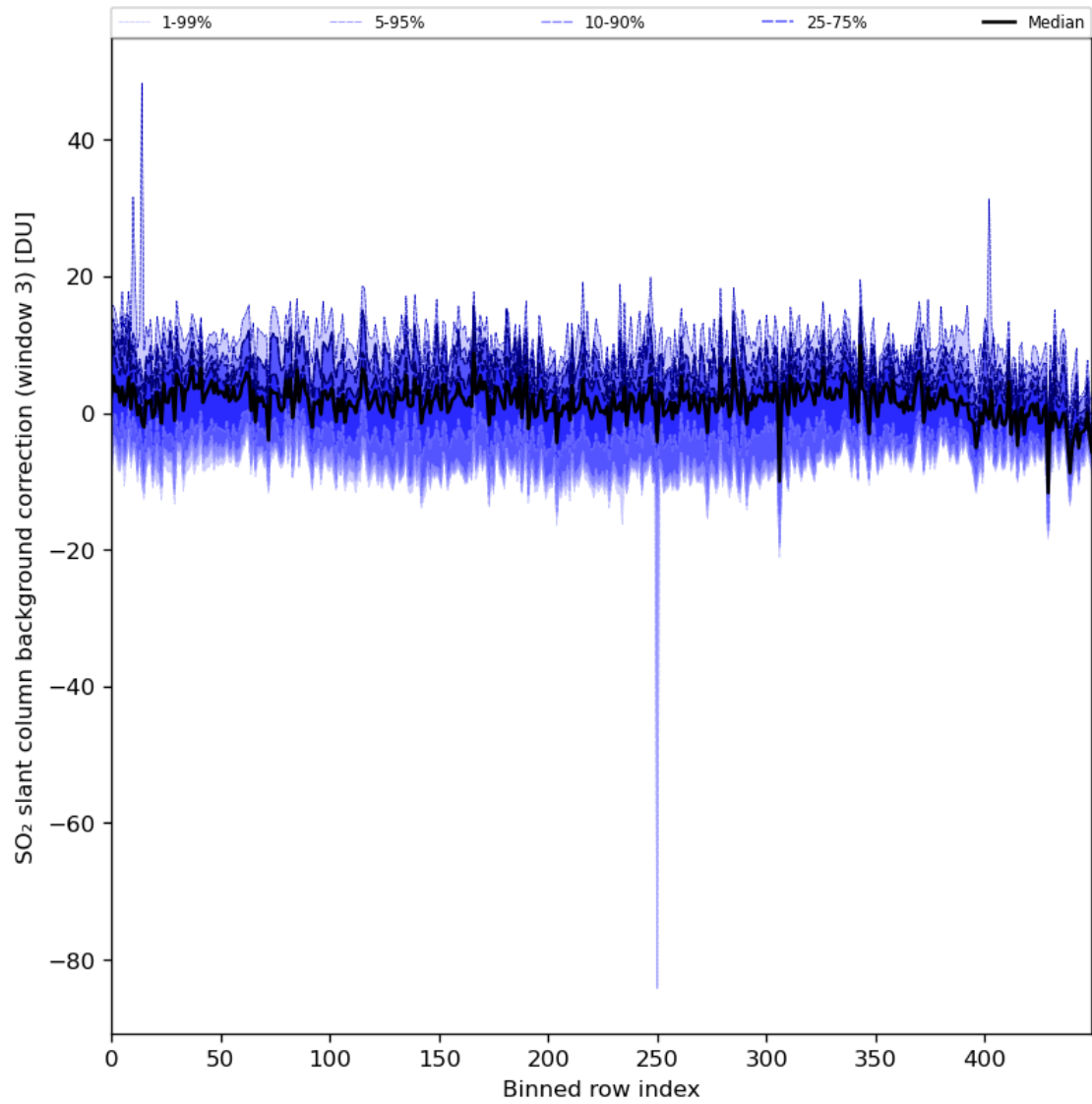
Figure 90: Along track statistics of “SO 2 slant column background correction (window 3)” for 2024-08-16 to 2024-08-18
