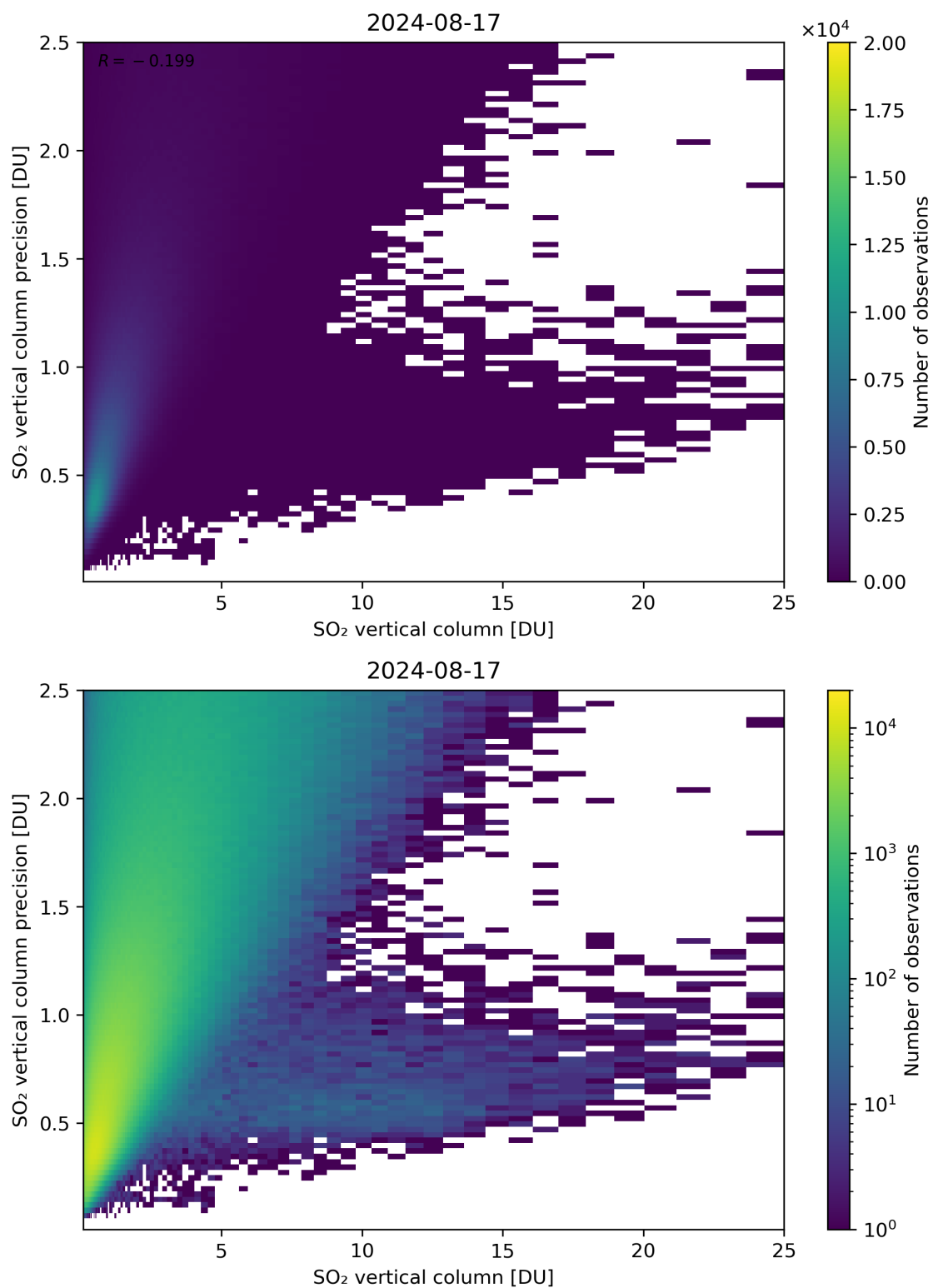
Figure 307: Scatter density plot of “SO 2 vertical column” against “SO 2 vertical column precision” for 2024-08-16 to 2024-08-18.
