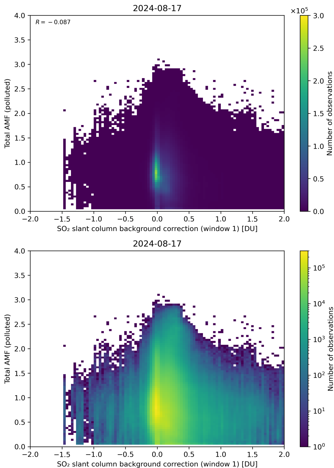
Figure 109: Scatter density plot of “SO 2 slant column background correction (window 1)” against “Total AMF (polluted)” for 2024-08-16 to 2024-08-18.
