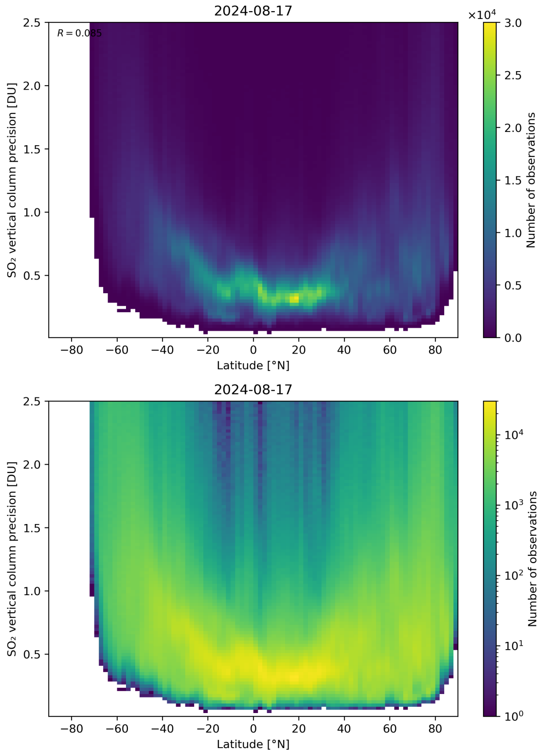
Figure 157: Scatter density plot of “Latitude” against “SO 2 vertical column precision” for 2024-08-16 to 2024-08-18.
