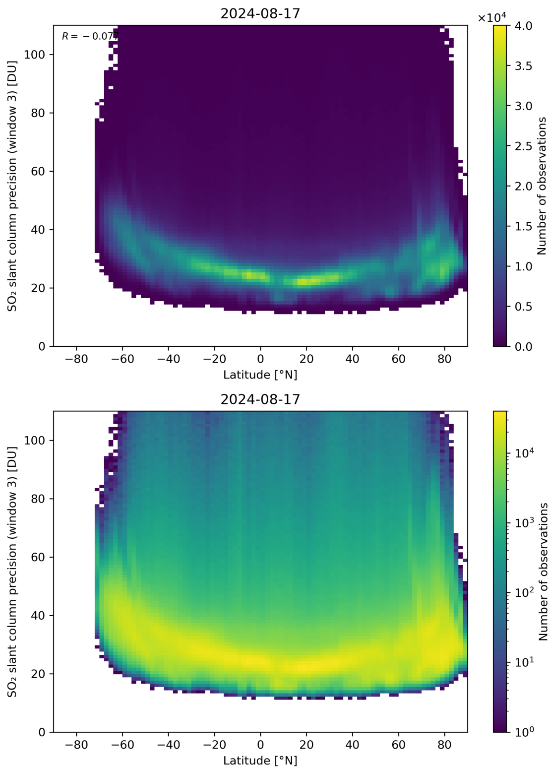
Figure 153: Scatter density plot of “Latitude” against “SO 2 slant column precision (window 3)” for 2024-08-16 to 2024-08-18.
