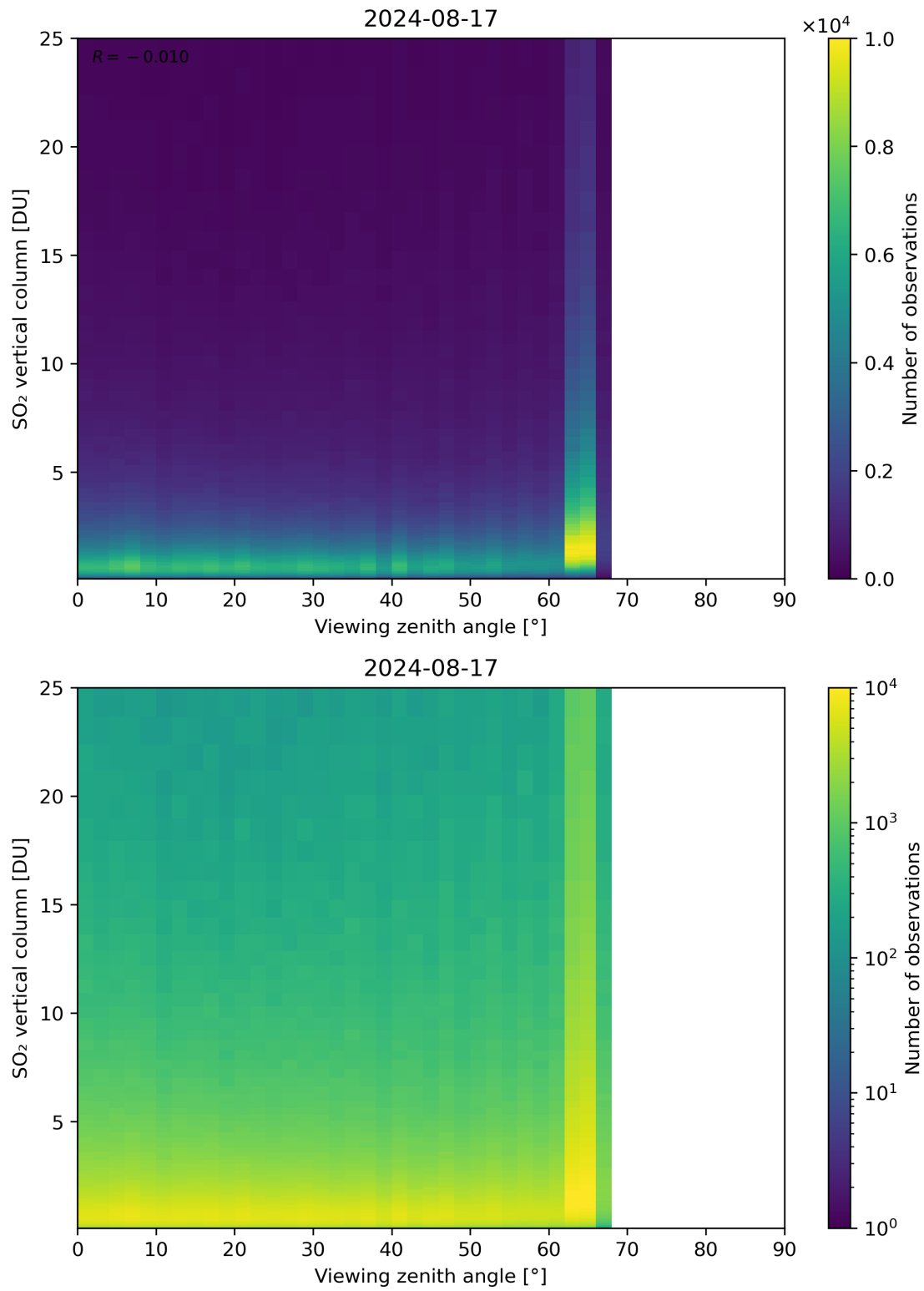
Figure 327: Scatter density plot of “Viewing zenith angle” against “SO 2 vertical column” for 2024-08-16 to 2024-08-18.
