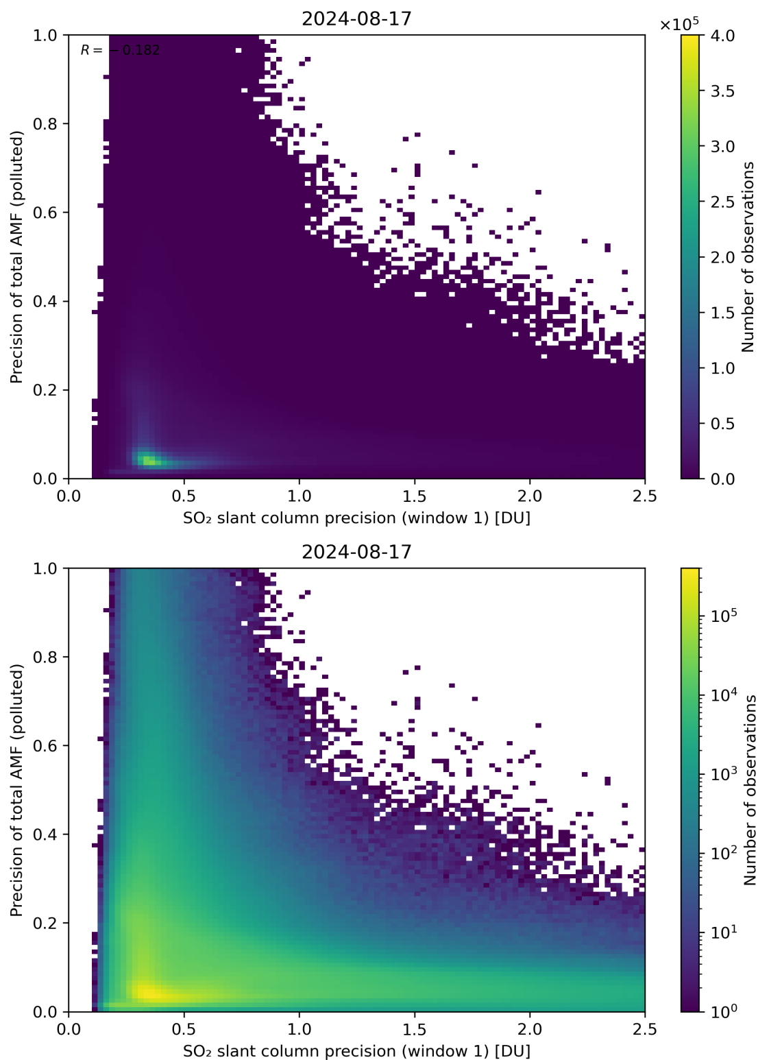
Figure 231: Scatter density plot of “SO 2 slant column precision (window 1)” against “Precision of total AMF (polluted)” for 2024-08-16 to 2024-08-18.
