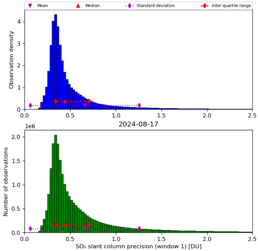
Figure 57: Histogram of “SO 2 slant column precision (window 1)” for 2024-08-16 to 2024-08-18
