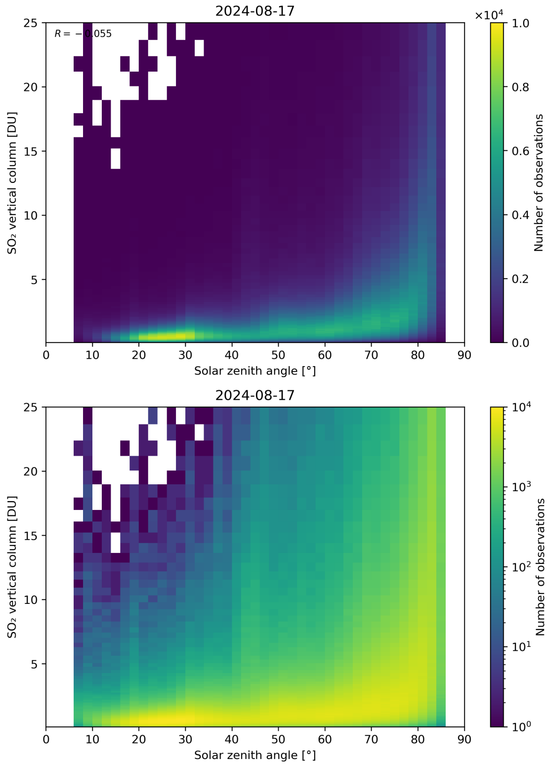
Figure 176: Scatter density plot of “Solar zenith angle” against “SO 2 vertical column” for 2024-08-16 to 2024-08-18.
