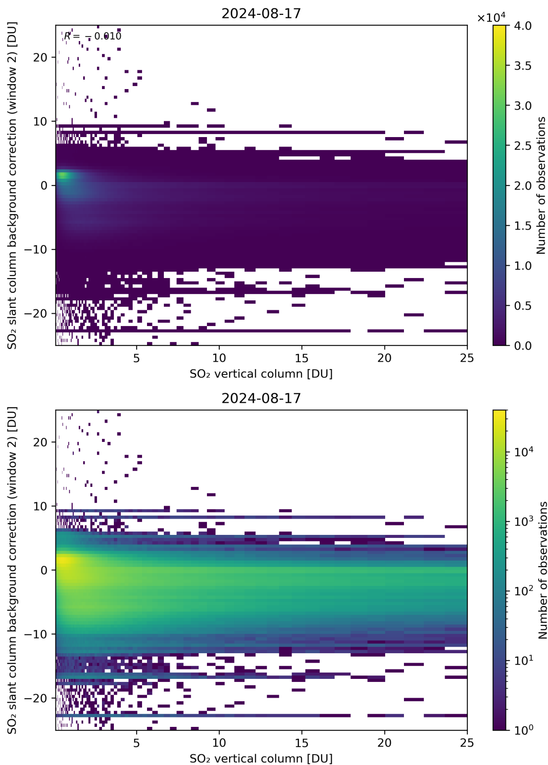
Figure 274: Scatter density plot of “SO 2 vertical column” against “SO 2 slant column background correction (window 2)” for 2024-08-16 to 2024-08-18.
