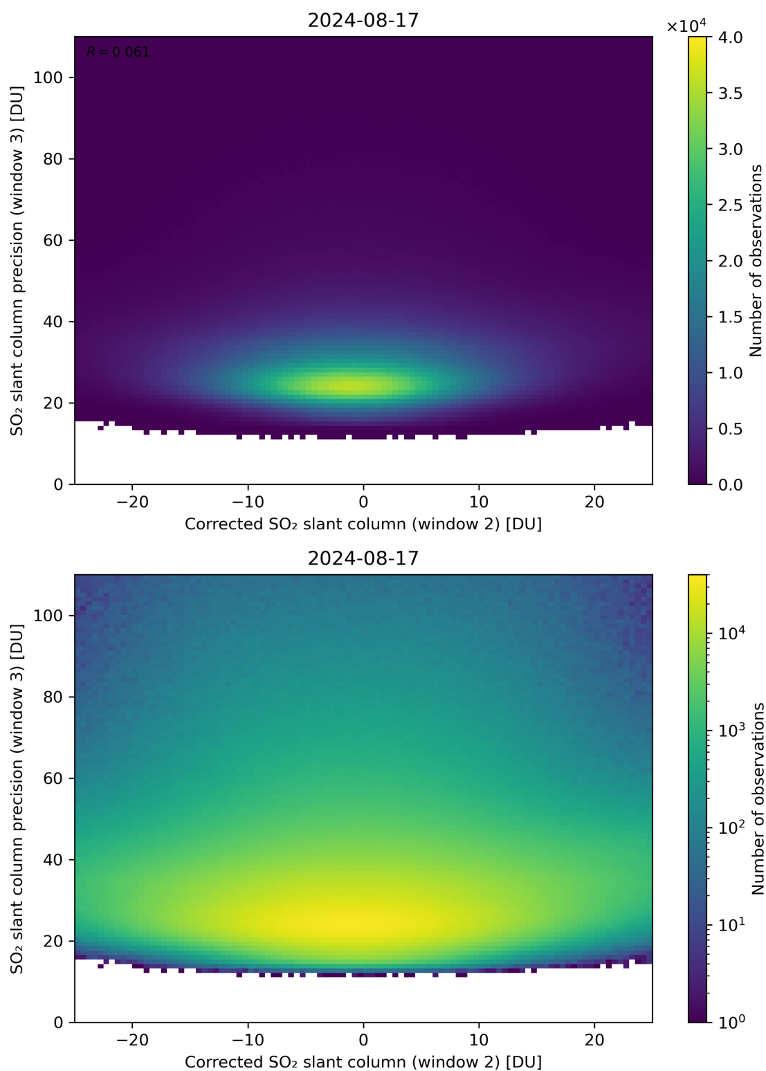
Figure 202: Scatter density plot of “Corrected SO 2 slant column (window 2)” against “SO 2 slant column precision (window 3)” for 2024-08-16 to 2024-08-18.
