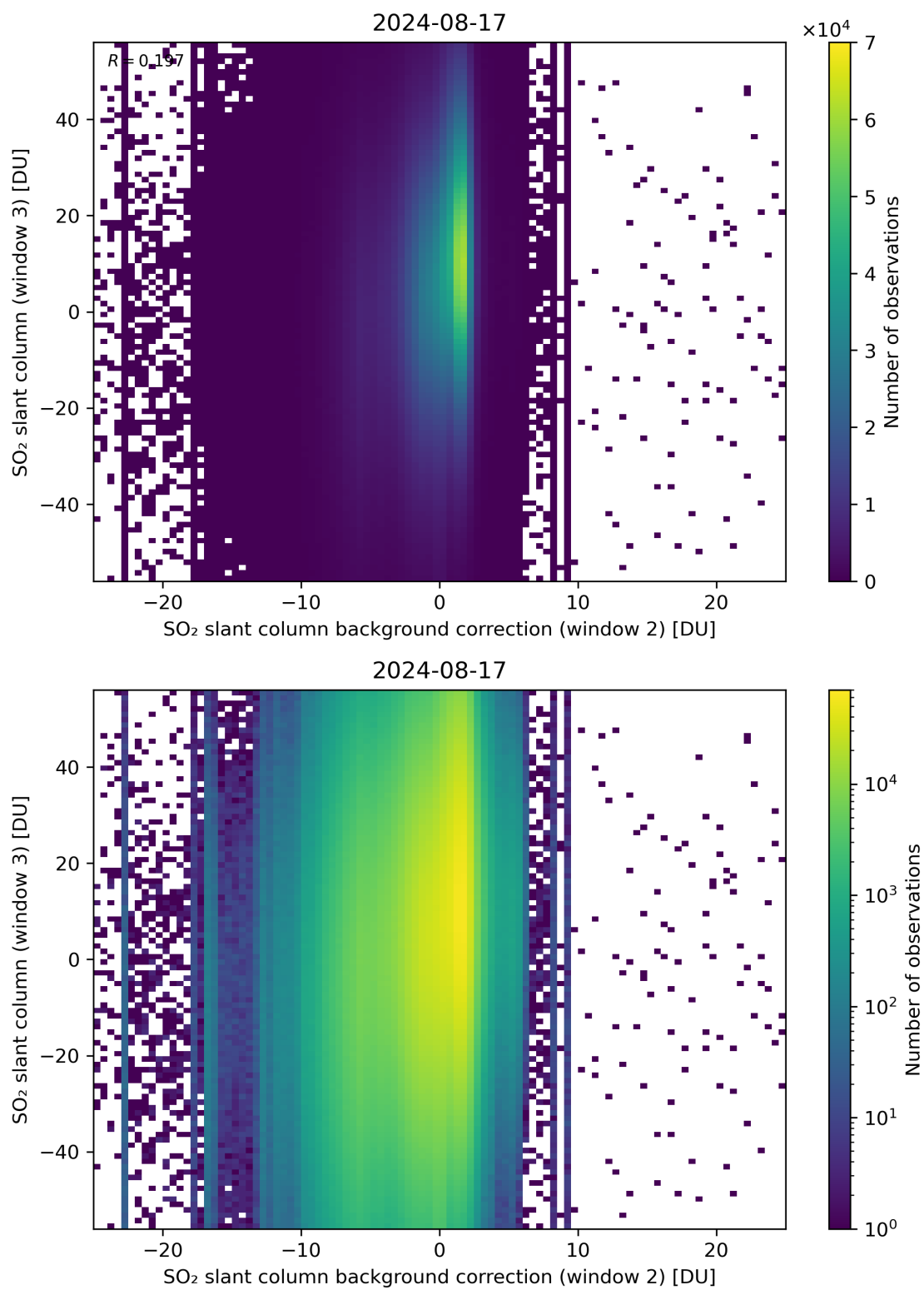
Figure 117: Scatter density plot of “SO 2 slant column background correction (window 2)” against “SO 2 slant column (window 3)” for 2024-08-16 to 2024-08-18.
