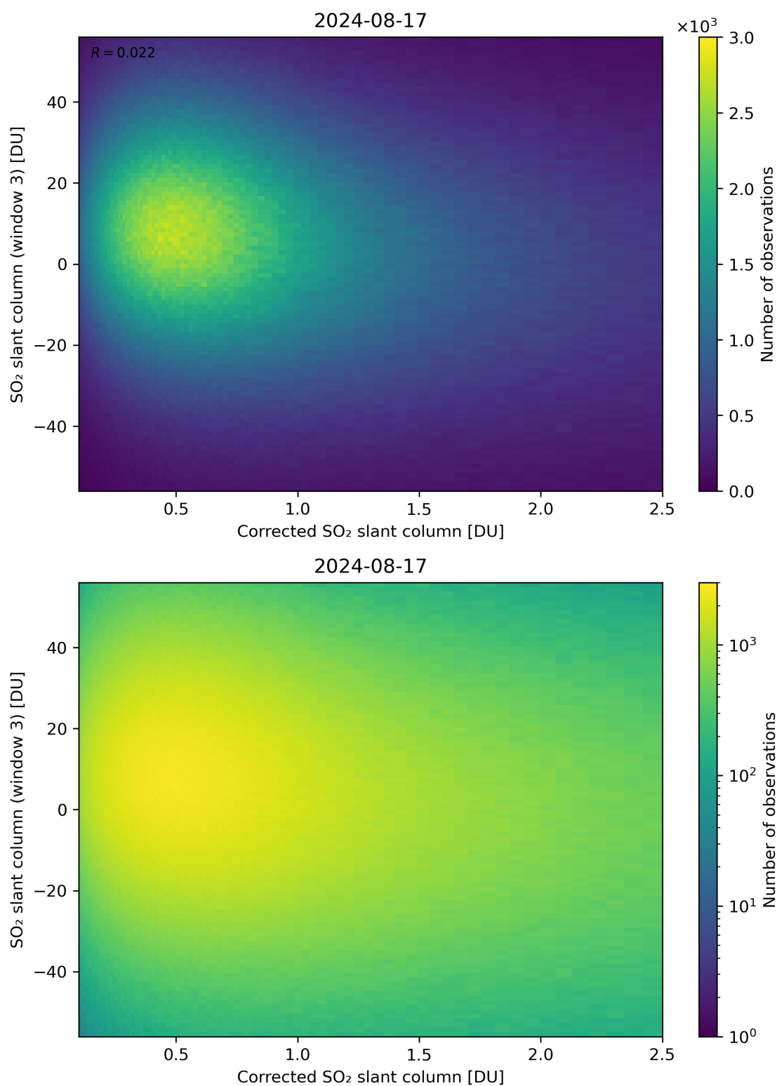
Figure 190: Scatter density plot of “Corrected SO 2 slant column” against “SO 2 slant column (window 3)” for 2024-08-16 to 2024-08-18.
