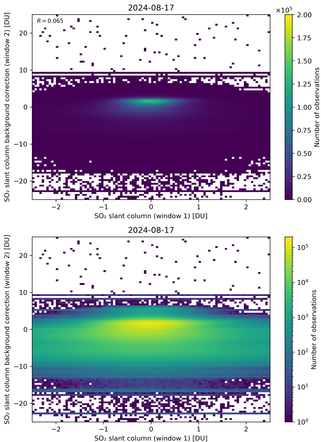
Figure 213: Scatter density plot of “SO 2 slant column (window 1)” against “SO 2 slant column background correction (window 2)” for 2024-08-16 to 2024-08-18.
