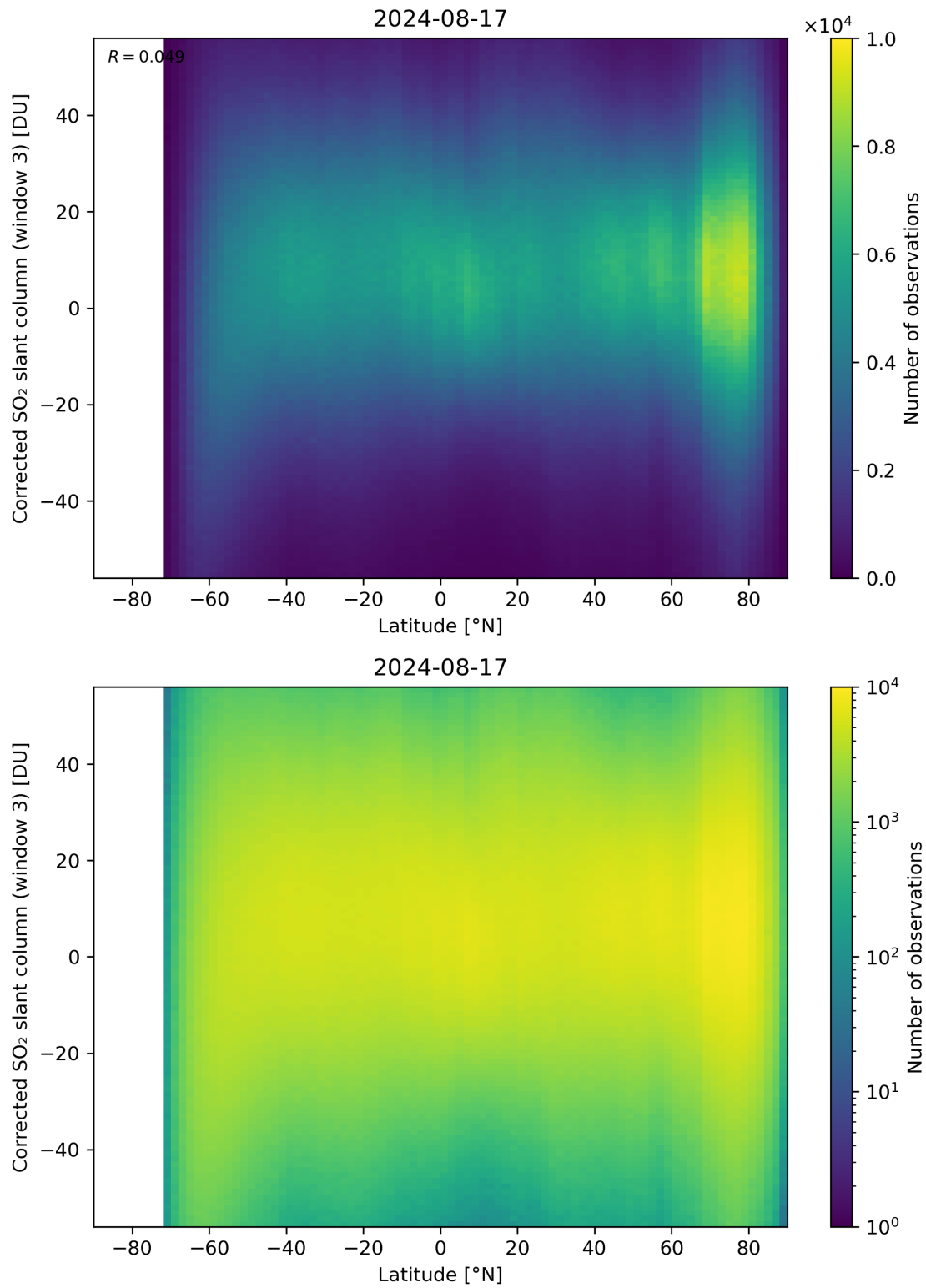
Figure 148: Scatter density plot of “Latitude” against “Corrected SO 2 slant column (window 3)” for 2024-08-16 to 2024-08-18.
