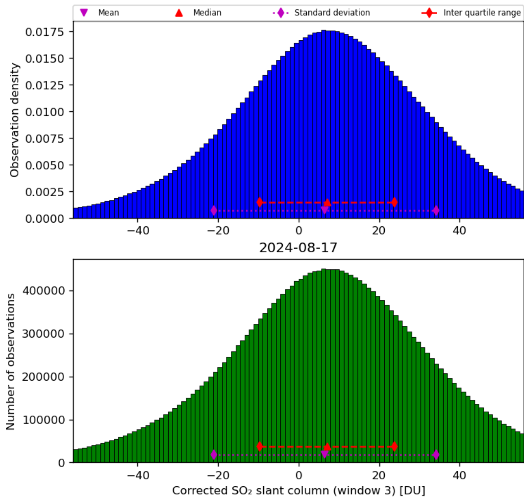
Figure 66: Histogram of "Corrected SO 2 slant column (window 3)" for 2024-08-16 to 2024-08-18
