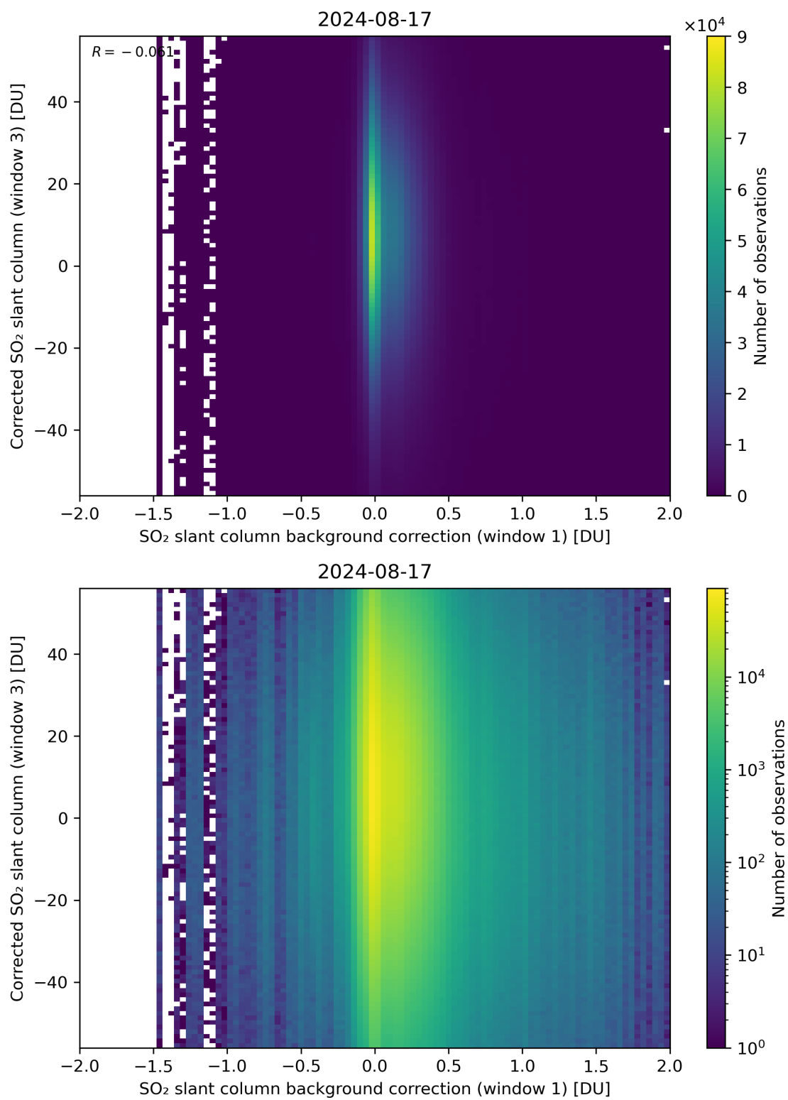
Figure 105: Scatter density plot of “SO 2 slant column background correction (window 1)” against “Corrected SO 2 slant column (window 3)” for 2024-08-16 to 2024-08-18.
