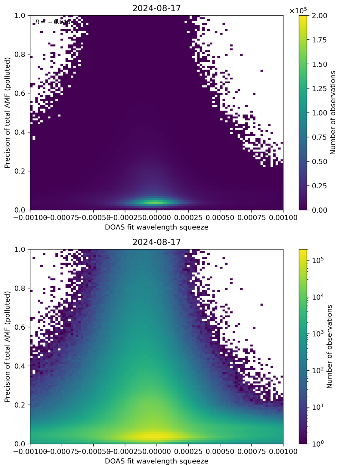
Figure 135: Scatter density plot of “DOAS fit wavelength squeeze” against “Precision of total AMF (polluted)” for 2024-08-16 to 2024-08-18.
