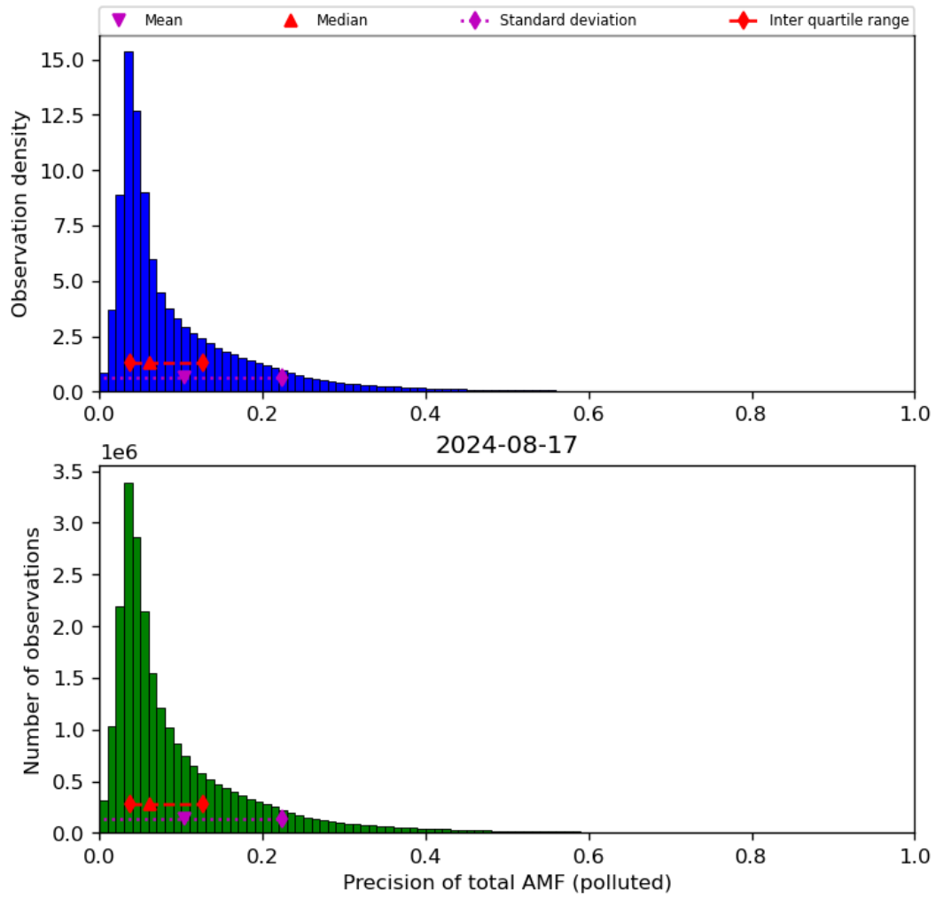
Figure 72: Histogram of “Precision of total AMF (polluted)” for 2024-08-16 to 2024-08-18
