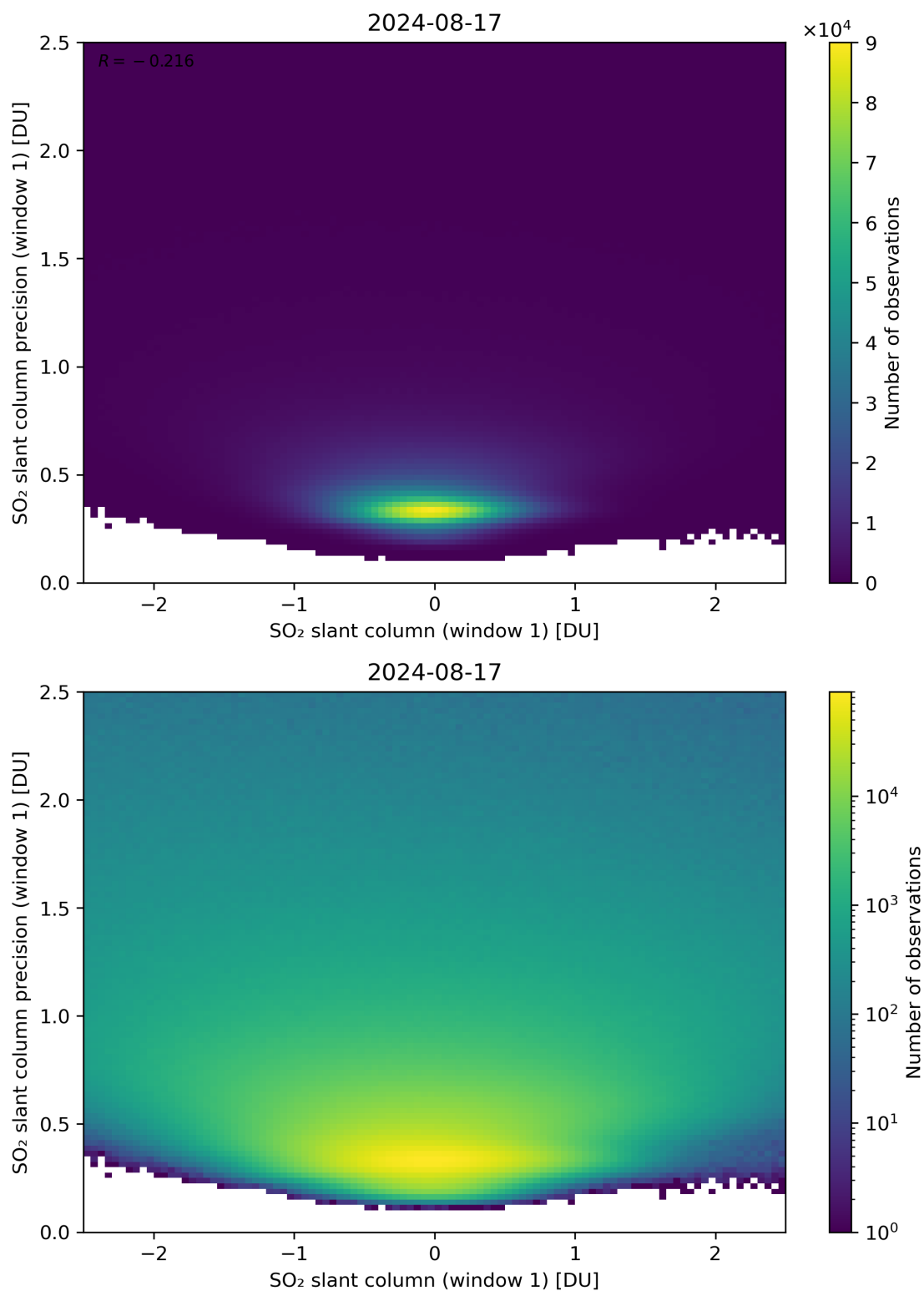
Figure 235: Scatter density plot of “SO 2 slant column (window 1)” against “SO 2 slant column precision (window 1)” for 2024-08-16 to 2024-08-18.
