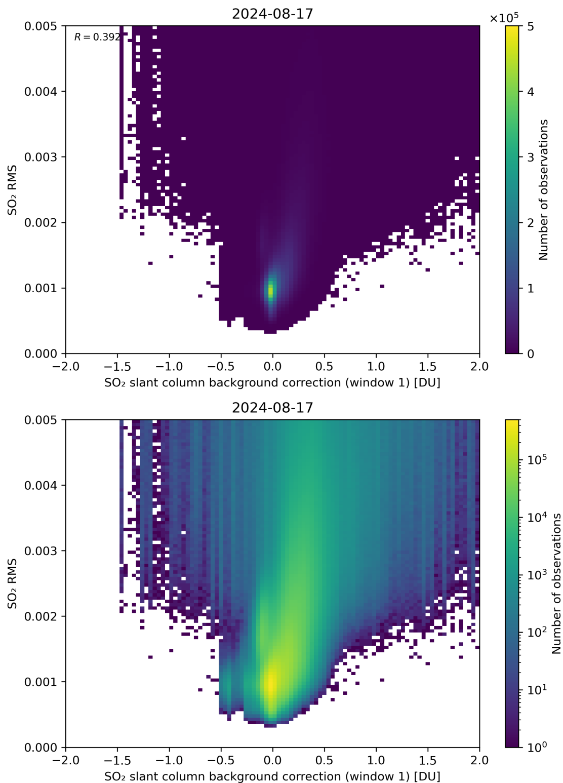
Figure 102: Scatter density plot of “SO 2 slant column background correction (window 1)” against “SO 2 RMS” for 2024-08-16 to 2024-08-18.
