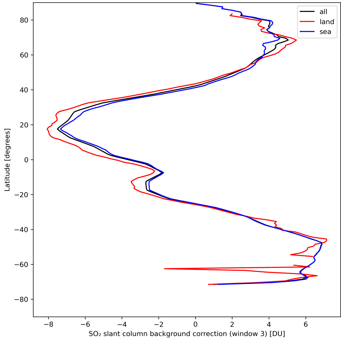
Figure 44: Zonal average of “SO 2 slant column background correction (window 3)” for 2024-08-16 to 2024-08-18.
