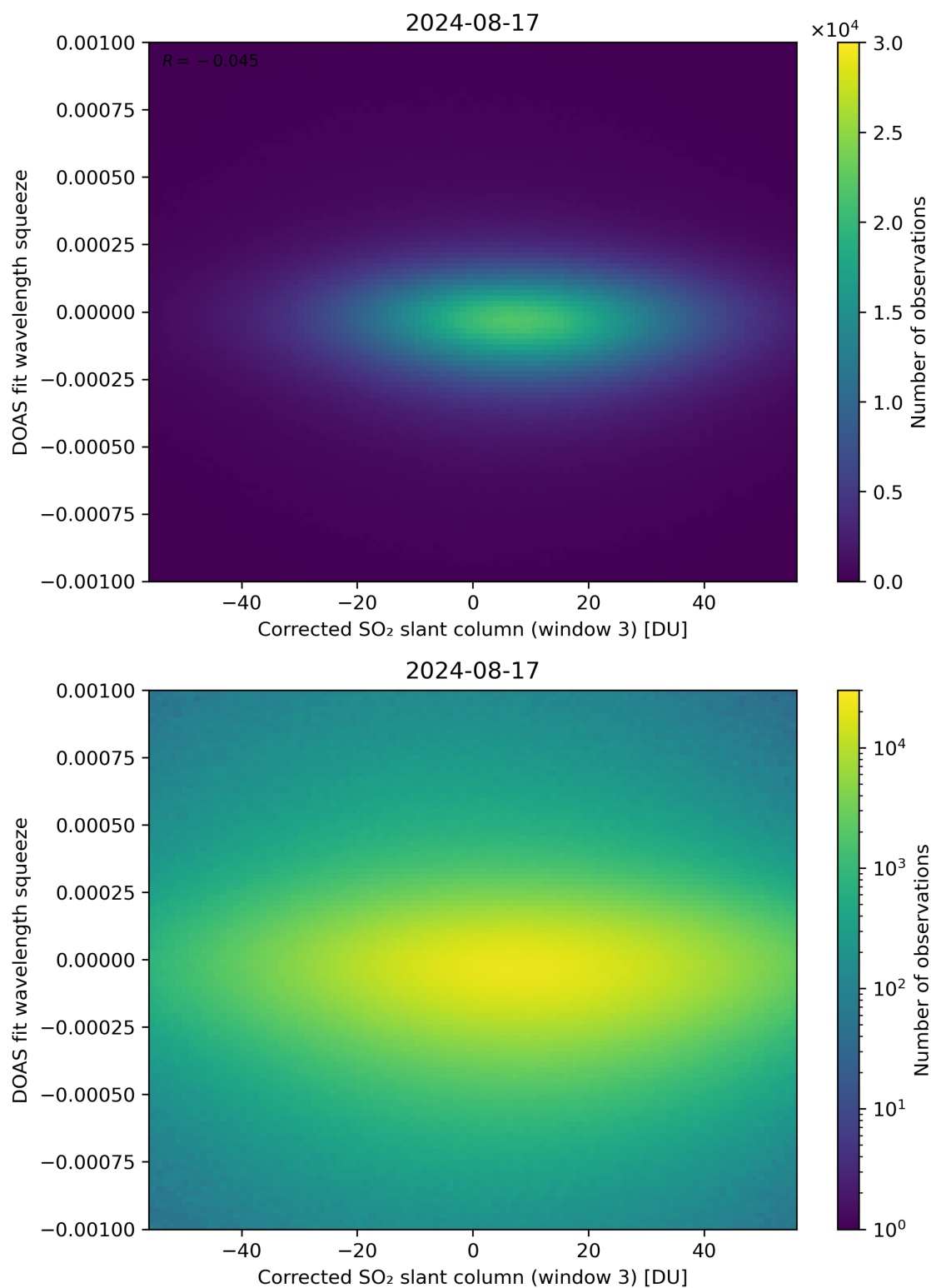
Figure 207: Scatter density plot of “Corrected SO 2 slant column (window 3)” against “DOAS fit wavelength squeeze” for 2024-08-16 to 2024-08-18.
