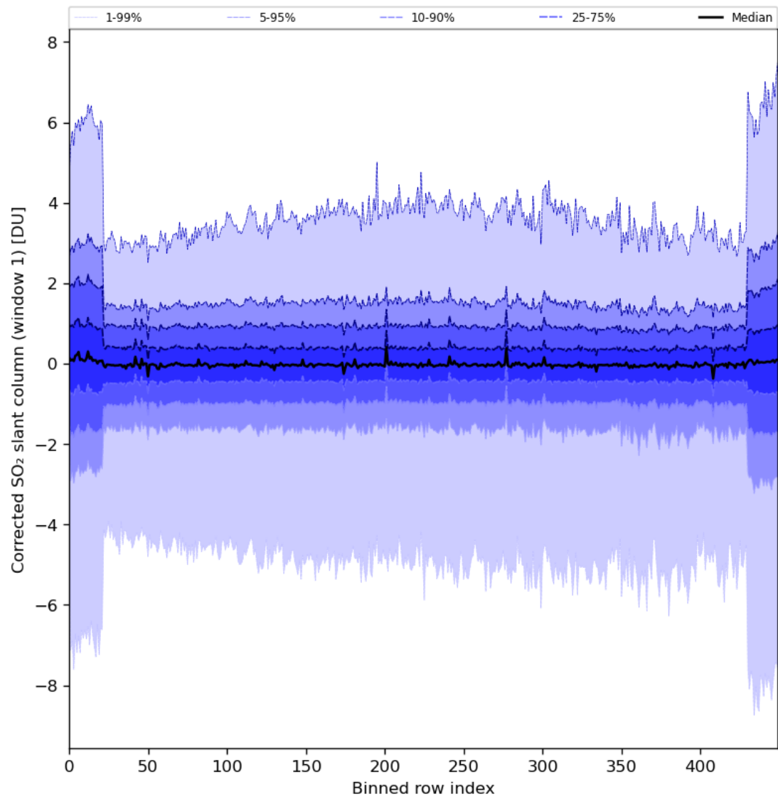
Figure 81: Along track statistics of "Corrected SO 2 slant column (window 1)" for 2024-08-16 to 2024-08-18
