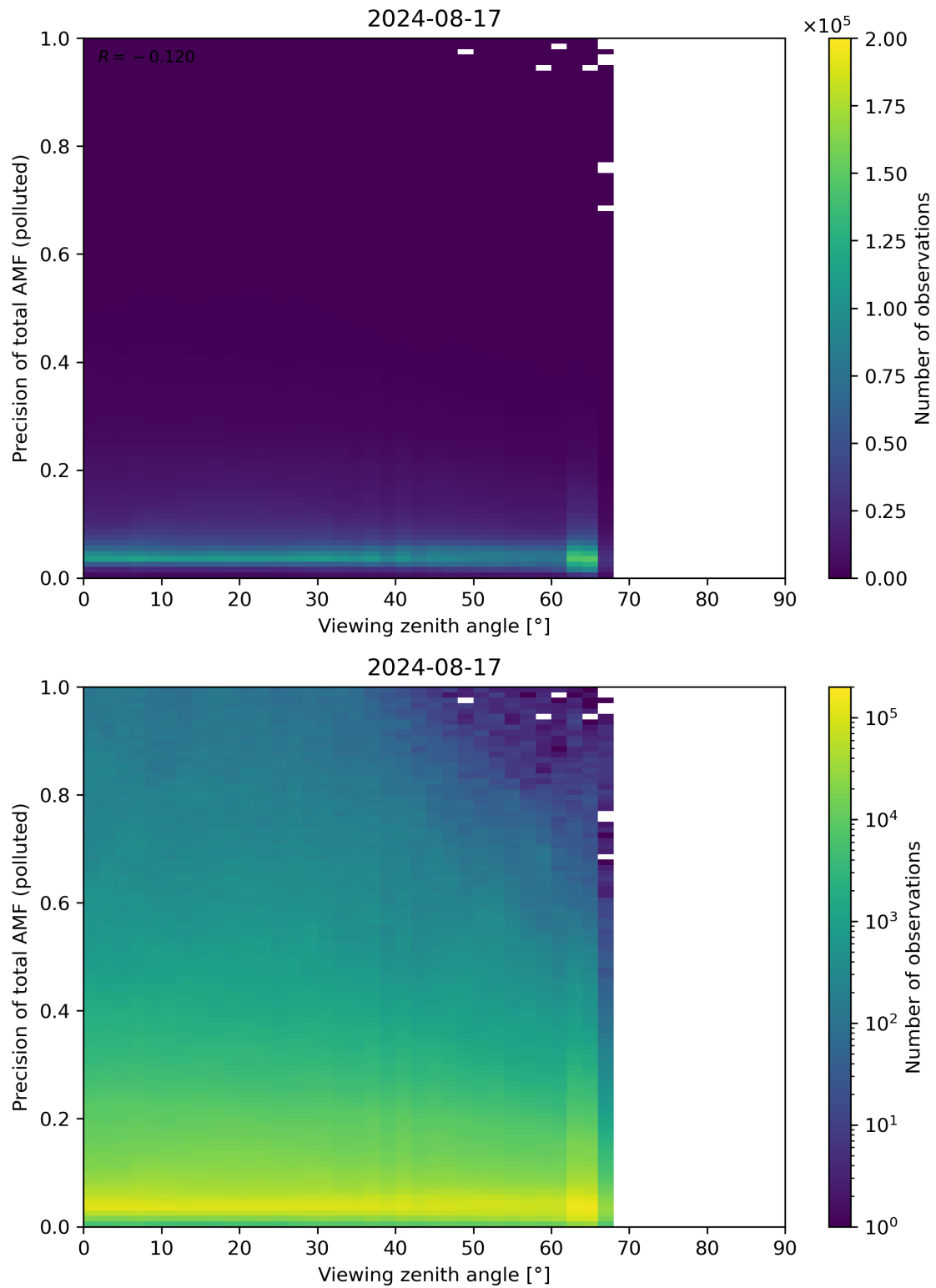
Figure 326: Scatter density plot of “Viewing zenith angle” against “Precision of total AMF (polluted)” for 2024-08-16 to 2024-08-18.
