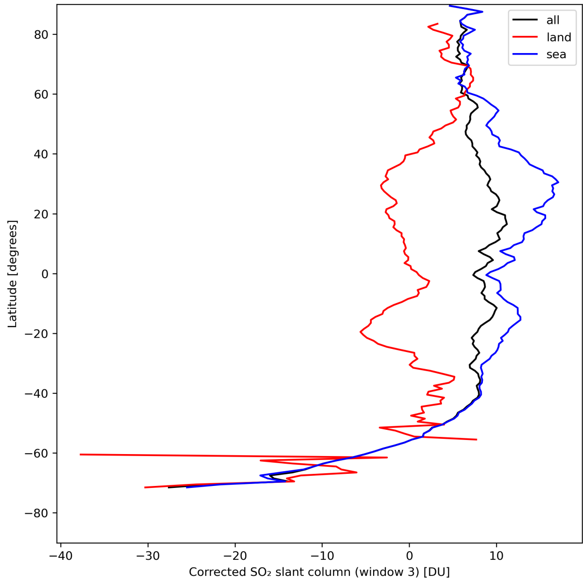
Figure 43: Zonal average of “Corrected SO 2 slant column (window 3)” for 2024-08-16 to 2024-08-18.
