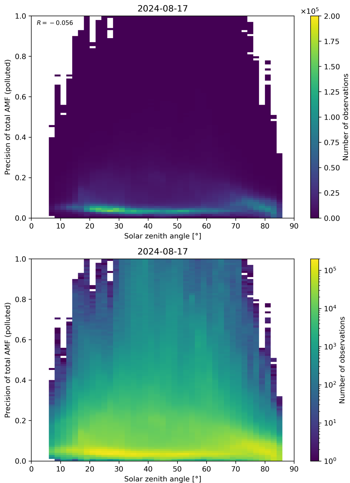
Figure 175: Scatter density plot of “Solar zenith angle” against “Precision of total AMF (polluted)” for 2024-08-16 to 2024-08-18.
