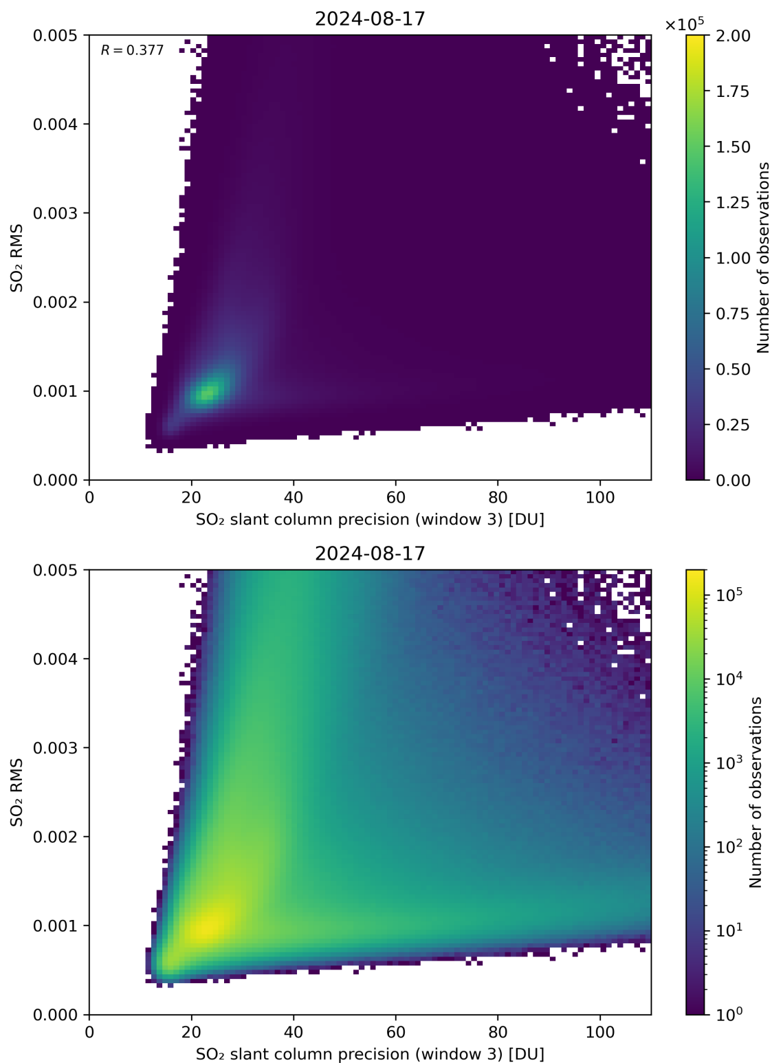
Figure 260: Scatter density plot of “SO 2 slant column precision (window 3)” against “SO 2 RMS” for 2024-08-16 to 2024-08-18.
