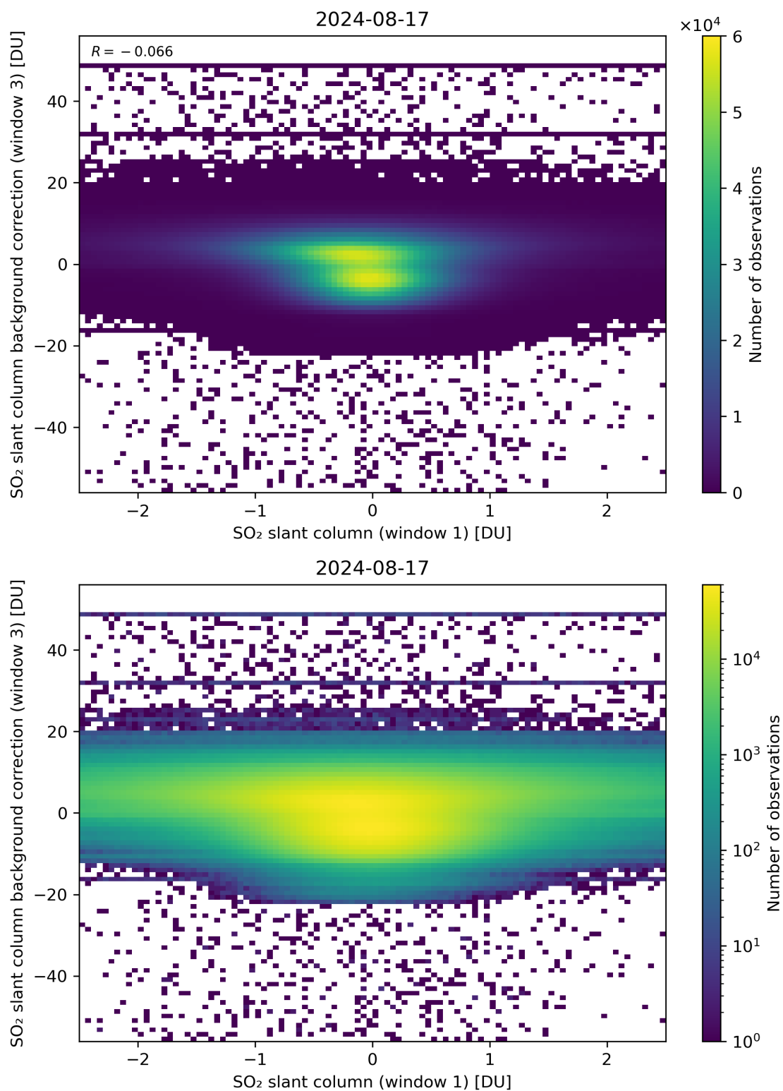
Figure 214: Scatter density plot of “SO 2 slant column (window 1)” against “SO 2 slant column background correction (window 3)” for 2024-08-16 to 2024-08-18.
