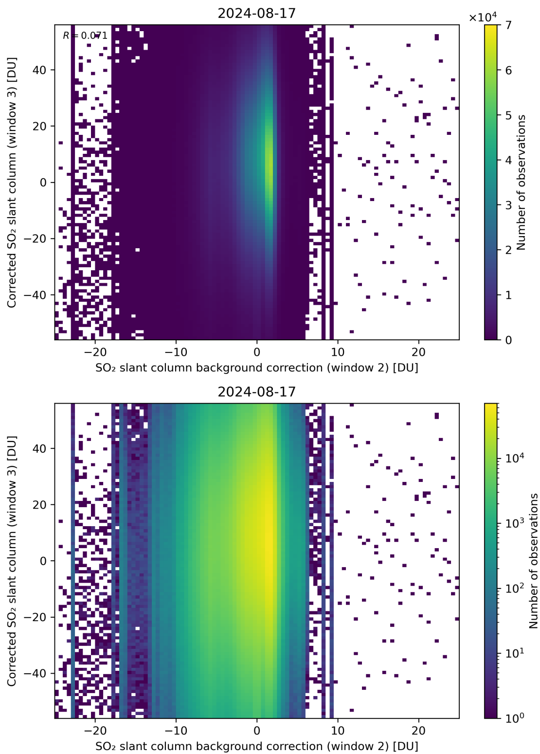
Figure 116: Scatter density plot of “SO 2 slant column background correction (window 2)” against “Corrected SO 2 slant column (window 3)” for 2024-08-16 to 2024-08-18.
