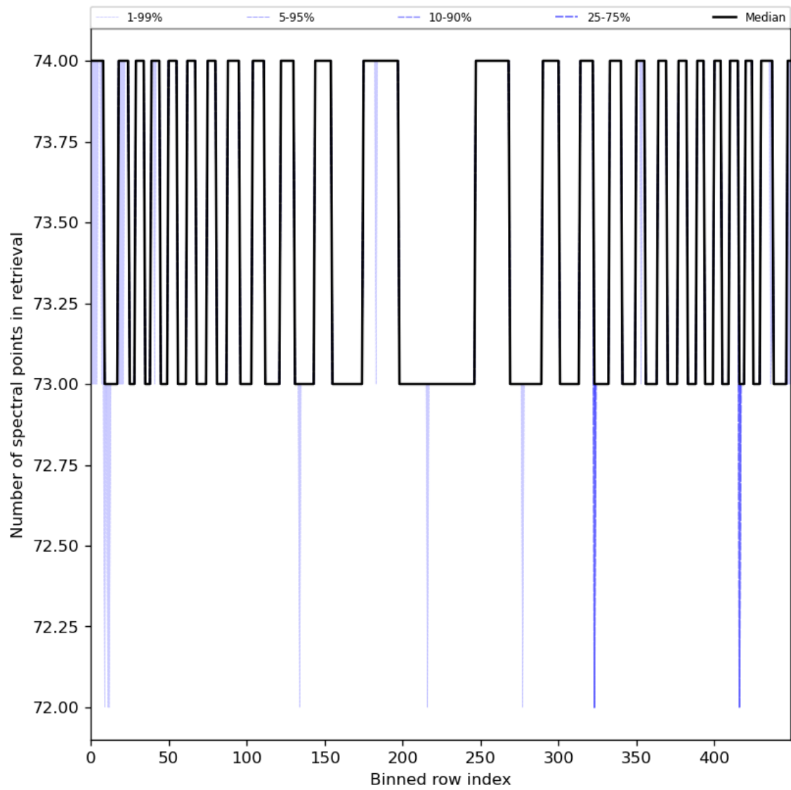
Figure 97: Along track statistics of “Number of spectral points in retrieval” for 2024-08-16 to 2024-08-18
