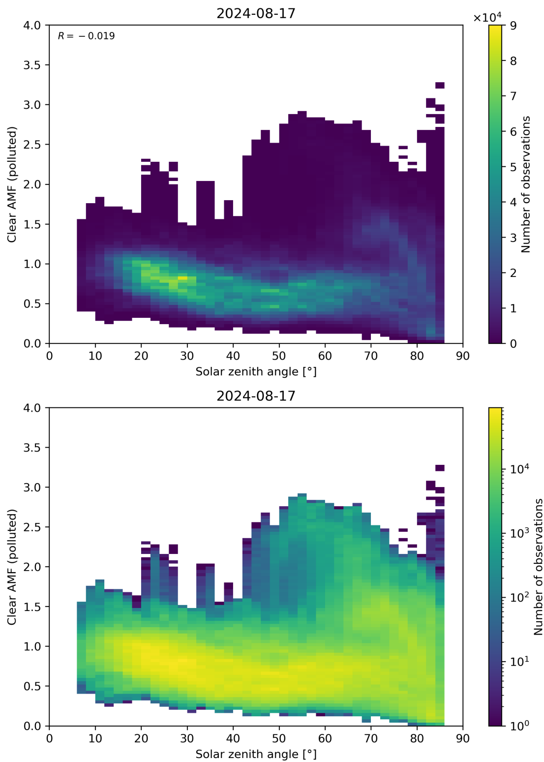
Figure 165: Scatter density plot of “Solar zenith angle” against “Clear AMF (polluted)” for 2024-08-16 to 2024-08-18.
