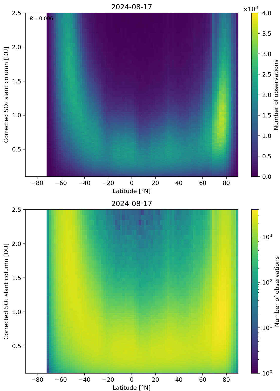
Figure 146: Scatter density plot of “Latitude” against “Corrected SO 2 slant column” for 2024-08-16 to 2024-08-18.
