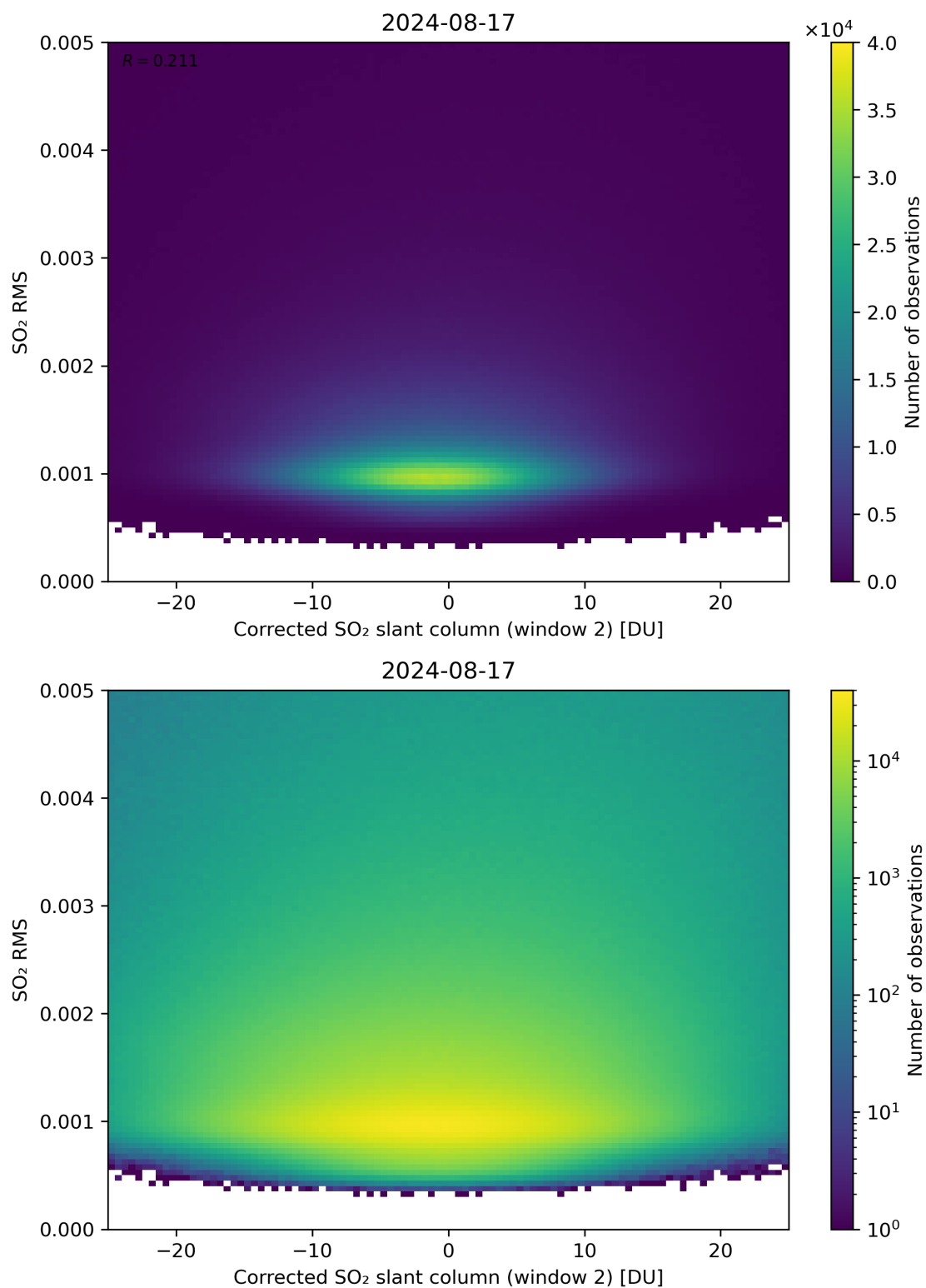
Figure 198: Scatter density plot of “Corrected SO 2 slant column (window 2)” against “SO 2 RMS” for 2024-08-16 to 2024-08-18.
