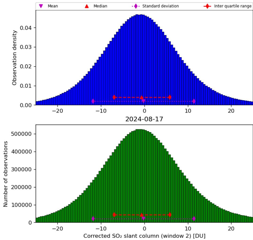
Figure 62: Histogram of “Corrected SO 2 slant column (window 2)” for 2024-08-16 to 2024-08-18
