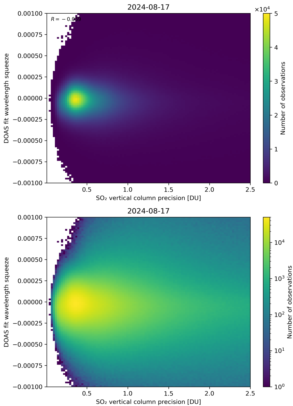
Figure 283: Scatter density plot of “SO 2 vertical column precision” against “DOAS fit wavelength squeeze” for 2024-08-16 to 2024-08-18.
