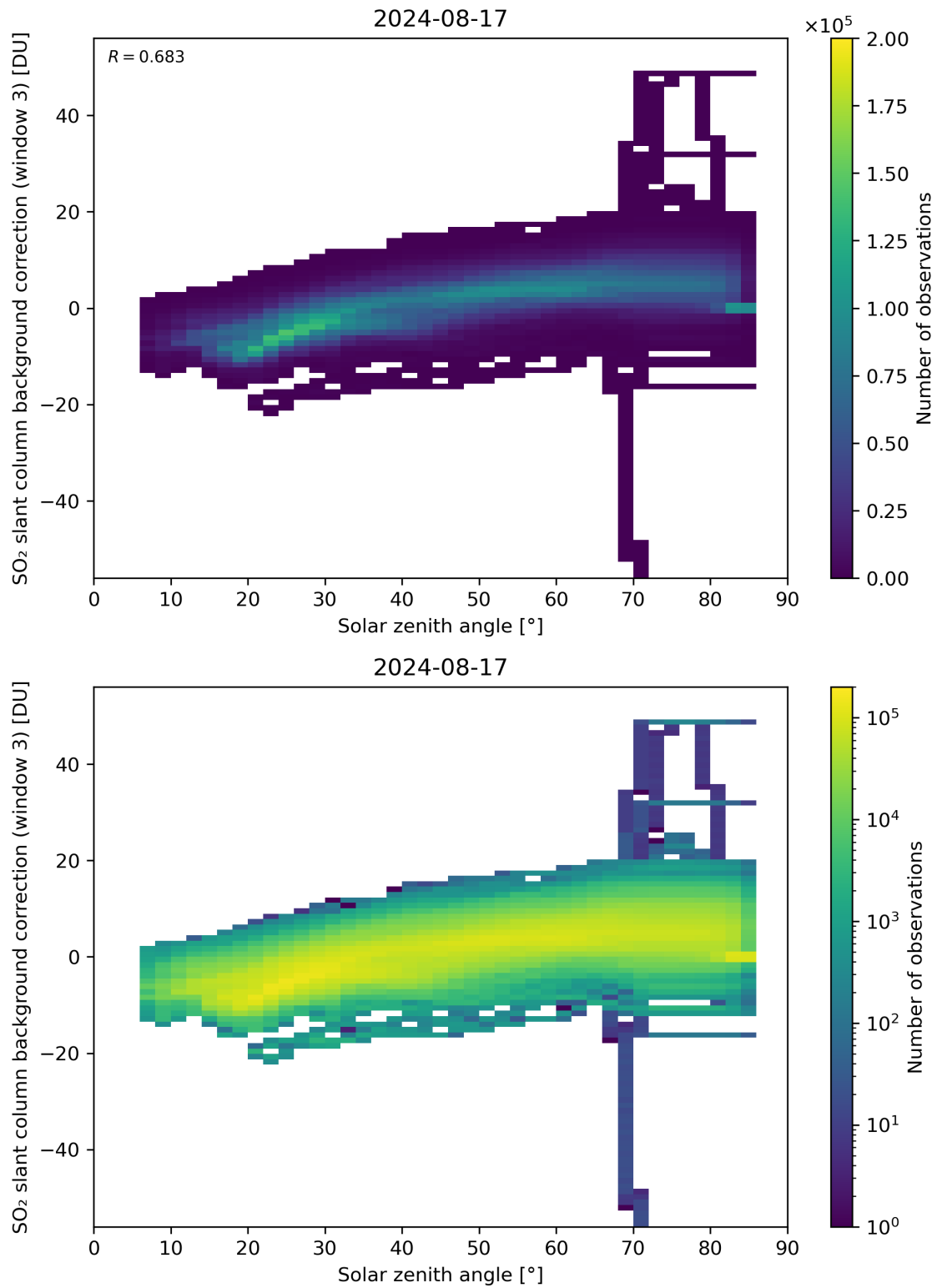
Figure 160: Scatter density plot of “Solar zenith angle” against “SO 2 slant column background correction (window 3)” for 2024-08-16 to 2024-08-18.
