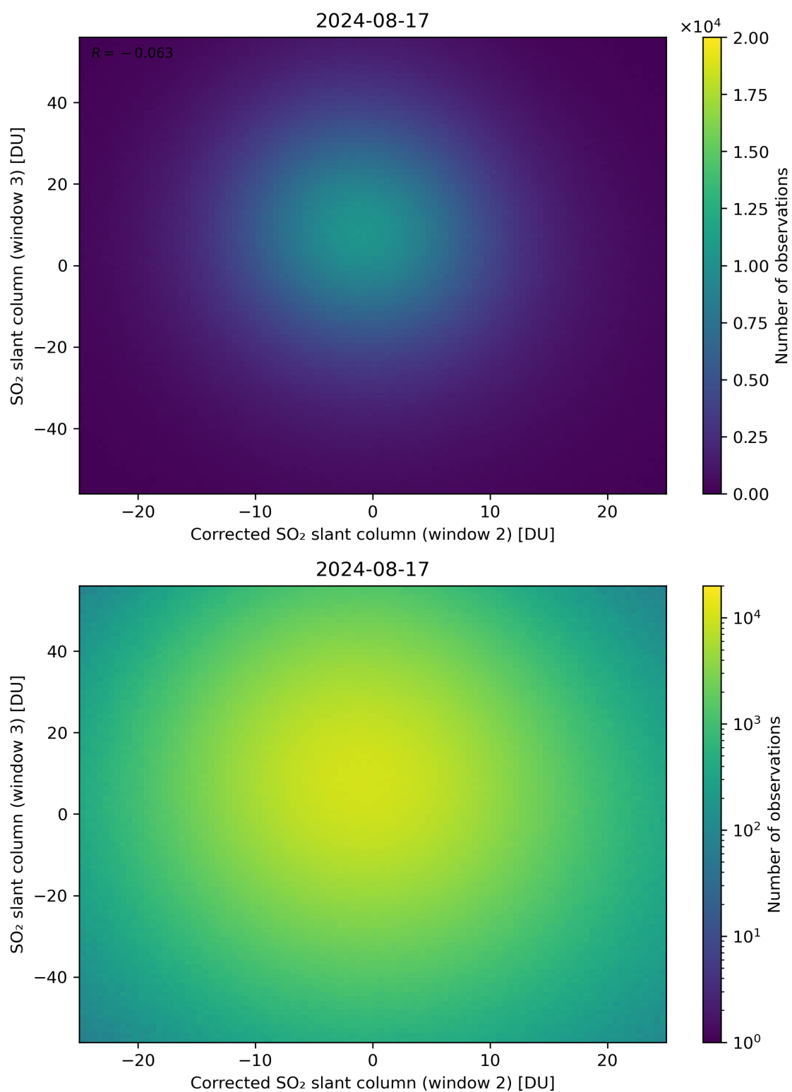
Figure 201: Scatter density plot of “Corrected SO 2 slant column (window 2)” against “SO 2 slant column (window 3)” for 2024-08-16 to 2024-08-18.
