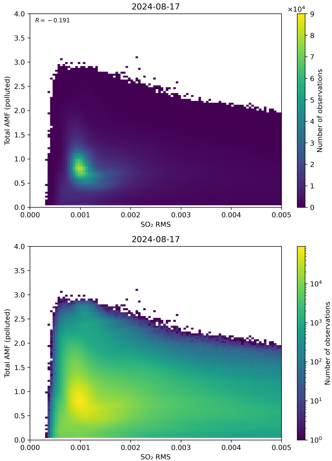
Figure 137: Scatter density plot of “SO 2 RMS” against “Total AMF (polluted)” for 2024-08-16 to 2024-08-18.
