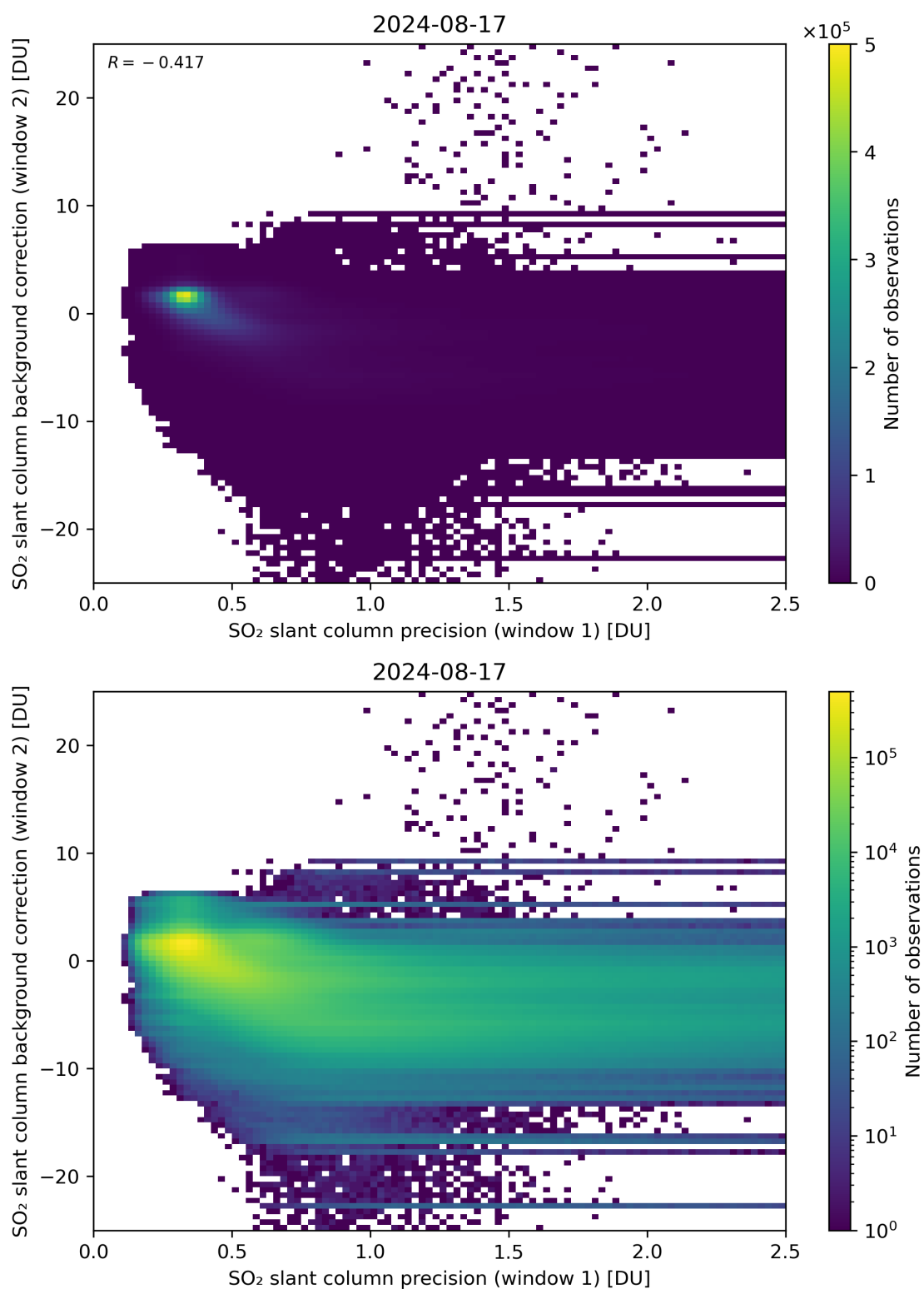
Figure 219: Scatter density plot of “SO 2 slant column precision (window 1)” against “SO 2 slant column background correction (window 2)” for 2024-08-16 to 2024-08-18.
