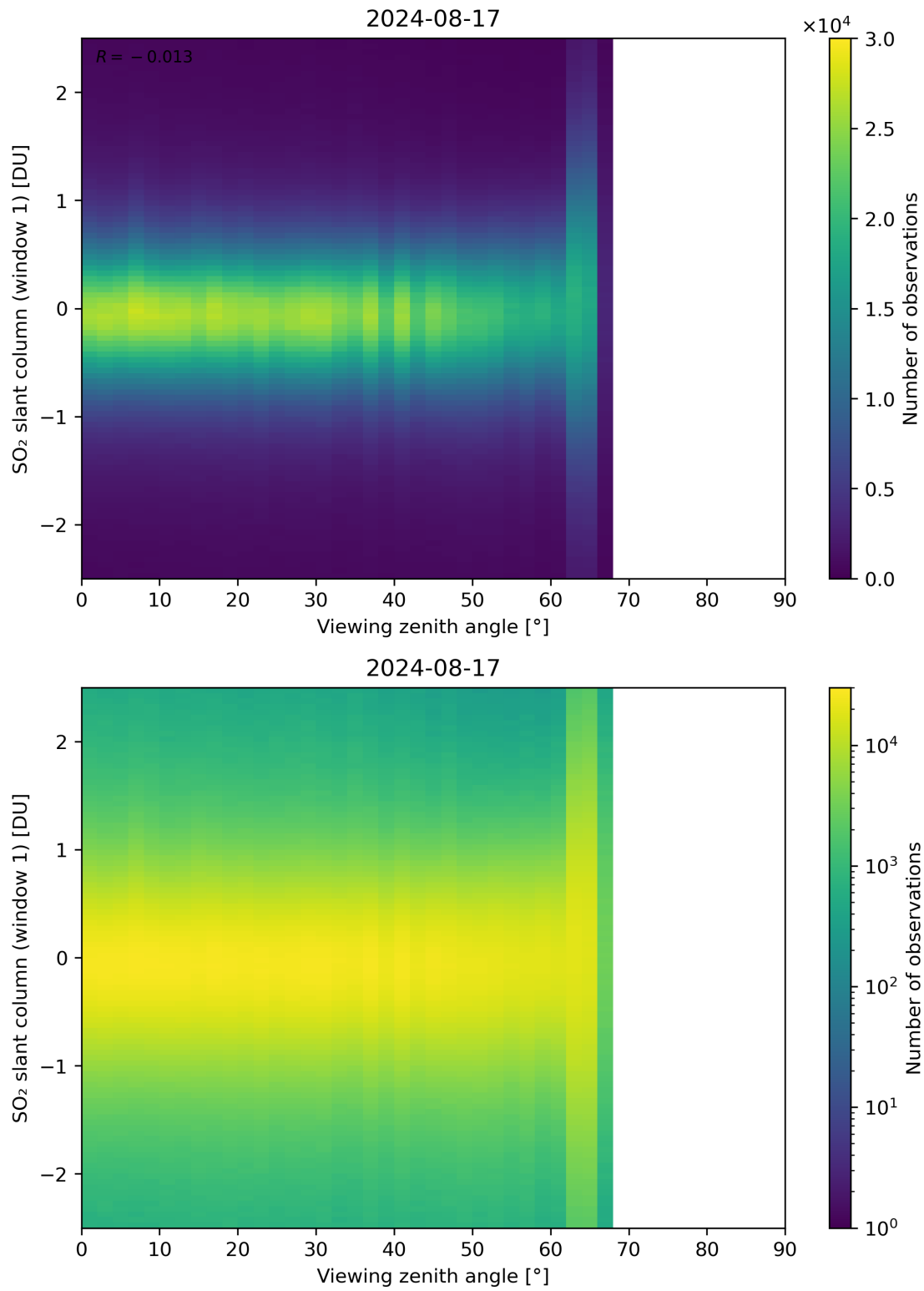
Figure 320: Scatter density plot of “Viewing zenith angle” against “SO 2 slant column (window 1)” for 2024-08-16 to 2024-08-18.
