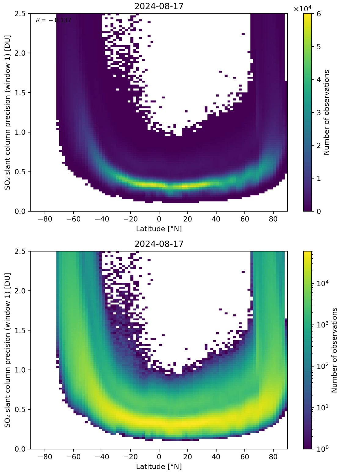
Figure 150: Scatter density plot of “Latitude” against “SO 2 slant column precision (window 1)” for 2024-08-16 to 2024-08-18.
