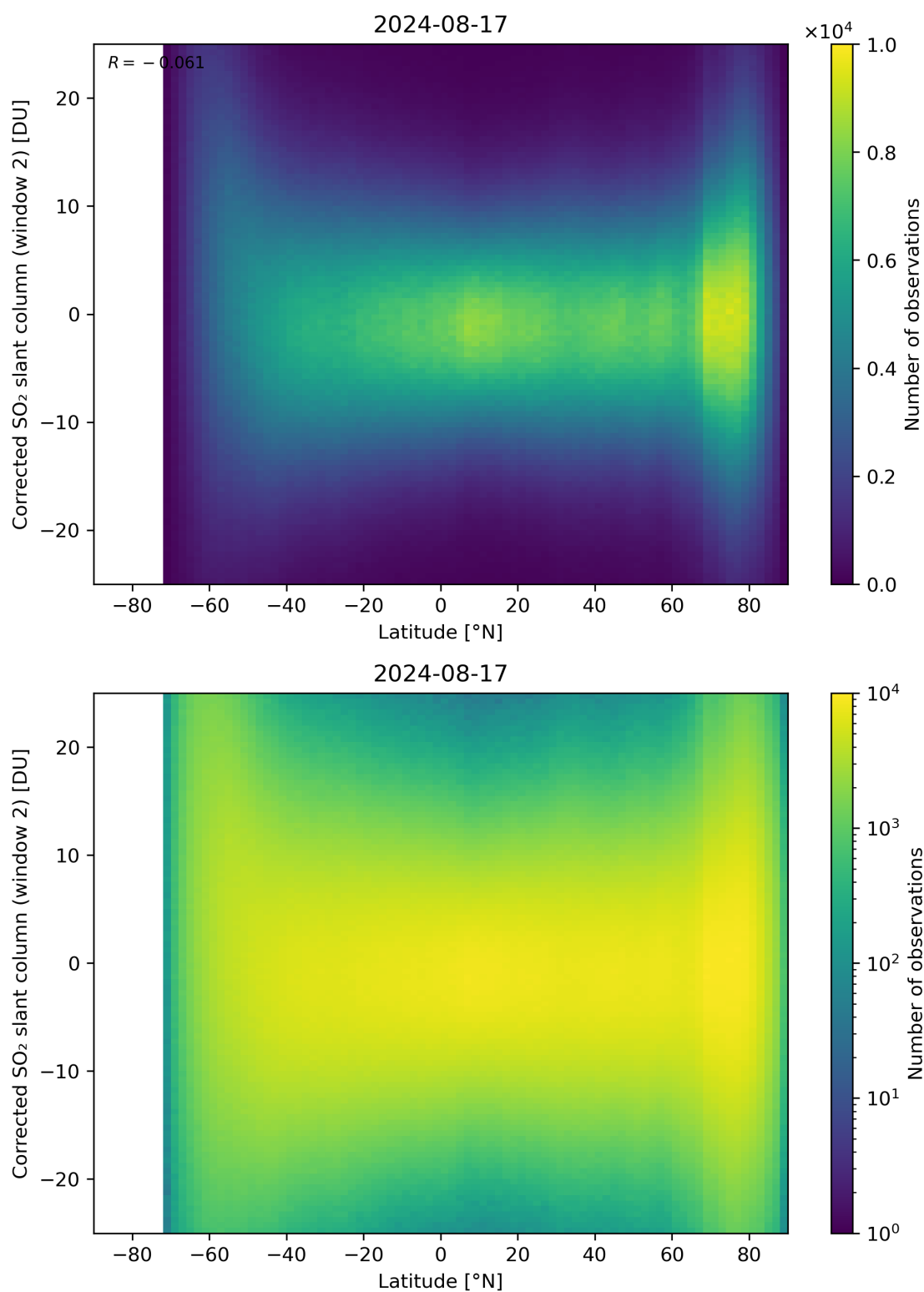
Figure 147: Scatter density plot of “Latitude” against “Corrected SO 2 slant column (window 2)” for 2024-08-16 to 2024-08-18.
