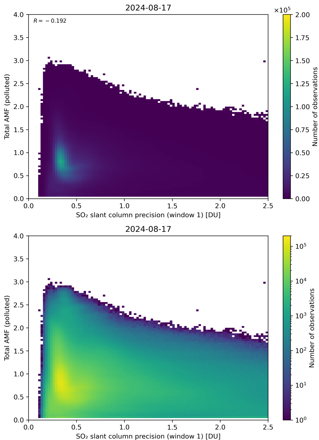
Figure 230: Scatter density plot of “SO 2 slant column precision (window 1)” against “Total AMF (polluted)” for 2024-08-16 to 2024-08-18.
