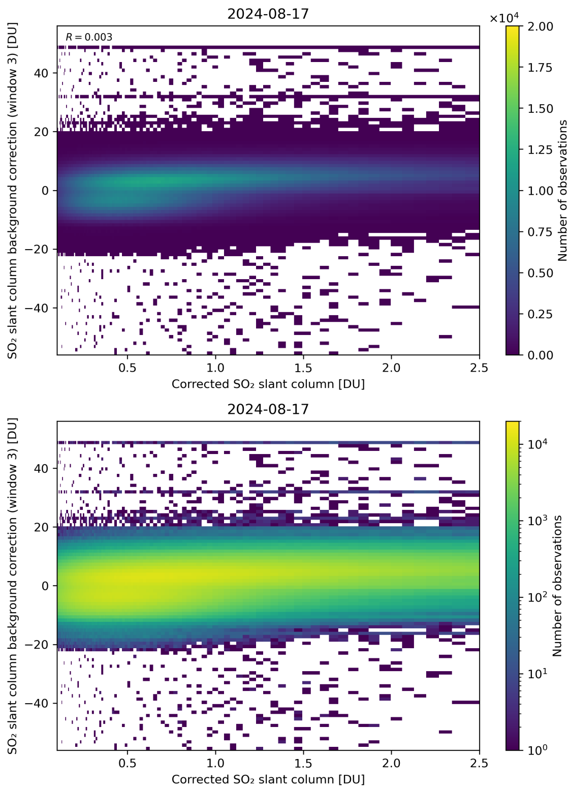
Figure 180: Scatter density plot of “Corrected SO 2 slant column” against “SO 2 slant column background correction (window 3)” for 2024-08-16 to 2024-08-18.
