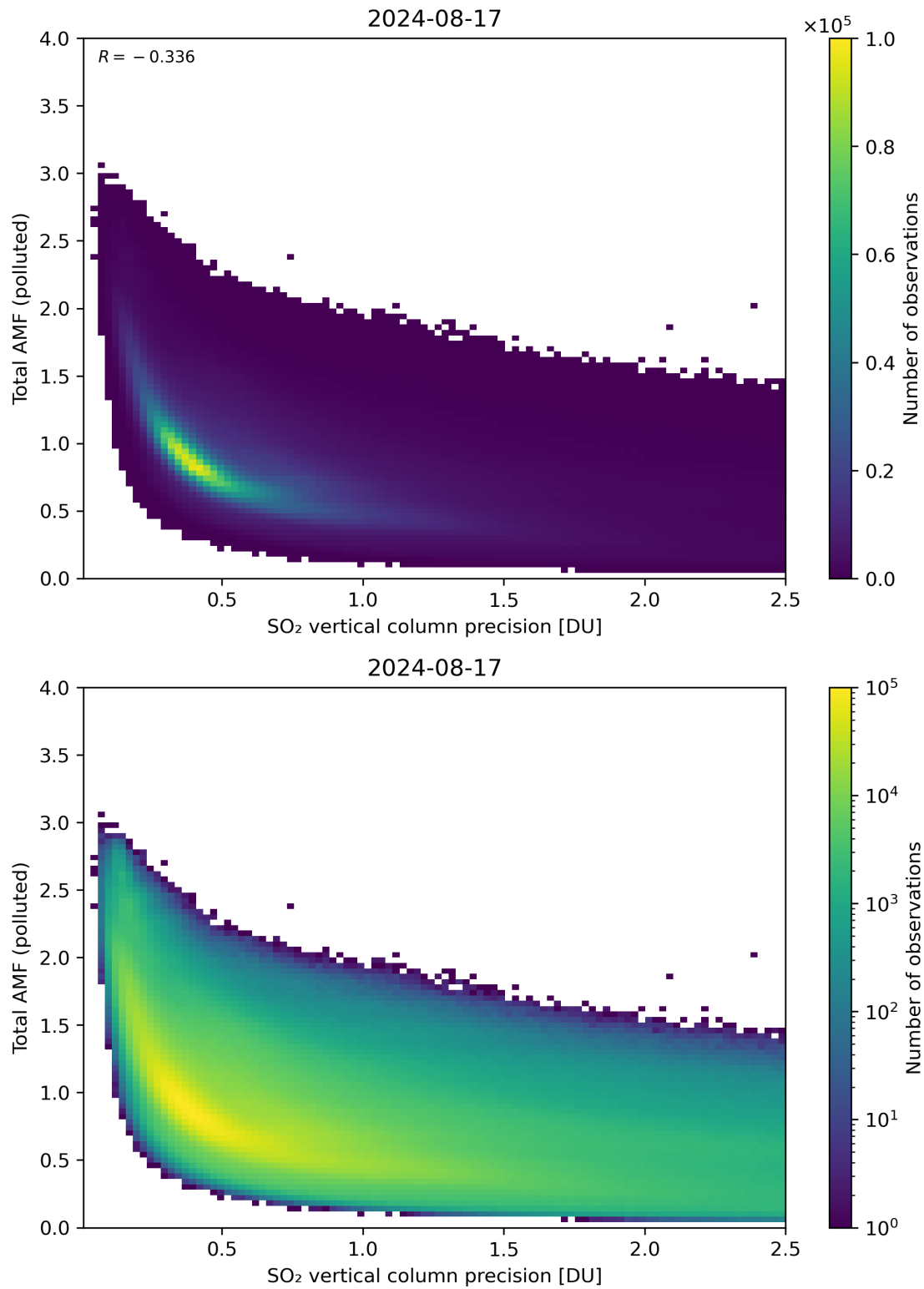
Figure 294: Scatter density plot of “SO 2 vertical column precision” against “Total AMF (polluted)” for 2024-08-16 to 2024-08-18.
