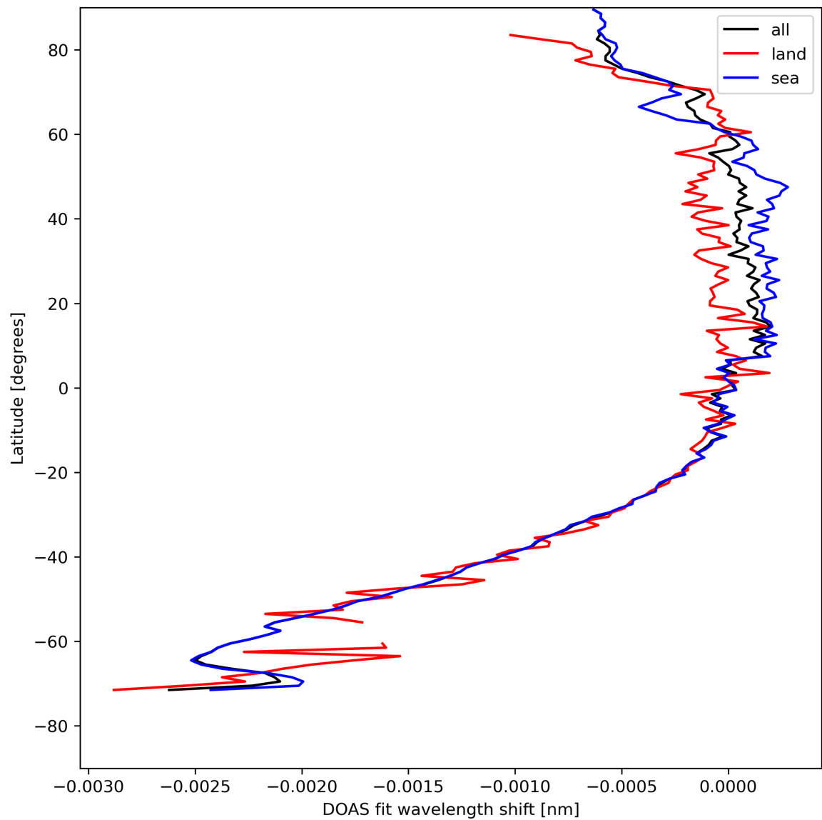
Figure 45: Zonal average of “DOAS fit wavelength shift” for 2024-08-16 to 2024-08-18.
