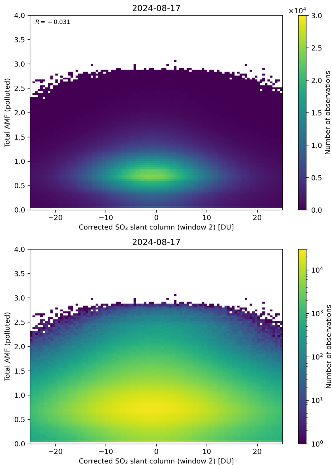
Figure 203: Scatter density plot of “Corrected SO 2 slant column (window 2)” against “Total AMF (polluted)” for 2024-08-16 to 2024-08-18.
