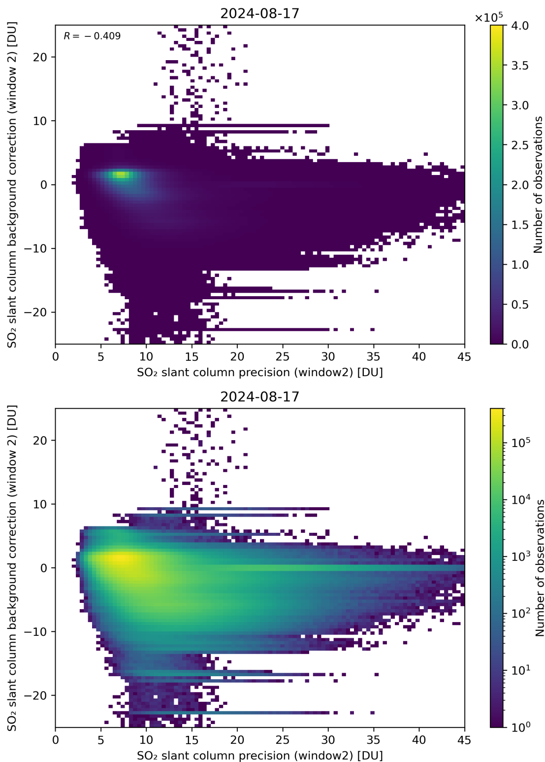
Figure 241: Scatter density plot of “SO 2 slant column precision (window2)” against “SO 2 slant column background correction (window 2)” for 2024-08-16 to 2024-08-18.
