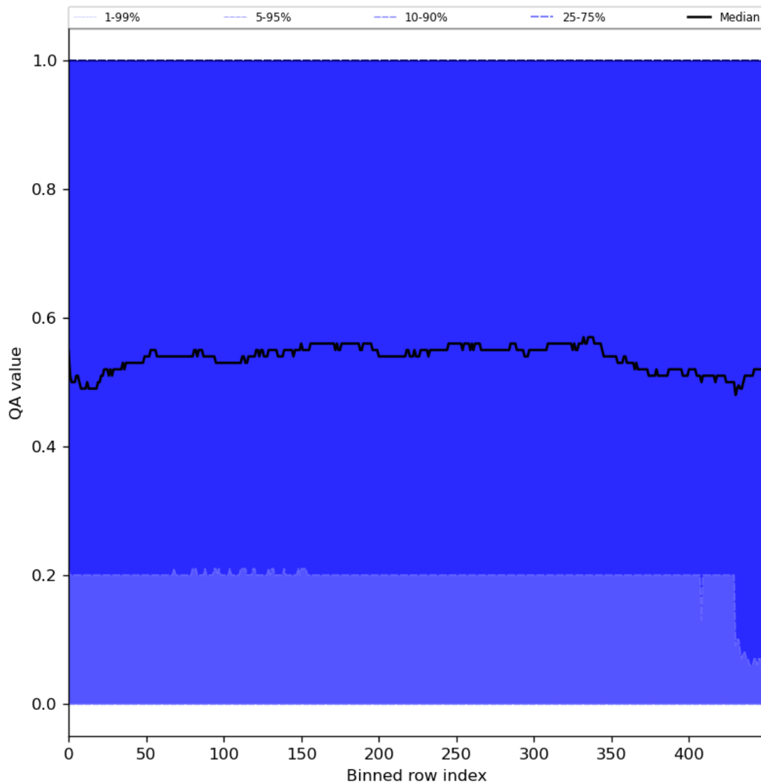
Figure 75: Along track statistics of “QA value” for 2024-08-16 to 2024-08-18
