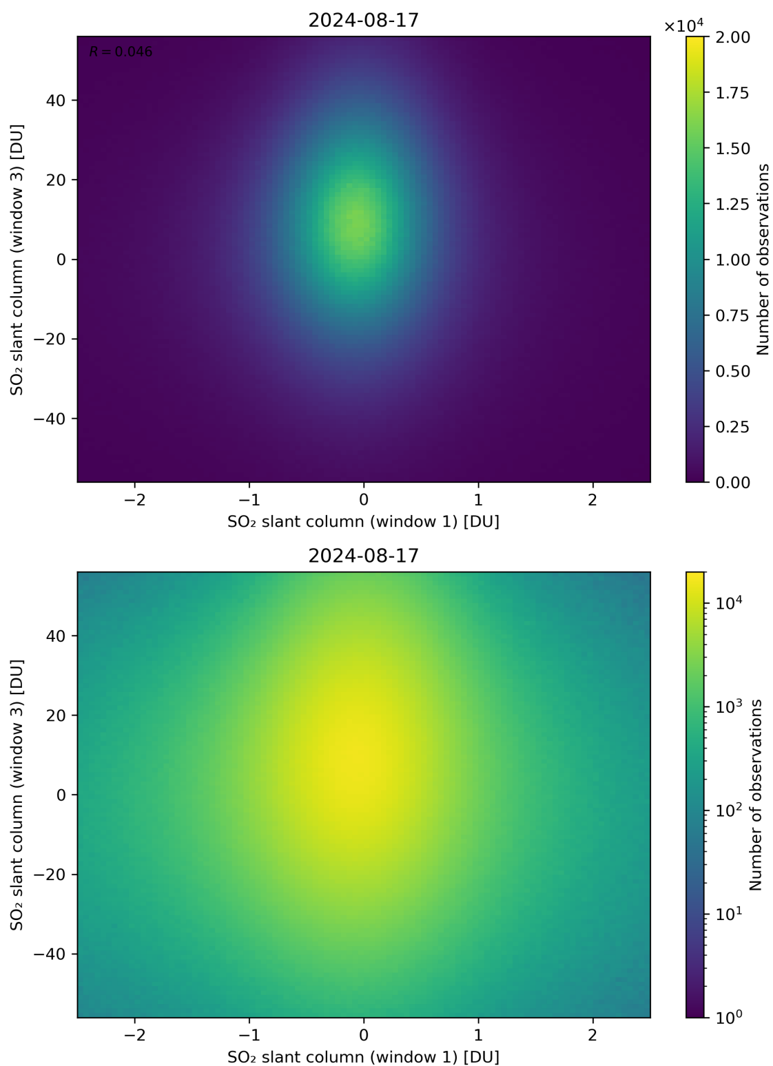
Figure 237: Scatter density plot of “SO 2 slant column (window 1)” against “SO 2 slant column (window 3)” for 2024-08-16 to 2024-08-18.
