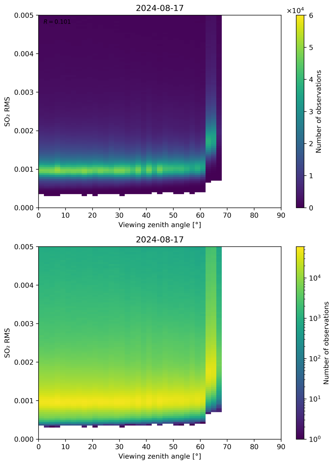
Figure 313: Scatter density plot of “Viewing zenith angle” against “SO 2 RMS” for 2024-08-16 to 2024-08-18.
