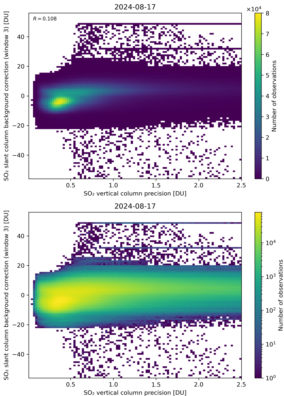
Figure 281: Scatter density plot of “SO 2 vertical column precision” against “SO 2 slant column background correction (window 3)” for 2024-08-16 to 2024-08-18.
