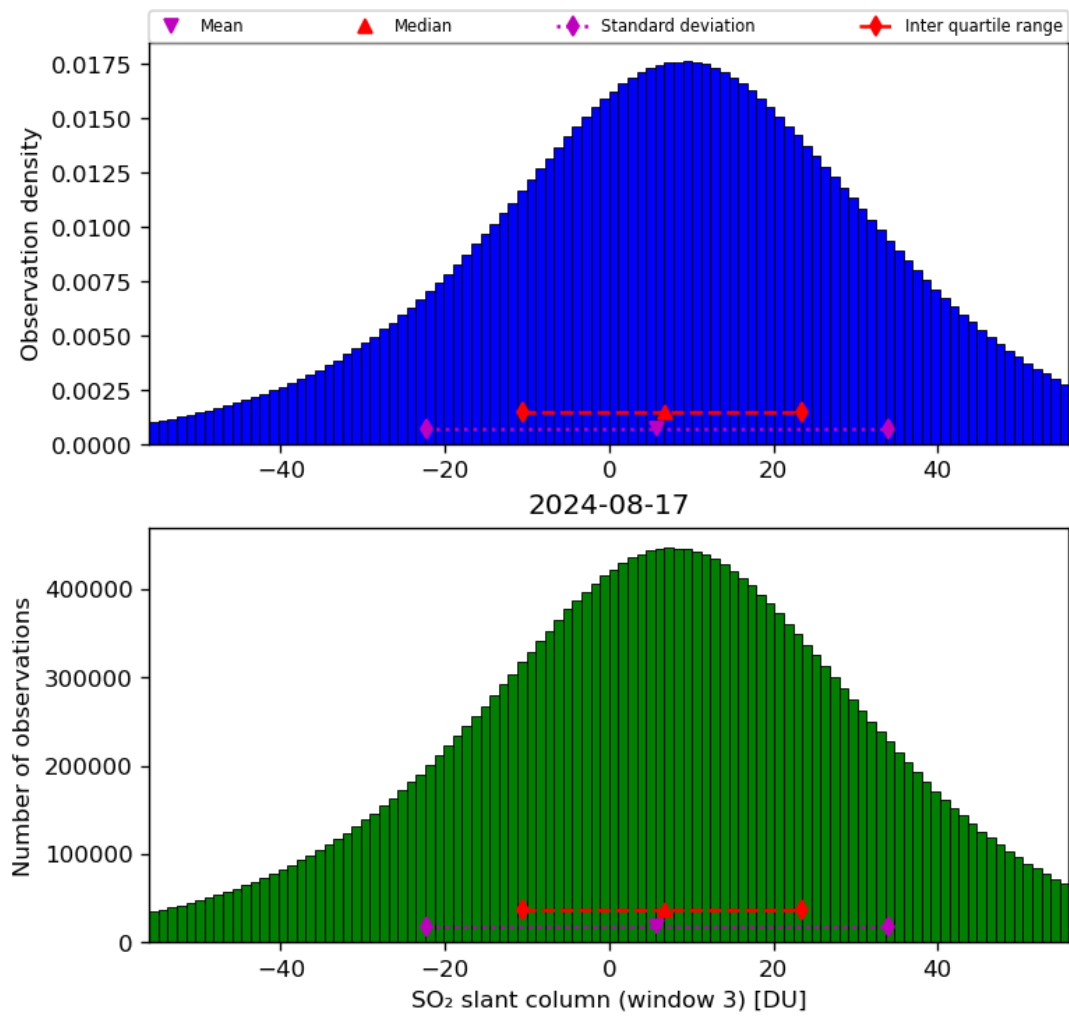
Figure 64: Histogram of “SO 2 slant column (window 3)” for 2024-08-16 to 2024-08-18
