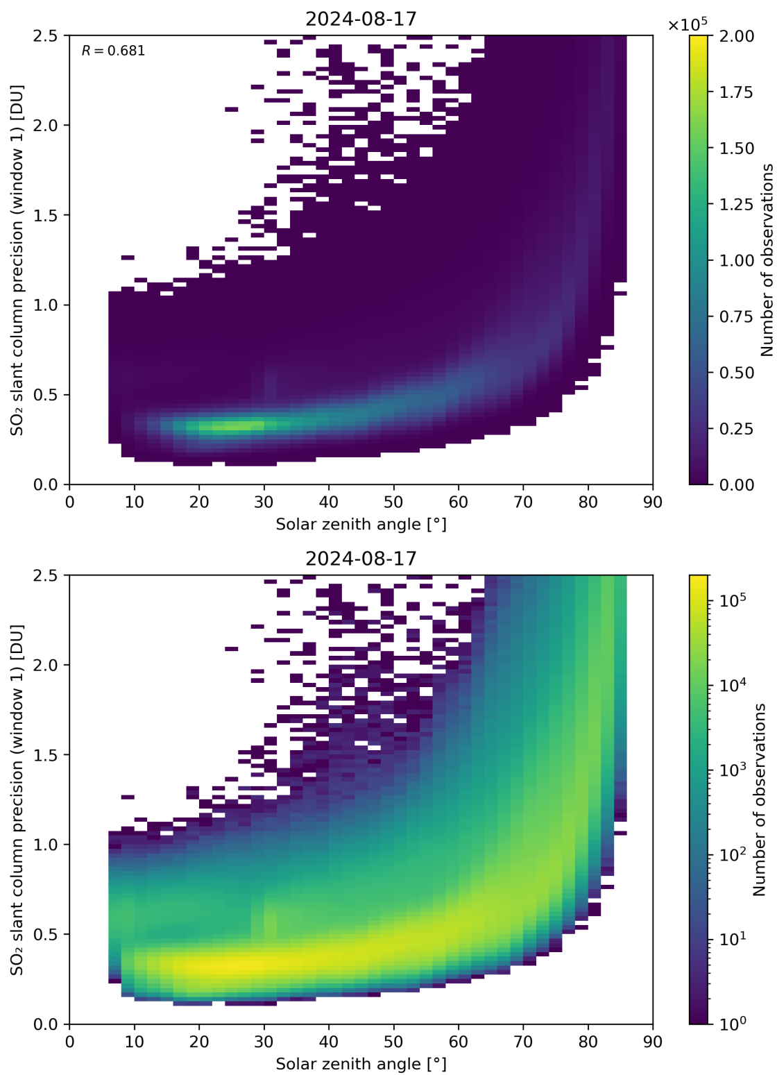
Figure 170: Scatter density plot of “Solar zenith angle” against “SO 2 slant column precision (window 1)” for 2024-08-16 to 2024-08-18.
