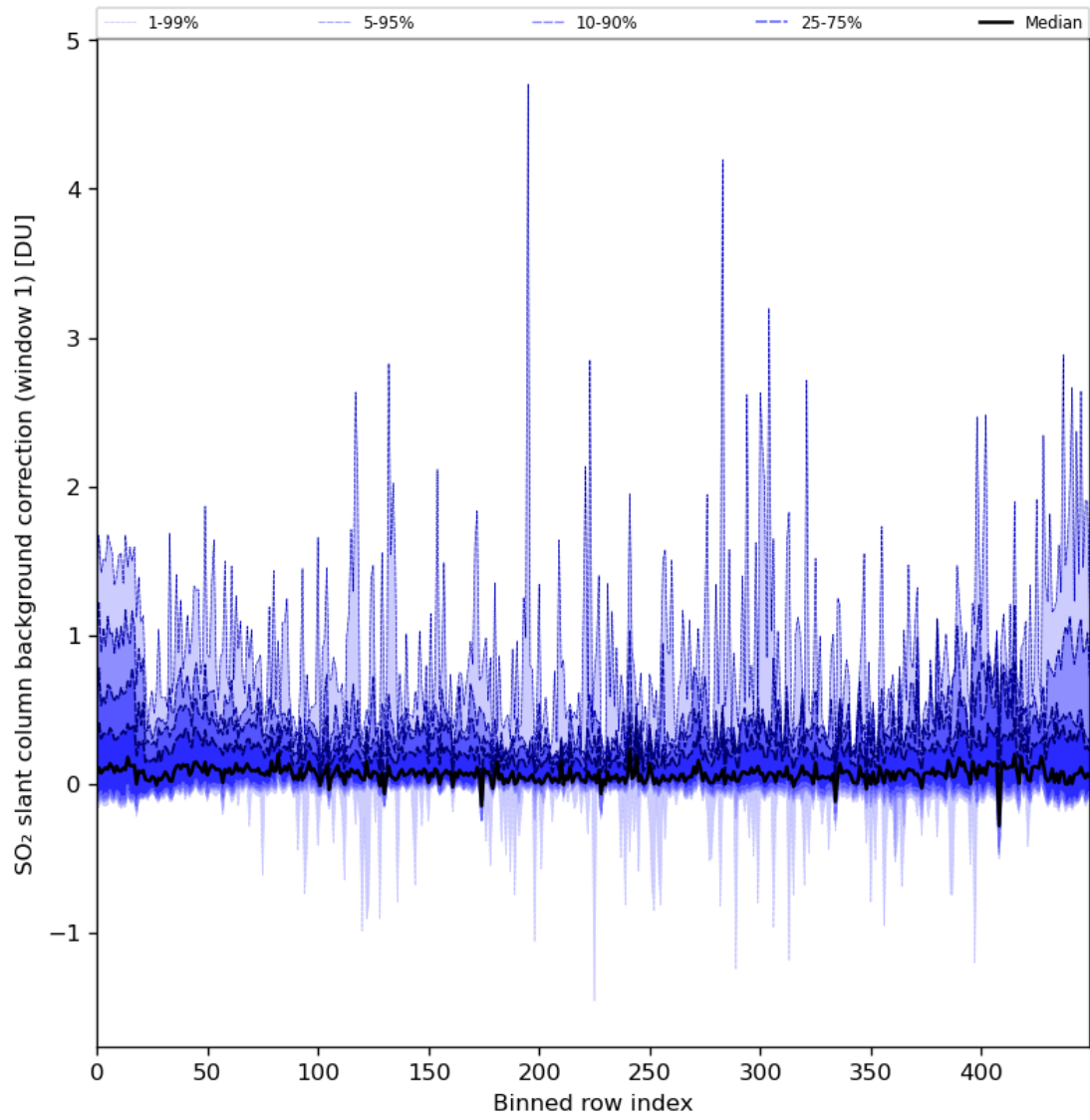
Figure 82: Along track statistics of “SO 2 slant column background correction (window 1)” for 2024-08-16 to 2024-08-18
