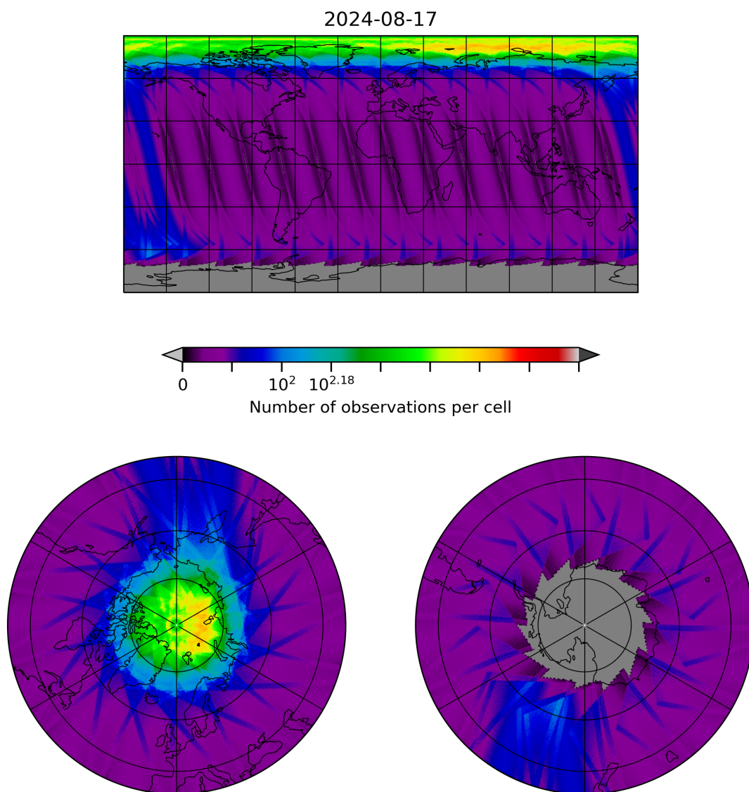
Figure 28: Map of the number of observations for 2024-08-16 to 2024-08-18
