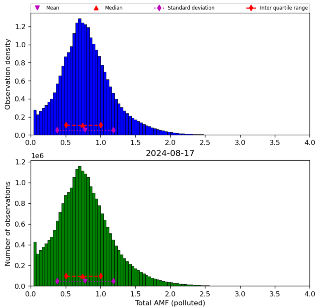
Figure 71: Histogram of “Total AMF (polluted)” for 2024-08-16 to 2024-08-18
