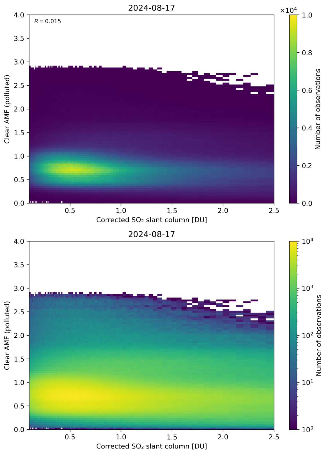
Figure 184: Scatter density plot of “Corrected SO 2 slant column” against “Clear AMF (polluted)” for 2024-08-16 to 2024-08-18.
