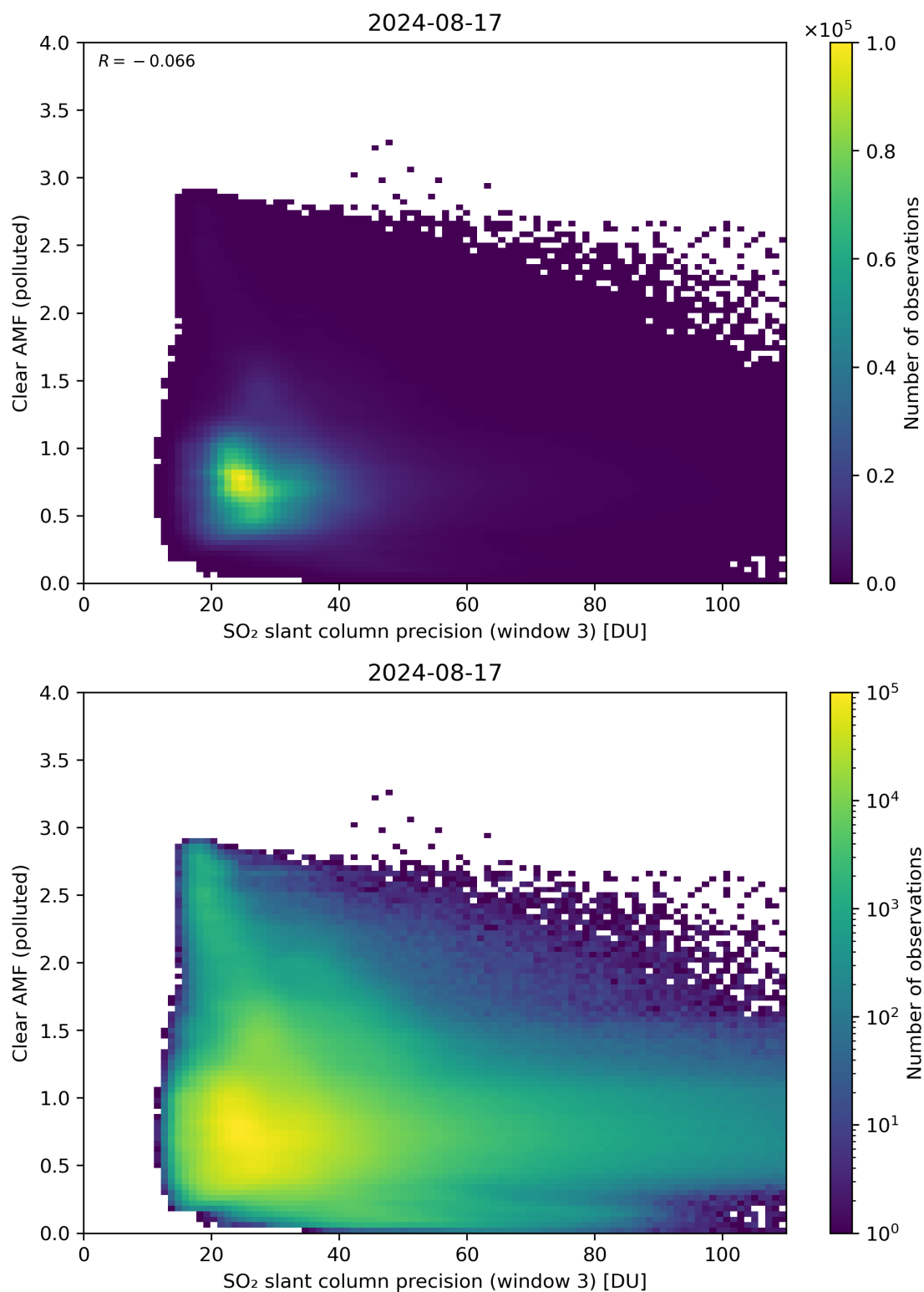
Figure 261: Scatter density plot of “SO 2 slant column precision (window 3)” against “Clear AMF (polluted)” for 2024-08-16 to 2024-08-18.
