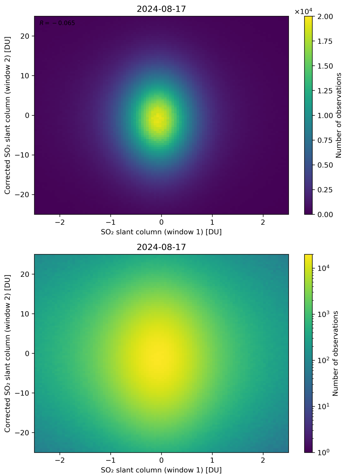
Figure 233: Scatter density plot of “SO 2 slant column (window 1)” against “Corrected SO 2 slant column (window 2)” for 2024-08-16 to 2024-08-18.
