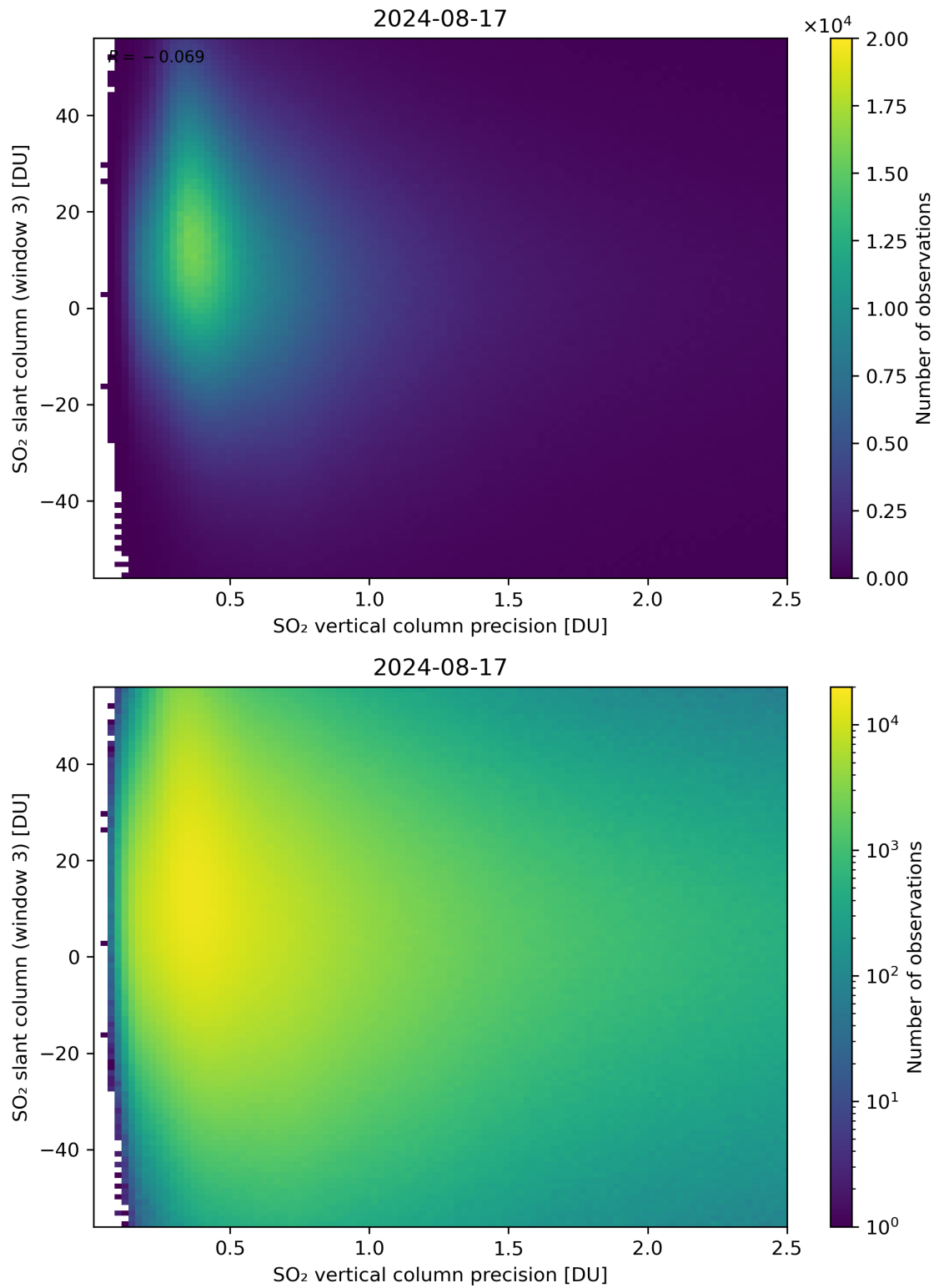
Figure 292: Scatter density plot of “SO 2 vertical column precision” against “SO 2 slant column (window 3)” for 2024-08-16 to 2024-08-18.
