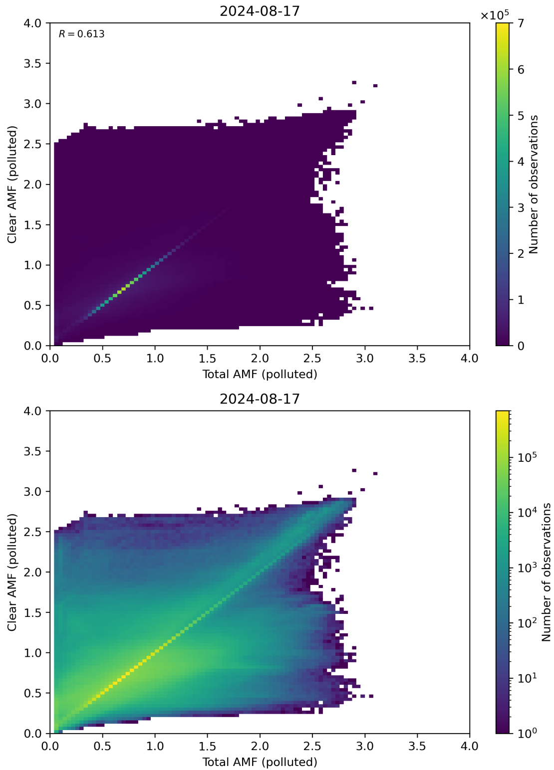
Figure 271: Scatter density plot of “Total AMF (polluted)” against “Clear AMF (polluted)” for 2024-08-16 to 2024-08-18.
