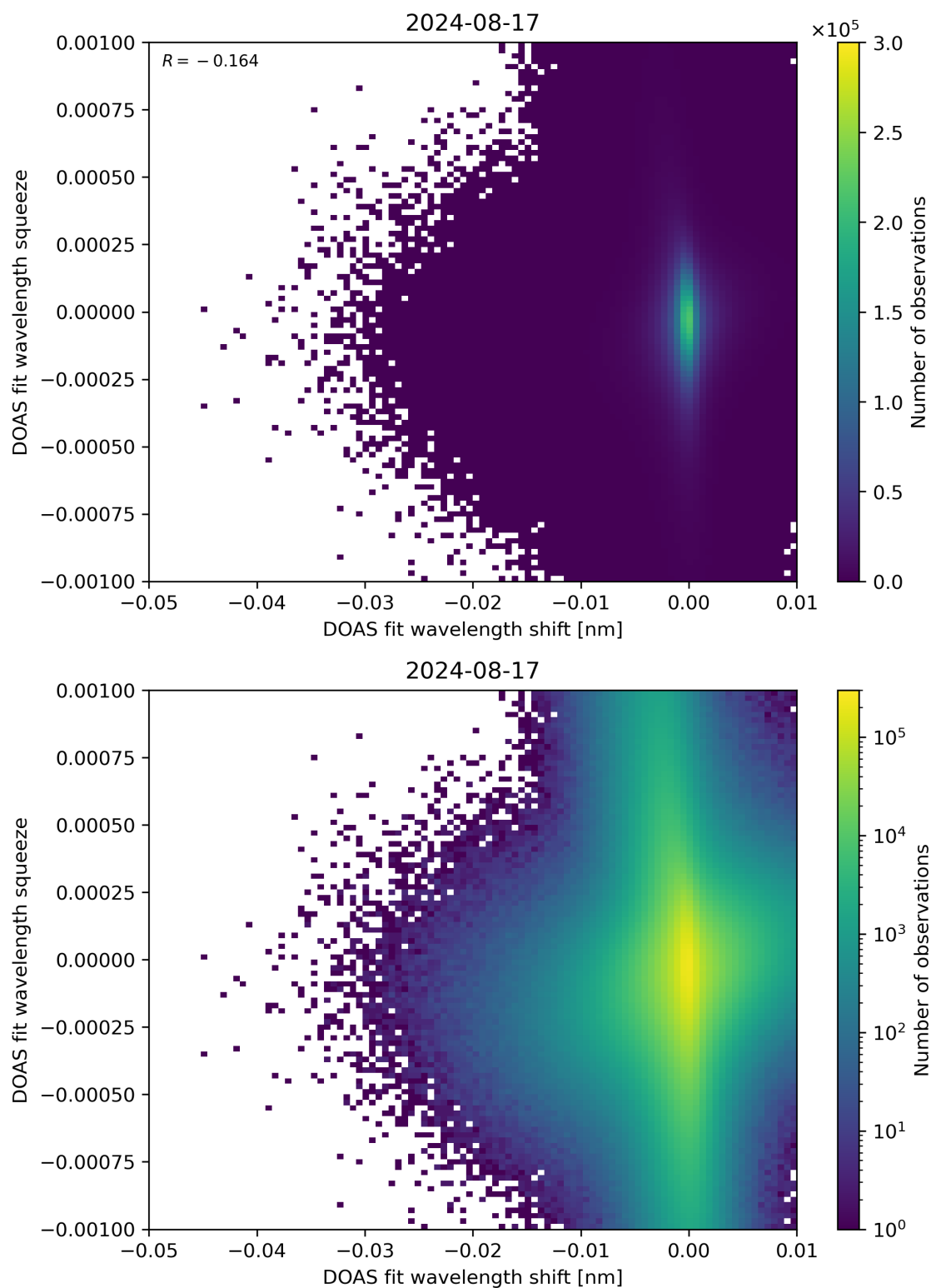
Figure 127: Scatter density plot of “DOAS fit wavelength shift” against “DOAS fit wavelength squeeze” for 2024-08-16 to 2024-08-18.
