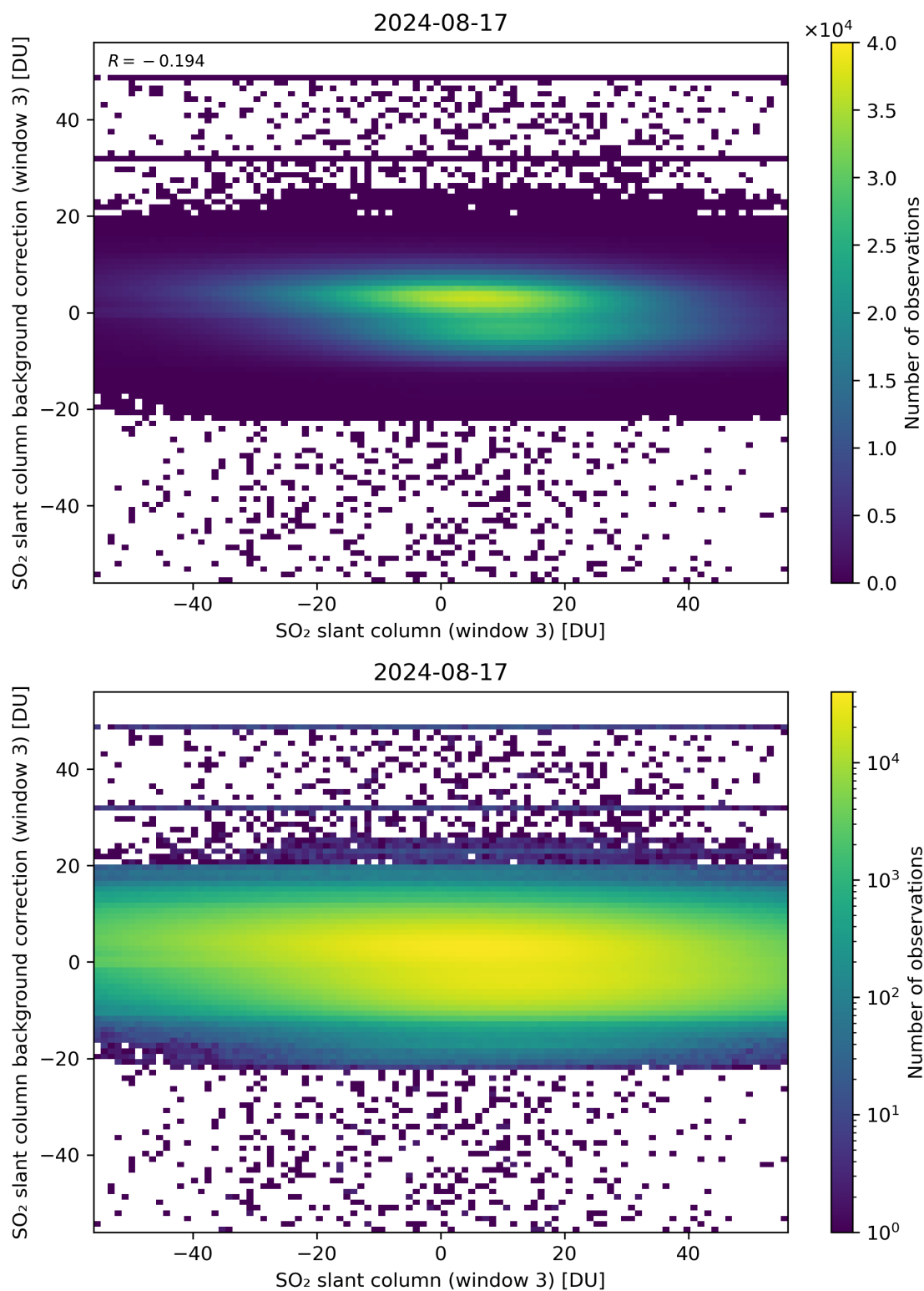
Figure 253: Scatter density plot of “SO 2 slant column (window 3)” against “SO 2 slant column background correction (window 3)” for 2024-08-16 to 2024-08-18.
