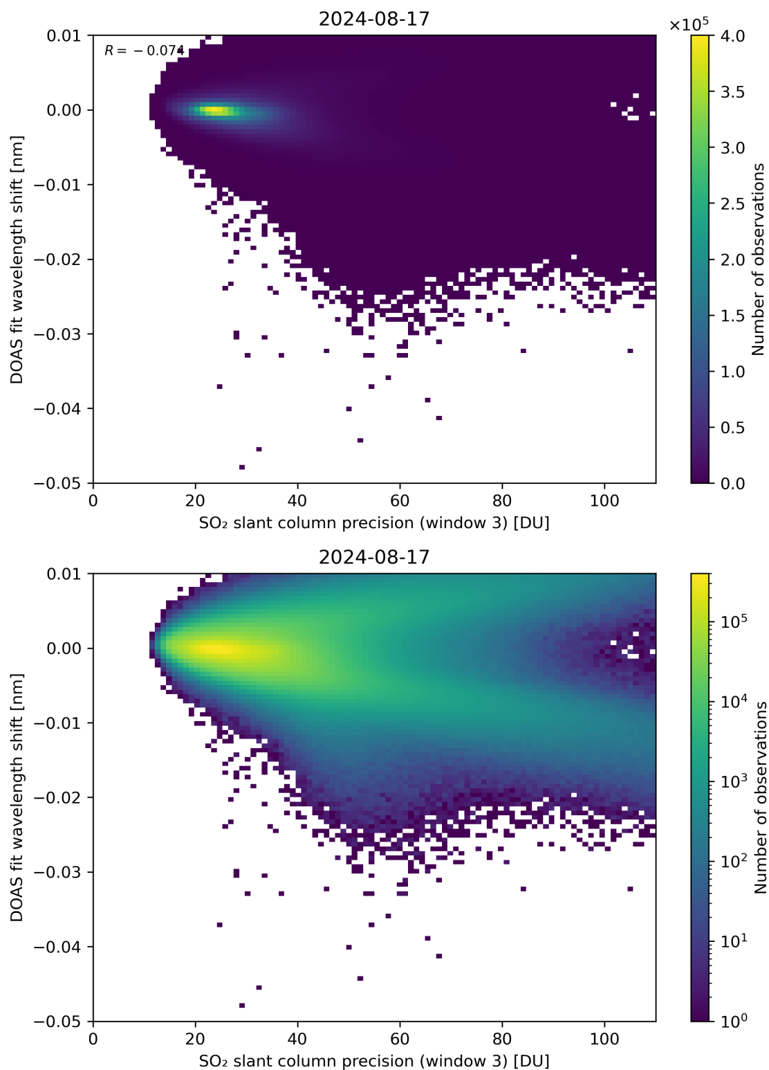
Figure 258: Scatter density plot of “SO 2 slant column precision (window 3)” against “DOAS fit wavelength shift” for 2024-08-16 to 2024-08-18.
