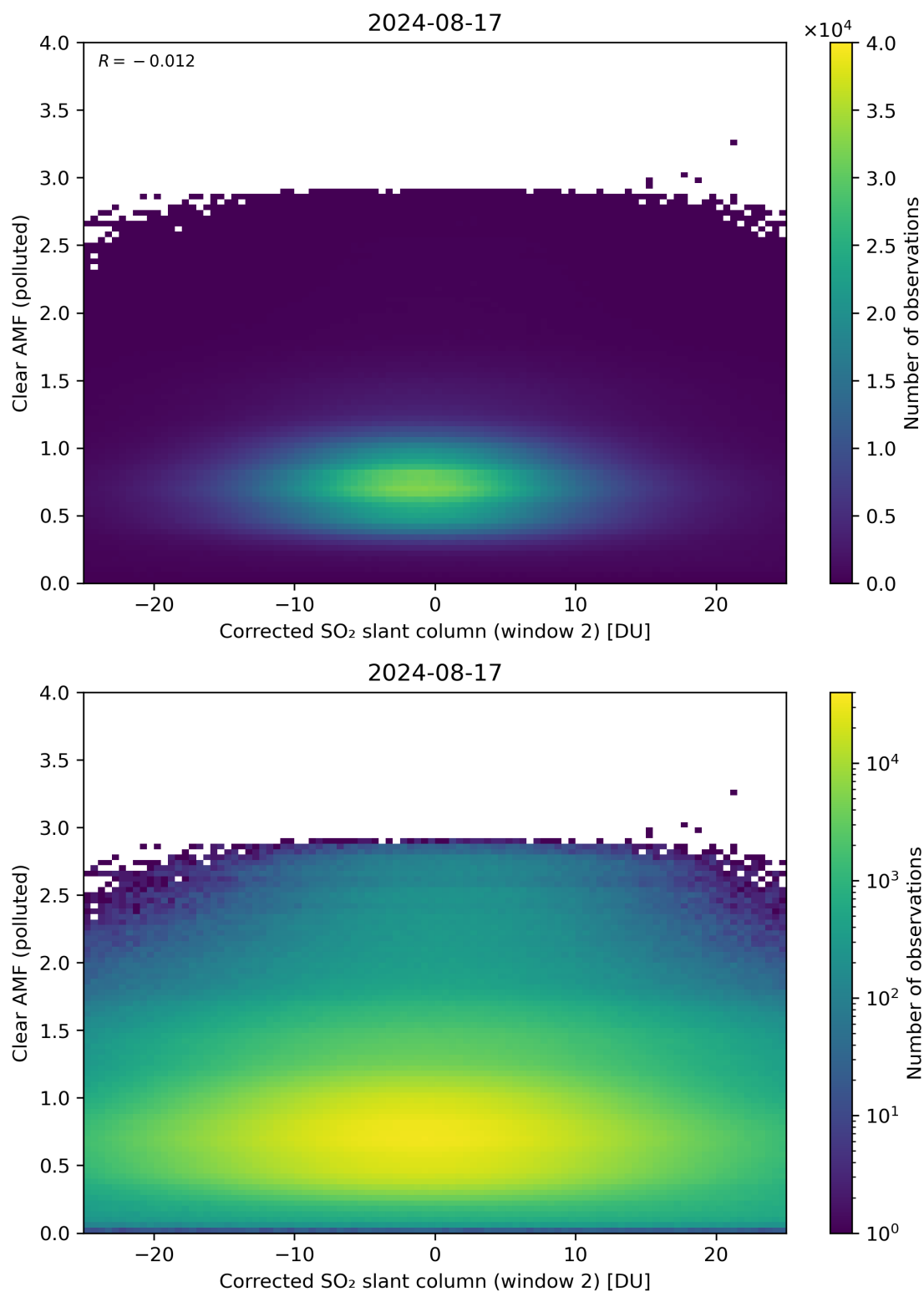
Figure 199: Scatter density plot of “Corrected SO 2 slant column (window 2)” against “Clear AMF (polluted)” for 2024-08-16 to 2024-08-18.
