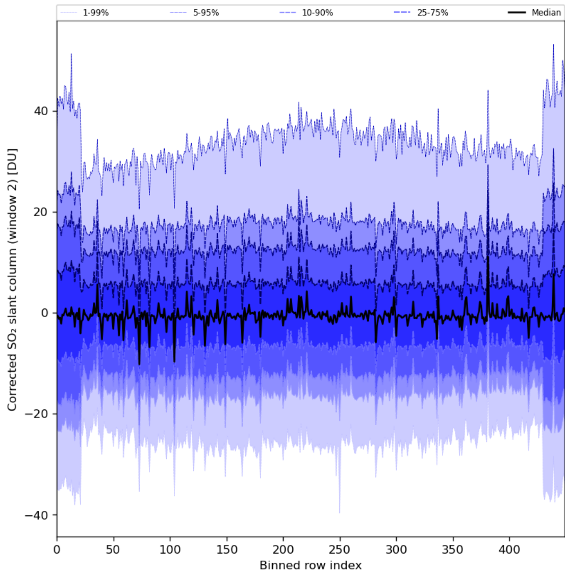
Figure 85: Along track statistics of “Corrected SO 2 slant column (window 2)” for 2024-08-16 to 2024-08-18
