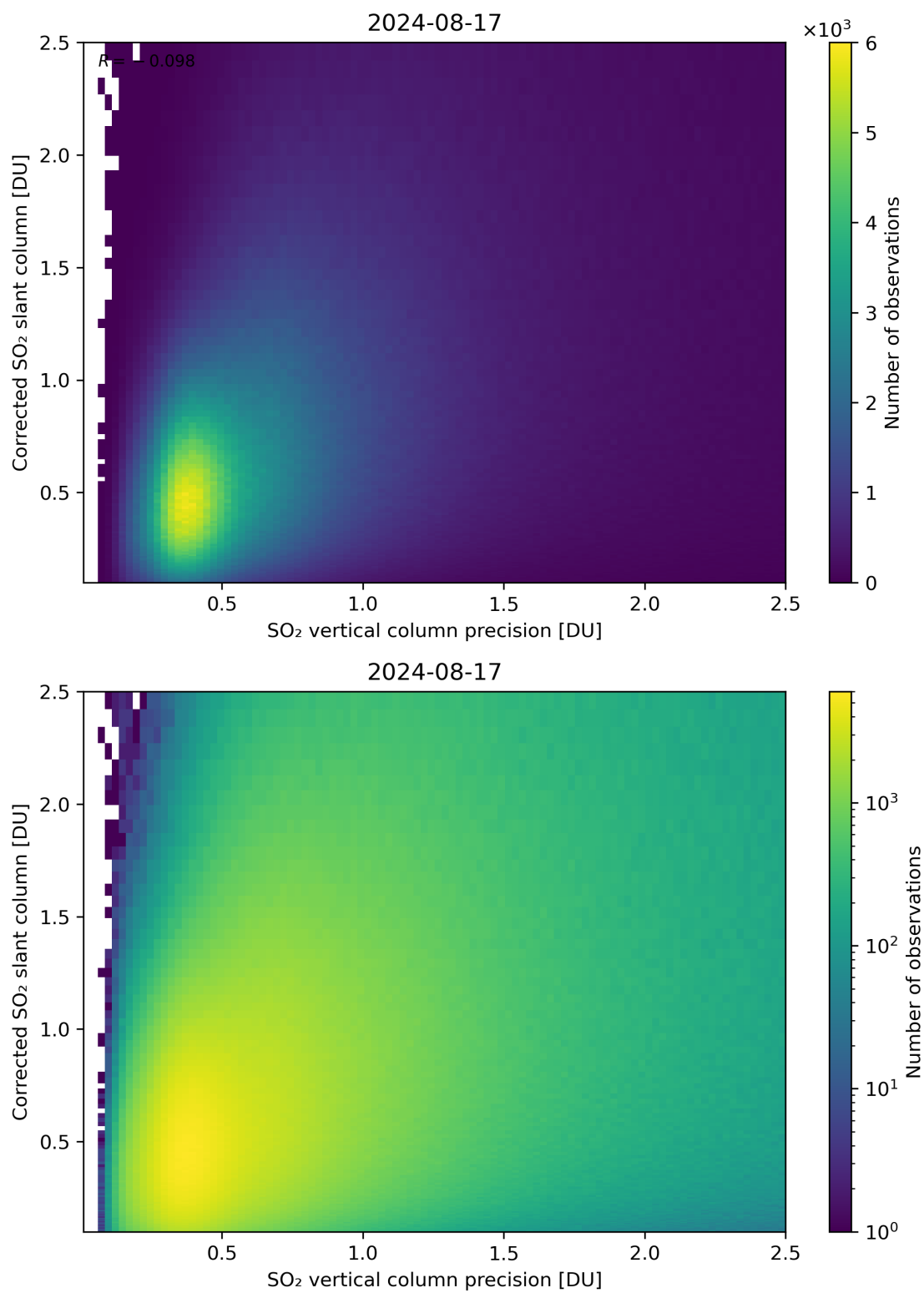
Figure 286: Scatter density plot of “SO 2 vertical column precision” against “Corrected SO 2 slant column” for 2024-08-16 to 2024-08-18.
