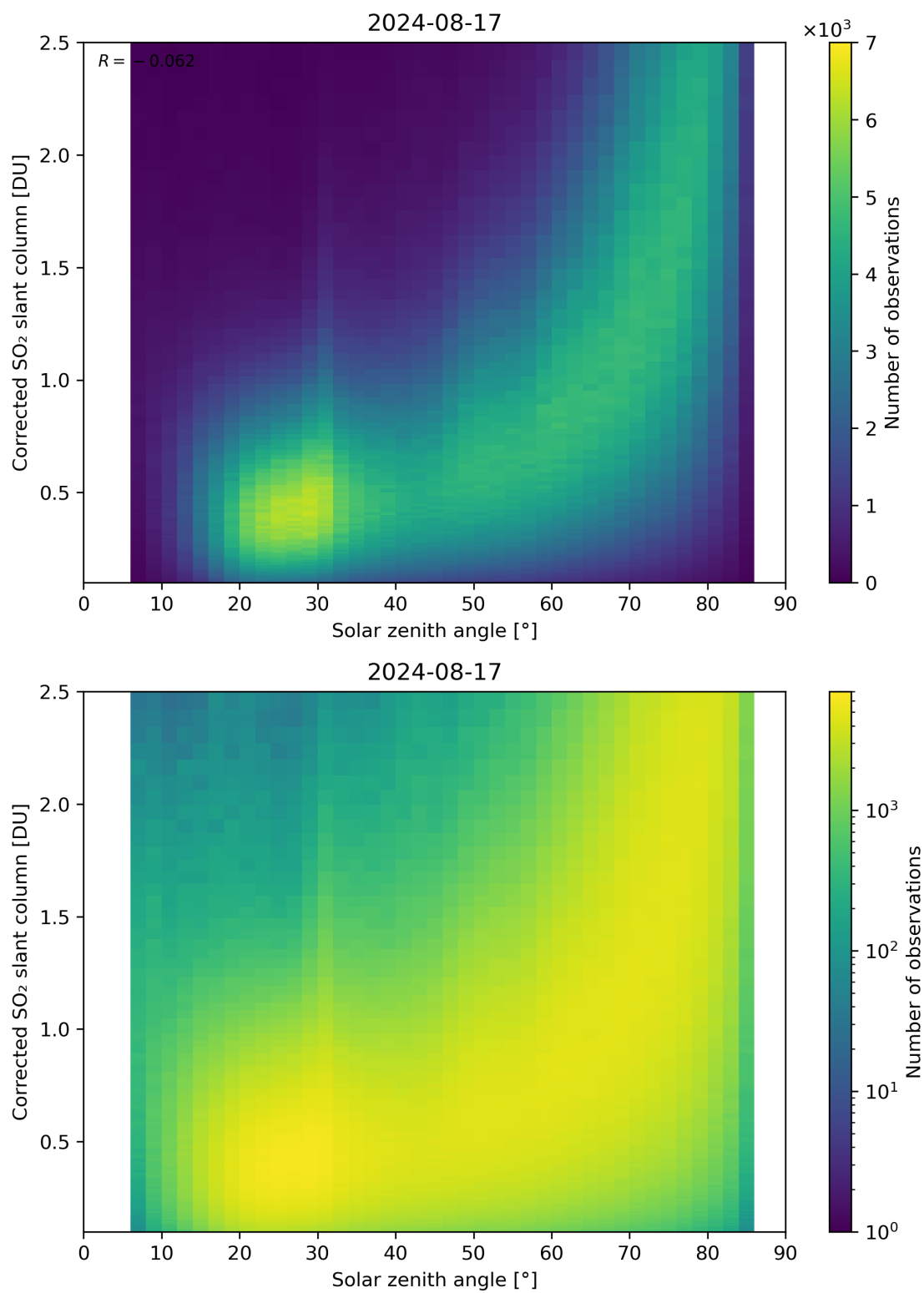
Figure 166: Scatter density plot of “Solar zenith angle” against “Corrected SO 2 slant column” for 2024-08-16 to 2024-08-18.
