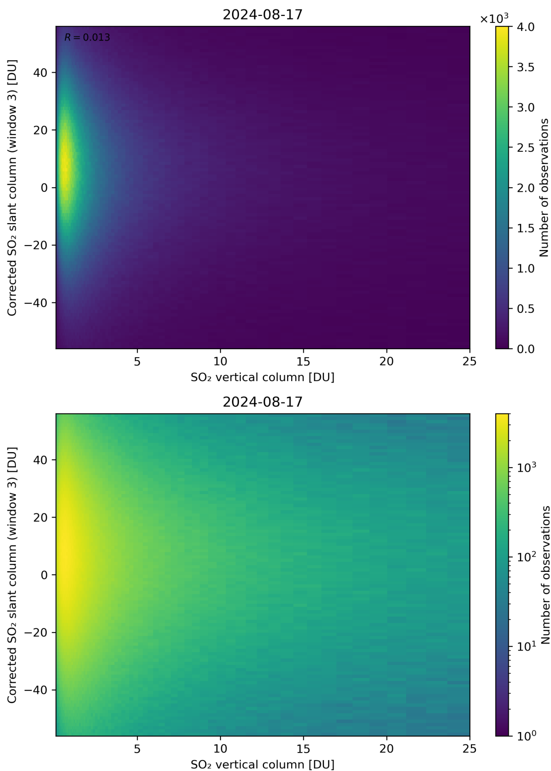
Figure 299: Scatter density plot of “SO 2 vertical column” against “Corrected SO 2 slant column (window 3)” for 2024-08-16 to 2024-08-18.
