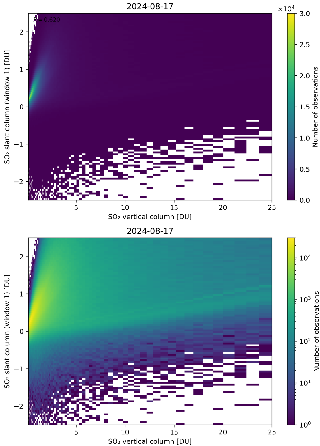
Figure 300: Scatter density plot of “SO 2 vertical column” against “SO 2 slant column (window 1)” for 2024-08-16 to 2024-08-18.
