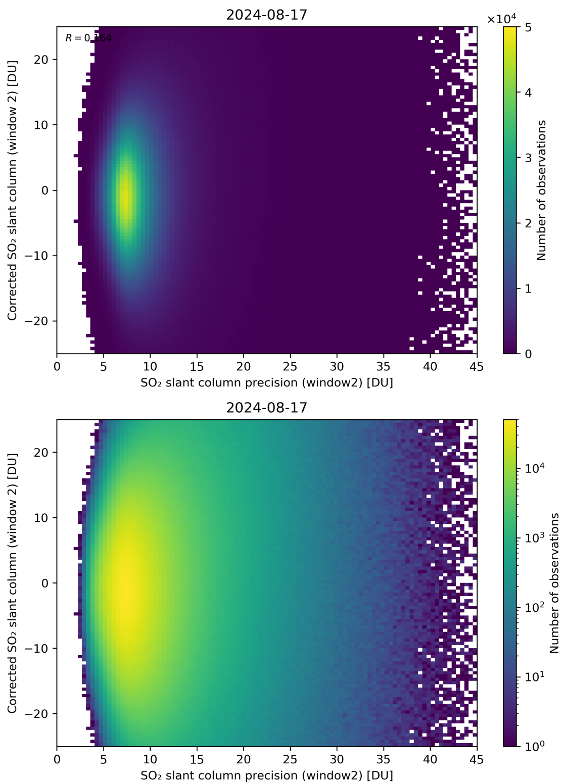
Figure 247: Scatter density plot of “SO 2 slant column precision (window2)” against “Corrected SO 2 slant column (window 2)” for 2024-08-16 to 2024-08-18.
