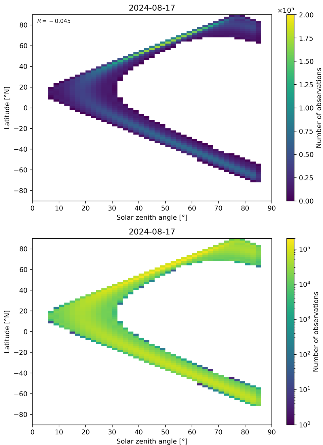
Figure 164: Scatter density plot of “Solar zenith angle” against “Latitude” for 2024-08-16 to 2024-08-18.
