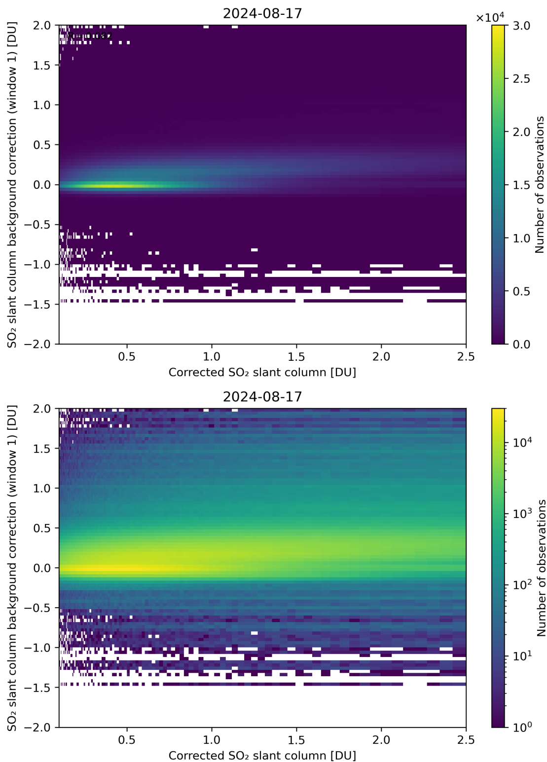
Figure 178: Scatter density plot of “Corrected SO 2 slant column” against “SO 2 slant column background correction (window 1)” for 2024-08-16 to 2024-08-18.
