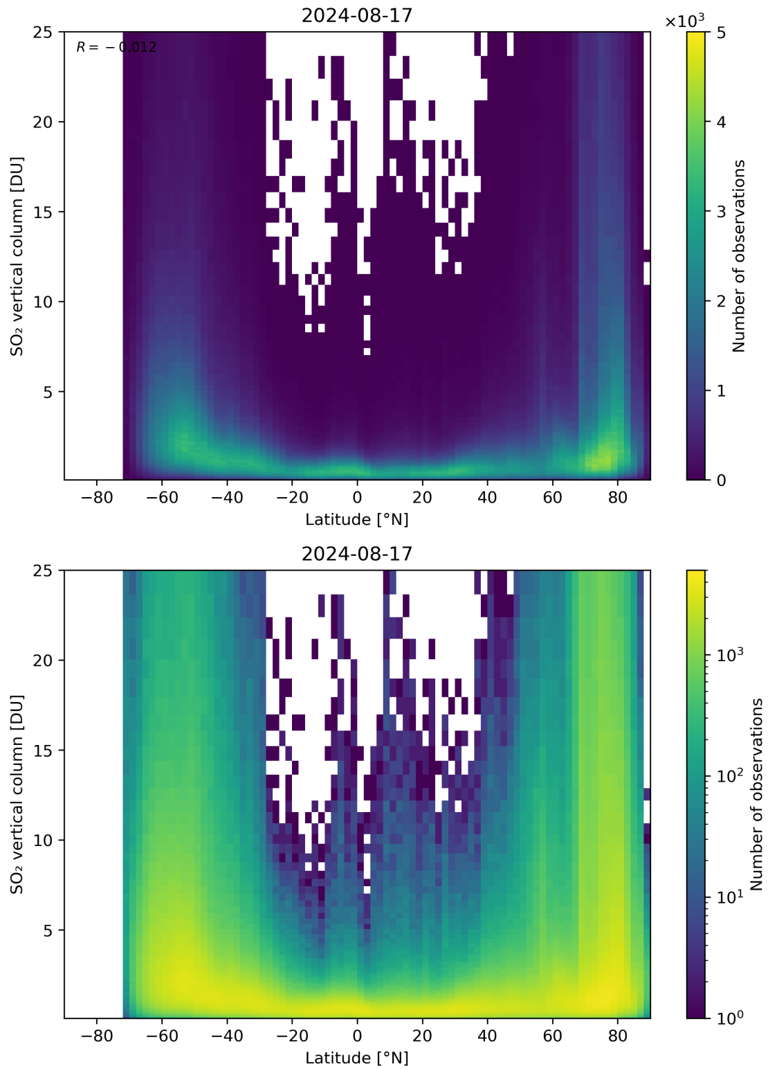
Figure 156: Scatter density plot of “Latitude” against “SO 2 vertical column” for 2024-08-16 to 2024-08-18.
