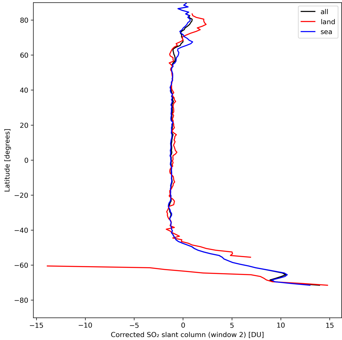
Figure 39: Zonal average of “Corrected SO 2 slant column (window 2)” for 2024-08-16 to 2024-08-18.
