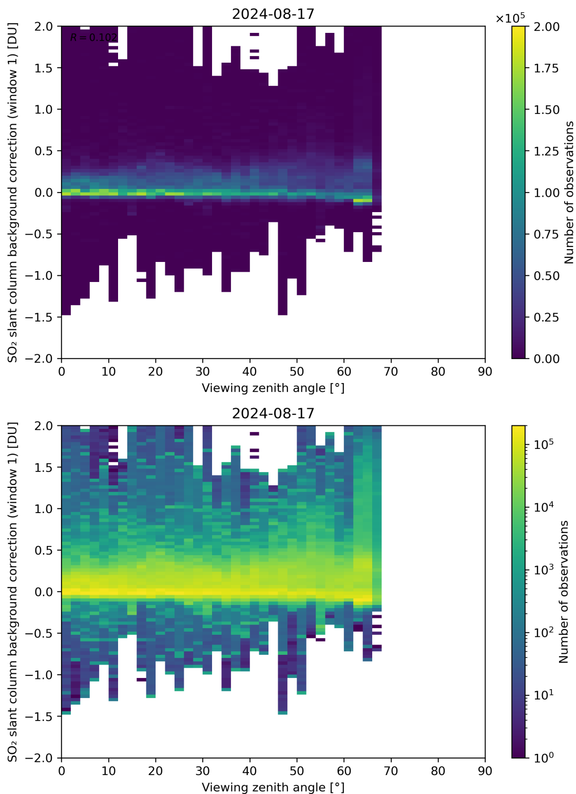
Figure 308: Scatter density plot of “Viewing zenith angle” against “SO 2 slant column background correction (window 1)” for 2024-08-16 to 2024-08-18.
