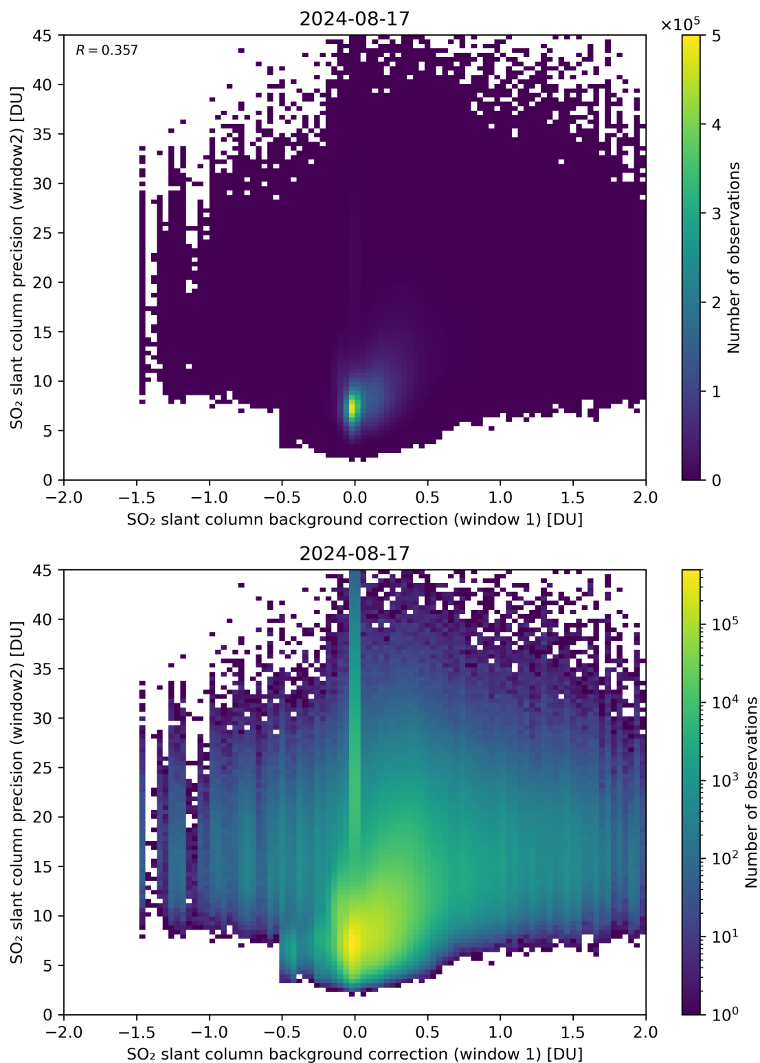
Figure 106: Scatter density plot of “SO 2 slant column background correction (window 1)” against “SO 2 slant column precision (window2)” for 2024-08-16 to 2024-08-18.
