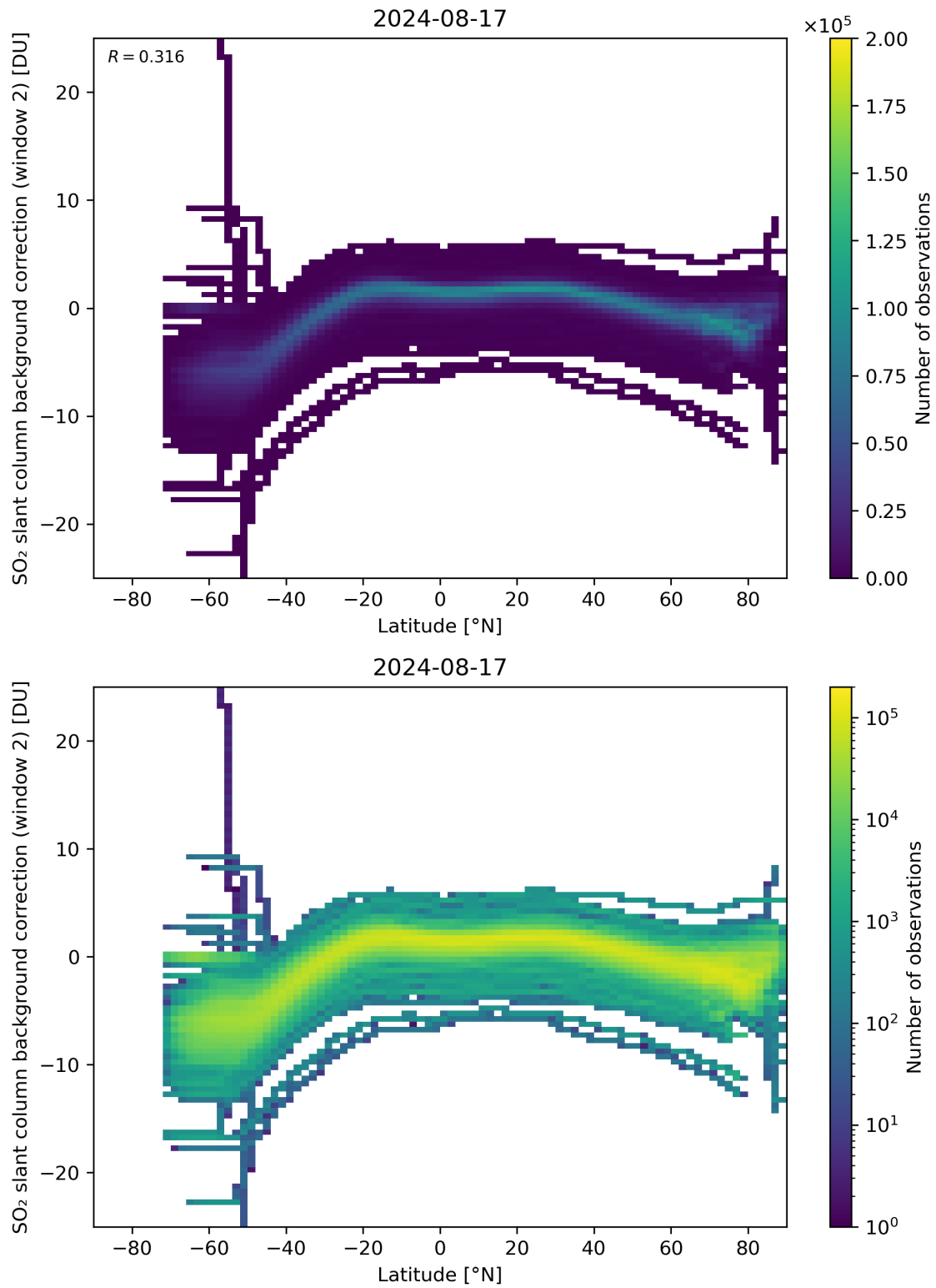
Figure 140: Scatter density plot of “Latitude” against “SO 2 slant column background correction (window 2)” for 2024-08-16 to 2024-08-18.
