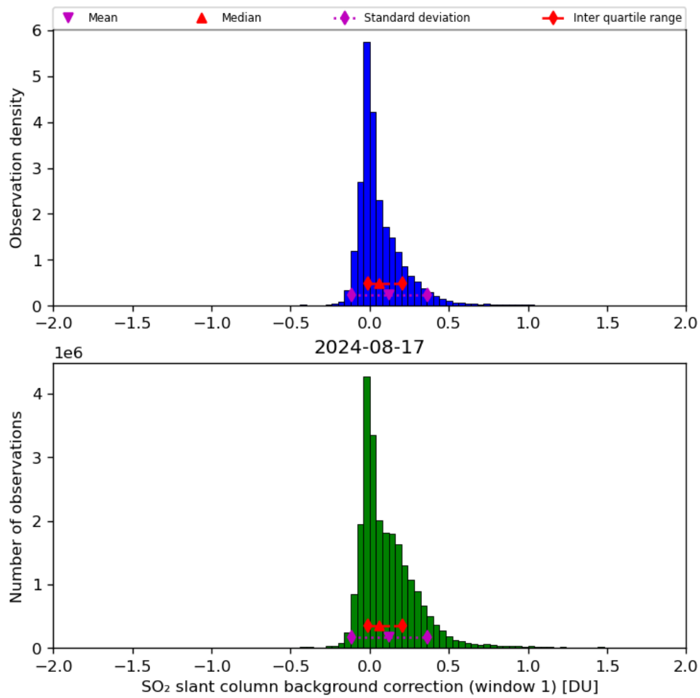
Figure 59: Histogram of “SO 2 slant column background correction (window 1)” for 2024-08-16 to 2024-08-18
