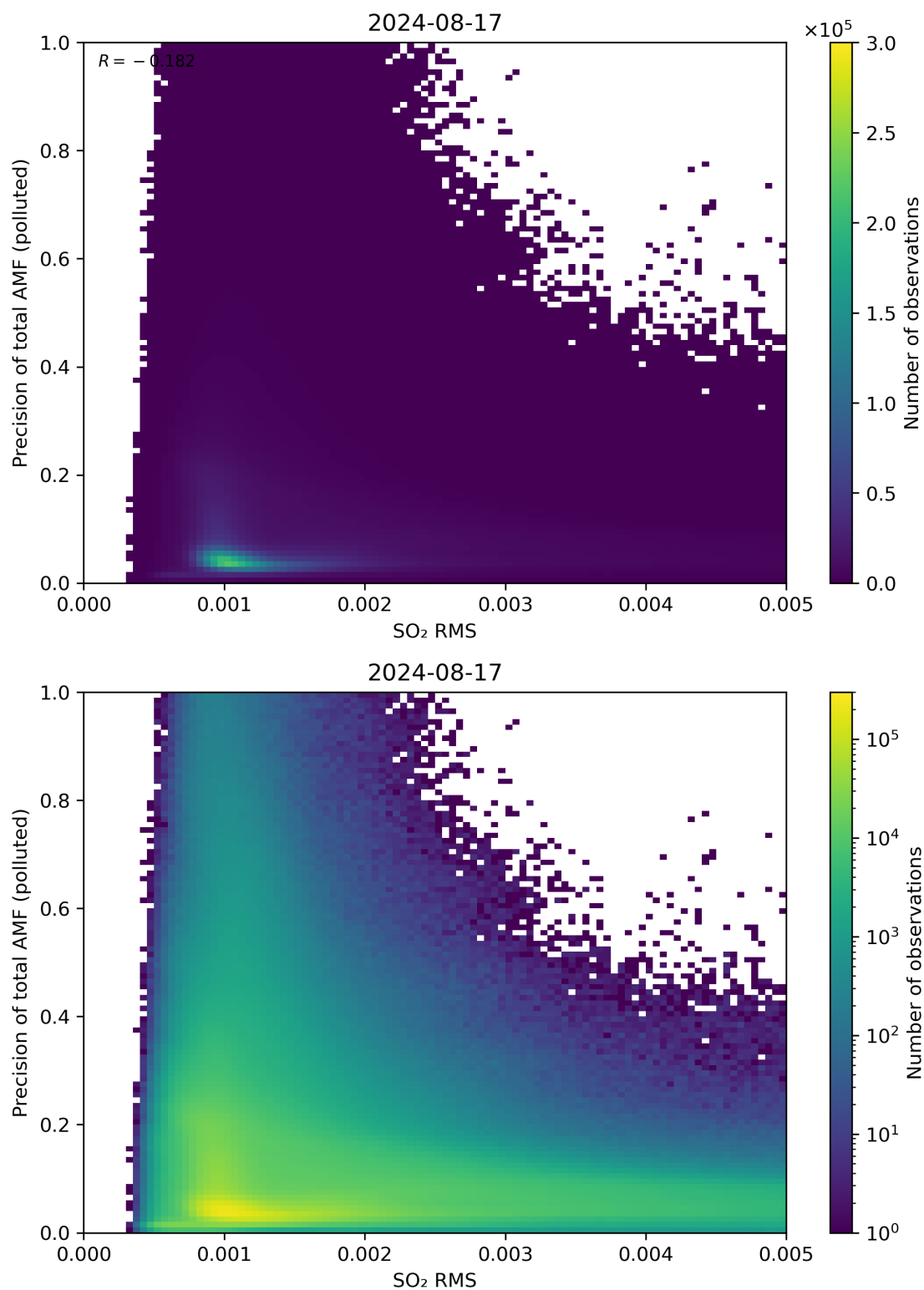
Figure 138: Scatter density plot of “SO 2 RMS” against “Precision of total AMF (polluted)” for 2024-08-16 to 2024-08-18.
