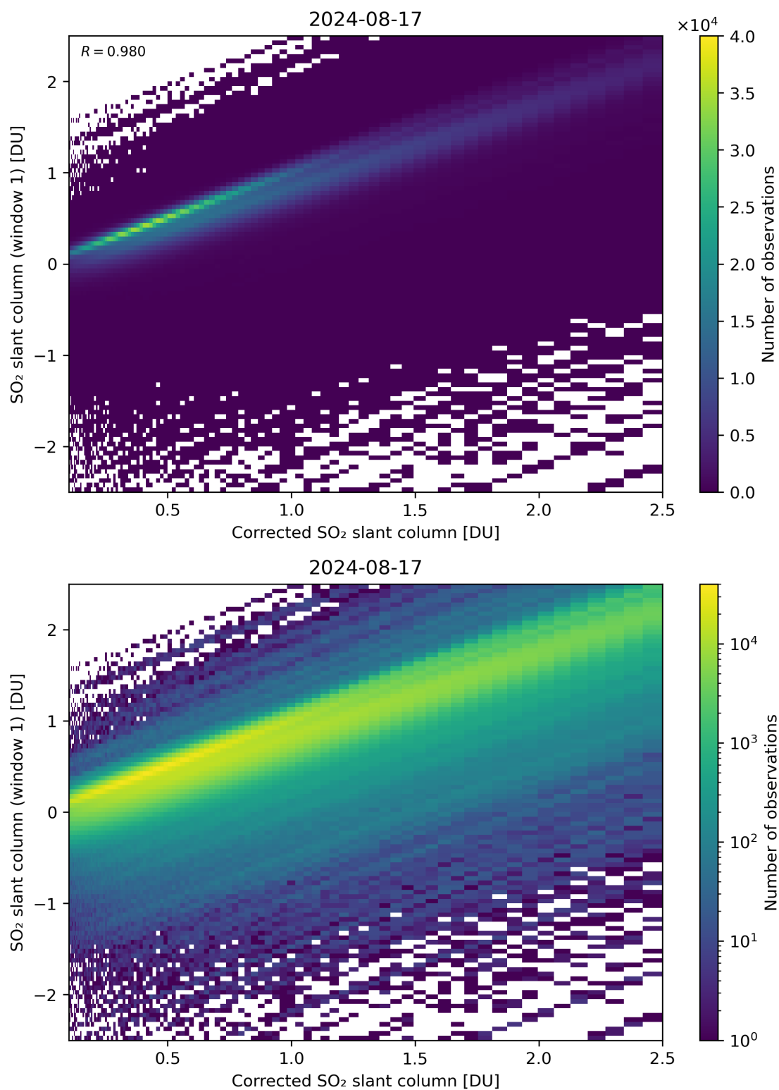
Figure 187: Scatter density plot of “Corrected SO 2 slant column” against “SO 2 slant column (window 1)” for 2024-08-16 to 2024-08-18.
