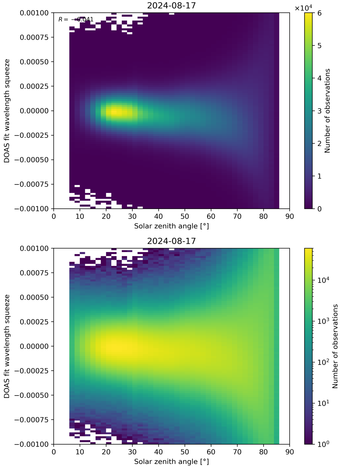
Figure 162: Scatter density plot of “Solar zenith angle” against “DOAS fit wavelength squeeze” for 2024-08-16 to 2024-08-18.
