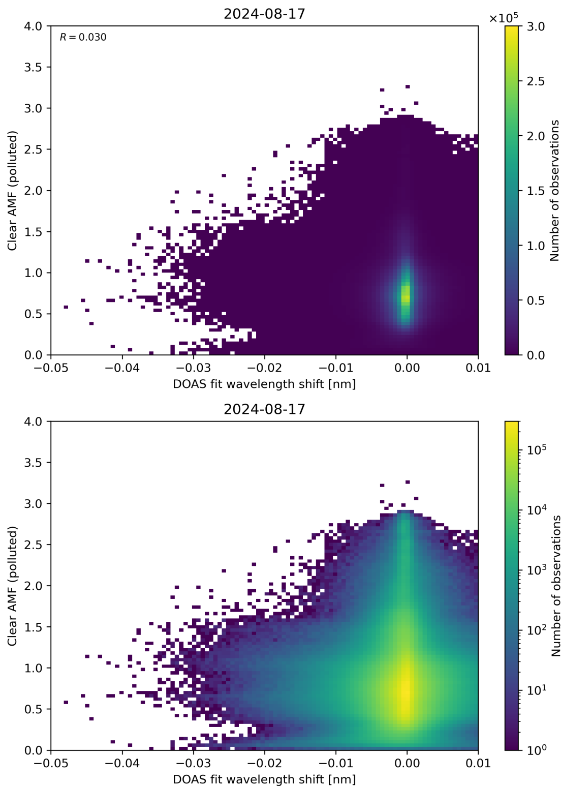
Figure 129: Scatter density plot of “DOAS fit wavelength shift” against “Clear AMF (polluted)” for 2024-08-16 to 2024-08-18.
