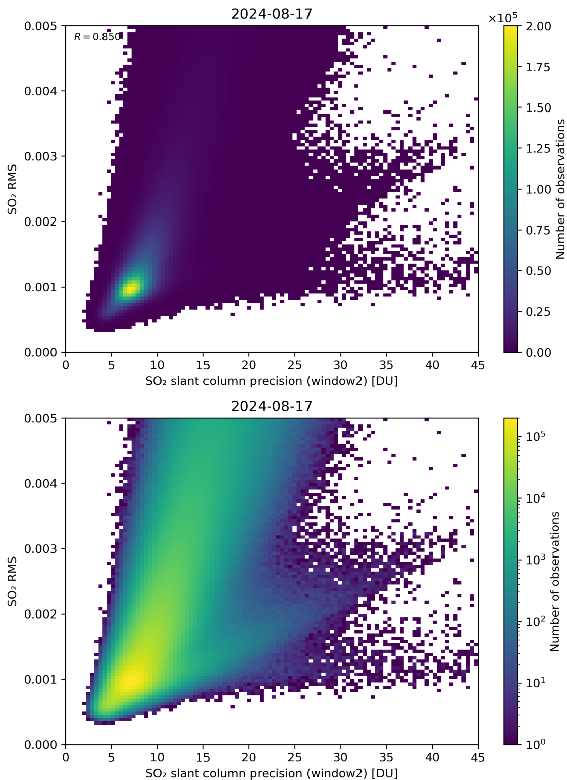
Figure 245: Scatter density plot of “SO 2 slant column precision (window2)” against “SO 2 RMS” for 2024-08-16 to 2024-08-18.
