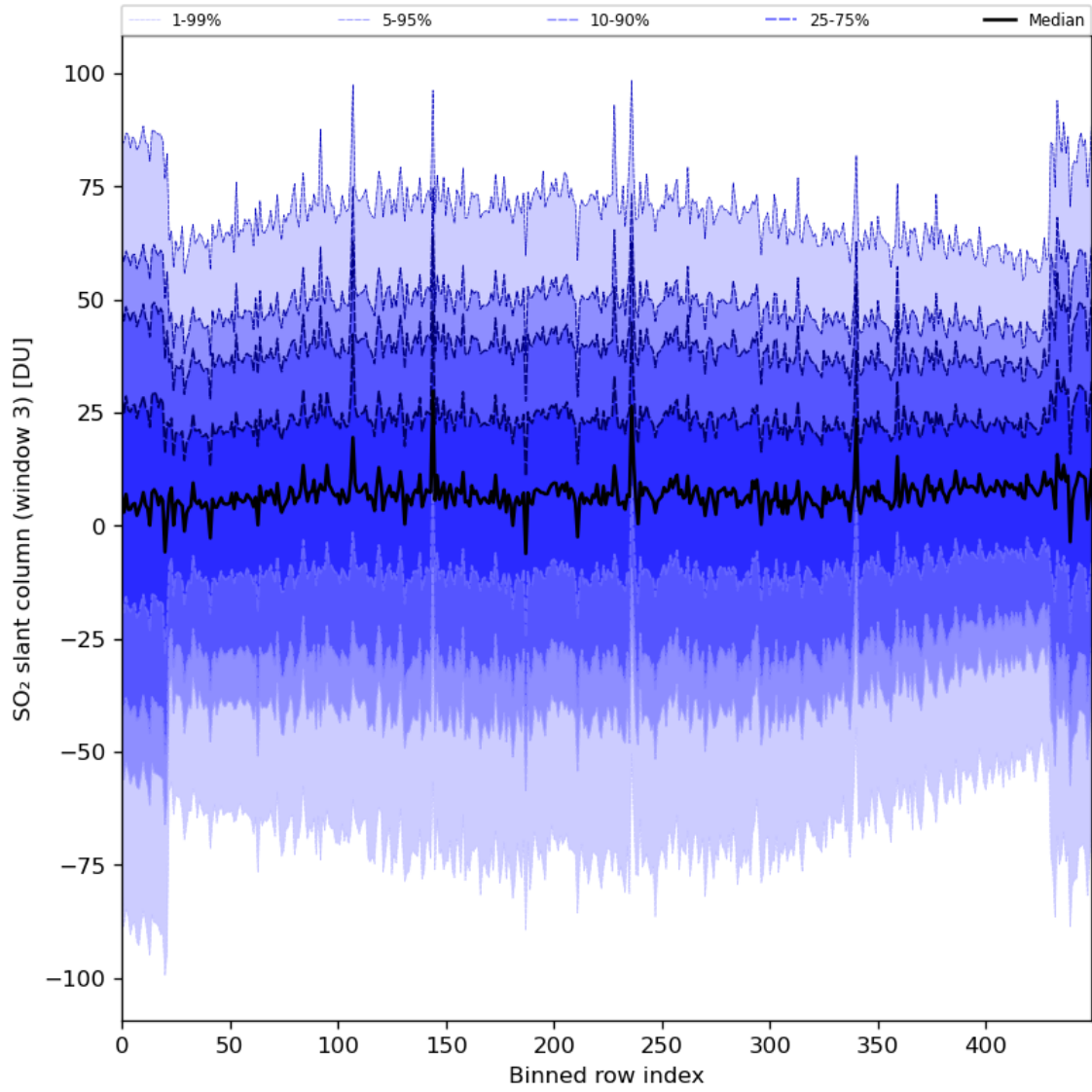
Figure 87: Along track statistics of “SO 2 slant column (window 3)” for 2024-08-16 to 2024-08-18
