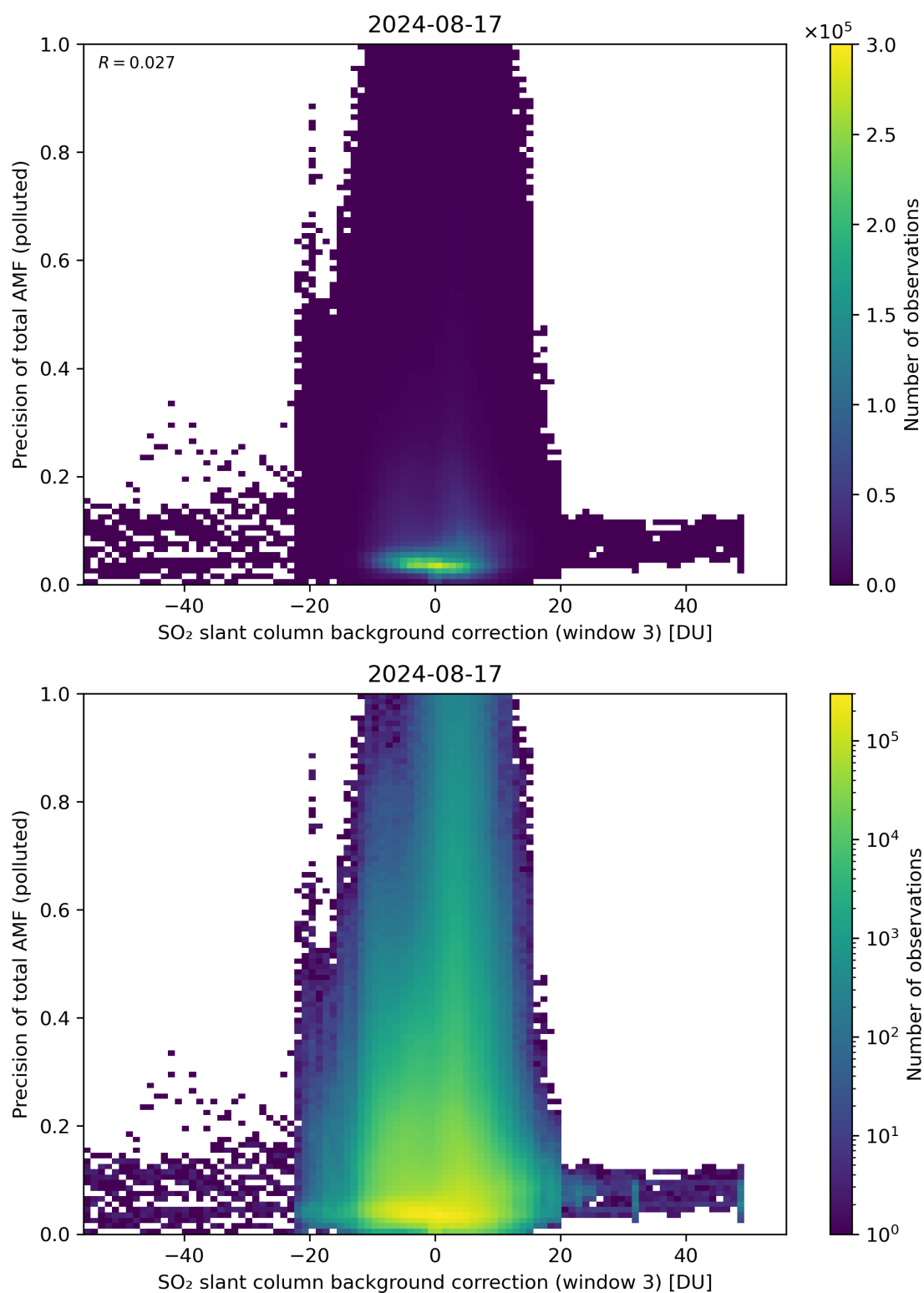
Figure 126: Scatter density plot of “SO 2 slant column background correction (window 3)” against “Precision of total AMF (polluted)” for 2024-08-16 to 2024-08-18.
