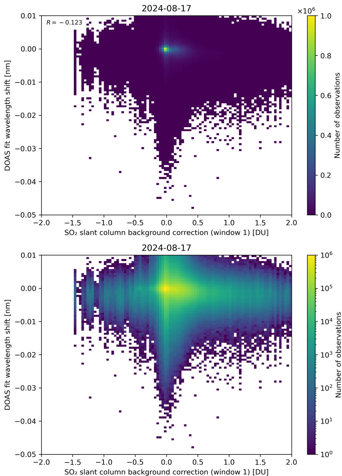
Figure 100: Scatter density plot of “SO 2 slant column background correction (window 1)” against “DOAS fit wavelength shift” for 2024-08-16 to 2024-08-18.
