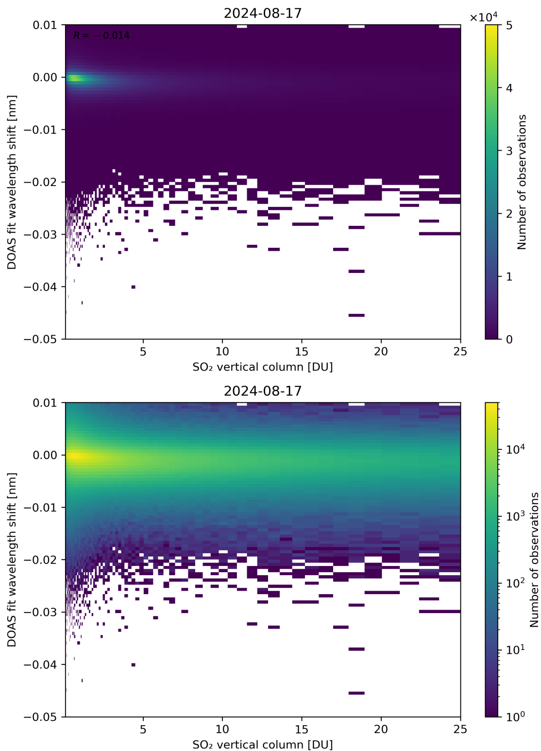
Figure 276: Scatter density plot of “SO 2 vertical column” against “DOAS fit wavelength shift” for 2024-08-16 to 2024-08-18.
