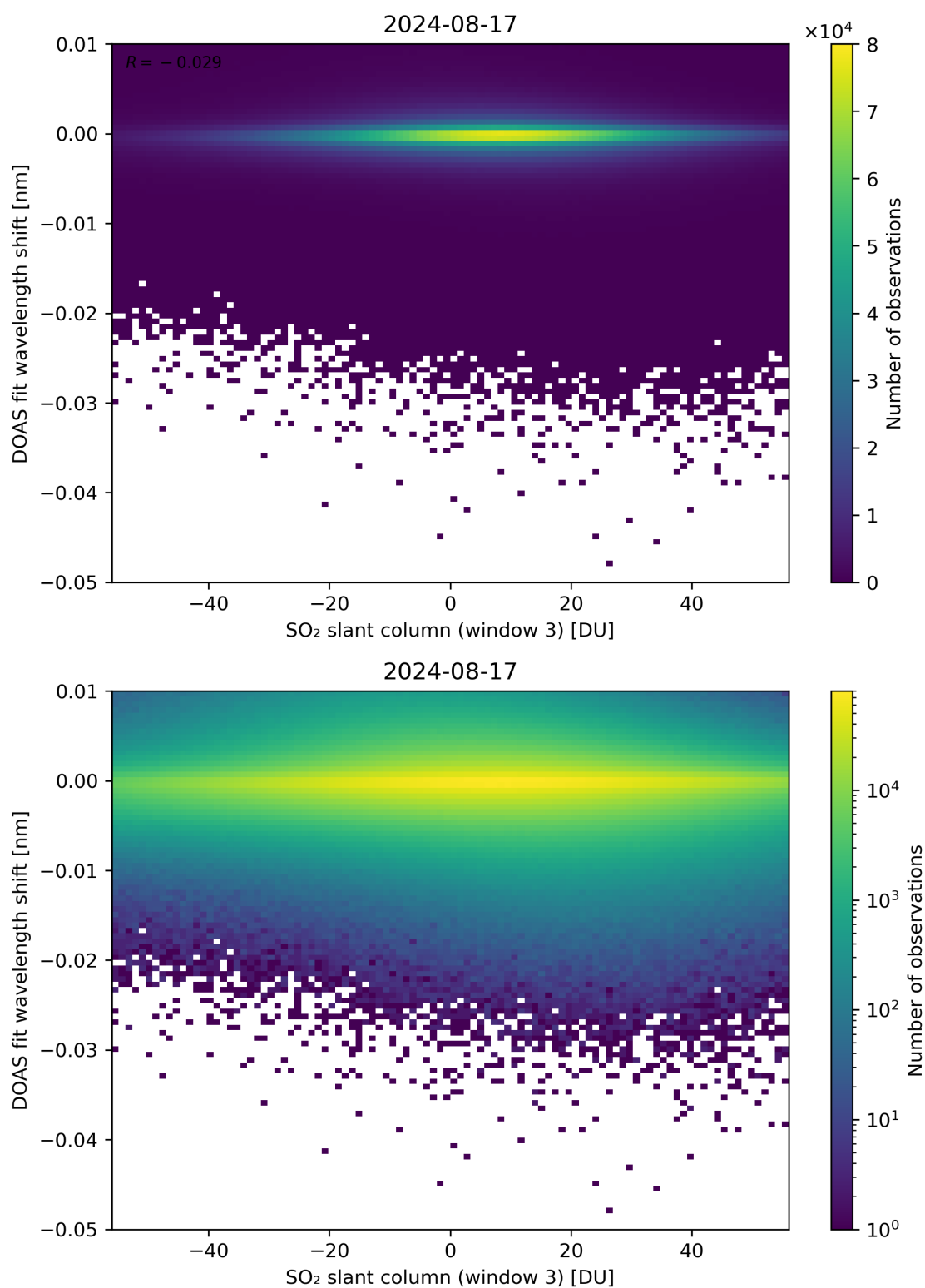
Figure 254: Scatter density plot of “SO 2 slant column (window 3)” against “DOAS fit wavelength shift” for 2024-08-16 to 2024-08-18.
