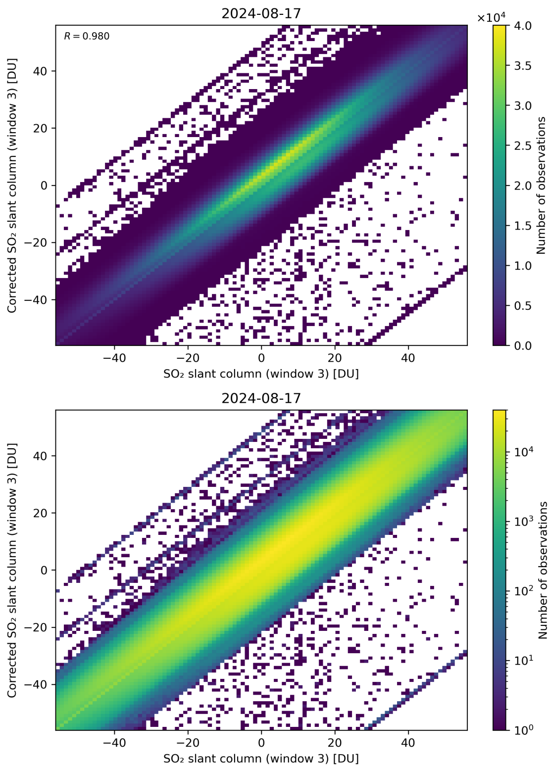
Figure 266: Scatter density plot of “SO 2 slant column (window 3)” against “Corrected SO 2 slant column (window 3)” for 2024-08-16 to 2024-08-18.
