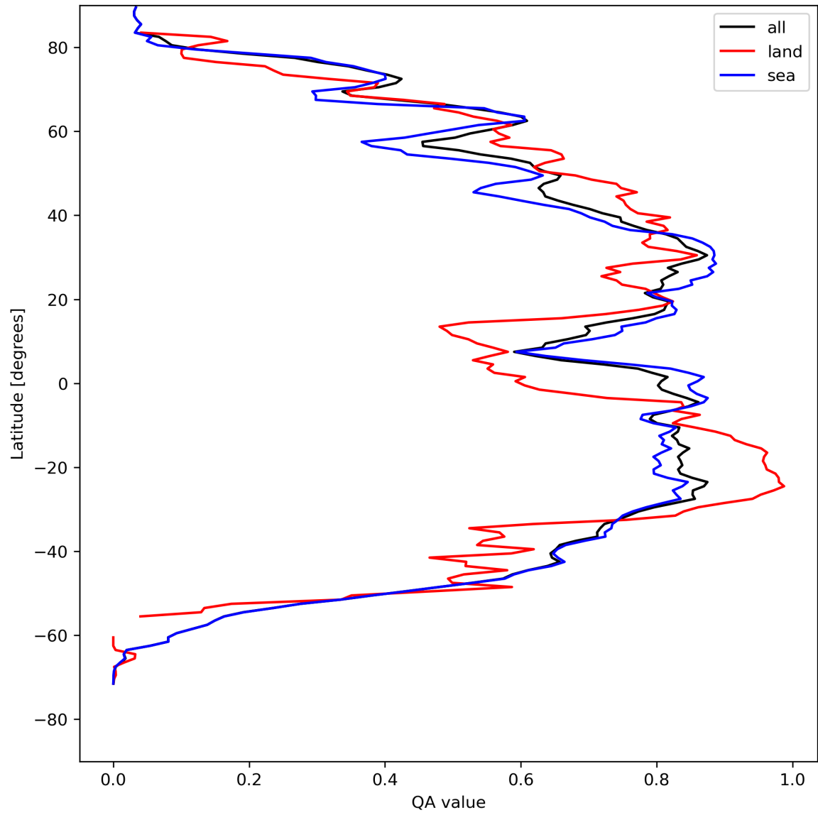
Figure 29: Zonal average of “QA value” for 2024-08-16 to 2024-08-18.
