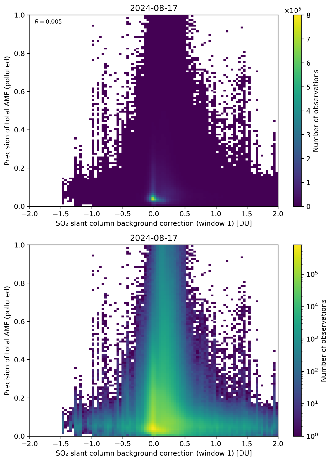
Figure 110: Scatter density plot of “SO 2 slant column background correction (window 1)” against “Precision of total AMF (polluted)” for 2024-08-16 to 2024-08-18.
