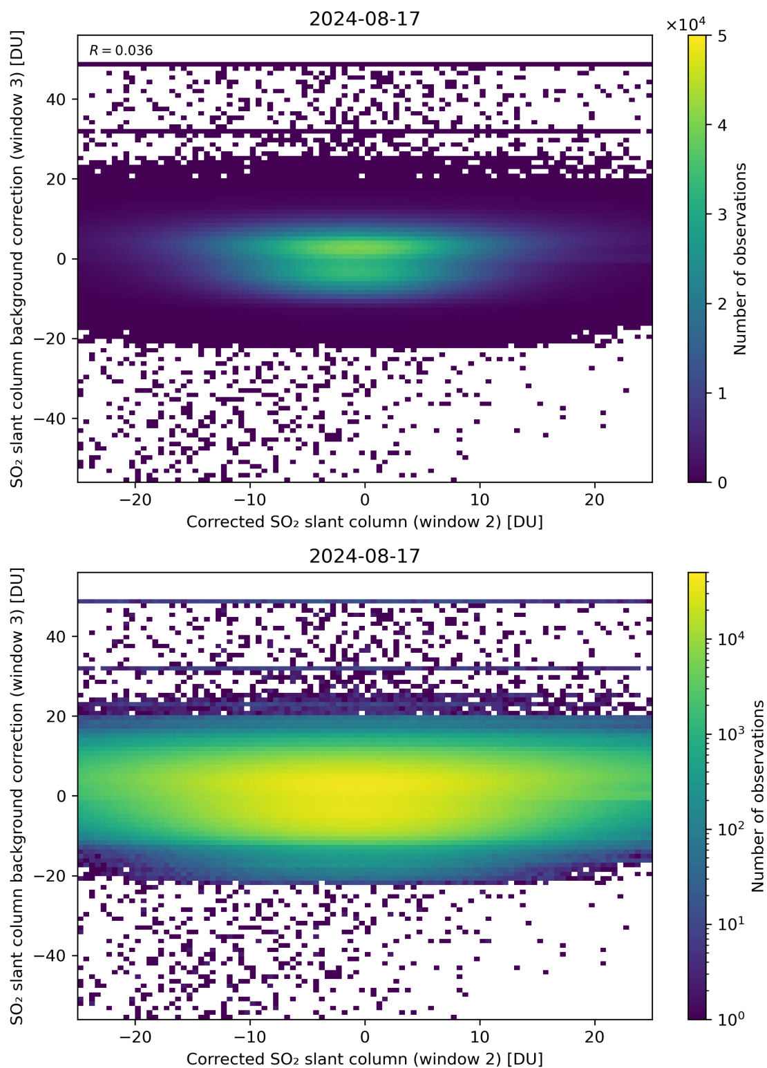
Figure 195: Scatter density plot of “Corrected SO 2 slant column (window 2)” against “SO 2 slant column background correction (window 3)” for 2024-08-16 to 2024-08-18.
