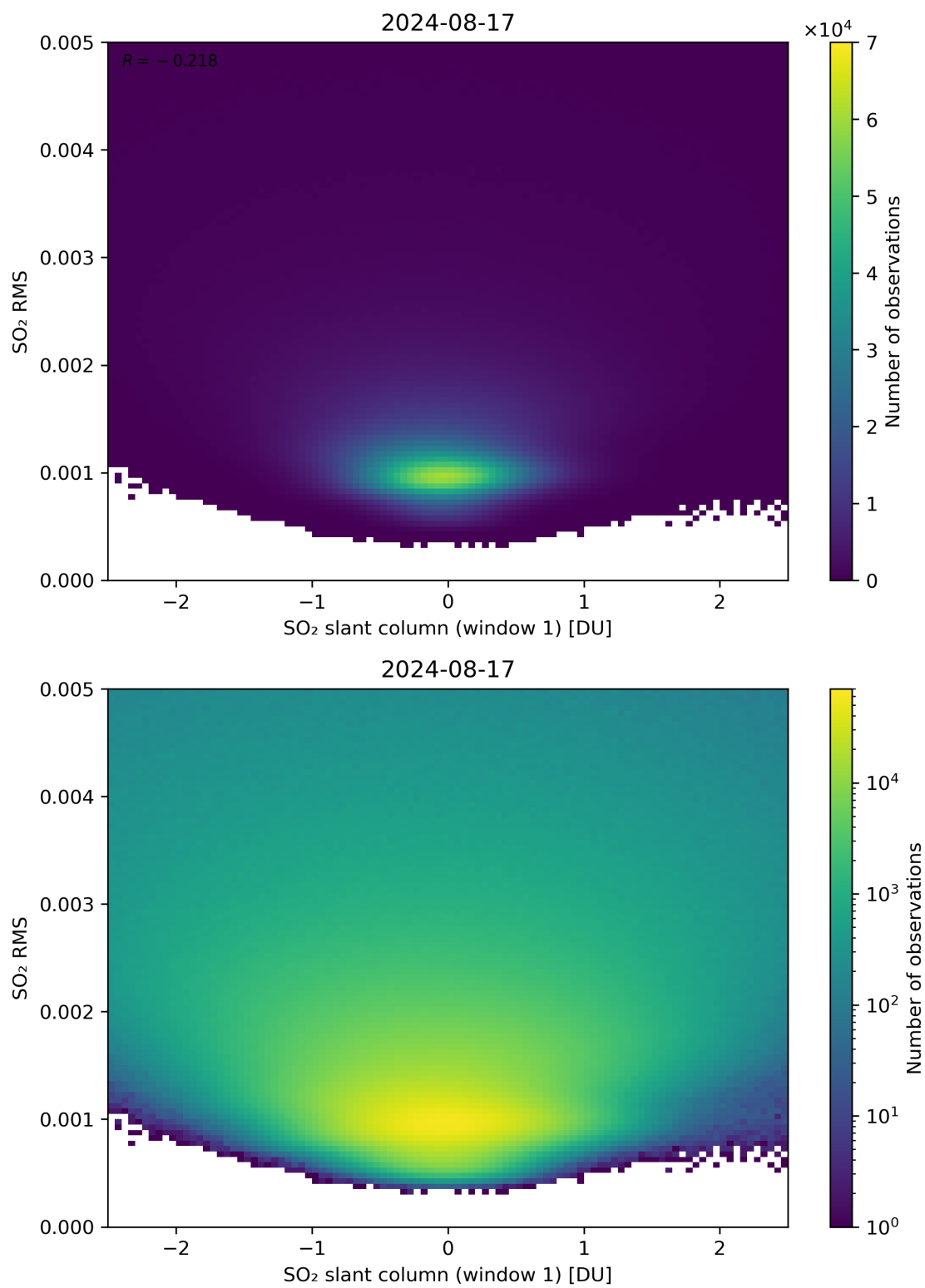
Figure 217: Scatter density plot of “SO 2 slant column (window 1)” against “SO 2 RMS” for 2024-08-16 to 2024-08-18.
