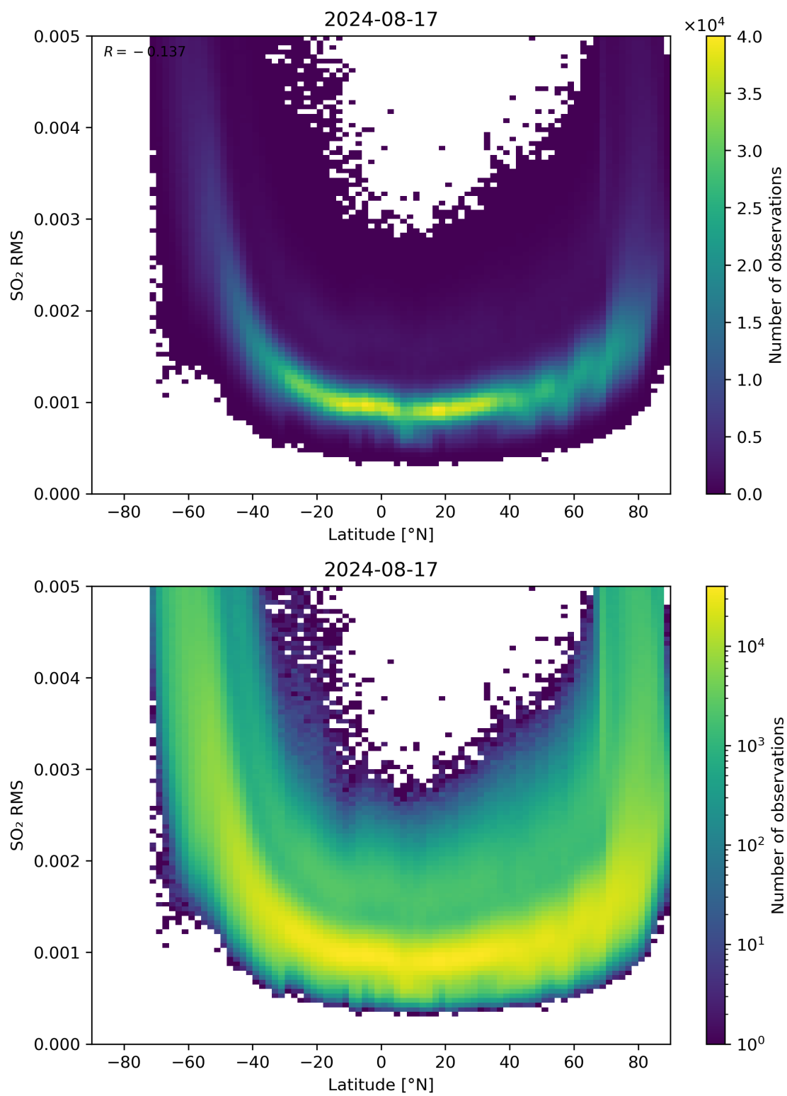
Figure 144: Scatter density plot of “Latitude” against “SO 2 RMS” for 2024-08-16 to 2024-08-18.
