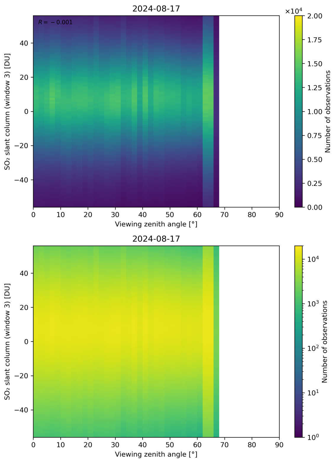
Figure 323: Scatter density plot of “Viewing zenith angle” against “SO 2 slant column (window 3)” for 2024-08-16 to 2024-08-18.
