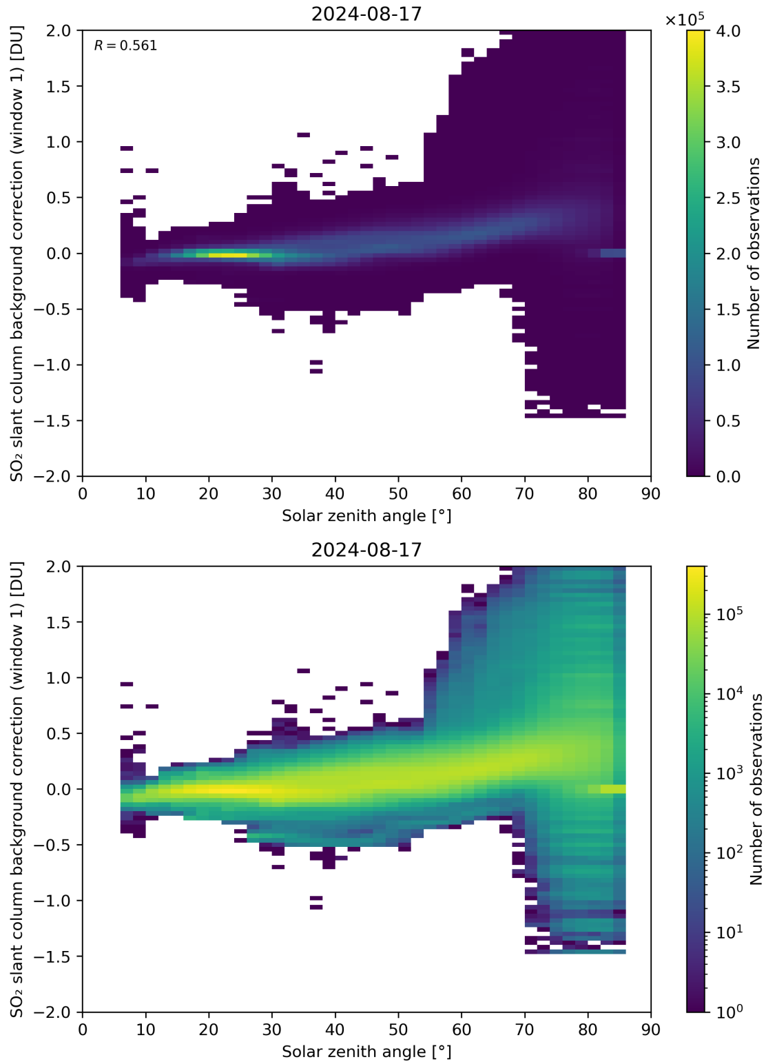
Figure 158: Scatter density plot of “Solar zenith angle” against “SO 2 slant column background correction (window 1)” for 2024-08-16 to 2024-08-18.
