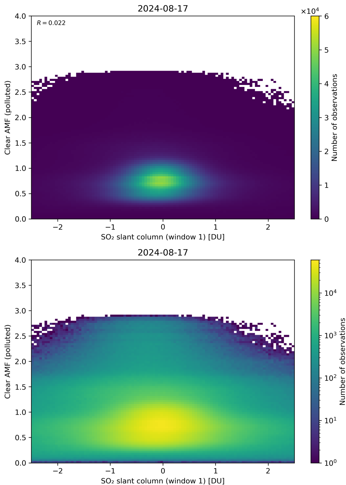
Figure 232: Scatter density plot of “SO 2 slant column (window 1)” against “Clear AMF (polluted)” for 2024-08-16 to 2024-08-18.
