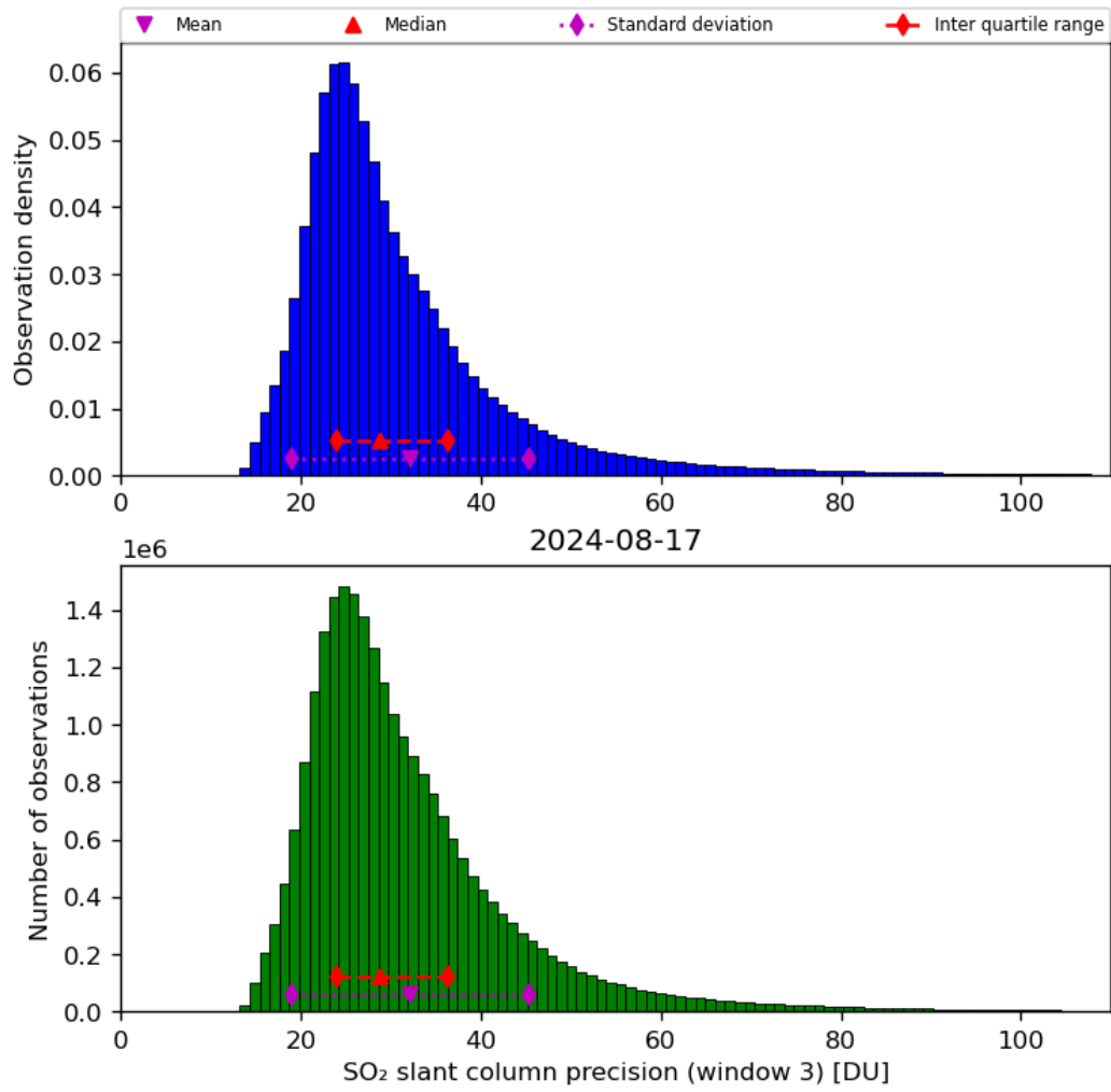
Figure 65: Histogram of “SO 2 slant column precision (window 3)” for 2024-08-16 to 2024-08-18
