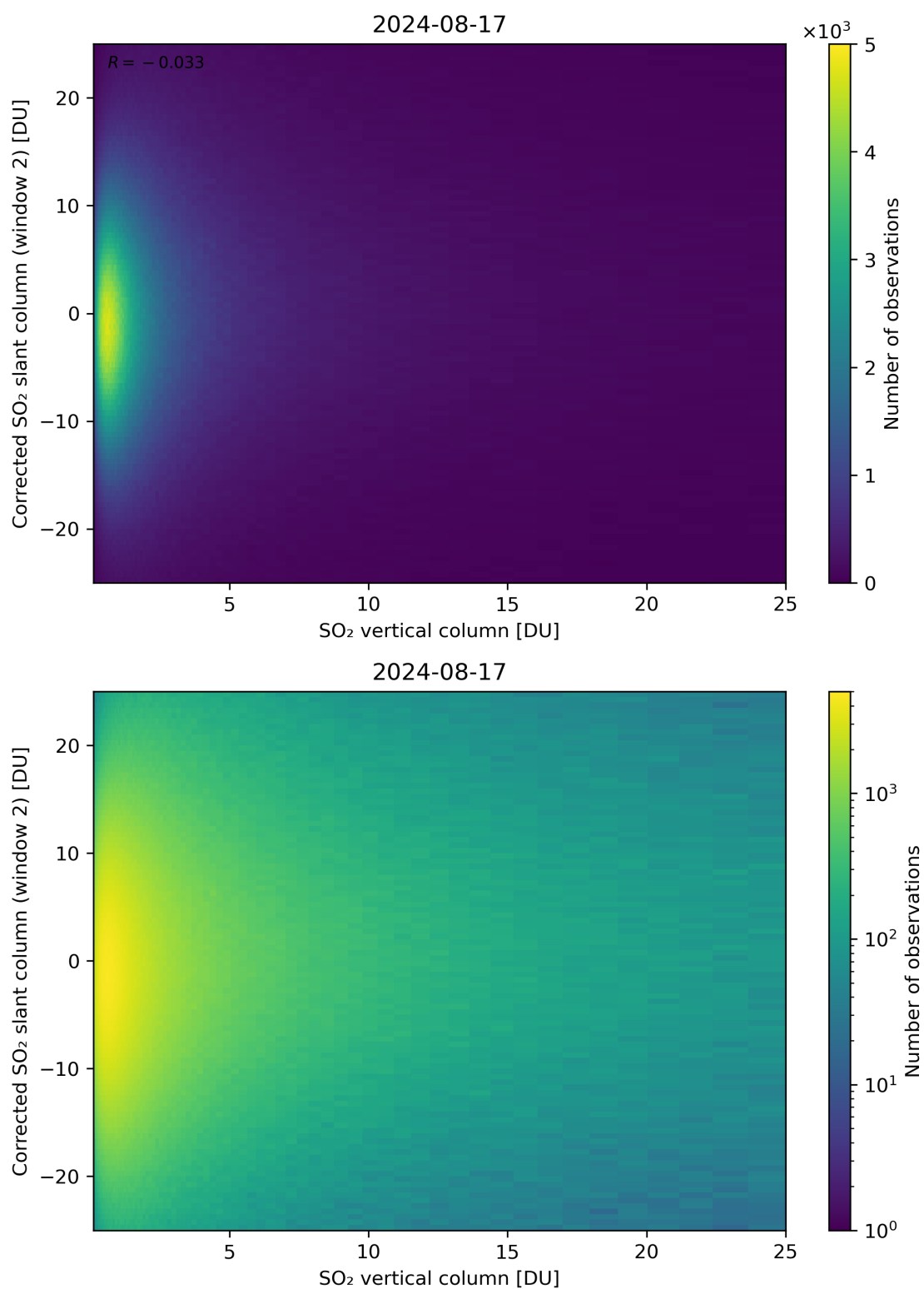
Figure 298: Scatter density plot of “SO 2 vertical column” against “Corrected SO 2 slant column (window 2)” for 2024-08-16 to 2024-08-18.
