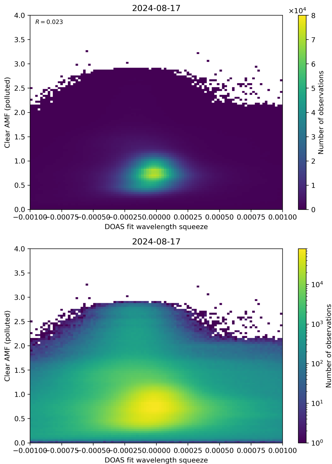
Figure 133: Scatter density plot of “DOAS fit wavelength squeeze” against “Clear AMF (polluted)” for 2024-08-16 to 2024-08-18.
