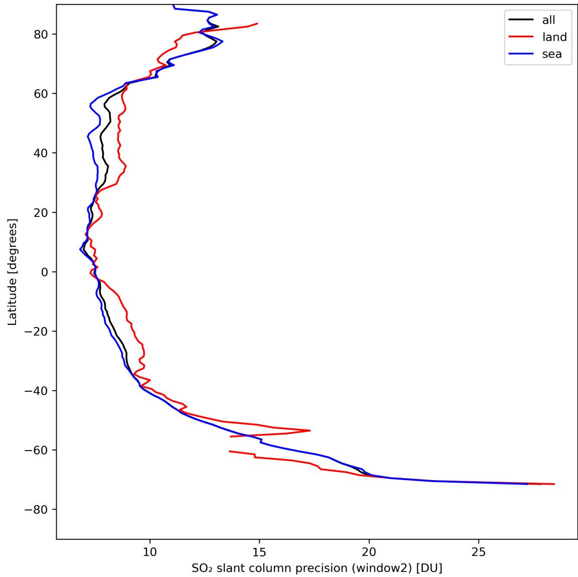
Figure 38: Zonal average of “SO 2 slant column precision (window2)” for 2024-08-16 to 2024-08-18.
