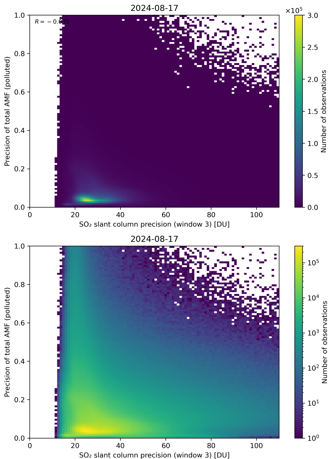
Figure 264: Scatter density plot of “SO 2 slant column precision (window 3)” against “Precision of total AMF (polluted)” for 2024-08-16 to 2024-08-18.
