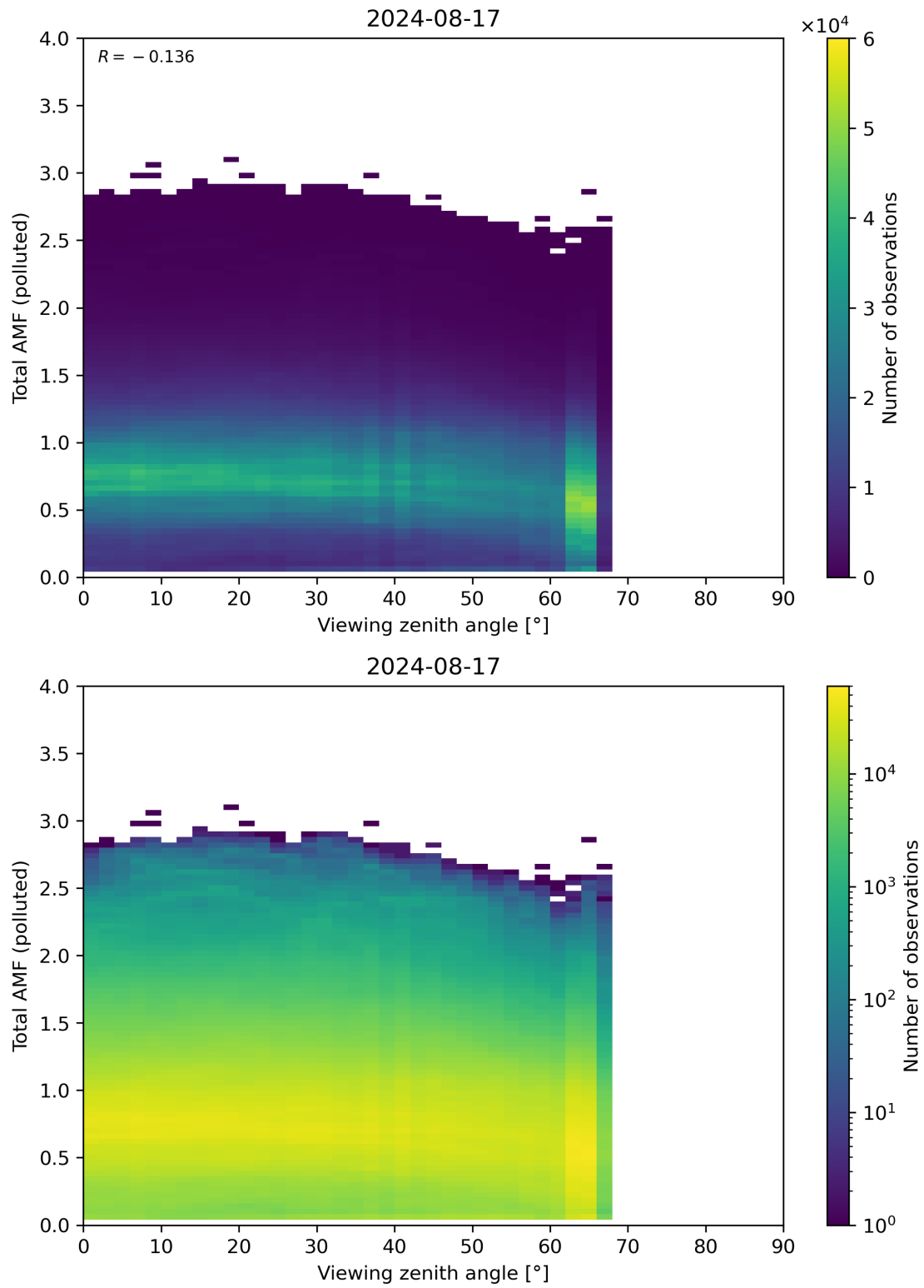
Figure 325: Scatter density plot of “Viewing zenith angle” against “Total AMF (polluted)” for 2024-08-16 to 2024-08-18.
