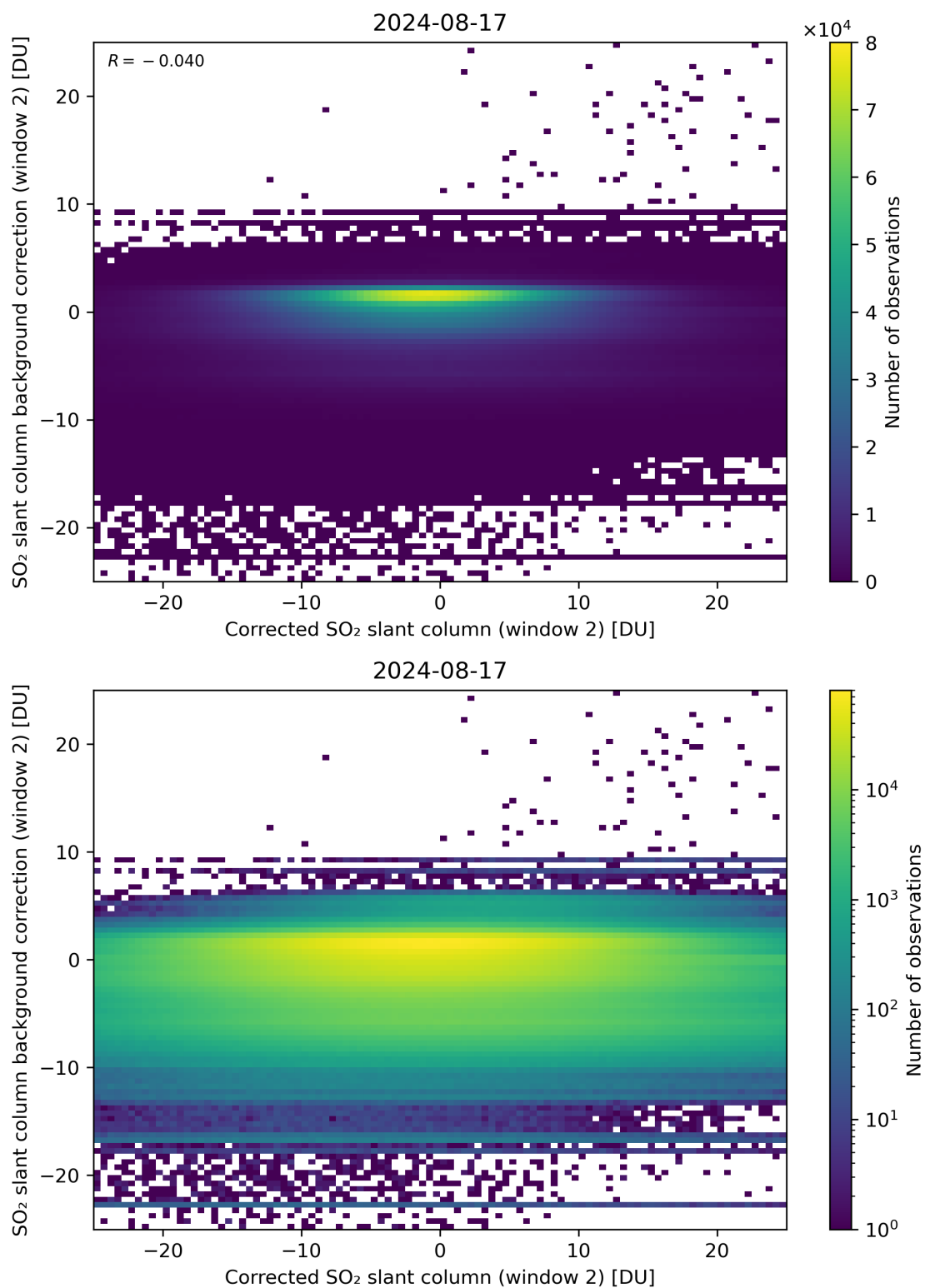
Figure 194: Scatter density plot of “Corrected SO 2 slant column (window 2)” against “SO 2 slant column background correction (window 2)” for 2024-08-16 to 2024-08-18.
