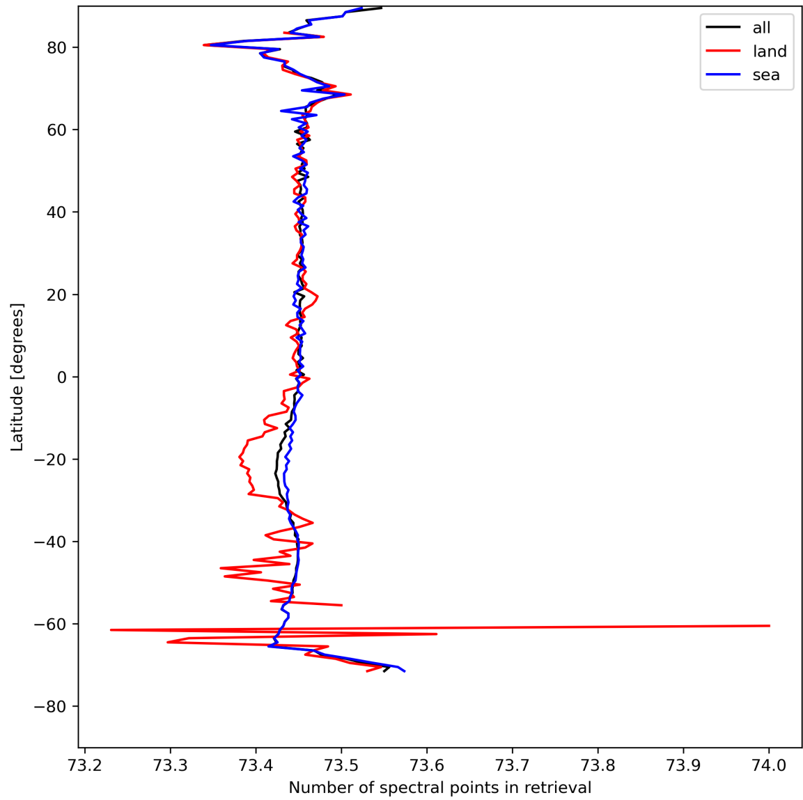
Figure 51: Zonal average of “Number of spectral points in retrieval” for 2024-08-16 to 2024-08-18.
