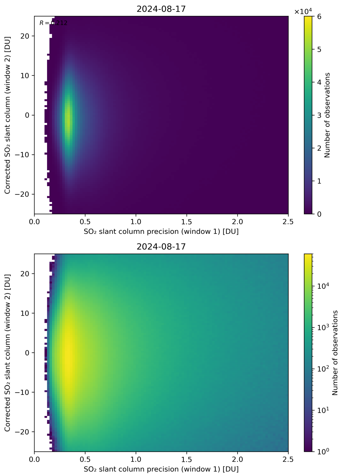
Figure 225: Scatter density plot of “SO 2 slant column precision (window 1)” against “Corrected SO 2 slant column (window 2)” for 2024-08-16 to 2024-08-18.
