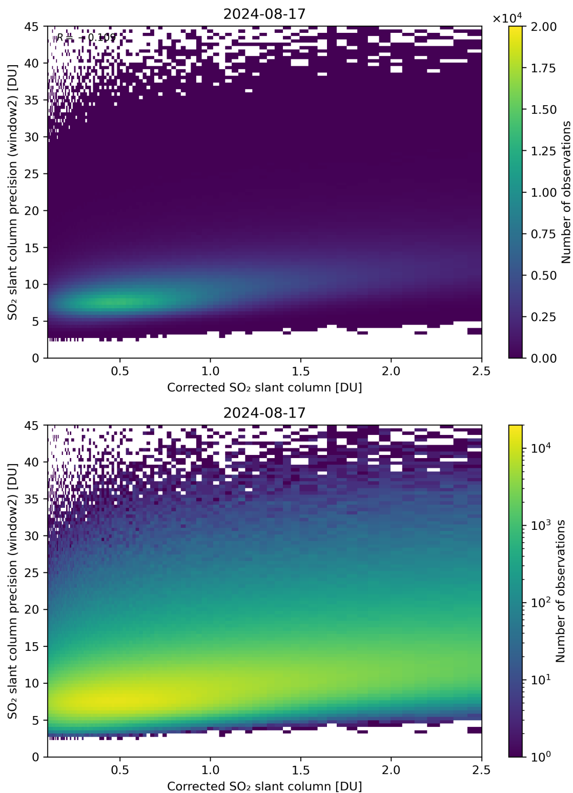
Figure 189: Scatter density plot of “Corrected SO 2 slant column” against “SO 2 slant column precision (window2)” for 2024-08-16 to 2024-08-18.
