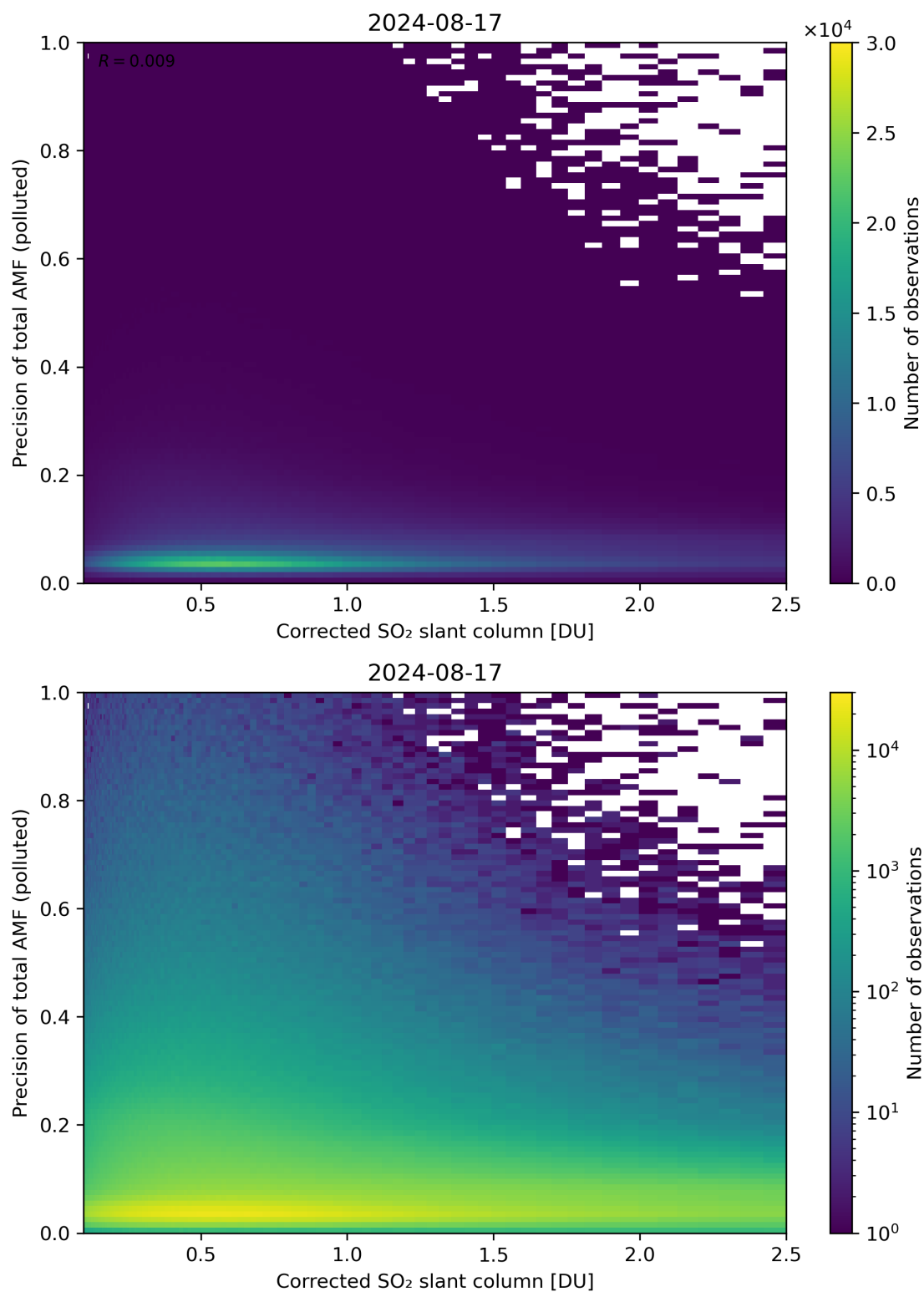
Figure 193: Scatter density plot of “Corrected SO 2 slant column” against “Precision of total AMF (polluted)” for 2024-08-16 to 2024-08-18.
