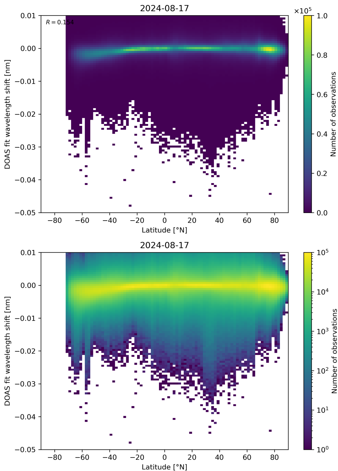
Figure 142: Scatter density plot of “Latitude” against “DOAS fit wavelength shift” for 2024-08-16 to 2024-08-18.
