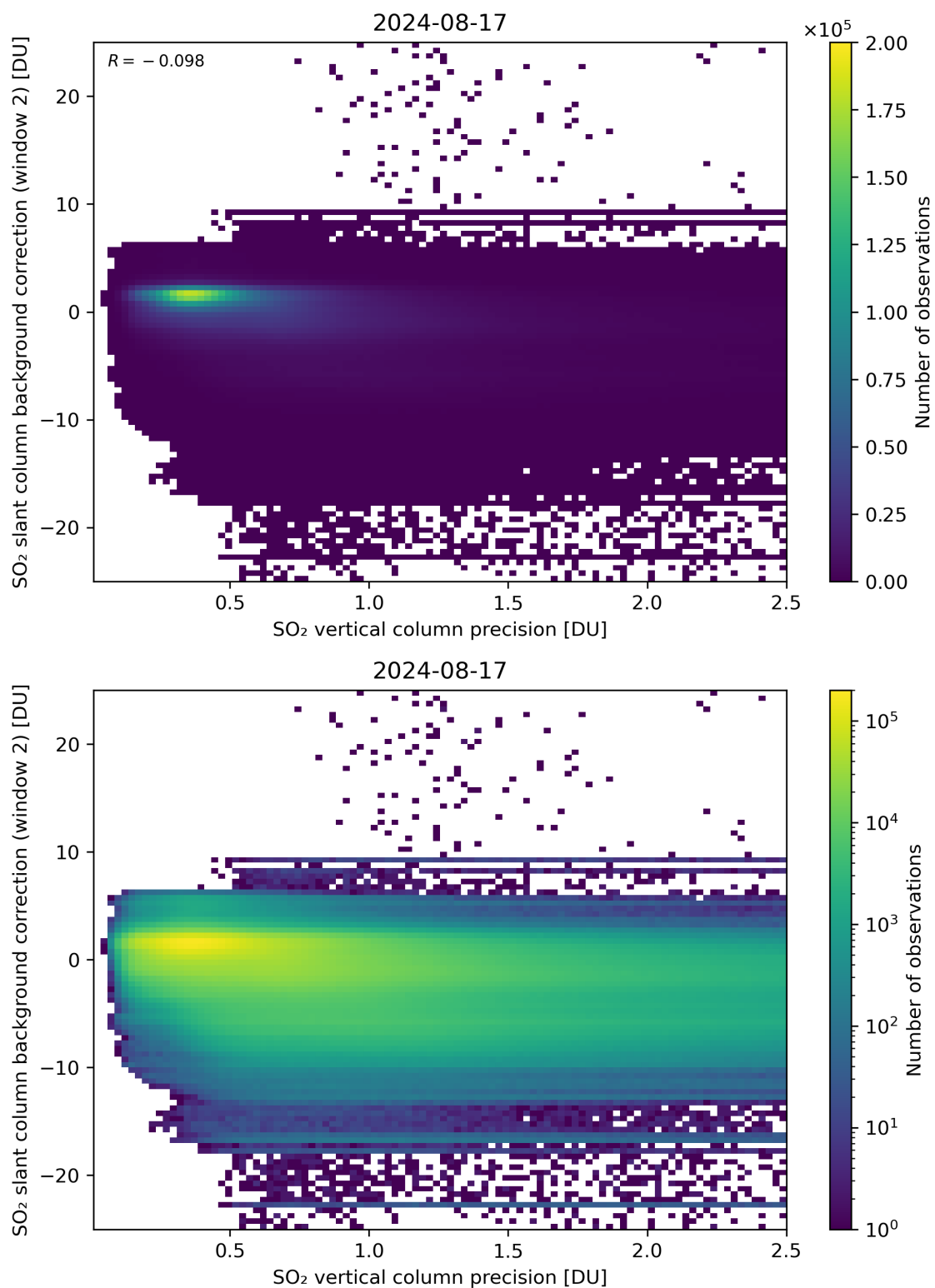
Figure 280: Scatter density plot of “SO 2 vertical column precision” against “SO 2 slant column background correction (window 2)” for 2024-08-16 to 2024-08-18.
