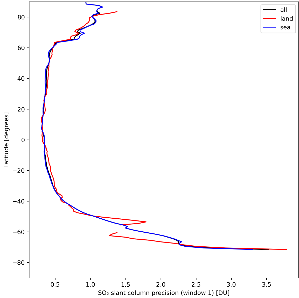
Figure 34: Zonal average of “SO 2 slant column precision (window 1)” for 2024-08-16 to 2024-08-18.
