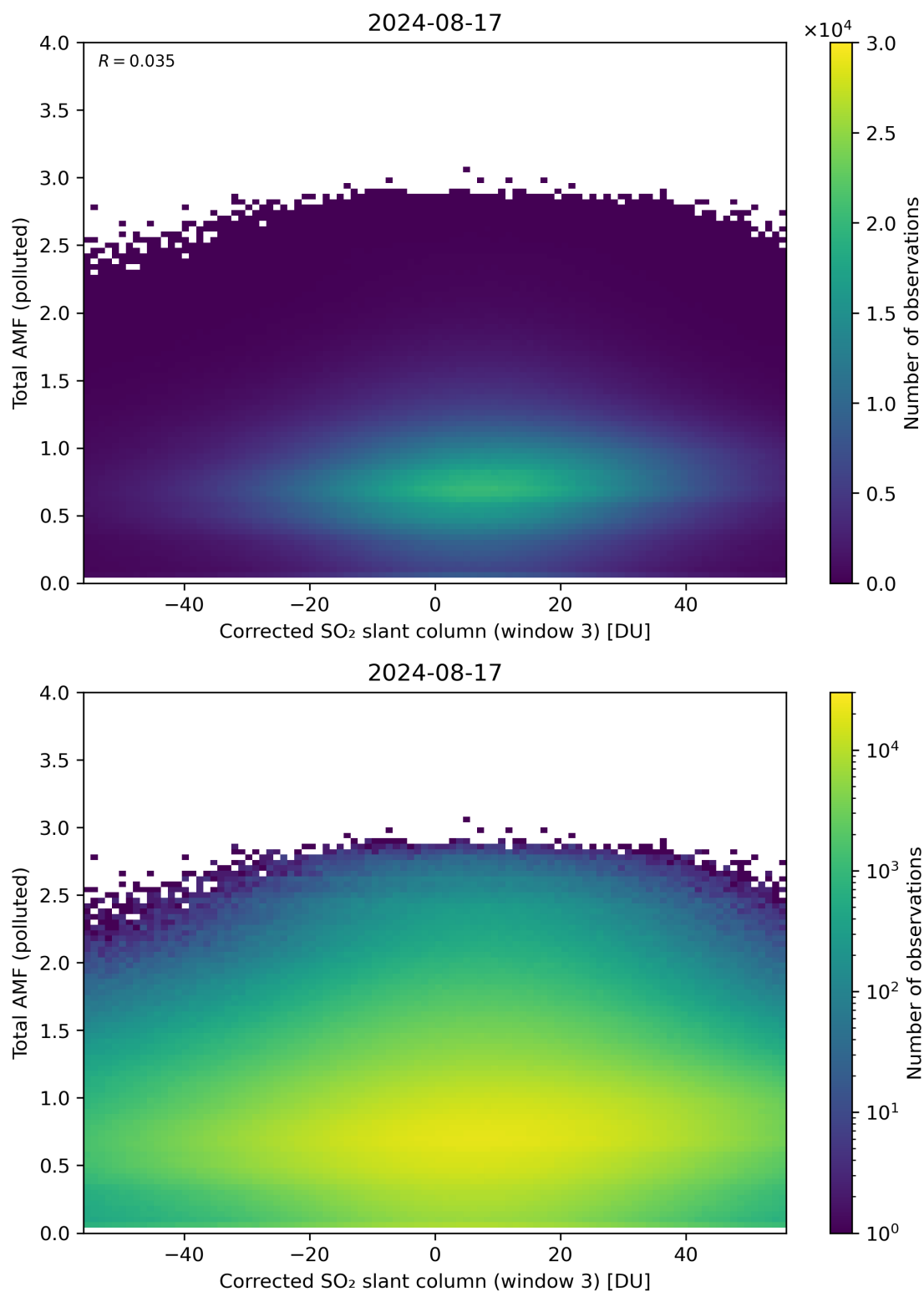
Figure 210: Scatter density plot of “Corrected SO 2 slant column (window 3)” against “Total AMF (polluted)” for 2024-08-16 to 2024-08-18.
