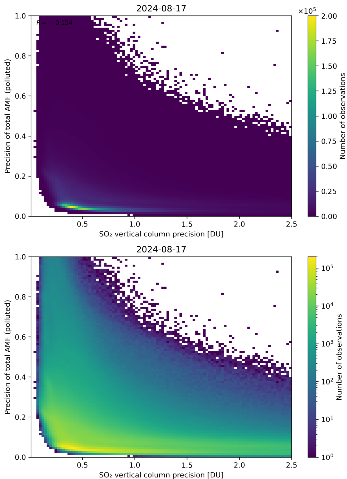
Figure 295: Scatter density plot of “SO 2 vertical column precision” against “Precision of total AMF (polluted)” for 2024-08-16 to 2024-08-18.
