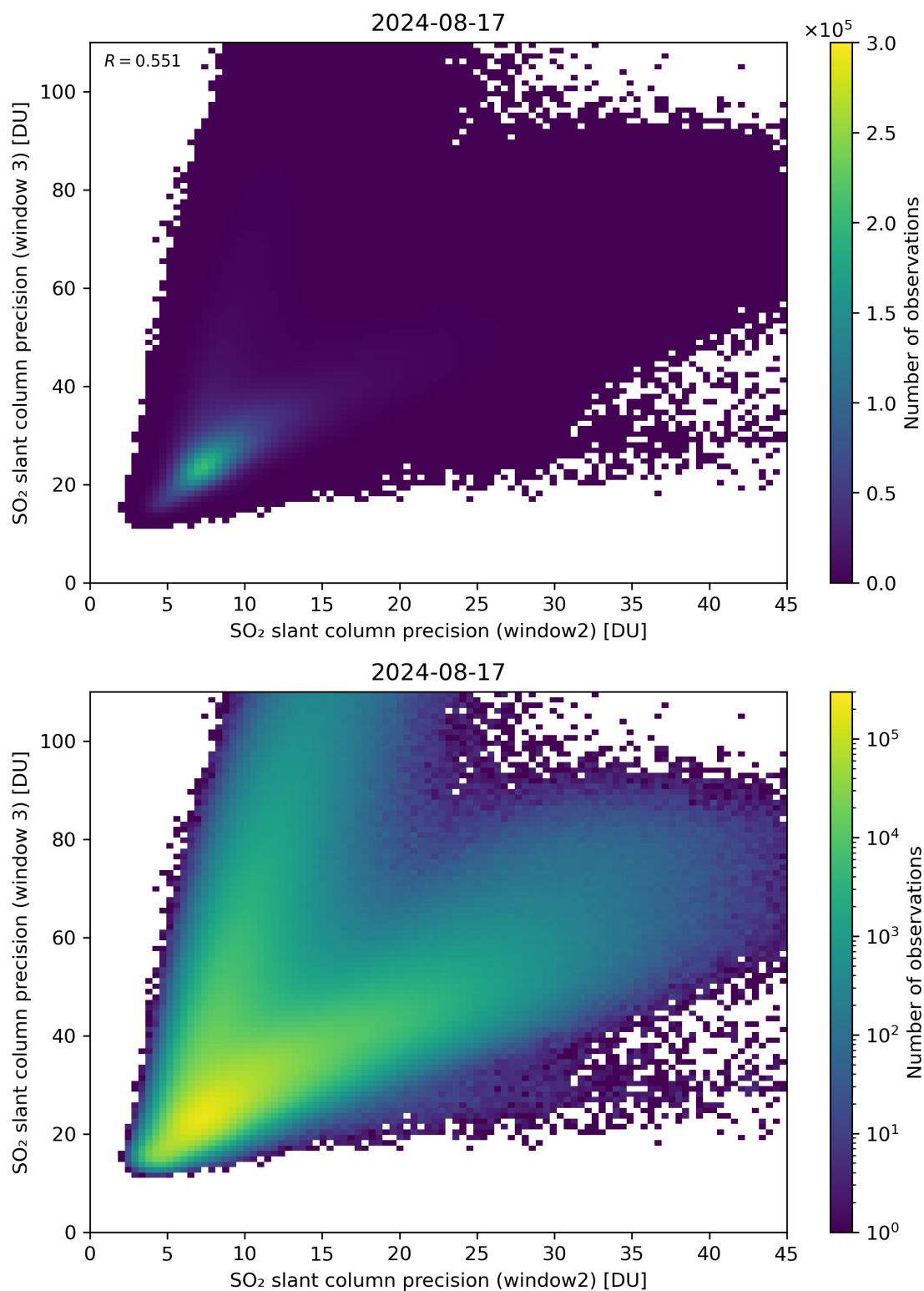
Figure 250: Scatter density plot of “SO 2 slant column precision (window2)” against “SO 2 slant column precision (window 3)” for 2024-08-16 to 2024-08-18.
