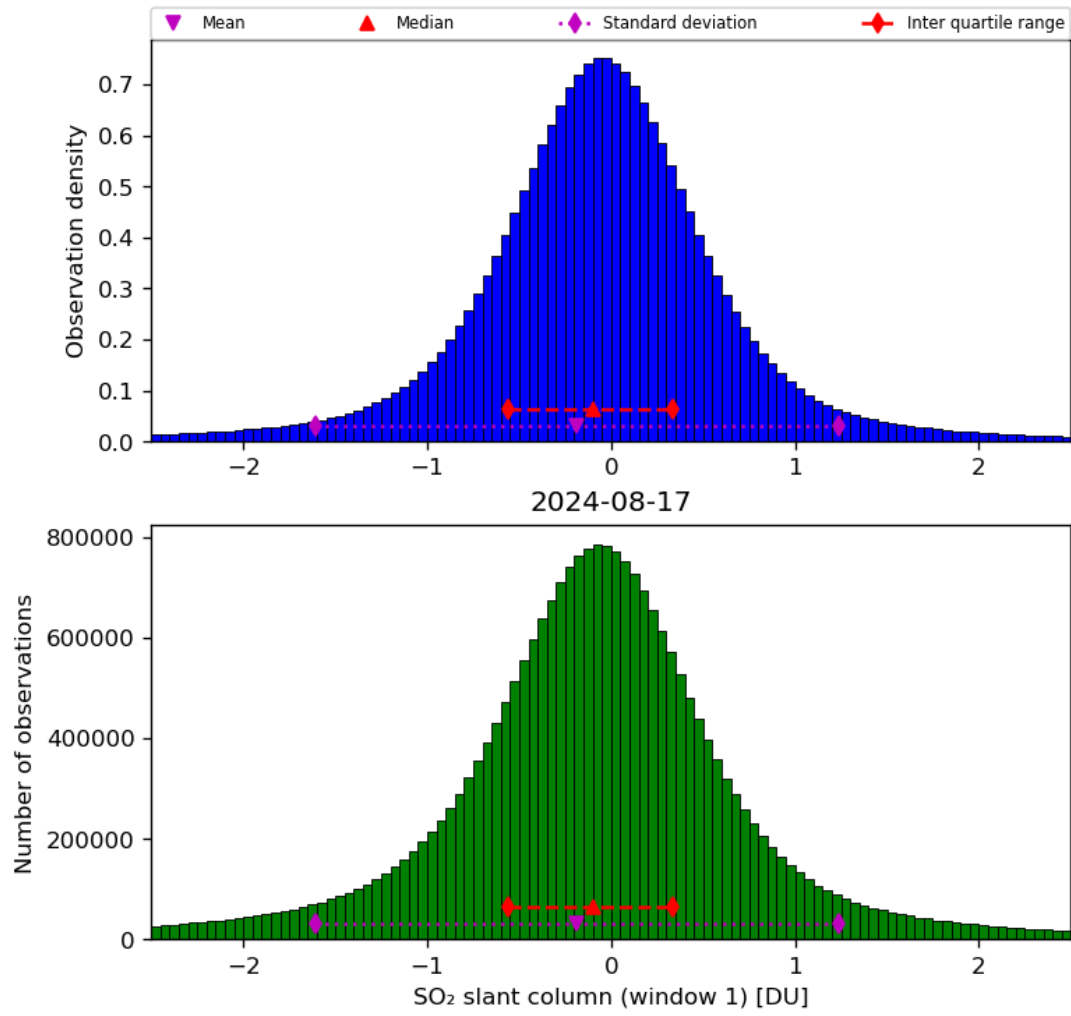
Figure 56: Histogram of “SO 2 slant column (window 1)” for 2024-08-16 to 2024-08-18
