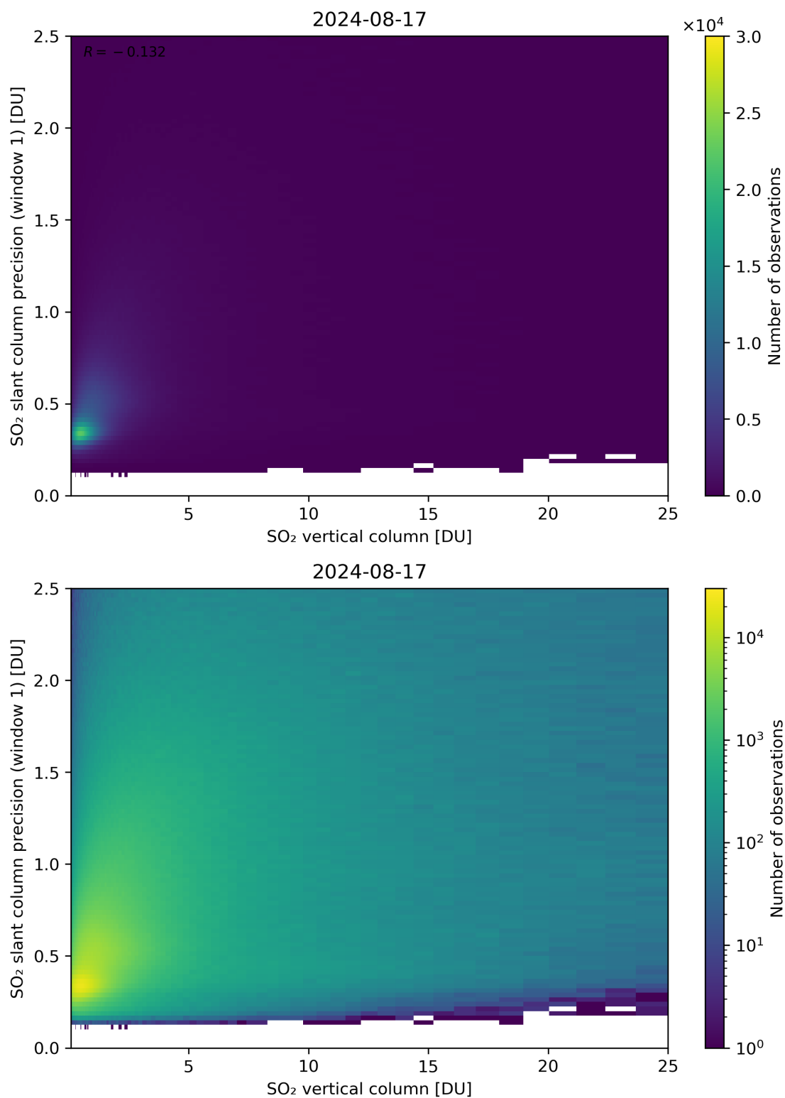
Figure 301: Scatter density plot of “SO 2 vertical column” against “SO 2 slant column precision (window 1)” for 2024-08-16 to 2024-08-18.
