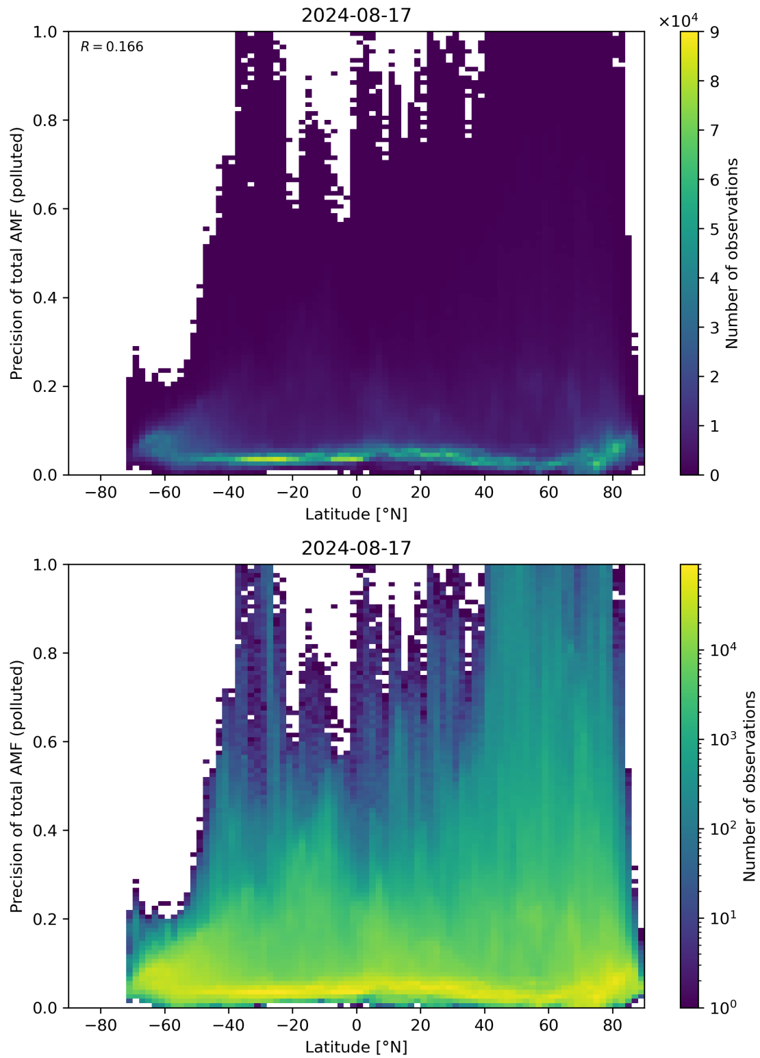
Figure 155: Scatter density plot of “Latitude” against “Precision of total AMF (polluted)” for 2024-08-16 to 2024-08-18.
