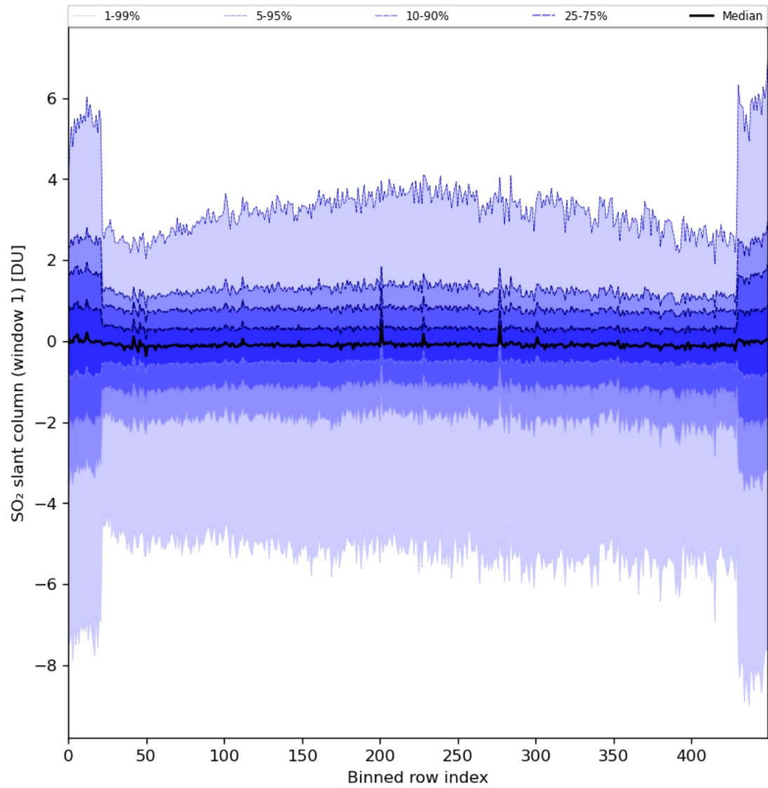
Figure 79: Along track statistics of “SO 2 slant column (window 1)” for 2024-08-16 to 2024-08-18
