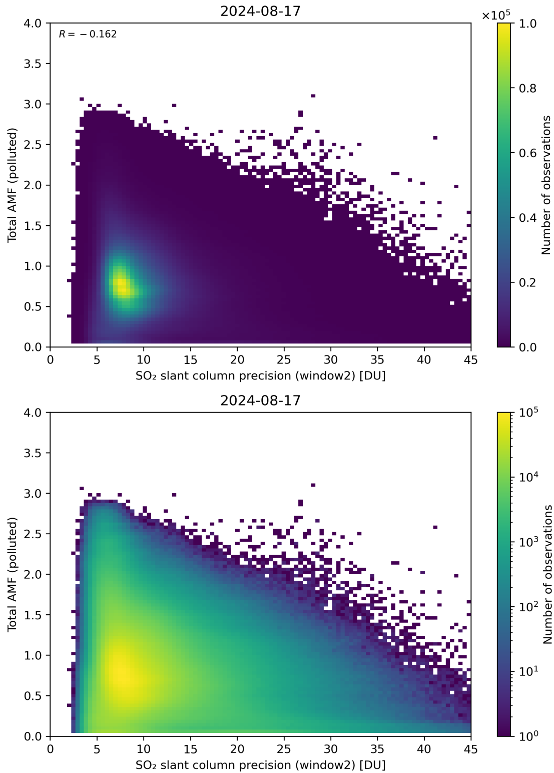
Figure 251: Scatter density plot of “SO 2 slant column precision (window2)” against “Total AMF (polluted)” for 2024-08-16 to 2024-08-18.
