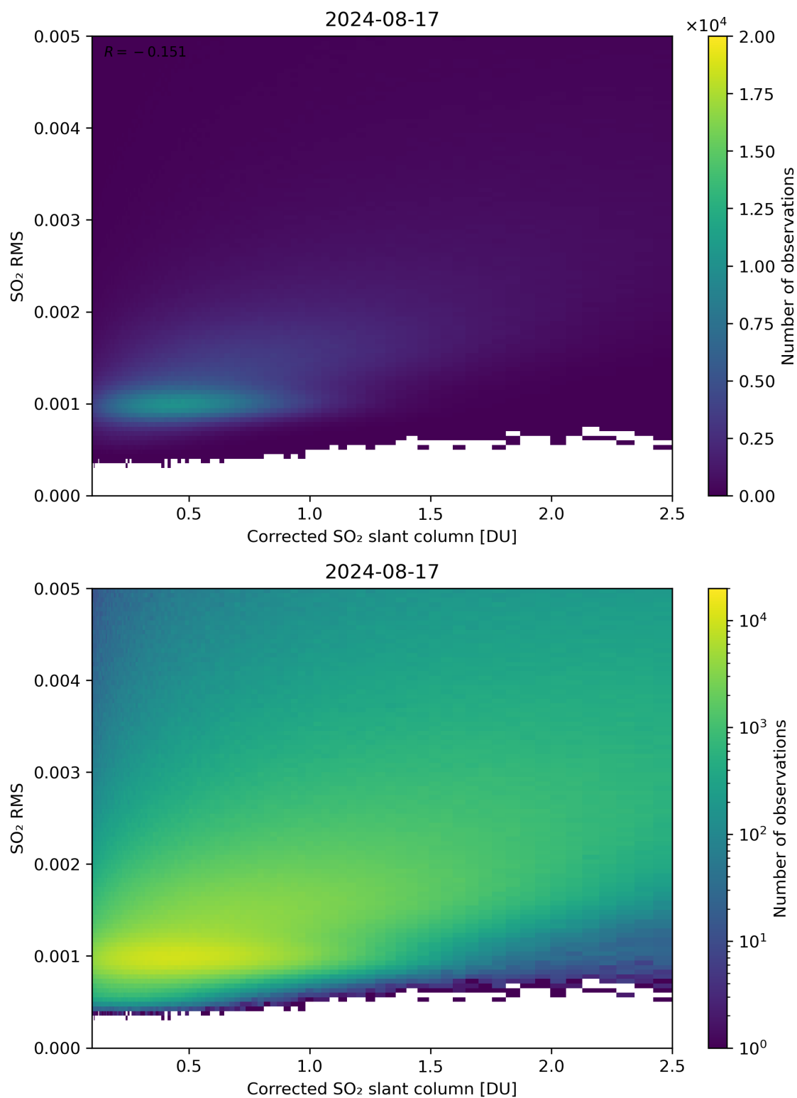
Figure 183: Scatter density plot of “Corrected SO 2 slant column” against “SO 2 RMS” for 2024-08-16 to 2024-08-18.
