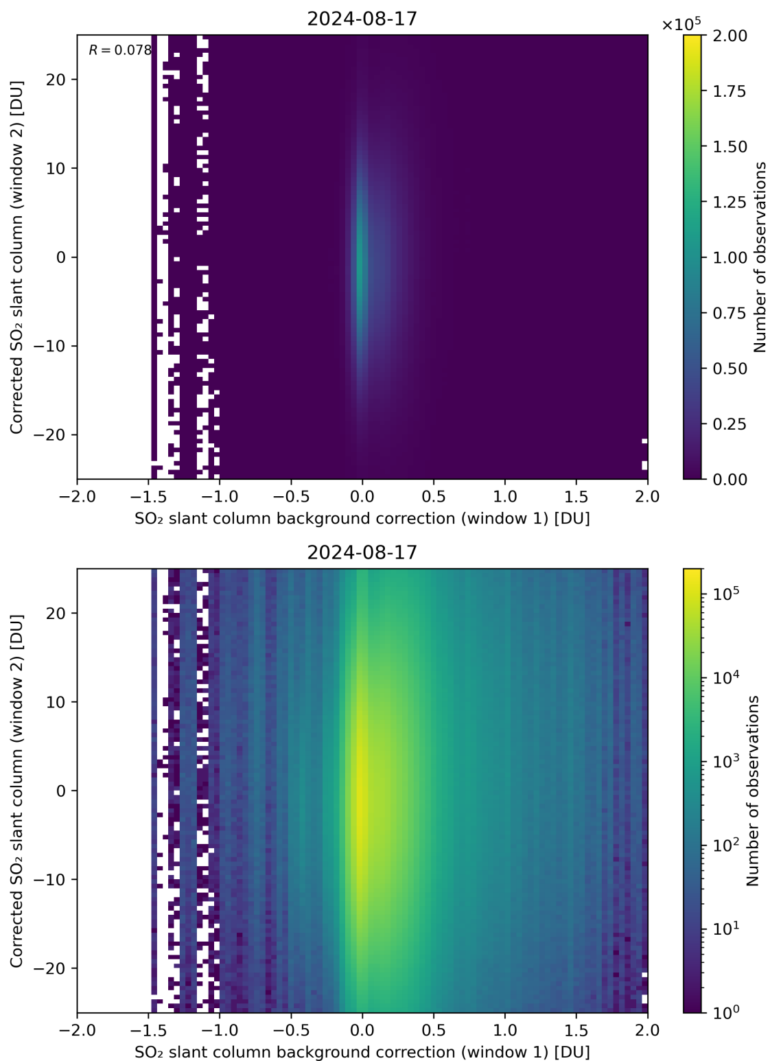
Figure 104: Scatter density plot of “SO 2 slant column background correction (window 1)” against “Corrected SO 2 slant column (window 2)” for 2024-08-16 to 2024-08-18.
