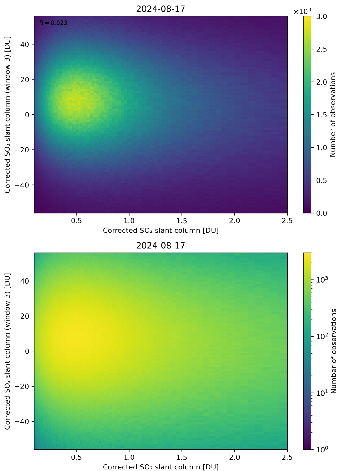
Figure 186: Scatter density plot of “Corrected SO 2 slant column” against “Corrected SO 2 slant column (window 3)” for 2024-08-16 to 2024-08-18.
