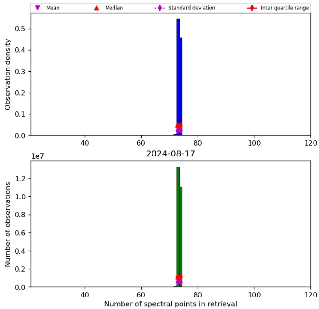
Figure 74: Histogram of “Number of spectral points in retrieval” for 2024-08-16 to 2024-08-18
