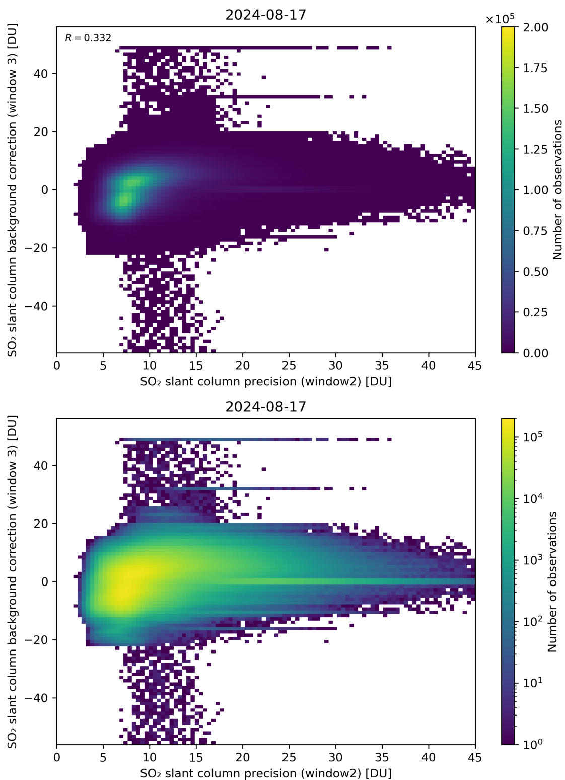
Figure 242: Scatter density plot of “SO 2 slant column precision (window2)” against “SO 2 slant column background correction (window 3)” for 2024-08-16 to 2024-08-18.
