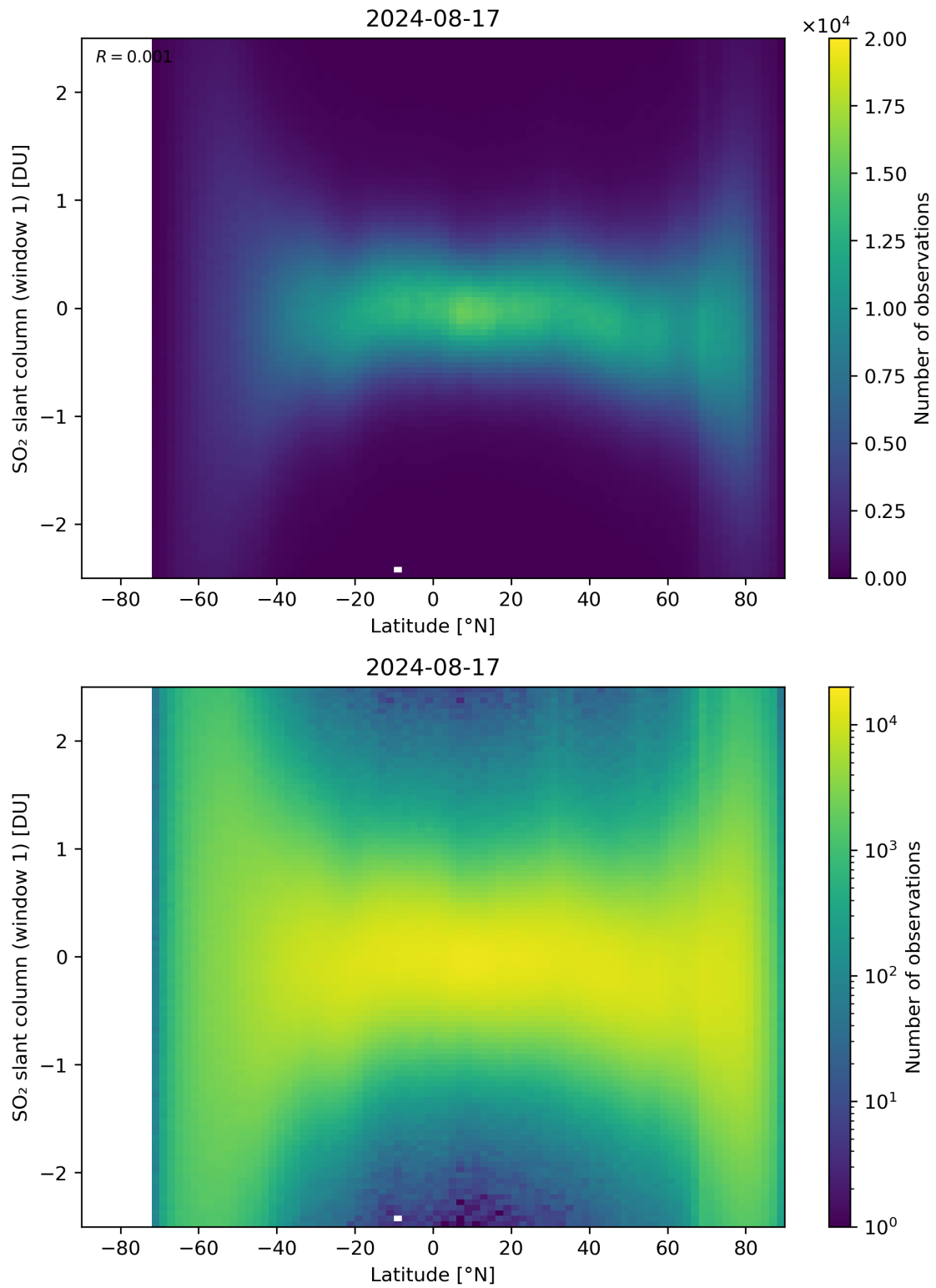
Figure 149: Scatter density plot of “Latitude” against “SO 2 slant column (window 1)” for 2024-08-16 to 2024-08-18.
