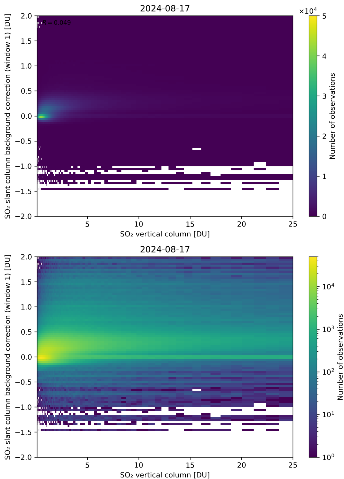
Figure 273: Scatter density plot of “SO 2 vertical column” against “SO 2 slant column background correction (window 1)” for 2024-08-16 to 2024-08-18.
