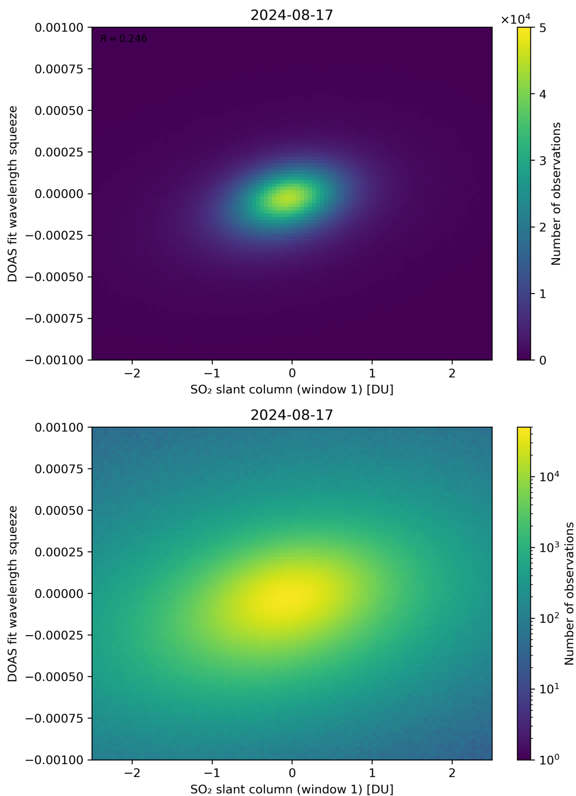
Figure 216: Scatter density plot of “SO 2 slant column (window 1)” against “DOAS fit wavelength squeeze” for 2024-08-16 to 2024-08-18.
