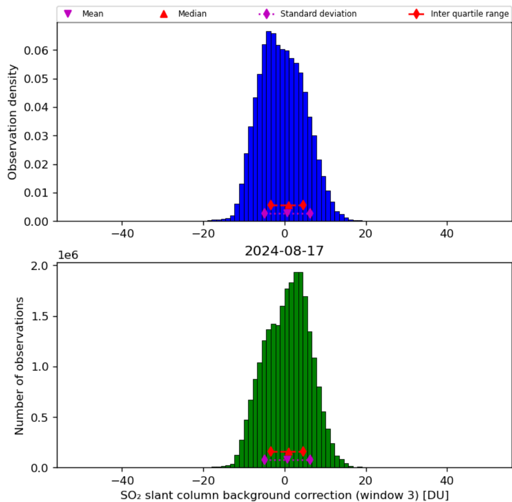
Figure 67: Histogram of “SO 2 slant column background correction (window 3)” for 2024-08-16 to 2024-08-18
