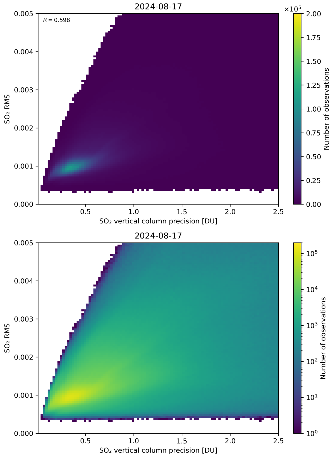
Figure 284: Scatter density plot of “SO 2 vertical column precision” against “SO 2 RMS” for 2024-08-16 to 2024-08-18.
