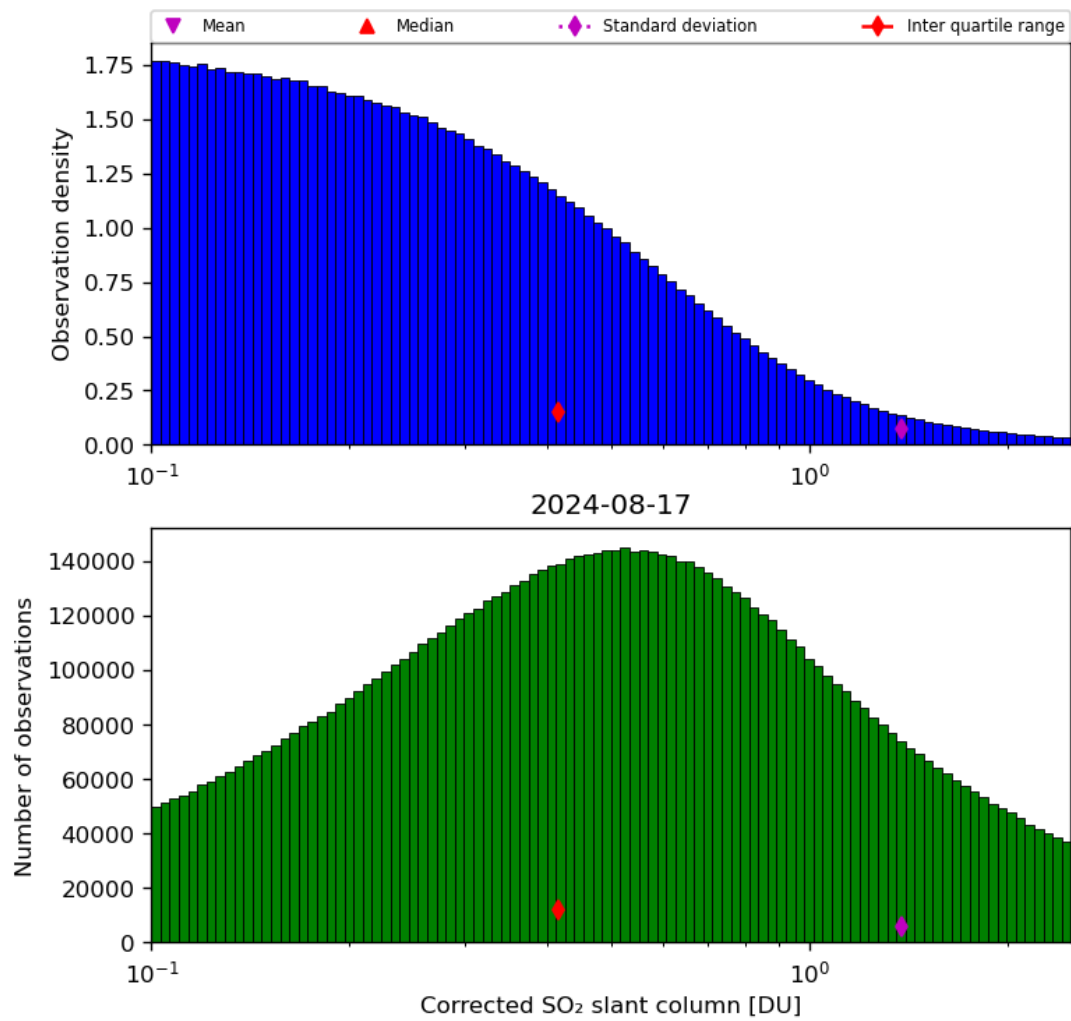
Figure 55: Histogram of “Corrected SO 2 slant column” for 2024-08-16 to 2024-08-18
