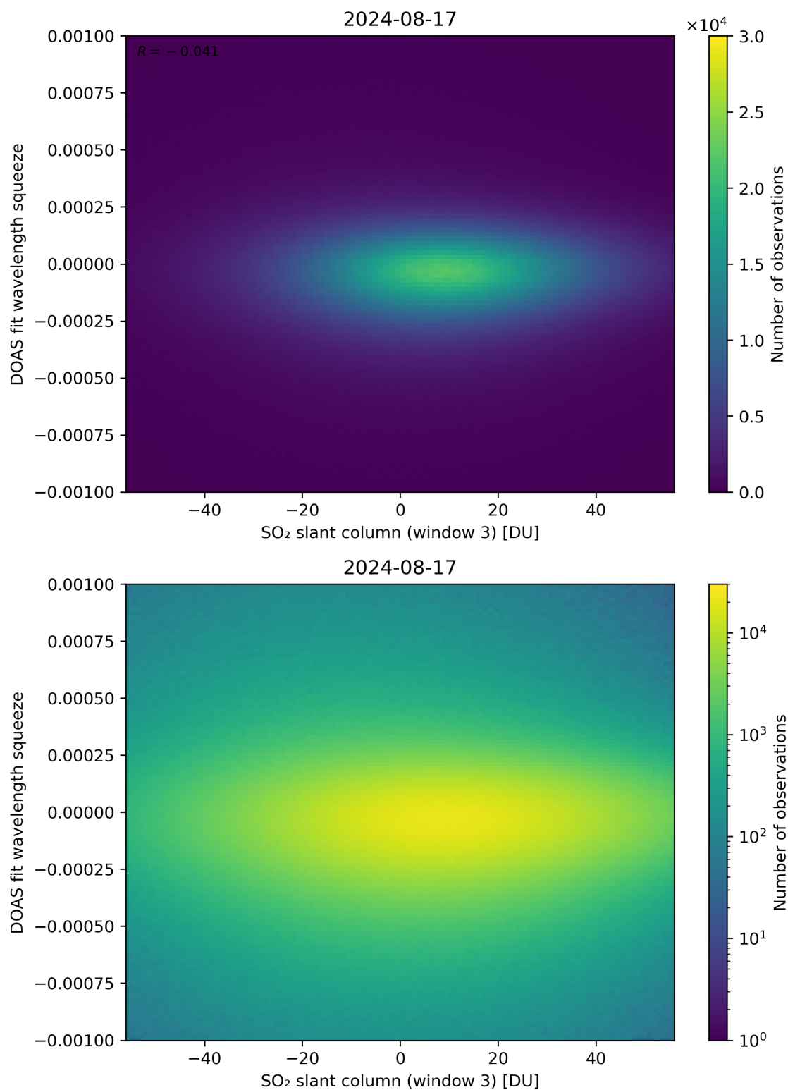
Figure 255: Scatter density plot of “SO 2 slant column (window 3)” against “DOAS fit wavelength squeeze” for 2024-08-16 to 2024-08-18.
