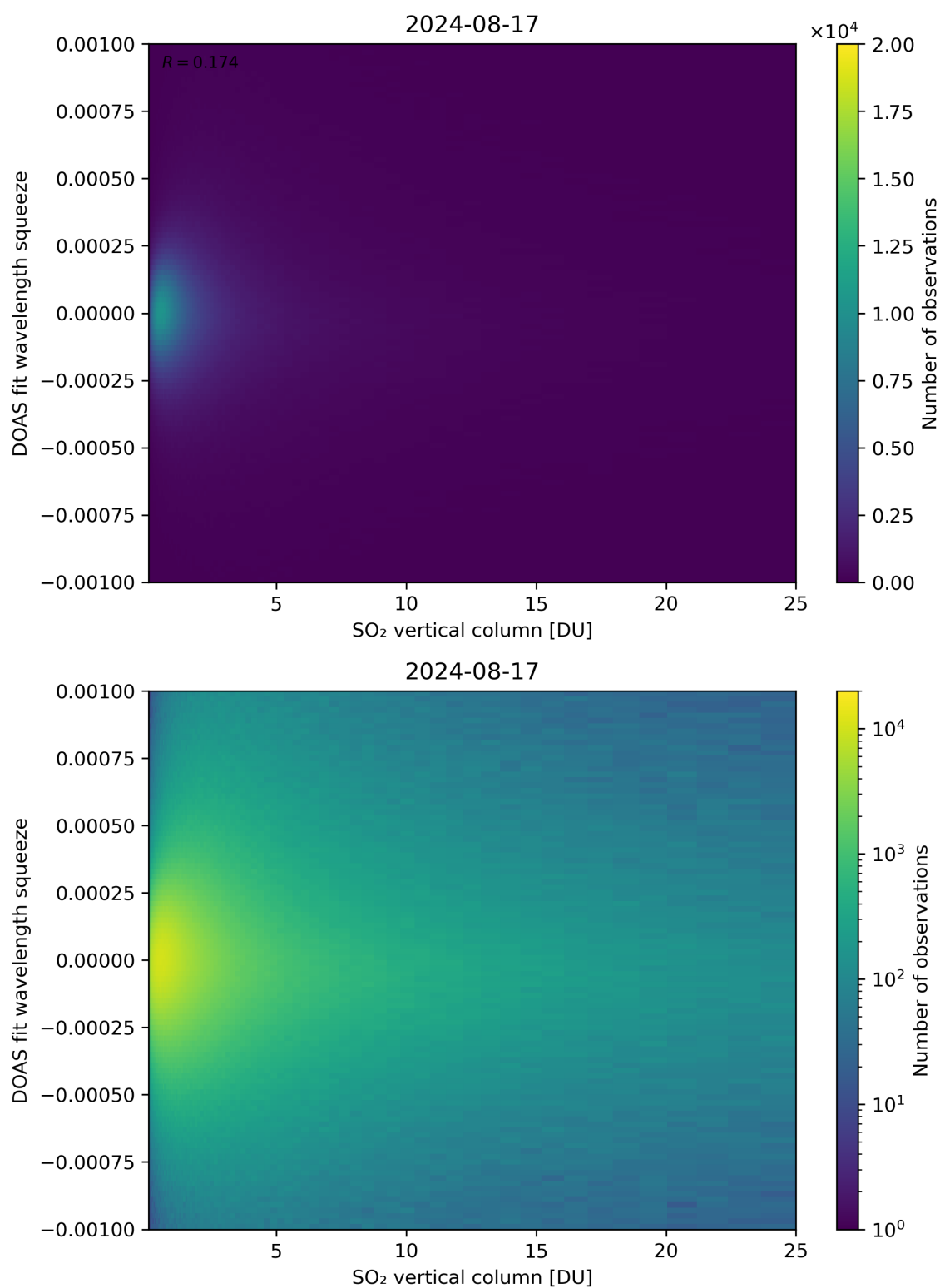
Figure 277: Scatter density plot of “SO 2 vertical column” against “DOAS fit wavelength squeeze” for 2024-08-16 to 2024-08-18.
