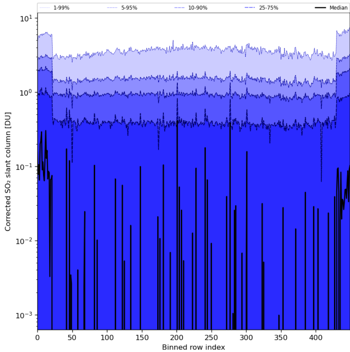
Figure 78: Along track statistics of “Corrected SO 2 slant column” for 2024-08-16 to 2024-08-18
