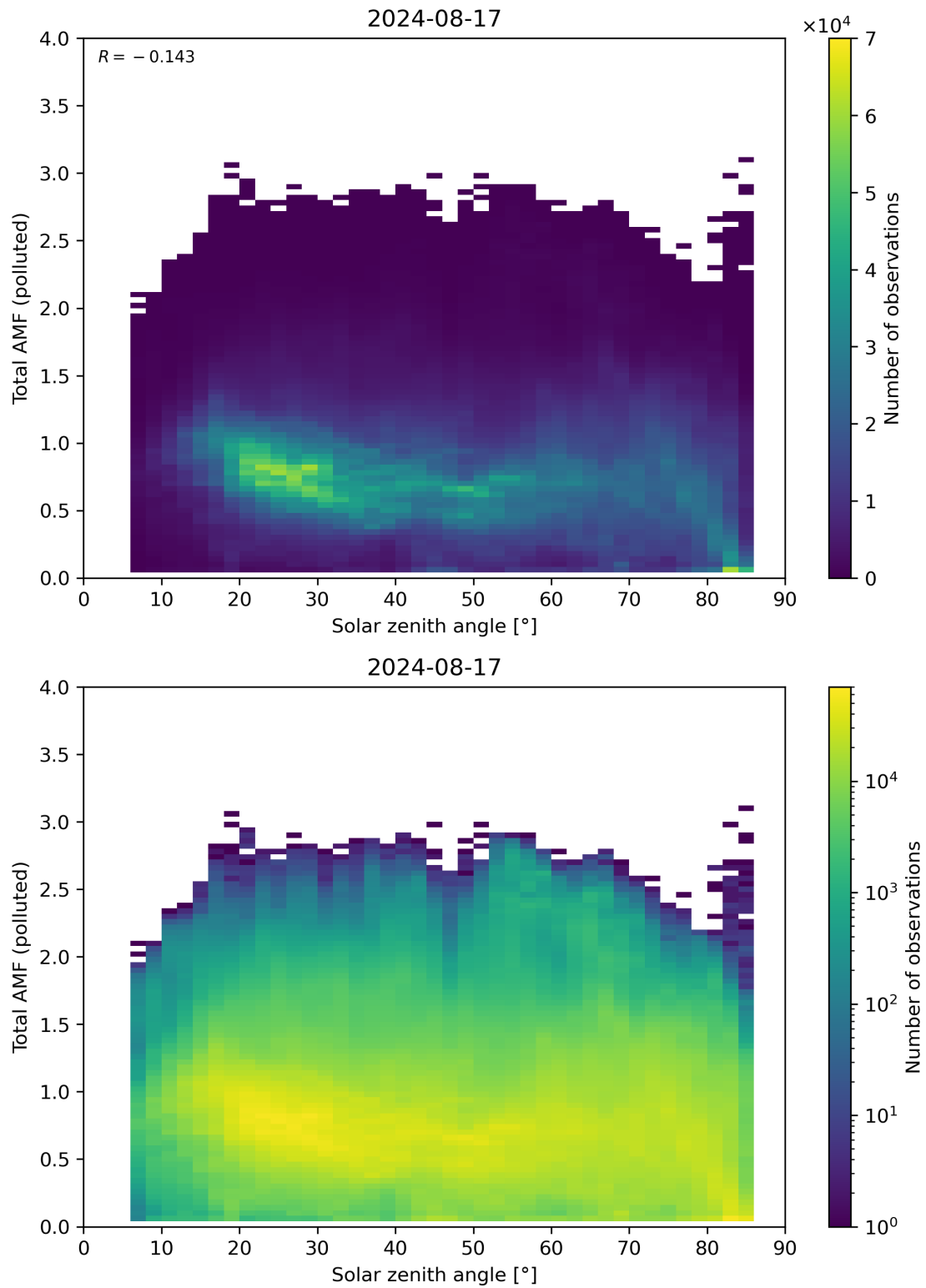
Figure 174: Scatter density plot of “Solar zenith angle” against “Total AMF (polluted)” for 2024-08-16 to 2024-08-18.
