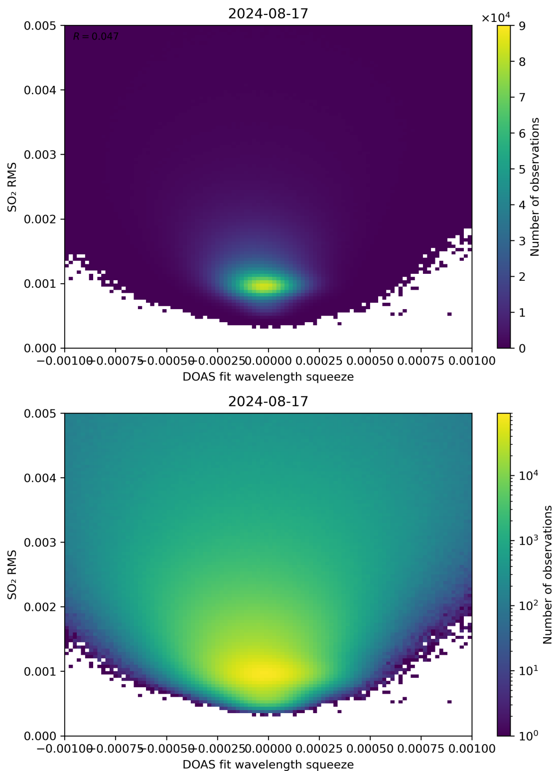
Figure 132: Scatter density plot of “DOAS fit wavelength squeeze” against “SO 2 RMS” for 2024-08-16 to 2024-08-18.
