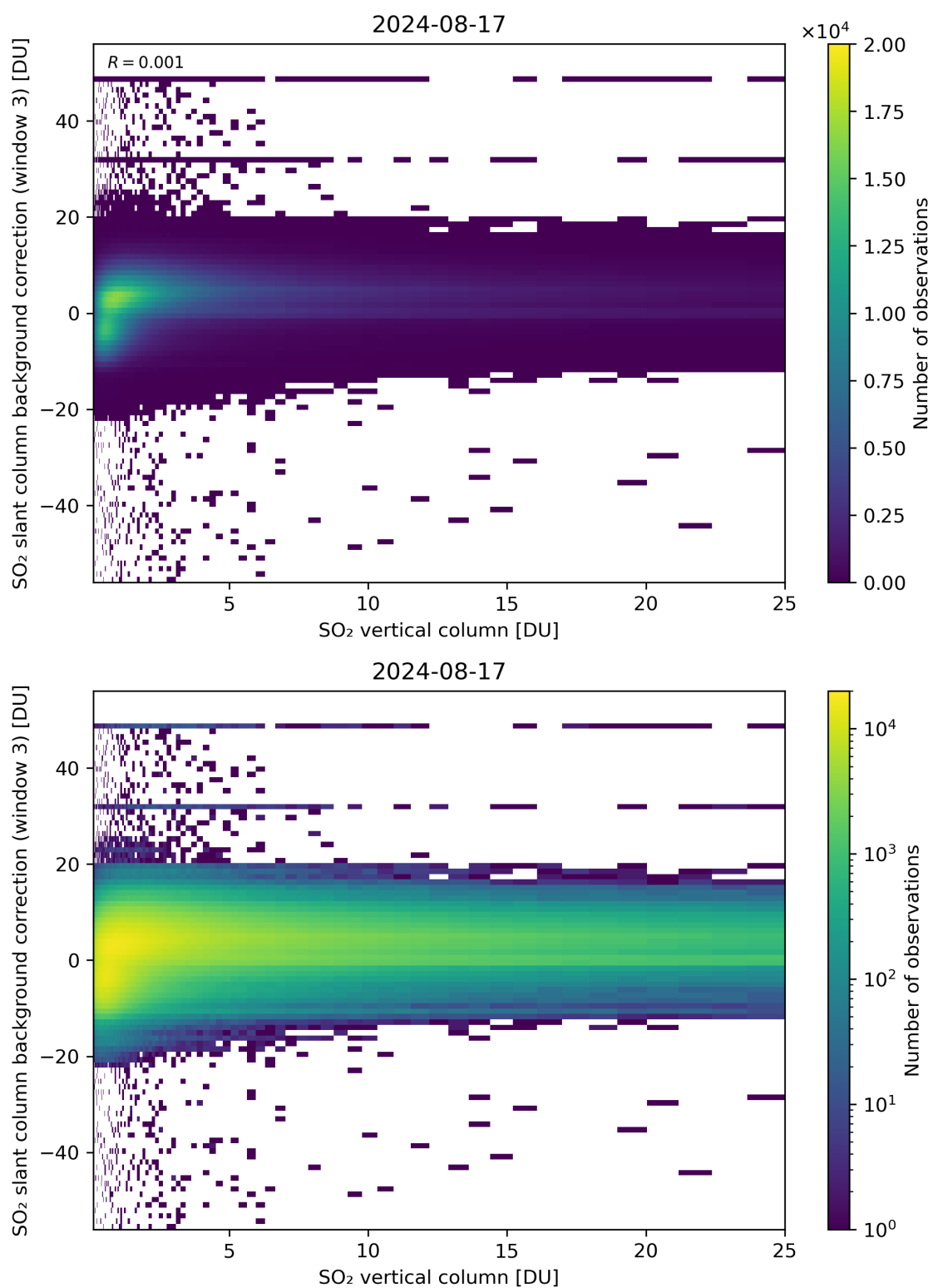
Figure 275: Scatter density plot of “SO 2 vertical column” against “SO 2 slant column background correction (window 3)” for 2024-08-16 to 2024-08-18.
