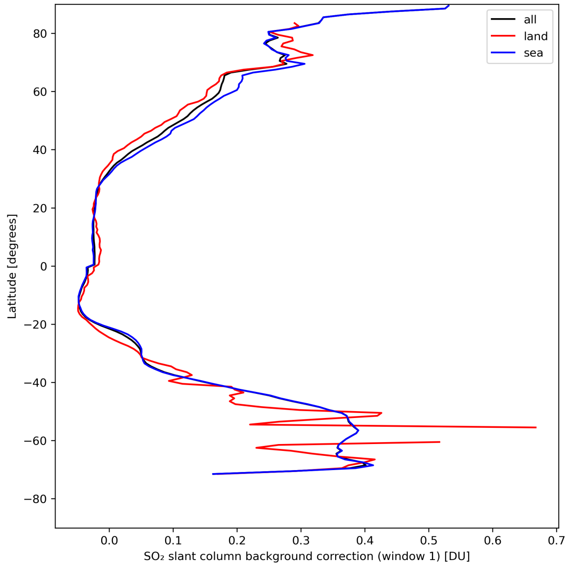
Figure 36: Zonal average of “SO 2 slant column background correction (window 1)” for 2024-08-16 to 2024-08-18.
