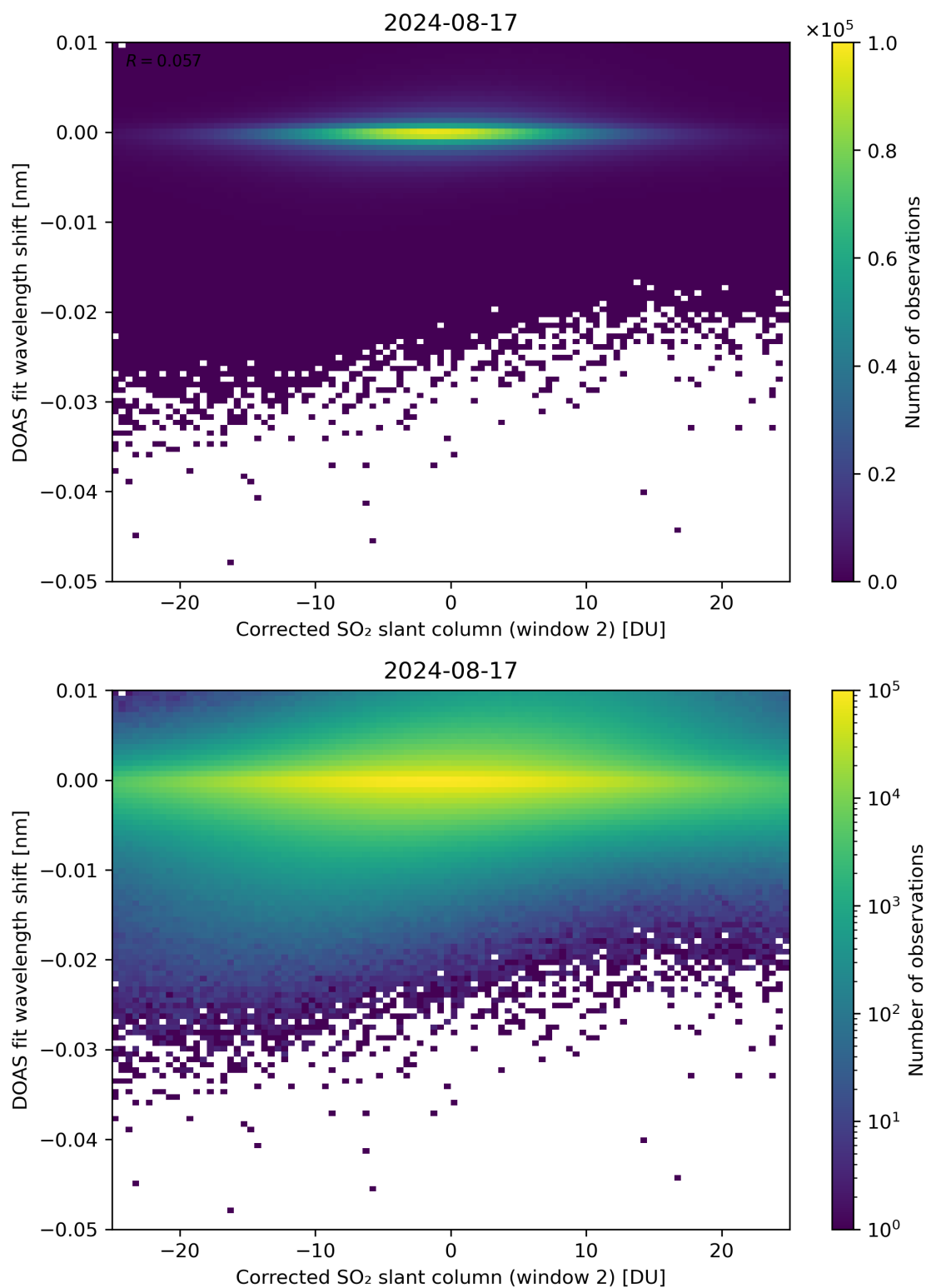
Figure 196: Scatter density plot of “Corrected SO 2 slant column (window 2)” against “DOAS fit wavelength shift” for 2024-08-16 to 2024-08-18.
