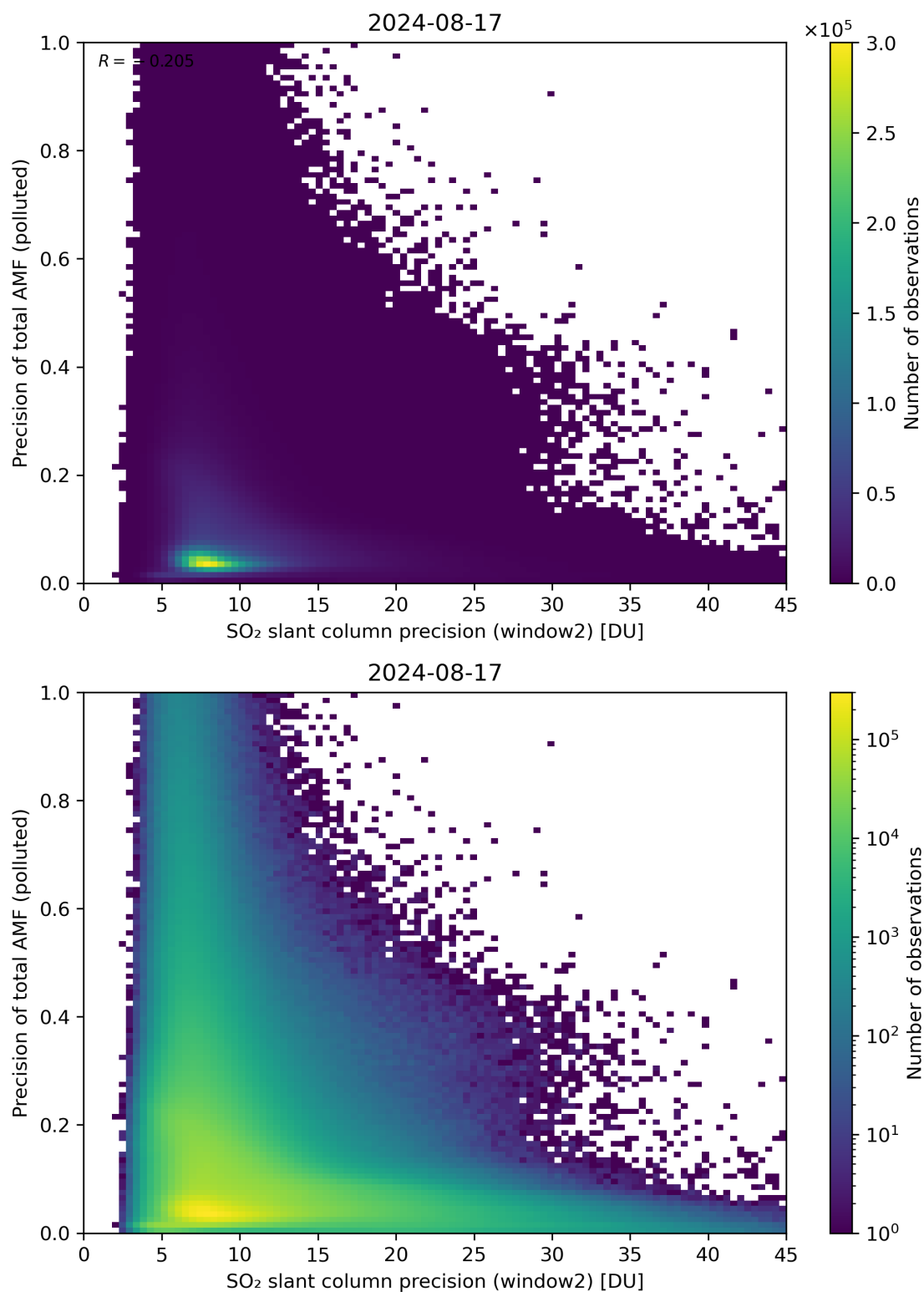
Figure 252: Scatter density plot of “SO 2 slant column precision (window2)” against “Precision of total AMF (polluted)” for 2024-08-16 to 2024-08-18.
