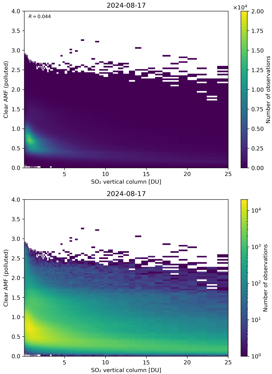
Figure 296: Scatter density plot of “SO 2 vertical column” against “Clear AMF (polluted)” for 2024-08-16 to 2024-08-18.
