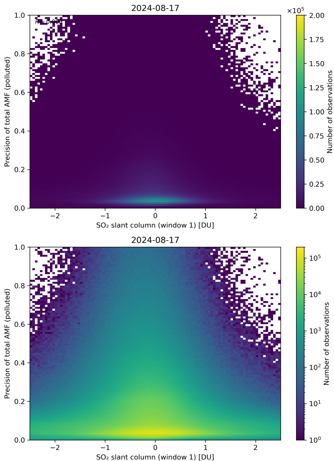
Figure 240: Scatter density plot of “SO 2 slant column (window 1)” against “Precision of total AMF (polluted)” for 2024-08-16 to 2024-08-18.
