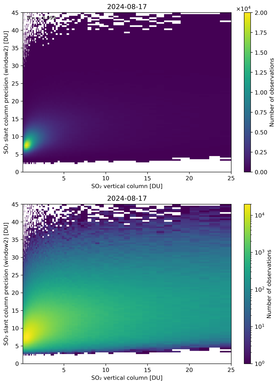
Figure 302: Scatter density plot of “SO 2 vertical column” against “SO 2 slant column precision (window2)” for 2024-08-16 to 2024-08-18.
