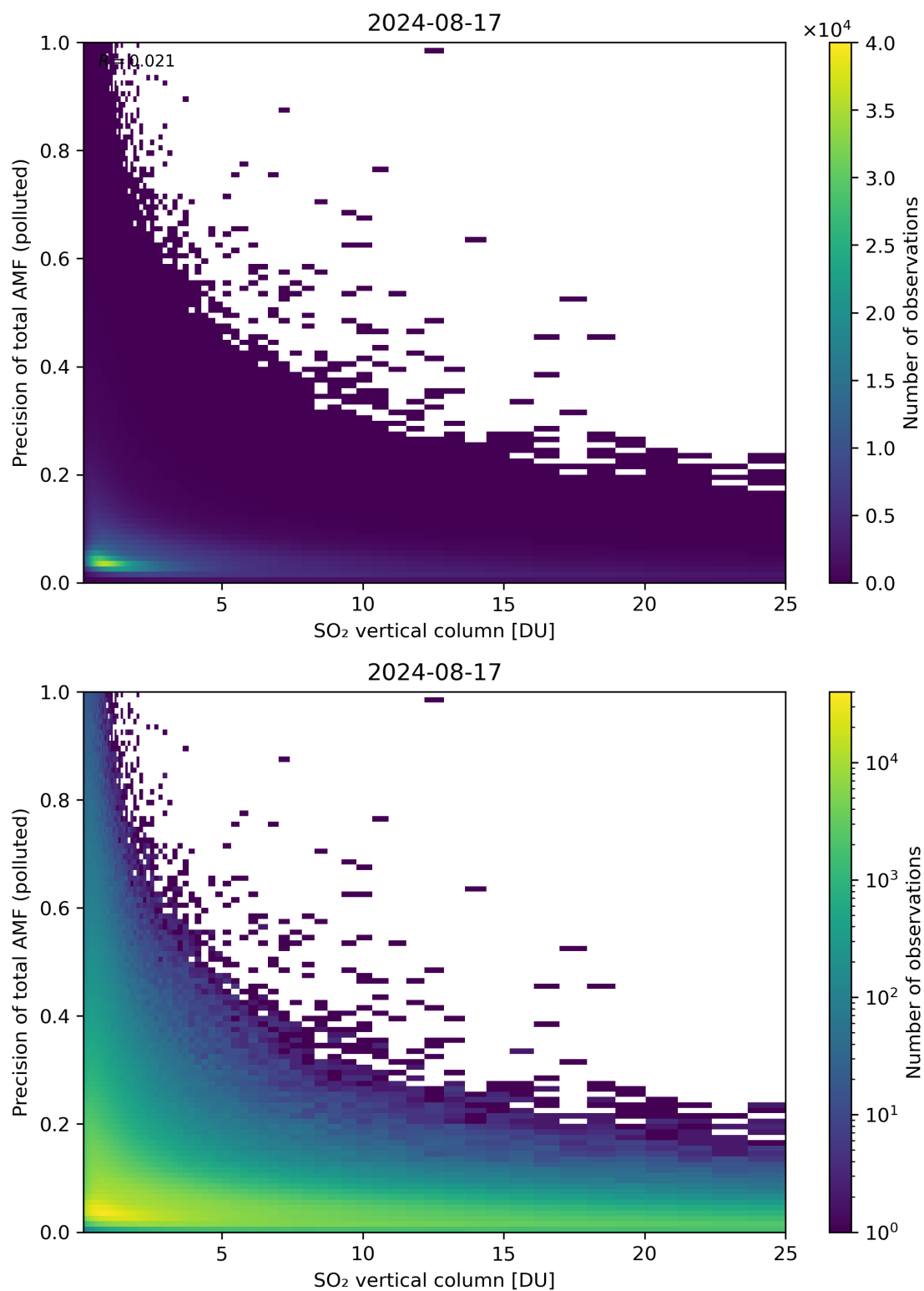
Figure 306: Scatter density plot of “SO 2 vertical column” against “Precision of total AMF (polluted)” for 2024-08-16 to 2024-08-18.
