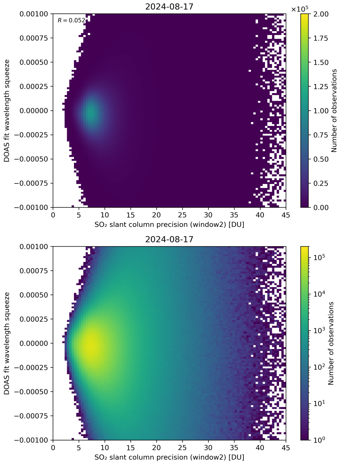
Figure 244: Scatter density plot of “SO 2 slant column precision (window2)” against “DOAS fit wavelength squeeze” for 2024-08-16 to 2024-08-18.
