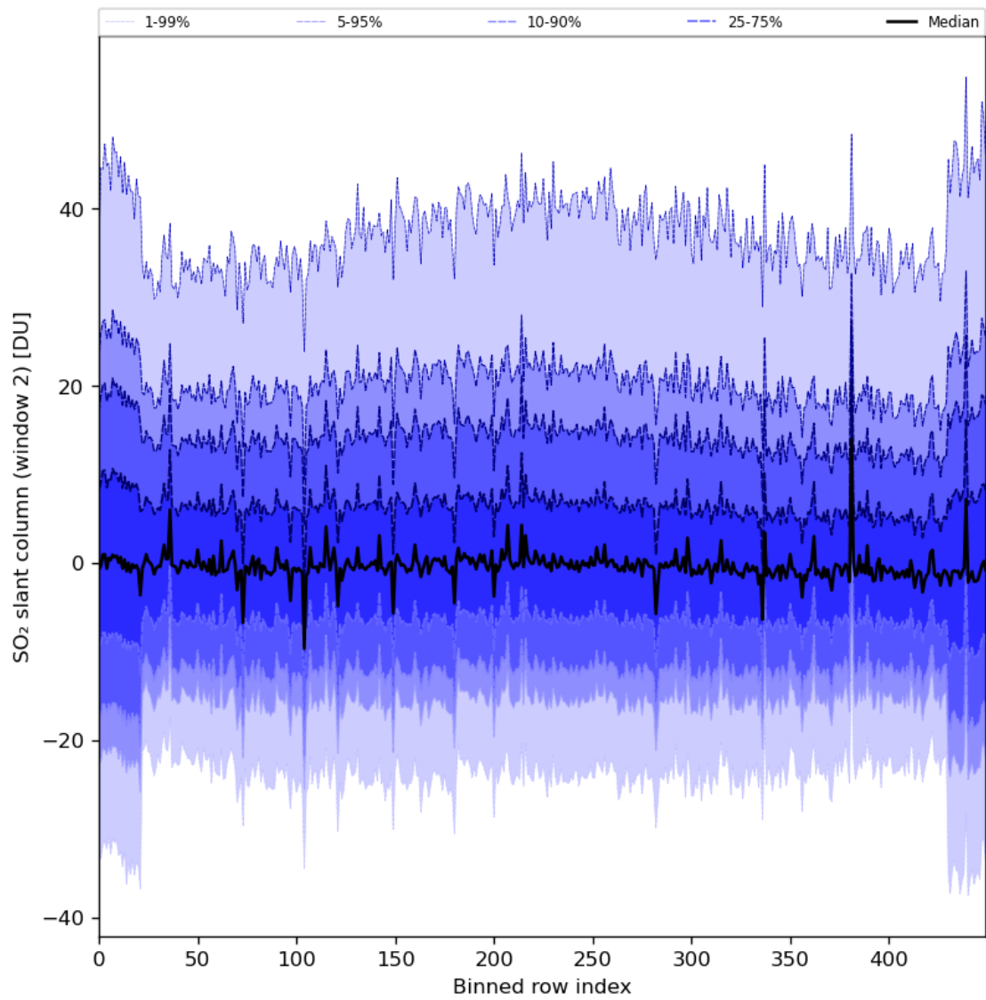
Figure 83: Along track statistics of “SO 2 slant column (window 2)” for 2024-08-16 to 2024-08-18
