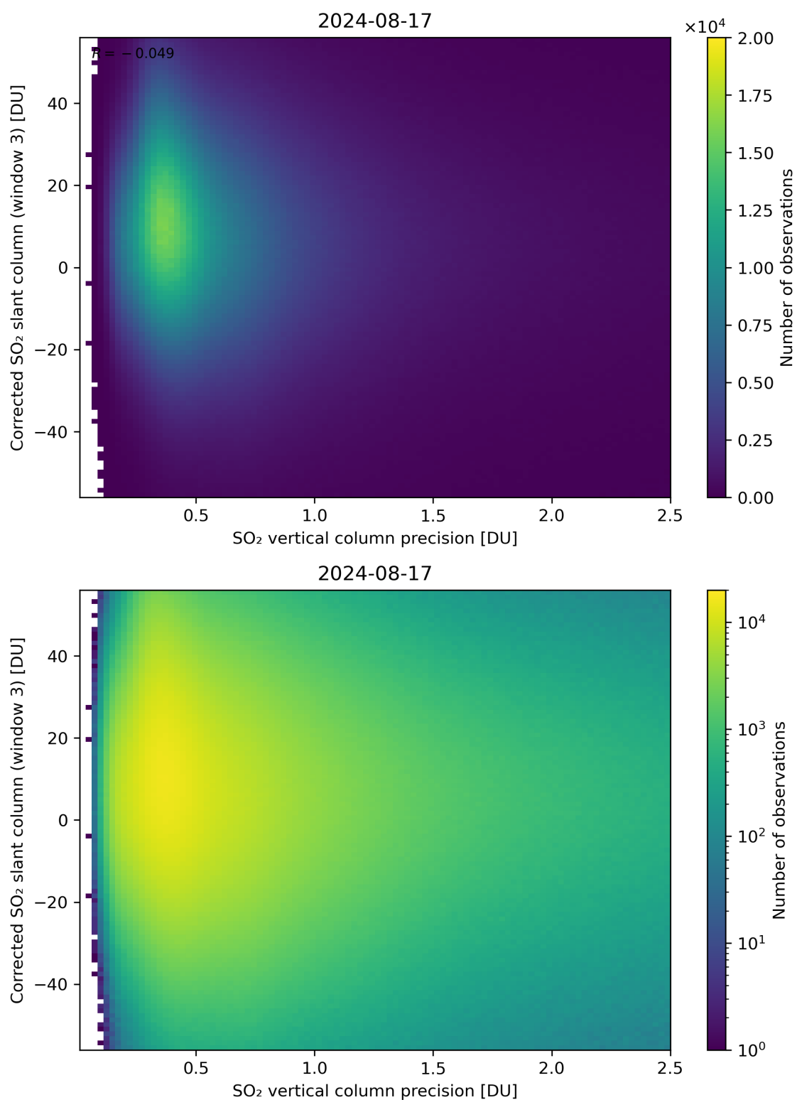
Figure 288: Scatter density plot of “SO 2 vertical column precision” against “Corrected SO 2 slant column (window 3)” for 2024-08-16 to 2024-08-18.
