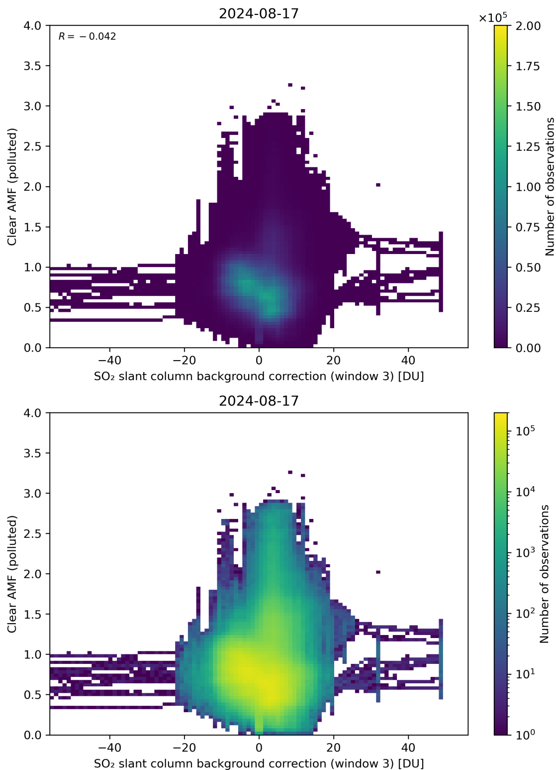
Figure 124: Scatter density plot of “SO 2 slant column background correction (window 3)” against “Clear AMF (polluted)” for 2024-08-16 to 2024-08-18.
