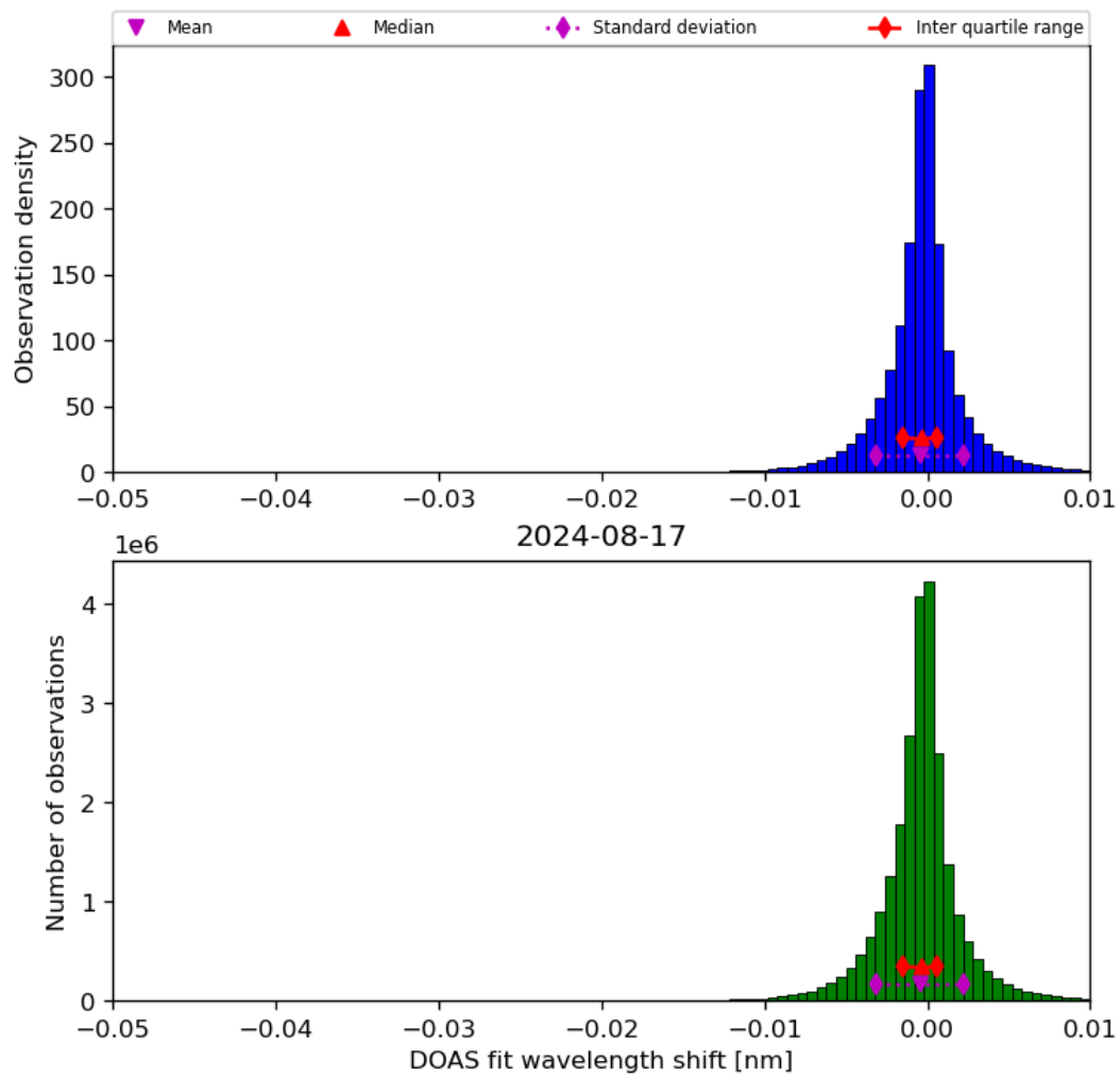
Figure 68: Histogram of “DOAS fit wavelength shift” for 2024-08-16 to 2024-08-18
