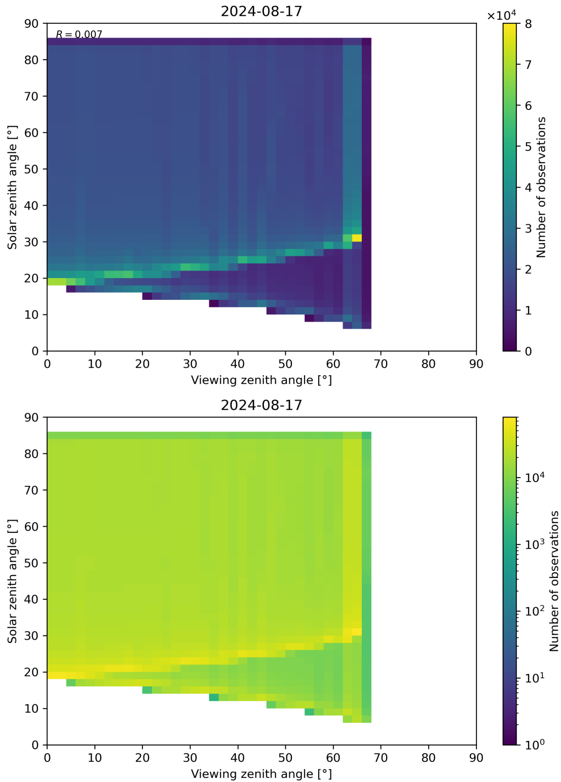
Figure 315: Scatter density plot of “Viewing zenith angle” against “Solar zenith angle” for 2024-08-16 to 2024-08-18.
