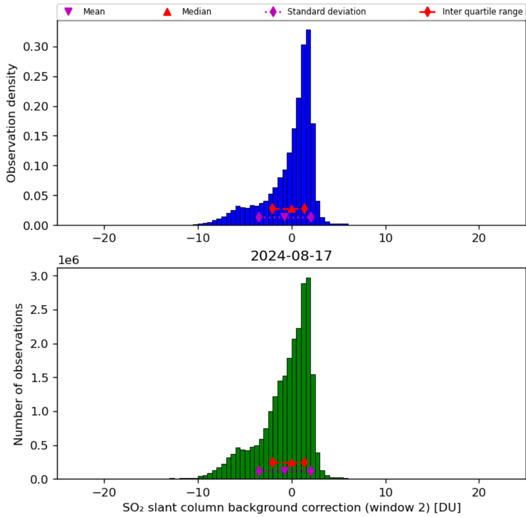
Figure 63: Histogram of “SO 2 slant column background correction (window 2)” for 2024-08-16 to 2024-08-18
