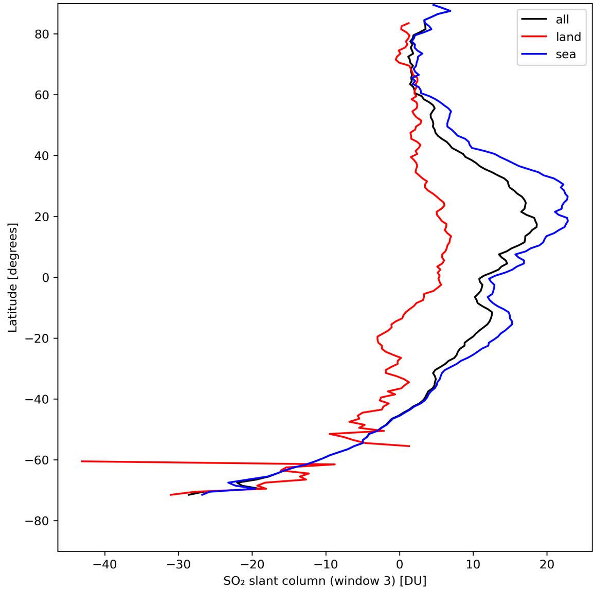
Figure 41: Zonal average of “SO 2 slant column (window 3)” for 2024-08-16 to 2024-08-18.
