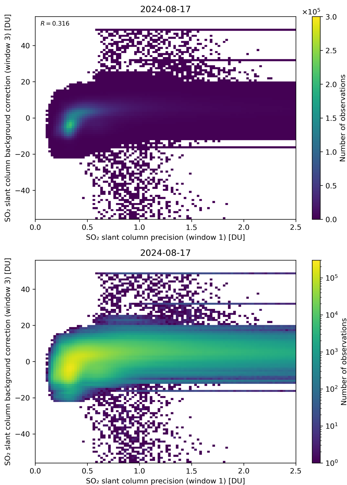
Figure 220: Scatter density plot of “SO 2 slant column precision (window 1)” against “SO 2 slant column background correction (window 3)” for 2024-08-16 to 2024-08-18.
