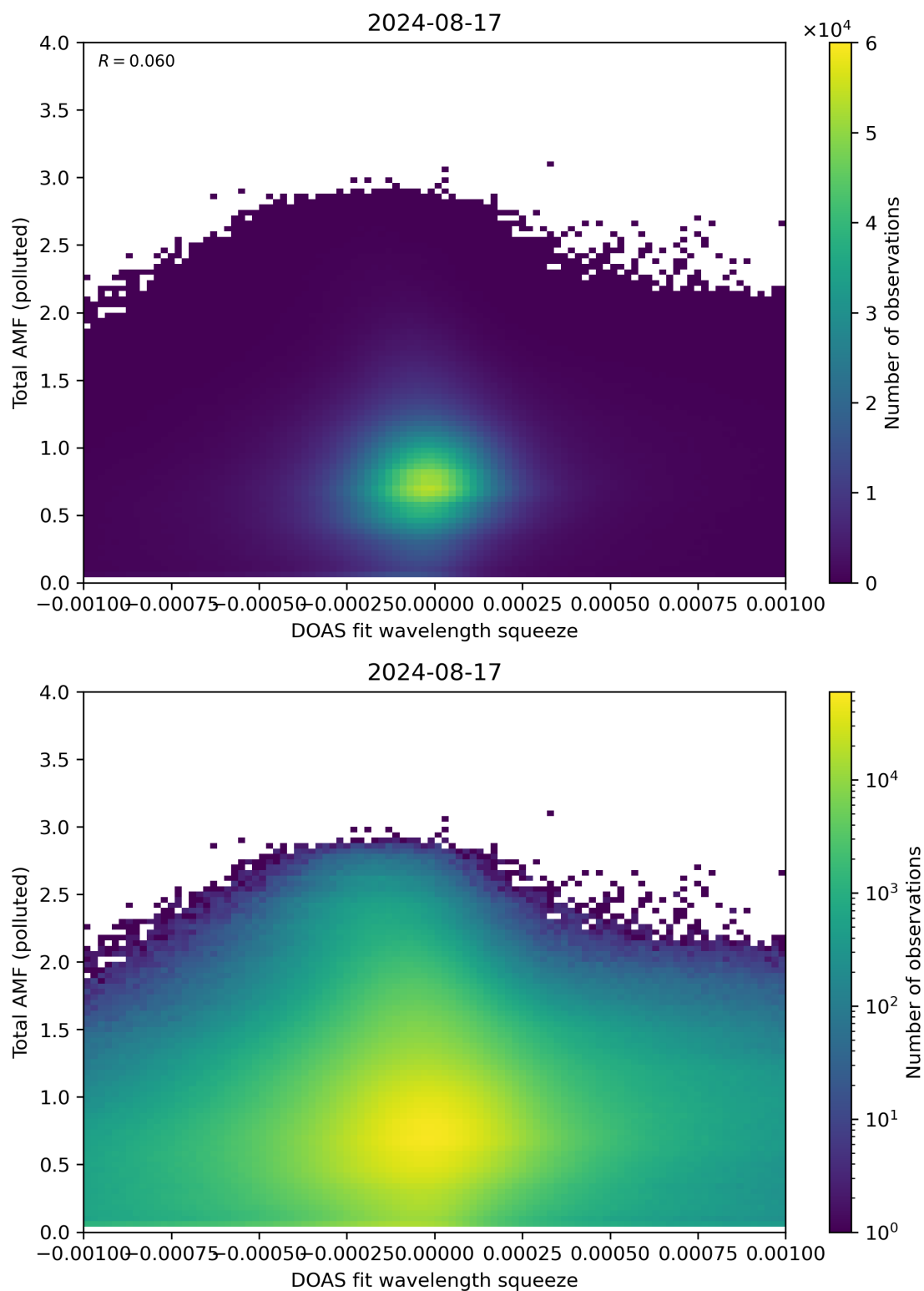
Figure 134: Scatter density plot of “DOAS fit wavelength squeeze” against “Total AMF (polluted)” for 2024-08-16 to 2024-08-18.
