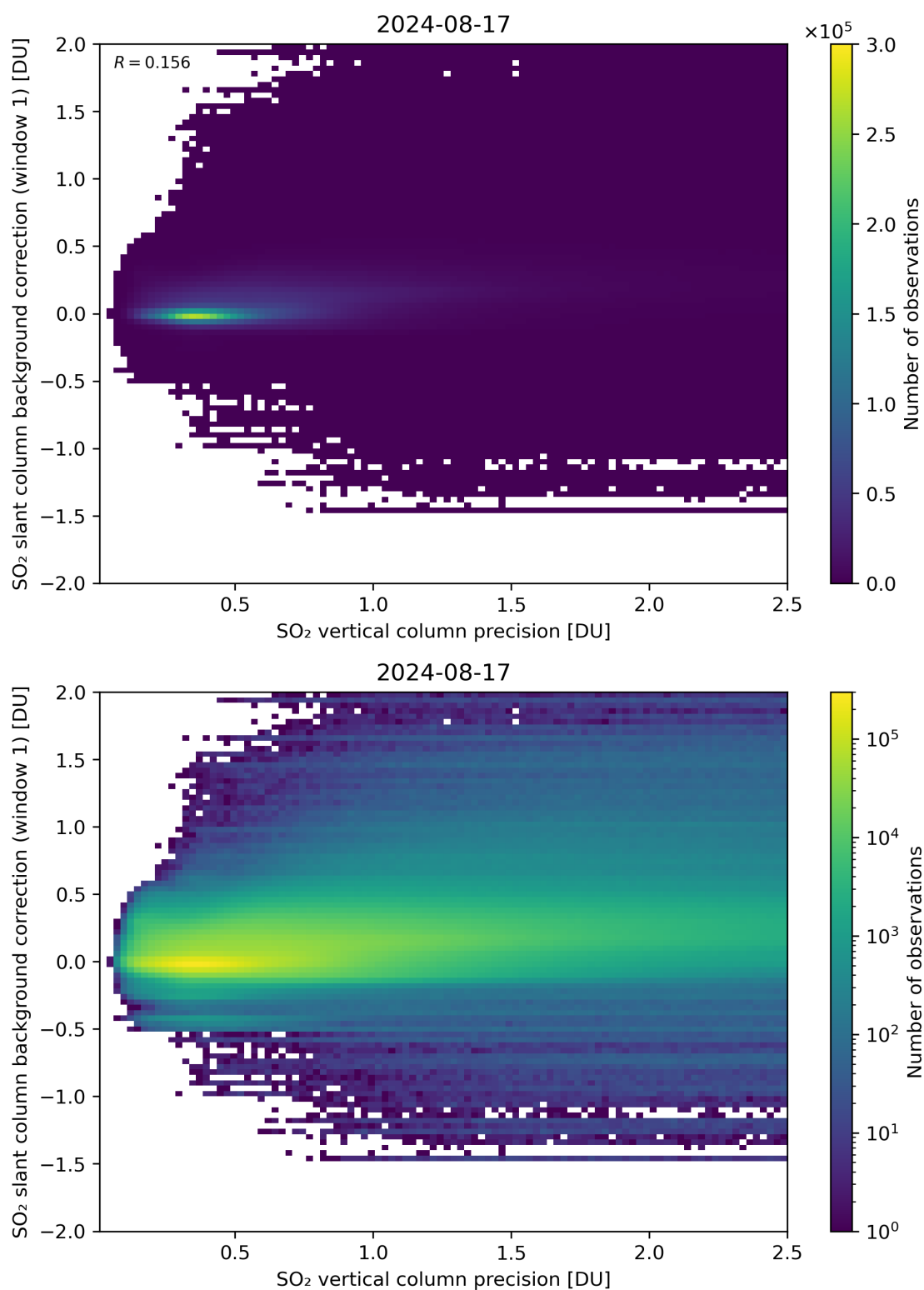
Figure 279: Scatter density plot of “SO 2 vertical column precision” against “SO 2 slant column background correction (window 1)” for 2024-08-16 to 2024-08-18.
