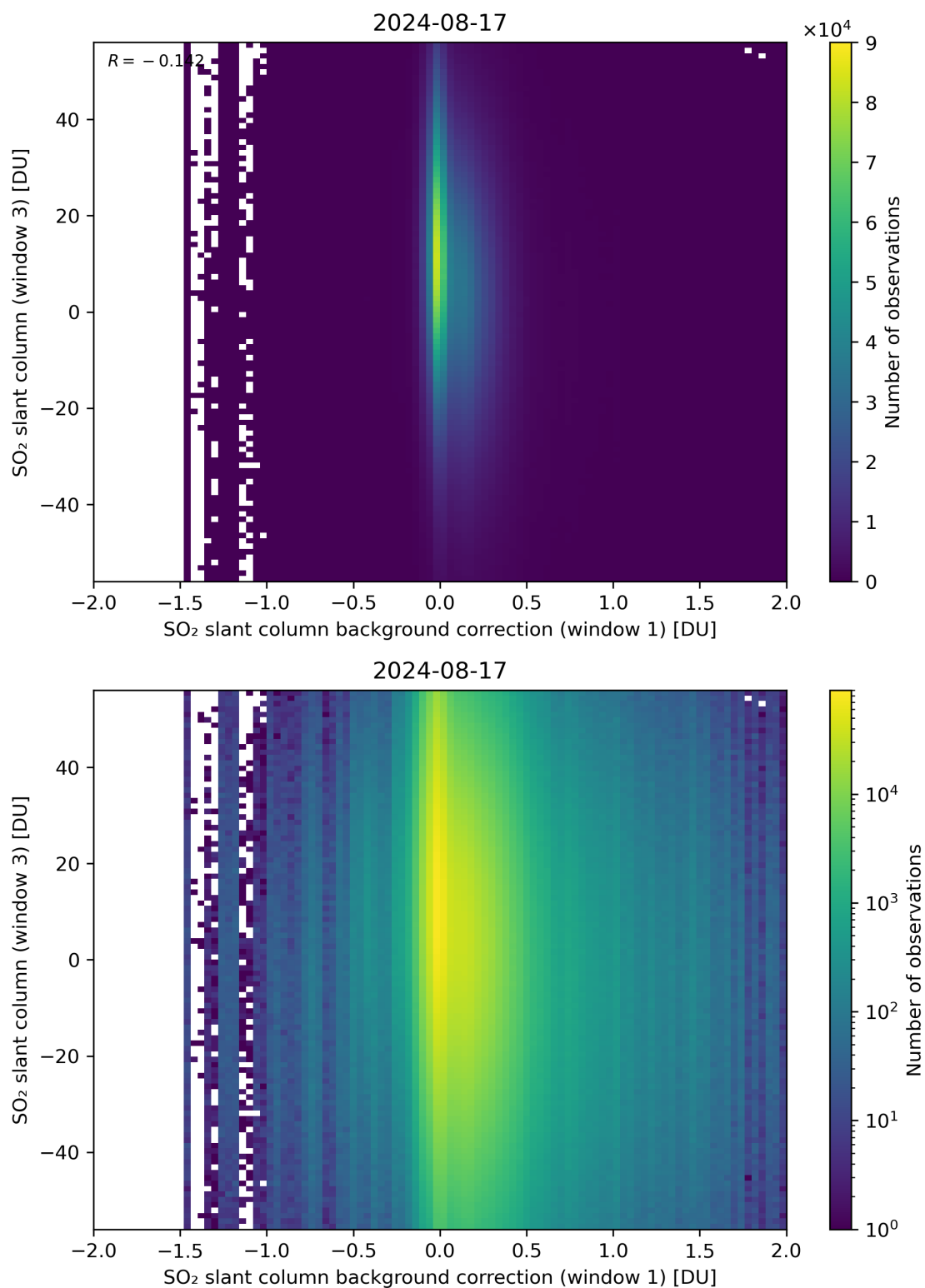
Figure 107: Scatter density plot of “SO 2 slant column background correction (window 1)” against “SO 2 slant column (window 3)” for 2024-08-16 to 2024-08-18.
