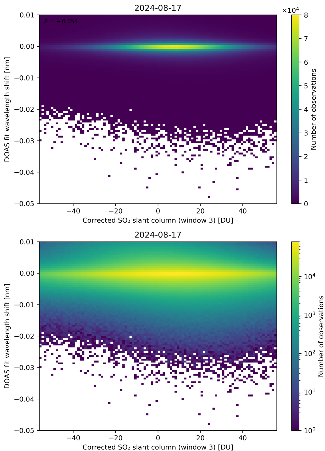
Figure 206: Scatter density plot of “Corrected SO 2 slant column (window 3)” against “DOAS fit wavelength shift” for 2024-08-16 to 2024-08-18.
