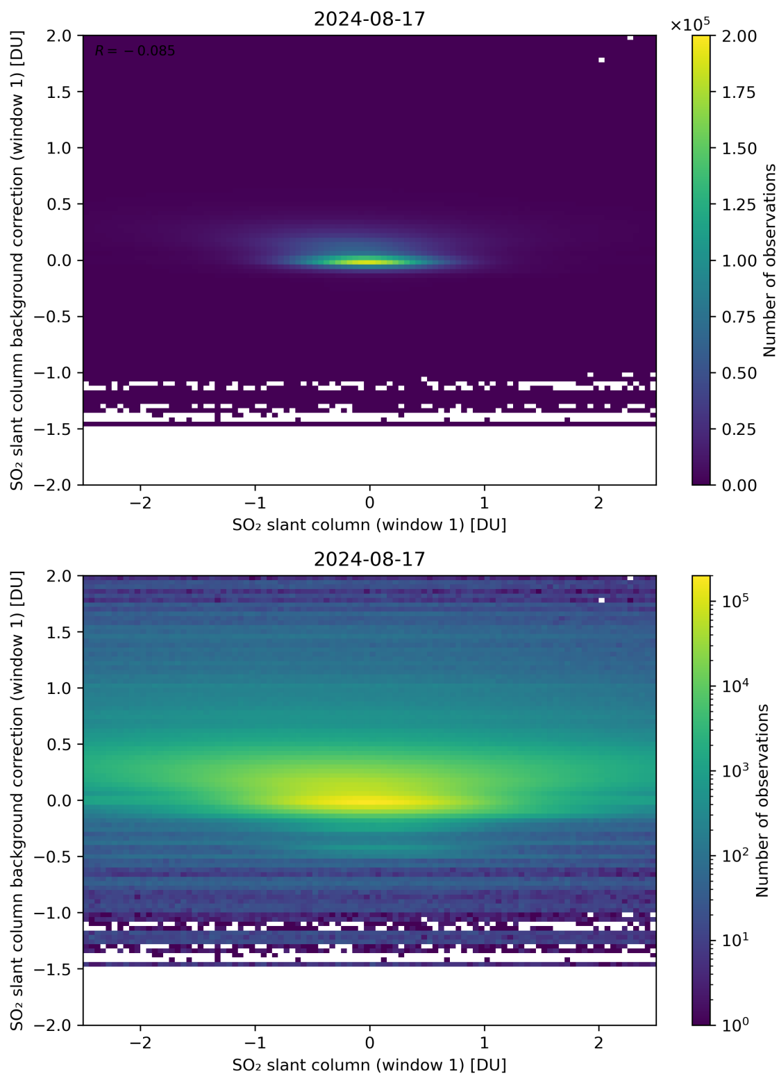
Figure 212: Scatter density plot of “SO 2 slant column (window 1)” against “SO 2 slant column background correction (window 1)” for 2024-08-16 to 2024-08-18.
