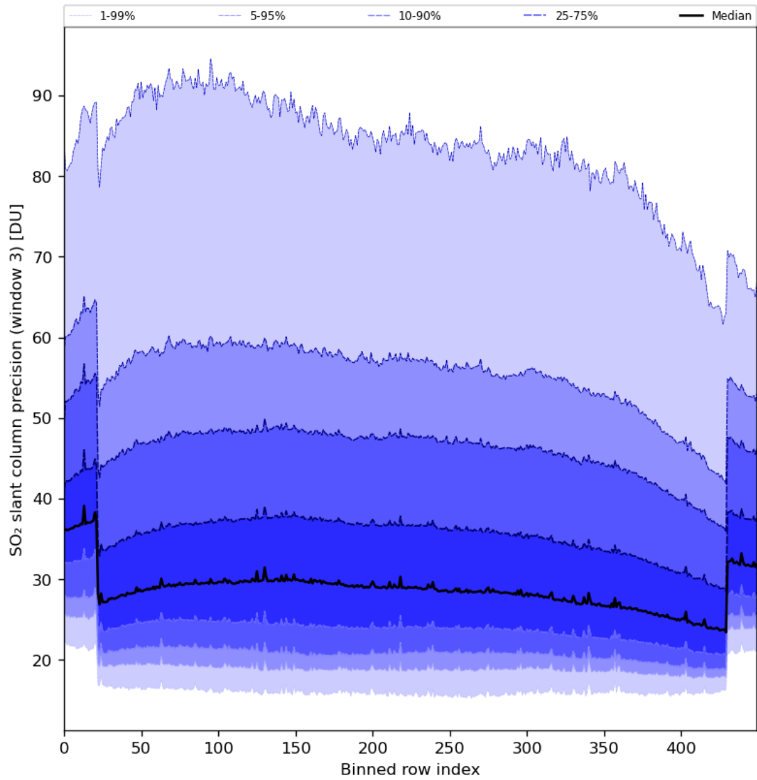
Figure 88: Along track statistics of “SO 2 slant column precision (window 3)” for 2024-08-16 to 2024-08-18
