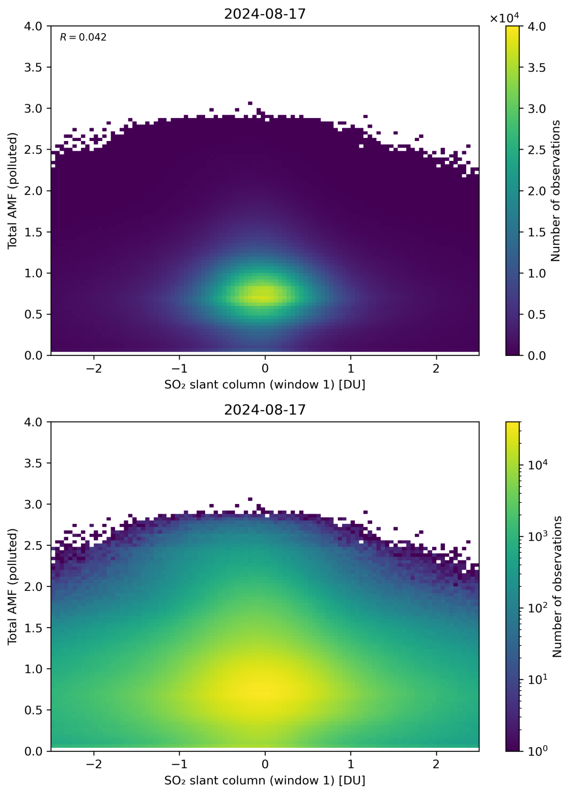
Figure 239: Scatter density plot of “SO 2 slant column (window 1)” against “Total AMF (polluted)” for 2024-08-16 to 2024-08-18.
