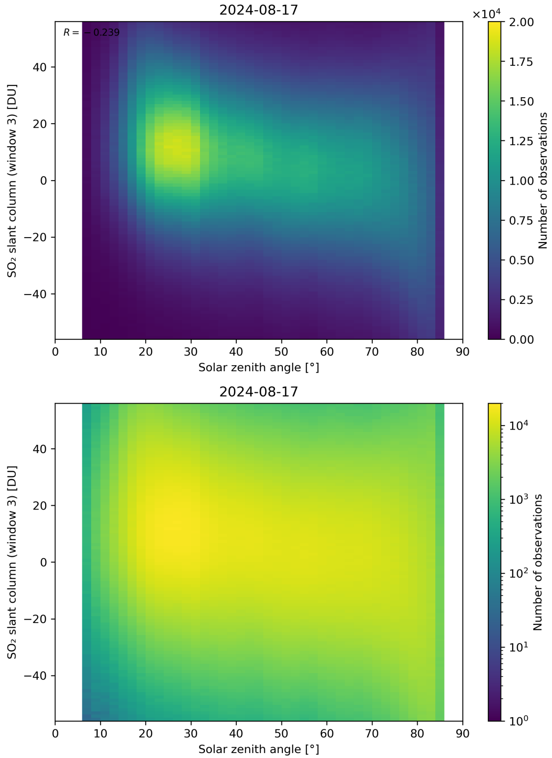
Figure 172: Scatter density plot of “Solar zenith angle” against “SO 2 slant column (window 3)” for 2024-08-16 to 2024-08-18.
