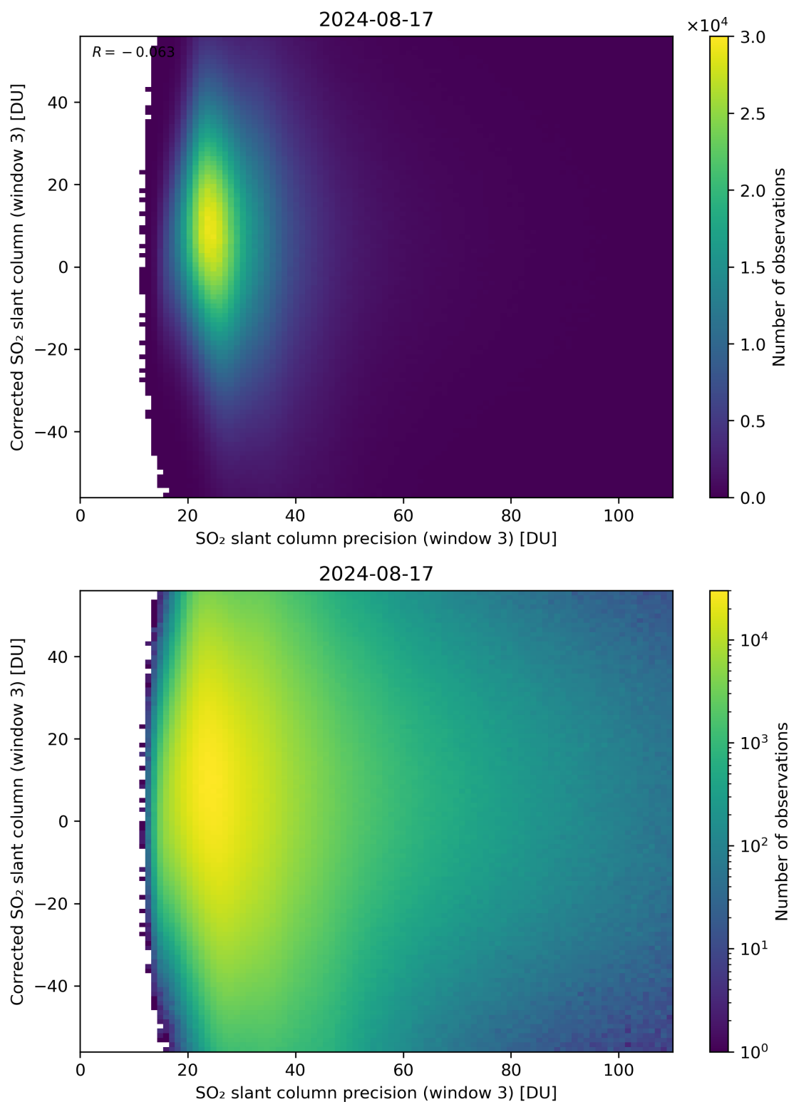
Figure 262: Scatter density plot of “SO 2 slant column precision (window 3)” against “Corrected SO 2 slant column (window 3)” for 2024-08-16 to 2024-08-18.
