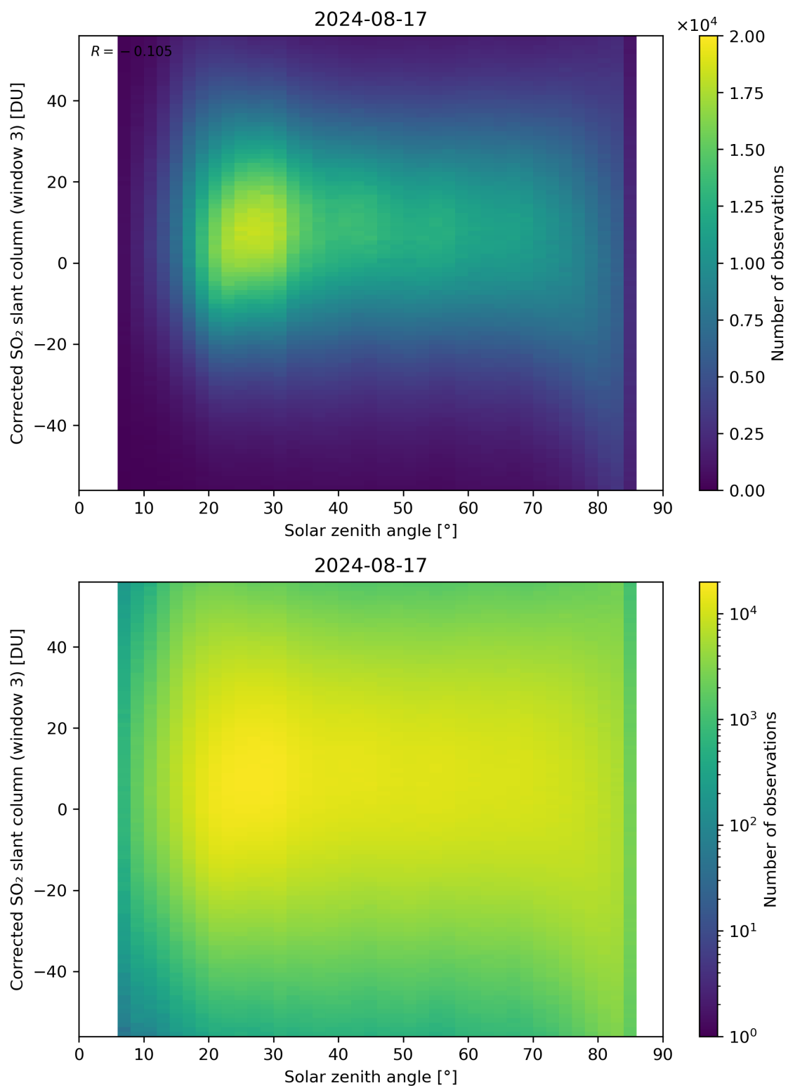
Figure 168: Scatter density plot of “Solar zenith angle” against “Corrected SO 2 slant column (window 3)” for 2024-08-16 to 2024-08-18.
