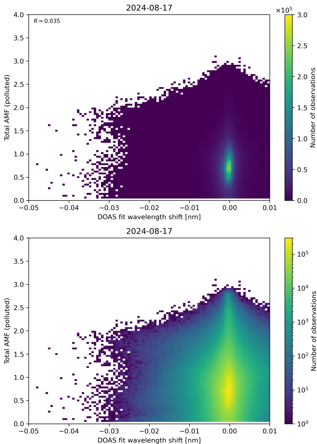
Figure 130: Scatter density plot of “DOAS fit wavelength shift” against “Total AMF (polluted)” for 2024-08-16 to 2024-08-18.
