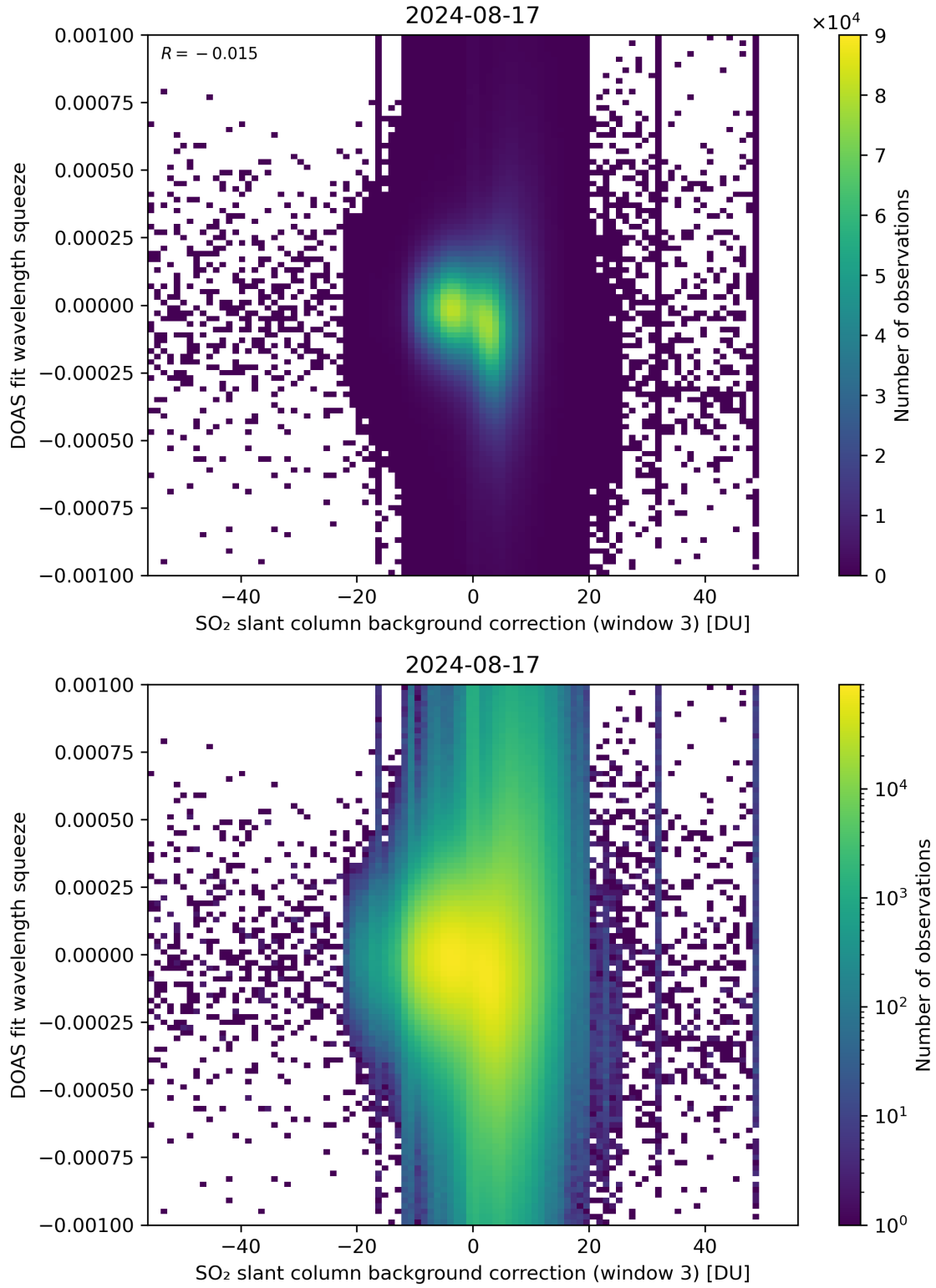
Figure 122: Scatter density plot of “SO 2 slant column background correction (window 3)” against “DOAS fit wavelength squeeze” for 2024-08-16 to 2024-08-18.
