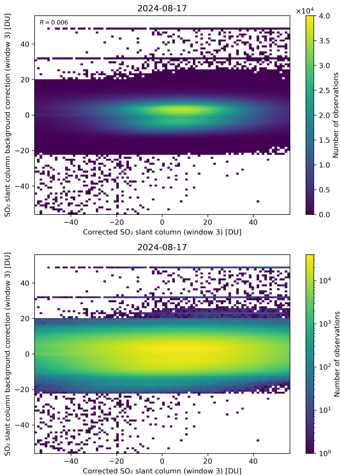
Figure 205: Scatter density plot of “Corrected SO 2 slant column (window 3)” against “SO 2 slant column background correction (window 3)” for 2024-08-16 to 2024-08-18.
