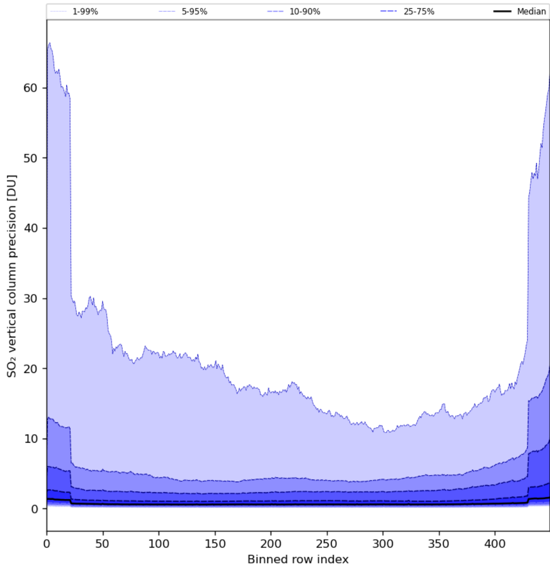
Figure 77: Along track statistics of “SO 2 vertical column precision” for 2024-08-16 to 2024-08-18
