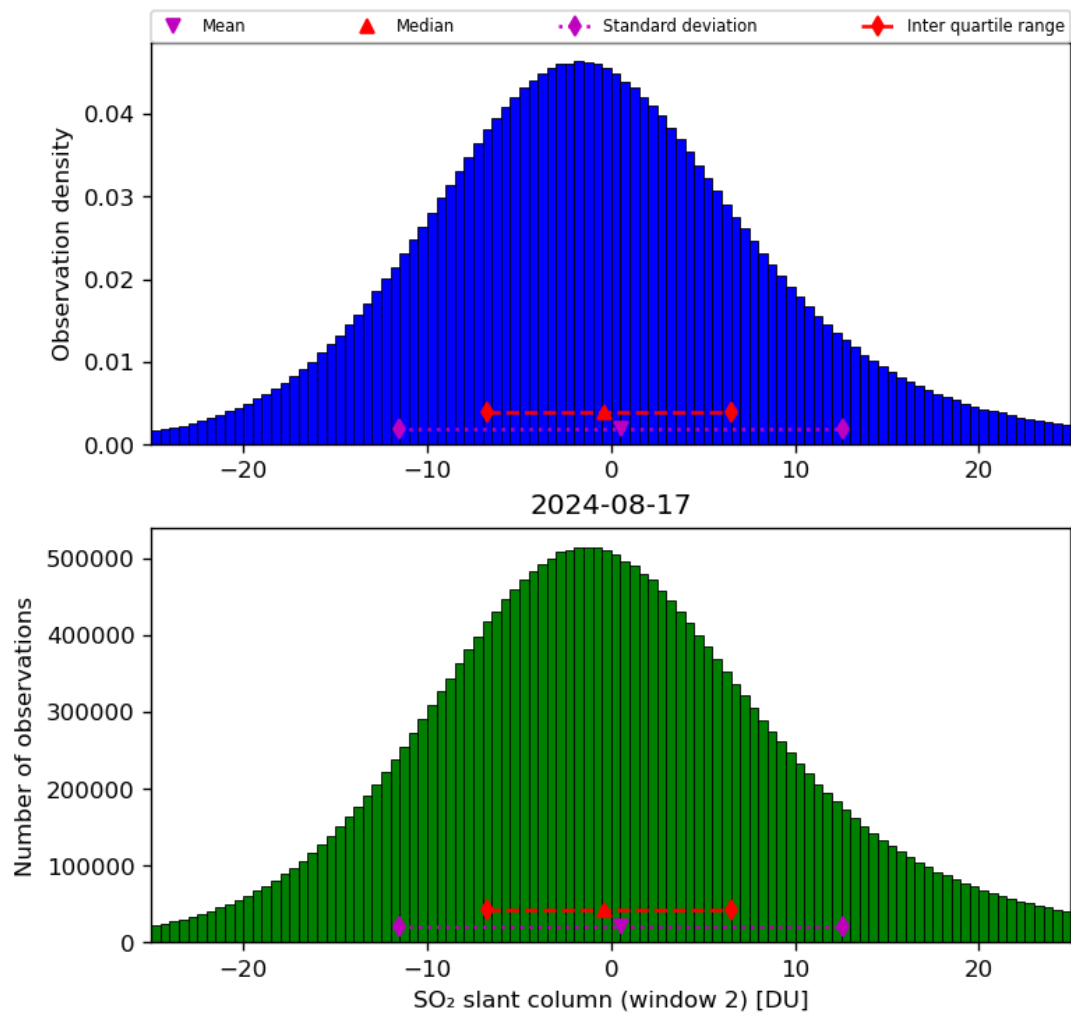
Figure 60: Histogram of “SO 2 slant column (window 2)” for 2024-08-16 to 2024-08-18
