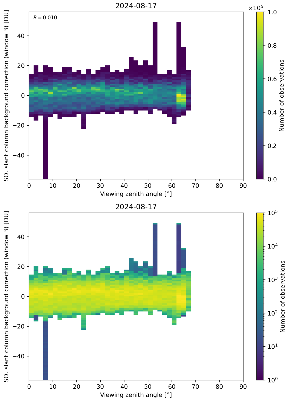
Figure 310: Scatter density plot of “Viewing zenith angle” against “SO 2 slant column background correction (window 3)” for 2024-08-16 to 2024-08-18.
