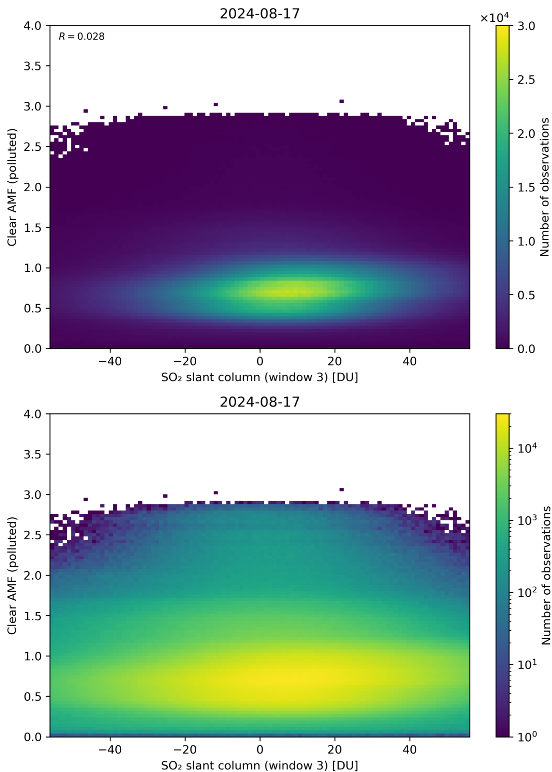
Figure 265: Scatter density plot of “SO 2 slant column (window 3)” against “Clear AMF (polluted)” for 2024-08-16 to 2024-08-18.
