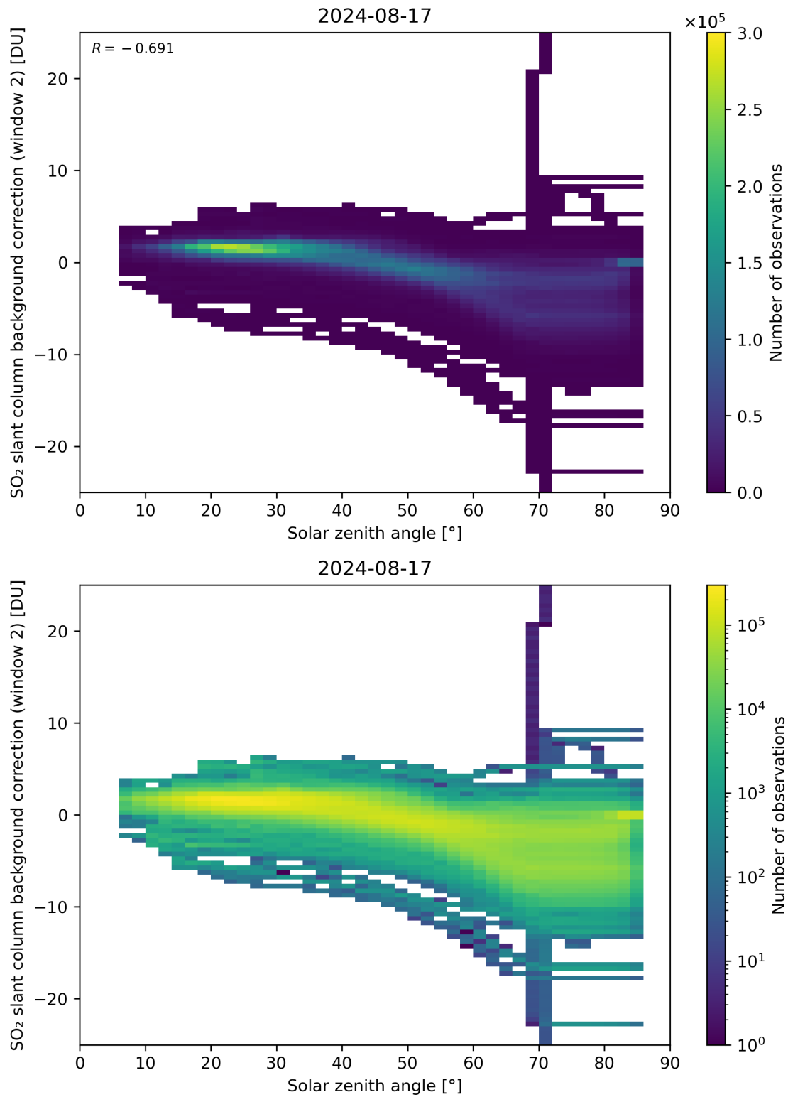
Figure 159: Scatter density plot of “Solar zenith angle” against “SO 2 slant column background correction (window 2)” for 2024-08-16 to 2024-08-18.
