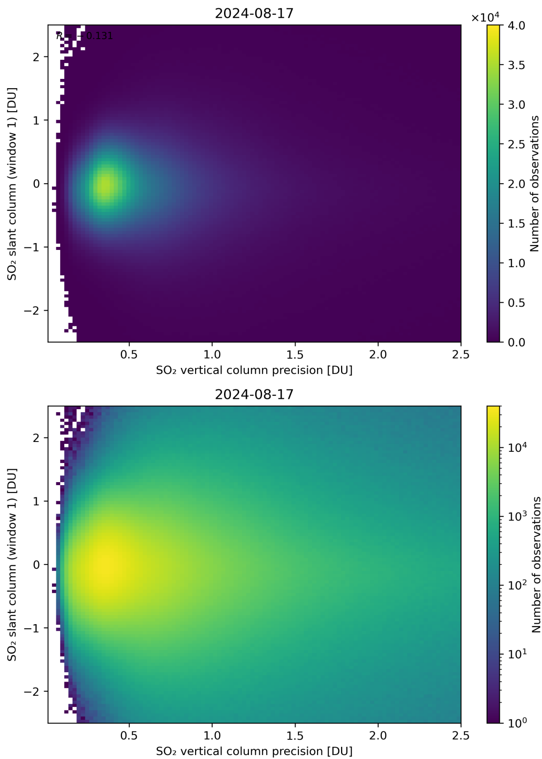
Figure 289: Scatter density plot of “SO 2 vertical column precision” against “SO 2 slant column (window 1)” for 2024-08-16 to 2024-08-18.
