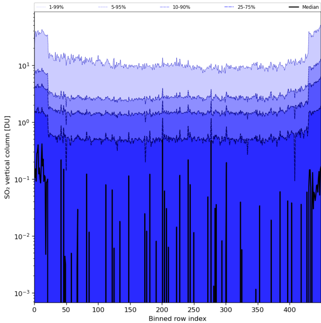
Figure 76: Along track statistics of “SO 2 vertical column” for 2024-08-16 to 2024-08-18
