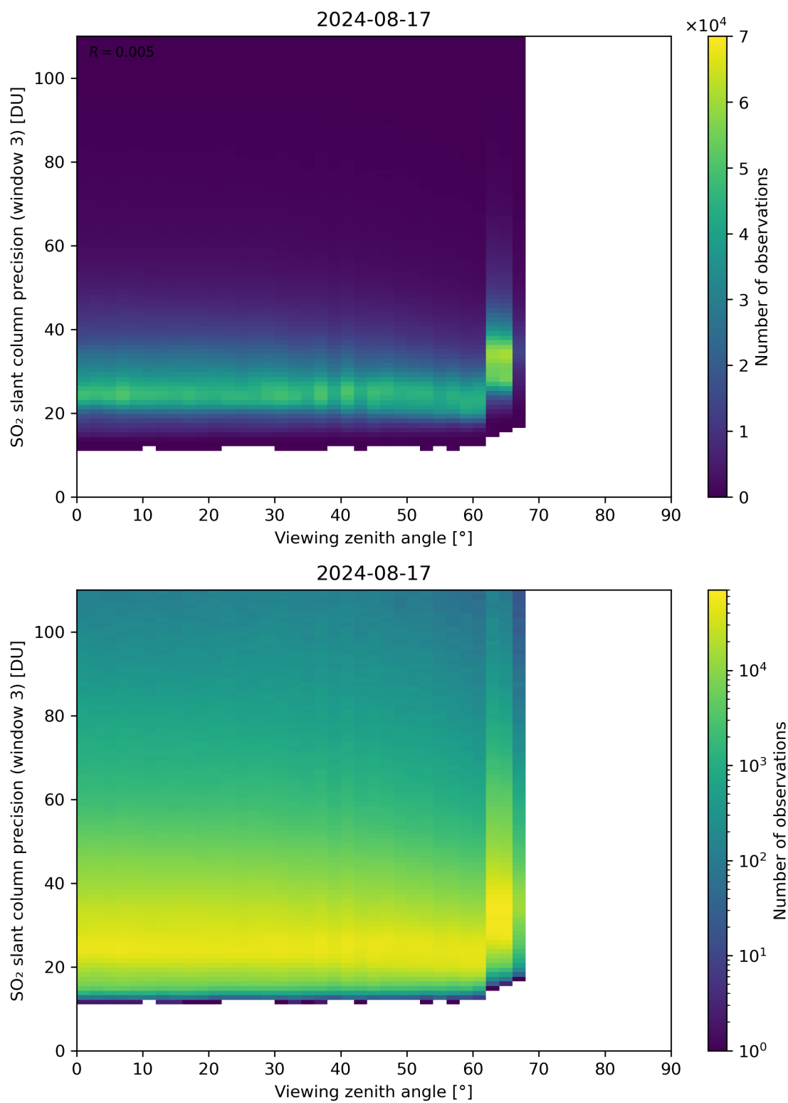
Figure 324: Scatter density plot of “Viewing zenith angle” against “SO 2 slant column precision (window 3)” for 2024-08-16 to 2024-08-18.
