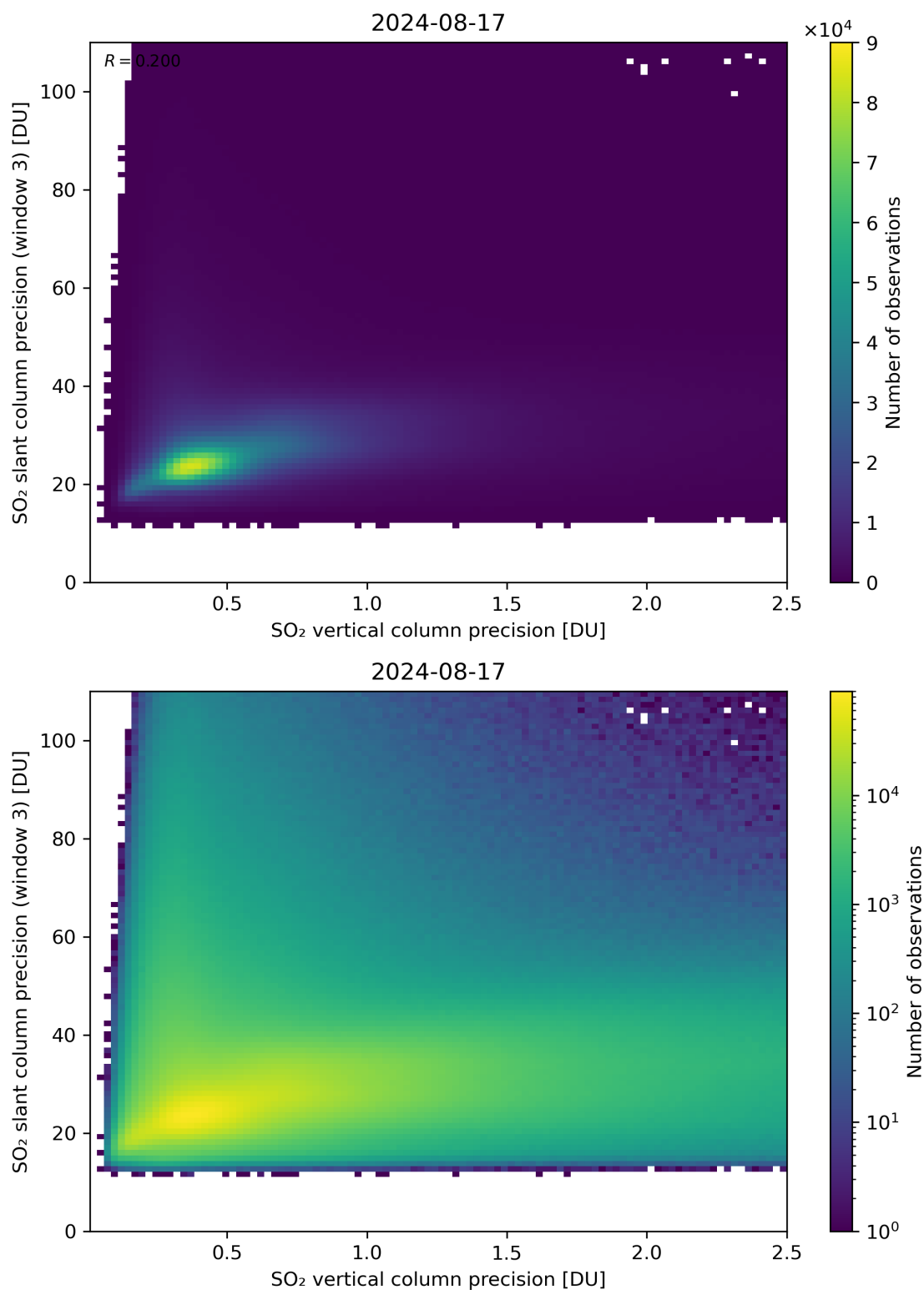
Figure 293: Scatter density plot of “SO 2 vertical column precision” against “SO 2 slant column precision (window 3)” for 2024-08-16 to 2024-08-18.
