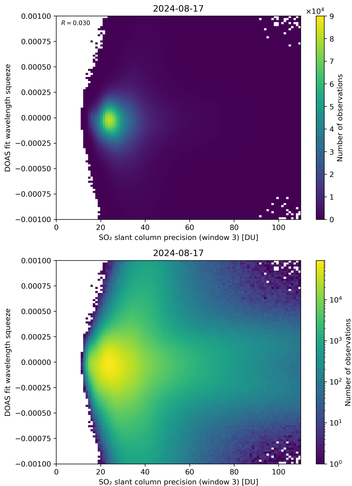
Figure 259: Scatter density plot of “SO 2 slant column precision (window 3)” against “DOAS fit wavelength squeeze” for 2024-08-16 to 2024-08-18.
