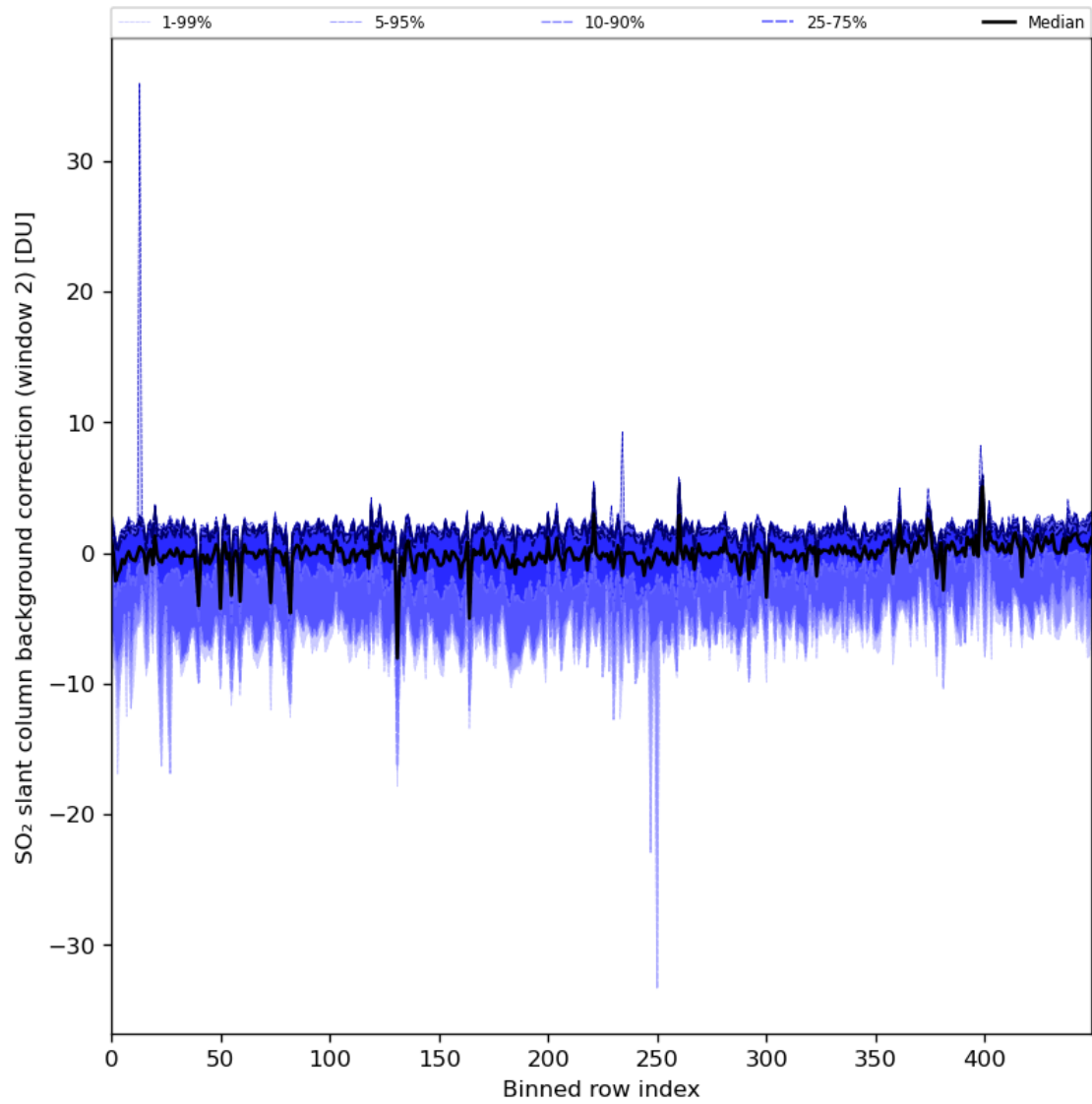
Figure 86: Along track statistics of “SO 2 slant column background correction (window 2)” for 2024-08-16 to 2024-08-18
