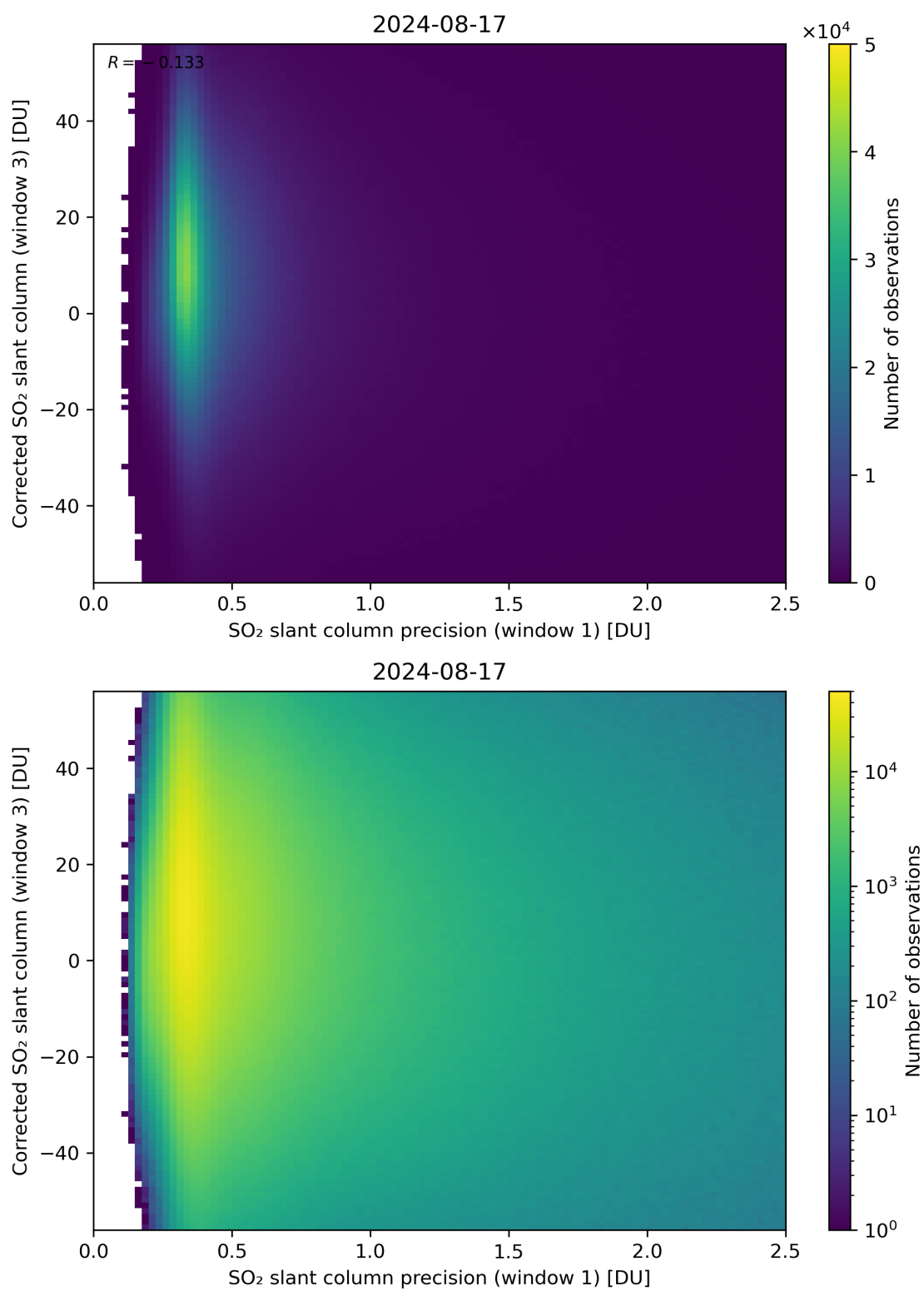
Figure 226: Scatter density plot of “SO 2 slant column precision (window 1)” against “Corrected SO 2 slant column (window 3)” for 2024-08-16 to 2024-08-18.
