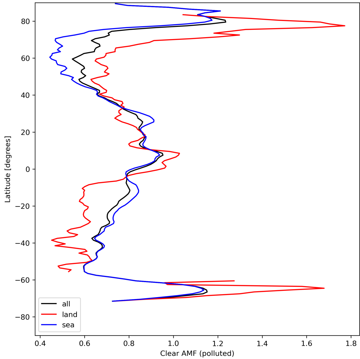
Figure 50: Zonal average of “Clear AMF (polluted)” for 2024-08-16 to 2024-08-18.
