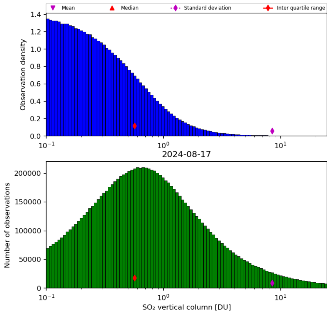
Figure 53: Histogram of “SO 2 vertical column” for 2024-08-16 to 2024-08-18
