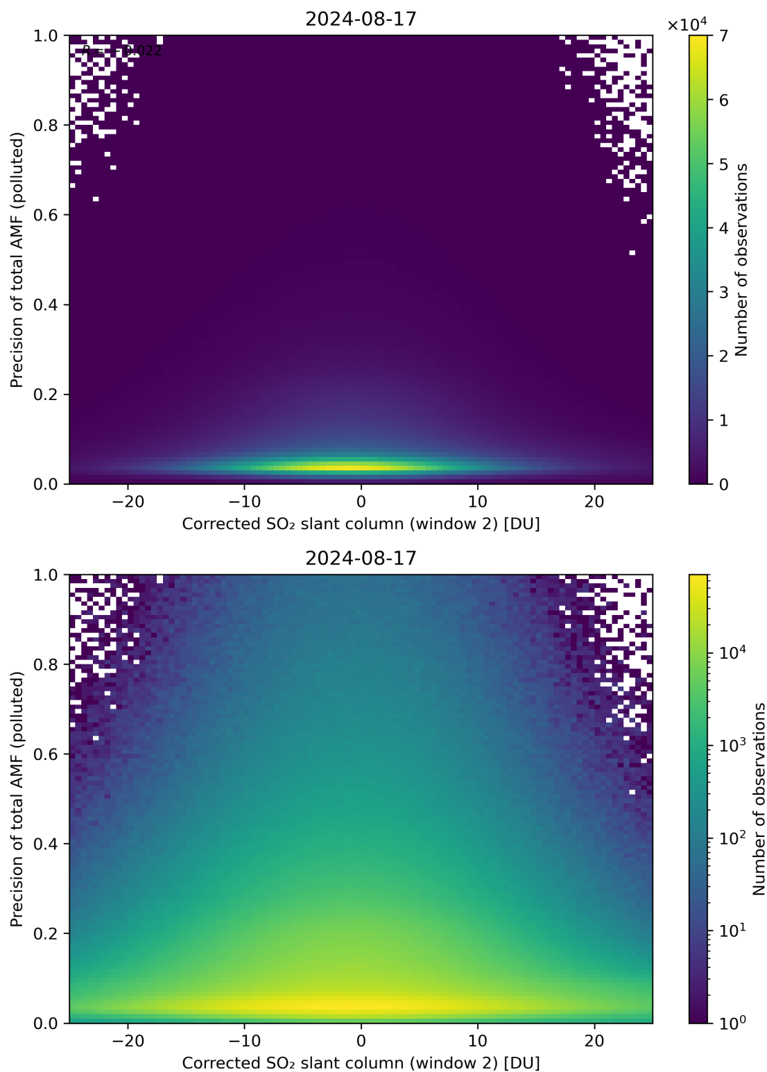
Figure 204: Scatter density plot of “Corrected SO 2 slant column (window 2)” against “Precision of total AMF (polluted)” for 2024-08-16 to 2024-08-18.
