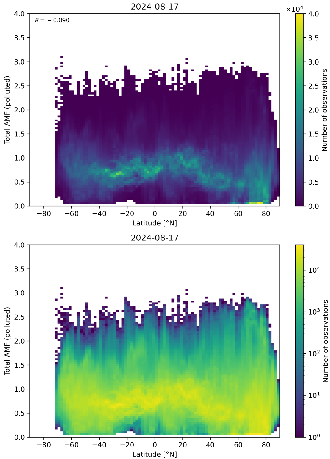
Figure 154: Scatter density plot of “Latitude” against “Total AMF (polluted)” for 2024-08-16 to 2024-08-18.
