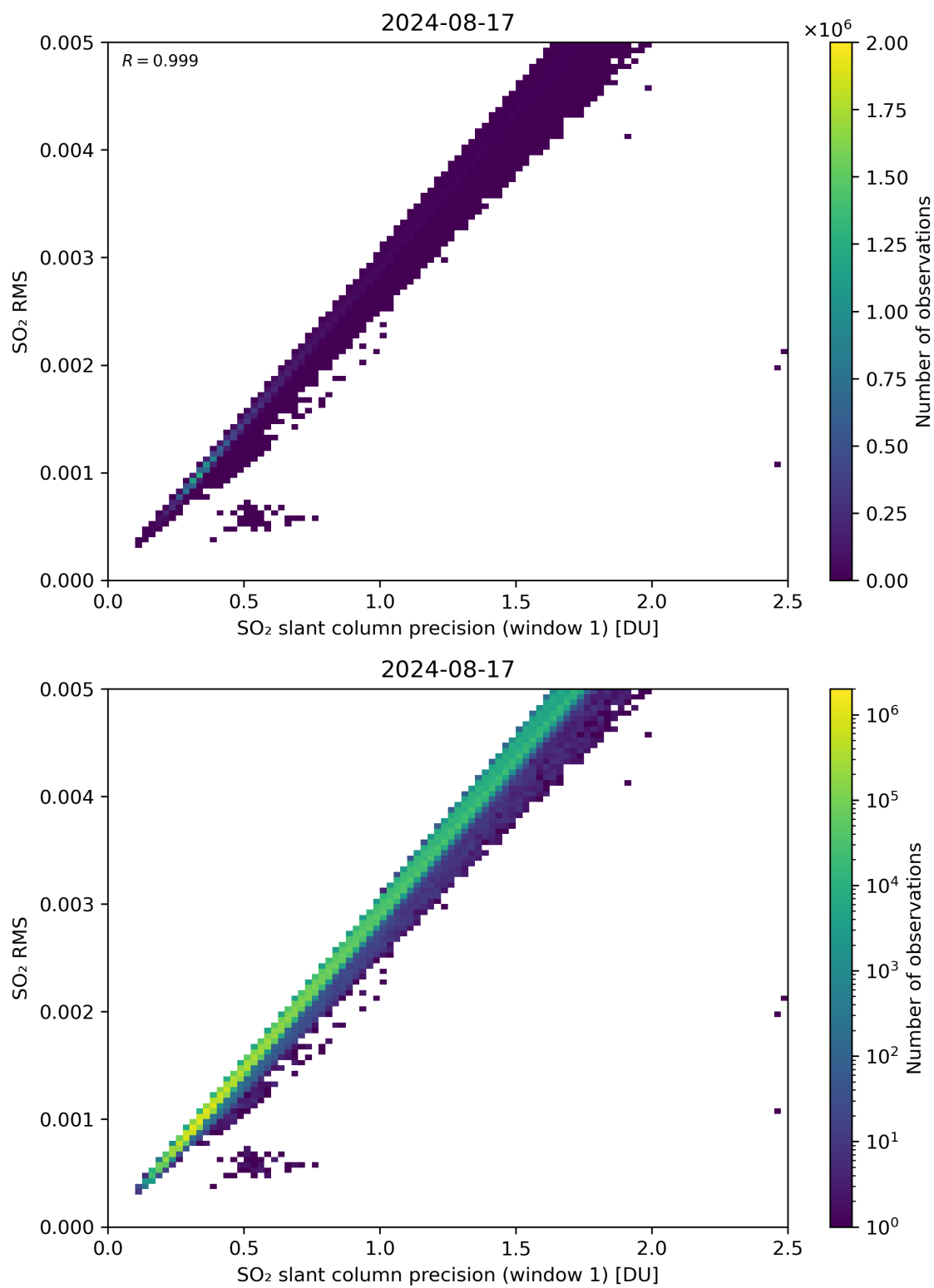
Figure 223: Scatter density plot of “SO 2 slant column precision (window 1)” against “SO 2 RMS” for 2024-08-16 to 2024-08-18.
