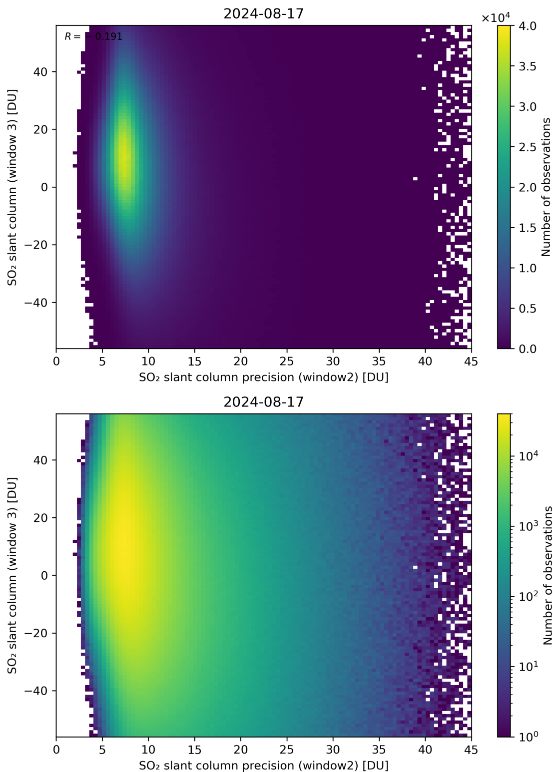
Figure 249: Scatter density plot of “SO 2 slant column precision (window2)” against “SO 2 slant column (window 3)” for 2024-08-16 to 2024-08-18.
