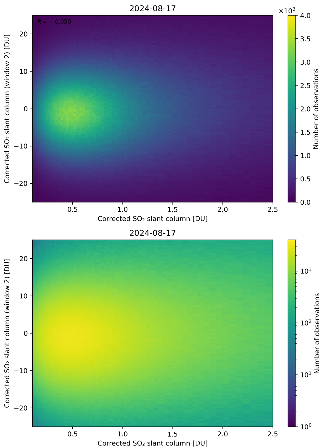
Figure 185: Scatter density plot of “Corrected SO 2 slant column” against “Corrected SO 2 slant column (window 2)” for 2024-08-16 to 2024-08-18.
