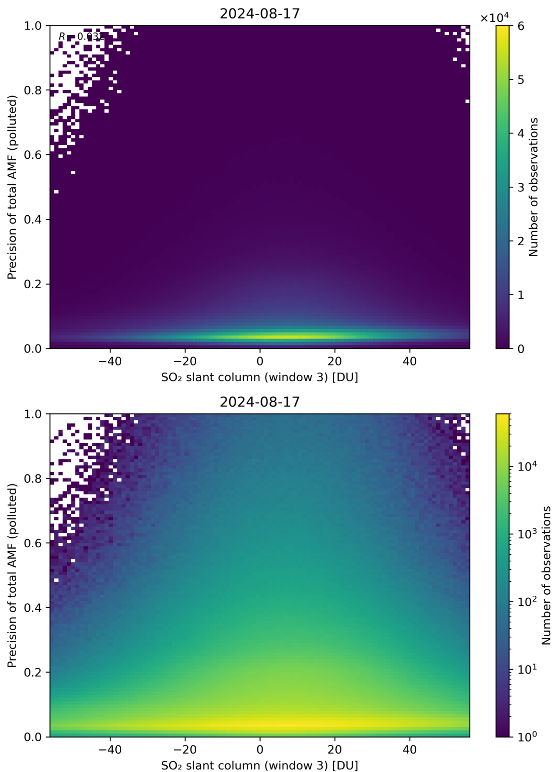
Figure 269: Scatter density plot of “SO 2 slant column (window 3)” against “Precision of total AMF (polluted)” for 2024-08-16 to 2024-08-18.
