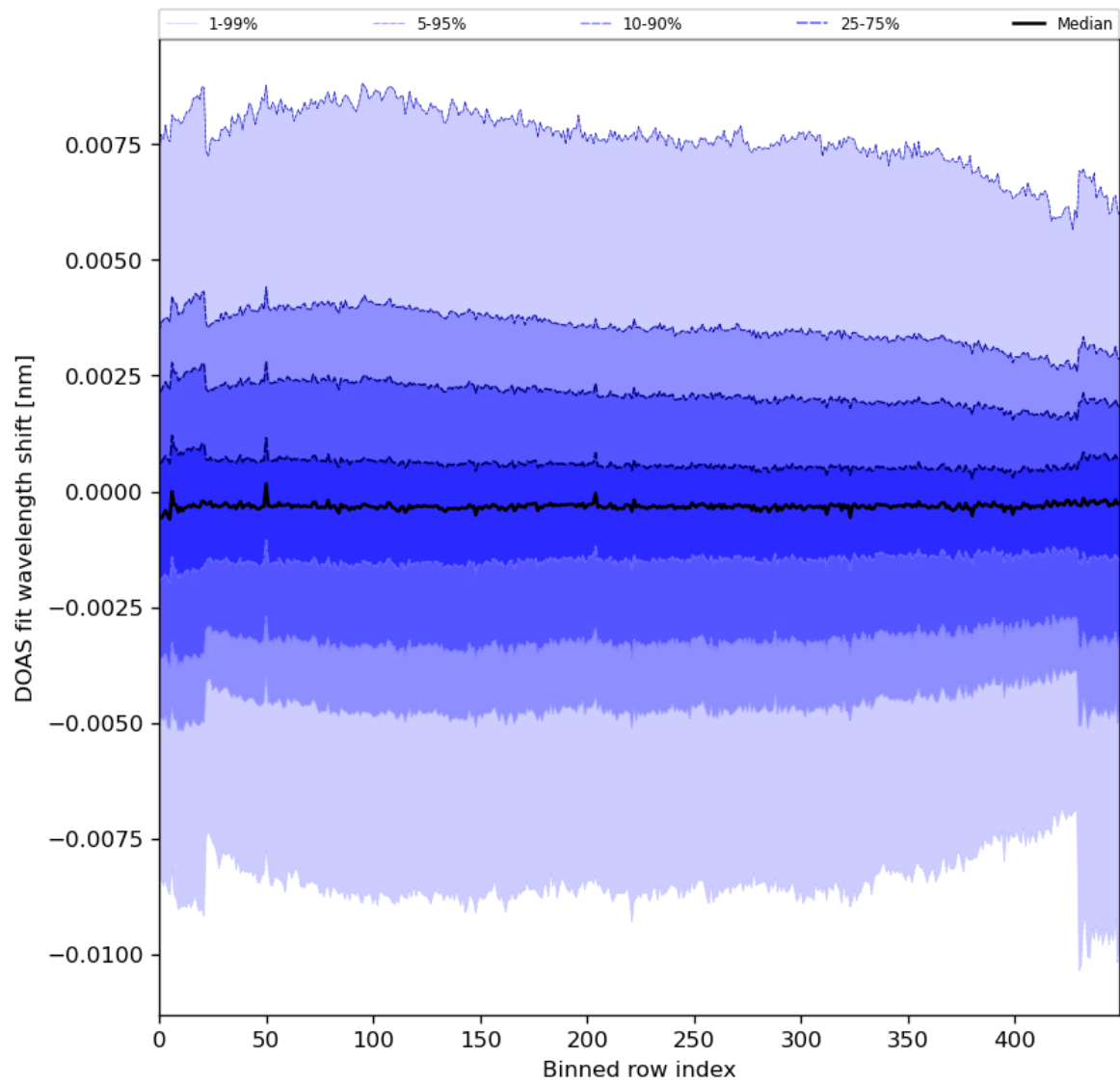
Figure 91: Along track statistics of “DOAS fit wavelength shift” for 2024-08-16 to 2024-08-18
