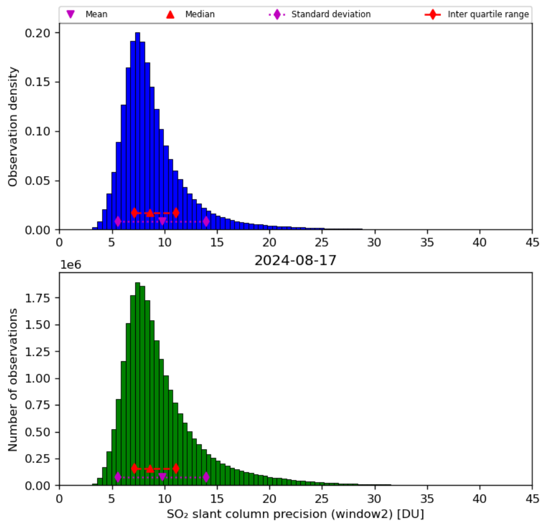
Figure 61: Histogram of “SO 2 slant column precision (window2)” for 2024-08-16 to 2024-08-18
