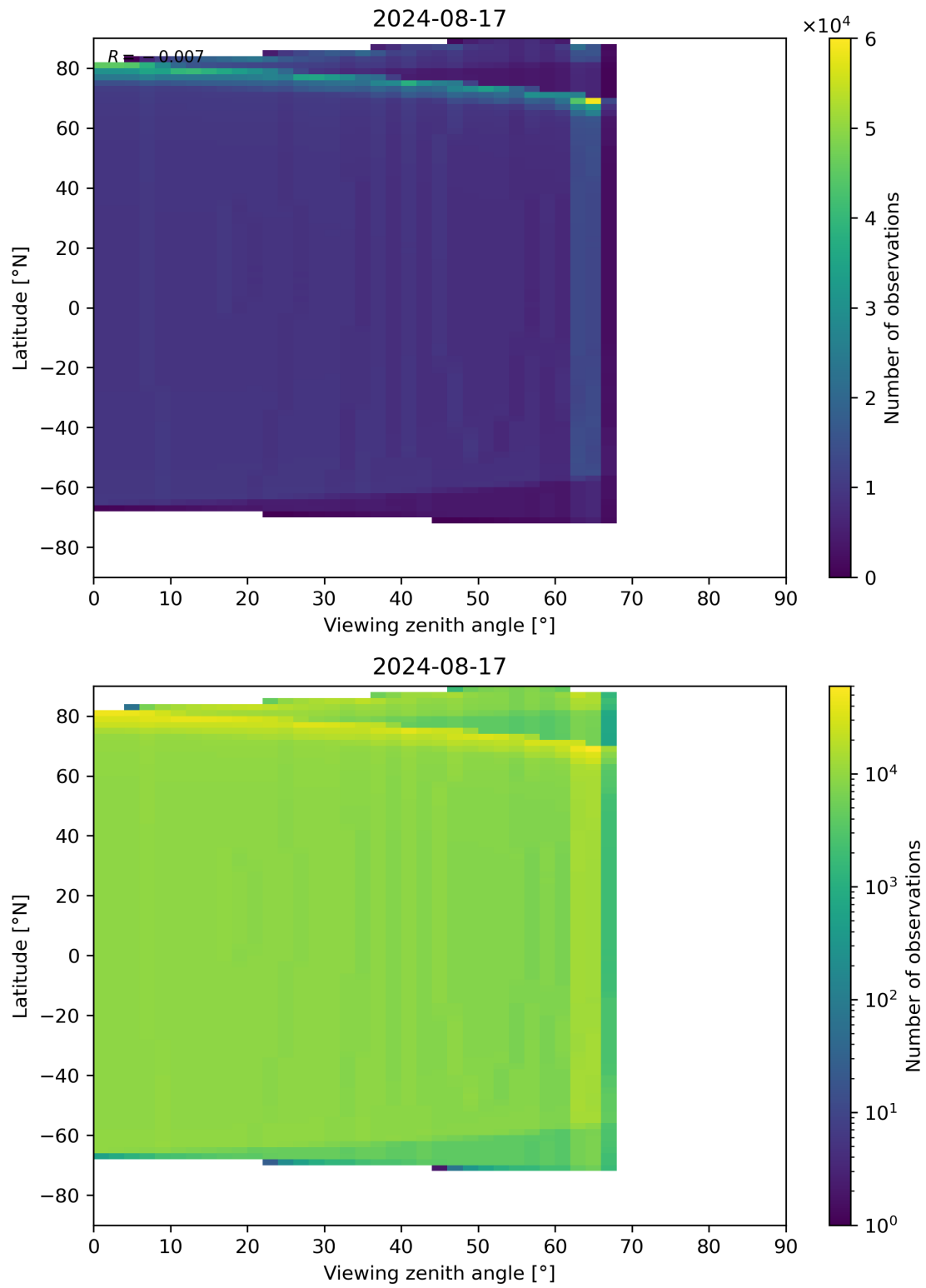
Figure 314: Scatter density plot of “Viewing zenith angle” against “Latitude” for 2024-08-16 to 2024-08-18.
