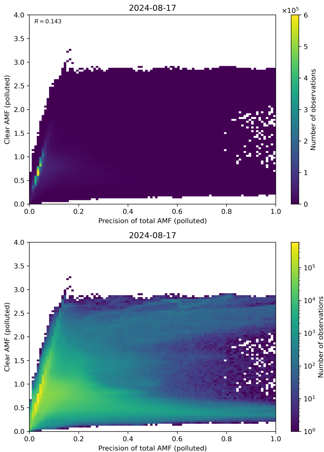
Figure 270: Scatter density plot of “Precision of total AMF (polluted)” against “Clear AMF (polluted)” for 2024-08-16 to 2024-08-18.
