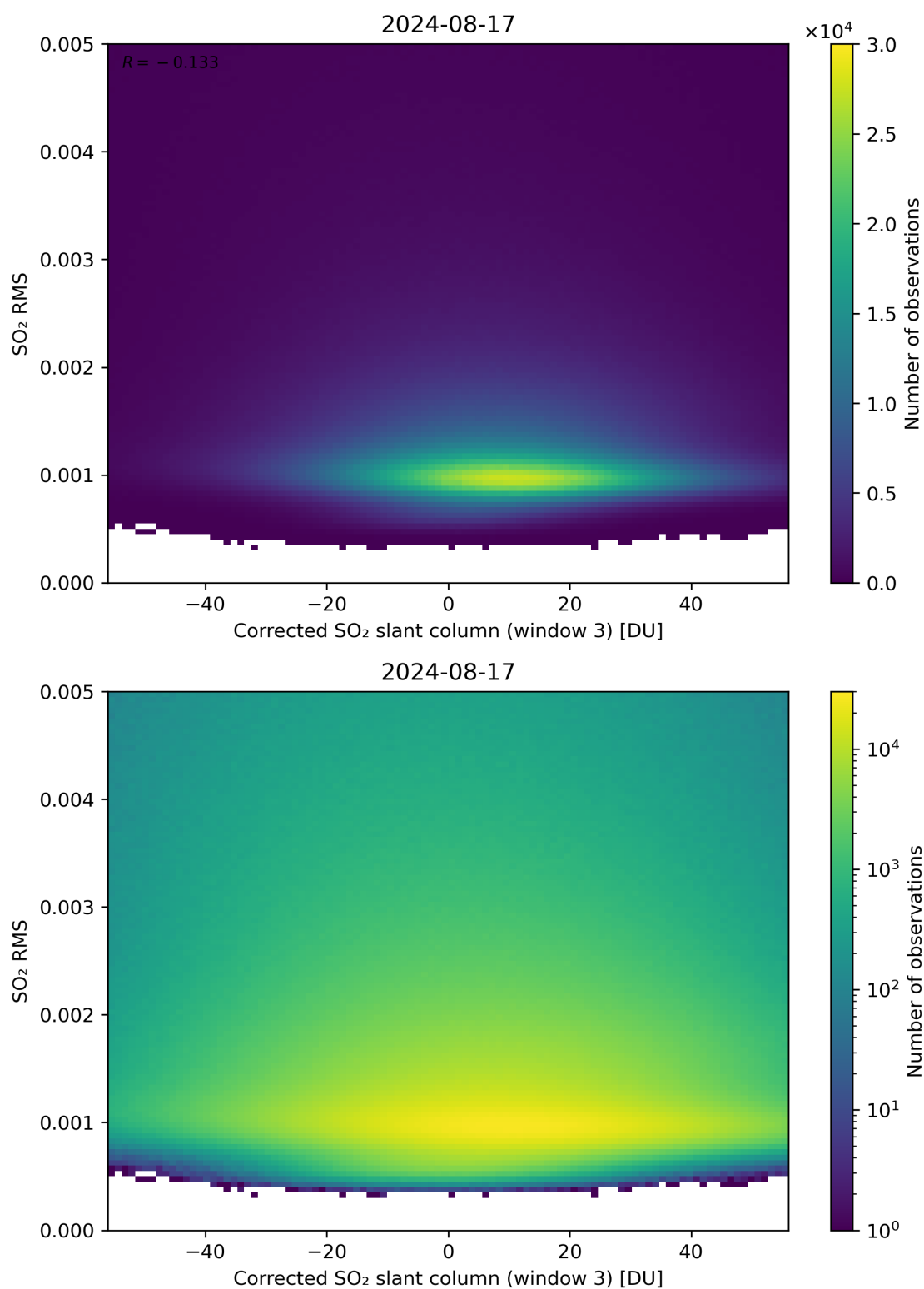
Figure 208: Scatter density plot of “Corrected SO 2 slant column (window 3)” against “SO 2 RMS” for 2024-08-16 to 2024-08-18.
