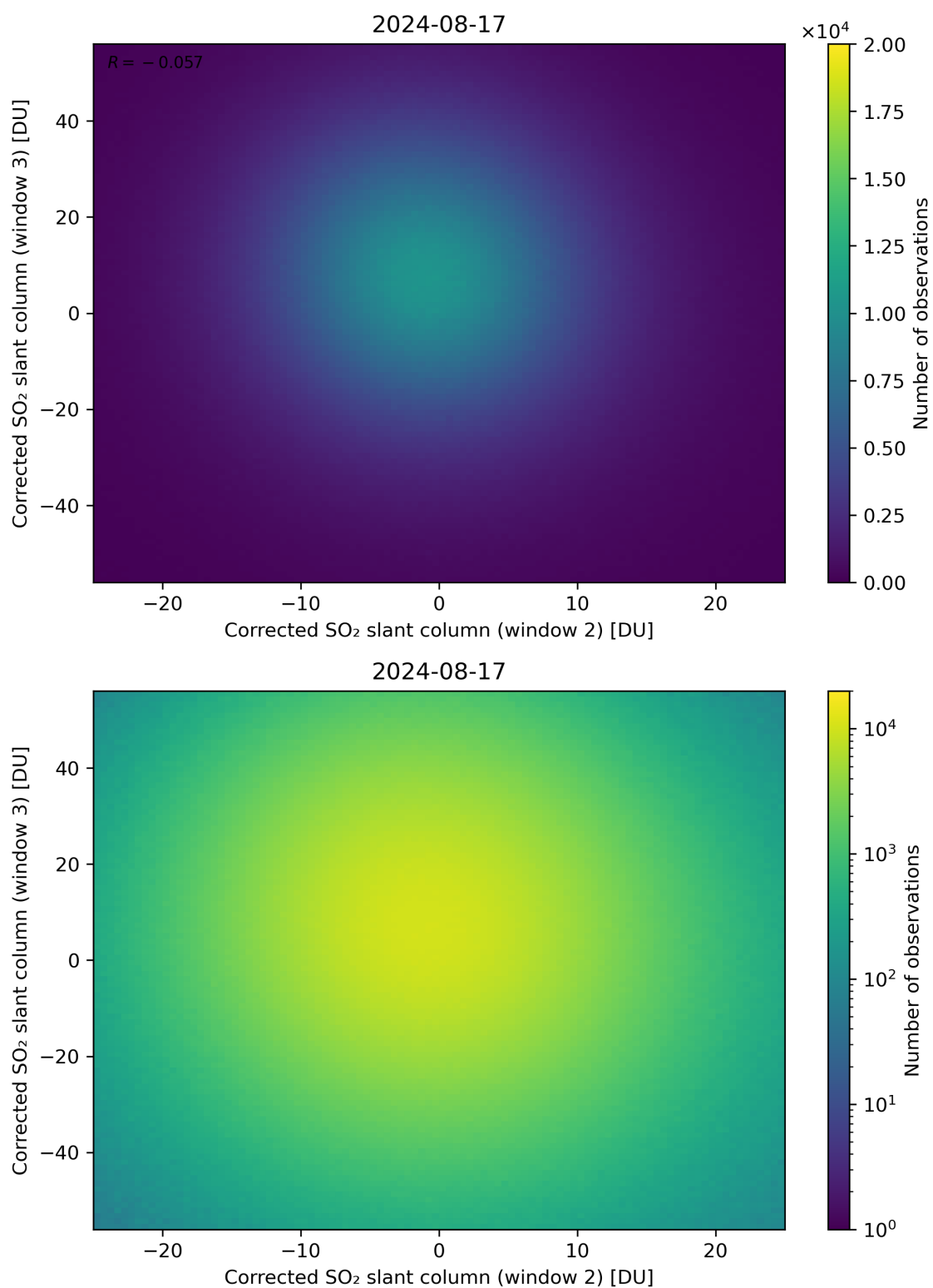
Figure 200: Scatter density plot of “Corrected SO 2 slant column (window 2)” against “Corrected SO 2 slant column (window 3)” for 2024-08-16 to 2024-08-18.
