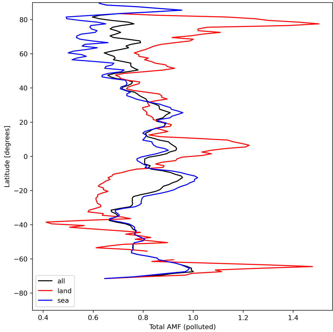
Figure 48: Zonal average of “Total AMF (polluted)” for 2024-08-16 to 2024-08-18.
