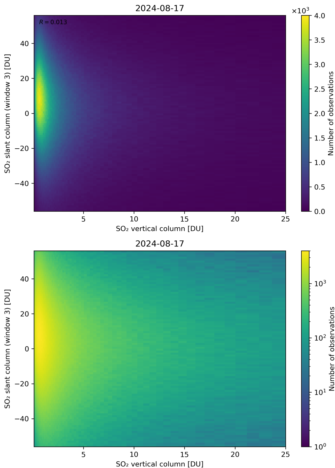
Figure 303: Scatter density plot of “SO 2 vertical column” against “SO 2 slant column (window 3)” for 2024-08-16 to 2024-08-18.
