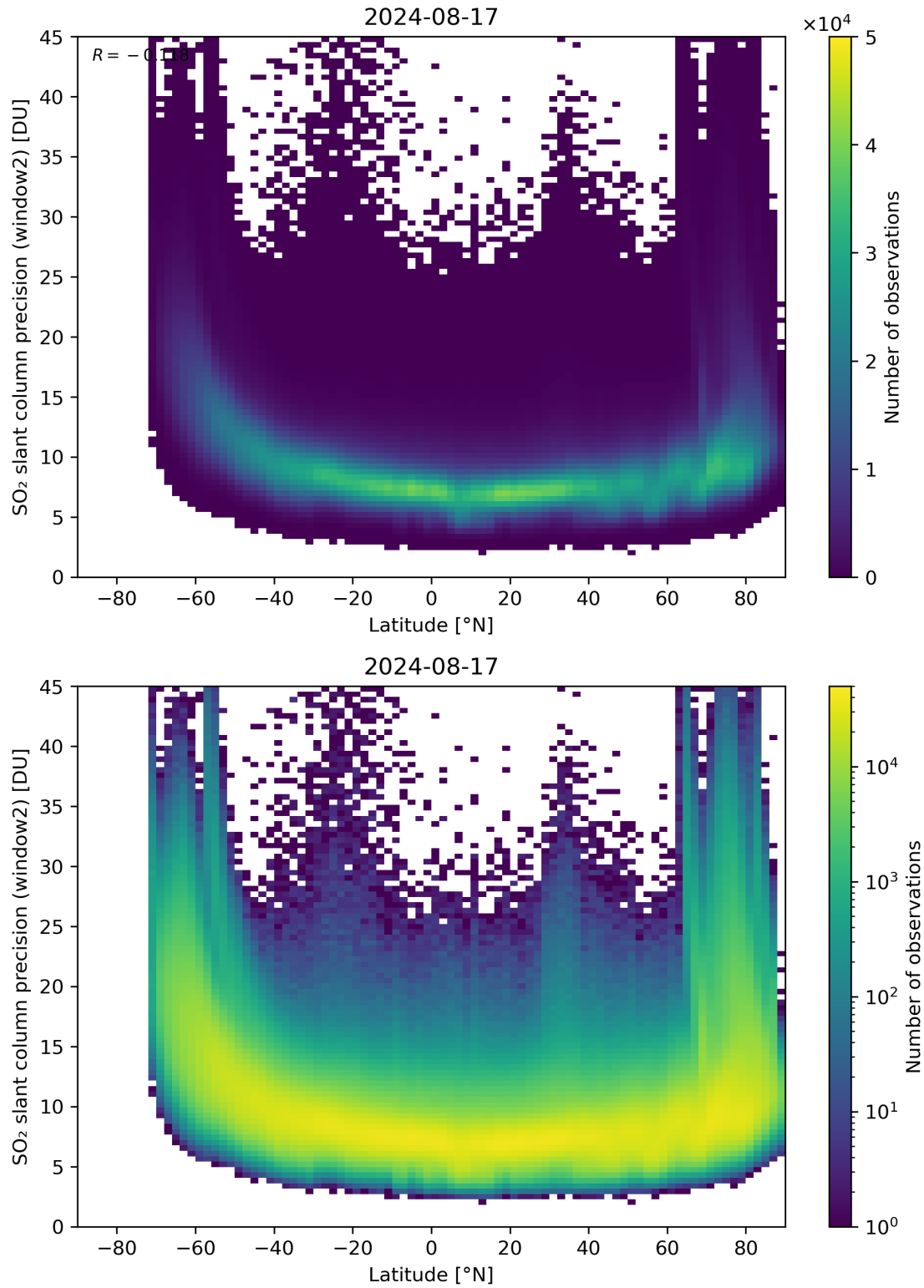
Figure 151: Scatter density plot of “Latitude” against “SO 2 slant column precision (window2)” for 2024-08-16 to 2024-08-18.
