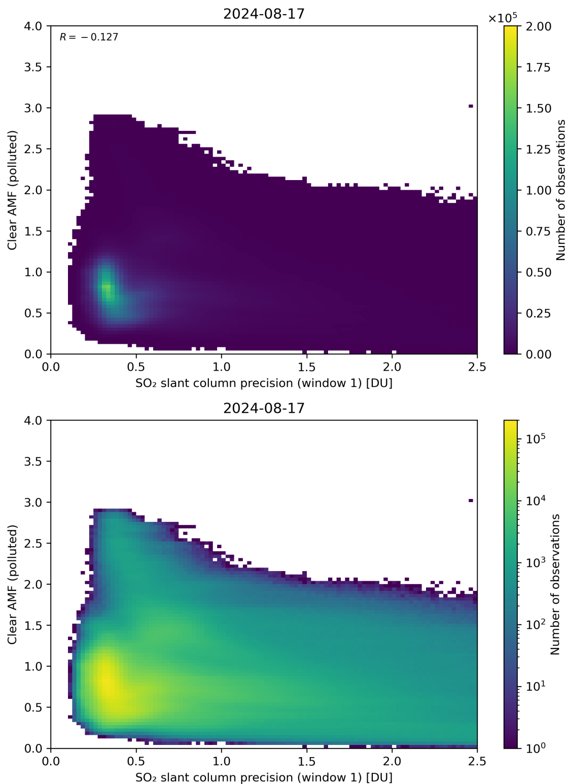
Figure 224: Scatter density plot of “SO 2 slant column precision (window 1)” against “Clear AMF (polluted)” for 2024-08-16 to 2024-08-18.
