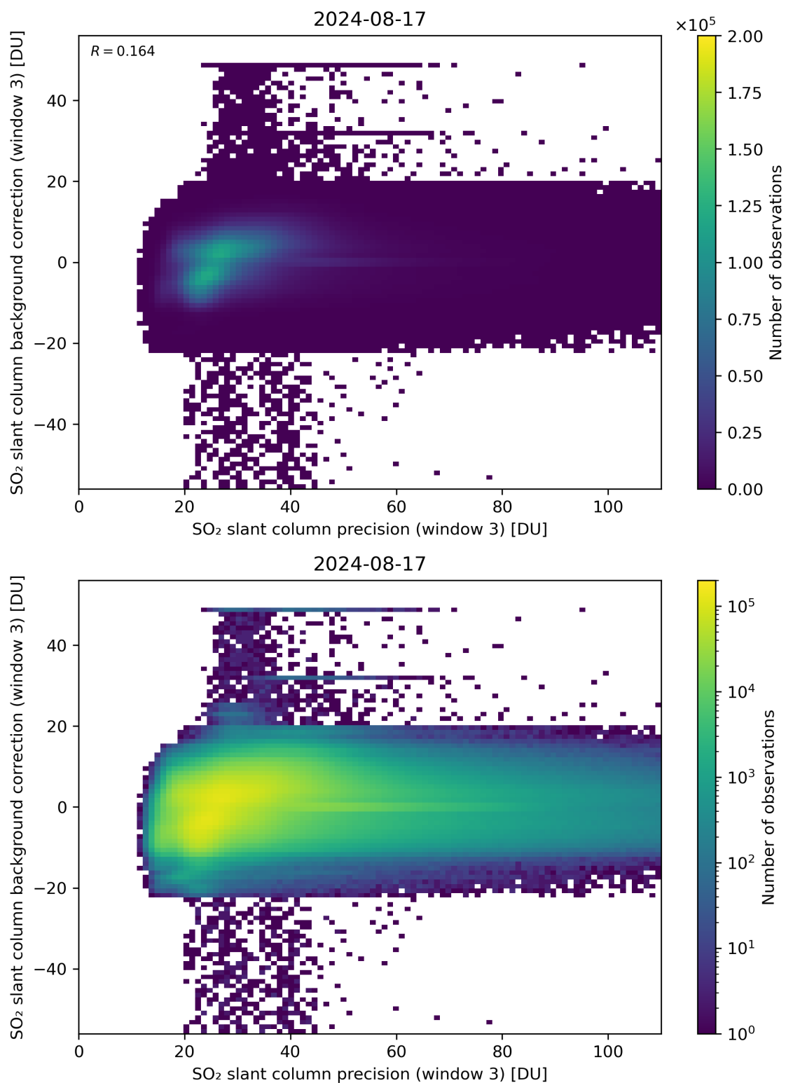
Figure 257: Scatter density plot of “SO 2 slant column precision (window 3)” against “SO 2 slant column background correction (window 3)” for 2024-08-16 to 2024-08-18.
