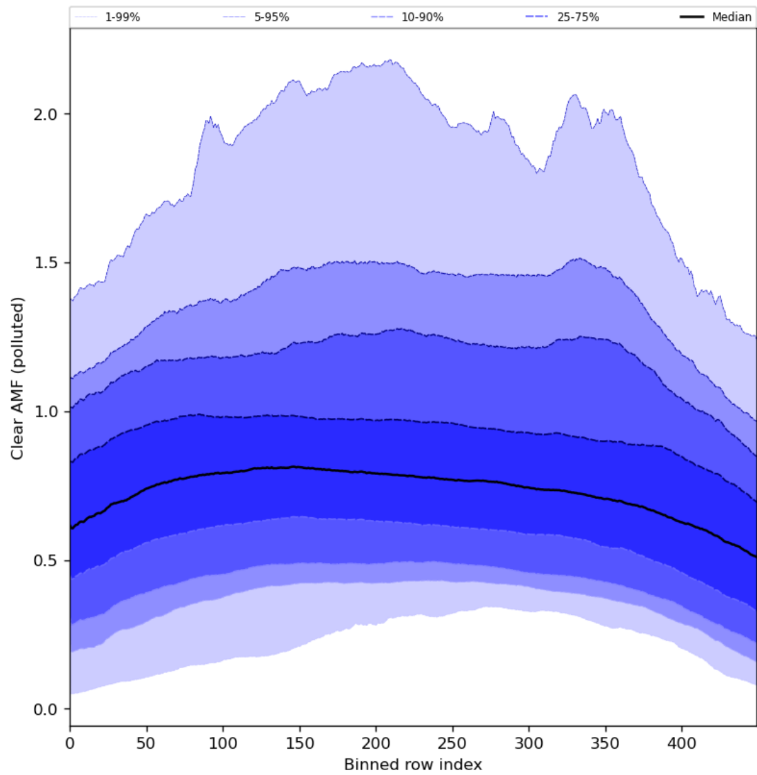
Figure 96: Along track statistics of “Clear AMF (polluted)” for 2024-08-16 to 2024-08-18
