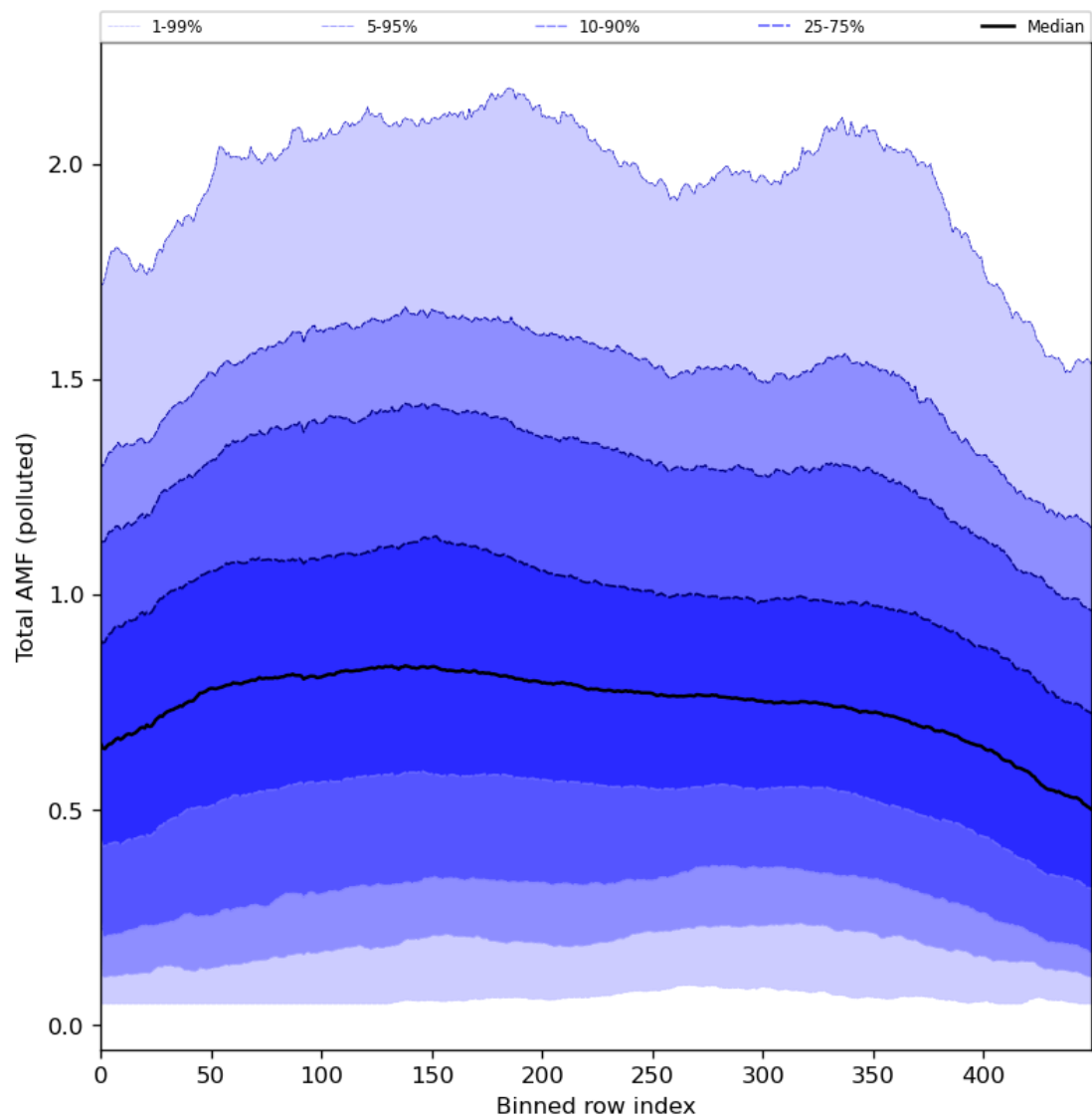
Figure 94: Along track statistics of “Total AMF (polluted)” for 2024-08-16 to 2024-08-18
