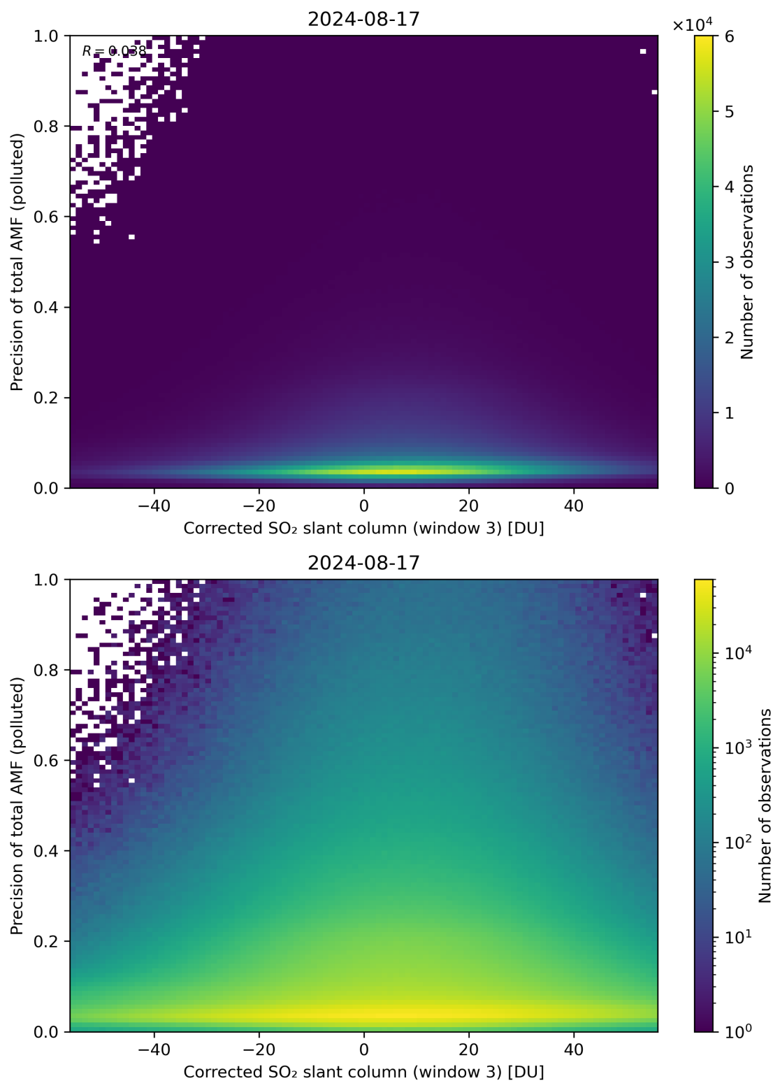
Figure 211: Scatter density plot of “Corrected SO 2 slant column (window 3)” against “Precision of total AMF (polluted)” for 2024-08-16 to 2024-08-18.
