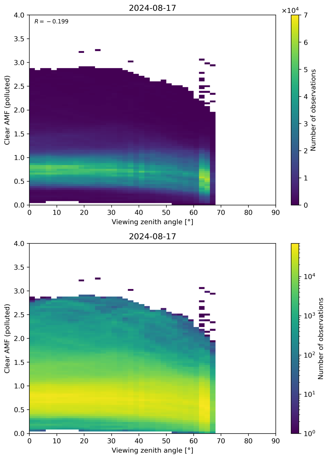
Figure 316: Scatter density plot of “Viewing zenith angle” against “Clear AMF (polluted)” for 2024-08-16 to 2024-08-18.
