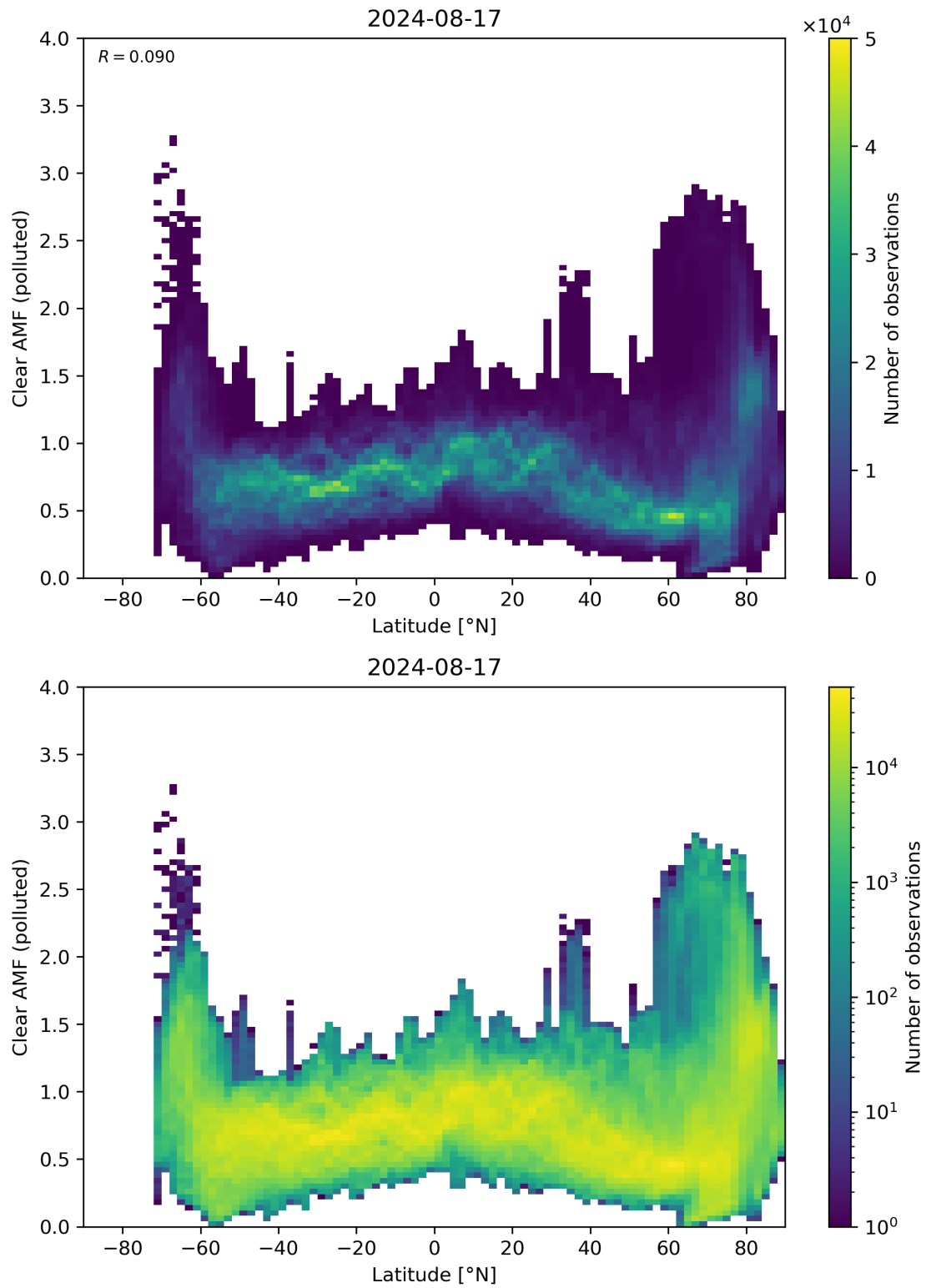
Figure 145: Scatter density plot of “Latitude” against “Clear AMF (polluted)” for 2024-08-16 to 2024-08-18.
