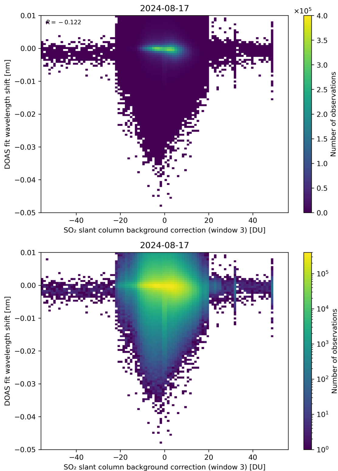
Figure 121: Scatter density plot of “SO 2 slant column background correction (window 3)” against “DOAS fit wavelength shift” for 2024-08-16 to 2024-08-18.
