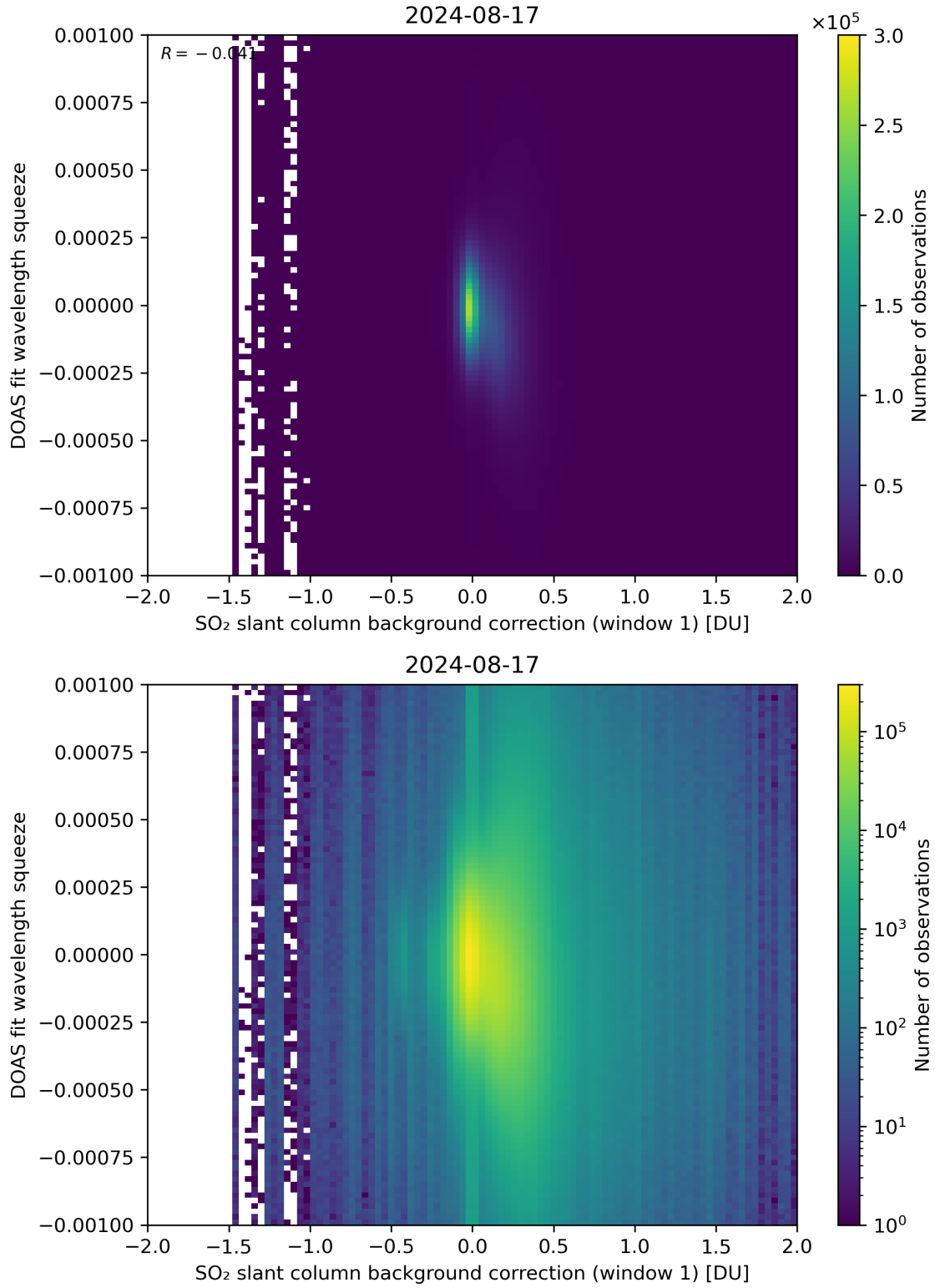
Figure 101: Scatter density plot of “SO 2 slant column background correction (window 1)” against “DOAS fit wavelength squeeze” for 2024-08-16 to 2024-08-18.
