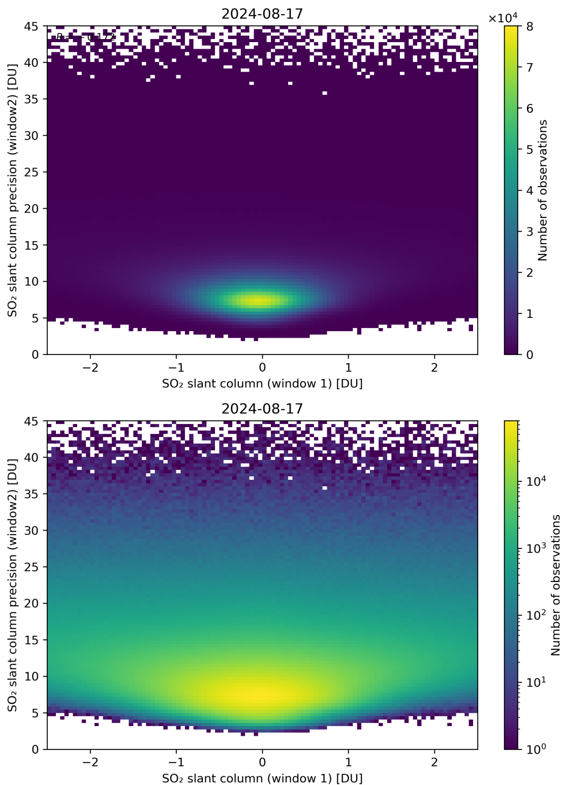
Figure 236: Scatter density plot of “SO 2 slant column (window 1)” against “SO 2 slant column precision (window2)” for 2024-08-16 to 2024-08-18.
