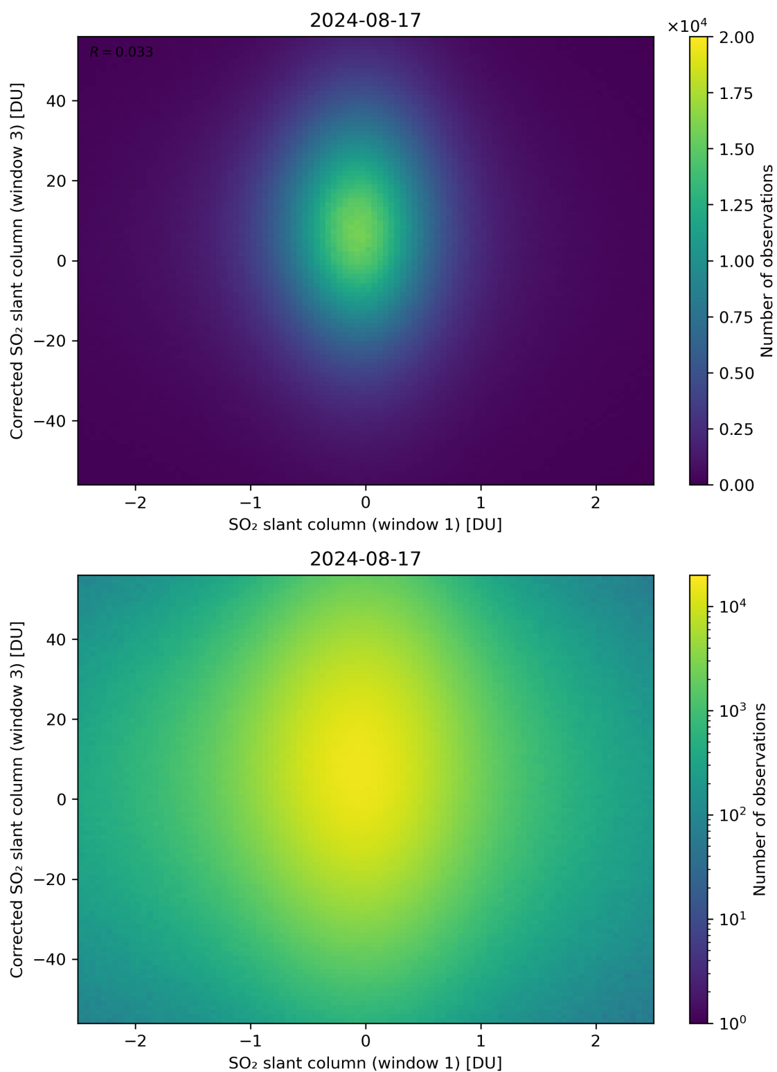
Figure 234: Scatter density plot of “SO 2 slant column (window 1)” against “Corrected SO 2 slant column (window 3)” for 2024-08-16 to 2024-08-18.
