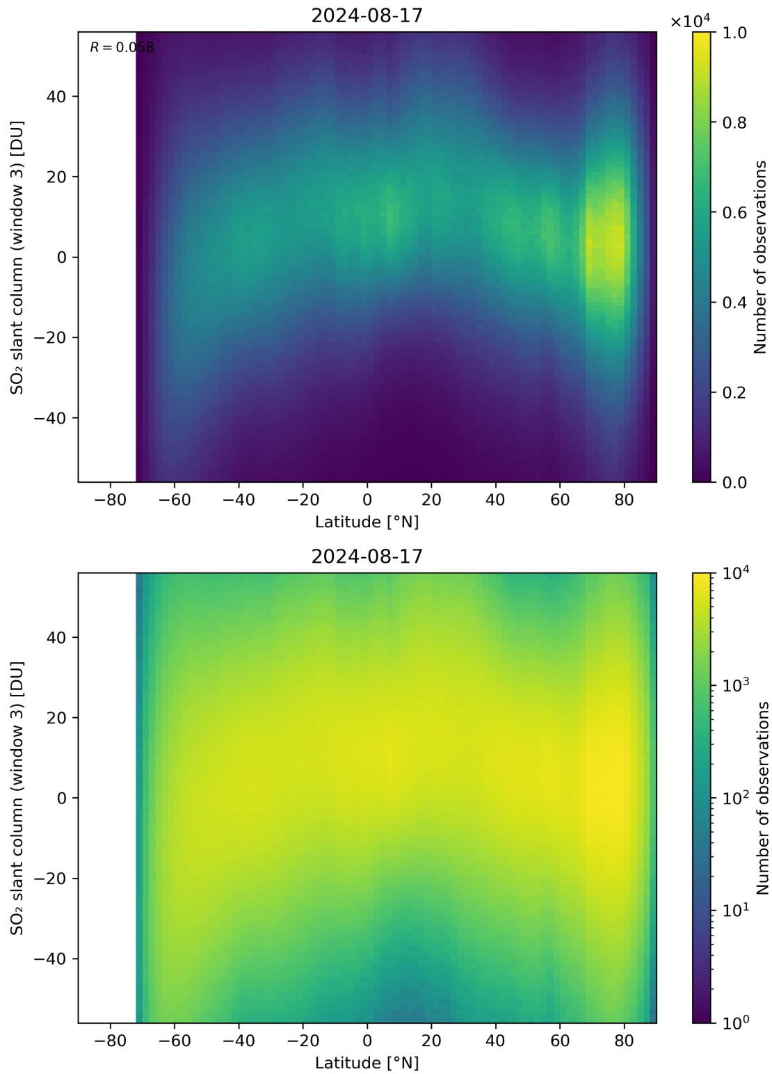
Figure 152: Scatter density plot of “Latitude” against “SO 2 slant column (window 3)” for 2024-08-16 to 2024-08-18.
