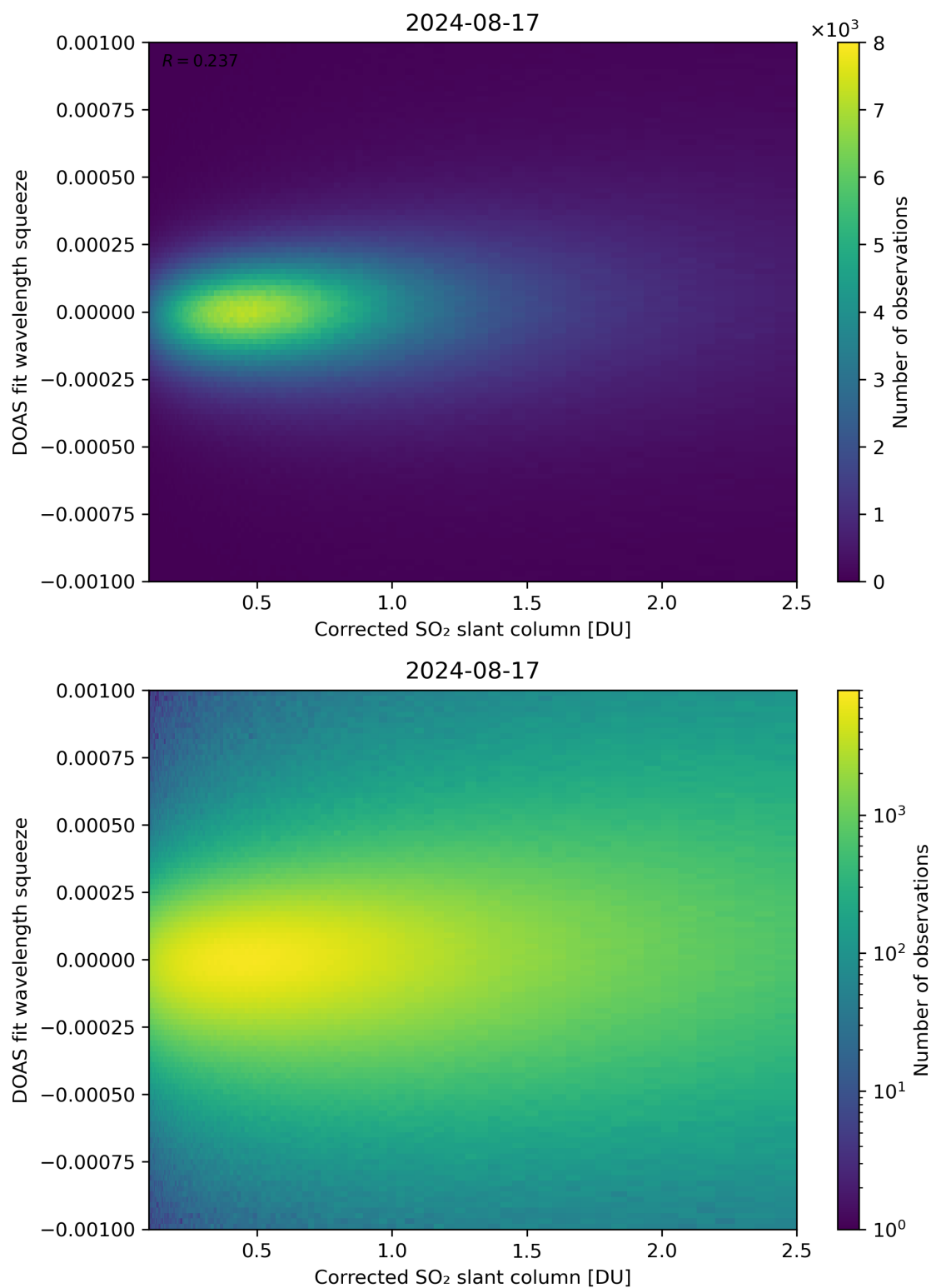
Figure 182: Scatter density plot of “Corrected SO 2 slant column” against “DOAS fit wavelength squeeze” for 2024-08-16 to 2024-08-18.
