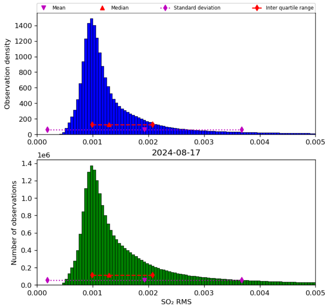
Figure 70: Histogram of “SO 2 RMS” for 2024-08-16 to 2024-08-18
