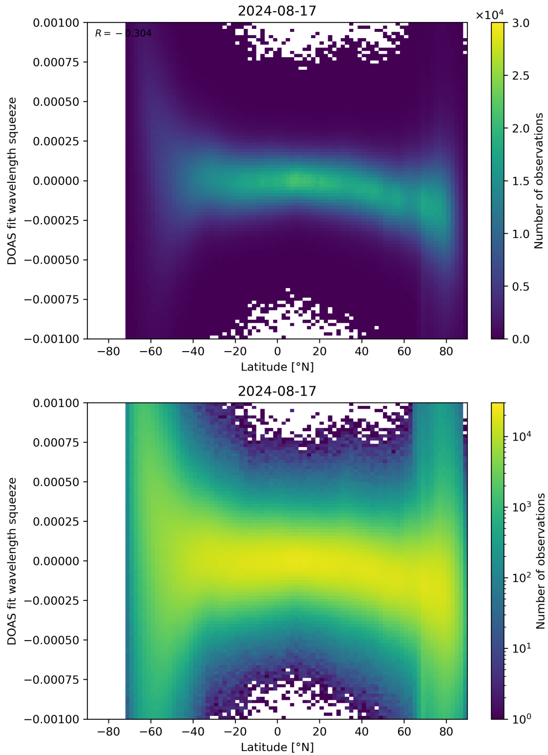
Figure 143: Scatter density plot of “Latitude” against “DOAS fit wavelength squeeze” for 2024-08-16 to 2024-08-18.
