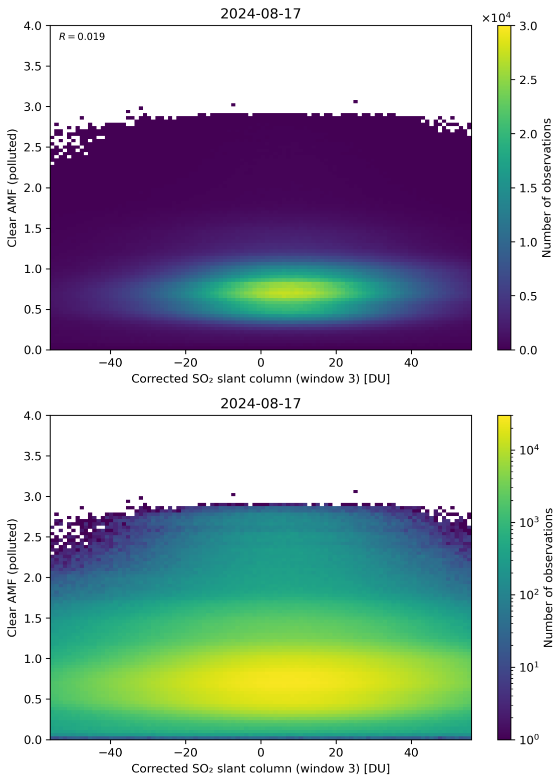
Figure 209: Scatter density plot of “Corrected SO 2 slant column (window 3)” against “Clear AMF (polluted)” for 2024-08-16 to 2024-08-18.
