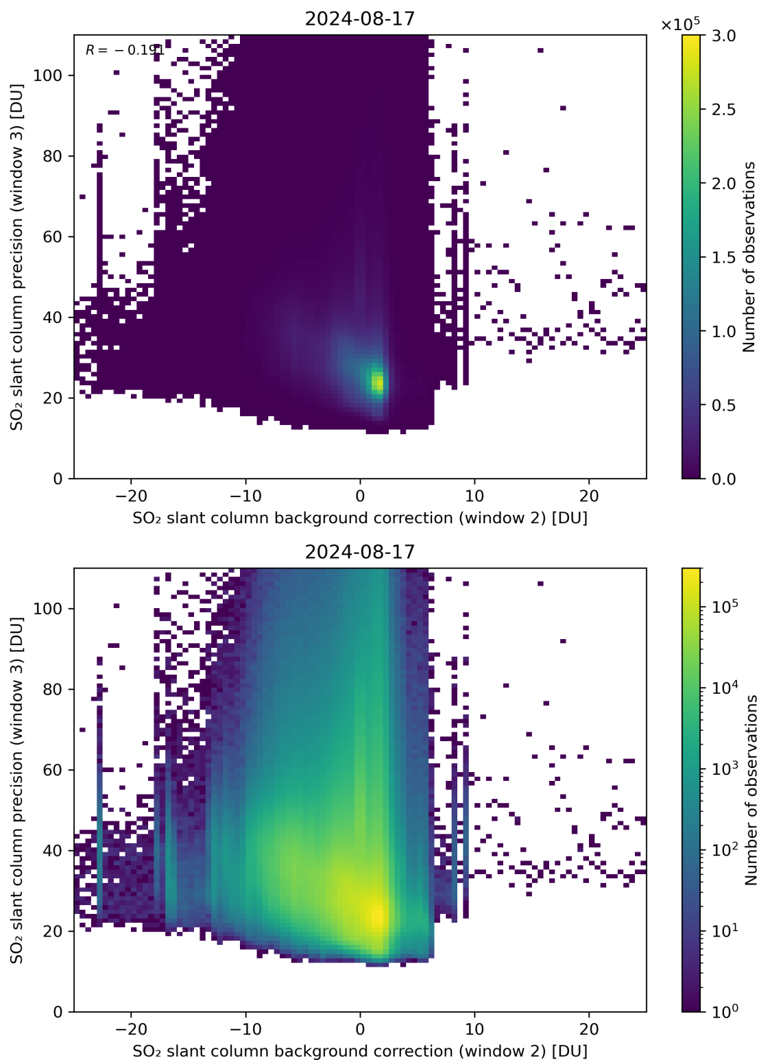
Figure 118: Scatter density plot of “SO 2 slant column background correction (window 2)” against “SO 2 slant column precision (window 3)” for 2024-08-16 to 2024-08-18.
