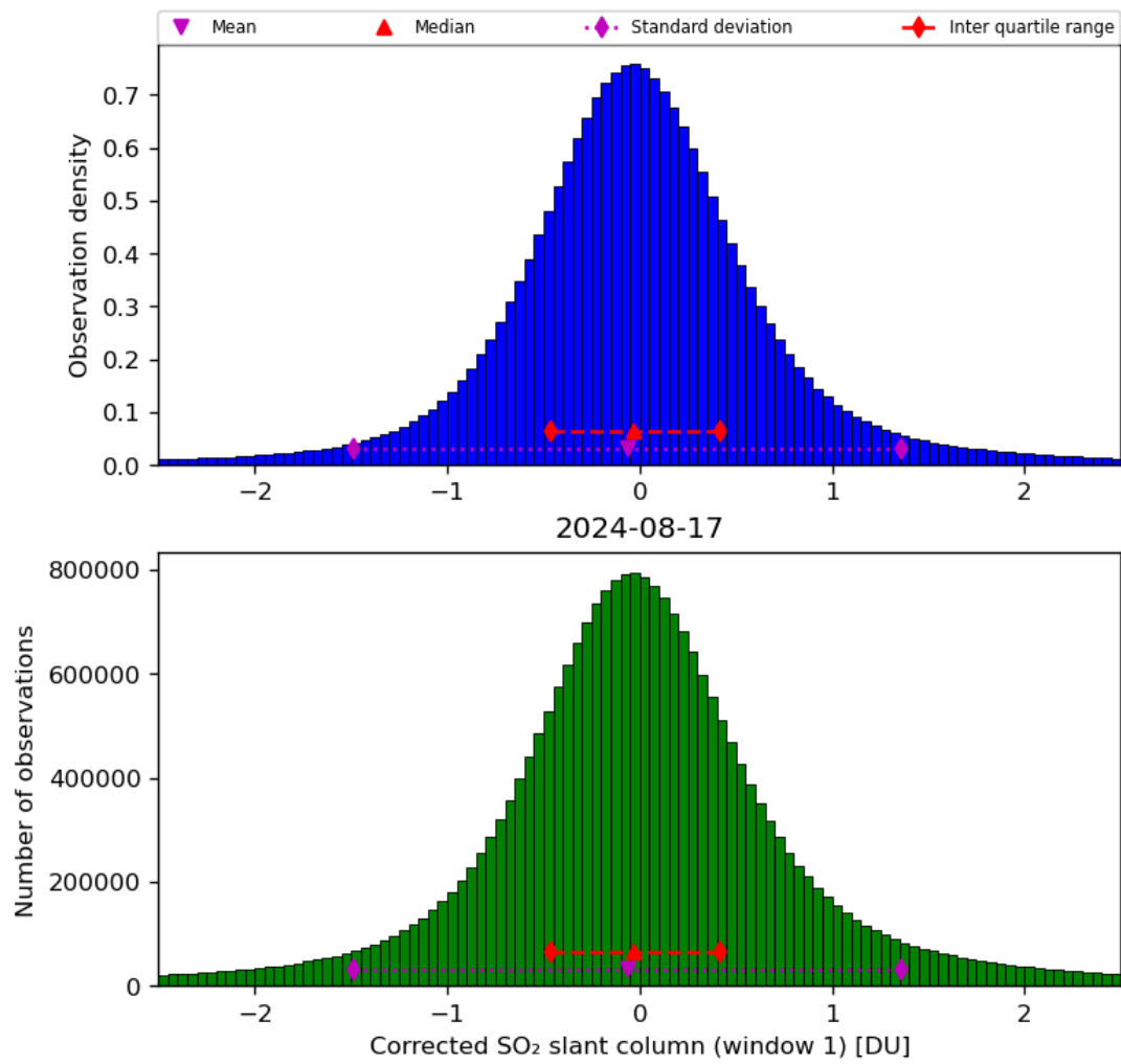
Figure 58: Histogram of “Corrected SO 2 slant column (window 1)” for 2024-08-16 to 2024-08-18
