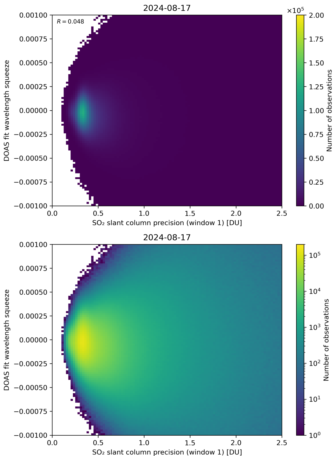
Figure 222: Scatter density plot of “SO 2 slant column precision (window 1)” against “DOAS fit wavelength squeeze” for 2024-08-16 to 2024-08-18.
