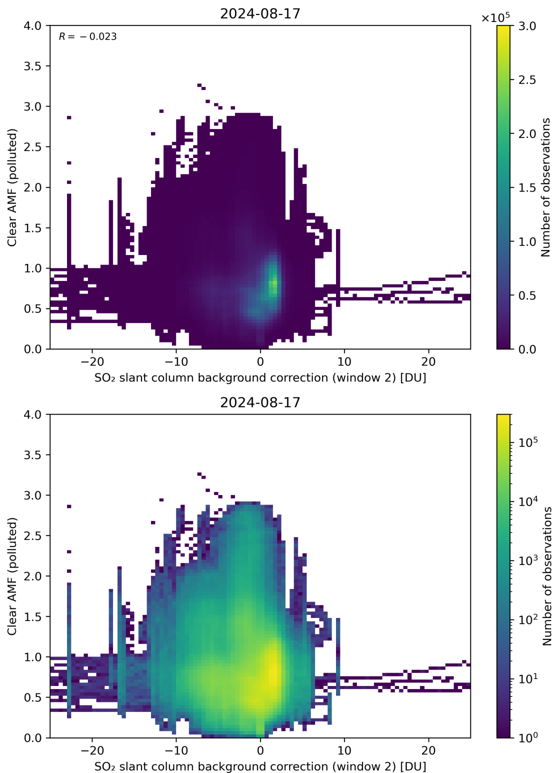
Figure 115: Scatter density plot of “SO 2 slant column background correction (window 2)” against “Clear AMF (polluted)” for 2024-08-16 to 2024-08-18.
