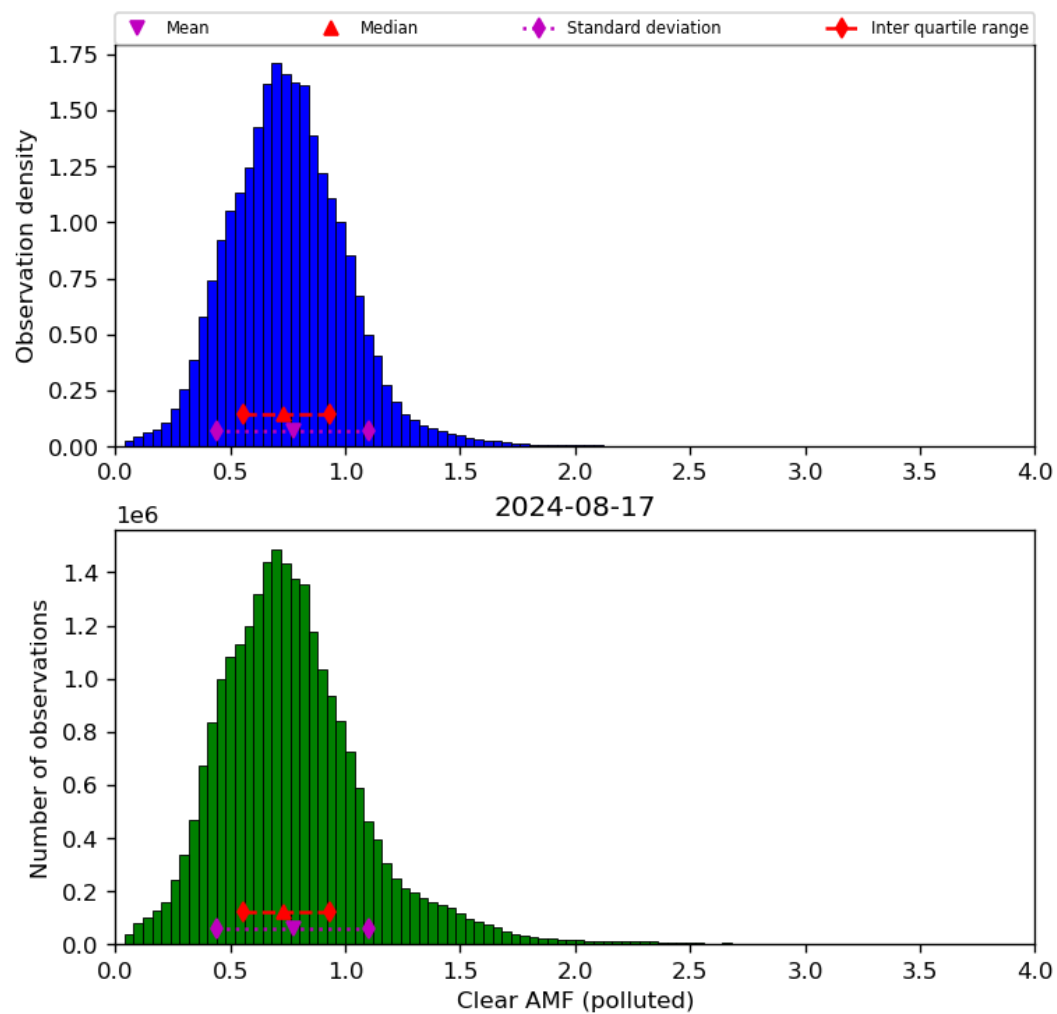
Figure 73: Histogram of “Clear AMF (polluted)” for 2024-08-16 to 2024-08-18
