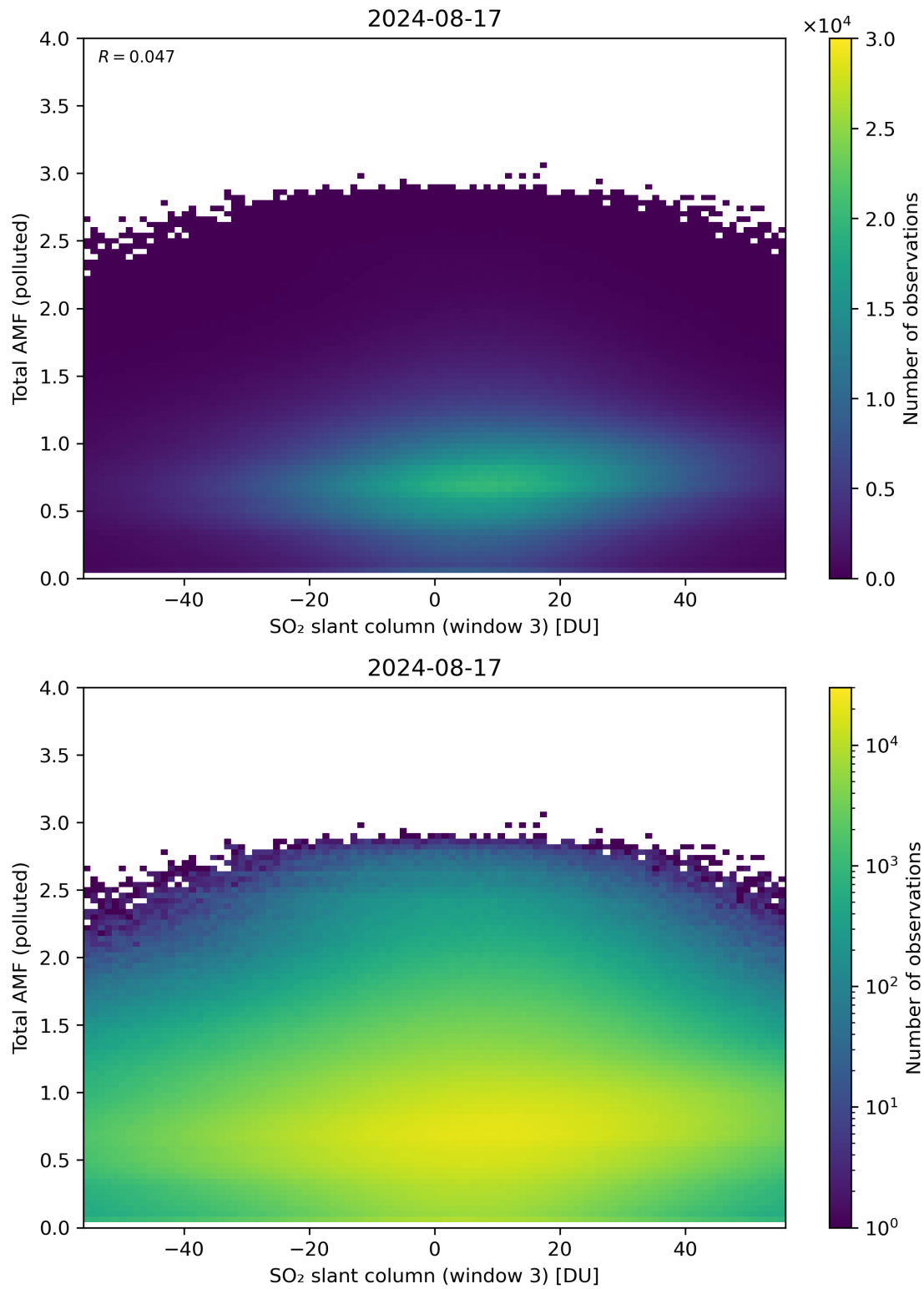
Figure 268: Scatter density plot of “SO 2 slant column (window 3)” against “Total AMF (polluted)” for 2024-08-16 to 2024-08-18.
