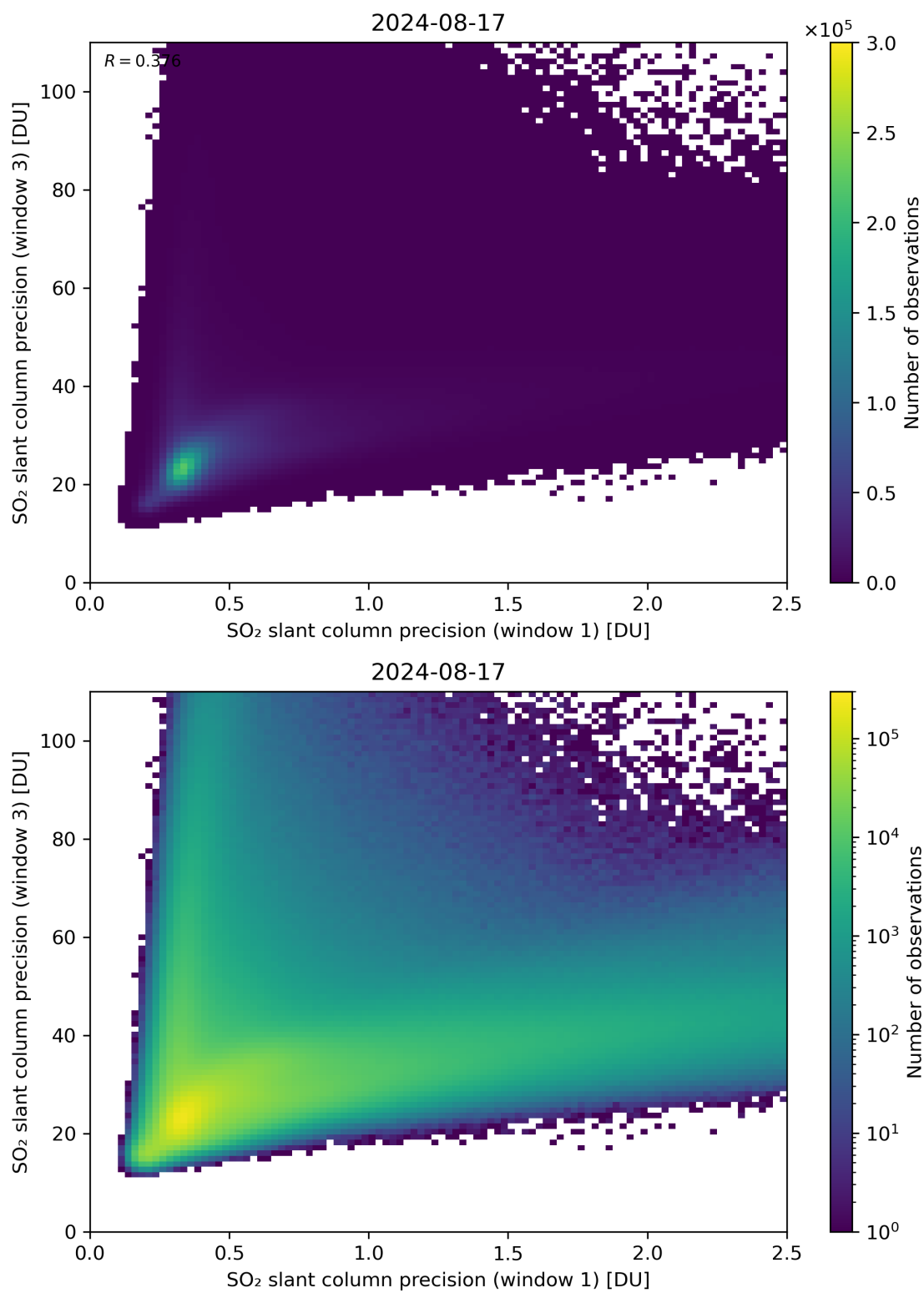
Figure 229: Scatter density plot of “SO 2 slant column precision (window 1)” against “SO 2 slant column precision (window 3)” for 2024-08-16 to 2024-08-18.
