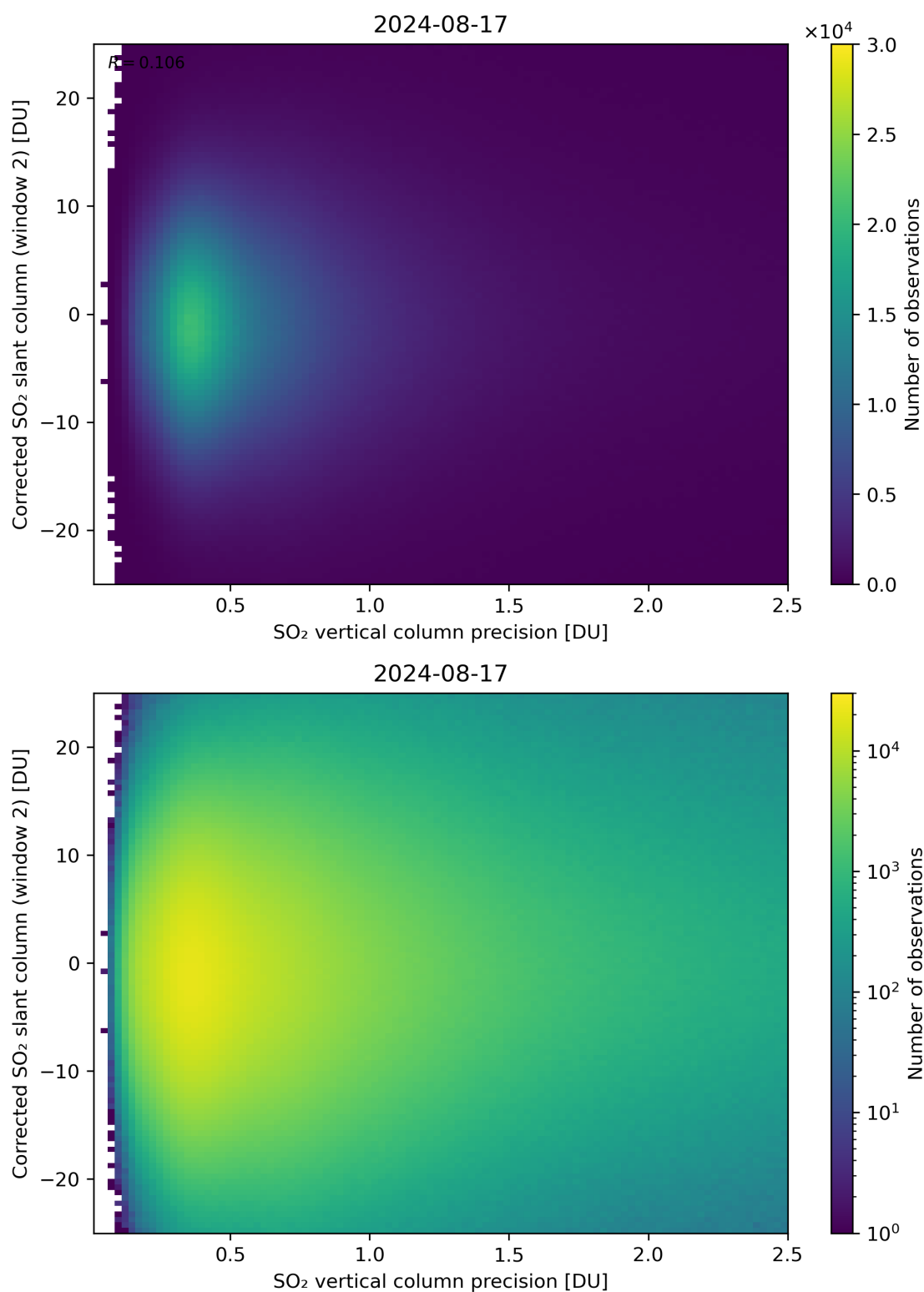
Figure 287: Scatter density plot of “SO 2 vertical column precision” against “Corrected SO 2 slant column (window 2)” for 2024-08-16 to 2024-08-18.
