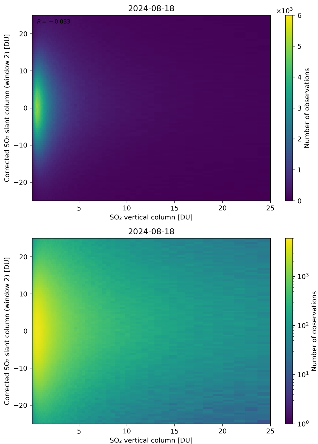
Figure 298: Scatter density plot of “SO 2 vertical column” against “Corrected SO 2 slant column (window 2)” for 2024-08-17 to 2024-08-19.
