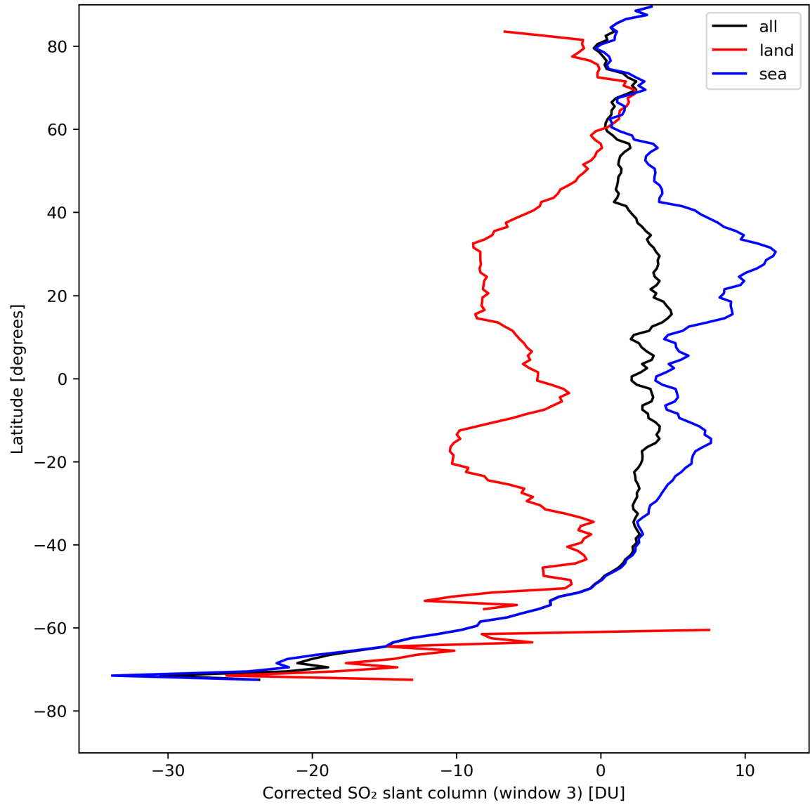
Figure 43: Zonal average of “Corrected SO 2 slant column (window 3)” for 2024-08-17 to 2024-08-19.
