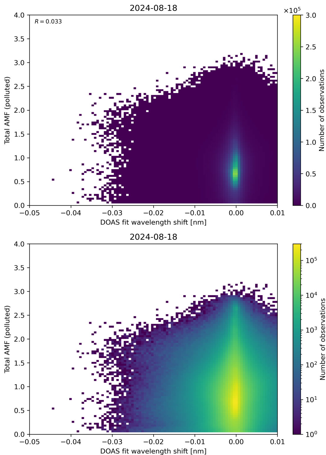
Figure 130: Scatter density plot of “DOAS fit wavelength shift” against “Total AMF (polluted)” for 2024-08-17 to 2024-08-19.
