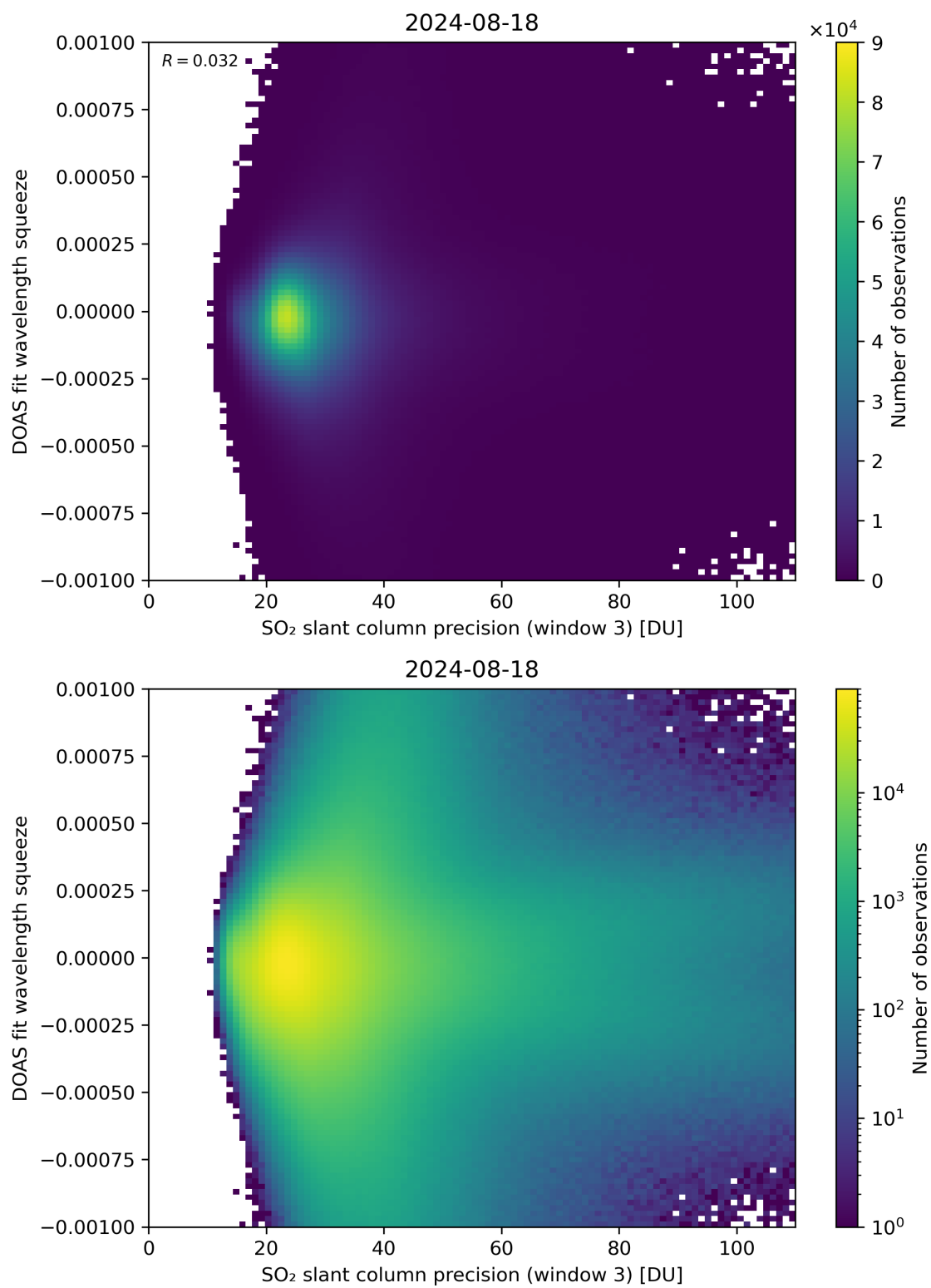
Figure 259: Scatter density plot of “SO 2 slant column precision (window 3)” against “DOAS fit wavelength squeeze” for 2024-08-17 to 2024-08-19.
