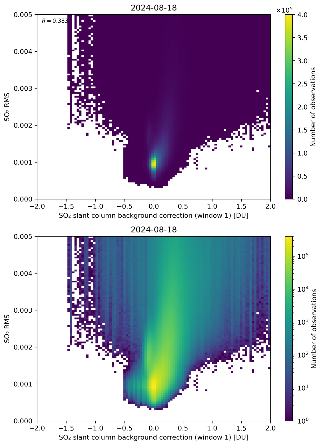
Figure 102: Scatter density plot of “SO 2 slant column background correction (window 1)” against “SO 2 RMS” for 2024-08-17 to 2024-08-19.
