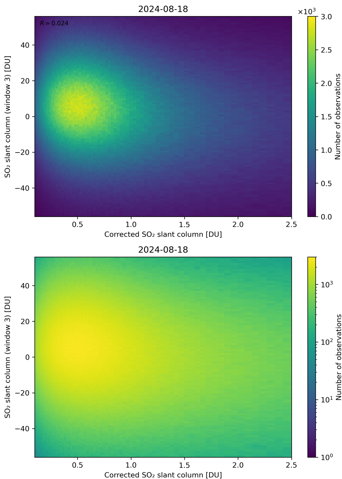
Figure 190: Scatter density plot of “Corrected SO 2 slant column” against “SO 2 slant column (window 3)” for 2024-08-17 to 2024-08-19.
