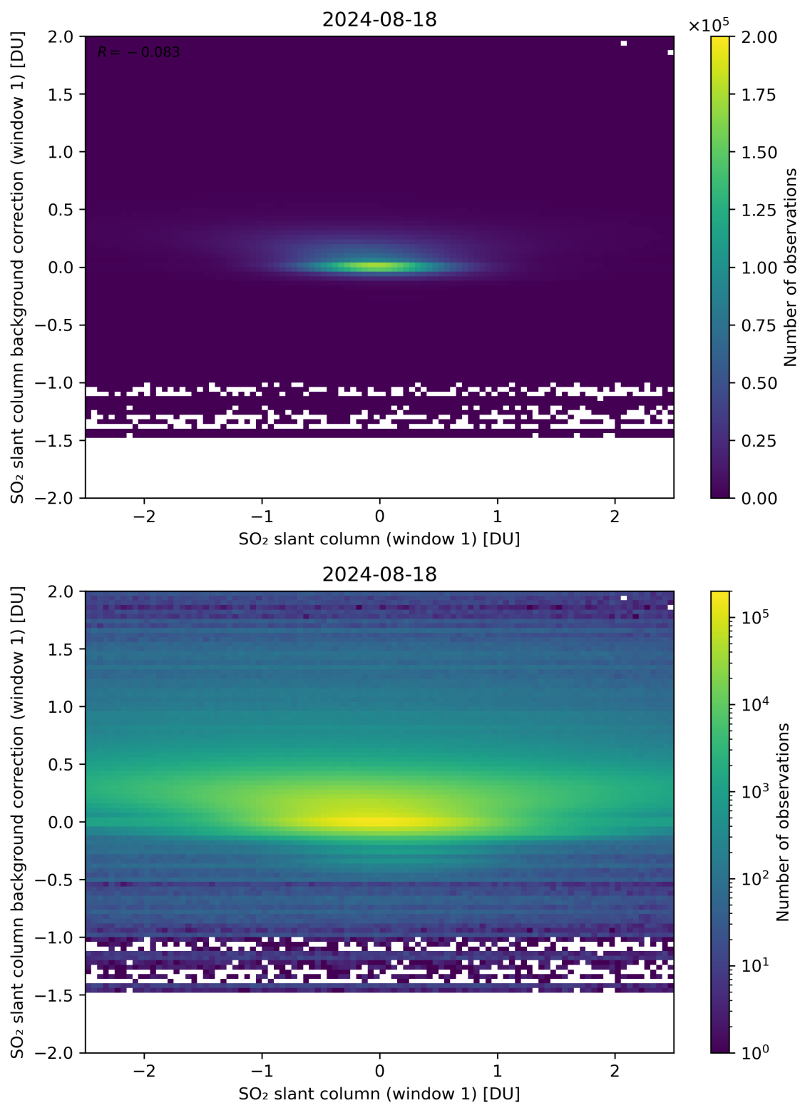
Figure 212: Scatter density plot of “SO 2 slant column (window 1)” against “SO 2 slant column background correction (window 1)” for 2024-08-17 to 2024-08-19.
