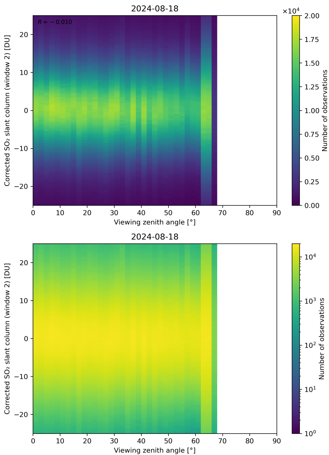
Figure 318: Scatter density plot of “Viewing zenith angle” against “Corrected SO 2 slant column (window 2)” for 2024-08-17 to 2024-08-19.
