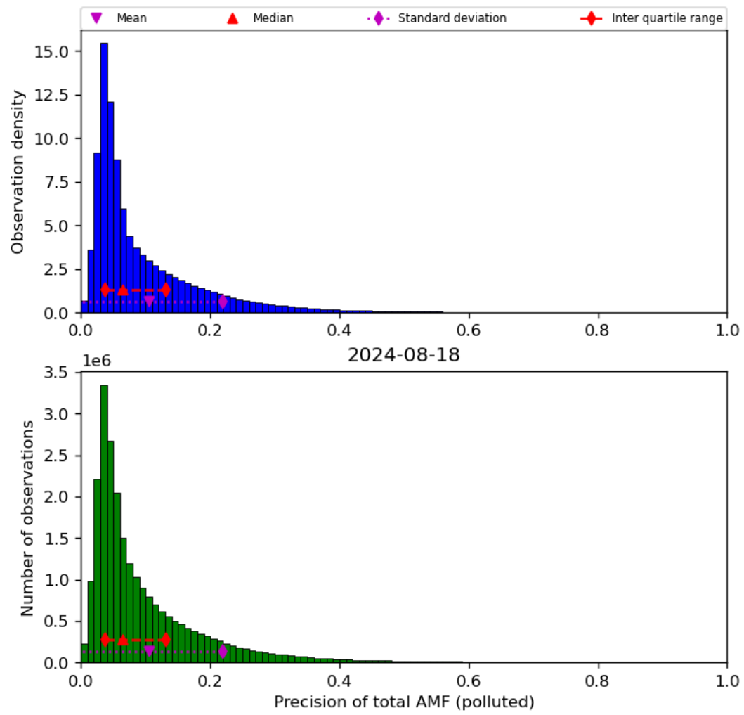
Figure 72: Histogram of “Precision of total AMF (polluted)” for 2024-08-17 to 2024-08-19
