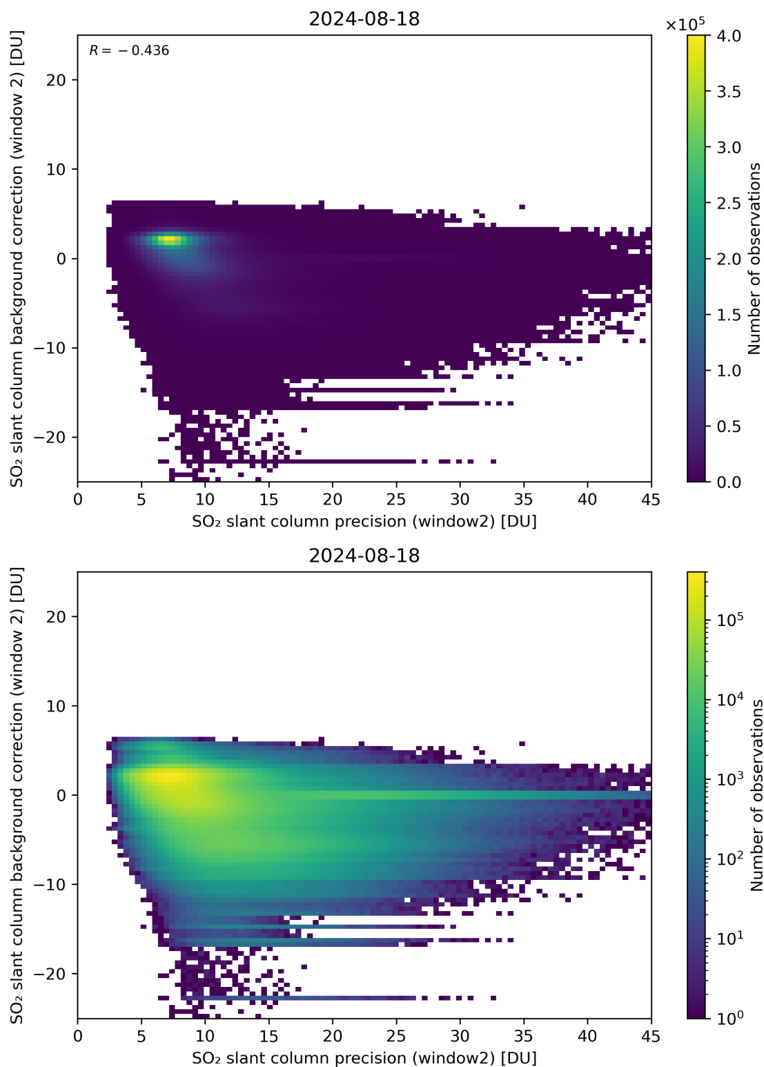
Figure 241: Scatter density plot of “SO 2 slant column precision (window2)” against “SO 2 slant column background correction (window 2)” for 2024-08-17 to 2024-08-19.
