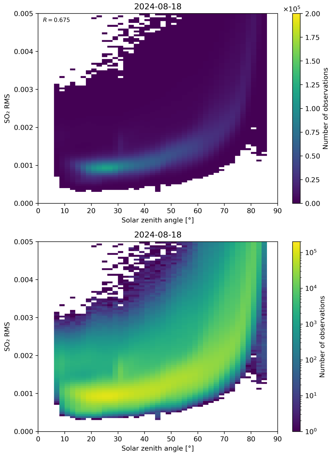
Figure 163: Scatter density plot of “Solar zenith angle” against “SO 2 RMS” for 2024-08-17 to 2024-08-19.
