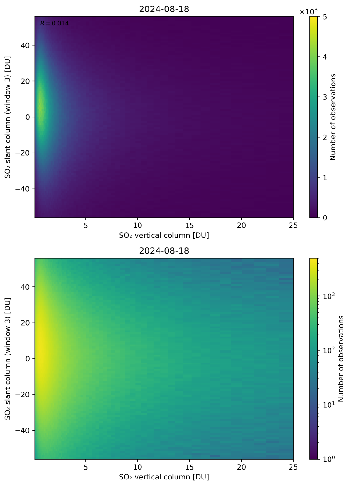
Figure 303: Scatter density plot of “SO 2 vertical column” against “SO 2 slant column (window 3)” for 2024-08-17 to 2024-08-19.
