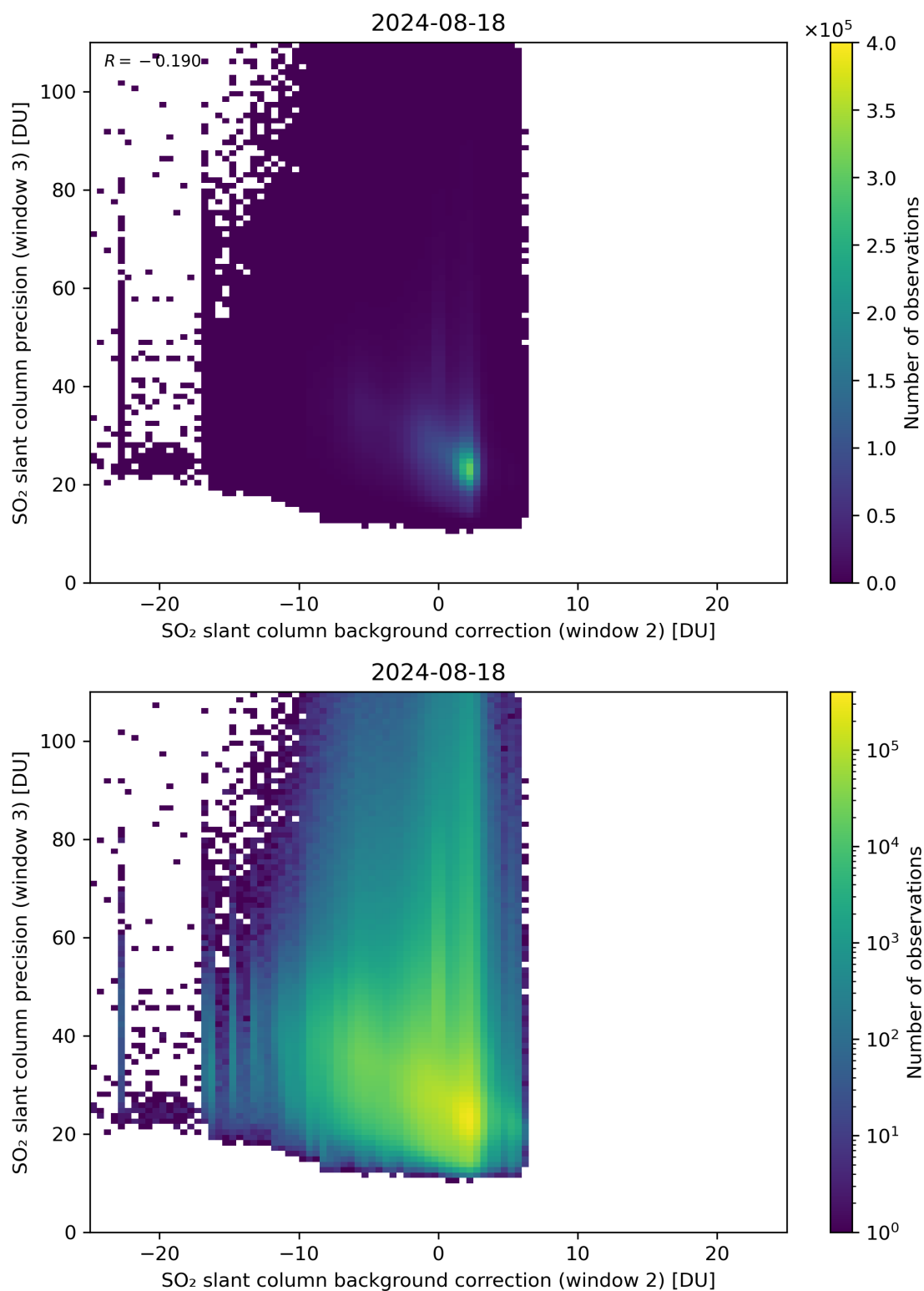
Figure 118: Scatter density plot of “SO 2 slant column background correction (window 2)” against “SO 2 slant column precision (window 3)” for 2024-08-17 to 2024-08-19.
