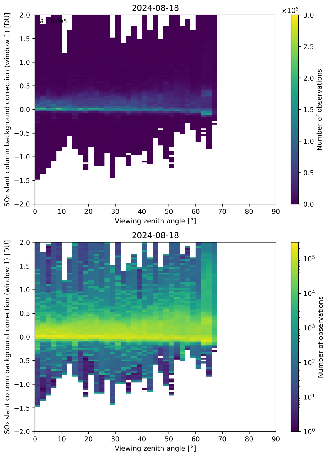
Figure 308: Scatter density plot of “Viewing zenith angle” against “SO 2 slant column background correction (window 1)” for 2024-08-17 to 2024-08-19.
