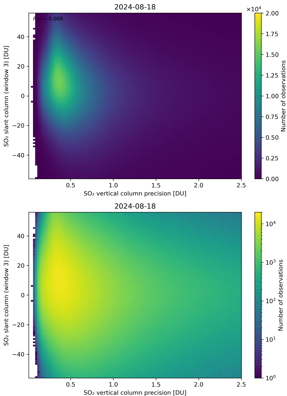
Figure 292: Scatter density plot of “SO 2 vertical column precision” against “SO 2 slant column (window 3)” for 2024-08-17 to 2024-08-19.
