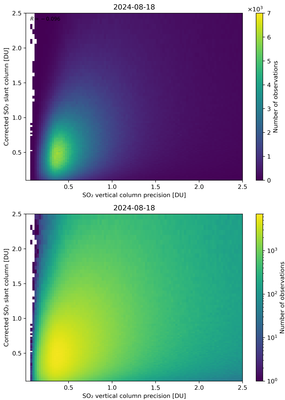
Figure 286: Scatter density plot of “SO 2 vertical column precision” against “Corrected SO 2 slant column” for 2024-08-17 to 2024-08-19.
