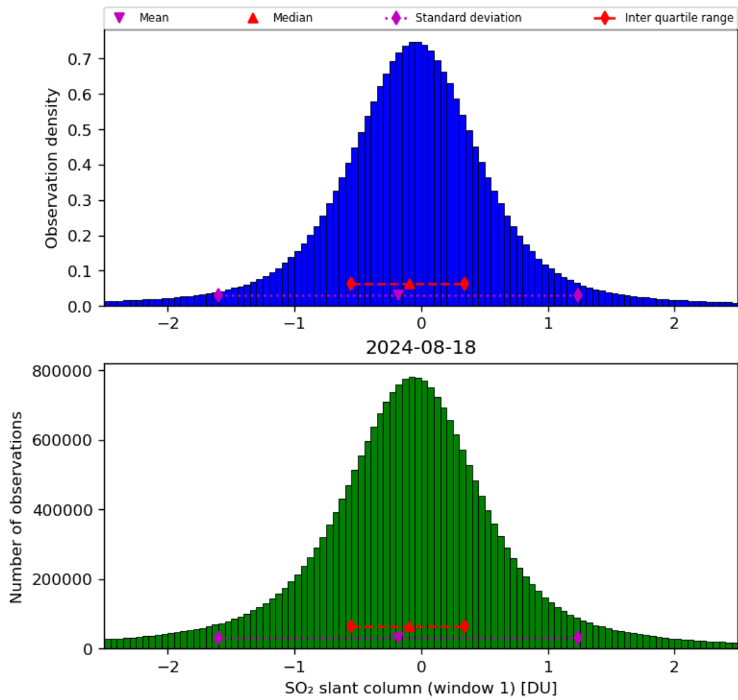
Figure 56: Histogram of “SO 2 slant column (window 1)” for 2024-08-17 to 2024-08-19
