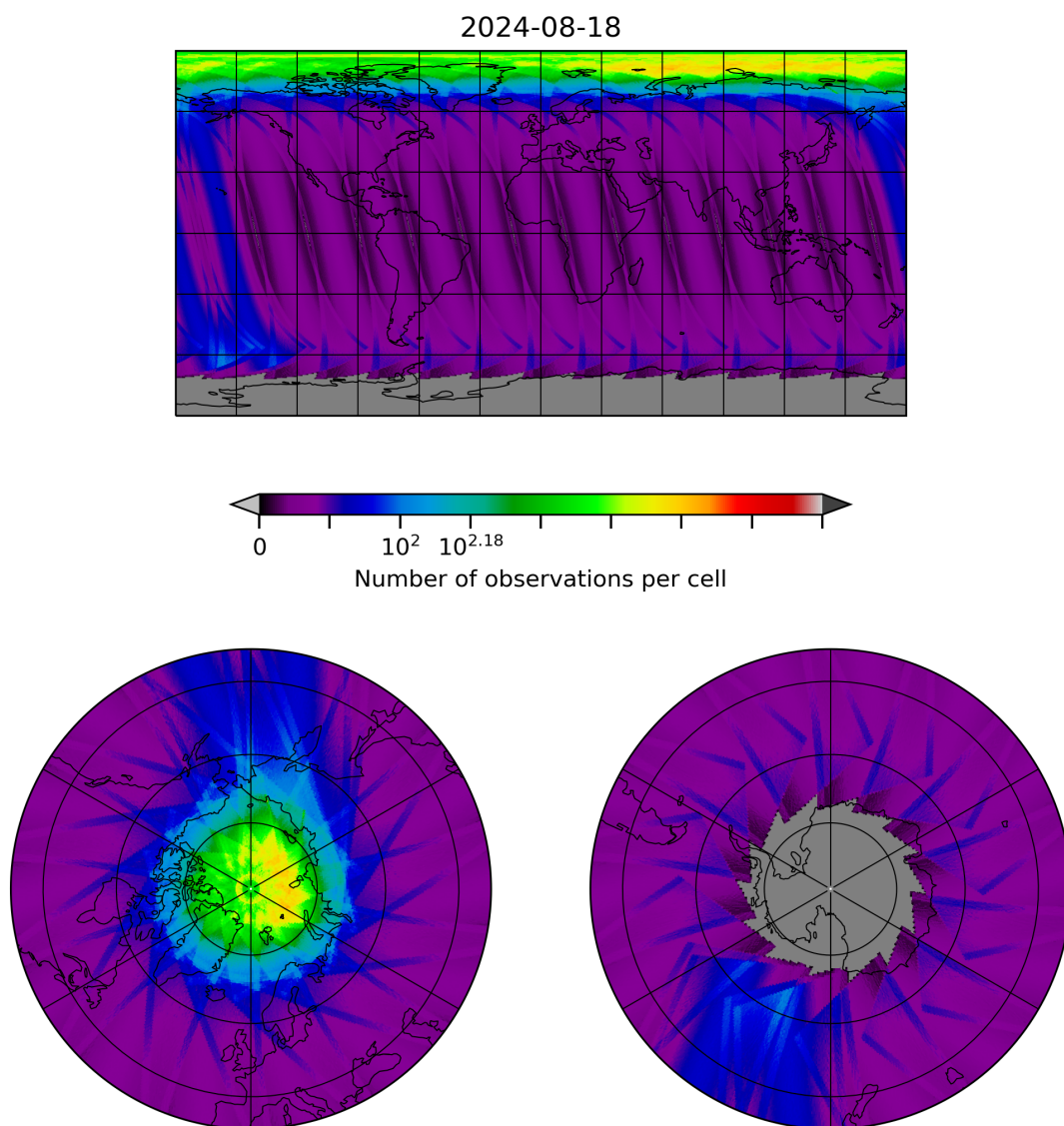
Figure 28: Map of the number of observations for 2024-08-17 to 2024-08-19
