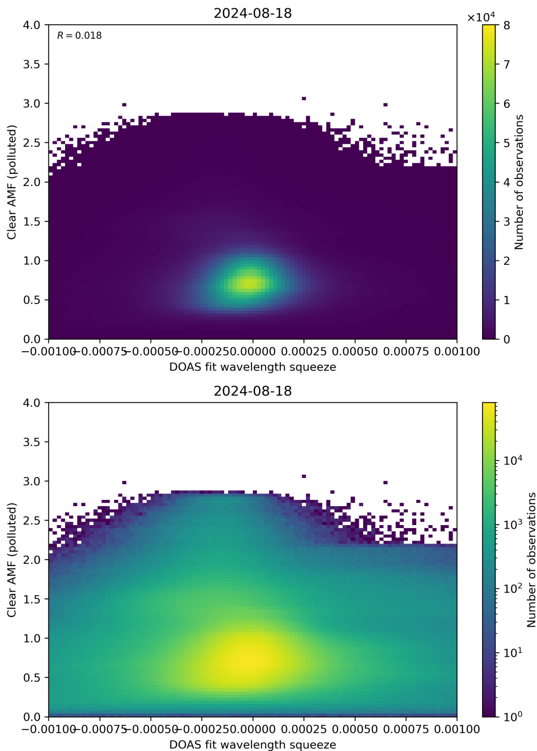
Figure 133: Scatter density plot of “DOAS fit wavelength squeeze” against “Clear AMF (polluted)” for 2024-08-17 to 2024-08-19.
