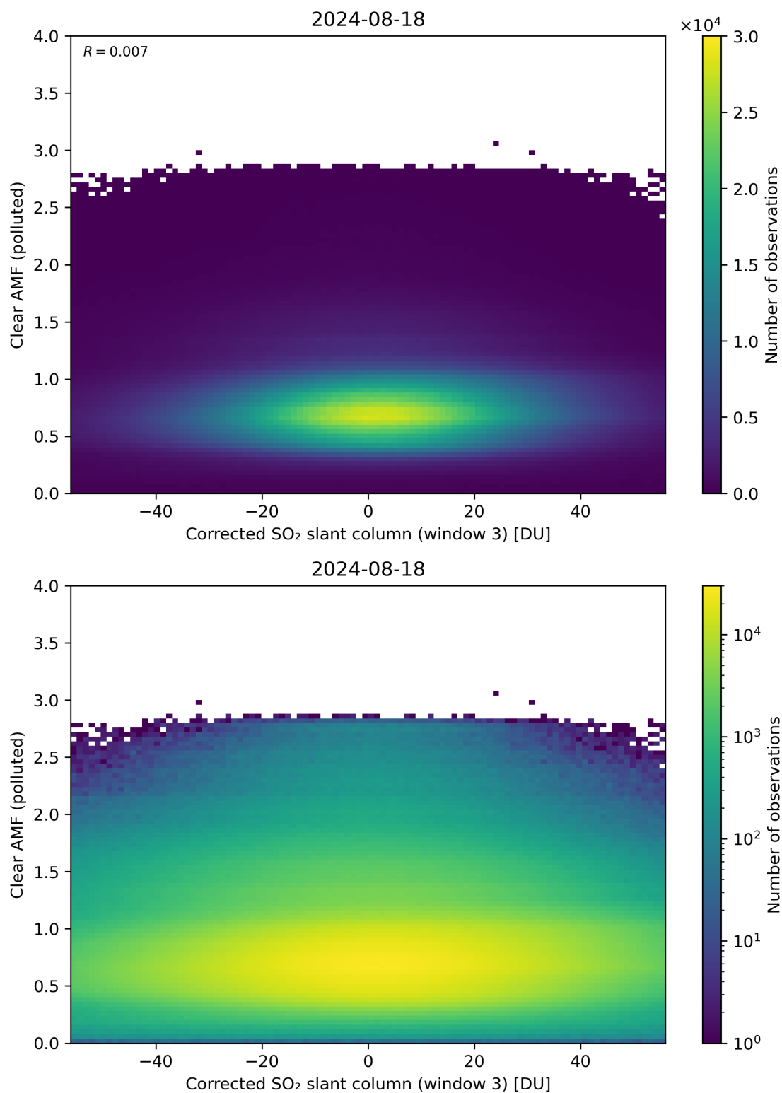
Figure 209: Scatter density plot of “Corrected SO 2 slant column (window 3)” against “Clear AMF (polluted)” for 2024-08-17 to 2024-08-19.
