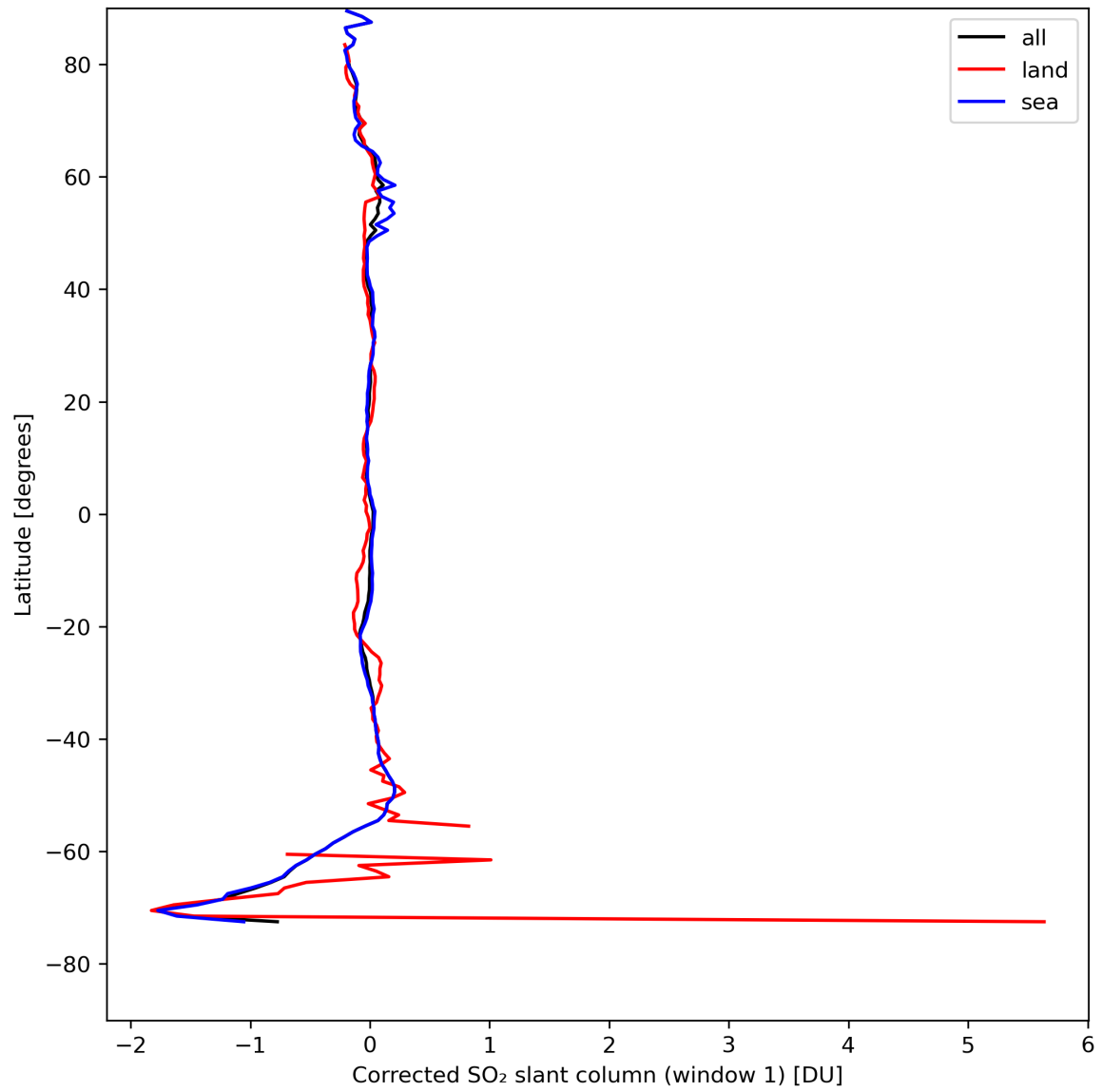
Figure 35: Zonal average of “Corrected SO 2 slant column (window 1)” for 2024-08-17 to 2024-08-19.
