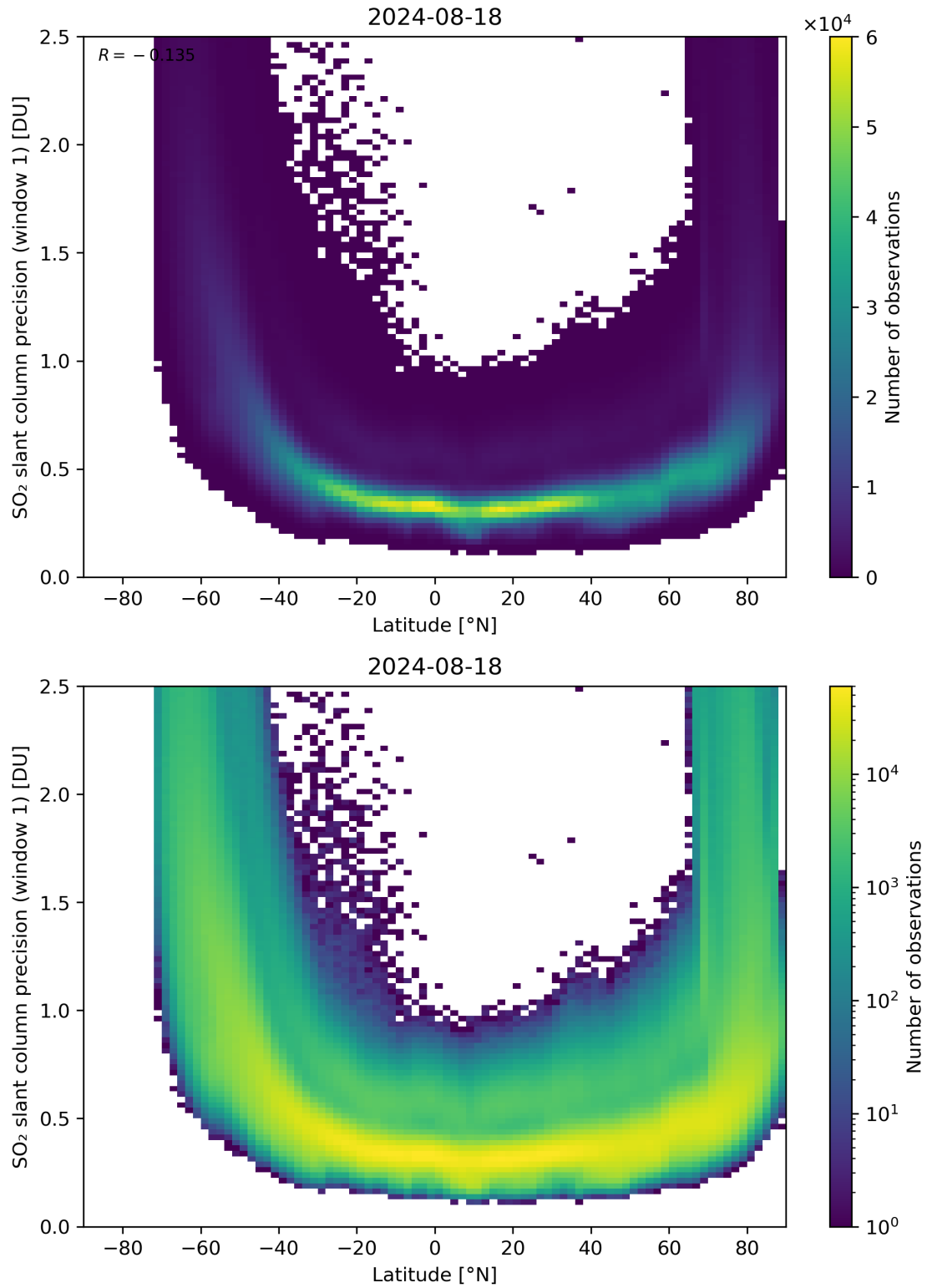
Figure 150: Scatter density plot of “Latitude” against “SO 2 slant column precision (window 1)” for 2024-08-17 to 2024-08-19.
