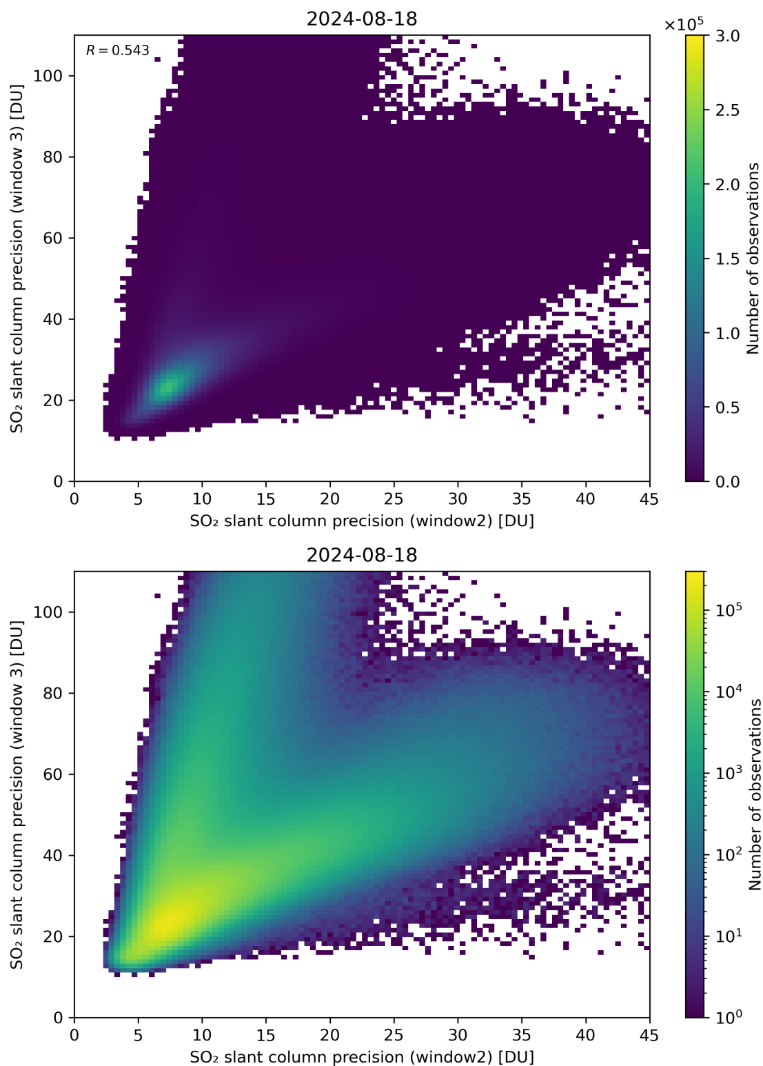
Figure 250: Scatter density plot of “SO 2 slant column precision (window2)” against “SO 2 slant column precision (window 3)” for 2024-08-17 to 2024-08-19.
