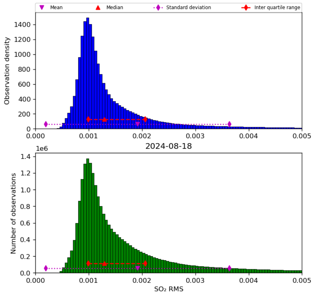
Figure 70: Histogram of “SO 2 RMS” for 2024-08-17 to 2024-08-19
