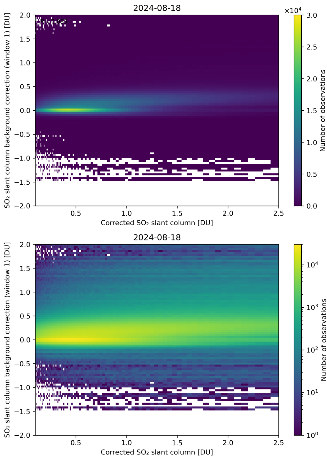
Figure 178: Scatter density plot of “Corrected SO 2 slant column” against “SO 2 slant column background correction (window 1)” for 2024-08-17 to 2024-08-19.
