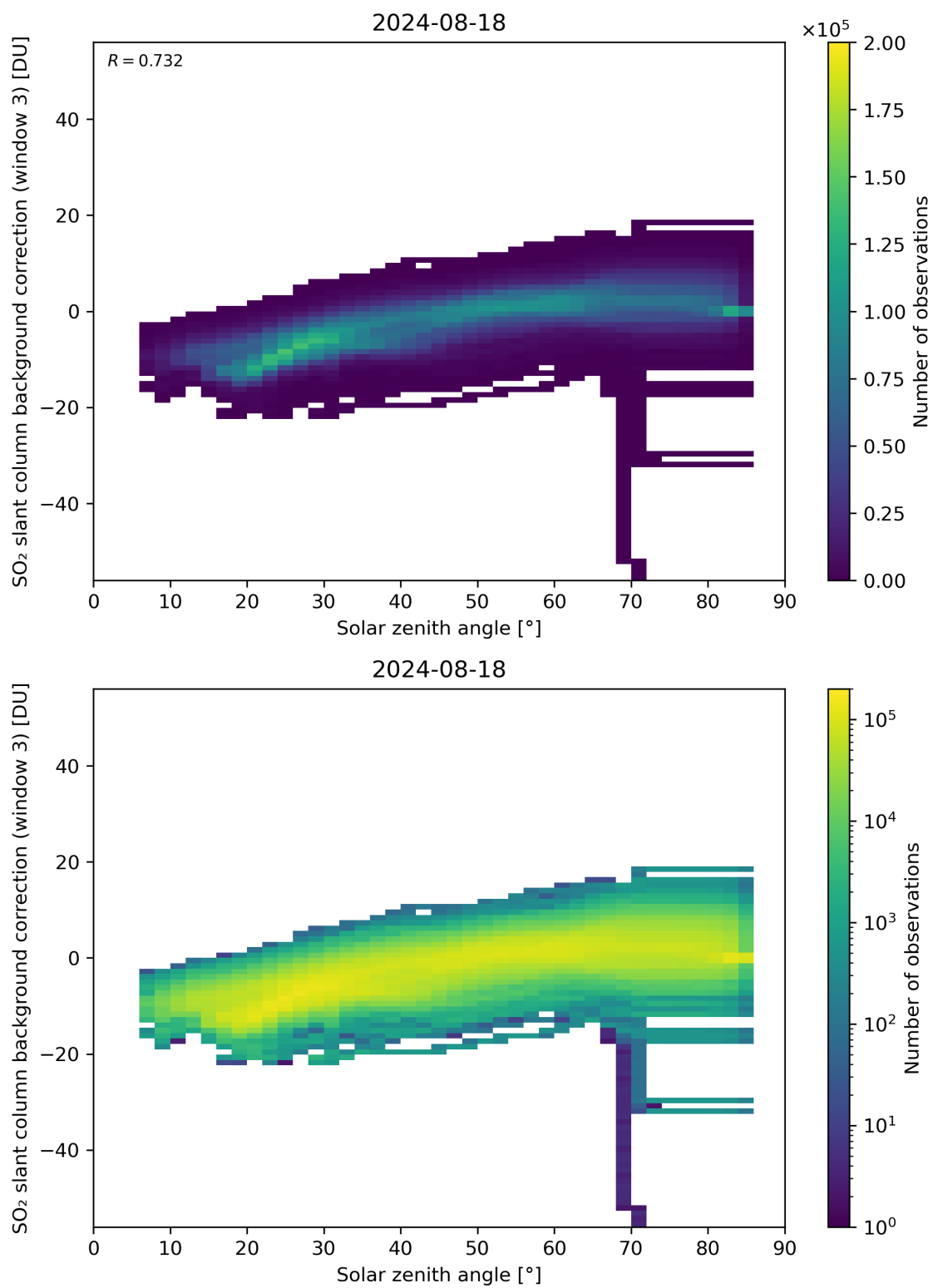
Figure 160: Scatter density plot of “Solar zenith angle” against “SO 2 slant column background correction (window 3)” for 2024-08-17 to 2024-08-19.
