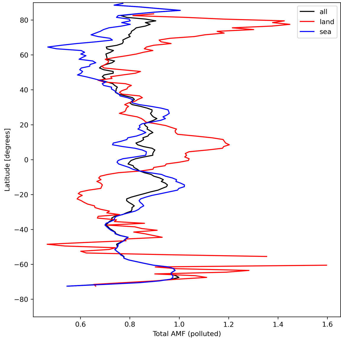
Figure 48: Zonal average of “Total AMF (polluted)” for 2024-08-17 to 2024-08-19.
