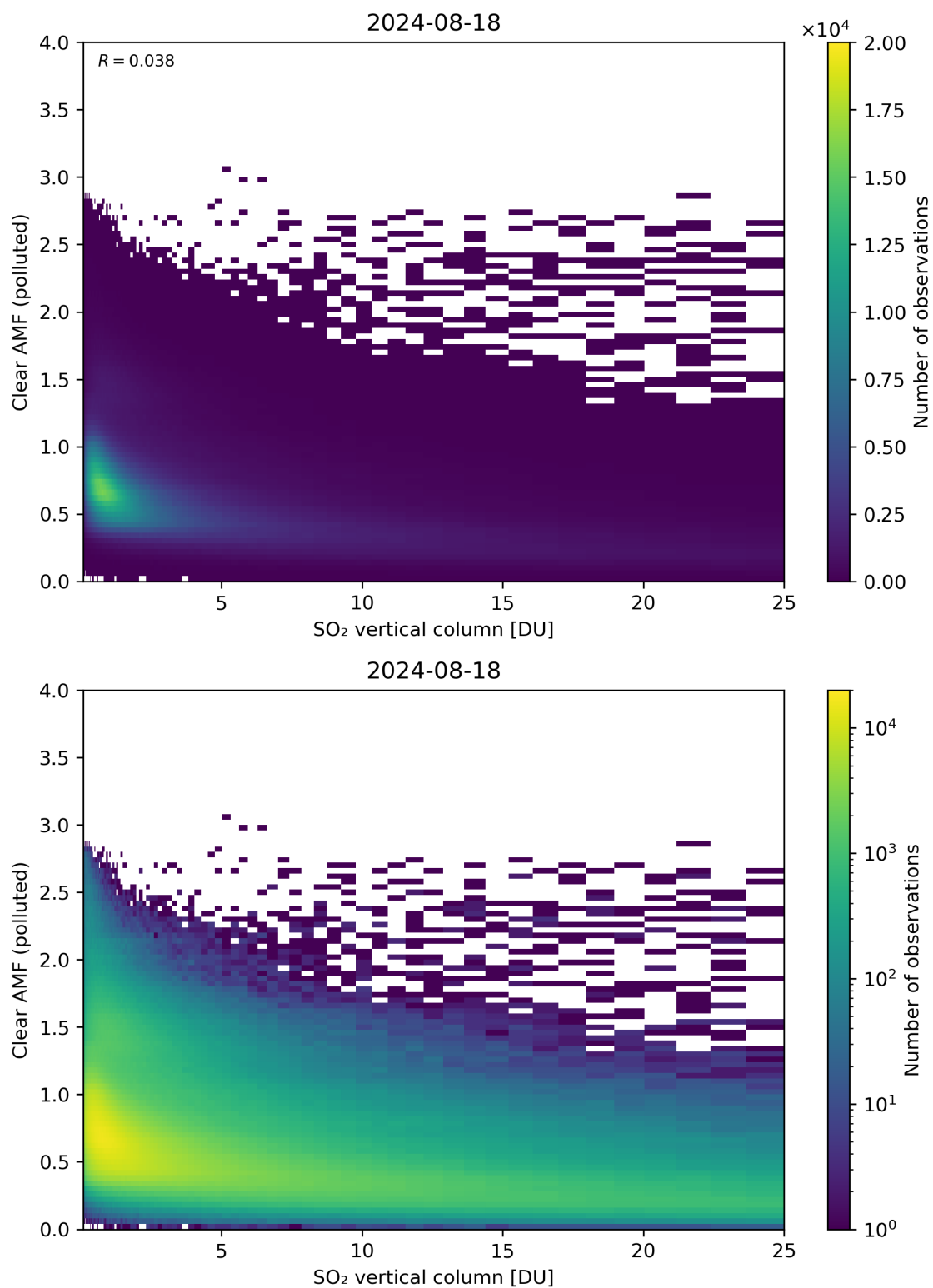
Figure 296: Scatter density plot of “SO 2 vertical column” against “Clear AMF (polluted)” for 2024-08-17 to 2024-08-19.
