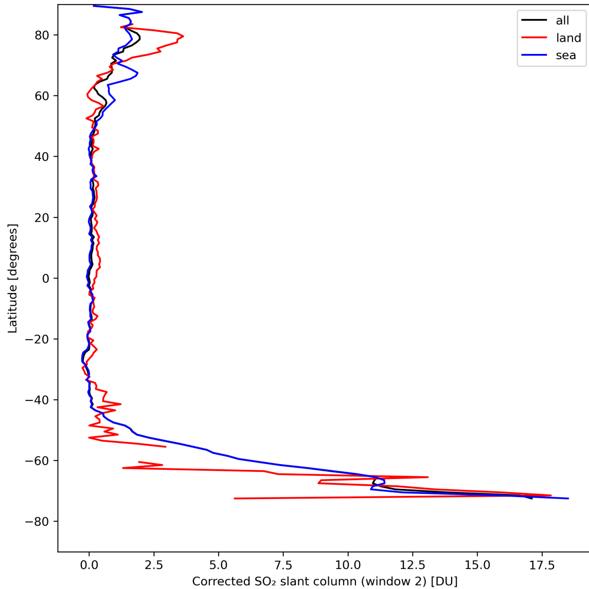
Figure 39: Zonal average of “Corrected SO 2 slant column (window 2)” for 2024-08-17 to 2024-08-19.
