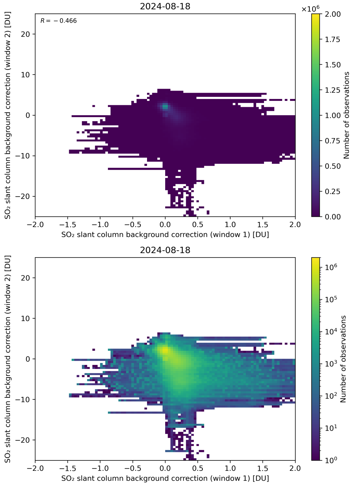
Figure 98: Scatter density plot of “SO 2 slant column background correction (window 1)” against “SO 2 slant column background correction (window 2)” for 2024-08-17 to 2024-08-19.
