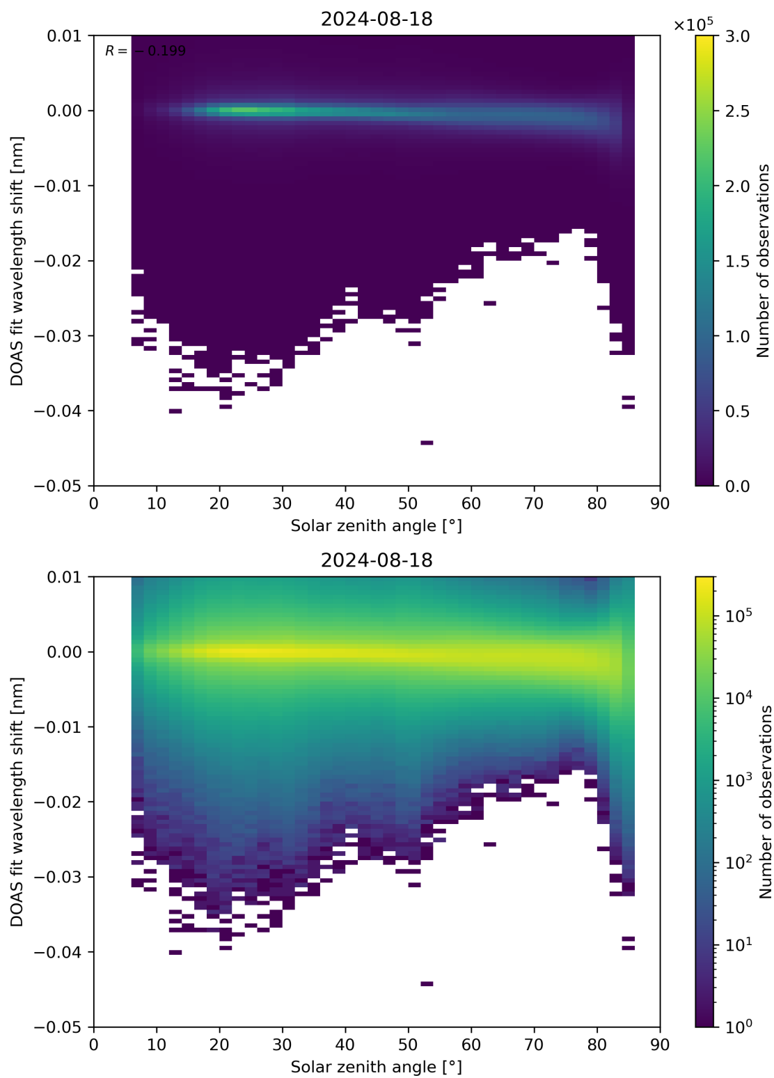
Figure 161: Scatter density plot of “Solar zenith angle” against “DOAS fit wavelength shift” for 2024-08-17 to 2024-08-19.
