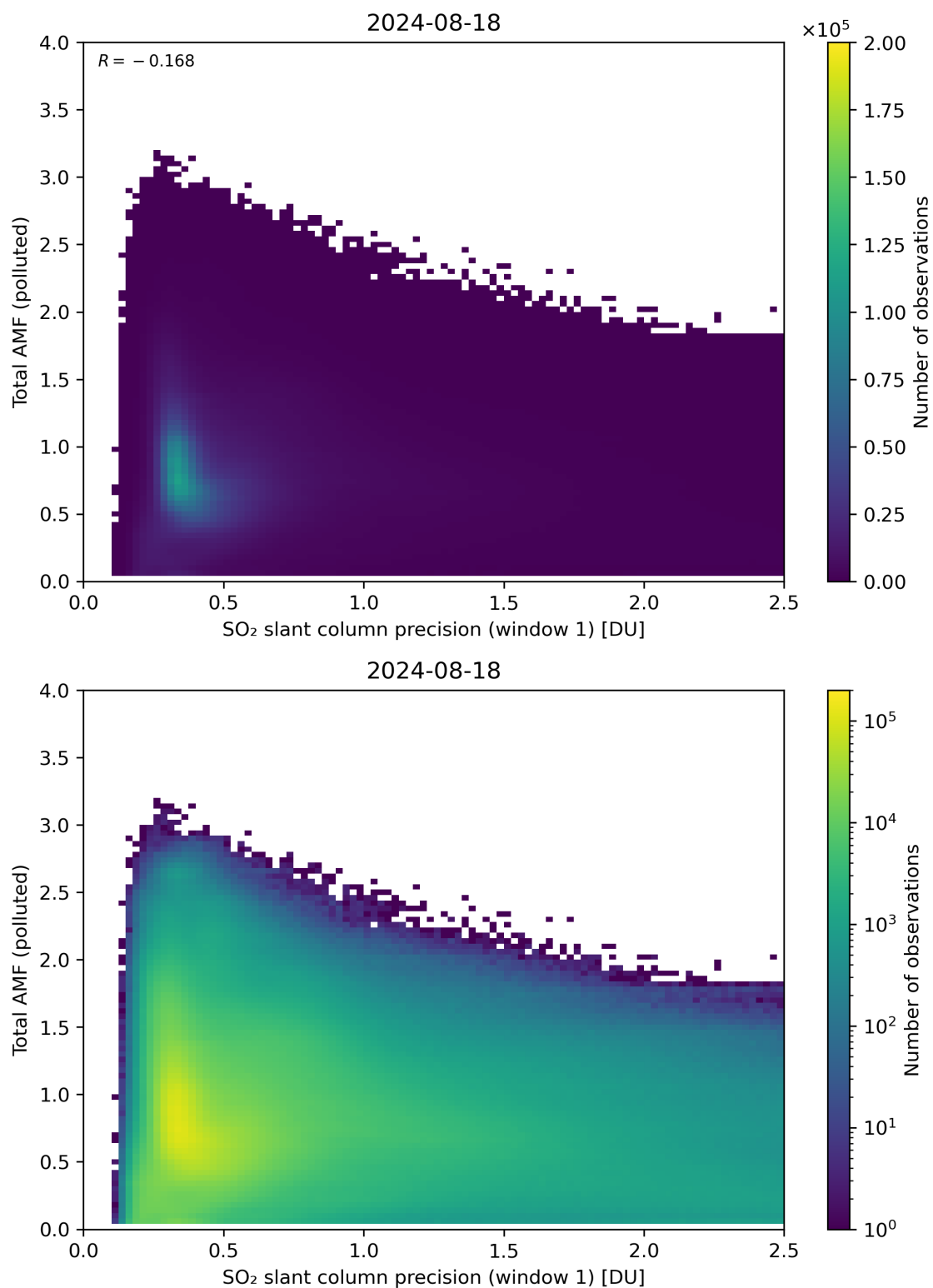
Figure 230: Scatter density plot of “SO 2 slant column precision (window 1)” against “Total AMF (polluted)” for 2024-08-17 to 2024-08-19.
