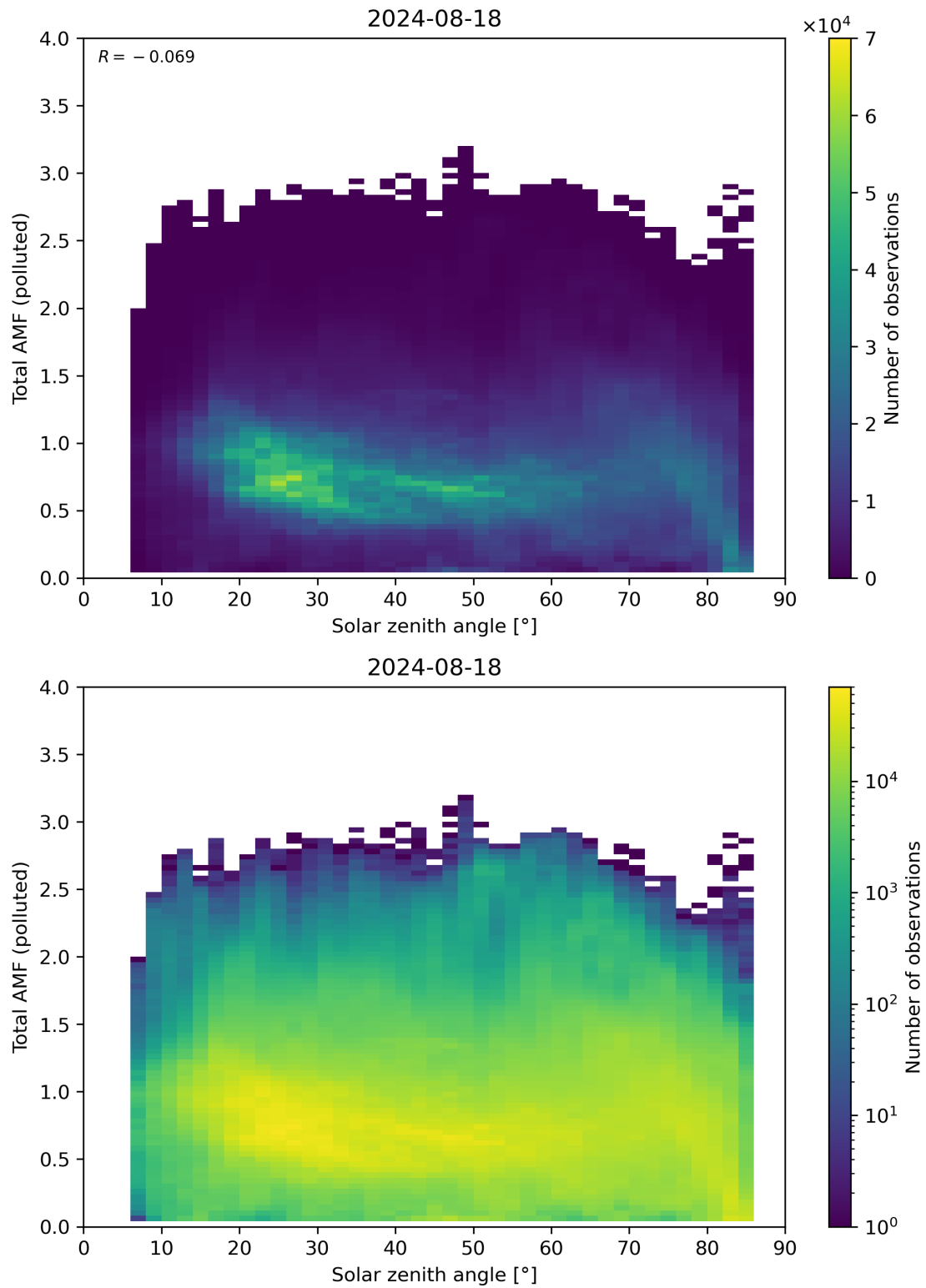
Figure 174: Scatter density plot of “Solar zenith angle” against “Total AMF (polluted)” for 2024-08-17 to 2024-08-19.
