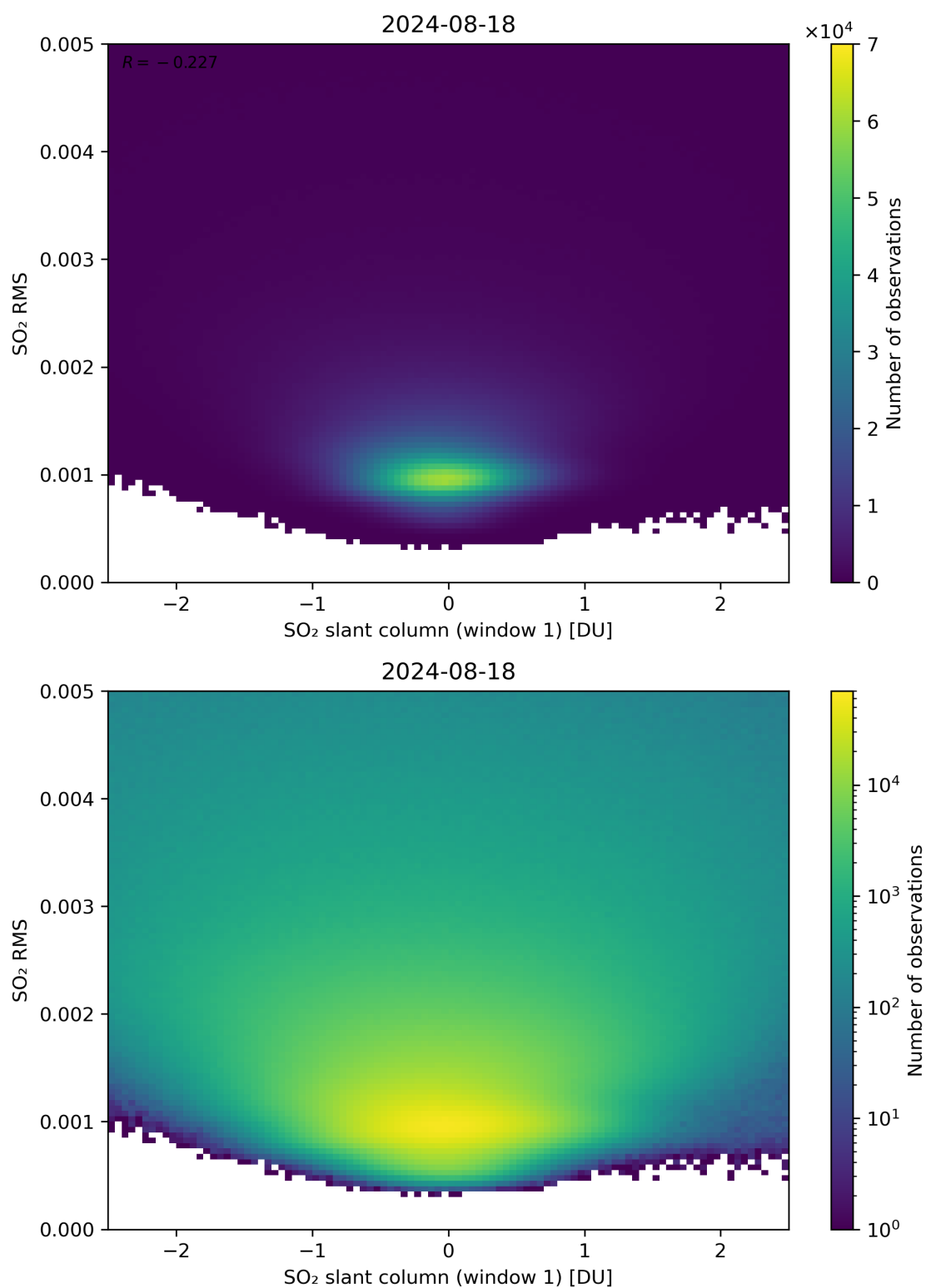
Figure 217: Scatter density plot of “SO 2 slant column (window 1)” against “SO 2 RMS” for 2024-08-17 to 2024-08-19.
