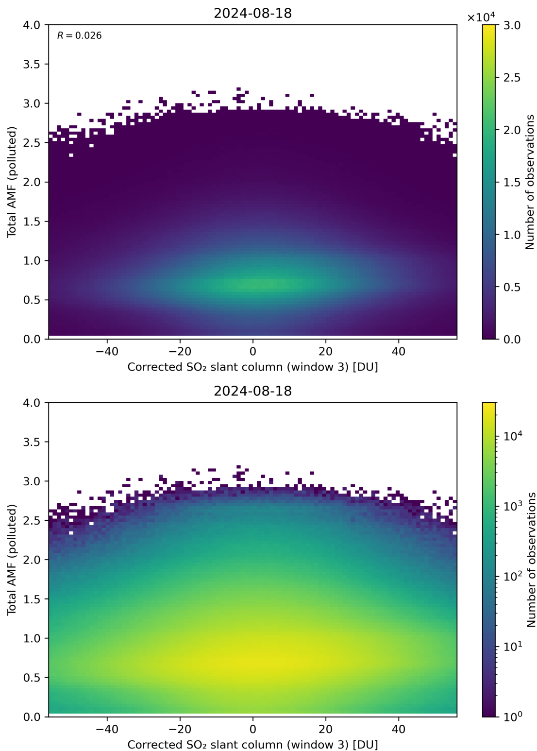
Figure 210: Scatter density plot of “Corrected SO 2 slant column (window 3)” against “Total AMF (polluted)” for 2024-08-17 to 2024-08-19.
