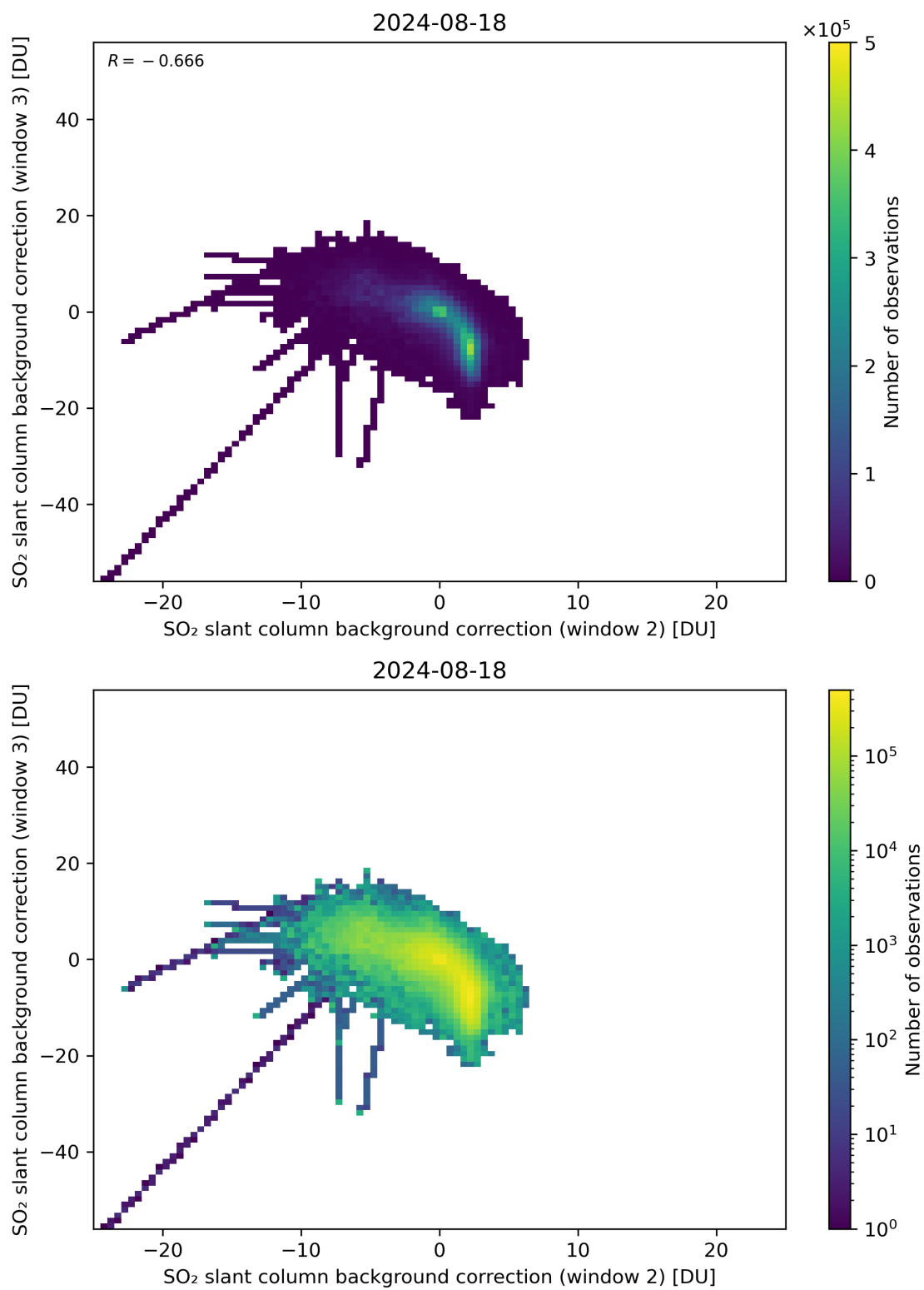
Figure 111: Scatter density plot of “SO 2 slant column background correction (window 2)” against “SO 2 slant column background correction (window 3)” for 2024-08-17 to 2024-08-19.
