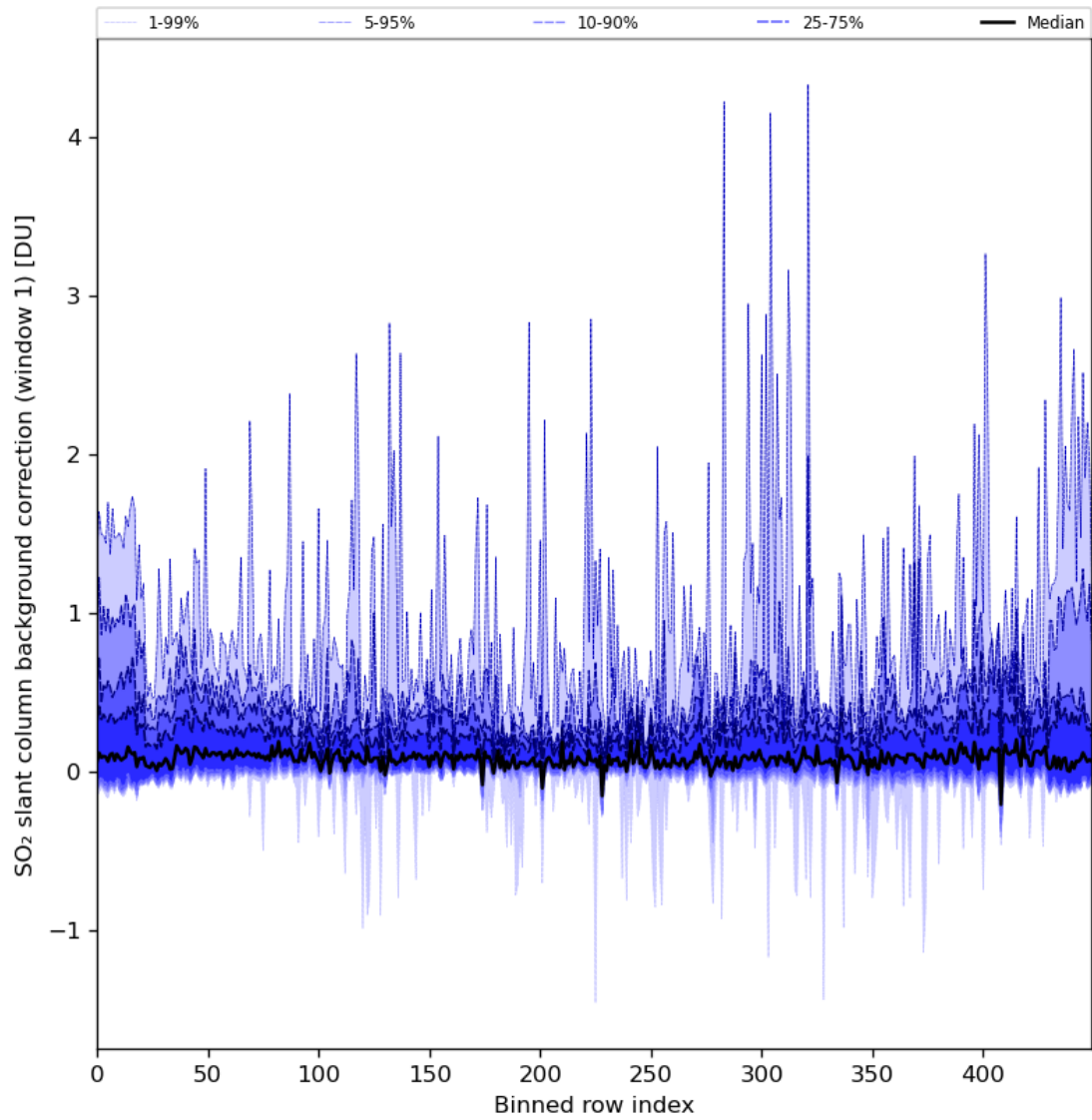
Figure 82: Along track statistics of “SO 2 slant column background correction (window 1)” for 2024-08-17 to 2024-08-19
