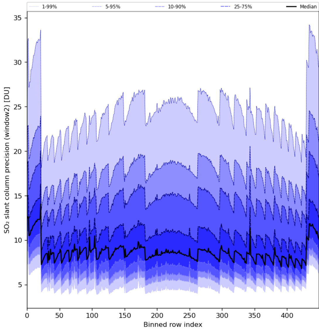
Figure 84: Along track statistics of “SO 2 slant column precision (window2)” for 2024-08-17 to 2024-08-19
