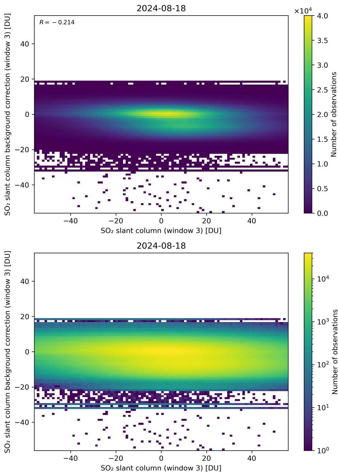
Figure 253: Scatter density plot of “SO 2 slant column (window 3)” against “SO 2 slant column background correction (window 3)” for 2024-08-17 to 2024-08-19.
