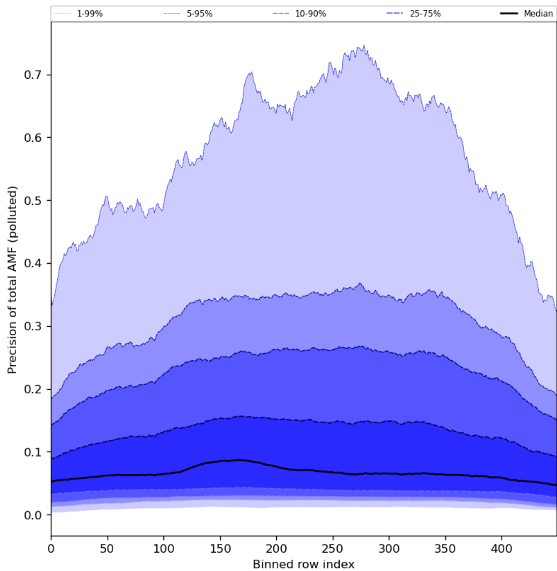
Figure 95: Along track statistics of “Precision of total AMF (polluted)” for 2024-08-17 to 2024-08-19
