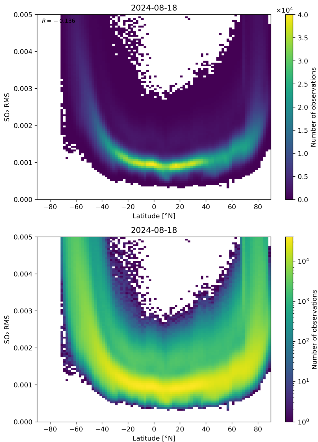
Figure 144: Scatter density plot of “Latitude” against “SO 2 RMS” for 2024-08-17 to 2024-08-19.
