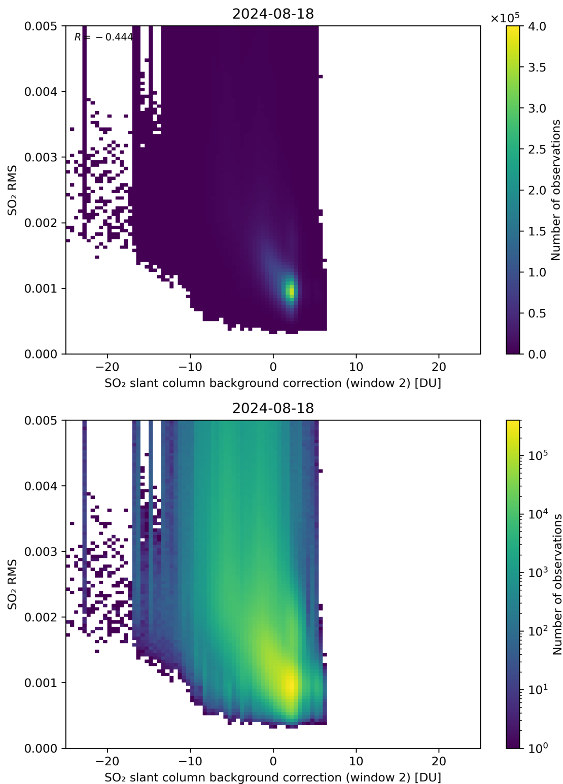
Figure 114: Scatter density plot of “SO 2 slant column background correction (window 2)” against “SO 2 RMS” for 2024-08-17 to 2024-08-19.
