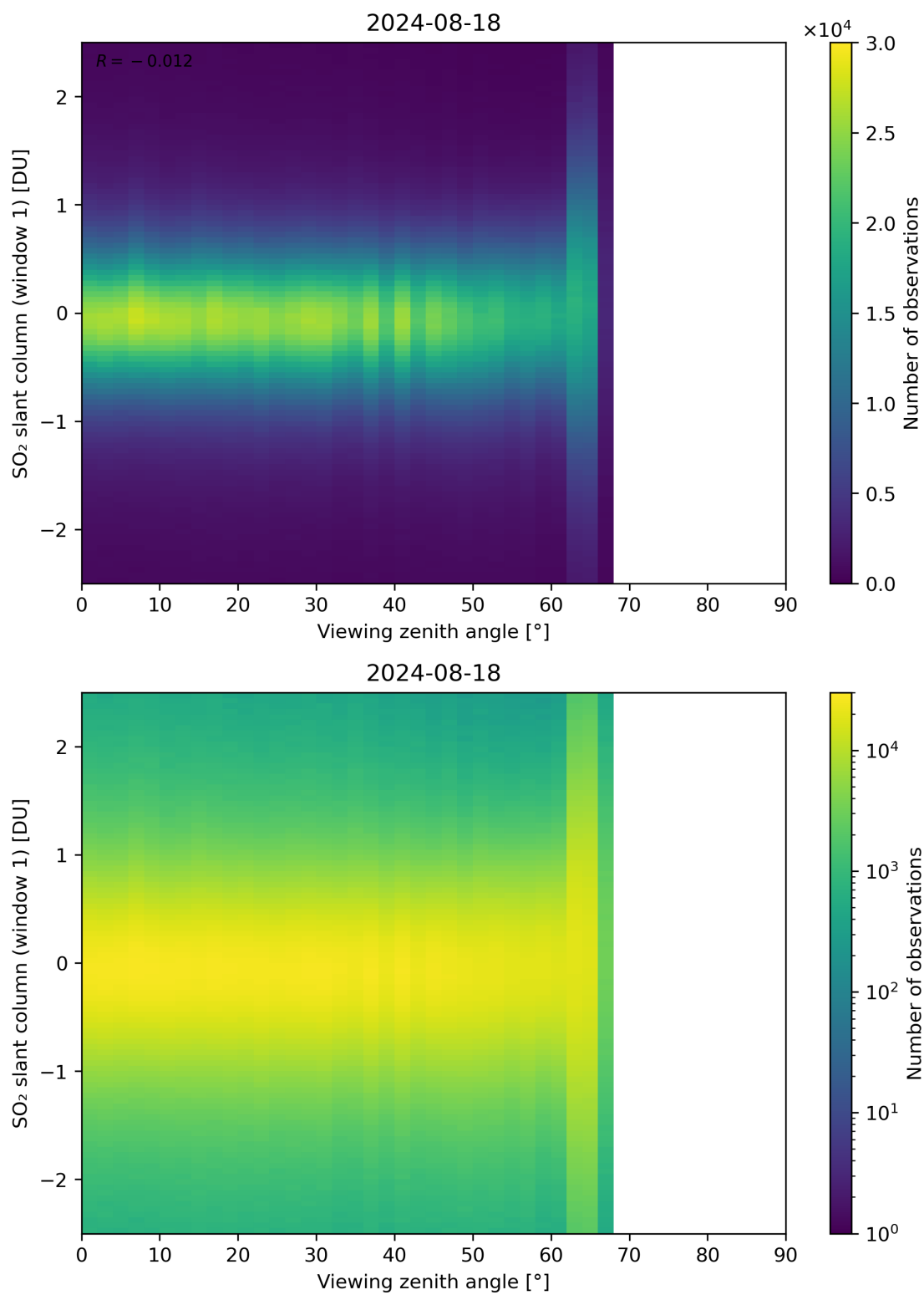
Figure 320: Scatter density plot of “Viewing zenith angle” against “SO 2 slant column (window 1)” for 2024-08-17 to 2024-08-19.
