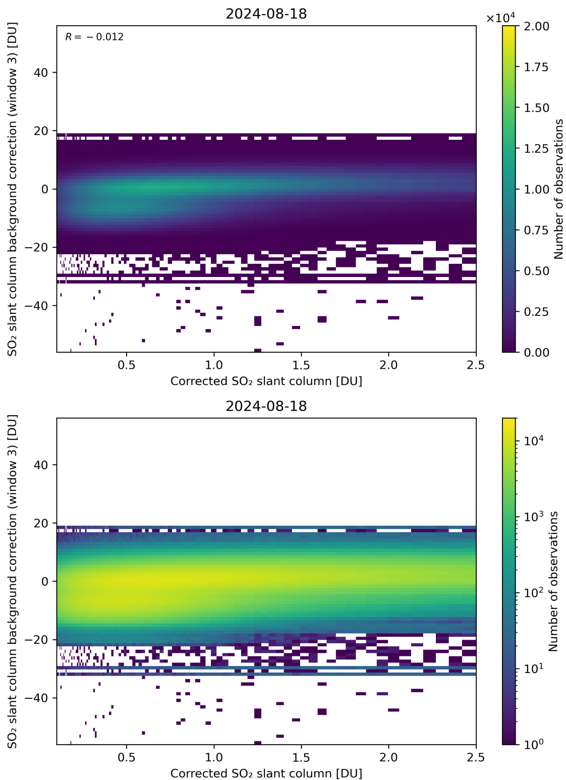
Figure 180: Scatter density plot of “Corrected SO 2 slant column” against “SO 2 slant column background correction (window 3)” for 2024-08-17 to 2024-08-19.
