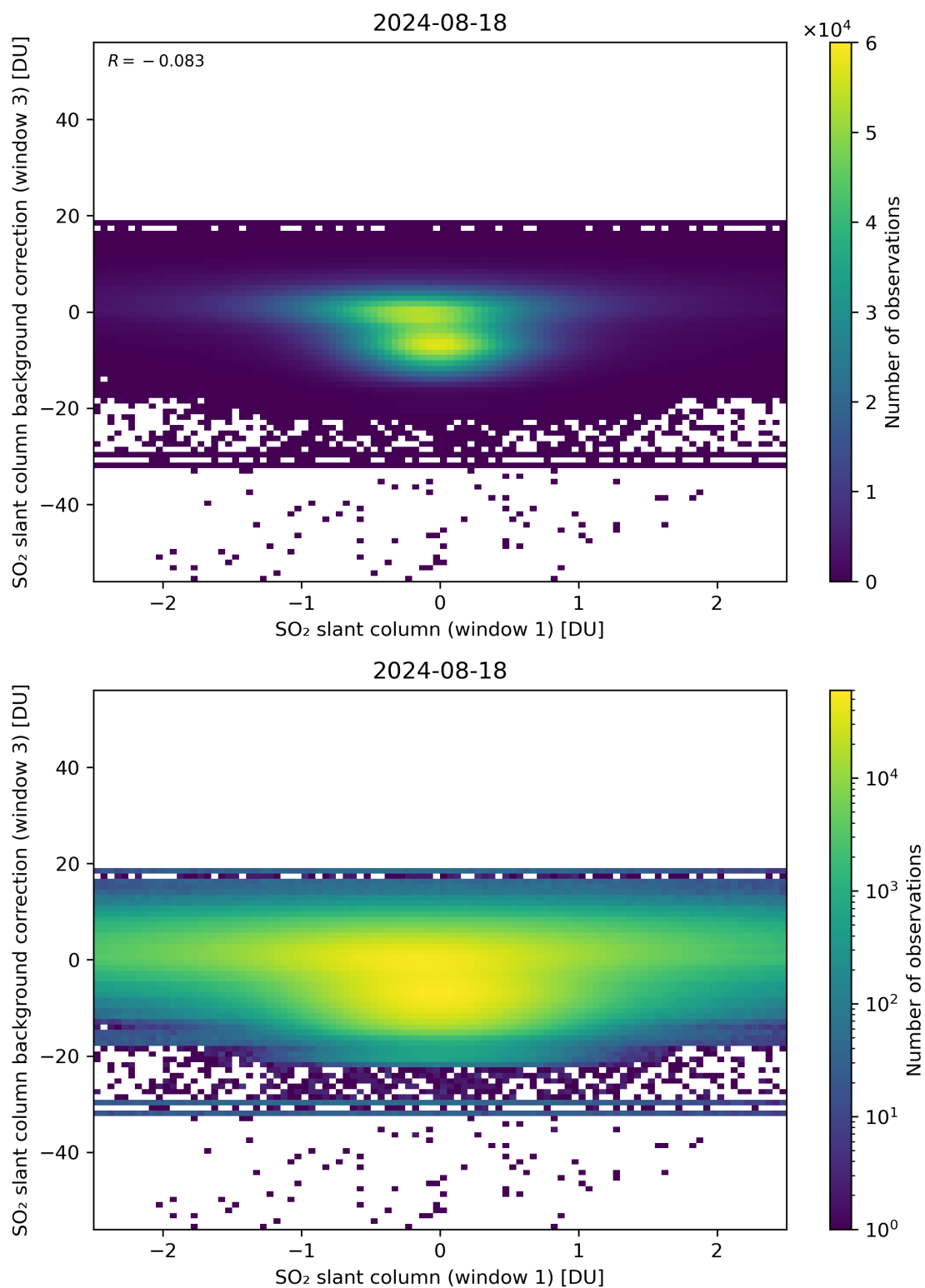
Figure 214: Scatter density plot of “SO 2 slant column (window 1)” against “SO 2 slant column background correction (window 3)” for 2024-08-17 to 2024-08-19.
