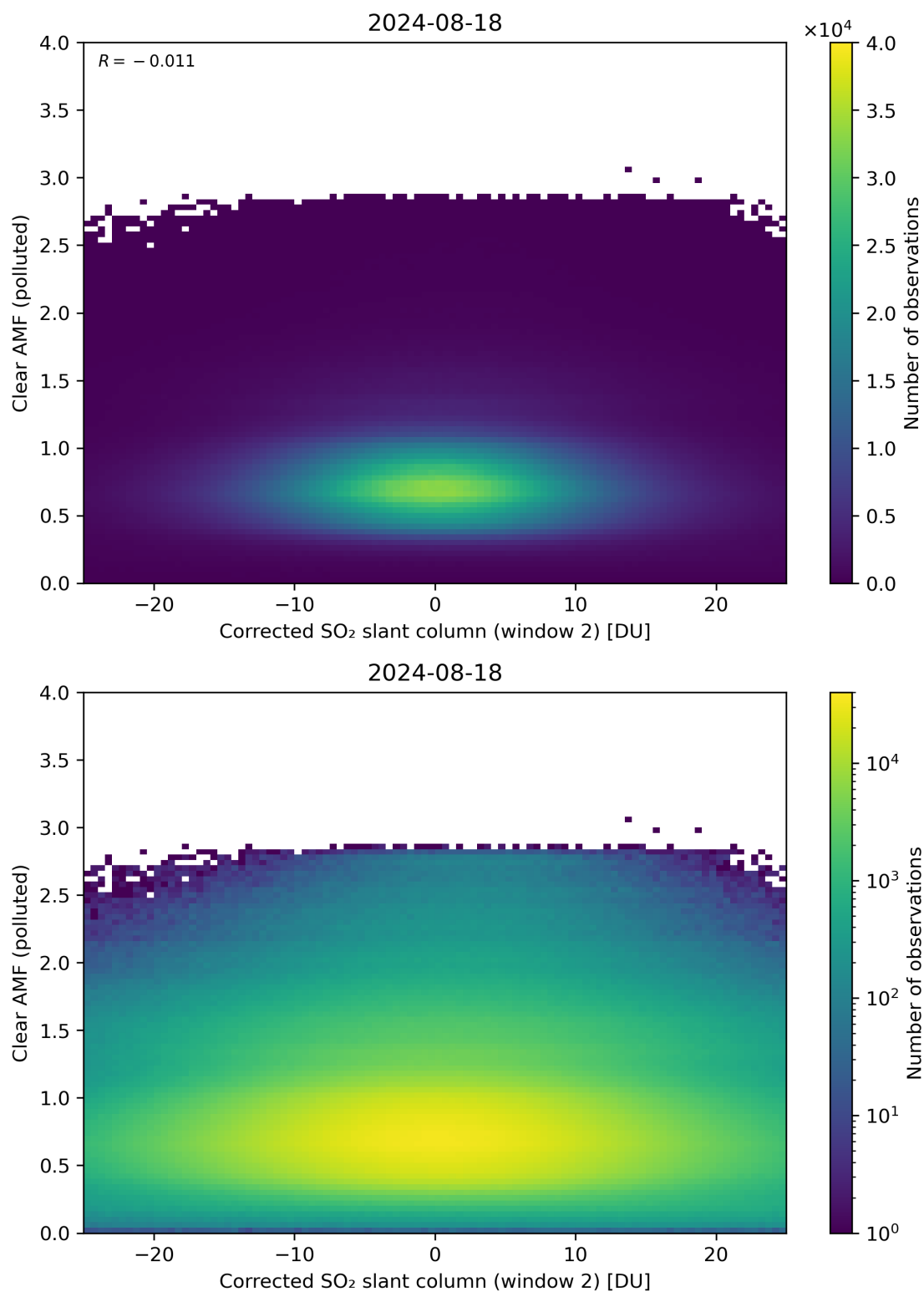
Figure 199: Scatter density plot of “Corrected SO 2 slant column (window 2)” against “Clear AMF (polluted)” for 2024-08-17 to 2024-08-19.
