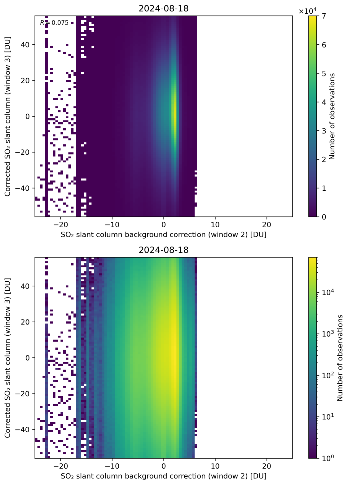
Figure 116: Scatter density plot of “SO 2 slant column background correction (window 2)” against “Corrected SO 2 slant column (window 3)” for 2024-08-17 to 2024-08-19.
