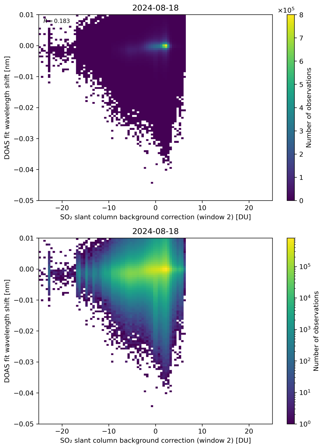
Figure 112: Scatter density plot of “SO 2 slant column background correction (window 2)” against “DOAS fit wavelength shift” for 2024-08-17 to 2024-08-19.
