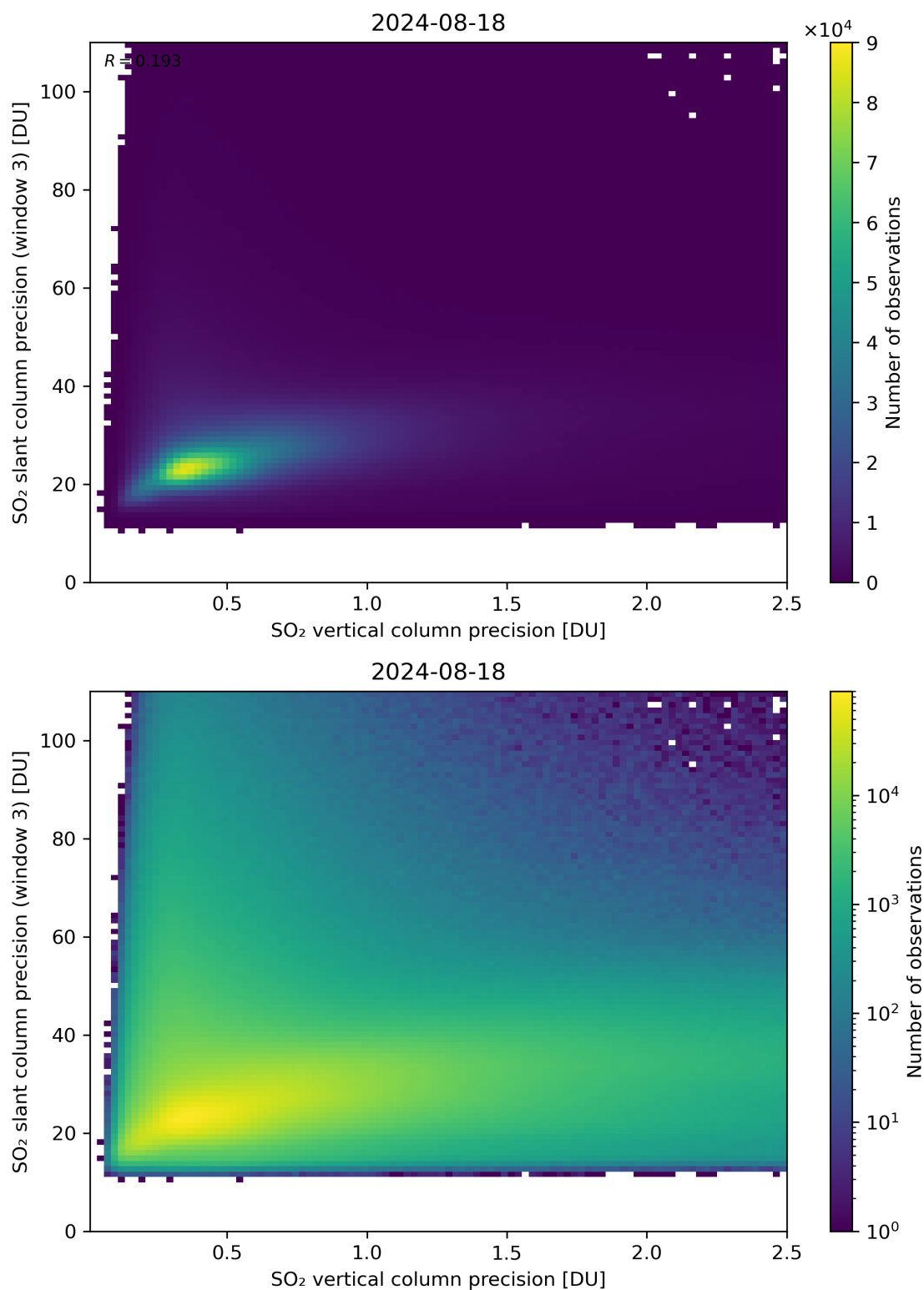
Figure 293: Scatter density plot of “SO 2 vertical column precision” against “SO 2 slant column precision (window 3)” for 2024-08-17 to 2024-08-19.
