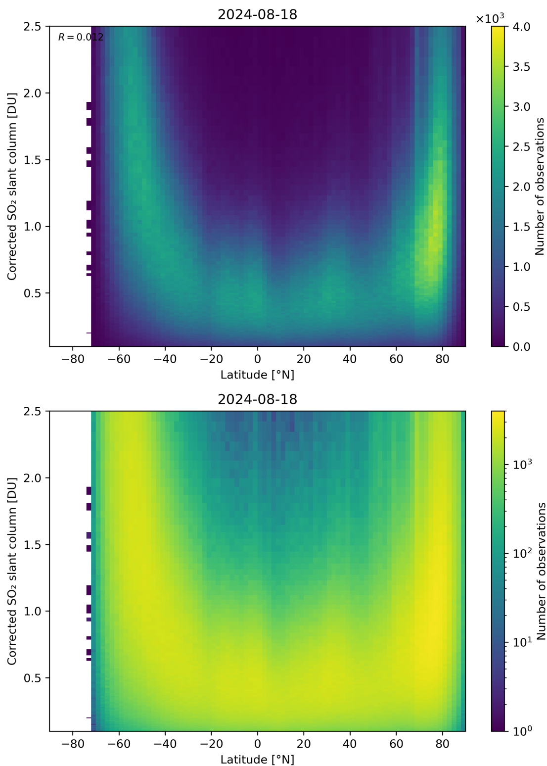
Figure 146: Scatter density plot of “Latitude” against “Corrected SO 2 slant column” for 2024-08-17 to 2024-08-19.
