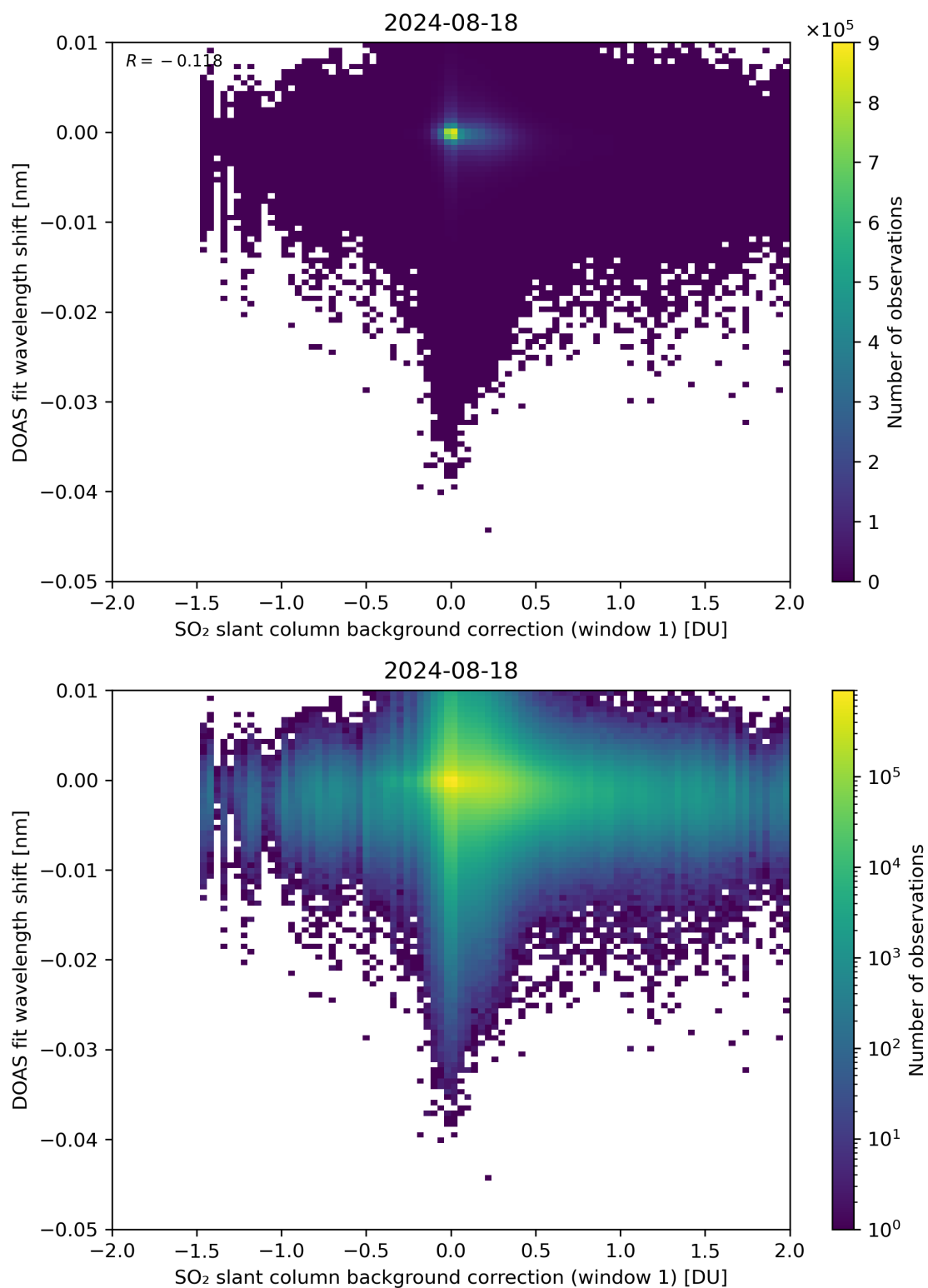
Figure 100: Scatter density plot of “SO 2 slant column background correction (window 1)” against “DOAS fit wavelength shift” for 2024-08-17 to 2024-08-19.
