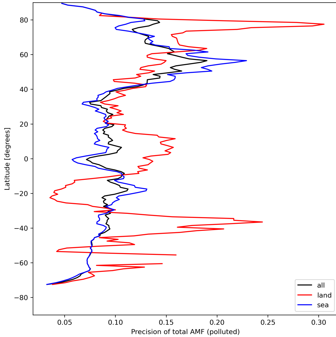
Figure 49: Zonal average of “Precision of total AMF (polluted)” for 2024-08-17 to 2024-08-19.
