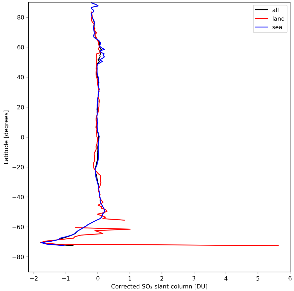
Figure 32: Zonal average of “Corrected SO 2 slant column” for 2024-08-17 to 2024-08-19.
