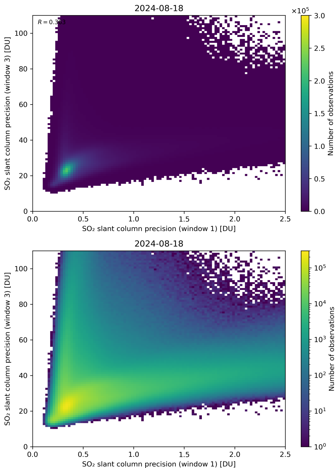
Figure 229: Scatter density plot of “SO 2 slant column precision (window 1)” against “SO 2 slant column precision (window 3)” for 2024-08-17 to 2024-08-19.
