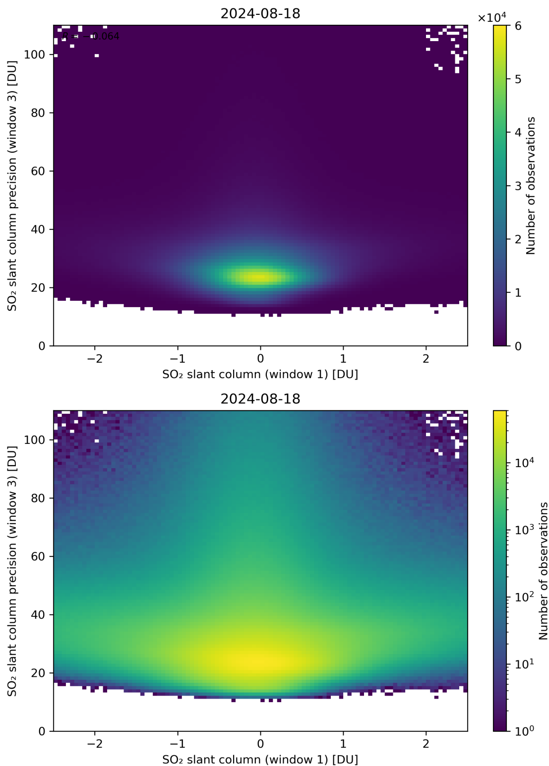
Figure 238: Scatter density plot of “SO 2 slant column (window 1)” against “SO 2 slant column precision (window 3)” for 2024-08-17 to 2024-08-19.
