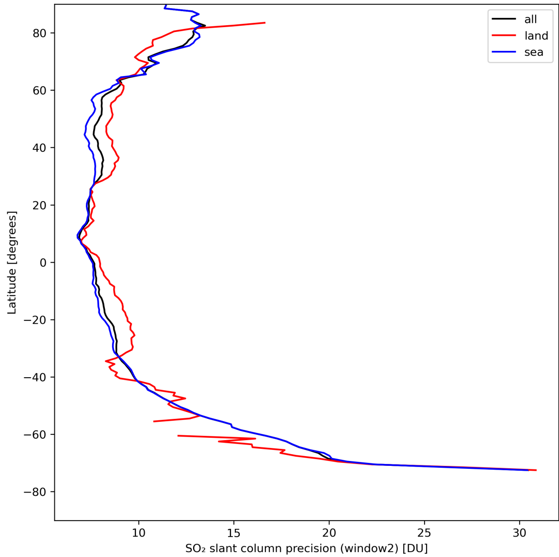
Figure 38: Zonal average of “SO 2 slant column precision (window2)” for 2024-08-17 to 2024-08-19.
