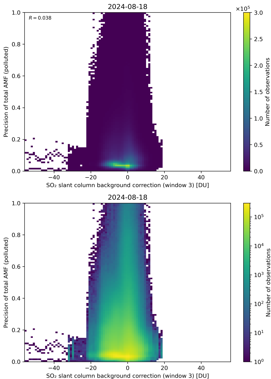
Figure 126: Scatter density plot of “SO 2 slant column background correction (window 3)” against “Precision of total AMF (polluted)” for 2024-08-17 to 2024-08-19.
