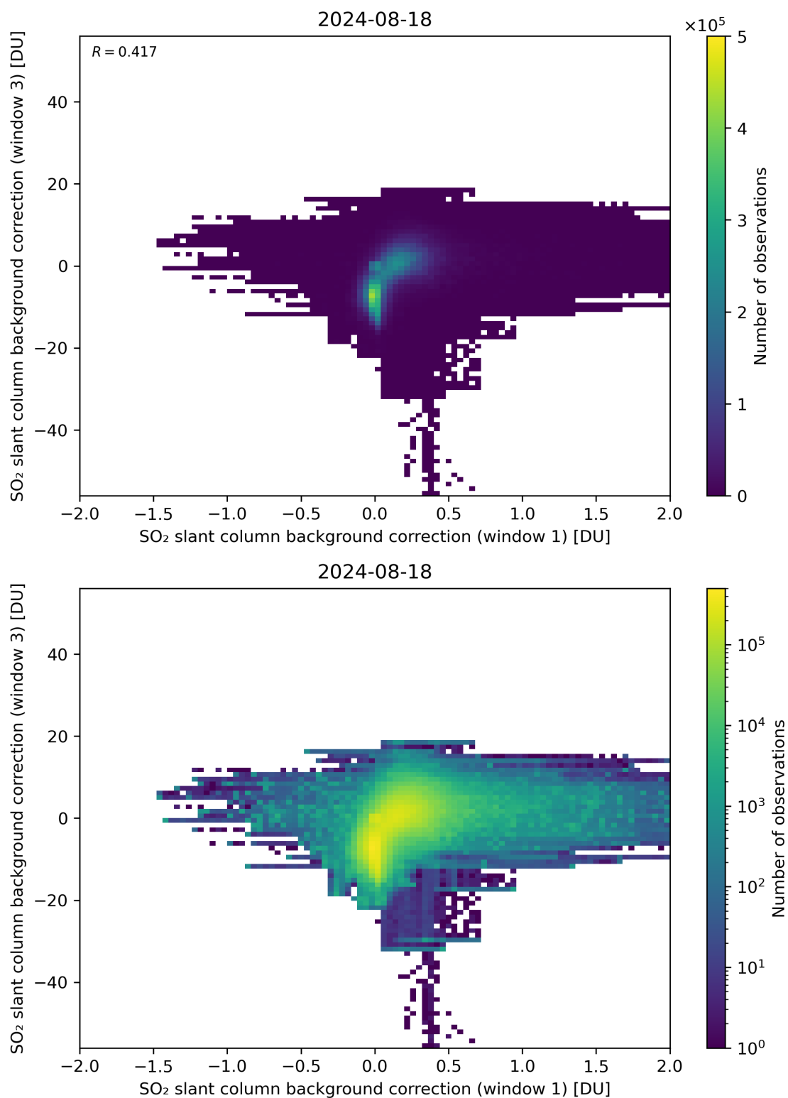
Figure 99: Scatter density plot of “SO 2 slant column background correction (window 1)” against “SO 2 slant column background correction (window 3)” for 2024-08-17 to 2024-08-19.
