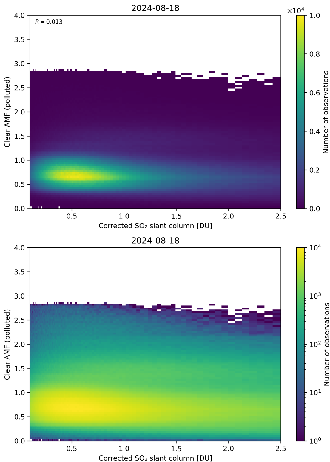
Figure 184: Scatter density plot of “Corrected SO 2 slant column” against “Clear AMF (polluted)” for 2024-08-17 to 2024-08-19.
