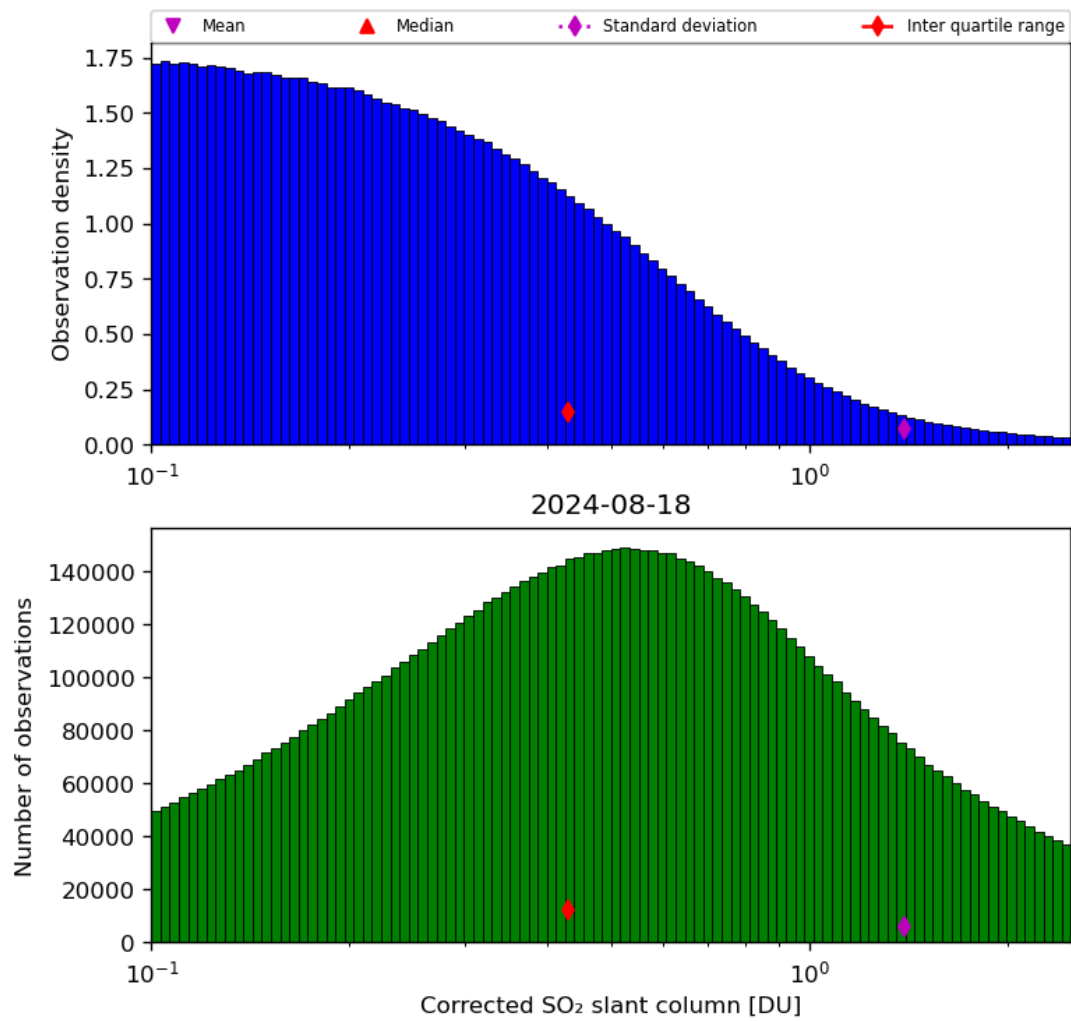
Figure 55: Histogram of “Corrected SO 2 slant column” for 2024-08-17 to 2024-08-19
