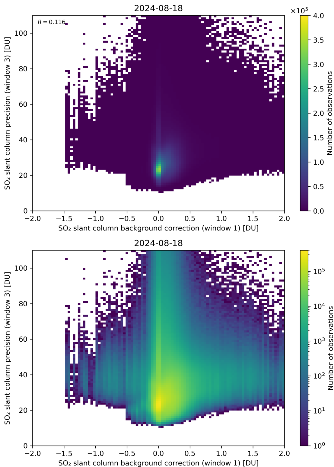
Figure 108: Scatter density plot of “SO 2 slant column background correction (window 1)” against “SO 2 slant column precision (window 3)” for 2024-08-17 to 2024-08-19.
