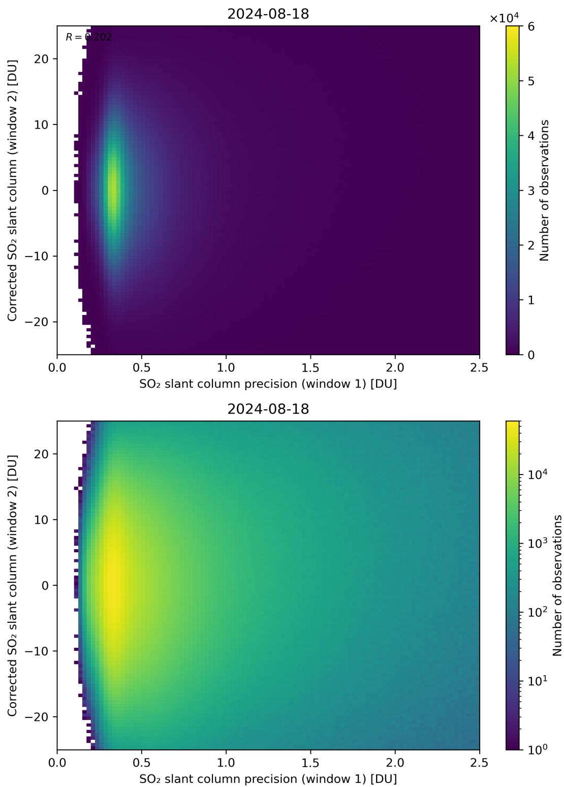
Figure 225: Scatter density plot of “SO 2 slant column precision (window 1)” against “Corrected SO 2 slant column (window 2)” for 2024-08-17 to 2024-08-19.
