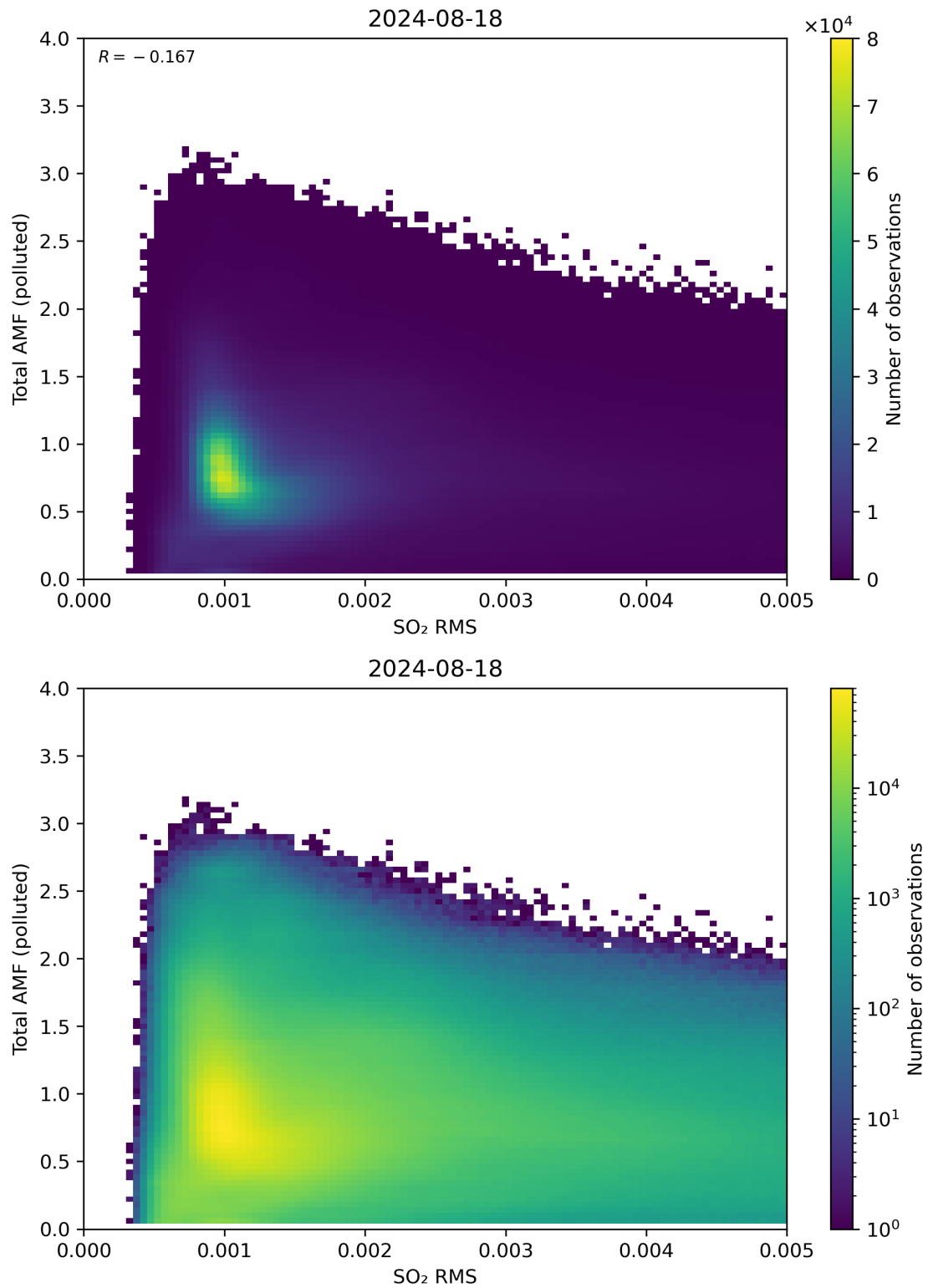
Figure 137: Scatter density plot of “SO 2 RMS” against “Total AMF (polluted)” for 2024-08-17 to 2024-08-19.
