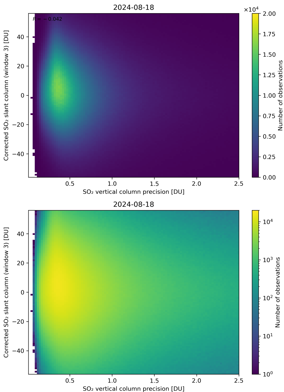
Figure 288: Scatter density plot of “SO 2 vertical column precision” against “Corrected SO 2 slant column (window 3)” for 2024-08-17 to 2024-08-19.
