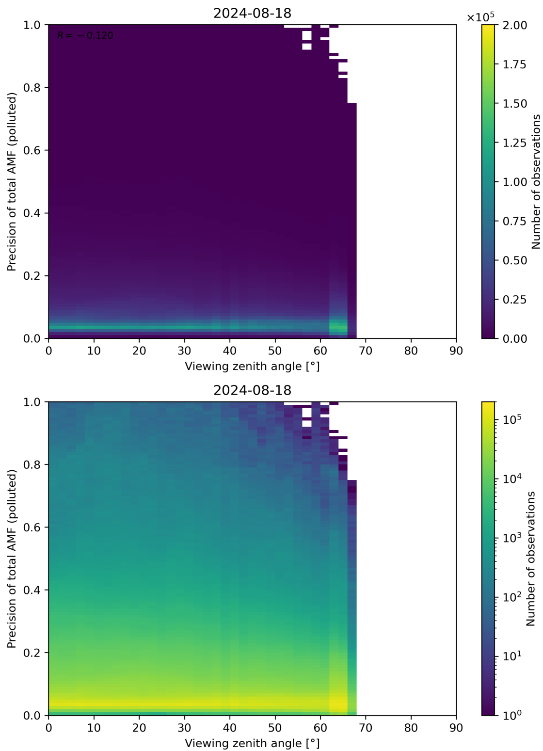
Figure 326: Scatter density plot of “Viewing zenith angle” against “Precision of total AMF (polluted)” for 2024-08-17 to 2024-08-19.
