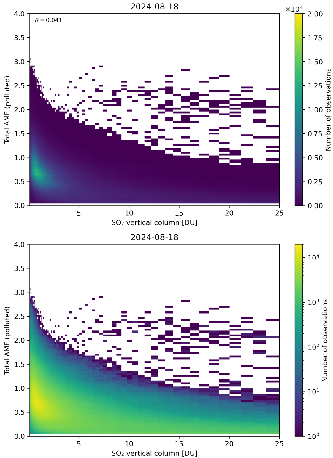
Figure 305: Scatter density plot of “SO 2 vertical column” against “Total AMF (polluted)” for 2024-08-17 to 2024-08-19.
