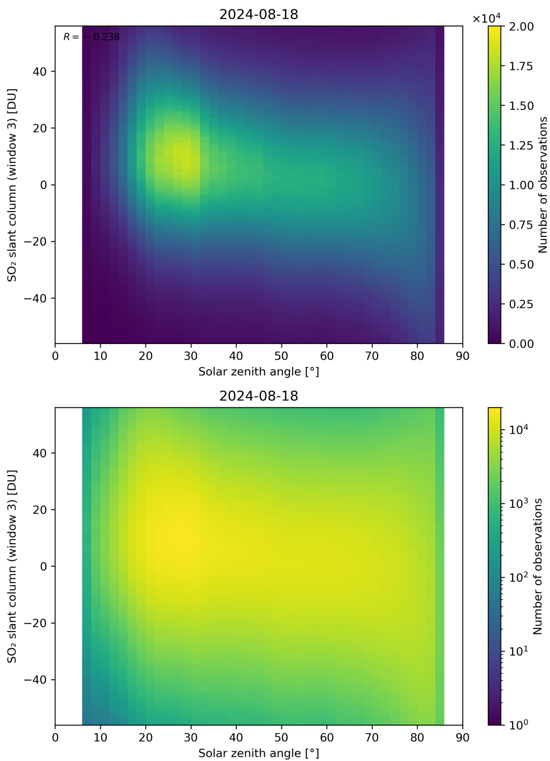
Figure 172: Scatter density plot of “Solar zenith angle” against “SO 2 slant column (window 3)” for 2024-08-17 to 2024-08-19.
