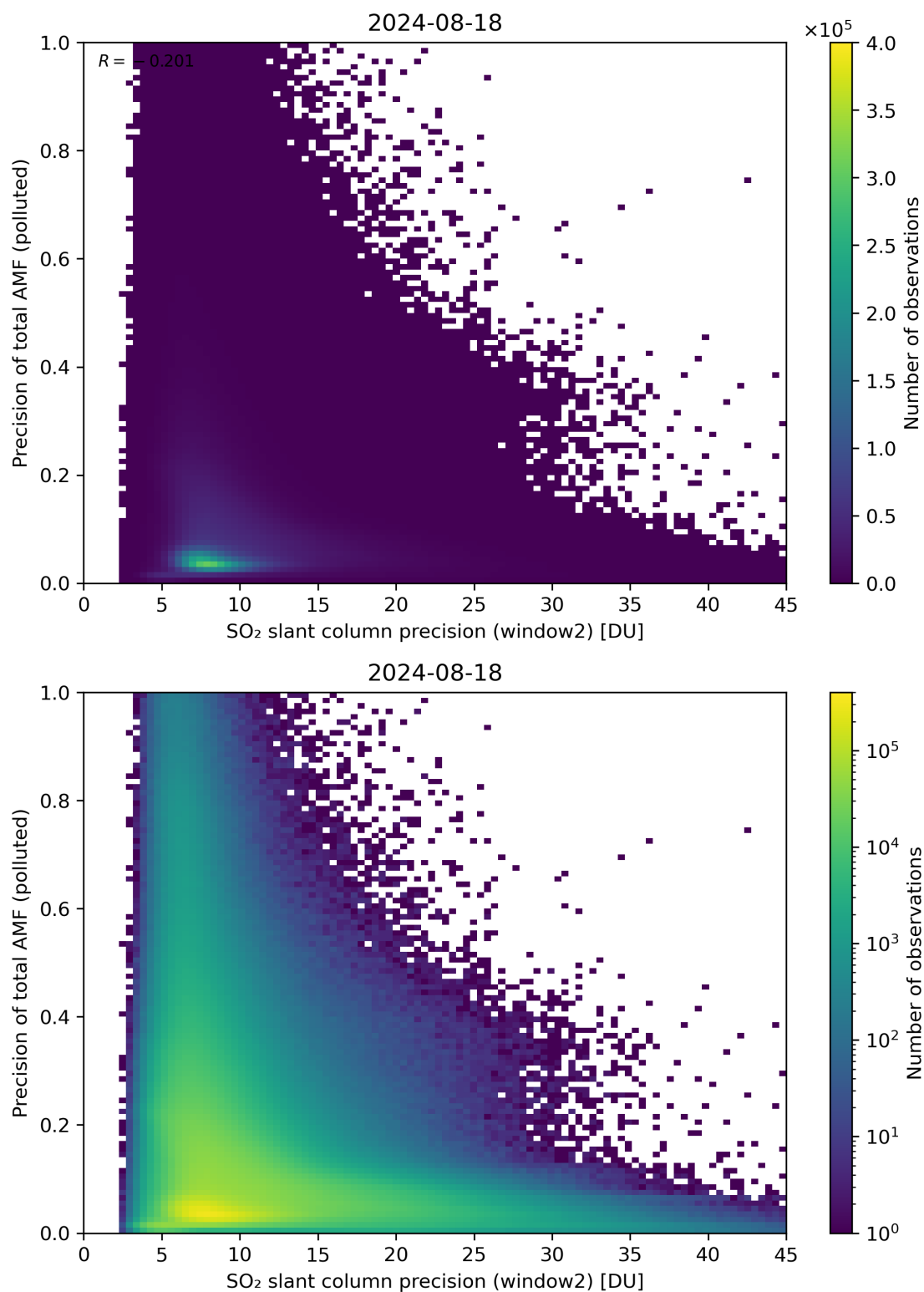
Figure 252: Scatter density plot of “SO 2 slant column precision (window2)” against “Precision of total AMF (polluted)” for 2024-08-17 to 2024-08-19.
