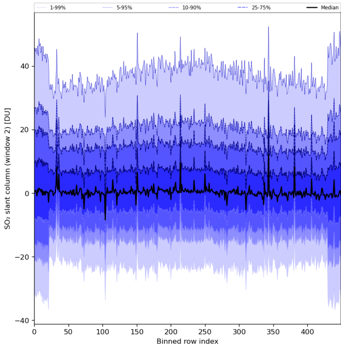
Figure 83: Along track statistics of “SO 2 slant column (window 2)” for 2024-08-17 to 2024-08-19
