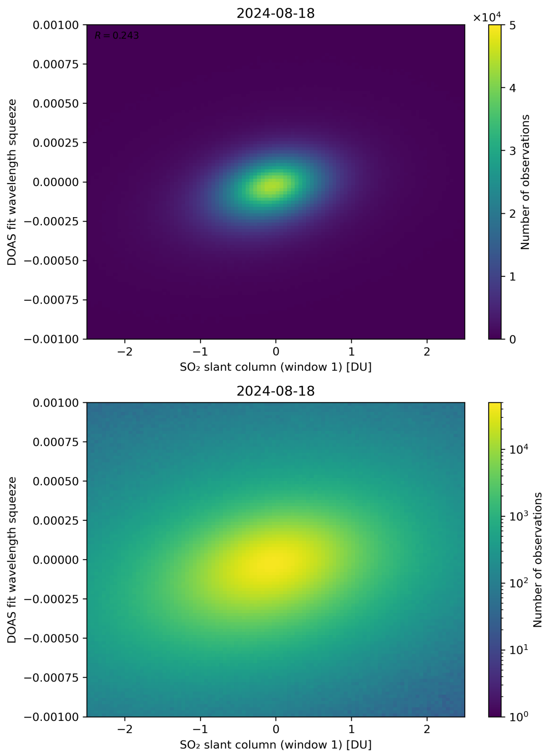
Figure 216: Scatter density plot of “SO 2 slant column (window 1)” against “DOAS fit wavelength squeeze” for 2024-08-17 to 2024-08-19.
