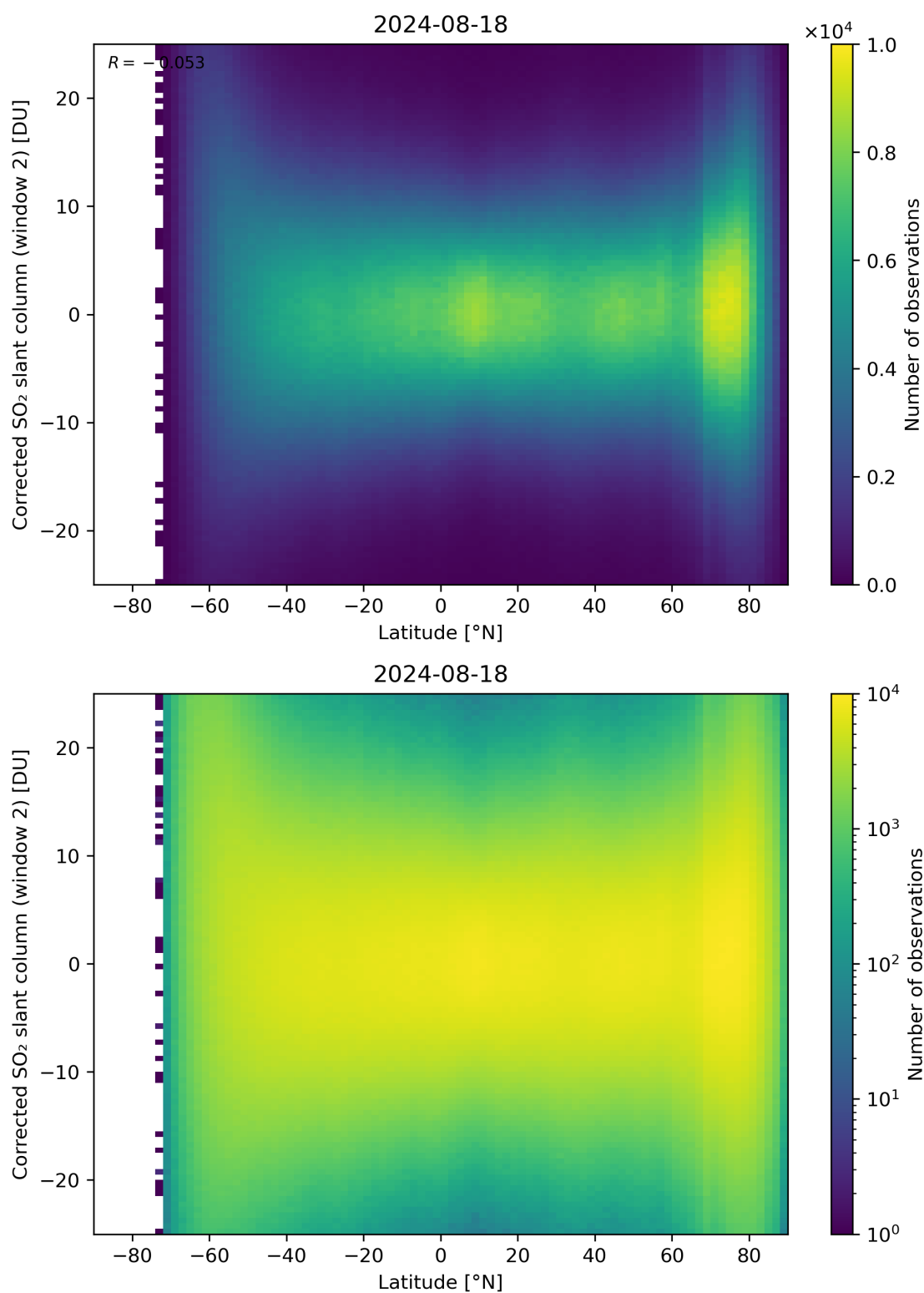
Figure 147: Scatter density plot of “Latitude” against “Corrected SO 2 slant column (window 2)” for 2024-08-17 to 2024-08-19.
