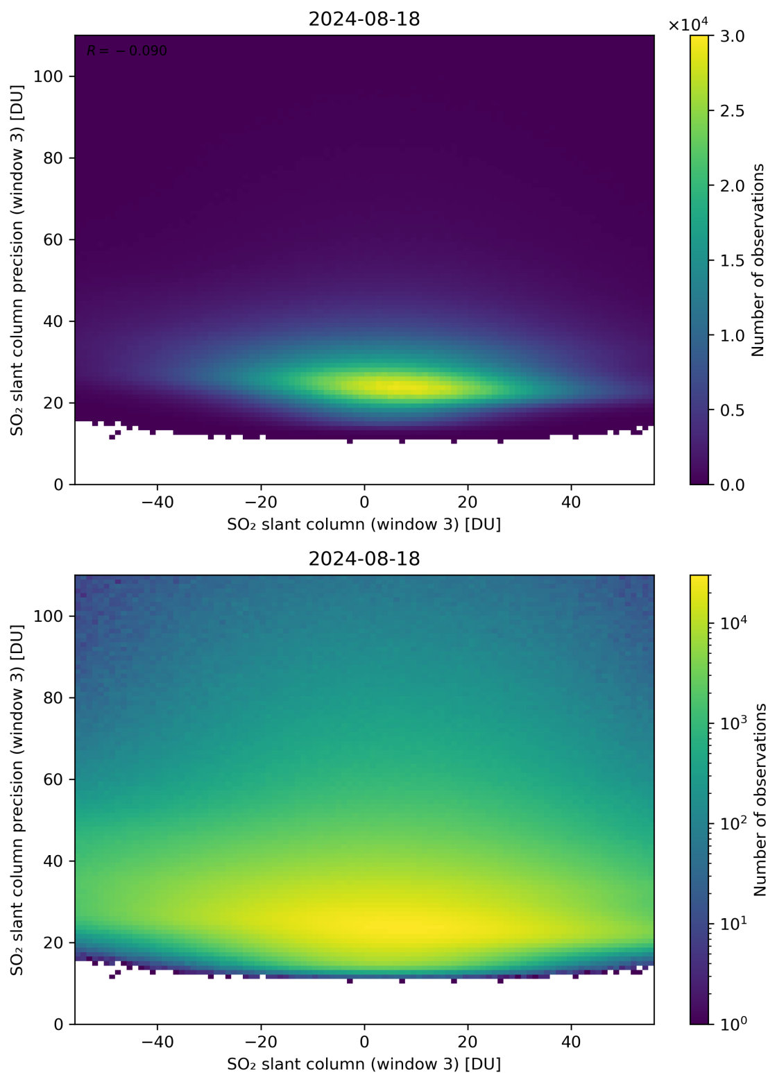
Figure 267: Scatter density plot of “SO 2 slant column (window 3)” against “SO 2 slant column precision (window 3)” for 2024-08-17 to 2024-08-19.
