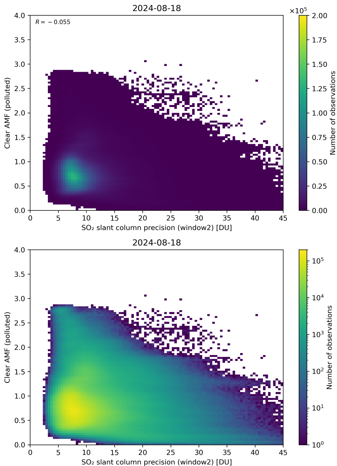
Figure 246: Scatter density plot of “SO 2 slant column precision (window2)” against “Clear AMF (polluted)” for 2024-08-17 to 2024-08-19.
