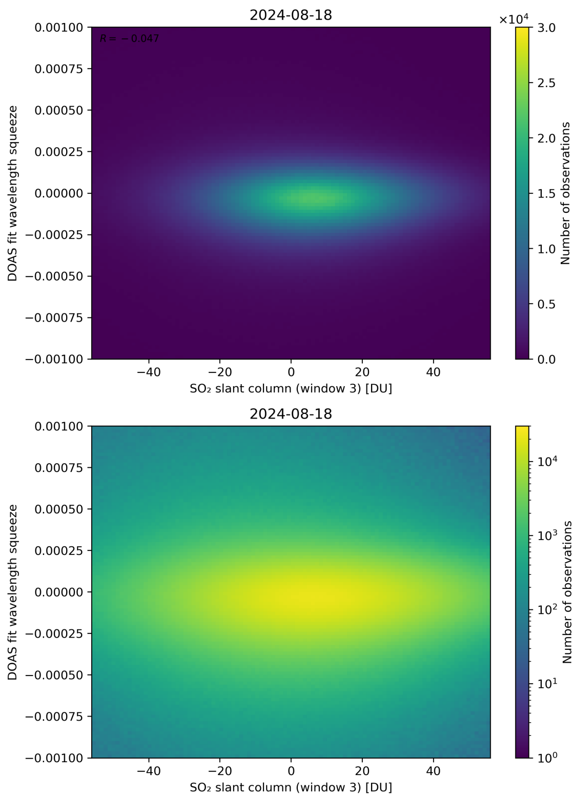
Figure 255: Scatter density plot of “SO 2 slant column (window 3)” against “DOAS fit wavelength squeeze” for 2024-08-17 to 2024-08-19.
