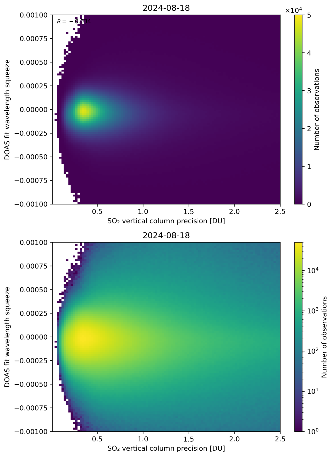
Figure 283: Scatter density plot of “SO 2 vertical column precision” against “DOAS fit wavelength squeeze” for 2024-08-17 to 2024-08-19.
