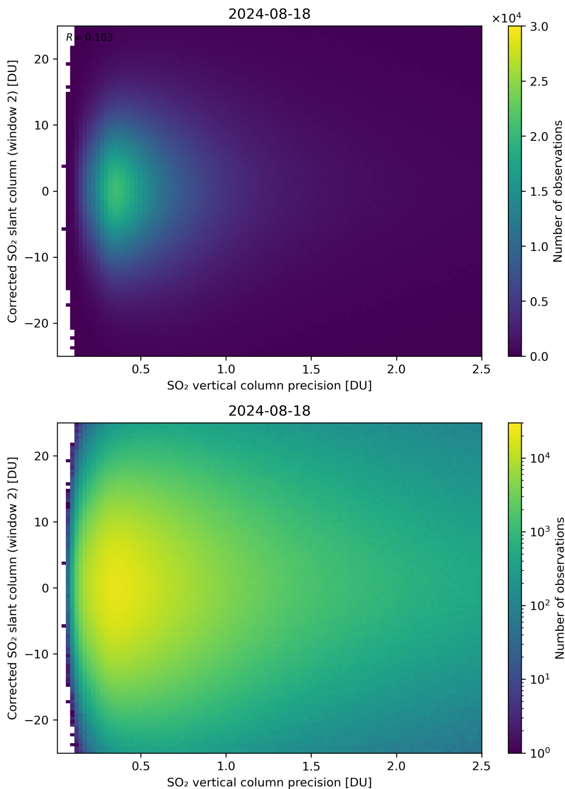
Figure 287: Scatter density plot of “SO 2 vertical column precision” against “Corrected SO 2 slant column (window 2)” for 2024-08-17 to 2024-08-19.
