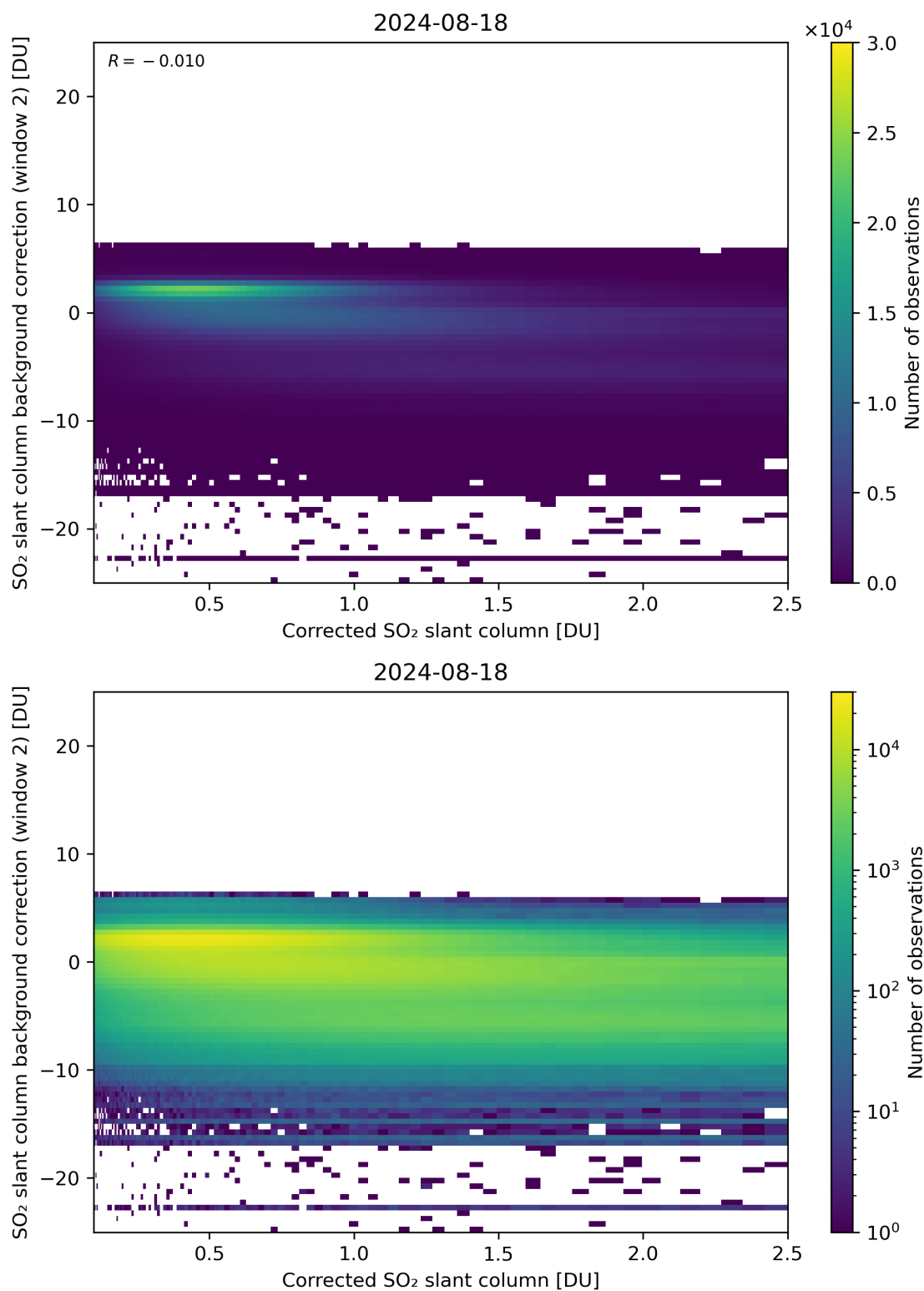
Figure 179: Scatter density plot of “Corrected SO 2 slant column” against “SO 2 slant column background correction (window 2)” for 2024-08-17 to 2024-08-19.
