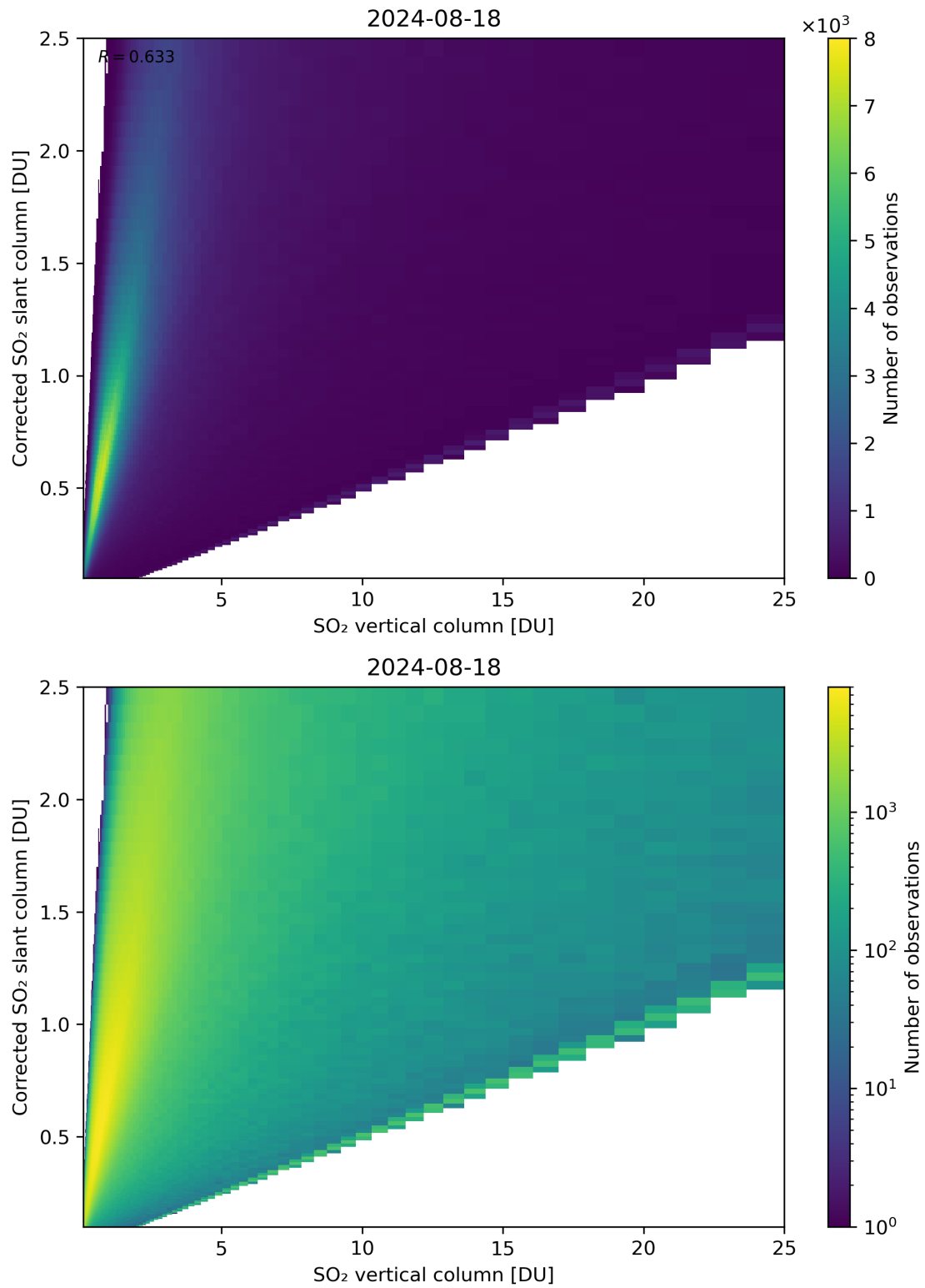
Figure 297: Scatter density plot of “SO 2 vertical column” against “Corrected SO 2 slant column” for 2024-08-17 to 2024-08-19.
