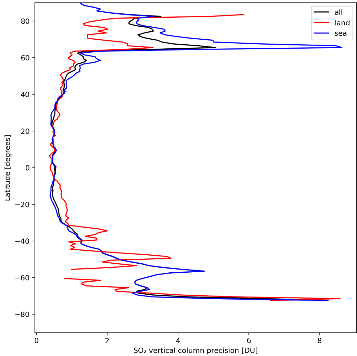
Figure 31: Zonal average of “SO 2 vertical column precision” for 2024-08-17 to 2024-08-19.
