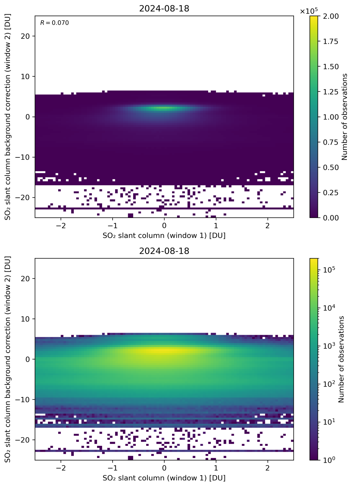
Figure 213: Scatter density plot of “SO 2 slant column (window 1)” against “SO 2 slant column background correction (window 2)” for 2024-08-17 to 2024-08-19.
