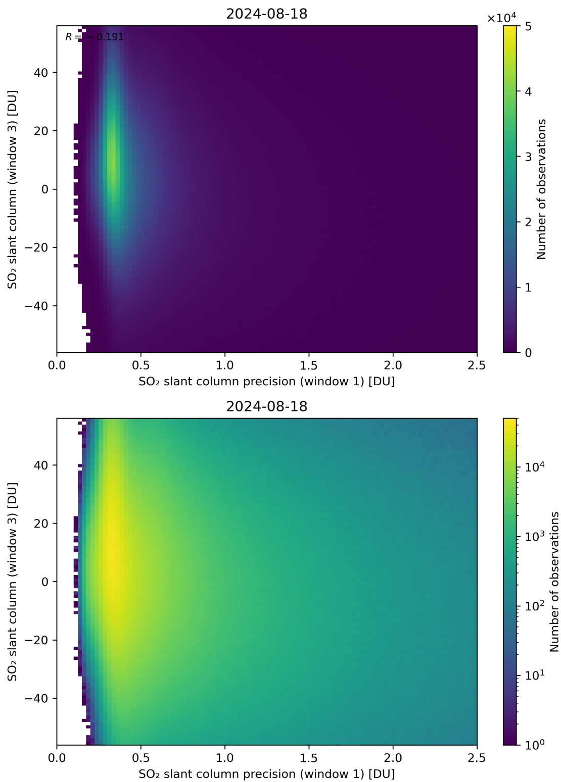
Figure 228: Scatter density plot of “SO 2 slant column precision (window 1)” against “SO 2 slant column (window 3)” for 2024-08-17 to 2024-08-19.
