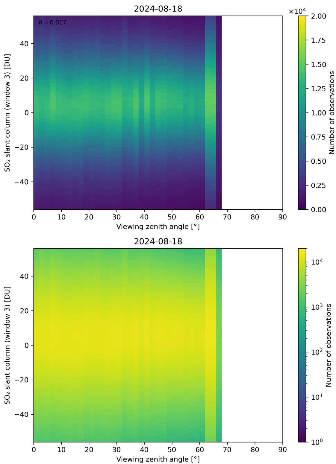
Figure 323: Scatter density plot of “Viewing zenith angle” against “SO 2 slant column (window 3)” for 2024-08-17 to 2024-08-19.
