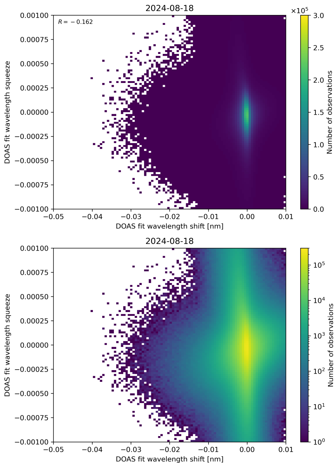
Figure 127: Scatter density plot of “DOAS fit wavelength shift” against “DOAS fit wavelength squeeze” for 2024-08-17 to 2024-08-19.
