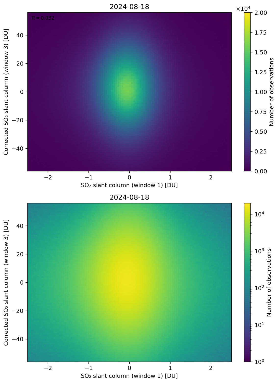
Figure 234: Scatter density plot of “SO 2 slant column (window 1)” against “Corrected SO 2 slant column (window 3)” for 2024-08-17 to 2024-08-19.
