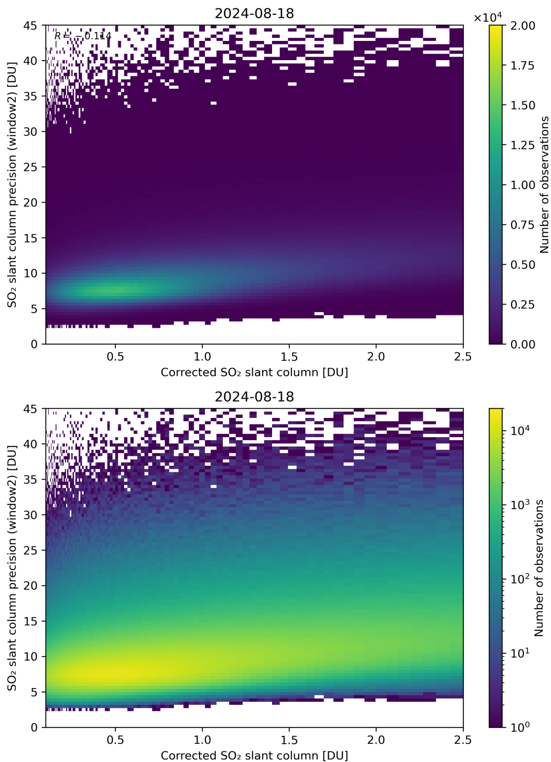
Figure 189: Scatter density plot of “Corrected SO 2 slant column” against “SO 2 slant column precision (window2)” for 2024-08-17 to 2024-08-19.
