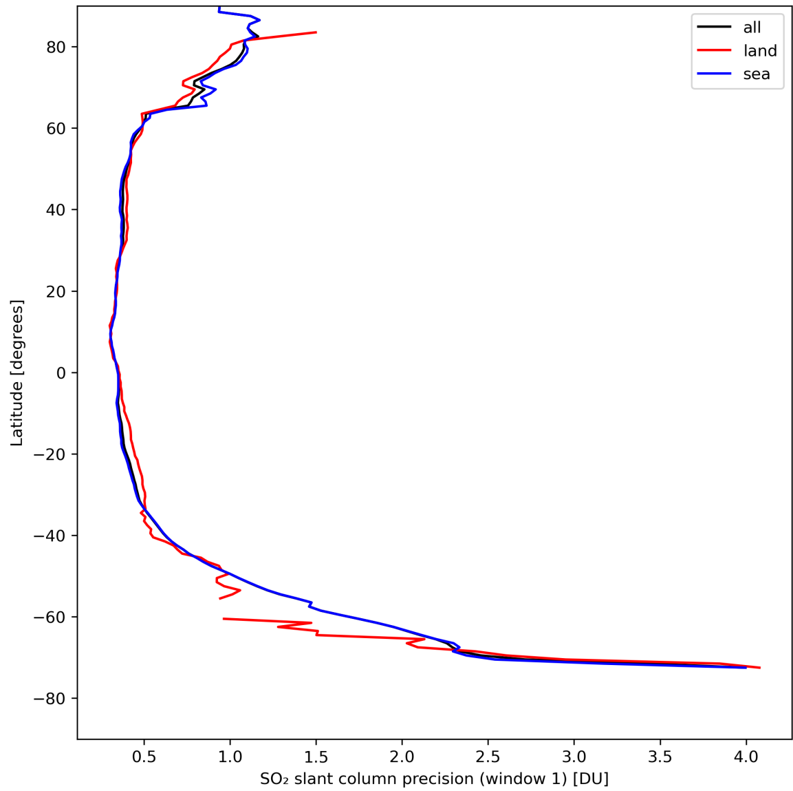
Figure 34: Zonal average of “SO 2 slant column precision (window 1)” for 2024-08-17 to 2024-08-19.
