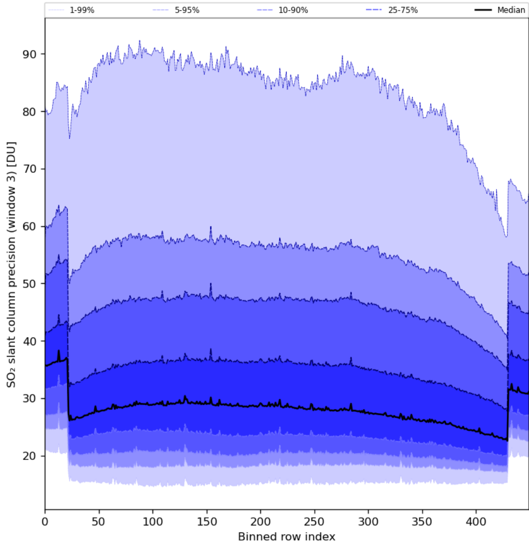
Figure 88: Along track statistics of “SO 2 slant column precision (window 3)” for 2024-08-17 to 2024-08-19
