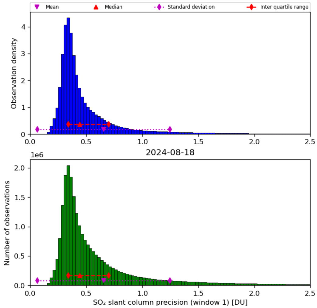
Figure 57: Histogram of “SO 2 slant column precision (window 1)” for 2024-08-17 to 2024-08-19
