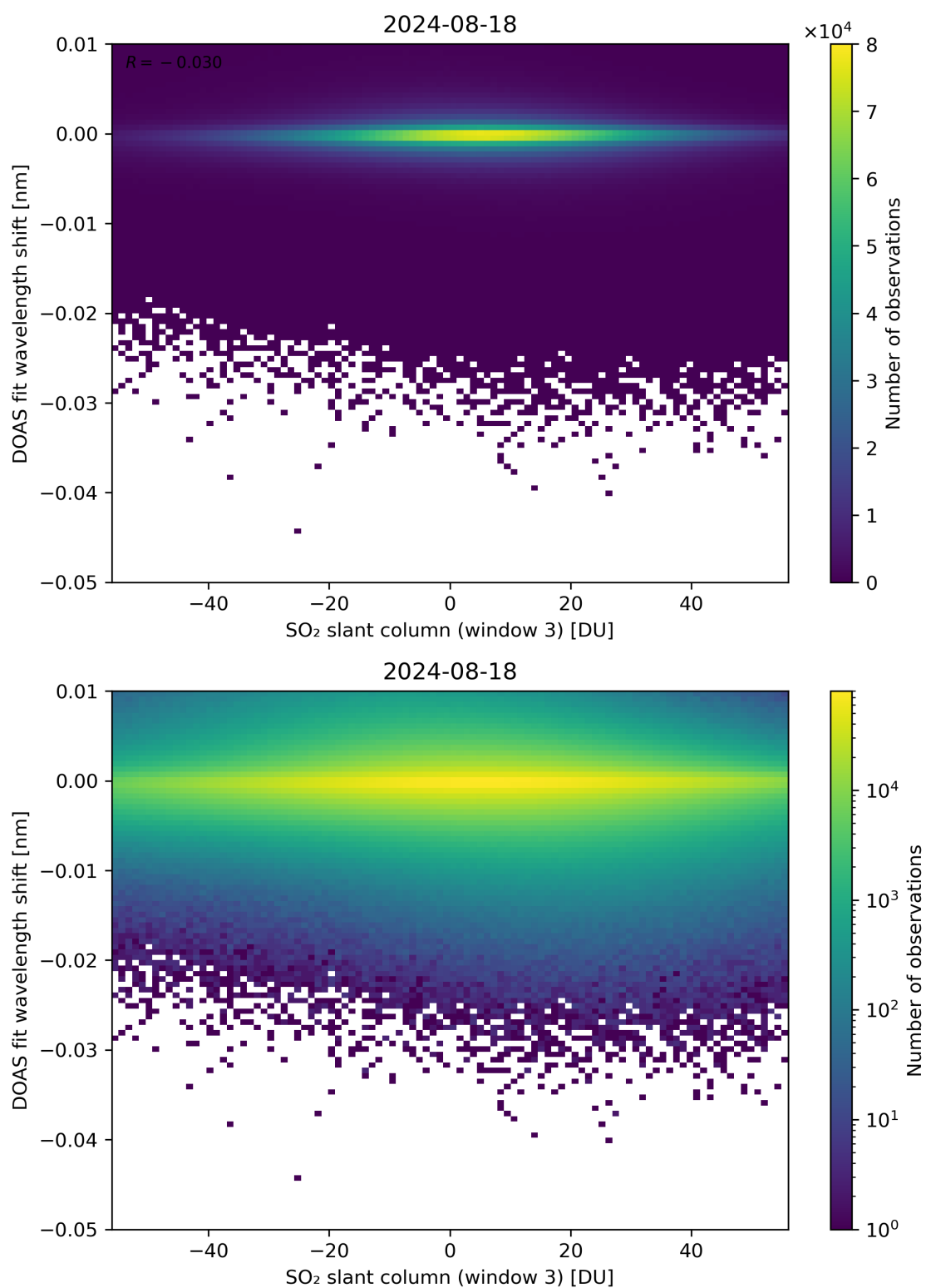
Figure 254: Scatter density plot of “SO 2 slant column (window 3)” against “DOAS fit wavelength shift” for 2024-08-17 to 2024-08-19.
