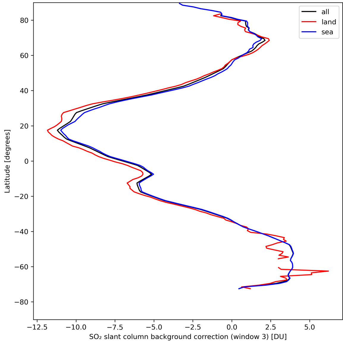
Figure 44: Zonal average of “SO 2 slant column background correction (window 3)” for 2024-08-17 to 2024-08-19.
