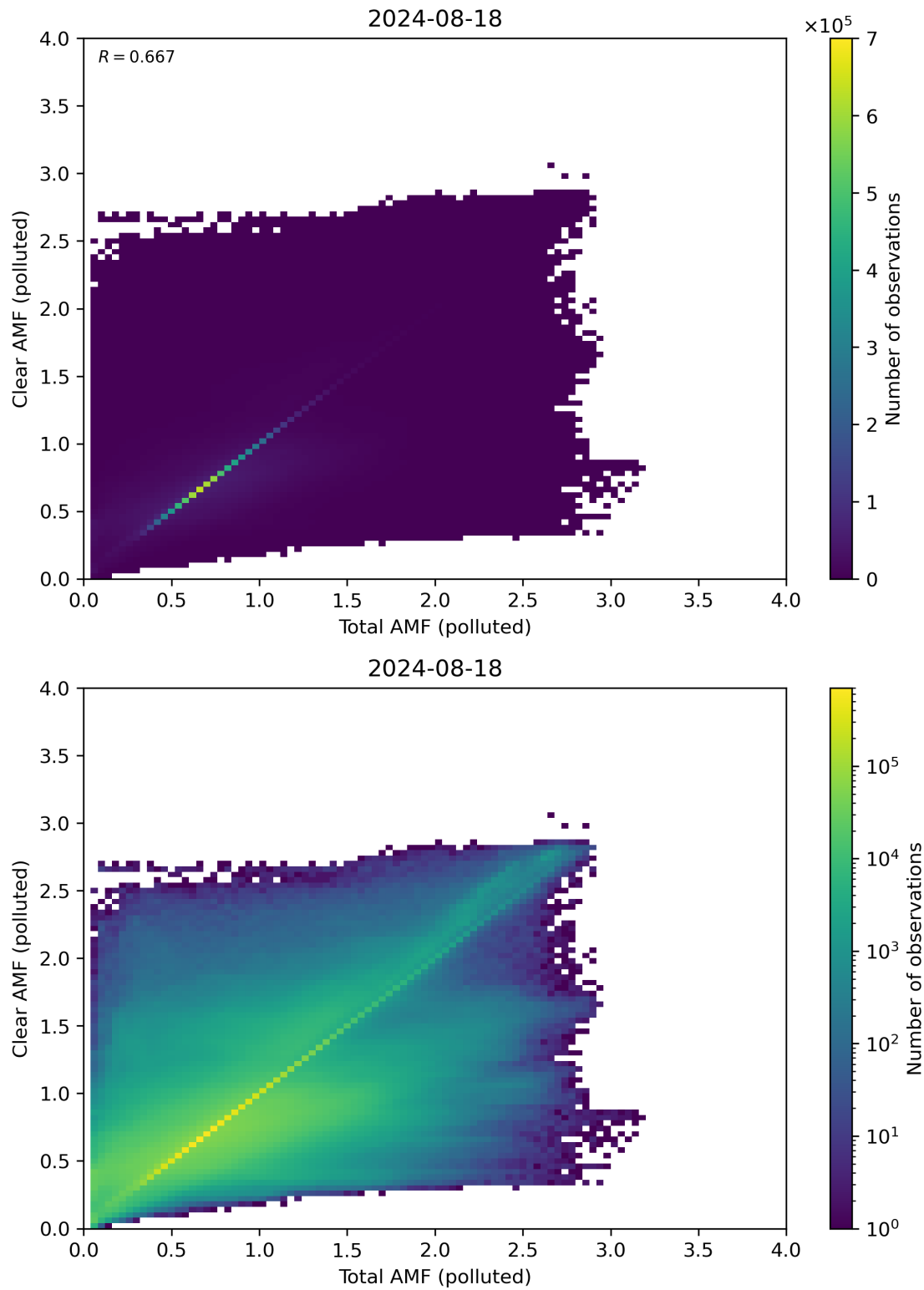
Figure 271: Scatter density plot of “Total AMF (polluted)” against “Clear AMF (polluted)” for 2024-08-17 to 2024-08-19.
