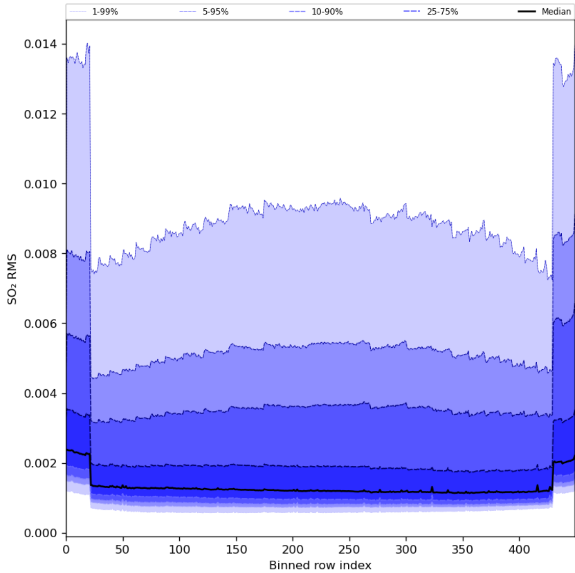
Figure 93: Along track statistics of “SO 2 RMS” for 2024-08-17 to 2024-08-19
