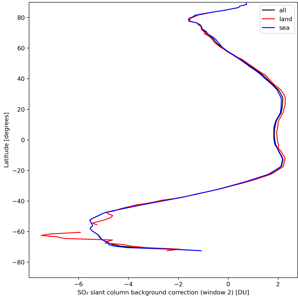
Figure 40: Zonal average of “SO 2 slant column background correction (window 2)” for 2024-08-17 to 2024-08-19.
