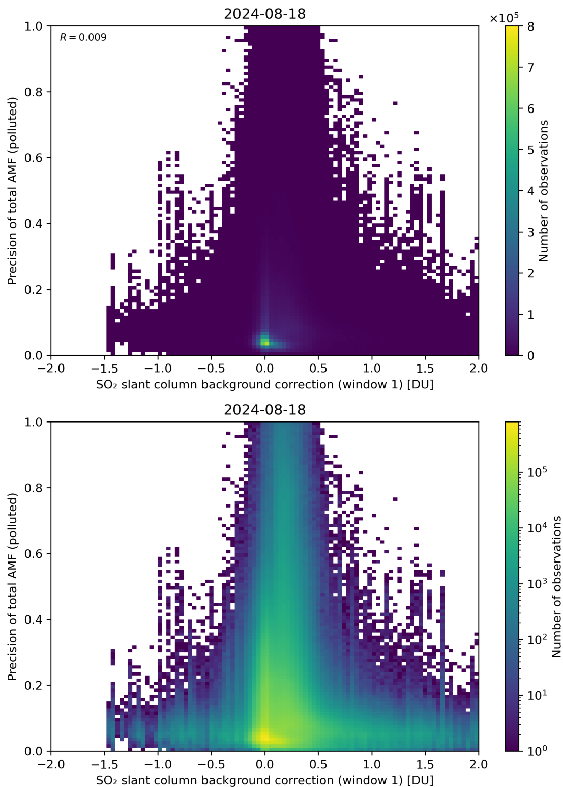
Figure 110: Scatter density plot of “SO 2 slant column background correction (window 1)” against “Precision of total AMF (polluted)” for 2024-08-17 to 2024-08-19.
