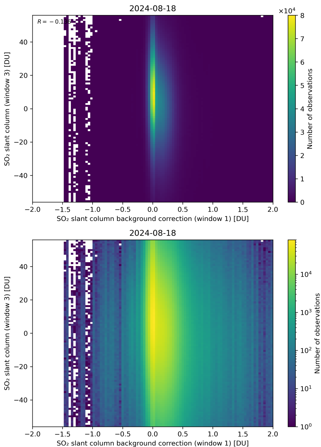
Figure 107: Scatter density plot of “SO 2 slant column background correction (window 1)” against “SO 2 slant column (window 3)” for 2024-08-17 to 2024-08-19.
