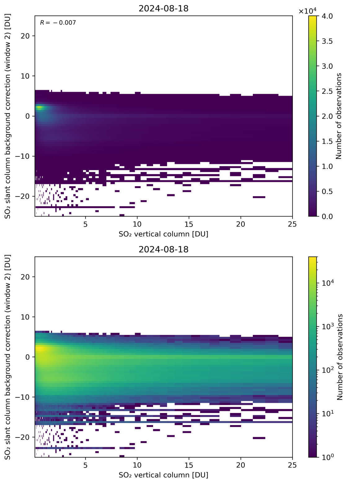
Figure 274: Scatter density plot of “SO 2 vertical column” against “SO 2 slant column background correction (window 2)” for 2024-08-17 to 2024-08-19.
