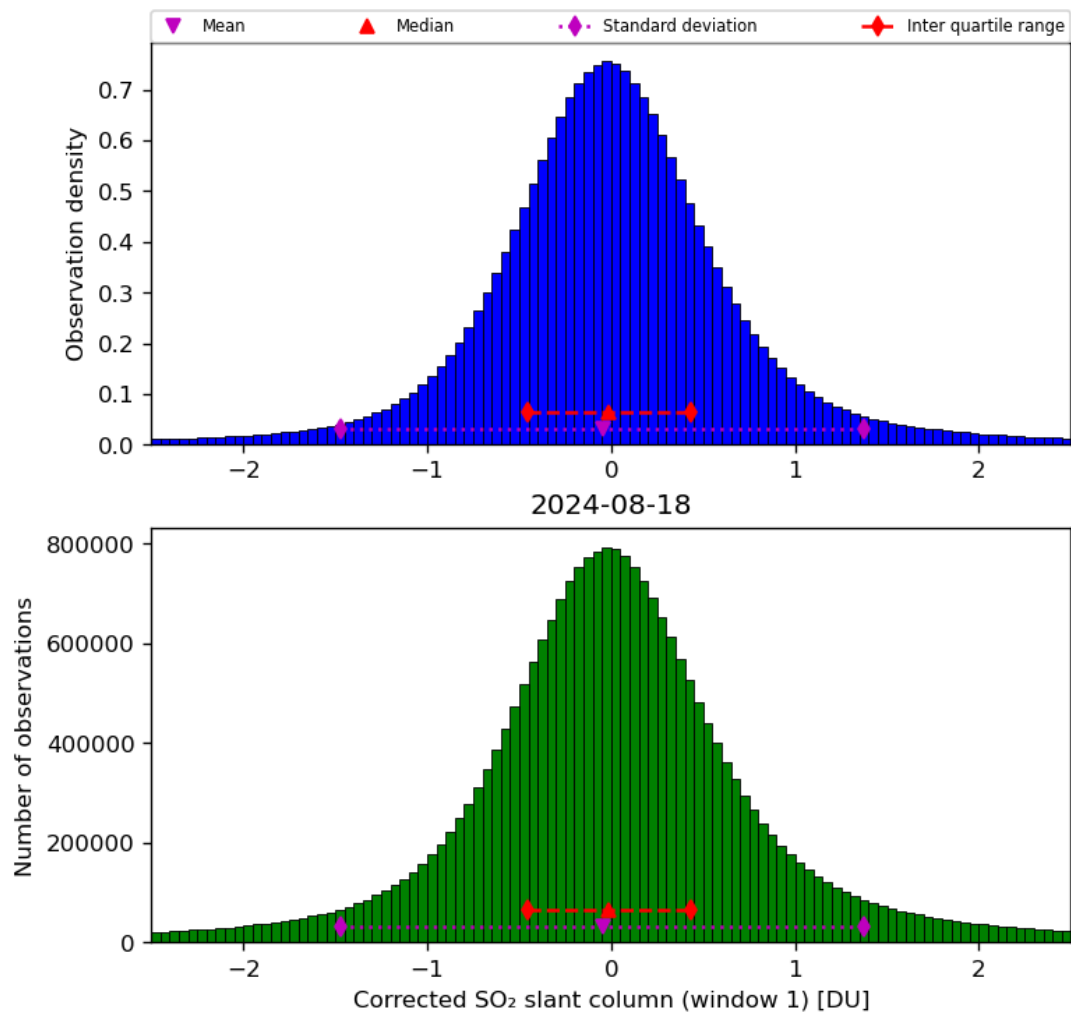
Figure 58: Histogram of “Corrected SO 2 slant column (window 1)” for 2024-08-17 to 2024-08-19
