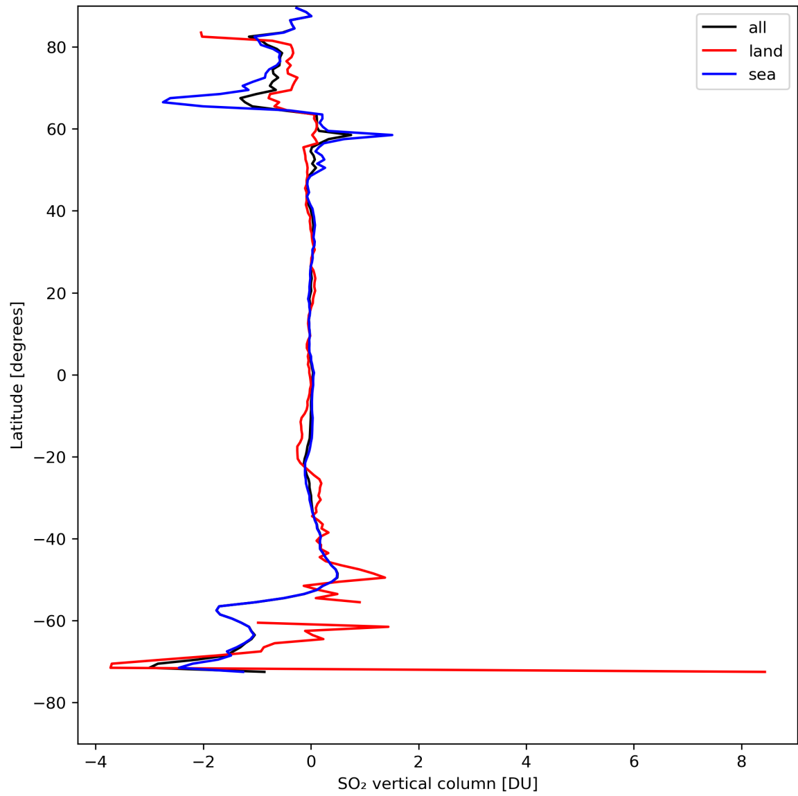
Figure 30: Zonal average of “SO 2 vertical column” for 2024-08-17 to 2024-08-19.
