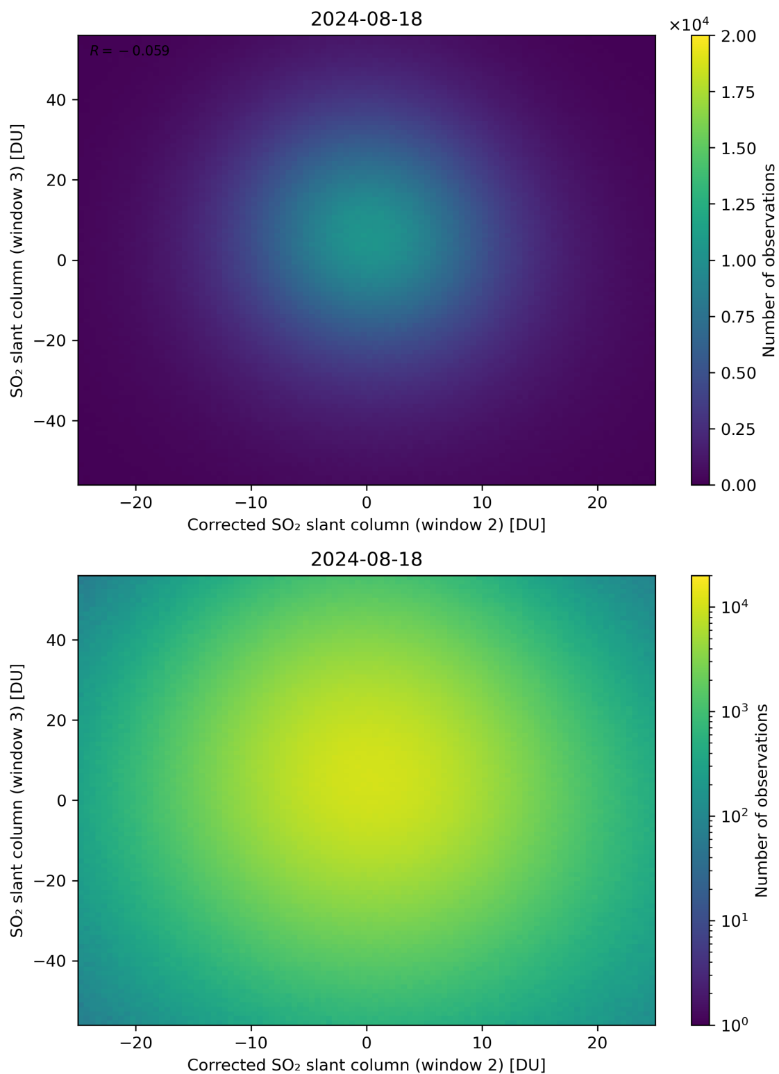
Figure 201: Scatter density plot of “Corrected SO 2 slant column (window 2)” against “SO 2 slant column (window 3)” for 2024-08-17 to 2024-08-19.
