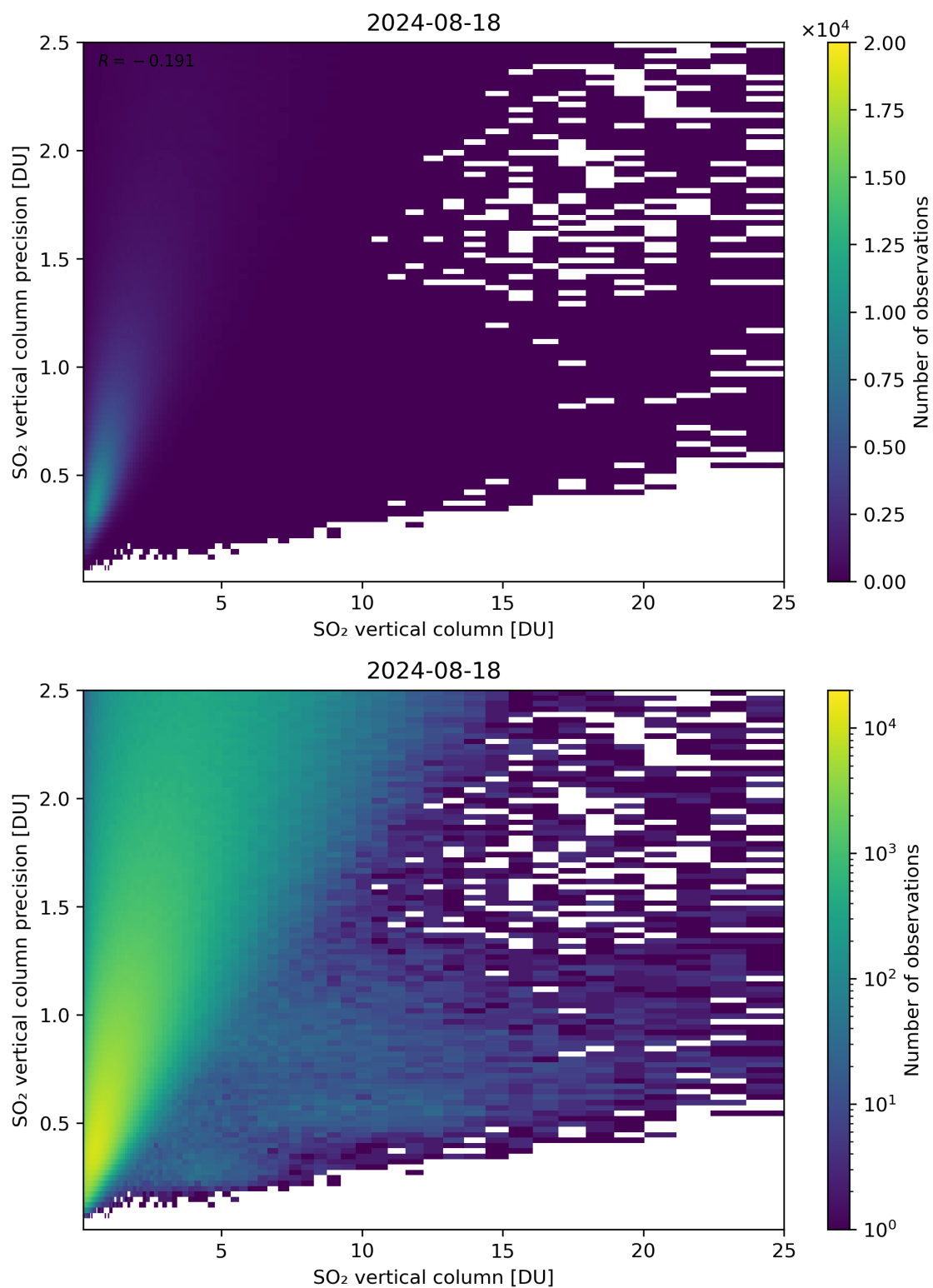
Figure 307: Scatter density plot of “SO 2 vertical column” against “SO 2 vertical column precision” for 2024-08-17 to 2024-08-19.
