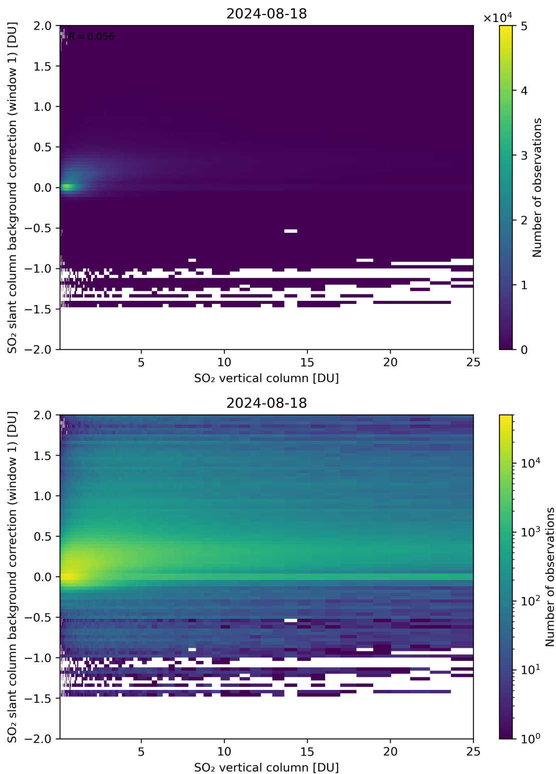
Figure 273: Scatter density plot of “SO 2 vertical column” against “SO 2 slant column background correction (window 1)” for 2024-08-17 to 2024-08-19.
