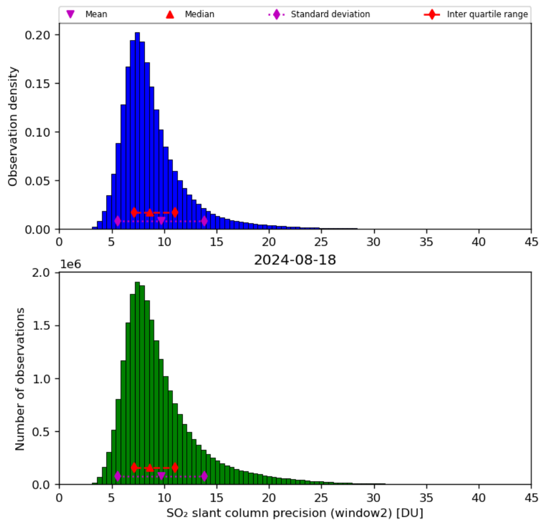
Figure 61: Histogram of “SO 2 slant column precision (window2)” for 2024-08-17 to 2024-08-19
