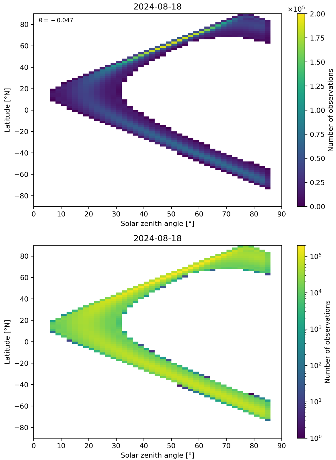
Figure 164: Scatter density plot of “Solar zenith angle” against “Latitude” for 2024-08-17 to 2024-08-19.
