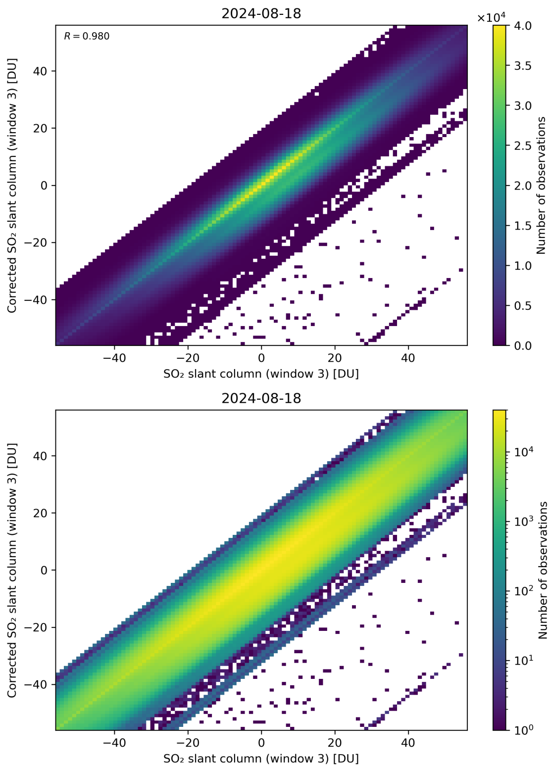
Figure 266: Scatter density plot of “SO 2 slant column (window 3)” against “Corrected SO 2 slant column (window 3)” for 2024-08-17 to 2024-08-19.
