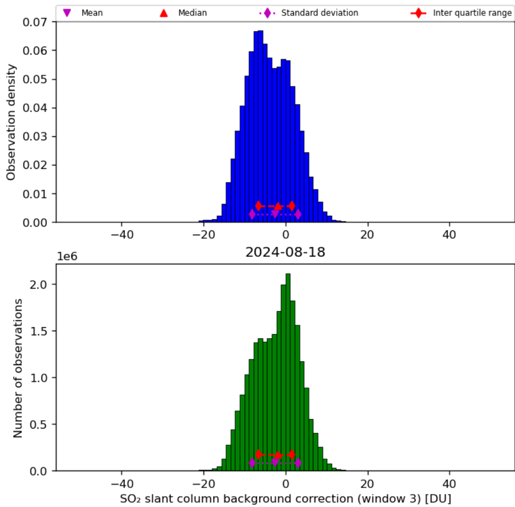
Figure 67: Histogram of “SO 2 slant column background correction (window 3)” for 2024-08-17 to 2024-08-19
