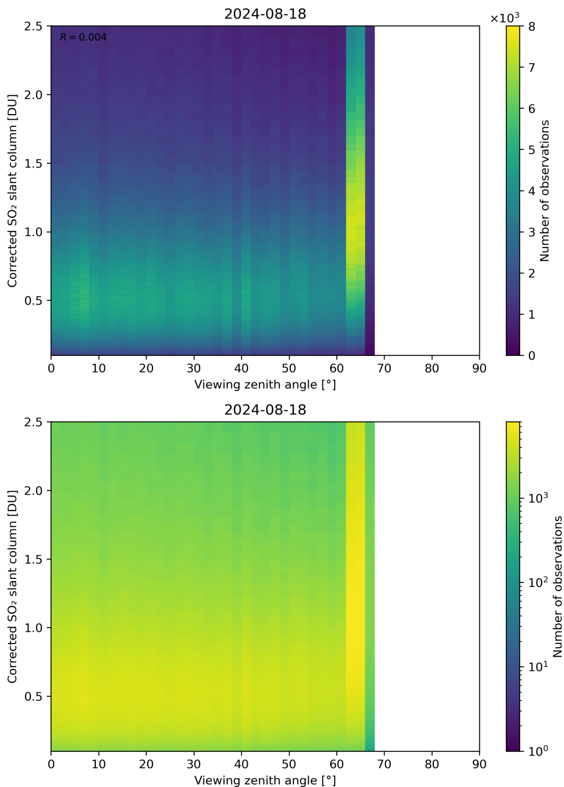
Figure 317: Scatter density plot of “Viewing zenith angle” against “Corrected SO 2 slant column” for 2024-08-17 to 2024-08-19.
