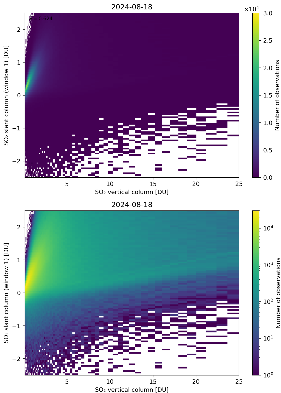
Figure 300: Scatter density plot of “SO 2 vertical column” against “SO 2 slant column (window 1)” for 2024-08-17 to 2024-08-19.
