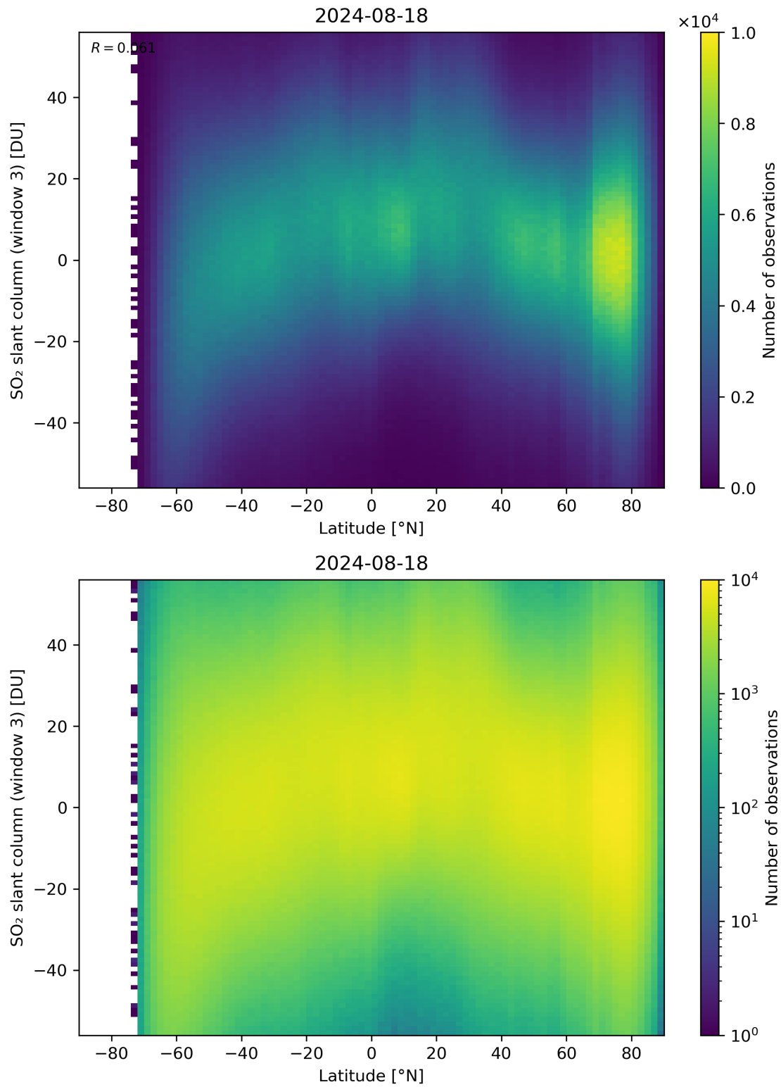
Figure 152: Scatter density plot of “Latitude” against “SO 2 slant column (window 3)” for 2024-08-17 to 2024-08-19.
