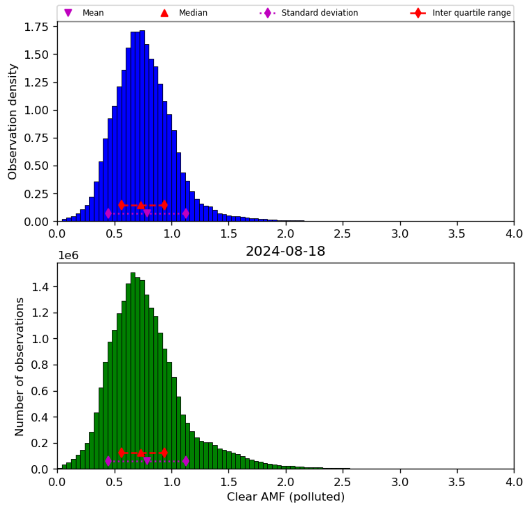
Figure 73: Histogram of “Clear AMF (polluted)” for 2024-08-17 to 2024-08-19
