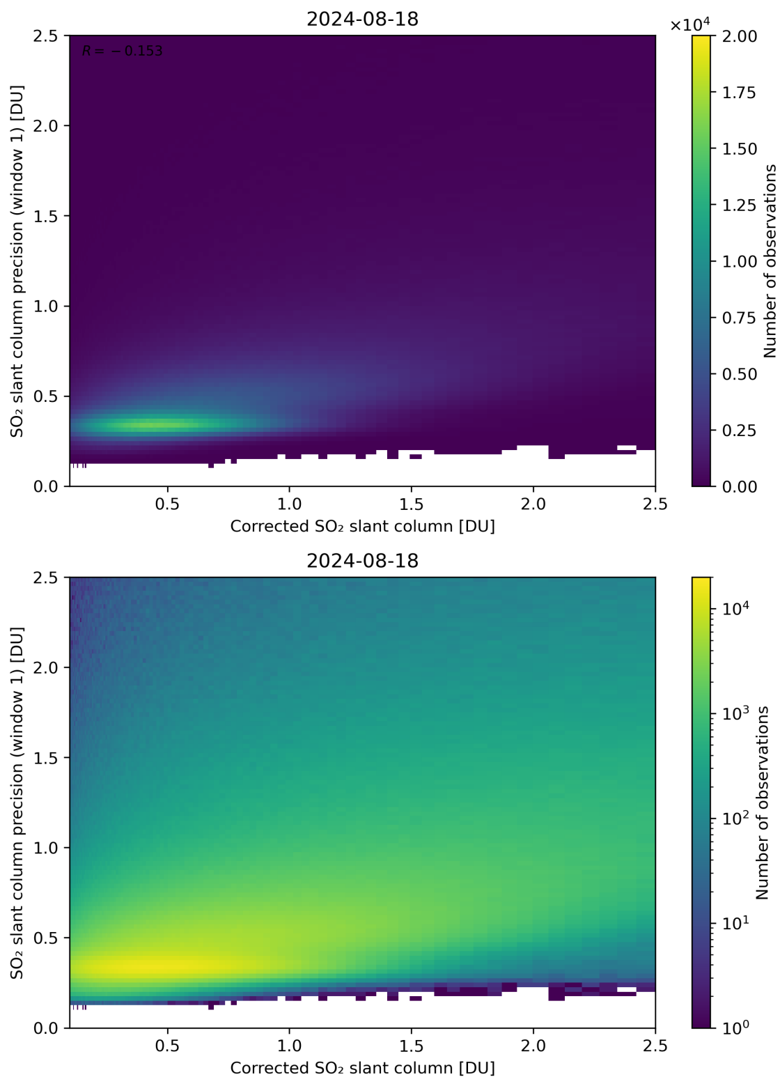
Figure 188: Scatter density plot of “Corrected SO 2 slant column” against “SO 2 slant column precision (window 1)” for 2024-08-17 to 2024-08-19.
