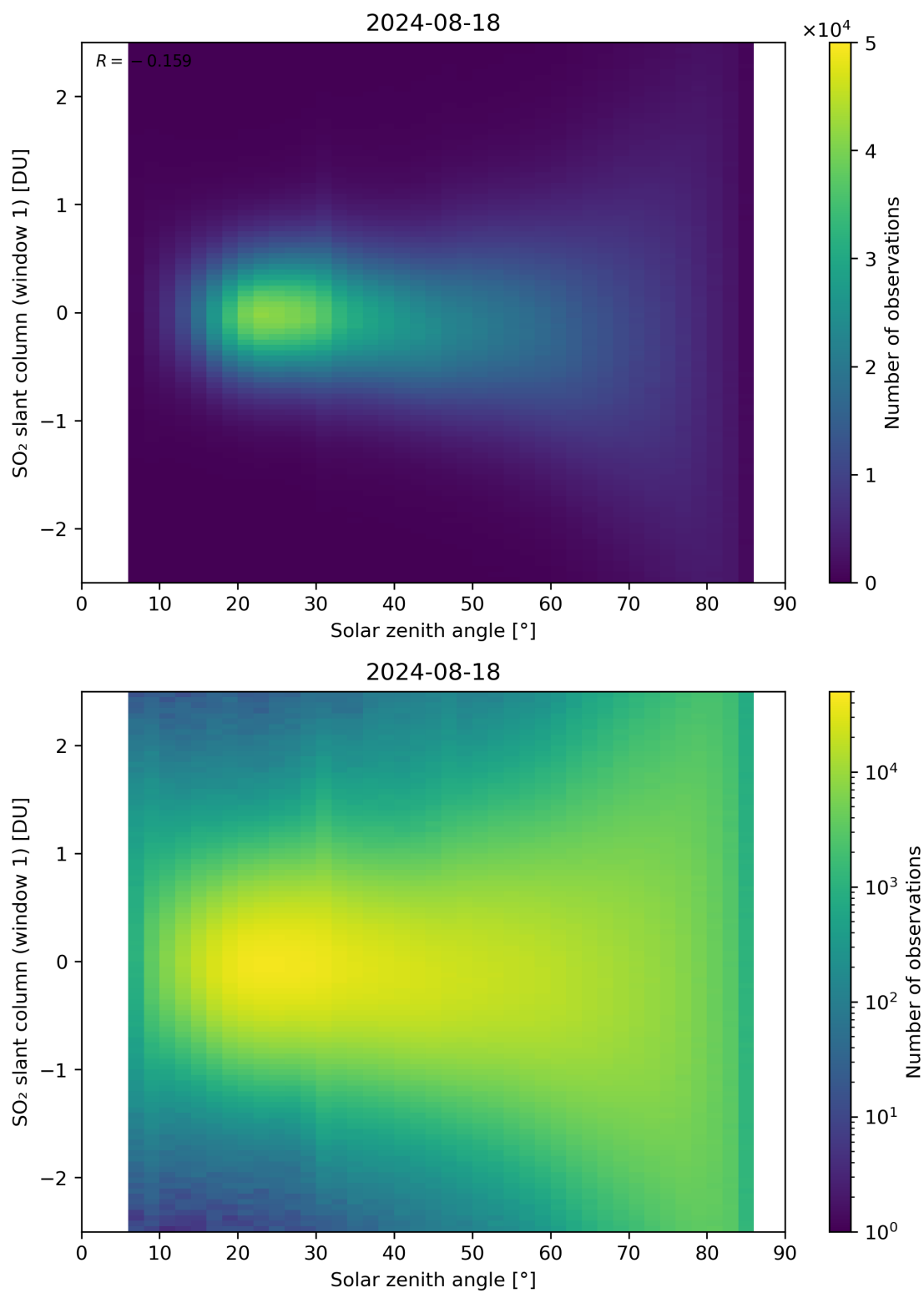
Figure 169: Scatter density plot of “Solar zenith angle” against “SO 2 slant column (window 1)” for 2024-08-17 to 2024-08-19.
