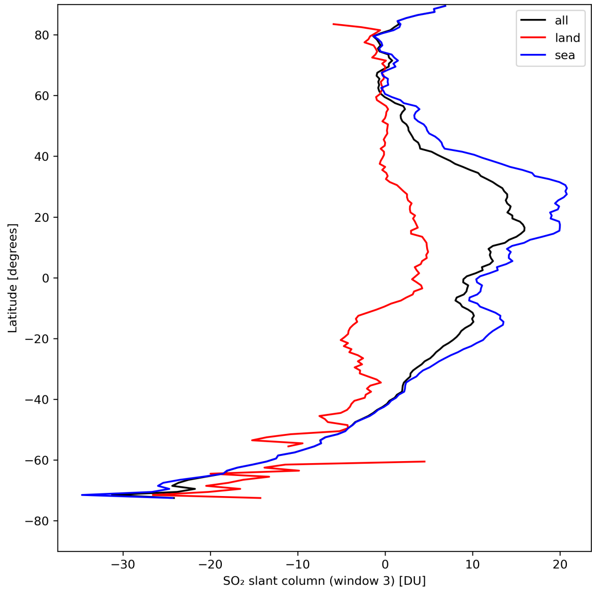
Figure 41: Zonal average of “SO 2 slant column (window 3)” for 2024-08-17 to 2024-08-19.
