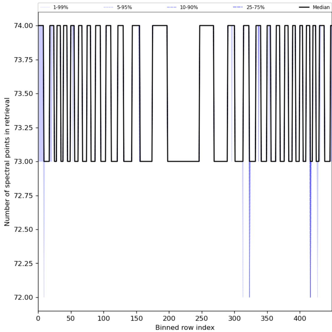
Figure 97: Along track statistics of “Number of spectral points in retrieval” for 2024-08-17 to 2024-08-19
