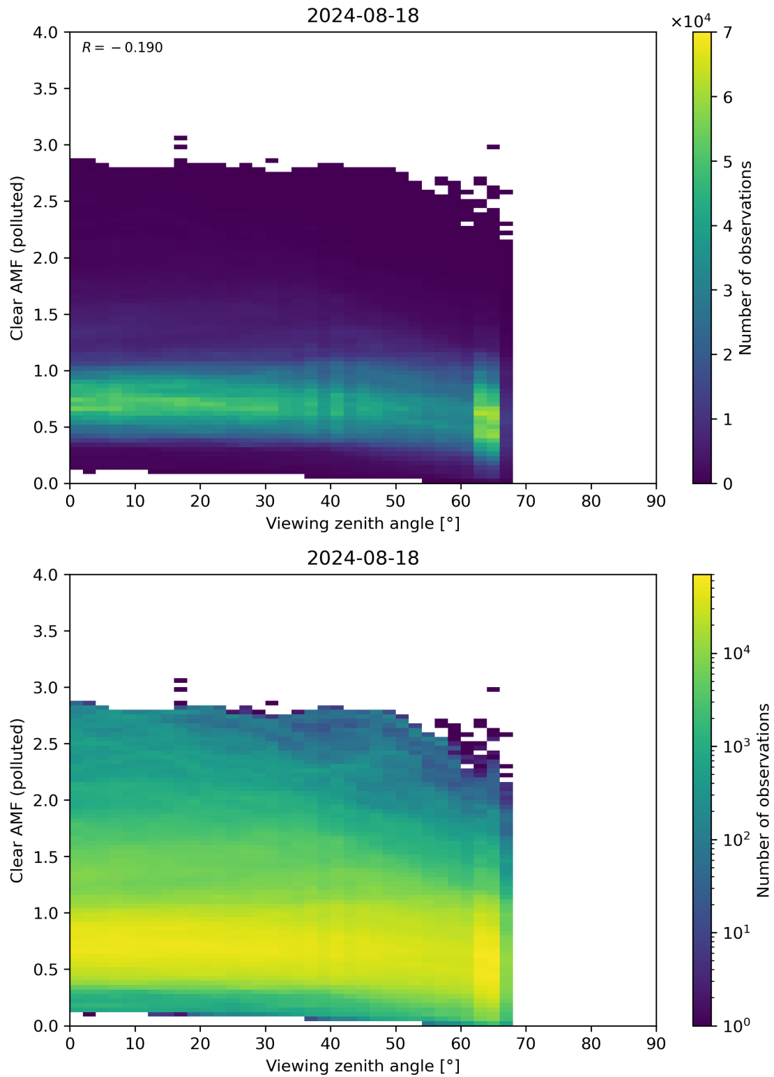
Figure 316: Scatter density plot of “Viewing zenith angle” against “Clear AMF (polluted)” for 2024-08-17 to 2024-08-19.
