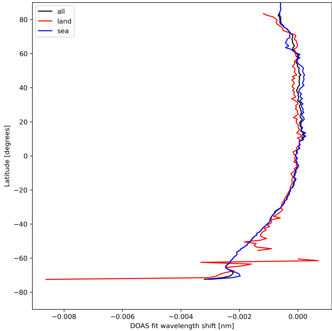
Figure 45: Zonal average of “DOAS fit wavelength shift” for 2024-08-17 to 2024-08-19.
