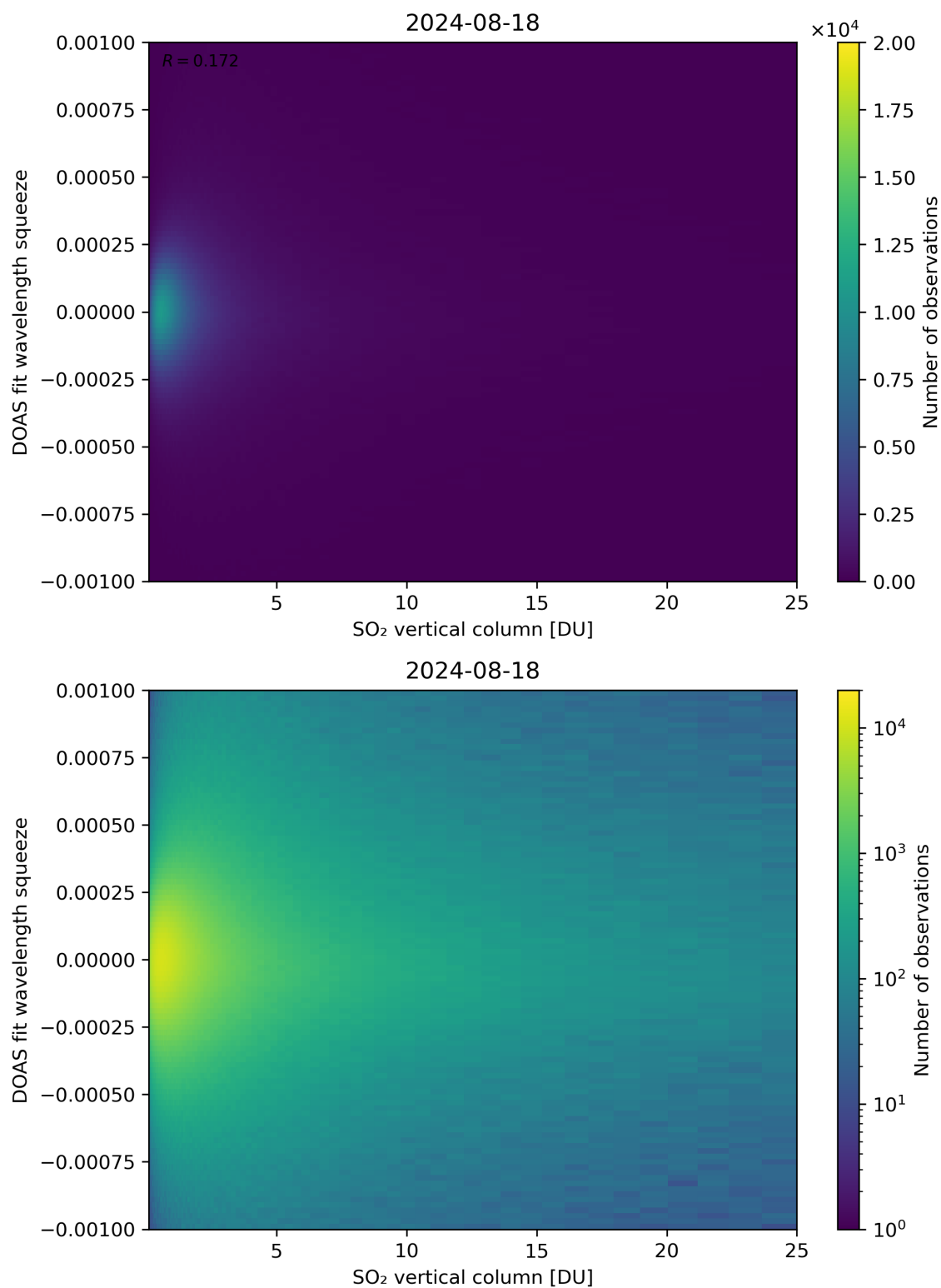
Figure 277: Scatter density plot of “SO 2 vertical column” against “DOAS fit wavelength squeeze” for 2024-08-17 to 2024-08-19.
