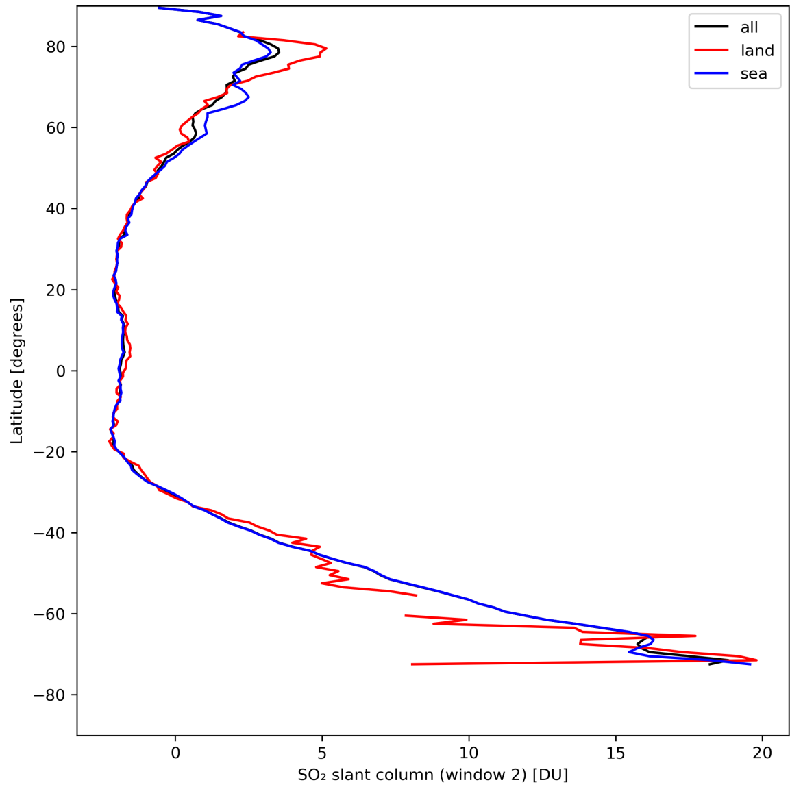
Figure 37: Zonal average of “SO 2 slant column (window 2)” for 2024-08-17 to 2024-08-19.
