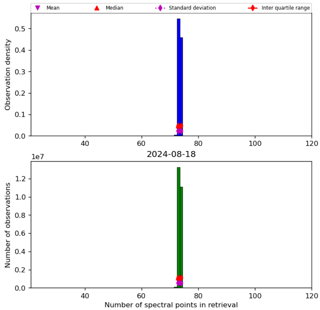
Figure 74: Histogram of “Number of spectral points in retrieval” for 2024-08-17 to 2024-08-19
