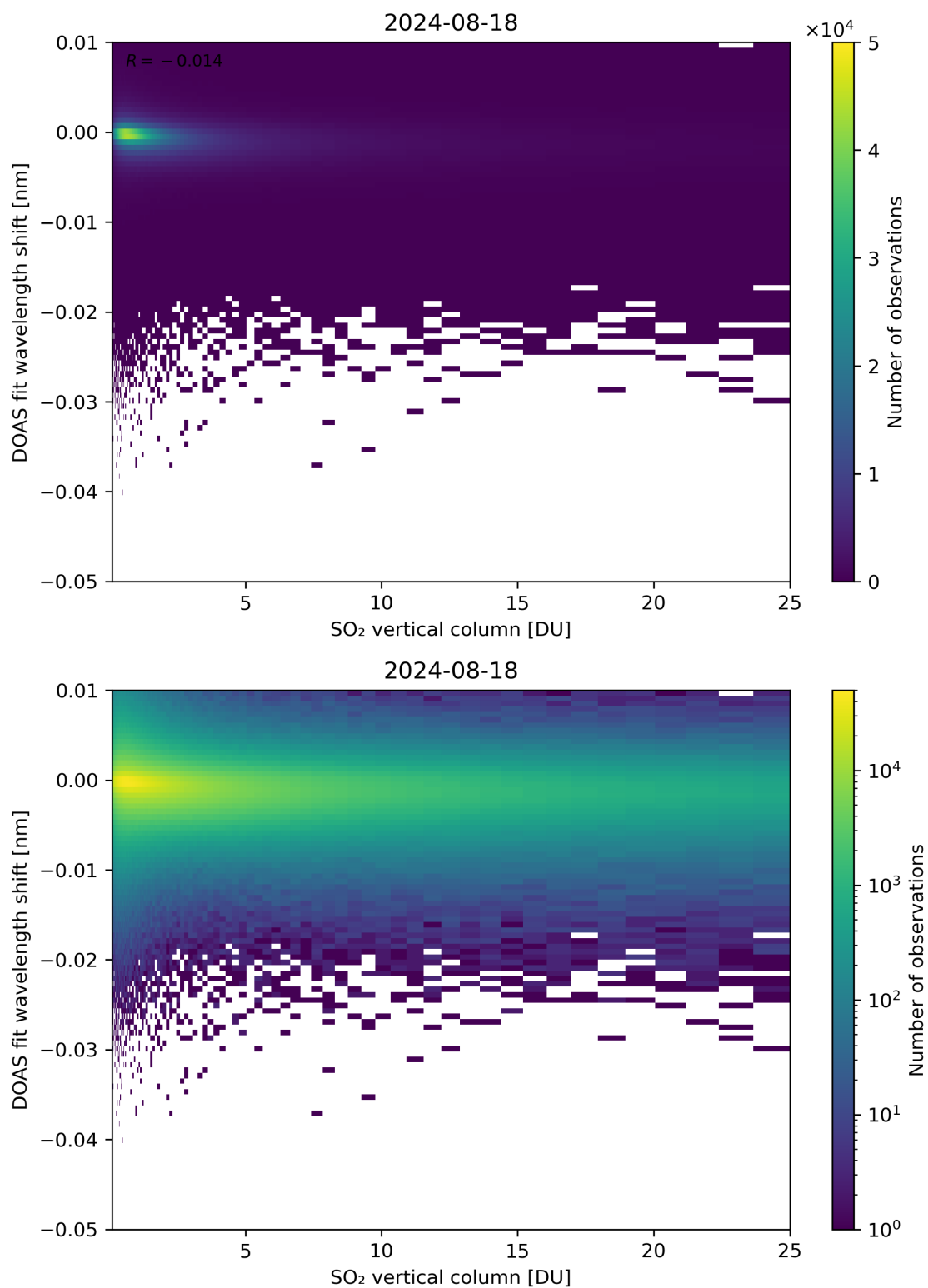
Figure 276: Scatter density plot of “SO 2 vertical column” against “DOAS fit wavelength shift” for 2024-08-17 to 2024-08-19.
