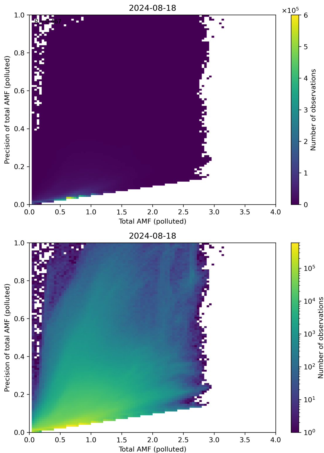
Figure 272: Scatter density plot of “Total AMF (polluted)” against “Precision of total AMF (polluted)” for 2024-08-17 to 2024-08-19.
