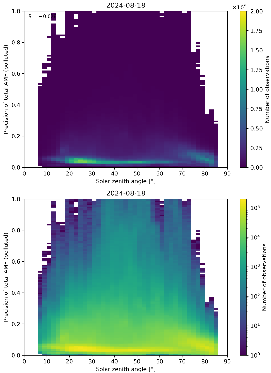
Figure 175: Scatter density plot of “Solar zenith angle” against “Precision of total AMF (polluted)” for 2024-08-17 to 2024-08-19.
