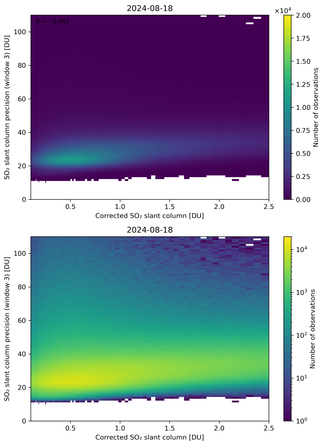
Figure 191: Scatter density plot of “Corrected SO 2 slant column” against “SO 2 slant column precision (window 3)” for 2024-08-17 to 2024-08-19.
