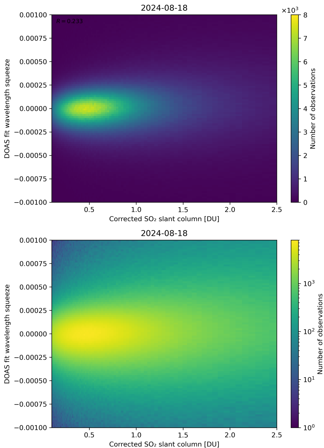
Figure 182: Scatter density plot of “Corrected SO 2 slant column” against “DOAS fit wavelength squeeze” for 2024-08-17 to 2024-08-19.
