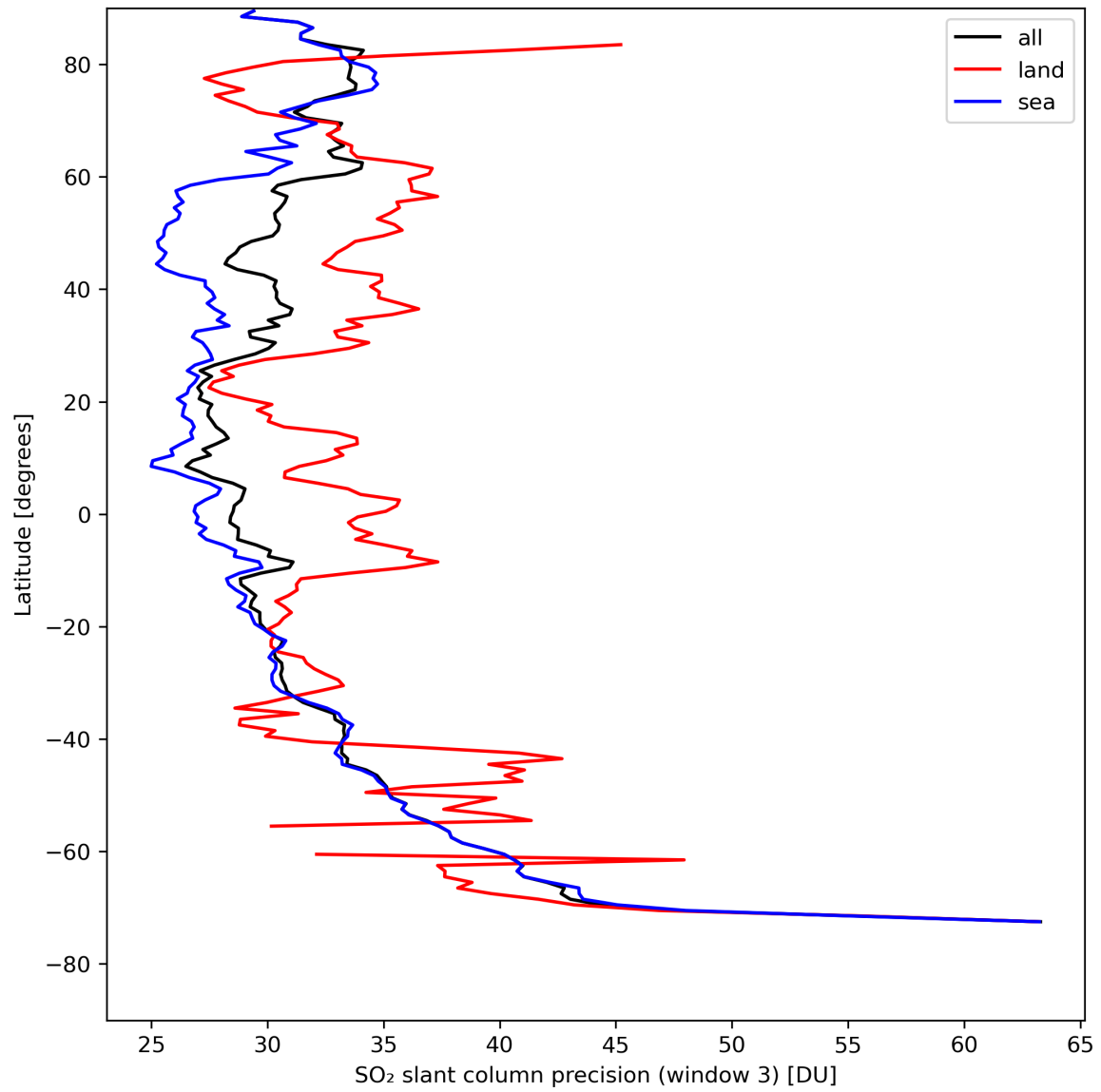
Figure 42: Zonal average of “SO 2 slant column precision (window 3)” for 2024-08-17 to 2024-08-19.
