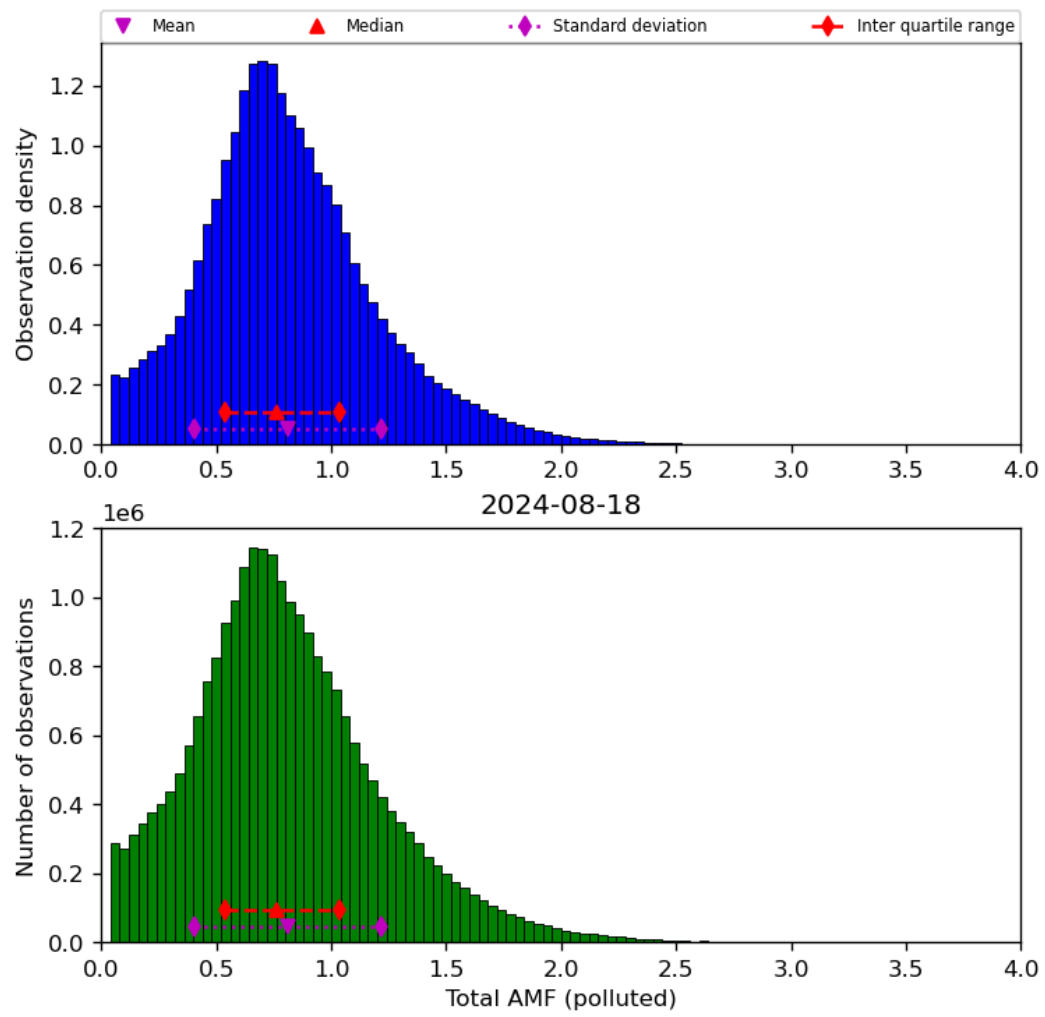
Figure 71: Histogram of “Total AMF (polluted)” for 2024-08-17 to 2024-08-19
