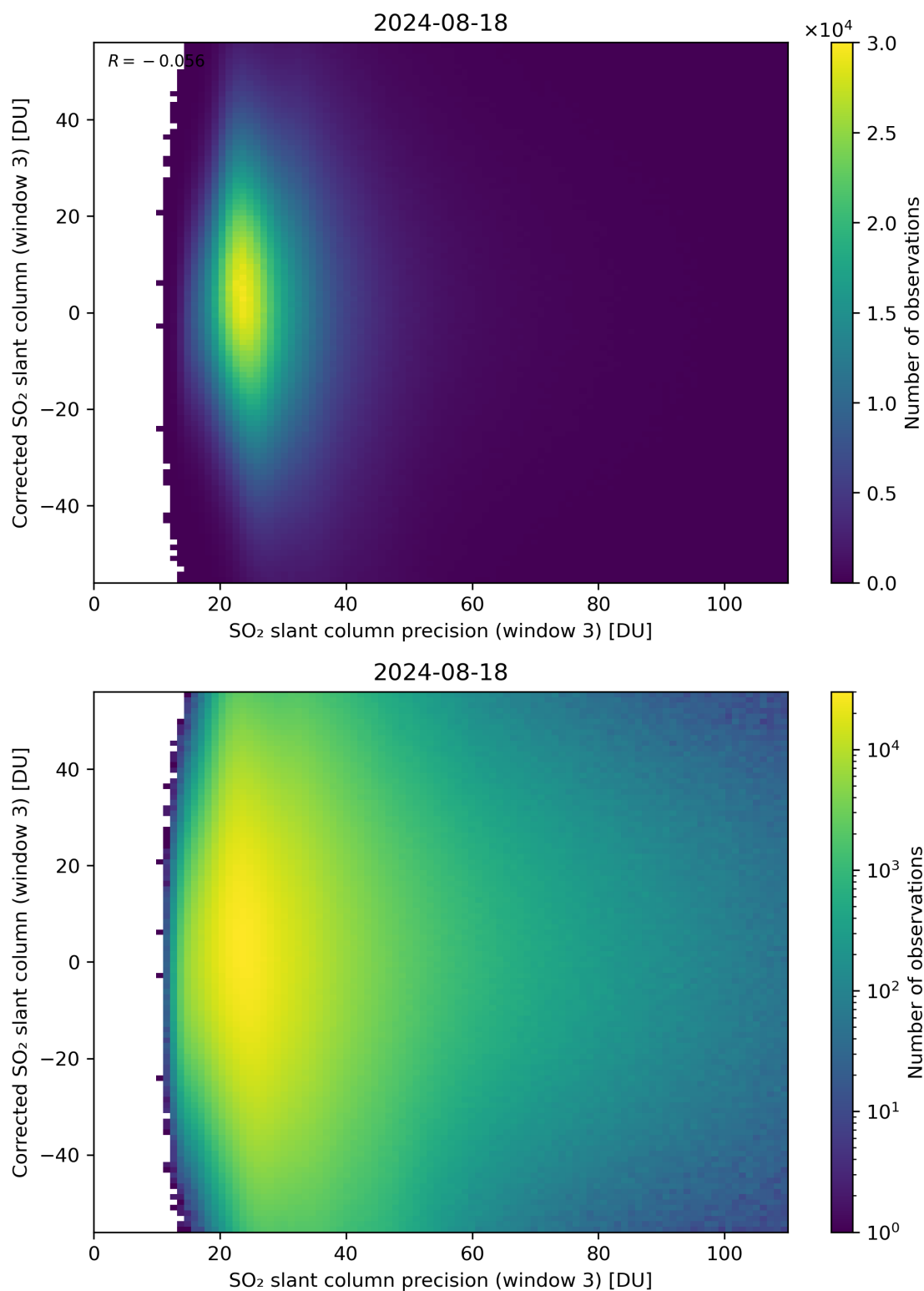
Figure 262: Scatter density plot of “SO 2 slant column precision (window 3)” against “Corrected SO 2 slant column (window 3)” for 2024-08-17 to 2024-08-19.
