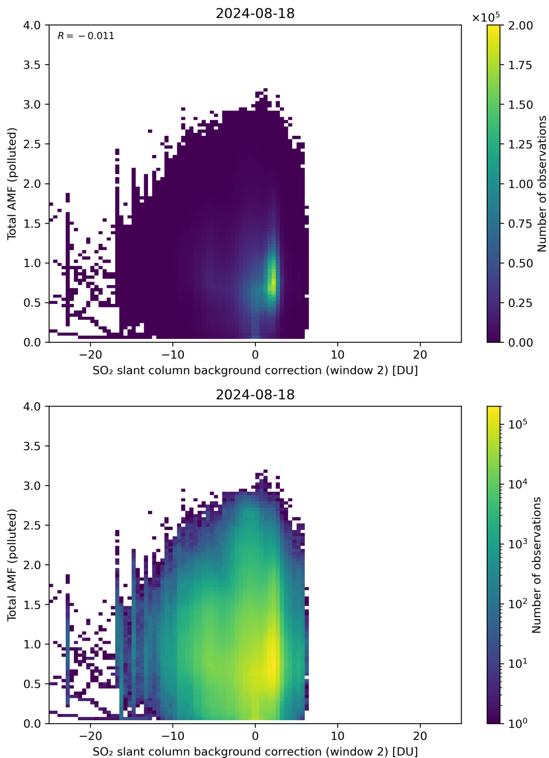
Figure 119: Scatter density plot of “SO 2 slant column background correction (window 2)” against “Total AMF (polluted)” for 2024-08-17 to 2024-08-19.
