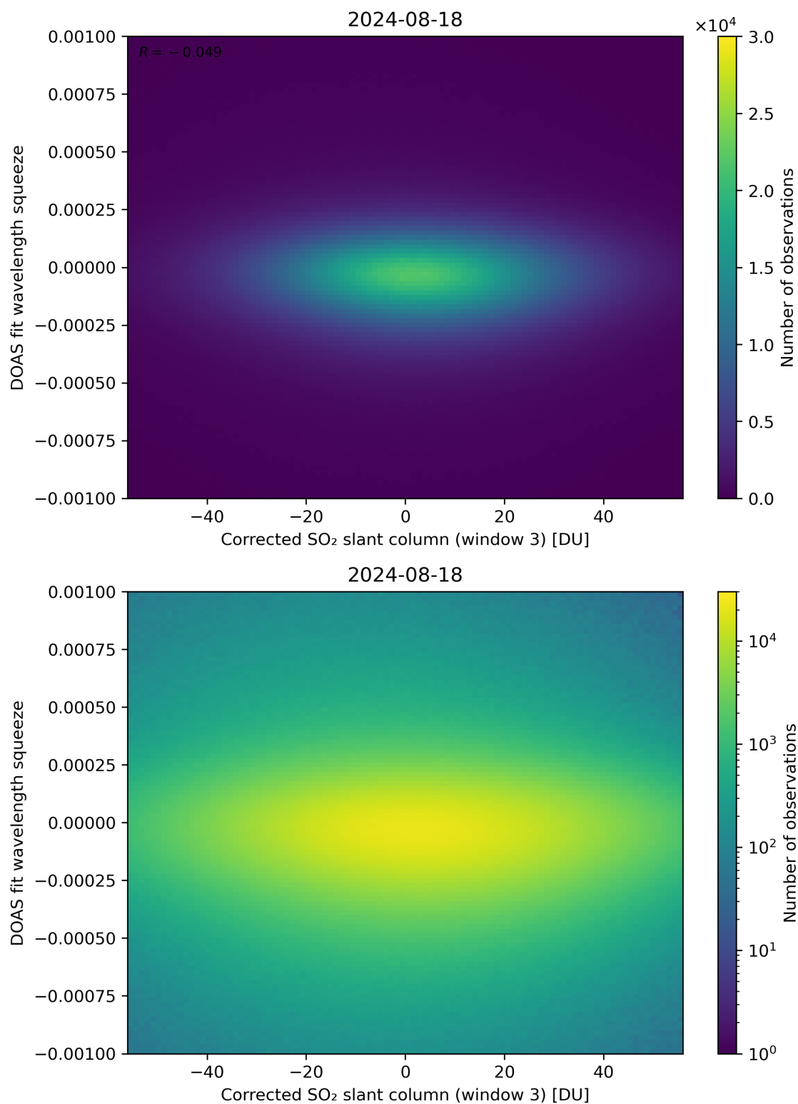
Figure 207: Scatter density plot of “Corrected SO 2 slant column (window 3)” against “DOAS fit wavelength squeeze” for 2024-08-17 to 2024-08-19.
