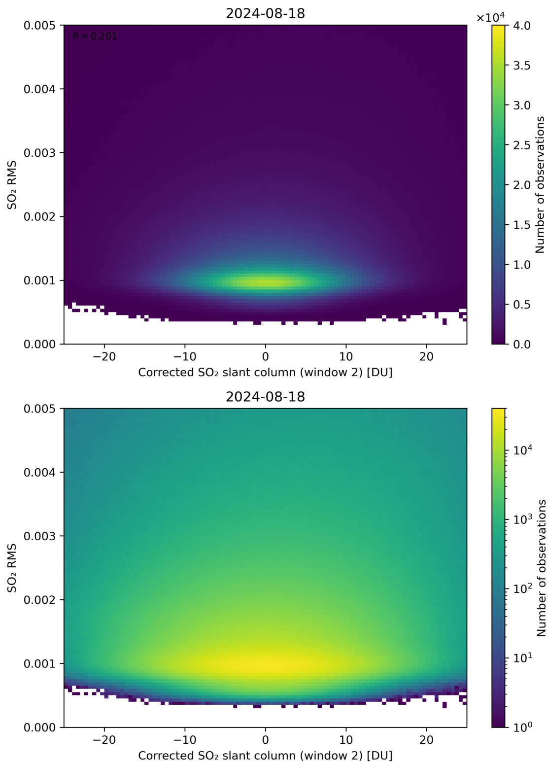
Figure 198: Scatter density plot of “Corrected SO 2 slant column (window 2)” against “SO 2 RMS” for 2024-08-17 to 2024-08-19.
