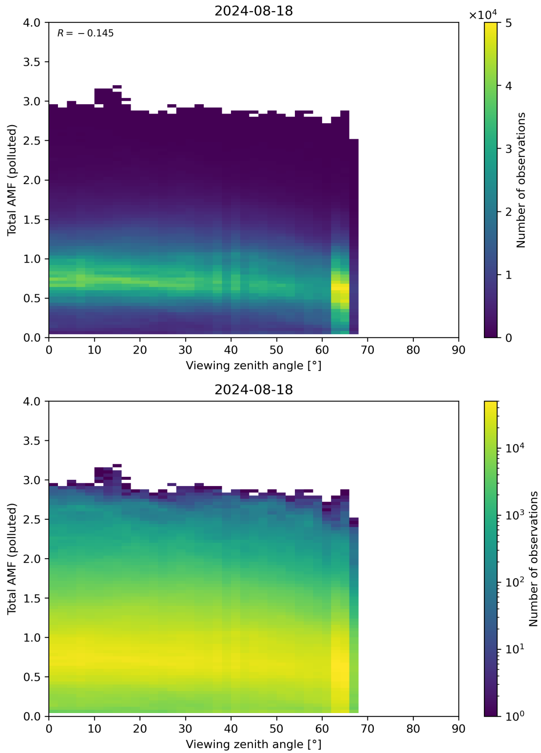
Figure 325: Scatter density plot of “Viewing zenith angle” against “Total AMF (polluted)” for 2024-08-17 to 2024-08-19.
