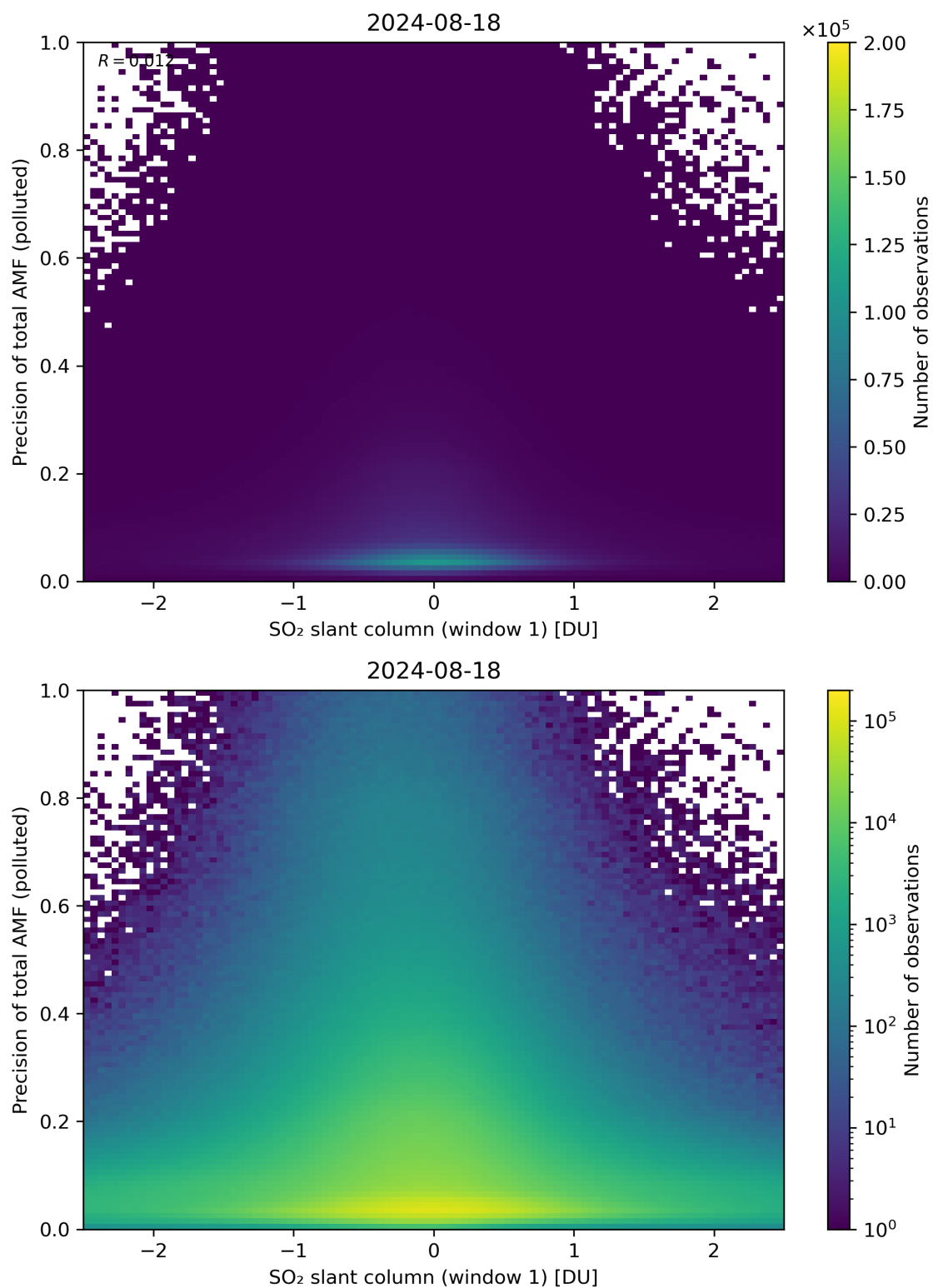
Figure 240: Scatter density plot of “SO 2 slant column (window 1)” against “Precision of total AMF (polluted)” for 2024-08-17 to 2024-08-19.
