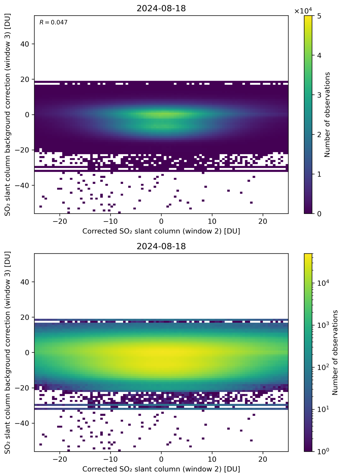
Figure 195: Scatter density plot of “Corrected SO 2 slant column (window 2)” against “SO 2 slant column background correction (window 3)” for 2024-08-17 to 2024-08-19.
