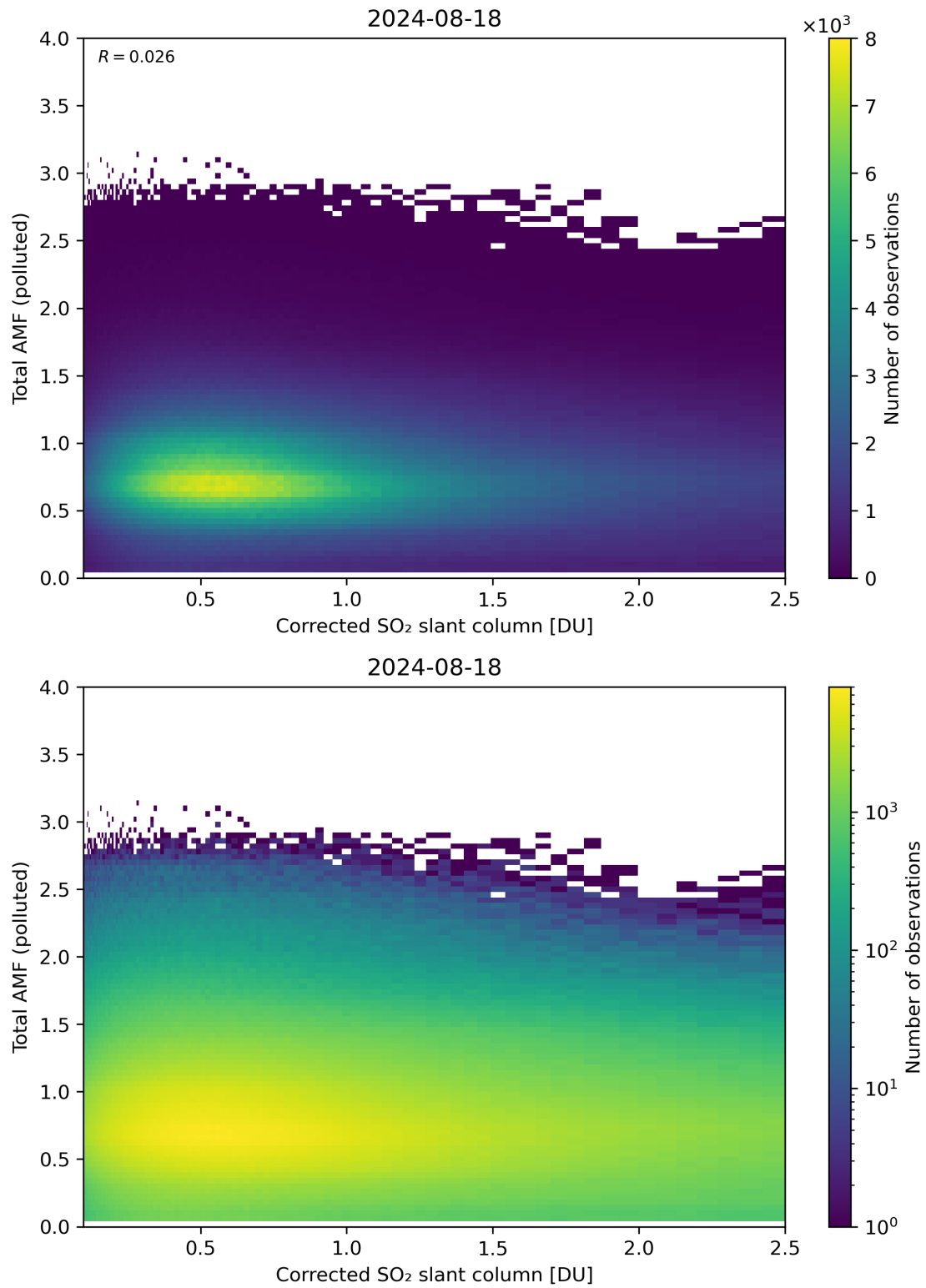
Figure 192: Scatter density plot of “Corrected SO 2 slant column” against “Total AMF (polluted)” for 2024-08-17 to 2024-08-19.
