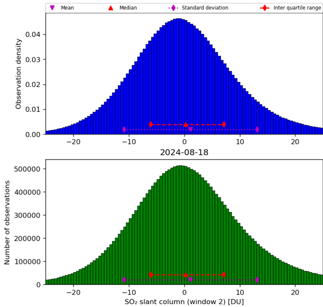
Figure 60: Histogram of “SO 2 slant column (window 2)” for 2024-08-17 to 2024-08-19
