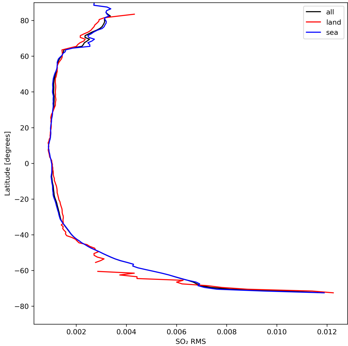
Figure 47: Zonal average of “SO 2 RMS” for 2024-08-17 to 2024-08-19.
