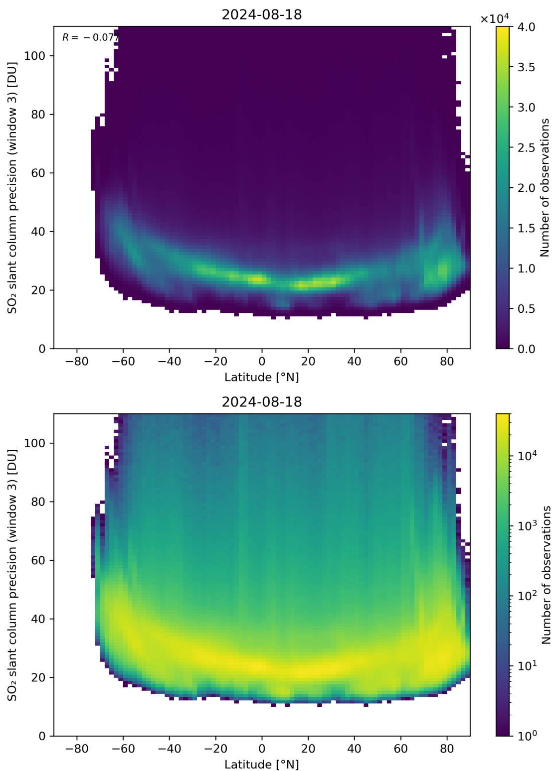
Figure 153: Scatter density plot of “Latitude” against “SO 2 slant column precision (window 3)” for 2024-08-17 to 2024-08-19.
