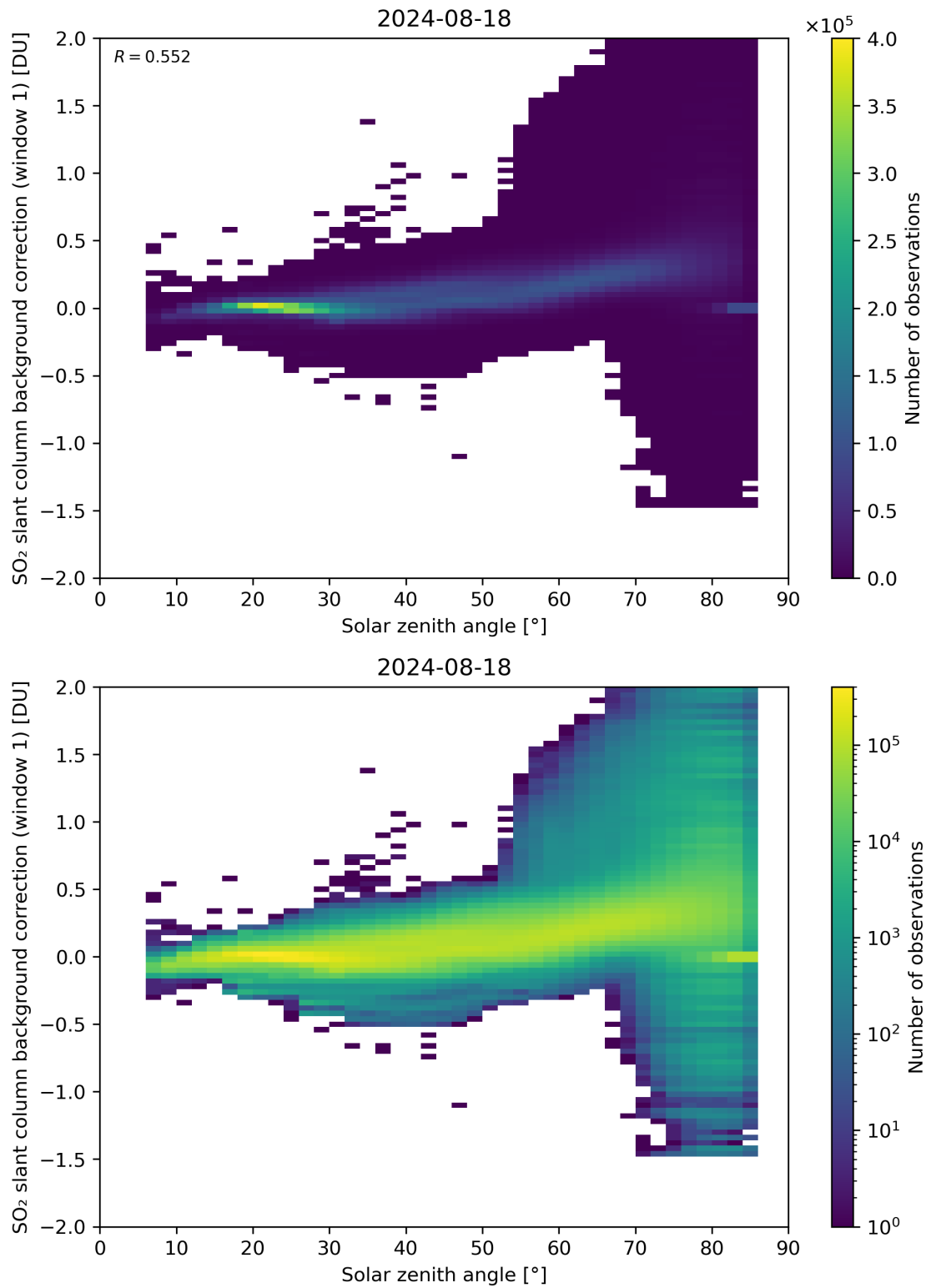
Figure 158: Scatter density plot of “Solar zenith angle” against “SO 2 slant column background correction (window 1)” for 2024-08-17 to 2024-08-19.
