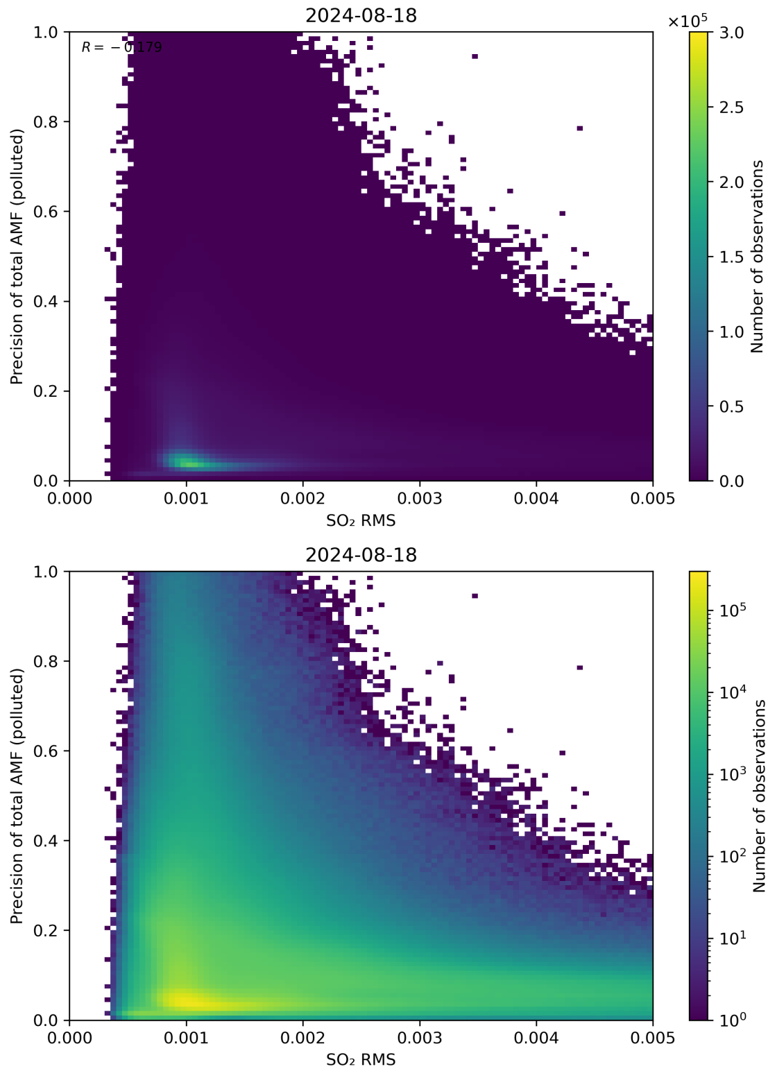
Figure 138: Scatter density plot of “SO 2 RMS” against “Precision of total AMF (polluted)” for 2024-08-17 to 2024-08-19.
