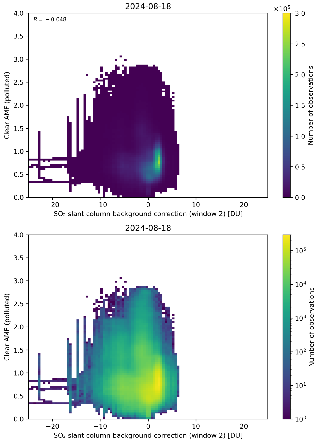
Figure 115: Scatter density plot of “SO 2 slant column background correction (window 2)” against “Clear AMF (polluted)” for 2024-08-17 to 2024-08-19.
