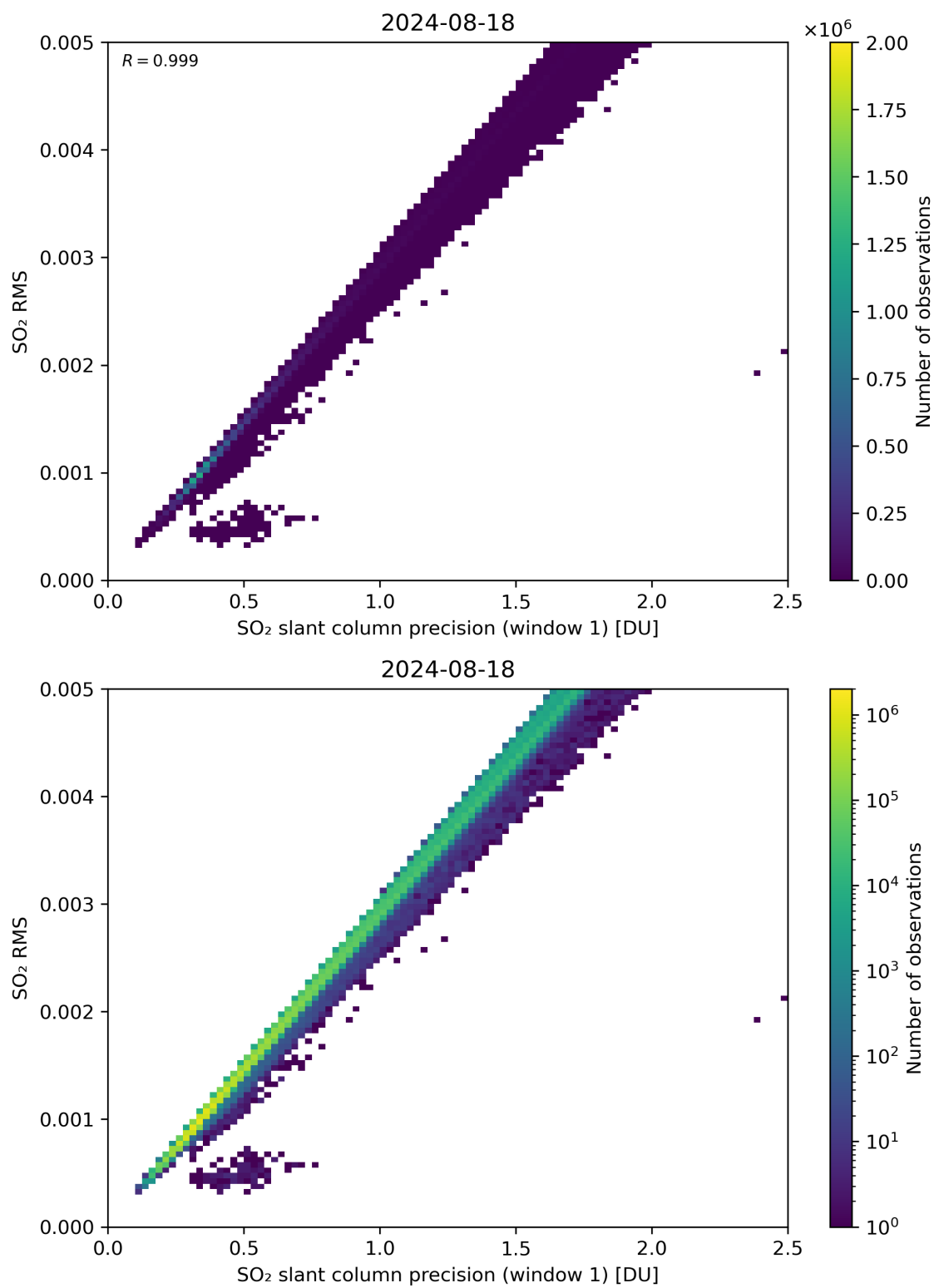
Figure 223: Scatter density plot of “SO 2 slant column precision (window 1)” against “SO 2 RMS” for 2024-08-17 to 2024-08-19.
