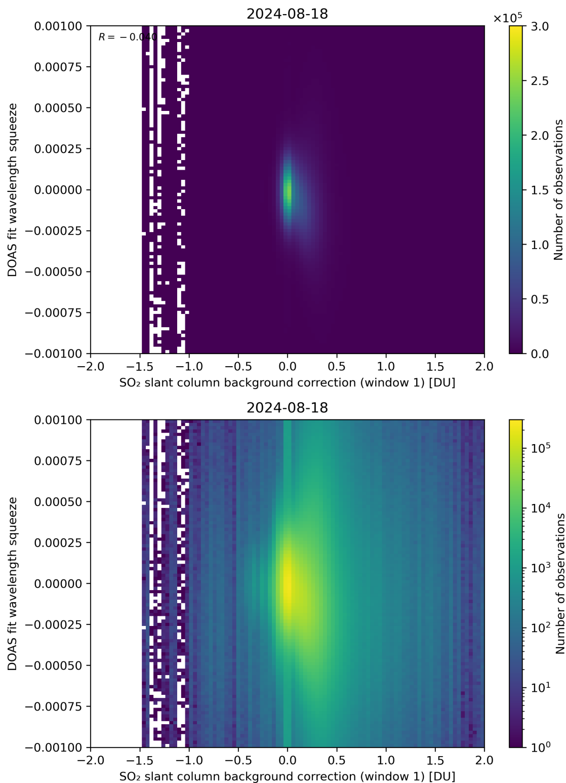
Figure 101: Scatter density plot of “SO 2 slant column background correction (window 1)” against “DOAS fit wavelength squeeze” for 2024-08-17 to 2024-08-19.
