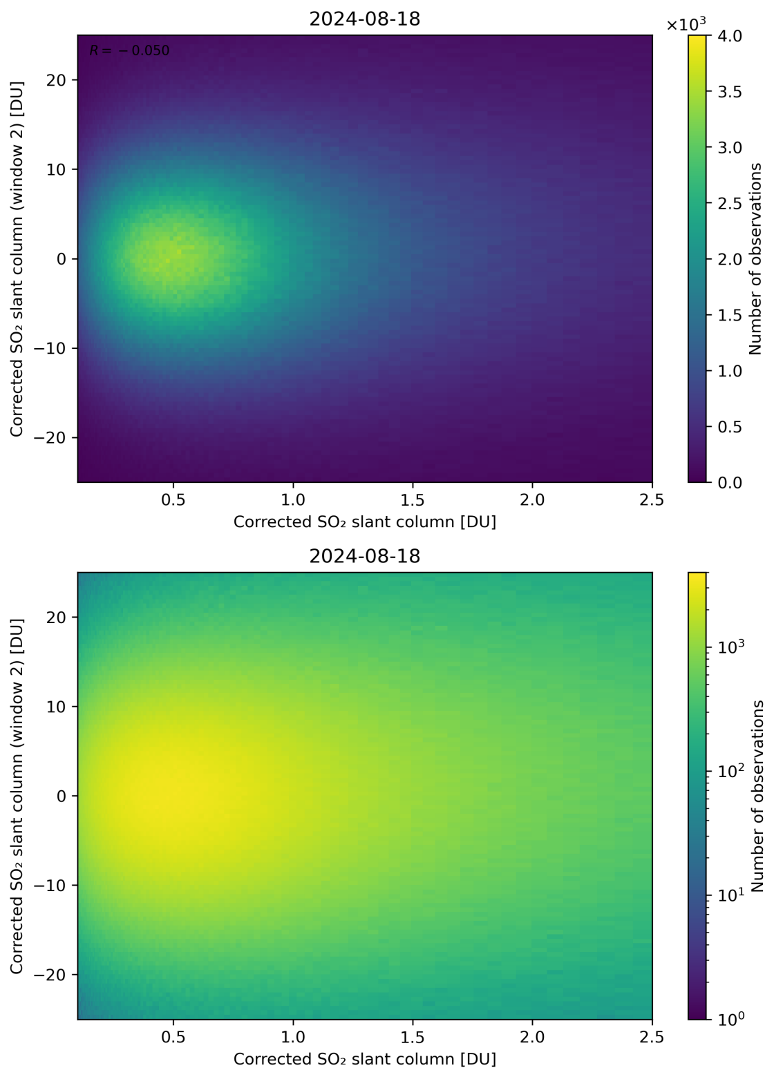
Figure 185: Scatter density plot of “Corrected SO 2 slant column” against “Corrected SO 2 slant column (window 2)” for 2024-08-17 to 2024-08-19.
