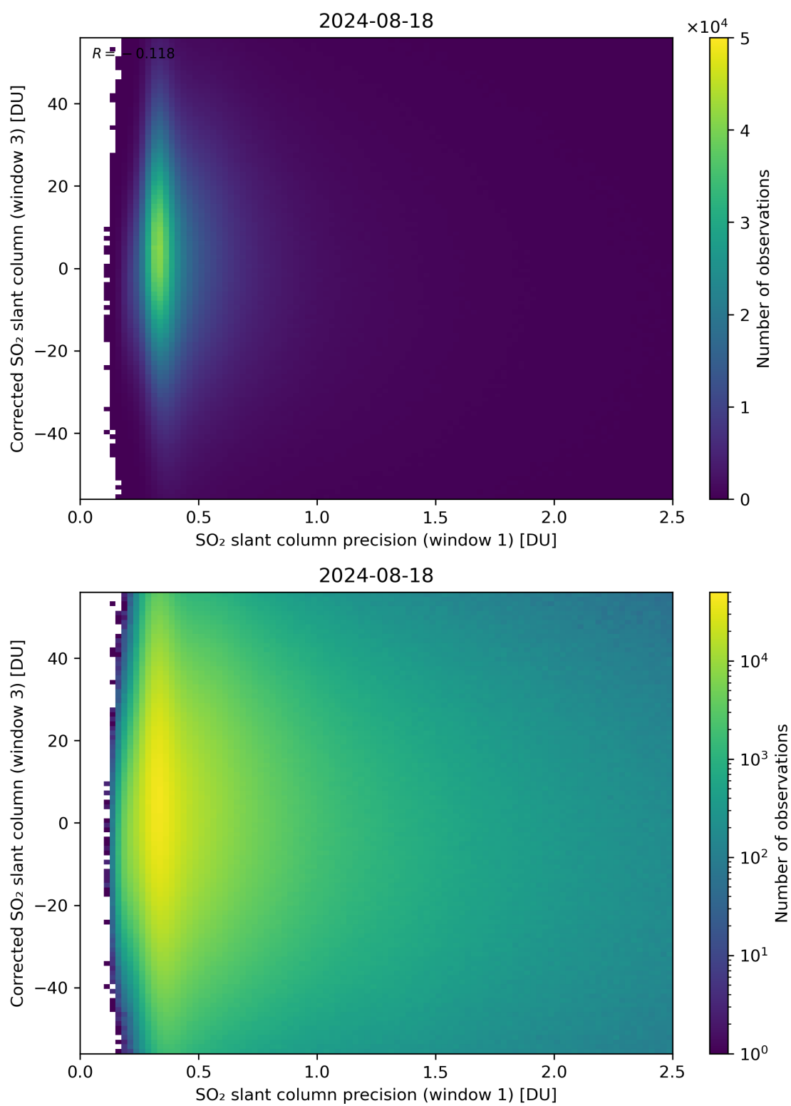
Figure 226: Scatter density plot of “SO 2 slant column precision (window 1)” against “Corrected SO 2 slant column (window 3)” for 2024-08-17 to 2024-08-19.
