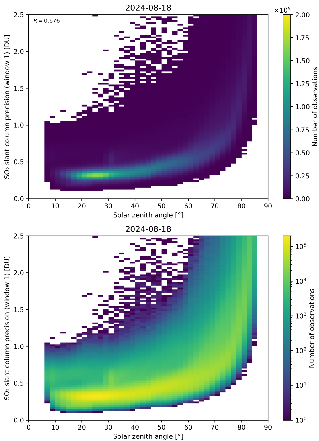
Figure 170: Scatter density plot of “Solar zenith angle” against “SO 2 slant column precision (window 1)” for 2024-08-17 to 2024-08-19.
