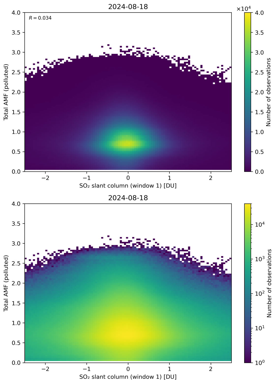
Figure 239: Scatter density plot of “SO 2 slant column (window 1)” against “Total AMF (polluted)” for 2024-08-17 to 2024-08-19.
