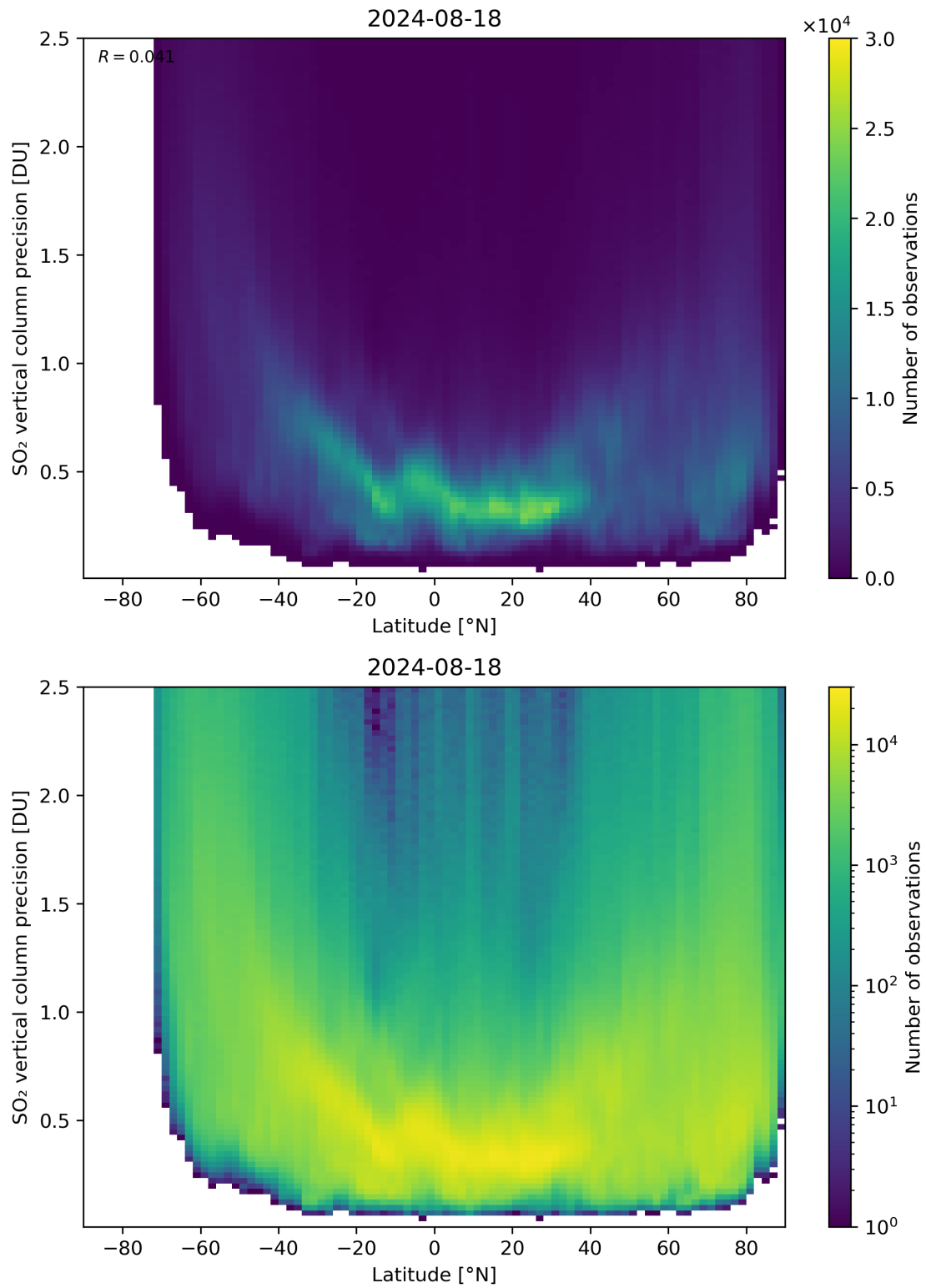
Figure 157: Scatter density plot of “Latitude” against “SO 2 vertical column precision” for 2024-08-17 to 2024-08-19.
