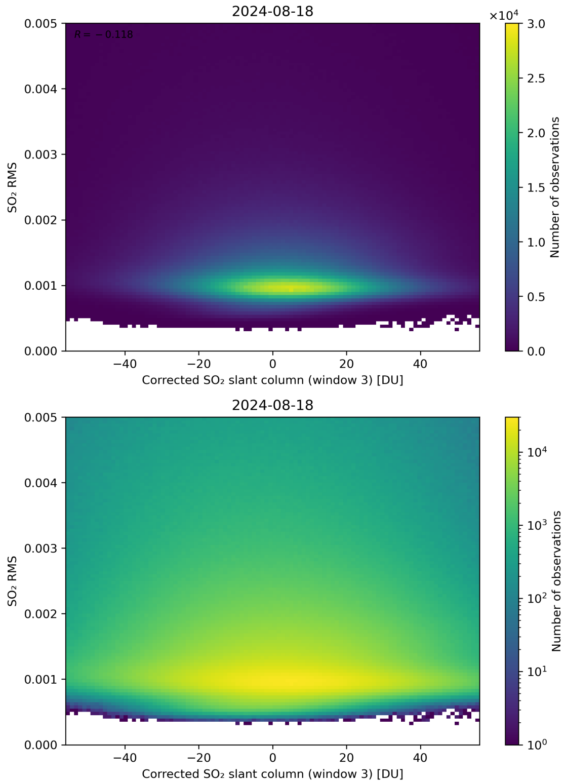
Figure 208: Scatter density plot of “Corrected SO 2 slant column (window 3)” against “SO 2 RMS” for 2024-08-17 to 2024-08-19.
