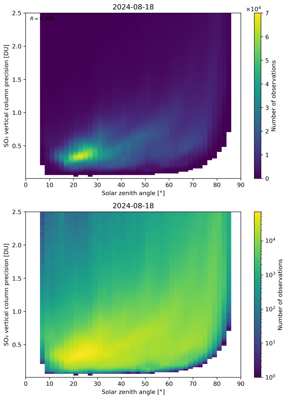
Figure 177: Scatter density plot of “Solar zenith angle” against “SO 2 vertical column precision” for 2024-08-17 to 2024-08-19.
