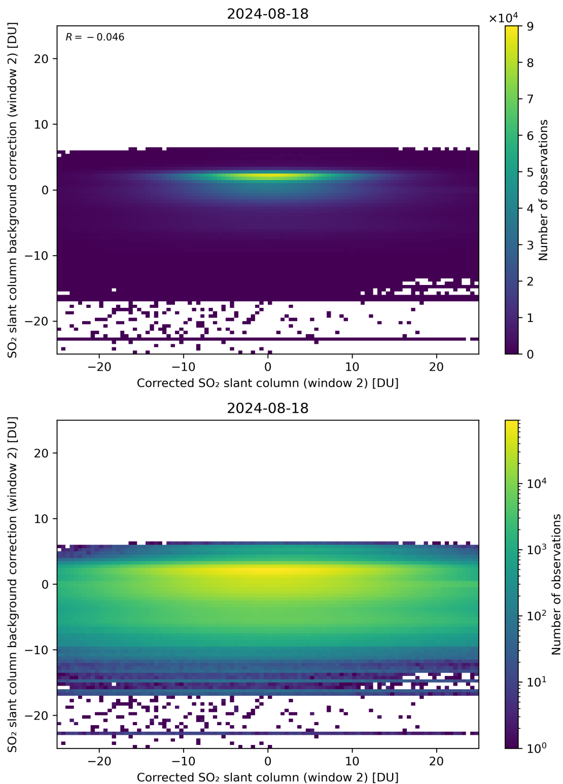
Figure 194: Scatter density plot of “Corrected SO 2 slant column (window 2)” against “SO 2 slant column background correction (window 2)” for 2024-08-17 to 2024-08-19.
