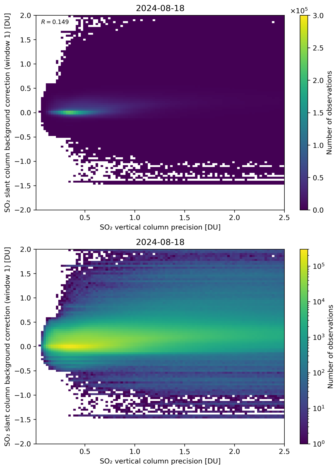
Figure 279: Scatter density plot of “SO 2 vertical column precision” against “SO 2 slant column background correction (window 1)” for 2024-08-17 to 2024-08-19.
