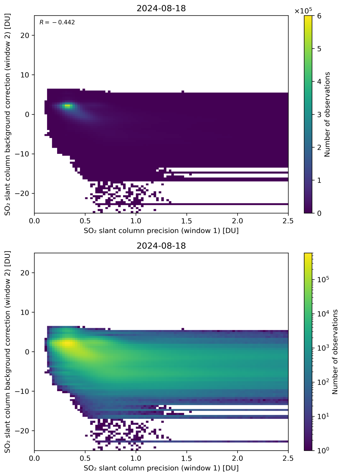
Figure 219: Scatter density plot of “SO 2 slant column precision (window 1)” against “SO 2 slant column background correction (window 2)” for 2024-08-17 to 2024-08-19.
