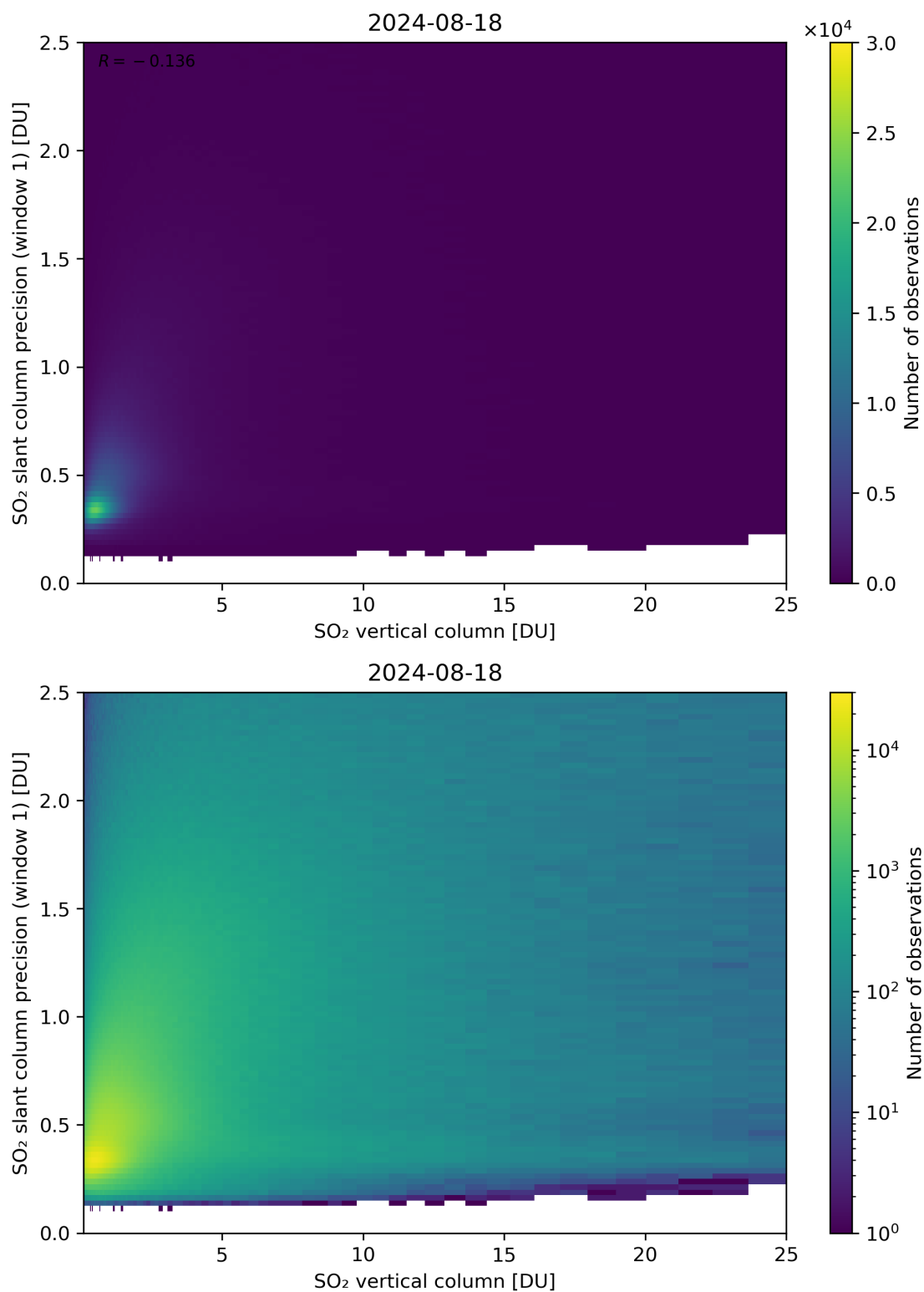
Figure 301: Scatter density plot of “SO 2 vertical column” against “SO 2 slant column precision (window 1)” for 2024-08-17 to 2024-08-19.
