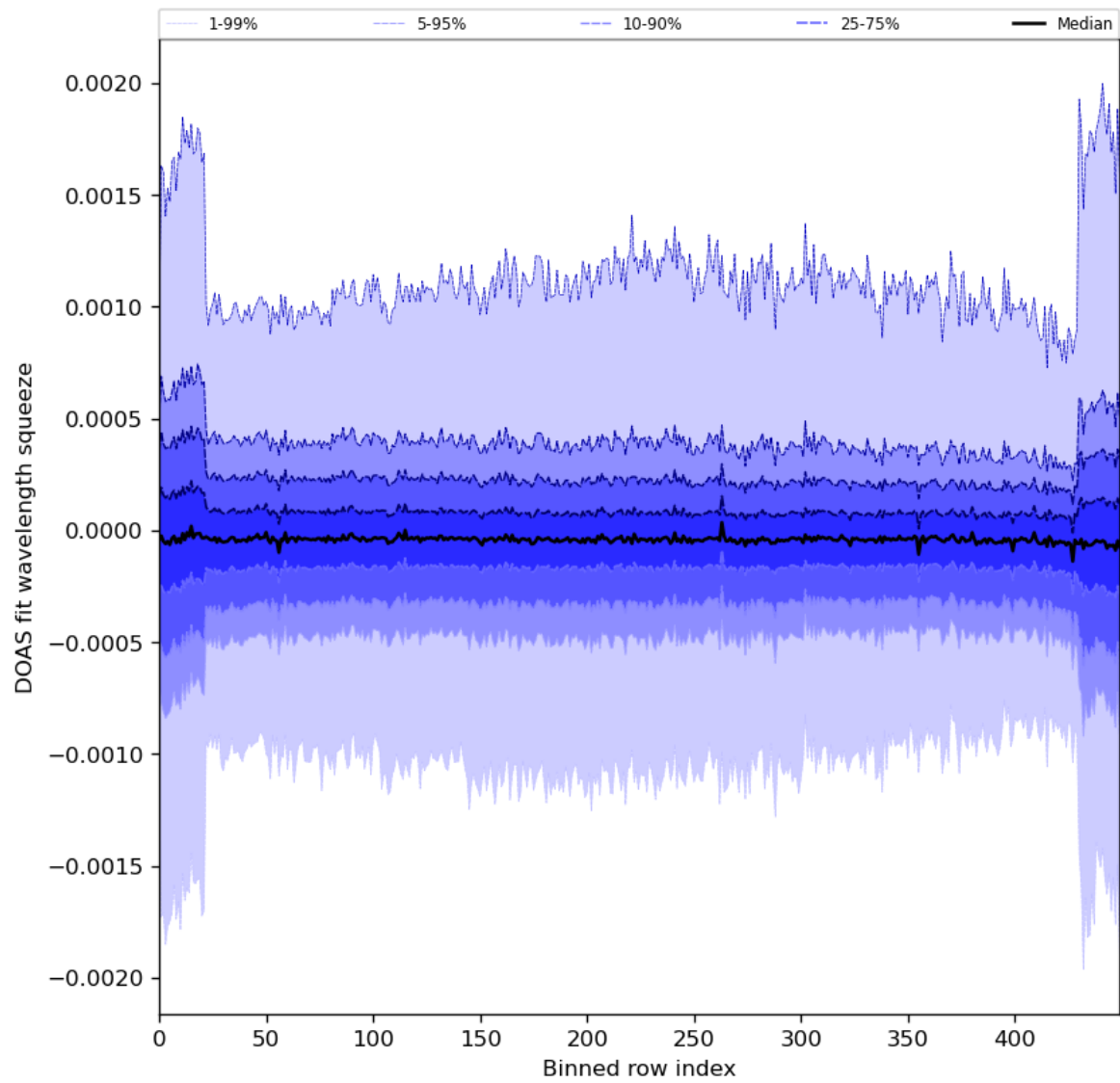
Figure 92: Along track statistics of “DOAS fit wavelength squeeze” for 2024-08-17 to 2024-08-19
