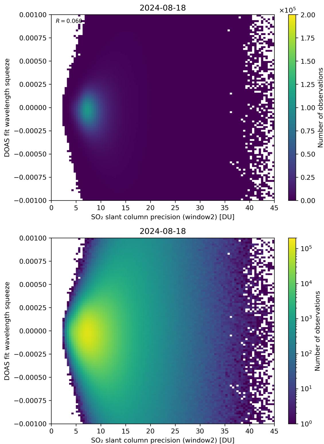
Figure 244: Scatter density plot of “SO 2 slant column precision (window2)” against “DOAS fit wavelength squeeze” for 2024-08-17 to 2024-08-19.
