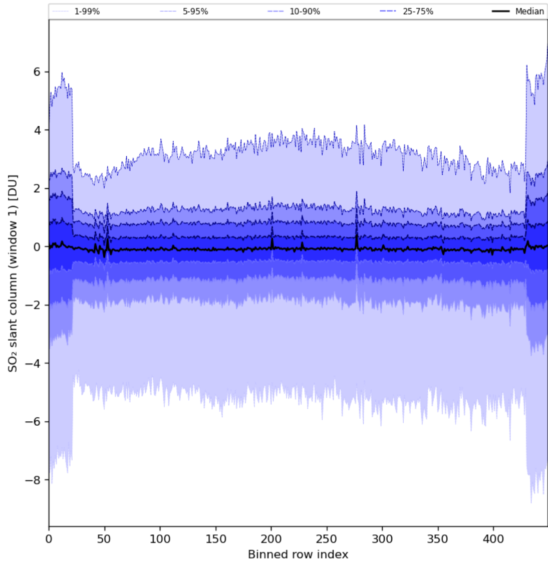
Figure 79: Along track statistics of “SO 2 slant column (window 1)” for 2024-08-17 to 2024-08-19
