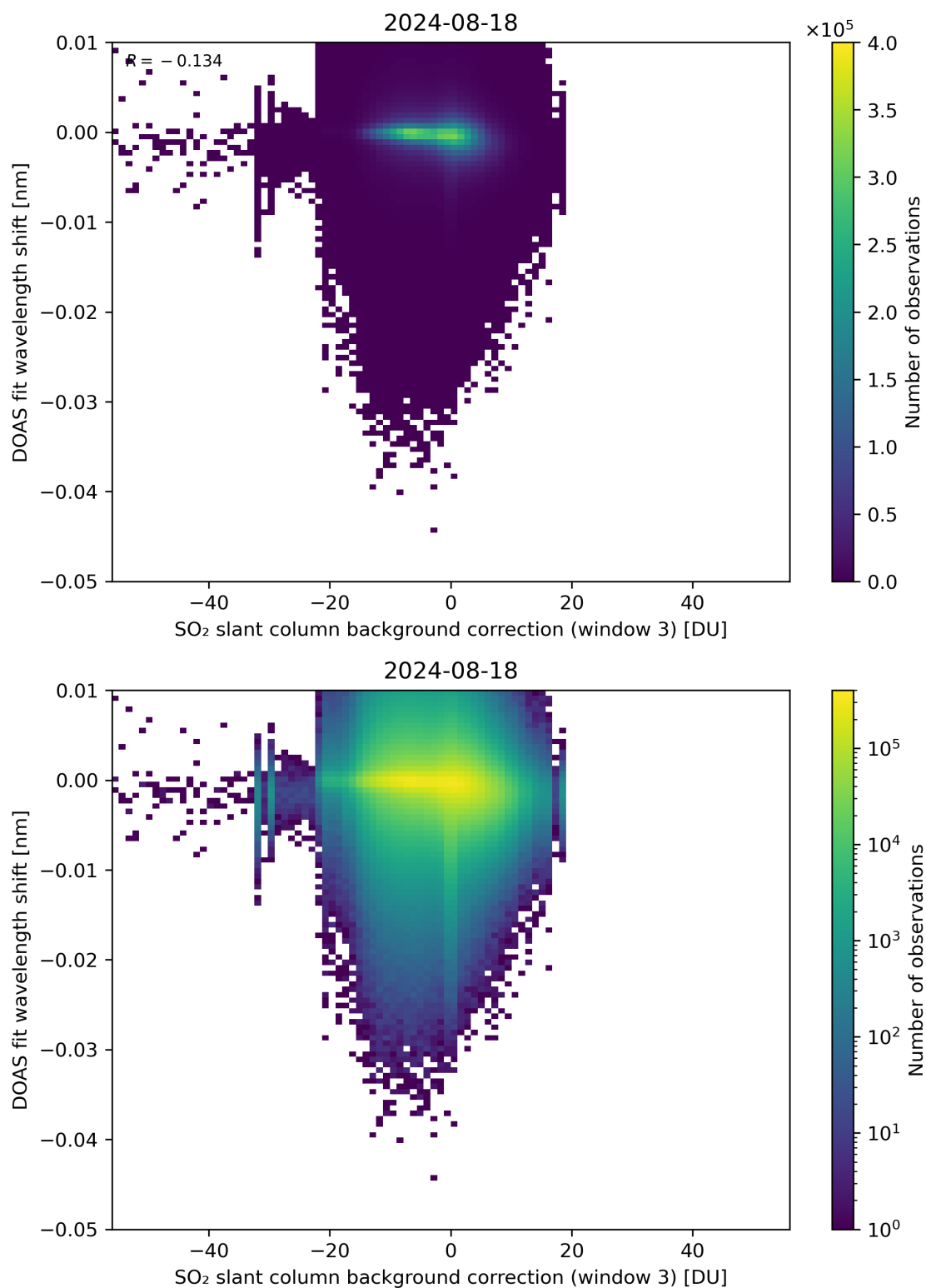
Figure 121: Scatter density plot of “SO 2 slant column background correction (window 3)” against “DOAS fit wavelength shift” for 2024-08-17 to 2024-08-19.
