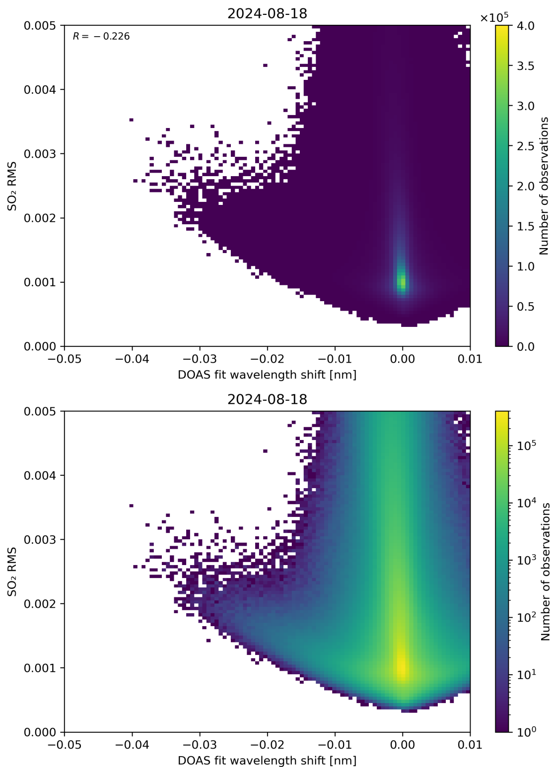
Figure 128: Scatter density plot of “DOAS fit wavelength shift” against “SO 2 RMS” for 2024-08-17 to 2024-08-19.
