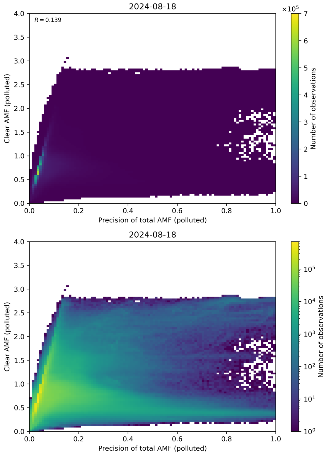
Figure 270: Scatter density plot of “Precision of total AMF (polluted)” against “Clear AMF (polluted)” for 2024-08-17 to 2024-08-19.
