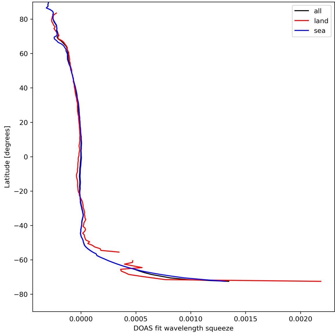
Figure 46: Zonal average of “DOAS fit wavelength squeeze” for 2024-08-17 to 2024-08-19.
