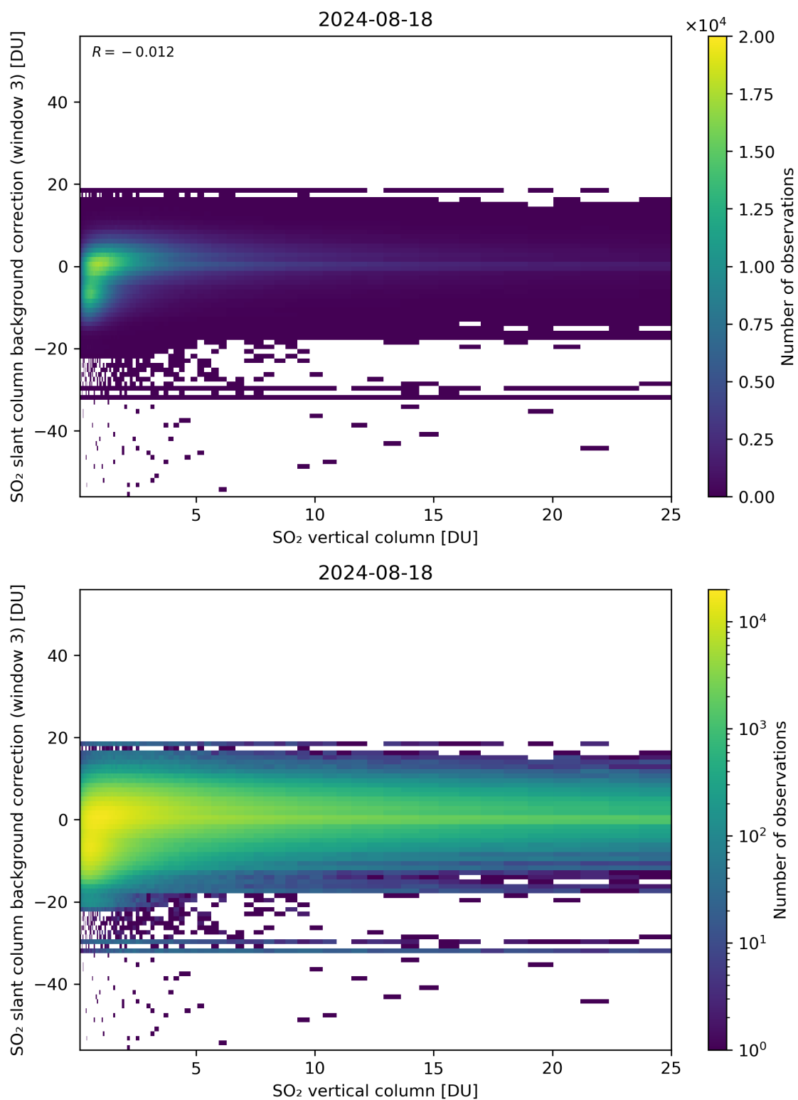
Figure 275: Scatter density plot of “SO 2 vertical column” against “SO 2 slant column background correction (window 3)” for 2024-08-17 to 2024-08-19.
