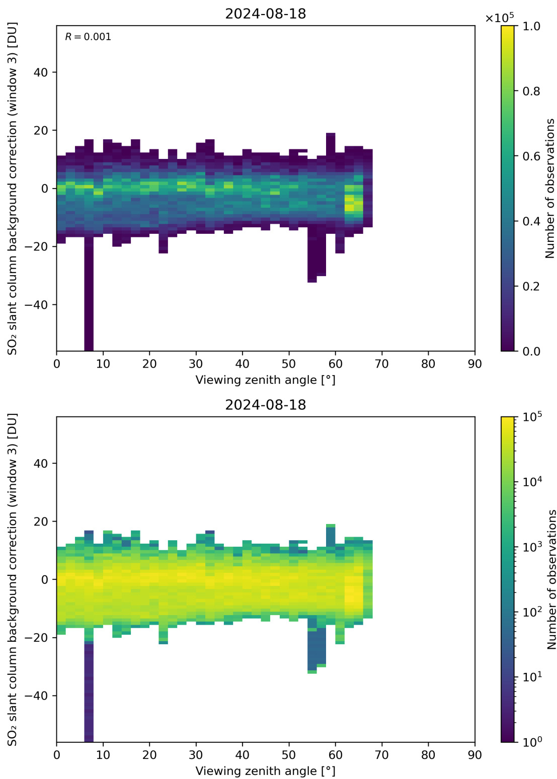
Figure 310: Scatter density plot of “Viewing zenith angle” against “SO 2 slant column background correction (window 3)” for 2024-08-17 to 2024-08-19.
