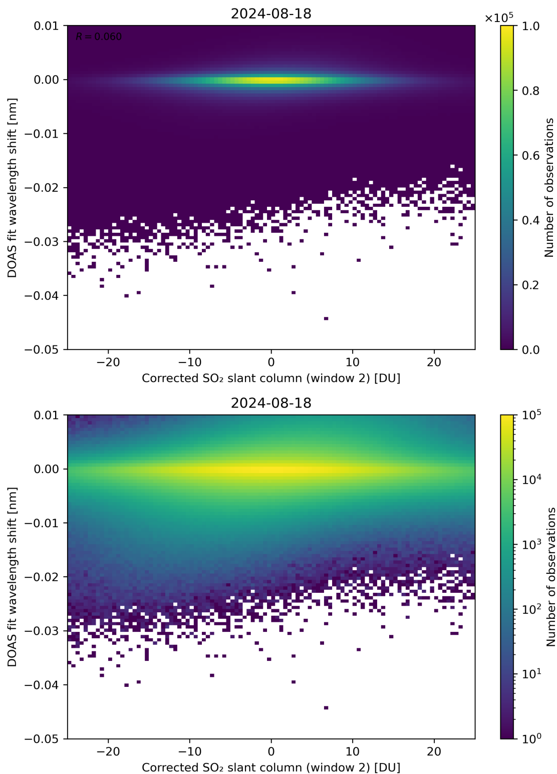
Figure 196: Scatter density plot of “Corrected SO 2 slant column (window 2)” against “DOAS fit wavelength shift” for 2024-08-17 to 2024-08-19.
