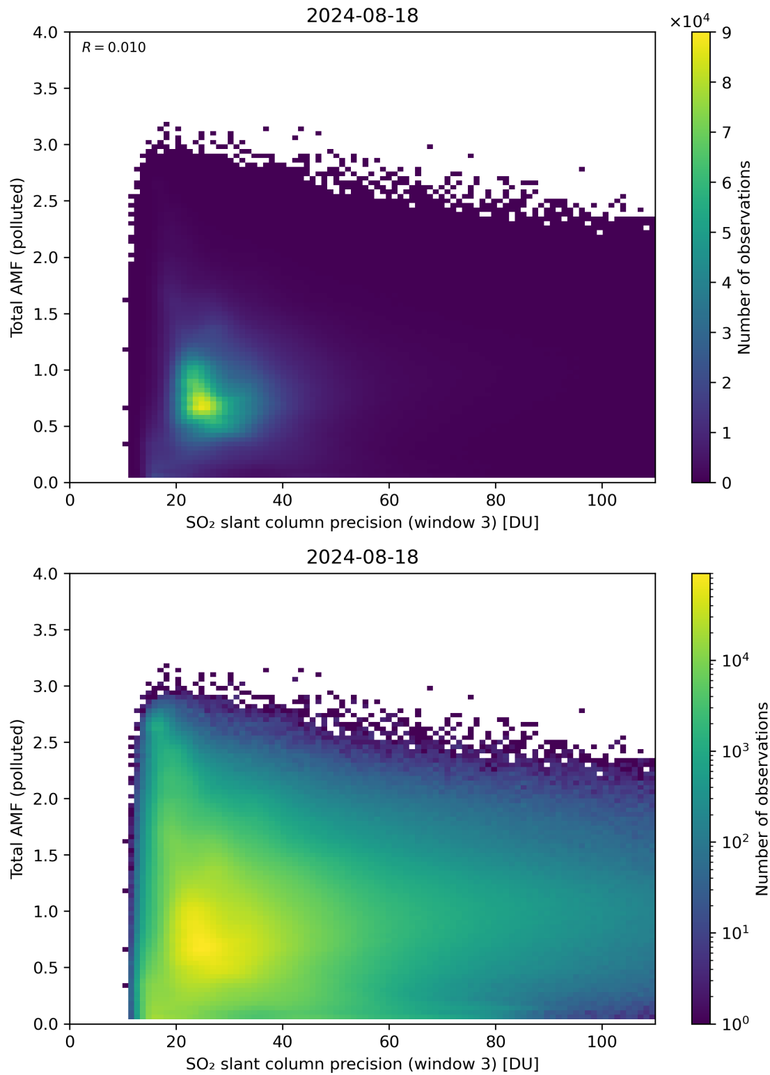
Figure 263: Scatter density plot of “SO 2 slant column precision (window 3)” against “Total AMF (polluted)” for 2024-08-17 to 2024-08-19.
