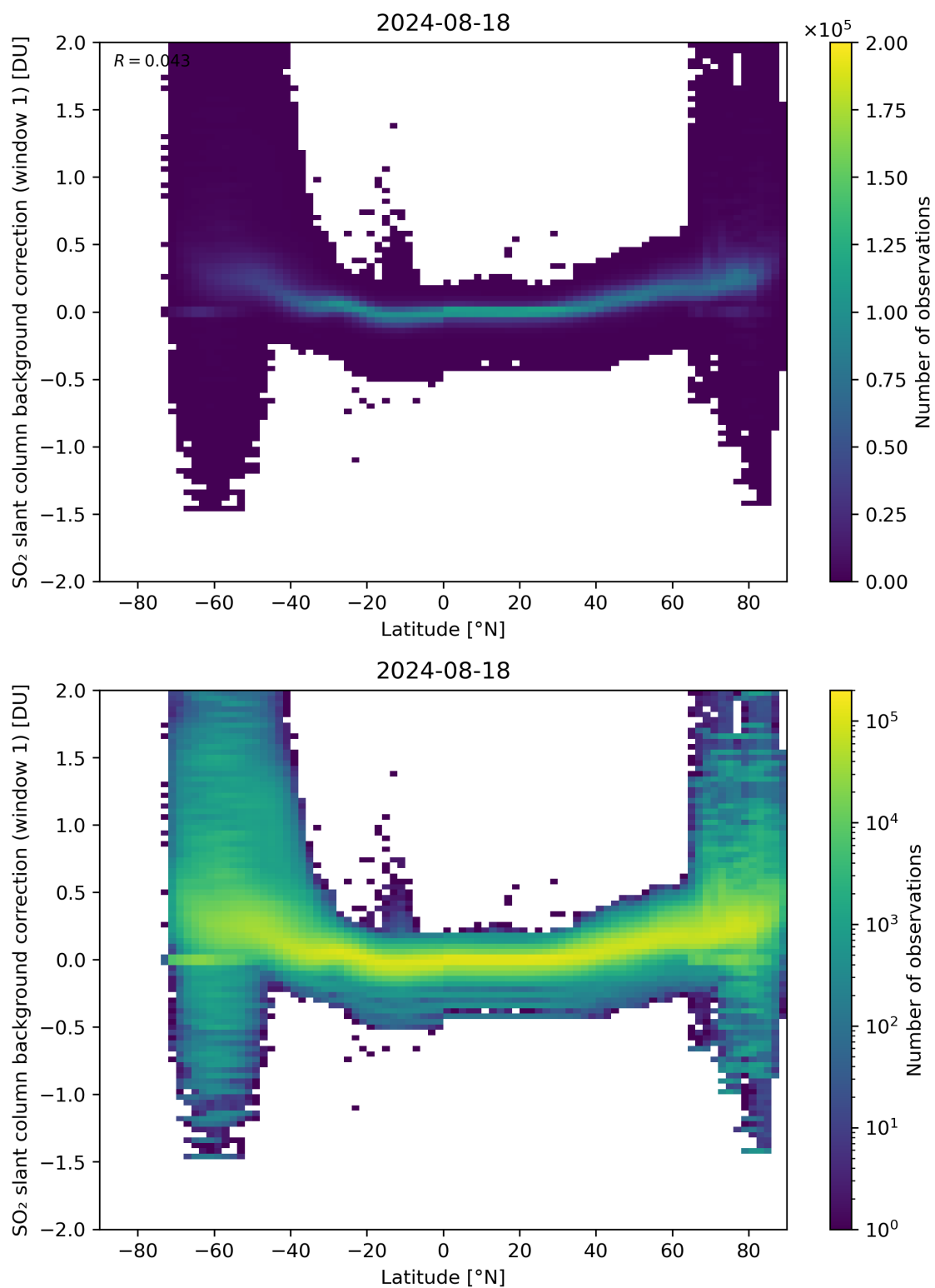
Figure 139: Scatter density plot of “Latitude” against “SO 2 slant column background correction (window 1)” for 2024-08-17 to 2024-08-19.
