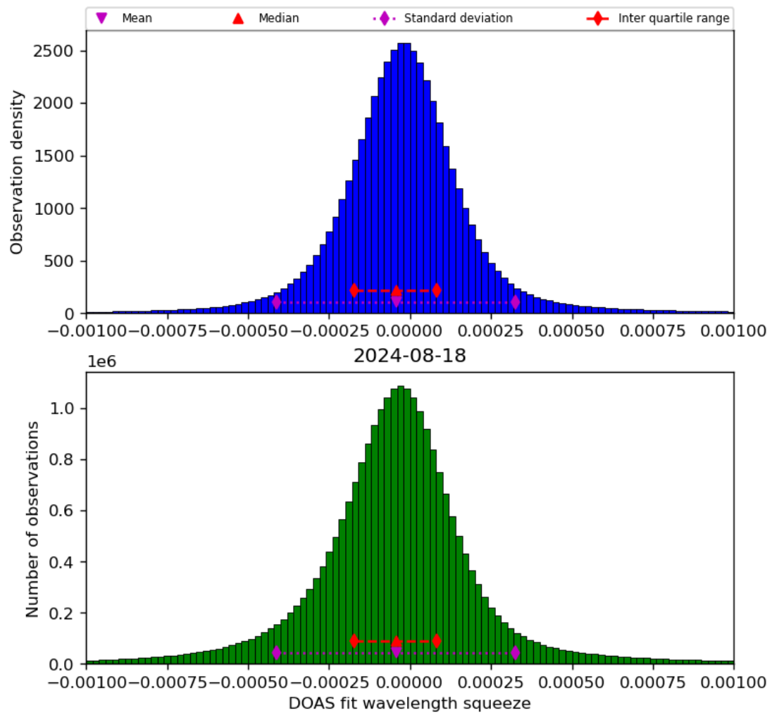
Figure 69: Histogram of “DOAS fit wavelength squeeze” for 2024-08-17 to 2024-08-19
