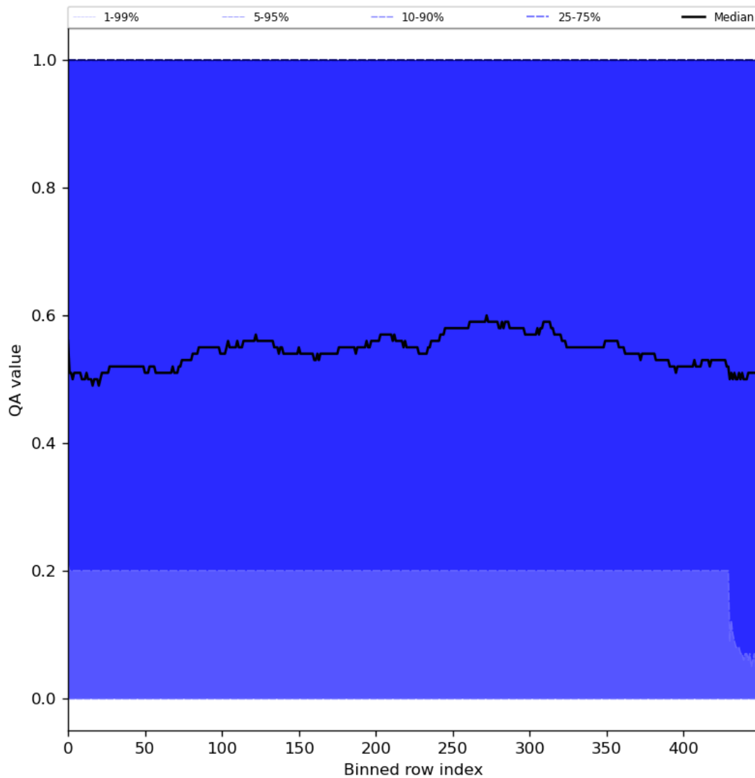
Figure 75: Along track statistics of “QA value” for 2024-08-17 to 2024-08-19
