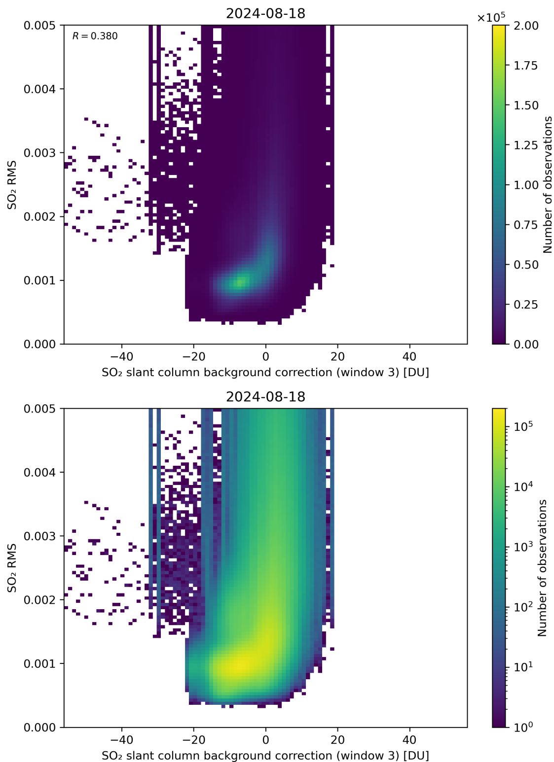
Figure 123: Scatter density plot of “SO 2 slant column background correction (window 3)” against “SO 2 RMS” for 2024-08-17 to 2024-08-19.
