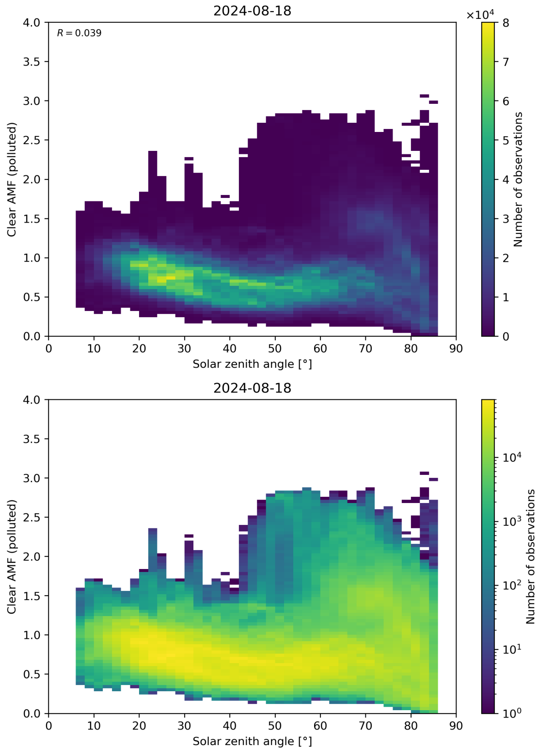
Figure 165: Scatter density plot of “Solar zenith angle” against “Clear AMF (polluted)” for 2024-08-17 to 2024-08-19.
