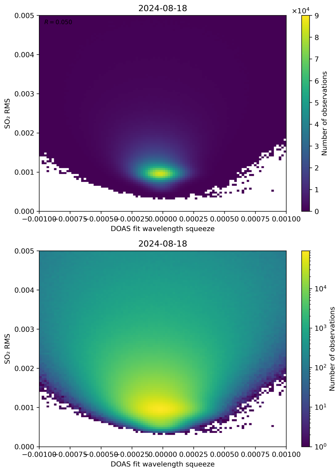
Figure 132: Scatter density plot of “DOAS fit wavelength squeeze” against “SO 2 RMS” for 2024-08-17 to 2024-08-19.
