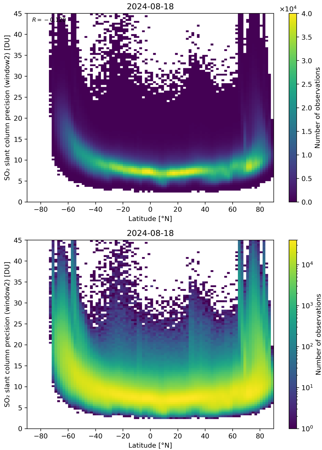
Figure 151: Scatter density plot of “Latitude” against “SO 2 slant column precision (window2)” for 2024-08-17 to 2024-08-19.
