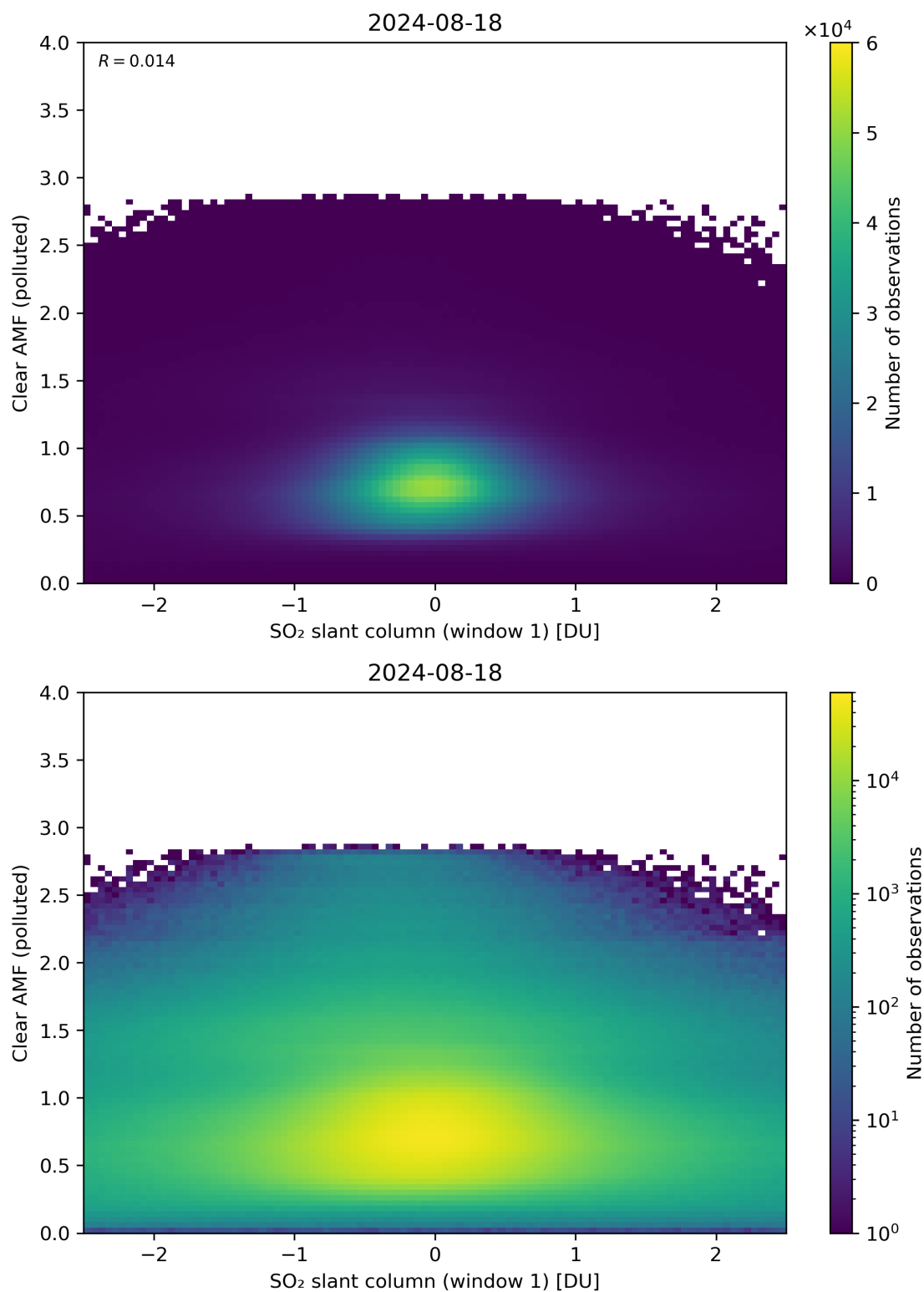
Figure 232: Scatter density plot of “SO 2 slant column (window 1)” against “Clear AMF (polluted)” for 2024-08-17 to 2024-08-19.
