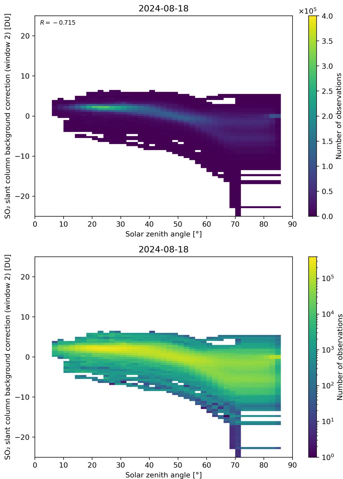
Figure 159: Scatter density plot of “Solar zenith angle” against “SO 2 slant column background correction (window 2)” for 2024-08-17 to 2024-08-19.
