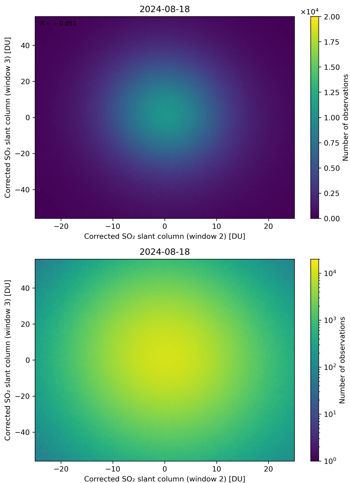
Figure 200: Scatter density plot of “Corrected SO 2 slant column (window 2)” against “Corrected SO 2 slant column (window 3)” for 2024-08-17 to 2024-08-19.
