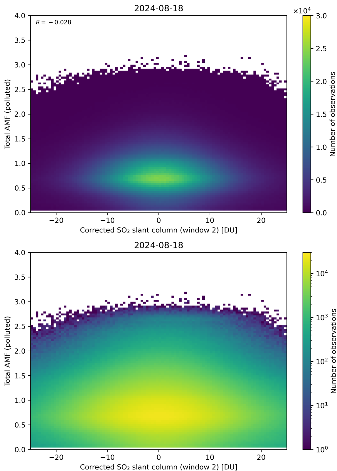
Figure 203: Scatter density plot of “Corrected SO 2 slant column (window 2)” against “Total AMF (polluted)” for 2024-08-17 to 2024-08-19.
