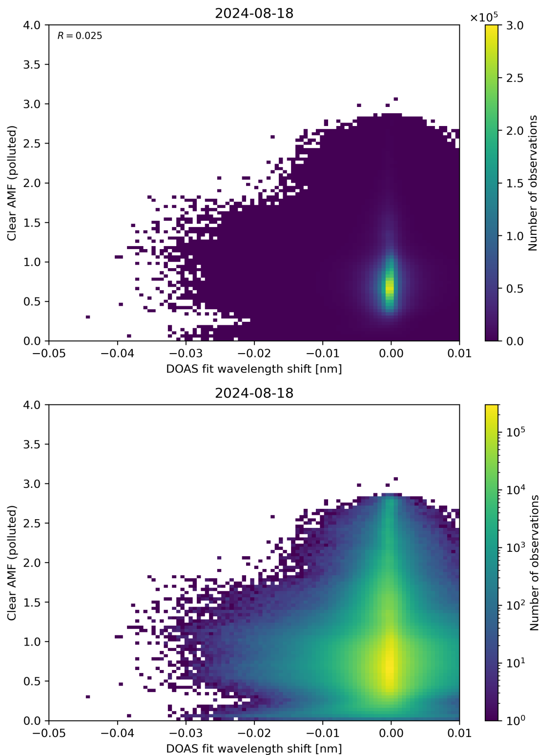
Figure 129: Scatter density plot of “DOAS fit wavelength shift” against “Clear AMF (polluted)” for 2024-08-17 to 2024-08-19.
