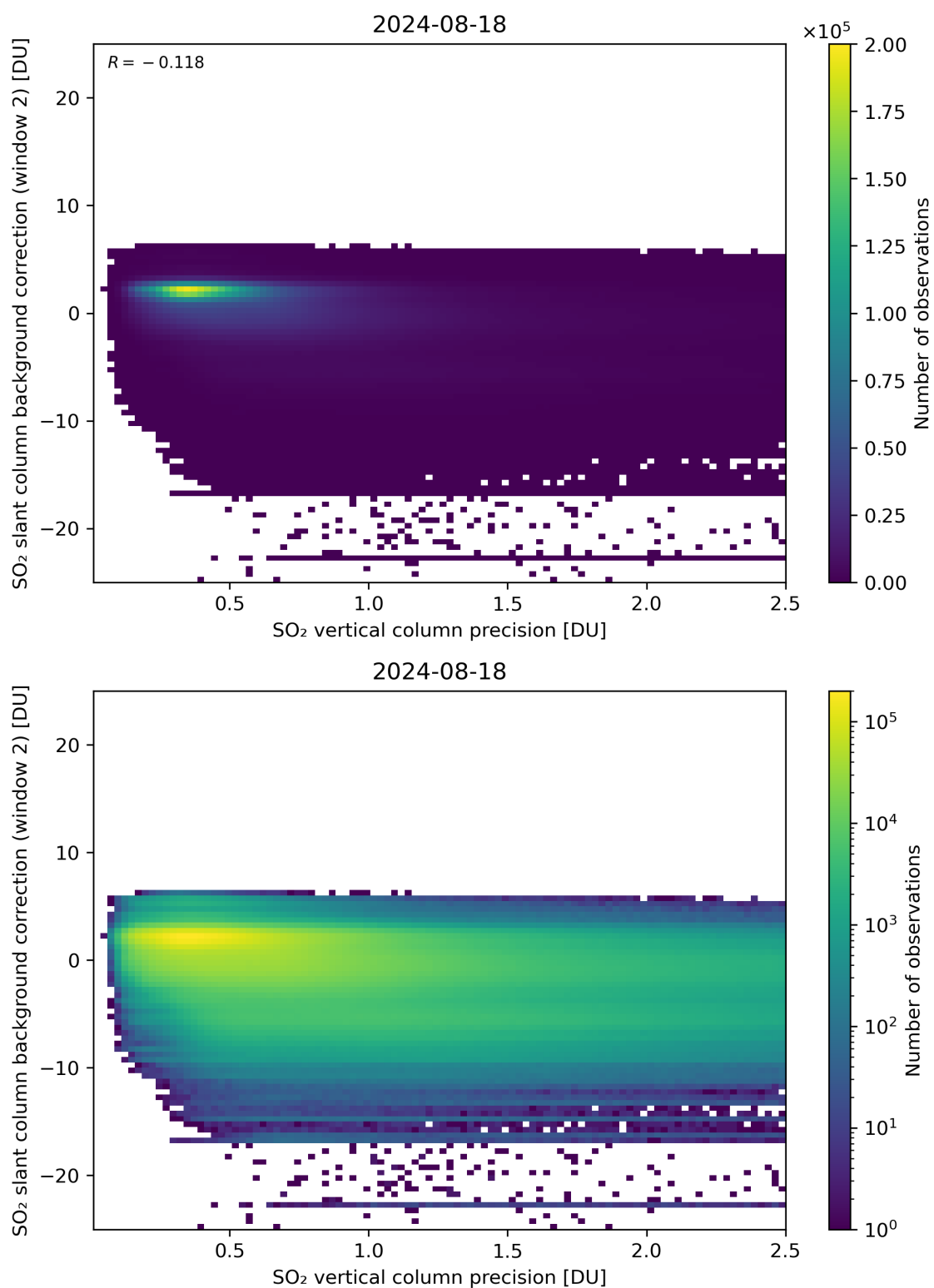
Figure 280: Scatter density plot of “SO 2 vertical column precision” against “SO 2 slant column background correction (window 2)” for 2024-08-17 to 2024-08-19.
