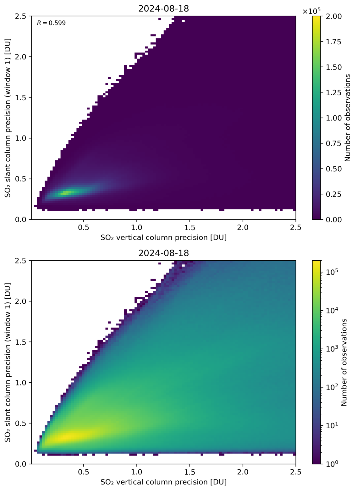
Figure 290: Scatter density plot of “SO 2 vertical column precision” against “SO 2 slant column precision (window 1)” for 2024-08-17 to 2024-08-19.
