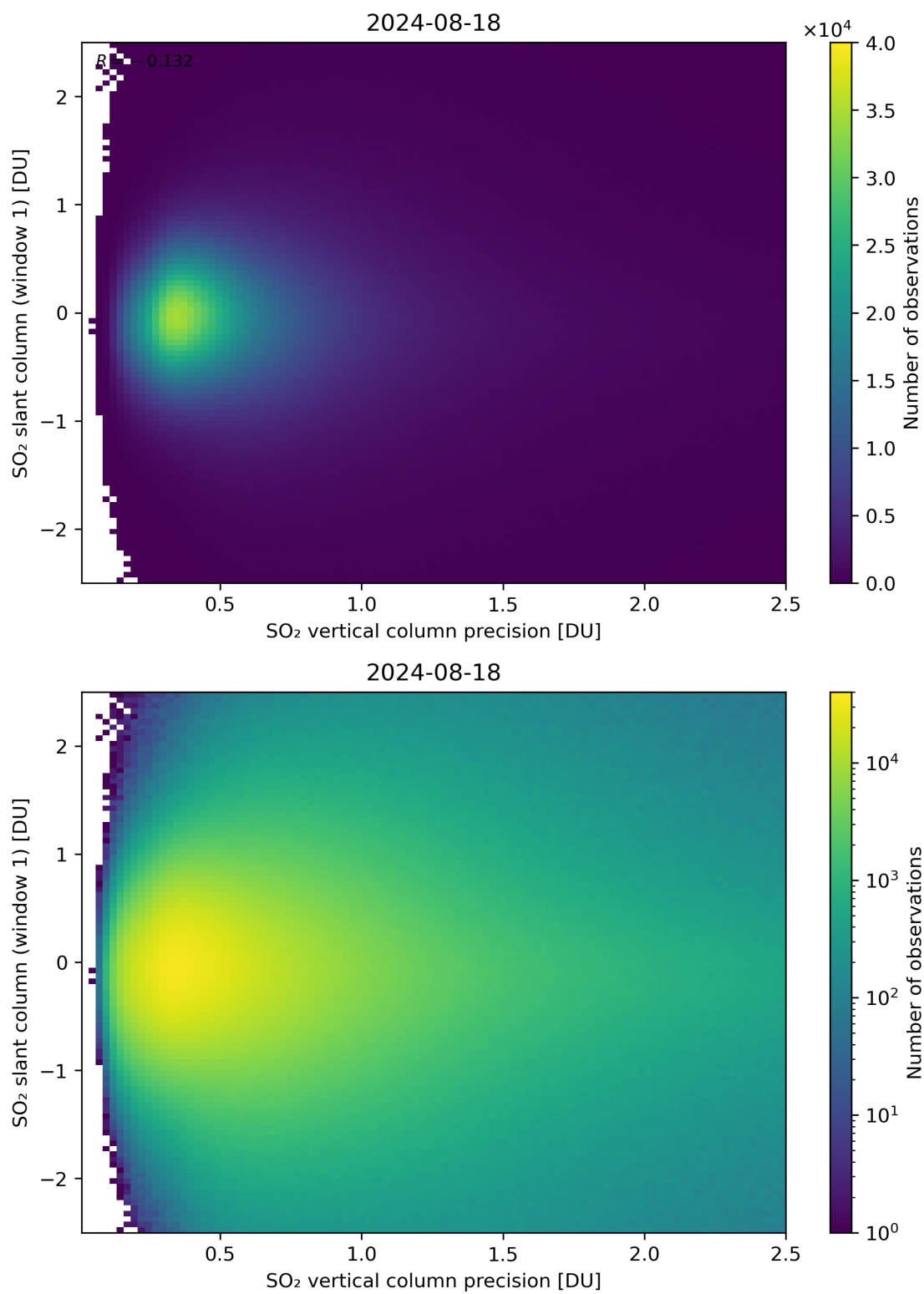
Figure 289: Scatter density plot of “SO 2 vertical column precision” against “SO 2 slant column (window 1)” for 2024-08-17 to 2024-08-19.
