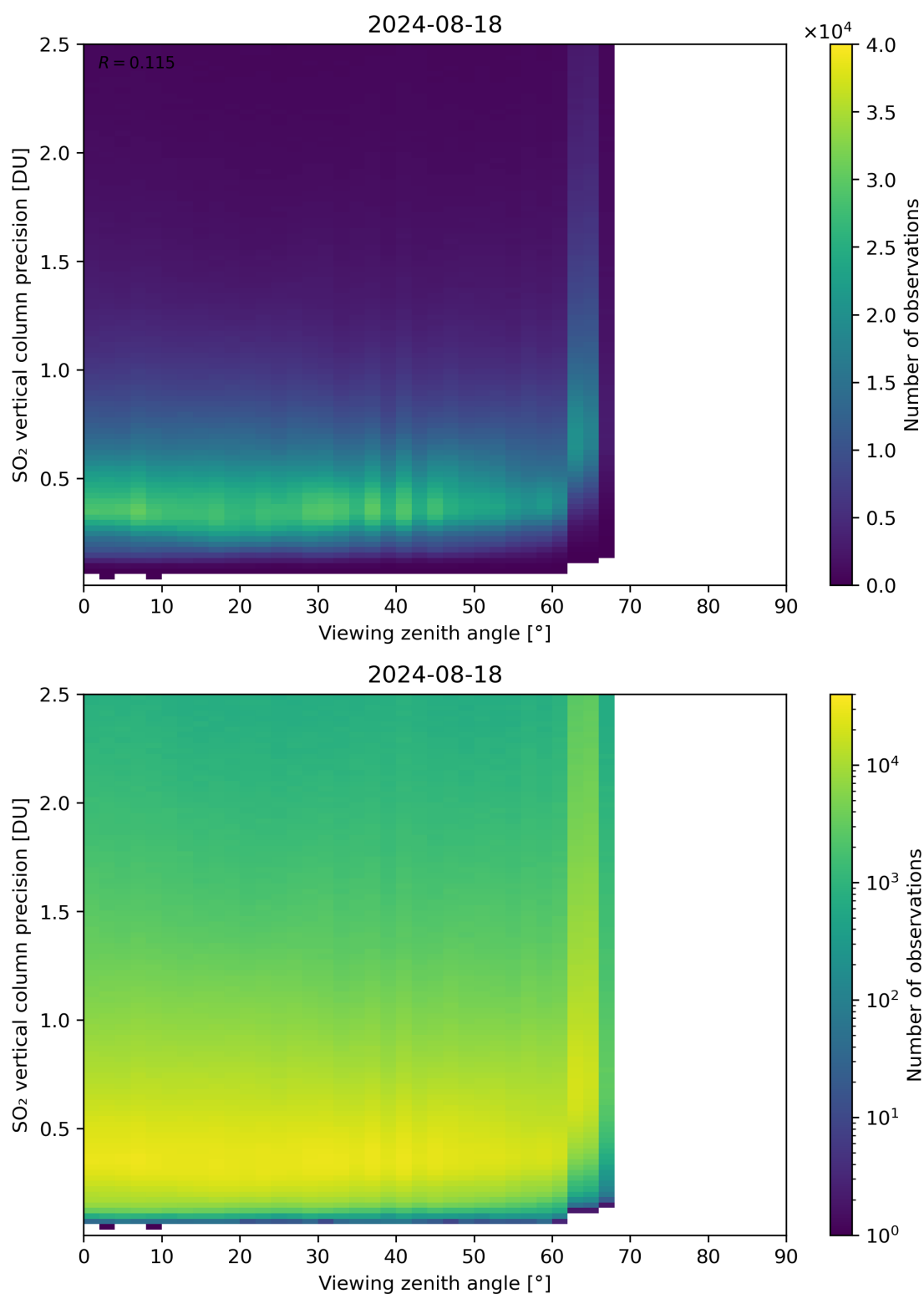
Figure 328: Scatter density plot of “Viewing zenith angle” against “SO 2 vertical column precision” for 2024-08-17 to 2024-08-19.
