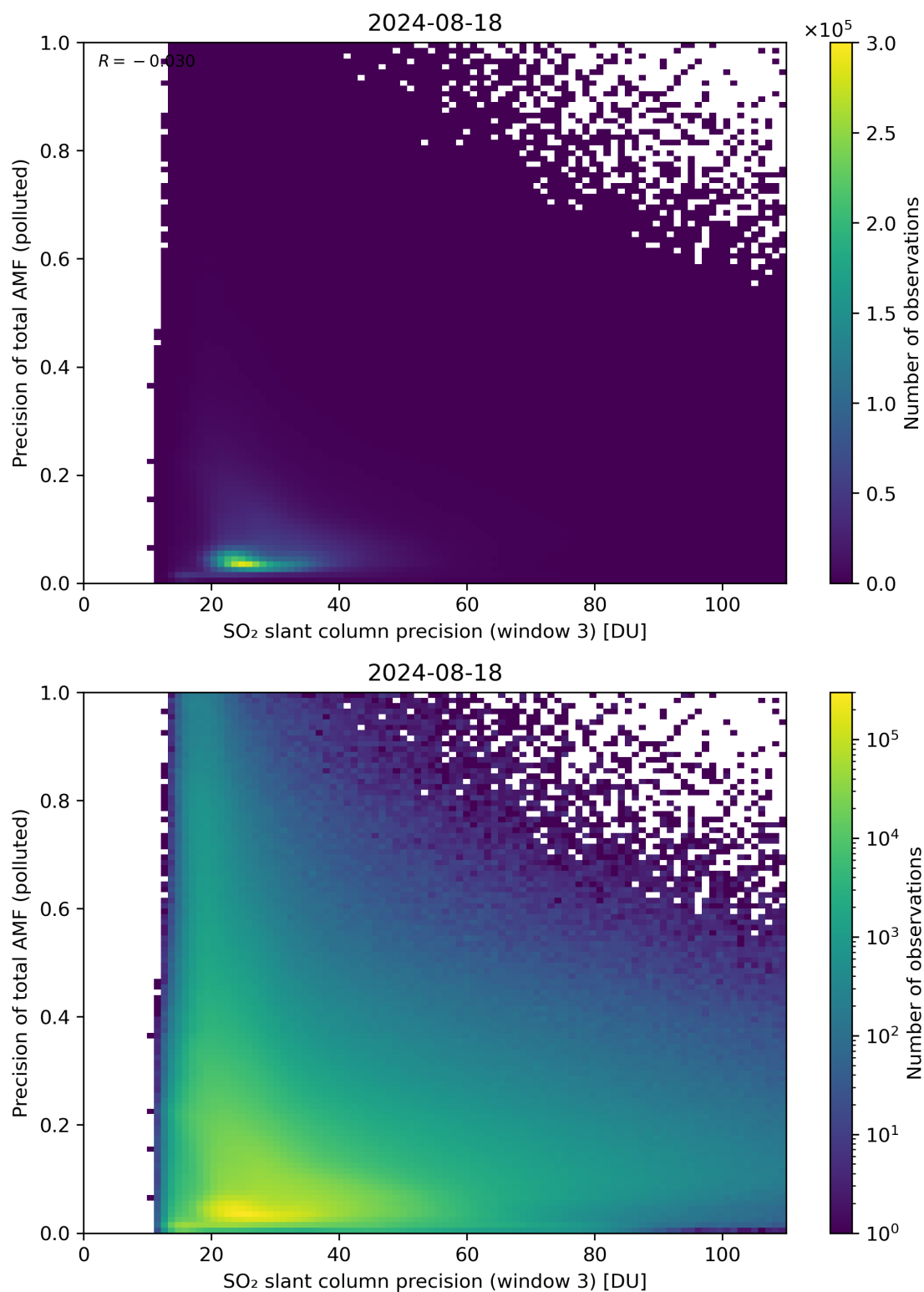
Figure 264: Scatter density plot of “SO 2 slant column precision (window 3)” against “Precision of total AMF (polluted)” for 2024-08-17 to 2024-08-19.
