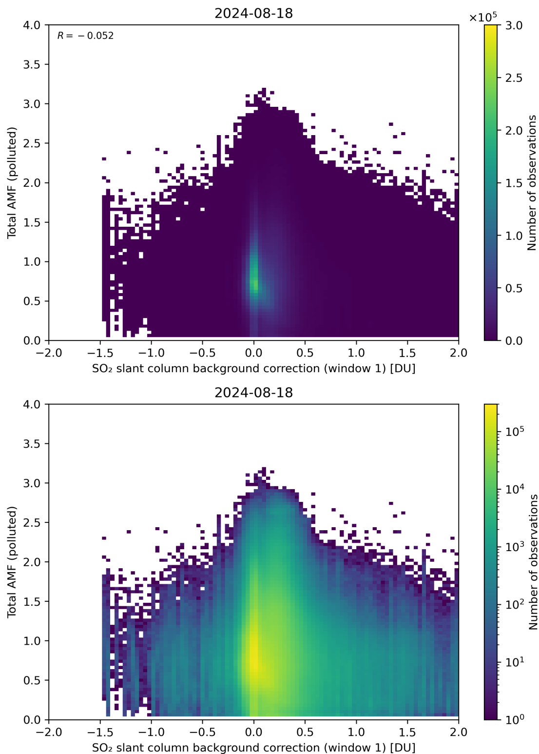
Figure 109: Scatter density plot of “SO 2 slant column background correction (window 1)” against “Total AMF (polluted)” for 2024-08-17 to 2024-08-19.
