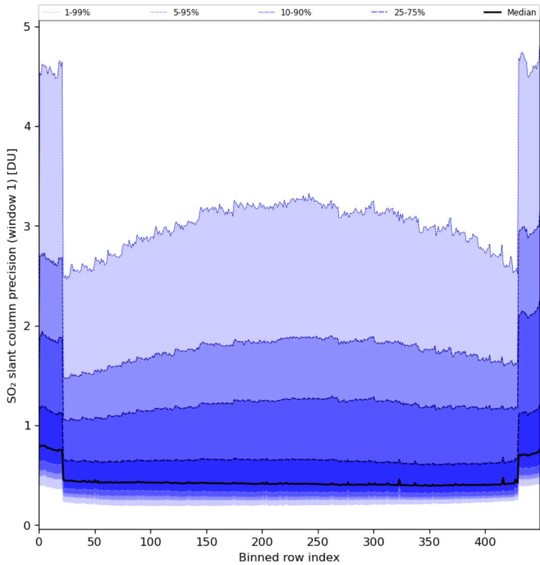
Figure 80: Along track statistics of “SO 2 slant column precision (window 1)” for 2024-08-17 to 2024-08-19
