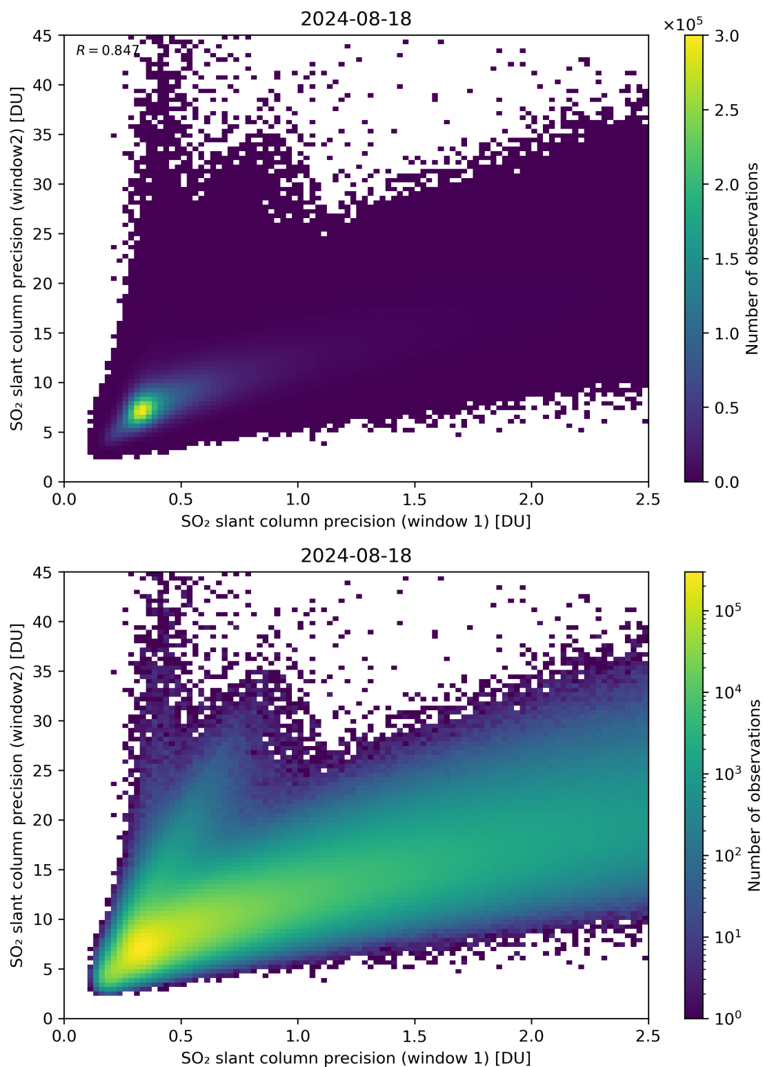
Figure 227: Scatter density plot of “SO 2 slant column precision (window 1)” against “SO 2 slant column precision (window2)” for 2024-08-17 to 2024-08-19.
