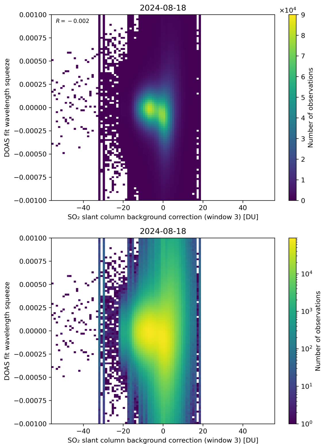
Figure 122: Scatter density plot of “SO 2 slant column background correction (window 3)” against “DOAS fit wavelength squeeze” for 2024-08-17 to 2024-08-19.
