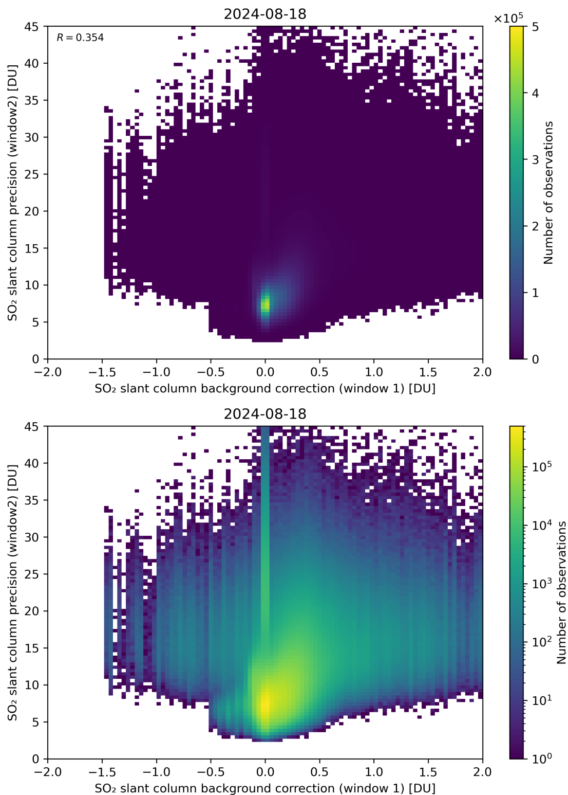
Figure 106: Scatter density plot of “SO 2 slant column background correction (window 1)” against “SO 2 slant column precision (window2)” for 2024-08-17 to 2024-08-19.
