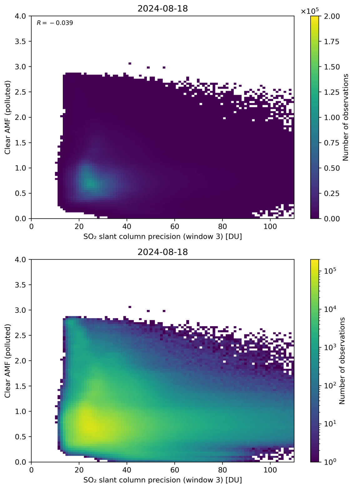
Figure 261: Scatter density plot of “SO 2 slant column precision (window 3)” against “Clear AMF (polluted)” for 2024-08-17 to 2024-08-19.
