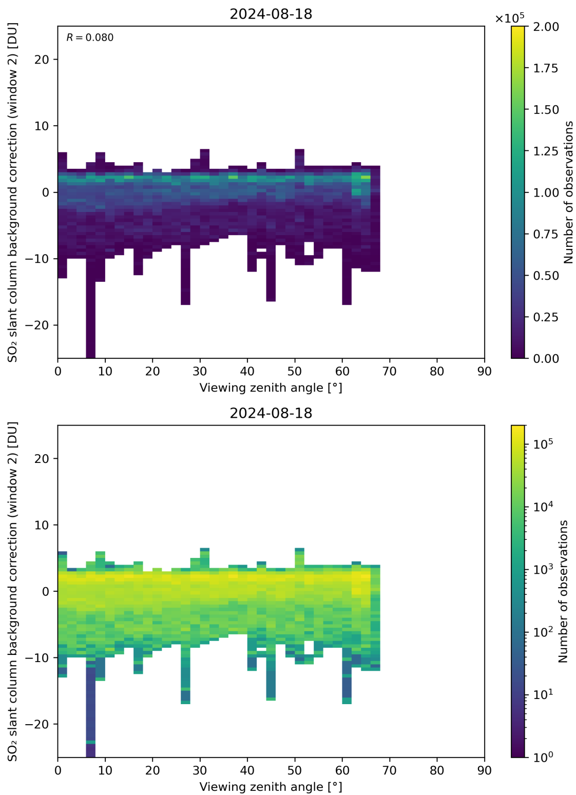
Figure 309: Scatter density plot of “Viewing zenith angle” against “SO 2 slant column background correction (window 2)” for 2024-08-17 to 2024-08-19.
