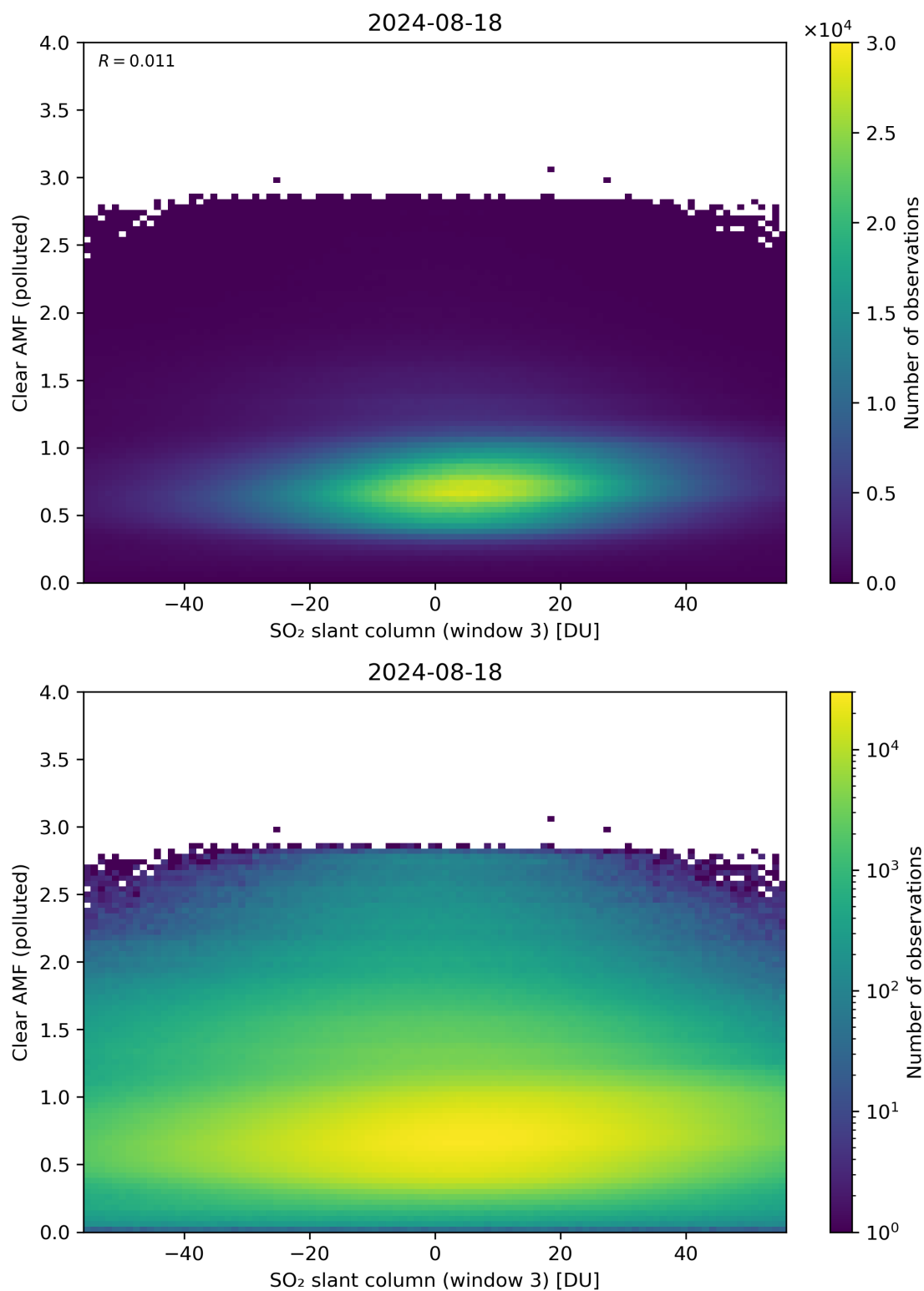
Figure 265: Scatter density plot of “SO 2 slant column (window 3)” against “Clear AMF (polluted)” for 2024-08-17 to 2024-08-19.
