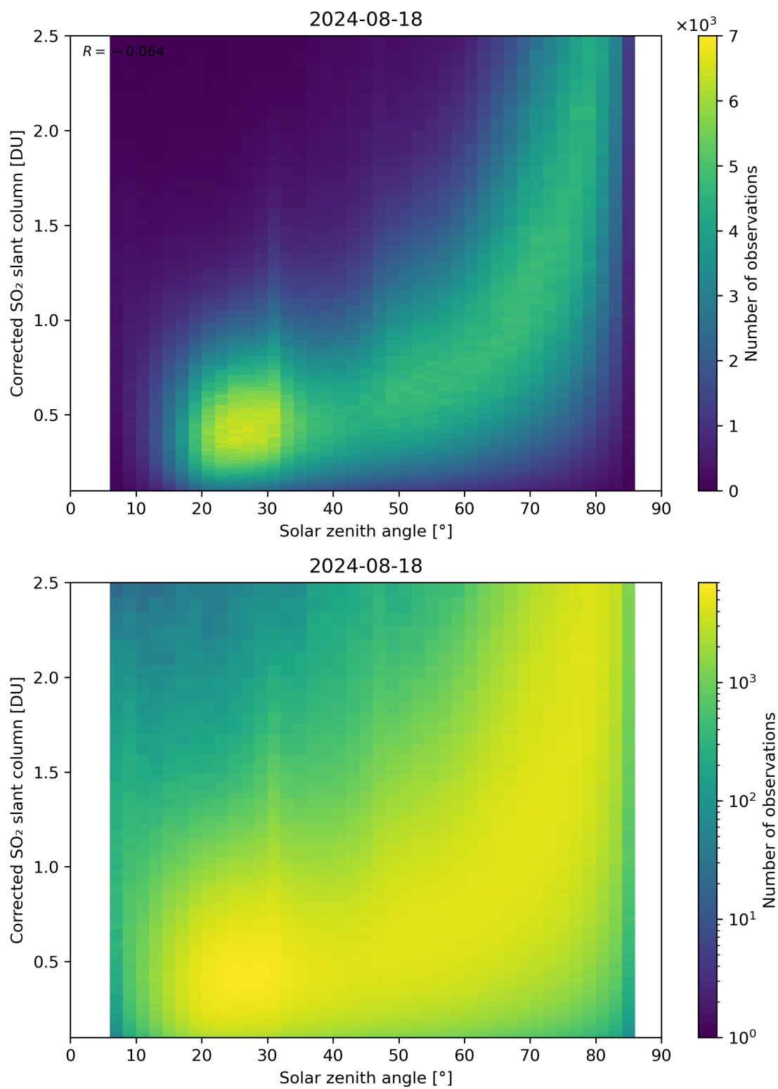
Figure 166: Scatter density plot of “Solar zenith angle” against “Corrected SO 2 slant column” for 2024-08-17 to 2024-08-19.
