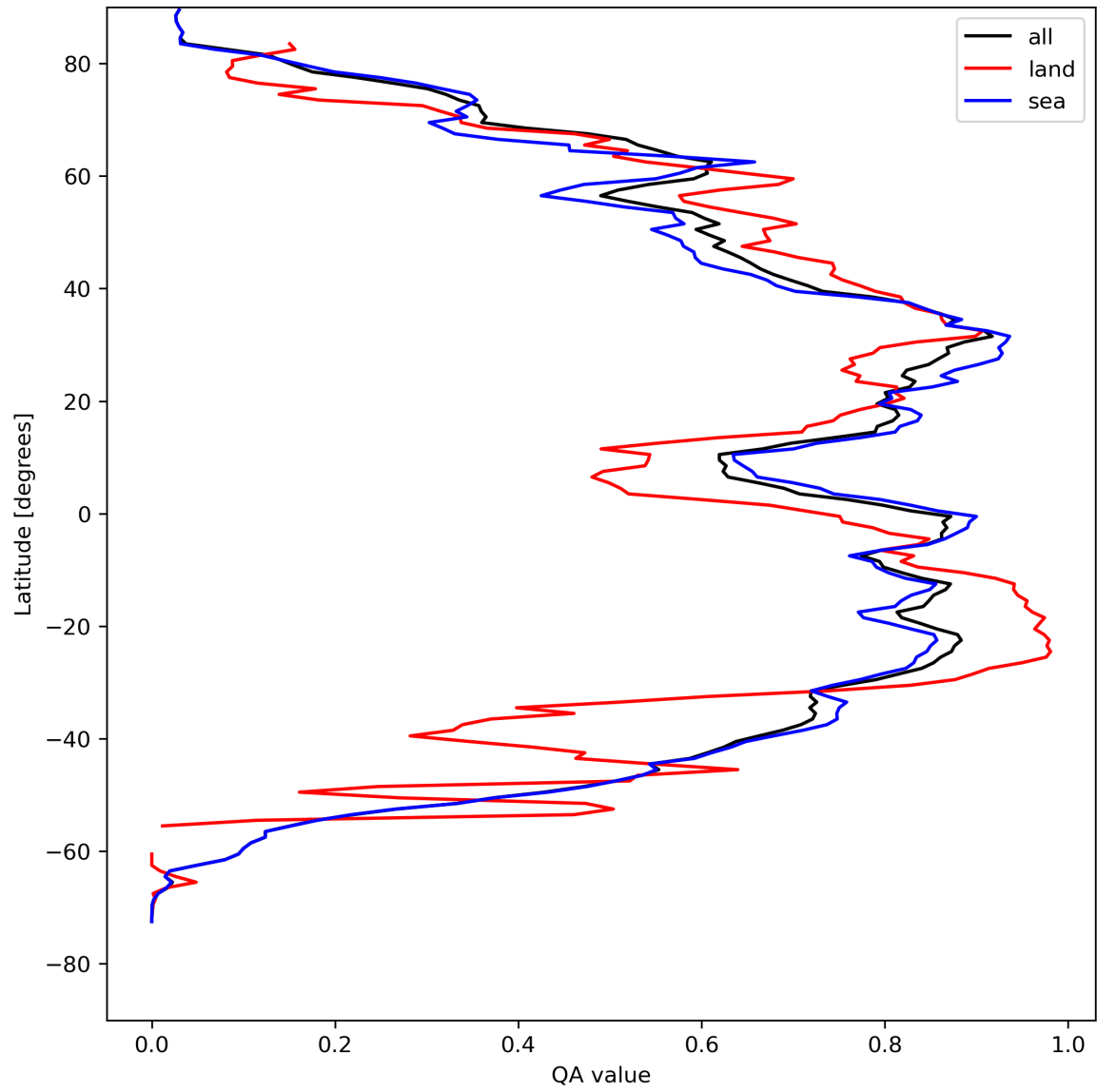
Figure 29: Zonal average of “QA value” for 2024-08-17 to 2024-08-19.
