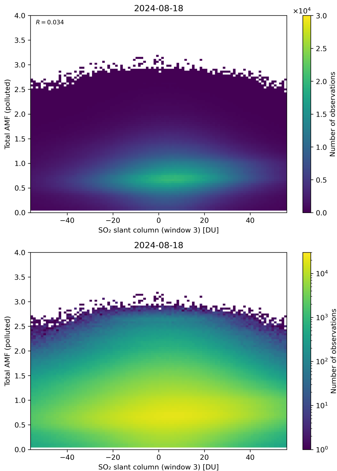
Figure 268: Scatter density plot of “SO 2 slant column (window 3)” against “Total AMF (polluted)” for 2024-08-17 to 2024-08-19.
