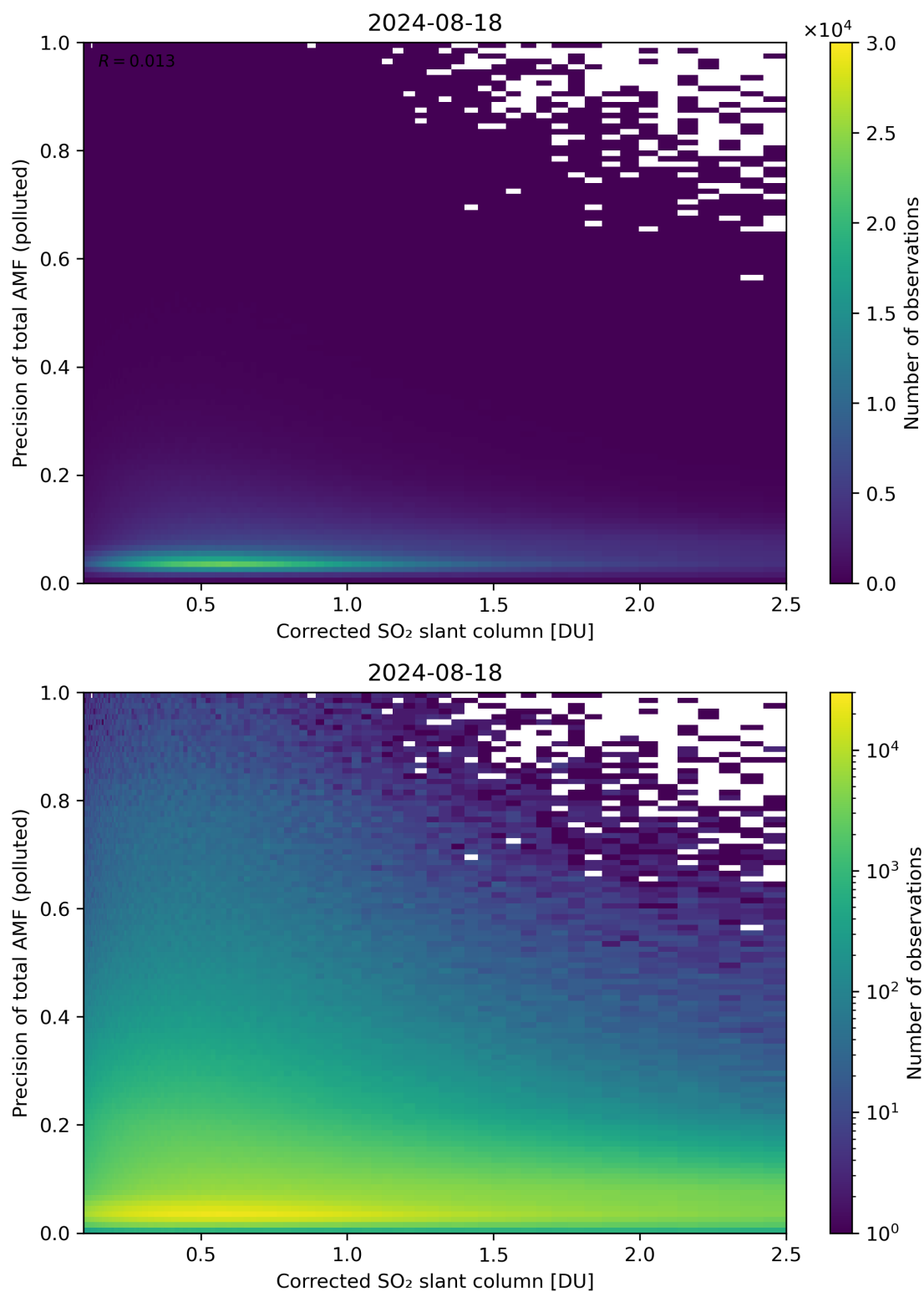
Figure 193: Scatter density plot of “Corrected SO 2 slant column” against “Precision of total AMF (polluted)” for 2024-08-17 to 2024-08-19.
