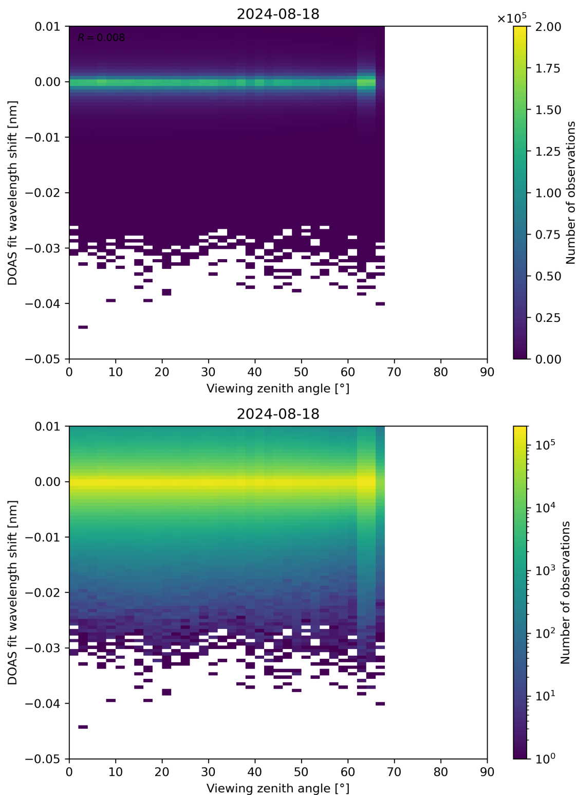
Figure 311: Scatter density plot of “Viewing zenith angle” against “DOAS fit wavelength shift” for 2024-08-17 to 2024-08-19.
