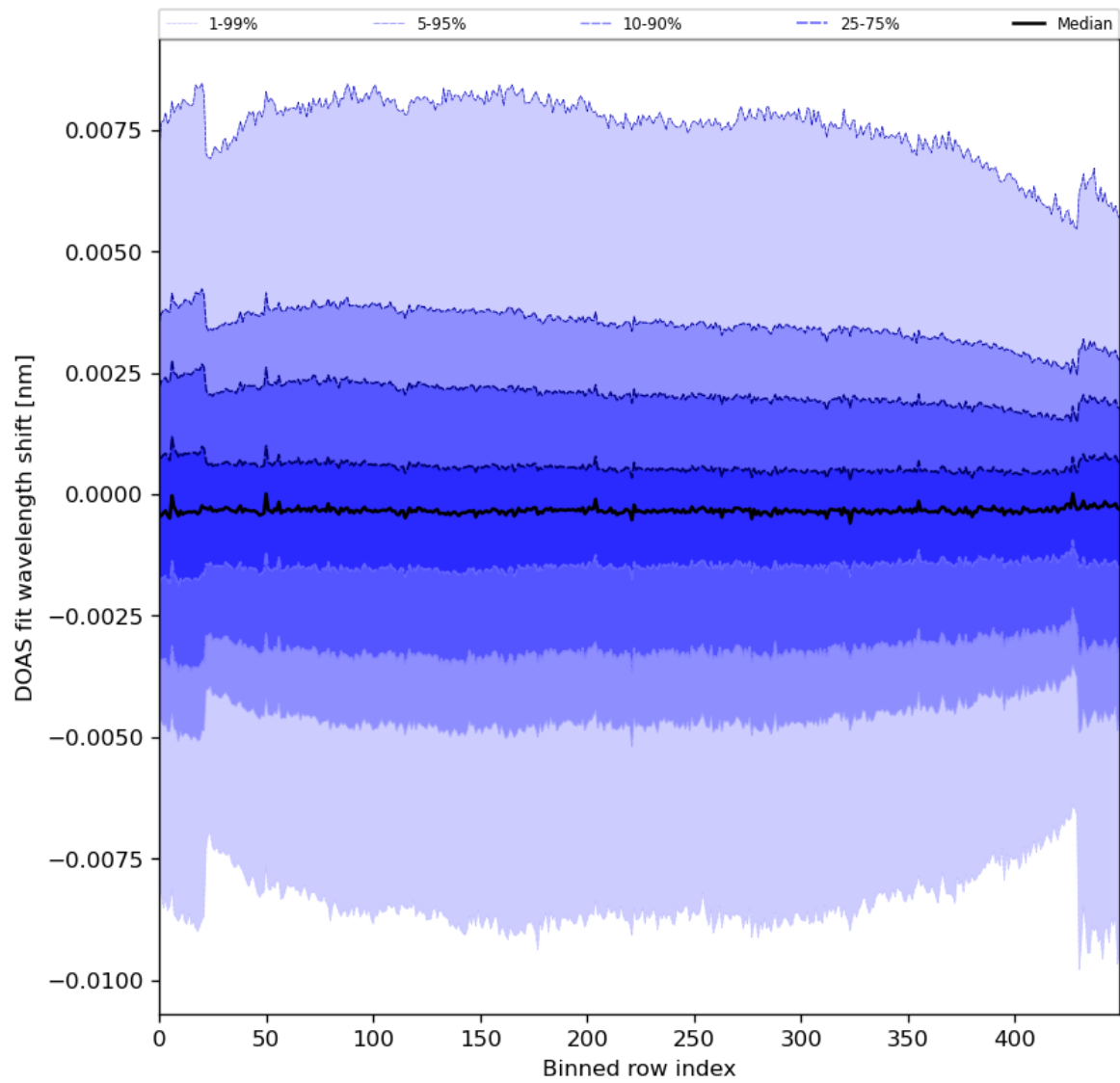
Figure 91: Along track statistics of “DOAS fit wavelength shift” for 2024-08-17 to 2024-08-19
