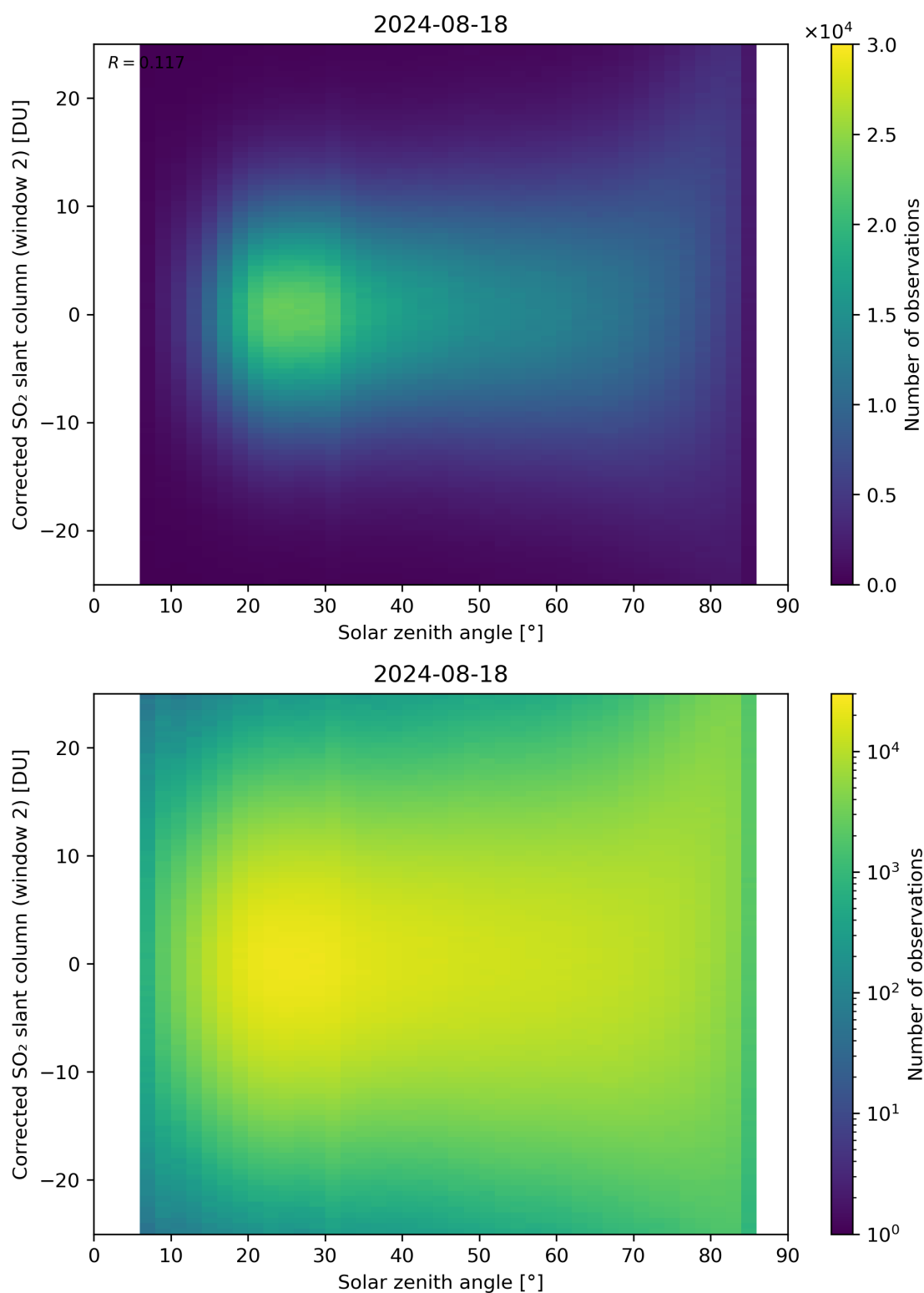
Figure 167: Scatter density plot of “Solar zenith angle” against “Corrected SO 2 slant column (window 2)” for 2024-08-17 to 2024-08-19.
