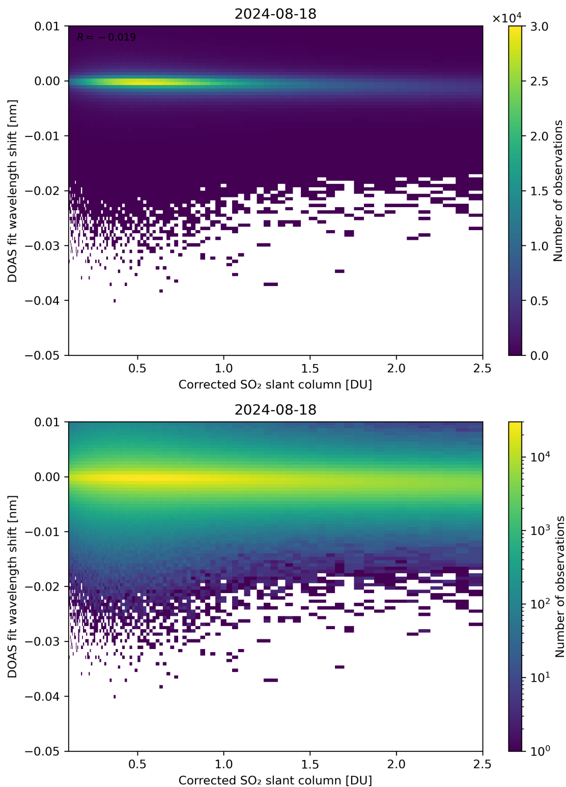
Figure 181: Scatter density plot of “Corrected SO 2 slant column” against “DOAS fit wavelength shift” for 2024-08-17 to 2024-08-19.
