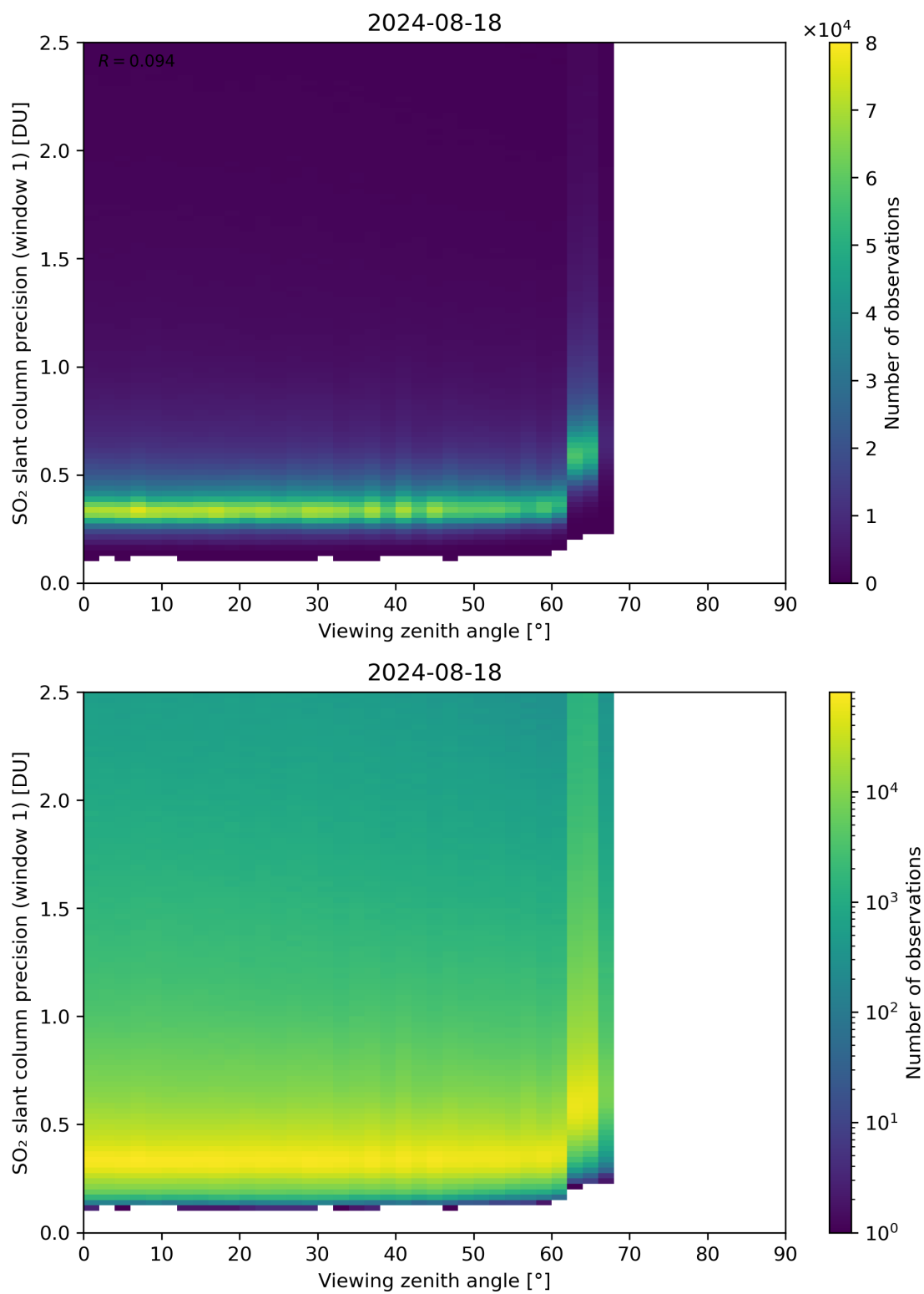
Figure 321: Scatter density plot of “Viewing zenith angle” against “SO 2 slant column precision (window 1)” for 2024-08-17 to 2024-08-19.
