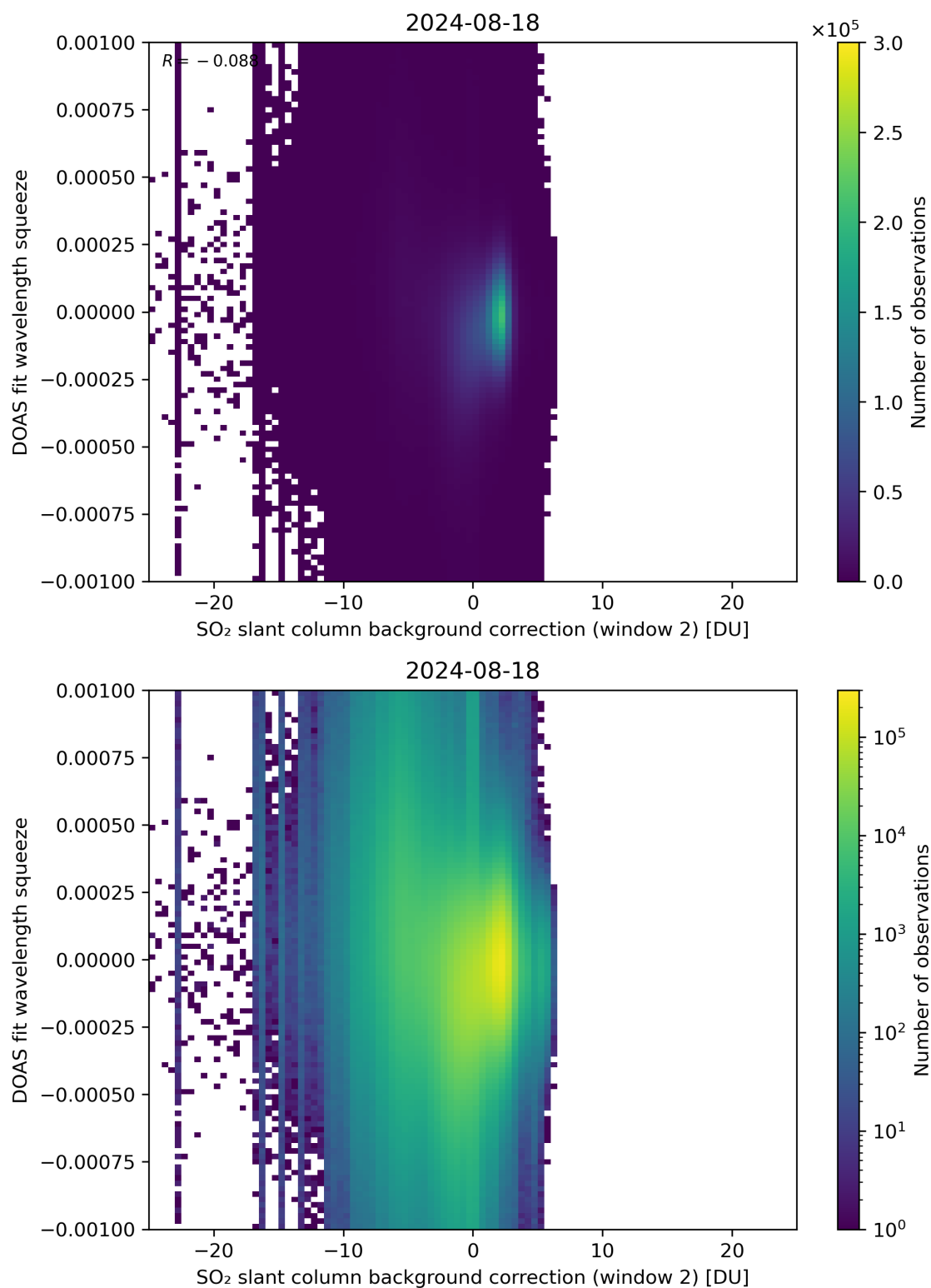
Figure 113: Scatter density plot of “SO 2 slant column background correction (window 2)” against “DOAS fit wavelength squeeze” for 2024-08-17 to 2024-08-19.
