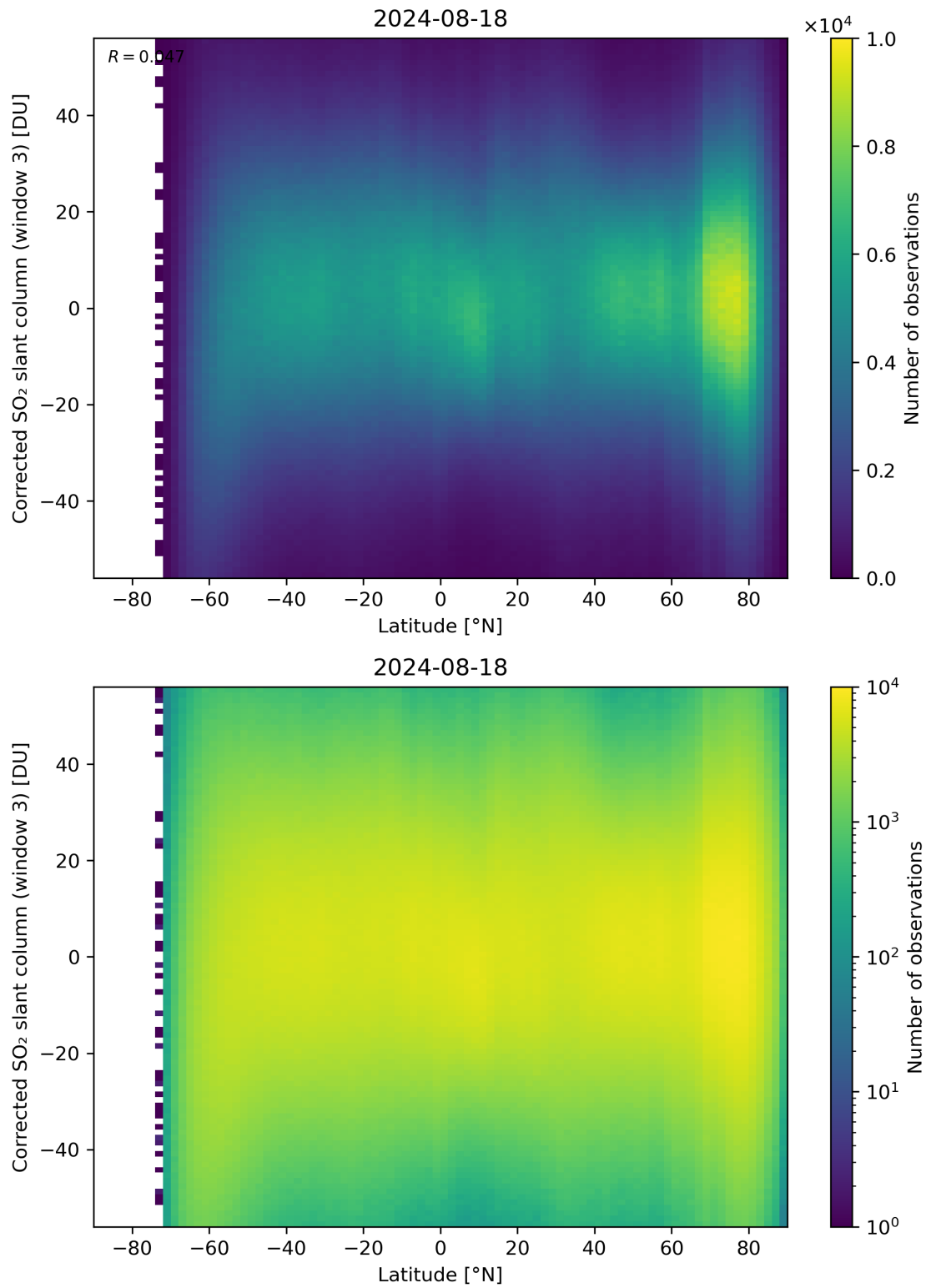
Figure 148: Scatter density plot of “Latitude” against “Corrected SO 2 slant column (window 3)” for 2024-08-17 to 2024-08-19.
