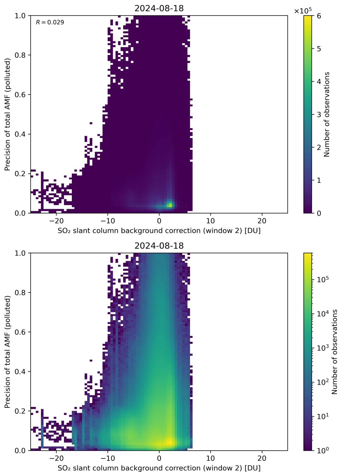
Figure 120: Scatter density plot of “SO 2 slant column background correction (window 2)” against “Precision of total AMF (polluted)” for 2024-08-17 to 2024-08-19.
