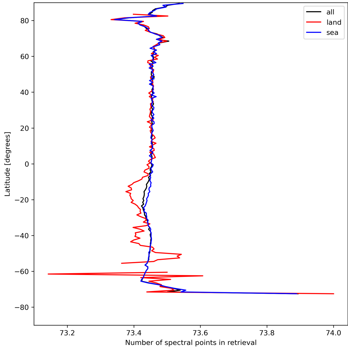
Figure 51: Zonal average of “Number of spectral points in retrieval” for 2024-08-17 to 2024-08-19.
