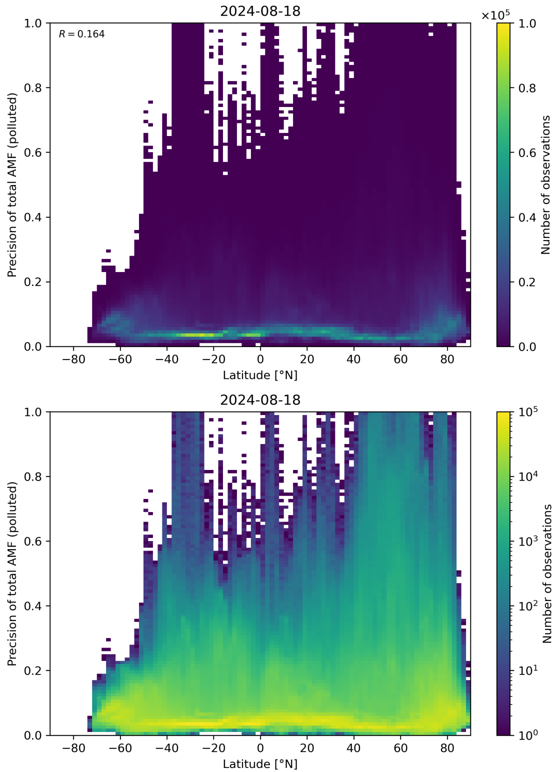
Figure 155: Scatter density plot of “Latitude” against “Precision of total AMF (polluted)” for 2024-08-17 to 2024-08-19.
