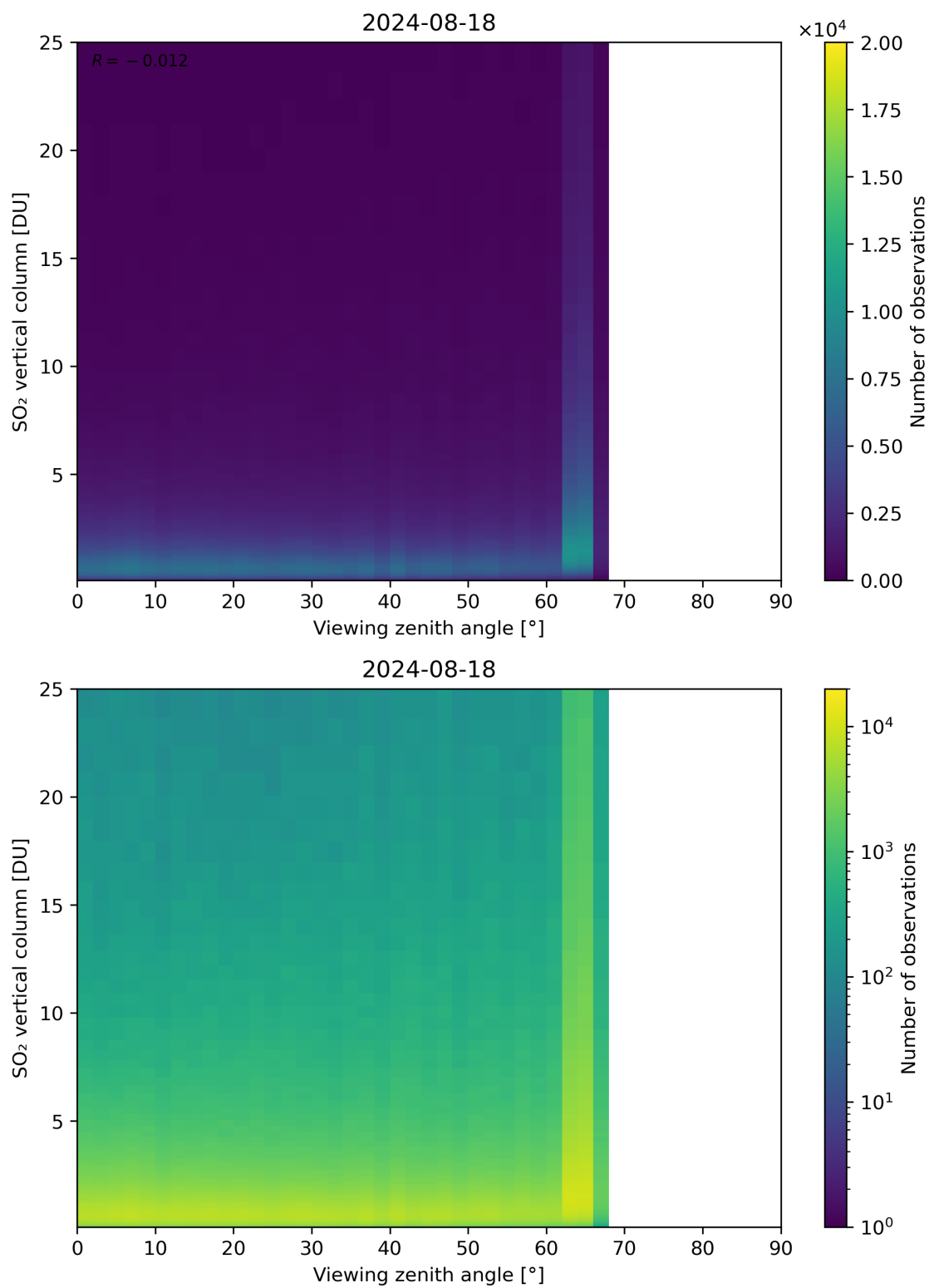
Figure 327: Scatter density plot of “Viewing zenith angle” against “SO 2 vertical column” for 2024-08-17 to 2024-08-19.
