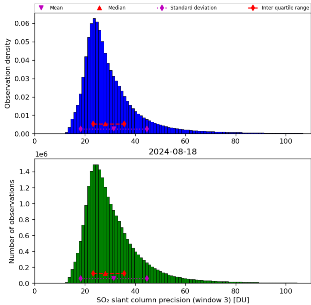
Figure 65: Histogram of “SO 2 slant column precision (window 3)” for 2024-08-17 to 2024-08-19
