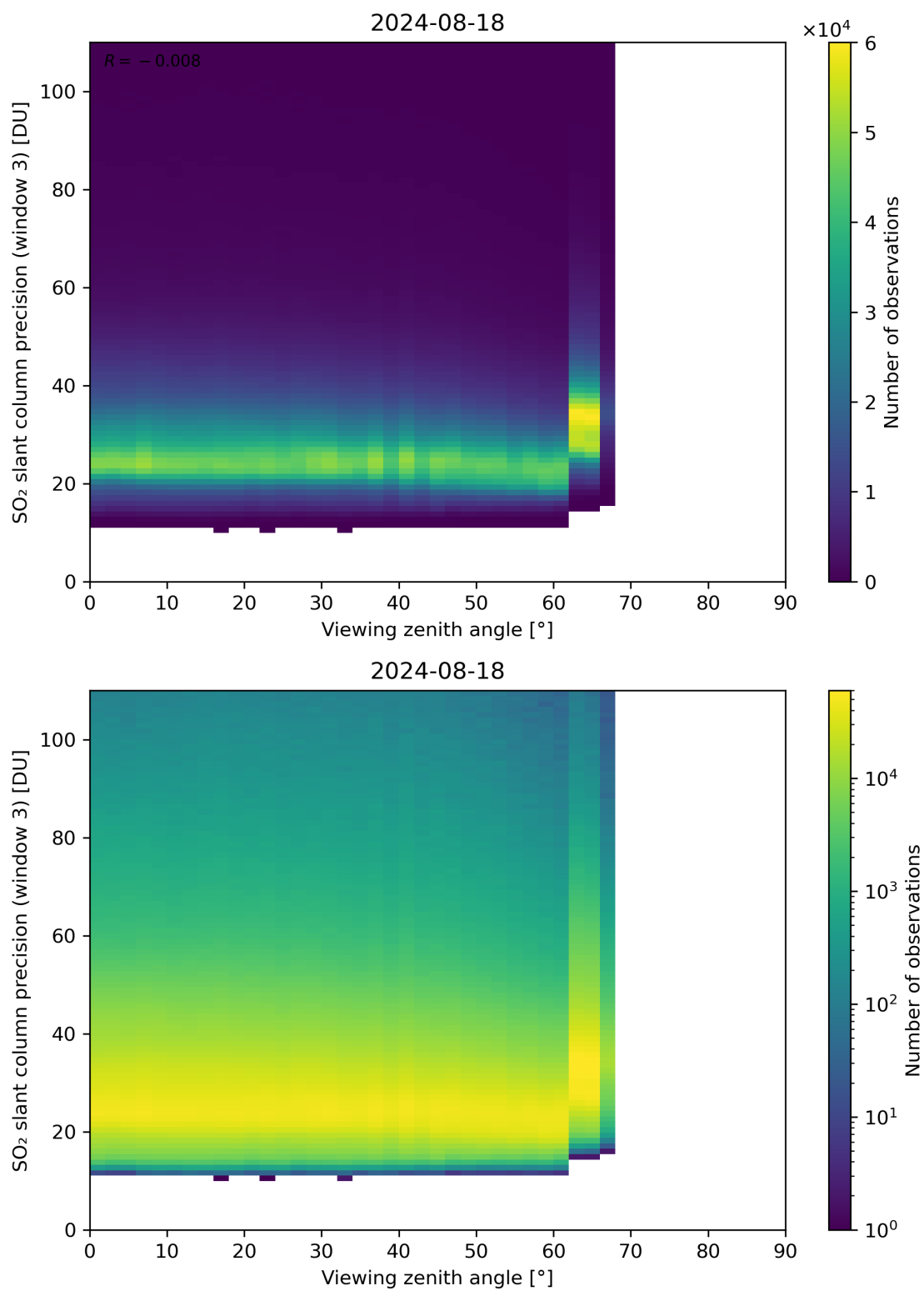
Figure 324: Scatter density plot of “Viewing zenith angle” against “SO 2 slant column precision (window 3)” for 2024-08-17 to 2024-08-19.
