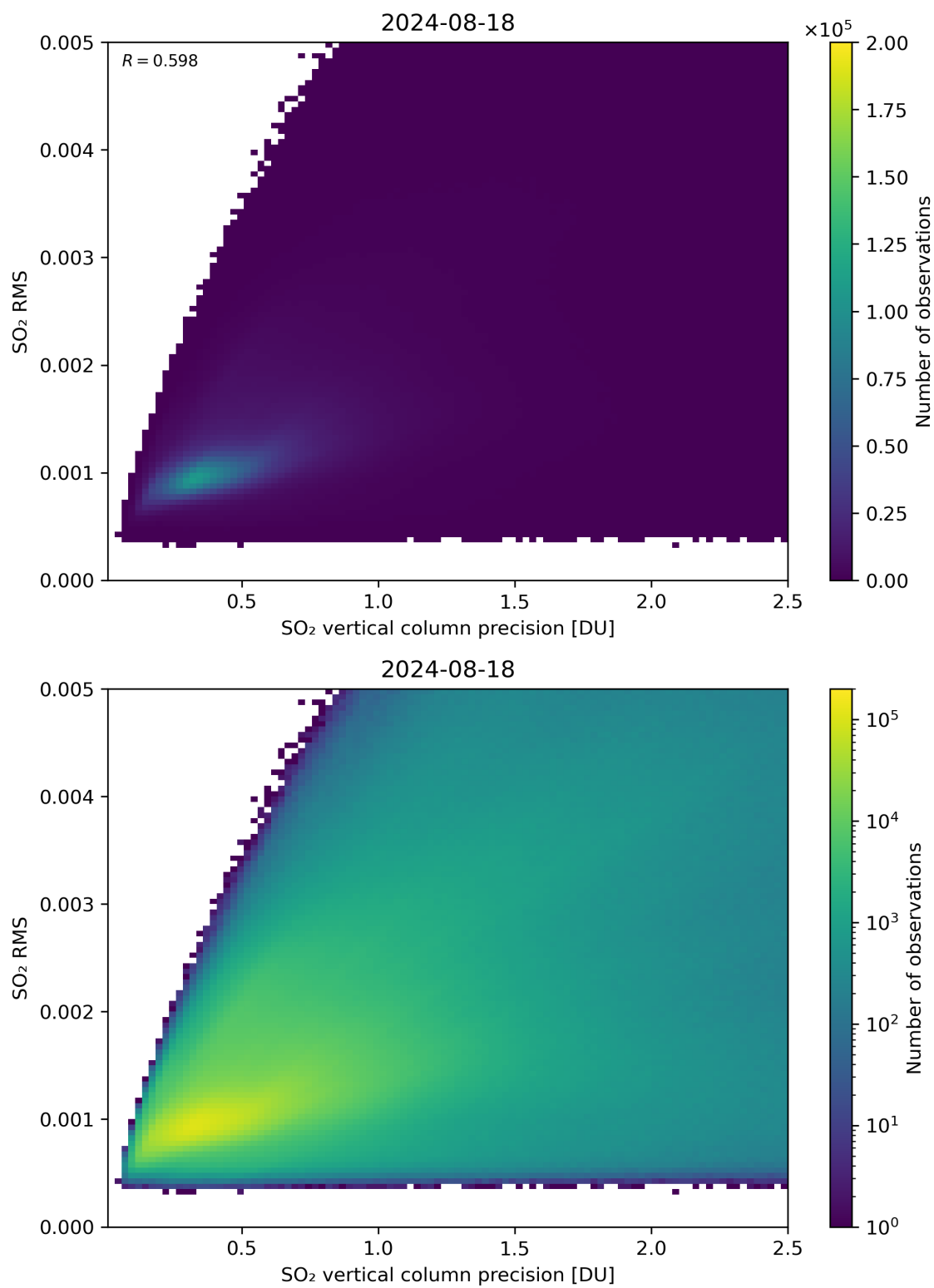
Figure 284: Scatter density plot of “SO 2 vertical column precision” against “SO 2 RMS” for 2024-08-17 to 2024-08-19.
