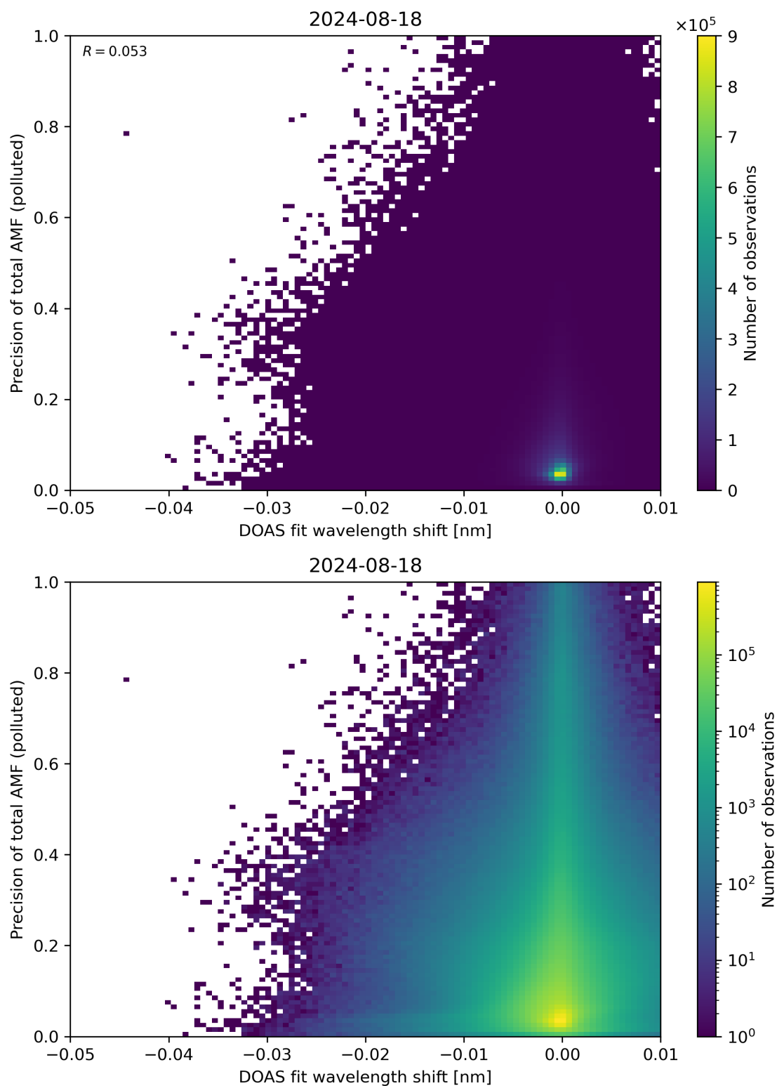
Figure 131: Scatter density plot of “DOAS fit wavelength shift” against “Precision of total AMF (polluted)” for 2024-08-17 to 2024-08-19.
