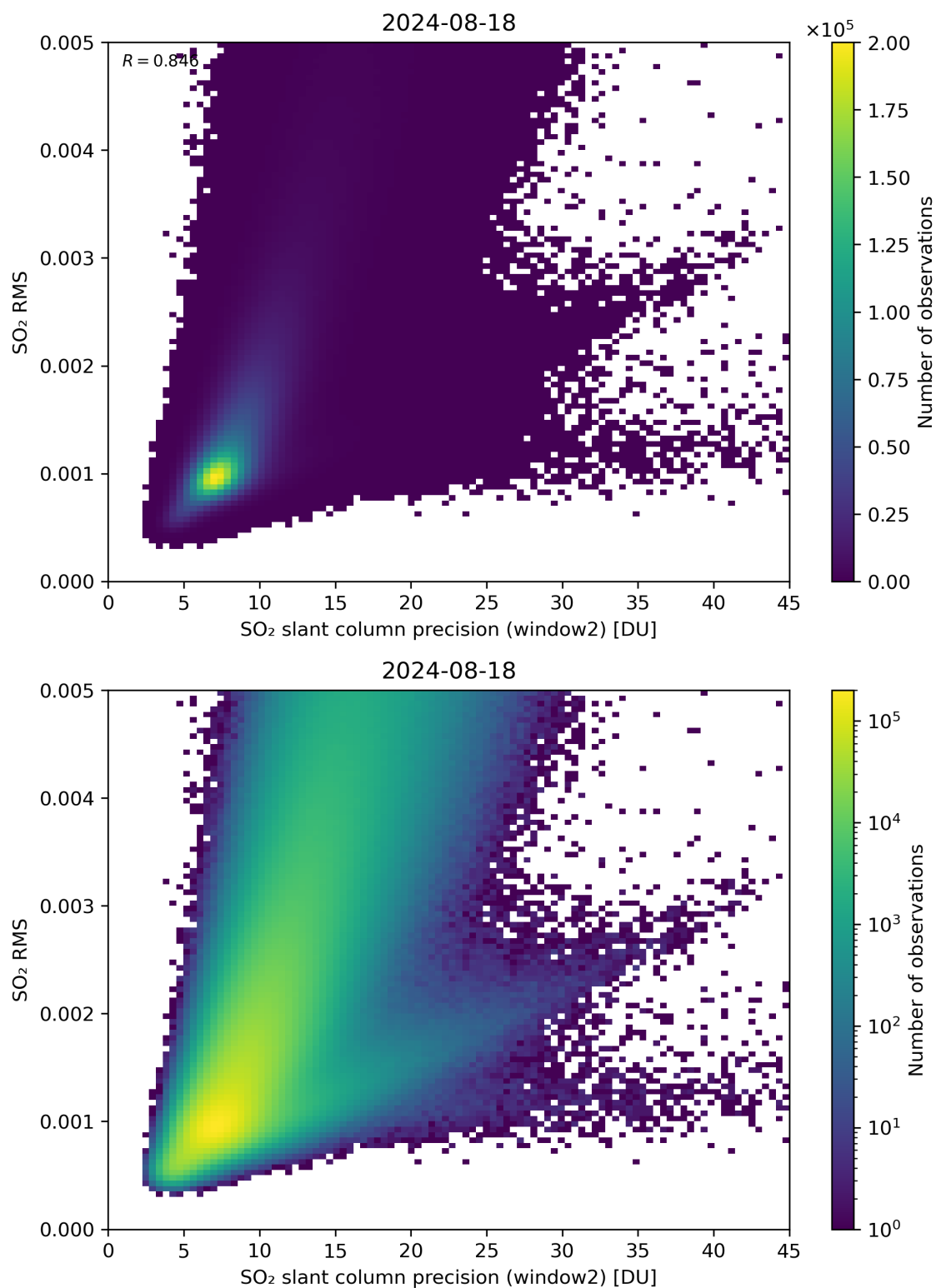
Figure 245: Scatter density plot of “SO 2 slant column precision (window2)” against “SO 2 RMS” for 2024-08-17 to 2024-08-19.
