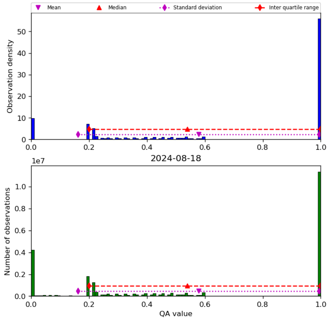
Figure 52: Histogram of “QA value” for 2024-08-17 to 2024-08-19
