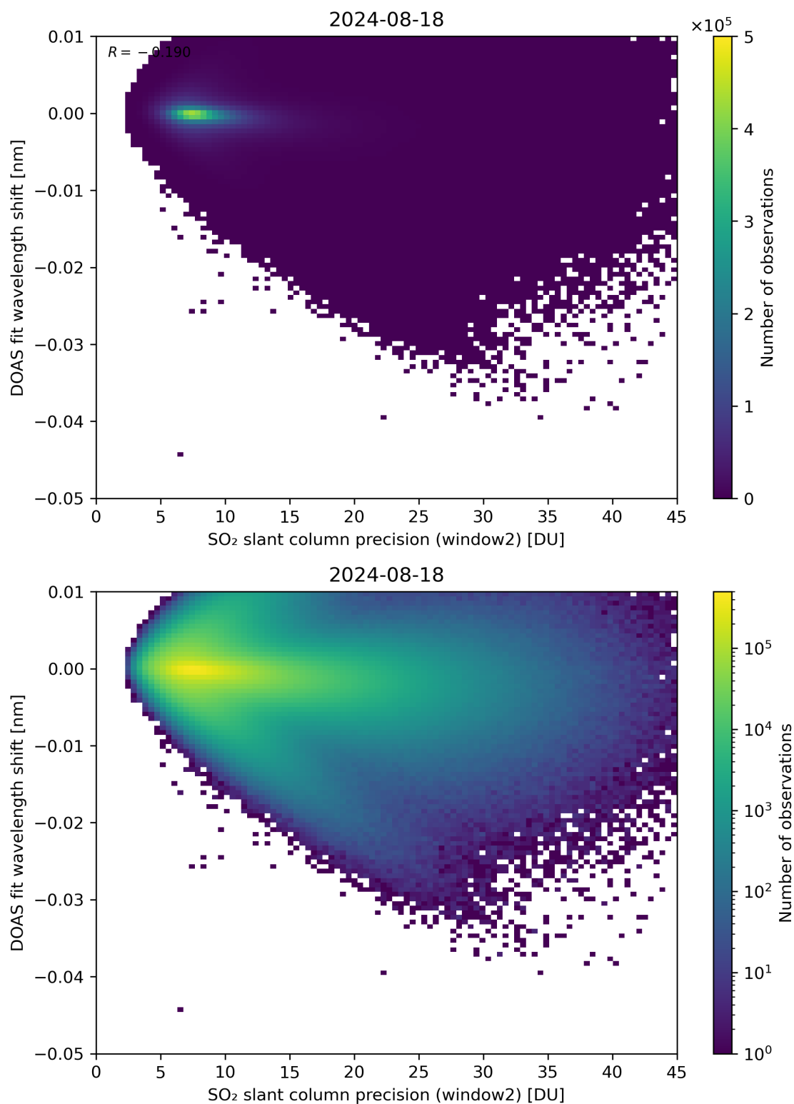
Figure 243: Scatter density plot of “SO 2 slant column precision (window2)” against “DOAS fit wavelength shift” for 2024-08-17 to 2024-08-19.
