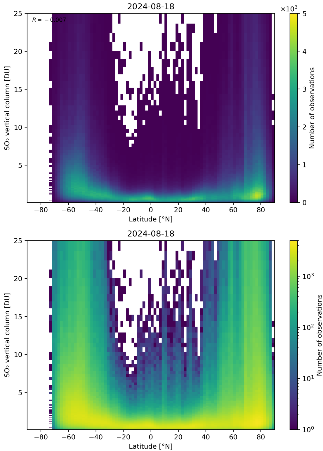
Figure 156: Scatter density plot of “Latitude” against “SO 2 vertical column” for 2024-08-17 to 2024-08-19.
