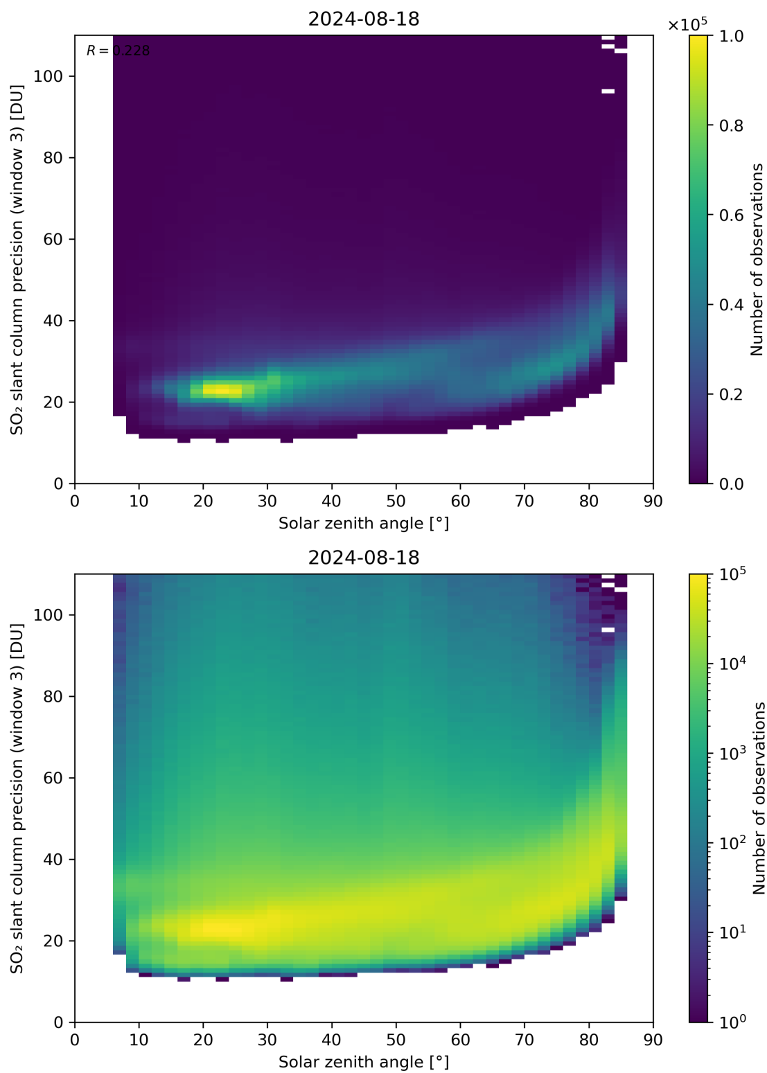
Figure 173: Scatter density plot of “Solar zenith angle” against “SO 2 slant column precision (window 3)” for 2024-08-17 to 2024-08-19.
