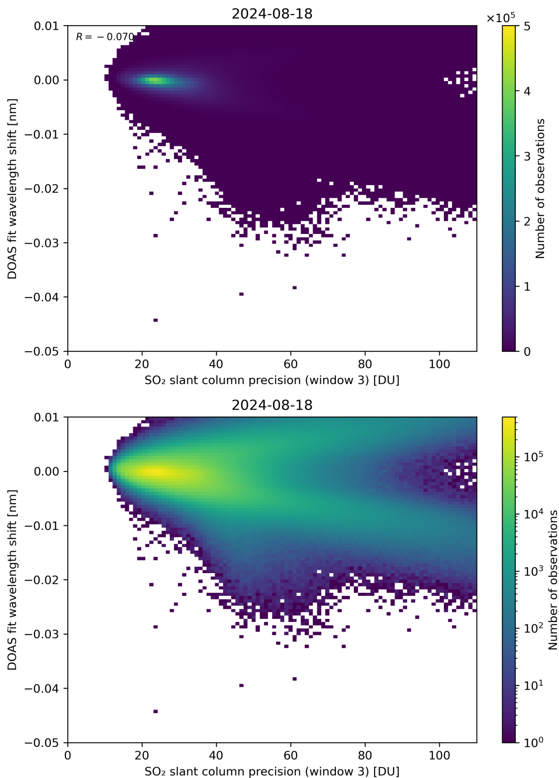
Figure 258: Scatter density plot of “SO 2 slant column precision (window 3)” against “DOAS fit wavelength shift” for 2024-08-17 to 2024-08-19.
