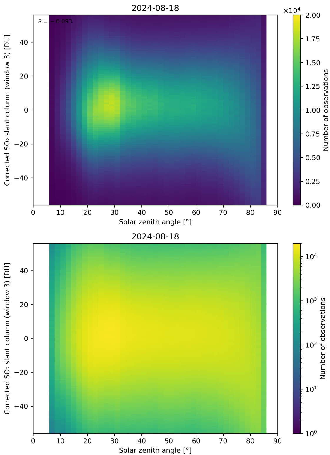
Figure 168: Scatter density plot of “Solar zenith angle” against “Corrected SO 2 slant column (window 3)” for 2024-08-17 to 2024-08-19.
