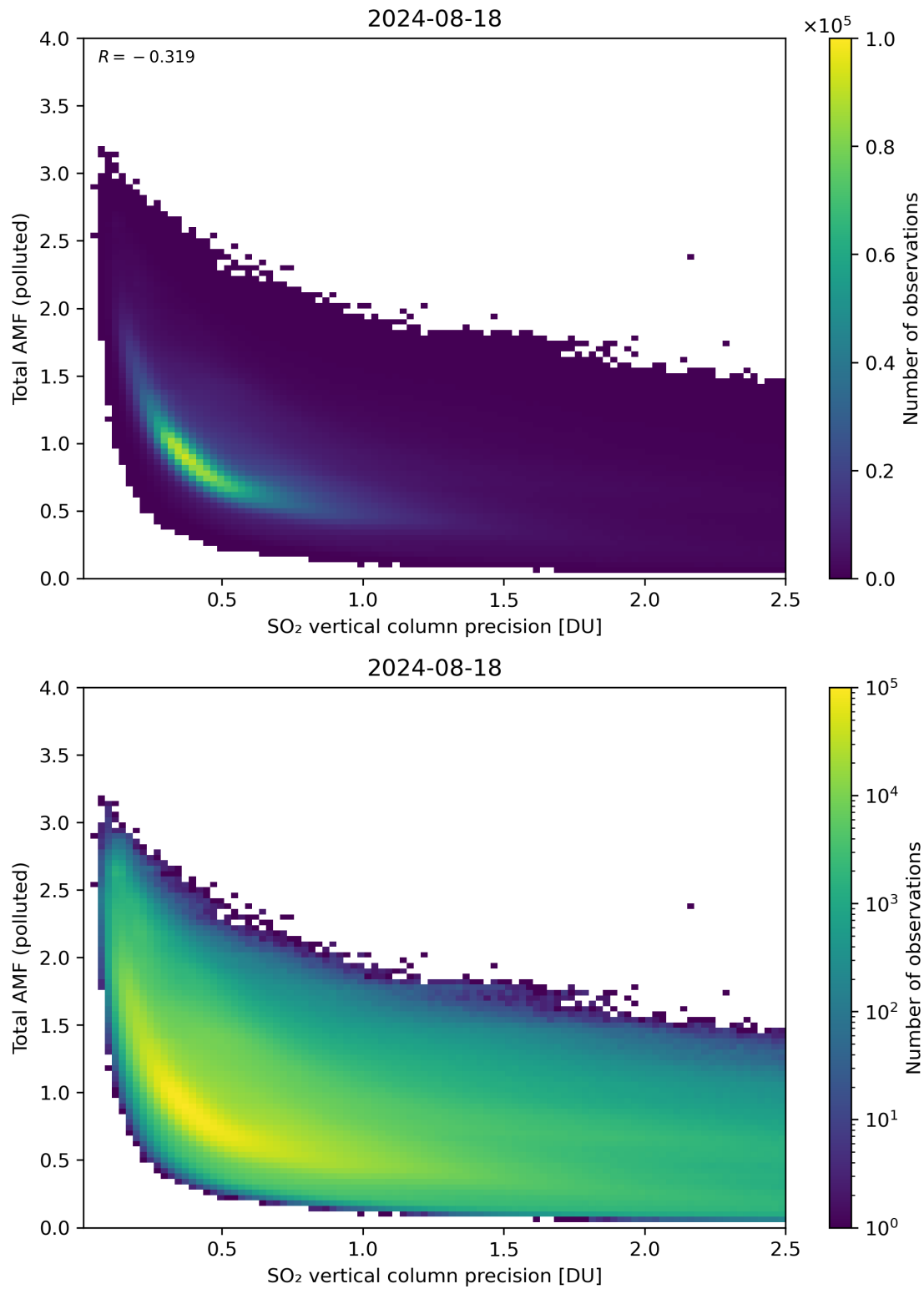
Figure 294: Scatter density plot of “SO 2 vertical column precision” against “Total AMF (polluted)” for 2024-08-17 to 2024-08-19.
