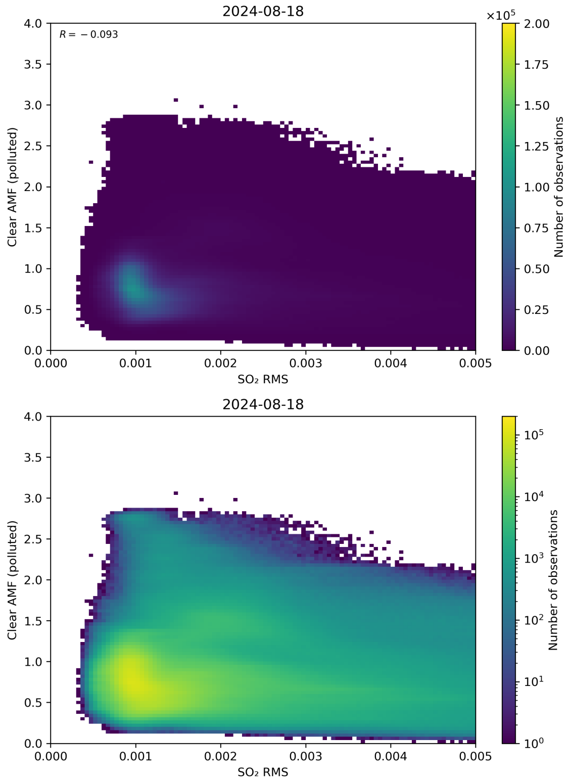
Figure 136: Scatter density plot of “SO 2 RMS” against “Clear AMF (polluted)” for 2024-08-17 to 2024-08-19.
