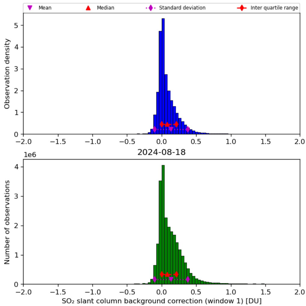
Figure 59: Histogram of “SO 2 slant column background correction (window 1)” for 2024-08-17 to 2024-08-19
