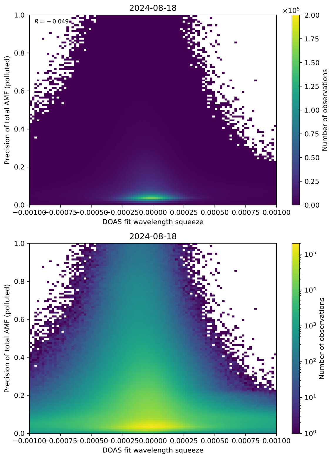
Figure 135: Scatter density plot of “DOAS fit wavelength squeeze” against “Precision of total AMF (polluted)” for 2024-08-17 to 2024-08-19.
