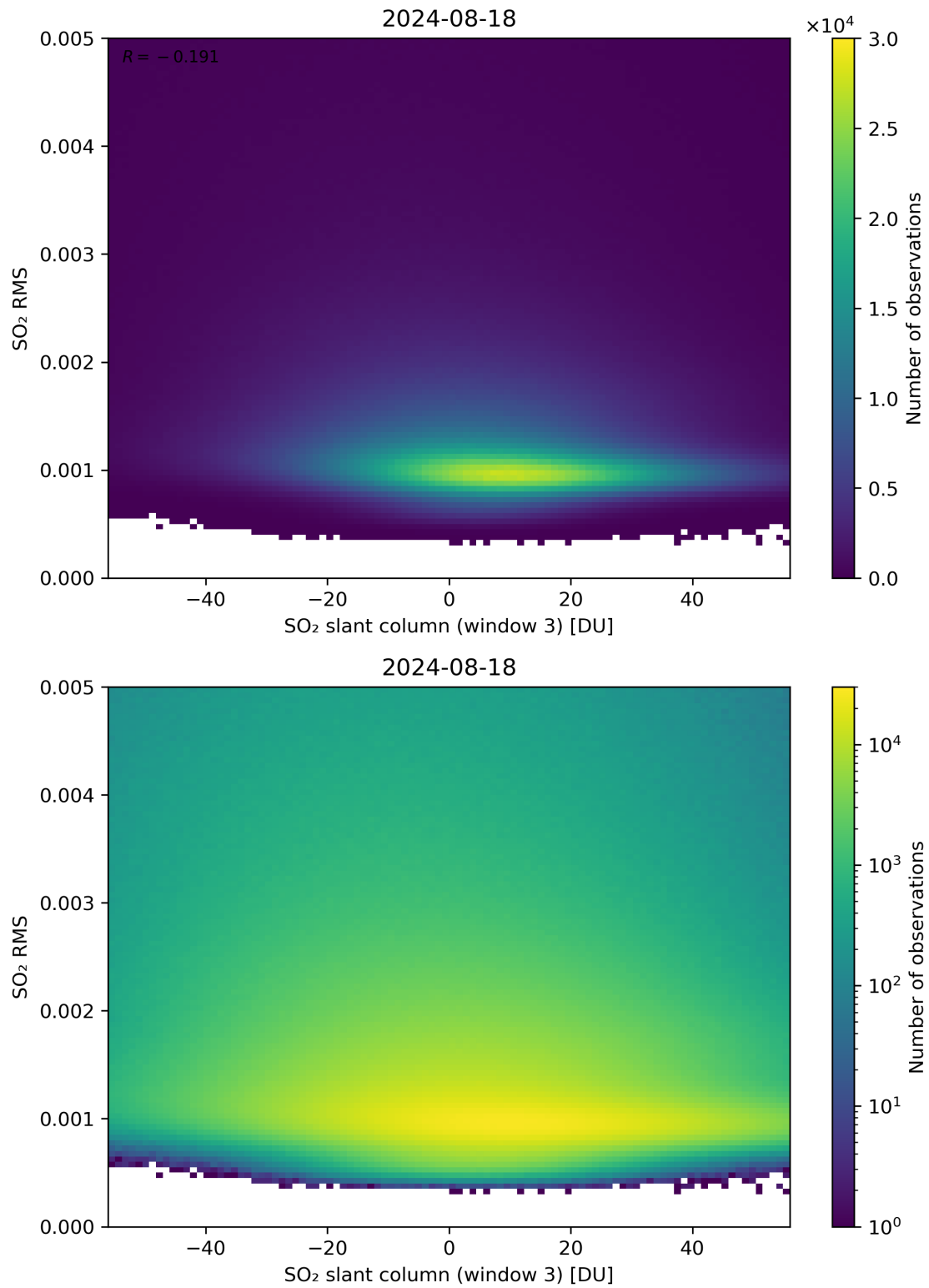
Figure 256: Scatter density plot of “SO 2 slant column (window 3)” against “SO 2 RMS” for 2024-08-17 to 2024-08-19.
