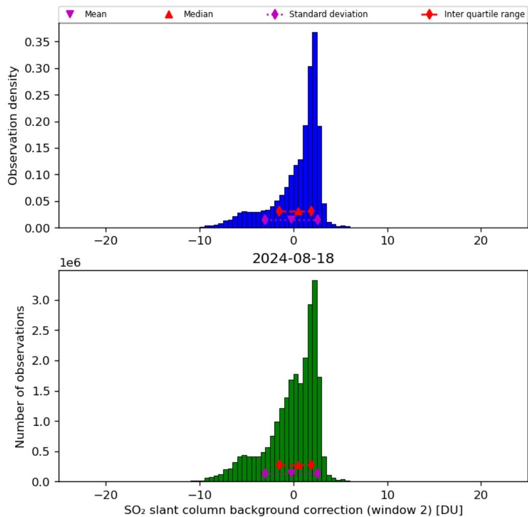
Figure 63: Histogram of “SO 2 slant column background correction (window 2)” for 2024-08-17 to 2024-08-19
