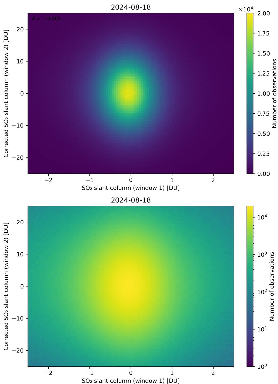
Figure 233: Scatter density plot of “SO 2 slant column (window 1)” against “Corrected SO 2 slant column (window 2)” for 2024-08-17 to 2024-08-19.
