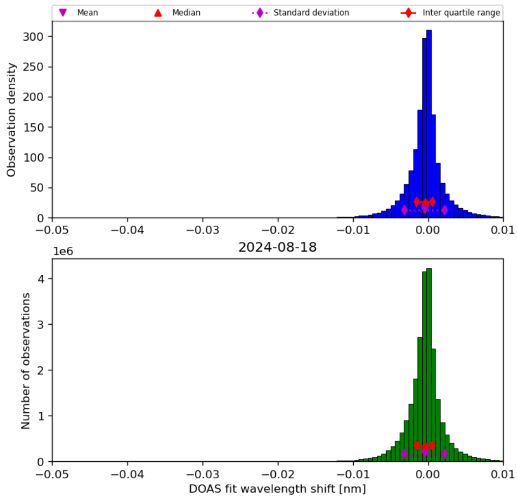
Figure 68: Histogram of “DOAS fit wavelength shift” for 2024-08-17 to 2024-08-19
