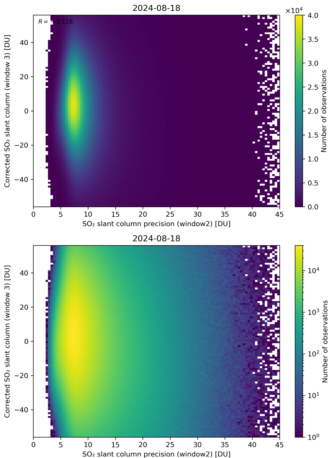
Figure 248: Scatter density plot of “SO 2 slant column precision (window2)” against “Corrected SO 2 slant column (window 3)” for 2024-08-17 to 2024-08-19.
