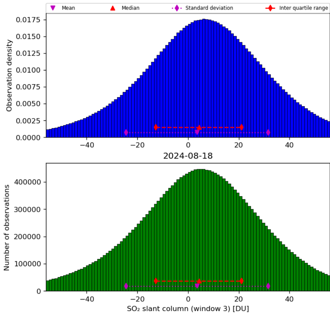
Figure 64: Histogram of “SO 2 slant column (window 3)” for 2024-08-17 to 2024-08-19
