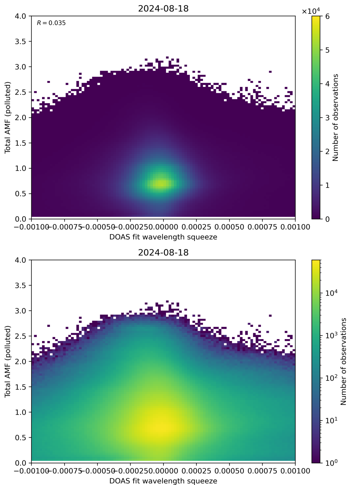
Figure 134: Scatter density plot of “DOAS fit wavelength squeeze” against “Total AMF (polluted)” for 2024-08-17 to 2024-08-19.
