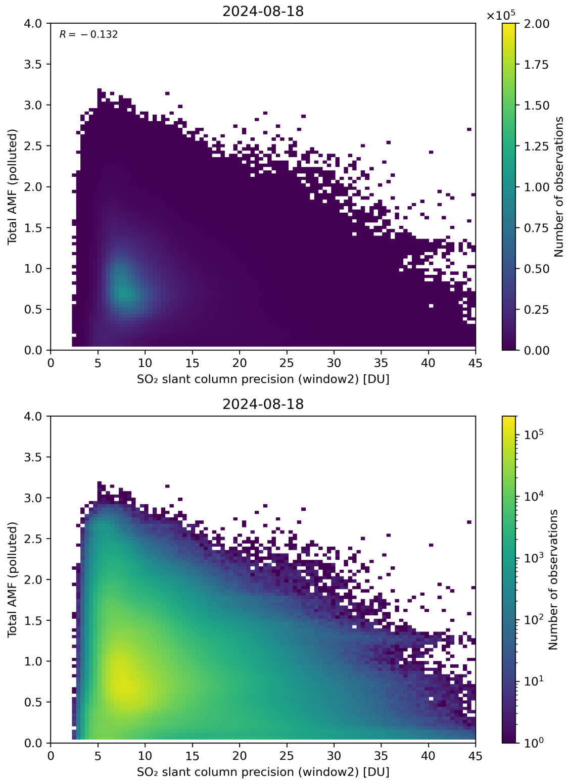
Figure 251: Scatter density plot of “SO 2 slant column precision (window2)” against “Total AMF (polluted)” for 2024-08-17 to 2024-08-19.
