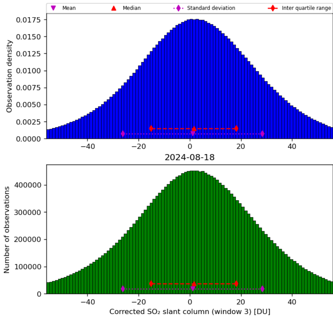
Figure 66: Histogram of “Corrected SO 2 slant column (window 3)” for 2024-08-17 to 2024-08-19
