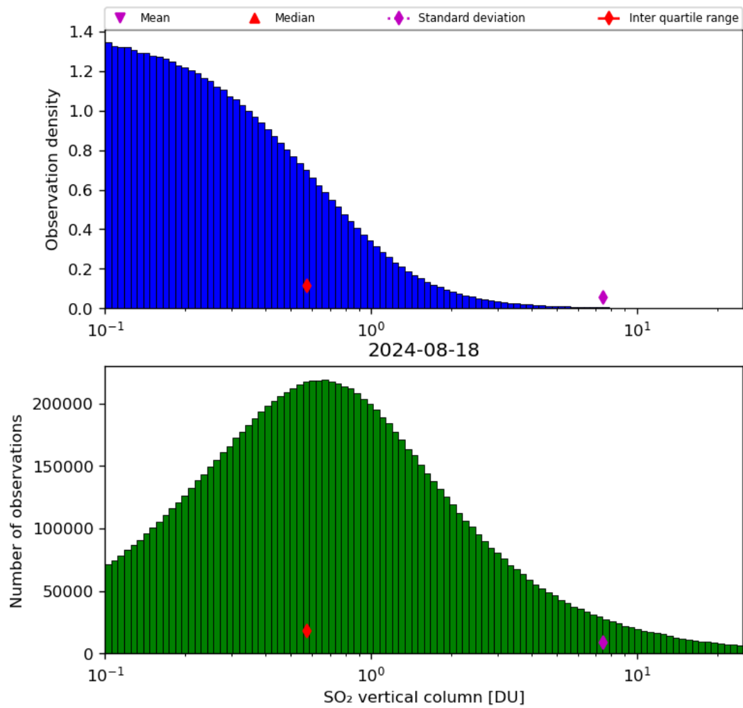
Figure 53: Histogram of “SO 2 vertical column” for 2024-08-17 to 2024-08-19
