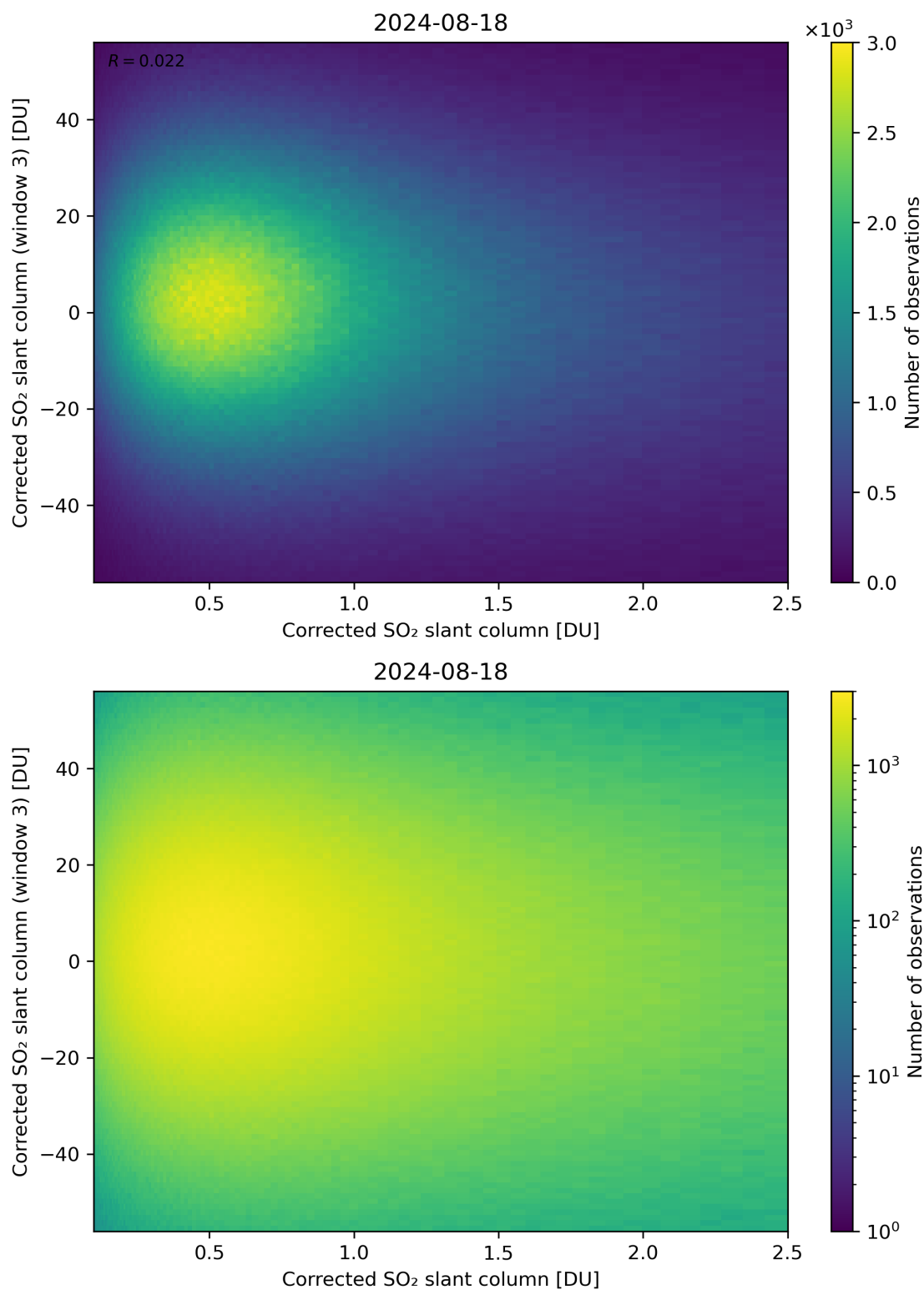
Figure 186: Scatter density plot of “Corrected SO 2 slant column” against “Corrected SO 2 slant column (window 3)” for 2024-08-17 to 2024-08-19.
