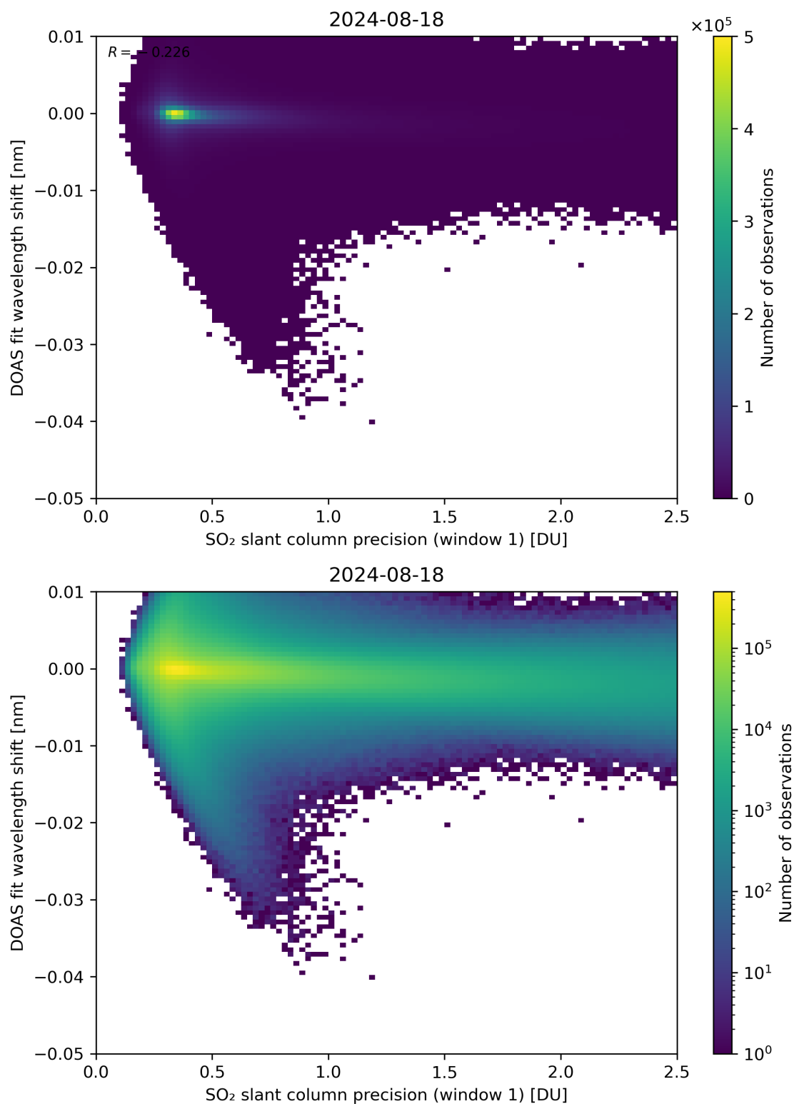
Figure 221: Scatter density plot of “SO 2 slant column precision (window 1)” against “DOAS fit wavelength shift” for 2024-08-17 to 2024-08-19.
