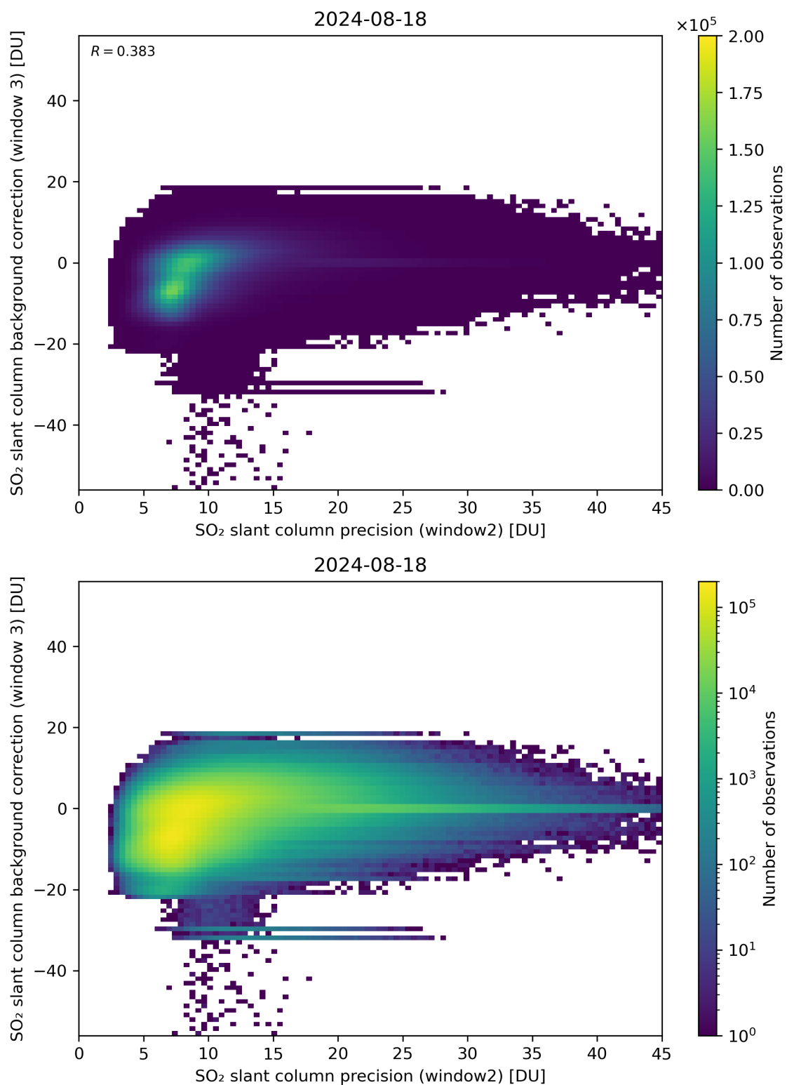
Figure 242: Scatter density plot of “SO 2 slant column precision (window2)” against “SO 2 slant column background correction (window 3)” for 2024-08-17 to 2024-08-19.
