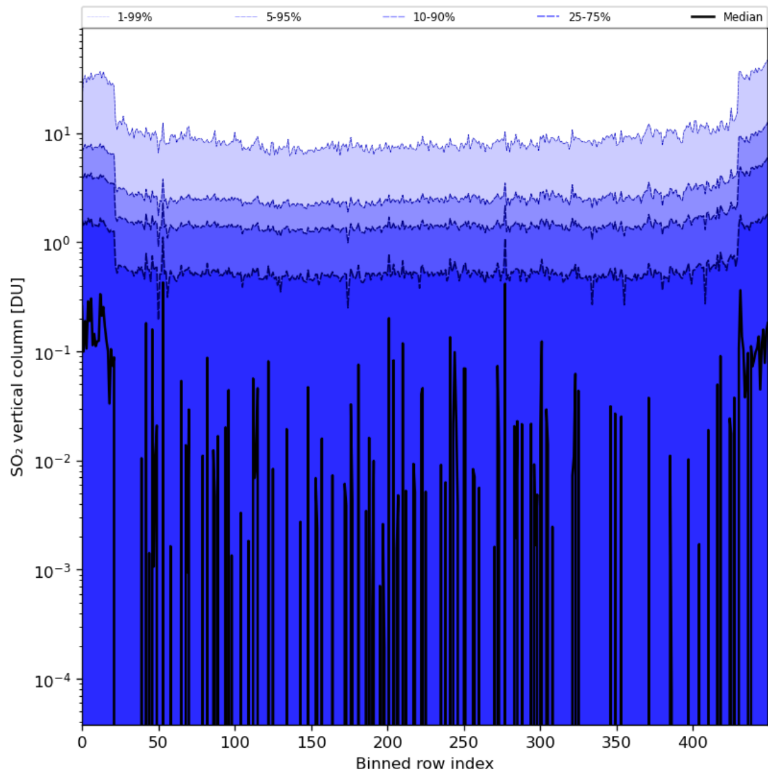
Figure 76: Along track statistics of “SO 2 vertical column” for 2024-08-17 to 2024-08-19
