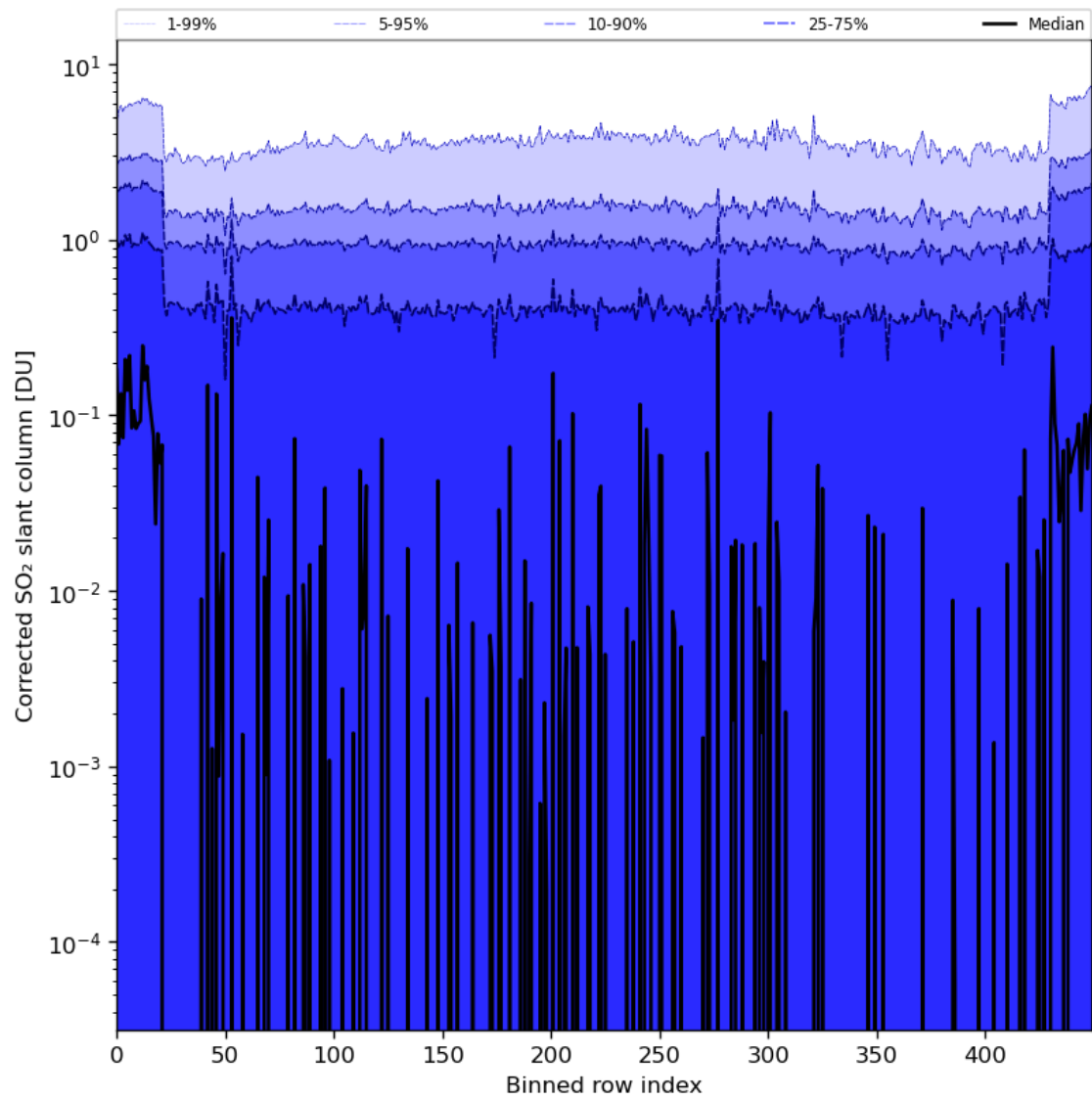
Figure 78: Along track statistics of “Corrected SO 2 slant column” for 2024-08-17 to 2024-08-19
