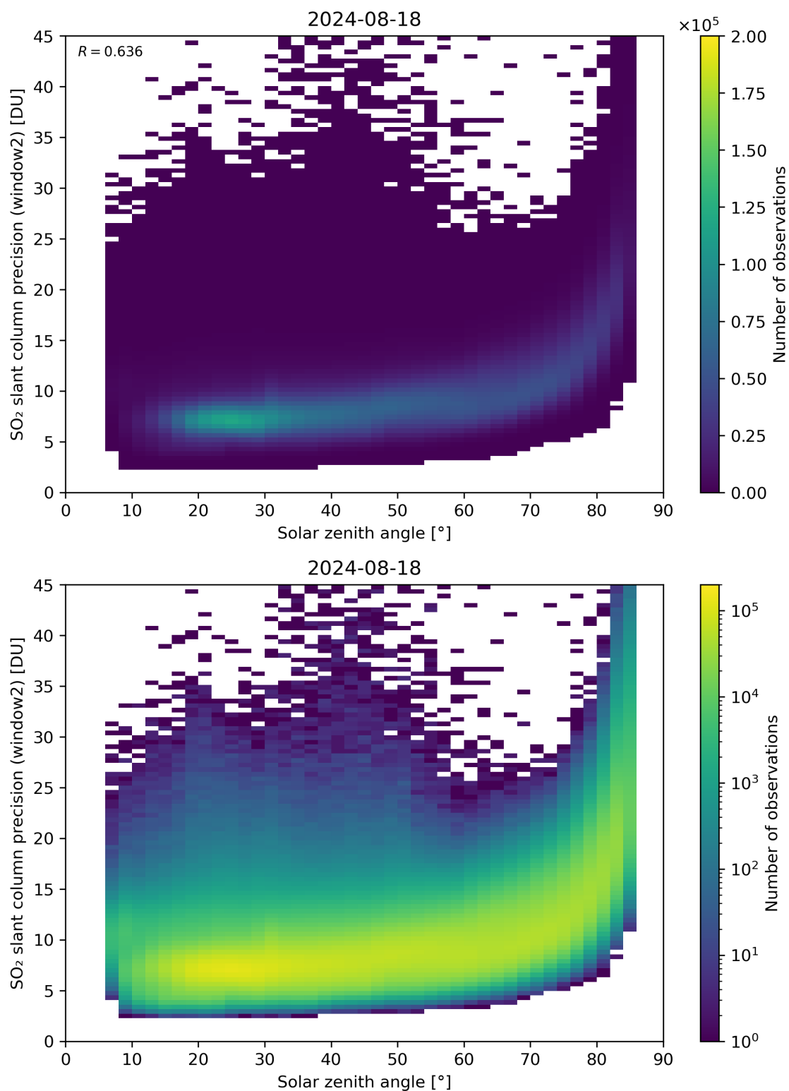
Figure 171: Scatter density plot of “Solar zenith angle” against “SO 2 slant column precision (window2)” for 2024-08-17 to 2024-08-19.
