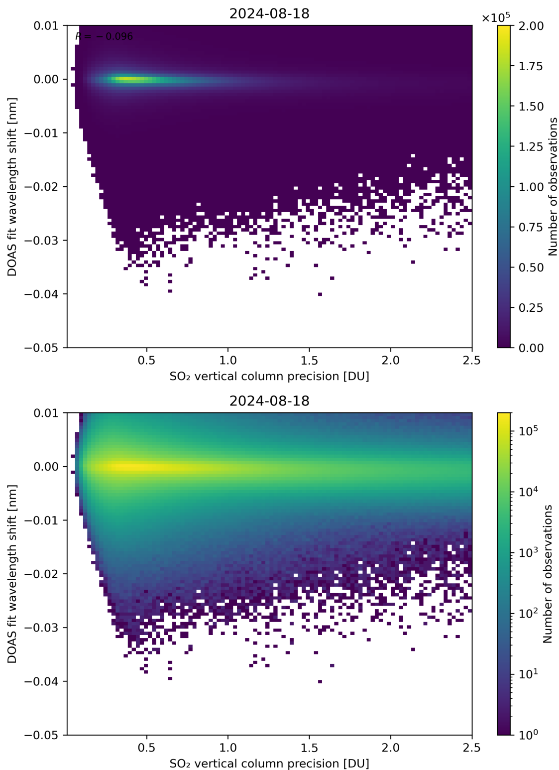
Figure 282: Scatter density plot of “SO 2 vertical column precision” against “DOAS fit wavelength shift” for 2024-08-17 to 2024-08-19.
