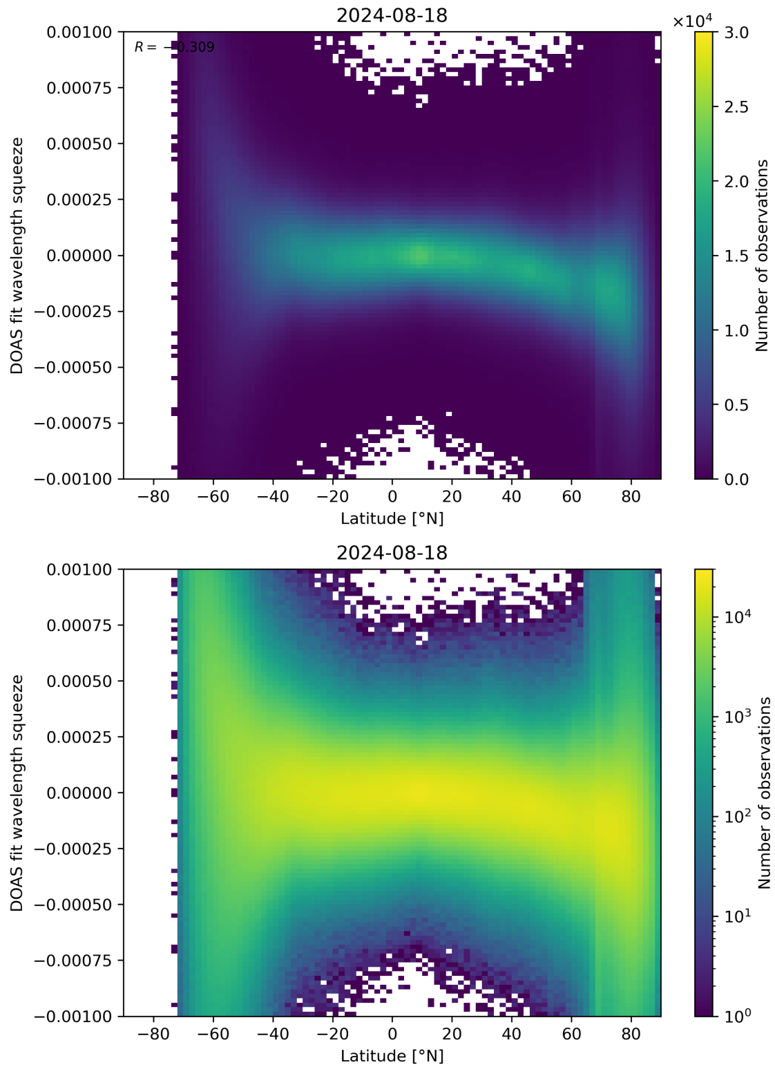
Figure 143: Scatter density plot of “Latitude” against “DOAS fit wavelength squeeze” for 2024-08-17 to 2024-08-19.
