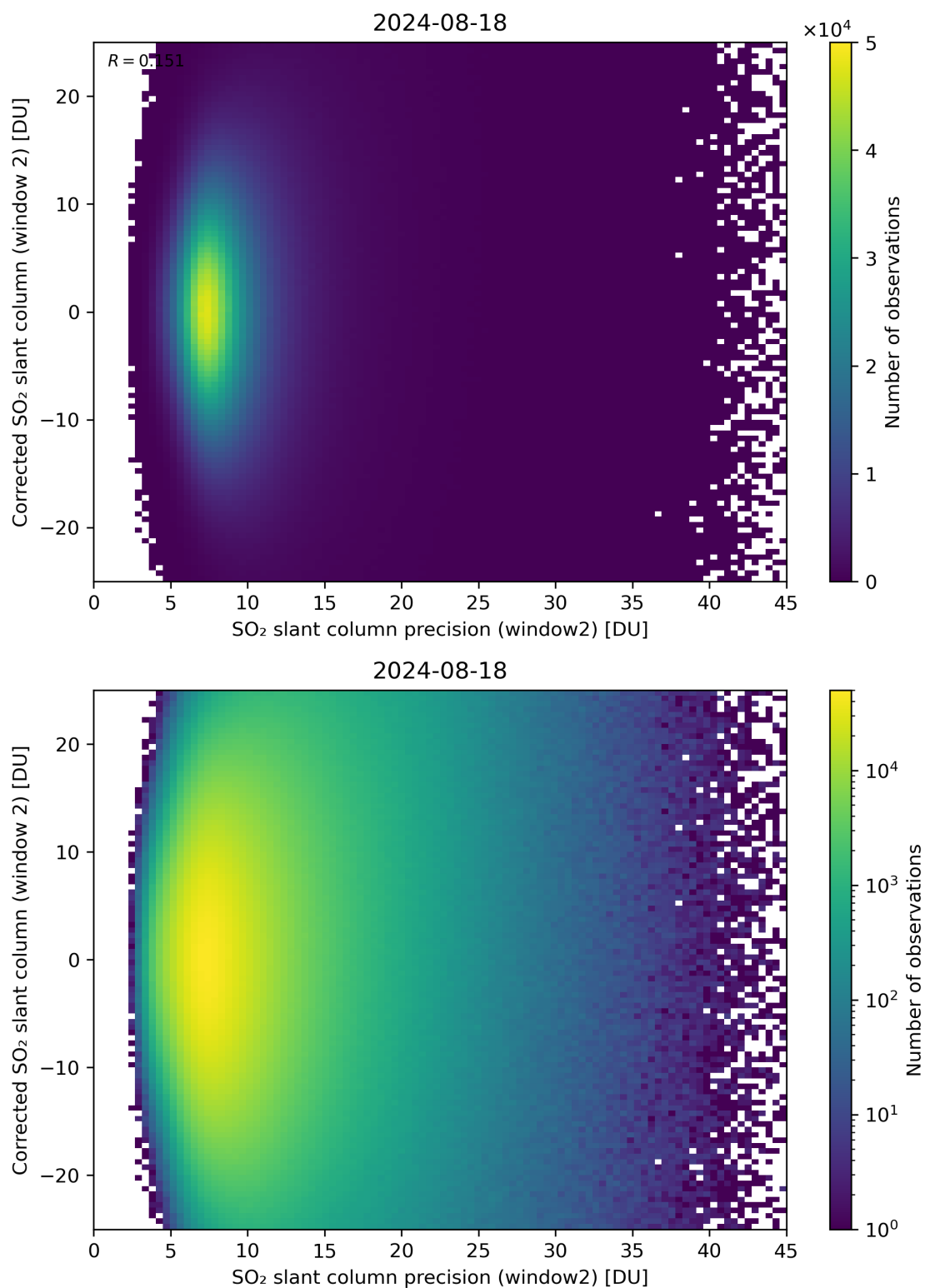
Figure 247: Scatter density plot of “SO 2 slant column precision (window2)” against “Corrected SO 2 slant column (window 2)” for 2024-08-17 to 2024-08-19.
