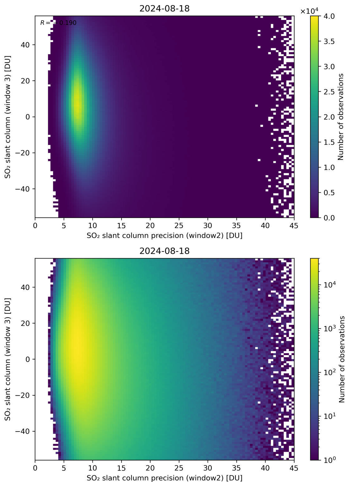
Figure 249: Scatter density plot of “SO 2 slant column precision (window2)” against “SO 2 slant column (window 3)” for 2024-08-17 to 2024-08-19.
