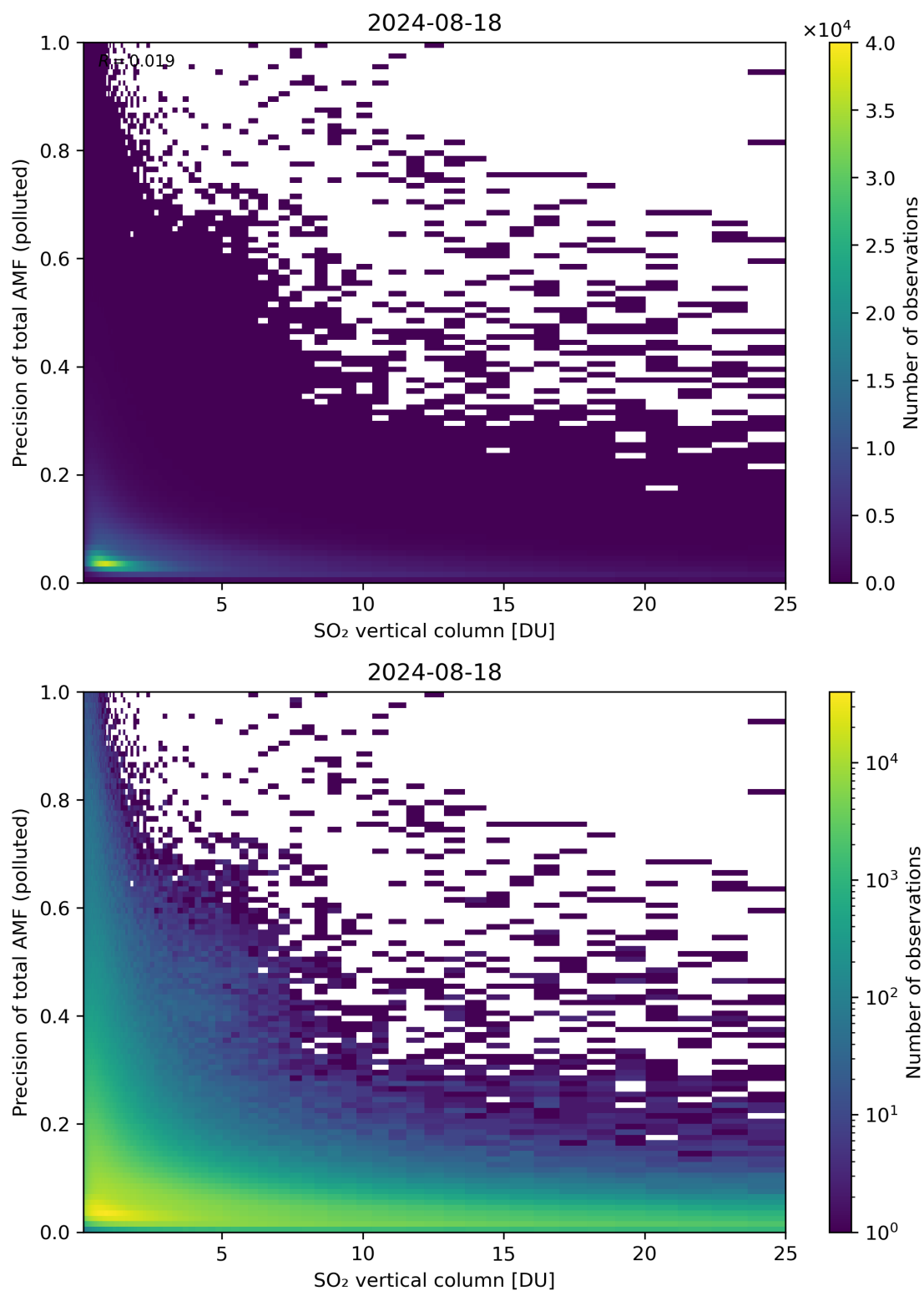
Figure 306: Scatter density plot of “SO 2 vertical column” against “Precision of total AMF (polluted)” for 2024-08-17 to 2024-08-19.
