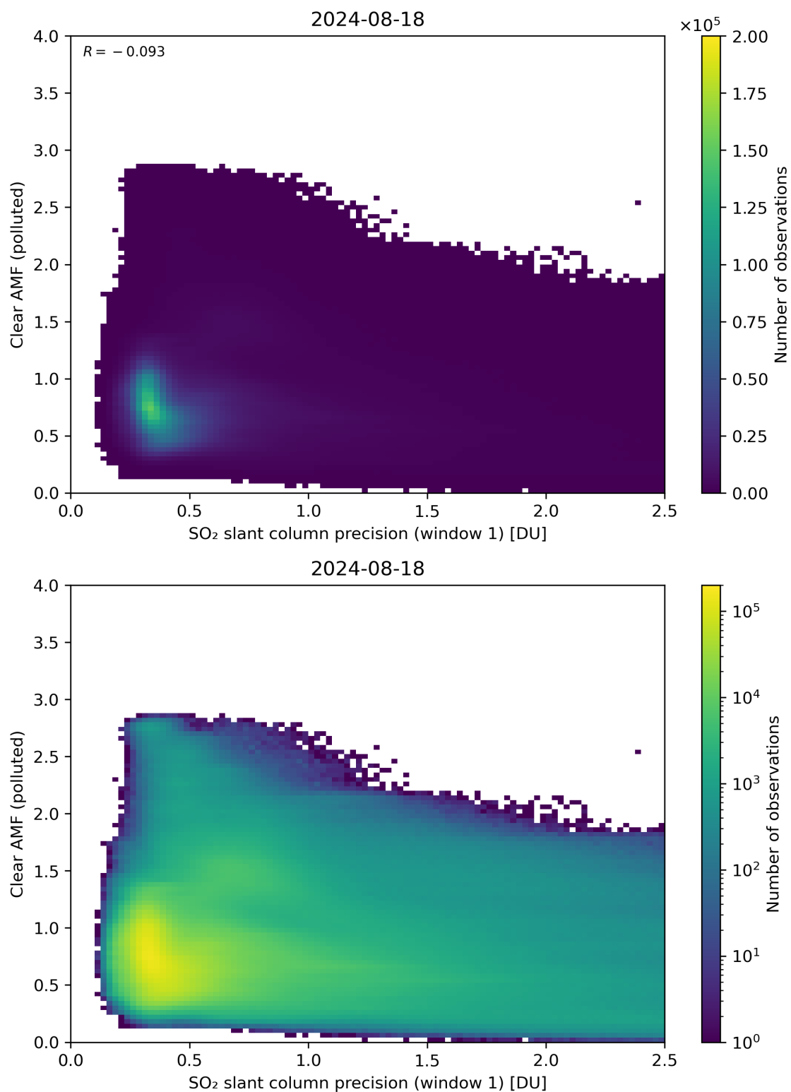
Figure 224: Scatter density plot of “SO 2 slant column precision (window 1)” against “Clear AMF (polluted)” for 2024-08-17 to 2024-08-19.
