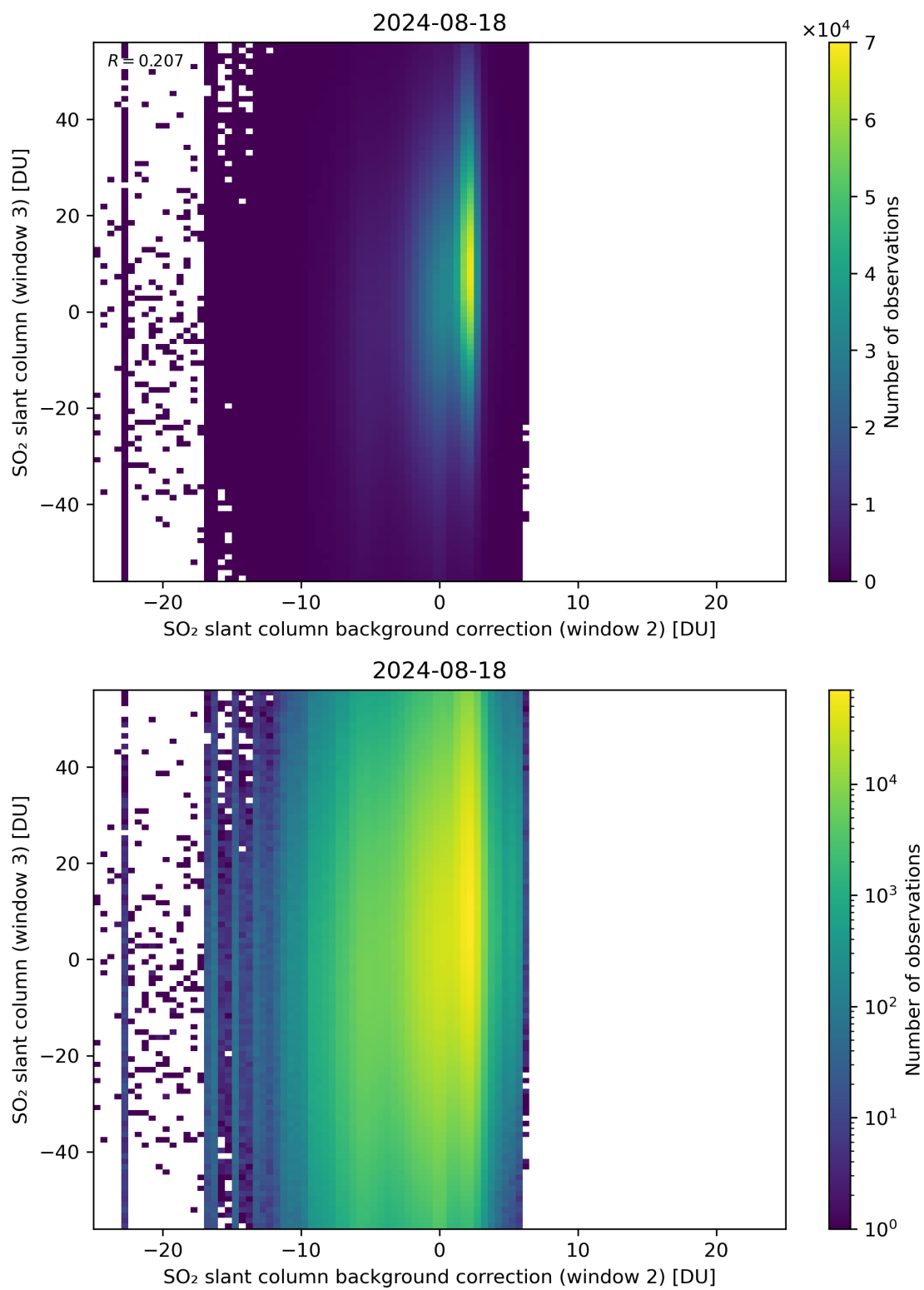
Figure 117: Scatter density plot of “SO 2 slant column background correction (window 2)” against “SO 2 slant column (window 3)” for 2024-08-17 to 2024-08-19.
