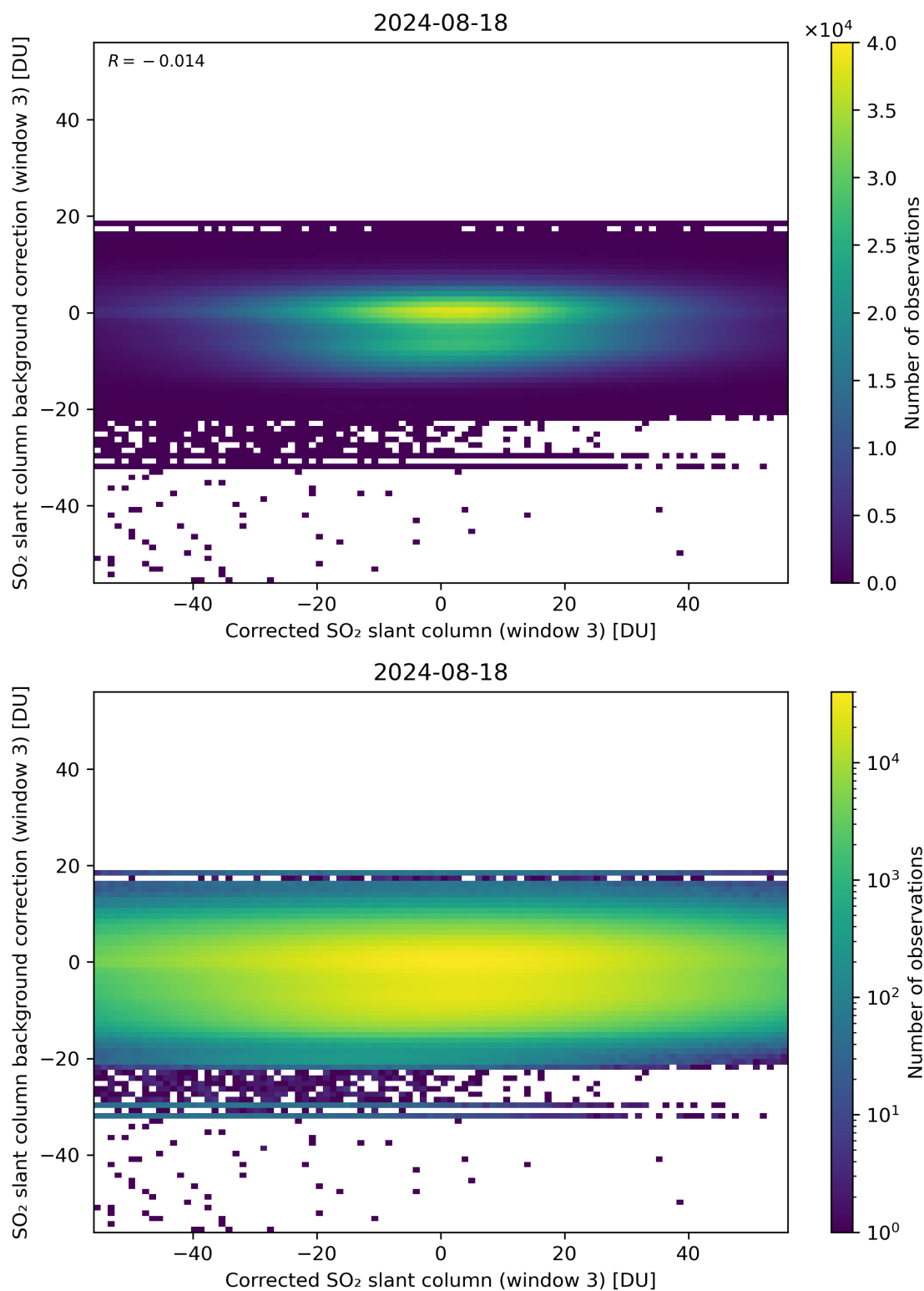
Figure 205: Scatter density plot of “Corrected SO 2 slant column (window 3)” against “SO 2 slant column background correction (window 3)” for 2024-08-17 to 2024-08-19.
