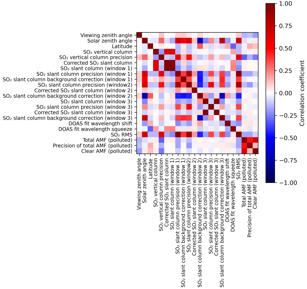
Figure 2: Map of correlation matrix for 2024-08-17 to 2024-08-19.
