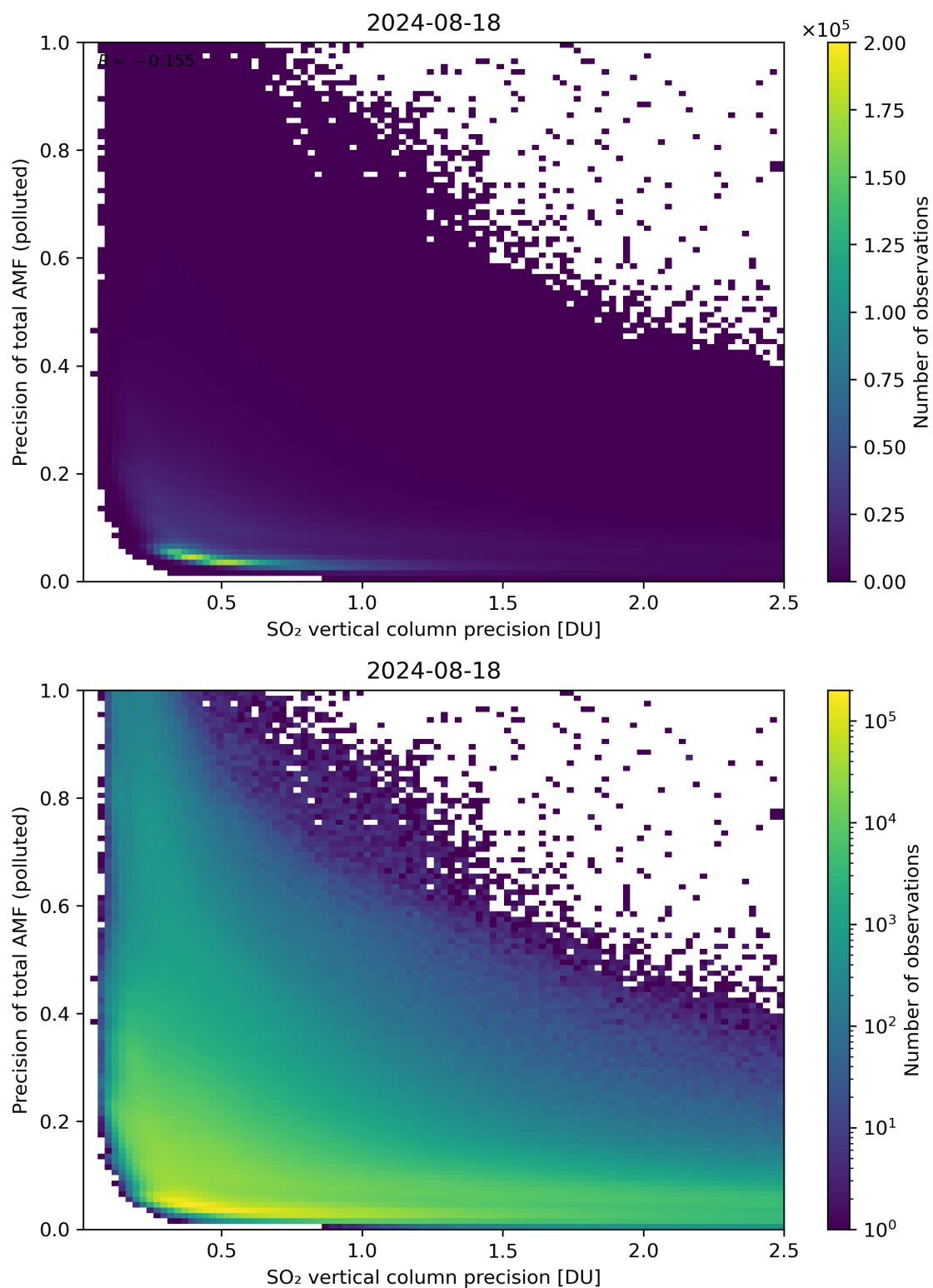
Figure 295: Scatter density plot of “SO 2 vertical column precision” against “Precision of total AMF (polluted)” for 2024-08-17 to 2024-08-19.
