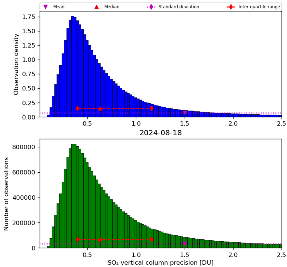
Figure 54: Histogram of “SO 2 vertical column precision” for 2024-08-17 to 2024-08-19
