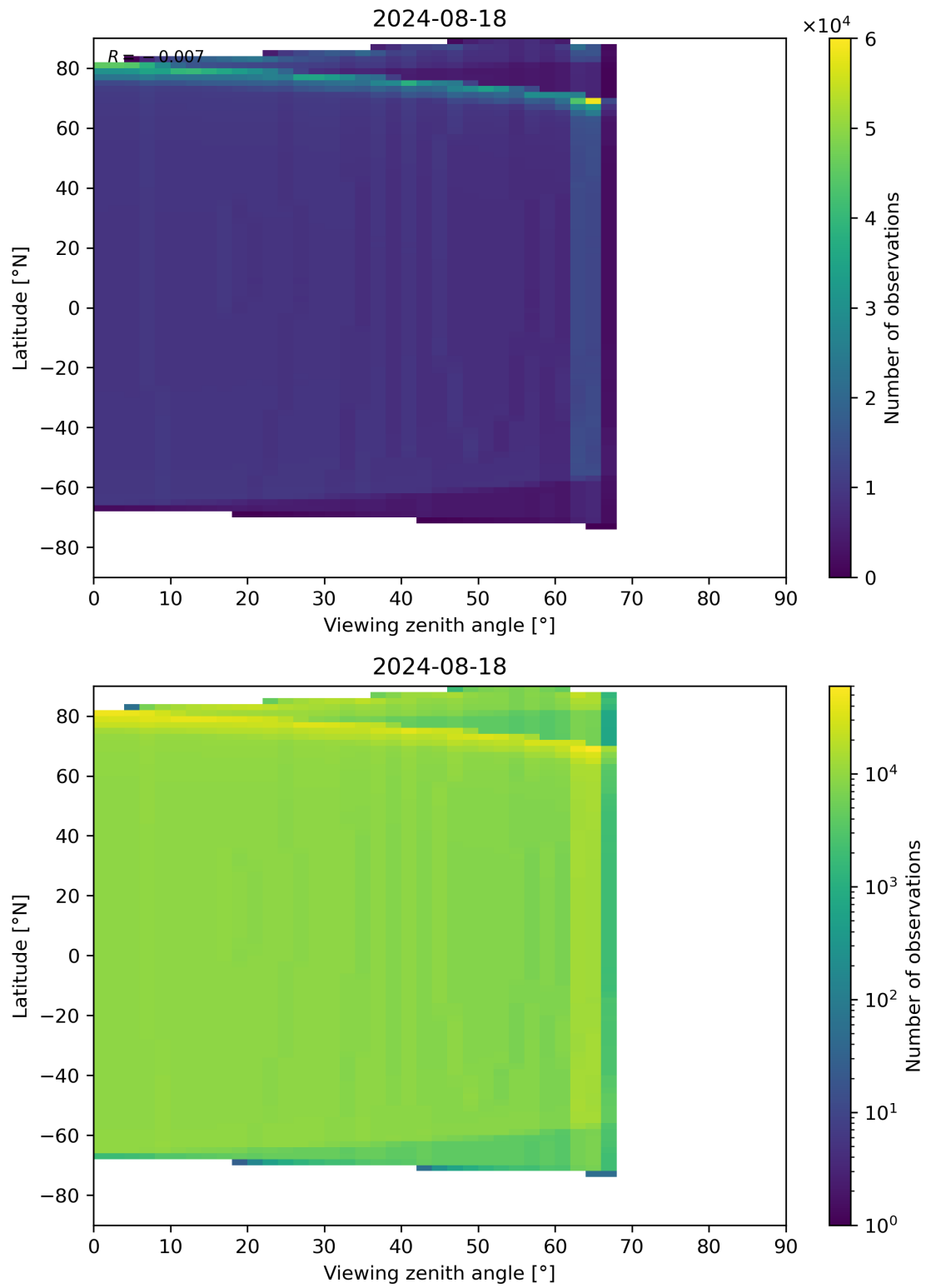
Figure 314: Scatter density plot of “Viewing zenith angle” against “Latitude” for 2024-08-17 to 2024-08-19.
