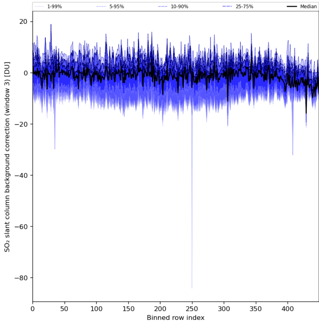
Figure 90: Along track statistics of “SO 2 slant column background correction (window 3)” for 2024-08-17 to 2024-08-19
