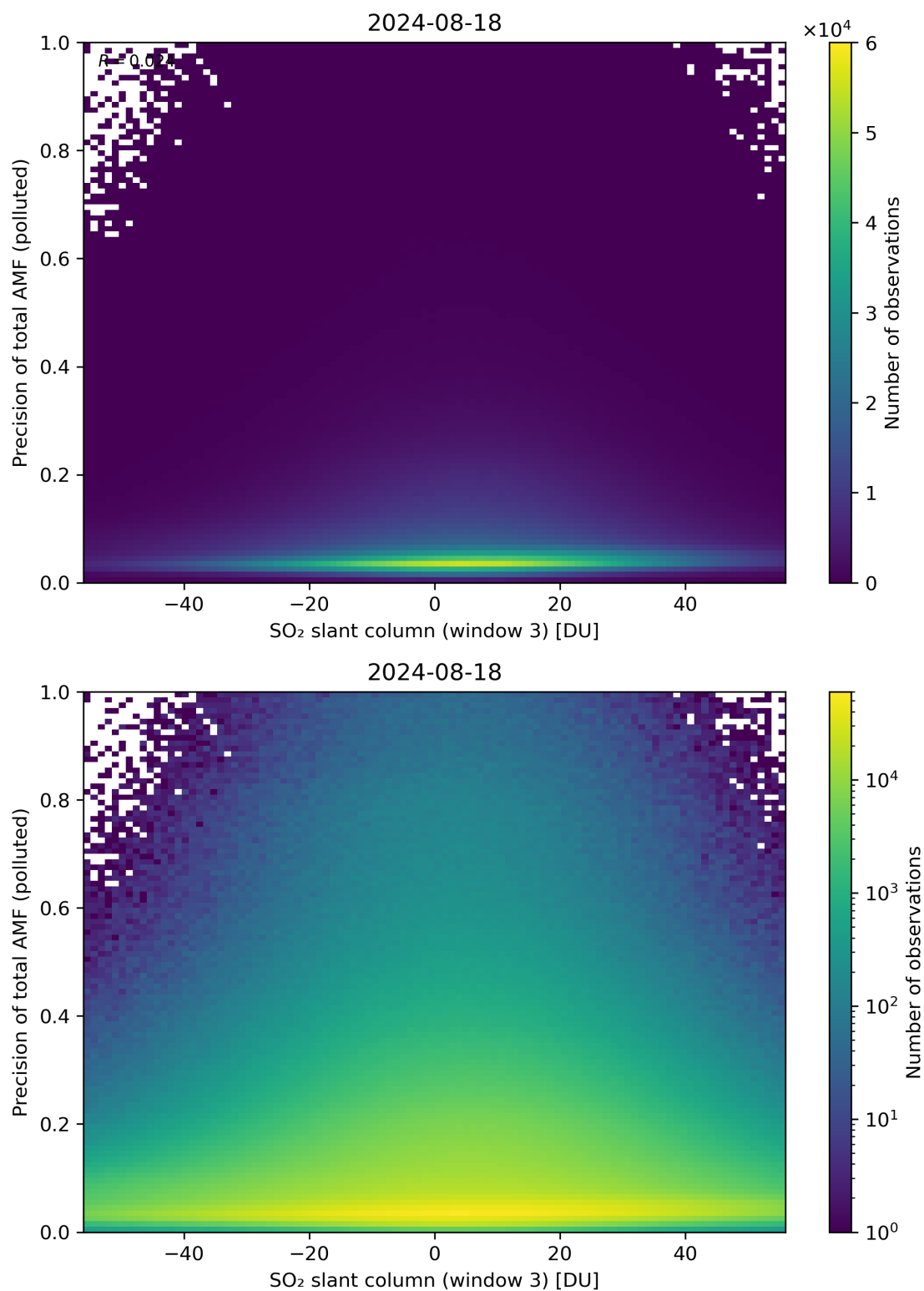
Figure 269: Scatter density plot of “SO 2 slant column (window 3)” against “Precision of total AMF (polluted)” for 2024-08-17 to 2024-08-19.
