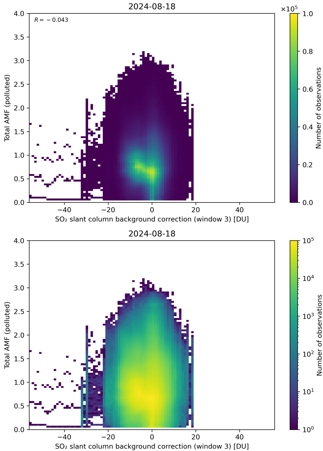
Figure 125: Scatter density plot of “SO 2 slant column background correction (window 3)” against “Total AMF (polluted)” for 2024-08-17 to 2024-08-19.
