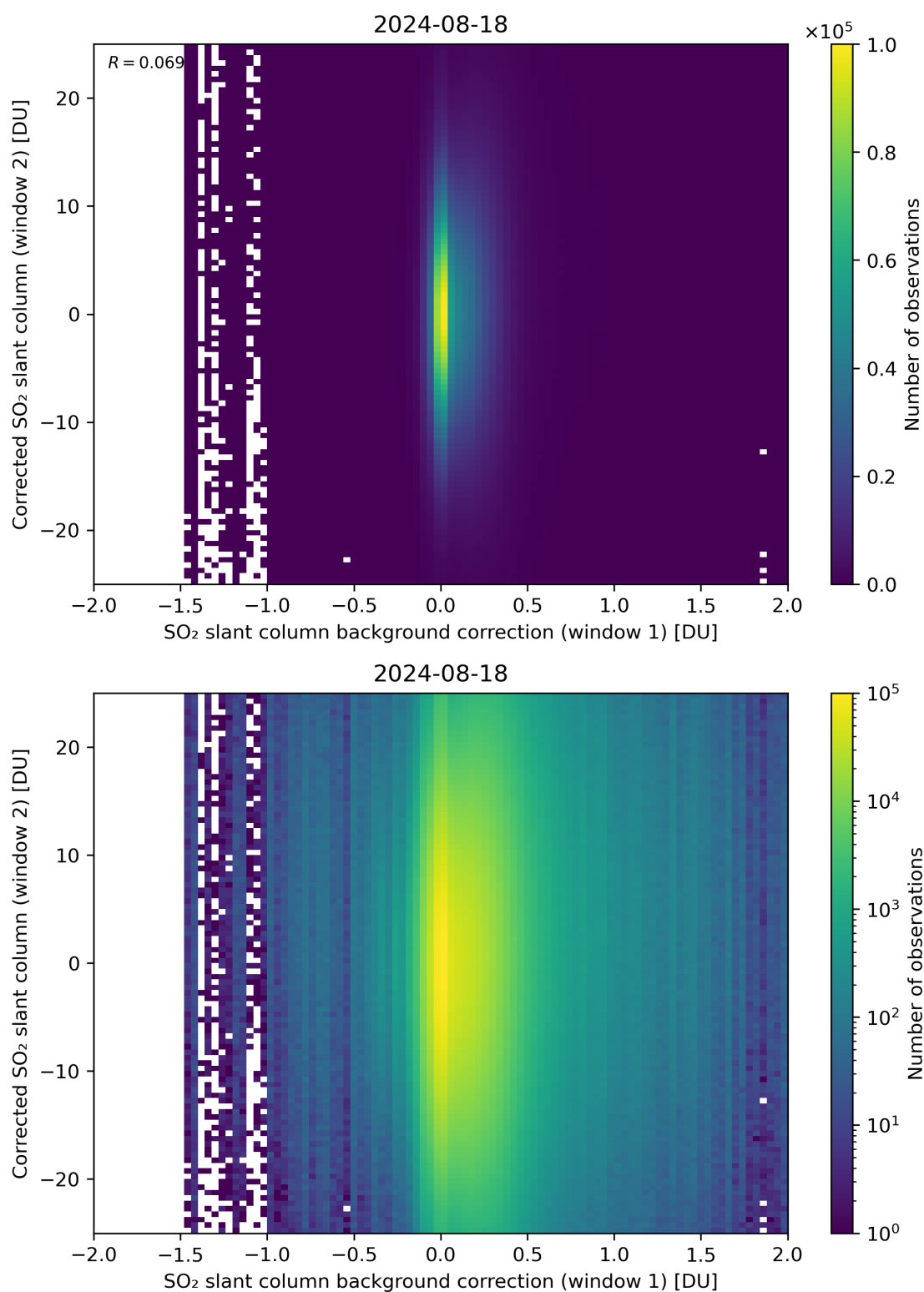
Figure 104: Scatter density plot of “SO 2 slant column background correction (window 1)” against “Corrected SO 2 slant column (window 2)” for 2024-08-17 to 2024-08-19.
