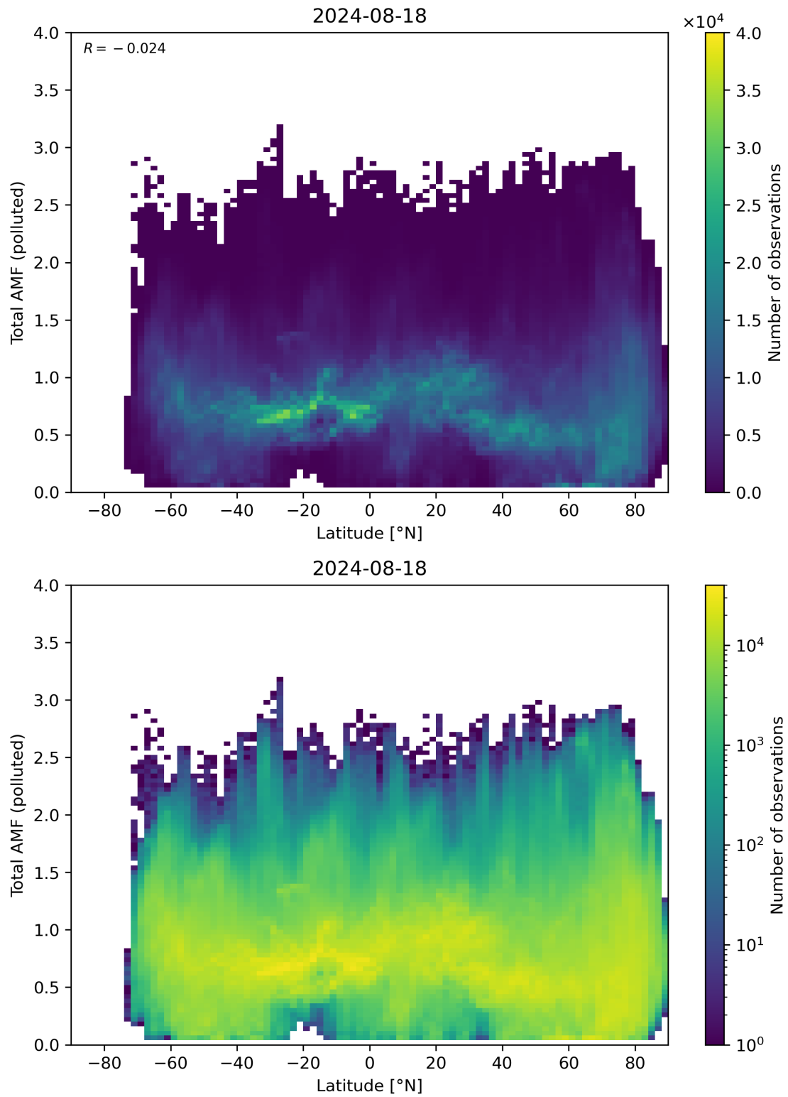
Figure 154: Scatter density plot of “Latitude” against “Total AMF (polluted)” for 2024-08-17 to 2024-08-19.
