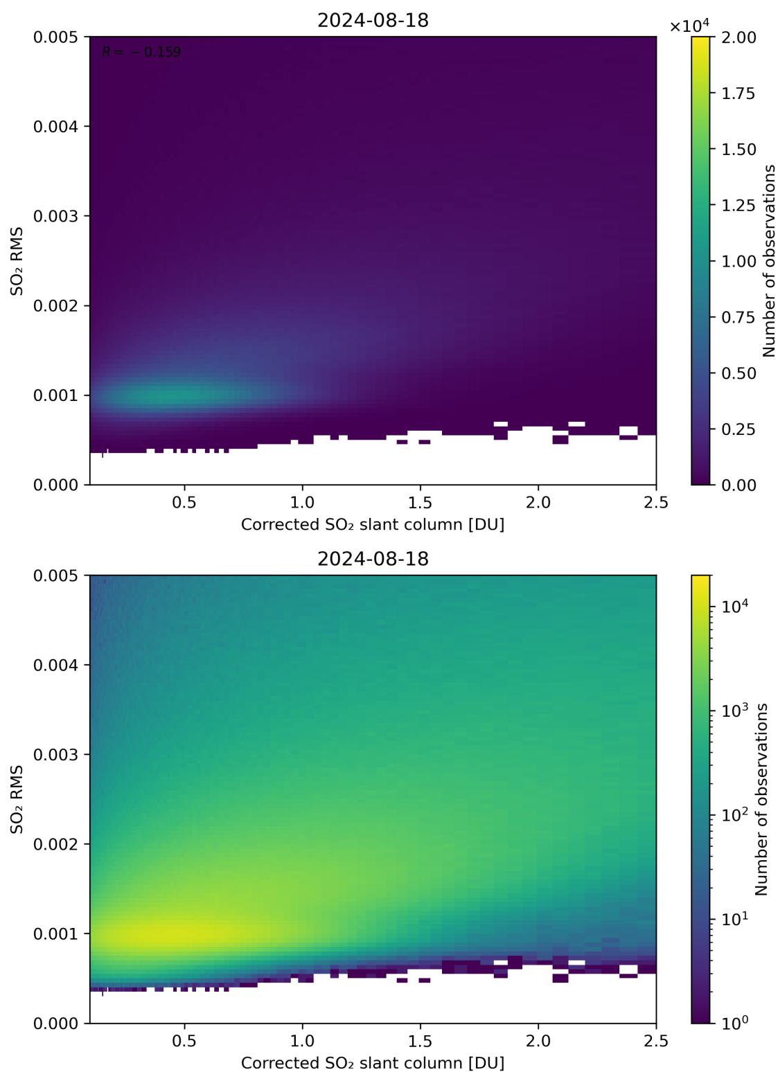
Figure 183: Scatter density plot of “Corrected SO 2 slant column” against “SO 2 RMS” for 2024-08-17 to 2024-08-19.
