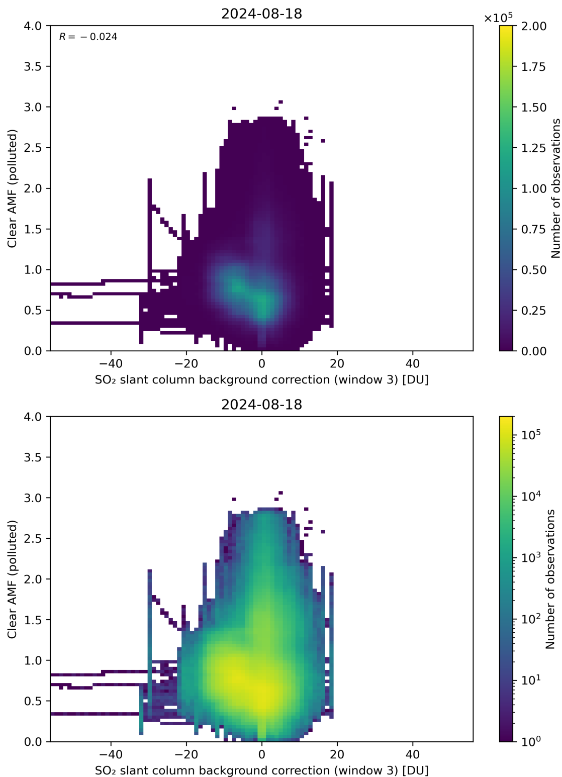
Figure 124: Scatter density plot of “SO 2 slant column background correction (window 3)” against “Clear AMF (polluted)” for 2024-08-17 to 2024-08-19.
