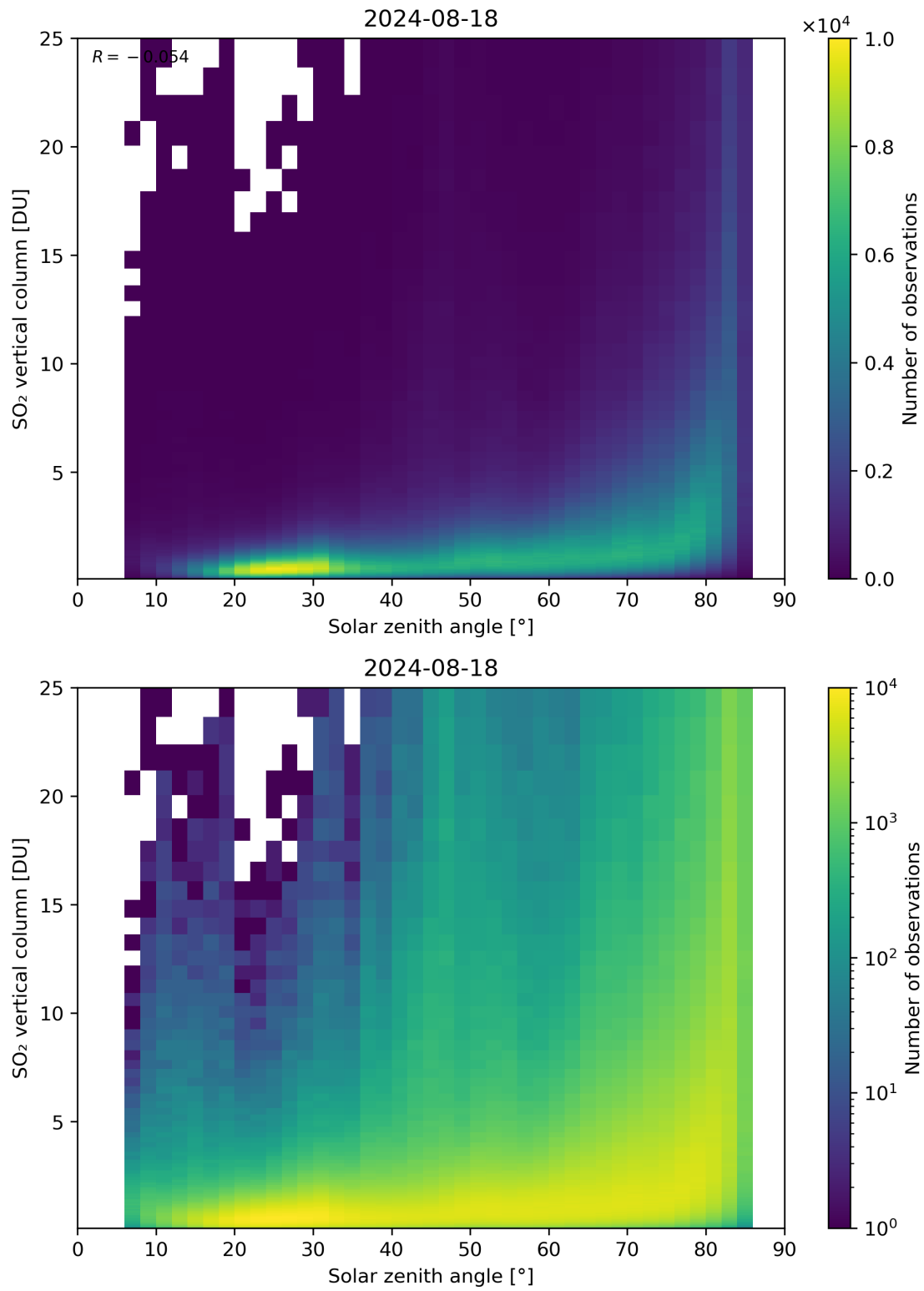
Figure 176: Scatter density plot of “Solar zenith angle” against “SO 2 vertical column” for 2024-08-17 to 2024-08-19.
