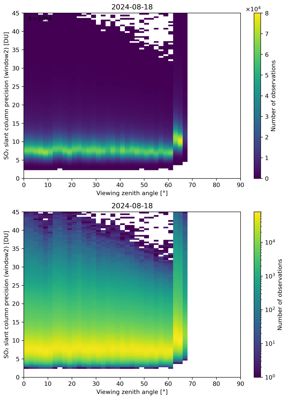
Figure 322: Scatter density plot of “Viewing zenith angle” against “SO 2 slant column precision (window2)” for 2024-08-17 to 2024-08-19.
