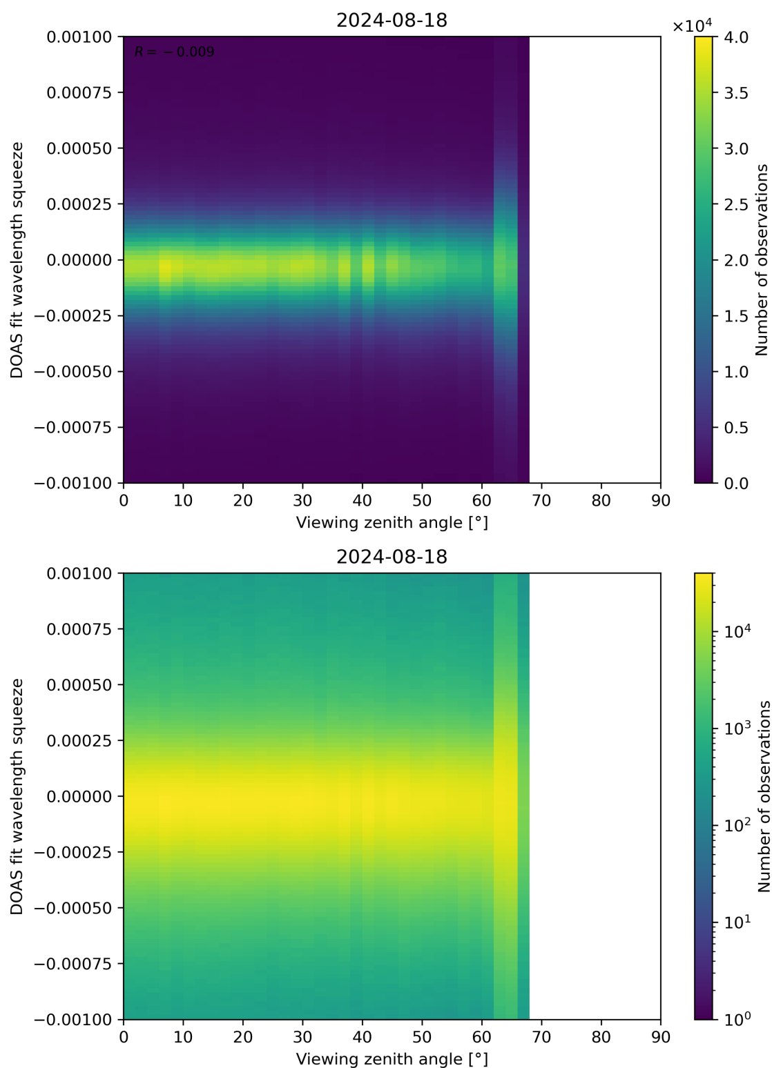
Figure 312: Scatter density plot of “Viewing zenith angle” against “DOAS fit wavelength squeeze” for 2024-08-17 to 2024-08-19.
