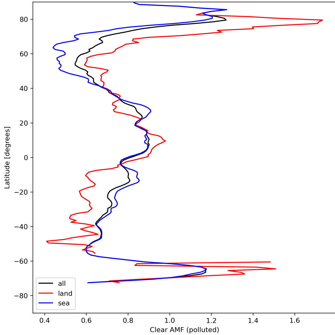
Figure 50: Zonal average of “Clear AMF (polluted)” for 2024-08-17 to 2024-08-19.
