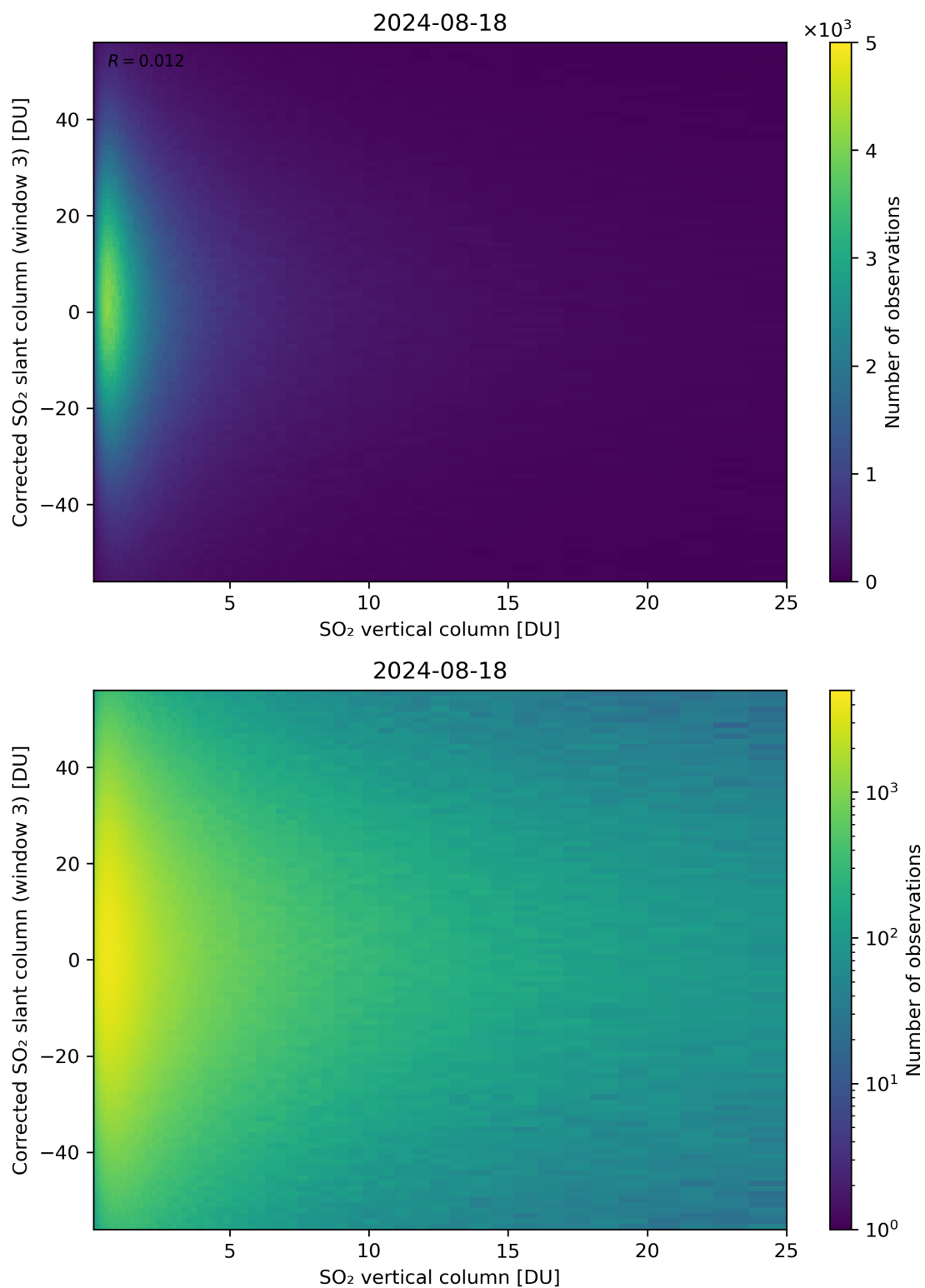
Figure 299: Scatter density plot of “SO 2 vertical column” against “Corrected SO 2 slant column (window 3)” for 2024-08-17 to 2024-08-19.
