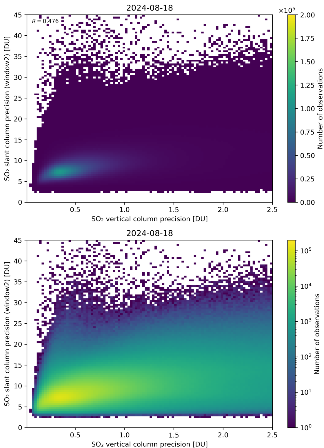
Figure 291: Scatter density plot of “SO 2 vertical column precision” against “SO 2 slant column precision (window2)” for 2024-08-17 to 2024-08-19.
