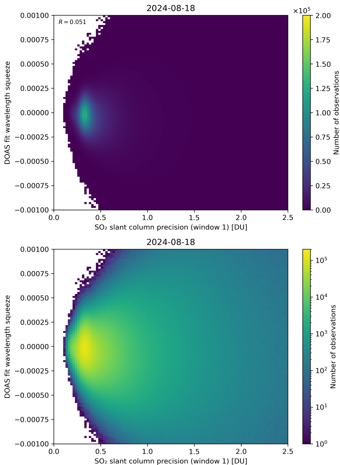
Figure 222: Scatter density plot of “SO 2 slant column precision (window 1)” against “DOAS fit wavelength squeeze” for 2024-08-17 to 2024-08-19.
