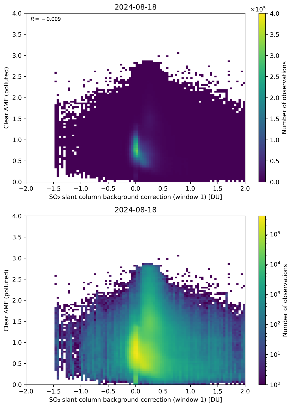
Figure 103: Scatter density plot of “SO 2 slant column background correction (window 1)” against “Clear AMF (polluted)” for 2024-08-17 to 2024-08-19.
