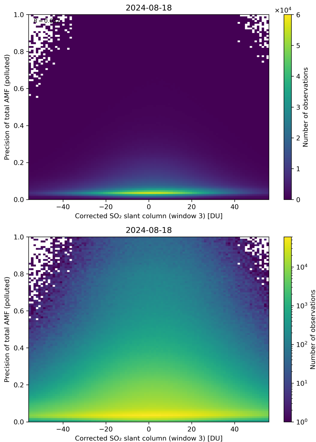
Figure 211: Scatter density plot of “Corrected SO 2 slant column (window 3)” against “Precision of total AMF (polluted)” for 2024-08-17 to 2024-08-19.
