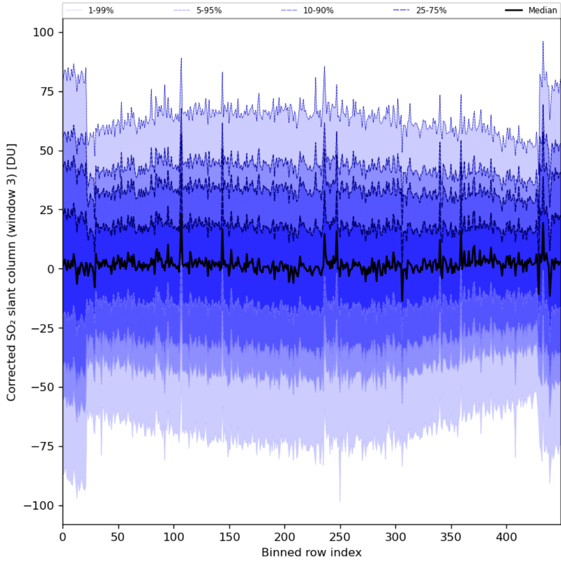
Figure 89: Along track statistics of “Corrected SO 2 slant column (window 3)” for 2024-08-17 to 2024-08-19
