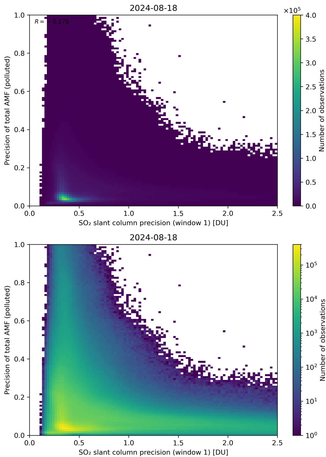
Figure 231: Scatter density plot of “SO 2 slant column precision (window 1)” against “Precision of total AMF (polluted)” for 2024-08-17 to 2024-08-19.
