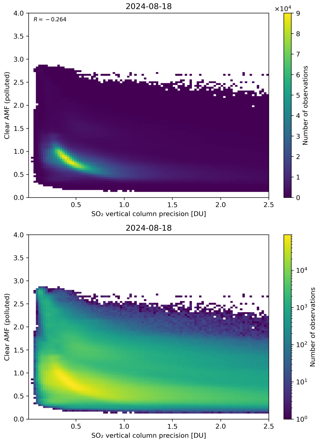
Figure 285: Scatter density plot of “SO 2 vertical column precision” against “Clear AMF (polluted)” for 2024-08-17 to 2024-08-19.
