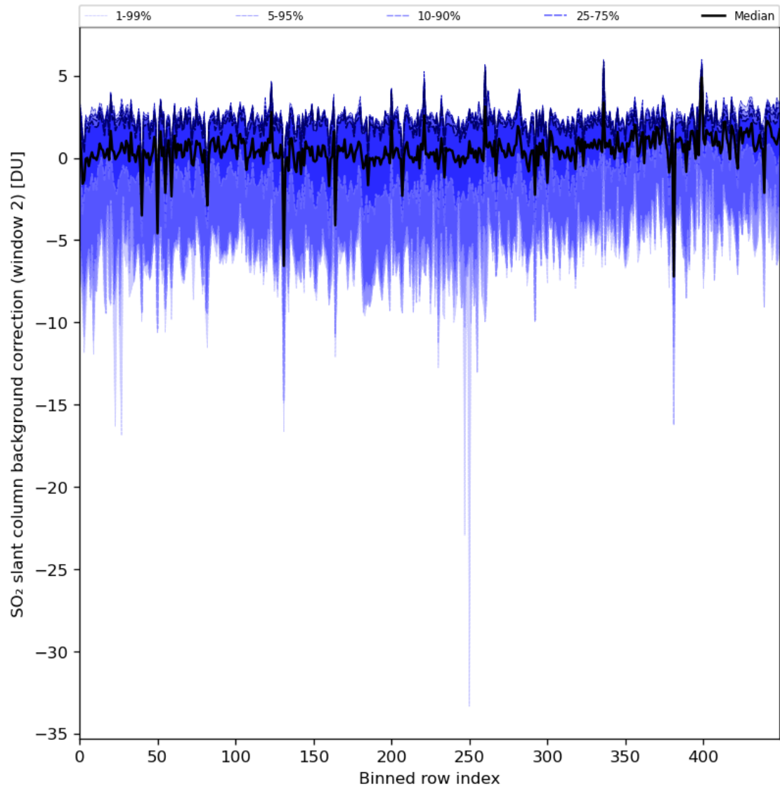
Figure 86: Along track statistics of “SO 2 slant column background correction (window 2)” for 2024-08-17 to 2024-08-19
