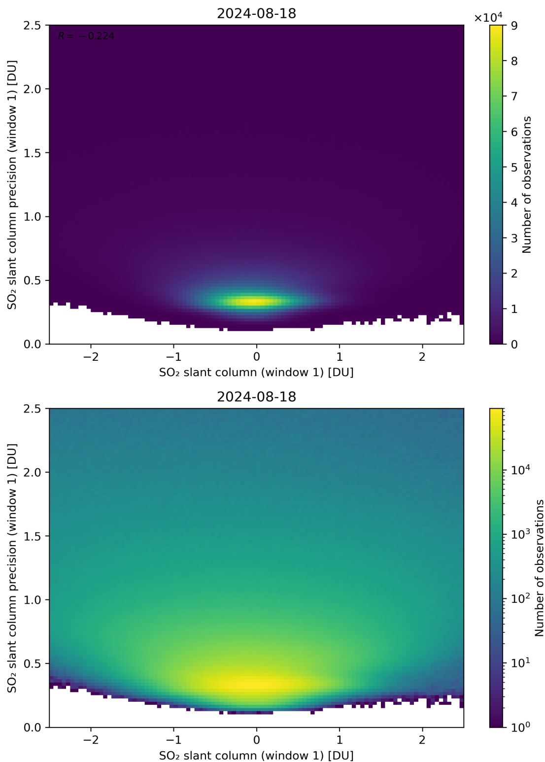
Figure 235: Scatter density plot of “SO 2 slant column (window 1)” against “SO 2 slant column precision (window 1)” for 2024-08-17 to 2024-08-19.
