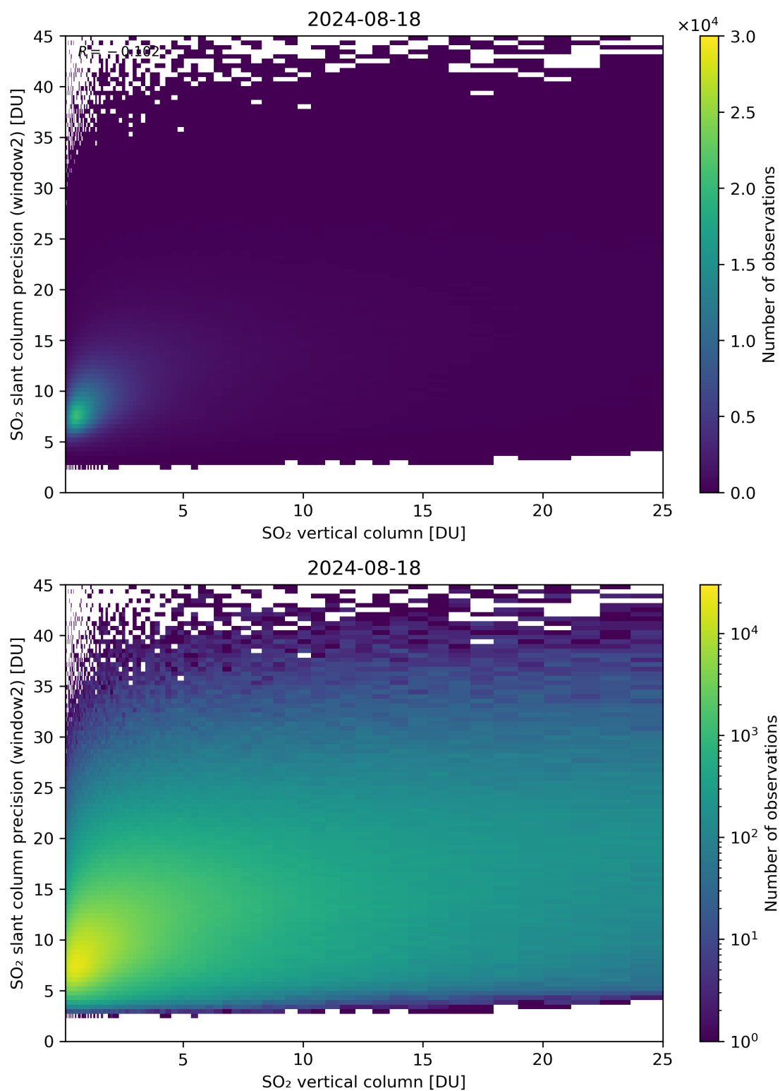
Figure 302: Scatter density plot of “SO 2 vertical column” against “SO 2 slant column precision (window2)” for 2024-08-17 to 2024-08-19.
