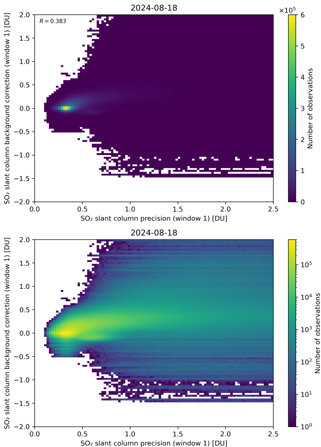
Figure 218: Scatter density plot of “SO 2 slant column precision (window 1)” against “SO 2 slant column background correction (window 1)” for 2024-08-17 to 2024-08-19.
