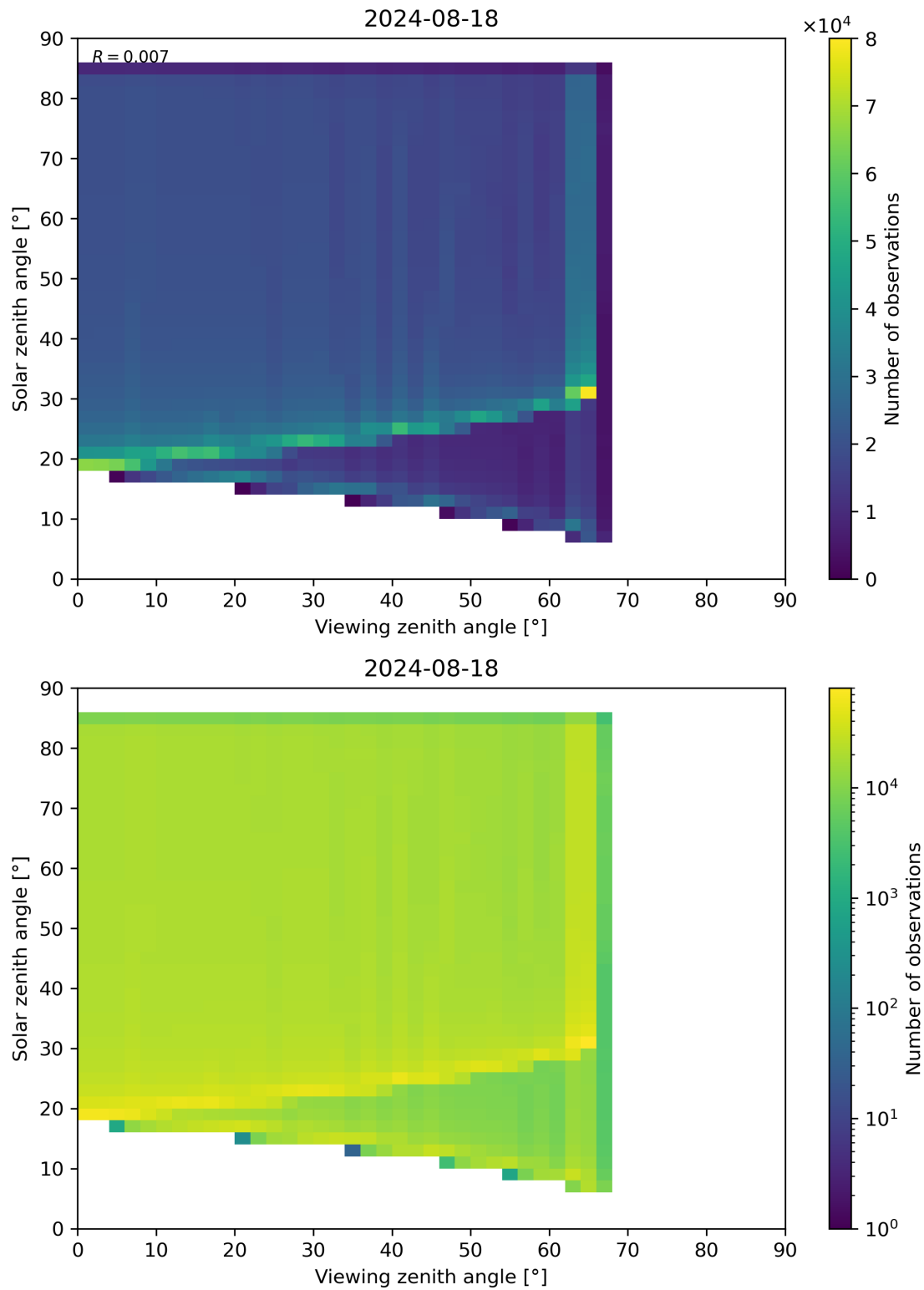
Figure 315: Scatter density plot of “Viewing zenith angle” against “Solar zenith angle” for 2024-08-17 to 2024-08-19.
