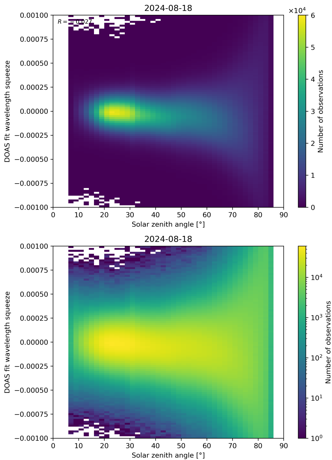
Figure 162: Scatter density plot of “Solar zenith angle” against “DOAS fit wavelength squeeze” for 2024-08-17 to 2024-08-19.
