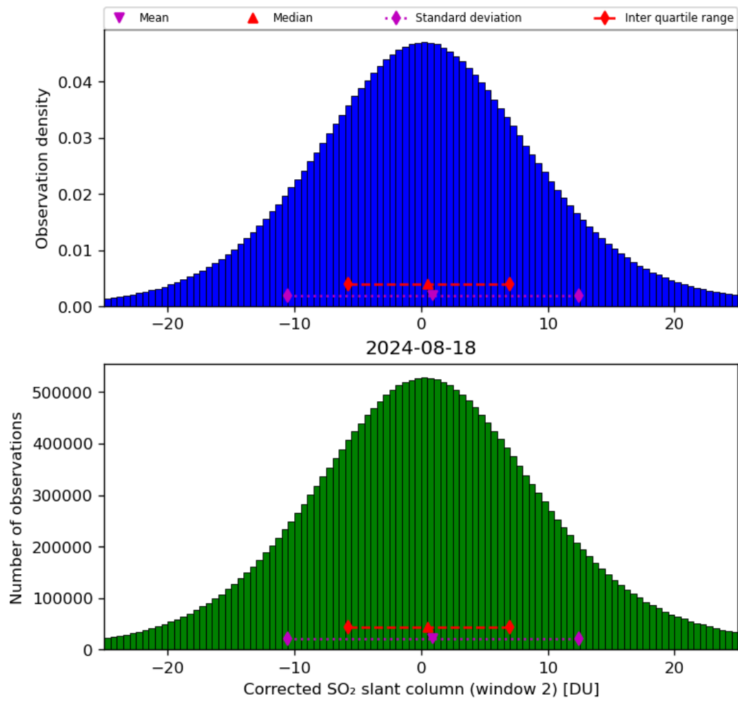
Figure 62: Histogram of “Corrected SO 2 slant column (window 2)” for 2024-08-17 to 2024-08-19
