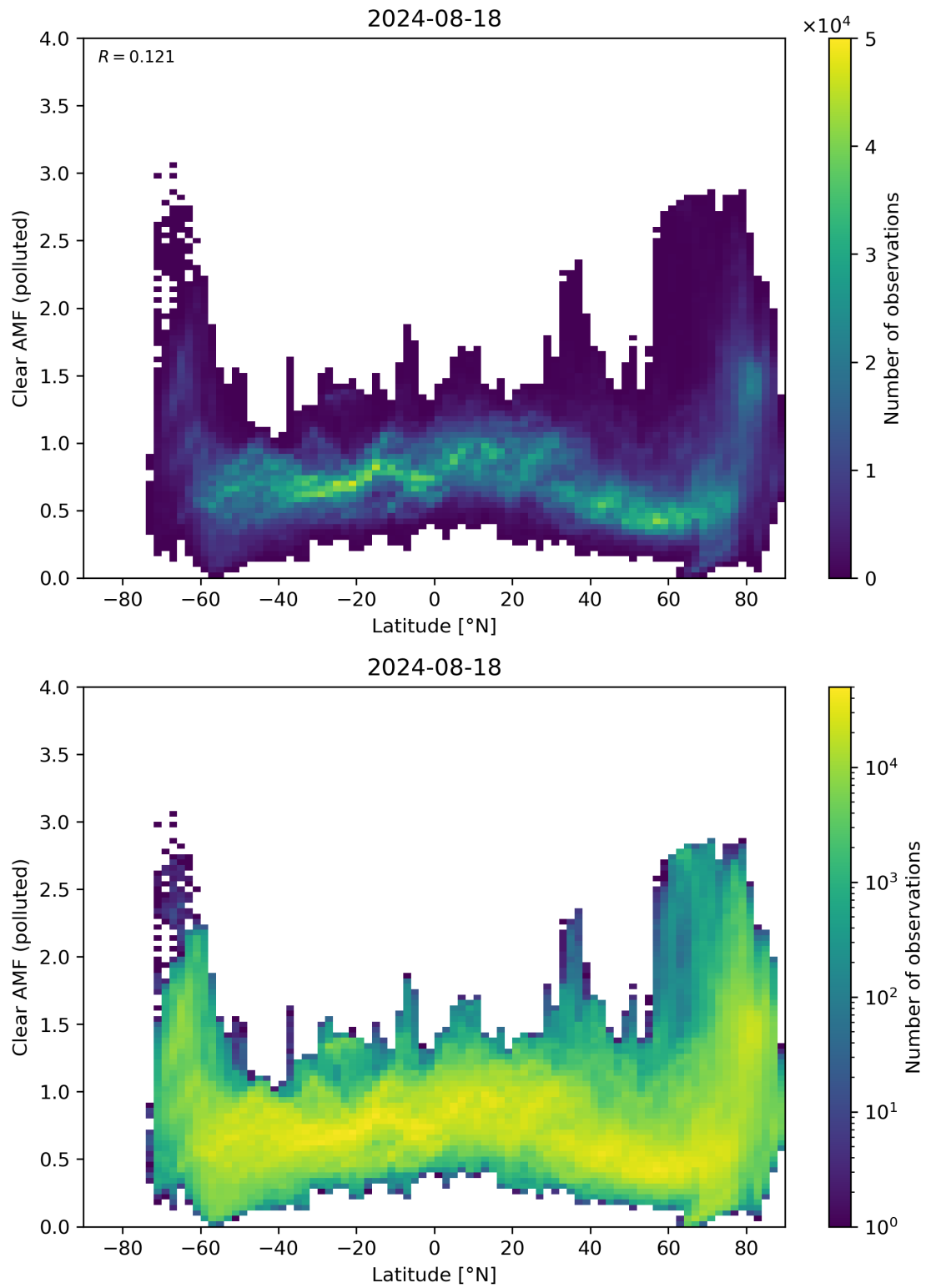
Figure 145: Scatter density plot of “Latitude” against “Clear AMF (polluted)” for 2024-08-17 to 2024-08-19.
