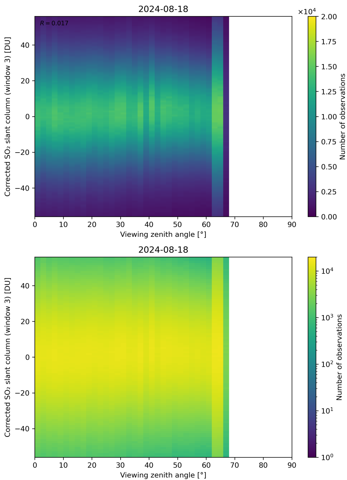
Figure 319: Scatter density plot of “Viewing zenith angle” against “Corrected SO 2 slant column (window 3)” for 2024-08-17 to 2024-08-19.
