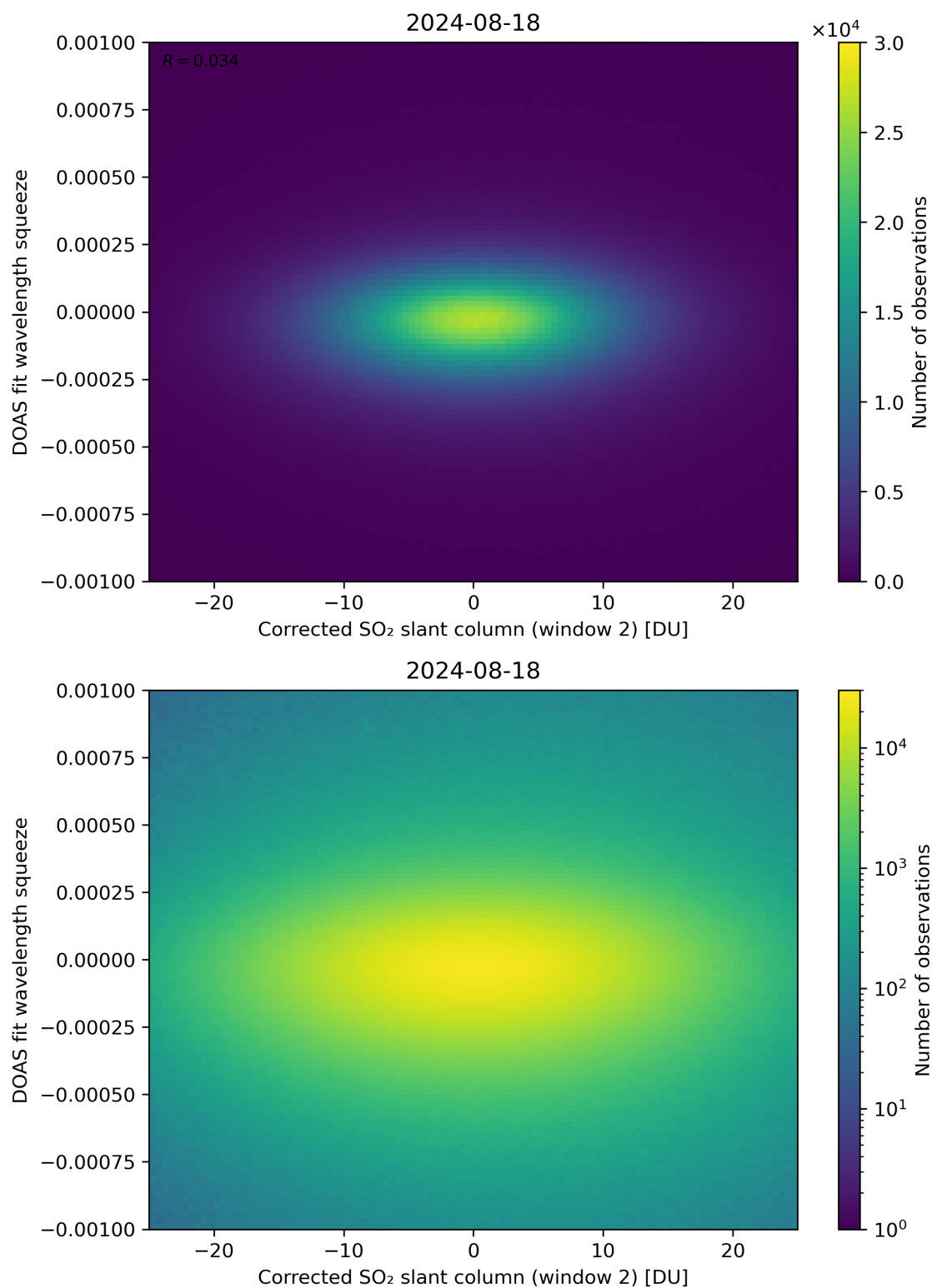
Figure 197: Scatter density plot of “Corrected SO 2 slant column (window 2)” against “DOAS fit wavelength squeeze” for 2024-08-17 to 2024-08-19.
