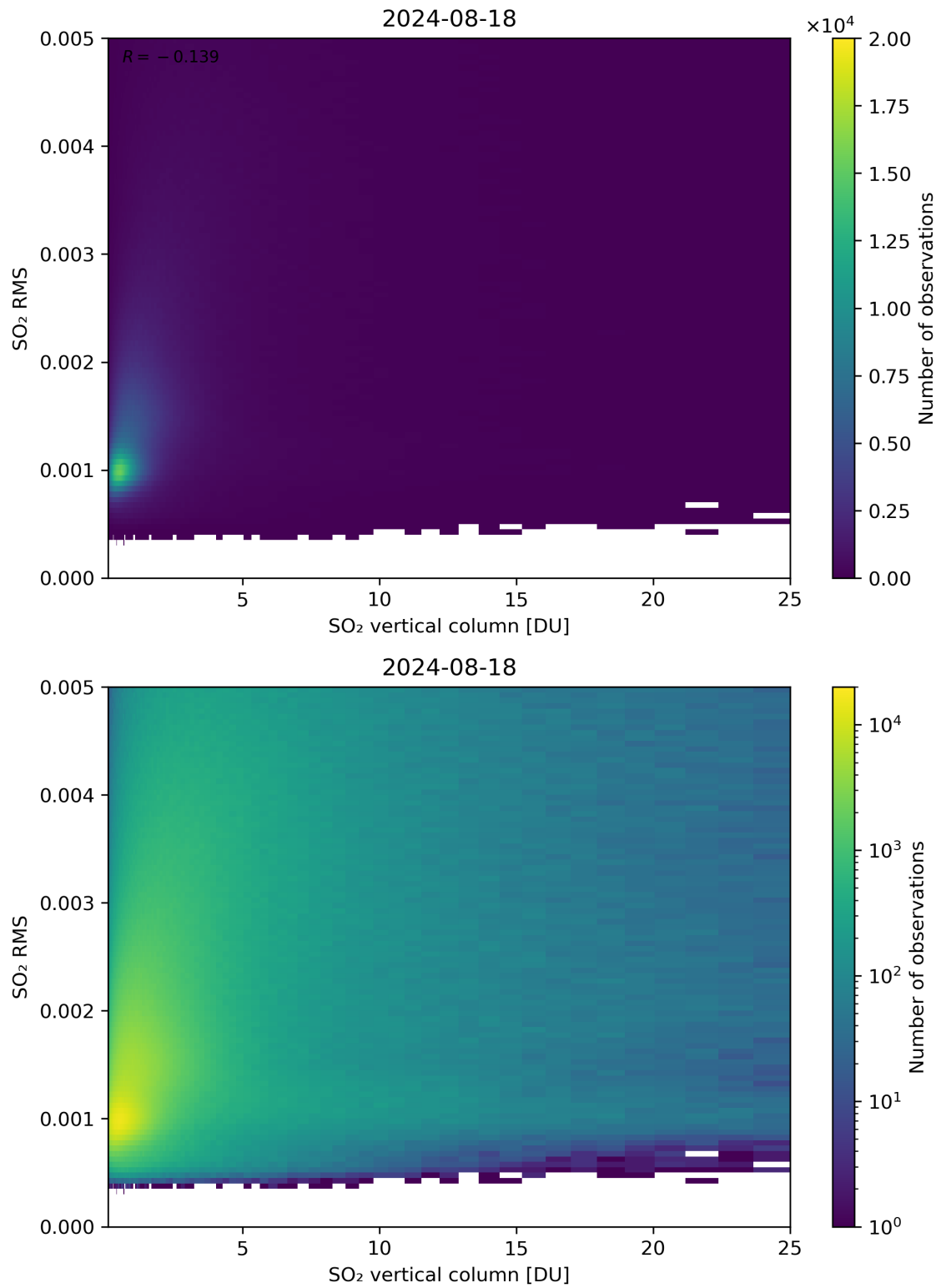
Figure 278: Scatter density plot of “SO 2 vertical column” against “SO 2 RMS” for 2024-08-17 to 2024-08-19.
