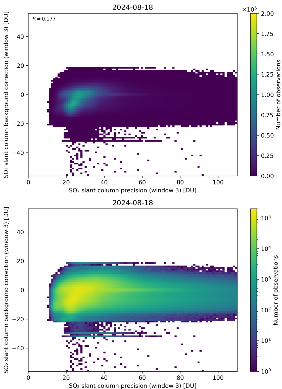
Figure 257: Scatter density plot of “SO 2 slant column precision (window 3)” against “SO 2 slant column background correction (window 3)” for 2024-08-17 to 2024-08-19.
