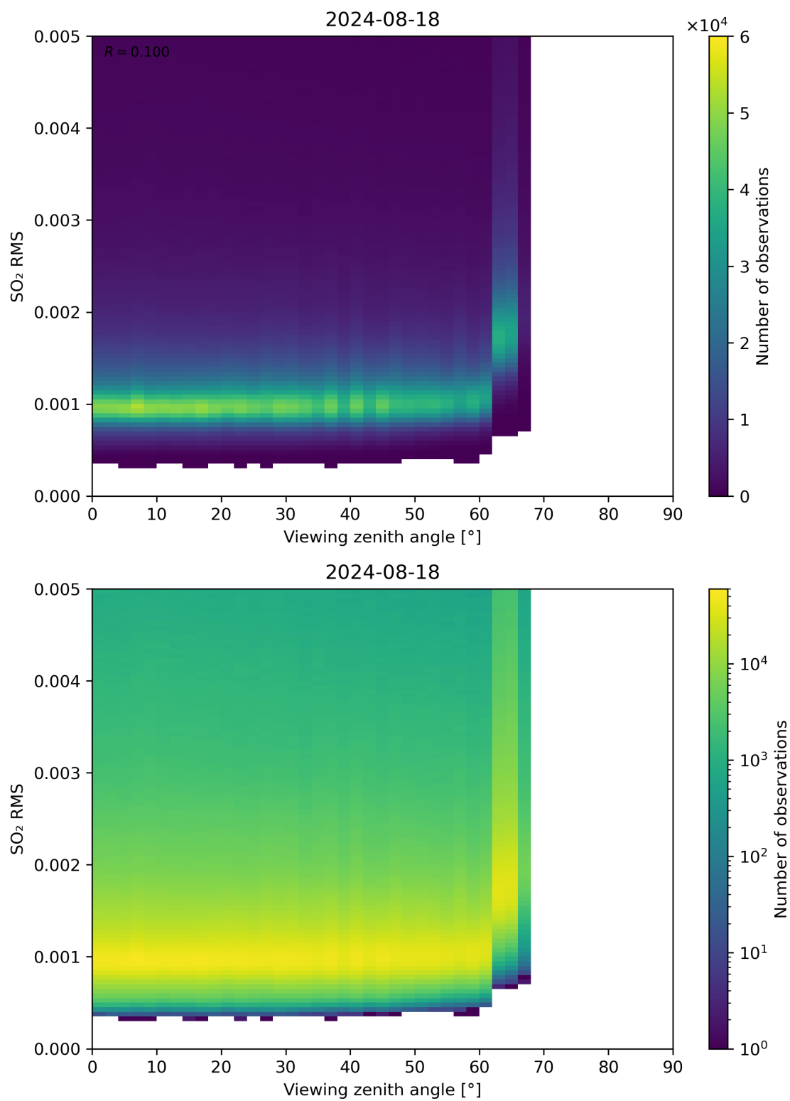
Figure 313: Scatter density plot of “Viewing zenith angle” against “SO 2 RMS” for 2024-08-17 to 2024-08-19.
