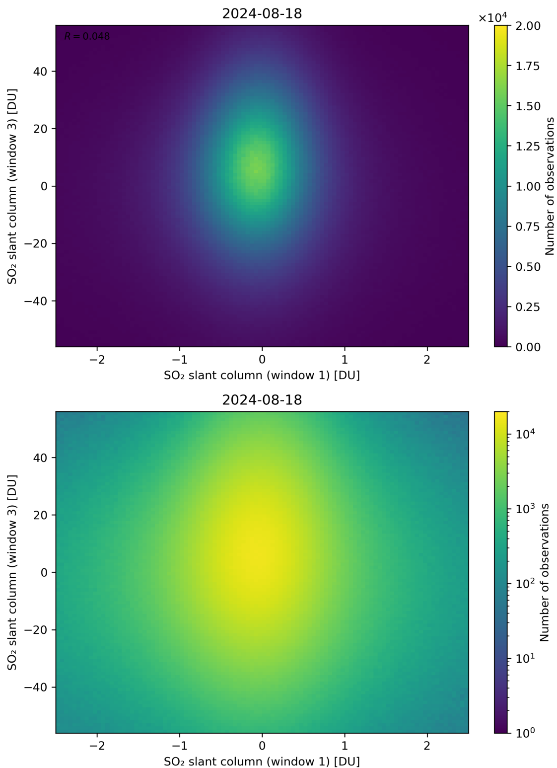
Figure 237: Scatter density plot of “SO 2 slant column (window 1)” against “SO 2 slant column (window 3)” for 2024-08-17 to 2024-08-19.
