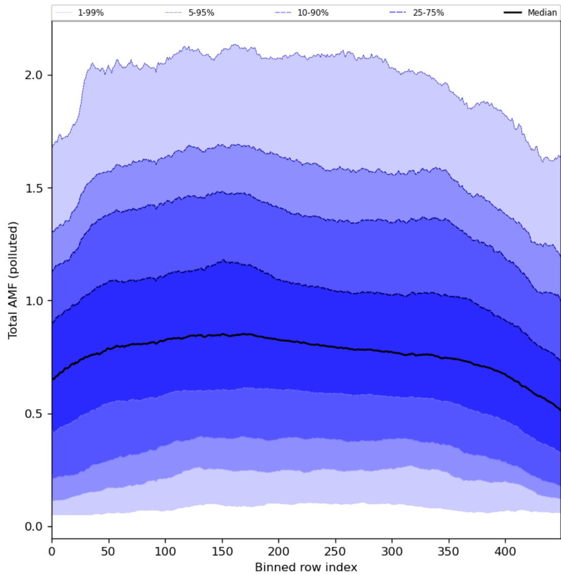
Figure 94: Along track statistics of “Total AMF (polluted)” for 2024-08-17 to 2024-08-19
