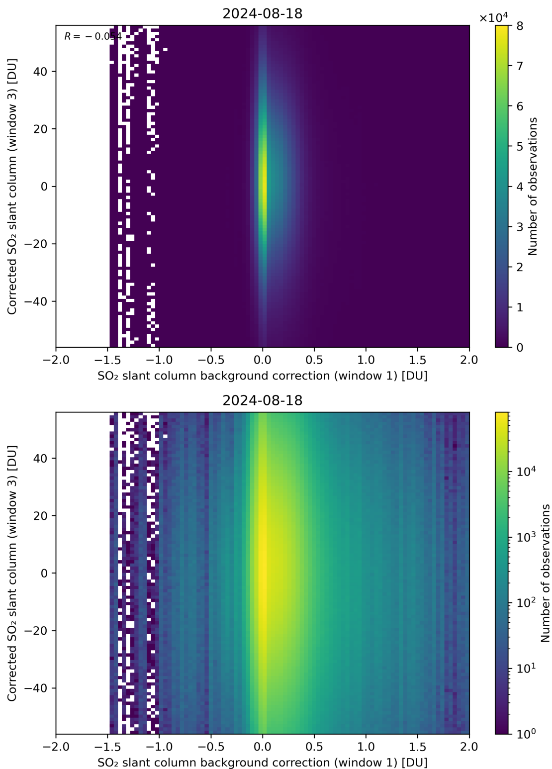
Figure 105: Scatter density plot of “SO 2 slant column background correction (window 1)” against “Corrected SO 2 slant column (window 3)” for 2024-08-17 to 2024-08-19.
