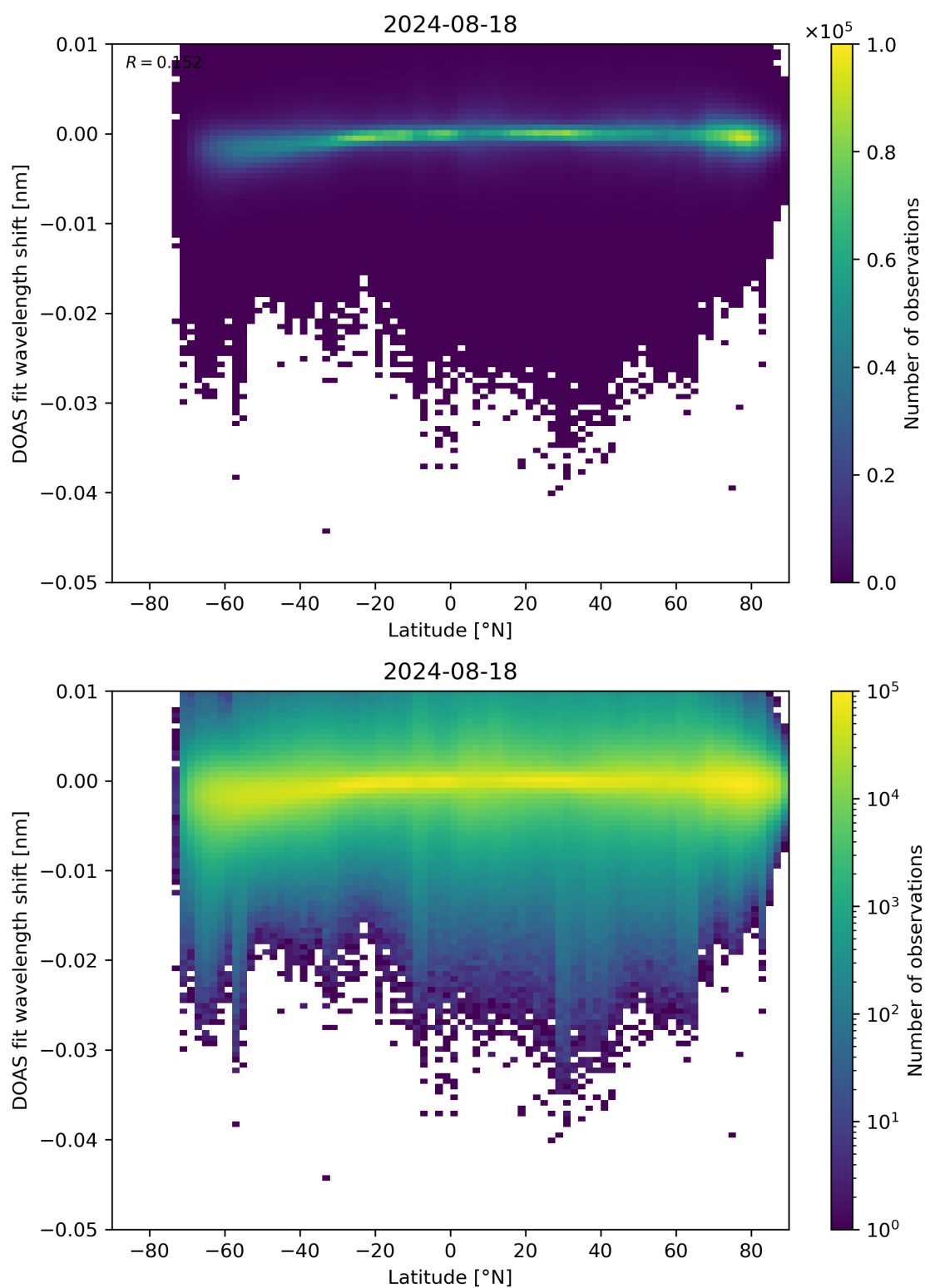
Figure 142: Scatter density plot of “Latitude” against “DOAS fit wavelength shift” for 2024-08-17 to 2024-08-19.
