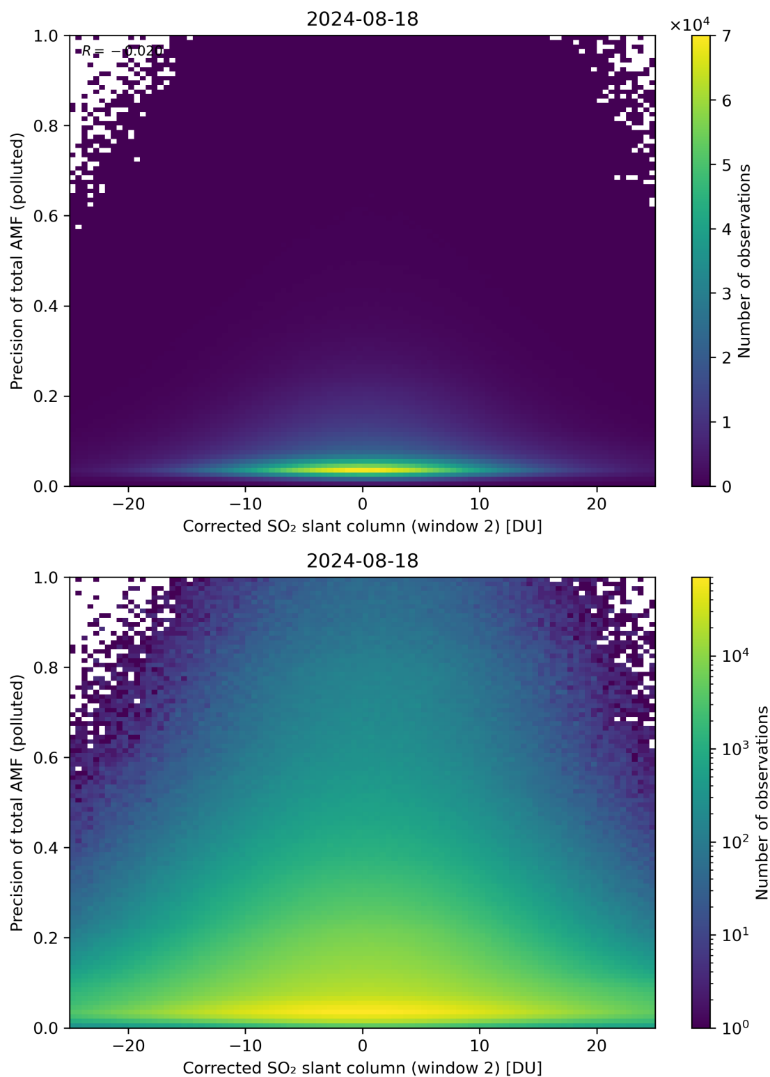
Figure 204: Scatter density plot of “Corrected SO 2 slant column (window 2)” against “Precision of total AMF (polluted)” for 2024-08-17 to 2024-08-19.
