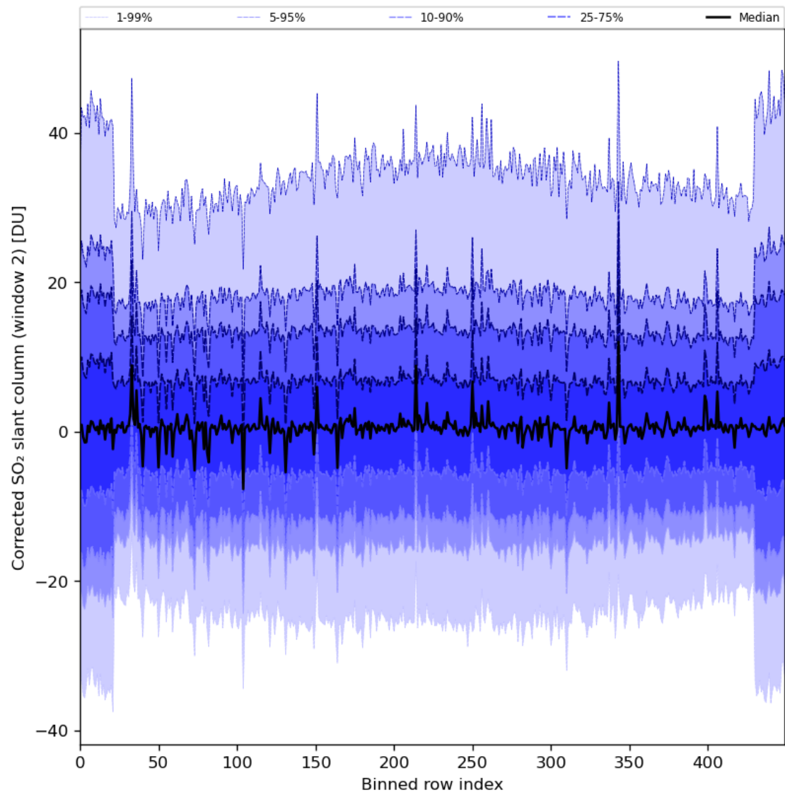
Figure 85: Along track statistics of “Corrected SO 2 slant column (window 2)” for 2024-08-17 to 2024-08-19
