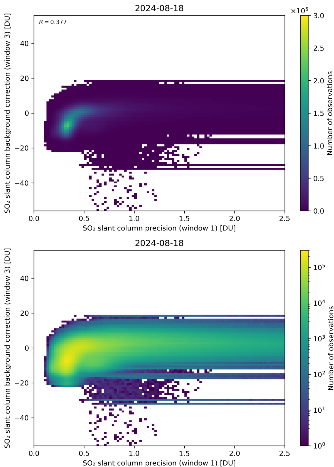
Figure 220: Scatter density plot of “SO 2 slant column precision (window 1)” against “SO 2 slant column background correction (window 3)” for 2024-08-17 to 2024-08-19.
