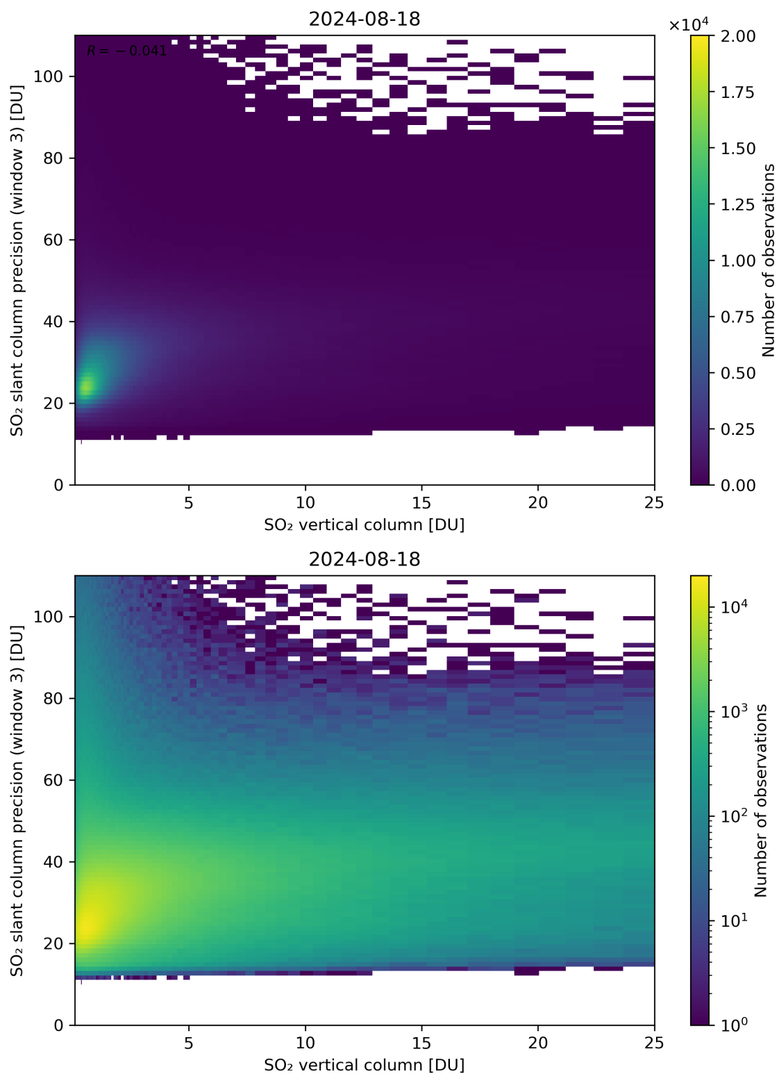
Figure 304: Scatter density plot of “SO 2 vertical column” against “SO 2 slant column precision (window 3)” for 2024-08-17 to 2024-08-19.
