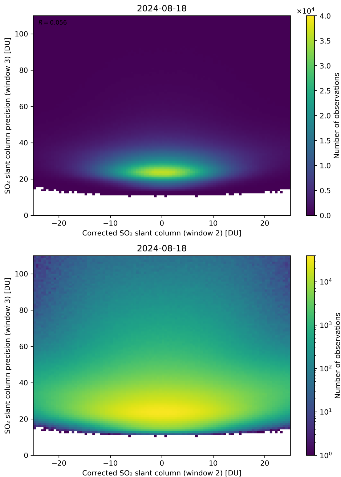
Figure 202: Scatter density plot of “Corrected SO 2 slant column (window 2)” against “SO 2 slant column precision (window 3)” for 2024-08-17 to 2024-08-19.
