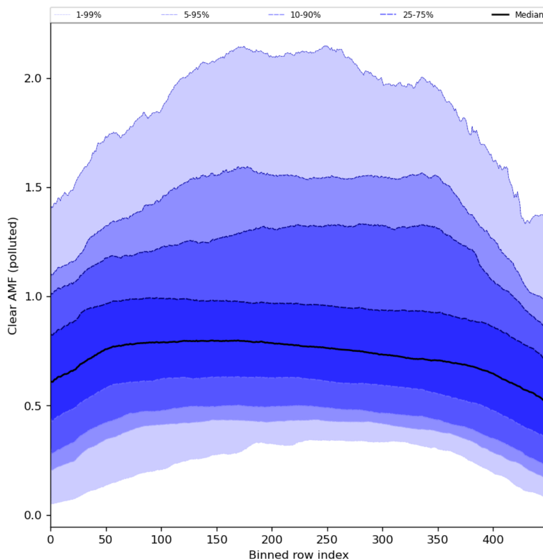
Figure 96: Along track statistics of “Clear AMF (polluted)” for 2024-08-17 to 2024-08-19
