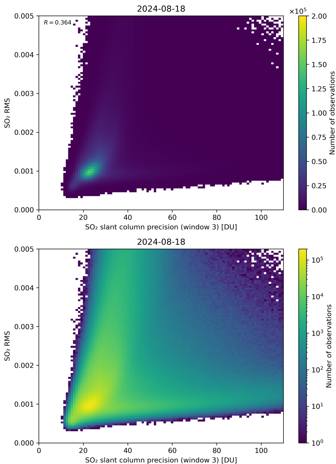
Figure 260: Scatter density plot of “SO 2 slant column precision (window 3)” against “SO 2 RMS” for 2024-08-17 to 2024-08-19.
