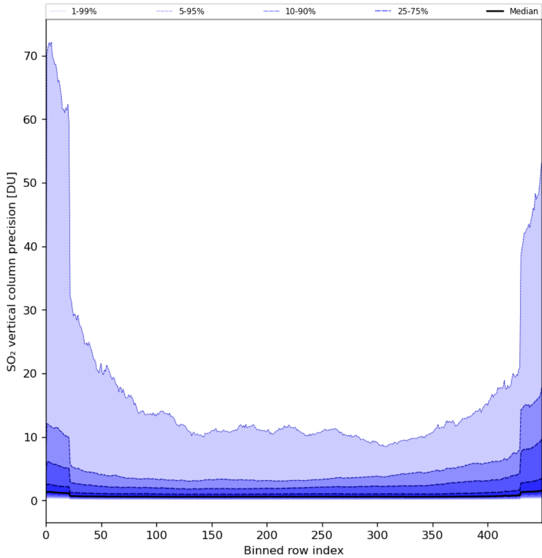
Figure 77: Along track statistics of “SO 2 vertical column precision” for 2024-08-17 to 2024-08-19
