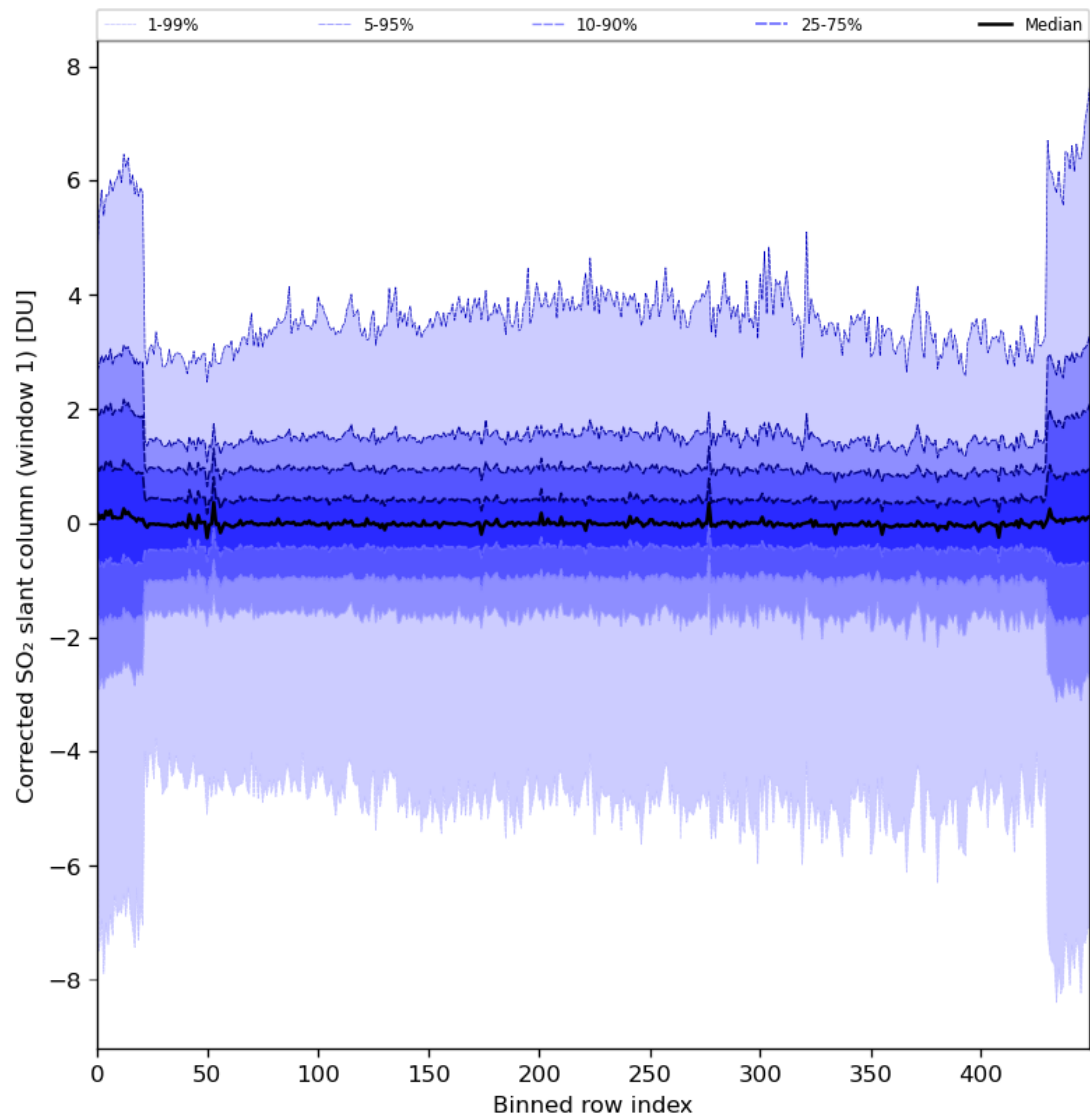
Figure 81: Along track statistics of “Corrected SO 2 slant column (window 1)” for 2024-08-17 to 2024-08-19
