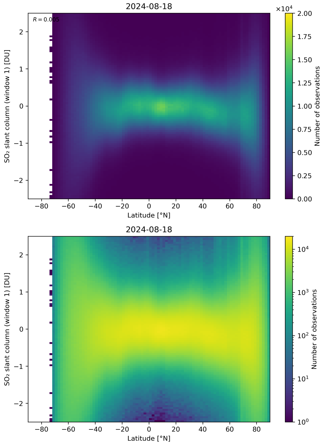
Figure 149: Scatter density plot of “Latitude” against “SO 2 slant column (window 1)” for 2024-08-17 to 2024-08-19.
