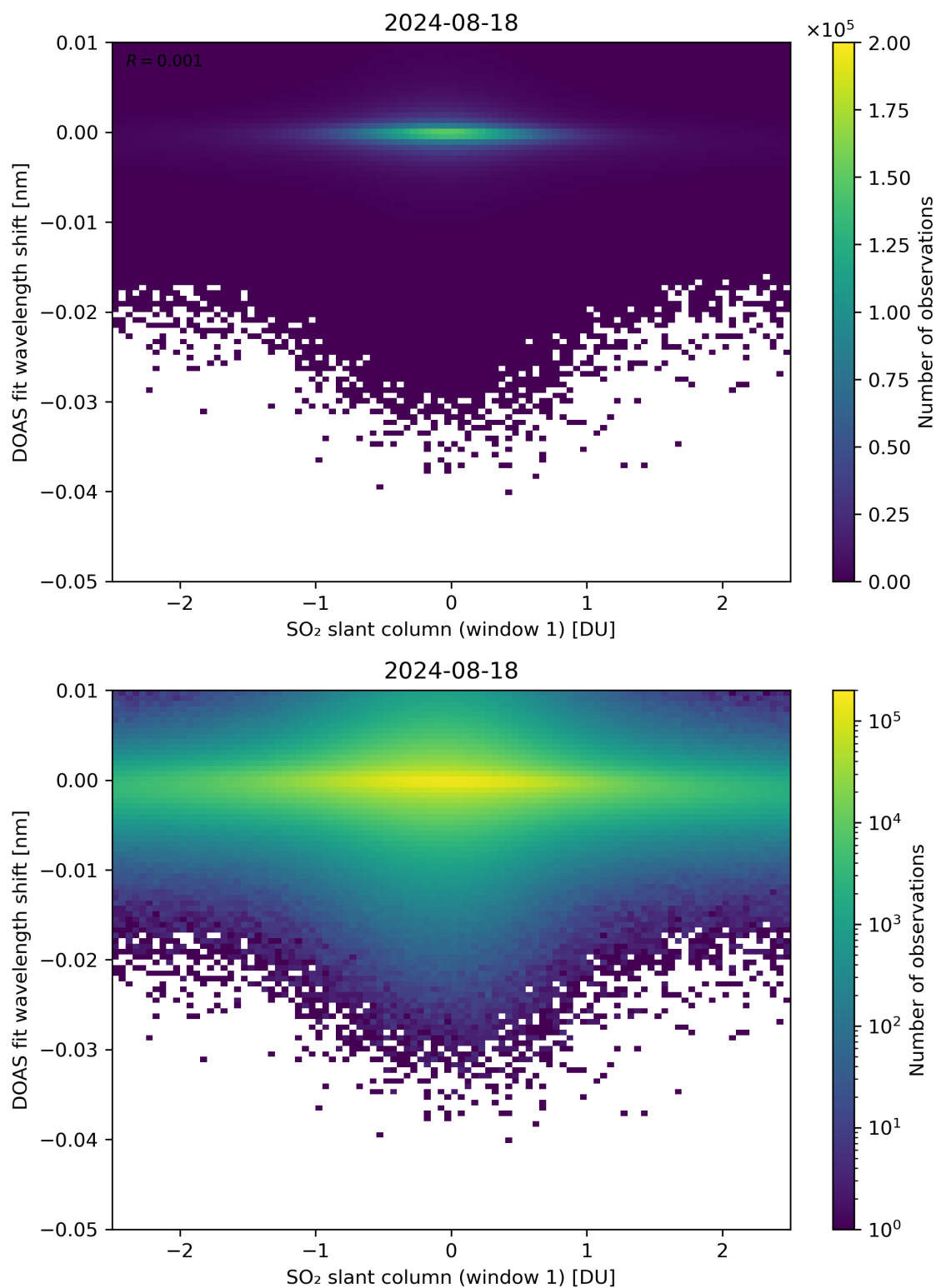
Figure 215: Scatter density plot of “SO 2 slant column (window 1)” against “DOAS fit wavelength shift” for 2024-08-17 to 2024-08-19.
