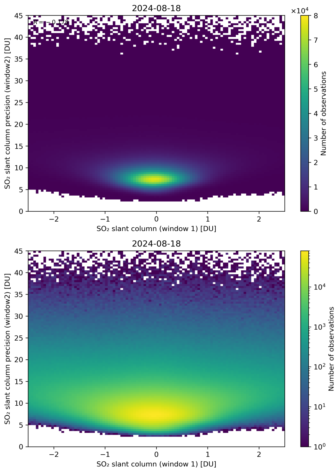
Figure 236: Scatter density plot of “SO 2 slant column (window 1)” against “SO 2 slant column precision (window2)” for 2024-08-17 to 2024-08-19.
