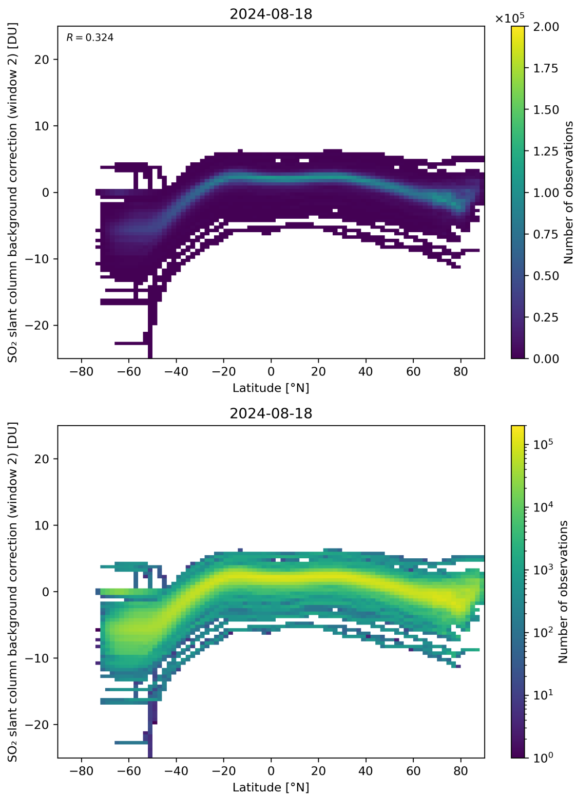
Figure 140: Scatter density plot of “Latitude” against “SO 2 slant column background correction (window 2)” for 2024-08-17 to 2024-08-19.
