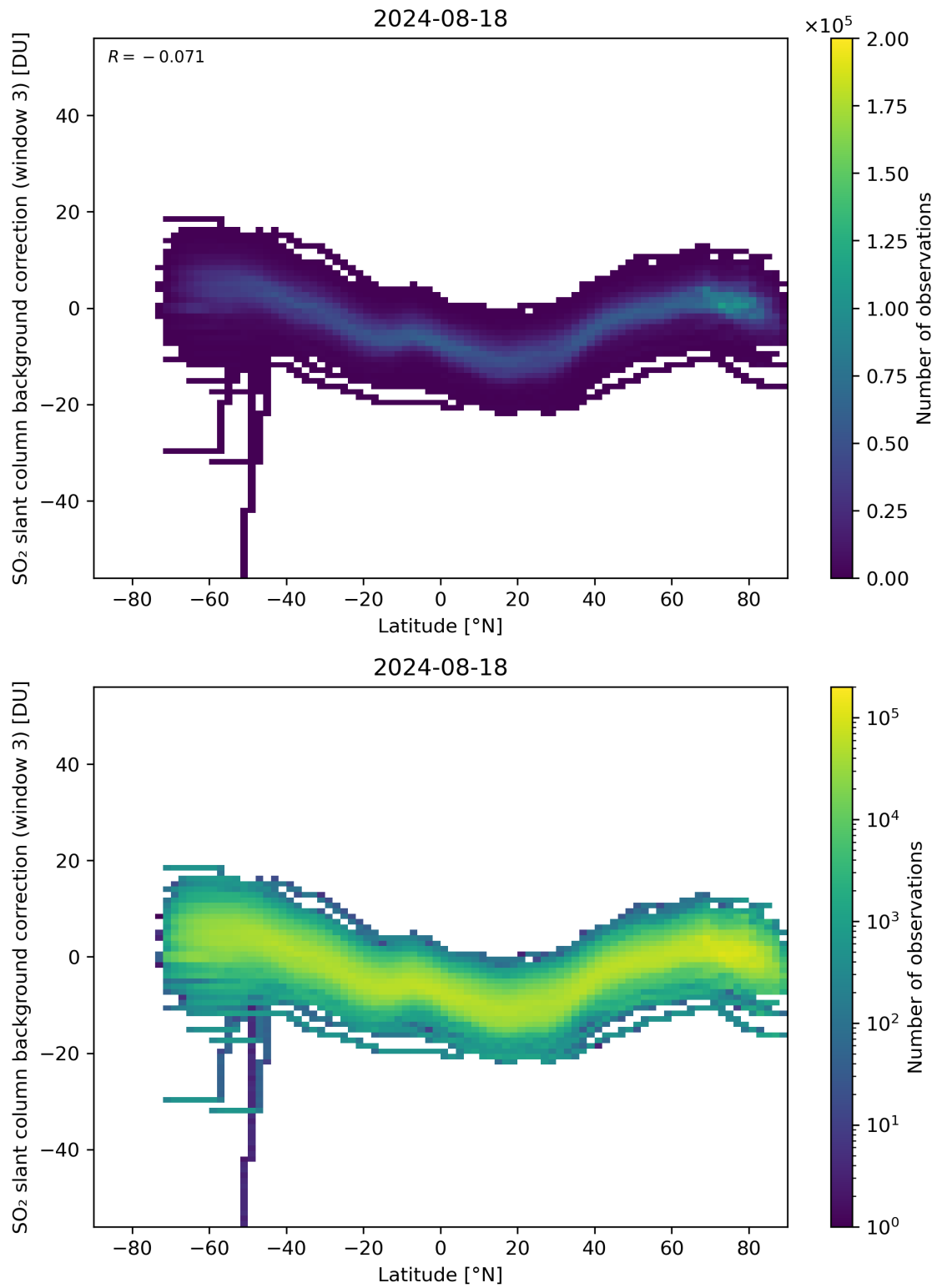
Figure 141: Scatter density plot of “Latitude” against “SO 2 slant column background correction (window 3)” for 2024-08-17 to 2024-08-19.
