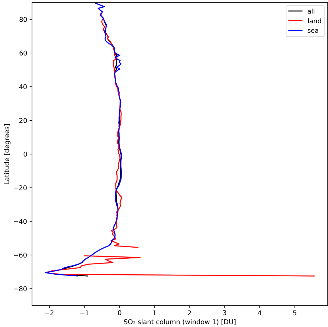
Figure 33: Zonal average of “SO 2 slant column (window 1)” for 2024-08-17 to 2024-08-19.
