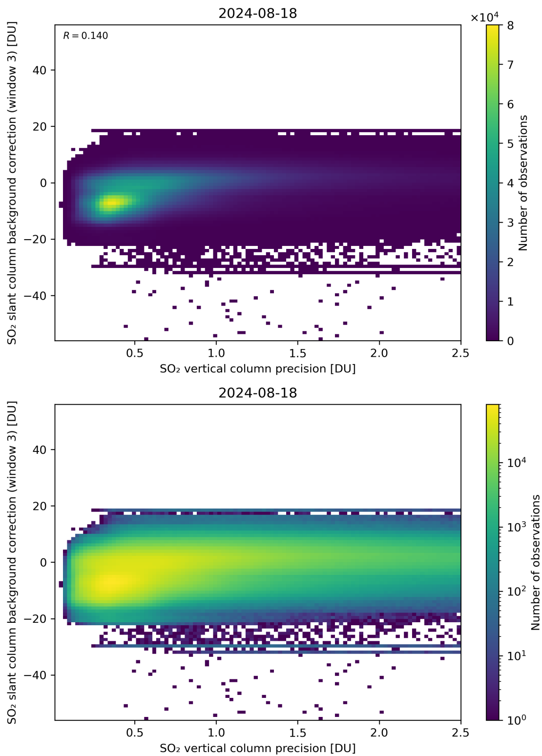
Figure 281: Scatter density plot of “SO 2 vertical column precision” against “SO 2 slant column background correction (window 3)” for 2024-08-17 to 2024-08-19.
