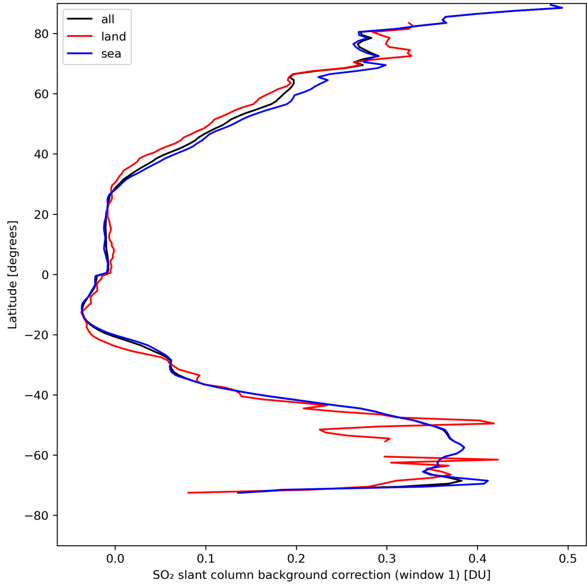
Figure 36: Zonal average of “SO 2 slant column background correction (window 1)” for 2024-08-17 to 2024-08-19.
