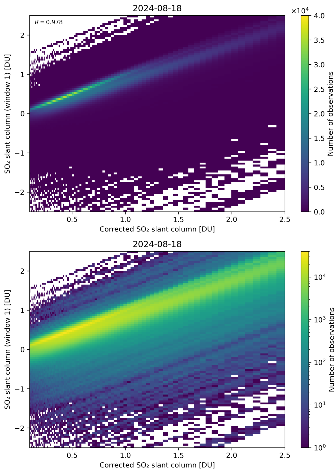
Figure 187: Scatter density plot of “Corrected SO 2 slant column” against “SO 2 slant column (window 1)” for 2024-08-17 to 2024-08-19.
