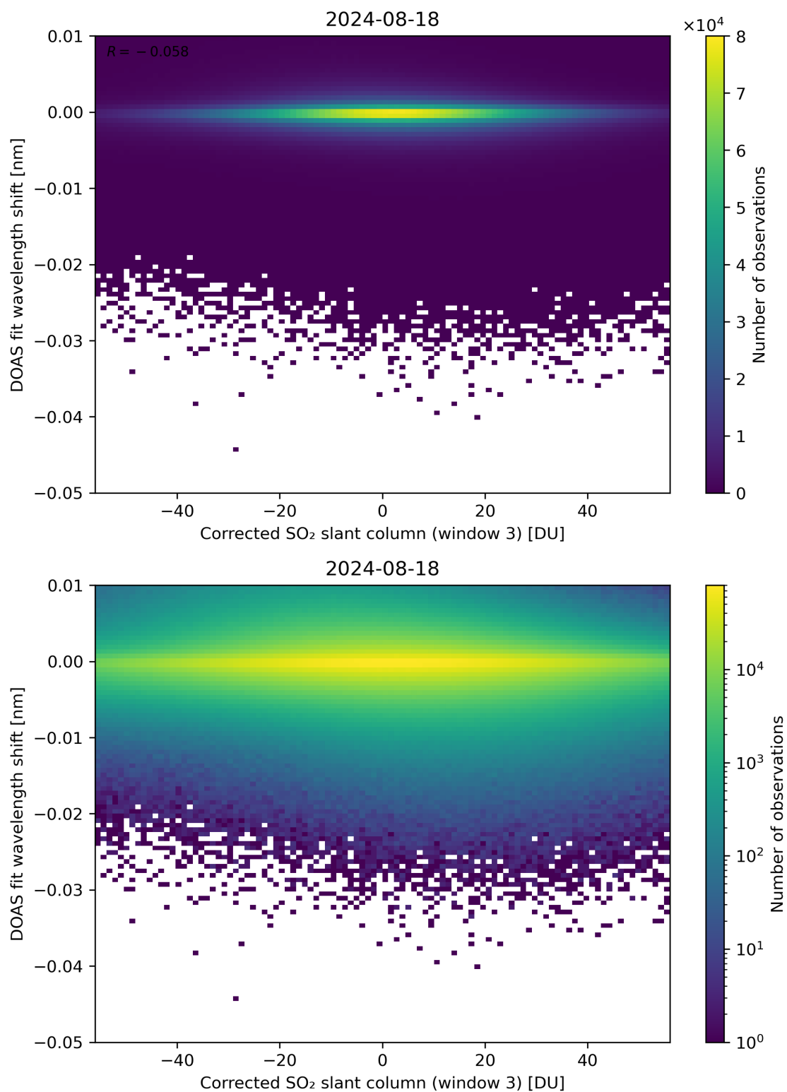
Figure 206: Scatter density plot of “Corrected SO 2 slant column (window 3)” against “DOAS fit wavelength shift” for 2024-08-17 to 2024-08-19.
