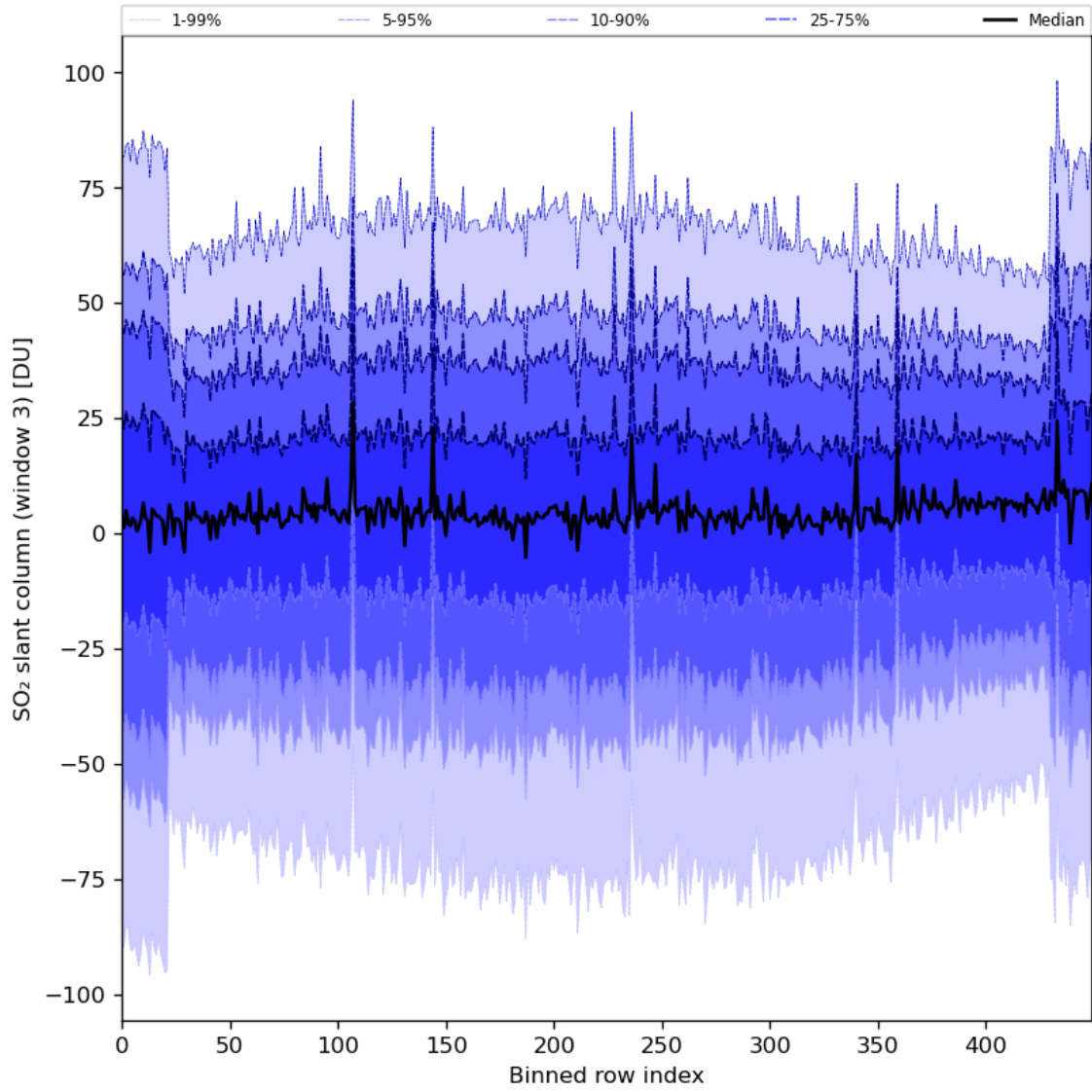
Figure 87: Along track statistics of “SO 2 slant column (window 3)” for 2024-08-17 to 2024-08-19
