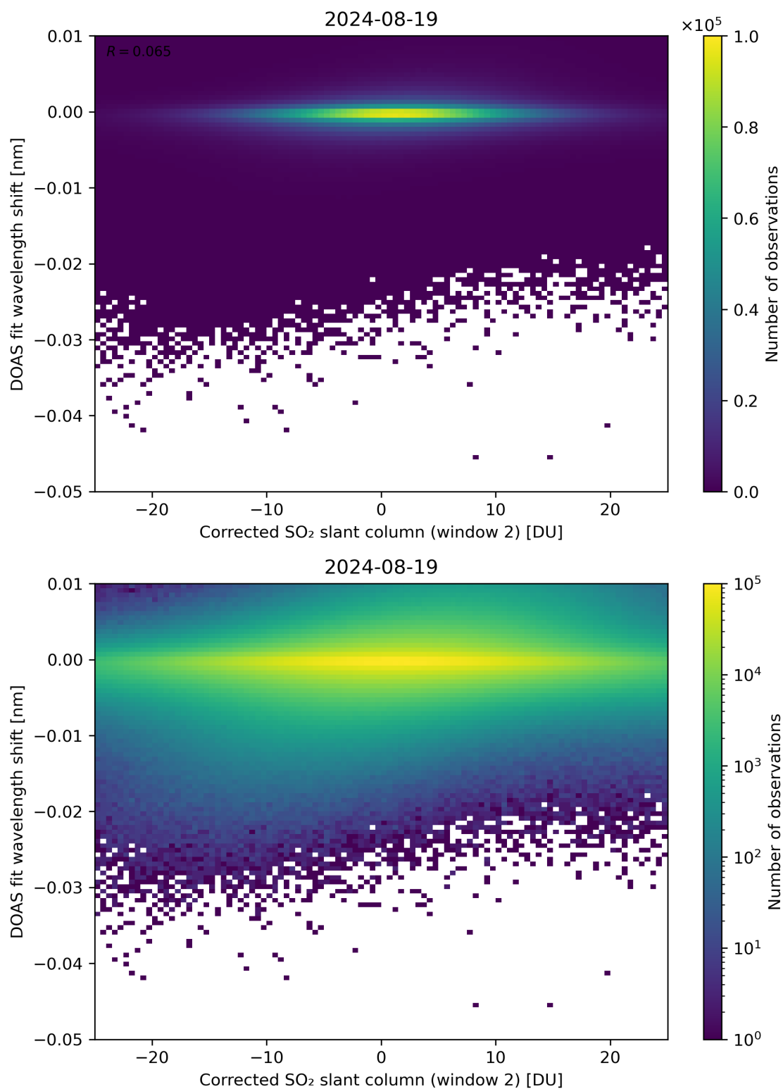
Figure 196: Scatter density plot of “Corrected SO 2 slant column (window 2)” against “DOAS fit wavelength shift” for 2024-08-18 to 2024-08-20.
