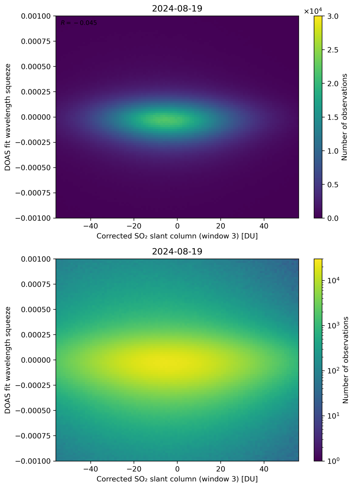
Figure 207: Scatter density plot of “Corrected SO 2 slant column (window 3)” against “DOAS fit wavelength squeeze” for 2024-08-18 to 2024-08-20.
