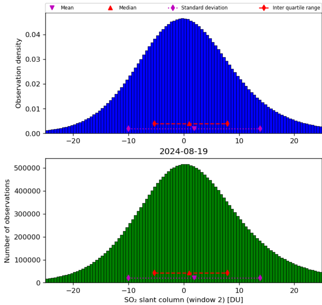
Figure 60: Histogram of “SO 2 slant column (window 2)” for 2024-08-18 to 2024-08-20
