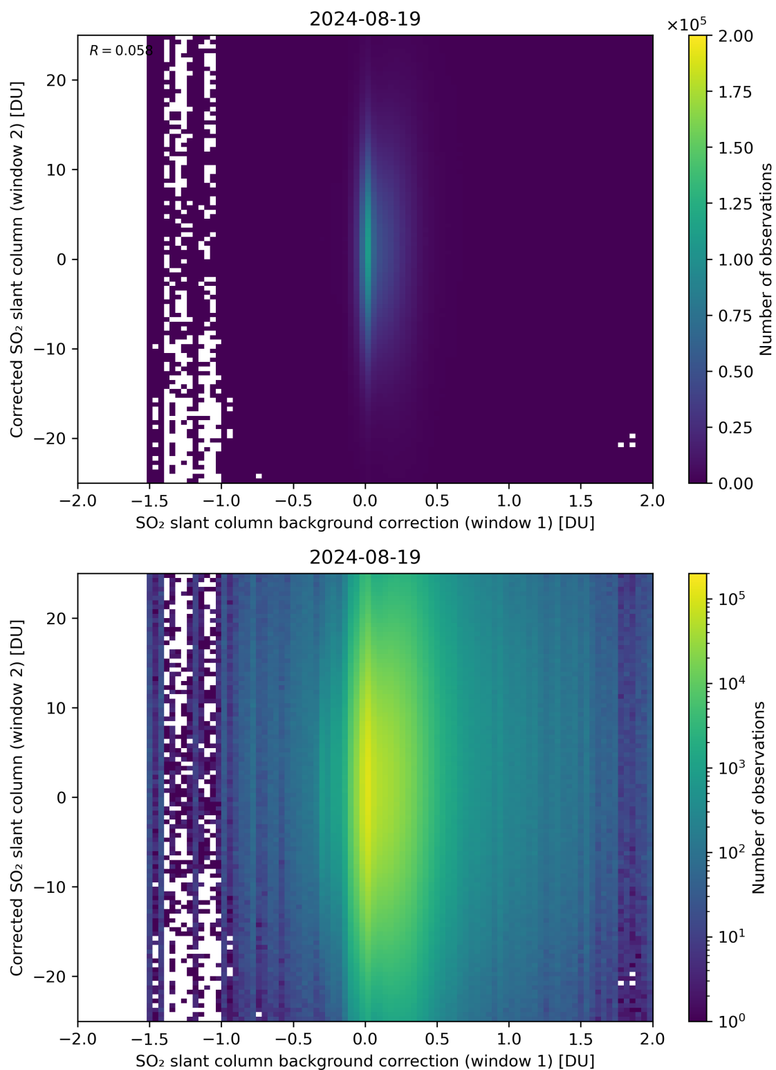
Figure 104: Scatter density plot of “SO 2 slant column background correction (window 1)” against “Corrected SO 2 slant column (window 2)” for 2024-08-18 to 2024-08-20.
