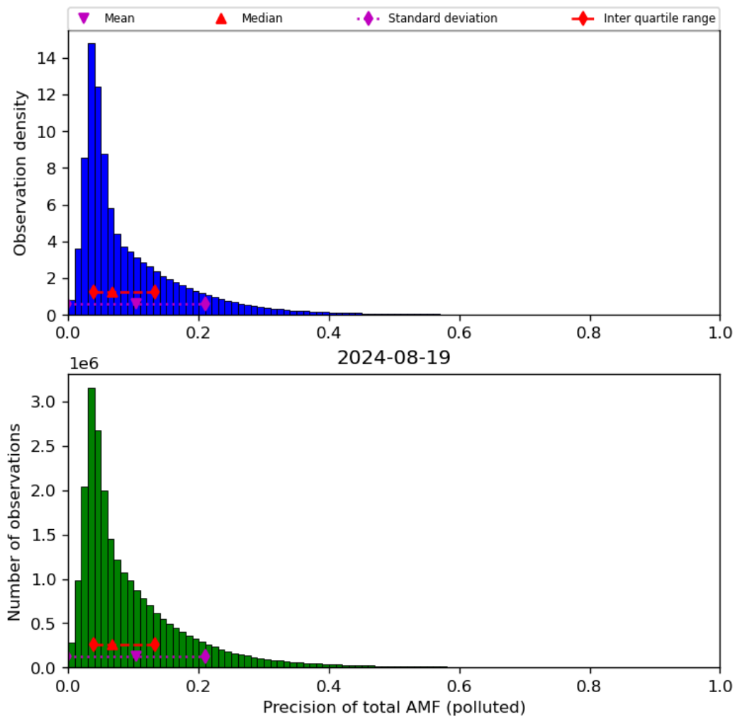
Figure 72: Histogram of “Precision of total AMF (polluted)” for 2024-08-18 to 2024-08-20
