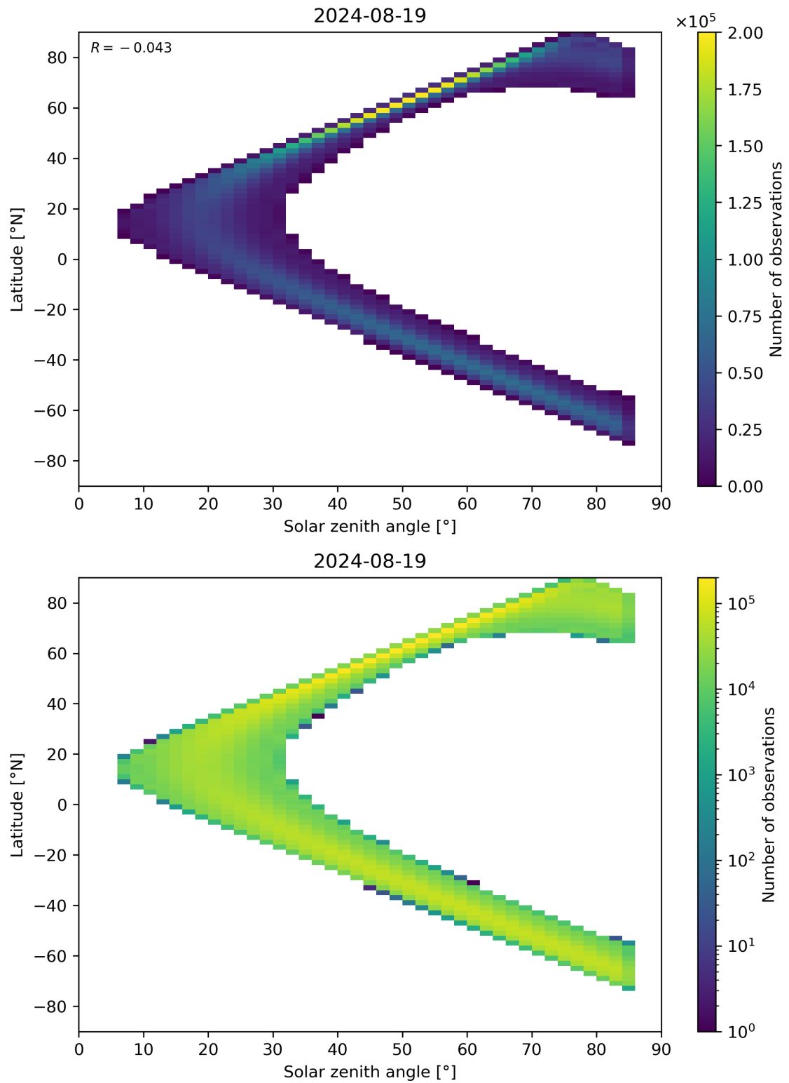
Figure 164: Scatter density plot of “Solar zenith angle” against “Latitude” for 2024-08-18 to 2024-08-20.
