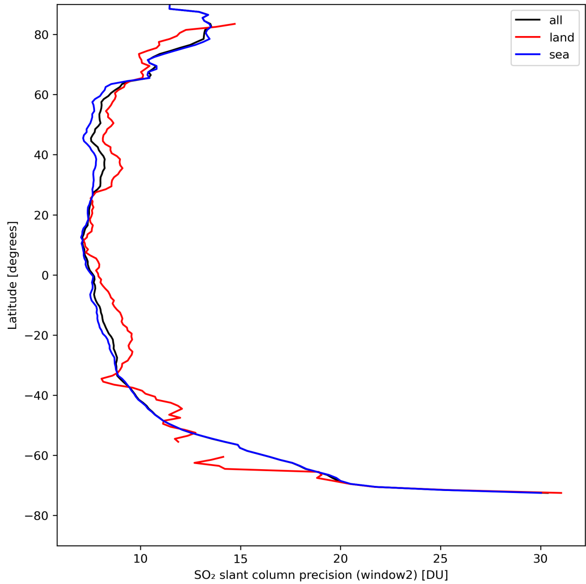
Figure 38: Zonal average of “SO 2 slant column precision (window2)” for 2024-08-18 to 2024-08-20.
