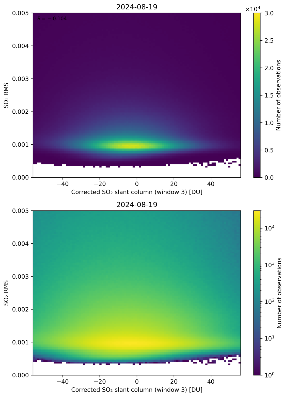
Figure 208: Scatter density plot of “Corrected SO 2 slant column (window 3)” against “SO 2 RMS” for 2024-08-18 to 2024-08-20.
