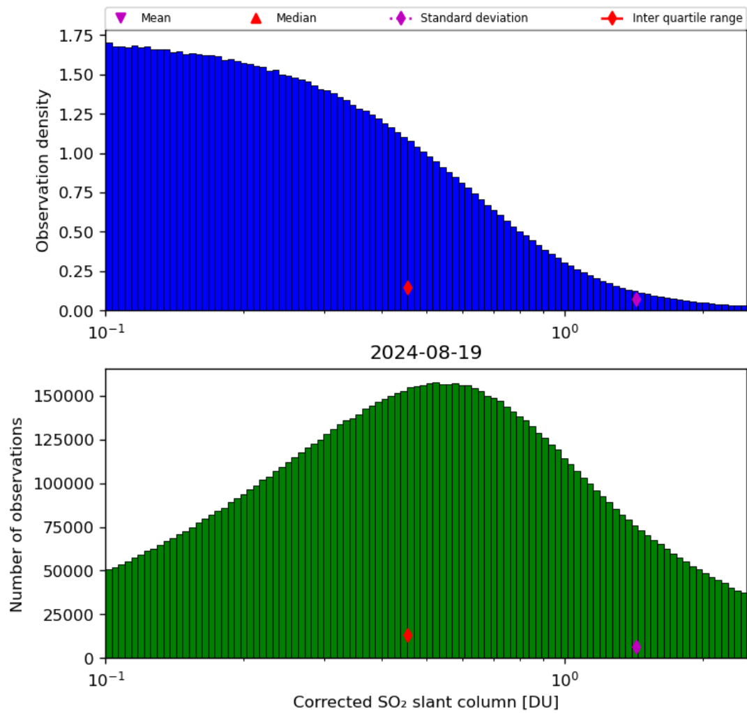
Figure 55: Histogram of “Corrected SO 2 slant column” for 2024-08-18 to 2024-08-20
