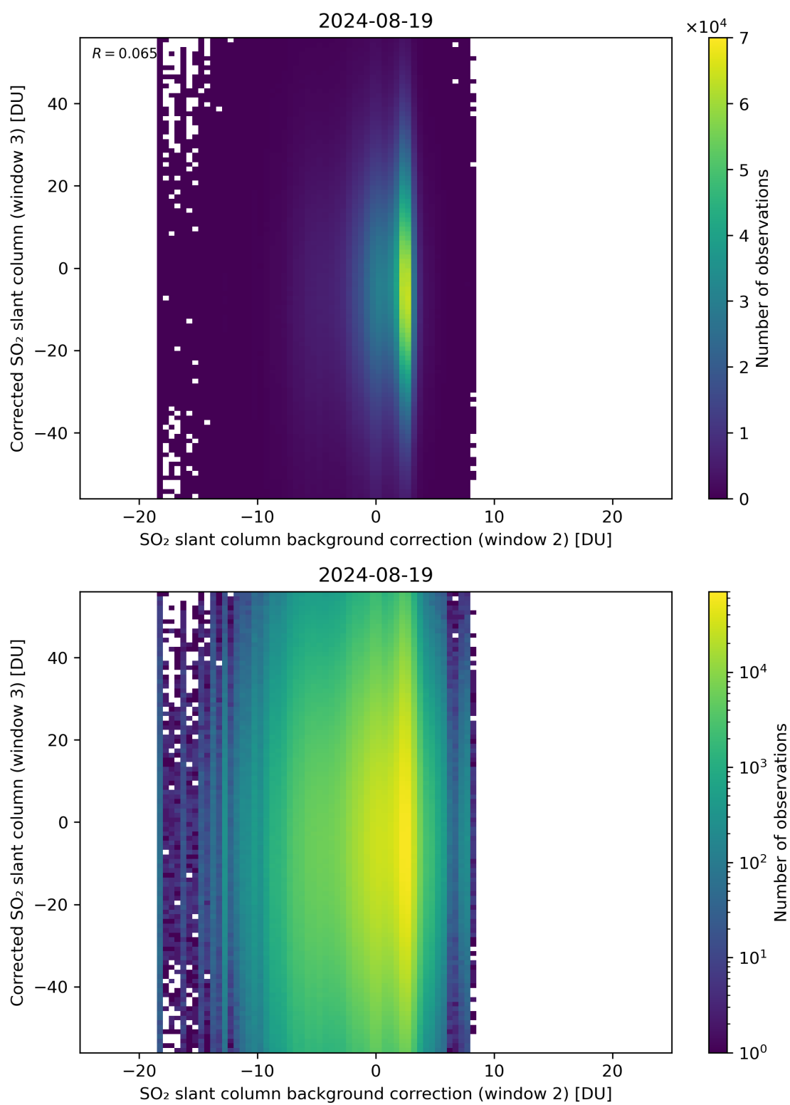
Figure 116: Scatter density plot of “SO 2 slant column background correction (window 2)” against “Corrected SO 2 slant column (window 3)” for 2024-08-18 to 2024-08-20.
