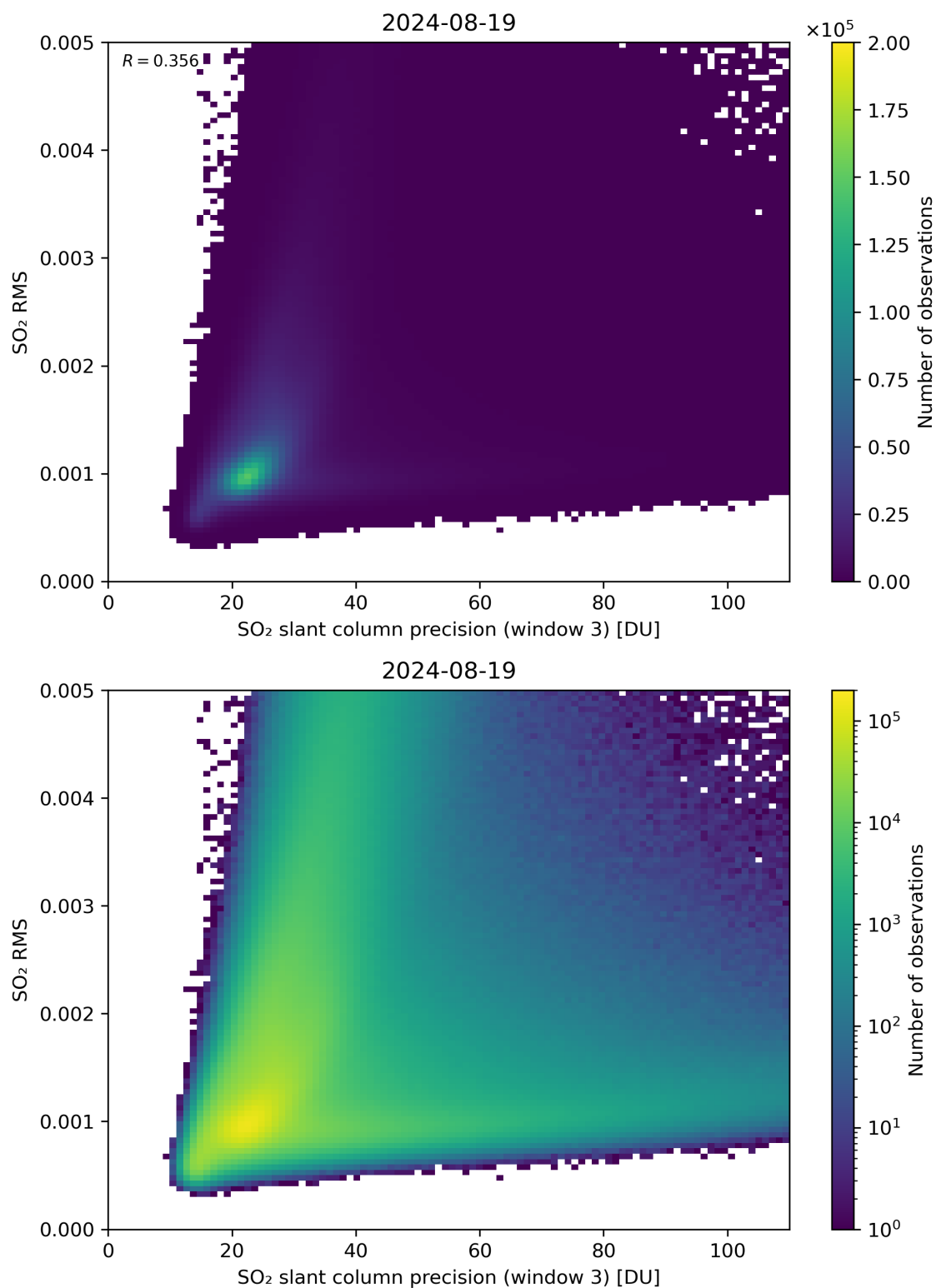
Figure 260: Scatter density plot of “SO 2 slant column precision (window 3)” against “SO 2 RMS” for 2024-08-18 to 2024-08-20.
