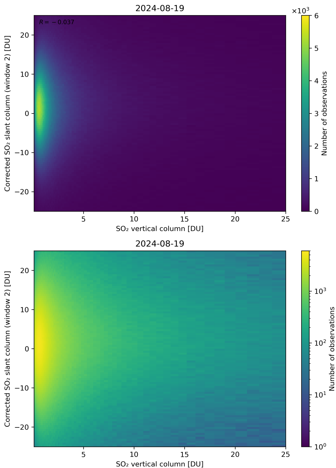
Figure 298: Scatter density plot of “SO 2 vertical column” against “Corrected SO 2 slant column (window 2)” for 2024-08-18 to 2024-08-20.
