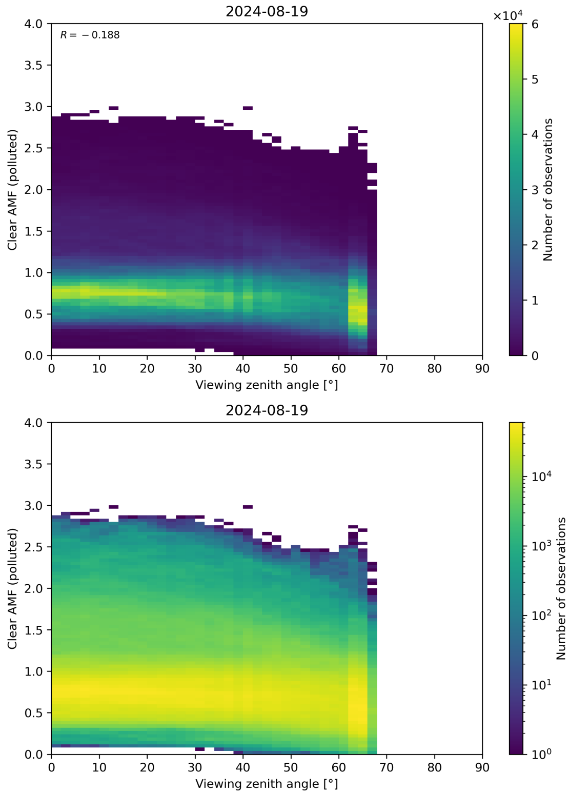
Figure 316: Scatter density plot of “Viewing zenith angle” against “Clear AMF (polluted)” for 2024-08-18 to 2024-08-20.
