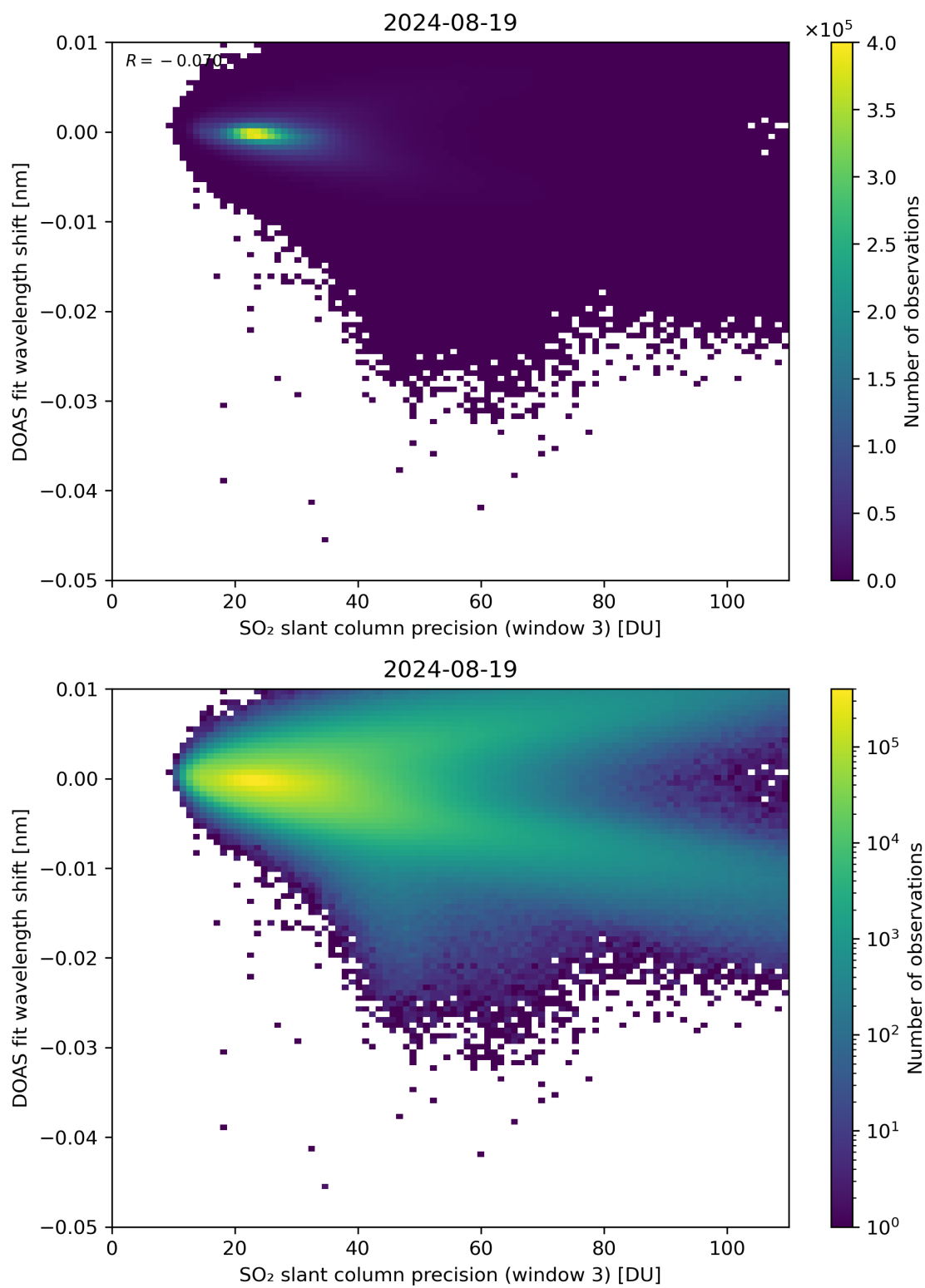
Figure 258: Scatter density plot of “SO 2 slant column precision (window 3)” against “DOAS fit wavelength shift” for 2024-08-18 to 2024-08-20.
