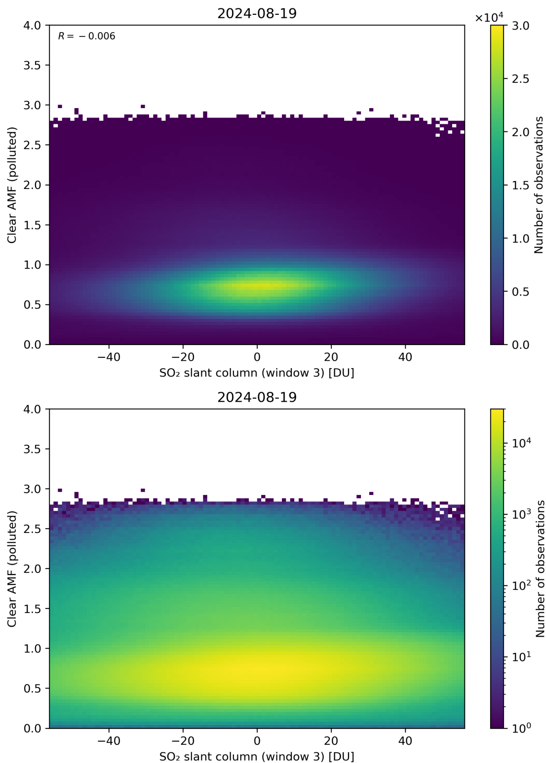
Figure 265: Scatter density plot of “SO 2 slant column (window 3)” against “Clear AMF (polluted)” for 2024-08-18 to 2024-08-20.
