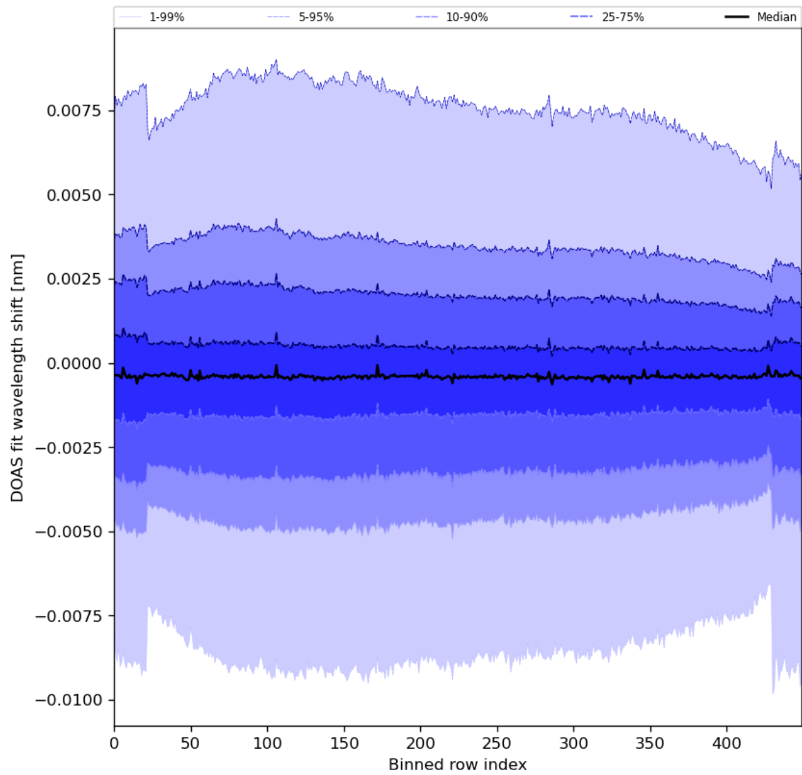
Figure 91: Along track statistics of “DOAS fit wavelength shift” for 2024-08-18 to 2024-08-20
