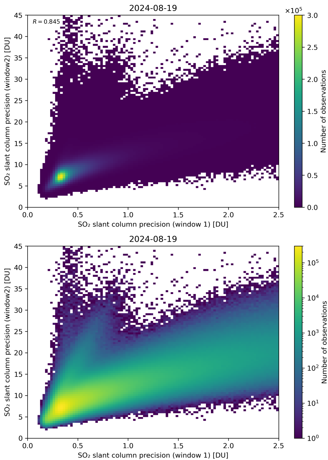
Figure 227: Scatter density plot of “SO 2 slant column precision (window 1)” against “SO 2 slant column precision (window 2)” for 2024-08-18 to 2024-08-20.
