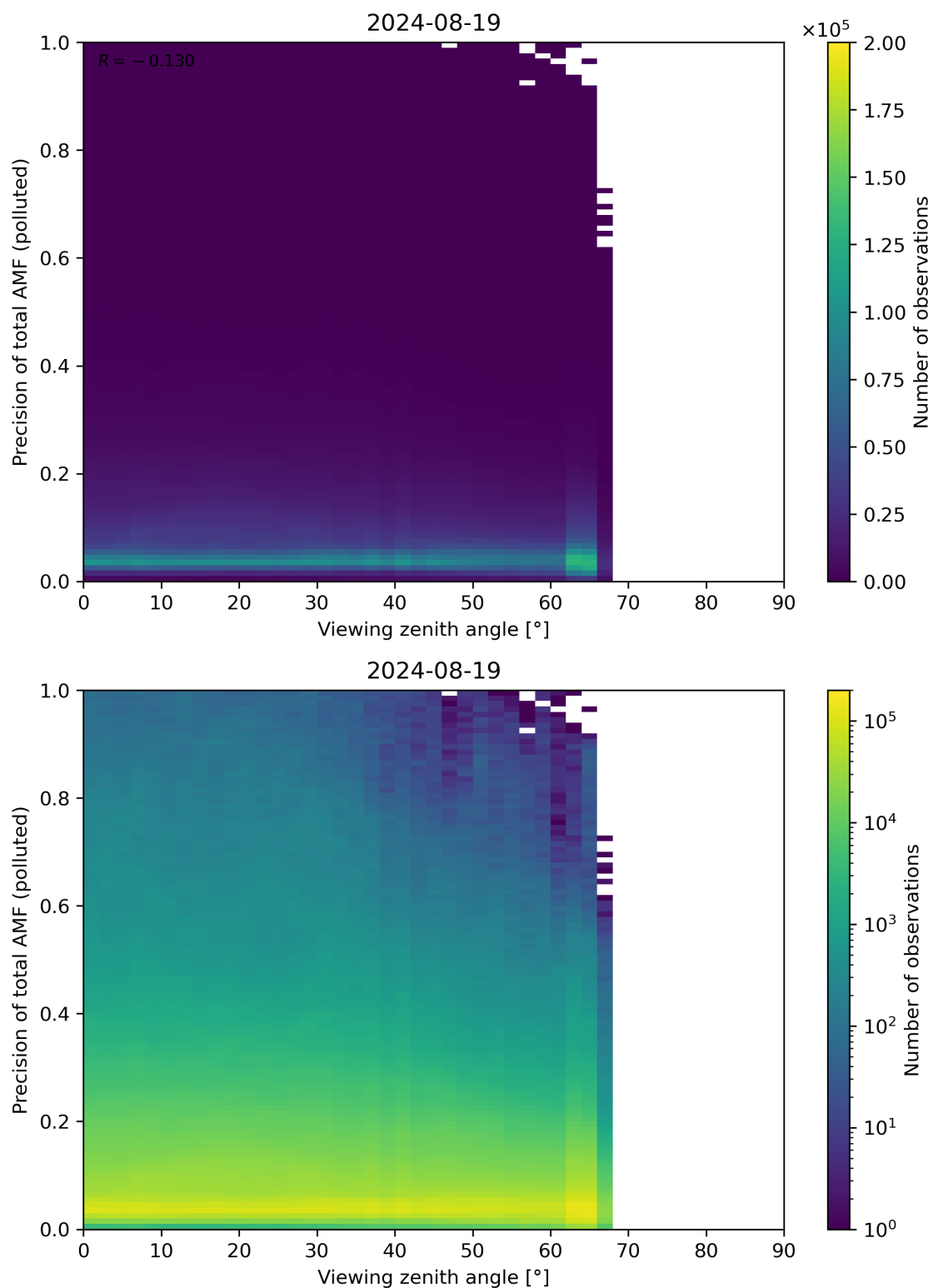
Figure 326: Scatter density plot of “Viewing zenith angle” against “Precision of total AMF (polluted)” for 2024-08-18 to 2024-08-20.
