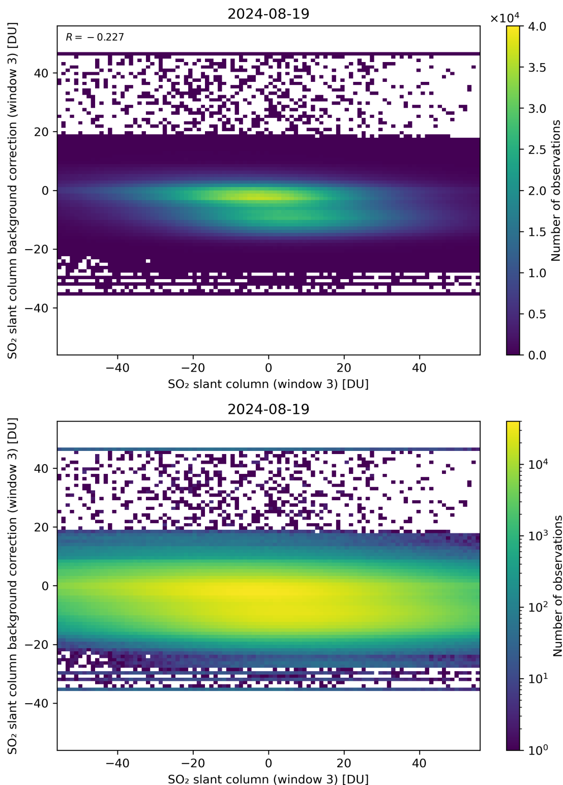
Figure 253: Scatter density plot of “SO 2 slant column (window 3)” against “SO 2 slant column background correction (window 3)” for 2024-08-18 to 2024-08-20.
