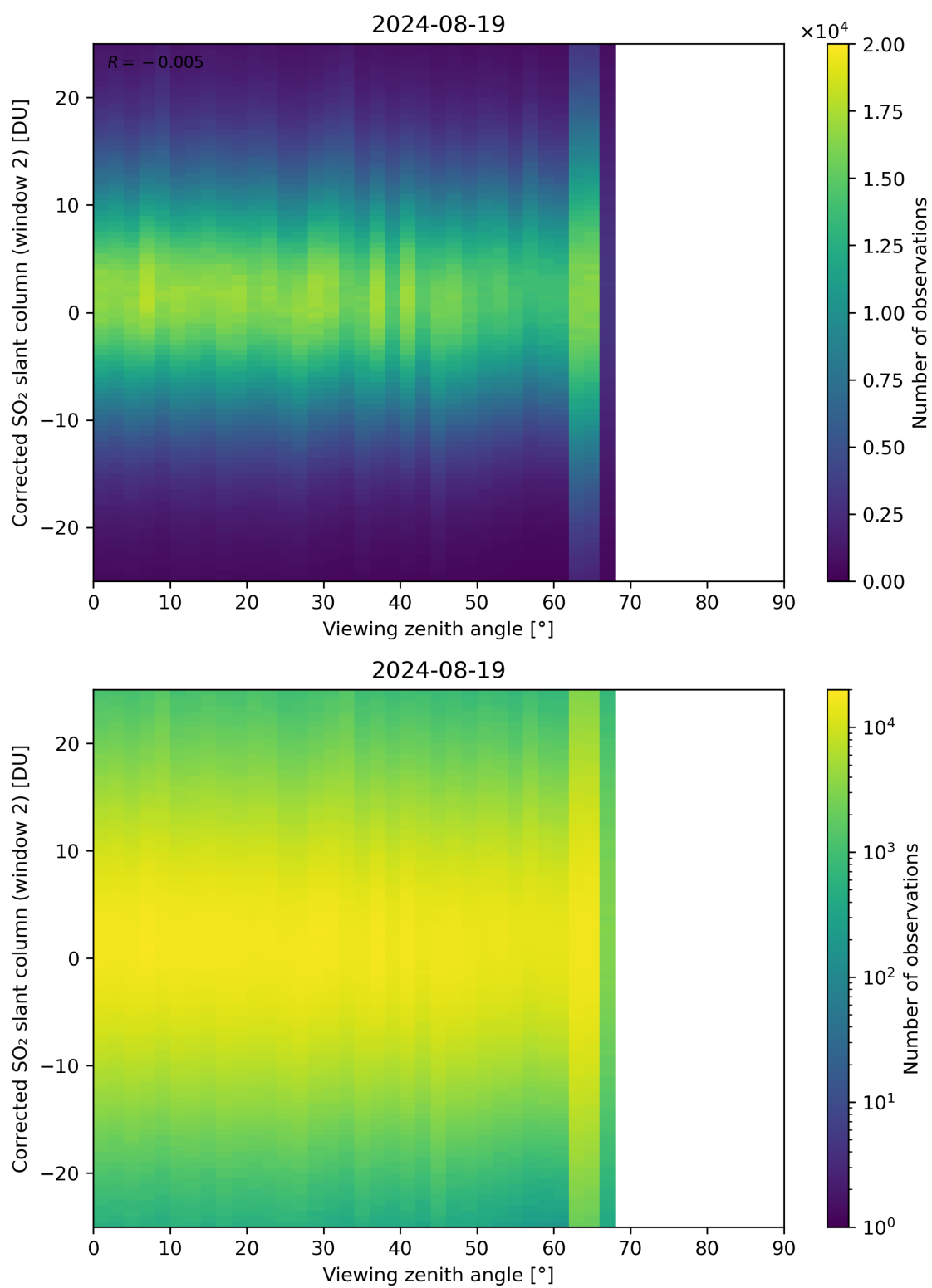
Figure 318: Scatter density plot of “Viewing zenith angle” against “Corrected SO 2 slant column (window 2)” for 2024-08-18 to 2024-08-20.
