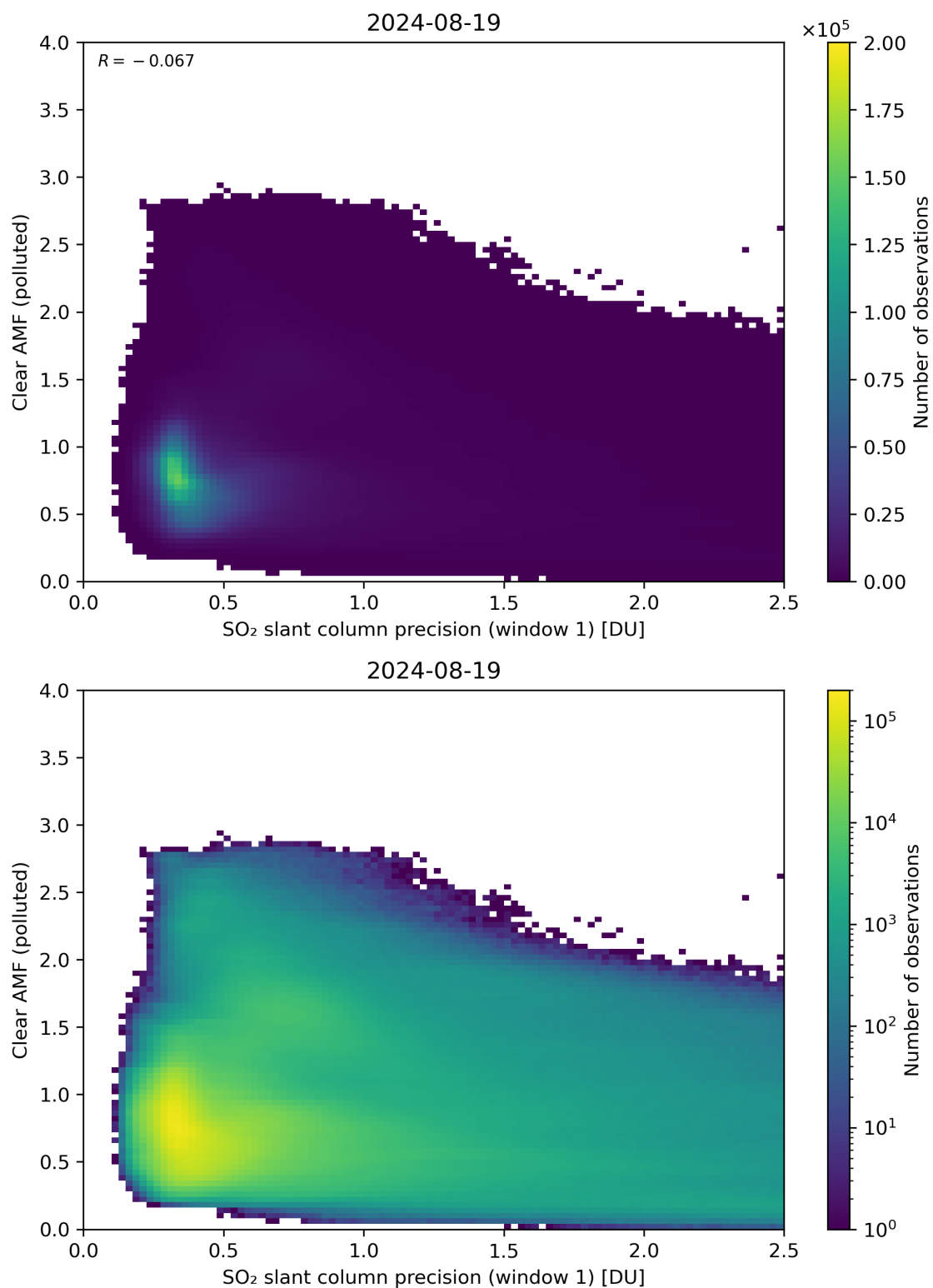
Figure 224: Scatter density plot of “SO 2 slant column precision (window 1)” against “Clear AMF (polluted)” for 2024-08-18 to 2024-08-20.
