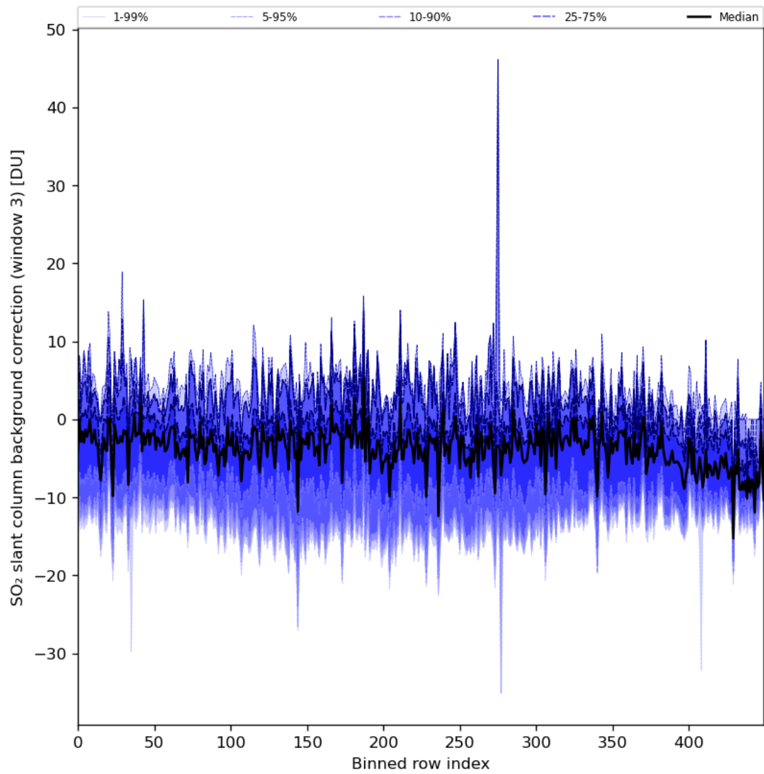
Figure 90: Along track statistics of “SO 2 slant column background correction (window 3)” for 2024-08-18 to 2024-08-20
