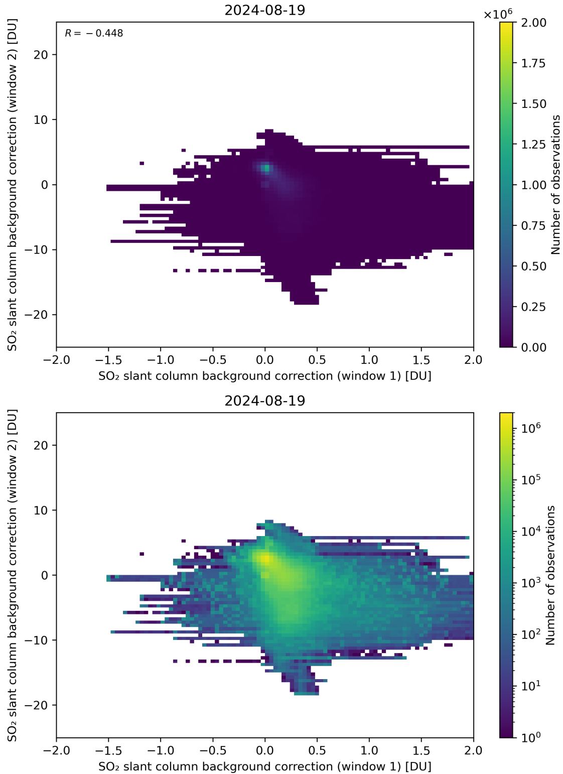
Figure 98: Scatter density plot of “SO 2 slant column background correction (window 1)” against “SO 2 slant column background correction (window 2)” for 2024-08-18 to 2024-08-20.
