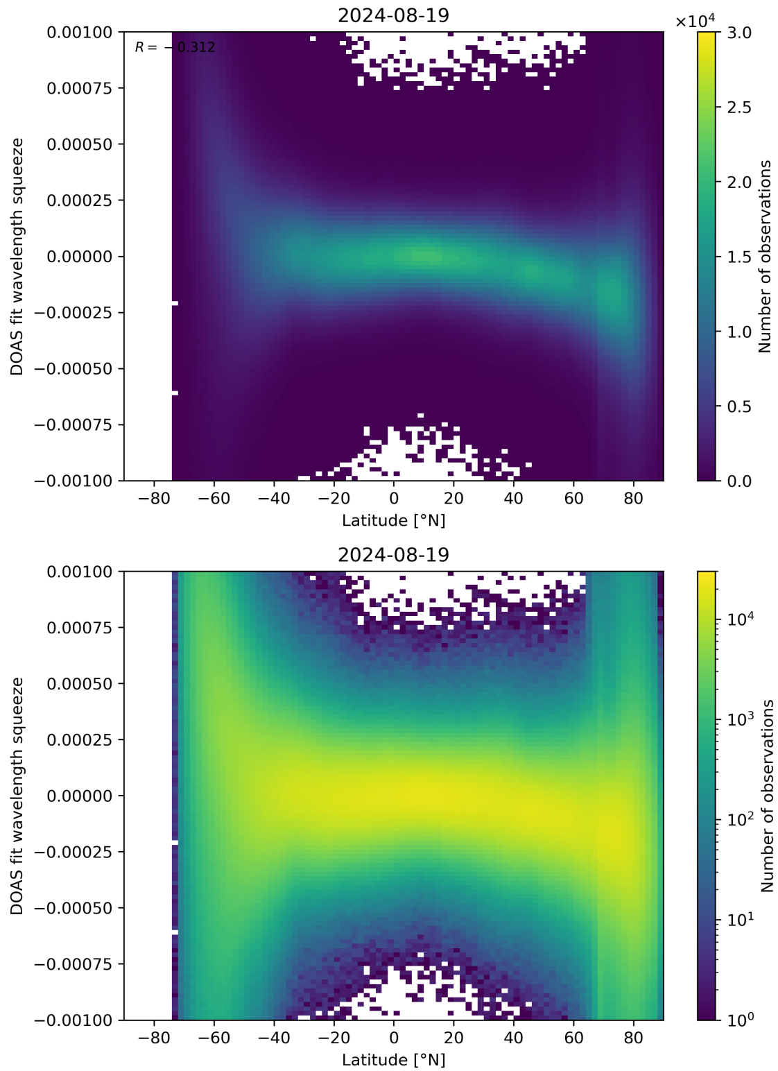
Figure 143: Scatter density plot of “Latitude” against “DOAS fit wavelength squeeze” for 2024-08-18 to 2024-08-20.
