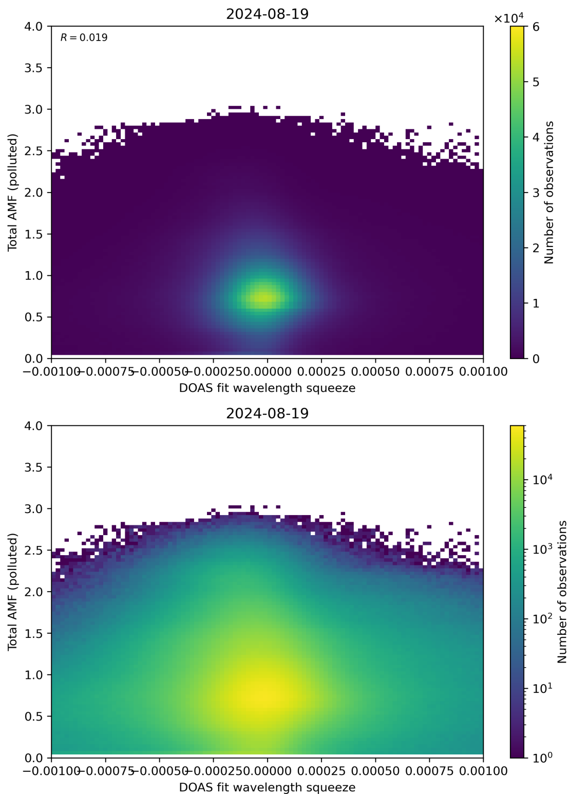
Figure 134: Scatter density plot of “DOAS fit wavelength squeeze” against “Total AMF (polluted)” for 2024-08-18 to 2024-08-20.
