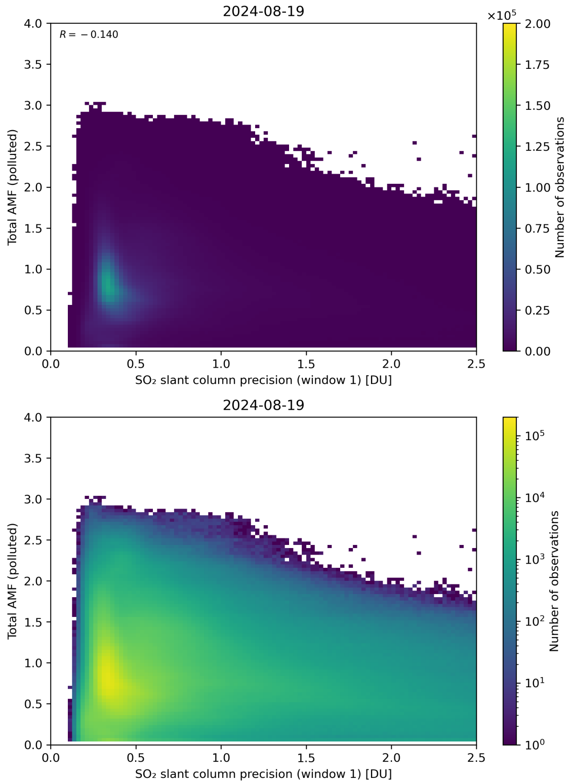
Figure 230: Scatter density plot of “SO 2 slant column precision (window 1)” against “Total AMF (polluted)” for 2024-08-18 to 2024-08-20.
