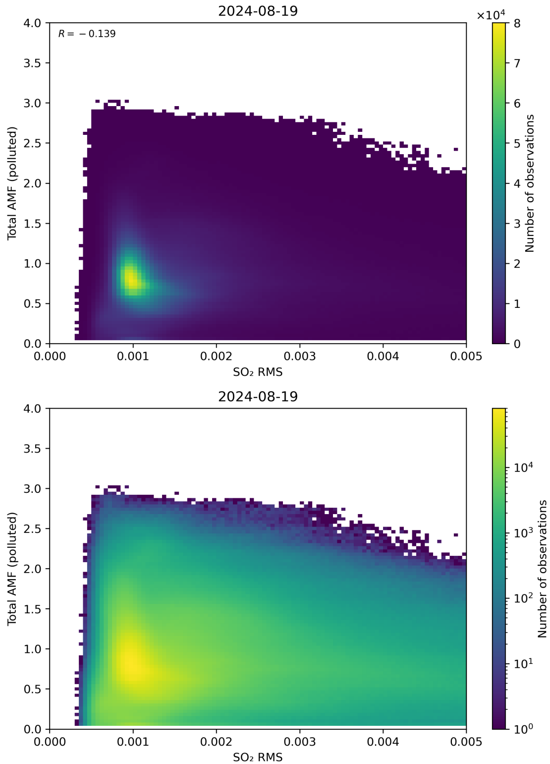
Figure 137: Scatter density plot of “SO 2 RMS” against “Total AMF (polluted)” for 2024-08-18 to 2024-08-20.
