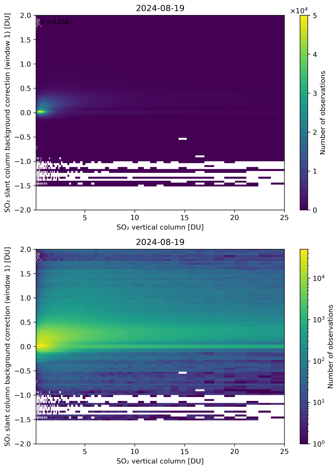
Figure 273: Scatter density plot of “SO 2 vertical column” against “SO 2 slant column background correction (window 1)” for 2024-08-18 to 2024-08-20.
