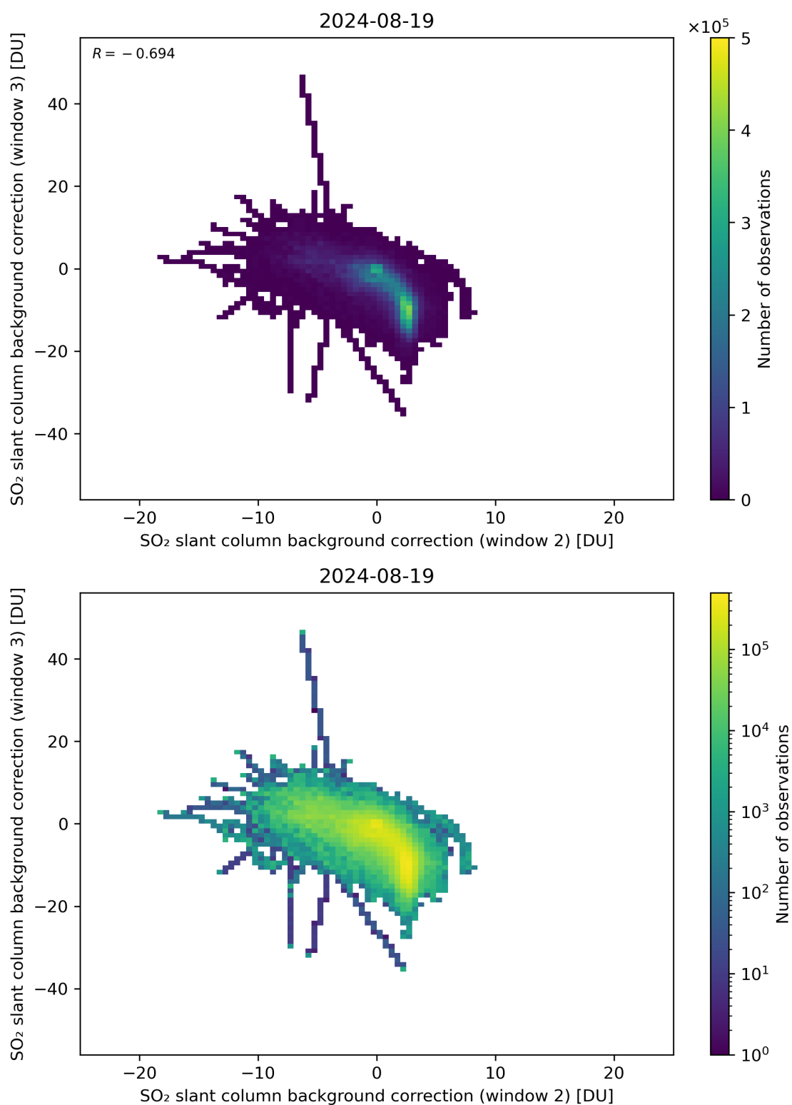
Figure 111: Scatter density plot of “SO 2 slant column background correction (window 2)” against “SO 2 slant column background correction (window 3)” for 2024-08-18 to 2024-08-20.
