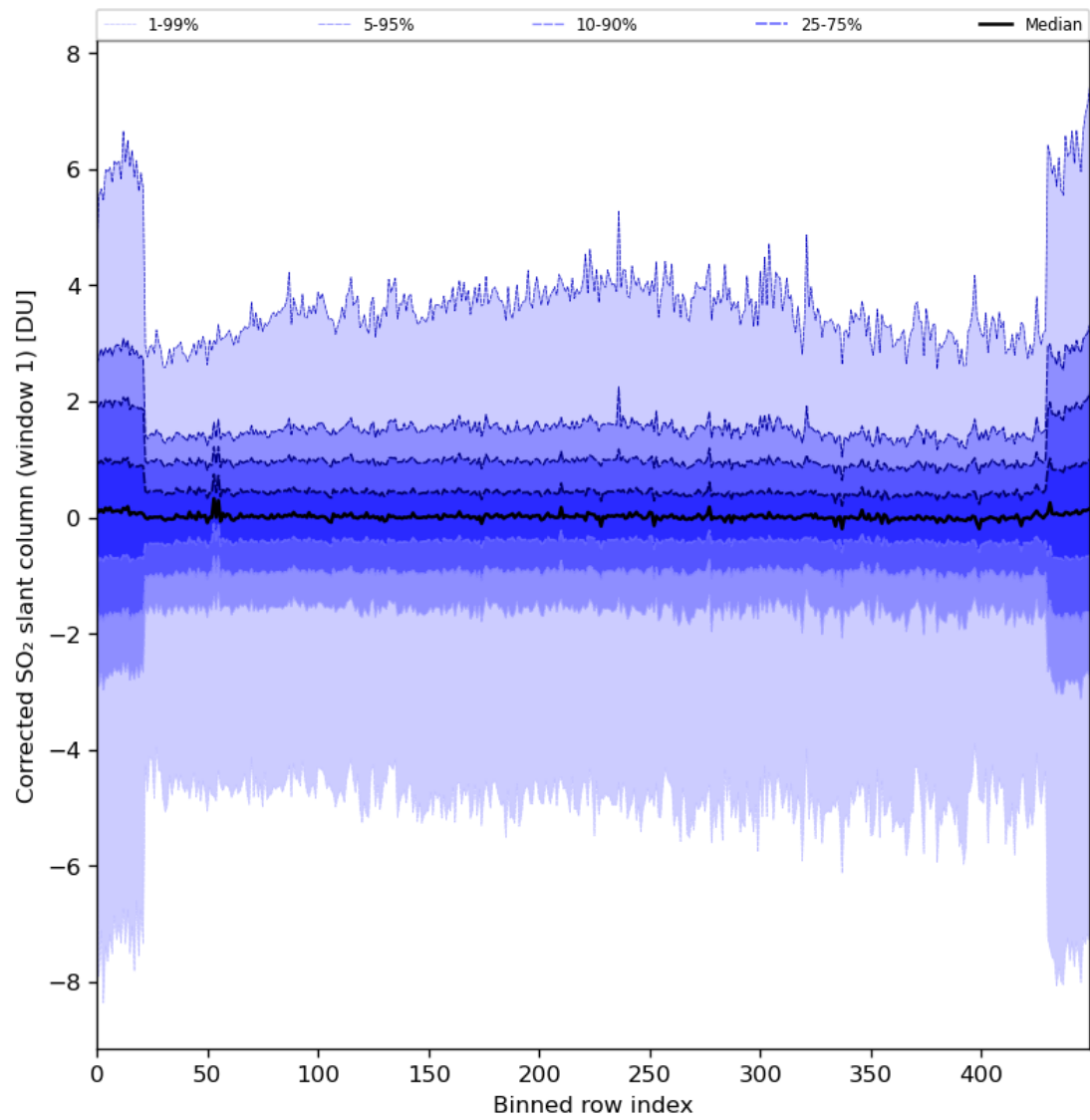
Figure 81: Along track statistics of “Corrected SO 2 slant column (window 1)” for 2024-08-18 to 2024-08-20
