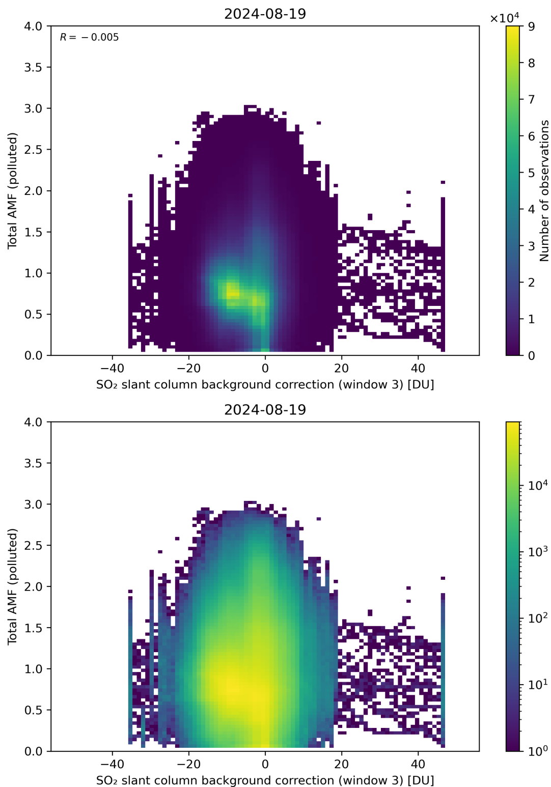
Figure 125: Scatter density plot of “SO 2 slant column background correction (window 3)” against “Total AMF (polluted)” for 2024-08-18 to 2024-08-20.
