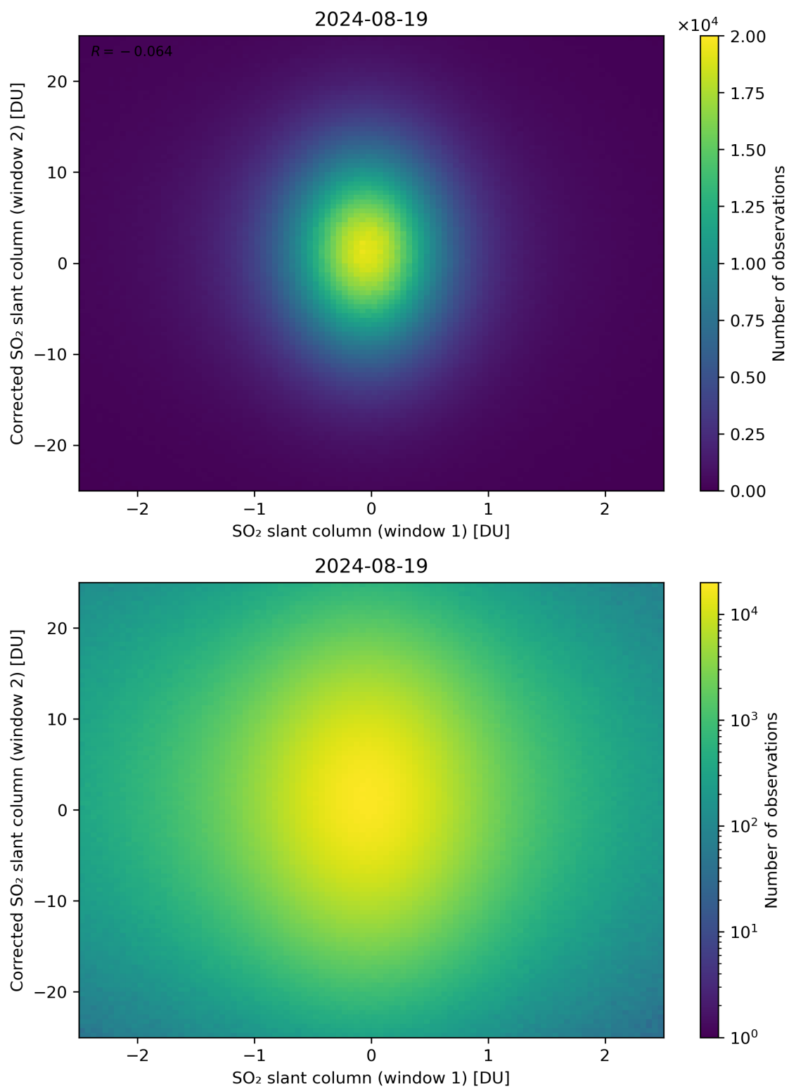
Figure 233: Scatter density plot of “SO 2 slant column (window 1)” against “Corrected SO 2 slant column (window 2)” for 2024-08-18 to 2024-08-20.
