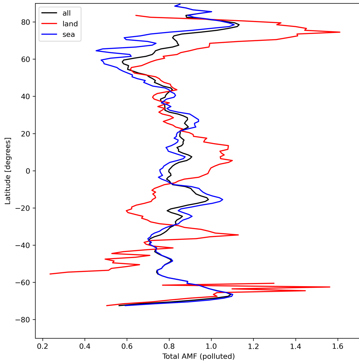
Figure 48: Zonal average of “Total AMF (polluted)” for 2024-08-18 to 2024-08-20.
