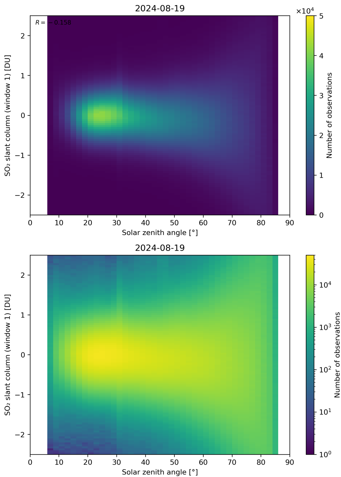
Figure 169: Scatter density plot of “Solar zenith angle” against “SO 2 slant column (window 1)” for 2024-08-18 to 2024-08-20.
