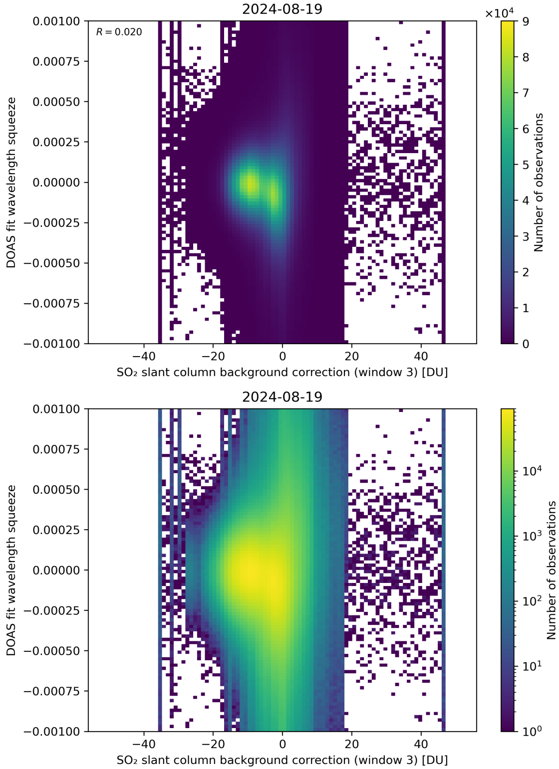
Figure 122: Scatter density plot of “SO 2 slant column background correction (window 3)” against “DOAS fit wavelength squeeze” for 2024-08-18 to 2024-08-20.
