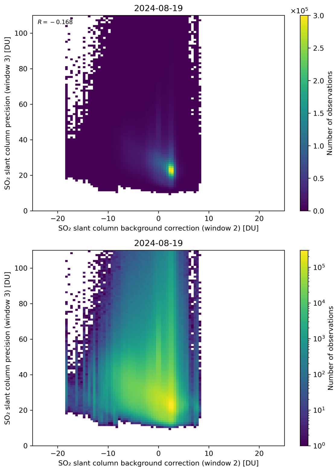
Figure 118: Scatter density plot of “SO 2 slant column background correction (window 2)” against “SO 2 slant column precision (window 3)” for 2024-08-18 to 2024-08-20.
