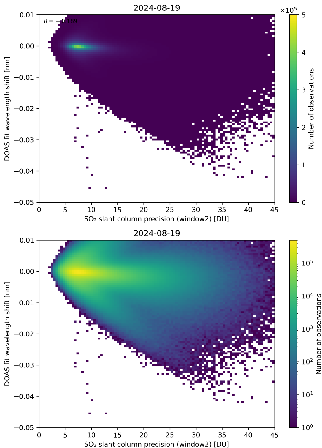
Figure 243: Scatter density plot of “SO 2 slant column precision (window2)” against “DOAS fit wavelength shift” for 2024-08-18 to 2024-08-20.
