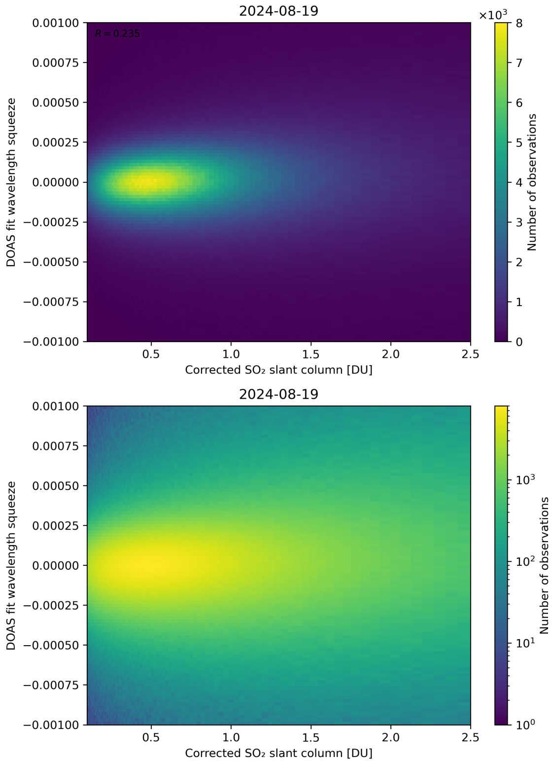
Figure 182: Scatter density plot of “Corrected SO 2 slant column” against “DOAS fit wavelength squeeze” for 2024-08-18 to 2024-08-20.
