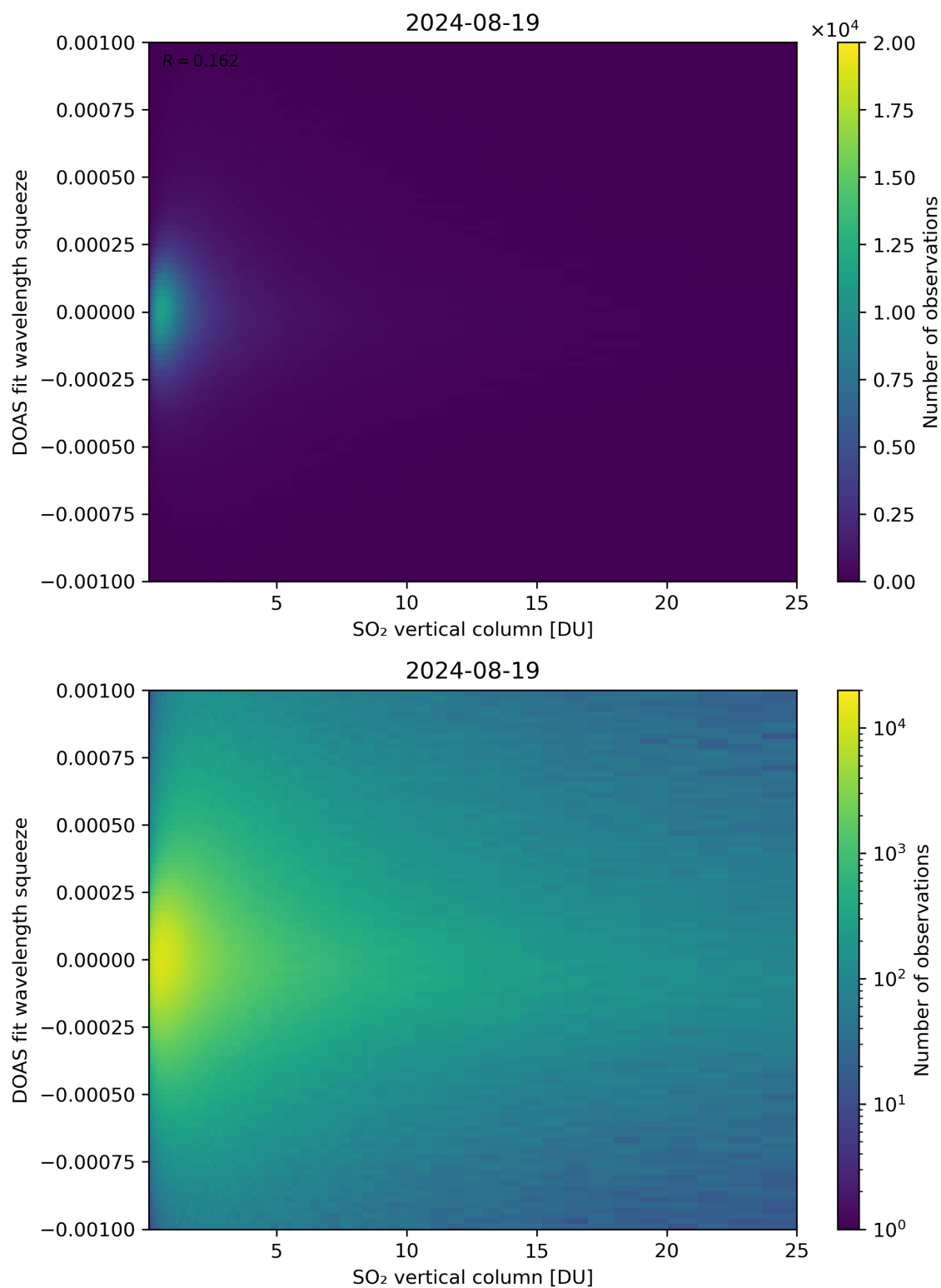
Figure 277: Scatter density plot of “SO 2 vertical column” against “DOAS fit wavelength squeeze” for 2024-08-18 to 2024-08-20.
