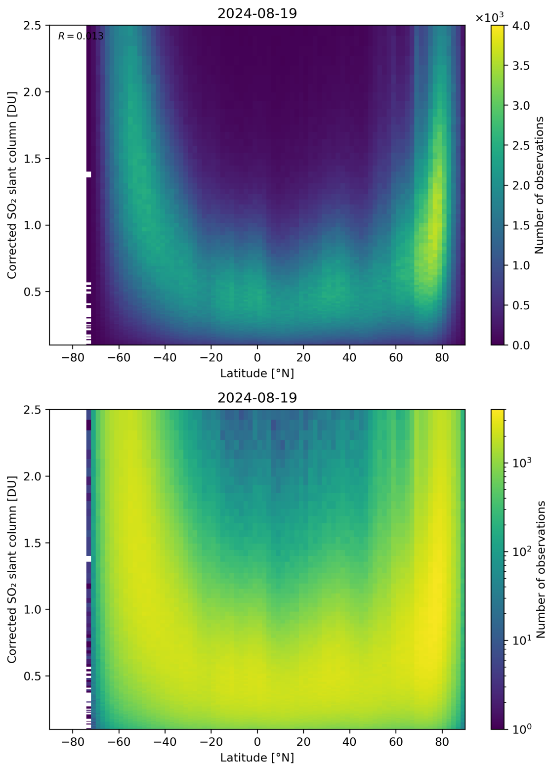
Figure 146: Scatter density plot of “Latitude” against “Corrected SO 2 slant column” for 2024-08-18 to 2024-08-20.
