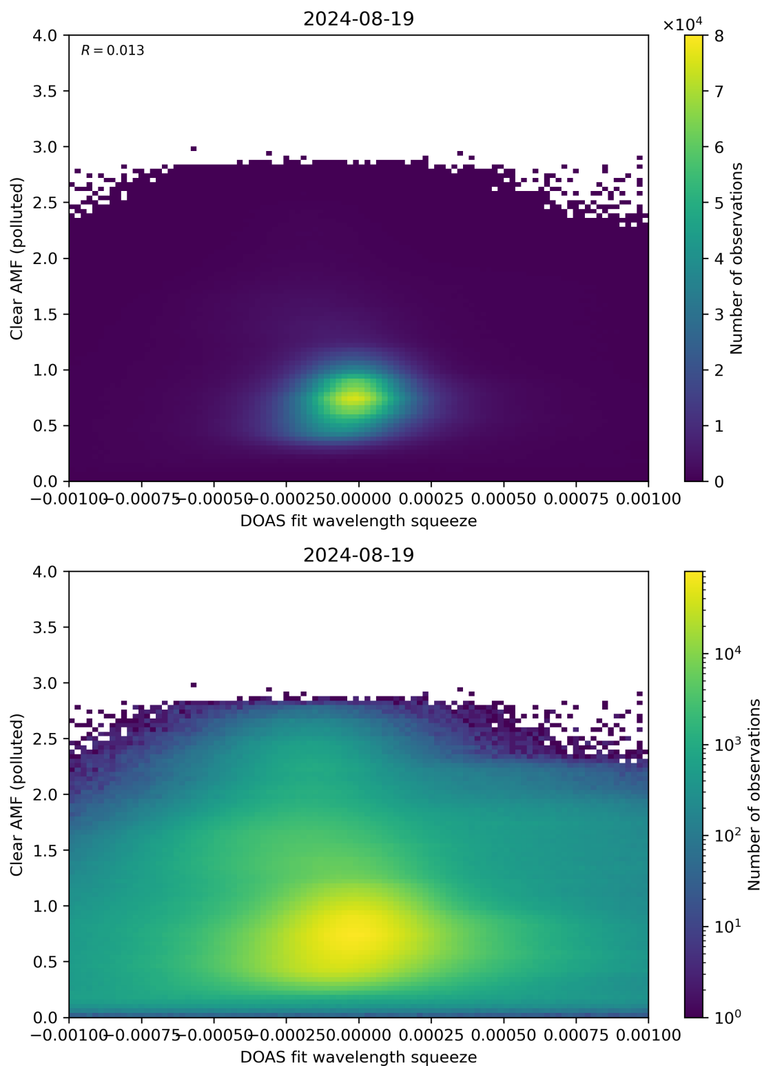
Figure 133: Scatter density plot of “DOAS fit wavelength squeeze” against “Clear AMF (polluted)” for 2024-08-18 to 2024-08-20.
