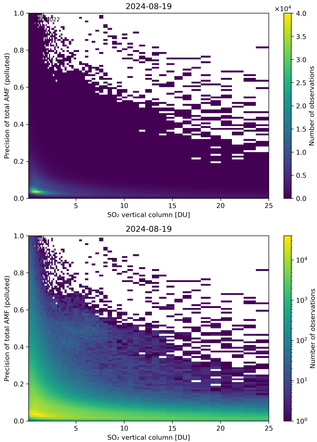
Figure 306: Scatter density plot of “SO 2 vertical column” against “Precision of total AMF (polluted)” for 2024-08-18 to 2024-08-20.
