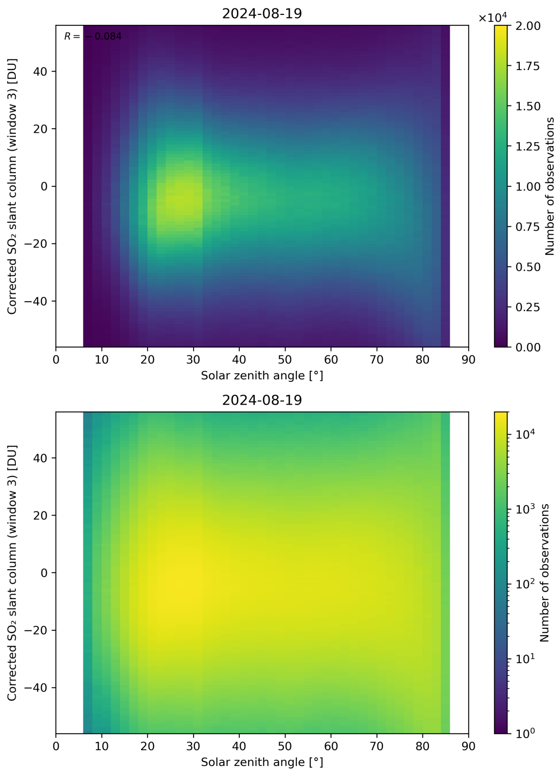
Figure 168: Scatter density plot of “Solar zenith angle” against “Corrected SO 2 slant column (window 3)” for 2024-08-18 to 2024-08-20.
