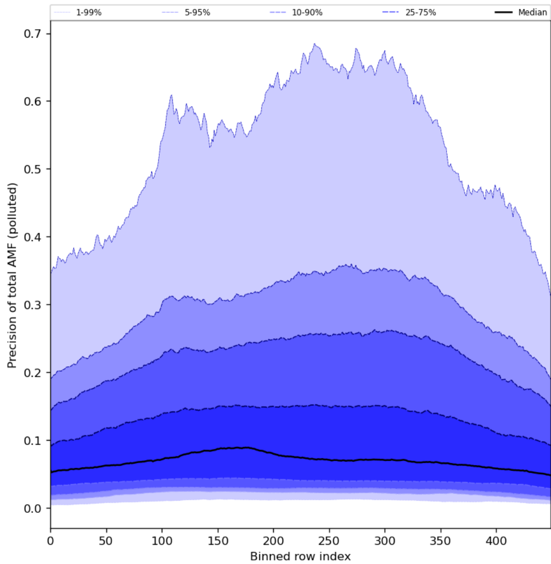
Figure 95: Along track statistics of “Precision of total AMF (polluted)” for 2024-08-18 to 2024-08-20
