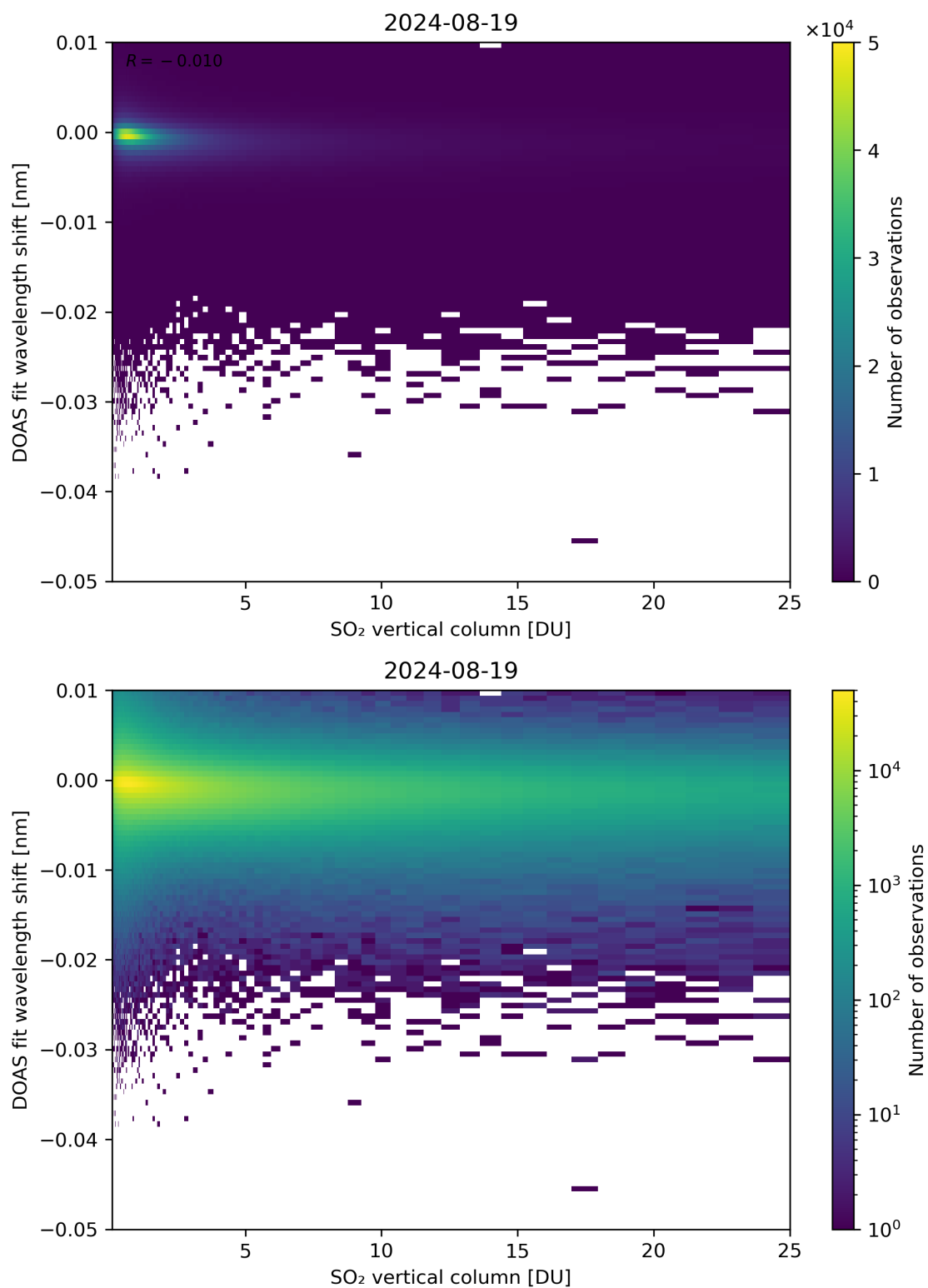
Figure 276: Scatter density plot of “SO 2 vertical column” against “DOAS fit wavelength shift” for 2024-08-18 to 2024-08-20.
