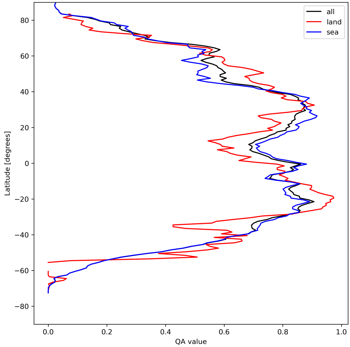
Figure 29: Zonal average of “QA value” for 2024-08-18 to 2024-08-20.
