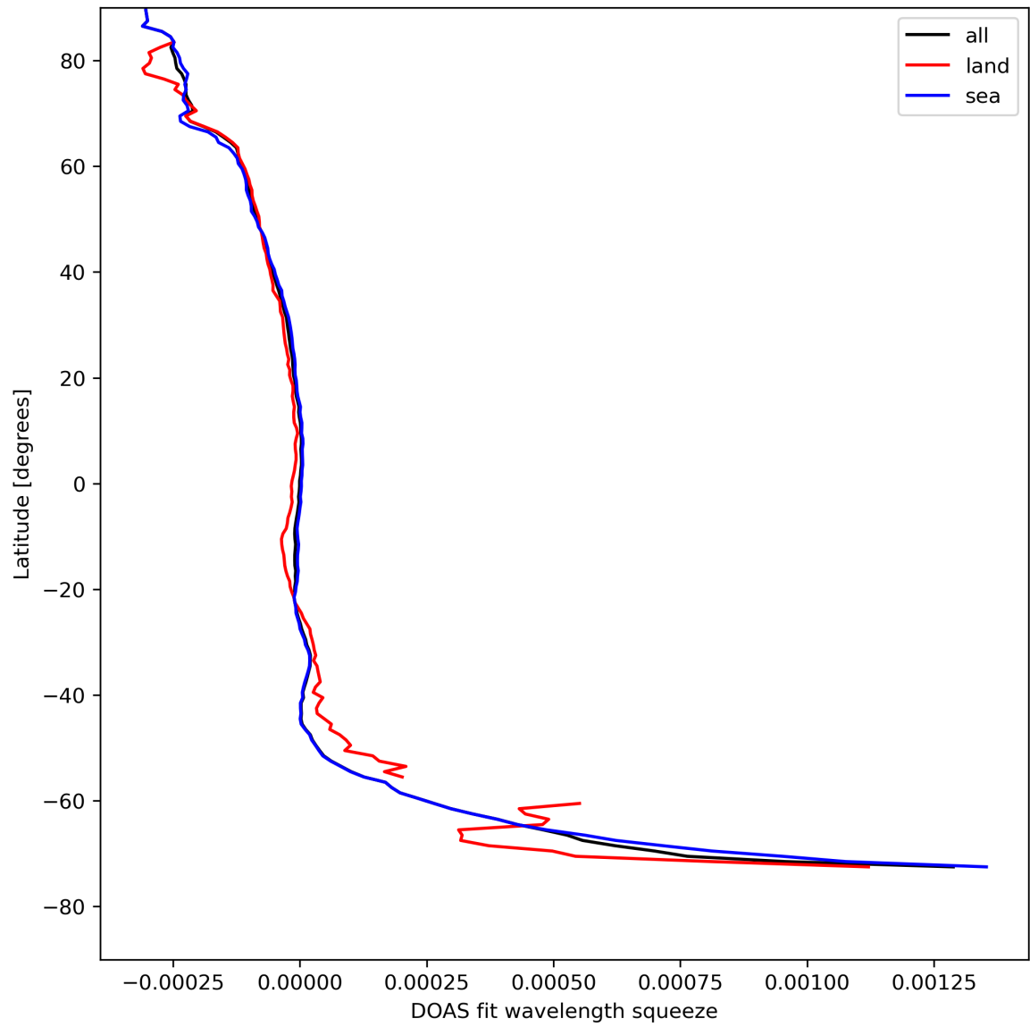
Figure 46: Zonal average of “DOAS fit wavelength squeeze” for 2024-08-18 to 2024-08-20.
