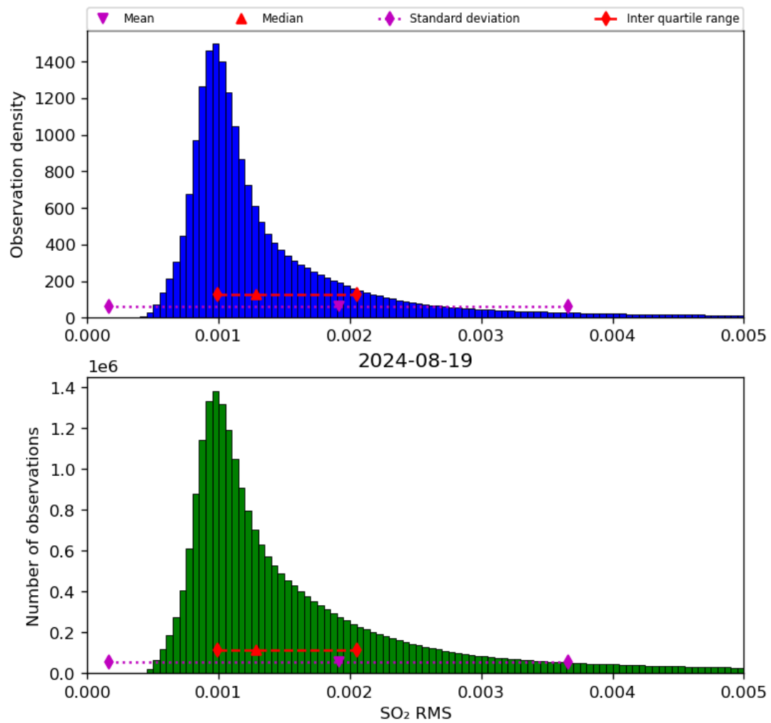
Figure 70: Histogram of “SO 2 RMS” for 2024-08-18 to 2024-08-20
