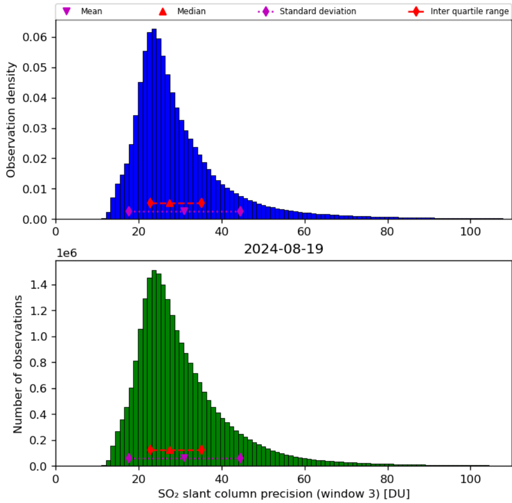
Figure 65: Histogram of “SO 2 slant column precision (window 3)” for 2024-08-18 to 2024-08-20
