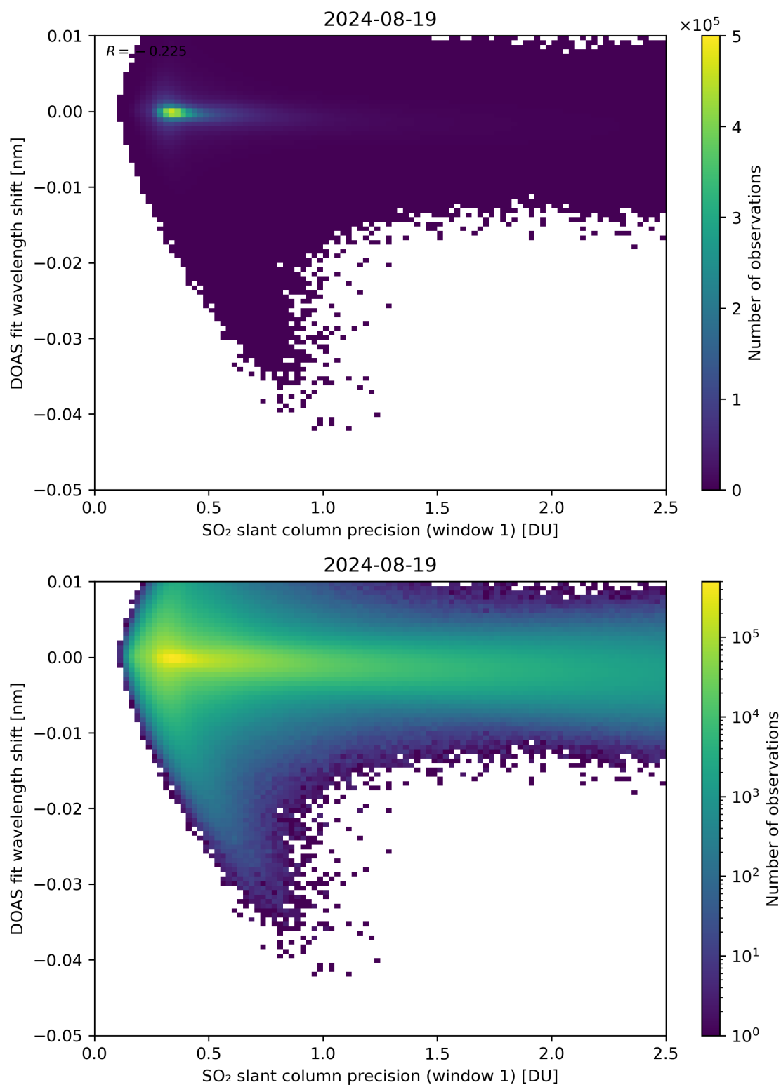
Figure 221: Scatter density plot of “SO 2 slant column precision (window 1)” against “DOAS fit wavelength shift” for 2024-08-18 to 2024-08-20.
