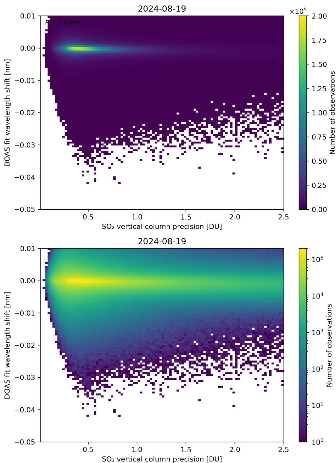
Figure 282: Scatter density plot of “SO 2 vertical column precision” against “DOAS fit wavelength shift” for 2024-08-18 to 2024-08-20.
