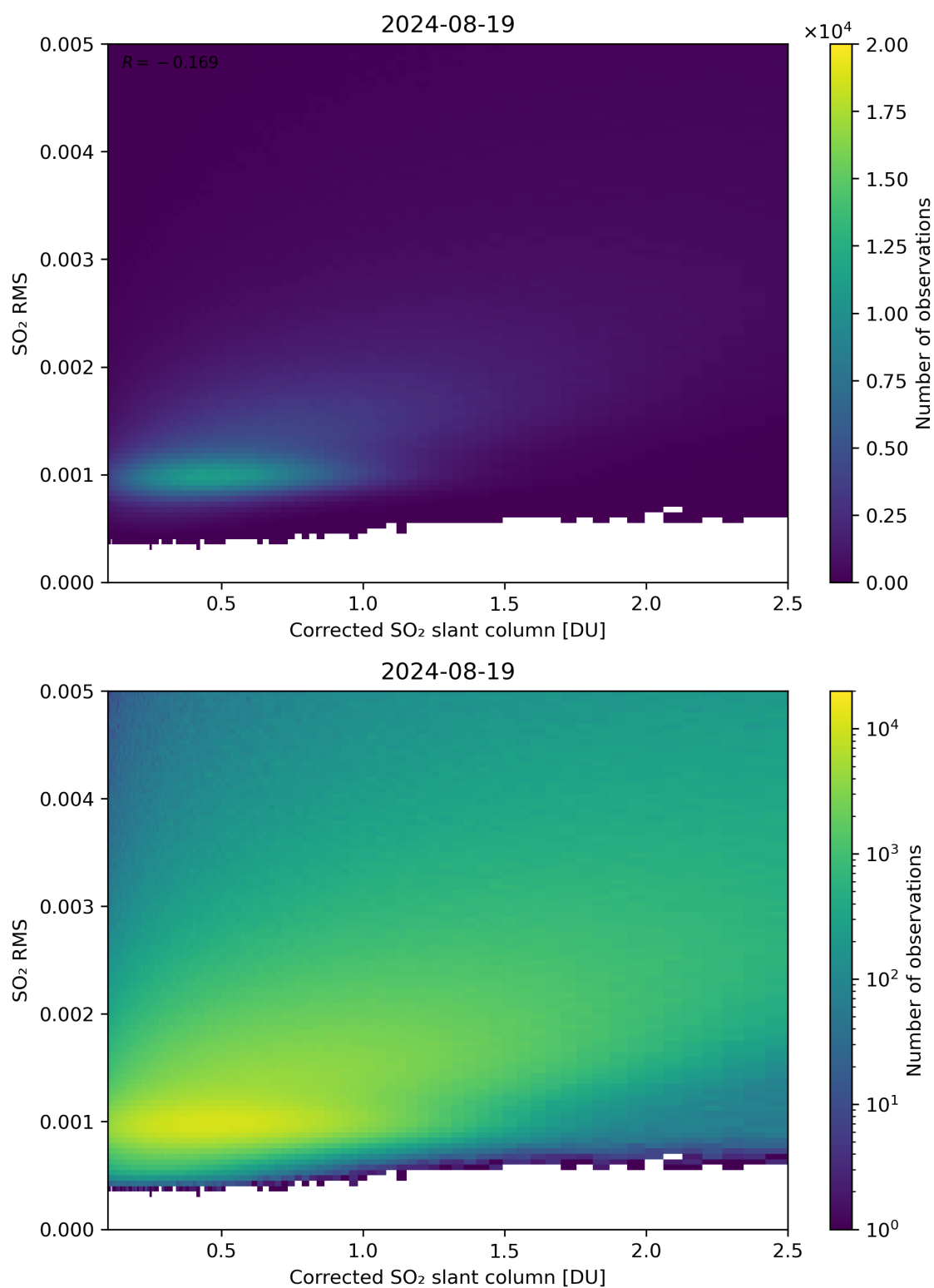
Figure 183: Scatter density plot of “Corrected SO 2 slant column” against “SO 2 RMS” for 2024-08-18 to 2024-08-20.
