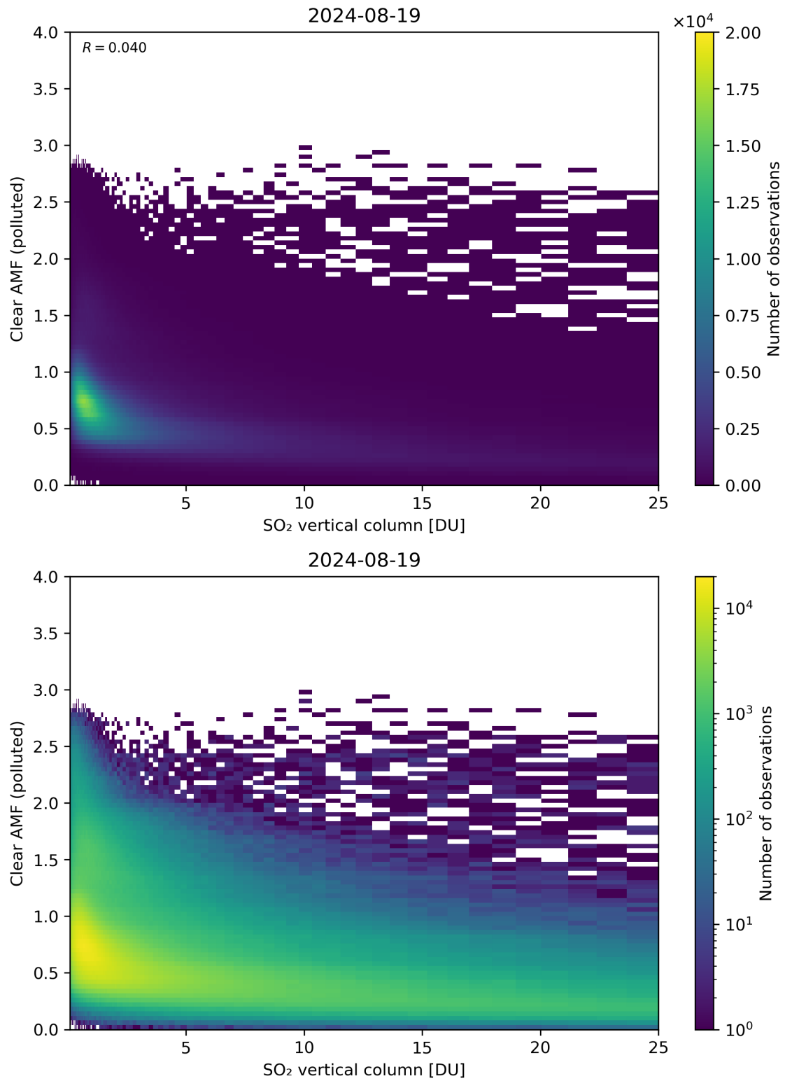
Figure 296: Scatter density plot of “SO 2 vertical column” against “Clear AMF (polluted)” for 2024-08-18 to 2024-08-20.
