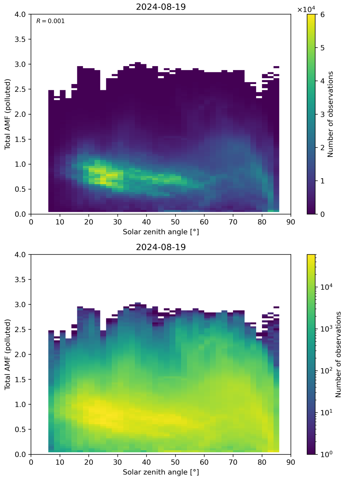
Figure 174: Scatter density plot of “Solar zenith angle” against “Total AMF (polluted)” for 2024-08-18 to 2024-08-20.
