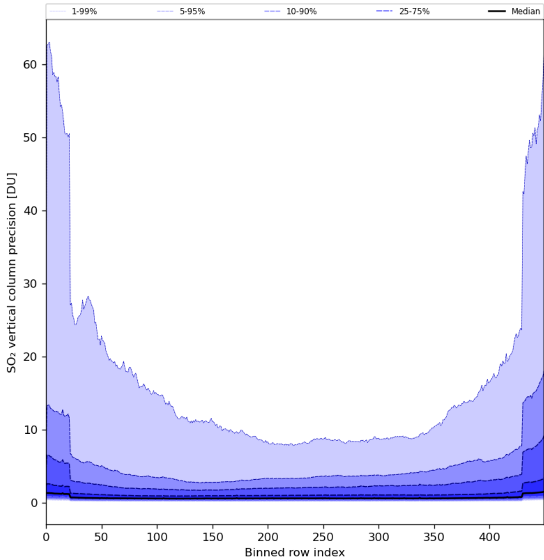
Figure 77: Along track statistics of “SO 2 vertical column precision” for 2024-08-18 to 2024-08-20
