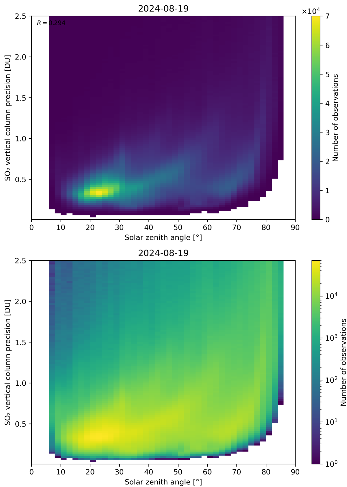
Figure 177: Scatter density plot of “Solar zenith angle” against “SO 2 vertical column precision” for 2024-08-18 to 2024-08-20.
