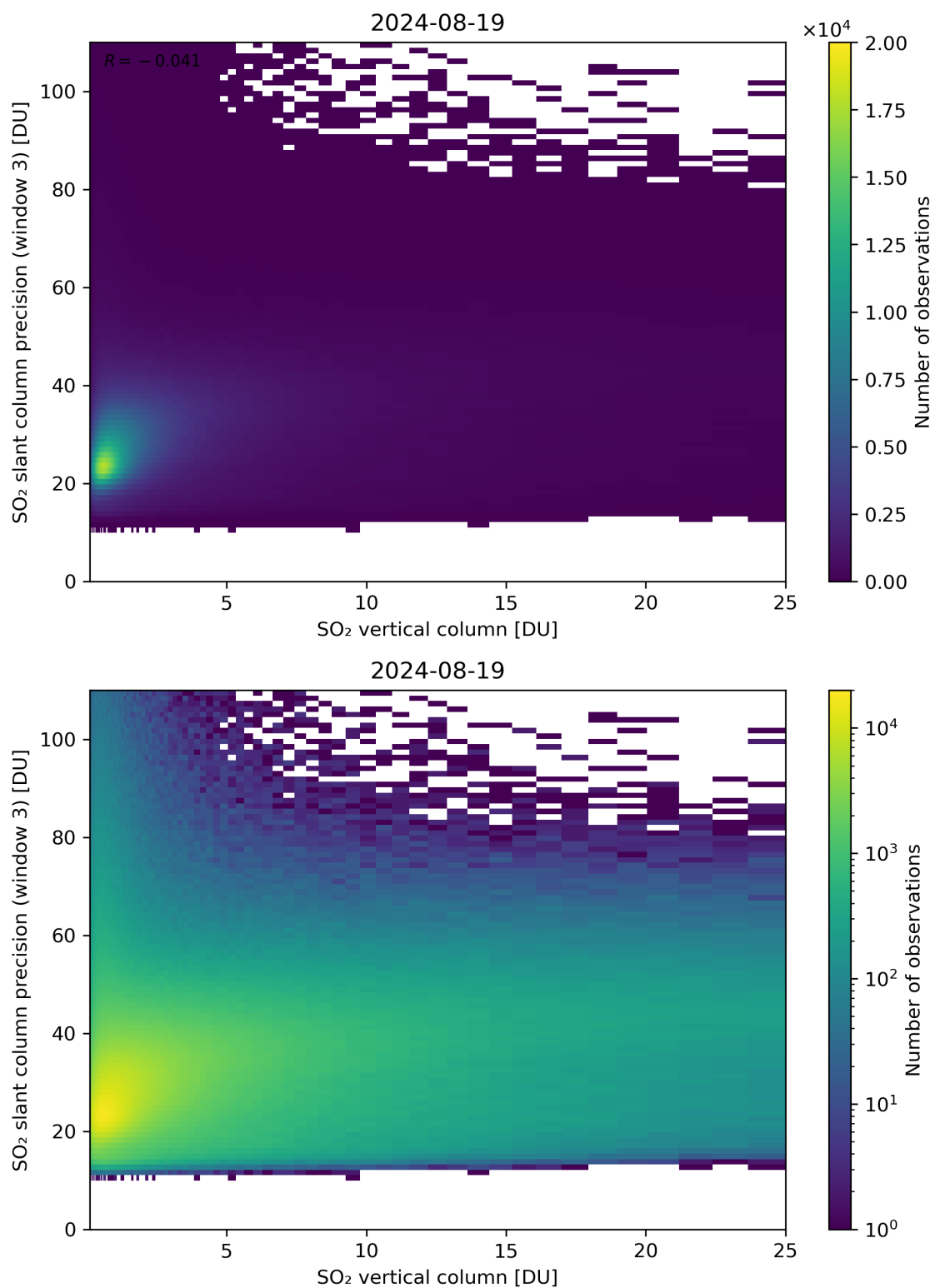
Figure 304: Scatter density plot of “SO 2 vertical column” against “SO 2 slant column precision (window 3)” for 2024-08-18 to 2024-08-20.
