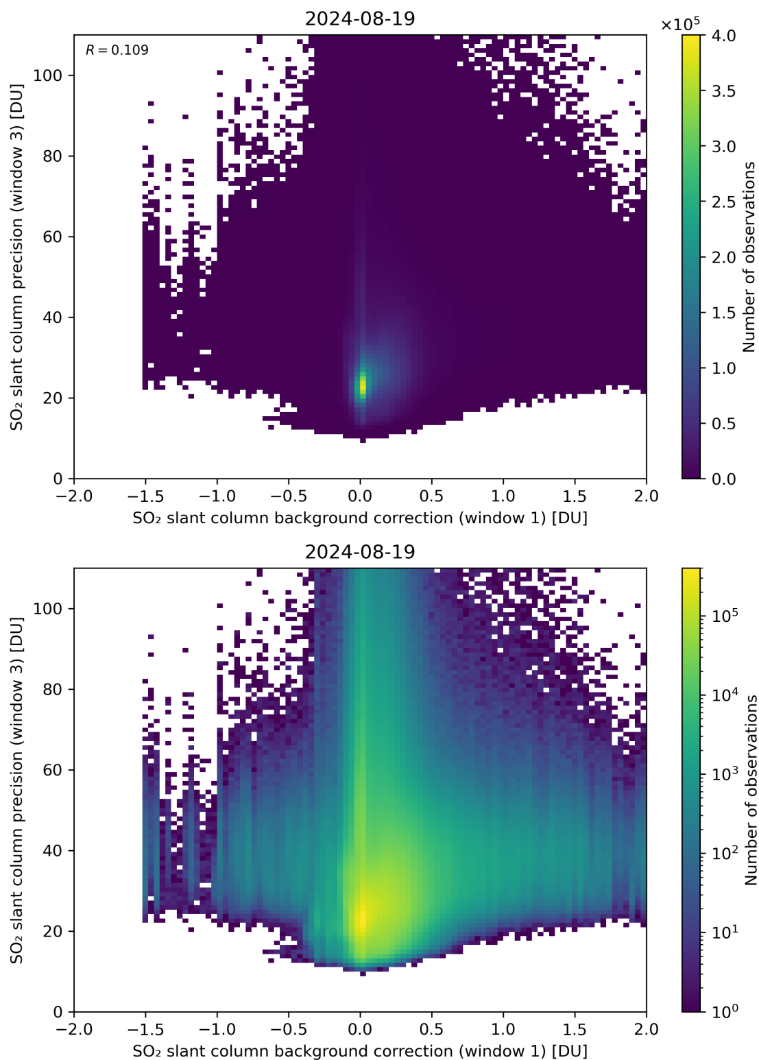
Figure 108: Scatter density plot of “SO 2 slant column background correction (window 1)” against “SO 2 slant column precision (window 3)” for 2024-08-18 to 2024-08-20.
