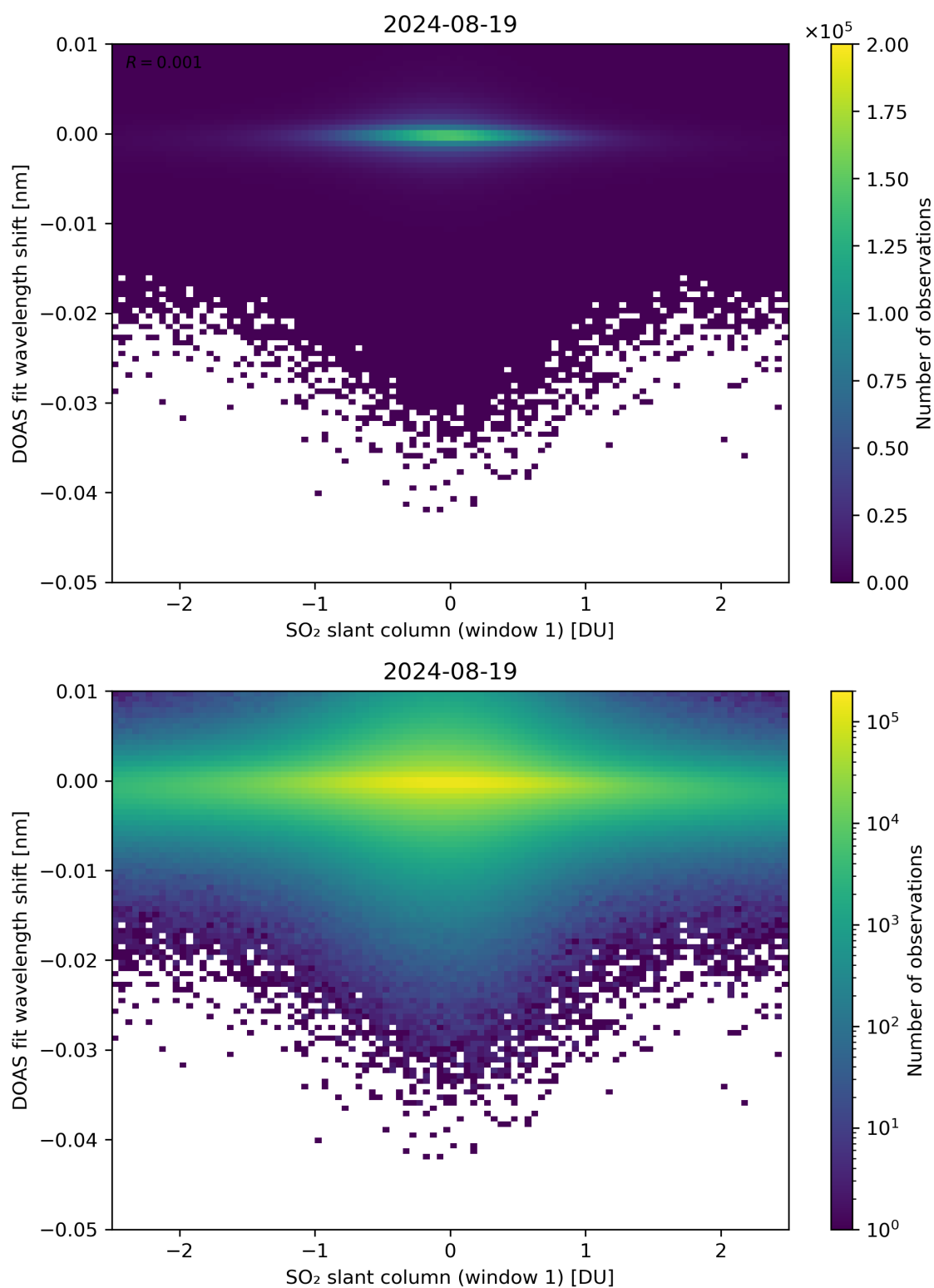
Figure 215: Scatter density plot of “SO 2 slant column (window 1)” against “DOAS fit wavelength shift” for 2024-08-18 to 2024-08-20.
