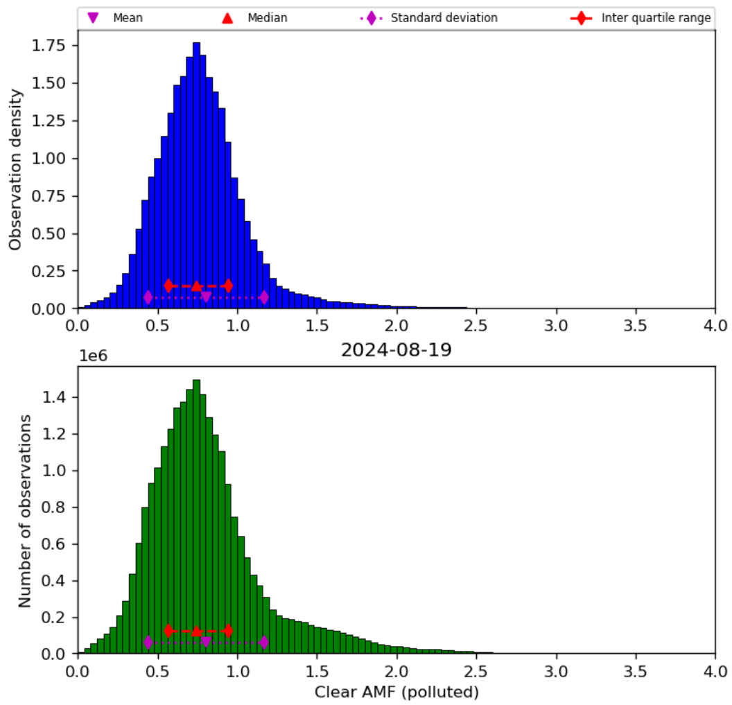
Figure 73: Histogram of “Clear AMF (polluted)” for 2024-08-18 to 2024-08-20
