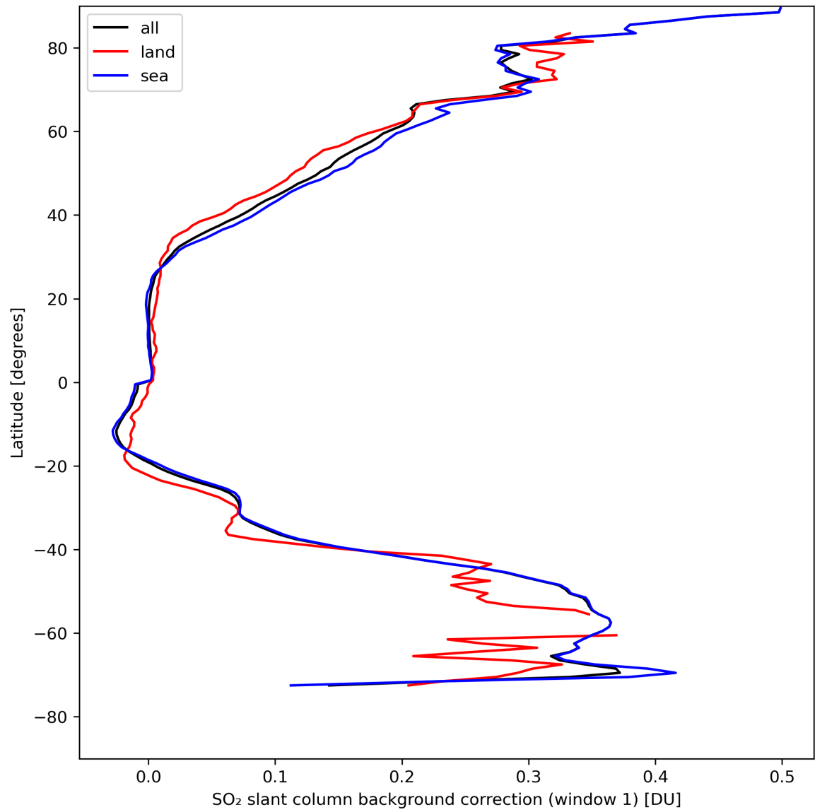
Figure 36: Zonal average of “SO 2 slant column background correction (window 1)” for 2024-08-18 to 2024-08-20.
