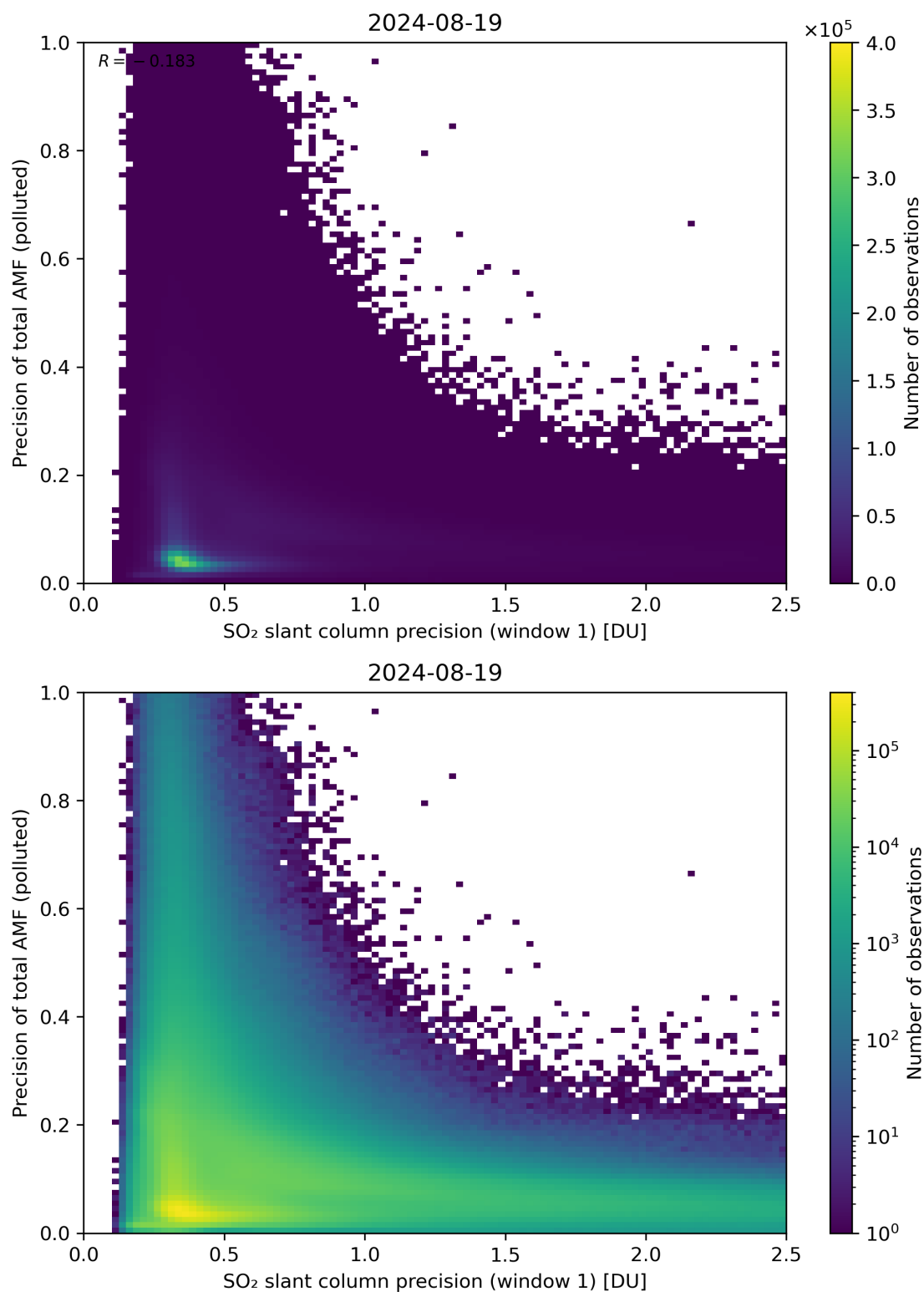
Figure 231: Scatter density plot of “SO 2 slant column precision (window 1)” against “Precision of total AMF (polluted)” for 2024-08-18 to 2024-08-20.
