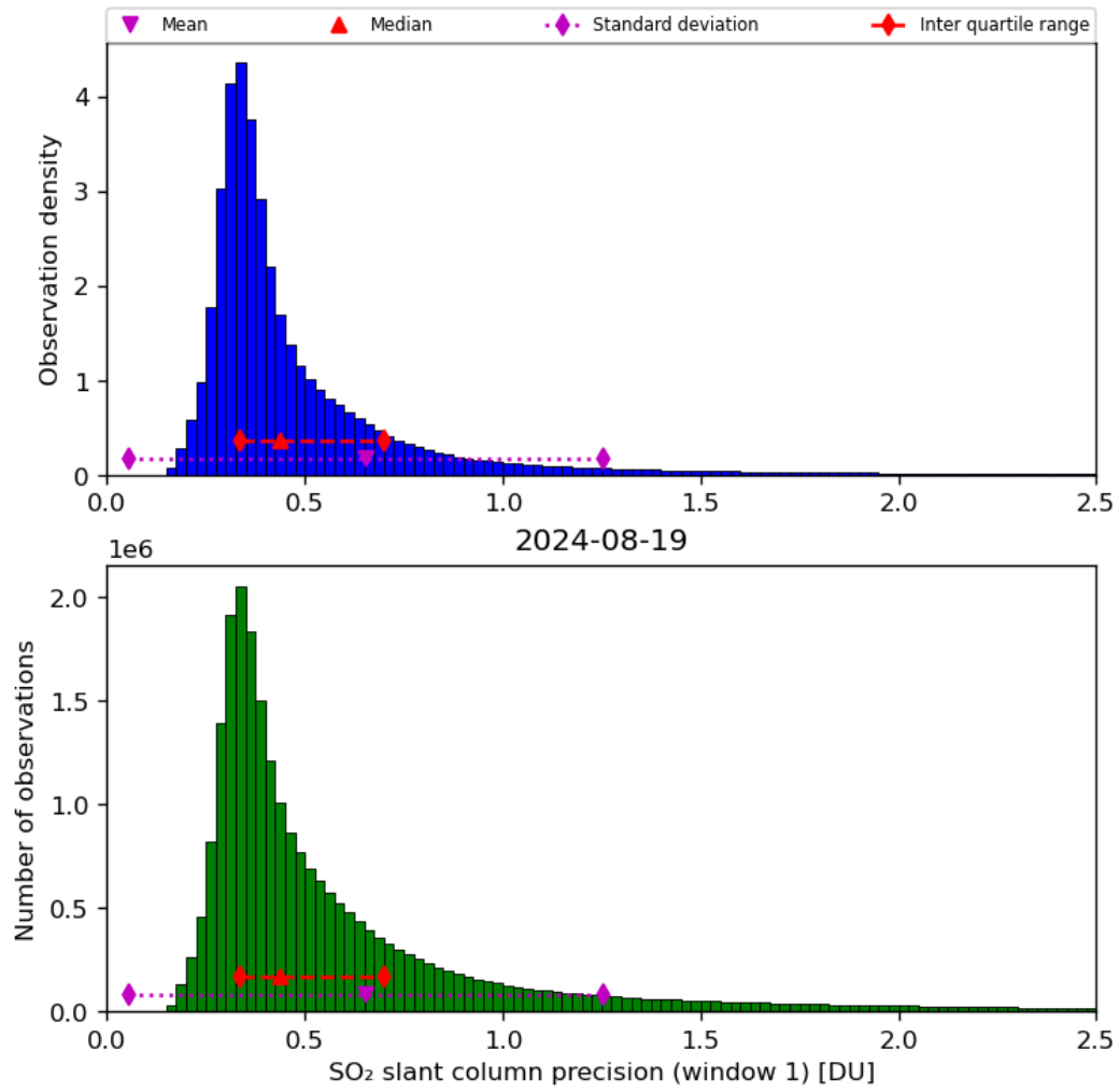
Figure 57: Histogram of “SO 2 slant column precision (window 1)” for 2024-08-18 to 2024-08-20
