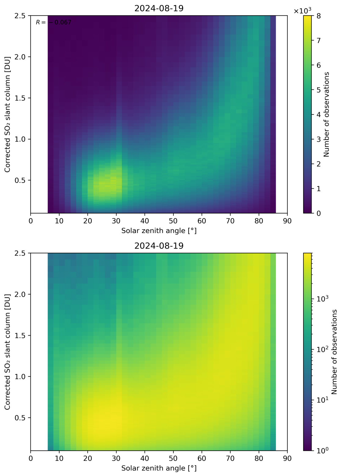
Figure 166: Scatter density plot of “Solar zenith angle” against “Corrected SO 2 slant column” for 2024-08-18 to 2024-08-20.
