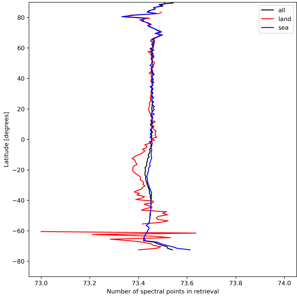
Figure 51: Zonal average of “Number of spectral points in retrieval” for 2024-08-18 to 2024-08-20.
