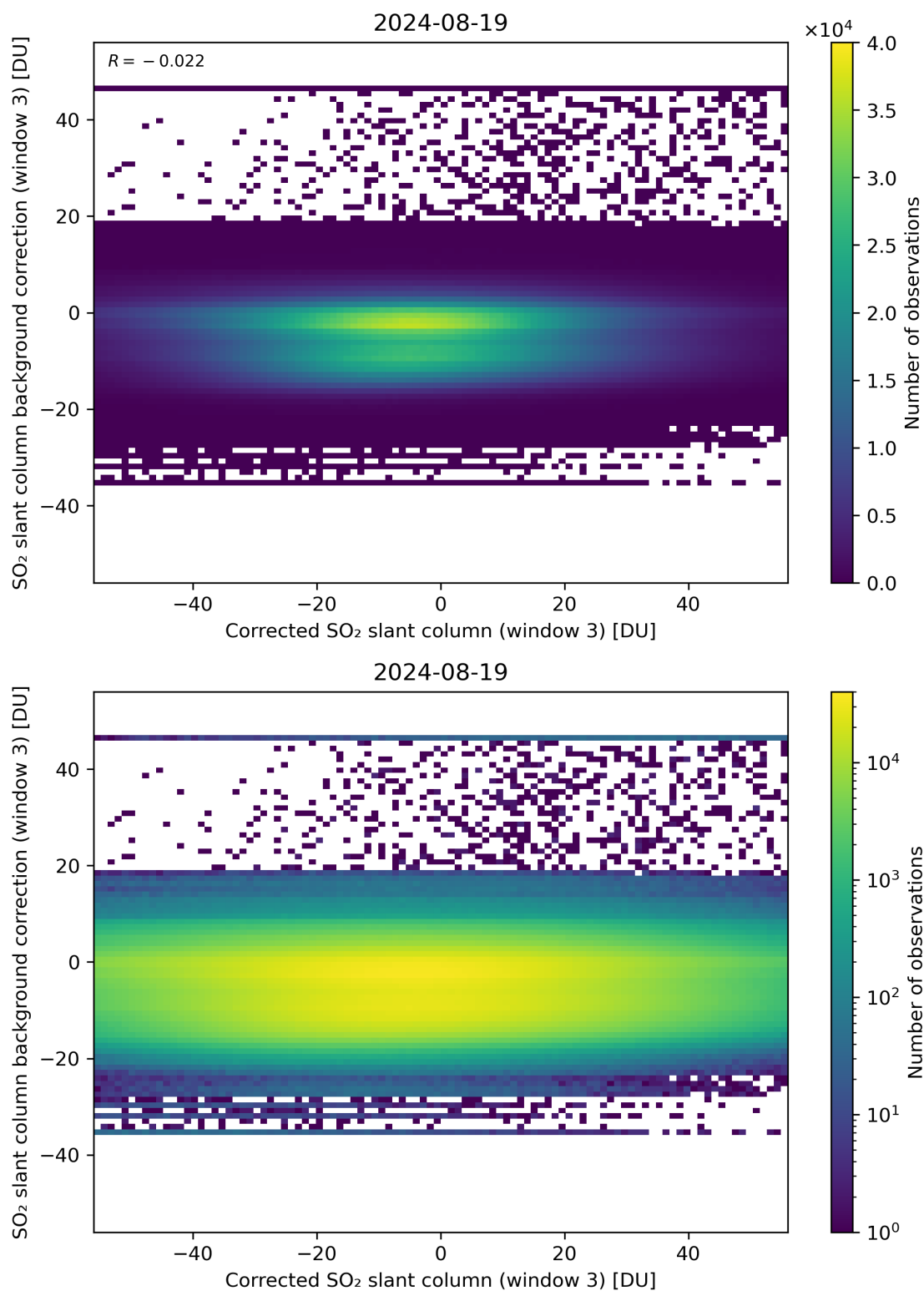
Figure 205: Scatter density plot of “Corrected SO 2 slant column (window 3)” against “SO 2 slant column background correction (window 3)” for 2024-08-18 to 2024-08-20.
