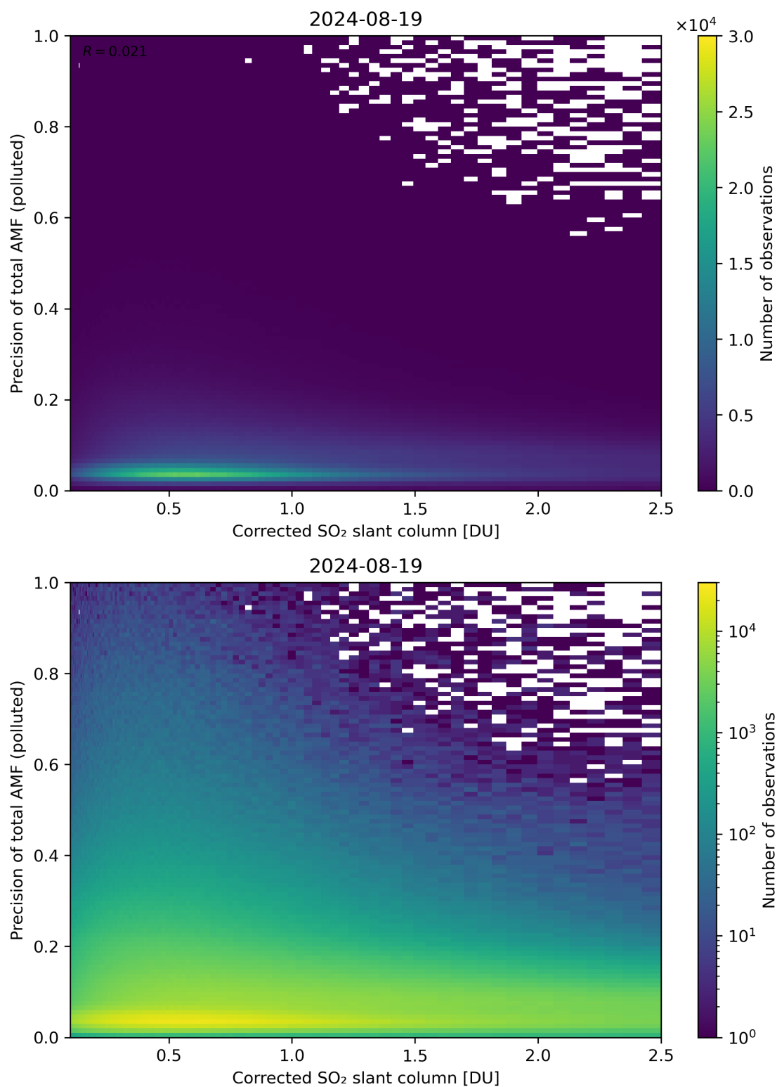
Figure 193: Scatter density plot of “Corrected SO 2 slant column” against “Precision of total AMF (polluted)” for 2024-08-18 to 2024-08-20.
