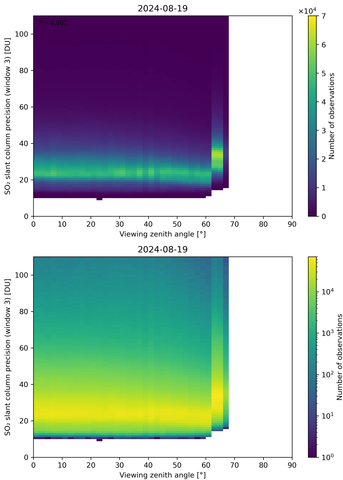
Figure 324: Scatter density plot of “Viewing zenith angle” against “SO 2 slant column precision (window 3)” for 2024-08-18 to 2024-08-20.
