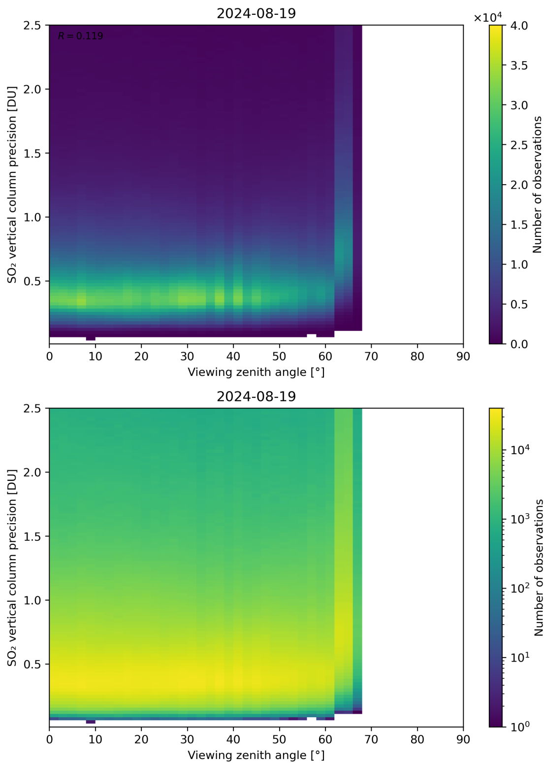
Figure 328: Scatter density plot of “Viewing zenith angle” against “SO 2 vertical column precision” for 2024-08-18 to 2024-08-20.
