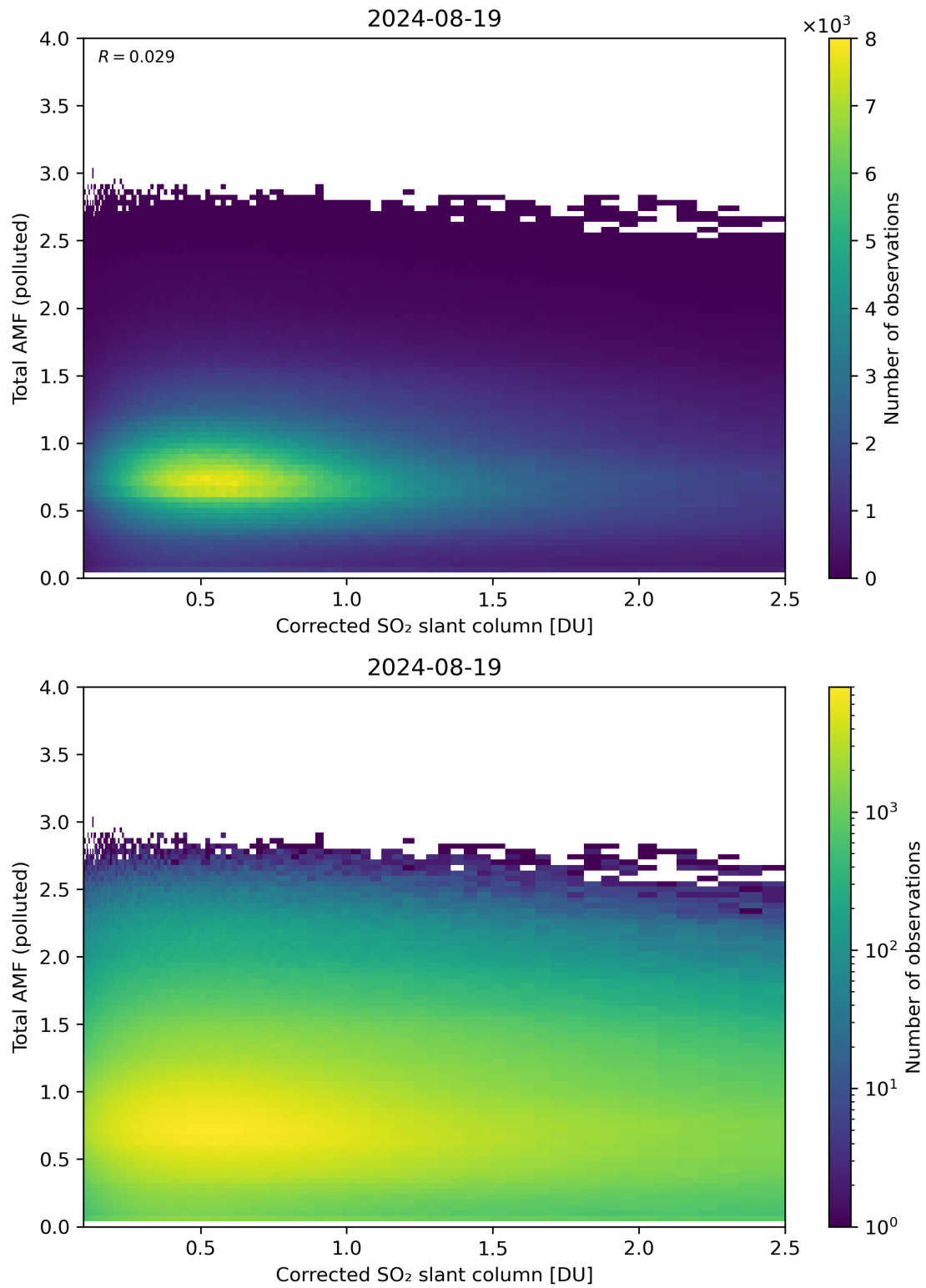
Figure 192: Scatter density plot of “Corrected SO 2 slant column” against “Total AMF (polluted)” for 2024-08-18 to 2024-08-20.
