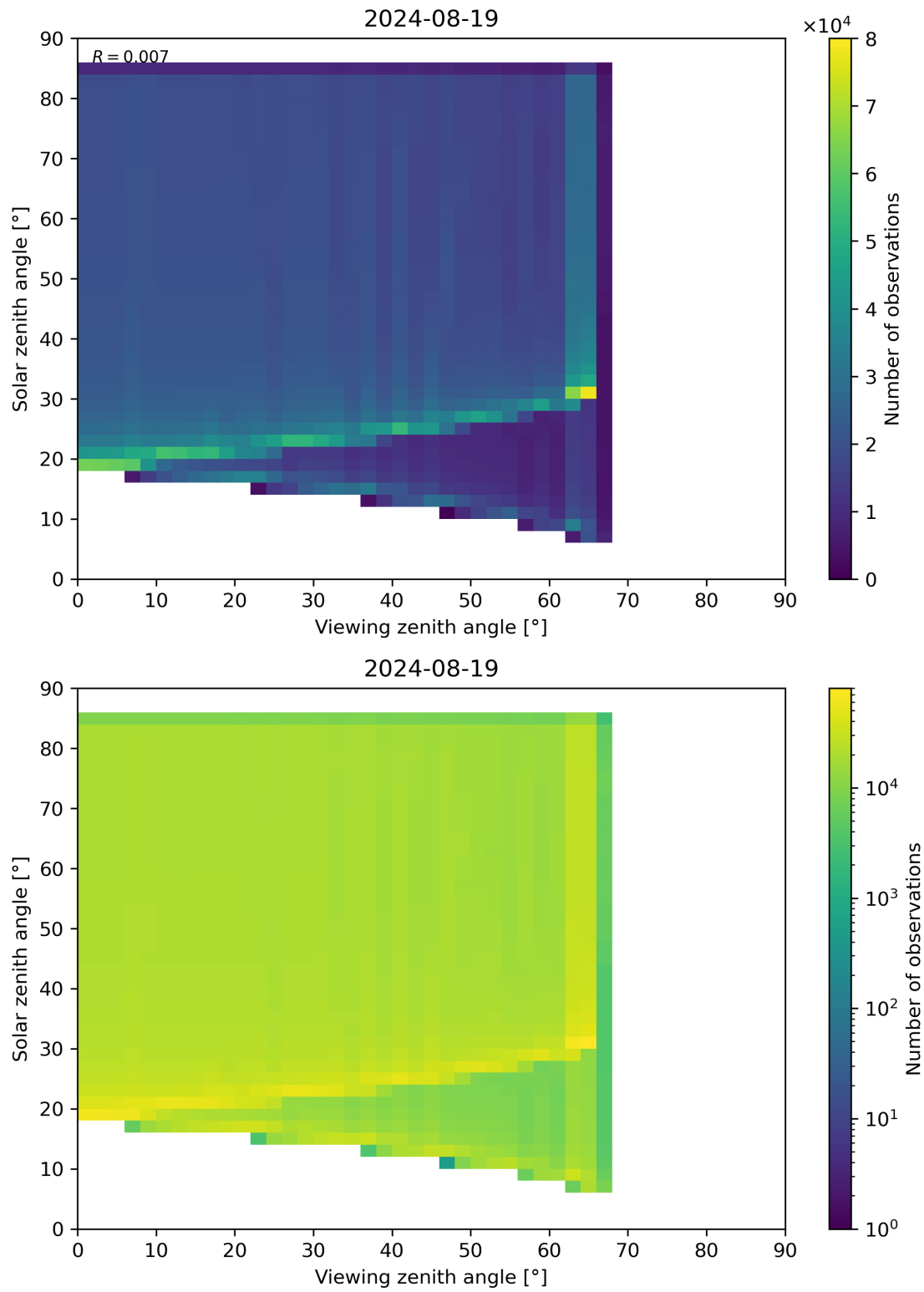
Figure 315: Scatter density plot of “Viewing zenith angle” against “Solar zenith angle” for 2024-08-18 to 2024-08-20.
