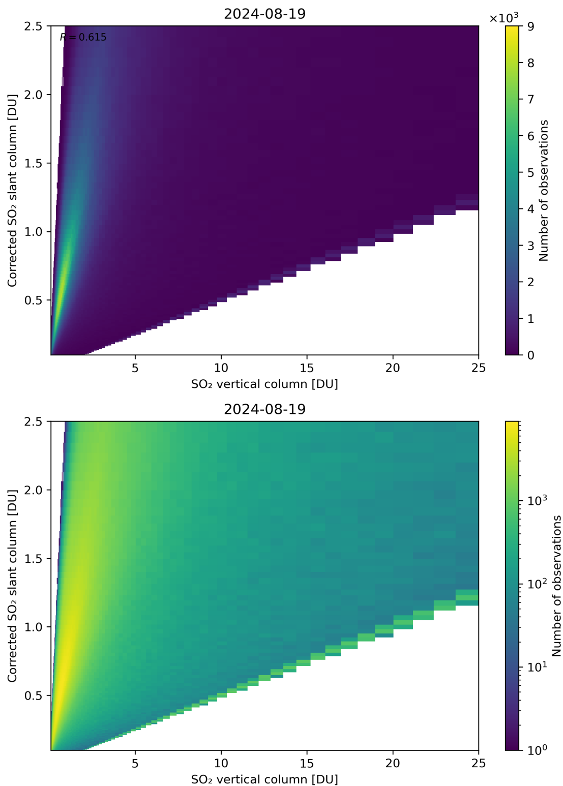
Figure 297: Scatter density plot of “SO 2 vertical column” against “Corrected SO 2 slant column” for 2024-08-18 to 2024-08-20.
