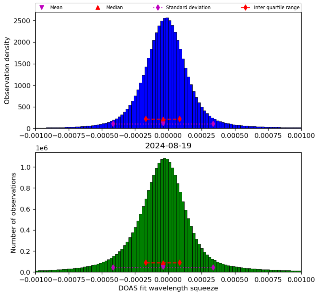
Figure 69: Histogram of “DOAS fit wavelength squeeze” for 2024-08-18 to 2024-08-20
