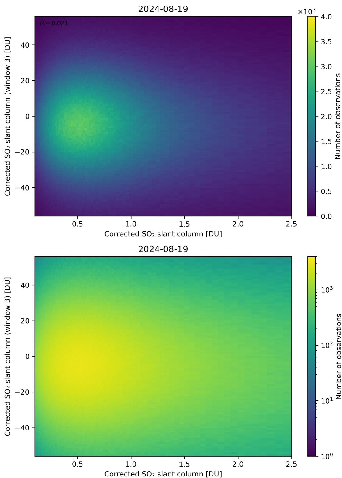
Figure 186: Scatter density plot of “Corrected SO 2 slant column” against “Corrected SO 2 slant column (window 3)” for 2024-08-18 to 2024-08-20.
