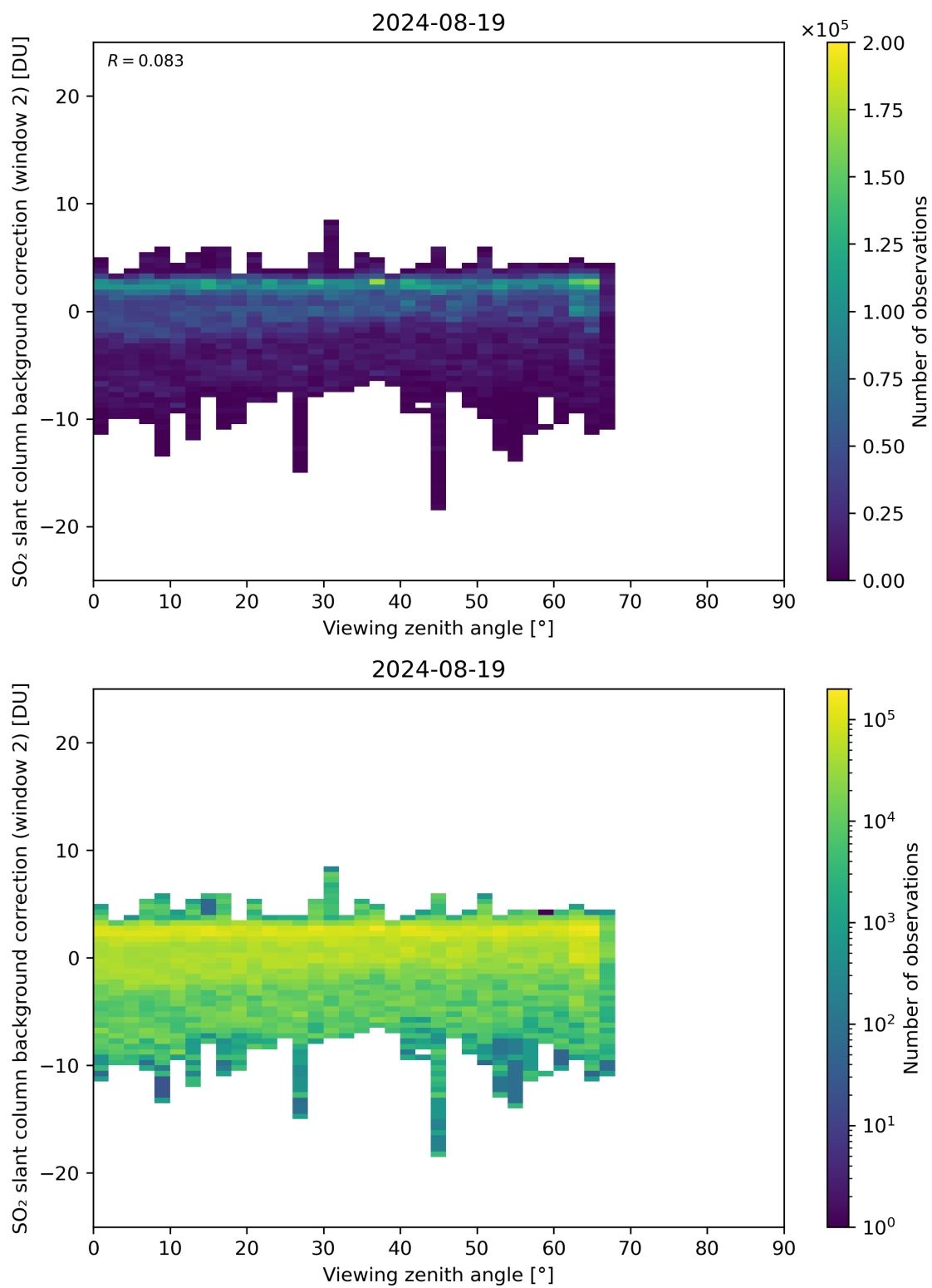
Figure 309: Scatter density plot of “Viewing zenith angle” against “SO 2 slant column background correction (window 2)” for 2024-08-18 to 2024-08-20.
