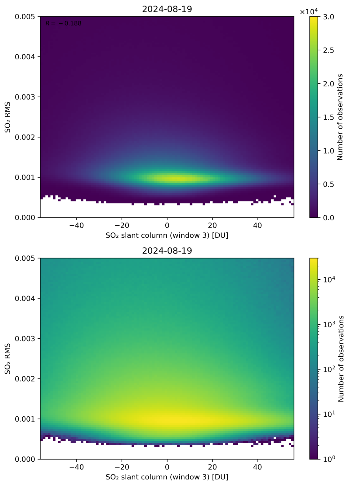
Figure 256: Scatter density plot of “SO 2 slant column (window 3)” against “SO 2 RMS” for 2024-08-18 to 2024-08-20.
