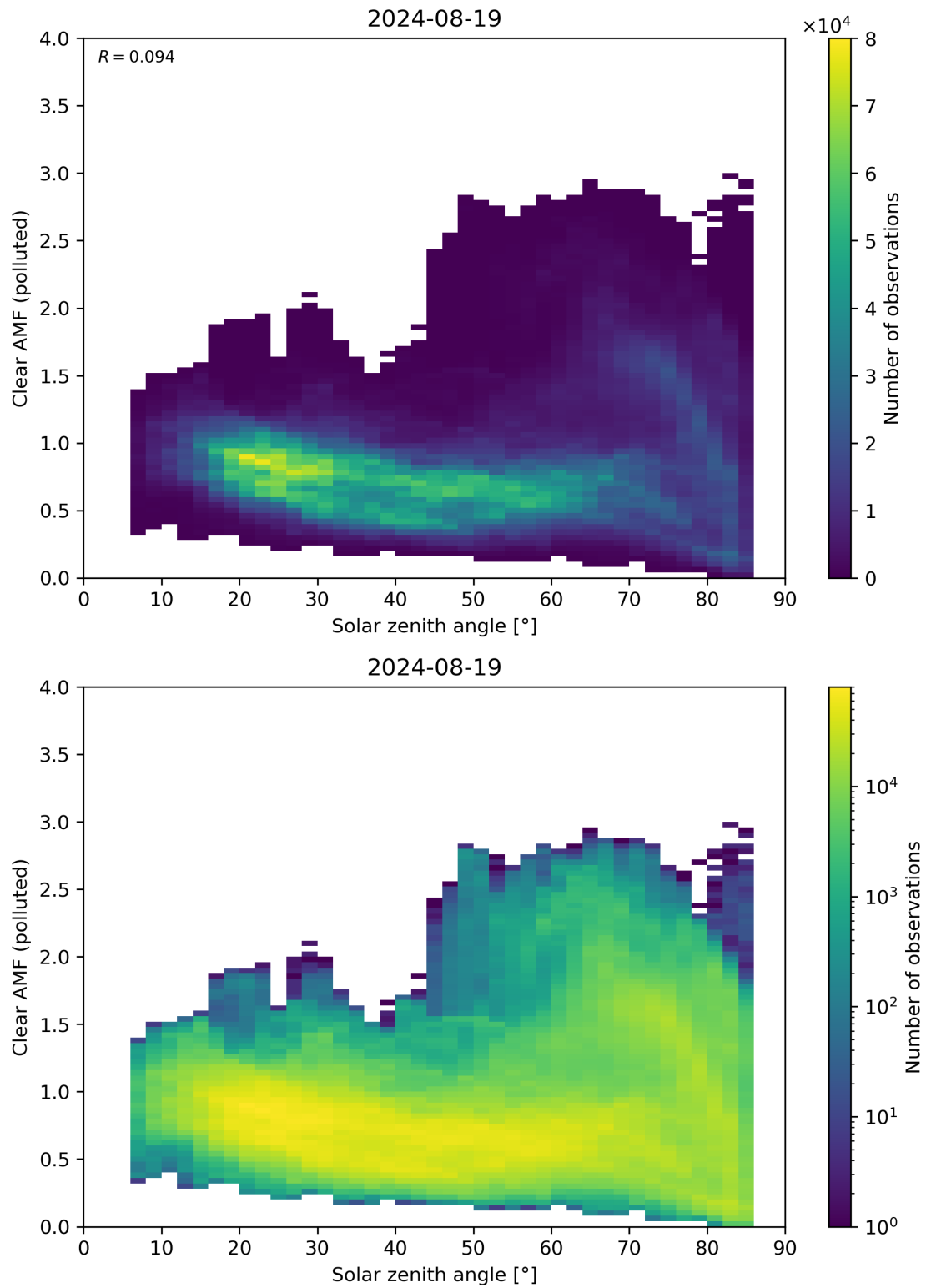
Figure 165: Scatter density plot of “Solar zenith angle” against “Clear AMF (polluted)” for 2024-08-18 to 2024-08-20.
