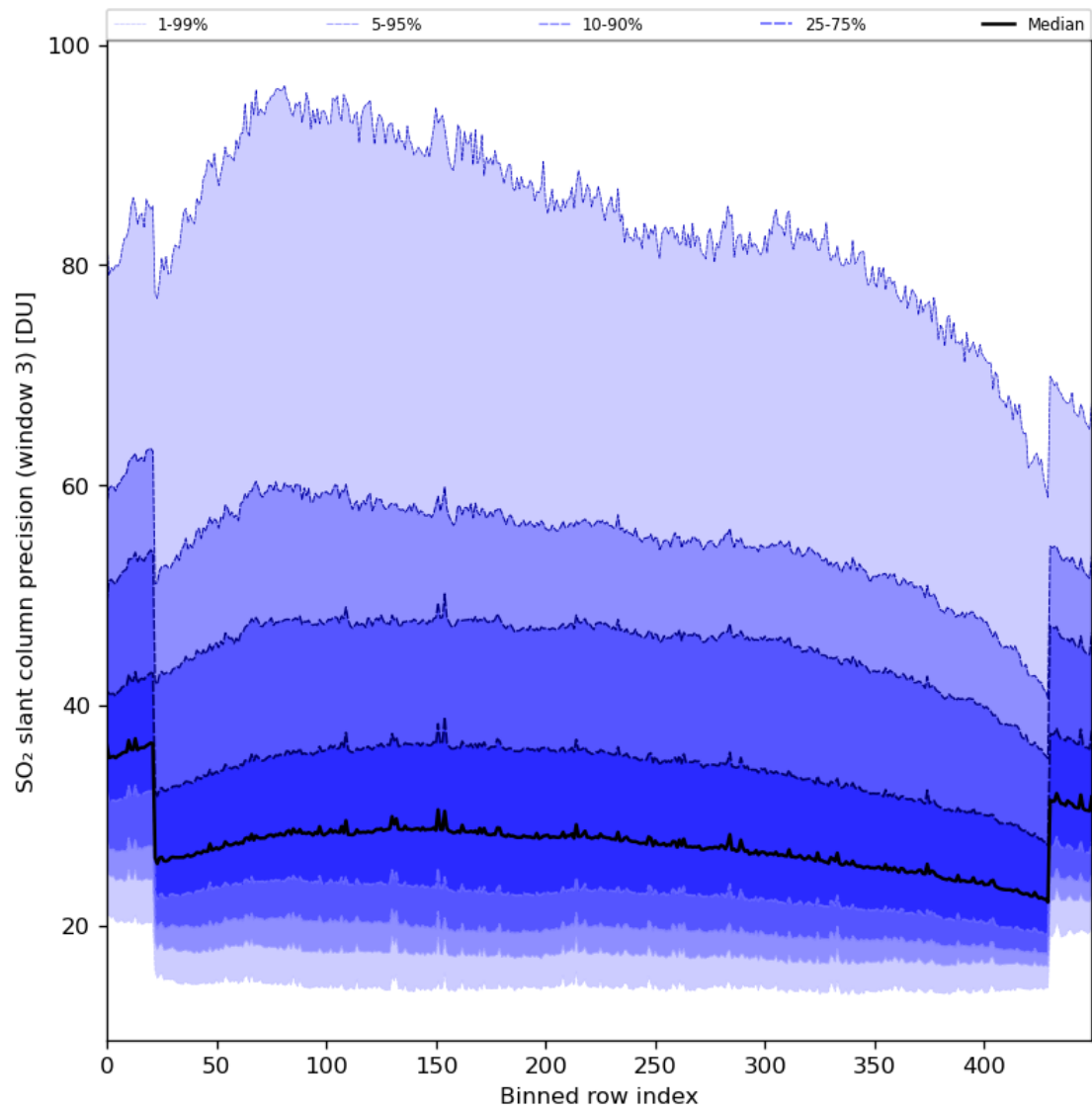
Figure 88: Along track statistics of “SO 2 slant column precision (window 3)” for 2024-08-18 to 2024-08-20
