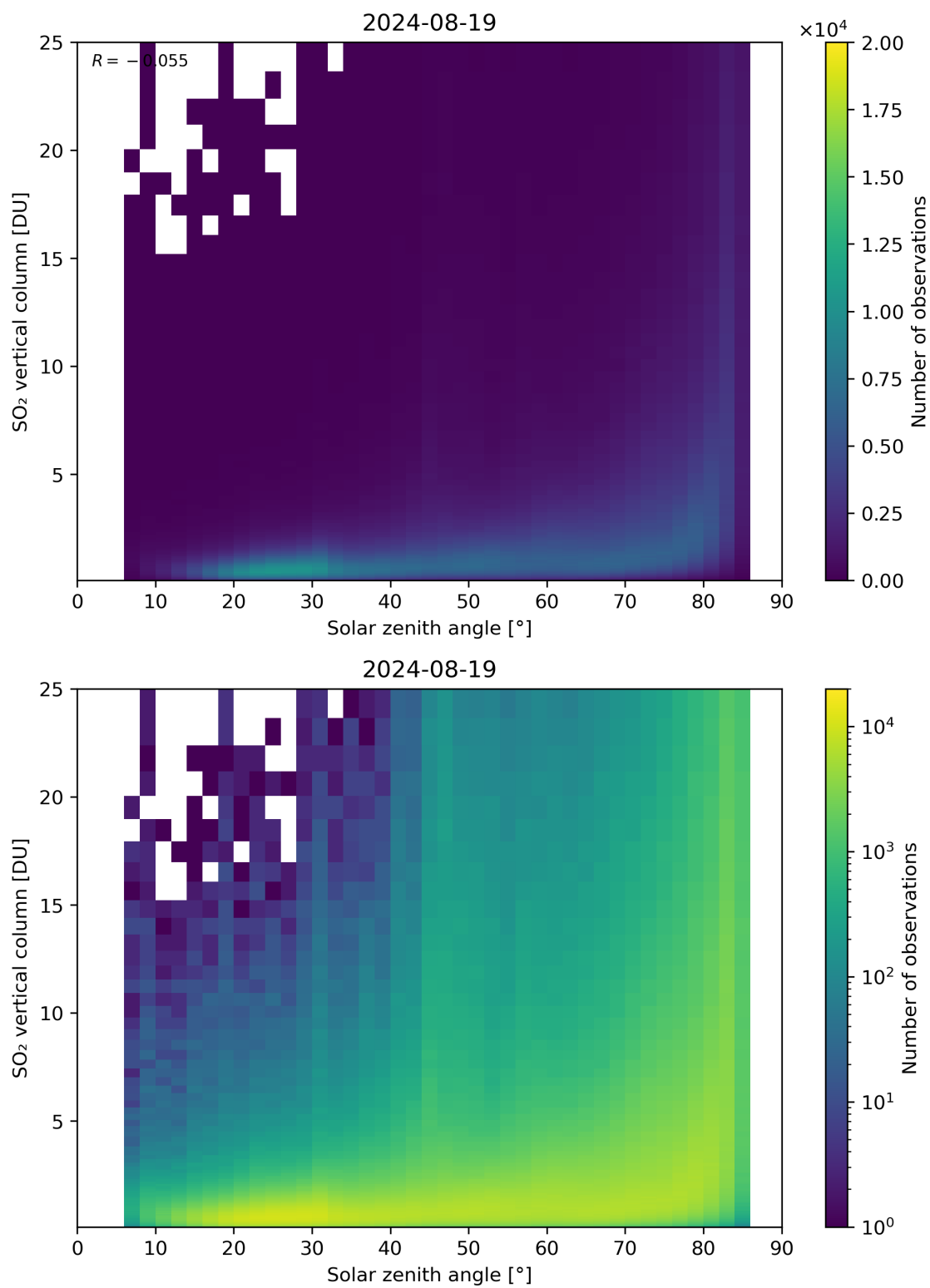
Figure 176: Scatter density plot of “Solar zenith angle” against “SO 2 vertical column” for 2024-08-18 to 2024-08-20.
