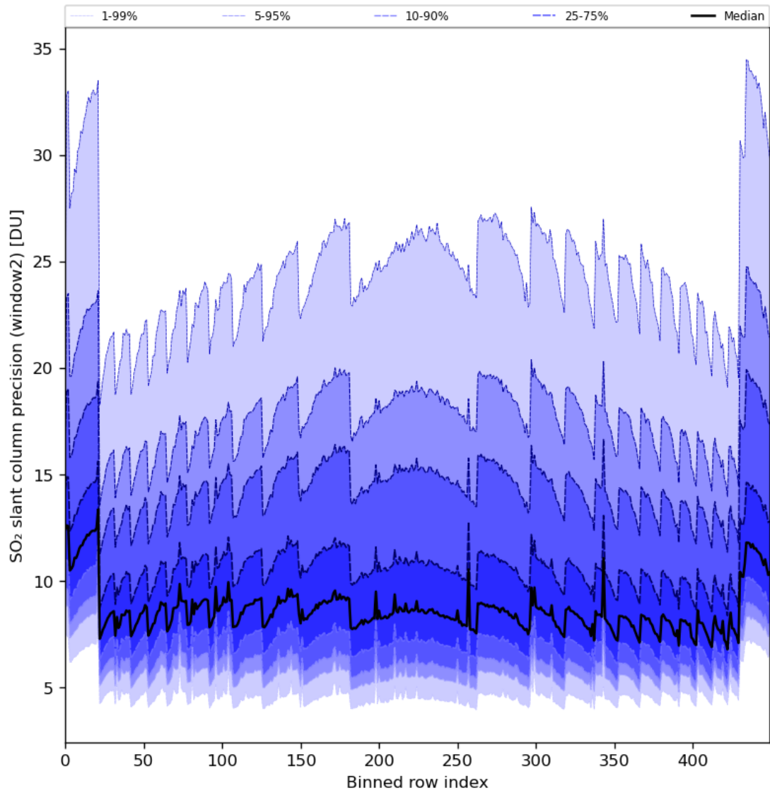
Figure 84: Along track statistics of “SO 2 slant column precision (window2)” for 2024-08-18 to 2024-08-20
