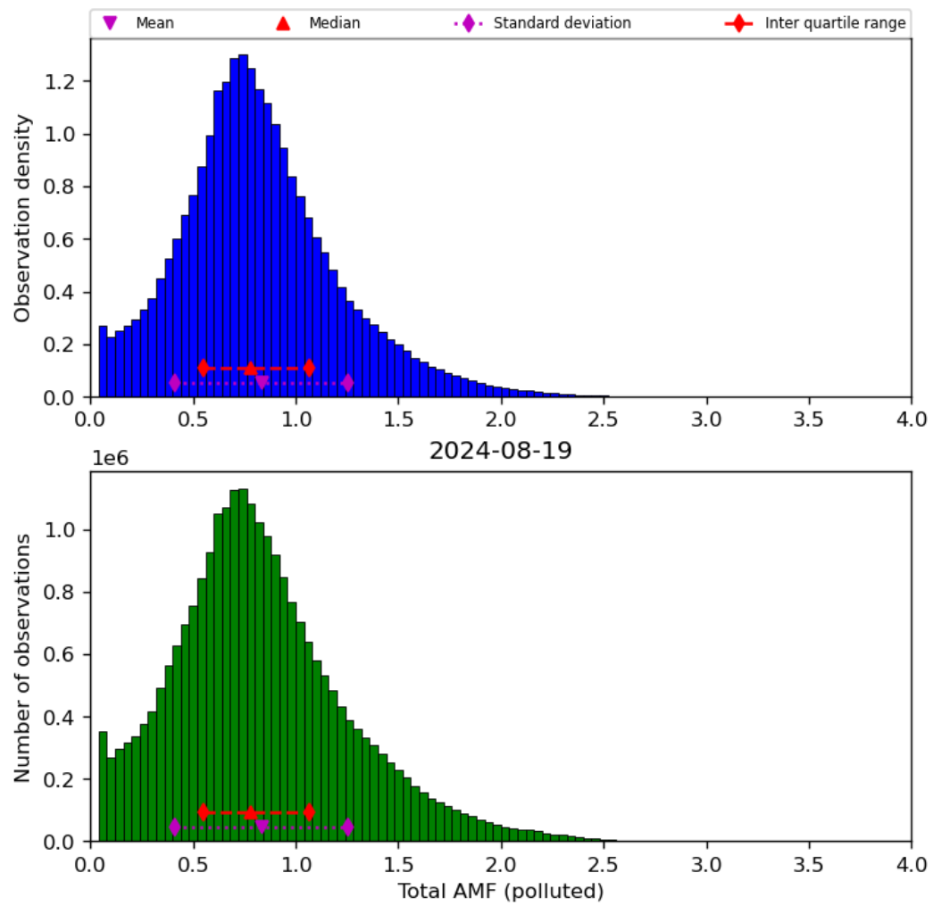
Figure 71: Histogram of “Total AMF (polluted)” for 2024-08-18 to 2024-08-20
