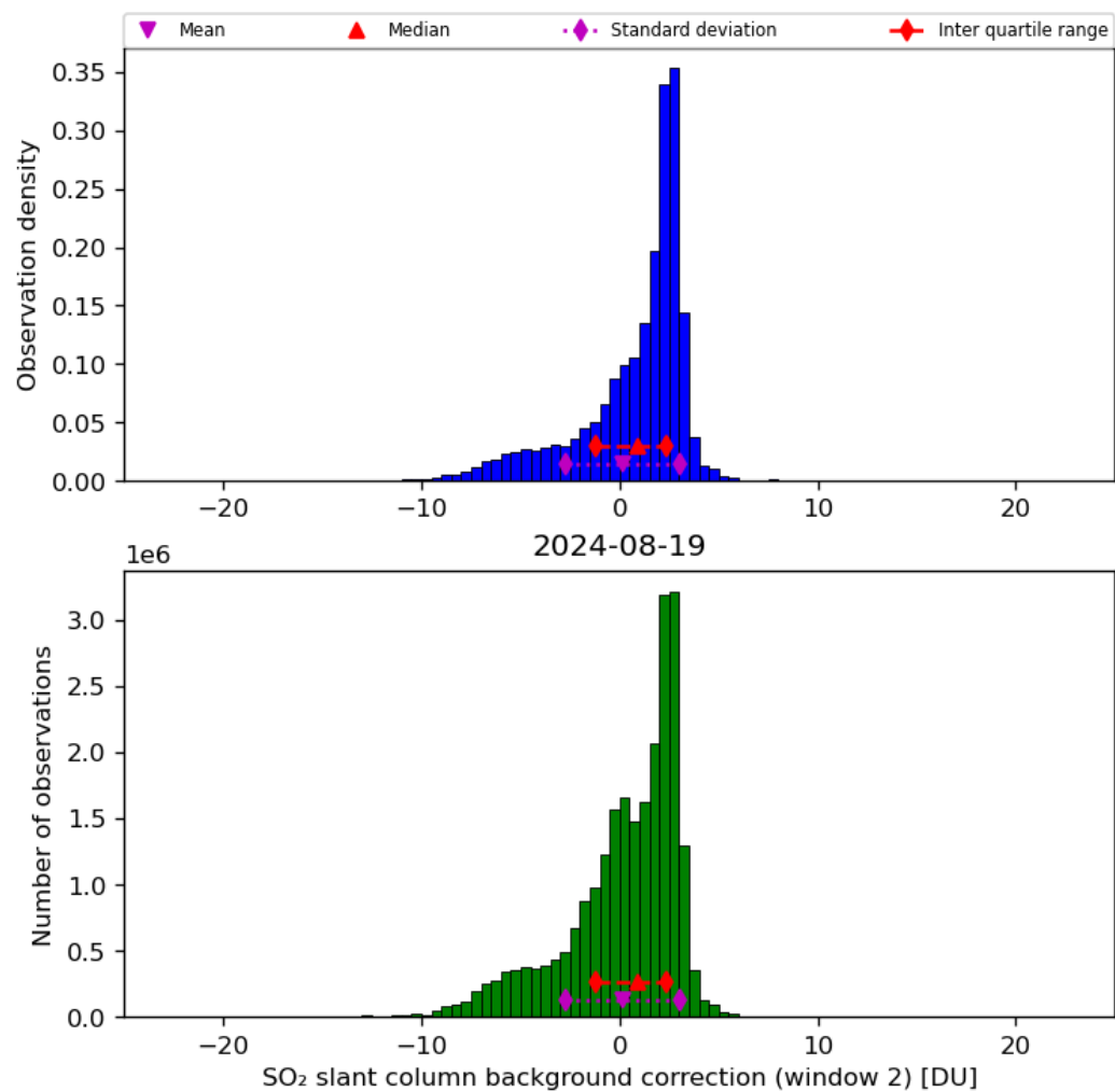
Figure 63: Histogram of “SO 2 slant column background correction (window 2)” for 2024-08-18 to 2024-08-20
