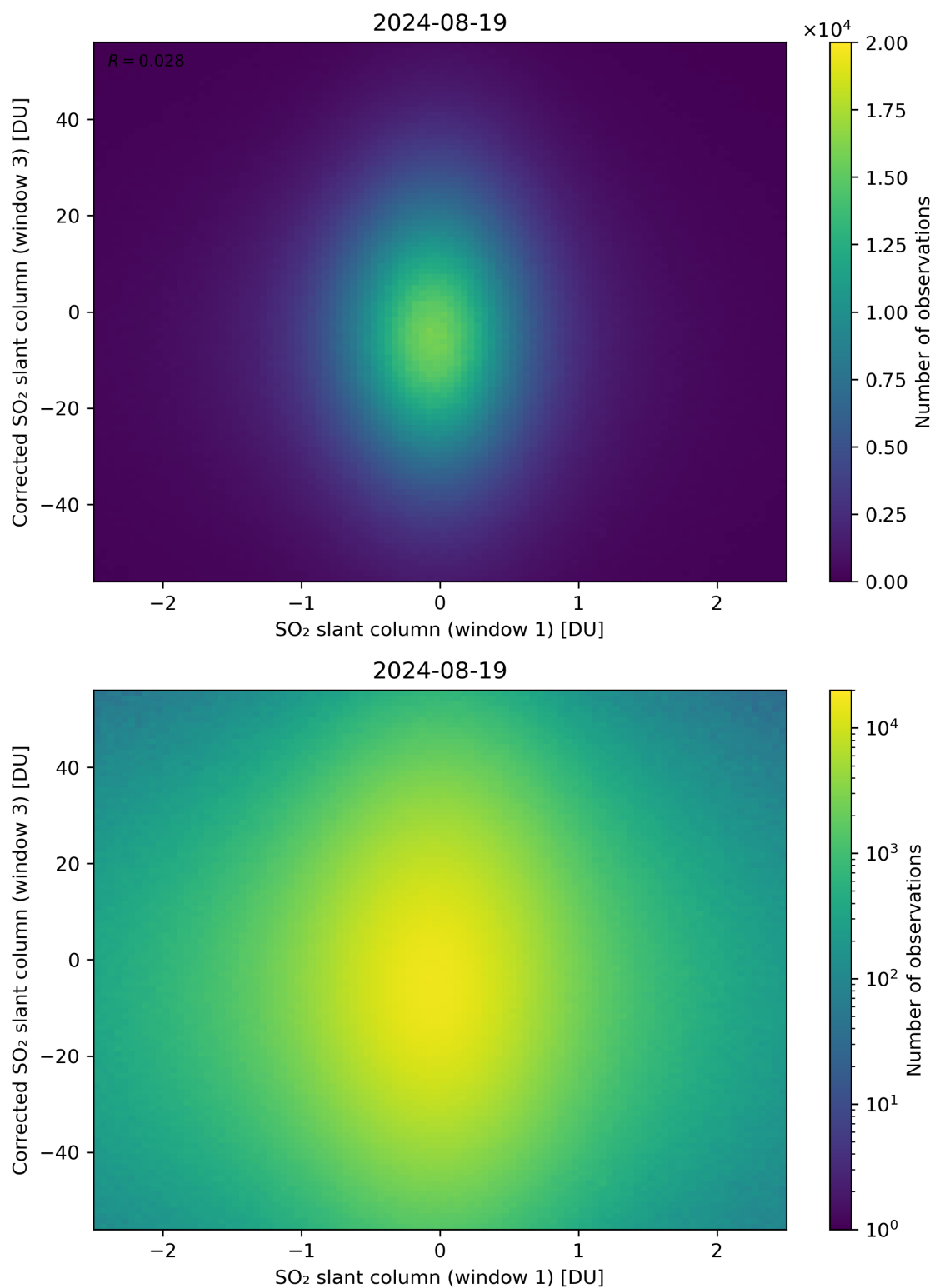
Figure 234: Scatter density plot of “SO 2 slant column (window 1)” against “Corrected SO 2 slant column (window 3)” for 2024-08-18 to 2024-08-20.
