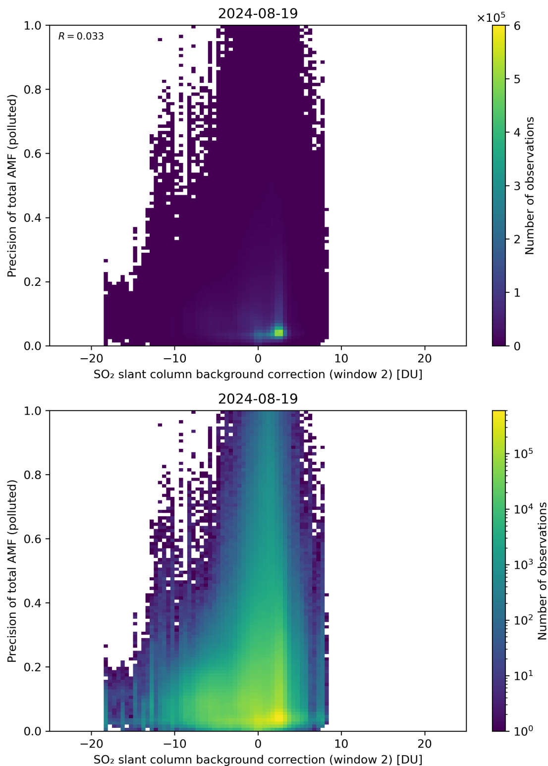
Figure 120: Scatter density plot of “SO 2 slant column background correction (window 2)” against “Precision of total AMF (polluted)” for 2024-08-18 to 2024-08-20.
