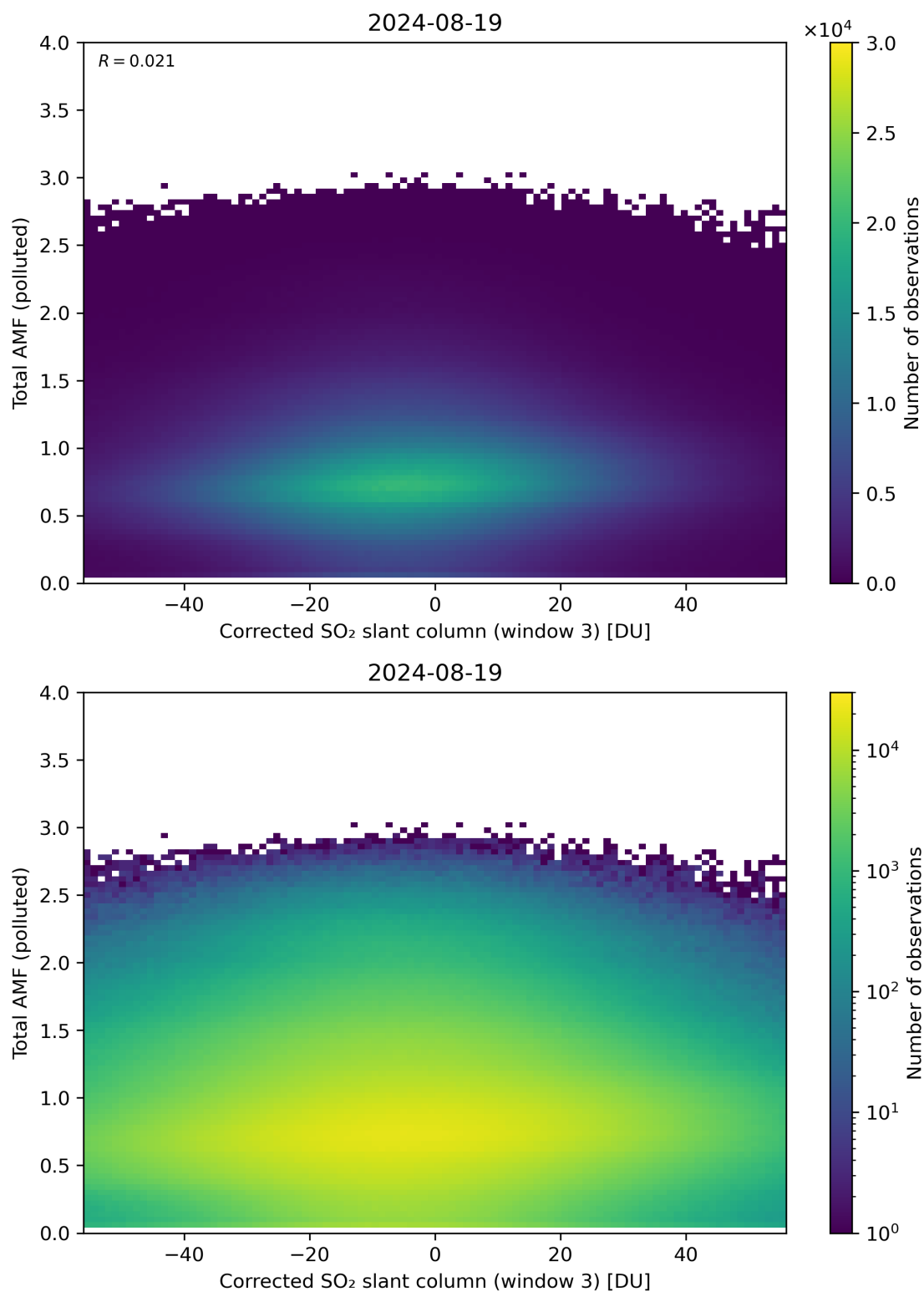
Figure 210: Scatter density plot of “Corrected SO 2 slant column (window 3)” against “Total AMF (polluted)” for 2024-08-18 to 2024-08-20.
