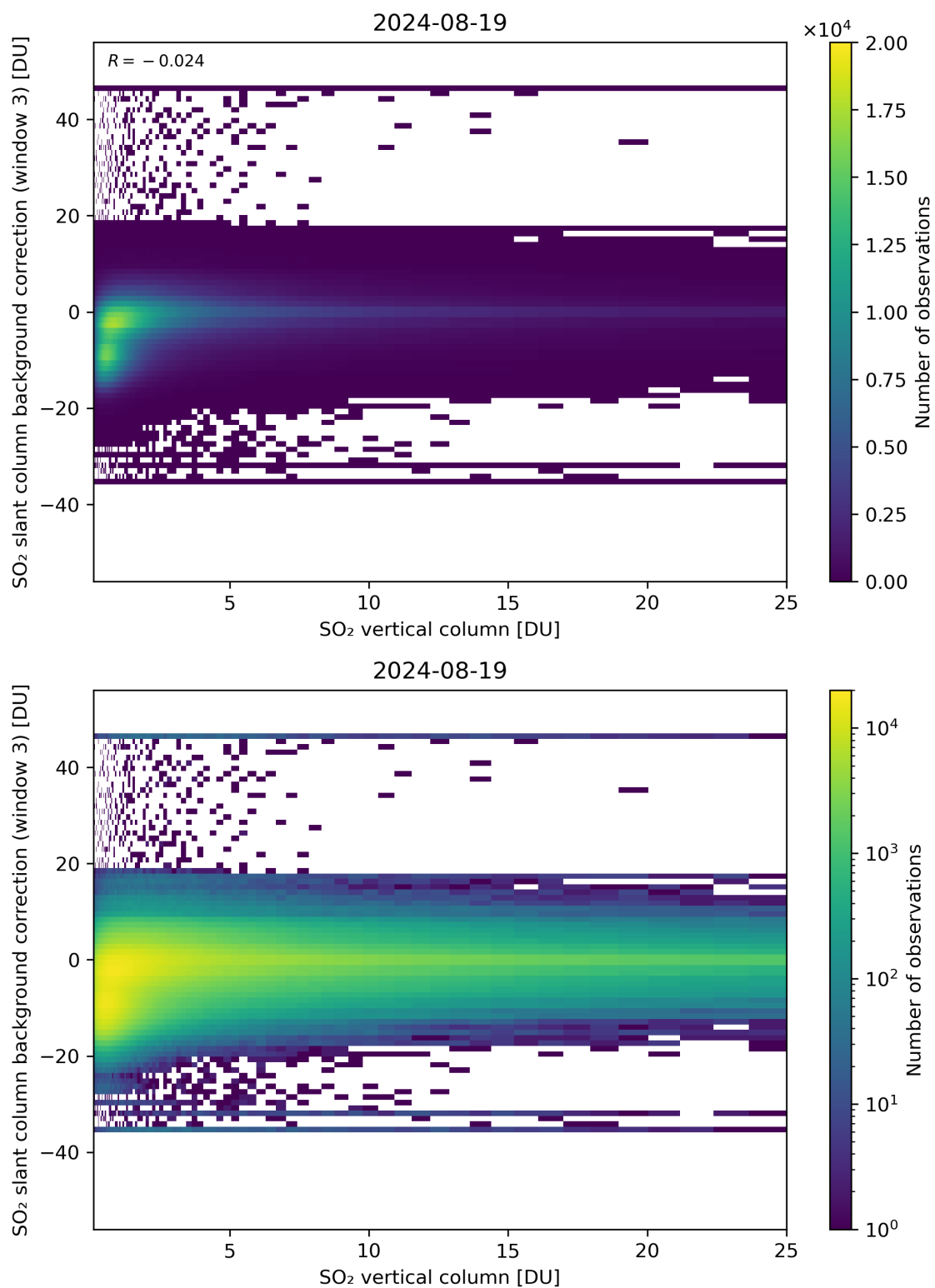
Figure 275: Scatter density plot of “SO 2 vertical column” against “SO 2 slant column background correction (window 3)” for 2024-08-18 to 2024-08-20.
