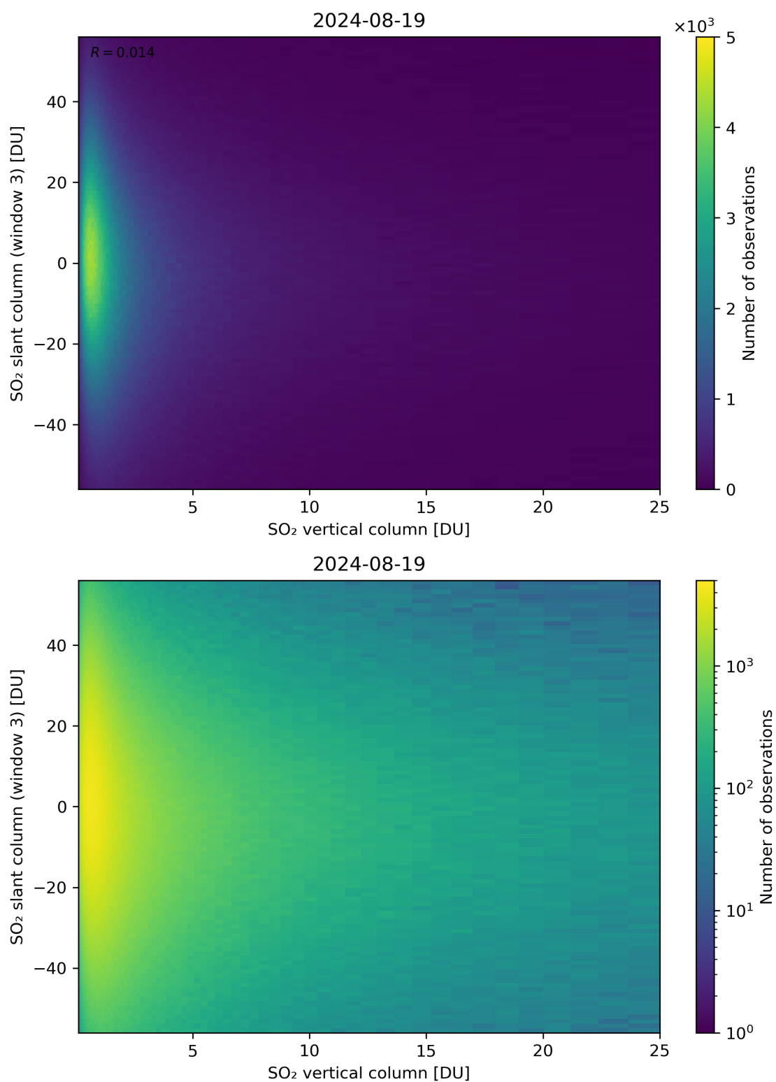
Figure 303: Scatter density plot of “SO 2 vertical column” against “SO 2 slant column (window 3)” for 2024-08-18 to 2024-08-20.
