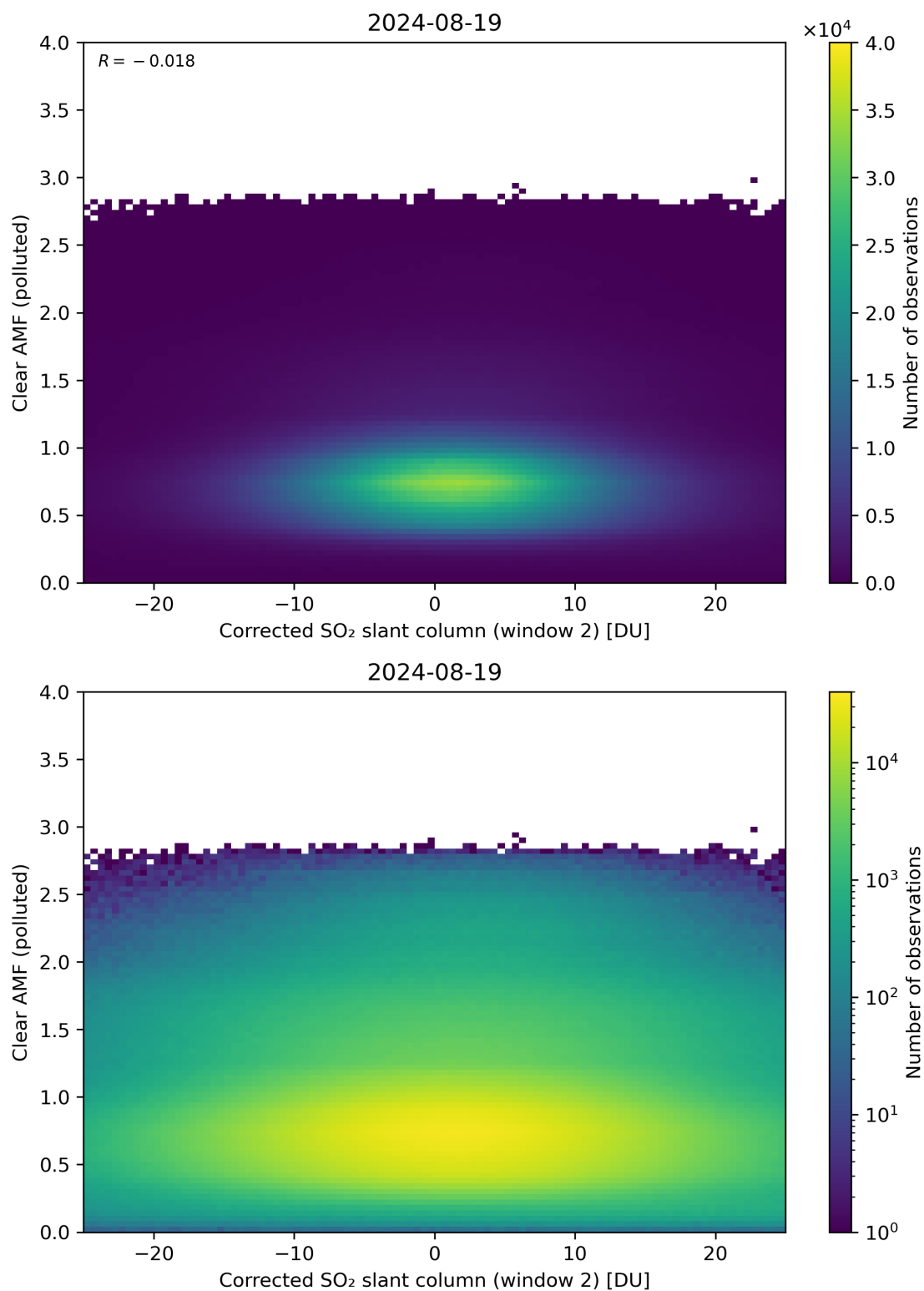
Figure 199: Scatter density plot of “Corrected SO 2 slant column (window 2)” against “Clear AMF (polluted)” for 2024-08-18 to 2024-08-20.
