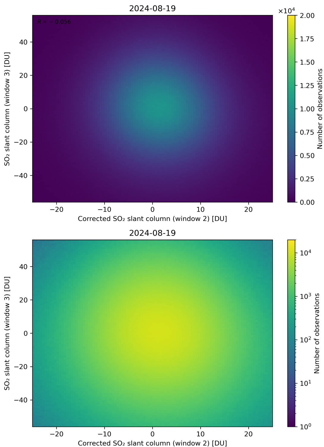
Figure 201: Scatter density plot of “Corrected SO 2 slant column (window 2)” against “SO 2 slant column (window 3)” for 2024-08-18 to 2024-08-20.
