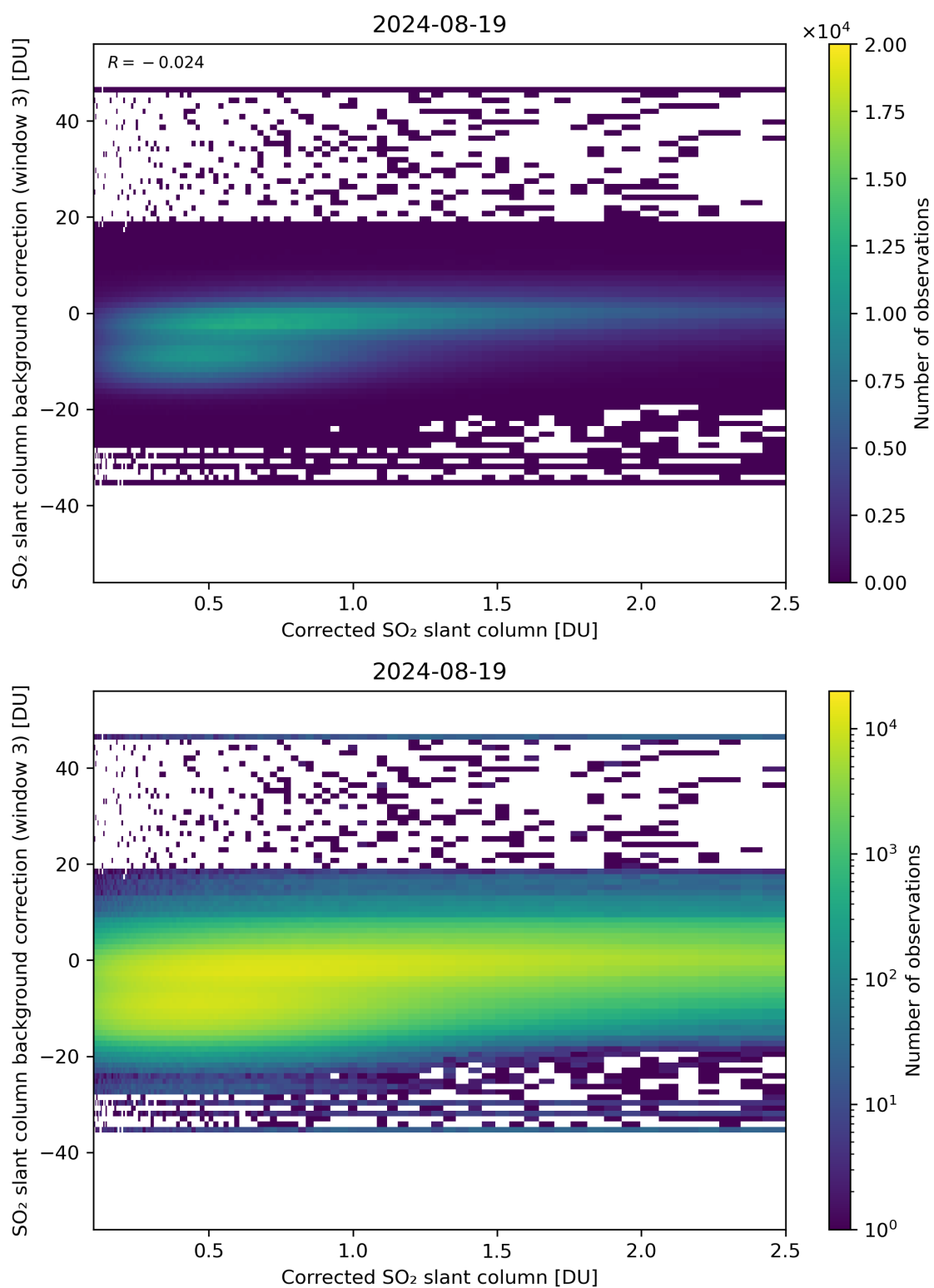
Figure 180: Scatter density plot of “Corrected SO 2 slant column” against “SO 2 slant column background correction (window 3)” for 2024-08-18 to 2024-08-20.
