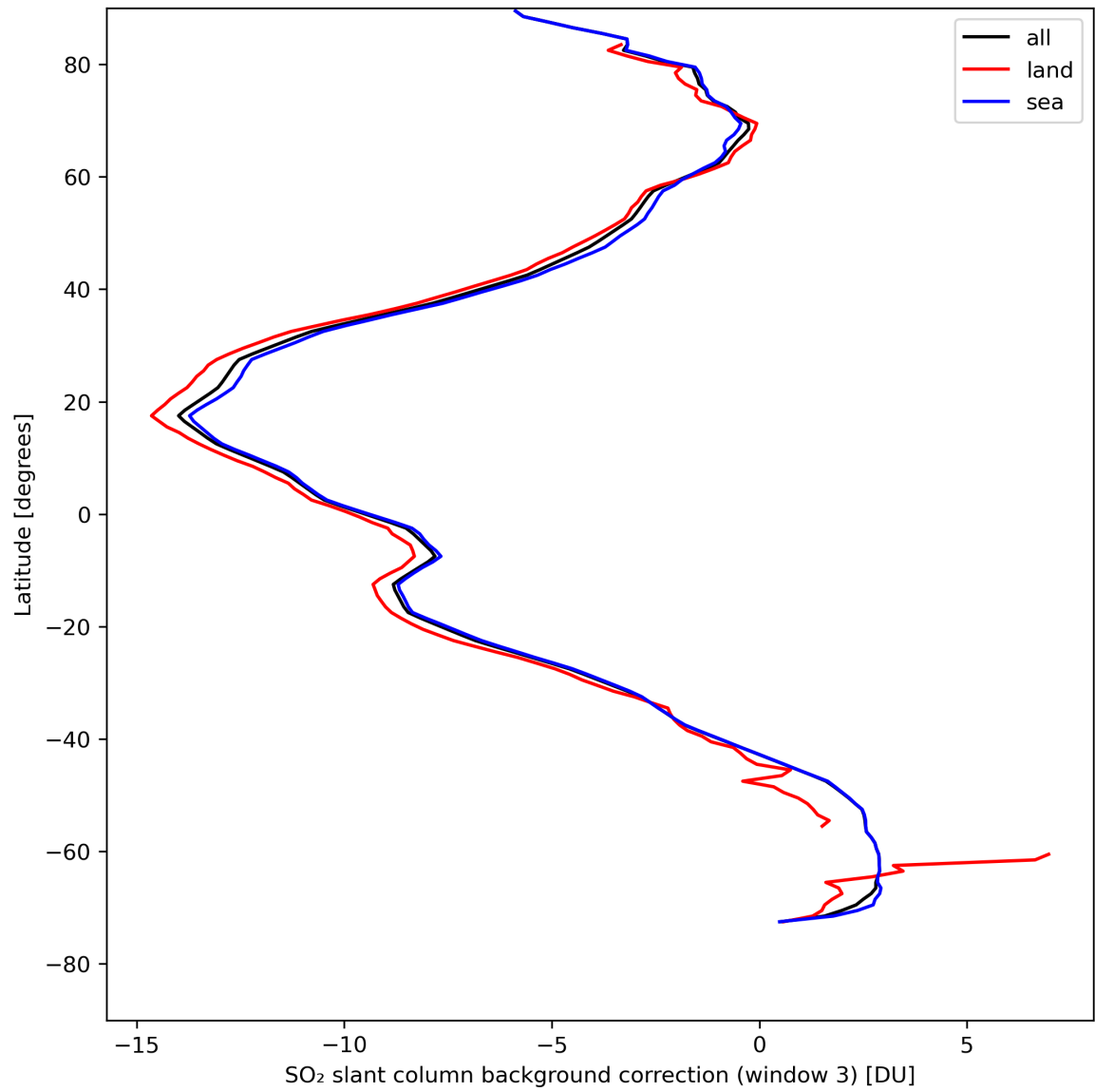
Figure 44: Zonal average of “SO 2 slant column background correction (window 3)” for 2024-08-18 to 2024-08-20.
