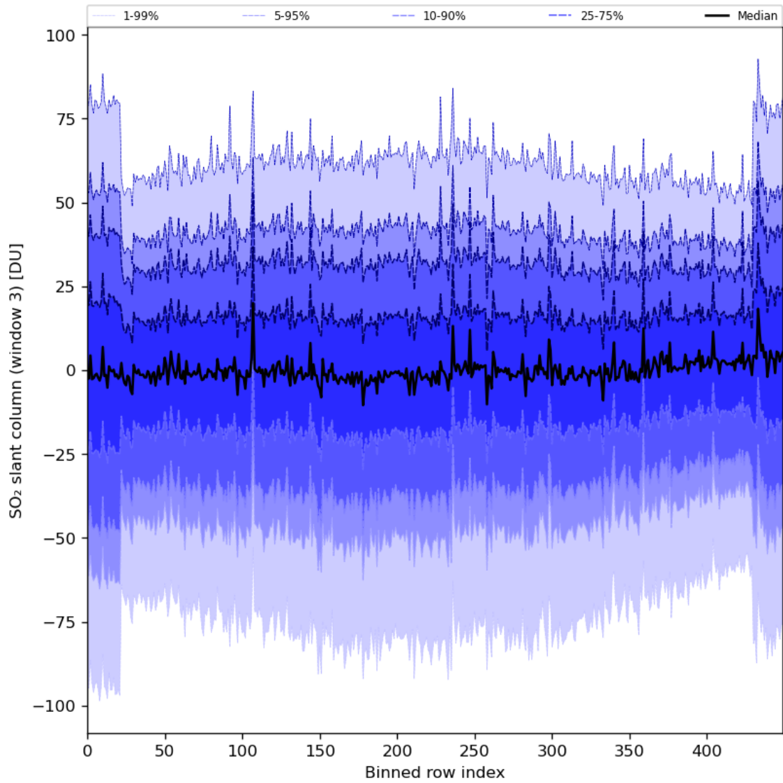
Figure 87: Along track statistics of “SO 2 slant column (window 3)” for 2024-08-18 to 2024-08-20
