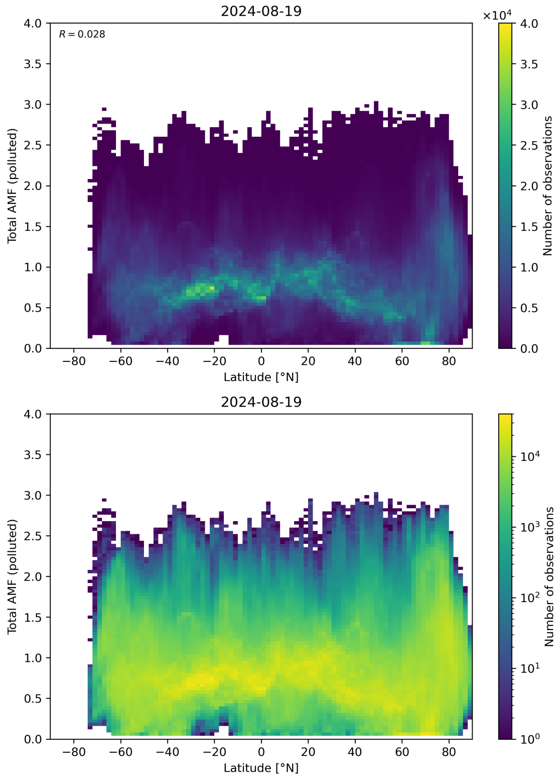
Figure 154: Scatter density plot of “Latitude” against “Total AMF (polluted)” for 2024-08-18 to 2024-08-20.
