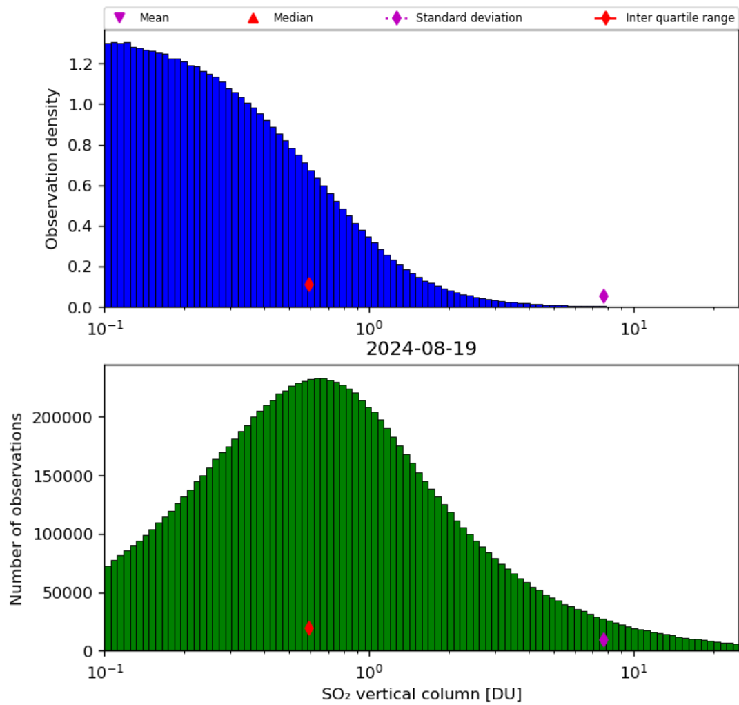
Figure 53: Histogram of “SO 2 vertical column” for 2024-08-18 to 2024-08-20
