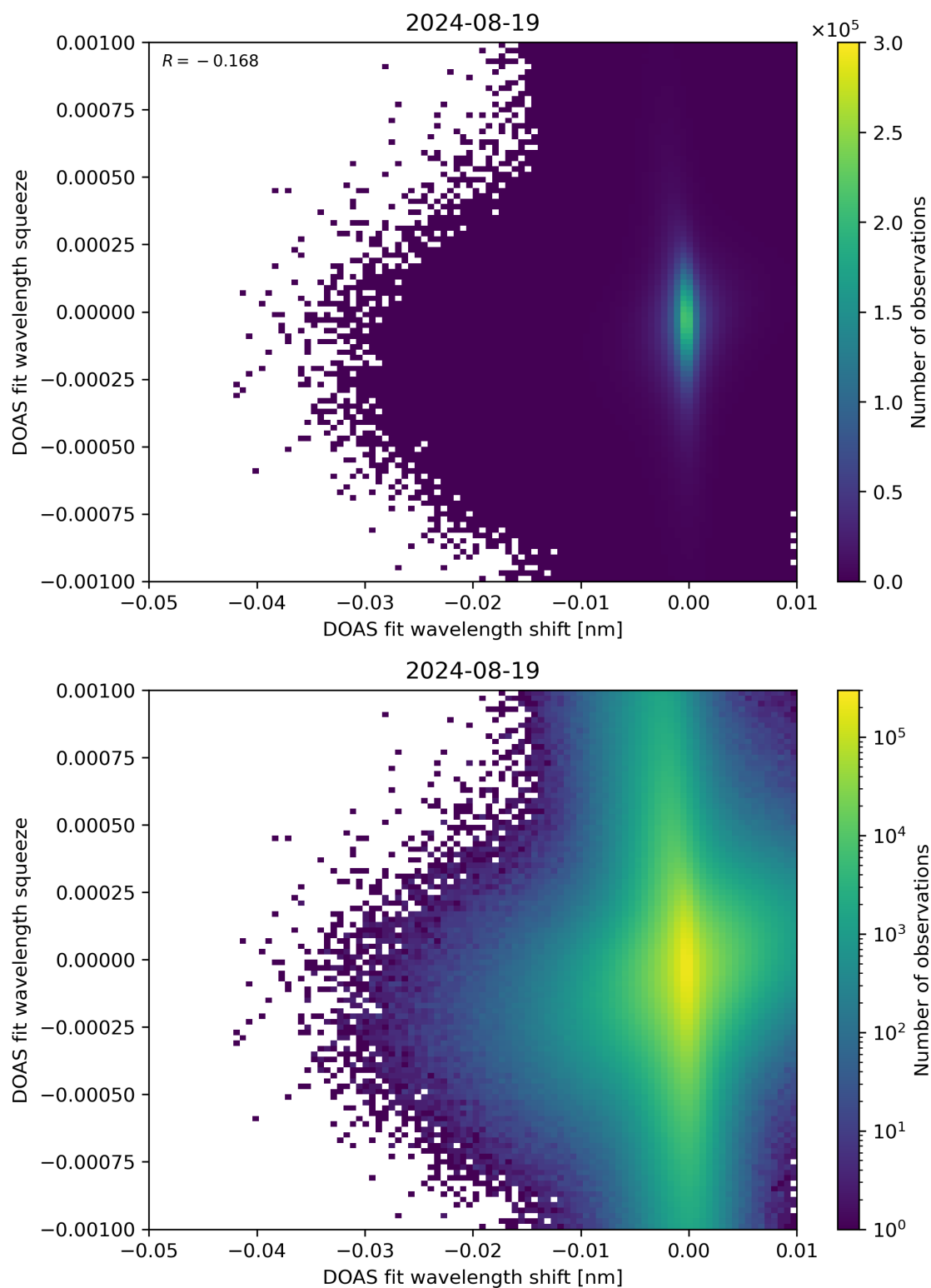
Figure 127: Scatter density plot of “DOAS fit wavelength shift” against “DOAS fit wavelength squeeze” for 2024-08-18 to 2024-08-20.
