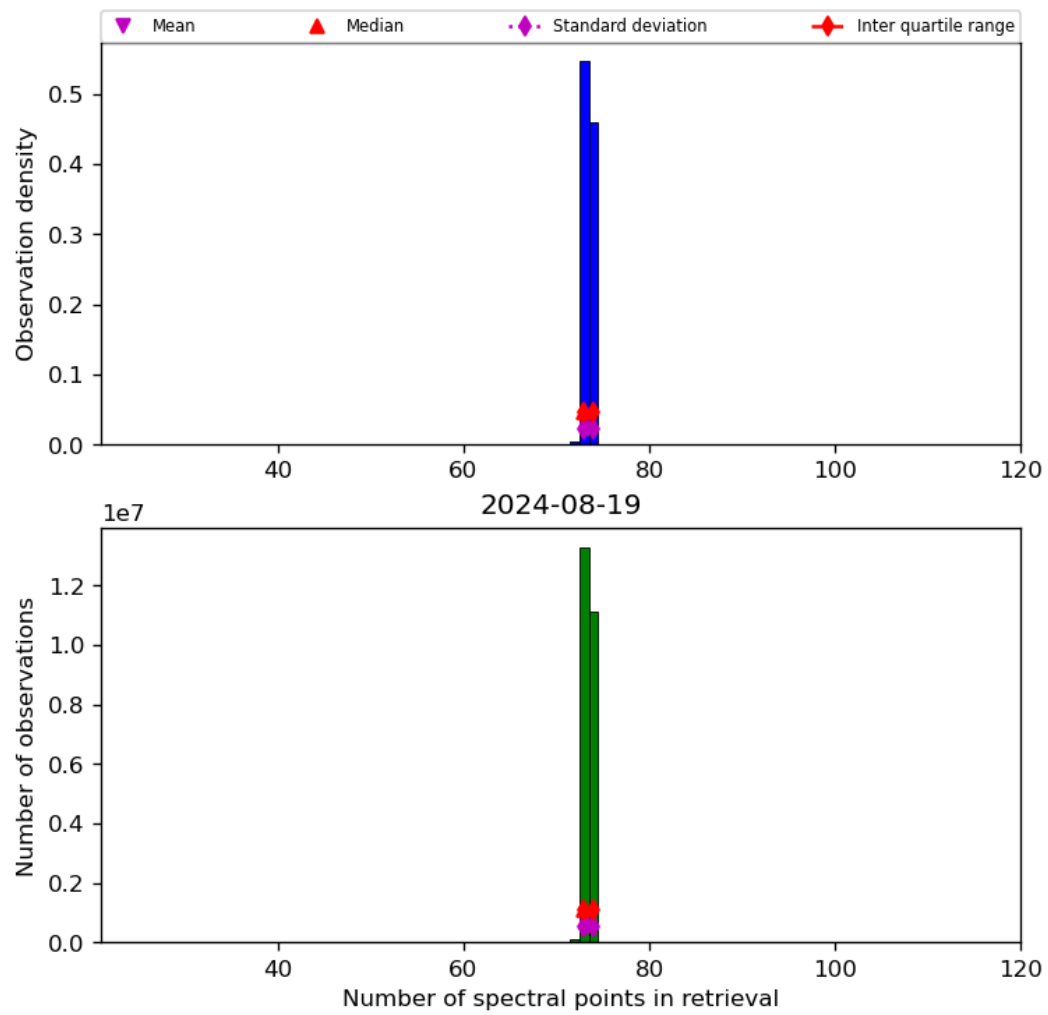
Figure 74: Histogram of “Number of spectral points in retrieval” for 2024-08-18 to 2024-08-20
