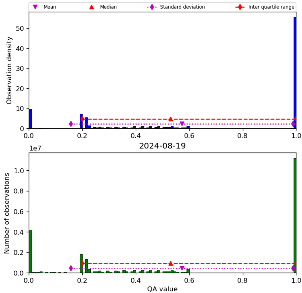
Figure 52: Histogram of “QA value” for 2024-08-18 to 2024-08-20
