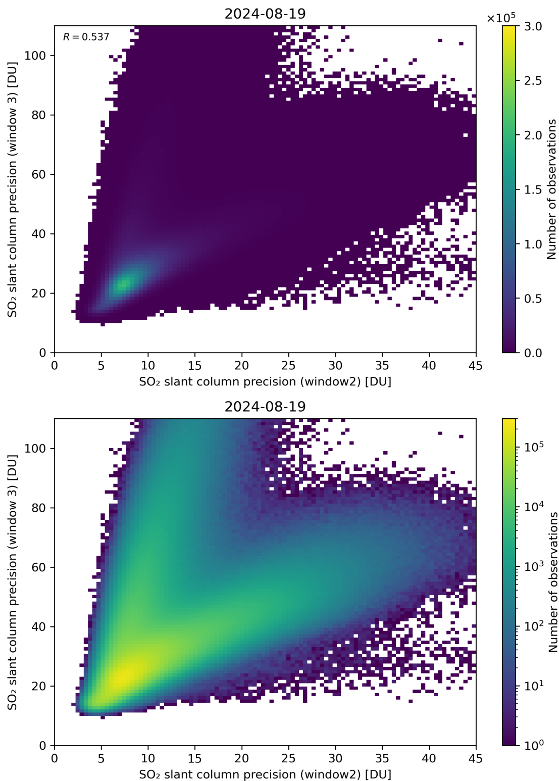
Figure 250: Scatter density plot of “SO 2 slant column precision (window2)” against “SO 2 slant column precision (window 3)” for 2024-08-18 to 2024-08-20.
