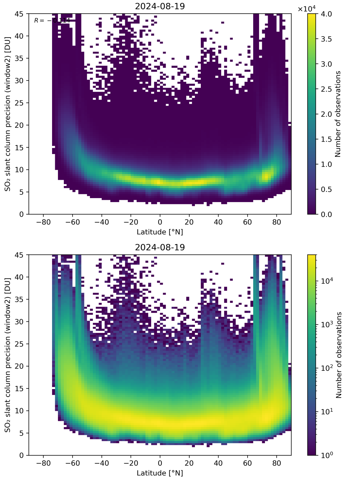
Figure 151: Scatter density plot of “Latitude” against “SO 2 slant column precision (window2)” for 2024-08-18 to 2024-08-20.
