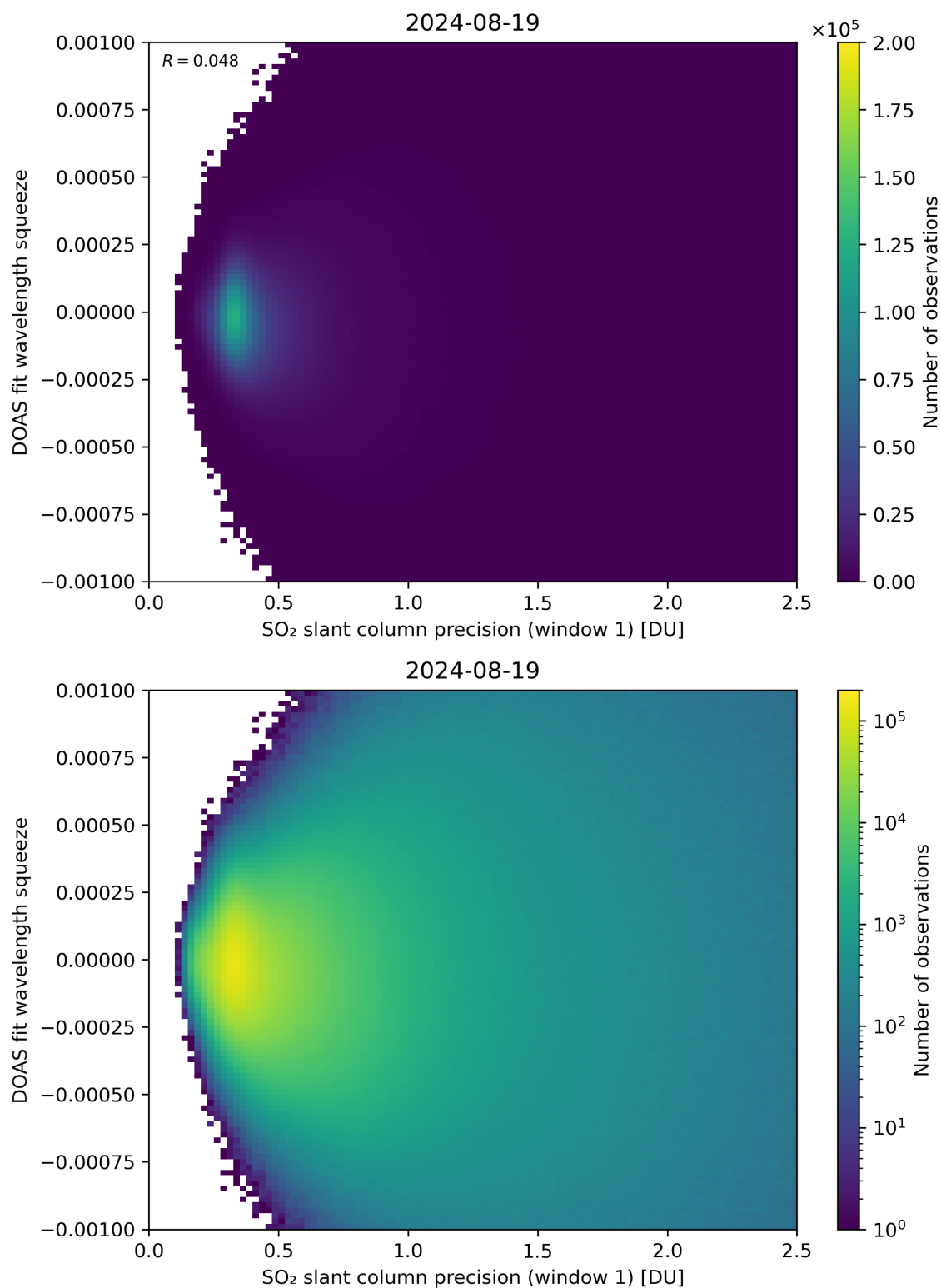
Figure 222: Scatter density plot of “SO 2 slant column precision (window 1)” against “DOAS fit wavelength squeeze” for 2024-08-18 to 2024-08-20.
