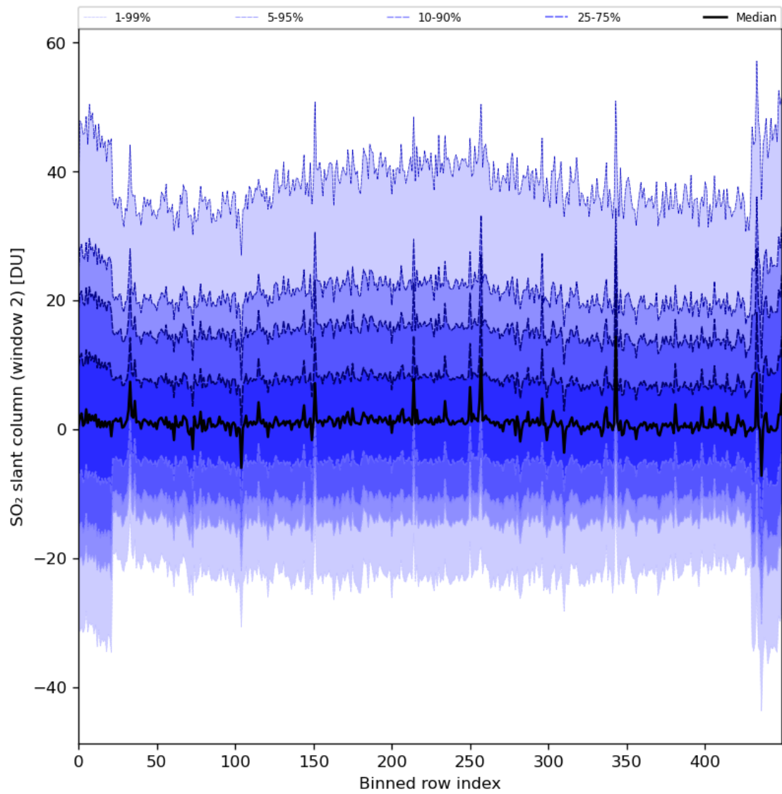
Figure 83: Along track statistics of “SO 2 slant column (window 2)” for 2024-08-18 to 2024-08-20
