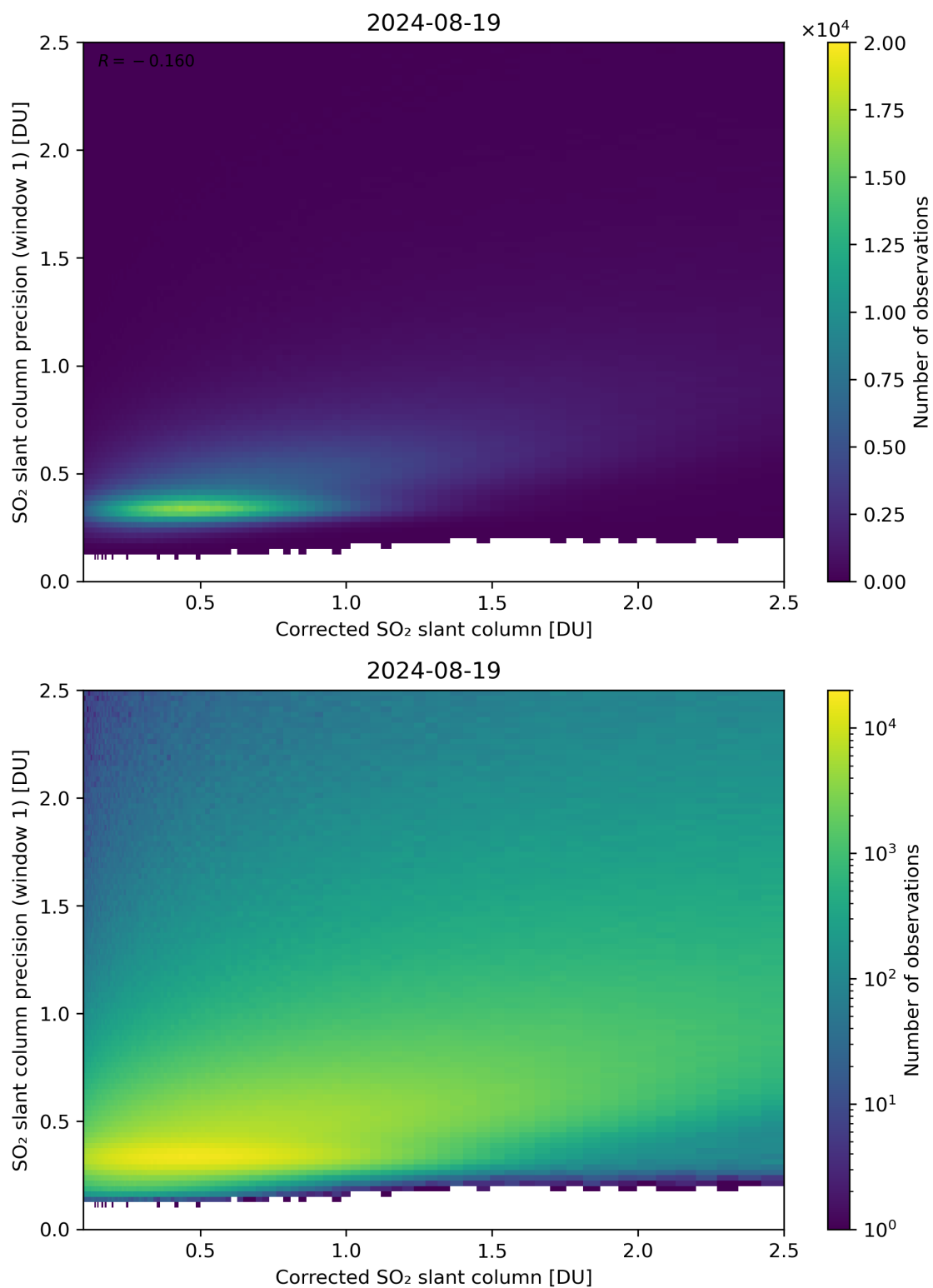
Figure 188: Scatter density plot of “Corrected SO 2 slant column” against “SO 2 slant column precision (window 1)” for 2024-08-18 to 2024-08-20.
