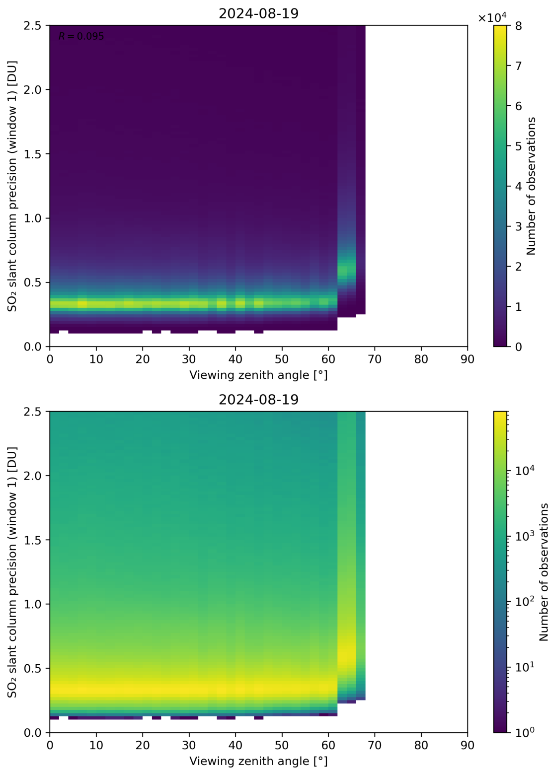
Figure 321: Scatter density plot of “Viewing zenith angle” against “SO 2 slant column precision (window 1)” for 2024-08-18 to 2024-08-20.
