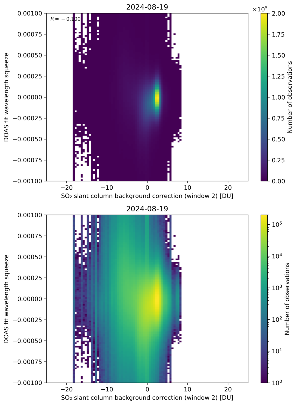
Figure 113: Scatter density plot of “SO 2 slant column background correction (window 2)” against “DOAS fit wavelength squeeze” for 2024-08-18 to 2024-08-20.
