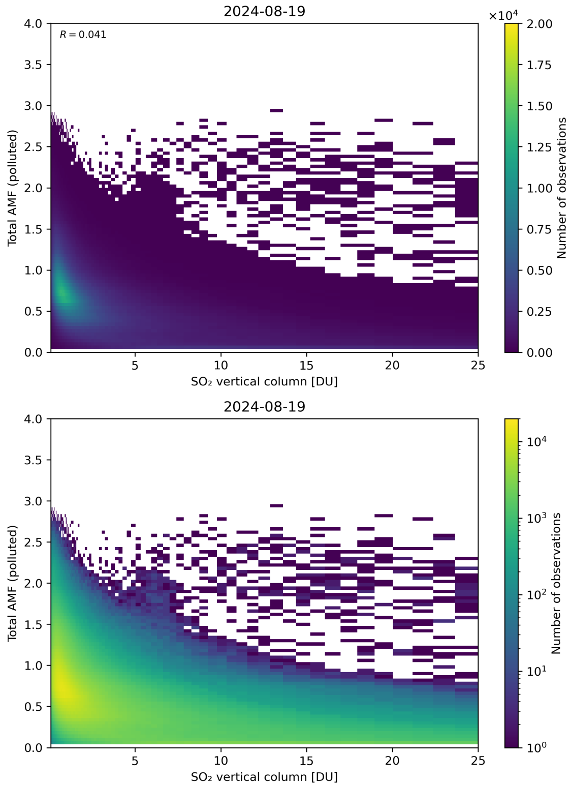
Figure 305: Scatter density plot of “SO 2 vertical column” against “Total AMF (polluted)” for 2024-08-18 to 2024-08-20.
