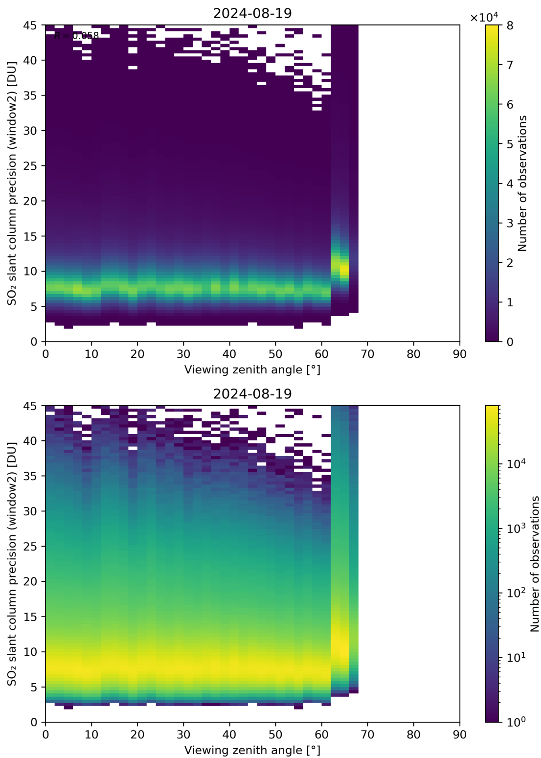
Figure 322: Scatter density plot of “Viewing zenith angle” against “SO 2 slant column precision (window2)” for 2024-08-18 to 2024-08-20.
