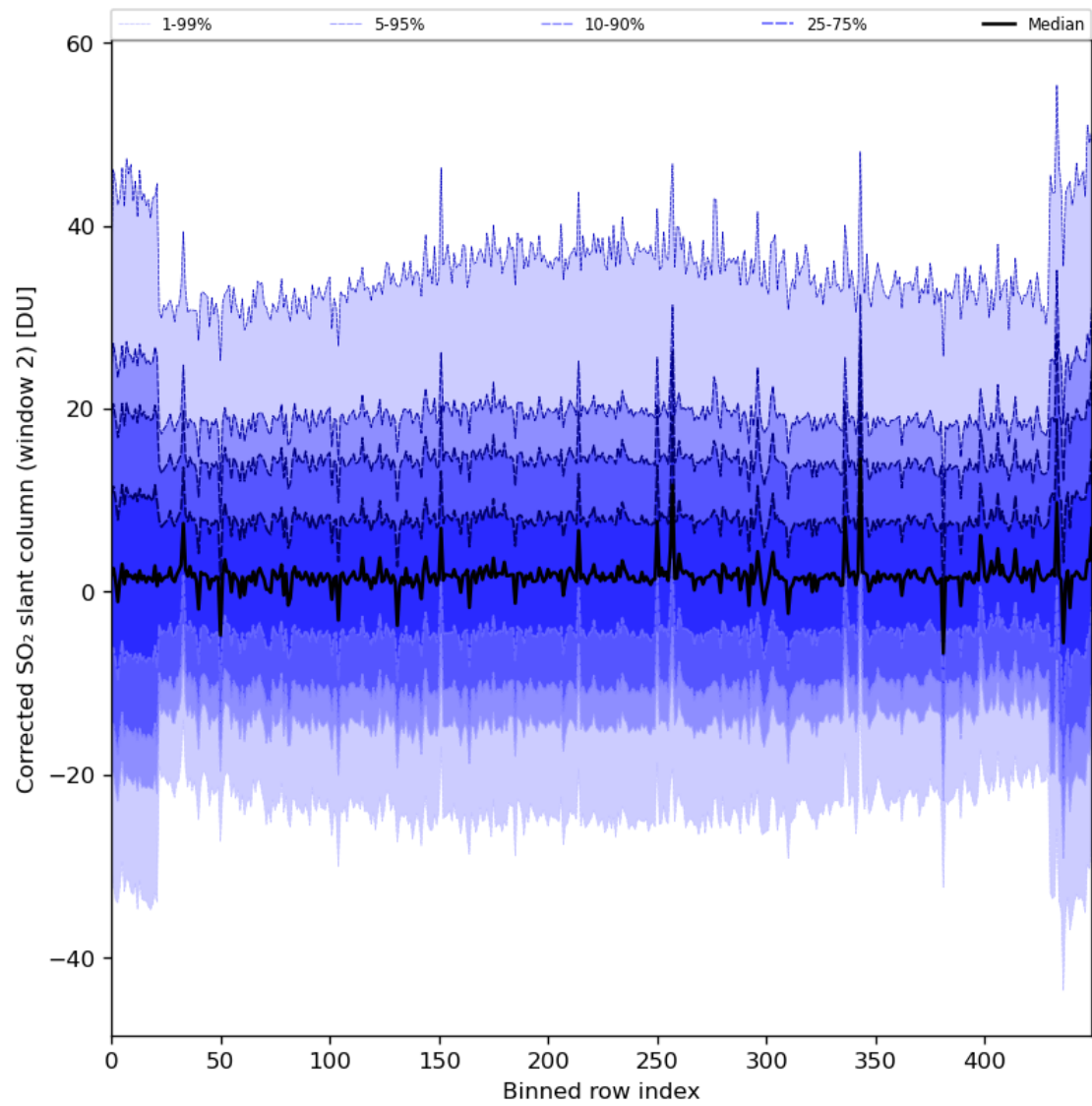
Figure 85: Along track statistics of “Corrected SO 2 slant column (window 2)” for 2024-08-18 to 2024-08-20
