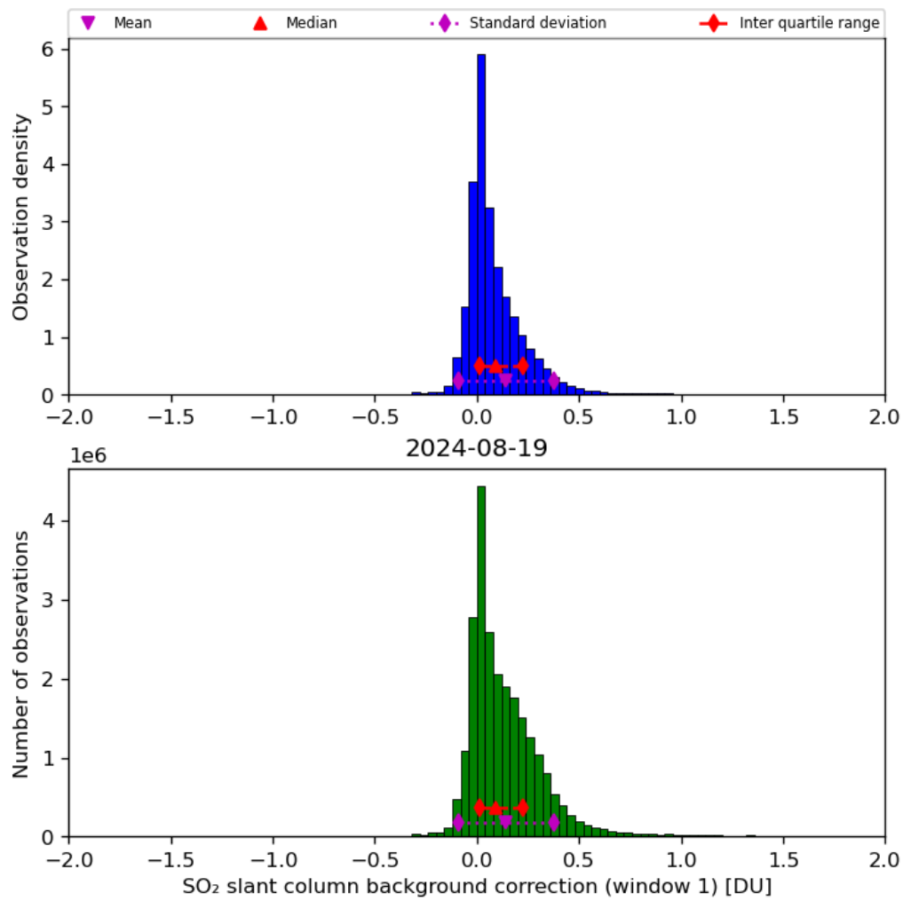
Figure 59: Histogram of “SO 2 slant column background correction (window 1)” for 2024-08-18 to 2024-08-20
