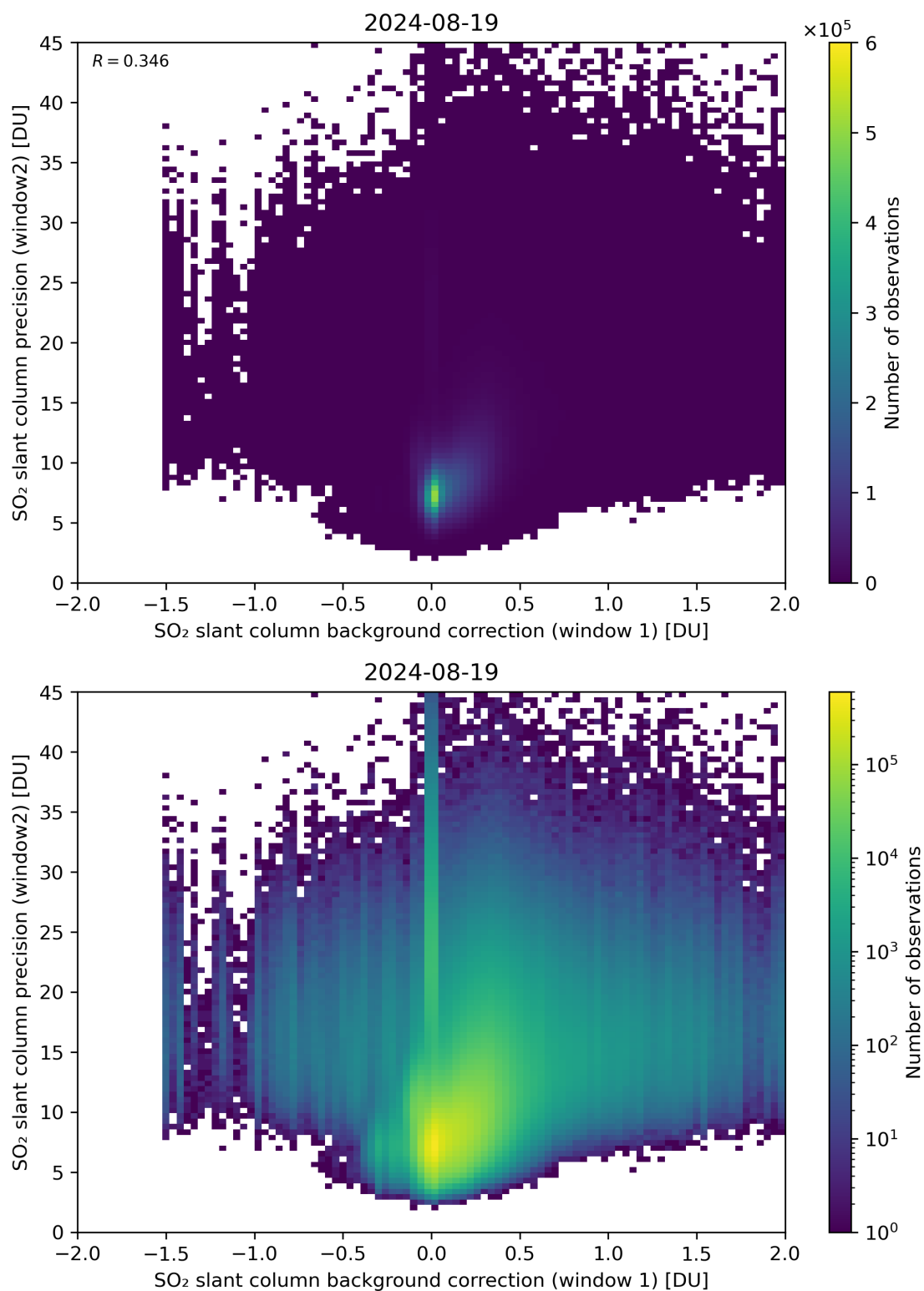
Figure 106: Scatter density plot of “SO 2 slant column background correction (window 1)” against “SO 2 slant column precision (window2)” for 2024-08-18 to 2024-08-20.
