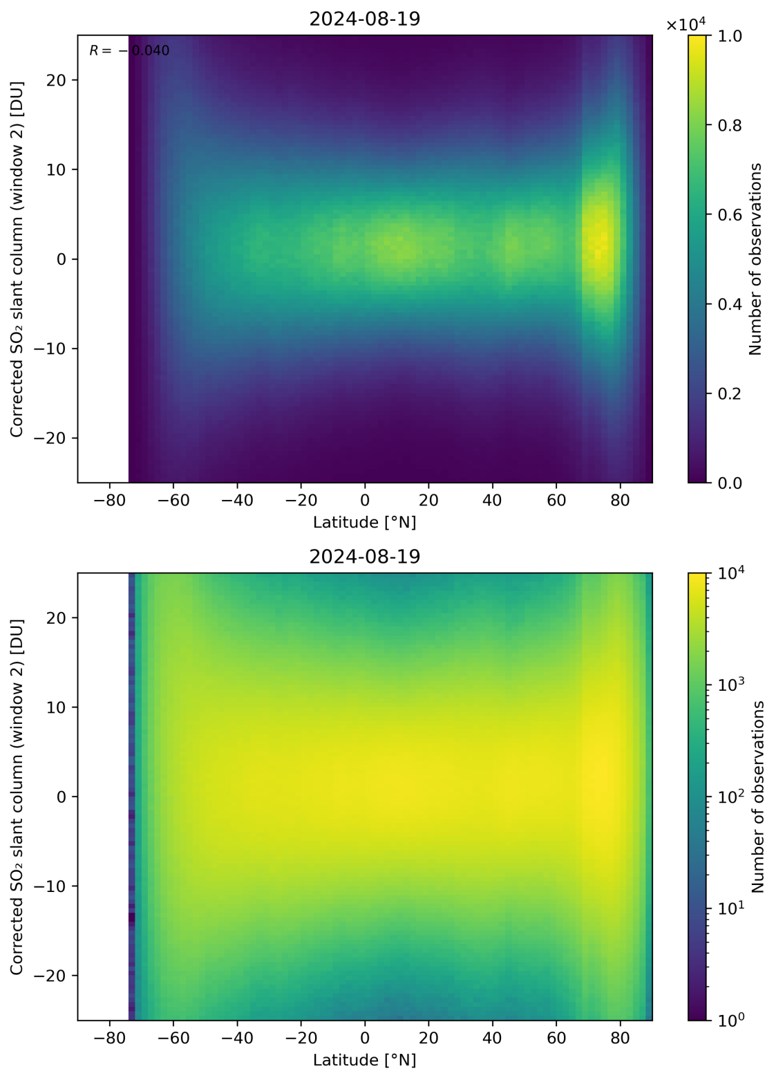
Figure 147: Scatter density plot of “Latitude” against “Corrected SO 2 slant column (window 2)” for 2024-08-18 to 2024-08-20.
