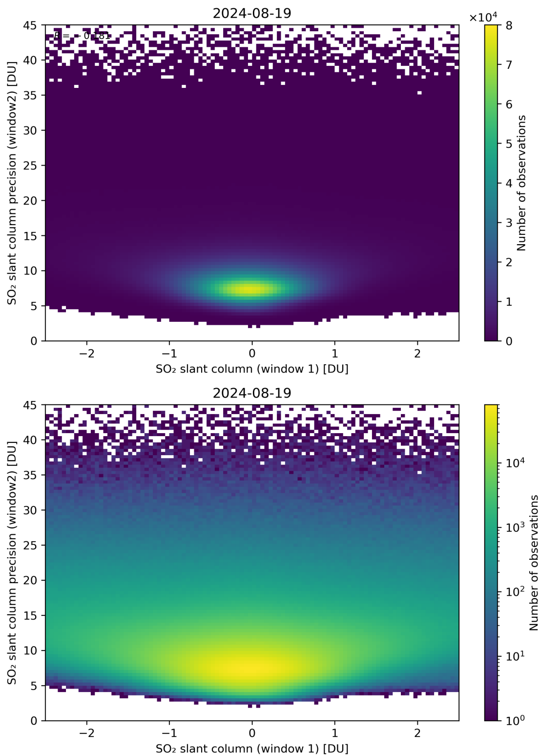
Figure 236: Scatter density plot of “SO 2 slant column (window 1)” against “SO 2 slant column precision (window2)” for 2024-08-18 to 2024-08-20.
