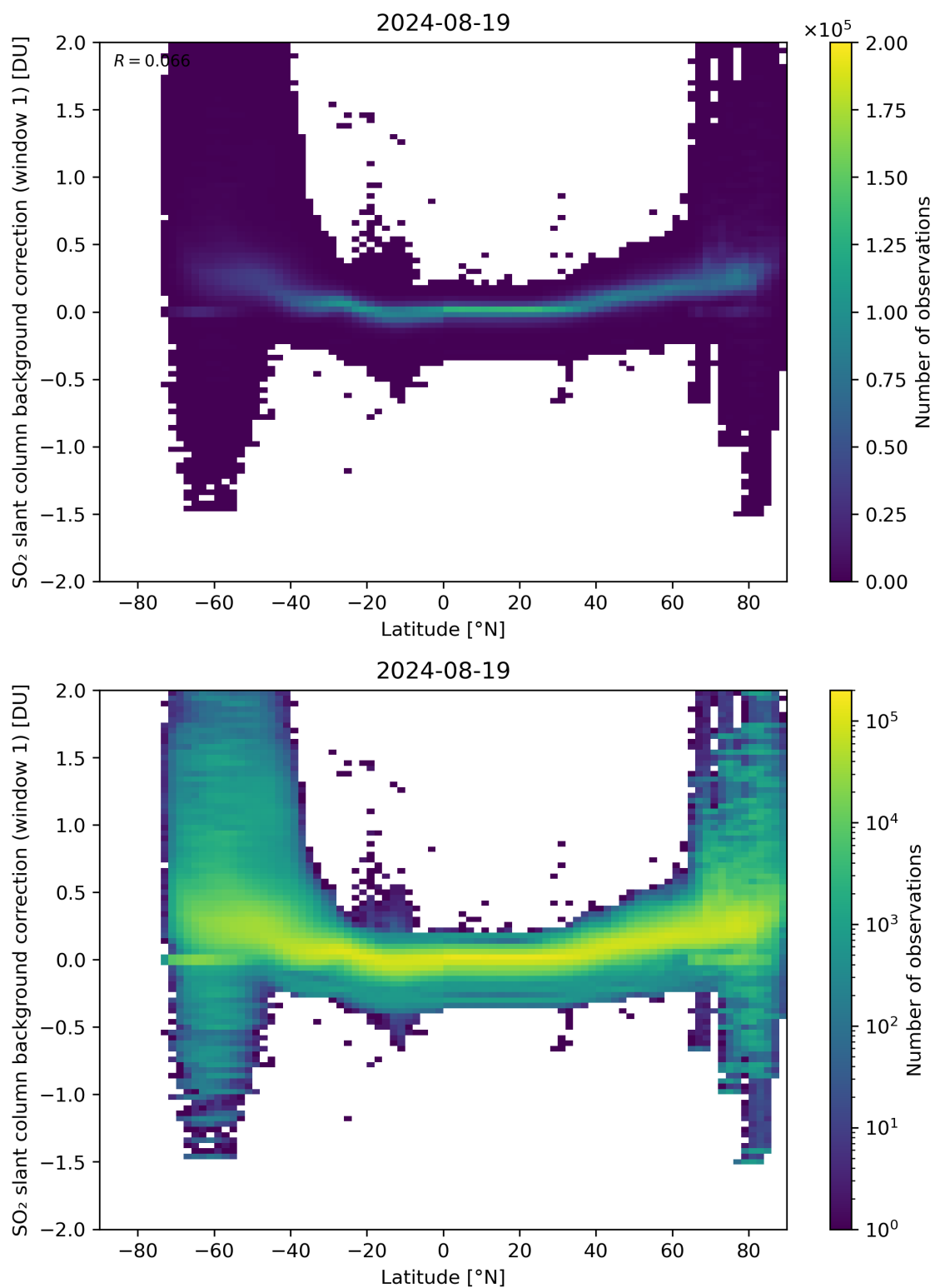
Figure 139: Scatter density plot of “Latitude” against “SO 2 slant column background correction (window 1)” for 2024-08-18 to 2024-08-20.
