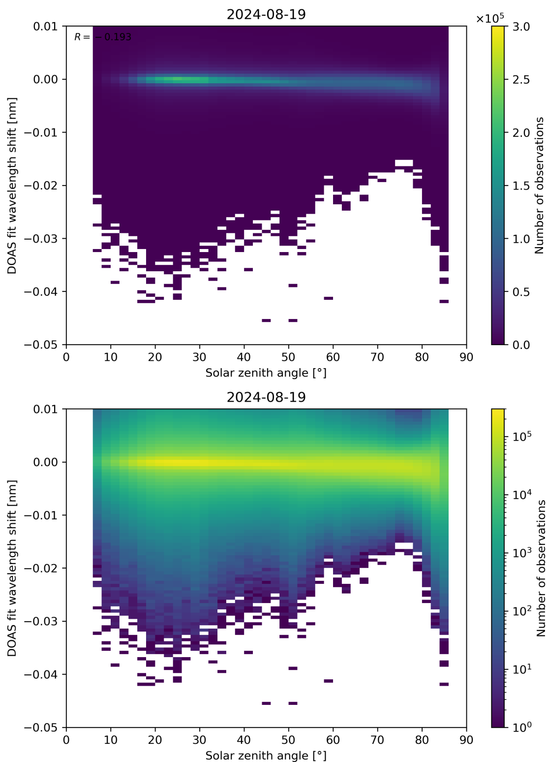
Figure 161: Scatter density plot of “Solar zenith angle” against “DOAS fit wavelength shift” for 2024-08-18 to 2024-08-20.
