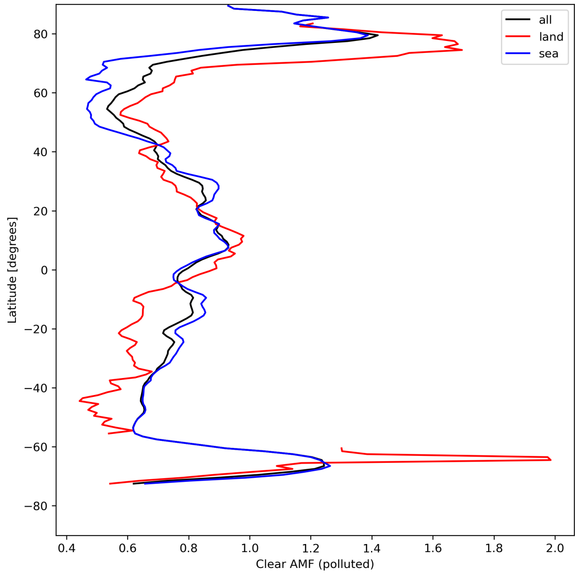
Figure 50: Zonal average of “Clear AMF (polluted)” for 2024-08-18 to 2024-08-20.
