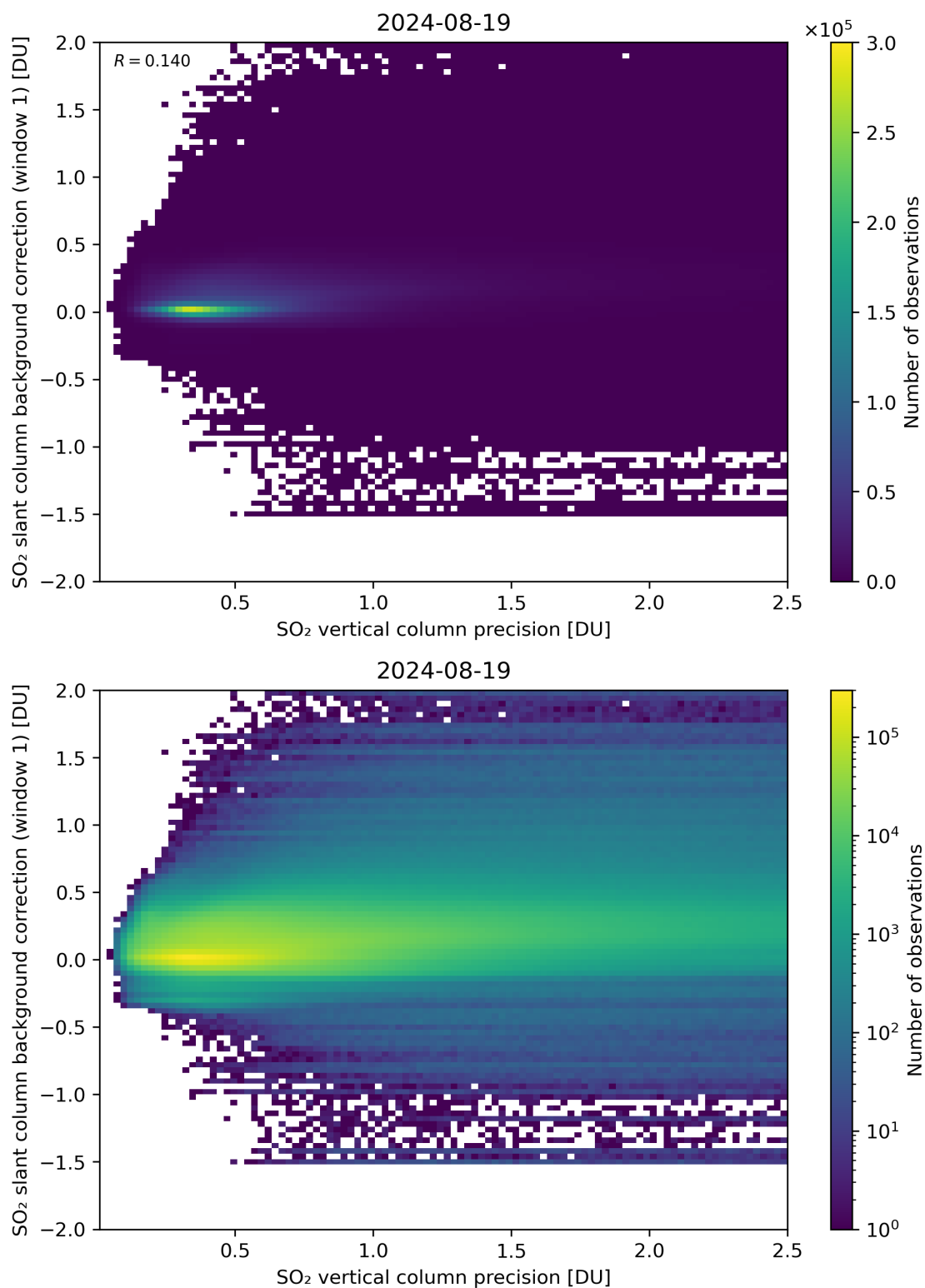
Figure 279: Scatter density plot of “SO 2 vertical column precision” against “SO 2 slant column background correction (window 1)” for 2024-08-18 to 2024-08-20.
