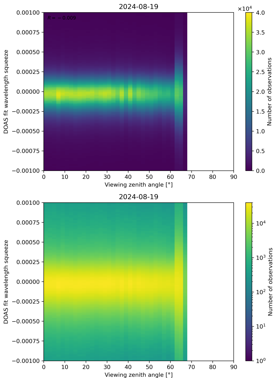
Figure 312: Scatter density plot of “Viewing zenith angle” against “DOAS fit wavelength squeeze” for 2024-08-18 to 2024-08-20.
