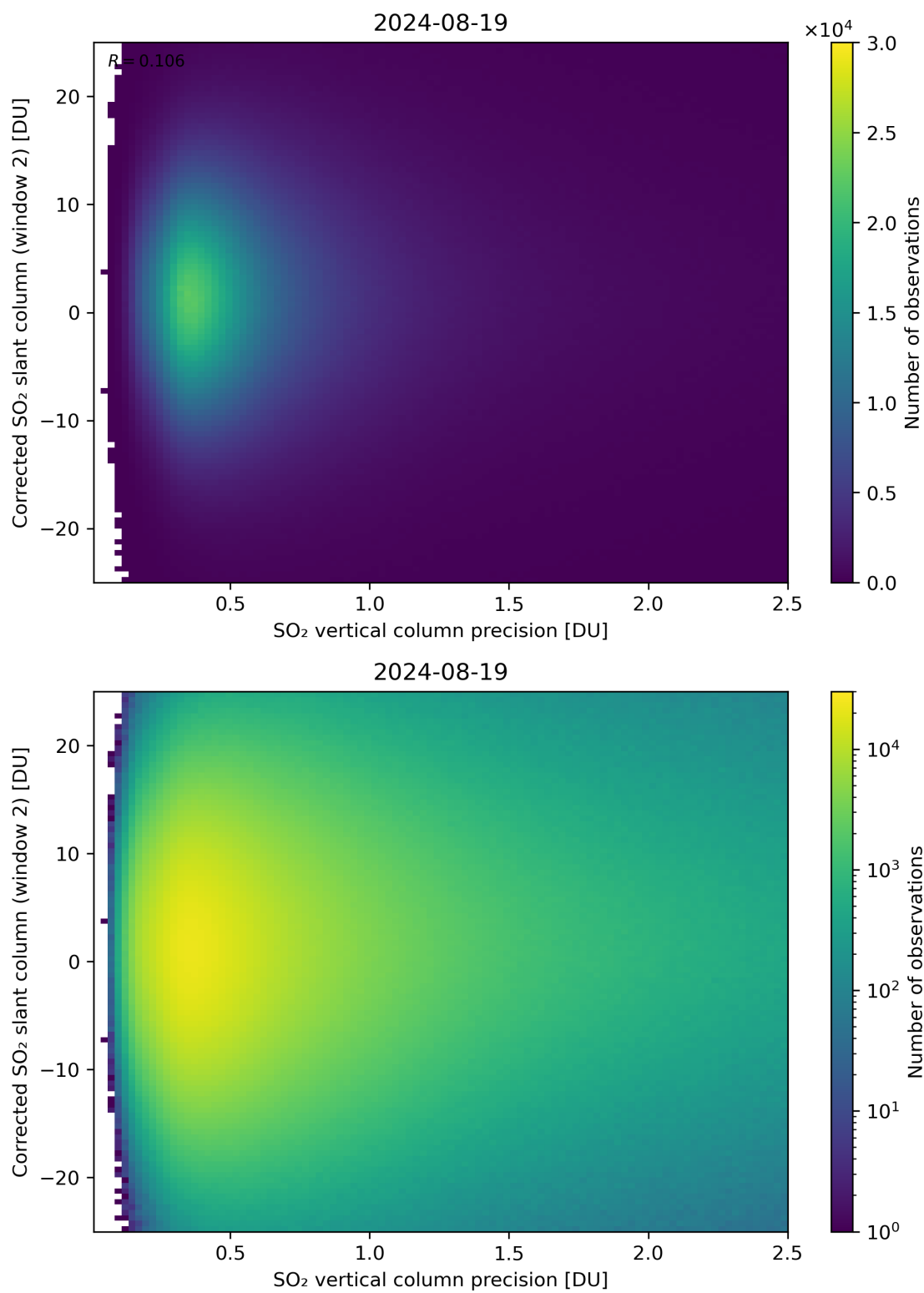
Figure 287: Scatter density plot of “SO 2 vertical column precision” against “Corrected SO 2 slant column (window 2)” for 2024-08-18 to 2024-08-20.
