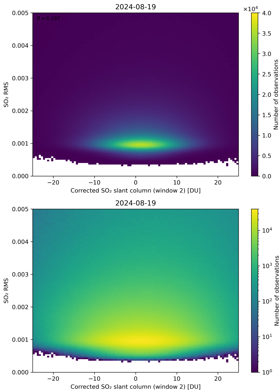
Figure 198: Scatter density plot of “Corrected SO 2 slant column (window 2)” against “SO 2 RMS” for 2024-08-18 to 2024-08-20.
