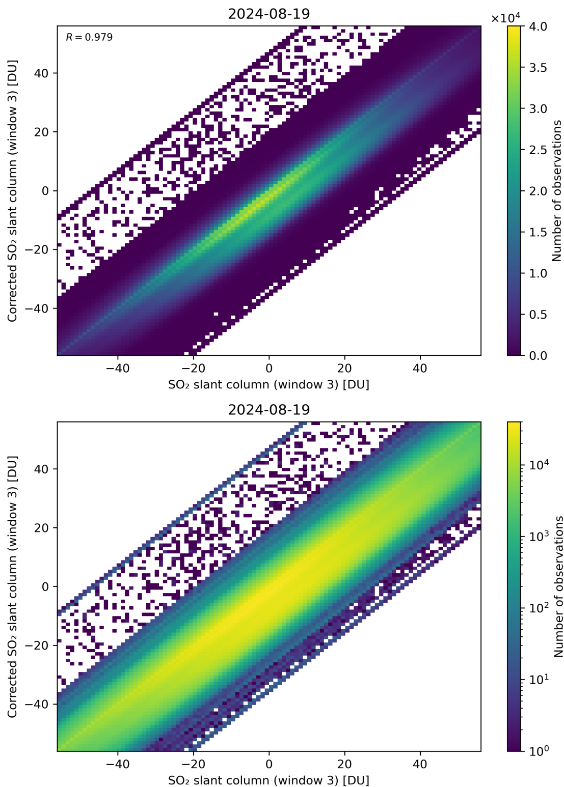
Figure 266: Scatter density plot of “SO 2 slant column (window 3)” against “Corrected SO 2 slant column (window 3)” for 2024-08-18 to 2024-08-20.
