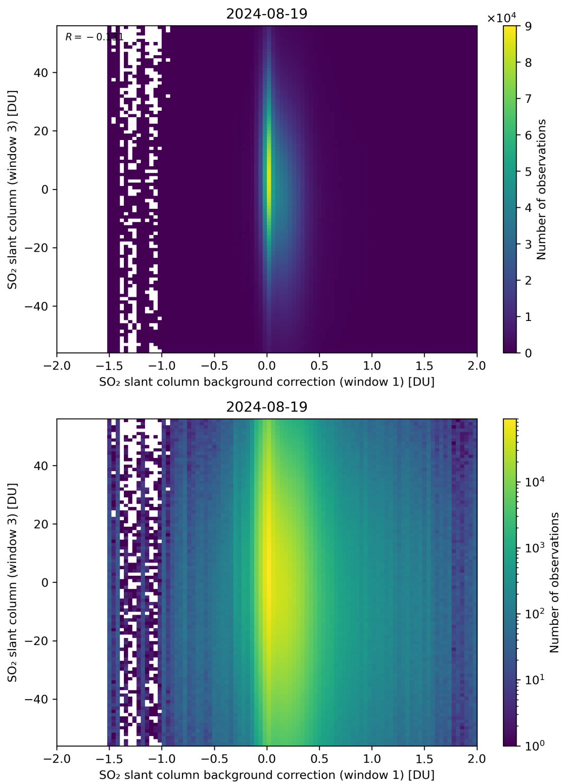
Figure 107: Scatter density plot of “SO 2 slant column background correction (window 1)” against “SO 2 slant column (window 3)” for 2024-08-18 to 2024-08-20.
