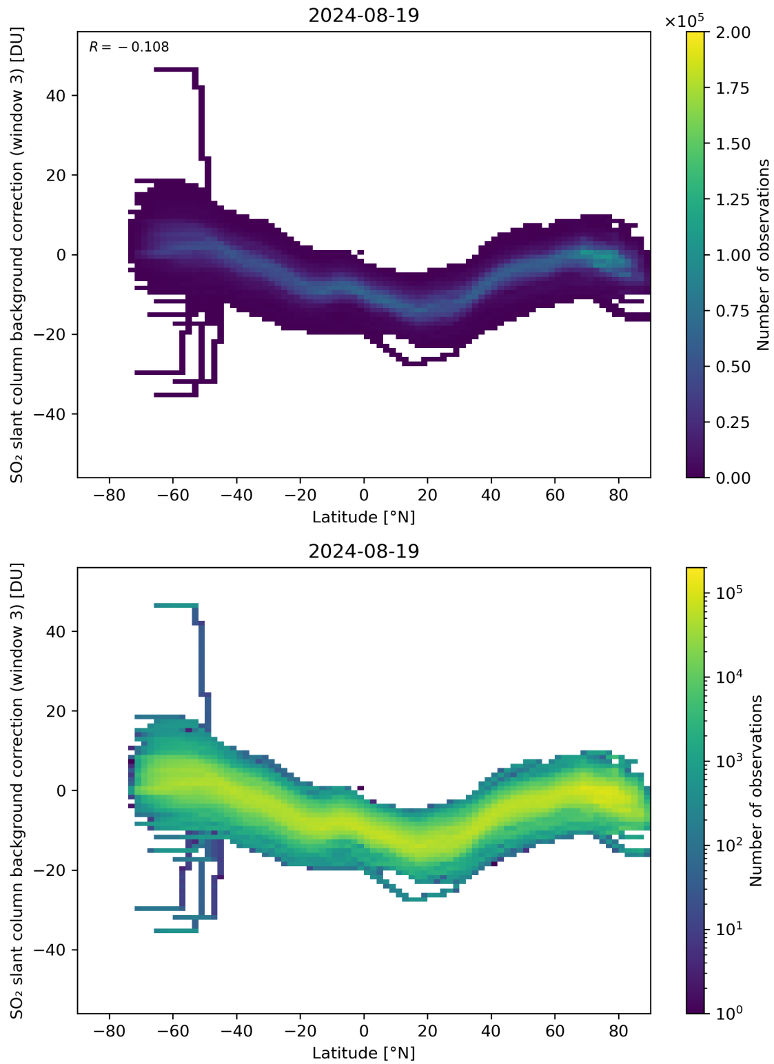
Figure 141: Scatter density plot of “Latitude” against “SO 2 slant column background correction (window 3)” for 2024-08-18 to 2024-08-20.
