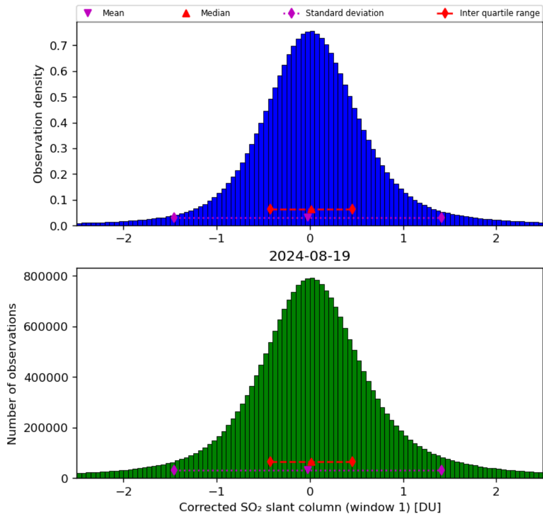
Figure 58: Histogram of “Corrected SO 2 slant column (window 1)” for 2024-08-18 to 2024-08-20
