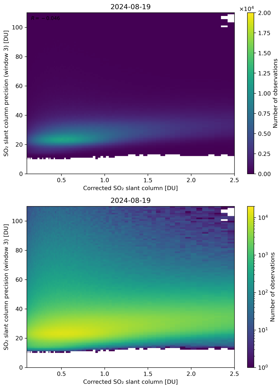
Figure 191: Scatter density plot of “Corrected SO 2 slant column” against “SO 2 slant column precision (window 3)” for 2024-08-18 to 2024-08-20.
