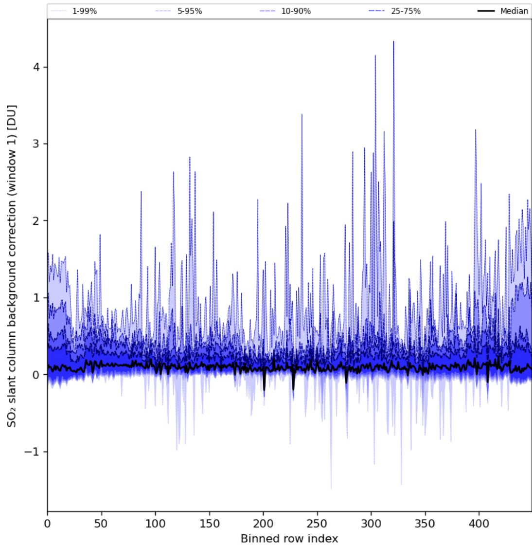
Figure 82: Along track statistics of “SO 2 slant column background correction (window 1)” for 2024-08-18 to 2024-08-20
