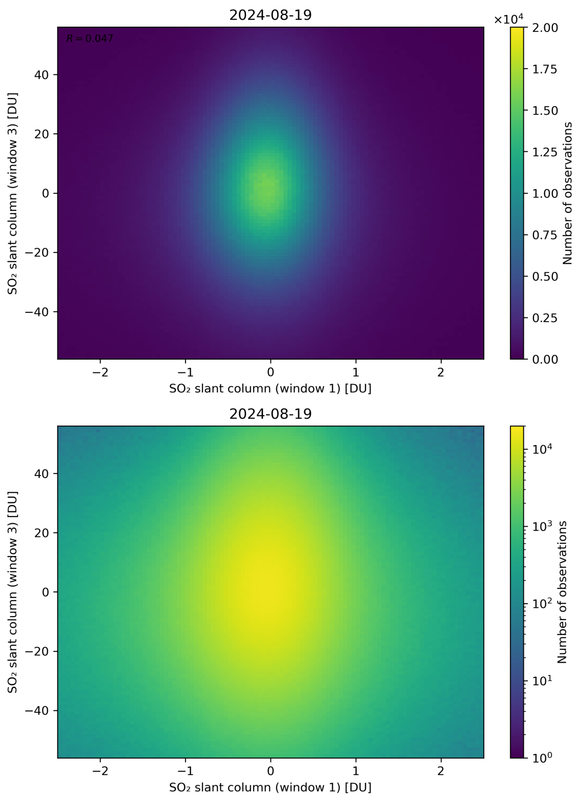
Figure 237: Scatter density plot of “SO 2 slant column (window 1)” against “SO 2 slant column (window 3)” for 2024-08-18 to 2024-08-20.
