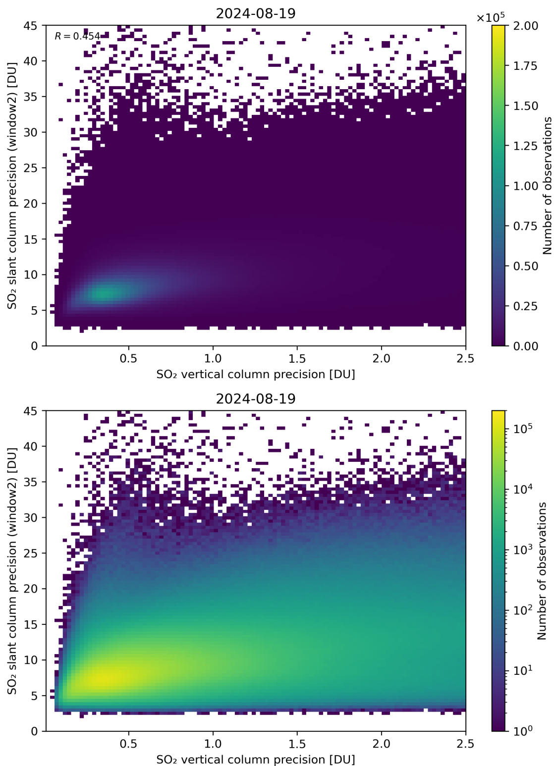
Figure 291: Scatter density plot of “SO 2 vertical column precision” against “SO 2 slant column precision (window2)” for 2024-08-18 to 2024-08-20.
