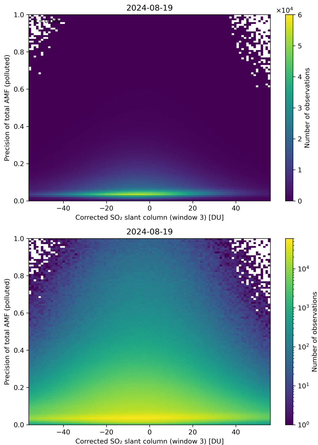
Figure 211: Scatter density plot of “Corrected SO 2 slant column (window 3)” against “Precision of total AMF (polluted)” for 2024-08-18 to 2024-08-20.
