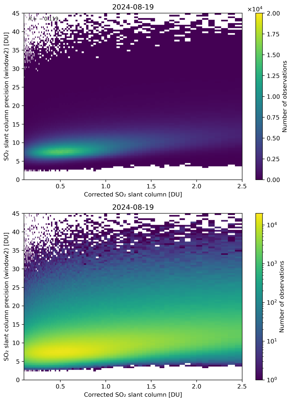
Figure 189: Scatter density plot of “Corrected SO 2 slant column” against “SO 2 slant column precision (window2)” for 2024-08-18 to 2024-08-20.
