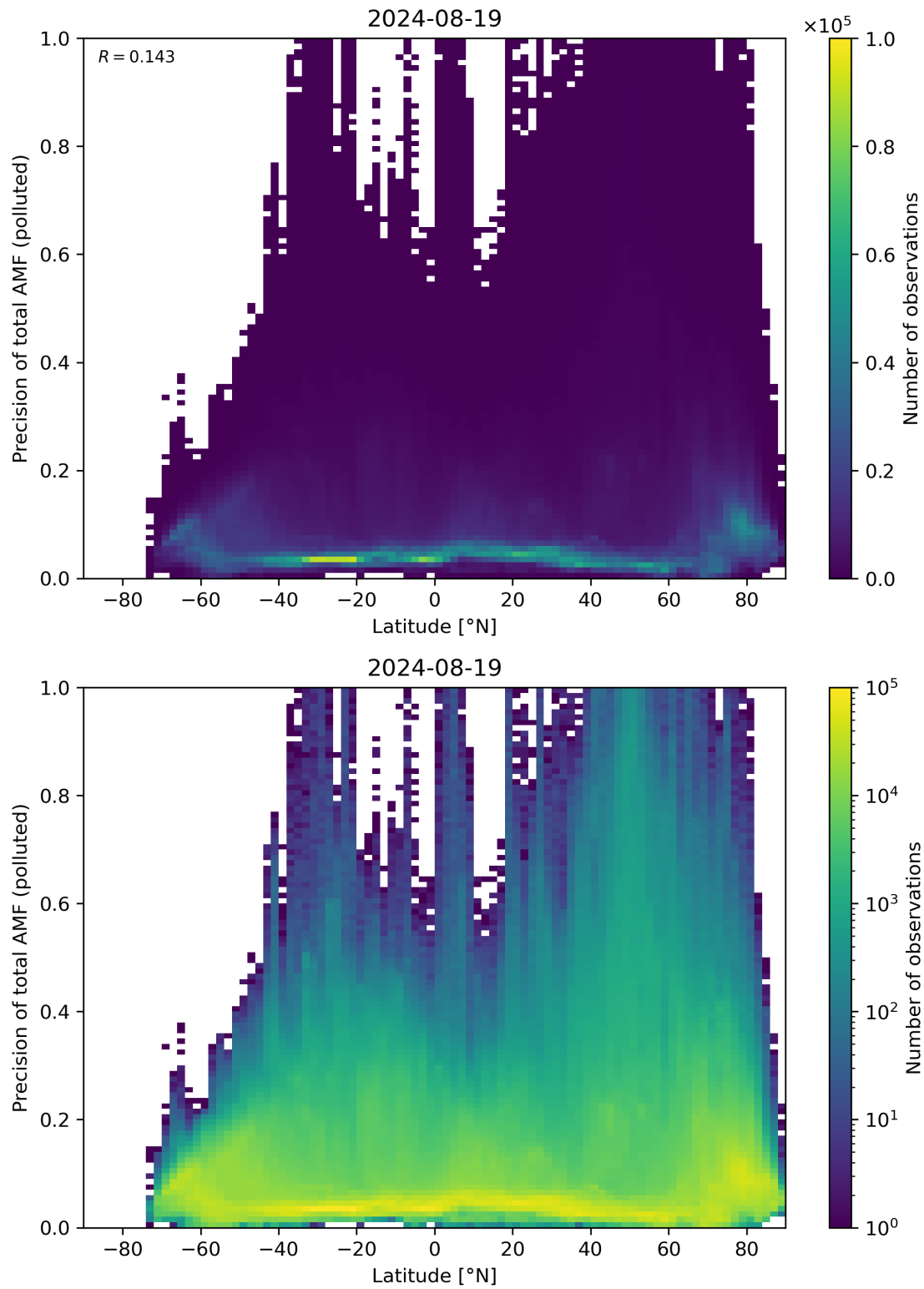
Figure 155: Scatter density plot of “Latitude” against “Precision of total AMF (polluted)” for 2024-08-18 to 2024-08-20.
