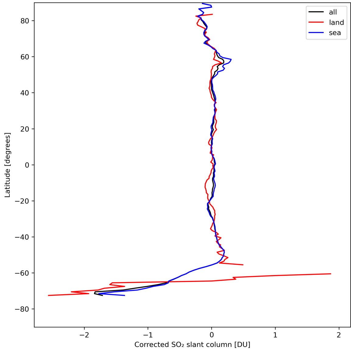
Figure 32: Zonal average of “Corrected SO 2 slant column” for 2024-08-18 to 2024-08-20.
