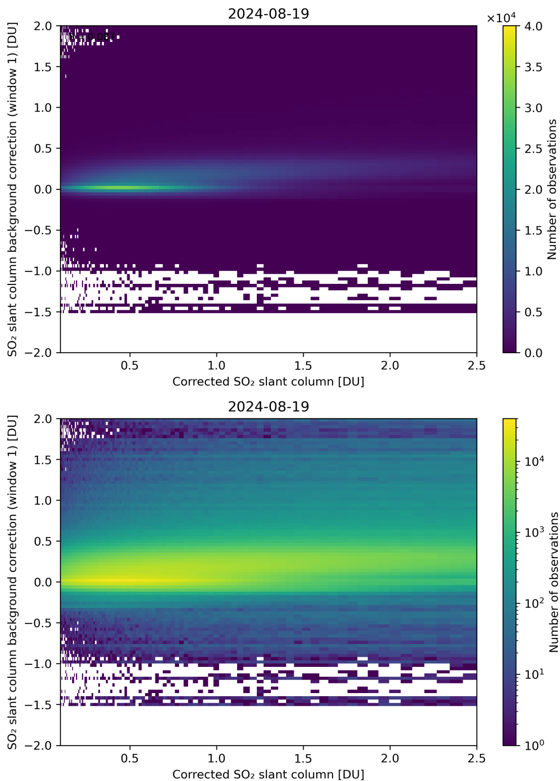
Figure 178: Scatter density plot of “Corrected SO 2 slant column” against “SO 2 slant column background correction (window 1)” for 2024-08-18 to 2024-08-20.
