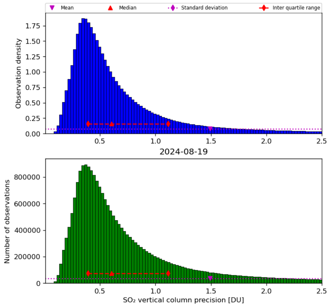
Figure 54: Histogram of “SO 2 vertical column precision” for 2024-08-18 to 2024-08-20
