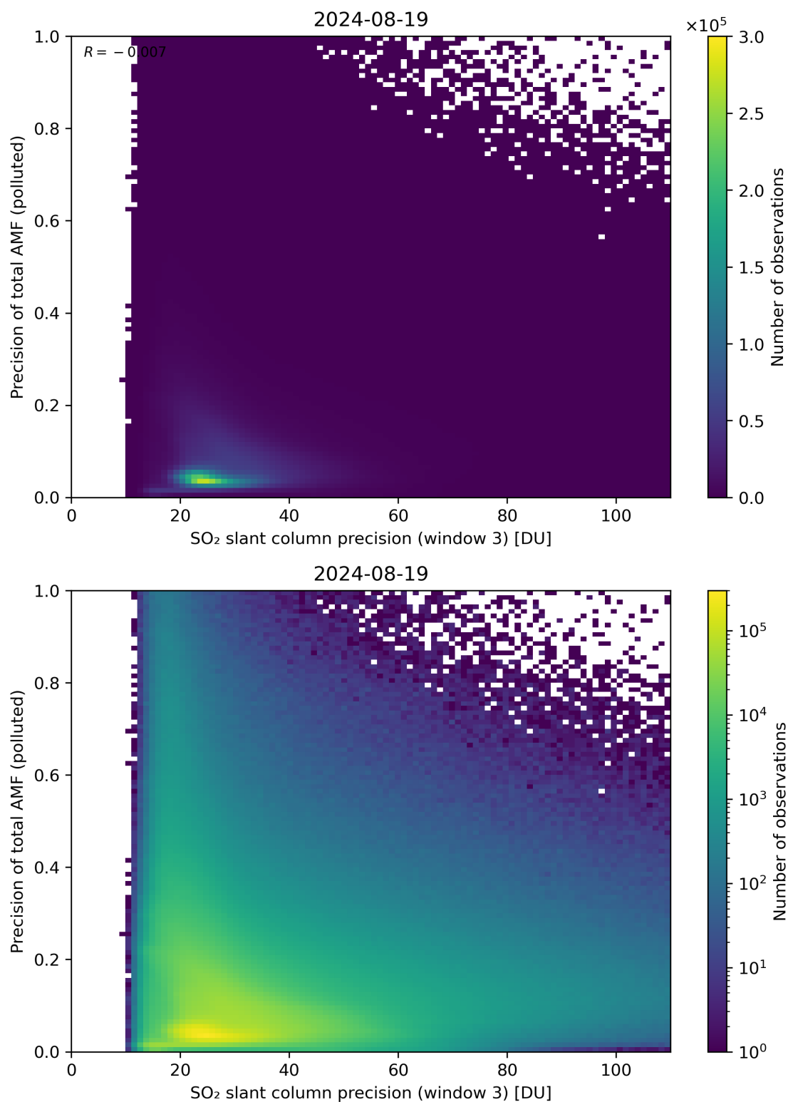
Figure 264: Scatter density plot of “SO 2 slant column precision (window 3)” against “Precision of total AMF (polluted)” for 2024-08-18 to 2024-08-20.
