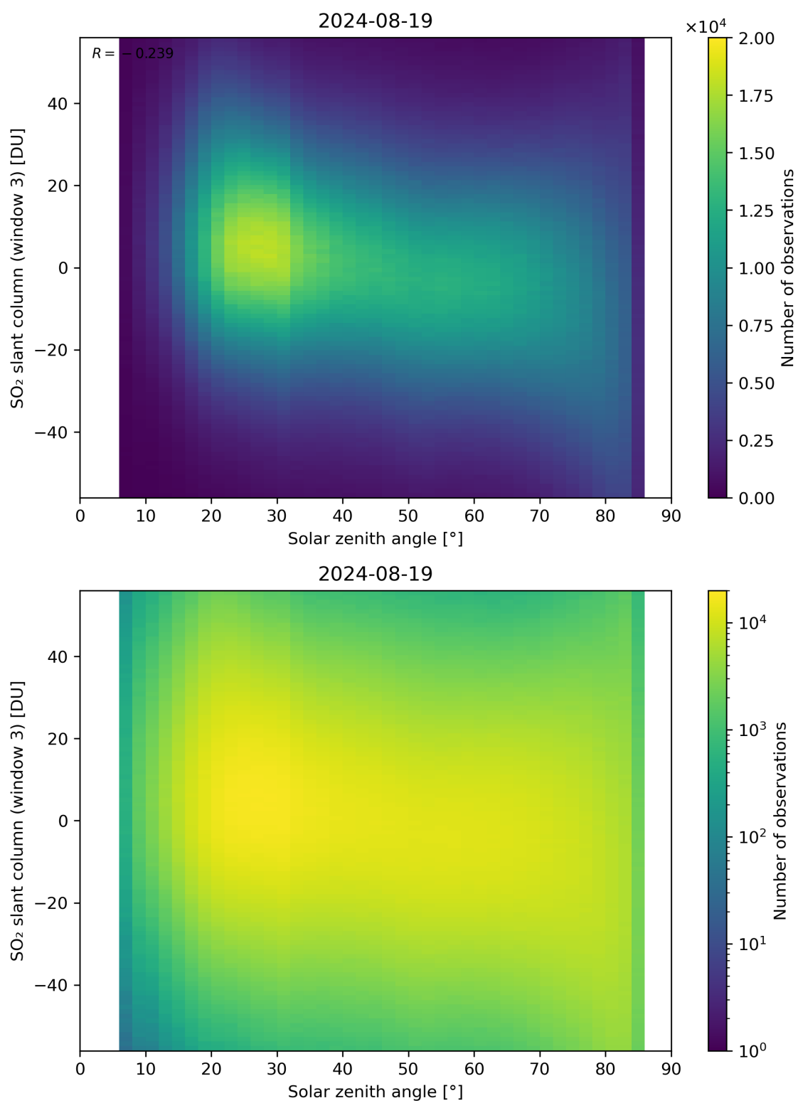
Figure 172: Scatter density plot of “Solar zenith angle” against “SO 2 slant column (window 3)” for 2024-08-18 to 2024-08-20.
