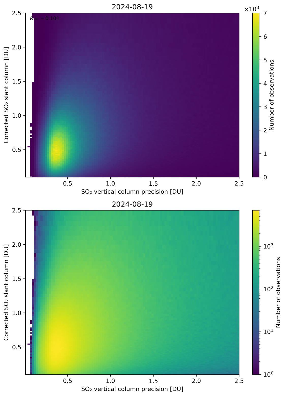
Figure 286: Scatter density plot of “SO 2 vertical column precision” against “Corrected SO 2 slant column” for 2024-08-18 to 2024-08-20.
