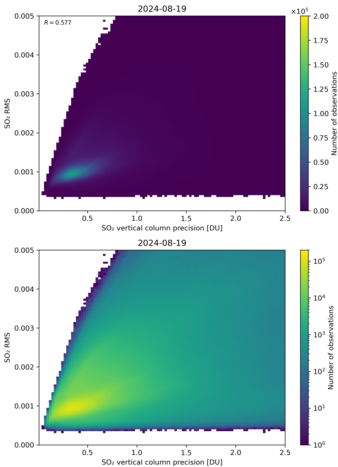
Figure 284: Scatter density plot of “SO 2 vertical column precision” against “SO 2 RMS” for 2024-08-18 to 2024-08-20.
