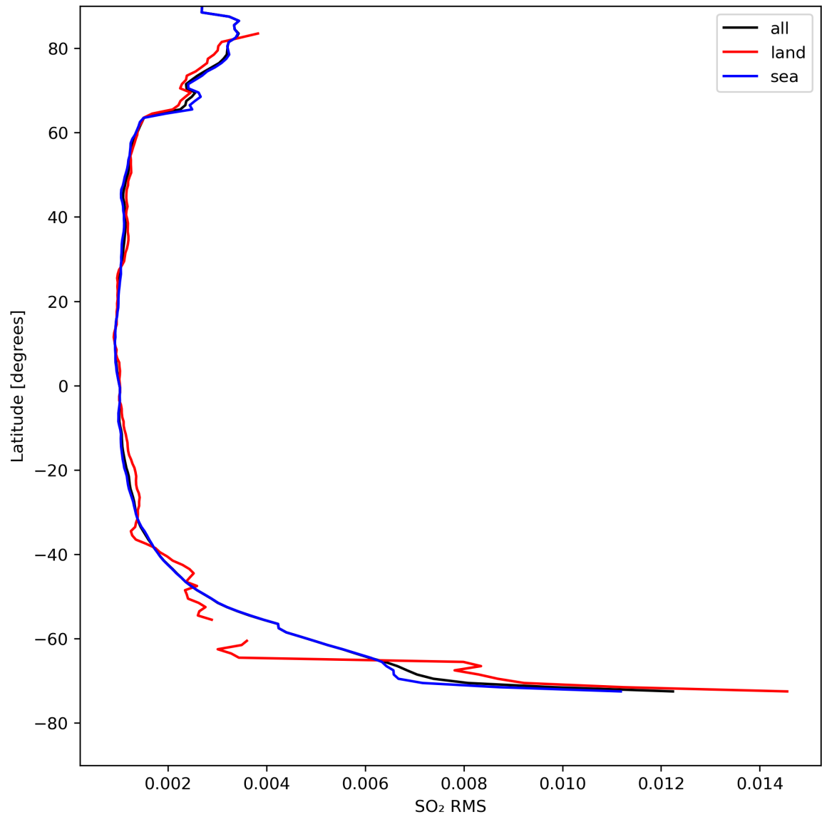
Figure 47: Zonal average of “SO 2 RMS” for 2024-08-18 to 2024-08-20.
