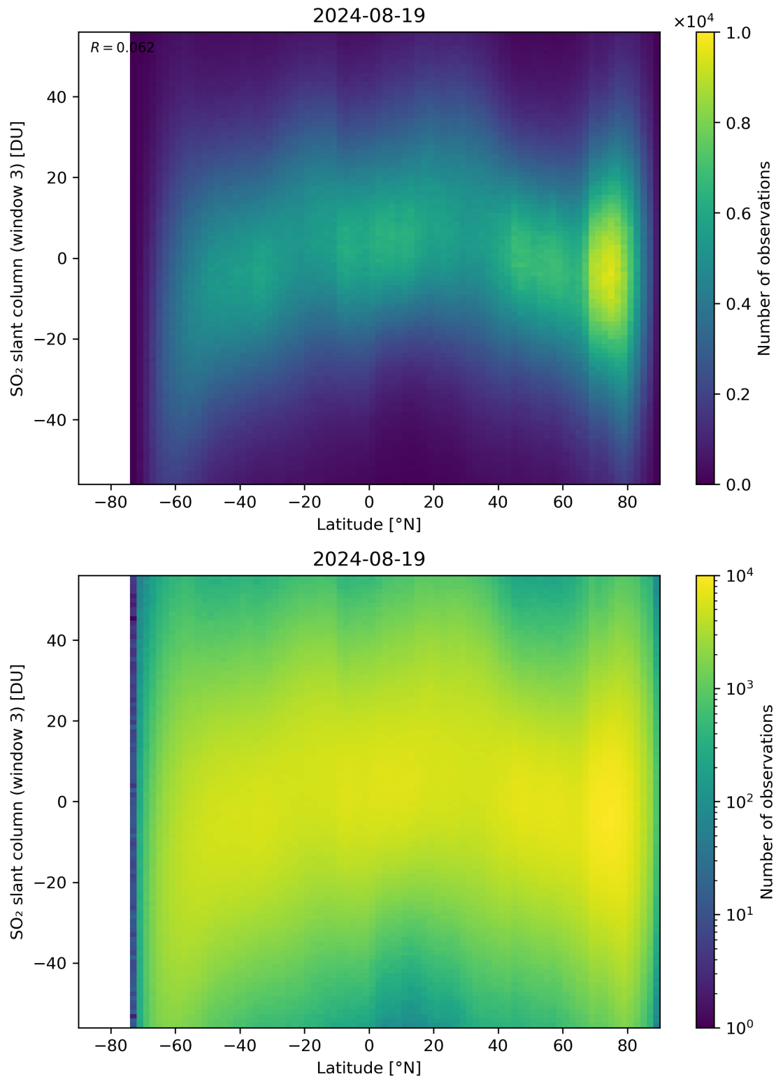
Figure 152: Scatter density plot of “Latitude” against “SO 2 slant column (window 3)” for 2024-08-18 to 2024-08-20.
