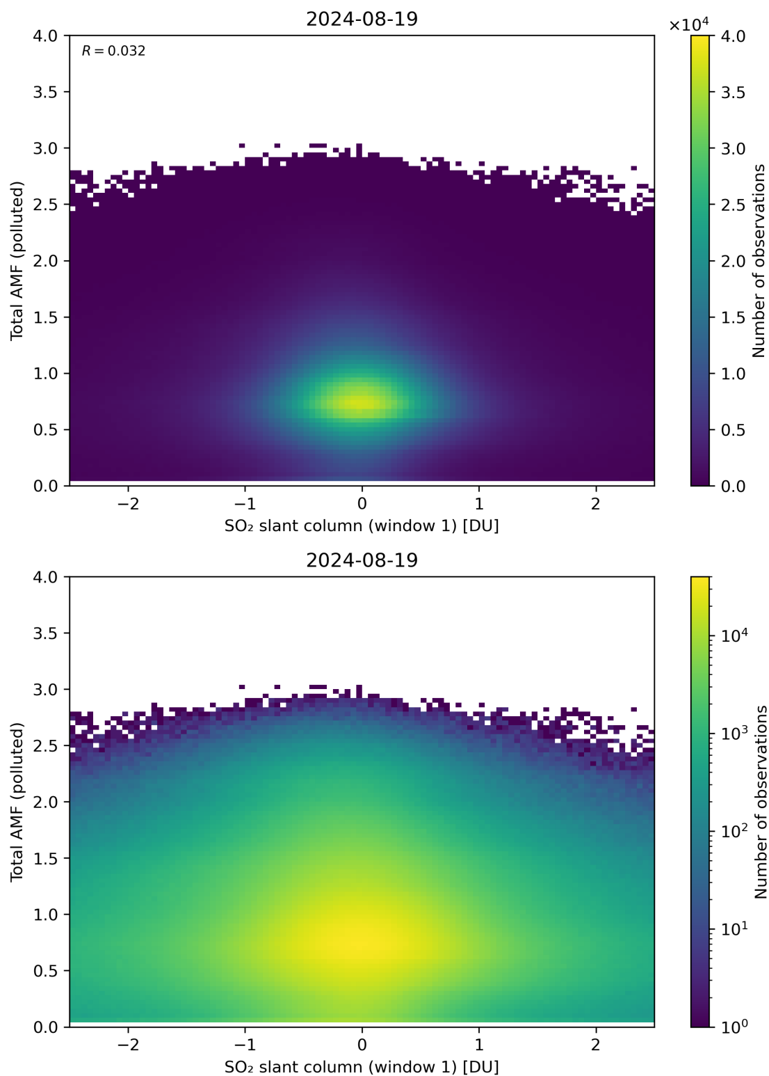
Figure 239: Scatter density plot of “SO 2 slant column (window 1)” against “Total AMF (polluted)” for 2024-08-18 to 2024-08-20.
