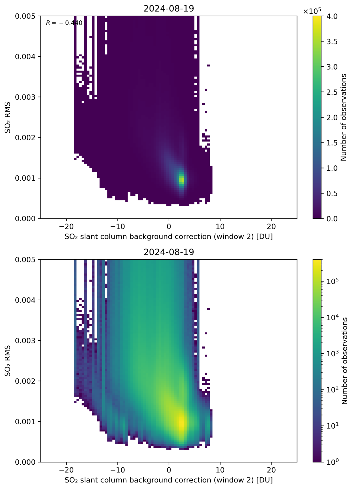
Figure 114: Scatter density plot of “SO 2 slant column background correction (window 2)” against “SO 2 RMS” for 2024-08-18 to 2024-08-20.
