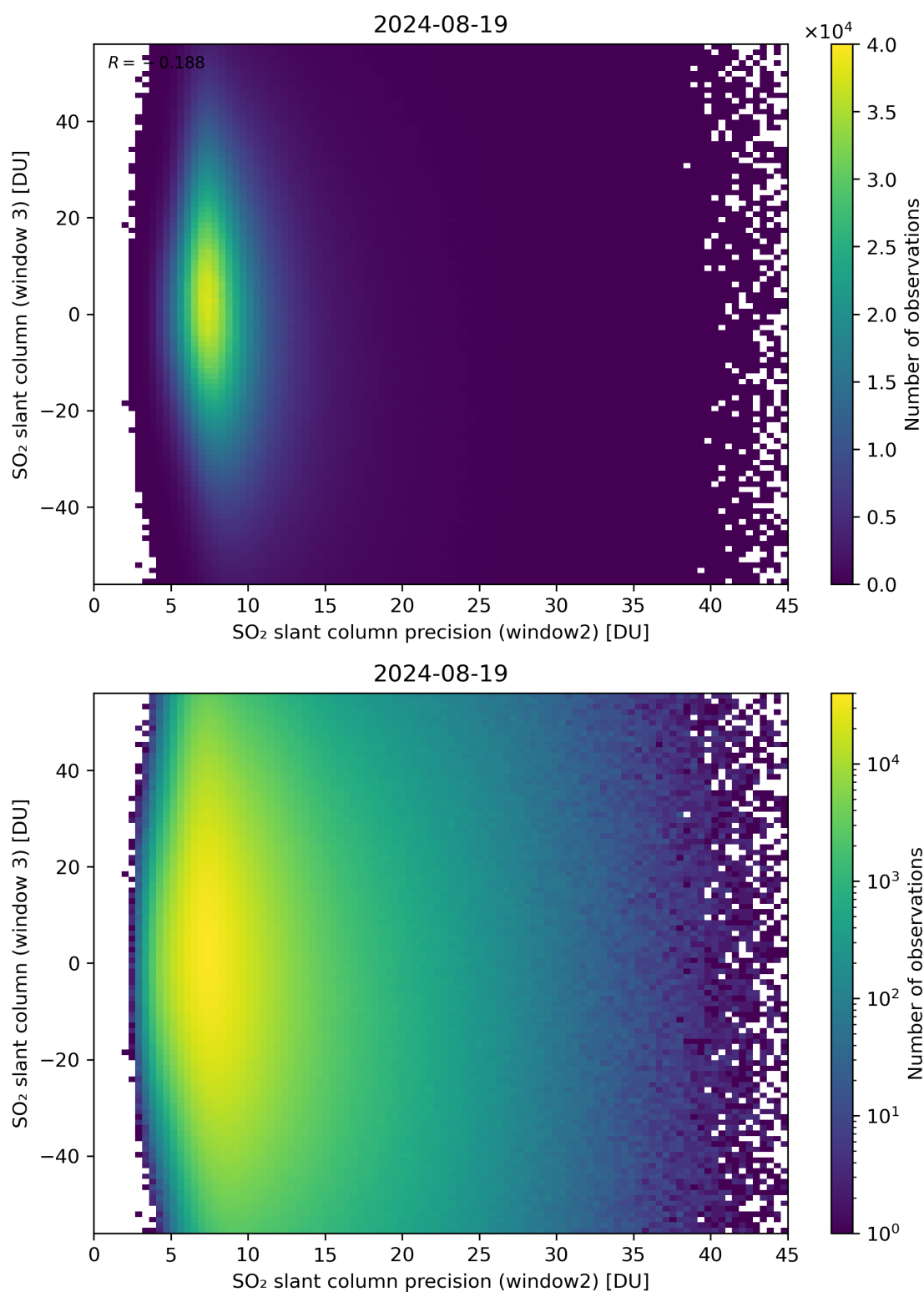
Figure 249: Scatter density plot of “SO 2 slant column precision (window2)” against “SO 2 slant column (window 3)” for 2024-08-18 to 2024-08-20.
