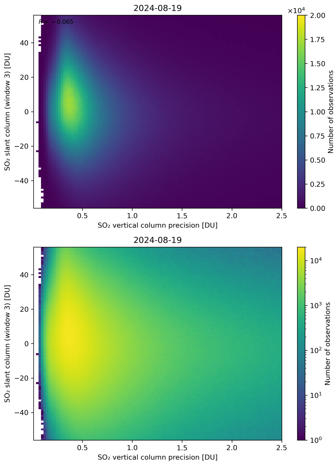
Figure 292: Scatter density plot of “SO 2 vertical column precision” against “SO 2 slant column (window 3)” for 2024-08-18 to 2024-08-20.
