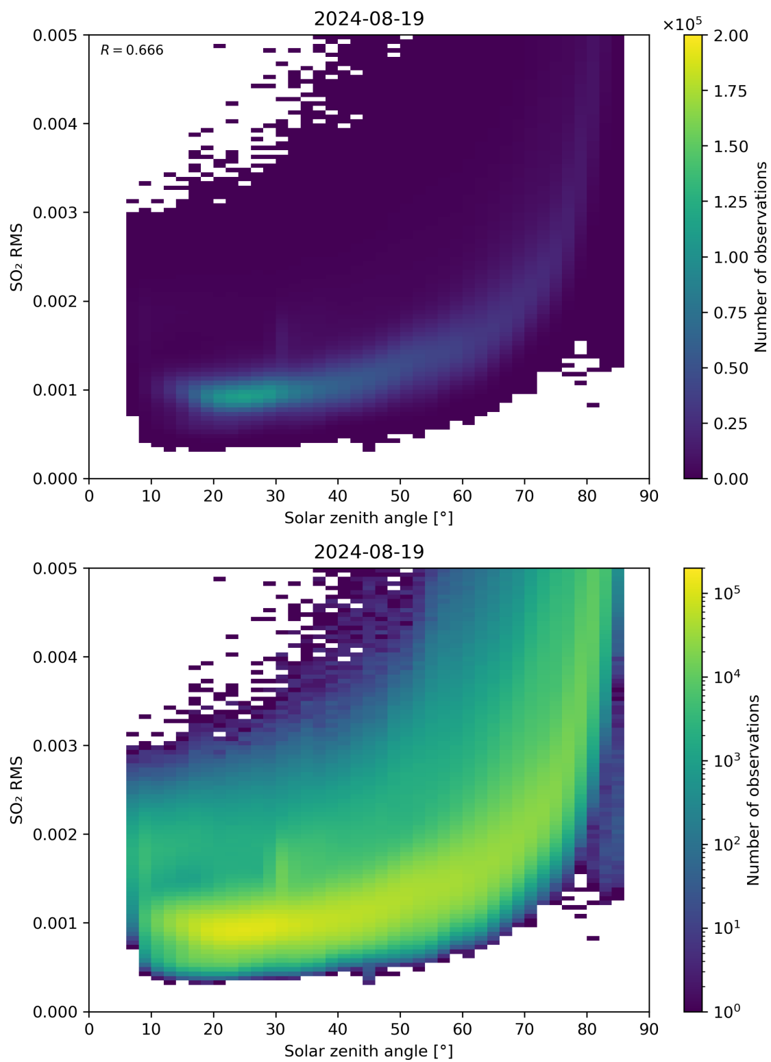
Figure 163: Scatter density plot of “Solar zenith angle” against “SO 2 RMS” for 2024-08-18 to 2024-08-20.
