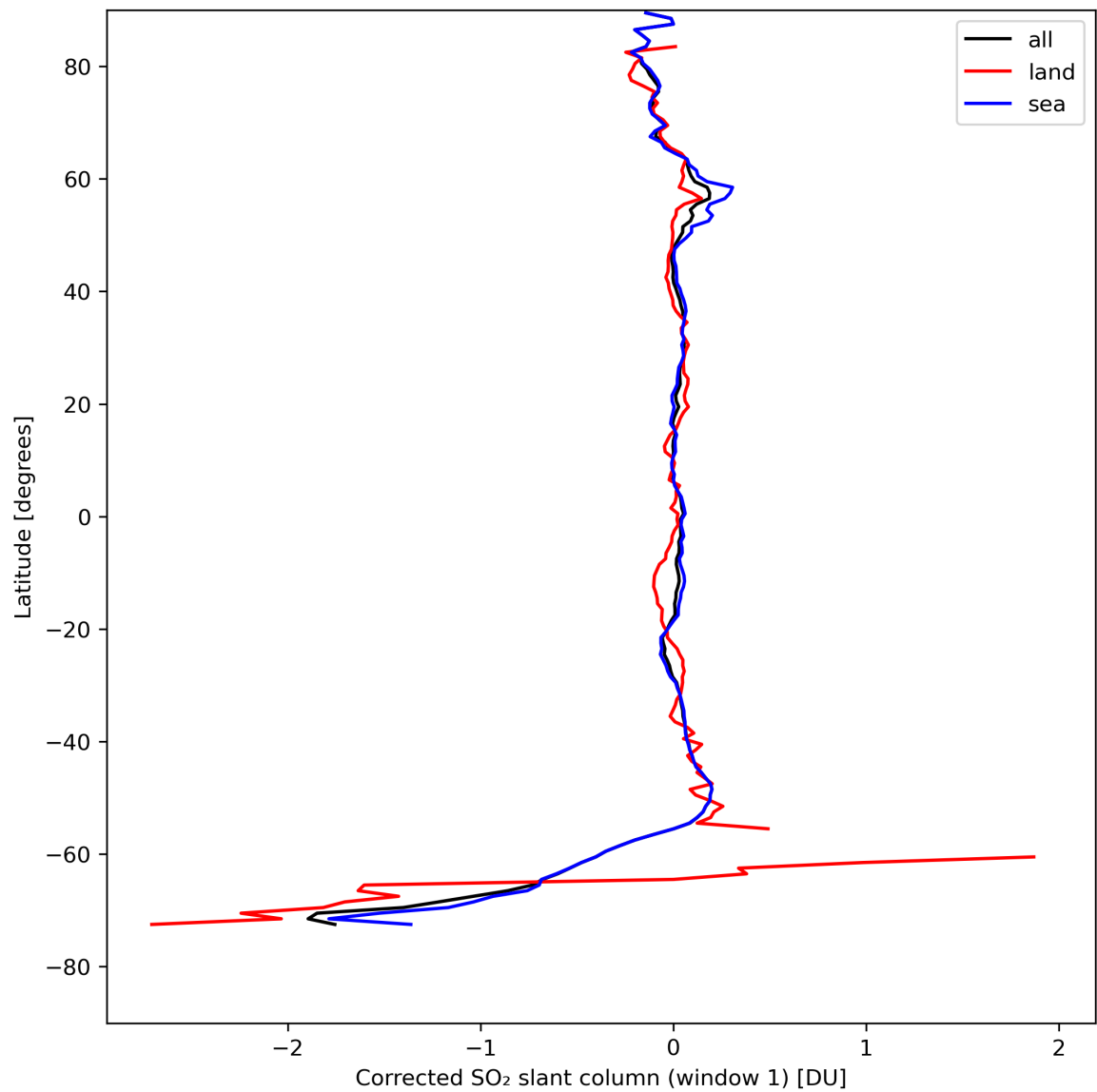
Figure 35: Zonal average of “Corrected SO 2 slant column (window 1)” for 2024-08-18 to 2024-08-20.
