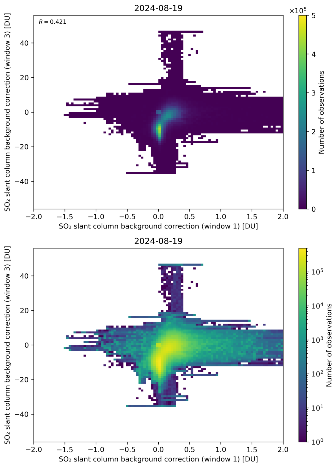
Figure 99: Scatter density plot of “SO 2 slant column background correction (window 1)” against “SO 2 slant column background correction (window 3)” for 2024-08-18 to 2024-08-20.
