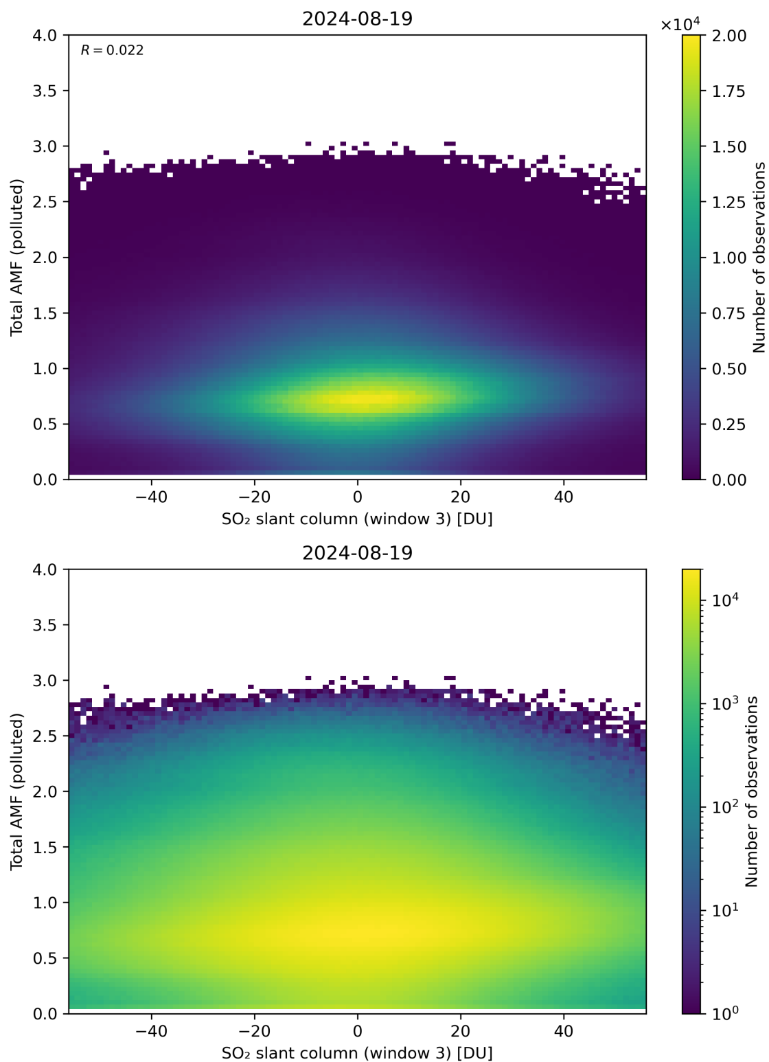
Figure 268: Scatter density plot of “SO 2 slant column (window 3)” against “Total AMF (polluted)” for 2024-08-18 to 2024-08-20.
