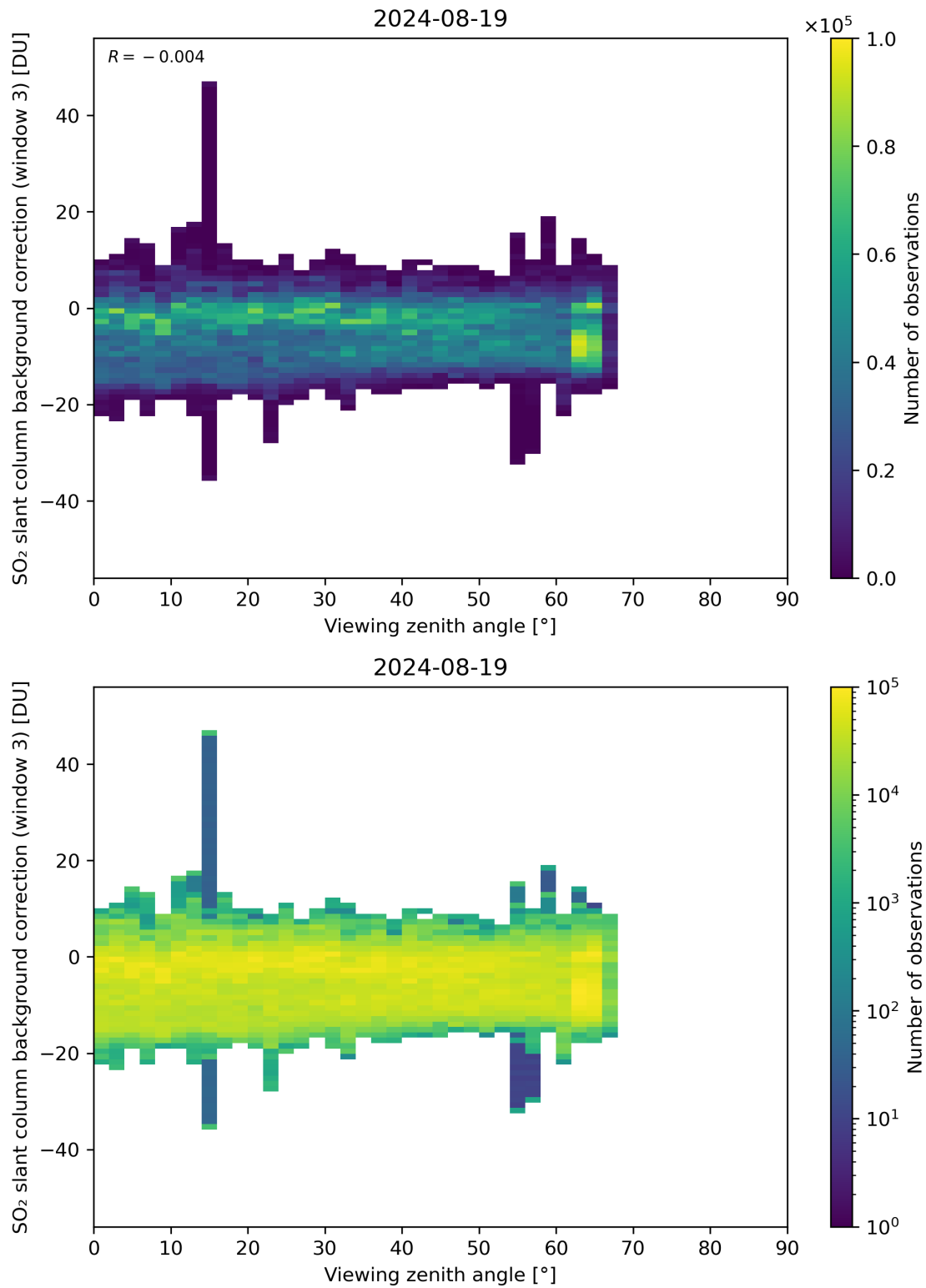
Figure 310: Scatter density plot of “Viewing zenith angle” against “SO 2 slant column background correction (window 3)” for 2024-08-18 to 2024-08-20.
