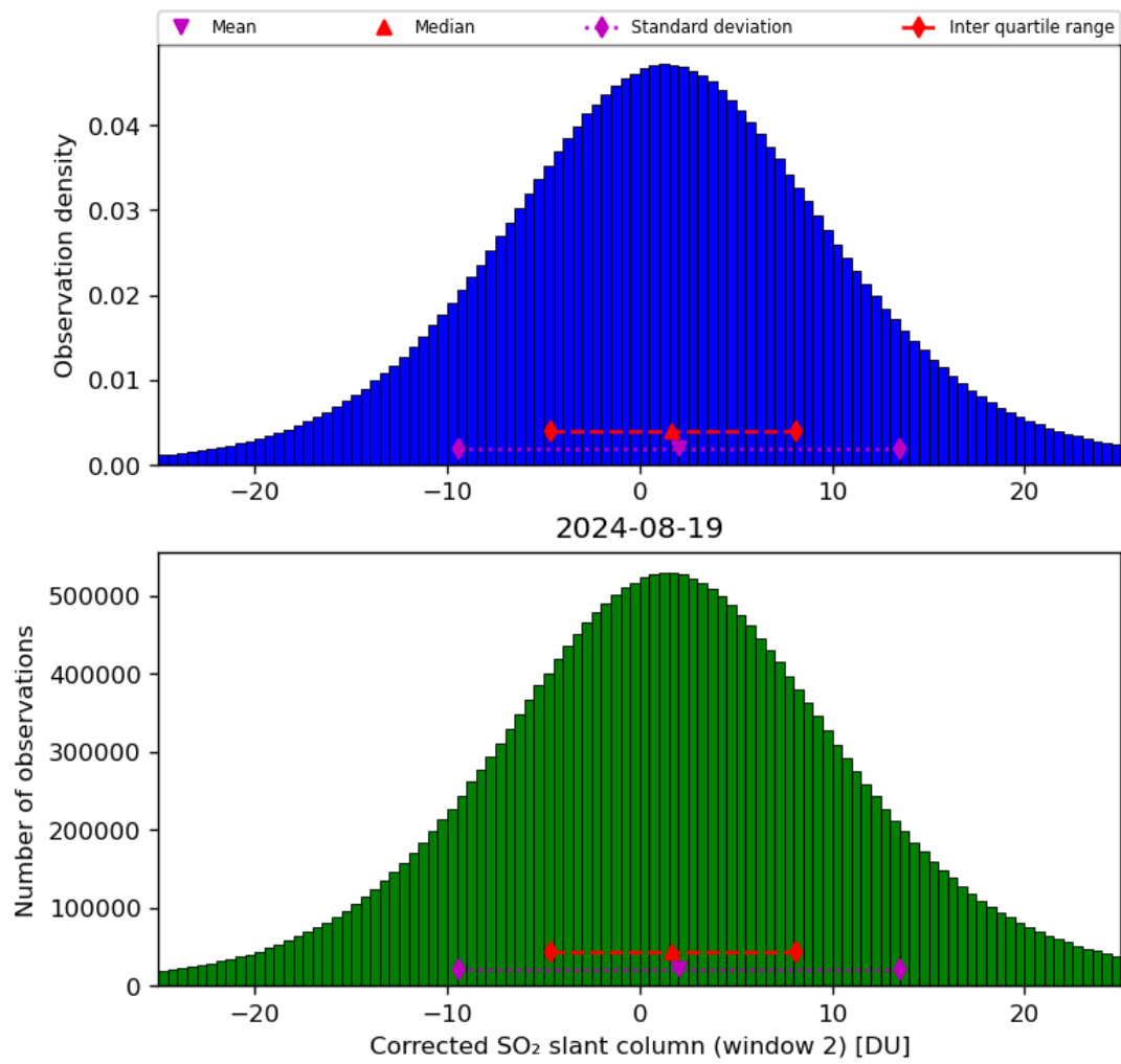
Figure 62: Histogram of “Corrected SO 2 slant column (window 2)” for 2024-08-18 to 2024-08-20
