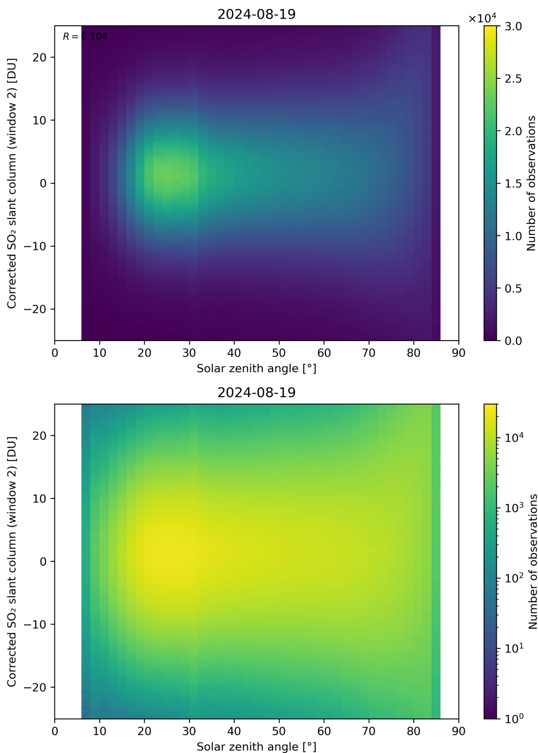
Figure 167: Scatter density plot of “Solar zenith angle” against “Corrected SO 2 slant column (window 2)” for 2024-08-18 to 2024-08-20.
