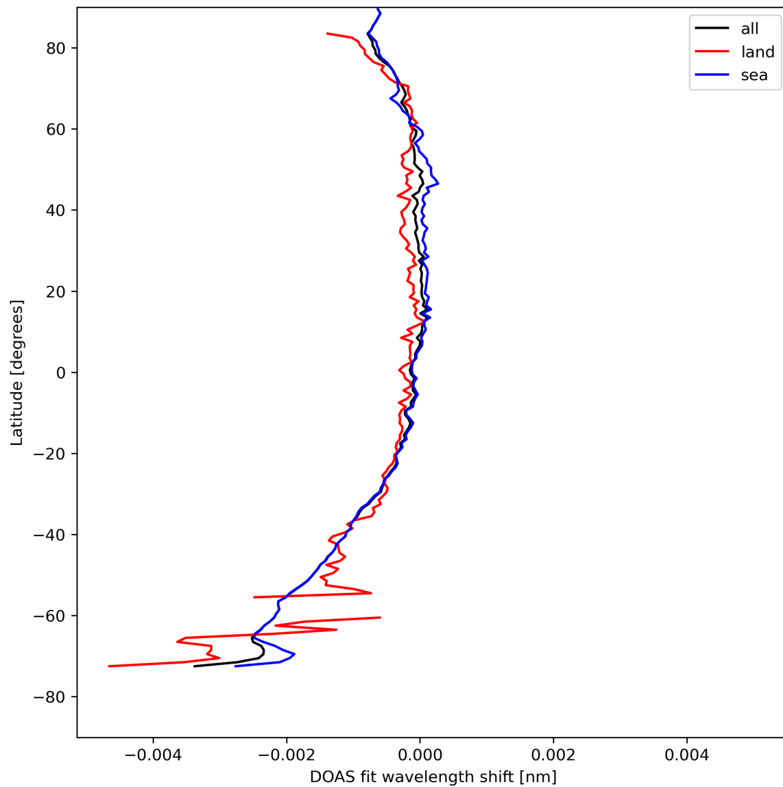
Figure 45: Zonal average of “DOAS fit wavelength shift” for 2024-08-18 to 2024-08-20.
