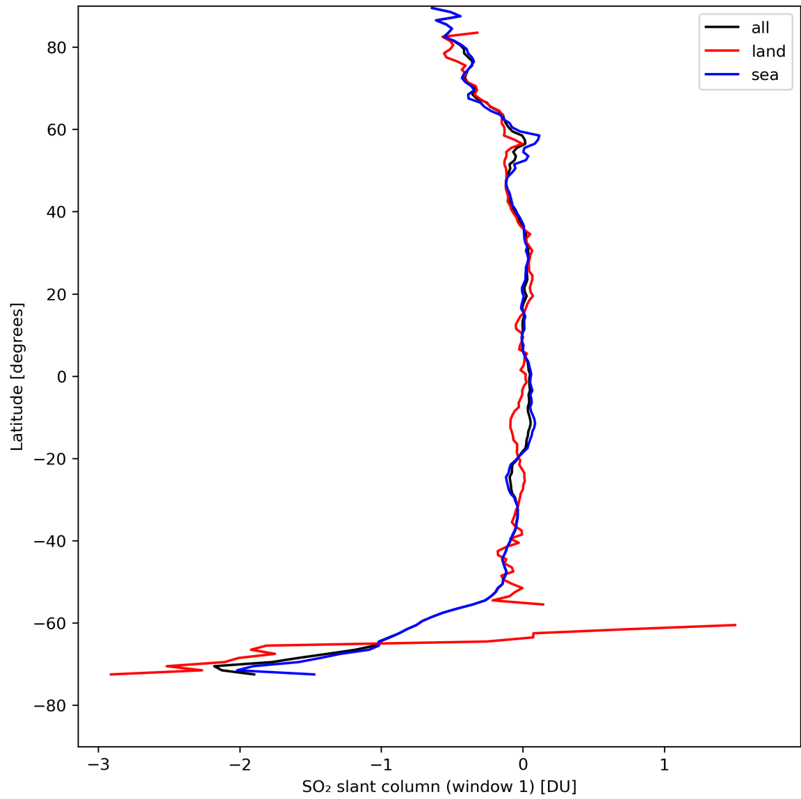
Figure 33: Zonal average of “SO 2 slant column (window 1)” for 2024-08-18 to 2024-08-20.
