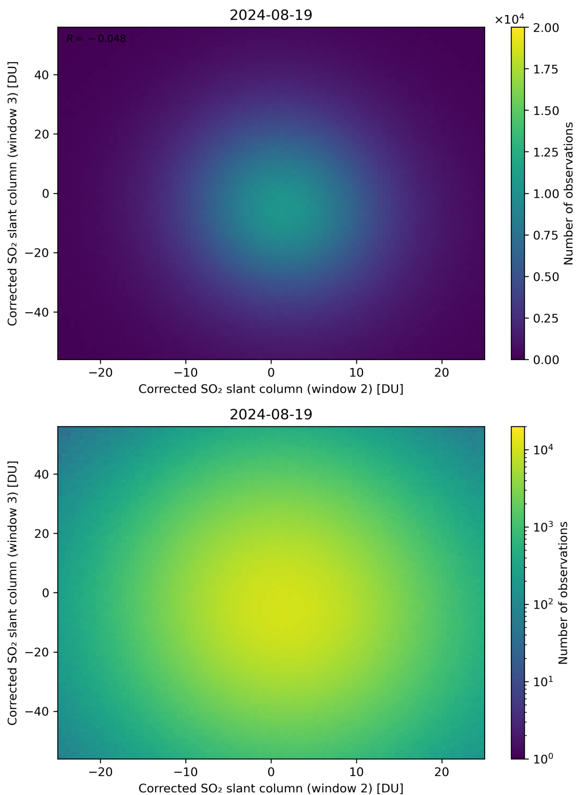
Figure 200: Scatter density plot of “Corrected SO 2 slant column (window 2)” against “Corrected SO 2 slant column (window 3)” for 2024-08-18 to 2024-08-20.
