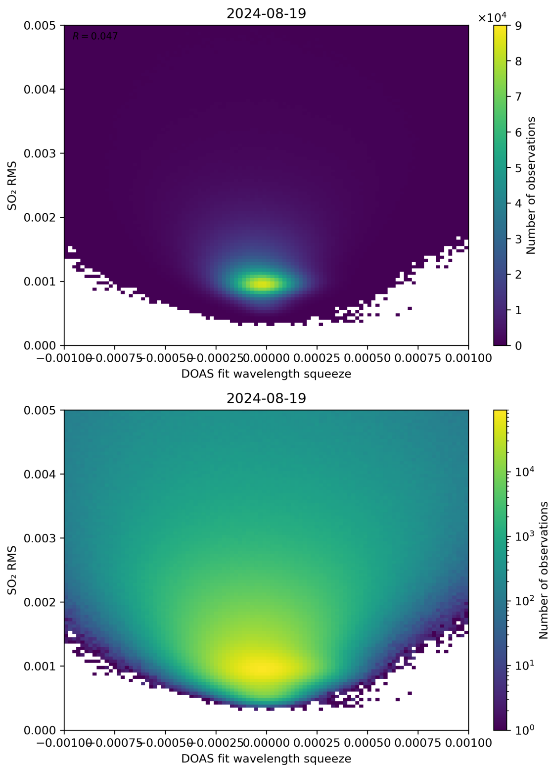
Figure 132: Scatter density plot of “DOAS fit wavelength squeeze” against “SO 2 RMS” for 2024-08-18 to 2024-08-20.
