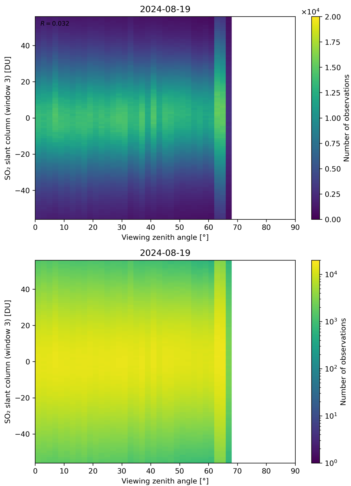
Figure 323: Scatter density plot of “Viewing zenith angle” against “SO 2 slant column (window 3)” for 2024-08-18 to 2024-08-20.
