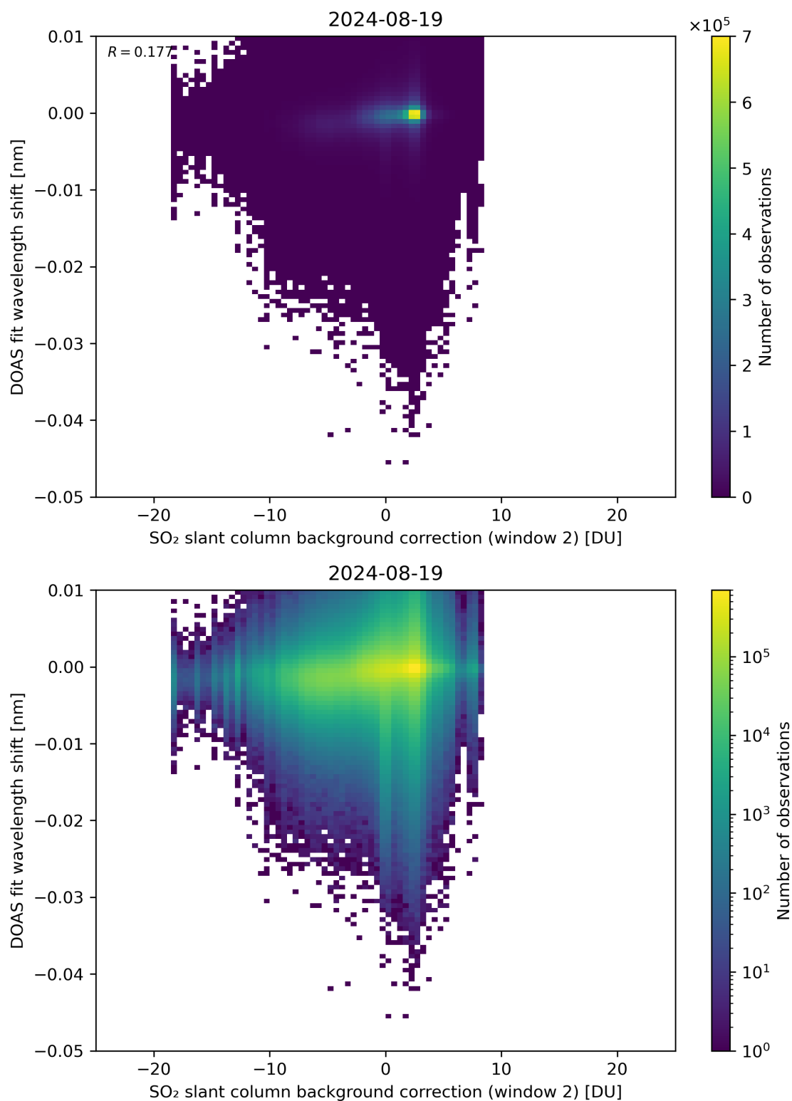
Figure 112: Scatter density plot of “SO 2 slant column background correction (window 2)” against “DOAS fit wavelength shift” for 2024-08-18 to 2024-08-20.
