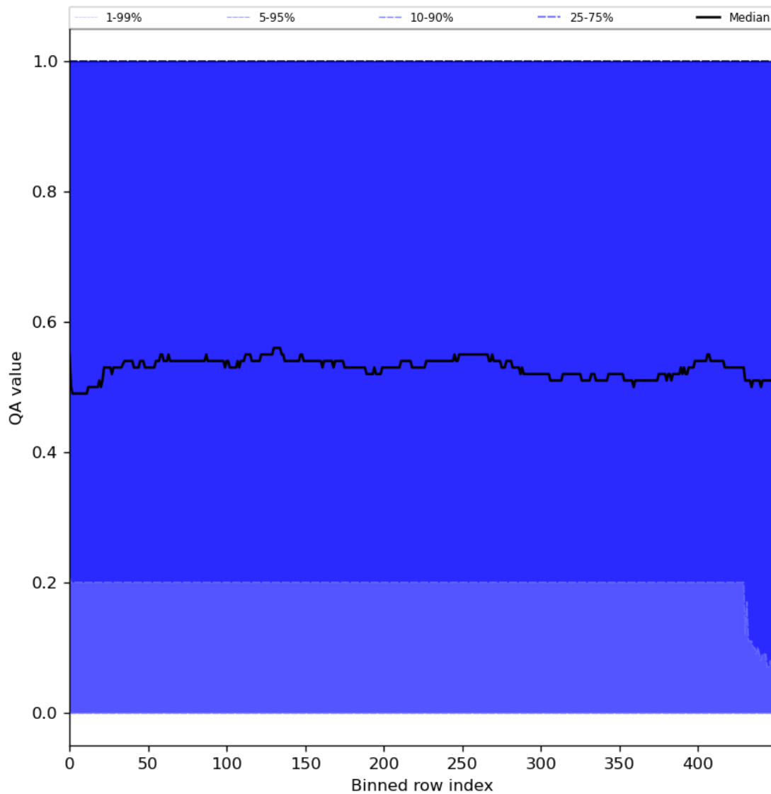
Figure 75: Along track statistics of “QA value” for 2024-08-18 to 2024-08-20
