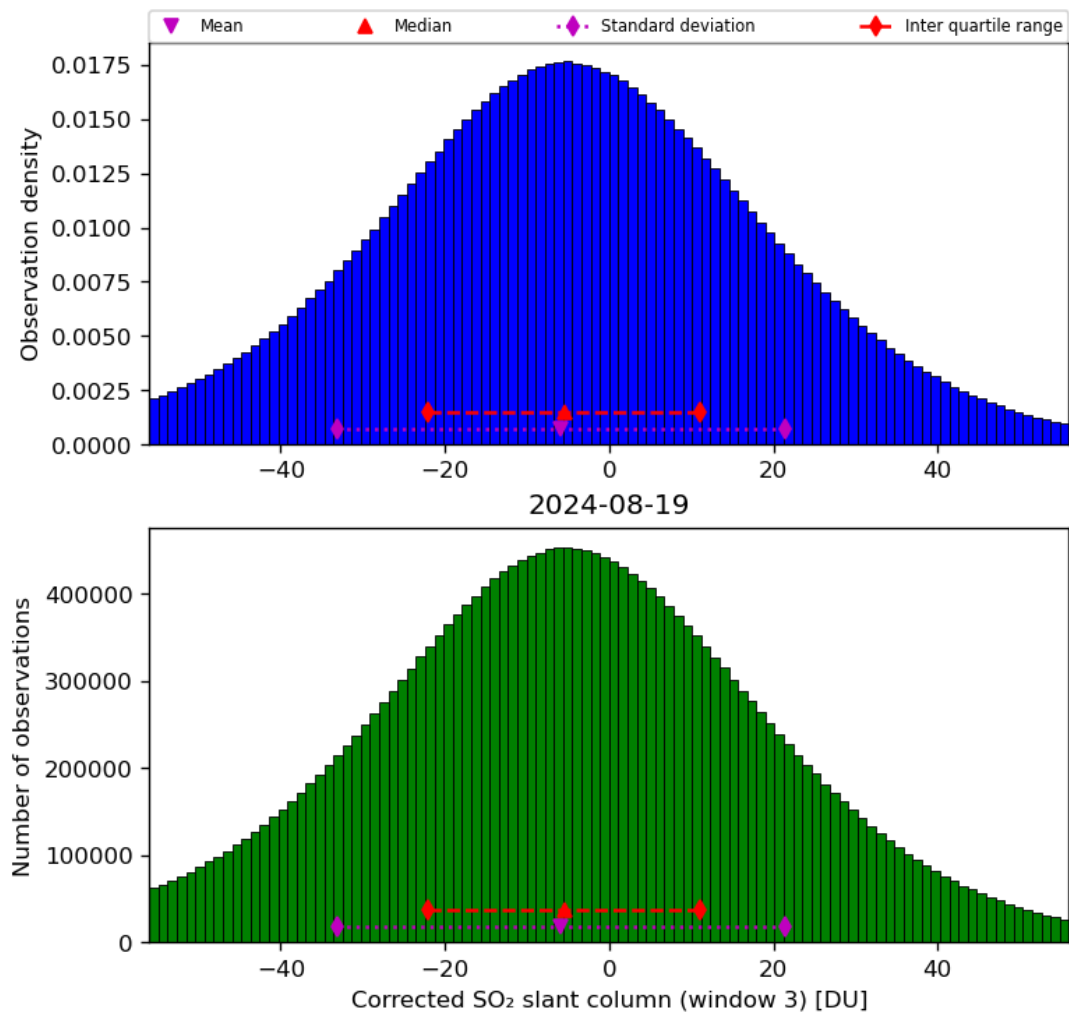
Figure 66: Histogram of “Corrected SO 2 slant column (window 3)” for 2024-08-18 to 2024-08-20
