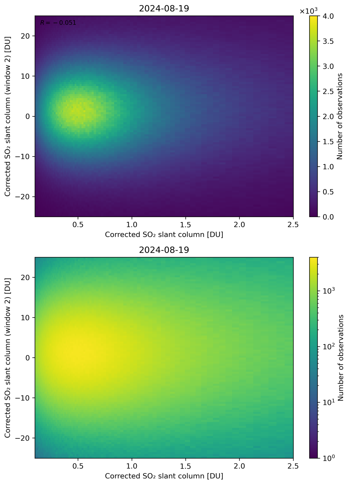
Figure 185: Scatter density plot of “Corrected SO 2 slant column” against “Corrected SO 2 slant column (window 2)” for 2024-08-18 to 2024-08-20.
