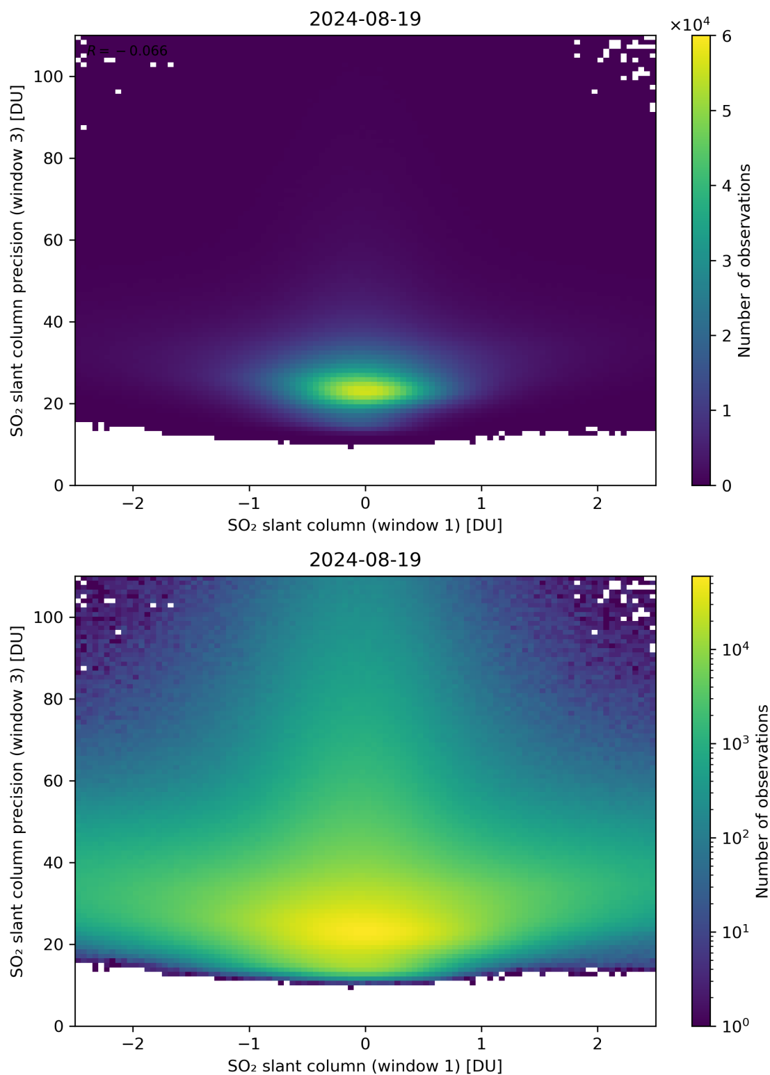
Figure 238: Scatter density plot of “SO 2 slant column (window 1)” against “SO 2 slant column precision (window 3)” for 2024-08-18 to 2024-08-20.
