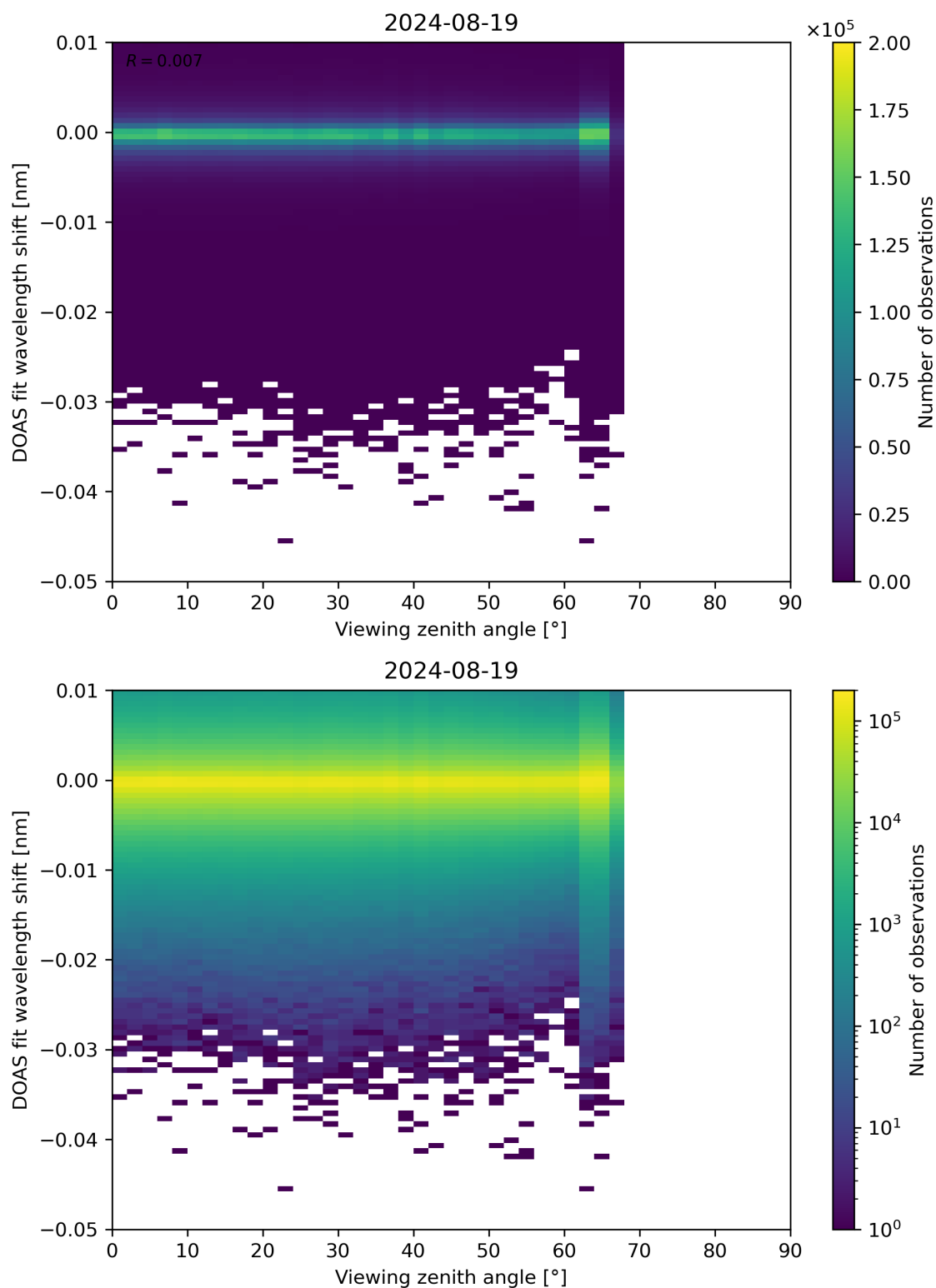
Figure 311: Scatter density plot of “Viewing zenith angle” against “DOAS fit wavelength shift” for 2024-08-18 to 2024-08-20.
