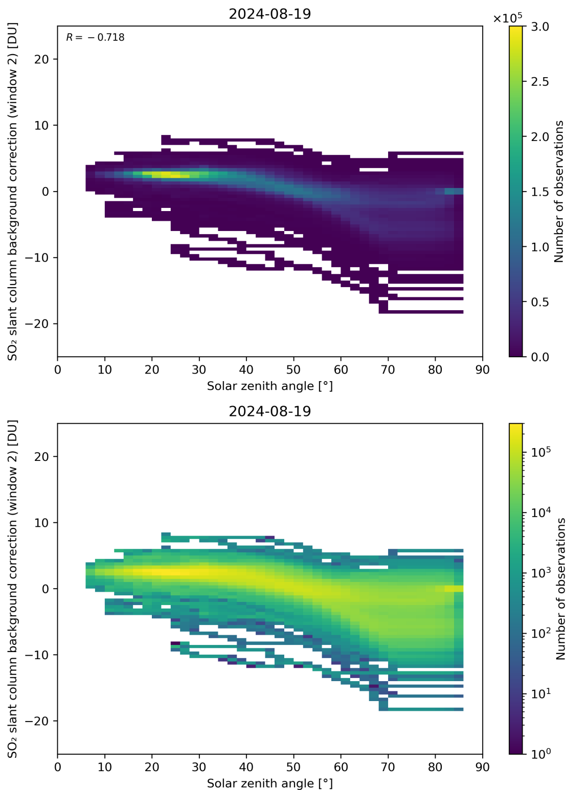
Figure 159: Scatter density plot of “Solar zenith angle” against “SO 2 slant column background correction (window 2)” for 2024-08-18 to 2024-08-20.
