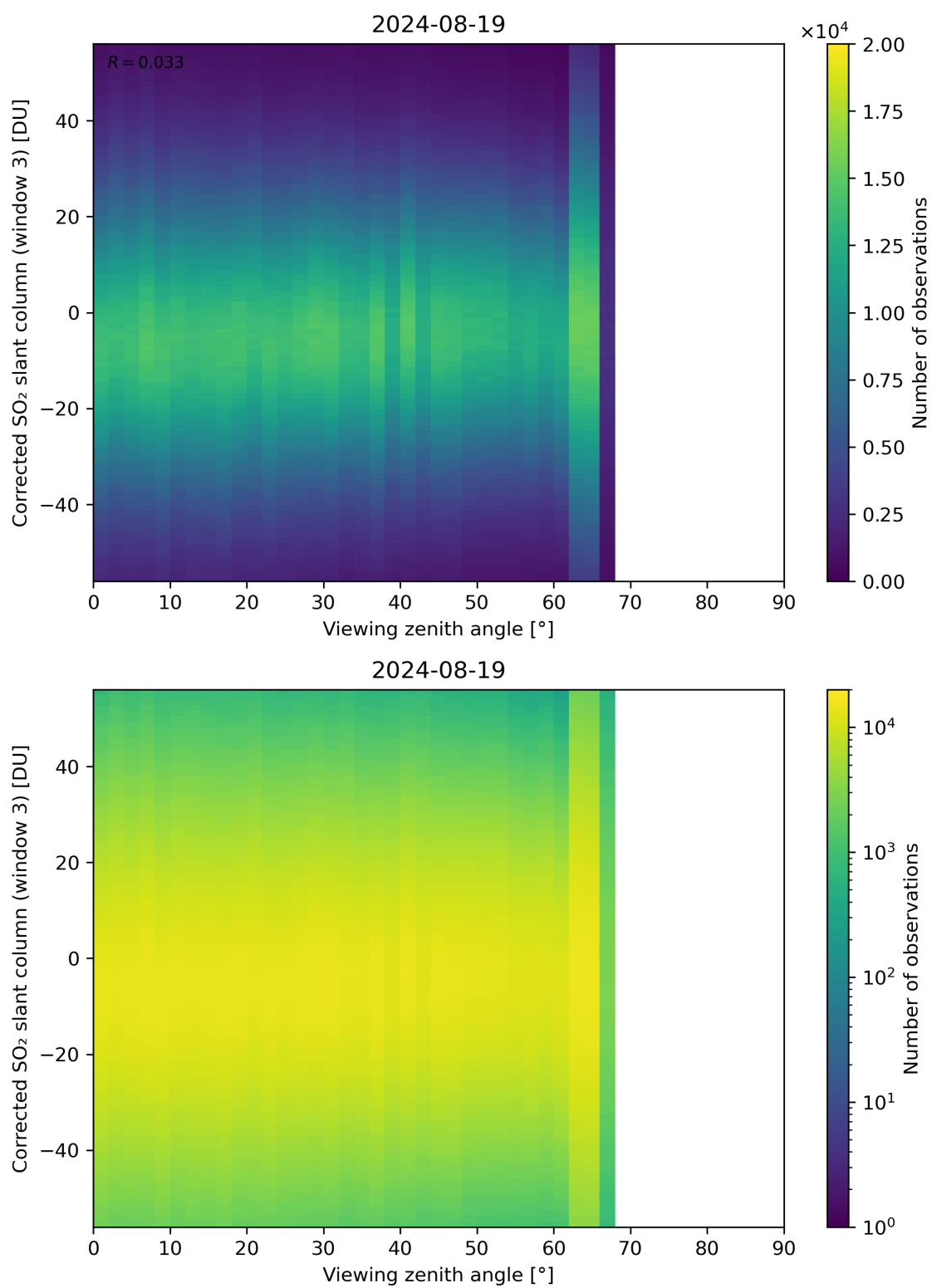
Figure 319: Scatter density plot of “Viewing zenith angle” against “Corrected SO 2 slant column (window 3)” for 2024-08-18 to 2024-08-20.
