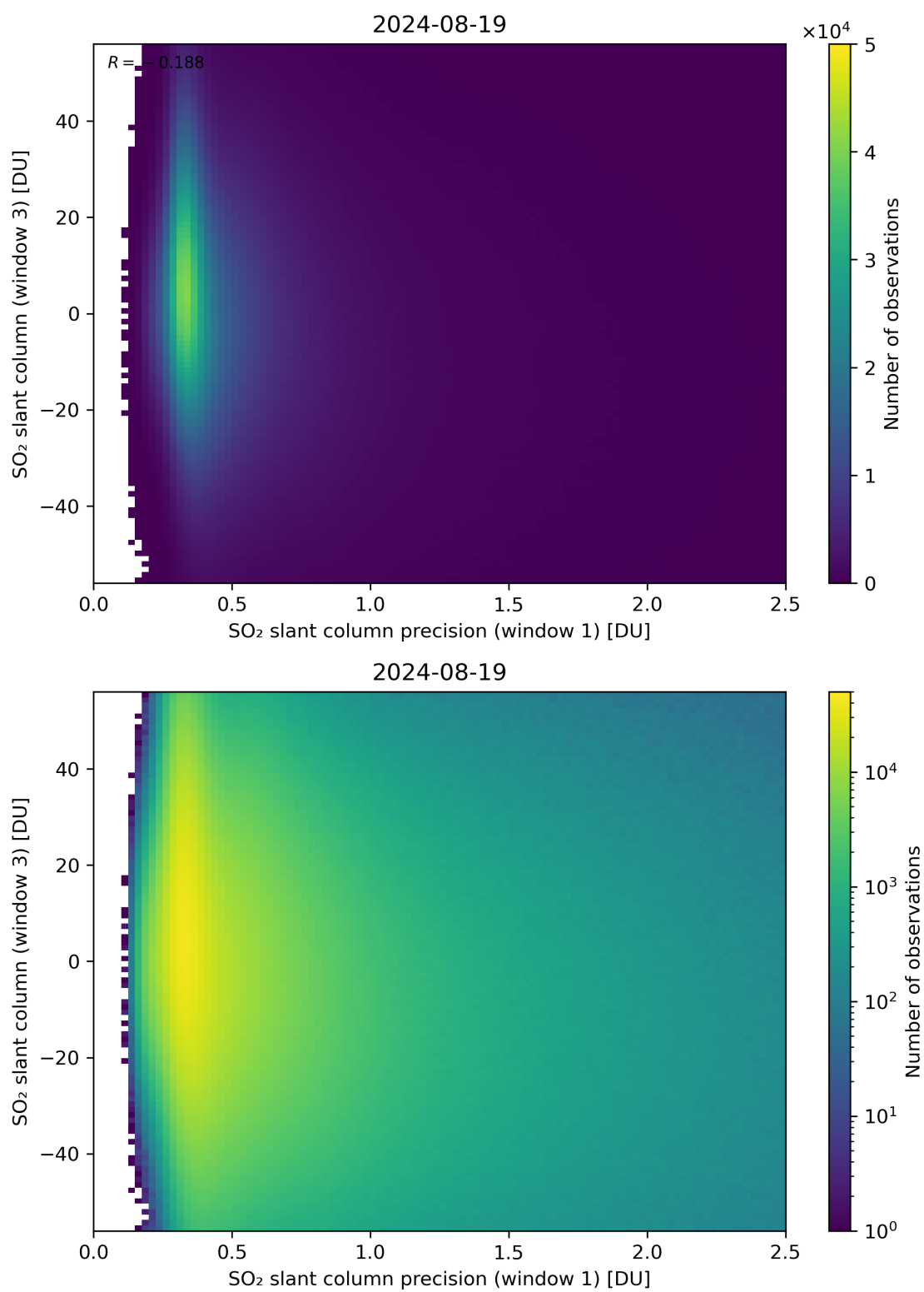
Figure 228: Scatter density plot of “SO 2 slant column precision (window 1)” against “SO 2 slant column (window 3)” for 2024-08-18 to 2024-08-20.
