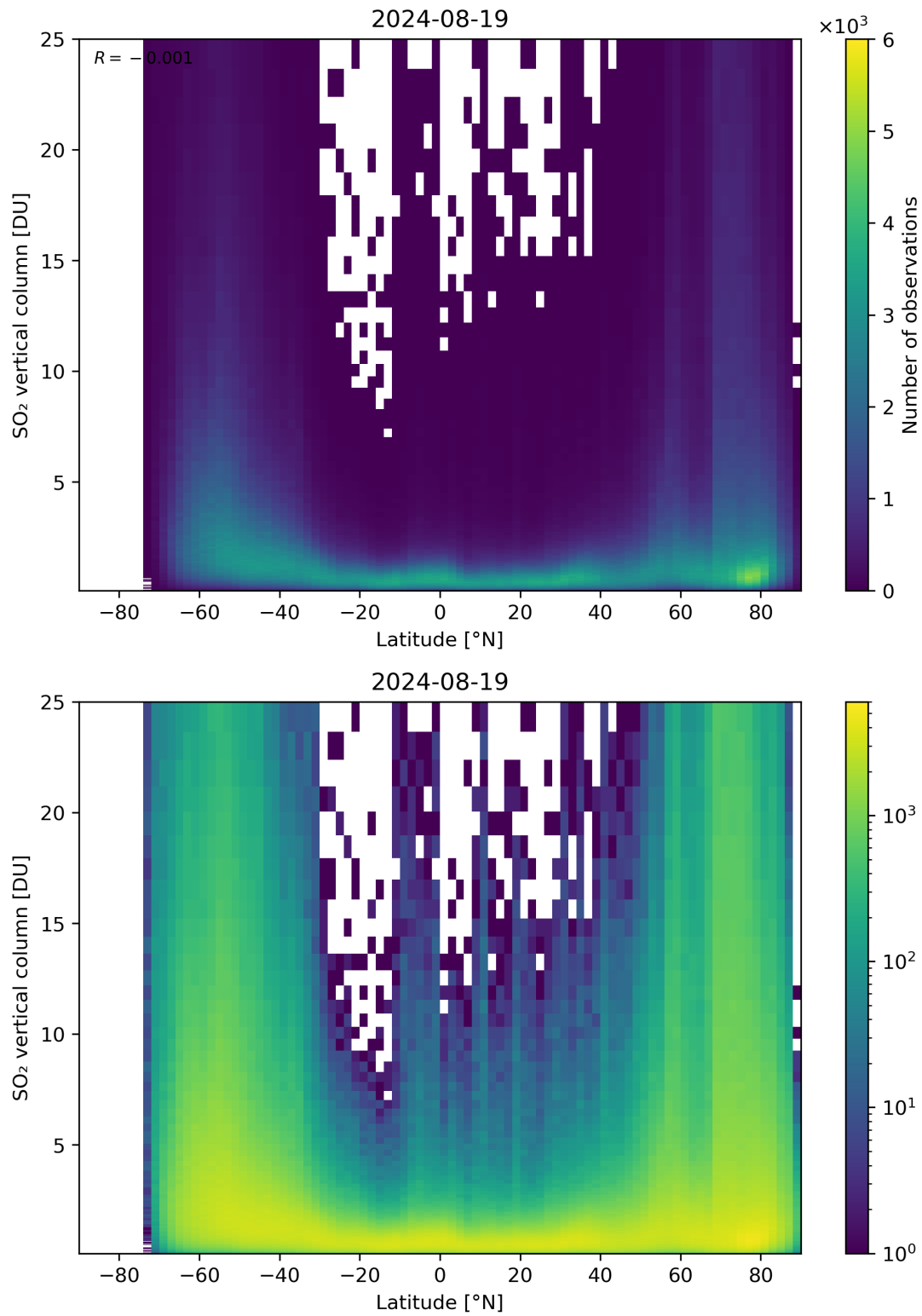
Figure 156: Scatter density plot of “Latitude” against “SO 2 vertical column” for 2024-08-18 to 2024-08-20.
