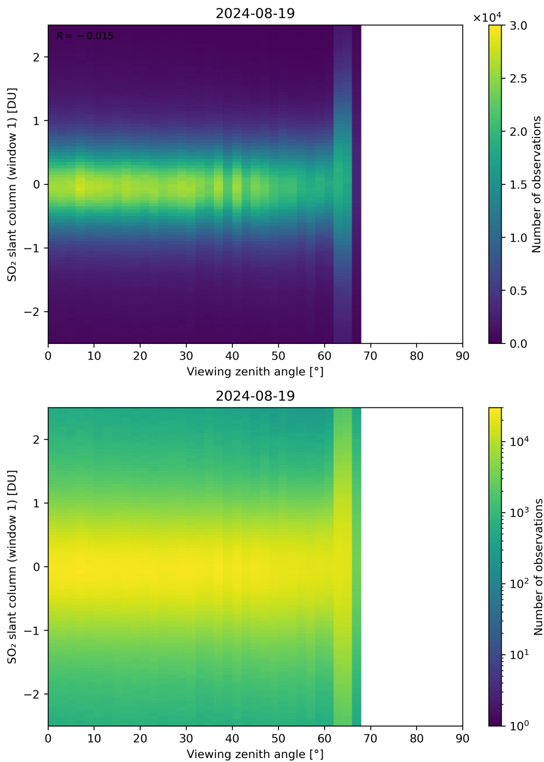
Figure 320: Scatter density plot of “Viewing zenith angle” against “SO 2 slant column (window 1)” for 2024-08-18 to 2024-08-20.
