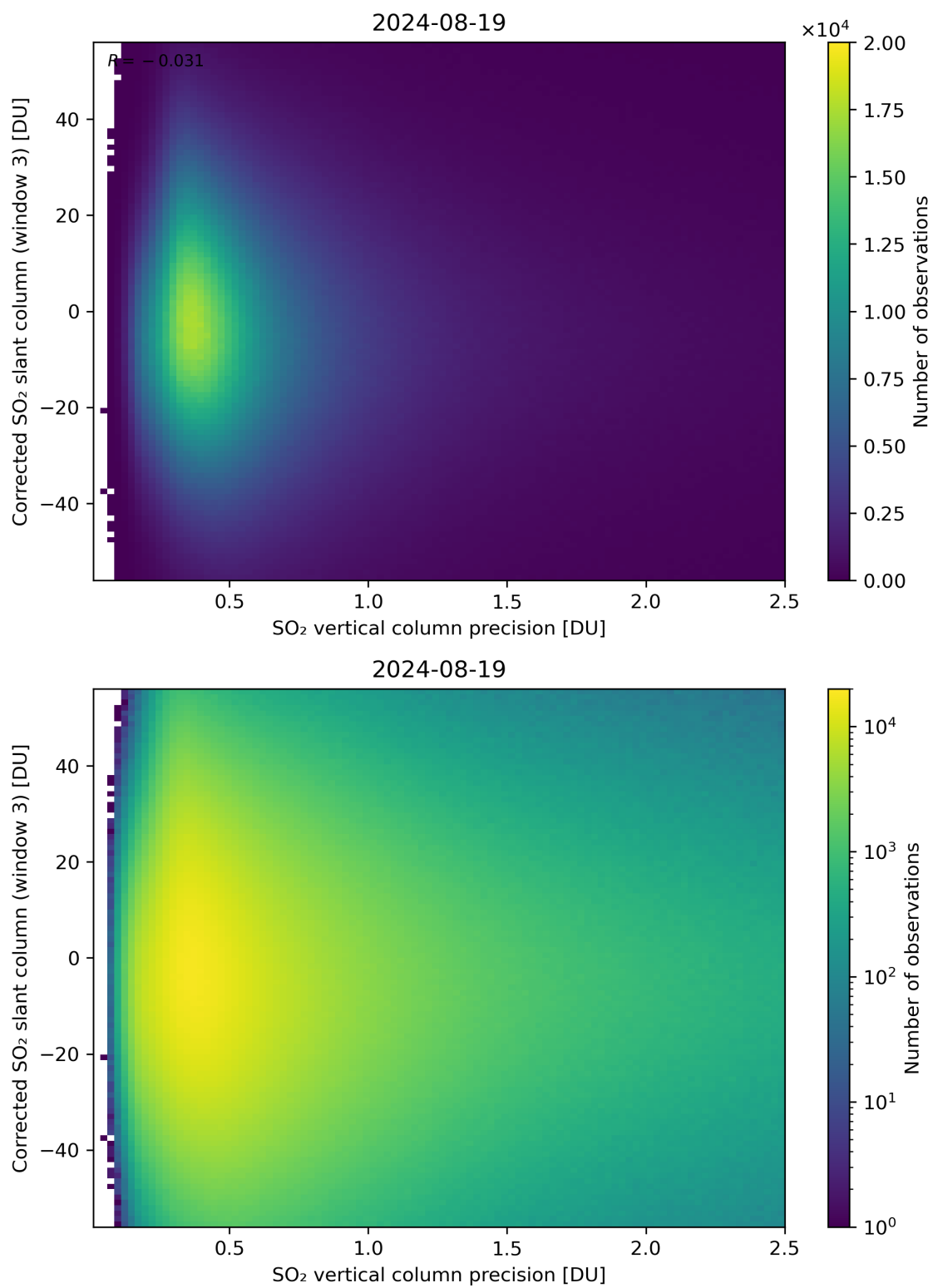
Figure 288: Scatter density plot of “SO 2 vertical column precision” against “Corrected SO 2 slant column (window 3)” for 2024-08-18 to 2024-08-20.
