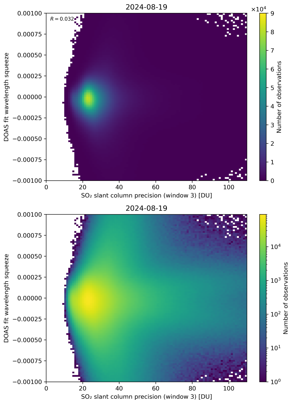
Figure 259: Scatter density plot of “SO 2 slant column precision (window 3)” against “DOAS fit wavelength squeeze” for 2024-08-18 to 2024-08-20.
