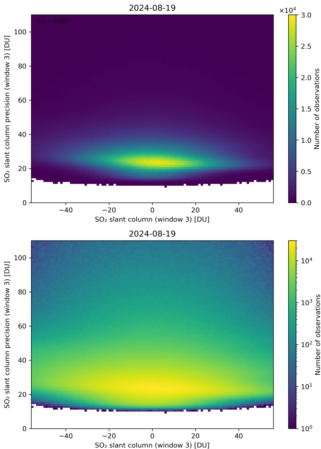
Figure 267: Scatter density plot of “SO 2 slant column (window 3)” against “SO 2 slant column precision (window 3)” for 2024-08-18 to 2024-08-20.
