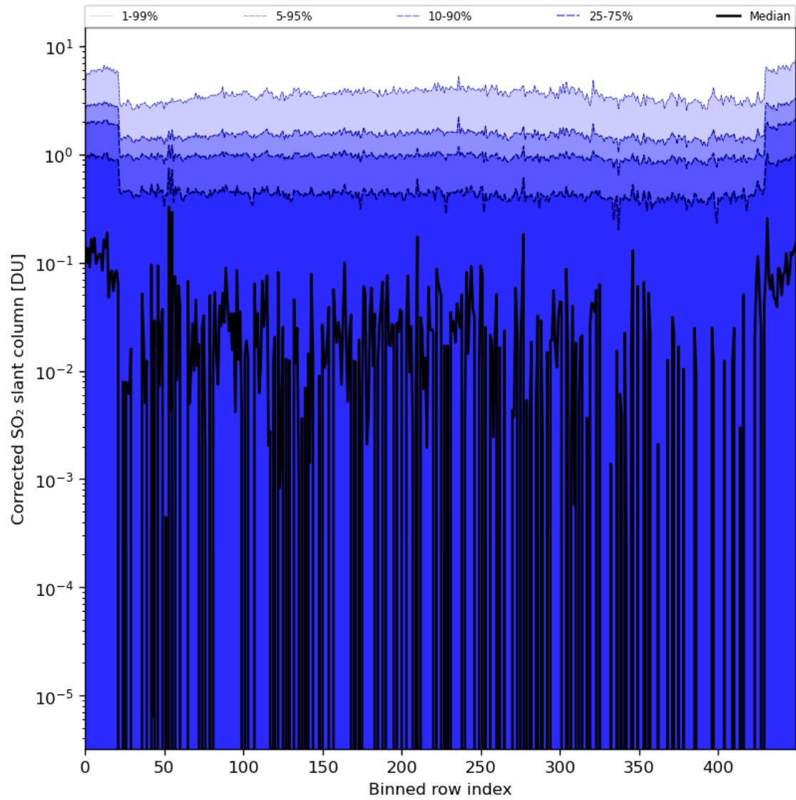
Figure 78: Along track statistics of “Corrected SO 2 slant column” for 2024-08-18 to 2024-08-20
