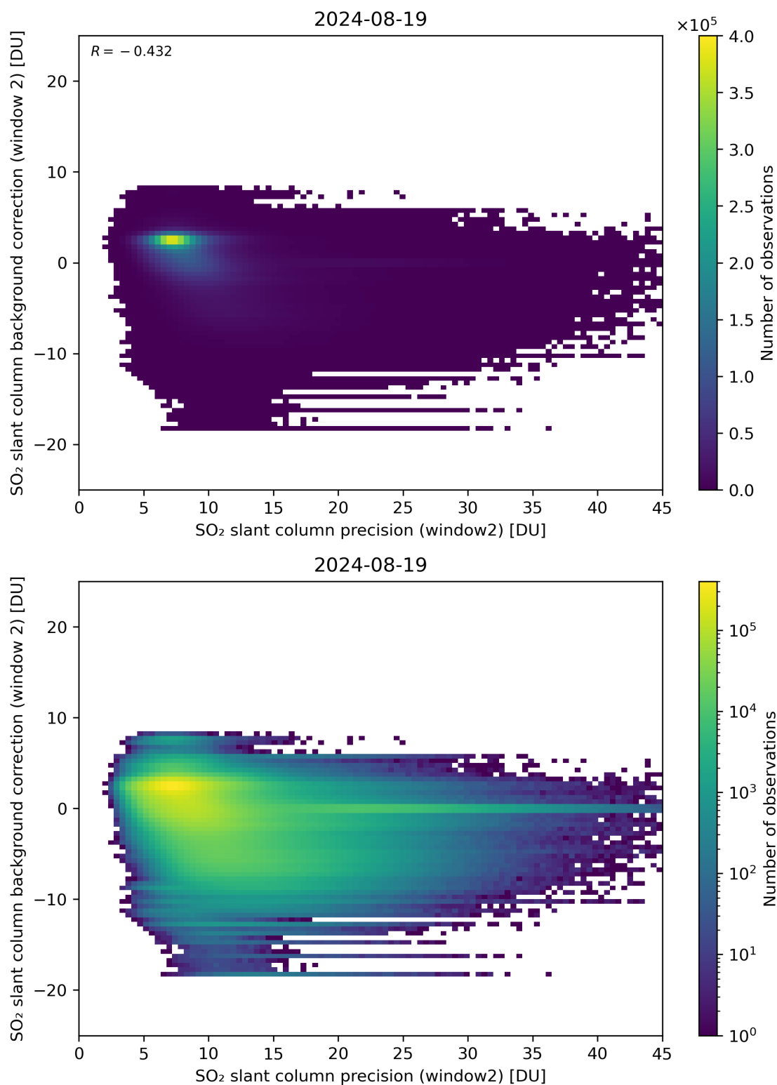
Figure 241: Scatter density plot of “SO 2 slant column precision (window2)” against “SO 2 slant column background correction (window 2)” for 2024-08-18 to 2024-08-20.
