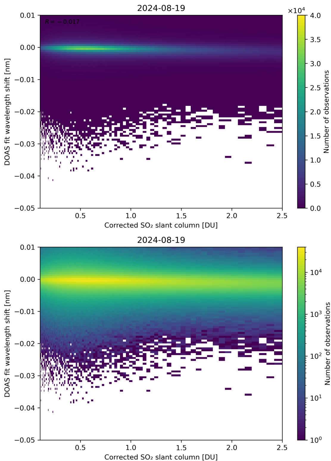
Figure 181: Scatter density plot of “Corrected SO 2 slant column” against “DOAS fit wavelength shift” for 2024-08-18 to 2024-08-20.
