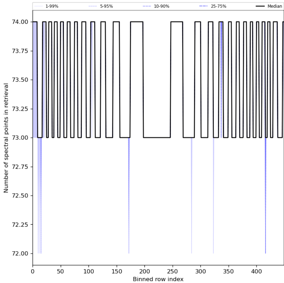
Figure 97: Along track statistics of “Number of spectral points in retrieval” for 2024-08-18 to 2024-08-20
