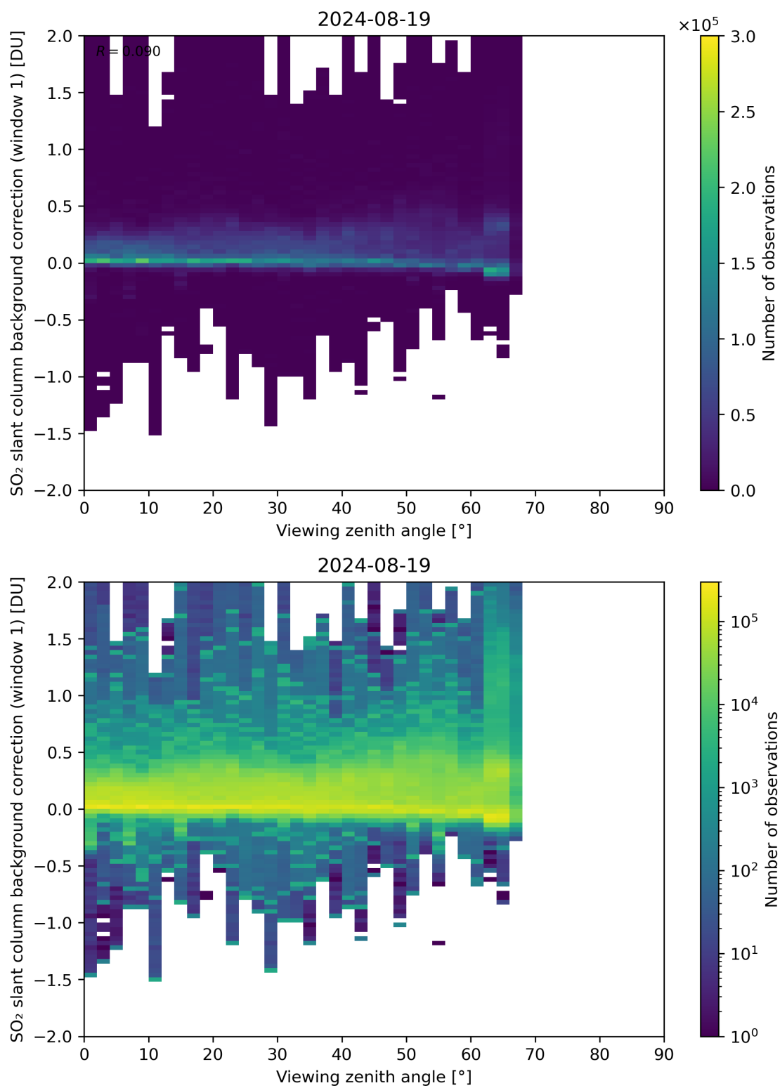
Figure 308: Scatter density plot of “Viewing zenith angle” against “SO 2 slant column background correction (window 1)” for 2024-08-18 to 2024-08-20.
