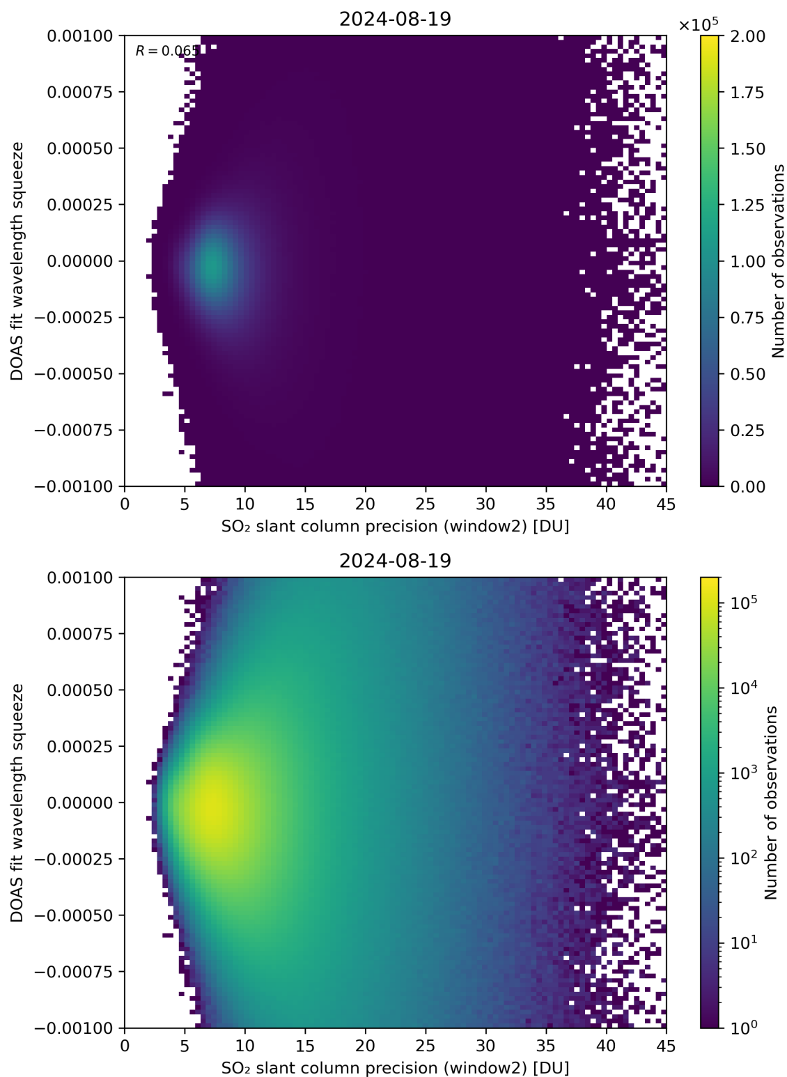
Figure 244: Scatter density plot of “SO 2 slant column precision (window2)” against “DOAS fit wavelength squeeze” for 2024-08-18 to 2024-08-20.
