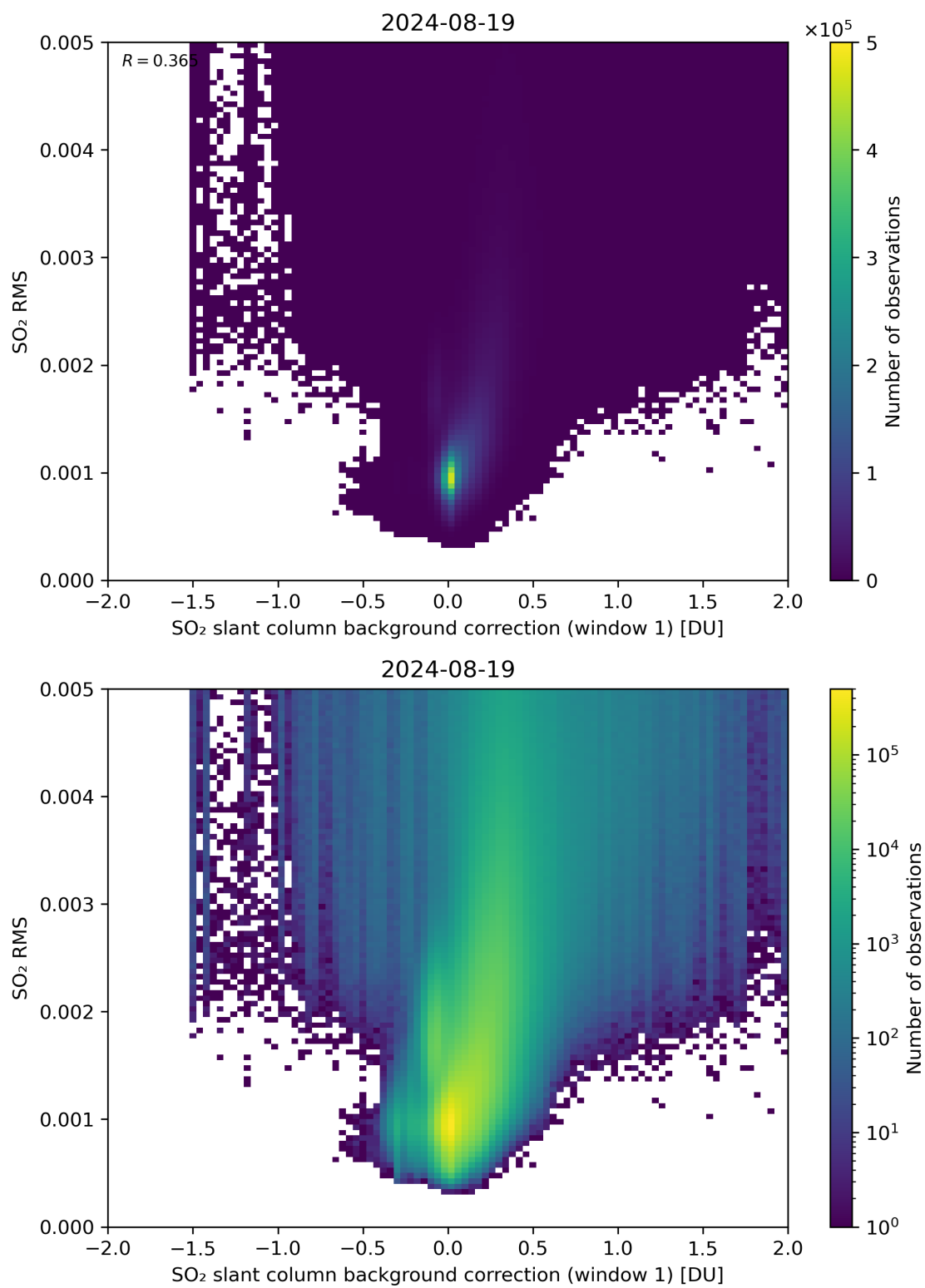
Figure 102: Scatter density plot of “SO 2 slant column background correction (window 1)” against “SO 2 RMS” for 2024-08-18 to 2024-08-20.
