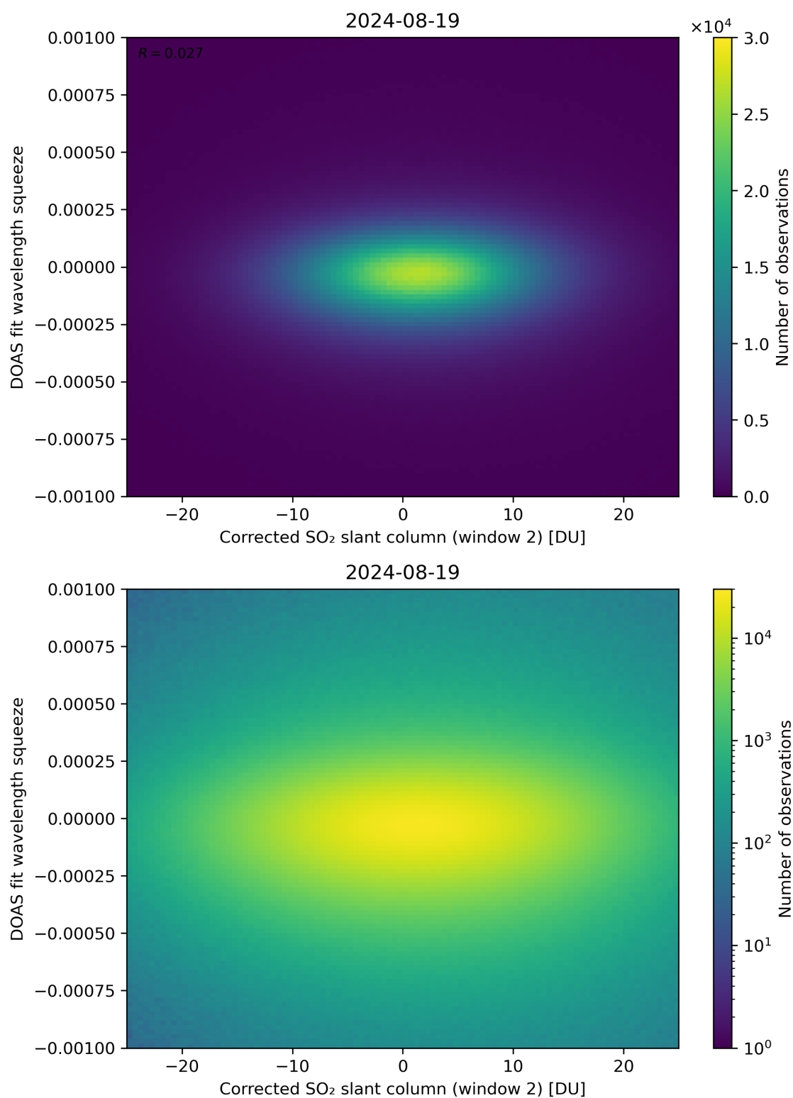
Figure 197: Scatter density plot of “Corrected SO 2 slant column (window 2)” against “DOAS fit wavelength squeeze” for 2024-08-18 to 2024-08-20.
