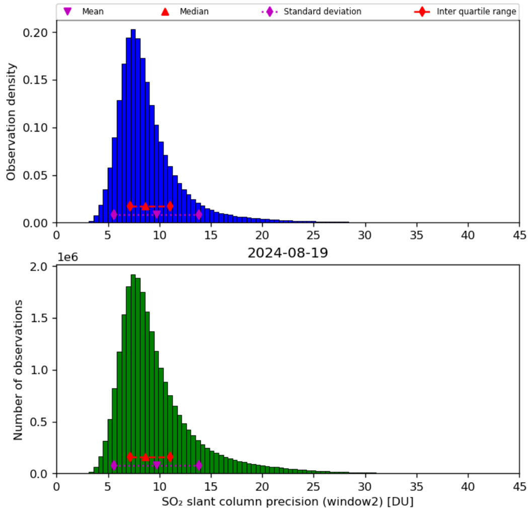
Figure 61: Histogram of “SO 2 slant column precision (window2)” for 2024-08-18 to 2024-08-20
