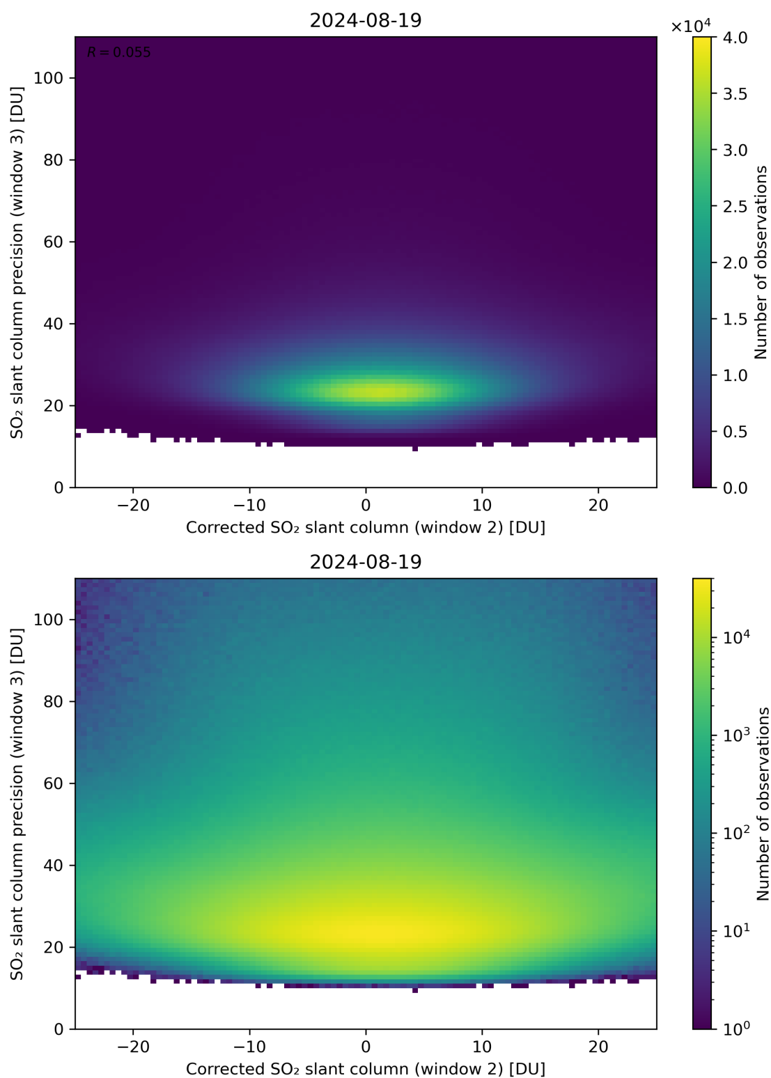
Figure 202: Scatter density plot of “Corrected SO 2 slant column (window 2)” against “SO 2 slant column precision (window 3)” for 2024-08-18 to 2024-08-20.
