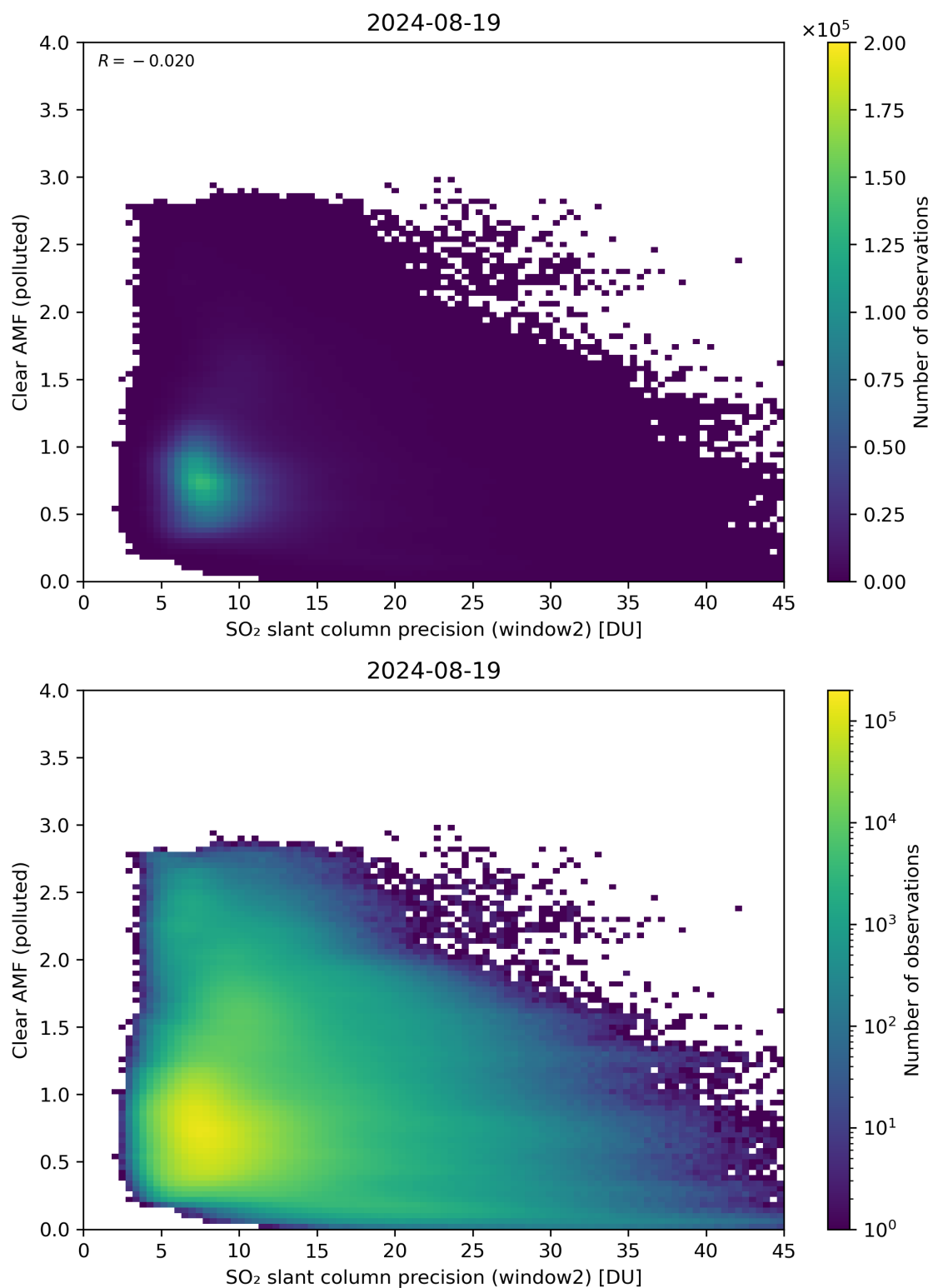
Figure 246: Scatter density plot of “SO 2 slant column precision (window2)” against “Clear AMF (polluted)” for 2024-08-18 to 2024-08-20.
