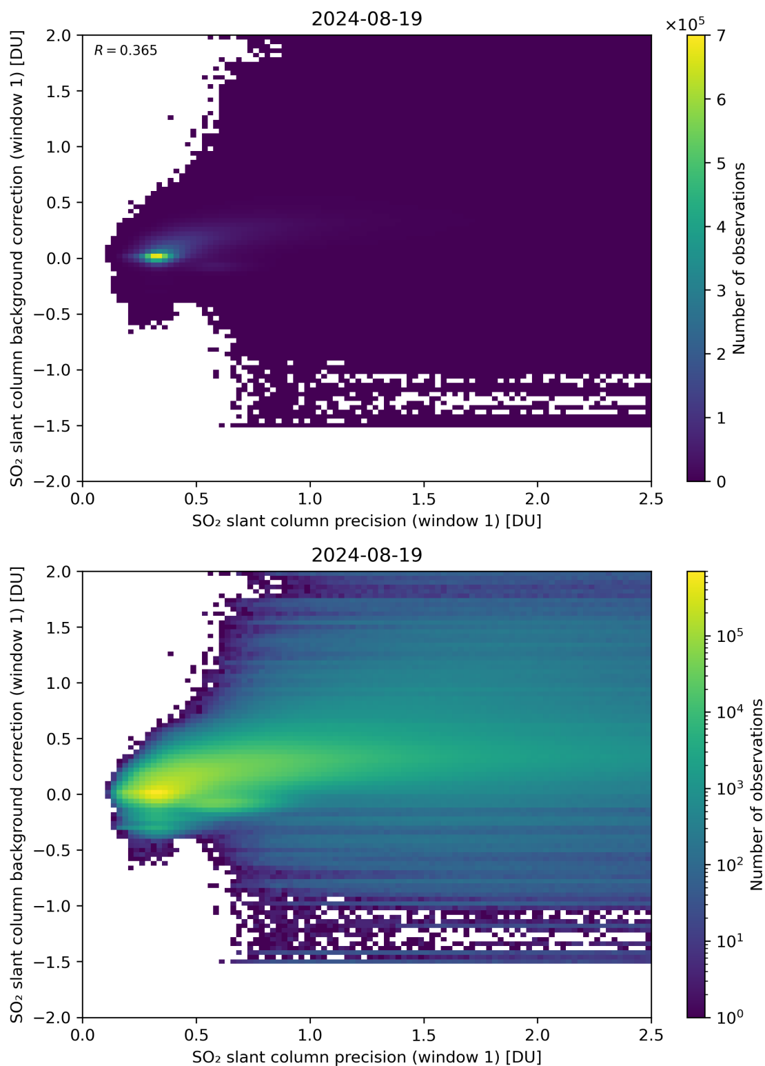
Figure 218: Scatter density plot of “SO 2 slant column precision (window 1)” against “SO 2 slant column background correction (window 1)” for 2024-08-18 to 2024-08-20.
