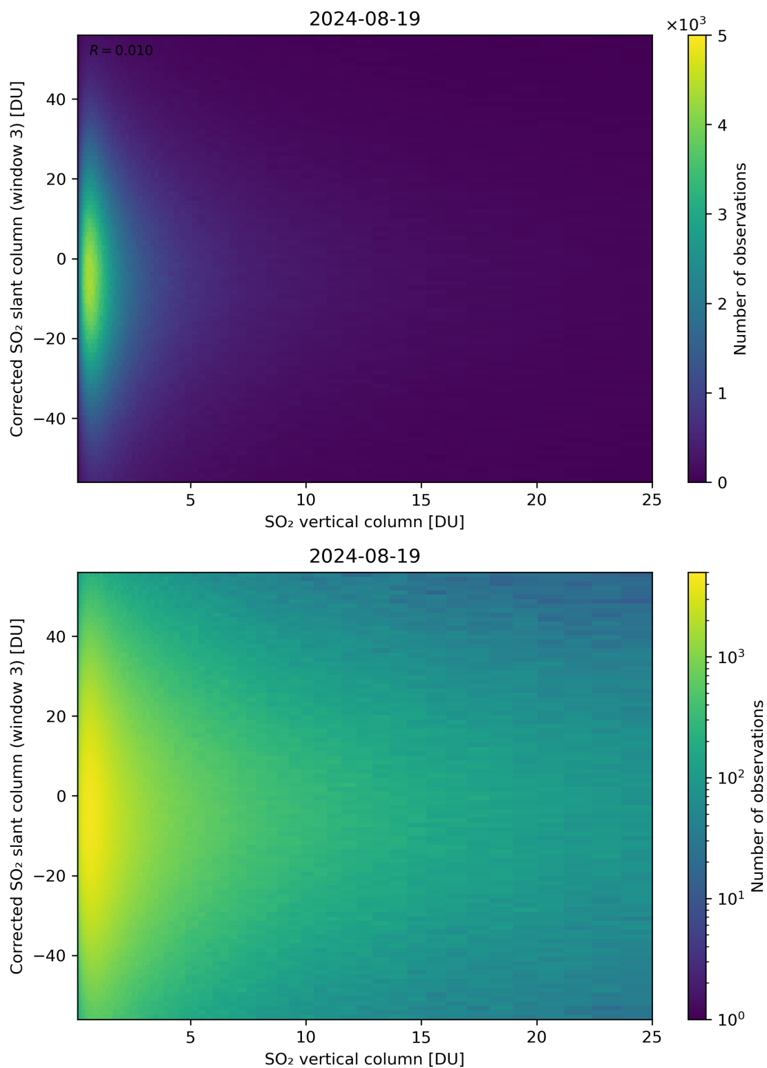
Figure 299: Scatter density plot of “SO 2 vertical column” against “Corrected SO 2 slant column (window 3)” for 2024-08-18 to 2024-08-20.
