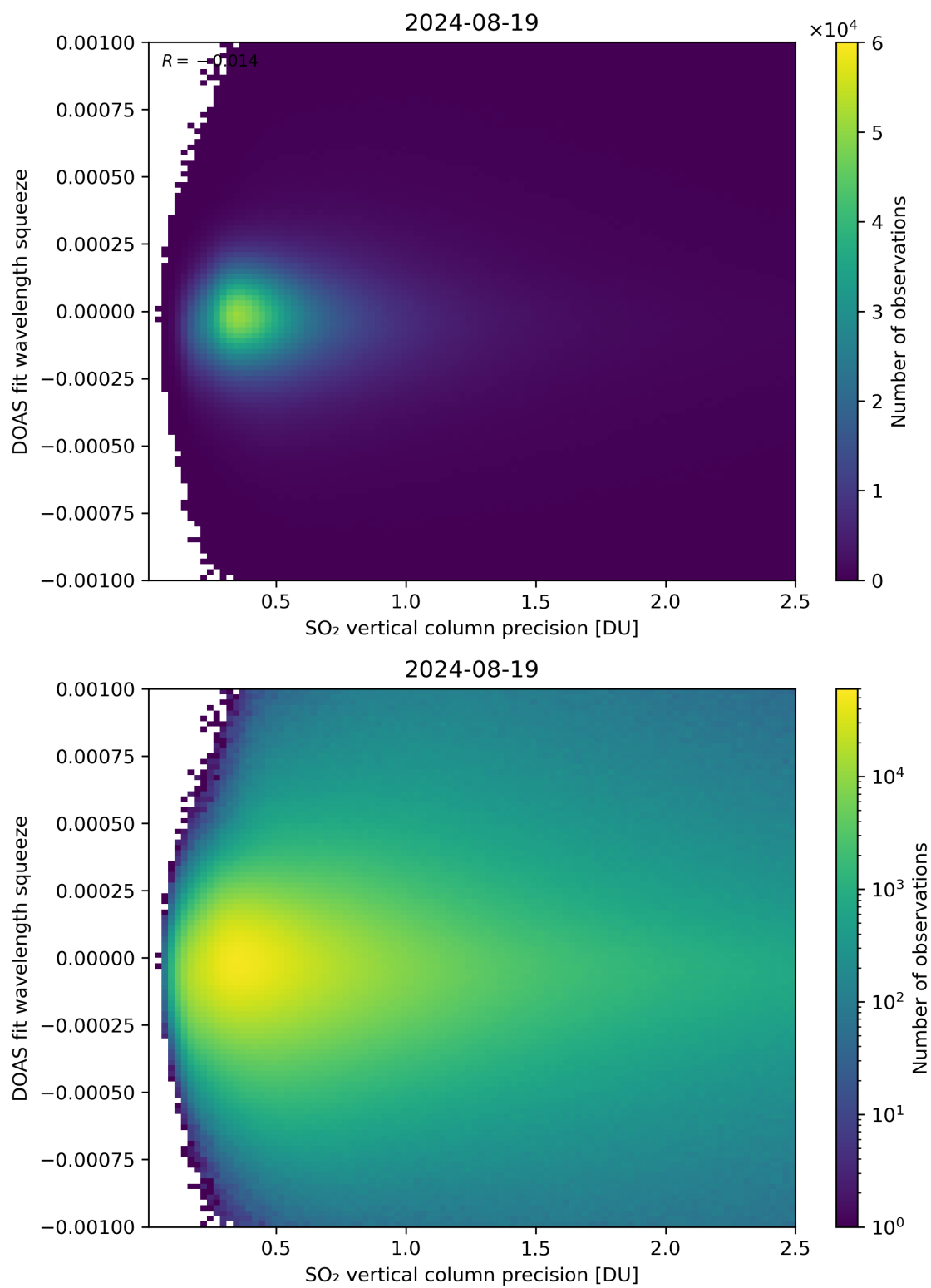
Figure 283: Scatter density plot of “SO 2 vertical column precision” against “DOAS fit wavelength squeeze” for 2024-08-18 to 2024-08-20.
