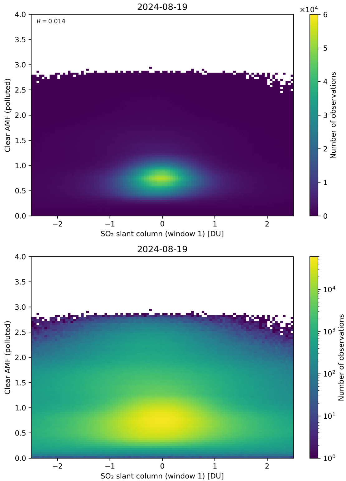
Figure 232: Scatter density plot of “SO 2 slant column (window 1)” against “Clear AMF (polluted)” for 2024-08-18 to 2024-08-20.
