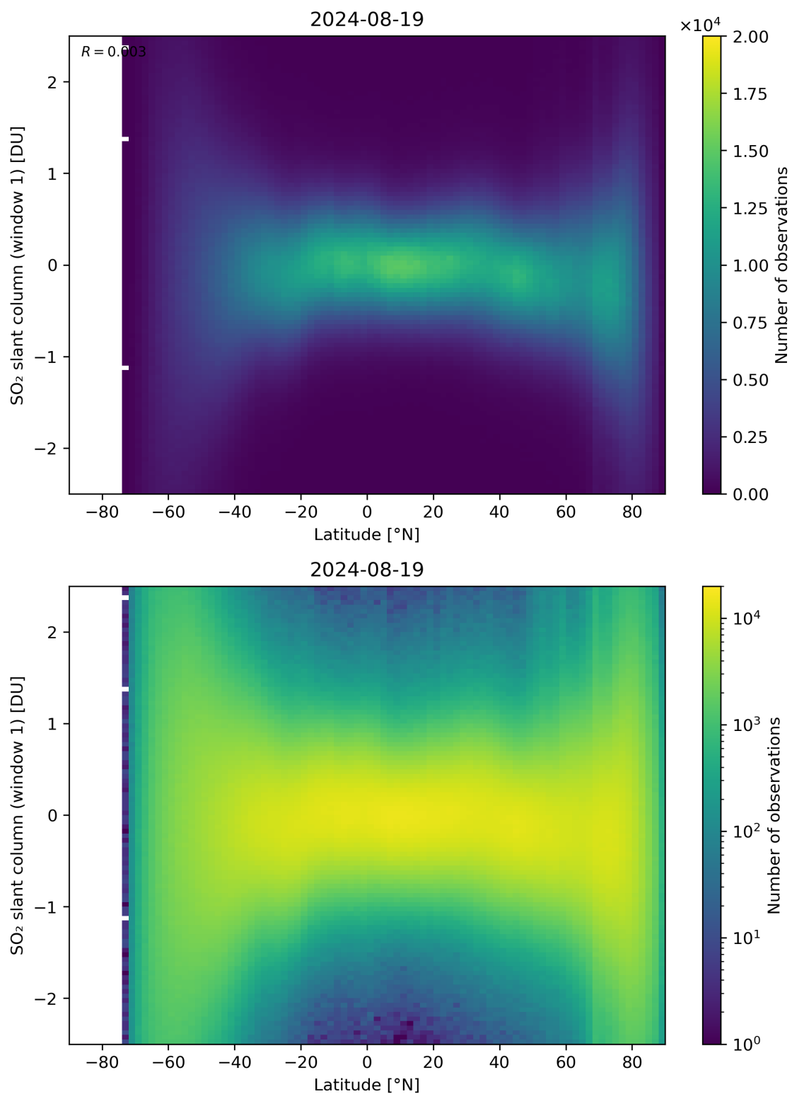
Figure 149: Scatter density plot of “Latitude” against “SO 2 slant column (window 1)” for 2024-08-18 to 2024-08-20.
