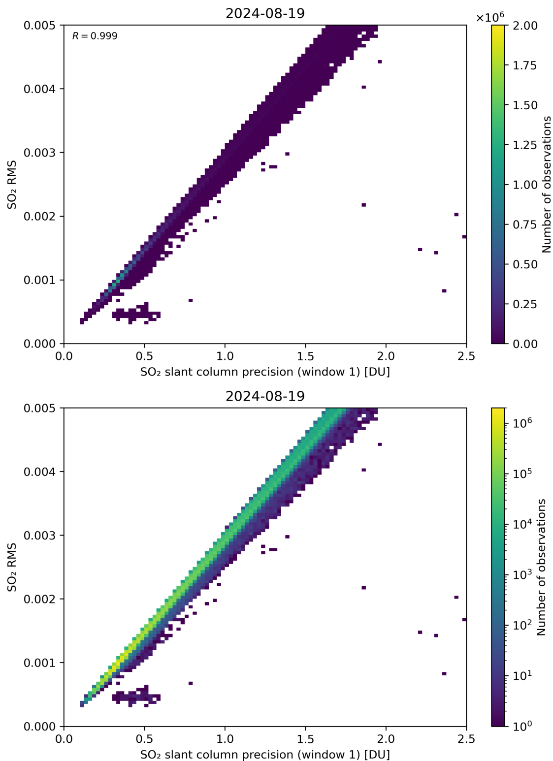
Figure 223: Scatter density plot of “SO 2 slant column precision (window 1)” against “SO 2 RMS” for 2024-08-18 to 2024-08-20.
