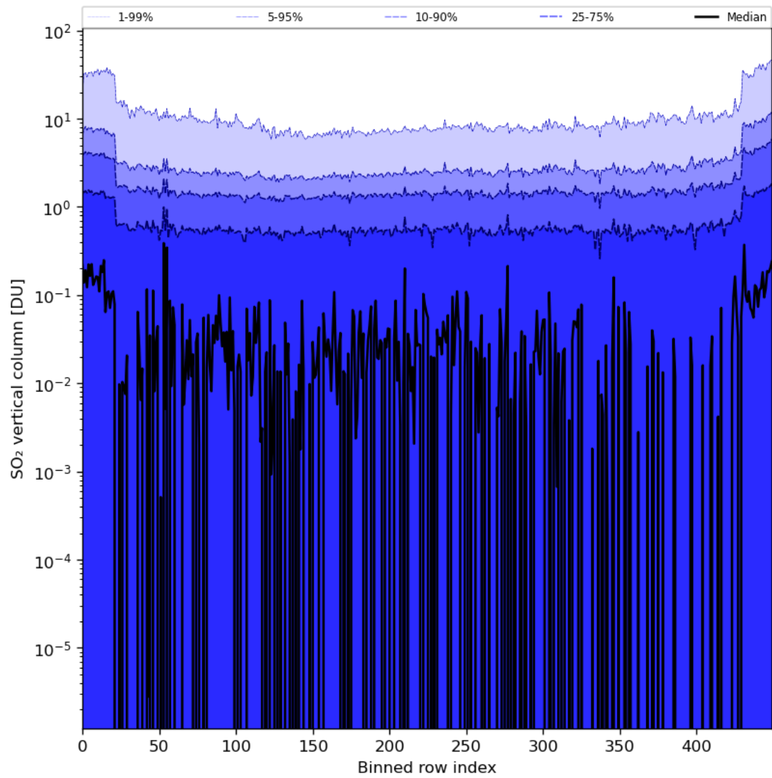
Figure 76: Along track statistics of “SO 2 vertical column” for 2024-08-18 to 2024-08-20
