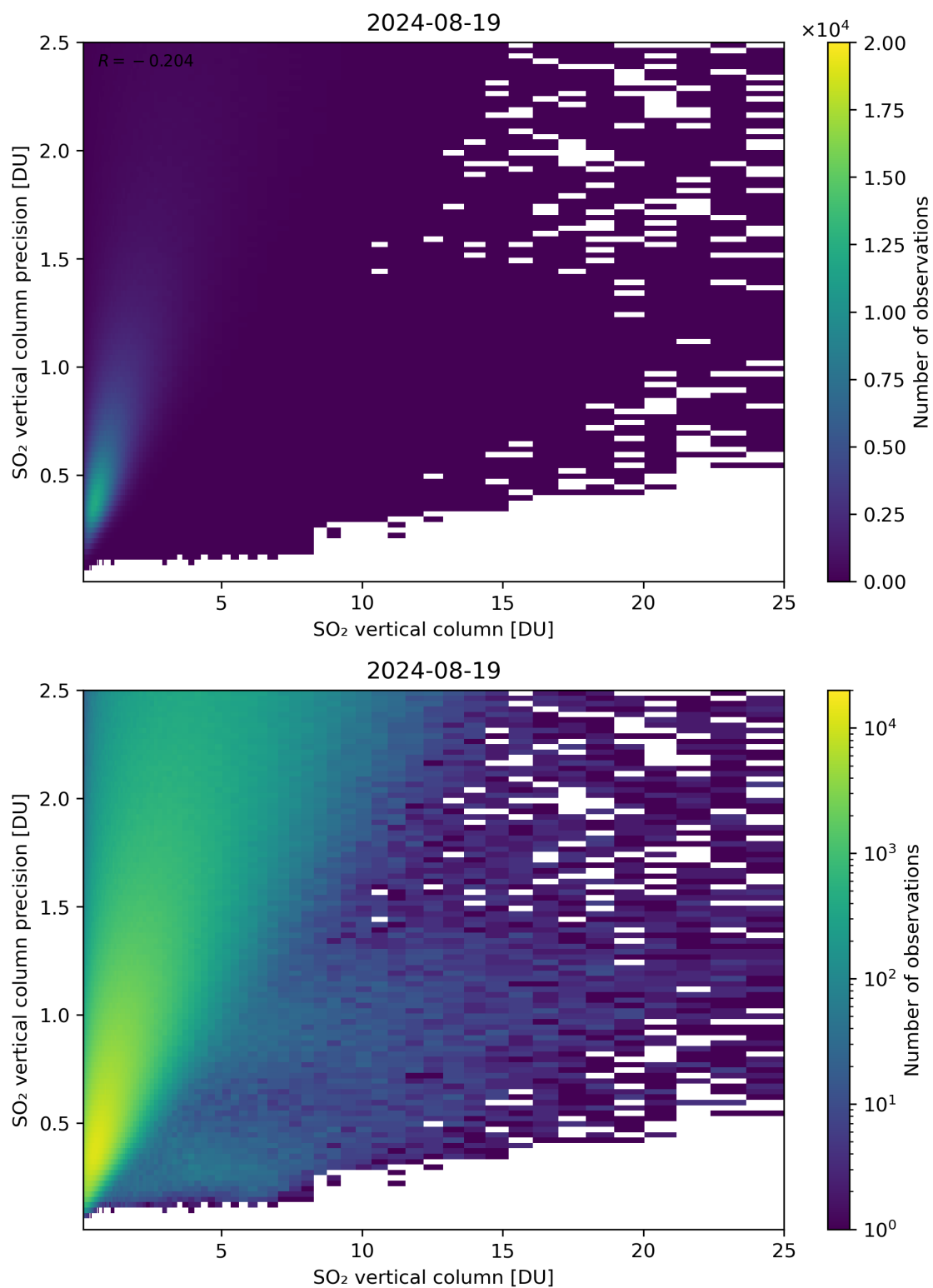
Figure 307: Scatter density plot of “SO 2 vertical column” against “SO 2 vertical column precision” for 2024-08-18 to 2024-08-20.
