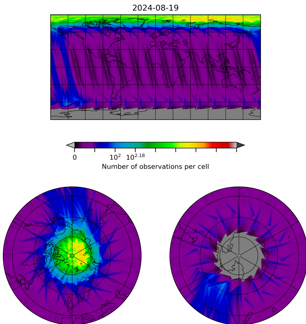
Figure 28: Map of the number of observations for 2024-08-18 to 2024-08-20
