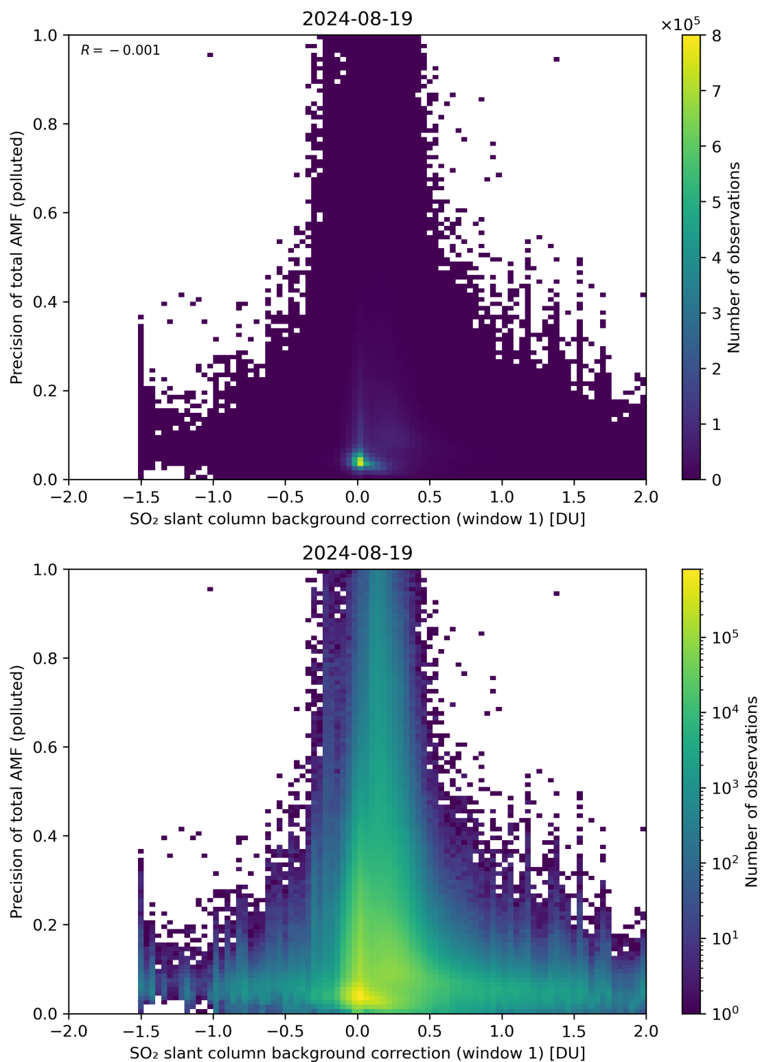
Figure 110: Scatter density plot of “SO 2 slant column background correction (window 1)” against “Precision of total AMF (polluted)” for 2024-08-18 to 2024-08-20.
