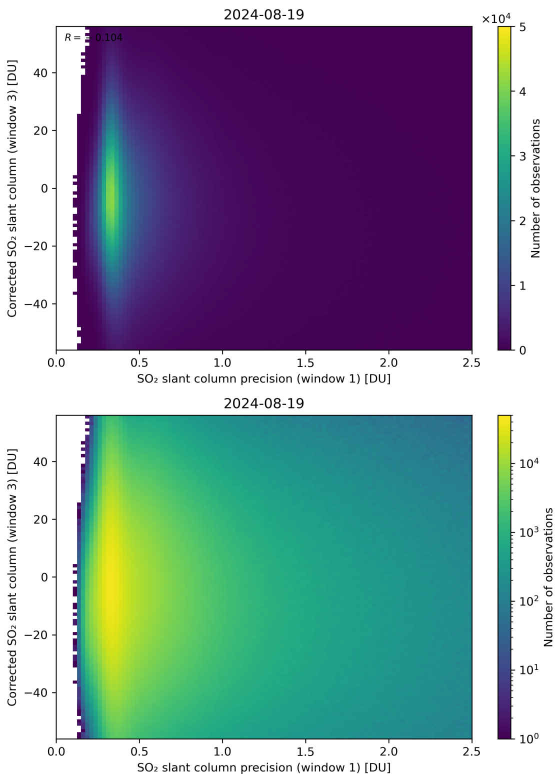
Figure 226: Scatter density plot of “SO 2 slant column precision (window 1)” against “Corrected SO 2 slant column (window 3)” for 2024-08-18 to 2024-08-20.
