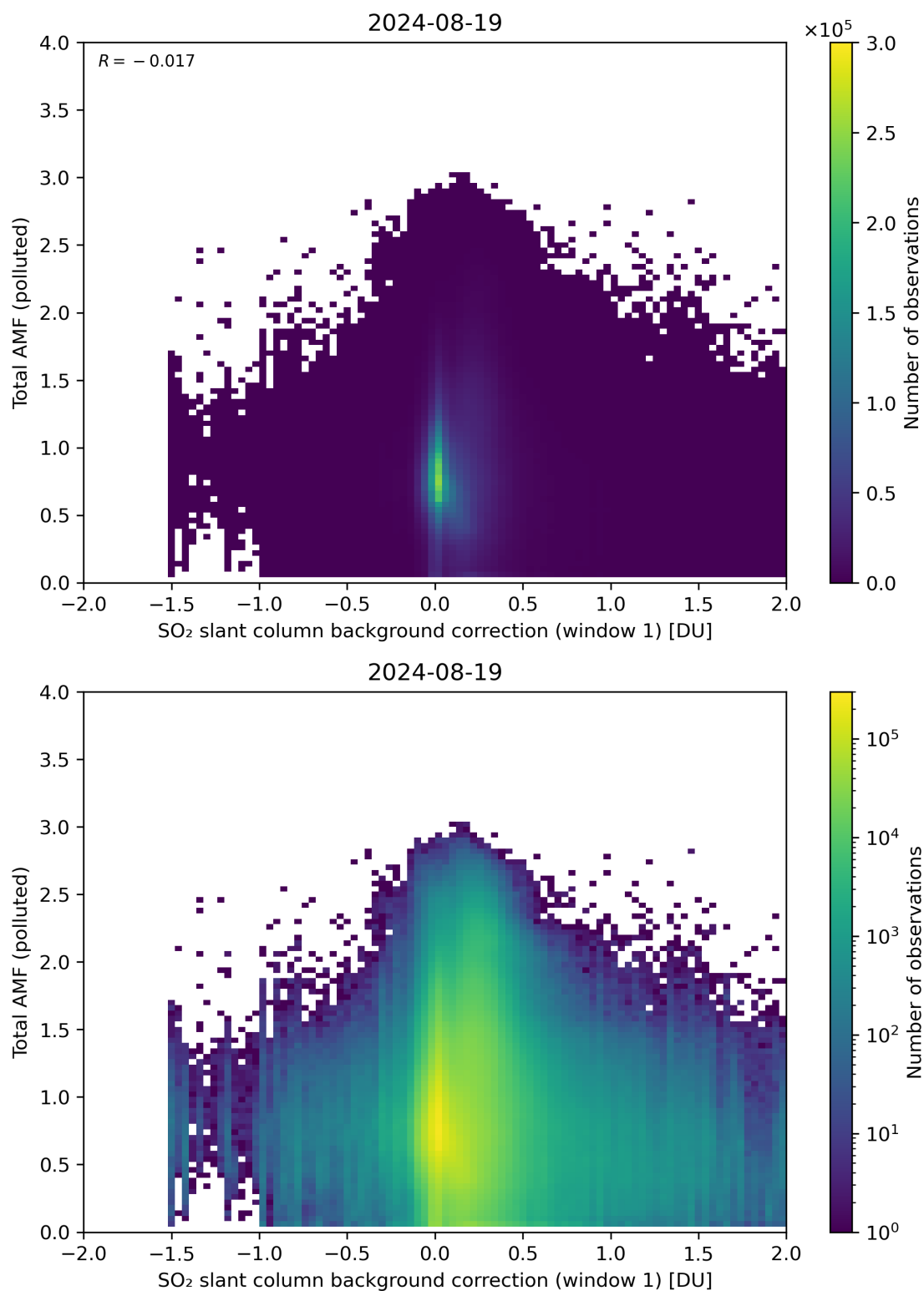
Figure 109: Scatter density plot of “SO 2 slant column background correction (window 1)” against “Total AMF (polluted)” for 2024-08-18 to 2024-08-20.
