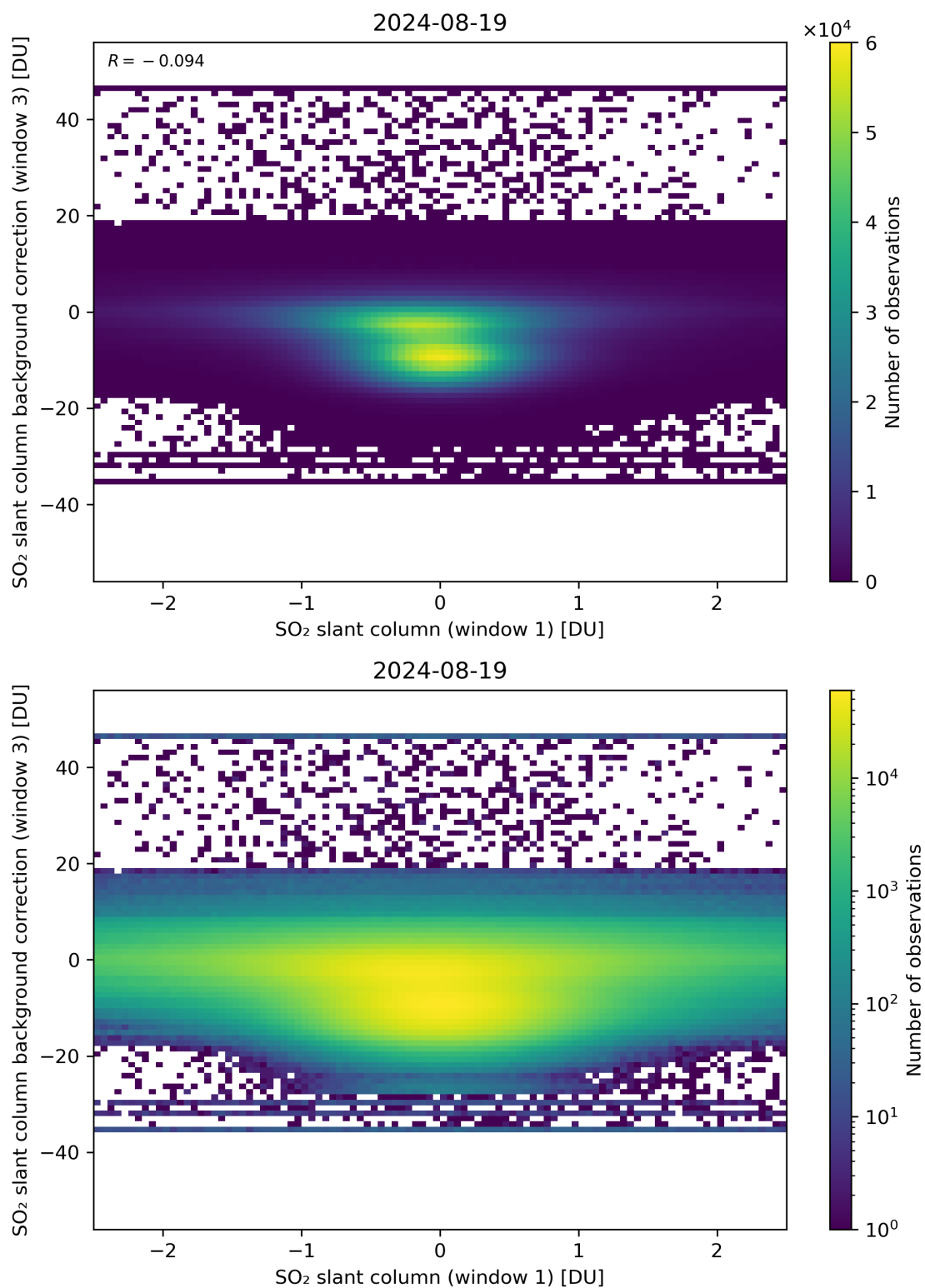
Figure 214: Scatter density plot of “SO 2 slant column (window 1)” against “SO 2 slant column background correction (window 3)” for 2024-08-18 to 2024-08-20.
