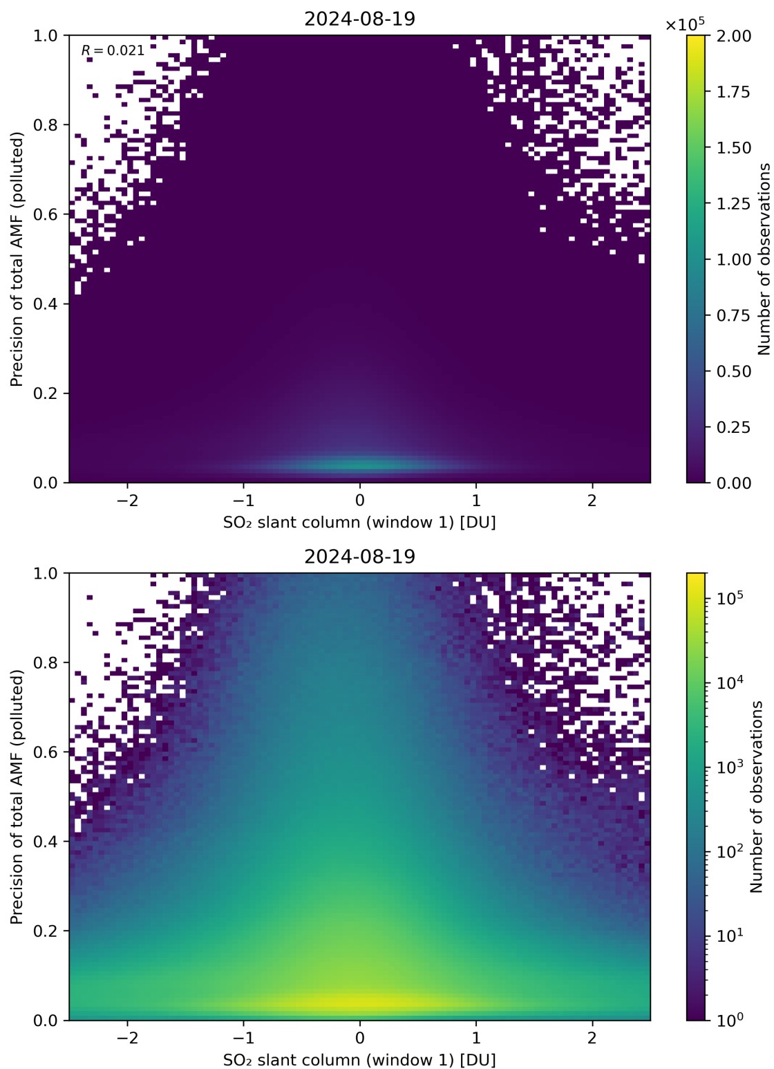
Figure 240: Scatter density plot of “SO 2 slant column (window 1)” against “Precision of total AMF (polluted)” for 2024-08-18 to 2024-08-20.
