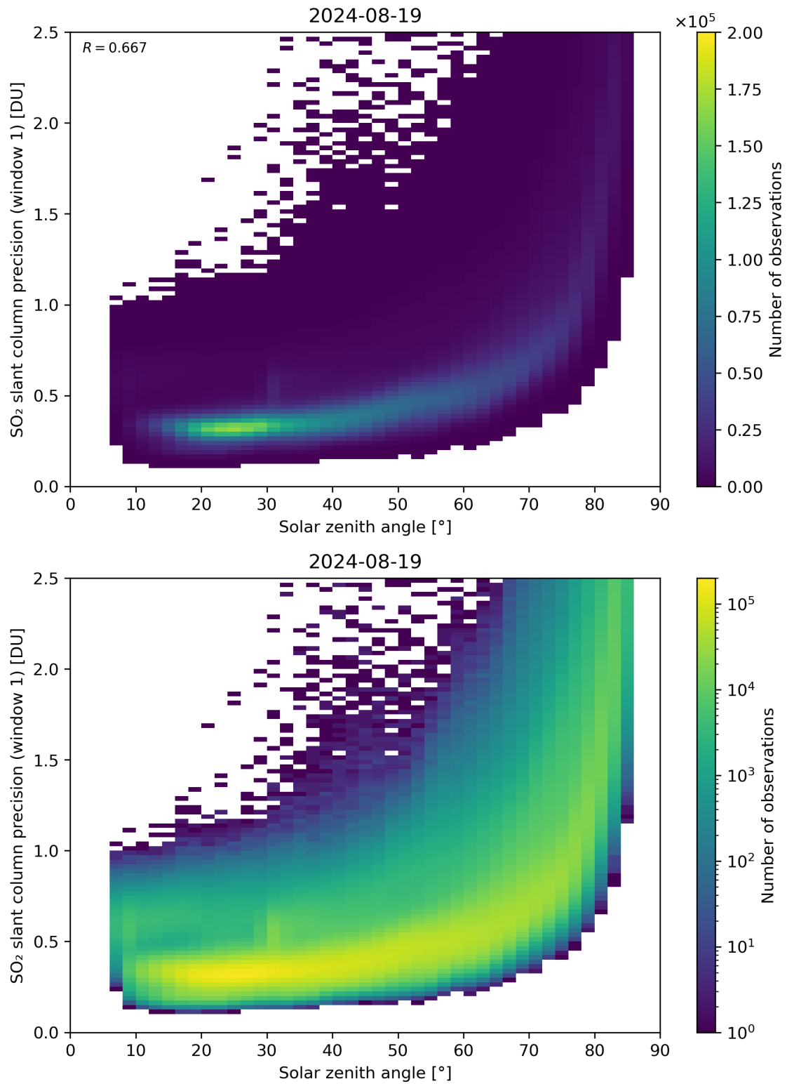
Figure 170: Scatter density plot of “Solar zenith angle” against “SO 2 slant column precision (window 1)” for 2024-08-18 to 2024-08-20.
