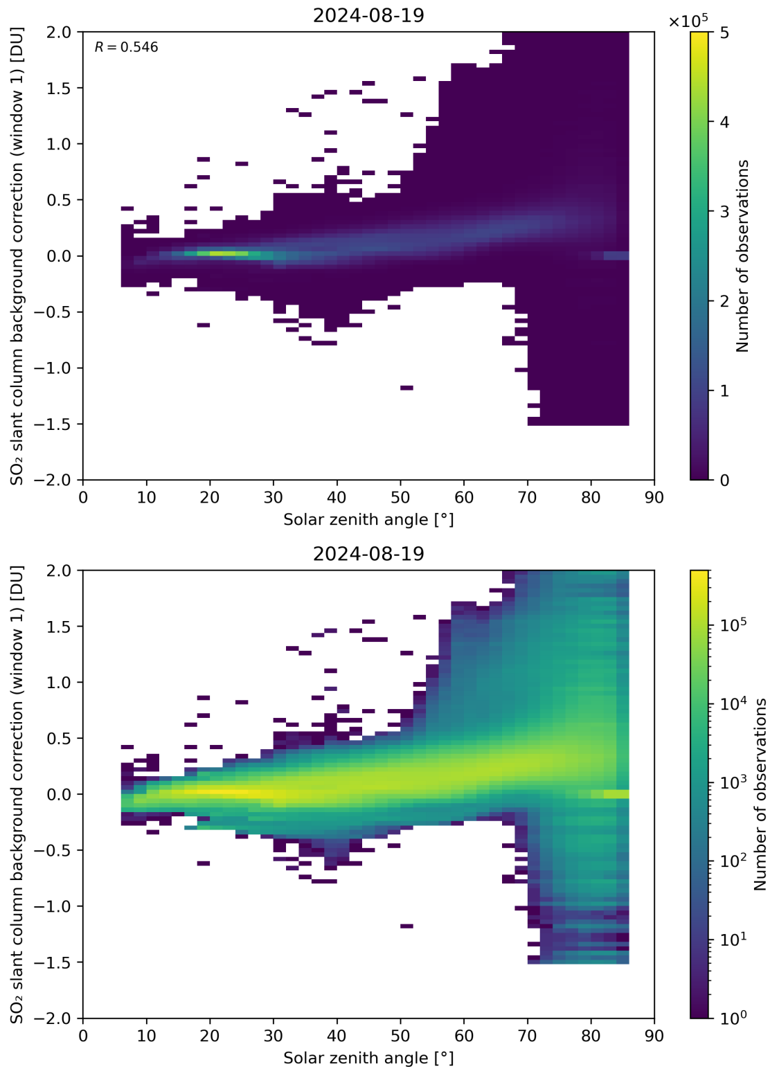
Figure 158: Scatter density plot of “Solar zenith angle” against “SO 2 slant column background correction (window 1)” for 2024-08-18 to 2024-08-20.
