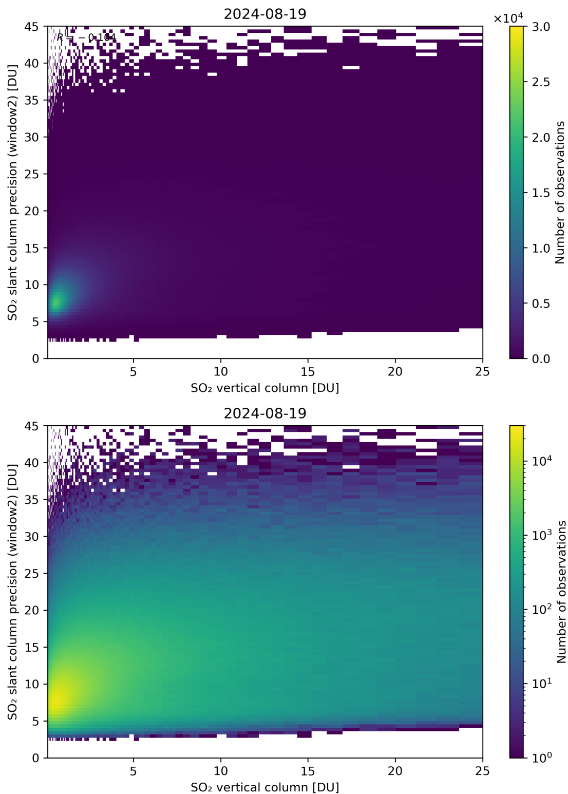
Figure 302: Scatter density plot of “SO 2 vertical column” against “SO 2 slant column precision (window2)” for 2024-08-18 to 2024-08-20.
