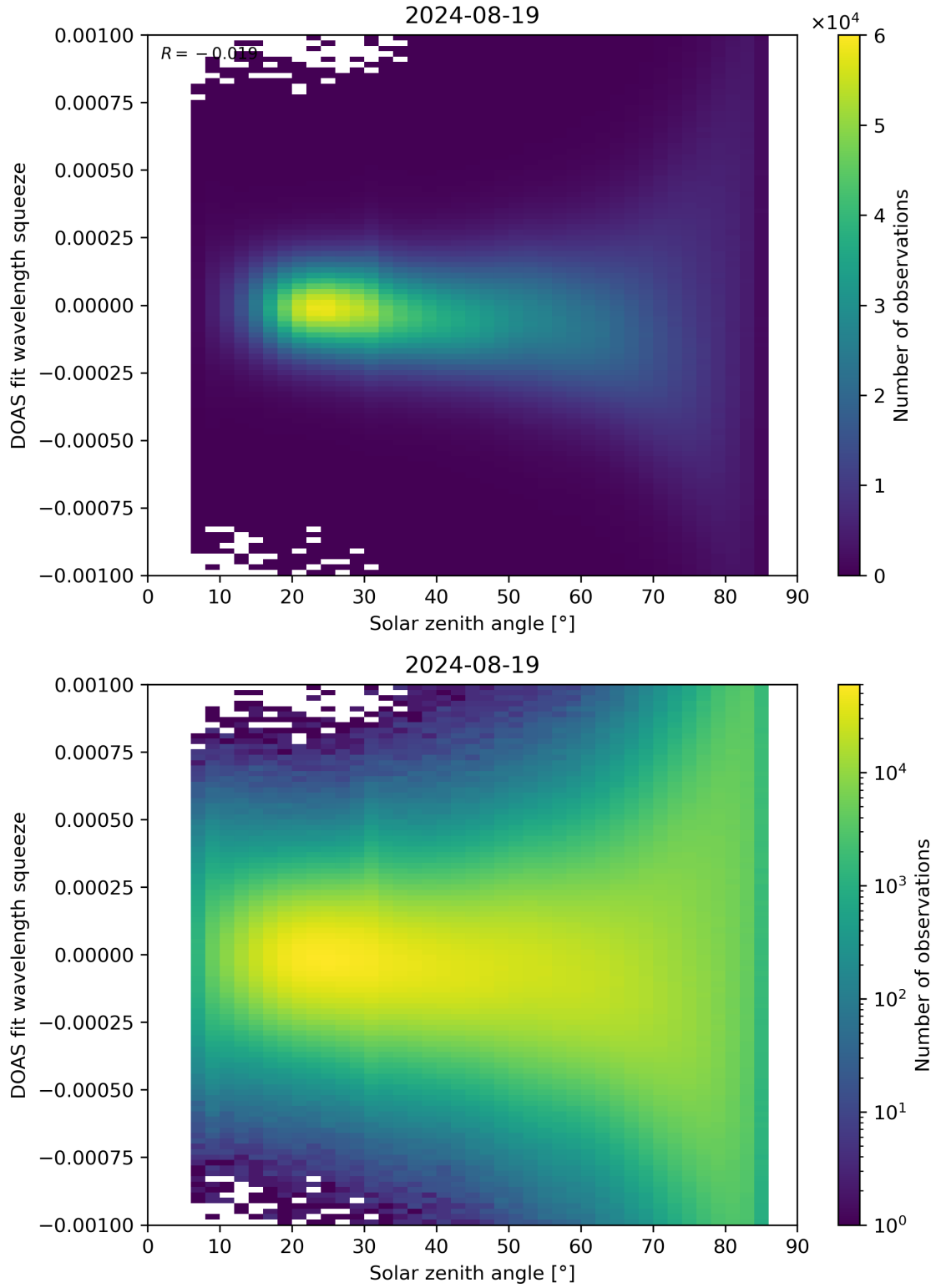
Figure 162: Scatter density plot of “Solar zenith angle” against “DOAS fit wavelength squeeze” for 2024-08-18 to 2024-08-20.
