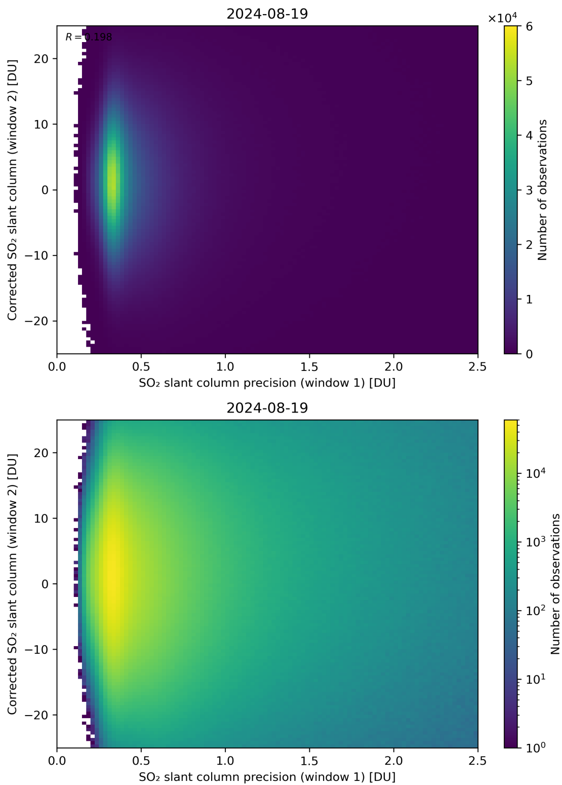
Figure 225: Scatter density plot of “SO 2 slant column precision (window 1)” against “Corrected SO 2 slant column (window 2)” for 2024-08-18 to 2024-08-20.
