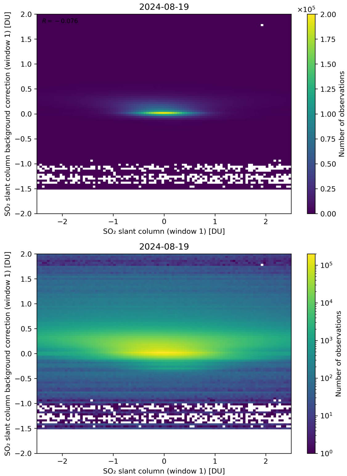
Figure 212: Scatter density plot of “SO 2 slant column (window 1)” against “SO 2 slant column background correction (window 1)” for 2024-08-18 to 2024-08-20.
