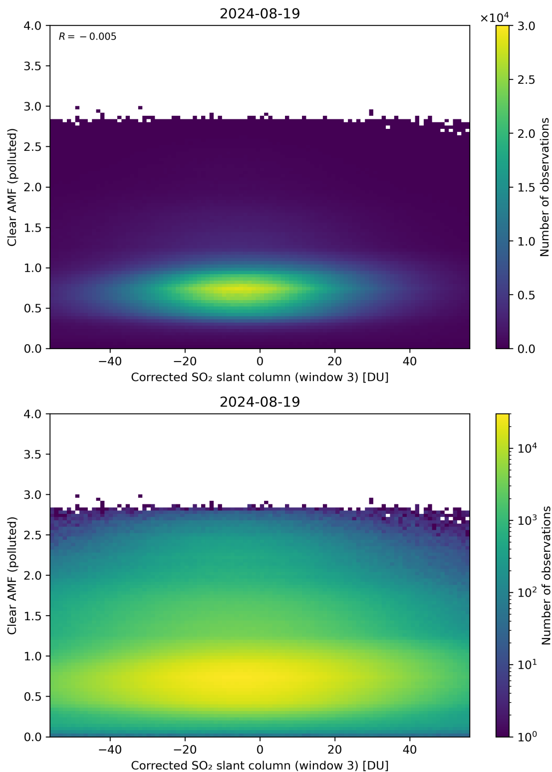
Figure 209: Scatter density plot of “Corrected SO 2 slant column (window 3)” against “Clear AMF (polluted)” for 2024-08-18 to 2024-08-20.
