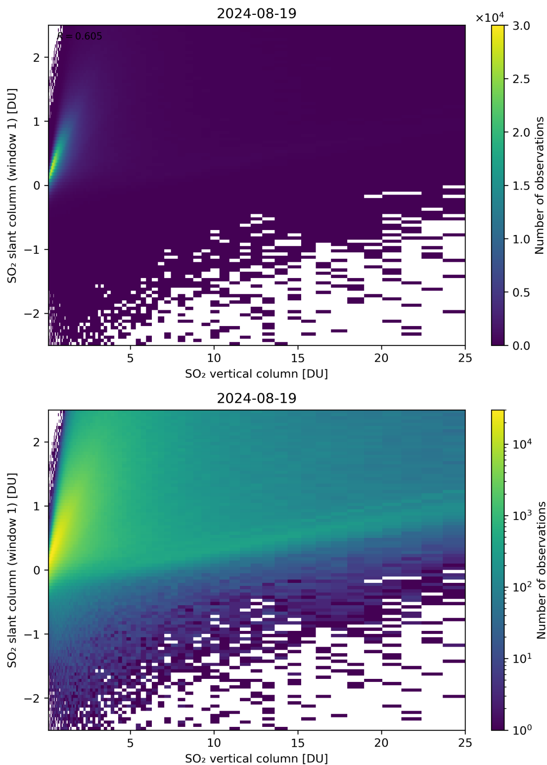
Figure 300: Scatter density plot of “SO 2 vertical column” against “SO 2 slant column (window 1)” for 2024-08-18 to 2024-08-20.
