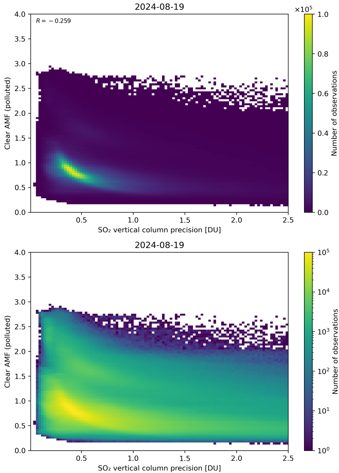
Figure 285: Scatter density plot of “SO 2 vertical column precision” against “Clear AMF (polluted)” for 2024-08-18 to 2024-08-20.
