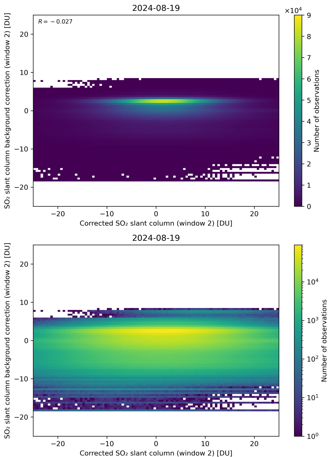
Figure 194: Scatter density plot of “Corrected SO 2 slant column (window 2)” against “SO 2 slant column background correction (window 2)” for 2024-08-18 to 2024-08-20.
