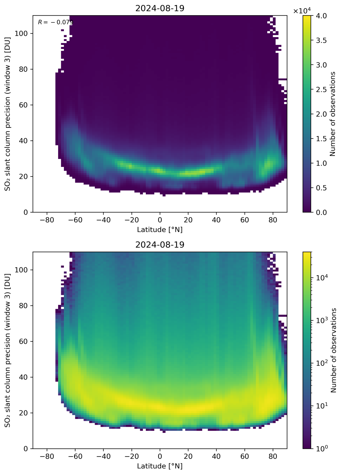
Figure 153: Scatter density plot of “Latitude” against “SO 2 slant column precision (window 3)” for 2024-08-18 to 2024-08-20.
