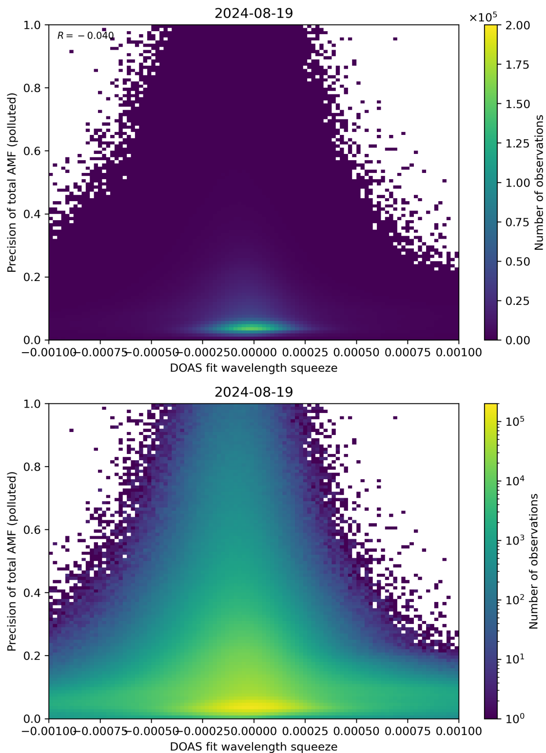
Figure 135: Scatter density plot of “DOAS fit wavelength squeeze” against “Precision of total AMF (polluted)” for 2024-08-18 to 2024-08-20.
