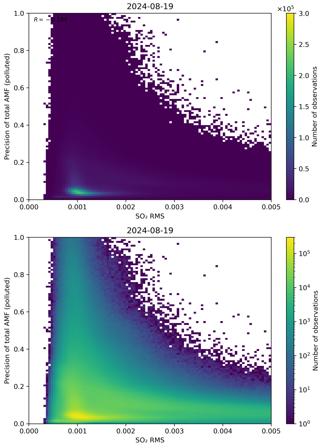
Figure 138: Scatter density plot of “SO 2 RMS” against “Precision of total AMF (polluted)” for 2024-08-18 to 2024-08-20.
