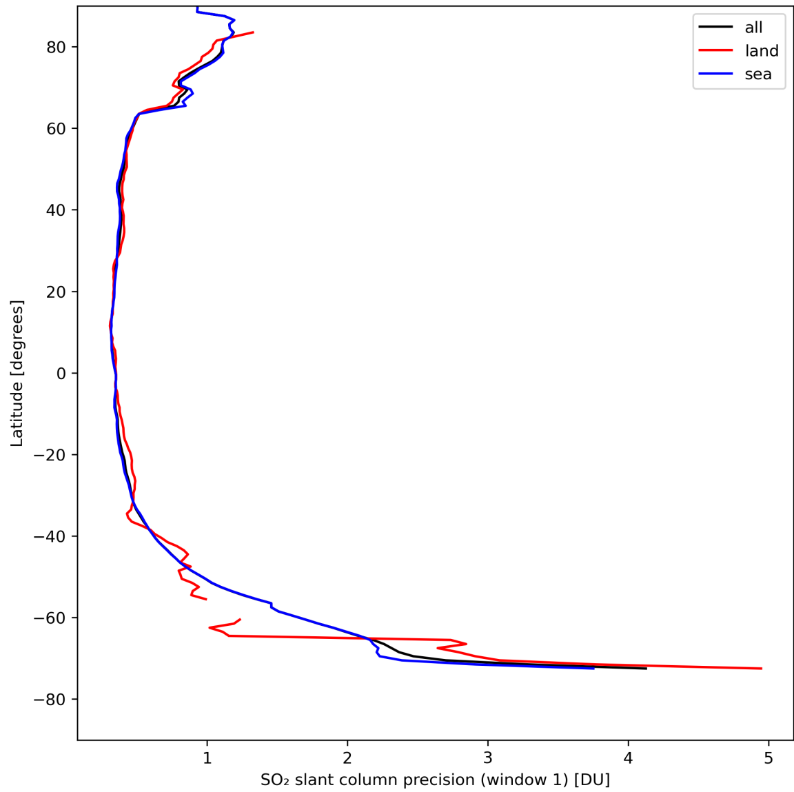
Figure 34: Zonal average of “SO 2 slant column precision (window 1)” for 2024-08-18 to 2024-08-20.
