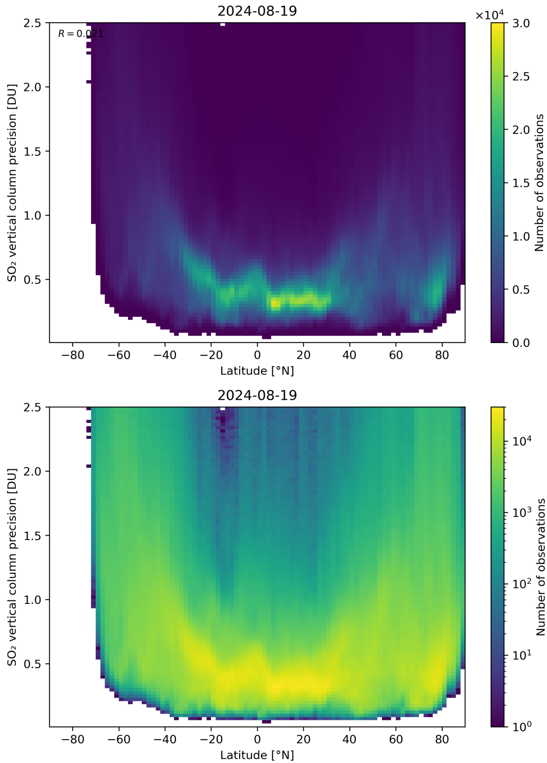
Figure 157: Scatter density plot of “Latitude” against “SO 2 vertical column precision” for 2024-08-18 to 2024-08-20.
