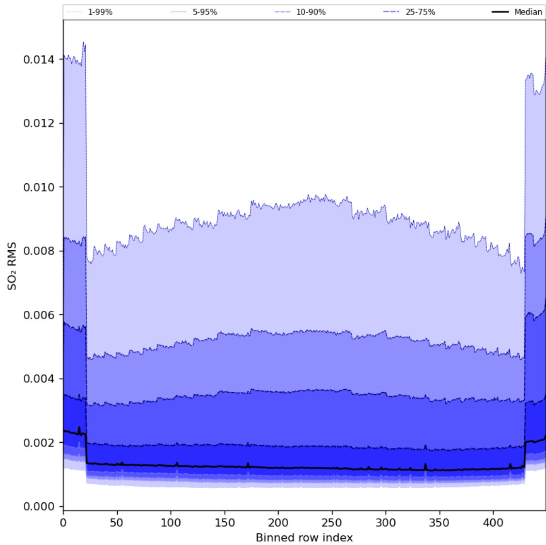
Figure 93: Along track statistics of “SO 2 RMS” for 2024-08-18 to 2024-08-20
