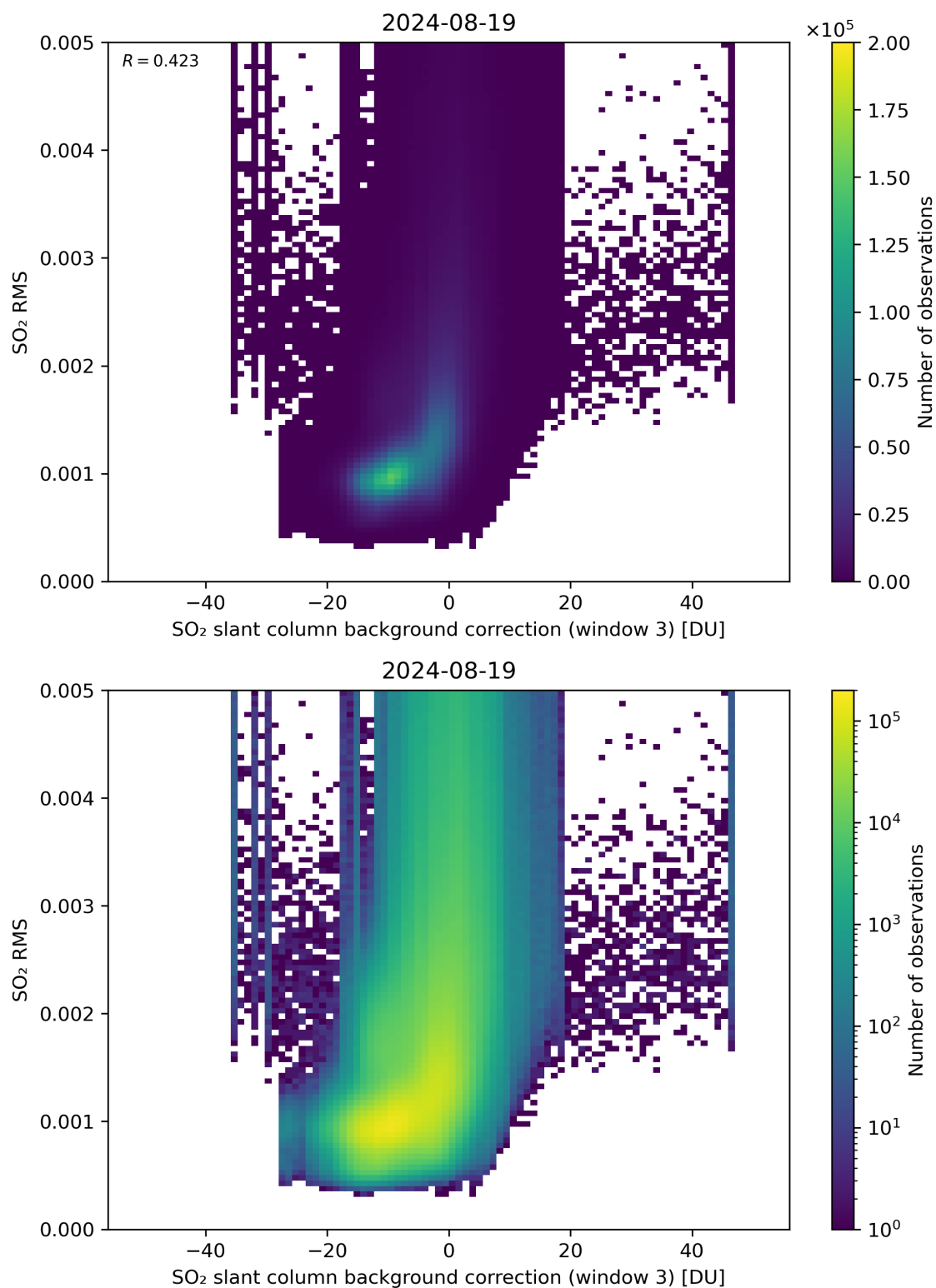
Figure 123: Scatter density plot of “SO 2 slant column background correction (window 3)” against “SO 2 RMS” for 2024-08-18 to 2024-08-20.
