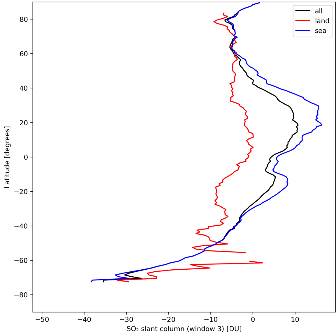
Figure 41: Zonal average of “SO 2 slant column (window 3)” for 2024-08-18 to 2024-08-20.
