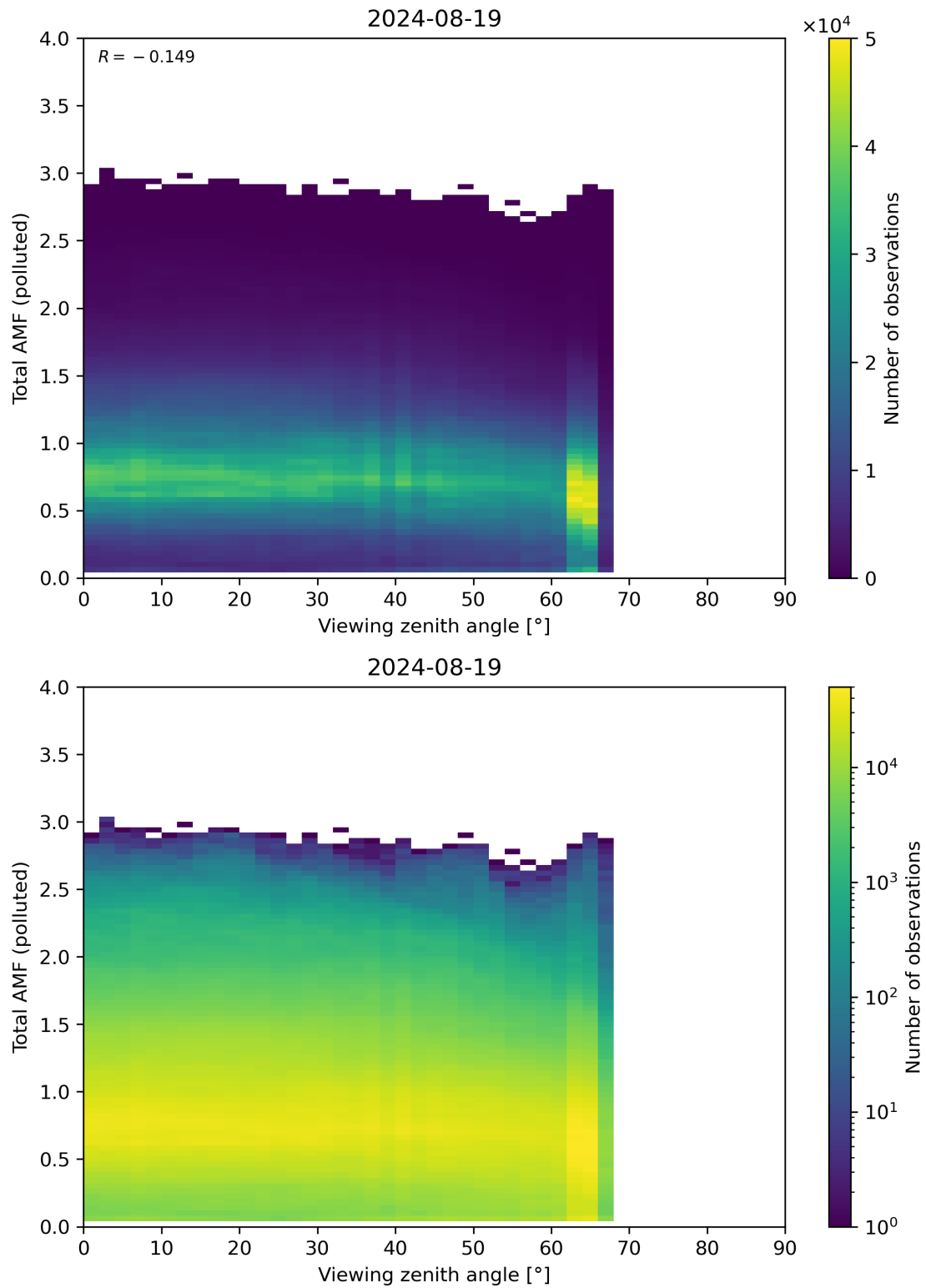
Figure 325: Scatter density plot of “Viewing zenith angle” against “Total AMF (polluted)” for 2024-08-18 to 2024-08-20.
