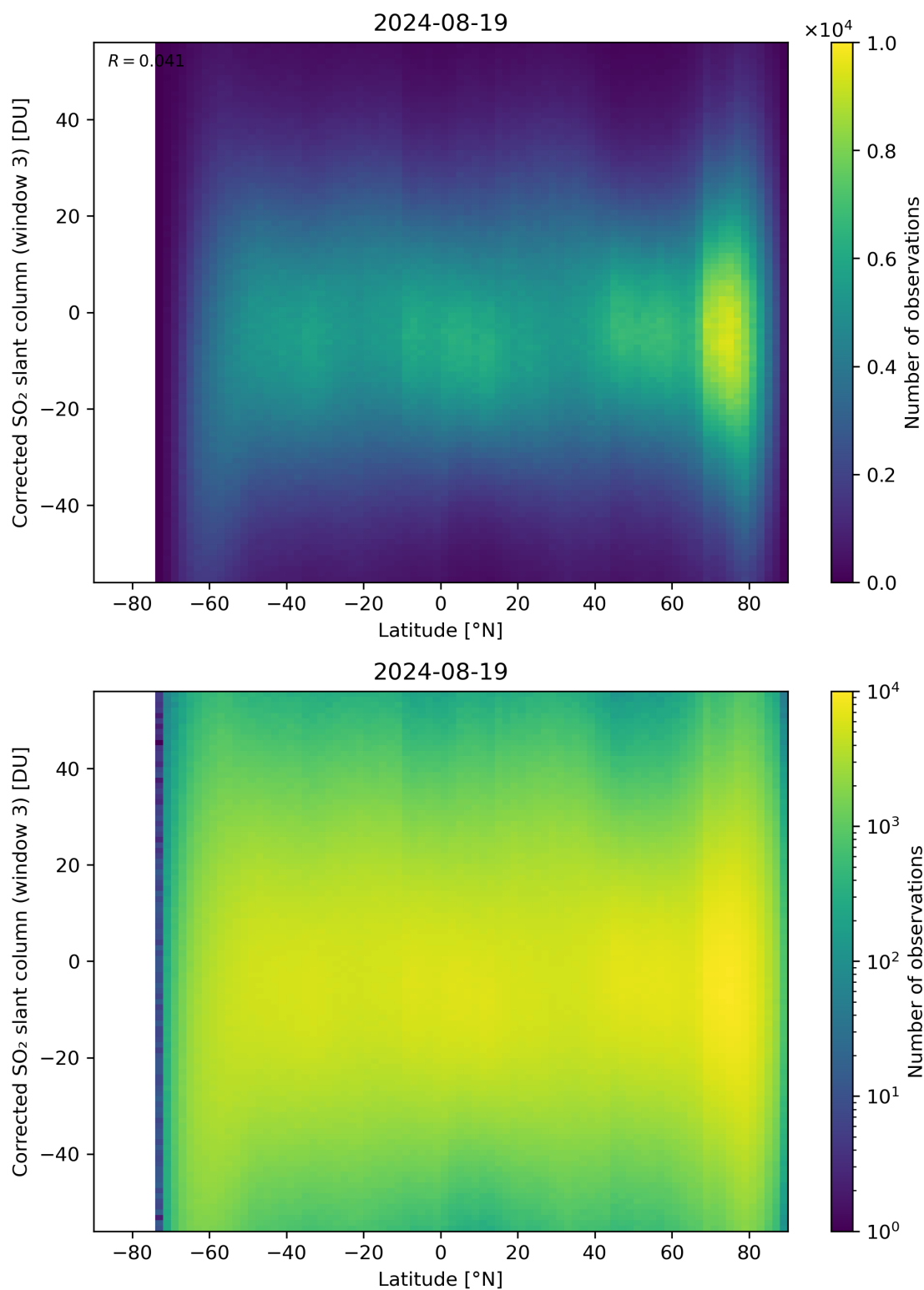
Figure 148: Scatter density plot of “Latitude” against “Corrected SO 2 slant column (window 3)” for 2024-08-18 to 2024-08-20.
