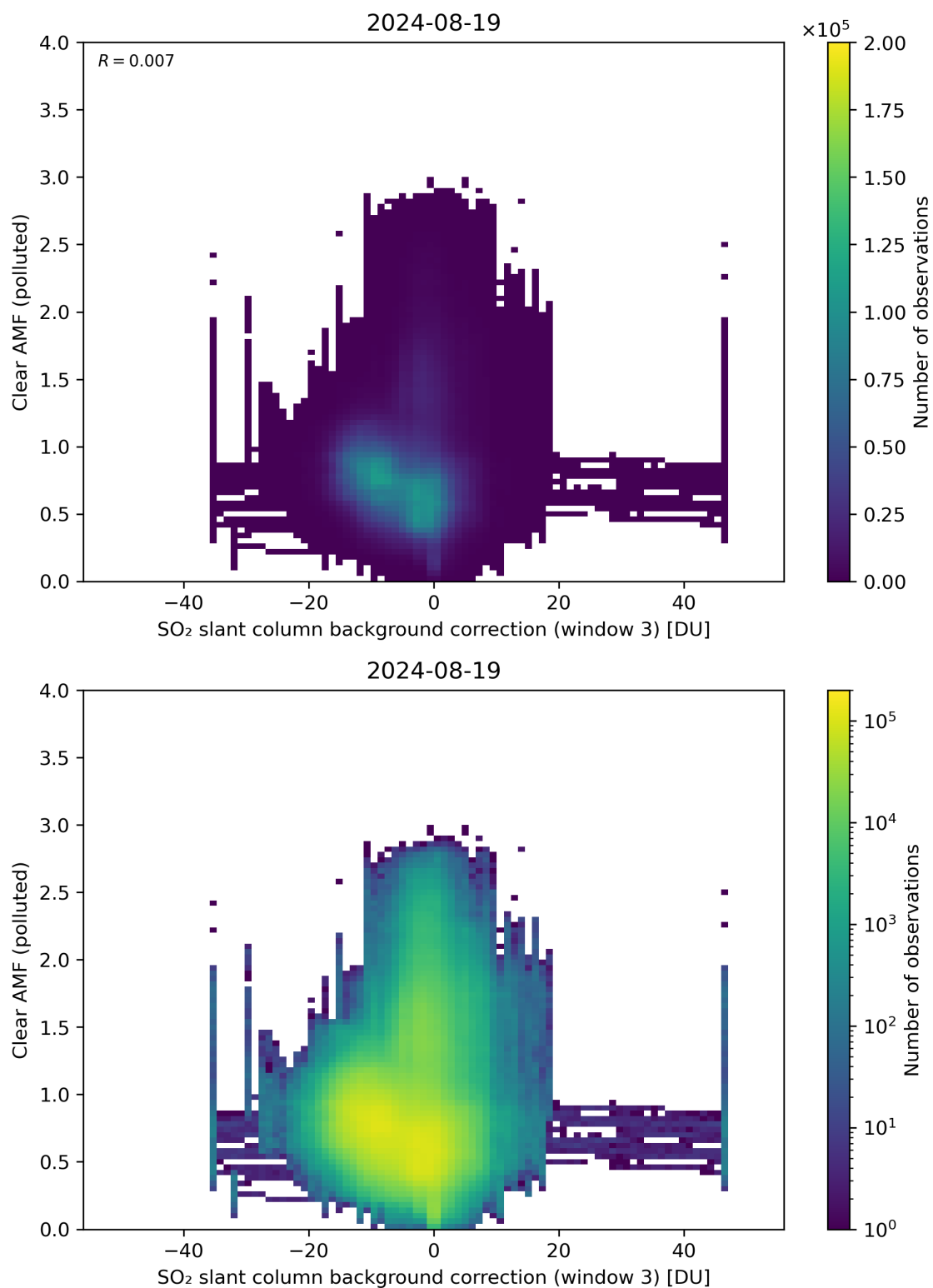
Figure 124: Scatter density plot of “SO 2 slant column background correction (window 3)” against “Clear AMF (polluted)” for 2024-08-18 to 2024-08-20.
