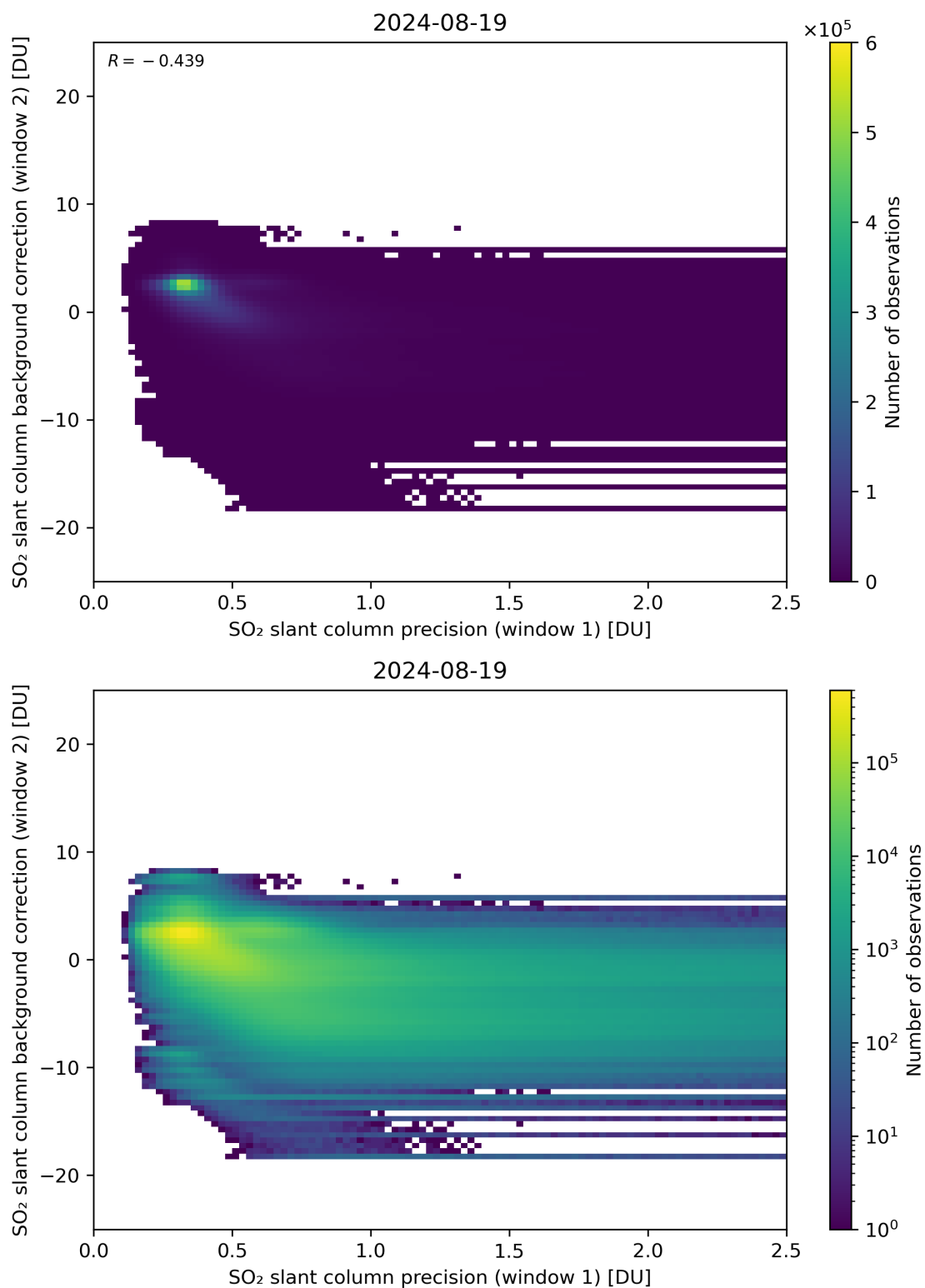
Figure 219: Scatter density plot of “SO 2 slant column precision (window 1)” against “SO 2 slant column background correction (window 2)” for 2024-08-18 to 2024-08-20.
