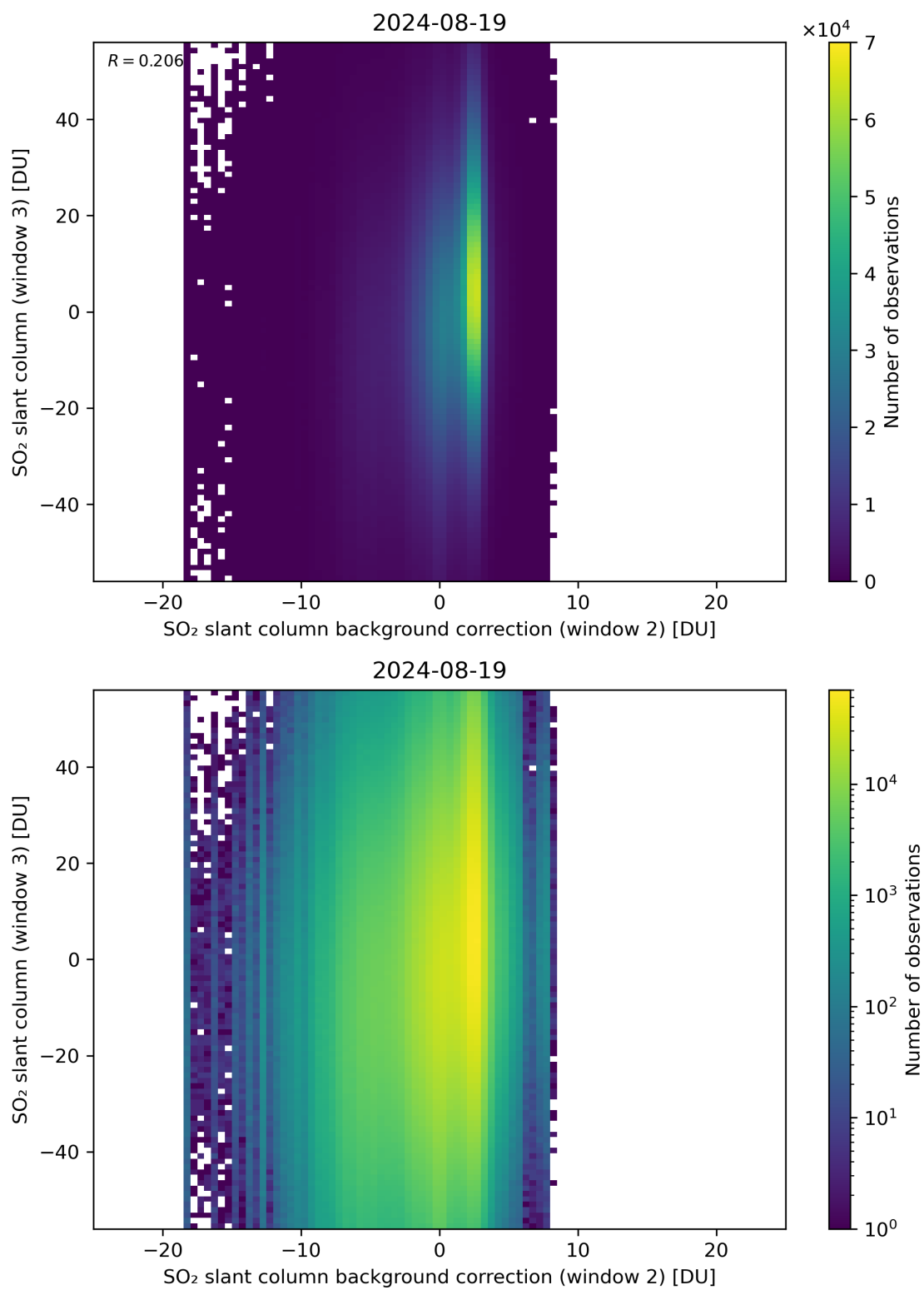
Figure 117: Scatter density plot of “SO 2 slant column background correction (window 2)” against “SO 2 slant column (window 3)” for 2024-08-18 to 2024-08-20.
