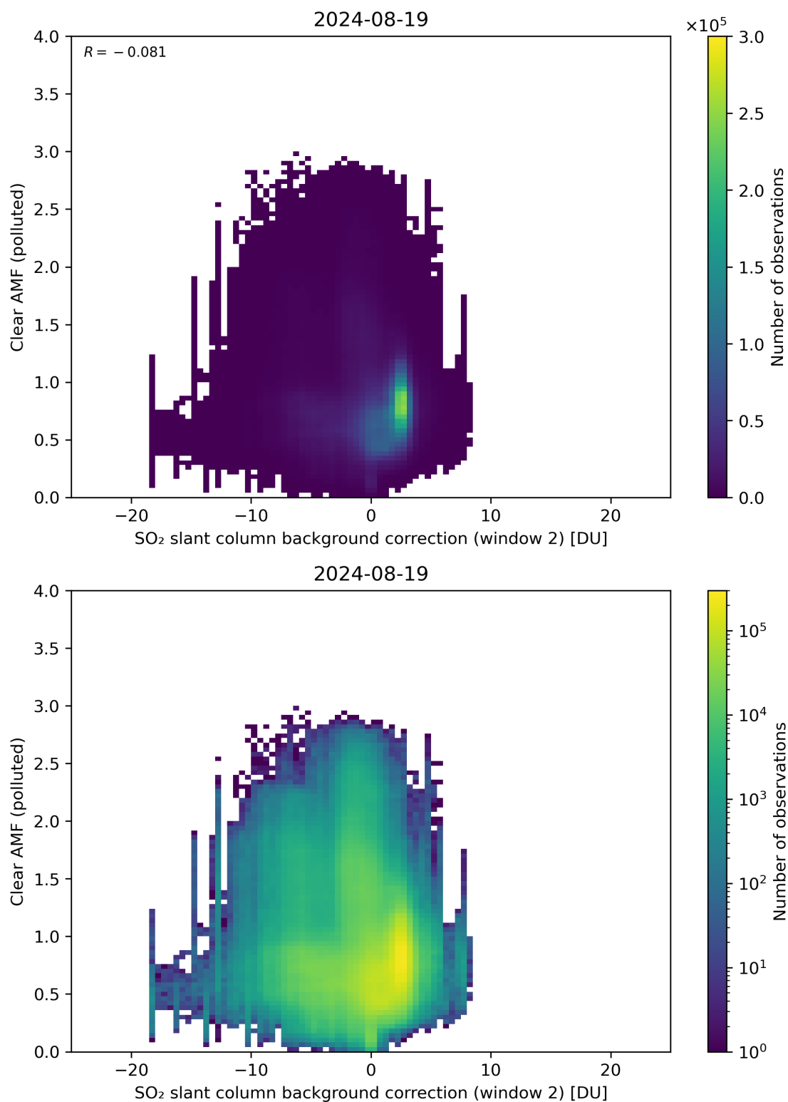
Figure 115: Scatter density plot of “SO 2 slant column background correction (window 2)” against “Clear AMF (polluted)” for 2024-08-18 to 2024-08-20.
