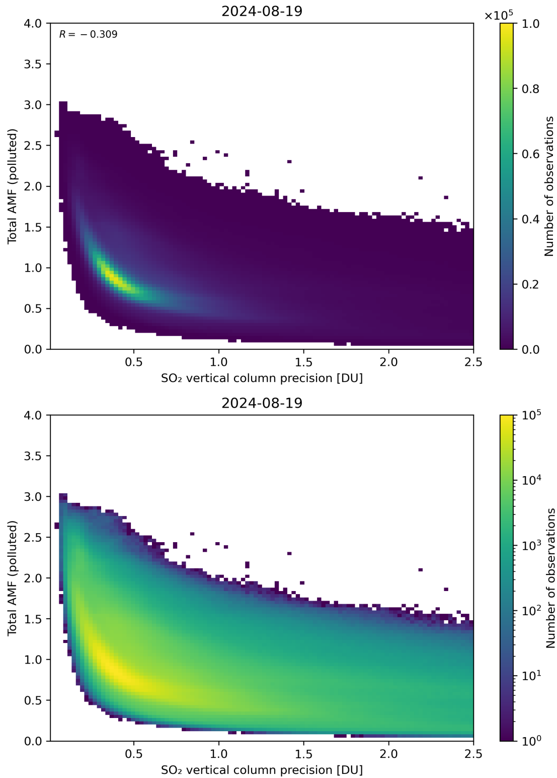
Figure 294: Scatter density plot of “SO 2 vertical column precision” against “Total AMF (polluted)” for 2024-08-18 to 2024-08-20.
