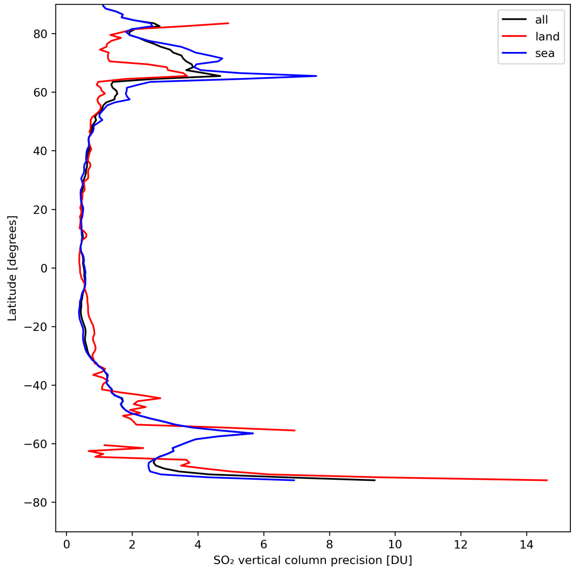
Figure 31: Zonal average of “SO 2 vertical column precision” for 2024-08-18 to 2024-08-20.
