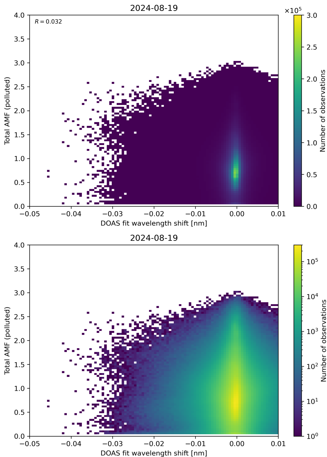
Figure 130: Scatter density plot of “DOAS fit wavelength shift” against “Total AMF (polluted)” for 2024-08-18 to 2024-08-20.
