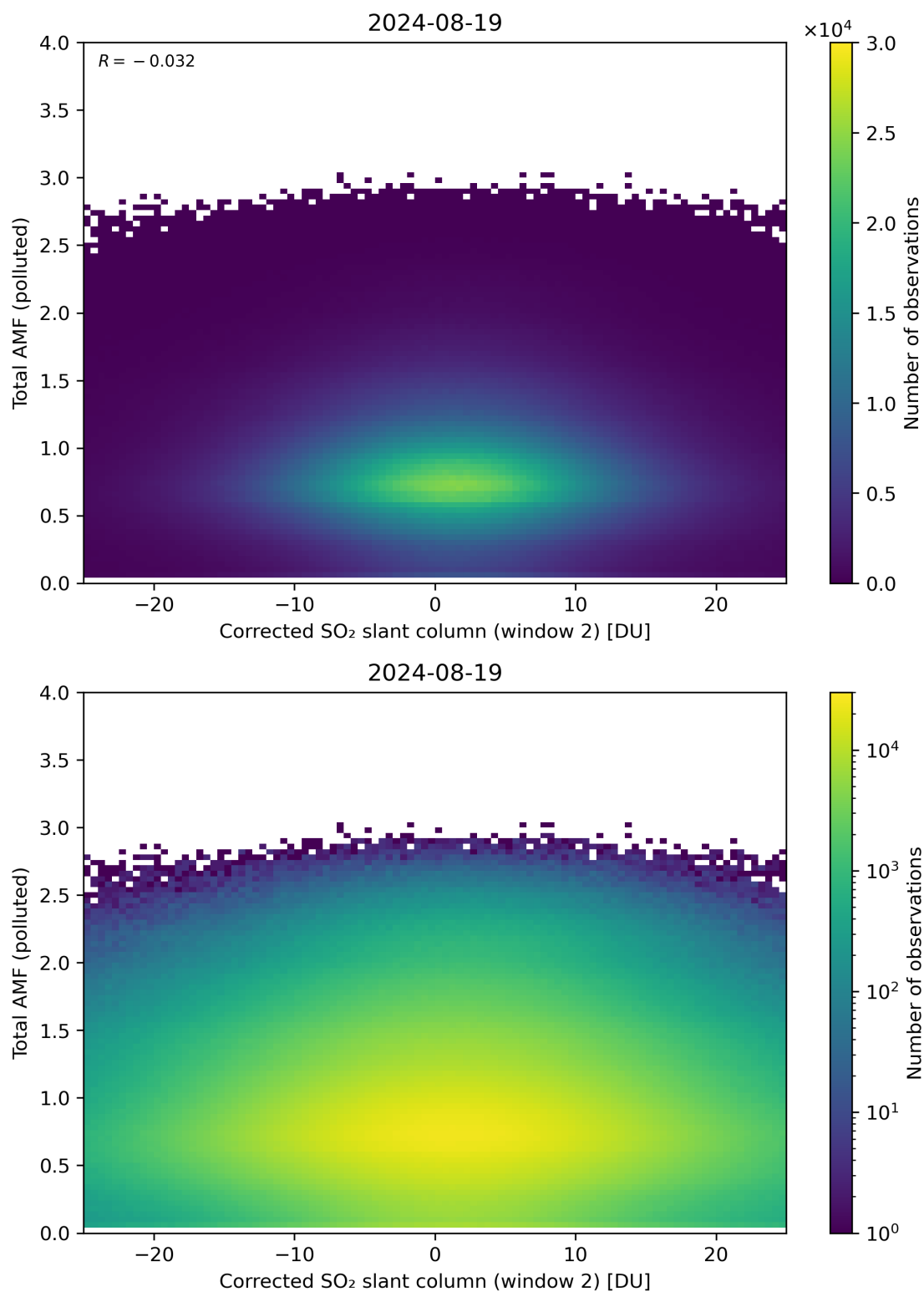
Figure 203: Scatter density plot of “Corrected SO 2 slant column (window 2)” against “Total AMF (polluted)” for 2024-08-18 to 2024-08-20.
