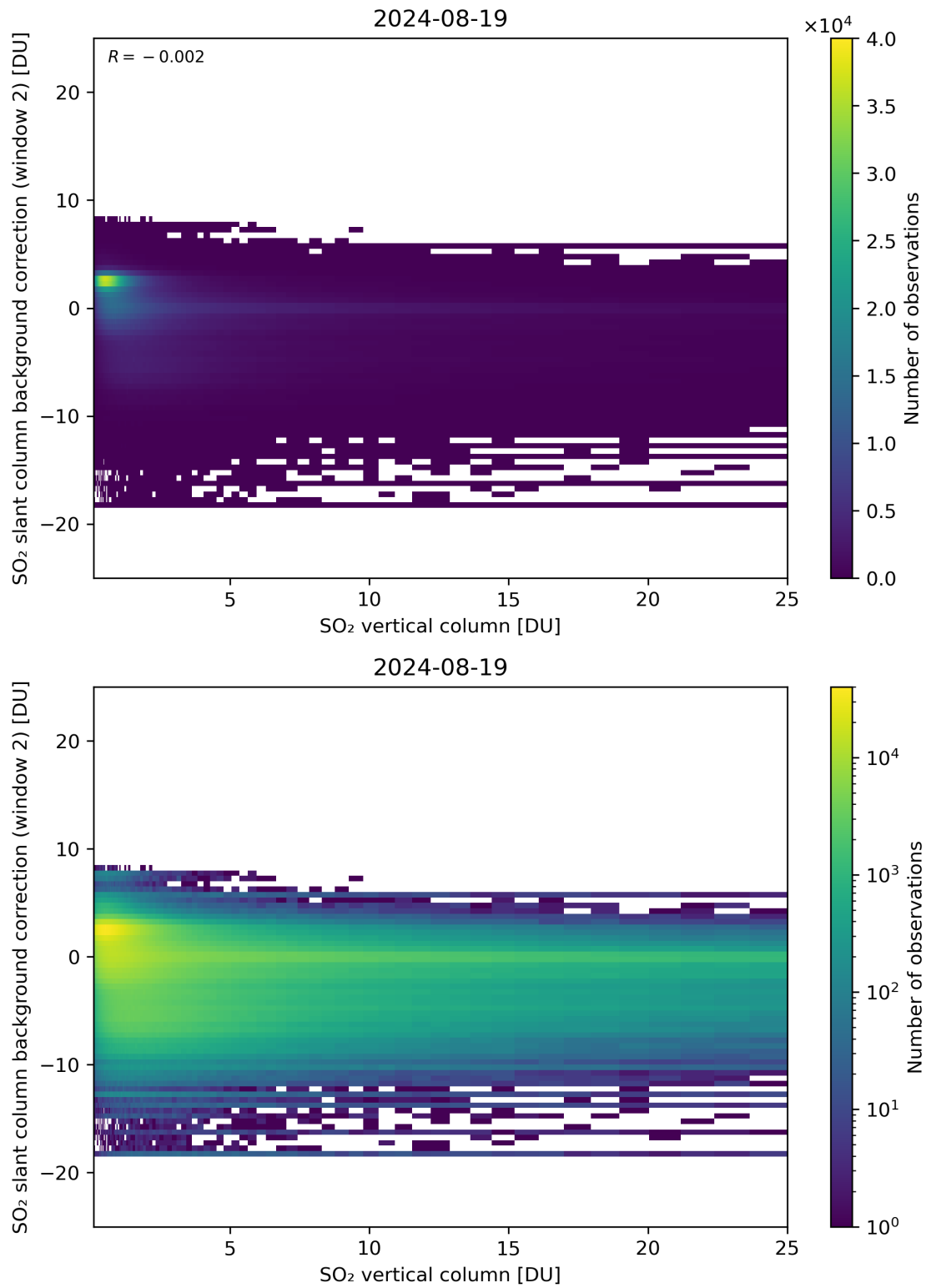
Figure 274: Scatter density plot of “SO 2 vertical column” against “SO 2 slant column background correction (window 2)” for 2024-08-18 to 2024-08-20.
