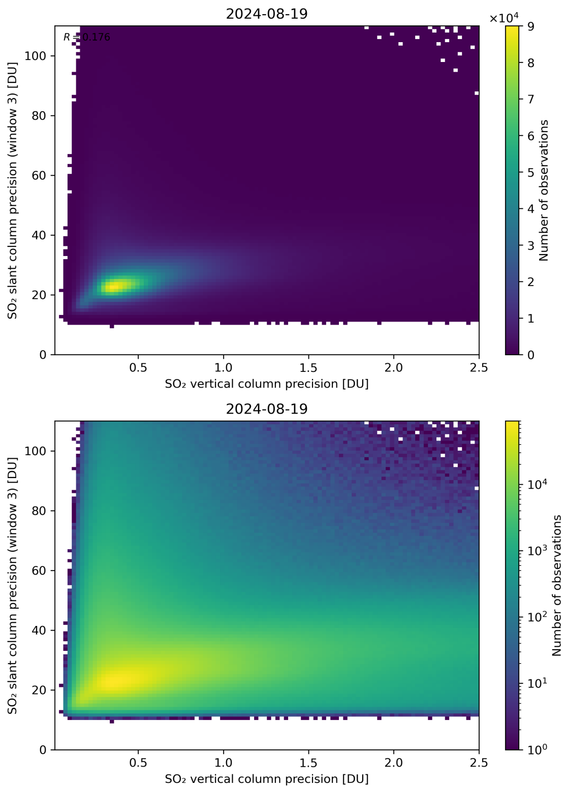
Figure 293: Scatter density plot of “SO 2 vertical column precision” against “SO 2 slant column precision (window 3)” for 2024-08-18 to 2024-08-20.
