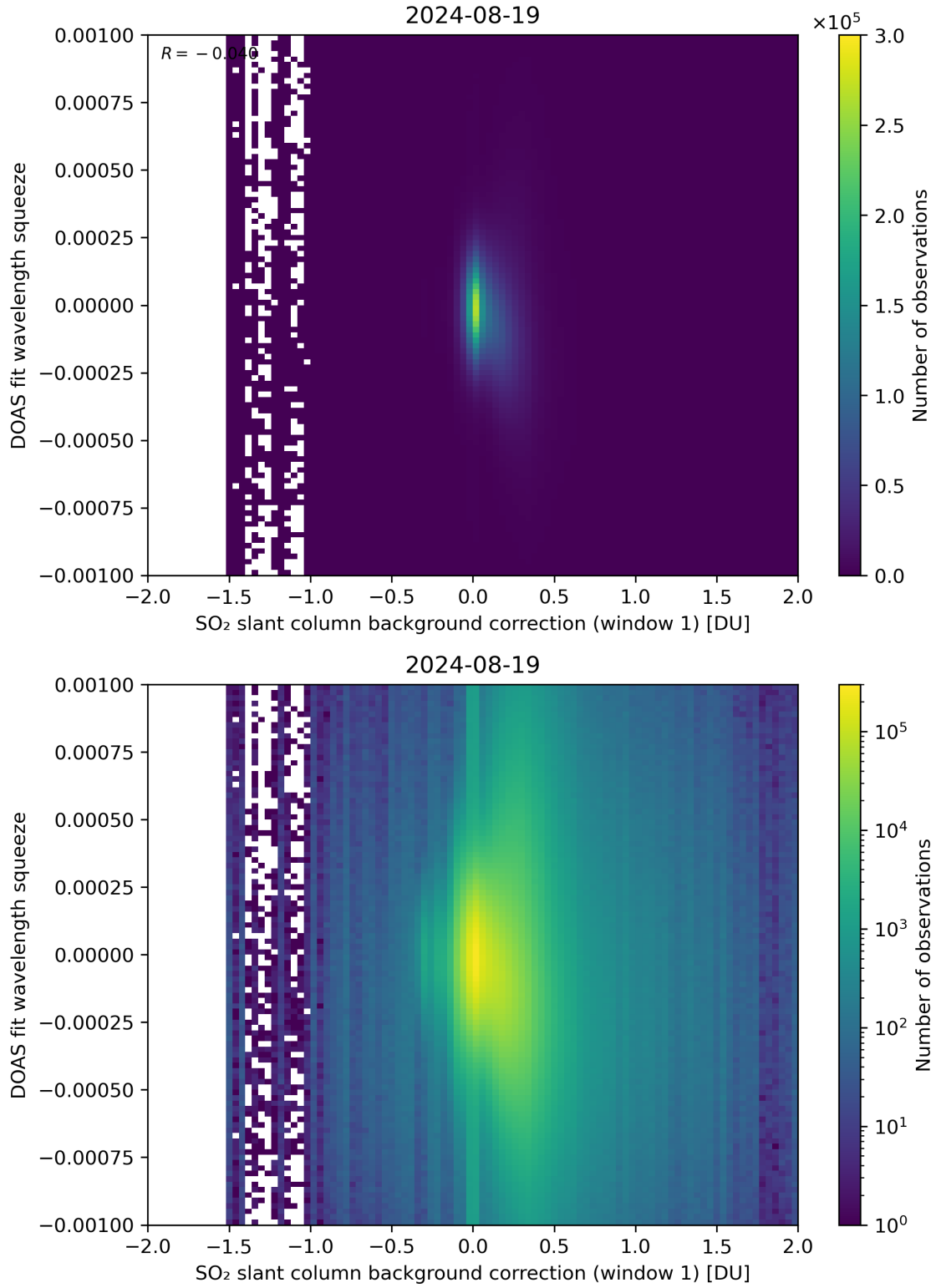
Figure 101: Scatter density plot of “SO 2 slant column background correction (window 1)” against “DOAS fit wavelength squeeze” for 2024-08-18 to 2024-08-20.
