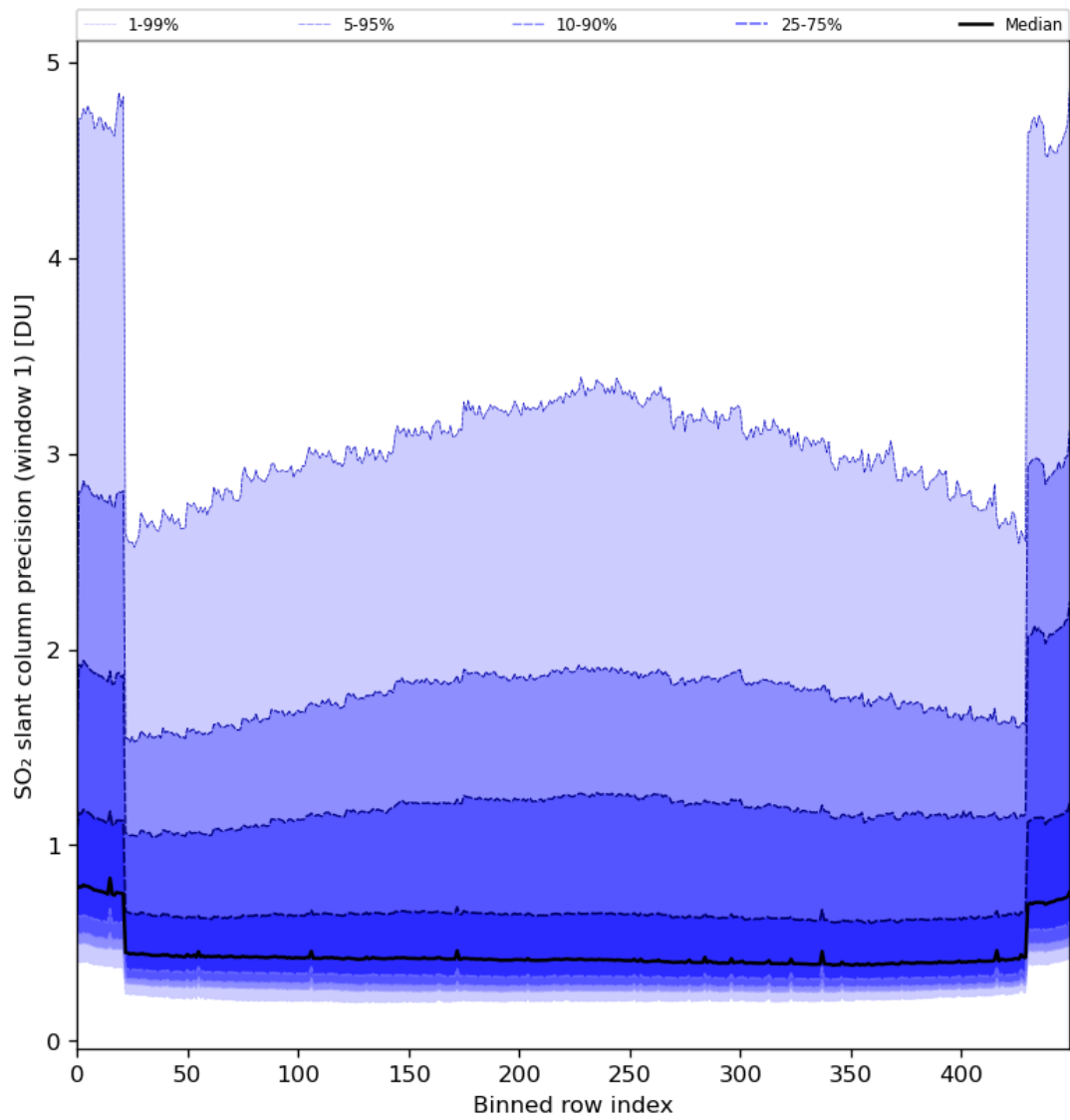
Figure 80: Along track statistics of “SO 2 slant column precision (window 1)” for 2024-08-18 to 2024-08-20
