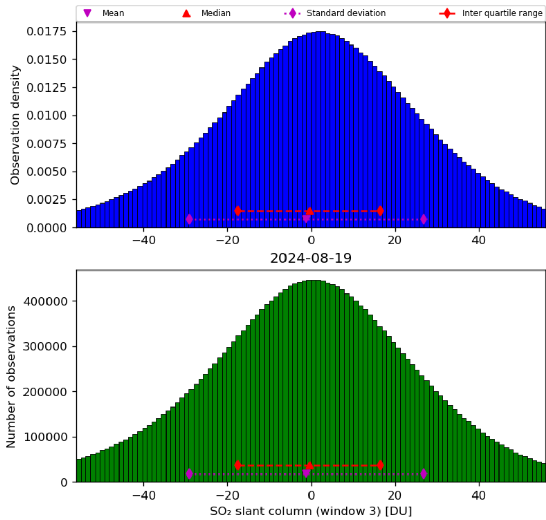
Figure 64: Histogram of “SO 2 slant column (window 3)” for 2024-08-18 to 2024-08-20
