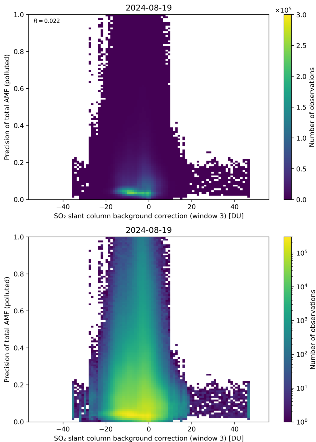
Figure 126: Scatter density plot of “SO 2 slant column background correction (window 3)” against “Precision of total AMF (polluted)” for 2024-08-18 to 2024-08-20.
