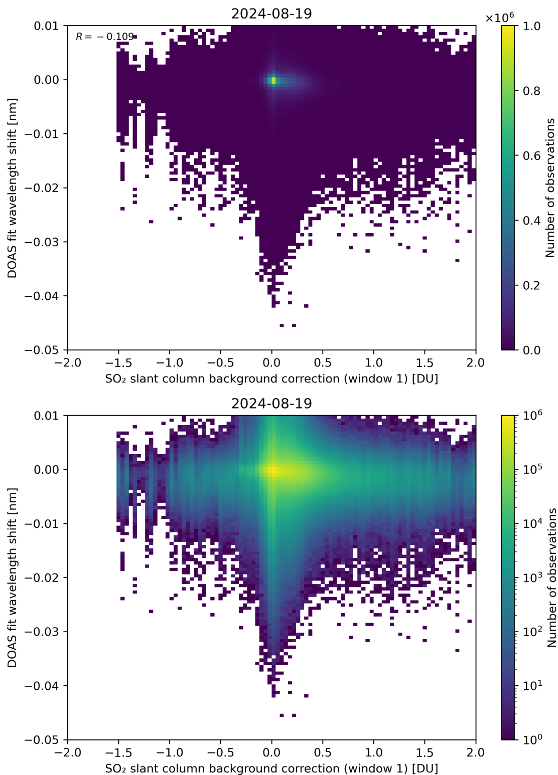
Figure 100: Scatter density plot of “SO 2 slant column background correction (window 1)” against “DOAS fit wavelength shift” for 2024-08-18 to 2024-08-20.
