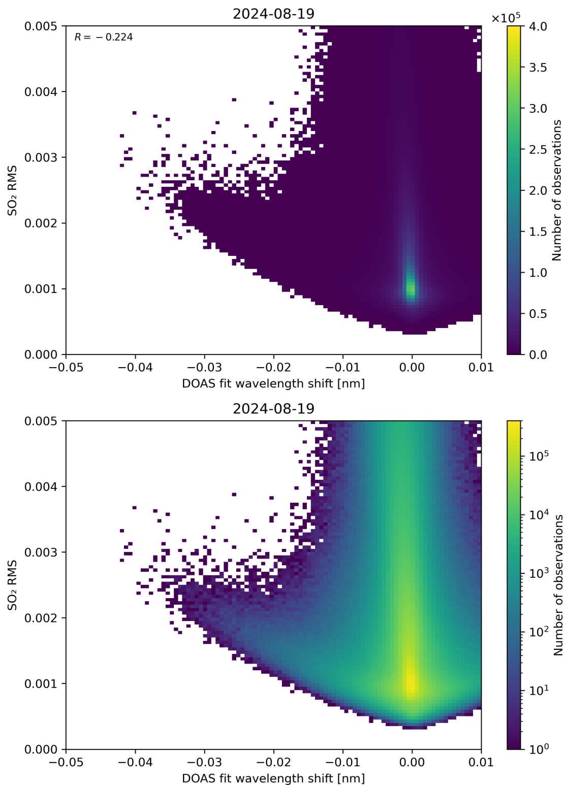
Figure 128: Scatter density plot of “DOAS fit wavelength shift” against “SO 2 RMS” for 2024-08-18 to 2024-08-20.
