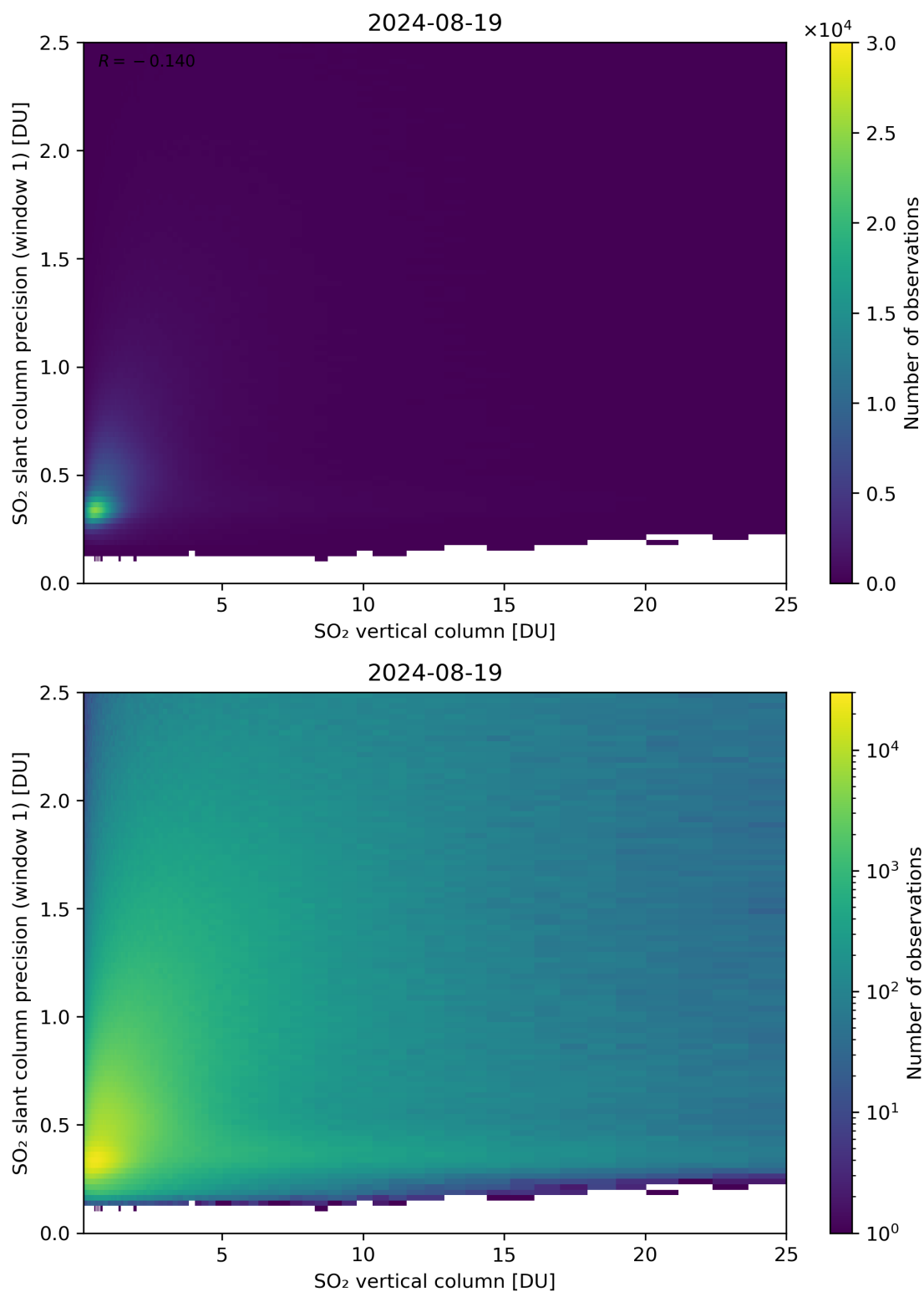
Figure 301: Scatter density plot of “SO 2 vertical column” against “SO 2 slant column precision (window 1)” for 2024-08-18 to 2024-08-20.
