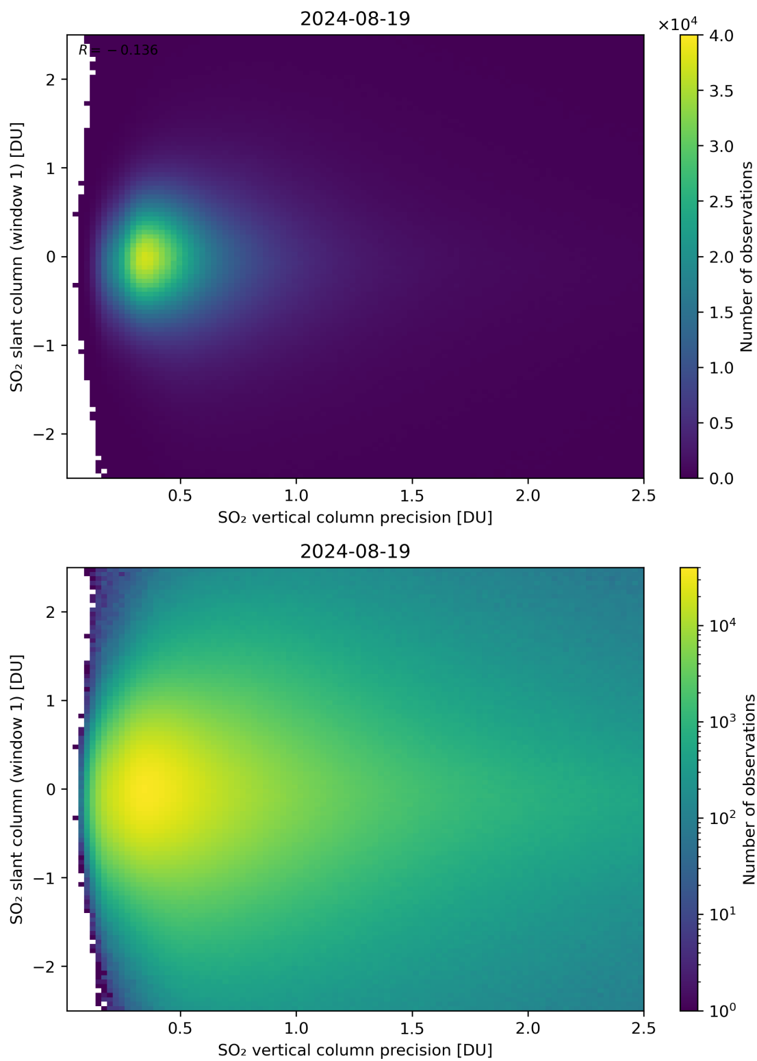
Figure 289: Scatter density plot of “SO 2 vertical column precision” against “SO 2 slant column (window 1)” for 2024-08-18 to 2024-08-20.
