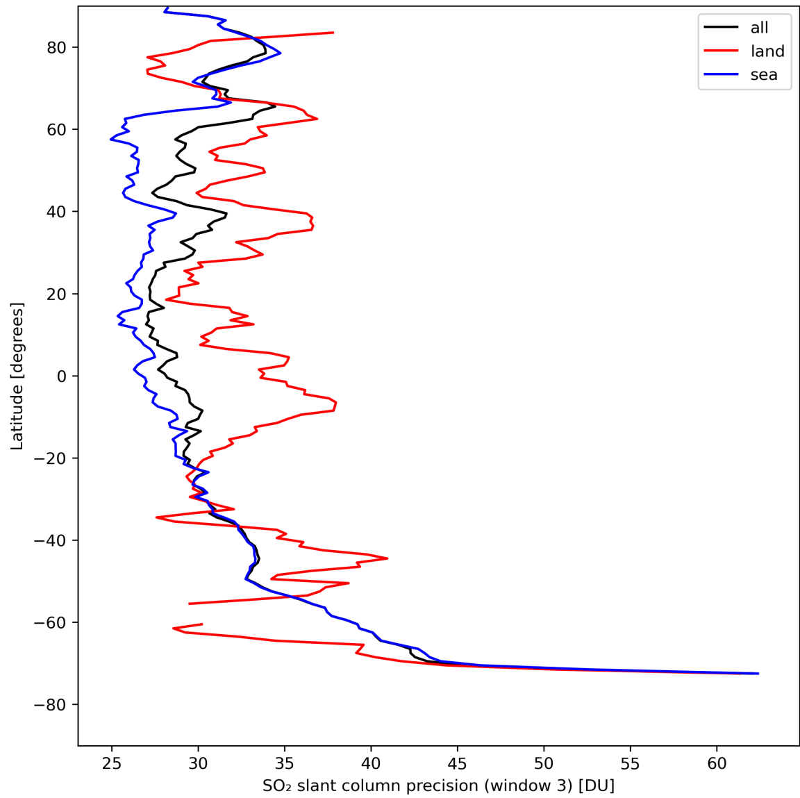
Figure 42: Zonal average of “SO 2 slant column precision (window 3)” for 2024-08-18 to 2024-08-20.
