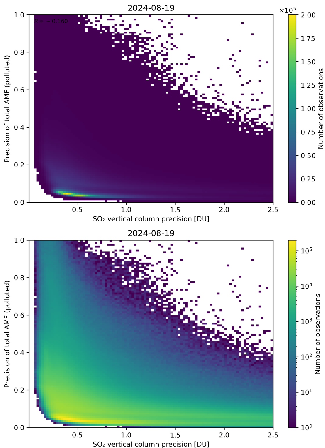
Figure 295: Scatter density plot of “SO 2 vertical column precision” against “Precision of total AMF (polluted)” for 2024-08-18 to 2024-08-20.
