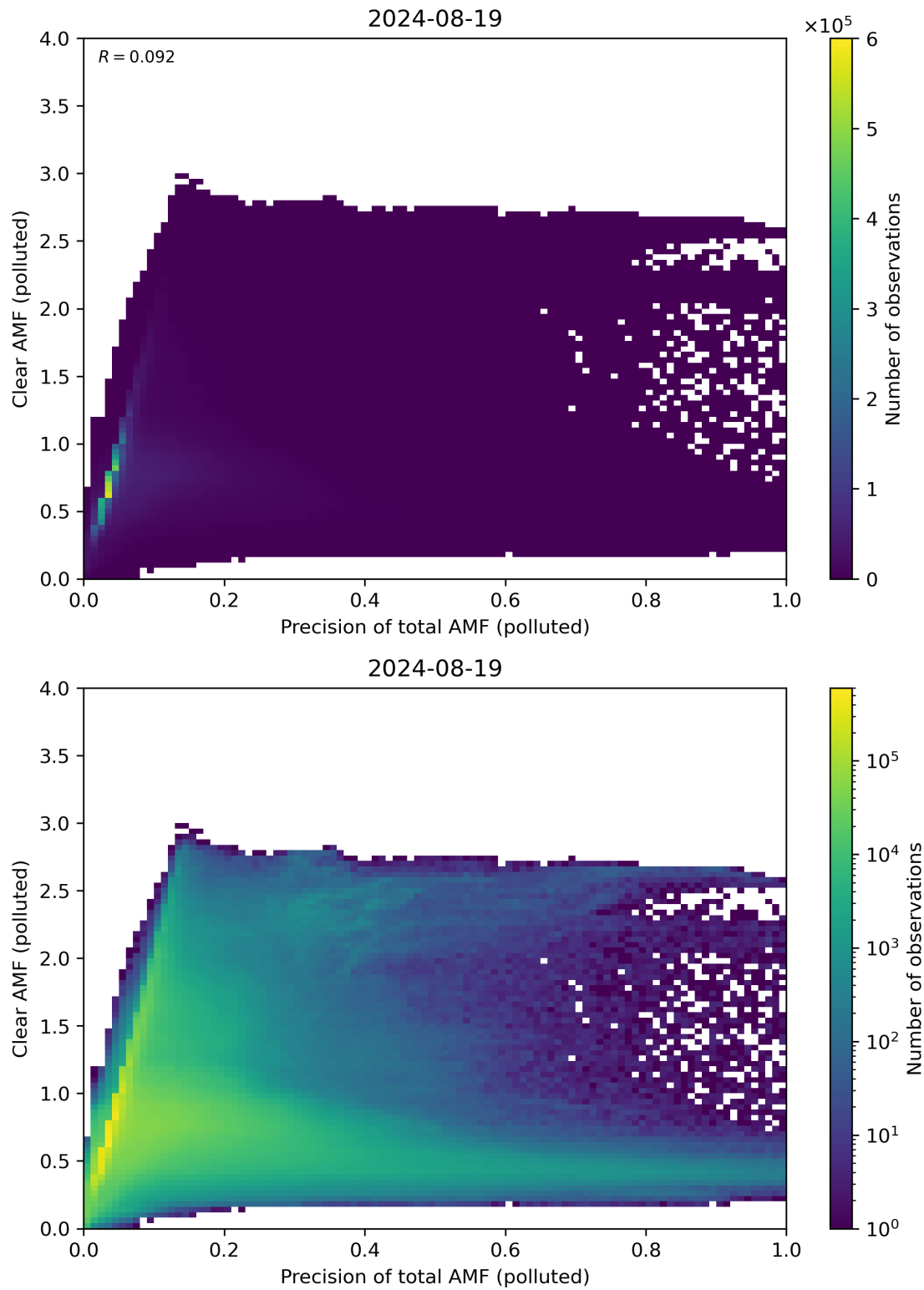
Figure 270: Scatter density plot of “Precision of total AMF (polluted)” against “Clear AMF (polluted)” for 2024-08-18 to 2024-08-20.
