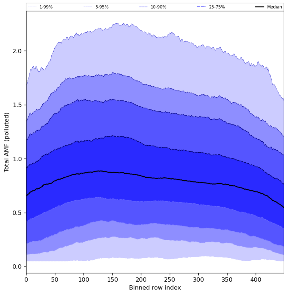
Figure 94: Along track statistics of “Total AMF (polluted)” for 2024-08-18 to 2024-08-20
