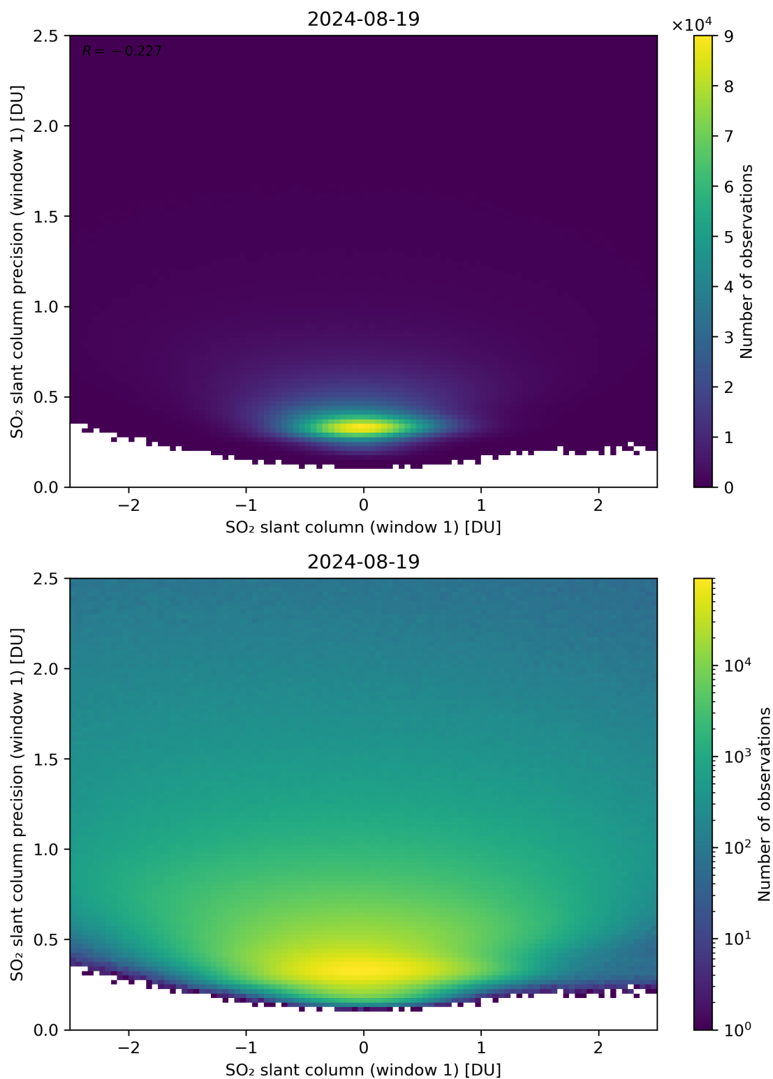
Figure 235: Scatter density plot of “SO 2 slant column (window 1)” against “SO 2 slant column precision (window 1)” for 2024-08-18 to 2024-08-20.
