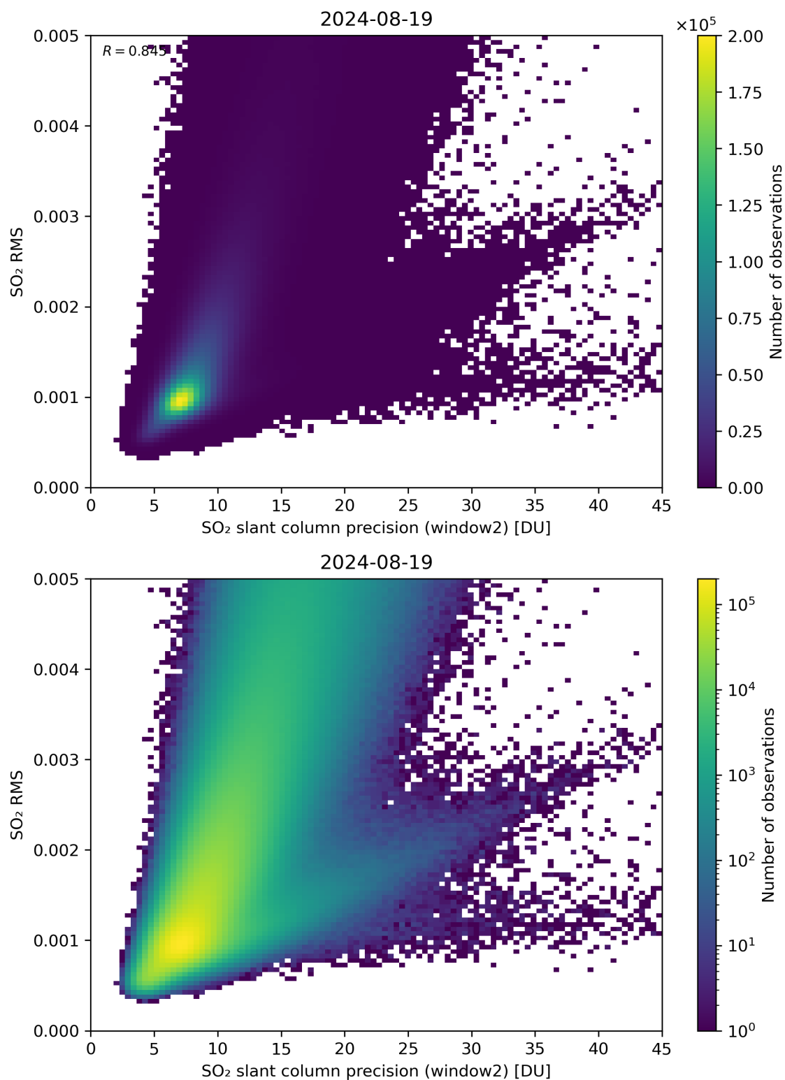
Figure 245: Scatter density plot of “SO 2 slant column precision (window2)” against “SO 2 RMS” for 2024-08-18 to 2024-08-20.
