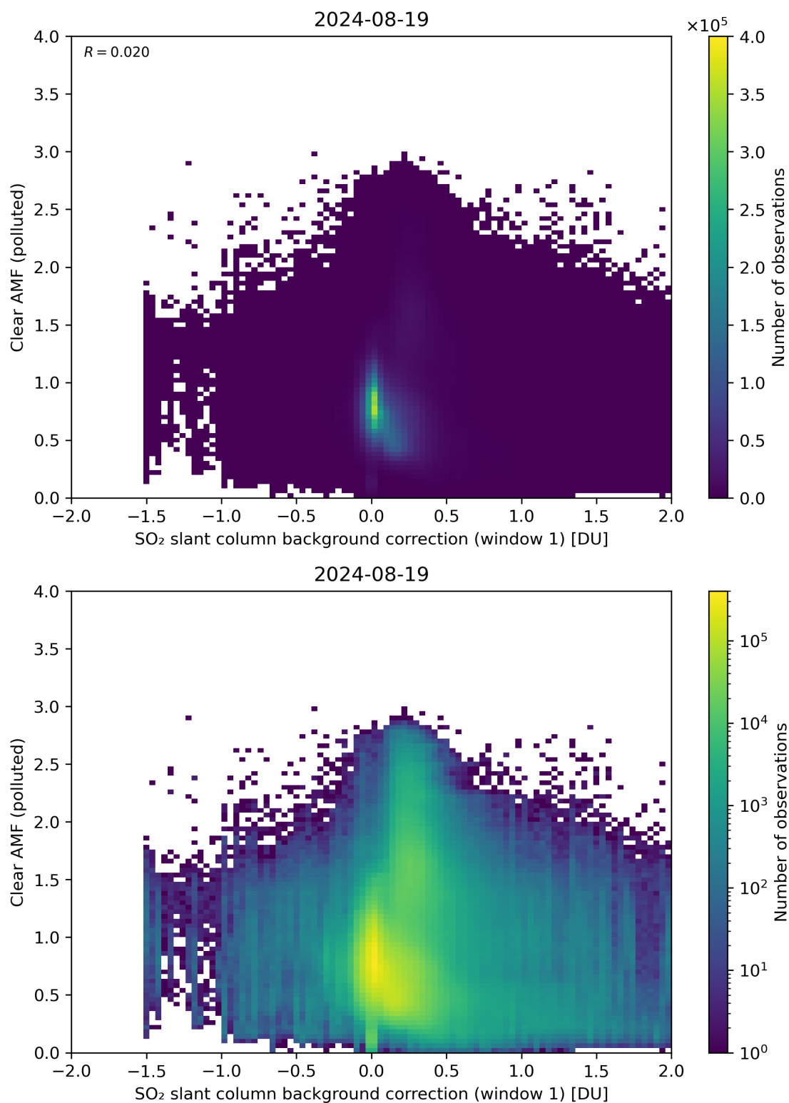
Figure 103: Scatter density plot of “SO 2 slant column background correction (window 1)” against “Clear AMF (polluted)” for 2024-08-18 to 2024-08-20.
