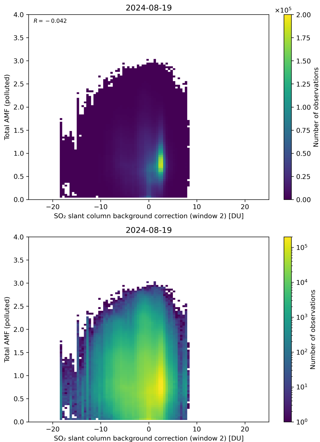
Figure 119: Scatter density plot of “SO 2 slant column background correction (window 2)” against “Total AMF (polluted)” for 2024-08-18 to 2024-08-20.
