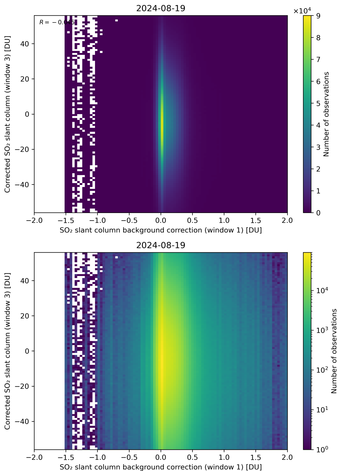
Figure 105: Scatter density plot of “SO 2 slant column background correction (window 1)” against “Corrected SO 2 slant column (window 3)” for 2024-08-18 to 2024-08-20.
