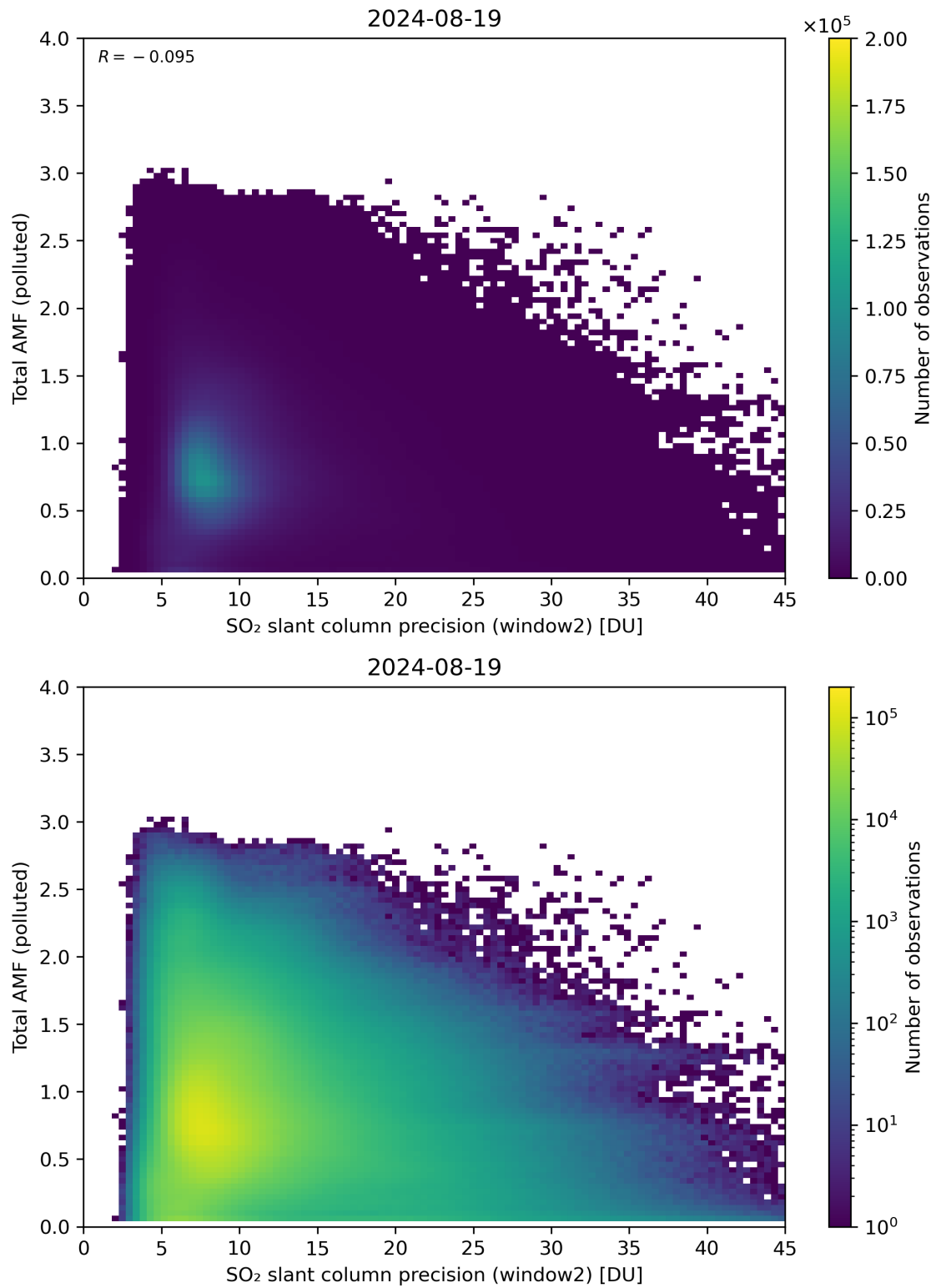
Figure 251: Scatter density plot of “SO 2 slant column precision (window2)” against “Total AMF (polluted)” for 2024-08-18 to 2024-08-20.
