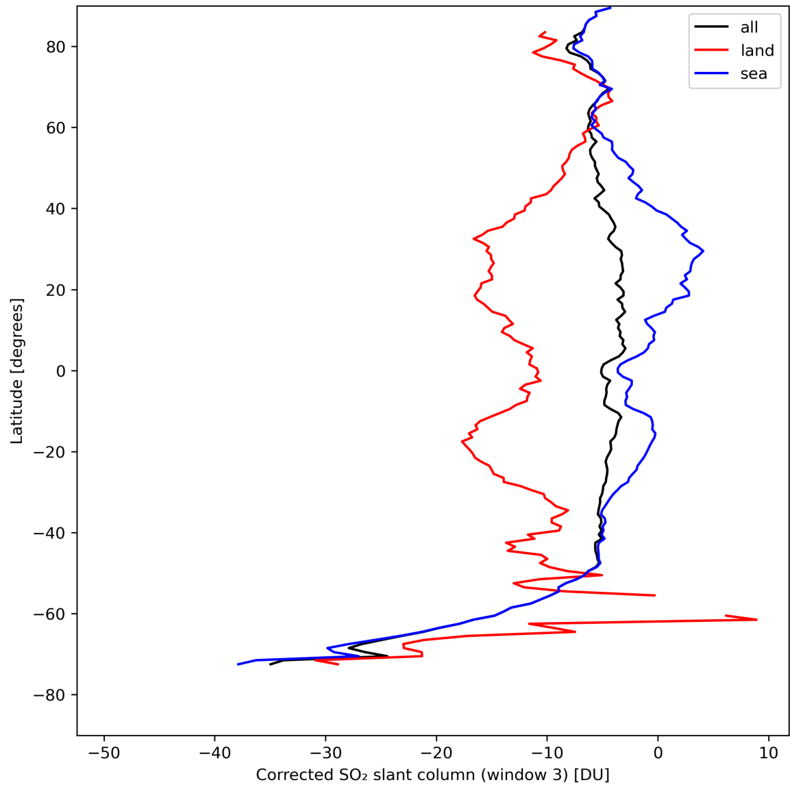
Figure 43: Zonal average of “Corrected SO 2 slant column (window 3)” for 2024-08-18 to 2024-08-20.
