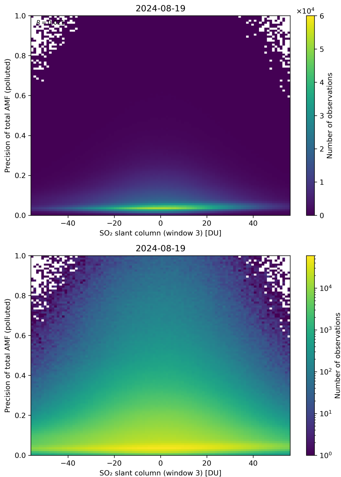
Figure 269: Scatter density plot of “SO 2 slant column (window 3)” against “Precision of total AMF (polluted)” for 2024-08-18 to 2024-08-20.
