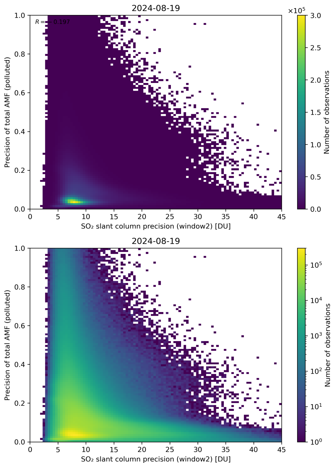
Figure 252: Scatter density plot of “SO 2 slant column precision (window2)” against “Precision of total AMF (polluted)” for 2024-08-18 to 2024-08-20.
