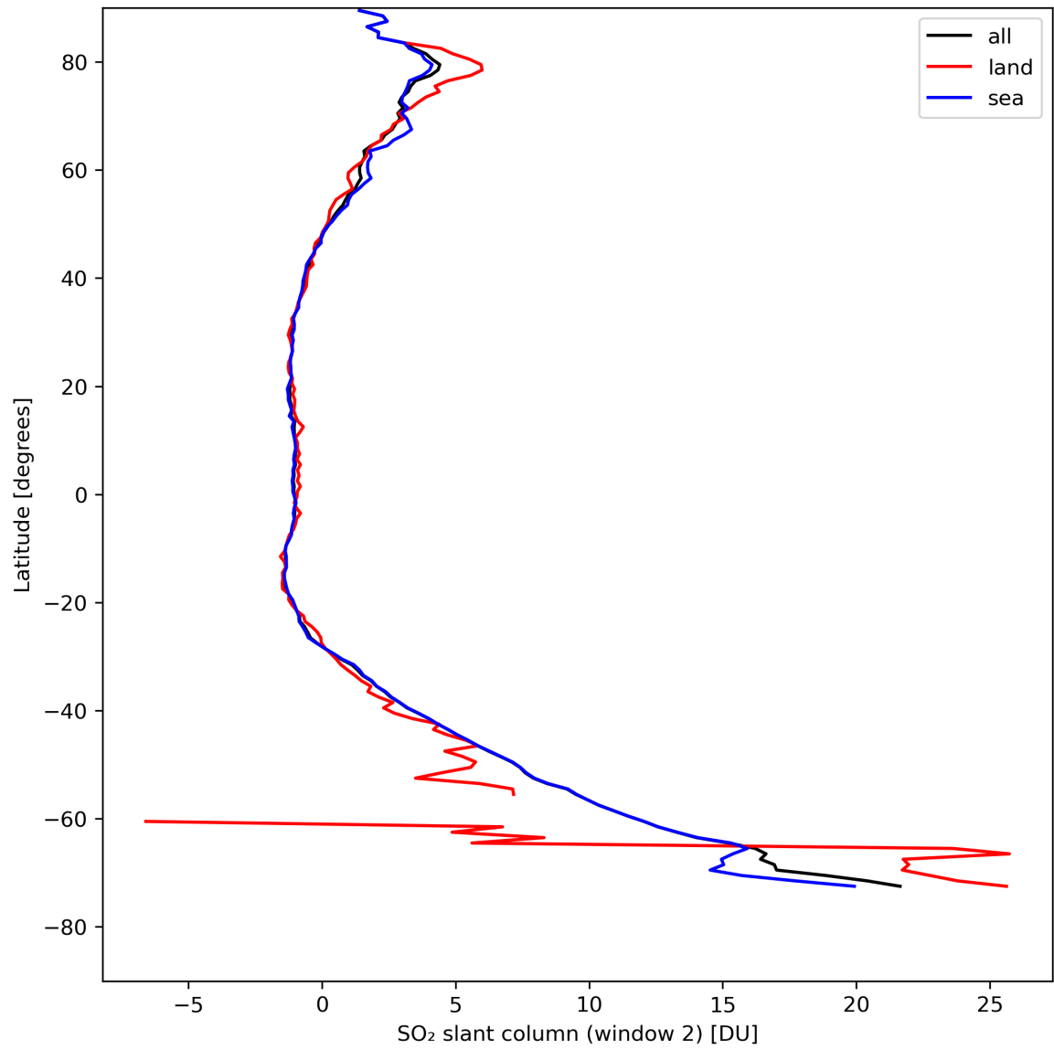
Figure 37: Zonal average of “SO 2 slant column (window 2)” for 2024-08-18 to 2024-08-20.
