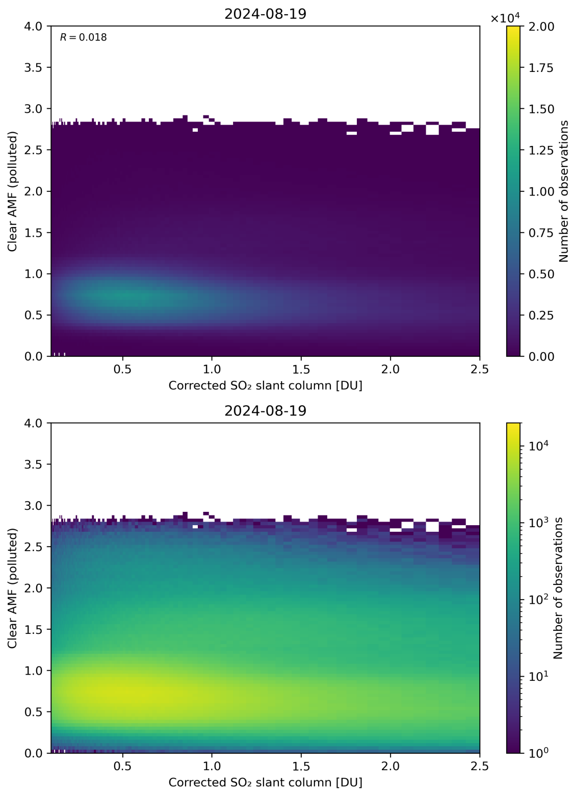
Figure 184: Scatter density plot of “Corrected SO 2 slant column” against “Clear AMF (polluted)” for 2024-08-18 to 2024-08-20.
