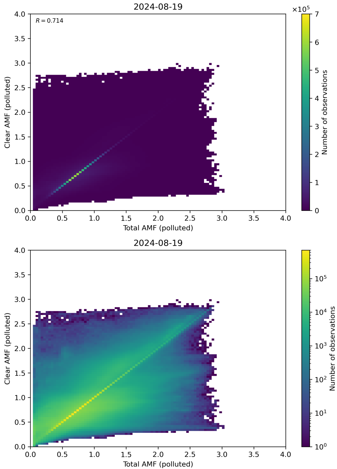
Figure 271: Scatter density plot of “Total AMF (polluted)” against “Clear AMF (polluted)” for 2024-08-18 to 2024-08-20.
