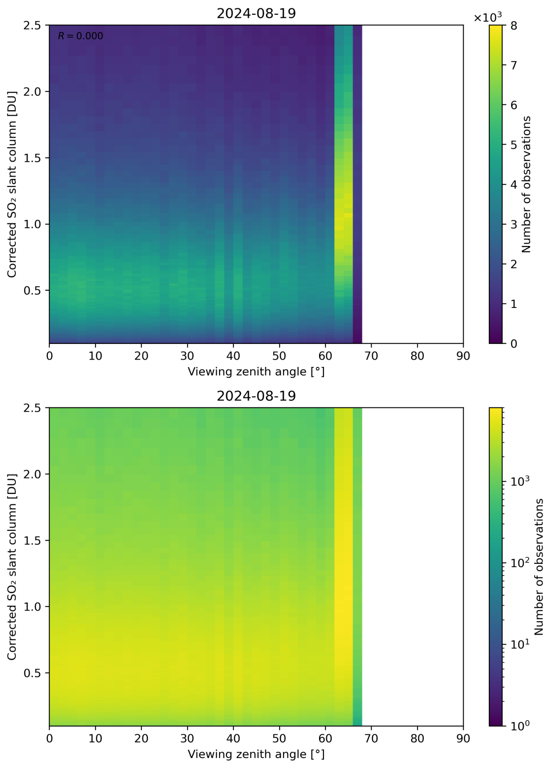
Figure 317: Scatter density plot of “Viewing zenith angle” against “Corrected SO 2 slant column” for 2024-08-18 to 2024-08-20.
