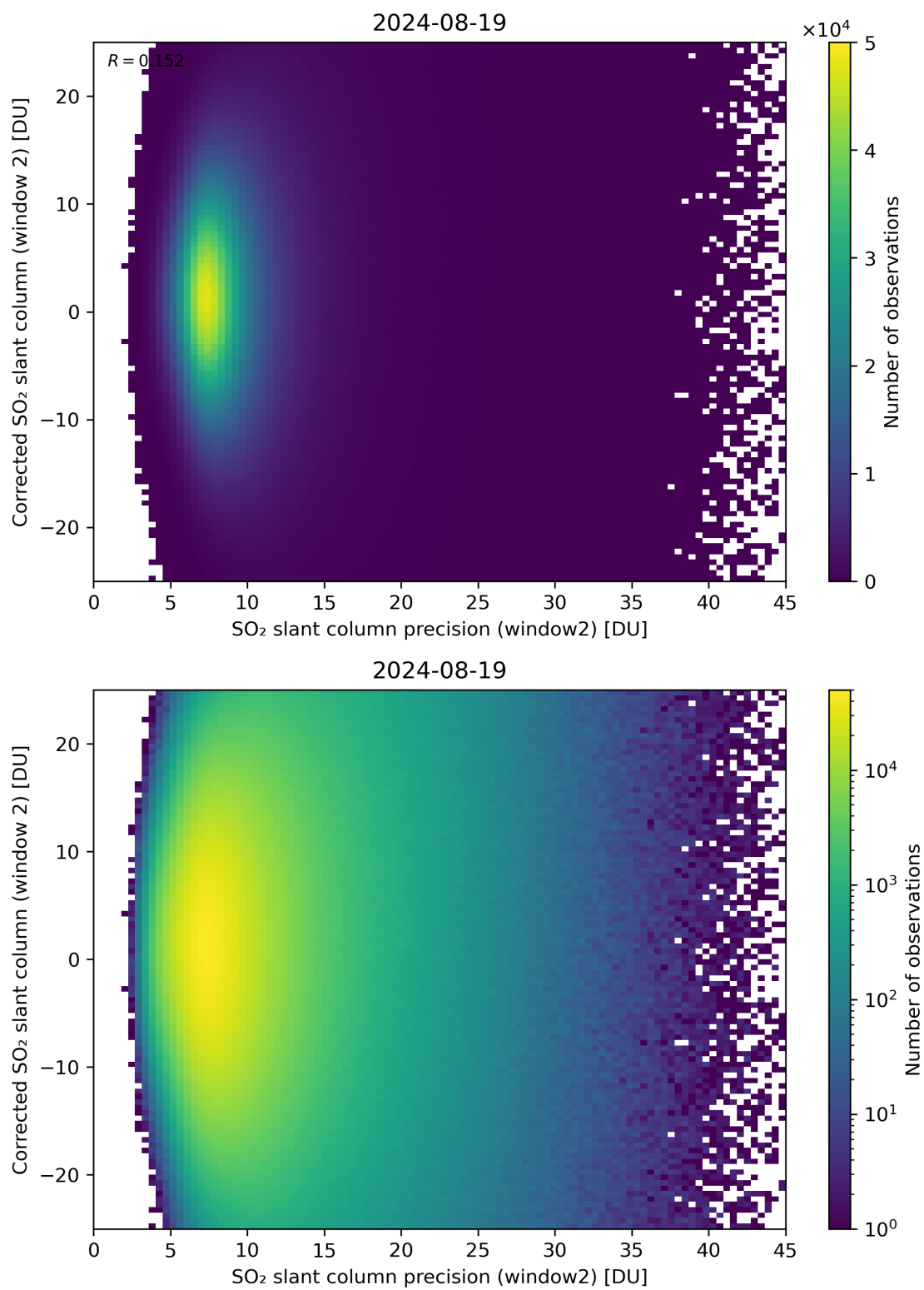
Figure 247: Scatter density plot of “SO 2 slant column precision (window2)” against “Corrected SO 2 slant column (window 2)” for 2024-08-18 to 2024-08-20.
