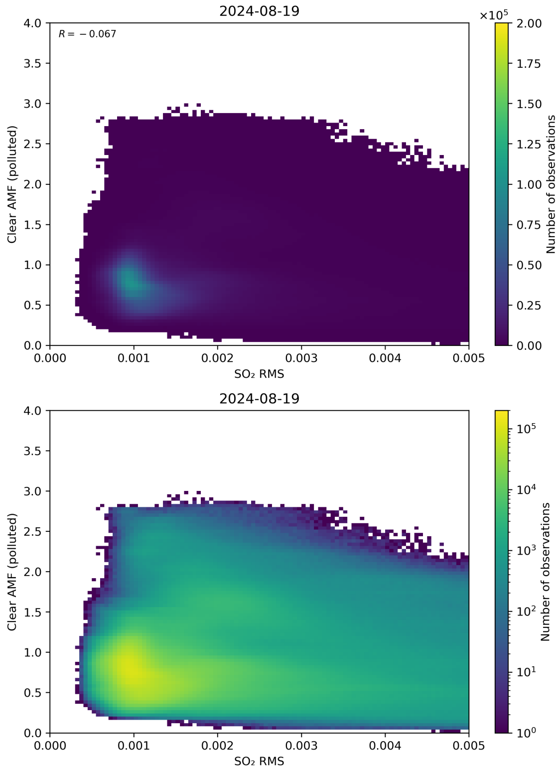
Figure 136: Scatter density plot of “SO 2 RMS” against “Clear AMF (polluted)” for 2024-08-18 to 2024-08-20.
