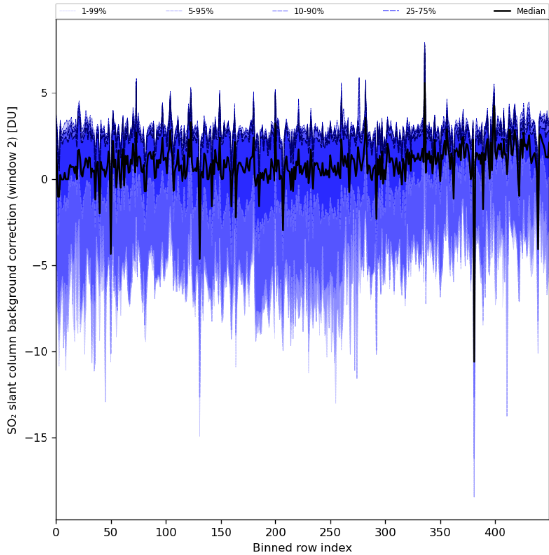
Figure 86: Along track statistics of “SO 2 slant column background correction (window 2)” for 2024-08-18 to 2024-08-20
