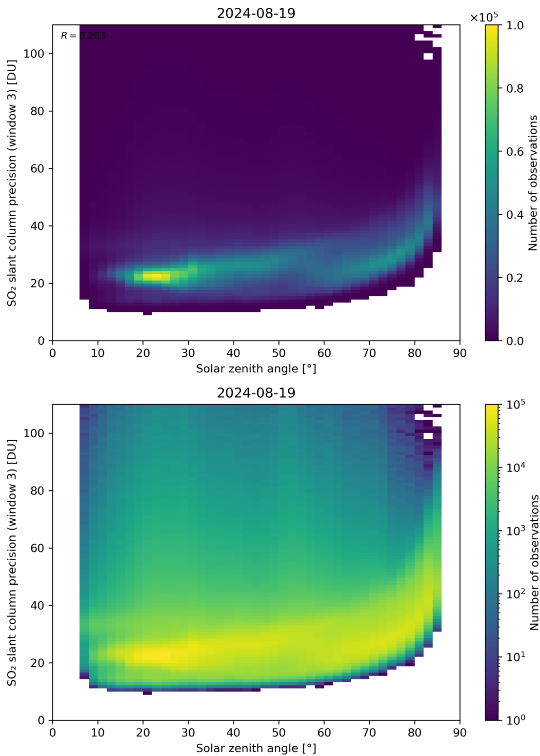
Figure 173: Scatter density plot of “Solar zenith angle” against “SO 2 slant column precision (window 3)” for 2024-08-18 to 2024-08-20.
