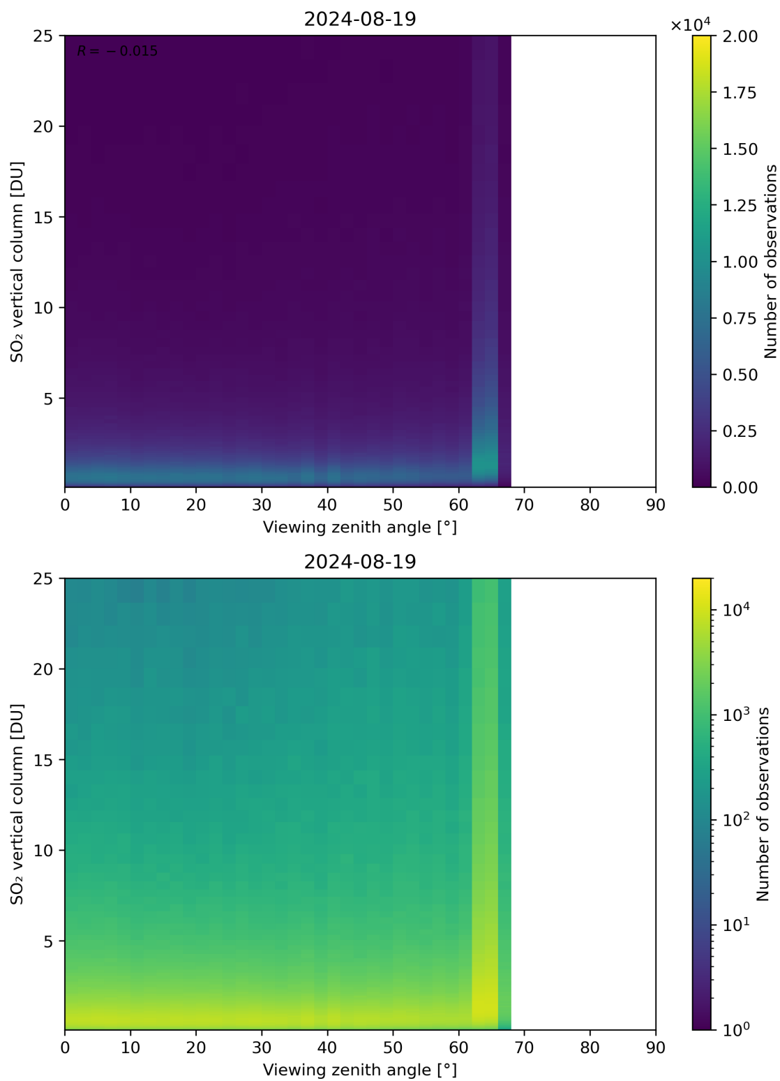
Figure 327: Scatter density plot of “Viewing zenith angle” against “SO 2 vertical column” for 2024-08-18 to 2024-08-20.
