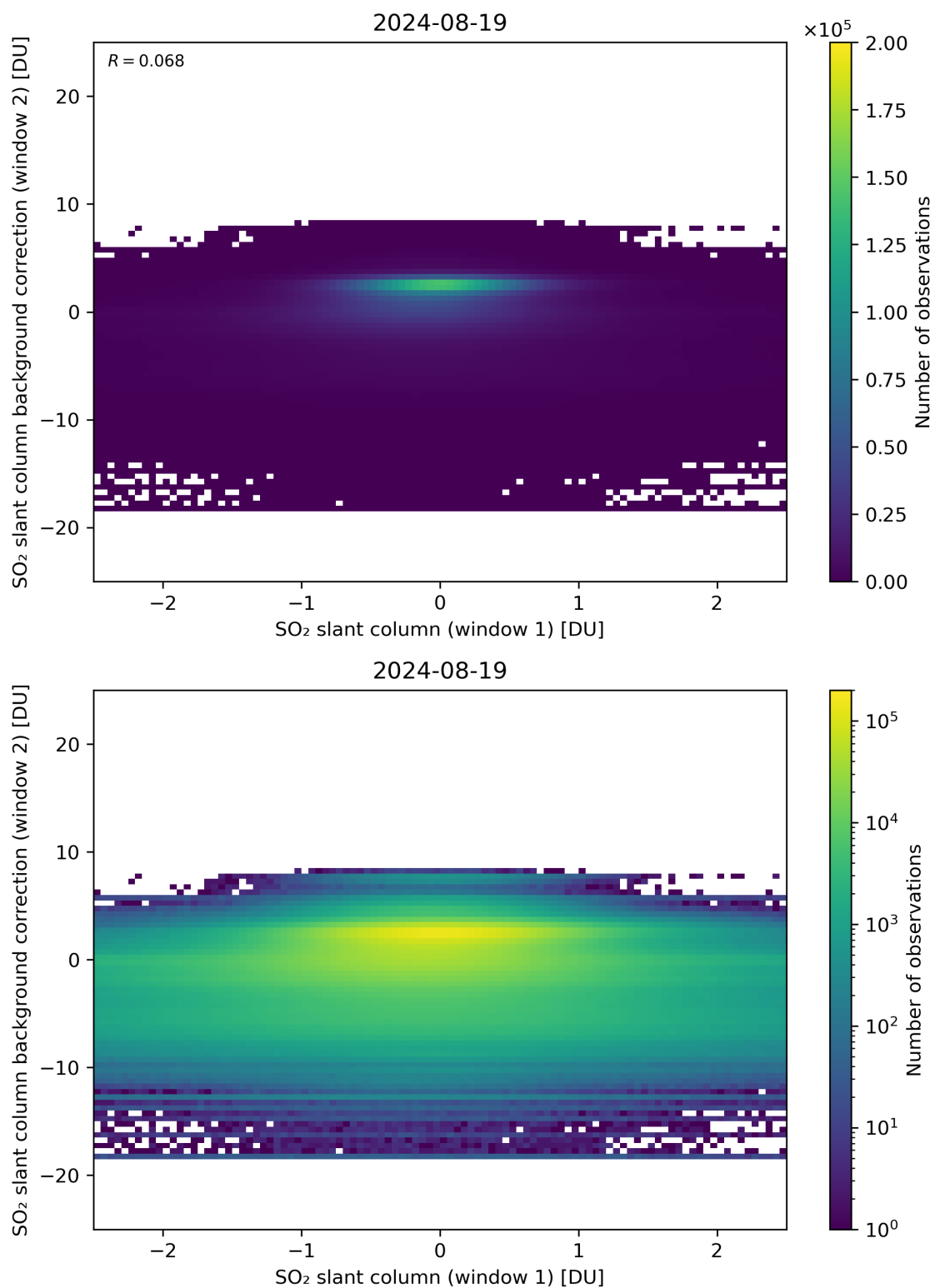
Figure 213: Scatter density plot of “SO 2 slant column (window 1)” against “SO 2 slant column background correction (window 2)” for 2024-08-18 to 2024-08-20.
