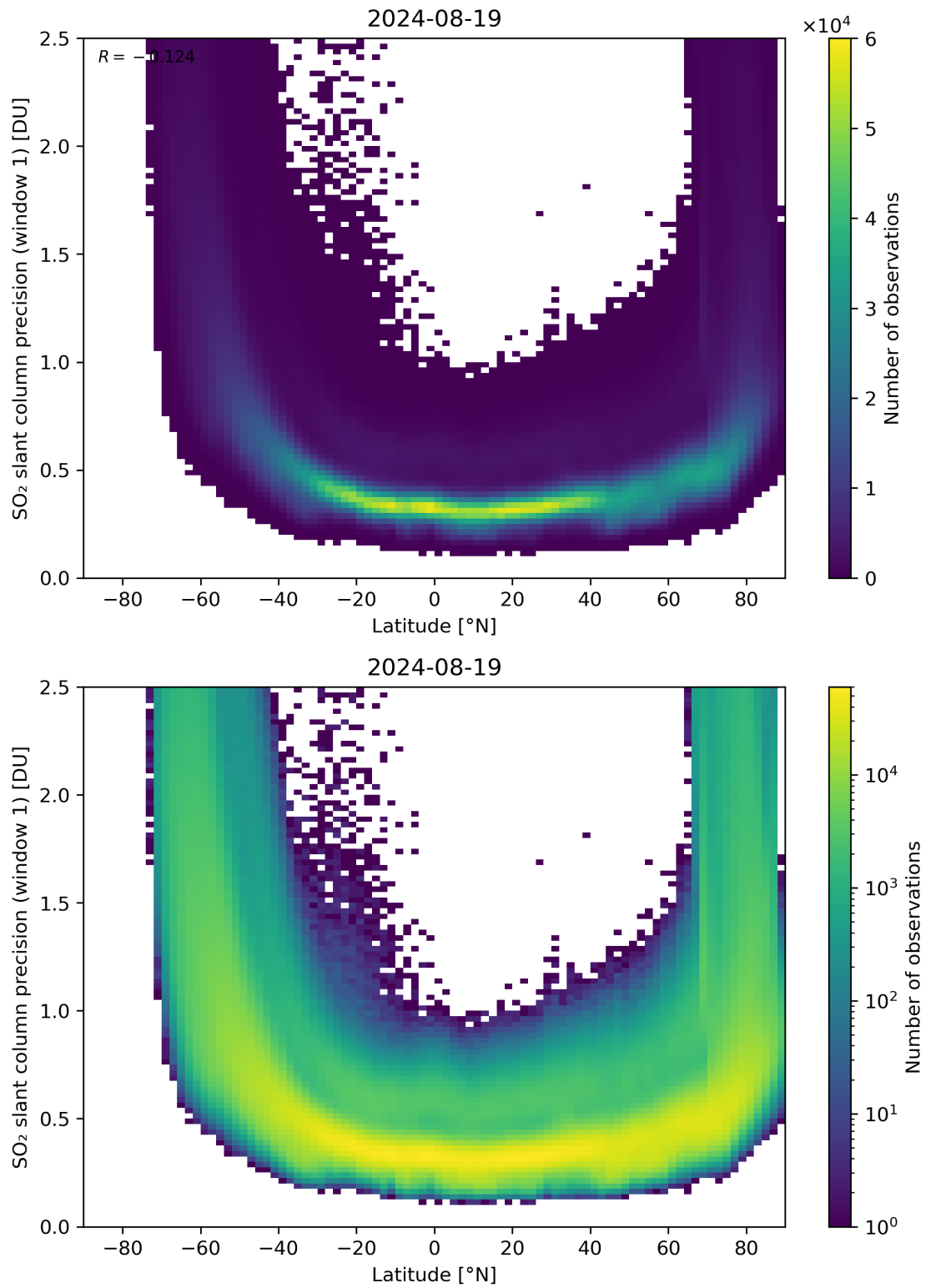
Figure 150: Scatter density plot of “Latitude” against “SO 2 slant column precision (window 1)” for 2024-08-18 to 2024-08-20.
