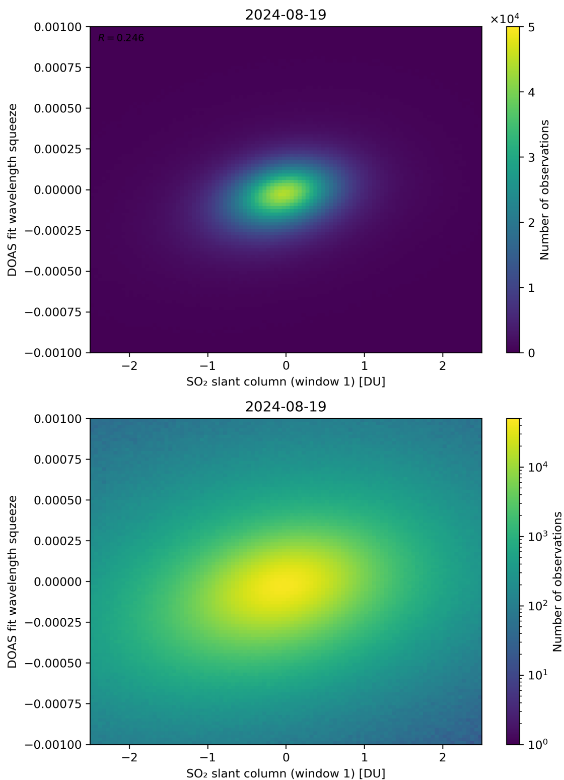
Figure 216: Scatter density plot of “SO 2 slant column (window 1)” against “DOAS fit wavelength squeeze” for 2024-08-18 to 2024-08-20.
