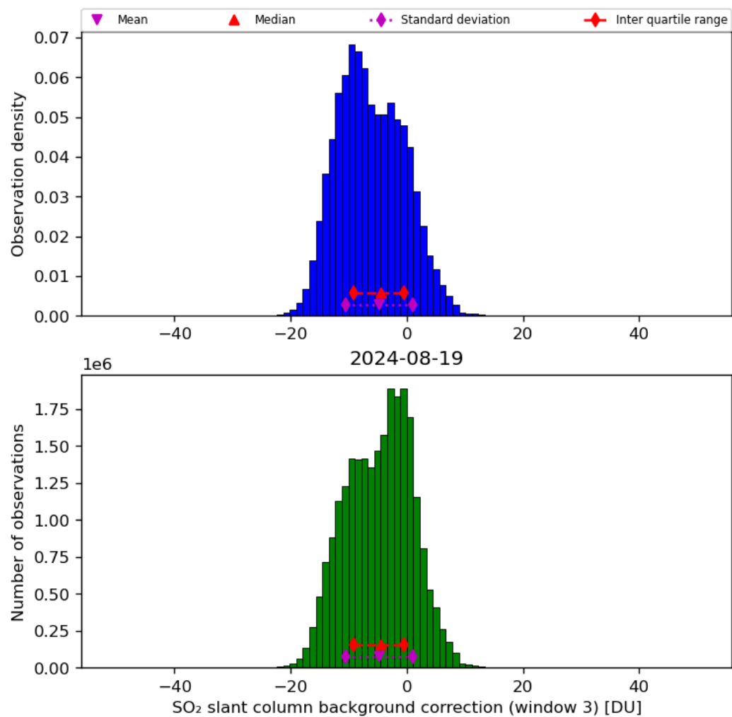
Figure 67: Histogram of “SO 2 slant column background correction (window 3)” for 2024-08-18 to 2024-08-20
