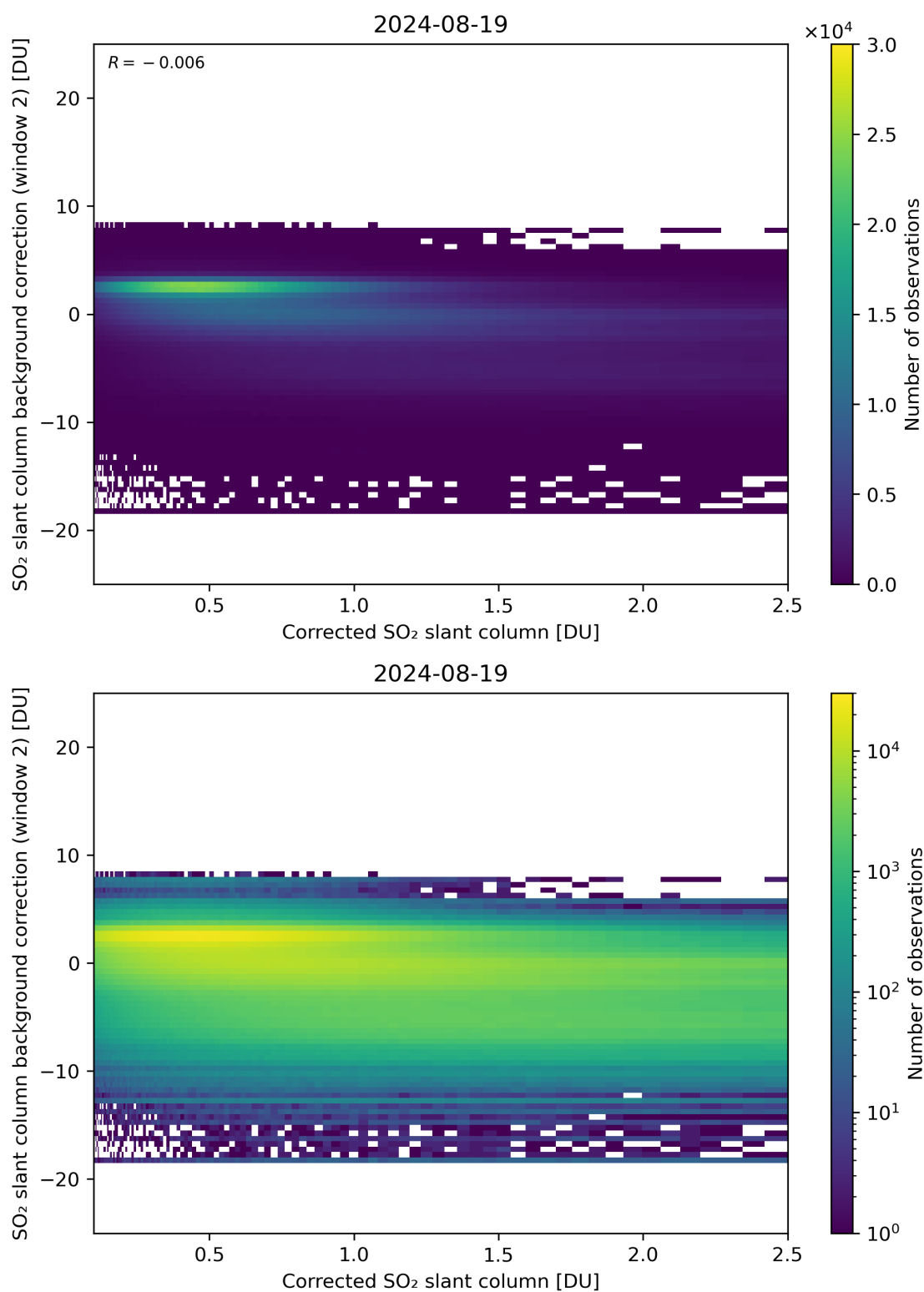
Figure 179: Scatter density plot of “Corrected SO 2 slant column” against “SO 2 slant column background correction (window 2)” for 2024-08-18 to 2024-08-20.
