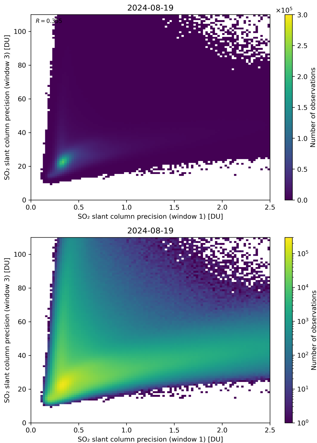
Figure 229: Scatter density plot of “SO 2 slant column precision (window 1)” against “SO 2 slant column precision (window 3)” for 2024-08-18 to 2024-08-20.
