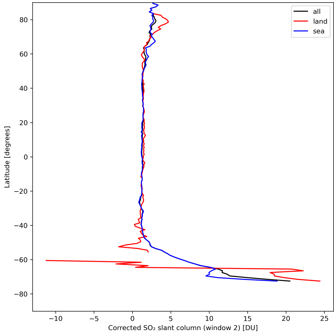
Figure 39: Zonal average of “Corrected SO 2 slant column (window 2)” for 2024-08-18 to 2024-08-20.
