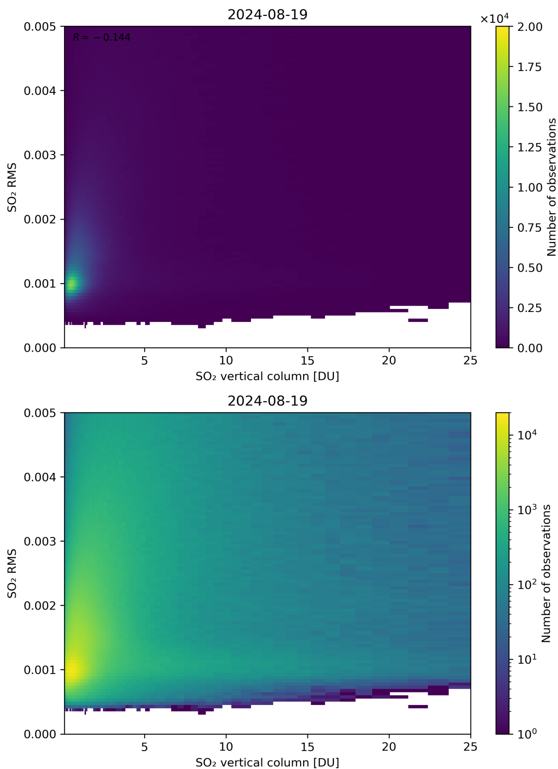
Figure 278: Scatter density plot of “SO 2 vertical column” against “SO 2 RMS” for 2024-08-18 to 2024-08-20.
