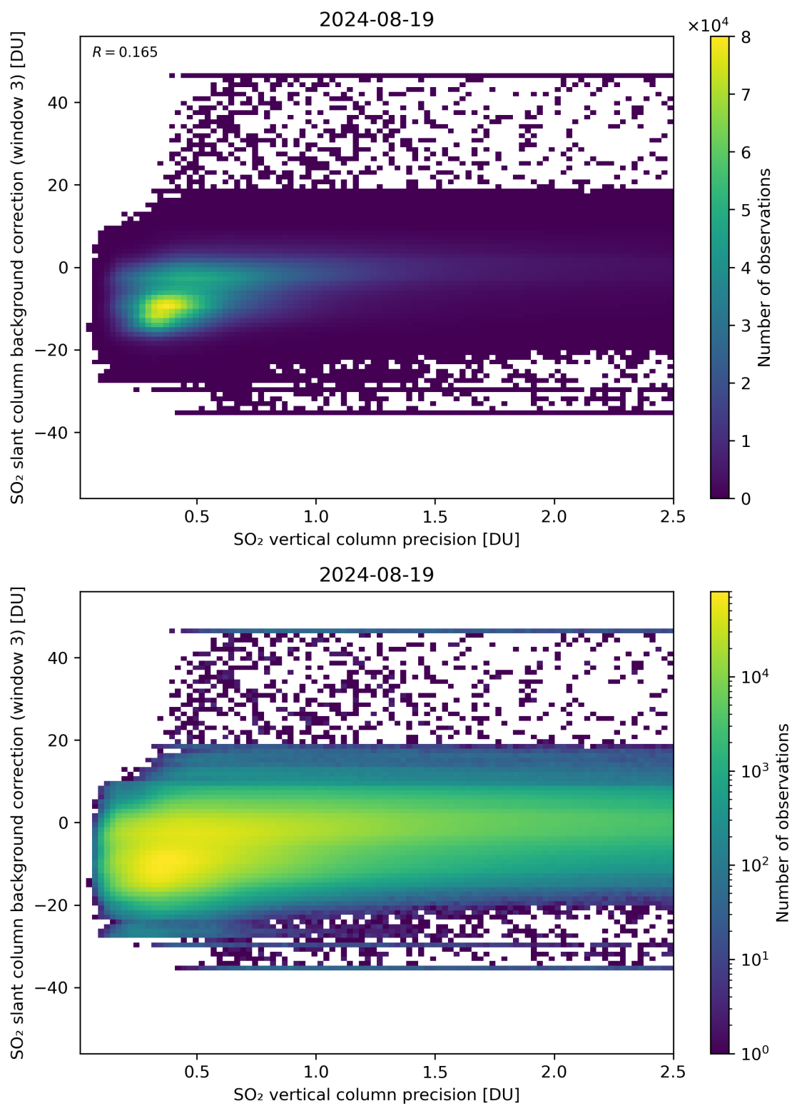
Figure 281: Scatter density plot of “SO 2 vertical column precision” against “SO 2 slant column background correction (window 3)” for 2024-08-18 to 2024-08-20.
