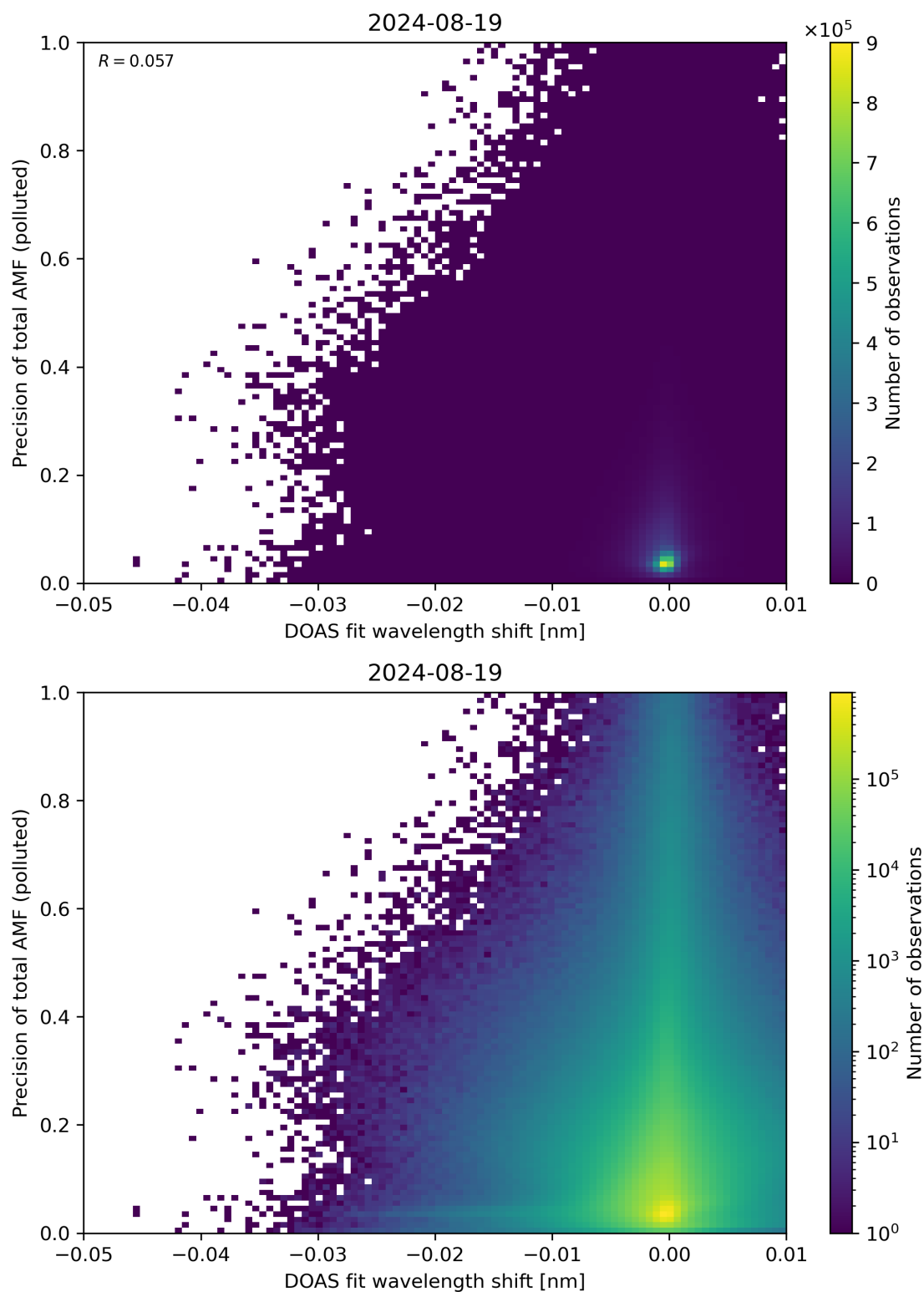
Figure 131: Scatter density plot of “DOAS fit wavelength shift” against “Precision of total AMF (polluted)” for 2024-08-18 to 2024-08-20.
