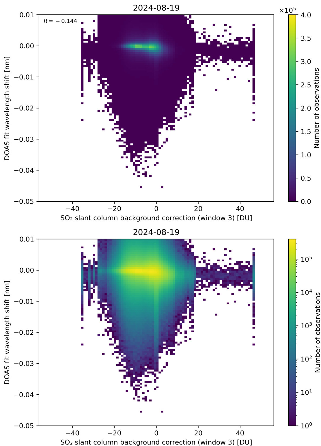
Figure 121: Scatter density plot of “SO 2 slant column background correction (window 3)” against “DOAS fit wavelength shift” for 2024-08-18 to 2024-08-20.
