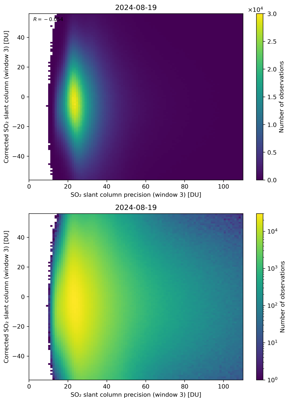
Figure 262: Scatter density plot of “SO 2 slant column precision (window 3)” against “Corrected SO 2 slant column (window 3)” for 2024-08-18 to 2024-08-20.
