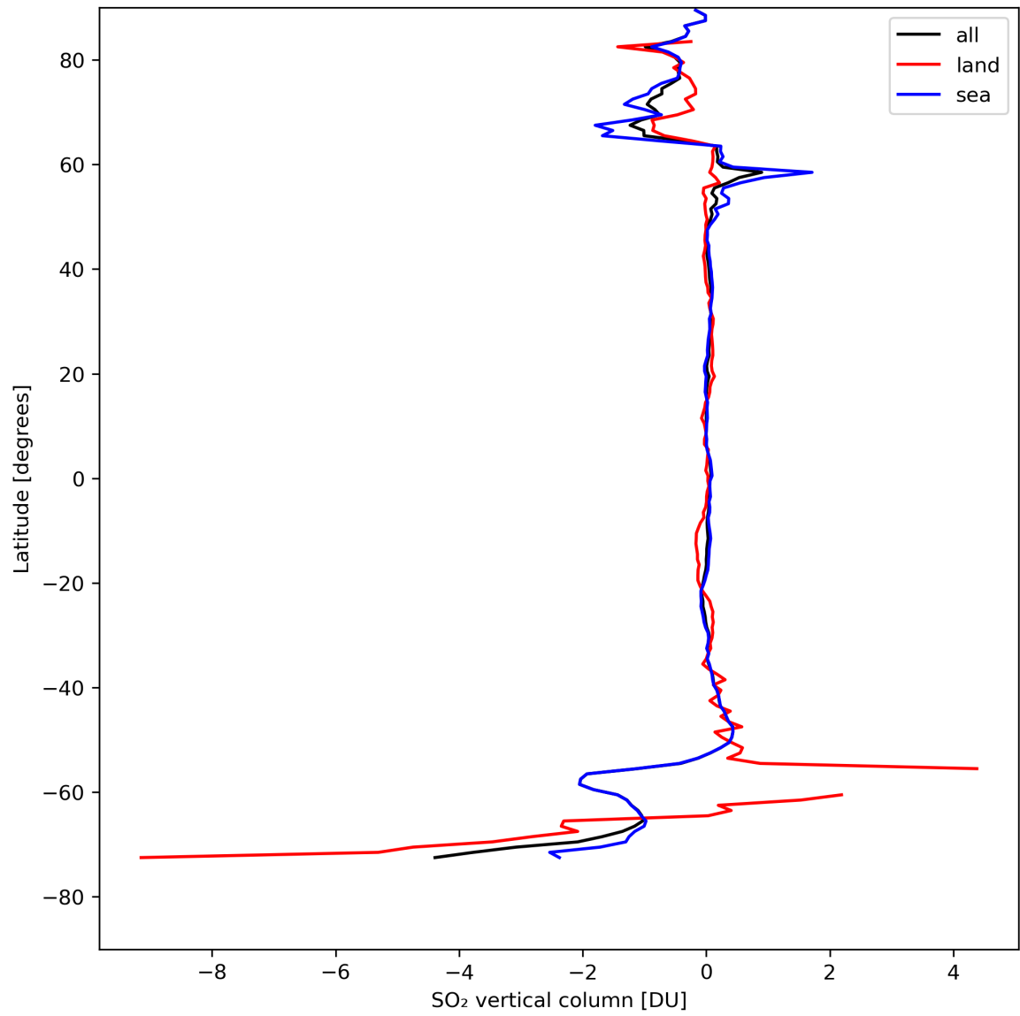
Figure 30: Zonal average of “SO 2 vertical column” for 2024-08-18 to 2024-08-20.
