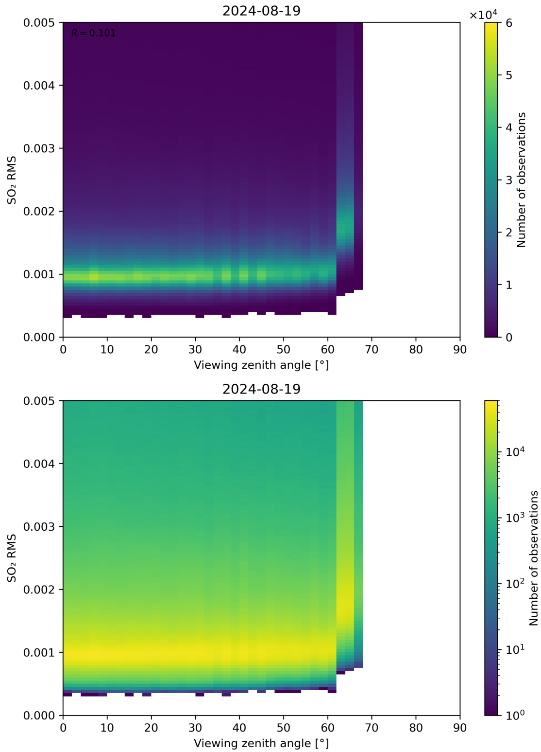
Figure 313: Scatter density plot of “Viewing zenith angle” against “SO 2 RMS” for 2024-08-18 to 2024-08-20.
