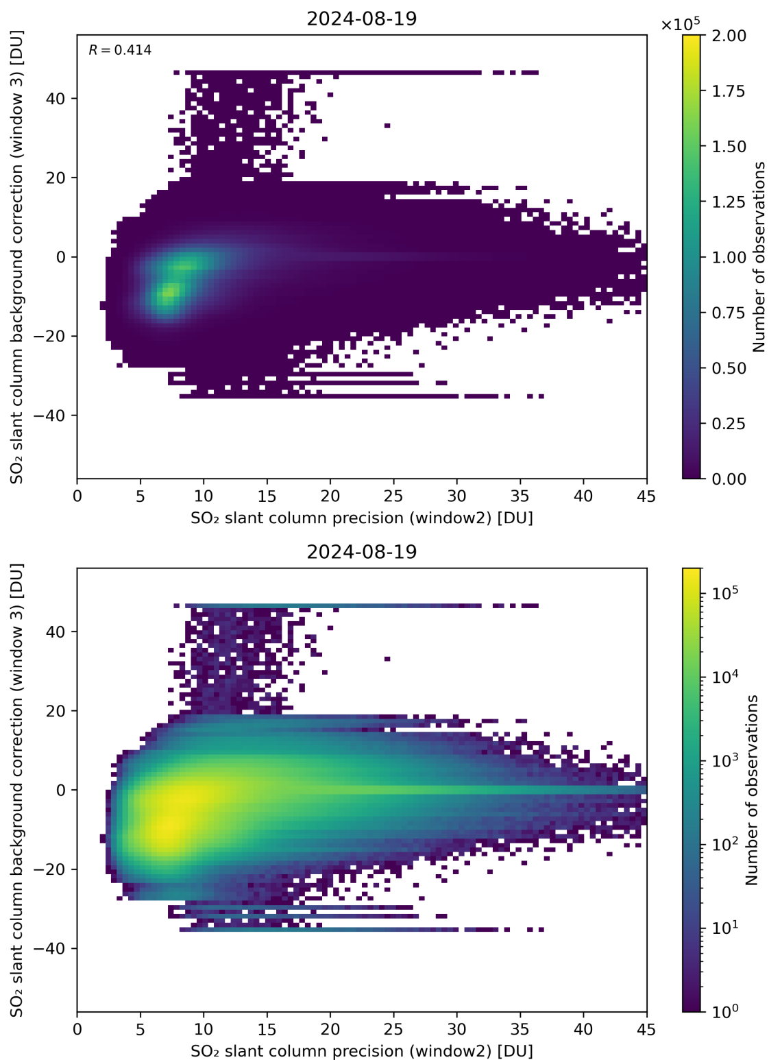
Figure 242: Scatter density plot of “SO 2 slant column precision (window2)” against “SO 2 slant column background correction (window 3)” for 2024-08-18 to 2024-08-20.
