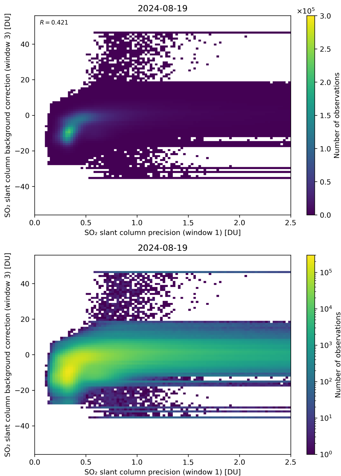
Figure 220: Scatter density plot of “SO 2 slant column precision (window 1)” against “SO 2 slant column background correction (window 3)” for 2024-08-18 to 2024-08-20.
