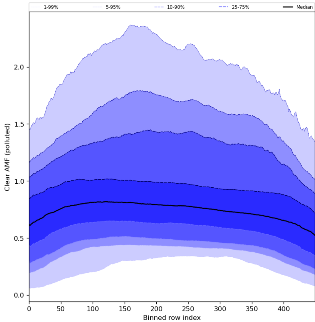
Figure 96: Along track statistics of “Clear AMF (polluted)” for 2024-08-18 to 2024-08-20
