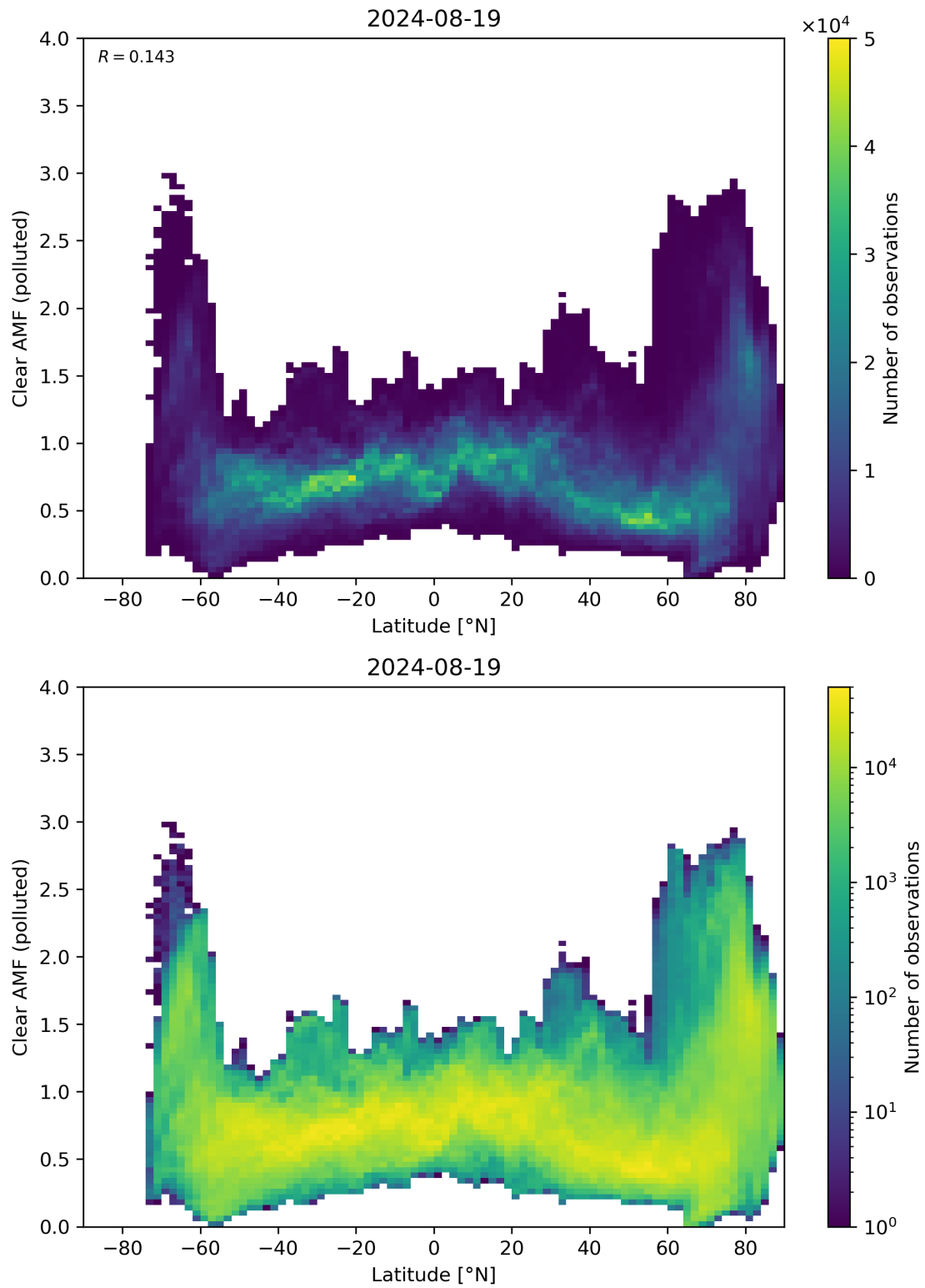
Figure 145: Scatter density plot of “Latitude” against “Clear AMF (polluted)” for 2024-08-18 to 2024-08-20.
