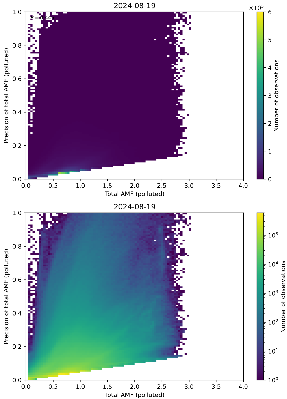
Figure 272: Scatter density plot of “Total AMF (polluted)” against “Precision of total AMF (polluted)” for 2024-08-18 to 2024-08-20.
