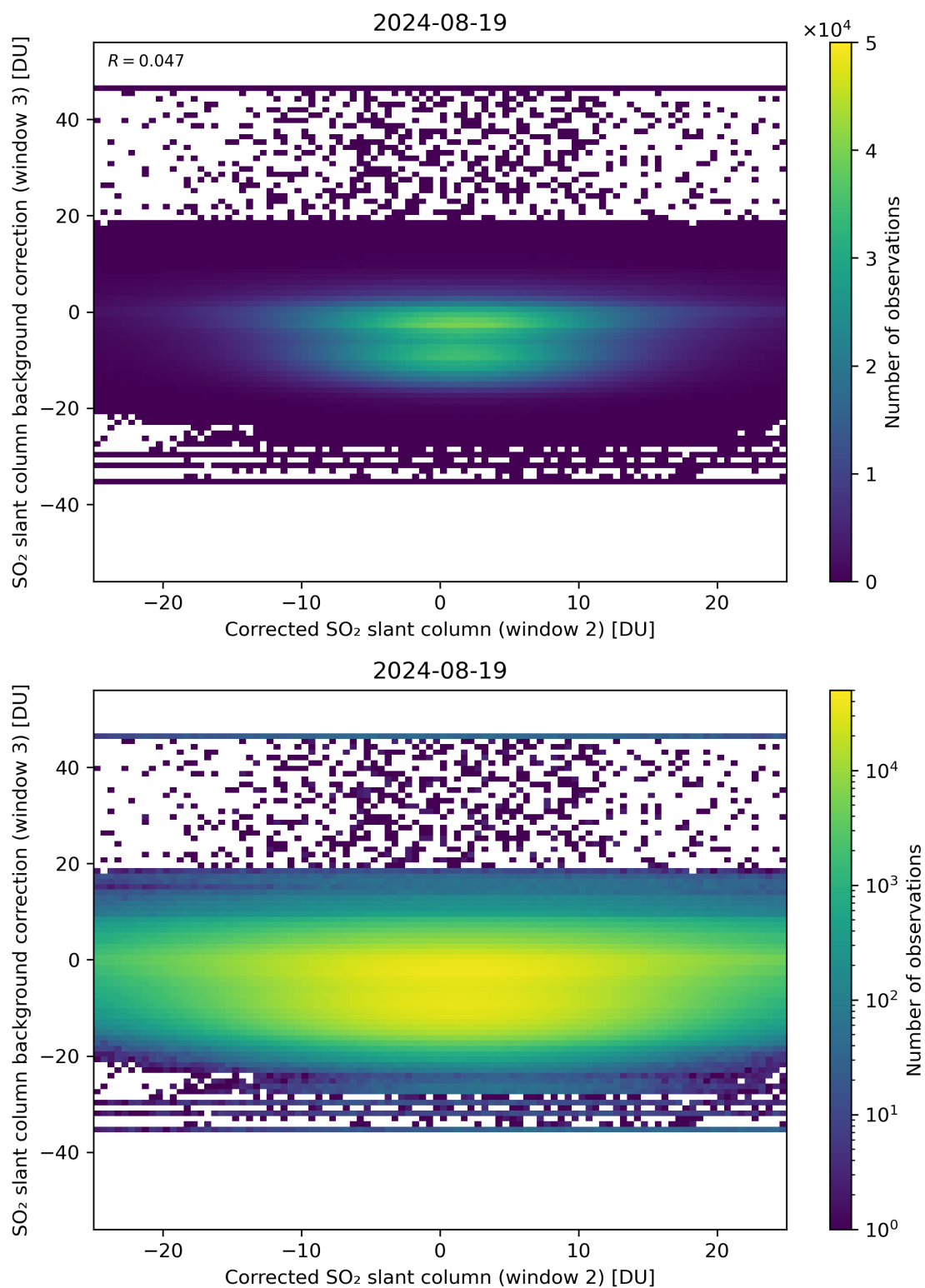
Figure 195: Scatter density plot of “Corrected SO 2 slant column (window 2)” against “SO 2 slant column background correction (window 3)” for 2024-08-18 to 2024-08-20.
