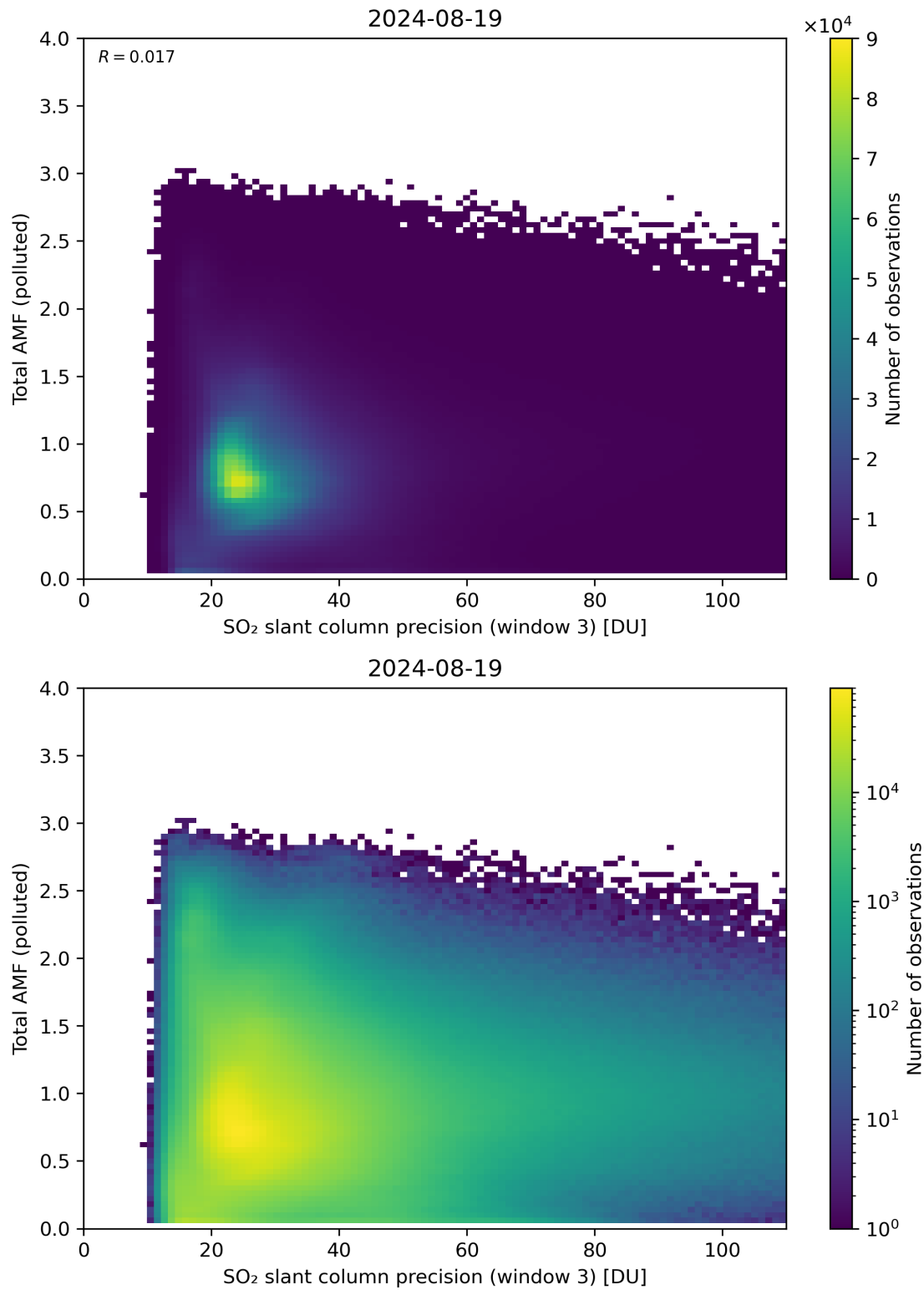
Figure 263: Scatter density plot of “SO 2 slant column precision (window 3)” against “Total AMF (polluted)” for 2024-08-18 to 2024-08-20.
