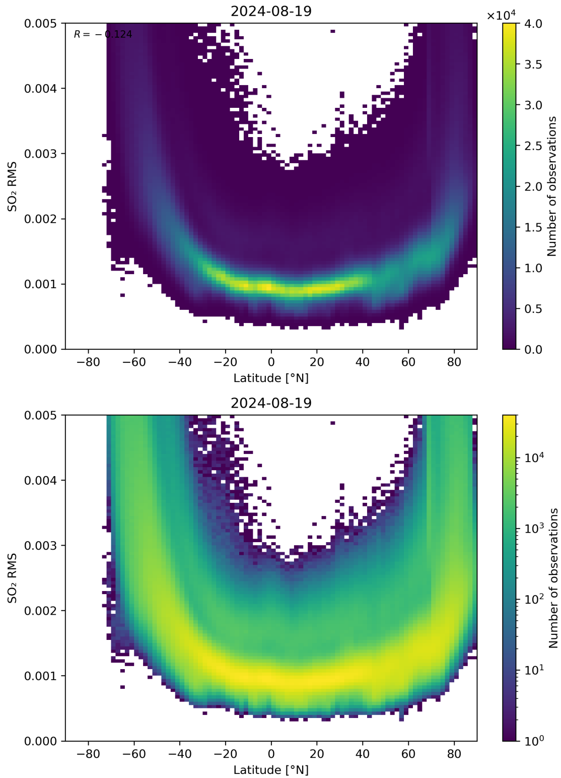
Figure 144: Scatter density plot of “Latitude” against “SO 2 RMS” for 2024-08-18 to 2024-08-20.
