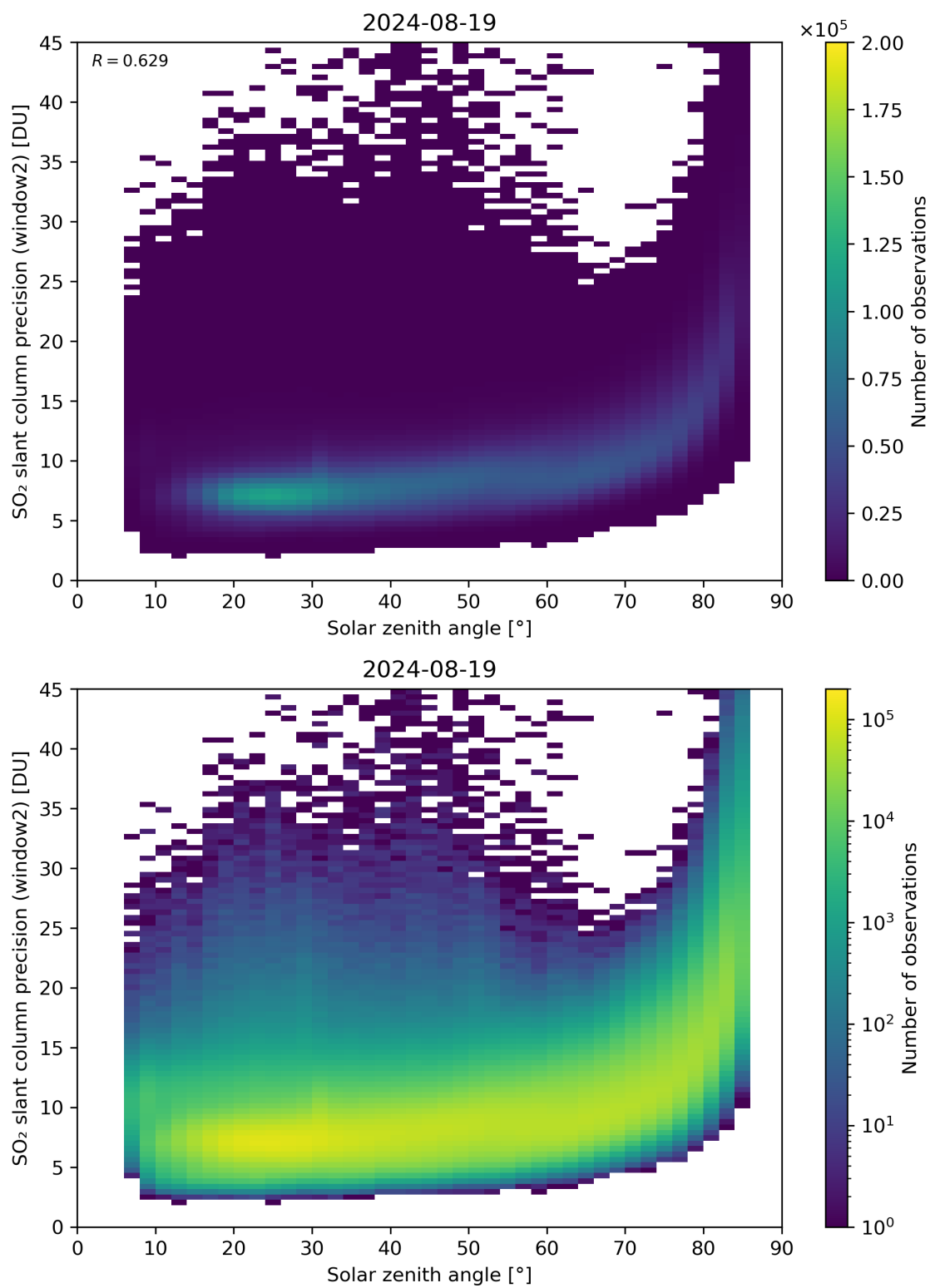
Figure 171: Scatter density plot of “Solar zenith angle” against “SO 2 slant column precision (window2)” for 2024-08-18 to 2024-08-20.
