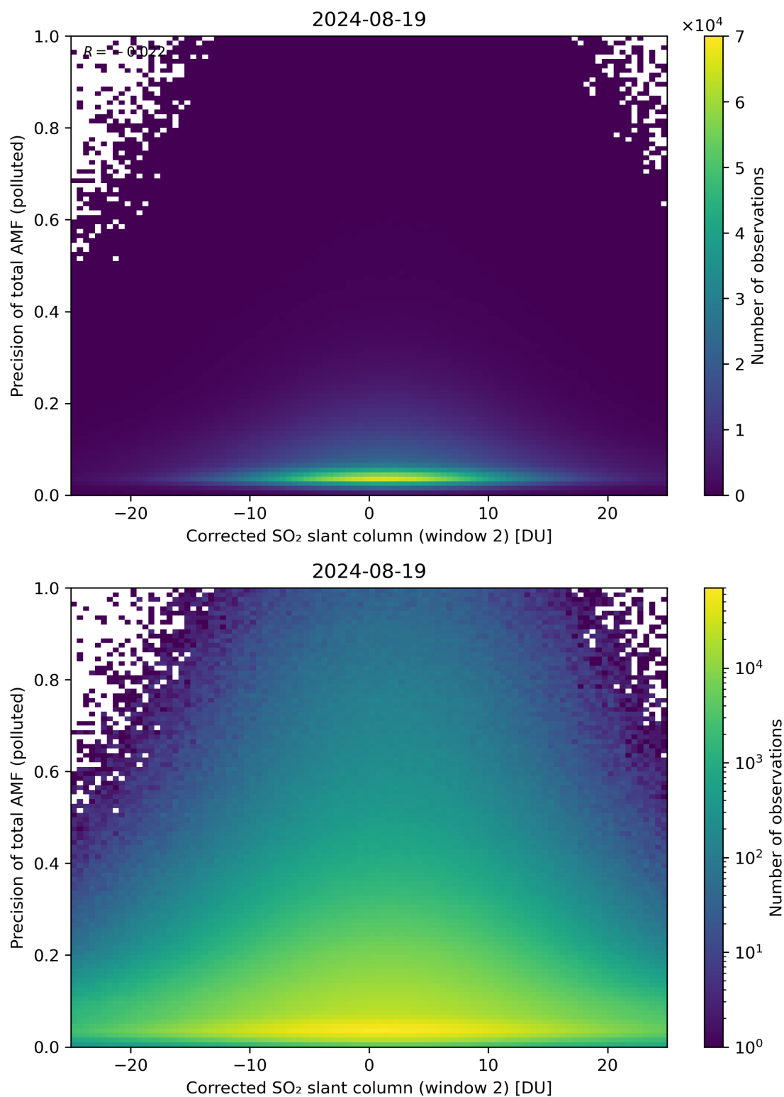
Figure 204: Scatter density plot of “Corrected SO 2 slant column (window 2)” against “Precision of total AMF (polluted)” for 2024-08-18 to 2024-08-20.
