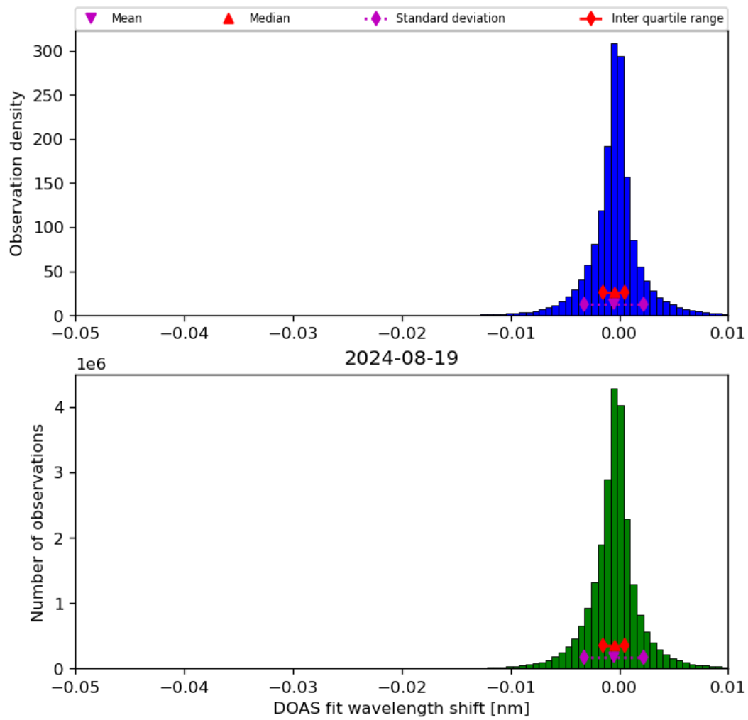
Figure 68: Histogram of “DOAS fit wavelength shift” for 2024-08-18 to 2024-08-20
