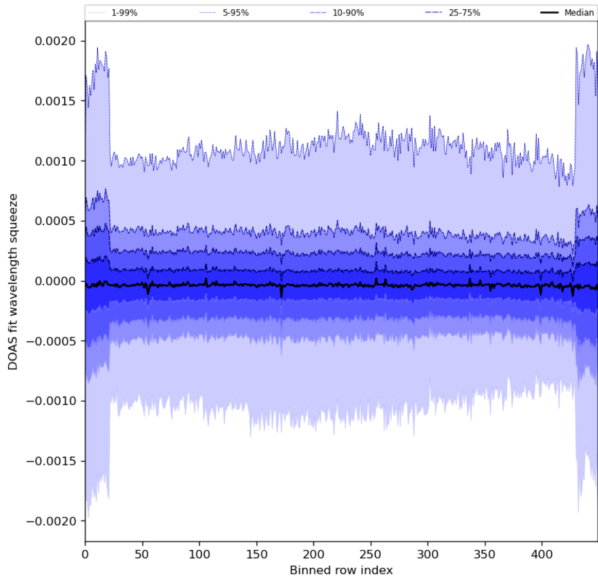
Figure 92: Along track statistics of “DOAS fit wavelength squeeze” for 2024-08-18 to 2024-08-20
