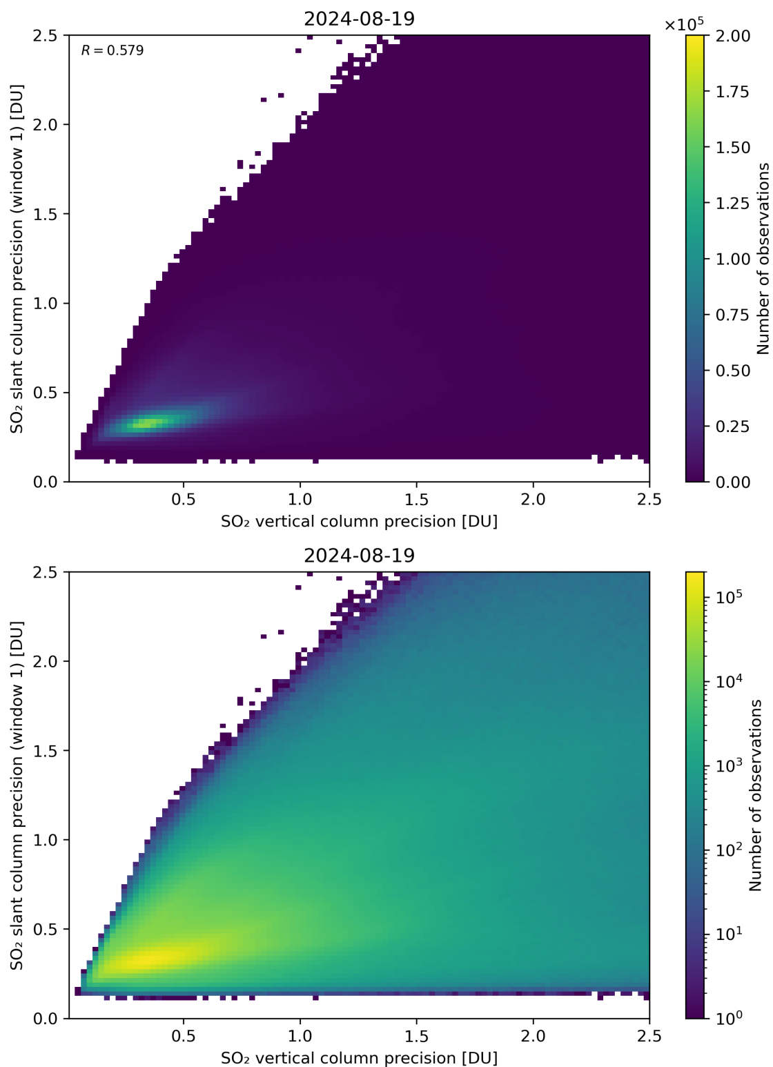
Figure 290: Scatter density plot of “SO 2 vertical column precision” against “SO 2 slant column precision (window 1)” for 2024-08-18 to 2024-08-20.
