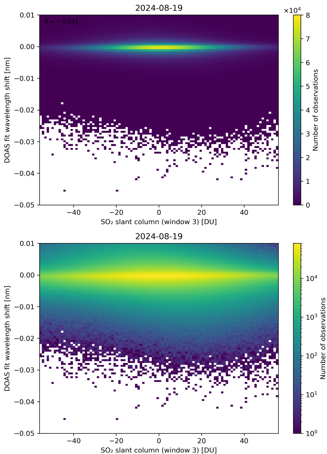
Figure 254: Scatter density plot of “SO 2 slant column (window 3)” against “DOAS fit wavelength shift” for 2024-08-18 to 2024-08-20.
