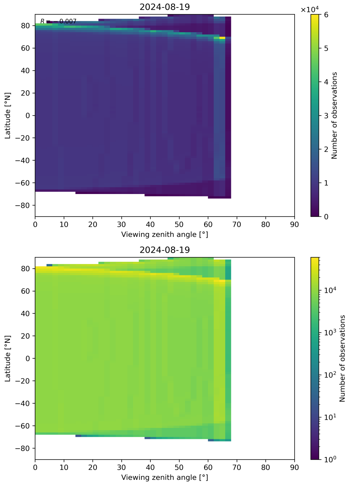
Figure 314: Scatter density plot of “Viewing zenith angle” against “Latitude” for 2024-08-18 to 2024-08-20.
