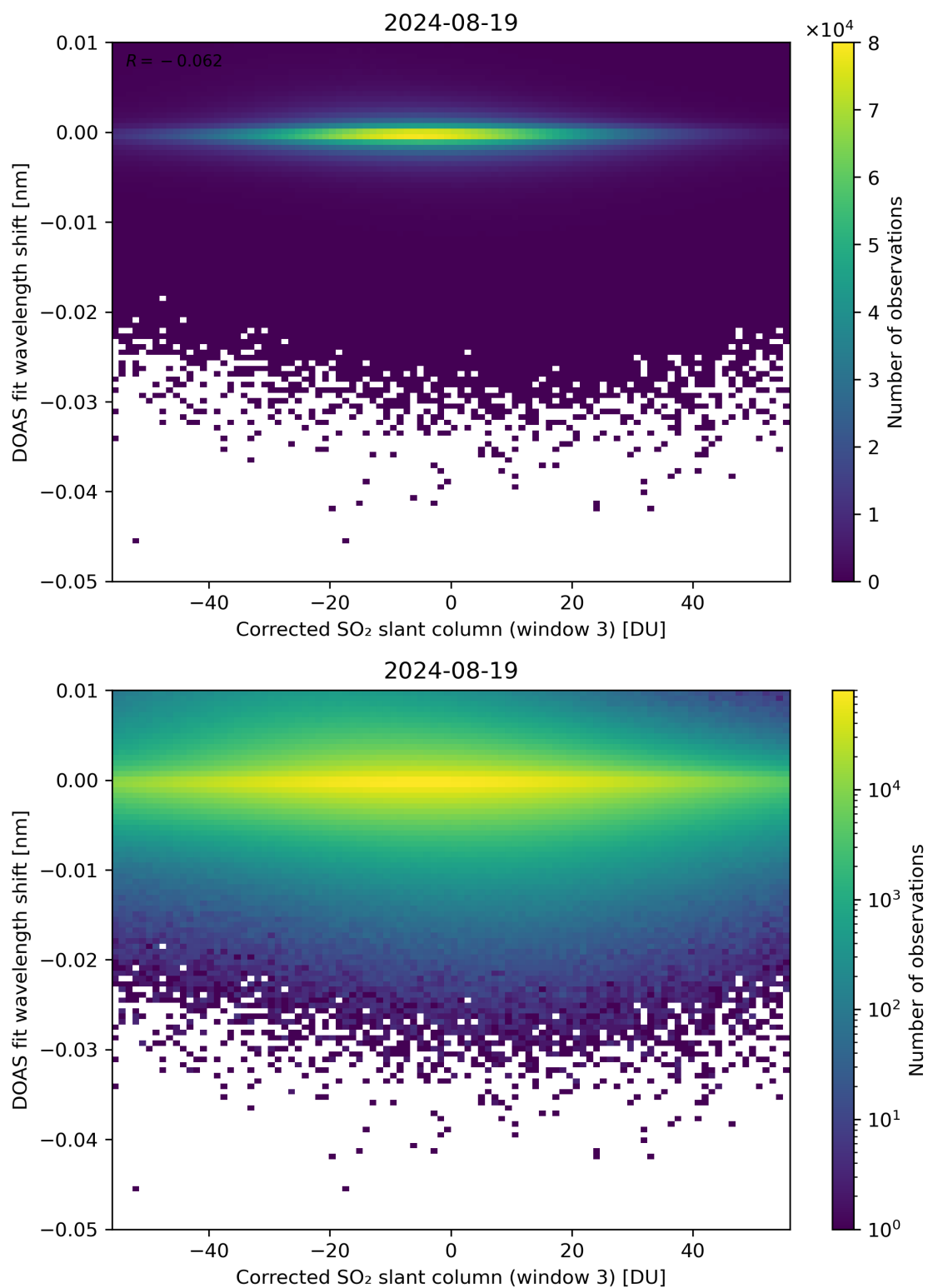
Figure 206: Scatter density plot of “Corrected SO 2 slant column (window 3)” against “DOAS fit wavelength shift” for 2024-08-18 to 2024-08-20.
