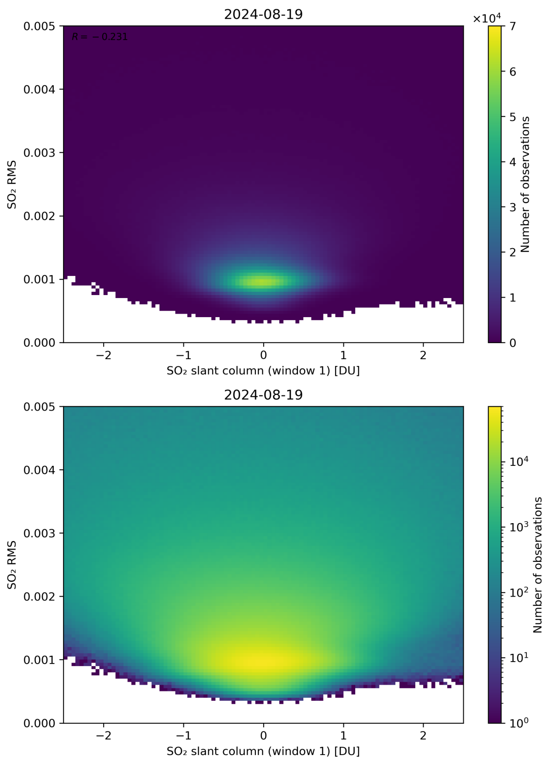
Figure 217: Scatter density plot of “SO 2 slant column (window 1)” against “SO 2 RMS” for 2024-08-18 to 2024-08-20.
