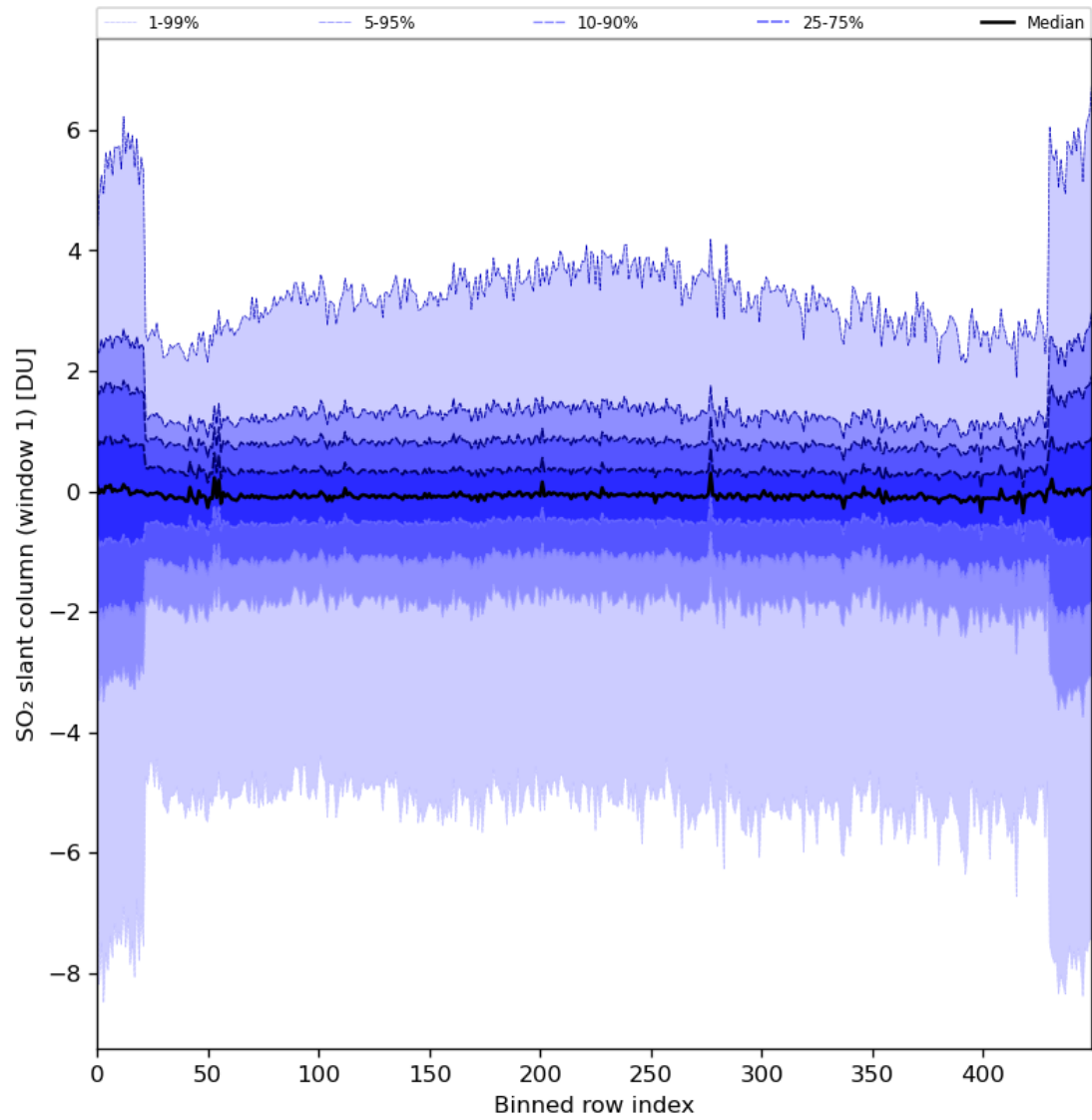
Figure 79: Along track statistics of “SO 2 slant column (window 1)” for 2024-08-18 to 2024-08-20
