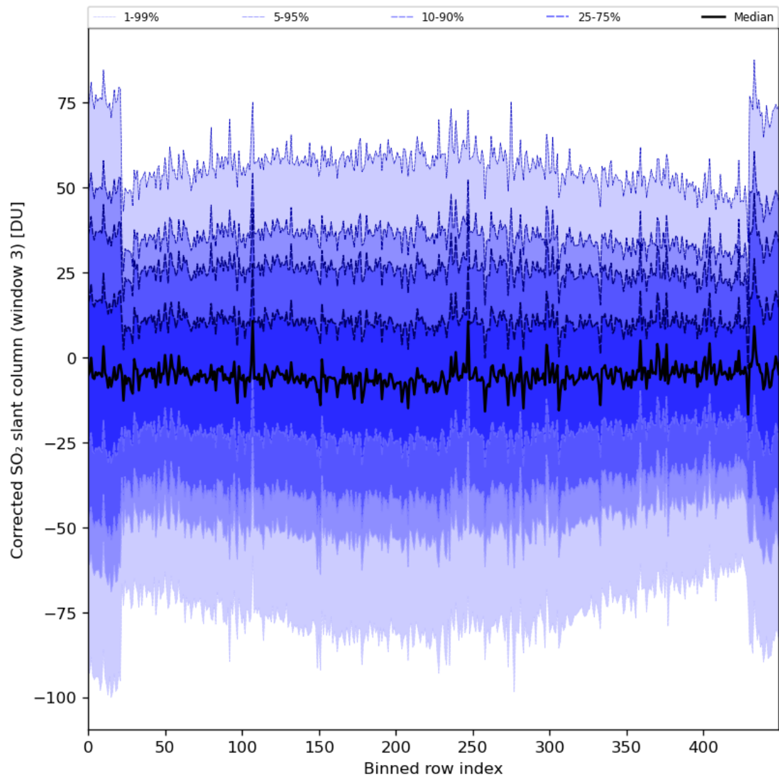
Figure 89: Along track statistics of “Corrected SO 2 slant column (window 3)” for 2024-08-18 to 2024-08-20
