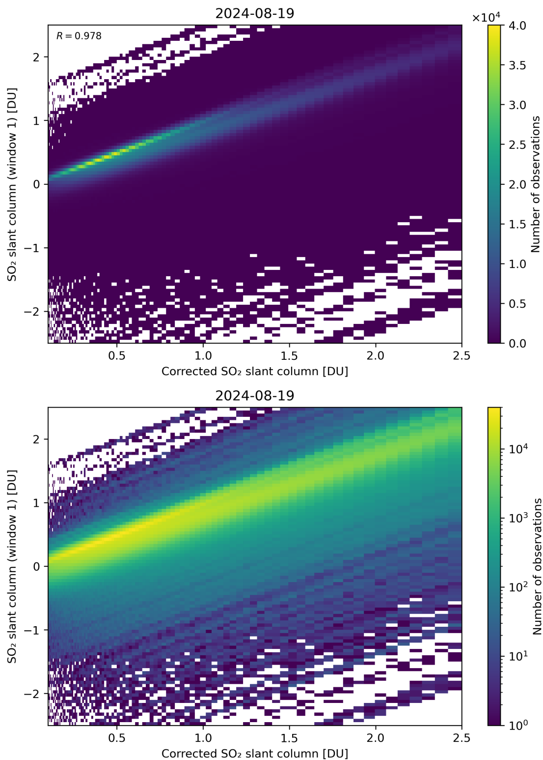
Figure 187: Scatter density plot of “Corrected SO 2 slant column” against “SO 2 slant column (window 1)” for 2024-08-18 to 2024-08-20.
