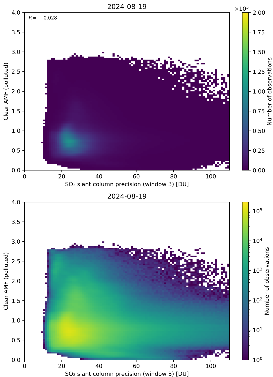
Figure 261: Scatter density plot of “SO 2 slant column precision (window 3)” against “Clear AMF (polluted)” for 2024-08-18 to 2024-08-20.
