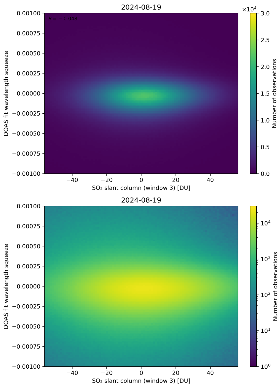
Figure 255: Scatter density plot of “SO 2 slant column (window 3)” against “DOAS fit wavelength squeeze” for 2024-08-18 to 2024-08-20.
