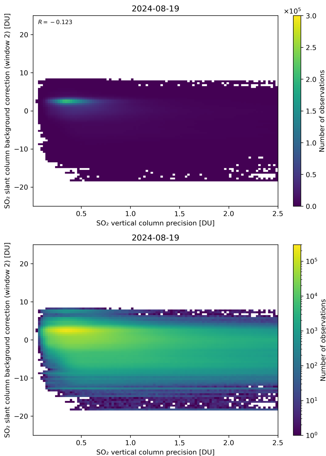
Figure 280: Scatter density plot of “SO 2 vertical column precision” against “SO 2 slant column background correction (window 2)” for 2024-08-18 to 2024-08-20.
