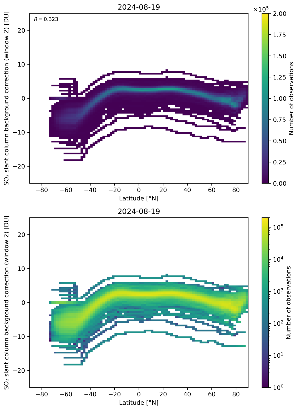
Figure 140: Scatter density plot of “Latitude” against “SO 2 slant column background correction (window 2)” for 2024-08-18 to 2024-08-20.
