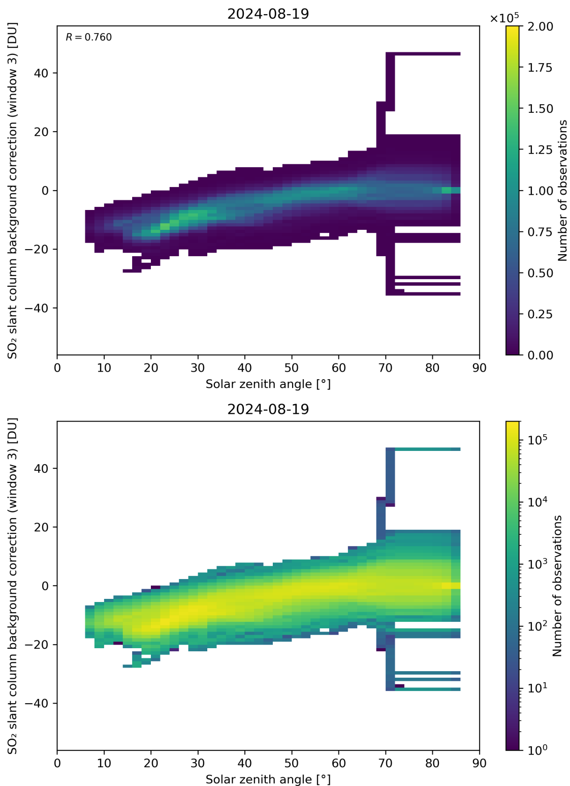
Figure 160: Scatter density plot of “Solar zenith angle” against “SO 2 slant column background correction (window 3)” for 2024-08-18 to 2024-08-20.
