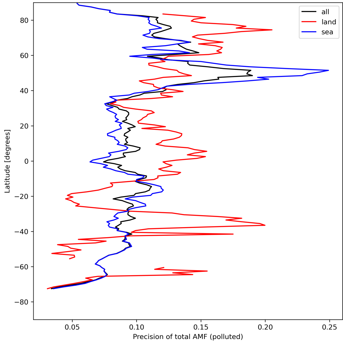
Figure 49: Zonal average of “Precision of total AMF (polluted)” for 2024-08-18 to 2024-08-20.
