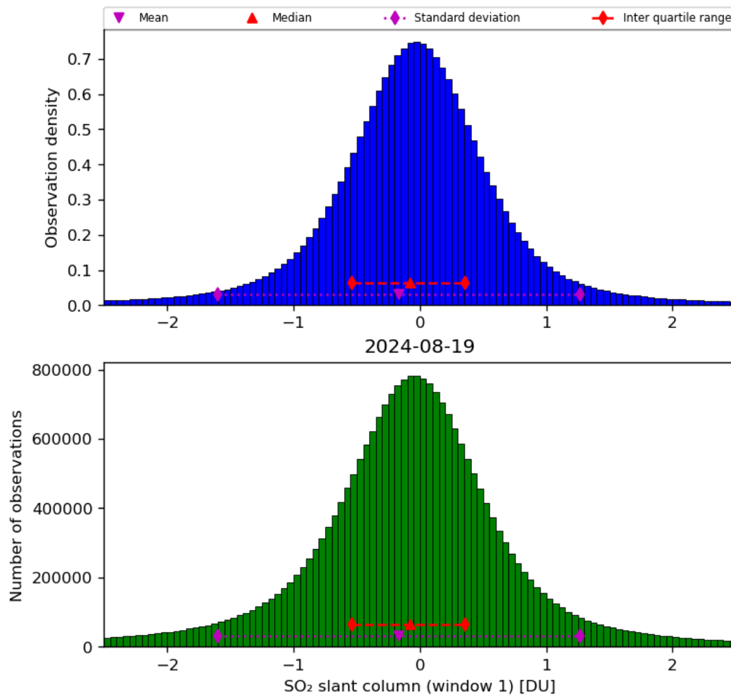
Figure 56: Histogram of “SO 2 slant column (window 1)” for 2024-08-18 to 2024-08-20
