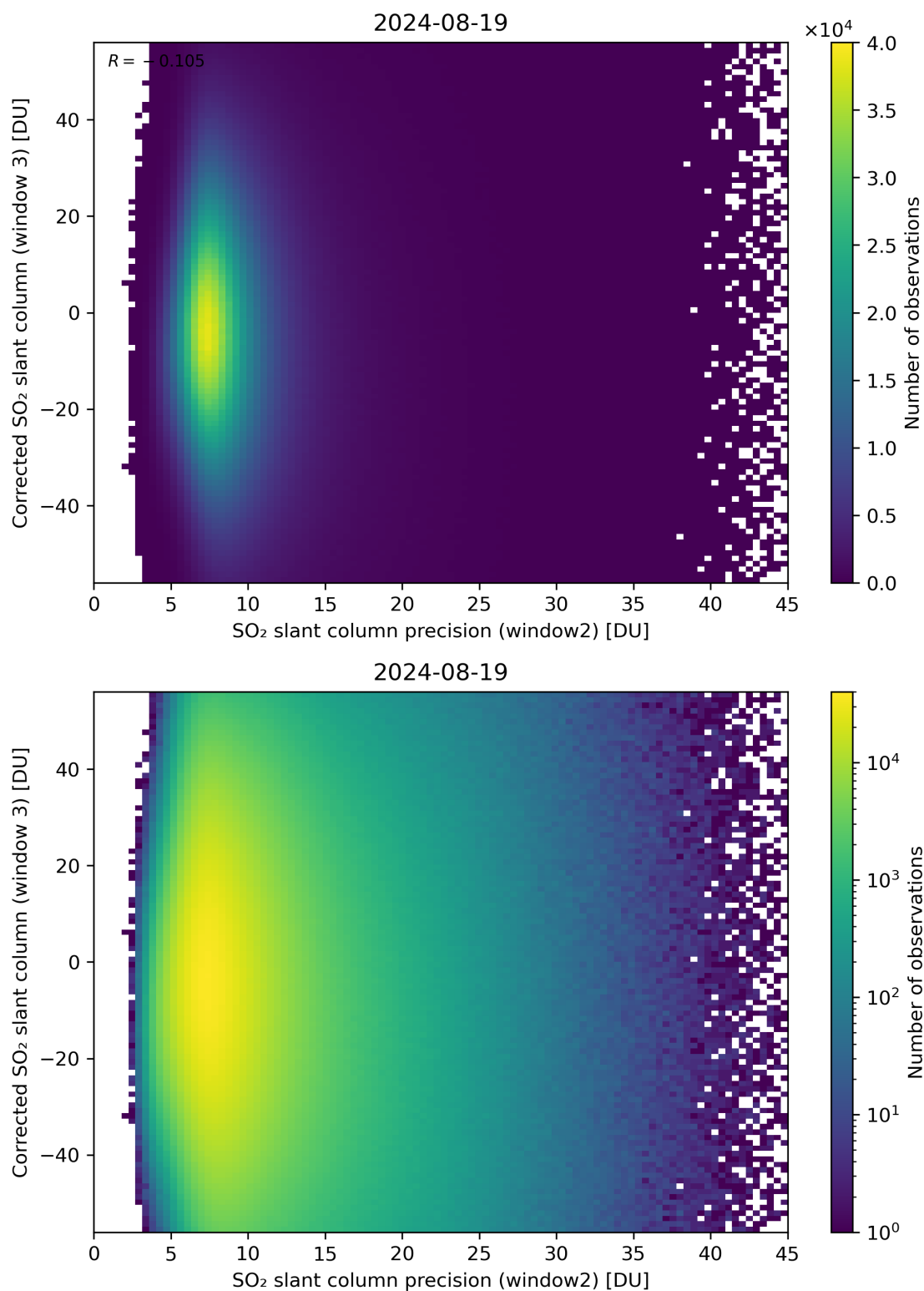
Figure 248: Scatter density plot of “SO 2 slant column precision (window2)” against “Corrected SO 2 slant column (window 3)” for 2024-08-18 to 2024-08-20.
