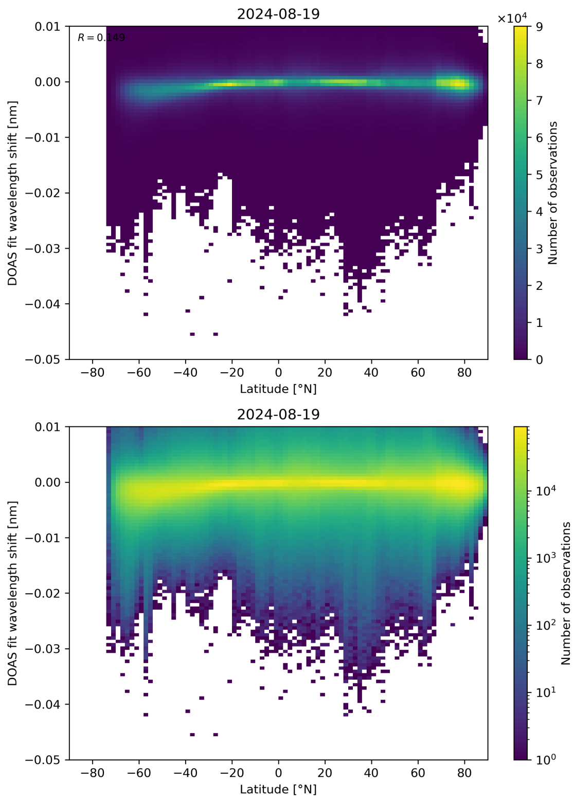
Figure 142: Scatter density plot of “Latitude” against “DOAS fit wavelength shift” for 2024-08-18 to 2024-08-20.
