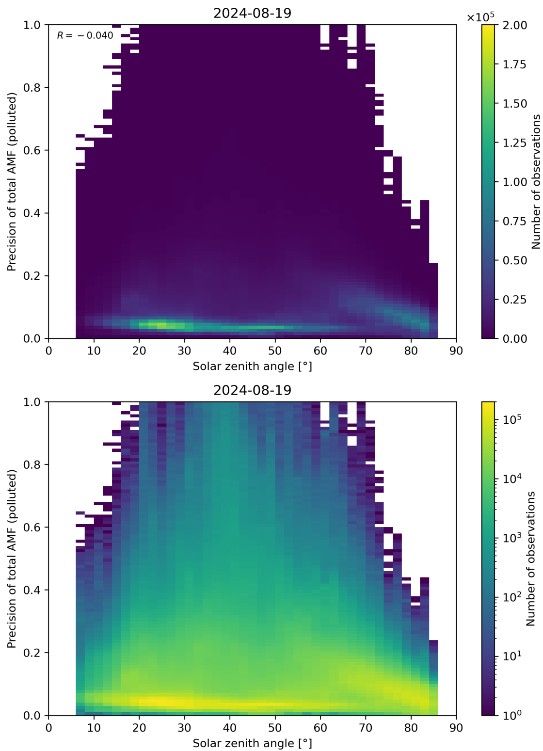
Figure 175: Scatter density plot of “Solar zenith angle” against “Precision of total AMF (polluted)” for 2024-08-18 to 2024-08-20.
