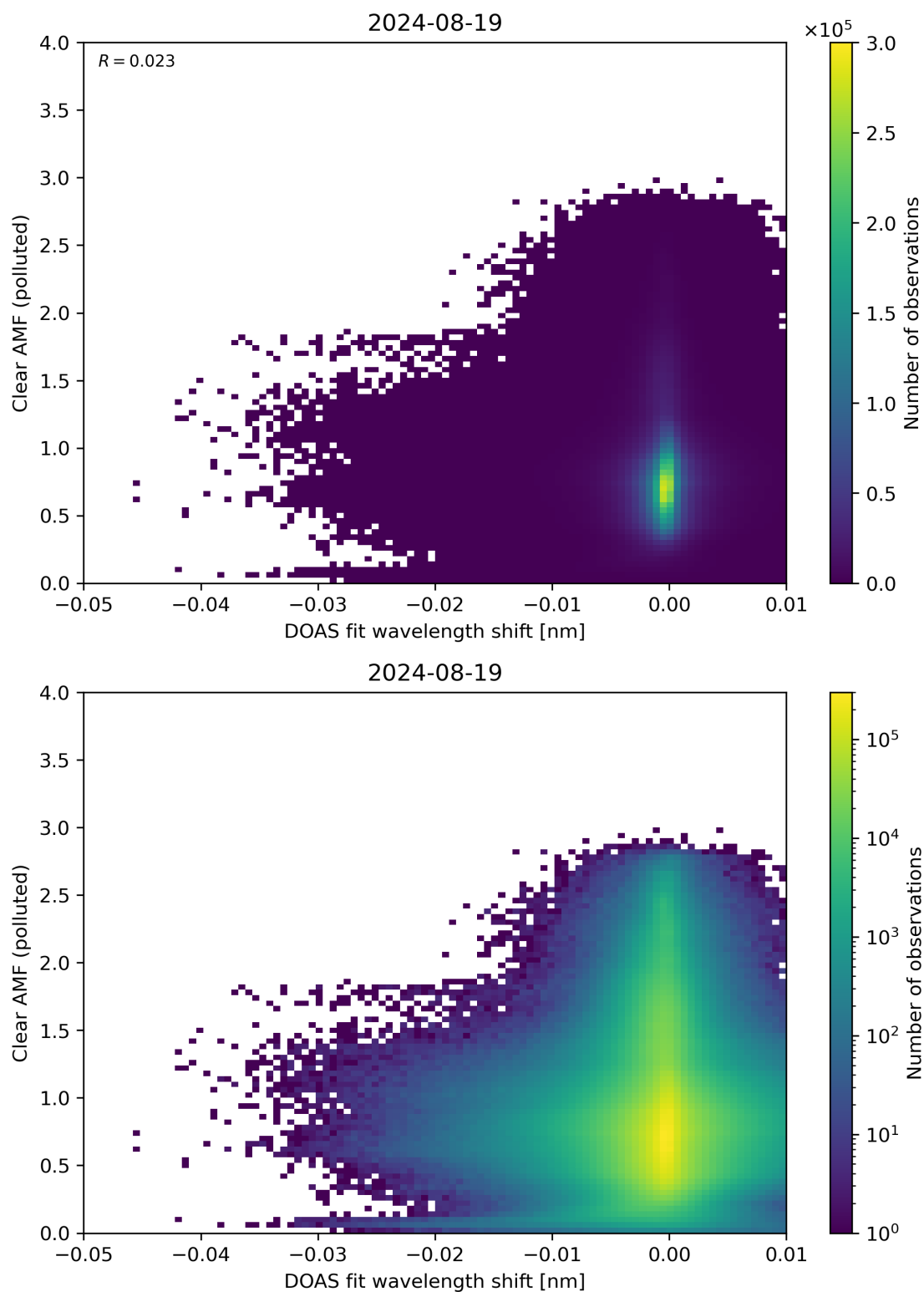
Figure 129: Scatter density plot of “DOAS fit wavelength shift” against “Clear AMF (polluted)” for 2024-08-18 to 2024-08-20.
