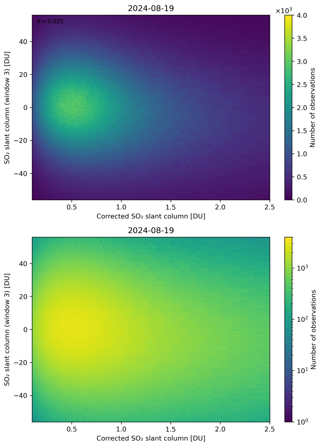
Figure 190: Scatter density plot of “Corrected SO 2 slant column” against “SO 2 slant column (window 3)” for 2024-08-18 to 2024-08-20.
