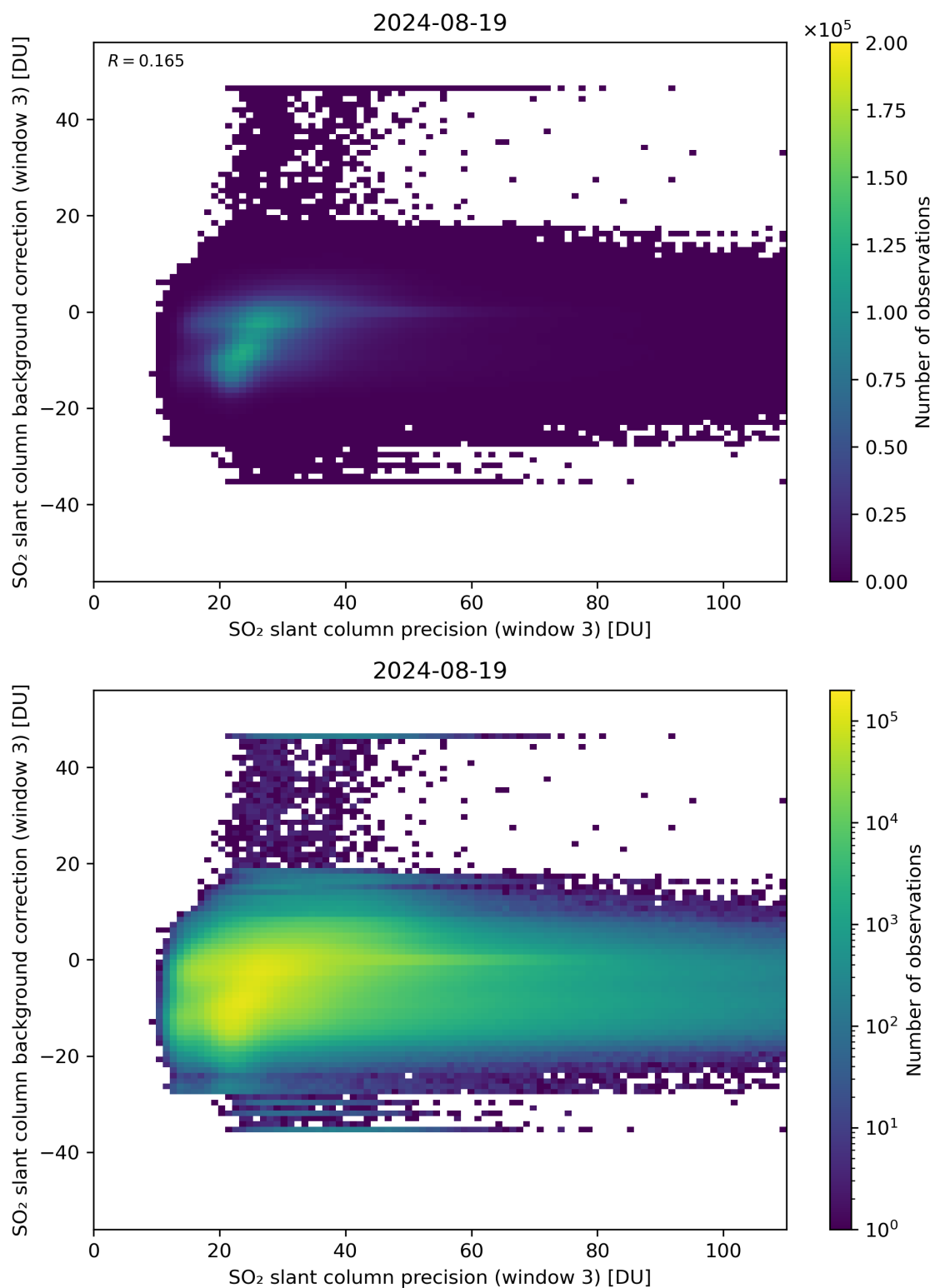
Figure 257: Scatter density plot of “SO 2 slant column precision (window 3)” against “SO 2 slant column background correction (window 3)” for 2024-08-18 to 2024-08-20.
