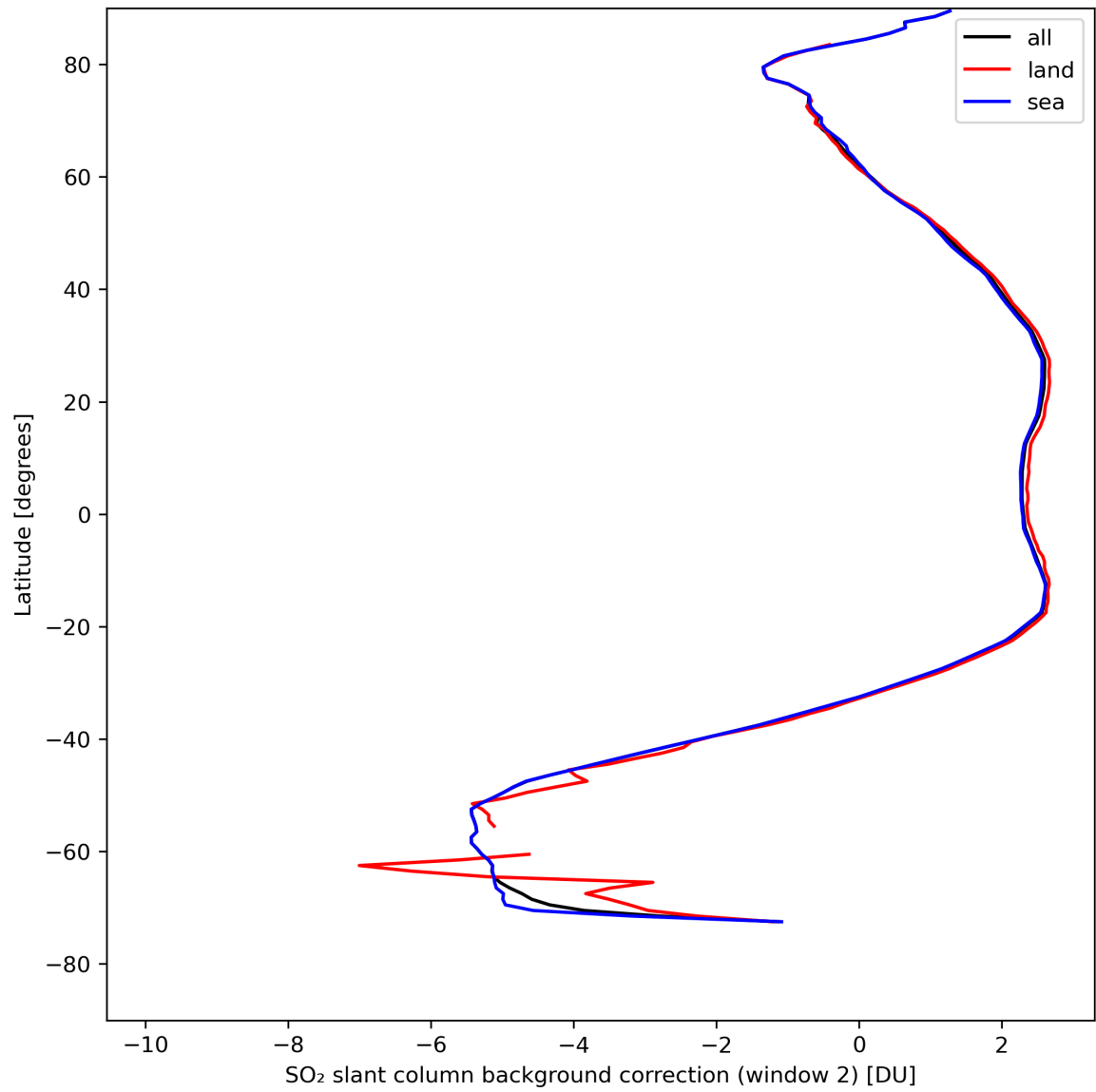
Figure 40: Zonal average of “SO 2 slant column background correction (window 2)” for 2024-08-18 to 2024-08-20.
