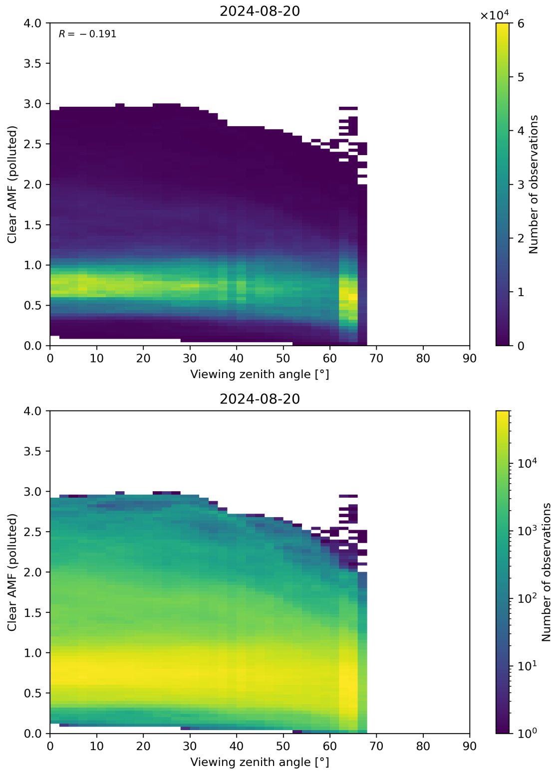
Figure 316: Scatter density plot of “Viewing zenith angle” against “Clear AMF (polluted)” for 2024-08-19 to 2024-08-21.
