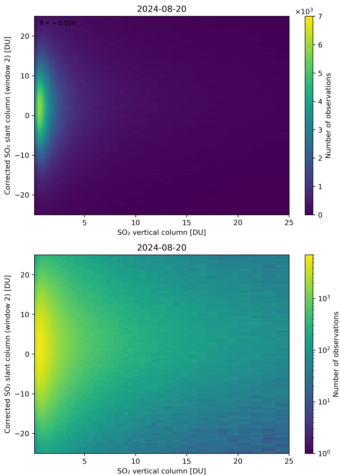
Figure 298: Scatter density plot of “SO 2 vertical column” against “Corrected SO 2 slant column (window 2)” for 2024-08-19 to 2024-08-21.
