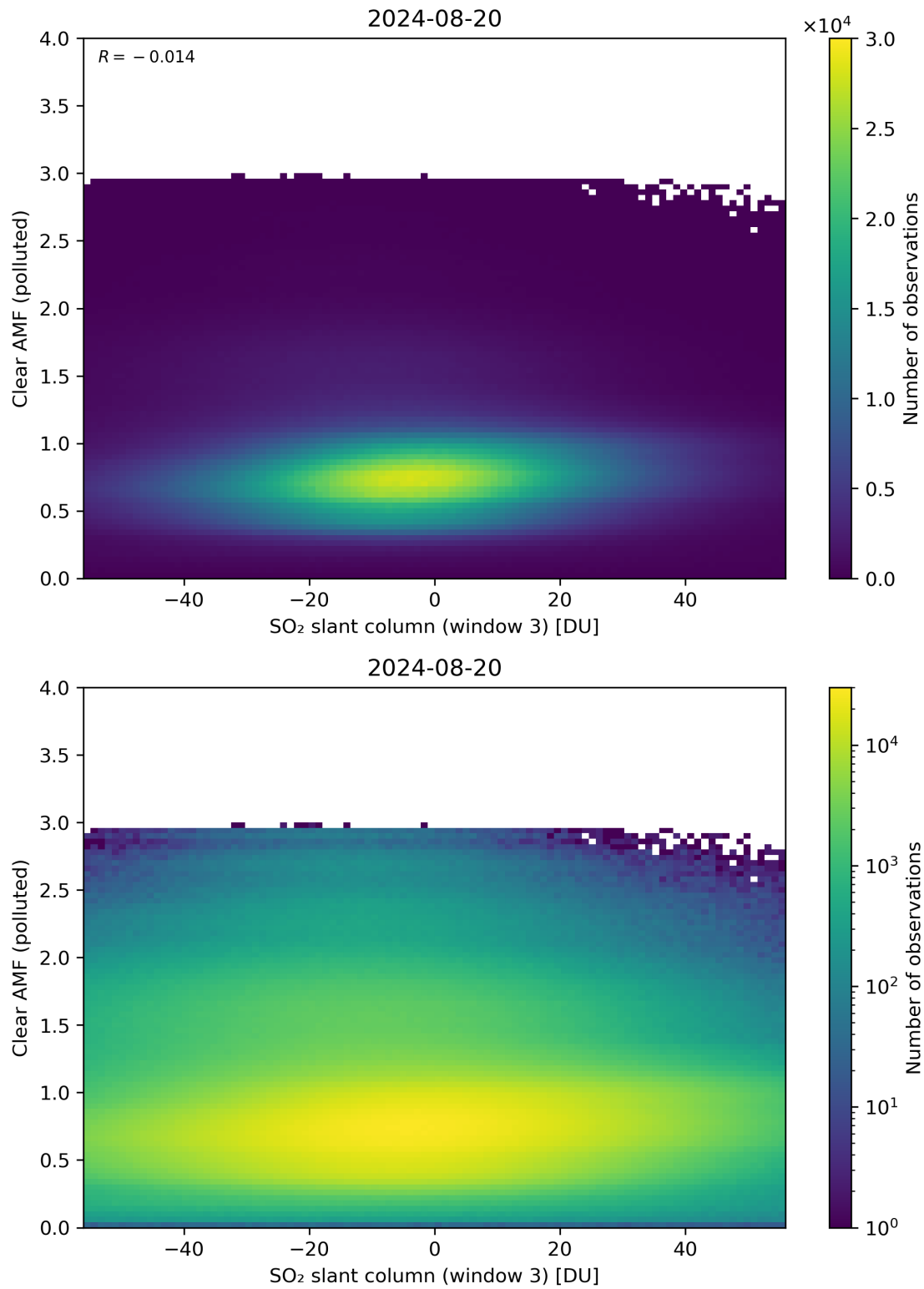
Figure 265: Scatter density plot of “SO 2 slant column (window 3)” against “Clear AMF (polluted)” for 2024-08-19 to 2024-08-21.
