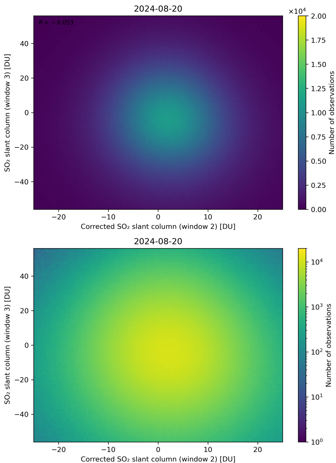
Figure 201: Scatter density plot of “Corrected SO 2 slant column (window 2)” against “SO 2 slant column (window 3)” for 2024-08-19 to 2024-08-21.
