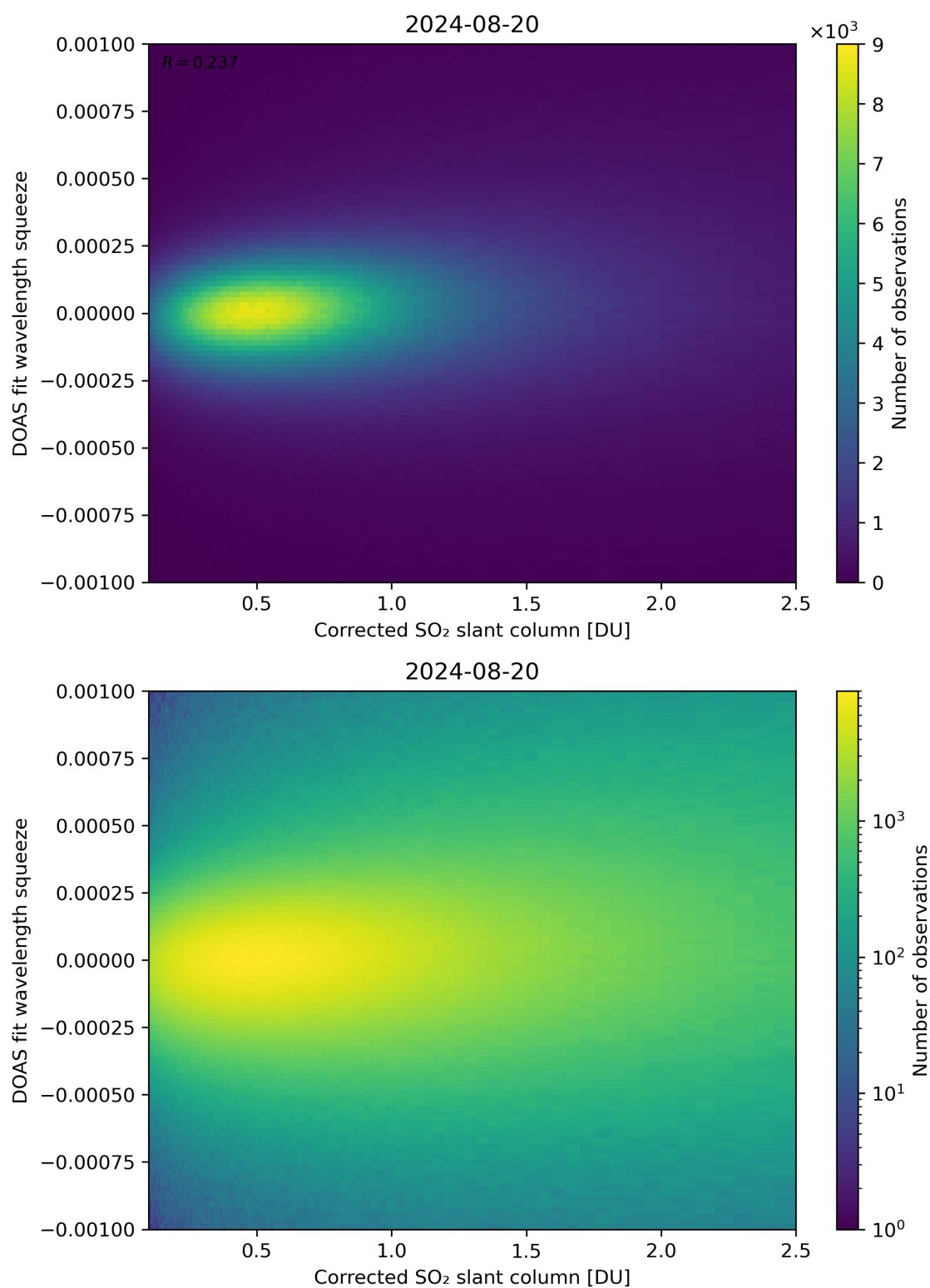
Figure 182: Scatter density plot of “Corrected SO 2 slant column” against “DOAS fit wavelength squeeze” for 2024-08-19 to 2024-08-21.
