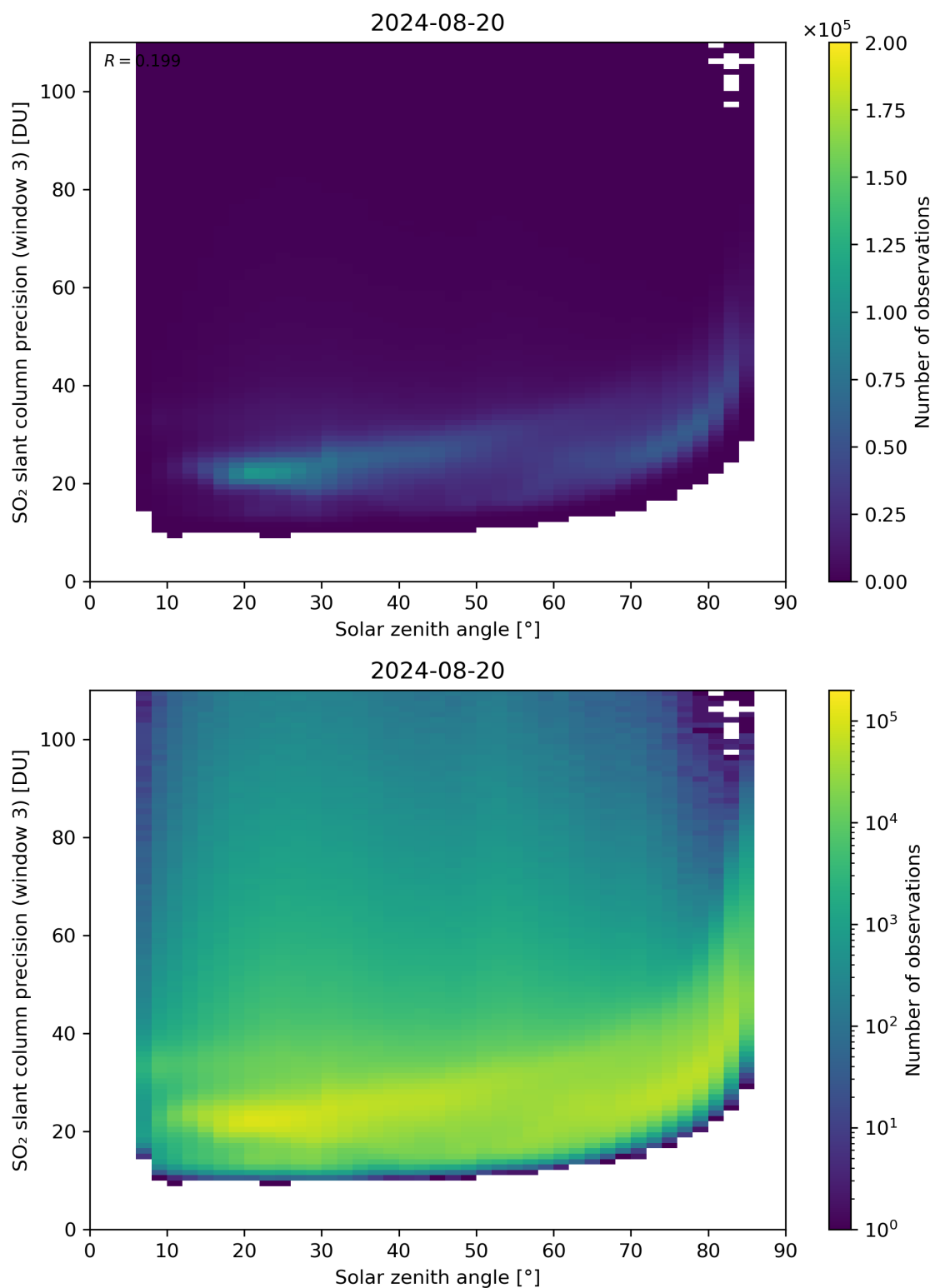
Figure 173: Scatter density plot of “Solar zenith angle” against “SO 2 slant column precision (window 3)” for 2024-08-19 to 2024-08-21.
