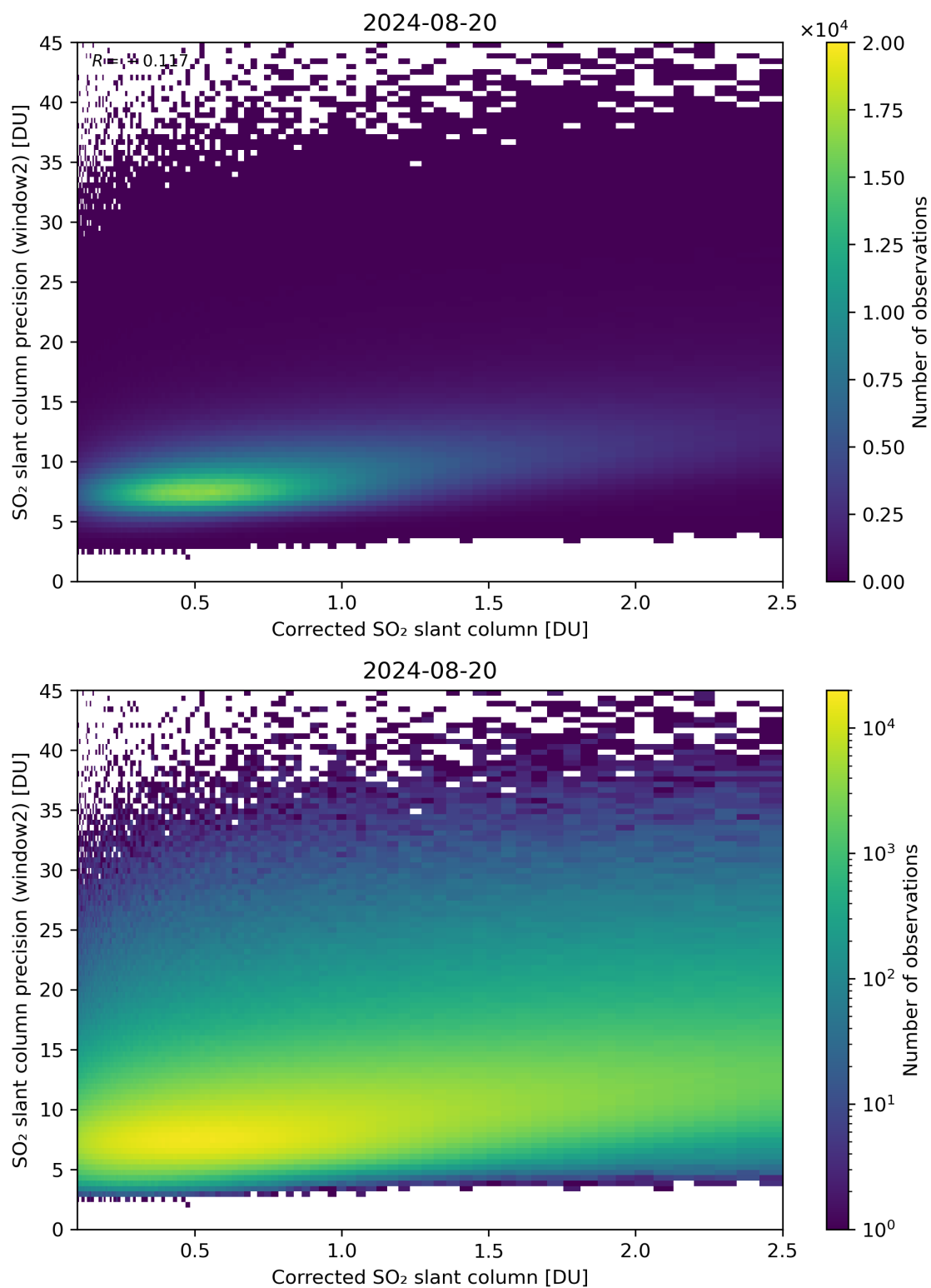
Figure 189: Scatter density plot of “Corrected SO 2 slant column” against “SO 2 slant column precision (window2)” for 2024-08-19 to 2024-08-21.
