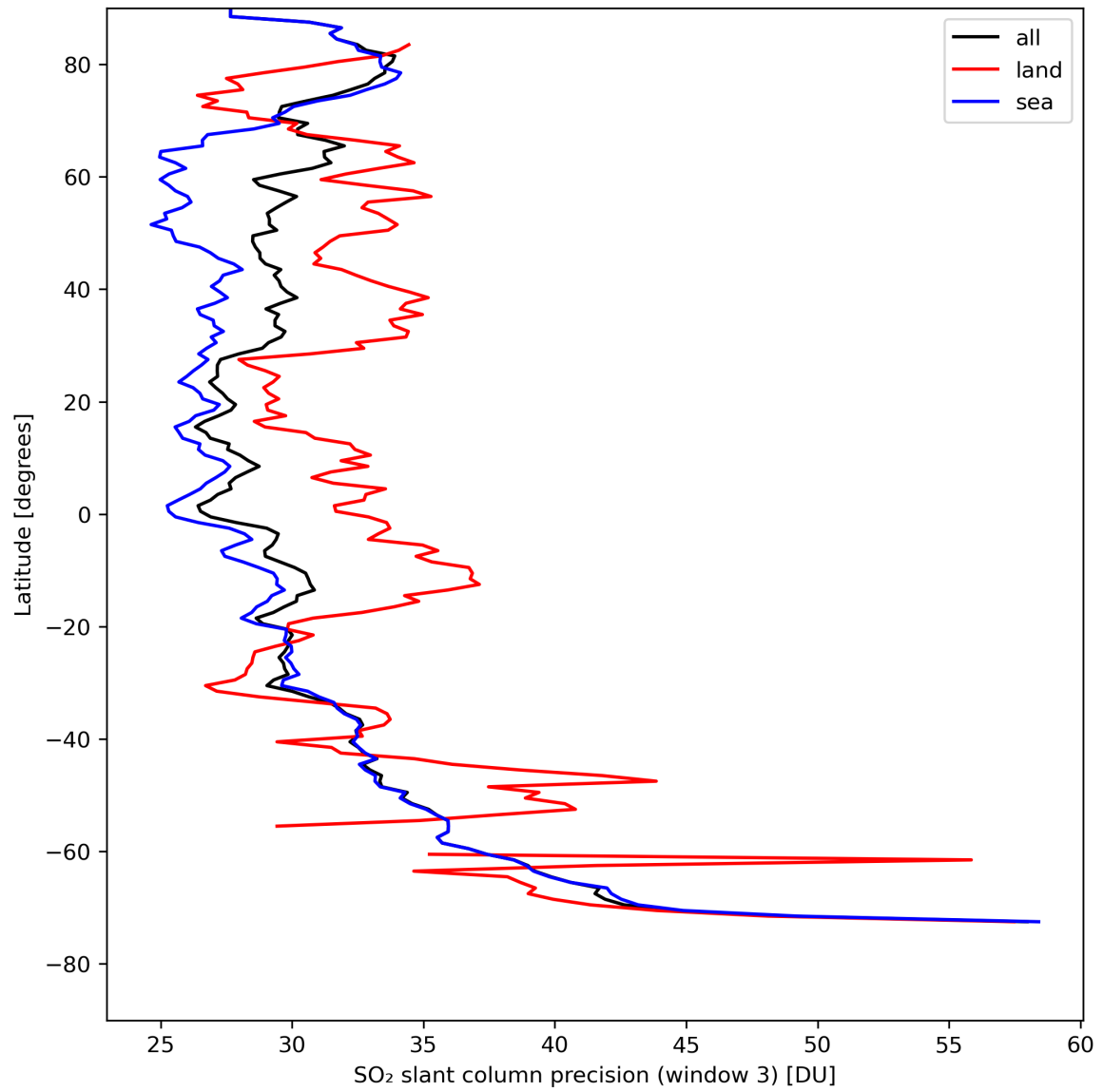
Figure 42: Zonal average of “SO 2 slant column precision (window 3)” for 2024-08-19 to 2024-08-21.
