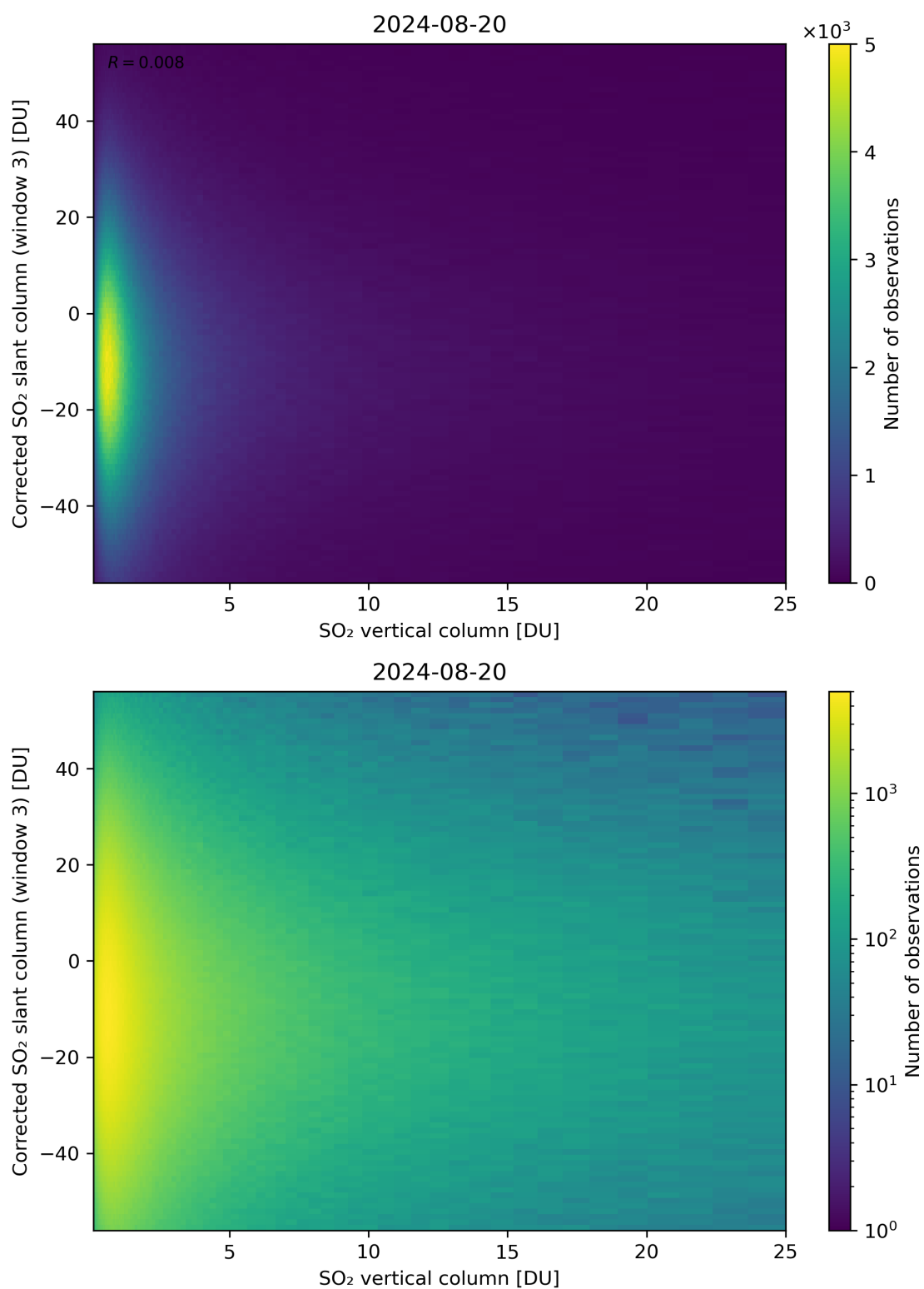
Figure 299: Scatter density plot of “SO 2 vertical column” against “Corrected SO 2 slant column (window 3)” for 2024-08-19 to 2024-08-21.
