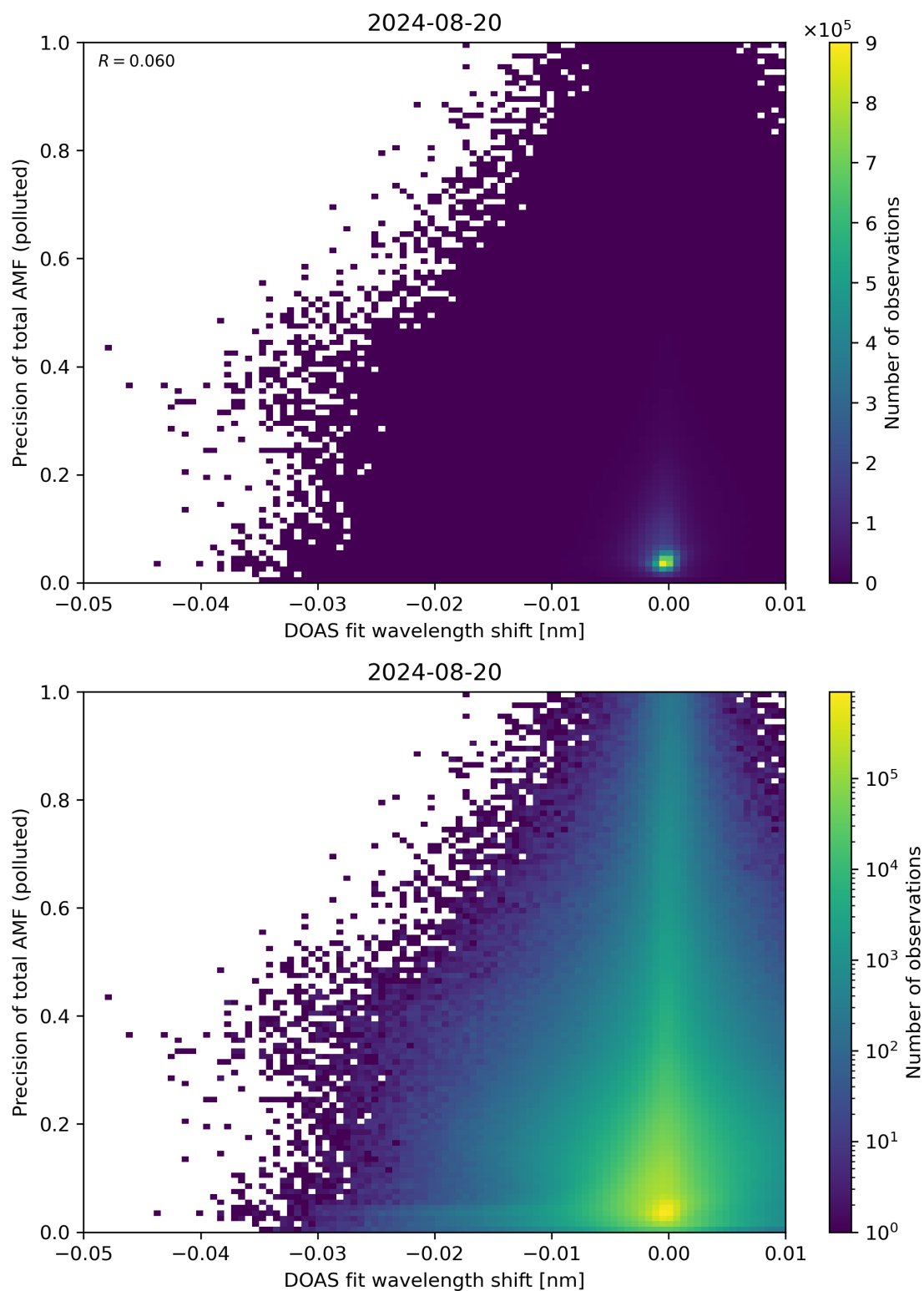
Figure 131: Scatter density plot of “DOAS fit wavelength shift” against “Precision of total AMF (polluted)” for 2024-08-19 to 2024-08-21.
