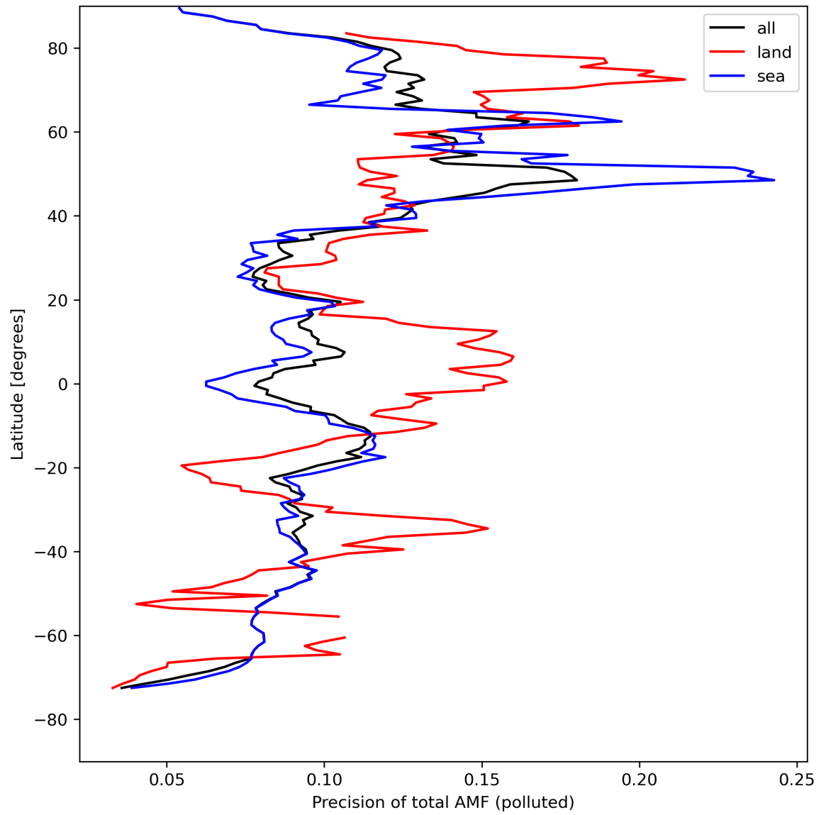
Figure 49: Zonal average of “Precision of total AMF (polluted)” for 2024-08-19 to 2024-08-21.
