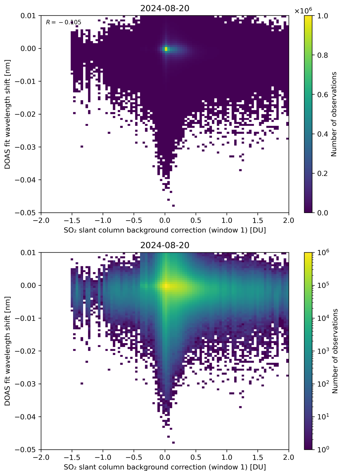
Figure 100: Scatter density plot of “SO 2 slant column background correction (window 1)” against “DOAS fit wavelength shift” for 2024-08-19 to 2024-08-21.
