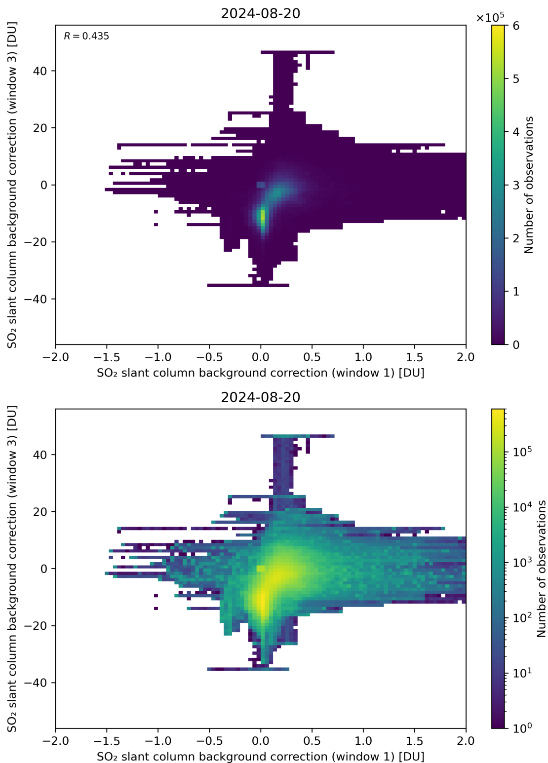
Figure 99: Scatter density plot of “SO 2 slant column background correction (window 1)” against “SO 2 slant column background correction (window 3)” for 2024-08-19 to 2024-08-21.
