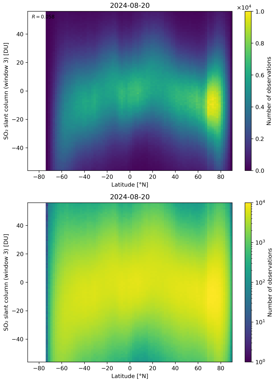
Figure 152: Scatter density plot of “Latitude” against “SO 2 slant column (window 3)” for 2024-08-19 to 2024-08-21.
