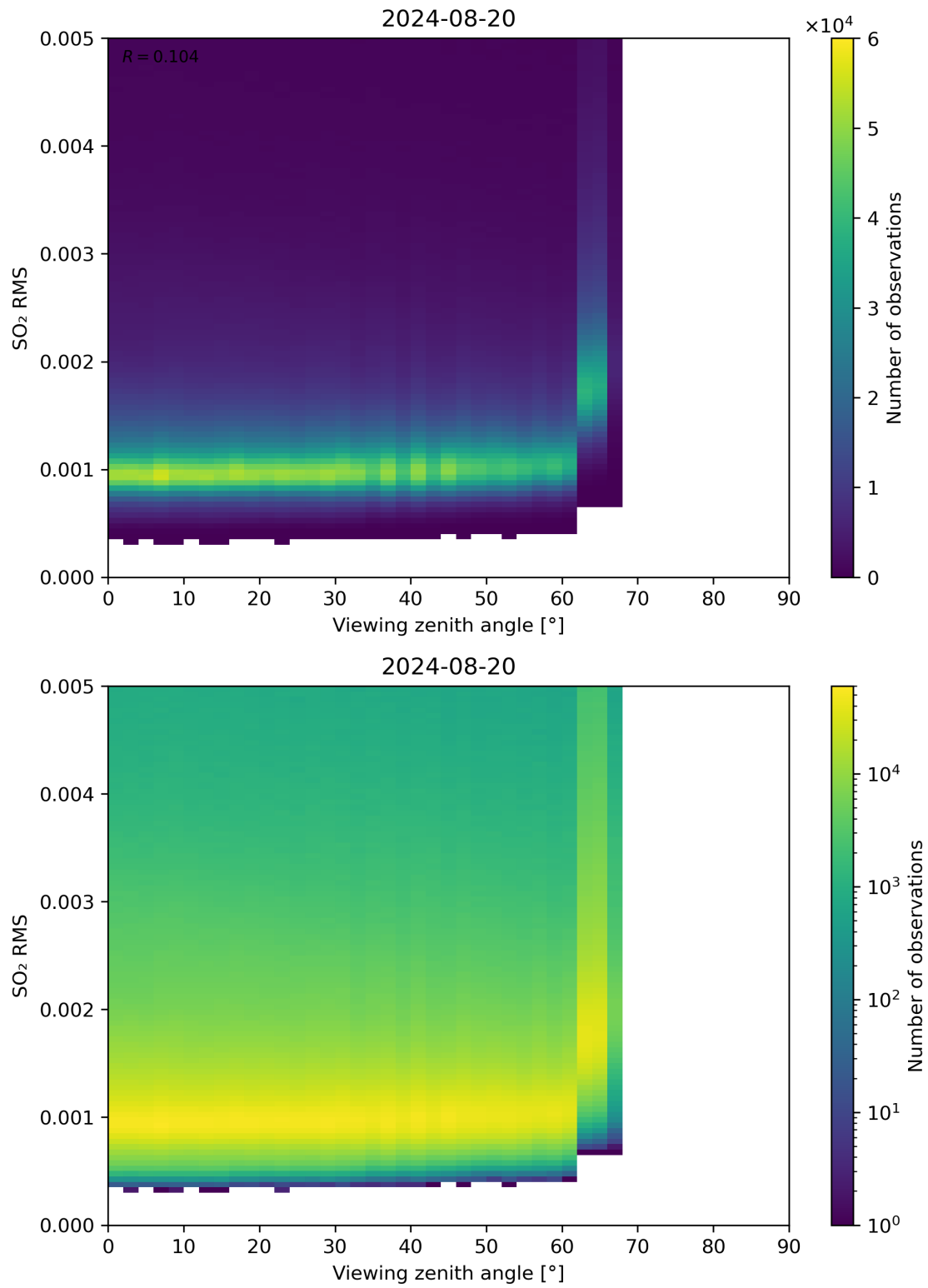
Figure 313: Scatter density plot of “Viewing zenith angle” against “SO 2 RMS” for 2024-08-19 to 2024-08-21.
