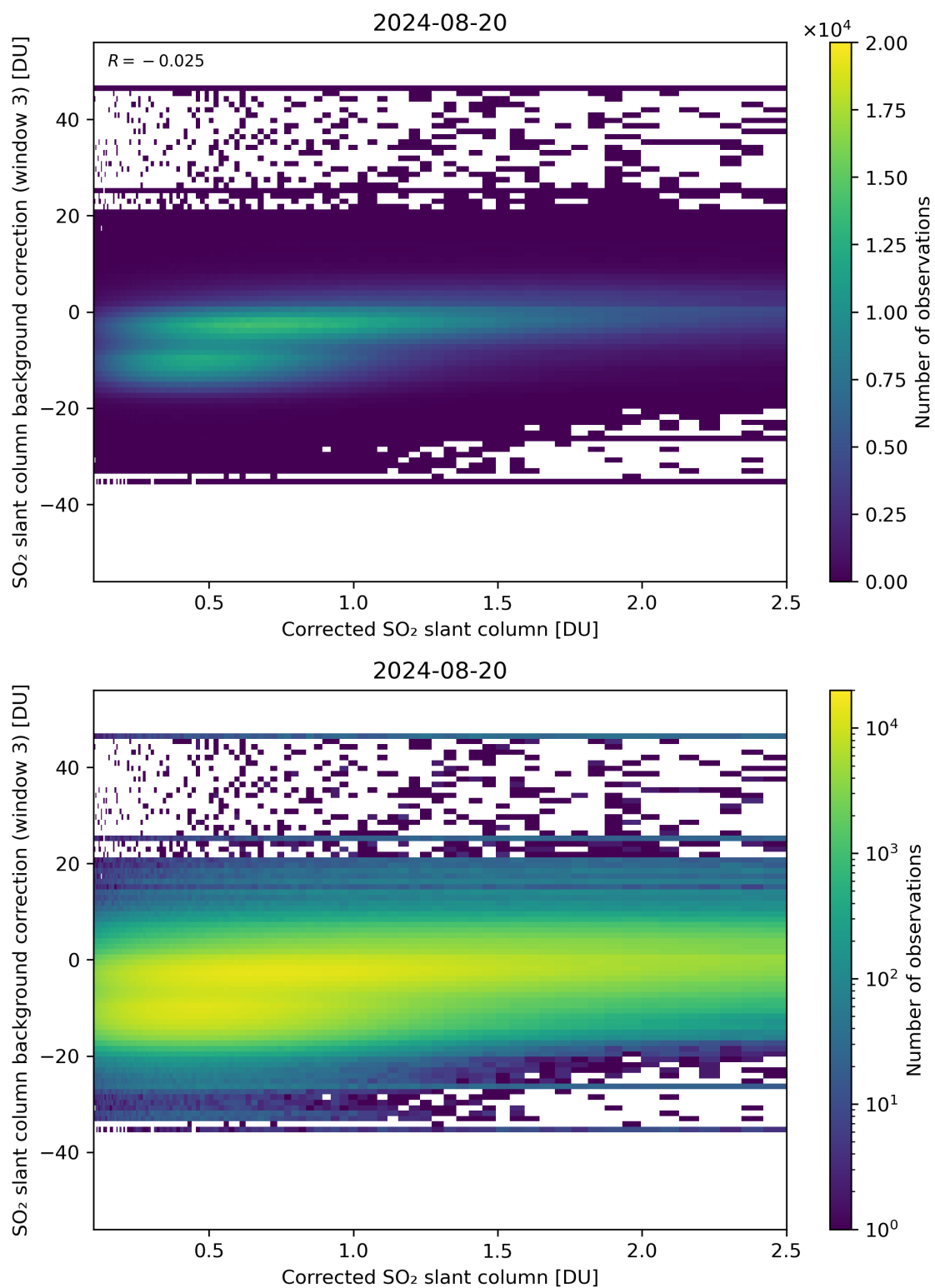
Figure 180: Scatter density plot of “Corrected SO 2 slant column” against “SO 2 slant column background correction (window 3)” for 2024-08-19 to 2024-08-21.
