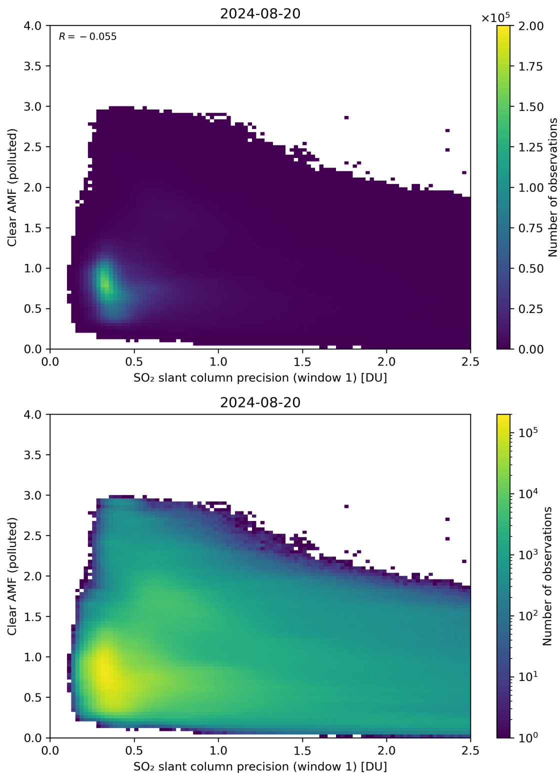
Figure 224: Scatter density plot of “SO 2 slant column precision (window 1)” against “Clear AMF (polluted)” for 2024-08-19 to 2024-08-21.
