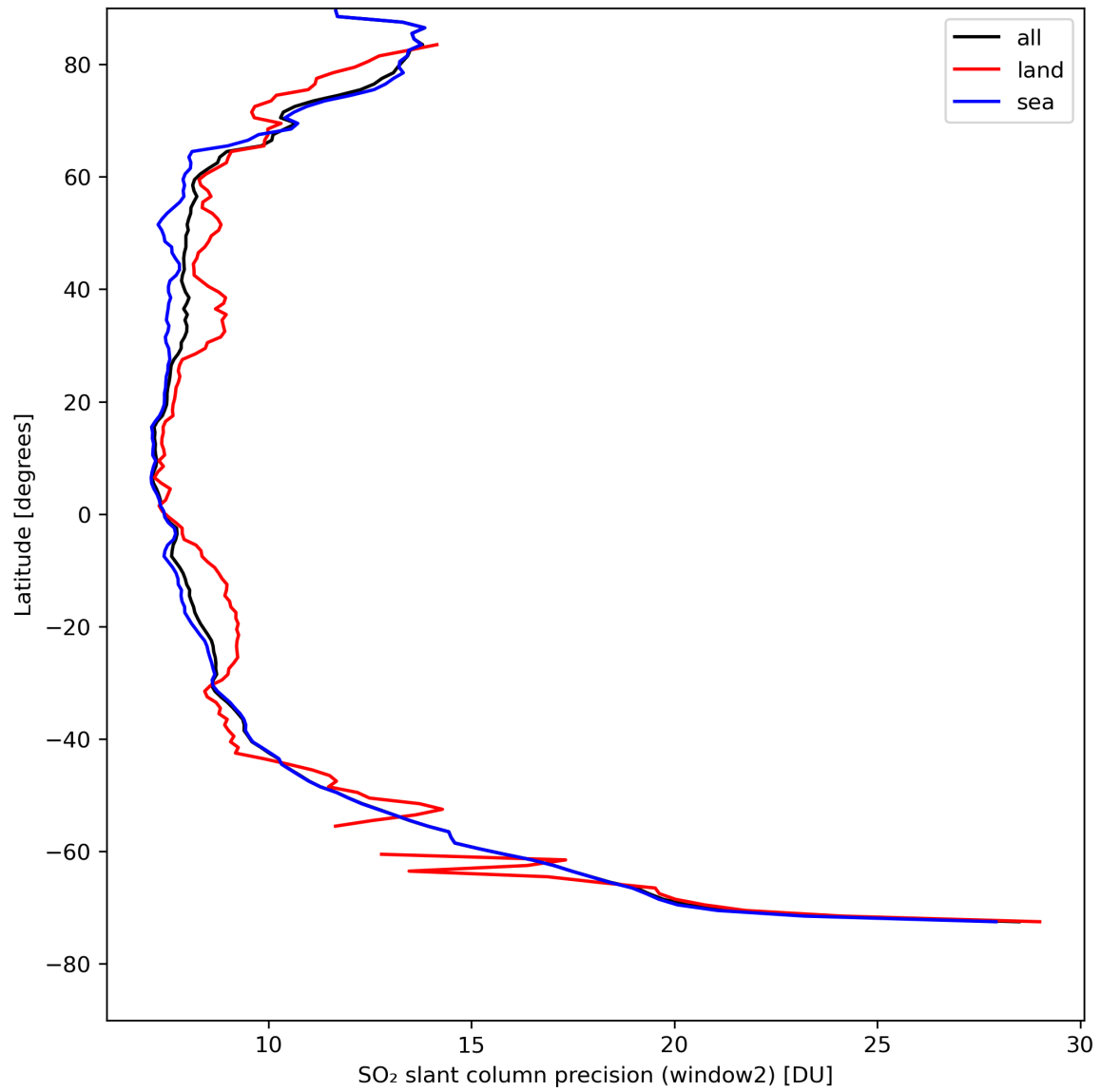
Figure 38: Zonal average of “SO 2 slant column precision (window2)” for 2024-08-19 to 2024-08-21.
