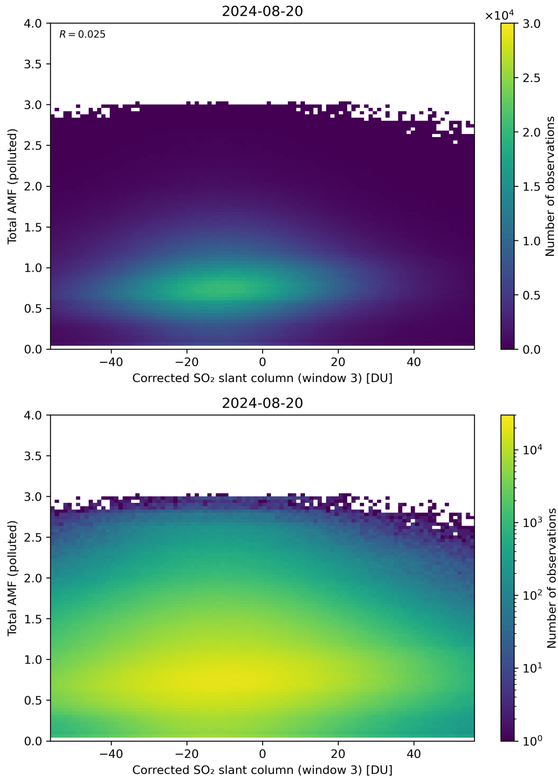
Figure 210: Scatter density plot of “Corrected SO 2 slant column (window 3)” against “Total AMF (polluted)” for 2024-08-19 to 2024-08-21.
