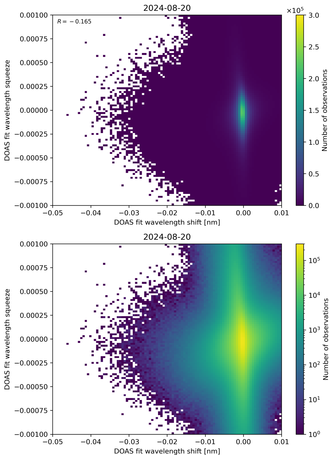
Figure 127: Scatter density plot of “DOAS fit wavelength shift” against “DOAS fit wavelength squeeze” for 2024-08-19 to 2024-08-21.
