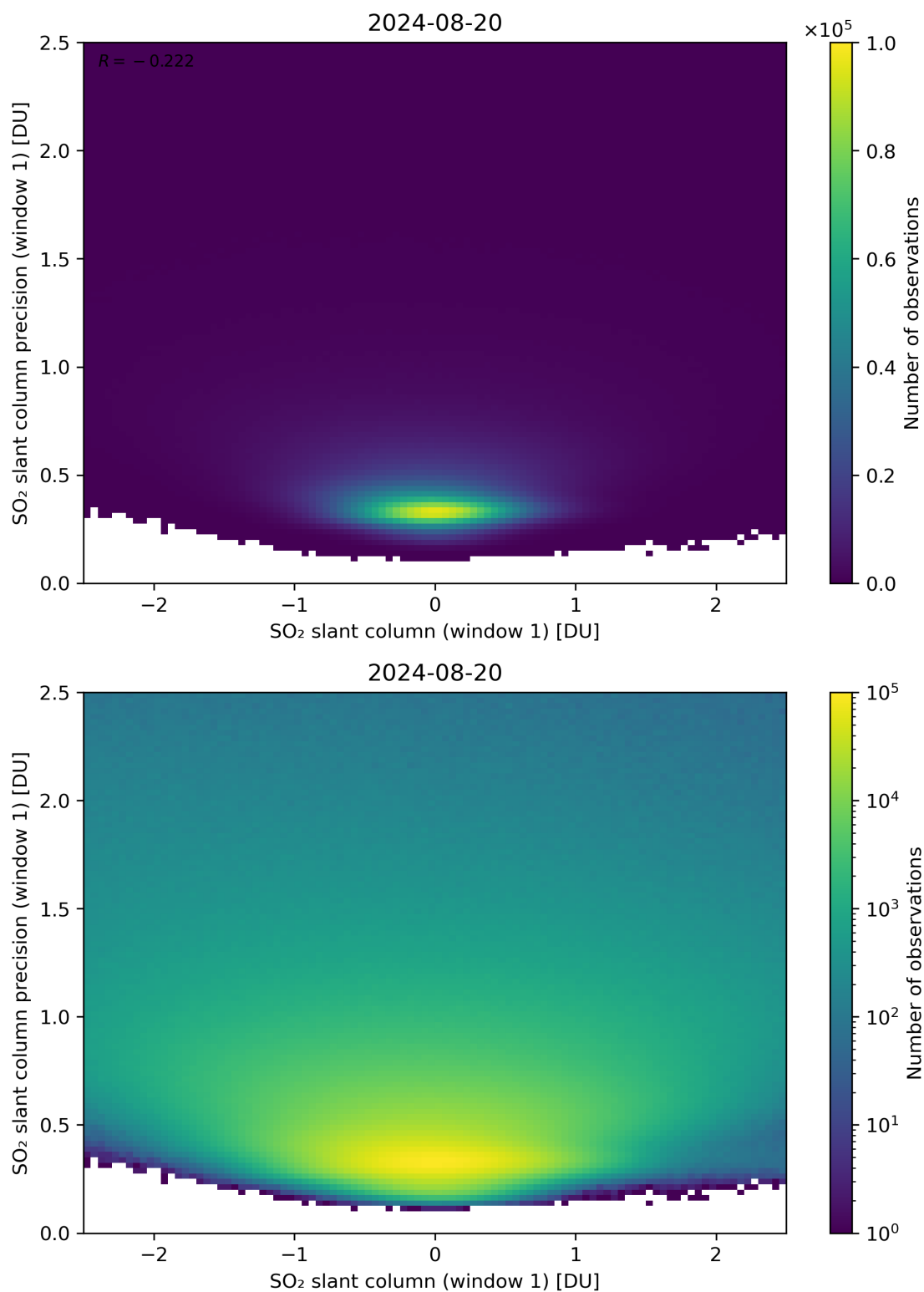
Figure 235: Scatter density plot of “SO 2 slant column (window 1)” against “SO 2 slant column precision (window 1)” for 2024-08-19 to 2024-08-21.
