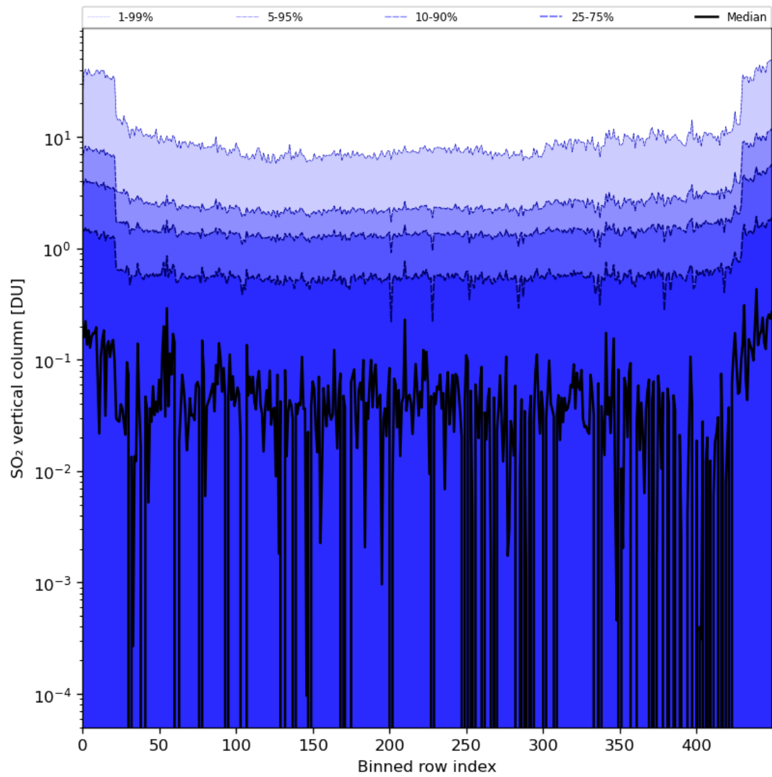
Figure 76: Along track statistics of “SO 2 vertical column” for 2024-08-19 to 2024-08-21
