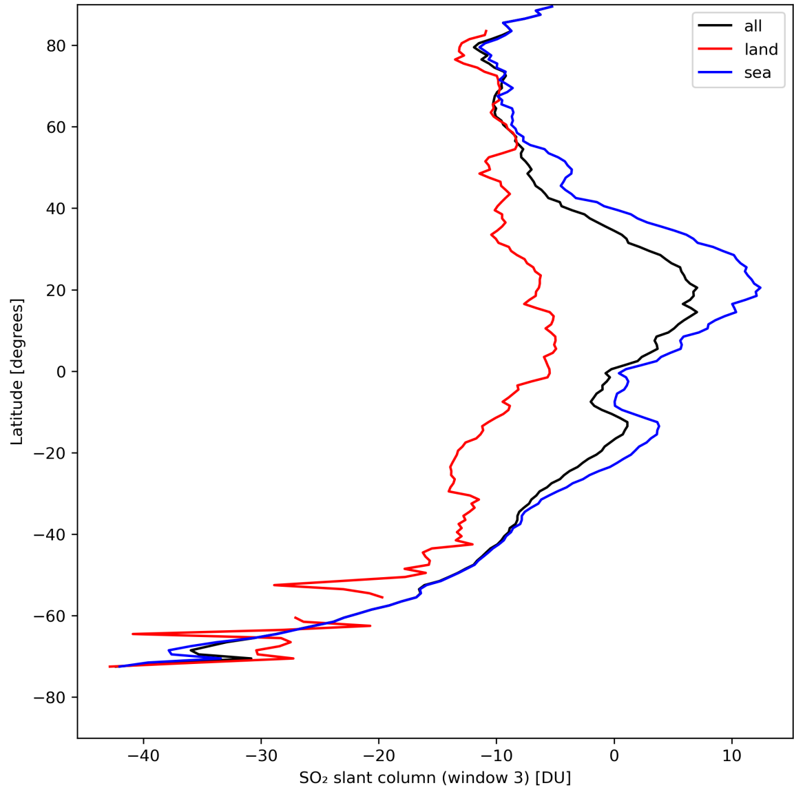
Figure 41: Zonal average of “SO 2 slant column (window 3)” for 2024-08-19 to 2024-08-21.
