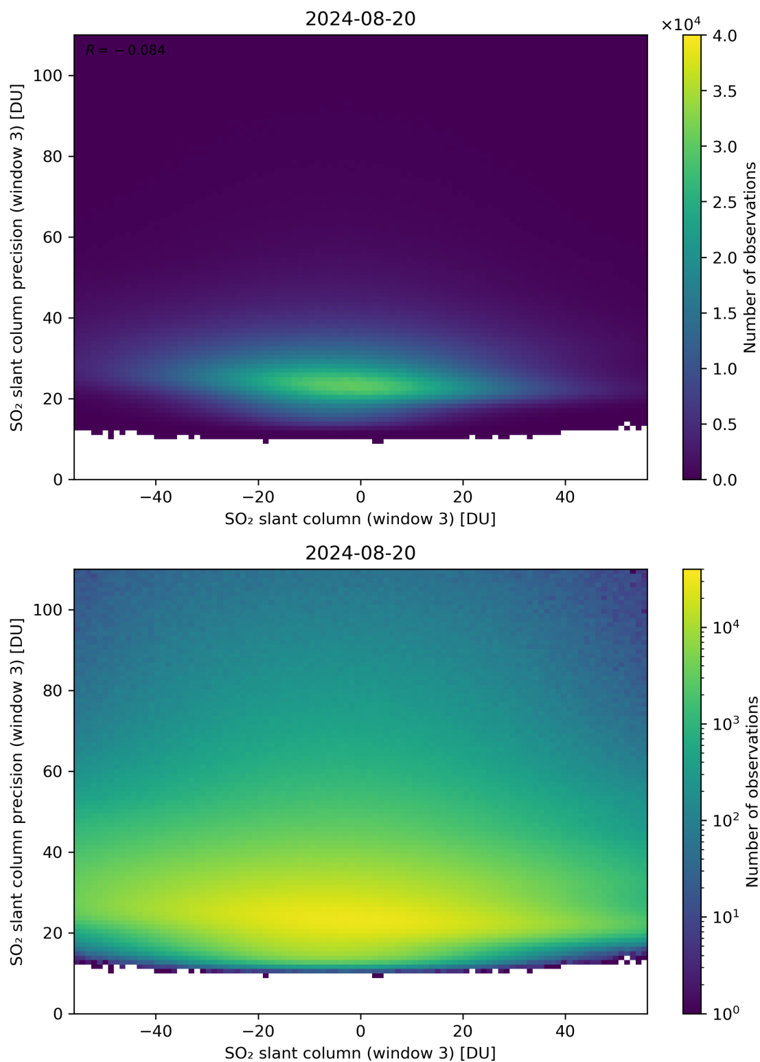
Figure 267: Scatter density plot of “SO 2 slant column (window 3)” against “SO 2 slant column precision (window 3)” for 2024-08-19 to 2024-08-21.
