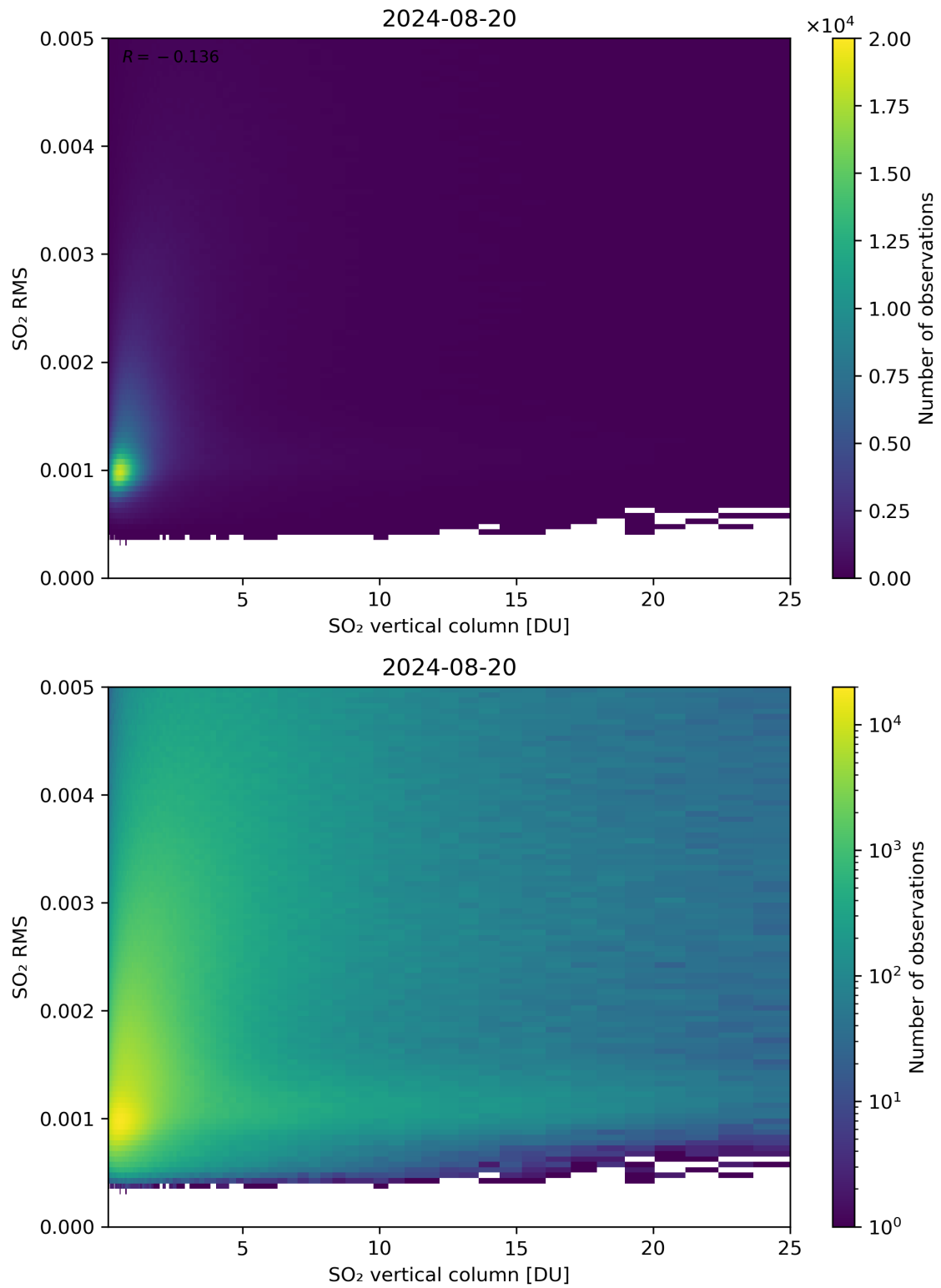
Figure 278: Scatter density plot of “SO 2 vertical column” against “SO 2 RMS” for 2024-08-19 to 2024-08-21.
