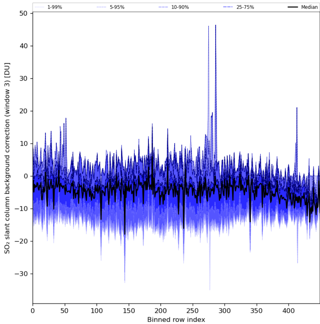
Figure 90: Along track statistics of “SO 2 slant column background correction (window 3)” for 2024-08-19 to 2024-08-21
