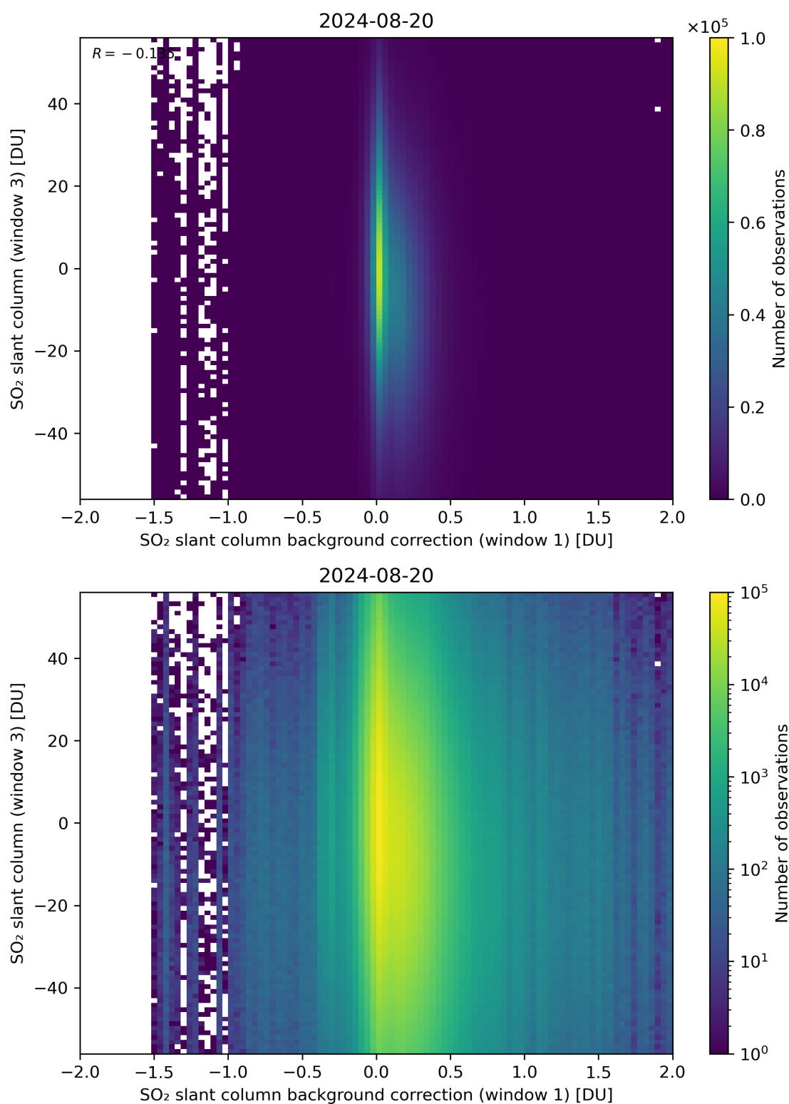
Figure 107: Scatter density plot of “SO 2 slant column background correction (window 1)” against “SO 2 slant column (window 3)” for 2024-08-19 to 2024-08-21.
