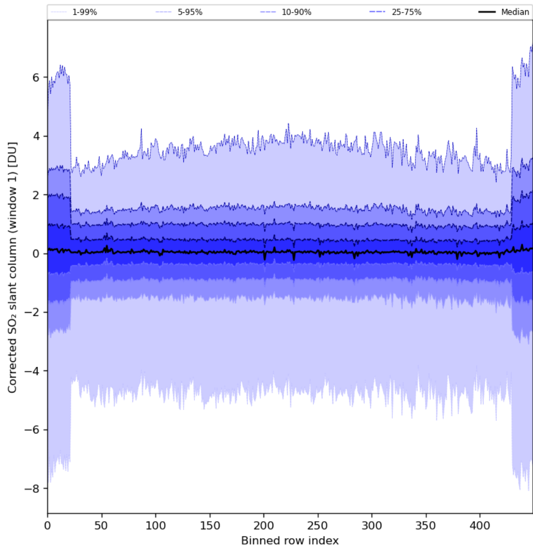
Figure 81: Along track statistics of “Corrected SO 2 slant column (window 1)” for 2024-08-19 to 2024-08-21
