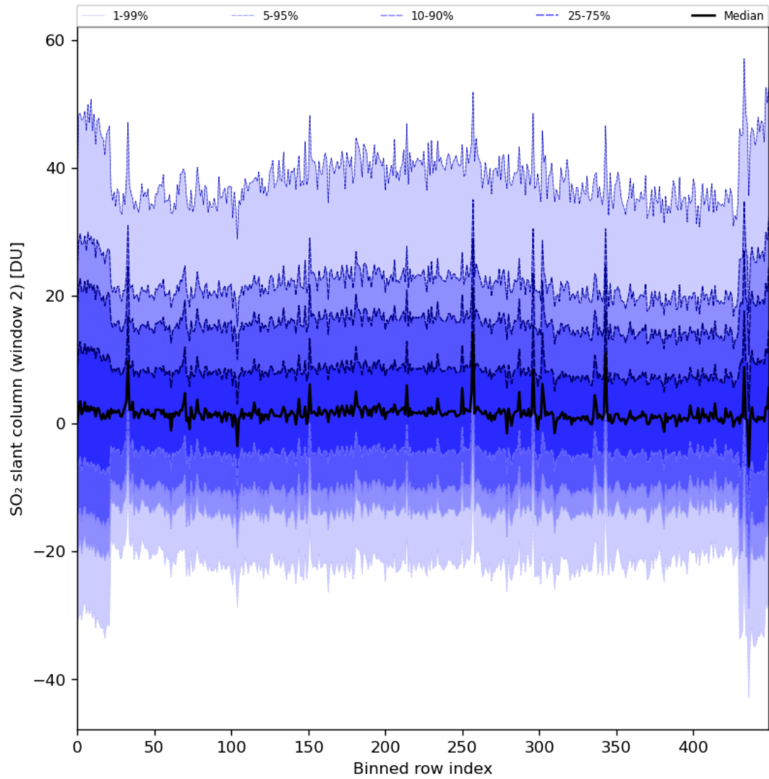
Figure 83: Along track statistics of “SO 2 slant column (window 2)” for 2024-08-19 to 2024-08-21
