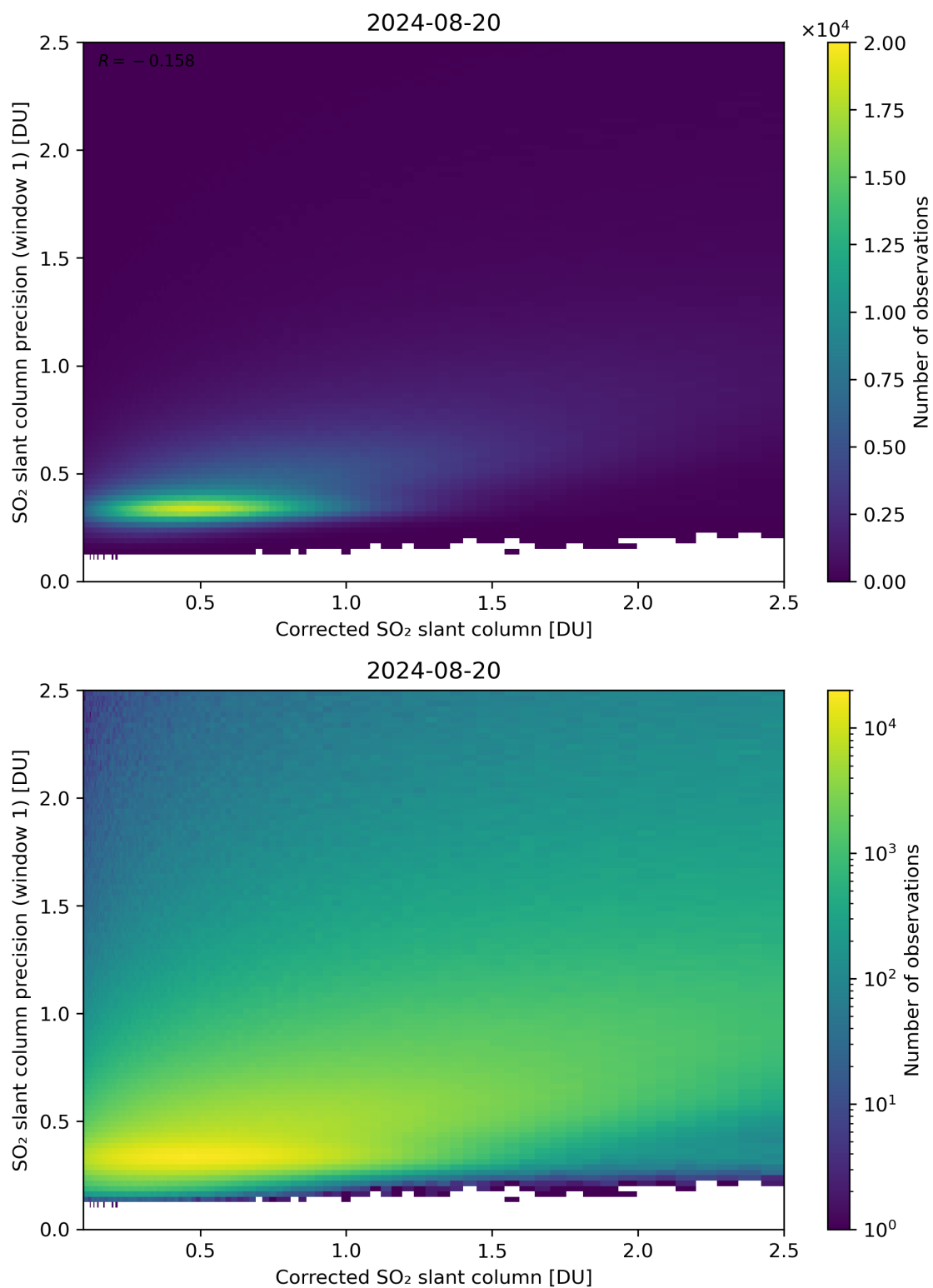
Figure 188: Scatter density plot of “Corrected SO 2 slant column” against “SO 2 slant column precision (window 1)” for 2024-08-19 to 2024-08-21.
