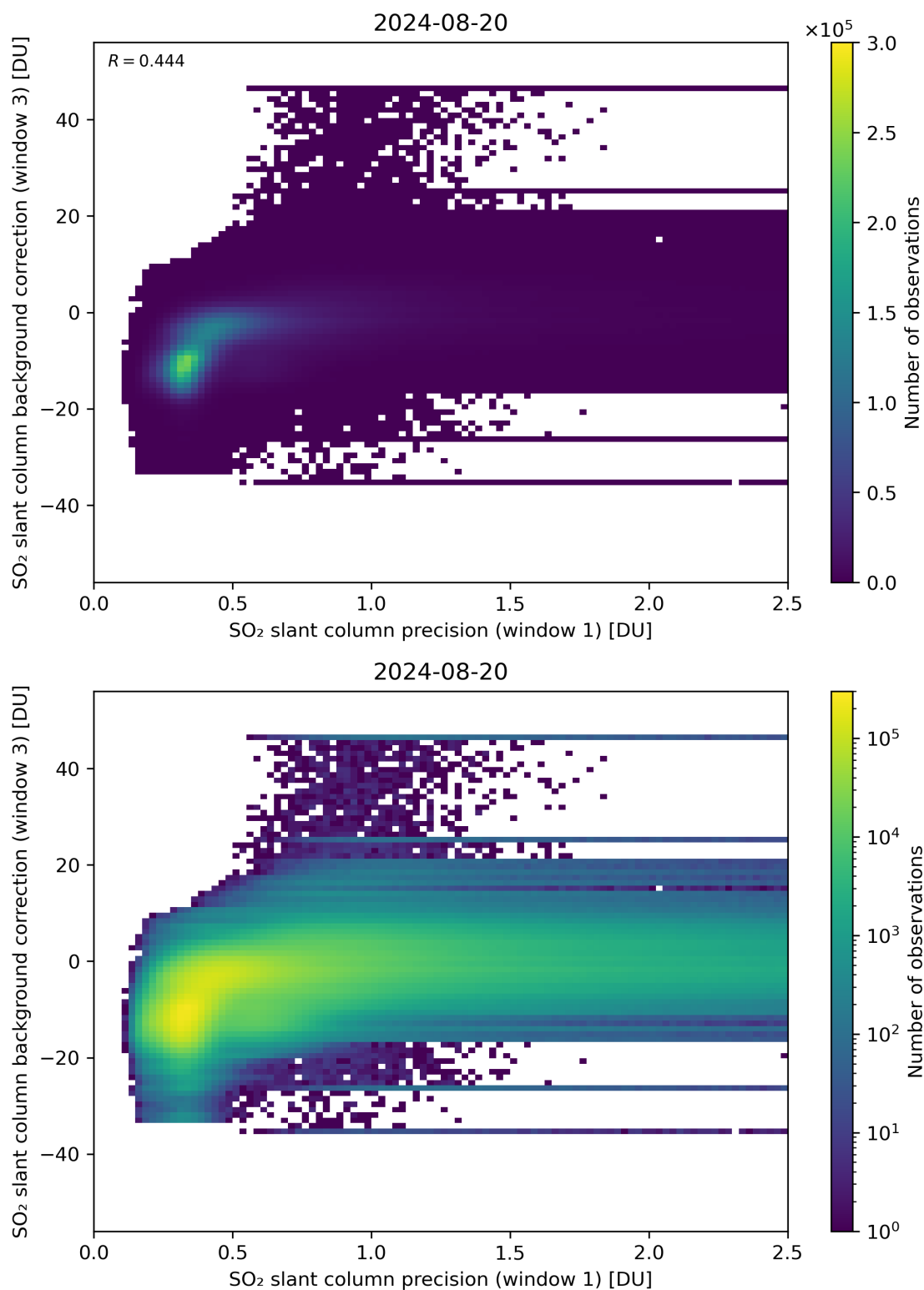
Figure 220: Scatter density plot of “SO 2 slant column precision (window 1)” against “SO 2 slant column background correction (window 3)” for 2024-08-19 to 2024-08-21.
