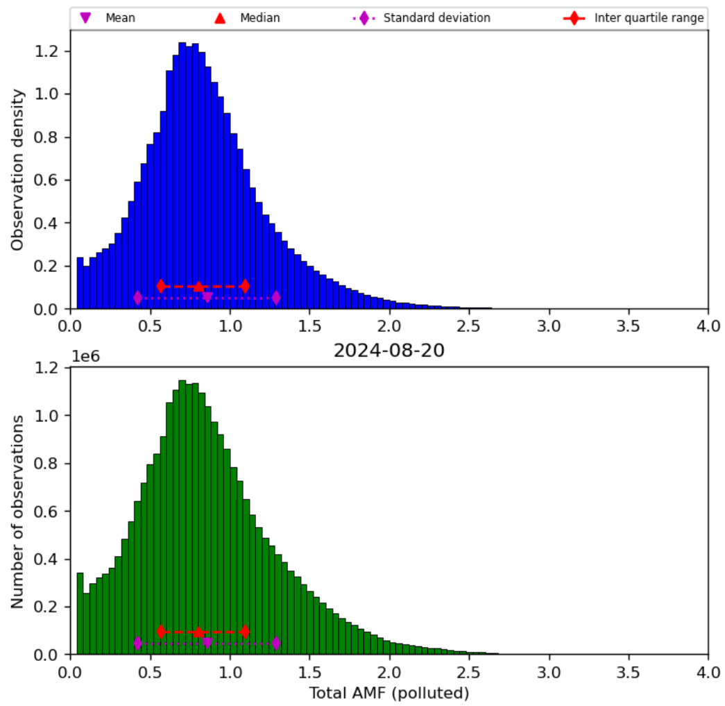
Figure 71: Histogram of “Total AMF (polluted)” for 2024-08-19 to 2024-08-21
