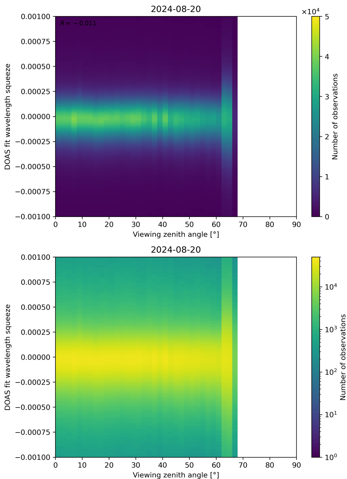
Figure 312: Scatter density plot of “Viewing zenith angle” against “DOAS fit wavelength squeeze” for 2024-08-19 to 2024-08-21.
