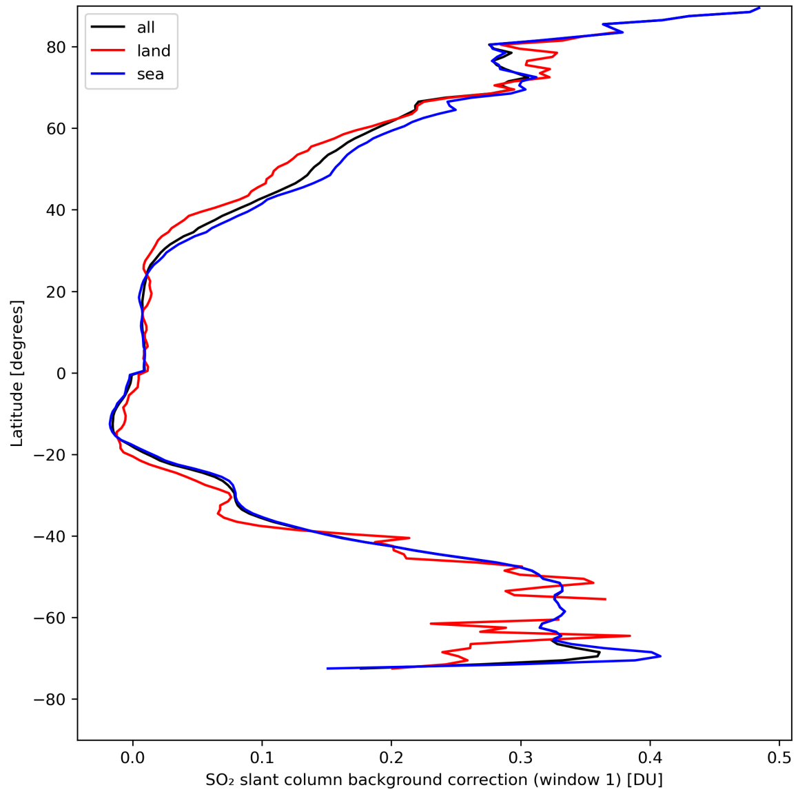
Figure 36: Zonal average of “SO 2 slant column background correction (window 1)” for 2024-08-19 to 2024-08-21.
