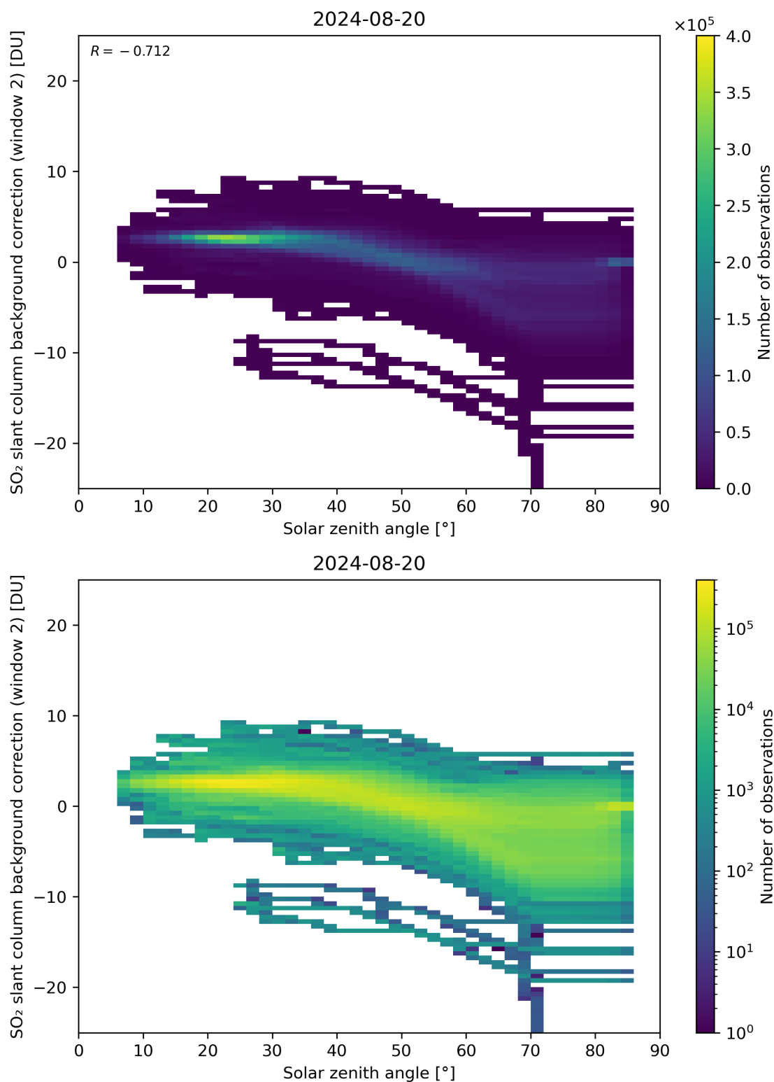
Figure 159: Scatter density plot of “Solar zenith angle” against “SO 2 slant column background correction (window 2)” for 2024-08-19 to 2024-08-21.
