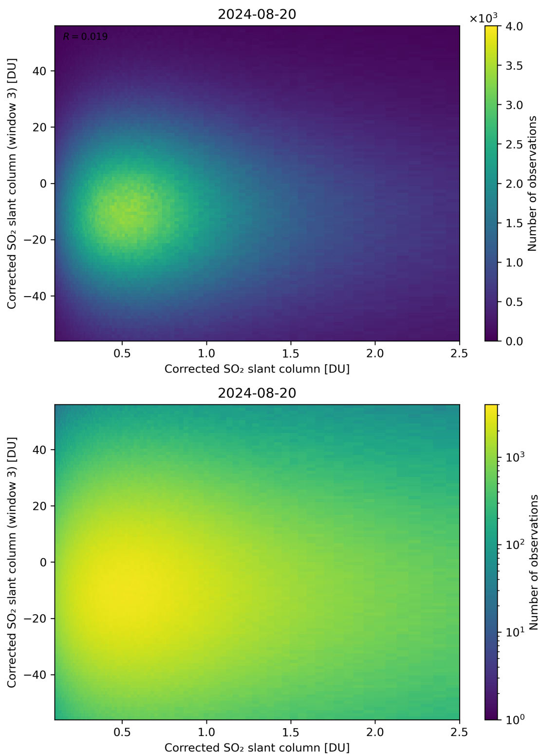
Figure 186: Scatter density plot of “Corrected SO 2 slant column” against “Corrected SO 2 slant column (window 3)” for 2024-08-19 to 2024-08-21.
