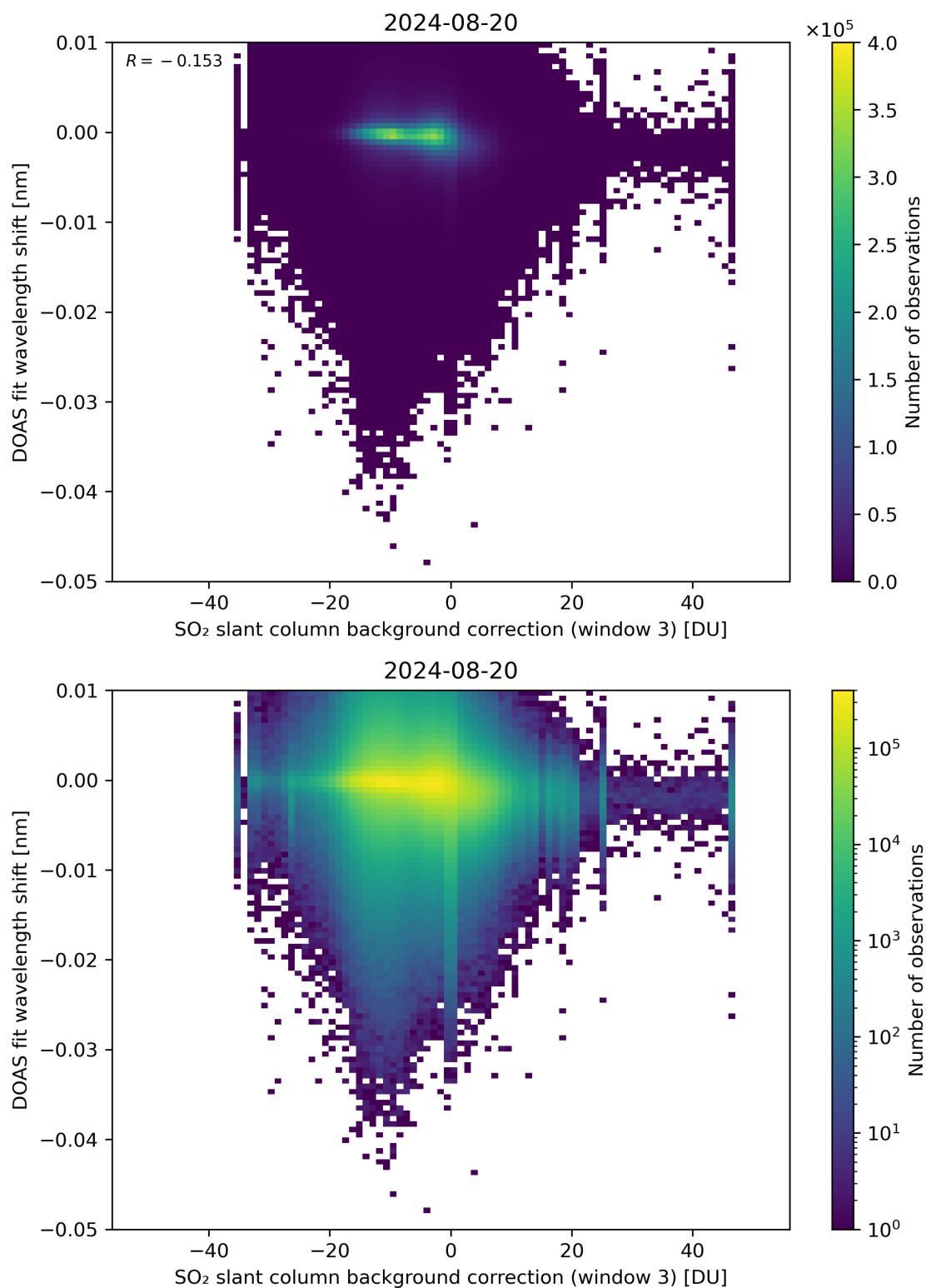
Figure 121: Scatter density plot of “SO 2 slant column background correction (window 3)” against “DOAS fit wavelength shift” for 2024-08-19 to 2024-08-21.
