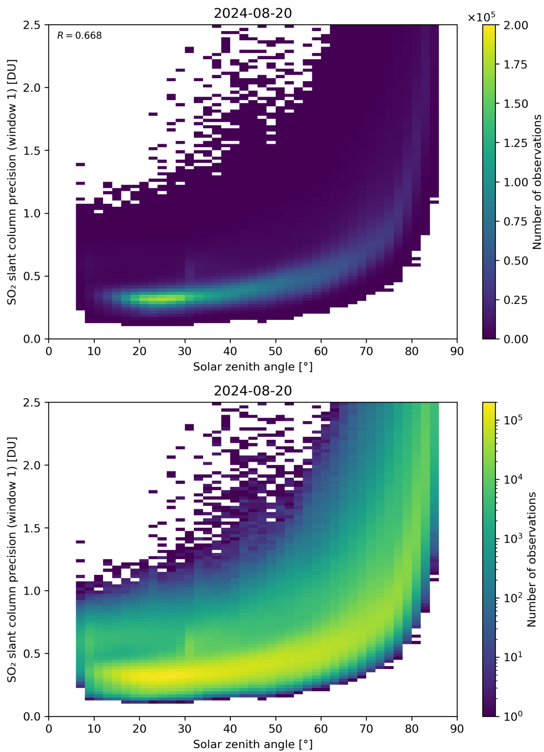
Figure 170: Scatter density plot of “Solar zenith angle” against “SO 2 slant column precision (window 1)” for 2024-08-19 to 2024-08-21.
