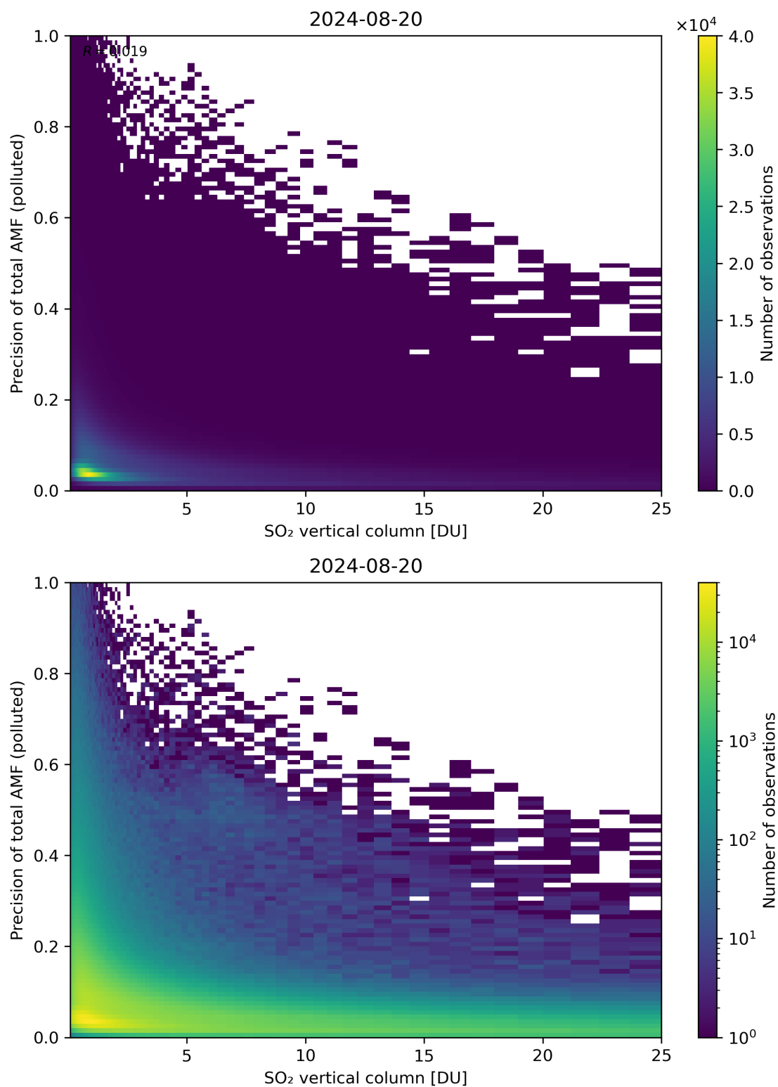
Figure 306: Scatter density plot of “SO 2 vertical column” against “Precision of total AMF (polluted)” for 2024-08-19 to 2024-08-21.
