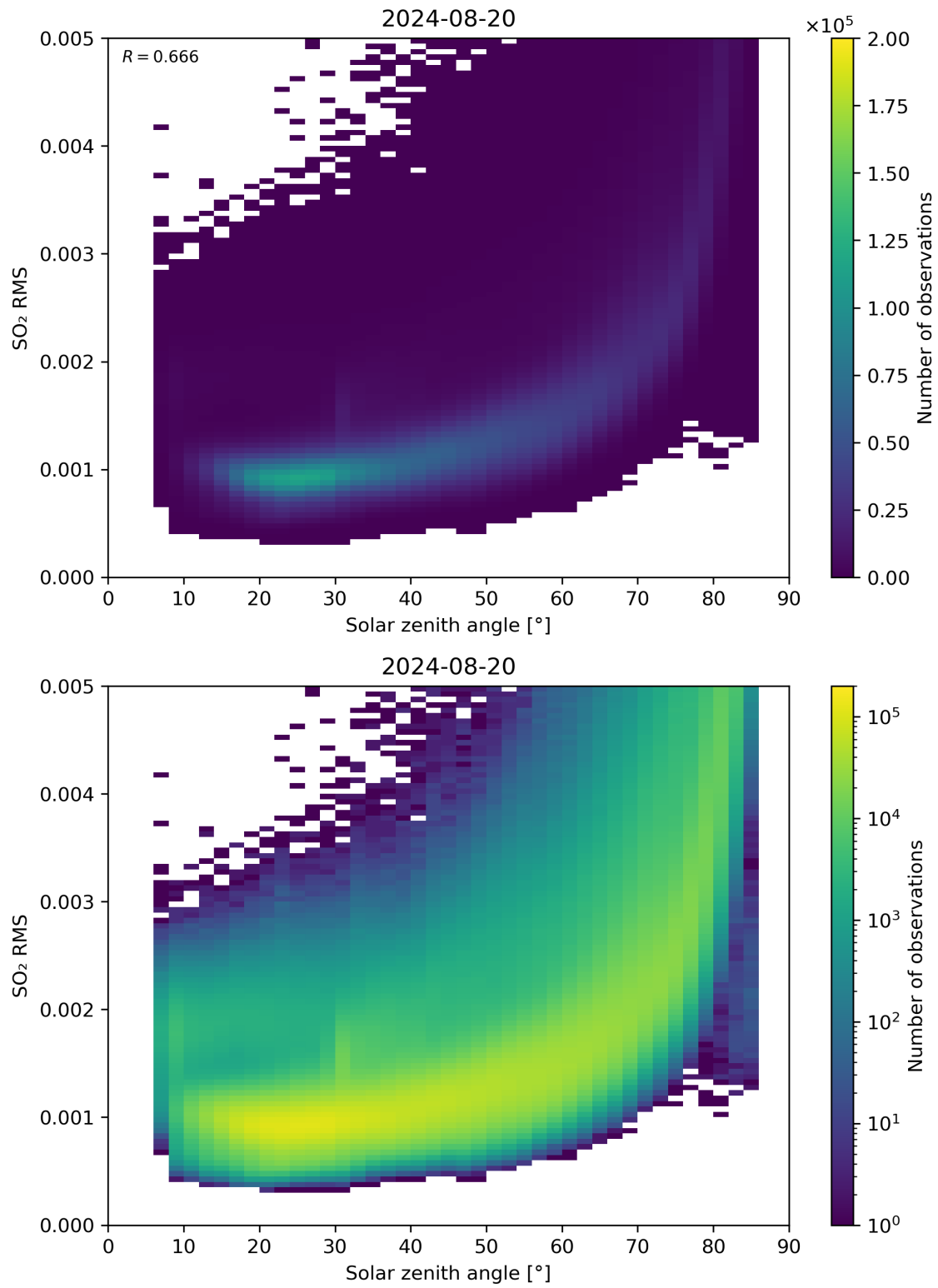
Figure 163: Scatter density plot of “Solar zenith angle” against “SO 2 RMS” for 2024-08-19 to 2024-08-21.
