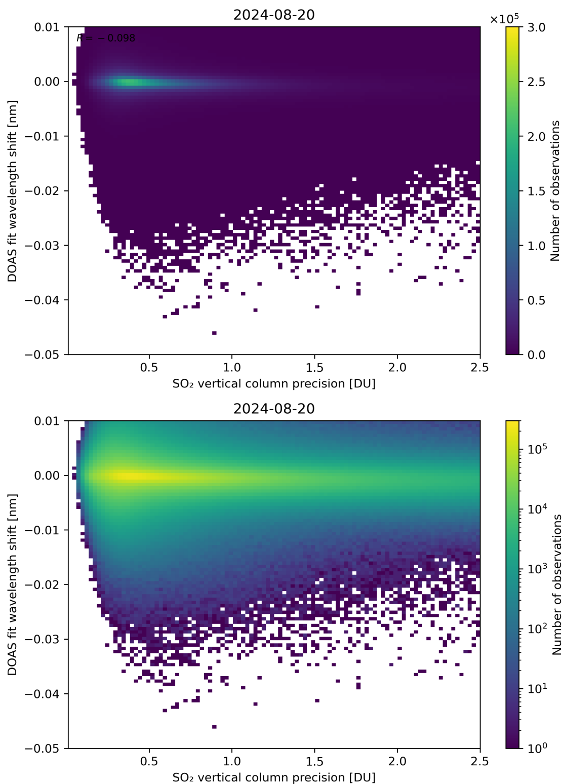
Figure 282: Scatter density plot of “SO 2 vertical column precision” against “DOAS fit wavelength shift” for 2024-08-19 to 2024-08-21.
