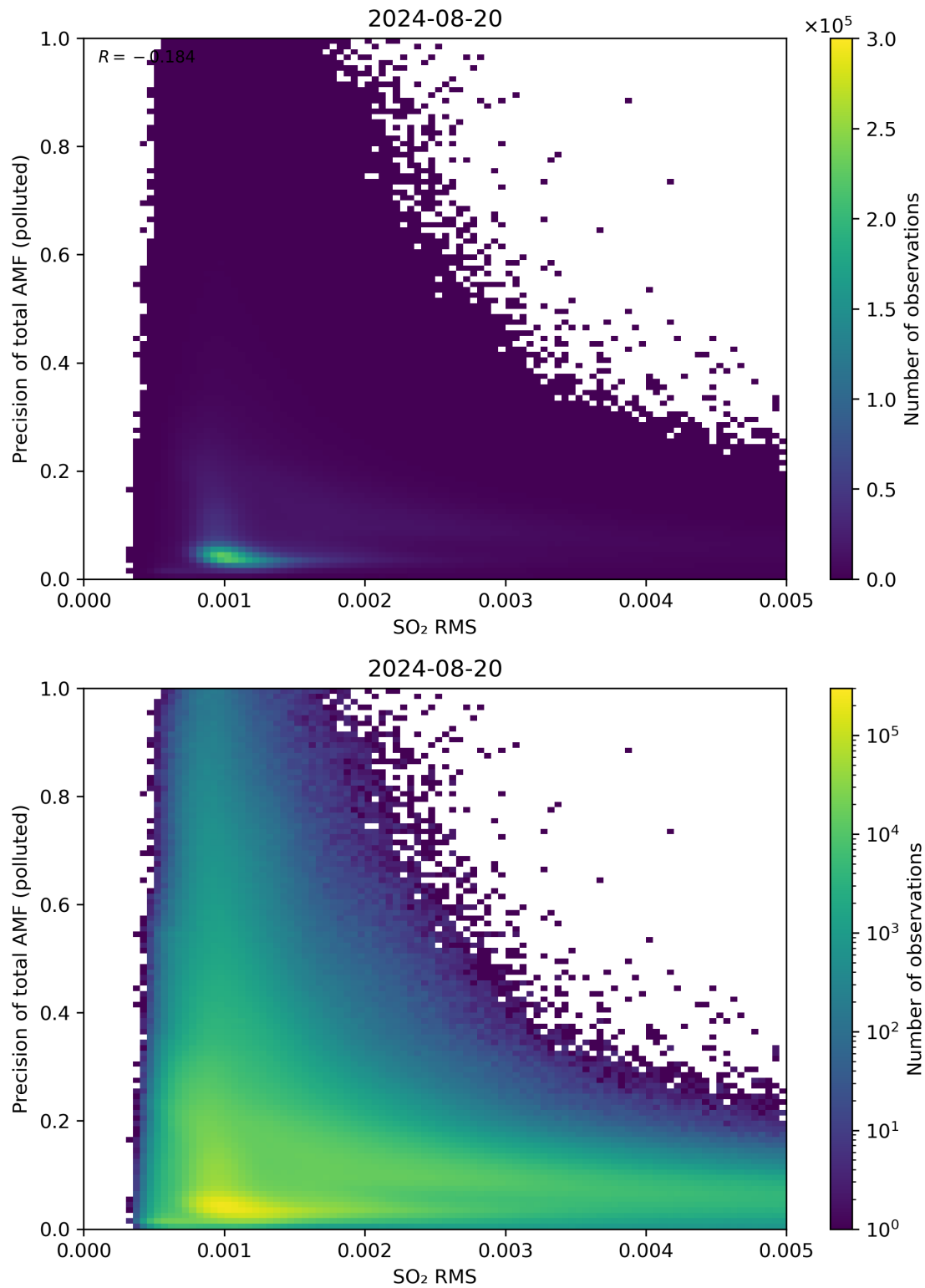
Figure 138: Scatter density plot of “SO 2 RMS” against “Precision of total AMF (polluted)” for 2024-08-19 to 2024-08-21.
