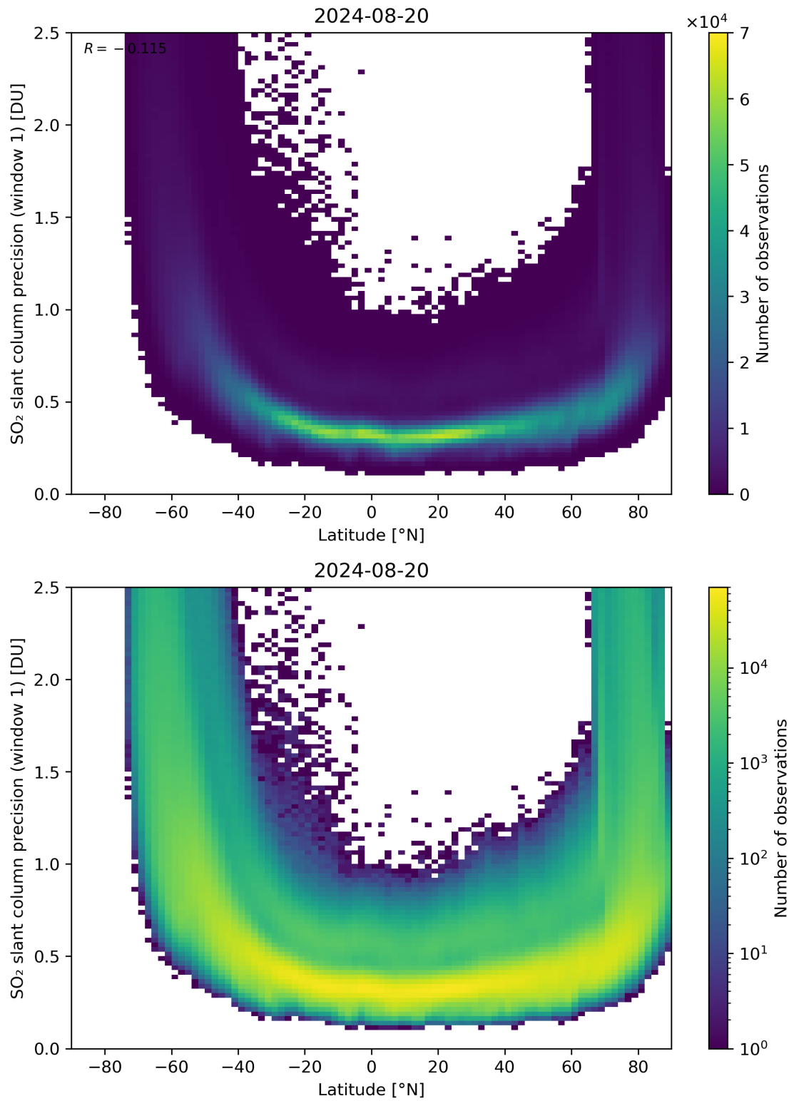
Figure 150: Scatter density plot of “Latitude” against “SO 2 slant column precision (window 1)” for 2024-08-19 to 2024-08-21.
