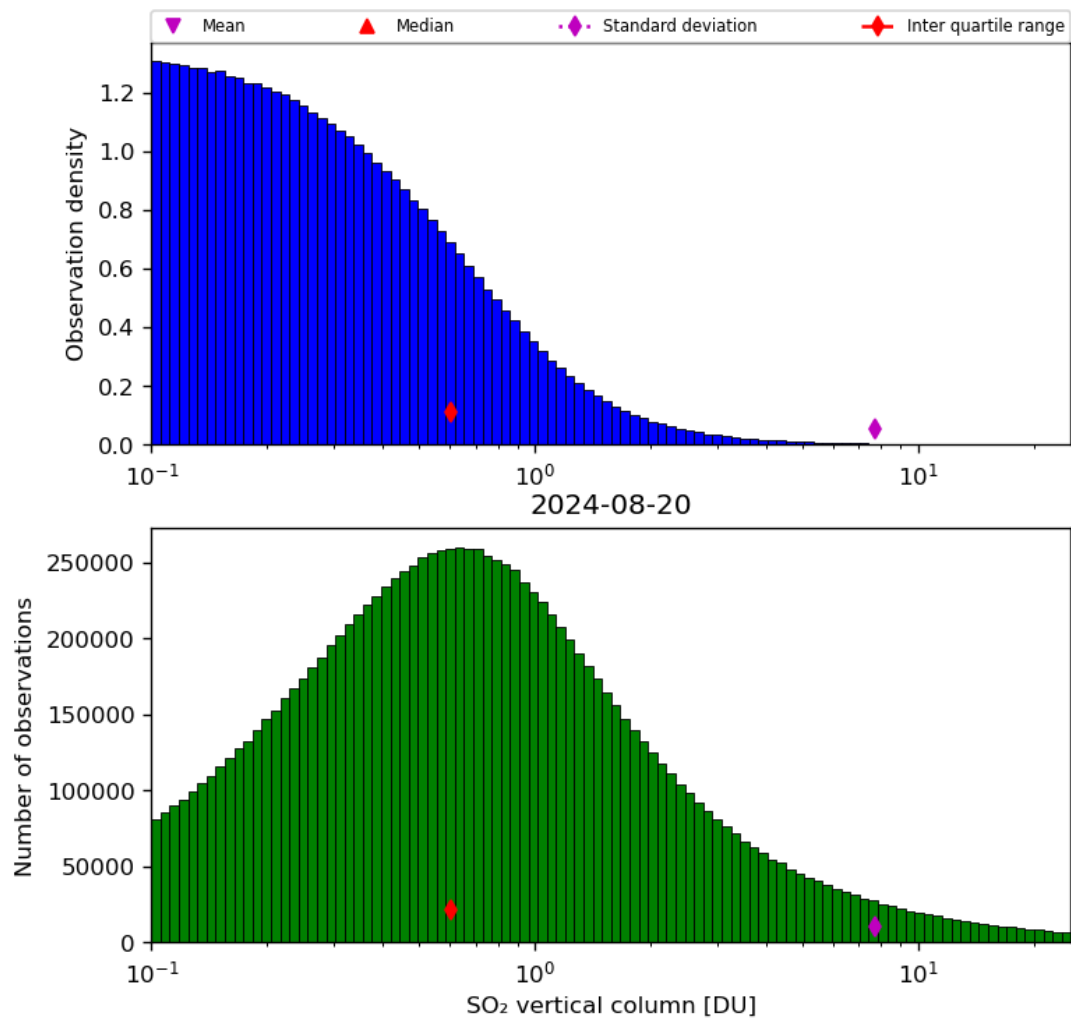
Figure 53: Histogram of “SO 2 vertical column” for 2024-08-19 to 2024-08-21
