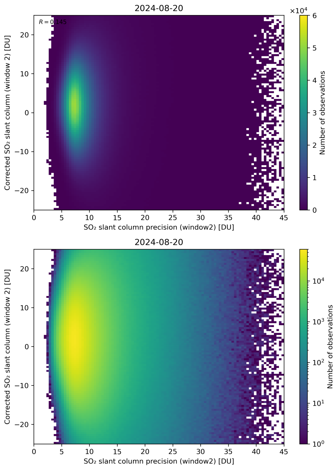
Figure 247: Scatter density plot of “SO 2 slant column precision (window2)” against “Corrected SO 2 slant column (window 2)” for 2024-08-19 to 2024-08-21.
