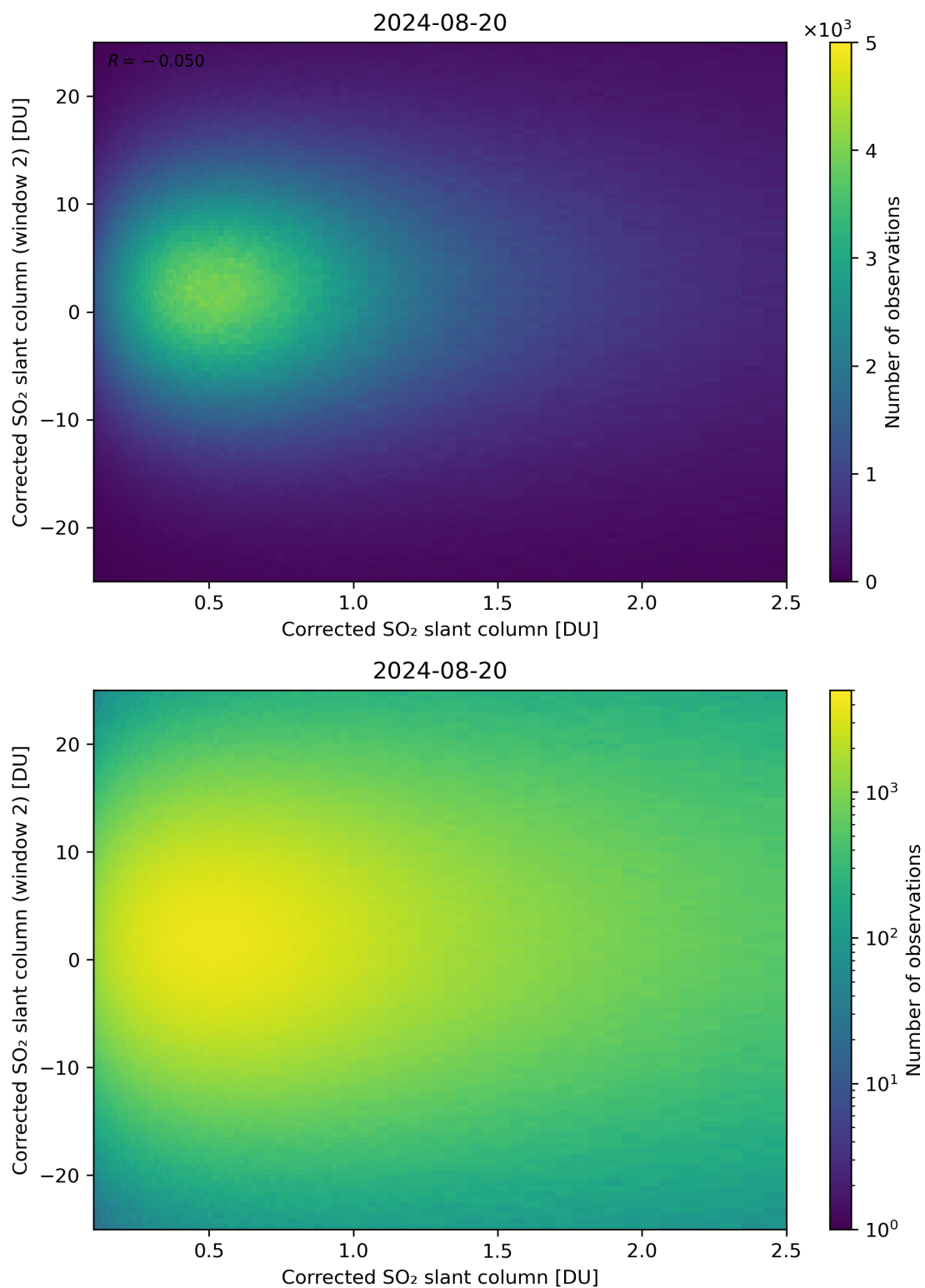
Figure 185: Scatter density plot of “Corrected SO 2 slant column” against “Corrected SO 2 slant column (window 2)” for 2024-08-19 to 2024-08-21.
