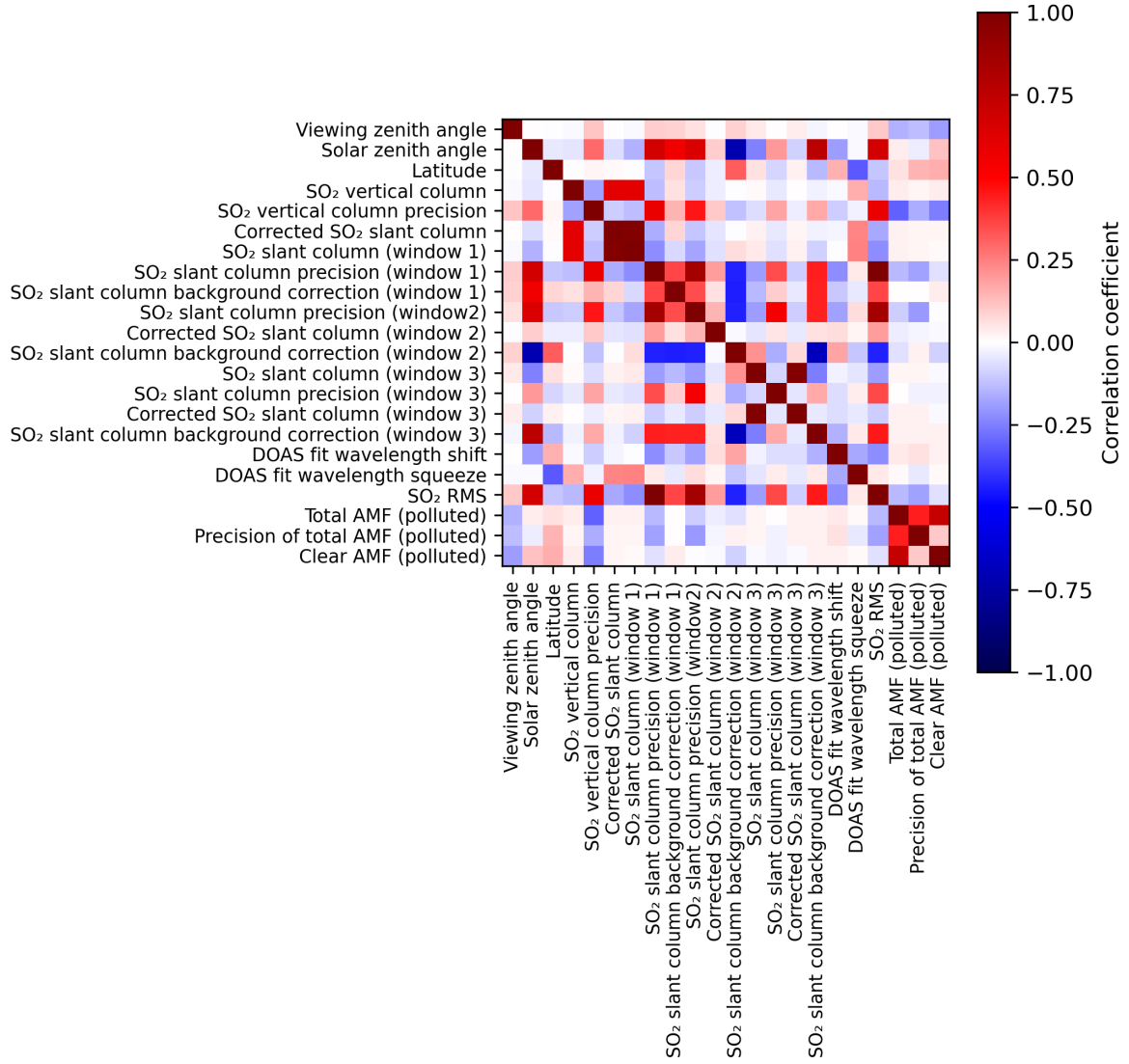
Figure 2: Map of correlation matrix for 2024-08-19 to 2024-08-21.
