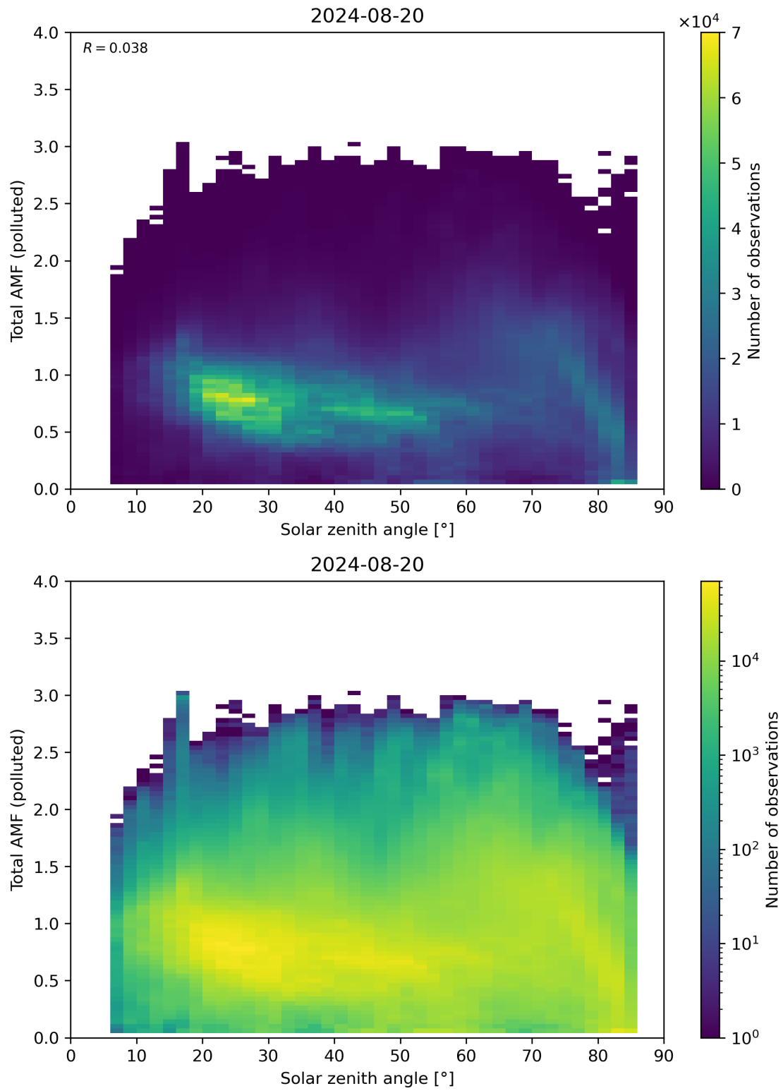
Figure 174: Scatter density plot of “Solar zenith angle” against “Total AMF (polluted)” for 2024-08-19 to 2024-08-21.
