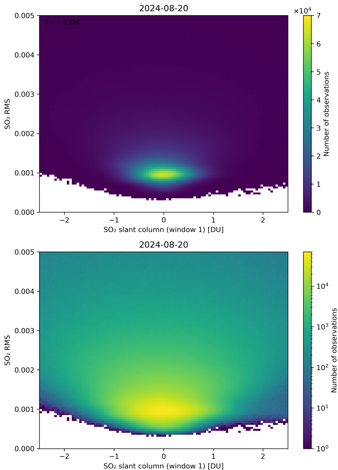
Figure 217: Scatter density plot of “SO 2 slant column (window 1)” against “SO 2 RMS” for 2024-08-19 to 2024-08-21.
