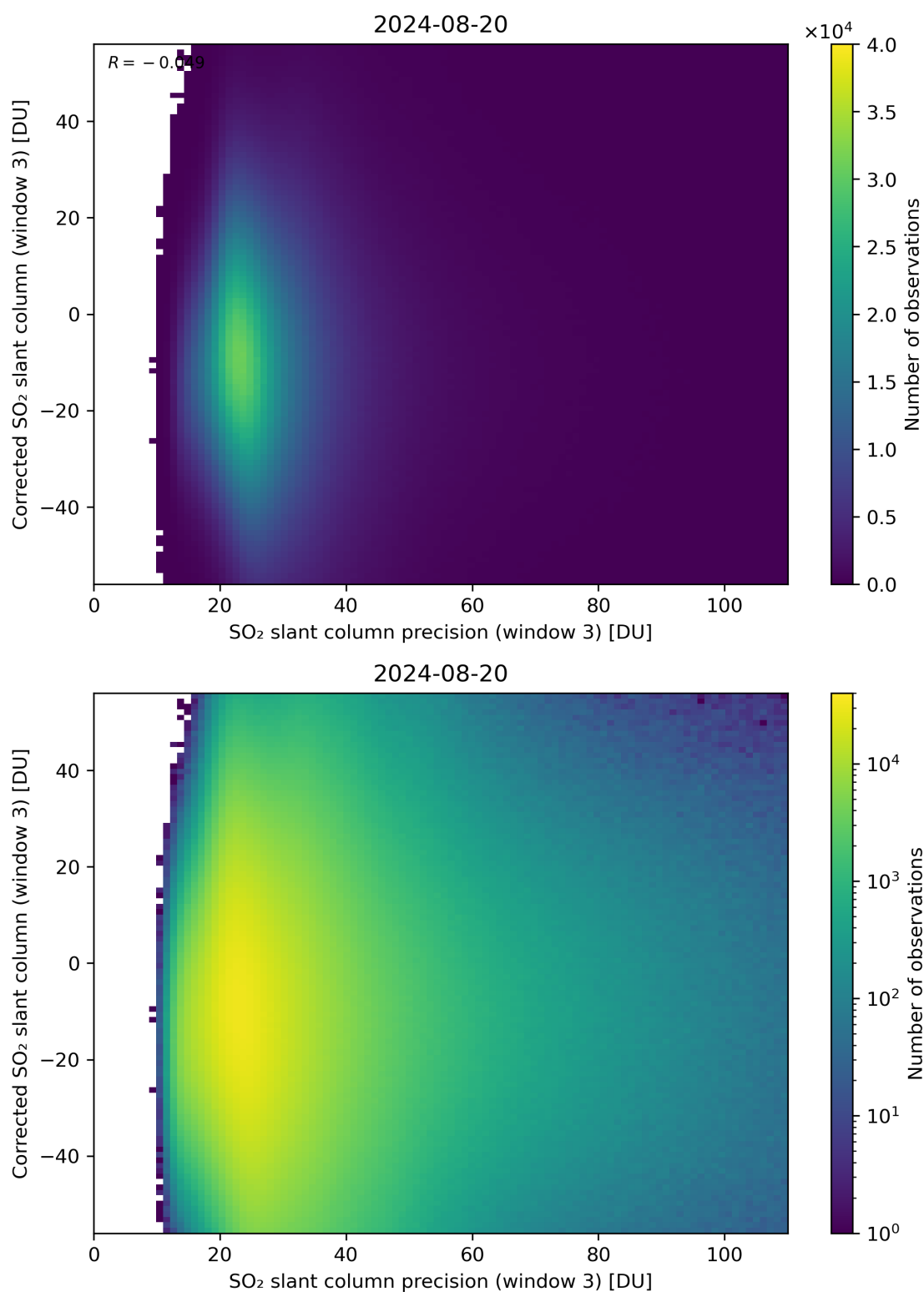
Figure 262: Scatter density plot of “SO 2 slant column precision (window 3)” against “Corrected SO 2 slant column (window 3)” for 2024-08-19 to 2024-08-21.
