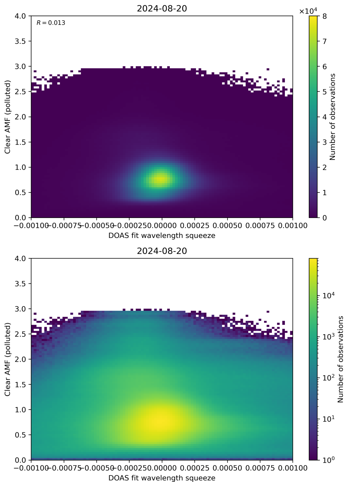
Figure 133: Scatter density plot of “DOAS fit wavelength squeeze” against “Clear AMF (polluted)” for 2024-08-19 to 2024-08-21.
