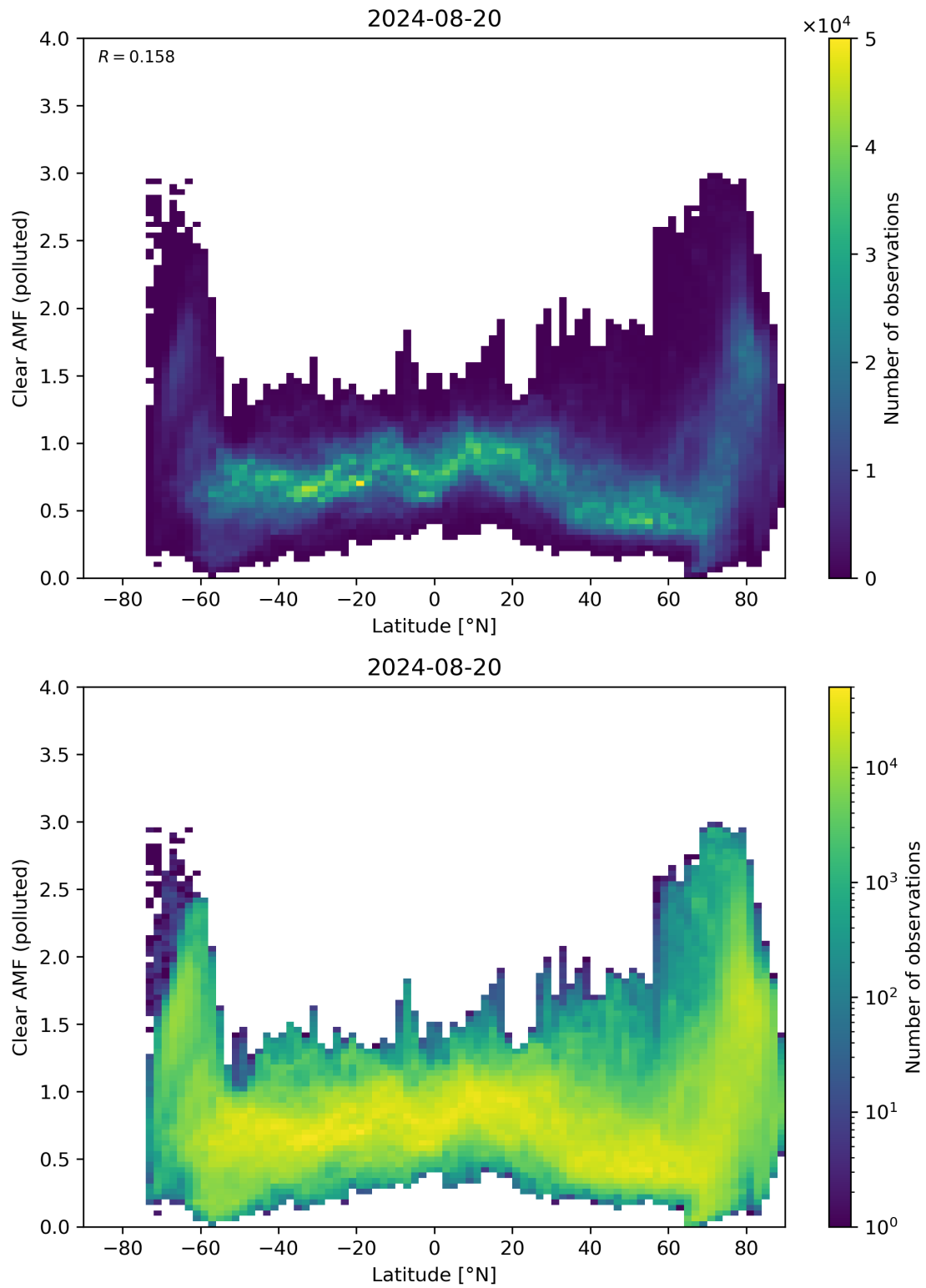
Figure 145: Scatter density plot of “Latitude” against “Clear AMF (polluted)” for 2024-08-19 to 2024-08-21.
