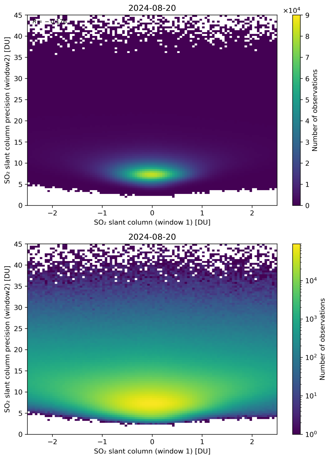
Figure 236: Scatter density plot of “SO 2 slant column (window 1)” against “SO 2 slant column precision (window2)” for 2024-08-19 to 2024-08-21.
