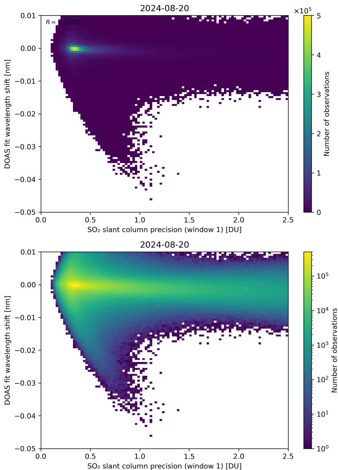
Figure 221: Scatter density plot of “SO 2 slant column precision (window 1)” against “DOAS fit wavelength shift” for 2024-08-19 to 2024-08-21.
