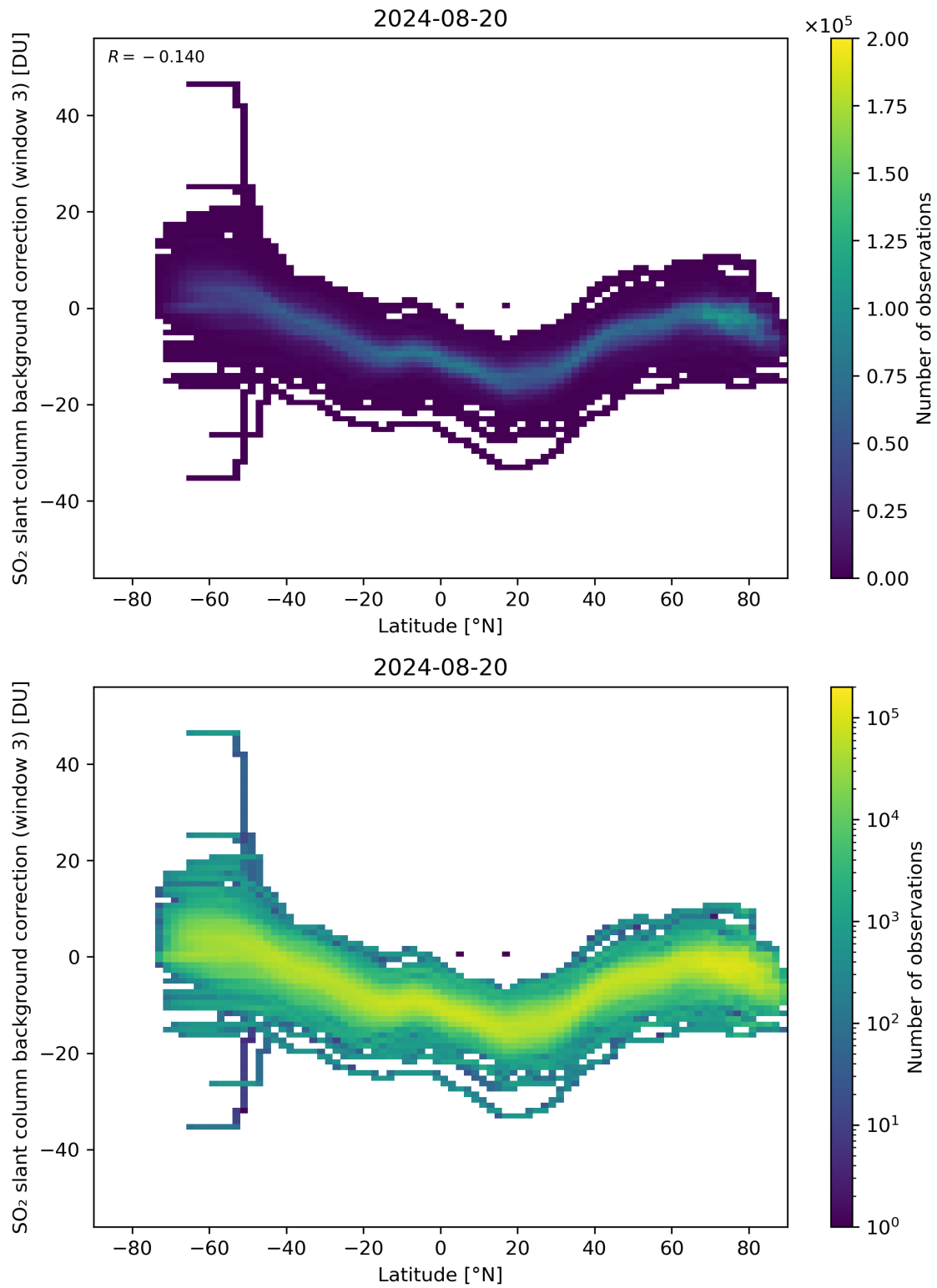
Figure 141: Scatter density plot of “Latitude” against “SO 2 slant column background correction (window 3)” for 2024-08-19 to 2024-08-21.
