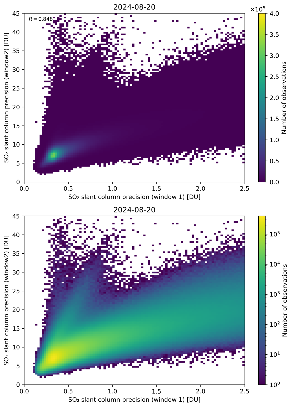
Figure 227: Scatter density plot of “SO 2 slant column precision (window 1)” against “SO 2 slant column precision (window2)” for 2024-08-19 to 2024-08-21.
