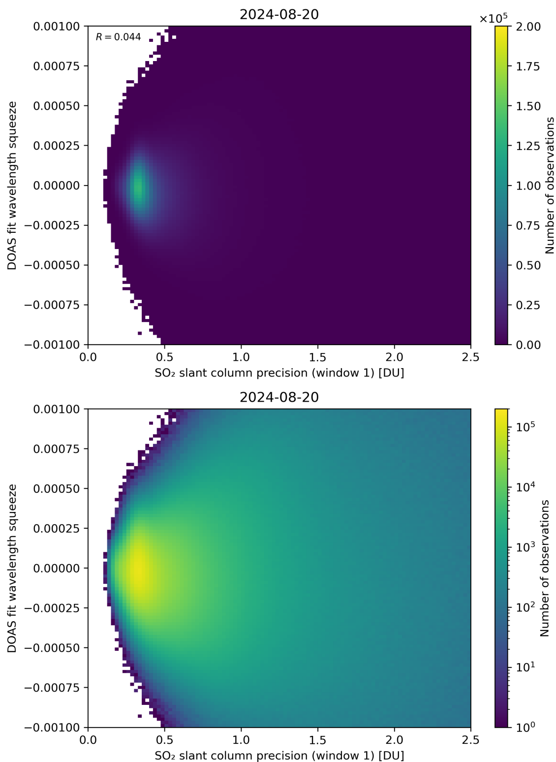
Figure 222: Scatter density plot of “SO 2 slant column precision (window 1)” against “DOAS fit wavelength squeeze” for 2024-08-19 to 2024-08-21.
