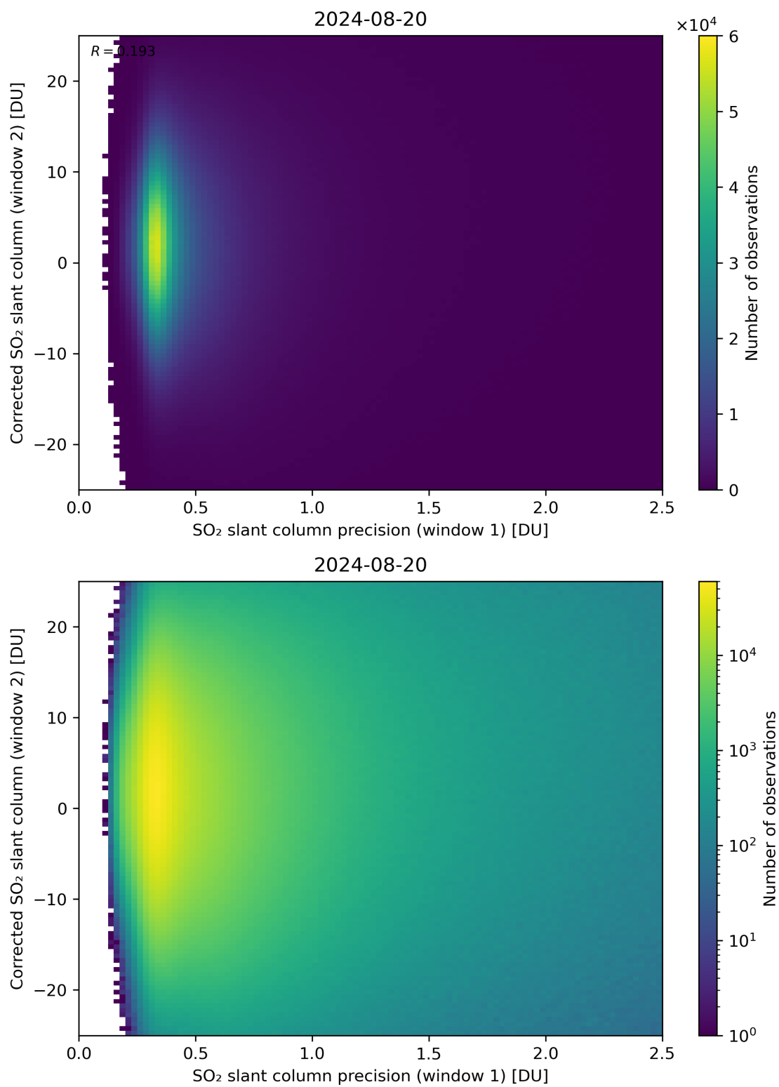
Figure 225: Scatter density plot of “SO 2 slant column precision (window 1)” against “Corrected SO 2 slant column (window 2)” for 2024-08-19 to 2024-08-21.
