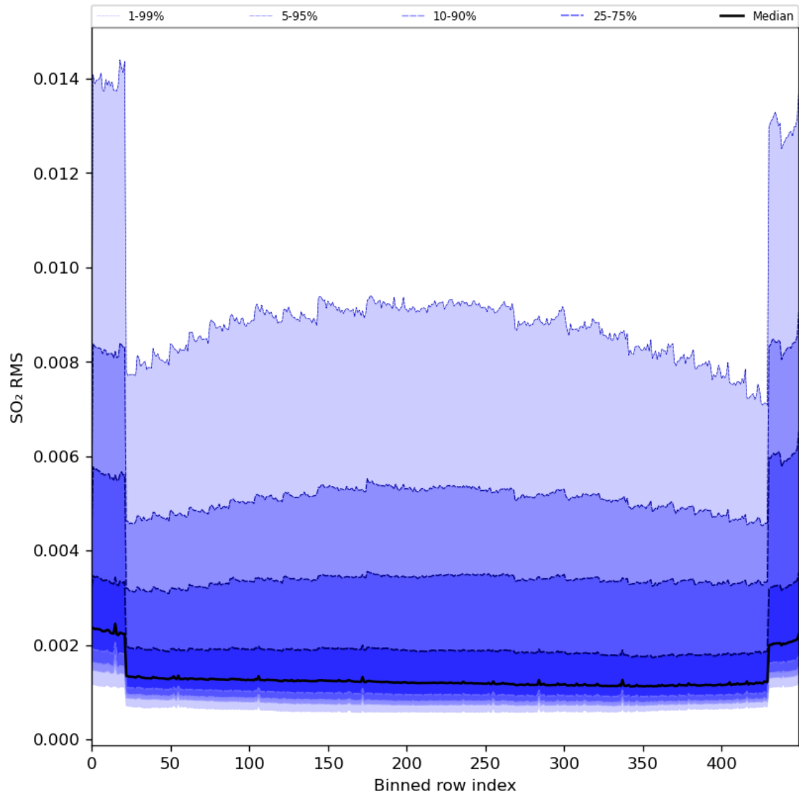
Figure 93: Along track statistics of “SO 2 RMS” for 2024-08-19 to 2024-08-21
