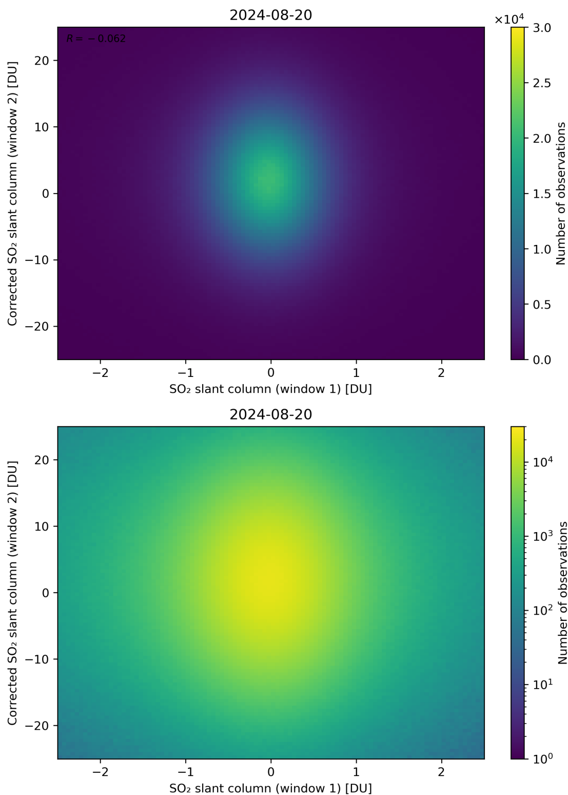
Figure 233: Scatter density plot of “SO 2 slant column (window 1)” against “Corrected SO 2 slant column (window 2)” for 2024-08-19 to 2024-08-21.
