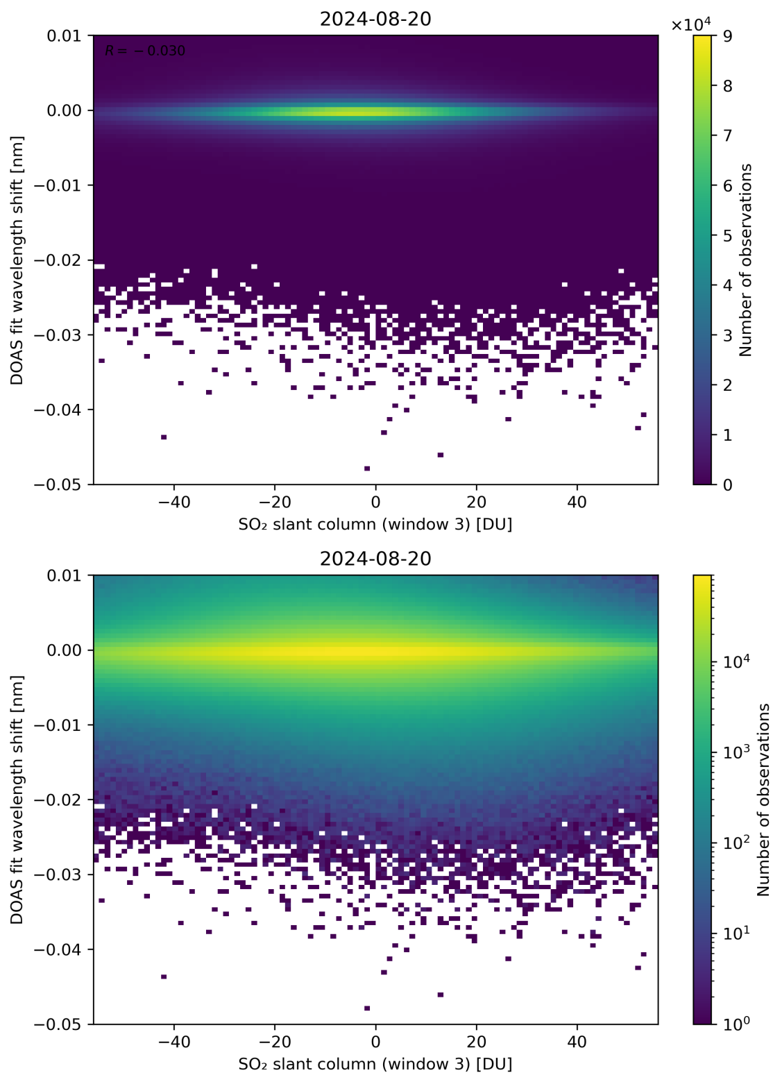
Figure 254: Scatter density plot of “SO 2 slant column (window 3)” against “DOAS fit wavelength shift” for 2024-08-19 to 2024-08-21.
