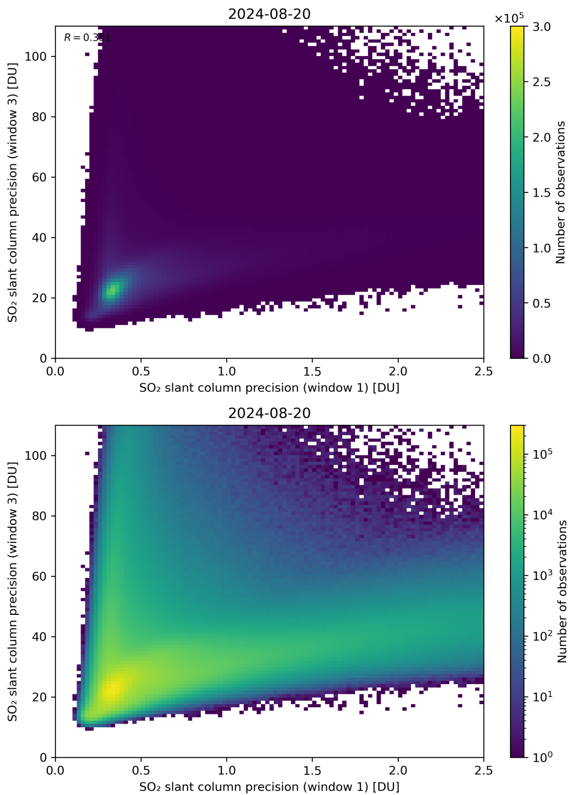
Figure 229: Scatter density plot of “SO 2 slant column precision (window 1)” against “SO 2 slant column precision (window 3)” for 2024-08-19 to 2024-08-21.
