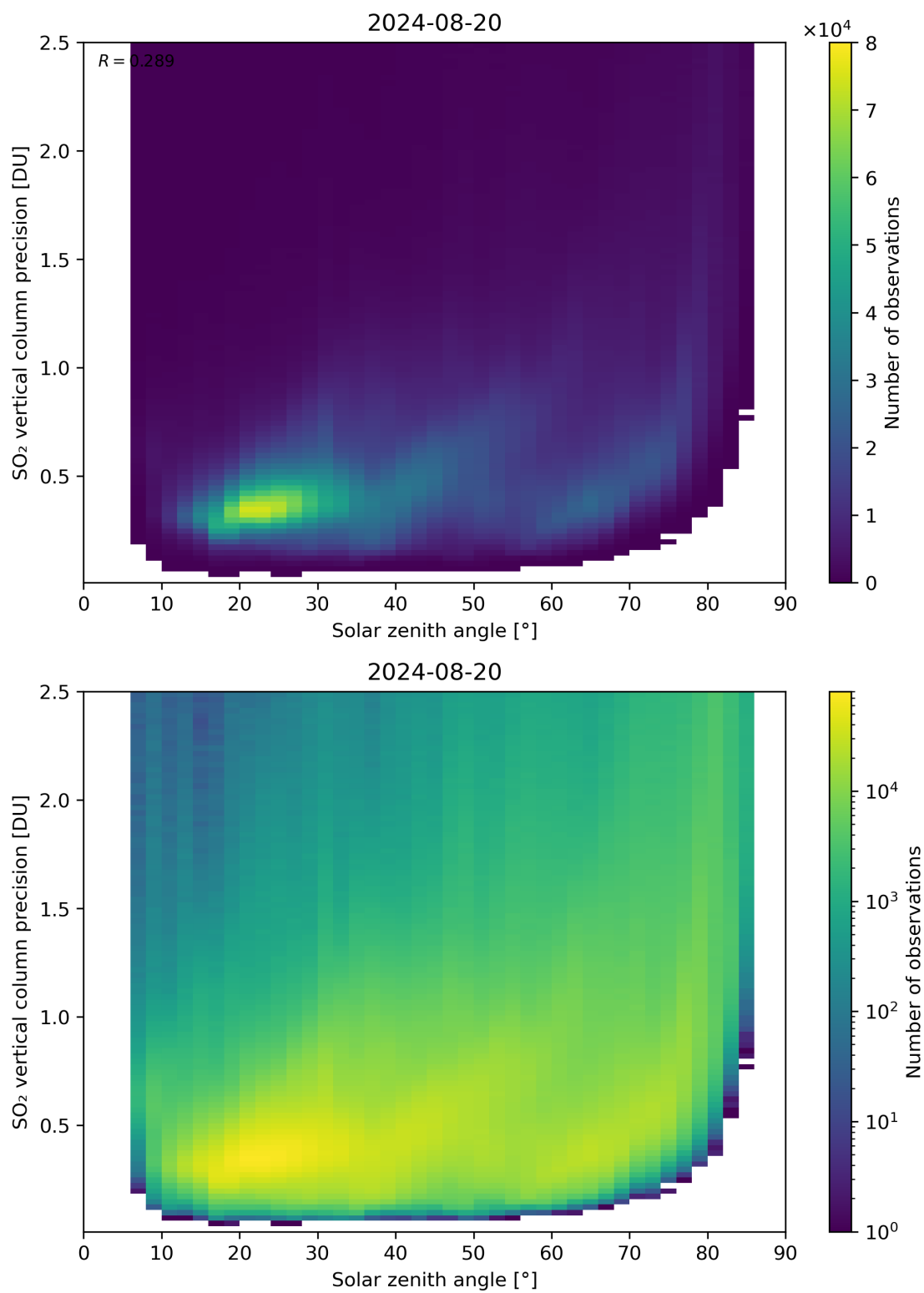
Figure 177: Scatter density plot of “Solar zenith angle” against “SO 2 vertical column precision” for 2024-08-19 to 2024-08-21.
