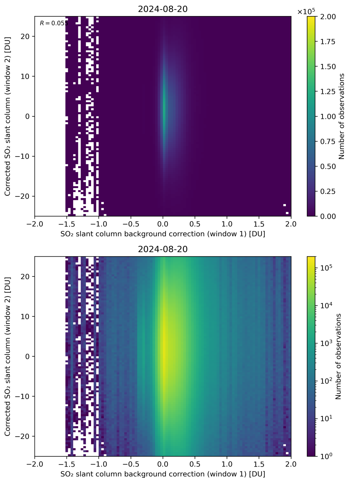
Figure 104: Scatter density plot of “SO 2 slant column background correction (window 1)” against “Corrected SO 2 slant column (window 2)” for 2024-08-19 to 2024-08-21.
