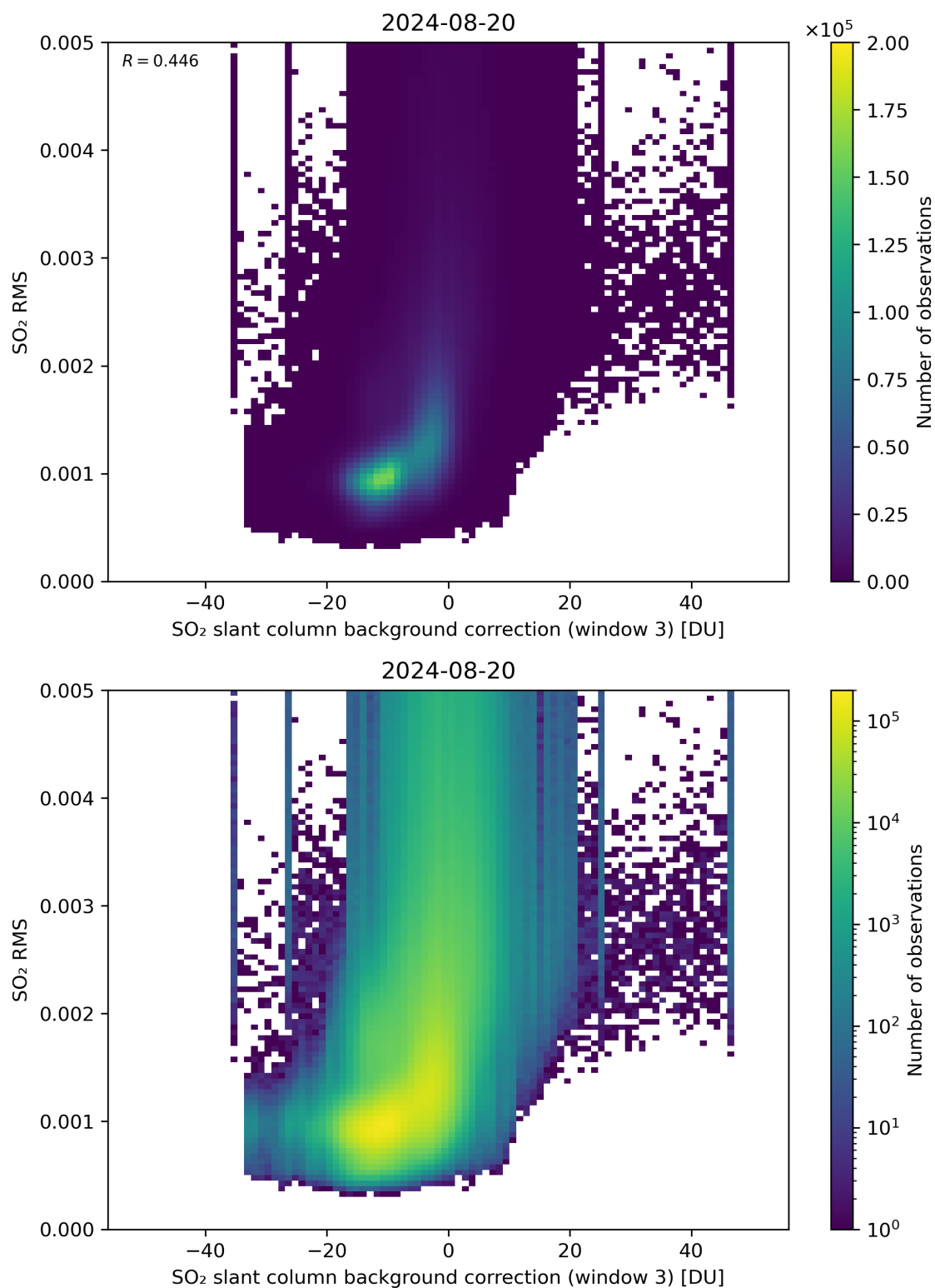
Figure 123: Scatter density plot of “SO 2 slant column background correction (window 3)” against “SO 2 RMS” for 2024-08-19 to 2024-08-21.
