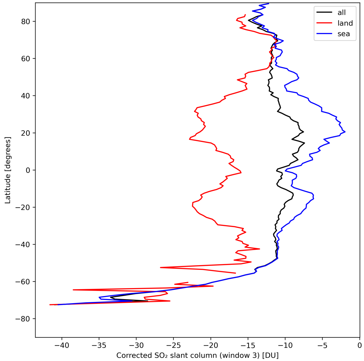
Figure 43: Zonal average of “Corrected SO 2 slant column (window 3)” for 2024-08-19 to 2024-08-21.
