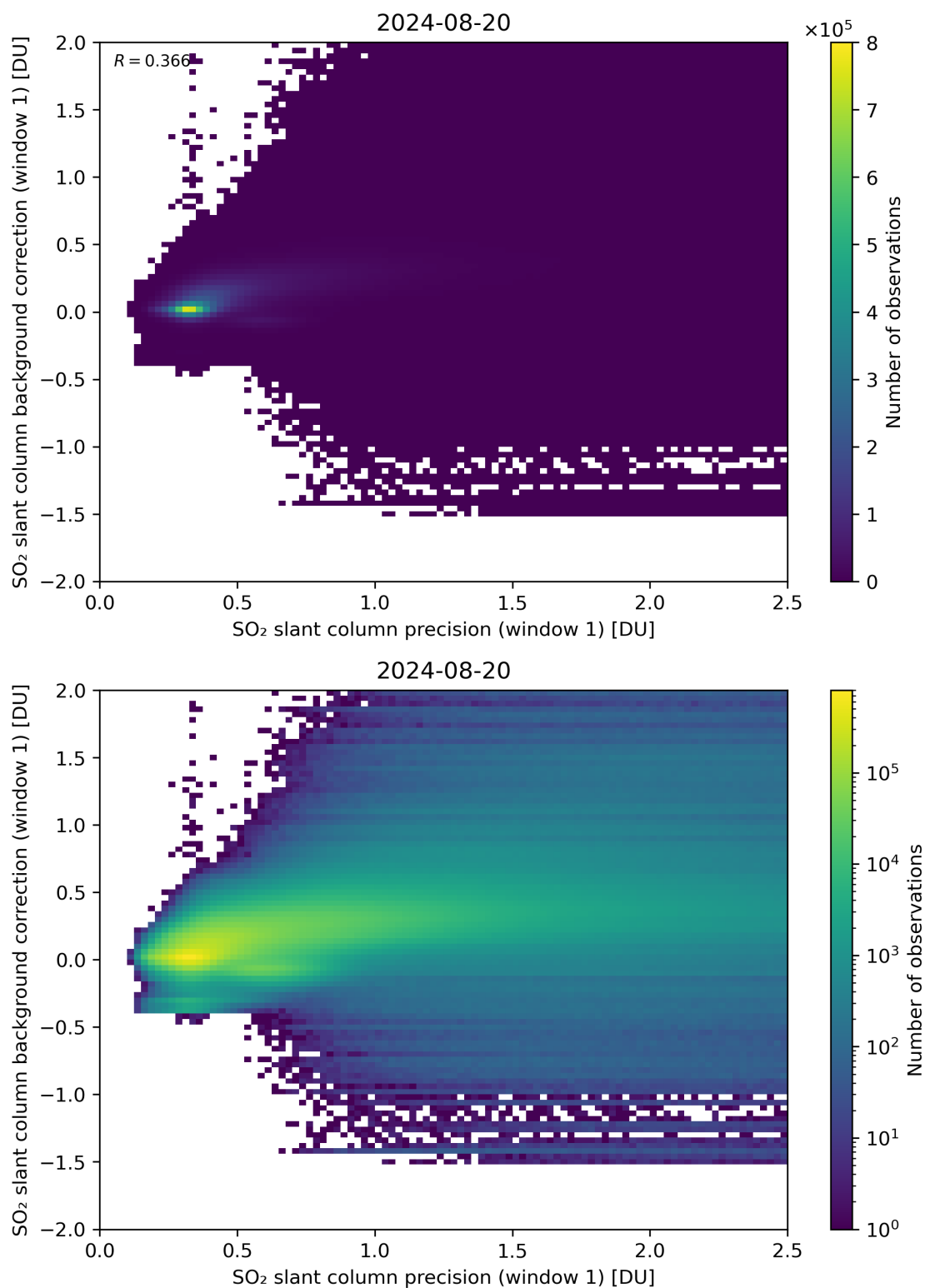
Figure 218: Scatter density plot of “SO 2 slant column precision (window 1)” against “SO 2 slant column background correction (window 1)” for 2024-08-19 to 2024-08-21.
