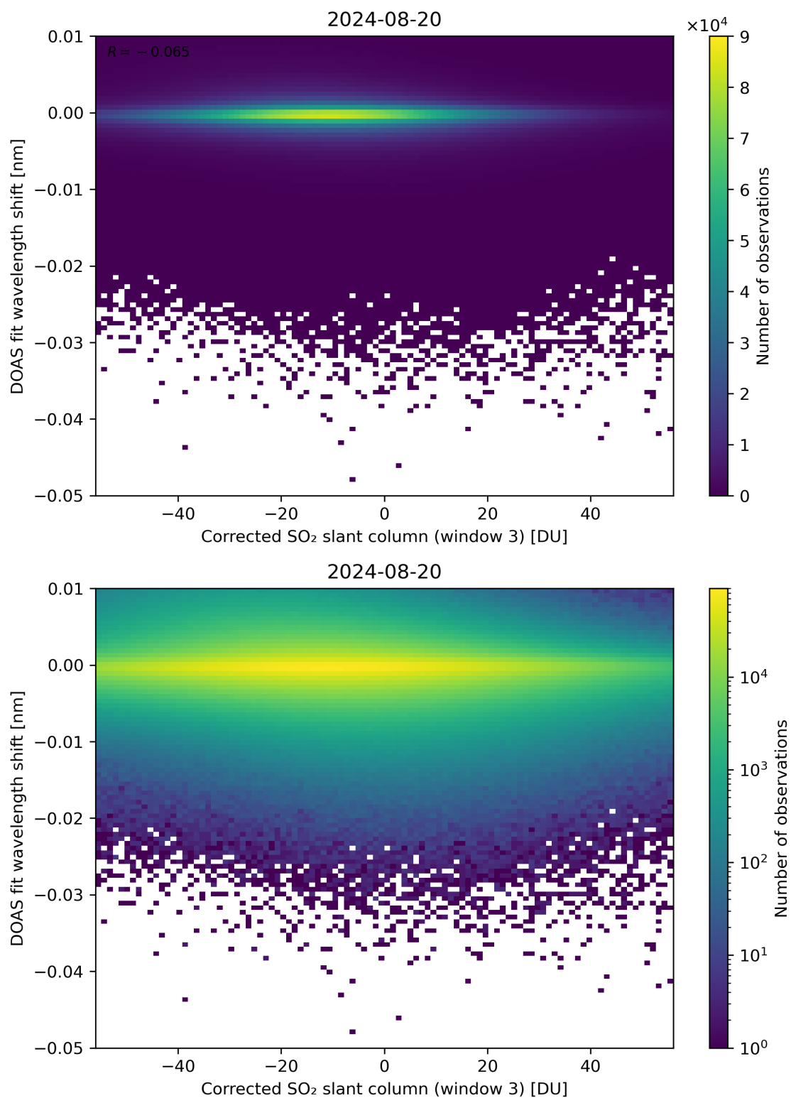
Figure 206: Scatter density plot of “Corrected SO 2 slant column (window 3)” against “DOAS fit wavelength shift” for 2024-08-19 to 2024-08-21.
