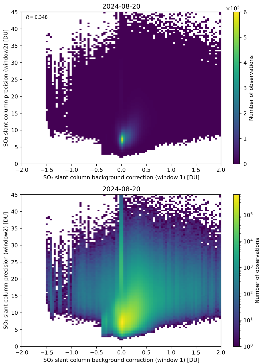
Figure 106: Scatter density plot of “SO 2 slant column background correction (window 1)” against “SO 2 slant column precision (window2)” for 2024-08-19 to 2024-08-21.
