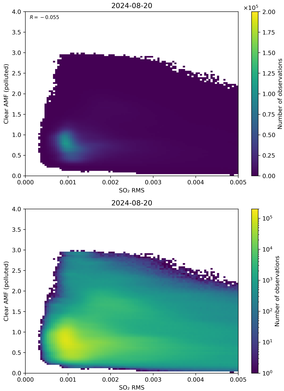
Figure 136: Scatter density plot of “SO 2 RMS” against “Clear AMF (polluted)” for 2024-08-19 to 2024-08-21.
