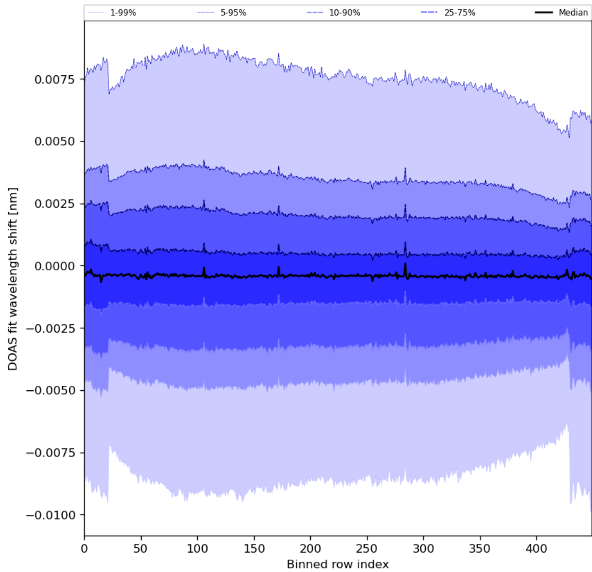
Figure 91: Along track statistics of “DOAS fit wavelength shift” for 2024-08-19 to 2024-08-21
