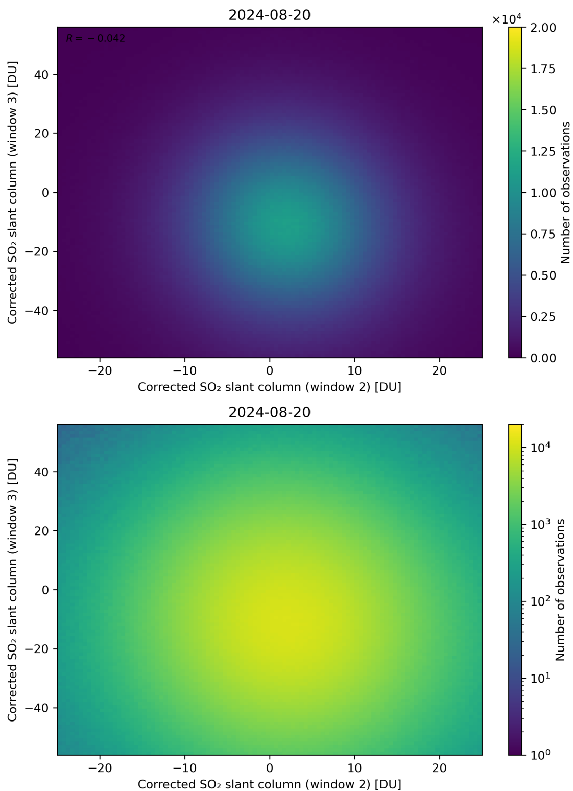
Figure 200: Scatter density plot of “Corrected SO 2 slant column (window 2)” against “Corrected SO 2 slant column (window 3)” for 2024-08-19 to 2024-08-21.
