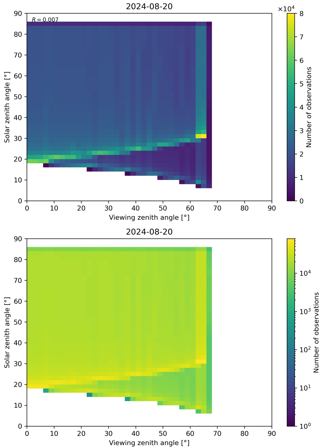
Figure 315: Scatter density plot of “Viewing zenith angle” against “Solar zenith angle” for 2024-08-19 to 2024-08-21.
