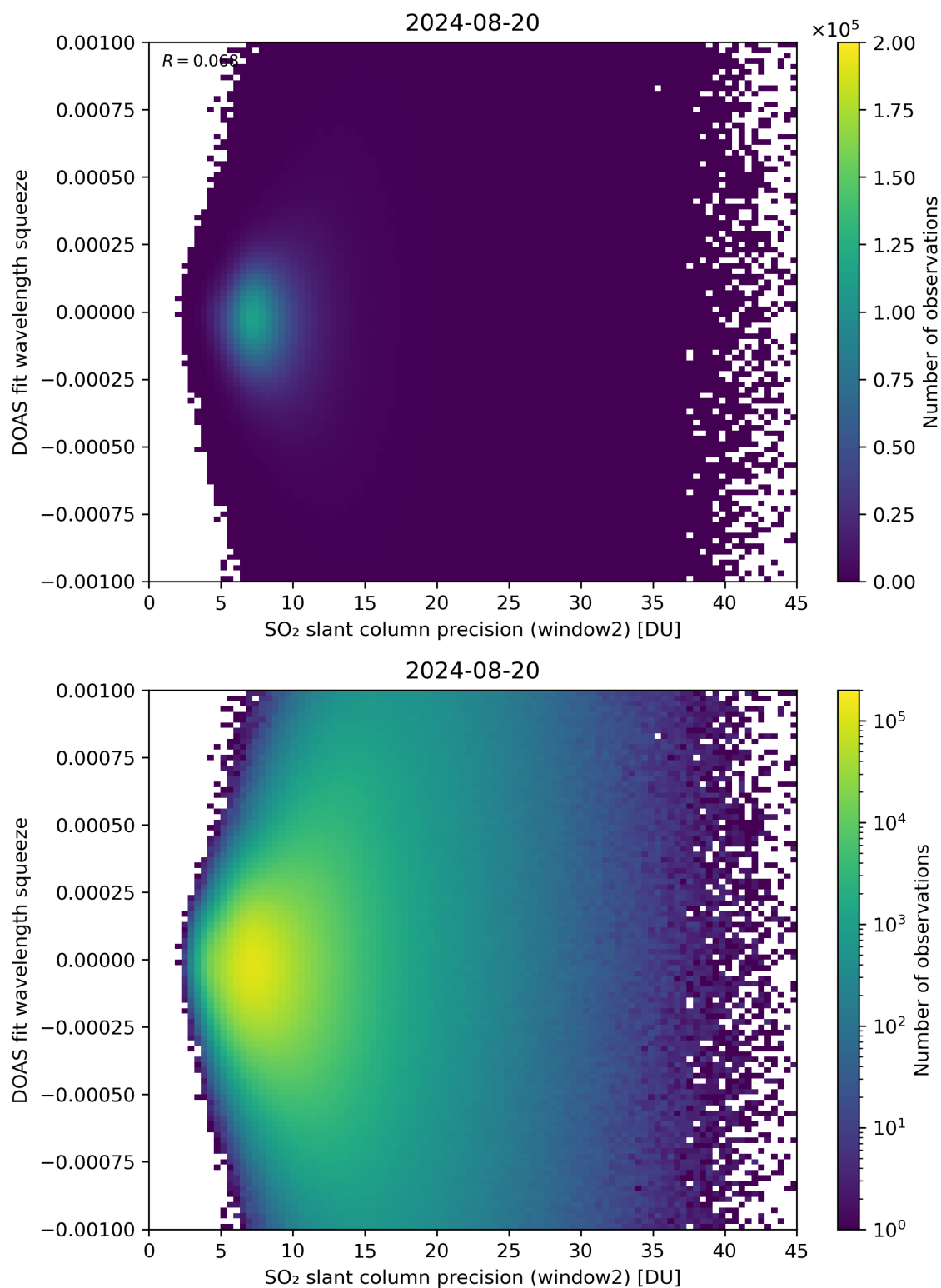
Figure 244: Scatter density plot of “SO 2 slant column precision (window2)” against “DOAS fit wavelength squeeze” for 2024-08-19 to 2024-08-21.
