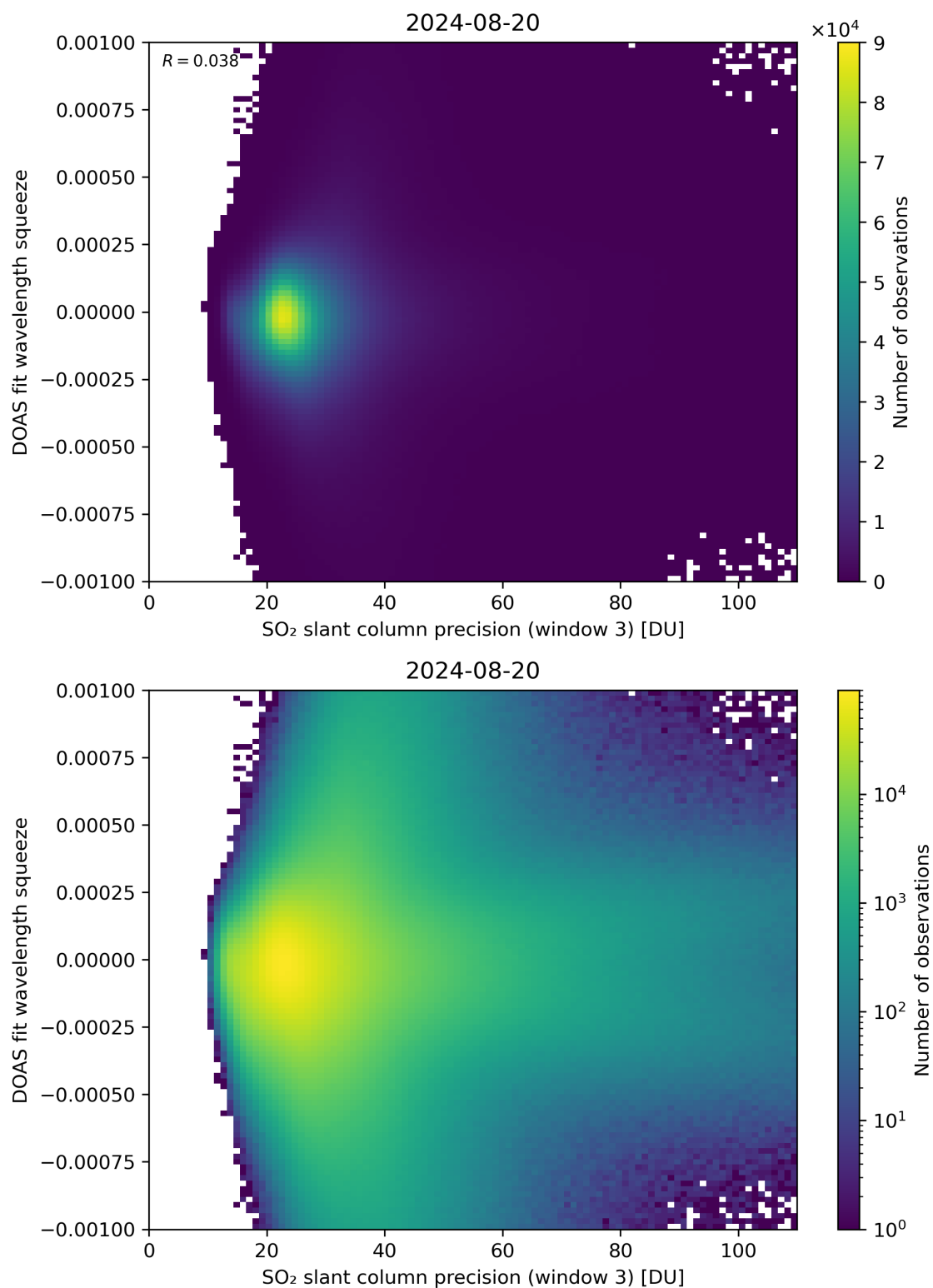
Figure 259: Scatter density plot of “SO 2 slant column precision (window 3)” against “DOAS fit wavelength squeeze” for 2024-08-19 to 2024-08-21.
