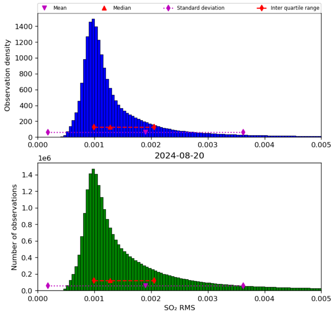
Figure 70: Histogram of “SO 2 RMS” for 2024-08-19 to 2024-08-21
