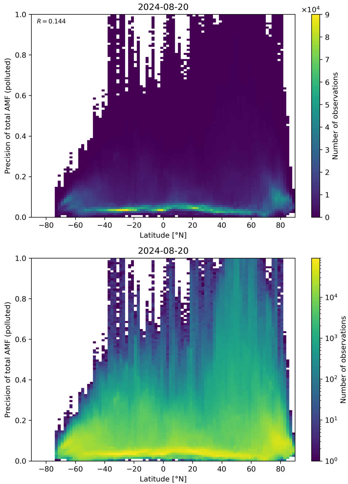
Figure 155: Scatter density plot of “Latitude” against “Precision of total AMF (polluted)” for 2024-08-19 to 2024-08-21.
