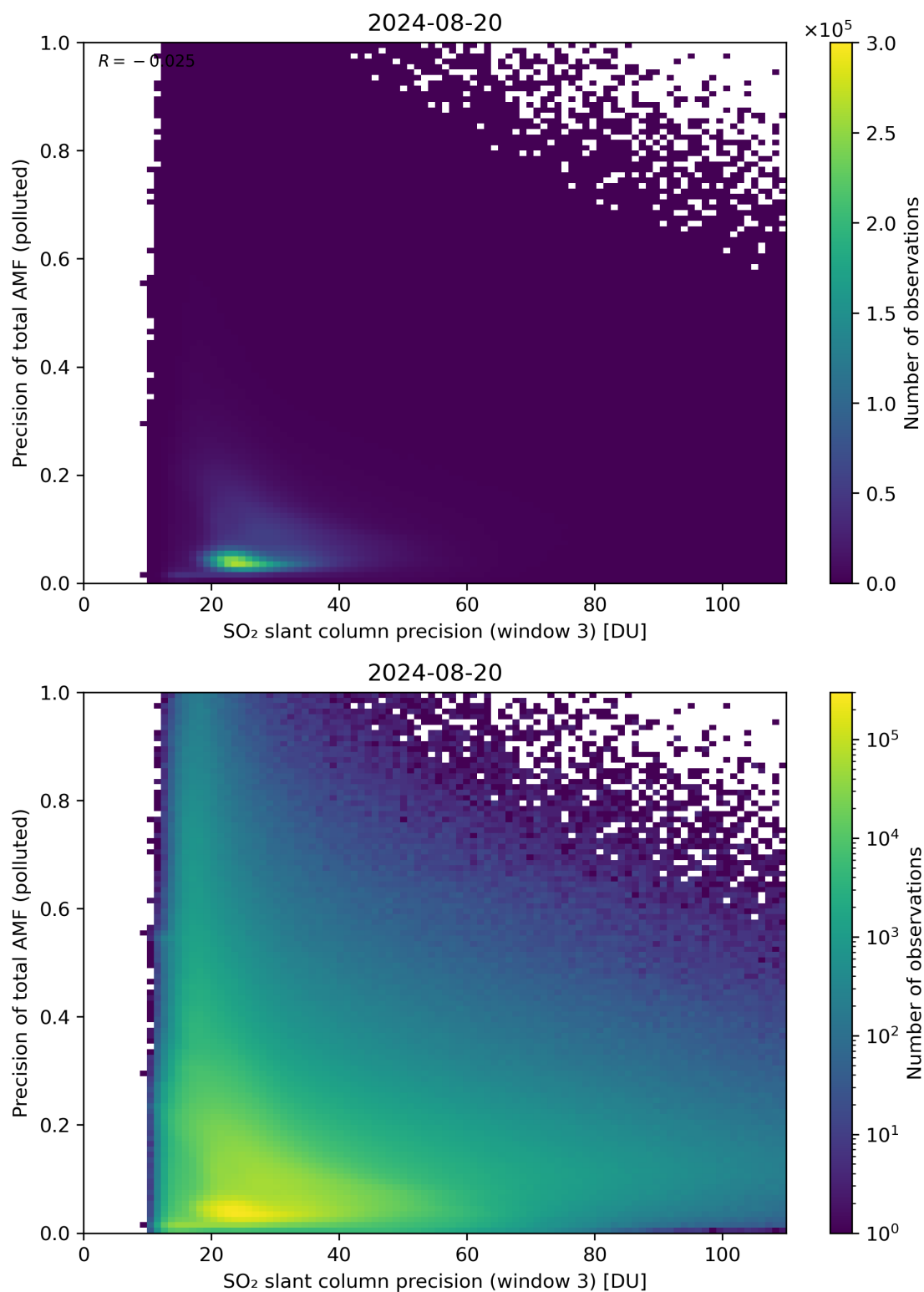
Figure 264: Scatter density plot of “SO 2 slant column precision (window 3)” against “Precision of total AMF (polluted)” for 2024-08-19 to 2024-08-21.
