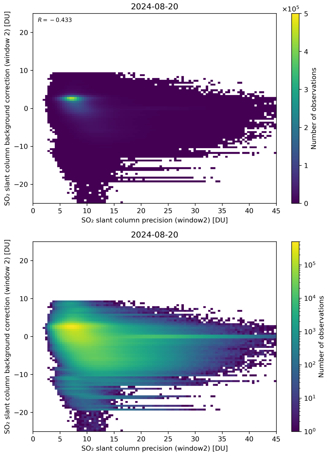
Figure 241: Scatter density plot of “SO 2 slant column precision (window2)” against “SO 2 slant column background correction (window 2)” for 2024-08-19 to 2024-08-21.
