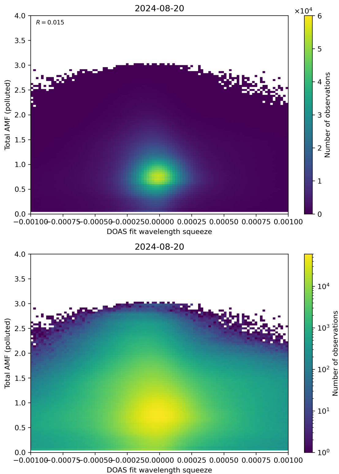
Figure 134: Scatter density plot of “DOAS fit wavelength squeeze” against “Total AMF (polluted)” for 2024-08-19 to 2024-08-21.
