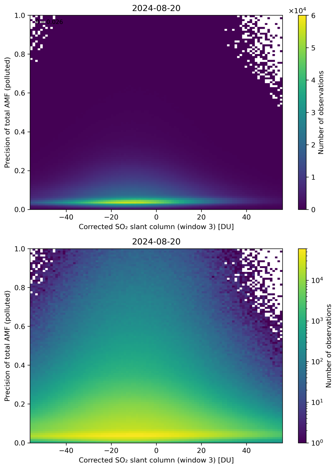
Figure 211: Scatter density plot of “Corrected SO 2 slant column (window 3)” against “Precision of total AMF (polluted)” for 2024-08-19 to 2024-08-21.
