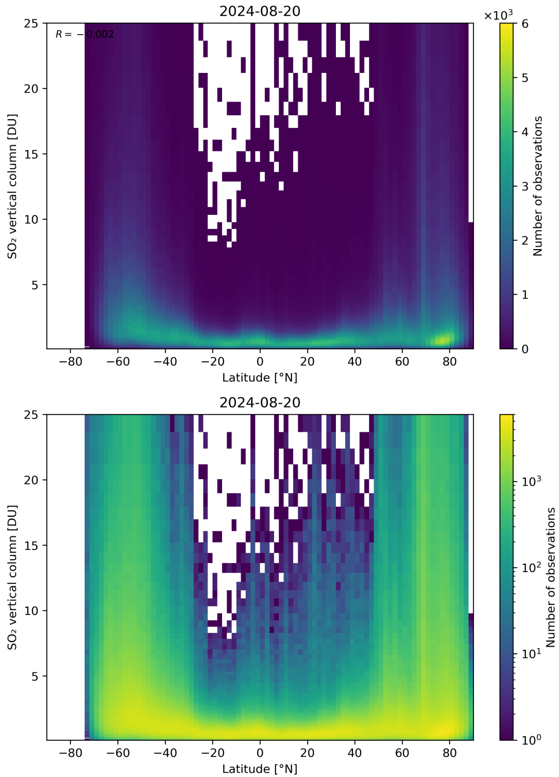
Figure 156: Scatter density plot of “Latitude” against “SO 2 vertical column” for 2024-08-19 to 2024-08-21.
