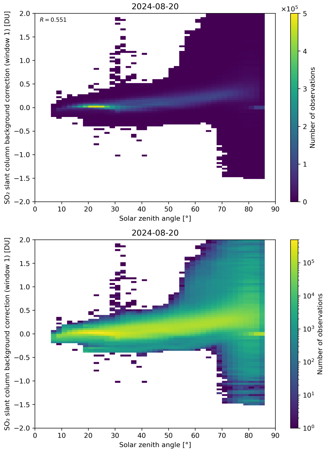
Figure 158: Scatter density plot of “Solar zenith angle” against “SO 2 slant column background correction (window 1)” for 2024-08-19 to 2024-08-21.
