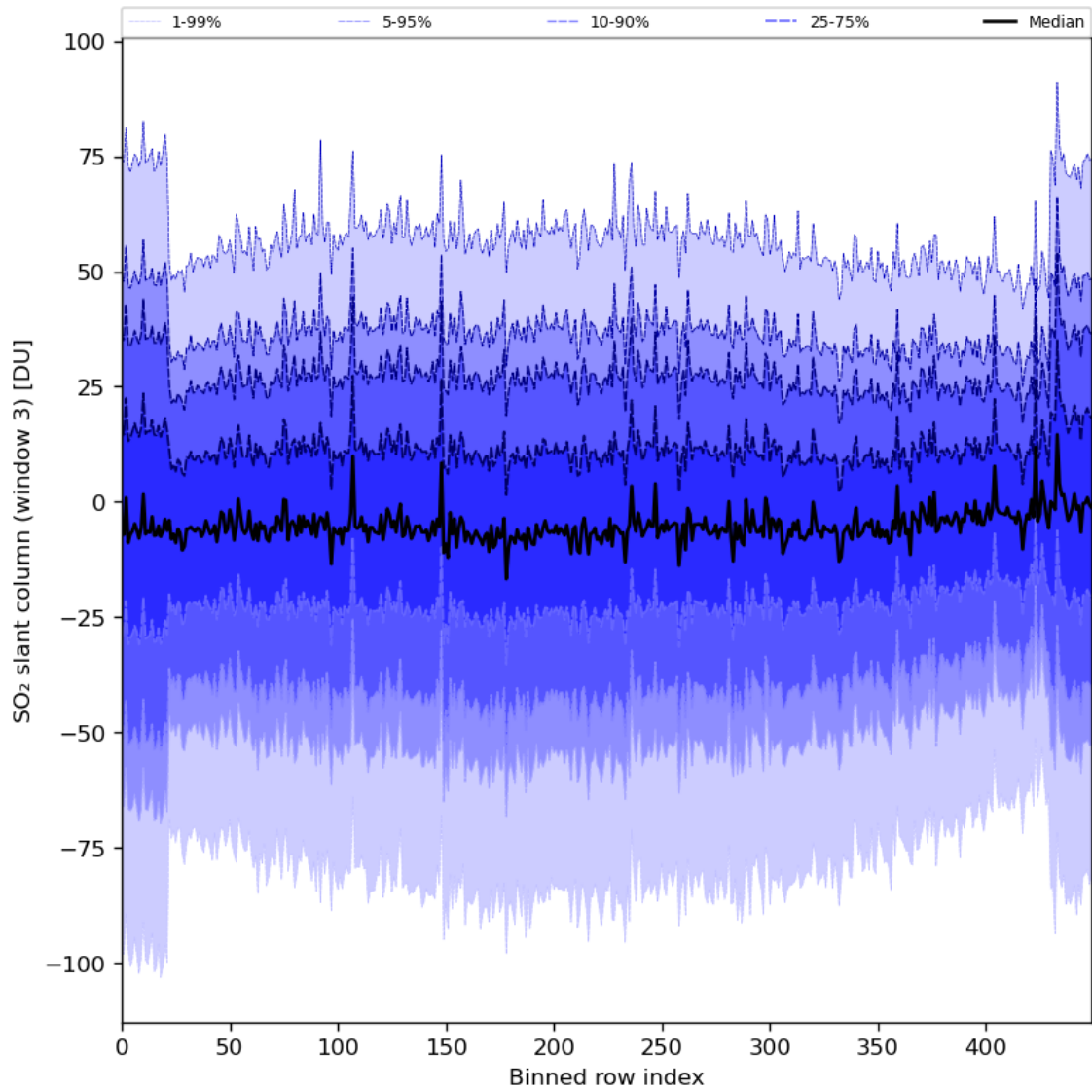
Figure 87: Along track statistics of "SO 2 slant column (window 3)" for 2024-08-19 to 2024-08-21
