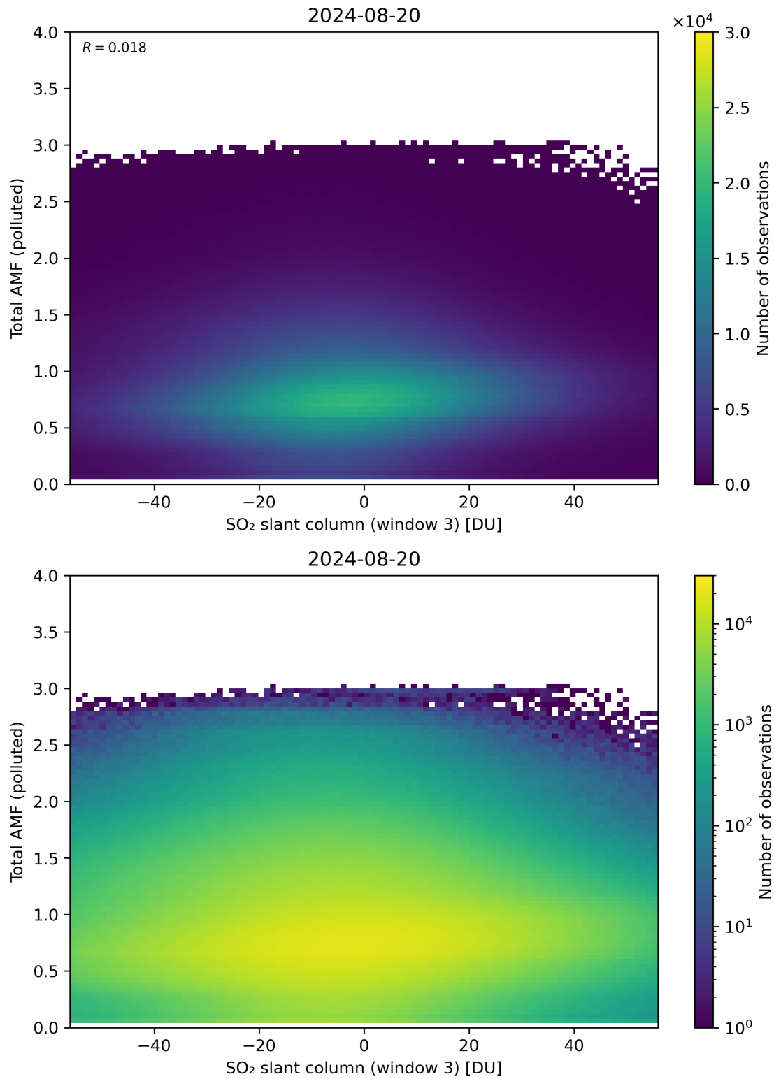
Figure 268: Scatter density plot of “SO 2 slant column (window 3)” against “Total AMF (polluted)” for 2024-08-19 to 2024-08-21.
