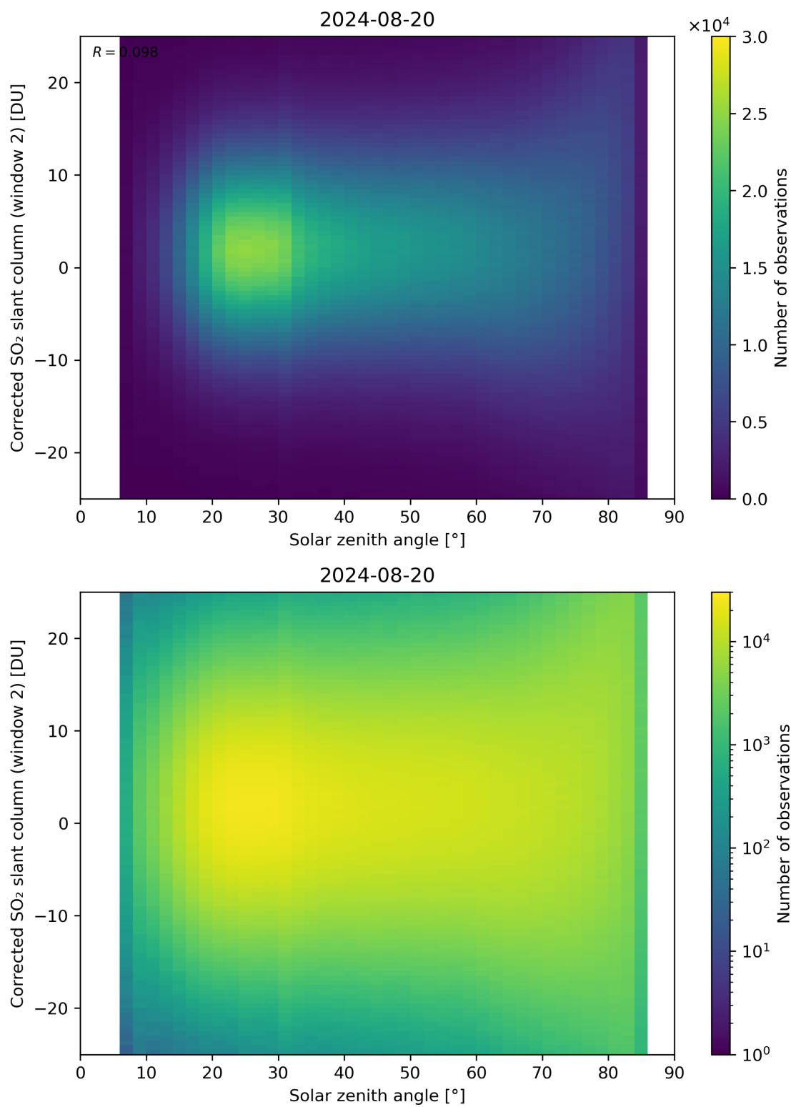
Figure 167: Scatter density plot of “Solar zenith angle” against “Corrected SO 2 slant column (window 2)” for 2024-08-19 to 2024-08-21.
