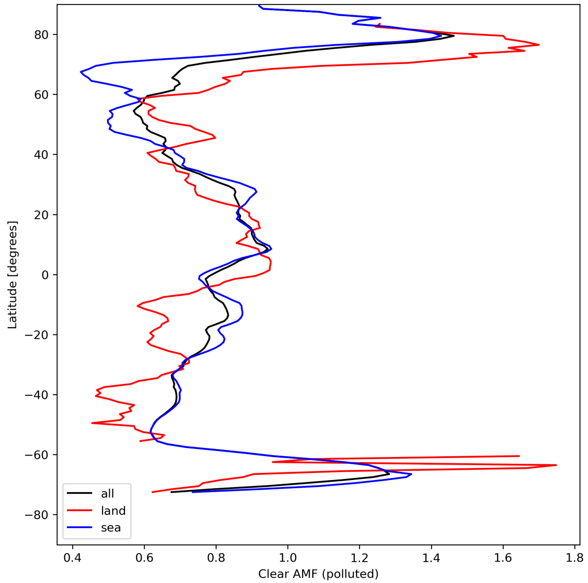
Figure 50: Zonal average of “Clear AMF (polluted)” for 2024-08-19 to 2024-08-21.
