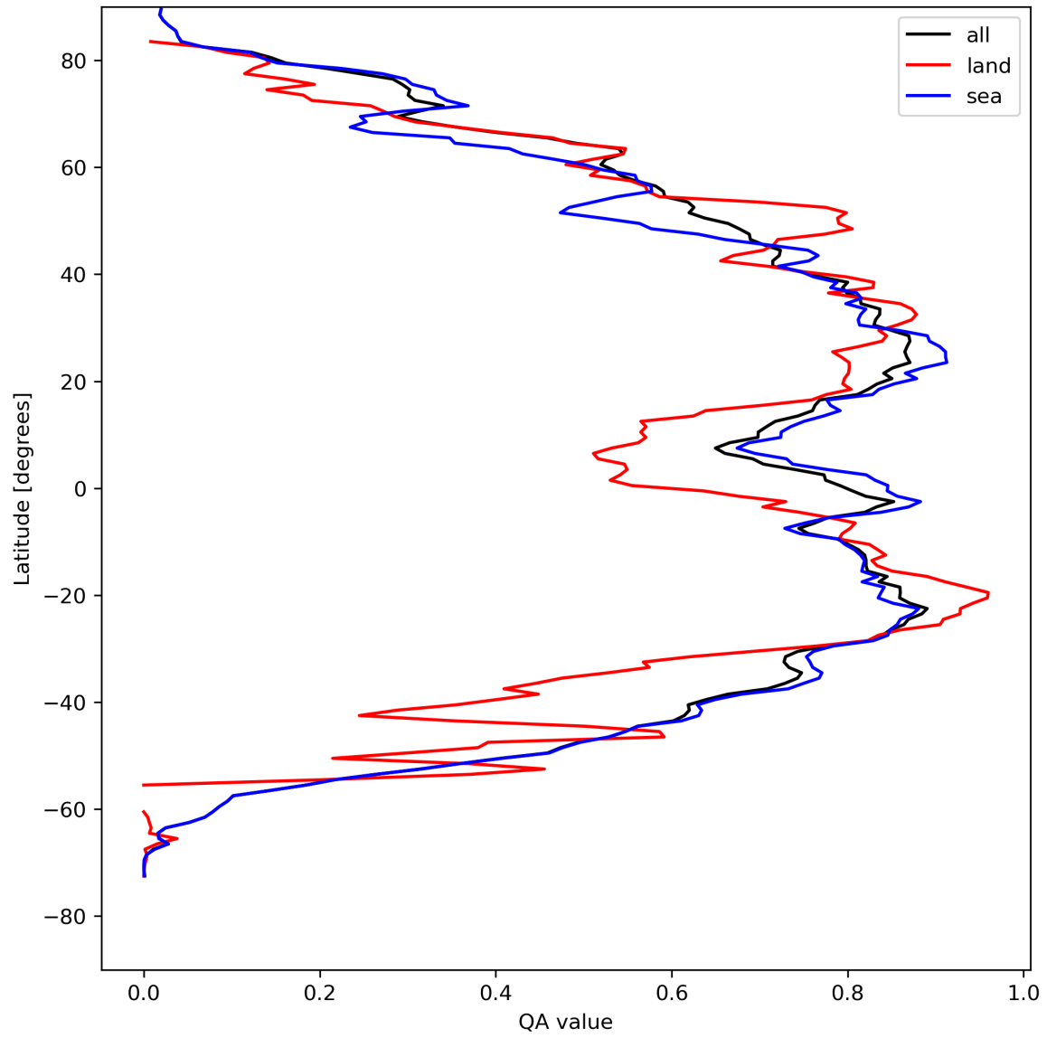
Figure 29: Zonal average of “QA value” for 2024-08-19 to 2024-08-21.
