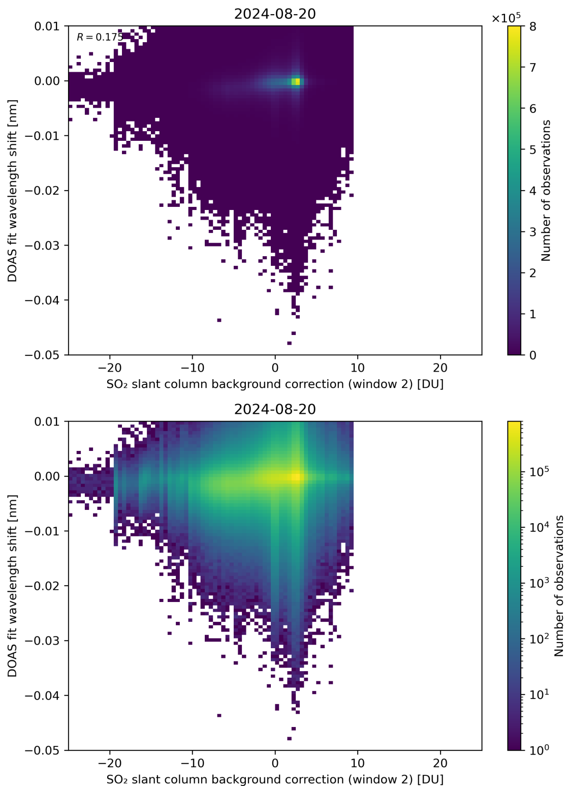
Figure 112: Scatter density plot of “SO 2 slant column background correction (window 2)” against “DOAS fit wavelength shift” for 2024-08-19 to 2024-08-21.
