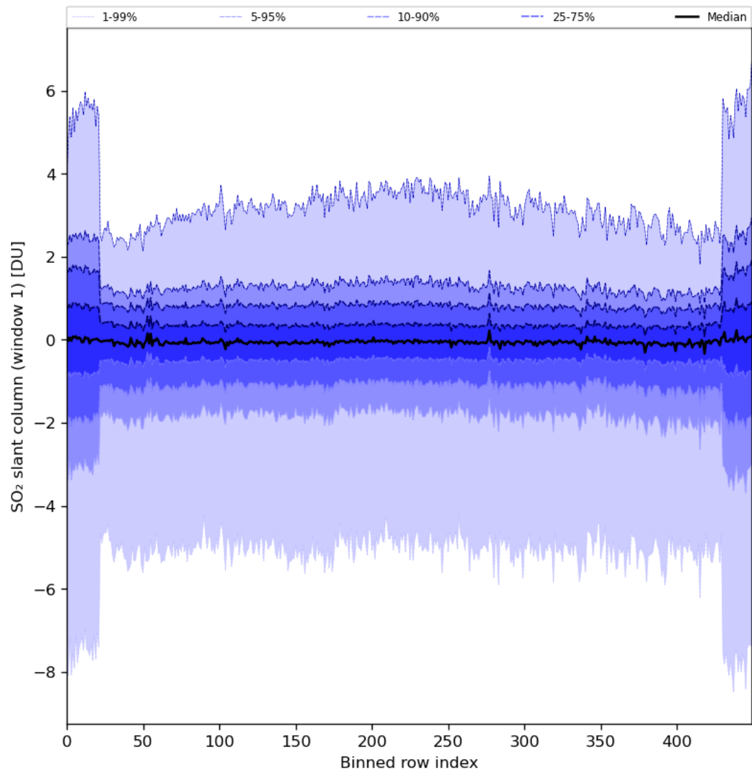
Figure 79: Along track statistics of “SO 2 slant column (window 1)” for 2024-08-19 to 2024-08-21
