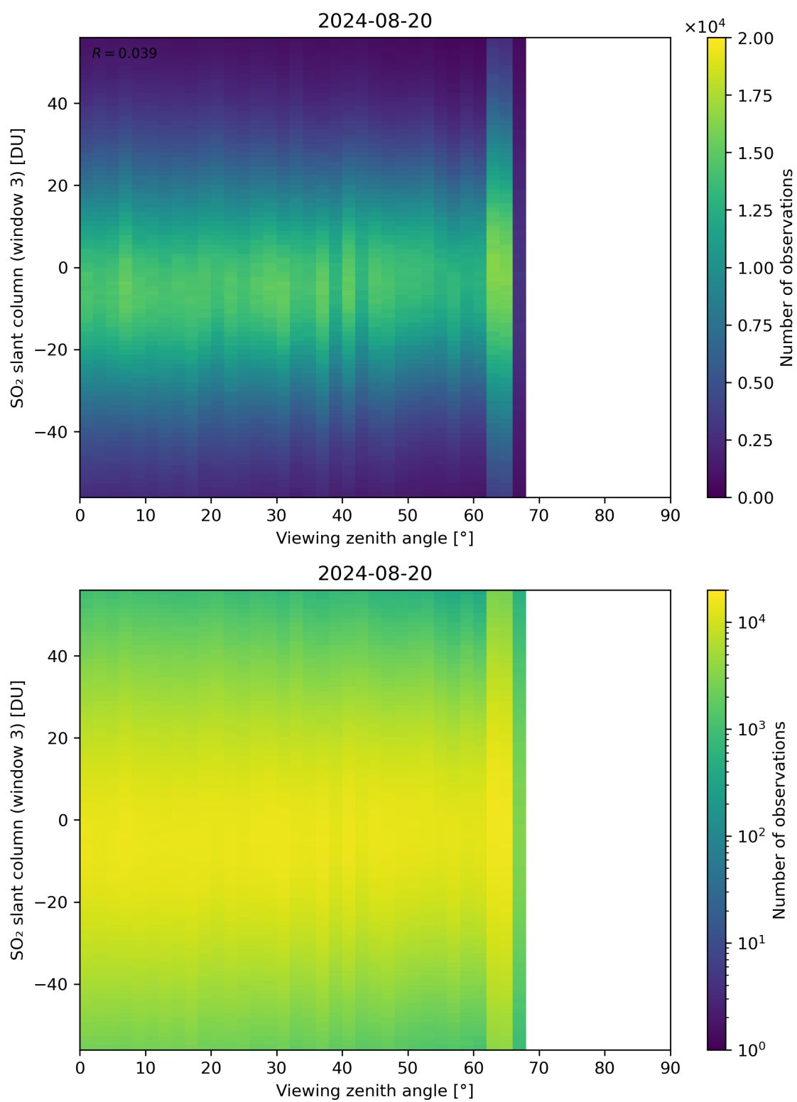
Figure 323: Scatter density plot of “Viewing zenith angle” against “SO 2 slant column (window 3)” for 2024-08-19 to 2024-08-21.
