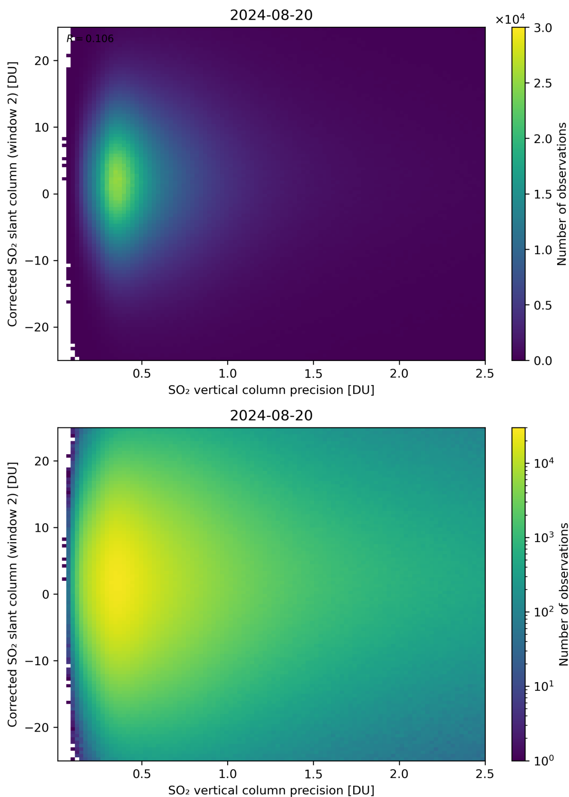
Figure 287: Scatter density plot of “SO 2 vertical column precision” against “Corrected SO 2 slant column (window 2)” for 2024-08-19 to 2024-08-21.
