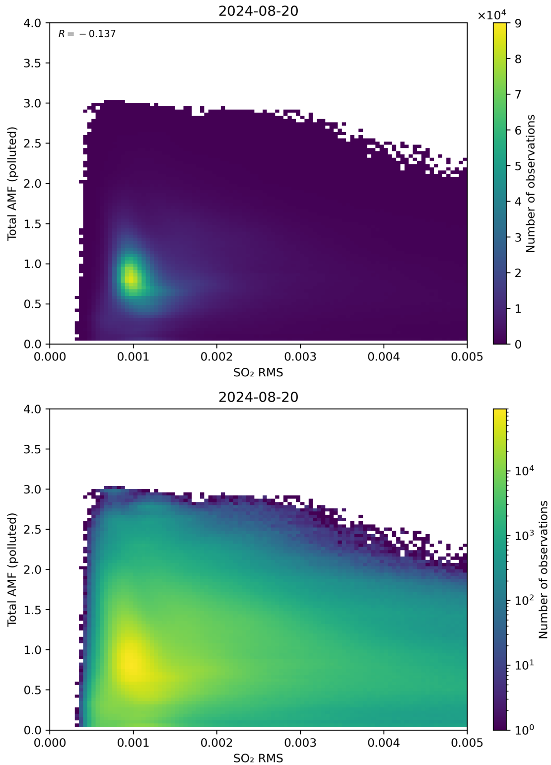
Figure 137: Scatter density plot of “SO 2 RMS” against “Total AMF (polluted)” for 2024-08-19 to 2024-08-21.
