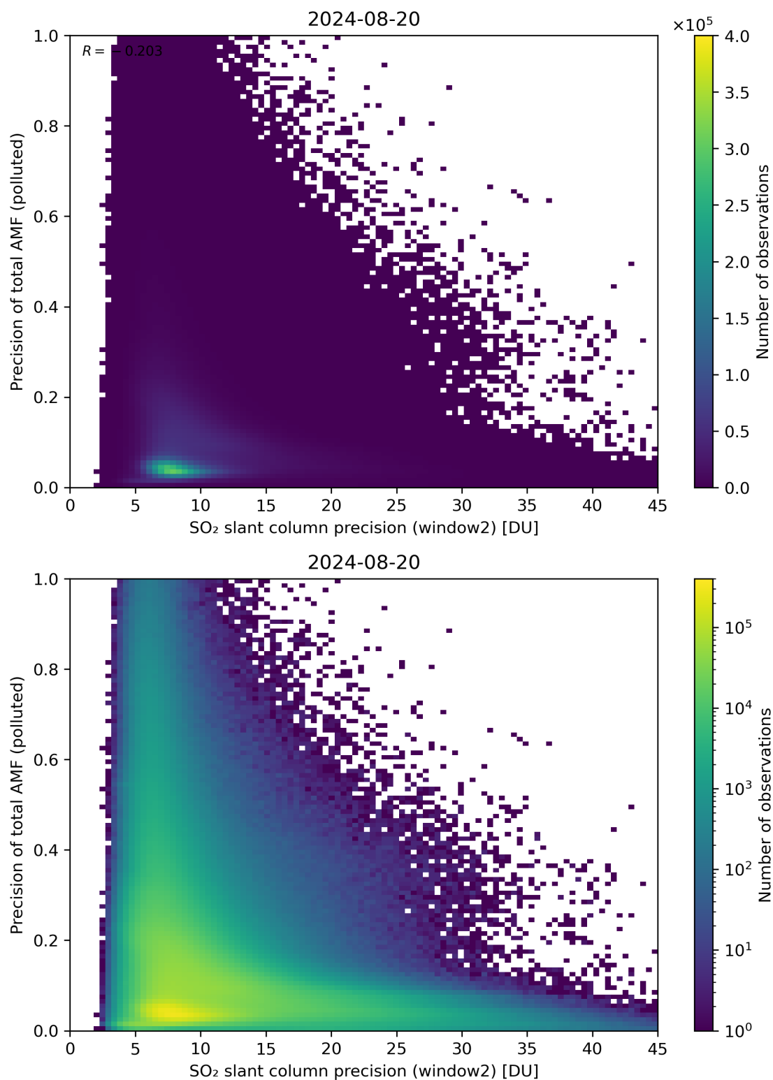
Figure 252: Scatter density plot of “SO 2 slant column precision (window2)” against “Precision of total AMF (polluted)” for 2024-08-19 to 2024-08-21.
