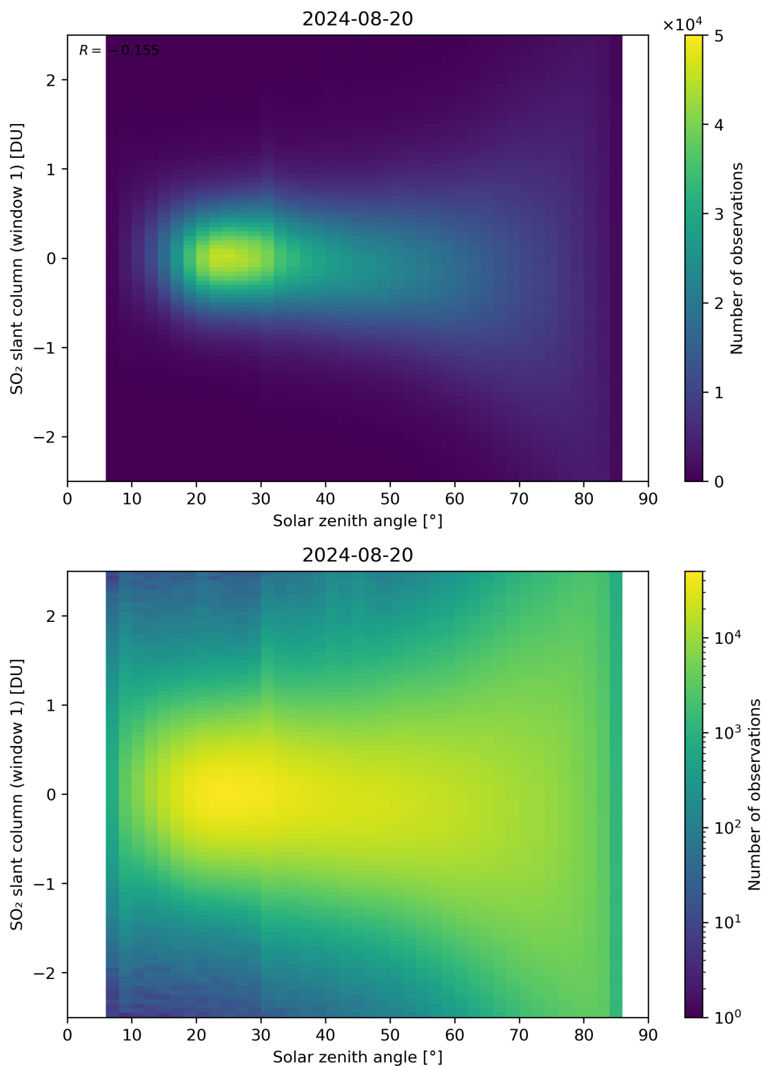
Figure 169: Scatter density plot of “Solar zenith angle” against “SO 2 slant column (window 1)” for 2024-08-19 to 2024-08-21.
