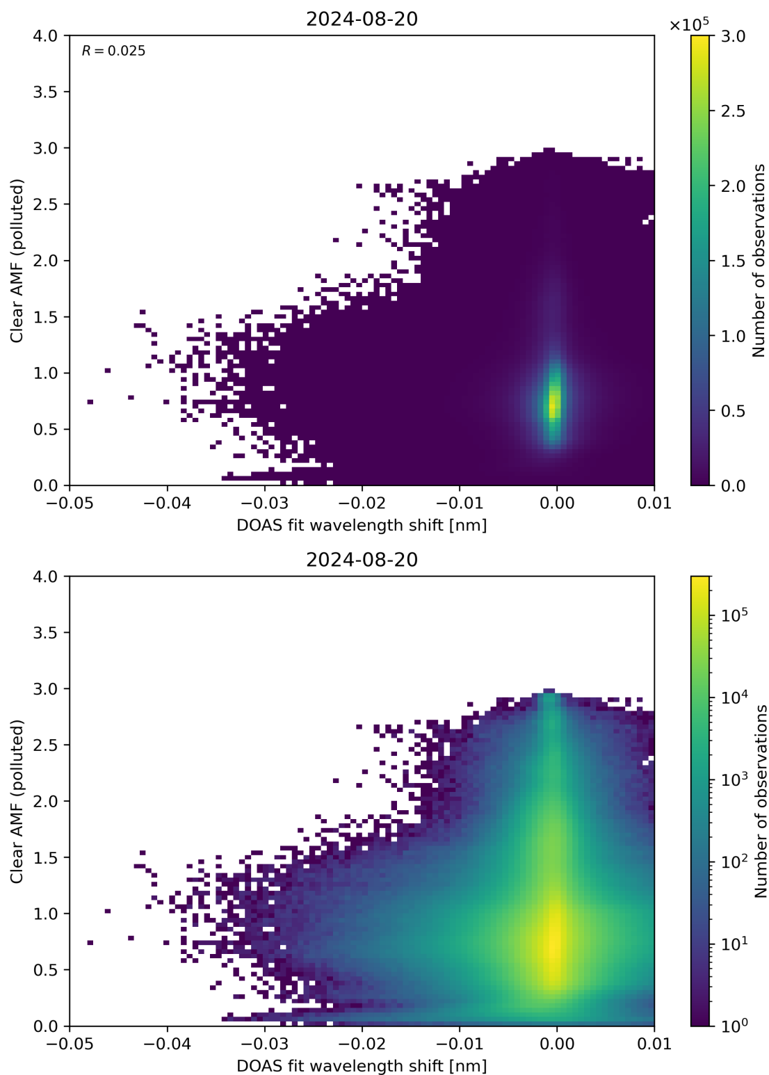
Figure 129: Scatter density plot of “DOAS fit wavelength shift” against “Clear AMF (polluted)” for 2024-08-19 to 2024-08-21.
