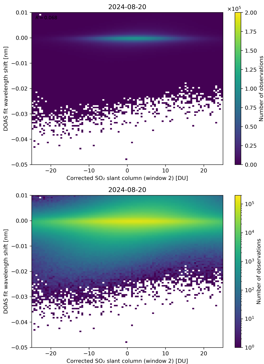
Figure 196: Scatter density plot of “Corrected SO 2 slant column (window 2)” against “DOAS fit wavelength shift” for 2024-08-19 to 2024-08-21.
