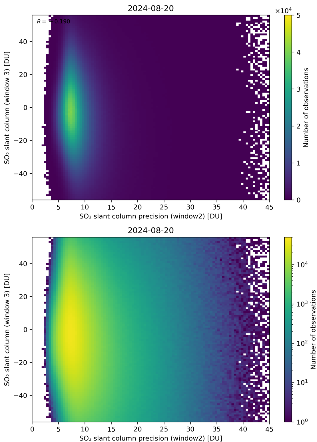
Figure 249: Scatter density plot of “SO 2 slant column precision (window2)” against “SO 2 slant column (window 3)” for 2024-08-19 to 2024-08-21.
