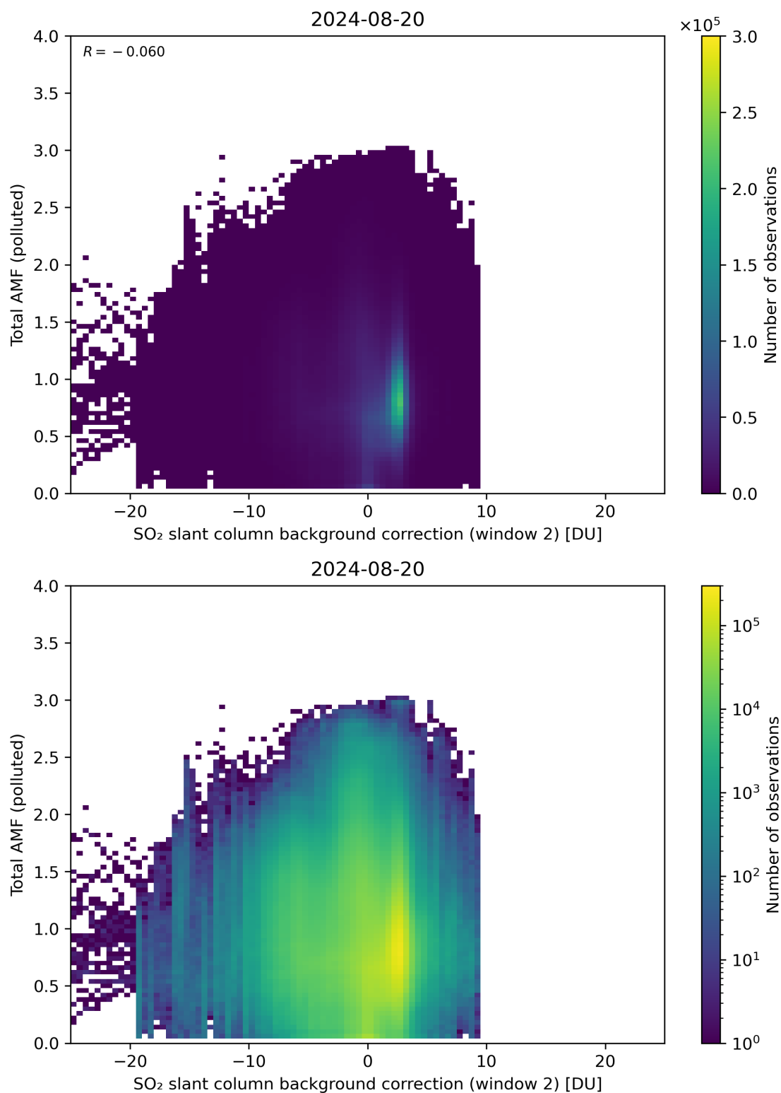
Figure 119: Scatter density plot of “SO 2 slant column background correction (window 2)” against “Total AMF (polluted)” for 2024-08-19 to 2024-08-21.
