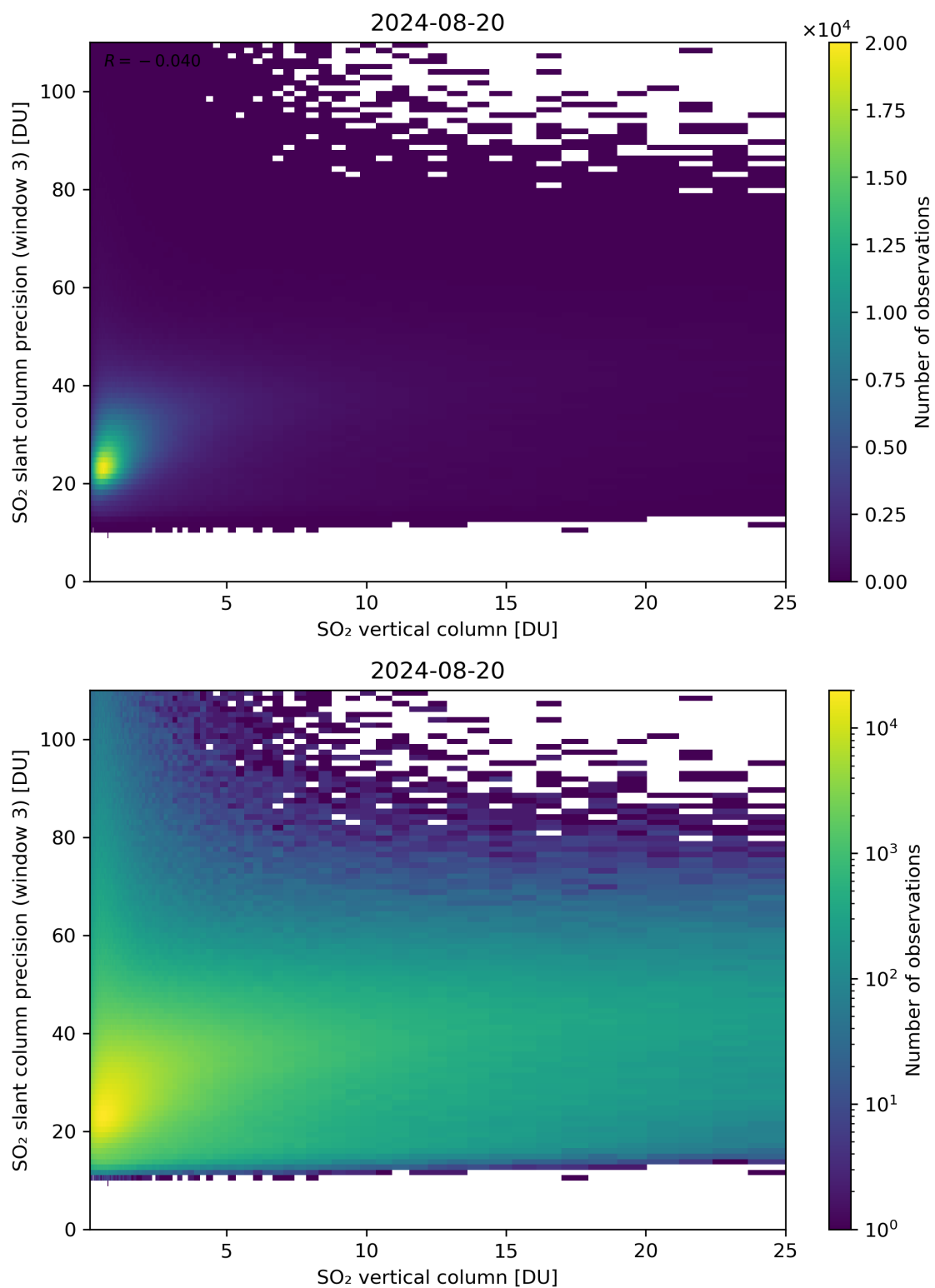
Figure 304: Scatter density plot of “SO 2 vertical column” against “SO 2 slant column precision (window 3)” for 2024-08-19 to 2024-08-21.
