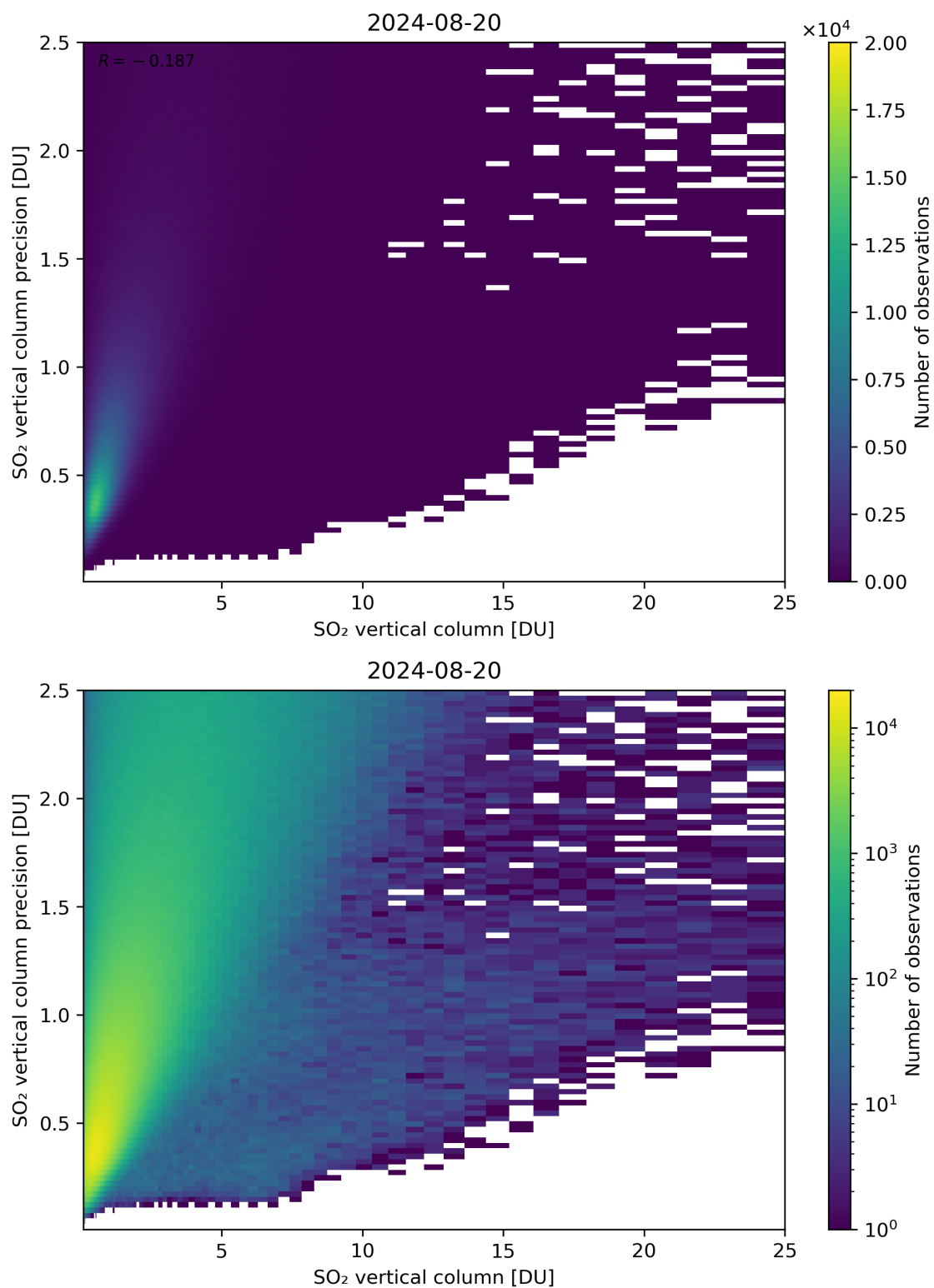
Figure 307: Scatter density plot of “SO 2 vertical column” against “SO 2 vertical column precision” for 2024-08-19 to 2024-08-21.
