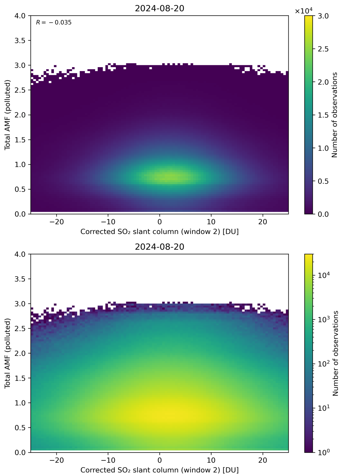
Figure 203: Scatter density plot of “Corrected SO 2 slant column (window 2)” against “Total AMF (polluted)” for 2024-08-19 to 2024-08-21.
