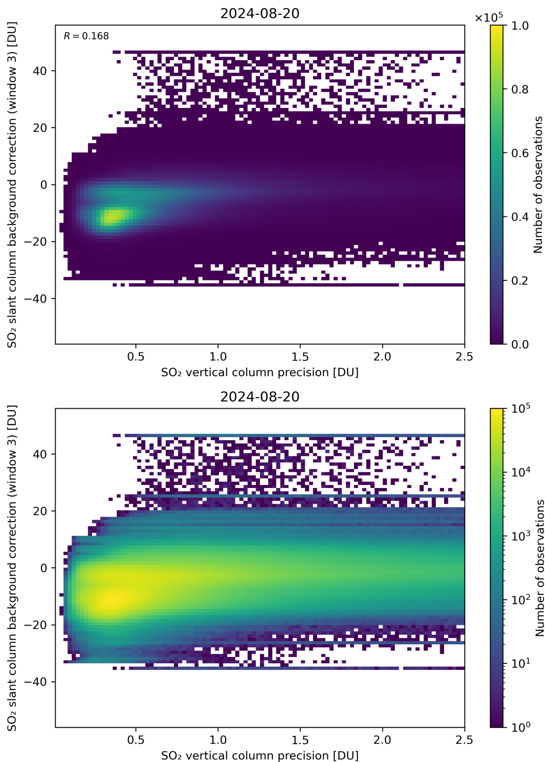
Figure 281: Scatter density plot of “SO 2 vertical column precision” against “SO 2 slant column background correction (window 3)” for 2024-08-19 to 2024-08-21.
