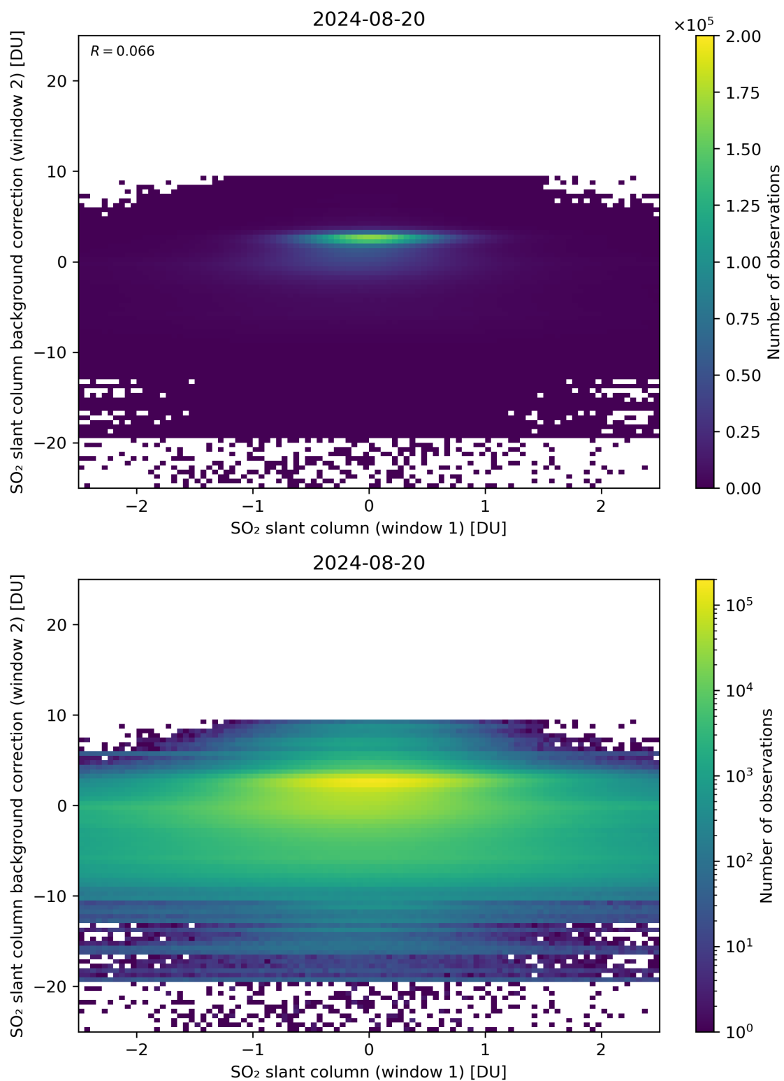
Figure 213: Scatter density plot of “SO 2 slant column (window 1)” against “SO 2 slant column background correction (window 2)” for 2024-08-19 to 2024-08-21.
