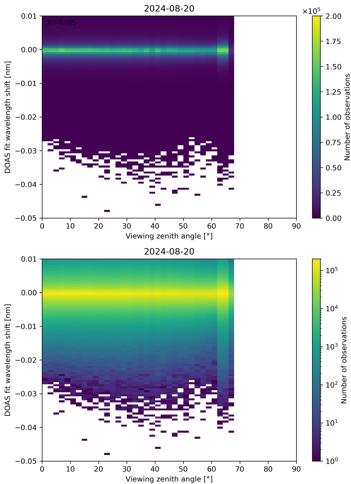
Figure 311: Scatter density plot of “Viewing zenith angle” against “DOAS fit wavelength shift” for 2024-08-19 to 2024-08-21.
