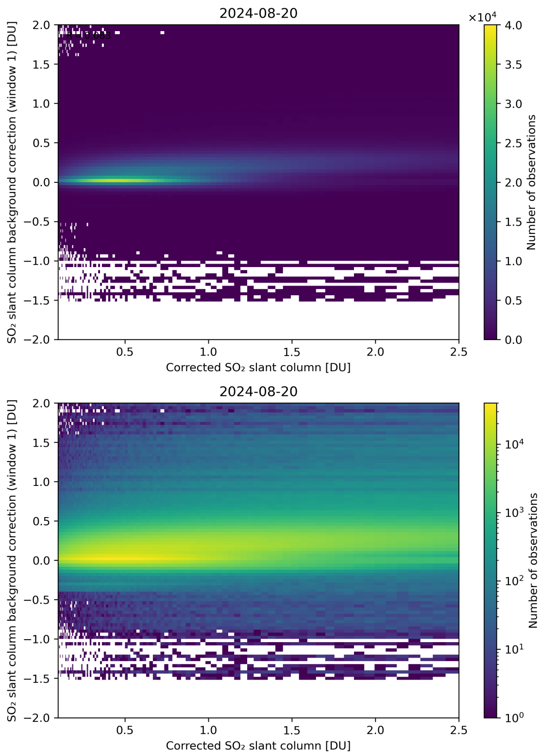
Figure 178: Scatter density plot of “Corrected SO 2 slant column” against “SO 2 slant column background correction (window 1)” for 2024-08-19 to 2024-08-21.
