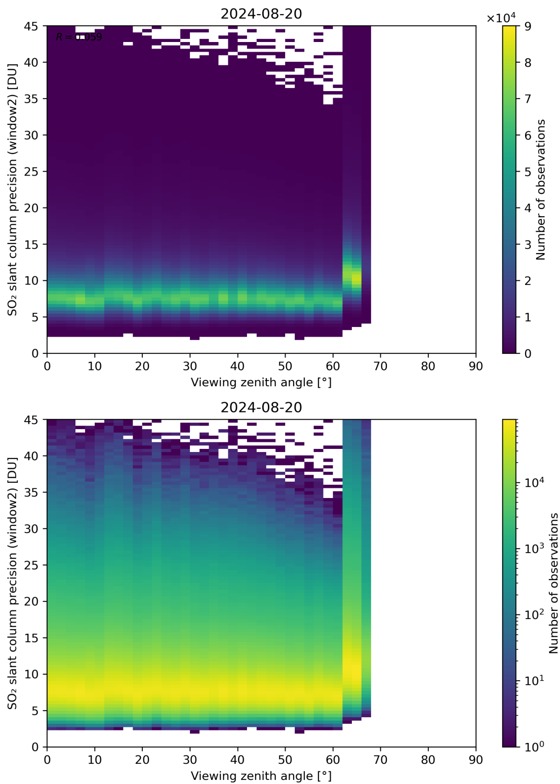
Figure 322: Scatter density plot of “Viewing zenith angle” against “SO 2 slant column precision (window2)” for 2024-08-19 to 2024-08-21.
