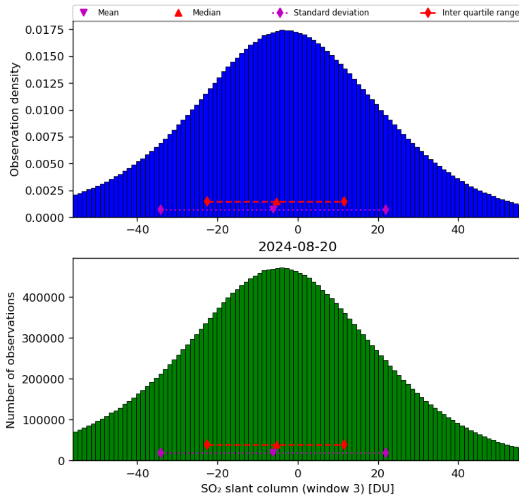
Figure 64: Histogram of “SO 2 slant column (window 3)” for 2024-08-19 to 2024-08-21
