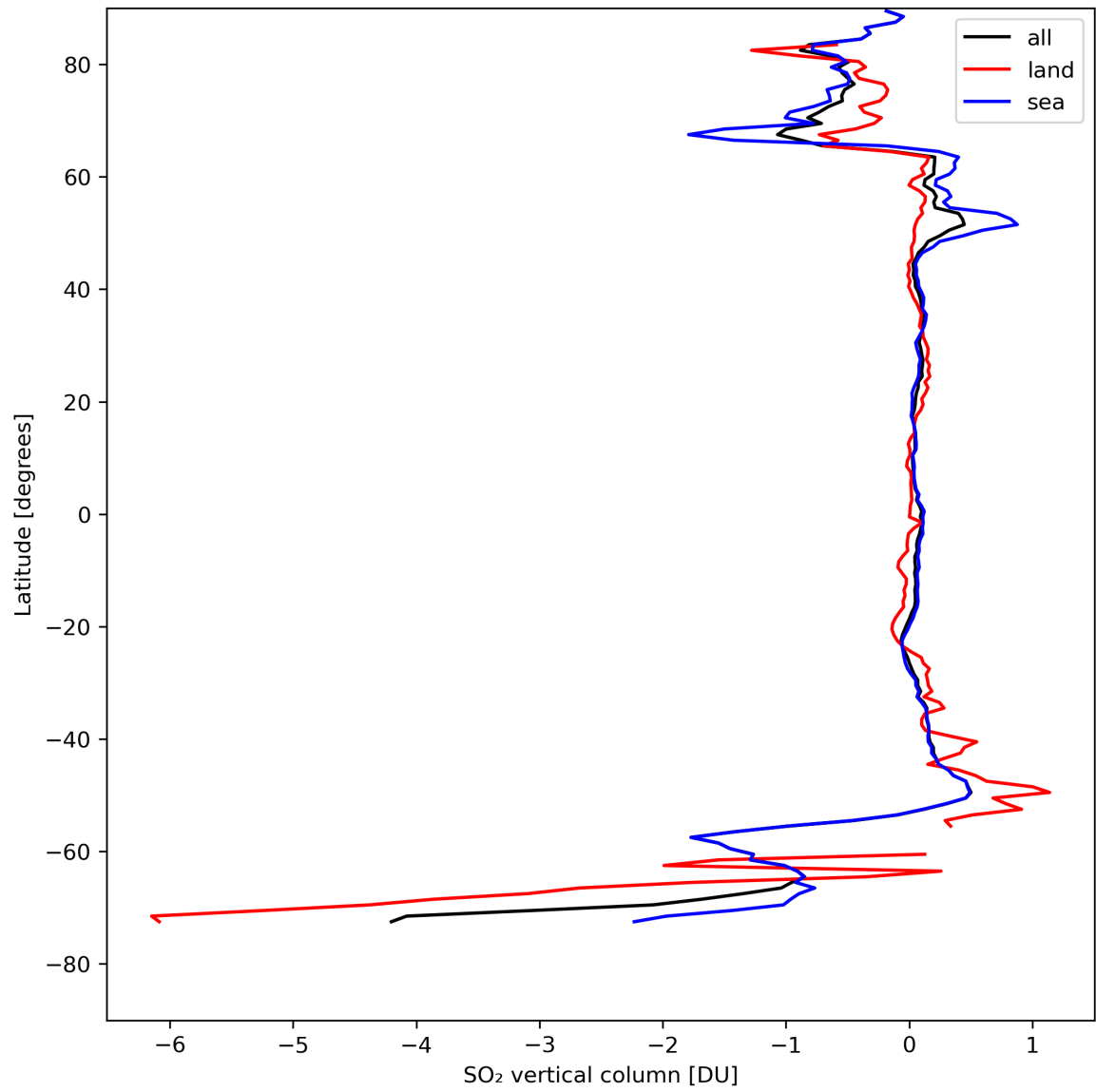
Figure 30: Zonal average of “SO 2 vertical column” for 2024-08-19 to 2024-08-21.
