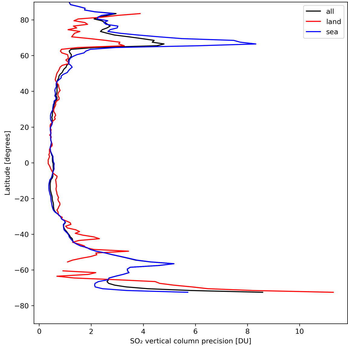
Figure 31: Zonal average of “SO 2 vertical column precision” for 2024-08-19 to 2024-08-21.
