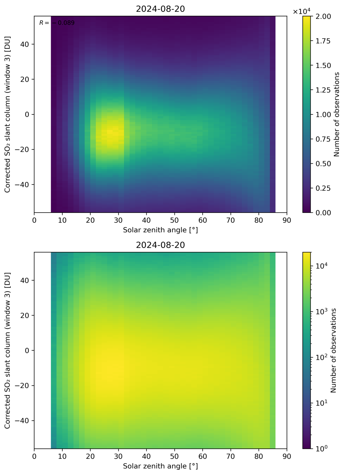
Figure 168: Scatter density plot of “Solar zenith angle” against “Corrected SO 2 slant column (window 3)” for 2024-08-19 to 2024-08-21.
