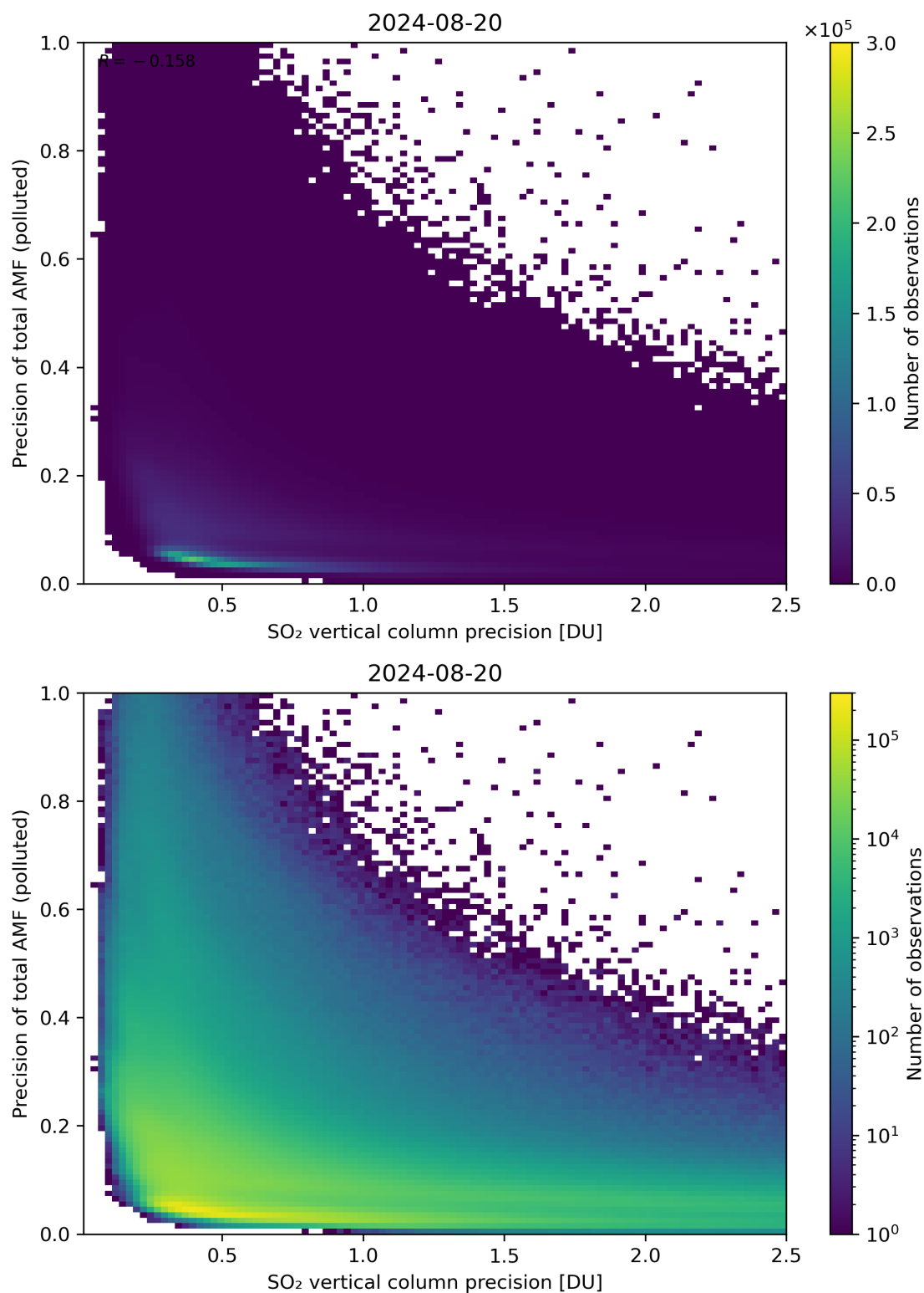
Figure 295: Scatter density plot of “SO 2 vertical column precision” against “Precision of total AMF (polluted)” for 2024-08-19 to 2024-08-21.
