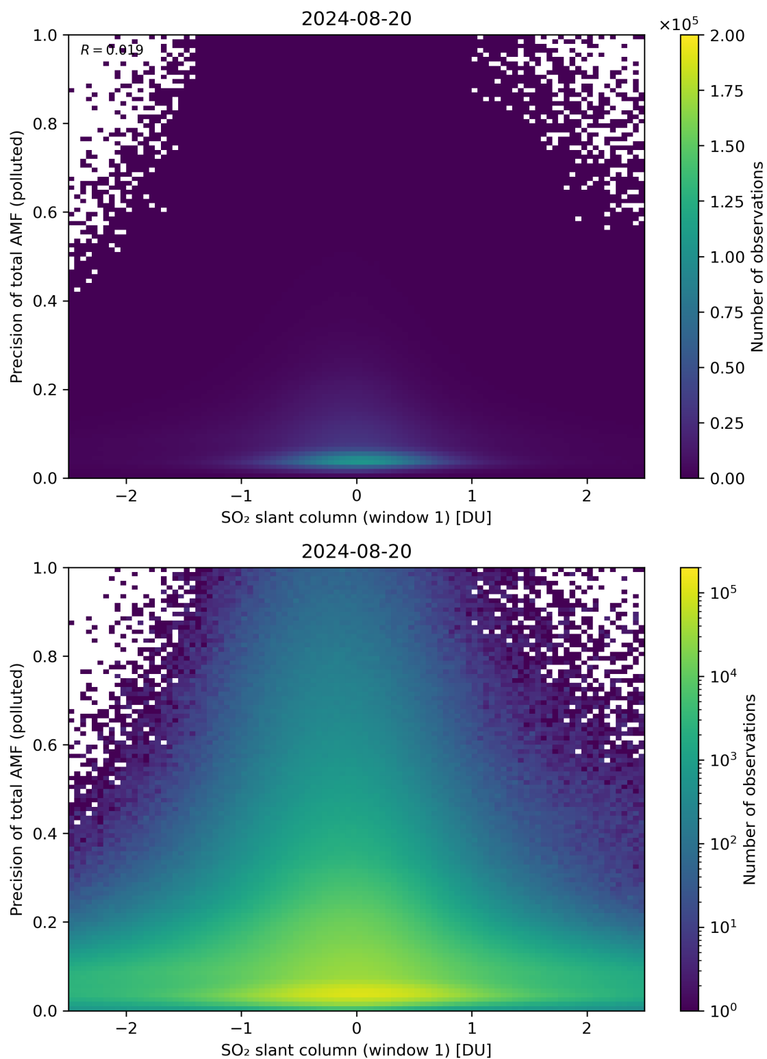
Figure 240: Scatter density plot of “SO 2 slant column (window 1)” against “Precision of total AMF (polluted)” for 2024-08-19 to 2024-08-21.
