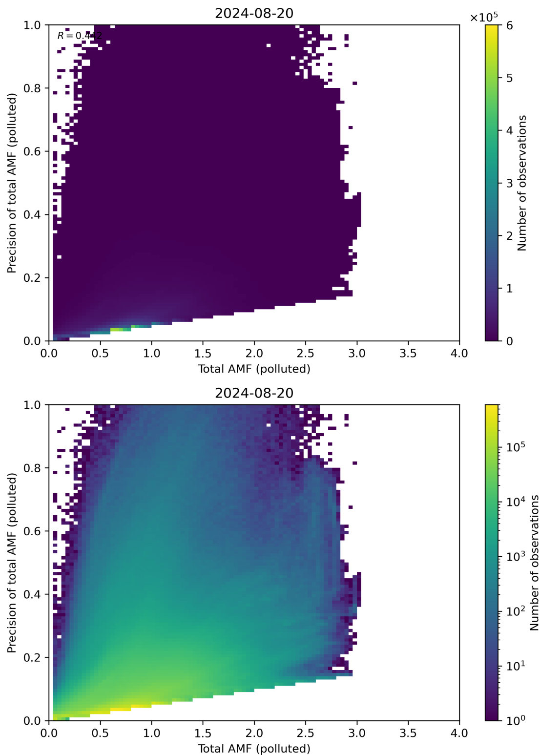
Figure 272: Scatter density plot of “Total AMF (polluted)” against “Precision of total AMF (polluted)” for 2024-08-19 to 2024-08-21.
