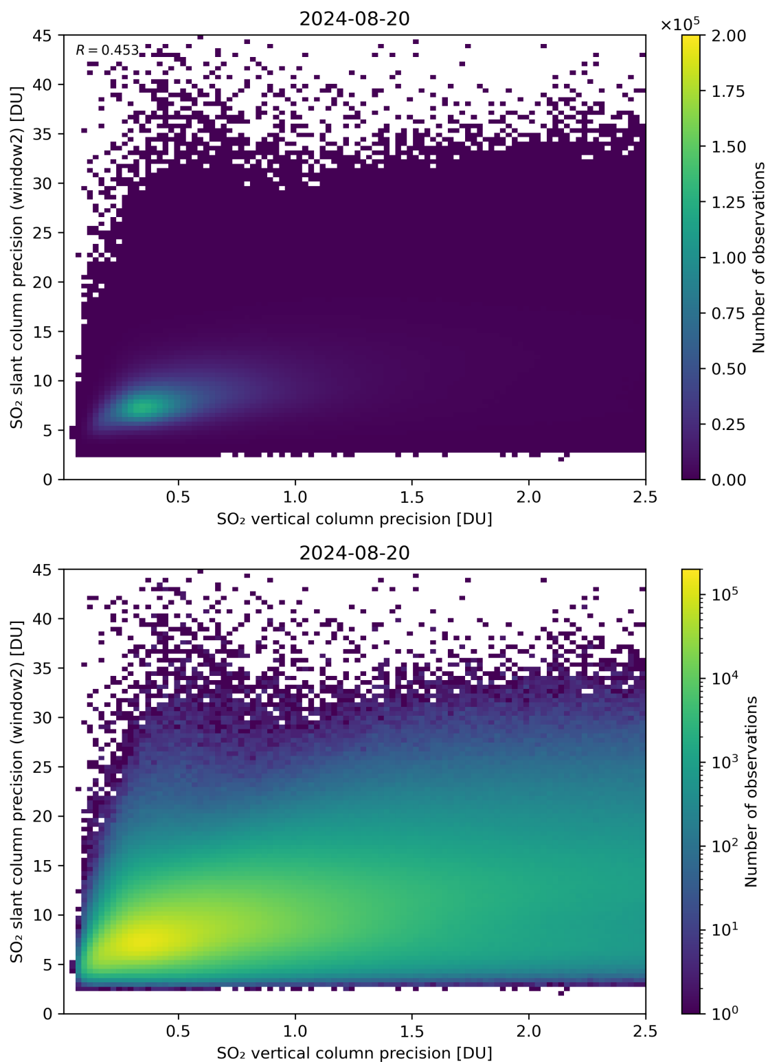
Figure 291: Scatter density plot of “SO 2 vertical column precision” against “SO 2 slant column precision (window2)” for 2024-08-19 to 2024-08-21.
