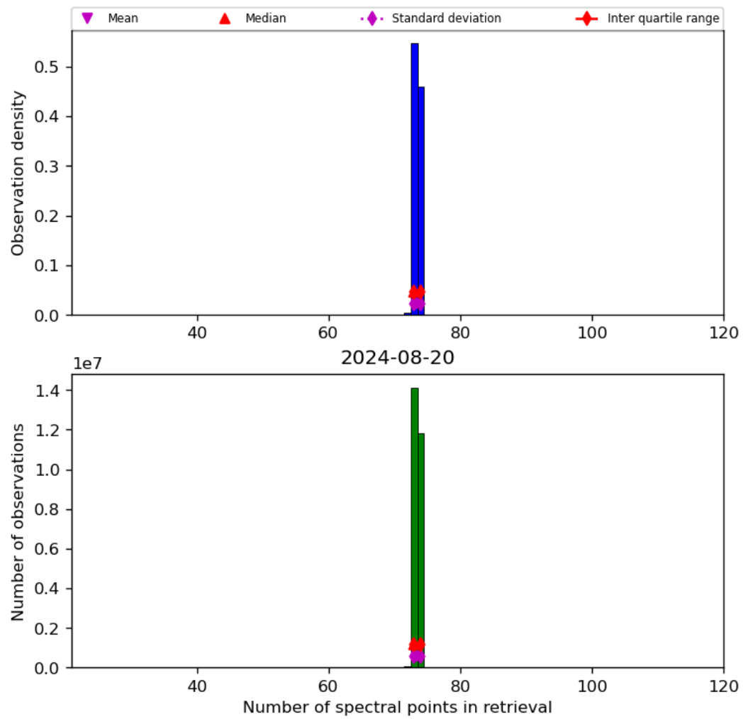
Figure 74: Histogram of “Number of spectral points in retrieval” for 2024-08-19 to 2024-08-21
