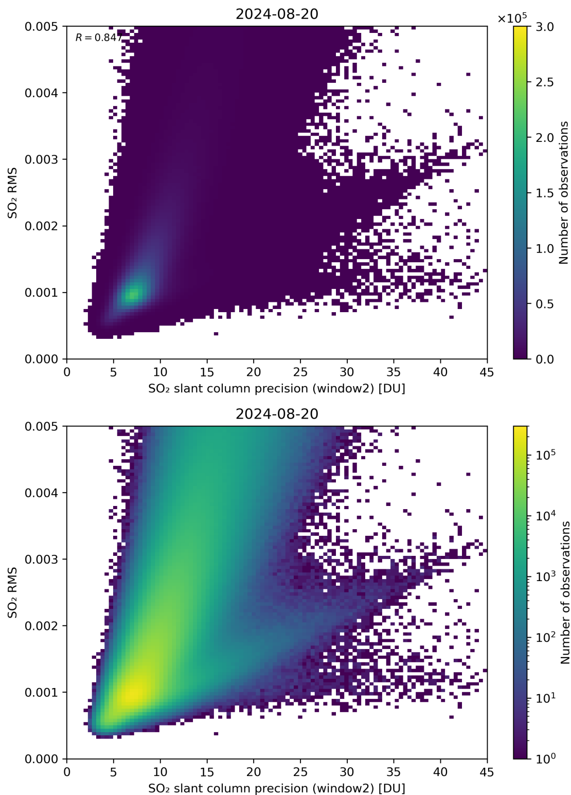
Figure 245: Scatter density plot of “SO 2 slant column precision (window2)” against “SO 2 RMS” for 2024-08-19 to 2024-08-21.
