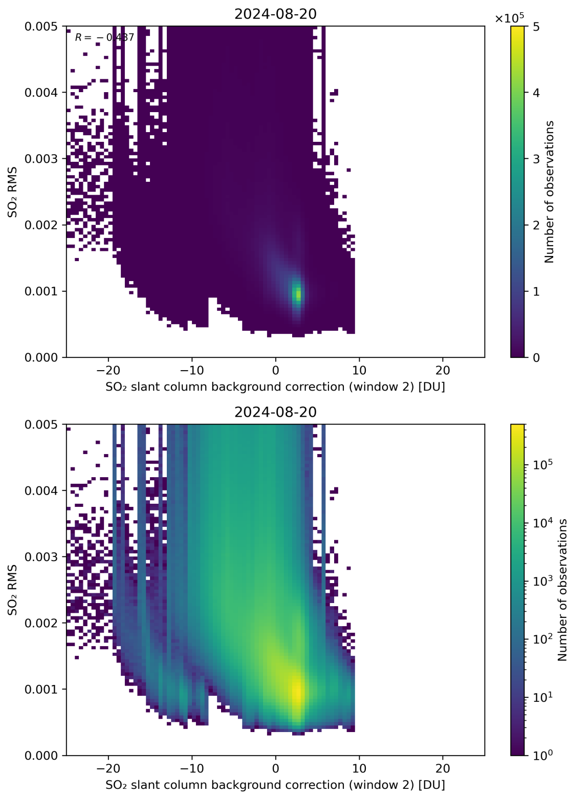
Figure 114: Scatter density plot of “SO 2 slant column background correction (window 2)” against “SO 2 RMS” for 2024-08-19 to 2024-08-21.
