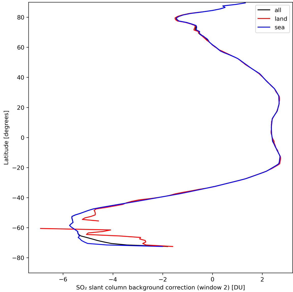
Figure 40: Zonal average of “SO 2 slant column background correction (window 2)” for 2024-08-19 to 2024-08-21.
