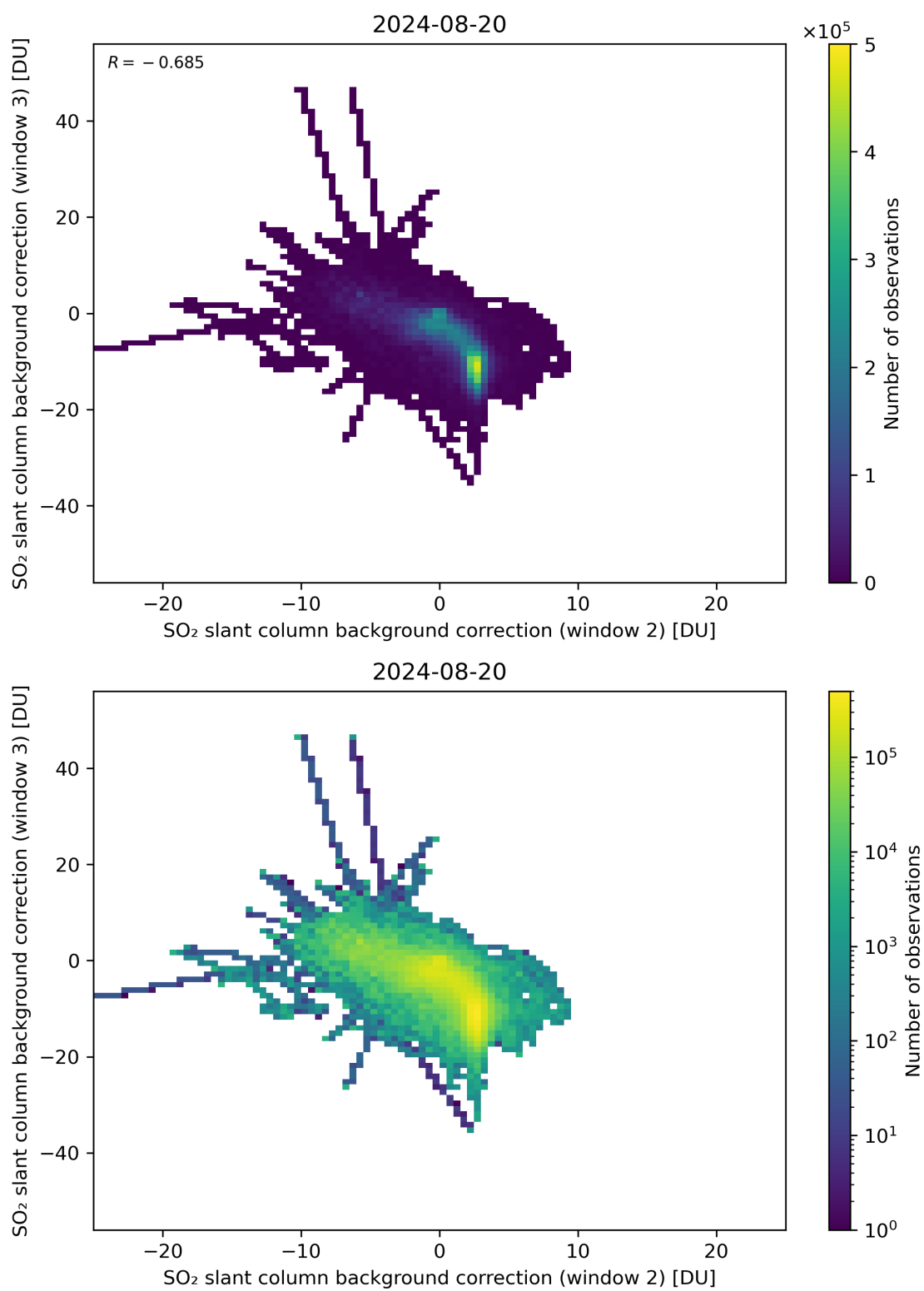
Figure 111: Scatter density plot of “SO 2 slant column background correction (window 2)” against “SO 2 slant column background correction (window 3)” for 2024-08-19 to 2024-08-21.
