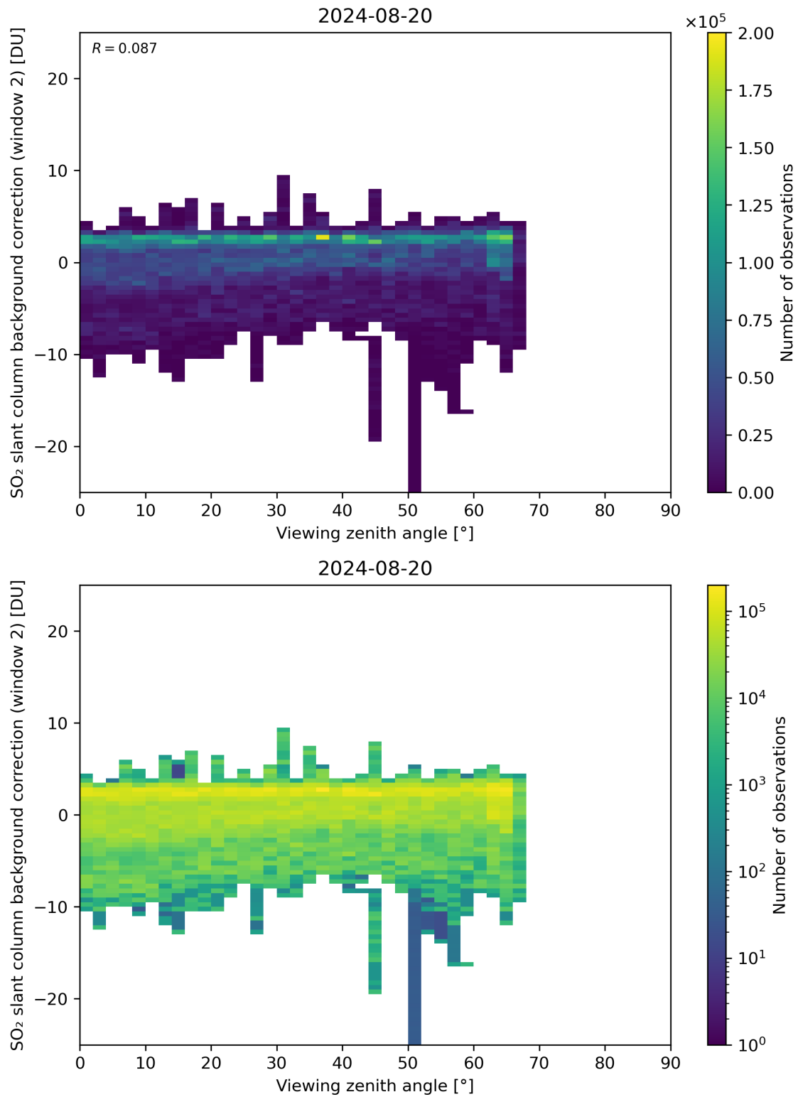
Figure 309: Scatter density plot of “Viewing zenith angle” against “SO 2 slant column background correction (window 2)” for 2024-08-19 to 2024-08-21.
