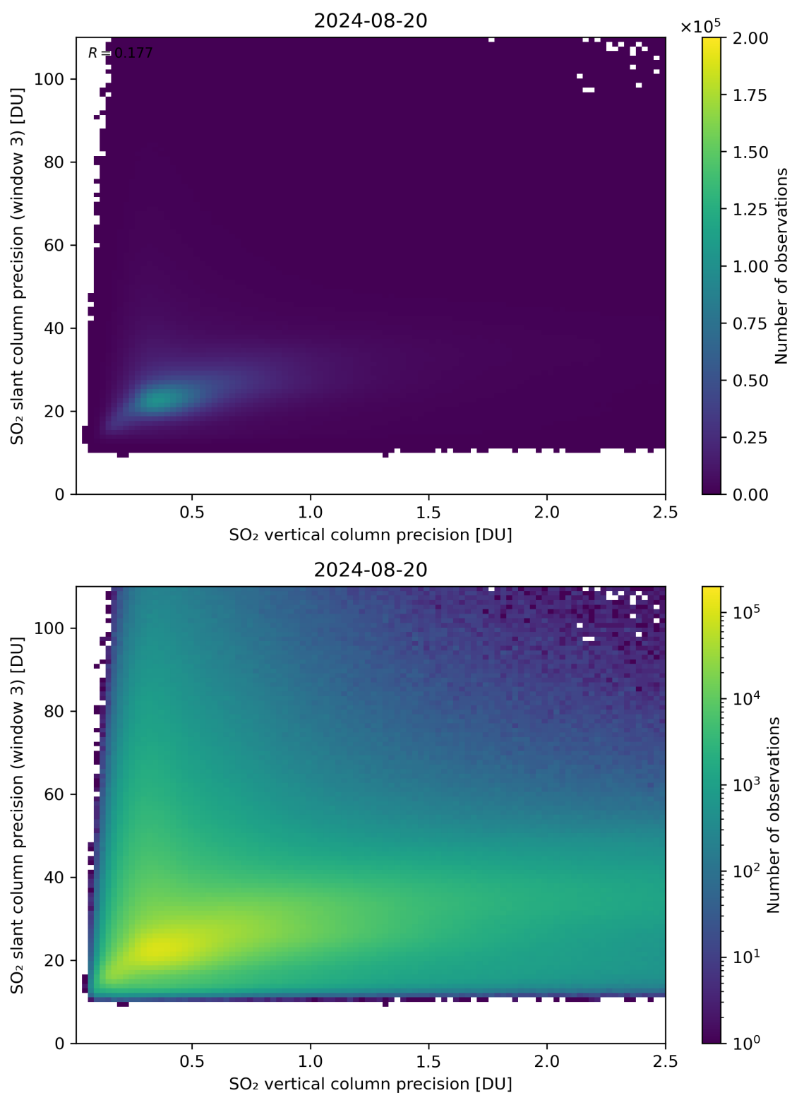
Figure 293: Scatter density plot of “SO 2 vertical column precision” against “SO 2 slant column precision (window 3)” for 2024-08-19 to 2024-08-21.
