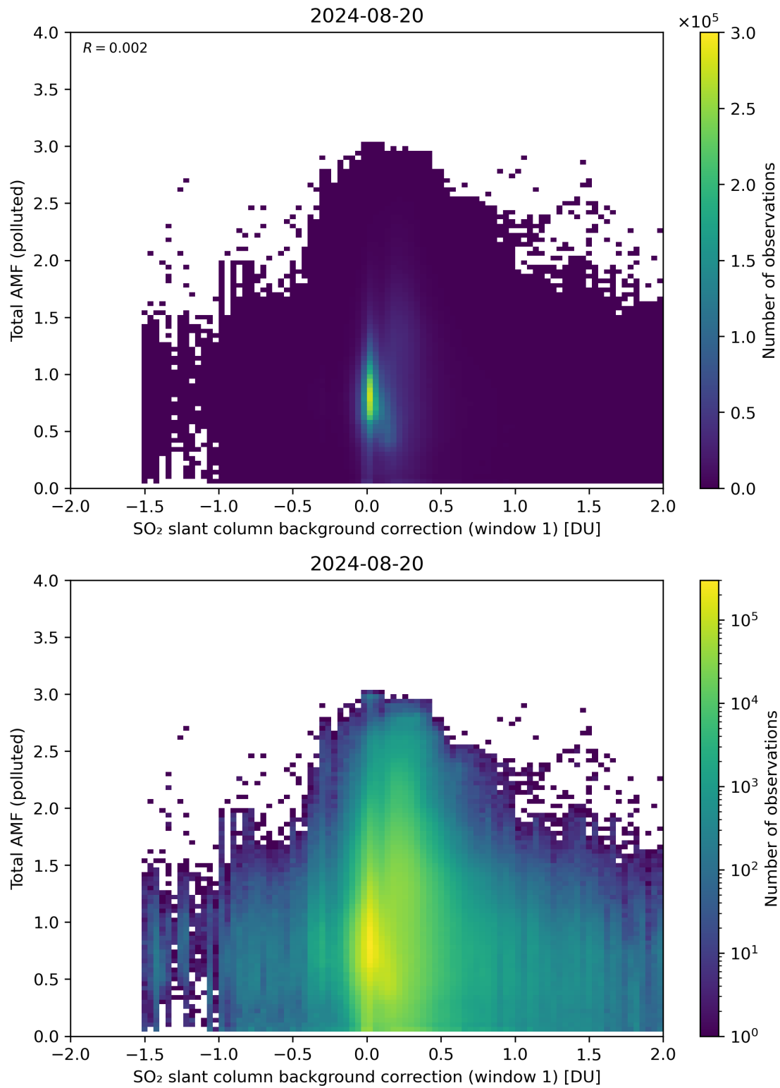
Figure 109: Scatter density plot of “SO 2 slant column background correction (window 1)” against “Total AMF (polluted)” for 2024-08-19 to 2024-08-21.
