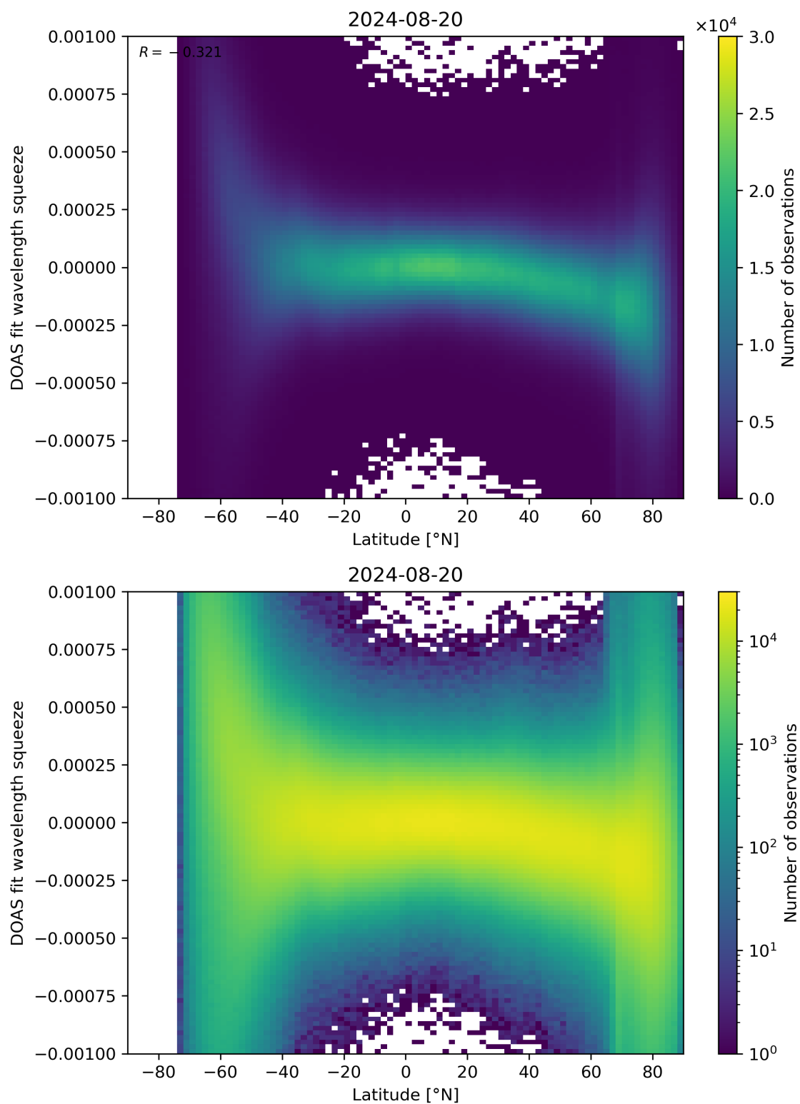
Figure 143: Scatter density plot of “Latitude” against “DOAS fit wavelength squeeze” for 2024-08-19 to 2024-08-21.
