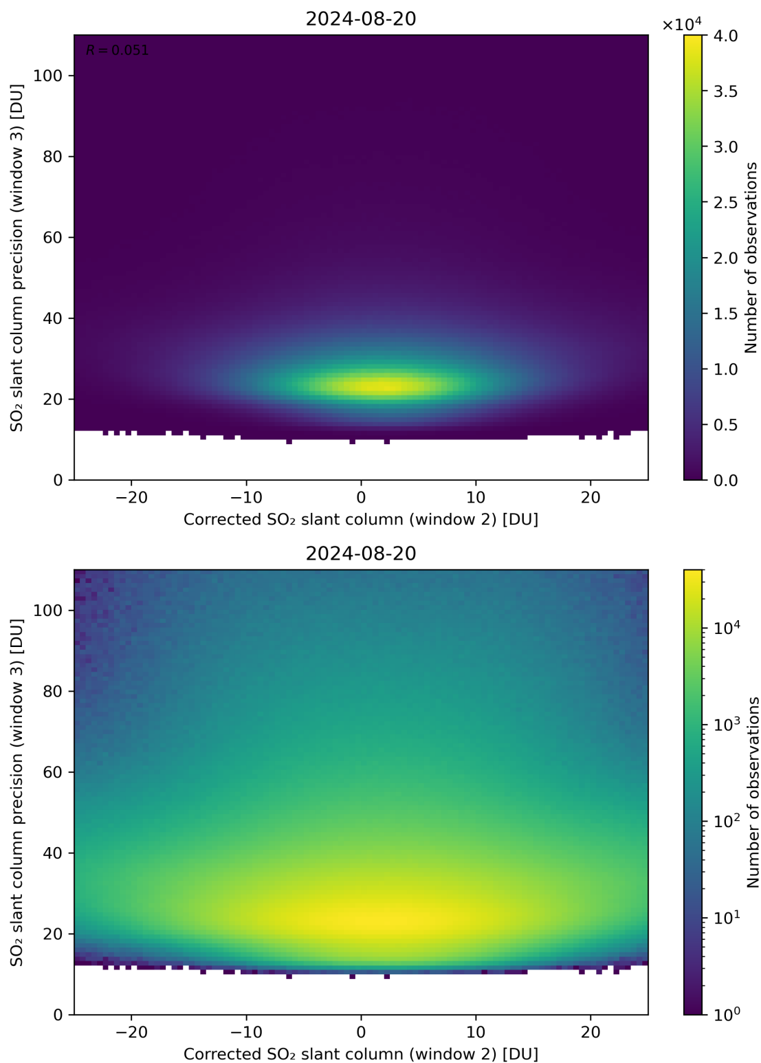
Figure 202: Scatter density plot of “Corrected SO 2 slant column (window 2)” against “SO 2 slant column precision (window 3)” for 2024-08-19 to 2024-08-21.
