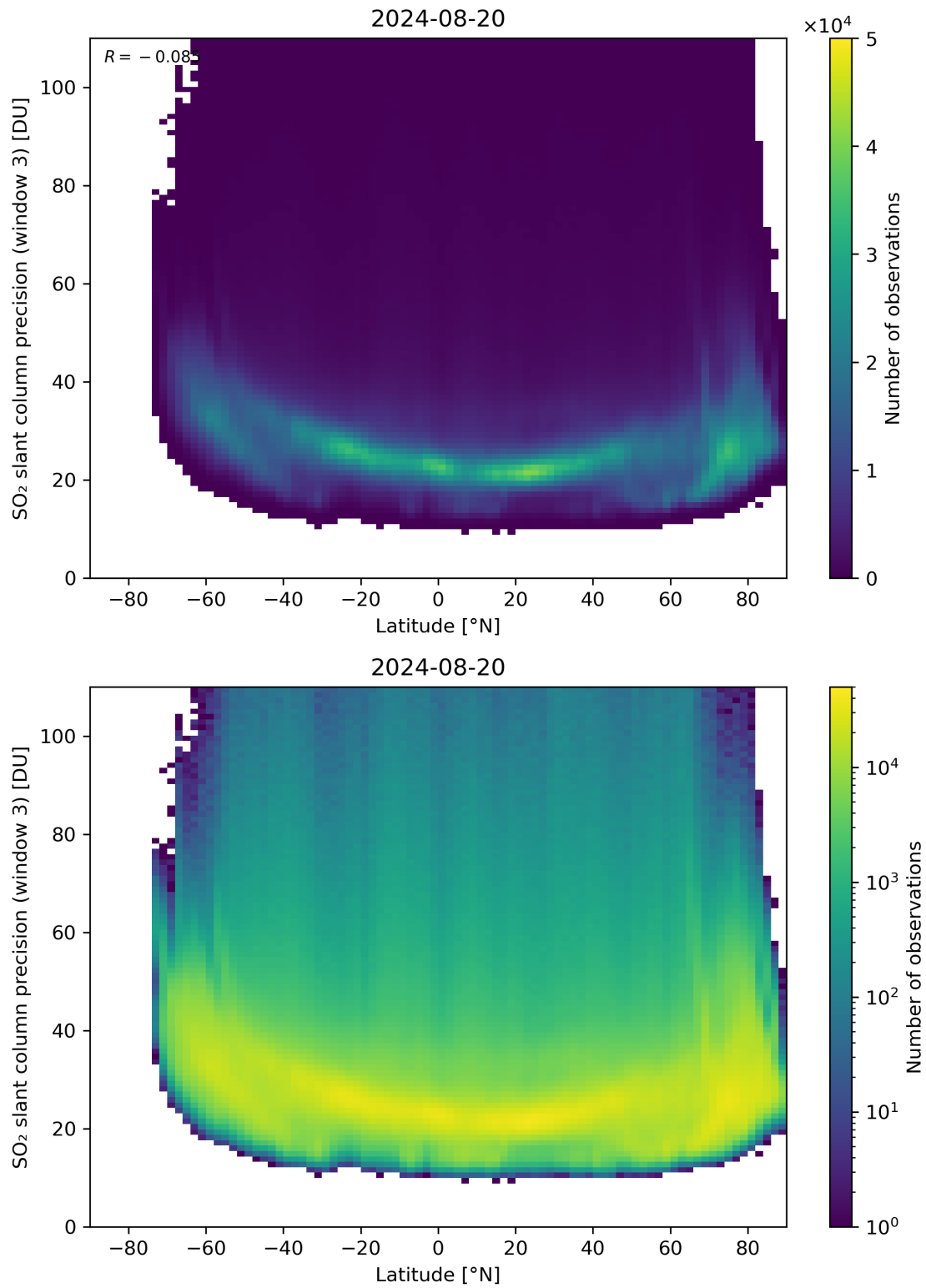
Figure 153: Scatter density plot of “Latitude” against “SO 2 slant column precision (window 3)” for 2024-08-19 to 2024-08-21.
