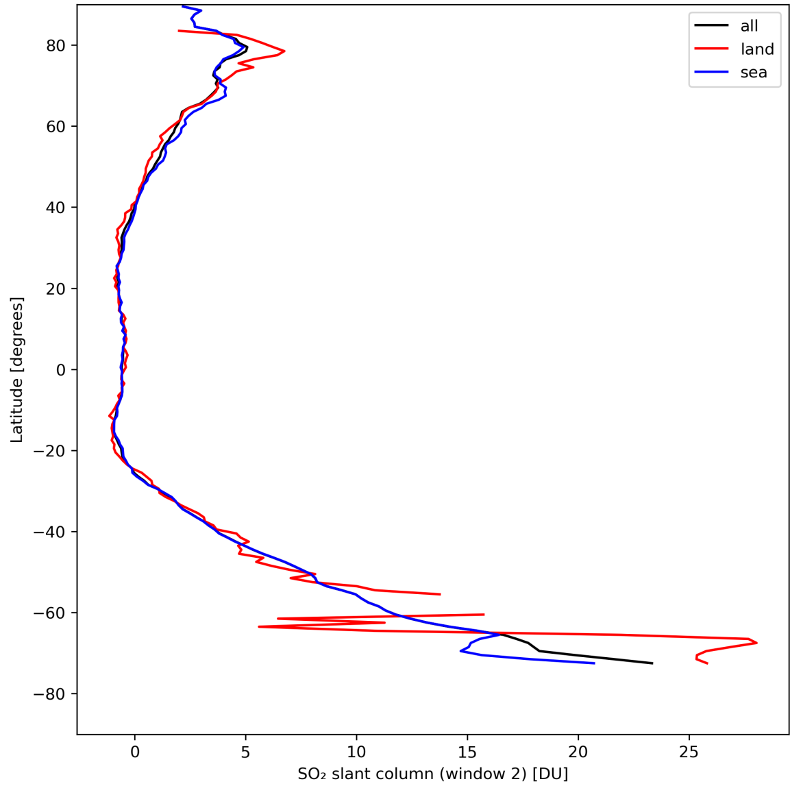
Figure 37: Zonal average of “SO 2 slant column (window 2)” for 2024-08-19 to 2024-08-21.
