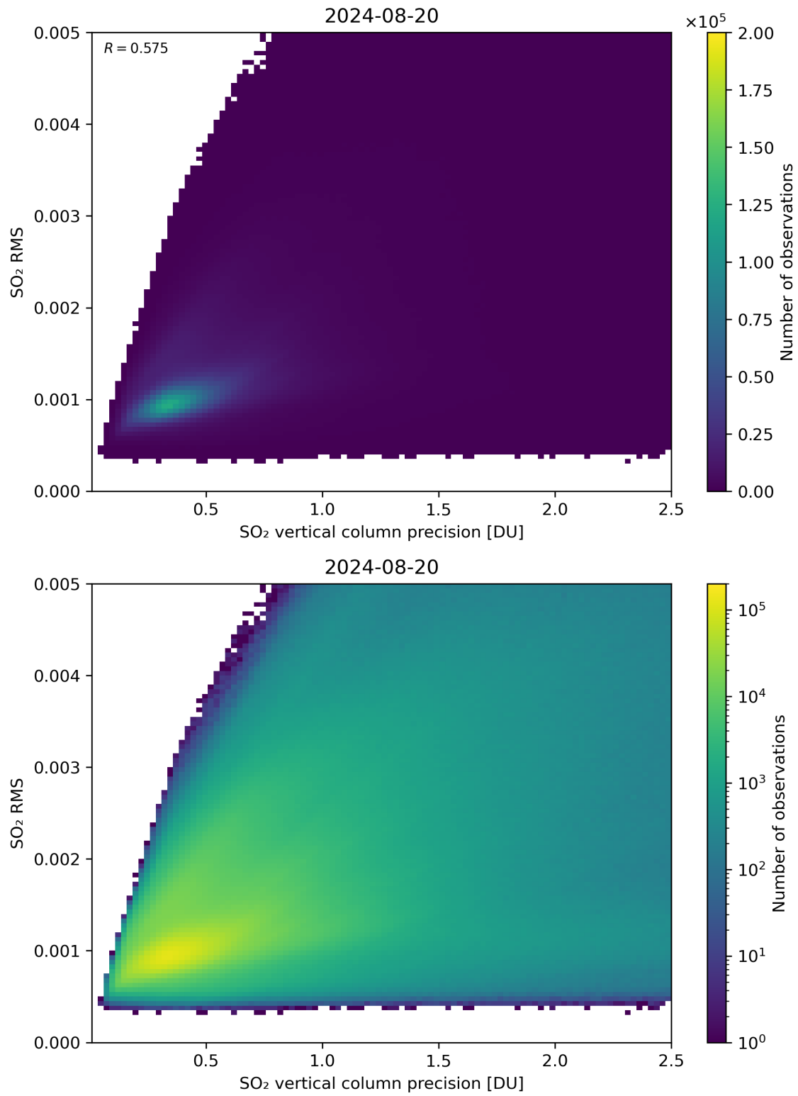
Figure 284: Scatter density plot of “SO 2 vertical column precision” against “SO 2 RMS” for 2024-08-19 to 2024-08-21.
