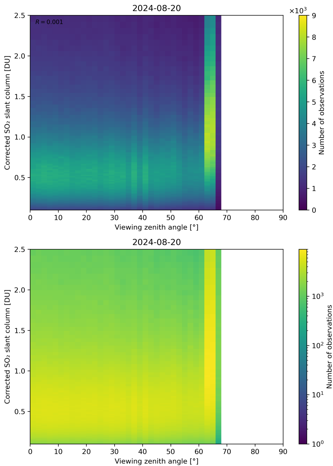
Figure 317: Scatter density plot of “Viewing zenith angle” against “Corrected SO 2 slant column” for 2024-08-19 to 2024-08-21.
