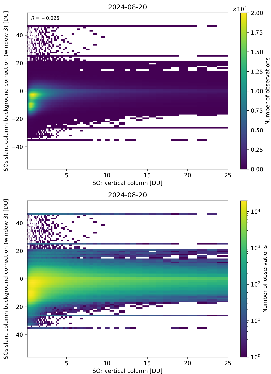
Figure 275: Scatter density plot of “SO 2 vertical column” against “SO 2 slant column background correction (window 3)” for 2024-08-19 to 2024-08-21.
