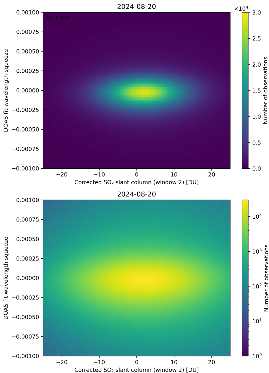
Figure 197: Scatter density plot of “Corrected SO 2 slant column (window 2)” against “DOAS fit wavelength squeeze” for 2024-08-19 to 2024-08-21.
