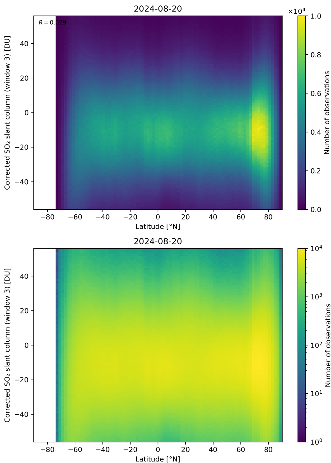
Figure 148: Scatter density plot of “Latitude” against “Corrected SO 2 slant column (window 3)” for 2024-08-19 to 2024-08-21.
