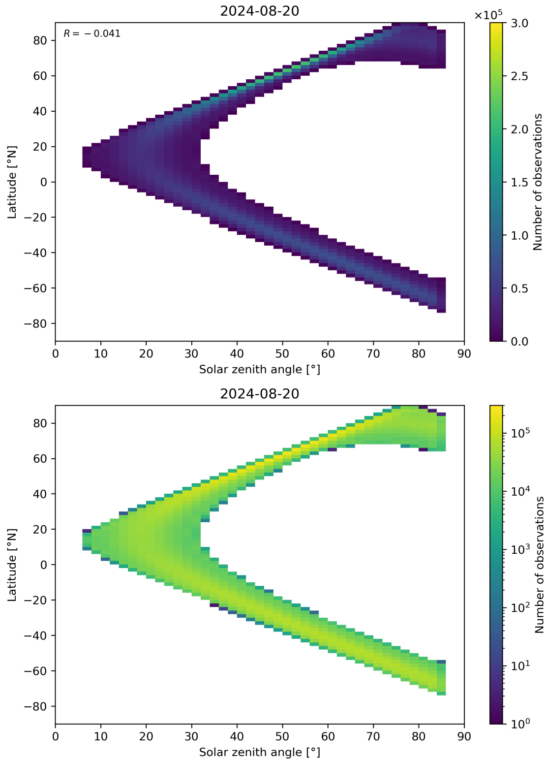
Figure 164: Scatter density plot of “Solar zenith angle” against “Latitude” for 2024-08-19 to 2024-08-21.
