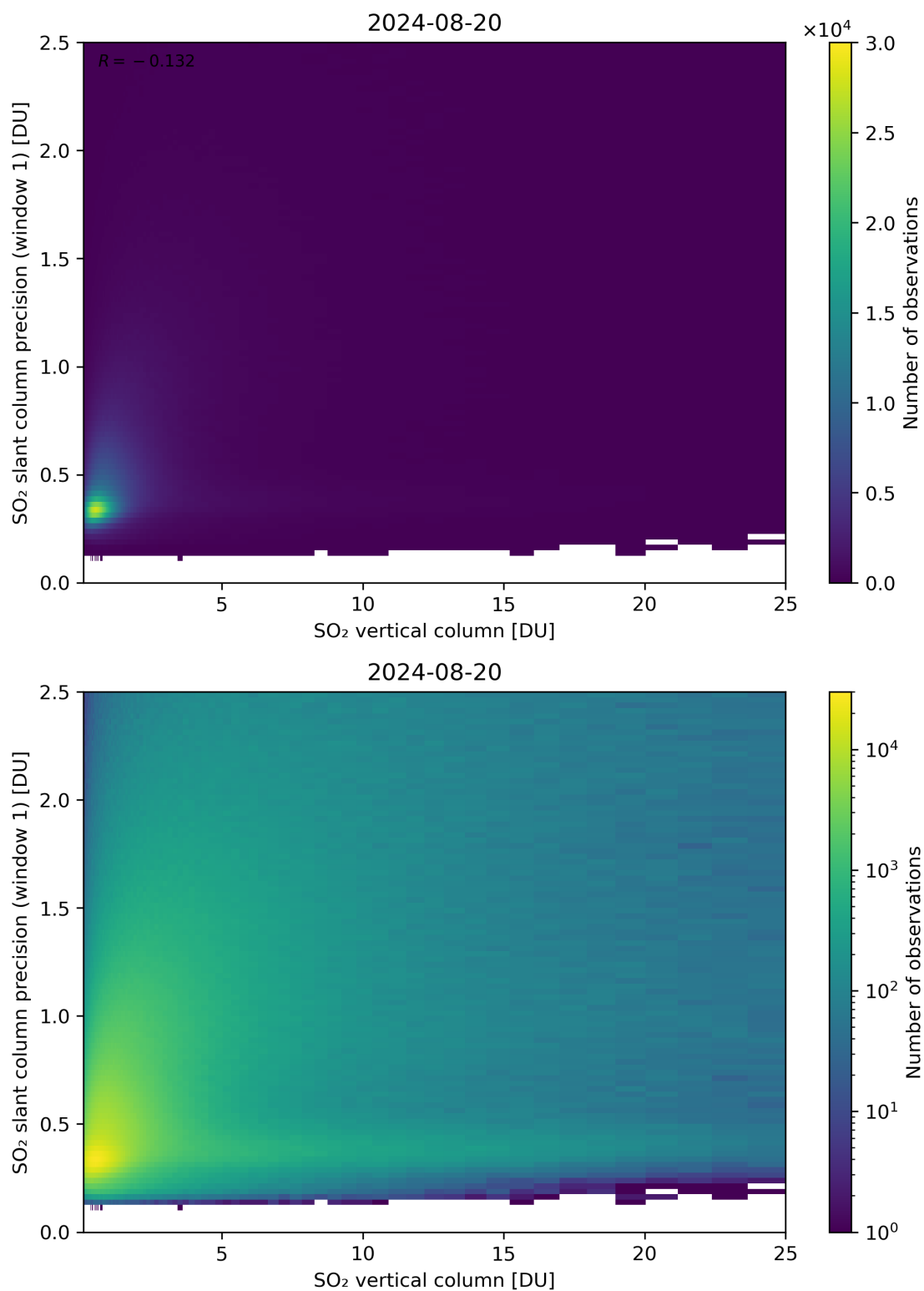
Figure 301: Scatter density plot of “SO 2 vertical column” against “SO 2 slant column precision (window 1)” for 2024-08-19 to 2024-08-21.
