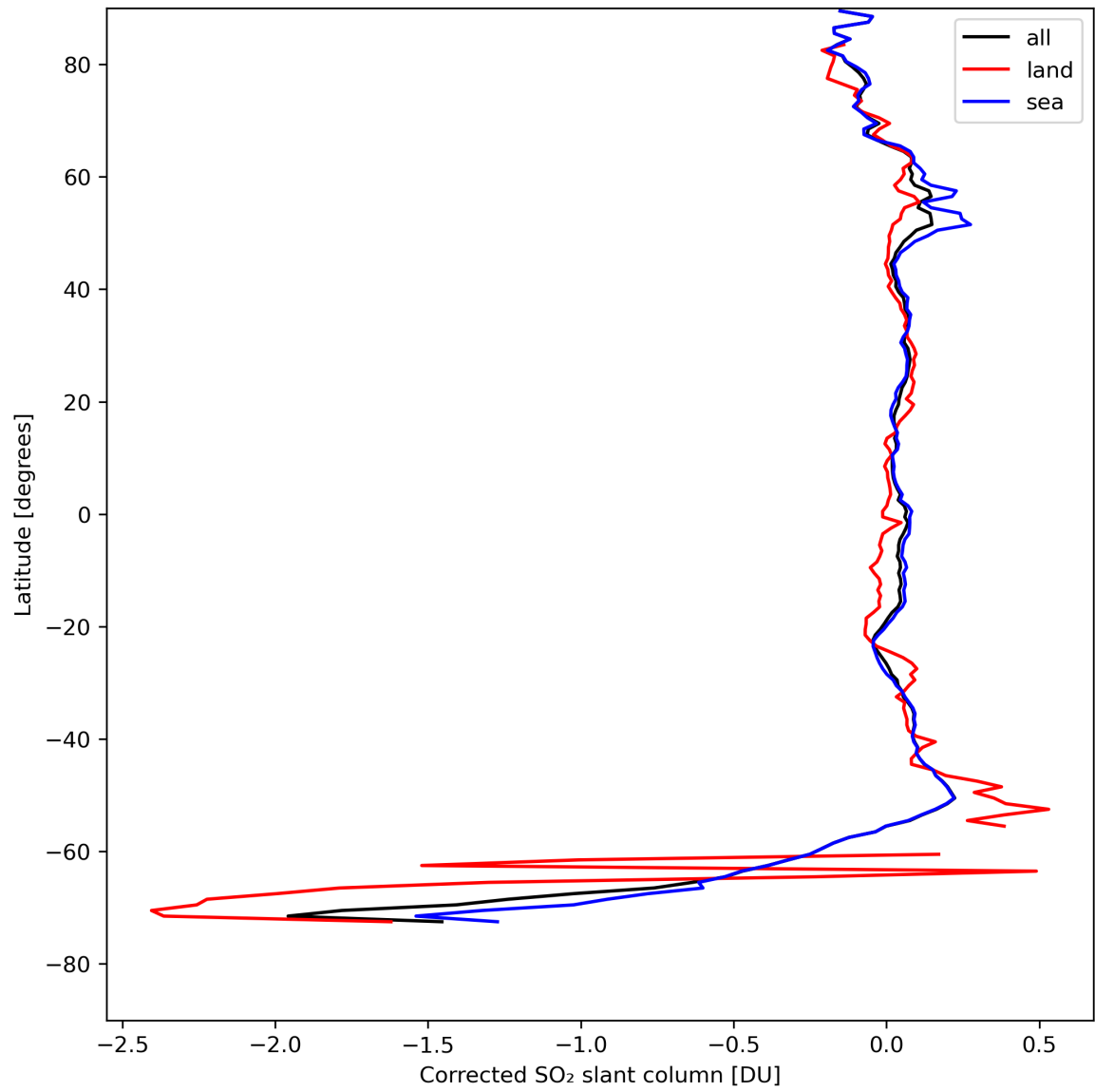
Figure 32: Zonal average of "Corrected SO 2 slant column" for 2024-08-19 to 2024-08-21.
