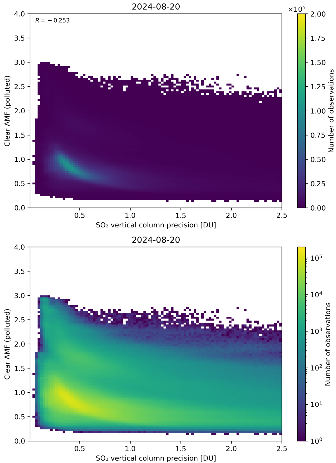
Figure 285: Scatter density plot of “SO 2 vertical column precision” against “Clear AMF (polluted)” for 2024-08-19 to 2024-08-21.
