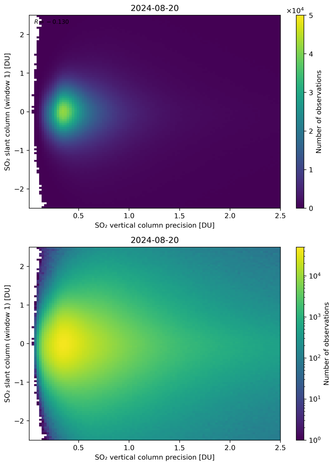
Figure 289: Scatter density plot of “SO 2 vertical column precision” against “SO 2 slant column (window 1)” for 2024-08-19 to 2024-08-21.
