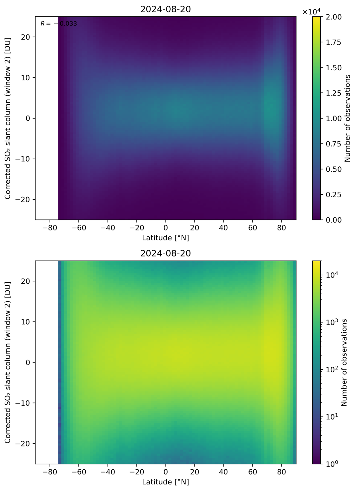
Figure 147: Scatter density plot of “Latitude” against “Corrected SO 2 slant column (window 2)” for 2024-08-19 to 2024-08-21.
