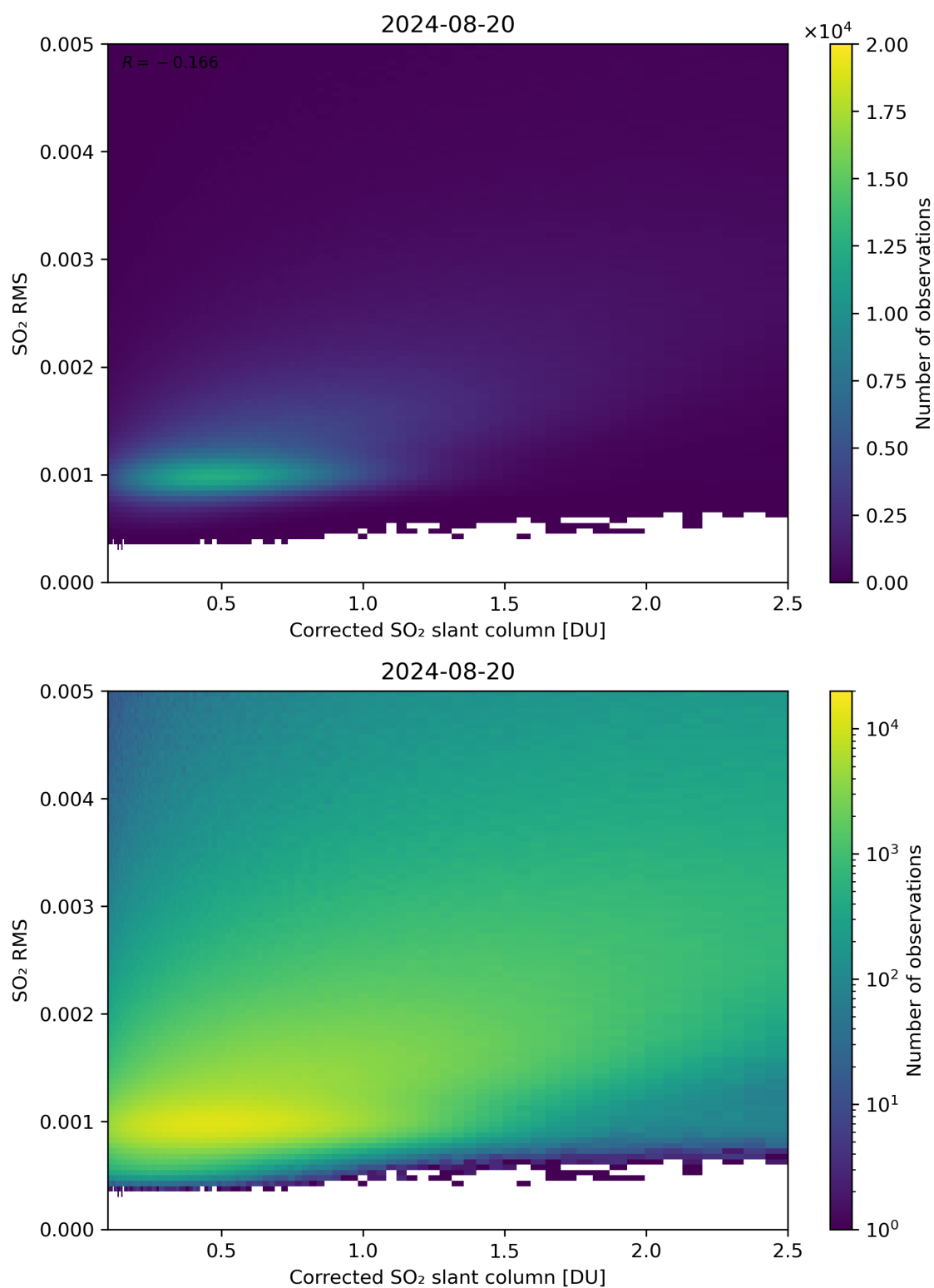
Figure 183: Scatter density plot of “Corrected SO 2 slant column” against “SO 2 RMS” for 2024-08-19 to 2024-08-21.
