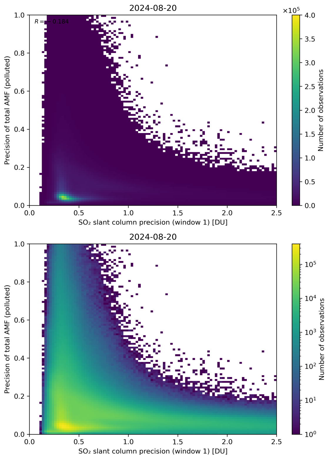
Figure 231: Scatter density plot of “SO 2 slant column precision (window 1)” against “Precision of total AMF (polluted)” for 2024-08-19 to 2024-08-21.
