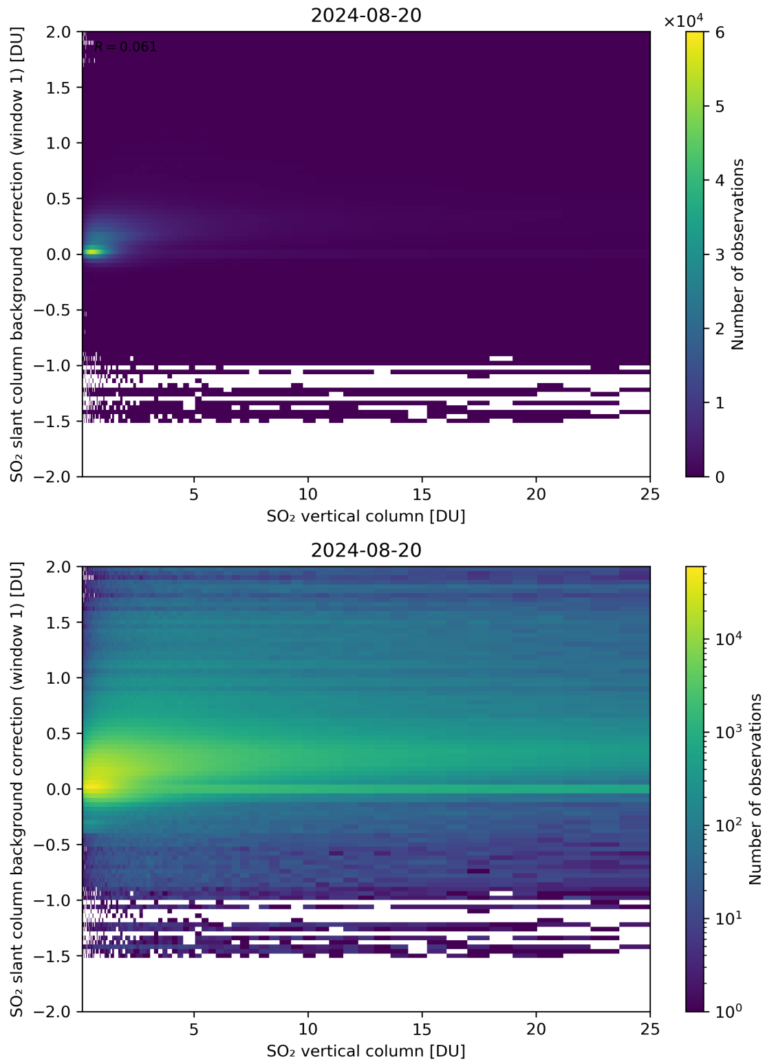
Figure 273: Scatter density plot of “SO 2 vertical column” against “SO 2 slant column background correction (window 1)” for 2024-08-19 to 2024-08-21.
