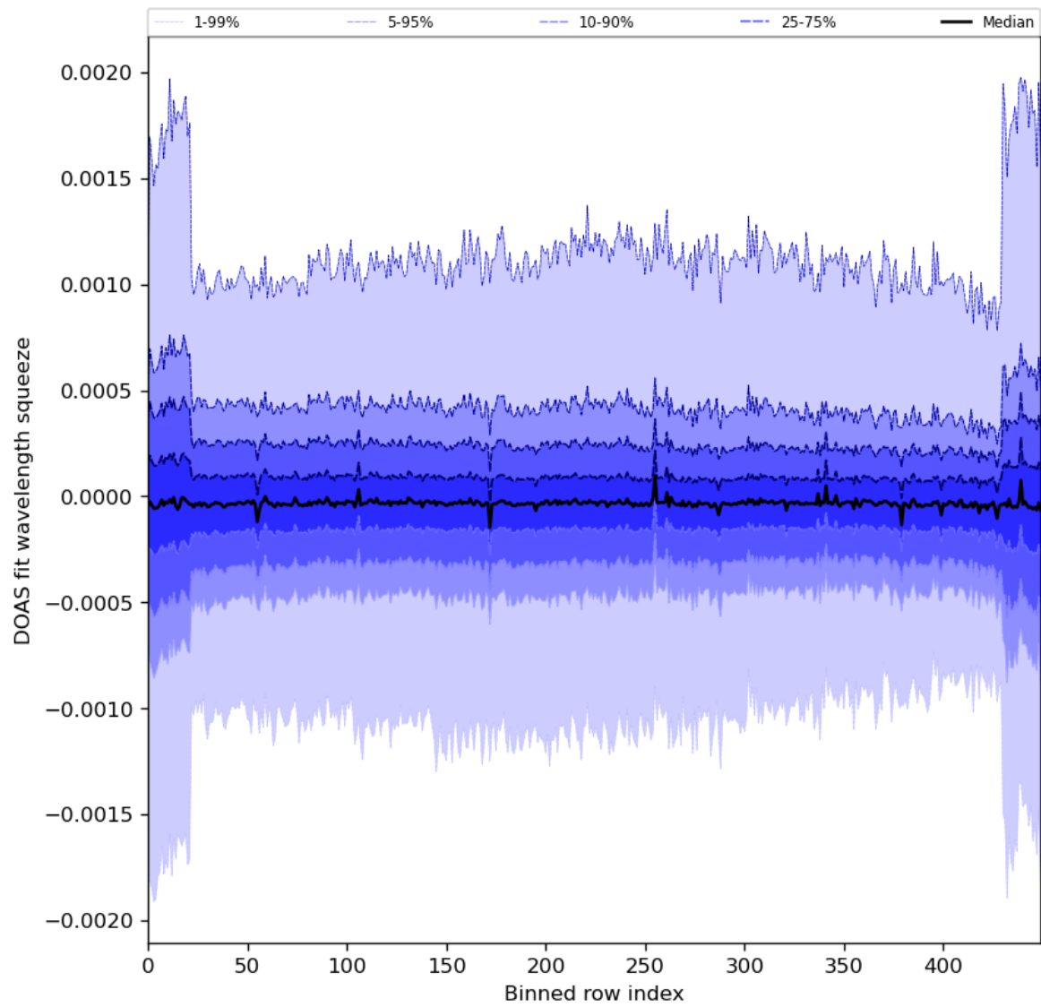
Figure 92: Along track statistics of “DOAS fit wavelength squeeze” for 2024-08-19 to 2024-08-21
