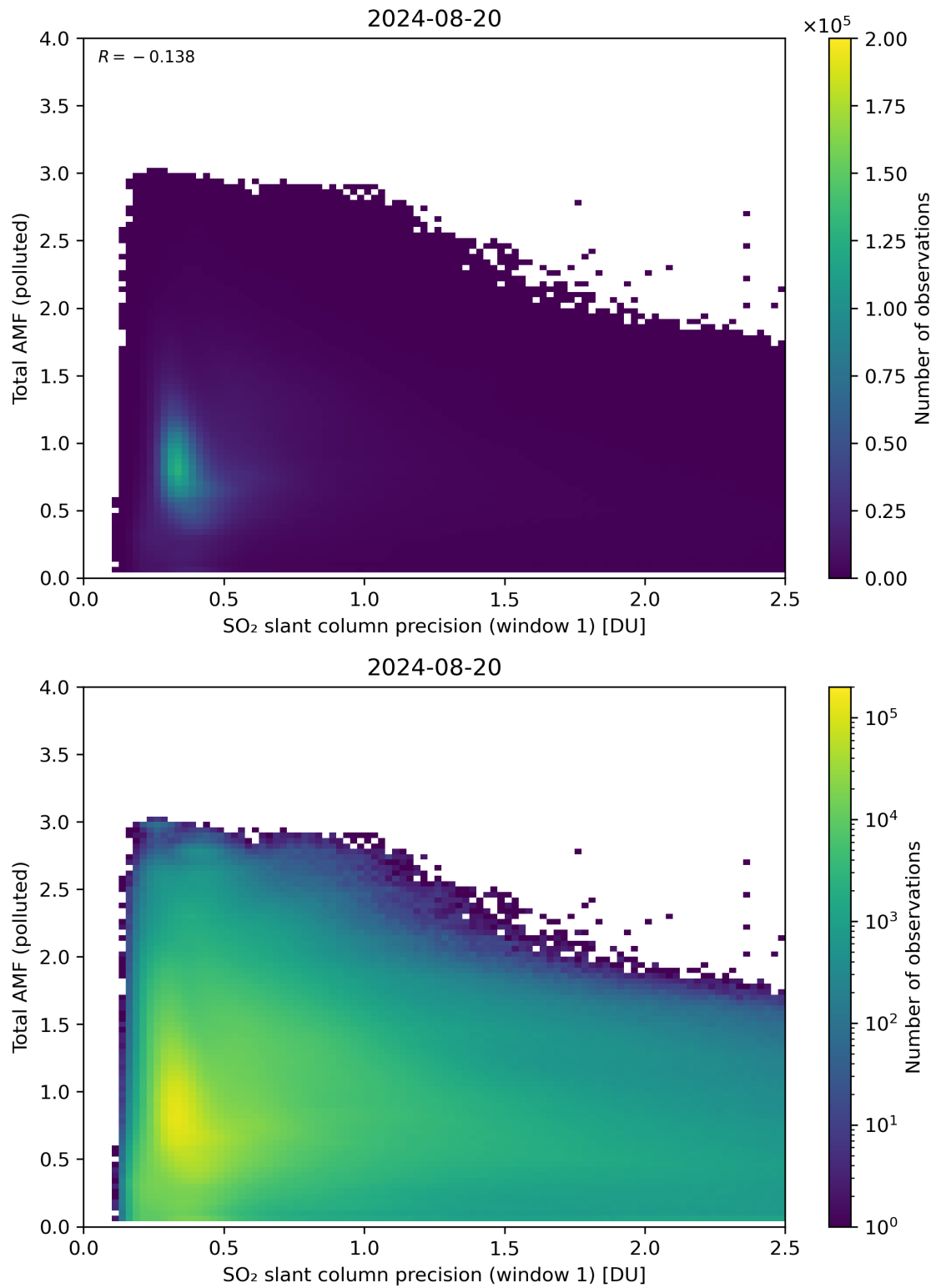
Figure 230: Scatter density plot of “SO 2 slant column precision (window 1)” against “Total AMF (polluted)” for 2024-08-19 to 2024-08-21.
