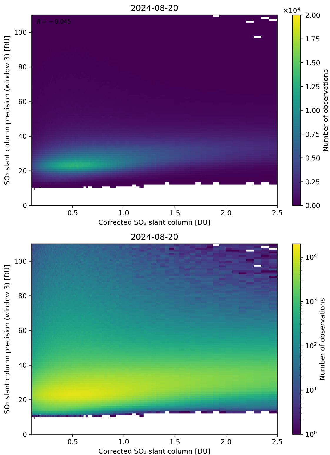
Figure 191: Scatter density plot of “Corrected SO 2 slant column” against “SO 2 slant column precision (window 3)” for 2024-08-19 to 2024-08-21.
