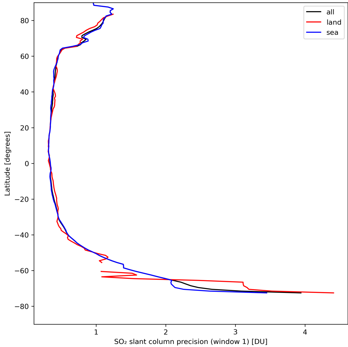
Figure 34: Zonal average of “SO 2 slant column precision (window 1)” for 2024-08-19 to 2024-08-21.
