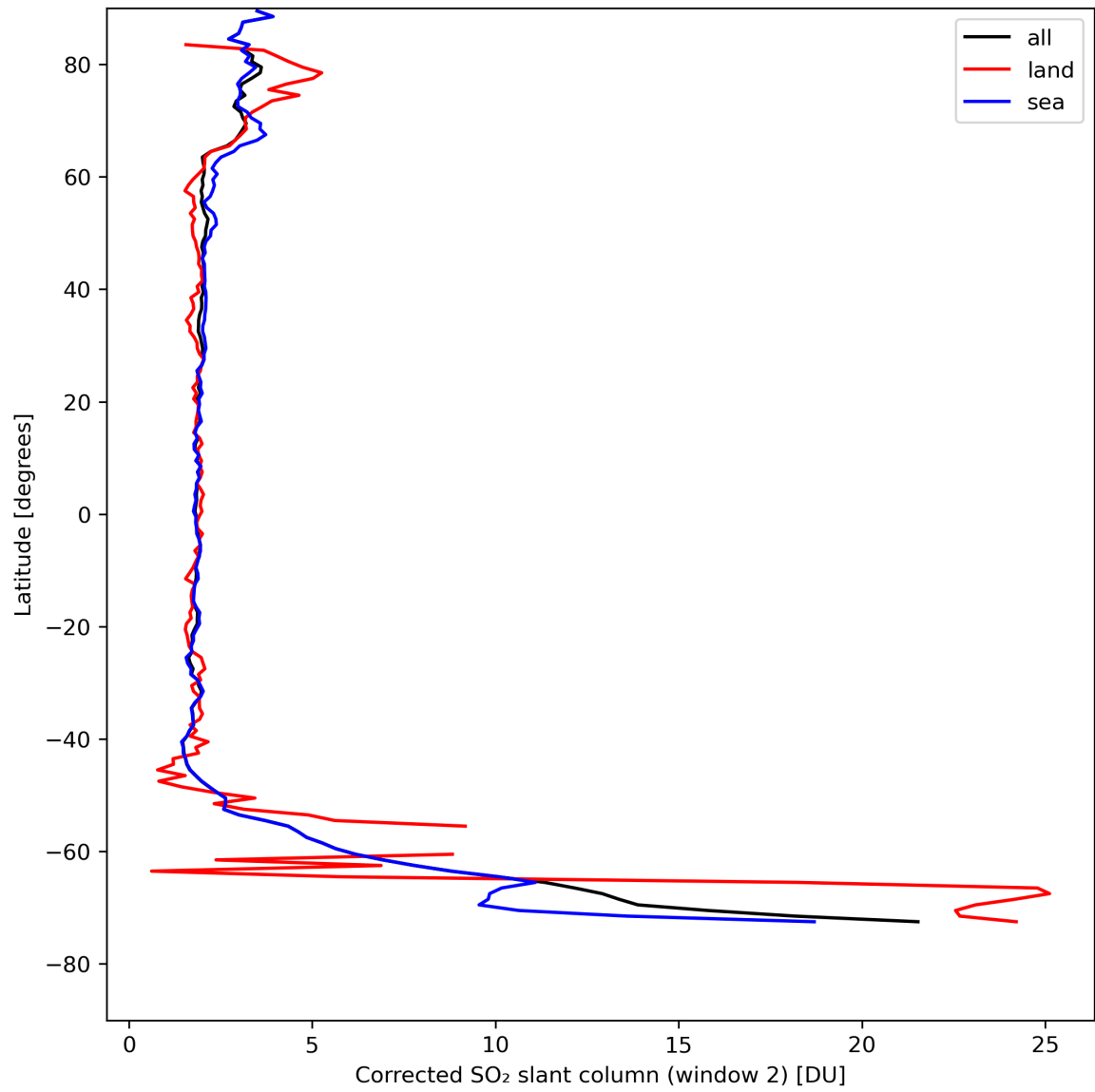
Figure 39: Zonal average of “Corrected SO 2 slant column (window 2)” for 2024-08-19 to 2024-08-21.
