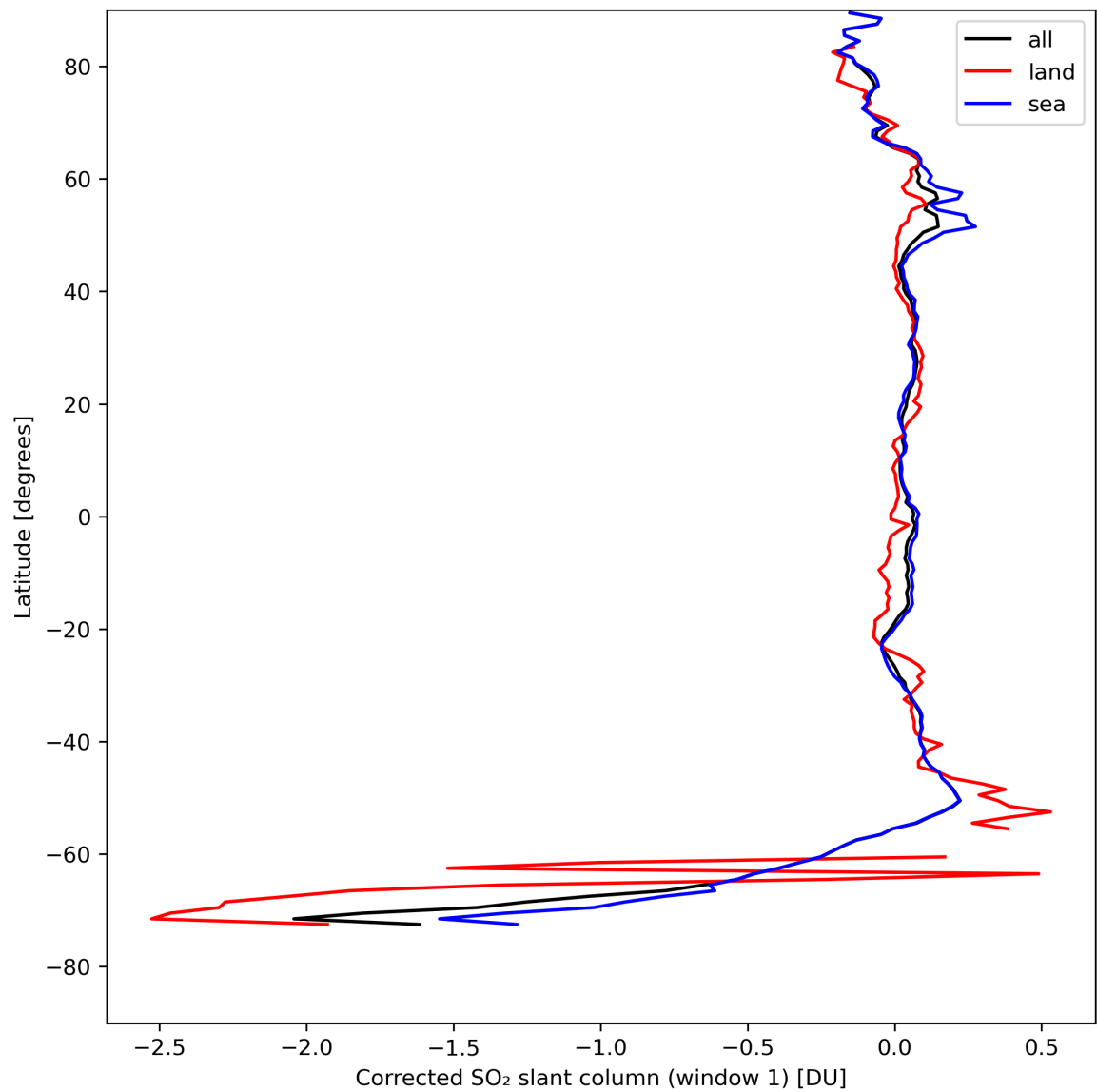
Figure 35: Zonal average of “Corrected SO 2 slant column (window 1)” for 2024-08-19 to 2024-08-21.
