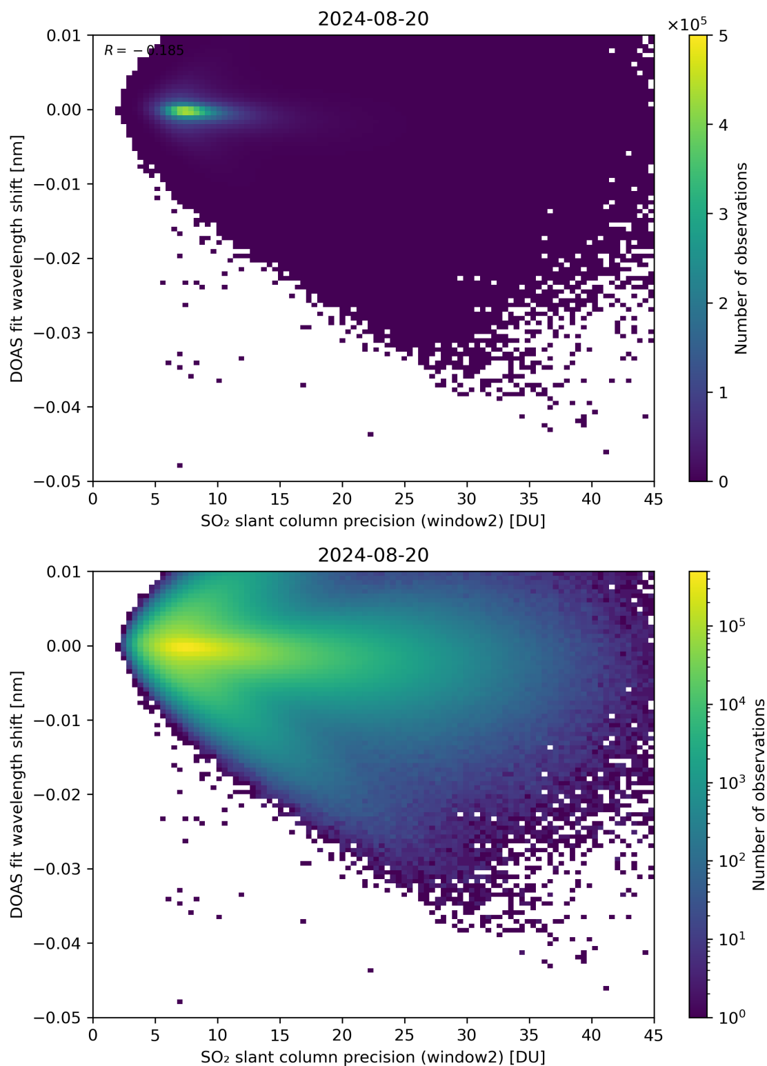
Figure 243: Scatter density plot of “SO 2 slant column precision (window2)” against “DOAS fit wavelength shift” for 2024-08-19 to 2024-08-21.
