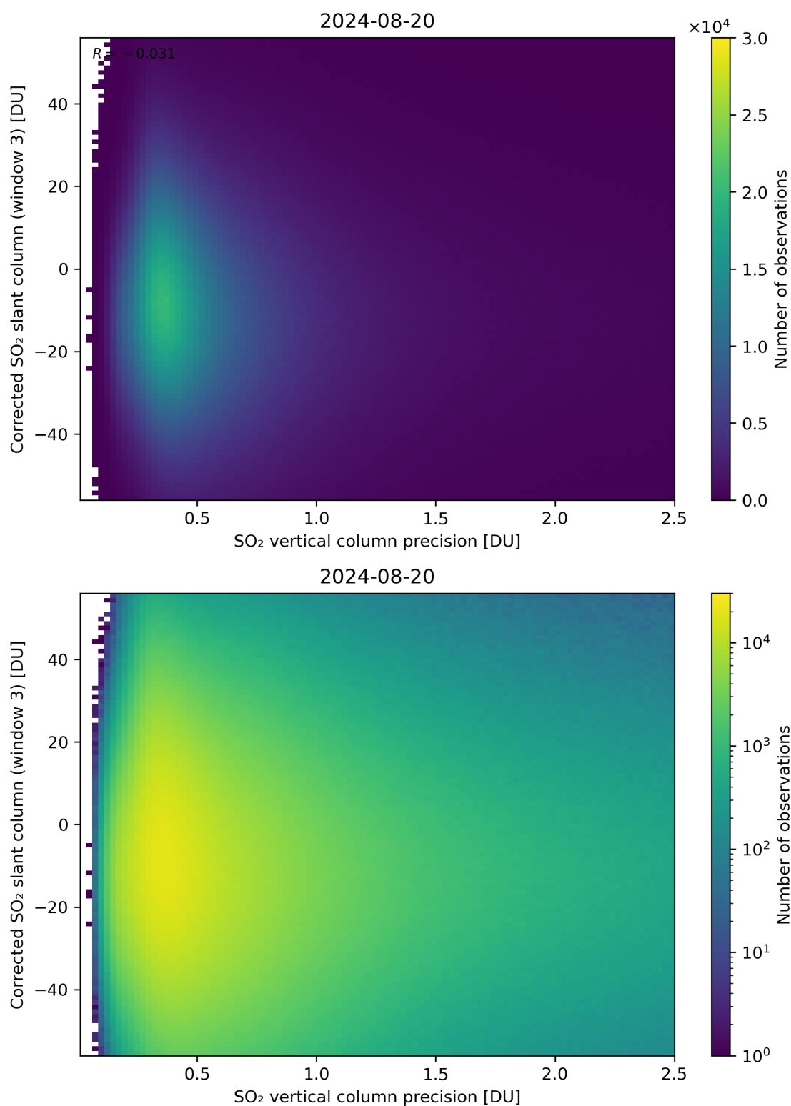
Figure 288: Scatter density plot of “SO 2 vertical column precision” against “Corrected SO 2 slant column (window 3)” for 2024-08-19 to 2024-08-21.
