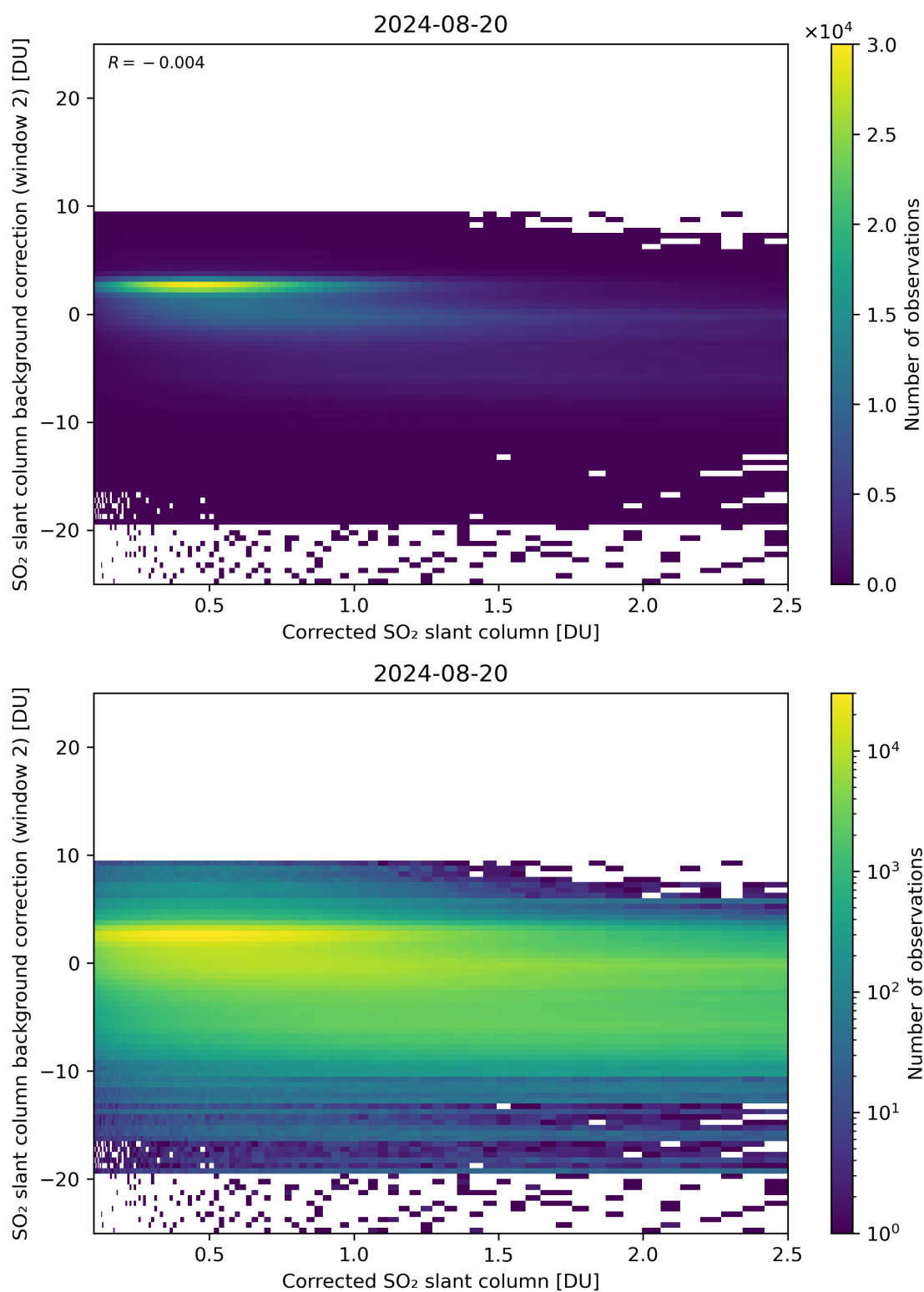
Figure 179: Scatter density plot of “Corrected SO 2 slant column” against “SO 2 slant column background correction (window 2)” for 2024-08-19 to 2024-08-21.
