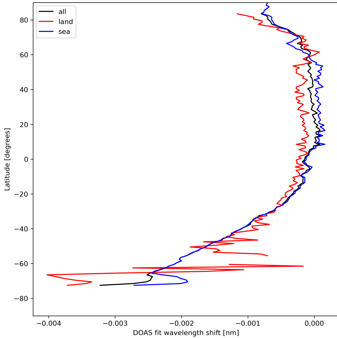
Figure 45: Zonal average of “DOAS fit wavelength shift” for 2024-08-19 to 2024-08-21.
