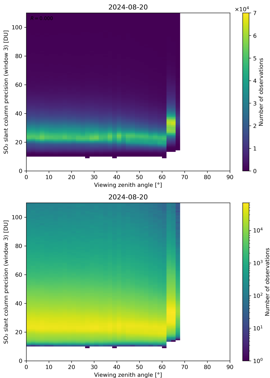
Figure 324: Scatter density plot of “Viewing zenith angle” against “SO 2 slant column precision (window 3)” for 2024-08-19 to 2024-08-21.
