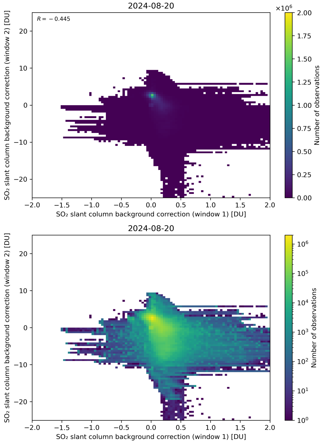
Figure 98: Scatter density plot of “SO 2 slant column background correction (window 1)” against “SO 2 slant column background correction (window 2)” for 2024-08-19 to 2024-08-21.
