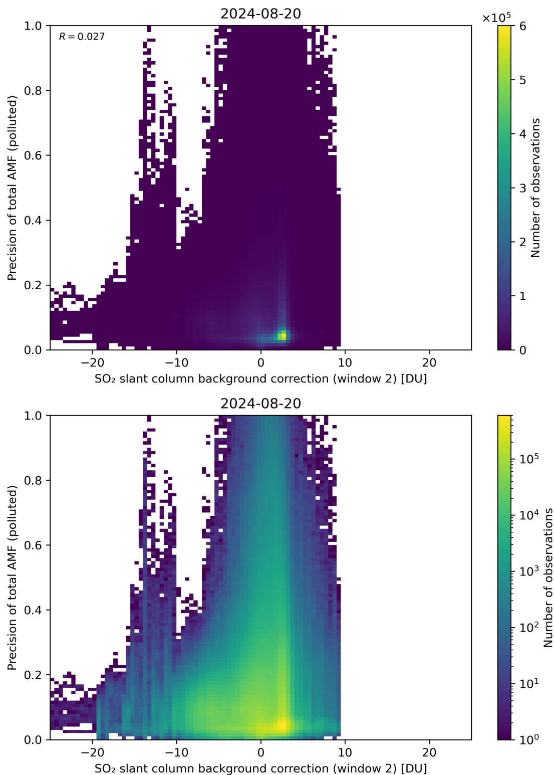
Figure 120: Scatter density plot of “SO 2 slant column background correction (window 2)” against “Precision of total AMF (polluted)” for 2024-08-19 to 2024-08-21.
