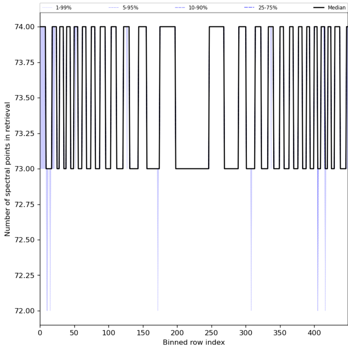
Figure 97: Along track statistics of “Number of spectral points in retrieval” for 2024-08-19 to 2024-08-21
