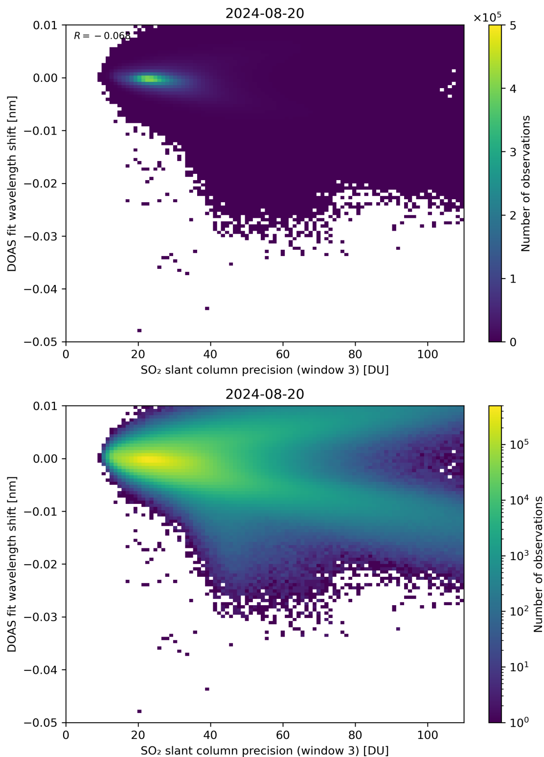
Figure 258: Scatter density plot of “SO 2 slant column precision (window 3)” against “DOAS fit wavelength shift” for 2024-08-19 to 2024-08-21.
