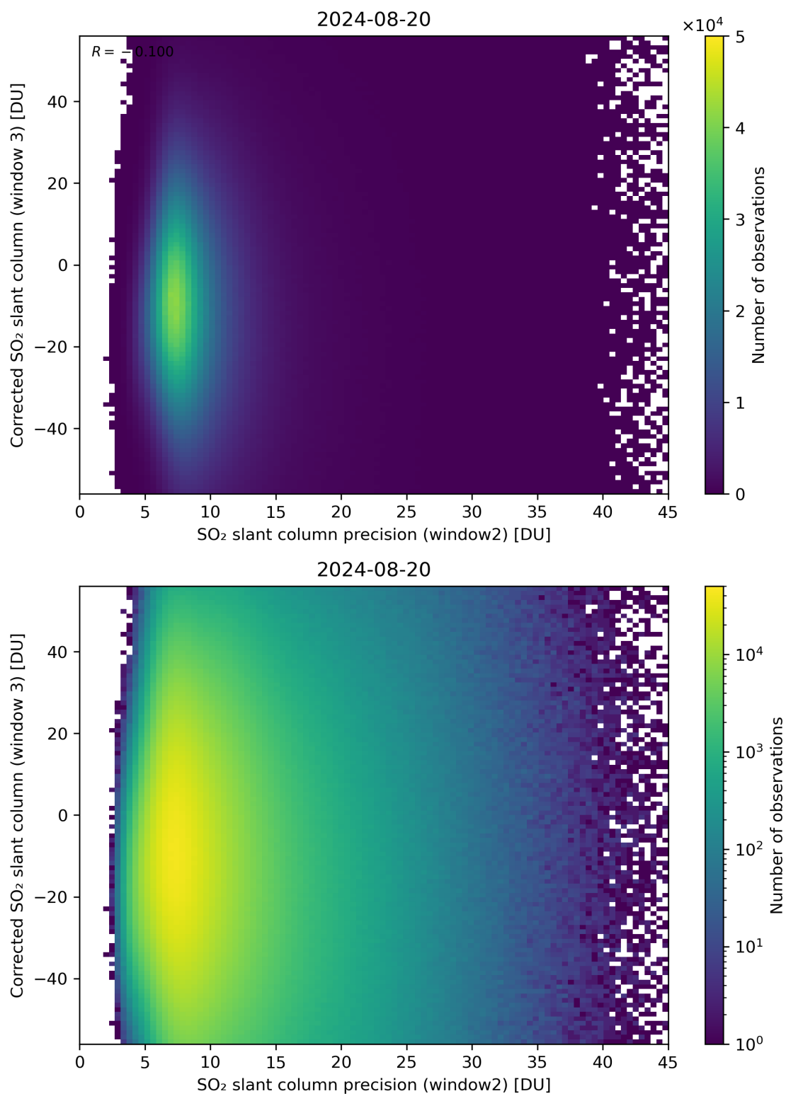
Figure 248: Scatter density plot of “SO 2 slant column precision (window2)” against “Corrected SO 2 slant column (window 3)” for 2024-08-19 to 2024-08-21.
