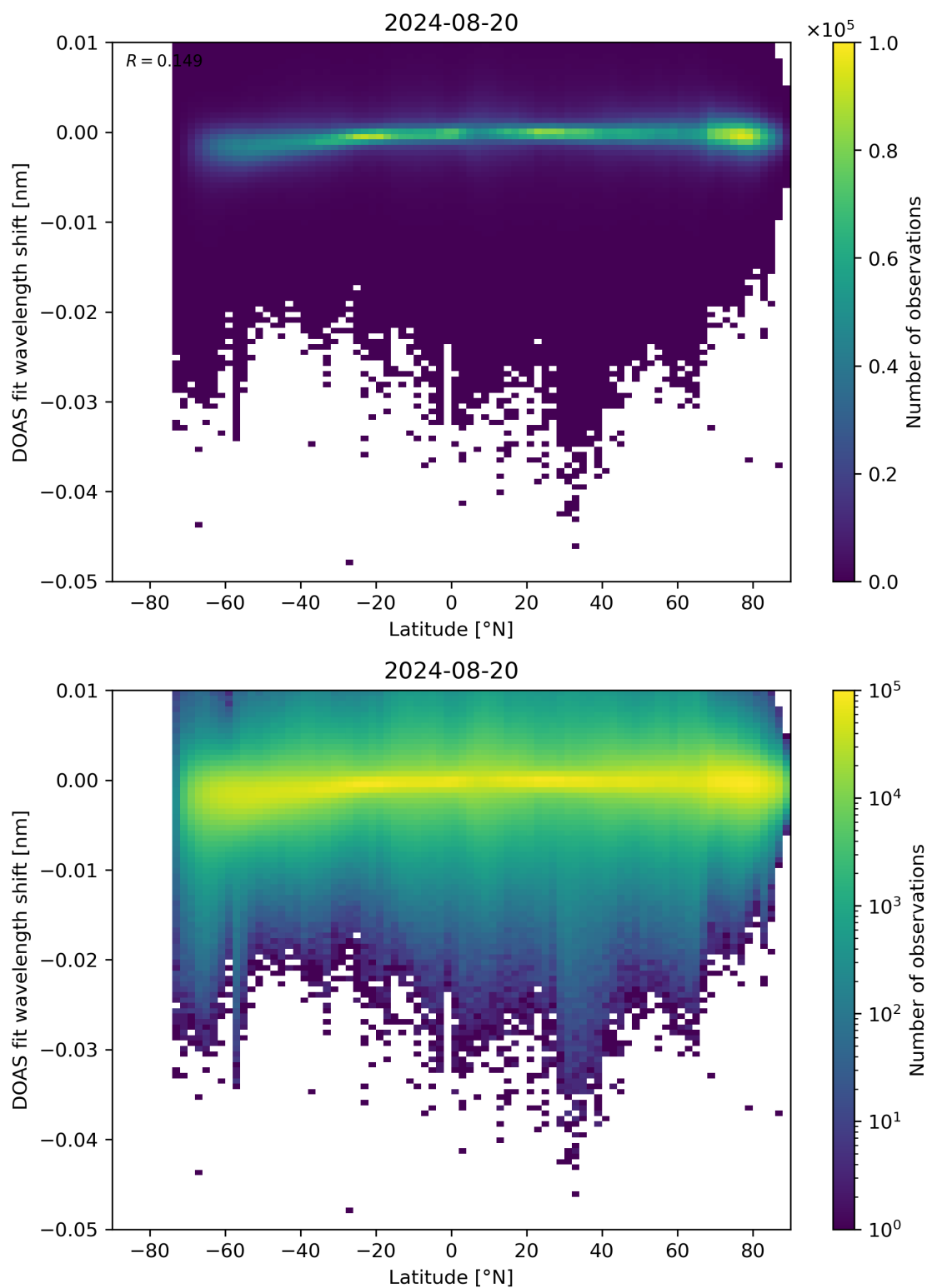
Figure 142: Scatter density plot of “Latitude” against “DOAS fit wavelength shift” for 2024-08-19 to 2024-08-21.
