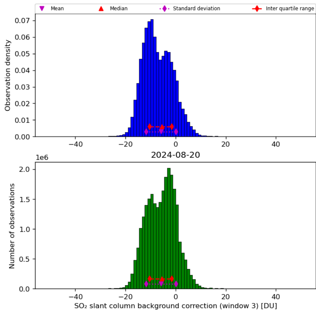
Figure 67: Histogram of “SO 2 slant column background correction (window 3)” for 2024-08-19 to 2024-08-21
