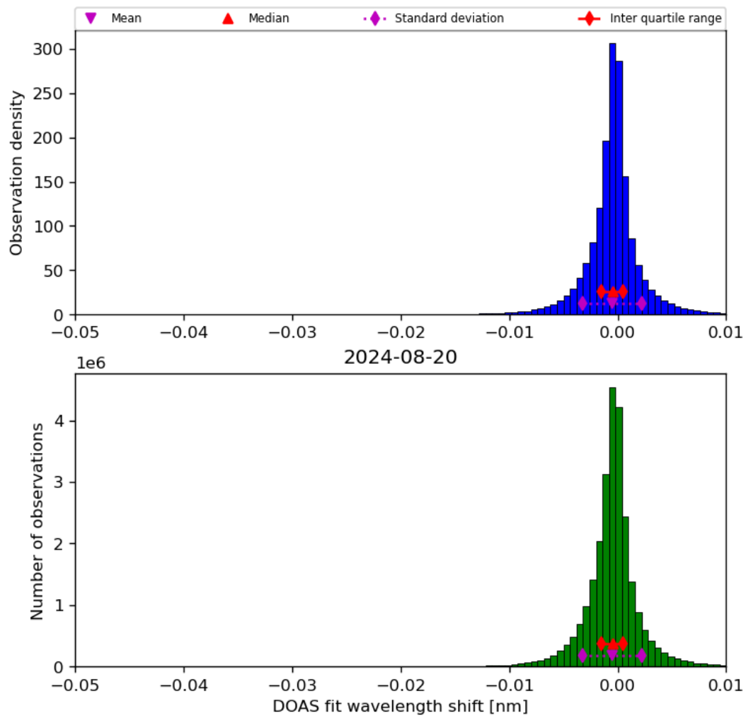
Figure 68: Histogram of “DOAS fit wavelength shift” for 2024-08-19 to 2024-08-21
