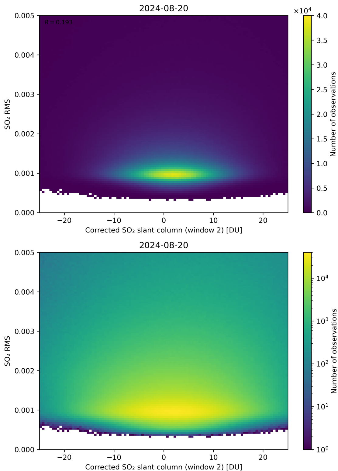
Figure 198: Scatter density plot of “Corrected SO 2 slant column (window 2)” against “SO 2 RMS” for 2024-08-19 to 2024-08-21.
