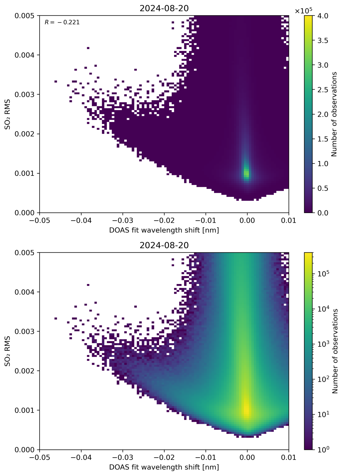
Figure 128: Scatter density plot of “DOAS fit wavelength shift” against “SO 2 RMS” for 2024-08-19 to 2024-08-21.
