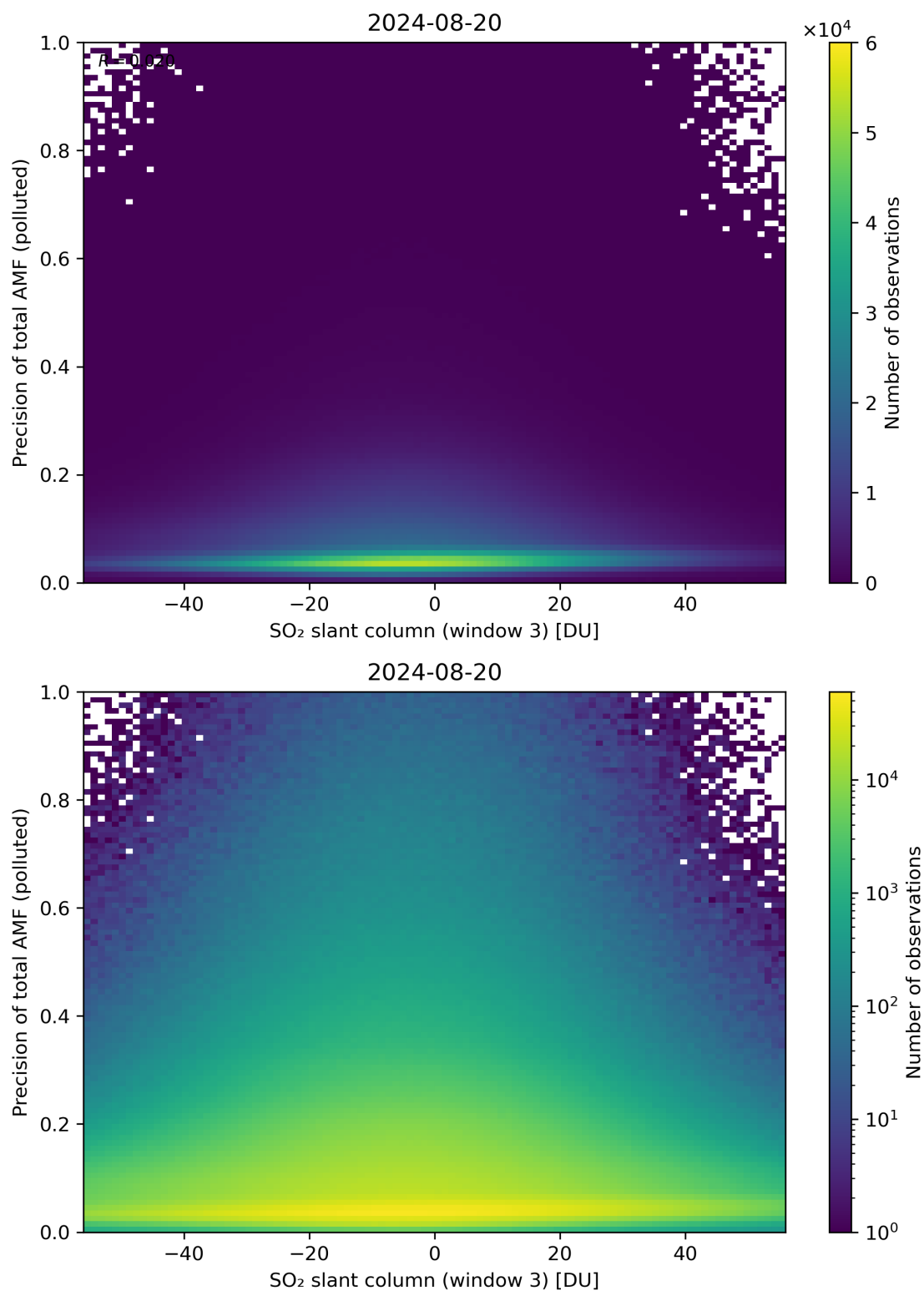
Figure 269: Scatter density plot of “SO 2 slant column (window 3)” against “Precision of total AMF (polluted)” for 2024-08-19 to 2024-08-21.
