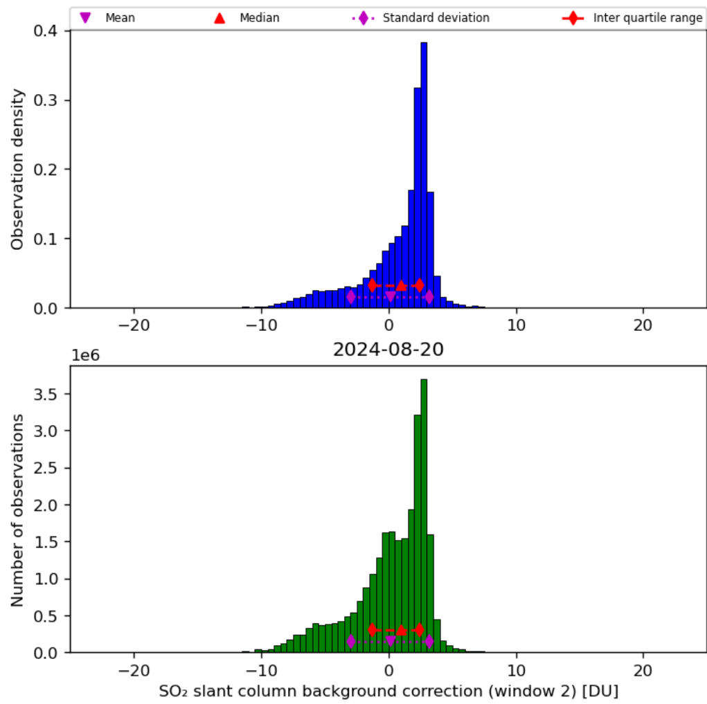
Figure 63: Histogram of “SO 2 slant column background correction (window 2)” for 2024-08-19 to 2024-08-21
