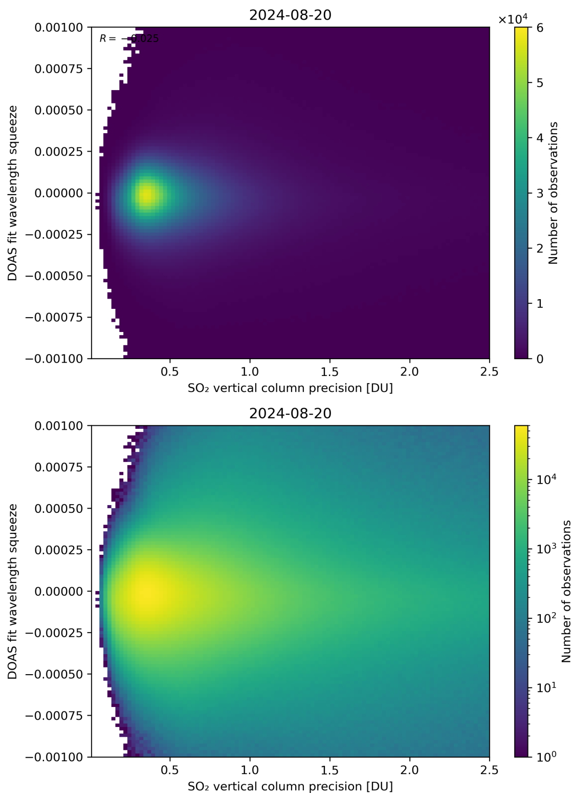
Figure 283: Scatter density plot of “SO 2 vertical column precision” against “DOAS fit wavelength squeeze” for 2024-08-19 to 2024-08-21.
