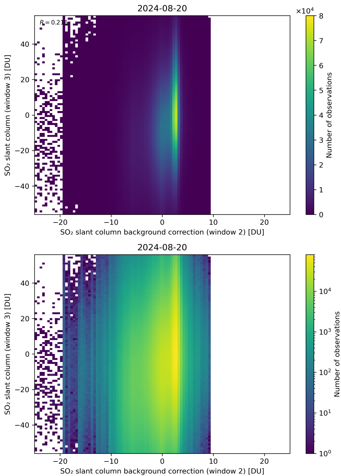
Figure 117: Scatter density plot of “SO 2 slant column background correction (window 2)” against “SO 2 slant column (window 3)” for 2024-08-19 to 2024-08-21.
