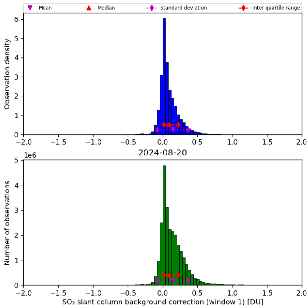
Figure 59: Histogram of “SO 2 slant column background correction (window 1)” for 2024-08-19 to 2024-08-21
