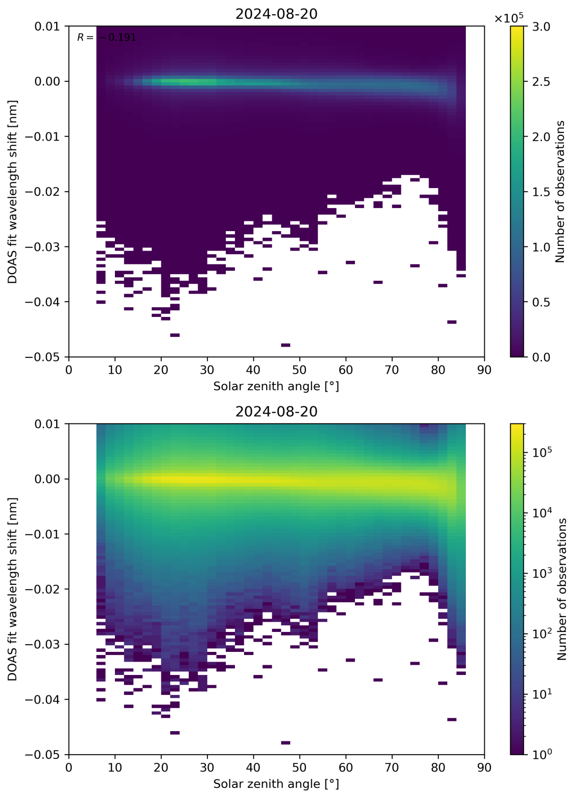
Figure 161: Scatter density plot of “Solar zenith angle” against “DOAS fit wavelength shift” for 2024-08-19 to 2024-08-21.
