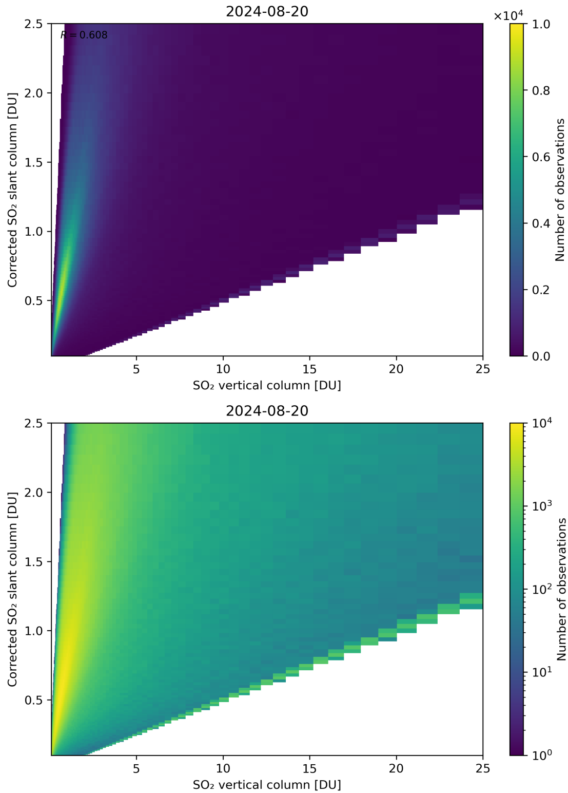
Figure 297: Scatter density plot of “SO 2 vertical column” against “Corrected SO 2 slant column” for 2024-08-19 to 2024-08-21.
