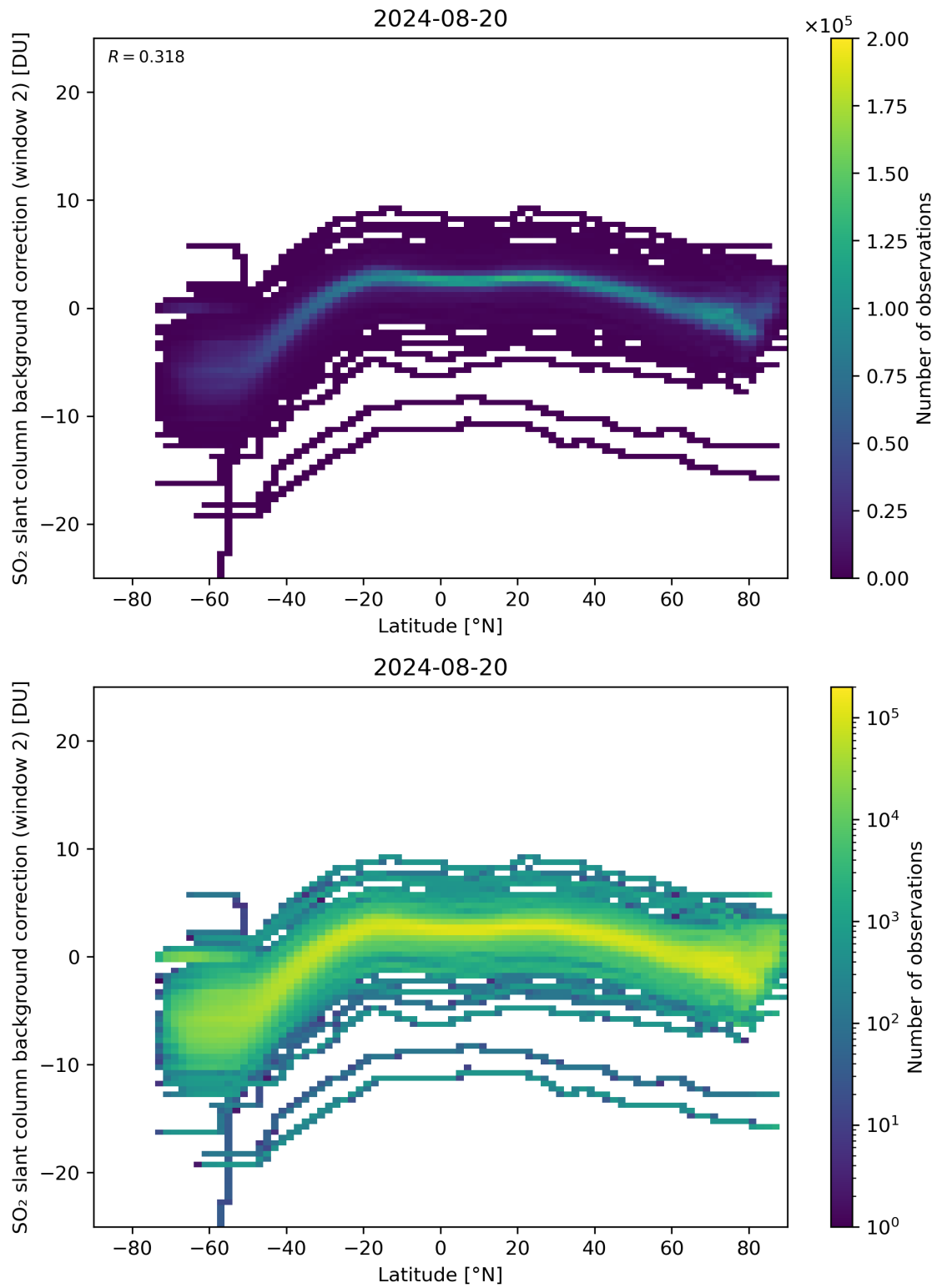
Figure 140: Scatter density plot of “Latitude” against “SO 2 slant column background correction (window 2)” for 2024-08-19 to 2024-08-21.
