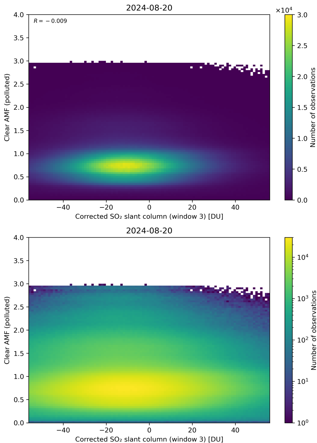
Figure 209: Scatter density plot of “Corrected SO 2 slant column (window 3)” against “Clear AMF (polluted)” for 2024-08-19 to 2024-08-21.
