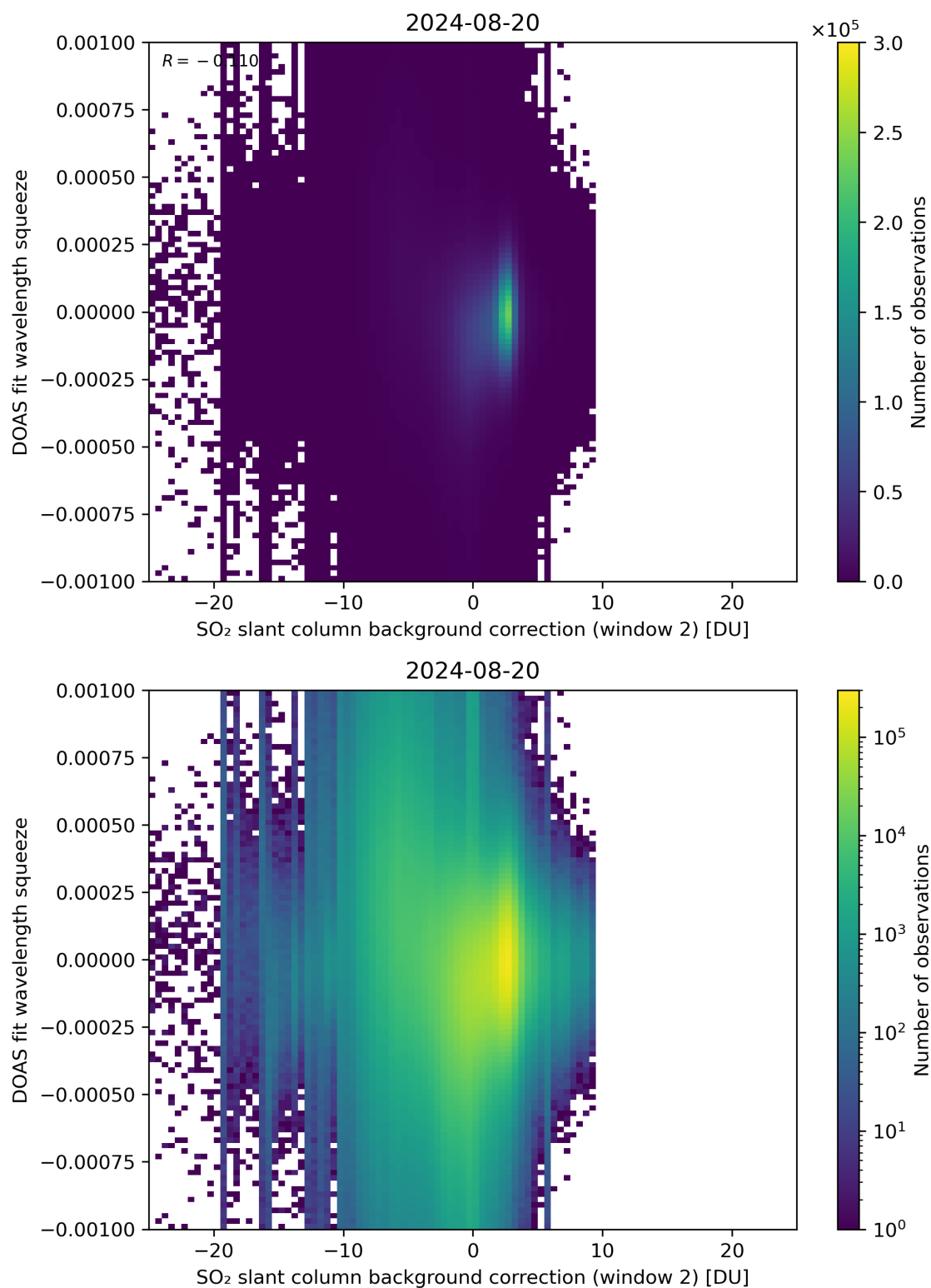
Figure 113: Scatter density plot of “SO 2 slant column background correction (window 2)” against “DOAS fit wavelength squeeze” for 2024-08-19 to 2024-08-21.
