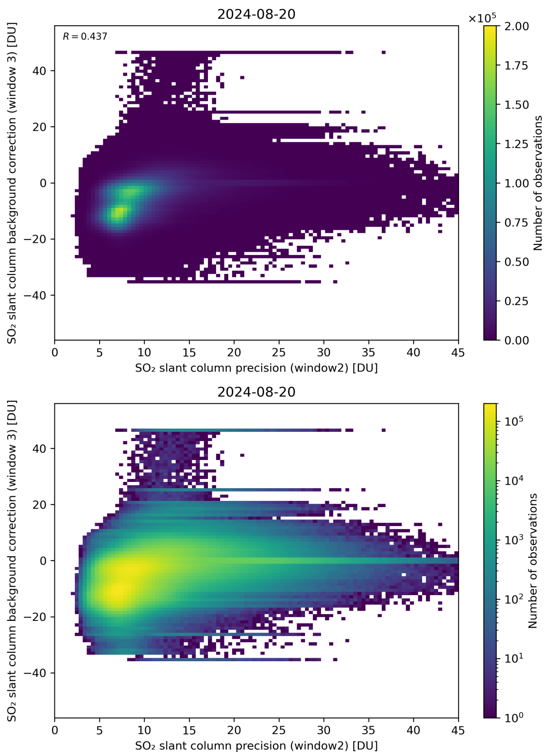
Figure 242: Scatter density plot of “SO 2 slant column precision (window2)” against “SO 2 slant column background correction (window 3)” for 2024-08-19 to 2024-08-21.
