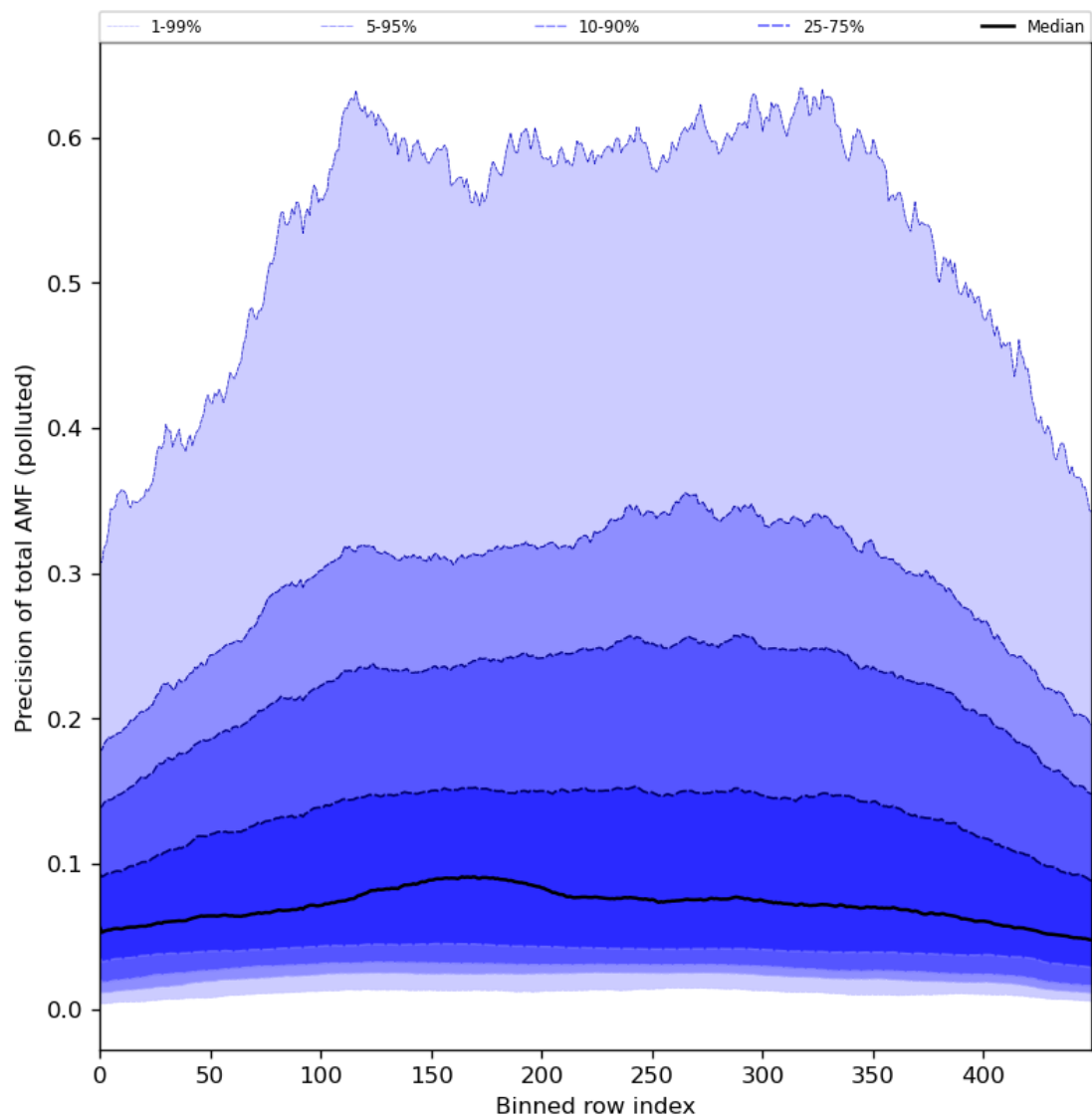
Figure 95: Along track statistics of “Precision of total AMF (polluted)” for 2024-08-19 to 2024-08-21
