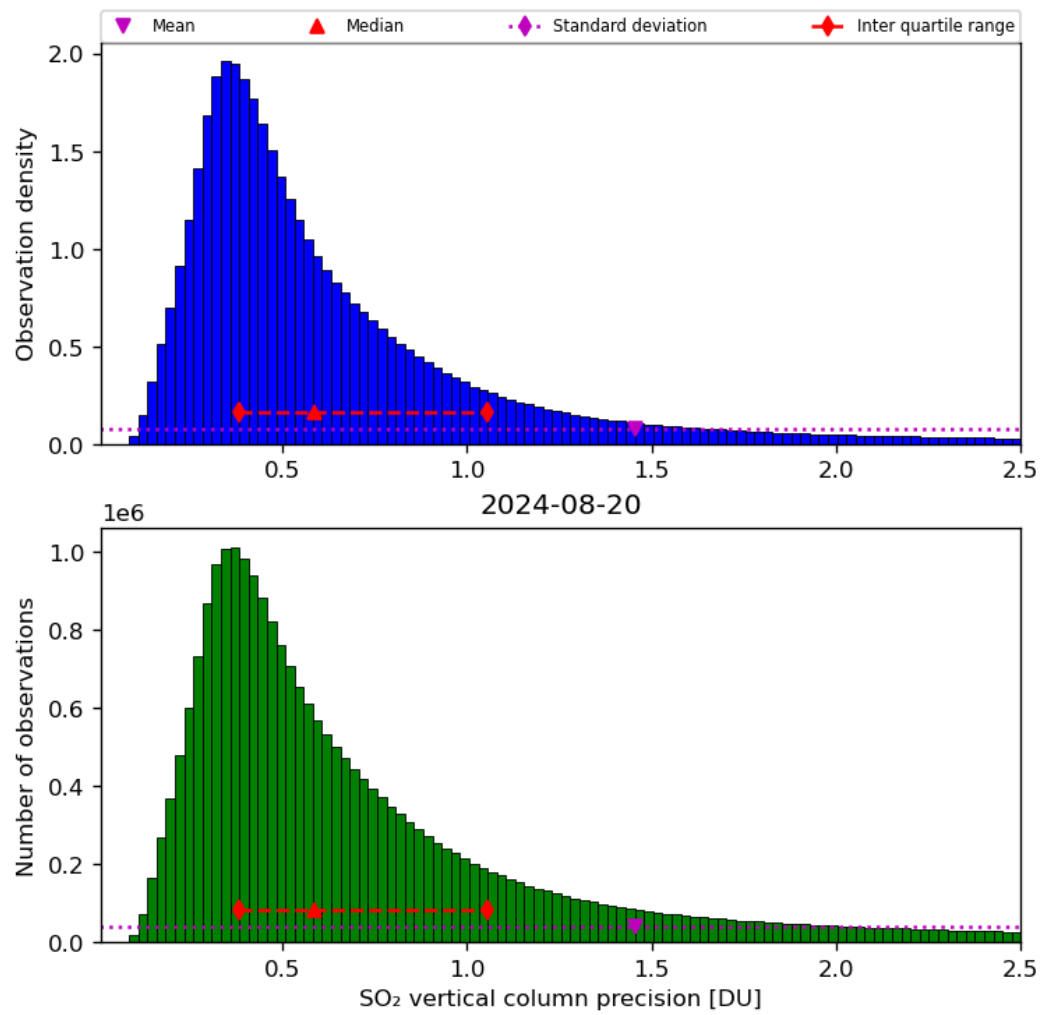
Figure 54: Histogram of “SO 2 vertical column precision” for 2024-08-19 to 2024-08-21
