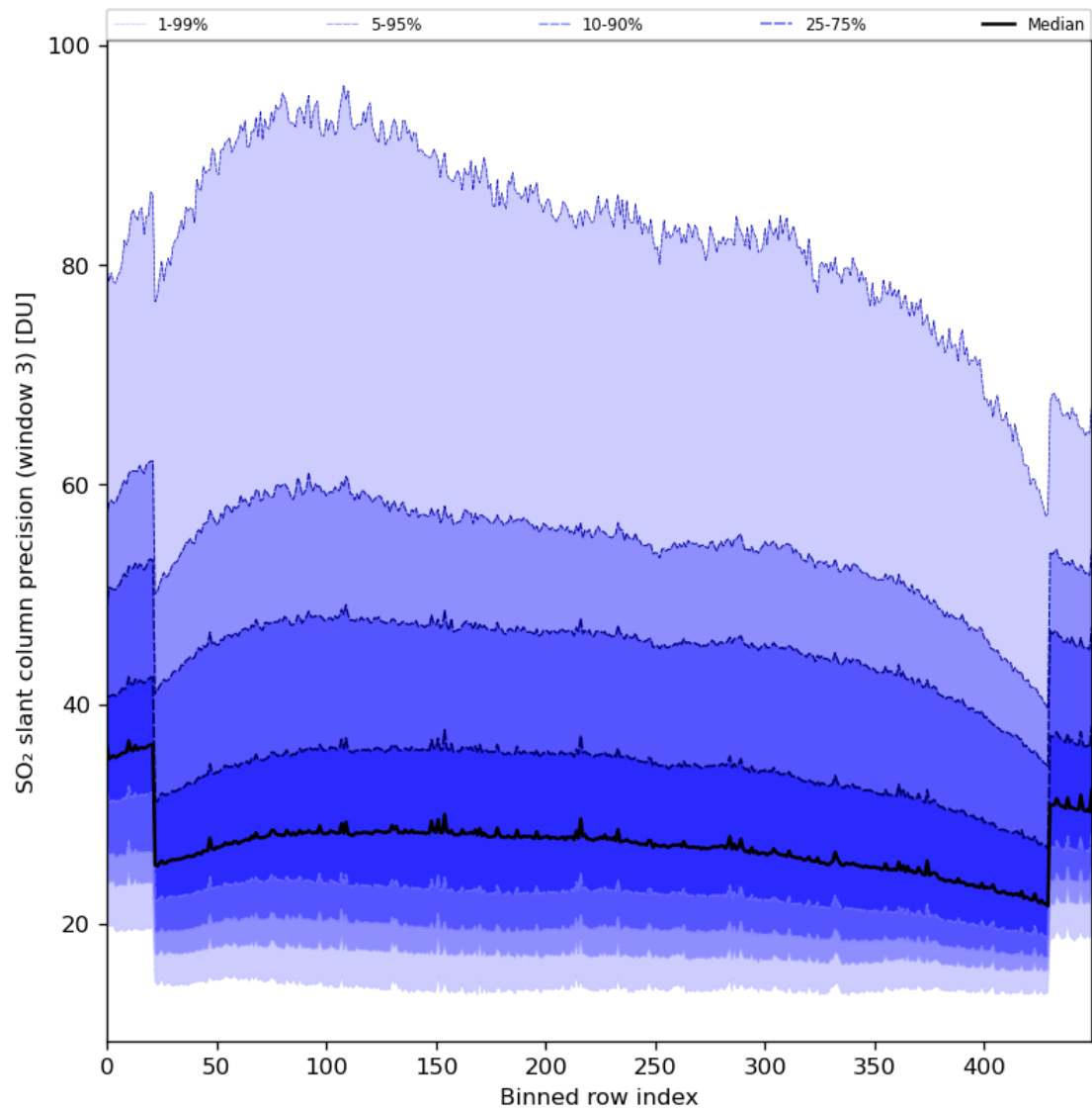
Figure 88: Along track statistics of “SO 2 slant column precision (window 3)” for 2024-08-19 to 2024-08-21
