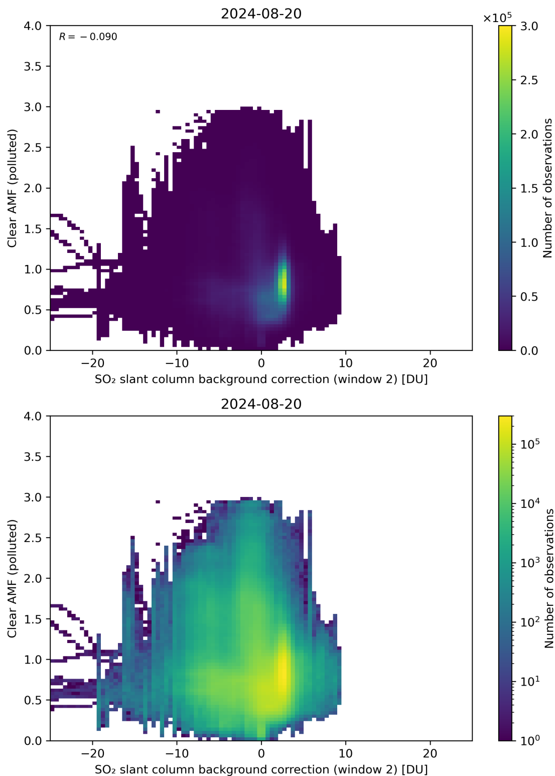
Figure 115: Scatter density plot of “SO 2 slant column background correction (window 2)” against “Clear AMF (polluted)” for 2024-08-19 to 2024-08-21.
