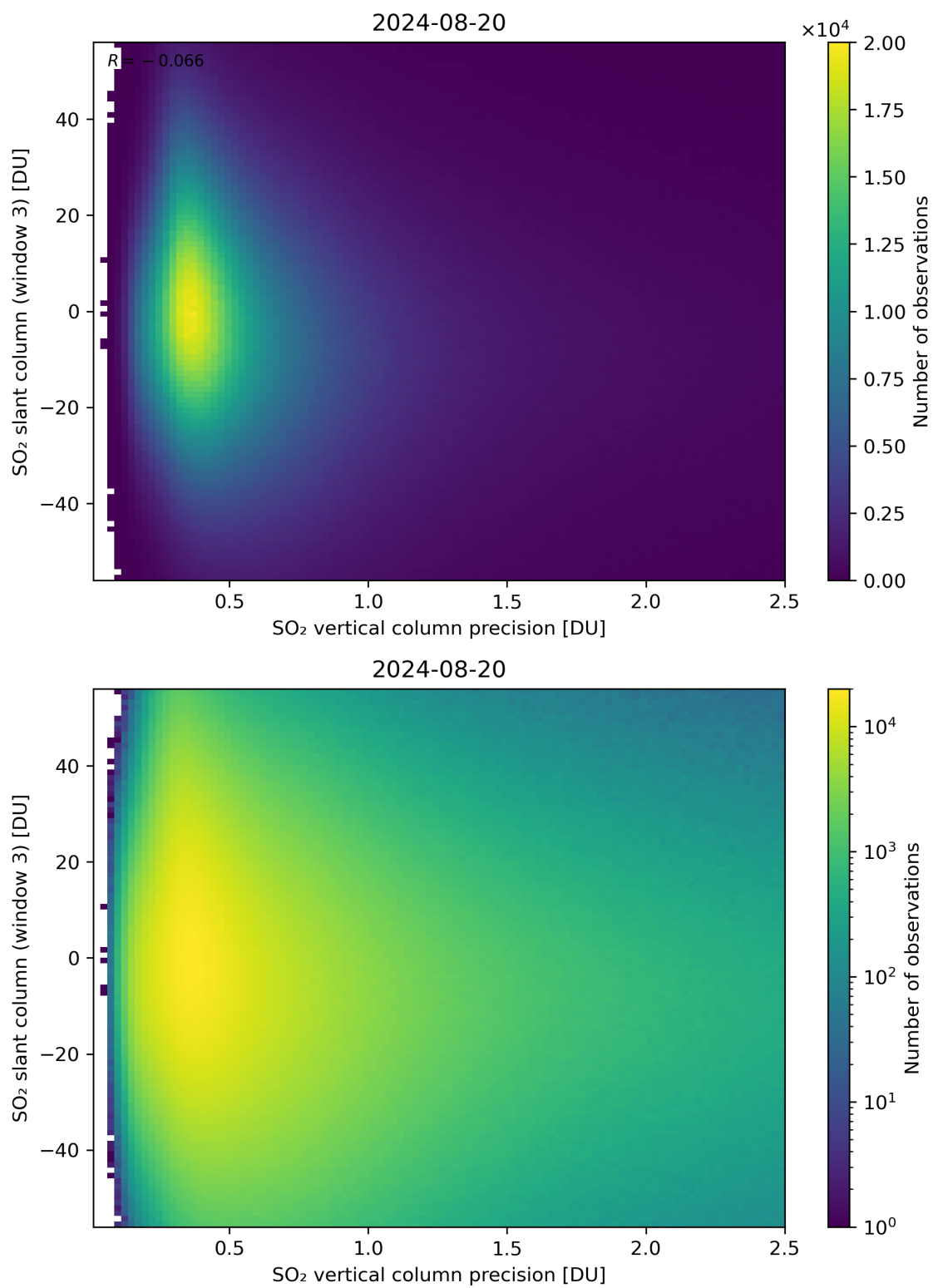
Figure 292: Scatter density plot of “SO 2 vertical column precision” against “SO 2 slant column (window 3)” for 2024-08-19 to 2024-08-21.
