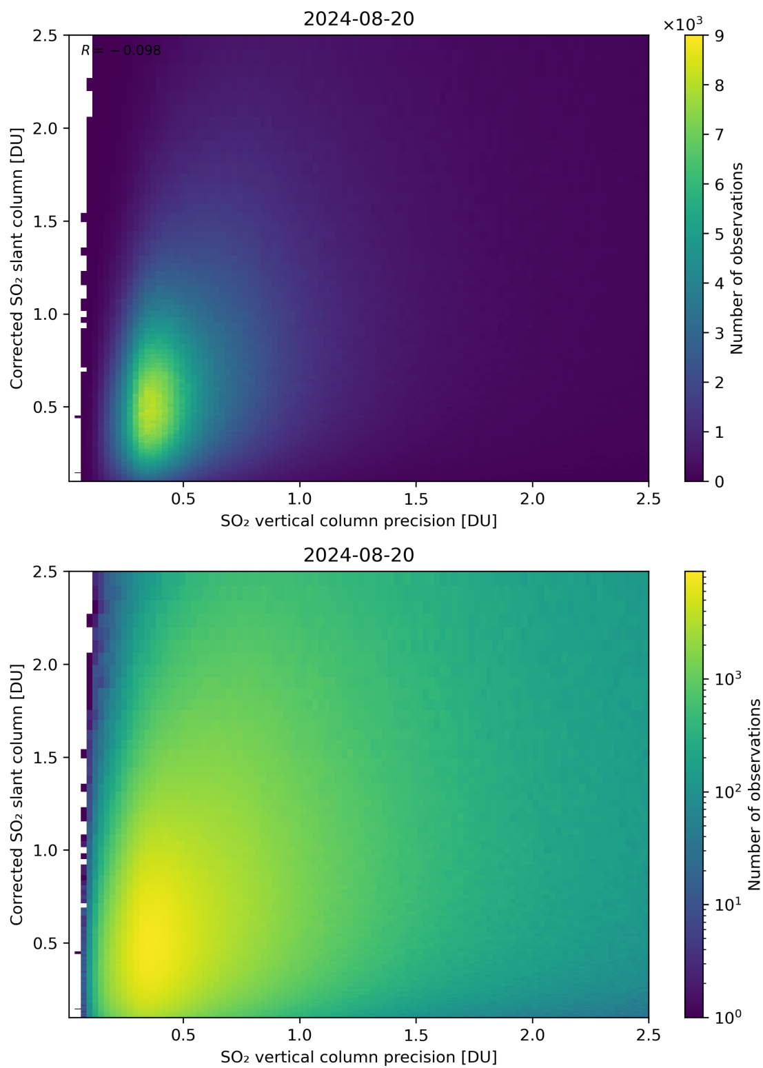
Figure 286: Scatter density plot of “SO 2 vertical column precision” against “Corrected SO 2 slant column” for 2024-08-19 to 2024-08-21.
