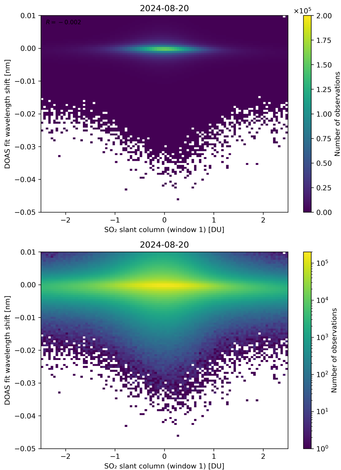
Figure 215: Scatter density plot of “SO 2 slant column (window 1)” against “DOAS fit wavelength shift” for 2024-08-19 to 2024-08-21.
