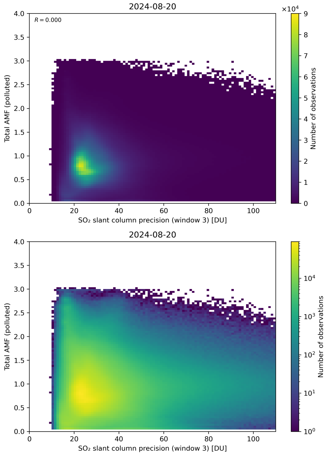
Figure 263: Scatter density plot of “SO 2 slant column precision (window 3)” against “Total AMF (polluted)” for 2024-08-19 to 2024-08-21.
