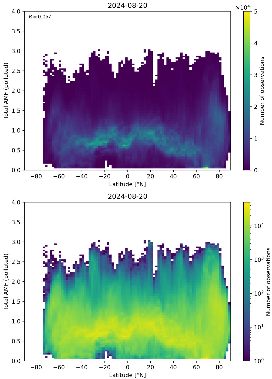
Figure 154: Scatter density plot of “Latitude” against “Total AMF (polluted)” for 2024-08-19 to 2024-08-21.
