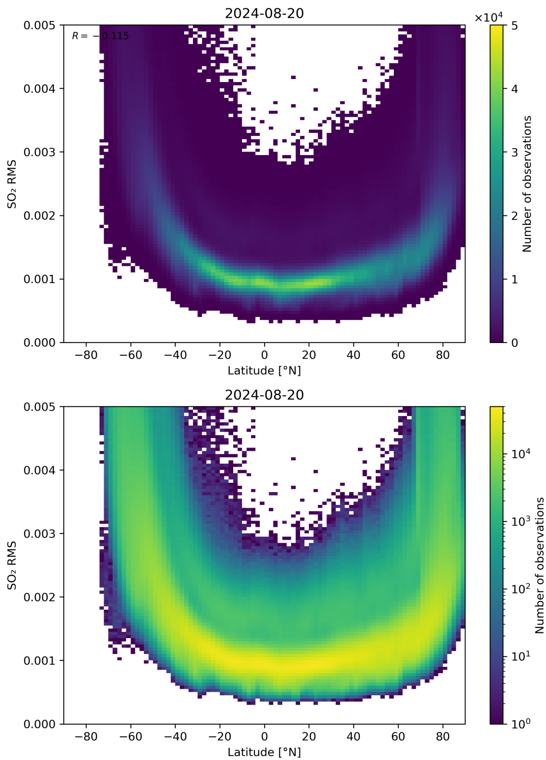
Figure 144: Scatter density plot of “Latitude” against “SO 2 RMS” for 2024-08-19 to 2024-08-21.
