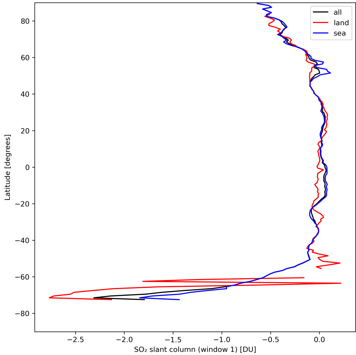
Figure 33: Zonal average of “SO 2 slant column (window 1)” for 2024-08-19 to 2024-08-21.
