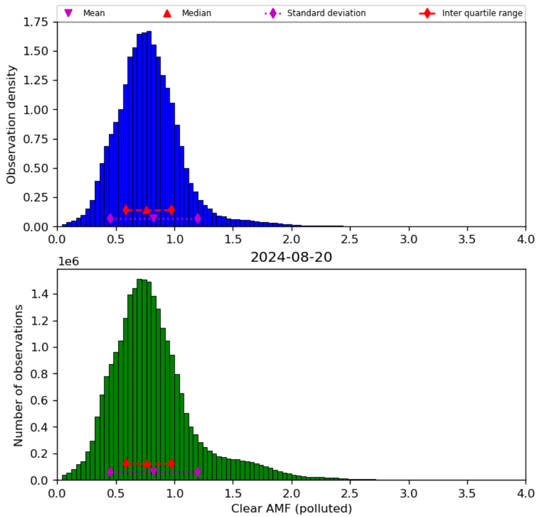
Figure 73: Histogram of “Clear AMF (polluted)” for 2024-08-19 to 2024-08-21
