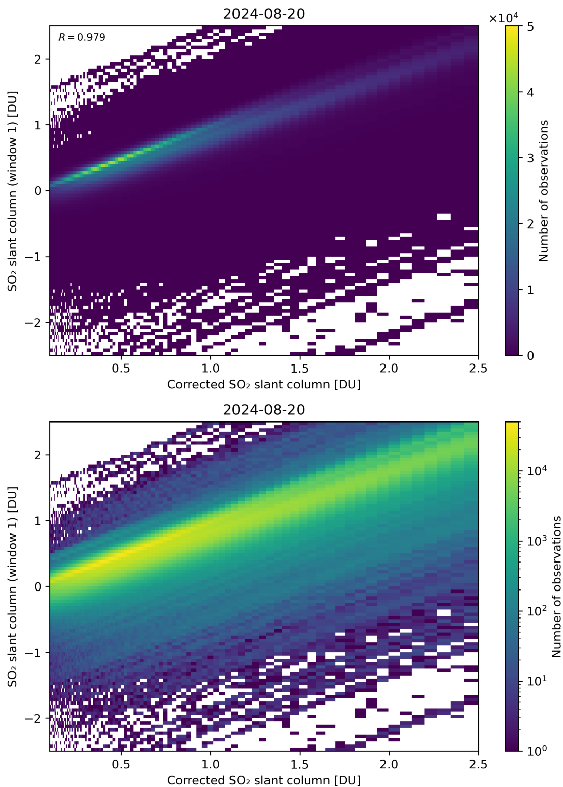
Figure 187: Scatter density plot of “Corrected SO 2 slant column” against “SO 2 slant column (window 1)” for 2024-08-19 to 2024-08-21.
