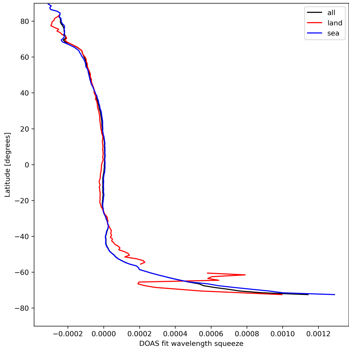
Figure 46: Zonal average of “DOAS fit wavelength squeeze” for 2024-08-19 to 2024-08-21.
