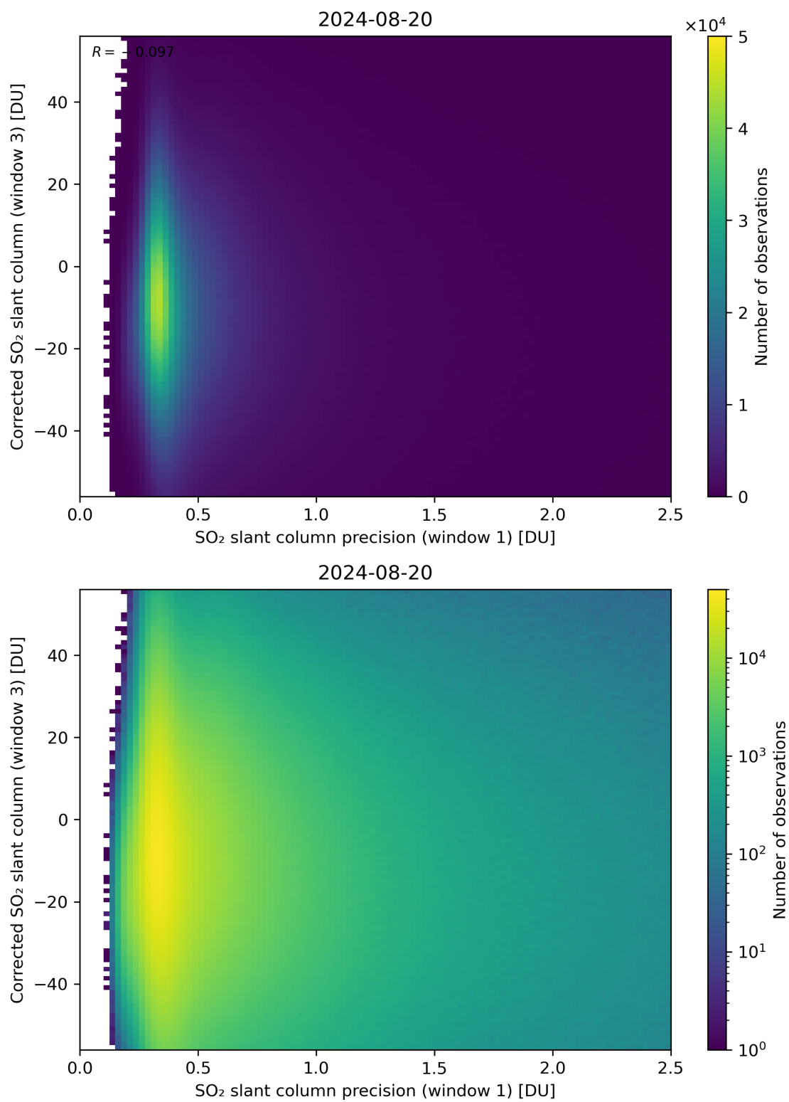
Figure 226: Scatter density plot of “SO 2 slant column precision (window 1)” against “Corrected SO 2 slant column (window 3)” for 2024-08-19 to 2024-08-21.
