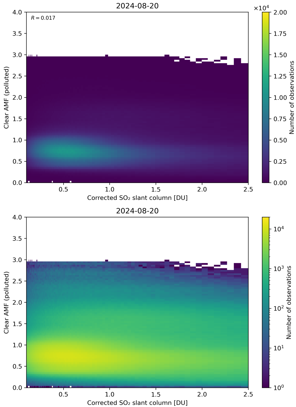
Figure 184: Scatter density plot of “Corrected SO 2 slant column” against “Clear AMF (polluted)” for 2024-08-19 to 2024-08-21.
