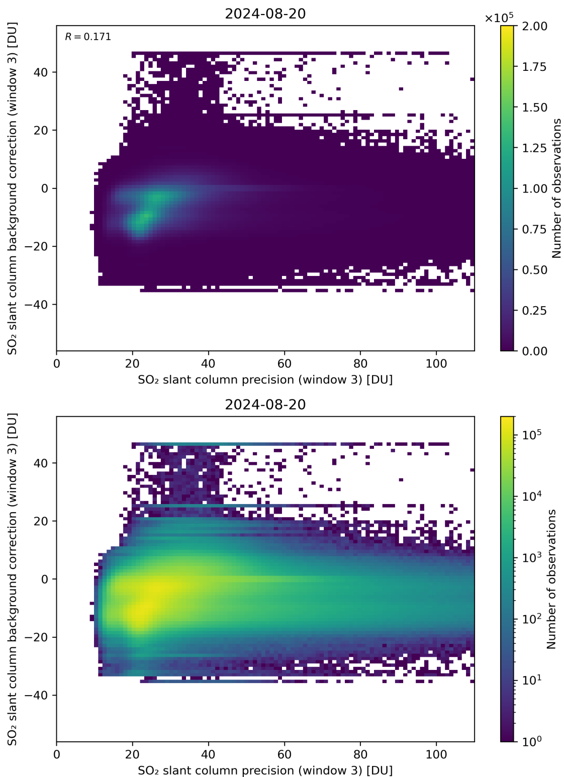
Figure 257: Scatter density plot of “SO 2 slant column precision (window 3)” against “SO 2 slant column background correction (window 3)” for 2024-08-19 to 2024-08-21.
