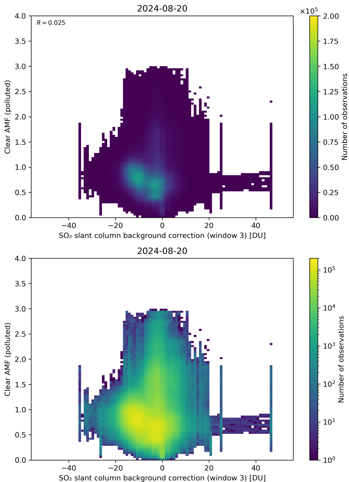
Figure 124: Scatter density plot of “SO 2 slant column background correction (window 3)” against “Clear AMF (polluted)” for 2024-08-19 to 2024-08-21.
