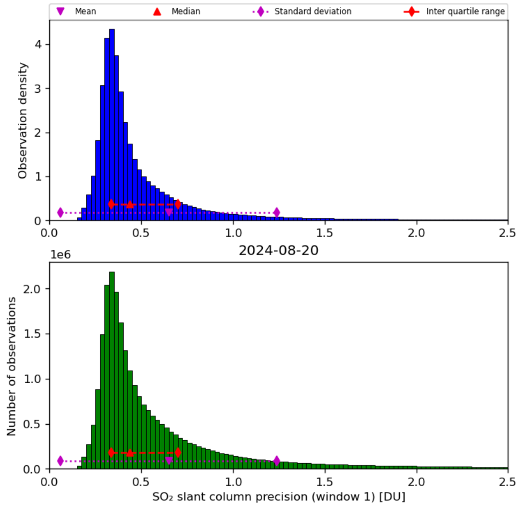
Figure 57: Histogram of “SO 2 slant column precision (window 1)” for 2024-08-19 to 2024-08-21
