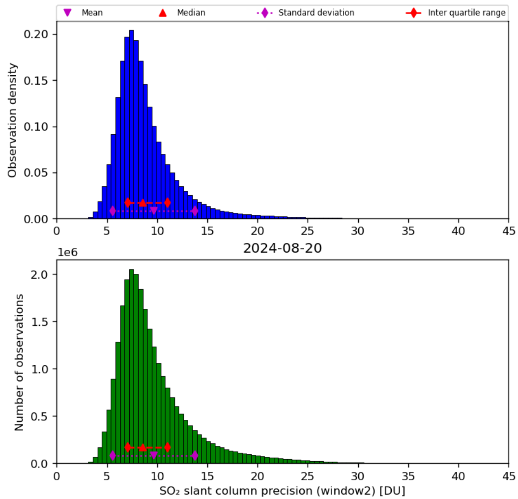
Figure 61: Histogram of “SO 2 slant column precision (window2)” for 2024-08-19 to 2024-08-21
