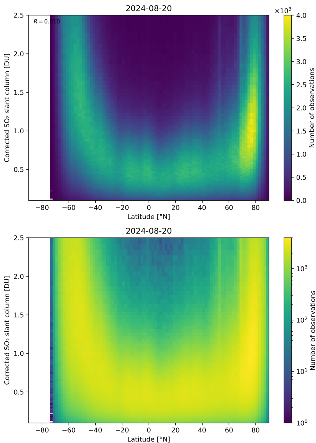
Figure 146: Scatter density plot of “Latitude” against “Corrected SO 2 slant column” for 2024-08-19 to 2024-08-21.
