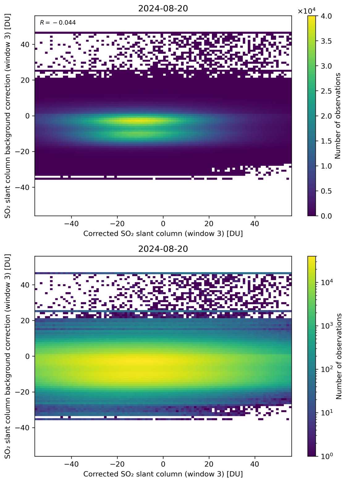
Figure 205: Scatter density plot of “Corrected SO 2 slant column (window 3)” against “SO 2 slant column background correction (window 3)” for 2024-08-19 to 2024-08-21.
