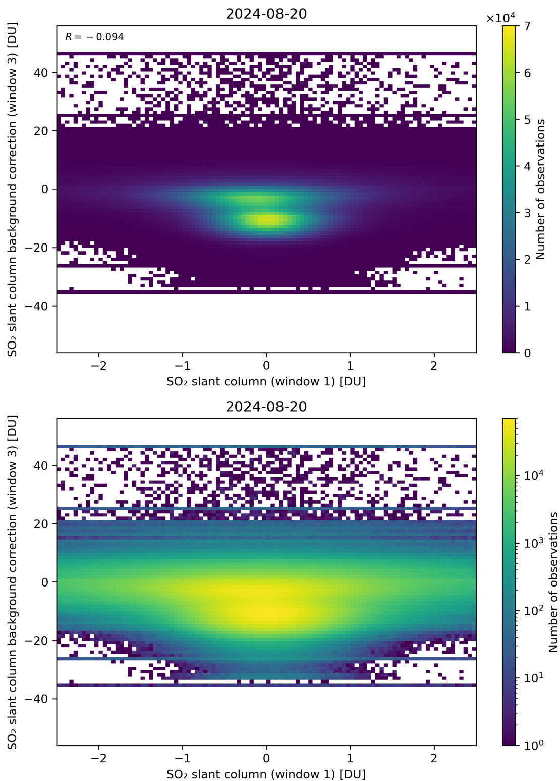
Figure 214: Scatter density plot of “SO 2 slant column (window 1)” against “SO 2 slant column background correction (window 3)” for 2024-08-19 to 2024-08-21.
