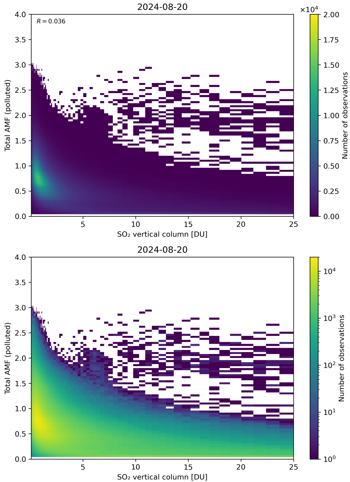
Figure 305: Scatter density plot of “SO 2 vertical column” against “Total AMF (polluted)” for 2024-08-19 to 2024-08-21.
