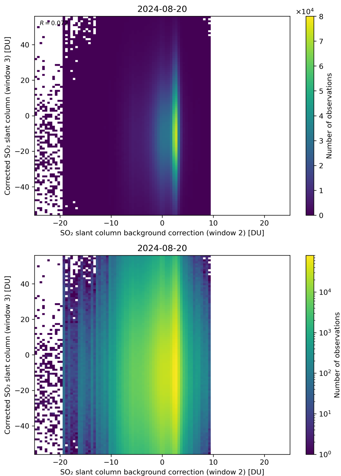
Figure 116: Scatter density plot of “SO 2 slant column background correction (window 2)” against “Corrected SO 2 slant column (window 3)” for 2024-08-19 to 2024-08-21.
