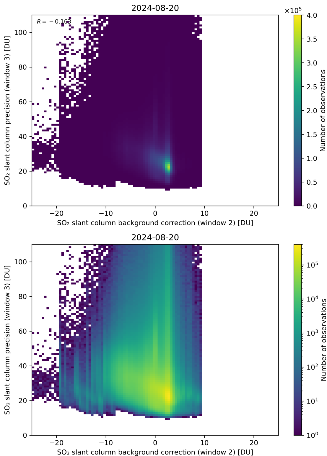
Figure 118: Scatter density plot of “SO 2 slant column background correction (window 2)” against “SO 2 slant column precision (window 3)” for 2024-08-19 to 2024-08-21.
