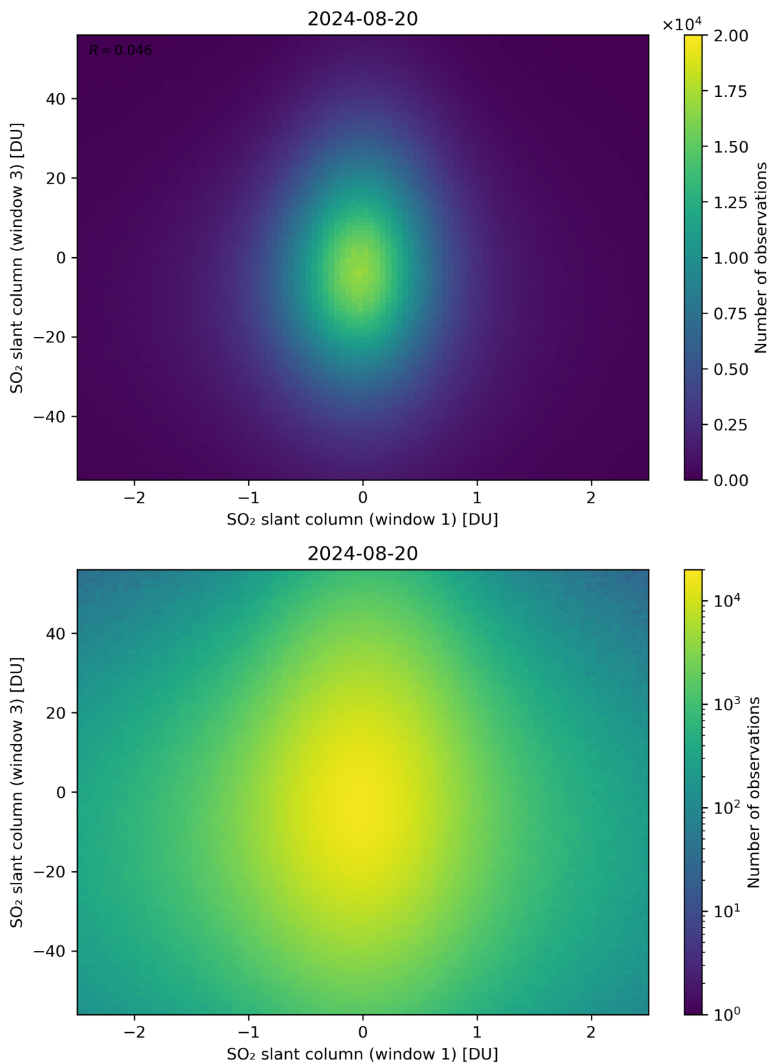
Figure 237: Scatter density plot of “SO 2 slant column (window 1)” against “SO 2 slant column (window 3)” for 2024-08-19 to 2024-08-21.
