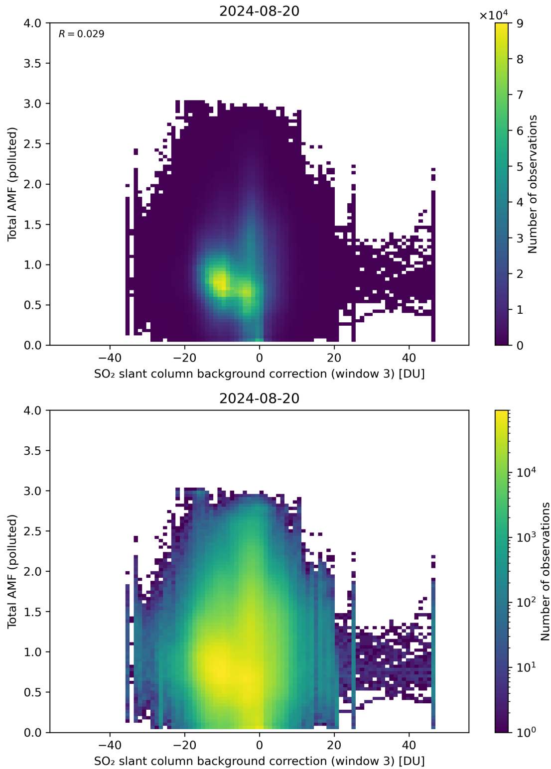
Figure 125: Scatter density plot of “SO 2 slant column background correction (window 3)” against “Total AMF (polluted)” for 2024-08-19 to 2024-08-21.
