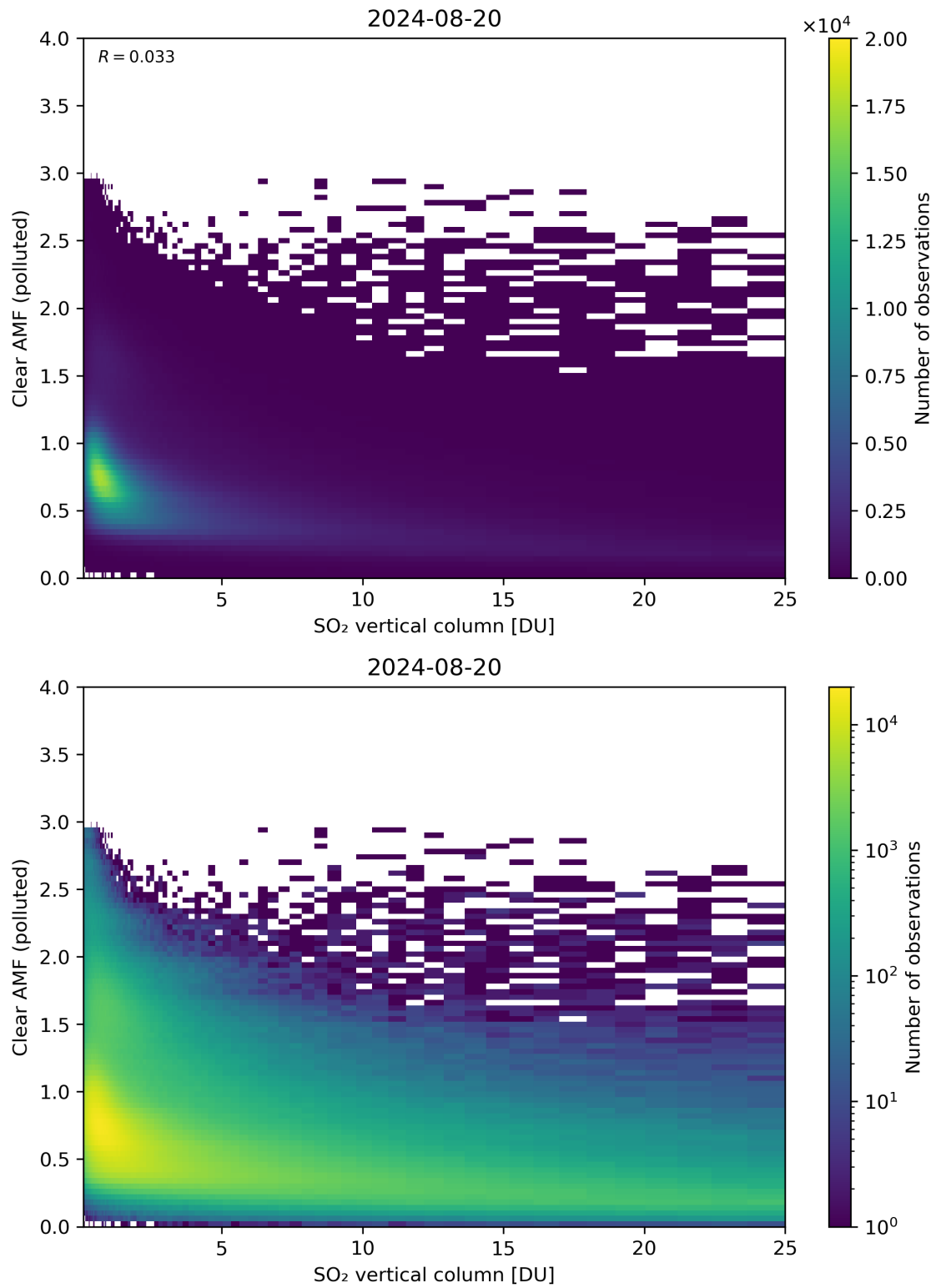
Figure 296: Scatter density plot of “SO 2 vertical column” against “Clear AMF (polluted)” for 2024-08-19 to 2024-08-21.
