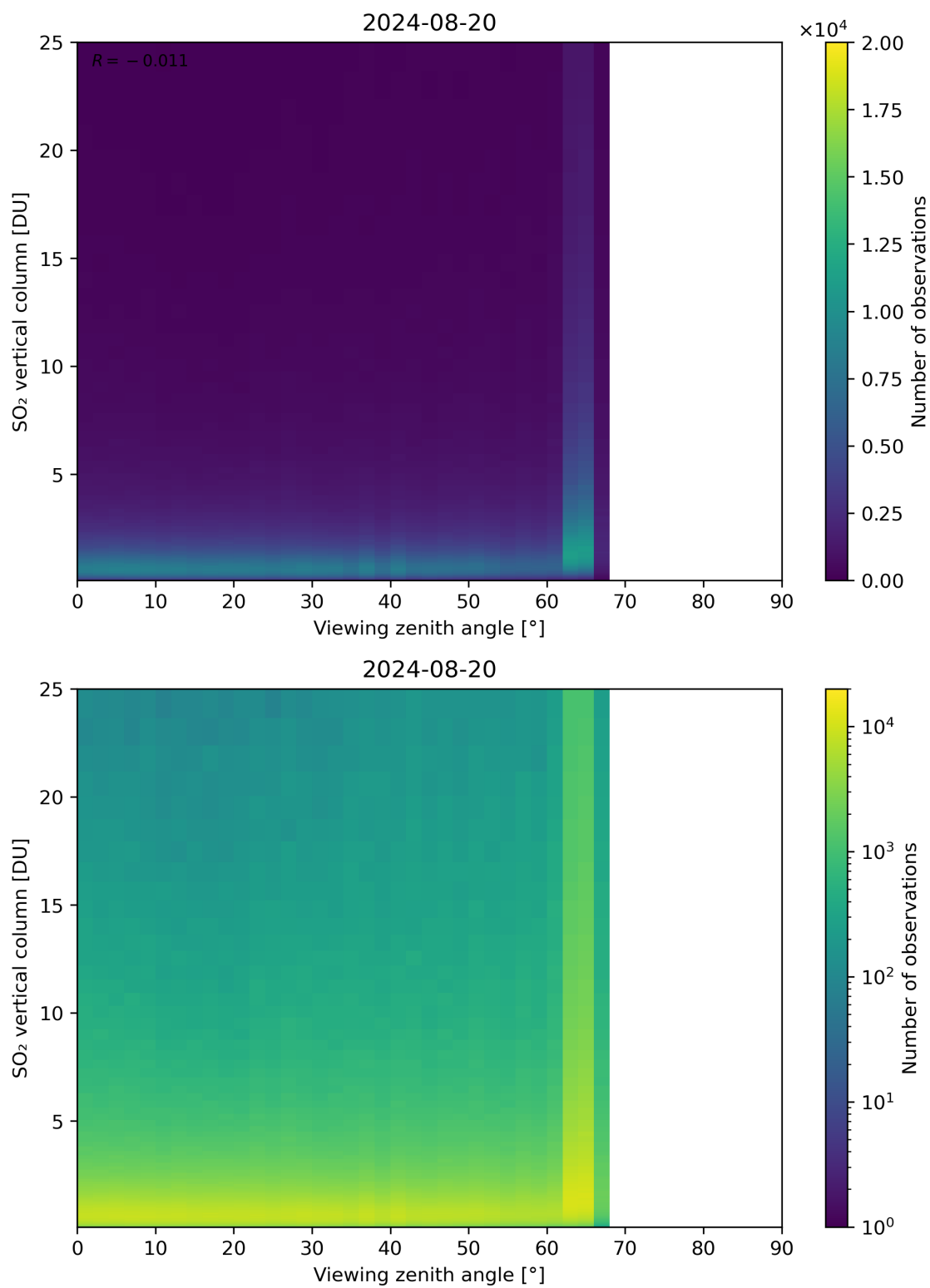
Figure 327: Scatter density plot of “Viewing zenith angle” against “SO 2 vertical column” for 2024-08-19 to 2024-08-21.
