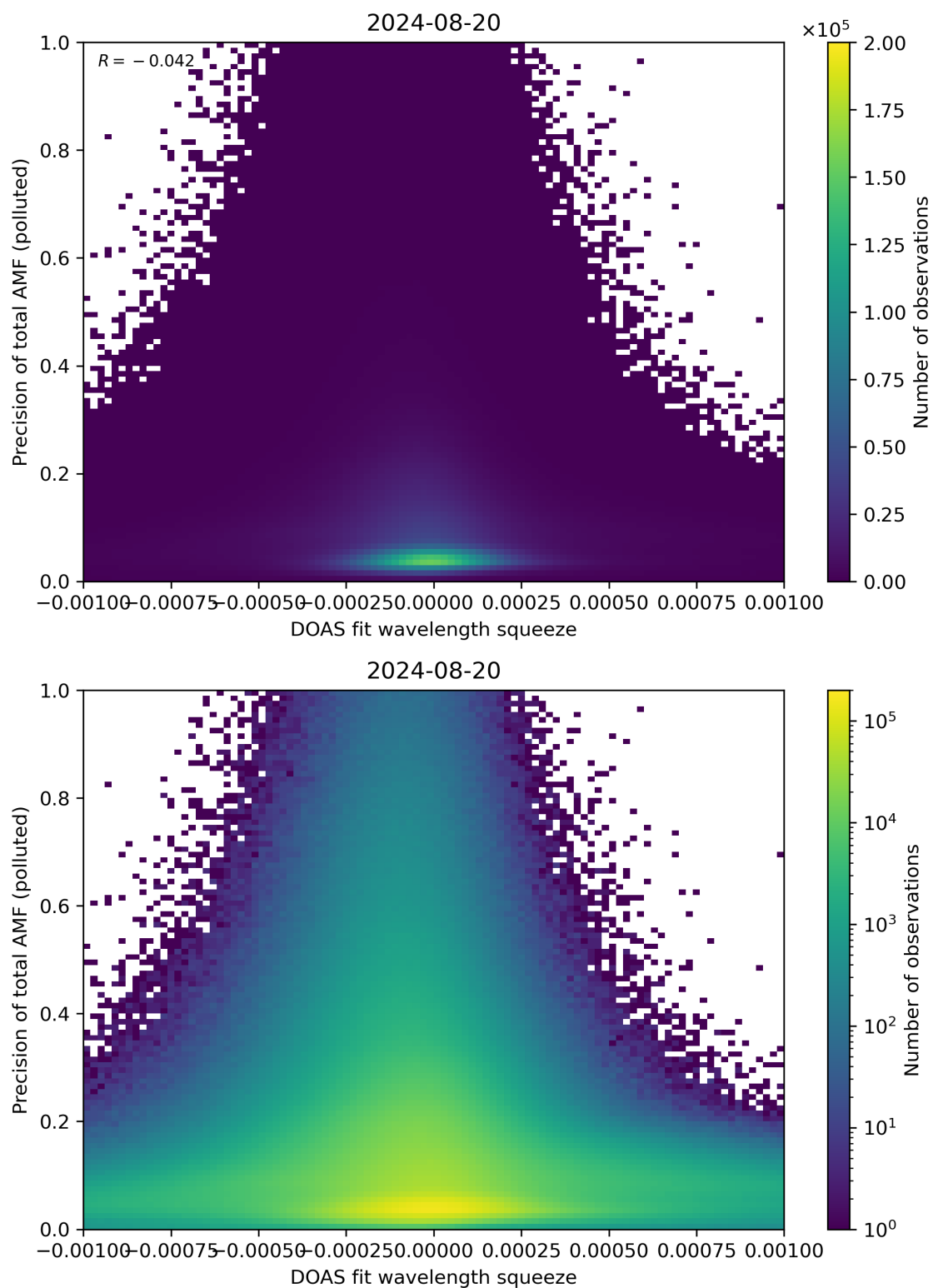
Figure 135: Scatter density plot of “DOAS fit wavelength squeeze” against “Precision of total AMF (polluted)” for 2024-08-19 to 2024-08-21.
