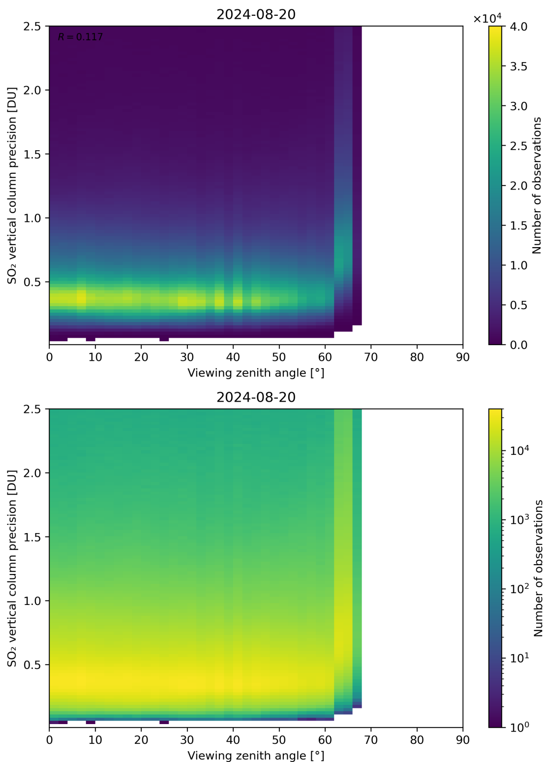
Figure 328: Scatter density plot of “Viewing zenith angle” against “SO 2 vertical column precision” for 2024-08-19 to 2024-08-21.
