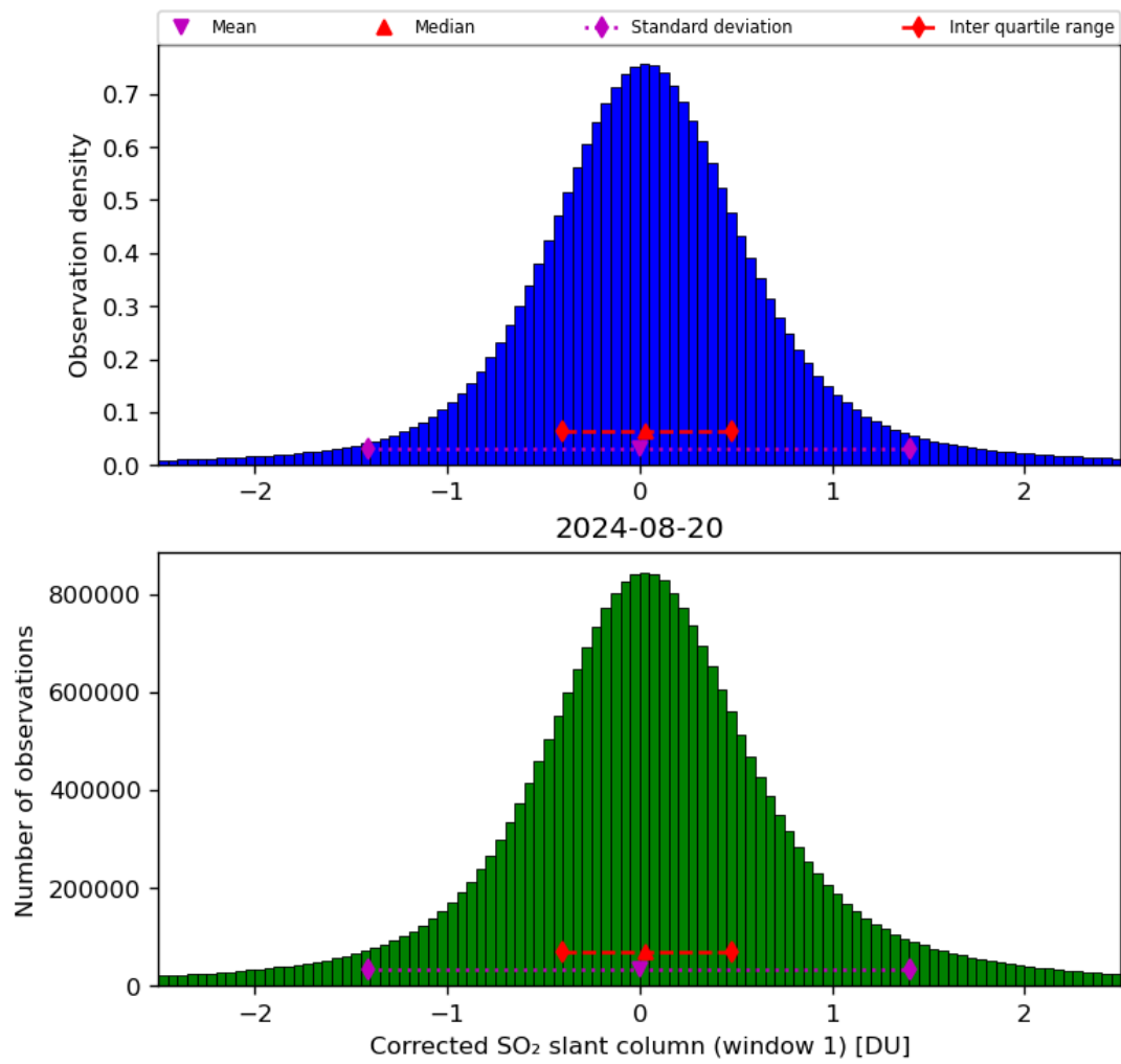
Figure 58: Histogram of “Corrected SO 2 slant column (window 1)” for 2024-08-19 to 2024-08-21
