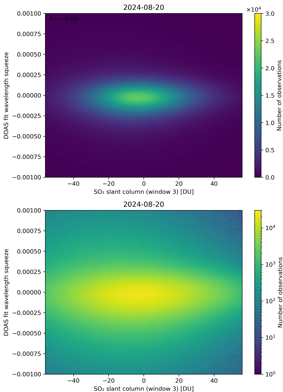
Figure 255: Scatter density plot of “SO 2 slant column (window 3)” against “DOAS fit wavelength squeeze” for 2024-08-19 to 2024-08-21.
