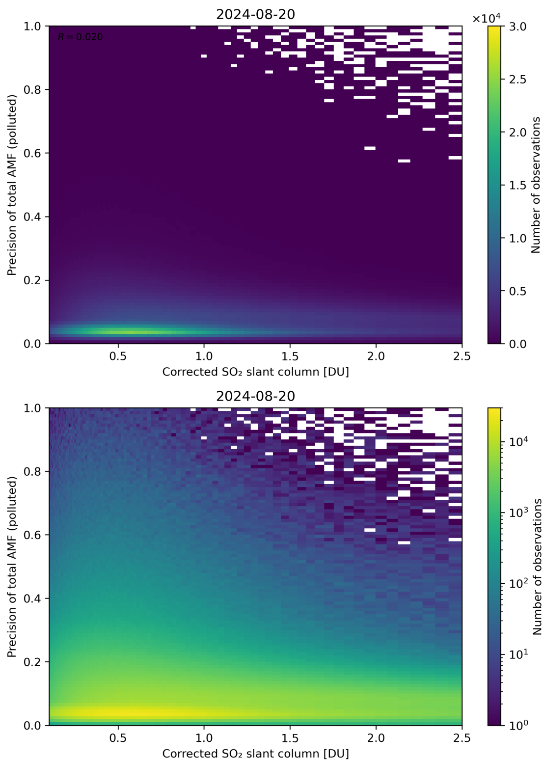
Figure 193: Scatter density plot of “Corrected SO 2 slant column” against “Precision of total AMF (polluted)” for 2024-08-19 to 2024-08-21.
