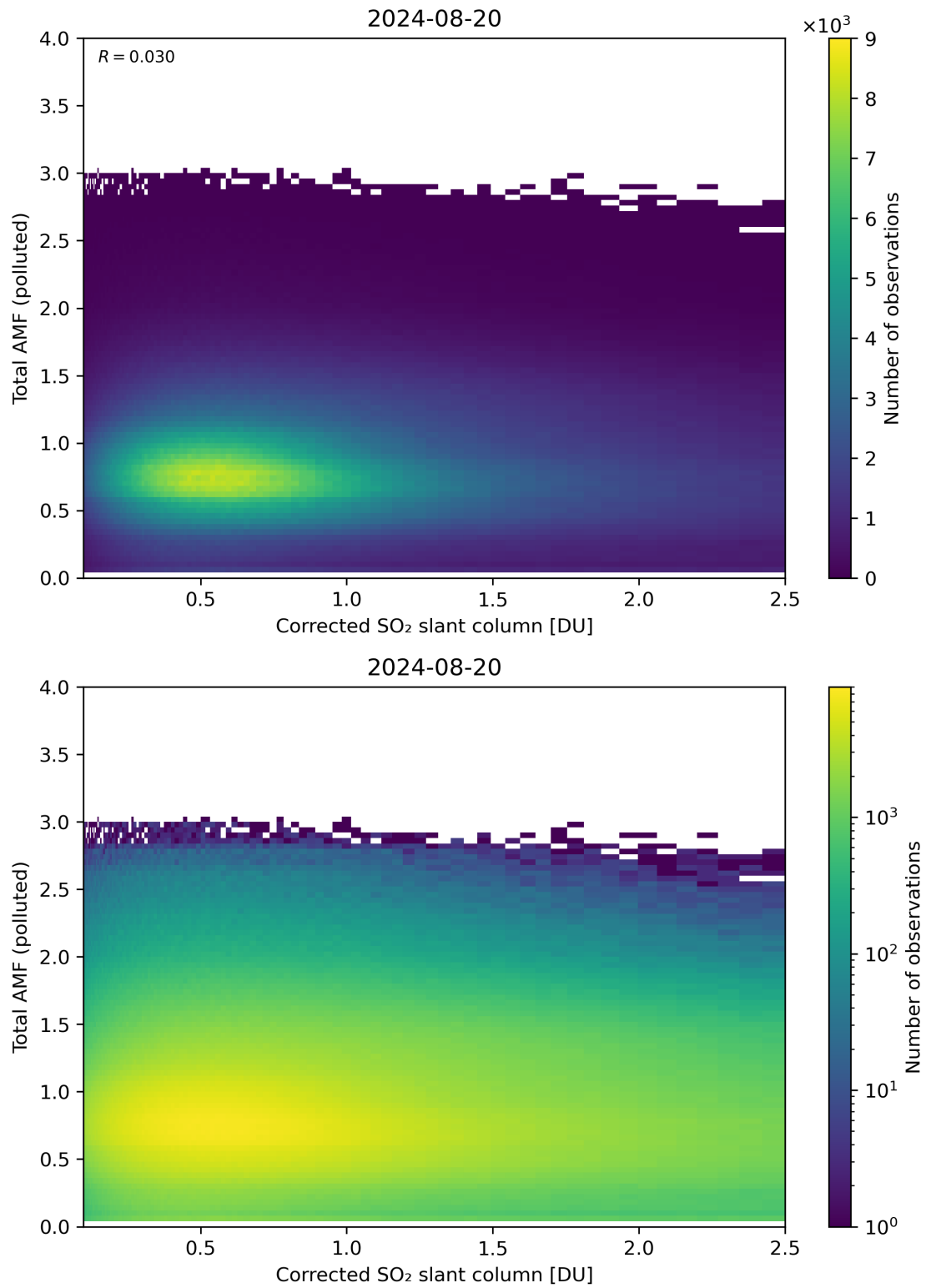
Figure 192: Scatter density plot of “Corrected SO 2 slant column” against “Total AMF (polluted)” for 2024-08-19 to 2024-08-21.
