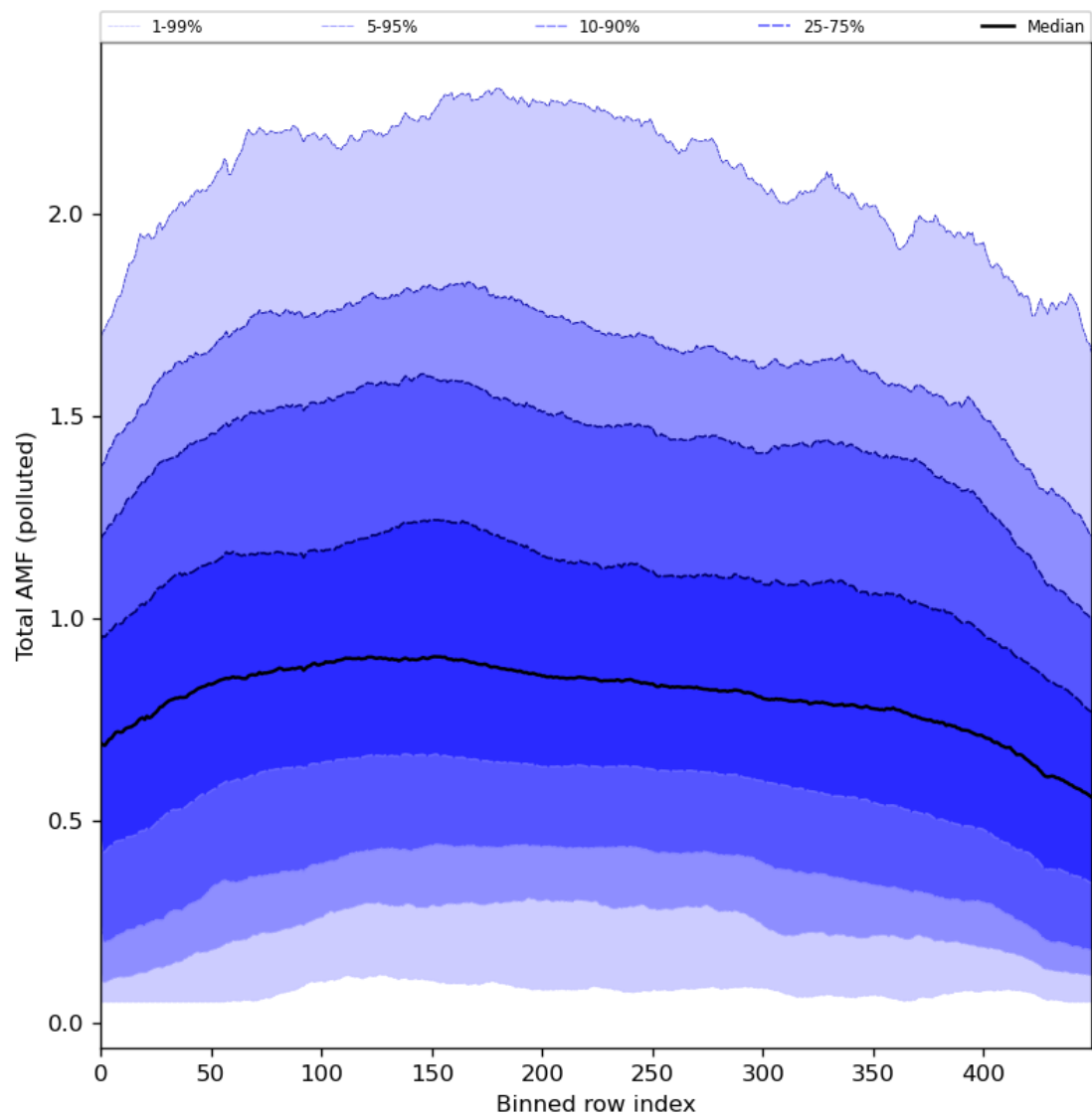
Figure 94: Along track statistics of “Total AMF (polluted)” for 2024-08-19 to 2024-08-21
