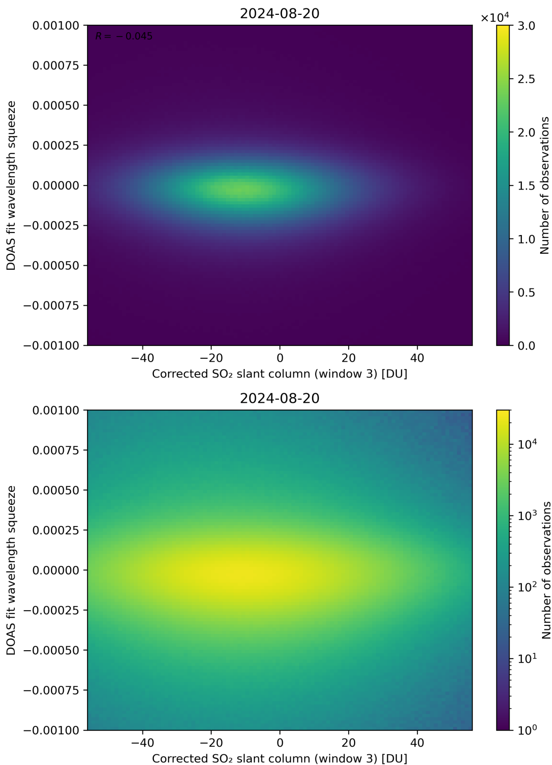
Figure 207: Scatter density plot of “Corrected SO 2 slant column (window 3)” against “DOAS fit wavelength squeeze” for 2024-08-19 to 2024-08-21.
