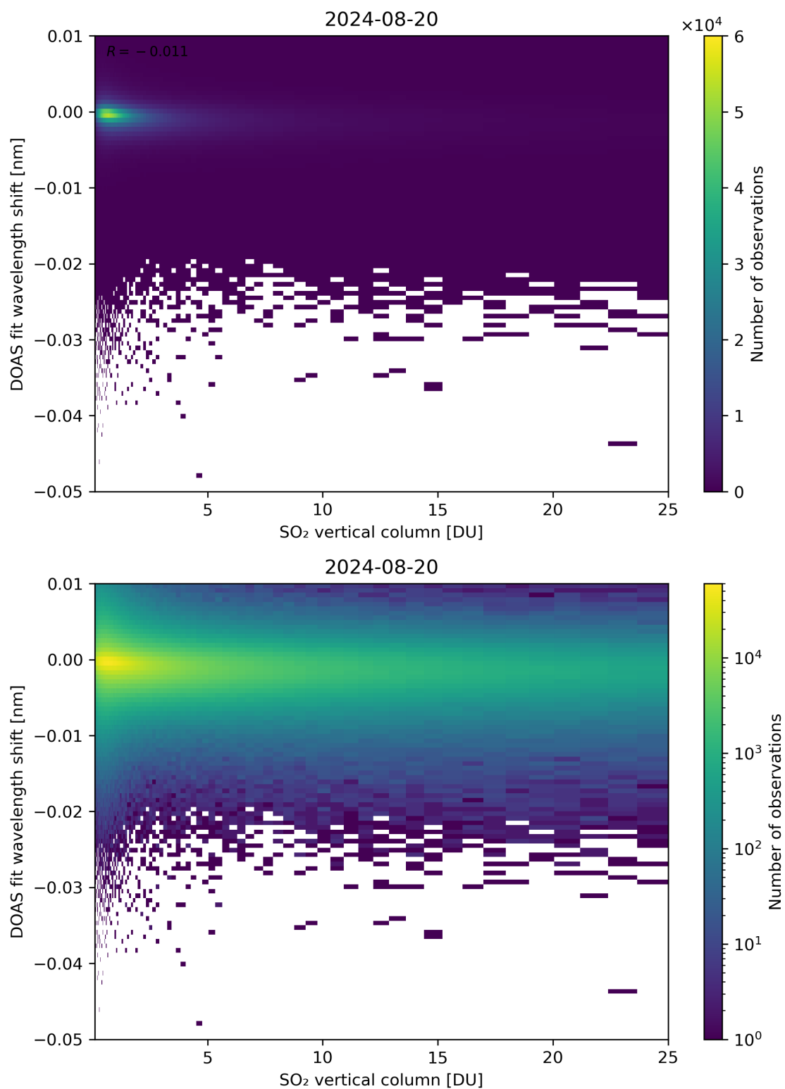
Figure 276: Scatter density plot of “SO 2 vertical column” against “DOAS fit wavelength shift” for 2024-08-19 to 2024-08-21.
