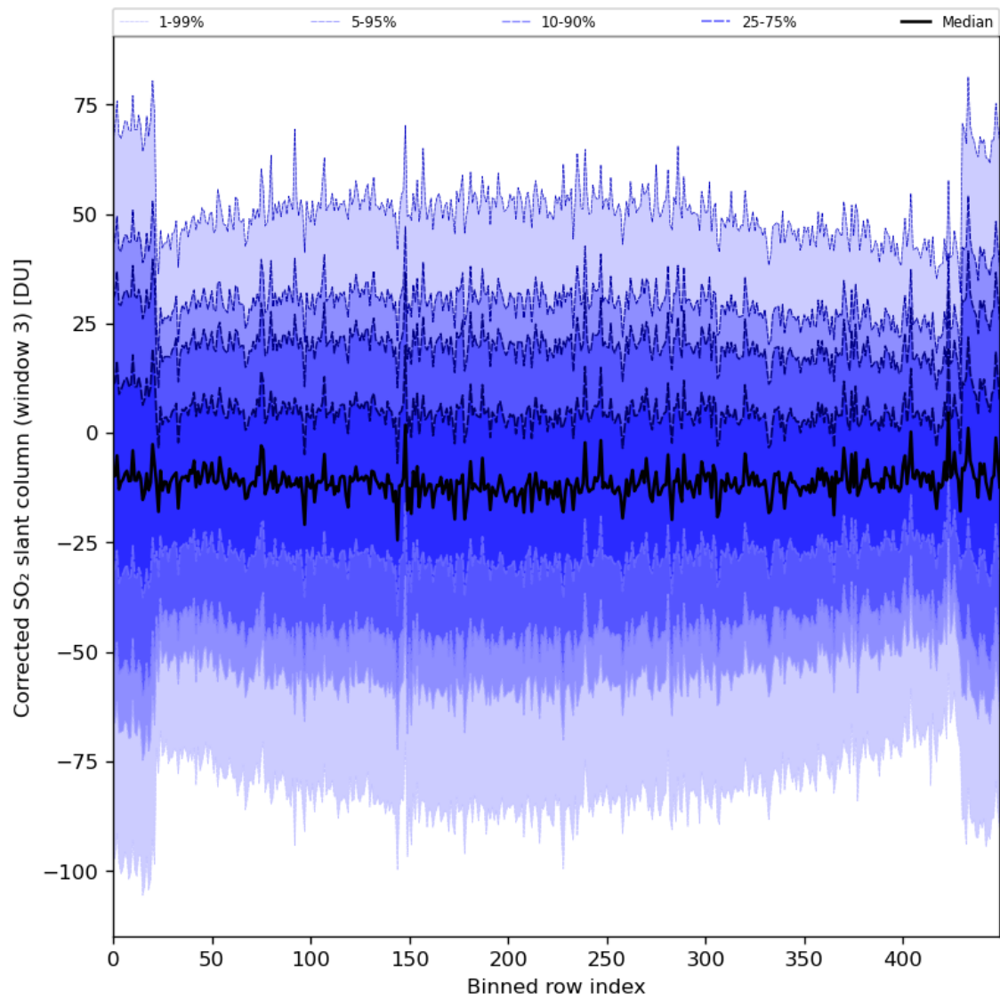
Figure 89: Along track statistics of “Corrected SO 2 slant column (window 3)” for 2024-08-19 to 2024-08-21
