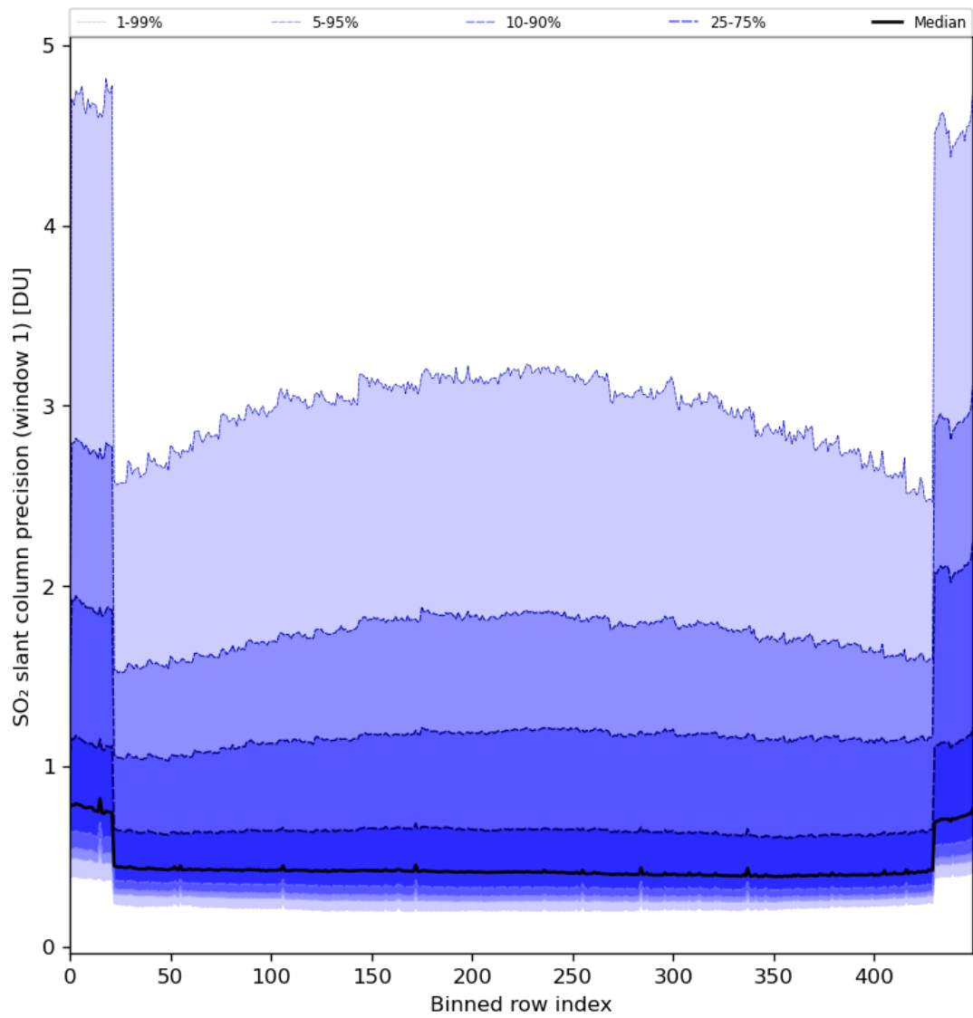
Figure 80: Along track statistics of “SO 2 slant column precision (window 1)” for 2024-08-19 to 2024-08-21
