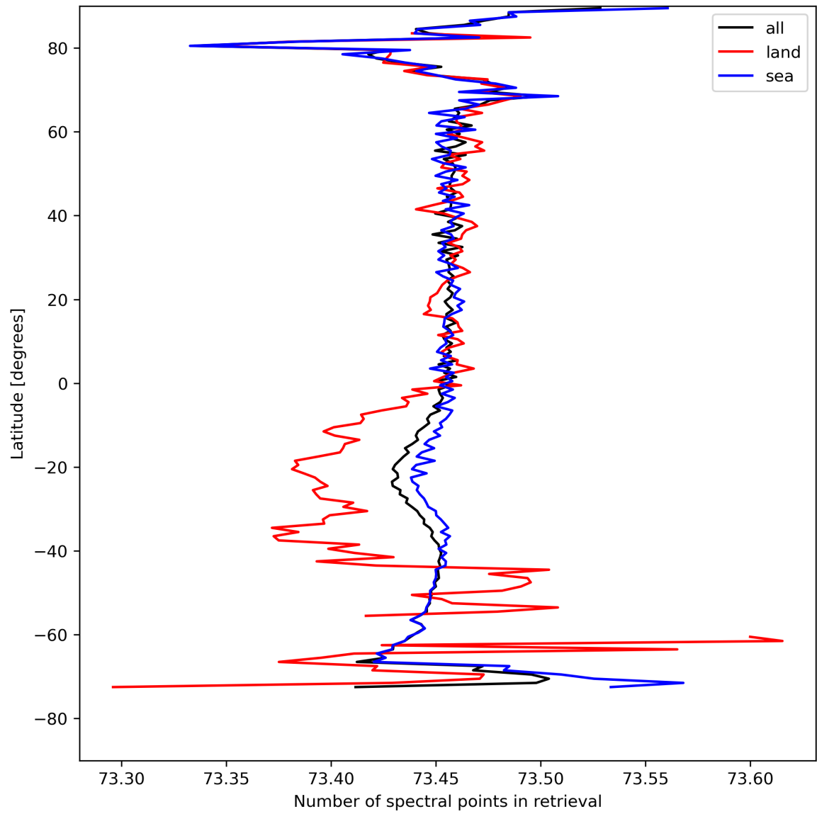
Figure 51: Zonal average of “Number of spectral points in retrieval” for 2024-08-19 to 2024-08-21.
