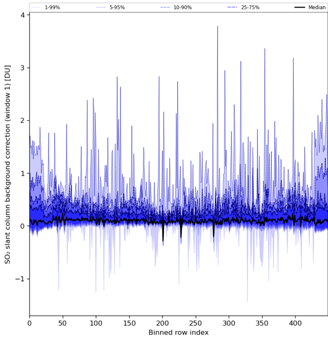
Figure 82: Along track statistics of “SO 2 slant column background correction (window 1)” for 2024-08-19 to 2024-08-21
