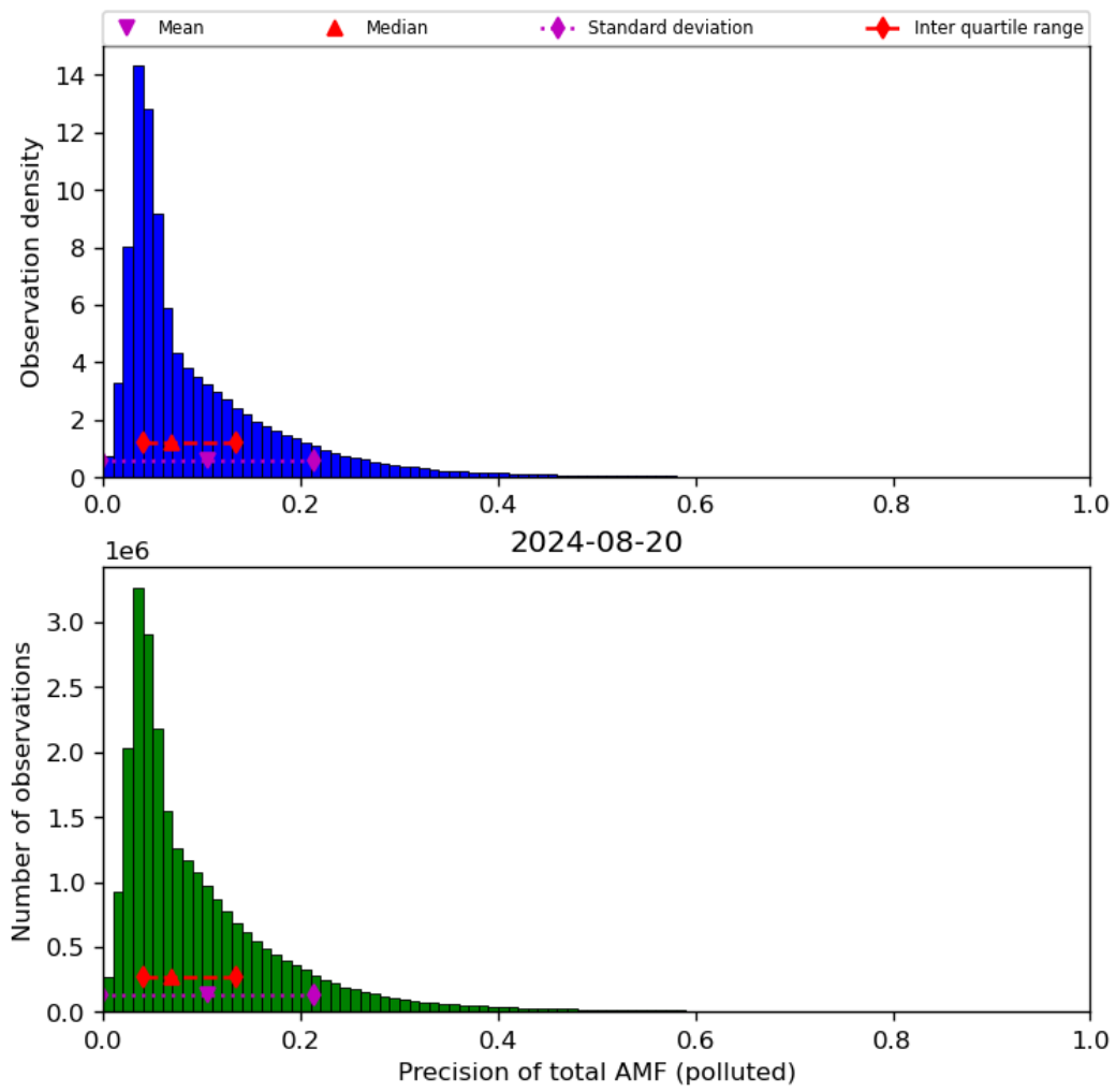
Figure 72: Histogram of “Precision of total AMF (polluted)” for 2024-08-19 to 2024-08-21
