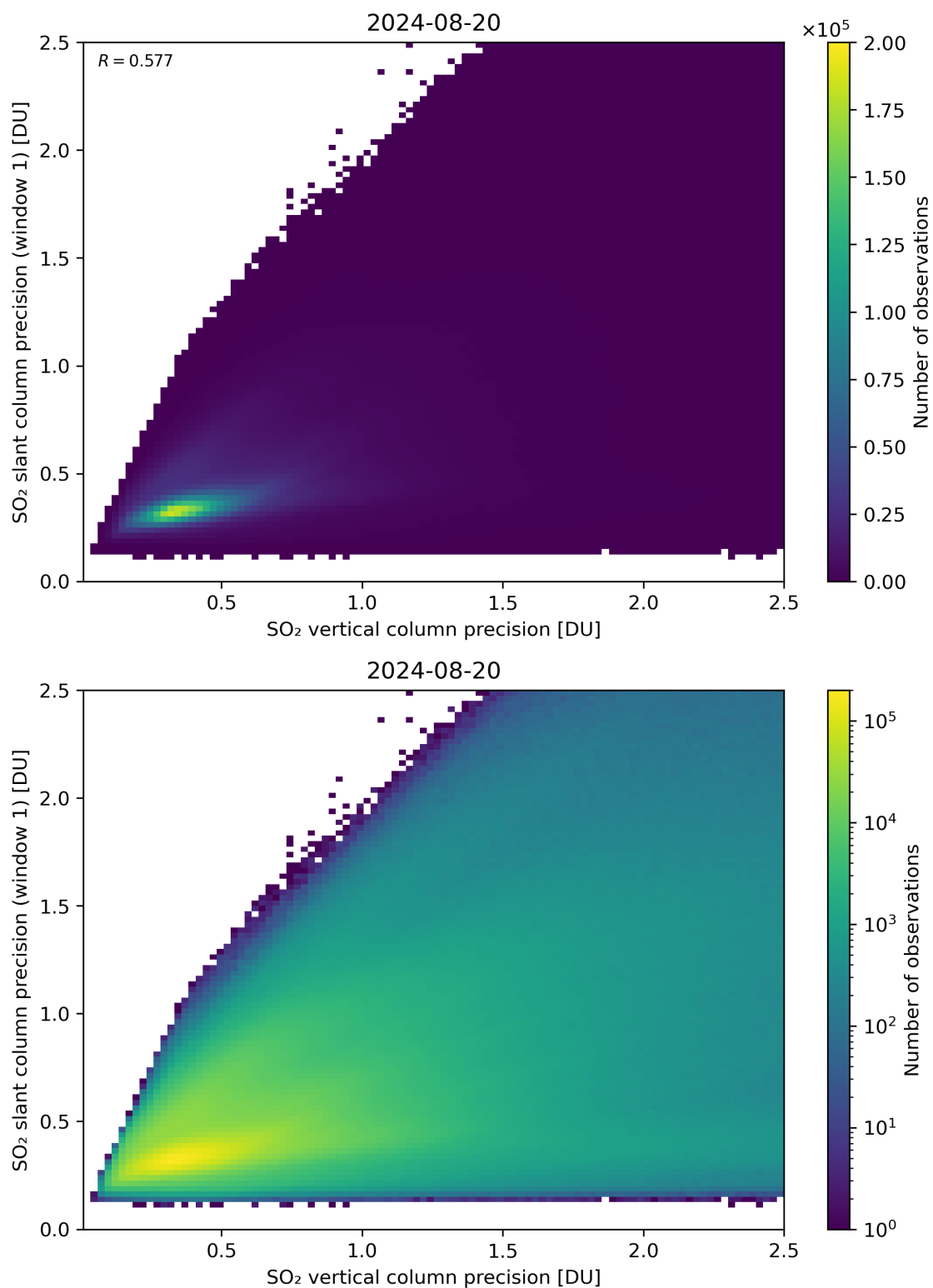
Figure 290: Scatter density plot of “SO 2 vertical column precision” against “SO 2 slant column precision (window 1)” for 2024-08-19 to 2024-08-21.
