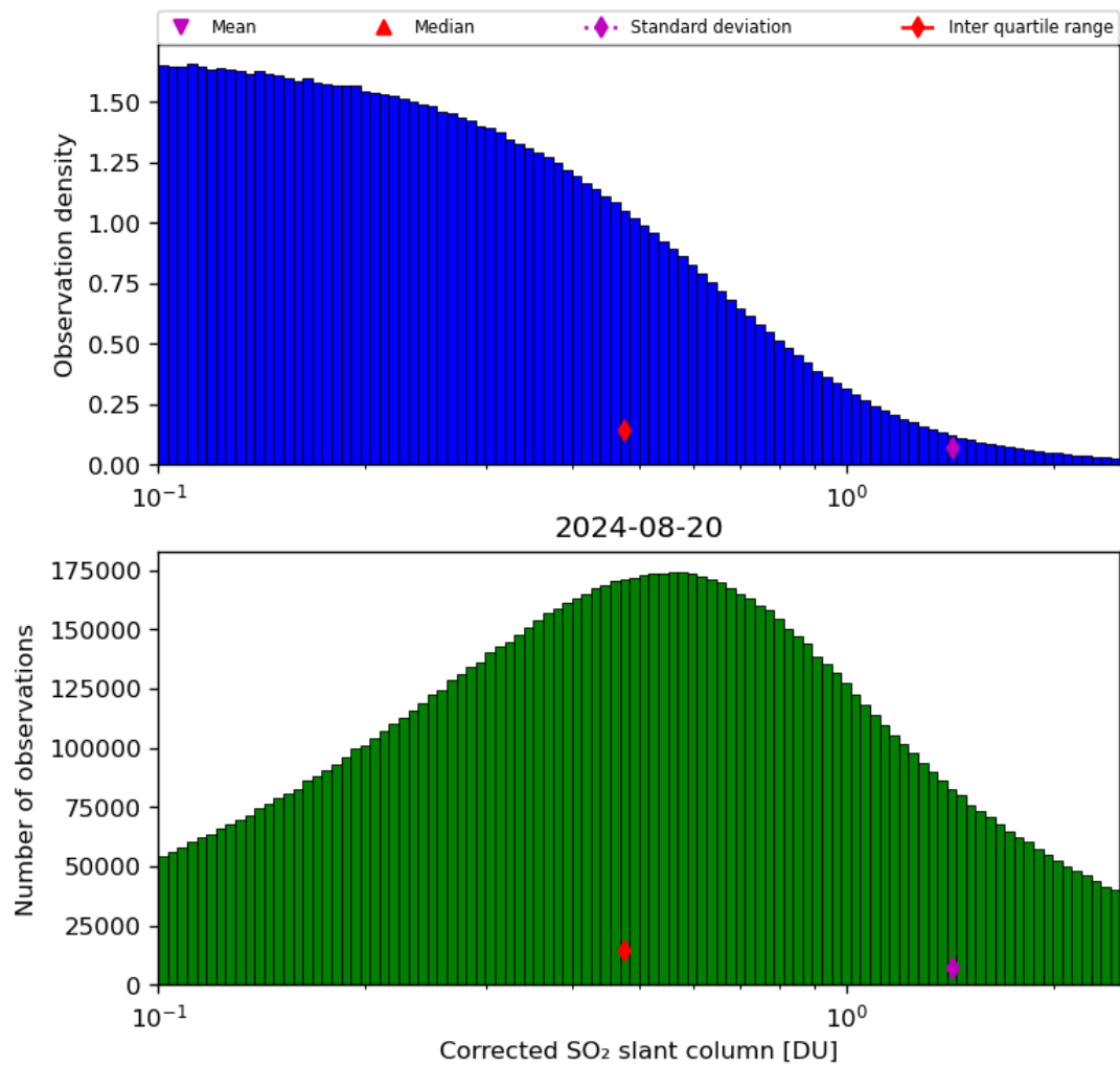
Figure 55: Histogram of “Corrected SO 2 slant column” for 2024-08-19 to 2024-08-21
