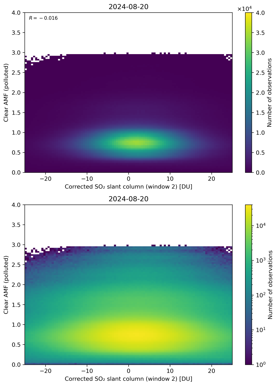
Figure 199: Scatter density plot of “Corrected SO 2 slant column (window 2)” against “Clear AMF (polluted)” for 2024-08-19 to 2024-08-21.
