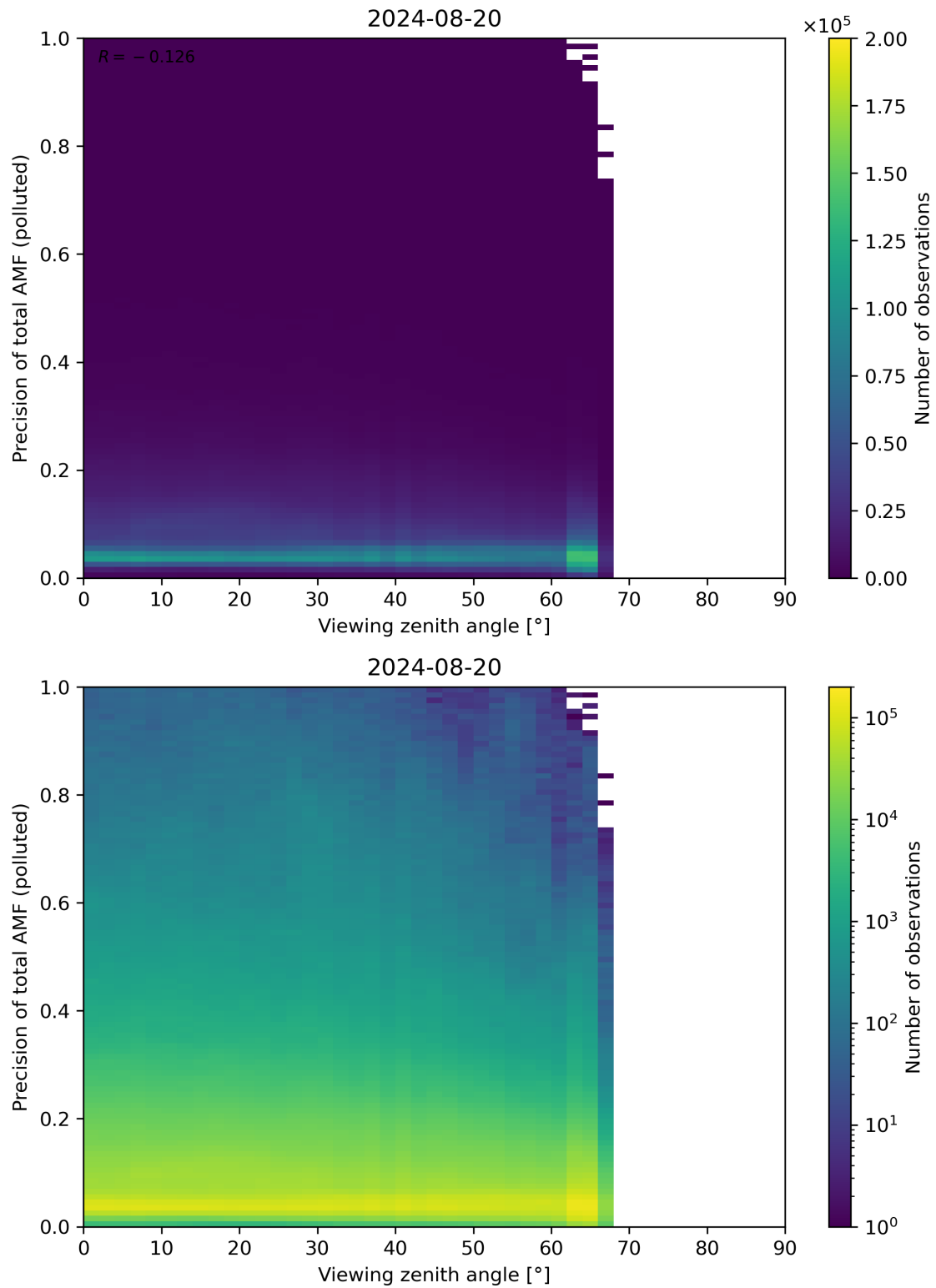
Figure 326: Scatter density plot of “Viewing zenith angle” against “Precision of total AMF (polluted)” for 2024-08-19 to 2024-08-21.
