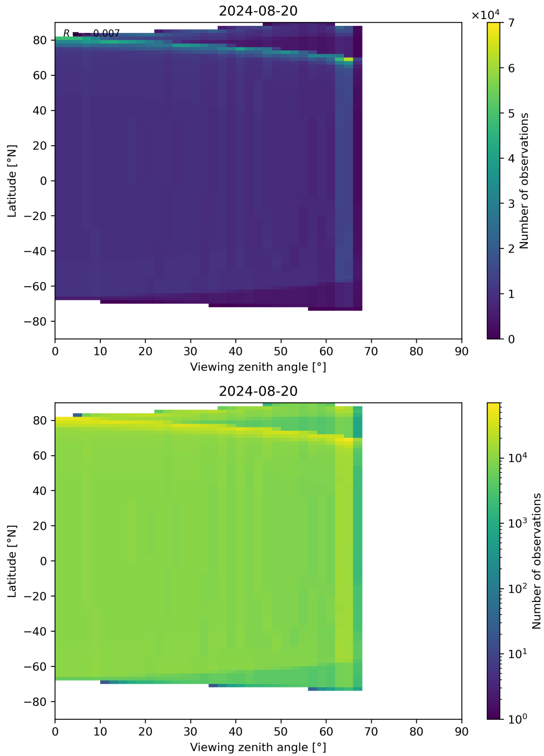
Figure 314: Scatter density plot of “Viewing zenith angle” against “Latitude” for 2024-08-19 to 2024-08-21.
