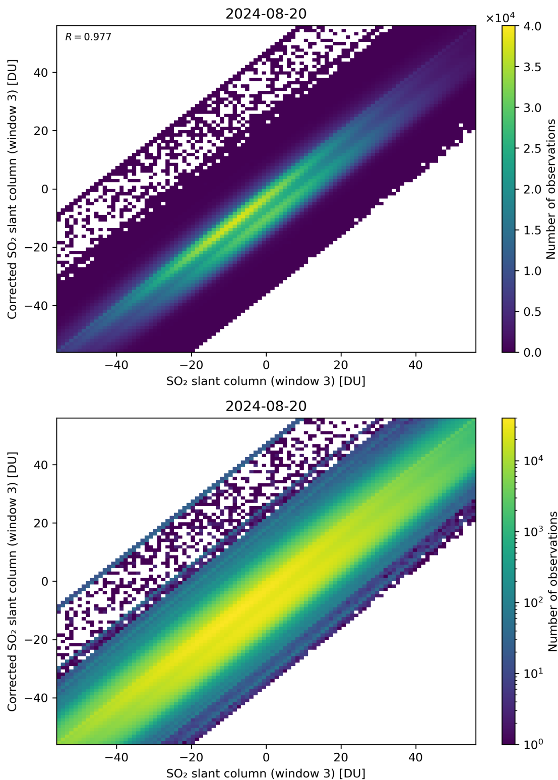
Figure 266: Scatter density plot of “SO 2 slant column (window 3)” against “Corrected SO 2 slant column (window 3)” for 2024-08-19 to 2024-08-21.
