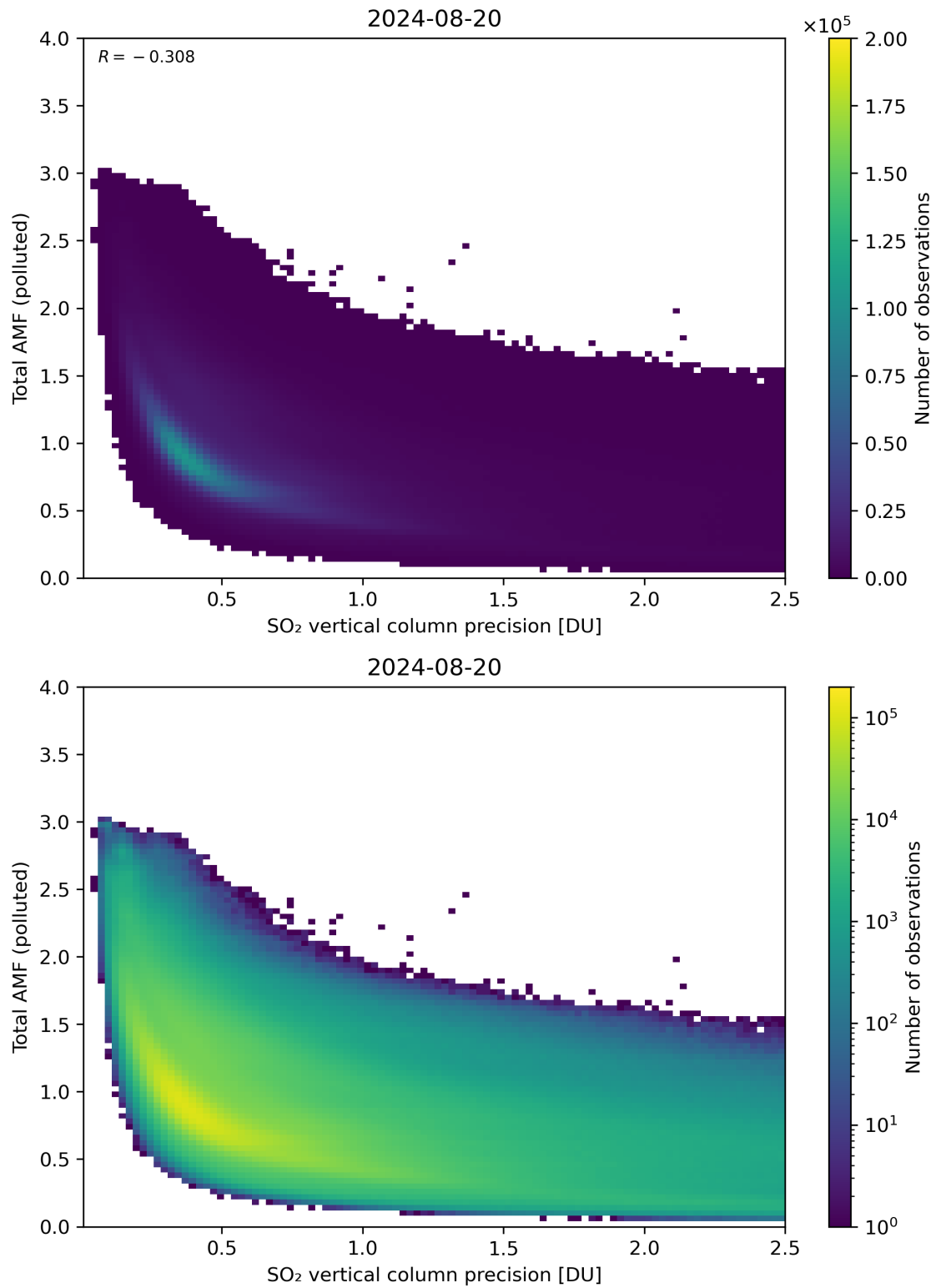
Figure 294: Scatter density plot of “SO 2 vertical column precision” against “Total AMF (polluted)” for 2024-08-19 to 2024-08-21.
