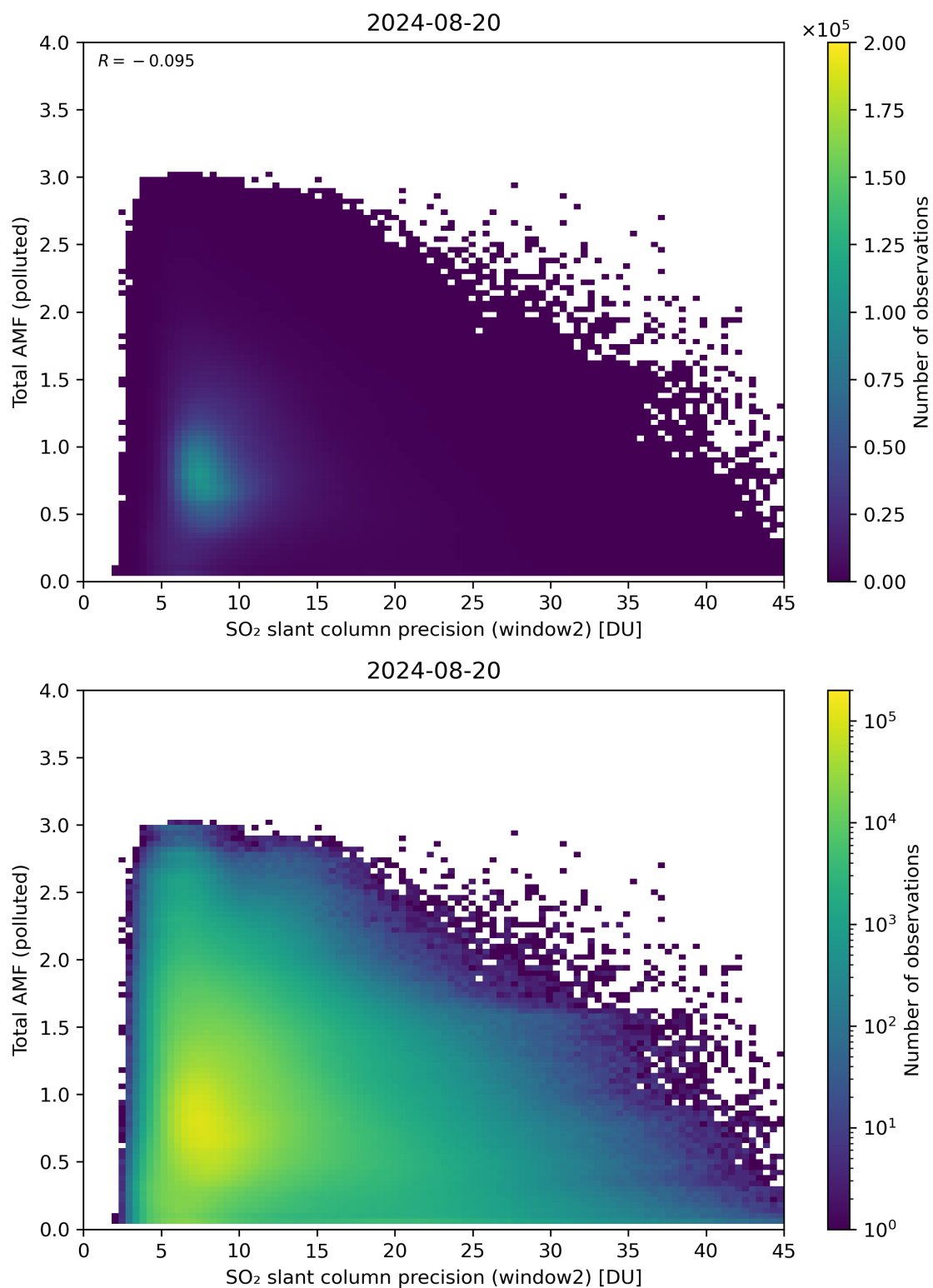
Figure 251: Scatter density plot of “SO 2 slant column precision (window2)” against “Total AMF (polluted)” for 2024-08-19 to 2024-08-21.
