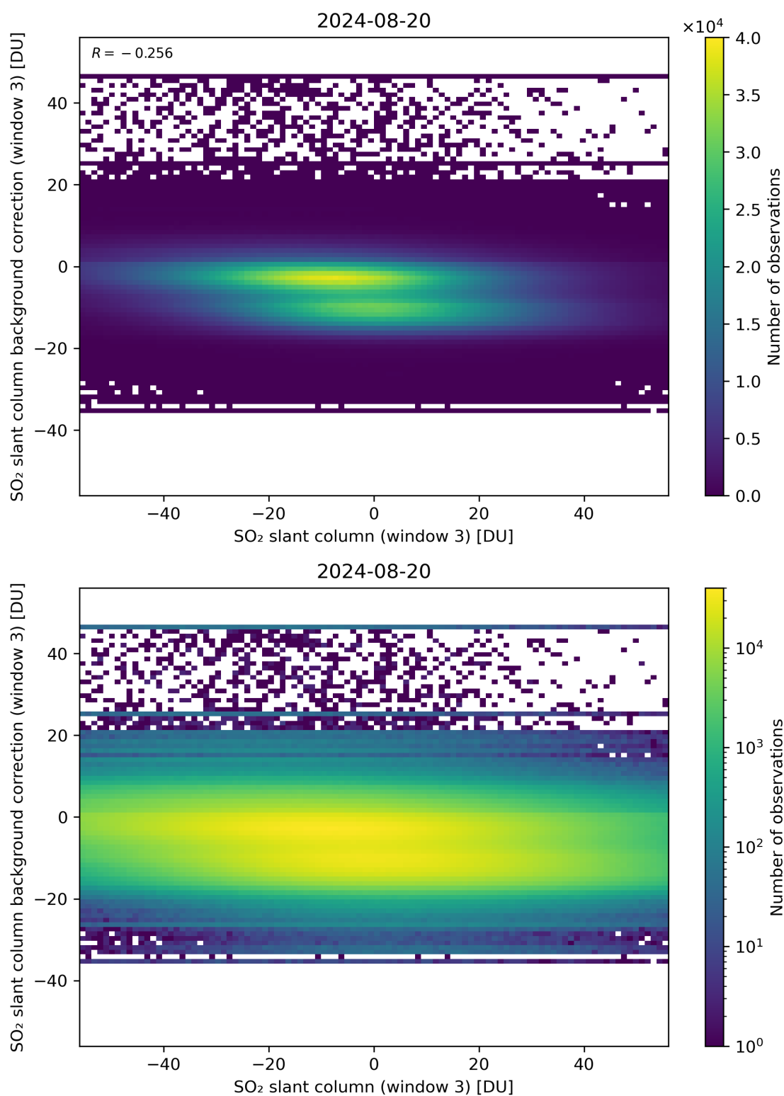
Figure 253: Scatter density plot of “SO 2 slant column (window 3)” against “SO 2 slant column background correction (window 3)” for 2024-08-19 to 2024-08-21.
