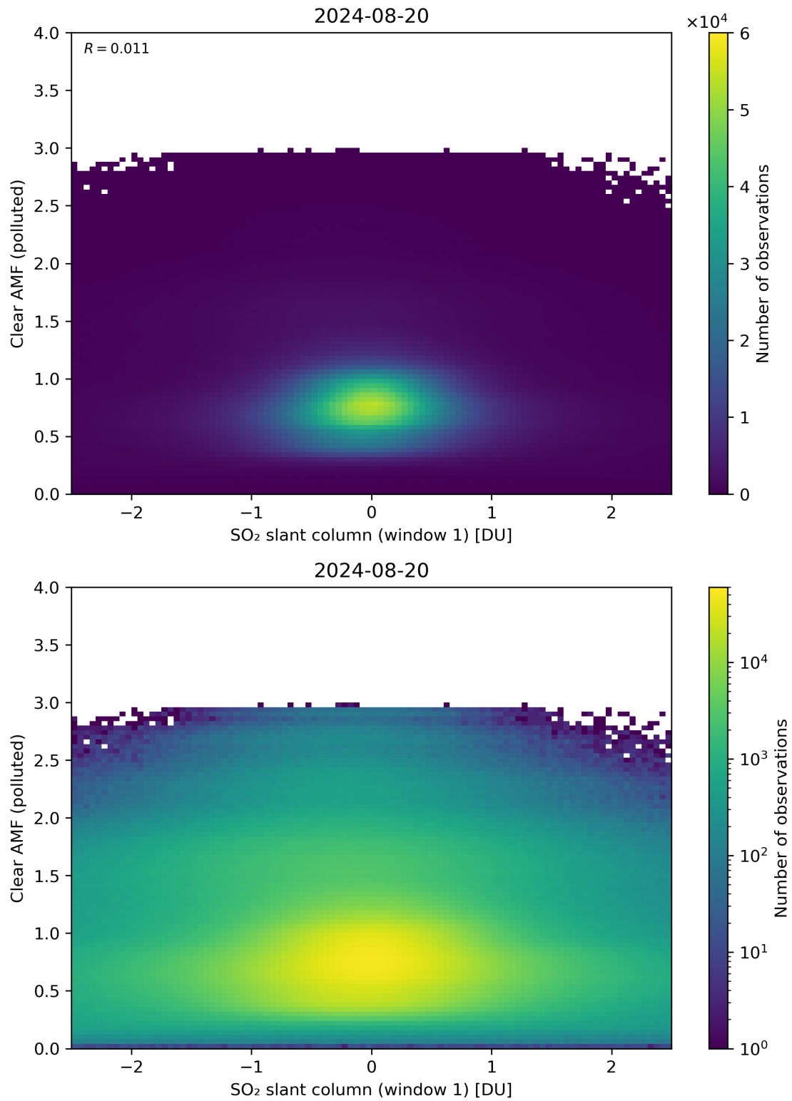
Figure 232: Scatter density plot of “SO 2 slant column (window 1)” against “Clear AMF (polluted)” for 2024-08-19 to 2024-08-21.
