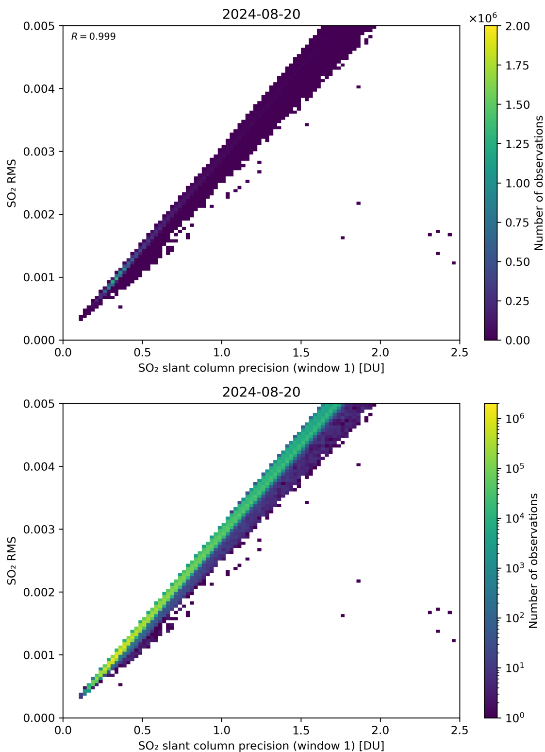
Figure 223: Scatter density plot of “SO 2 slant column precision (window 1)” against “SO 2 RMS” for 2024-08-19 to 2024-08-21.
