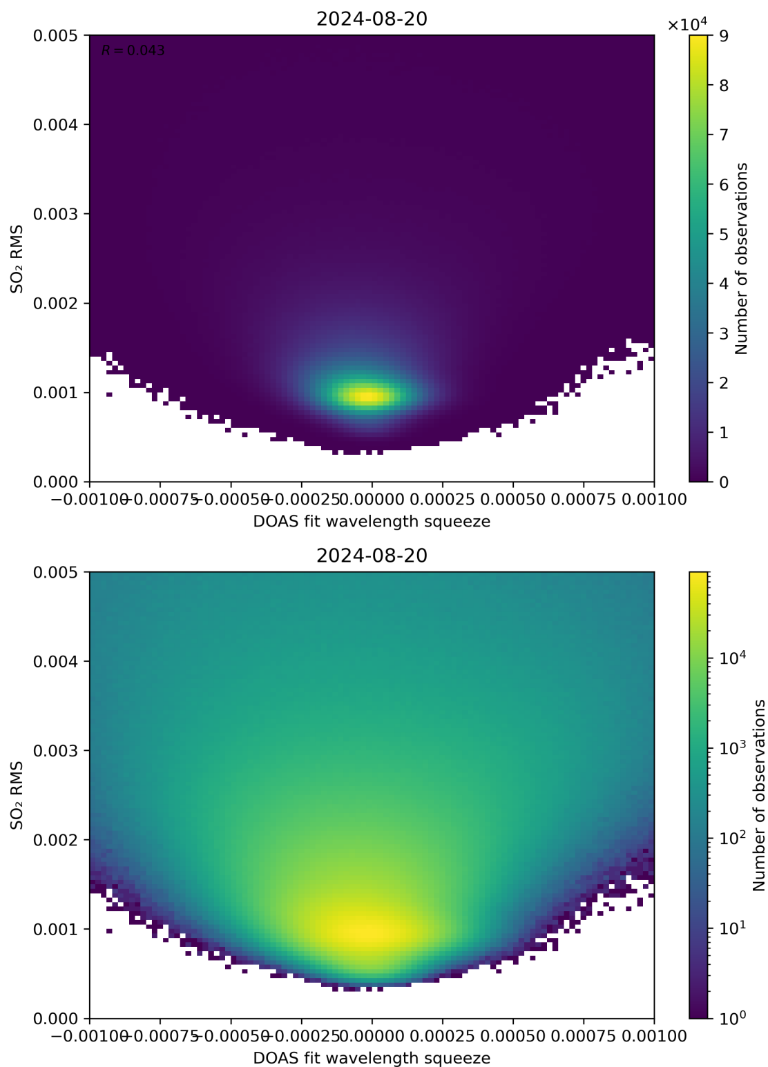
Figure 132: Scatter density plot of “DOAS fit wavelength squeeze” against “SO 2 RMS” for 2024-08-19 to 2024-08-21.
