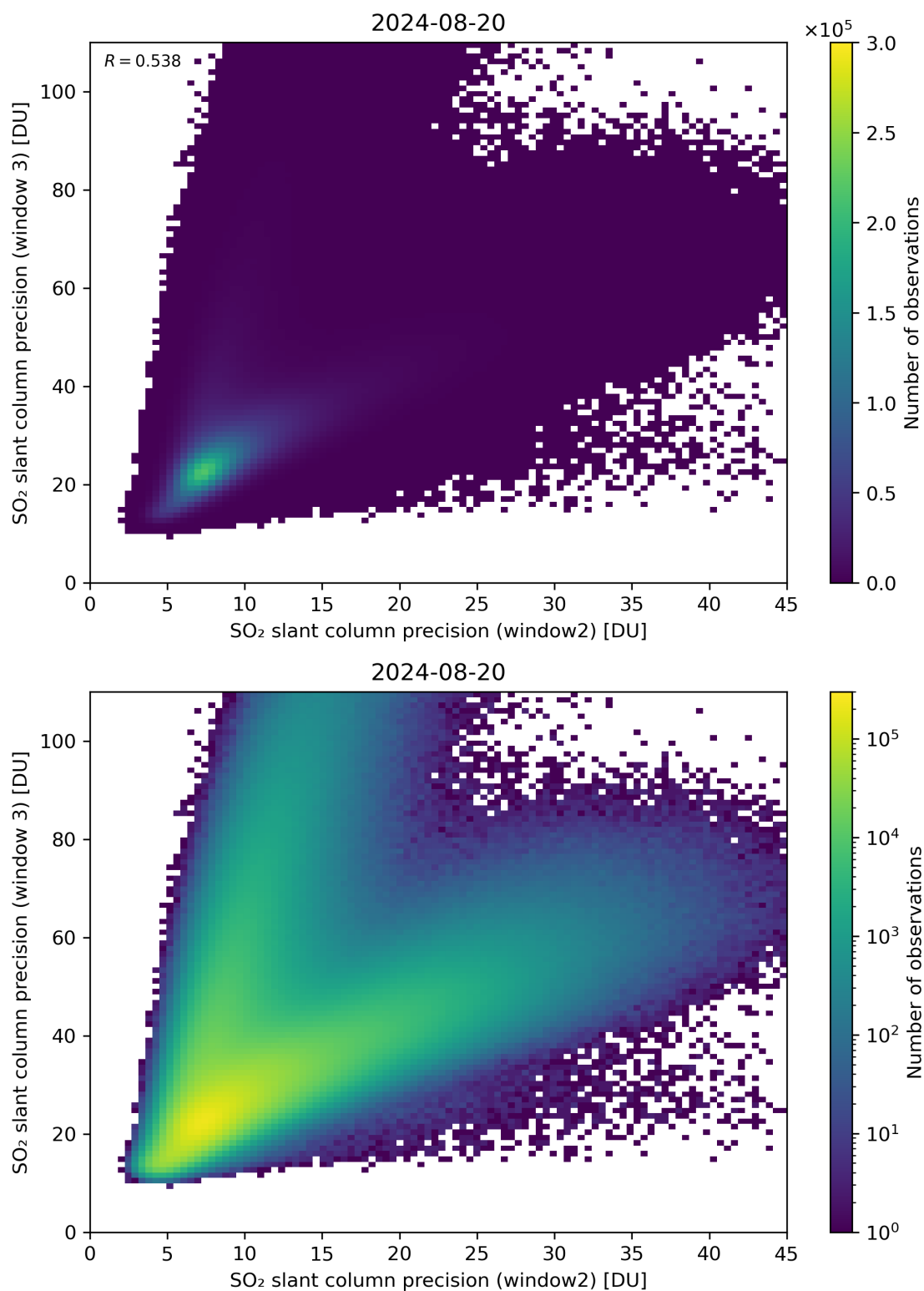
Figure 250: Scatter density plot of “SO 2 slant column precision (window2)” against “SO 2 slant column precision (window 3)” for 2024-08-19 to 2024-08-21.
