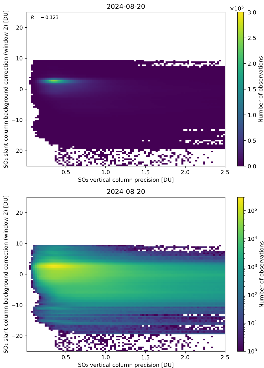
Figure 280: Scatter density plot of “SO 2 vertical column precision” against “SO 2 slant column background correction (window 2)” for 2024-08-19 to 2024-08-21.
