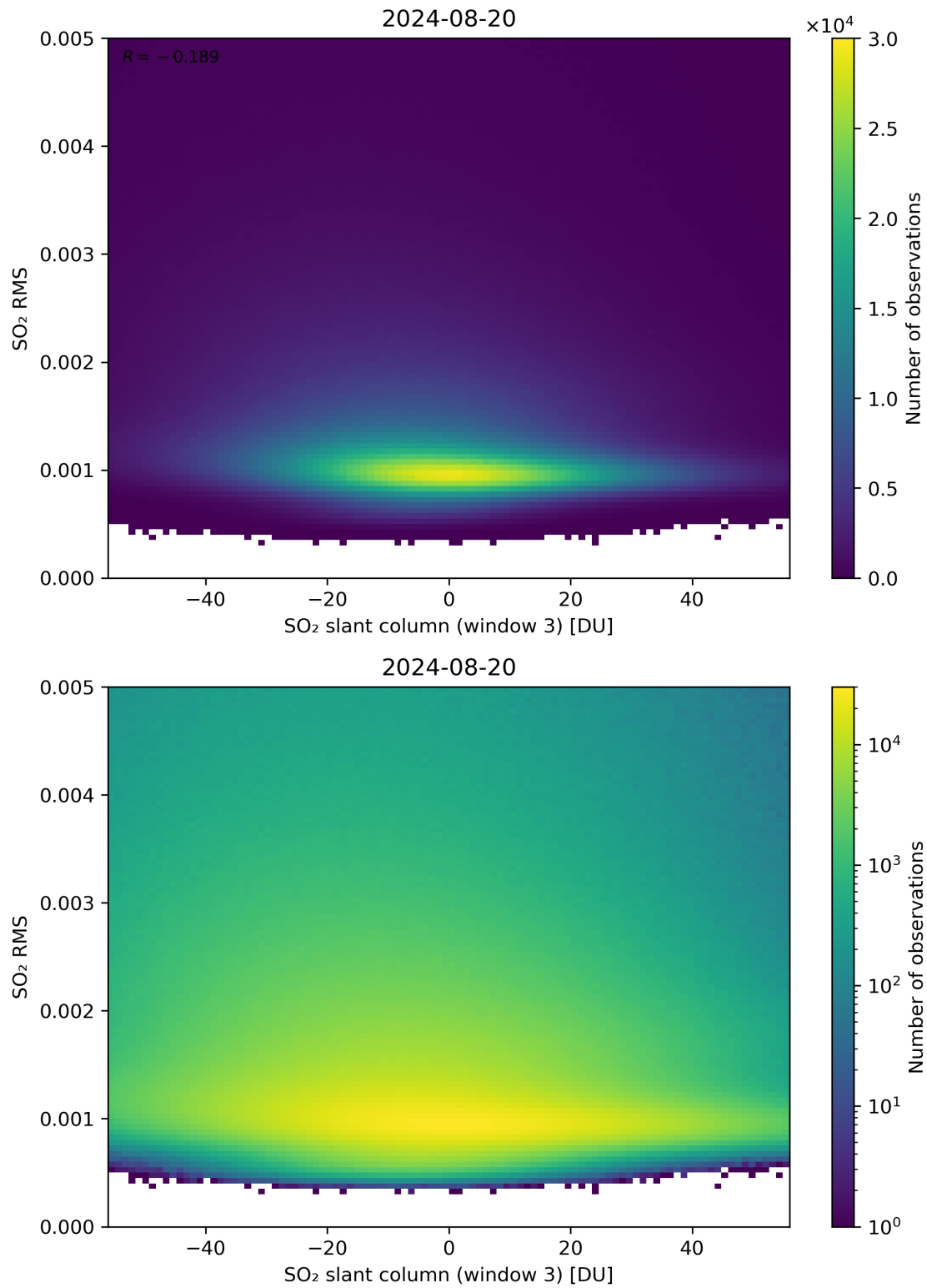
Figure 256: Scatter density plot of “SO 2 slant column (window 3)” against “SO 2 RMS” for 2024-08-19 to 2024-08-21.
