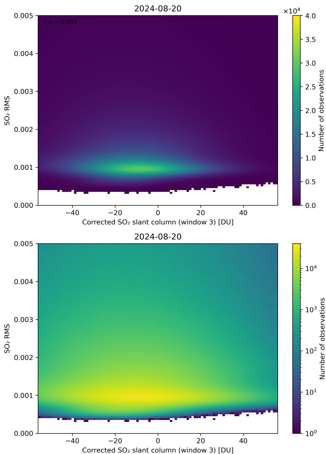
Figure 208: Scatter density plot of “Corrected SO 2 slant column (window 3)” against “SO 2 RMS” for 2024-08-19 to 2024-08-21.
