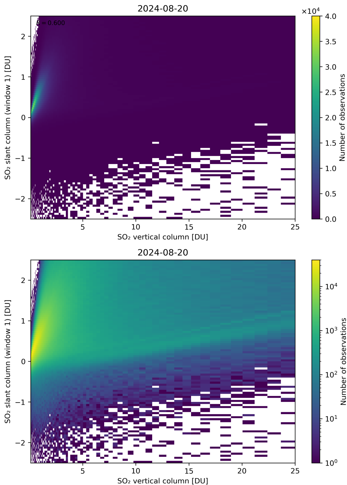
Figure 300: Scatter density plot of “SO 2 vertical column” against “SO 2 slant column (window 1)” for 2024-08-19 to 2024-08-21.
