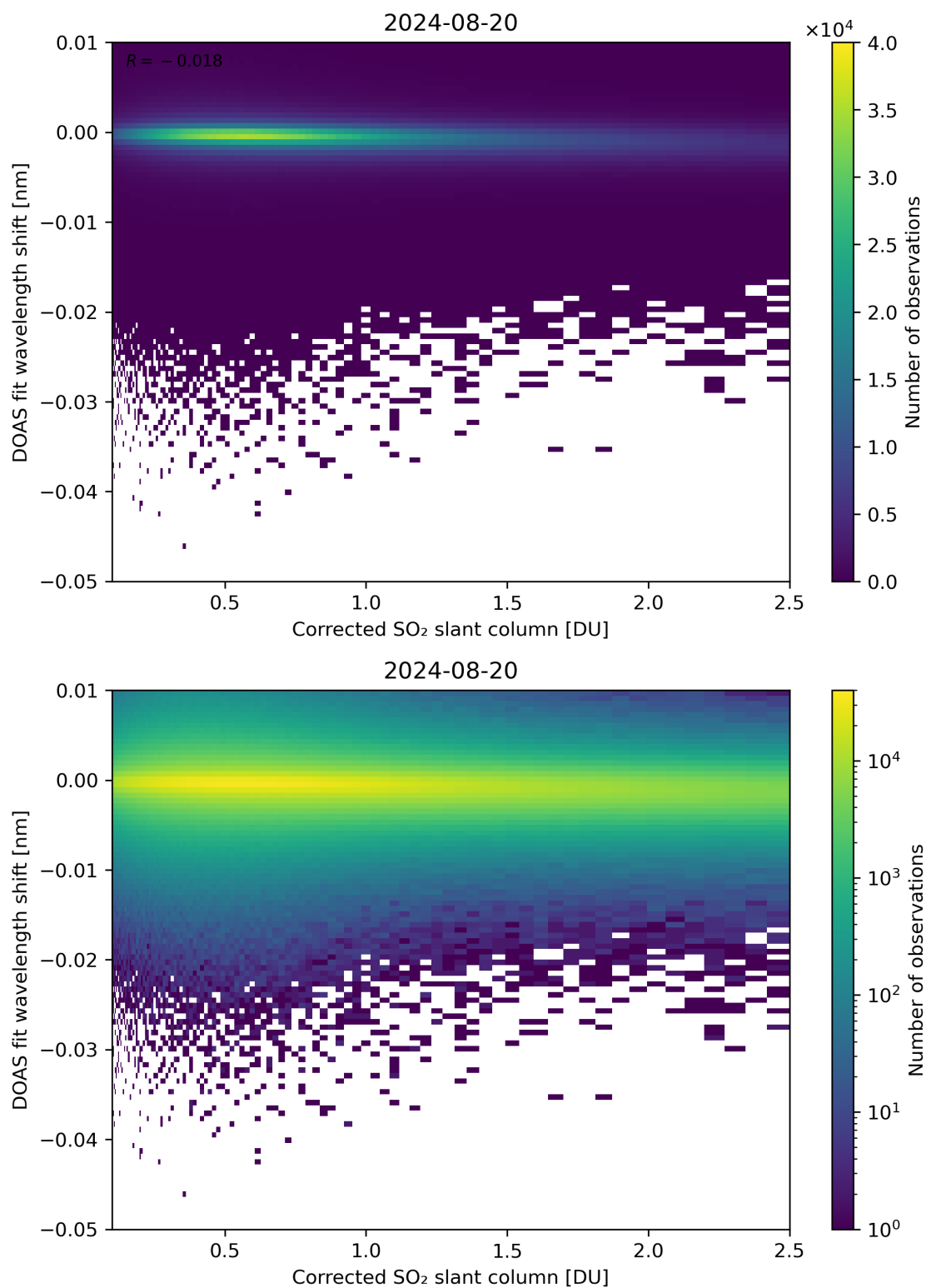
Figure 181: Scatter density plot of “Corrected SO 2 slant column” against “DOAS fit wavelength shift” for 2024-08-19 to 2024-08-21.
