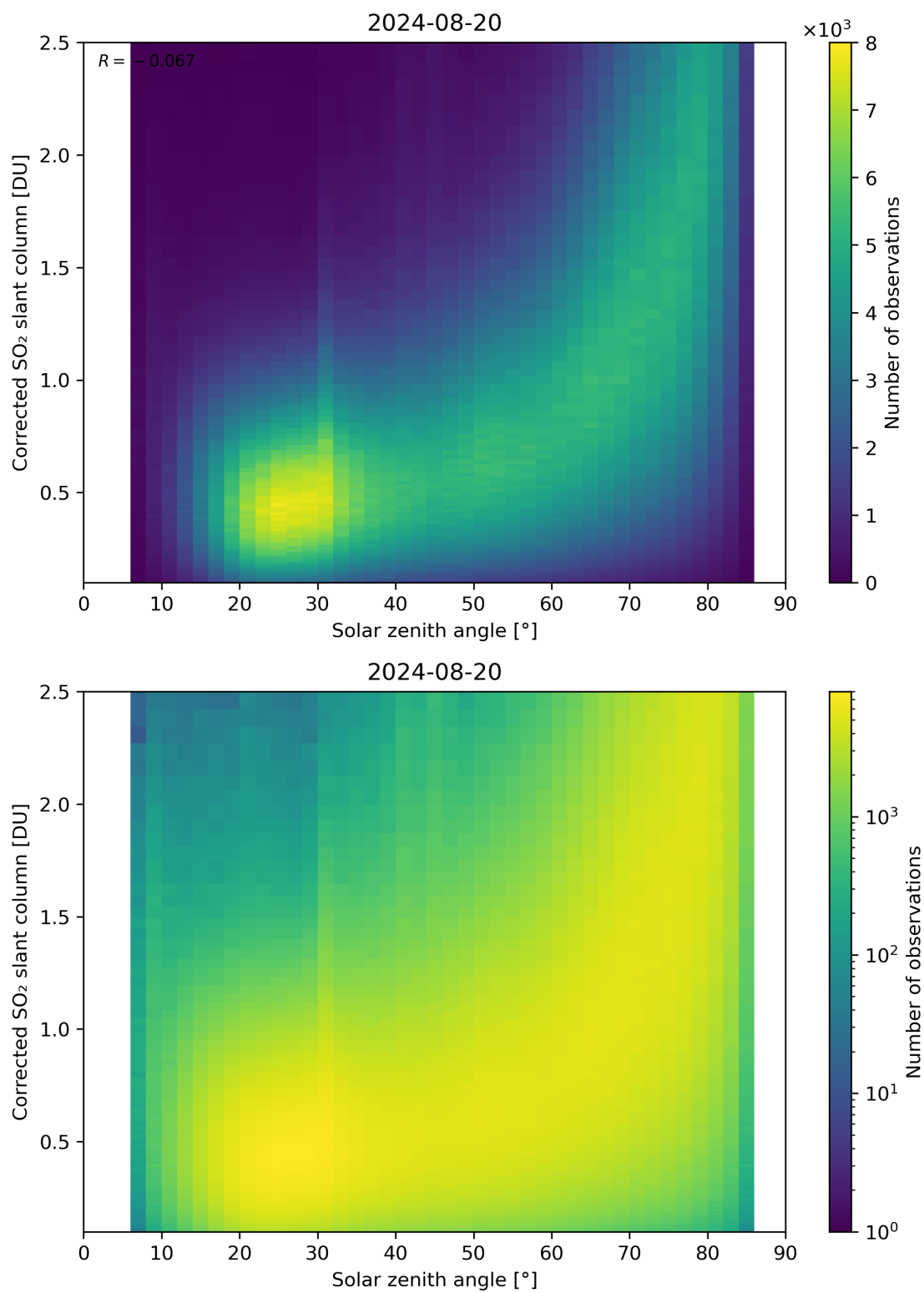
Figure 166: Scatter density plot of “Solar zenith angle” against “Corrected SO 2 slant column” for 2024-08-19 to 2024-08-21.
