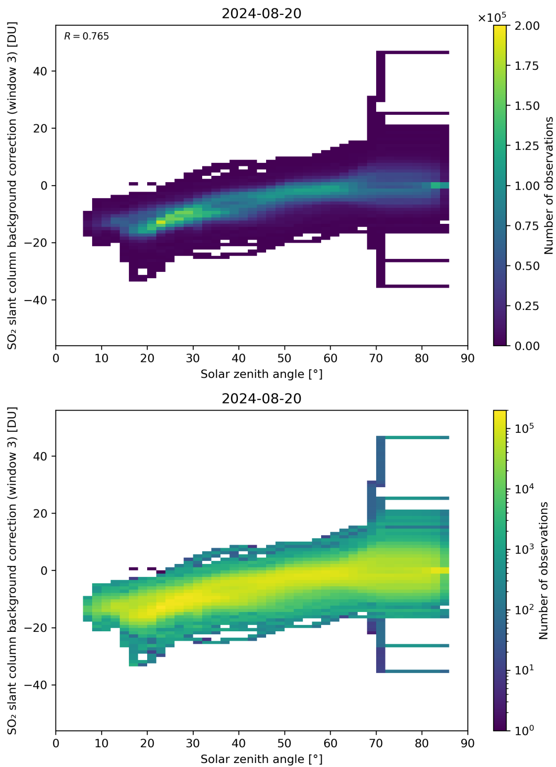
Figure 160: Scatter density plot of “Solar zenith angle” against “SO 2 slant column background correction (window 3)” for 2024-08-19 to 2024-08-21.
