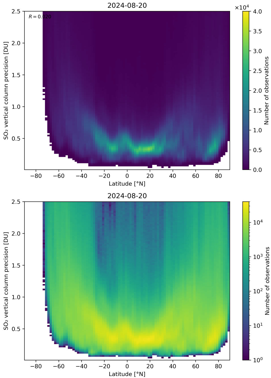
Figure 157: Scatter density plot of “Latitude” against “SO 2 vertical column precision” for 2024-08-19 to 2024-08-21.
