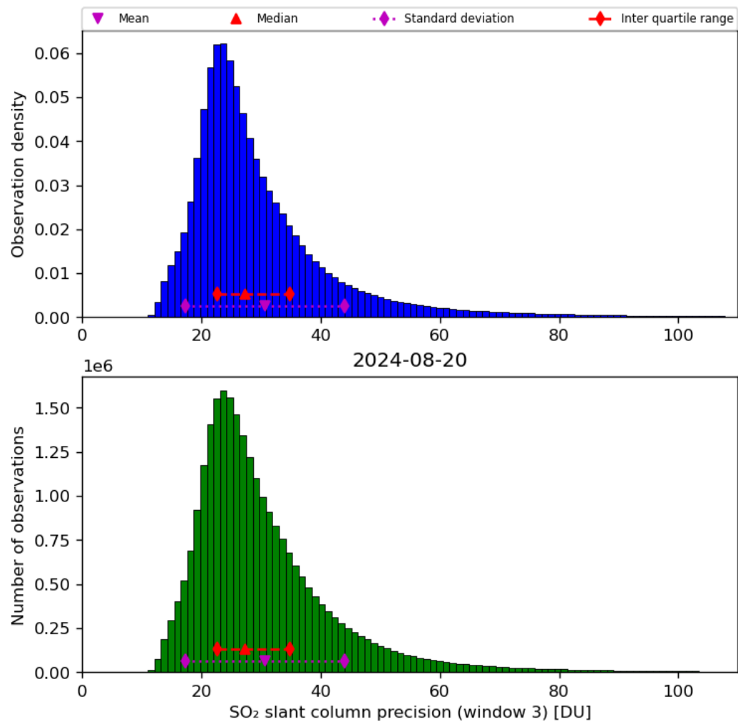
Figure 65: Histogram of “SO 2 slant column precision (window 3)” for 2024-08-19 to 2024-08-21
