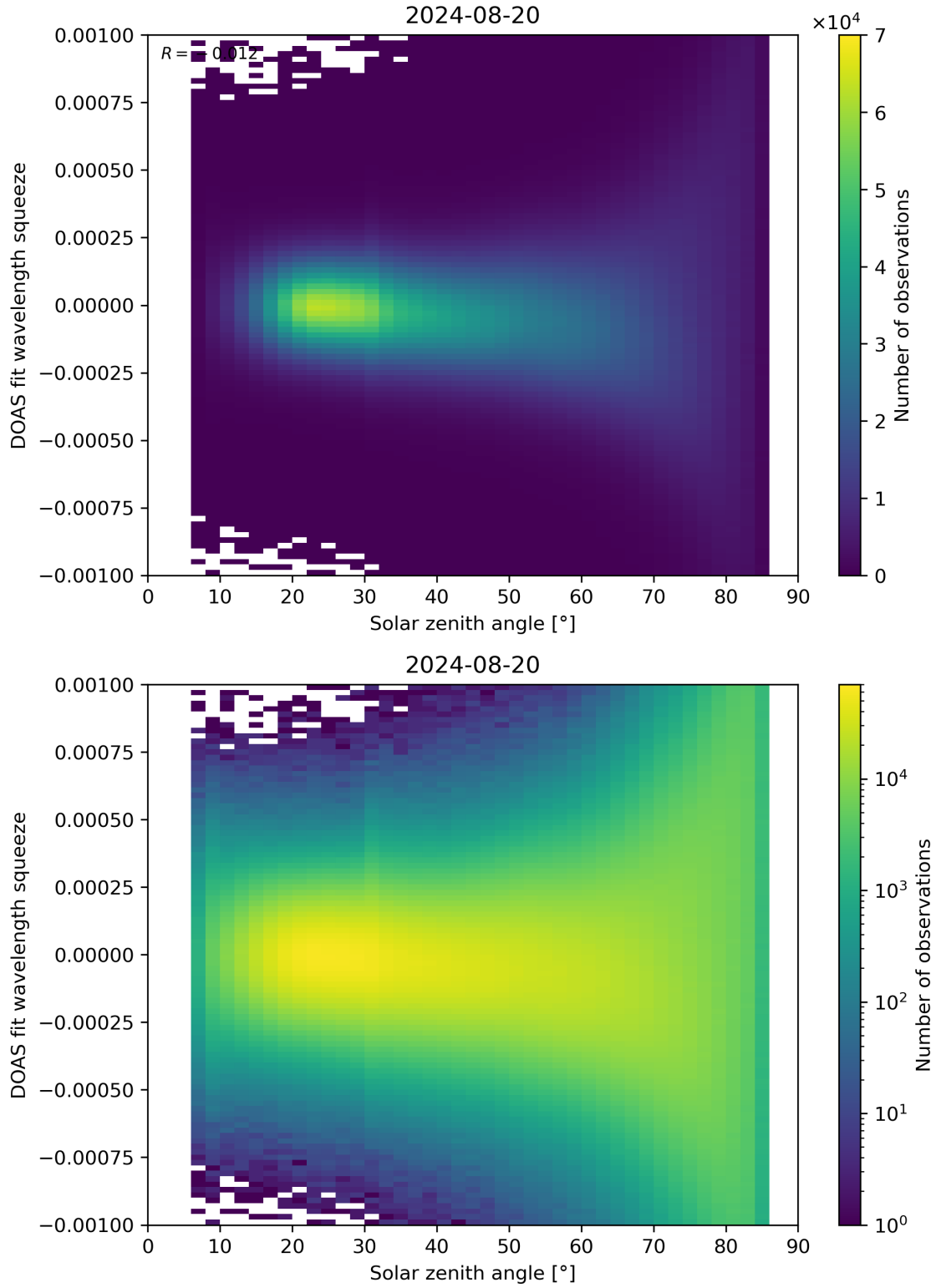
Figure 162: Scatter density plot of “Solar zenith angle” against “DOAS fit wavelength squeeze” for 2024-08-19 to 2024-08-21.
