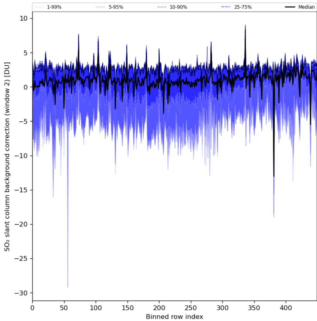
Figure 86: Along track statistics of “SO 2 slant column background correction (window 2)” for 2024-08-19 to 2024-08-21
