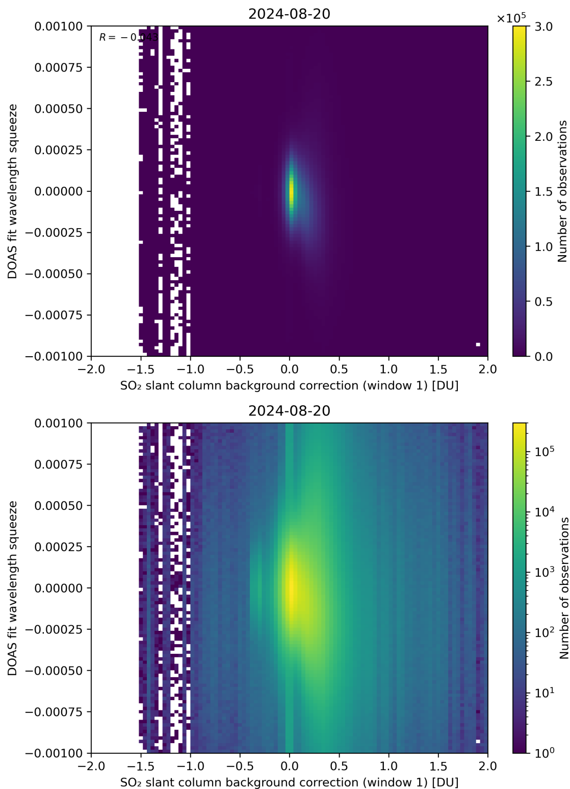
Figure 101: Scatter density plot of “SO 2 slant column background correction (window 1)” against “DOAS fit wavelength squeeze” for 2024-08-19 to 2024-08-21.
