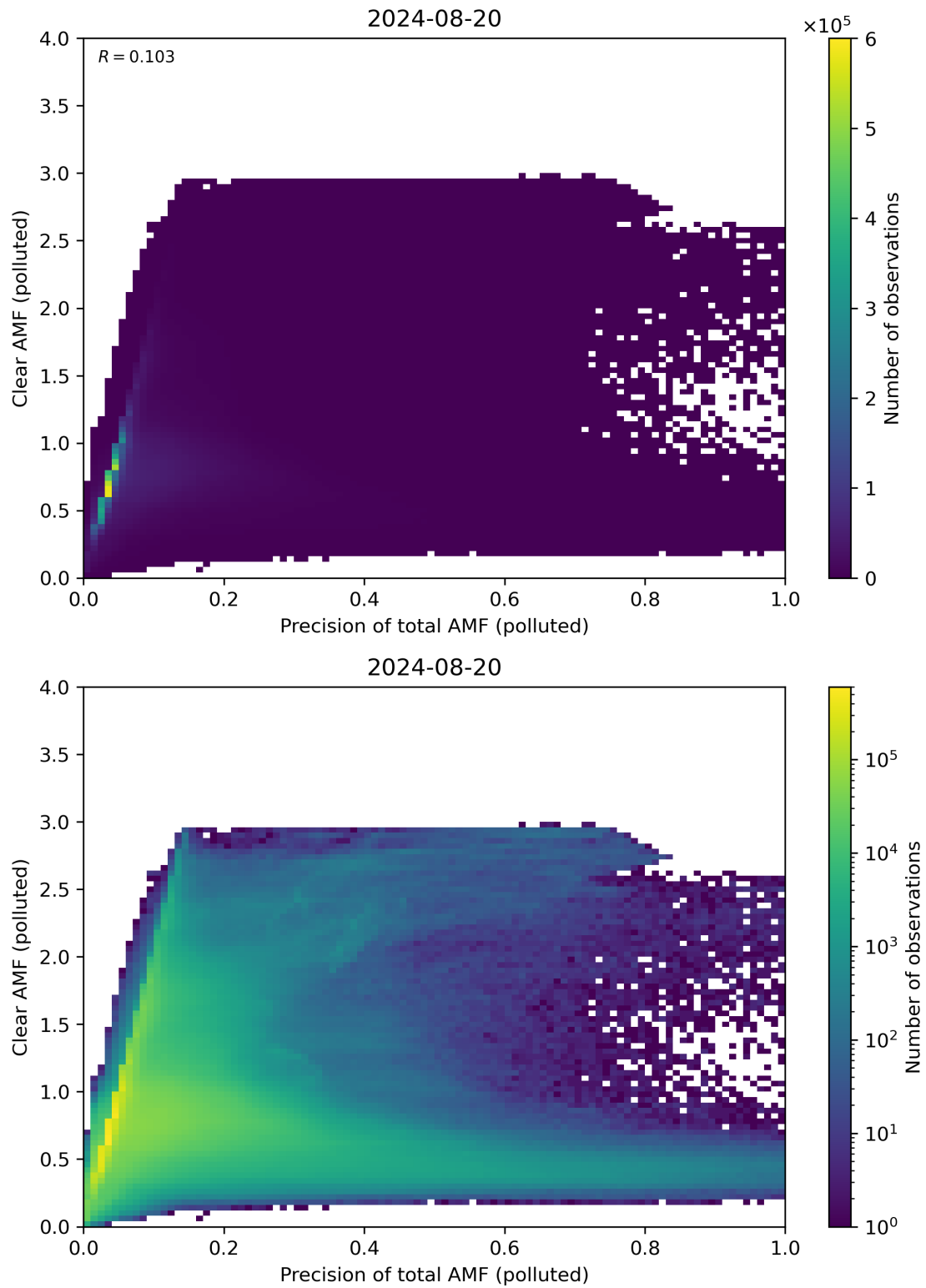
Figure 270: Scatter density plot of “Precision of total AMF (polluted)” against “Clear AMF (polluted)” for 2024-08-19 to 2024-08-21.
