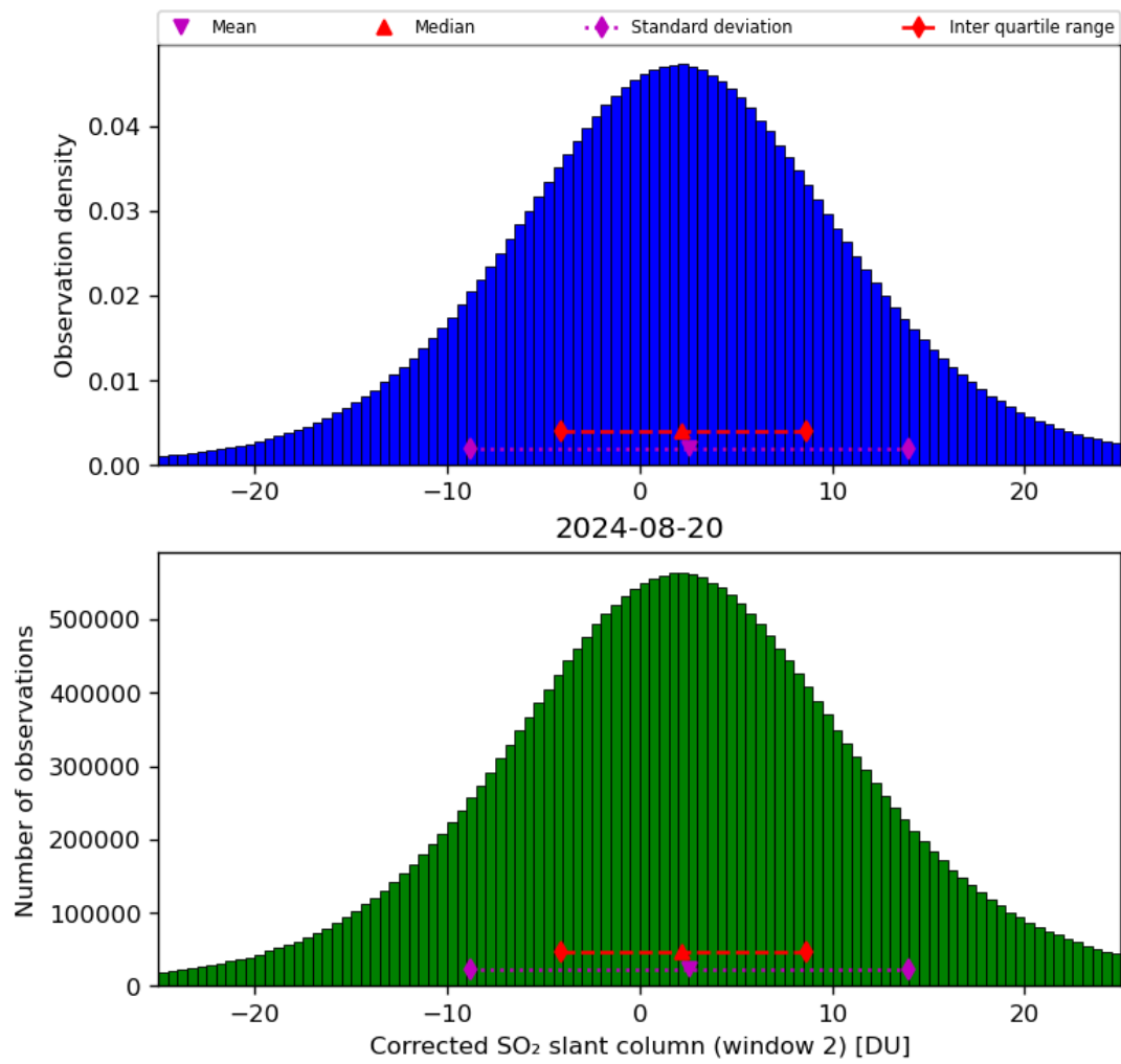
Figure 62: Histogram of “Corrected SO 2 slant column (window 2)” for 2024-08-19 to 2024-08-21
