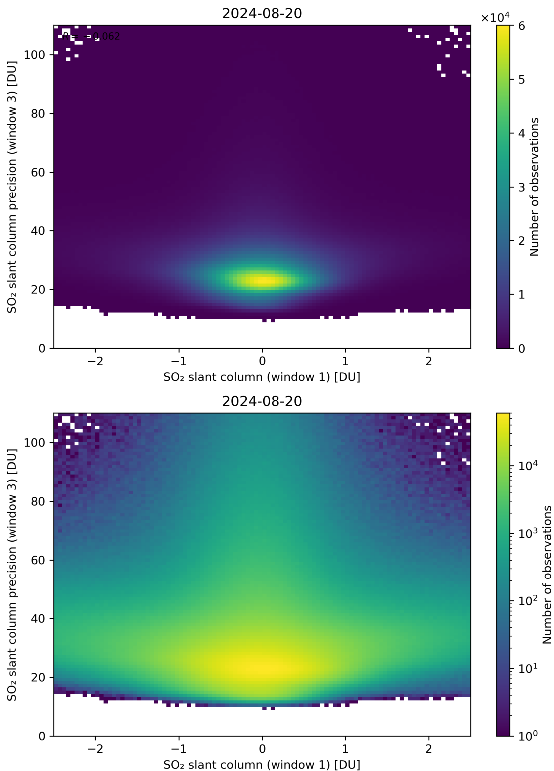
Figure 238: Scatter density plot of “SO 2 slant column (window 1)” against “SO 2 slant column precision (window 3)” for 2024-08-19 to 2024-08-21.
