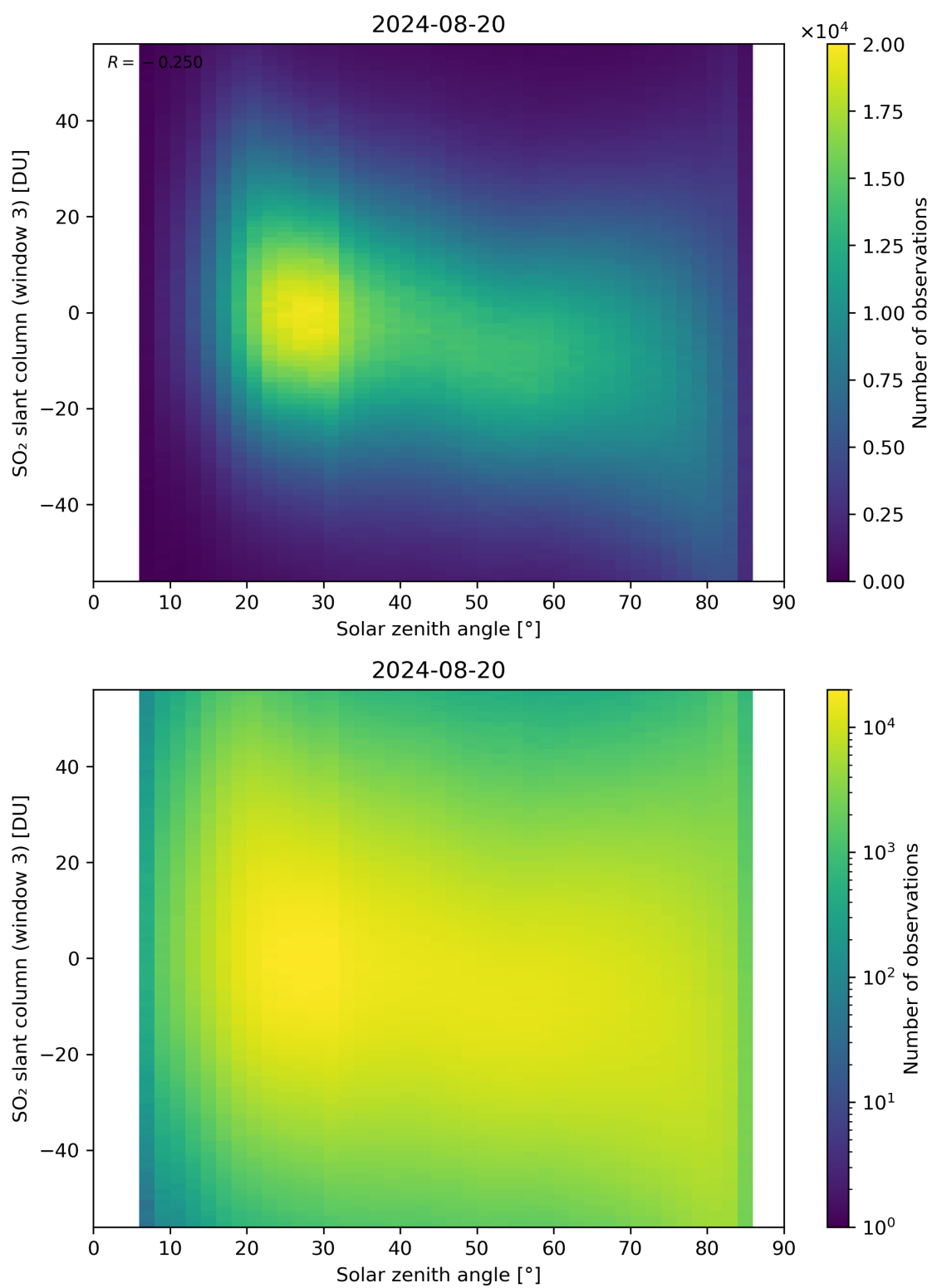
Figure 172: Scatter density plot of “Solar zenith angle” against “SO 2 slant column (window 3)” for 2024-08-19 to 2024-08-21.
