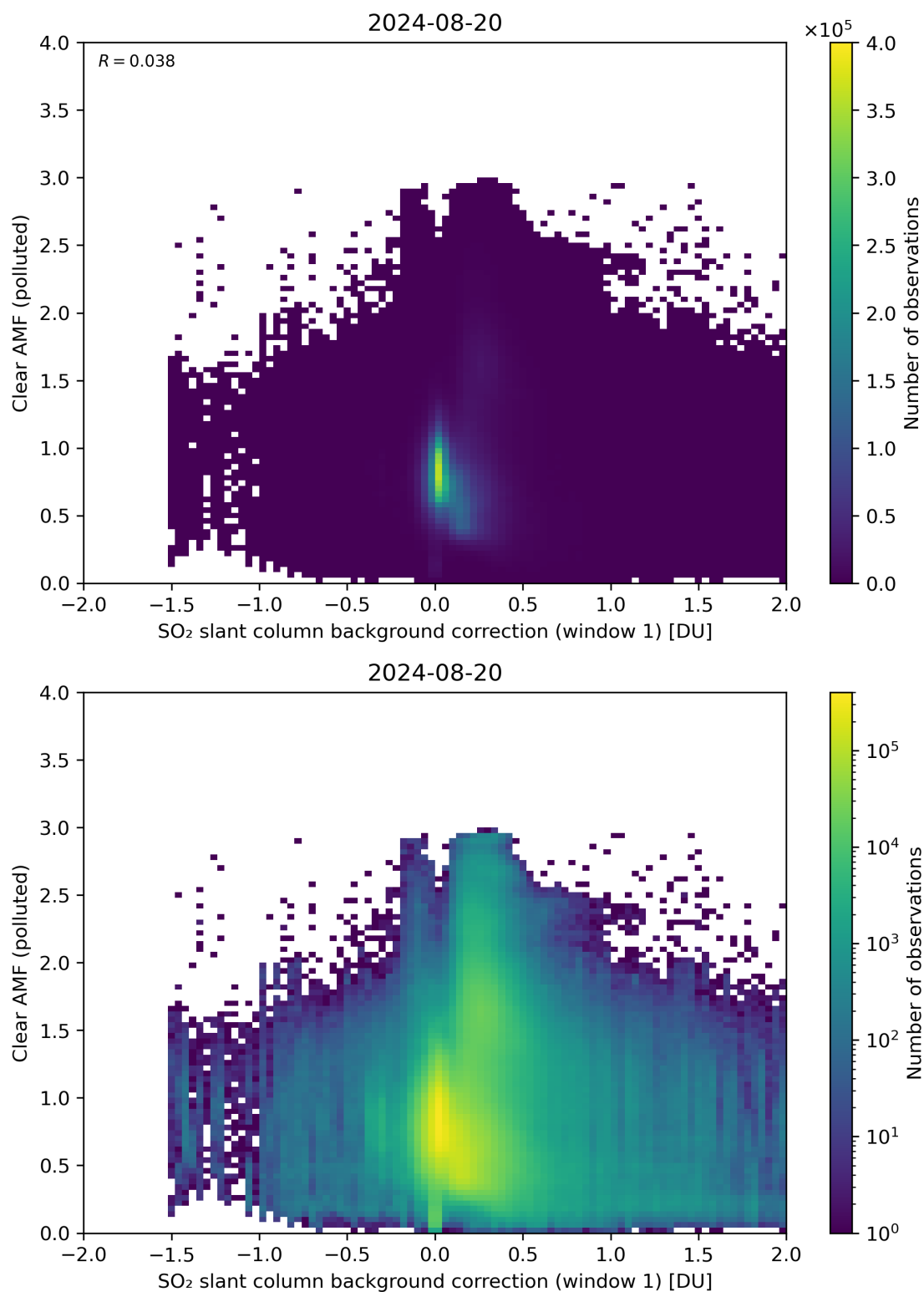
Figure 103: Scatter density plot of “SO 2 slant column background correction (window 1)” against “Clear AMF (polluted)” for 2024-08-19 to 2024-08-21.
