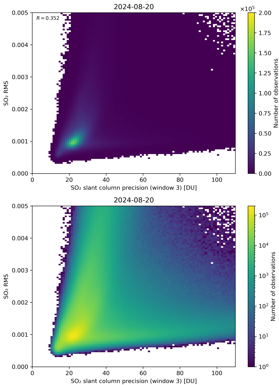
Figure 260: Scatter density plot of “SO 2 slant column precision (window 3)” against “SO 2 RMS” for 2024-08-19 to 2024-08-21.
