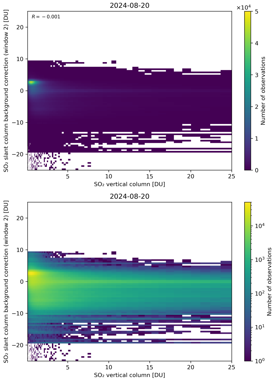
Figure 274: Scatter density plot of “SO 2 vertical column” against “SO 2 slant column background correction (window 2)” for 2024-08-19 to 2024-08-21.
