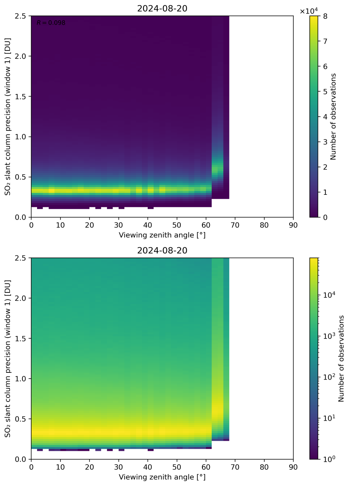
Figure 321: Scatter density plot of “Viewing zenith angle” against “SO 2 slant column precision (window 1)” for 2024-08-19 to 2024-08-21.
