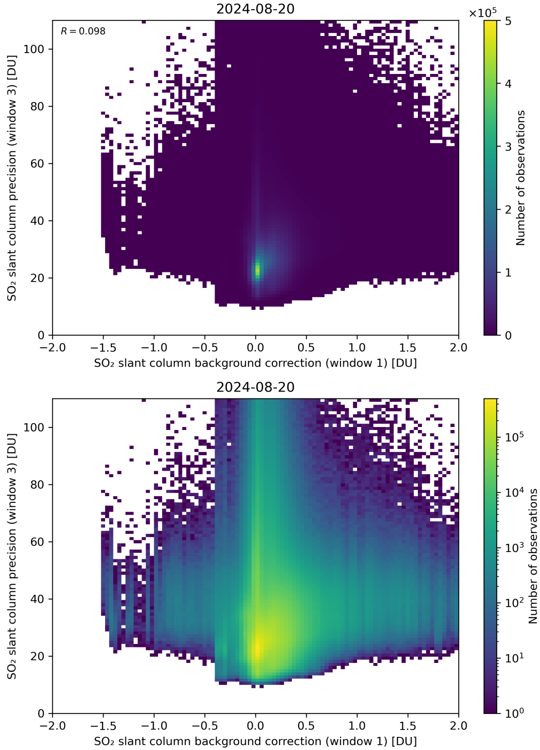
Figure 108: Scatter density plot of “SO 2 slant column background correction (window 1)” against “SO 2 slant column precision (window 3)” for 2024-08-19 to 2024-08-21.
