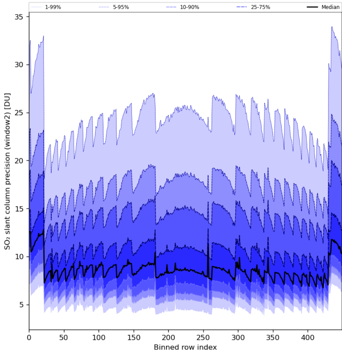
Figure 84: Along track statistics of “SO 2 slant column precision (window2)” for 2024-08-19 to 2024-08-21
