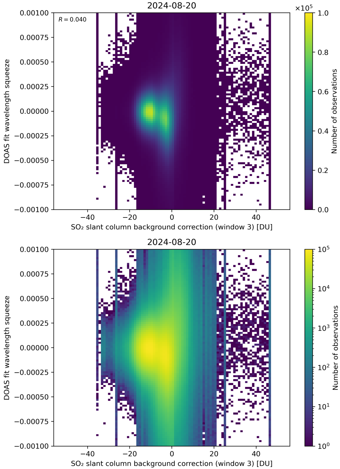
Figure 122: Scatter density plot of “SO 2 slant column background correction (window 3)” against “DOAS fit wavelength squeeze” for 2024-08-19 to 2024-08-21.
