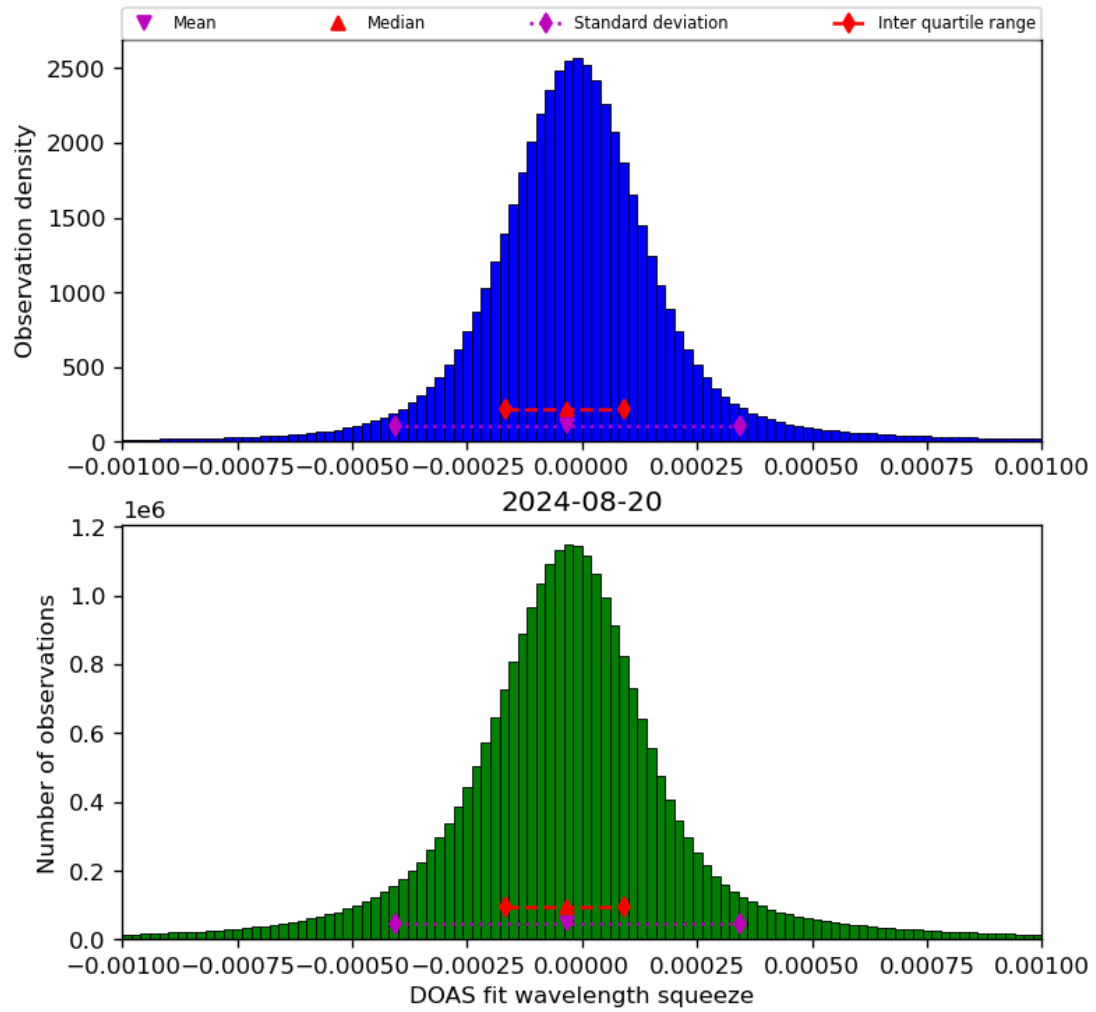
Figure 69: Histogram of “DOAS fit wavelength squeeze” for 2024-08-19 to 2024-08-21
