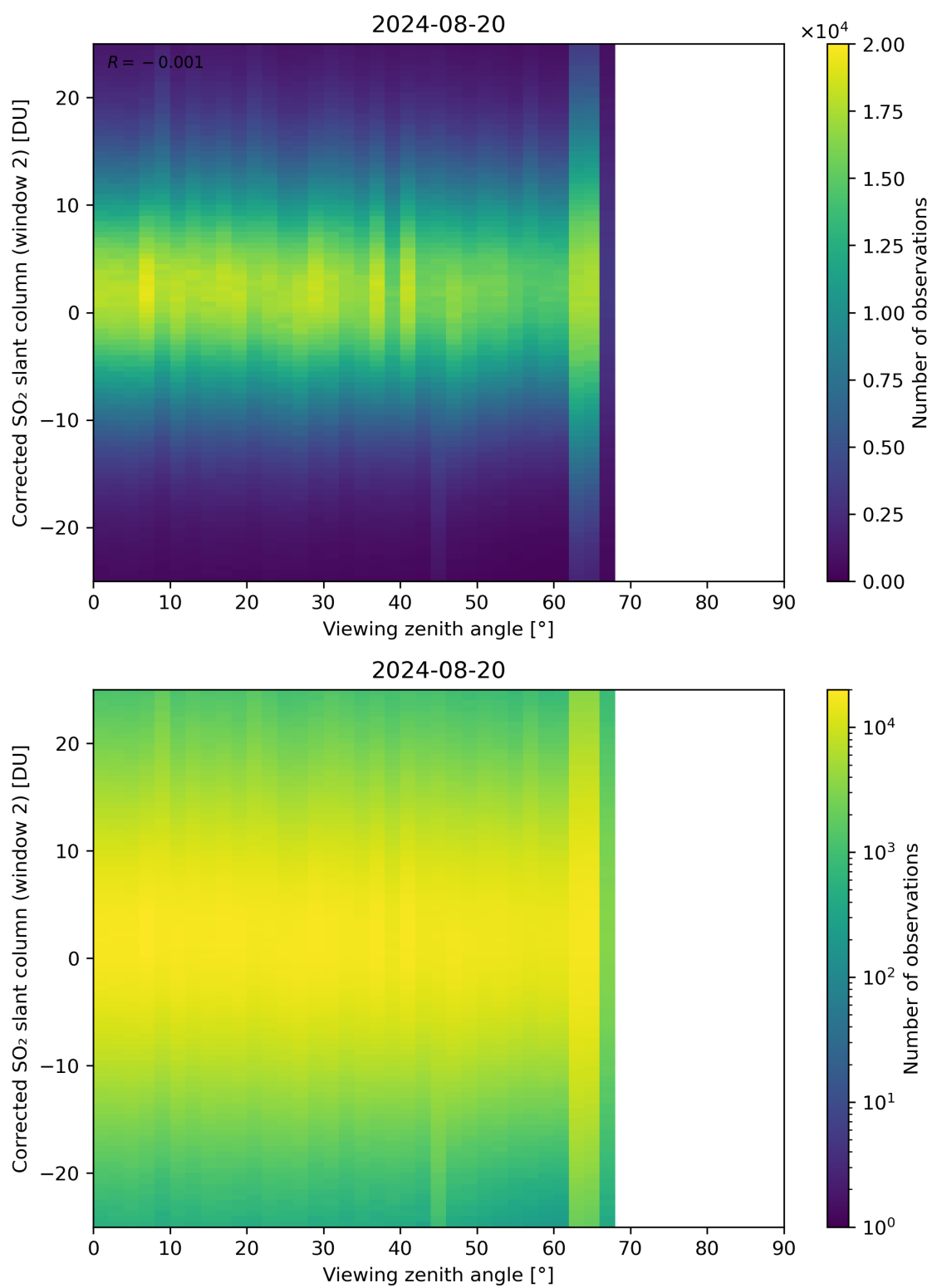
Figure 318: Scatter density plot of “Viewing zenith angle” against “Corrected SO 2 slant column (window 2)” for 2024-08-19 to 2024-08-21.
