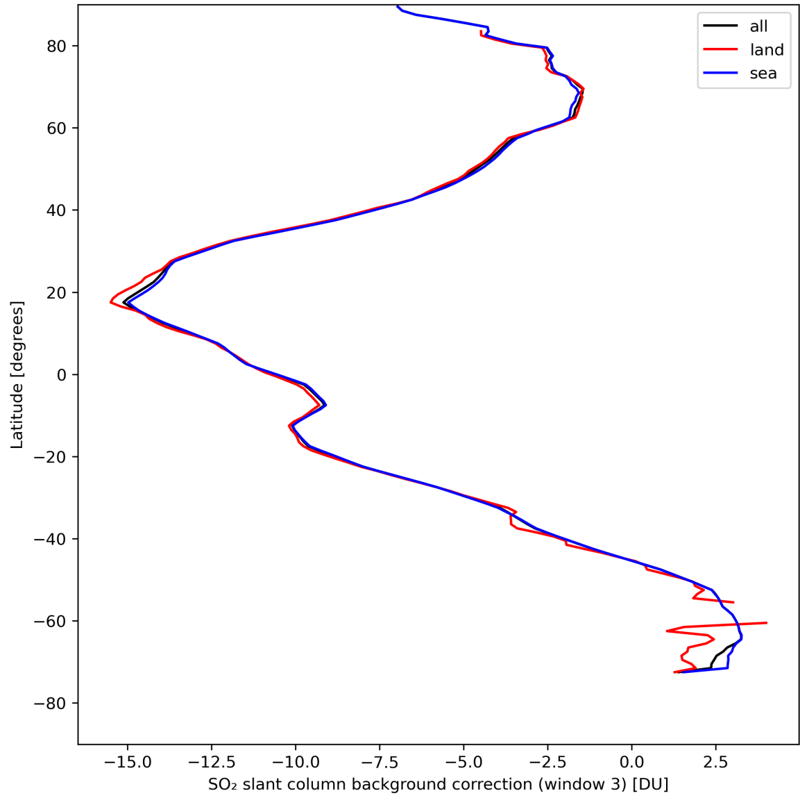
Figure 44: Zonal average of “SO 2 slant column background correction (window 3)” for 2024-08-19 to 2024-08-21.
