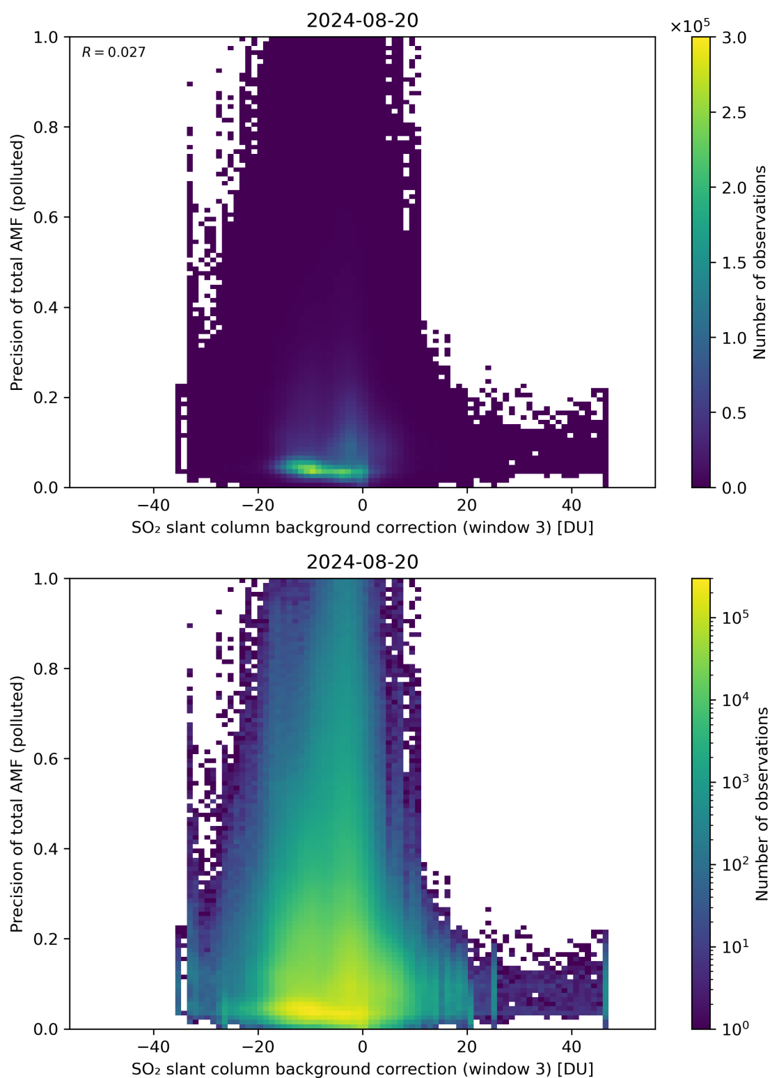
Figure 126: Scatter density plot of “SO 2 slant column background correction (window 3)” against “Precision of total AMF (polluted)” for 2024-08-19 to 2024-08-21.
