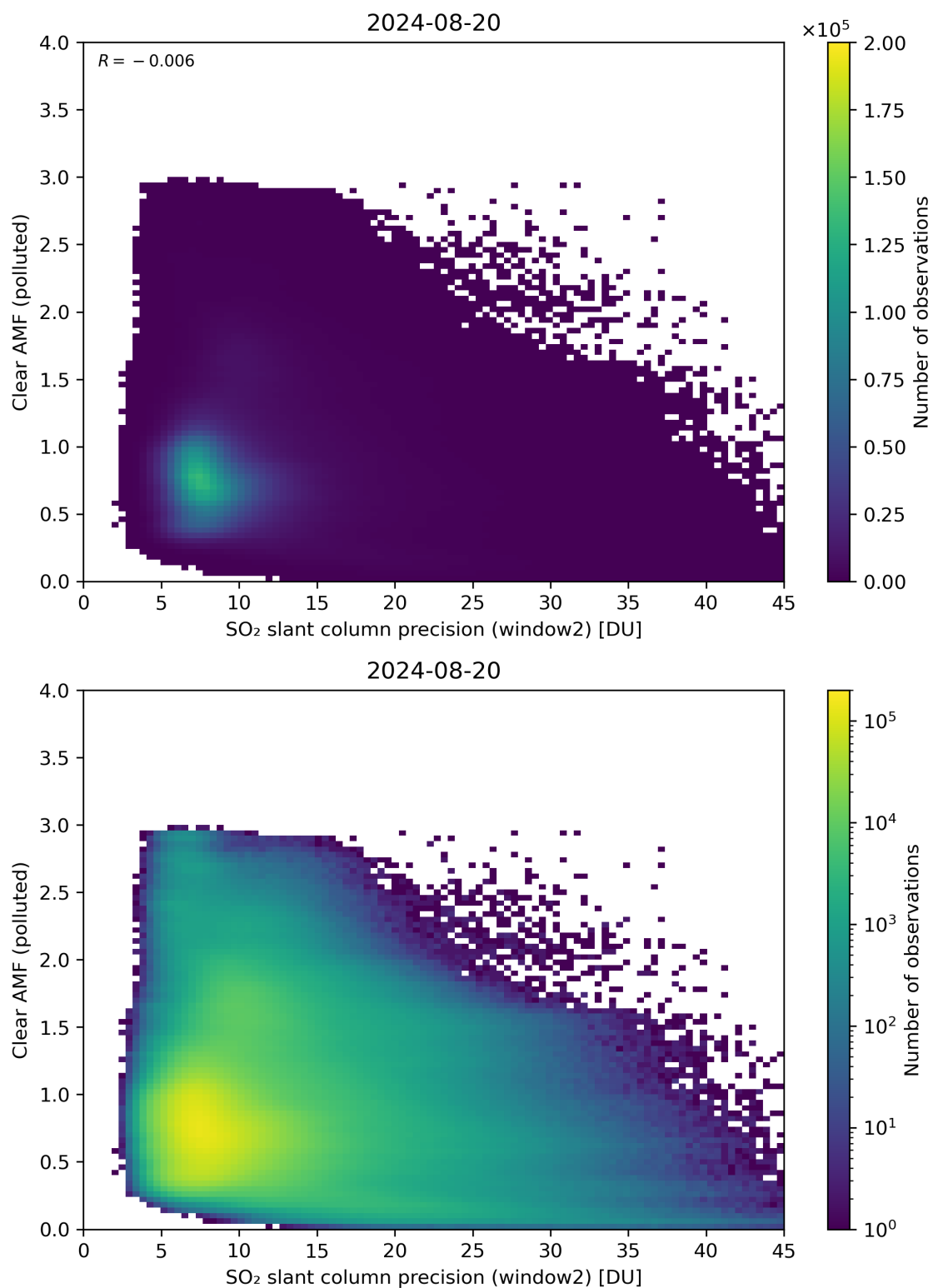
Figure 246: Scatter density plot of “SO 2 slant column precision (window2)” against “Clear AMF (polluted)” for 2024-08-19 to 2024-08-21.
