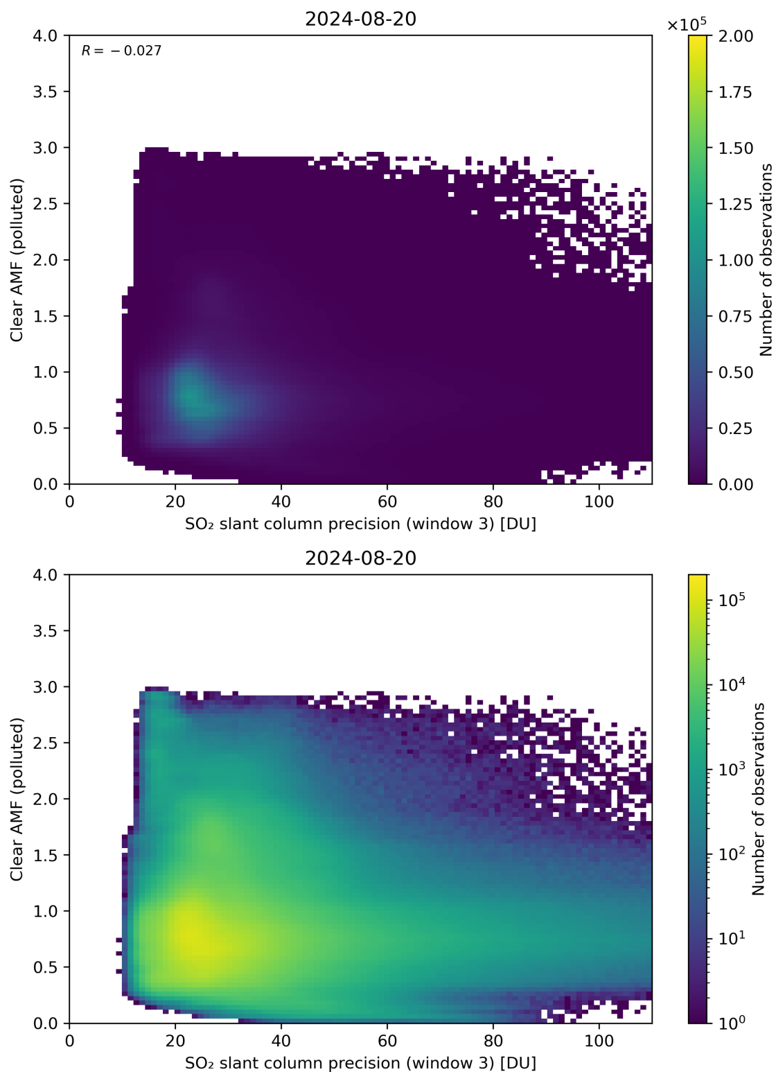
Figure 261: Scatter density plot of “SO 2 slant column precision (window 3)” against “Clear AMF (polluted)” for 2024-08-19 to 2024-08-21.
