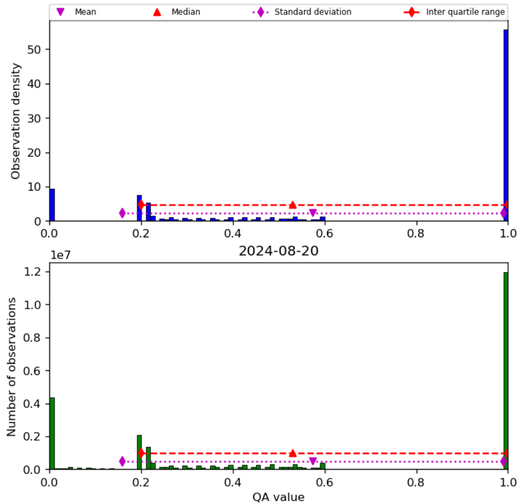
Figure 52: Histogram of “QA value” for 2024-08-19 to 2024-08-21
