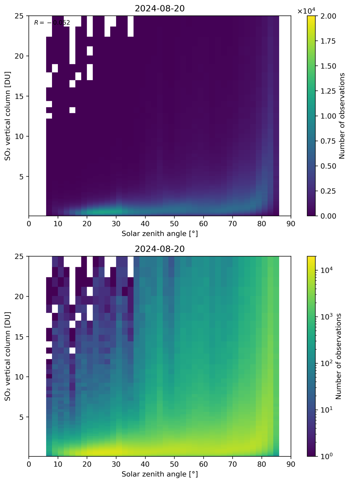
Figure 176: Scatter density plot of “Solar zenith angle” against “SO 2 vertical column” for 2024-08-19 to 2024-08-21.
