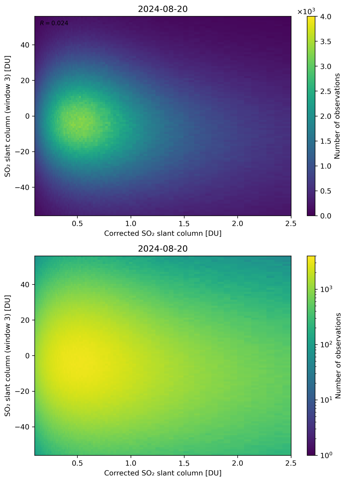
Figure 190: Scatter density plot of “Corrected SO 2 slant column” against “SO 2 slant column (window 3)” for 2024-08-19 to 2024-08-21.
