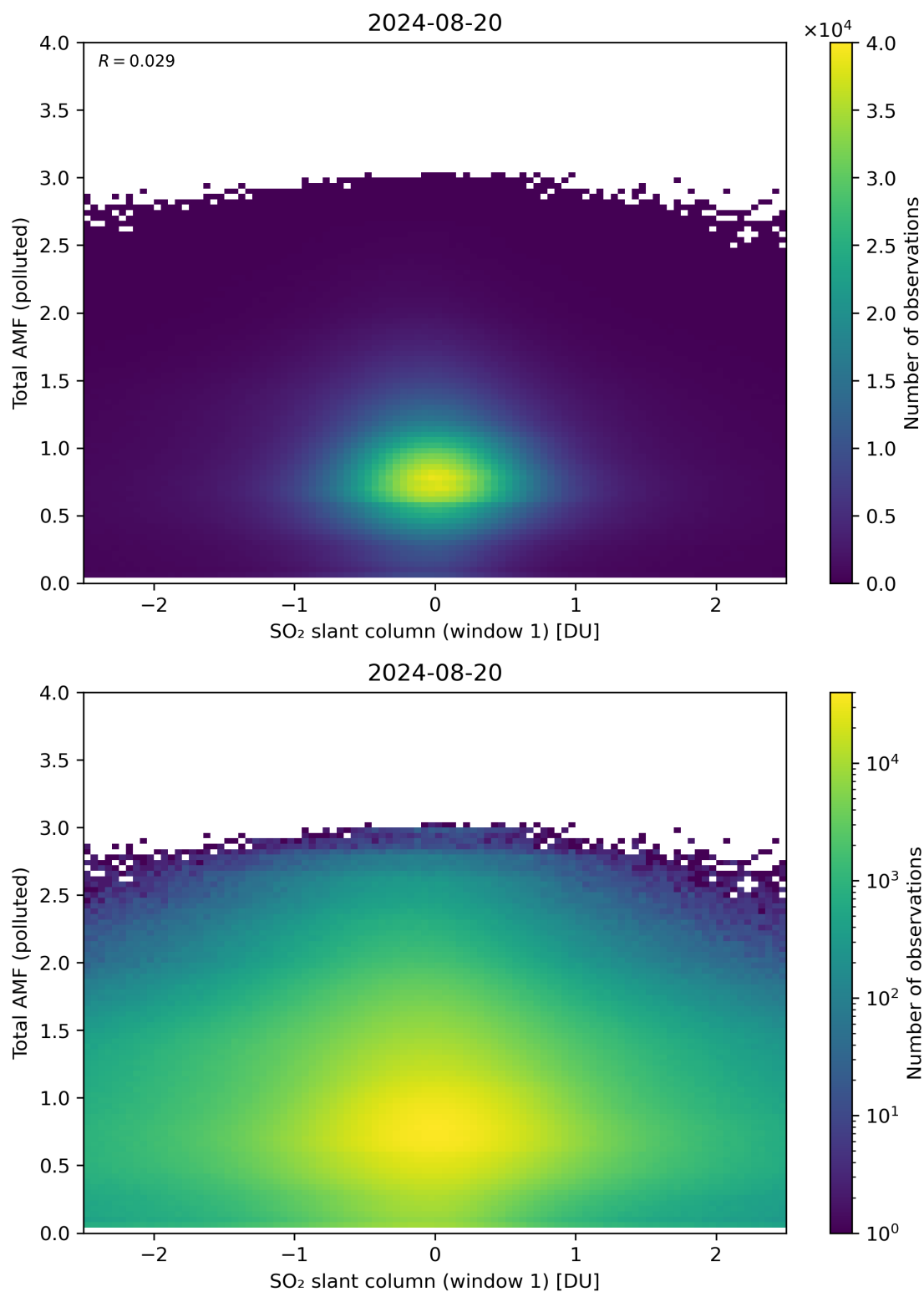
Figure 239: Scatter density plot of “SO 2 slant column (window 1)” against “Total AMF (polluted)” for 2024-08-19 to 2024-08-21.
