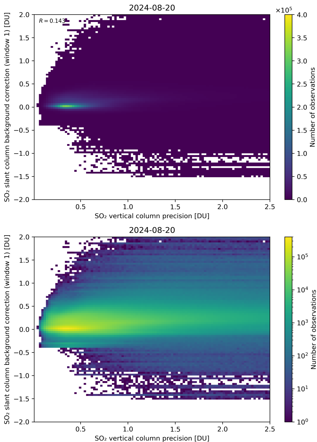
Figure 279: Scatter density plot of “SO 2 vertical column precision” against “SO 2 slant column background correction (window 1)” for 2024-08-19 to 2024-08-21.
