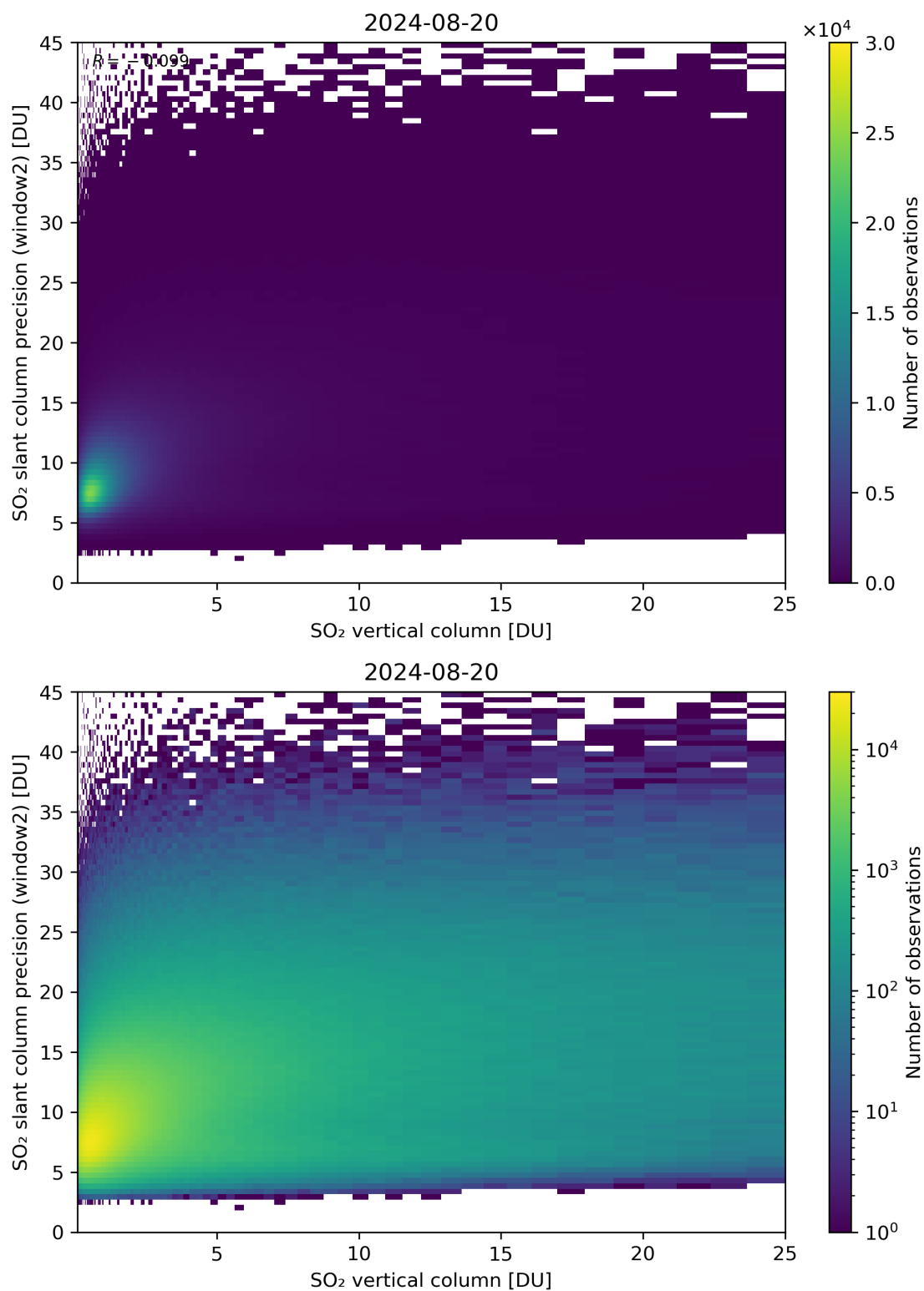
Figure 302: Scatter density plot of “SO 2 vertical column” against “SO 2 slant column precision (window2)” for 2024-08-19 to 2024-08-21.
