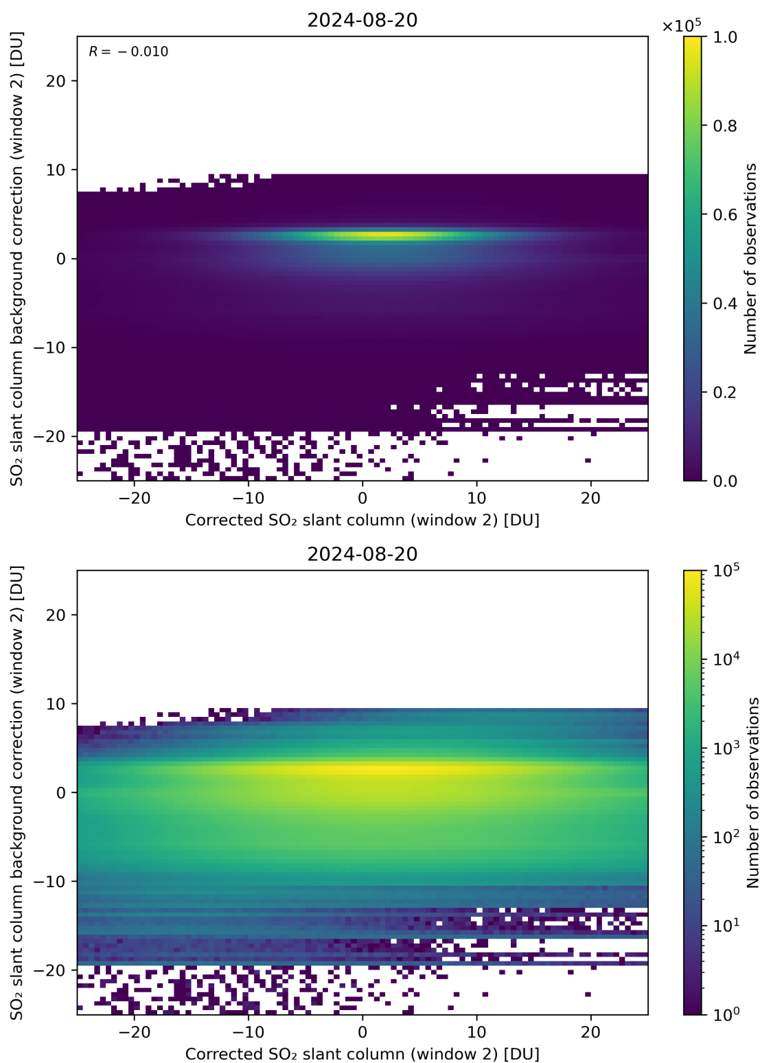
Figure 194: Scatter density plot of “Corrected SO 2 slant column (window 2)” against “SO 2 slant column background correction (window 2)” for 2024-08-19 to 2024-08-21.
