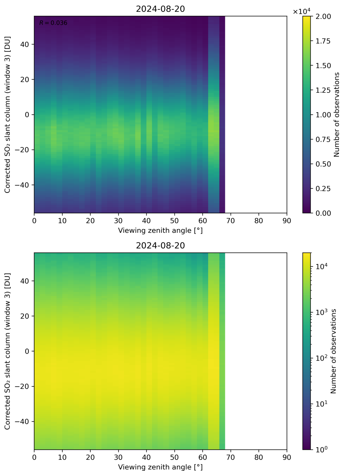
Figure 319: Scatter density plot of “Viewing zenith angle” against “Corrected SO 2 slant column (window 3)” for 2024-08-19 to 2024-08-21.
