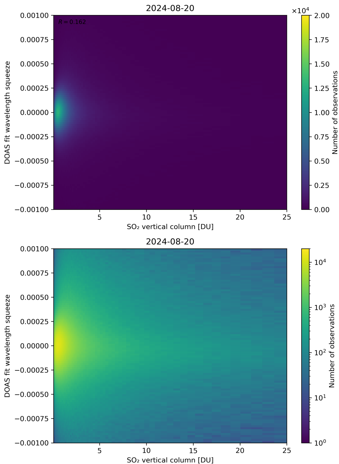
Figure 277: Scatter density plot of “SO 2 vertical column” against “DOAS fit wavelength squeeze” for 2024-08-19 to 2024-08-21.
