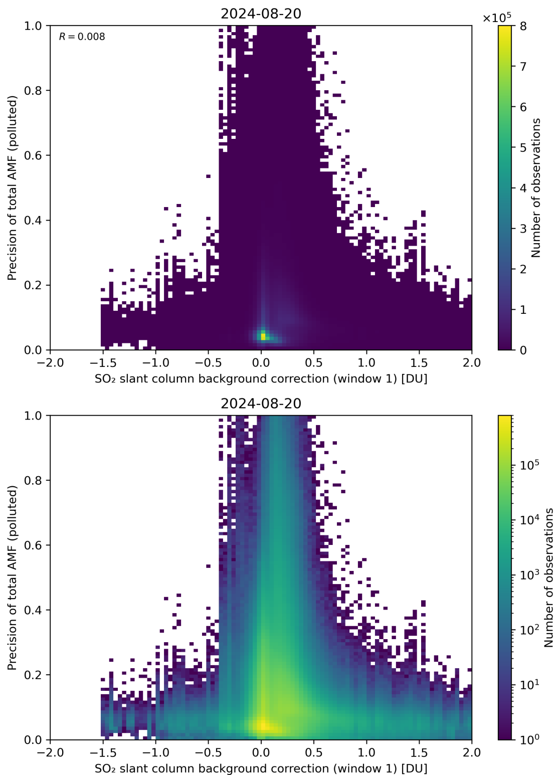
Figure 110: Scatter density plot of “SO 2 slant column background correction (window 1)” against “Precision of total AMF (polluted)” for 2024-08-19 to 2024-08-21.
