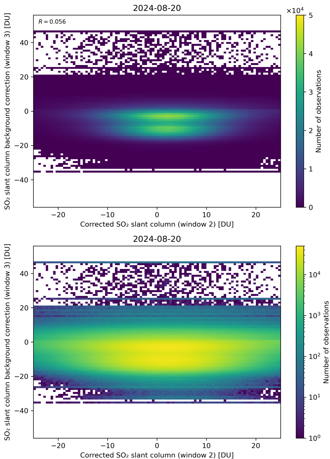
Figure 195: Scatter density plot of “Corrected SO 2 slant column (window 2)” against “SO 2 slant column background correction (window 3)” for 2024-08-19 to 2024-08-21.
