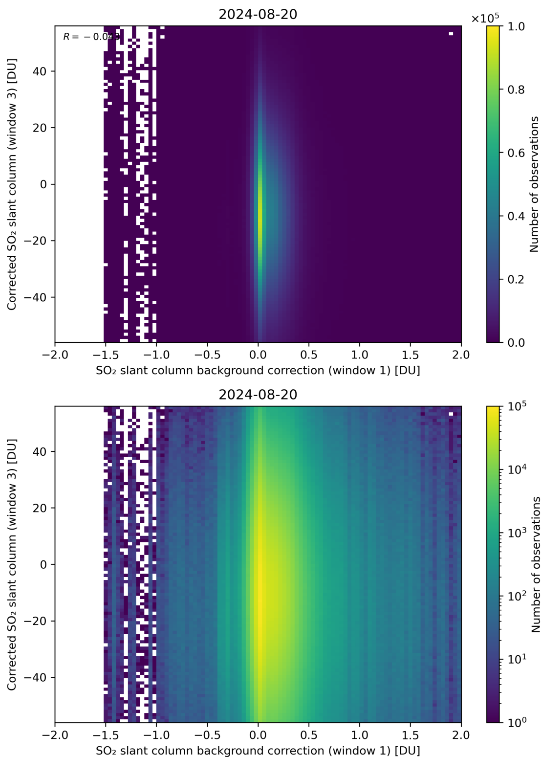
Figure 105: Scatter density plot of “SO 2 slant column background correction (window 1)” against “Corrected SO 2 slant column (window 3)” for 2024-08-19 to 2024-08-21.
