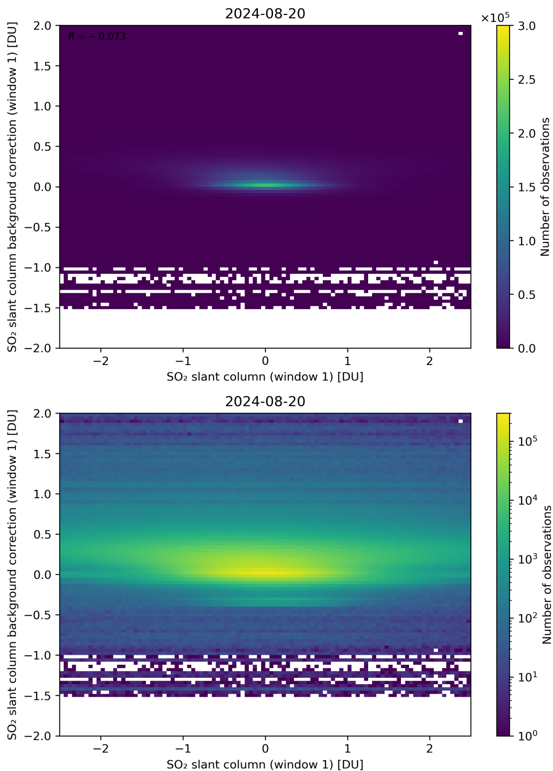
Figure 212: Scatter density plot of “SO 2 slant column (window 1)” against “SO 2 slant column background correction (window 1)” for 2024-08-19 to 2024-08-21.
