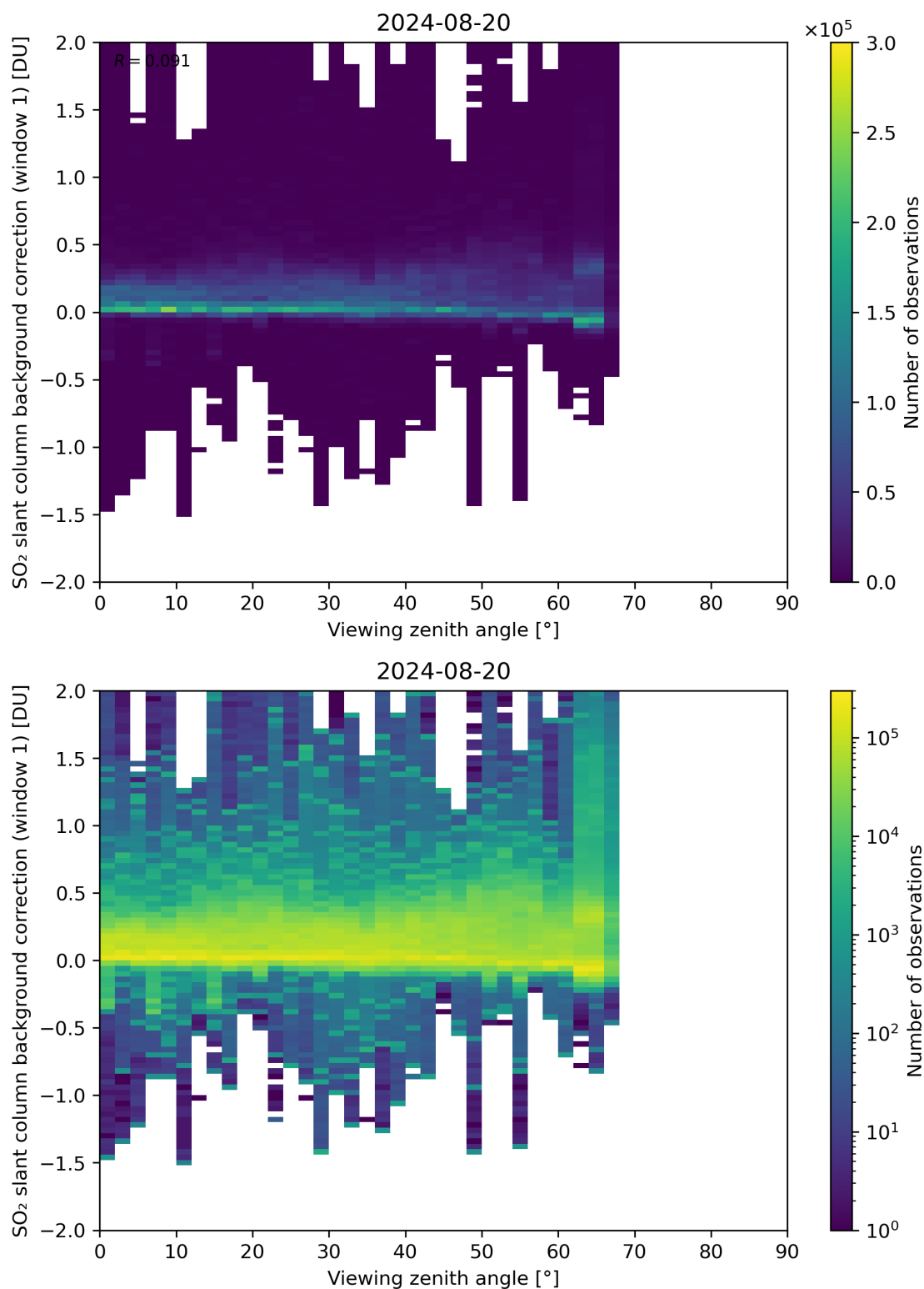
Figure 308: Scatter density plot of “Viewing zenith angle” against “SO 2 slant column background correction (window 1)” for 2024-08-19 to 2024-08-21.
