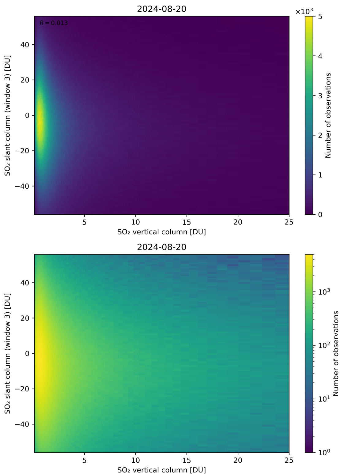
Figure 303: Scatter density plot of “SO 2 vertical column” against “SO 2 slant column (window 3)” for 2024-08-19 to 2024-08-21.
