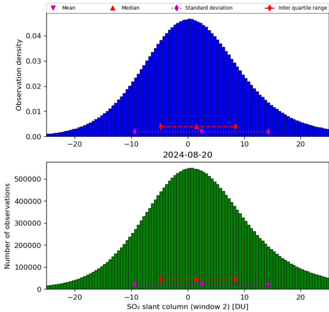
Figure 60: Histogram of “SO 2 slant column (window 2)” for 2024-08-19 to 2024-08-21
