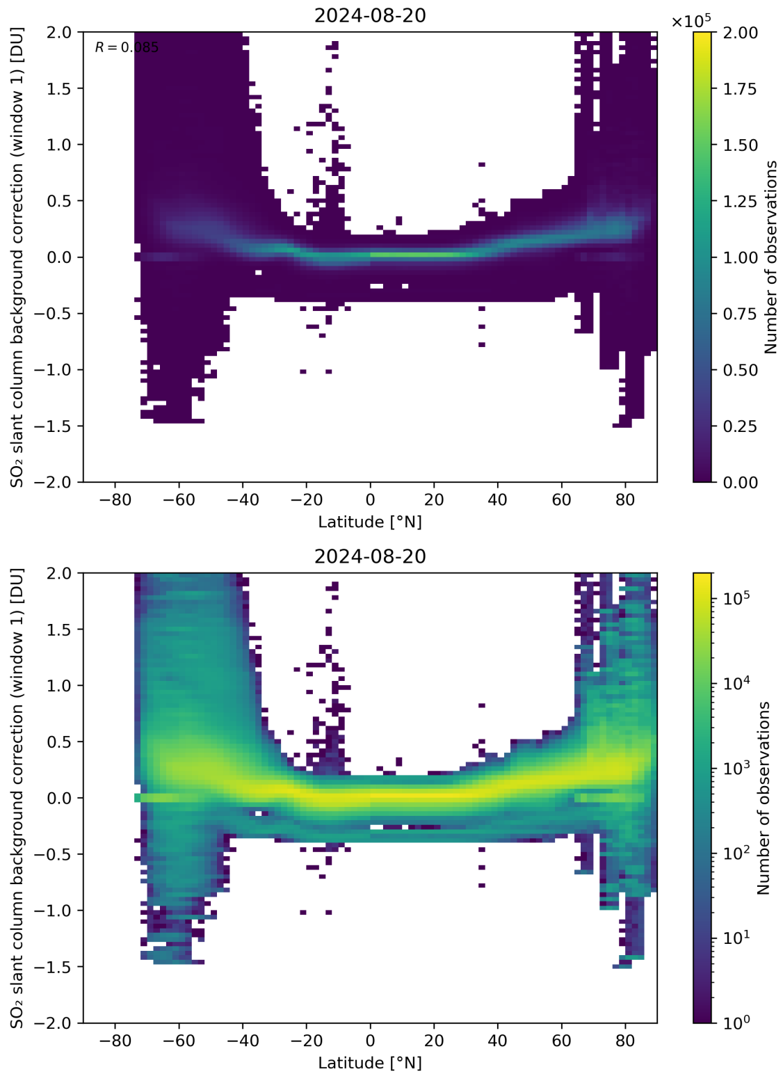
Figure 139: Scatter density plot of “Latitude” against “SO 2 slant column background correction (window 1)” for 2024-08-19 to 2024-08-21.
