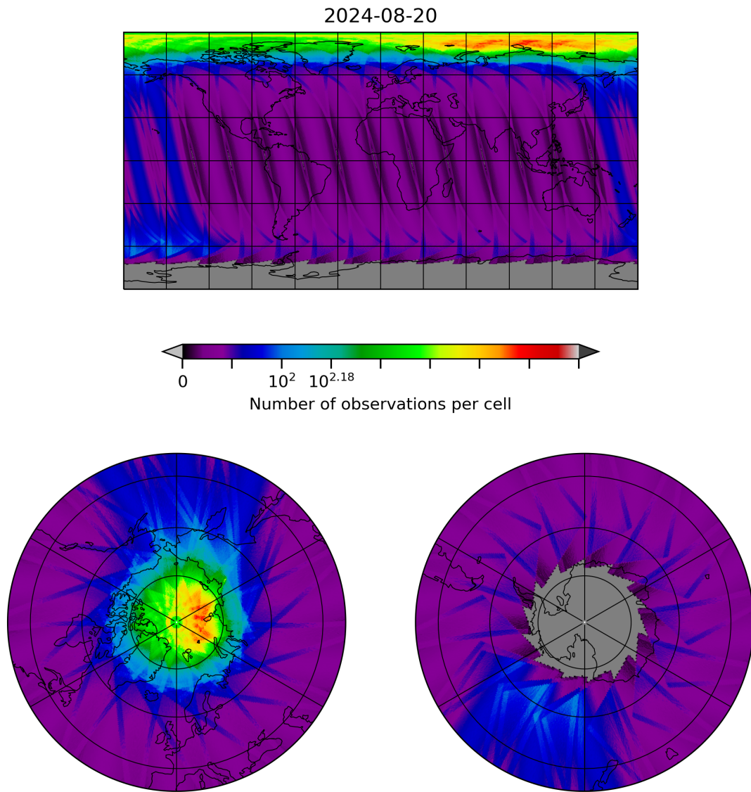
Figure 28: Map of the number of observations for 2024-08-19 to 2024-08-21
