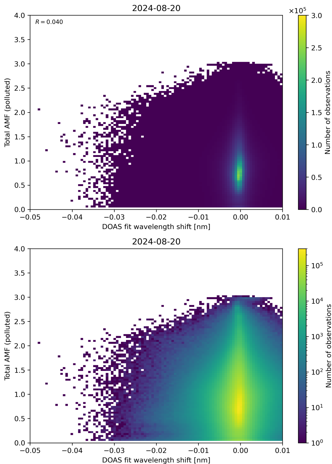
Figure 130: Scatter density plot of “DOAS fit wavelength shift” against “Total AMF (polluted)” for 2024-08-19 to 2024-08-21.
