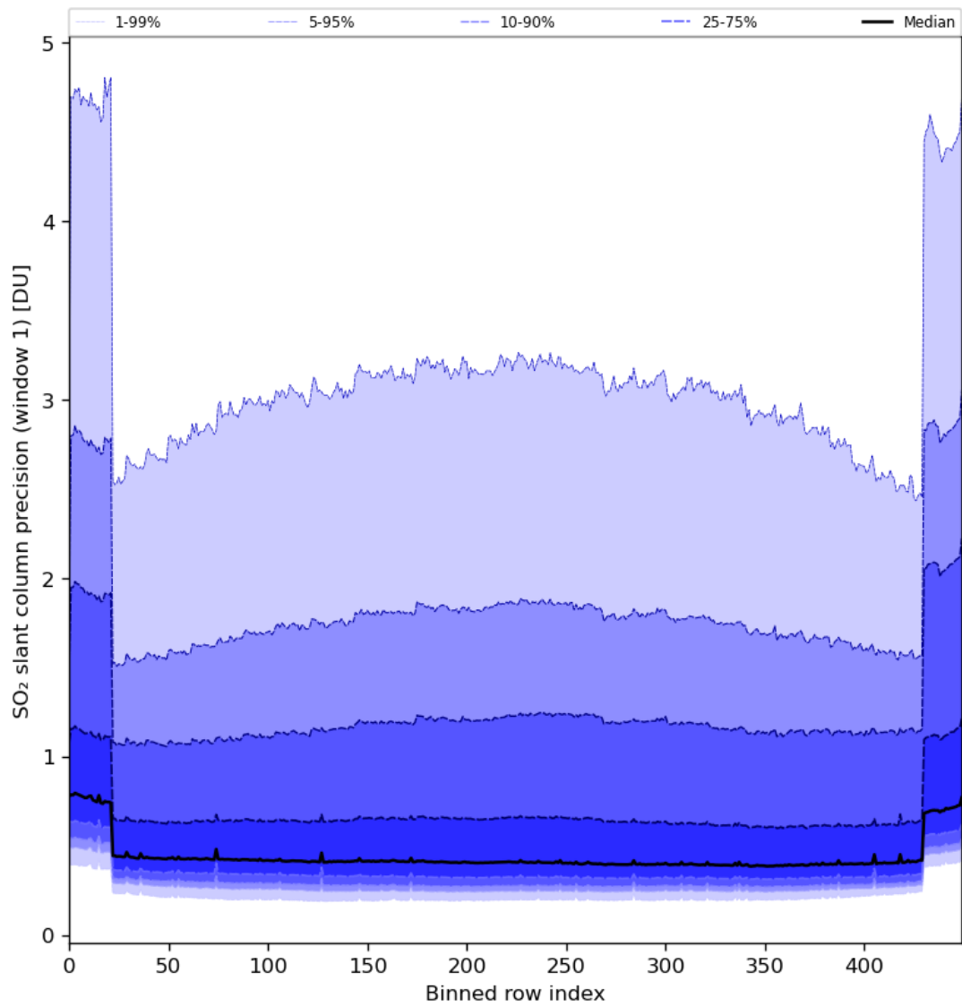
Figure 80: Along track statistics of “SO 2 slant column precision (window 1)” for 2024-08-21 to 2024-08-22
