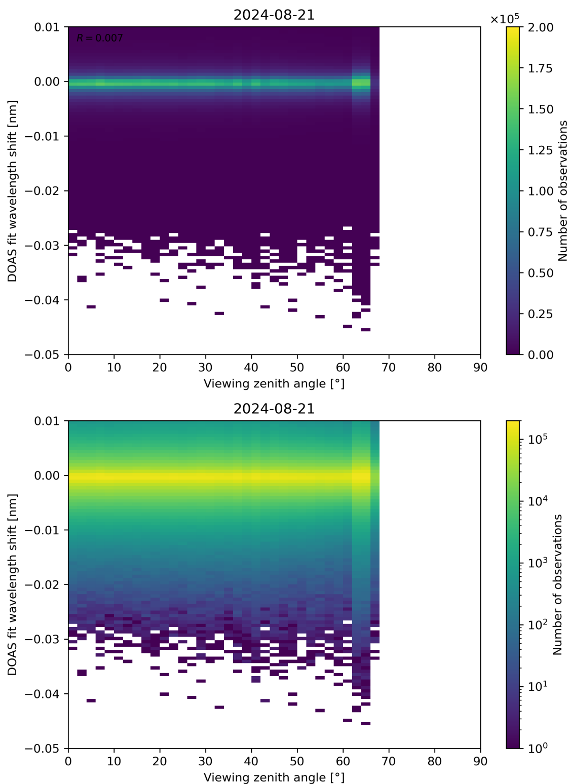
Figure 311: Scatter density plot of “Viewing zenith angle” against “DOAS fit wavelength shift” for 2024-08-21 to 2024-08-22.
