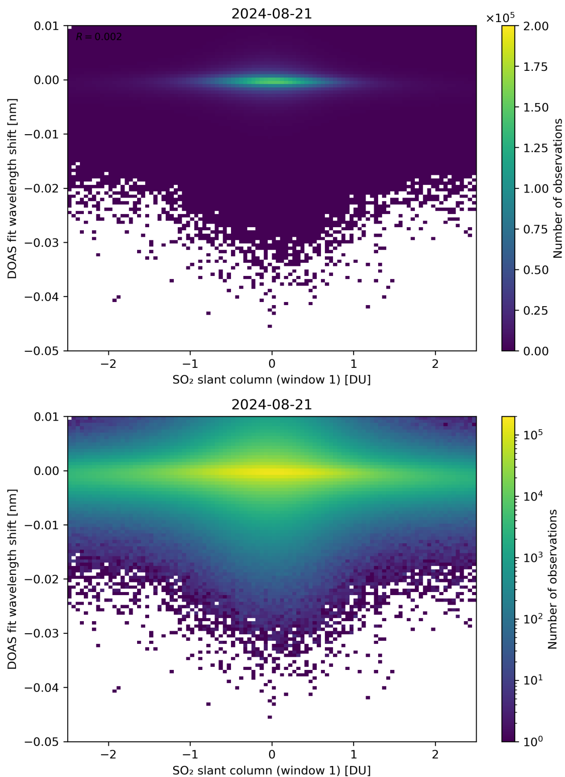
Figure 215: Scatter density plot of “SO 2 slant column (window 1)” against “DOAS fit wavelength shift” for 2024-08-21 to 2024-08-22.
