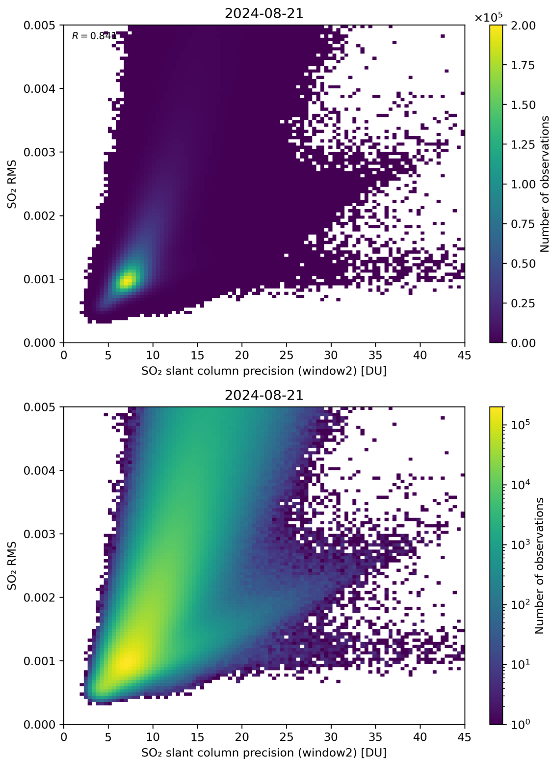
Figure 245: Scatter density plot of “SO 2 slant column precision (window2)” against “SO 2 RMS” for 2024-08-21 to 2024-08-22.
