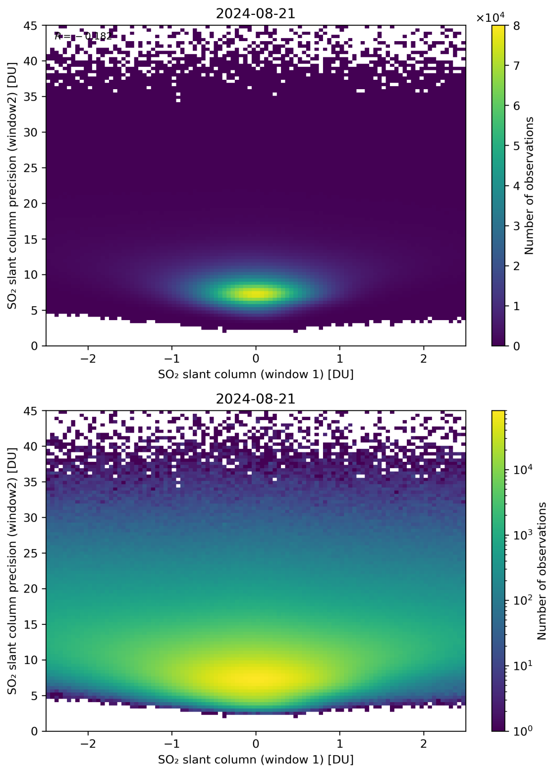
Figure 236: Scatter density plot of “SO 2 slant column (window 1)” against “SO 2 slant column precision (window2)” for 2024-08-21 to 2024-08-22.
