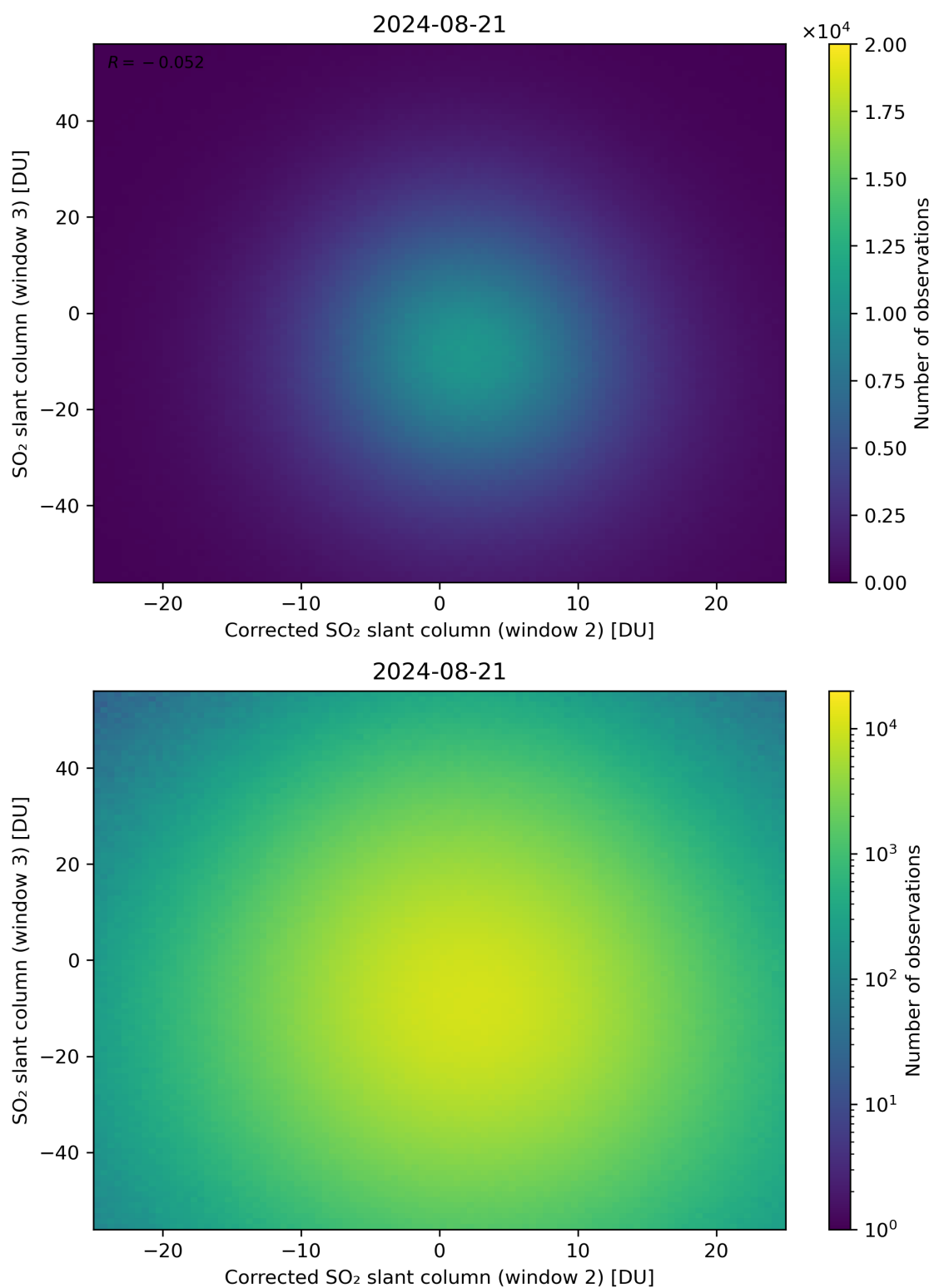
Figure 201: Scatter density plot of “Corrected SO 2 slant column (window 2)” against “SO 2 slant column (window 3)” for 2024-08-21 to 2024-08-22.
