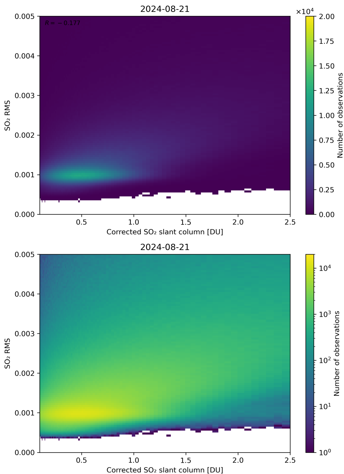
Figure 183: Scatter density plot of “Corrected SO 2 slant column” against “SO 2 RMS” for 2024-08-21 to 2024-08-22.
