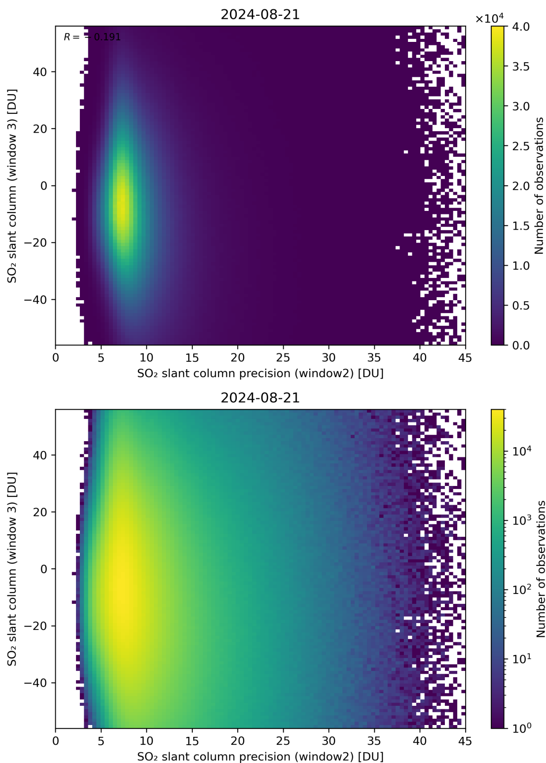
Figure 249: Scatter density plot of “SO 2 slant column precision (window2)” against “SO 2 slant column (window 3)” for 2024-08-21 to 2024-08-22.
