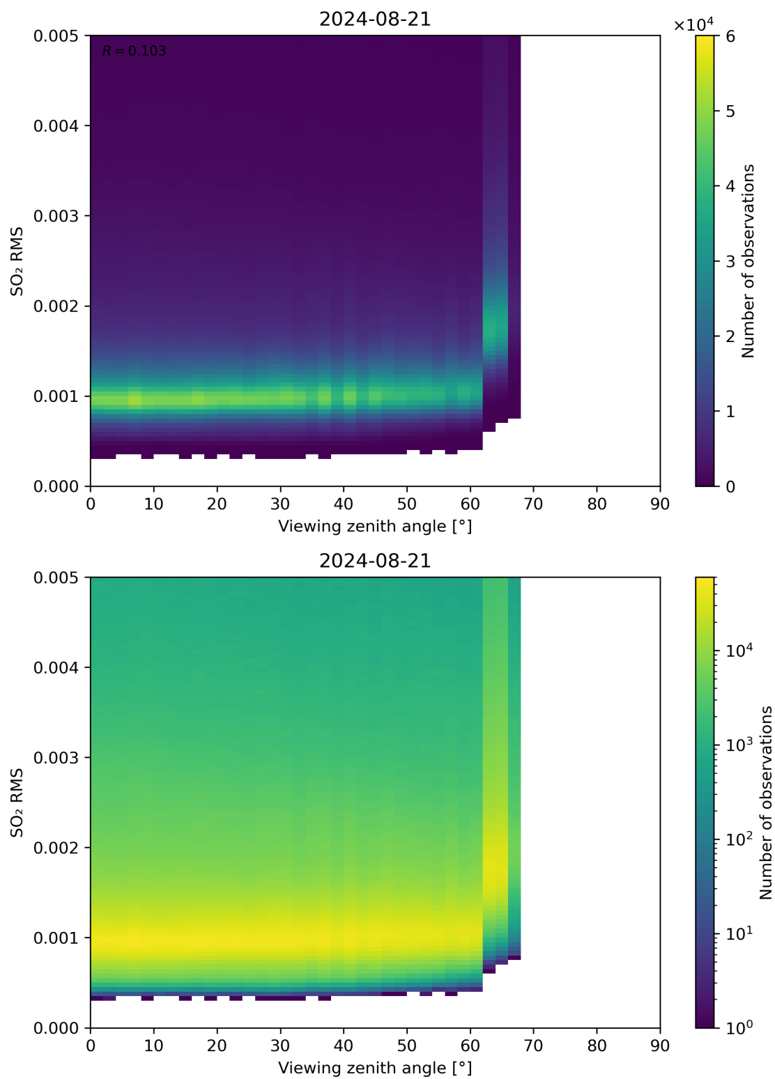
Figure 313: Scatter density plot of “Viewing zenith angle” against “SO 2 RMS” for 2024-08-21 to 2024-08-22.
