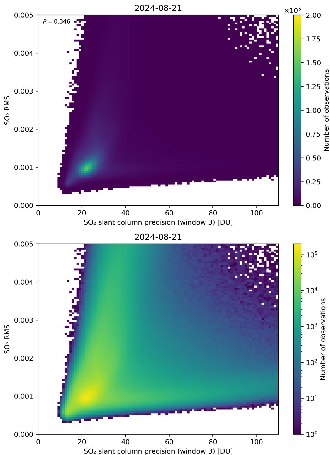
Figure 260: Scatter density plot of “SO 2 slant column precision (window 3)” against “SO 2 RMS” for 2024-08-21 to 2024-08-22.
