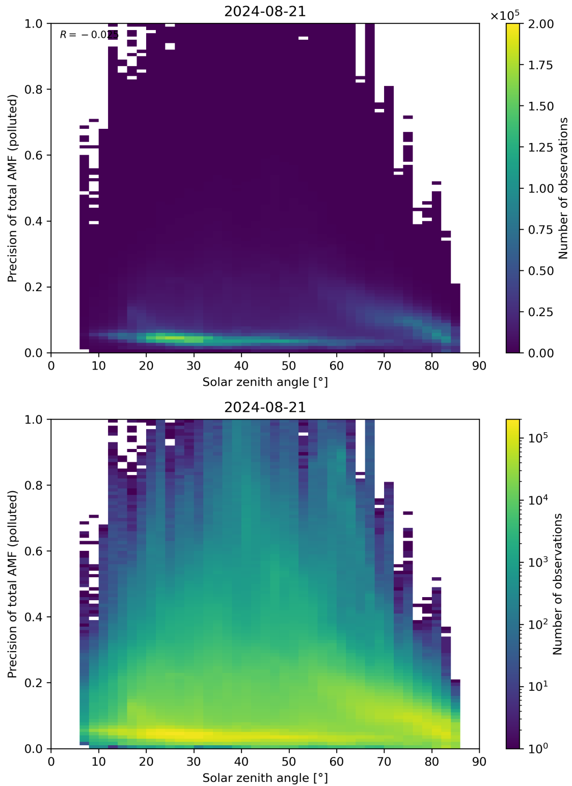
Figure 175: Scatter density plot of “Solar zenith angle” against “Precision of total AMF (polluted)” for 2024-08-21 to 2024-08-22.
