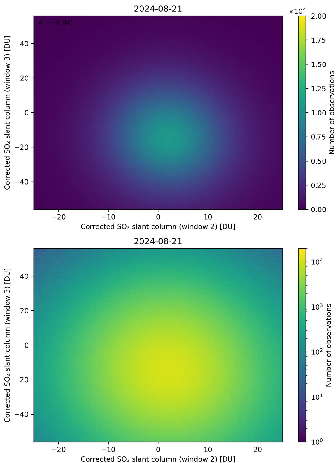
Figure 200: Scatter density plot of “Corrected SO 2 slant column (window 2)” against “Corrected SO 2 slant column (window 3)” for 2024-08-21 to 2024-08-22.
