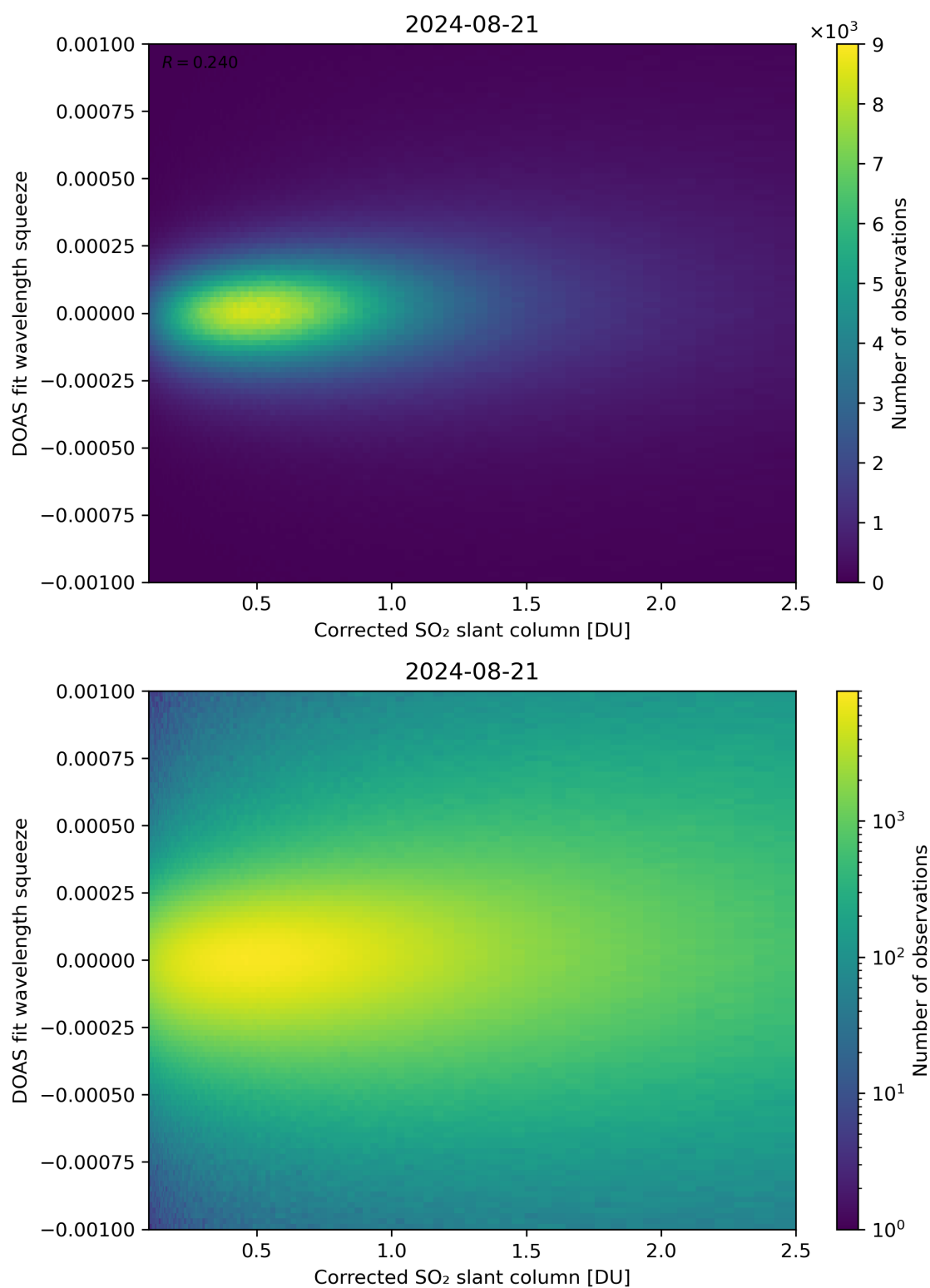
Figure 182: Scatter density plot of “Corrected SO 2 slant column” against “DOAS fit wavelength squeeze” for 2024-08-21 to 2024-08-22.
