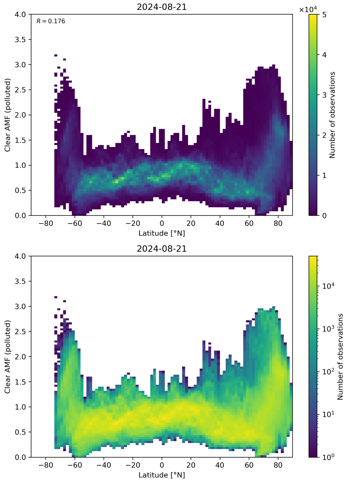
Figure 145: Scatter density plot of “Latitude” against “Clear AMF (polluted)” for 2024-08-21 to 2024-08-22.
