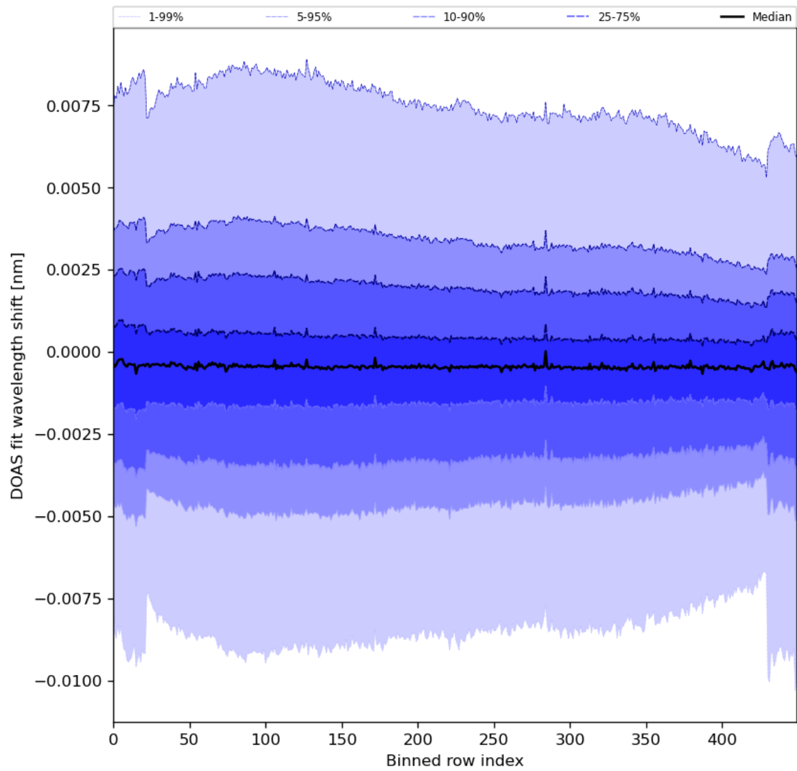
Figure 91: Along track statistics of “DOAS fit wavelength shift” for 2024-08-21 to 2024-08-22
