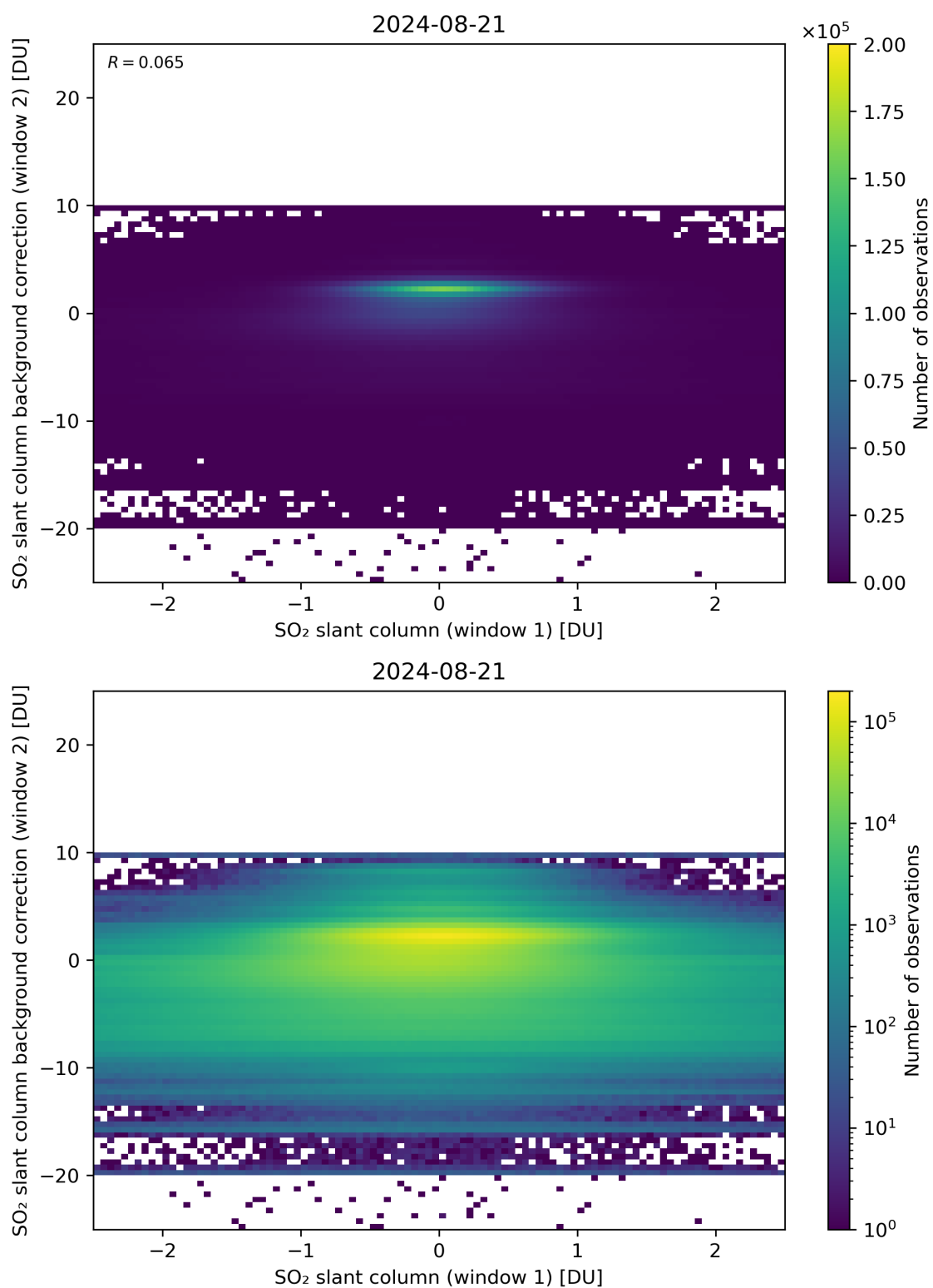
Figure 213: Scatter density plot of “SO 2 slant column (window 1)” against “SO 2 slant column background correction (window 2)” for 2024-08-21 to 2024-08-22.
