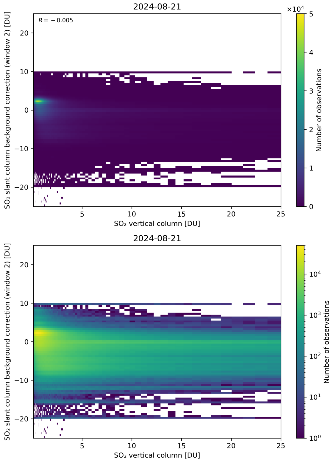
Figure 274: Scatter density plot of “SO 2 vertical column” against “SO 2 slant column background correction (window 2)” for 2024-08-21 to 2024-08-22.
