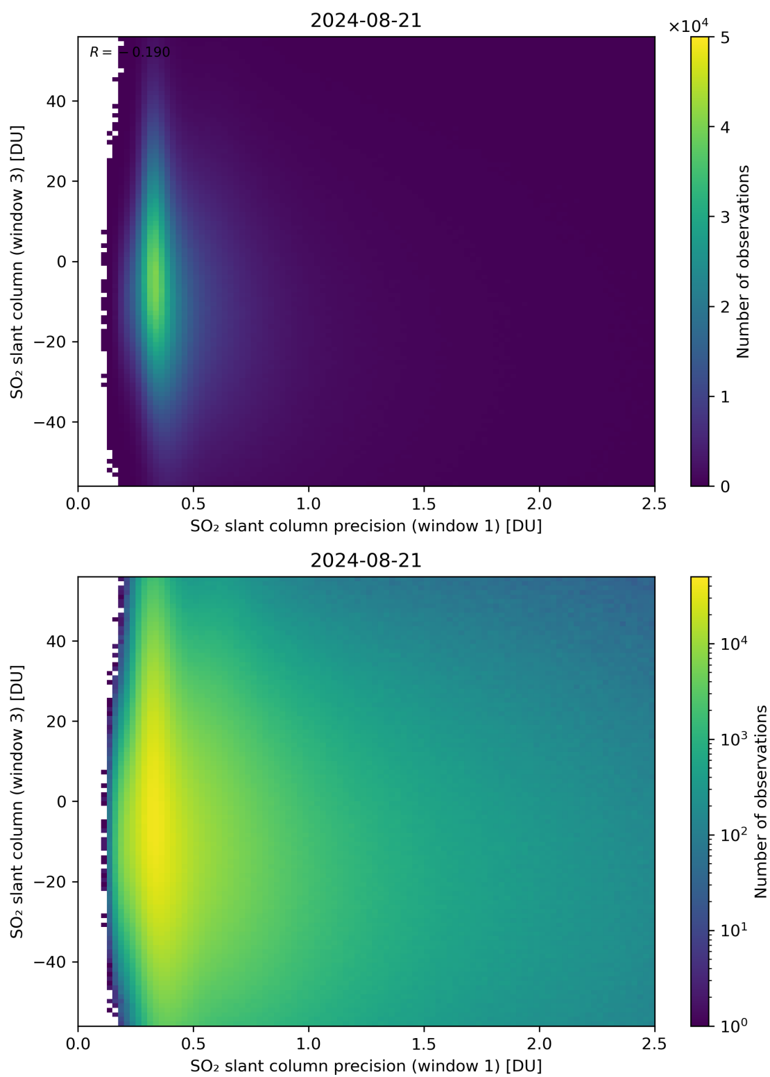
Figure 228: Scatter density plot of “SO 2 slant column precision (window 1)” against “SO 2 slant column (window 3)” for 2024-08-21 to 2024-08-22.
