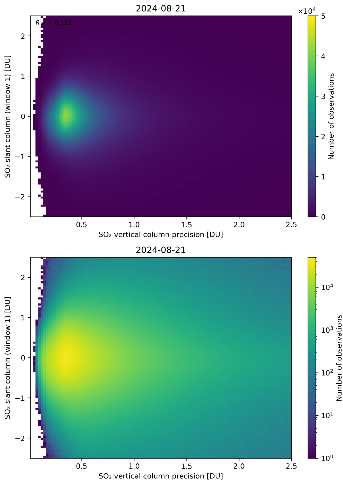
Figure 289: Scatter density plot of “SO 2 vertical column precision” against “SO 2 slant column (window 1)” for 2024-08-21 to 2024-08-22.
