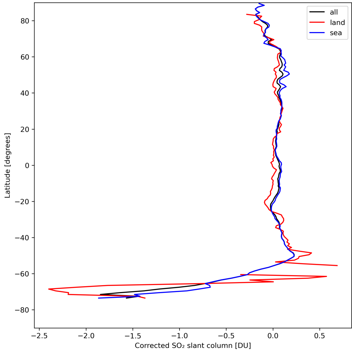
Figure 32: Zonal average of "Corrected SO 2 slant column" for 2024-08-21 to 2024-08-22.
