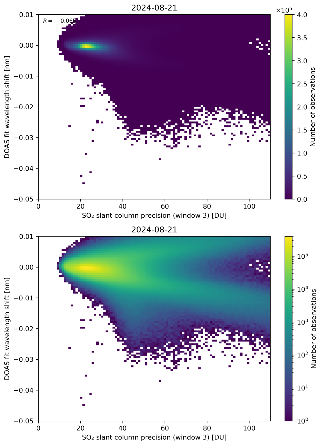
Figure 258: Scatter density plot of “SO 2 slant column precision (window 3)” against “DOAS fit wavelength shift” for 2024-08-21 to 2024-08-22.
