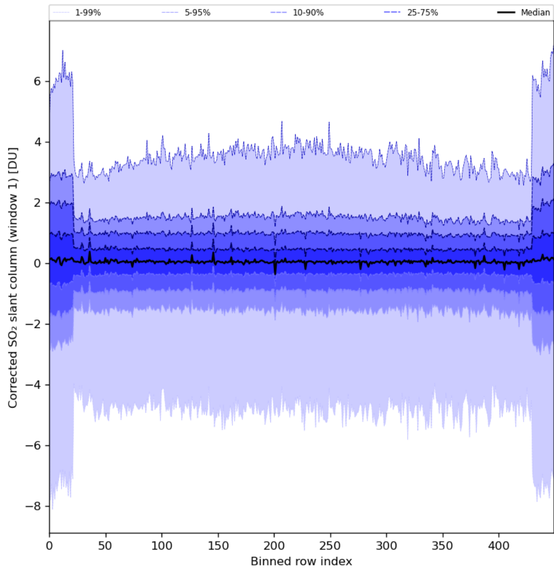
Figure 81: Along track statistics of “Corrected SO 2 slant column (window 1)” for 2024-08-21 to 2024-08-22
