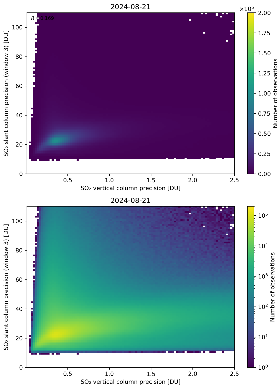
Figure 293: Scatter density plot of “SO 2 vertical column precision” against “SO 2 slant column precision (window 3)” for 2024-08-21 to 2024-08-22.
