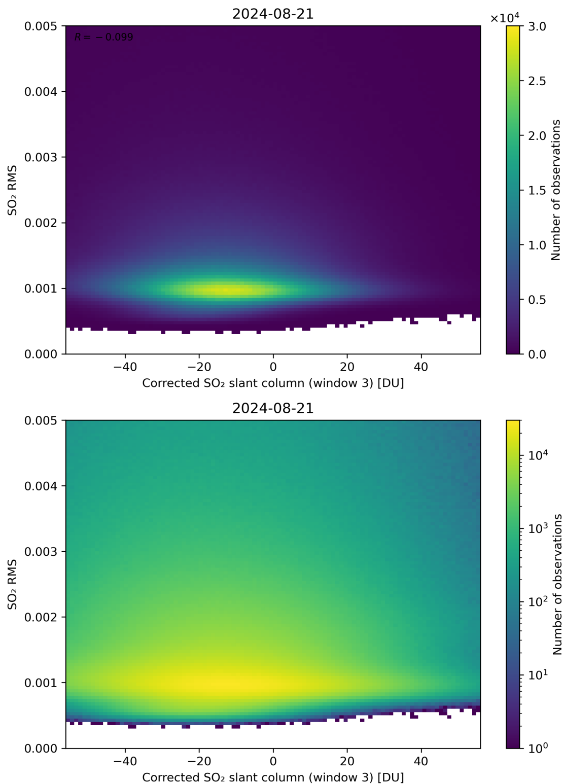
Figure 208: Scatter density plot of “Corrected SO 2 slant column (window 3)” against “SO 2 RMS” for 2024-08-21 to 2024-08-22.
