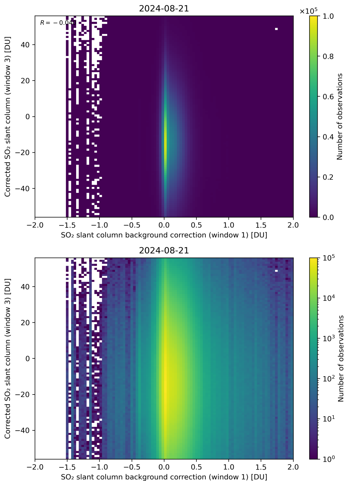
Figure 105: Scatter density plot of “SO 2 slant column background correction (window 1)” against “Corrected SO 2 slant column (window 3)” for 2024-08-21 to 2024-08-22.
