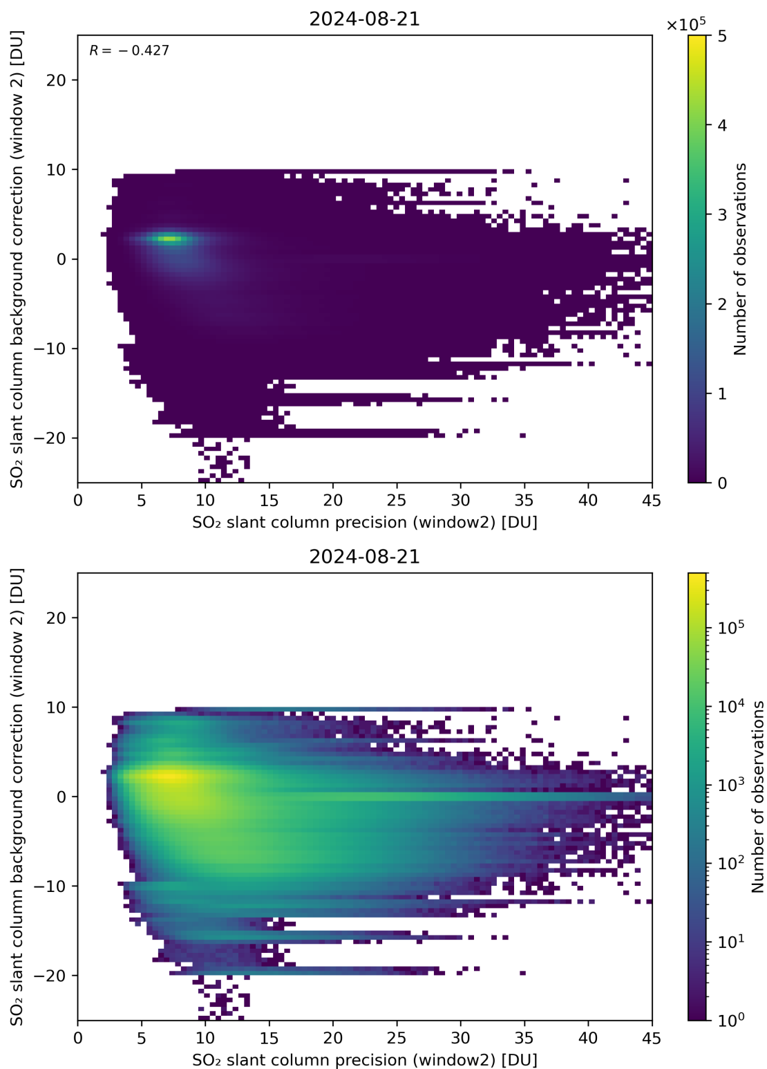
Figure 241: Scatter density plot of “SO 2 slant column precision (window2)” against “SO 2 slant column background correction (window 2)” for 2024-08-21 to 2024-08-22.
