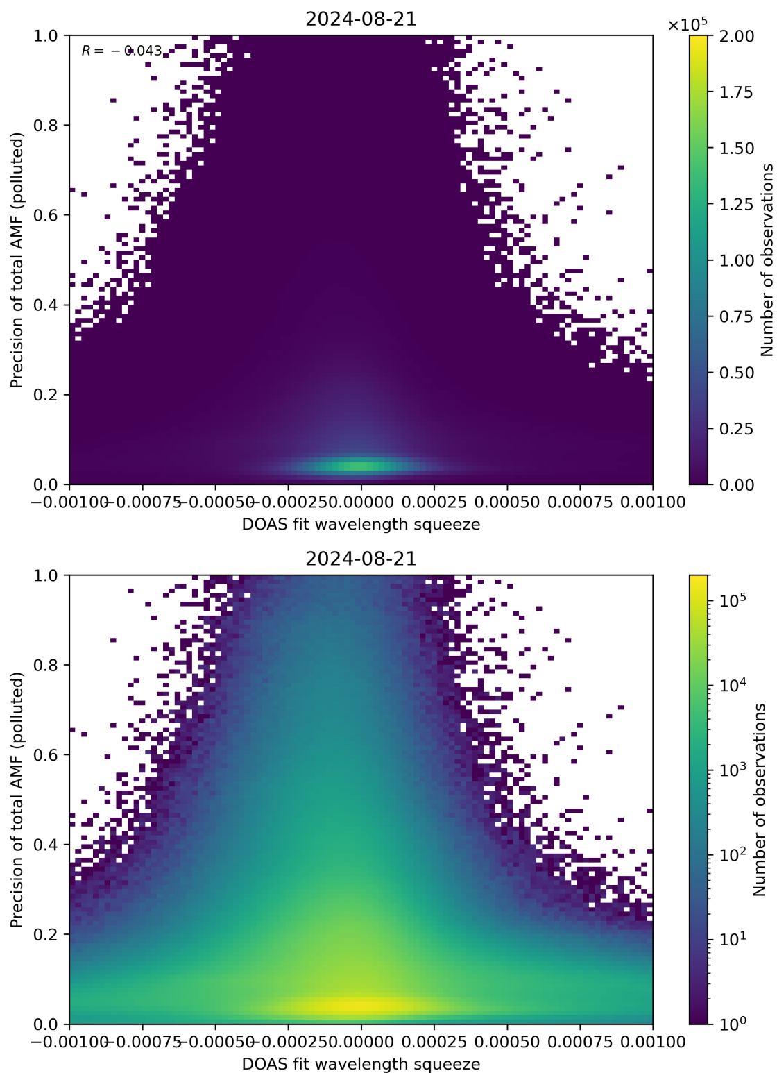
Figure 135: Scatter density plot of “DOAS fit wavelength squeeze” against “Precision of total AMF (polluted)” for 2024-08-21 to 2024-08-22.
