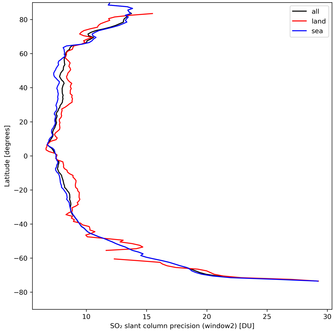
Figure 38: Zonal average of “SO 2 slant column precision (window2)” for 2024-08-21 to 2024-08-22.
