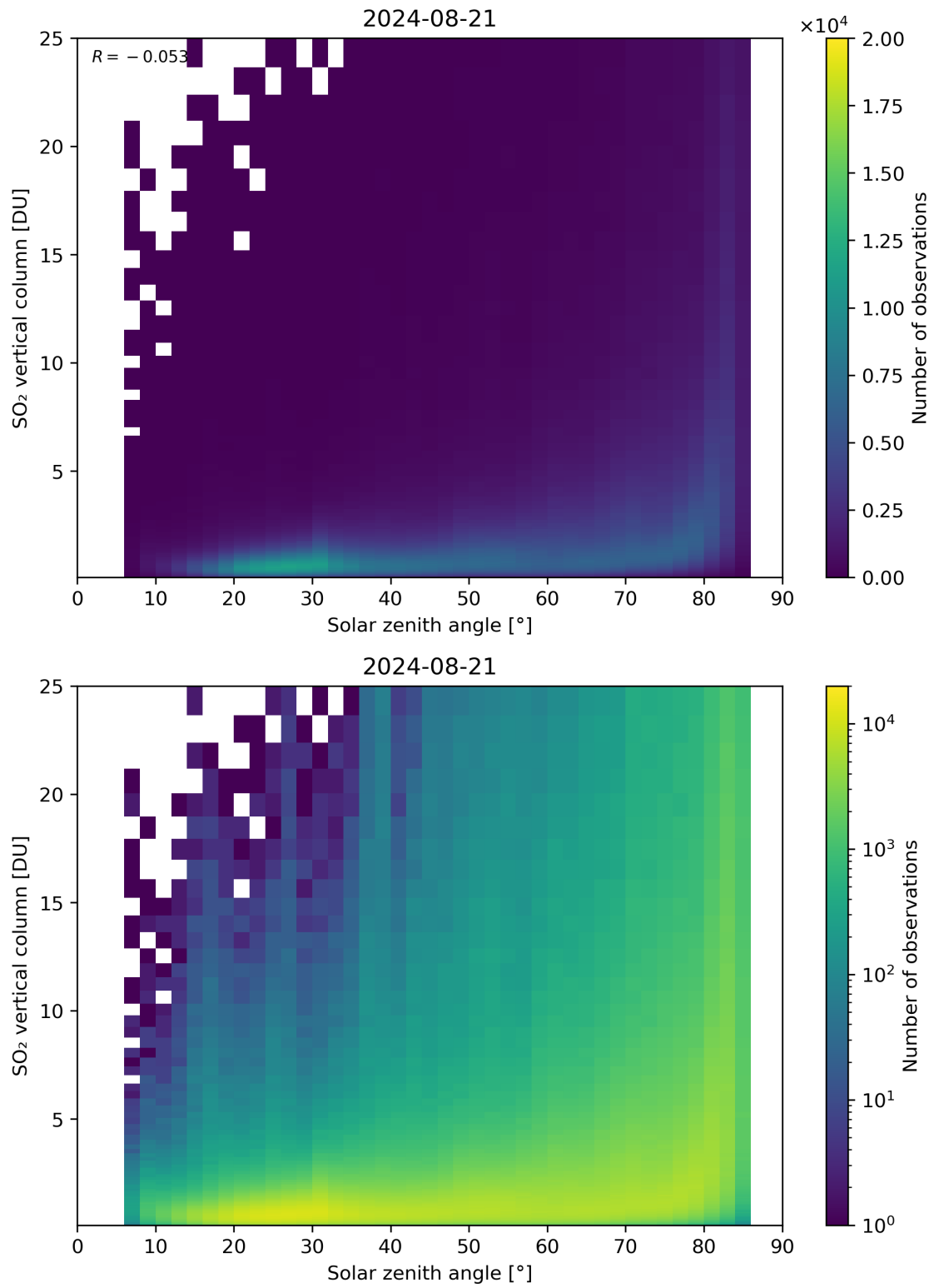
Figure 176: Scatter density plot of “Solar zenith angle” against “SO 2 vertical column” for 2024-08-21 to 2024-08-22.
