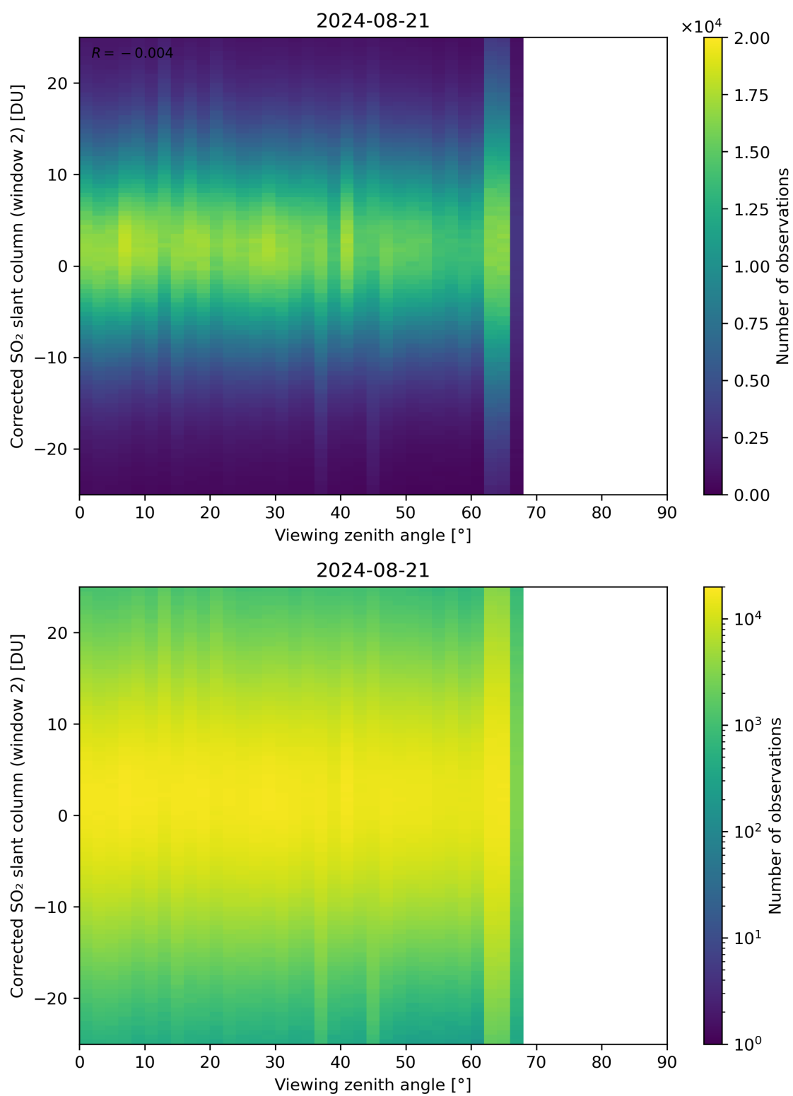
Figure 318: Scatter density plot of “Viewing zenith angle” against “Corrected SO 2 slant column (window 2)” for 2024-08-21 to 2024-08-22.
