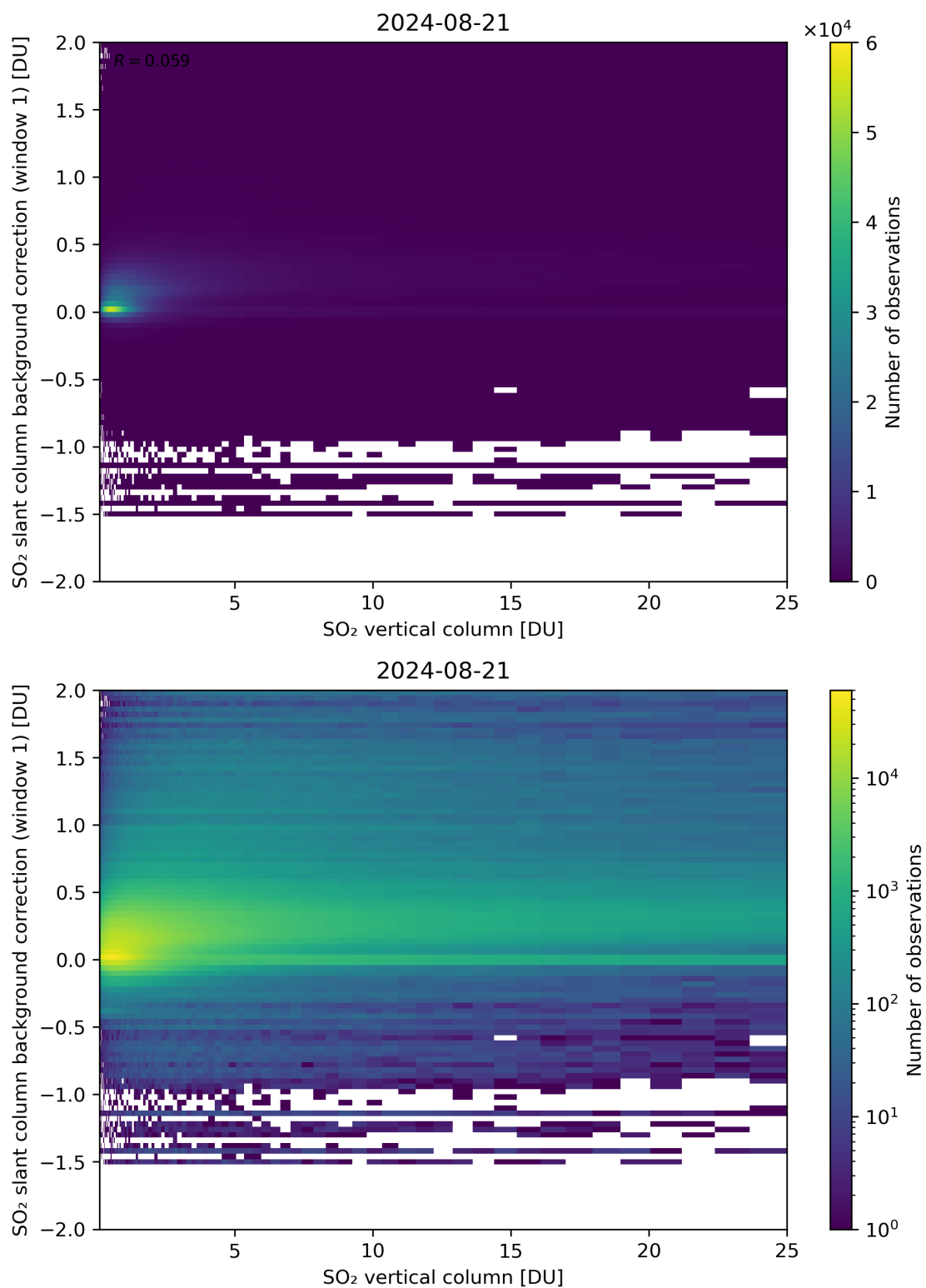
Figure 273: Scatter density plot of “SO 2 vertical column” against “SO 2 slant column background correction (window 1)” for 2024-08-21 to 2024-08-22.
