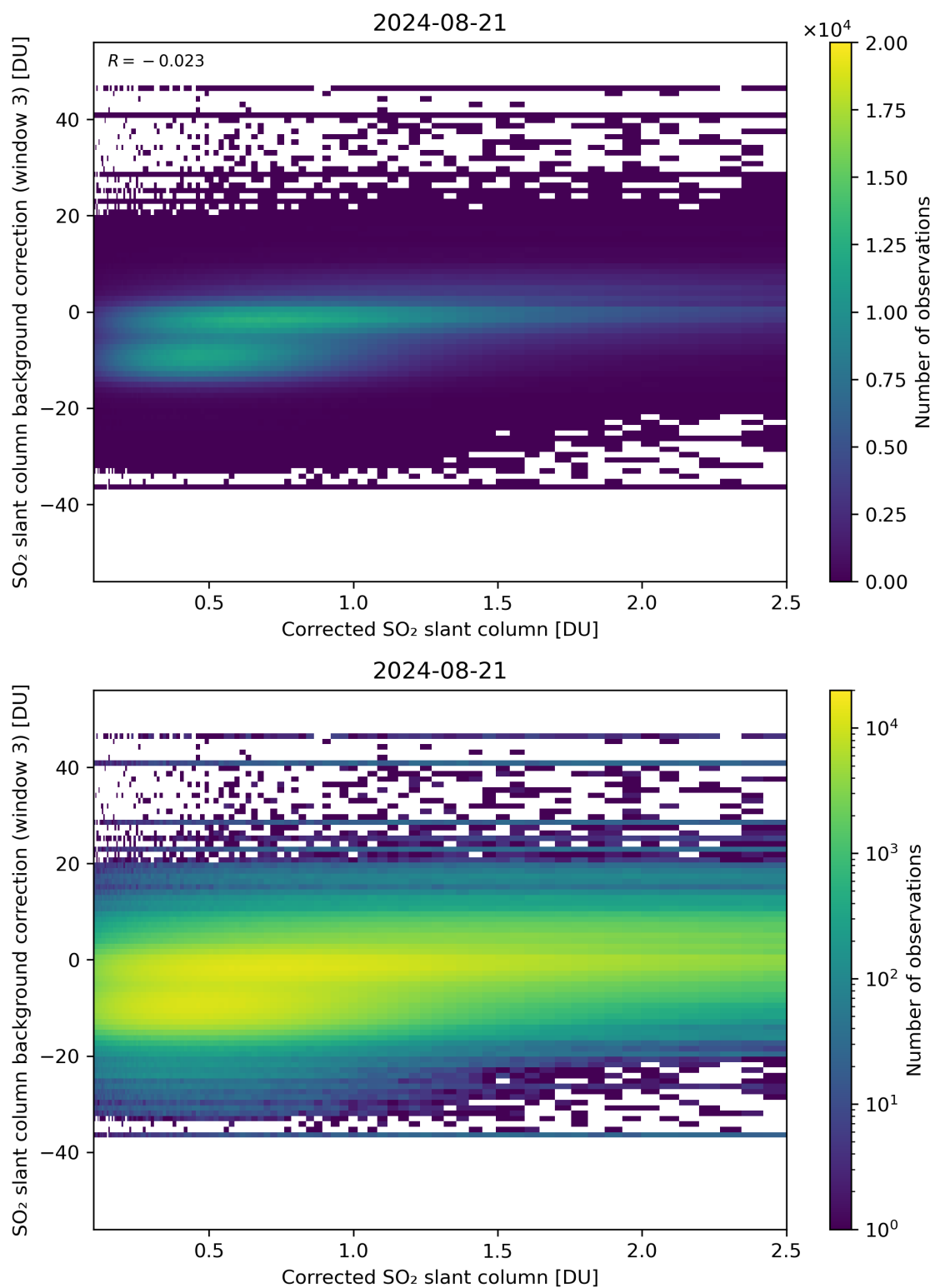
Figure 180: Scatter density plot of “Corrected SO 2 slant column” against “SO 2 slant column background correction (window 3)” for 2024-08-21 to 2024-08-22.
