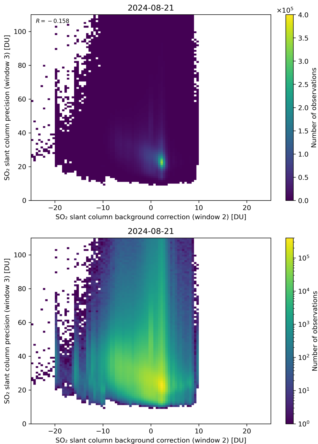
Figure 118: Scatter density plot of “SO 2 slant column background correction (window 2)” against “SO 2 slant column precision (window 3)” for 2024-08-21 to 2024-08-22.
