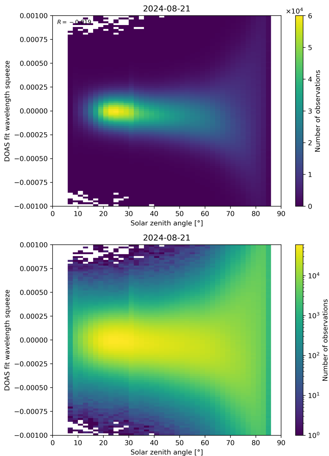
Figure 162: Scatter density plot of “Solar zenith angle” against “DOAS fit wavelength squeeze” for 2024-08-21 to 2024-08-22.
