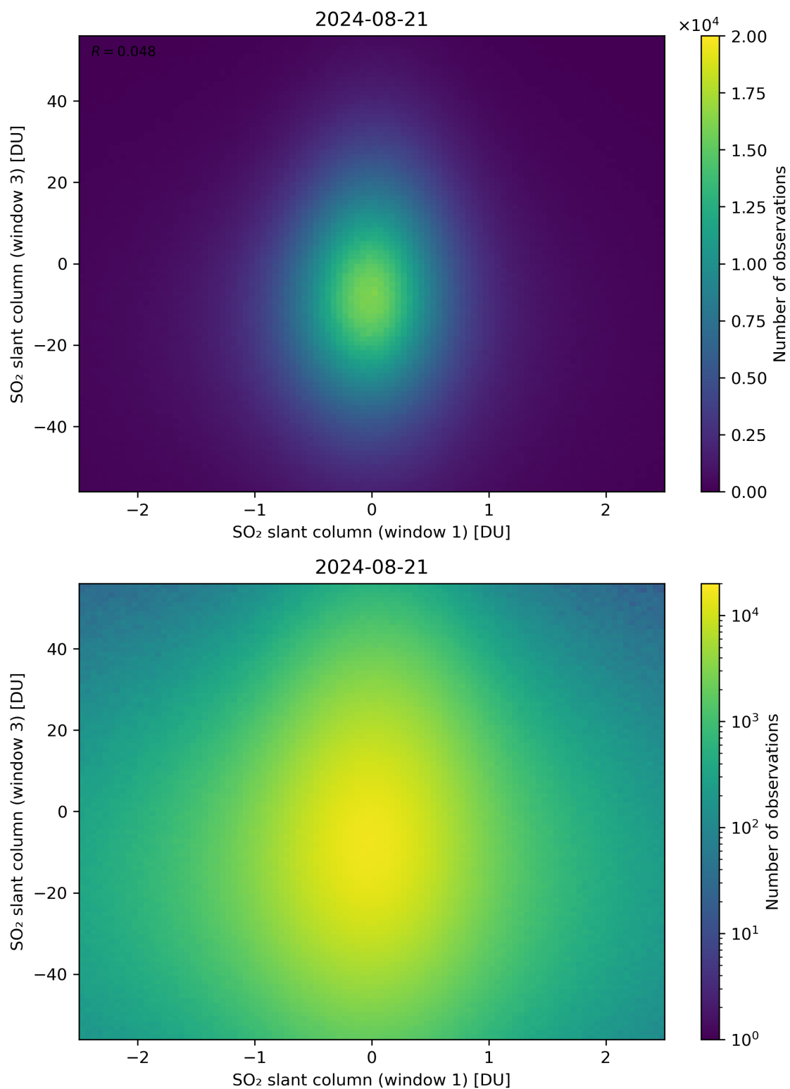
Figure 237: Scatter density plot of “SO 2 slant column (window 1)” against “SO 2 slant column (window 3)” for 2024-08-21 to 2024-08-22.
