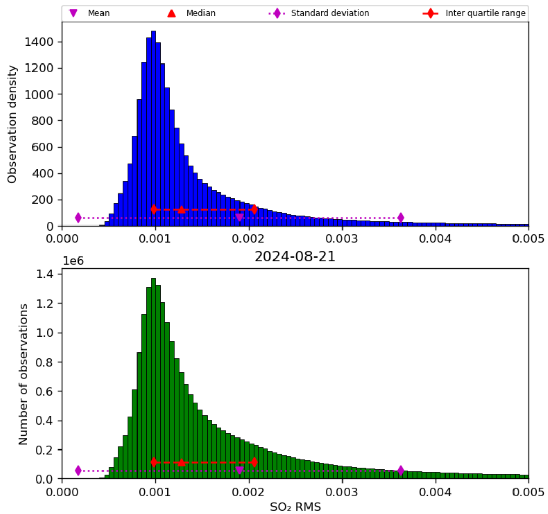
Figure 70: Histogram of “SO 2 RMS” for 2024-08-21 to 2024-08-22
