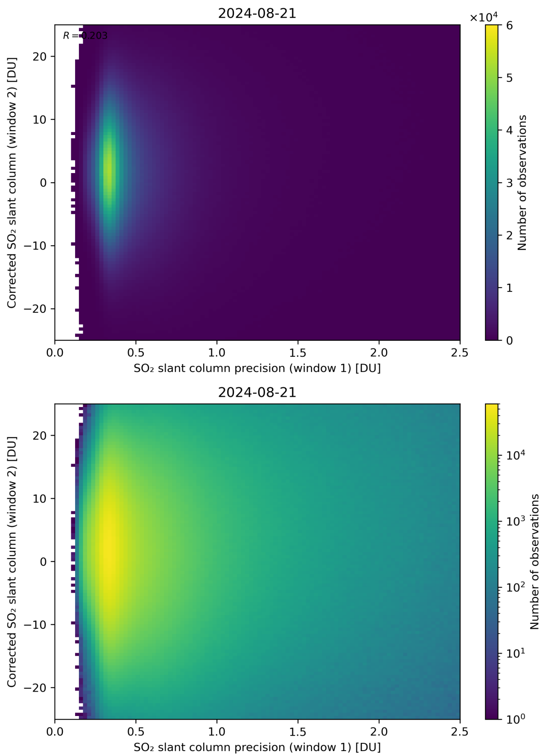
Figure 225: Scatter density plot of “SO 2 slant column precision (window 1)” against “Corrected SO 2 slant column (window 2)” for 2024-08-21 to 2024-08-22.
