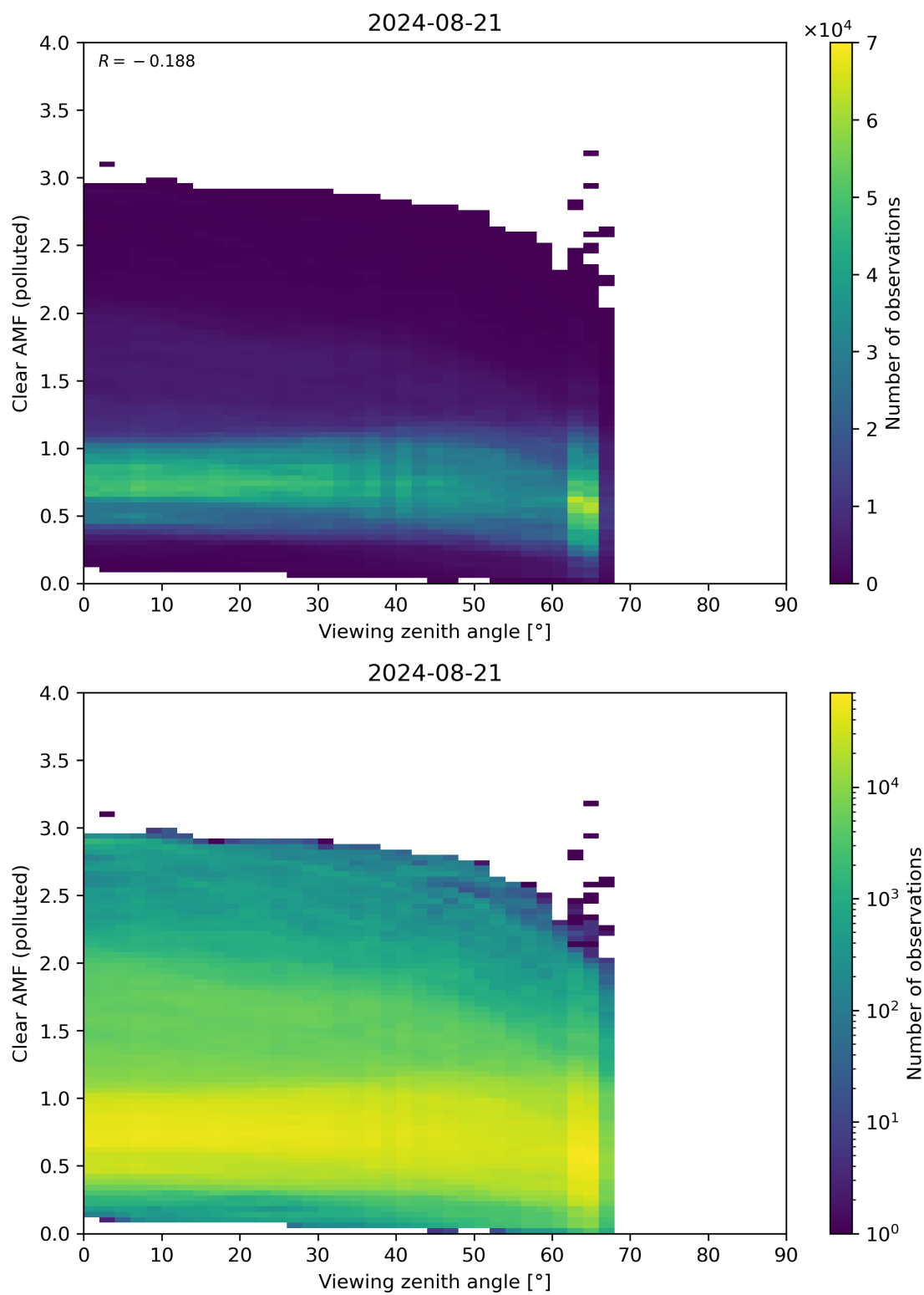
Figure 316: Scatter density plot of “Viewing zenith angle” against “Clear AMF (polluted)” for 2024-08-21 to 2024-08-22.
