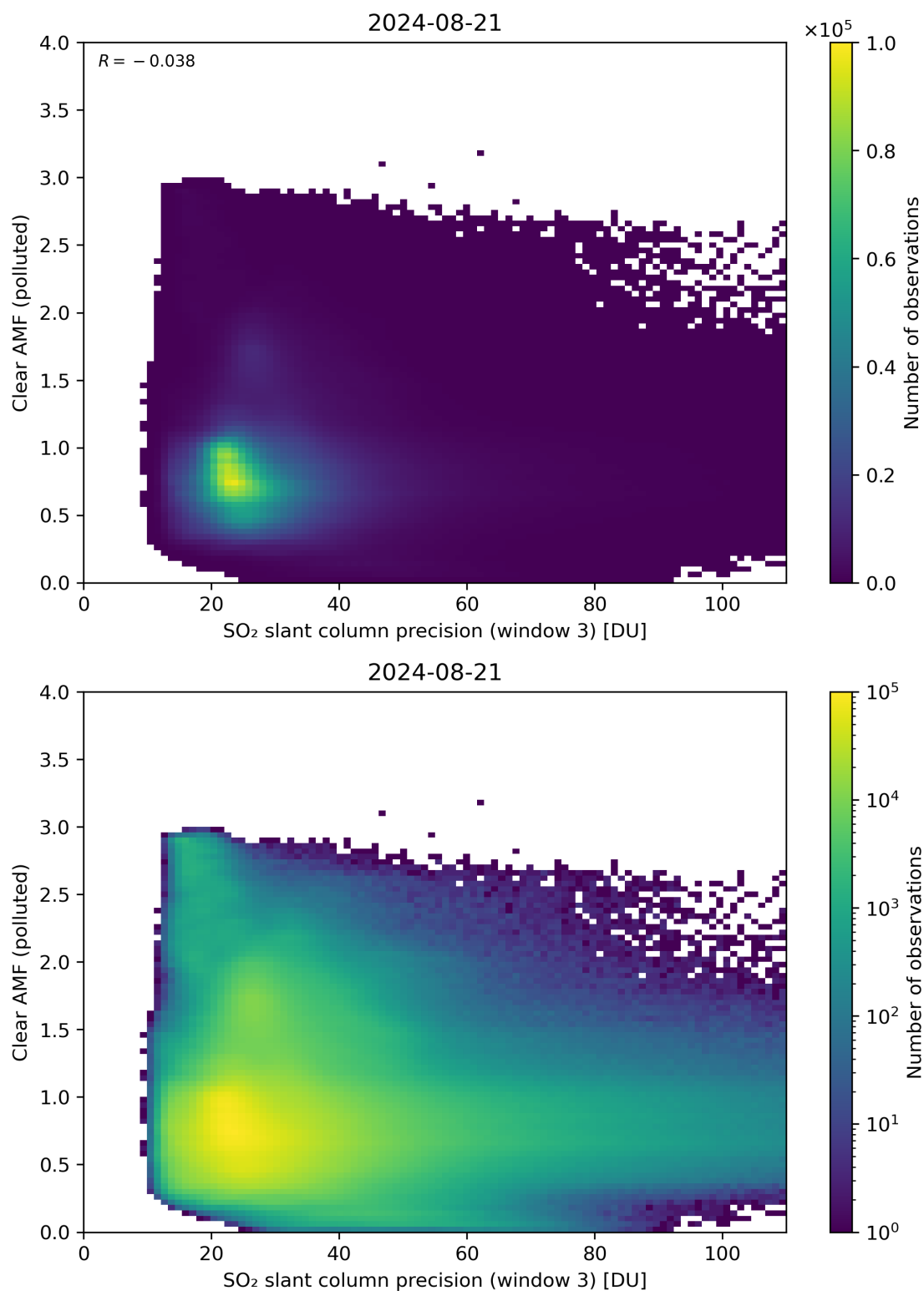
Figure 261: Scatter density plot of “SO 2 slant column precision (window 3)” against “Clear AMF (polluted)” for 2024-08-21 to 2024-08-22.
