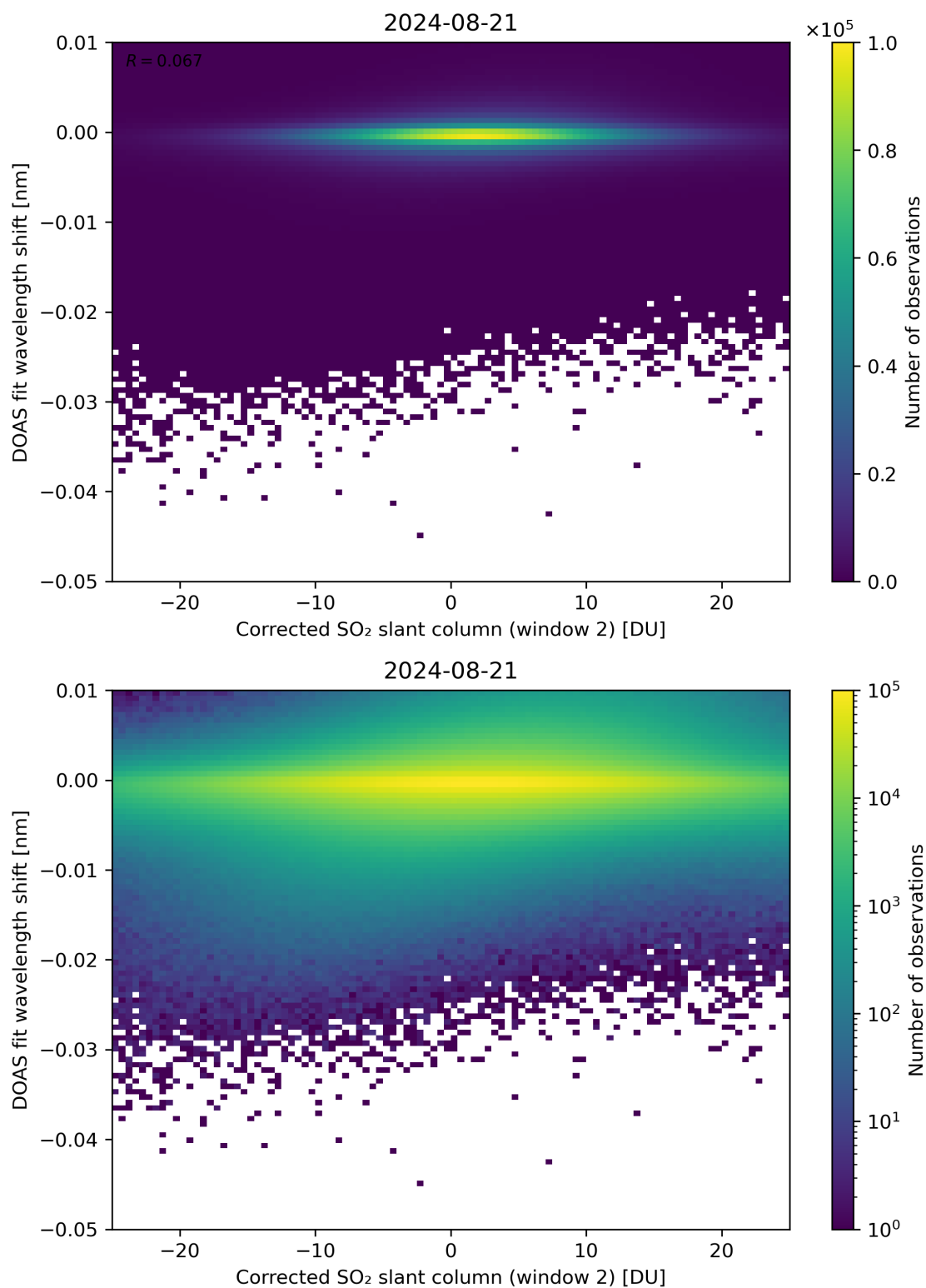
Figure 196: Scatter density plot of “Corrected SO 2 slant column (window 2)” against “DOAS fit wavelength shift” for 2024-08-21 to 2024-08-22.
