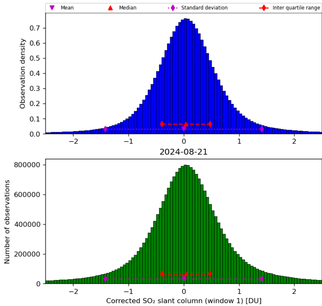
Figure 58: Histogram of “Corrected SO 2 slant column (window 1)” for 2024-08-21 to 2024-08-22
