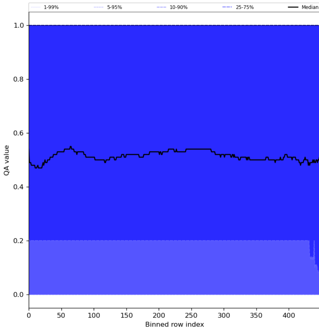
Figure 75: Along track statistics of “QA value” for 2024-08-21 to 2024-08-22
