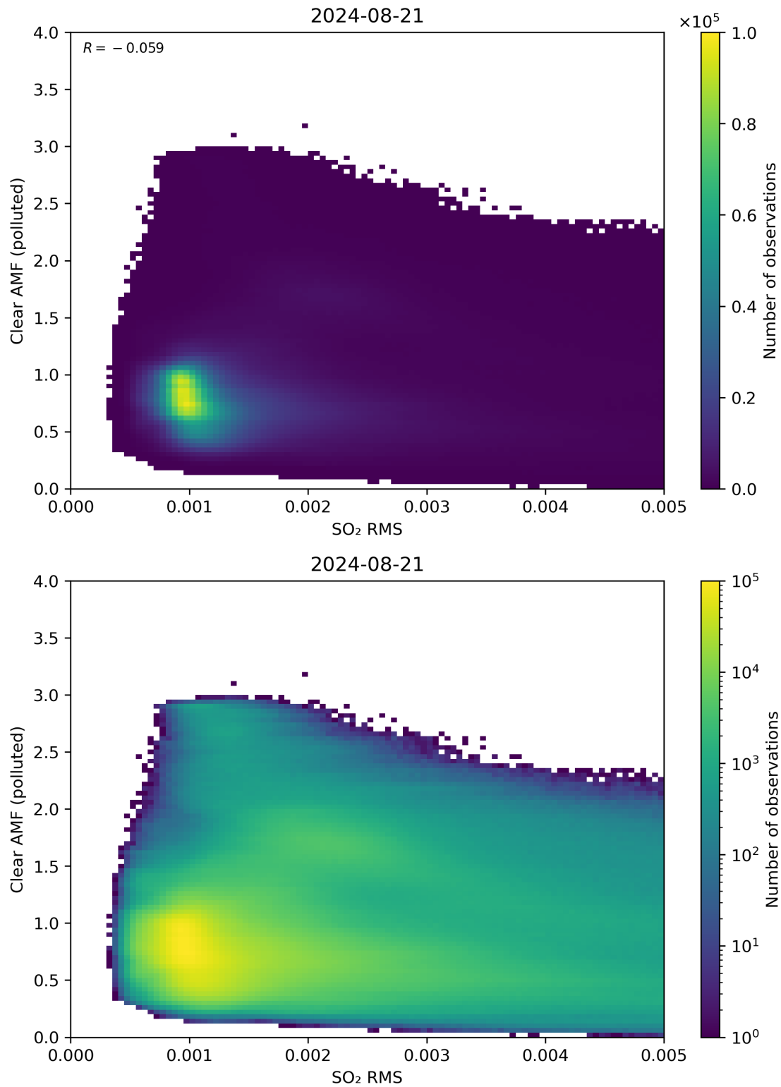
Figure 136: Scatter density plot of “SO 2 RMS” against “Clear AMF (polluted)” for 2024-08-21 to 2024-08-22.
