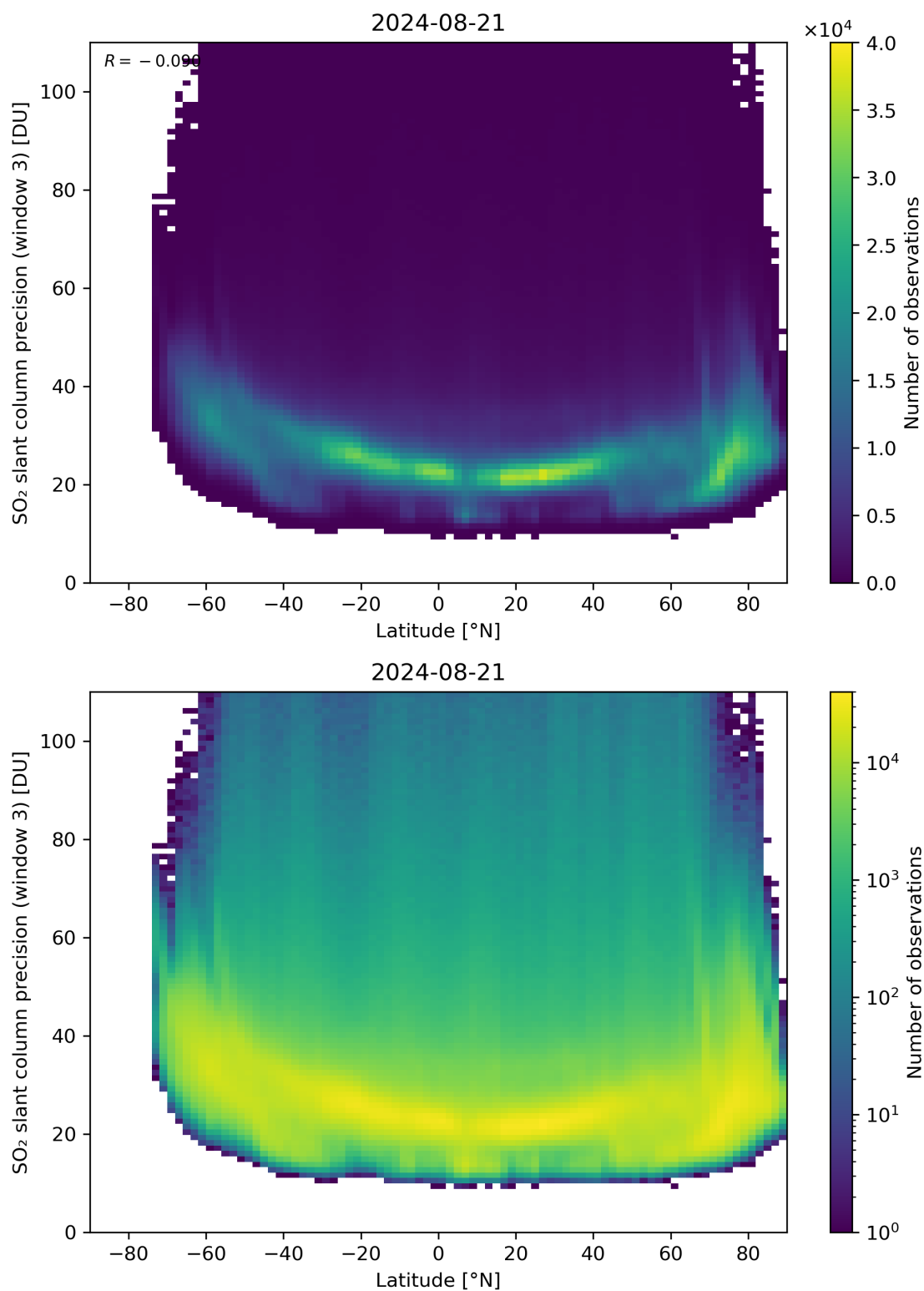
Figure 153: Scatter density plot of “Latitude” against “SO 2 slant column precision (window 3)” for 2024-08-21 to 2024-08-22.
