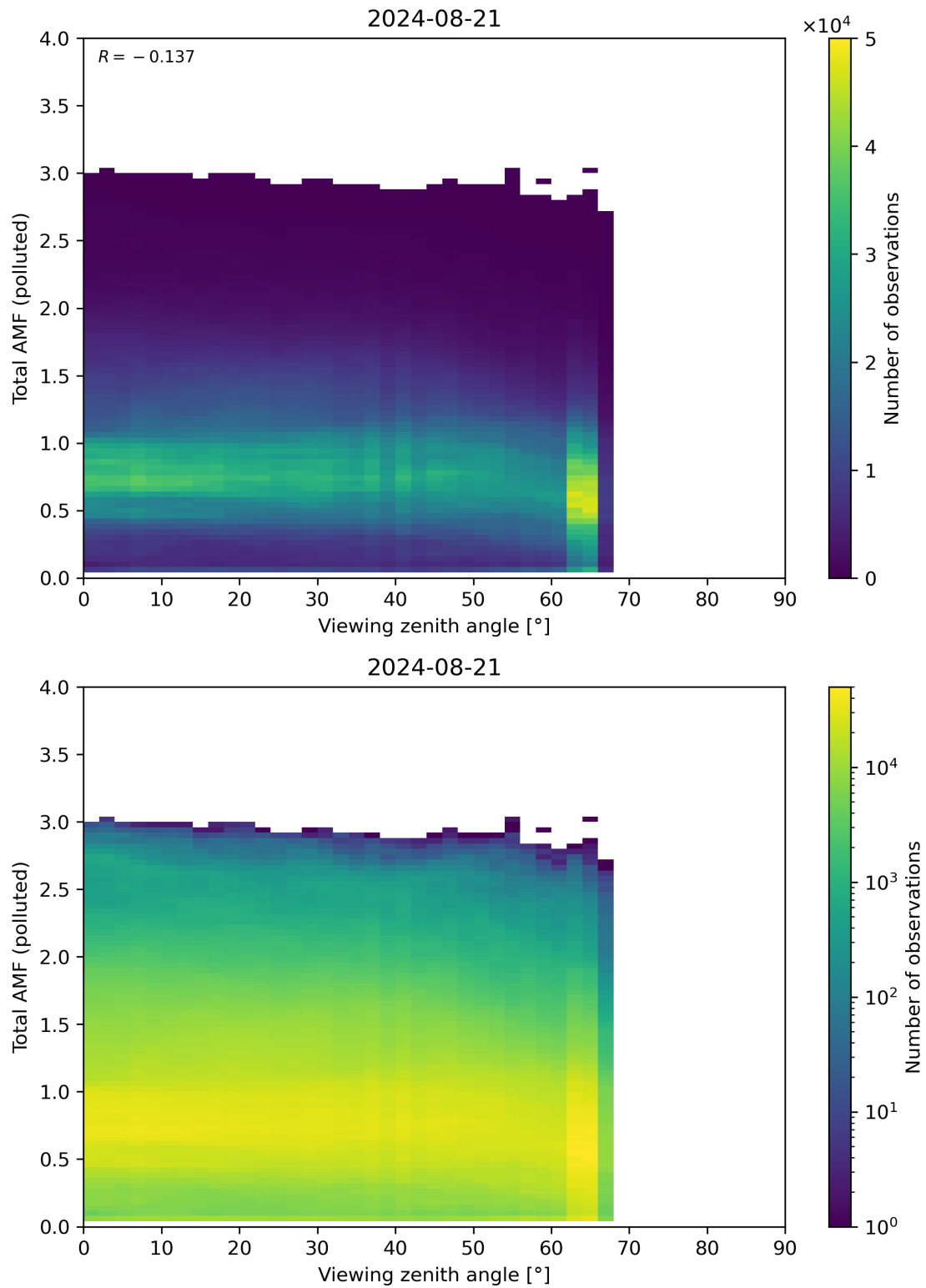
Figure 325: Scatter density plot of “Viewing zenith angle” against “Total AMF (polluted)” for 2024-08-21 to 2024-08-22.
