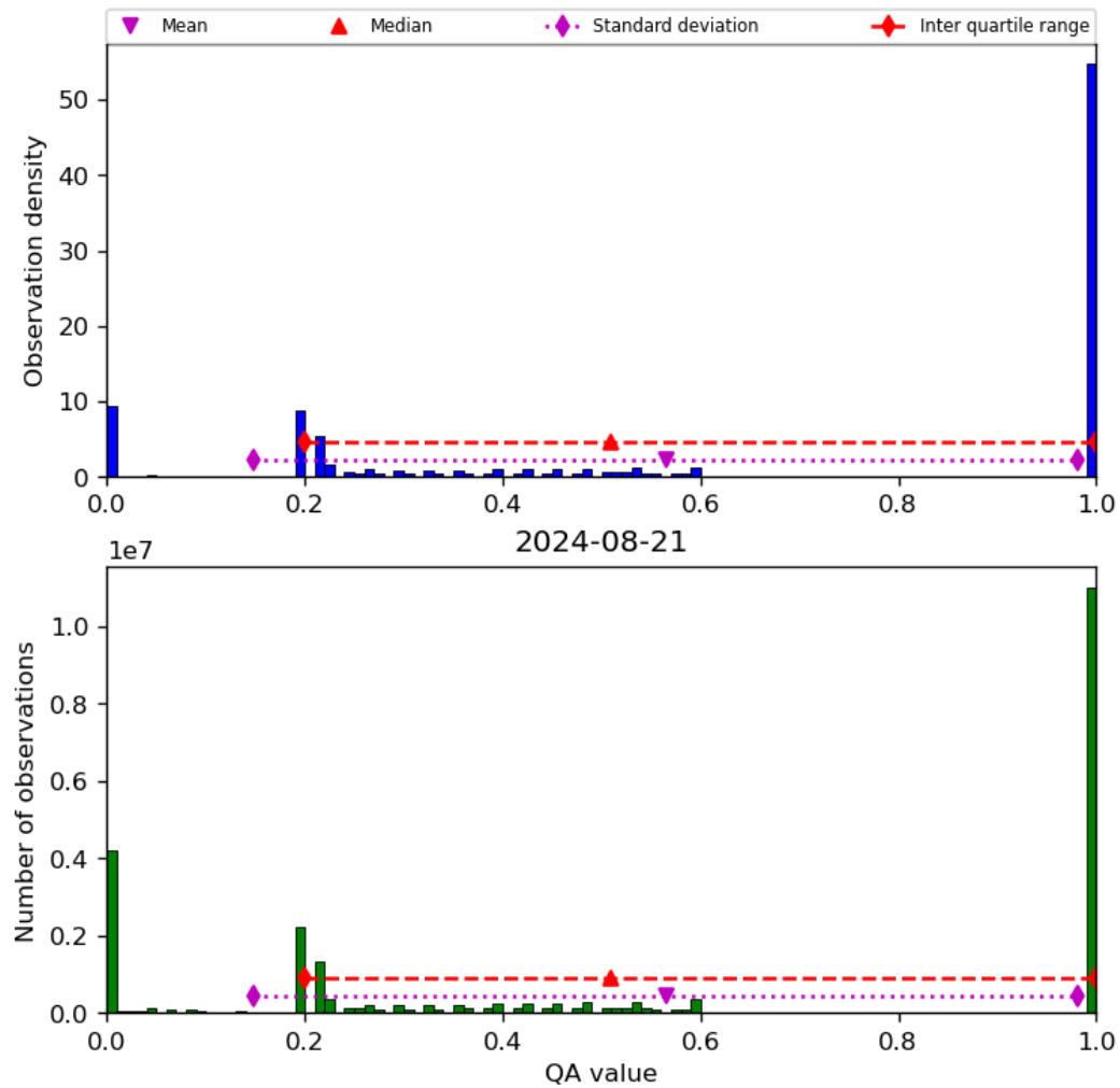
Figure 52: Histogram of “QA value” for 2024-08-21 to 2024-08-22
