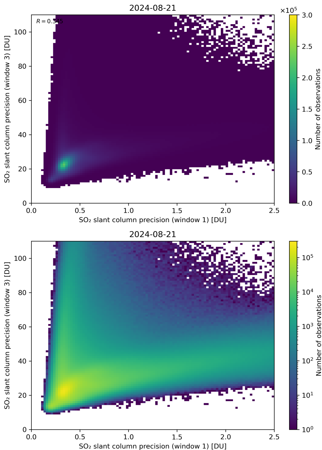
Figure 229: Scatter density plot of “SO 2 slant column precision (window 1)” against “SO 2 slant column precision (window 3)” for 2024-08-21 to 2024-08-22.
