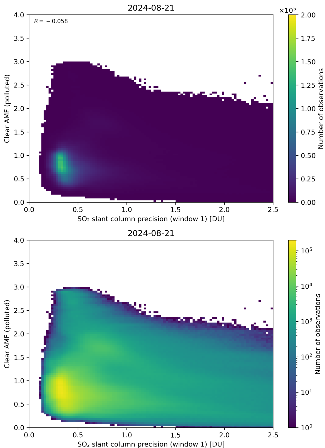
Figure 224: Scatter density plot of “SO 2 slant column precision (window 1)” against “Clear AMF (polluted)” for 2024-08-21 to 2024-08-22.
