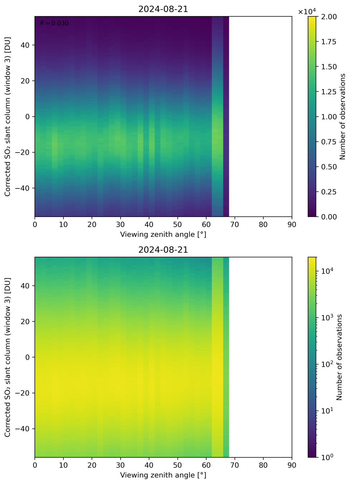
Figure 319: Scatter density plot of “Viewing zenith angle” against “Corrected SO 2 slant column (window 3)” for 2024-08-21 to 2024-08-22.
