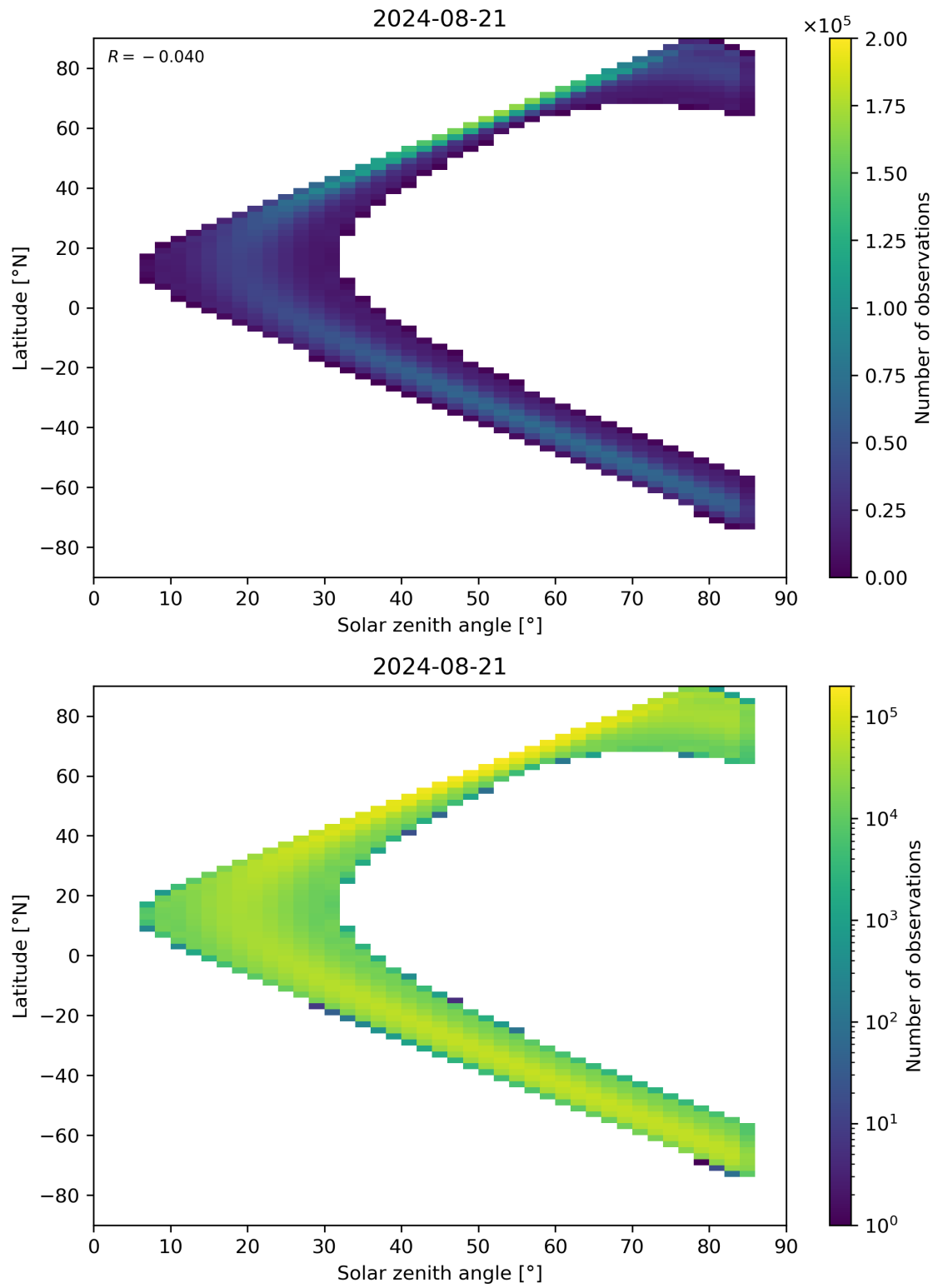
Figure 164: Scatter density plot of “Solar zenith angle” against “Latitude” for 2024-08-21 to 2024-08-22.
