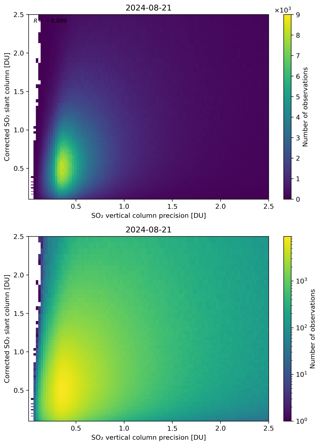
Figure 286: Scatter density plot of “SO 2 vertical column precision” against “Corrected SO 2 slant column” for 2024-08-21 to 2024-08-22.
