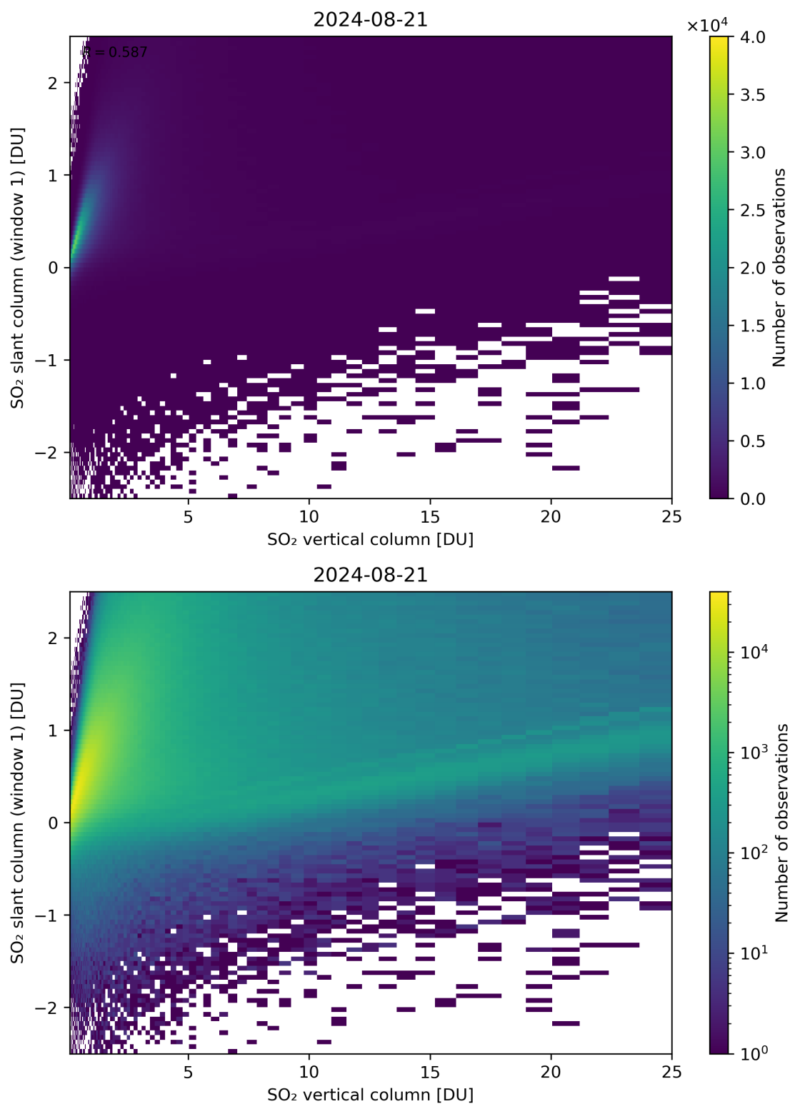
Figure 300: Scatter density plot of “SO 2 vertical column” against “SO 2 slant column (window 1)” for 2024-08-21 to 2024-08-22.
