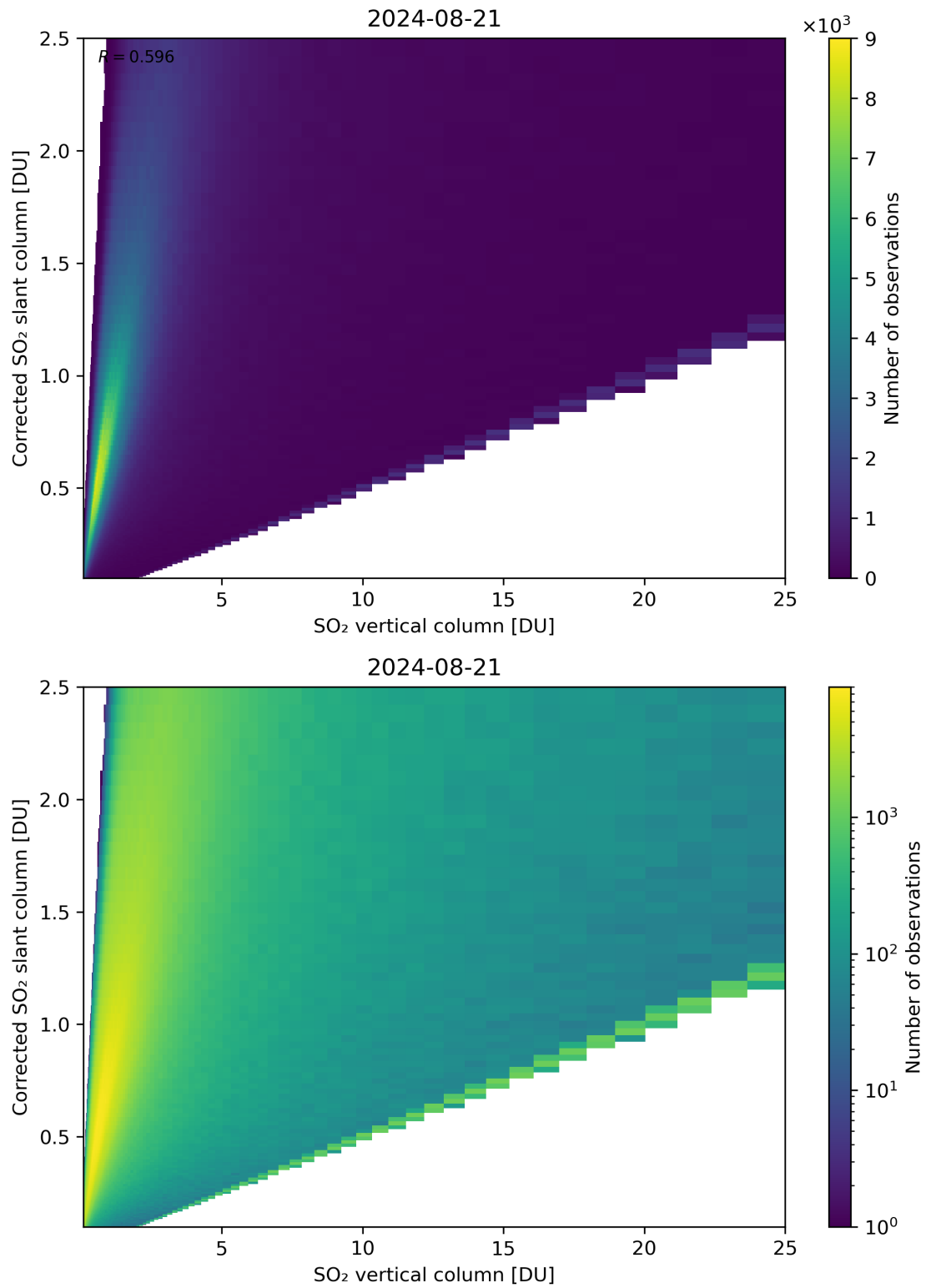
Figure 297: Scatter density plot of “SO 2 vertical column” against “Corrected SO 2 slant column” for 2024-08-21 to 2024-08-22.
