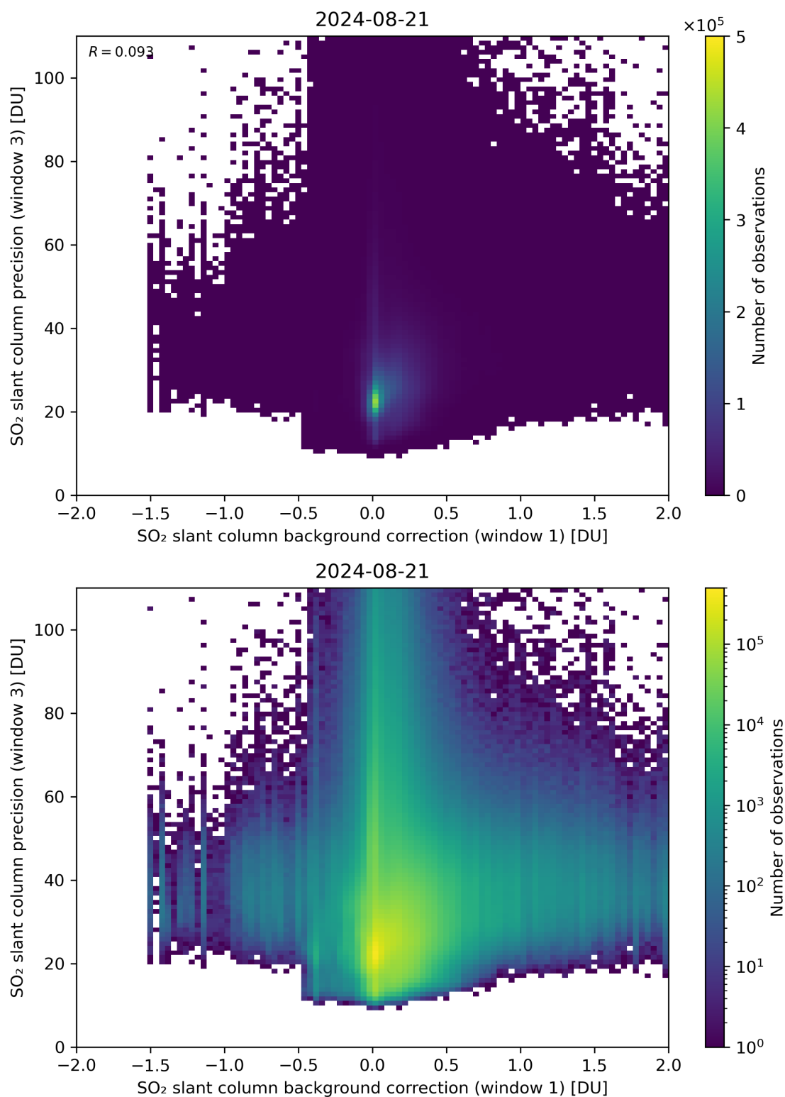
Figure 108: Scatter density plot of “SO 2 slant column background correction (window 1)” against “SO 2 slant column precision (window 3)” for 2024-08-21 to 2024-08-22.
