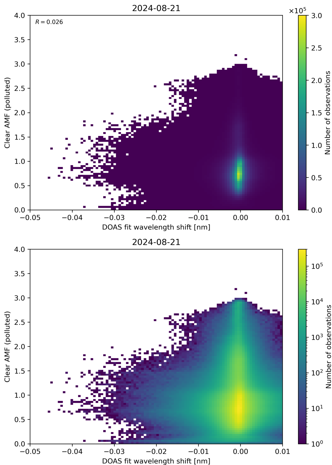
Figure 129: Scatter density plot of “DOAS fit wavelength shift” against “Clear AMF (polluted)” for 2024-08-21 to 2024-08-22.
