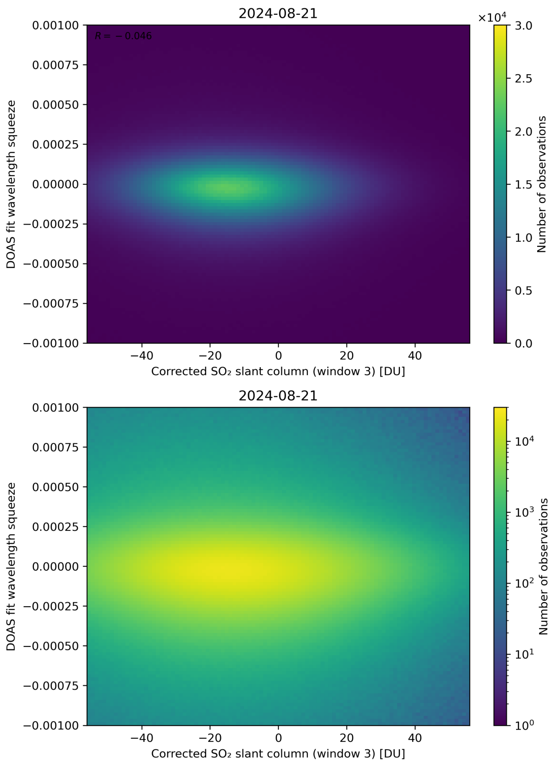
Figure 207: Scatter density plot of “Corrected SO 2 slant column (window 3)” against “DOAS fit wavelength squeeze” for 2024-08-21 to 2024-08-22.
