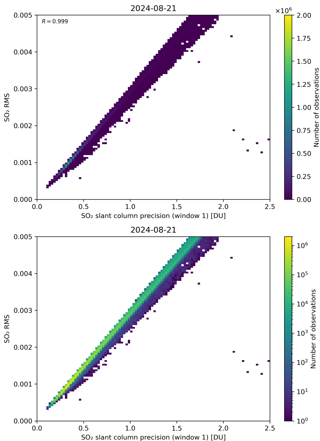
Figure 223: Scatter density plot of “SO 2 slant column precision (window 1)” against “SO 2 RMS” for 2024-08-21 to 2024-08-22.
