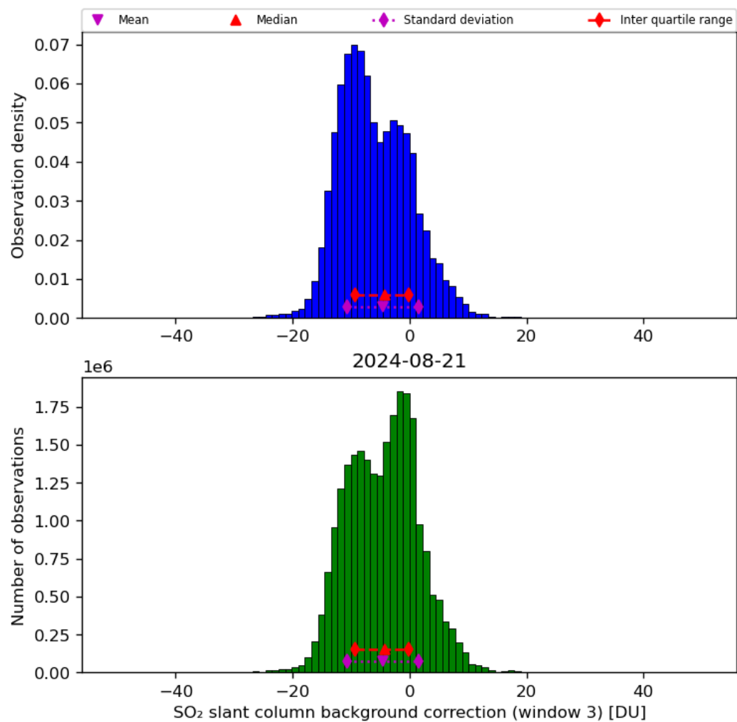
Figure 67: Histogram of “SO 2 slant column background correction (window 3)” for 2024-08-21 to 2024-08-22
