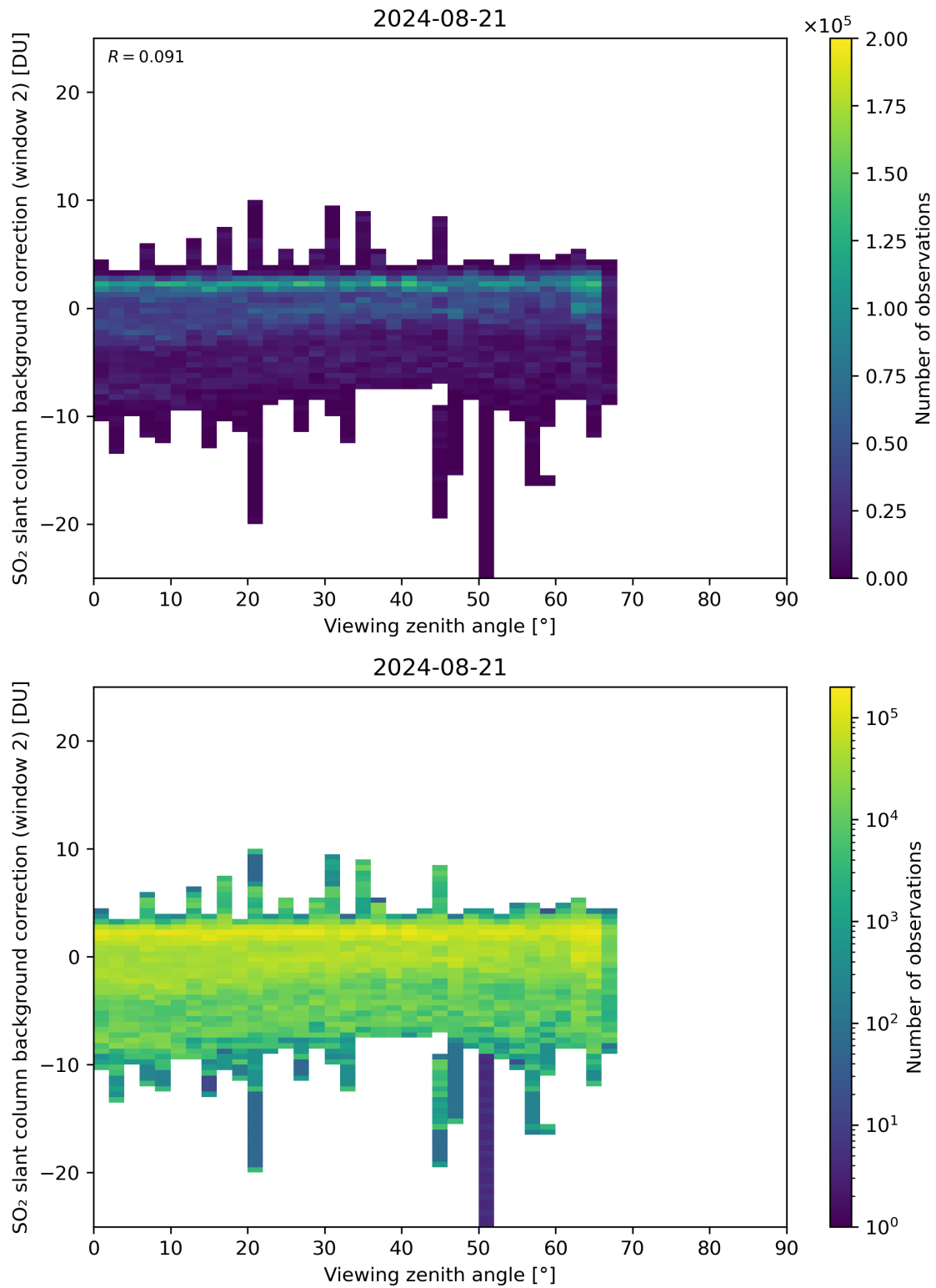
Figure 309: Scatter density plot of “Viewing zenith angle” against “SO 2 slant column background correction (window 2)” for 2024-08-21 to 2024-08-22.
