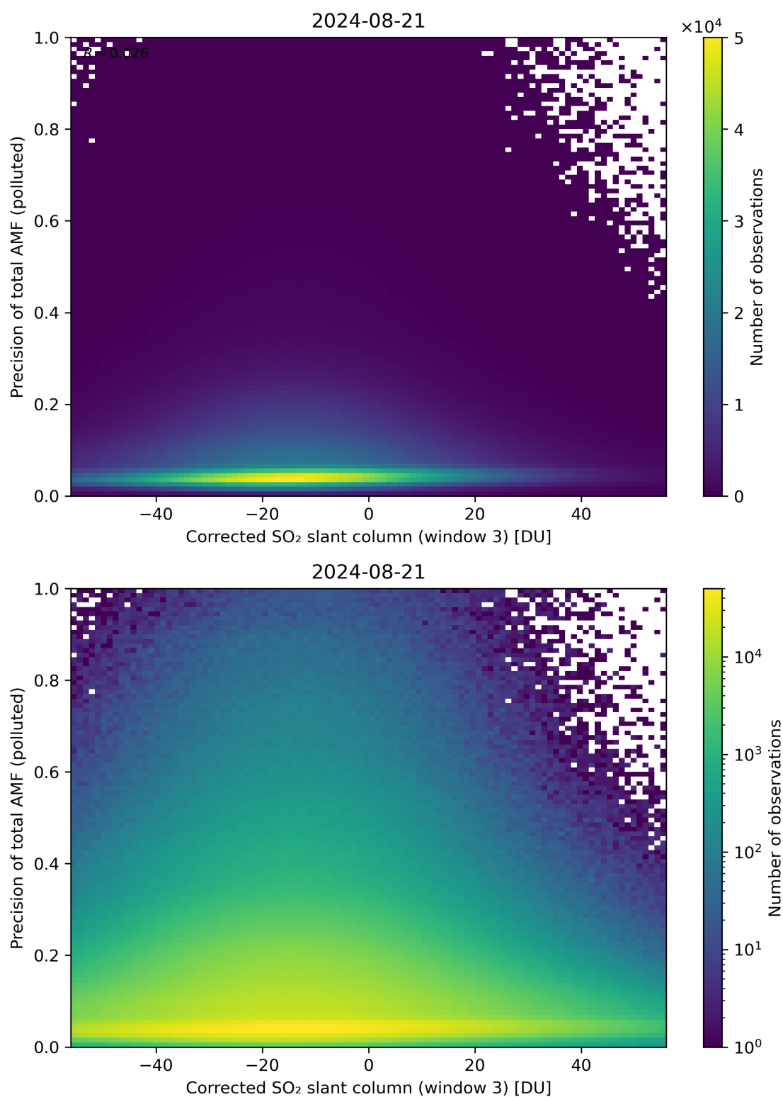
Figure 211: Scatter density plot of “Corrected SO 2 slant column (window 3)” against “Precision of total AMF (polluted)” for 2024-08-21 to 2024-08-22.
