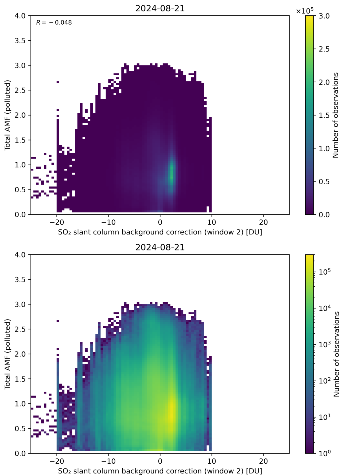
Figure 119: Scatter density plot of “SO 2 slant column background correction (window 2)” against “Total AMF (polluted)” for 2024-08-21 to 2024-08-22.
