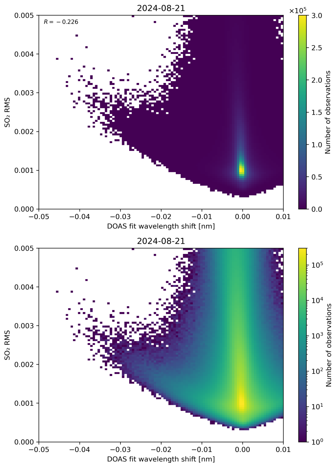
Figure 128: Scatter density plot of “DOAS fit wavelength shift” against “SO 2 RMS” for 2024-08-21 to 2024-08-22.
