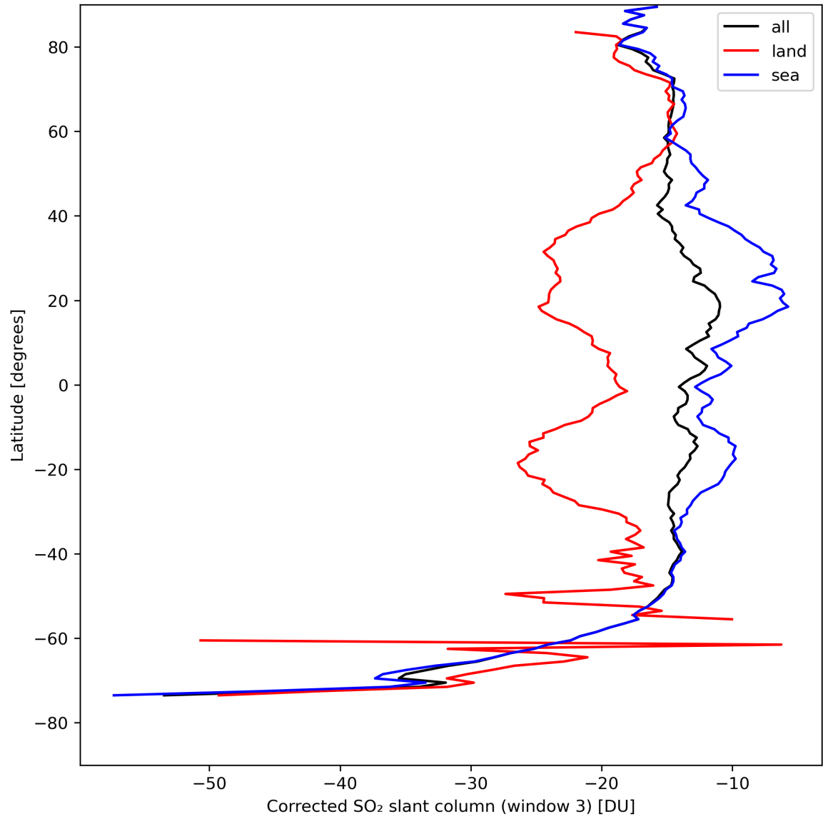
Figure 43: Zonal average of “Corrected SO 2 slant column (window 3)” for 2024-08-21 to 2024-08-22.
