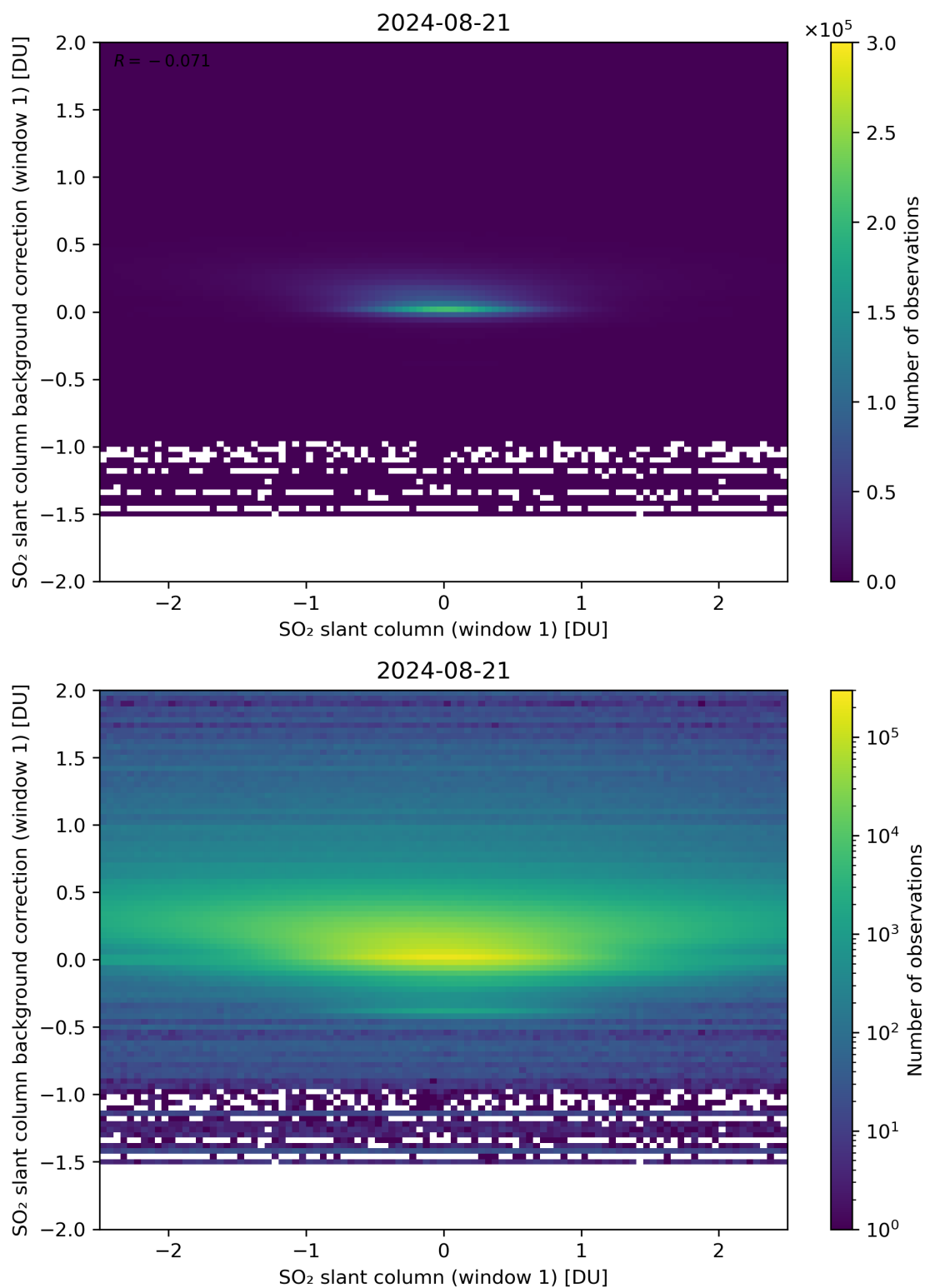
Figure 212: Scatter density plot of “SO 2 slant column (window 1)” against “SO 2 slant column background correction (window 1)” for 2024-08-21 to 2024-08-22.
