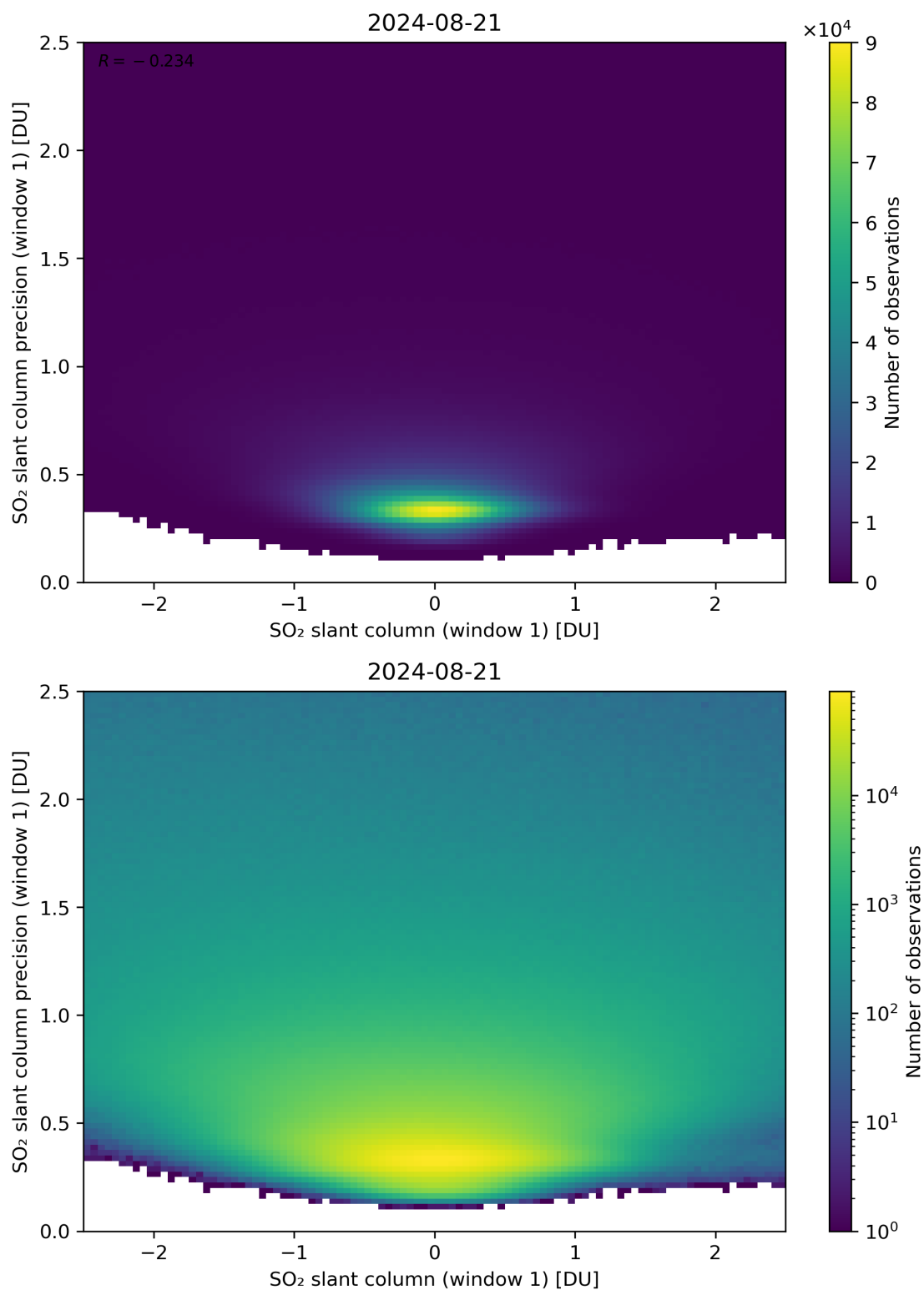
Figure 235: Scatter density plot of “SO 2 slant column (window 1)” against “SO 2 slant column precision (window 1)” for 2024-08-21 to 2024-08-22.
