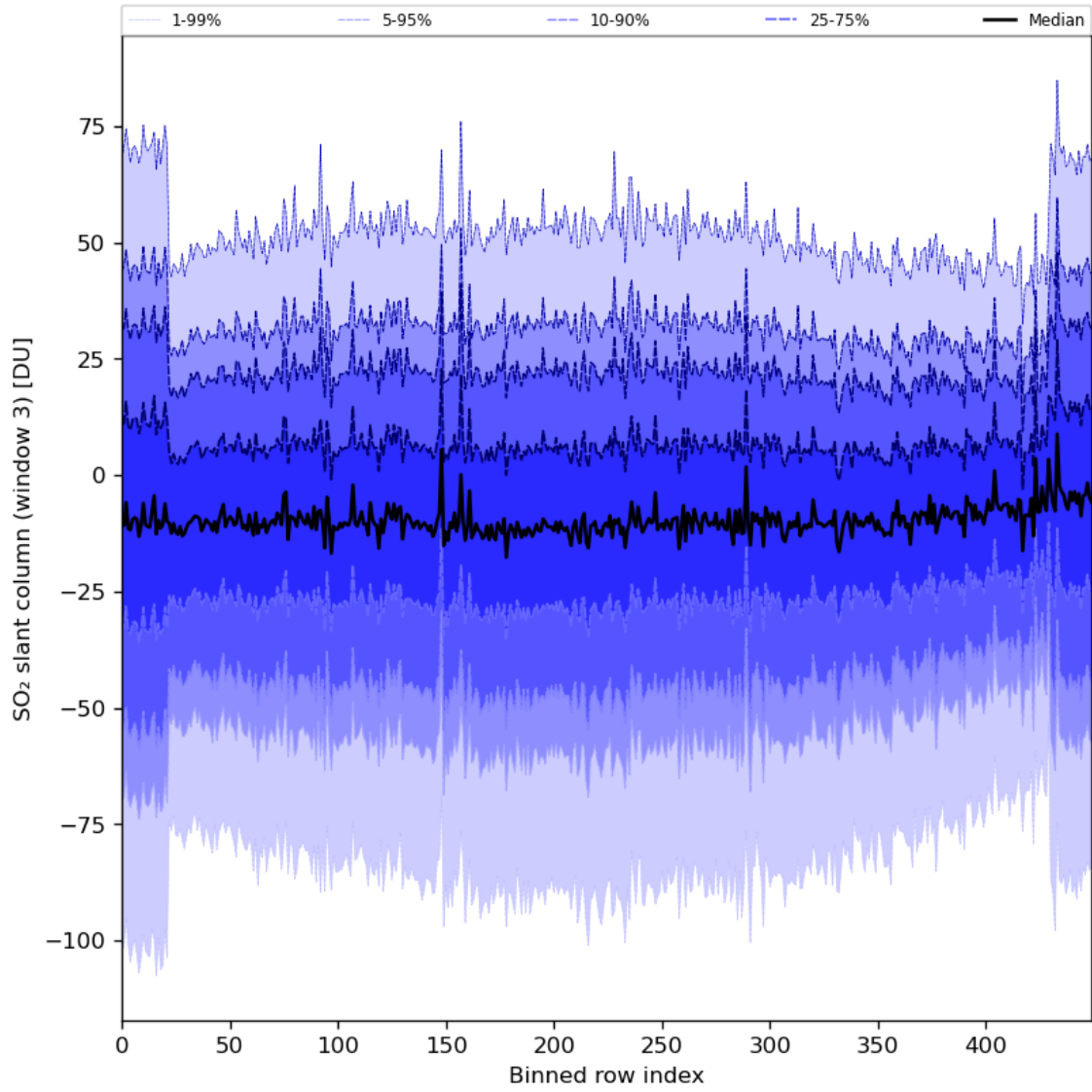
Figure 87: Along track statistics of "SO 2 slant column (window 3)" for 2024-08-21 to 2024-08-22
