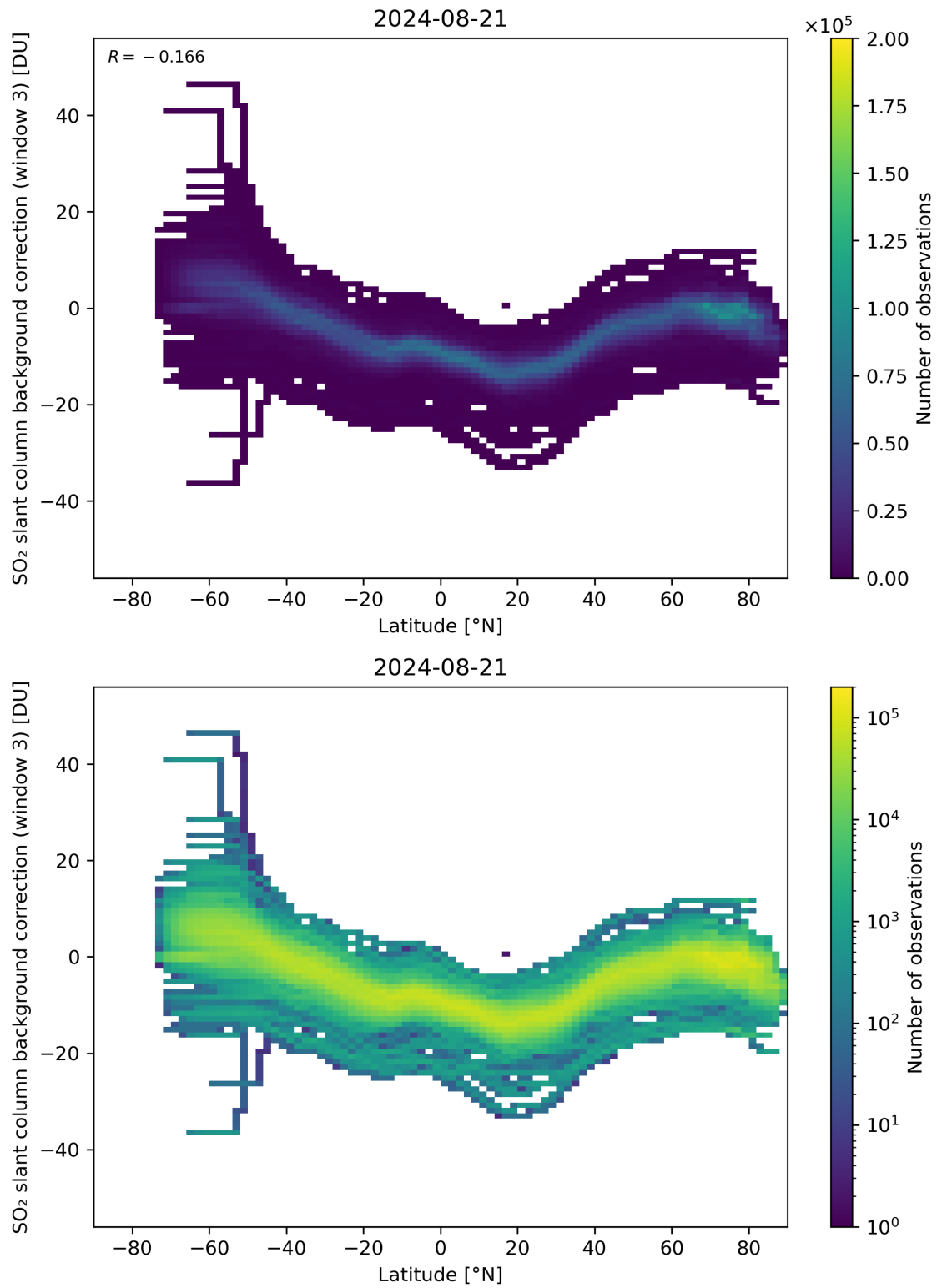
Figure 141: Scatter density plot of “Latitude” against “SO 2 slant column background correction (window 3)” for 2024-08-21 to 2024-08-22.
