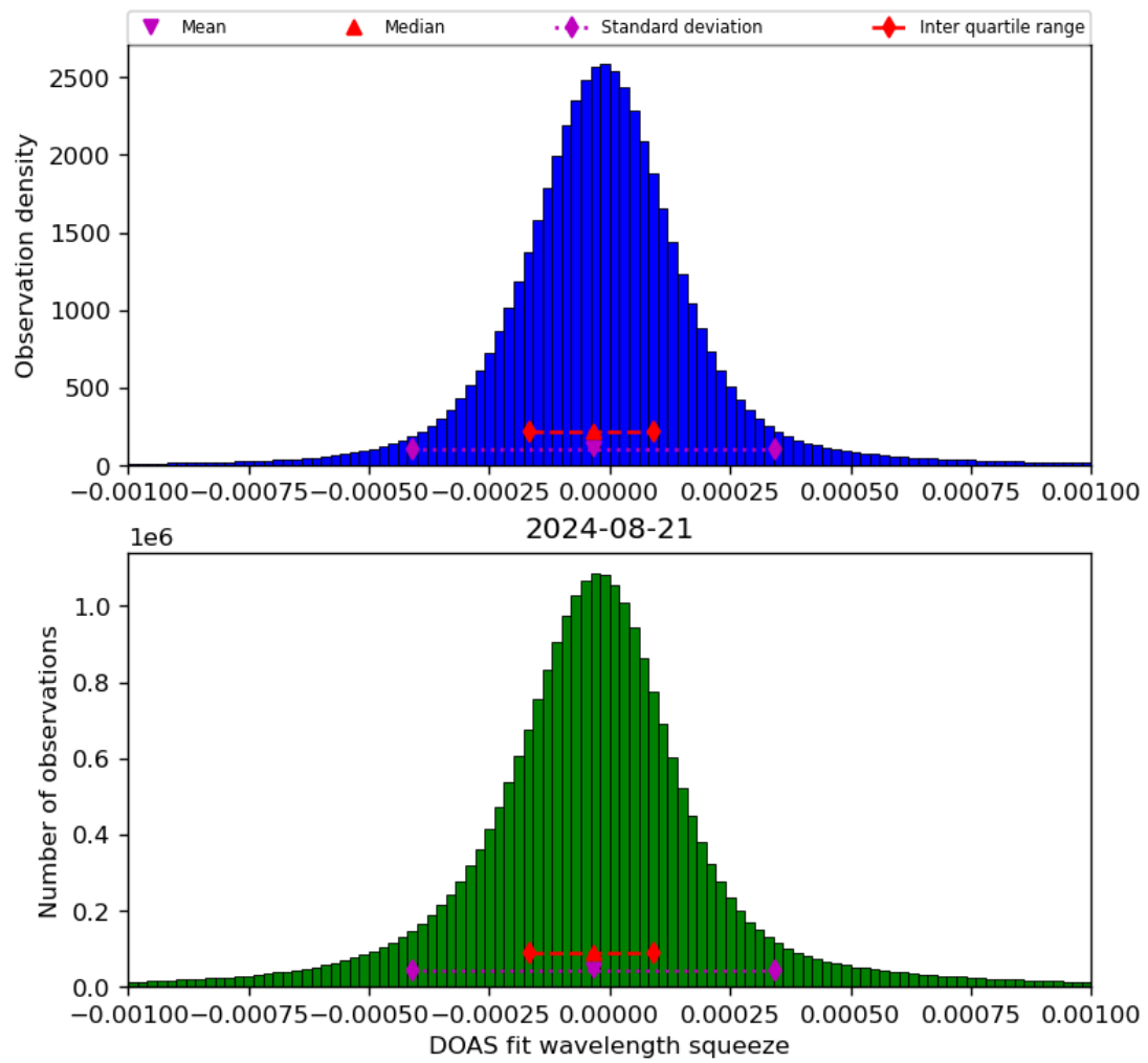
Figure 69: Histogram of “DOAS fit wavelength squeeze” for 2024-08-21 to 2024-08-22
