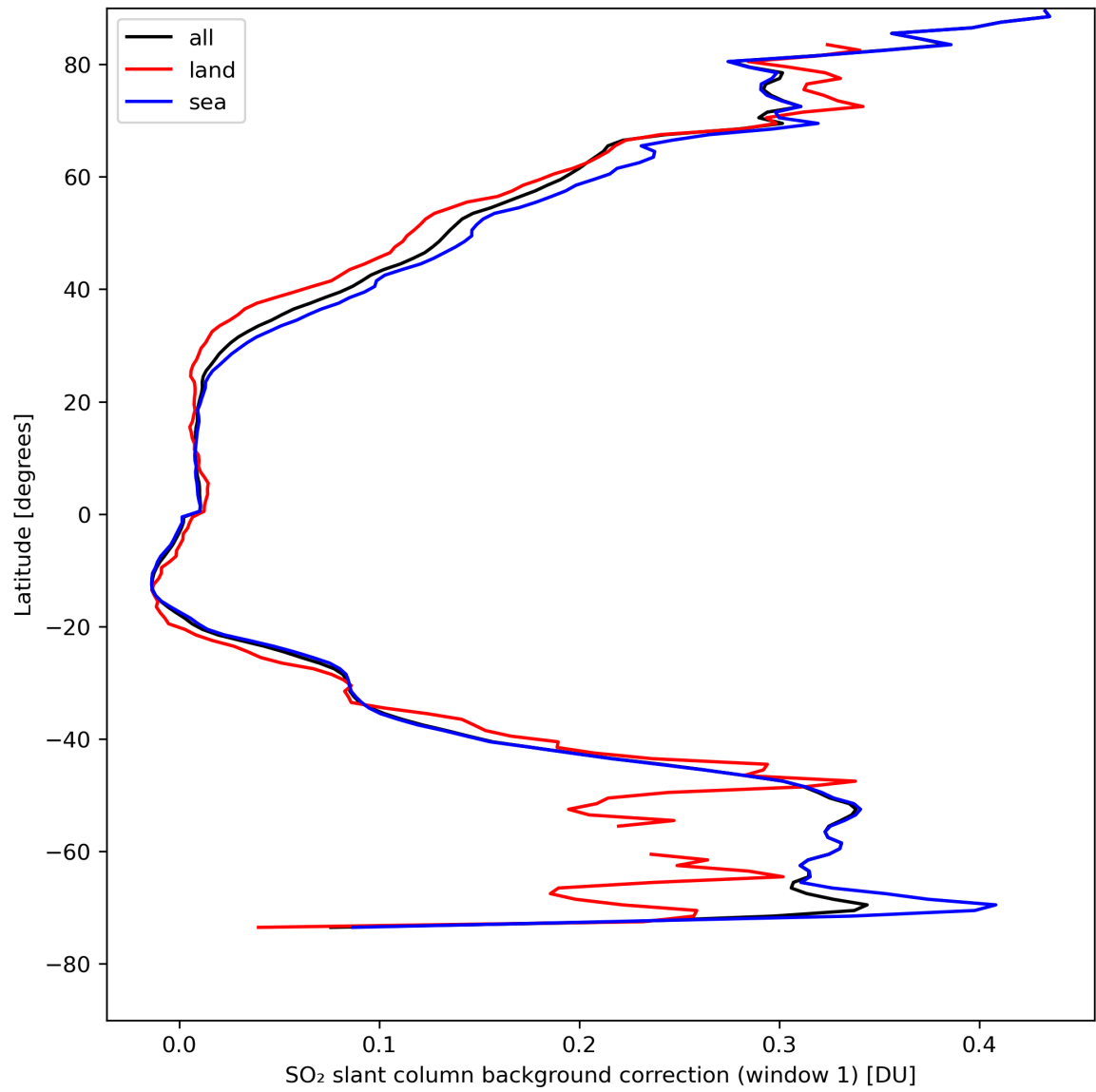
Figure 36: Zonal average of “SO 2 slant column background correction (window 1)” for 2024-08-21 to 2024-08-22.
