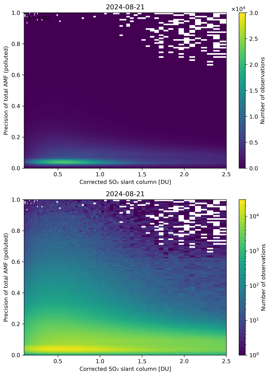
Figure 193: Scatter density plot of “Corrected SO 2 slant column” against “Precision of total AMF (polluted)” for 2024-08-21 to 2024-08-22.
