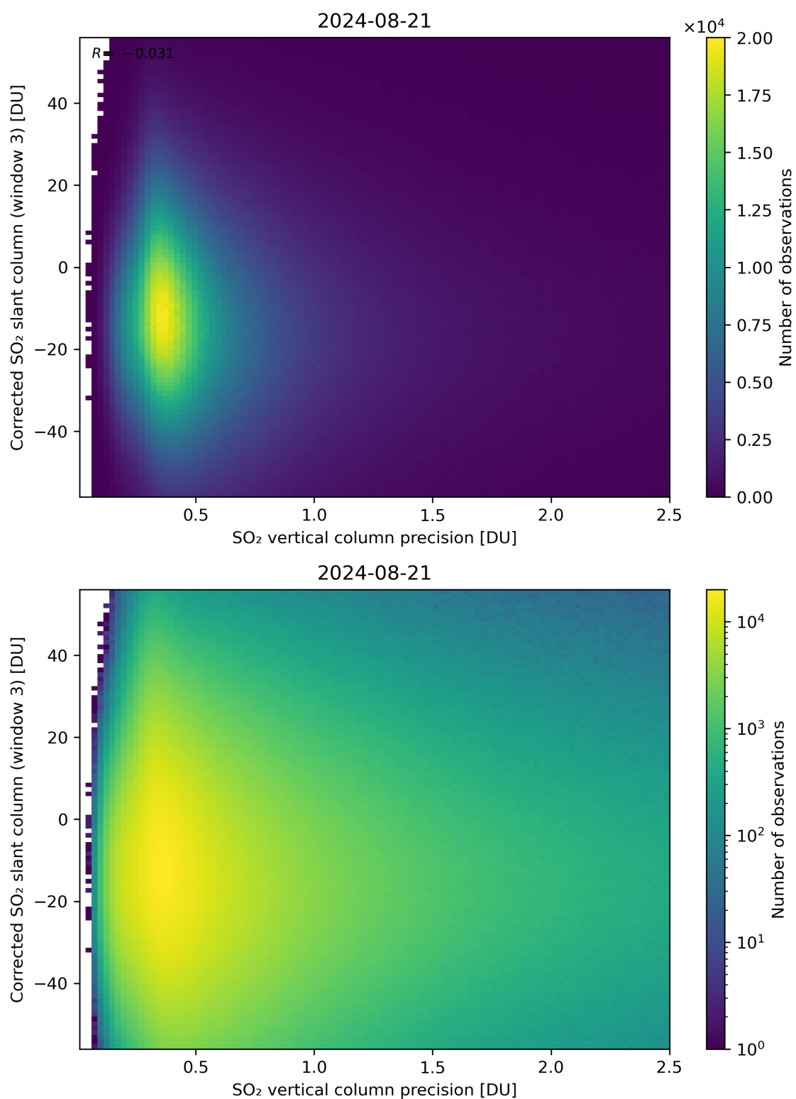
Figure 288: Scatter density plot of “SO 2 vertical column precision” against “Corrected SO 2 slant column (window 3)” for 2024-08-21 to 2024-08-22.
