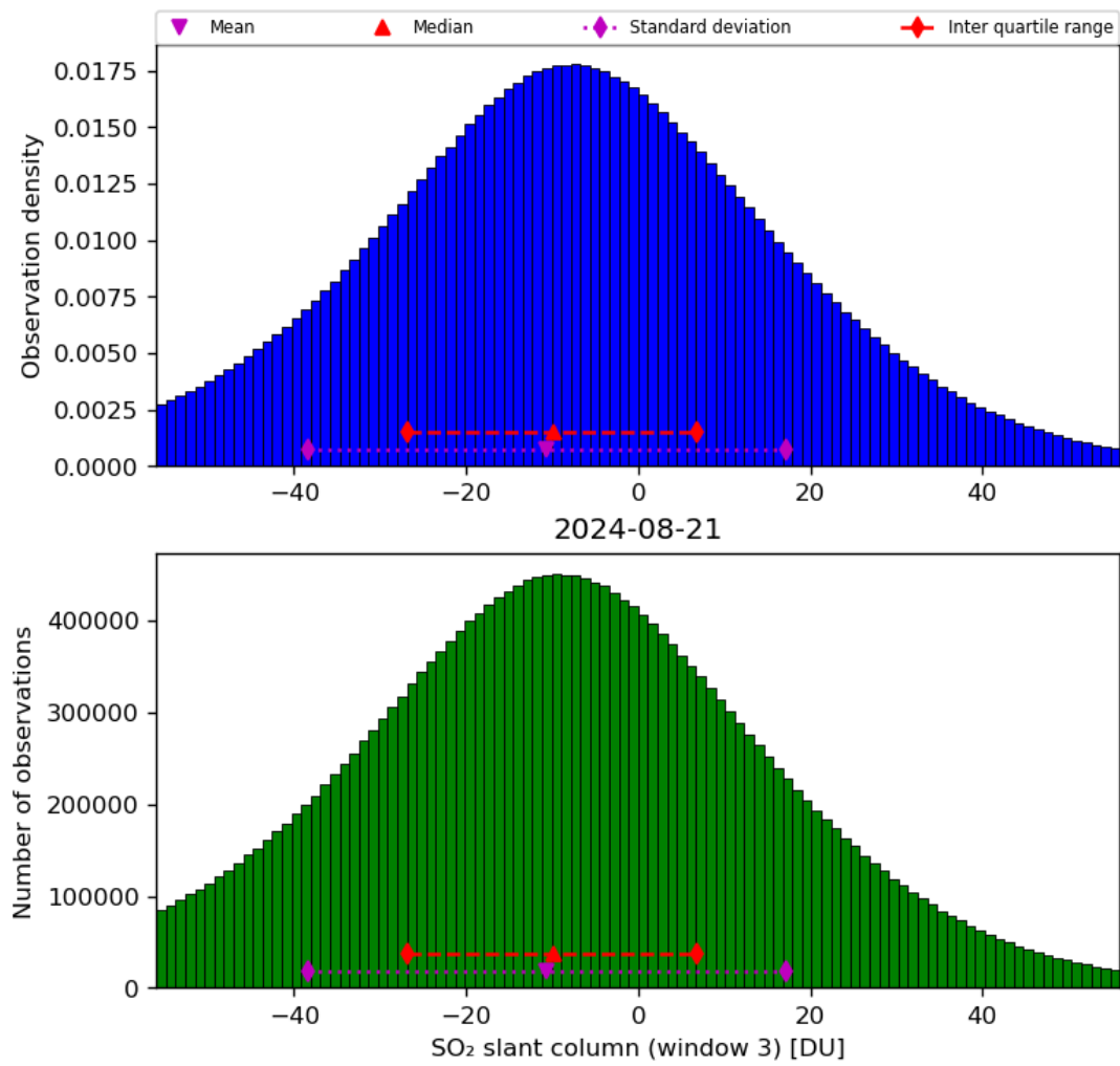
Figure 64: Histogram of “SO 2 slant column (window 3)” for 2024-08-21 to 2024-08-22
