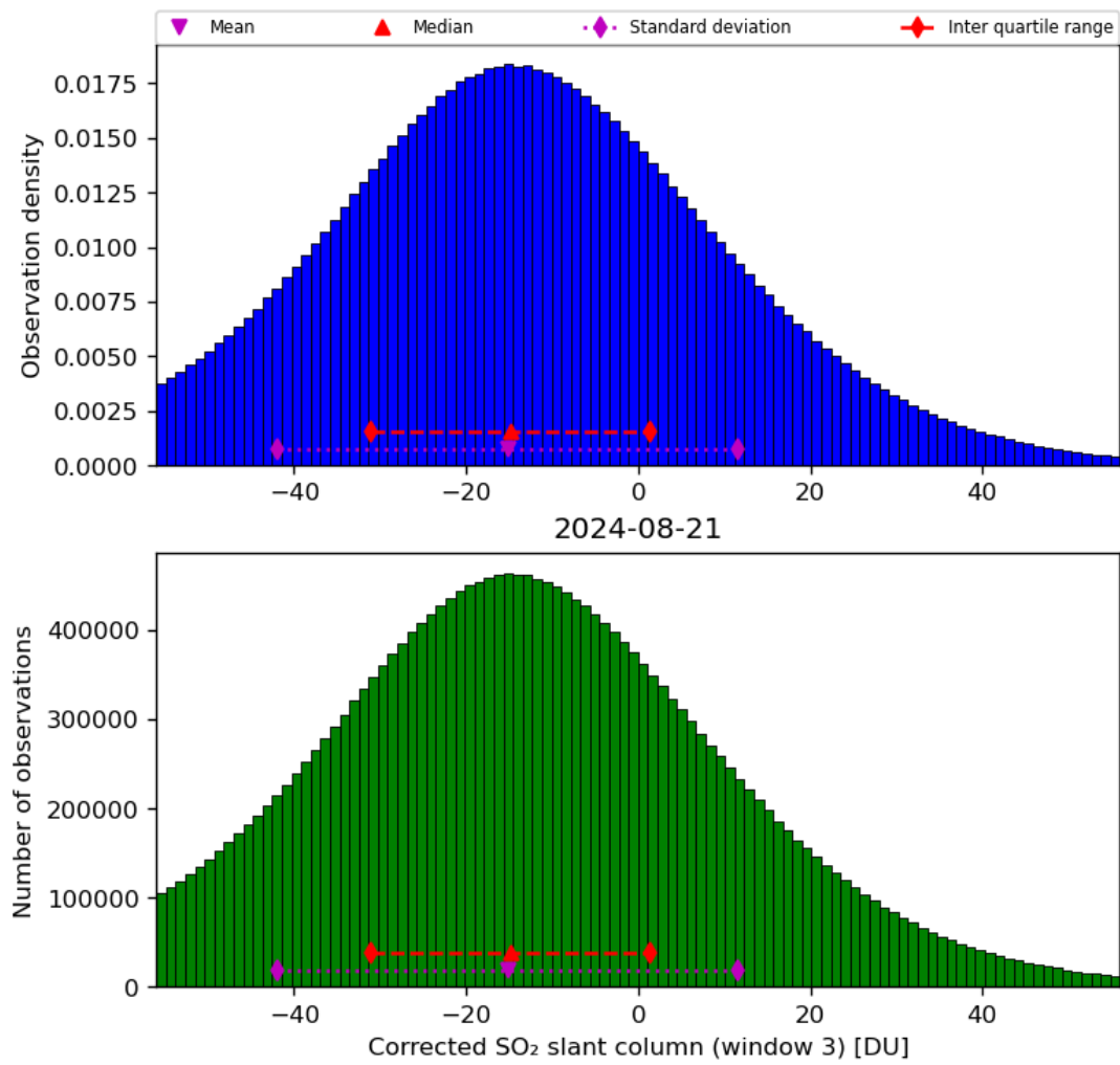
Figure 66: Histogram of “Corrected SO 2 slant column (window 3)” for 2024-08-21 to 2024-08-22
