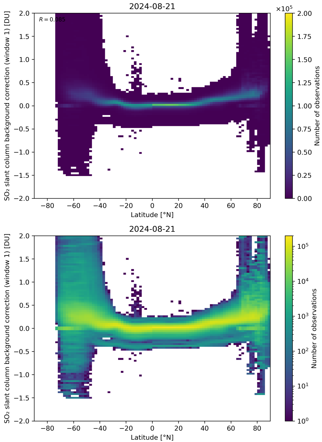
Figure 139: Scatter density plot of “Latitude” against “SO 2 slant column background correction (window 1)” for 2024-08-21 to 2024-08-22.
