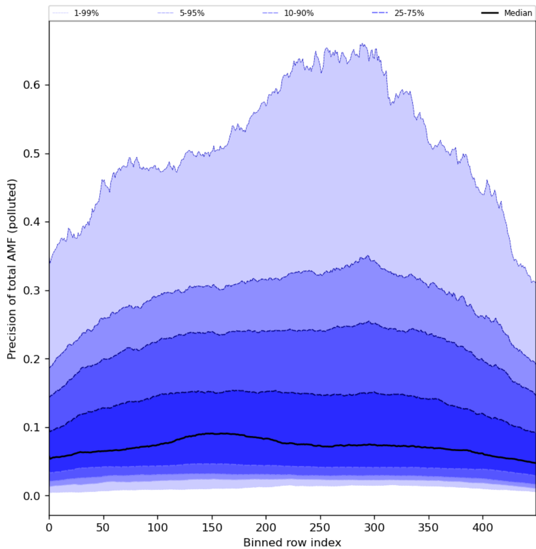
Figure 95: Along track statistics of “Precision of total AMF (polluted)” for 2024-08-21 to 2024-08-22
