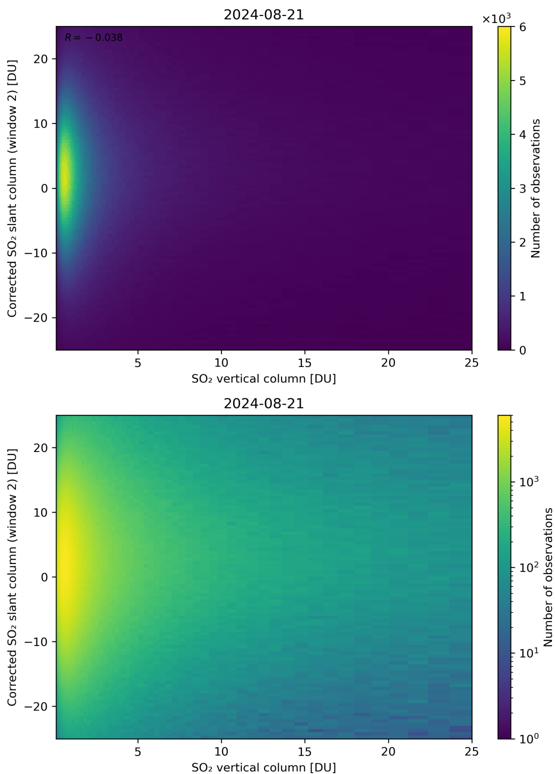
Figure 298: Scatter density plot of “SO 2 vertical column” against “Corrected SO 2 slant column (window 2)” for 2024-08-21 to 2024-08-22.
