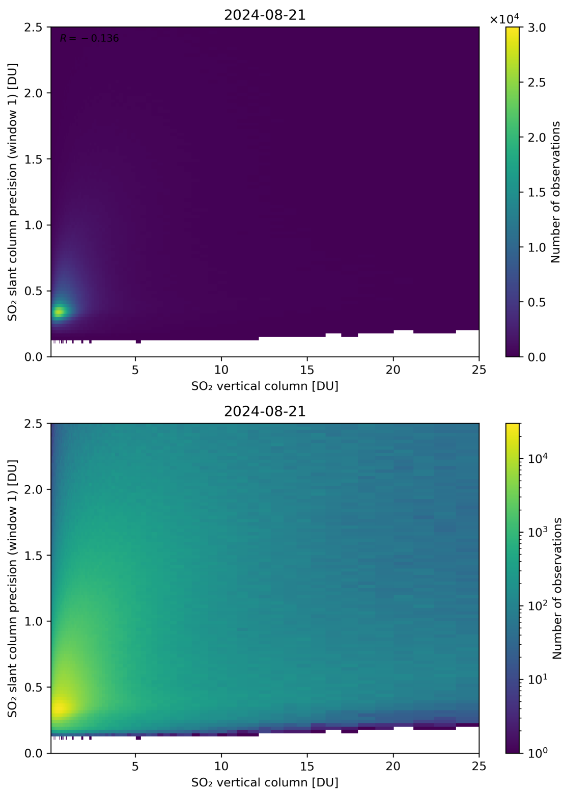
Figure 301: Scatter density plot of “SO 2 vertical column” against “SO 2 slant column precision (window 1)” for 2024-08-21 to 2024-08-22.
