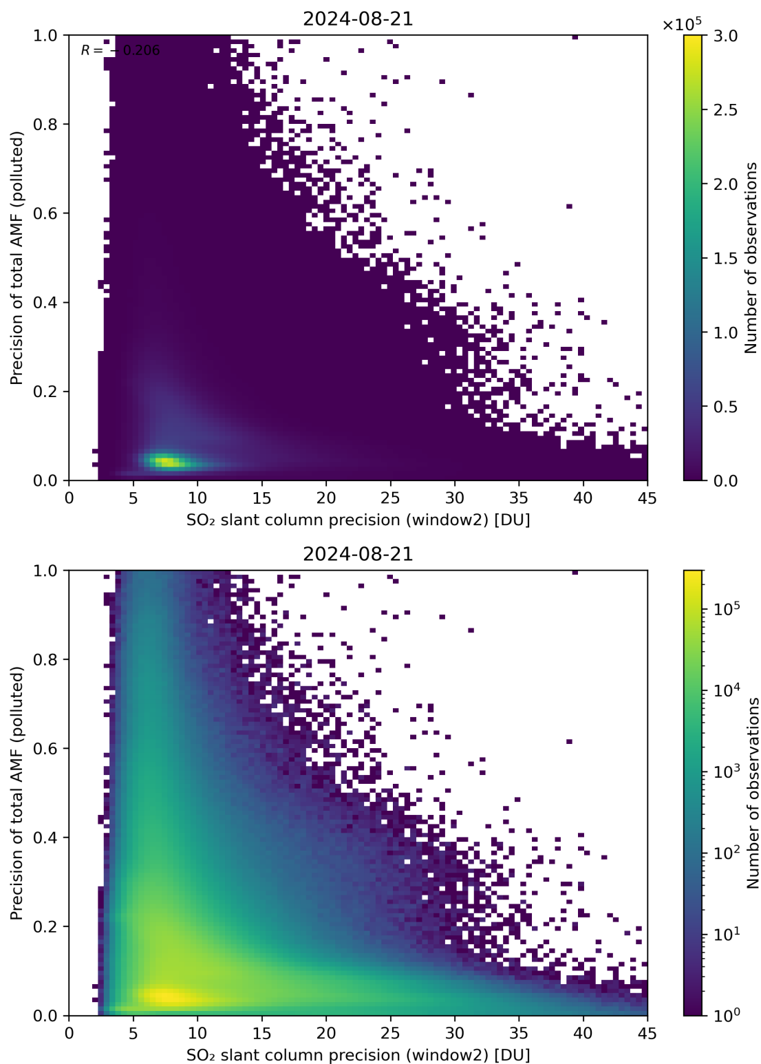
Figure 252: Scatter density plot of “SO 2 slant column precision (window2)” against “Precision of total AMF (polluted)” for 2024-08-21 to 2024-08-22.
