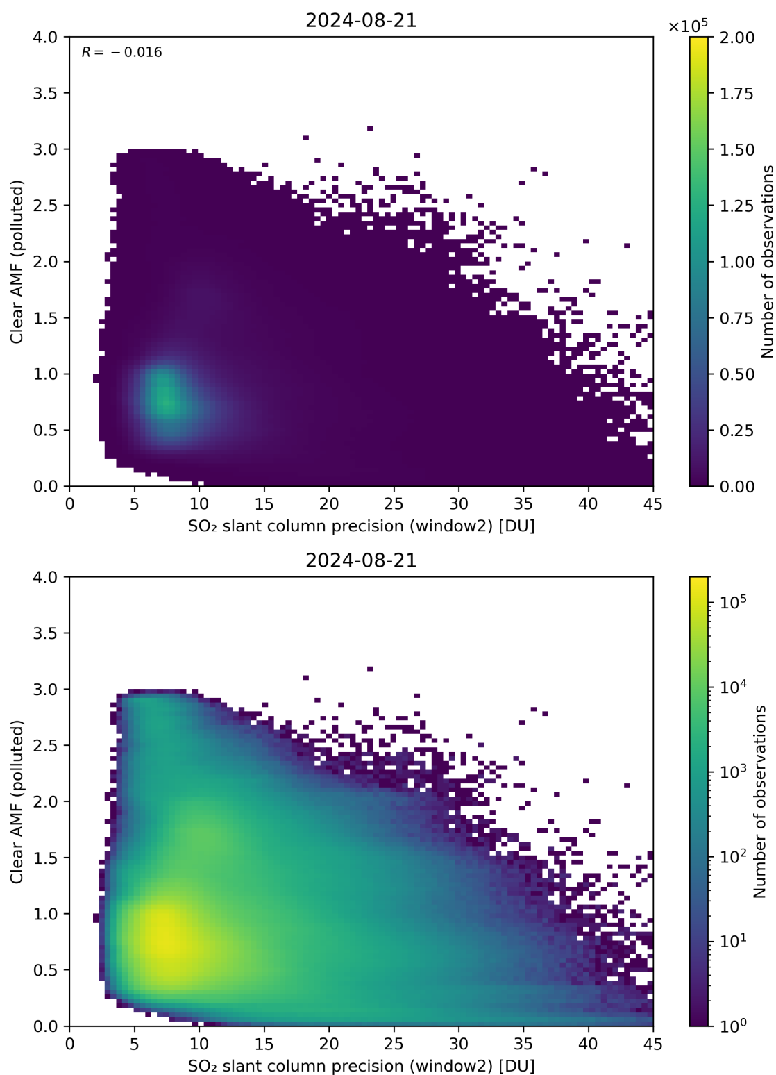
Figure 246: Scatter density plot of “SO 2 slant column precision (window2)” against “Clear AMF (polluted)” for 2024-08-21 to 2024-08-22.
