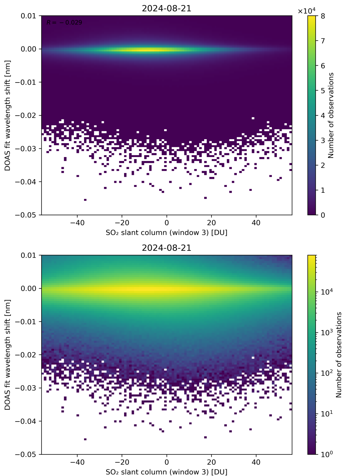
Figure 254: Scatter density plot of “SO 2 slant column (window 3)” against “DOAS fit wavelength shift” for 2024-08-21 to 2024-08-22.
