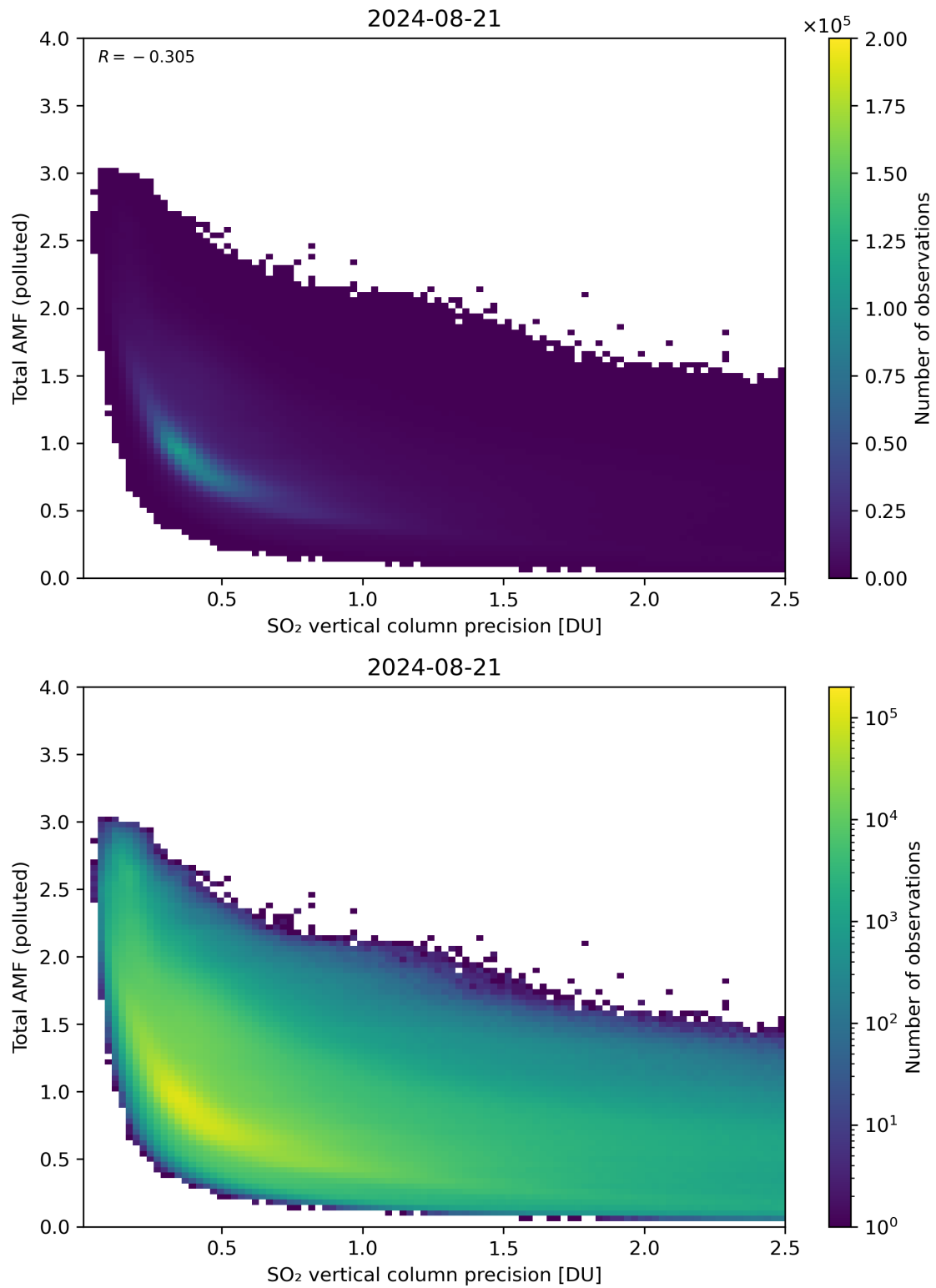
Figure 294: Scatter density plot of “SO 2 vertical column precision” against “Total AMF (polluted)” for 2024-08-21 to 2024-08-22.
