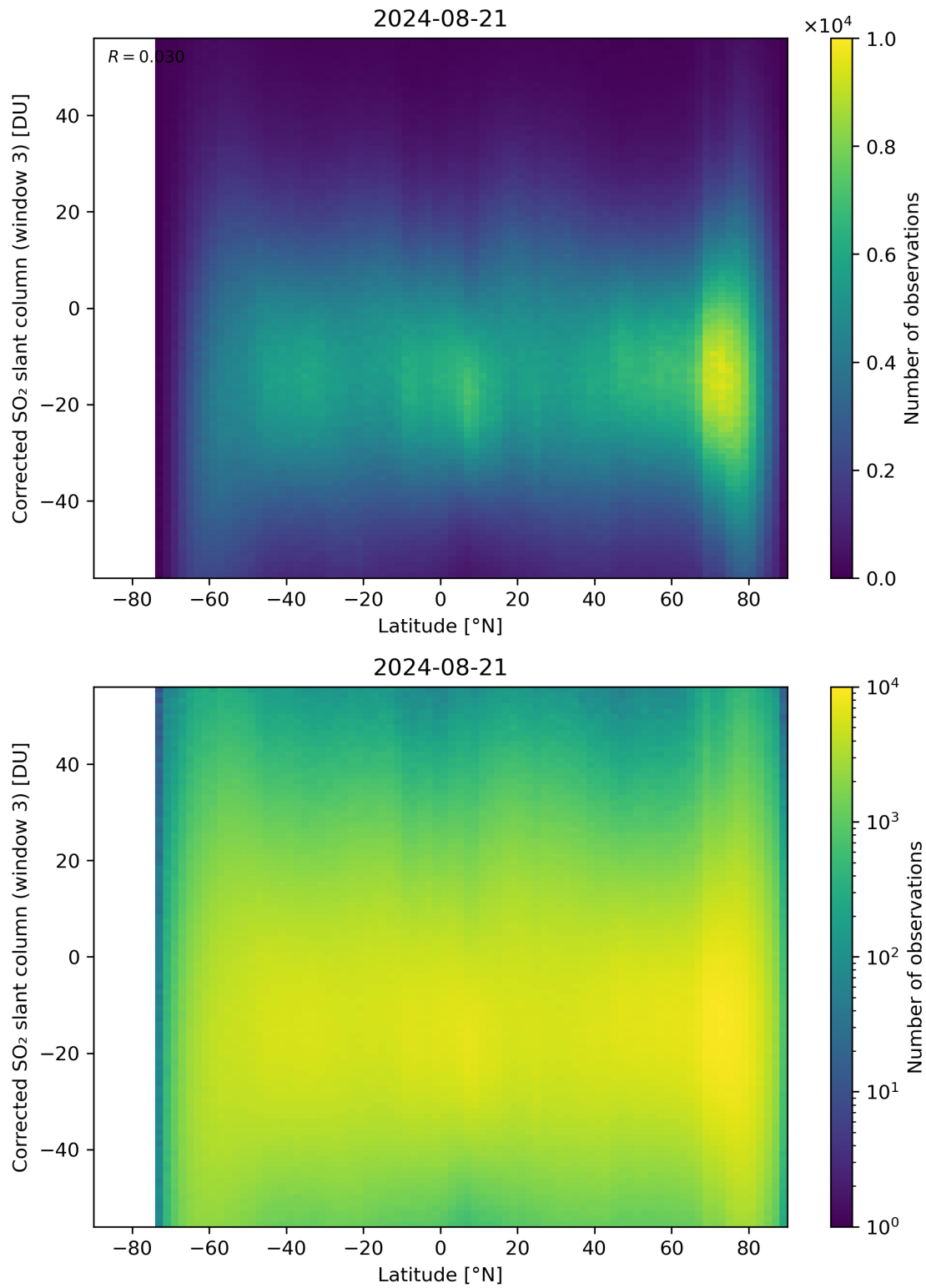
Figure 148: Scatter density plot of “Latitude” against “Corrected SO 2 slant column (window 3)” for 2024-08-21 to 2024-08-22.
