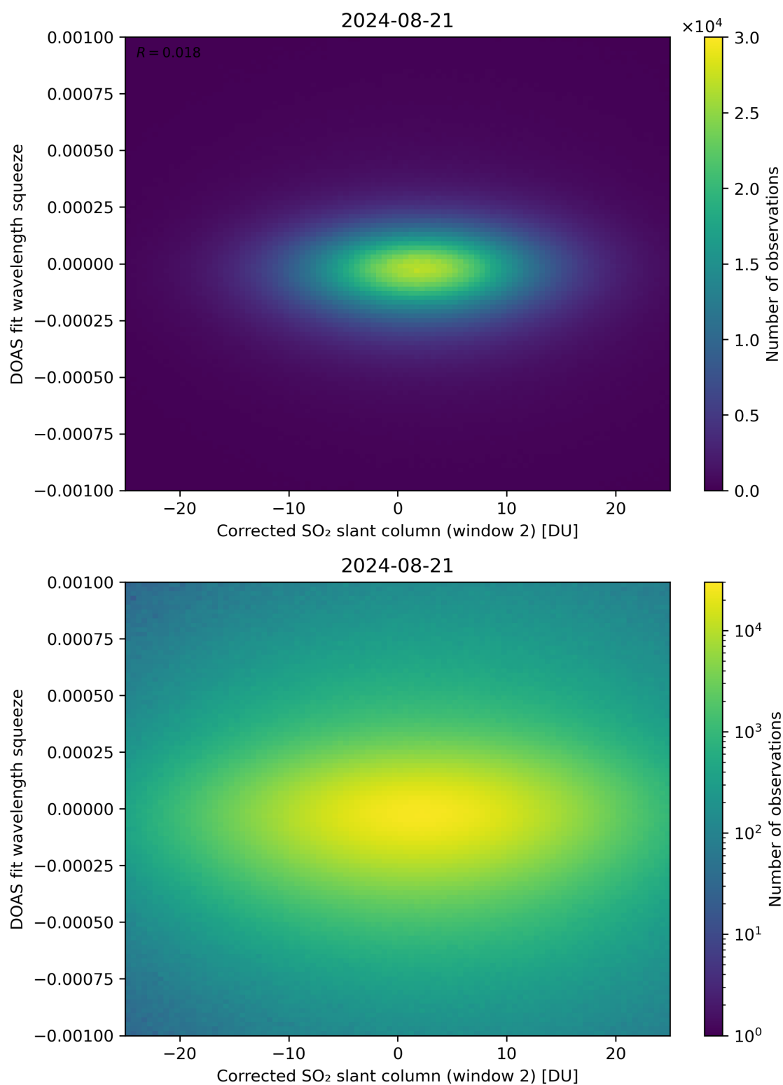
Figure 197: Scatter density plot of “Corrected SO 2 slant column (window 2)” against “DOAS fit wavelength squeeze” for 2024-08-21 to 2024-08-22.
