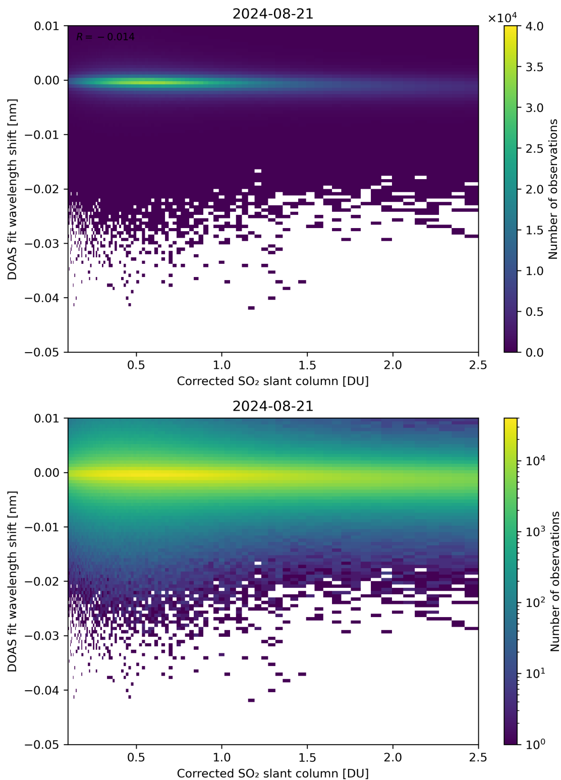
Figure 181: Scatter density plot of “Corrected SO 2 slant column” against “DOAS fit wavelength shift” for 2024-08-21 to 2024-08-22.
