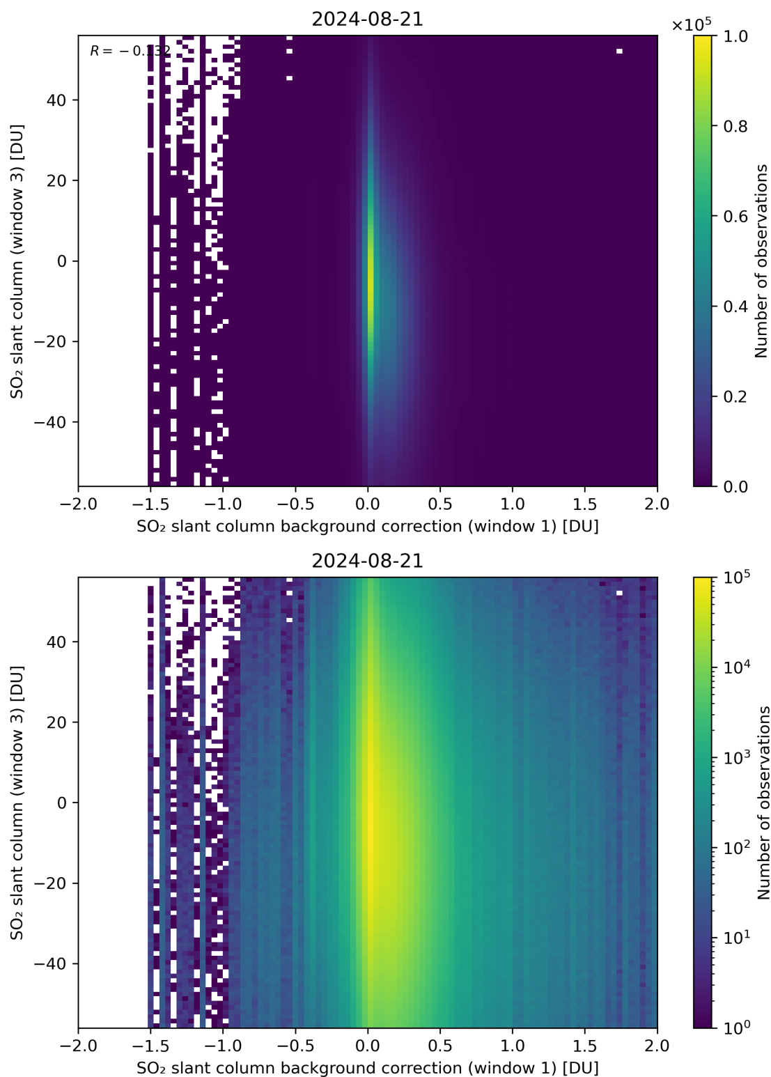
Figure 107: Scatter density plot of “SO 2 slant column background correction (window 1)” against “SO 2 slant column (window 3)” for 2024-08-21 to 2024-08-22.
