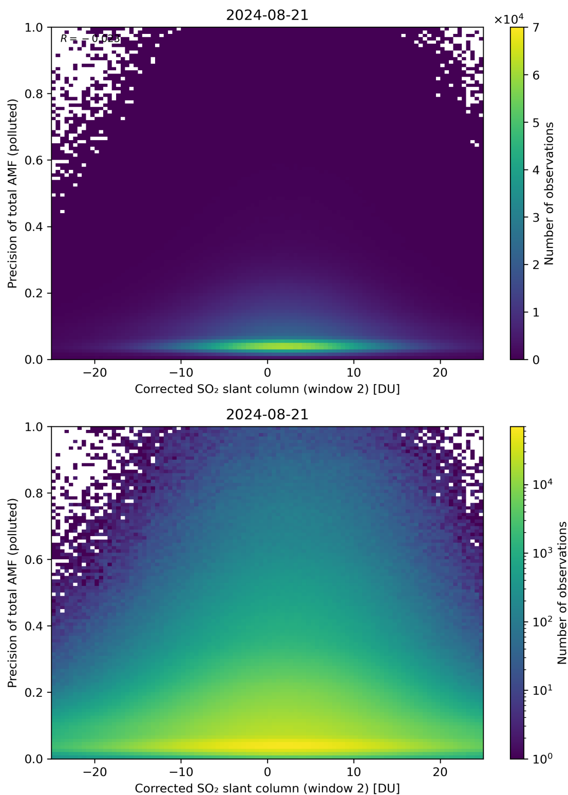
Figure 204: Scatter density plot of “Corrected SO 2 slant column (window 2)” against “Precision of total AMF (polluted)” for 2024-08-21 to 2024-08-22.
