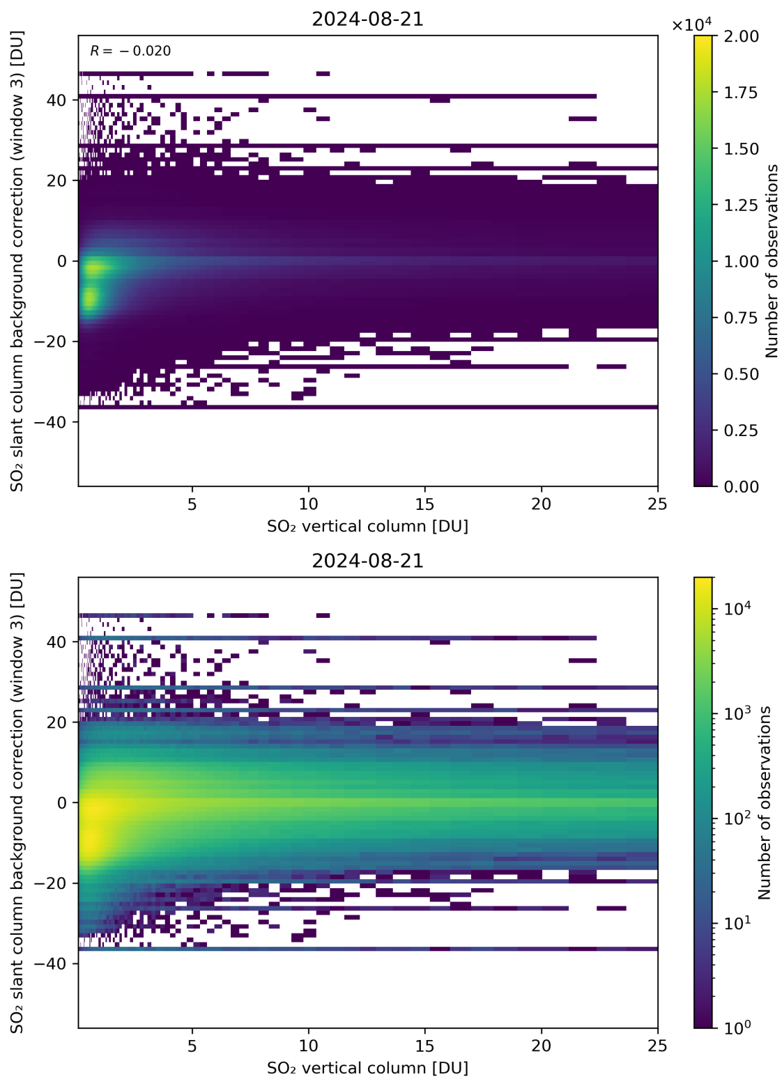
Figure 275: Scatter density plot of “SO 2 vertical column” against “SO 2 slant column background correction (window 3)” for 2024-08-21 to 2024-08-22.
