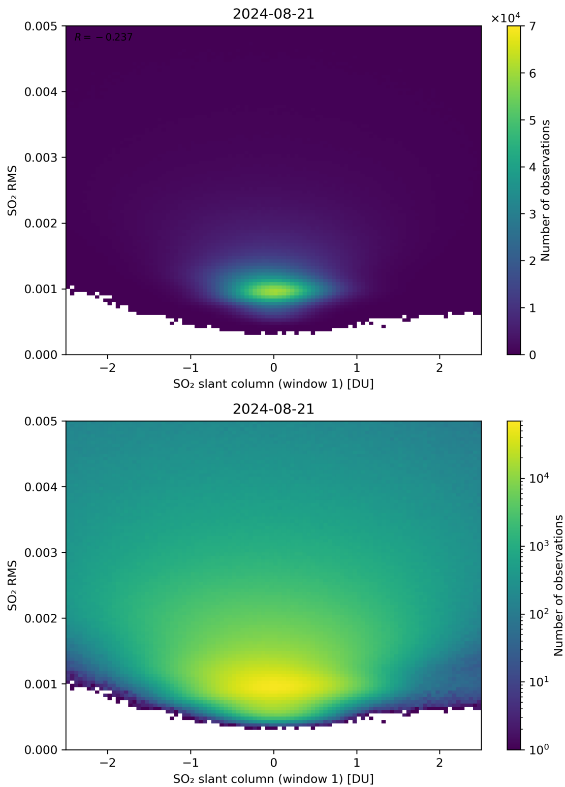
Figure 217: Scatter density plot of “SO 2 slant column (window 1)” against “SO 2 RMS” for 2024-08-21 to 2024-08-22.
