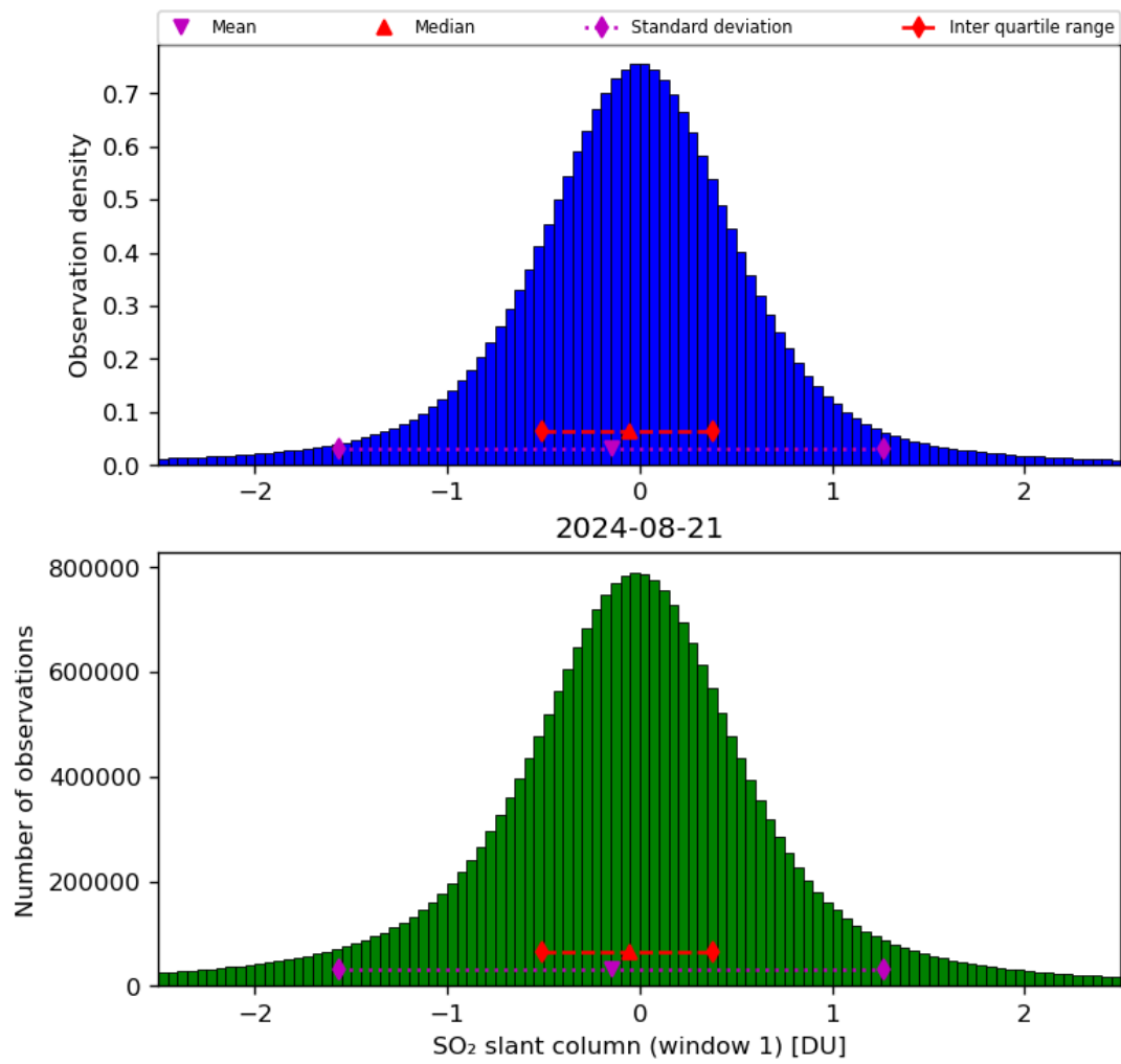
Figure 56: Histogram of “SO 2 slant column (window 1)” for 2024-08-21 to 2024-08-22
