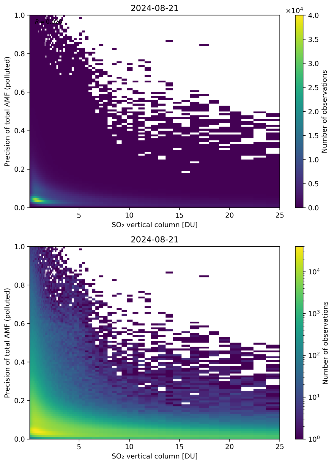
Figure 306: Scatter density plot of “SO 2 vertical column” against “Precision of total AMF (polluted)” for 2024-08-21 to 2024-08-22.
