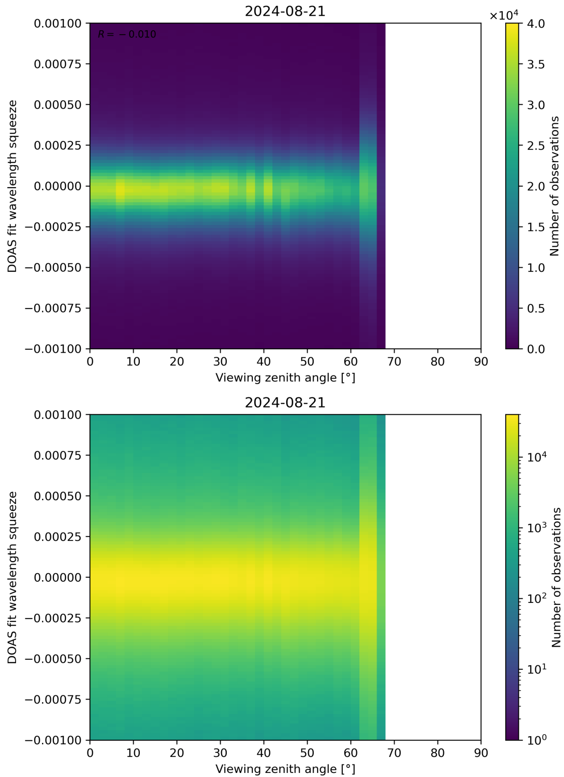
Figure 312: Scatter density plot of “Viewing zenith angle” against “DOAS fit wavelength squeeze” for 2024-08-21 to 2024-08-22.
