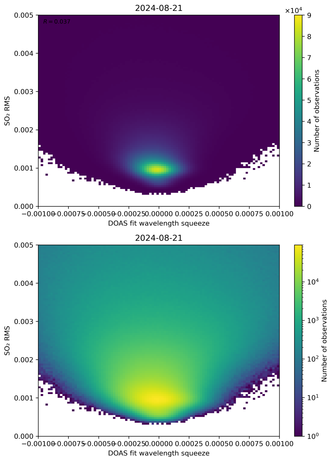
Figure 132: Scatter density plot of “DOAS fit wavelength squeeze” against “SO 2 RMS” for 2024-08-21 to 2024-08-22.
