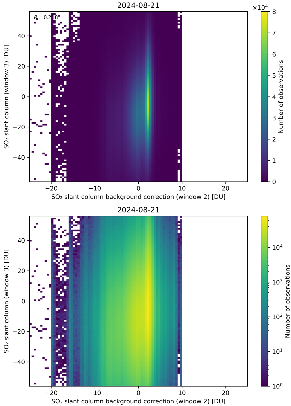
Figure 117: Scatter density plot of “SO 2 slant column background correction (window 2)” against “SO 2 slant column (window 3)” for 2024-08-21 to 2024-08-22.
