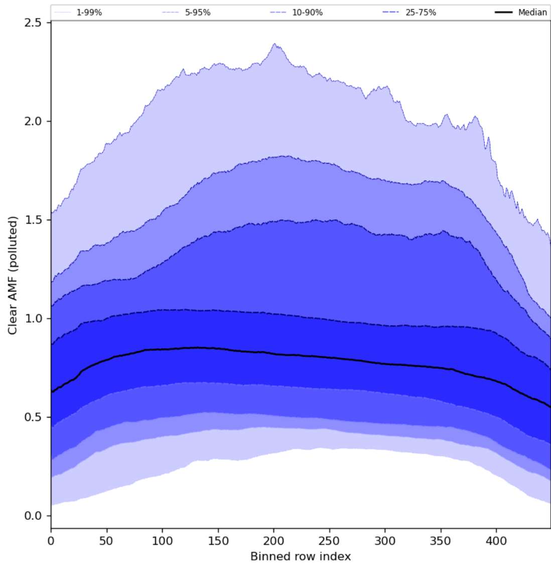
Figure 96: Along track statistics of “Clear AMF (polluted)” for 2024-08-21 to 2024-08-22
