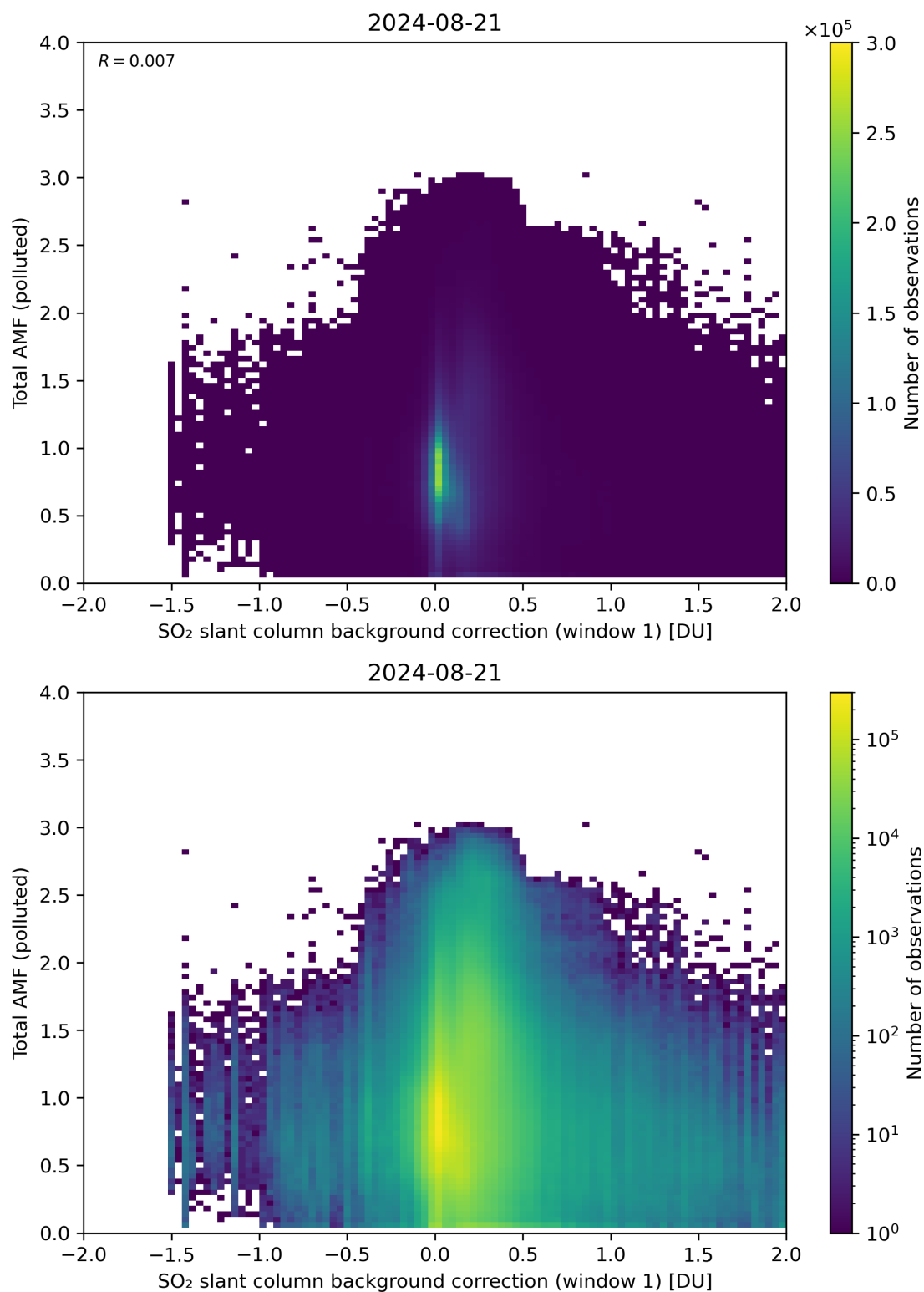
Figure 109: Scatter density plot of “SO 2 slant column background correction (window 1)” against “Total AMF (polluted)” for 2024-08-21 to 2024-08-22.
