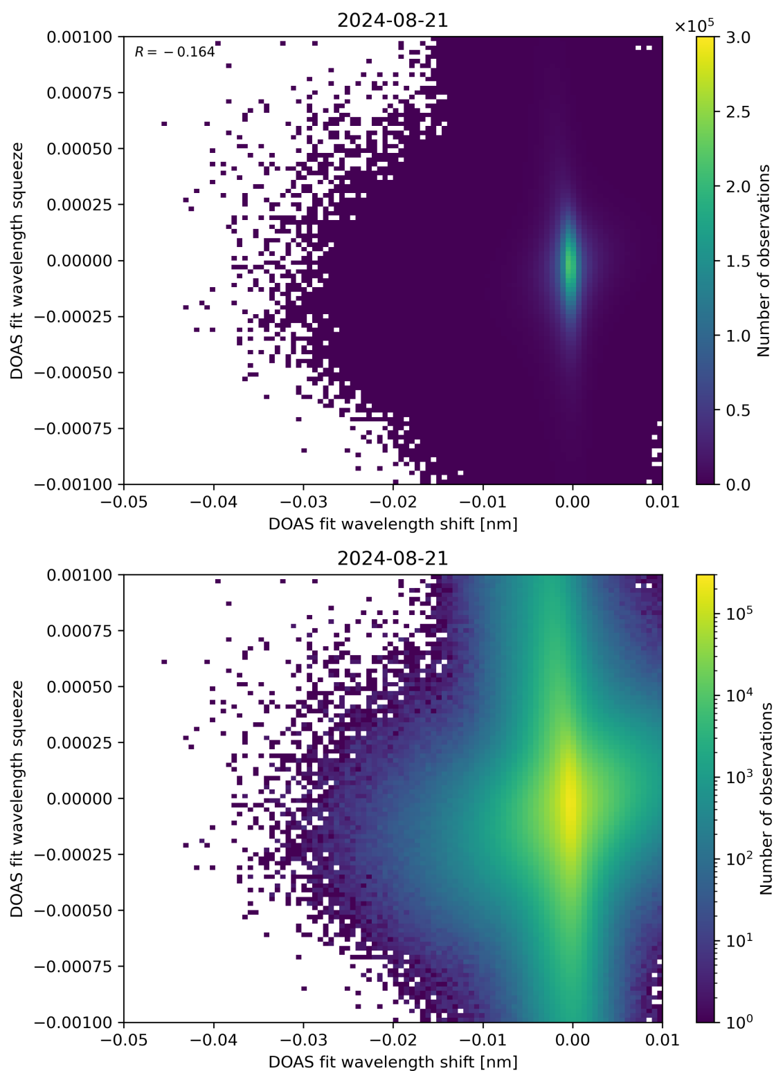
Figure 127: Scatter density plot of “DOAS fit wavelength shift” against “DOAS fit wavelength squeeze” for 2024-08-21 to 2024-08-22.
