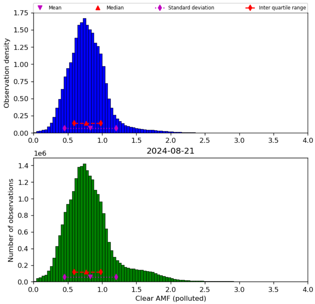
Figure 73: Histogram of “Clear AMF (polluted)” for 2024-08-21 to 2024-08-22
