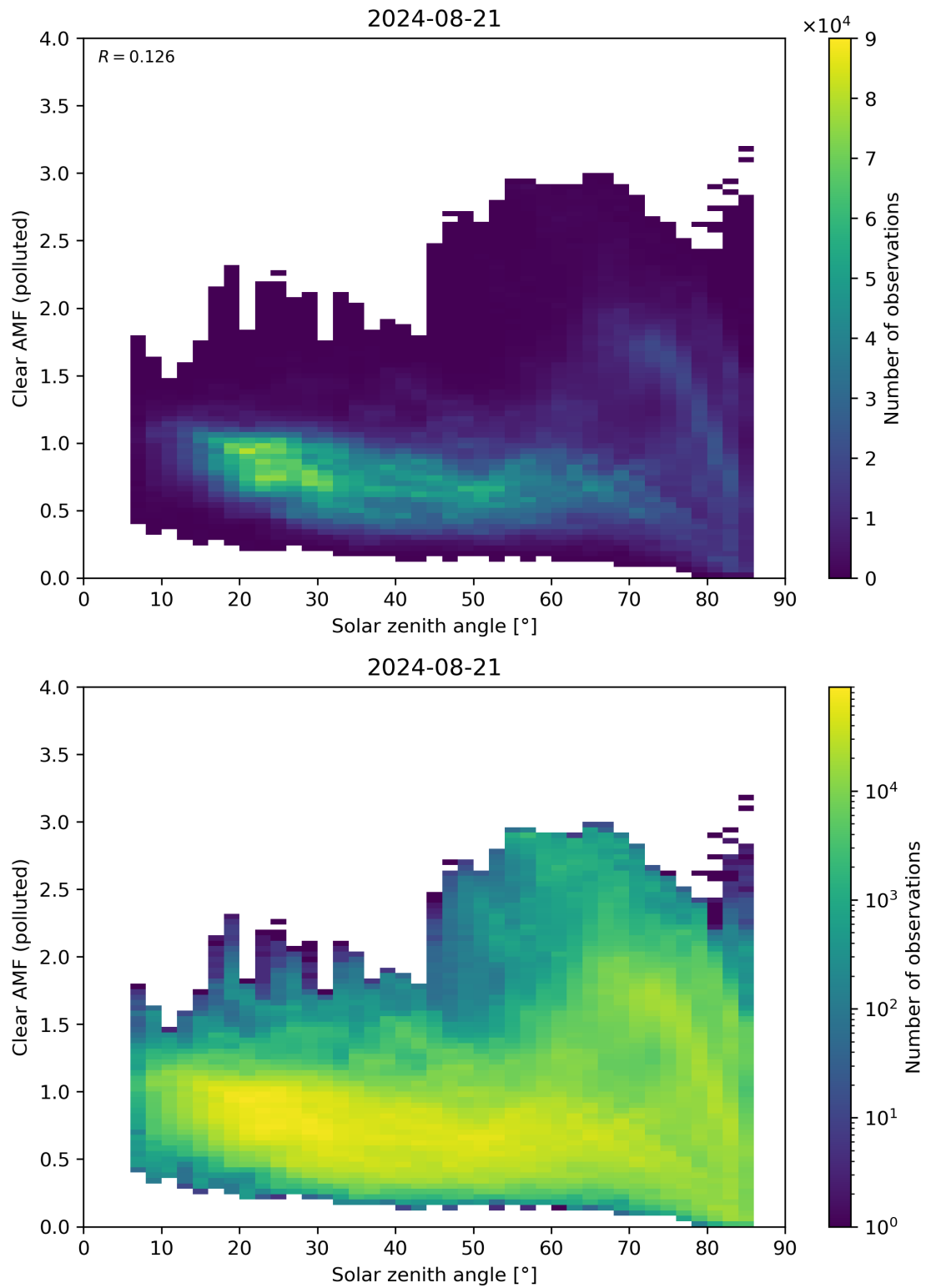
Figure 165: Scatter density plot of “Solar zenith angle” against “Clear AMF (polluted)” for 2024-08-21 to 2024-08-22.
