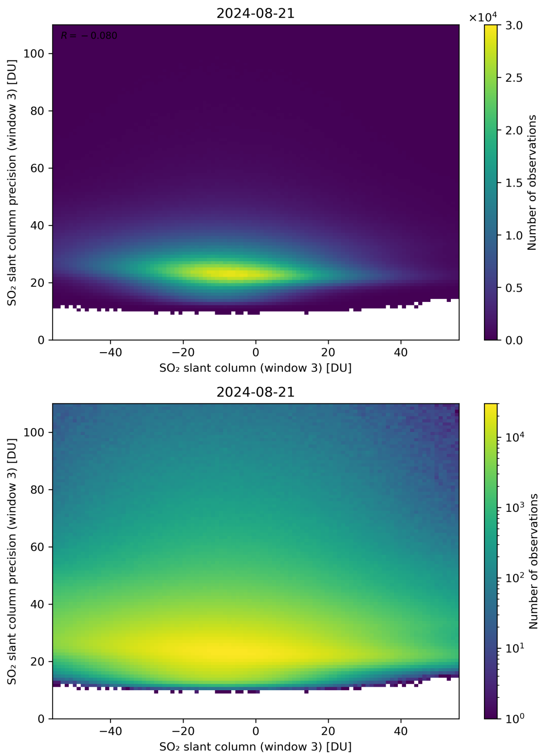
Figure 267: Scatter density plot of “SO 2 slant column (window 3)” against “SO 2 slant column precision (window 3)” for 2024-08-21 to 2024-08-22.
