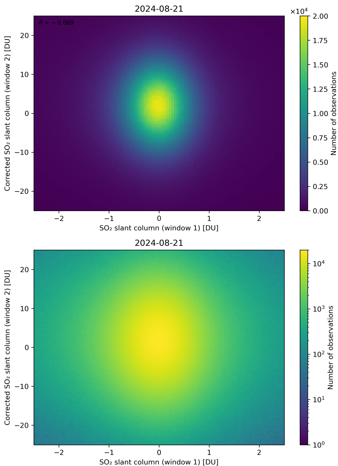
Figure 233: Scatter density plot of “SO 2 slant column (window 1)” against “Corrected SO 2 slant column (window 2)” for 2024-08-21 to 2024-08-22.
