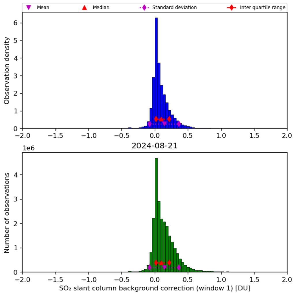
Figure 59: Histogram of “SO 2 slant column background correction (window 1)” for 2024-08-21 to 2024-08-22
