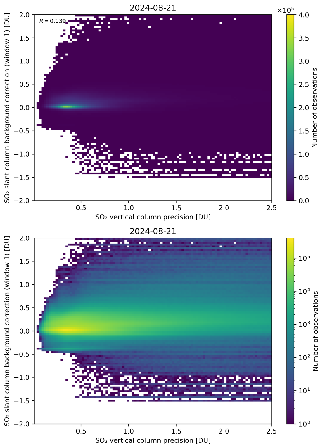
Figure 279: Scatter density plot of “SO 2 vertical column precision” against “SO 2 slant column background correction (window 1)” for 2024-08-21 to 2024-08-22.
