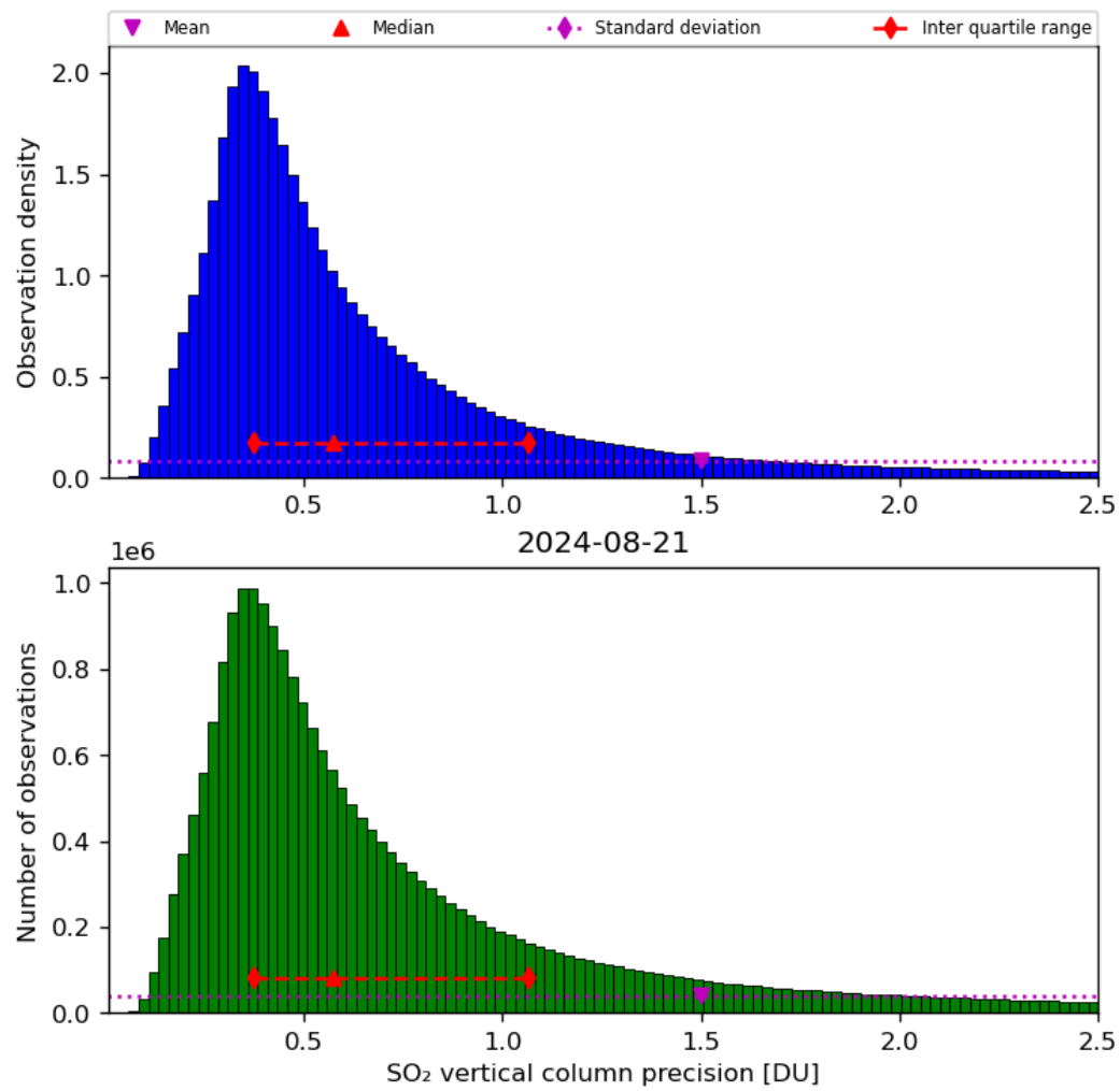
Figure 54: Histogram of “SO 2 vertical column precision” for 2024-08-21 to 2024-08-22
