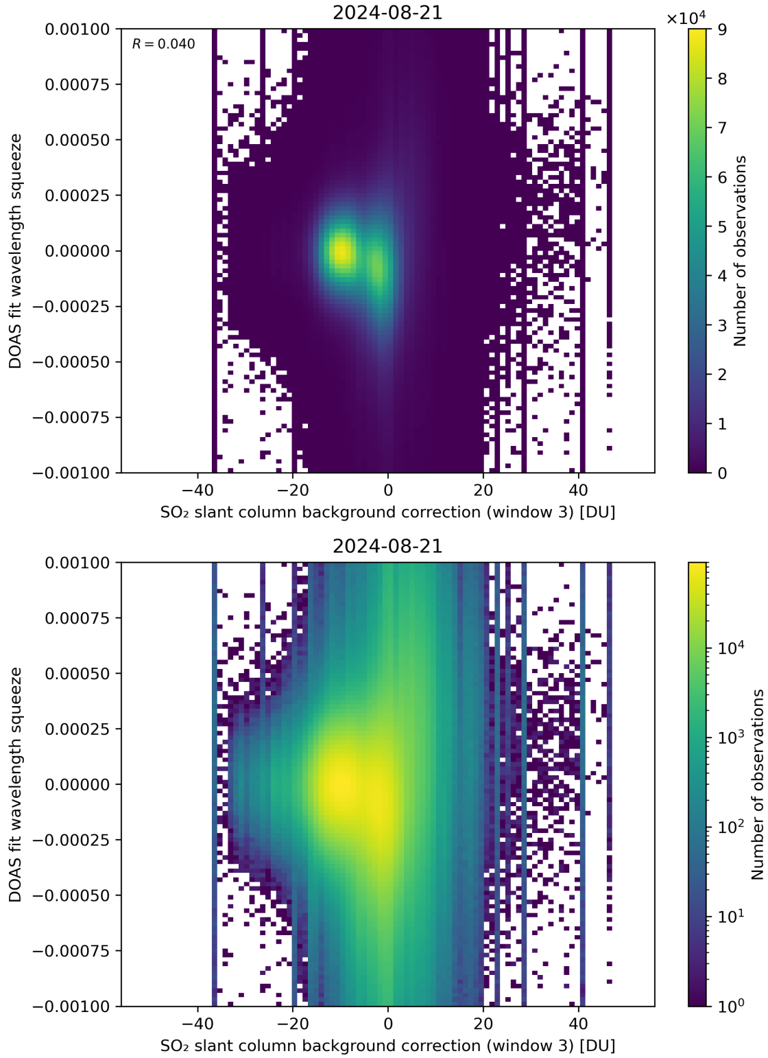
Figure 122: Scatter density plot of “SO 2 slant column background correction (window 3)” against “DOAS fit wavelength squeeze” for 2024-08-21 to 2024-08-22.
