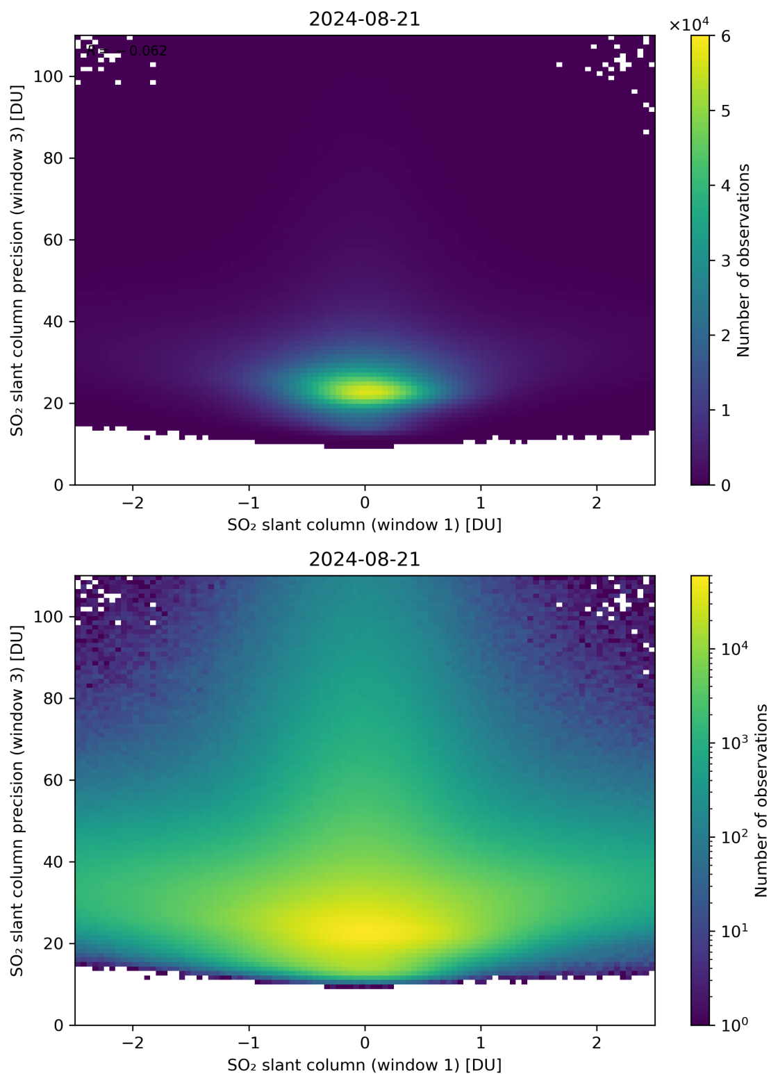
Figure 238: Scatter density plot of “SO 2 slant column (window 1)” against “SO 2 slant column precision (window 3)” for 2024-08-21 to 2024-08-22.
