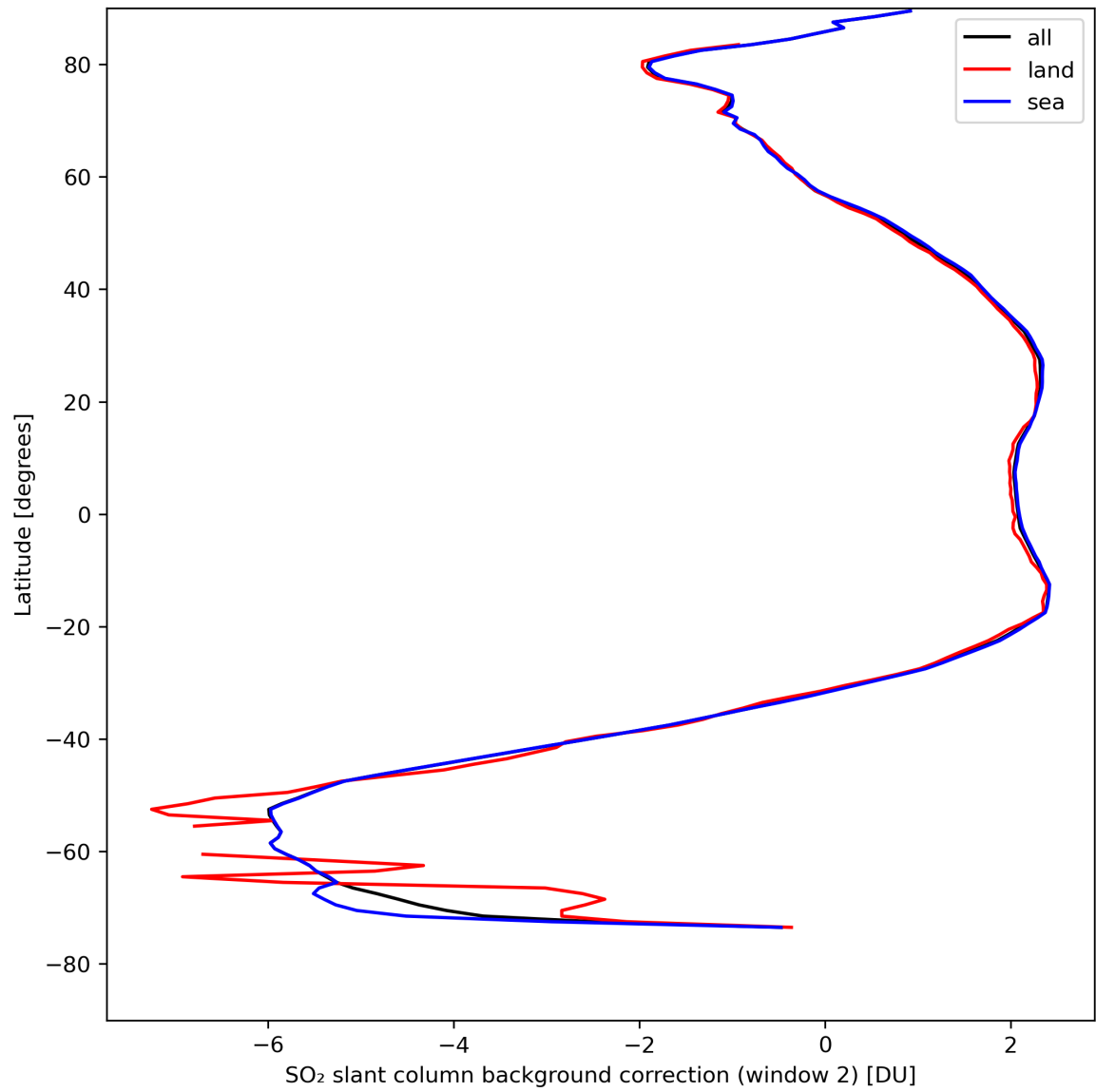
Figure 40: Zonal average of “SO 2 slant column background correction (window 2)” for 2024-08-21 to 2024-08-22.
