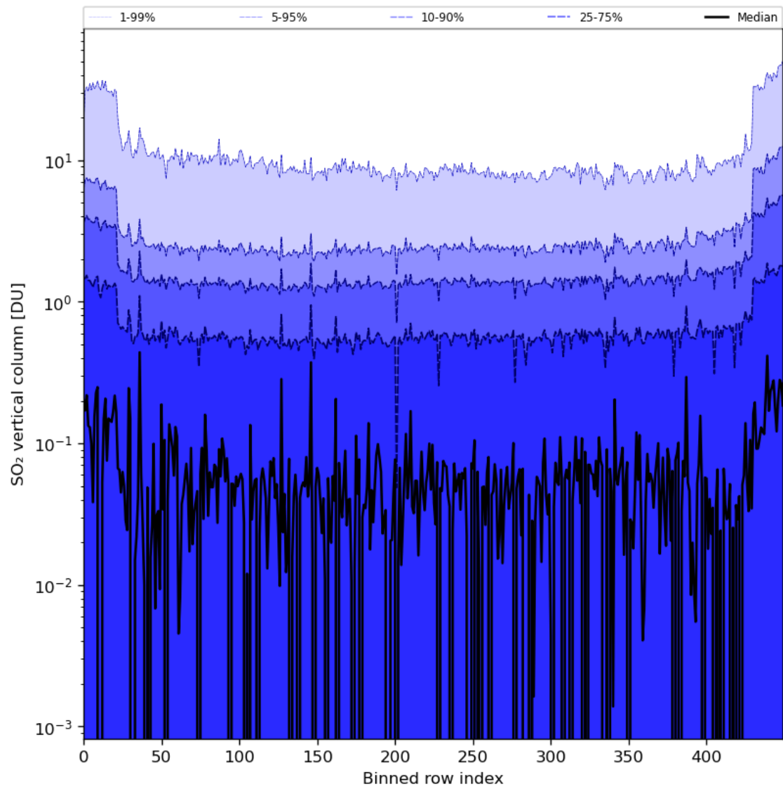
Figure 76: Along track statistics of “SO 2 vertical column” for 2024-08-21 to 2024-08-22
