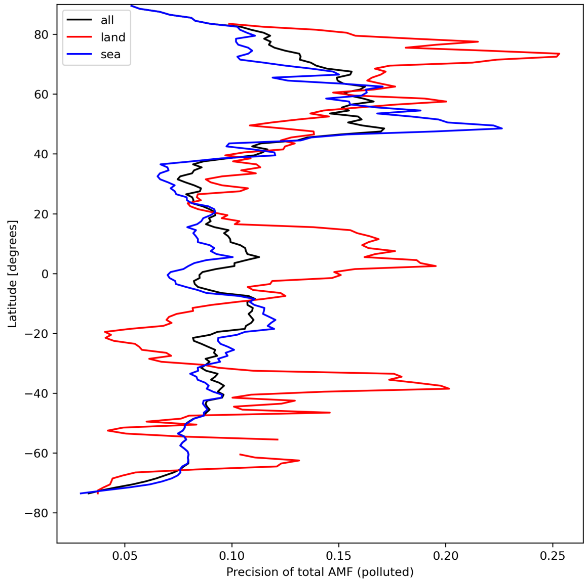
Figure 49: Zonal average of “Precision of total AMF (polluted)” for 2024-08-21 to 2024-08-22.
