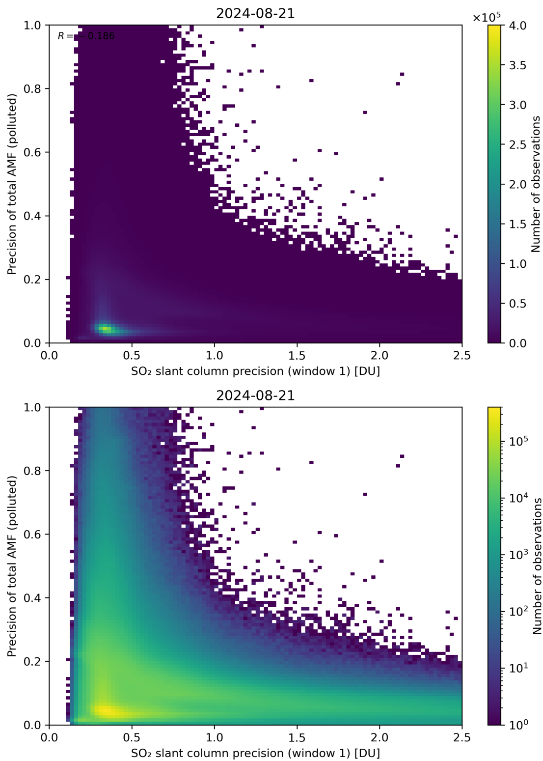
Figure 231: Scatter density plot of “SO 2 slant column precision (window 1)” against “Precision of total AMF (polluted)” for 2024-08-21 to 2024-08-22.
