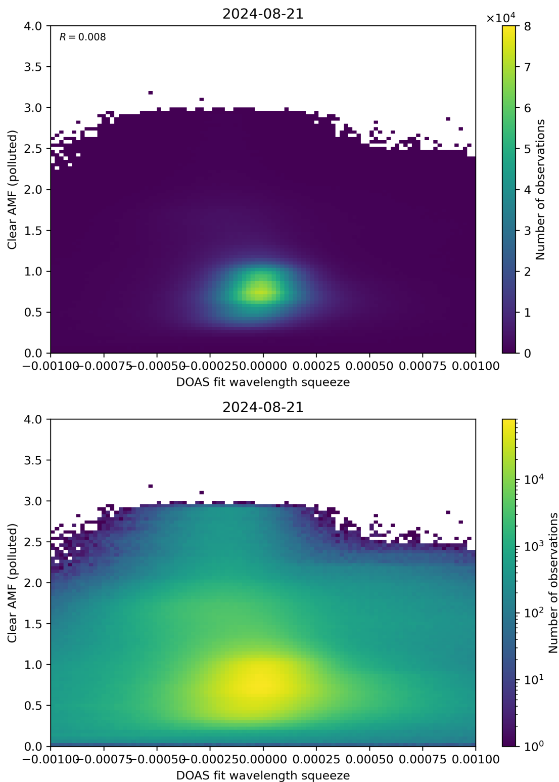
Figure 133: Scatter density plot of “DOAS fit wavelength squeeze” against “Clear AMF (polluted)” for 2024-08-21 to 2024-08-22.
