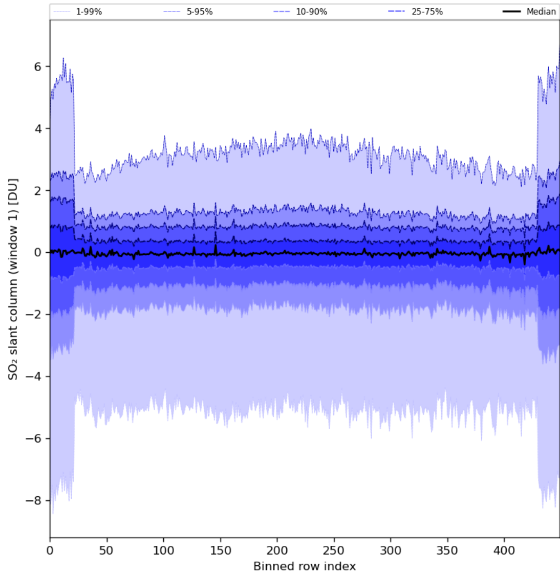
Figure 79: Along track statistics of “SO 2 slant column (window 1)” for 2024-08-21 to 2024-08-22
