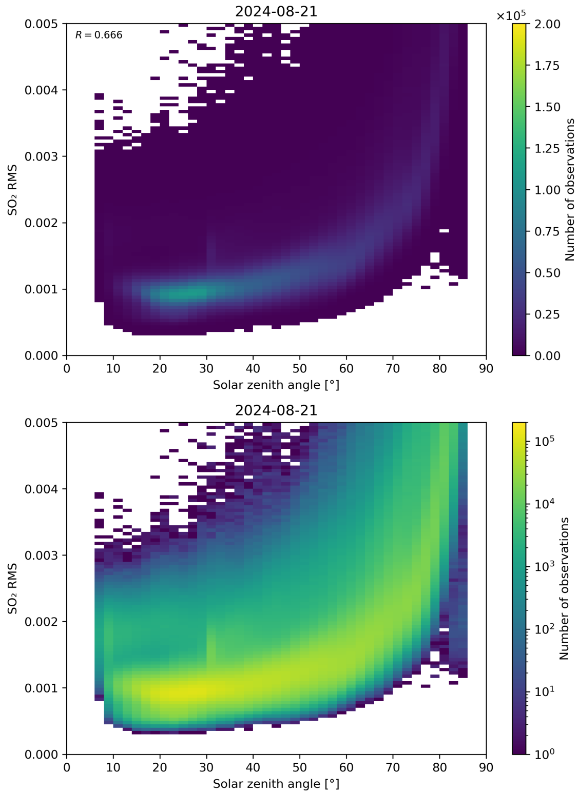
Figure 163: Scatter density plot of “Solar zenith angle” against “SO 2 RMS” for 2024-08-21 to 2024-08-22.
