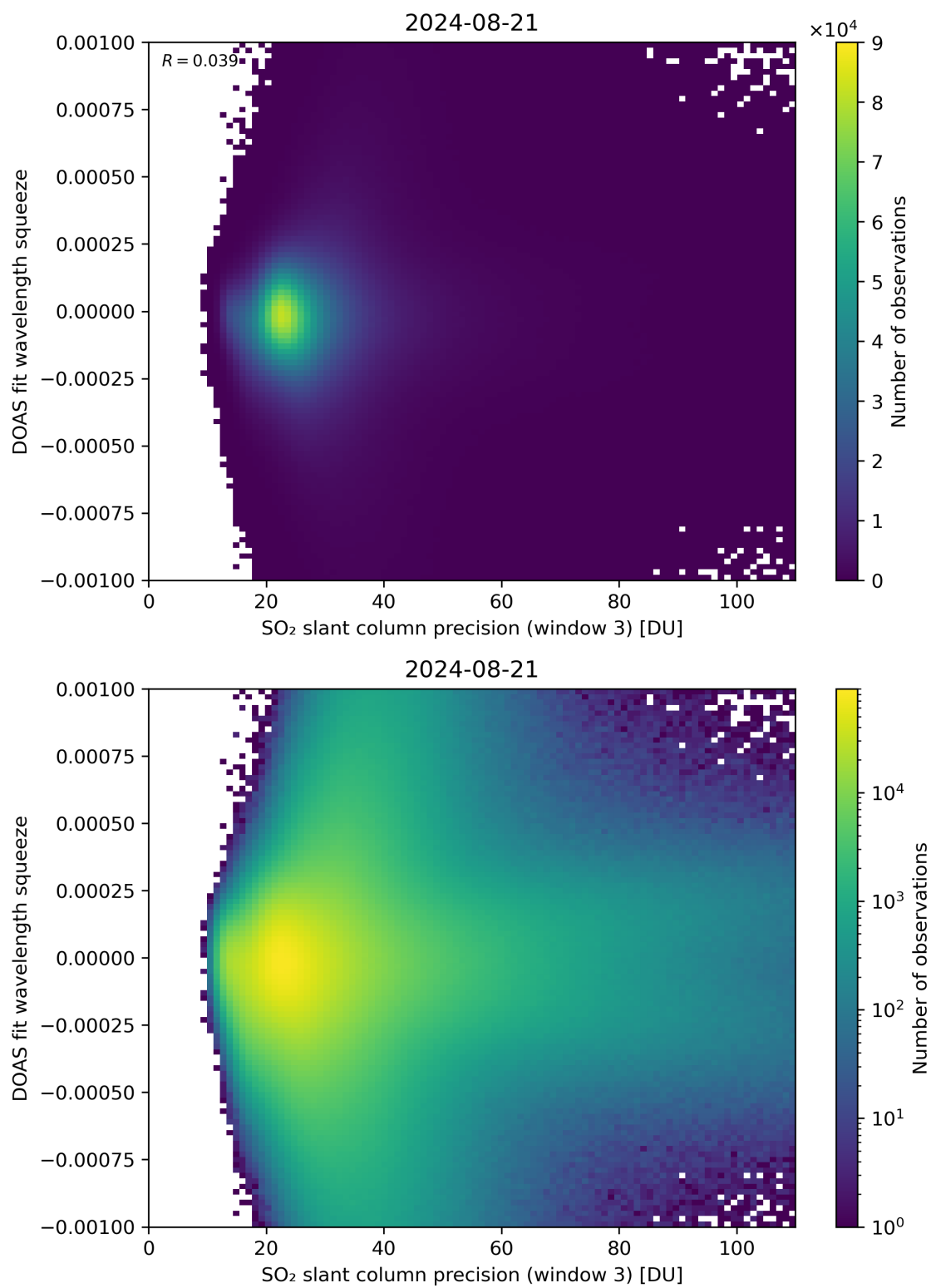
Figure 259: Scatter density plot of “SO 2 slant column precision (window 3)” against “DOAS fit wavelength squeeze” for 2024-08-21 to 2024-08-22.
