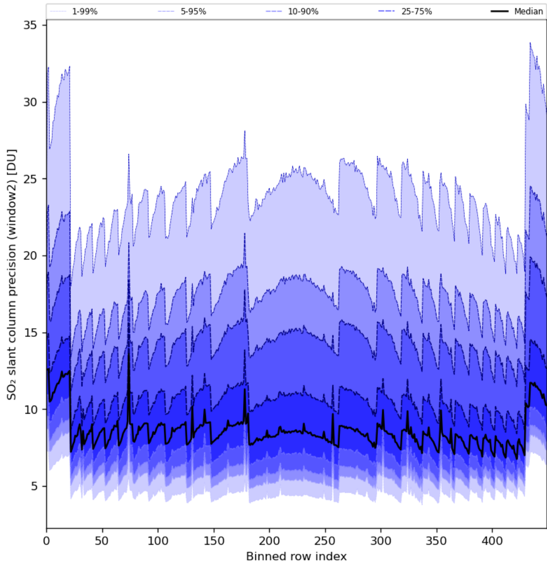
Figure 84: Along track statistics of “SO 2 slant column precision (window2)” for 2024-08-21 to 2024-08-22
