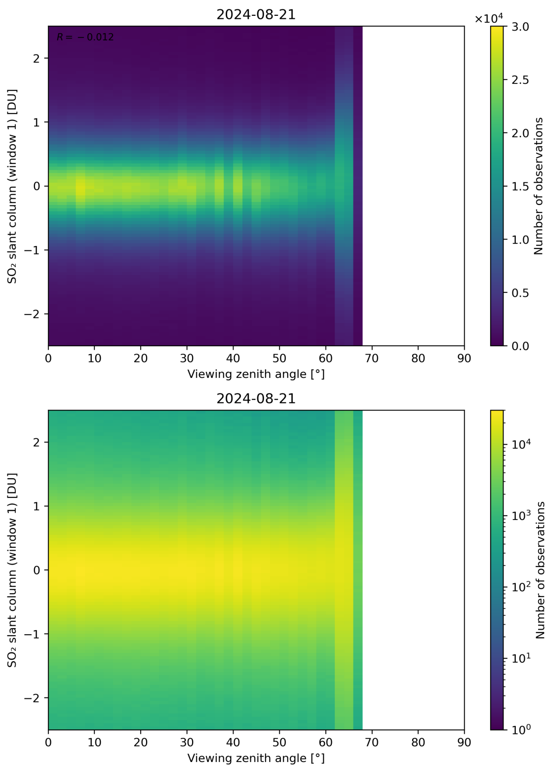
Figure 320: Scatter density plot of “Viewing zenith angle” against “SO 2 slant column (window 1)” for 2024-08-21 to 2024-08-22.
