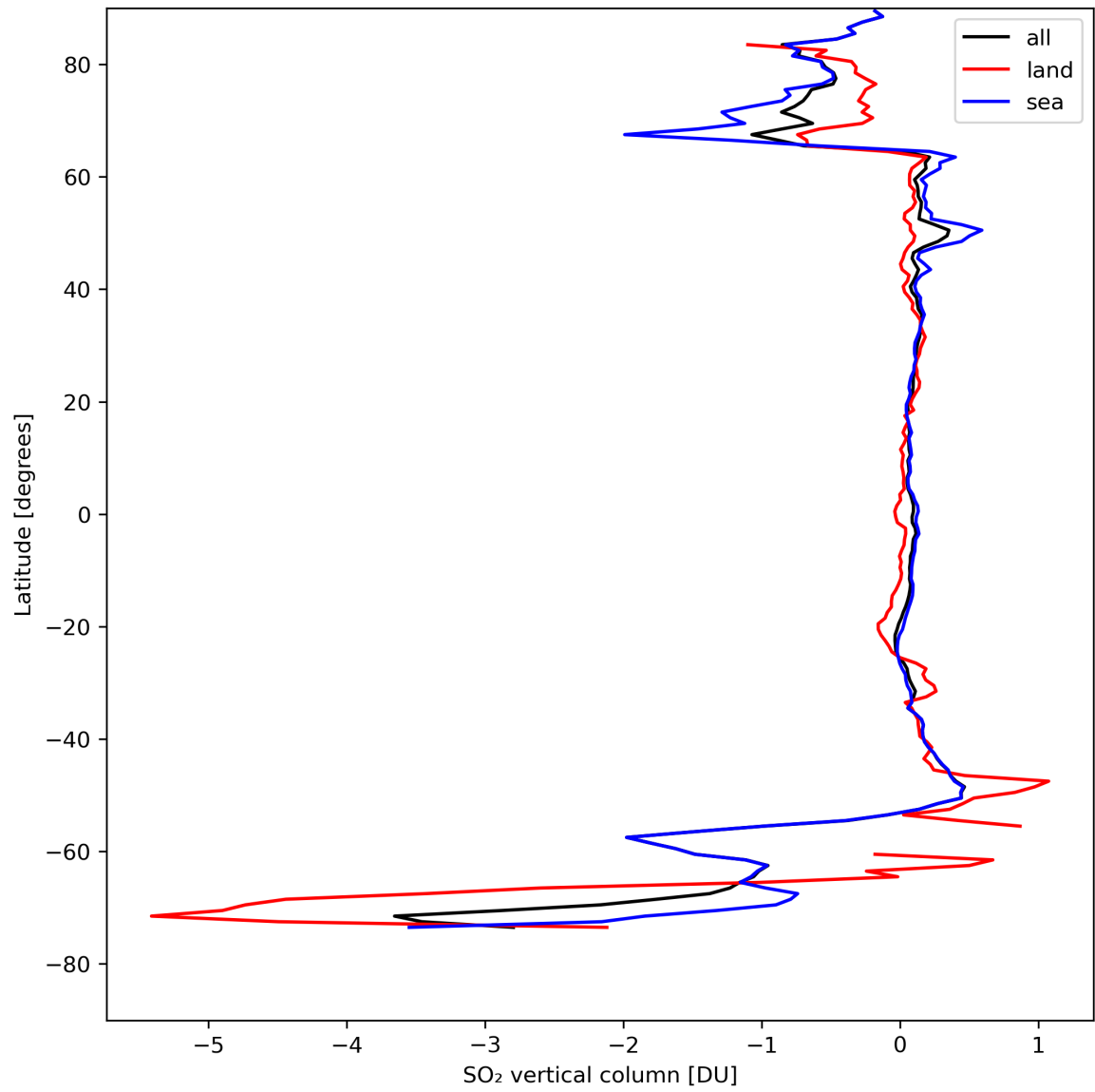
Figure 30: Zonal average of “SO 2 vertical column” for 2024-08-21 to 2024-08-22.
