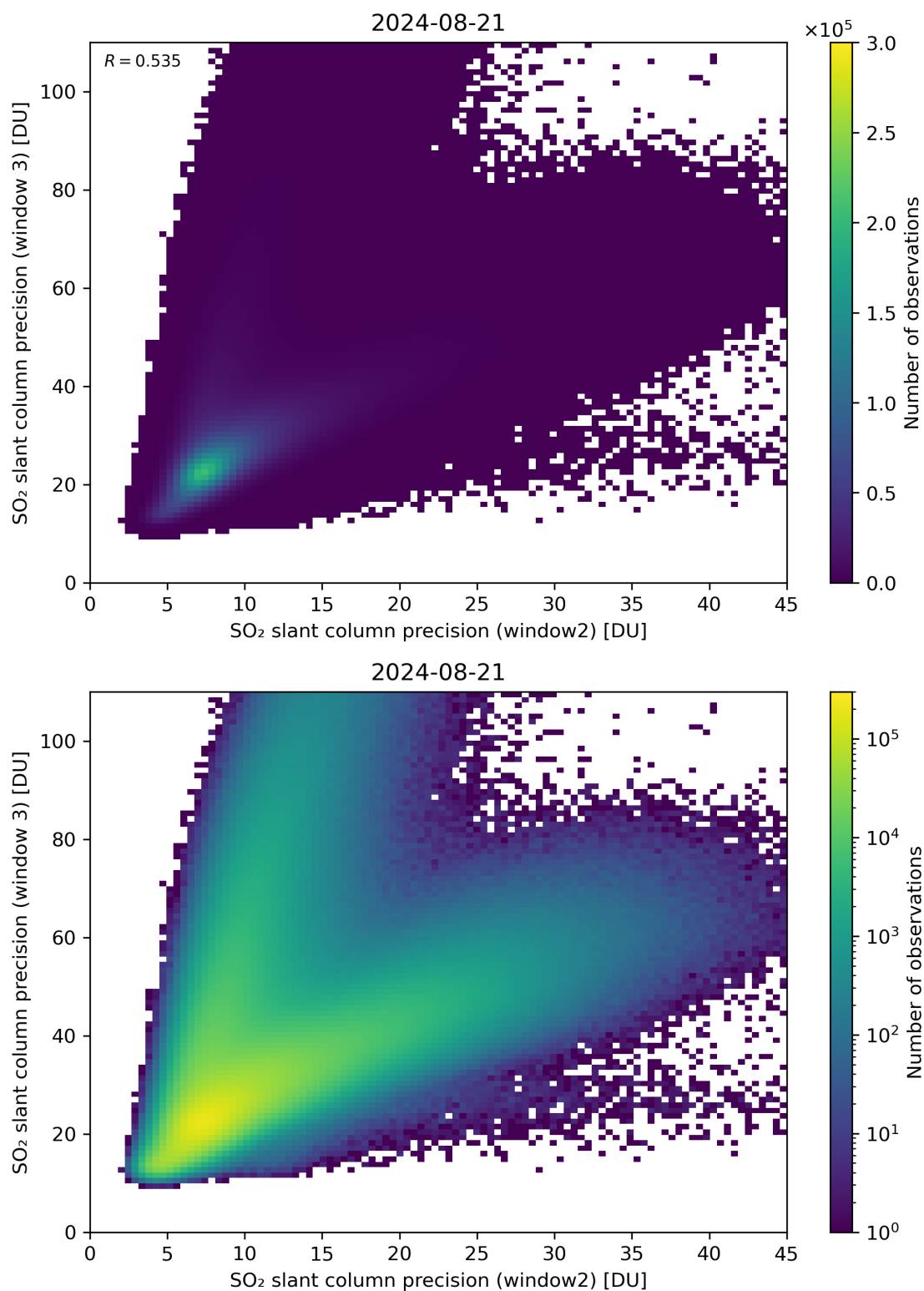
Figure 250: Scatter density plot of “SO 2 slant column precision (window2)” against “SO 2 slant column precision (window 3)” for 2024-08-21 to 2024-08-22.
