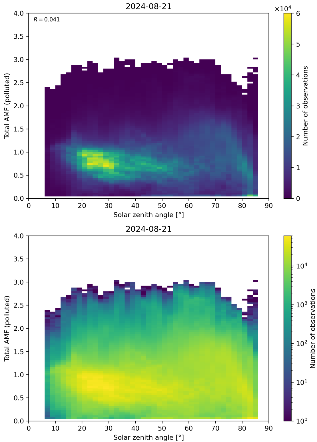
Figure 174: Scatter density plot of “Solar zenith angle” against “Total AMF (polluted)” for 2024-08-21 to 2024-08-22.
