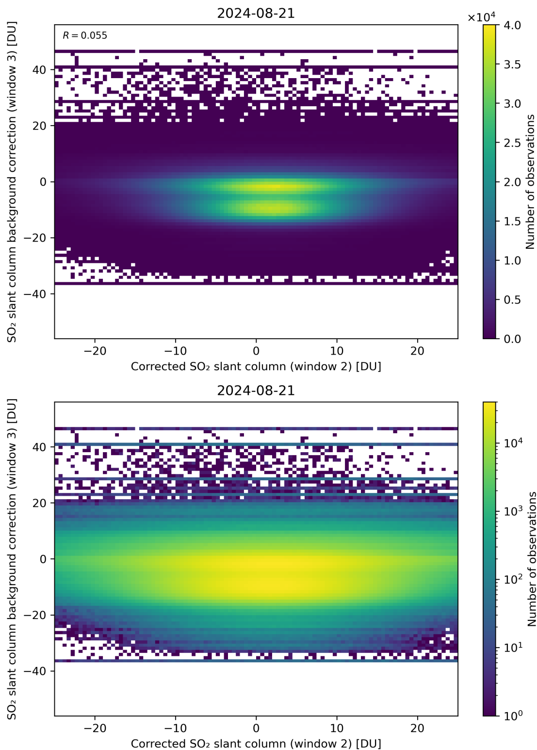
Figure 195: Scatter density plot of “Corrected SO 2 slant column (window 2)” against “SO 2 slant column background correction (window 3)” for 2024-08-21 to 2024-08-22.
