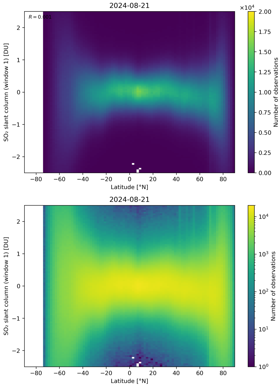
Figure 149: Scatter density plot of “Latitude” against “SO 2 slant column (window 1)” for 2024-08-21 to 2024-08-22.
