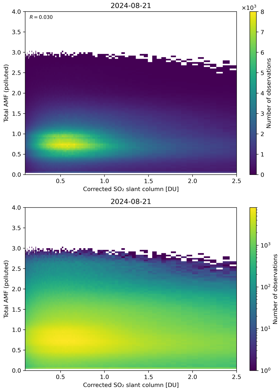
Figure 192: Scatter density plot of “Corrected SO 2 slant column” against “Total AMF (polluted)” for 2024-08-21 to 2024-08-22.
