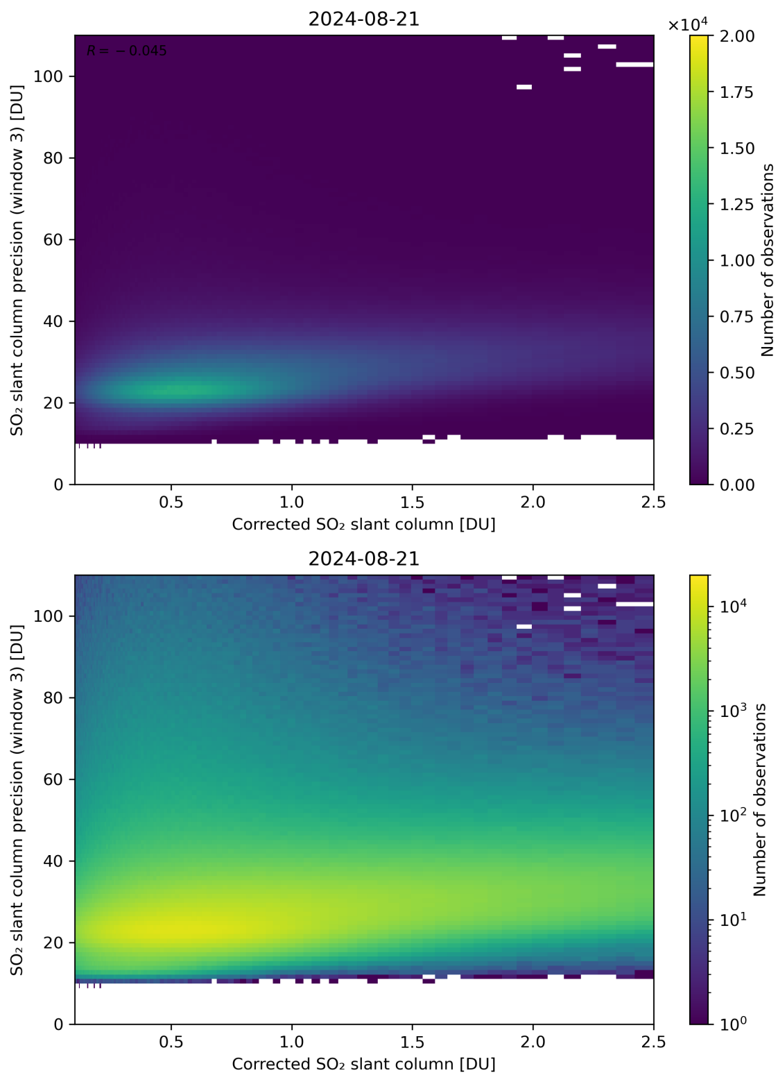
Figure 191: Scatter density plot of “Corrected SO 2 slant column” against “SO 2 slant column precision (window 3)” for 2024-08-21 to 2024-08-22.
