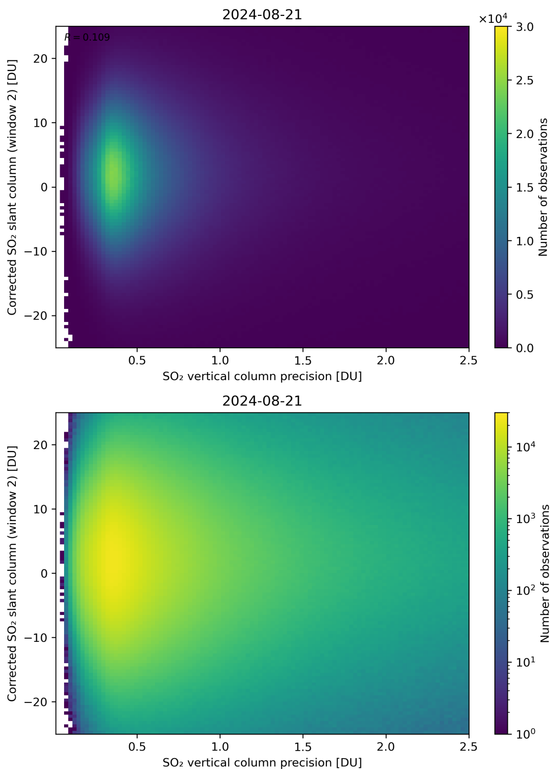
Figure 287: Scatter density plot of “SO 2 vertical column precision” against “Corrected SO 2 slant column (window 2)” for 2024-08-21 to 2024-08-22.
