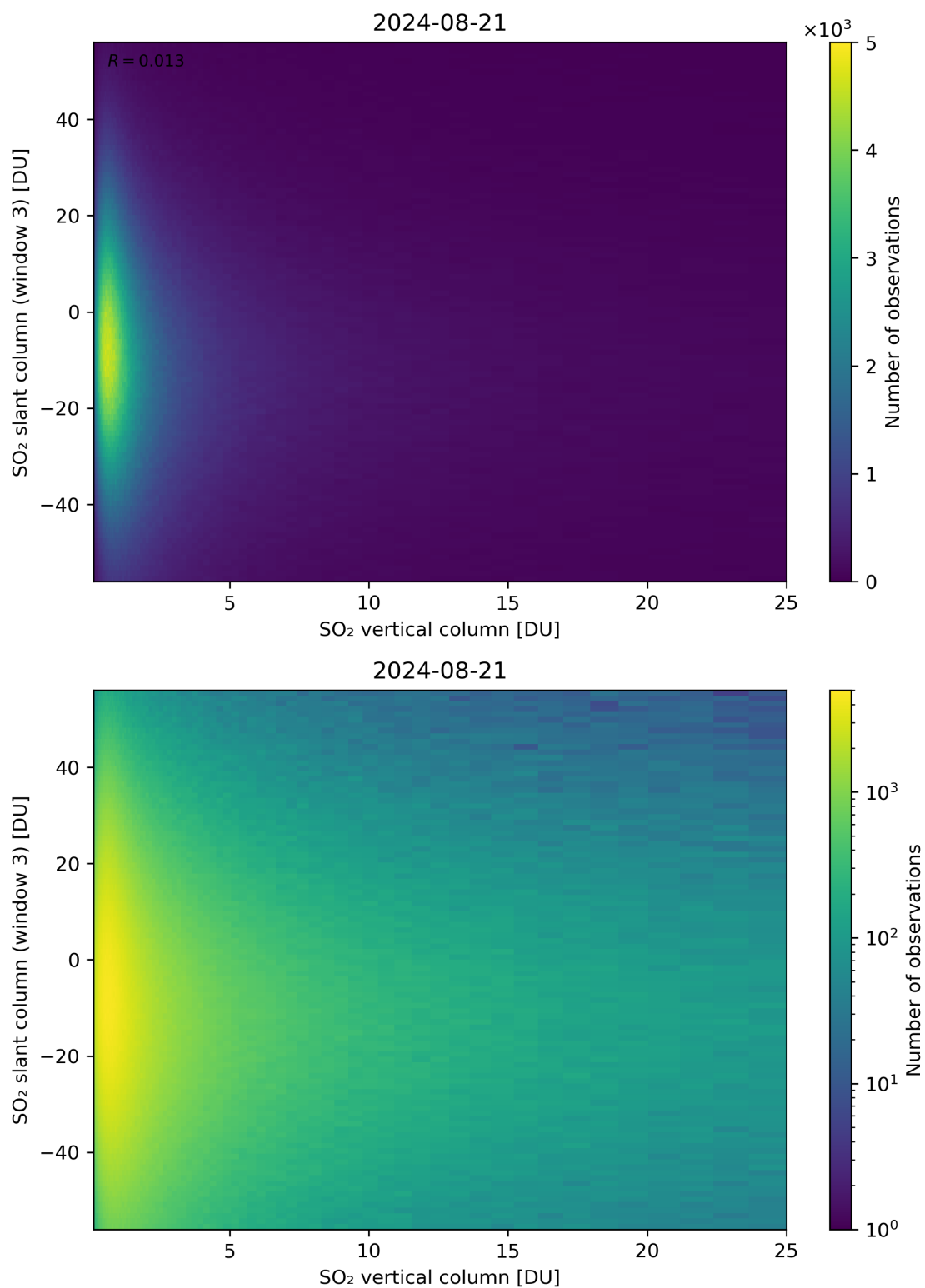
Figure 303: Scatter density plot of “SO 2 vertical column” against “SO 2 slant column (window 3)” for 2024-08-21 to 2024-08-22.
