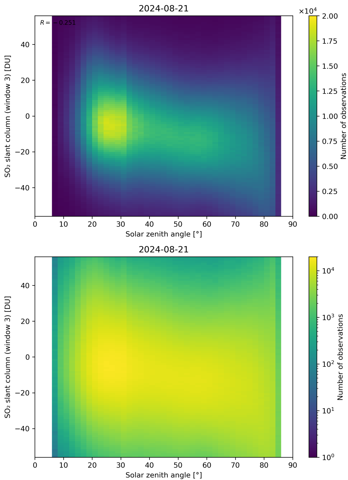
Figure 172: Scatter density plot of “Solar zenith angle” against “SO 2 slant column (window 3)” for 2024-08-21 to 2024-08-22.
