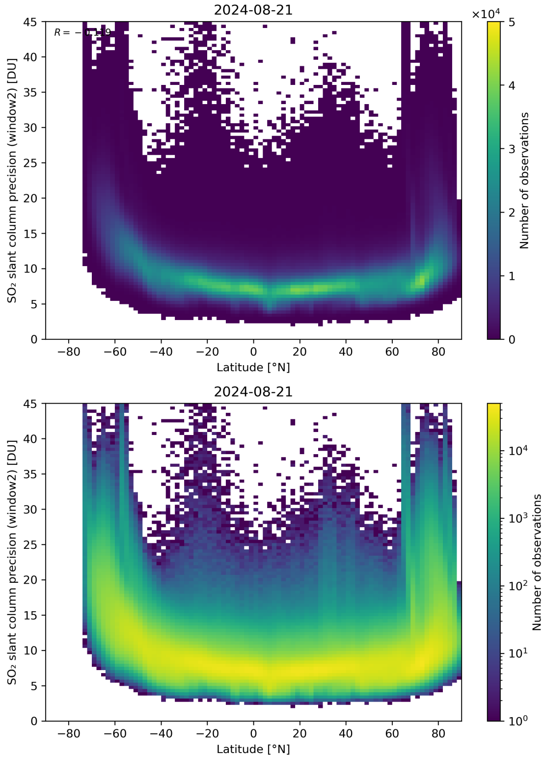
Figure 151: Scatter density plot of “Latitude” against “SO 2 slant column precision (window2)” for 2024-08-21 to 2024-08-22.
