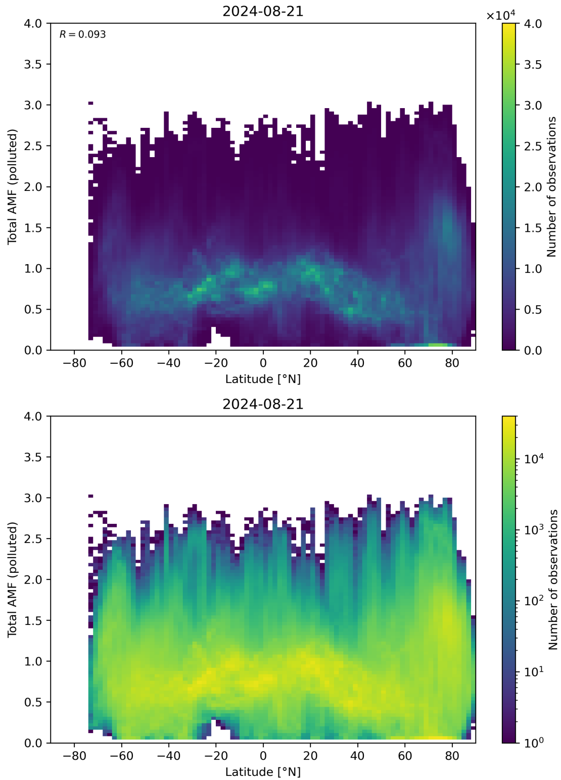
Figure 154: Scatter density plot of “Latitude” against “Total AMF (polluted)” for 2024-08-21 to 2024-08-22.
