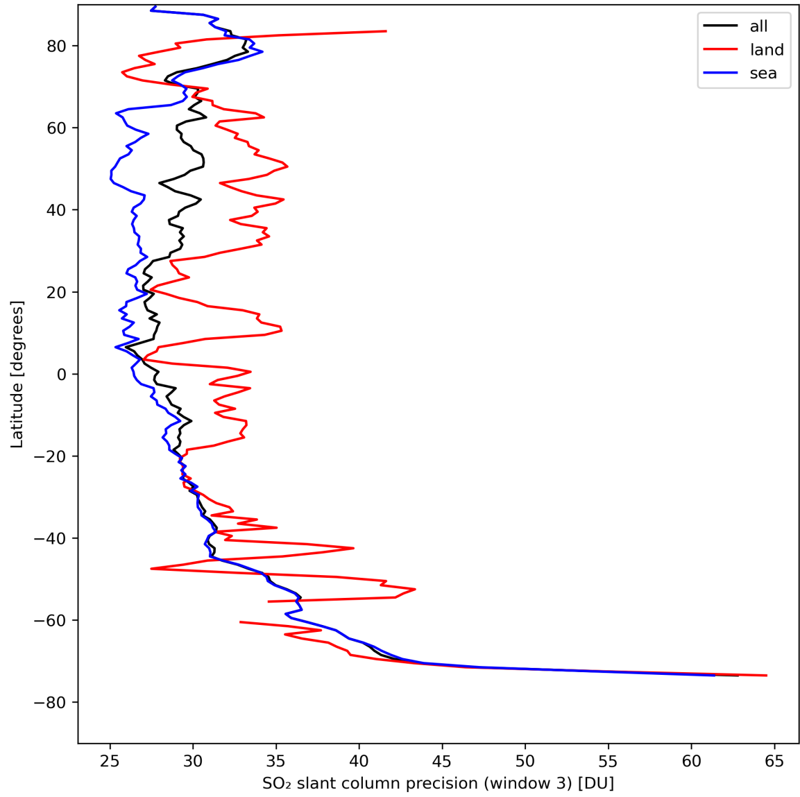
Figure 42: Zonal average of “SO 2 slant column precision (window 3)” for 2024-08-21 to 2024-08-22.
