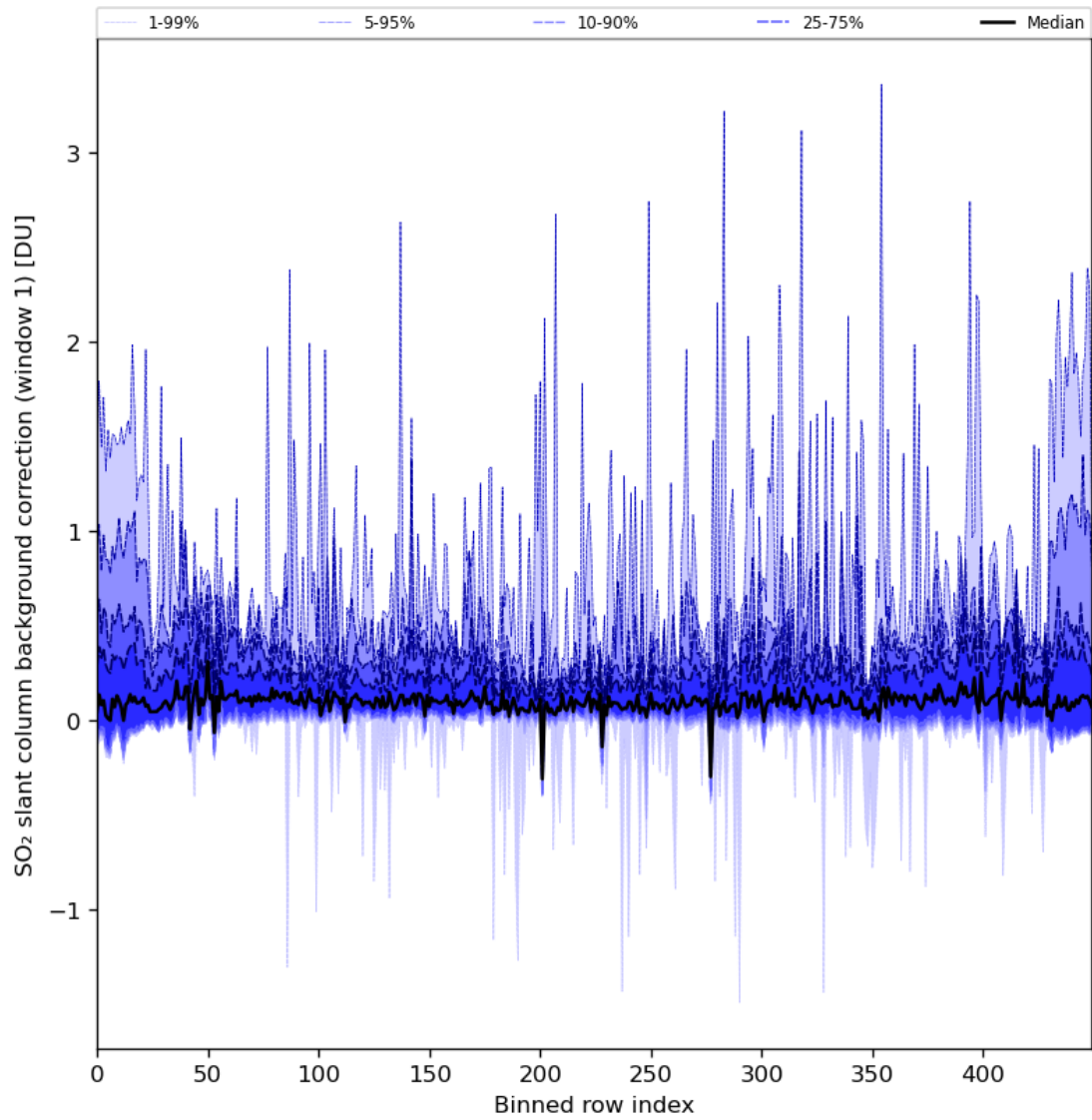
Figure 82: Along track statistics of “SO 2 slant column background correction (window 1)” for 2024-08-21 to 2024-08-22
