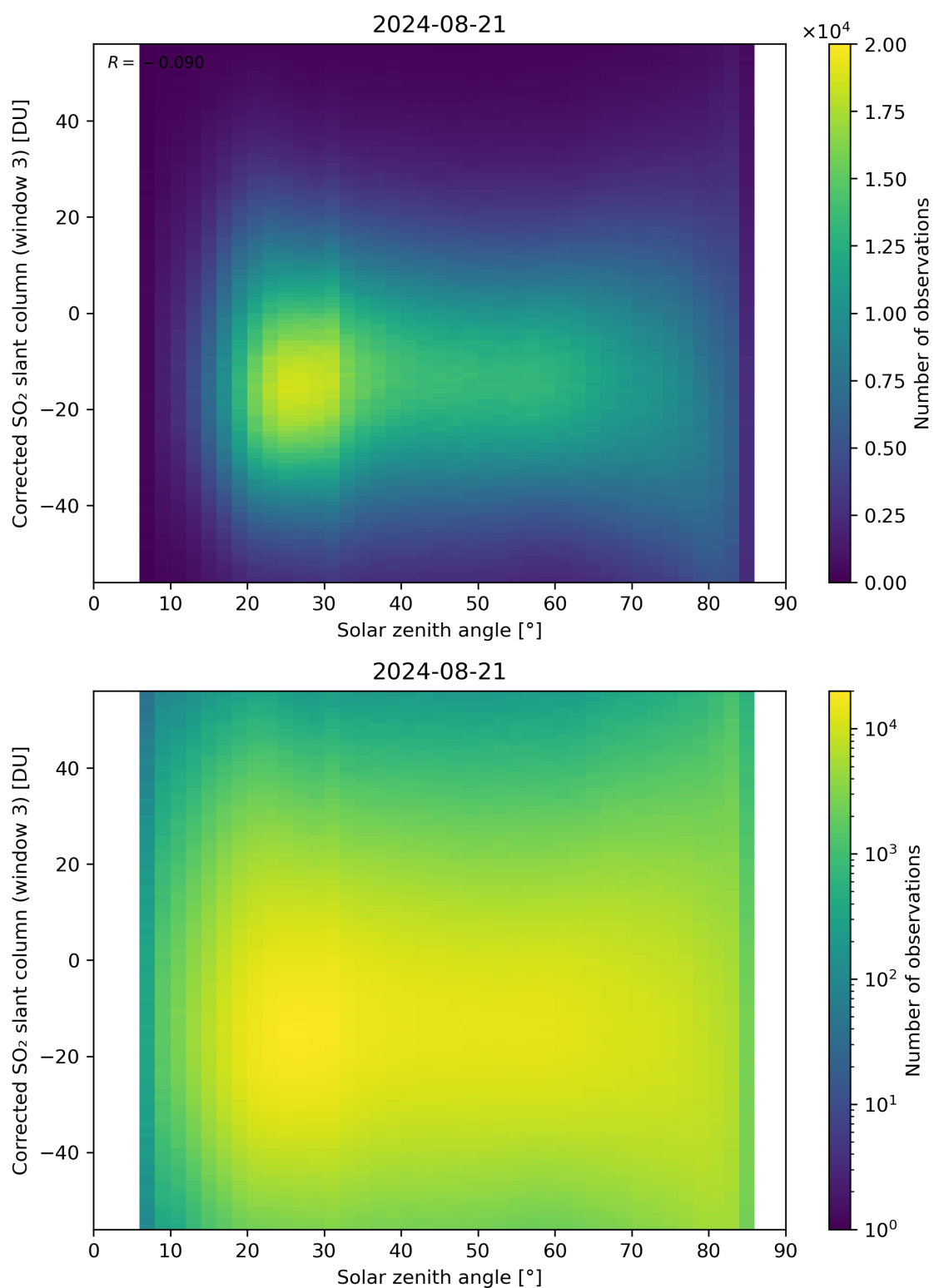
Figure 168: Scatter density plot of “Solar zenith angle” against “Corrected SO 2 slant column (window 3)” for 2024-08-21 to 2024-08-22.
