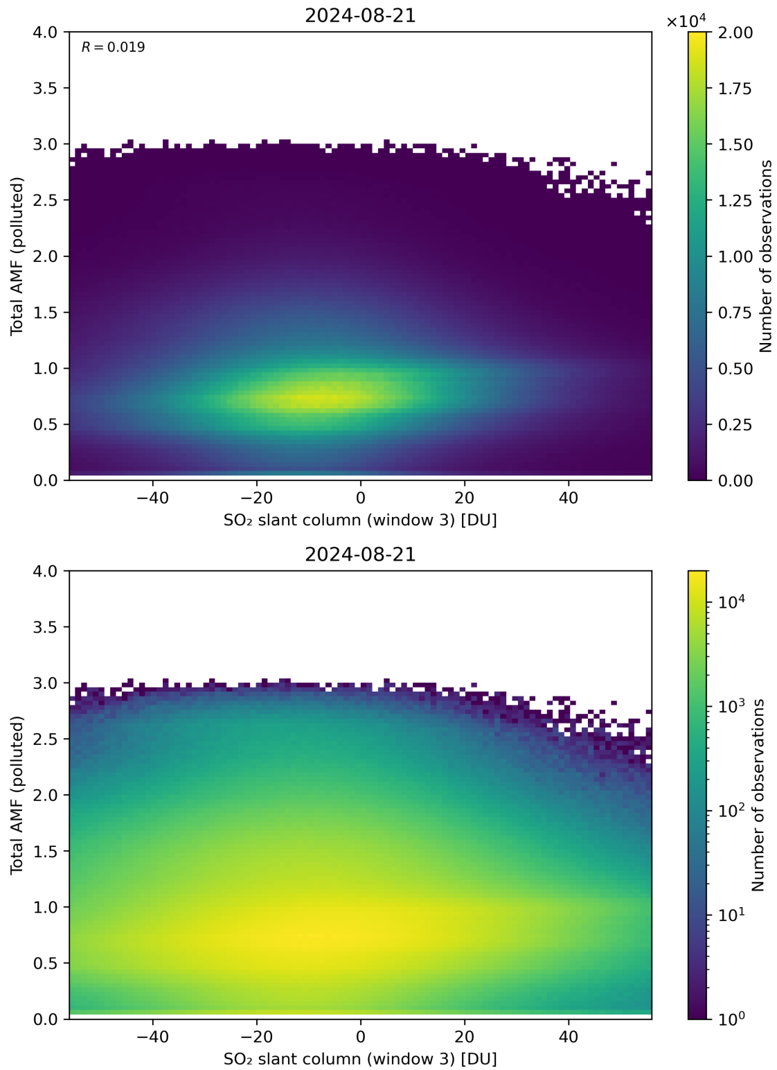
Figure 268: Scatter density plot of “SO 2 slant column (window 3)” against “Total AMF (polluted)” for 2024-08-21 to 2024-08-22.
