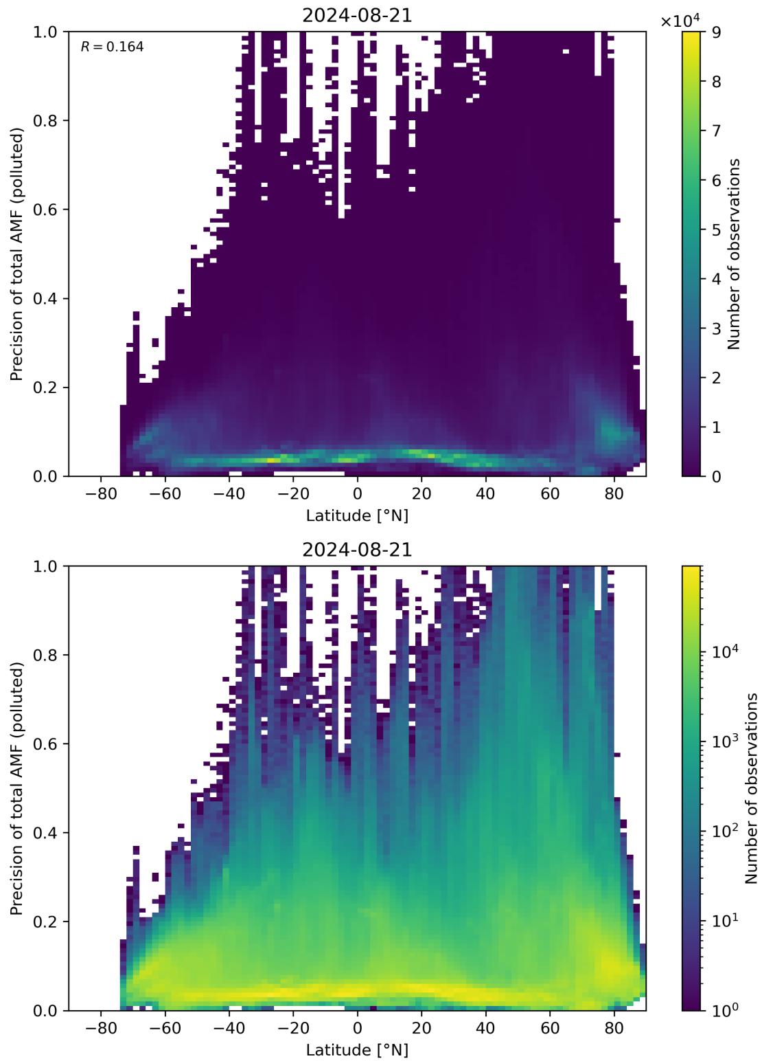
Figure 155: Scatter density plot of “Latitude” against “Precision of total AMF (polluted)” for 2024-08-21 to 2024-08-22.
