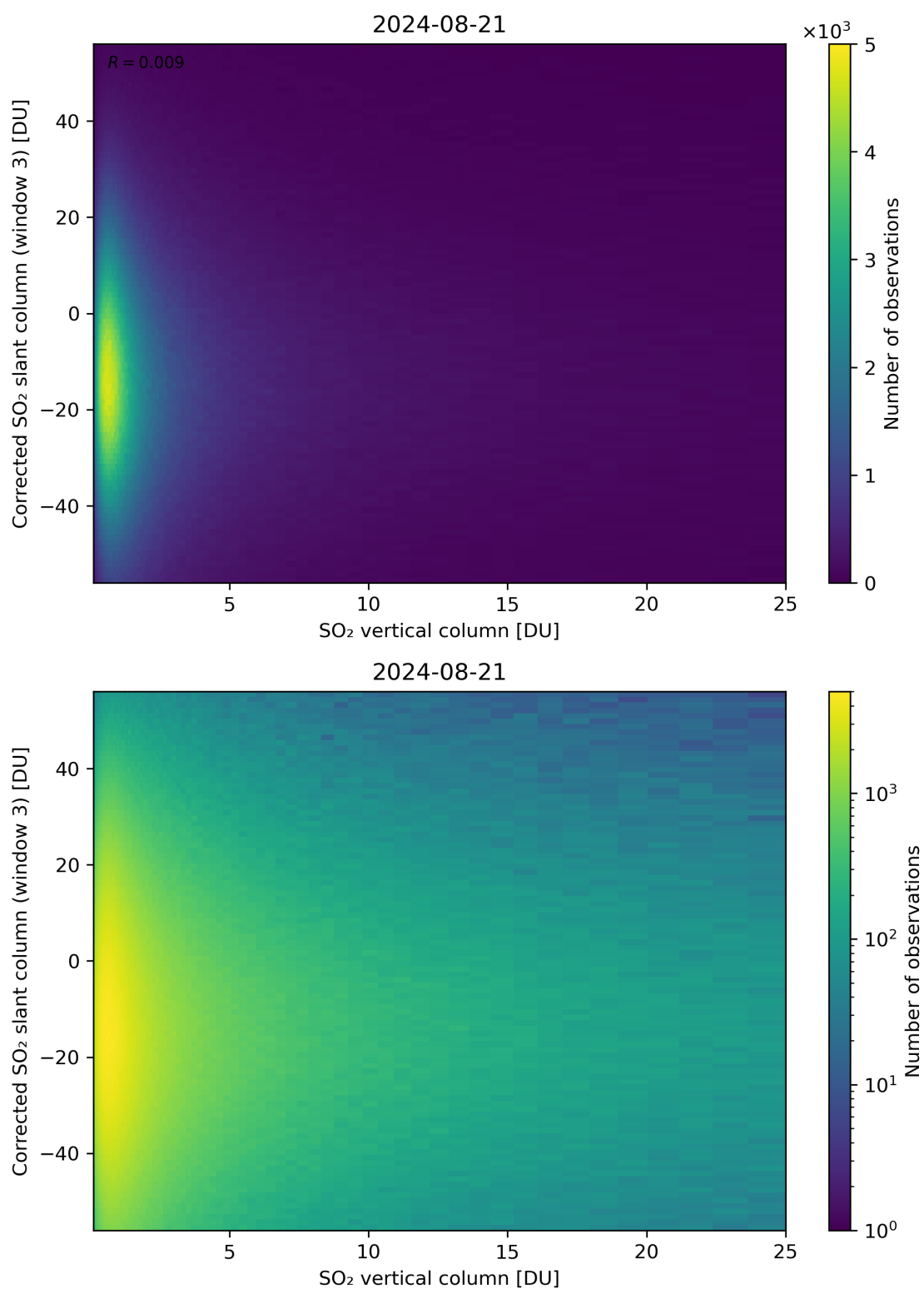
Figure 299: Scatter density plot of “SO 2 vertical column” against “Corrected SO 2 slant column (window 3)” for 2024-08-21 to 2024-08-22.
