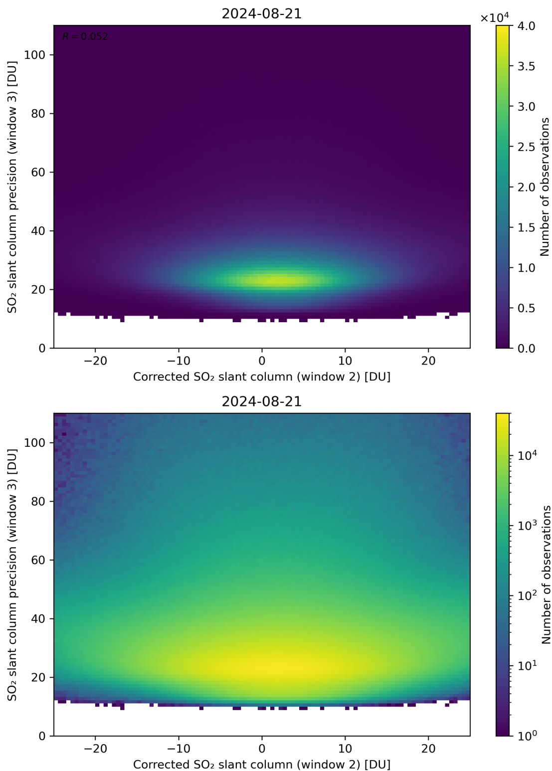
Figure 202: Scatter density plot of “Corrected SO 2 slant column (window 2)” against “SO 2 slant column precision (window 3)” for 2024-08-21 to 2024-08-22.
