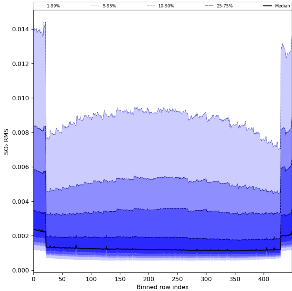
Figure 93: Along track statistics of “SO 2 RMS” for 2024-08-21 to 2024-08-22
