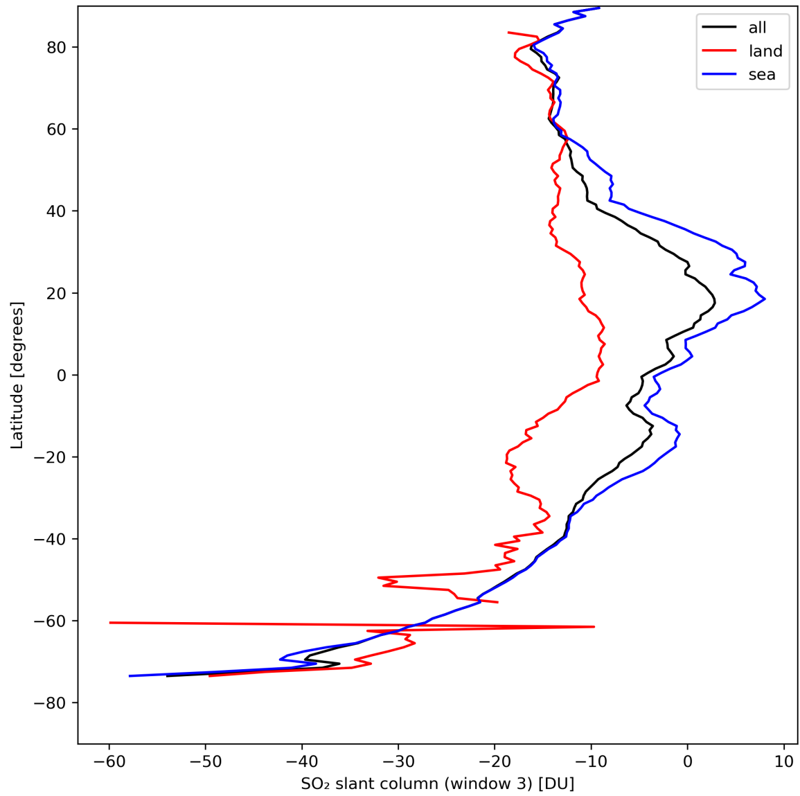
Figure 41: Zonal average of “SO 2 slant column (window 3)” for 2024-08-21 to 2024-08-22.
