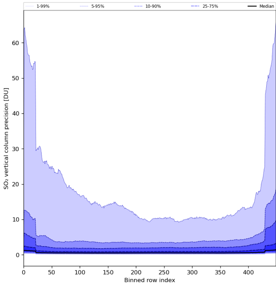
Figure 77: Along track statistics of “SO 2 vertical column precision” for 2024-08-21 to 2024-08-22
