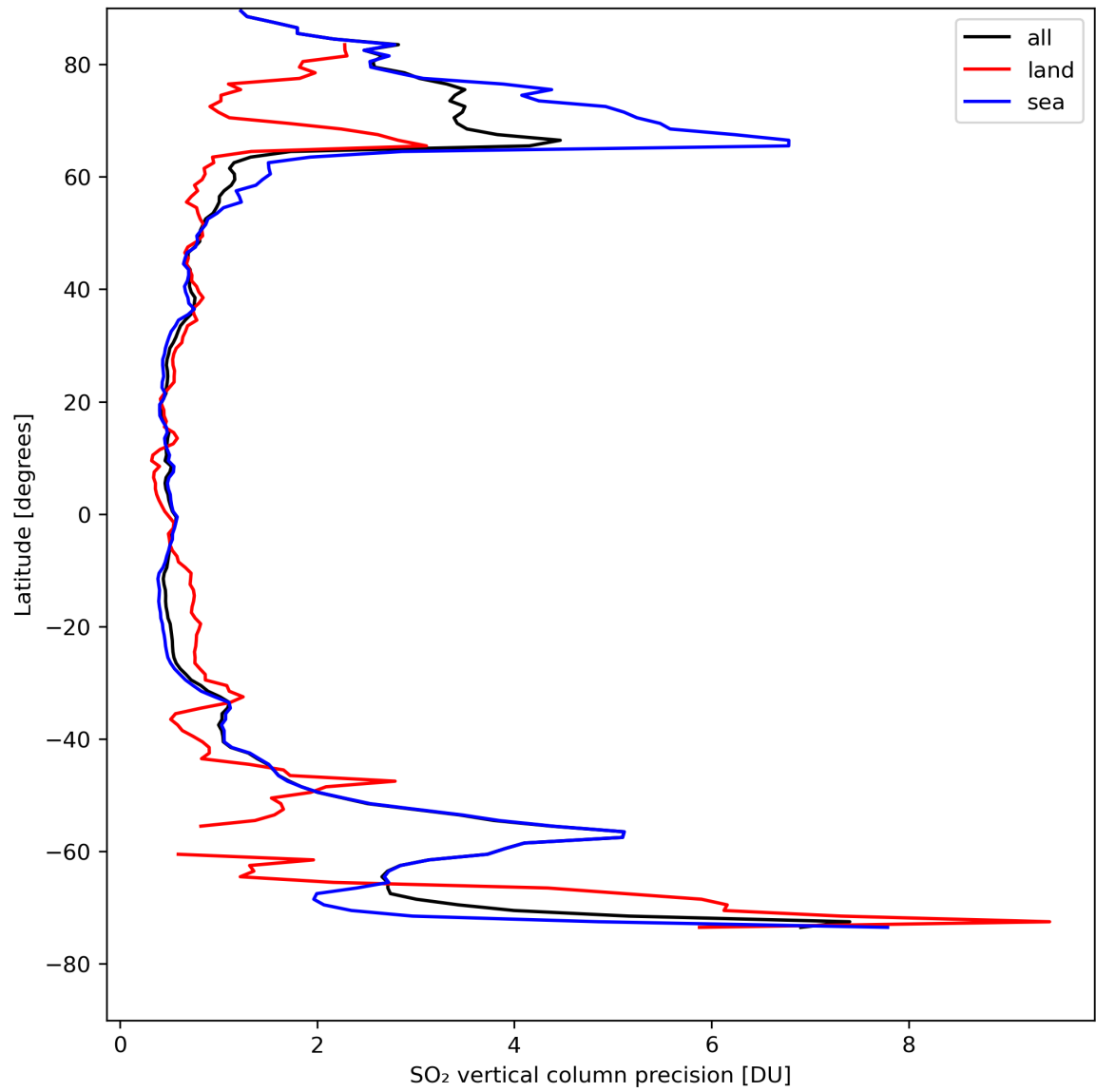
Figure 31: Zonal average of “SO 2 vertical column precision” for 2024-08-21 to 2024-08-22.
