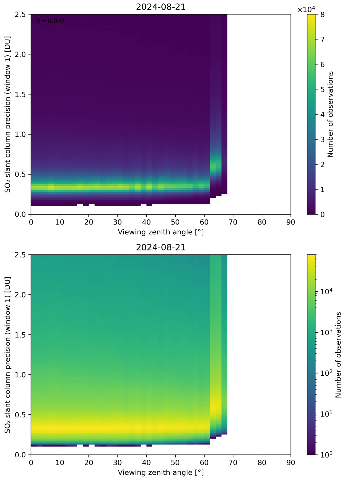
Figure 321: Scatter density plot of “Viewing zenith angle” against “SO 2 slant column precision (window 1)” for 2024-08-21 to 2024-08-22.
