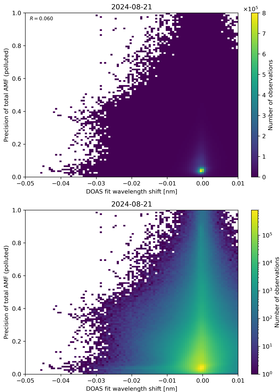
Figure 131: Scatter density plot of “DOAS fit wavelength shift” against “Precision of total AMF (polluted)” for 2024-08-21 to 2024-08-22.
