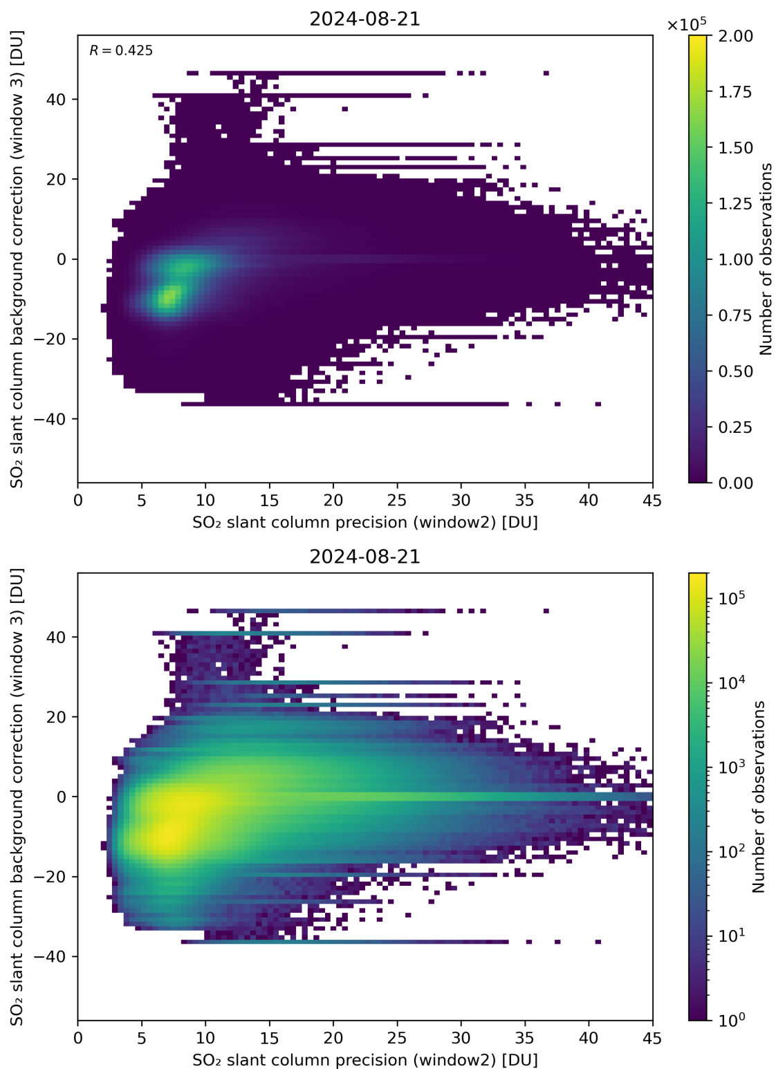
Figure 242: Scatter density plot of “SO 2 slant column precision (window2)” against “SO 2 slant column background correction (window 3)” for 2024-08-21 to 2024-08-22.
