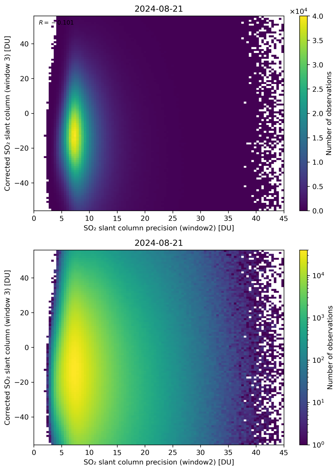
Figure 248: Scatter density plot of “SO 2 slant column precision (window2)” against “Corrected SO 2 slant column (window 3)” for 2024-08-21 to 2024-08-22.
