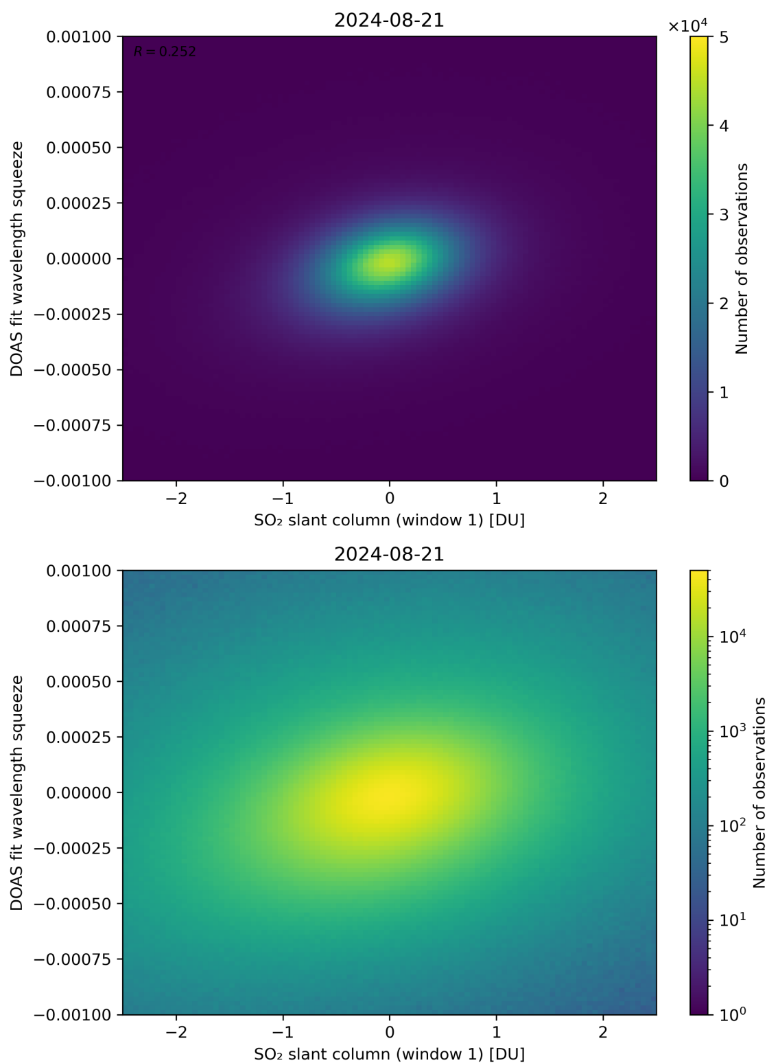
Figure 216: Scatter density plot of “SO 2 slant column (window 1)” against “DOAS fit wavelength squeeze” for 2024-08-21 to 2024-08-22.
