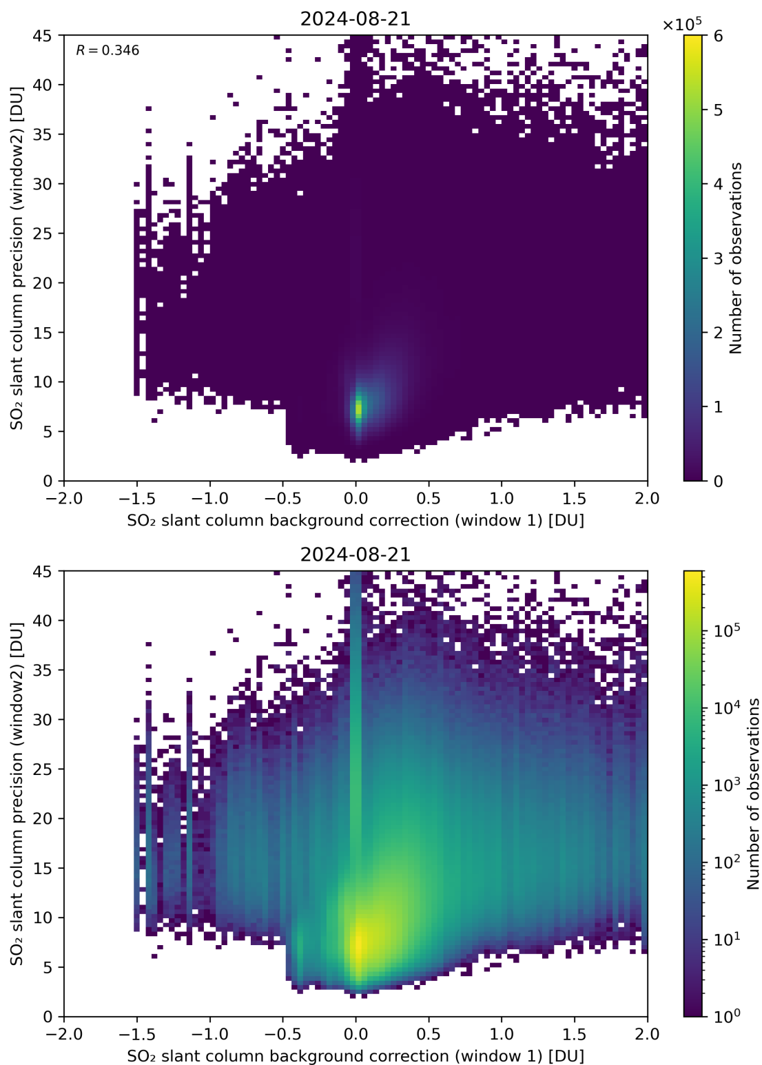
Figure 106: Scatter density plot of “SO 2 slant column background correction (window 1)” against “SO 2 slant column precision (window2)” for 2024-08-21 to 2024-08-22.
