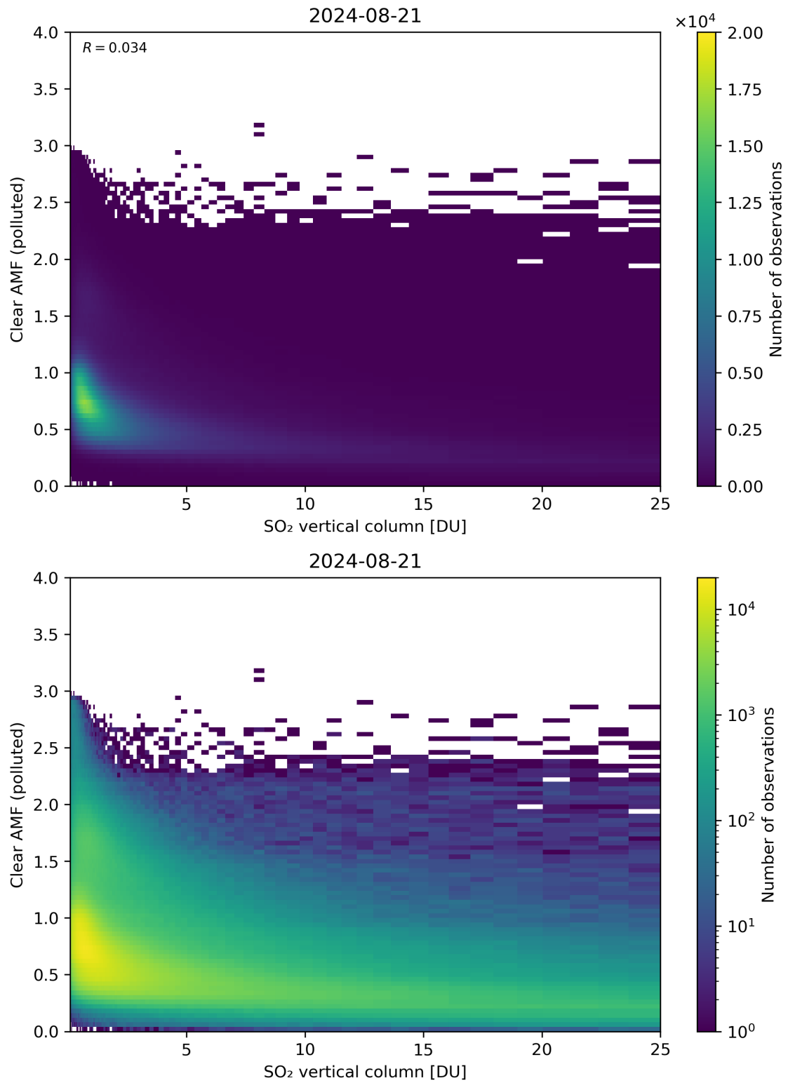
Figure 296: Scatter density plot of “SO 2 vertical column” against “Clear AMF (polluted)” for 2024-08-21 to 2024-08-22.
