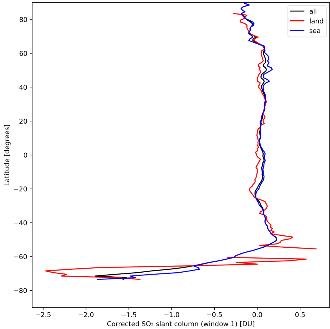
Figure 35: Zonal average of “Corrected SO 2 slant column (window 1)” for 2024-08-21 to 2024-08-22.
