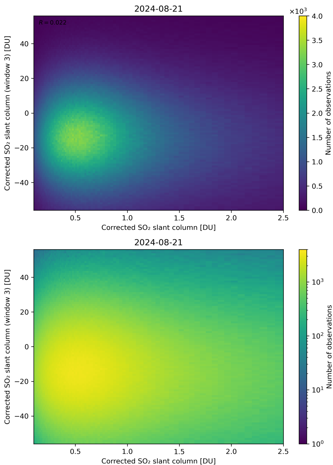
Figure 186: Scatter density plot of “Corrected SO 2 slant column” against “Corrected SO 2 slant column (window 3)” for 2024-08-21 to 2024-08-22.
