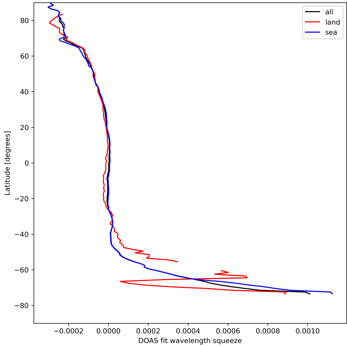
Figure 46: Zonal average of “DOAS fit wavelength squeeze” for 2024-08-21 to 2024-08-22.
