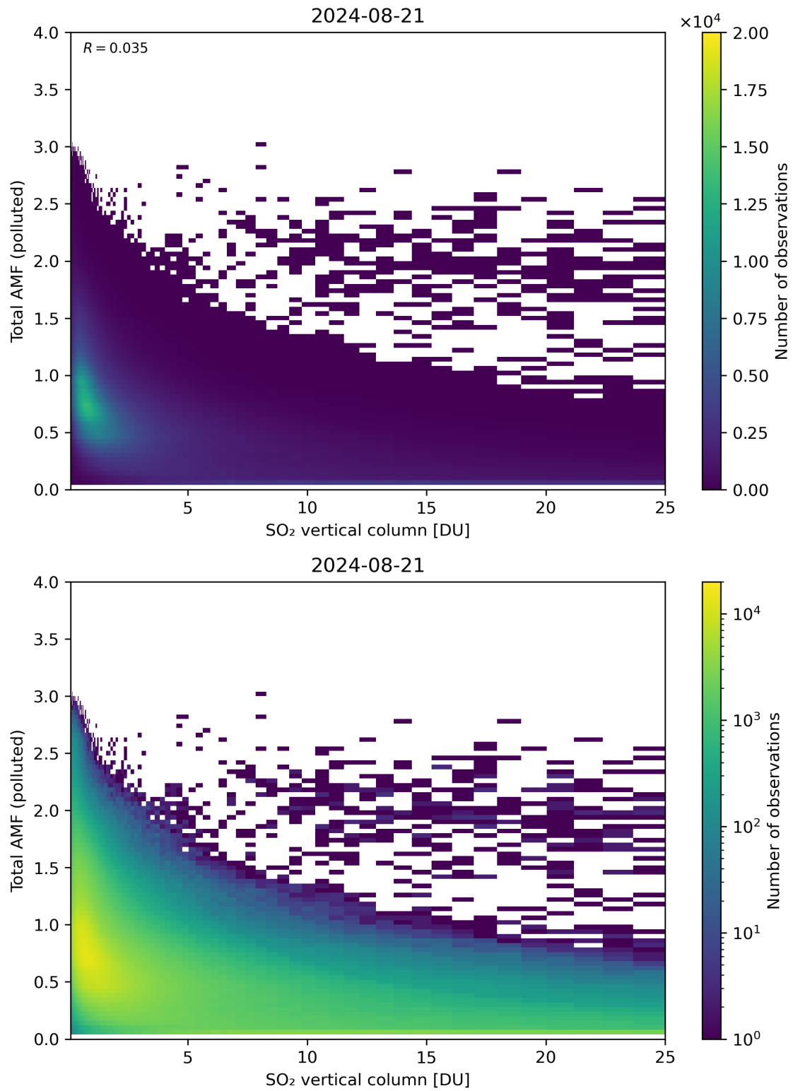
Figure 305: Scatter density plot of “SO 2 vertical column” against “Total AMF (polluted)” for 2024-08-21 to 2024-08-22.
