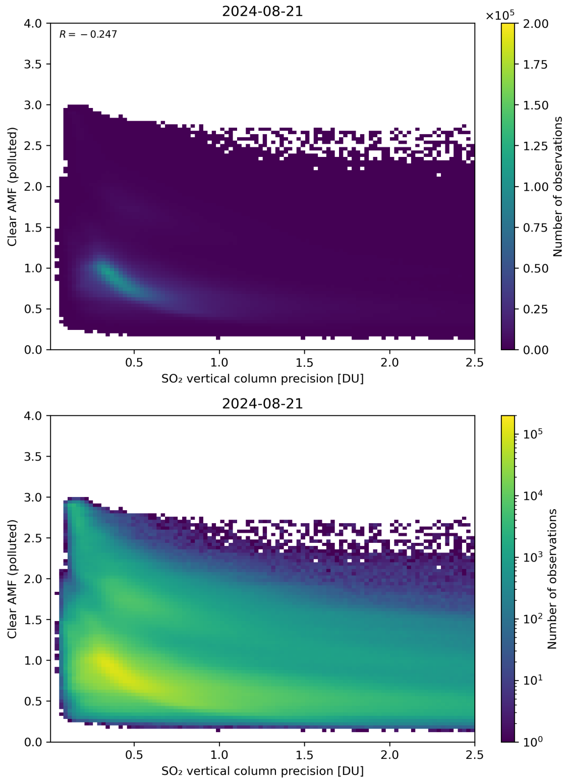
Figure 285: Scatter density plot of “SO 2 vertical column precision” against “Clear AMF (polluted)” for 2024-08-21 to 2024-08-22.
