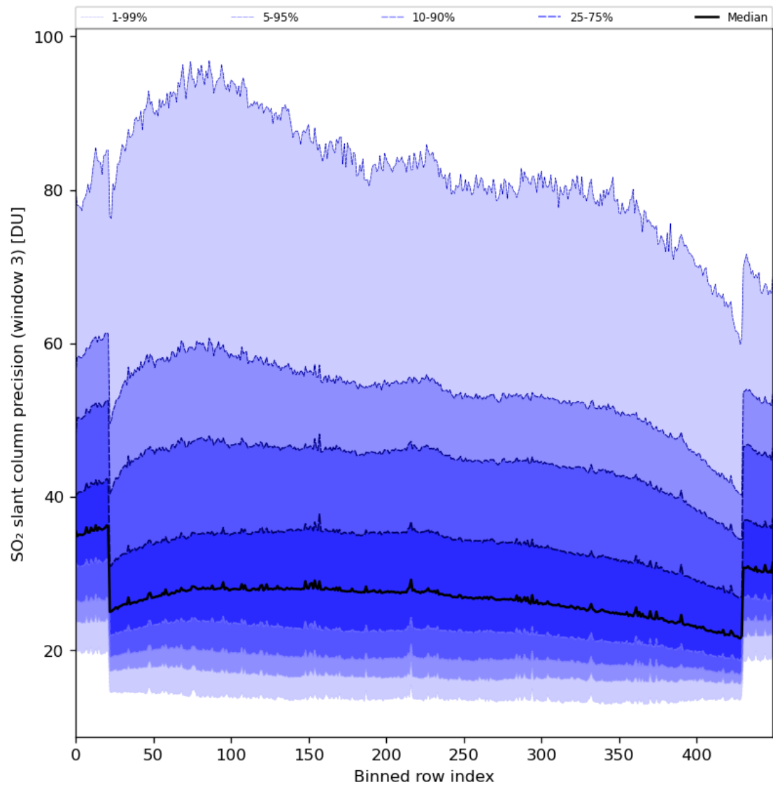
Figure 88: Along track statistics of “SO 2 slant column precision (window 3)” for 2024-08-21 to 2024-08-22
