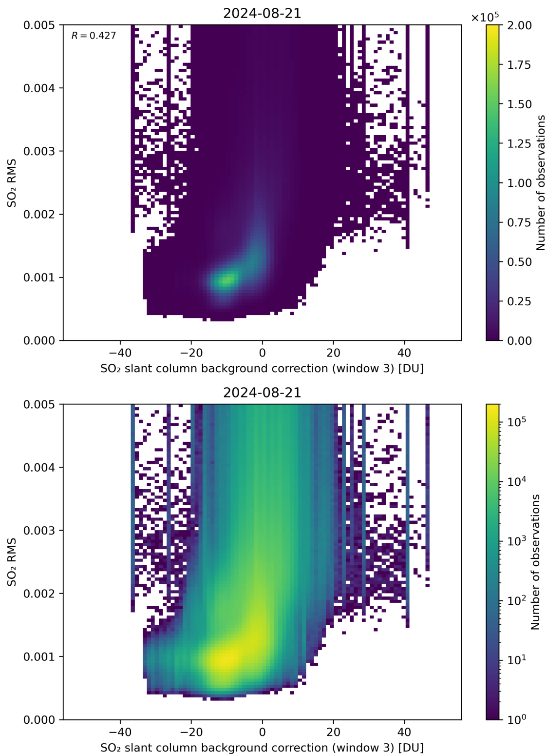
Figure 123: Scatter density plot of “SO 2 slant column background correction (window 3)” against “SO 2 RMS” for 2024-08-21 to 2024-08-22.
