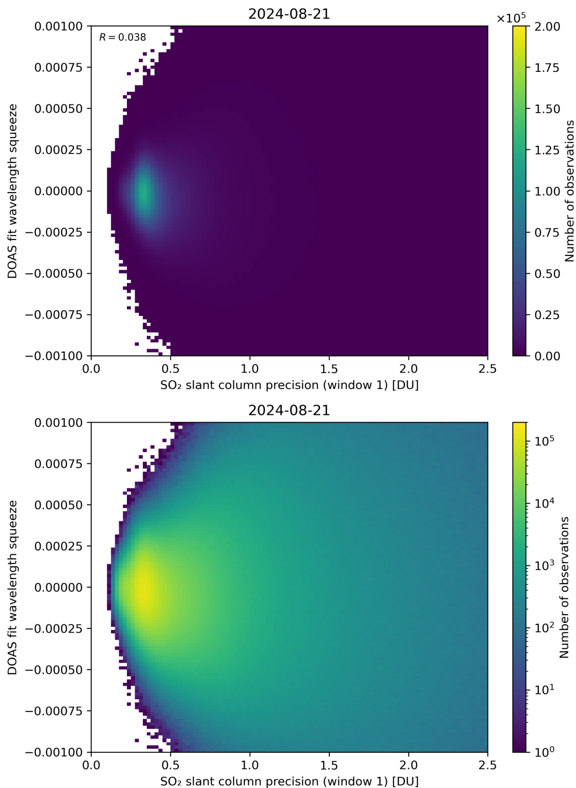
Figure 222: Scatter density plot of “SO 2 slant column precision (window 1)” against “DOAS fit wavelength squeeze” for 2024-08-21 to 2024-08-22.
