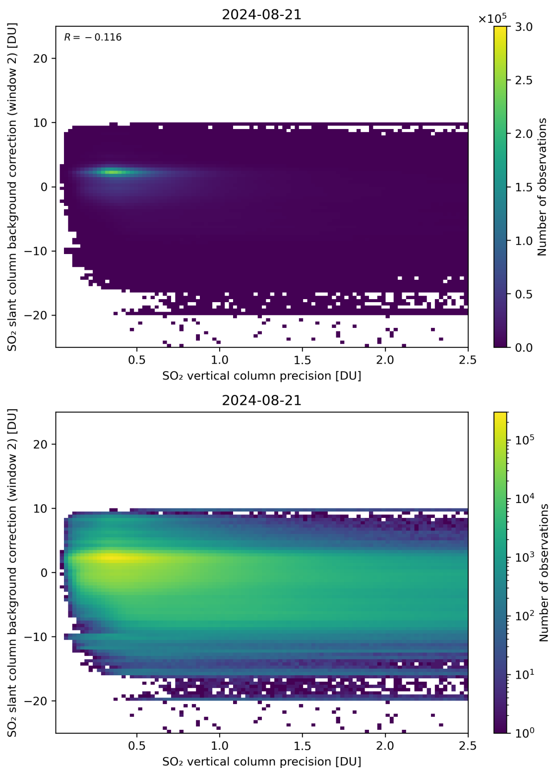
Figure 280: Scatter density plot of “SO 2 vertical column precision” against “SO 2 slant column background correction (window 2)” for 2024-08-21 to 2024-08-22.
