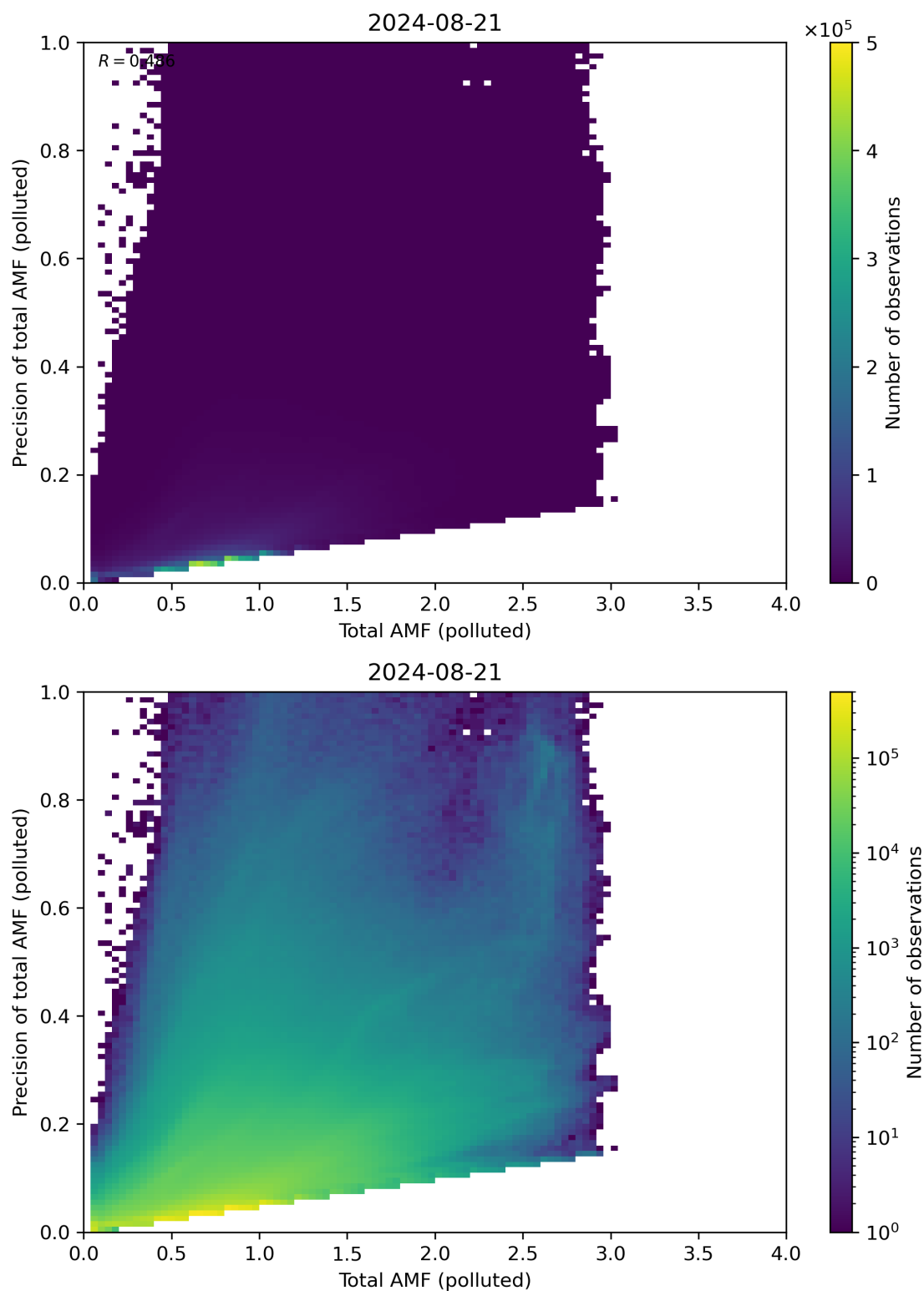
Figure 272: Scatter density plot of “Total AMF (polluted)” against “Precision of total AMF (polluted)” for 2024-08-21 to 2024-08-22.
