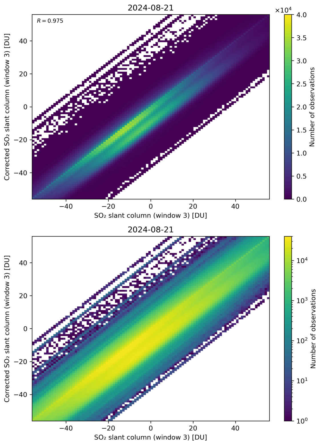
Figure 266: Scatter density plot of “SO 2 slant column (window 3)” against “Corrected SO 2 slant column (window 3)” for 2024-08-21 to 2024-08-22.
