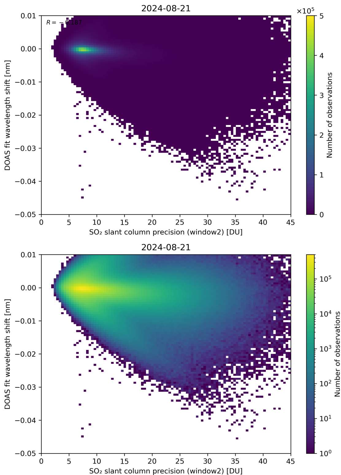
Figure 243: Scatter density plot of “SO 2 slant column precision (window2)” against “DOAS fit wavelength shift” for 2024-08-21 to 2024-08-22.
