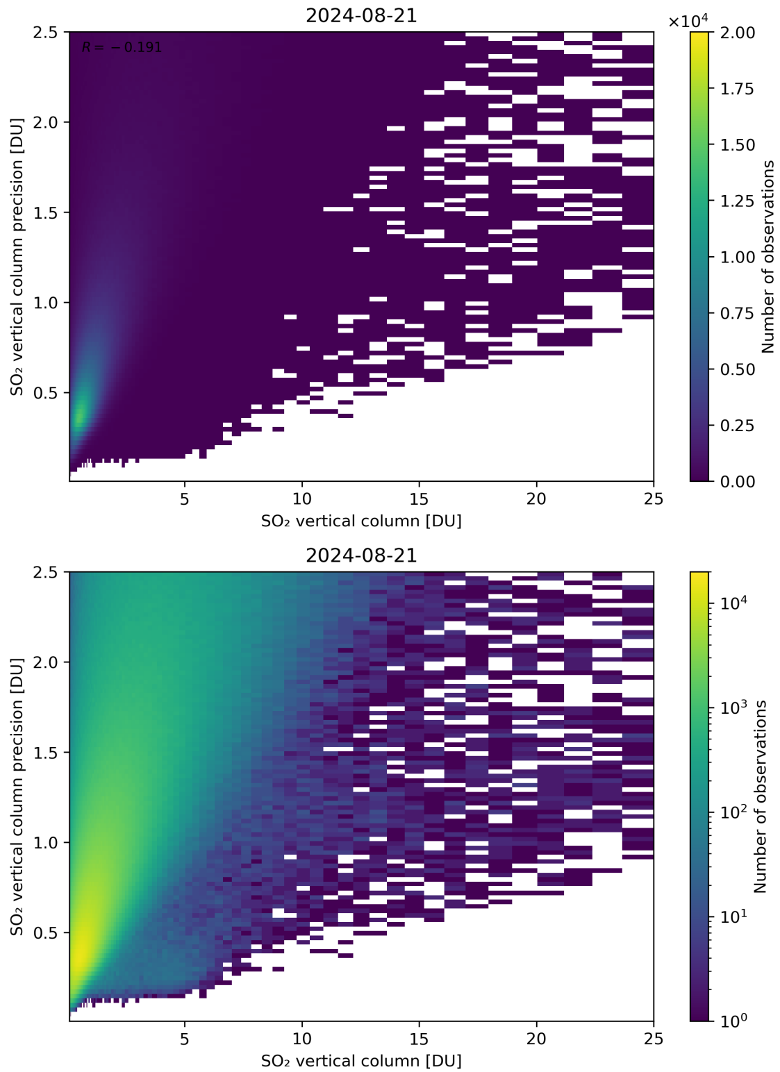
Figure 307: Scatter density plot of “SO 2 vertical column” against “SO 2 vertical column precision” for 2024-08-21 to 2024-08-22.
