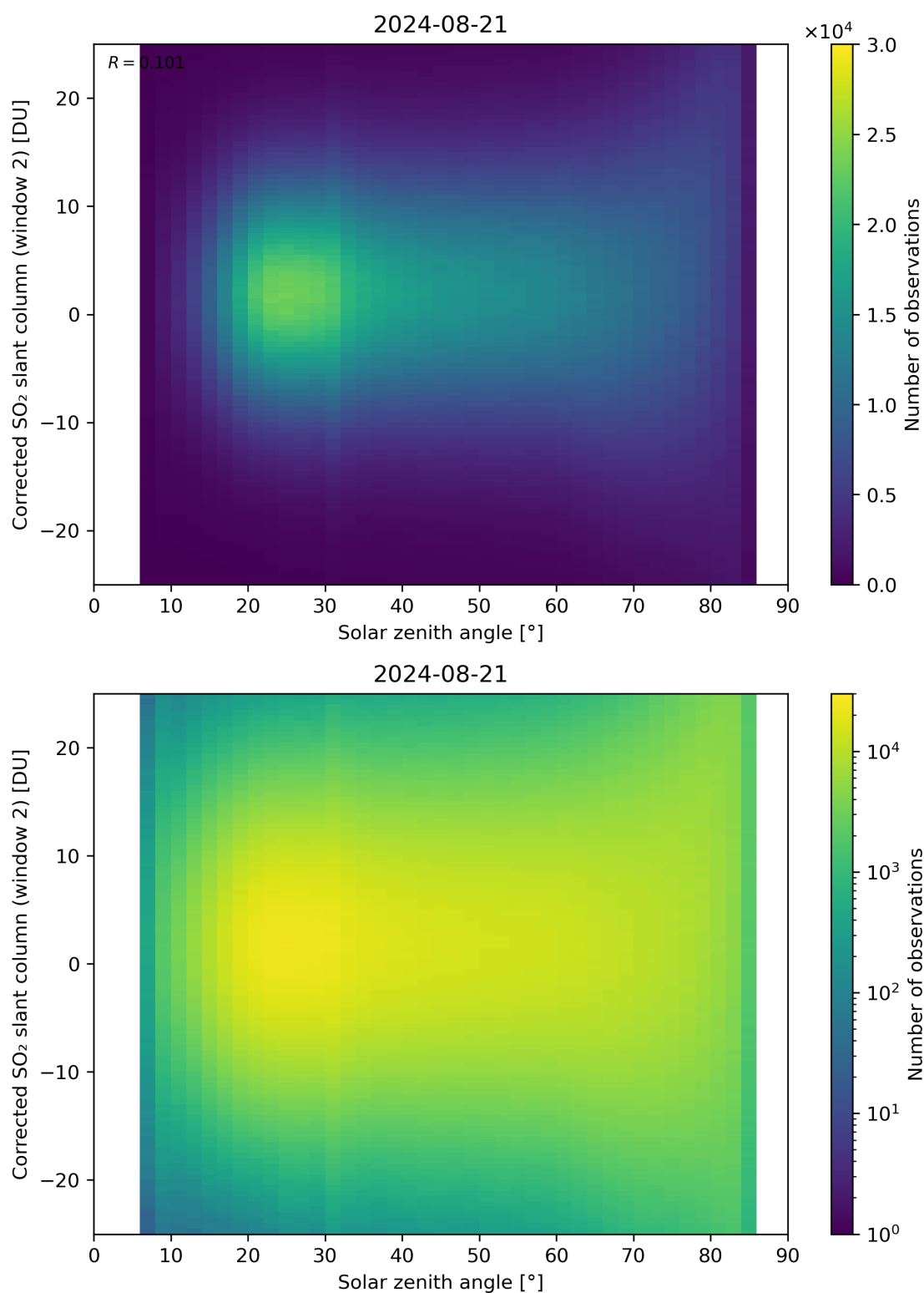
Figure 167: Scatter density plot of “Solar zenith angle” against “Corrected SO 2 slant column (window 2)” for 2024-08-21 to 2024-08-22.
