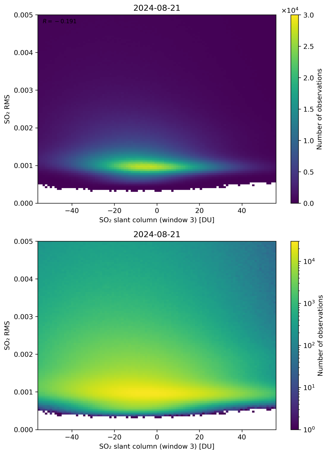
Figure 256: Scatter density plot of “SO 2 slant column (window 3)” against “SO 2 RMS” for 2024-08-21 to 2024-08-22.
