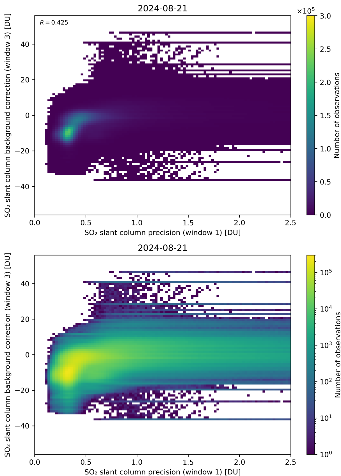
Figure 220: Scatter density plot of “SO 2 slant column precision (window 1)” against “SO 2 slant column background correction (window 3)” for 2024-08-21 to 2024-08-22.
