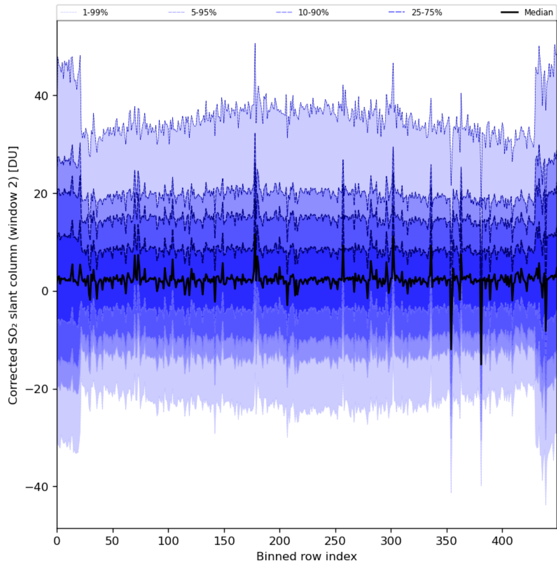
Figure 85: Along track statistics of “Corrected SO 2 slant column (window 2)” for 2024-08-21 to 2024-08-22
