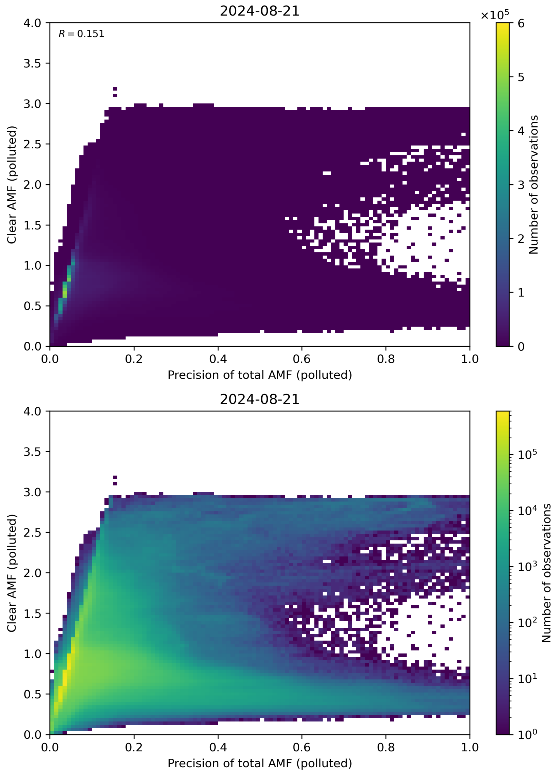
Figure 270: Scatter density plot of “Precision of total AMF (polluted)” against “Clear AMF (polluted)” for 2024-08-21 to 2024-08-22.
