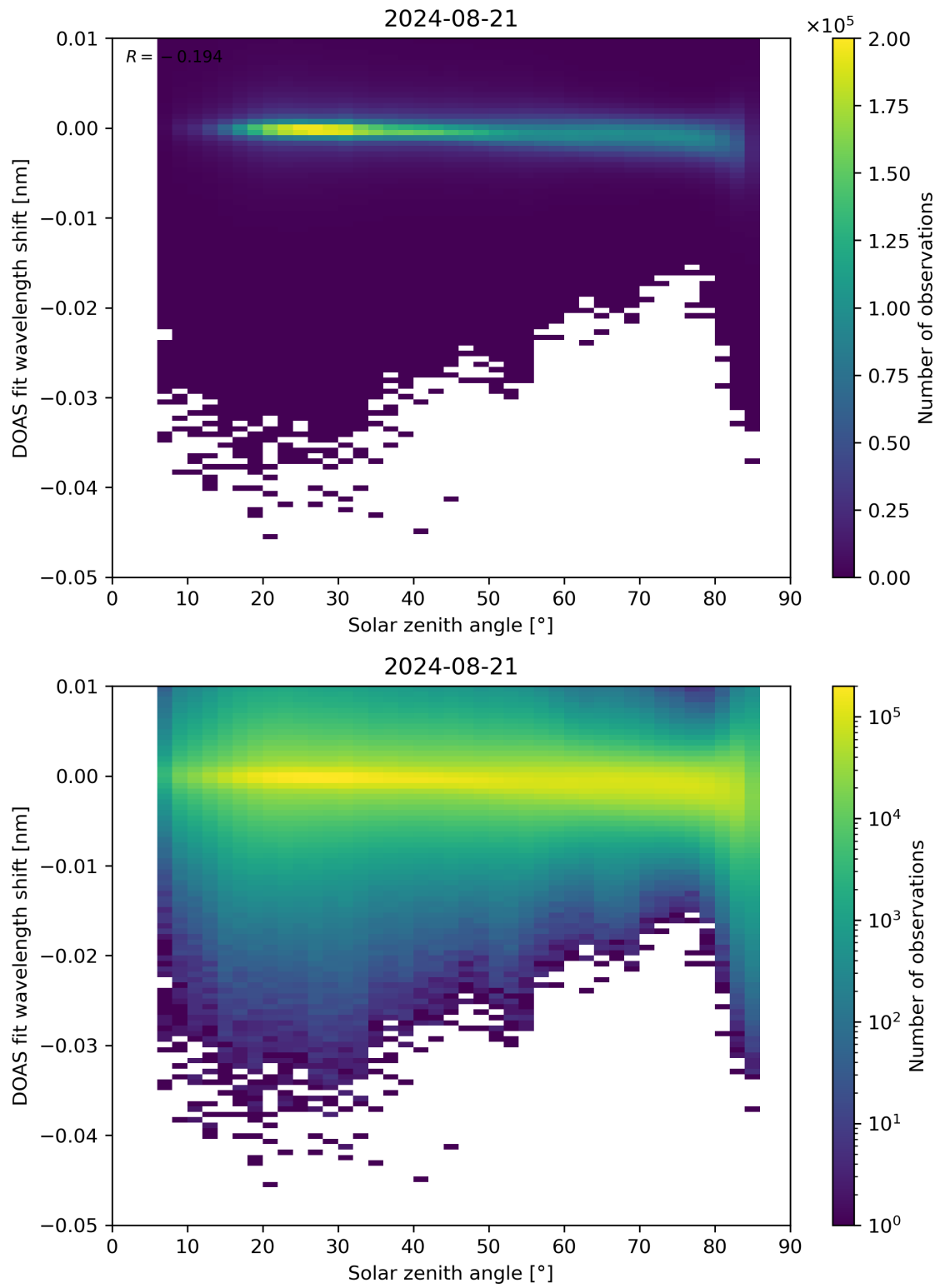
Figure 161: Scatter density plot of “Solar zenith angle” against “DOAS fit wavelength shift” for 2024-08-21 to 2024-08-22.
