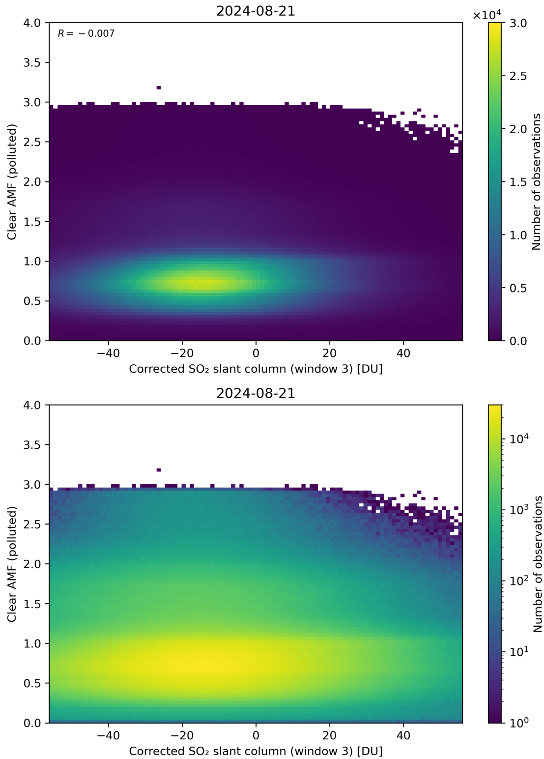
Figure 209: Scatter density plot of “Corrected SO 2 slant column (window 3)” against “Clear AMF (polluted)” for 2024-08-21 to 2024-08-22.
