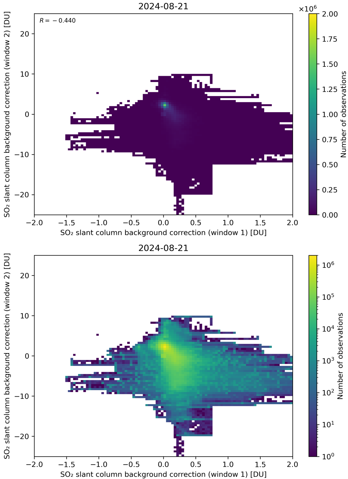
Figure 98: Scatter density plot of “SO 2 slant column background correction (window 1)” against “SO 2 slant column background correction (window 2)” for 2024-08-21 to 2024-08-22.
