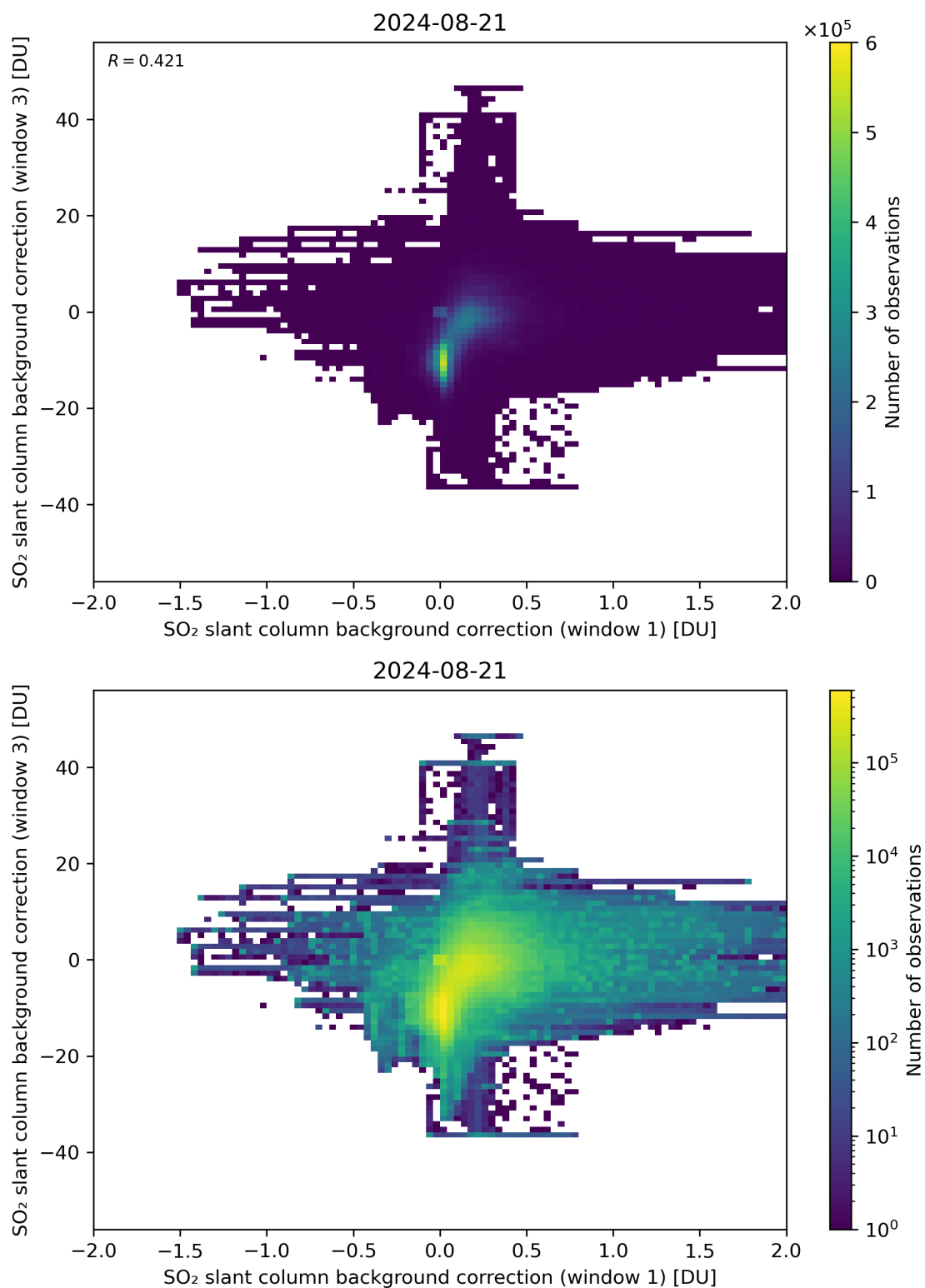
Figure 99: Scatter density plot of “SO 2 slant column background correction (window 1)” against “SO 2 slant column background correction (window 3)” for 2024-08-21 to 2024-08-22.
