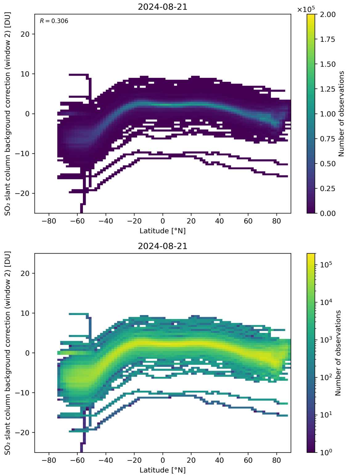
Figure 140: Scatter density plot of “Latitude” against “SO 2 slant column background correction (window 2)” for 2024-08-21 to 2024-08-22.
