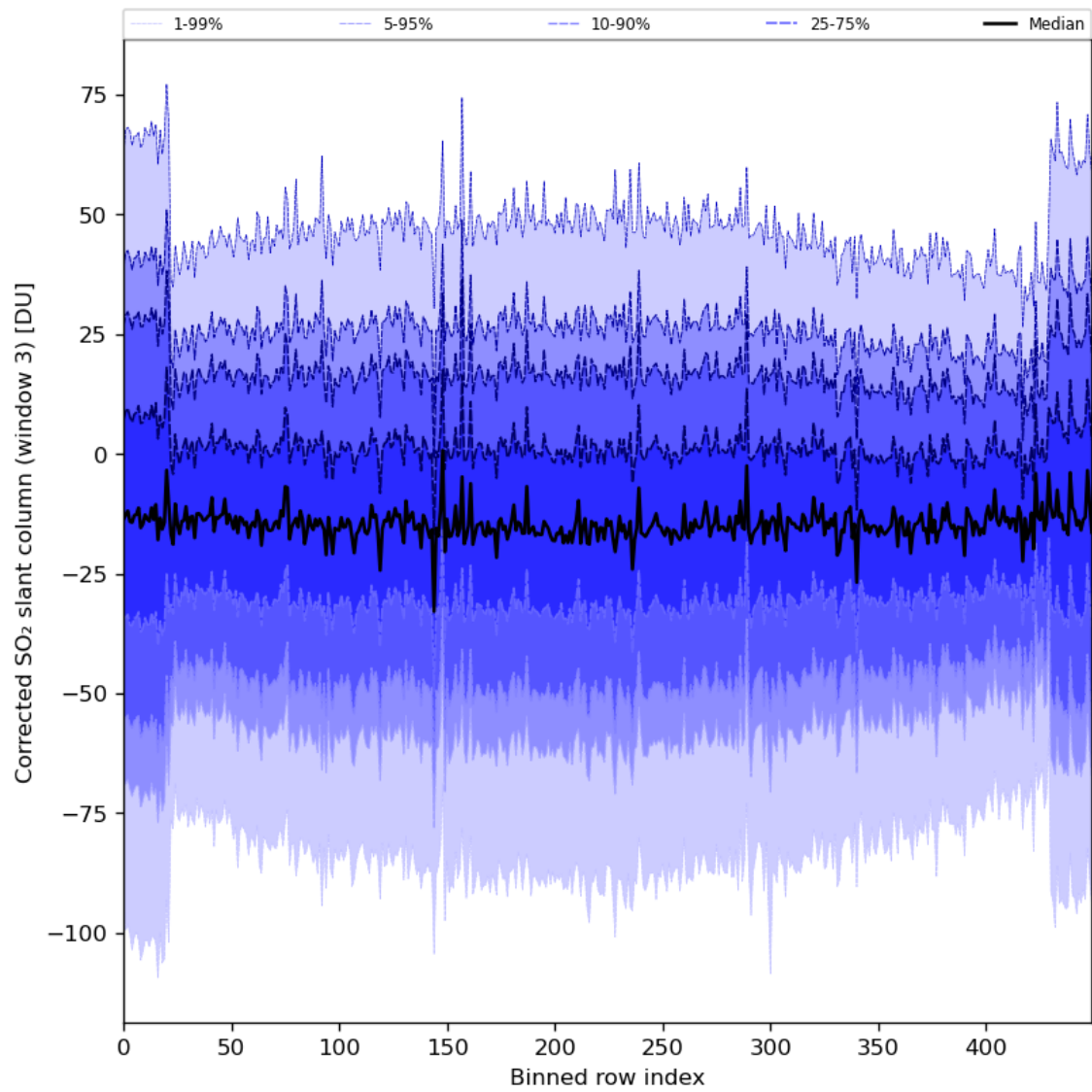
Figure 89: Along track statistics of “Corrected SO 2 slant column (window 3)” for 2024-08-21 to 2024-08-22
