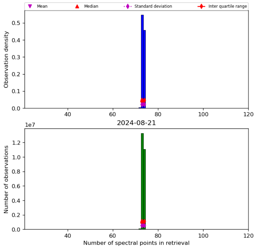
Figure 74: Histogram of “Number of spectral points in retrieval” for 2024-08-21 to 2024-08-22
