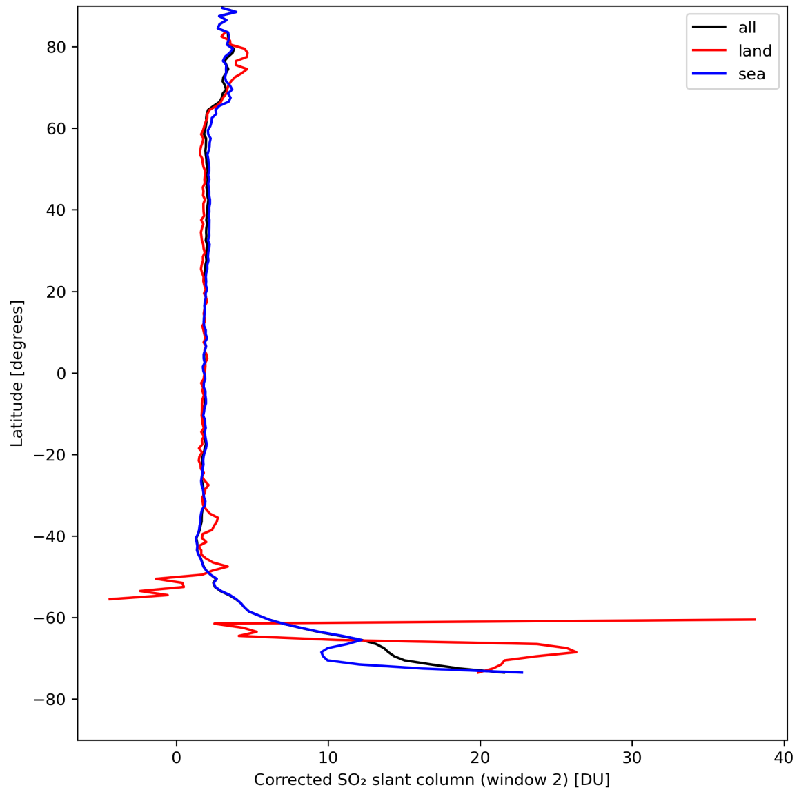
Figure 39: Zonal average of “Corrected SO 2 slant column (window 2)” for 2024-08-21 to 2024-08-22.
