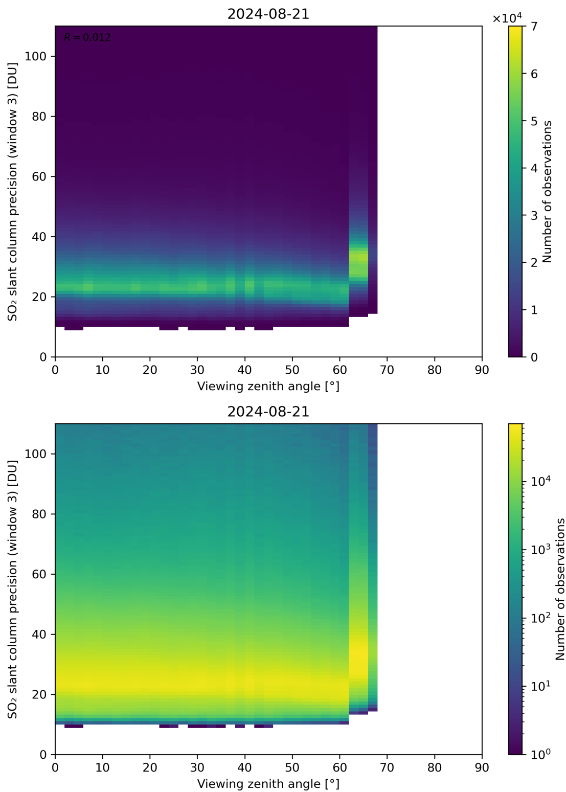
Figure 324: Scatter density plot of “Viewing zenith angle” against “SO 2 slant column precision (window 3)” for 2024-08-21 to 2024-08-22.
