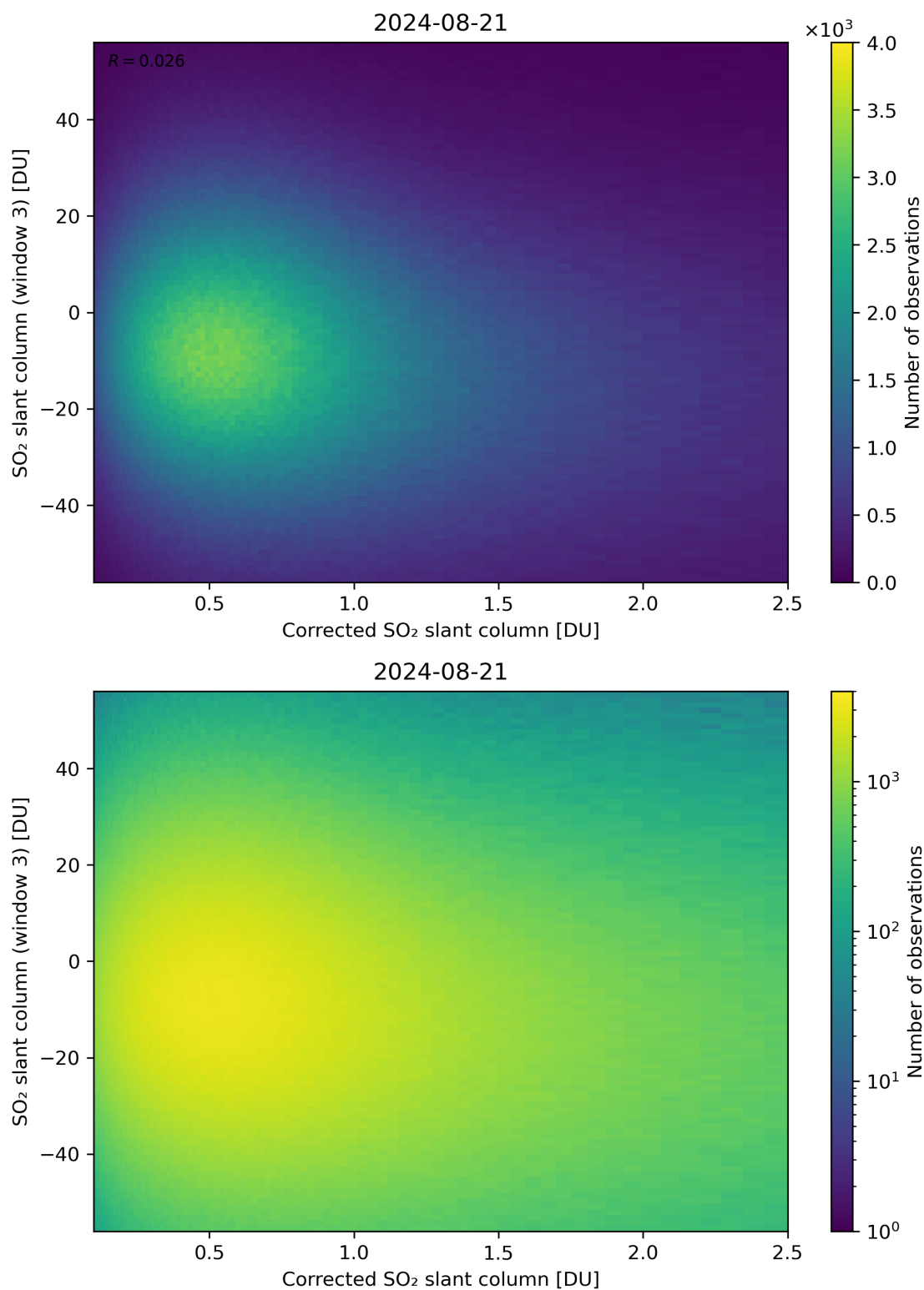
Figure 190: Scatter density plot of “Corrected SO 2 slant column” against “SO 2 slant column (window 3)” for 2024-08-21 to 2024-08-22.
