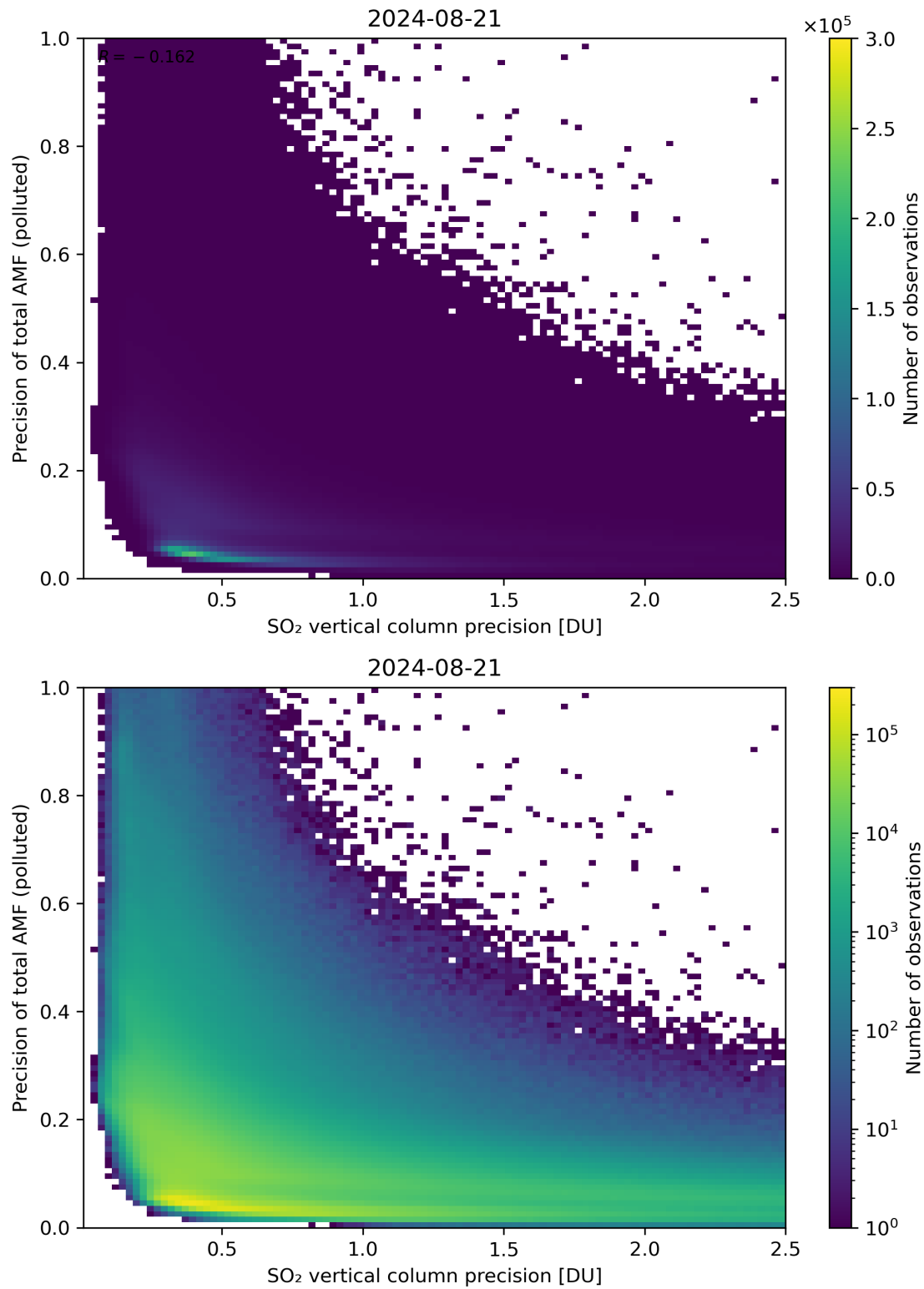
Figure 295: Scatter density plot of “SO 2 vertical column precision” against “Precision of total AMF (polluted)” for 2024-08-21 to 2024-08-22.
