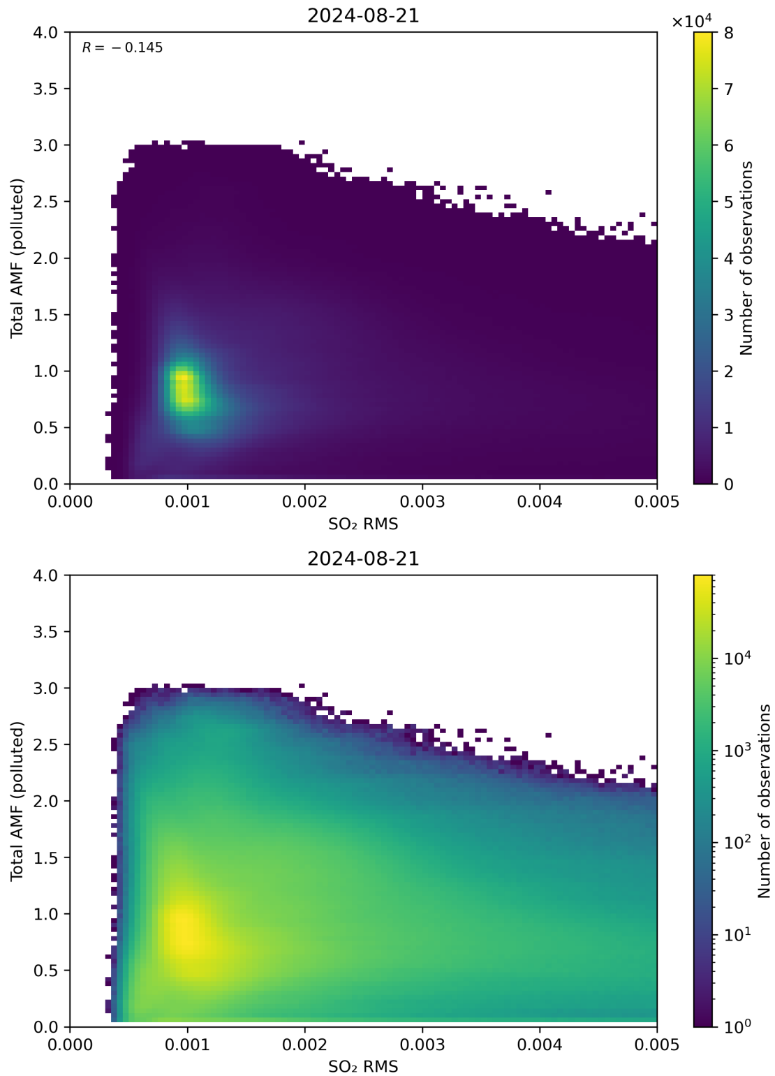
Figure 137: Scatter density plot of “SO 2 RMS” against “Total AMF (polluted)” for 2024-08-21 to 2024-08-22.
