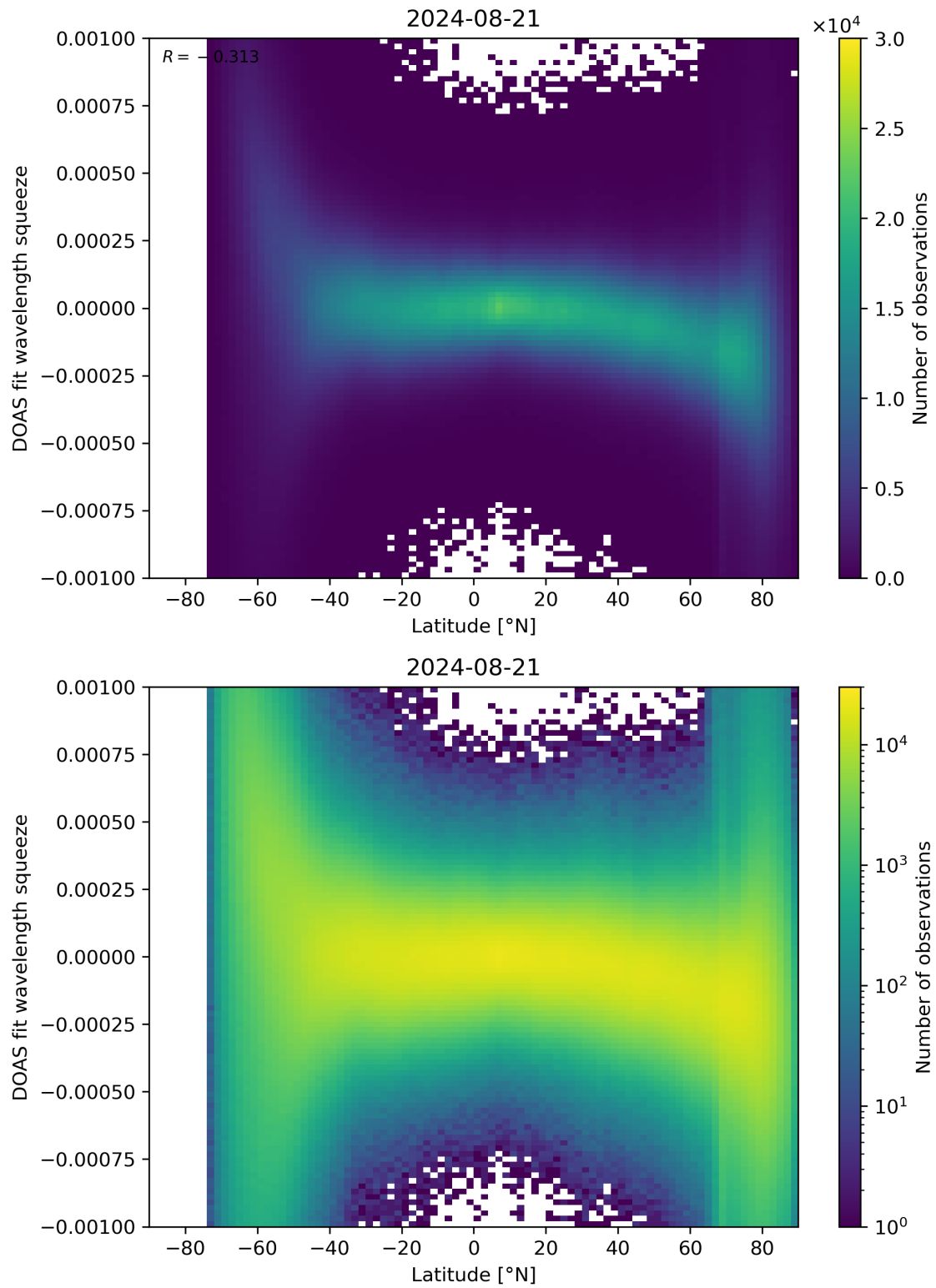
Figure 143: Scatter density plot of “Latitude” against “DOAS fit wavelength squeeze” for 2024-08-21 to 2024-08-22.
