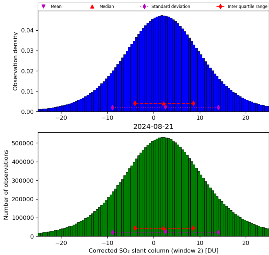
Figure 62: Histogram of “Corrected SO 2 slant column (window 2)” for 2024-08-21 to 2024-08-22
