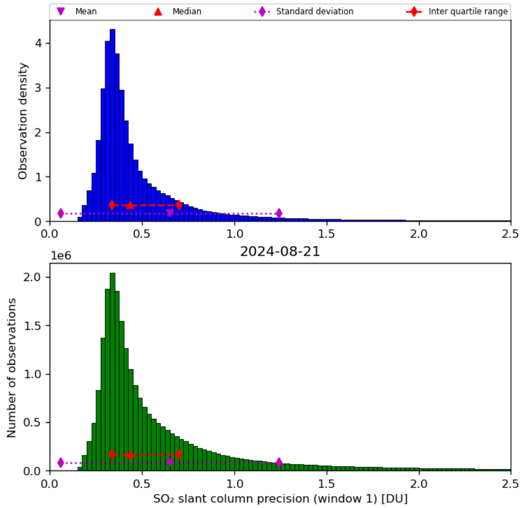
Figure 57: Histogram of “SO 2 slant column precision (window 1)” for 2024-08-21 to 2024-08-22
