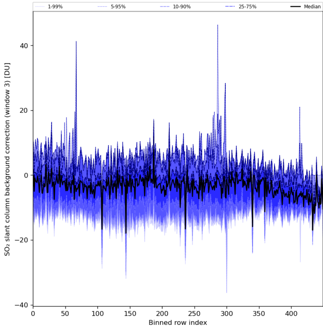
Figure 90: Along track statistics of “SO 2 slant column background correction (window 3)” for 2024-08-21 to 2024-08-22
