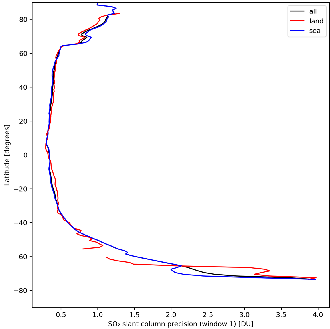
Figure 34: Zonal average of “SO 2 slant column precision (window 1)” for 2024-08-21 to 2024-08-22.
