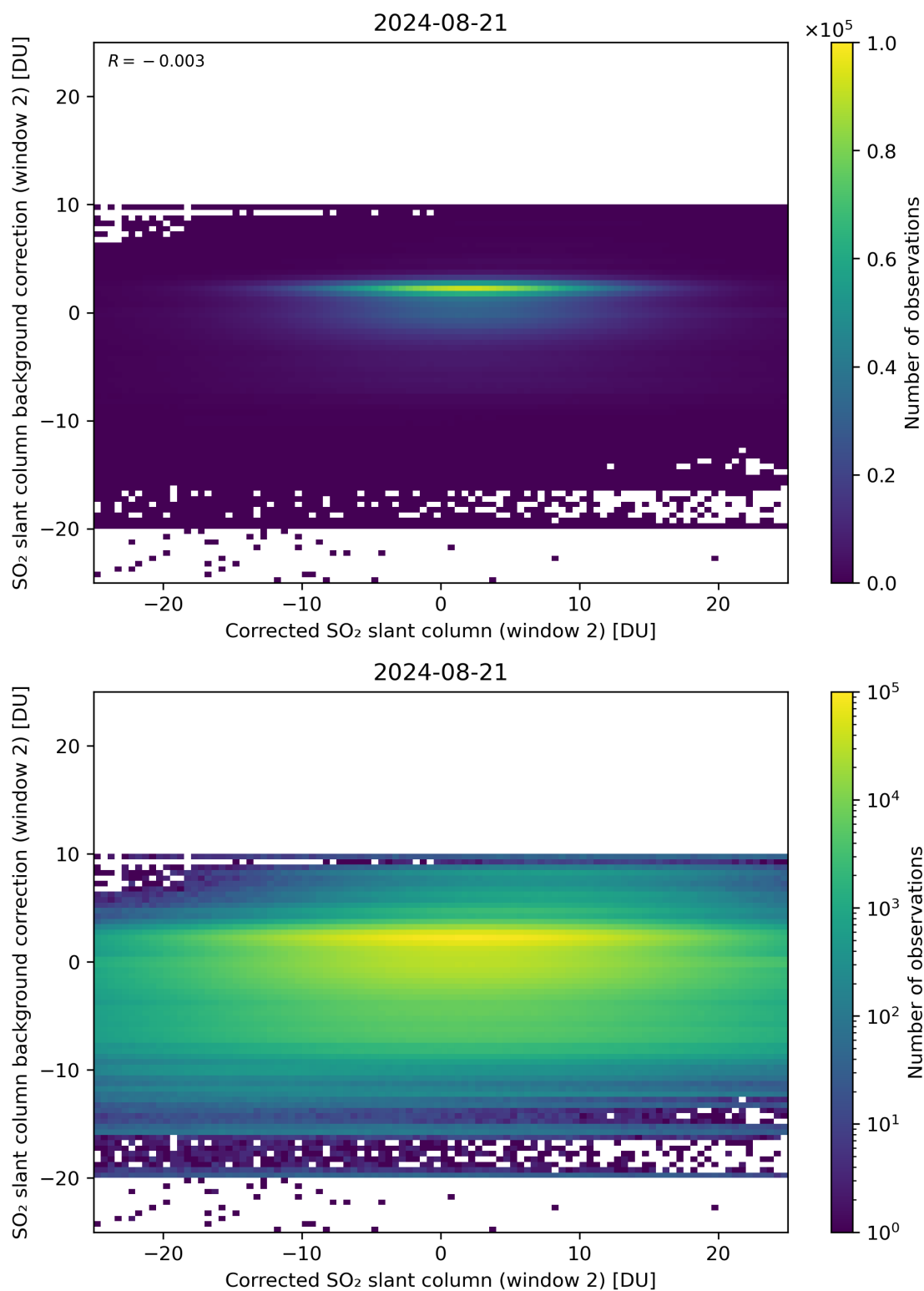
Figure 194: Scatter density plot of “Corrected SO 2 slant column (window 2)” against “SO 2 slant column background correction (window 2)” for 2024-08-21 to 2024-08-22.
