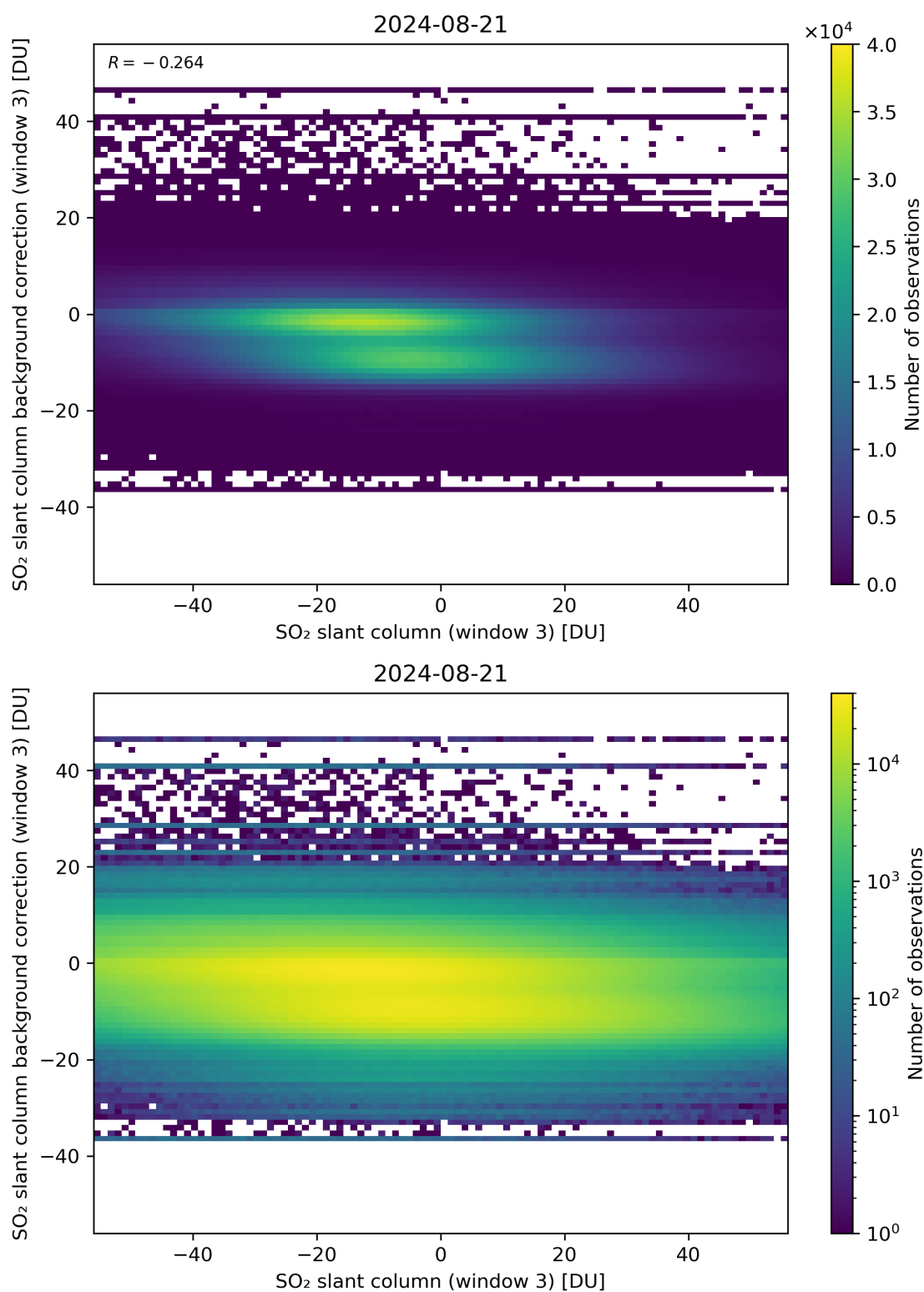
Figure 253: Scatter density plot of “SO 2 slant column (window 3)” against “SO 2 slant column background correction (window 3)” for 2024-08-21 to 2024-08-22.
