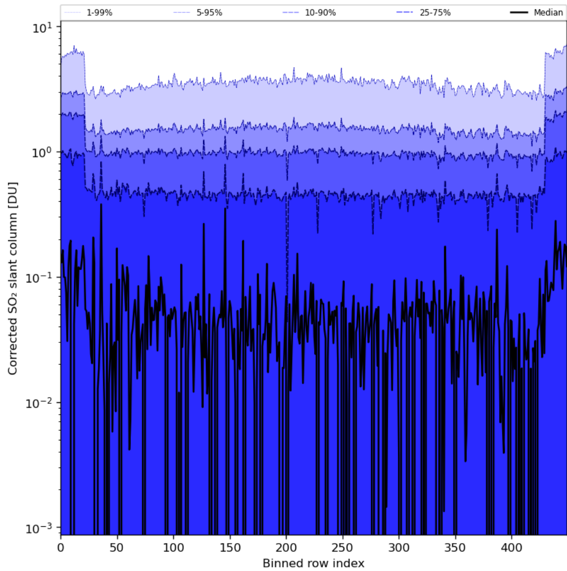
Figure 78: Along track statistics of “Corrected SO 2 slant column” for 2024-08-21 to 2024-08-22
