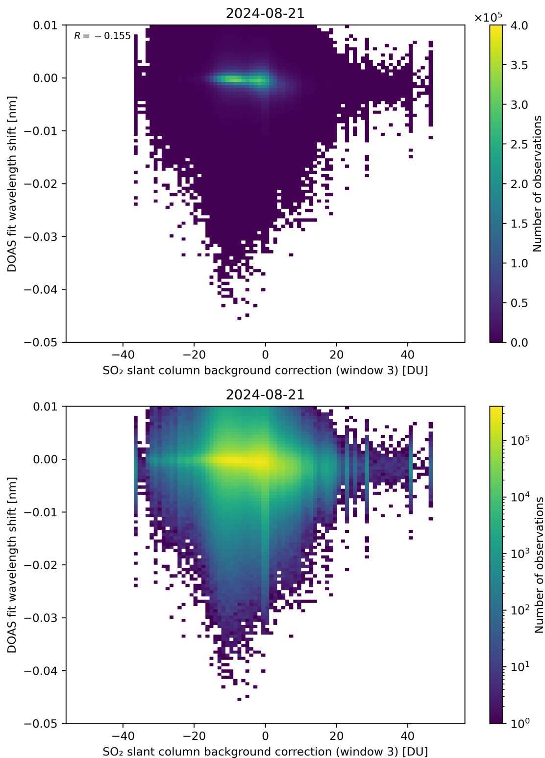
Figure 121: Scatter density plot of “SO 2 slant column background correction (window 3)” against “DOAS fit wavelength shift” for 2024-08-21 to 2024-08-22.
