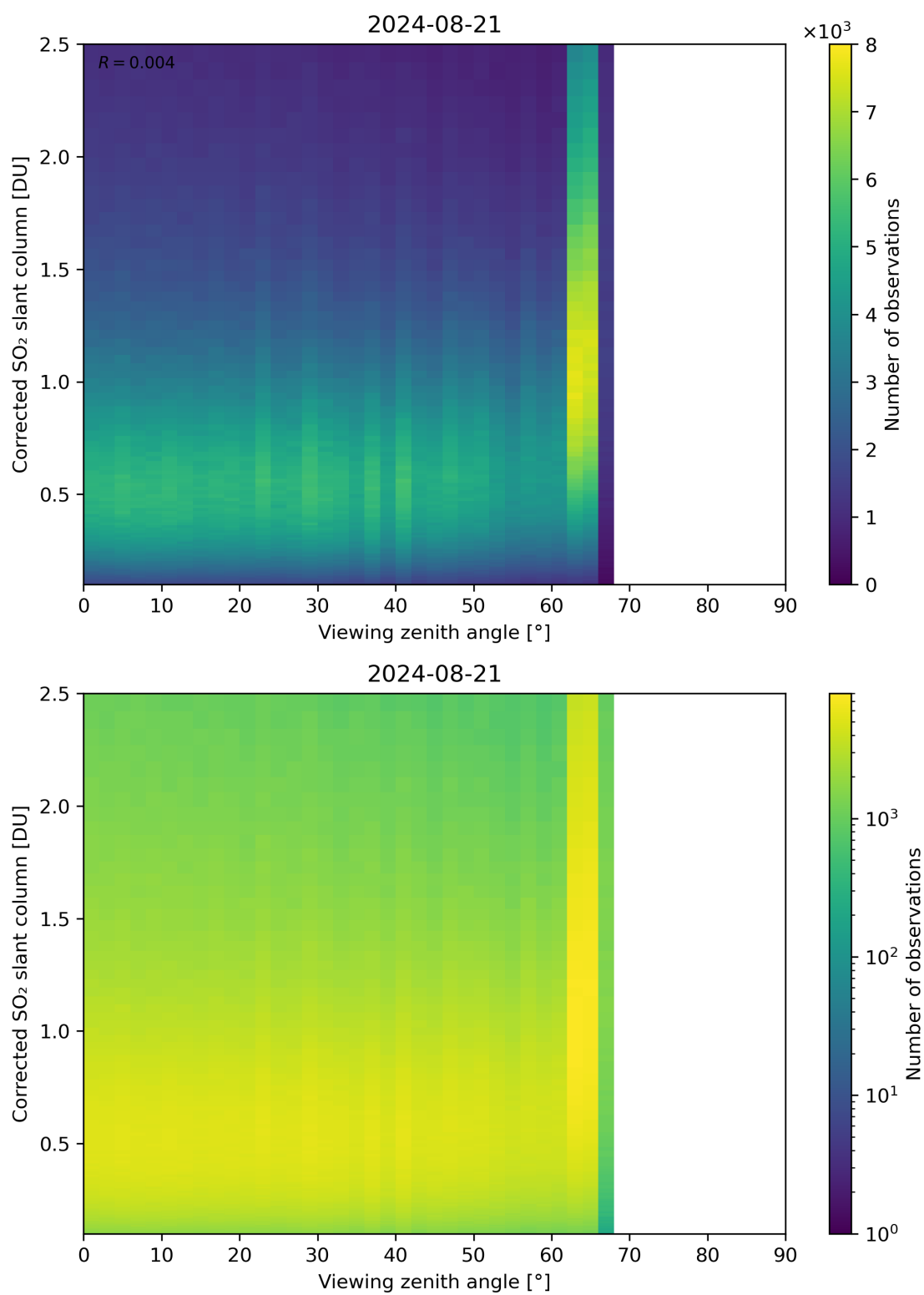
Figure 317: Scatter density plot of “Viewing zenith angle” against “Corrected SO 2 slant column” for 2024-08-21 to 2024-08-22.
