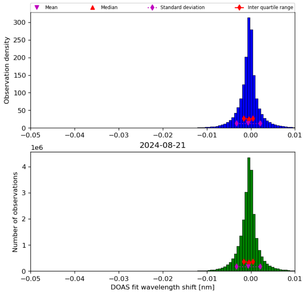
Figure 68: Histogram of “DOAS fit wavelength shift” for 2024-08-21 to 2024-08-22
