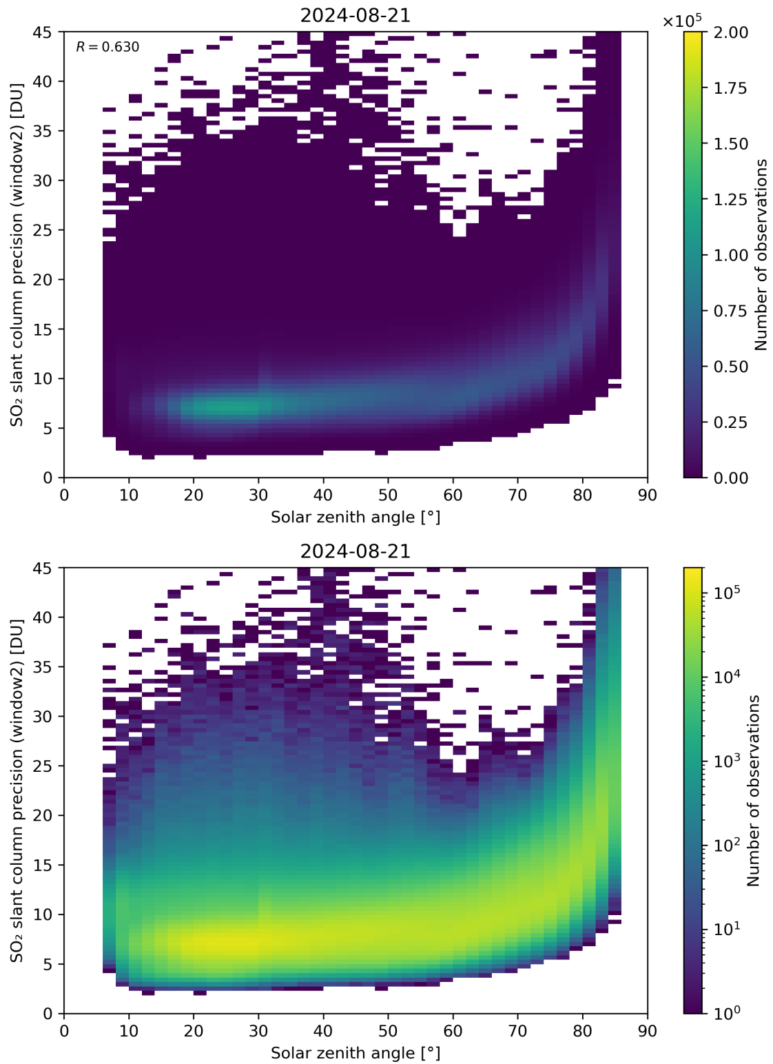
Figure 171: Scatter density plot of “Solar zenith angle” against “SO 2 slant column precision (window2)” for 2024-08-21 to 2024-08-22.
