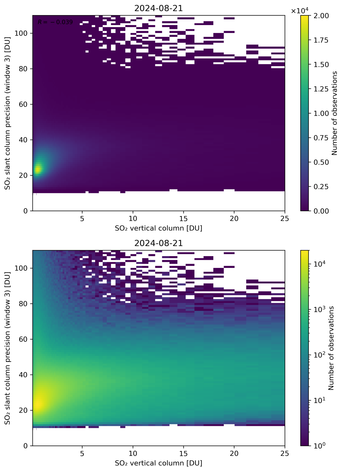
Figure 304: Scatter density plot of “SO 2 vertical column” against “SO 2 slant column precision (window 3)” for 2024-08-21 to 2024-08-22.
