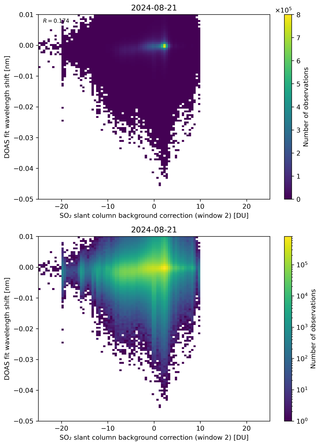
Figure 112: Scatter density plot of “SO 2 slant column background correction (window 2)” against “DOAS fit wavelength shift” for 2024-08-21 to 2024-08-22.
