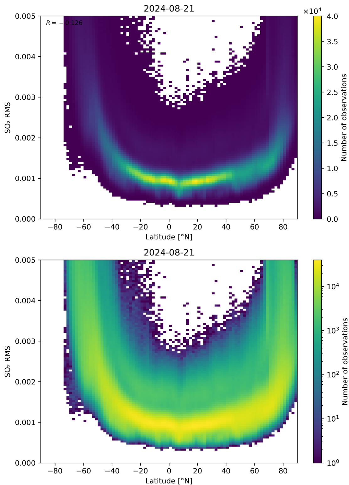
Figure 144: Scatter density plot of “Latitude” against “SO 2 RMS” for 2024-08-21 to 2024-08-22.
