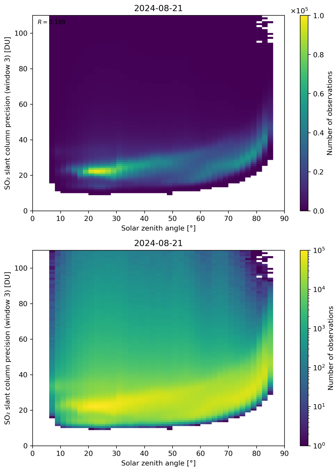
Figure 173: Scatter density plot of “Solar zenith angle” against “SO 2 slant column precision (window 3)” for 2024-08-21 to 2024-08-22.
