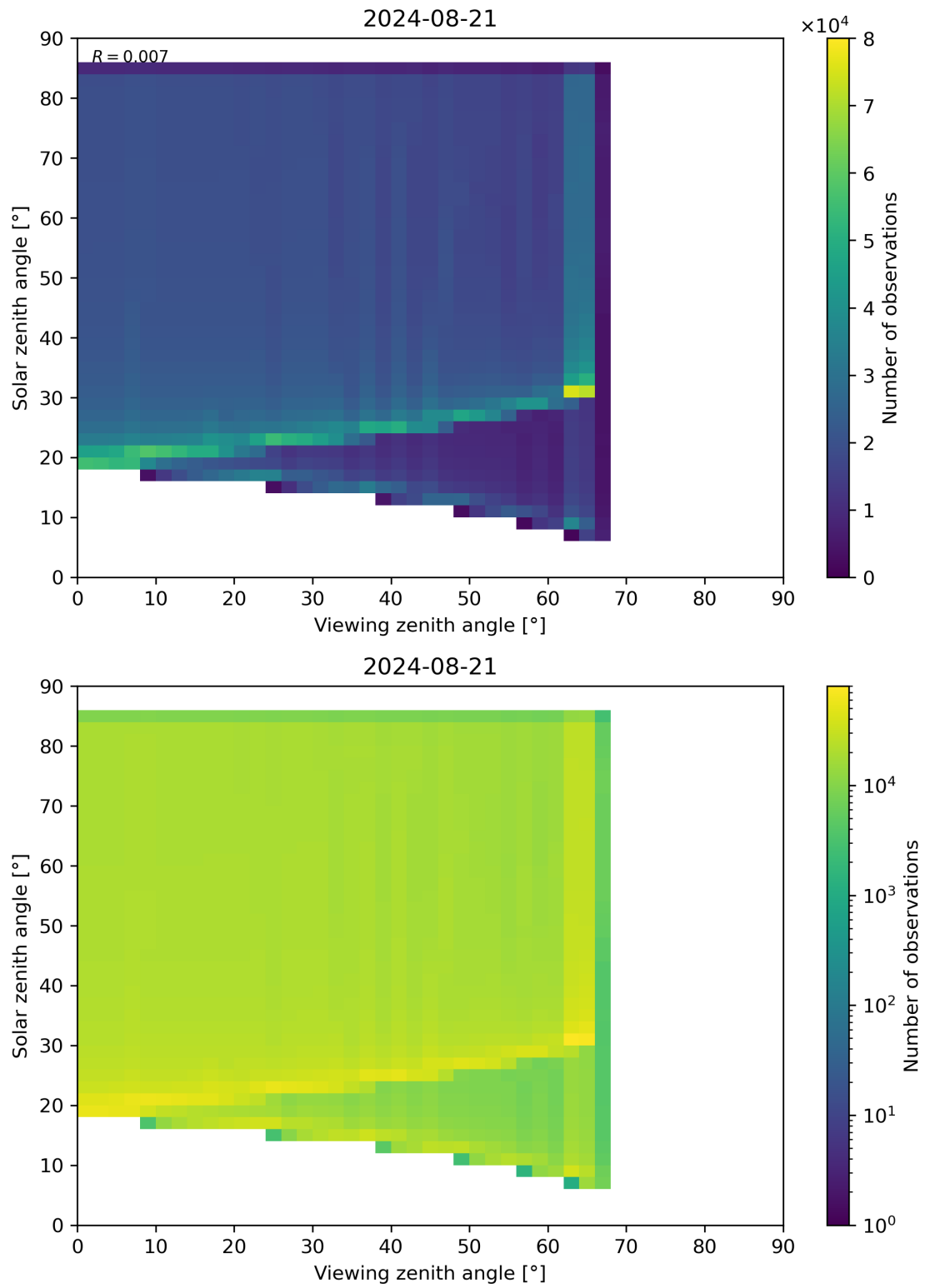
Figure 315: Scatter density plot of “Viewing zenith angle” against “Solar zenith angle” for 2024-08-21 to 2024-08-22.
