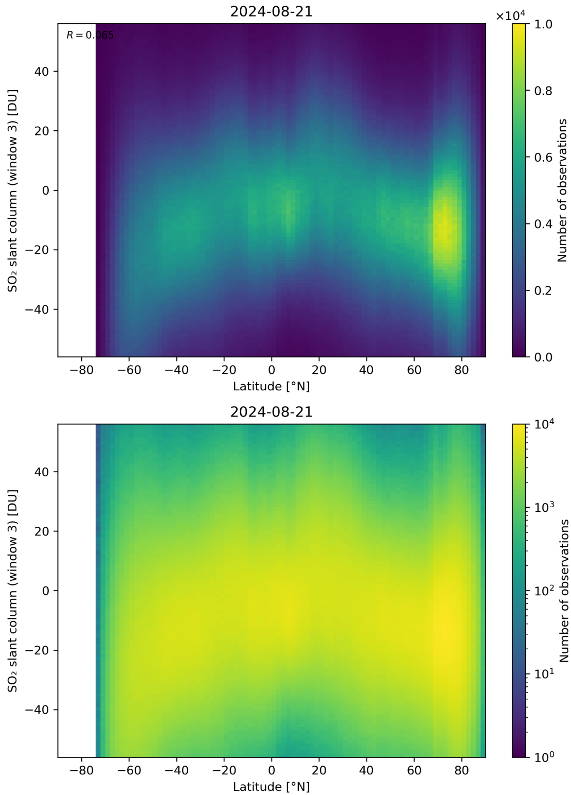
Figure 152: Scatter density plot of “Latitude” against “SO 2 slant column (window 3)” for 2024-08-21 to 2024-08-22.
