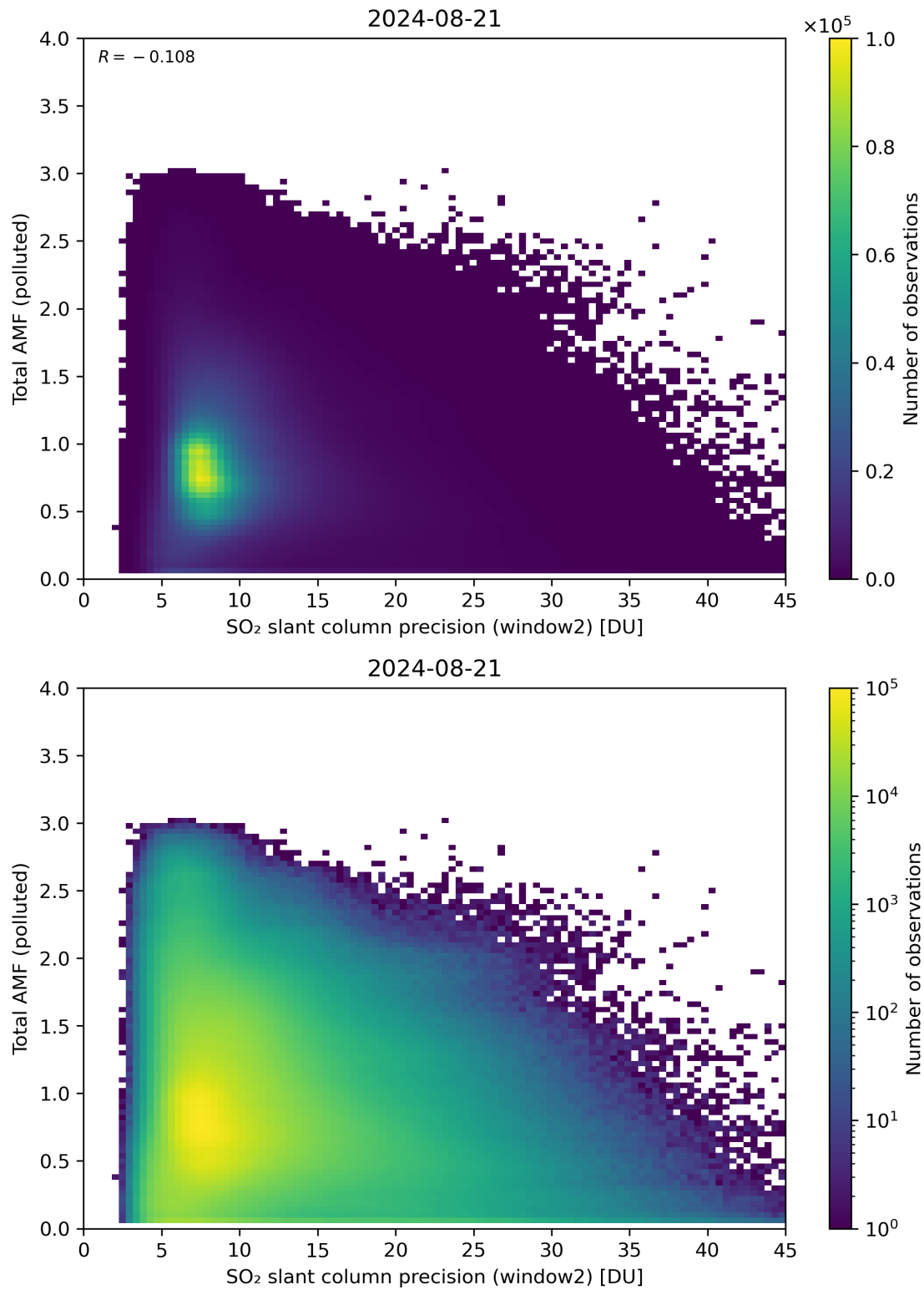
Figure 251: Scatter density plot of “SO 2 slant column precision (window2)” against “Total AMF (polluted)” for 2024-08-21 to 2024-08-22.
