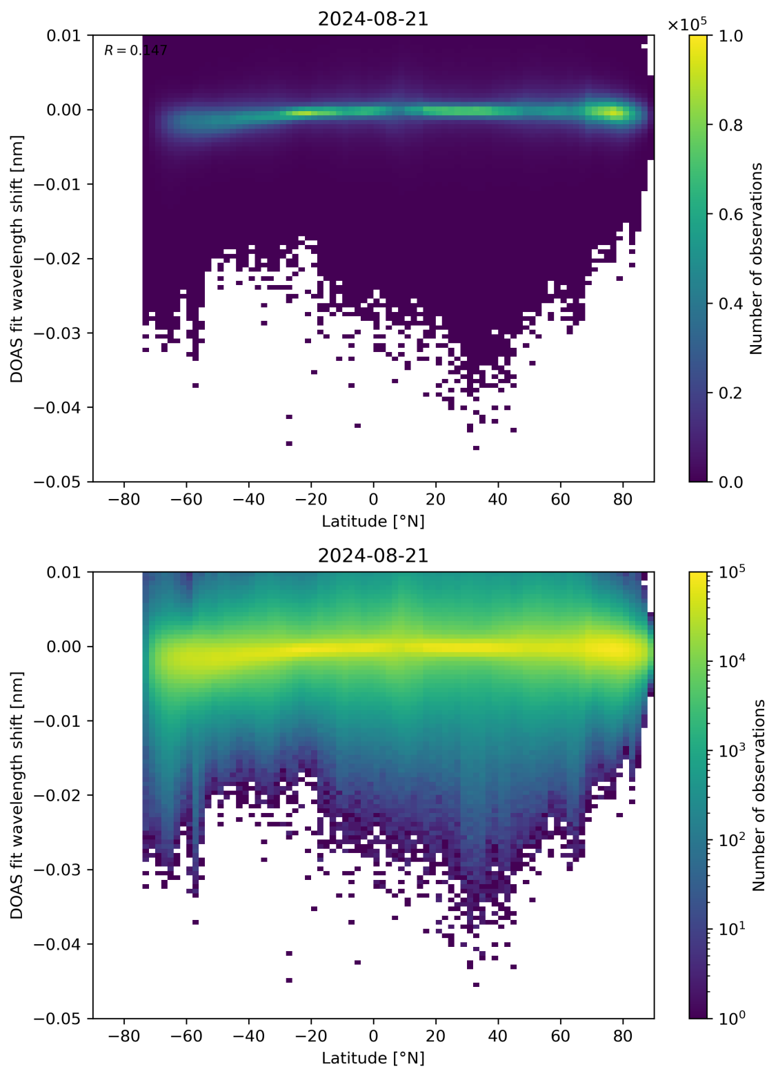
Figure 142: Scatter density plot of “Latitude” against “DOAS fit wavelength shift” for 2024-08-21 to 2024-08-22.
