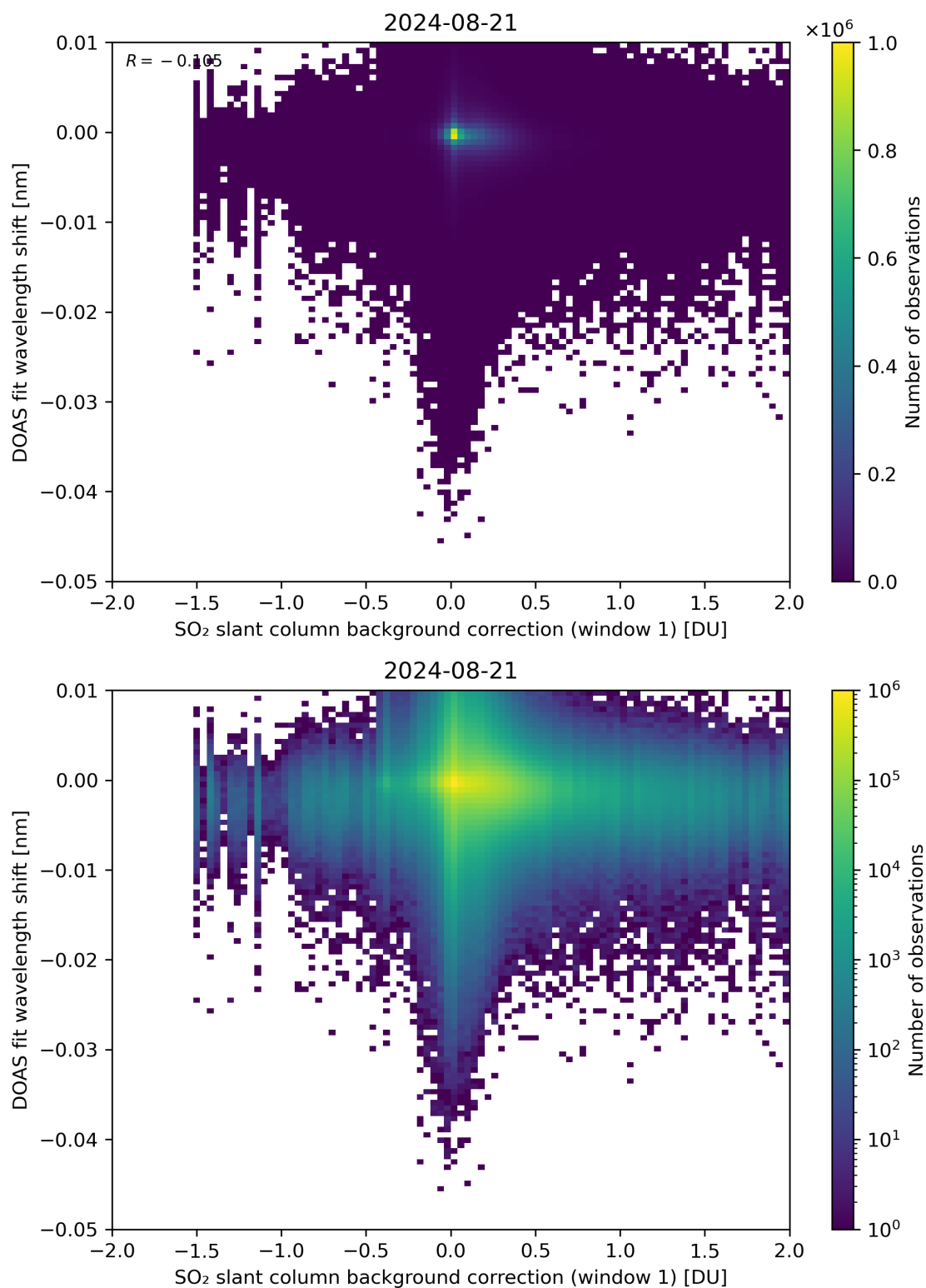
Figure 100: Scatter density plot of “SO 2 slant column background correction (window 1)” against “DOAS fit wavelength shift” for 2024-08-21 to 2024-08-22.
