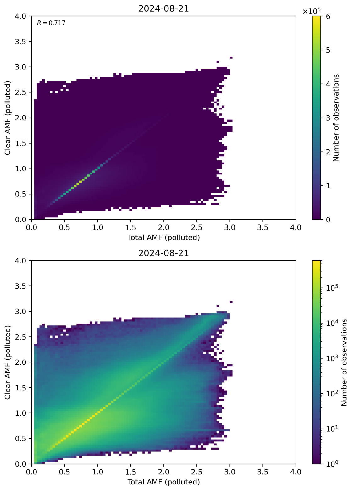
Figure 271: Scatter density plot of “Total AMF (polluted)” against “Clear AMF (polluted)” for 2024-08-21 to 2024-08-22.
