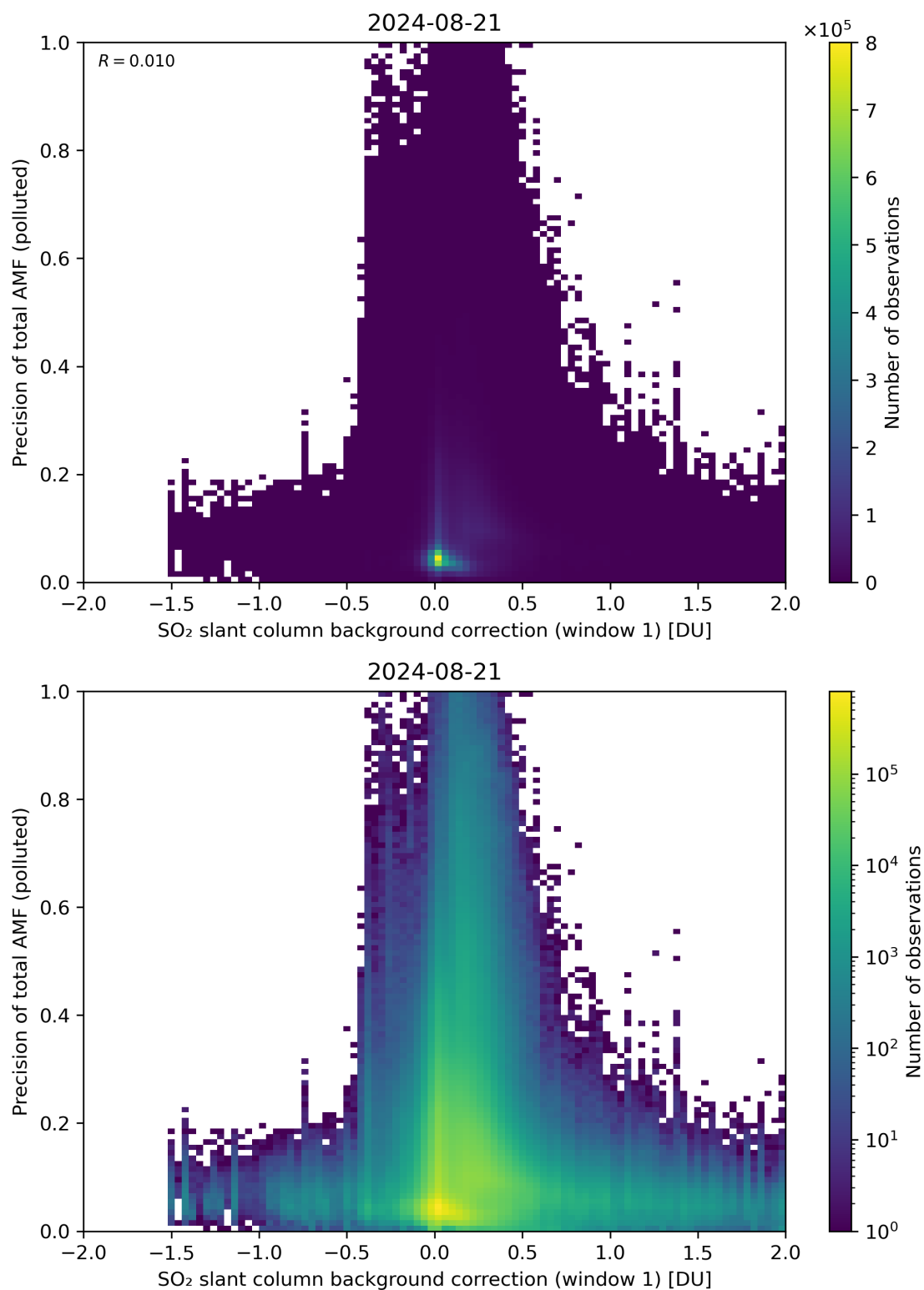
Figure 110: Scatter density plot of “SO 2 slant column background correction (window 1)” against “Precision of total AMF (polluted)” for 2024-08-21 to 2024-08-22.
