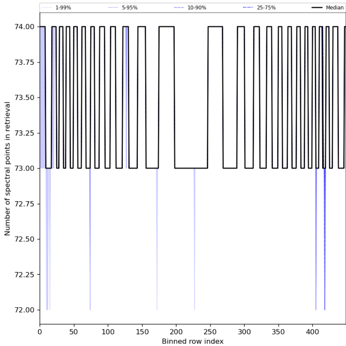
Figure 97: Along track statistics of “Number of spectral points in retrieval” for 2024-08-21 to 2024-08-22
