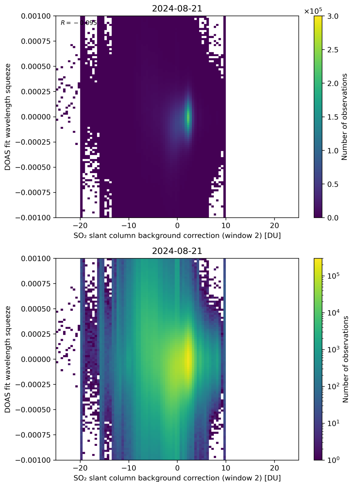
Figure 113: Scatter density plot of “SO 2 slant column background correction (window 2)” against “DOAS fit wavelength squeeze” for 2024-08-21 to 2024-08-22.
