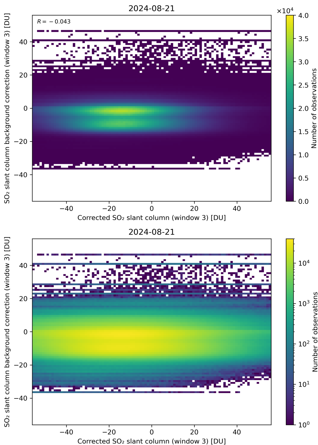
Figure 205: Scatter density plot of “Corrected SO 2 slant column (window 3)” against “SO 2 slant column background correction (window 3)” for 2024-08-21 to 2024-08-22.
