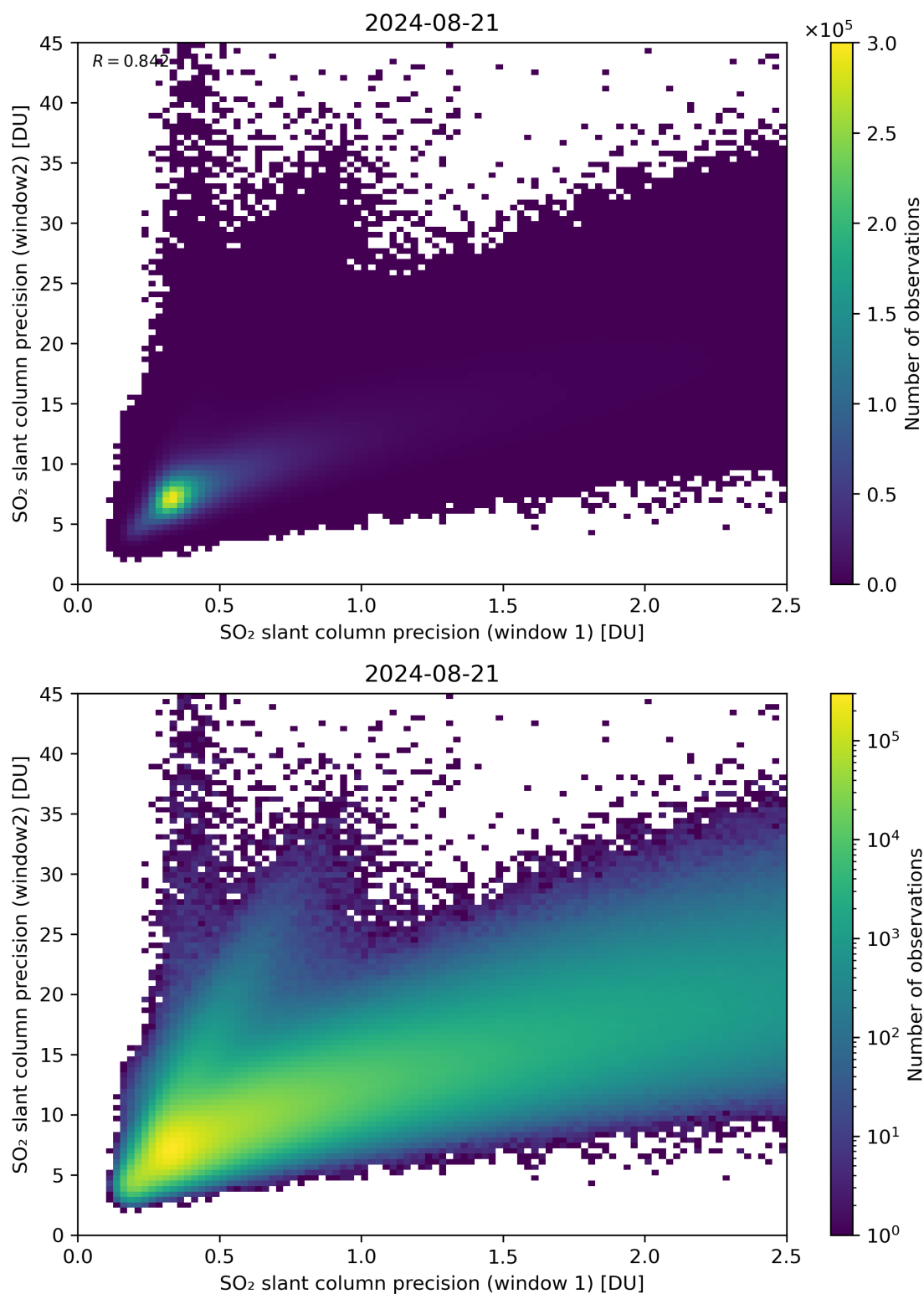
Figure 227: Scatter density plot of “SO 2 slant column precision (window 1)” against “SO 2 slant column precision (window2)” for 2024-08-21 to 2024-08-22.
