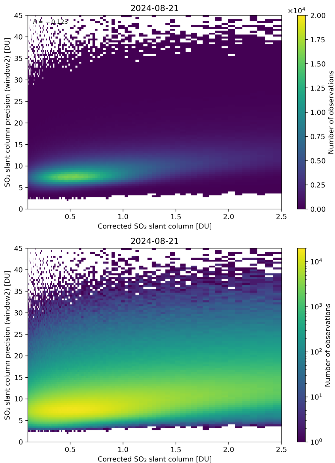
Figure 189: Scatter density plot of “Corrected SO 2 slant column” against “SO 2 slant column precision (window2)” for 2024-08-21 to 2024-08-22.
