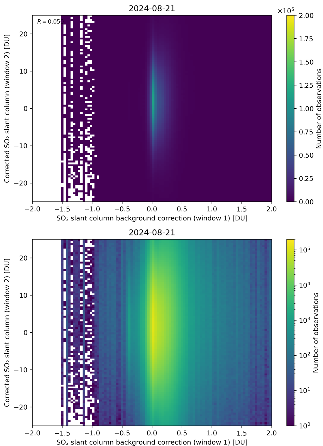
Figure 104: Scatter density plot of “SO 2 slant column background correction (window 1)” against “Corrected SO 2 slant column (window 2)” for 2024-08-21 to 2024-08-22.
