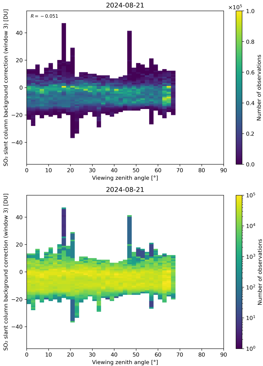
Figure 310: Scatter density plot of “Viewing zenith angle” against “SO 2 slant column background correction (window 3)” for 2024-08-21 to 2024-08-22.
