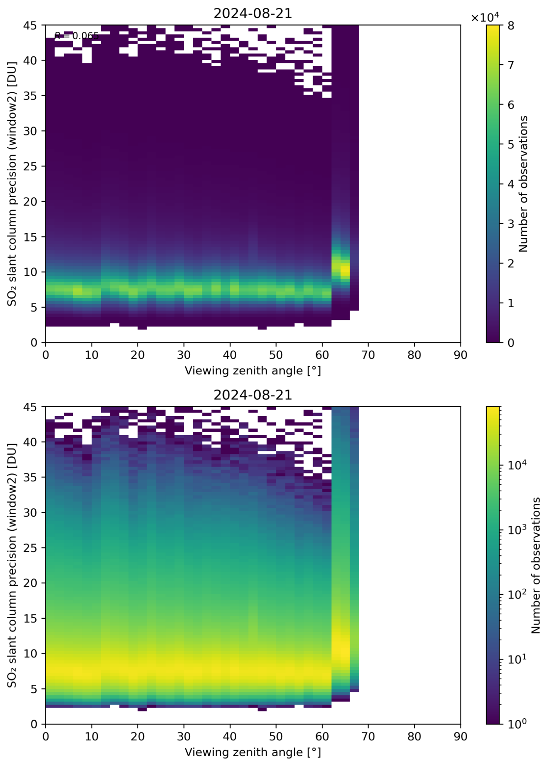
Figure 322: Scatter density plot of “Viewing zenith angle” against “SO 2 slant column precision (window2)” for 2024-08-21 to 2024-08-22.
