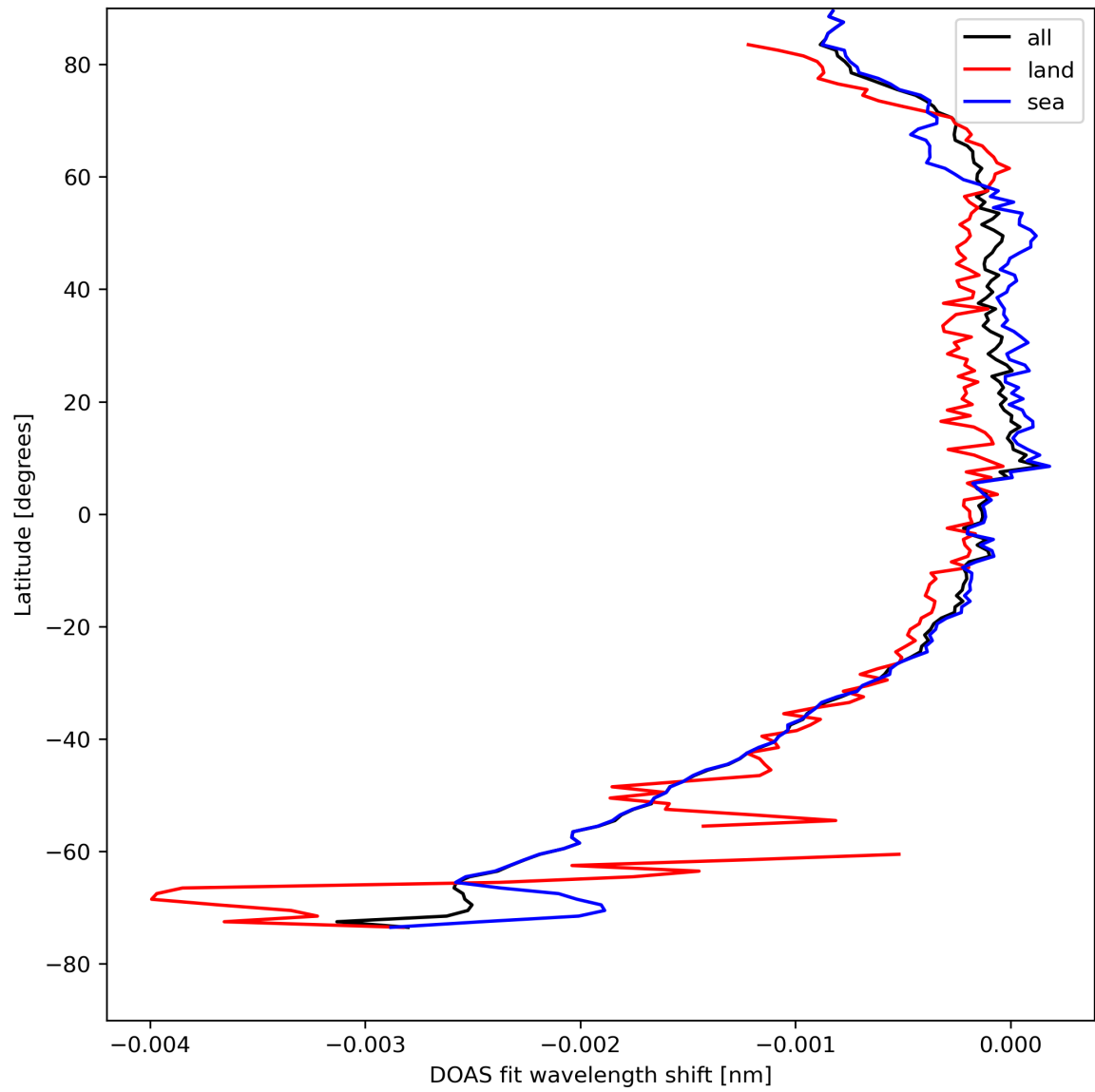
Figure 45: Zonal average of “DOAS fit wavelength shift” for 2024-08-21 to 2024-08-22.
