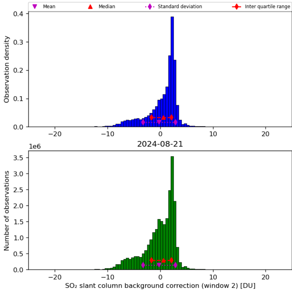
Figure 63: Histogram of “SO 2 slant column background correction (window 2)” for 2024-08-21 to 2024-08-22
