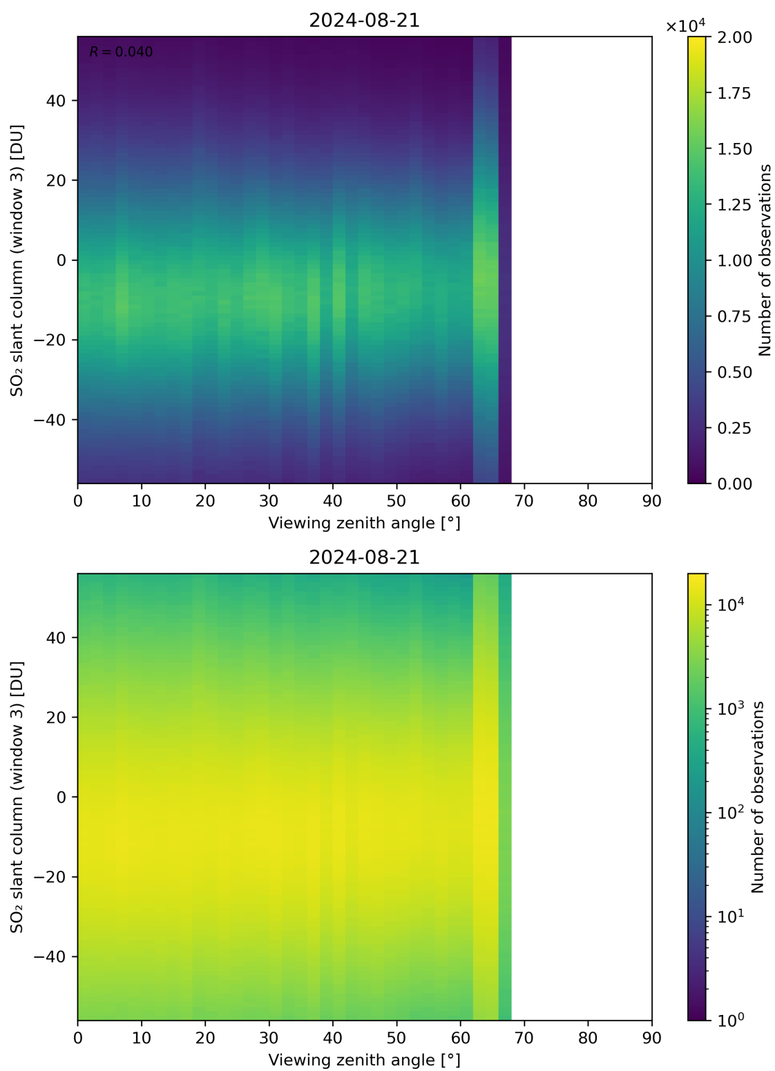
Figure 323: Scatter density plot of “Viewing zenith angle” against “SO 2 slant column (window 3)” for 2024-08-21 to 2024-08-22.
