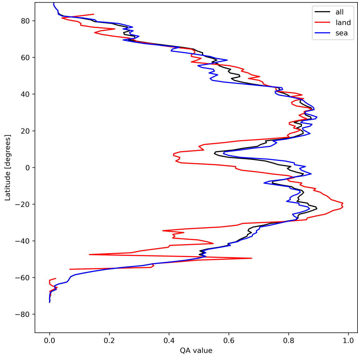
Figure 29: Zonal average of “QA value” for 2024-08-21 to 2024-08-22.
