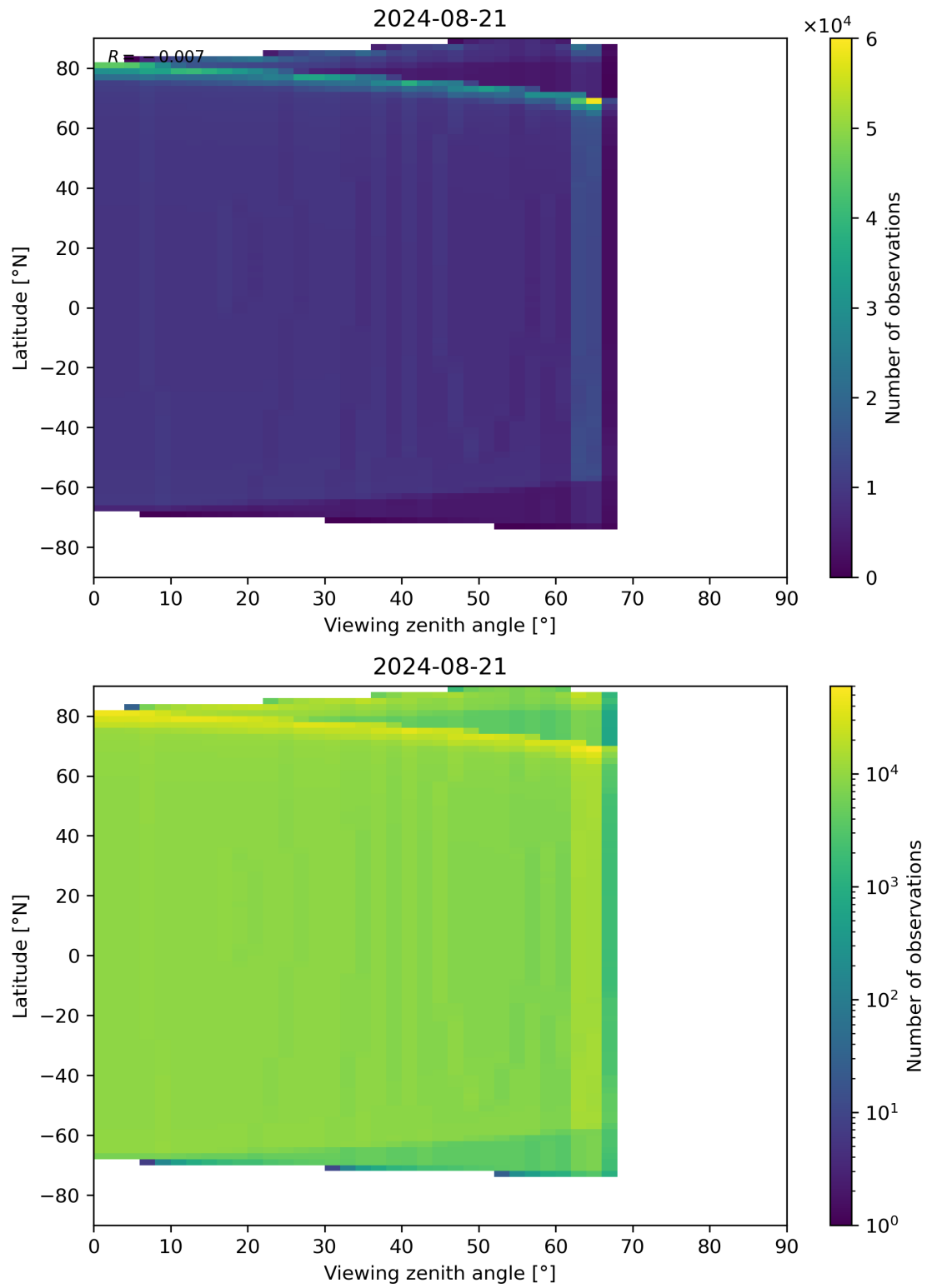
Figure 314: Scatter density plot of “Viewing zenith angle” against “Latitude” for 2024-08-21 to 2024-08-22.
