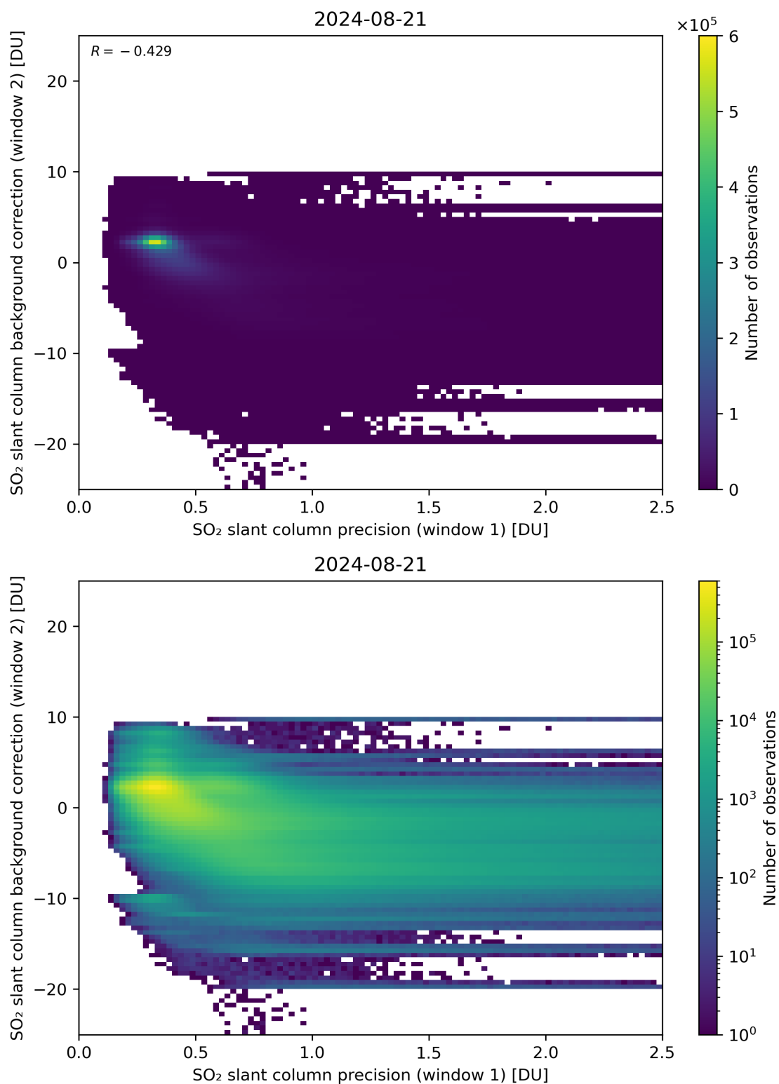
Figure 219: Scatter density plot of “SO 2 slant column precision (window 1)” against “SO 2 slant column background correction (window 2)” for 2024-08-21 to 2024-08-22.
