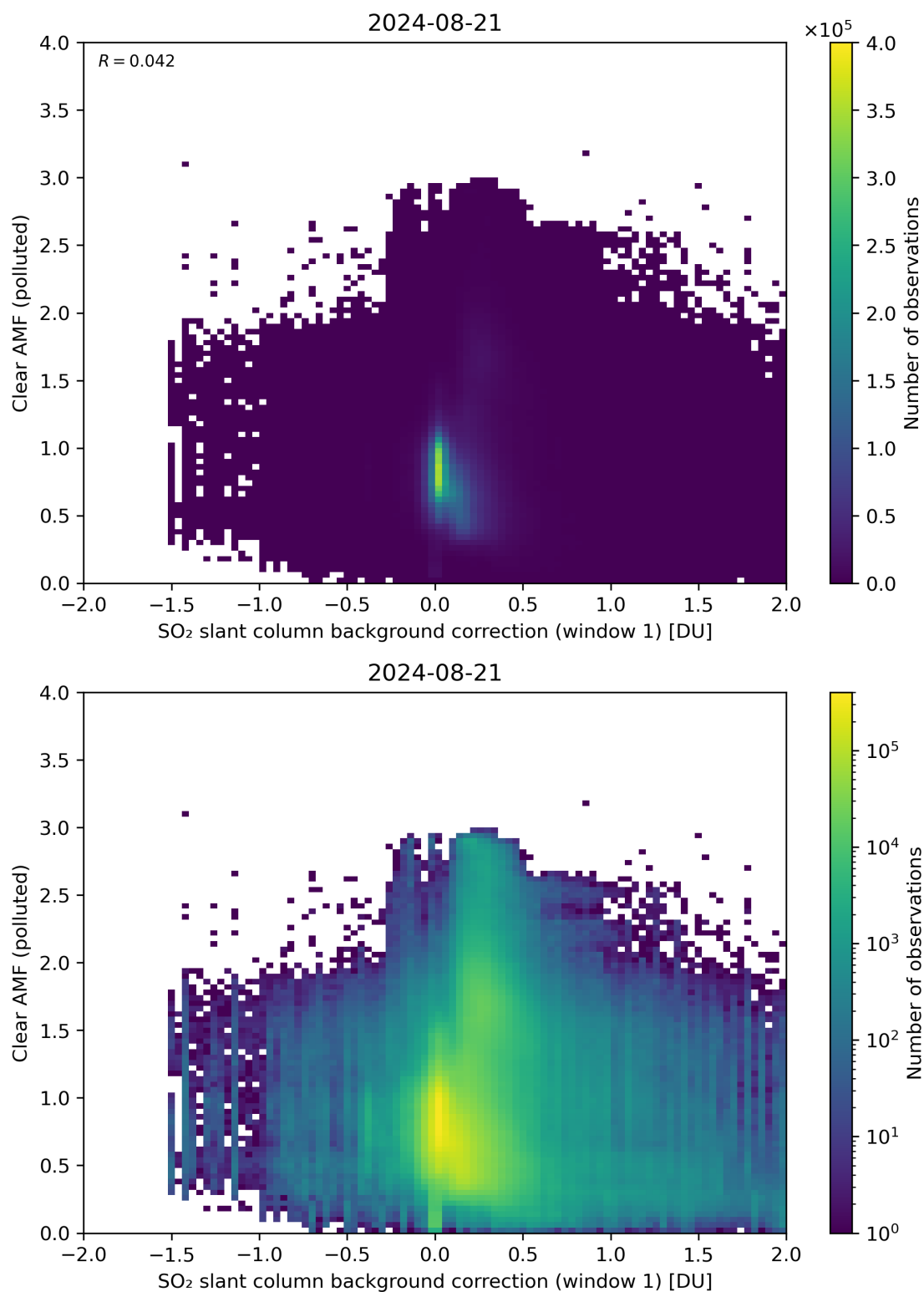
Figure 103: Scatter density plot of “SO 2 slant column background correction (window 1)” against “Clear AMF (polluted)” for 2024-08-21 to 2024-08-22.
