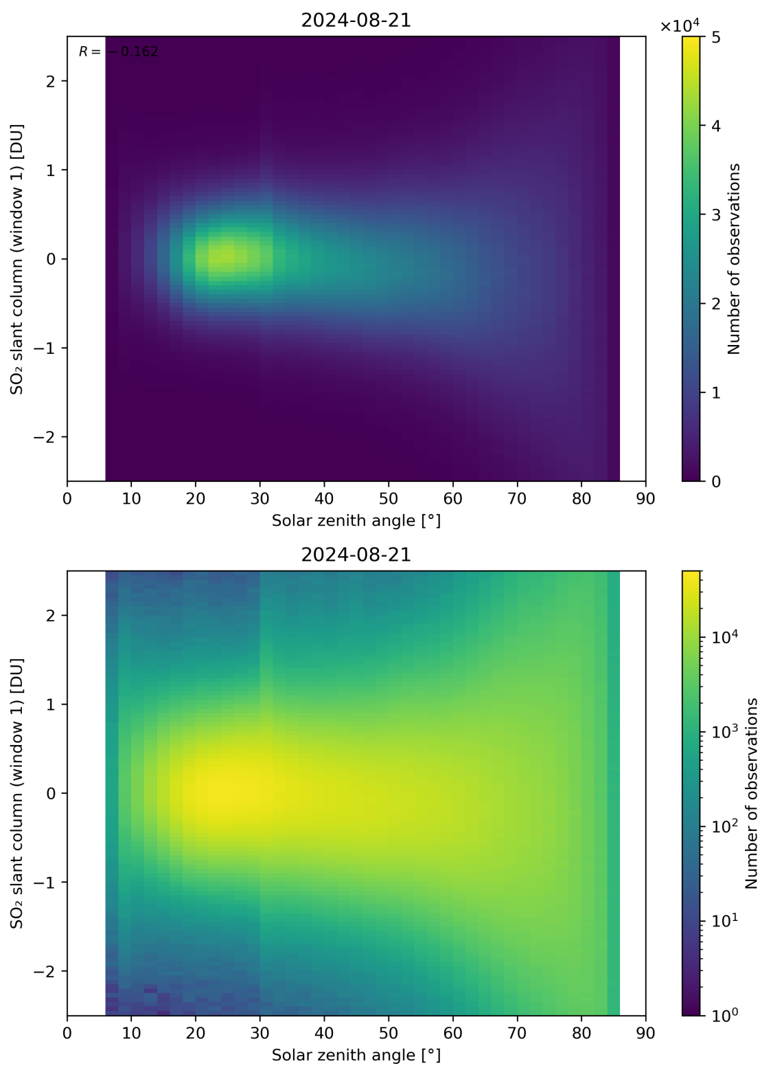
Figure 169: Scatter density plot of “Solar zenith angle” against “SO 2 slant column (window 1)” for 2024-08-21 to 2024-08-22.
