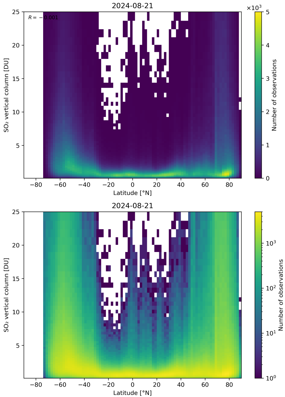
Figure 156: Scatter density plot of “Latitude” against “SO 2 vertical column” for 2024-08-21 to 2024-08-22.
