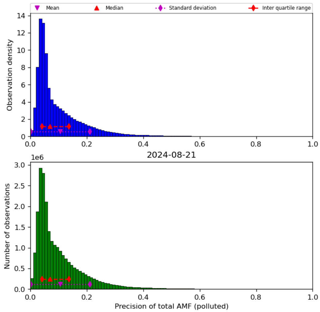
Figure 72: Histogram of “Precision of total AMF (polluted)” for 2024-08-21 to 2024-08-22
