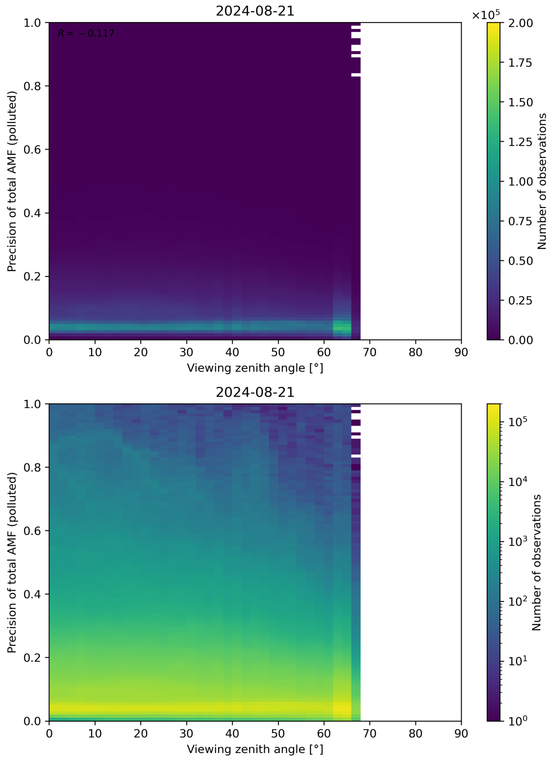
Figure 326: Scatter density plot of “Viewing zenith angle” against “Precision of total AMF (polluted)” for 2024-08-21 to 2024-08-22.
