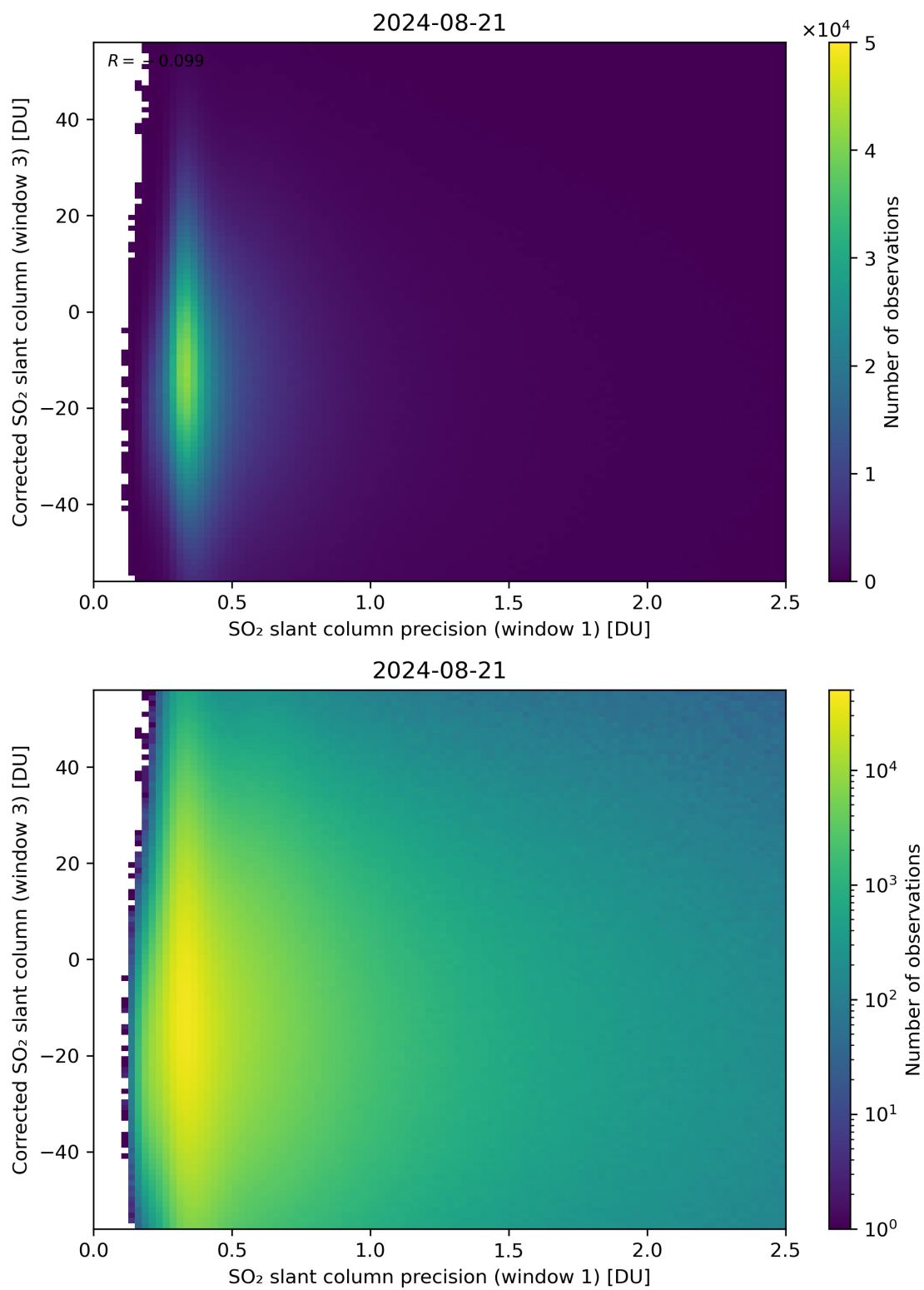
Figure 226: Scatter density plot of “SO 2 slant column precision (window 1)” against “Corrected SO 2 slant column (window 3)” for 2024-08-21 to 2024-08-22.
