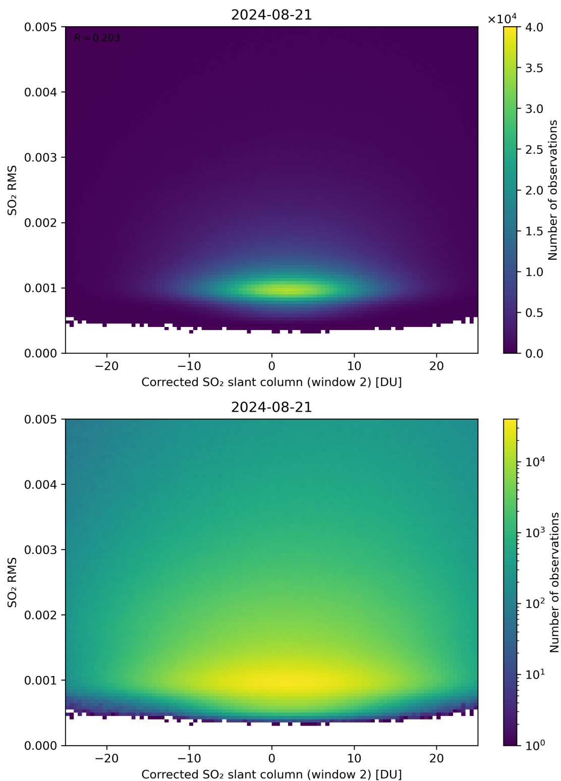
Figure 198: Scatter density plot of “Corrected SO 2 slant column (window 2)” against “SO 2 RMS” for 2024-08-21 to 2024-08-22.
