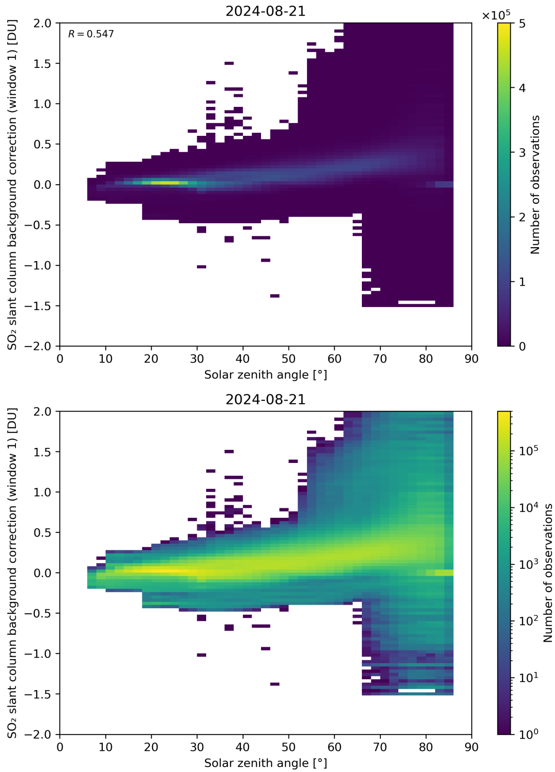
Figure 158: Scatter density plot of “Solar zenith angle” against “SO 2 slant column background correction (window 1)” for 2024-08-21 to 2024-08-22.
