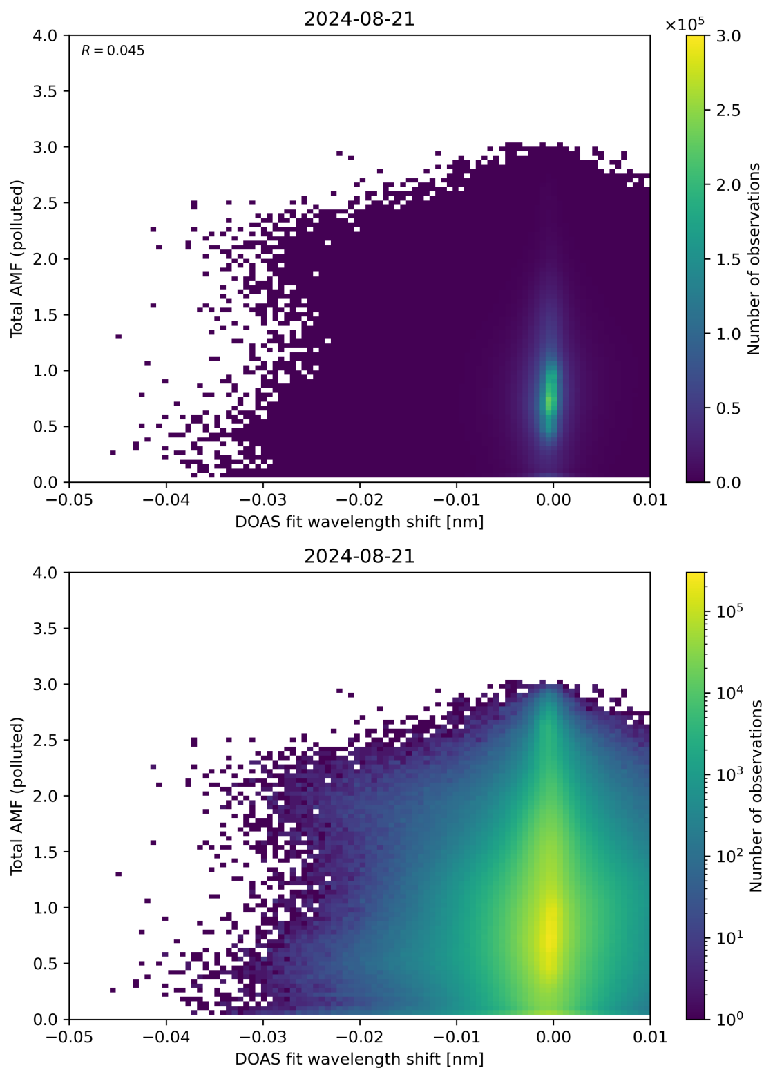
Figure 130: Scatter density plot of “DOAS fit wavelength shift” against “Total AMF (polluted)” for 2024-08-21 to 2024-08-22.
