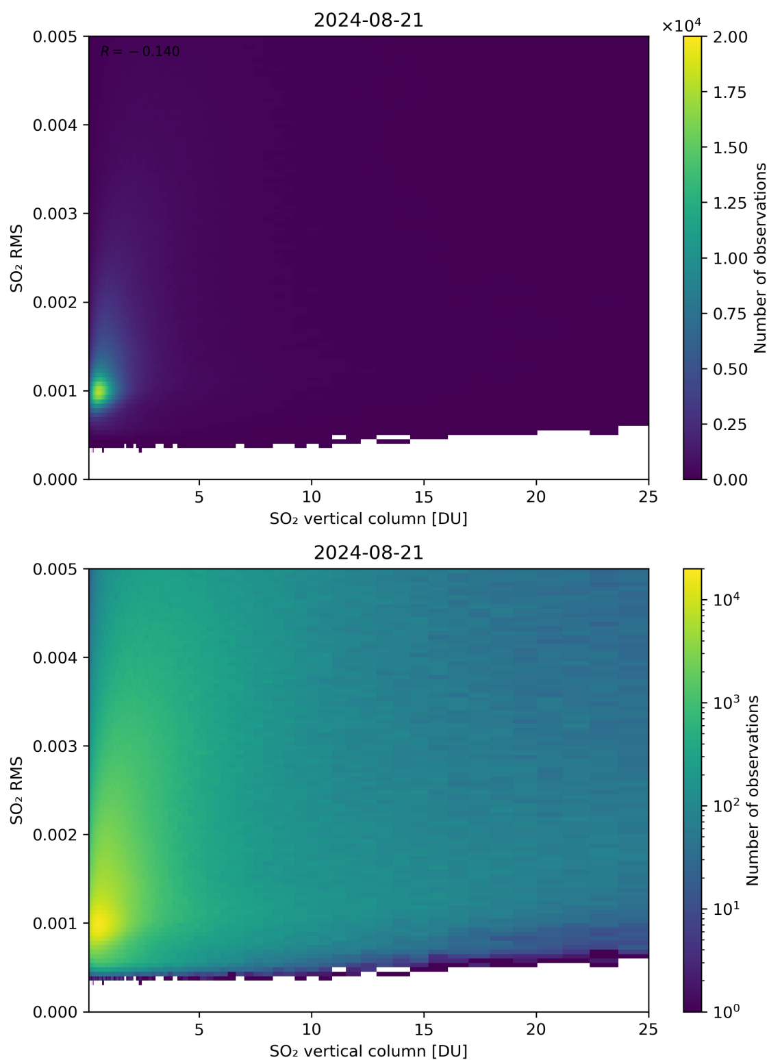
Figure 278: Scatter density plot of “SO 2 vertical column” against “SO 2 RMS” for 2024-08-21 to 2024-08-22.
