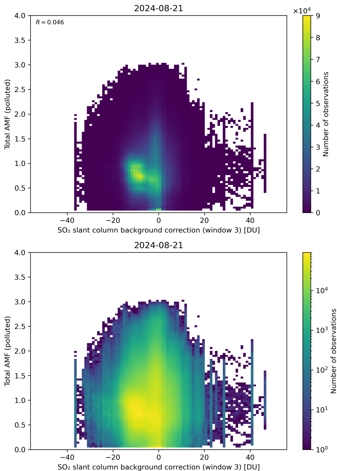
Figure 125: Scatter density plot of “SO 2 slant column background correction (window 3)” against “Total AMF (polluted)” for 2024-08-21 to 2024-08-22.
