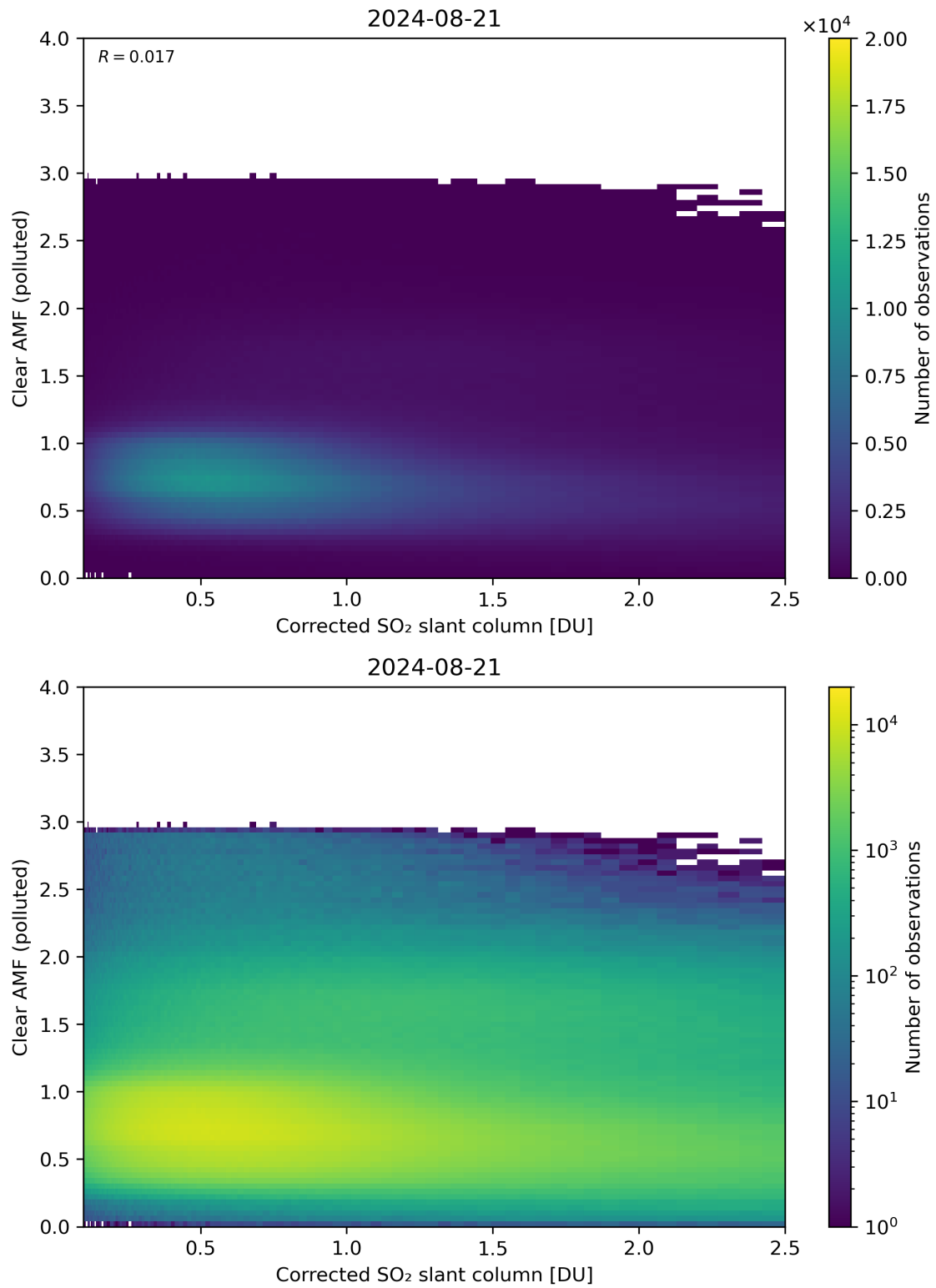
Figure 184: Scatter density plot of “Corrected SO 2 slant column” against “Clear AMF (polluted)” for 2024-08-21 to 2024-08-22.
