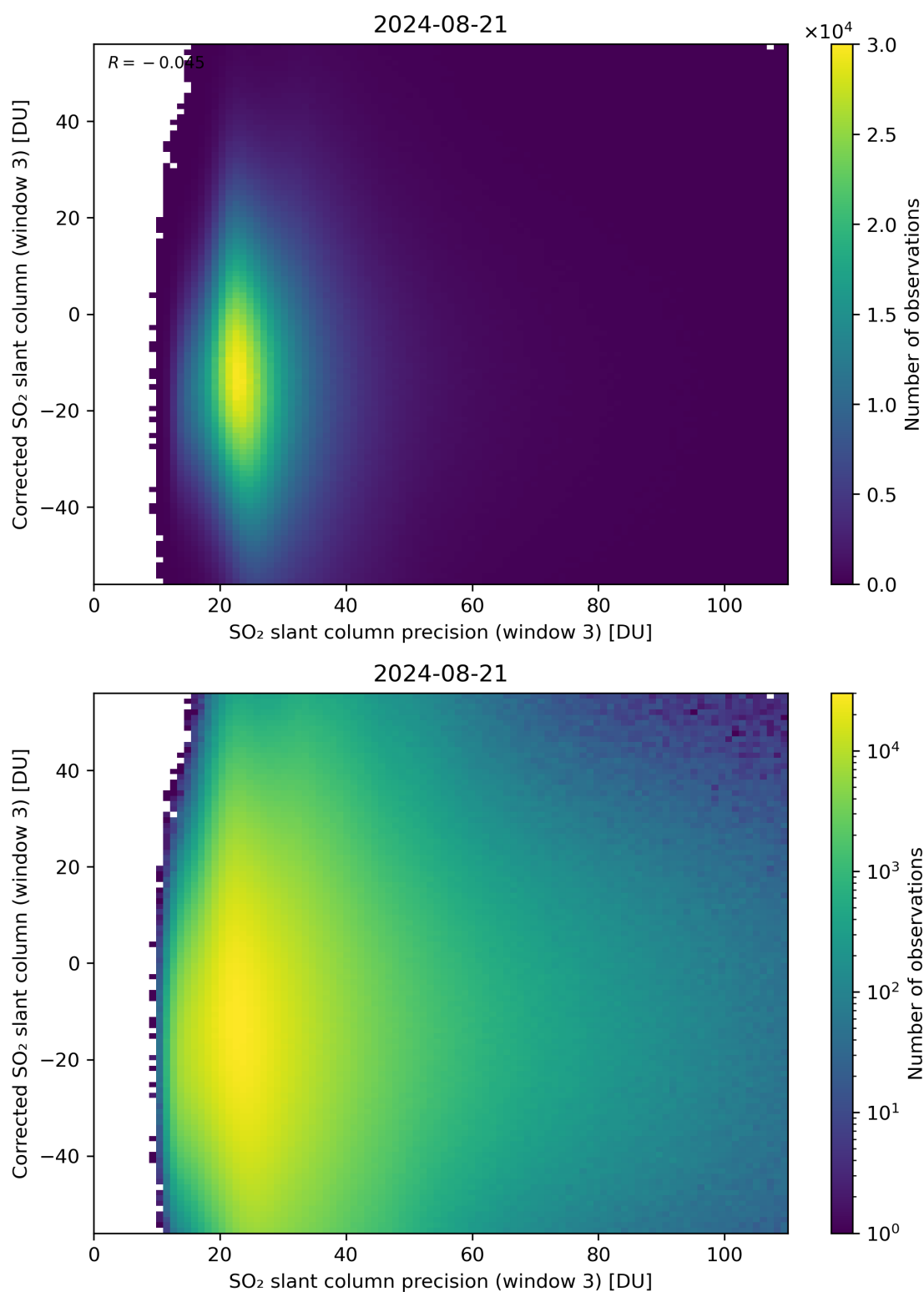
Figure 262: Scatter density plot of “SO 2 slant column precision (window 3)” against “Corrected SO 2 slant column (window 3)” for 2024-08-21 to 2024-08-22.
