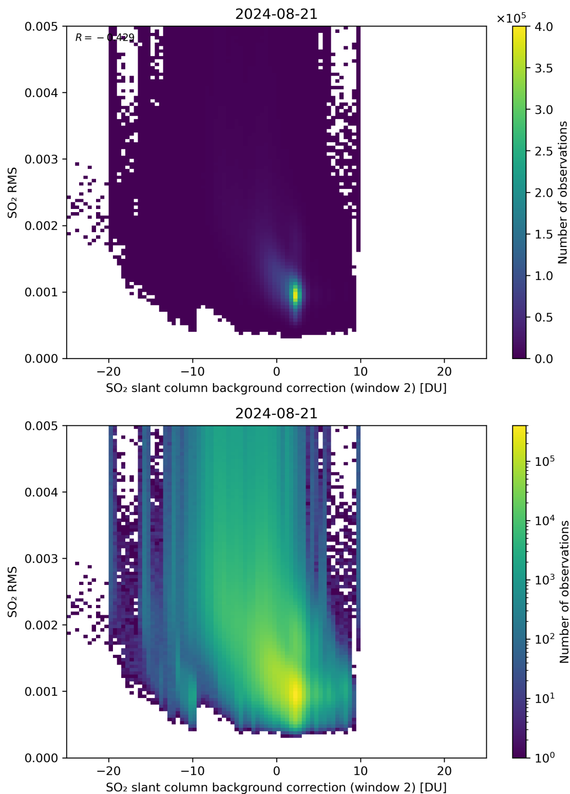
Figure 114: Scatter density plot of “SO 2 slant column background correction (window 2)” against “SO 2 RMS” for 2024-08-21 to 2024-08-22.
