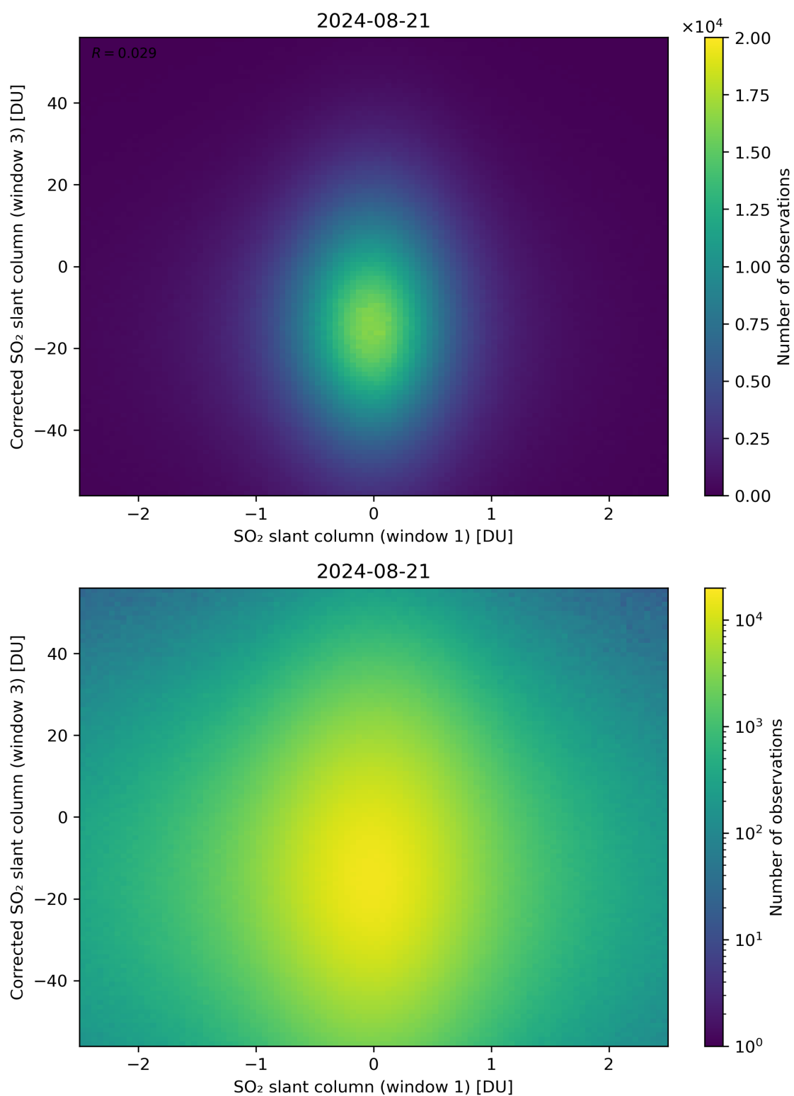
Figure 234: Scatter density plot of “SO 2 slant column (window 1)” against “Corrected SO 2 slant column (window 3)” for 2024-08-21 to 2024-08-22.
