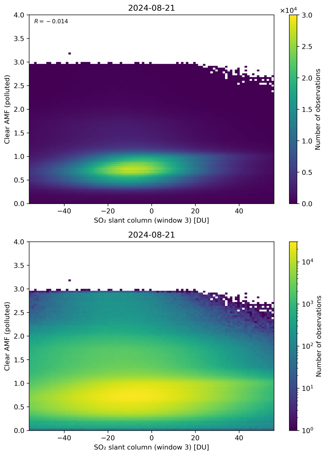
Figure 265: Scatter density plot of “SO 2 slant column (window 3)” against “Clear AMF (polluted)” for 2024-08-21 to 2024-08-22.
