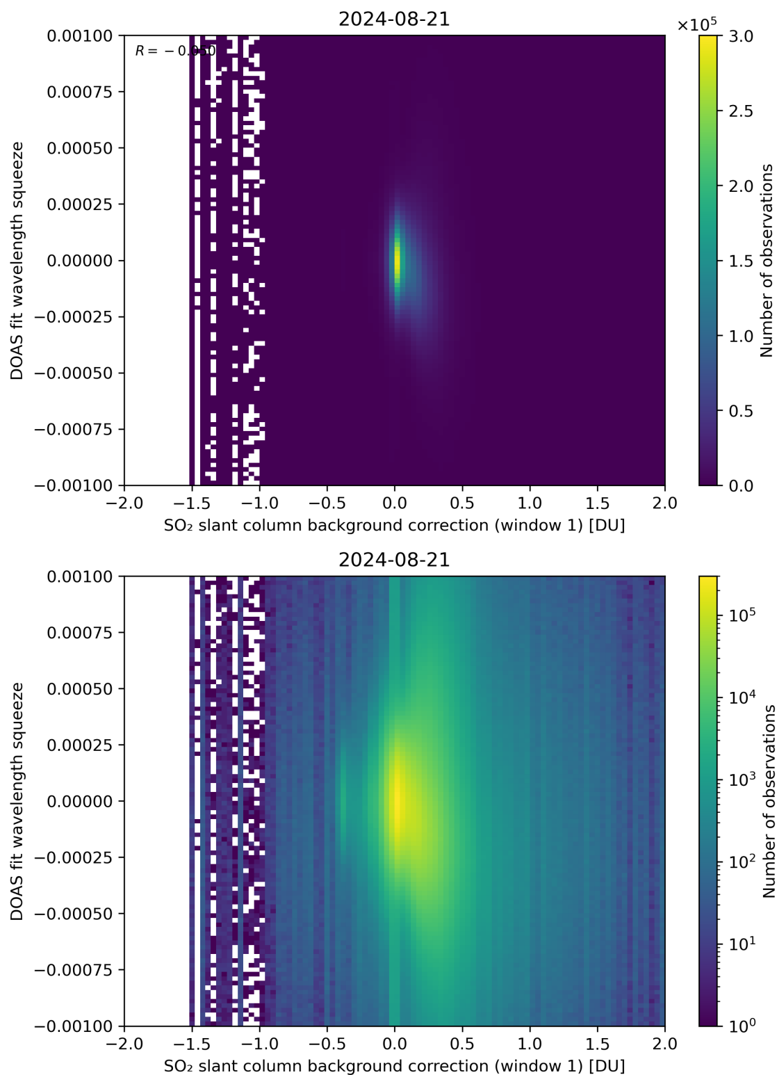
Figure 101: Scatter density plot of “SO 2 slant column background correction (window 1)” against “DOAS fit wavelength squeeze” for 2024-08-21 to 2024-08-22.
