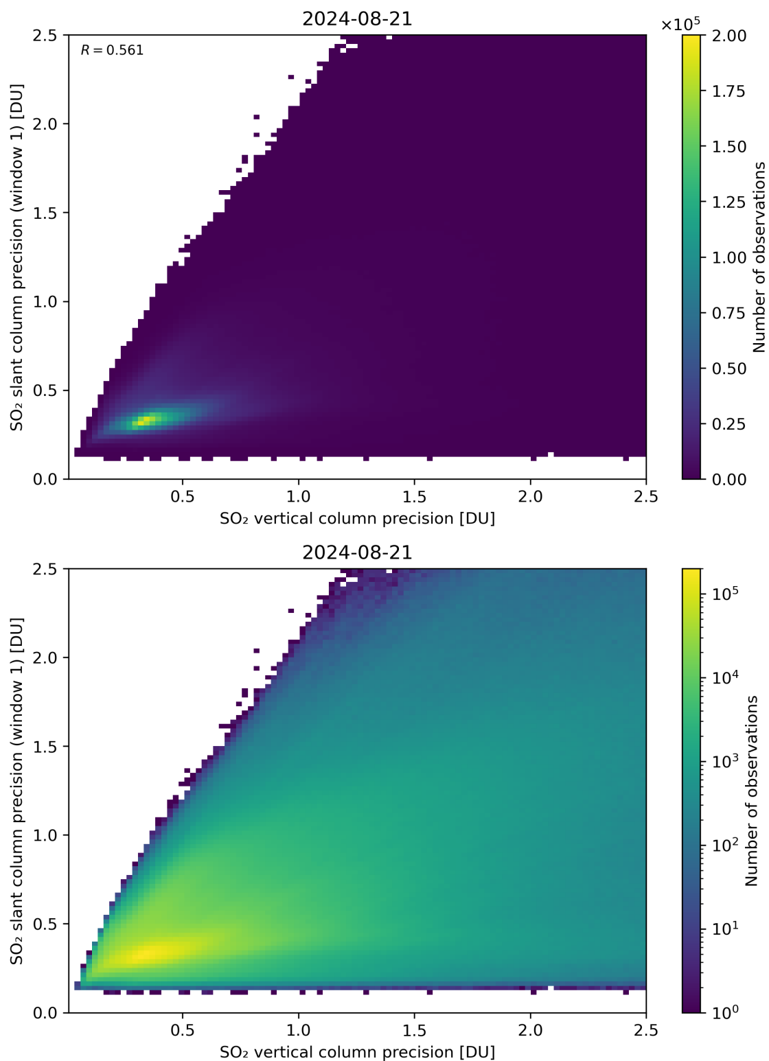
Figure 290: Scatter density plot of “SO 2 vertical column precision” against “SO 2 slant column precision (window 1)” for 2024-08-21 to 2024-08-22.
