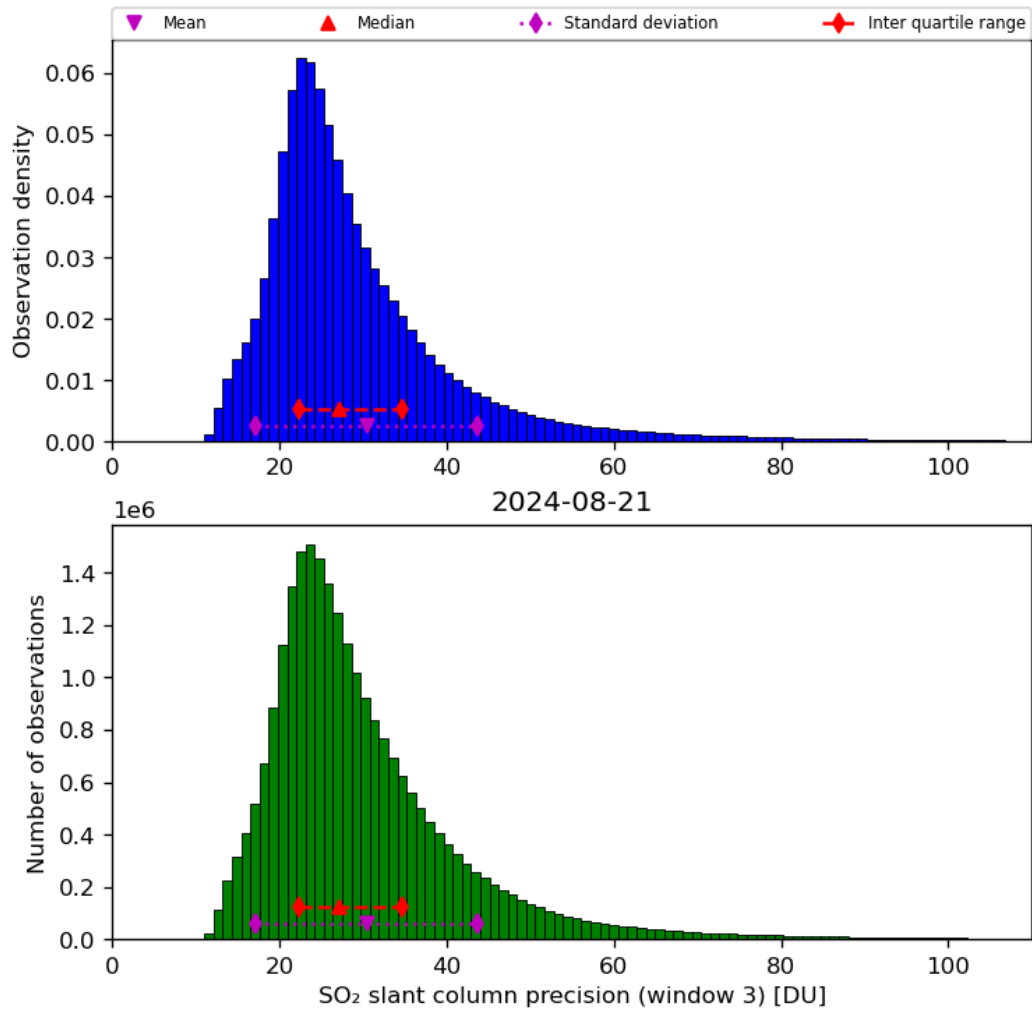
Figure 65: Histogram of “SO 2 slant column precision (window 3)” for 2024-08-21 to 2024-08-22
