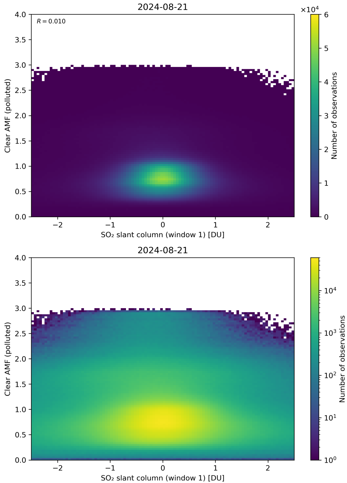
Figure 232: Scatter density plot of “SO 2 slant column (window 1)” against “Clear AMF (polluted)” for 2024-08-21 to 2024-08-22.
