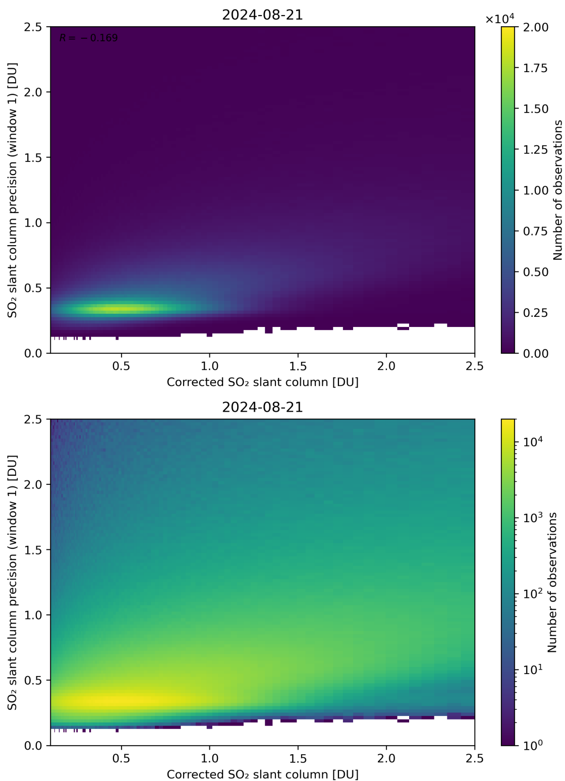
Figure 188: Scatter density plot of “Corrected SO 2 slant column” against “SO 2 slant column precision (window 1)” for 2024-08-21 to 2024-08-22.
