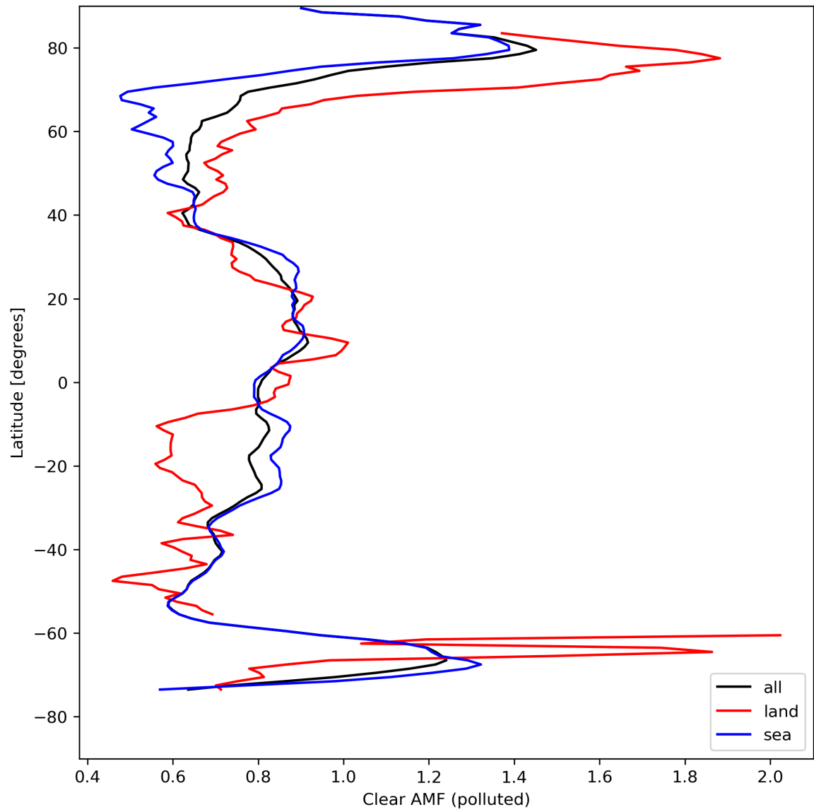
Figure 50: Zonal average of “Clear AMF (polluted)” for 2024-08-21 to 2024-08-22.
