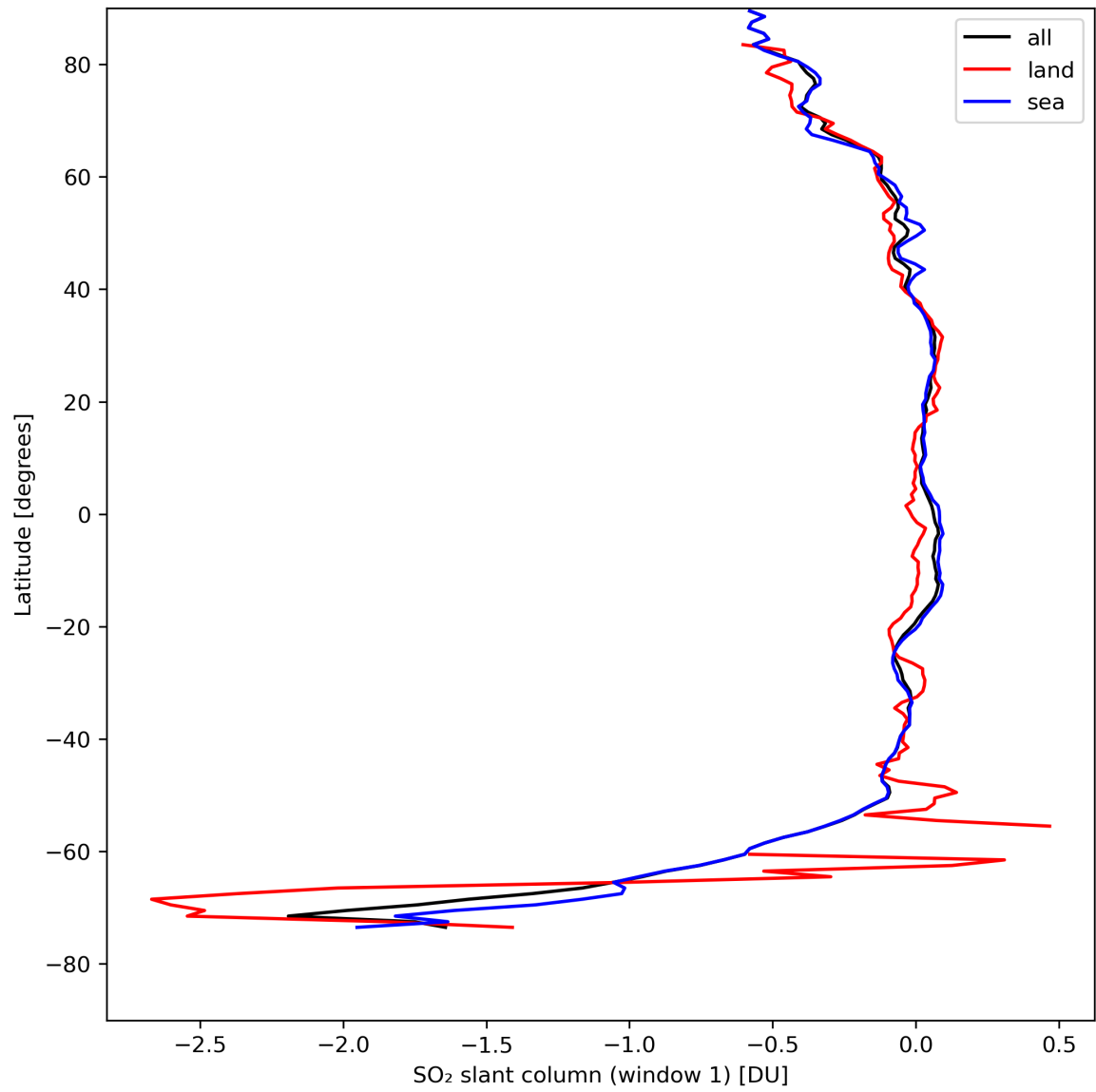
Figure 33: Zonal average of “SO 2 slant column (window 1)” for 2024-08-21 to 2024-08-22.
