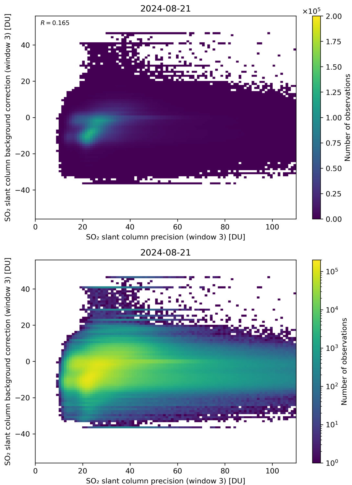
Figure 257: Scatter density plot of “SO 2 slant column precision (window 3)” against “SO 2 slant column background correction (window 3)” for 2024-08-21 to 2024-08-22.
