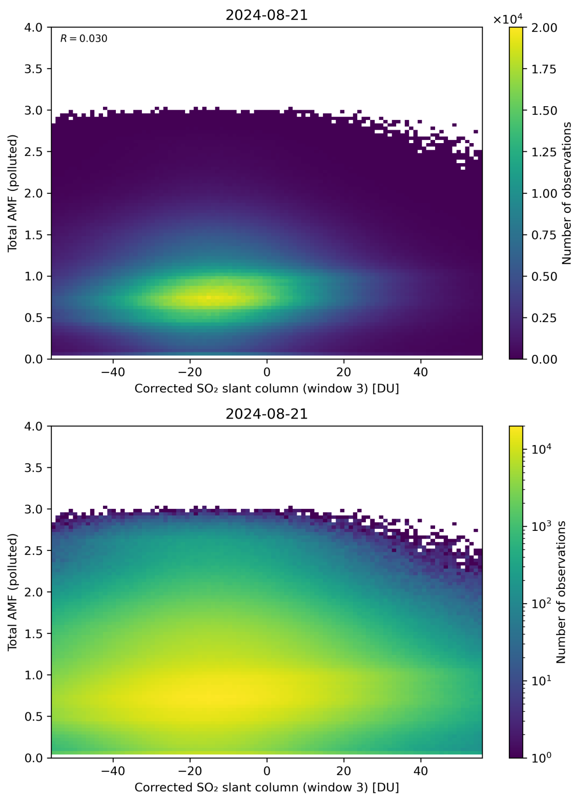
Figure 210: Scatter density plot of “Corrected SO 2 slant column (window 3)” against “Total AMF (polluted)” for 2024-08-21 to 2024-08-22.
