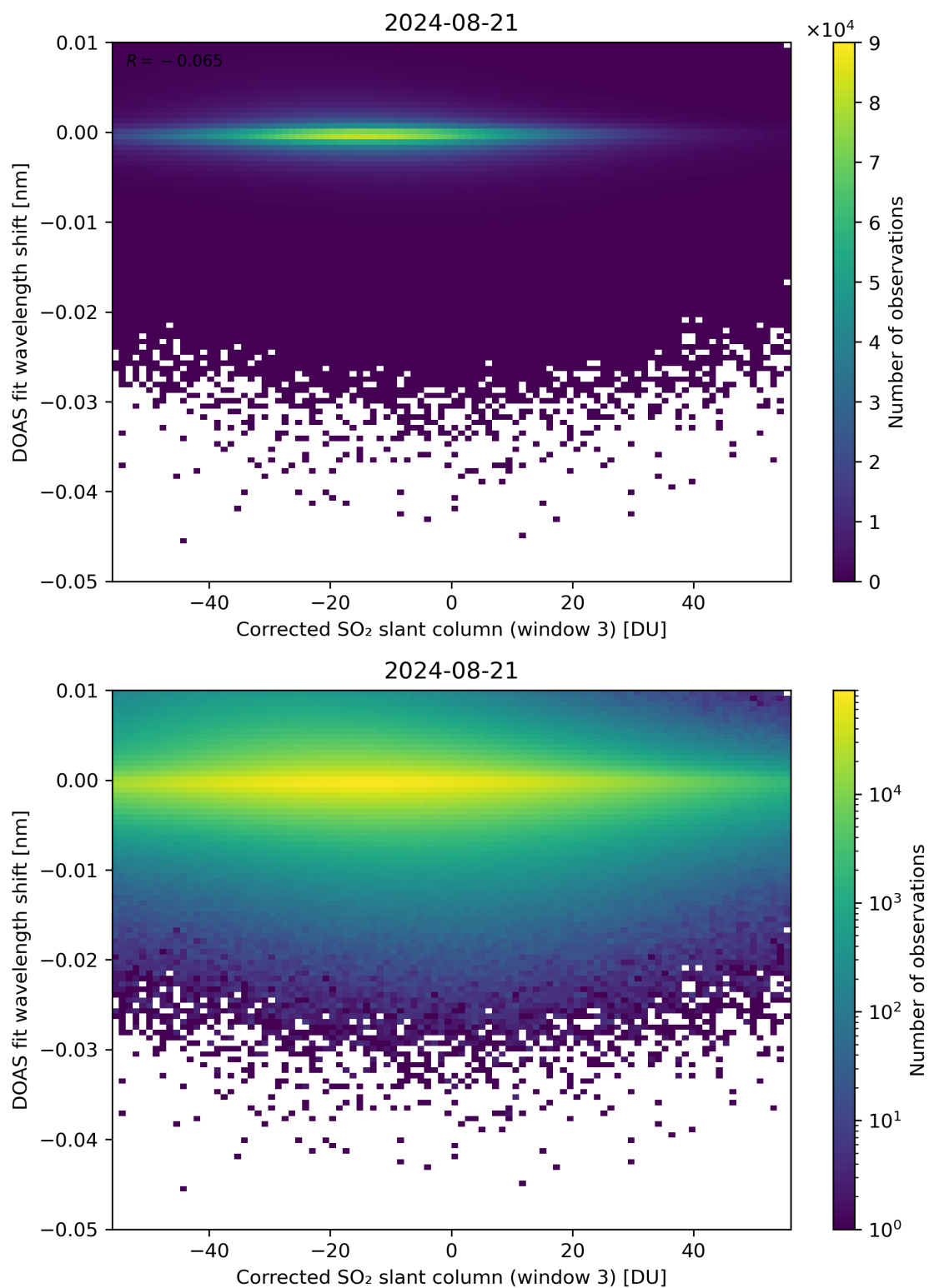
Figure 206: Scatter density plot of “Corrected SO 2 slant column (window 3)” against “DOAS fit wavelength shift” for 2024-08-21 to 2024-08-22.
