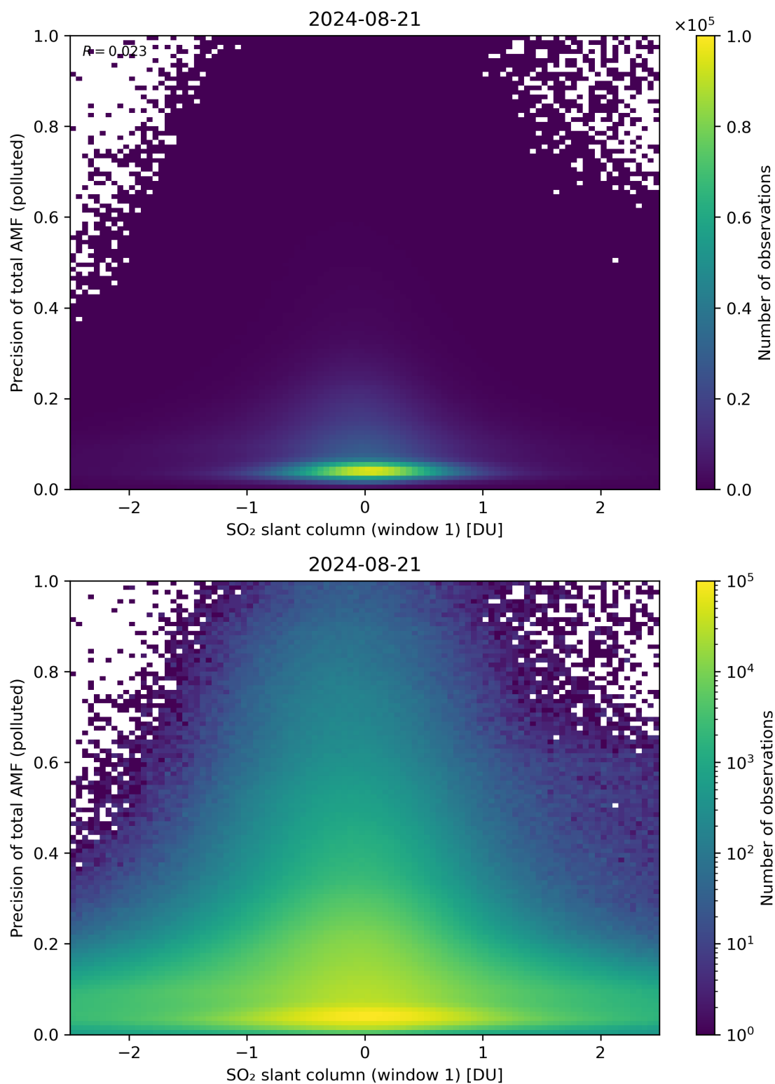
Figure 240: Scatter density plot of “SO 2 slant column (window 1)” against “Precision of total AMF (polluted)” for 2024-08-21 to 2024-08-22.
