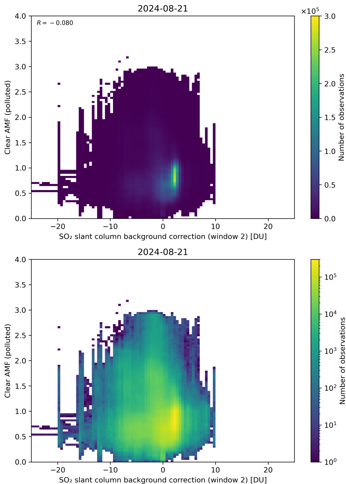
Figure 115: Scatter density plot of “SO 2 slant column background correction (window 2)” against “Clear AMF (polluted)” for 2024-08-21 to 2024-08-22.
