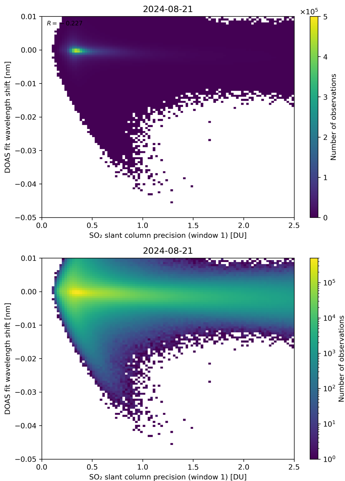
Figure 221: Scatter density plot of “SO 2 slant column precision (window 1)” against “DOAS fit wavelength shift” for 2024-08-21 to 2024-08-22.
