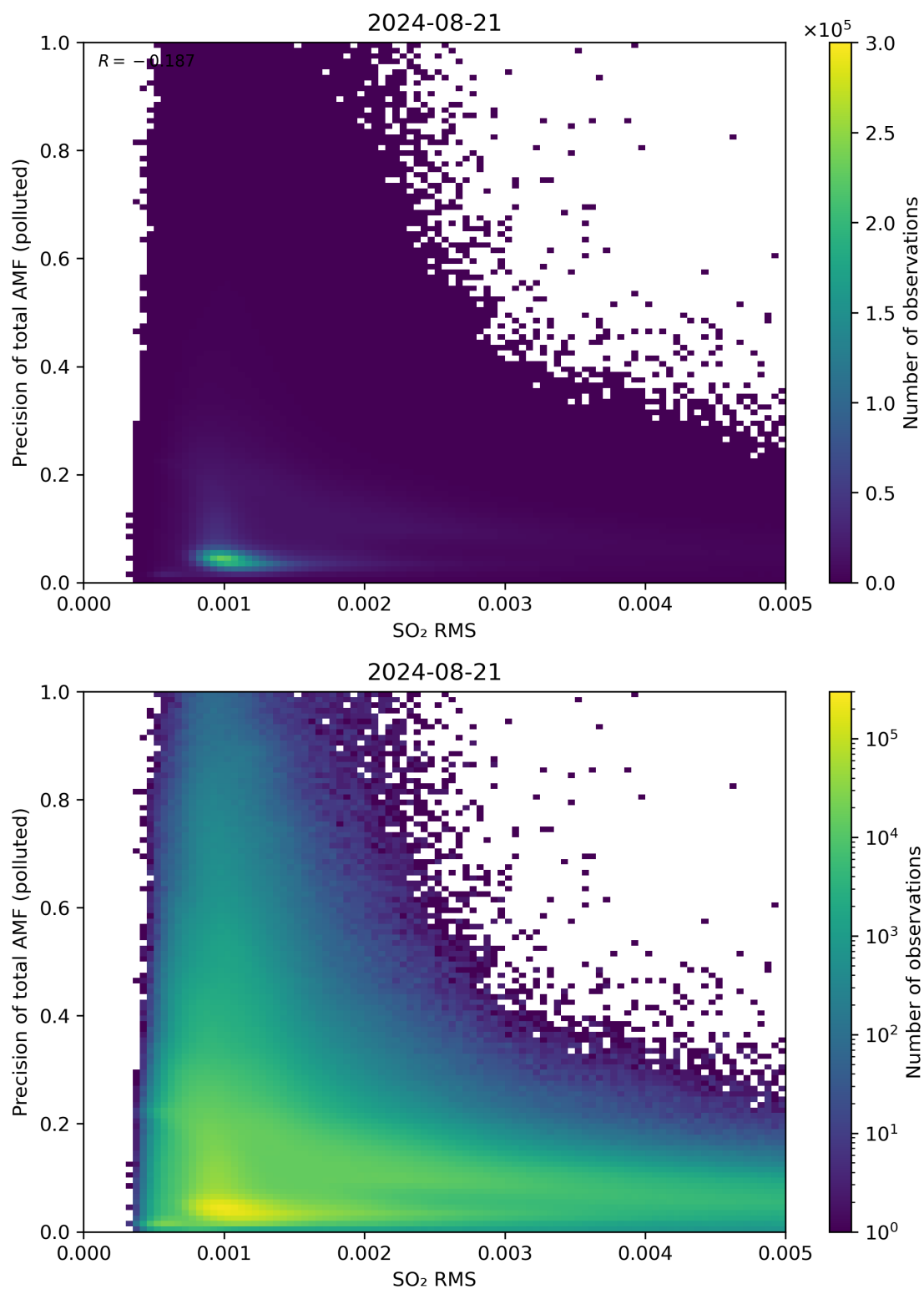
Figure 138: Scatter density plot of “SO 2 RMS” against “Precision of total AMF (polluted)” for 2024-08-21 to 2024-08-22.
