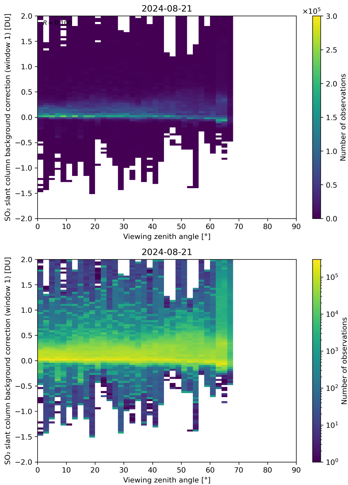
Figure 308: Scatter density plot of “Viewing zenith angle” against “SO 2 slant column background correction (window 1)” for 2024-08-21 to 2024-08-22.
