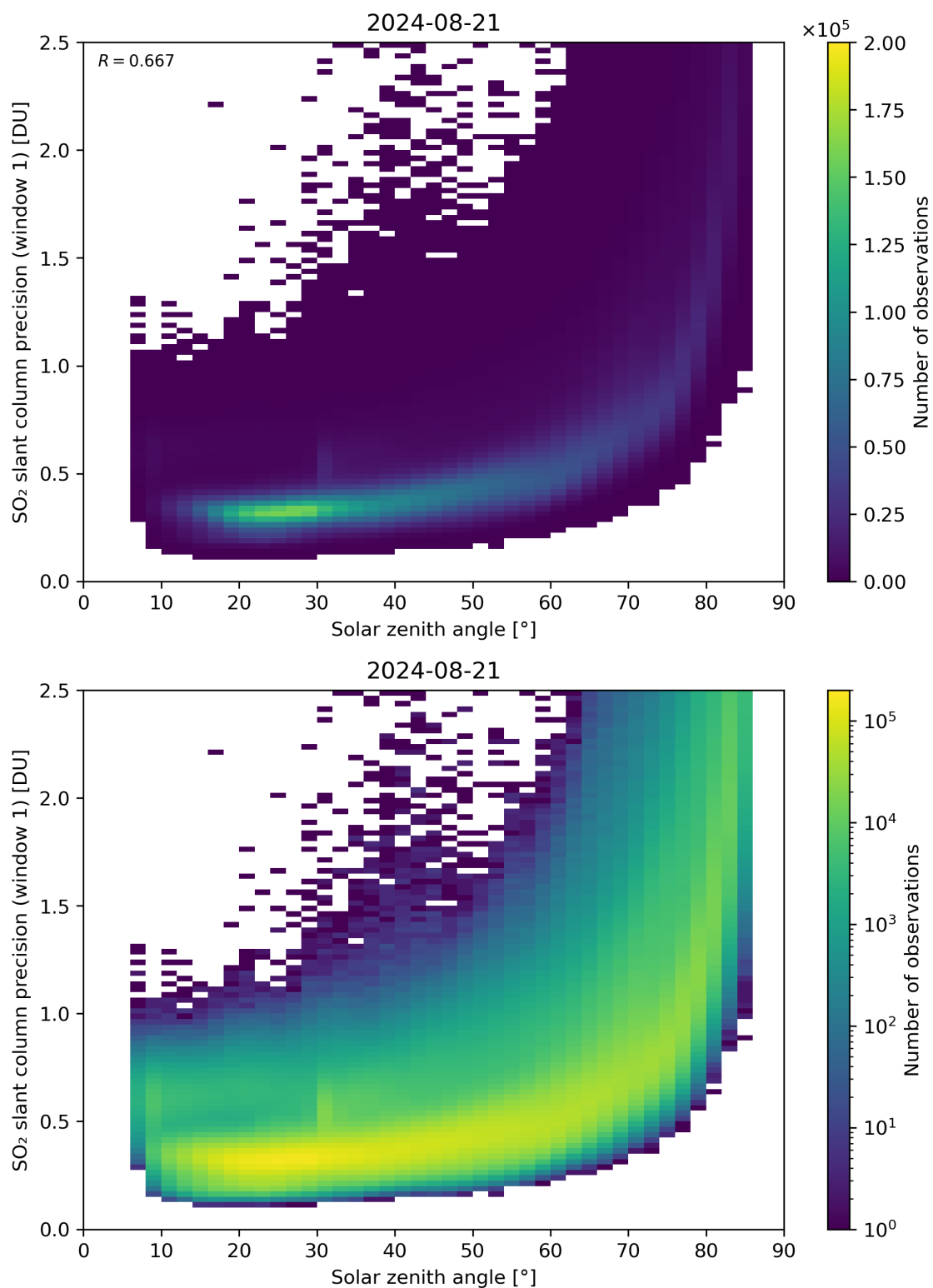
Figure 170: Scatter density plot of “Solar zenith angle” against “SO 2 slant column precision (window 1)” for 2024-08-21 to 2024-08-22.
