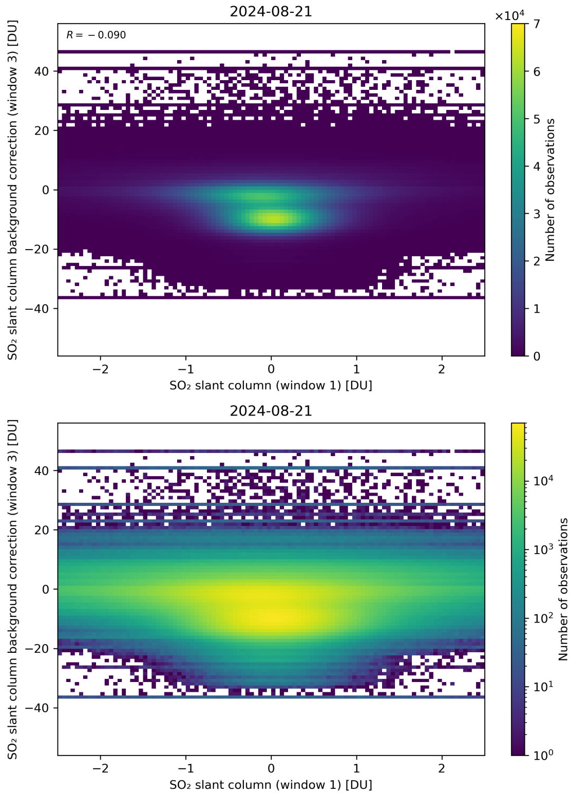
Figure 214: Scatter density plot of “SO 2 slant column (window 1)” against “SO 2 slant column background correction (window 3)” for 2024-08-21 to 2024-08-22.
