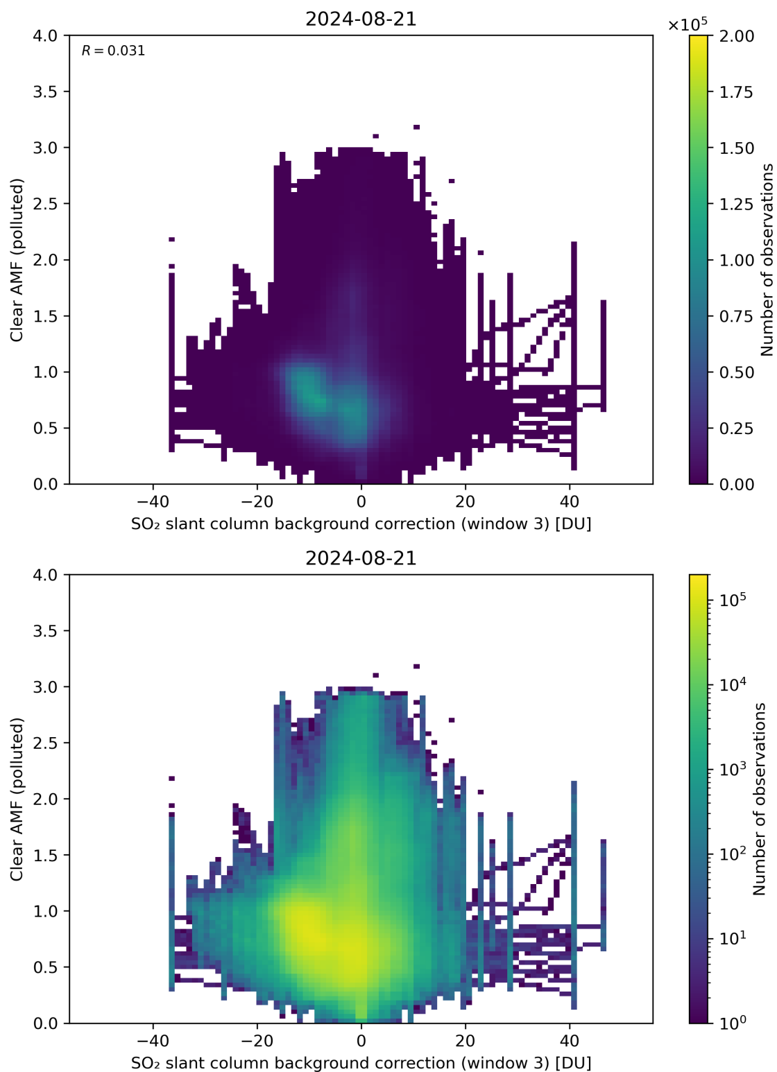
Figure 124: Scatter density plot of “SO 2 slant column background correction (window 3)” against “Clear AMF (polluted)” for 2024-08-21 to 2024-08-22.
