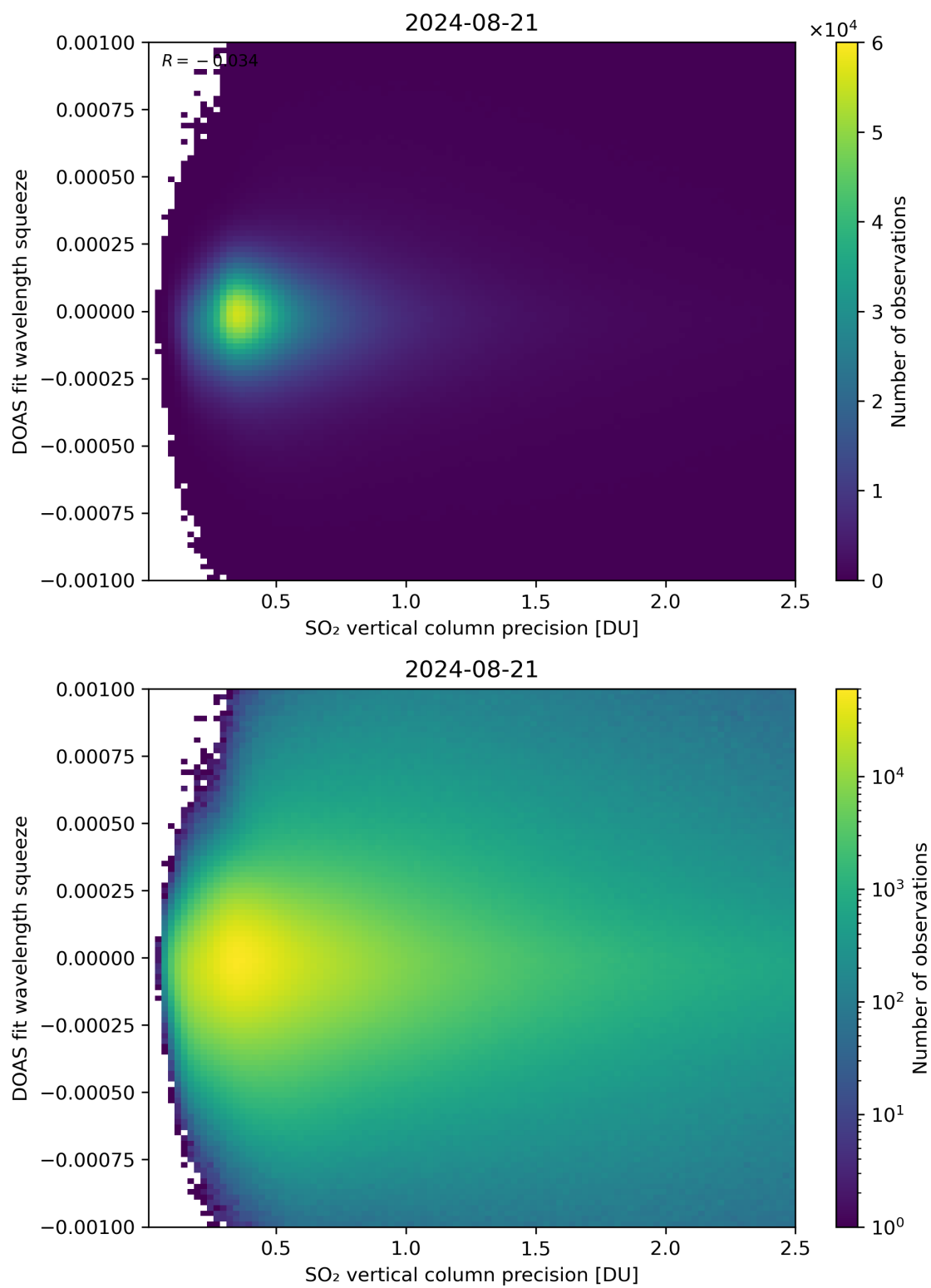
Figure 283: Scatter density plot of “SO 2 vertical column precision” against “DOAS fit wavelength squeeze” for 2024-08-21 to 2024-08-22.
