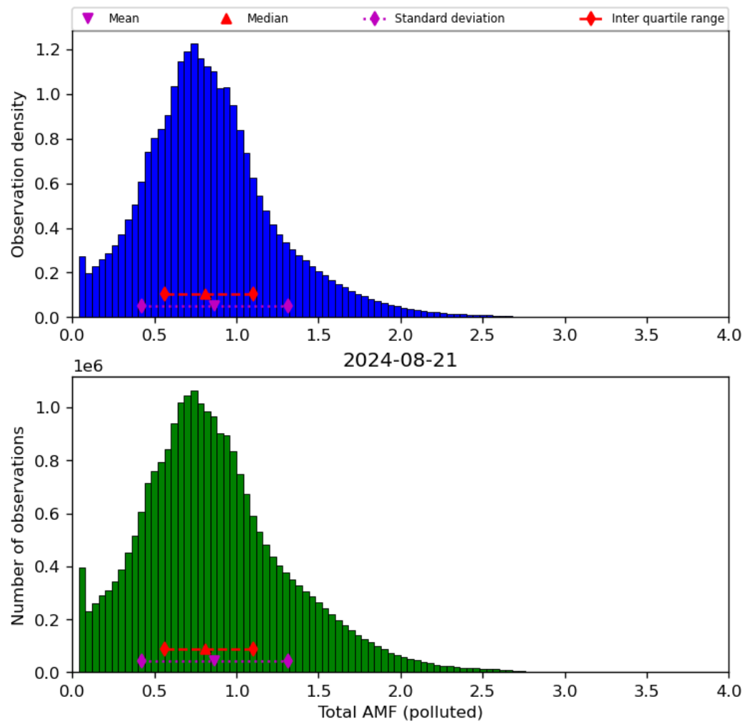
Figure 71: Histogram of “Total AMF (polluted)” for 2024-08-21 to 2024-08-22
