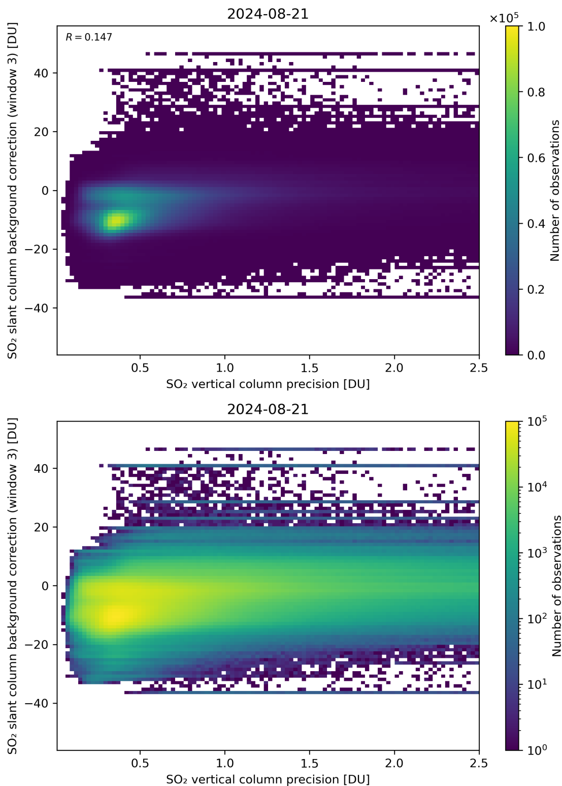
Figure 281: Scatter density plot of “SO 2 vertical column precision” against “SO 2 slant column background correction (window 3)” for 2024-08-21 to 2024-08-22.
