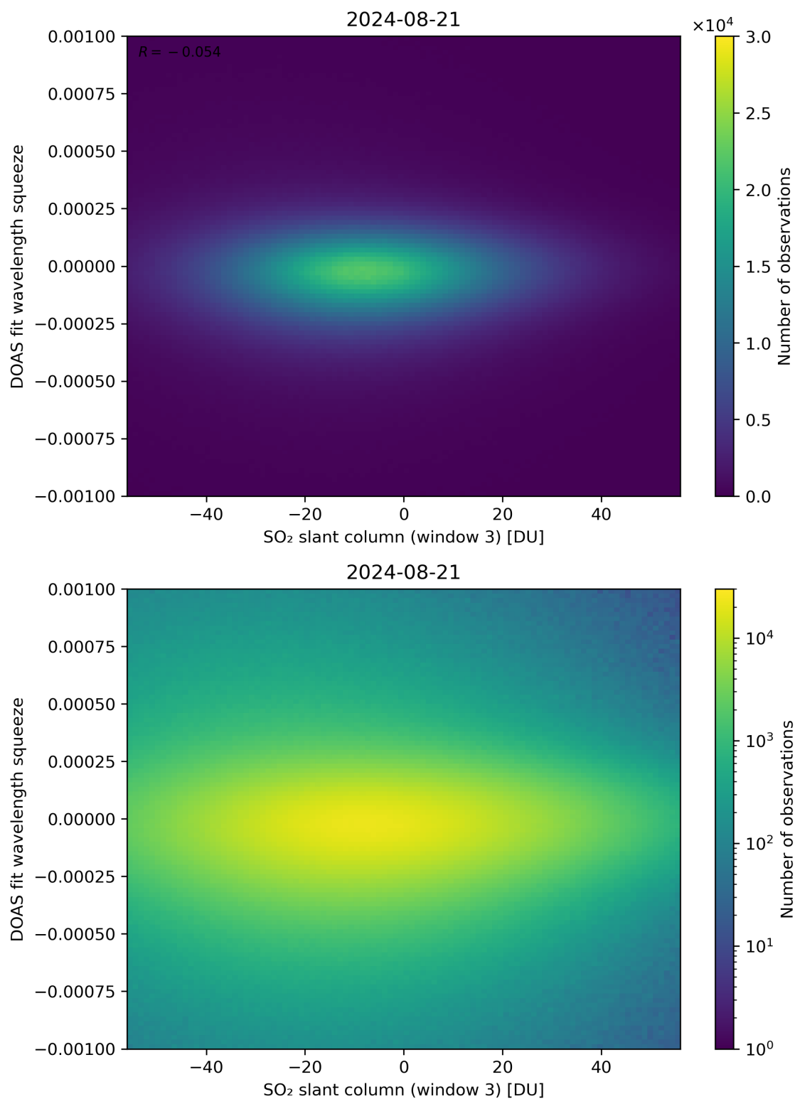
Figure 255: Scatter density plot of “SO 2 slant column (window 3)” against “DOAS fit wavelength squeeze” for 2024-08-21 to 2024-08-22.
