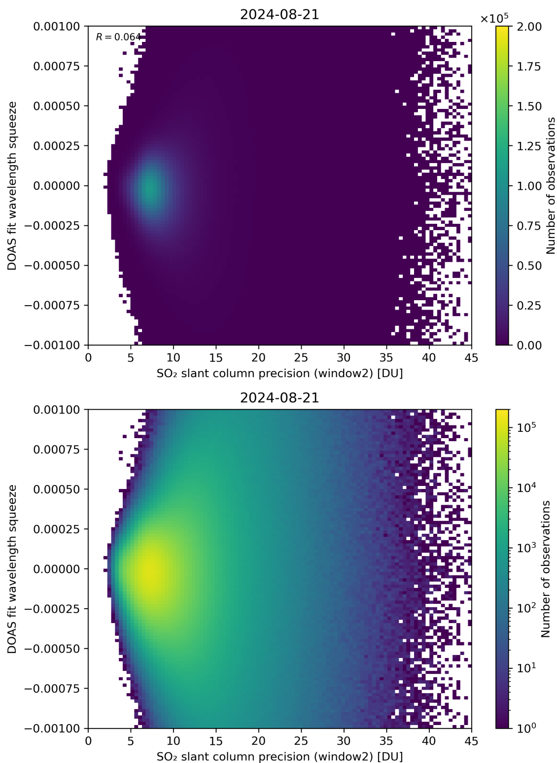
Figure 244: Scatter density plot of “SO 2 slant column precision (window2)” against “DOAS fit wavelength squeeze” for 2024-08-21 to 2024-08-22.
