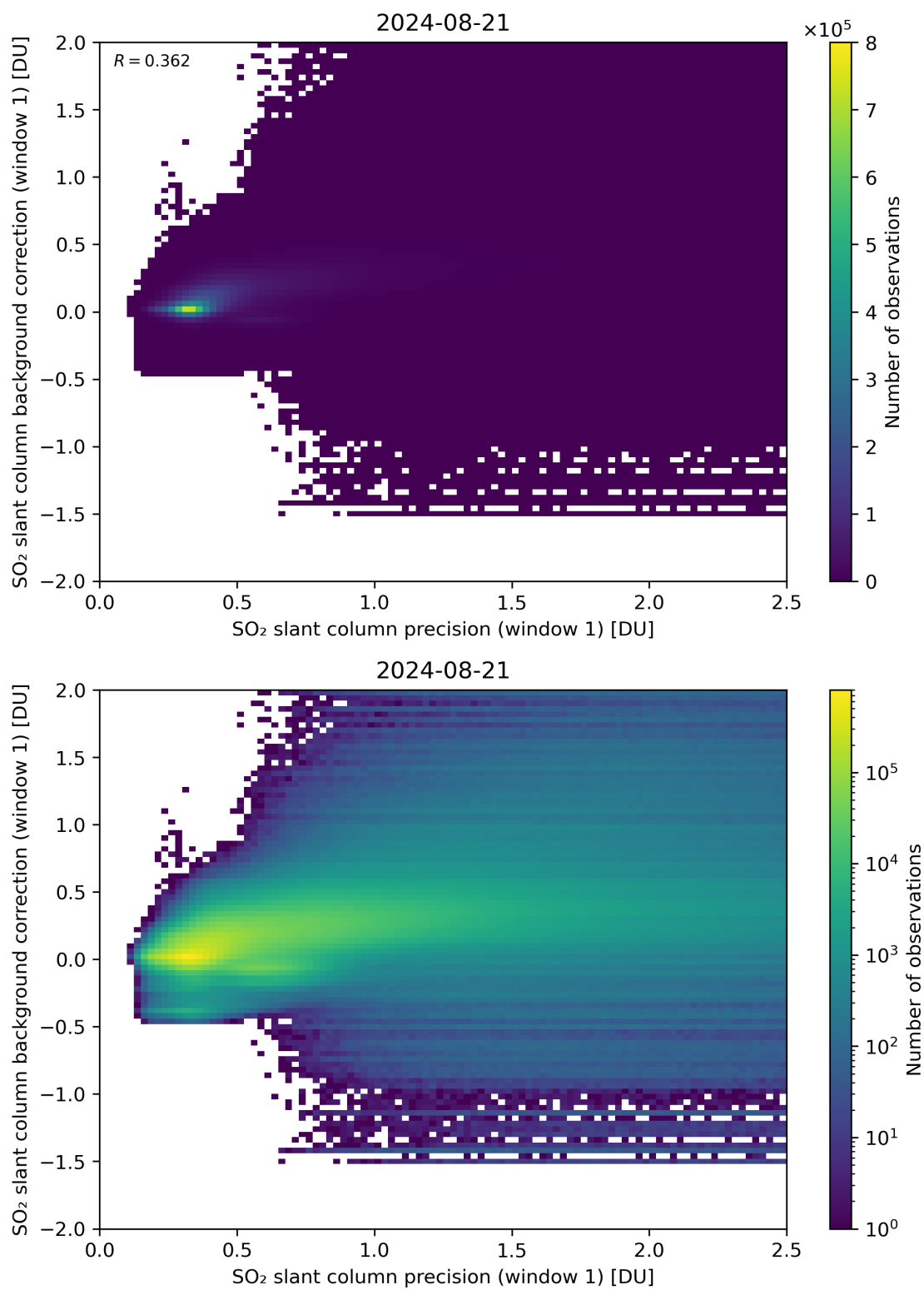
Figure 218: Scatter density plot of “SO 2 slant column precision (window 1)” against “SO 2 slant column background correction (window 1)” for 2024-08-21 to 2024-08-22.
