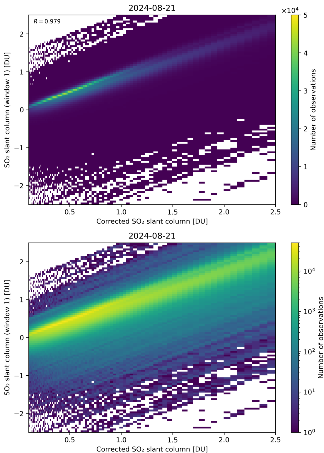
Figure 187: Scatter density plot of “Corrected SO 2 slant column” against “SO 2 slant column (window 1)” for 2024-08-21 to 2024-08-22.
