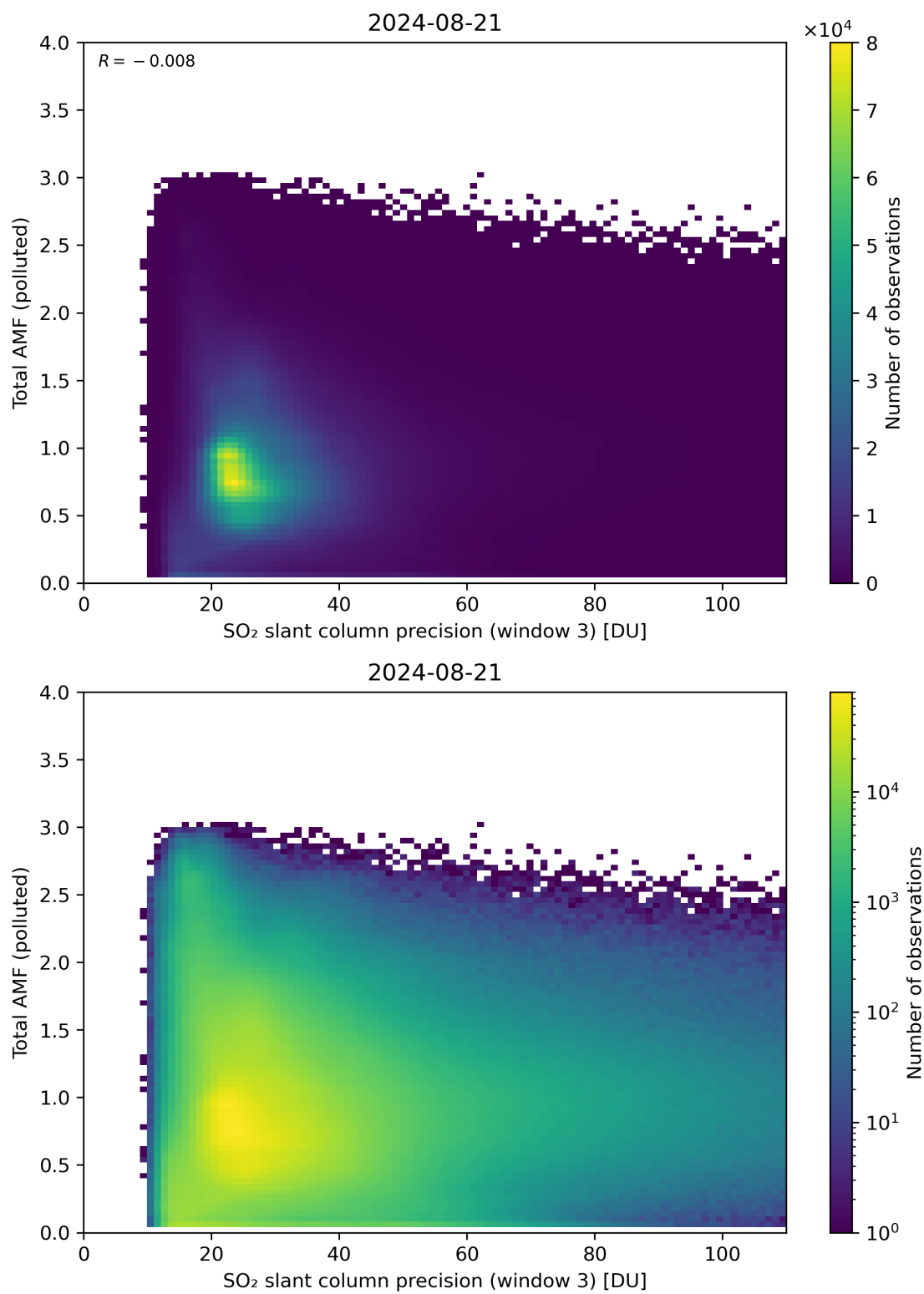
Figure 263: Scatter density plot of “SO 2 slant column precision (window 3)” against “Total AMF (polluted)” for 2024-08-21 to 2024-08-22.
