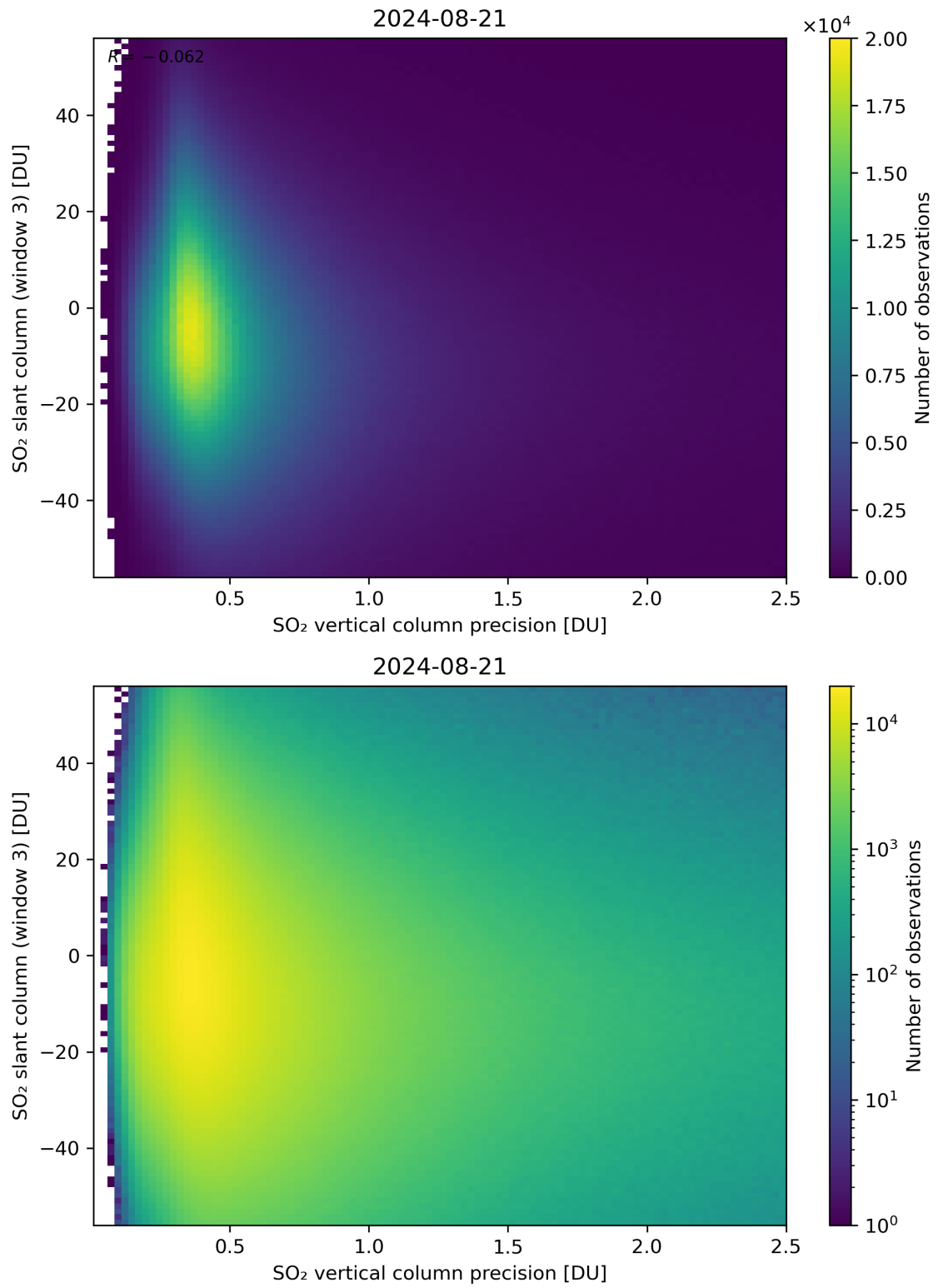
Figure 292: Scatter density plot of “SO 2 vertical column precision” against “SO 2 slant column (window 3)” for 2024-08-21 to 2024-08-22.
