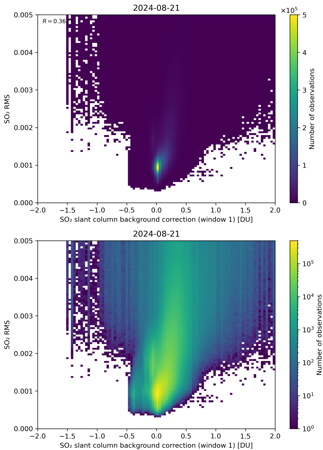
Figure 102: Scatter density plot of “SO 2 slant column background correction (window 1)” against “SO 2 RMS” for 2024-08-21 to 2024-08-22.
