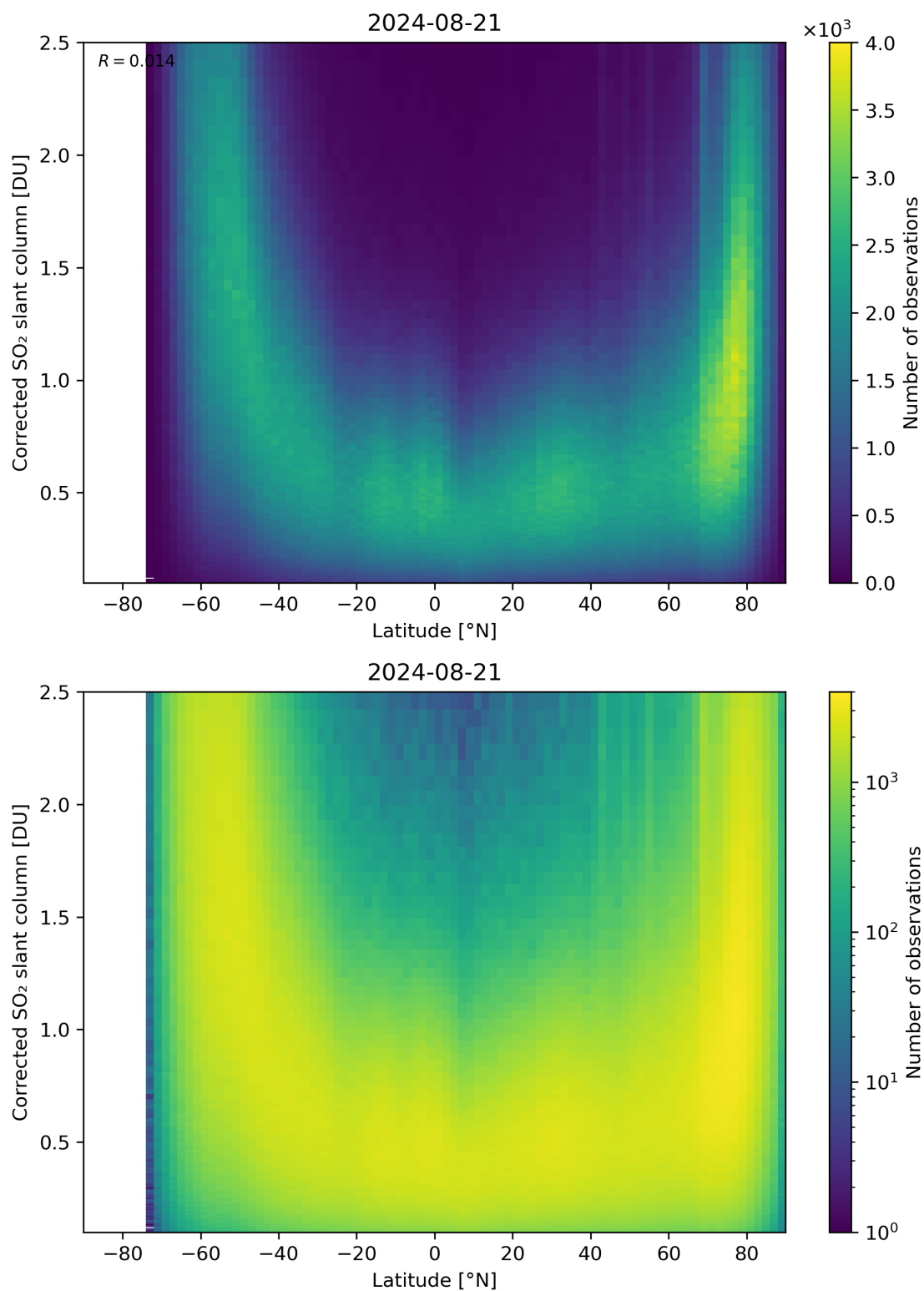
Figure 146: Scatter density plot of “Latitude” against “Corrected SO 2 slant column” for 2024-08-21 to 2024-08-22.
