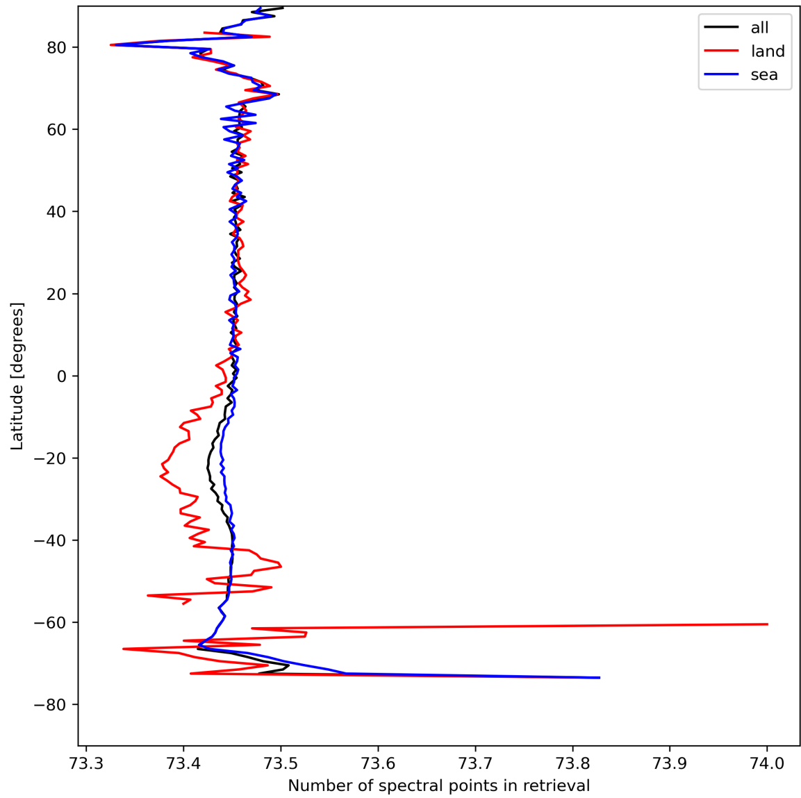
Figure 51: Zonal average of “Number of spectral points in retrieval” for 2024-08-21 to 2024-08-22.
