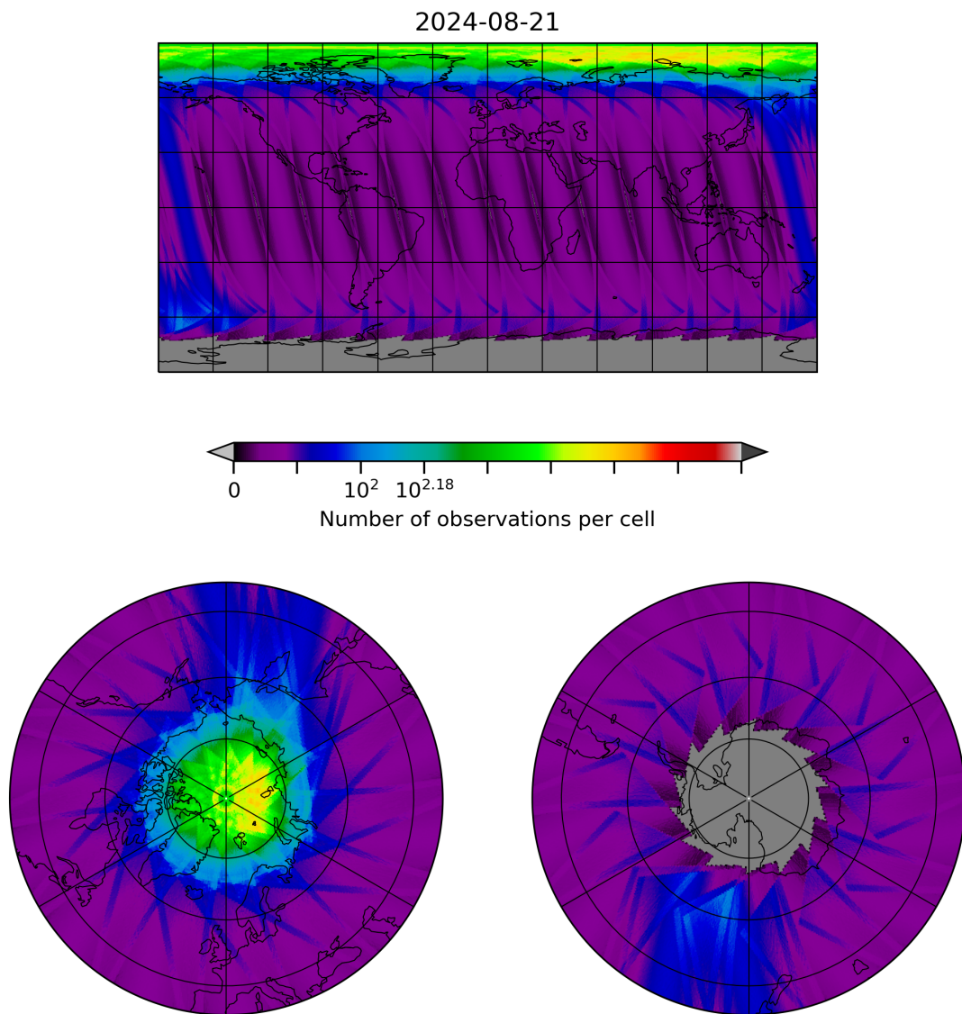
Figure 28: Map of the number of observations for 2024-08-21 to 2024-08-22
