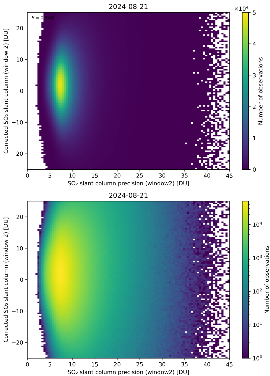
Figure 247: Scatter density plot of “SO 2 slant column precision (window2)” against “Corrected SO 2 slant column (window 2)” for 2024-08-21 to 2024-08-22.
