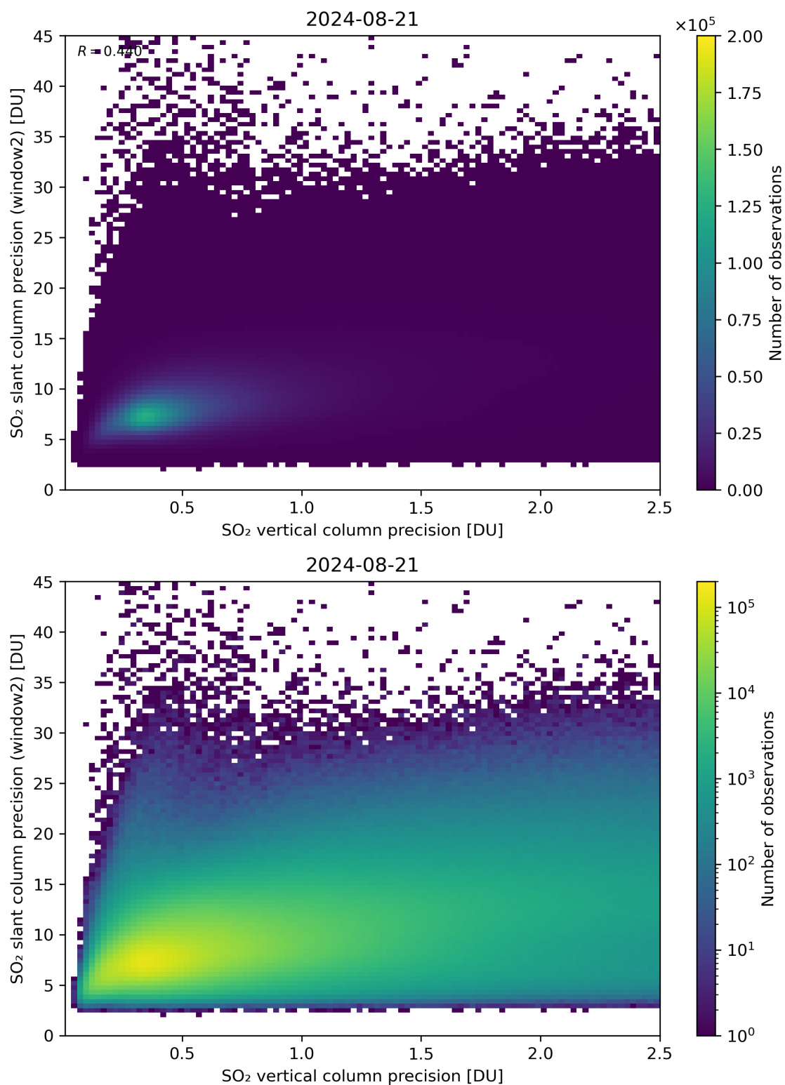
Figure 291: Scatter density plot of “SO 2 vertical column precision” against “SO 2 slant column precision (window2)” for 2024-08-21 to 2024-08-22.
