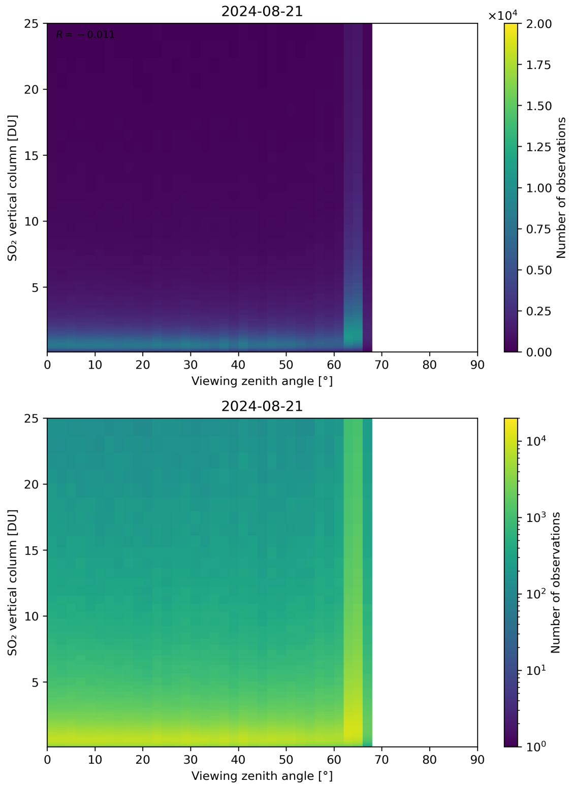
Figure 327: Scatter density plot of “Viewing zenith angle” against “SO 2 vertical column” for 2024-08-21 to 2024-08-22.
