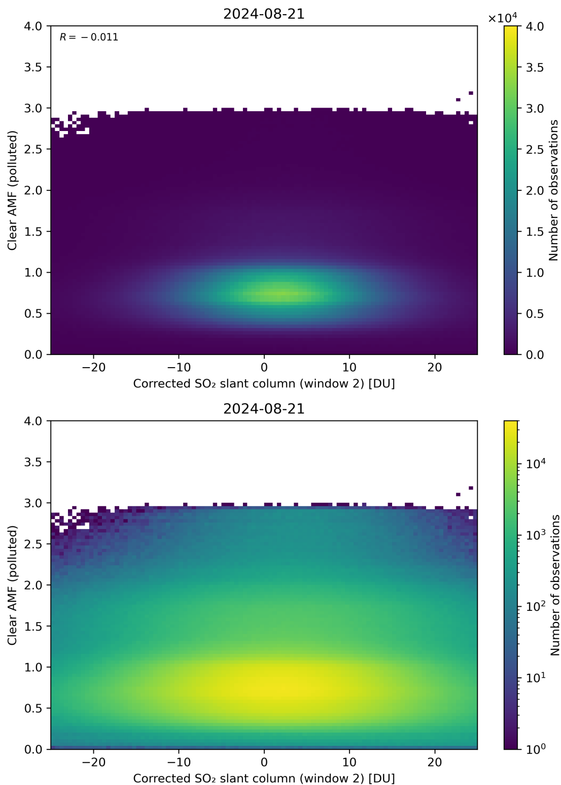
Figure 199: Scatter density plot of “Corrected SO 2 slant column (window 2)” against “Clear AMF (polluted)” for 2024-08-21 to 2024-08-22.
