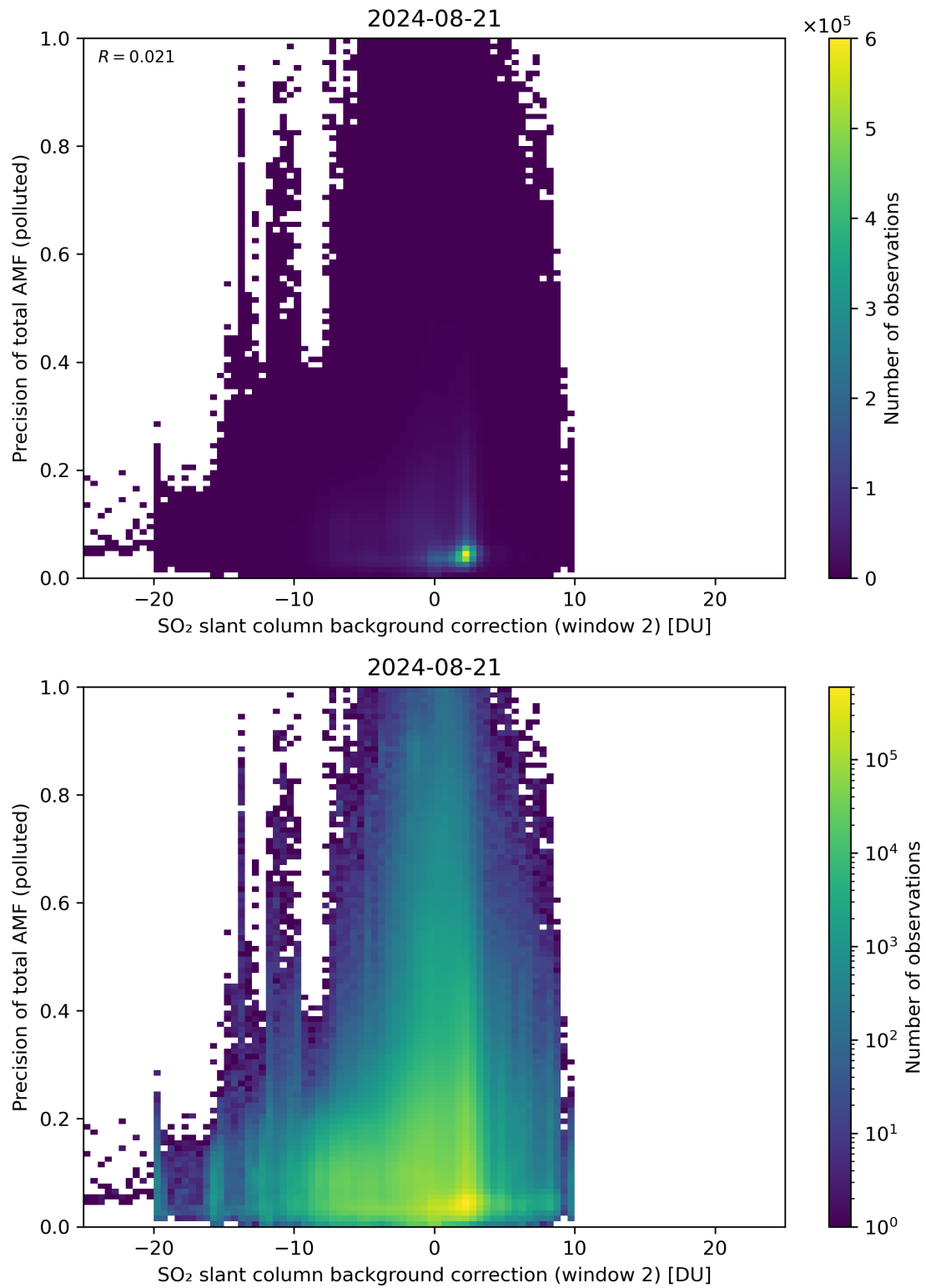
Figure 120: Scatter density plot of “SO 2 slant column background correction (window 2)” against “Precision of total AMF (polluted)” for 2024-08-21 to 2024-08-22.
