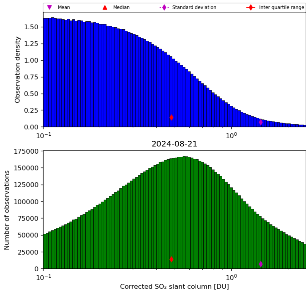
Figure 55: Histogram of “Corrected SO 2 slant column” for 2024-08-21 to 2024-08-22
