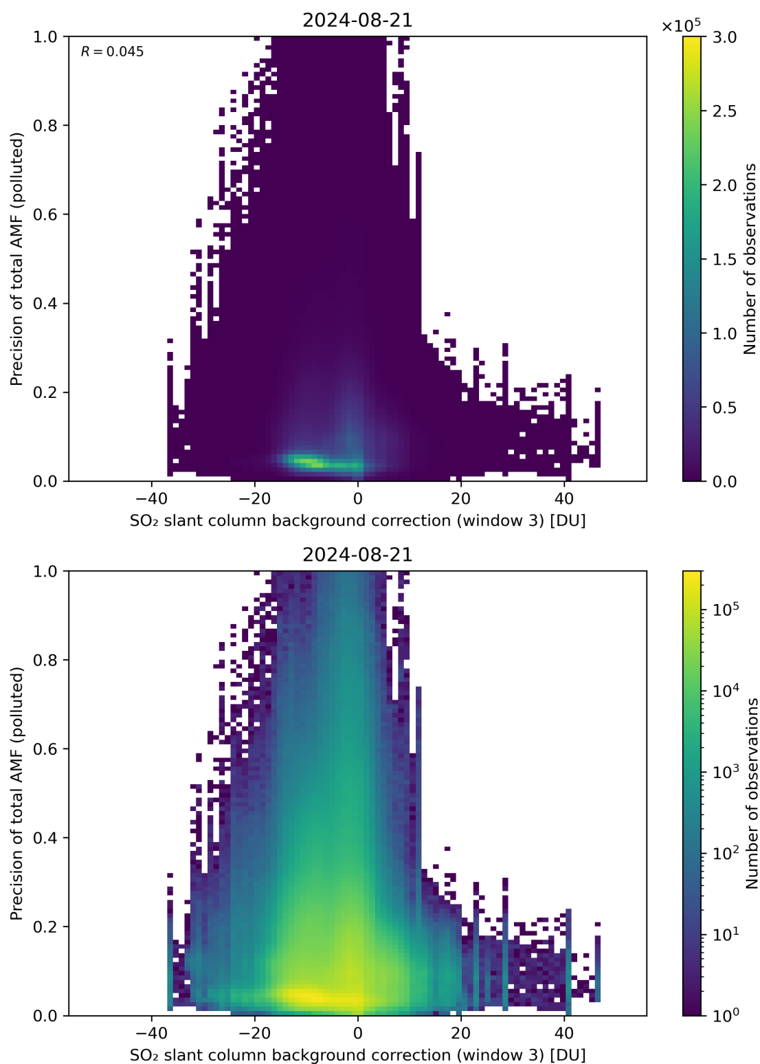
Figure 126: Scatter density plot of “SO 2 slant column background correction (window 3)” against “Precision of total AMF (polluted)” for 2024-08-21 to 2024-08-22.
