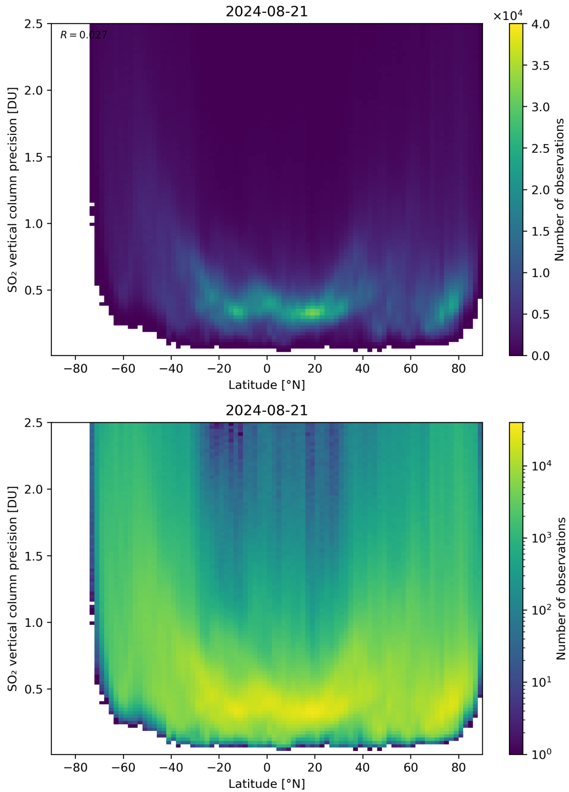
Figure 157: Scatter density plot of “Latitude” against “SO 2 vertical column precision” for 2024-08-21 to 2024-08-22.
