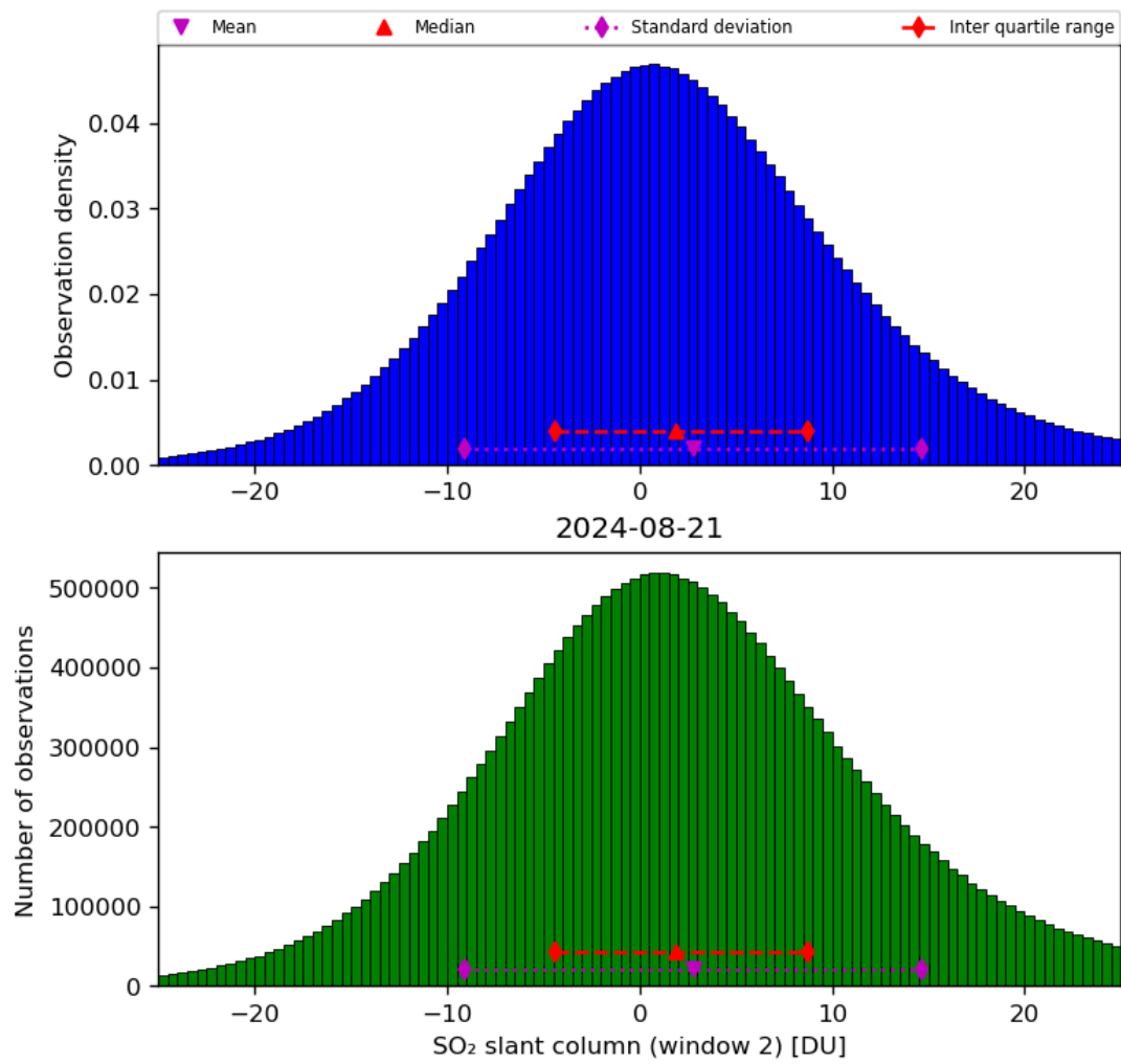
Figure 60: Histogram of “SO 2 slant column (window 2)” for 2024-08-21 to 2024-08-22
