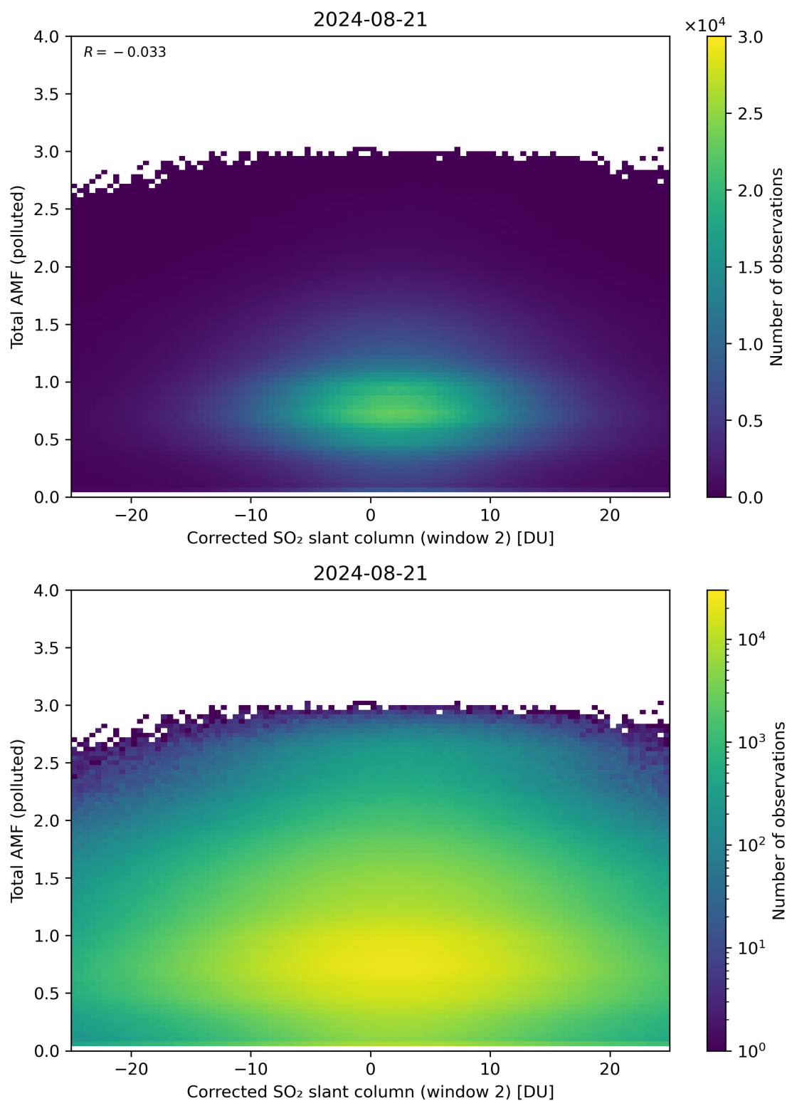
Figure 203: Scatter density plot of “Corrected SO 2 slant column (window 2)” against “Total AMF (polluted)” for 2024-08-21 to 2024-08-22.
