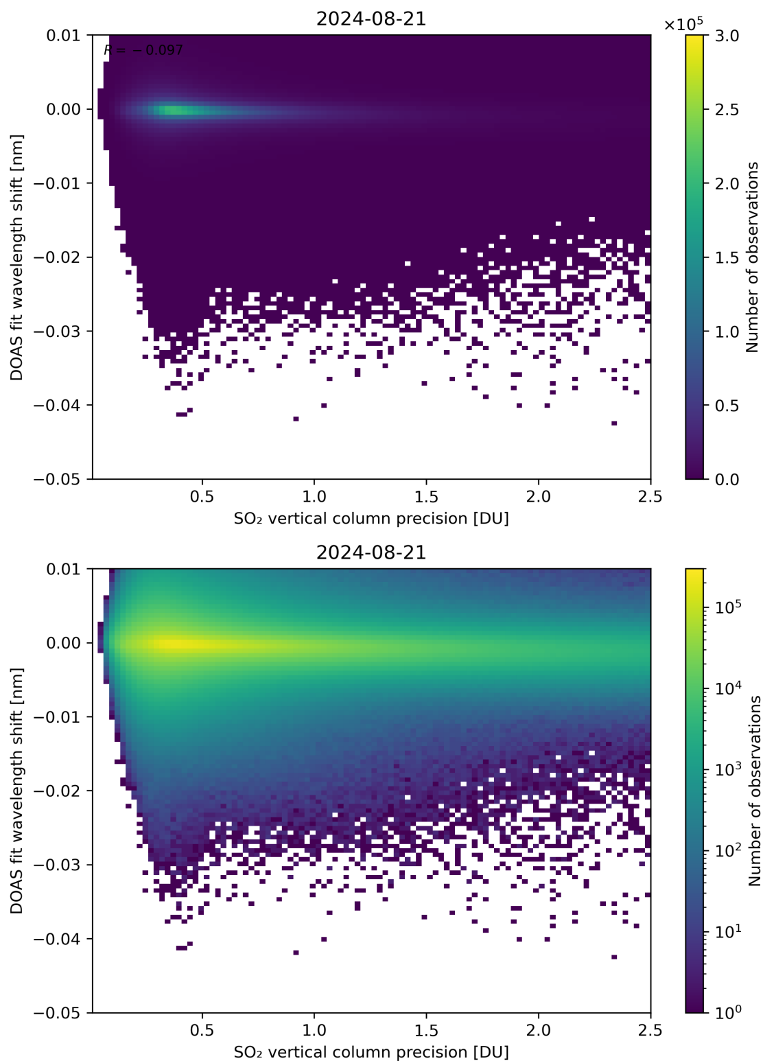
Figure 282: Scatter density plot of “SO 2 vertical column precision” against “DOAS fit wavelength shift” for 2024-08-21 to 2024-08-22.
