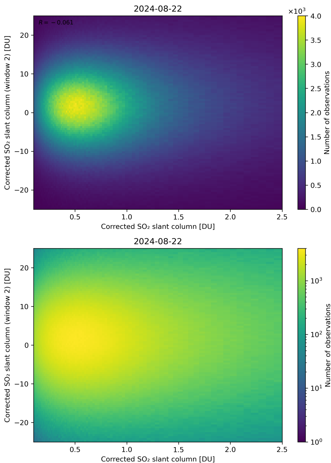
Figure 185: Scatter density plot of “Corrected SO 2 slant column” against “Corrected SO 2 slant column (window 2)” for 2024-08-22 to 2024-08-23.
