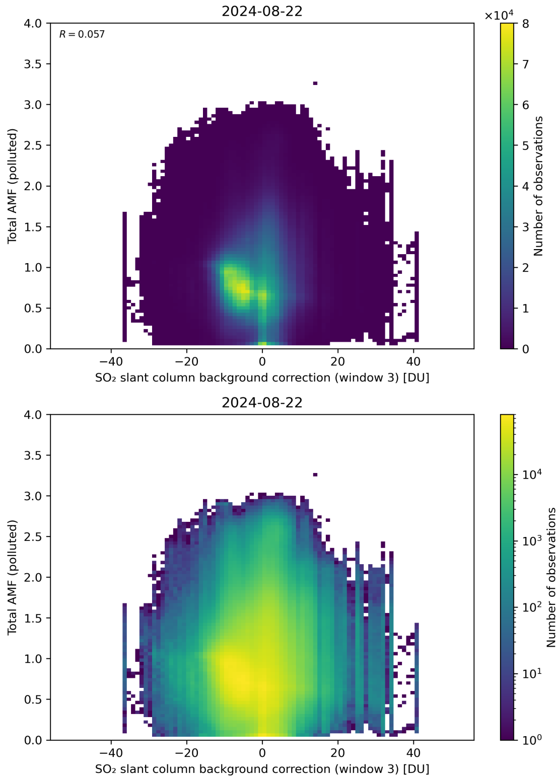
Figure 125: Scatter density plot of “SO 2 slant column background correction (window 3)” against “Total AMF (polluted)” for 2024-08-22 to 2024-08-23.
