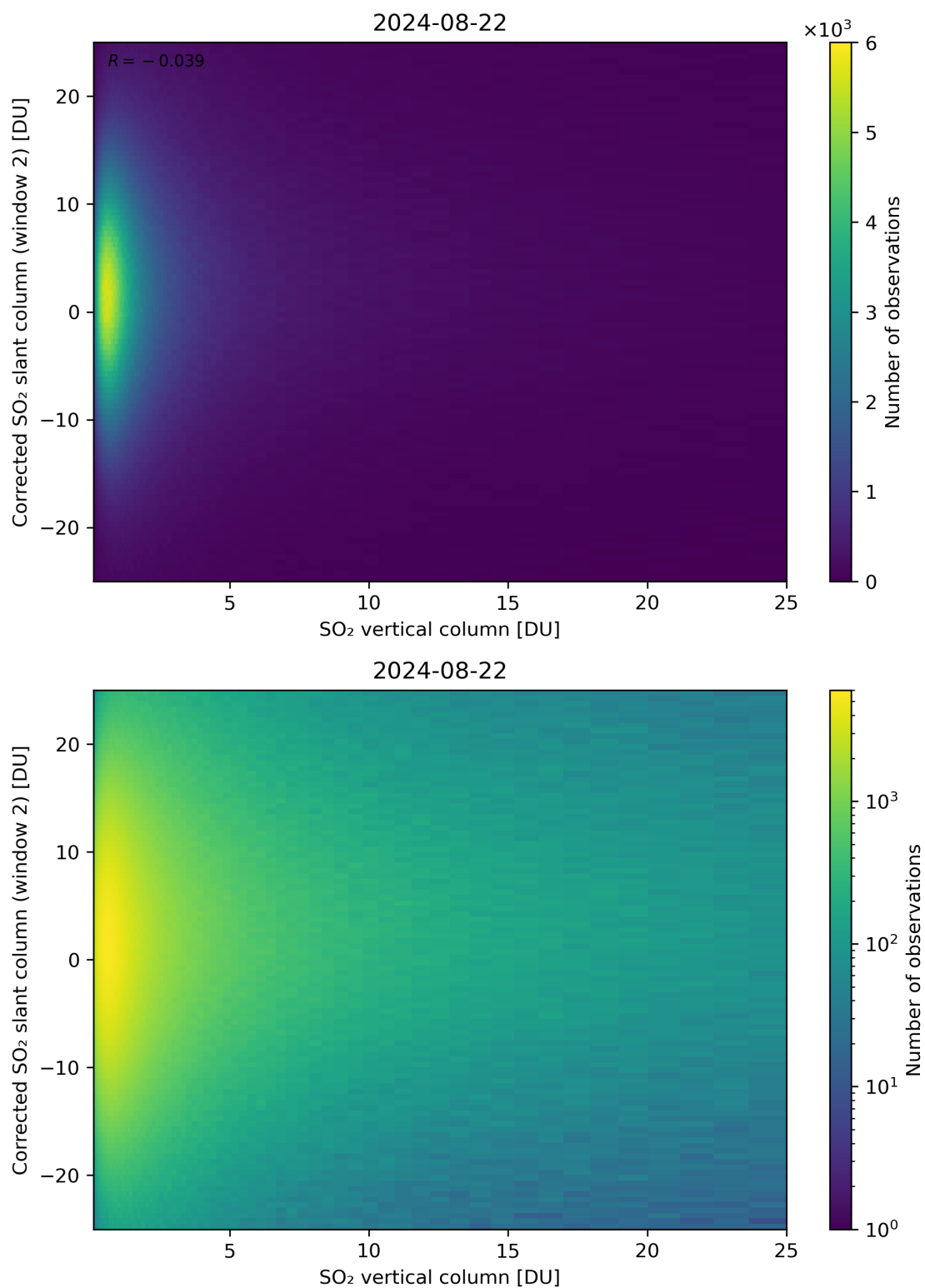
Figure 298: Scatter density plot of “SO 2 vertical column” against “Corrected SO 2 slant column (window 2)” for 2024-08-22 to 2024-08-23.
