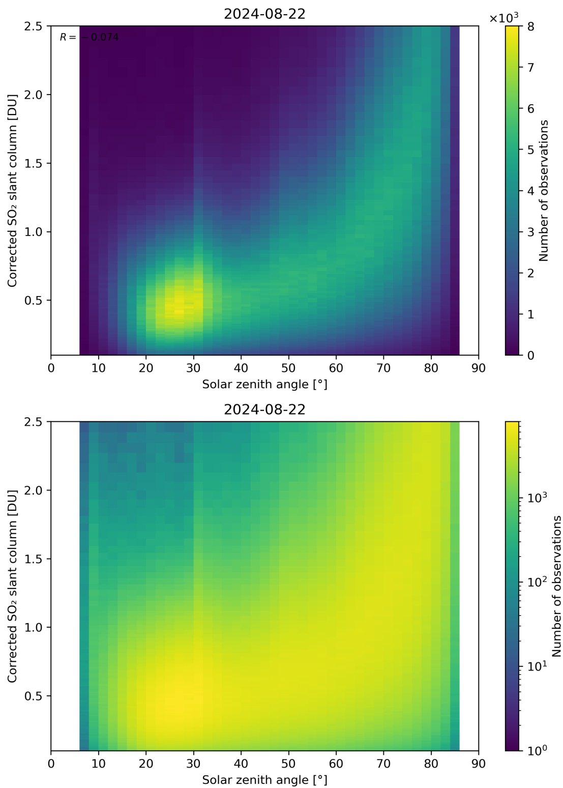
Figure 166: Scatter density plot of “Solar zenith angle” against “Corrected SO 2 slant column” for 2024-08-22 to 2024-08-23.
