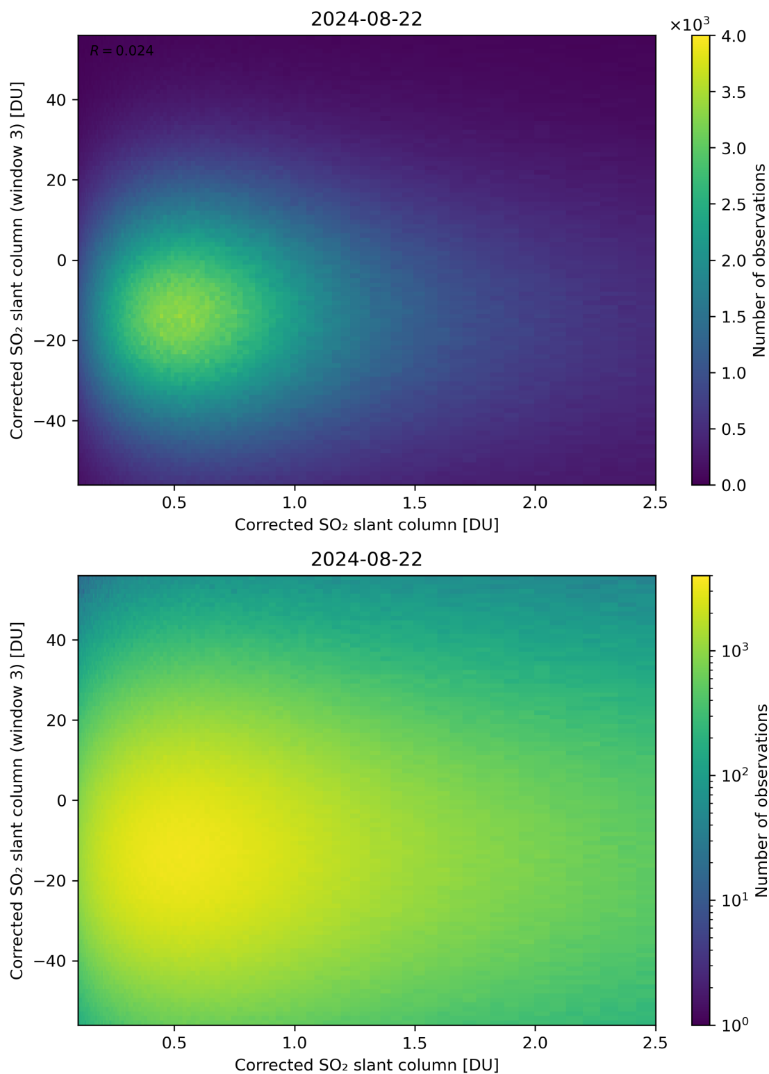
Figure 186: Scatter density plot of “Corrected SO 2 slant column” against “Corrected SO 2 slant column (window 3)” for 2024-08-22 to 2024-08-23.
