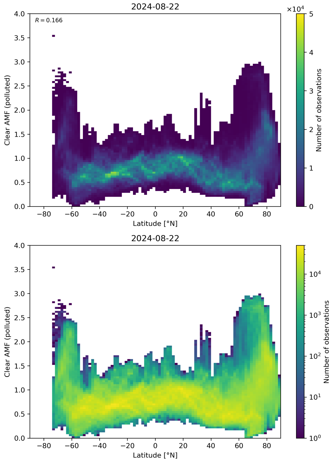
Figure 145: Scatter density plot of “Latitude” against “Clear AMF (polluted)” for 2024-08-22 to 2024-08-23.
