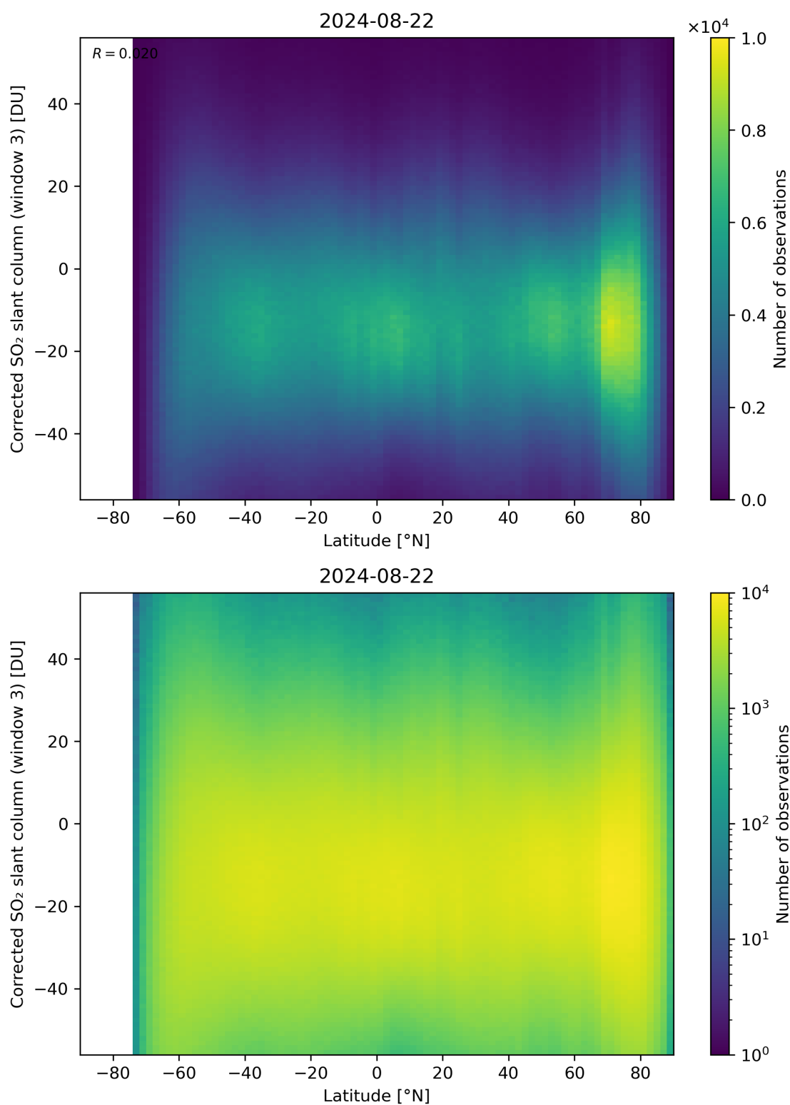
Figure 148: Scatter density plot of “Latitude” against “Corrected SO 2 slant column (window 3)” for 2024-08-22 to 2024-08-23.
