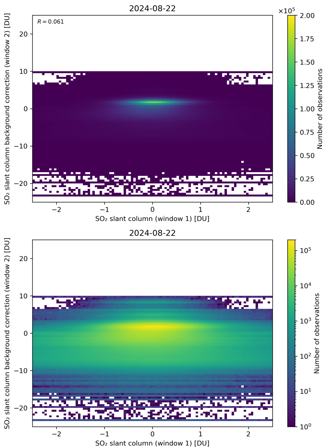
Figure 213: Scatter density plot of “SO 2 slant column (window 1)” against “SO 2 slant column background correction (window 2)” for 2024-08-22 to 2024-08-23.
