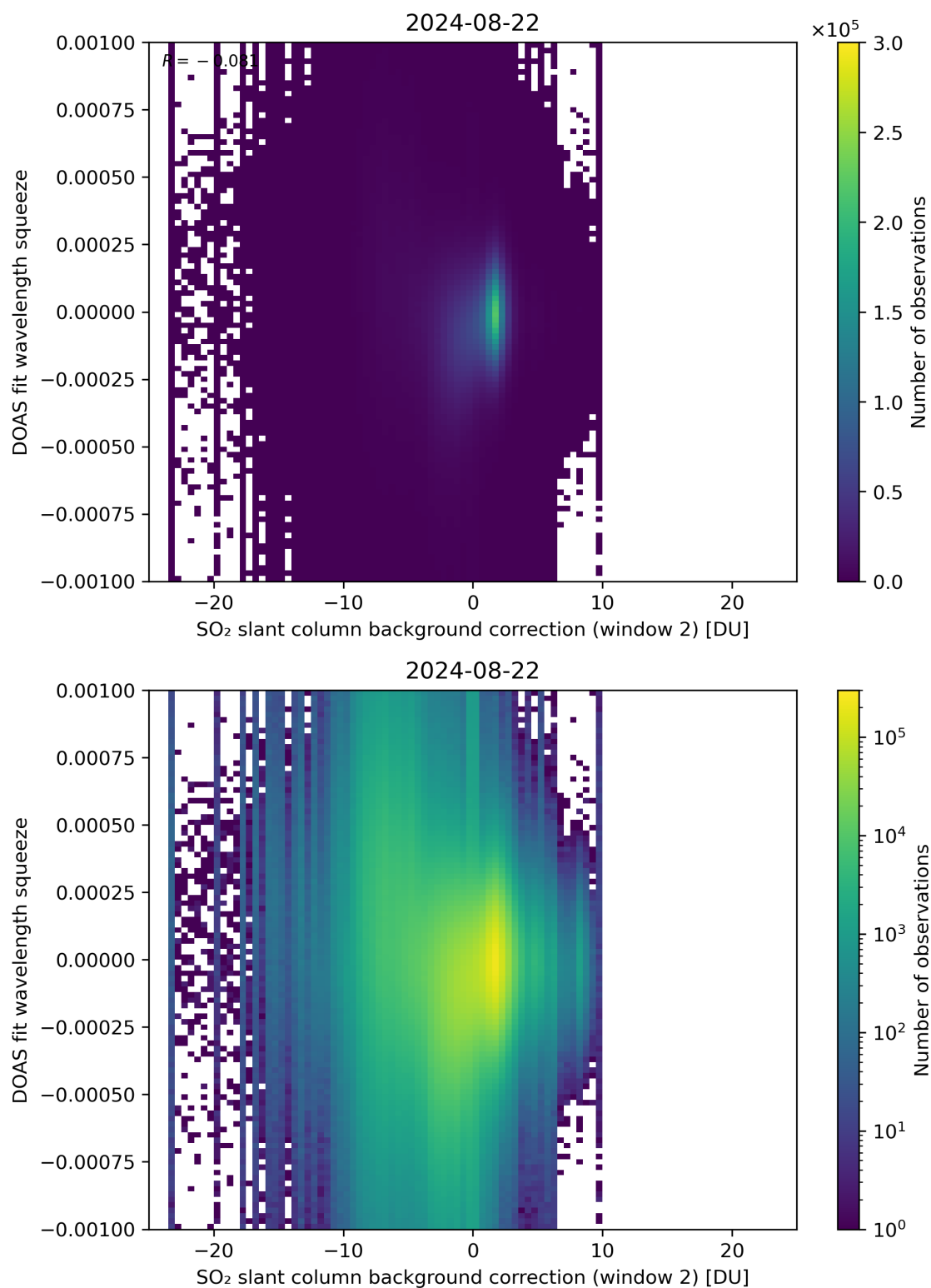
Figure 113: Scatter density plot of “SO 2 slant column background correction (window 2)” against “DOAS fit wavelength squeeze” for 2024-08-22 to 2024-08-23.
