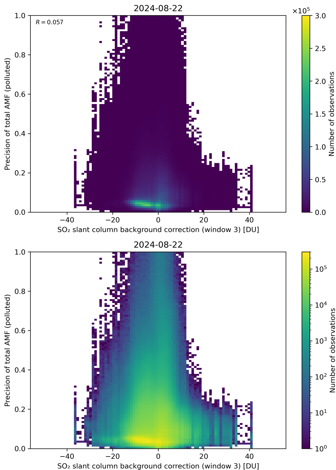
Figure 126: Scatter density plot of “SO 2 slant column background correction (window 3)” against “Precision of total AMF (polluted)” for 2024-08-22 to 2024-08-23.
