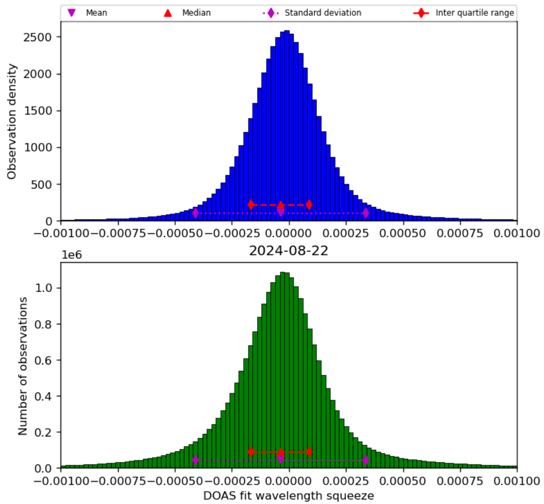
Figure 69: Histogram of “DOAS fit wavelength squeeze” for 2024-08-22 to 2024-08-23
