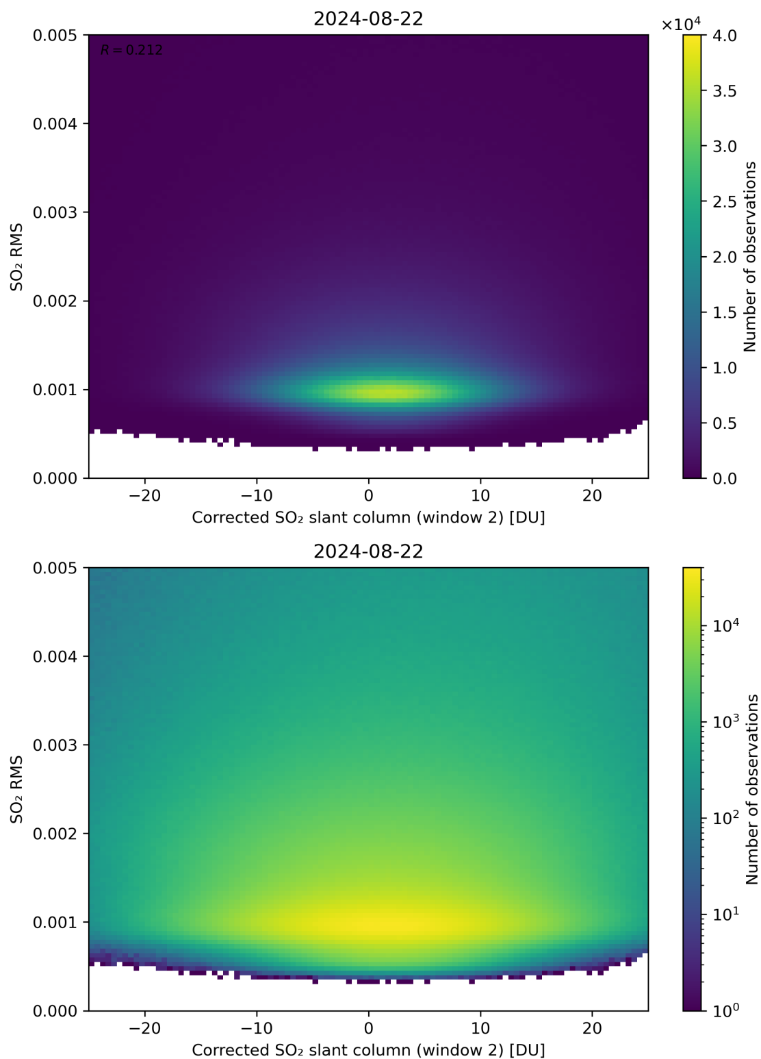
Figure 198: Scatter density plot of “Corrected SO 2 slant column (window 2)” against “SO 2 RMS” for 2024-08-22 to 2024-08-23.
