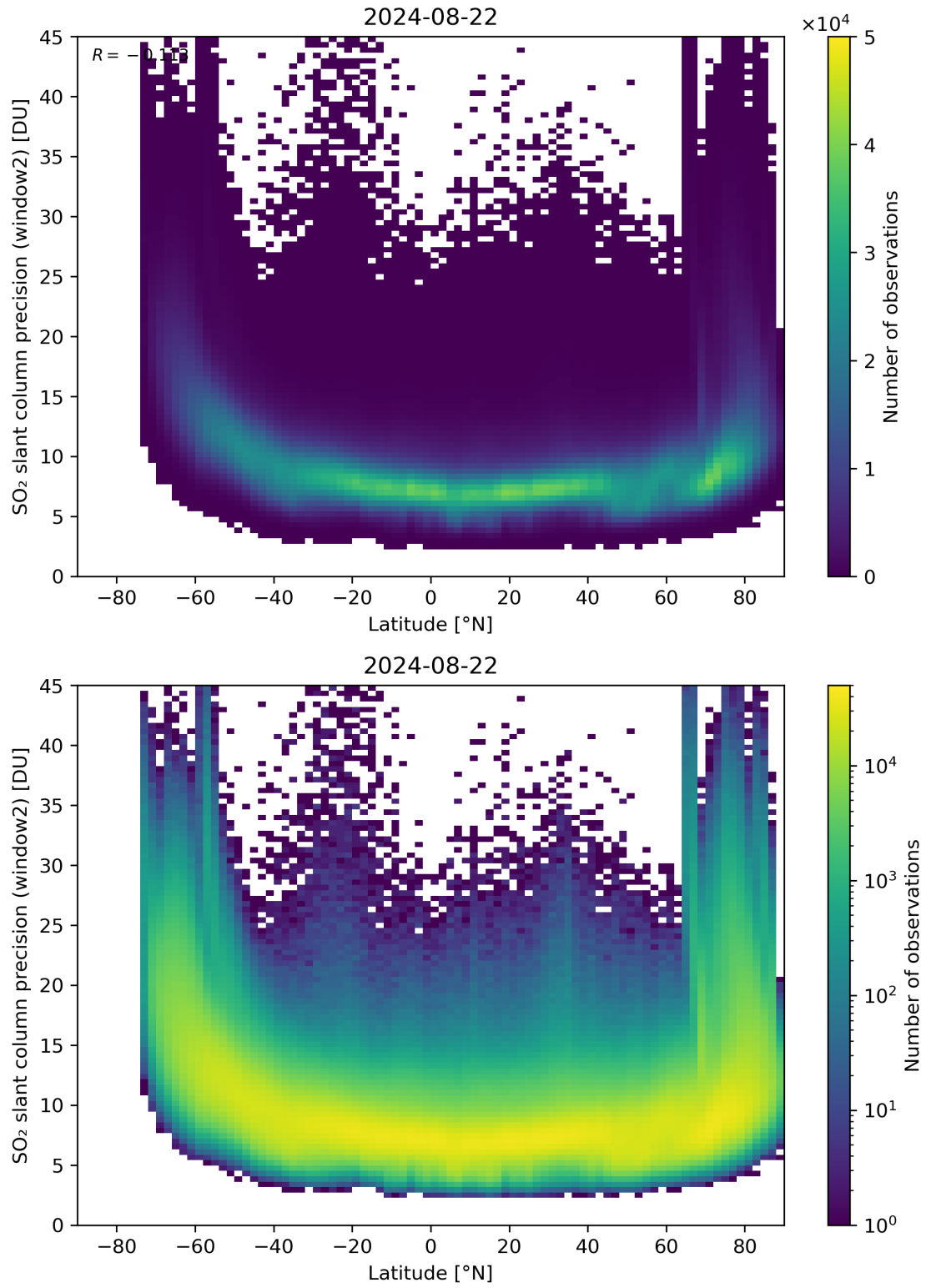
Figure 151: Scatter density plot of “Latitude” against “SO 2 slant column precision (window2)” for 2024-08-22 to 2024-08-23.
