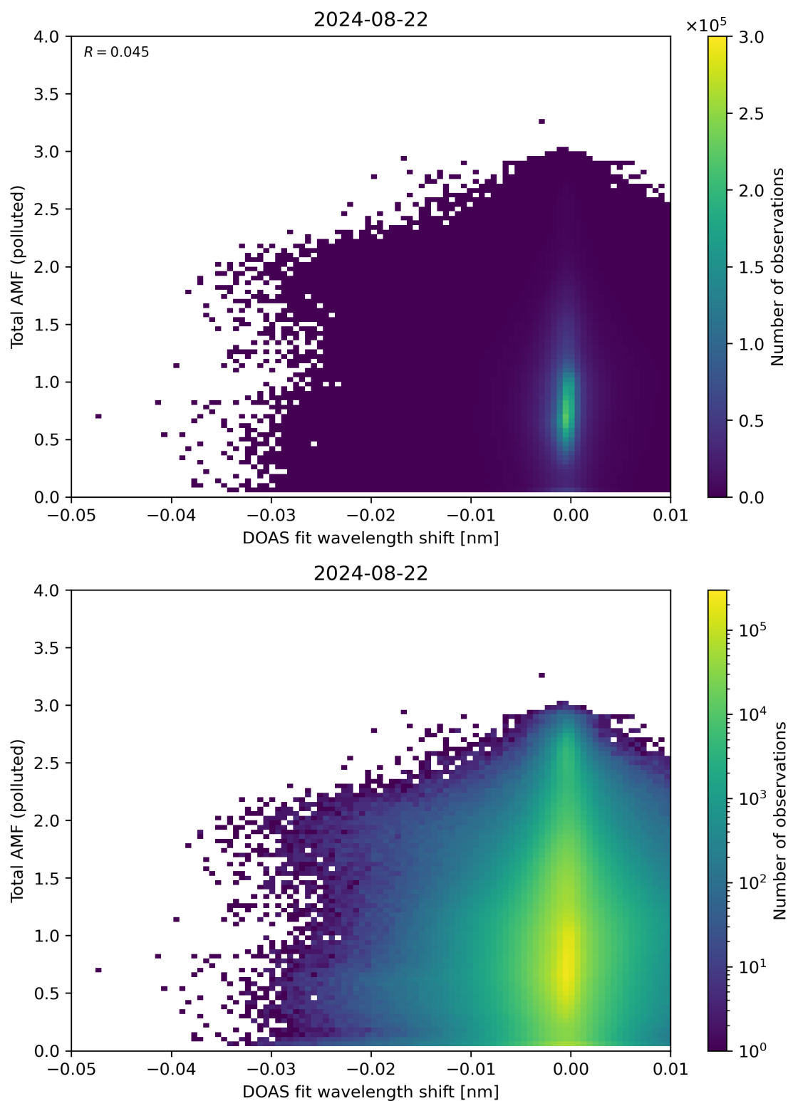
Figure 130: Scatter density plot of “DOAS fit wavelength shift” against “Total AMF (polluted)” for 2024-08-22 to 2024-08-23.
