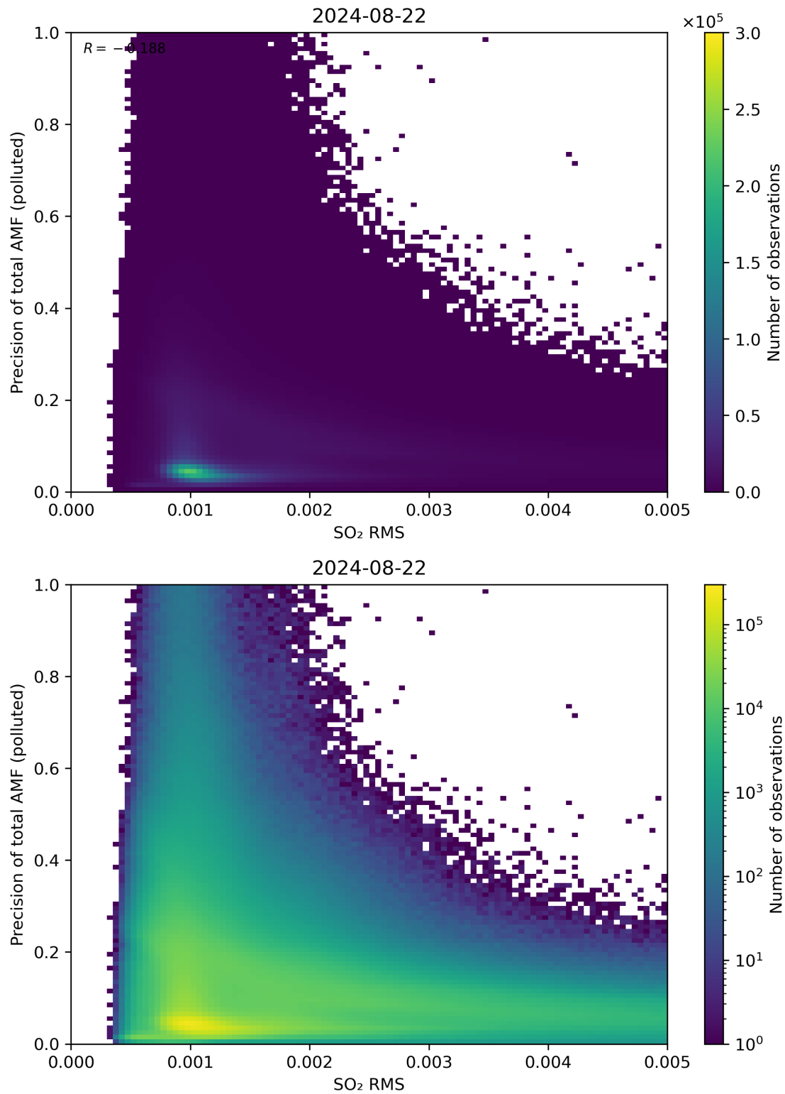
Figure 138: Scatter density plot of “SO 2 RMS” against “Precision of total AMF (polluted)” for 2024-08-22 to 2024-08-23.
