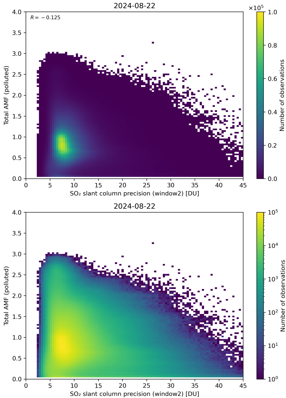
Figure 251: Scatter density plot of “SO 2 slant column precision (window2)” against “Total AMF (polluted)” for 2024-08-22 to 2024-08-23.
