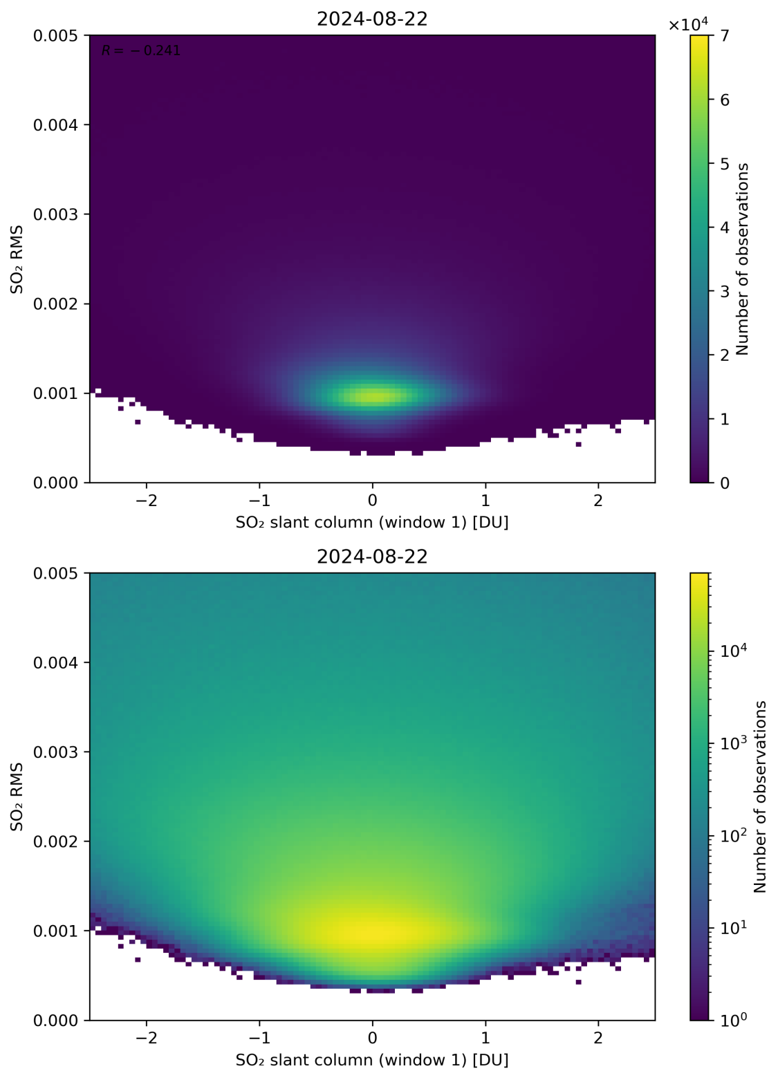
Figure 217: Scatter density plot of “SO 2 slant column (window 1)” against “SO 2 RMS” for 2024-08-22 to 2024-08-23.
