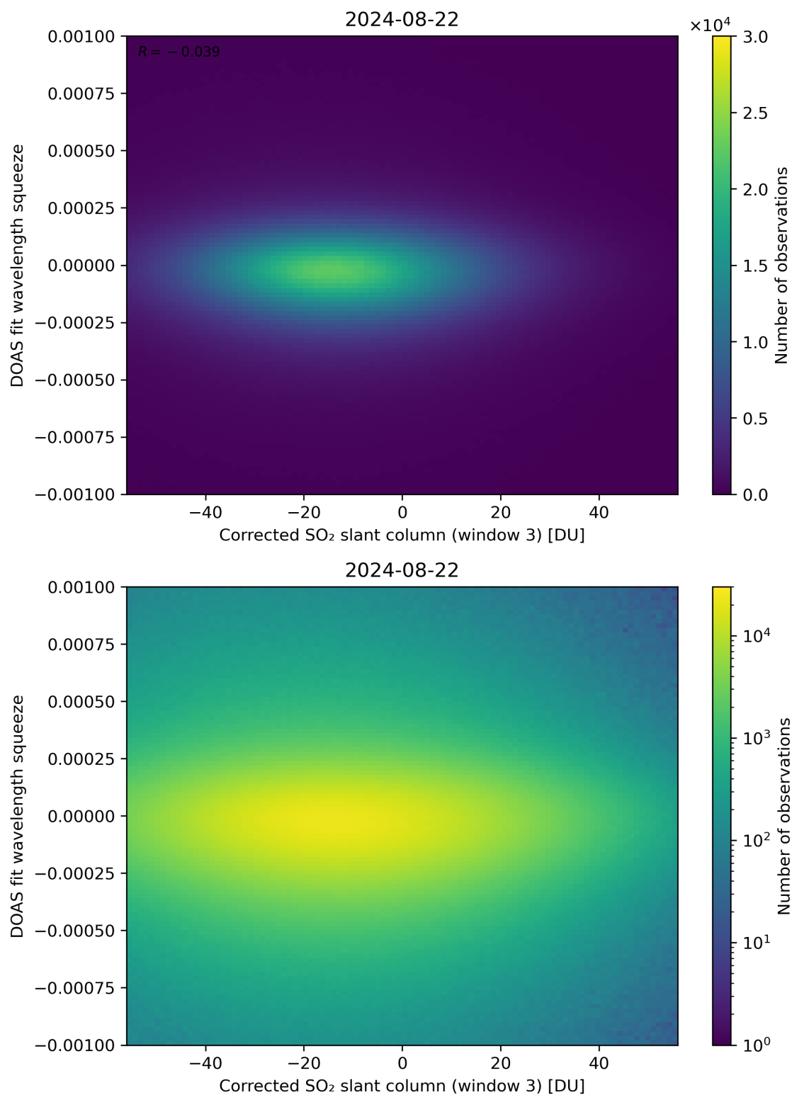
Figure 207: Scatter density plot of “Corrected SO 2 slant column (window 3)” against “DOAS fit wavelength squeeze” for 2024-08-22 to 2024-08-23.
