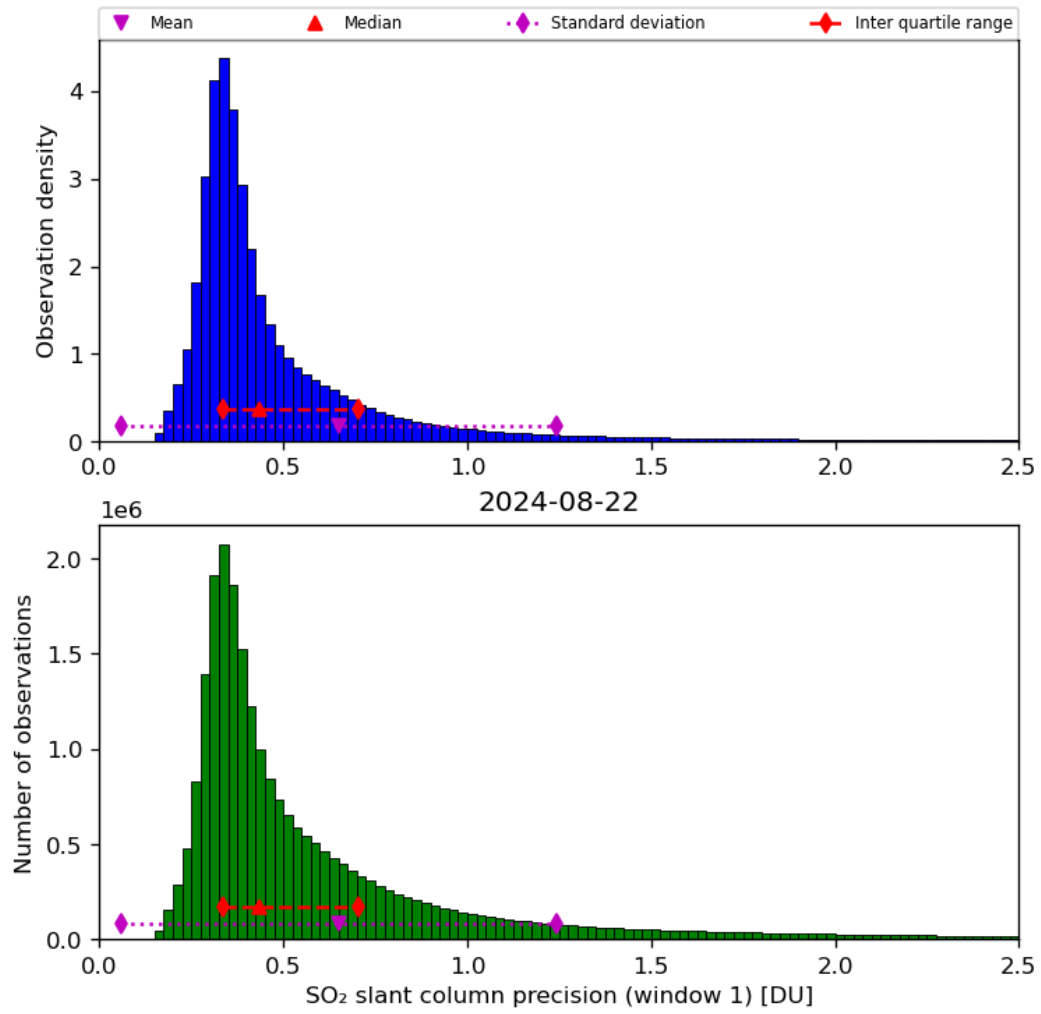
Figure 57: Histogram of “SO 2 slant column precision (window 1)” for 2024-08-22 to 2024-08-23
