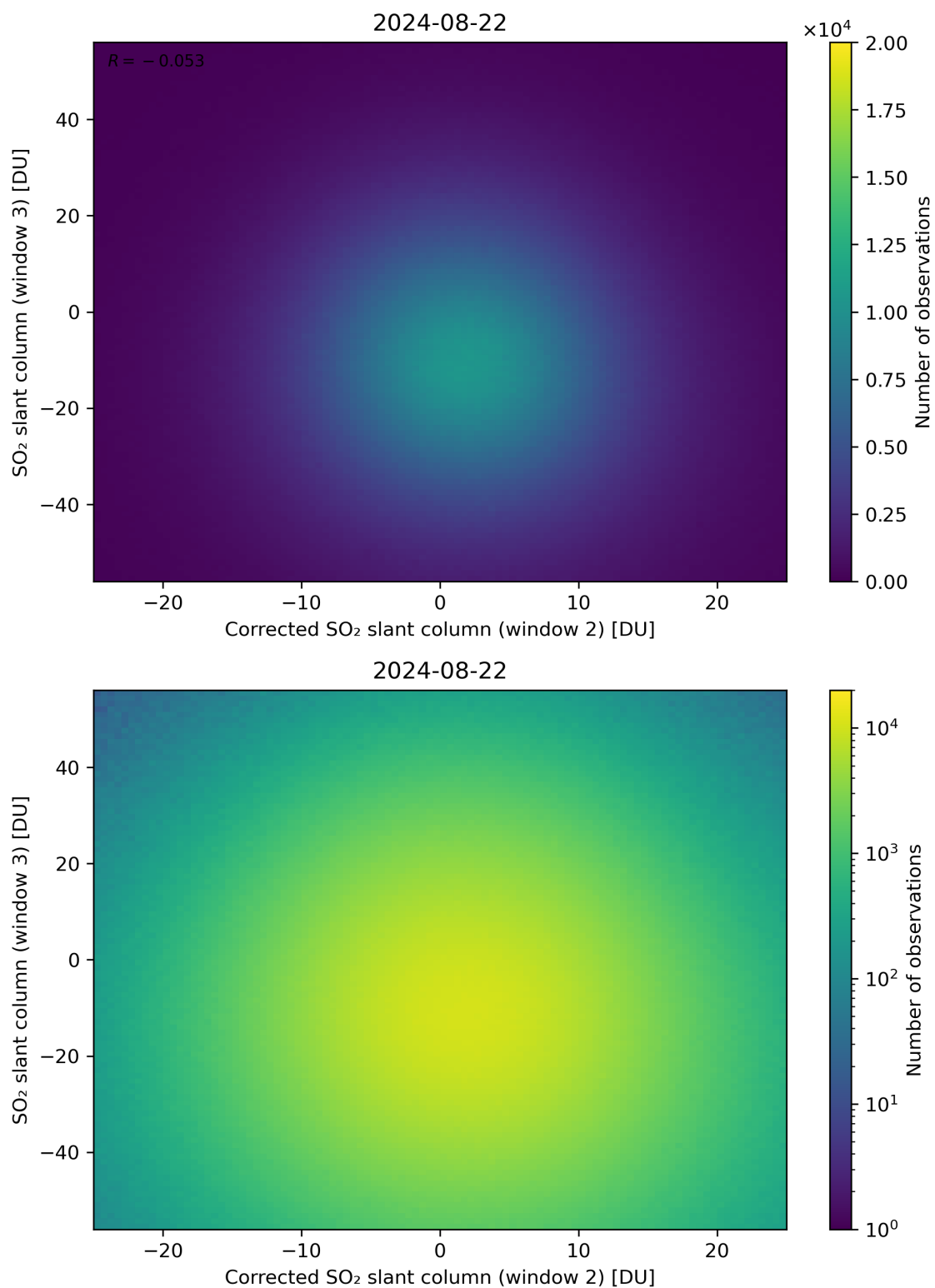
Figure 201: Scatter density plot of “Corrected SO 2 slant column (window 2)” against “SO 2 slant column (window 3)” for 2024-08-22 to 2024-08-23.
