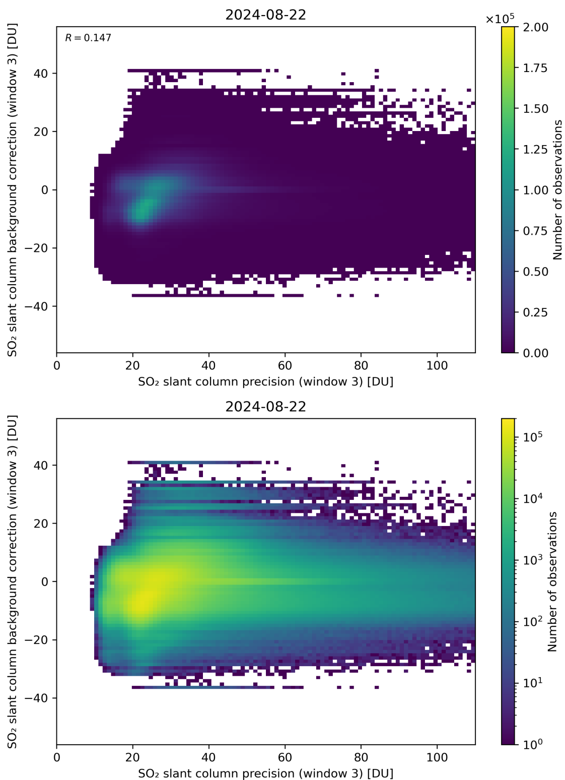
Figure 257: Scatter density plot of “SO 2 slant column precision (window 3)” against “SO 2 slant column background correction (window 3)” for 2024-08-22 to 2024-08-23.
