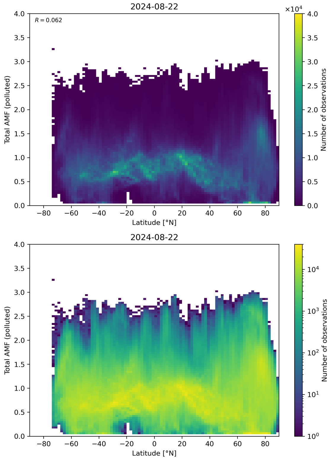
Figure 154: Scatter density plot of “Latitude” against “Total AMF (polluted)” for 2024-08-22 to 2024-08-23.
