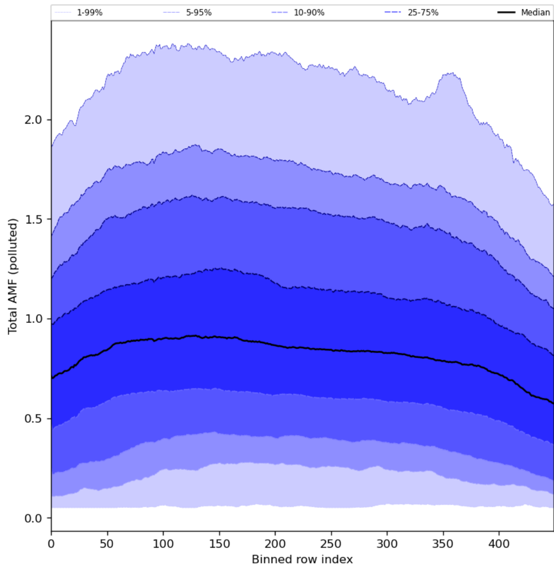
Figure 94: Along track statistics of “Total AMF (polluted)” for 2024-08-22 to 2024-08-23
