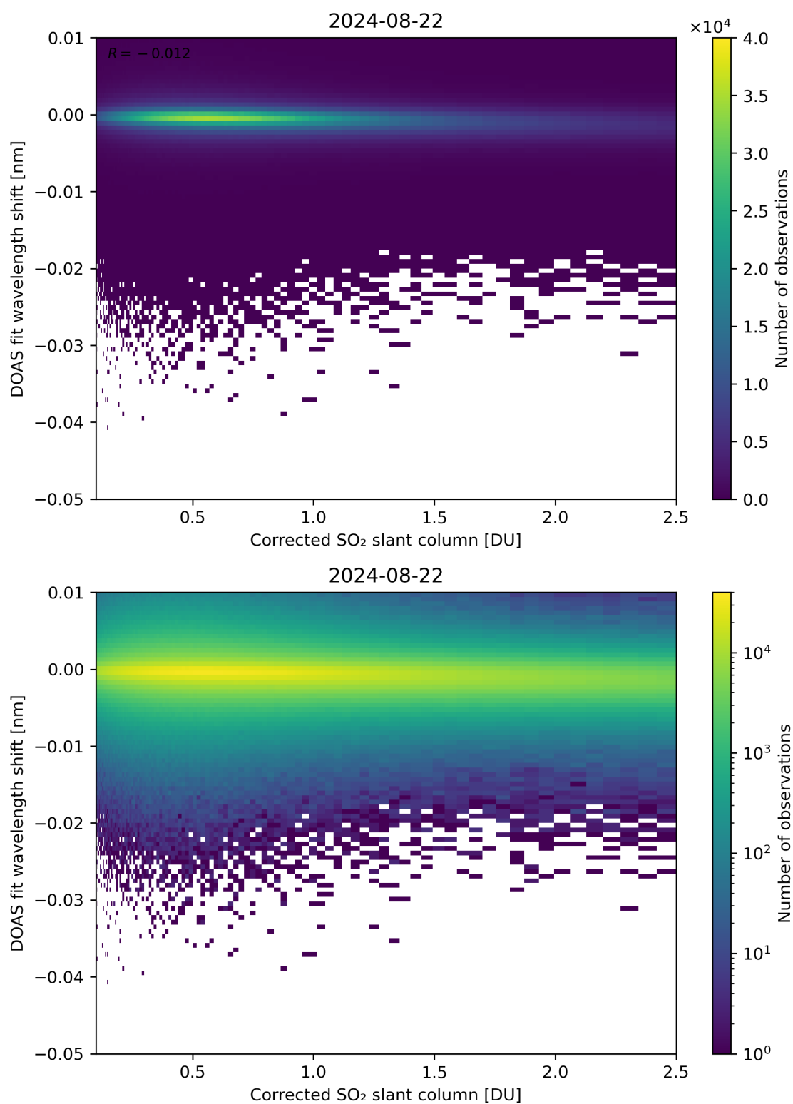
Figure 181: Scatter density plot of “Corrected SO 2 slant column” against “DOAS fit wavelength shift” for 2024-08-22 to 2024-08-23.
