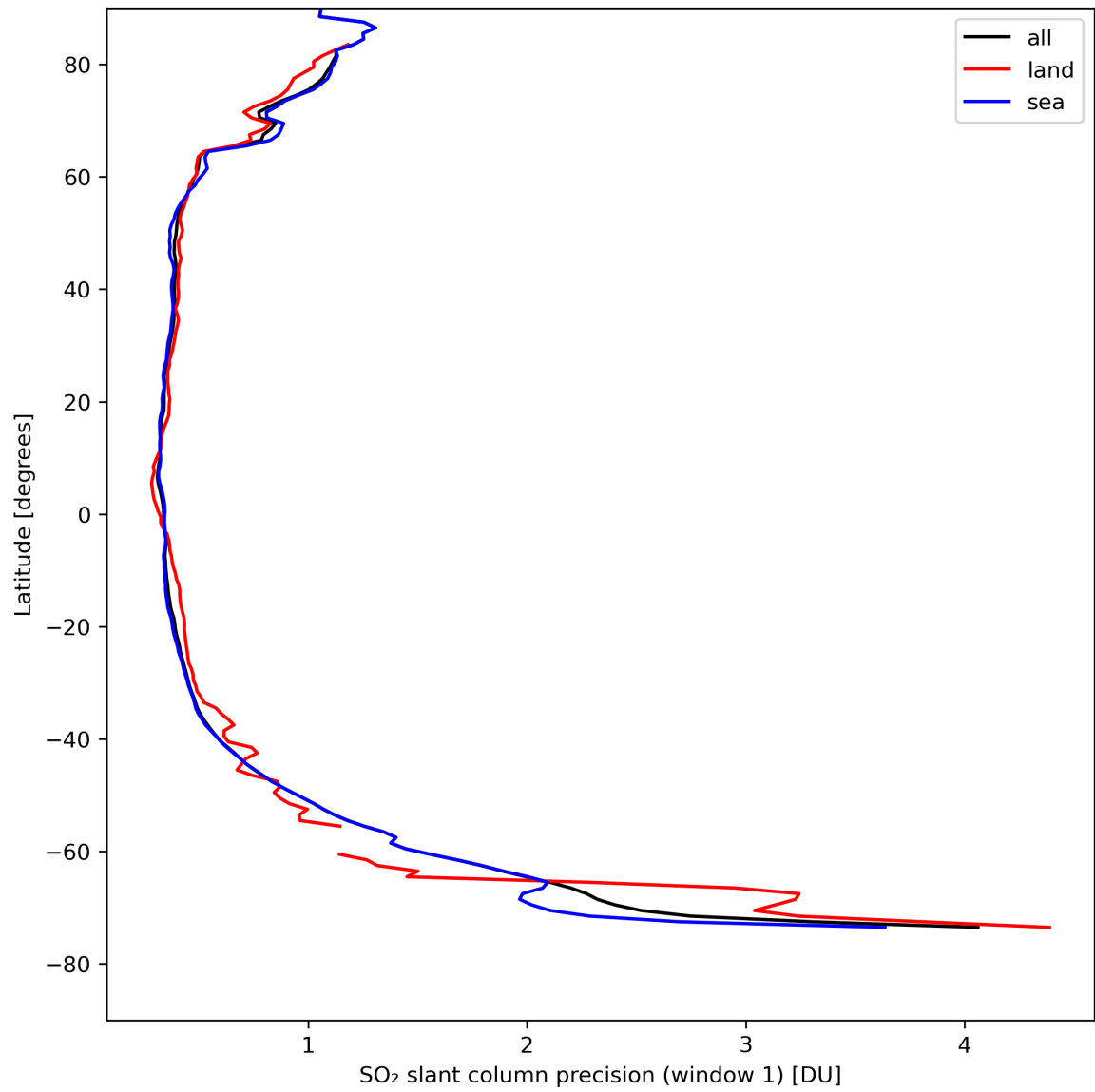
Figure 34: Zonal average of “SO 2 slant column precision (window 1)” for 2024-08-22 to 2024-08-23.
