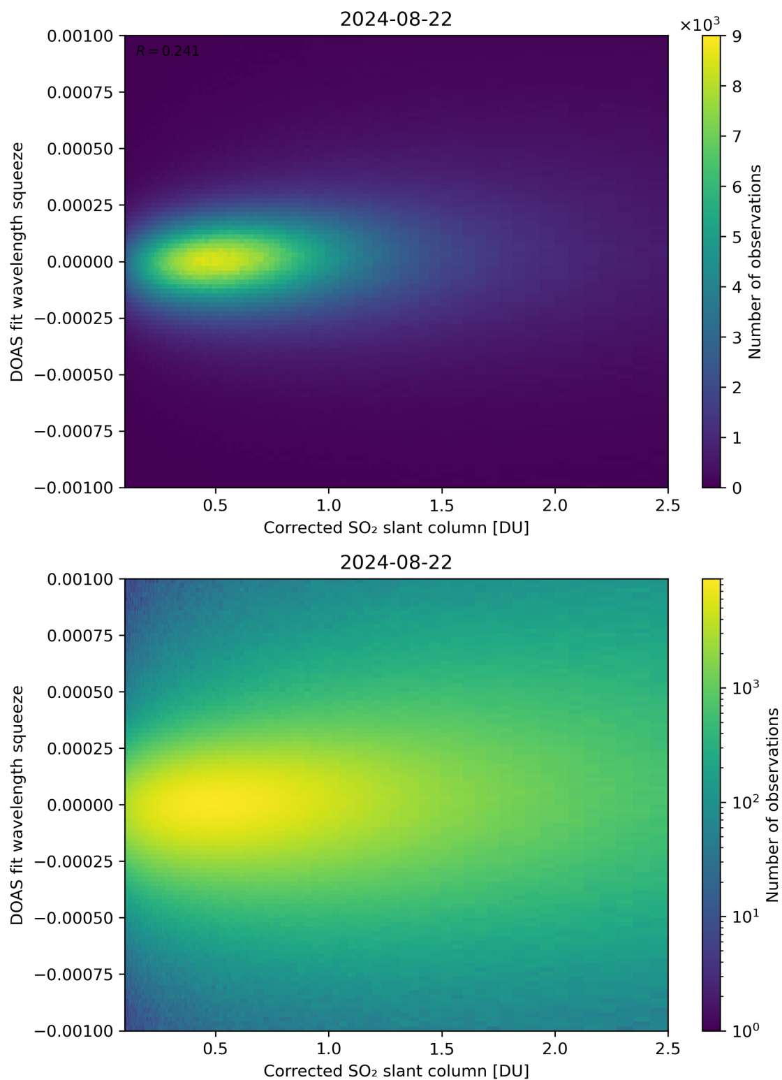
Figure 182: Scatter density plot of “Corrected SO 2 slant column” against “DOAS fit wavelength squeeze” for 2024-08-22 to 2024-08-23.
