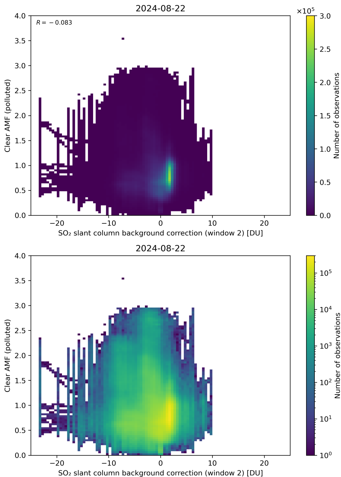
Figure 115: Scatter density plot of “SO 2 slant column background correction (window 2)” against “Clear AMF (polluted)” for 2024-08-22 to 2024-08-23.
