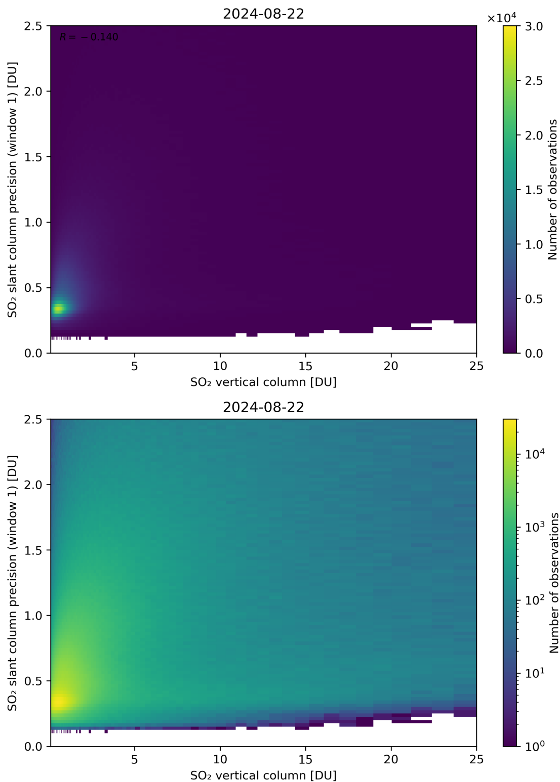
Figure 301: Scatter density plot of “SO 2 vertical column” against “SO 2 slant column precision (window 1)” for 2024-08-22 to 2024-08-23.
