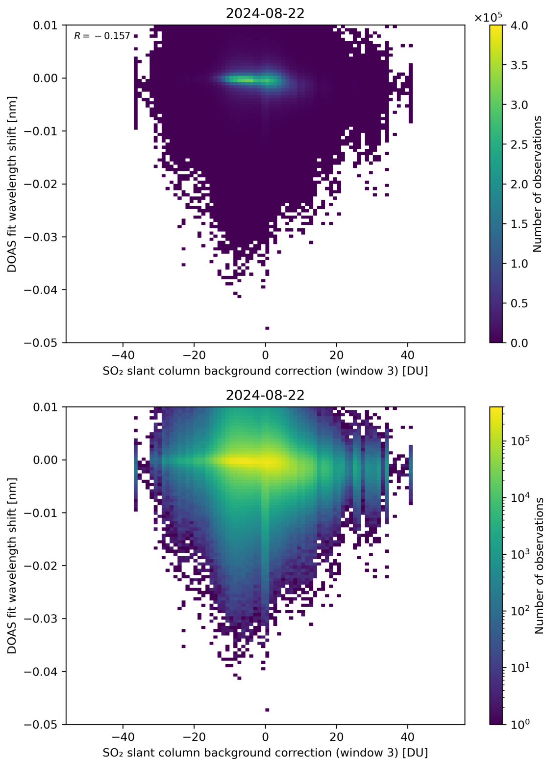
Figure 121: Scatter density plot of “SO 2 slant column background correction (window 3)” against “DOAS fit wavelength shift” for 2024-08-22 to 2024-08-23.
