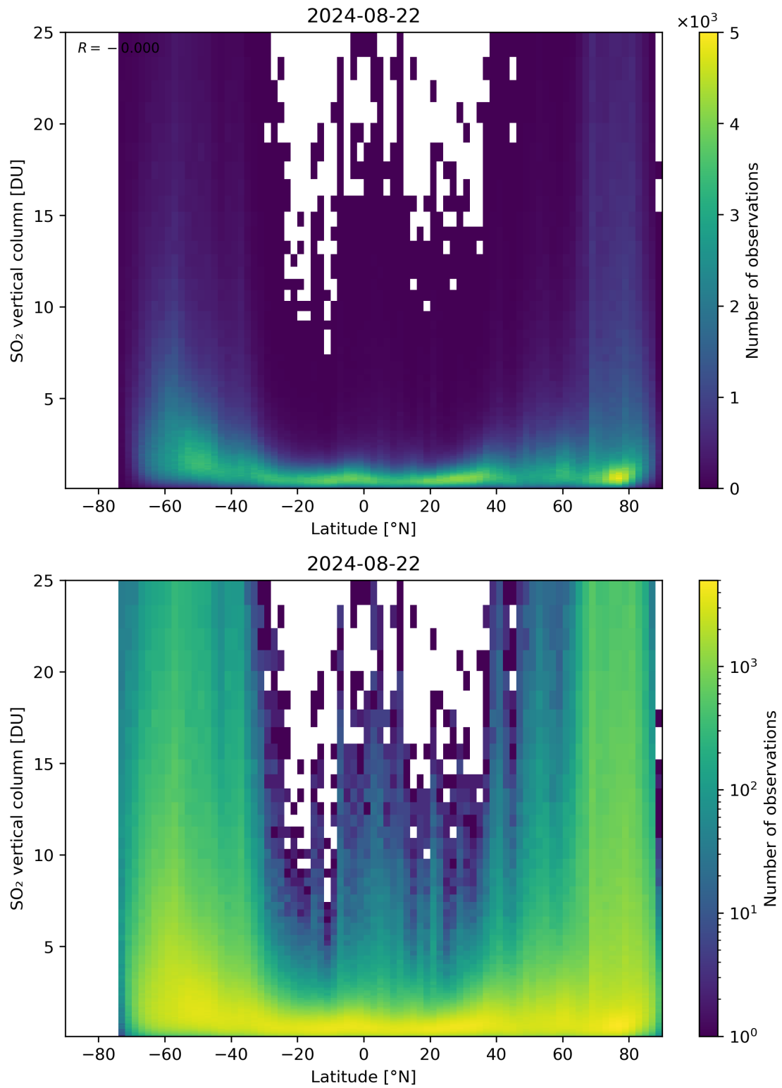
Figure 156: Scatter density plot of “Latitude” against “SO 2 vertical column” for 2024-08-22 to 2024-08-23.
