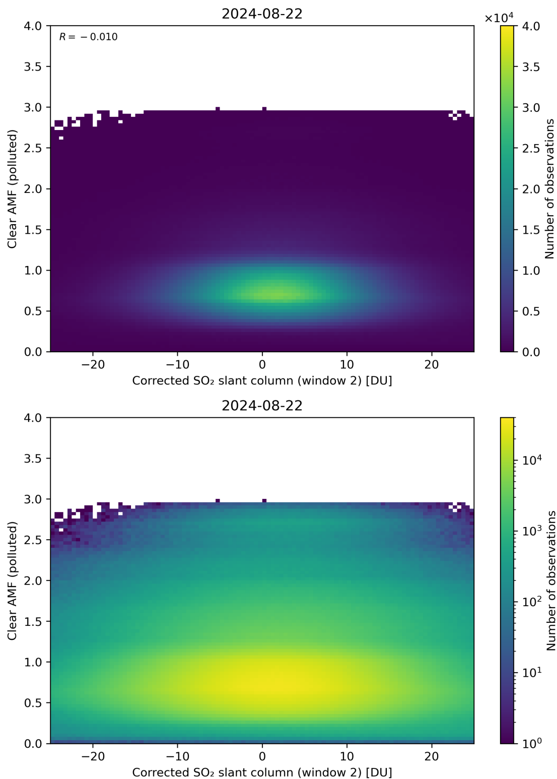
Figure 199: Scatter density plot of “Corrected SO 2 slant column (window 2)” against “Clear AMF (polluted)” for 2024-08-22 to 2024-08-23.
