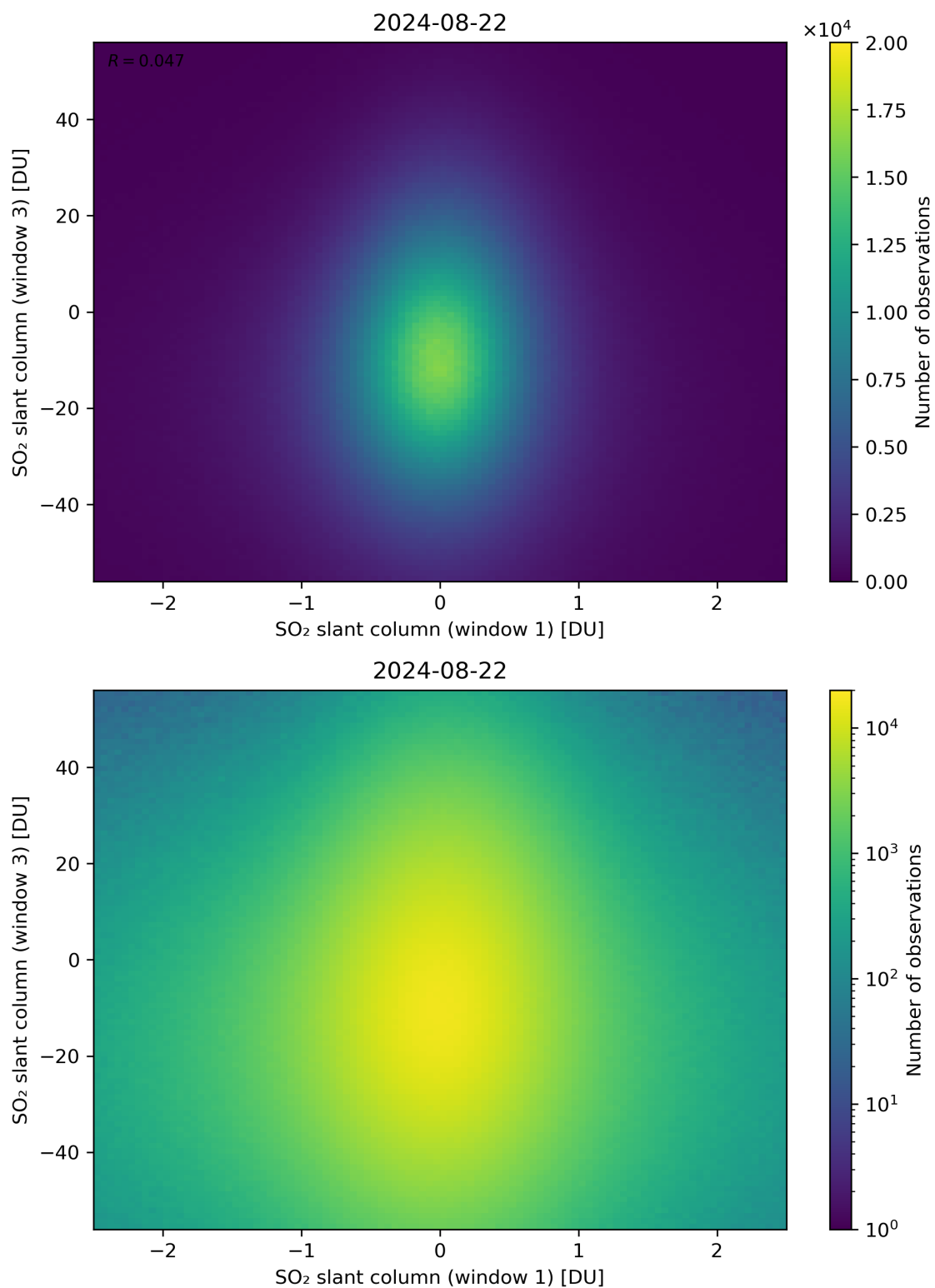
Figure 237: Scatter density plot of “SO 2 slant column (window 1)” against “SO 2 slant column (window 3)” for 2024-08-22 to 2024-08-23.
