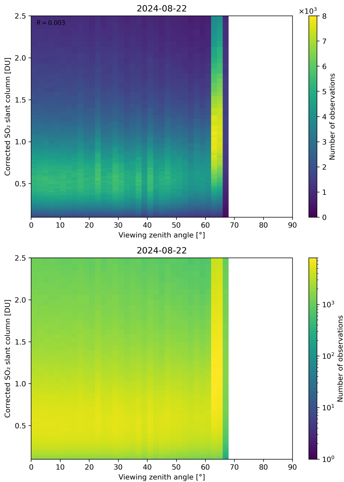
Figure 317: Scatter density plot of “Viewing zenith angle” against “Corrected SO 2 slant column” for 2024-08-22 to 2024-08-23.
