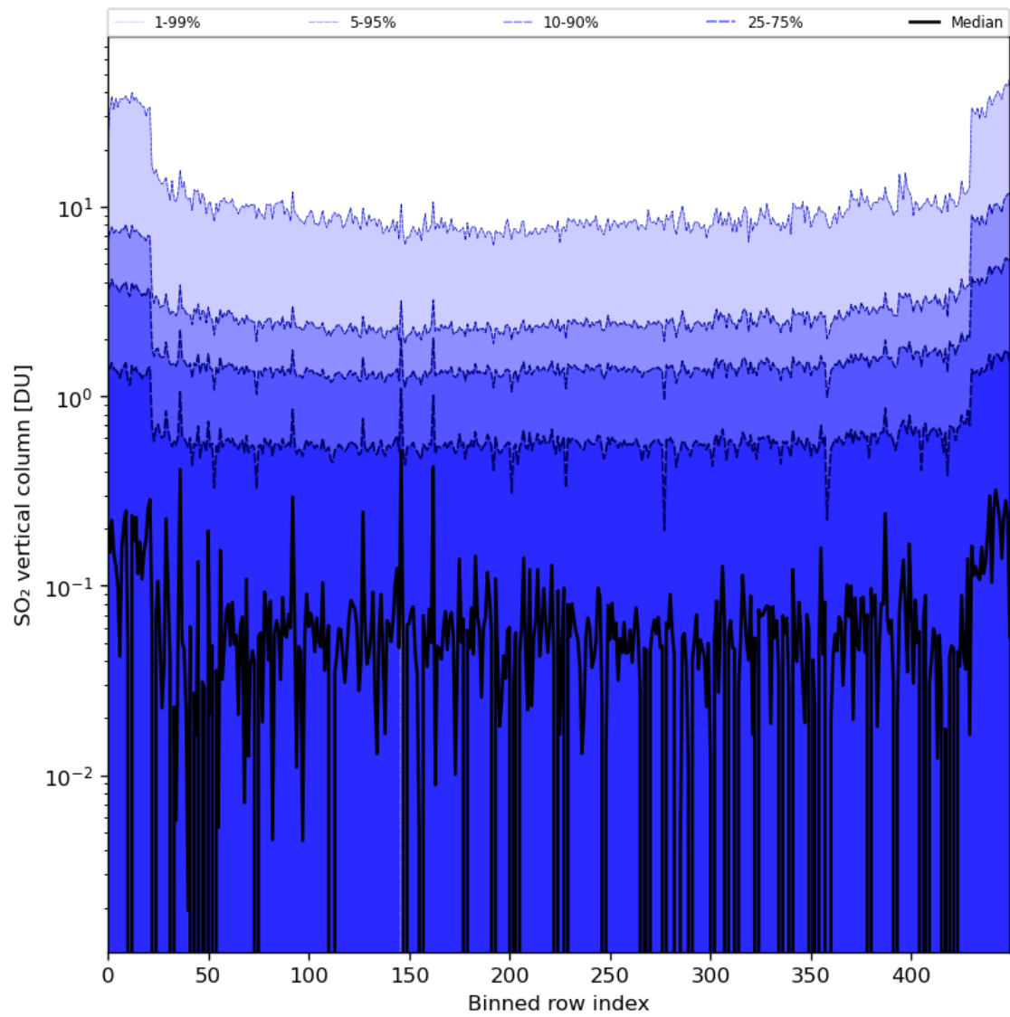
Figure 76: Along track statistics of “SO 2 vertical column” for 2024-08-22 to 2024-08-23
