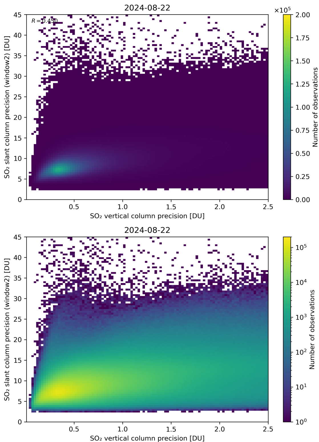
Figure 291: Scatter density plot of “SO 2 vertical column precision” against “SO 2 slant column precision (window2)” for 2024-08-22 to 2024-08-23.
