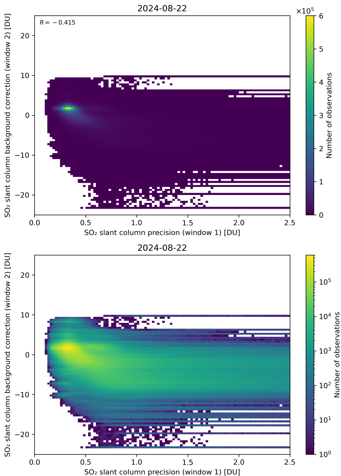
Figure 219: Scatter density plot of “SO 2 slant column precision (window 1)” against “SO 2 slant column background correction (window 2)” for 2024-08-22 to 2024-08-23.
