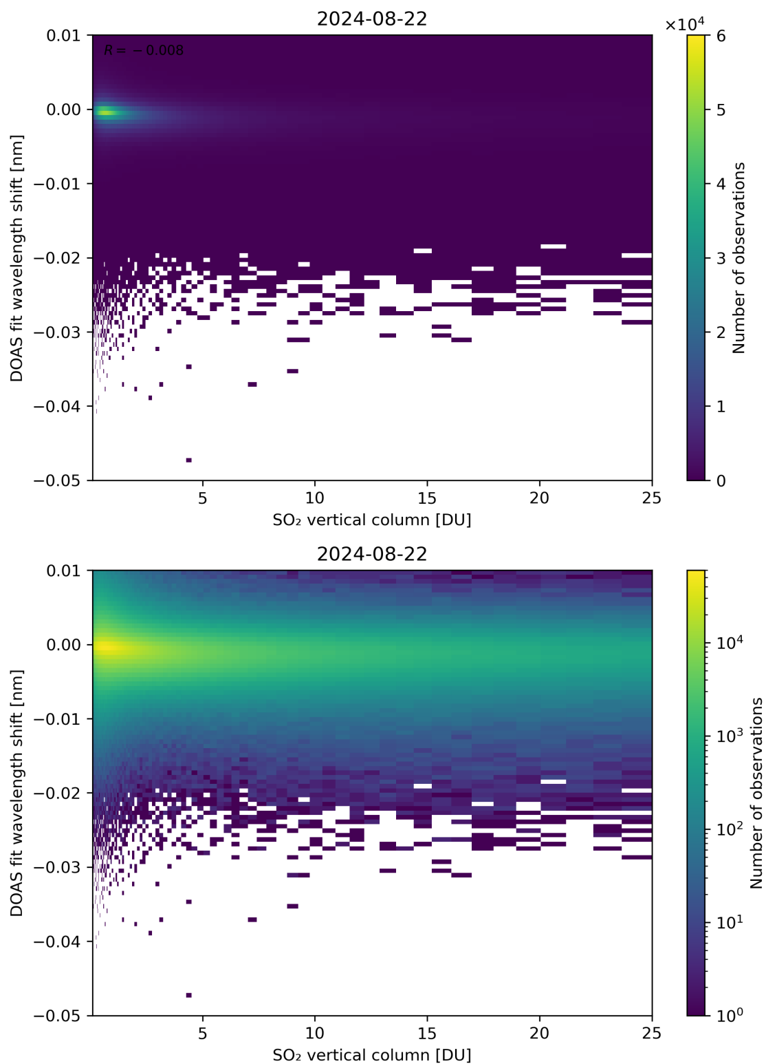
Figure 276: Scatter density plot of “SO 2 vertical column” against “DOAS fit wavelength shift” for 2024-08-22 to 2024-08-23.
