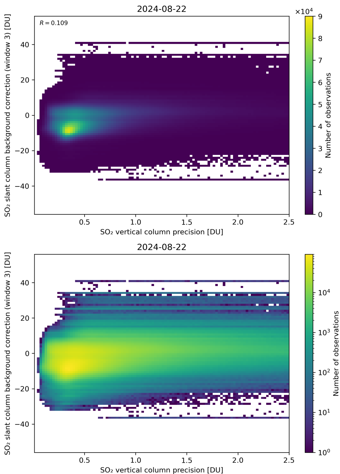
Figure 281: Scatter density plot of “SO 2 vertical column precision” against “SO 2 slant column background correction (window 3)” for 2024-08-22 to 2024-08-23.
