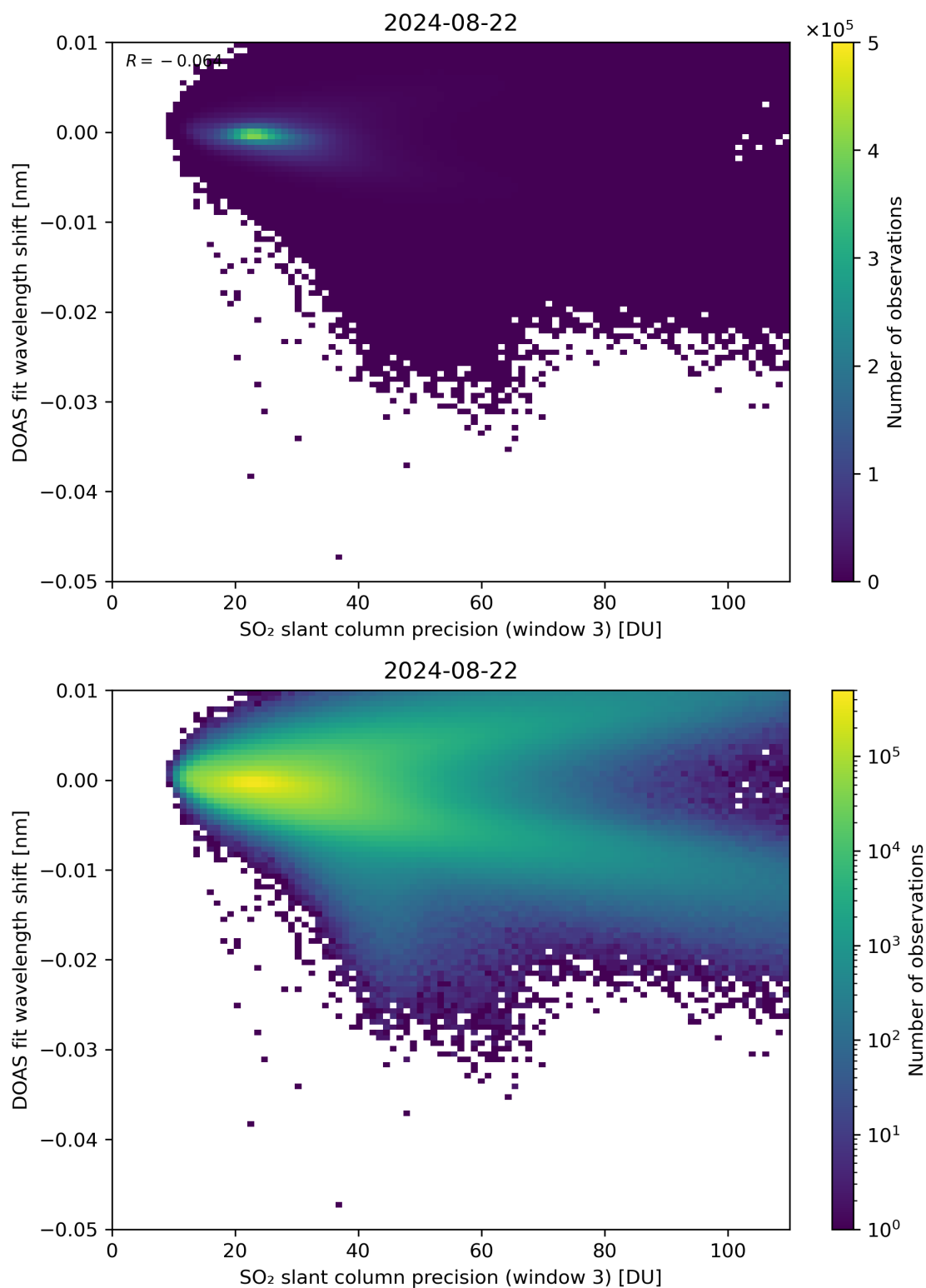
Figure 258: Scatter density plot of “SO 2 slant column precision (window 3)” against “DOAS fit wavelength shift” for 2024-08-22 to 2024-08-23.
