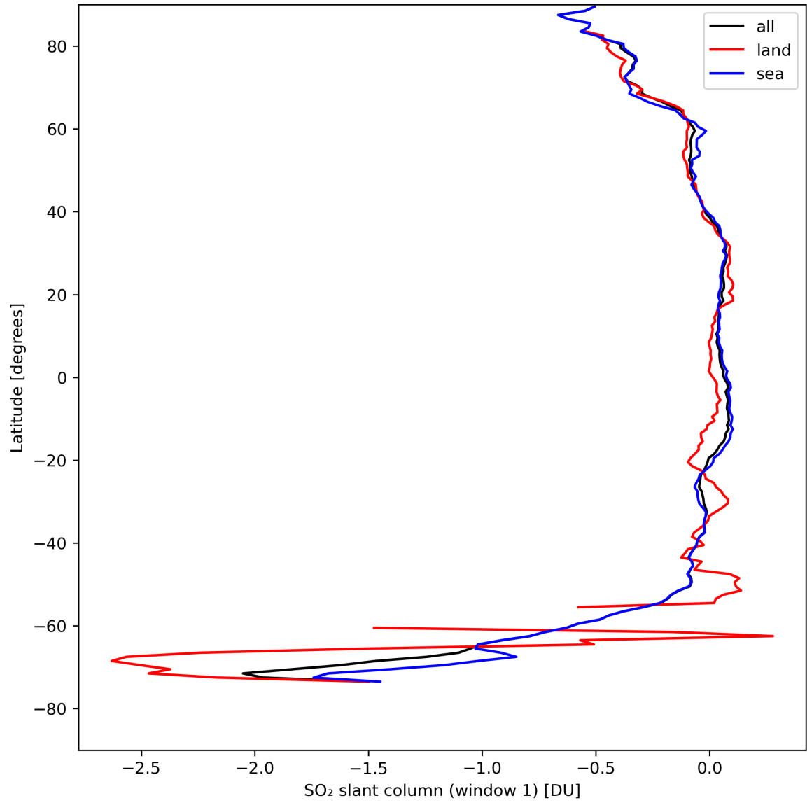
Figure 33: Zonal average of “SO 2 slant column (window 1)” for 2024-08-22 to 2024-08-23.
