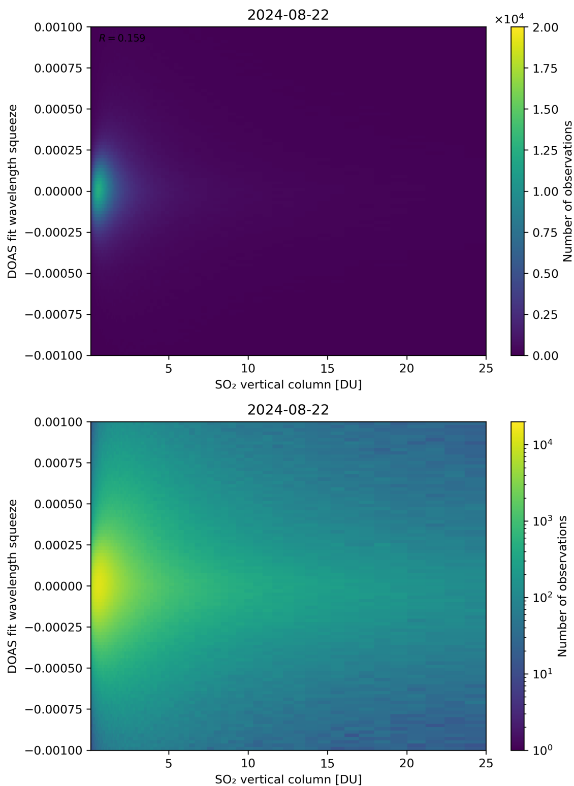
Figure 277: Scatter density plot of “SO 2 vertical column” against “DOAS fit wavelength squeeze” for 2024-08-22 to 2024-08-23.
