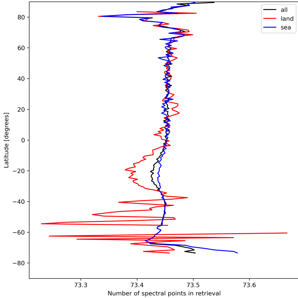
Figure 51: Zonal average of “Number of spectral points in retrieval” for 2024-08-22 to 2024-08-23.
