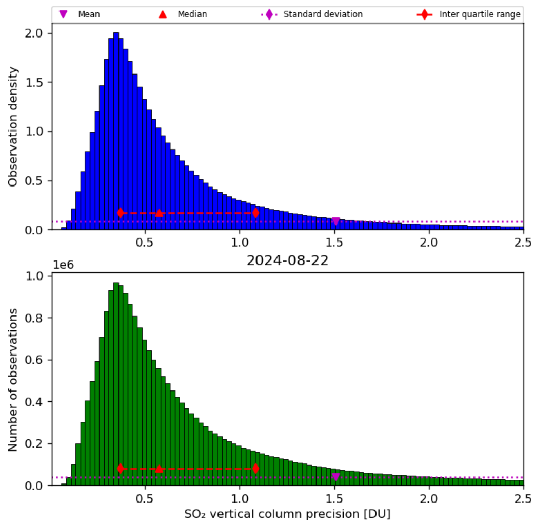
Figure 54: Histogram of “SO 2 vertical column precision” for 2024-08-22 to 2024-08-23
