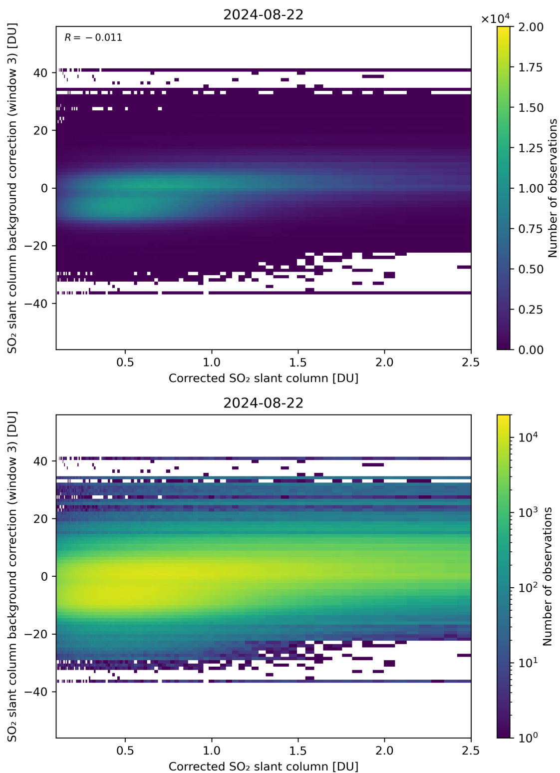
Figure 180: Scatter density plot of “Corrected SO 2 slant column” against “SO 2 slant column background correction (window 3)” for 2024-08-22 to 2024-08-23.
