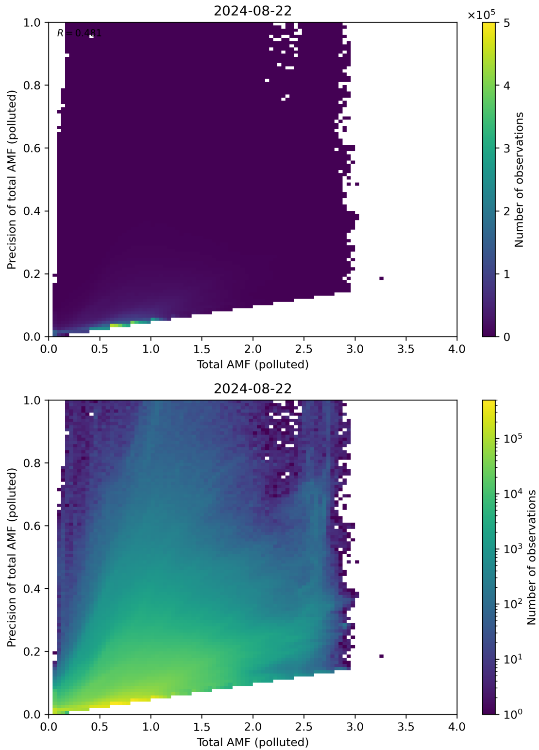
Figure 272: Scatter density plot of “Total AMF (polluted)” against “Precision of total AMF (polluted)” for 2024-08-22 to 2024-08-23.
