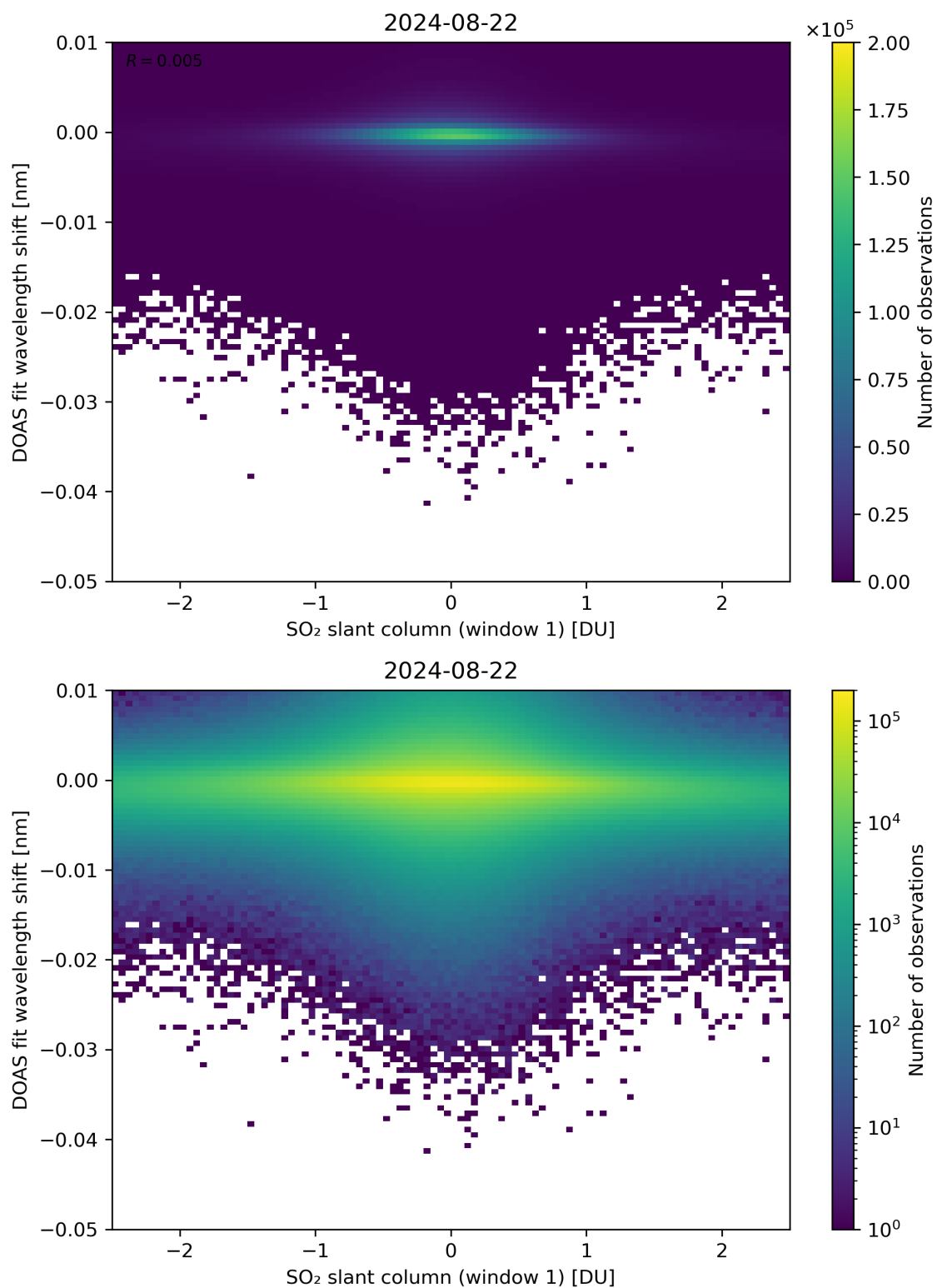
Figure 215: Scatter density plot of “SO 2 slant column (window 1)” against “DOAS fit wavelength shift” for 2024-08-22 to 2024-08-23.
