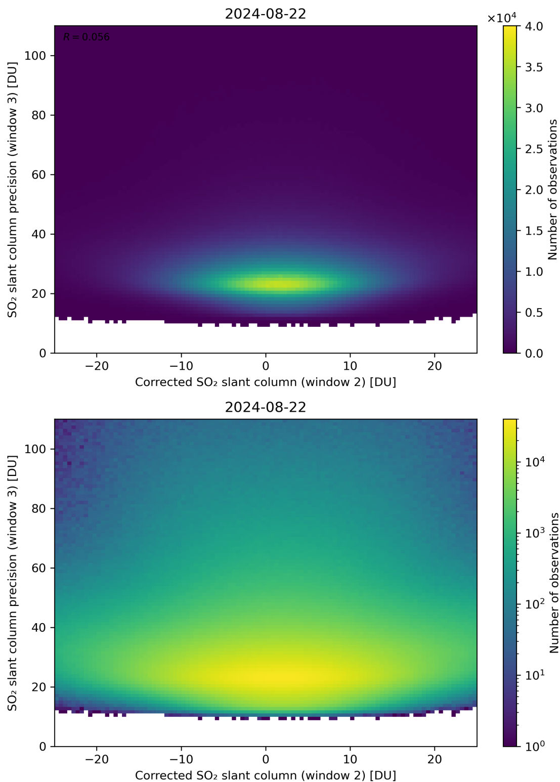
Figure 202: Scatter density plot of “Corrected SO 2 slant column (window 2)” against “SO 2 slant column precision (window 3)” for 2024-08-22 to 2024-08-23.
