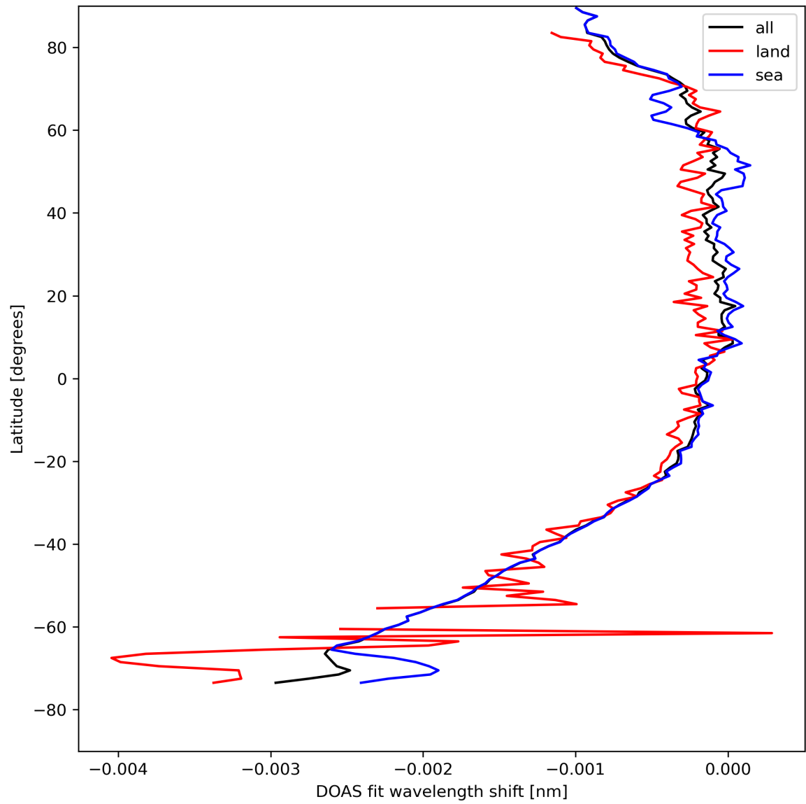
Figure 45: Zonal average of “DOAS fit wavelength shift” for 2024-08-22 to 2024-08-23.
