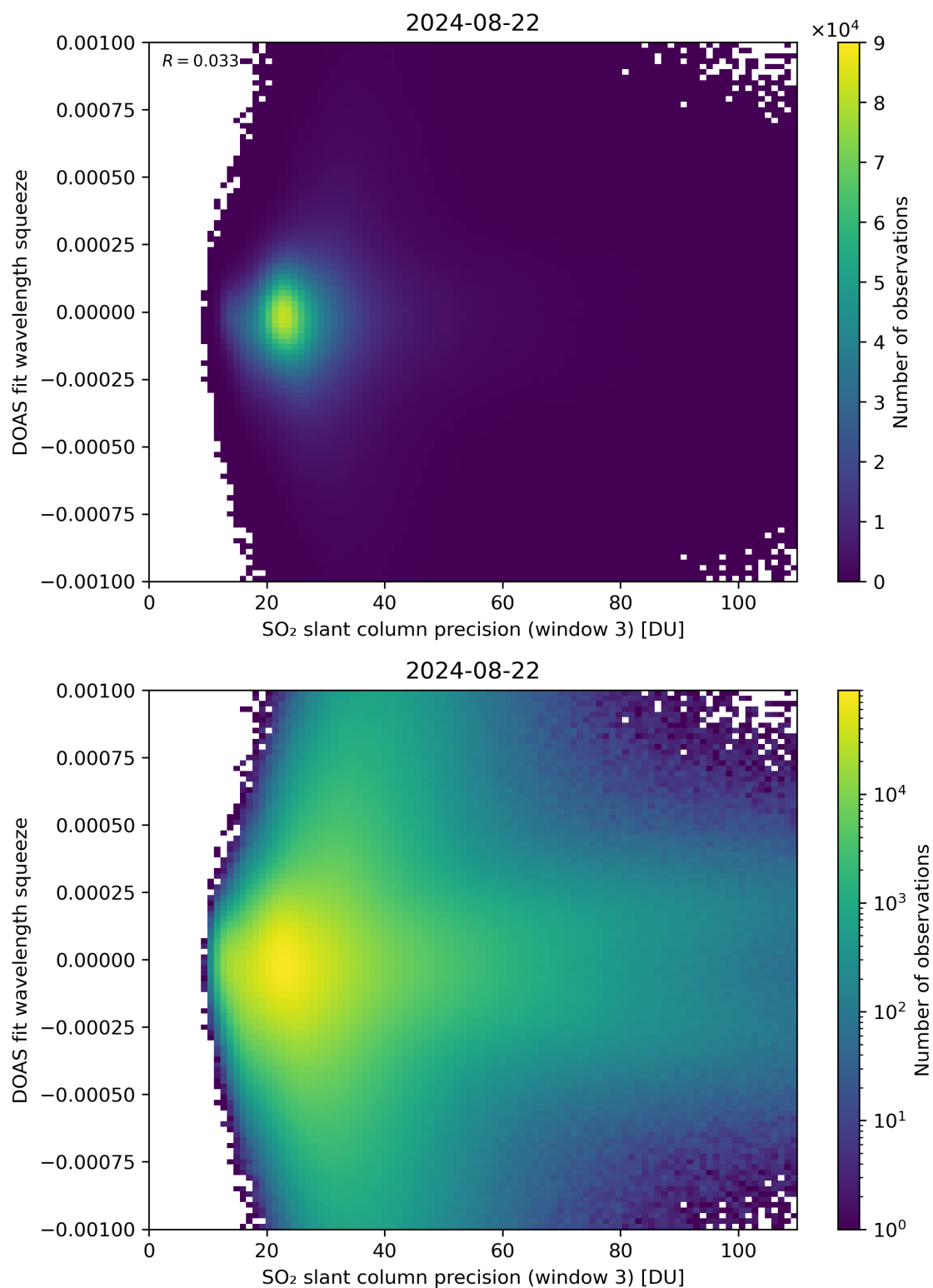
Figure 259: Scatter density plot of “SO 2 slant column precision (window 3)” against “DOAS fit wavelength squeeze” for 2024-08-22 to 2024-08-23.
