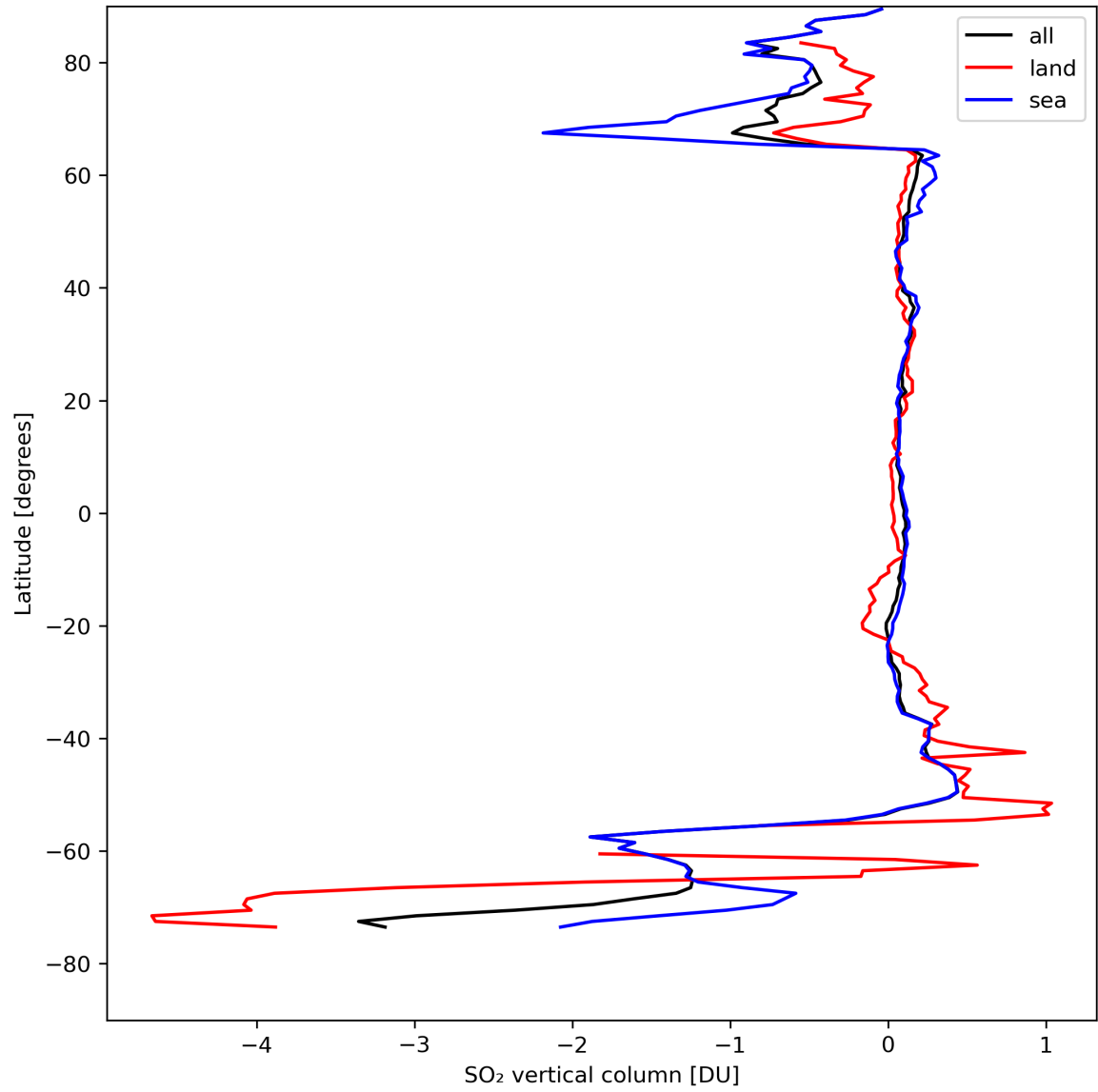
Figure 30: Zonal average of “SO 2 vertical column” for 2024-08-22 to 2024-08-23.
