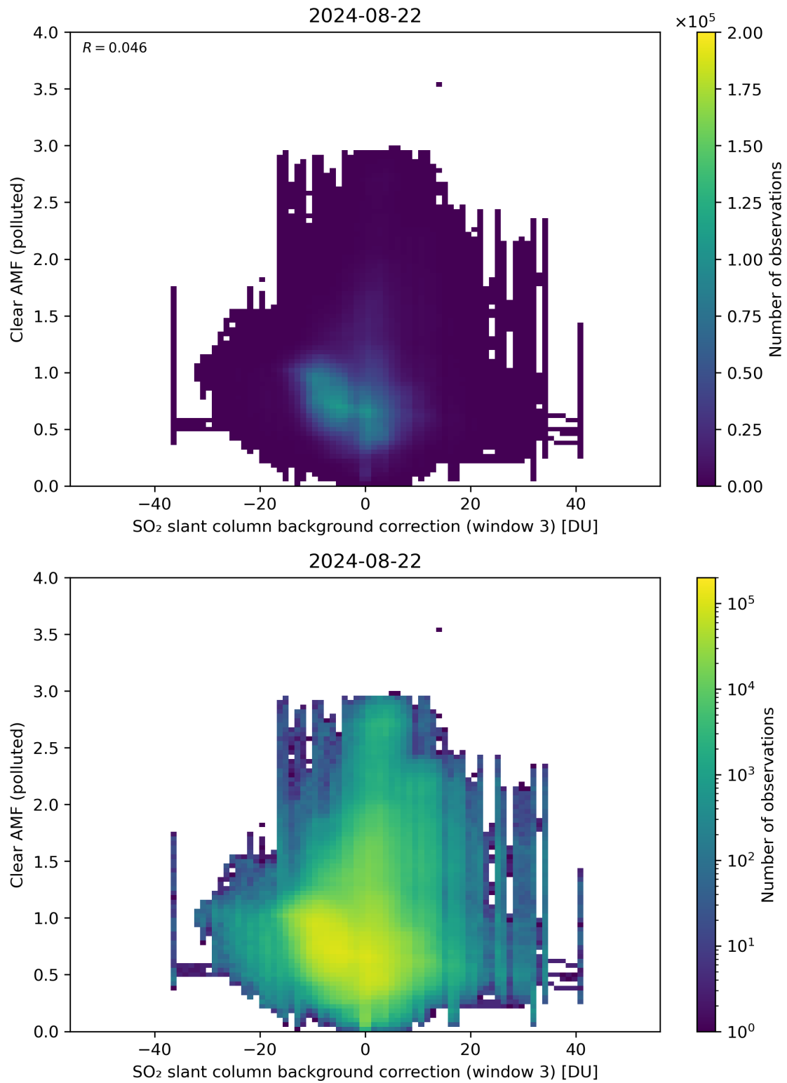
Figure 124: Scatter density plot of “SO 2 slant column background correction (window 3)” against “Clear AMF (polluted)” for 2024-08-22 to 2024-08-23.
