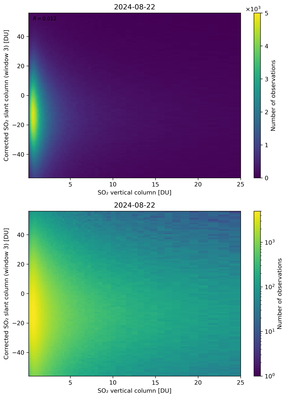
Figure 299: Scatter density plot of “SO 2 vertical column” against “Corrected SO 2 slant column (window 3)” for 2024-08-22 to 2024-08-23.
