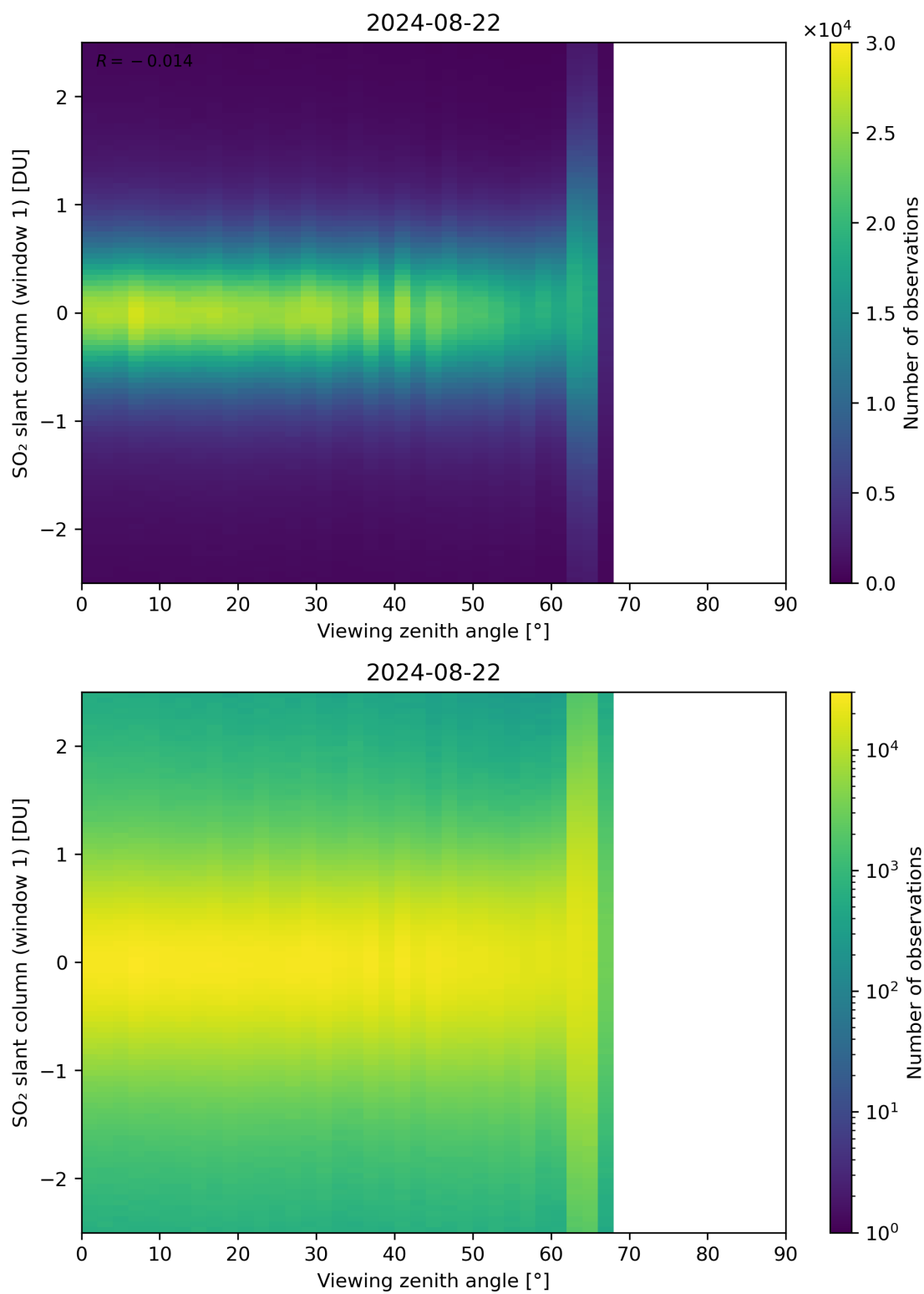
Figure 320: Scatter density plot of “Viewing zenith angle” against “SO 2 slant column (window 1)” for 2024-08-22 to 2024-08-23.
