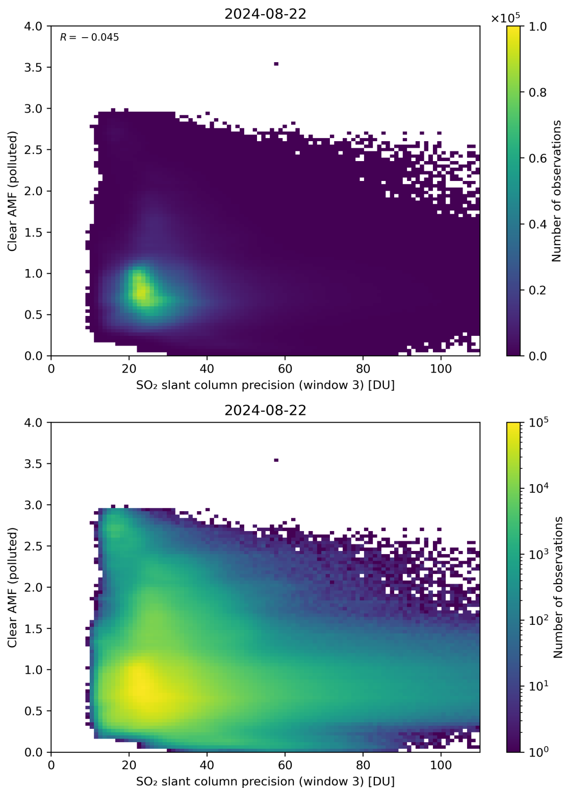
Figure 261: Scatter density plot of “SO 2 slant column precision (window 3)” against “Clear AMF (polluted)” for 2024-08-22 to 2024-08-23.
