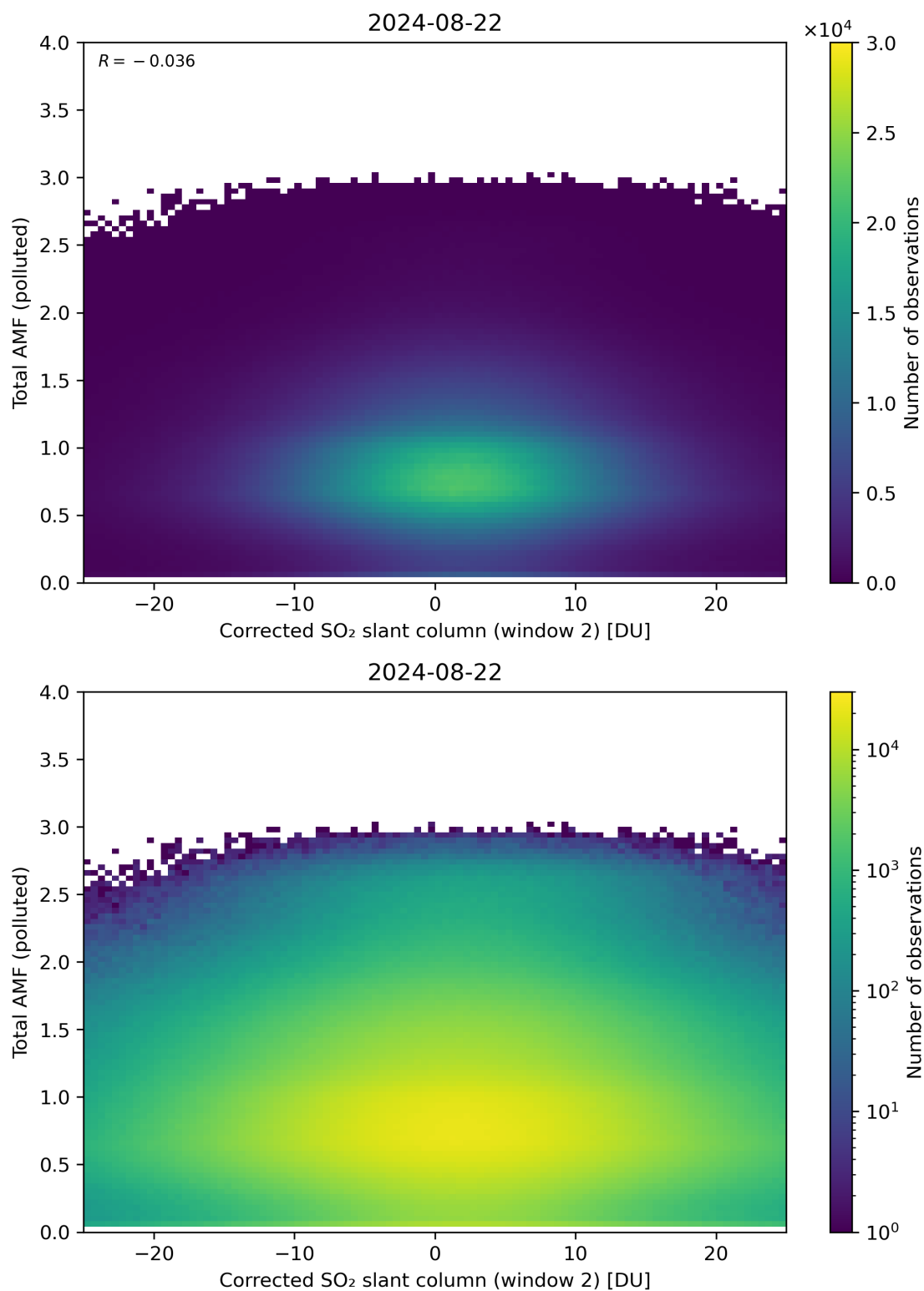
Figure 203: Scatter density plot of “Corrected SO 2 slant column (window 2)” against “Total AMF (polluted)” for 2024-08-22 to 2024-08-23.
