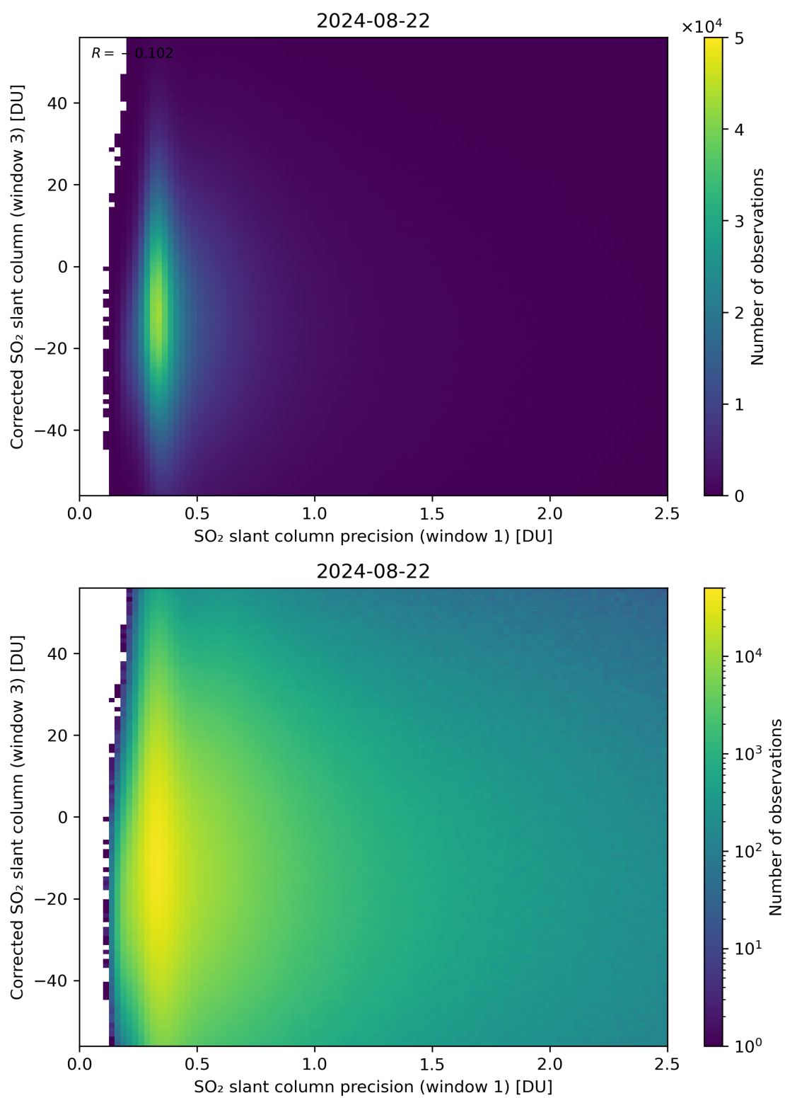
Figure 226: Scatter density plot of “SO 2 slant column precision (window 1)” against “Corrected SO 2 slant column (window 3)” for 2024-08-22 to 2024-08-23.
