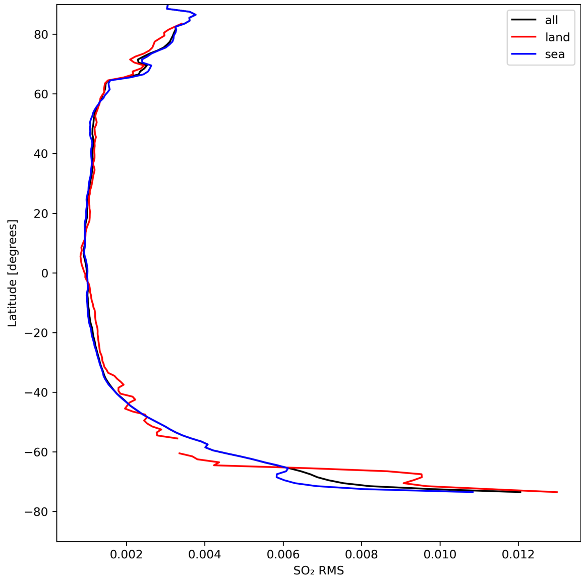
Figure 47: Zonal average of “SO 2 RMS” for 2024-08-22 to 2024-08-23.
