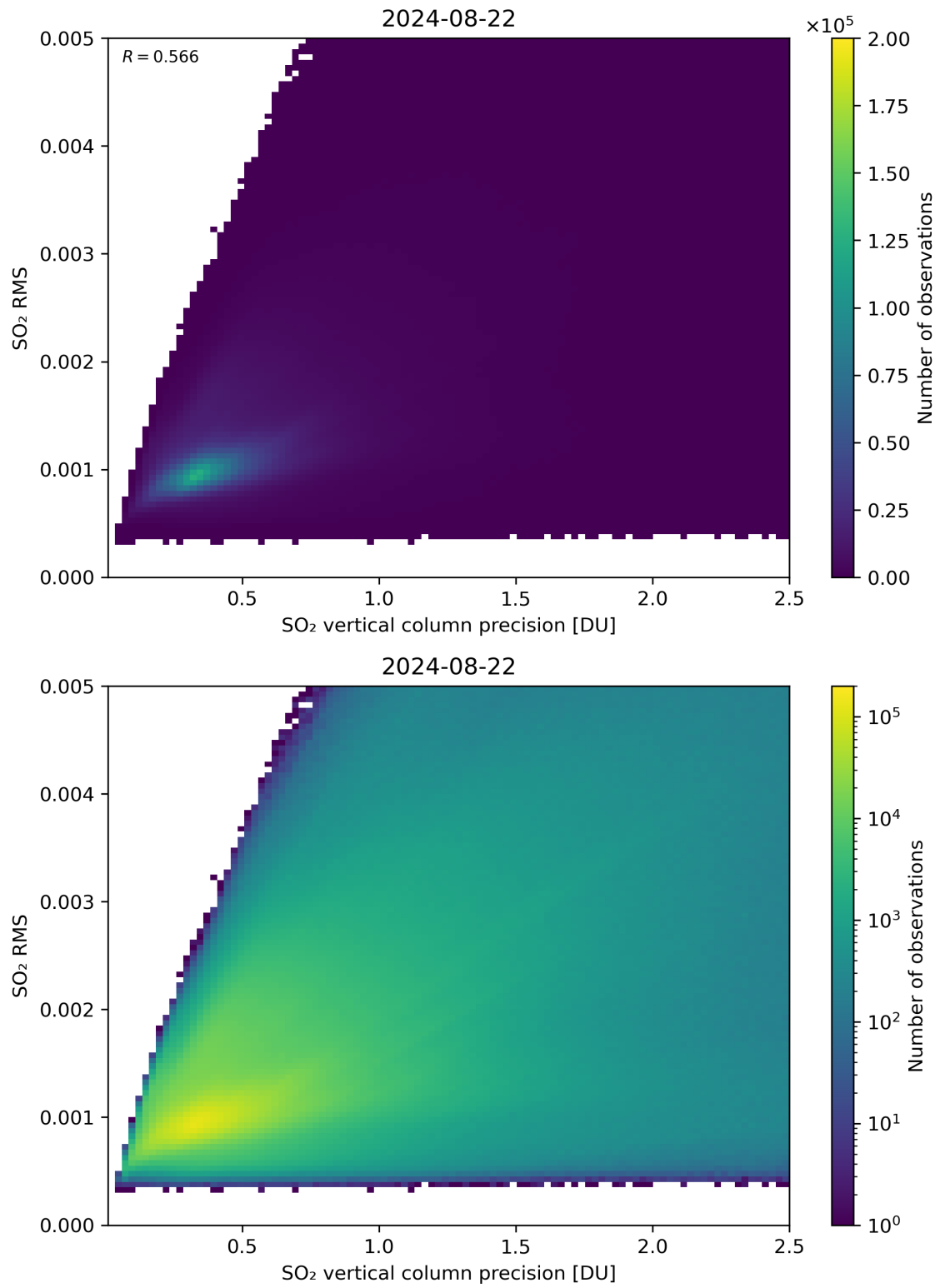
Figure 284: Scatter density plot of “SO 2 vertical column precision” against “SO 2 RMS” for 2024-08-22 to 2024-08-23.
