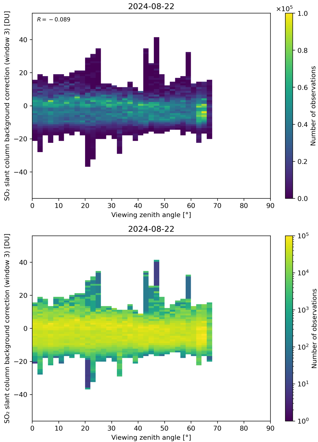
Figure 310: Scatter density plot of “Viewing zenith angle” against “SO 2 slant column background correction (window 3)” for 2024-08-22 to 2024-08-23.
