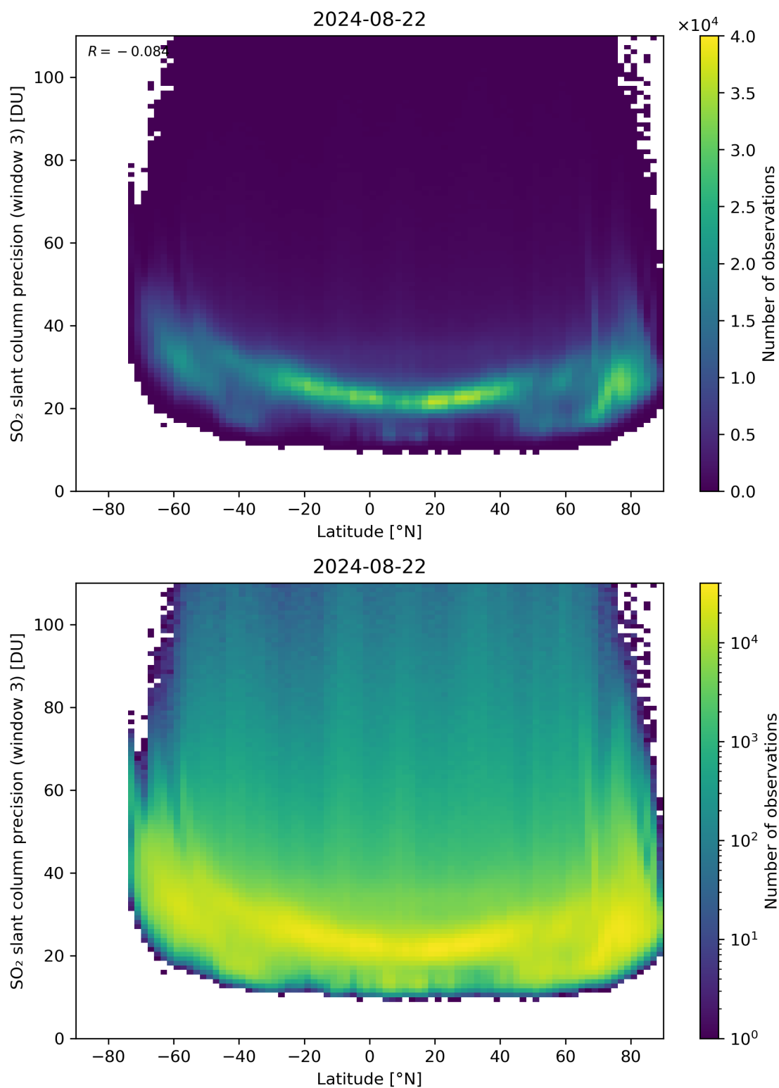
Figure 153: Scatter density plot of “Latitude” against “SO 2 slant column precision (window 3)” for 2024-08-22 to 2024-08-23.
