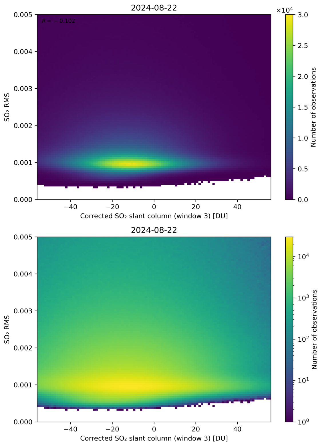
Figure 208: Scatter density plot of “Corrected SO 2 slant column (window 3)” against “SO 2 RMS” for 2024-08-22 to 2024-08-23.
