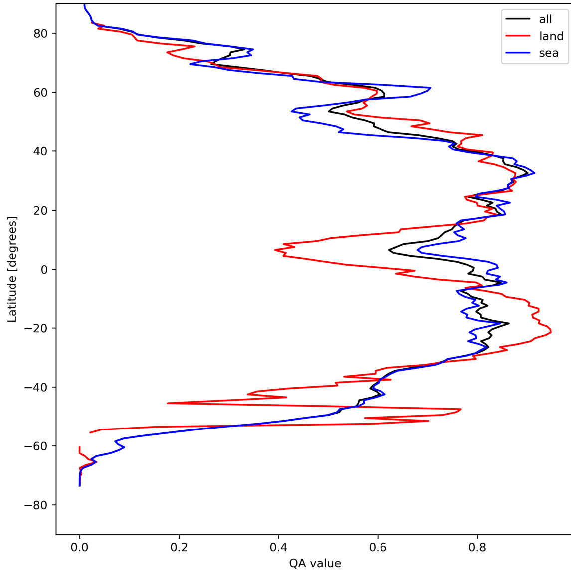
Figure 29: Zonal average of “QA value” for 2024-08-22 to 2024-08-23.
