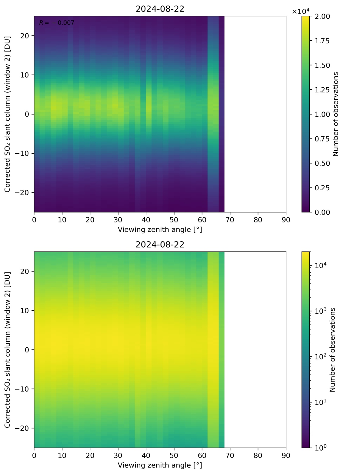
Figure 318: Scatter density plot of “Viewing zenith angle” against “Corrected SO 2 slant column (window 2)” for 2024-08-22 to 2024-08-23.
