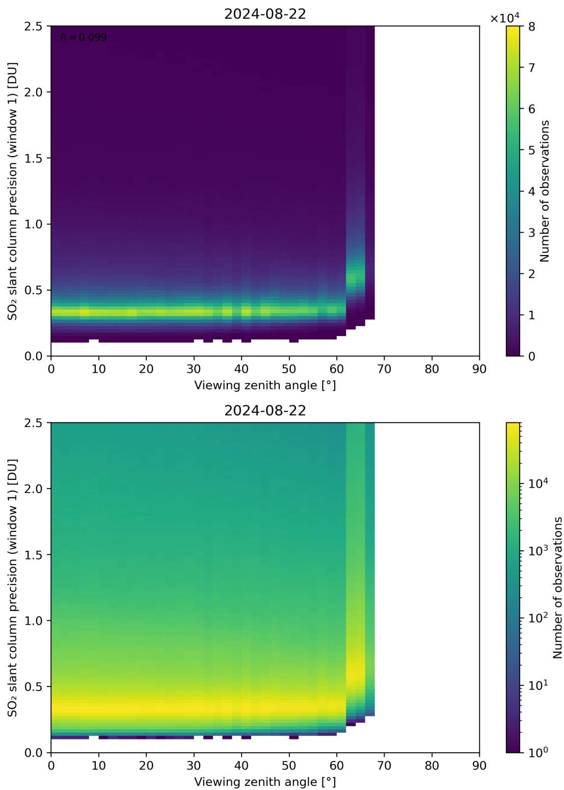
Figure 321: Scatter density plot of “Viewing zenith angle” against “SO 2 slant column precision (window 1)” for 2024-08-22 to 2024-08-23.
