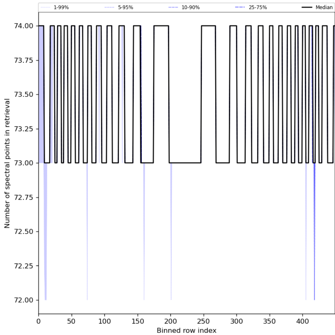
Figure 97: Along track statistics of “Number of spectral points in retrieval” for 2024-08-22 to 2024-08-23
