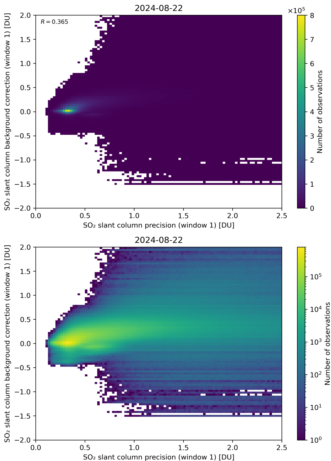
Figure 218: Scatter density plot of “SO 2 slant column precision (window 1)” against “SO 2 slant column background correction (window 1)” for 2024-08-22 to 2024-08-23.
