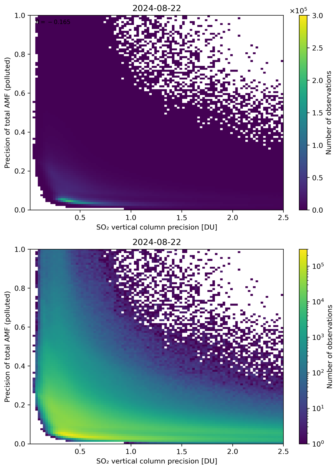
Figure 295: Scatter density plot of “SO 2 vertical column precision” against “Precision of total AMF (polluted)” for 2024-08-22 to 2024-08-23.
