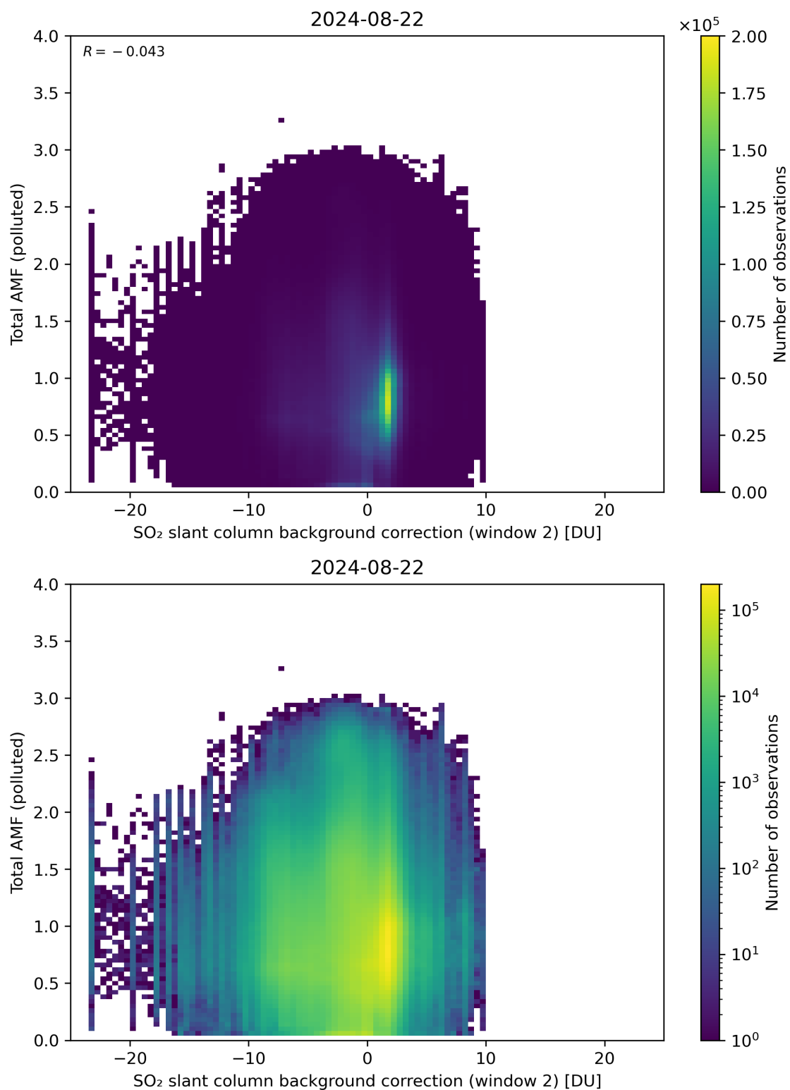
Figure 119: Scatter density plot of “SO 2 slant column background correction (window 2)” against “Total AMF (polluted)” for 2024-08-22 to 2024-08-23.
