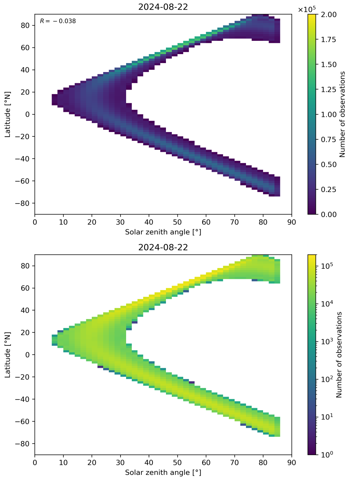
Figure 164: Scatter density plot of “Solar zenith angle” against “Latitude” for 2024-08-22 to 2024-08-23.
