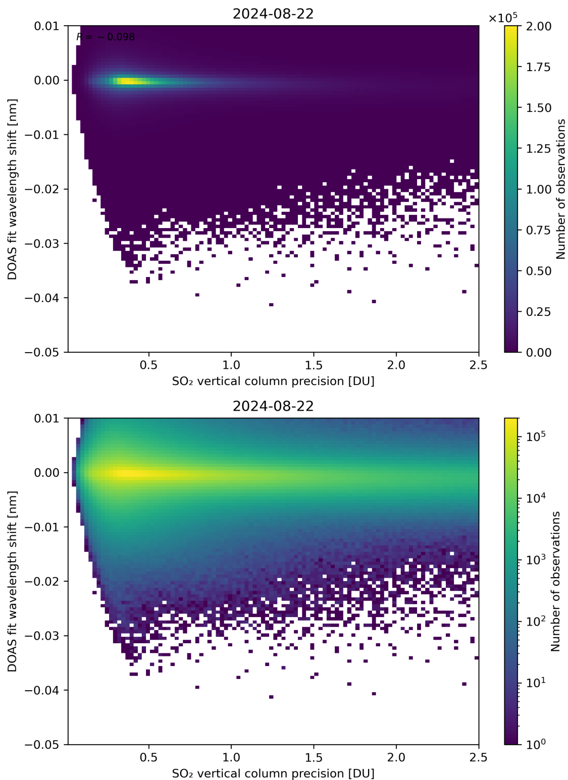
Figure 282: Scatter density plot of “SO 2 vertical column precision” against “DOAS fit wavelength shift” for 2024-08-22 to 2024-08-23.
