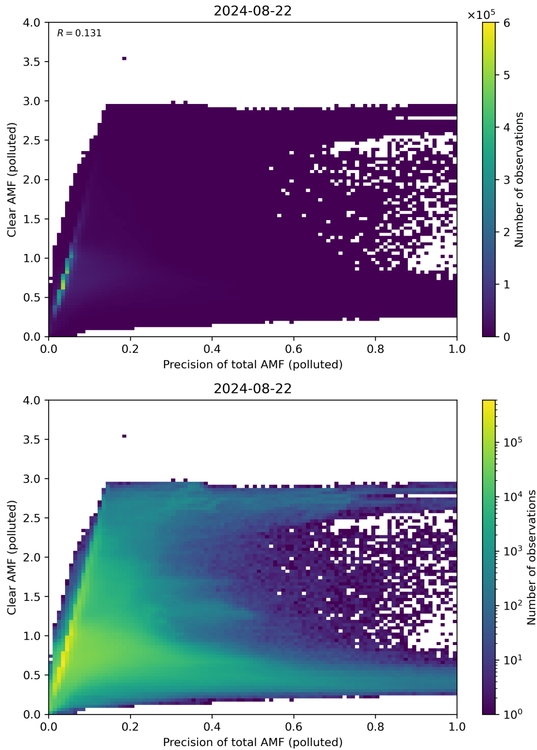
Figure 270: Scatter density plot of “Precision of total AMF (polluted)” against “Clear AMF (polluted)” for 2024-08-22 to 2024-08-23.
