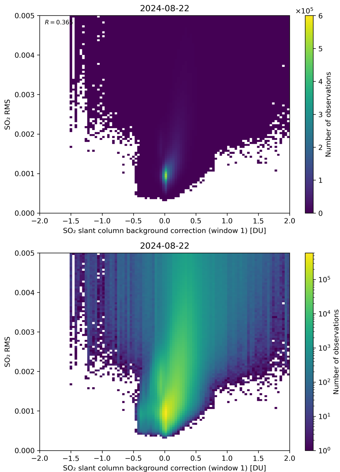
Figure 102: Scatter density plot of “SO 2 slant column background correction (window 1)” against “SO 2 RMS” for 2024-08-22 to 2024-08-23.
