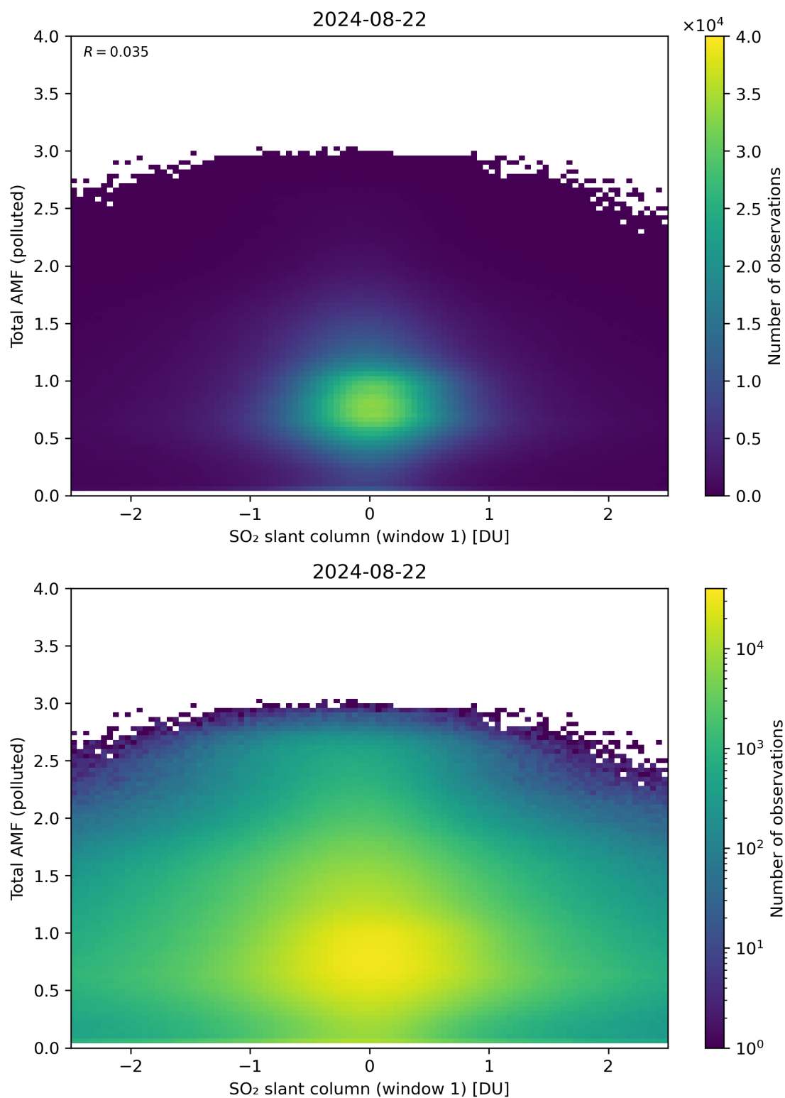
Figure 239: Scatter density plot of “SO 2 slant column (window 1)” against “Total AMF (polluted)” for 2024-08-22 to 2024-08-23.
