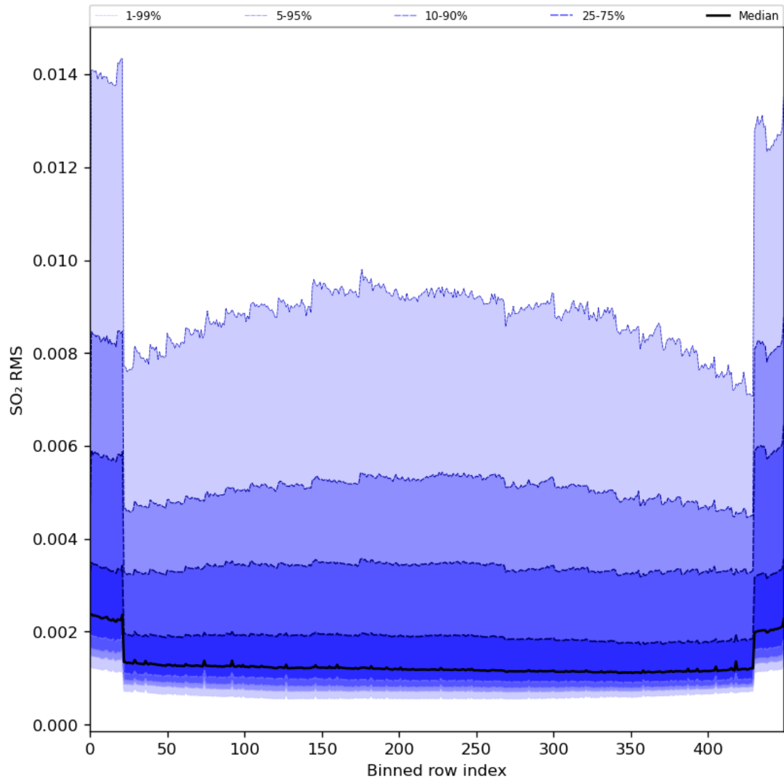
Figure 93: Along track statistics of “SO 2 RMS” for 2024-08-22 to 2024-08-23
