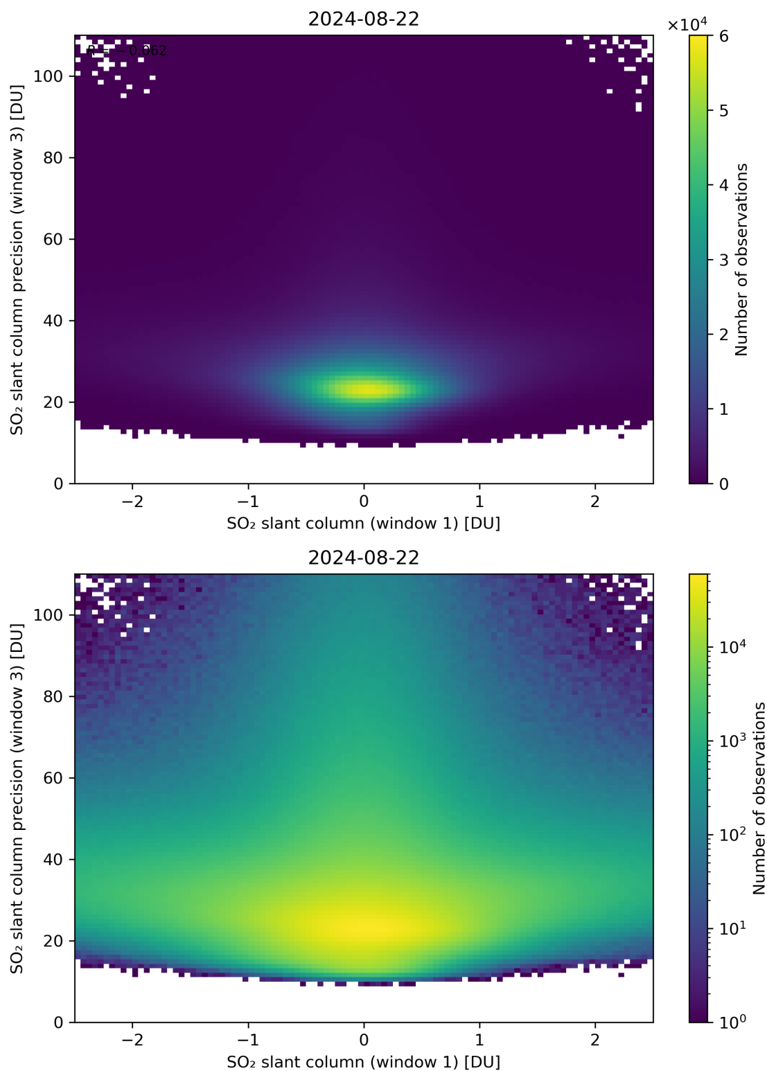
Figure 238: Scatter density plot of “SO 2 slant column (window 1)” against “SO 2 slant column precision (window 3)” for 2024-08-22 to 2024-08-23.
