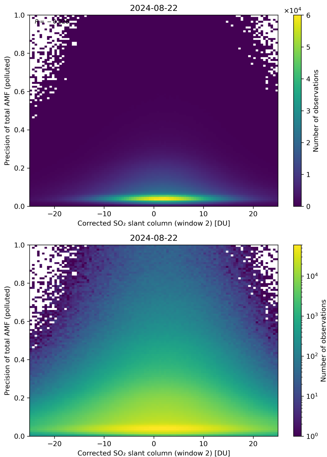
Figure 204: Scatter density plot of “Corrected SO 2 slant column (window 2)” against “Precision of total AMF (polluted)” for 2024-08-22 to 2024-08-23.
