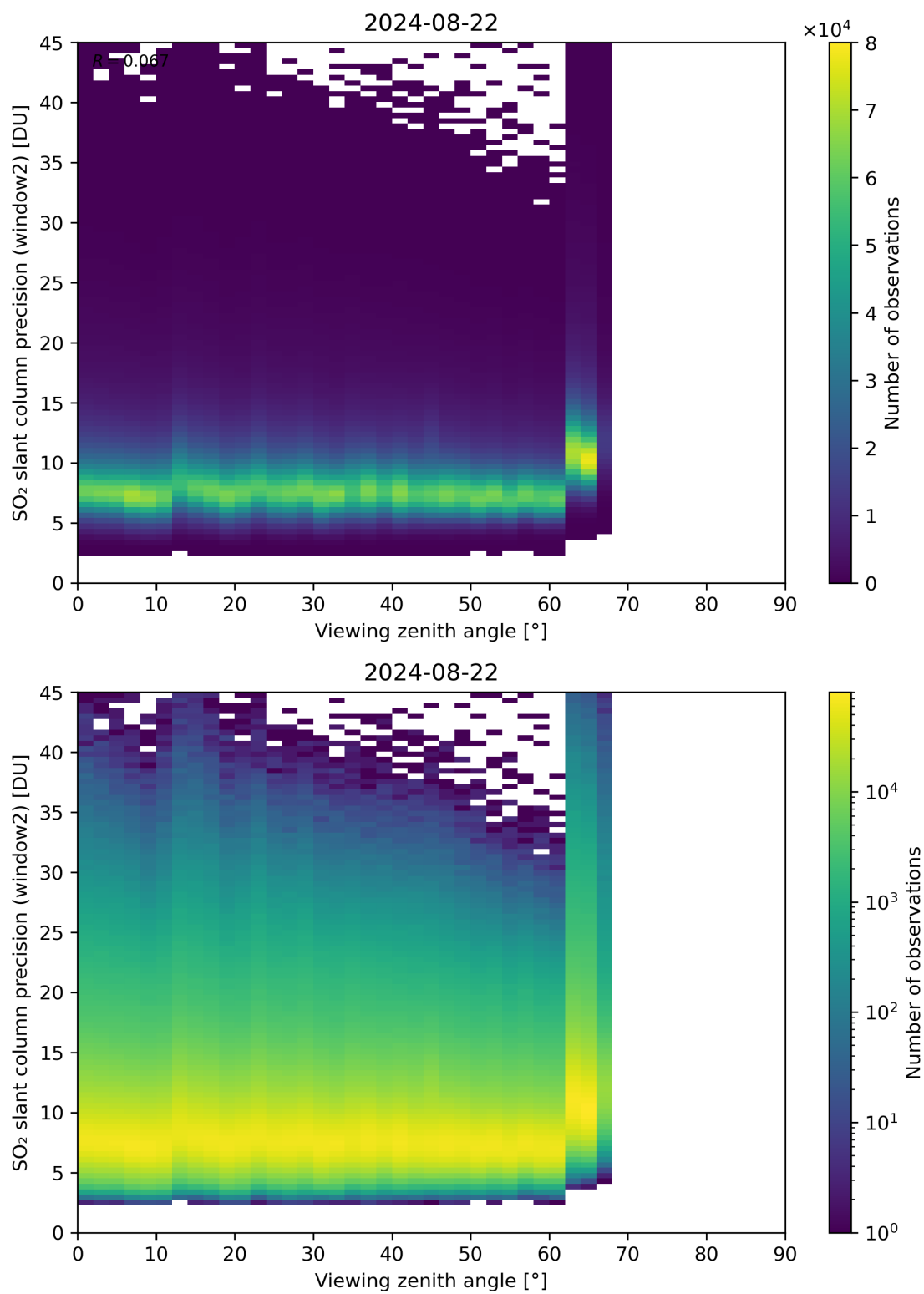
Figure 322: Scatter density plot of “Viewing zenith angle” against “SO 2 slant column precision (window2)” for 2024-08-22 to 2024-08-23.
