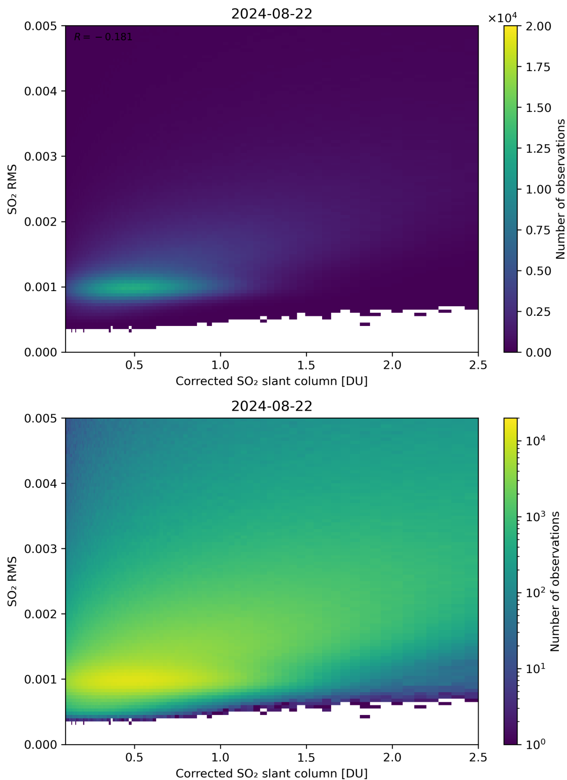
Figure 183: Scatter density plot of “Corrected SO 2 slant column” against “SO 2 RMS” for 2024-08-22 to 2024-08-23.
