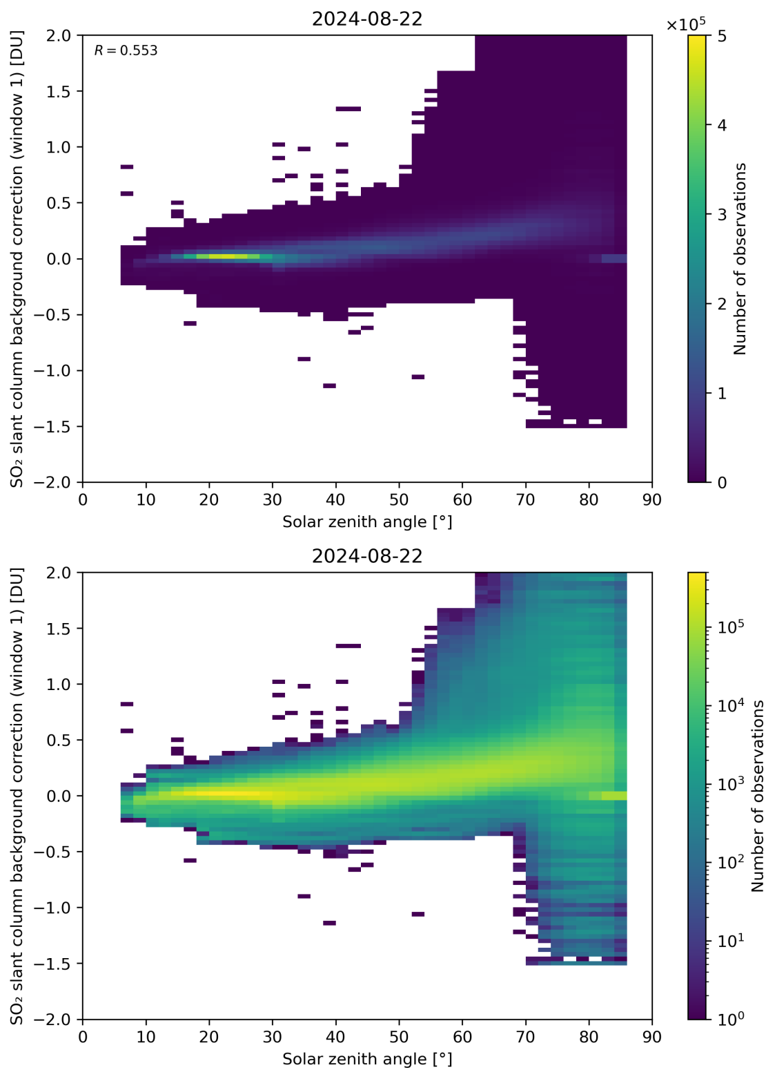
Figure 158: Scatter density plot of “Solar zenith angle” against “SO 2 slant column background correction (window 1)” for 2024-08-22 to 2024-08-23.
