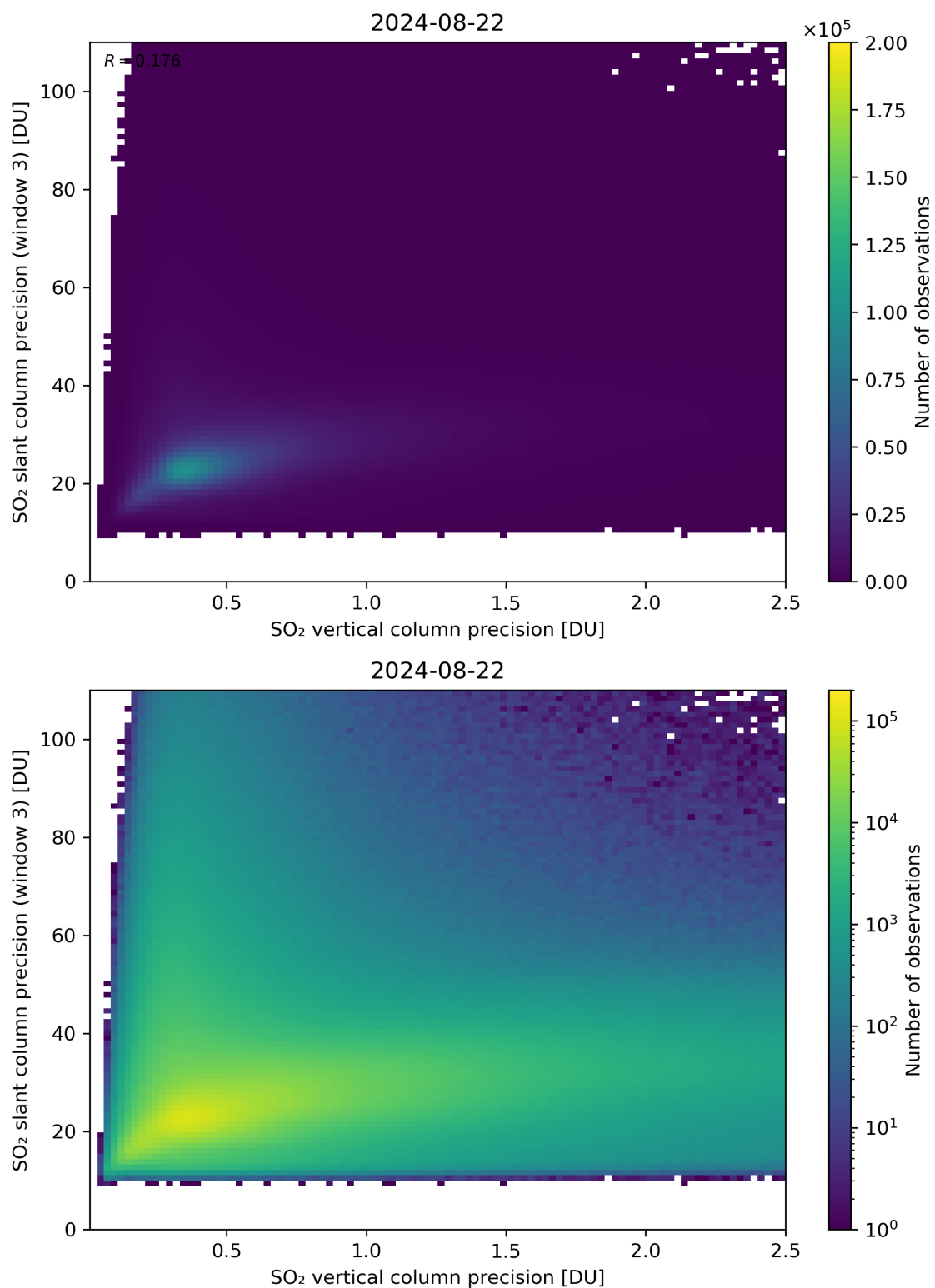
Figure 293: Scatter density plot of “SO 2 vertical column precision” against “SO 2 slant column precision (window 3)” for 2024-08-22 to 2024-08-23.
