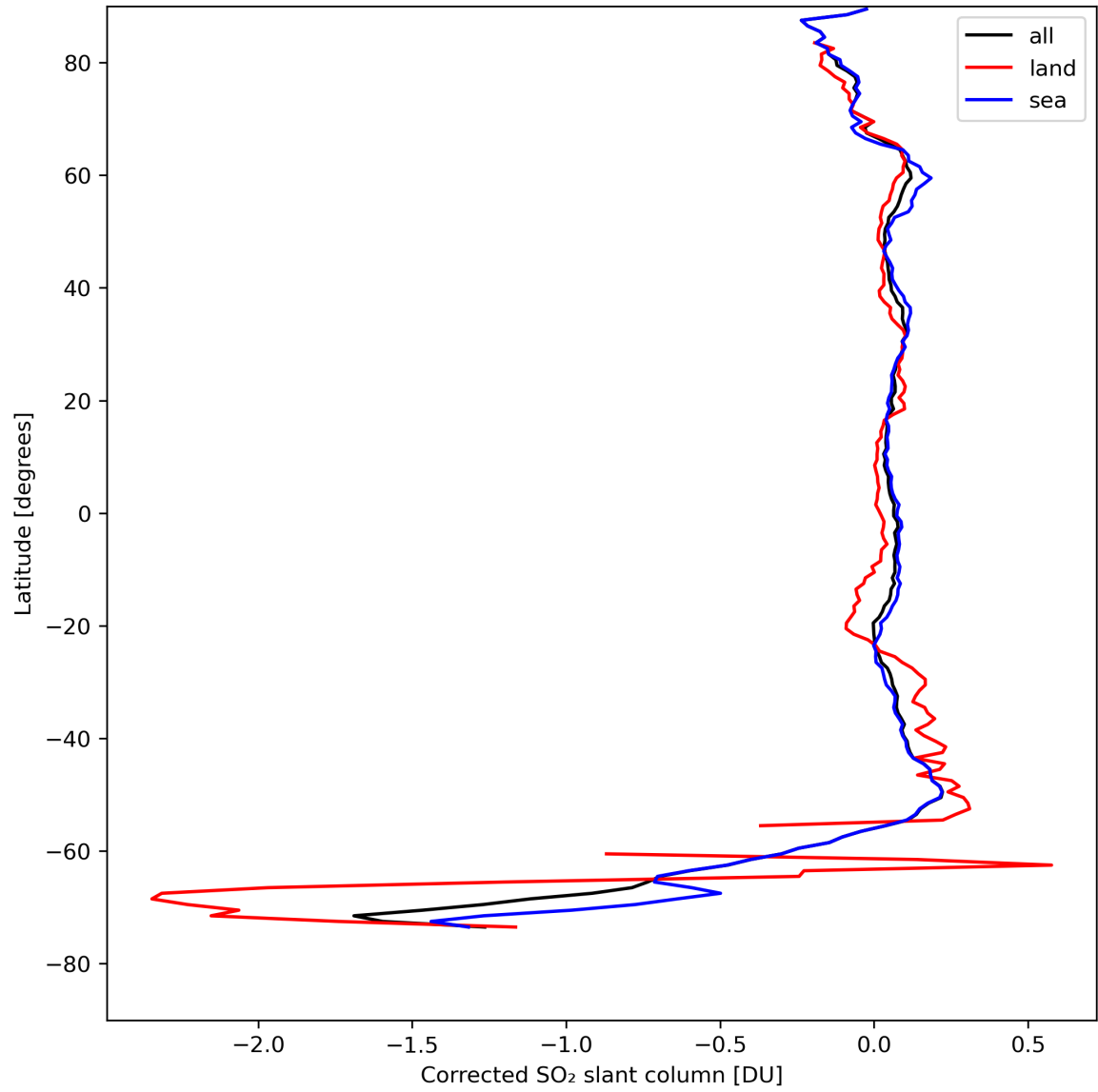
Figure 32: Zonal average of “Corrected SO 2 slant column” for 2024-08-22 to 2024-08-23.
