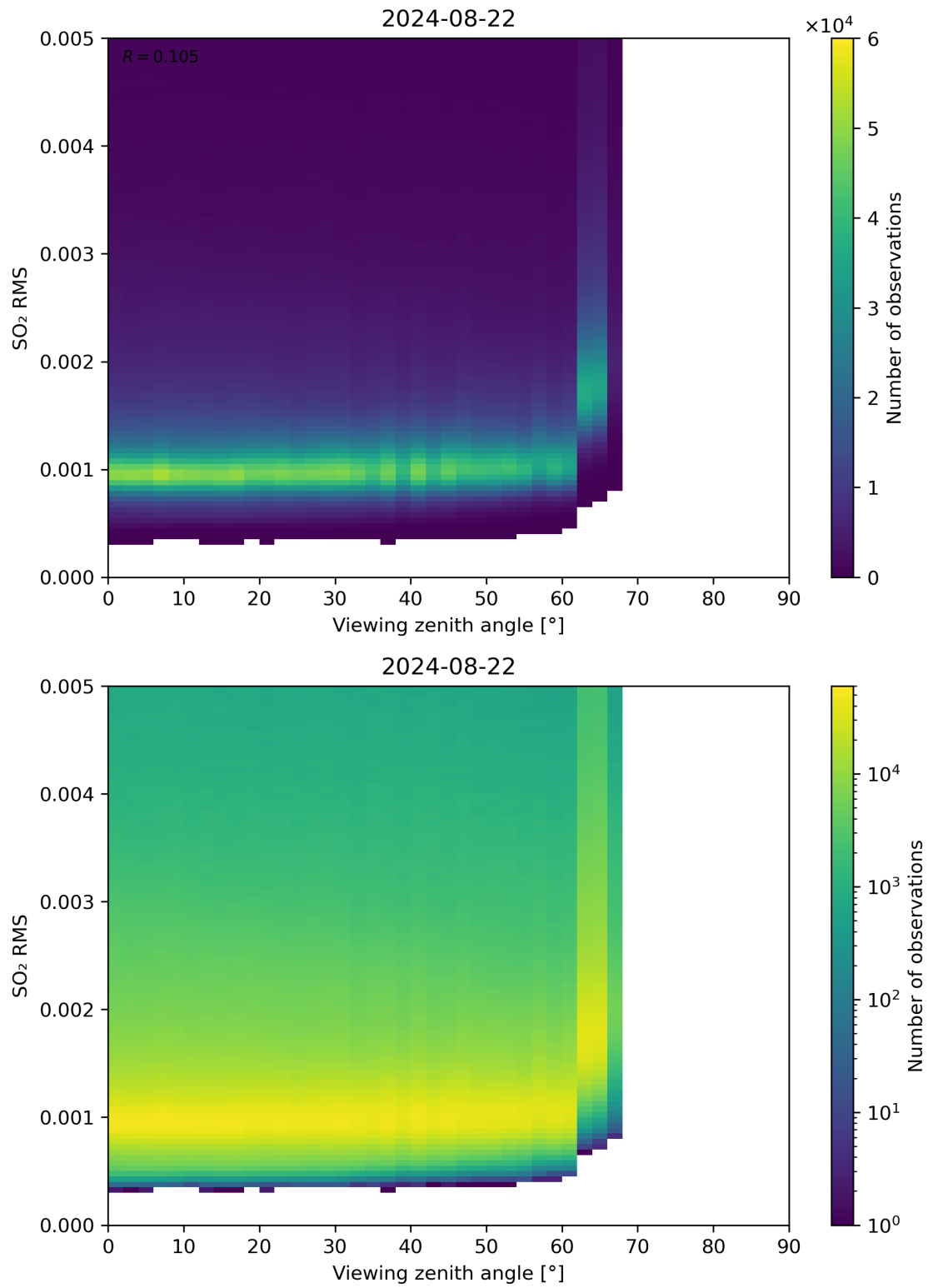
Figure 313: Scatter density plot of “Viewing zenith angle” against “SO 2 RMS” for 2024-08-22 to 2024-08-23.
