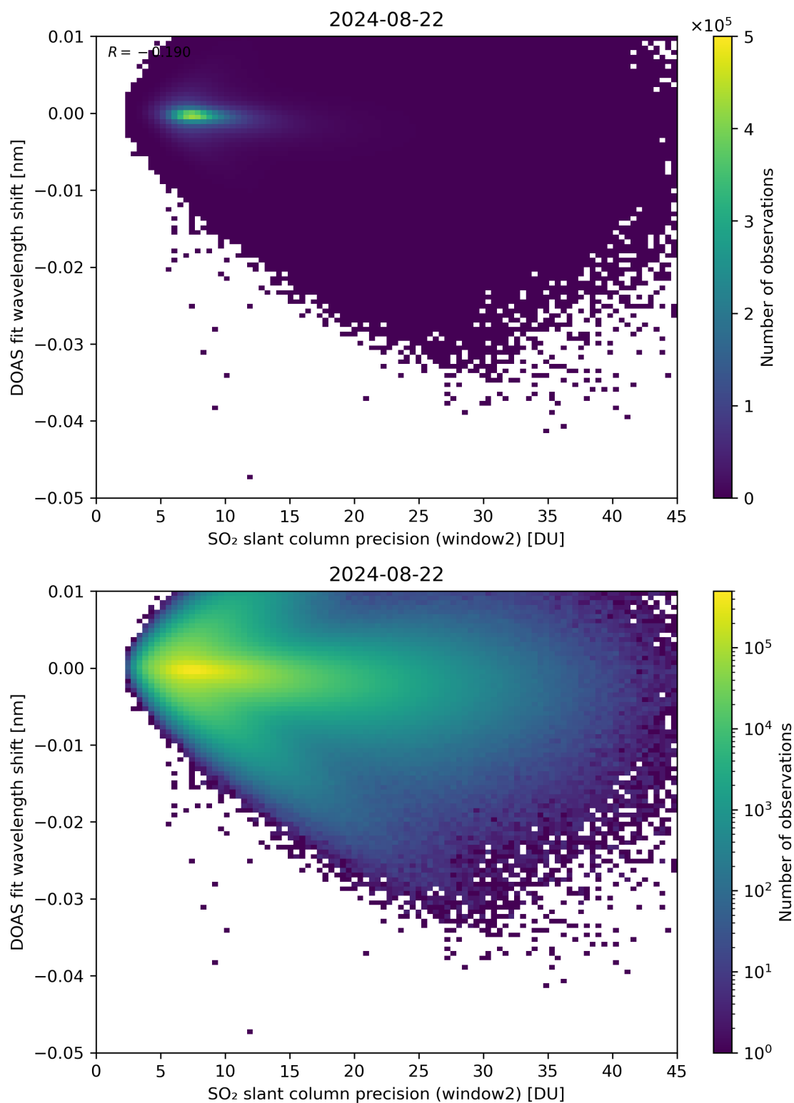
Figure 243: Scatter density plot of “SO 2 slant column precision (window2)” against “DOAS fit wavelength shift” for 2024-08-22 to 2024-08-23.
