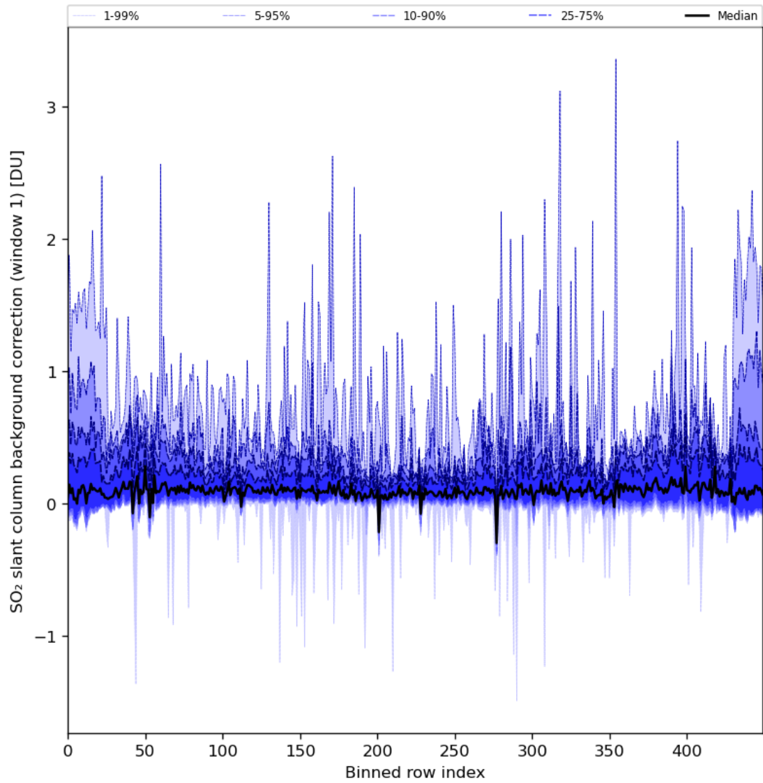
Figure 82: Along track statistics of “SO 2 slant column background correction (window 1)” for 2024-08-22 to 2024-08-23
