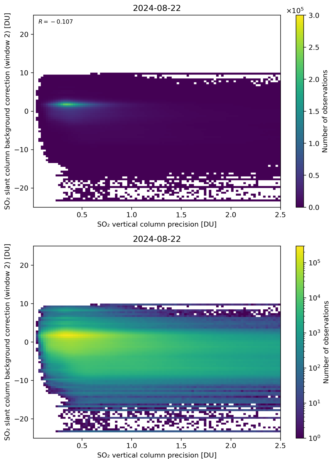
Figure 280: Scatter density plot of “SO 2 vertical column precision” against “SO 2 slant column background correction (window 2)” for 2024-08-22 to 2024-08-23.
