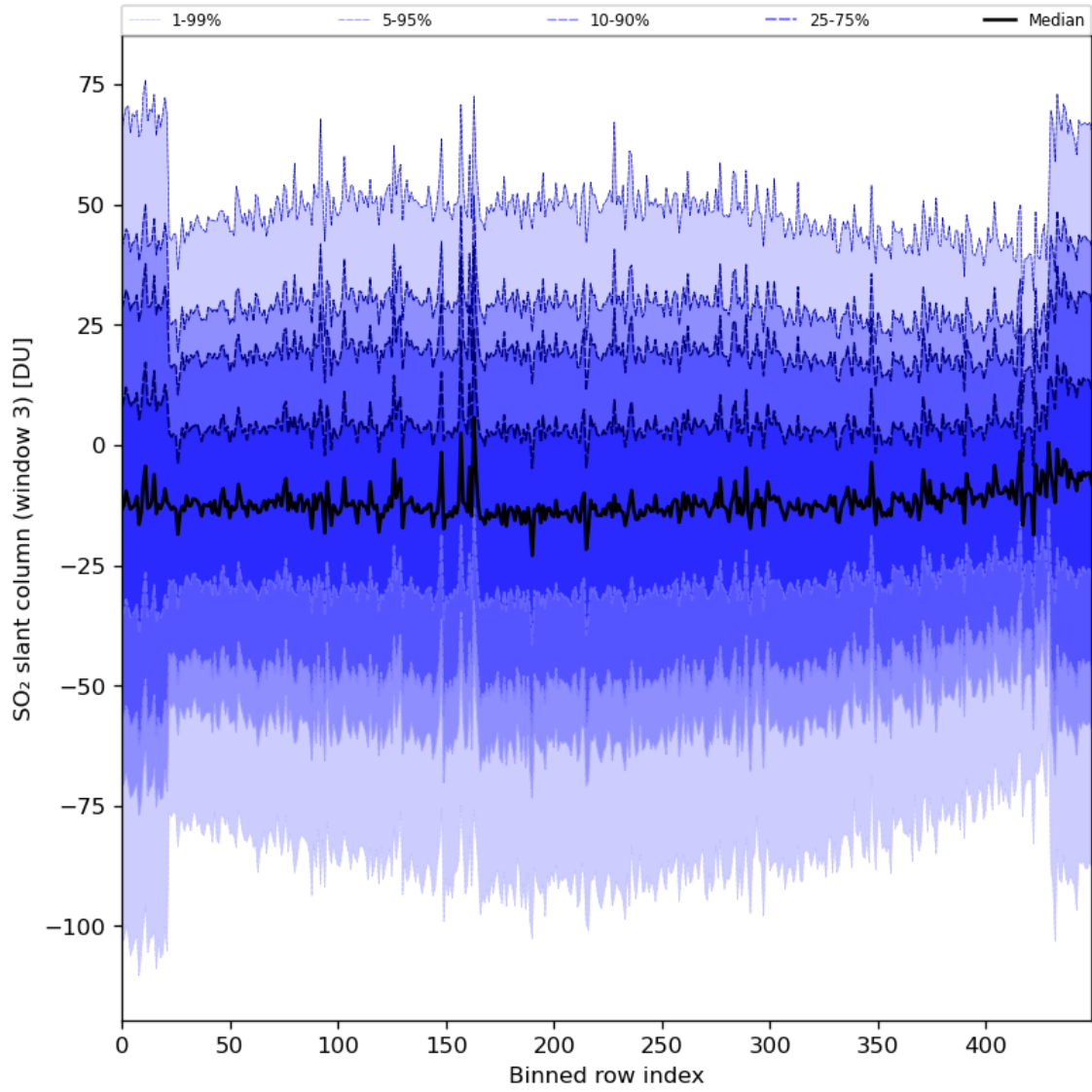
Figure 87: Along track statistics of “SO 2 slant column (window 3)” for 2024-08-22 to 2024-08-23
