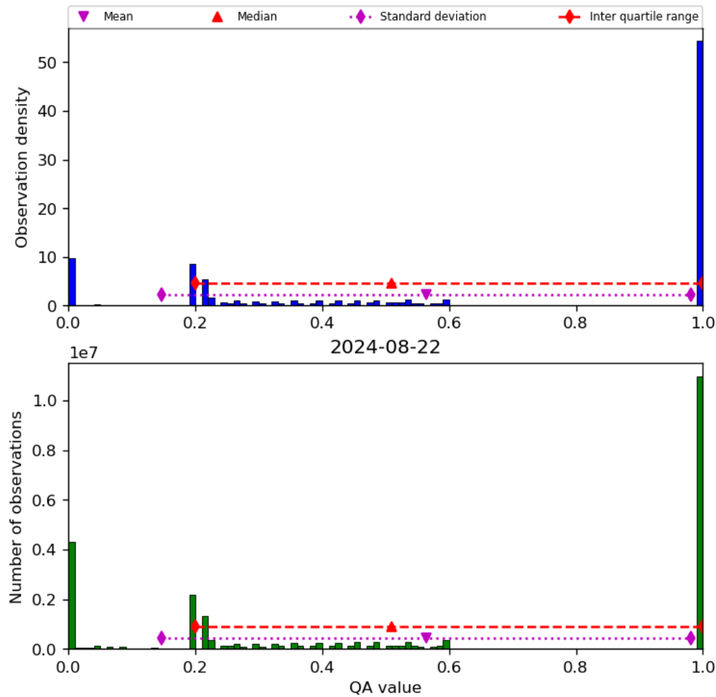
Figure 52: Histogram of “QA value” for 2024-08-22 to 2024-08-23
