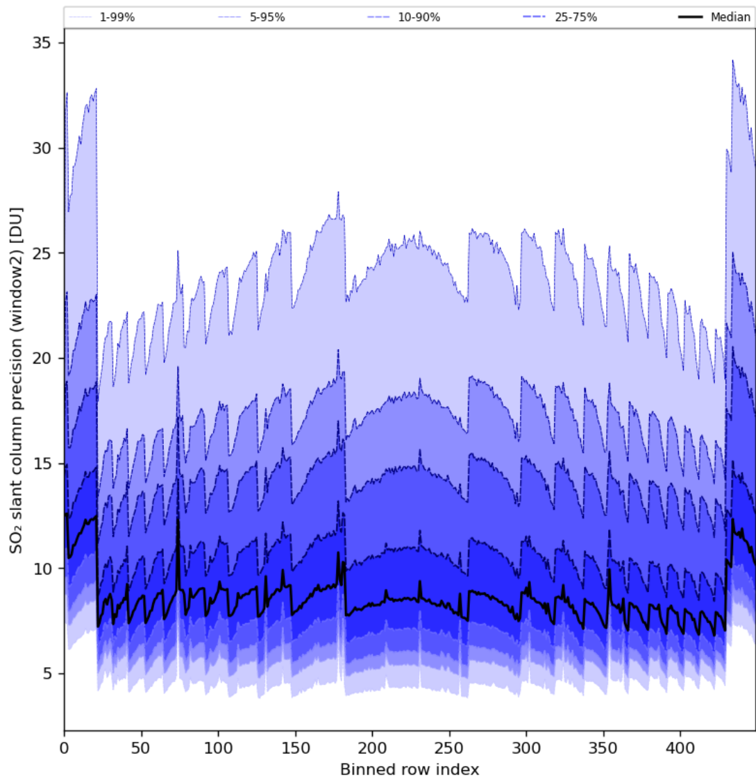
Figure 84: Along track statistics of “SO 2 slant column precision (window2)” for 2024-08-22 to 2024-08-23
