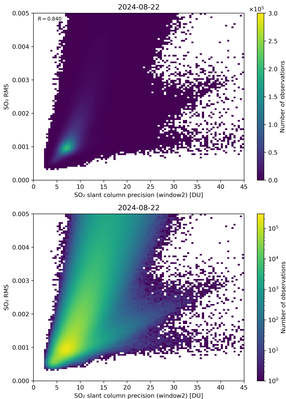
Figure 245: Scatter density plot of “SO 2 slant column precision (window2)” against “SO 2 RMS” for 2024-08-22 to 2024-08-23.
