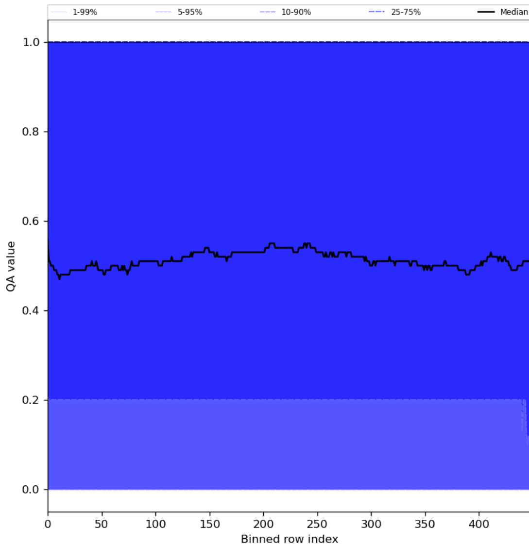
Figure 75: Along track statistics of “QA value” for 2024-08-22 to 2024-08-23
