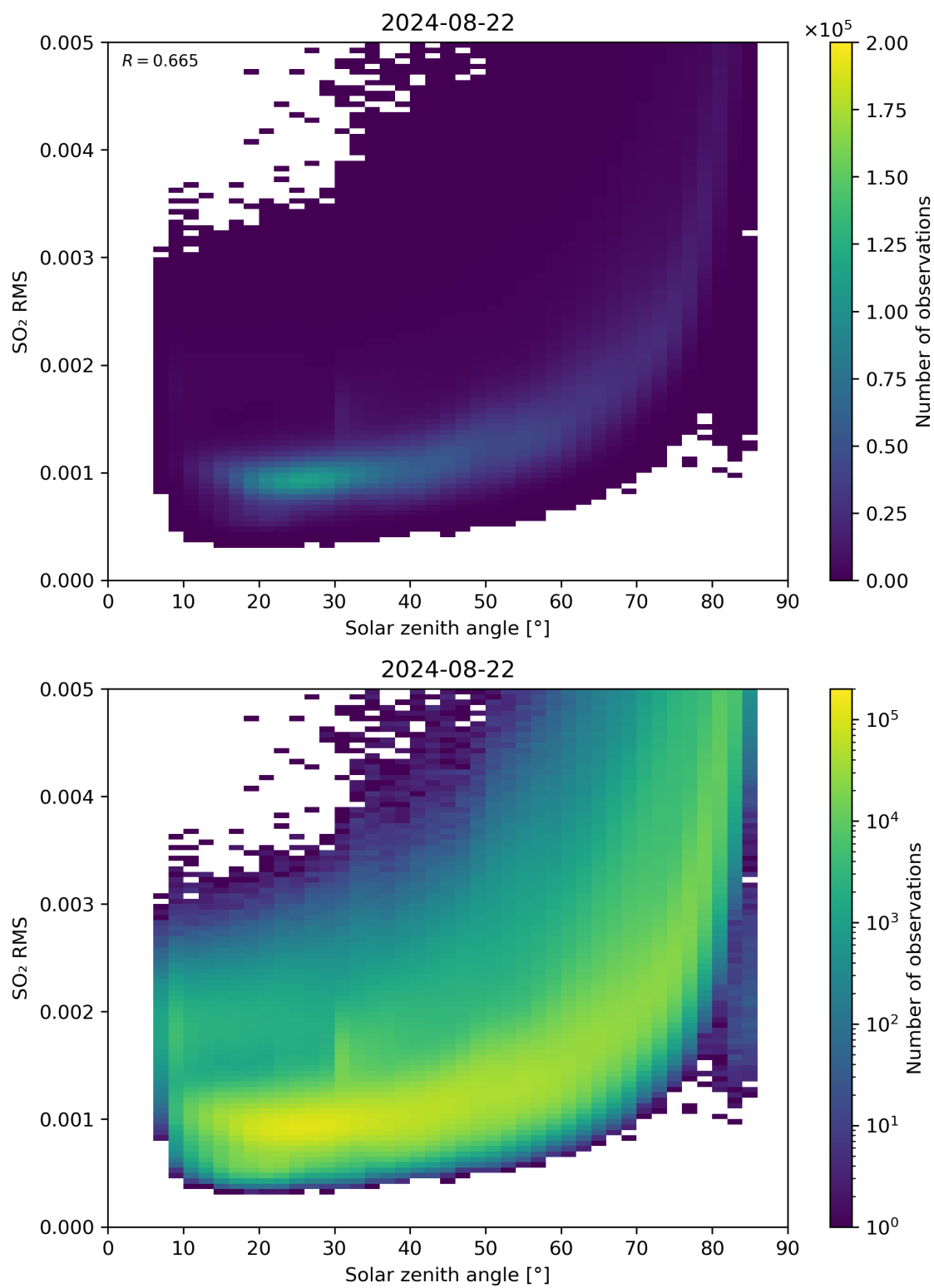
Figure 163: Scatter density plot of “Solar zenith angle” against “SO 2 RMS” for 2024-08-22 to 2024-08-23.
