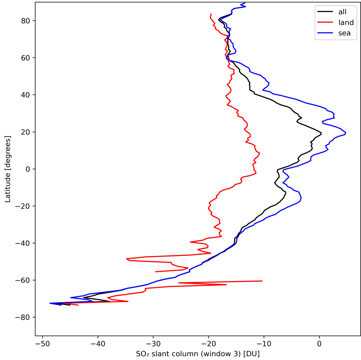
Figure 41: Zonal average of “SO 2 slant column (window 3)” for 2024-08-22 to 2024-08-23.
