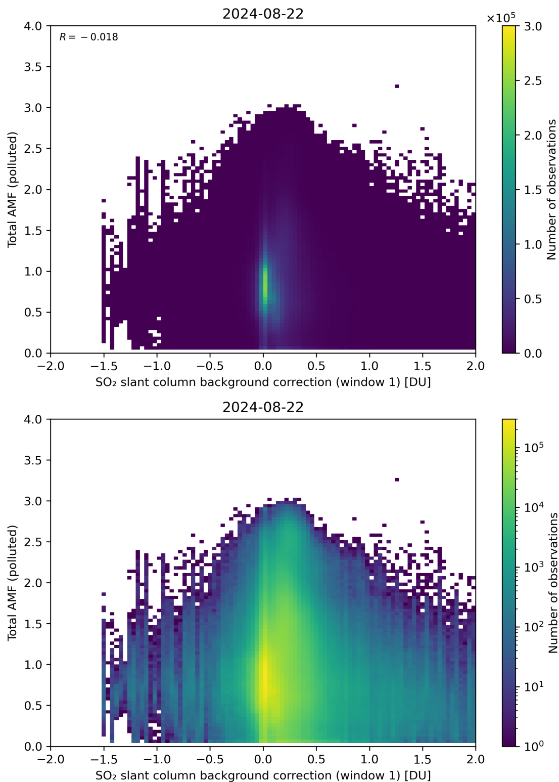
Figure 109: Scatter density plot of “SO 2 slant column background correction (window 1)” against “Total AMF (polluted)” for 2024-08-22 to 2024-08-23.
