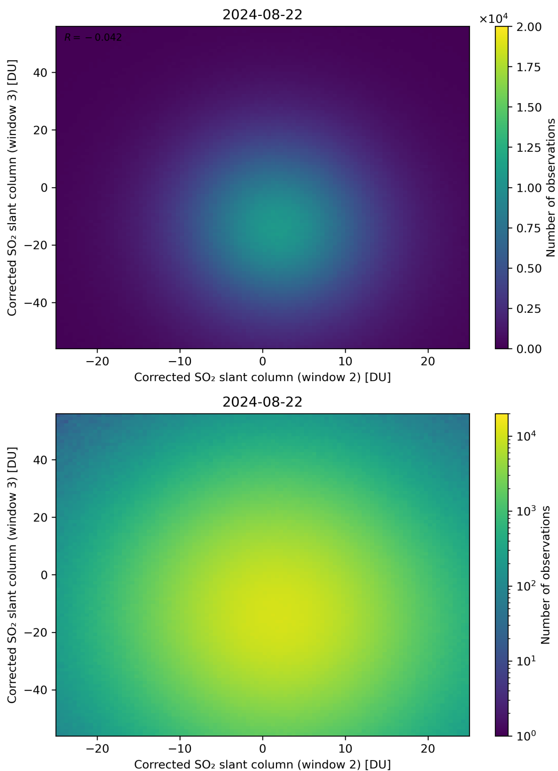
Figure 200: Scatter density plot of “Corrected SO 2 slant column (window 2)” against “Corrected SO 2 slant column (window 3)” for 2024-08-22 to 2024-08-23.
