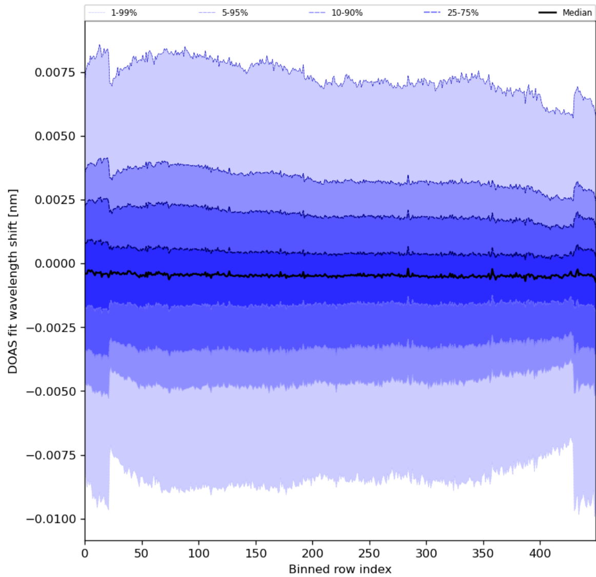
Figure 91: Along track statistics of “DOAS fit wavelength shift” for 2024-08-22 to 2024-08-23
