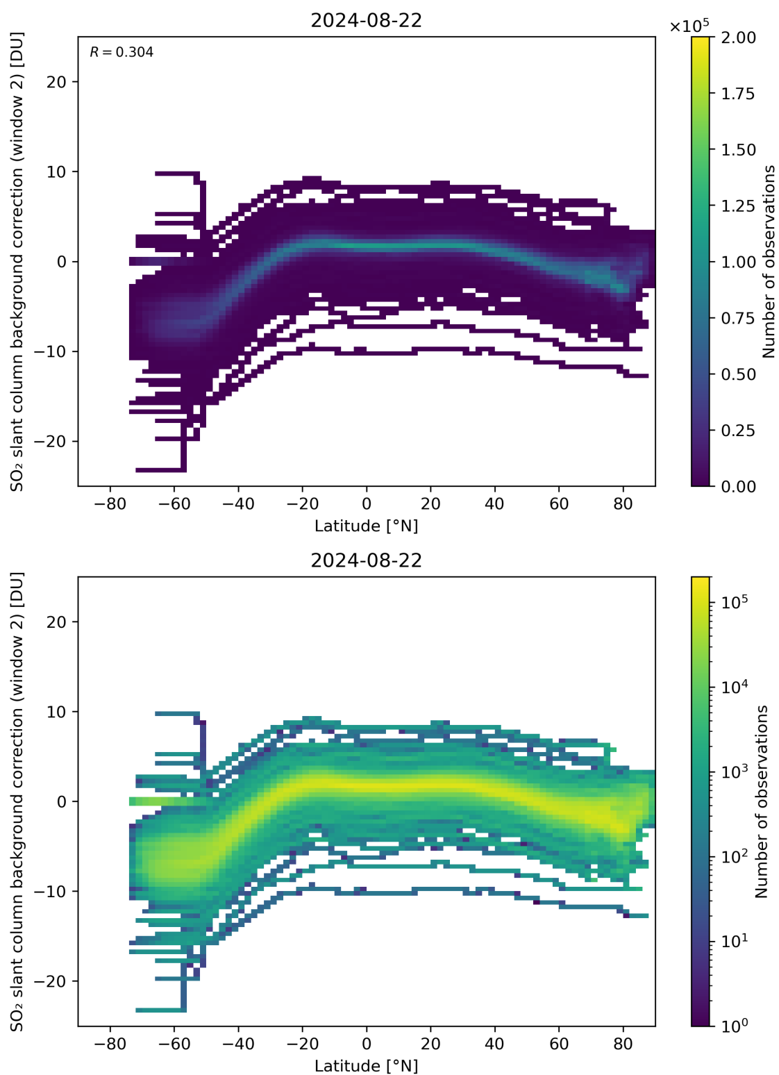
Figure 140: Scatter density plot of “Latitude” against “SO 2 slant column background correction (window 2)” for 2024-08-22 to 2024-08-23.
