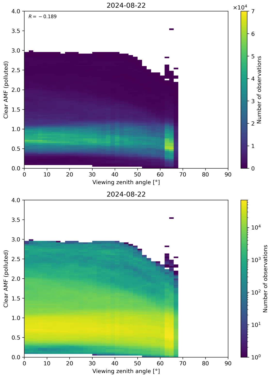
Figure 316: Scatter density plot of “Viewing zenith angle” against “Clear AMF (polluted)” for 2024-08-22 to 2024-08-23.
