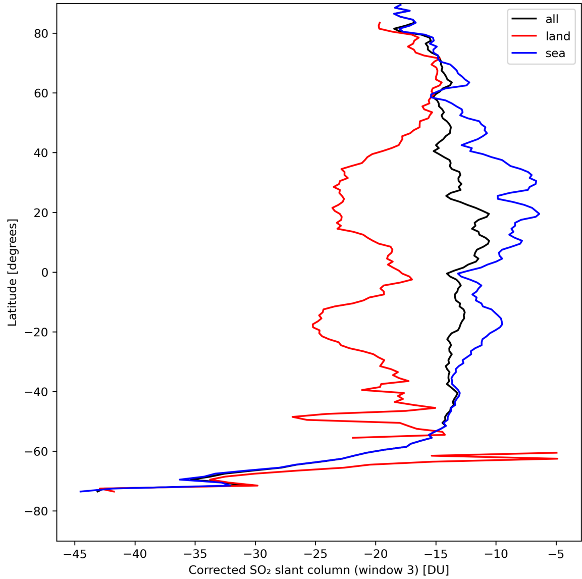
Figure 43: Zonal average of “Corrected SO 2 slant column (window 3)” for 2024-08-22 to 2024-08-23.
