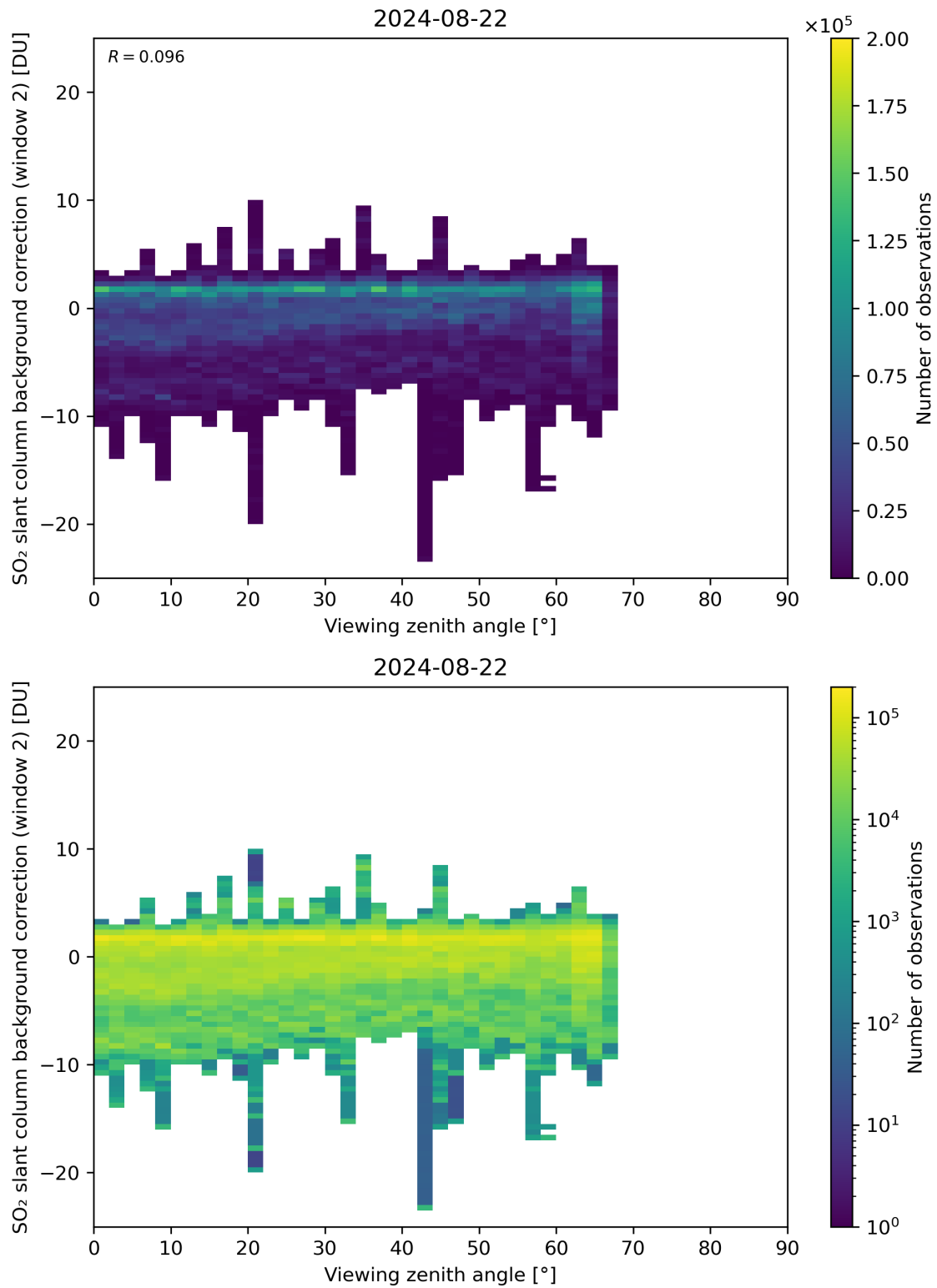
Figure 309: Scatter density plot of “Viewing zenith angle” against “SO 2 slant column background correction (window 2)” for 2024-08-22 to 2024-08-23.
