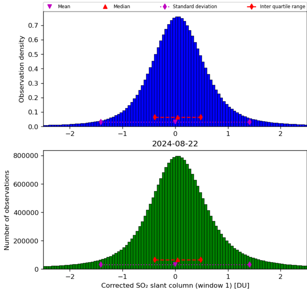
Figure 58: Histogram of “Corrected SO 2 slant column (window 1)” for 2024-08-22 to 2024-08-23
