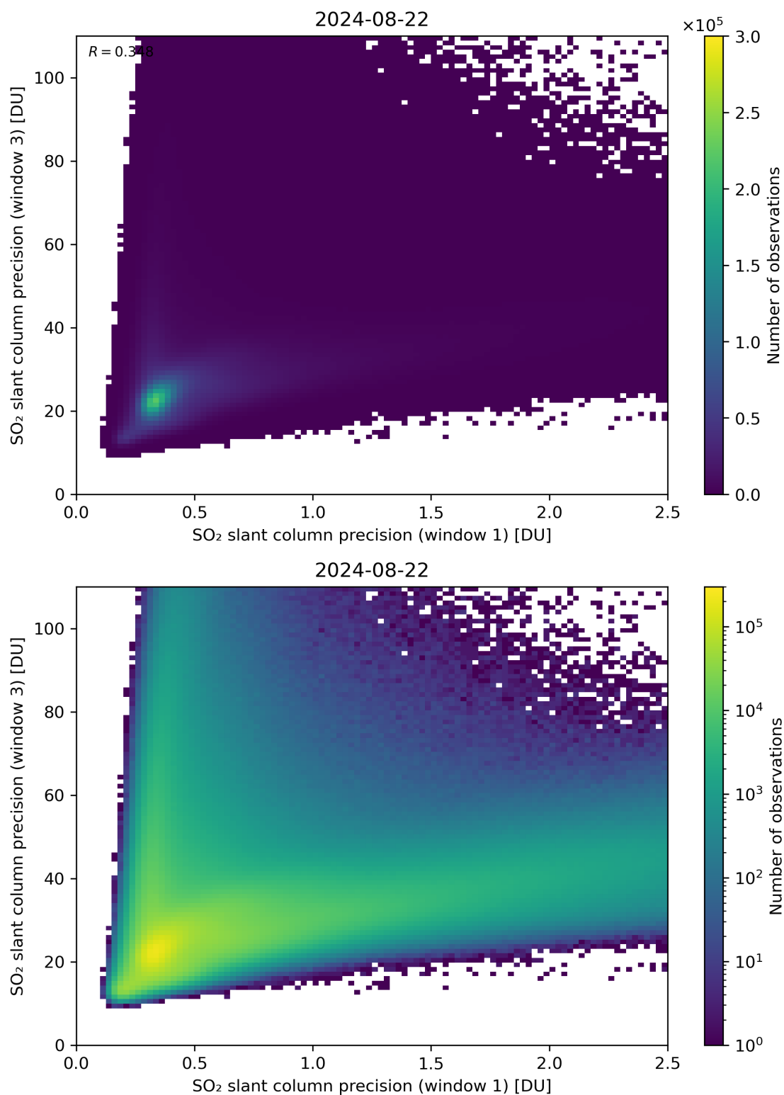
Figure 229: Scatter density plot of “SO 2 slant column precision (window 1)” against “SO 2 slant column precision (window 3)” for 2024-08-22 to 2024-08-23.
