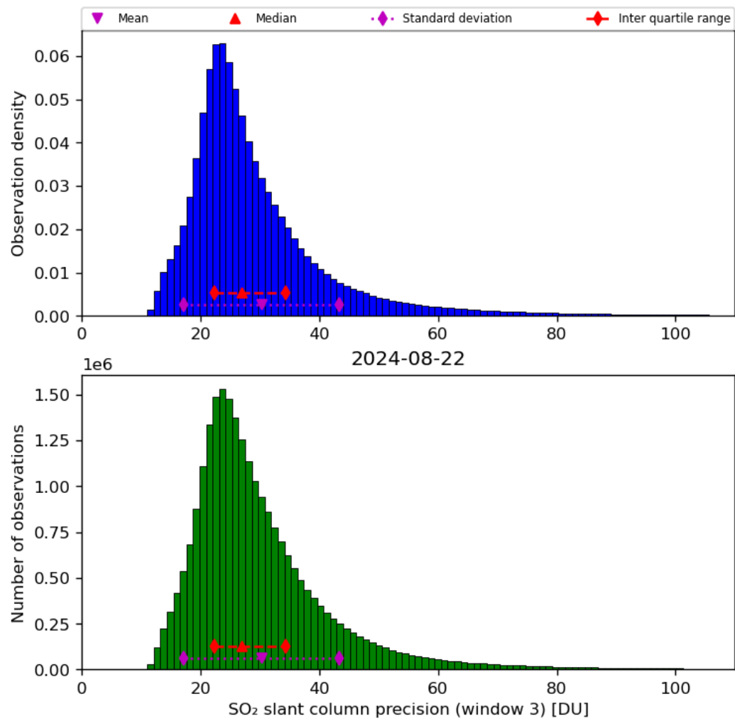
Figure 65: Histogram of “SO 2 slant column precision (window 3)” for 2024-08-22 to 2024-08-23
