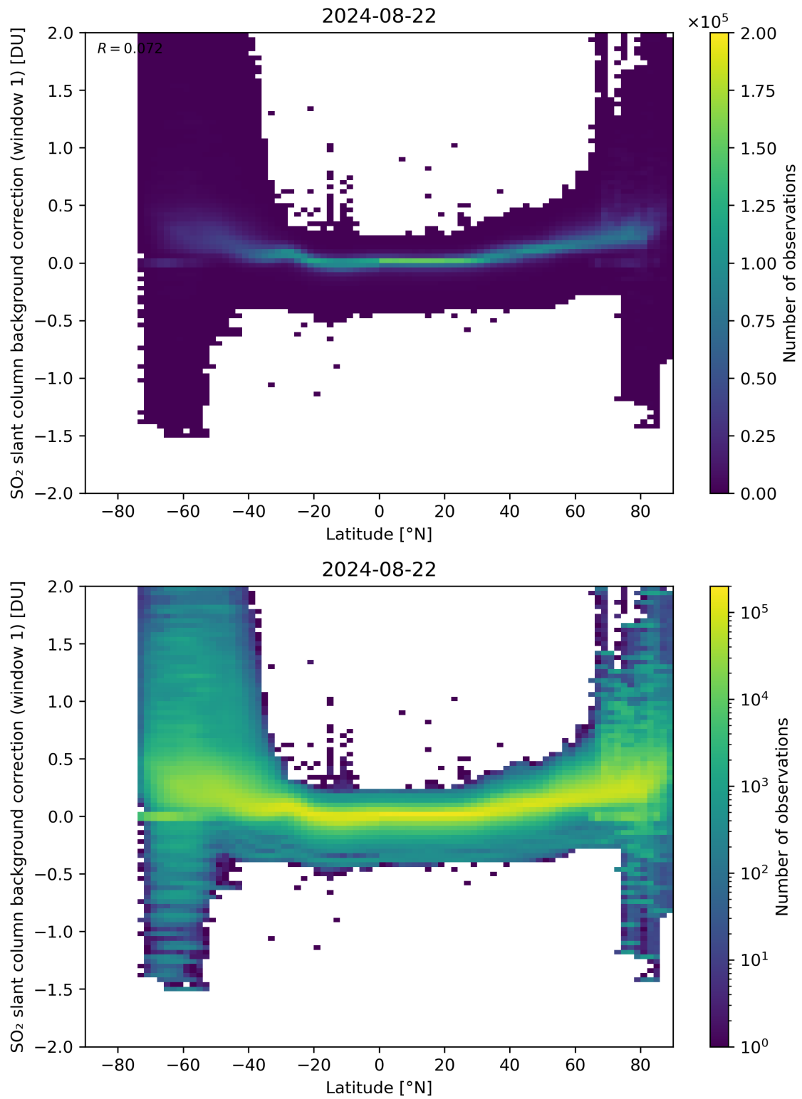
Figure 139: Scatter density plot of “Latitude” against “SO 2 slant column background correction (window 1)” for 2024-08-22 to 2024-08-23.
