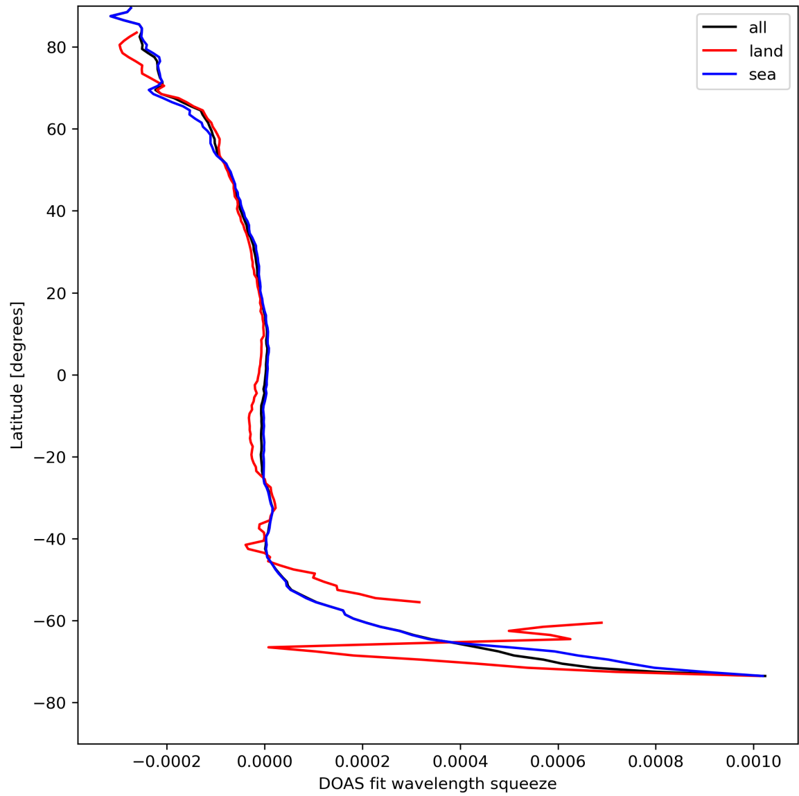
Figure 46: Zonal average of “DOAS fit wavelength squeeze” for 2024-08-22 to 2024-08-23.
