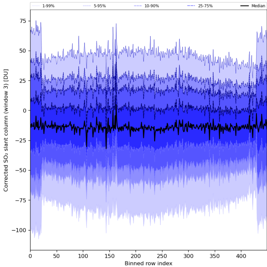
Figure 89: Along track statistics of “Corrected SO 2 slant column (window 3)” for 2024-08-22 to 2024-08-23
