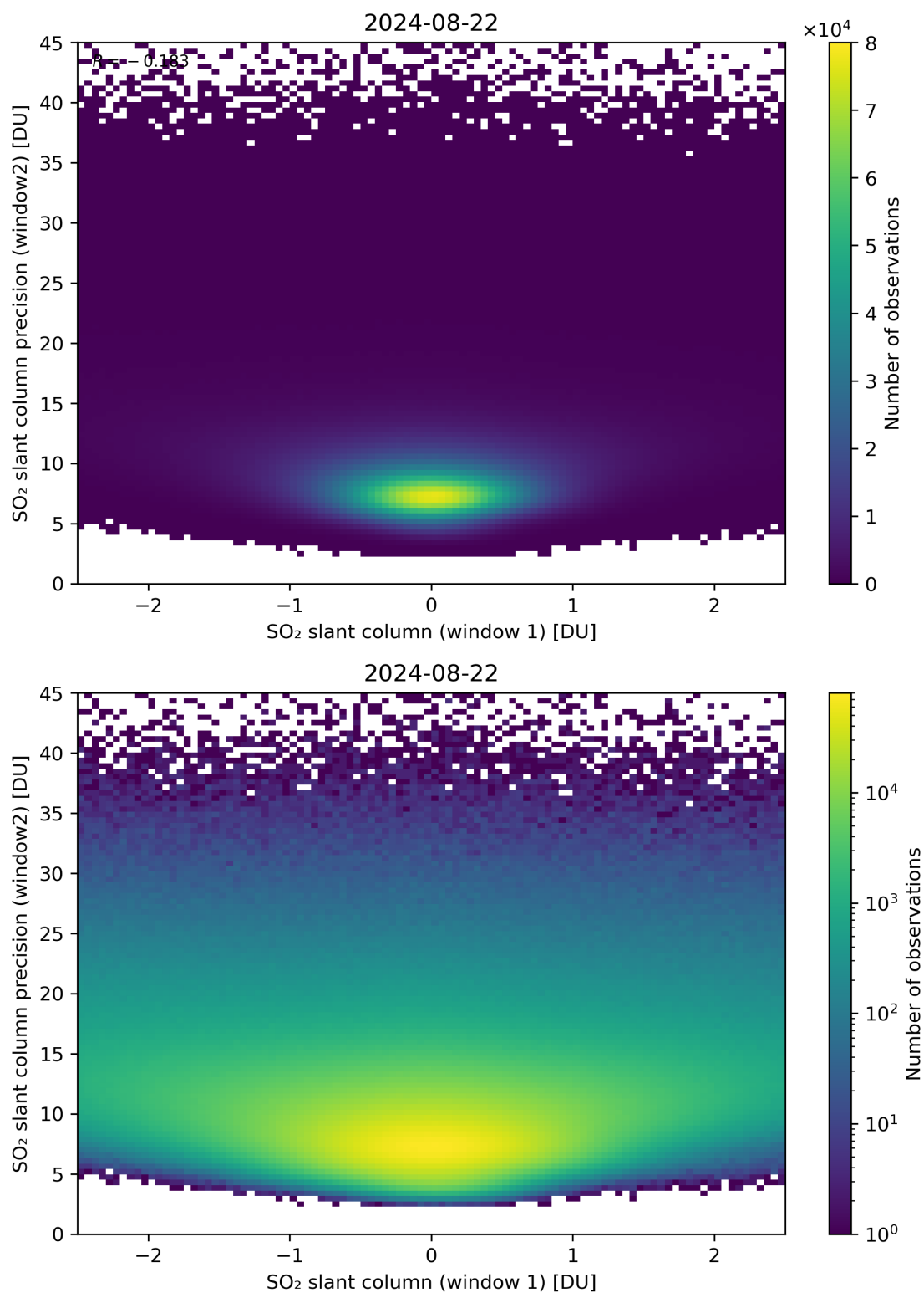
Figure 236: Scatter density plot of “SO 2 slant column (window 1)” against “SO 2 slant column precision (window2)” for 2024-08-22 to 2024-08-23.
