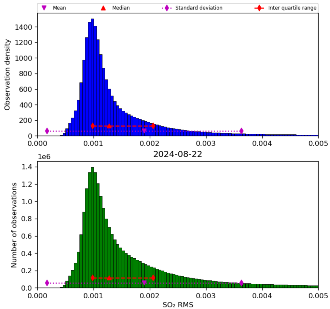
Figure 70: Histogram of “SO 2 RMS” for 2024-08-22 to 2024-08-23
