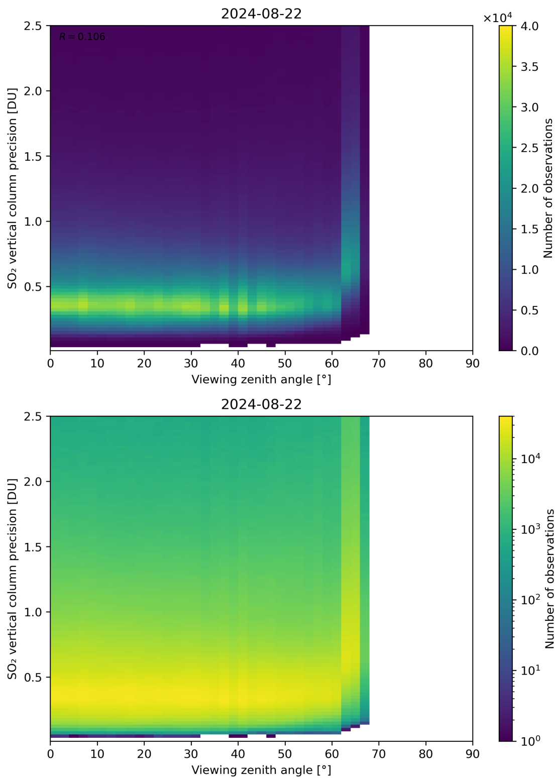
Figure 328: Scatter density plot of “Viewing zenith angle” against “SO 2 vertical column precision” for 2024-08-22 to 2024-08-23.
