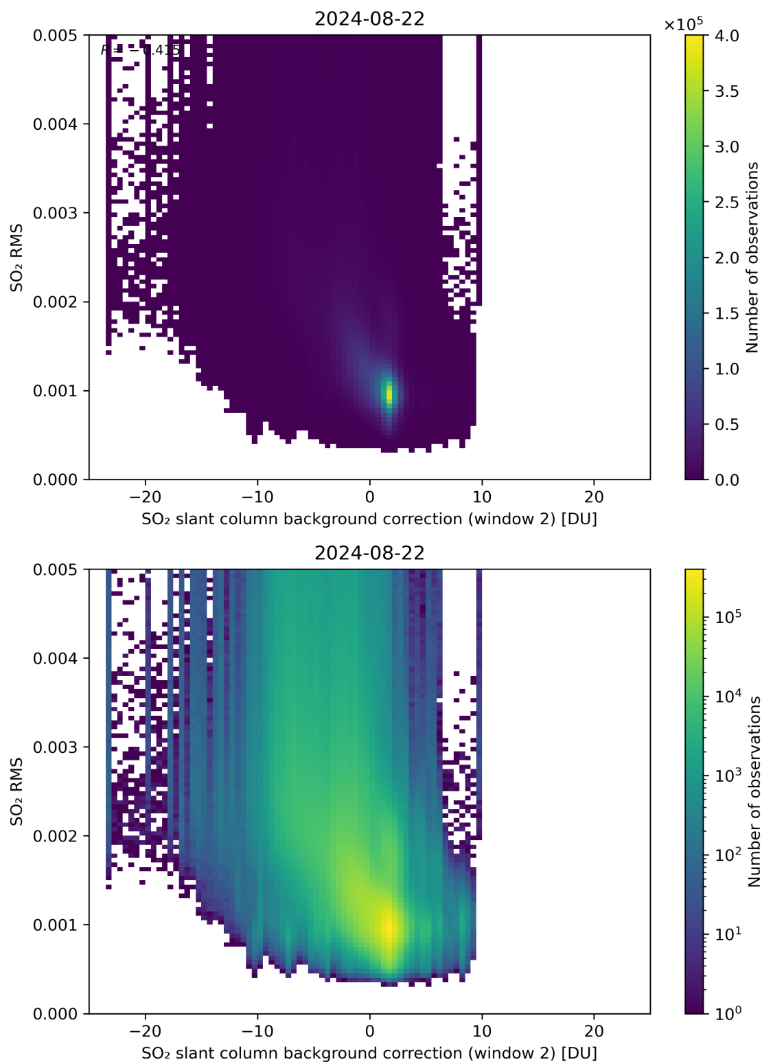
Figure 114: Scatter density plot of “SO 2 slant column background correction (window 2)” against “SO 2 RMS” for 2024-08-22 to 2024-08-23.
