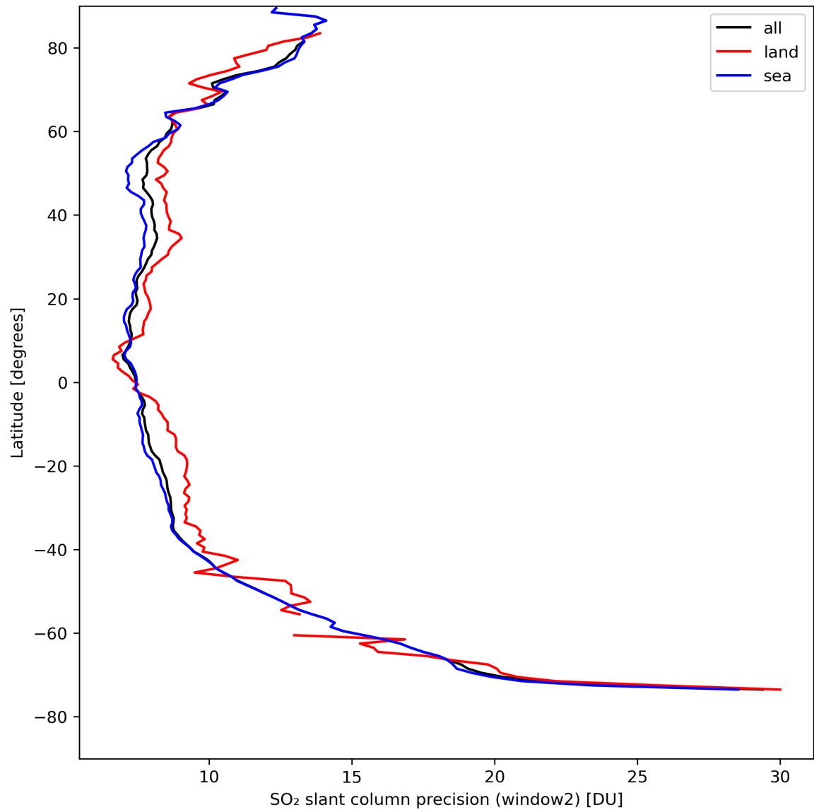
Figure 38: Zonal average of “SO 2 slant column precision (window2)” for 2024-08-22 to 2024-08-23.
