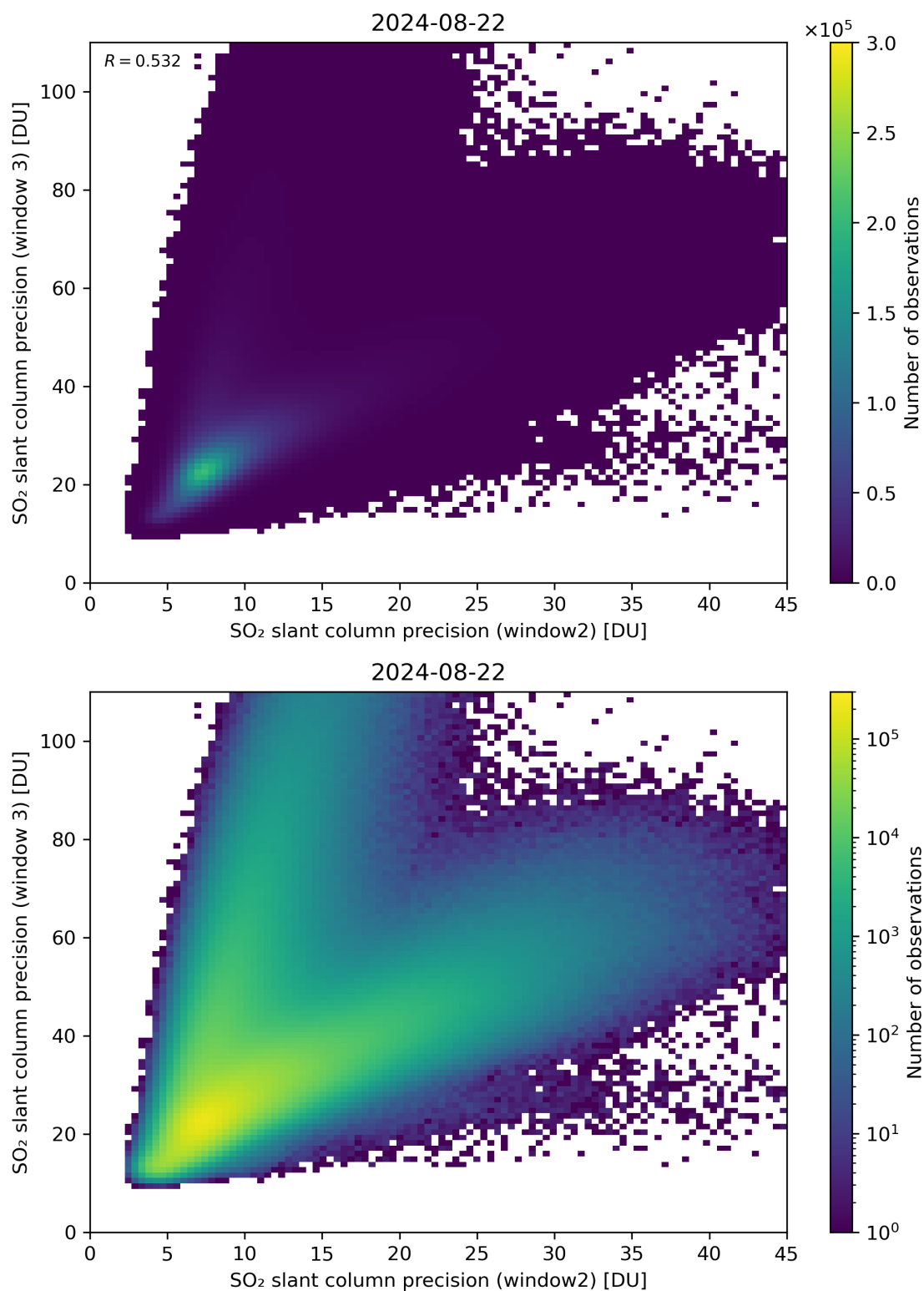
Figure 250: Scatter density plot of “SO 2 slant column precision (window2)” against “SO 2 slant column precision (window 3)” for 2024-08-22 to 2024-08-23.
