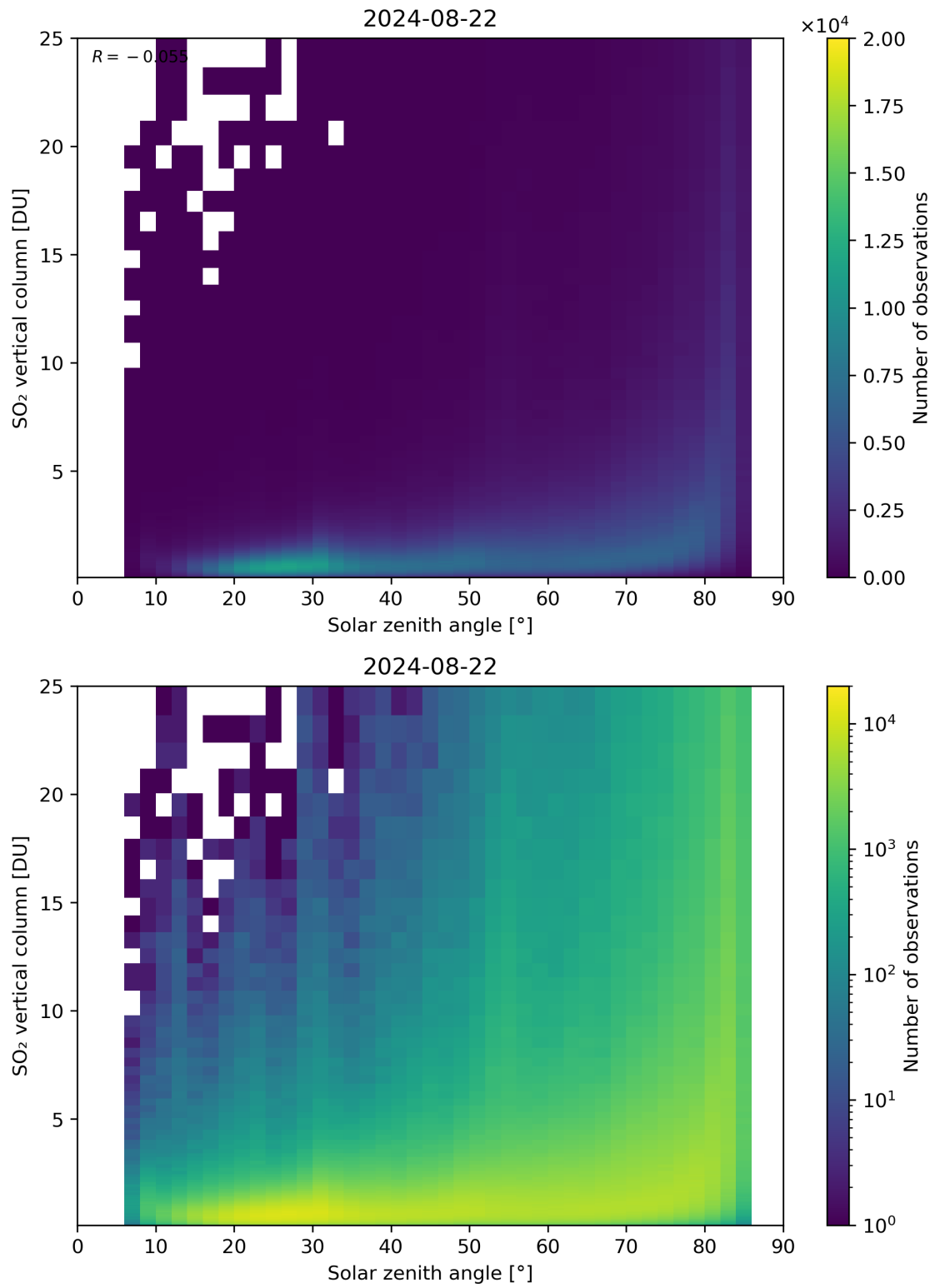
Figure 176: Scatter density plot of “Solar zenith angle” against “SO 2 vertical column” for 2024-08-22 to 2024-08-23.
