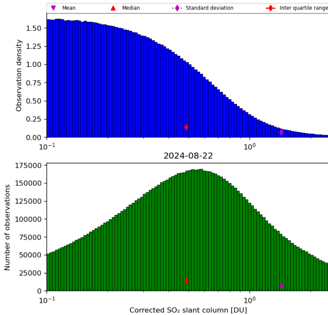
Figure 55: Histogram of “Corrected SO 2 slant column” for 2024-08-22 to 2024-08-23
