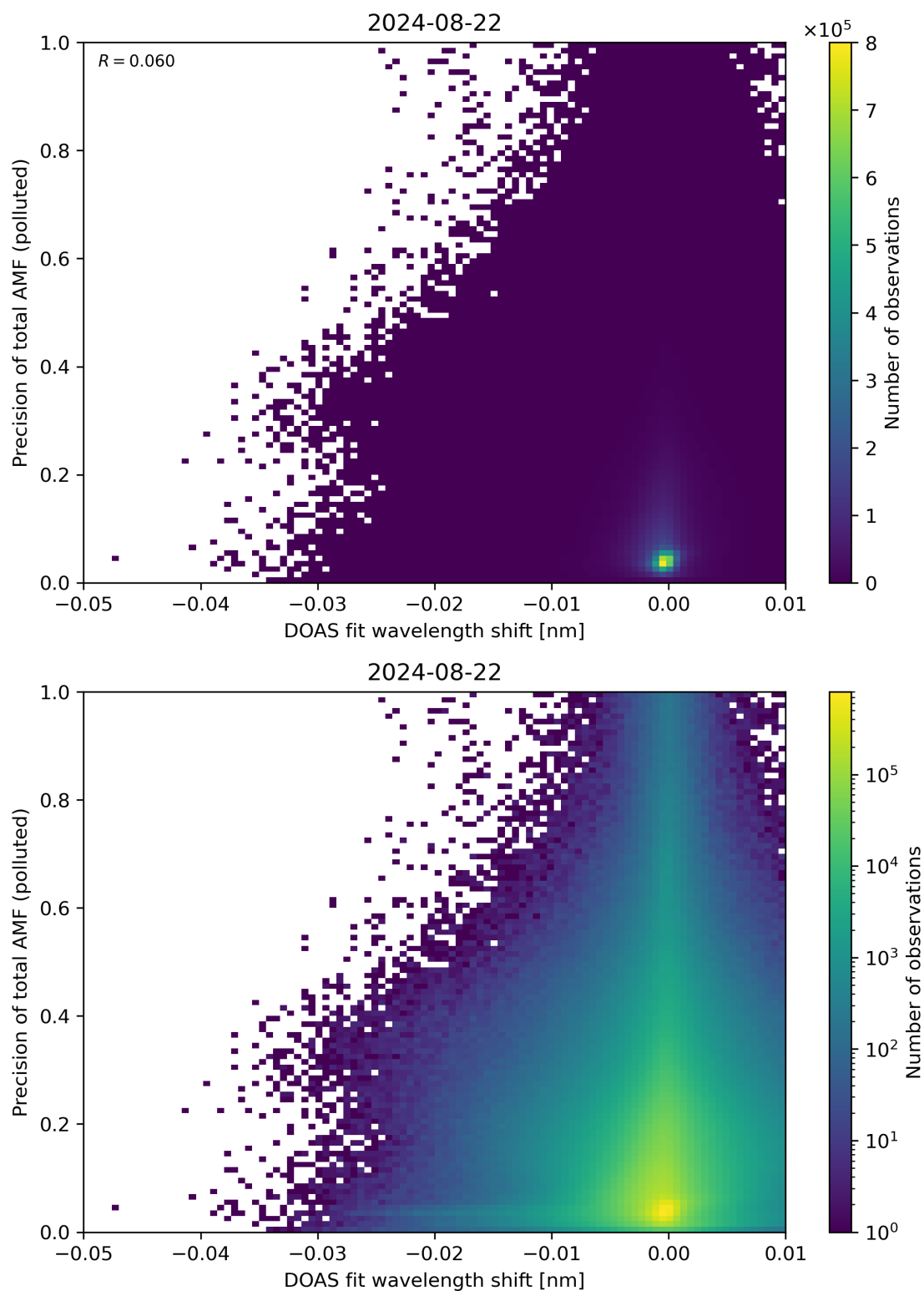
Figure 131: Scatter density plot of “DOAS fit wavelength shift” against “Precision of total AMF (polluted)” for 2024-08-22 to 2024-08-23.
