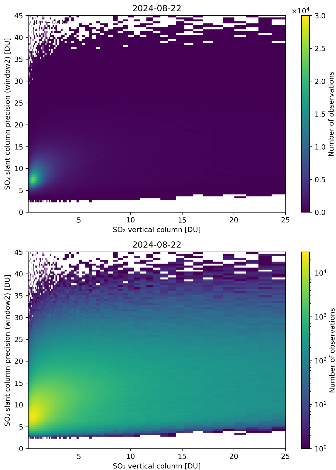
Figure 302: Scatter density plot of “SO 2 vertical column” against “SO 2 slant column precision (window2)” for 2024-08-22 to 2024-08-23.
