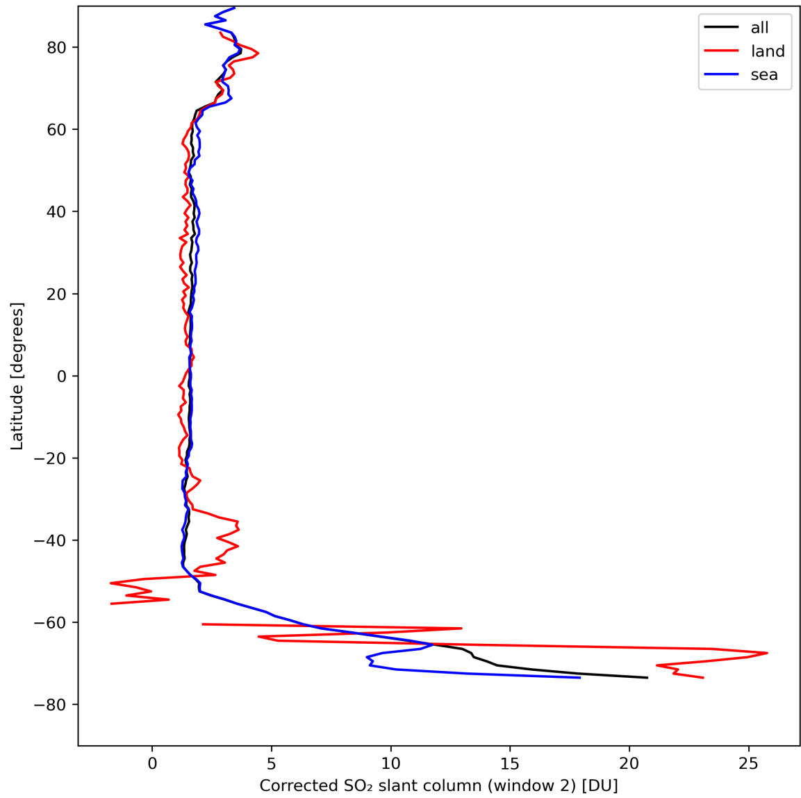
Figure 39: Zonal average of “Corrected SO 2 slant column (window 2)” for 2024-08-22 to 2024-08-23.
