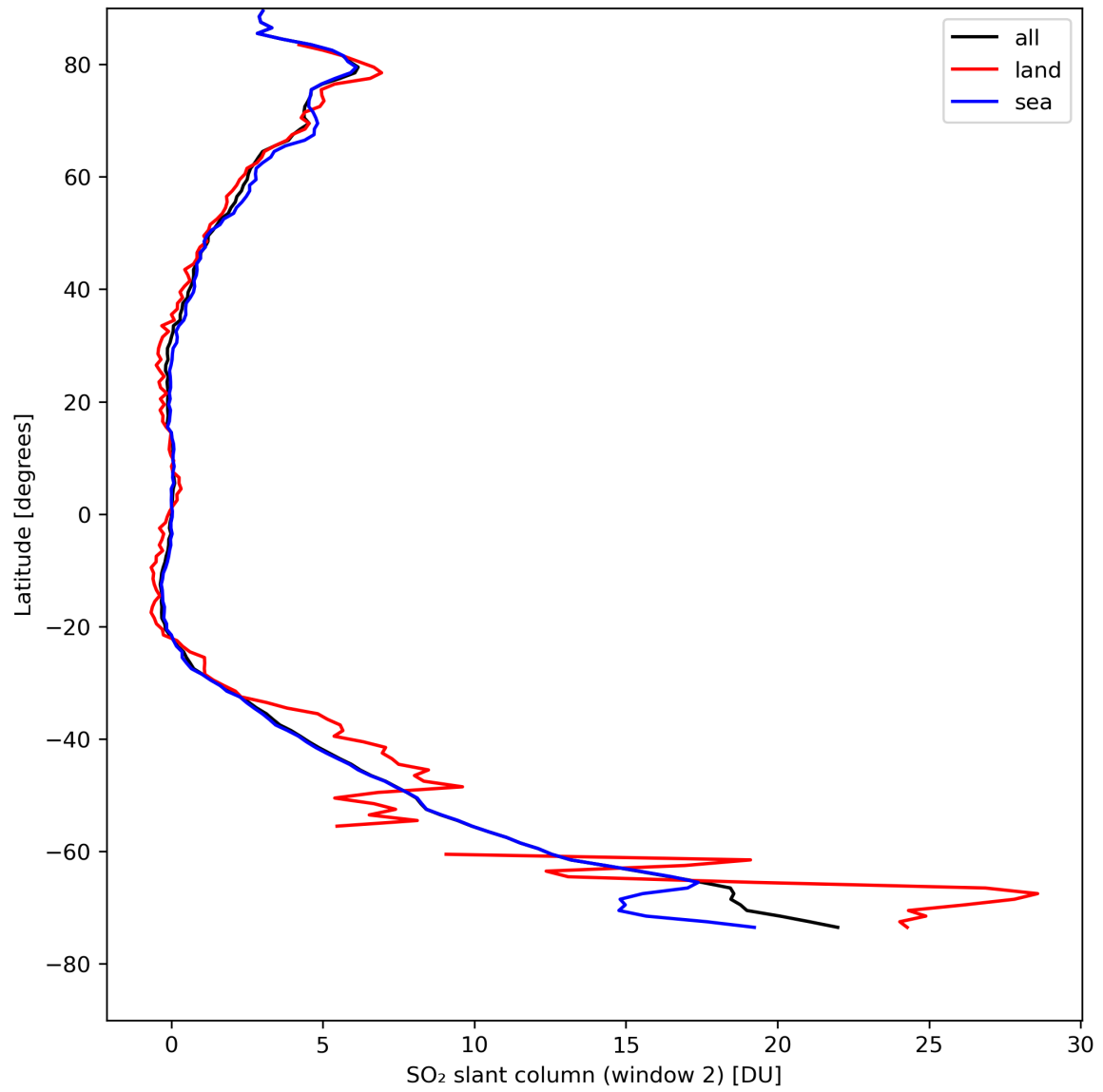
Figure 37: Zonal average of “SO 2 slant column (window 2)” for 2024-08-22 to 2024-08-23.
