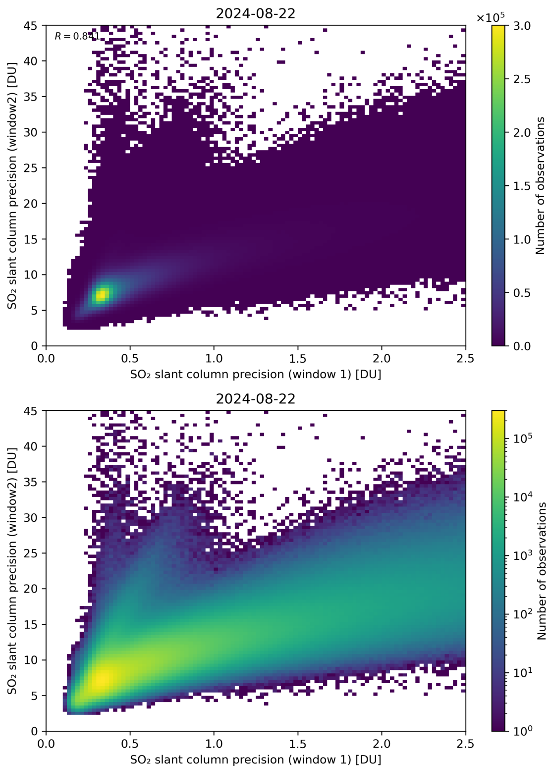
Figure 227: Scatter density plot of “SO 2 slant column precision (window 1)” against “SO 2 slant column precision (window2)” for 2024-08-22 to 2024-08-23.
