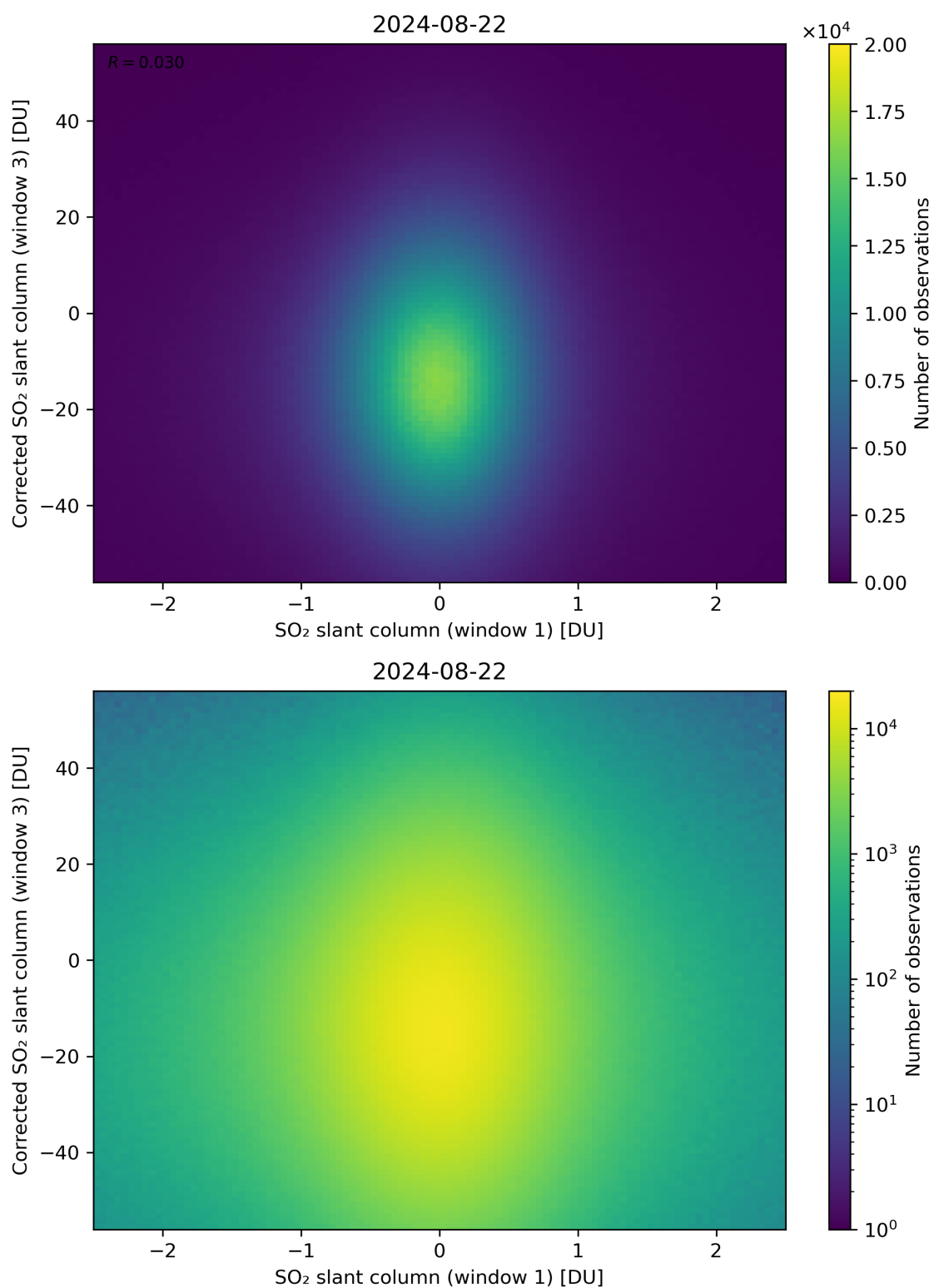
Figure 234: Scatter density plot of “SO 2 slant column (window 1)” against “Corrected SO 2 slant column (window 3)” for 2024-08-22 to 2024-08-23.
