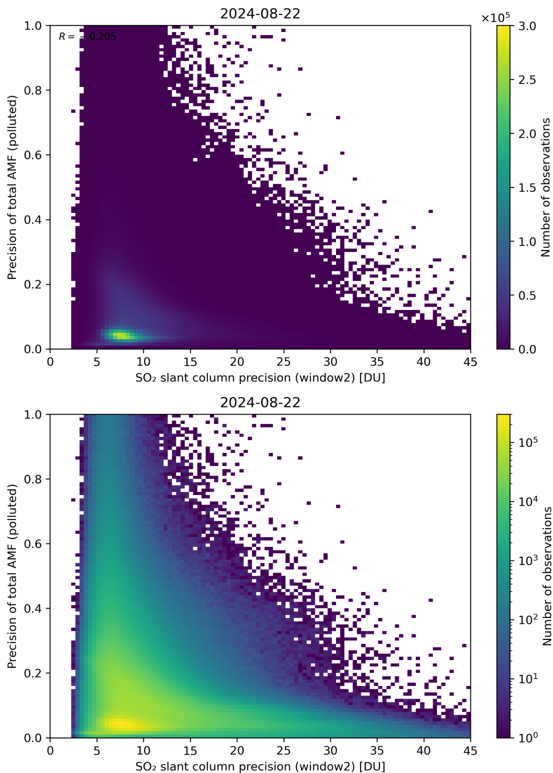
Figure 252: Scatter density plot of “SO 2 slant column precision (window2)” against “Precision of total AMF (polluted)” for 2024-08-22 to 2024-08-23.
