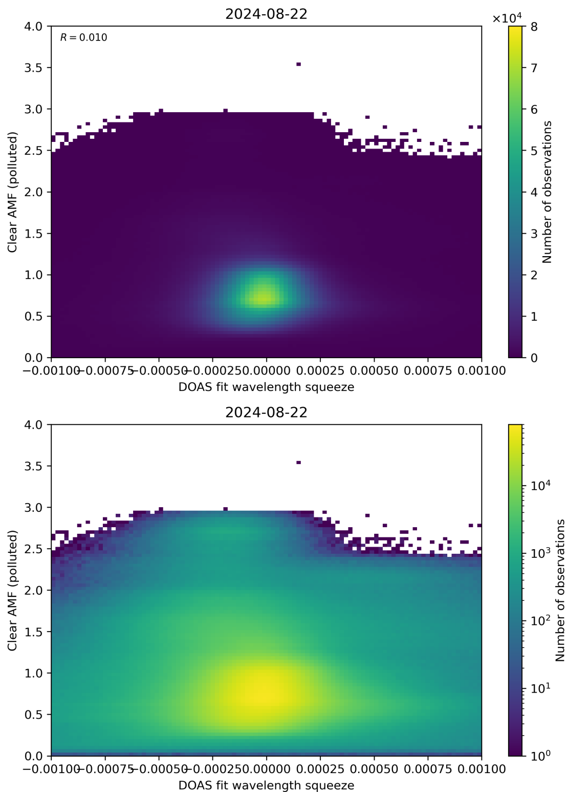
Figure 133: Scatter density plot of “DOAS fit wavelength squeeze” against “Clear AMF (polluted)” for 2024-08-22 to 2024-08-23.
