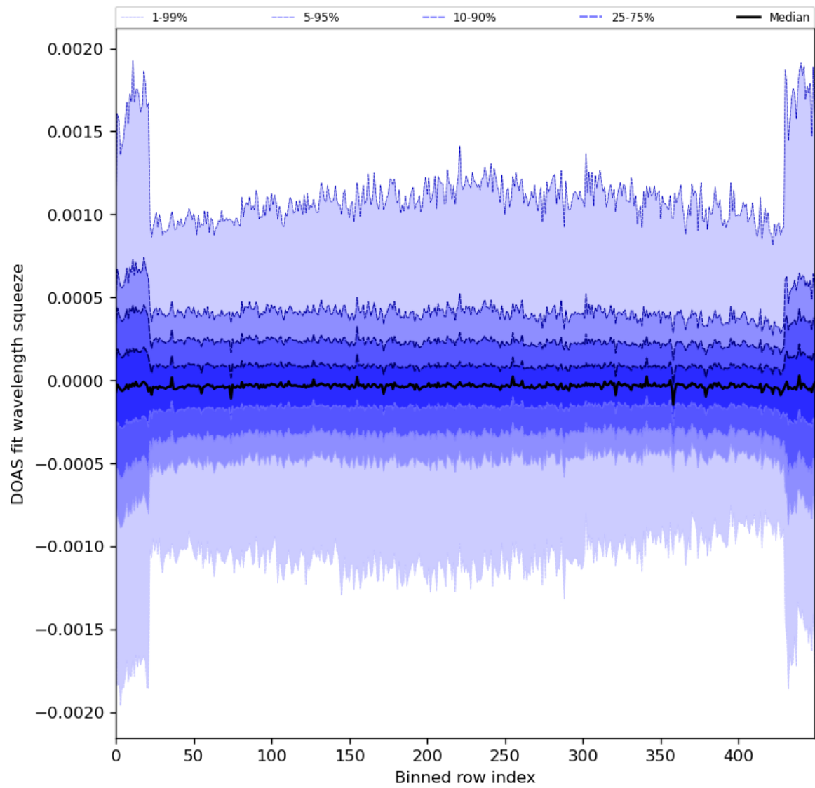
Figure 92: Along track statistics of “DOAS fit wavelength squeeze” for 2024-08-22 to 2024-08-23
