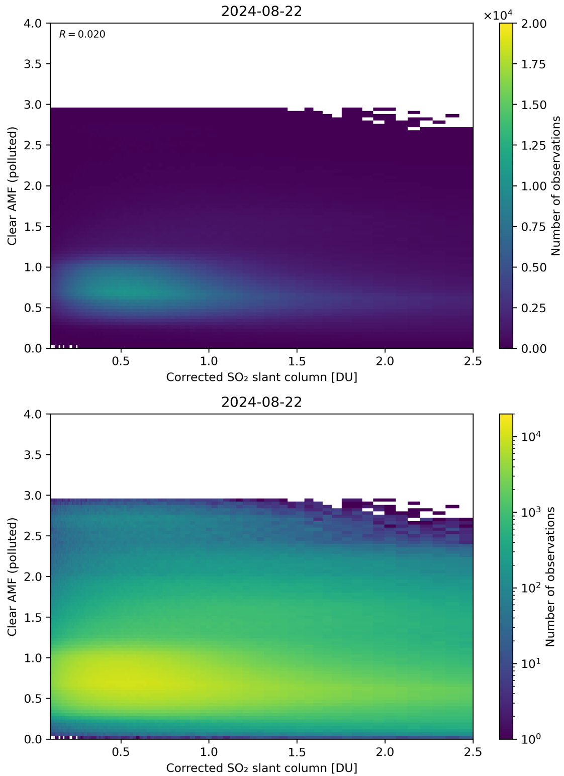
Figure 184: Scatter density plot of “Corrected SO 2 slant column” against “Clear AMF (polluted)” for 2024-08-22 to 2024-08-23.
