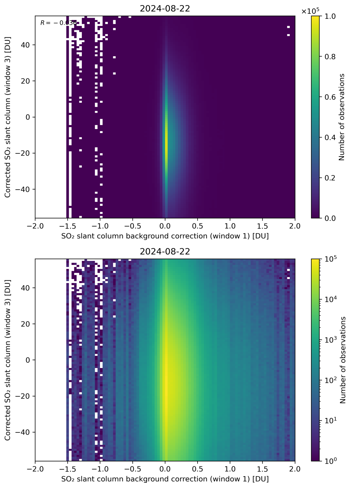
Figure 105: Scatter density plot of “SO 2 slant column background correction (window 1)” against “Corrected SO 2 slant column (window 3)” for 2024-08-22 to 2024-08-23.
