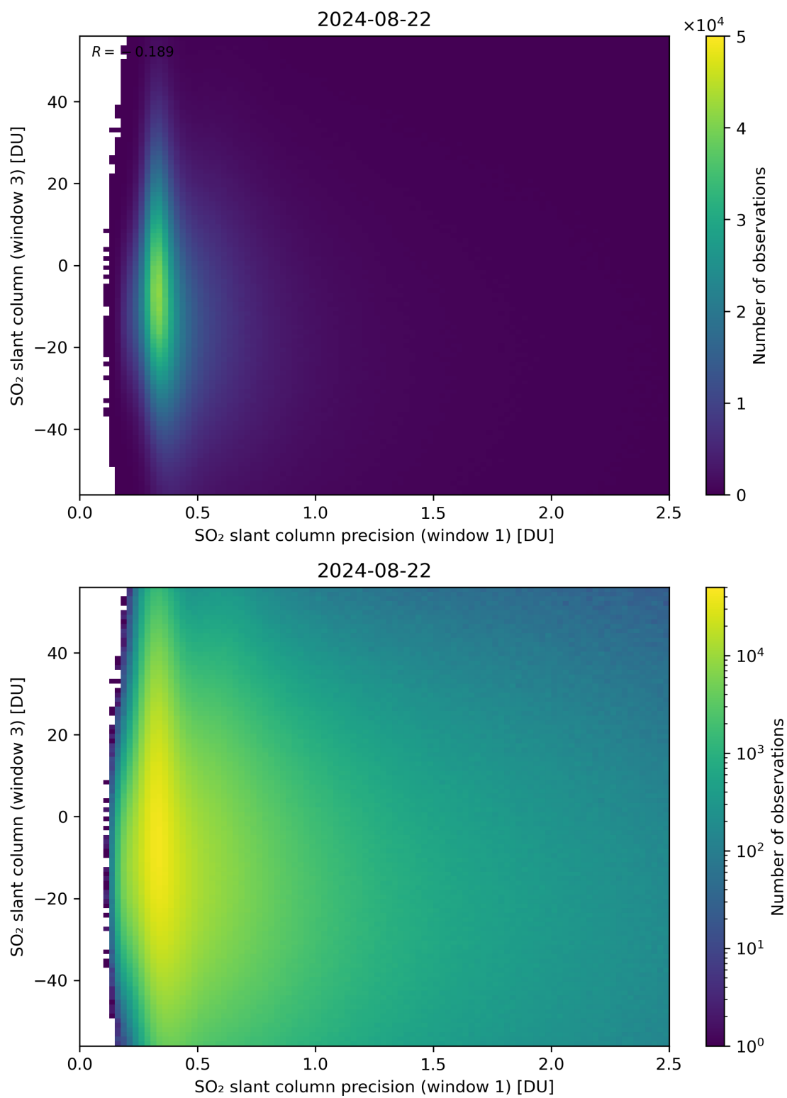
Figure 228: Scatter density plot of “SO 2 slant column precision (window 1)” against “SO 2 slant column (window 3)” for 2024-08-22 to 2024-08-23.
