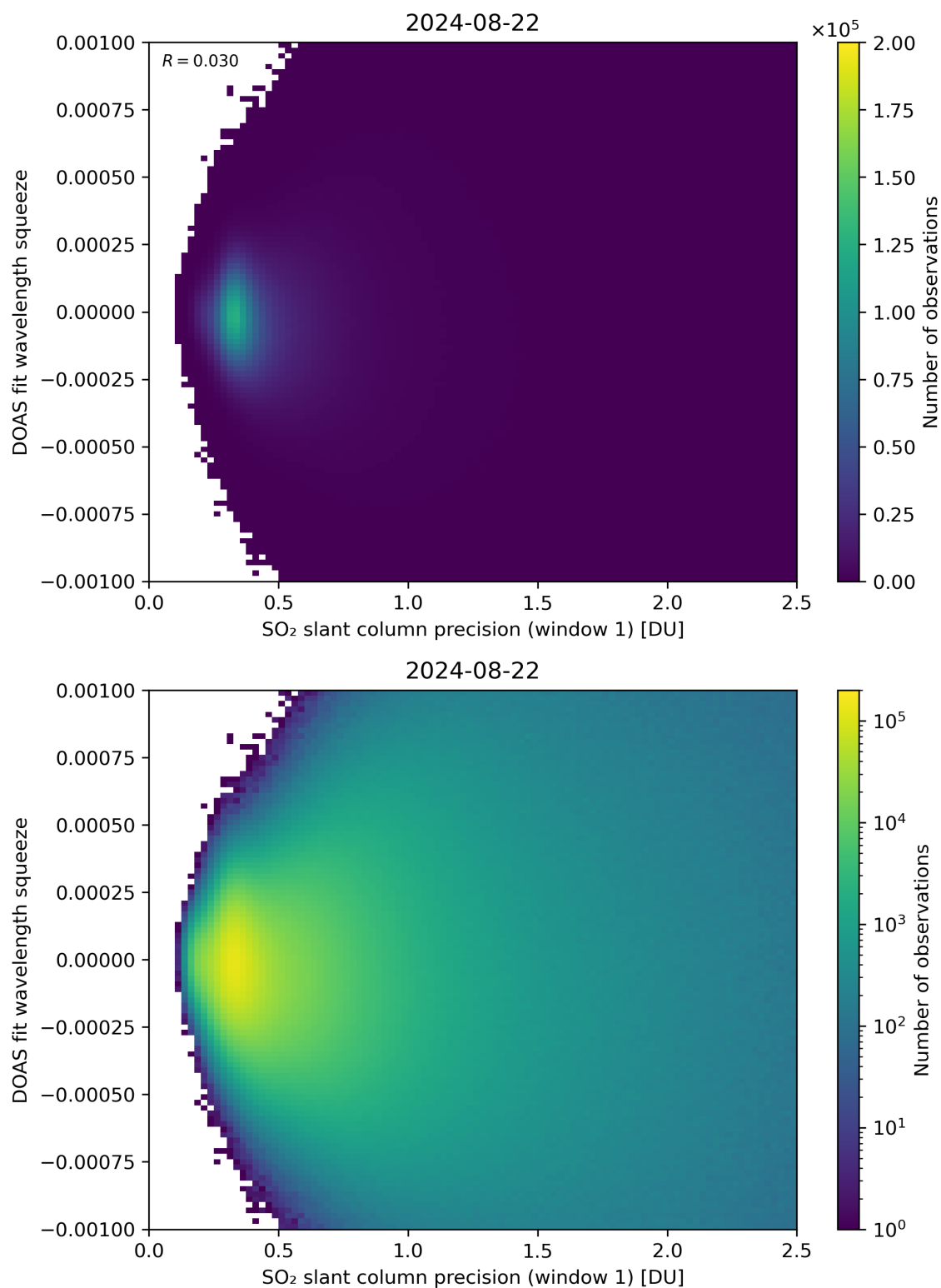
Figure 222: Scatter density plot of “SO 2 slant column precision (window 1)” against “DOAS fit wavelength squeeze” for 2024-08-22 to 2024-08-23.
