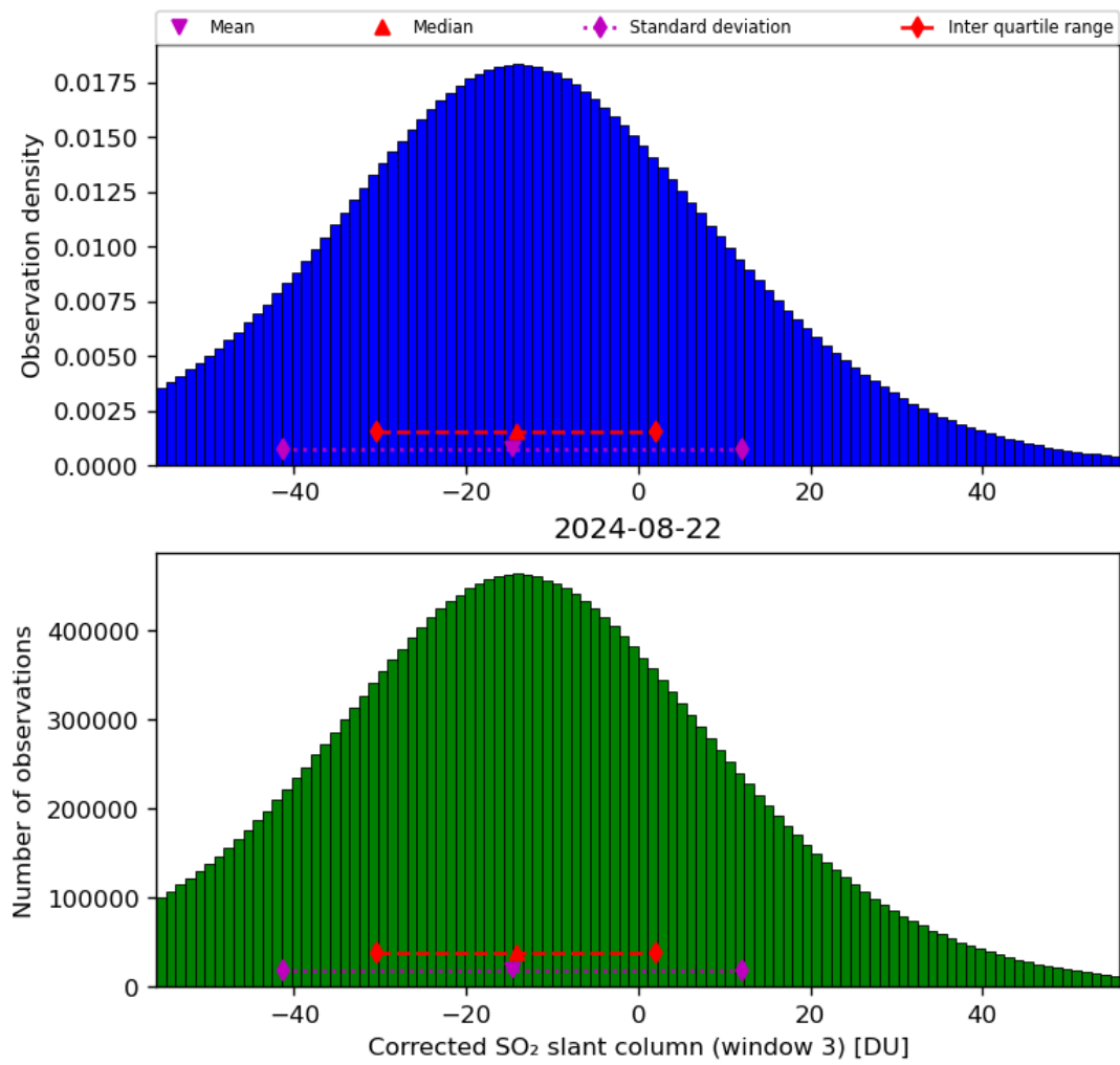
Figure 66: Histogram of “Corrected SO 2 slant column (window 3)” for 2024-08-22 to 2024-08-23
