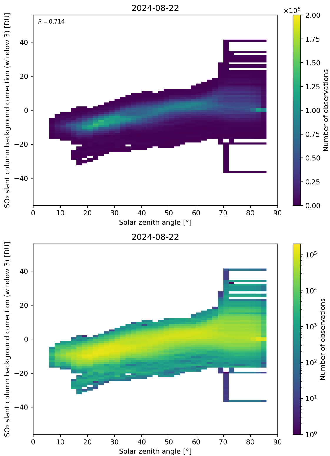
Figure 160: Scatter density plot of “Solar zenith angle” against “SO 2 slant column background correction (window 3)” for 2024-08-22 to 2024-08-23.
