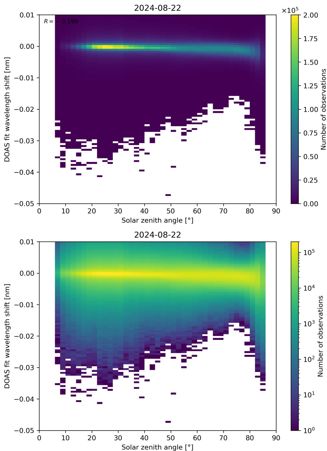
Figure 161: Scatter density plot of “Solar zenith angle” against “DOAS fit wavelength shift” for 2024-08-22 to 2024-08-23.
