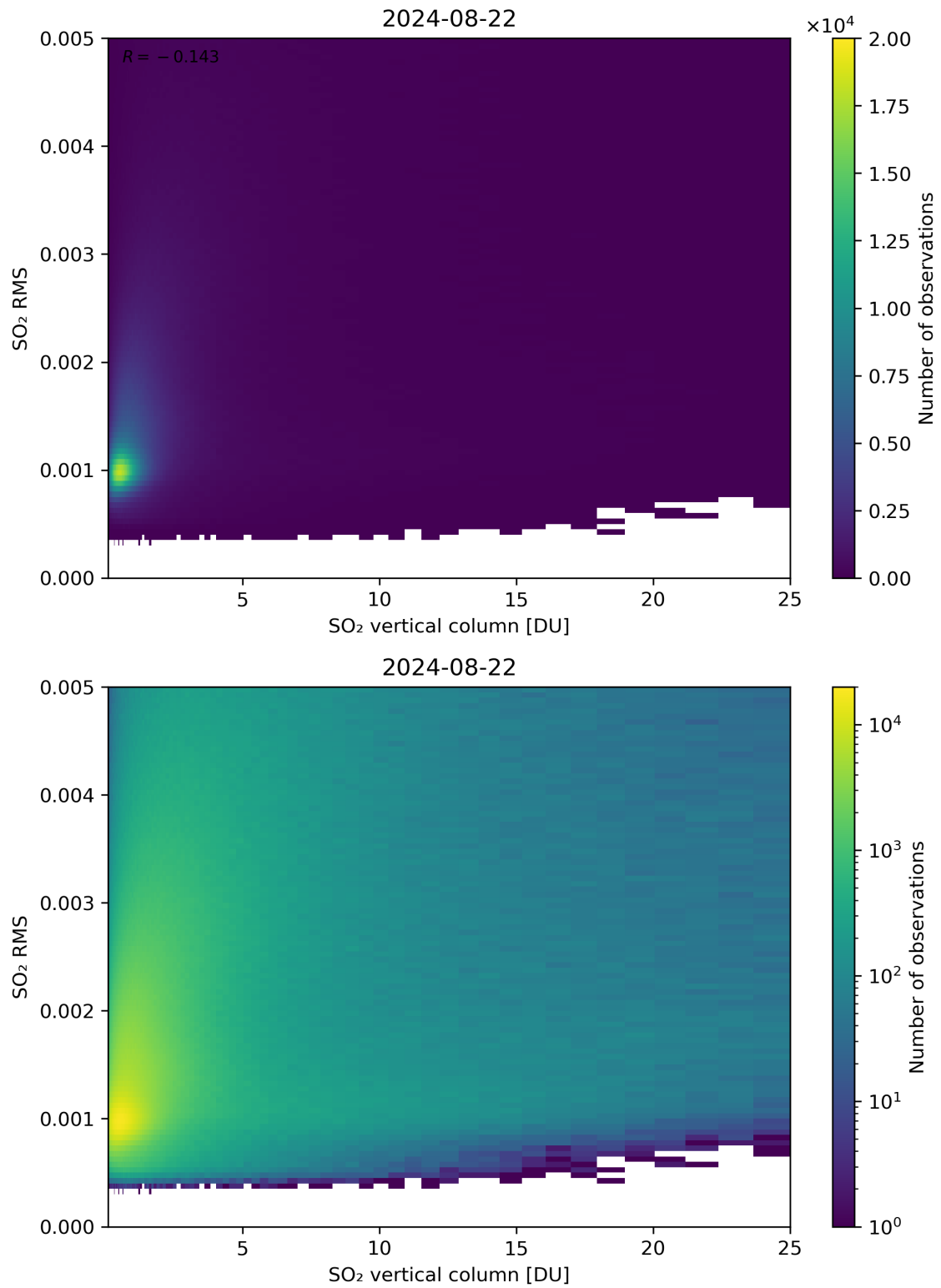
Figure 278: Scatter density plot of “SO 2 vertical column” against “SO 2 RMS” for 2024-08-22 to 2024-08-23.
