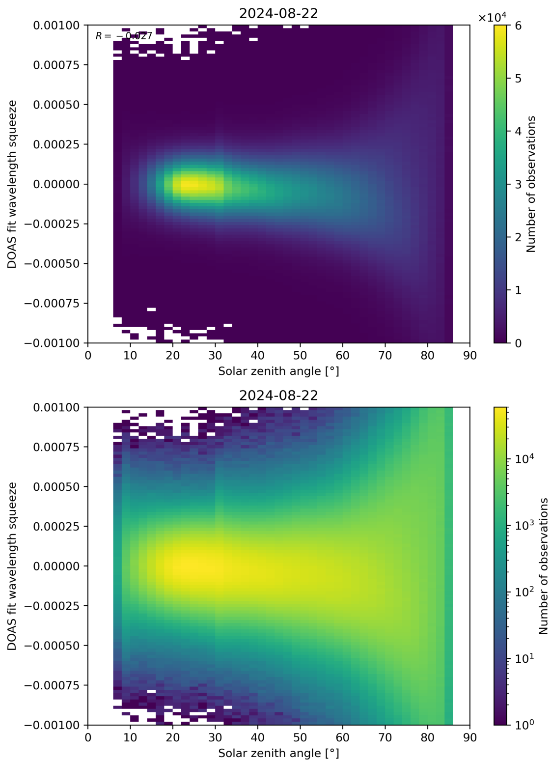
Figure 162: Scatter density plot of “Solar zenith angle” against “DOAS fit wavelength squeeze” for 2024-08-22 to 2024-08-23.
