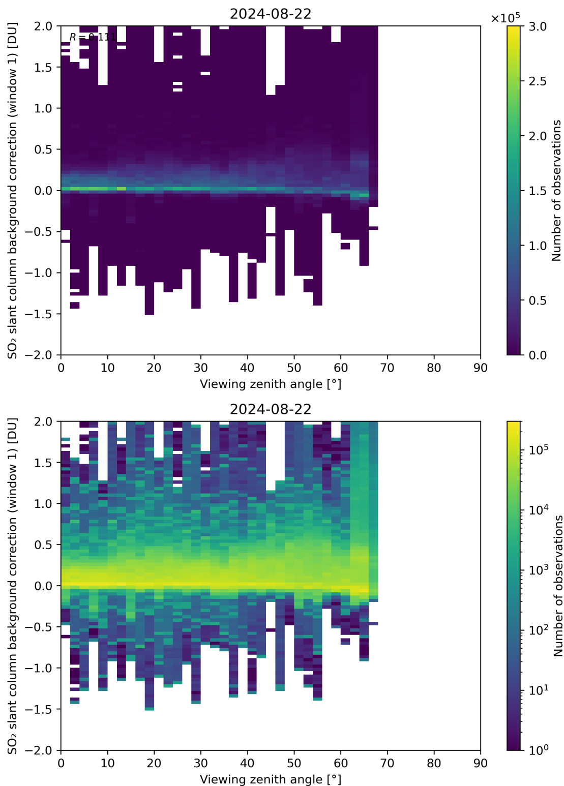
Figure 308: Scatter density plot of “Viewing zenith angle” against “SO 2 slant column background correction (window 1)” for 2024-08-22 to 2024-08-23.
