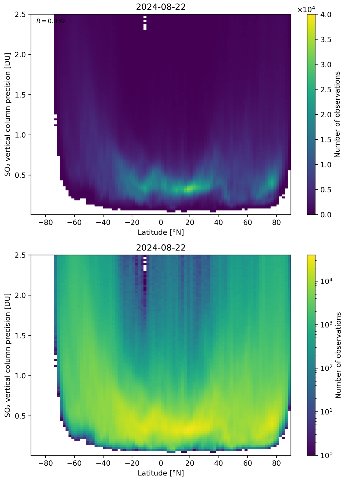
Figure 157: Scatter density plot of “Latitude” against “SO 2 vertical column precision” for 2024-08-22 to 2024-08-23.
