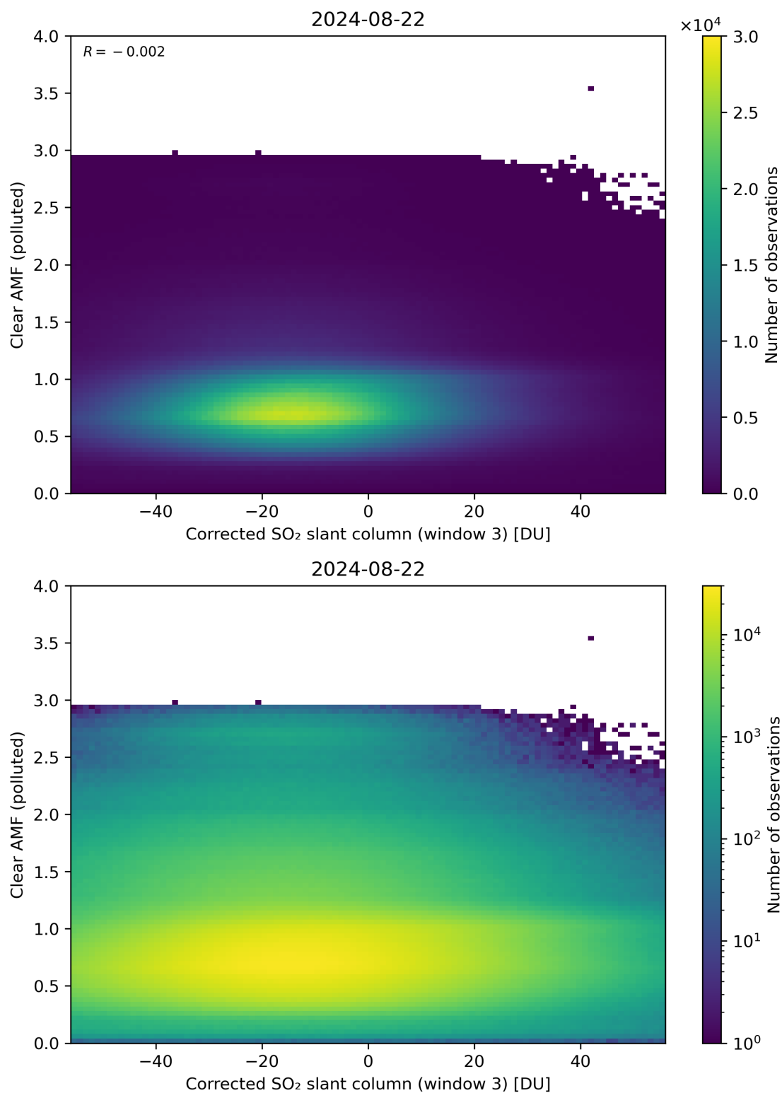
Figure 209: Scatter density plot of “Corrected SO 2 slant column (window 3)” against “Clear AMF (polluted)” for 2024-08-22 to 2024-08-23.
