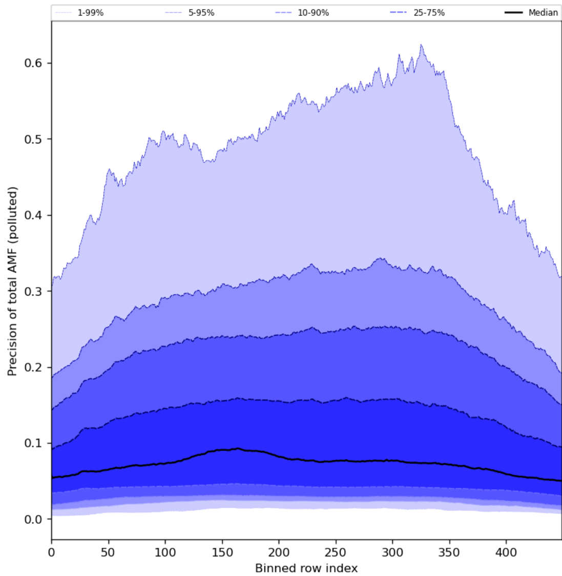
Figure 95: Along track statistics of “Precision of total AMF (polluted)” for 2024-08-22 to 2024-08-23
