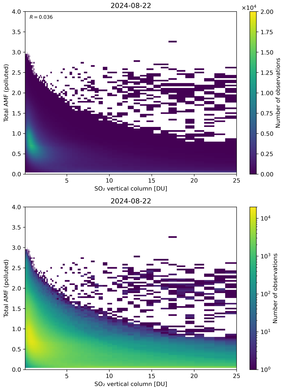
Figure 305: Scatter density plot of “SO 2 vertical column” against “Total AMF (polluted)” for 2024-08-22 to 2024-08-23.
