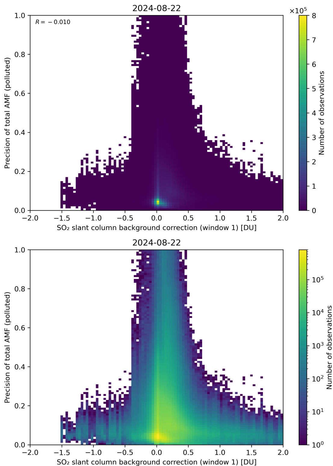
Figure 110: Scatter density plot of “SO 2 slant column background correction (window 1)” against “Precision of total AMF (polluted)” for 2024-08-22 to 2024-08-23.
