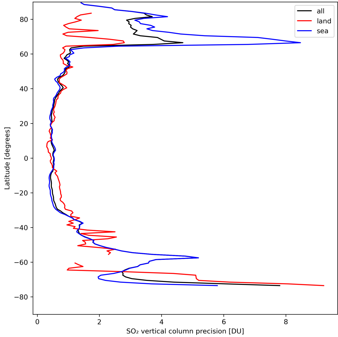
Figure 31: Zonal average of “SO 2 vertical column precision” for 2024-08-22 to 2024-08-23.
