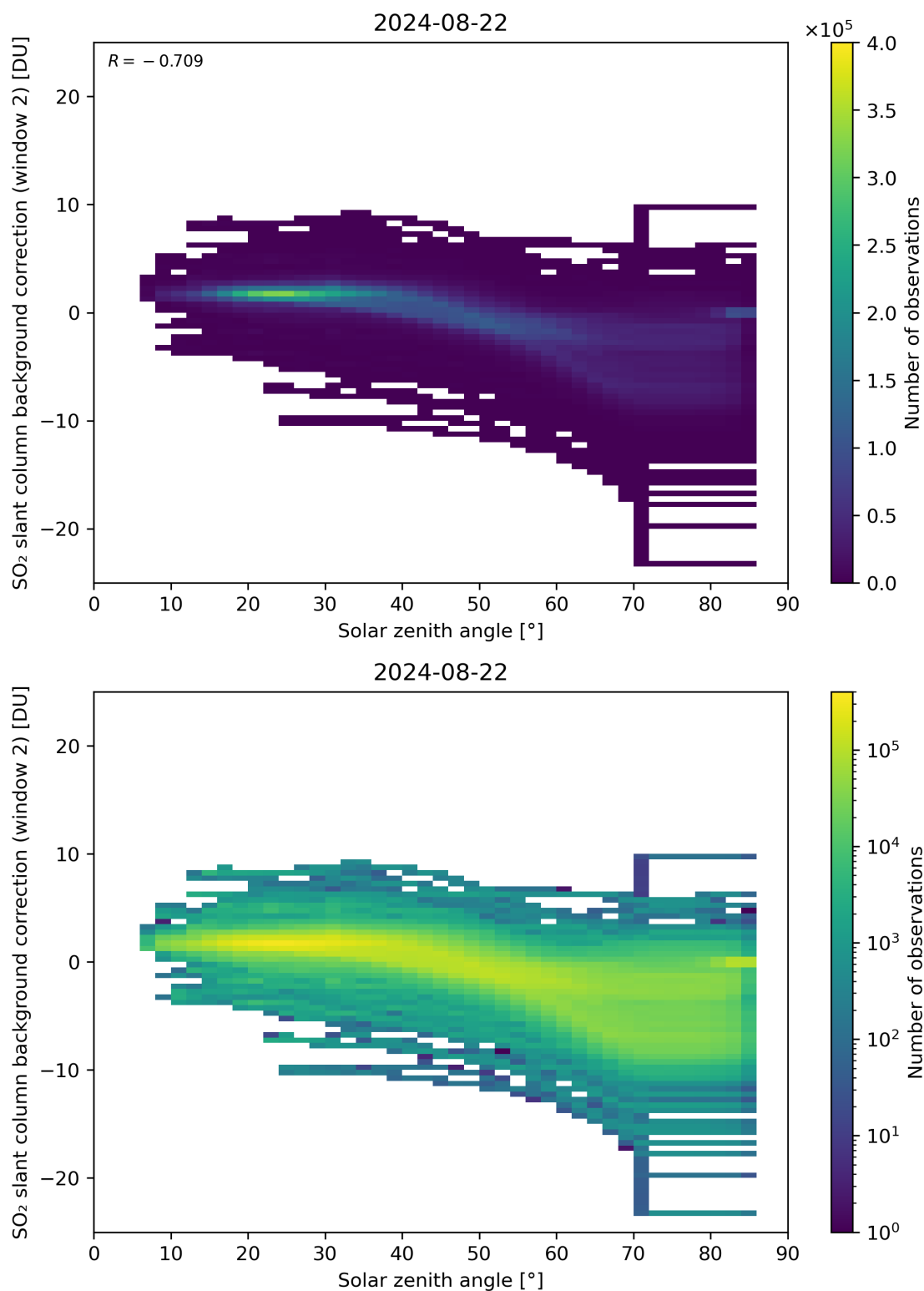
Figure 159: Scatter density plot of “Solar zenith angle” against “SO 2 slant column background correction (window 2)” for 2024-08-22 to 2024-08-23.
