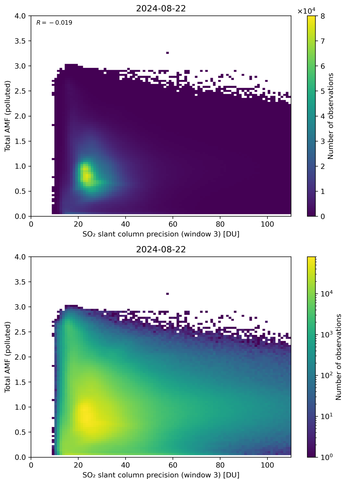
Figure 263: Scatter density plot of “SO 2 slant column precision (window 3)” against “Total AMF (polluted)” for 2024-08-22 to 2024-08-23.
