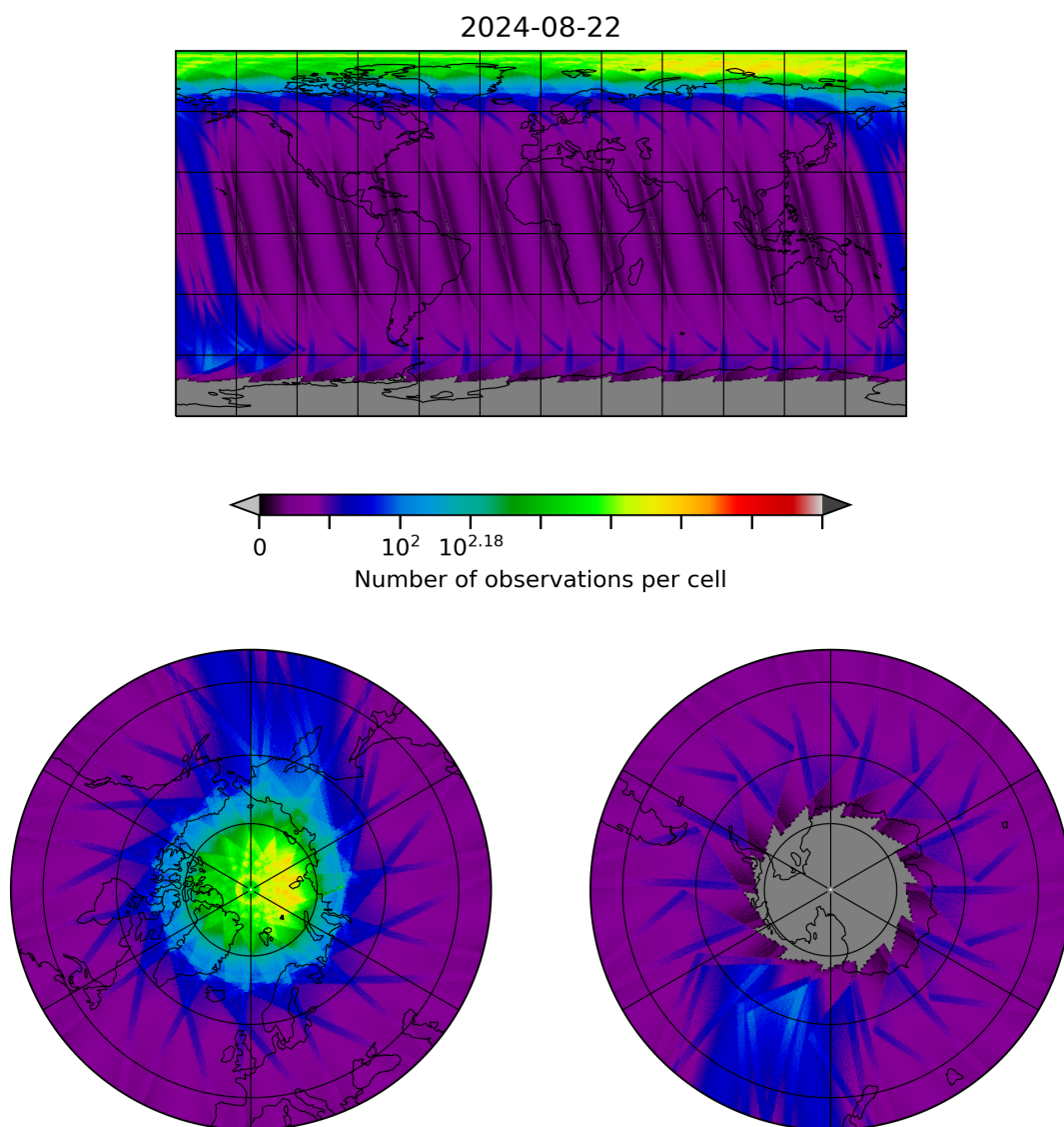
Figure 28: Map of the number of observations for 2024-08-22 to 2024-08-23
