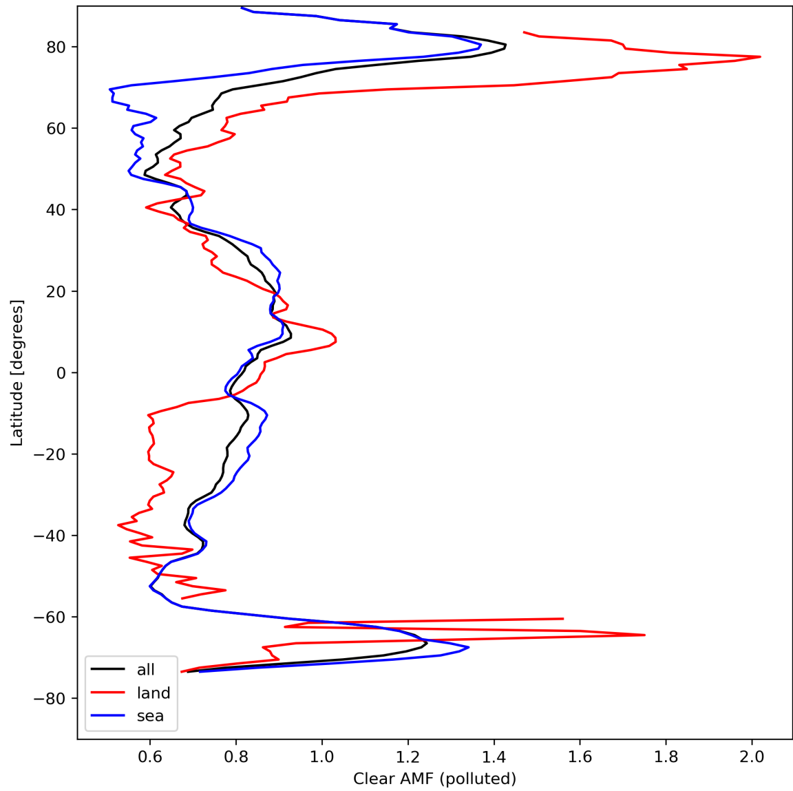
Figure 50: Zonal average of “Clear AMF (polluted)” for 2024-08-22 to 2024-08-23.
