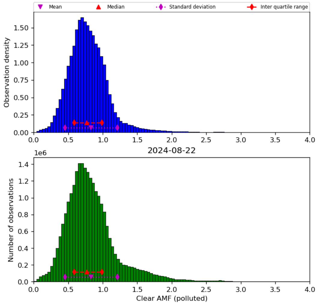
Figure 73: Histogram of “Clear AMF (polluted)” for 2024-08-22 to 2024-08-23
