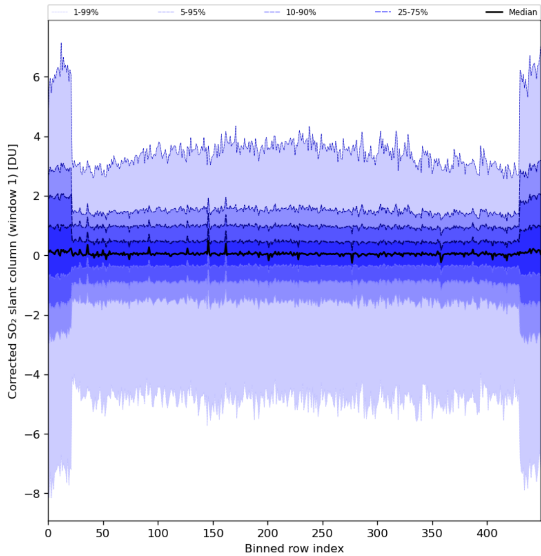
Figure 81: Along track statistics of “Corrected SO 2 slant column (window 1)” for 2024-08-22 to 2024-08-23
