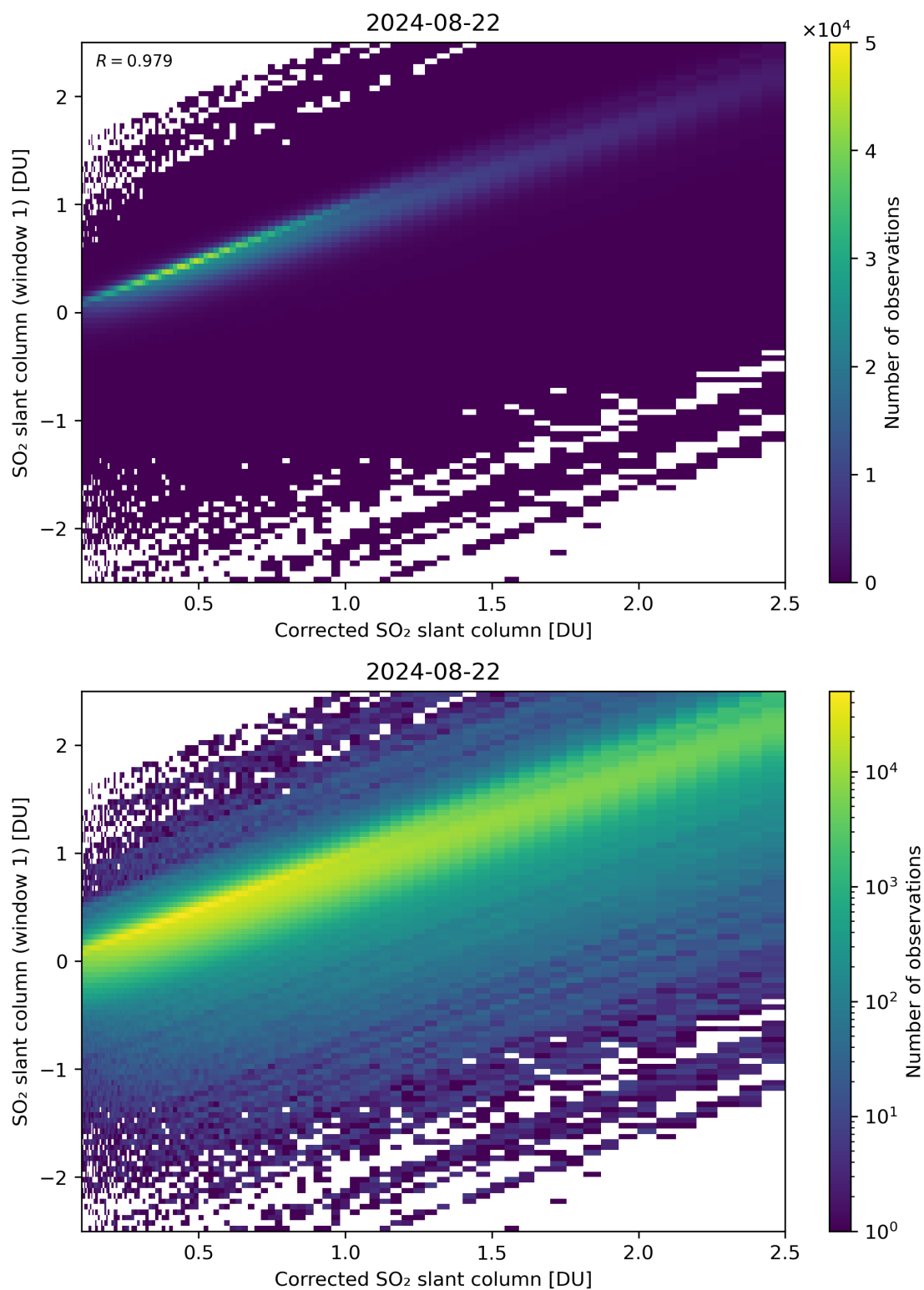
Figure 187: Scatter density plot of “Corrected SO 2 slant column” against “SO 2 slant column (window 1)” for 2024-08-22 to 2024-08-23.
