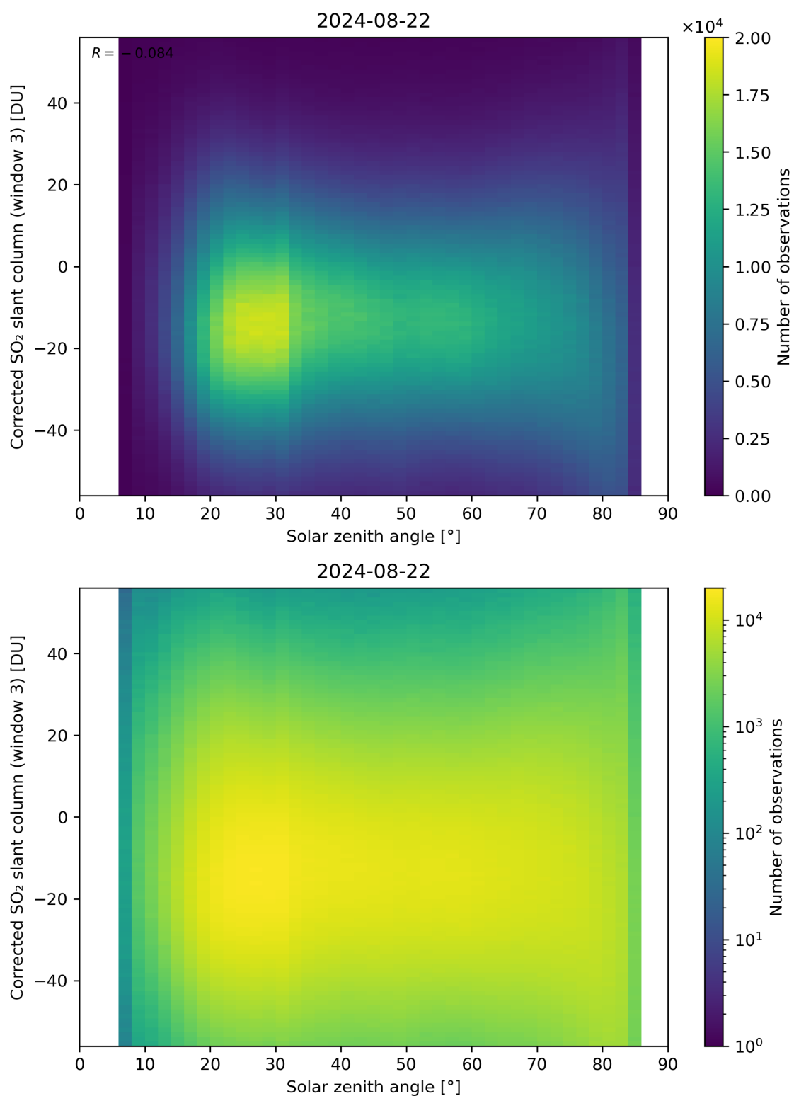
Figure 168: Scatter density plot of “Solar zenith angle” against “Corrected SO 2 slant column (window 3)” for 2024-08-22 to 2024-08-23.
