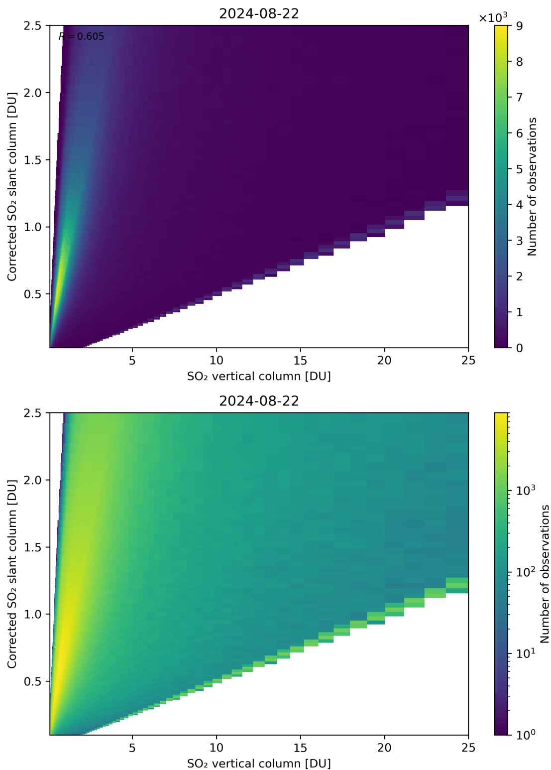
Figure 297: Scatter density plot of “SO 2 vertical column” against “Corrected SO 2 slant column” for 2024-08-22 to 2024-08-23.
