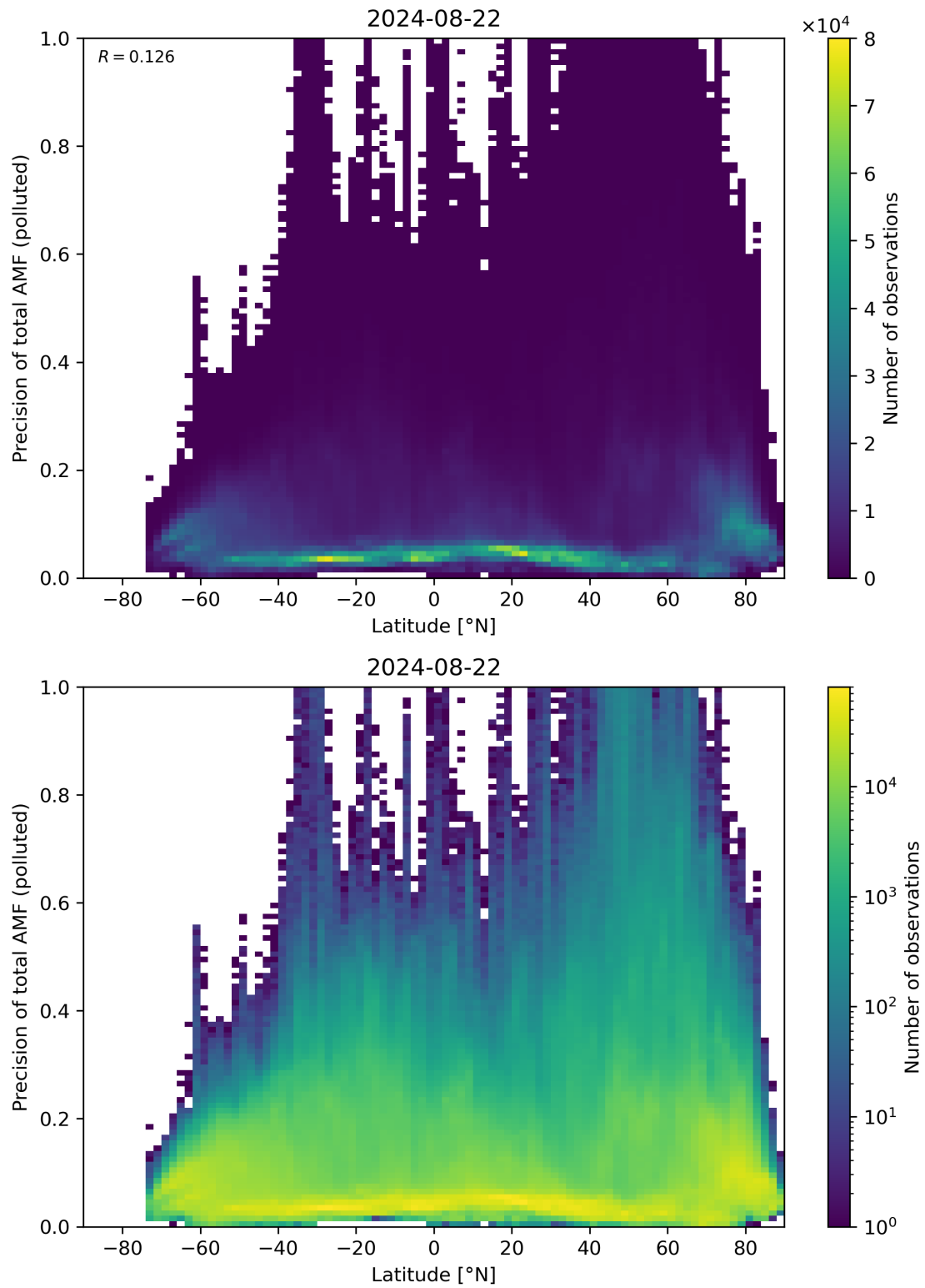
Figure 155: Scatter density plot of “Latitude” against “Precision of total AMF (polluted)” for 2024-08-22 to 2024-08-23.
