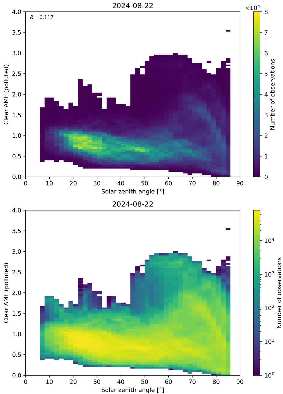
Figure 165: Scatter density plot of “Solar zenith angle” against “Clear AMF (polluted)” for 2024-08-22 to 2024-08-23.
