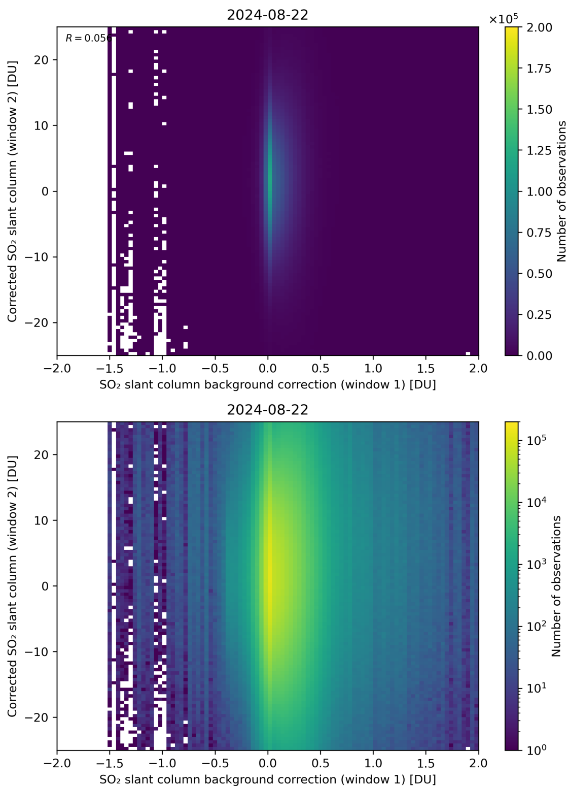
Figure 104: Scatter density plot of “SO 2 slant column background correction (window 1)” against “Corrected SO 2 slant column (window 2)” for 2024-08-22 to 2024-08-23.
