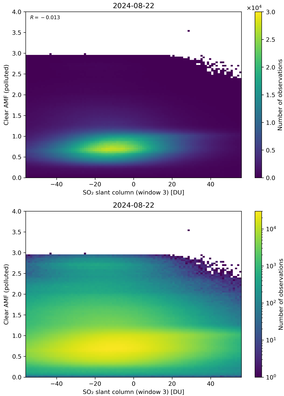
Figure 265: Scatter density plot of “SO 2 slant column (window 3)” against “Clear AMF (polluted)” for 2024-08-22 to 2024-08-23.
