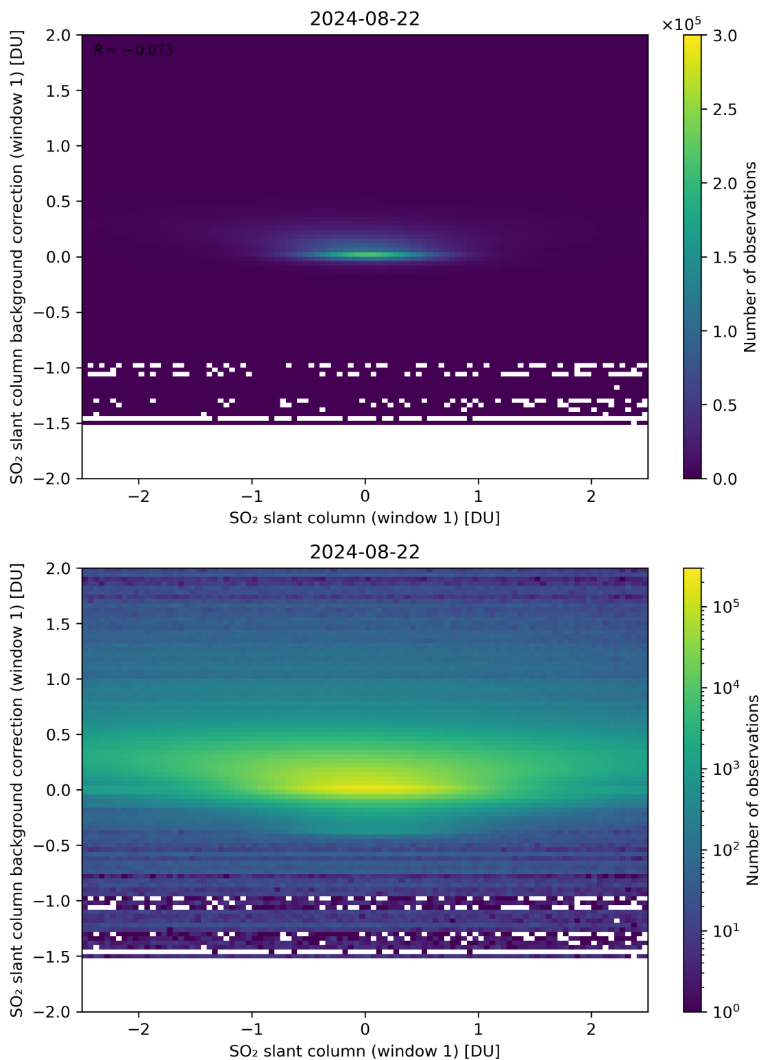
Figure 212: Scatter density plot of “SO 2 slant column (window 1)” against “SO 2 slant column background correction (window 1)” for 2024-08-22 to 2024-08-23.
