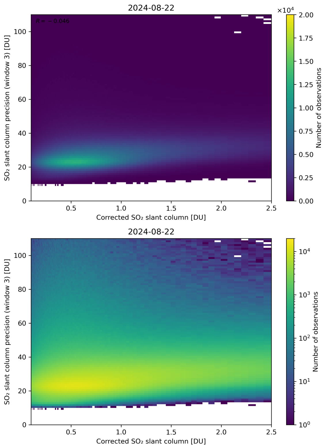
Figure 191: Scatter density plot of “Corrected SO 2 slant column” against “SO 2 slant column precision (window 3)” for 2024-08-22 to 2024-08-23.
