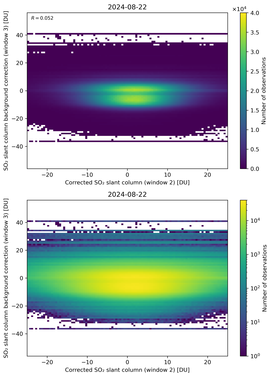
Figure 195: Scatter density plot of “Corrected SO 2 slant column (window 2)” against “SO 2 slant column background correction (window 3)” for 2024-08-22 to 2024-08-23.
