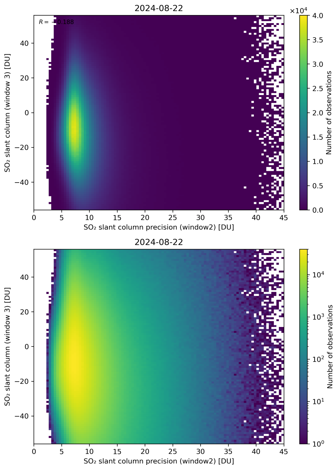
Figure 249: Scatter density plot of “SO 2 slant column precision (window2)” against “SO 2 slant column (window 3)” for 2024-08-22 to 2024-08-23.
