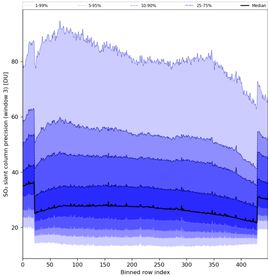
Figure 88: Along track statistics of “SO 2 slant column precision (window 3)” for 2024-08-22 to 2024-08-23
