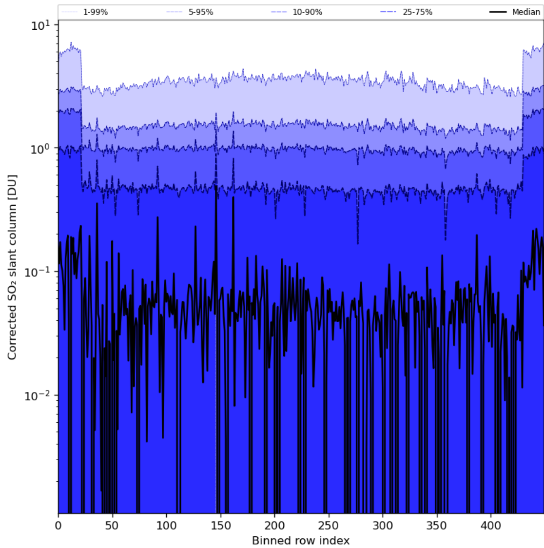
Figure 78: Along track statistics of “Corrected SO 2 slant column” for 2024-08-22 to 2024-08-23
