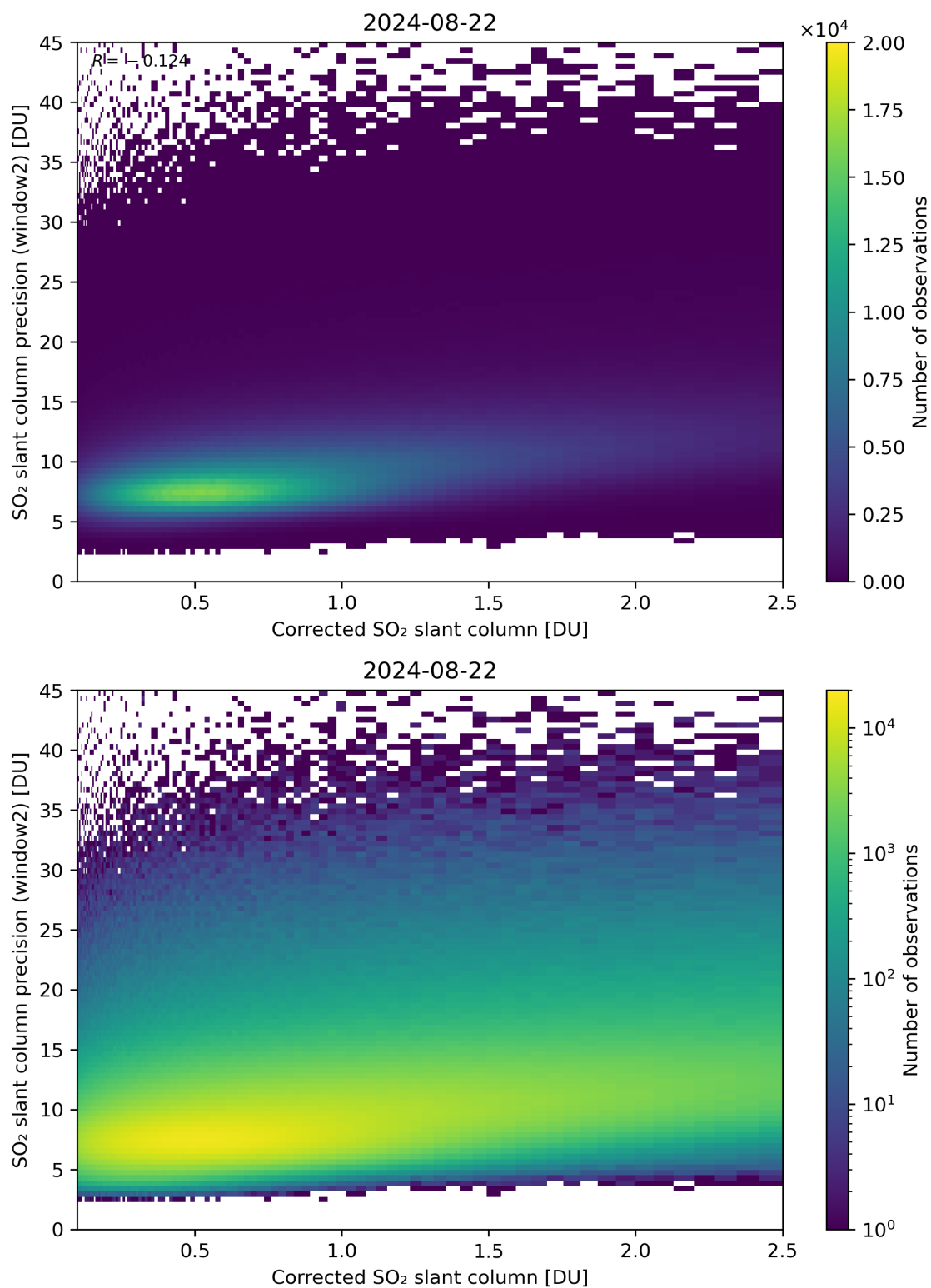
Figure 189: Scatter density plot of “Corrected SO 2 slant column” against “SO 2 slant column precision (window2)” for 2024-08-22 to 2024-08-23.
