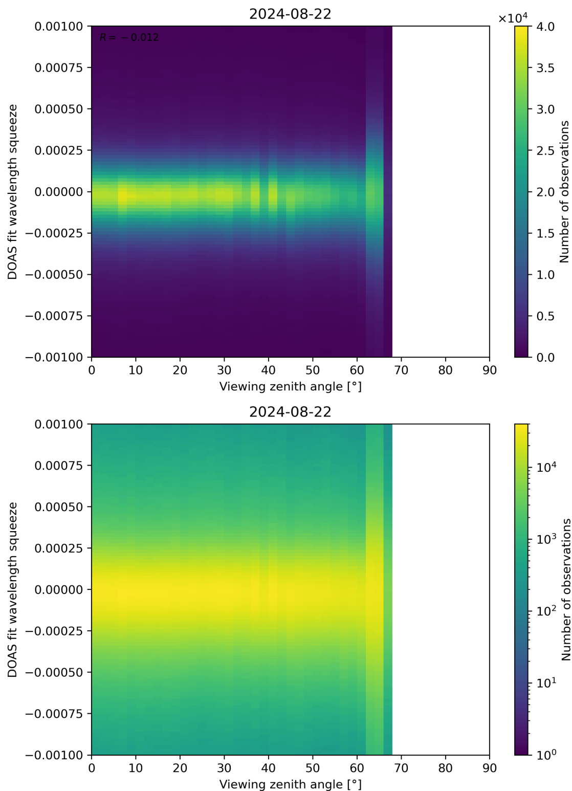
Figure 312: Scatter density plot of “Viewing zenith angle” against “DOAS fit wavelength squeeze” for 2024-08-22 to 2024-08-23.
