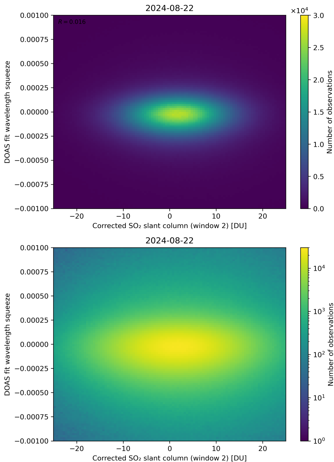
Figure 197: Scatter density plot of “Corrected SO 2 slant column (window 2)” against “DOAS fit wavelength squeeze” for 2024-08-22 to 2024-08-23.
