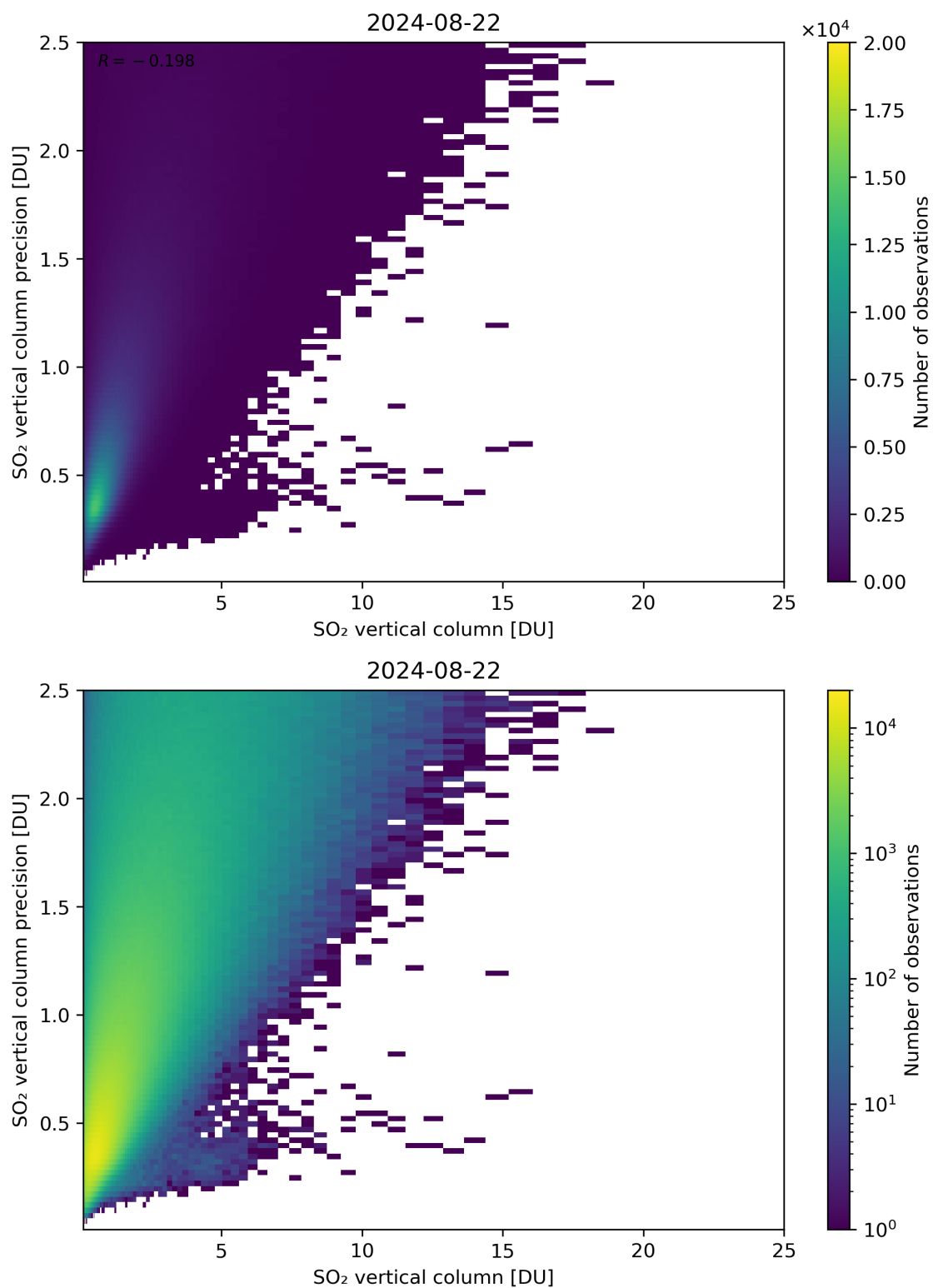
Figure 307: Scatter density plot of “SO 2 vertical column” against “SO 2 vertical column precision” for 2024-08-22 to 2024-08-23.
