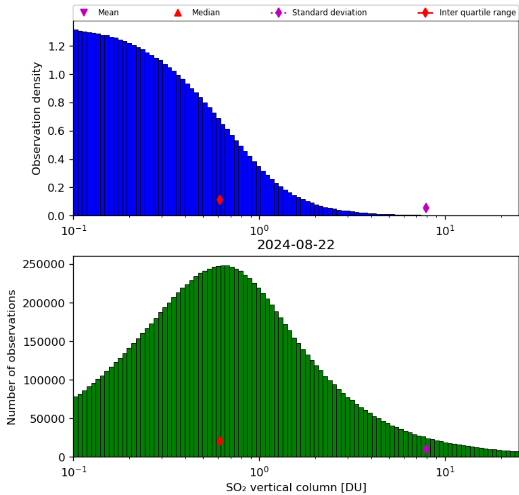
Figure 53: Histogram of “SO 2 vertical column” for 2024-08-22 to 2024-08-23
