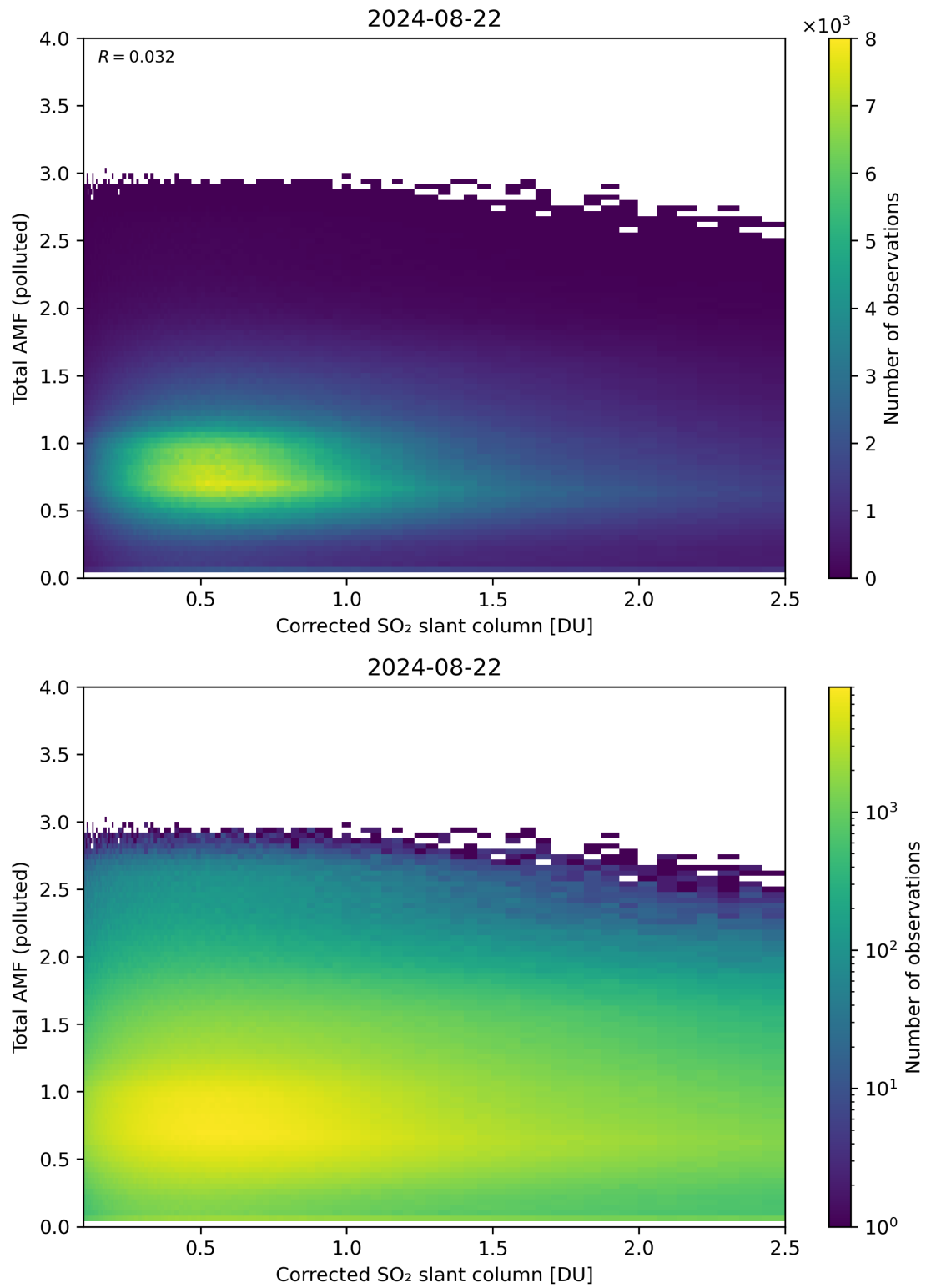
Figure 192: Scatter density plot of “Corrected SO 2 slant column” against “Total AMF (polluted)” for 2024-08-22 to 2024-08-23.
