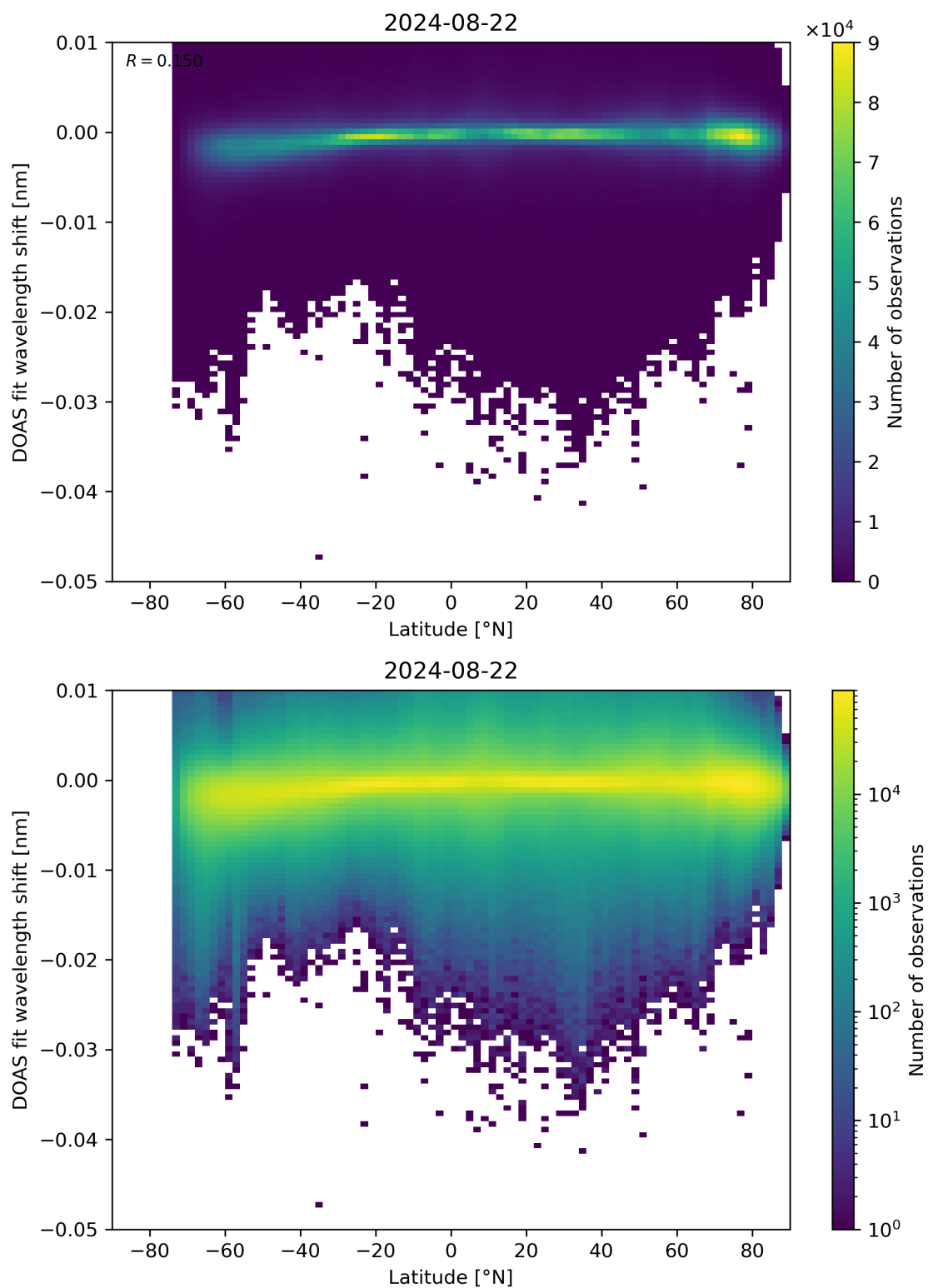
Figure 142: Scatter density plot of “Latitude” against “DOAS fit wavelength shift” for 2024-08-22 to 2024-08-23.
