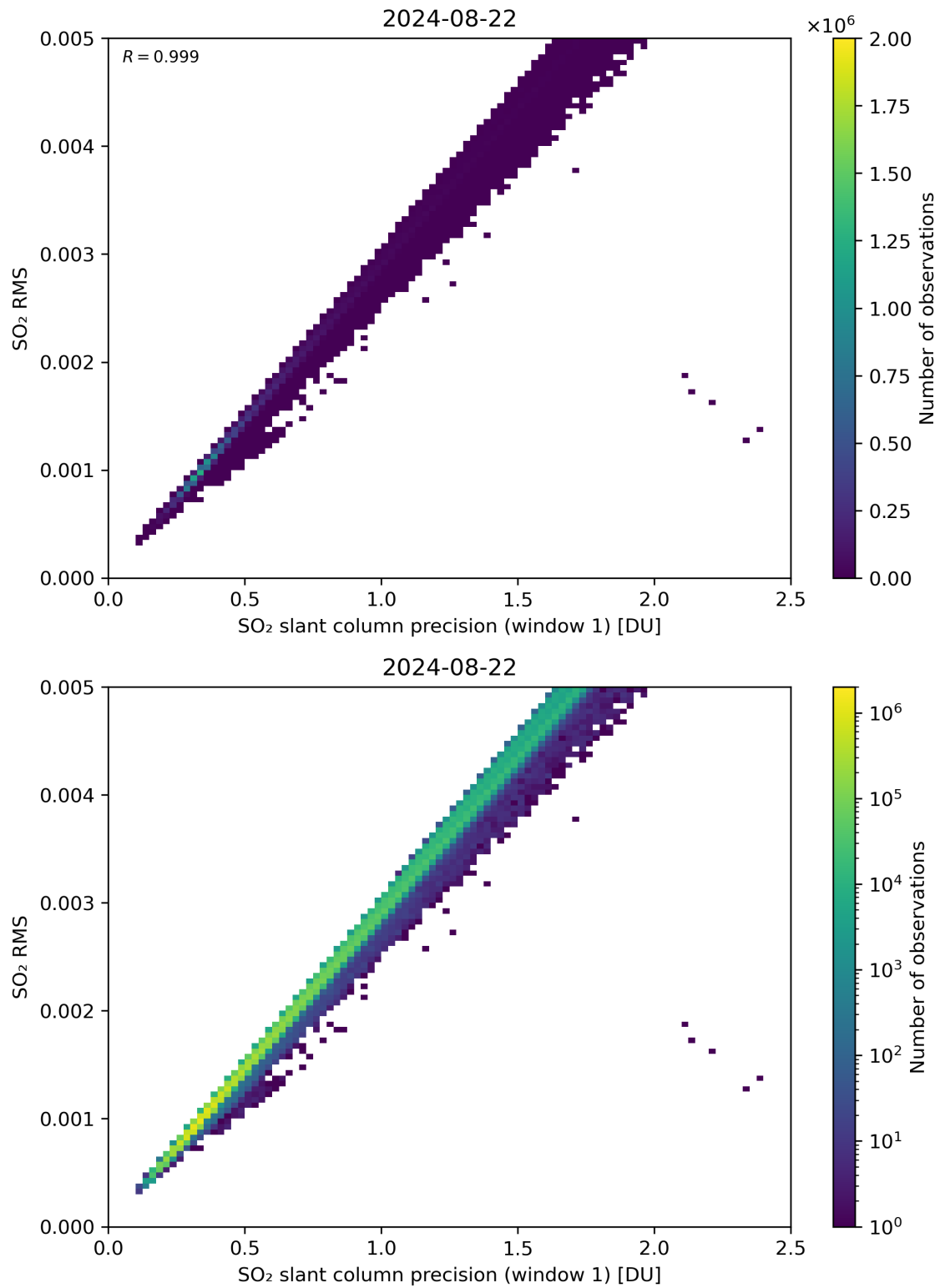
Figure 223: Scatter density plot of “SO 2 slant column precision (window 1)” against “SO 2 RMS” for 2024-08-22 to 2024-08-23.
