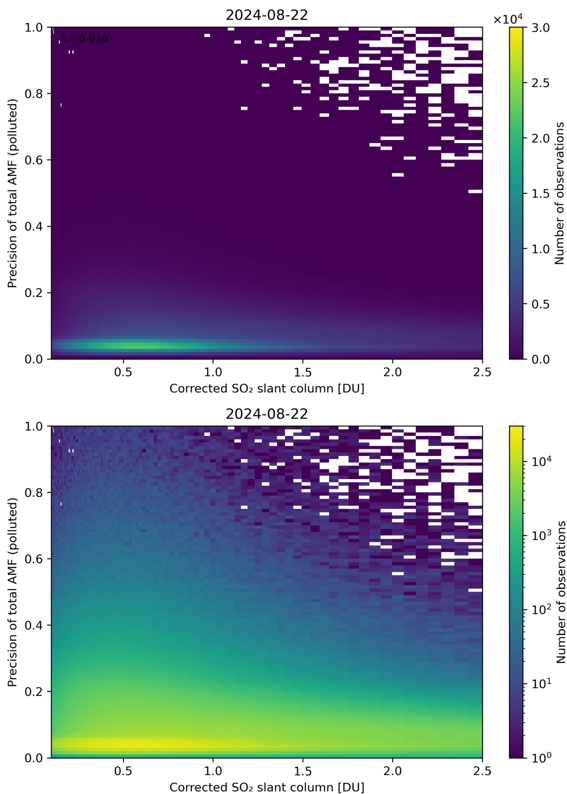
Figure 193: Scatter density plot of “Corrected SO 2 slant column” against “Precision of total AMF (polluted)” for 2024-08-22 to 2024-08-23.
