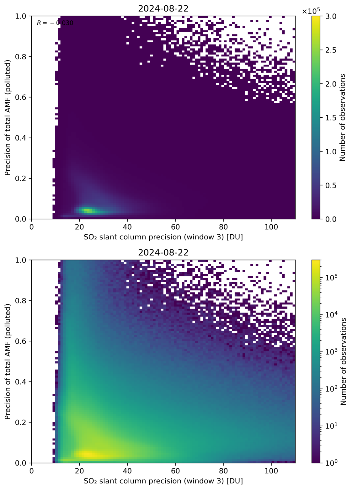
Figure 264: Scatter density plot of “SO 2 slant column precision (window 3)” against “Precision of total AMF (polluted)” for 2024-08-22 to 2024-08-23.
