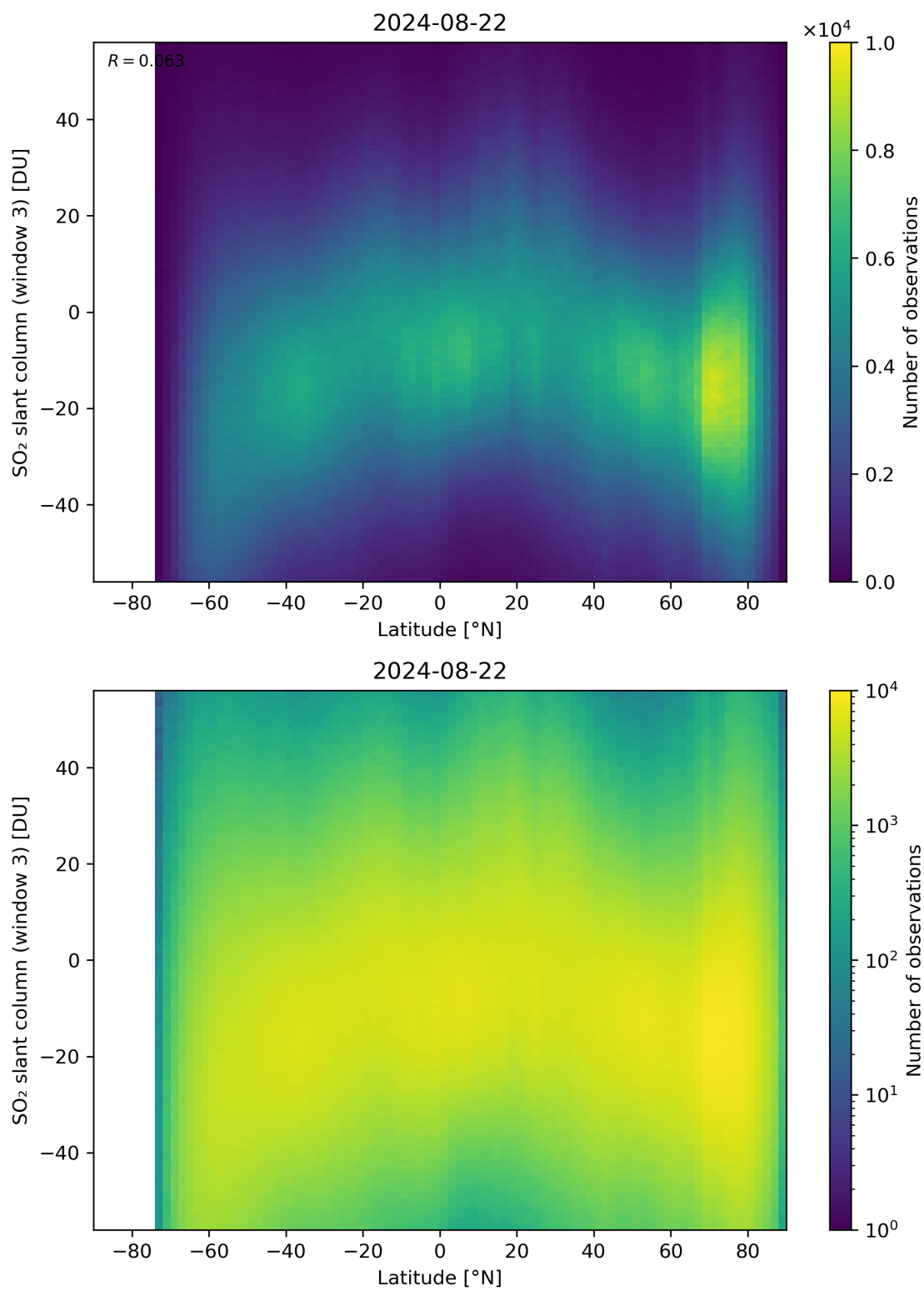
Figure 152: Scatter density plot of “Latitude” against “SO 2 slant column (window 3)” for 2024-08-22 to 2024-08-23.
