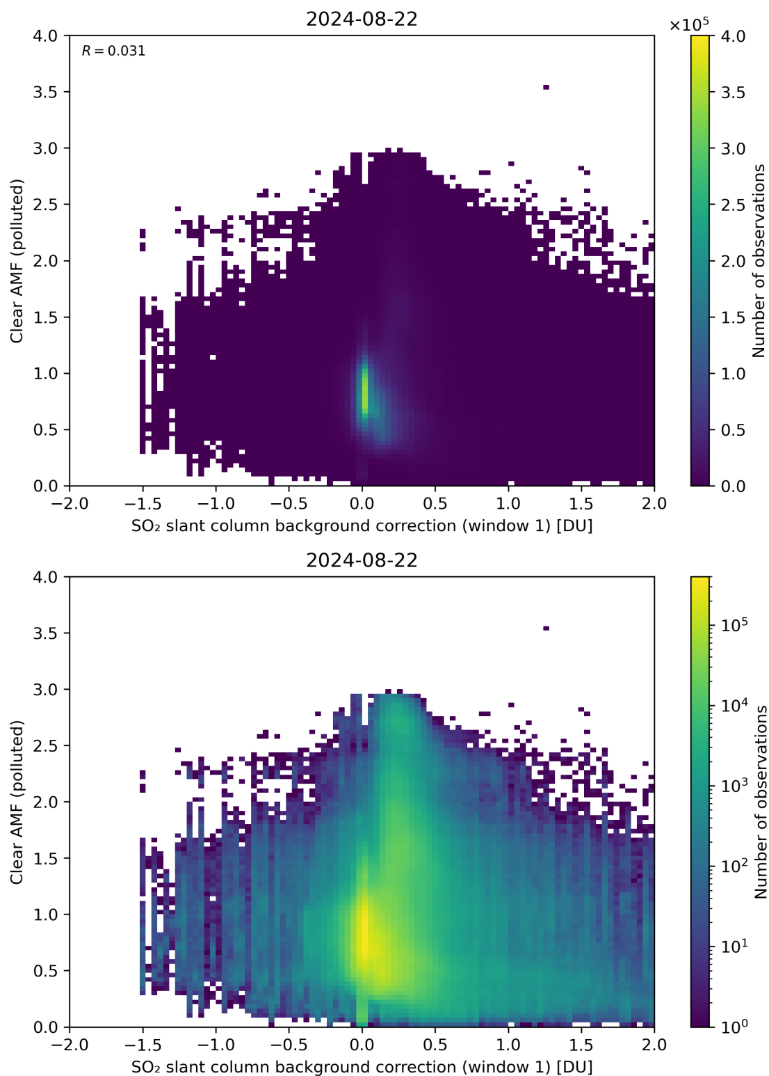
Figure 103: Scatter density plot of “SO 2 slant column background correction (window 1)” against “Clear AMF (polluted)” for 2024-08-22 to 2024-08-23.
