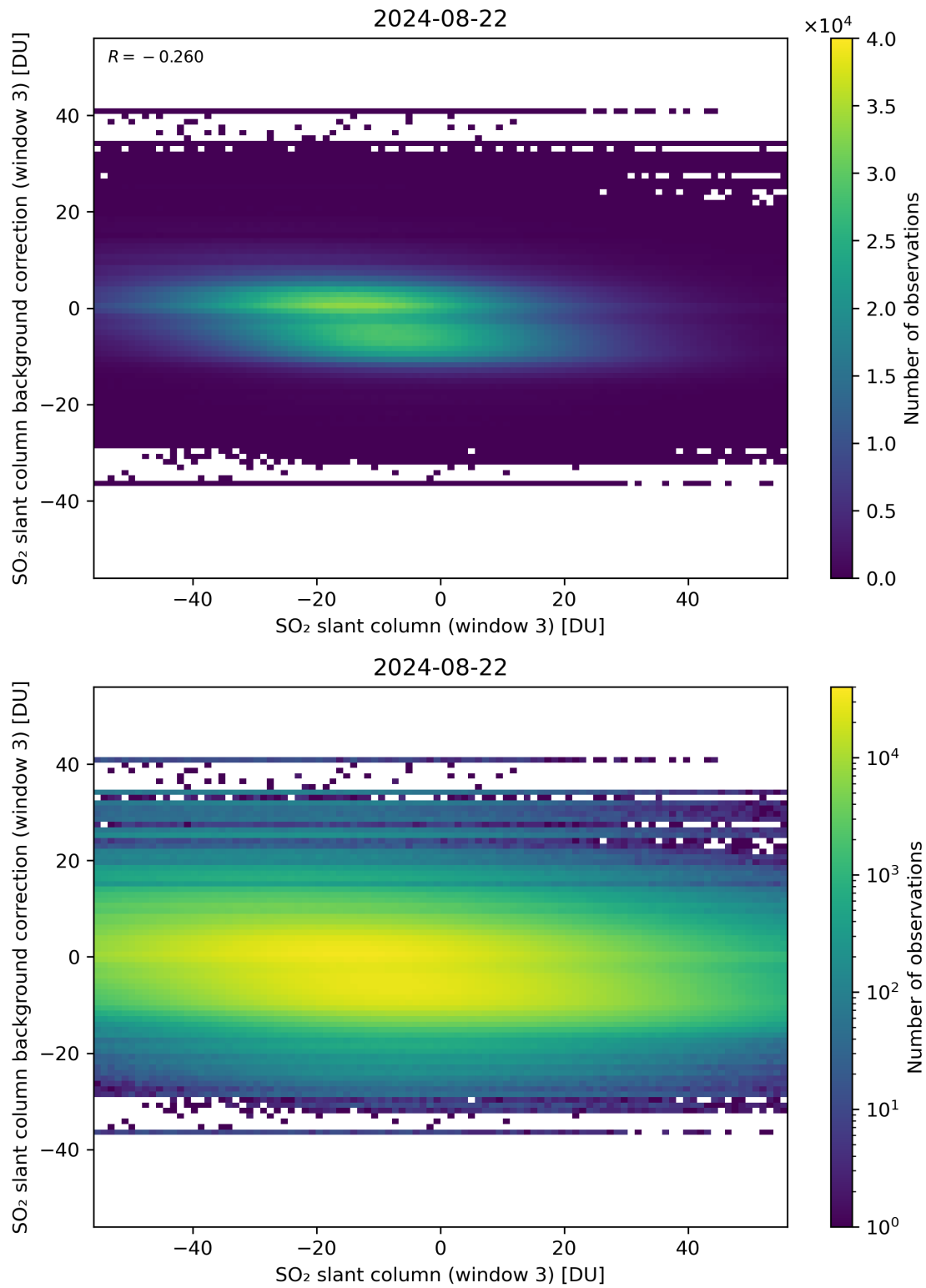
Figure 253: Scatter density plot of “SO 2 slant column (window 3)” against “SO 2 slant column background correction (window 3)” for 2024-08-22 to 2024-08-23.
