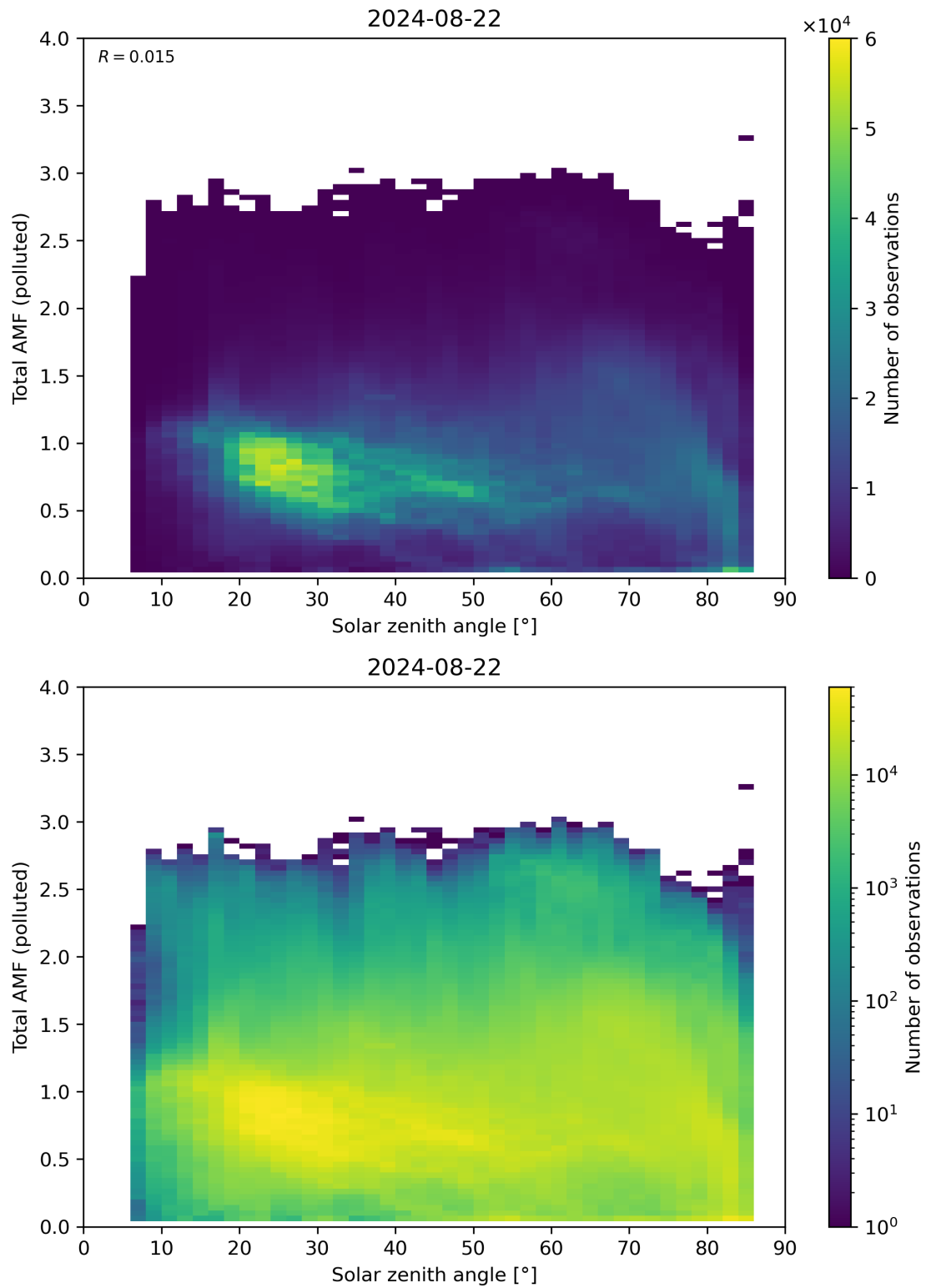
Figure 174: Scatter density plot of “Solar zenith angle” against “Total AMF (polluted)” for 2024-08-22 to 2024-08-23.
