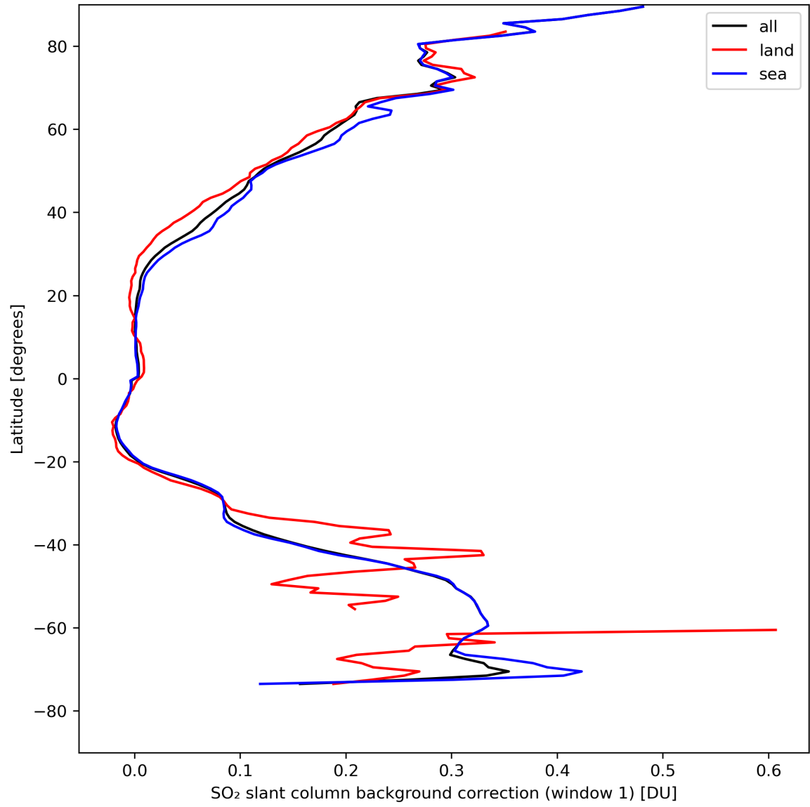
Figure 36: Zonal average of “SO 2 slant column background correction (window 1)” for 2024-08-22 to 2024-08-23.
