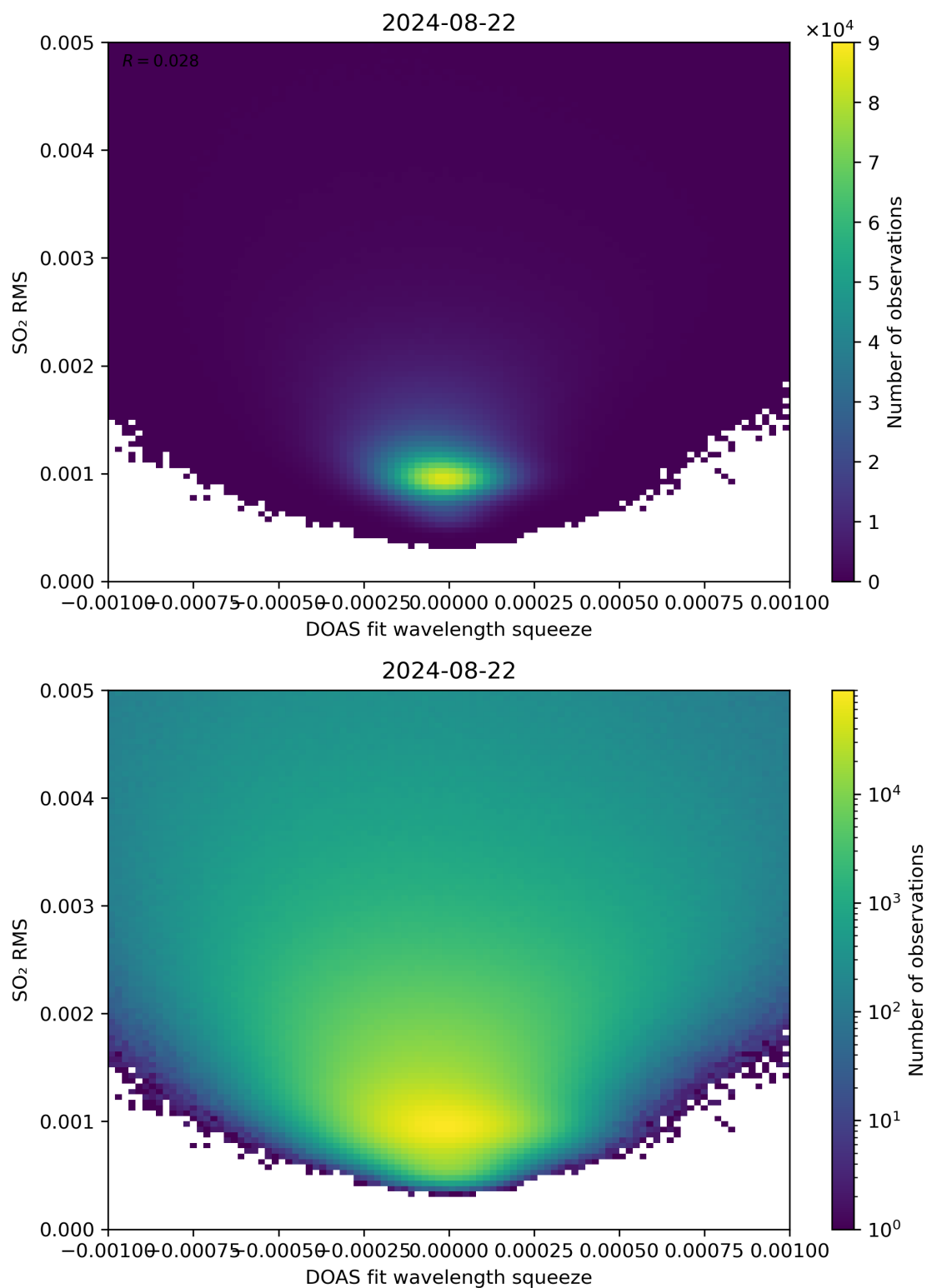
Figure 132: Scatter density plot of “DOAS fit wavelength squeeze” against “SO 2 RMS” for 2024-08-22 to 2024-08-23.
