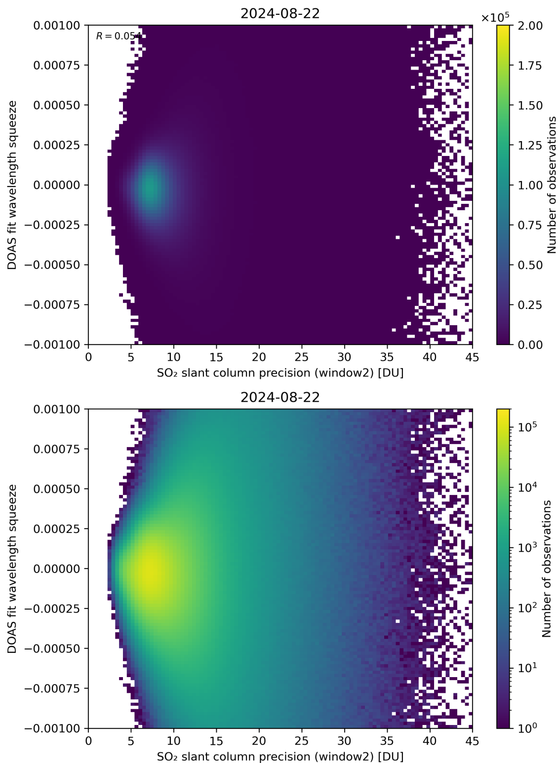
Figure 244: Scatter density plot of “SO 2 slant column precision (window2)” against “DOAS fit wavelength squeeze” for 2024-08-22 to 2024-08-23.
