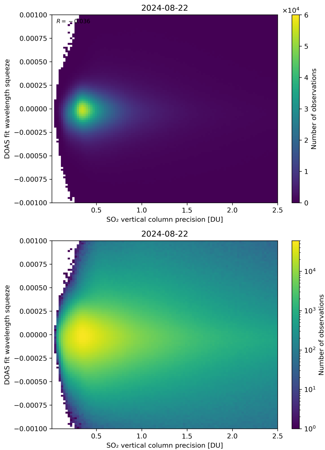
Figure 283: Scatter density plot of “SO 2 vertical column precision” against “DOAS fit wavelength squeeze” for 2024-08-22 to 2024-08-23.
