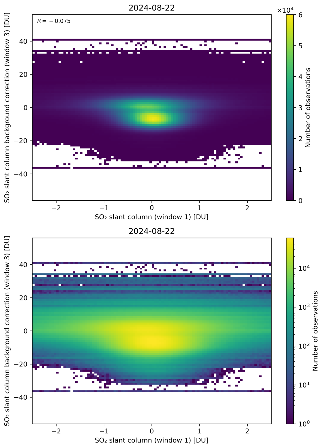
Figure 214: Scatter density plot of “SO 2 slant column (window 1)” against “SO 2 slant column background correction (window 3)” for 2024-08-22 to 2024-08-23.
