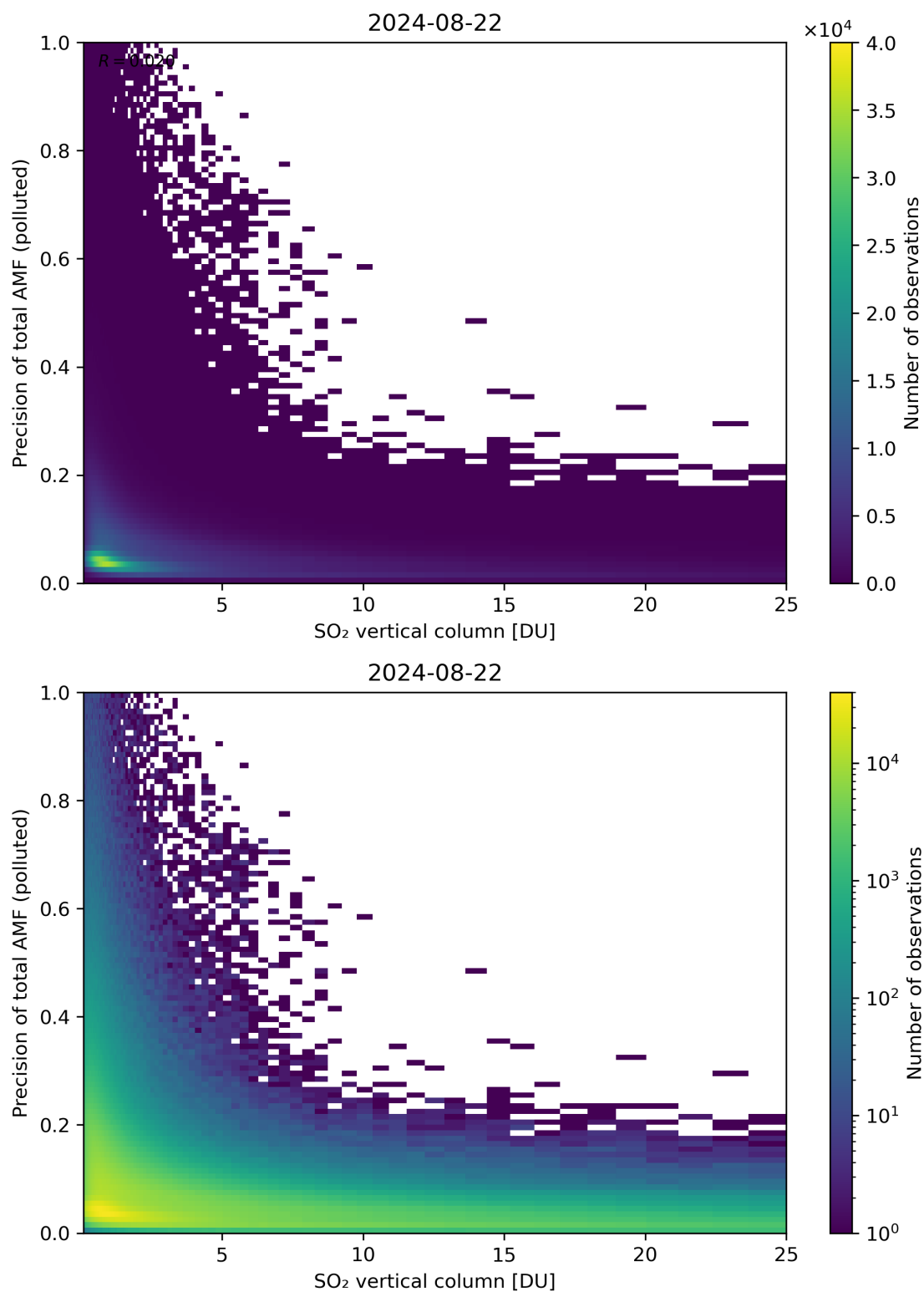
Figure 306: Scatter density plot of “SO 2 vertical column” against “Precision of total AMF (polluted)” for 2024-08-22 to 2024-08-23.
