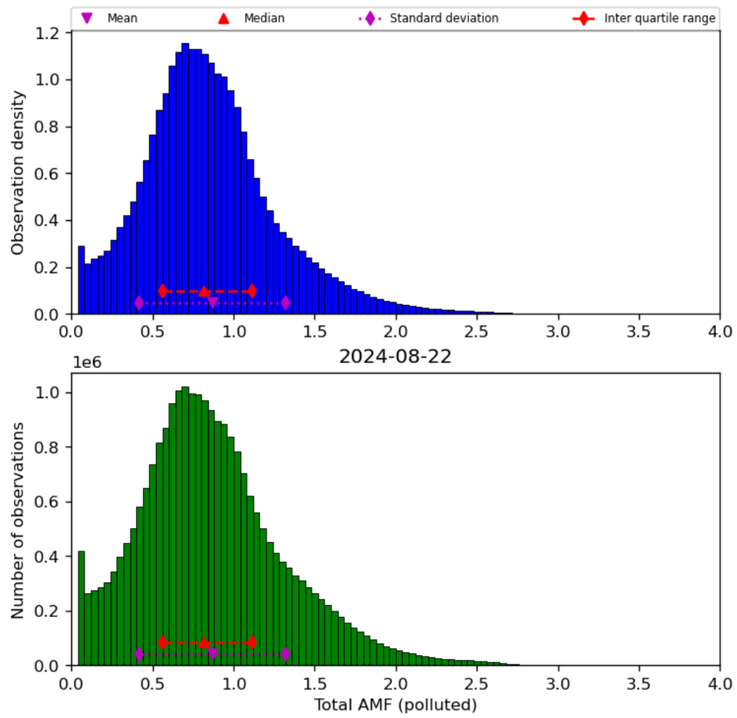
Figure 71: Histogram of “Total AMF (polluted)” for 2024-08-22 to 2024-08-23
