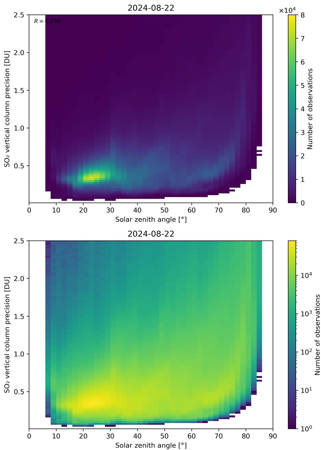
Figure 177: Scatter density plot of “Solar zenith angle” against “SO 2 vertical column precision” for 2024-08-22 to 2024-08-23.
