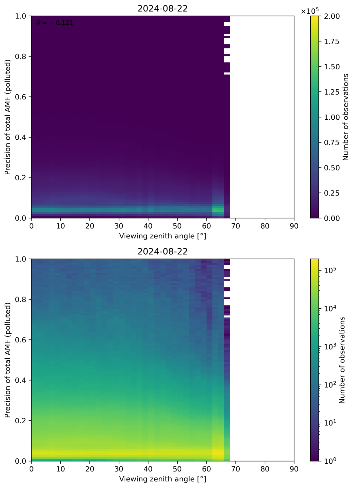
Figure 326: Scatter density plot of “Viewing zenith angle” against “Precision of total AMF (polluted)” for 2024-08-22 to 2024-08-23.
