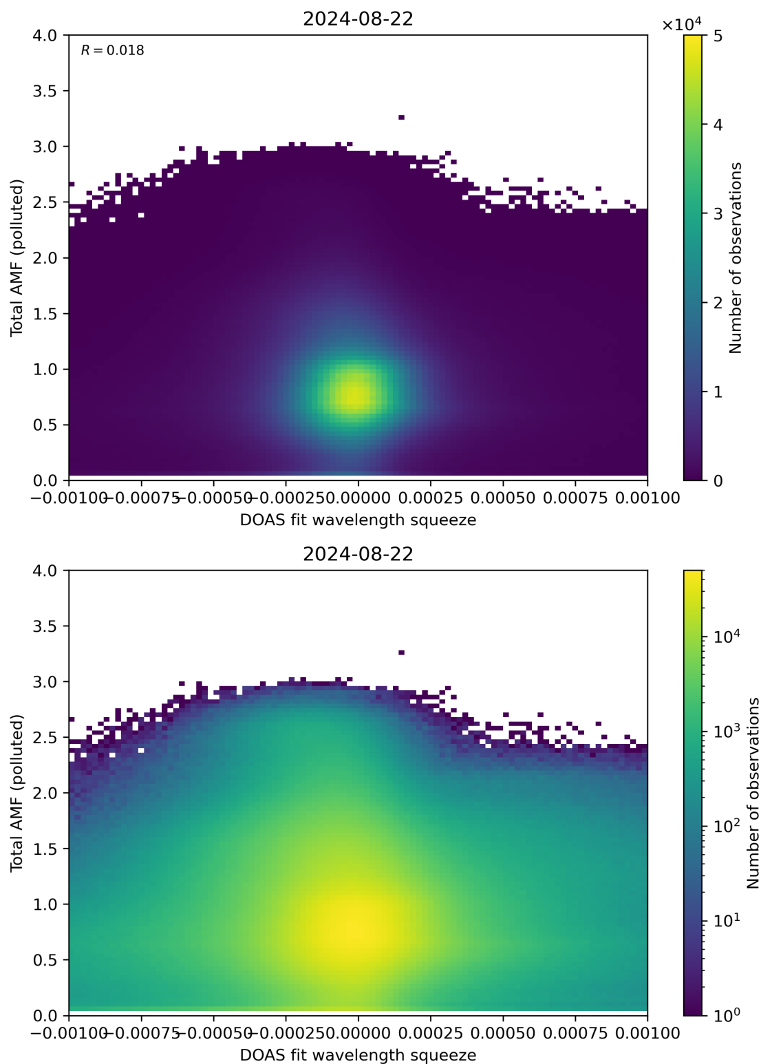
Figure 134: Scatter density plot of “DOAS fit wavelength squeeze” against “Total AMF (polluted)” for 2024-08-22 to 2024-08-23.
