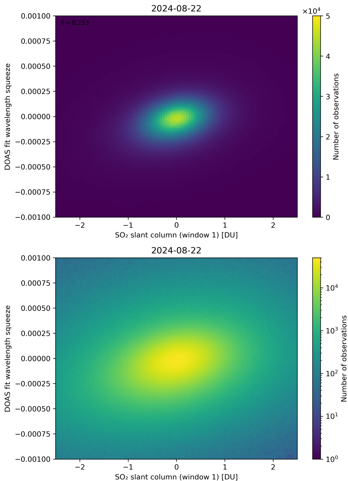
Figure 216: Scatter density plot of “SO 2 slant column (window 1)” against “DOAS fit wavelength squeeze” for 2024-08-22 to 2024-08-23.
