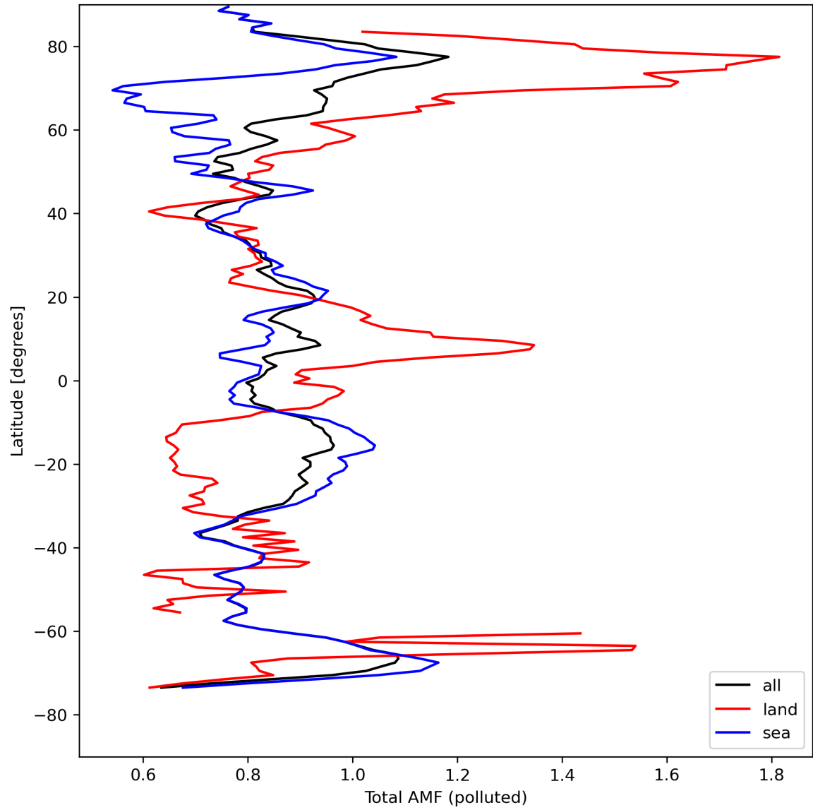
Figure 48: Zonal average of “Total AMF (polluted)” for 2024-08-22 to 2024-08-23.
