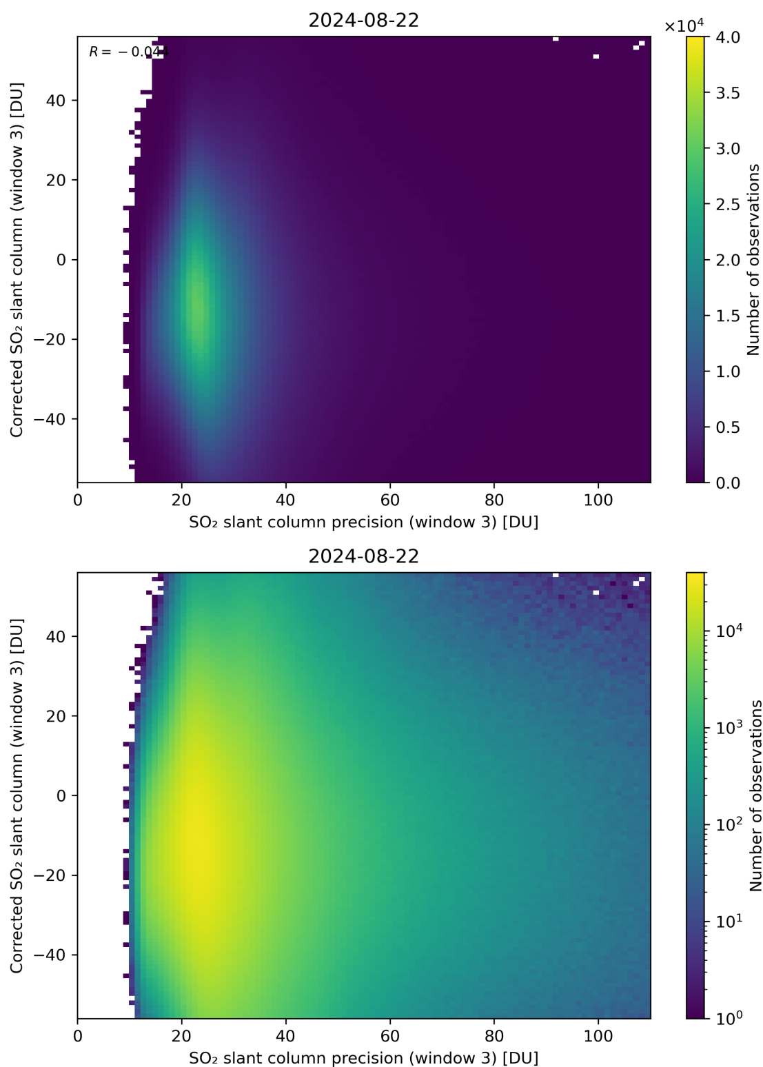
Figure 262: Scatter density plot of “SO 2 slant column precision (window 3)” against “Corrected SO 2 slant column (window 3)” for 2024-08-22 to 2024-08-23.
