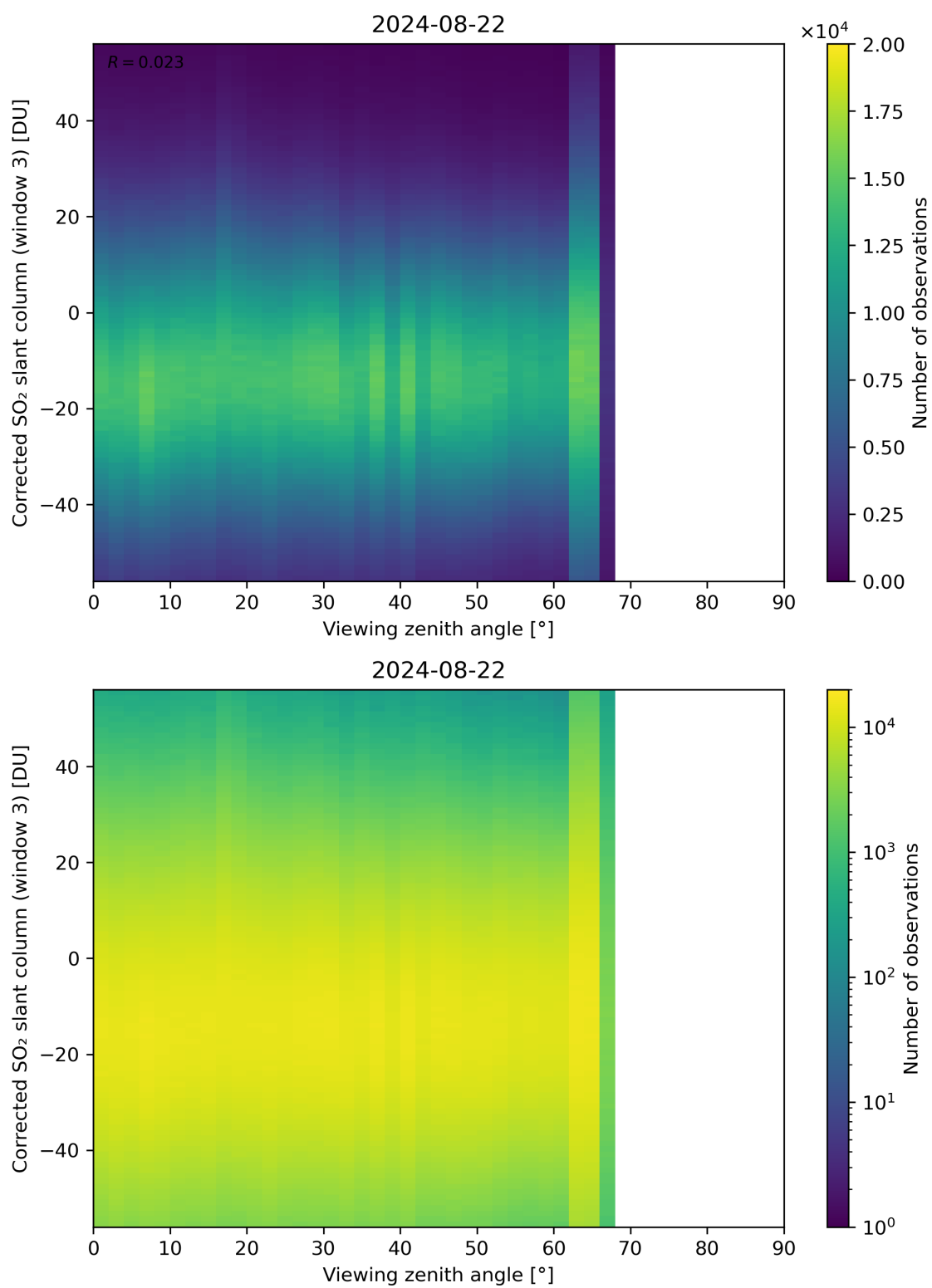
Figure 319: Scatter density plot of “Viewing zenith angle” against “Corrected SO 2 slant column (window 3)” for 2024-08-22 to 2024-08-23.
