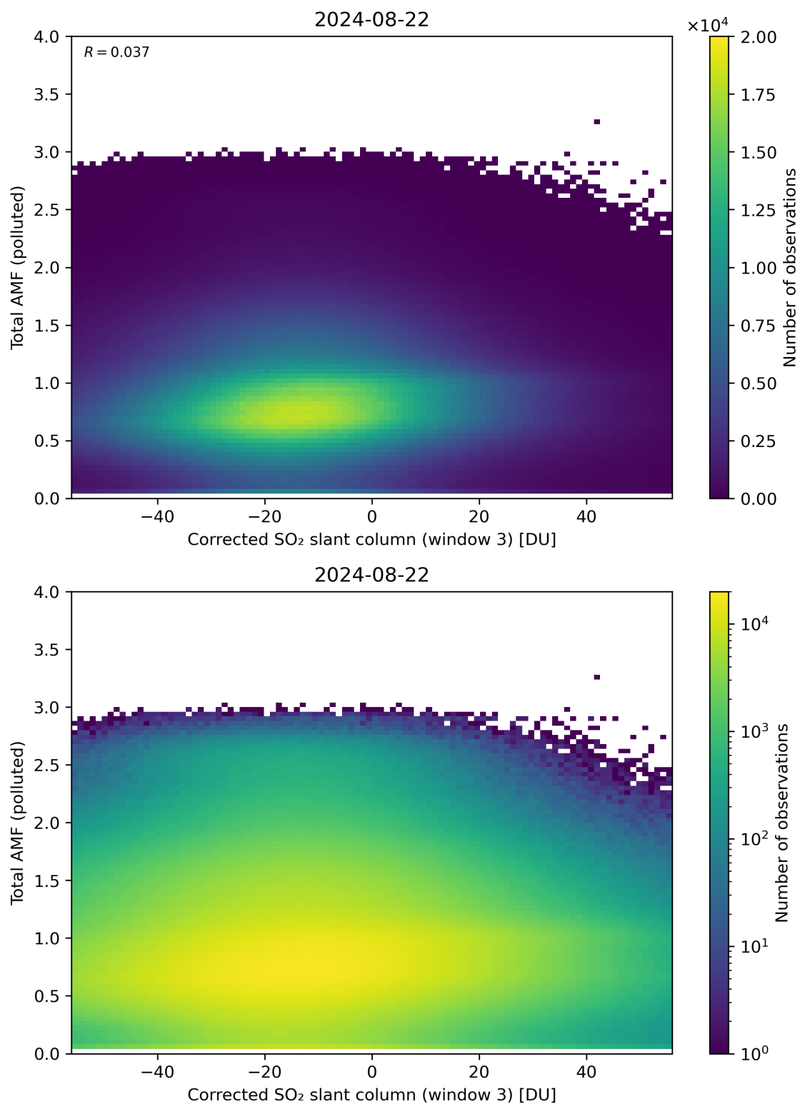
Figure 210: Scatter density plot of “Corrected SO 2 slant column (window 3)” against “Total AMF (polluted)” for 2024-08-22 to 2024-08-23.
