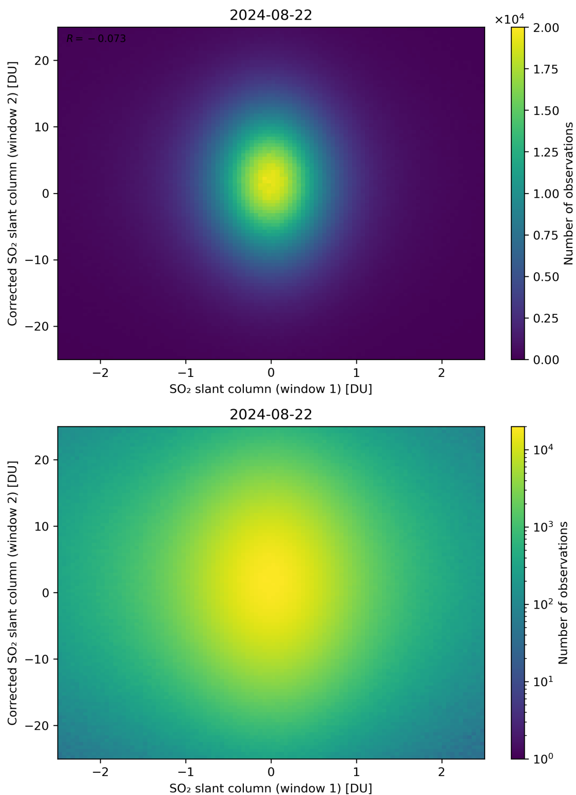
Figure 233: Scatter density plot of “SO 2 slant column (window 1)” against “Corrected SO 2 slant column (window 2)” for 2024-08-22 to 2024-08-23.
