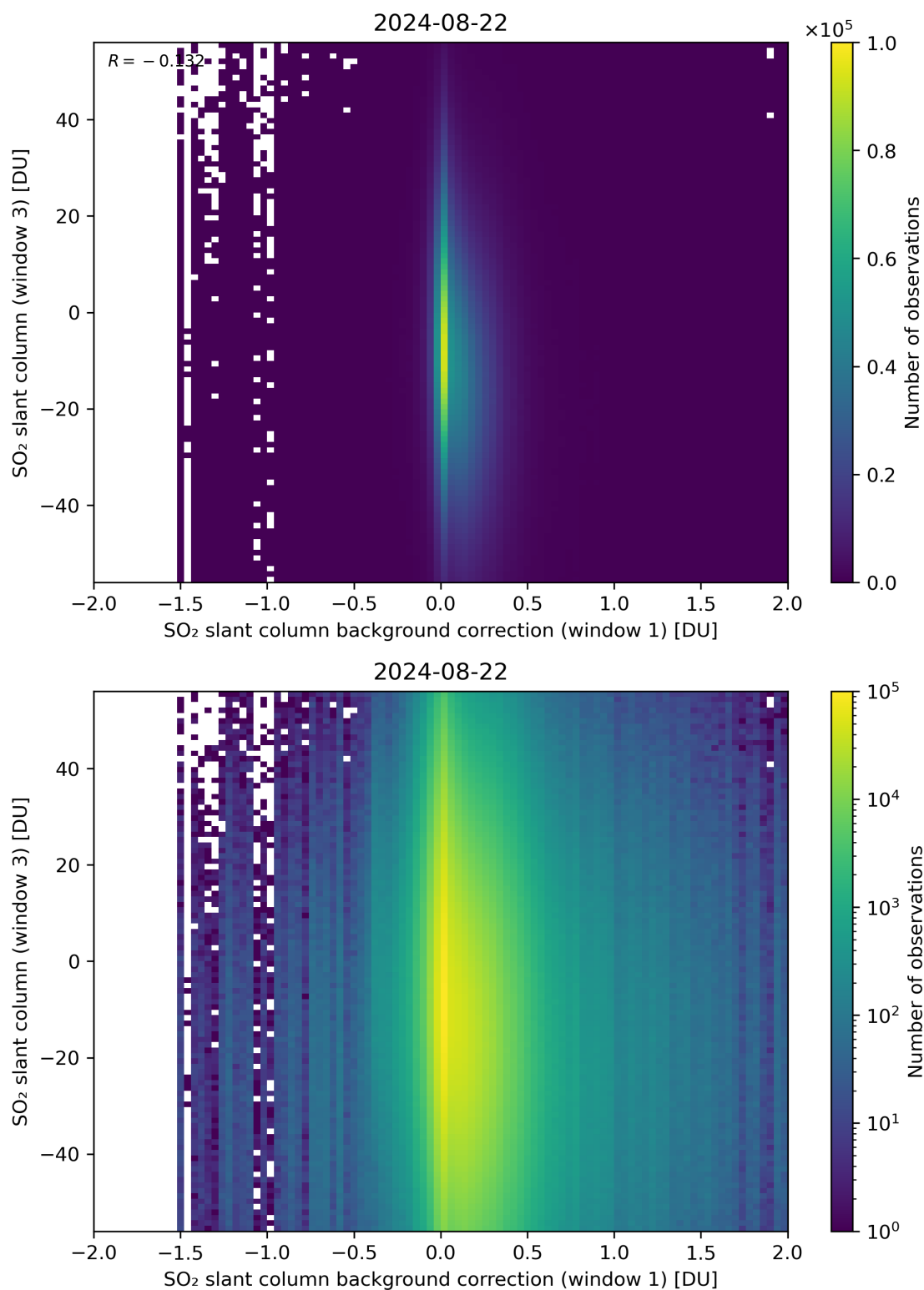
Figure 107: Scatter density plot of “SO 2 slant column background correction (window 1)” against “SO 2 slant column (window 3)” for 2024-08-22 to 2024-08-23.
