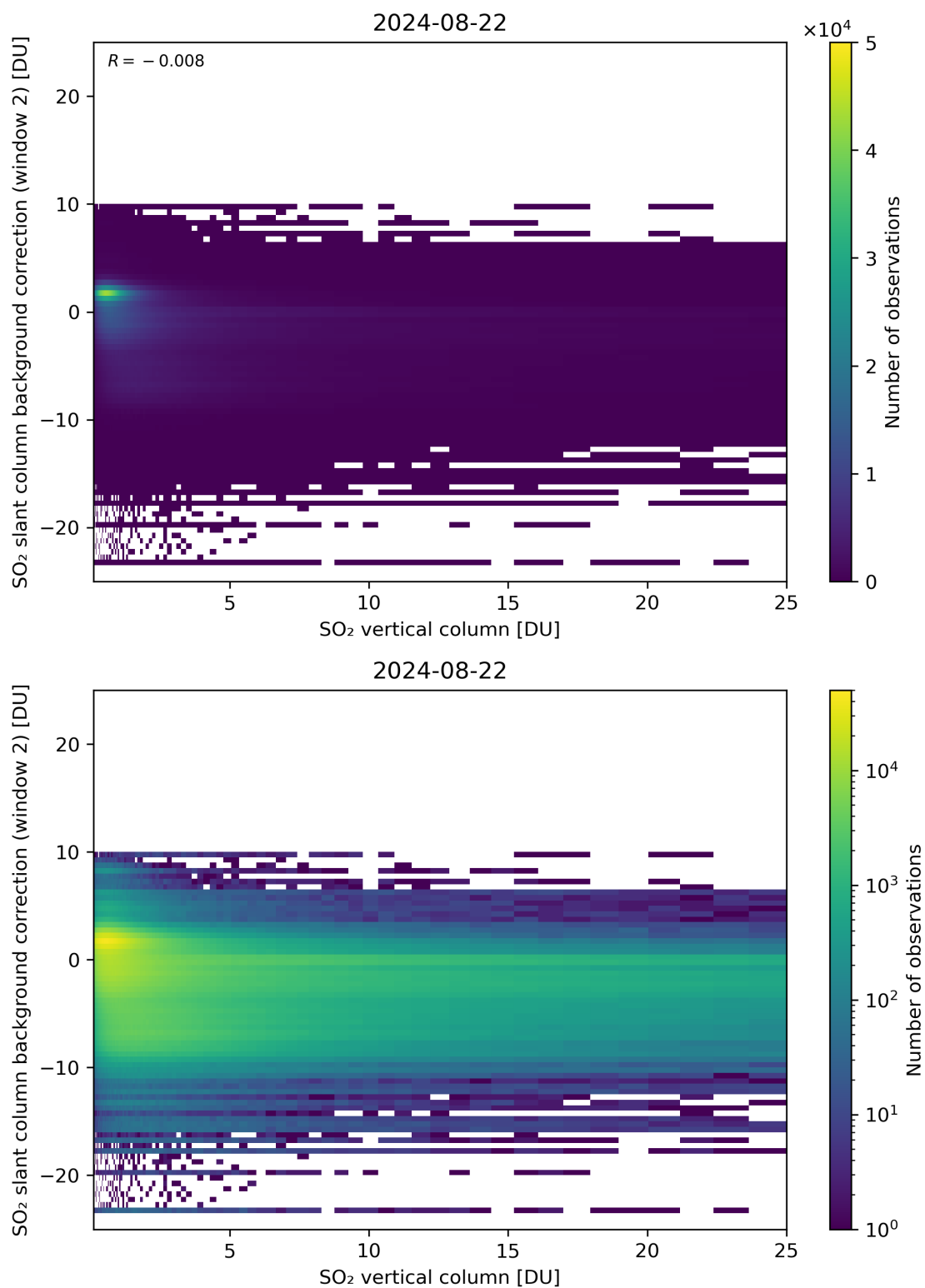
Figure 274: Scatter density plot of “SO 2 vertical column” against “SO 2 slant column background correction (window 2)” for 2024-08-22 to 2024-08-23.
