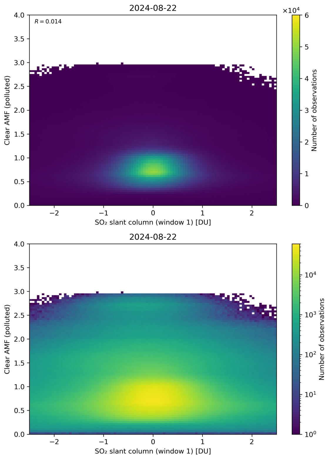
Figure 232: Scatter density plot of “SO 2 slant column (window 1)” against “Clear AMF (polluted)” for 2024-08-22 to 2024-08-23.
