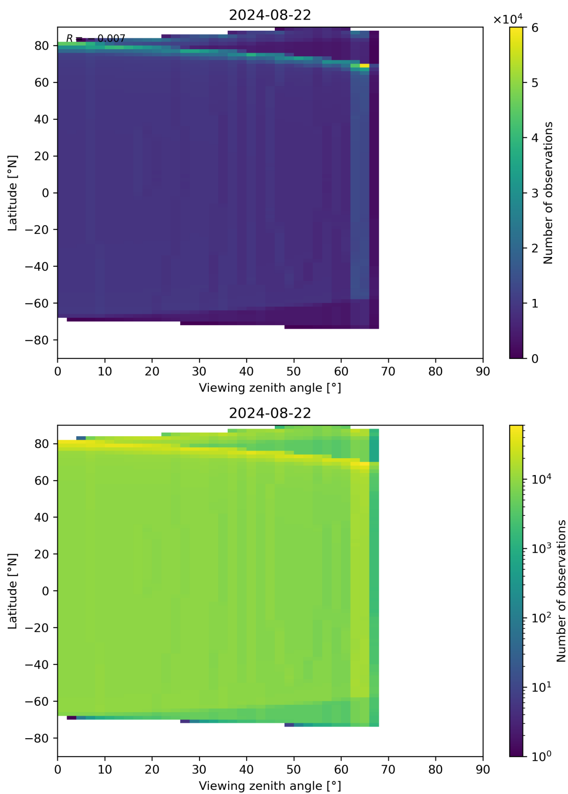
Figure 314: Scatter density plot of “Viewing zenith angle” against “Latitude” for 2024-08-22 to 2024-08-23.
