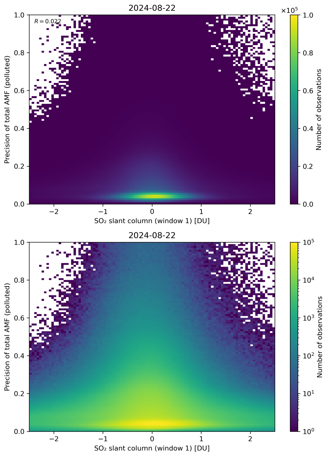
Figure 240: Scatter density plot of “SO 2 slant column (window 1)” against “Precision of total AMF (polluted)” for 2024-08-22 to 2024-08-23.
