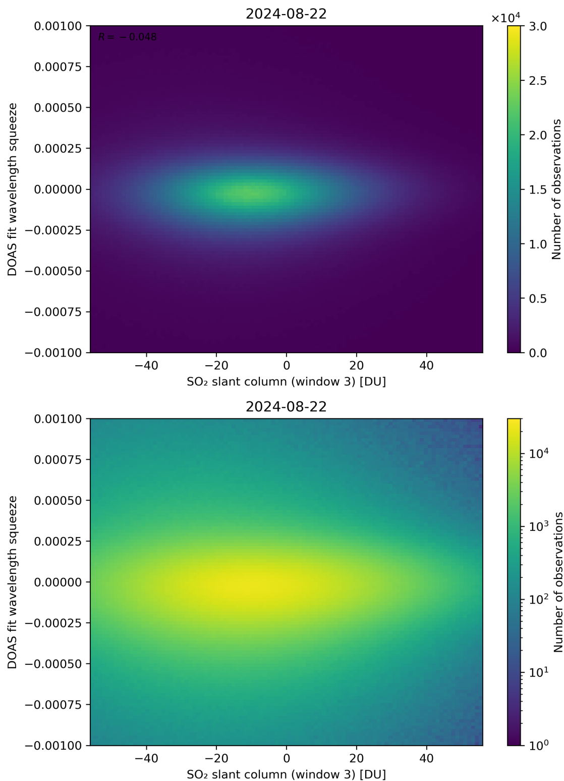
Figure 255: Scatter density plot of “SO 2 slant column (window 3)” against “DOAS fit wavelength squeeze” for 2024-08-22 to 2024-08-23.
