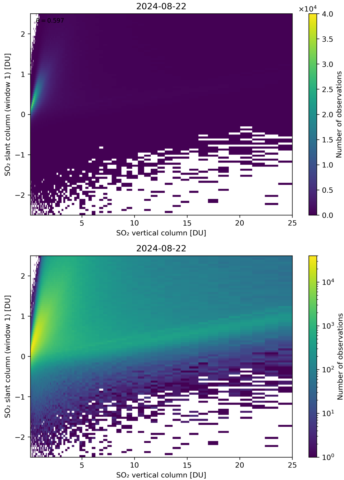
Figure 300: Scatter density plot of “SO 2 vertical column” against “SO 2 slant column (window 1)” for 2024-08-22 to 2024-08-23.
