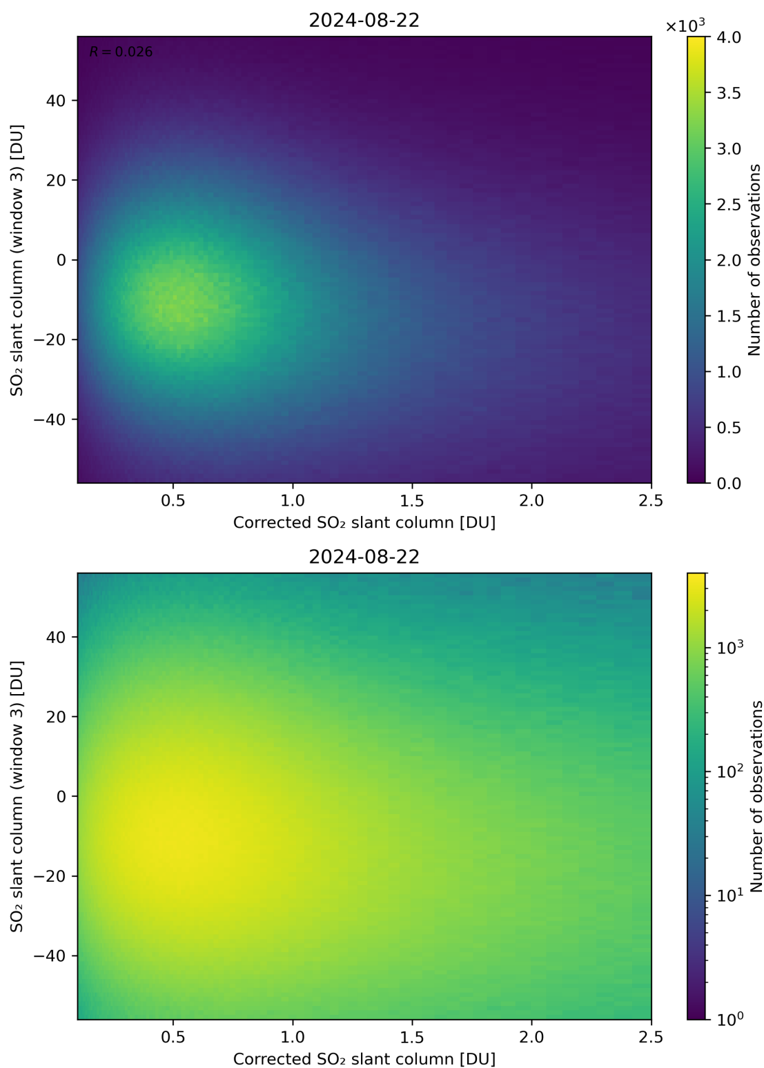
Figure 190: Scatter density plot of “Corrected SO 2 slant column” against “SO 2 slant column (window 3)” for 2024-08-22 to 2024-08-23.
