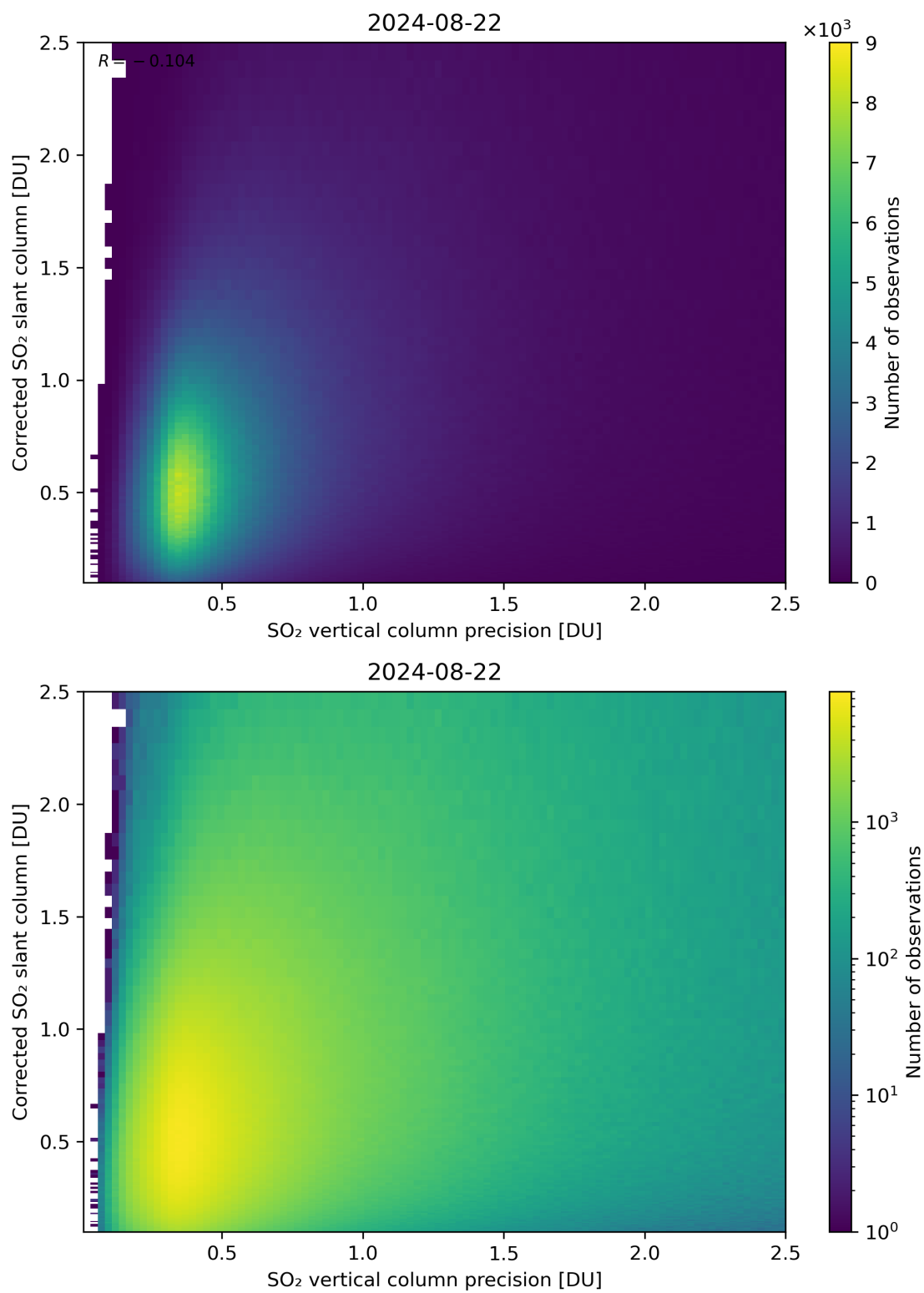
Figure 286: Scatter density plot of “SO 2 vertical column precision” against “Corrected SO 2 slant column” for 2024-08-22 to 2024-08-23.
