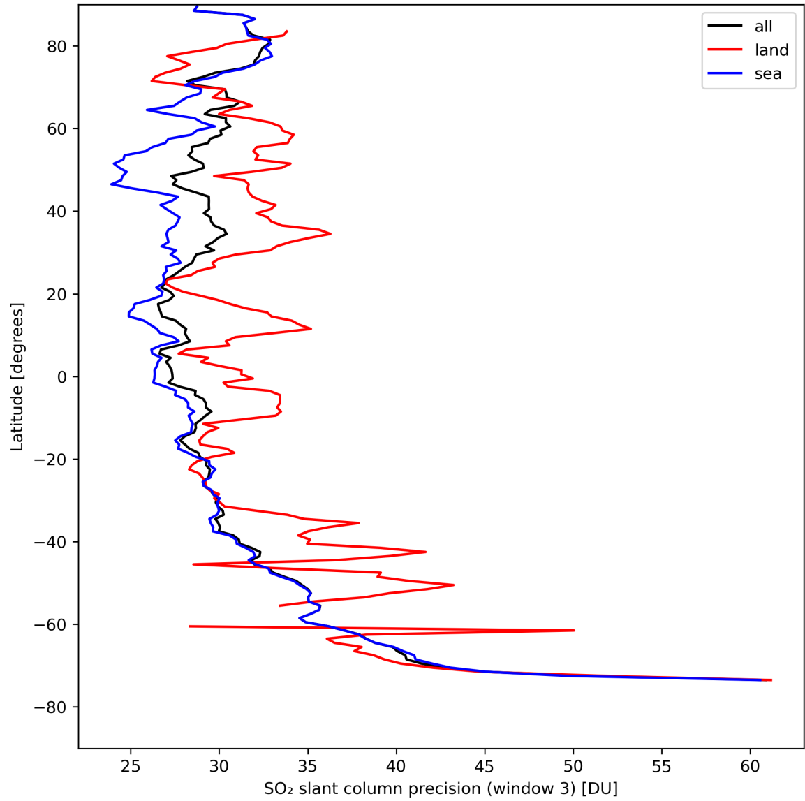
Figure 42: Zonal average of “SO 2 slant column precision (window 3)” for 2024-08-22 to 2024-08-23.
