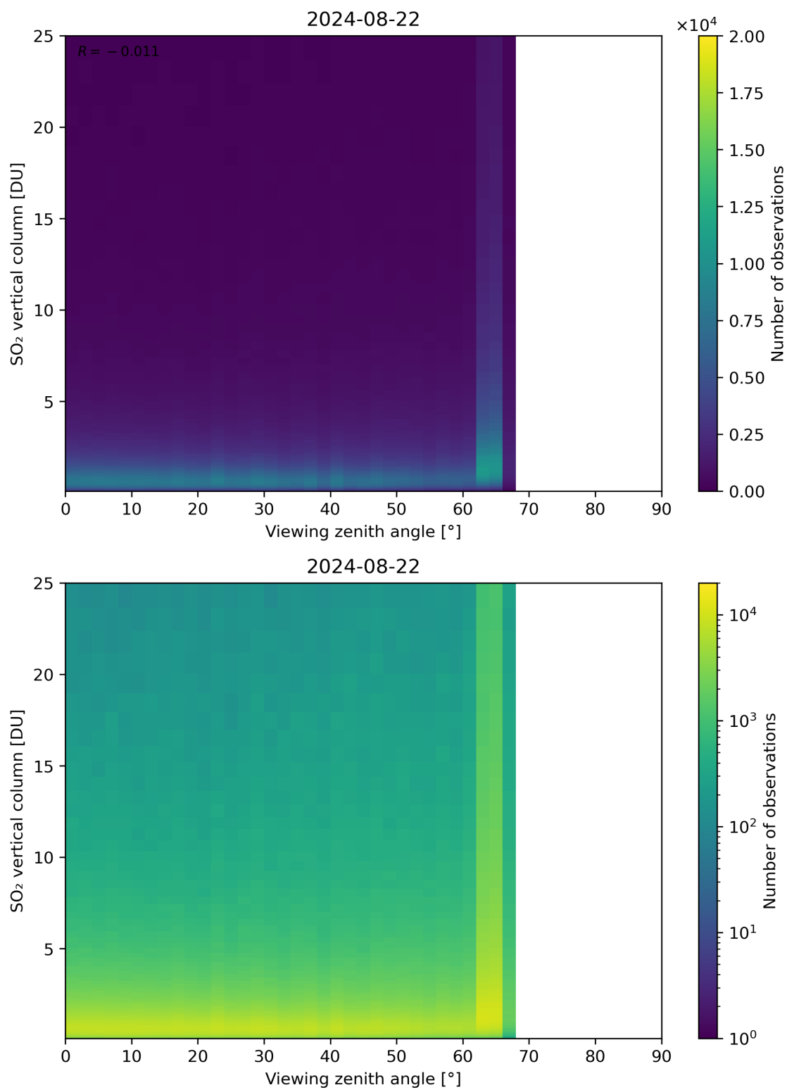
Figure 327: Scatter density plot of “Viewing zenith angle” against “SO 2 vertical column” for 2024-08-22 to 2024-08-23.
