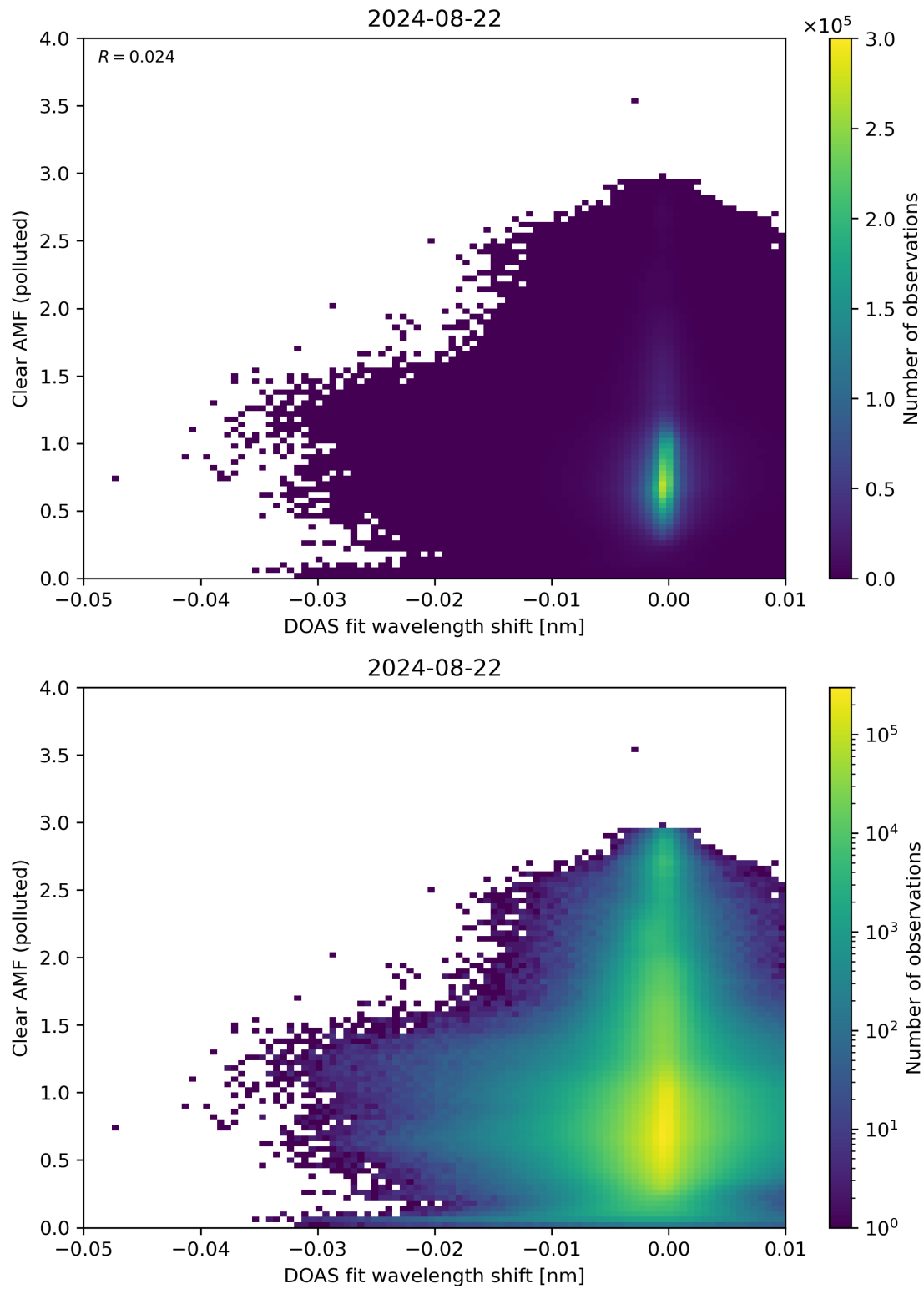
Figure 129: Scatter density plot of “DOAS fit wavelength shift” against “Clear AMF (polluted)” for 2024-08-22 to 2024-08-23.
