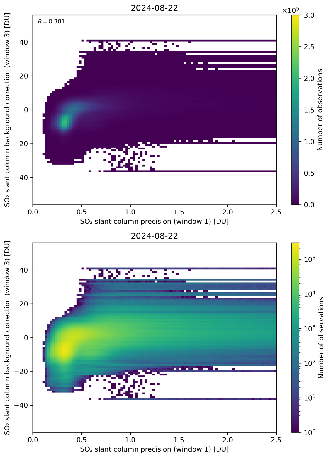
Figure 220: Scatter density plot of “SO 2 slant column precision (window 1)” against “SO 2 slant column background correction (window 3)” for 2024-08-22 to 2024-08-23.
