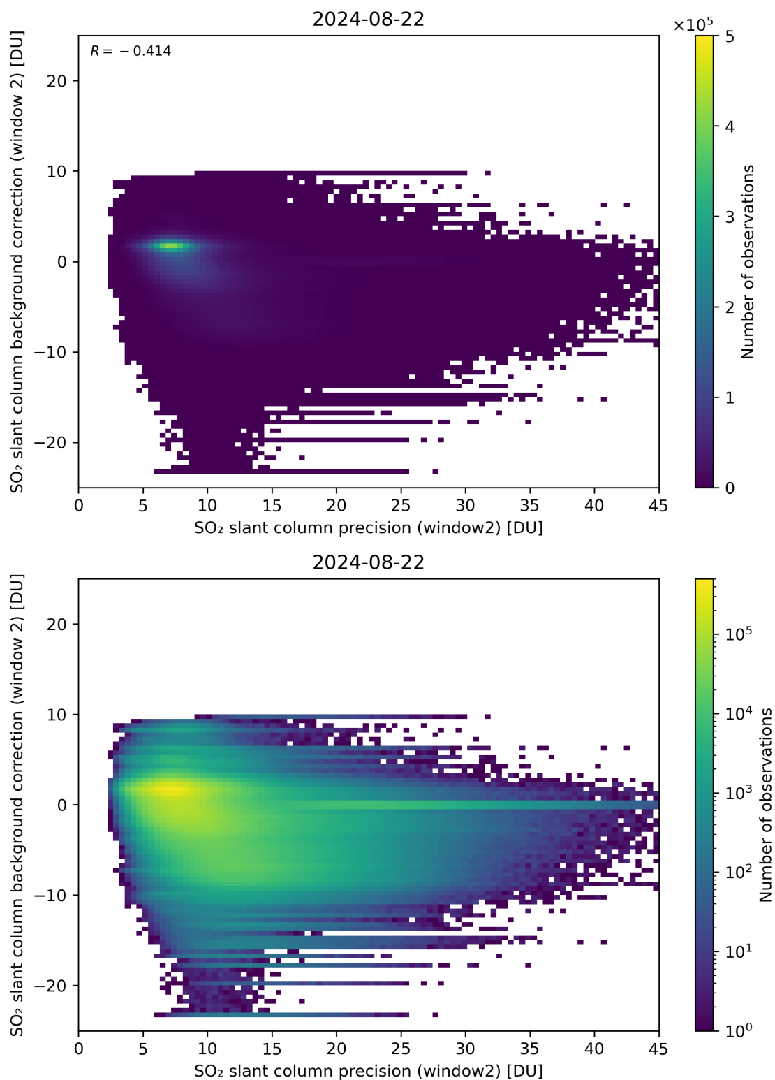
Figure 241: Scatter density plot of “SO 2 slant column precision (window2)” against “SO 2 slant column background correction (window 2)” for 2024-08-22 to 2024-08-23.
