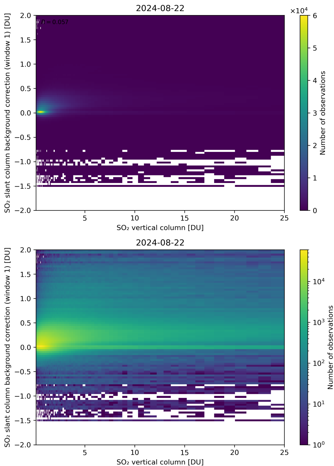
Figure 273: Scatter density plot of “SO 2 vertical column” against “SO 2 slant column background correction (window 1)” for 2024-08-22 to 2024-08-23.
