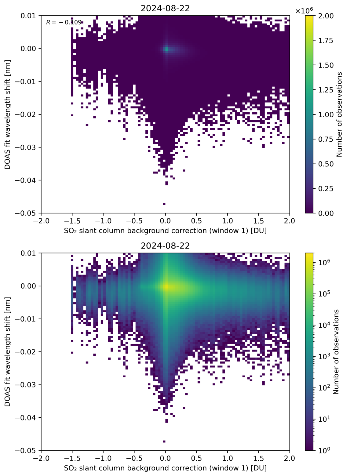
Figure 100: Scatter density plot of “SO 2 slant column background correction (window 1)” against “DOAS fit wavelength shift” for 2024-08-22 to 2024-08-23.
