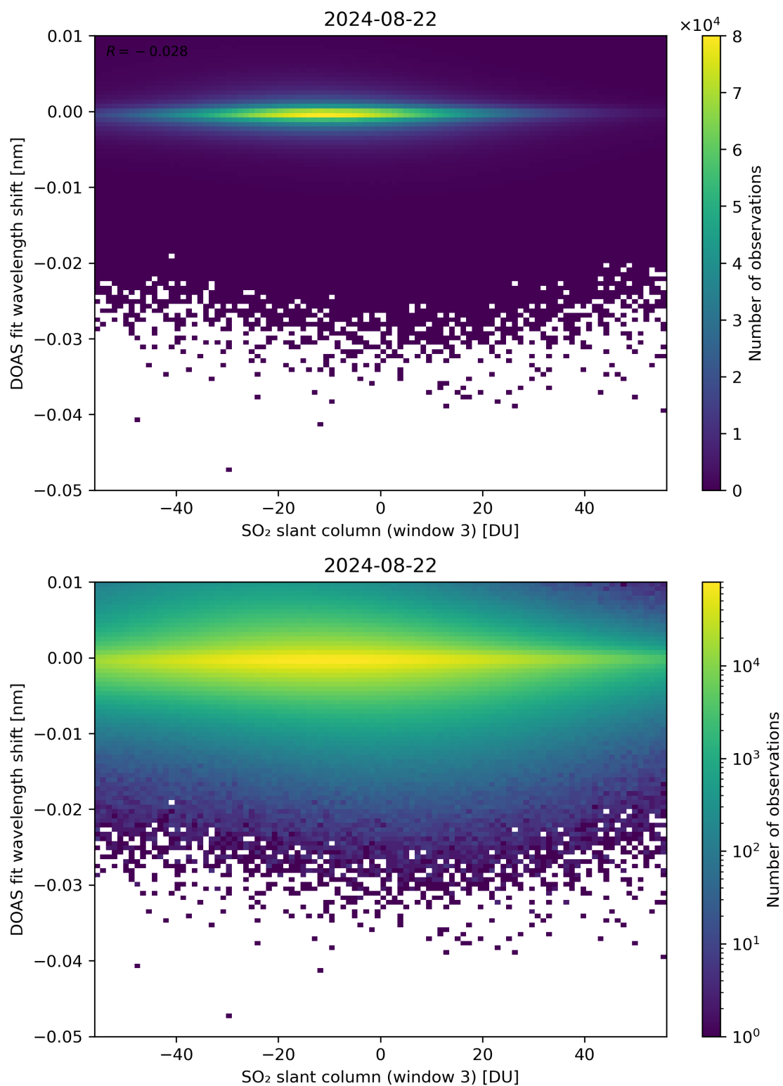
Figure 254: Scatter density plot of “SO 2 slant column (window 3)” against “DOAS fit wavelength shift” for 2024-08-22 to 2024-08-23.
