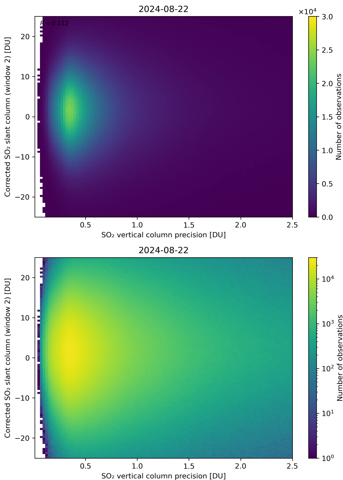
Figure 287: Scatter density plot of “SO 2 vertical column precision” against “Corrected SO 2 slant column (window 2)” for 2024-08-22 to 2024-08-23.
