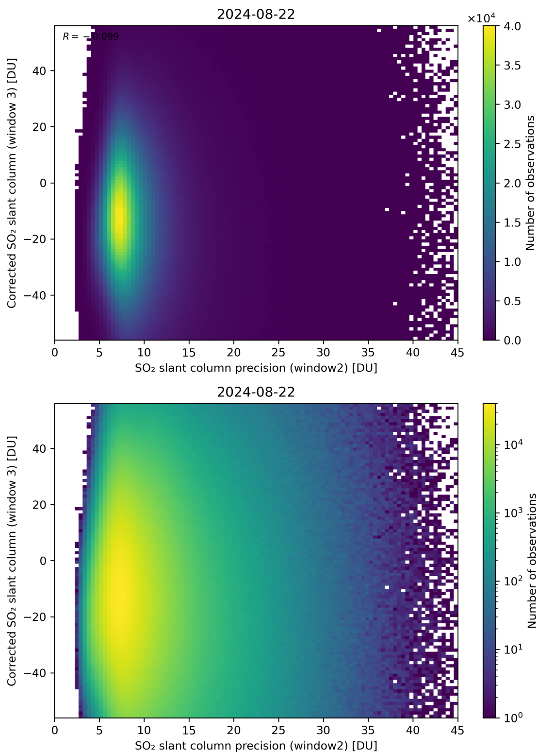
Figure 248: Scatter density plot of “SO 2 slant column precision (window2)” against “Corrected SO 2 slant column (window 3)” for 2024-08-22 to 2024-08-23.
