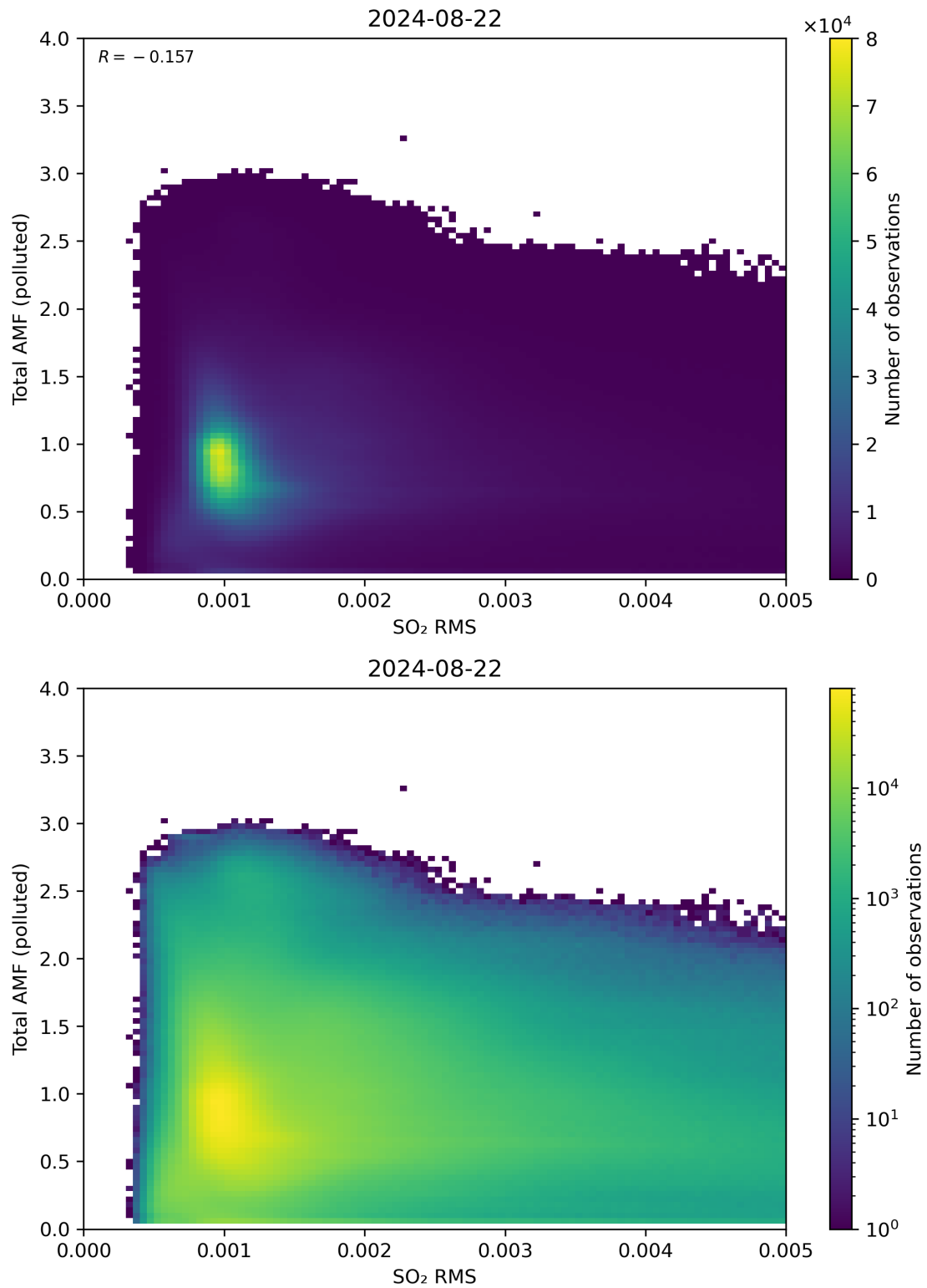
Figure 137: Scatter density plot of “SO 2 RMS” against “Total AMF (polluted)” for 2024-08-22 to 2024-08-23.
