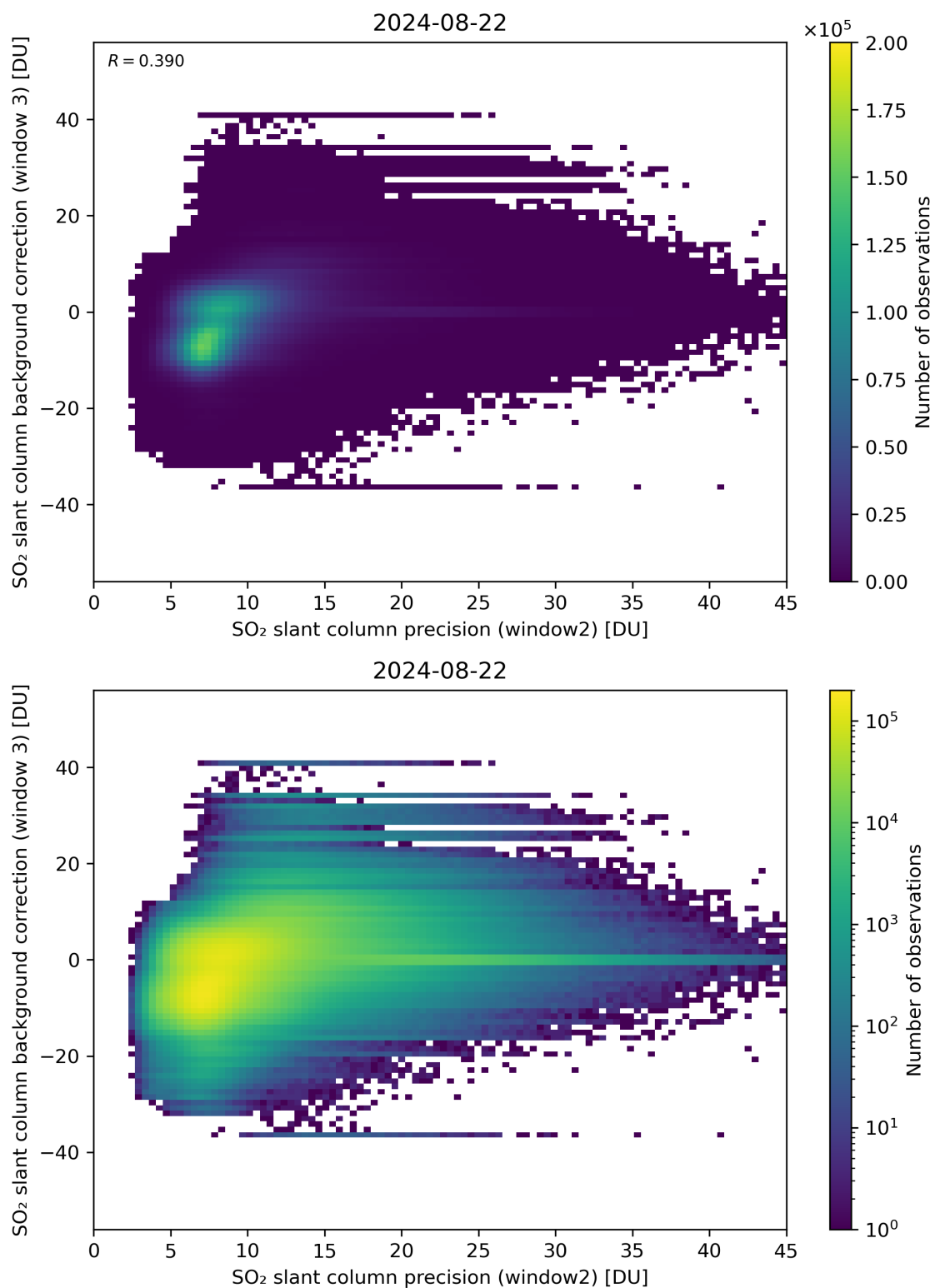
Figure 242: Scatter density plot of “SO 2 slant column precision (window2)” against “SO 2 slant column background correction (window 3)” for 2024-08-22 to 2024-08-23.
