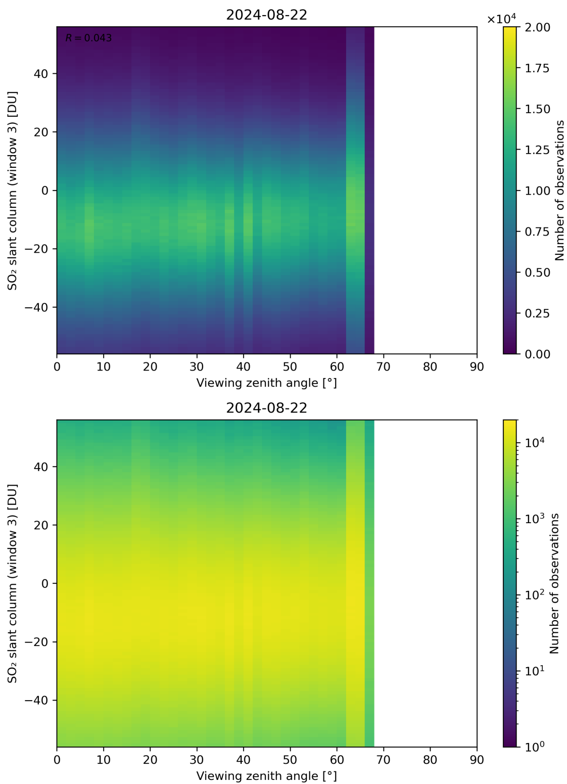
Figure 323: Scatter density plot of “Viewing zenith angle” against “SO 2 slant column (window 3)” for 2024-08-22 to 2024-08-23.
