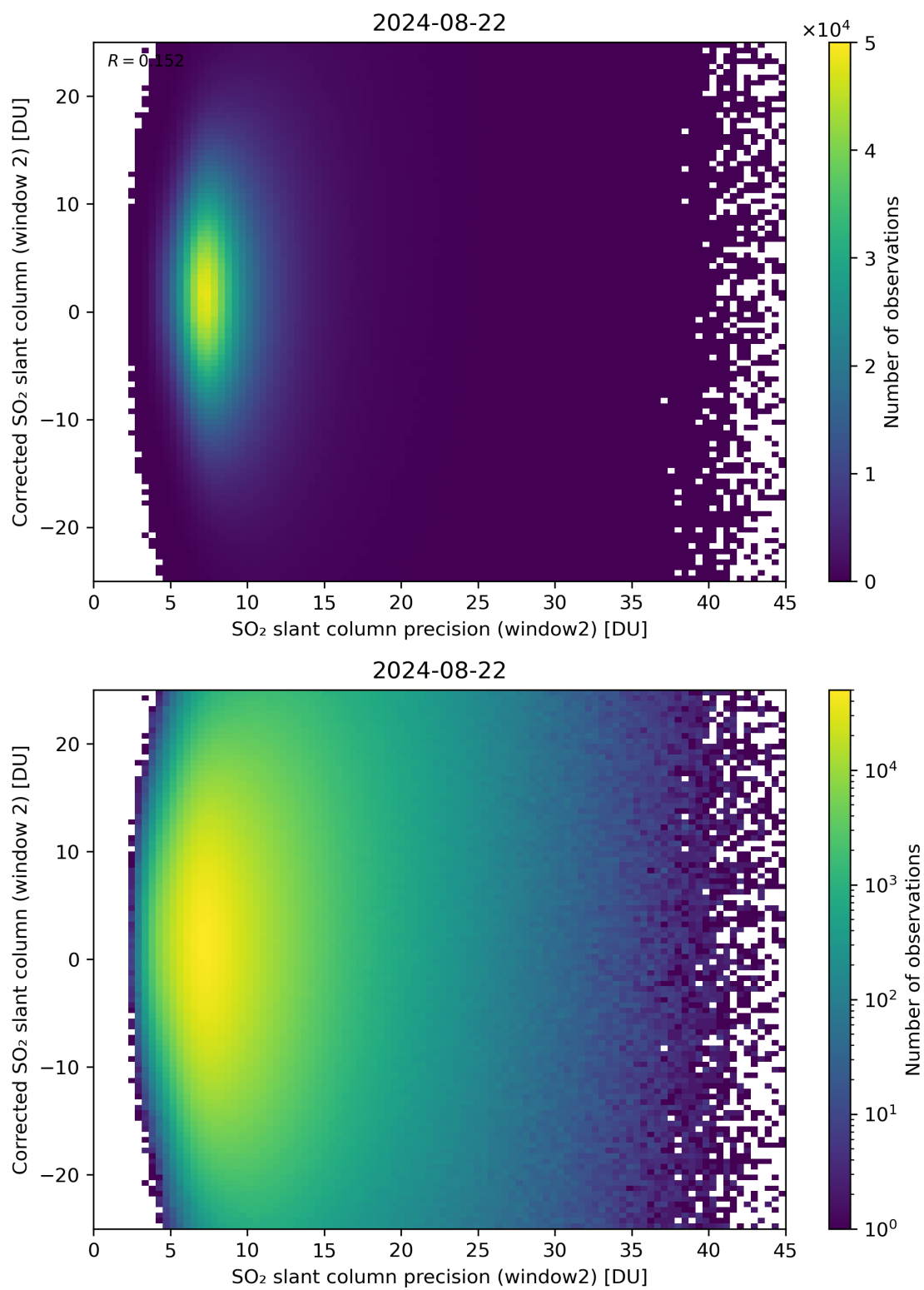
Figure 247: Scatter density plot of “SO 2 slant column precision (window2)” against “Corrected SO 2 slant column (window 2)” for 2024-08-22 to 2024-08-23.
