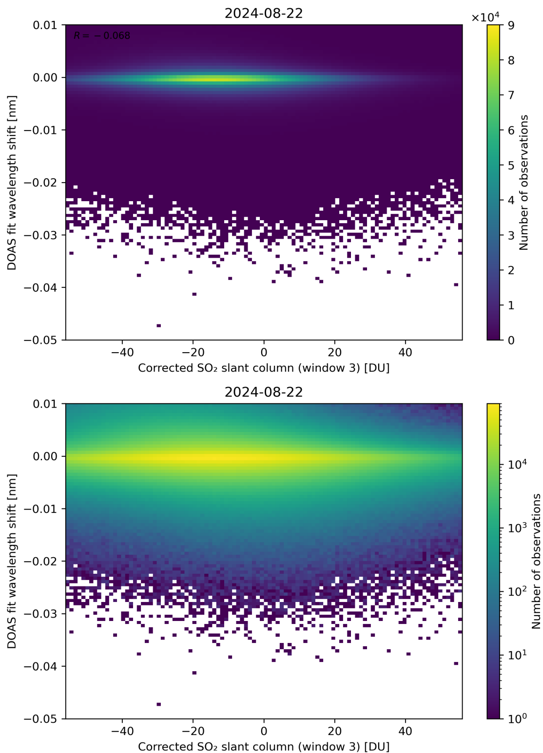
Figure 206: Scatter density plot of “Corrected SO 2 slant column (window 3)” against “DOAS fit wavelength shift” for 2024-08-22 to 2024-08-23.
