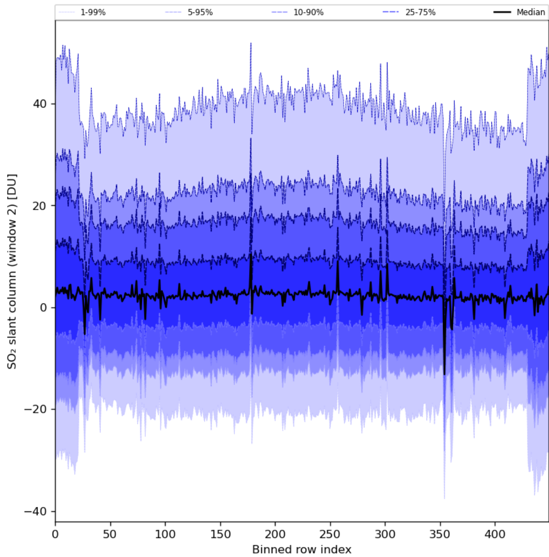
Figure 83: Along track statistics of “SO 2 slant column (window 2)” for 2024-08-22 to 2024-08-23
