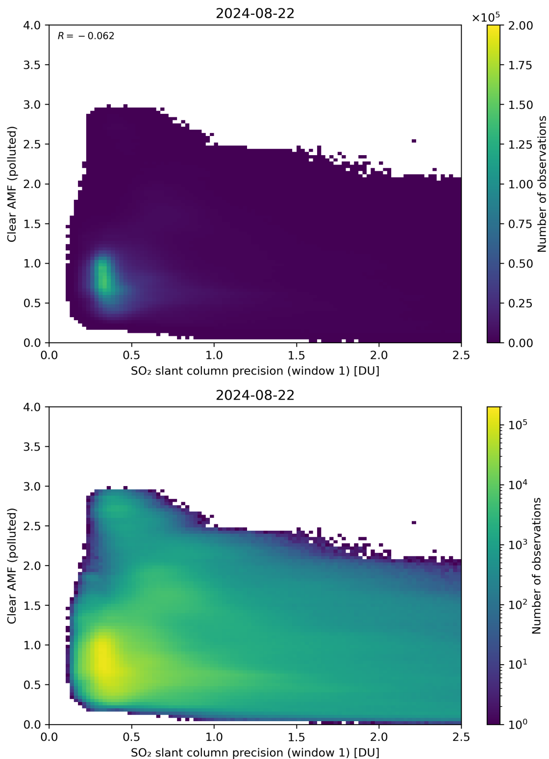
Figure 224: Scatter density plot of “SO 2 slant column precision (window 1)” against “Clear AMF (polluted)” for 2024-08-22 to 2024-08-23.
