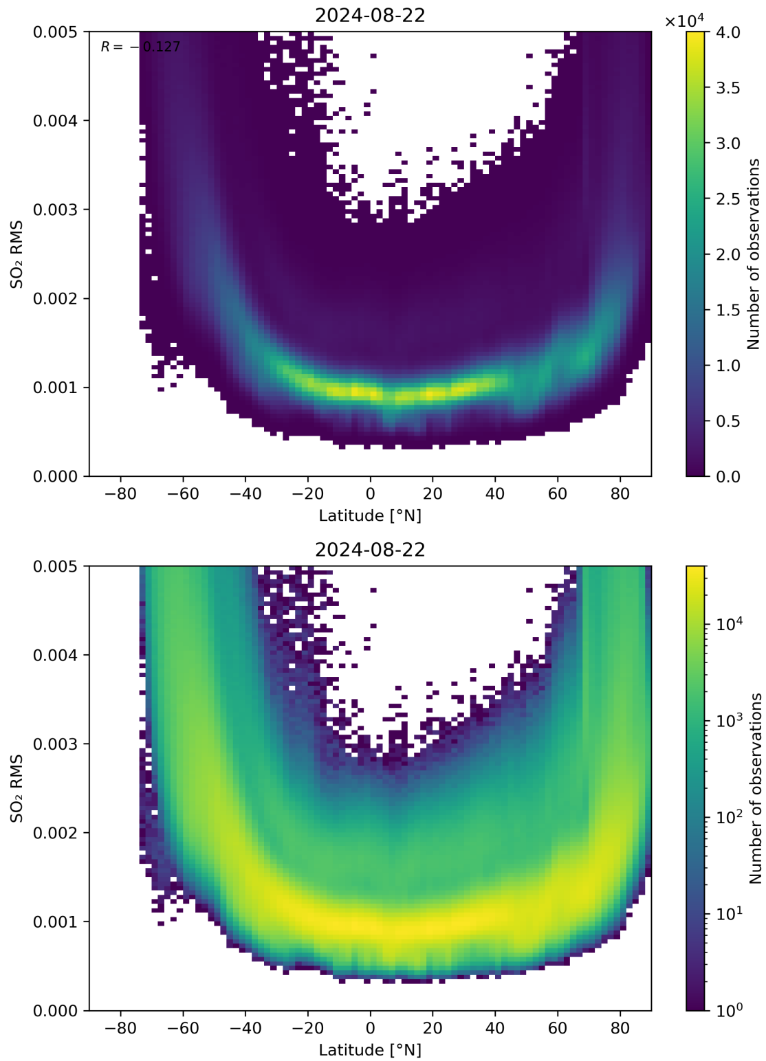
Figure 144: Scatter density plot of “Latitude” against “SO 2 RMS” for 2024-08-22 to 2024-08-23.
