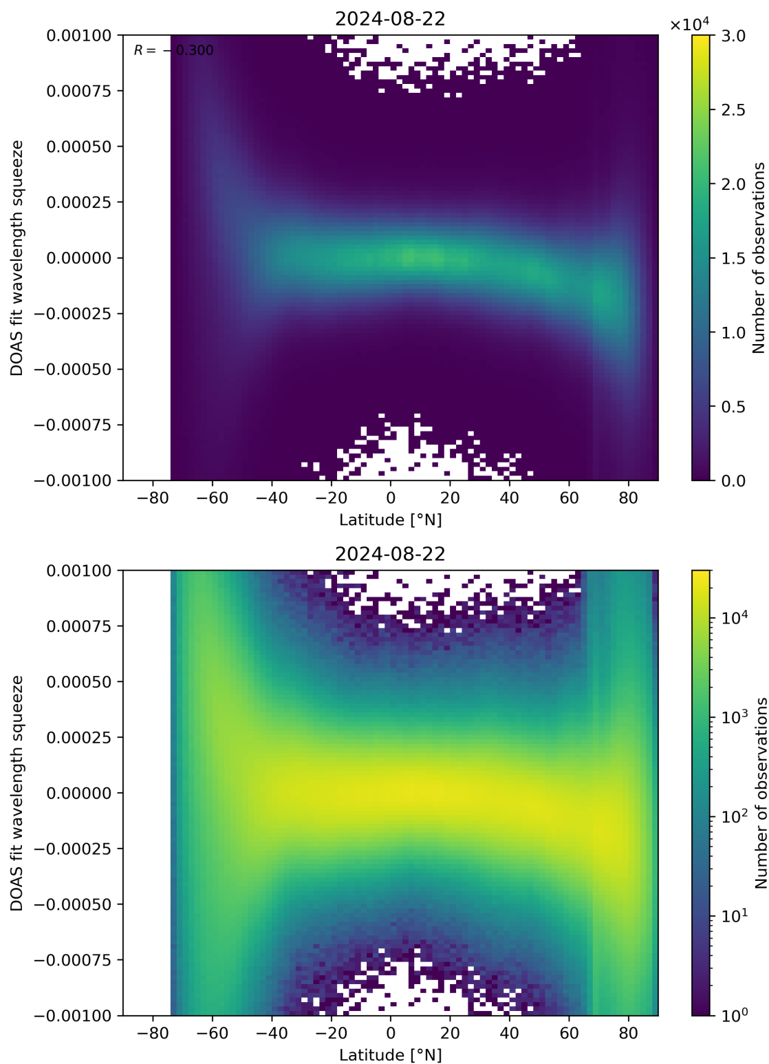
Figure 143: Scatter density plot of “Latitude” against “DOAS fit wavelength squeeze” for 2024-08-22 to 2024-08-23.
