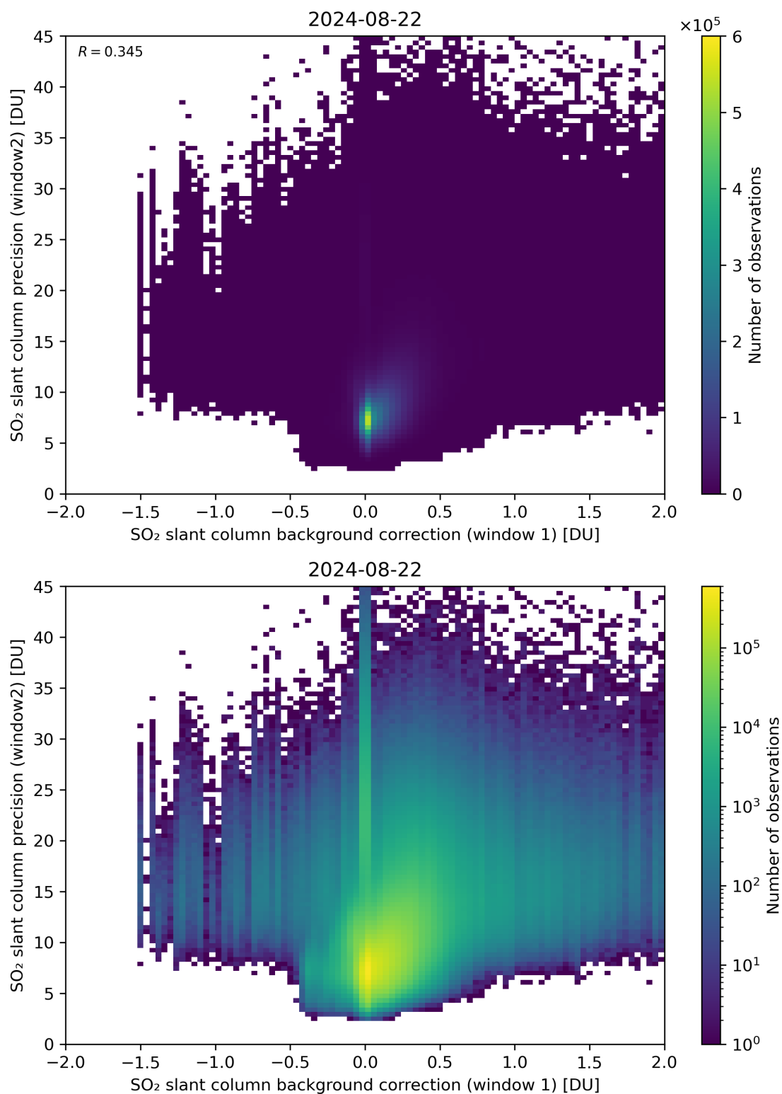
Figure 106: Scatter density plot of “SO 2 slant column background correction (window 1)” against “SO 2 slant column precision (window2)” for 2024-08-22 to 2024-08-23.
