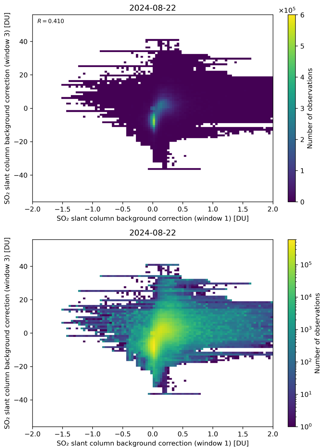
Figure 99: Scatter density plot of “SO 2 slant column background correction (window 1)” against “SO 2 slant column background correction (window 3)” for 2024-08-22 to 2024-08-23.
