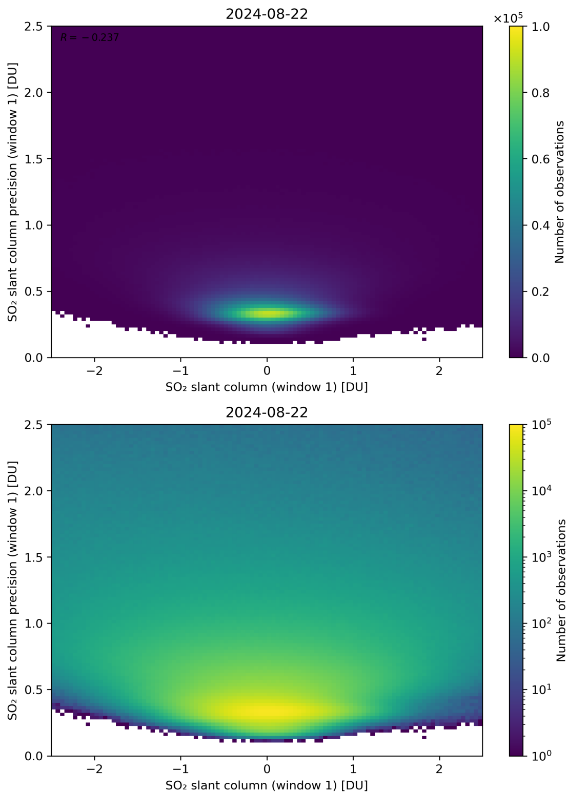
Figure 235: Scatter density plot of “SO 2 slant column (window 1)” against “SO 2 slant column precision (window 1)” for 2024-08-22 to 2024-08-23.
