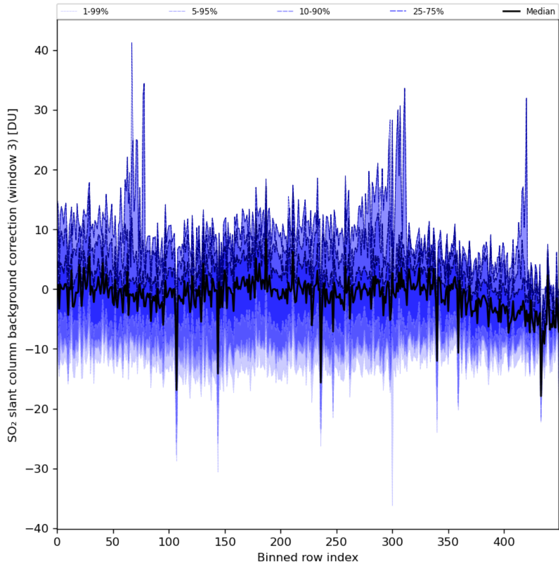
Figure 90: Along track statistics of “SO 2 slant column background correction (window 3)” for 2024-08-22 to 2024-08-23
