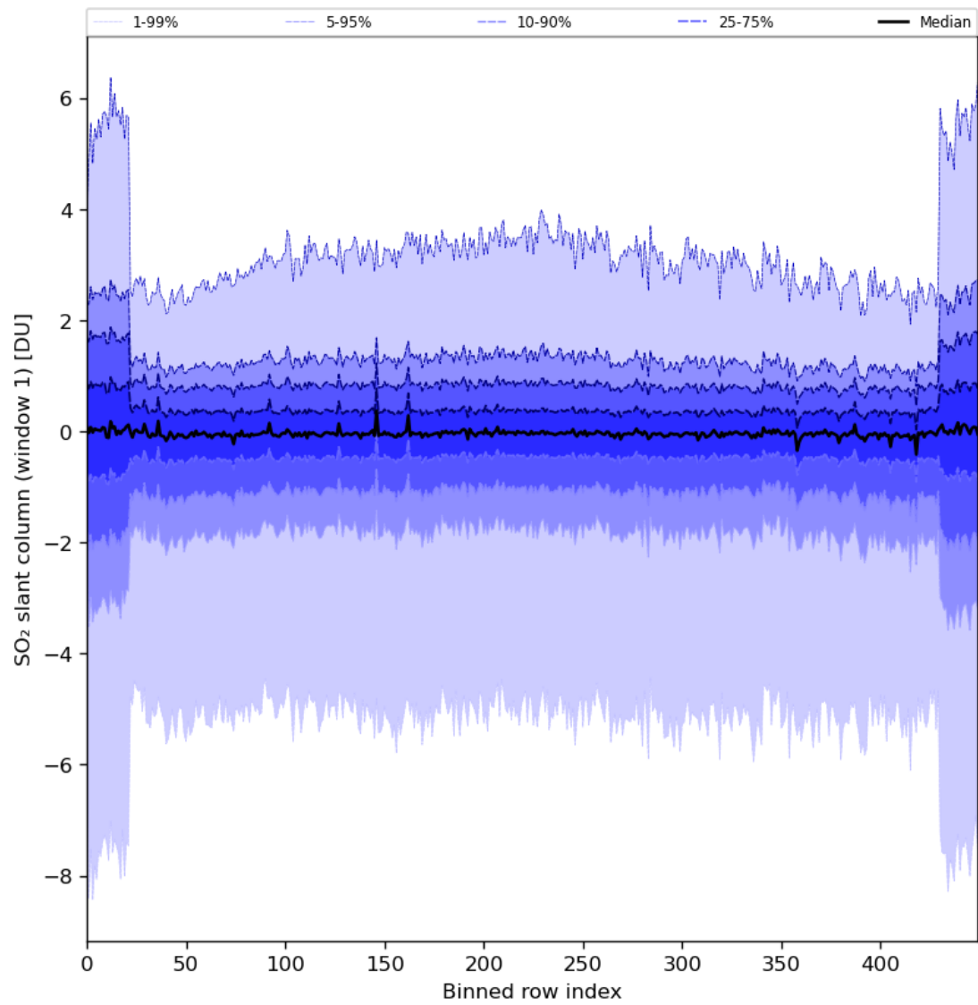
Figure 79: Along track statistics of “SO 2 slant column (window 1)” for 2024-08-22 to 2024-08-23
