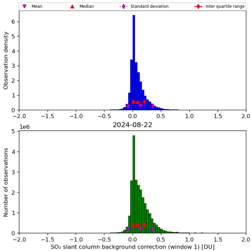
Figure 59: Histogram of “SO 2 slant column background correction (window 1)” for 2024-08-22 to 2024-08-23
