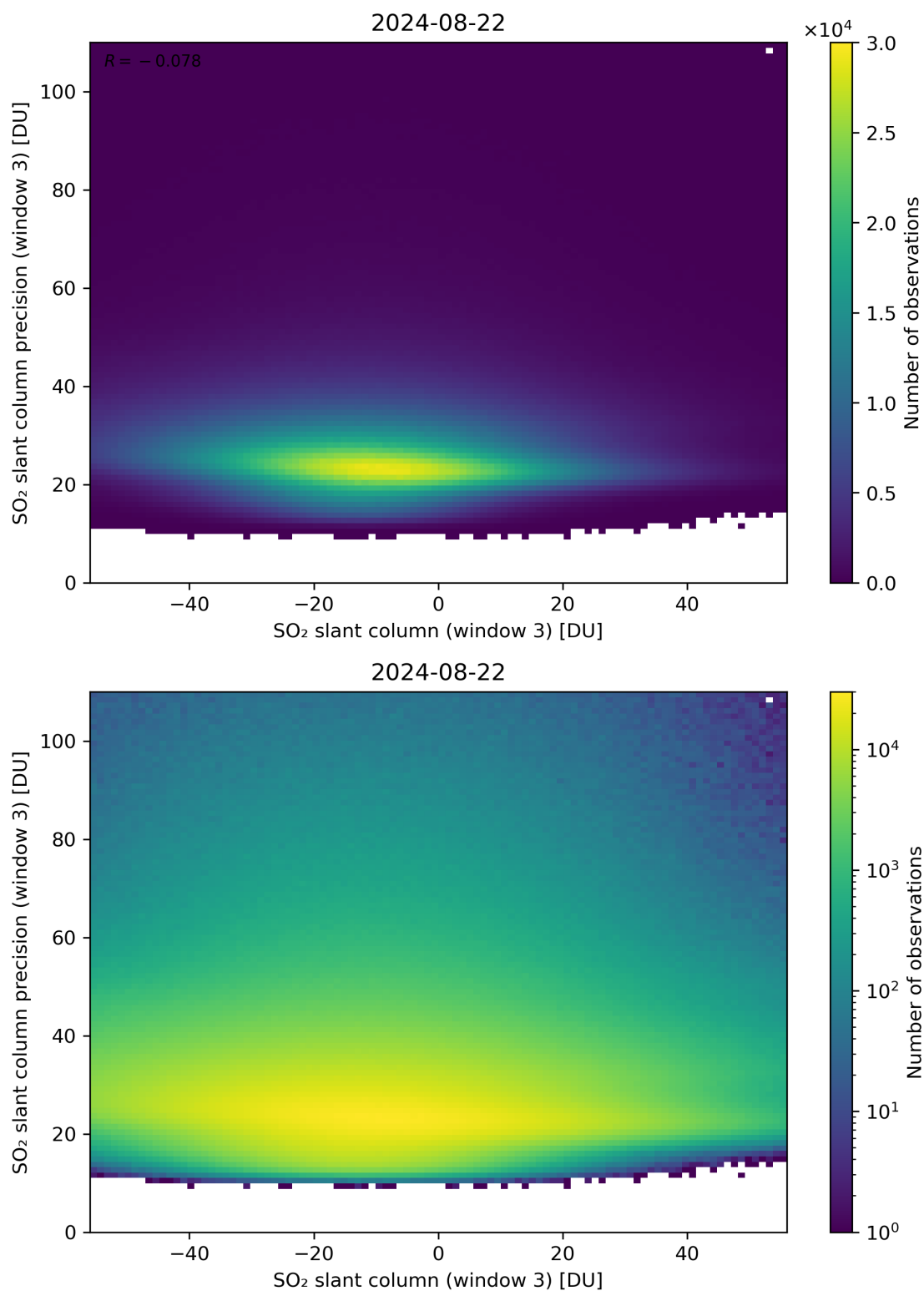
Figure 267: Scatter density plot of “SO 2 slant column (window 3)” against “SO 2 slant column precision (window 3)” for 2024-08-22 to 2024-08-23.
