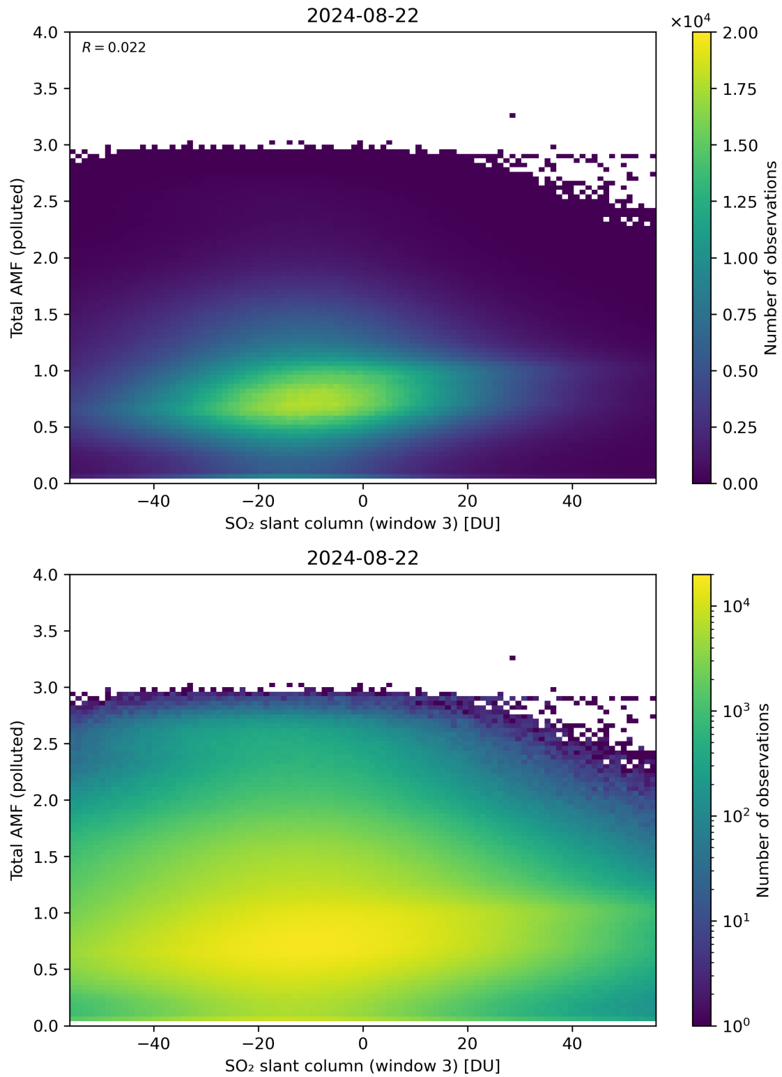
Figure 268: Scatter density plot of “SO 2 slant column (window 3)” against “Total AMF (polluted)” for 2024-08-22 to 2024-08-23.
