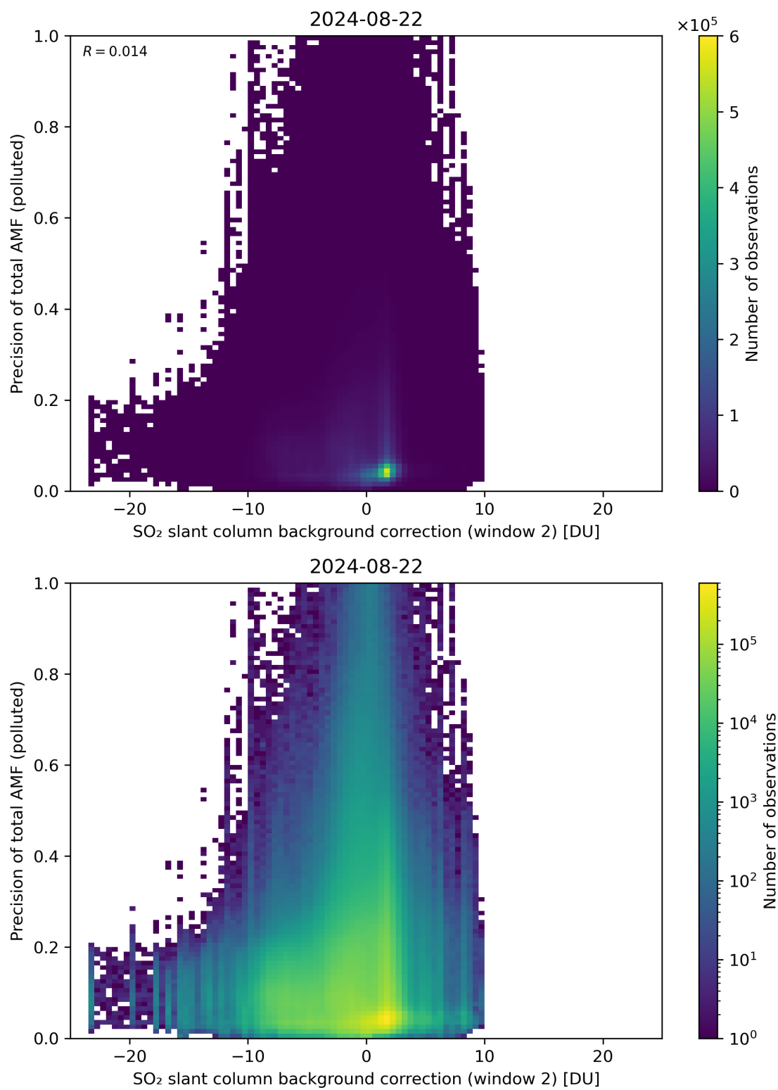
Figure 120: Scatter density plot of “SO 2 slant column background correction (window 2)” against “Precision of total AMF (polluted)” for 2024-08-22 to 2024-08-23.
