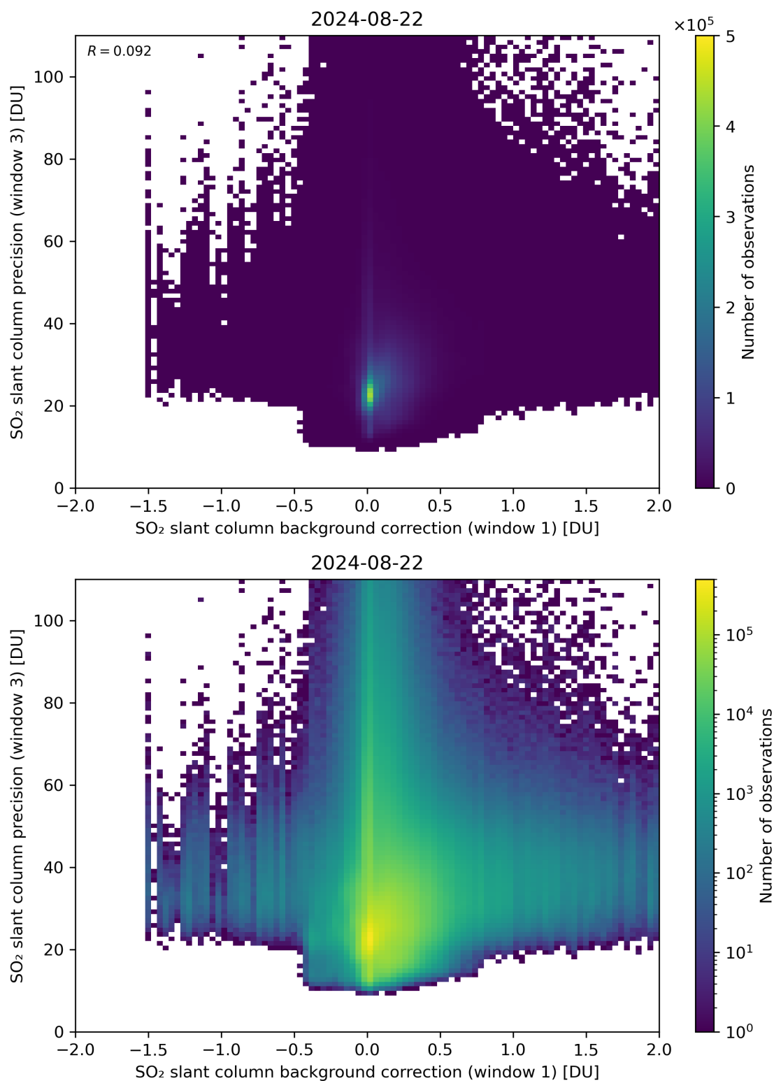
Figure 108: Scatter density plot of “SO 2 slant column background correction (window 1)” against “SO 2 slant column precision (window 3)” for 2024-08-22 to 2024-08-23.
