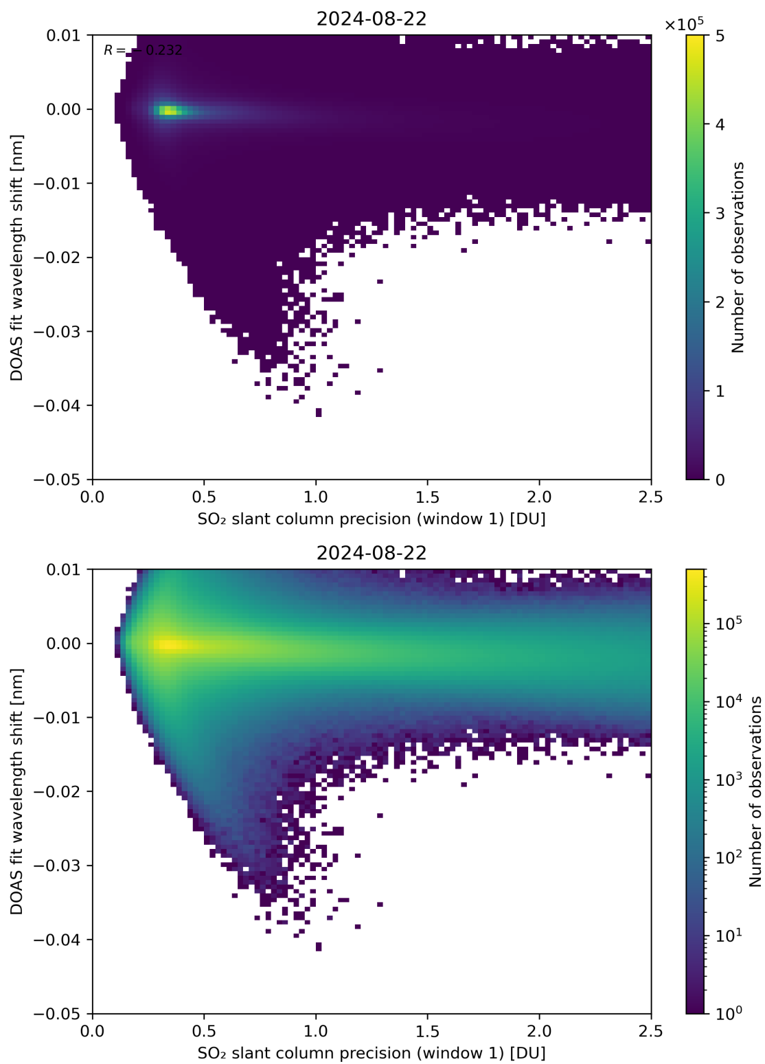
Figure 221: Scatter density plot of “SO 2 slant column precision (window 1)” against “DOAS fit wavelength shift” for 2024-08-22 to 2024-08-23.
