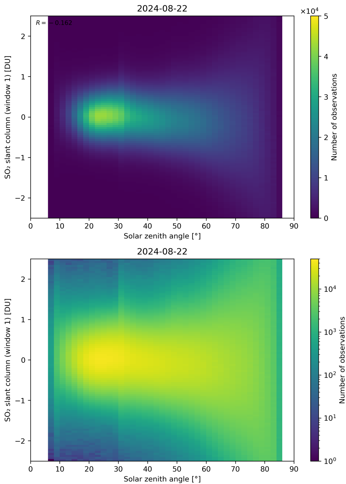
Figure 169: Scatter density plot of “Solar zenith angle” against “SO 2 slant column (window 1)” for 2024-08-22 to 2024-08-23.
