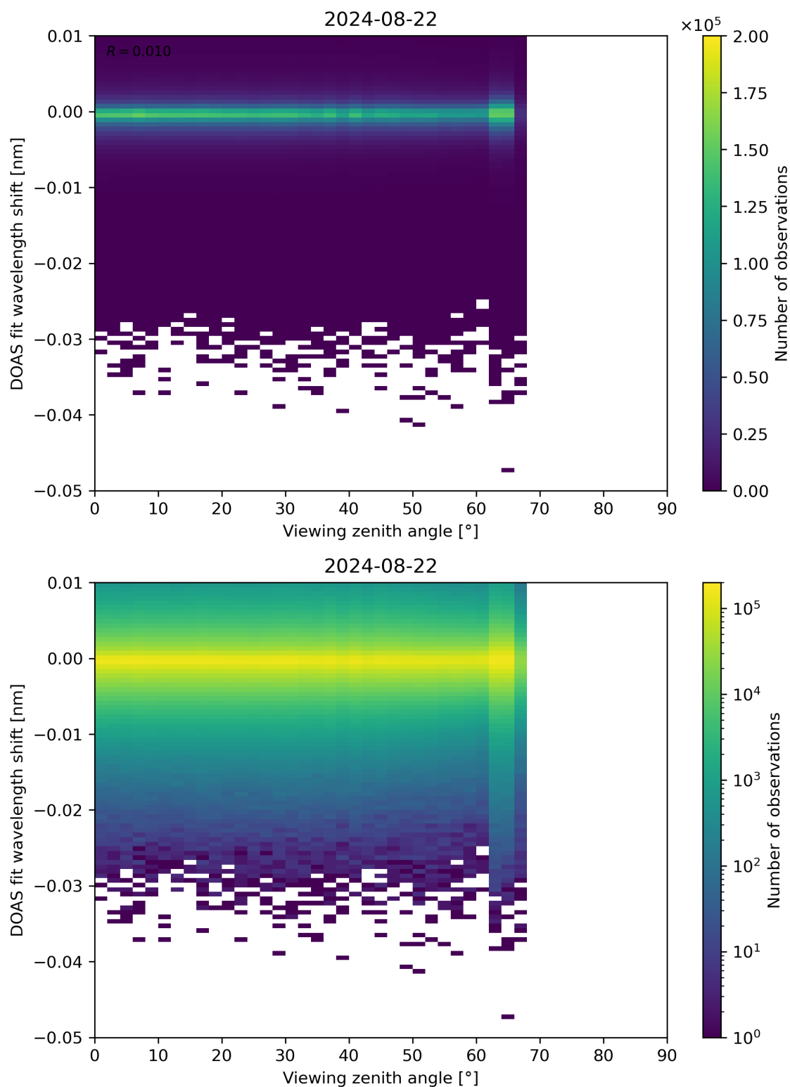
Figure 311: Scatter density plot of “Viewing zenith angle” against “DOAS fit wavelength shift” for 2024-08-22 to 2024-08-23.
