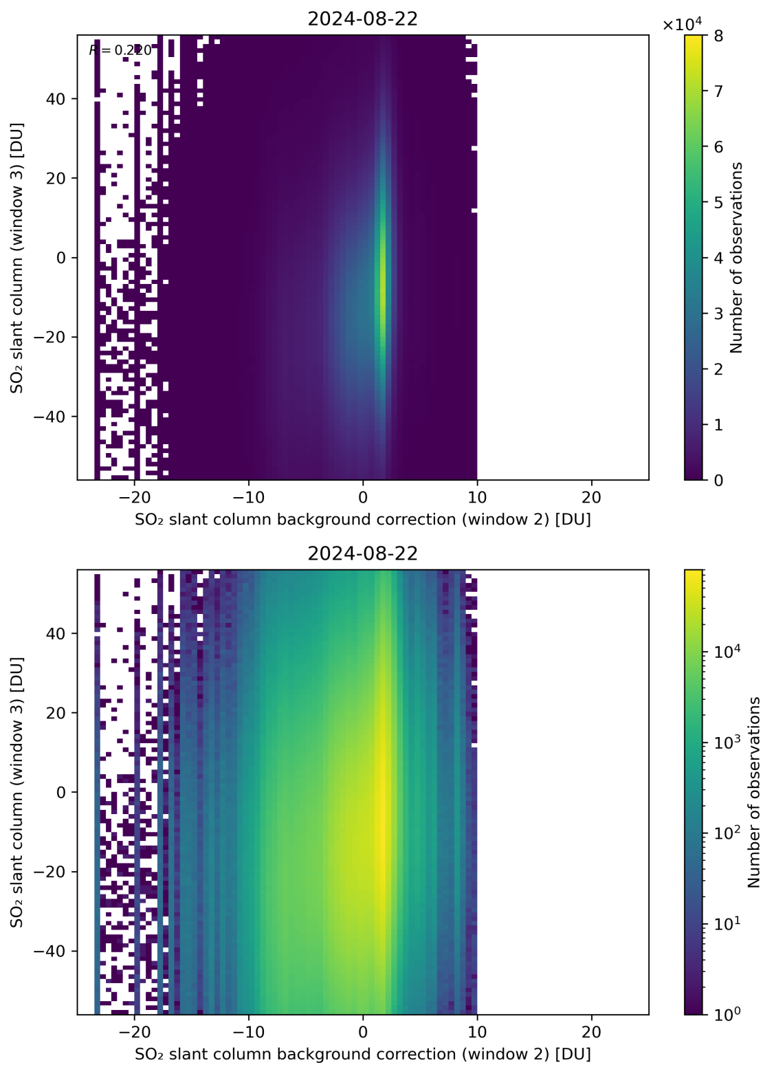
Figure 117: Scatter density plot of “SO 2 slant column background correction (window 2)” against “SO 2 slant column (window 3)” for 2024-08-22 to 2024-08-23.
