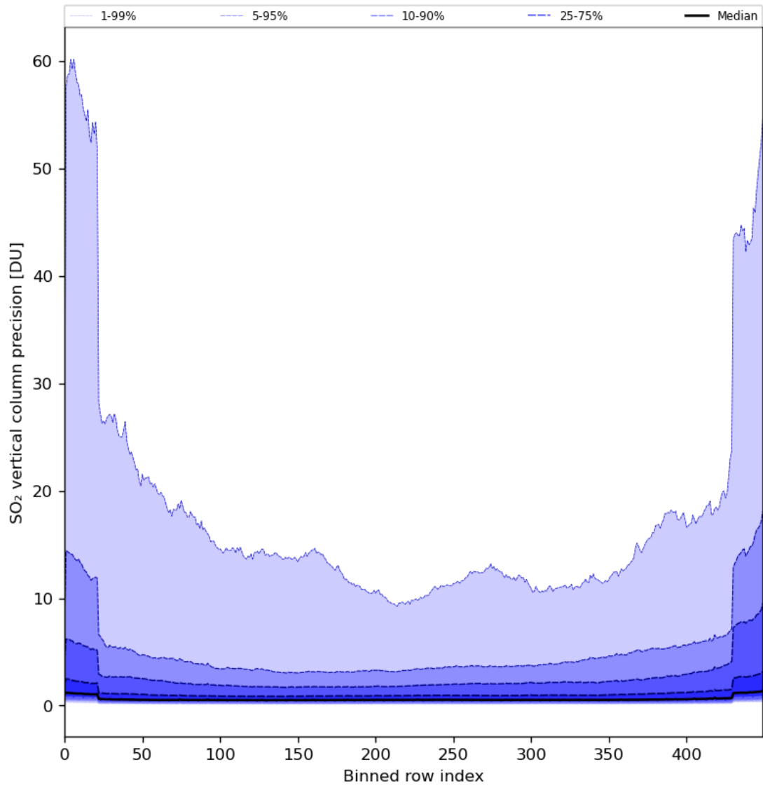
Figure 77: Along track statistics of “SO 2 vertical column precision” for 2024-08-22 to 2024-08-23
