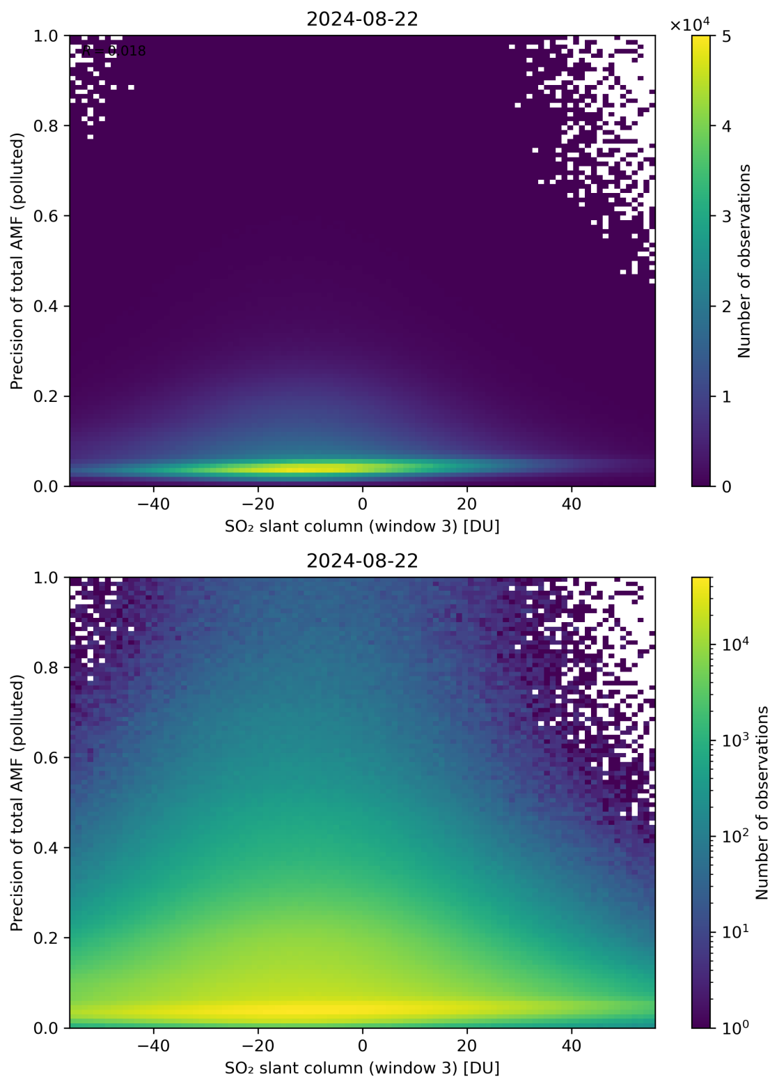
Figure 269: Scatter density plot of “SO 2 slant column (window 3)” against “Precision of total AMF (polluted)” for 2024-08-22 to 2024-08-23.
