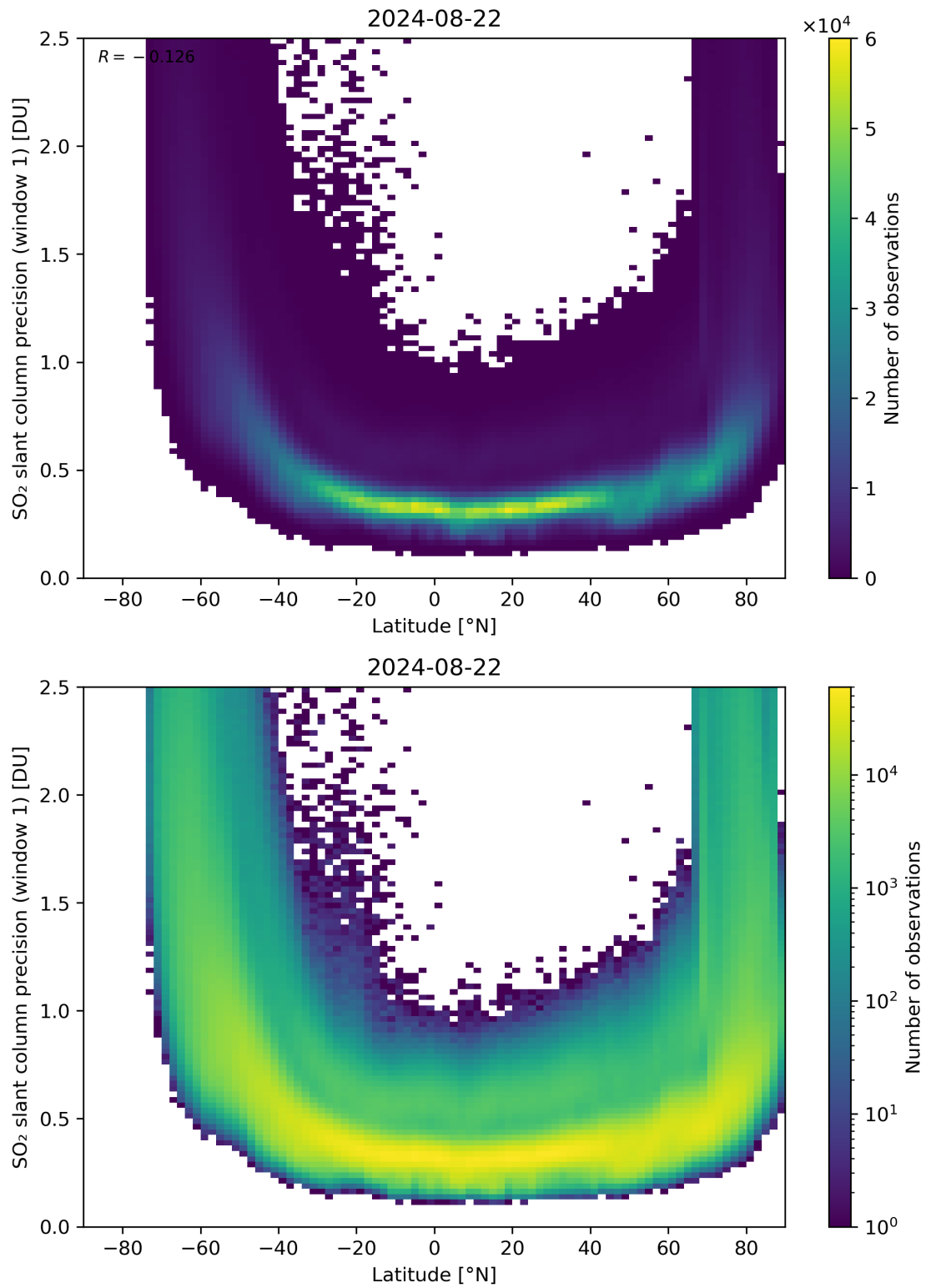
Figure 150: Scatter density plot of “Latitude” against “SO 2 slant column precision (window 1)” for 2024-08-22 to 2024-08-23.
