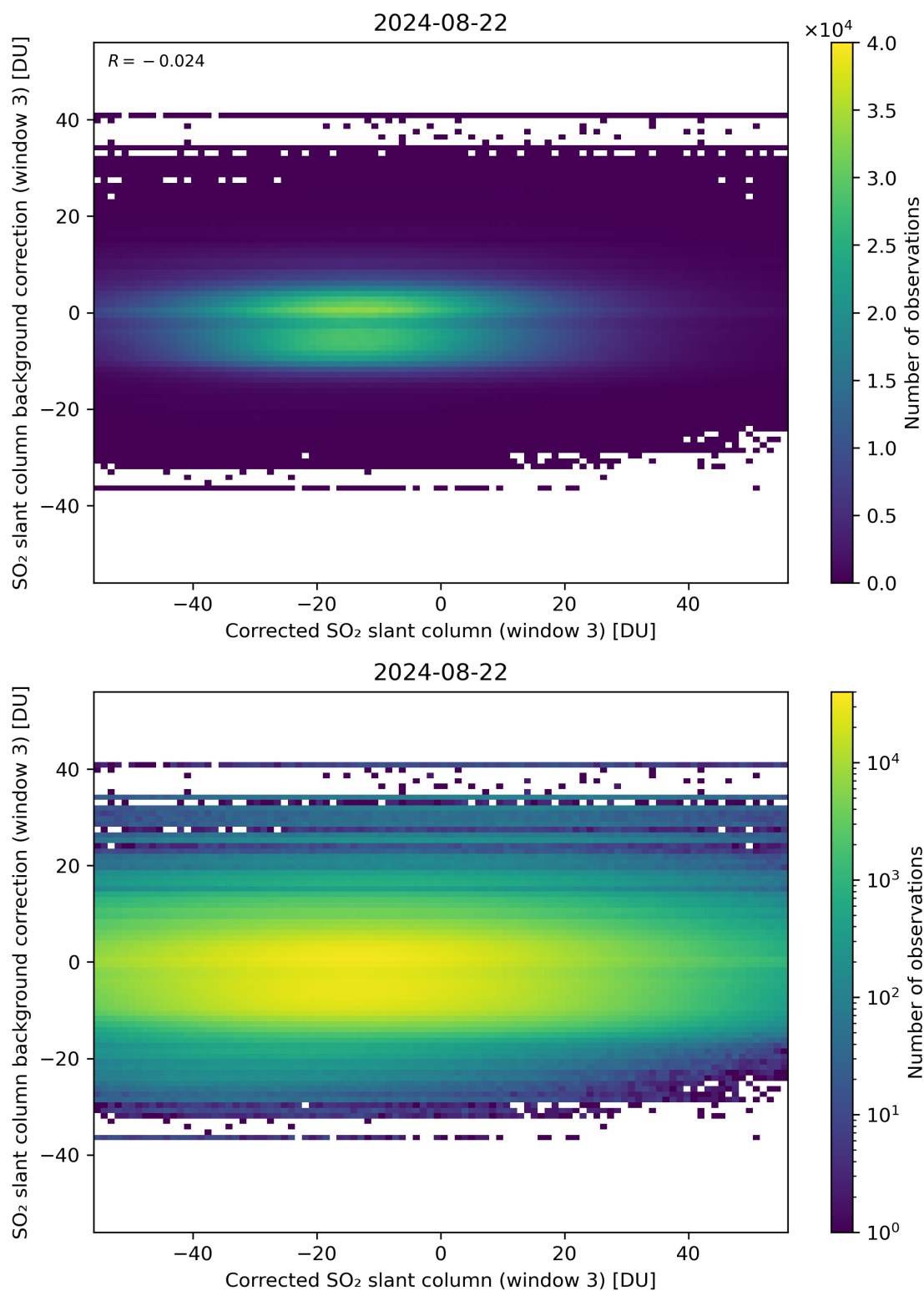
Figure 205: Scatter density plot of “Corrected SO 2 slant column (window 3)” against “SO 2 slant column background correction (window 3)” for 2024-08-22 to 2024-08-23.
