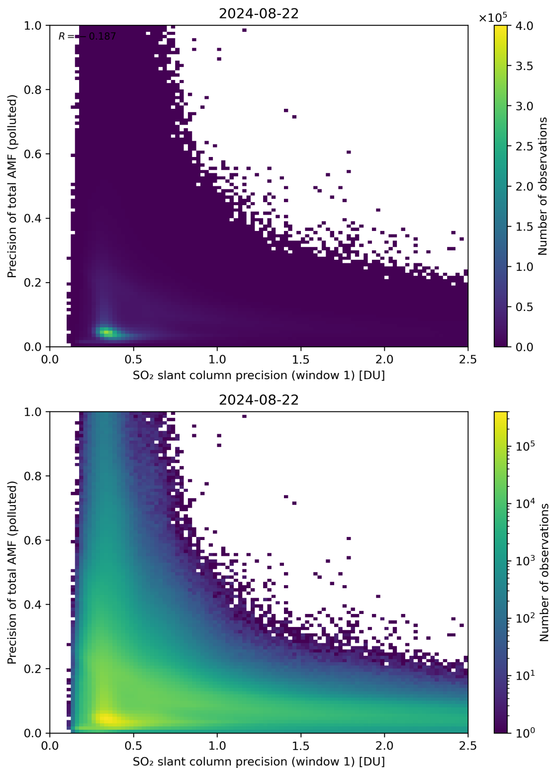
Figure 231: Scatter density plot of “SO 2 slant column precision (window 1)” against “Precision of total AMF (polluted)” for 2024-08-22 to 2024-08-23.
