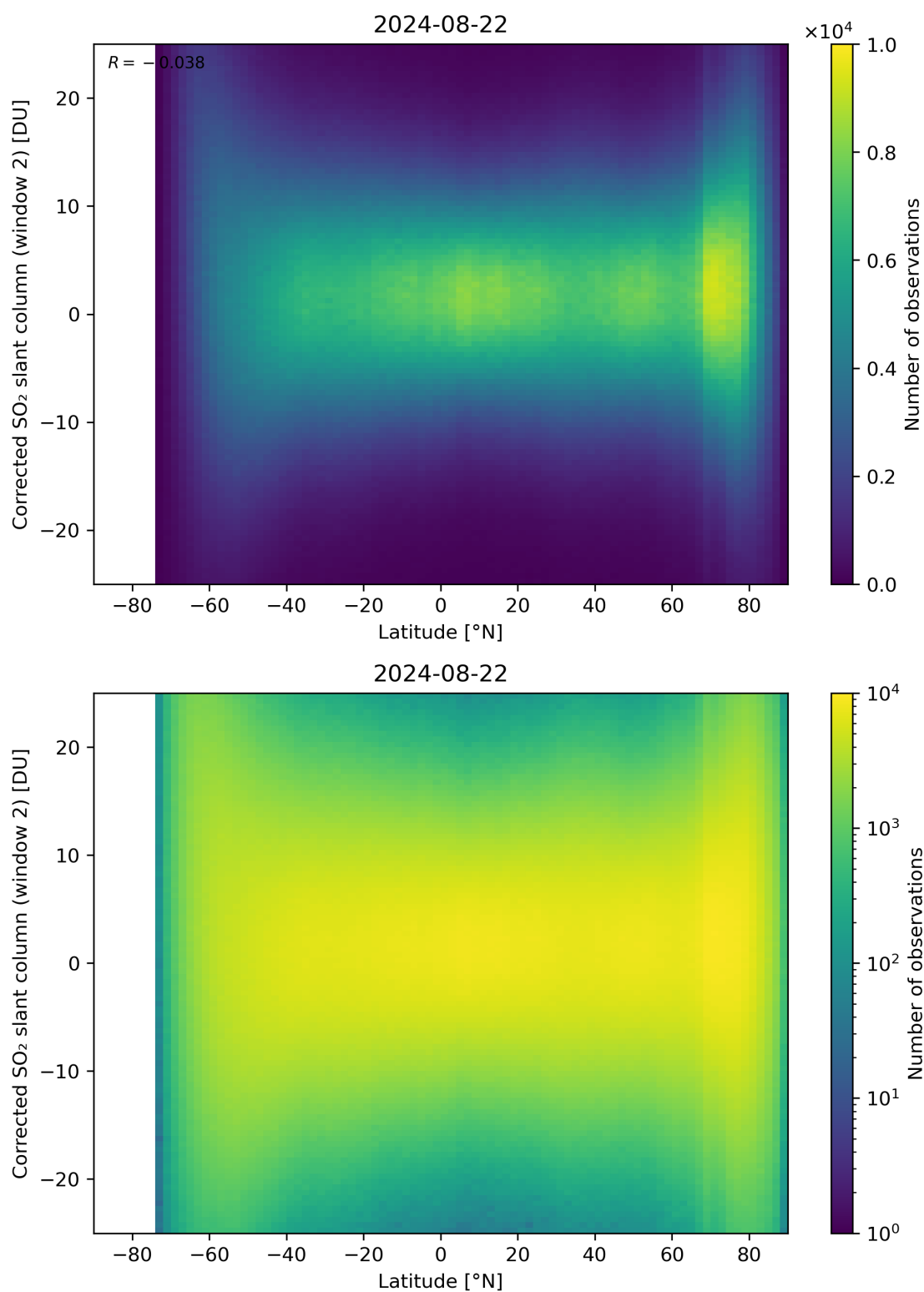
Figure 147: Scatter density plot of “Latitude” against “Corrected SO 2 slant column (window 2)” for 2024-08-22 to 2024-08-23.
