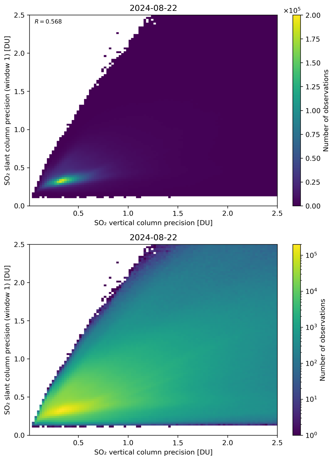
Figure 290: Scatter density plot of “SO 2 vertical column precision” against “SO 2 slant column precision (window 1)” for 2024-08-22 to 2024-08-23.
