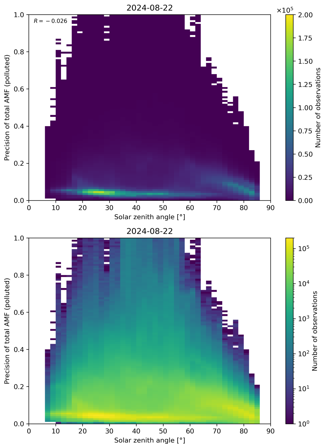
Figure 175: Scatter density plot of “Solar zenith angle” against “Precision of total AMF (polluted)” for 2024-08-22 to 2024-08-23.
