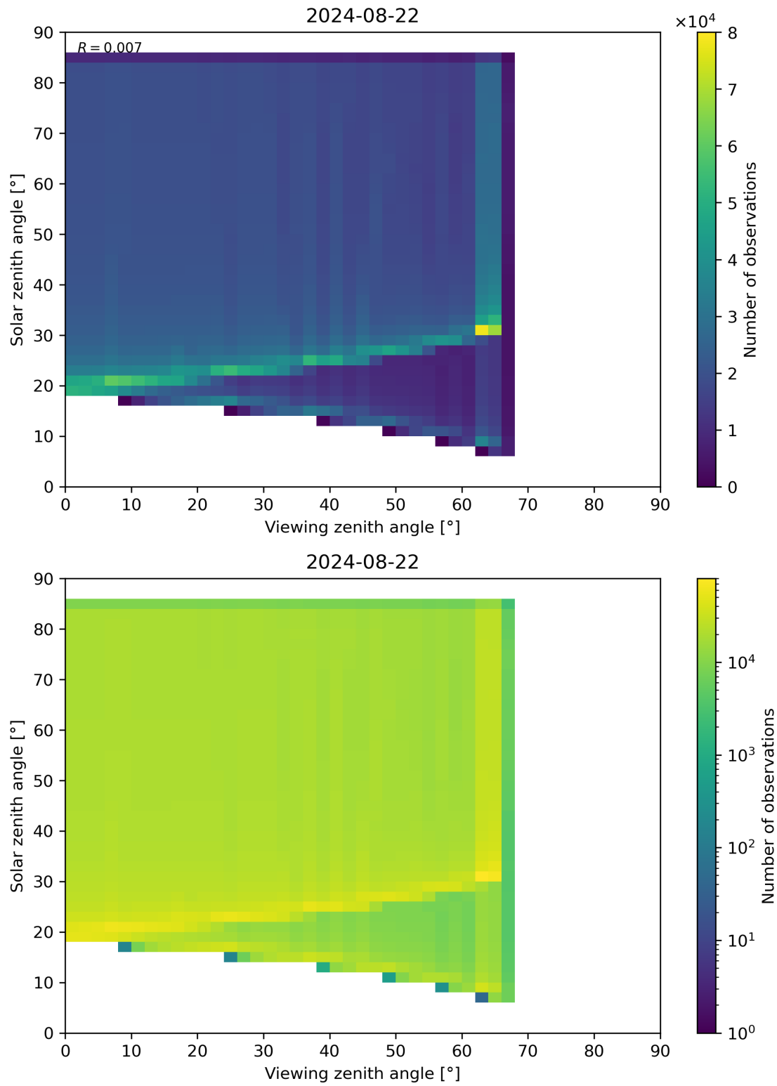
Figure 315: Scatter density plot of “Viewing zenith angle” against “Solar zenith angle” for 2024-08-22 to 2024-08-23.
