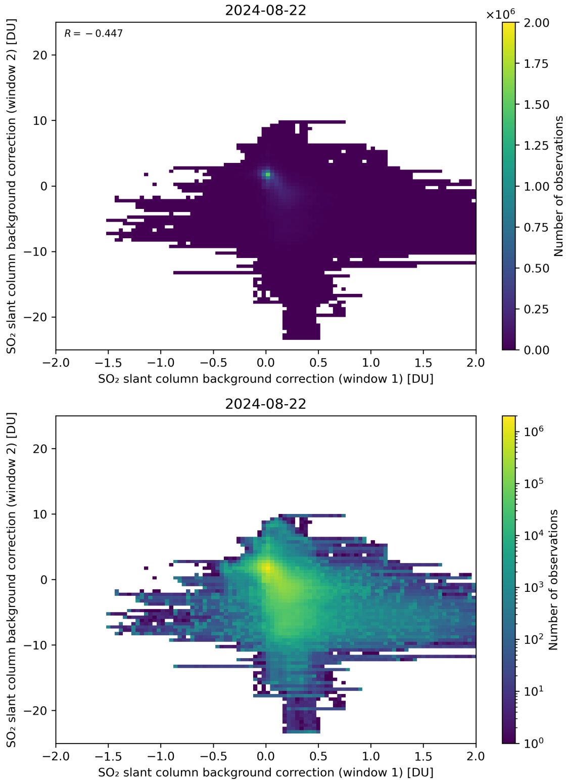
Figure 98: Scatter density plot of “SO 2 slant column background correction (window 1)” against “SO 2 slant column background correction (window 2)” for 2024-08-22 to 2024-08-23.
