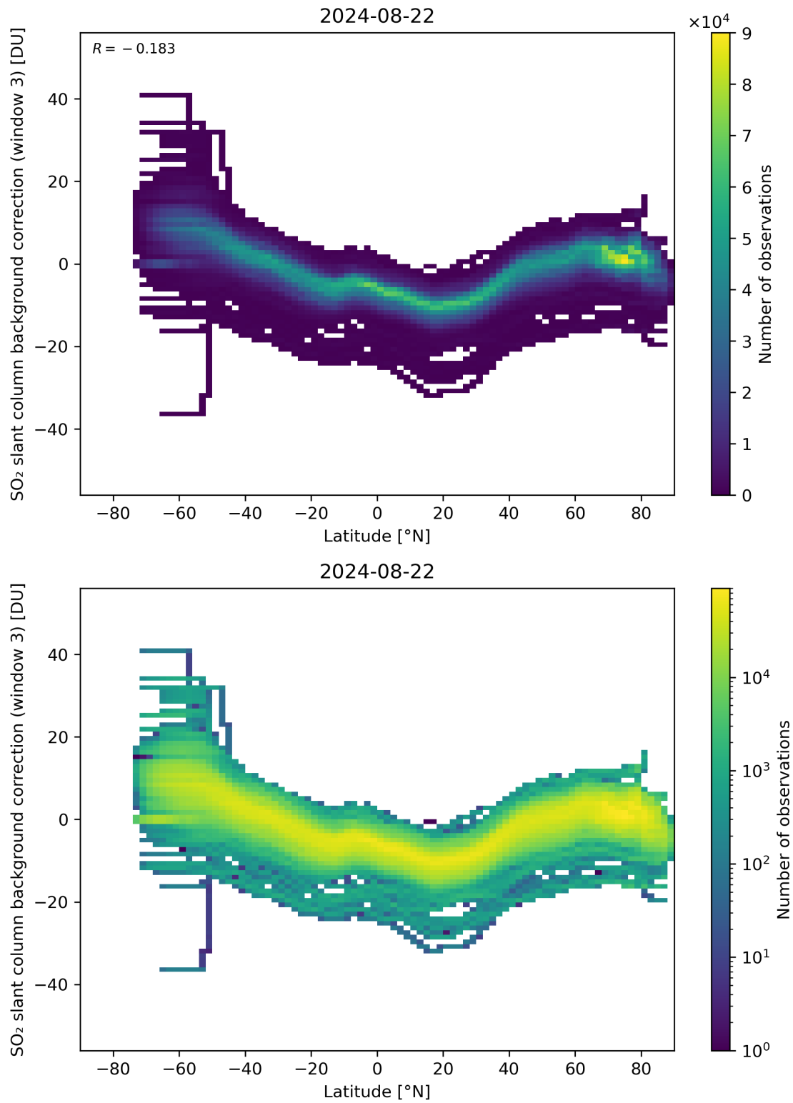
Figure 141: Scatter density plot of “Latitude” against “SO 2 slant column background correction (window 3)” for 2024-08-22 to 2024-08-23.
