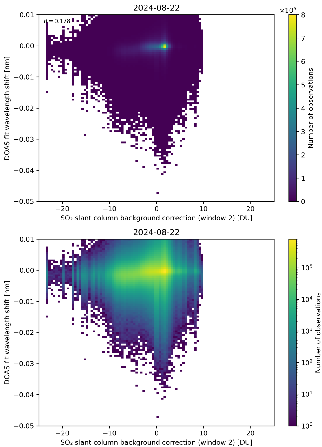
Figure 112: Scatter density plot of “SO 2 slant column background correction (window 2)” against “DOAS fit wavelength shift” for 2024-08-22 to 2024-08-23.
