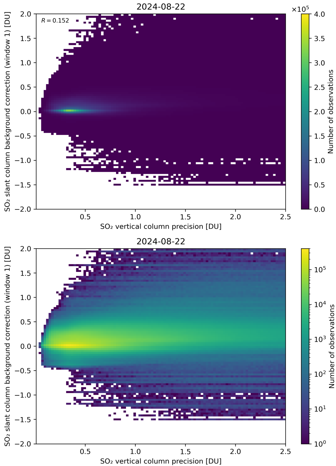
Figure 279: Scatter density plot of “SO 2 vertical column precision” against “SO 2 slant column background correction (window 1)” for 2024-08-22 to 2024-08-23.
