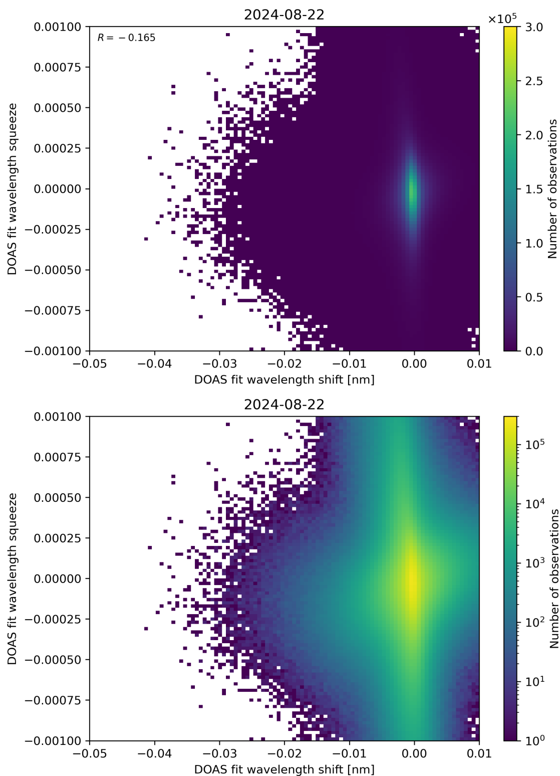
Figure 127: Scatter density plot of “DOAS fit wavelength shift” against “DOAS fit wavelength squeeze” for 2024-08-22 to 2024-08-23.
