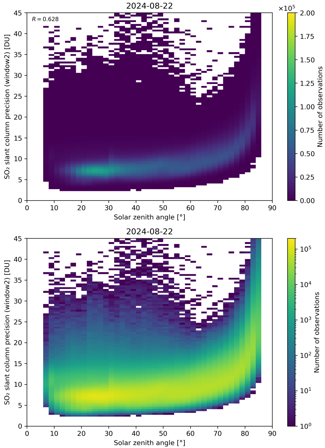
Figure 171: Scatter density plot of “Solar zenith angle” against “SO 2 slant column precision (window2)” for 2024-08-22 to 2024-08-23.
