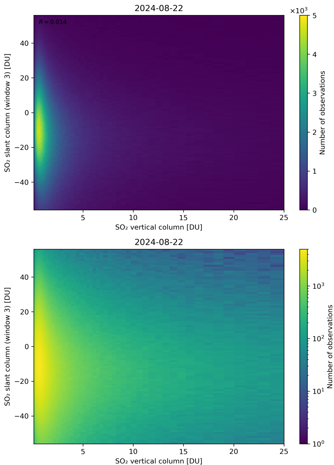
Figure 303: Scatter density plot of “SO 2 vertical column” against “SO 2 slant column (window 3)” for 2024-08-22 to 2024-08-23.
