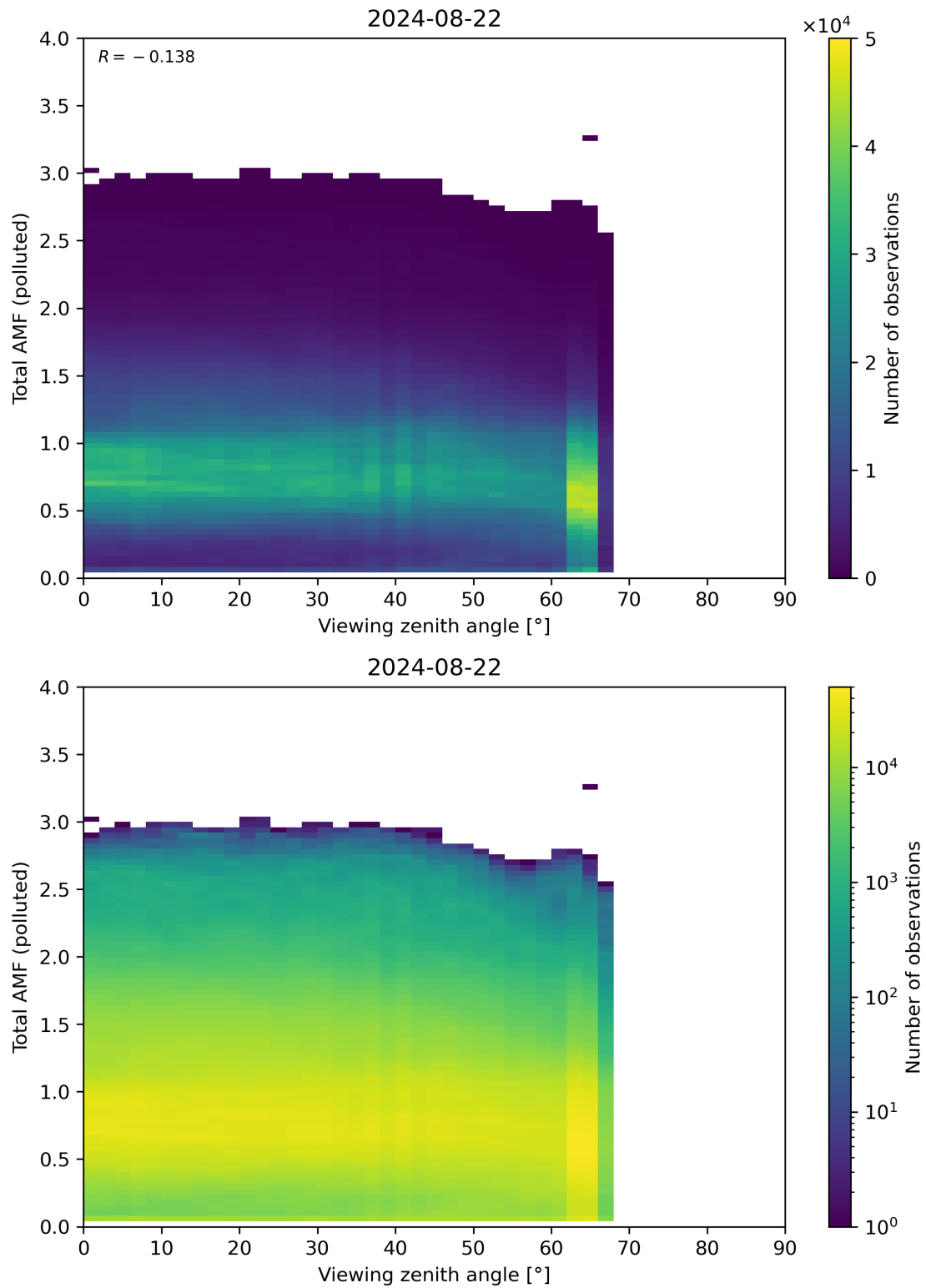
Figure 325: Scatter density plot of “Viewing zenith angle” against “Total AMF (polluted)” for 2024-08-22 to 2024-08-23.
