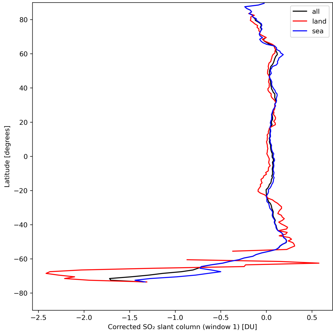
Figure 35: Zonal average of “Corrected SO 2 slant column (window 1)” for 2024-08-22 to 2024-08-23.
