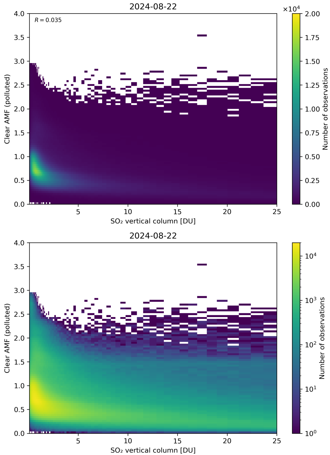
Figure 296: Scatter density plot of “SO 2 vertical column” against “Clear AMF (polluted)” for 2024-08-22 to 2024-08-23.
