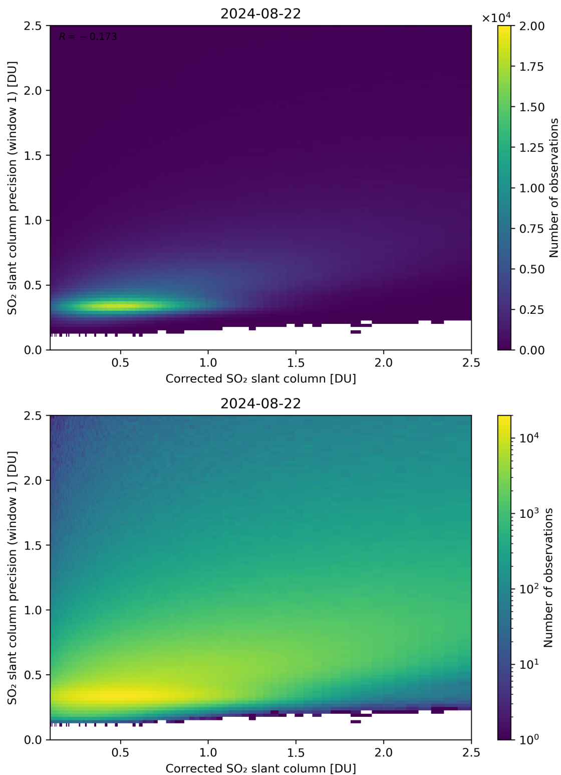
Figure 188: Scatter density plot of “Corrected SO 2 slant column” against “SO 2 slant column precision (window 1)” for 2024-08-22 to 2024-08-23.
