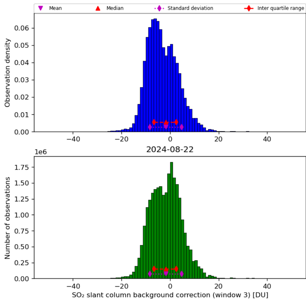
Figure 67: Histogram of “SO 2 slant column background correction (window 3)” for 2024-08-22 to 2024-08-23
