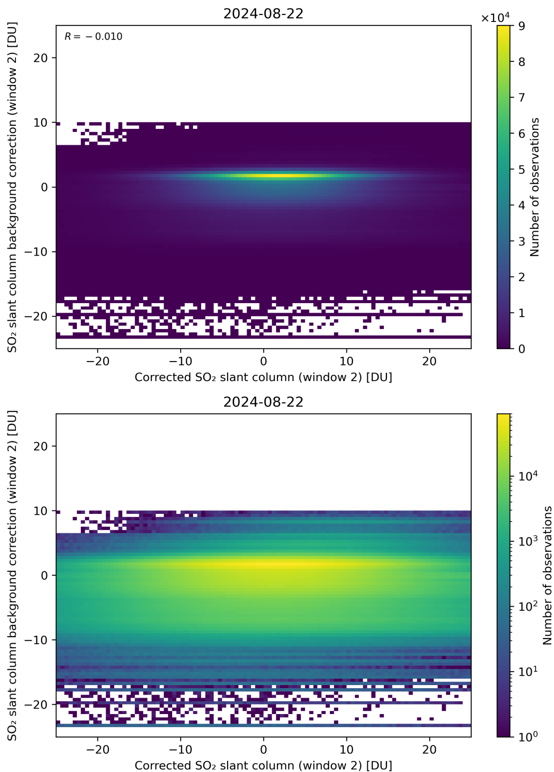
Figure 194: Scatter density plot of “Corrected SO 2 slant column (window 2)” against “SO 2 slant column background correction (window 2)” for 2024-08-22 to 2024-08-23.
