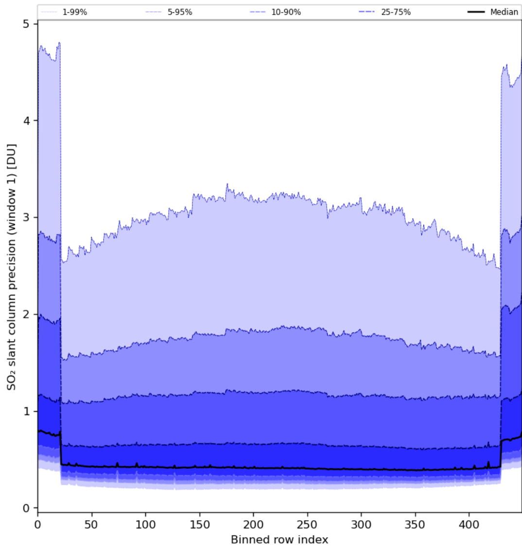
Figure 80: Along track statistics of “SO 2 slant column precision (window 1)” for 2024-08-22 to 2024-08-23
