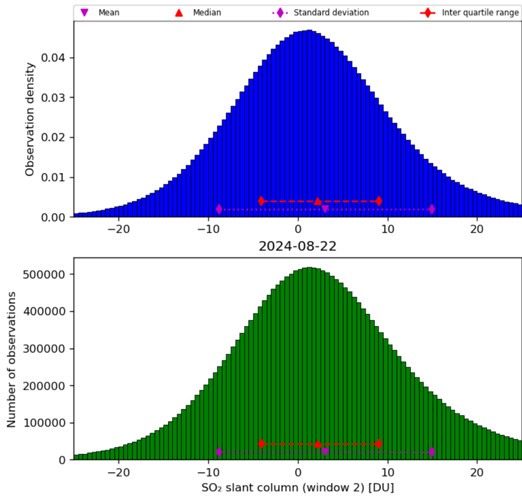
Figure 60: Histogram of “SO 2 slant column (window 2)” for 2024-08-22 to 2024-08-23
