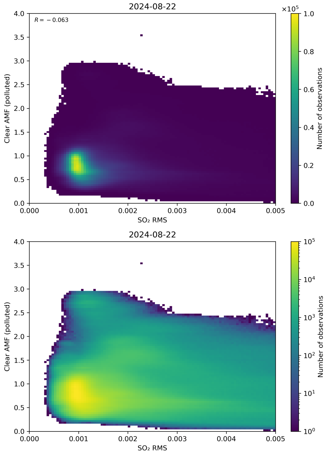
Figure 136: Scatter density plot of “SO 2 RMS” against “Clear AMF (polluted)” for 2024-08-22 to 2024-08-23.
