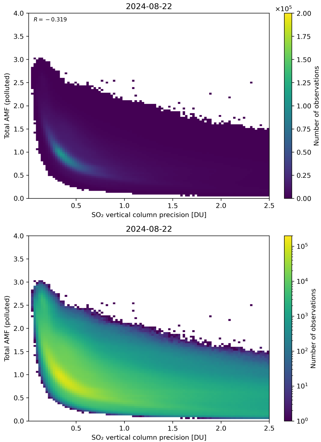
Figure 294: Scatter density plot of “SO 2 vertical column precision” against “Total AMF (polluted)” for 2024-08-22 to 2024-08-23.
