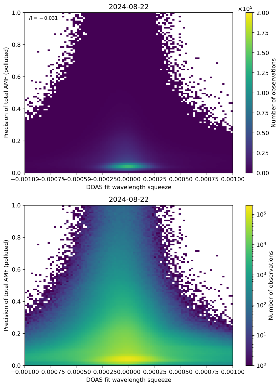
Figure 135: Scatter density plot of “DOAS fit wavelength squeeze” against “Precision of total AMF (polluted)” for 2024-08-22 to 2024-08-23.
