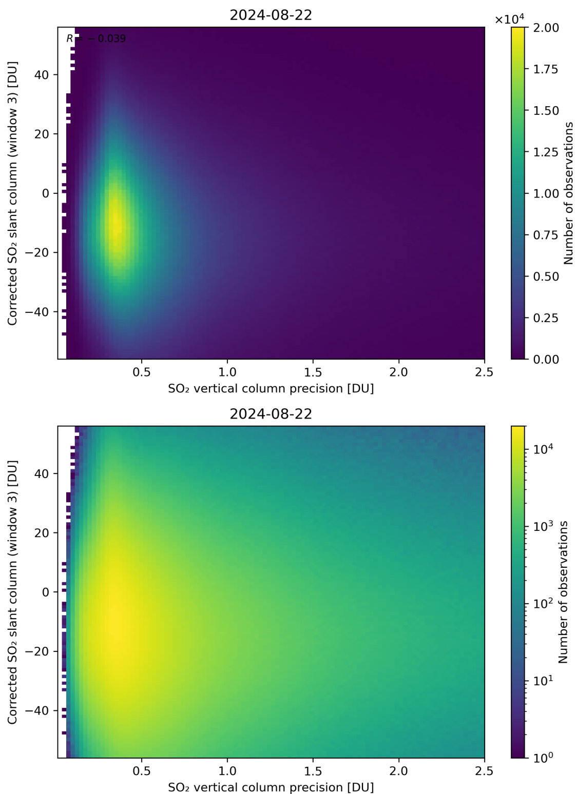
Figure 288: Scatter density plot of “SO 2 vertical column precision” against “Corrected SO 2 slant column (window 3)” for 2024-08-22 to 2024-08-23.
