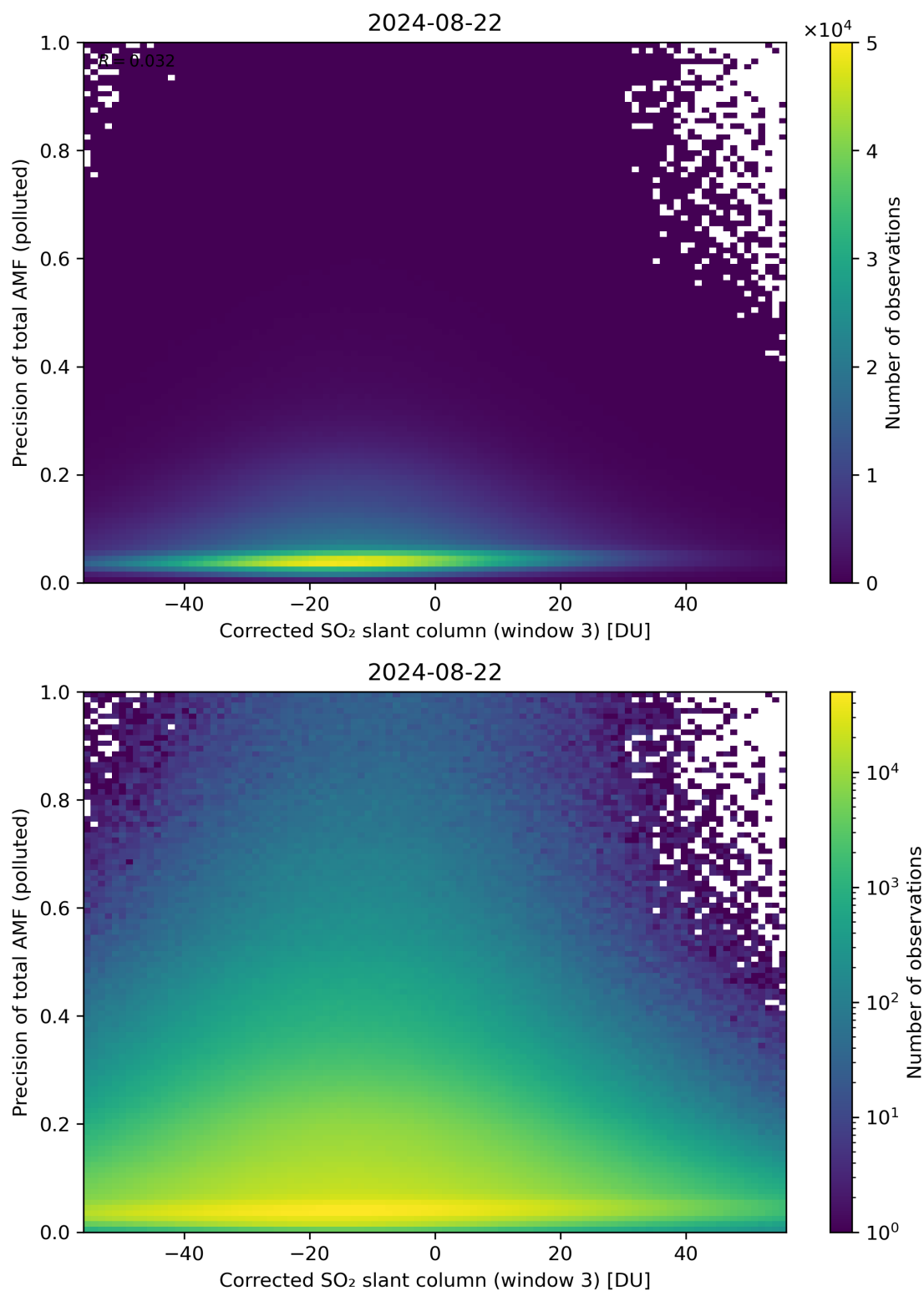
Figure 211: Scatter density plot of “Corrected SO 2 slant column (window 3)” against “Precision of total AMF (polluted)” for 2024-08-22 to 2024-08-23.
