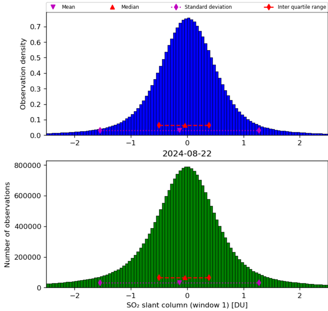
Figure 56: Histogram of “SO 2 slant column (window 1)” for 2024-08-22 to 2024-08-23
