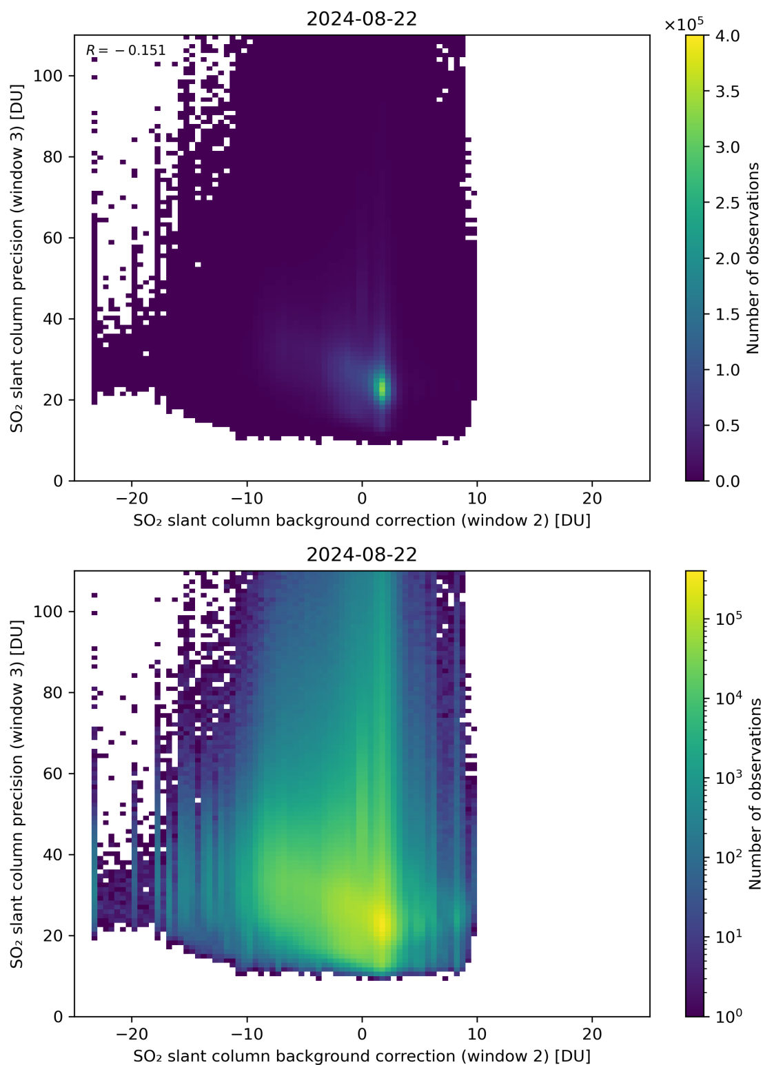
Figure 118: Scatter density plot of “SO 2 slant column background correction (window 2)” against “SO 2 slant column precision (window 3)” for 2024-08-22 to 2024-08-23.
