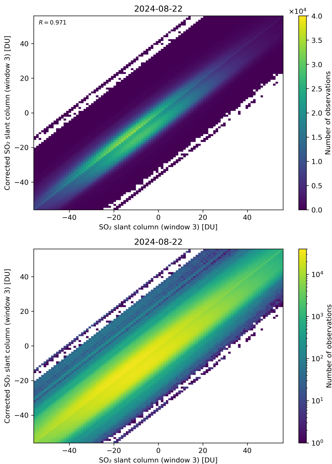
Figure 266: Scatter density plot of “SO 2 slant column (window 3)” against “Corrected SO 2 slant column (window 3)” for 2024-08-22 to 2024-08-23.
