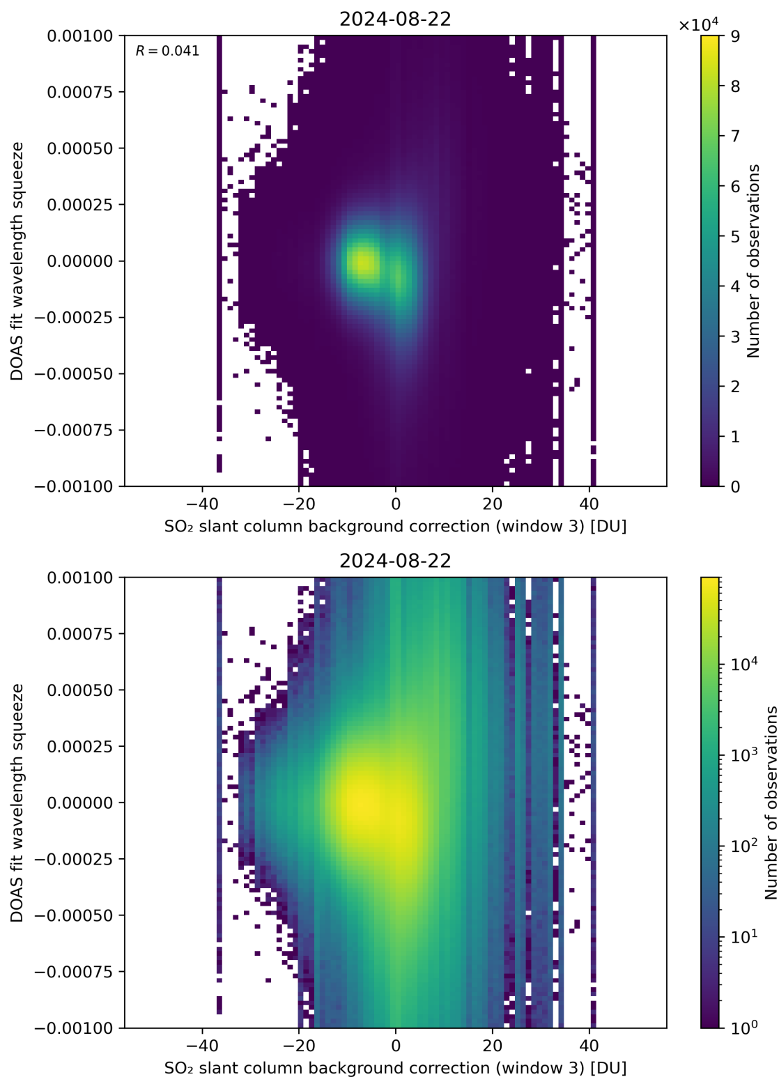
Figure 122: Scatter density plot of “SO 2 slant column background correction (window 3)” against “DOAS fit wavelength squeeze” for 2024-08-22 to 2024-08-23.
