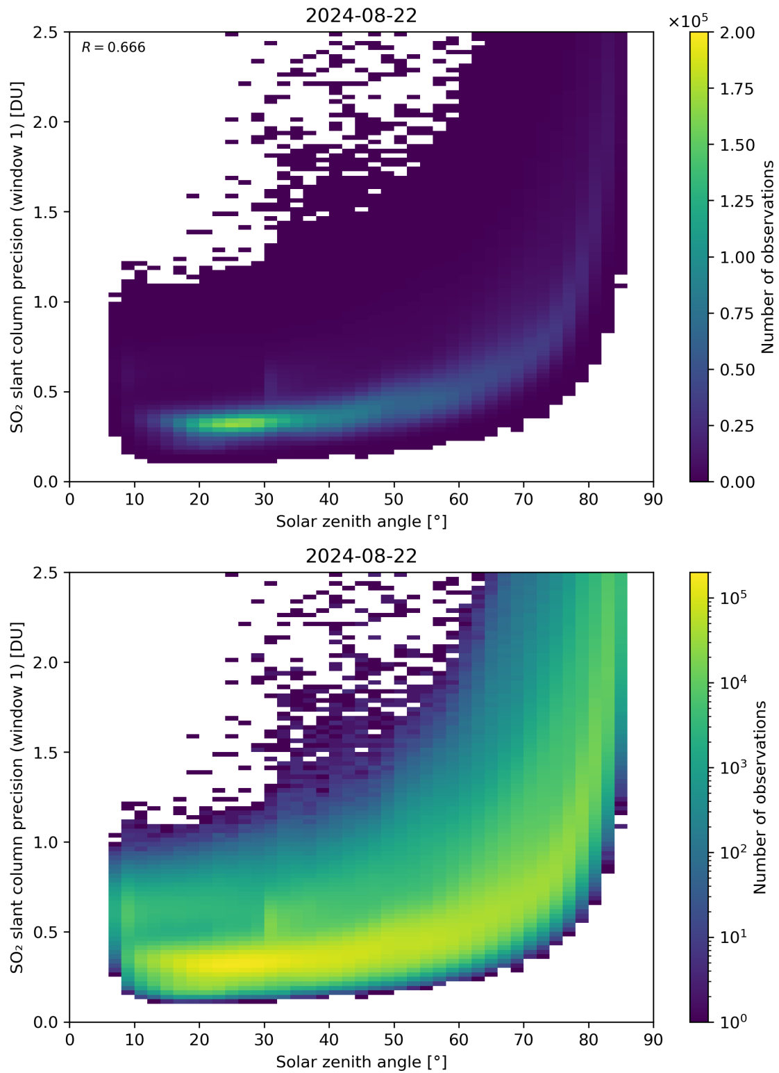
Figure 170: Scatter density plot of “Solar zenith angle” against “SO 2 slant column precision (window 1)” for 2024-08-22 to 2024-08-23.
