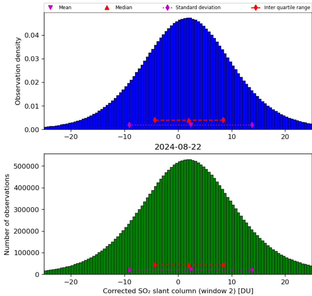
Figure 62: Histogram of “Corrected SO 2 slant column (window 2)” for 2024-08-22 to 2024-08-23
