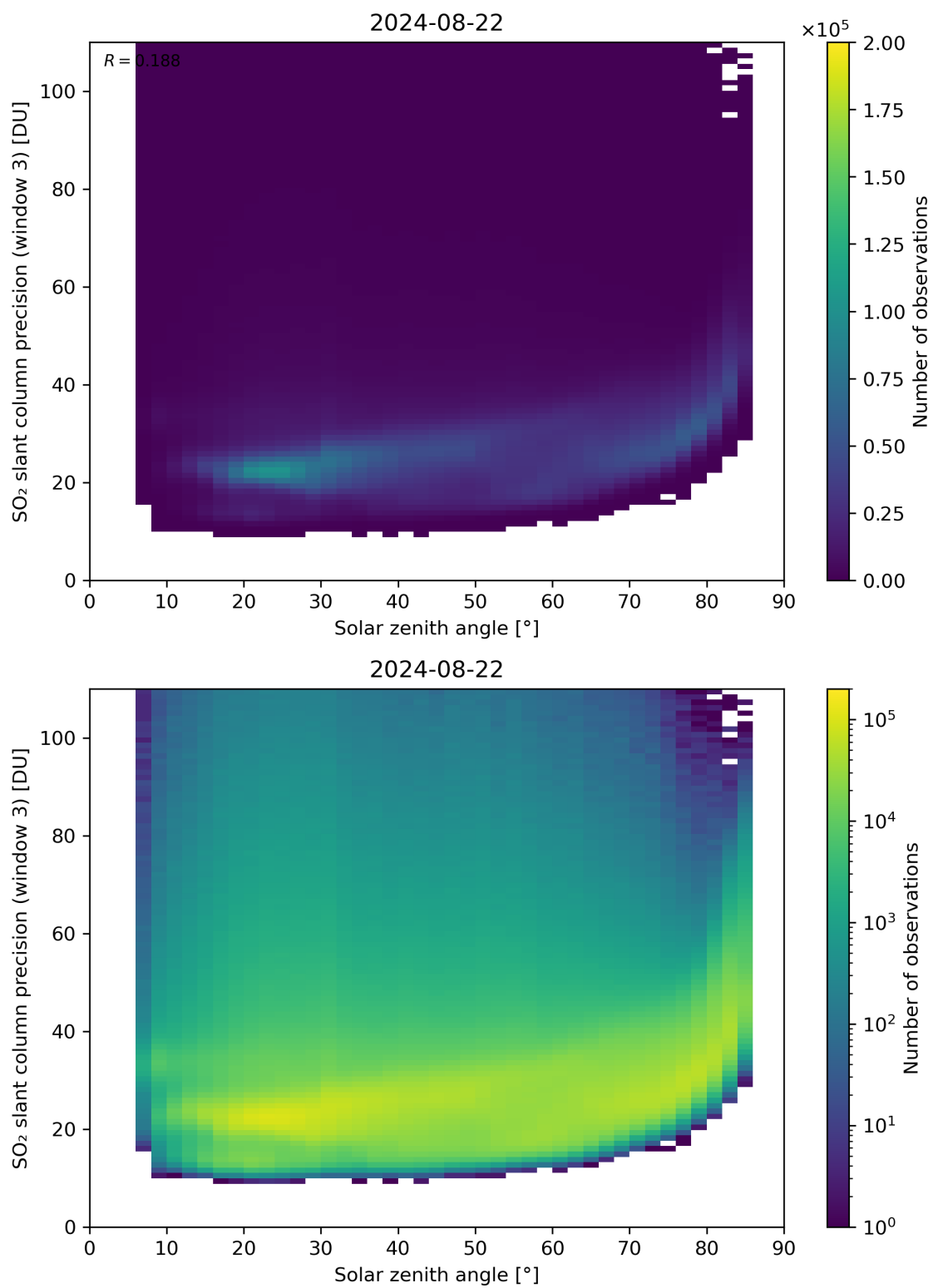
Figure 173: Scatter density plot of “Solar zenith angle” against “SO 2 slant column precision (window 3)” for 2024-08-22 to 2024-08-23.
