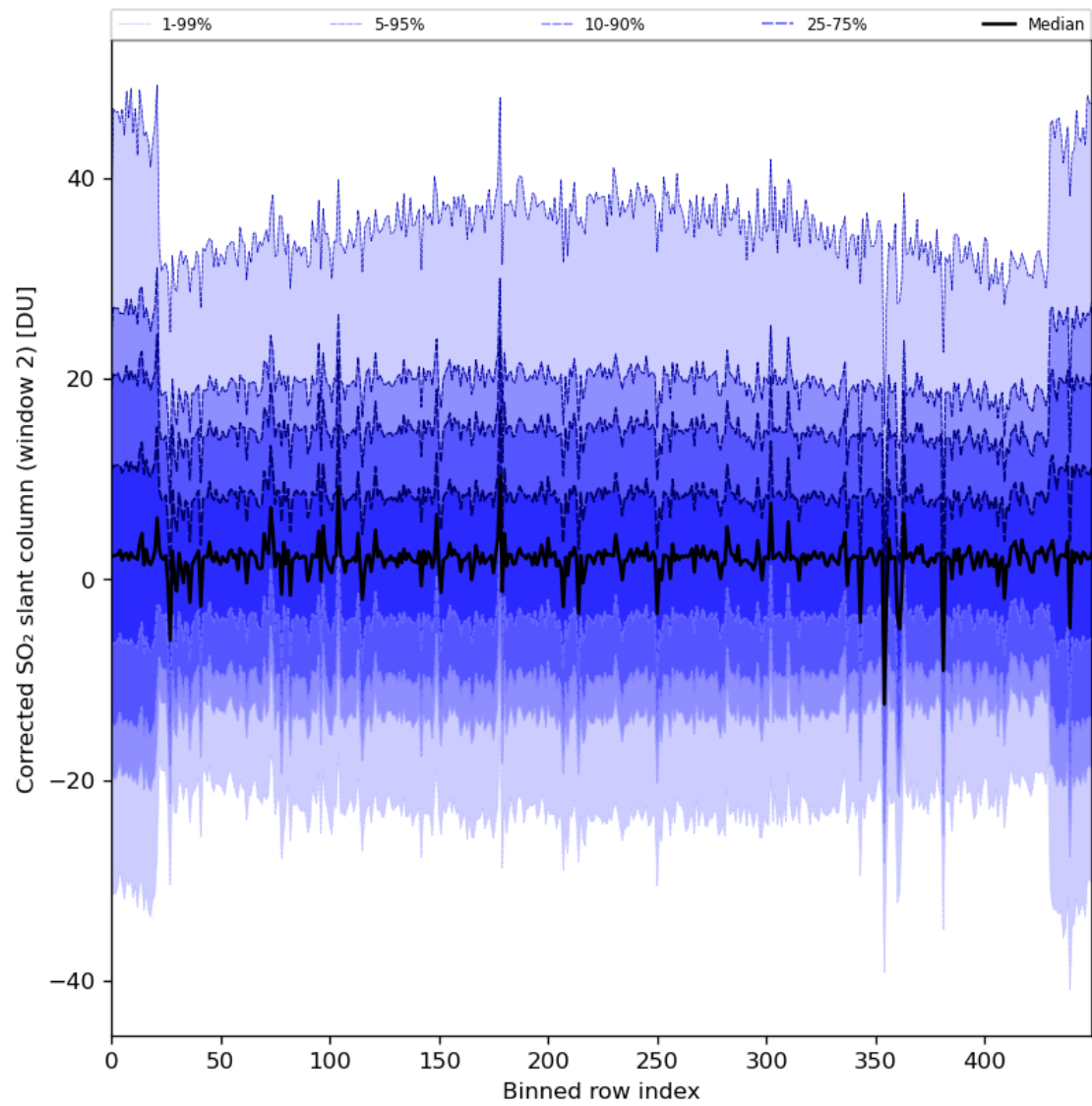
Figure 85: Along track statistics of “Corrected SO 2 slant column (window 2)” for 2024-08-22 to 2024-08-23
