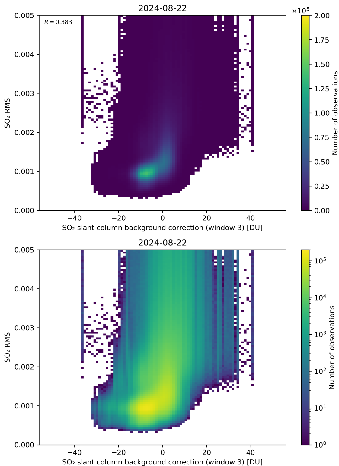
Figure 123: Scatter density plot of “SO 2 slant column background correction (window 3)” against “SO 2 RMS” for 2024-08-22 to 2024-08-23.
