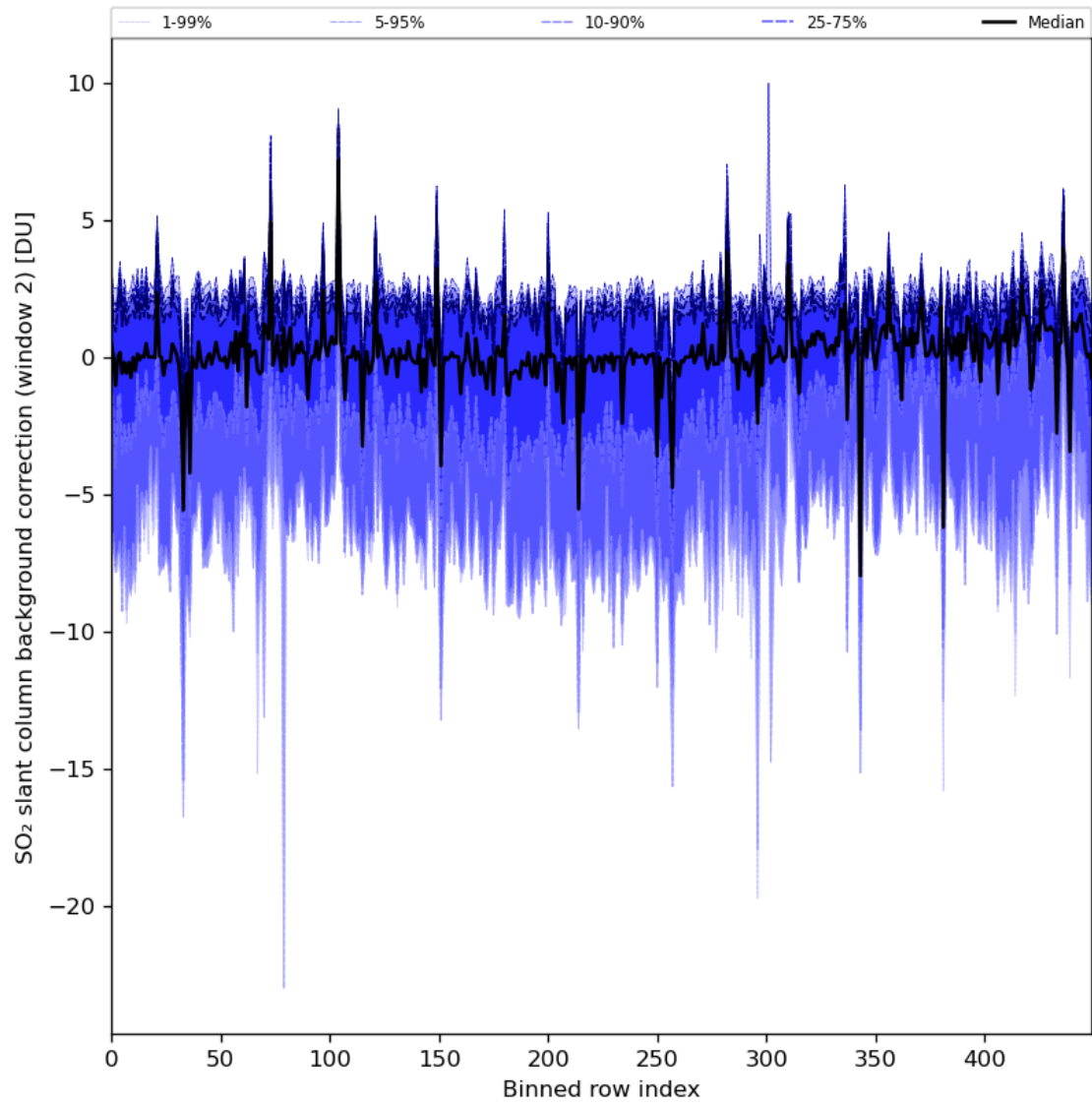
Figure 86: Along track statistics of “SO 2 slant column background correction (window 2)” for 2024-08-22 to 2024-08-23
