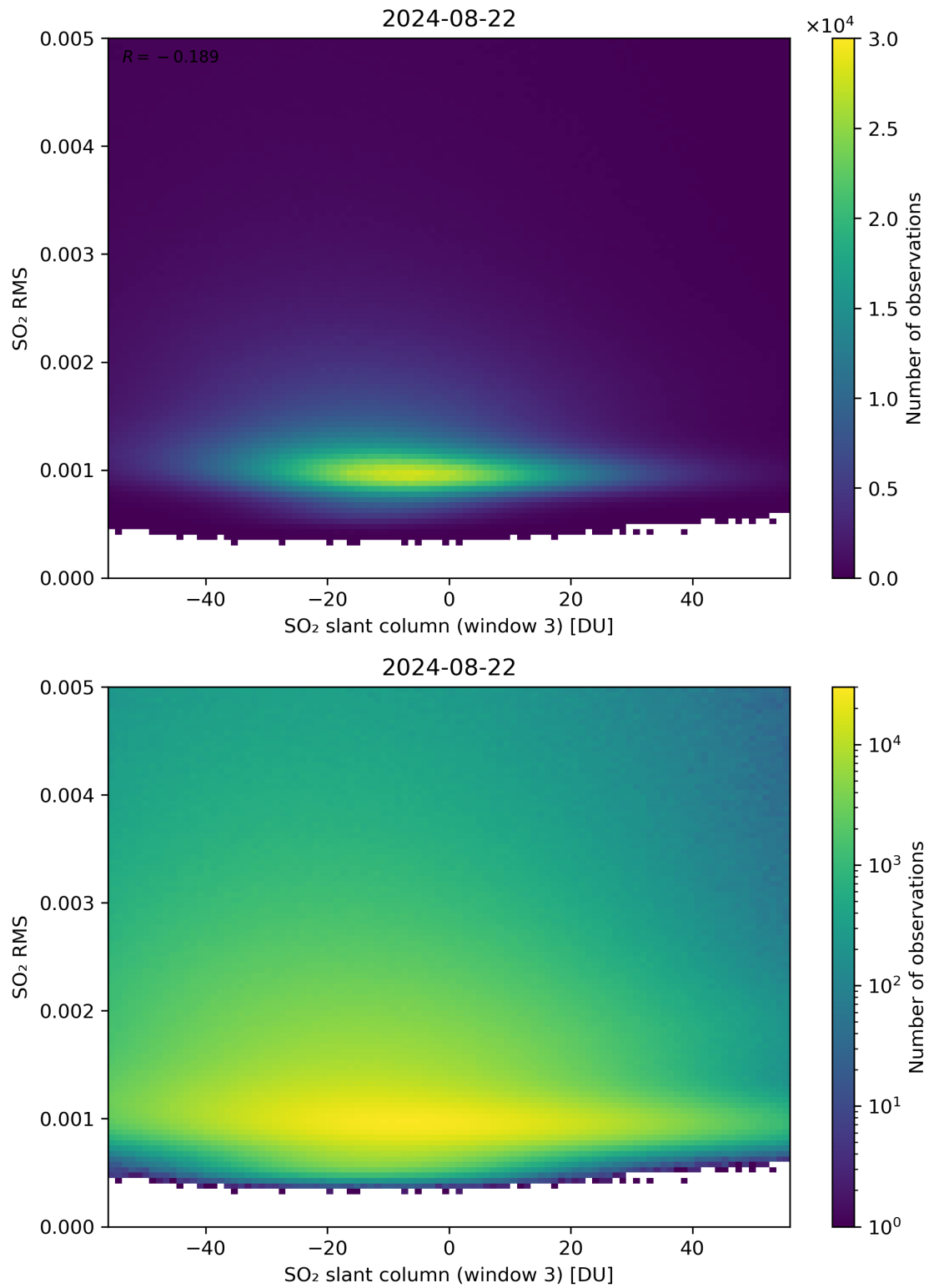
Figure 256: Scatter density plot of “SO 2 slant column (window 3)” against “SO 2 RMS” for 2024-08-22 to 2024-08-23.
