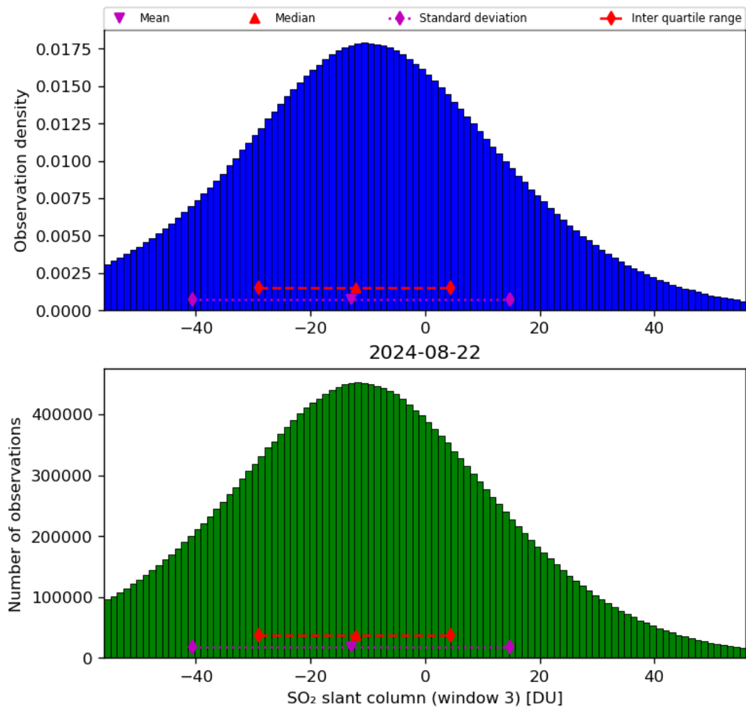
Figure 64: Histogram of “SO 2 slant column (window 3)” for 2024-08-22 to 2024-08-23
