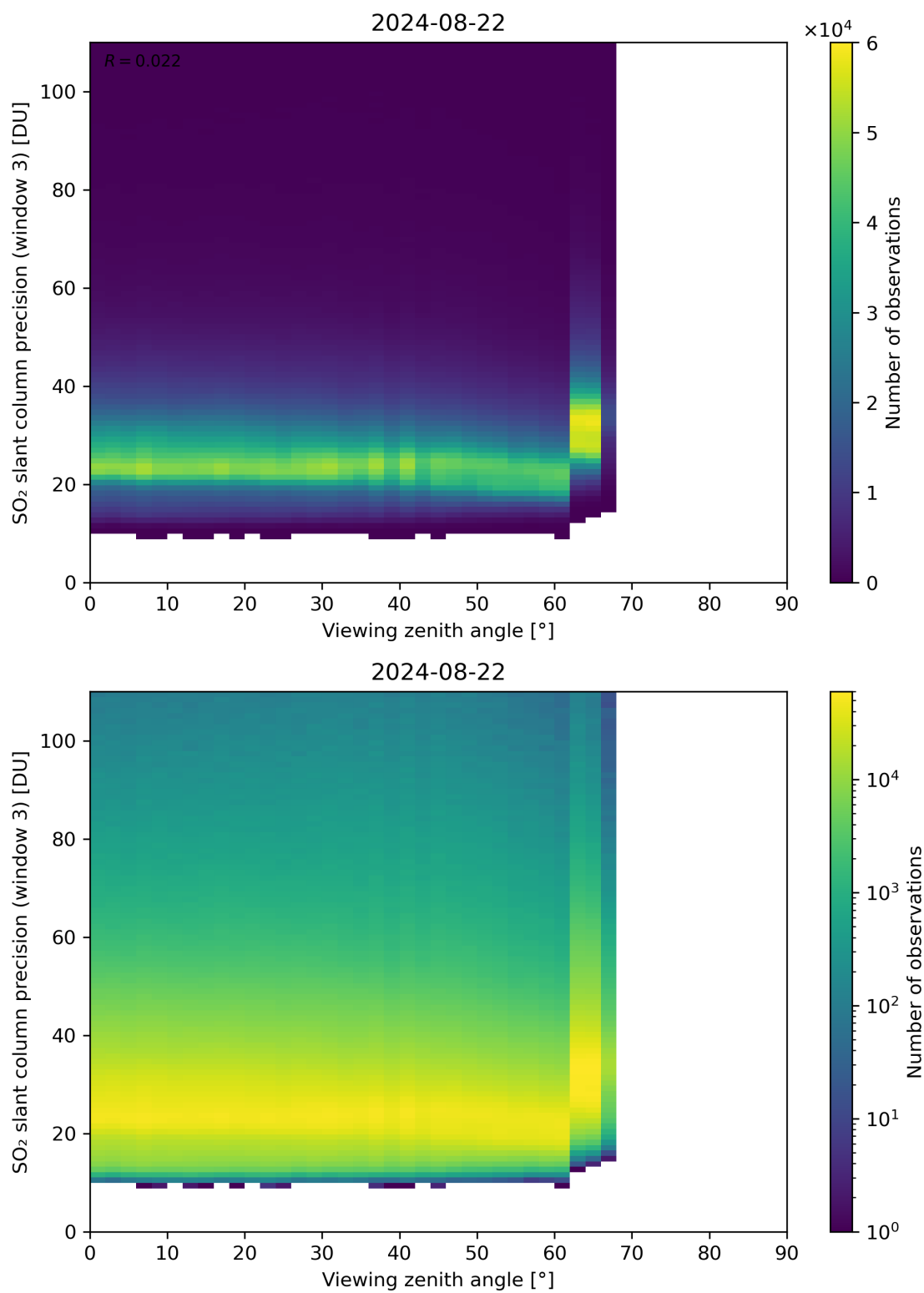
Figure 324: Scatter density plot of “Viewing zenith angle” against “SO 2 slant column precision (window 3)” for 2024-08-22 to 2024-08-23.
