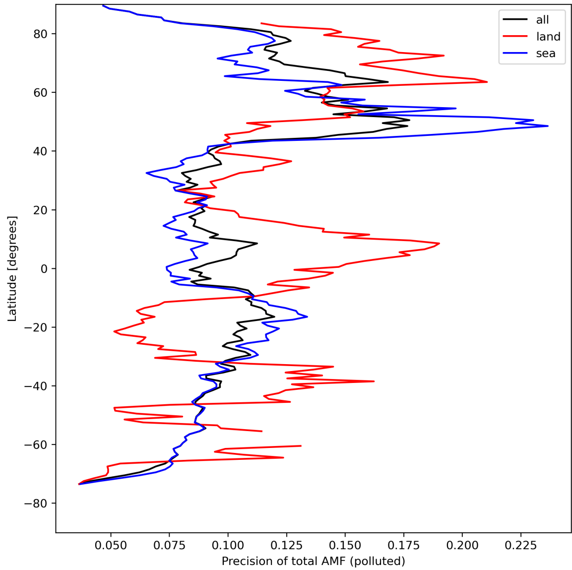
Figure 49: Zonal average of “Precision of total AMF (polluted)” for 2024-08-22 to 2024-08-23.
