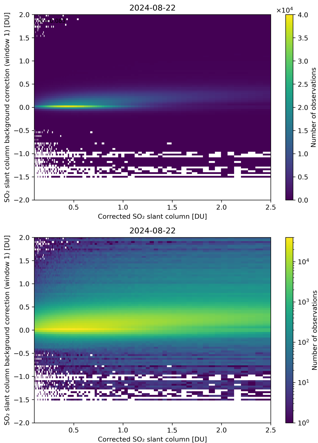
Figure 178: Scatter density plot of “Corrected SO 2 slant column” against “SO 2 slant column background correction (window 1)” for 2024-08-22 to 2024-08-23.
