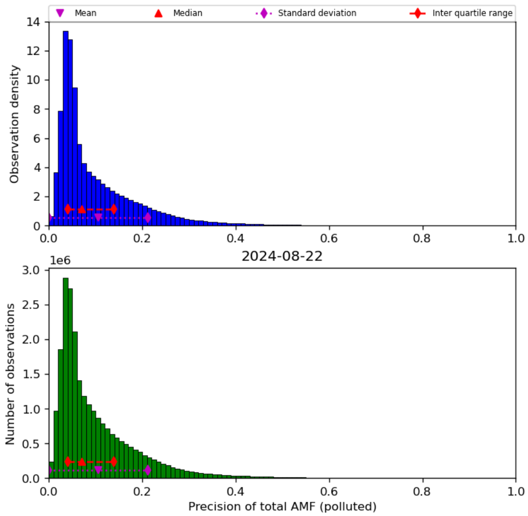
Figure 72: Histogram of “Precision of total AMF (polluted)” for 2024-08-22 to 2024-08-23
