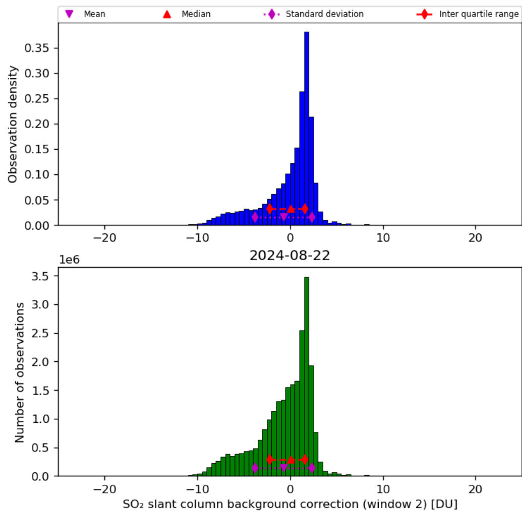
Figure 63: Histogram of “SO 2 slant column background correction (window 2)” for 2024-08-22 to 2024-08-23
