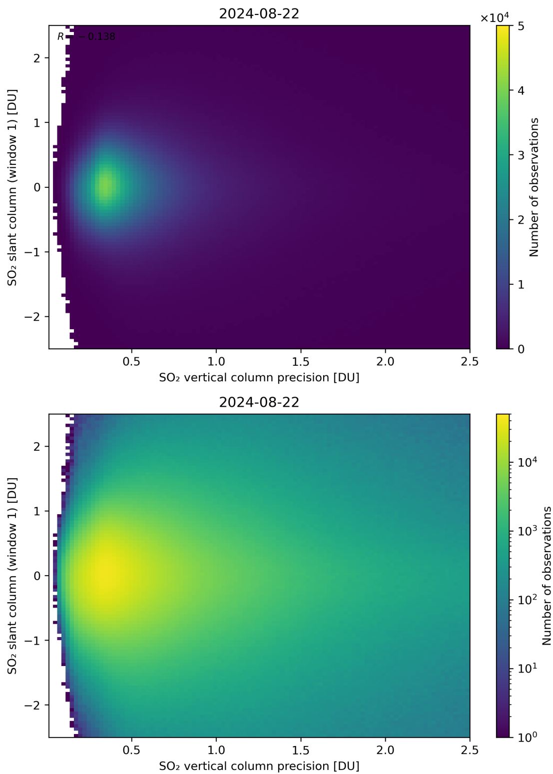
Figure 289: Scatter density plot of “SO 2 vertical column precision” against “SO 2 slant column (window 1)” for 2024-08-22 to 2024-08-23.
