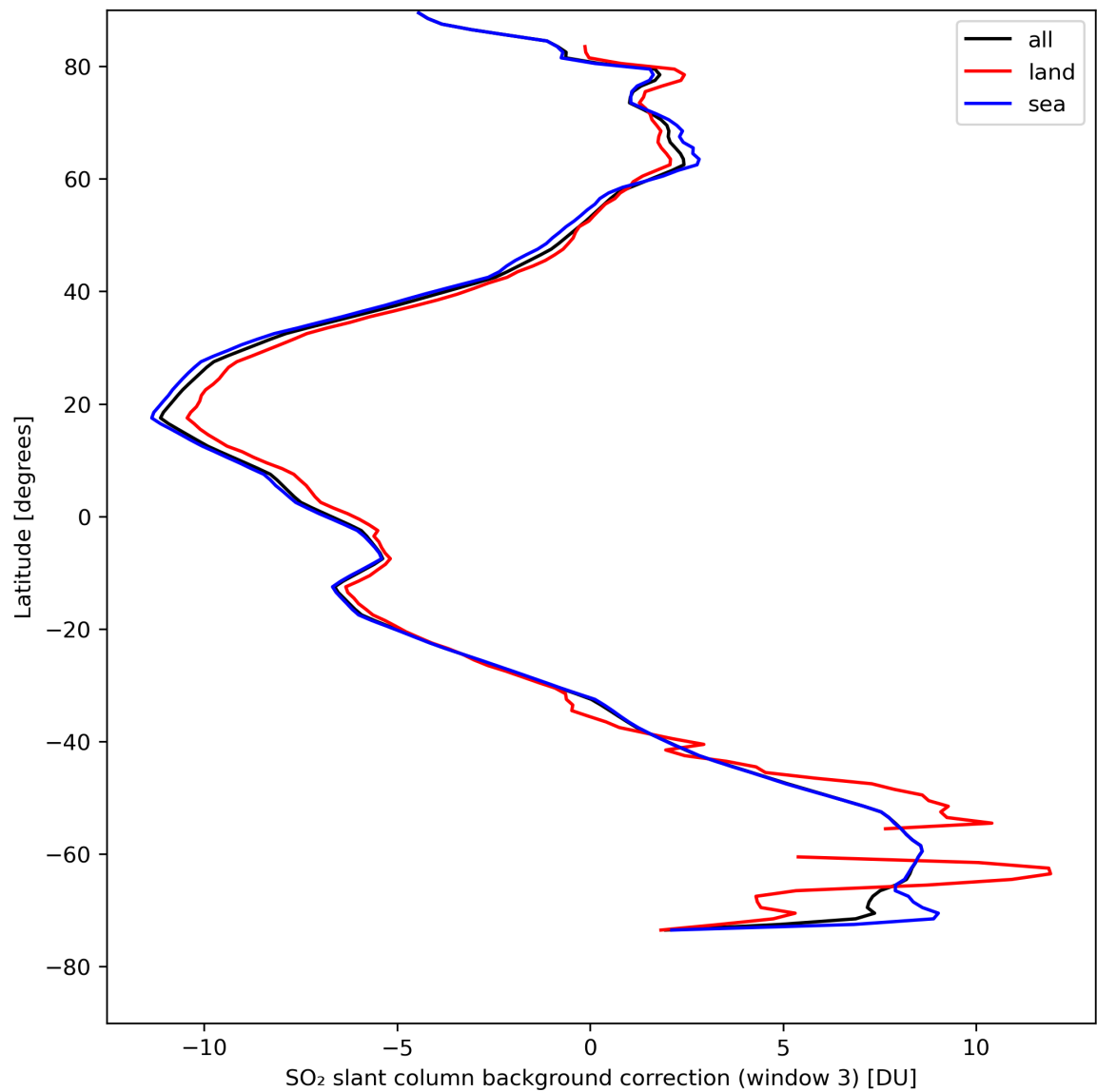
Figure 44: Zonal average of “SO 2 slant column background correction (window 3)” for 2024-08-22 to 2024-08-23.
