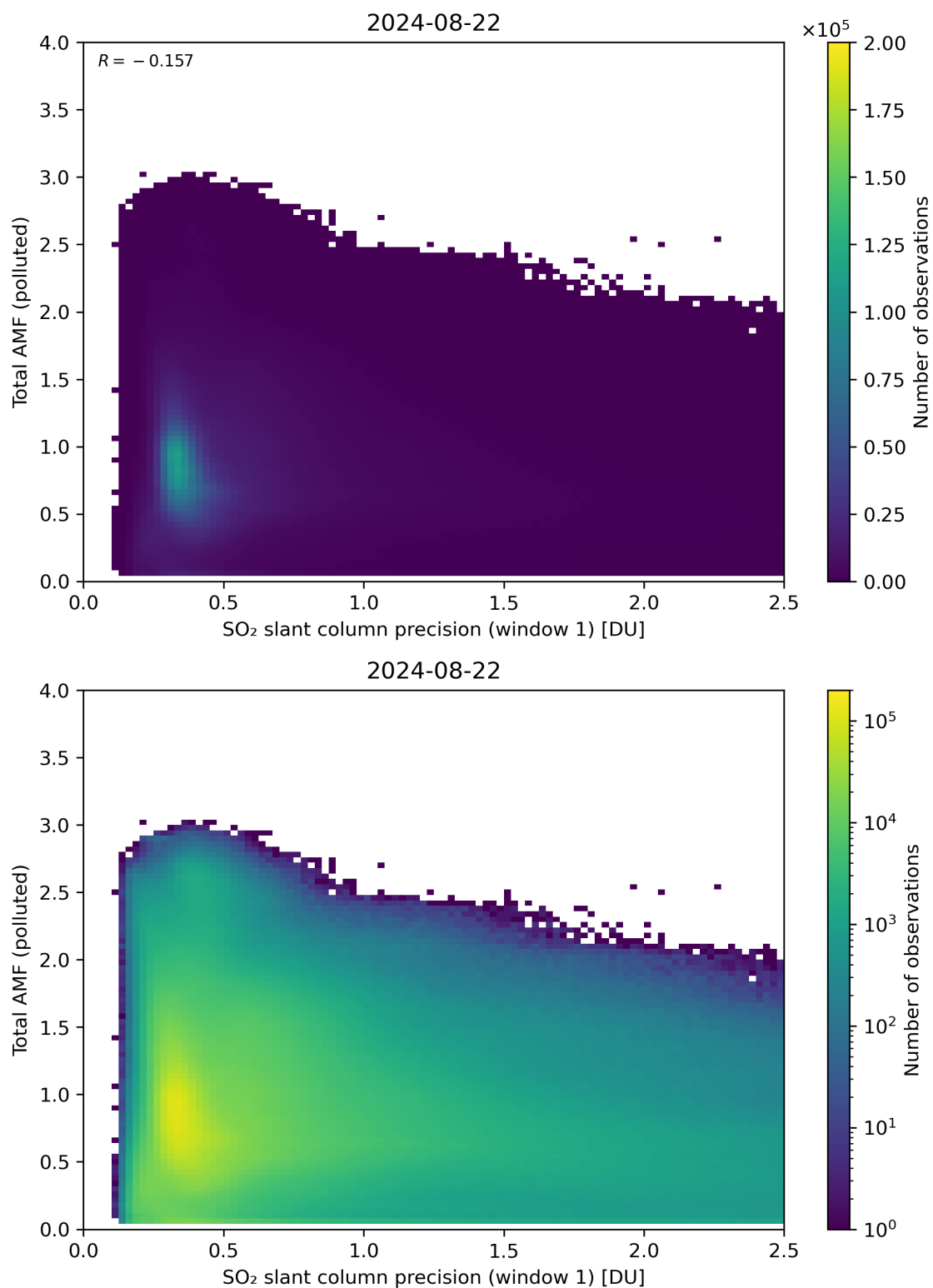
Figure 230: Scatter density plot of “SO 2 slant column precision (window 1)” against “Total AMF (polluted)” for 2024-08-22 to 2024-08-23.
