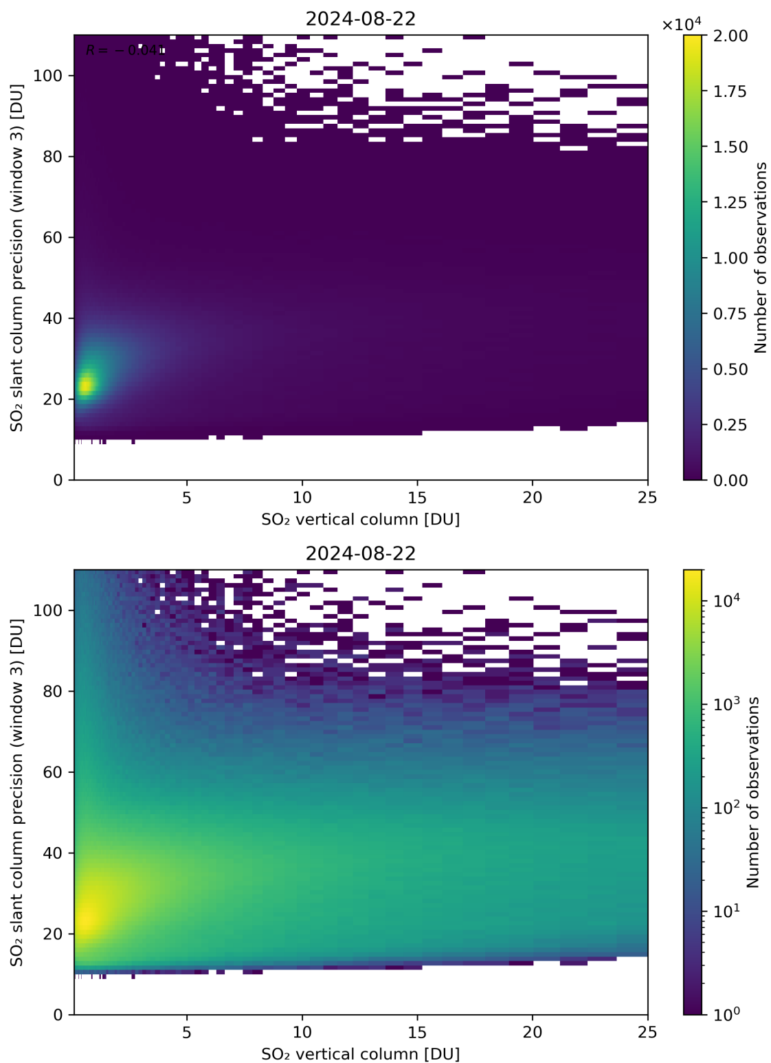
Figure 304: Scatter density plot of “SO 2 vertical column” against “SO 2 slant column precision (window 3)” for 2024-08-22 to 2024-08-23.
