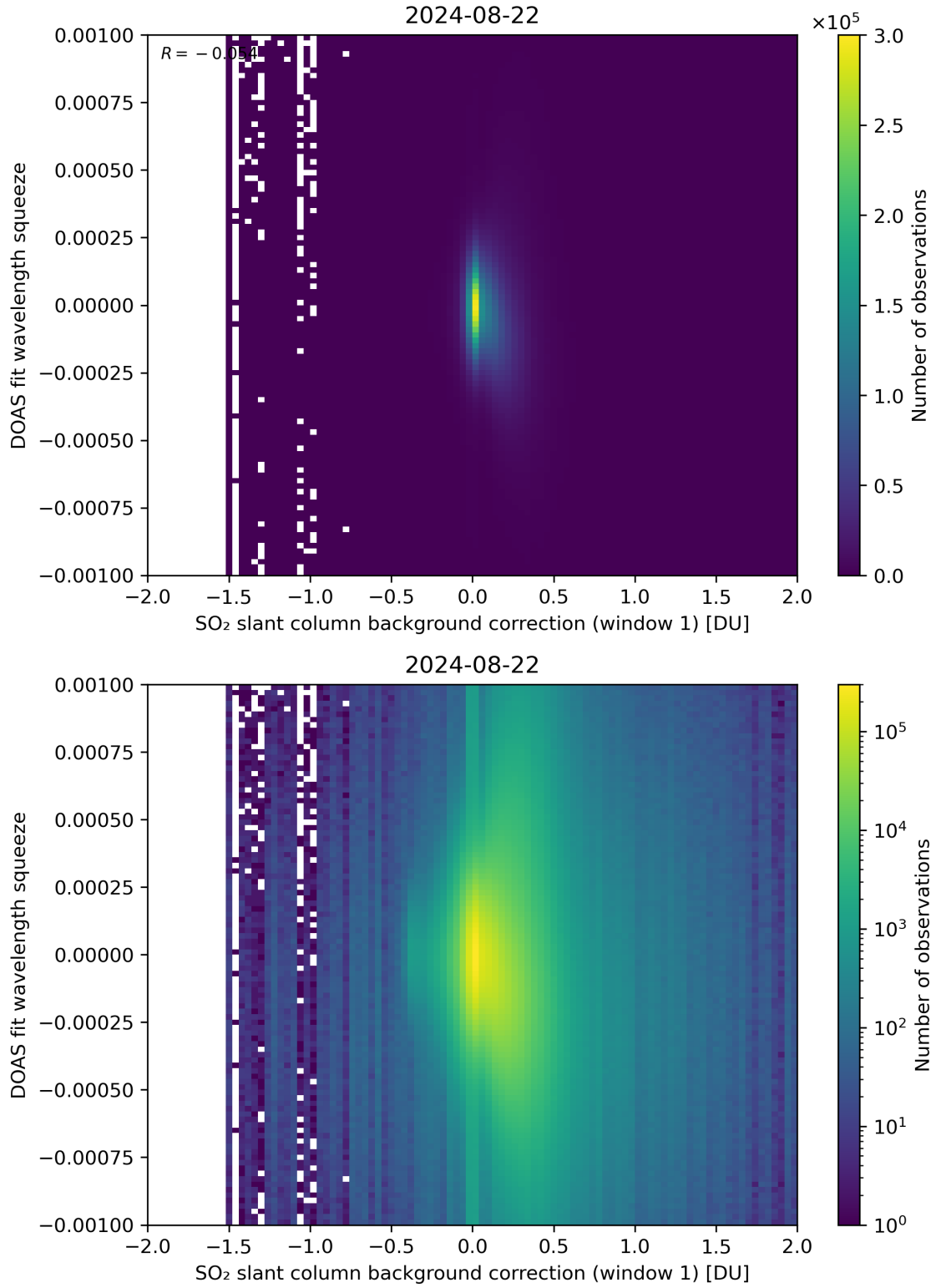
Figure 101: Scatter density plot of “SO 2 slant column background correction (window 1)” against “DOAS fit wavelength squeeze” for 2024-08-22 to 2024-08-23.
