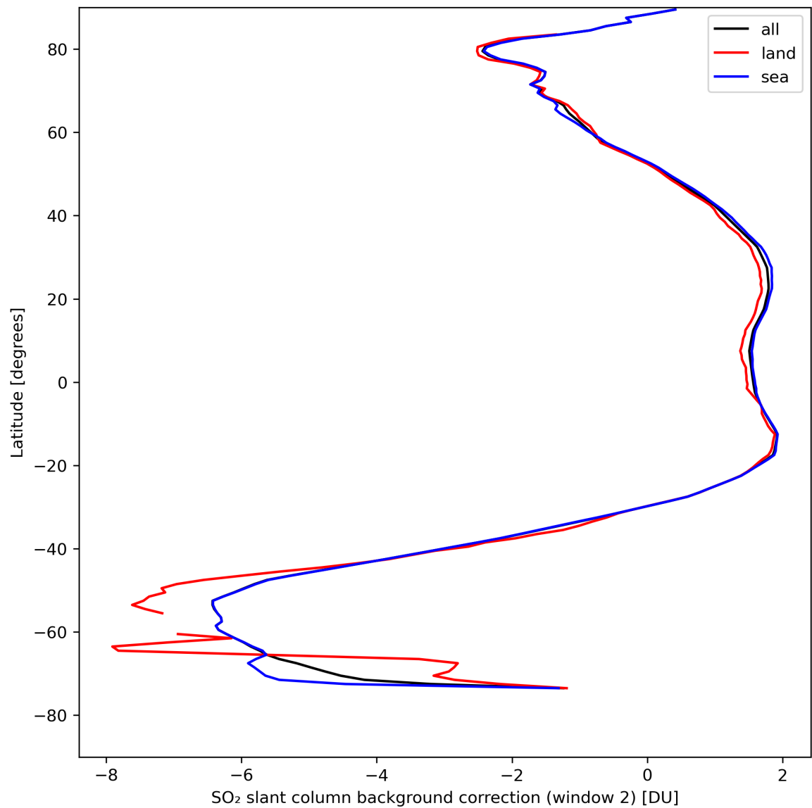
Figure 40: Zonal average of “SO 2 slant column background correction (window 2)” for 2024-08-22 to 2024-08-23.
