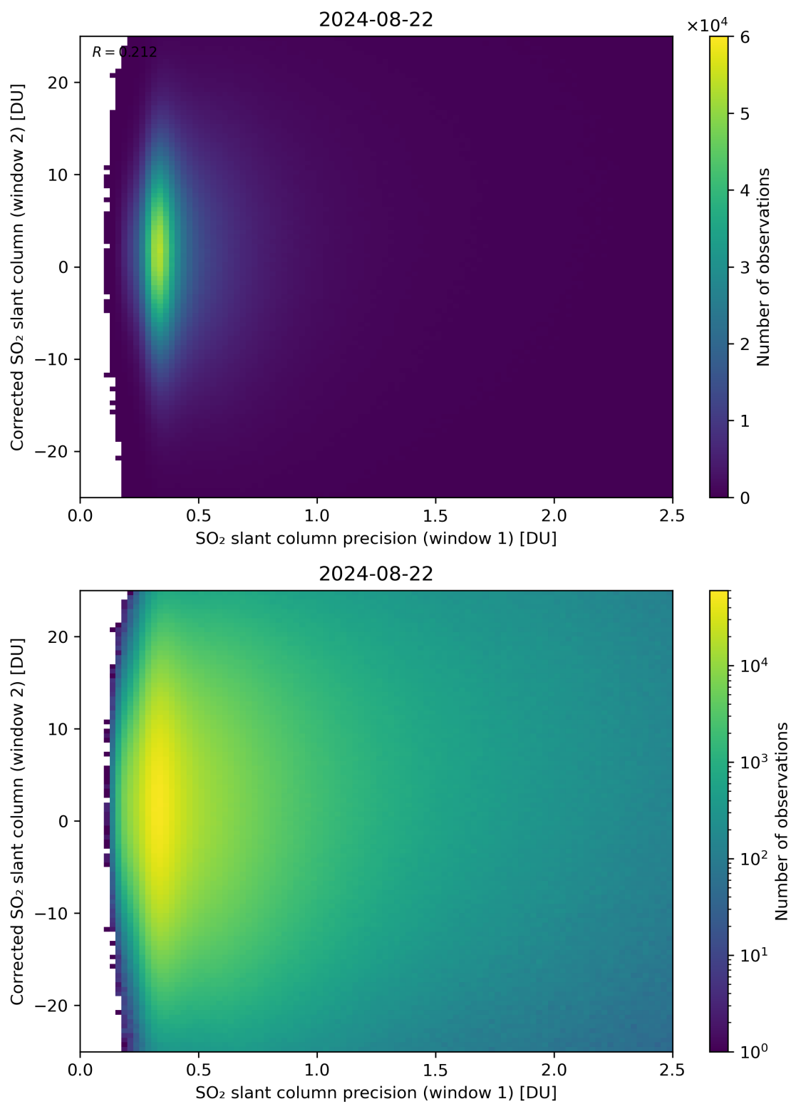
Figure 225: Scatter density plot of “SO 2 slant column precision (window 1)” against “Corrected SO 2 slant column (window 2)” for 2024-08-22 to 2024-08-23.
