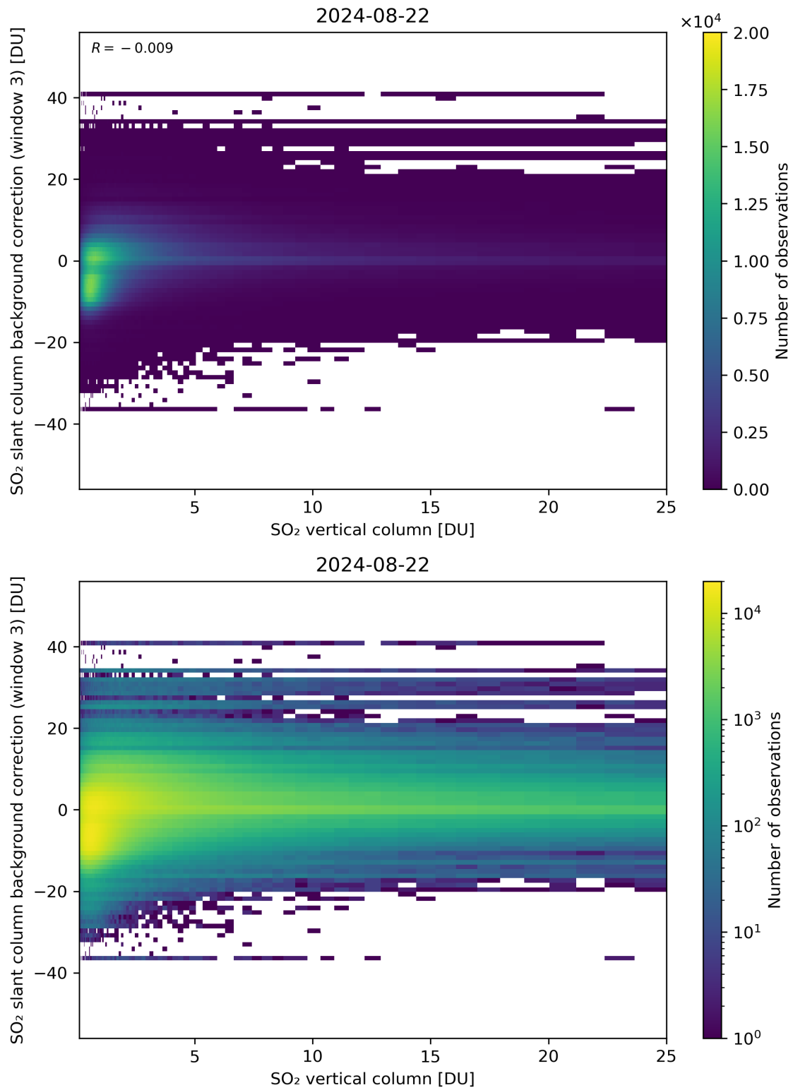
Figure 275: Scatter density plot of “SO 2 vertical column” against “SO 2 slant column background correction (window 3)” for 2024-08-22 to 2024-08-23.
