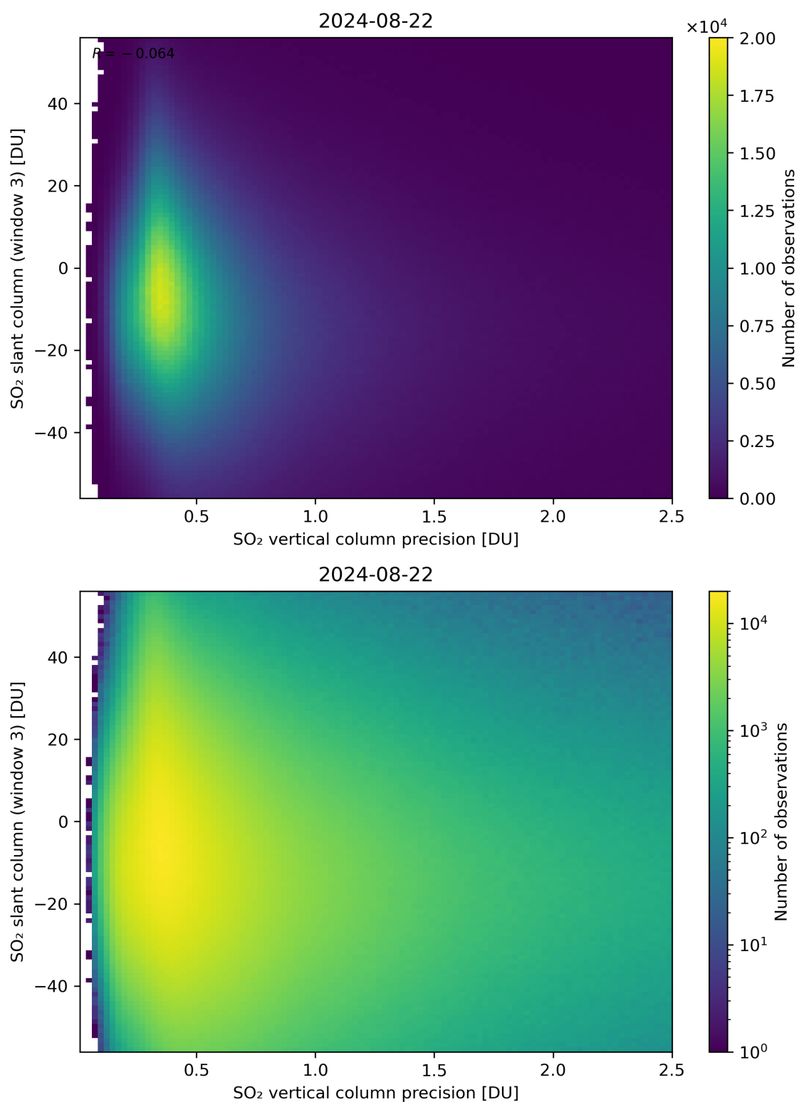
Figure 292: Scatter density plot of “SO 2 vertical column precision” against “SO 2 slant column (window 3)” for 2024-08-22 to 2024-08-23.
