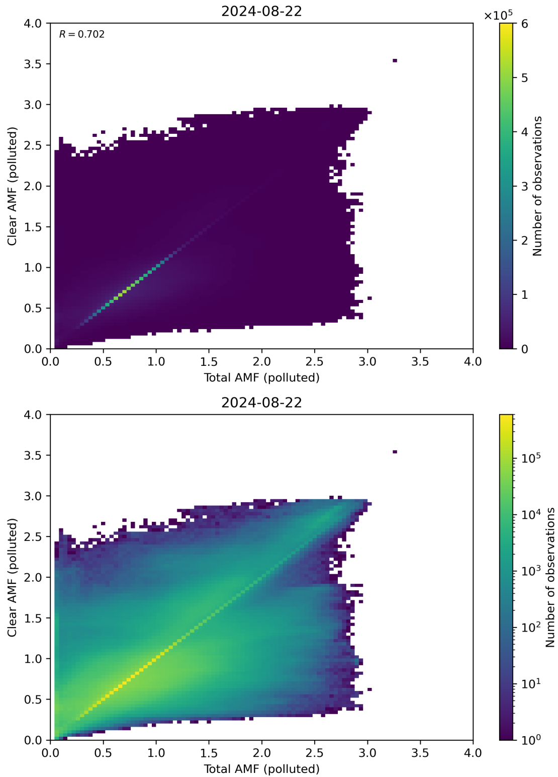
Figure 271: Scatter density plot of “Total AMF (polluted)” against “Clear AMF (polluted)” for 2024-08-22 to 2024-08-23.
