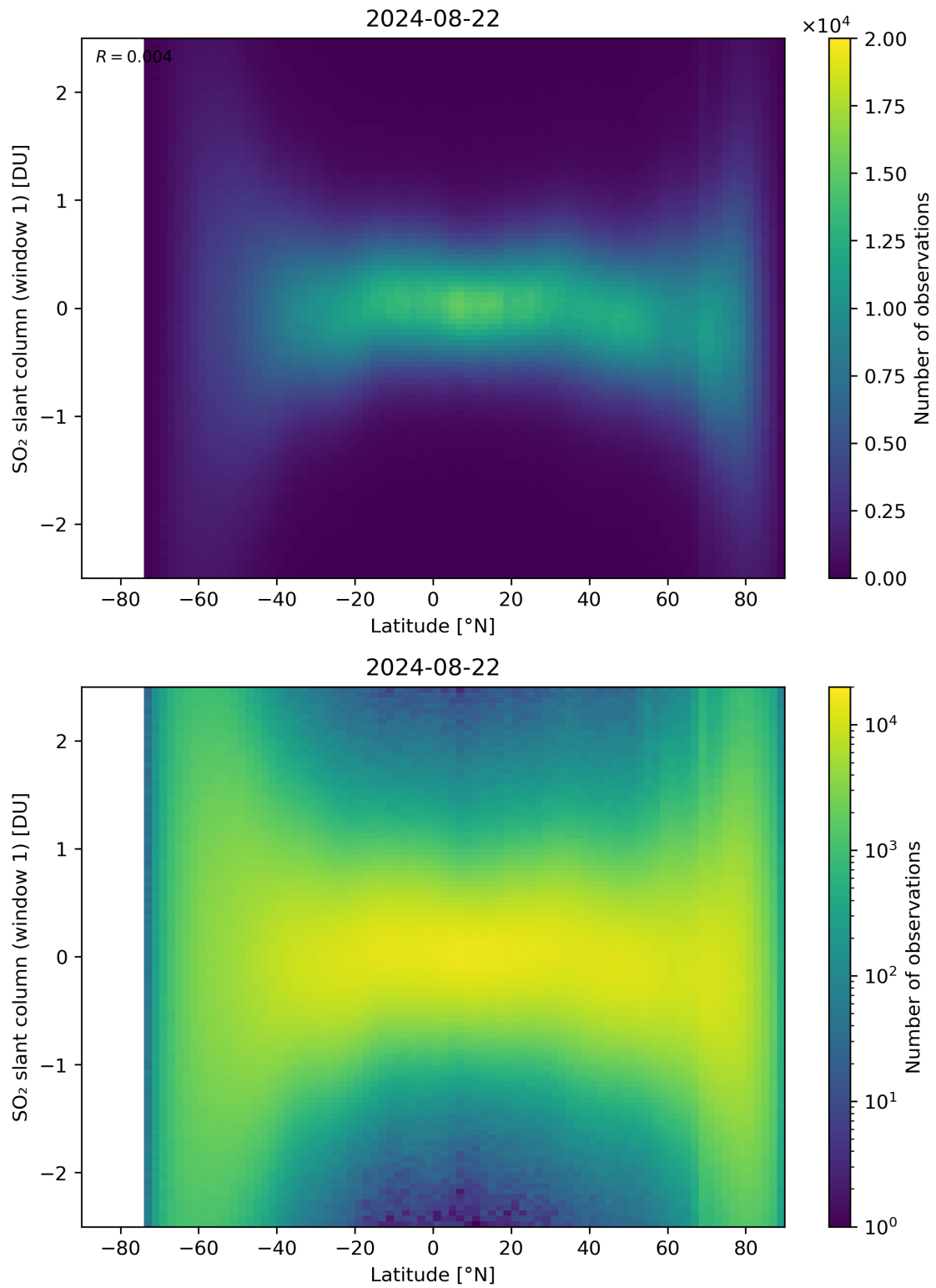
Figure 149: Scatter density plot of “Latitude” against “SO 2 slant column (window 1)” for 2024-08-22 to 2024-08-23.
