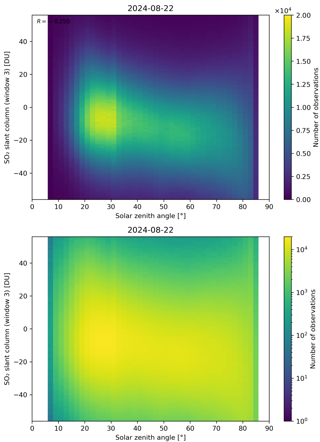
Figure 172: Scatter density plot of “Solar zenith angle” against “SO 2 slant column (window 3)” for 2024-08-22 to 2024-08-23.
