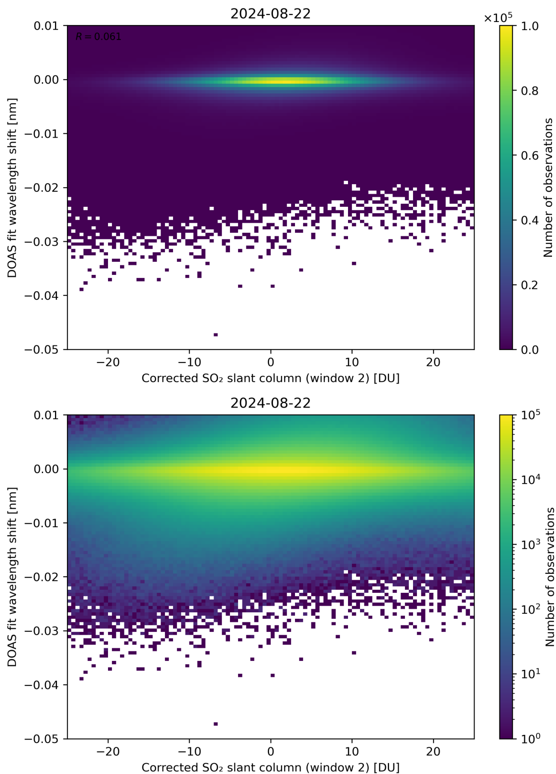
Figure 196: Scatter density plot of “Corrected SO 2 slant column (window 2)” against “DOAS fit wavelength shift” for 2024-08-22 to 2024-08-23.
