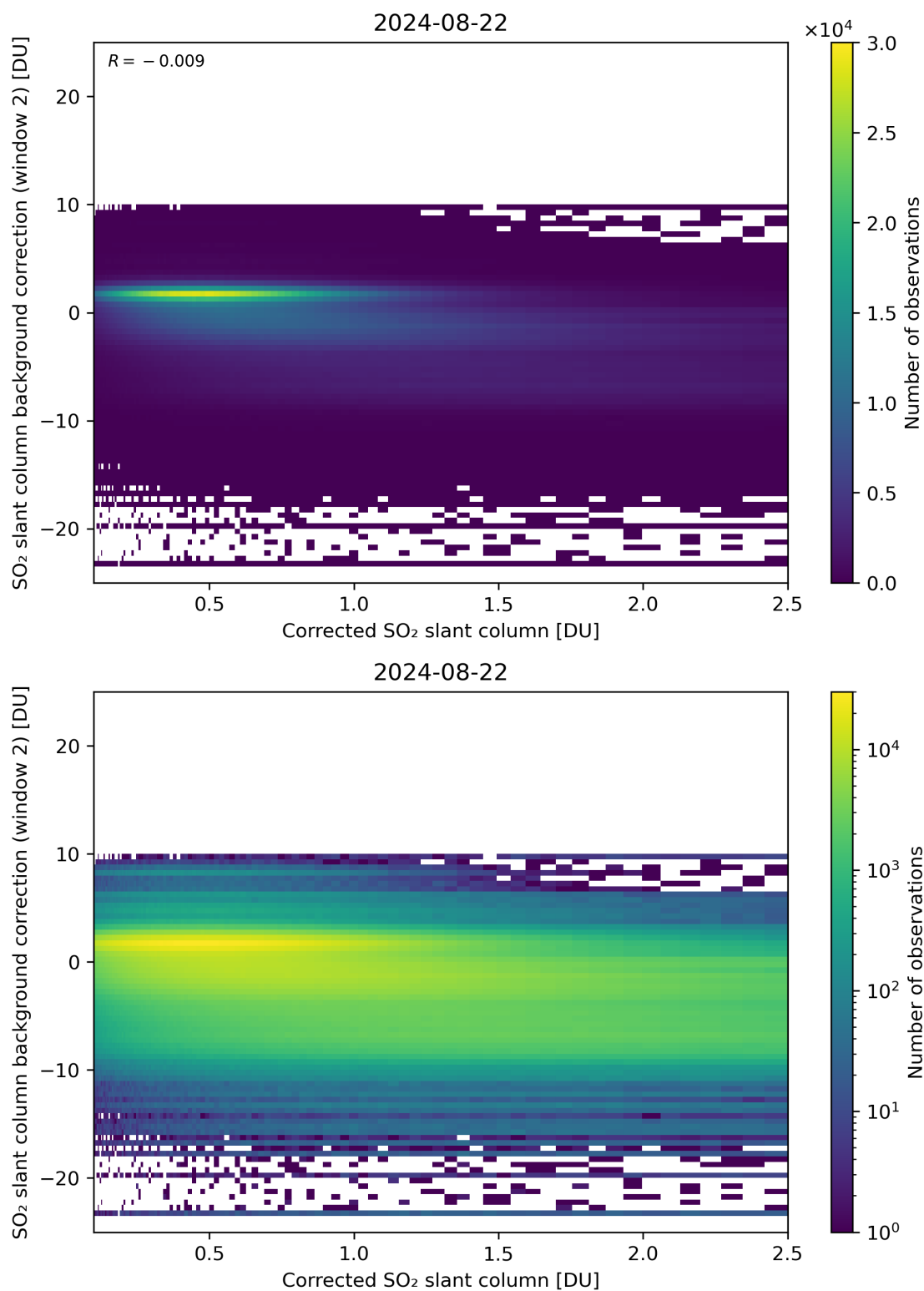
Figure 179: Scatter density plot of “Corrected SO 2 slant column” against “SO 2 slant column background correction (window 2)” for 2024-08-22 to 2024-08-23.
