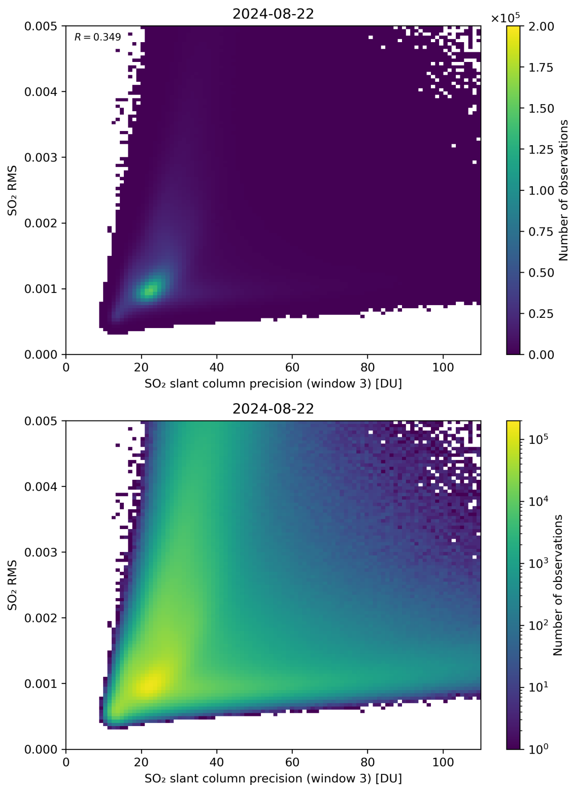
Figure 260: Scatter density plot of “SO 2 slant column precision (window 3)” against “SO 2 RMS” for 2024-08-22 to 2024-08-23.
