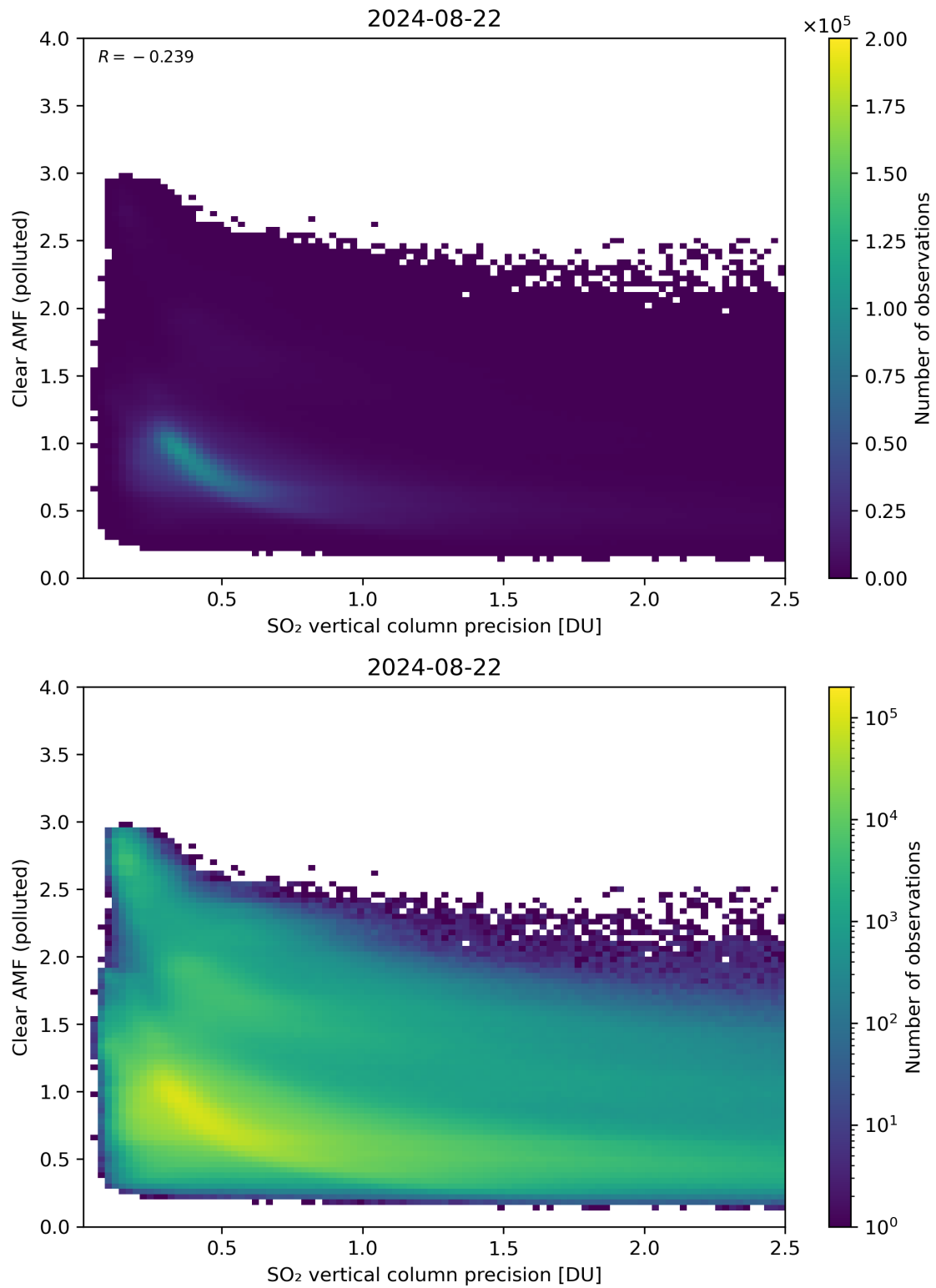
Figure 285: Scatter density plot of “SO 2 vertical column precision” against “Clear AMF (polluted)” for 2024-08-22 to 2024-08-23.
