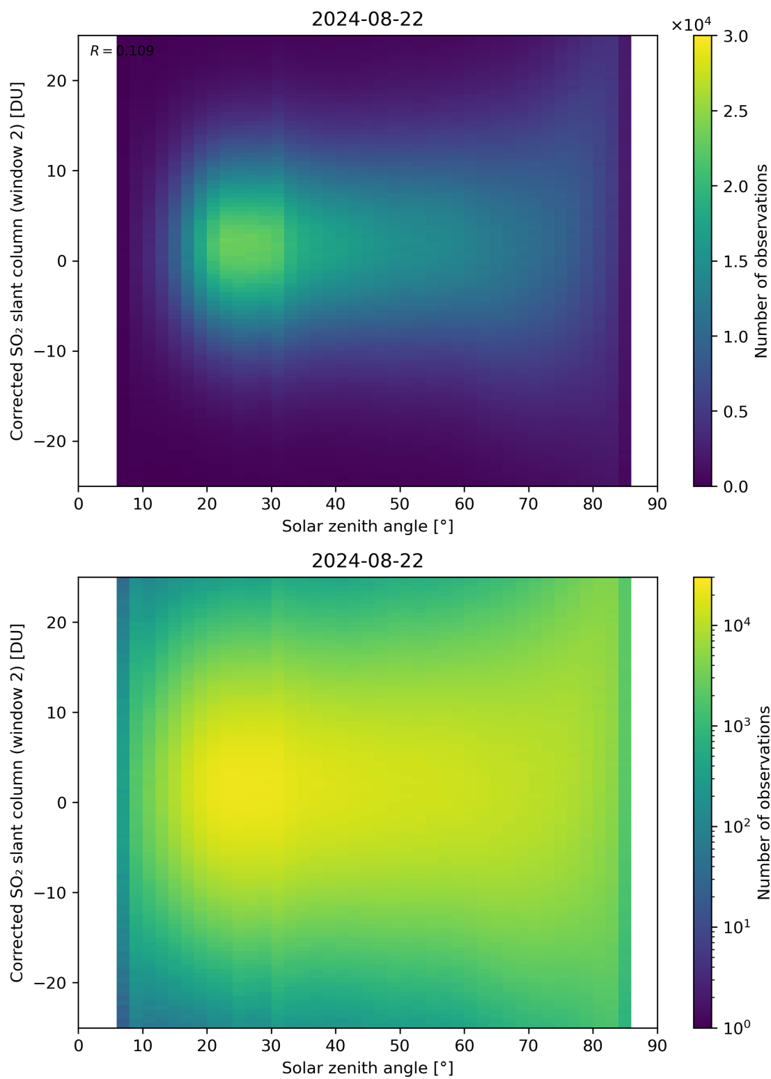
Figure 167: Scatter density plot of “Solar zenith angle” against “Corrected SO 2 slant column (window 2)” for 2024-08-22 to 2024-08-23.
