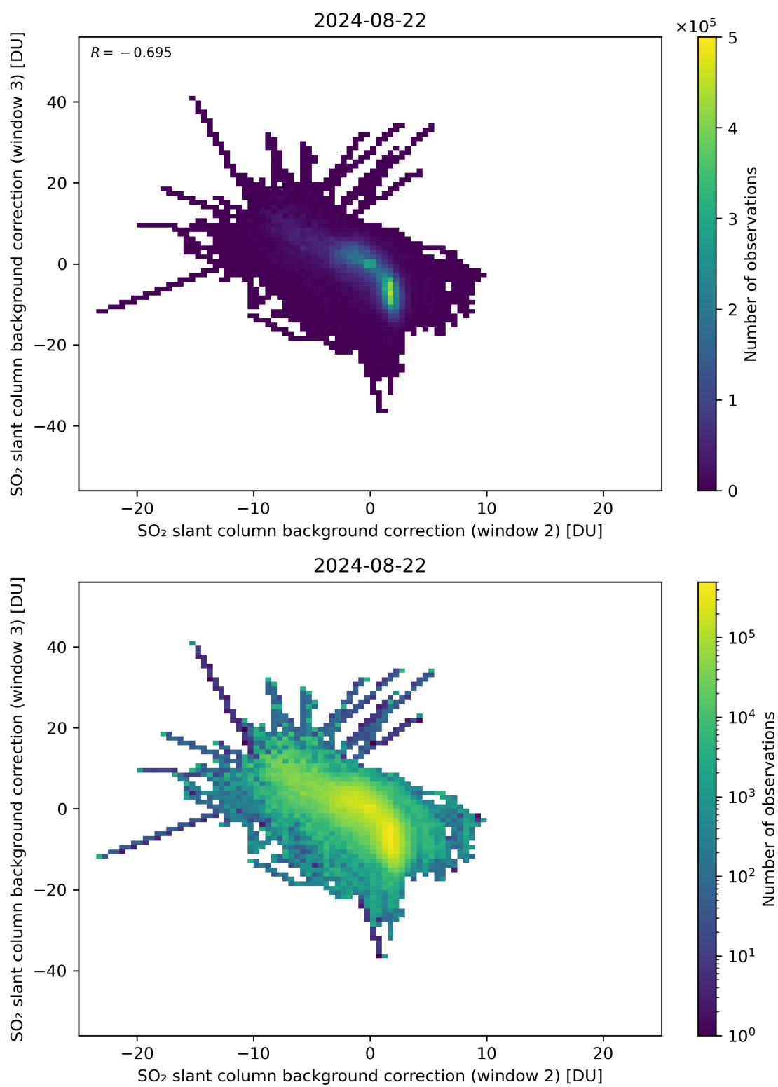
Figure 111: Scatter density plot of “SO 2 slant column background correction (window 2)” against “SO 2 slant column background correction (window 3)” for 2024-08-22 to 2024-08-23.
