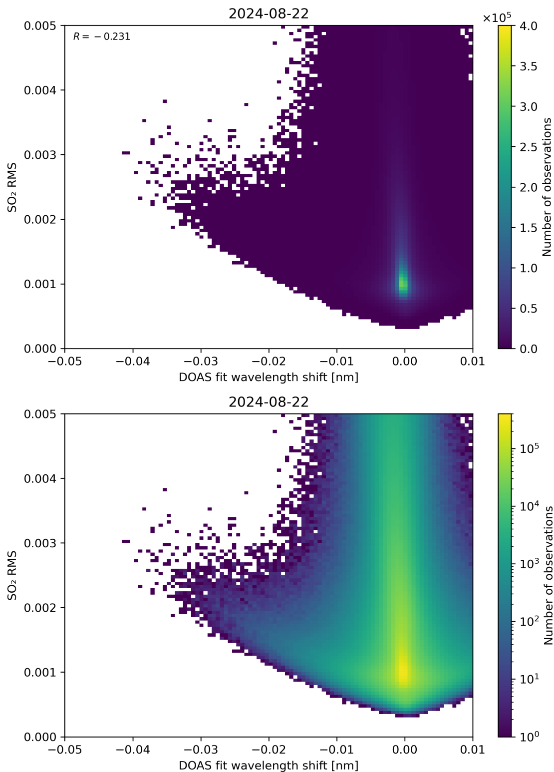
Figure 128: Scatter density plot of “DOAS fit wavelength shift” against “SO 2 RMS” for 2024-08-22 to 2024-08-23.
