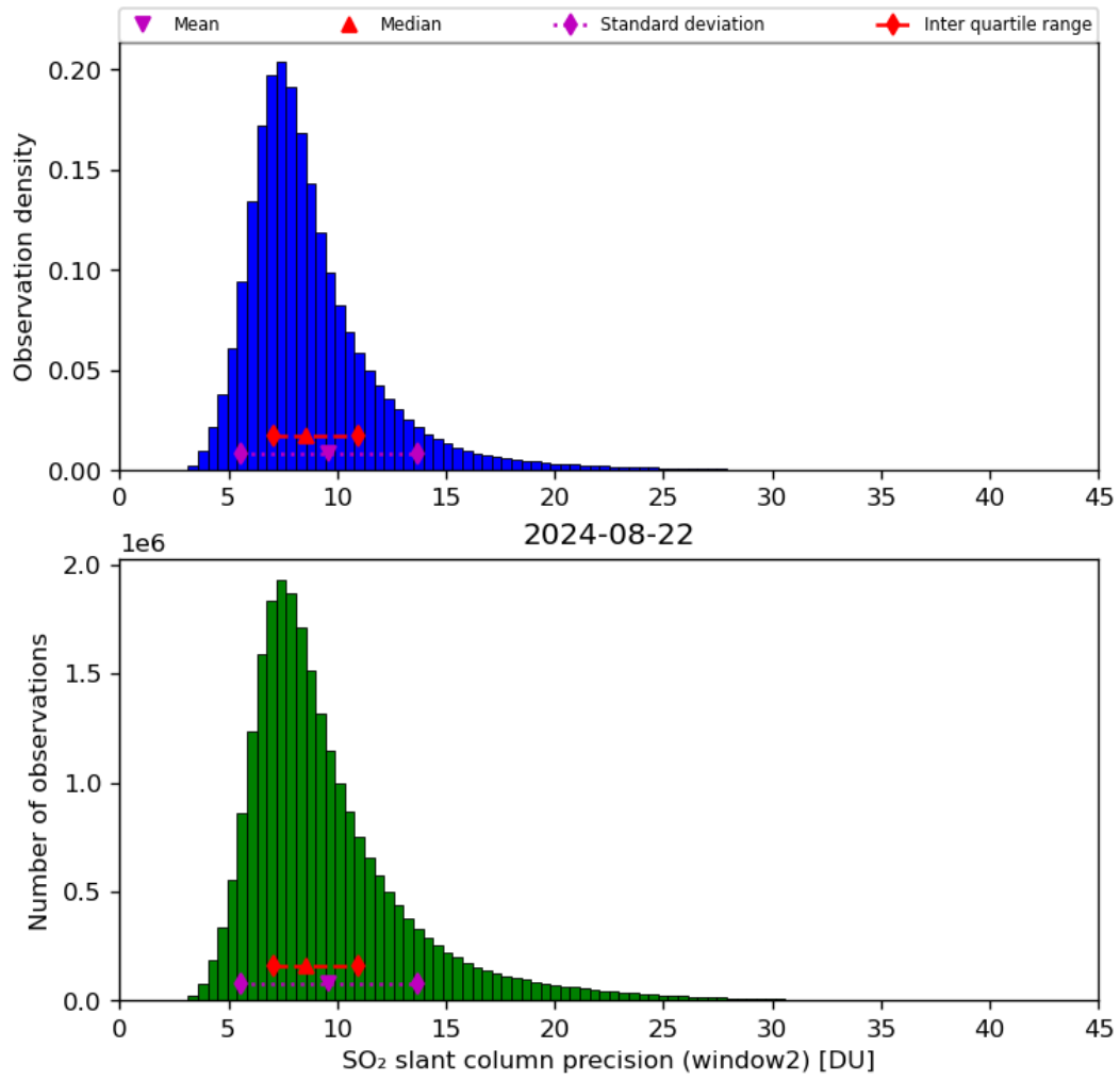
Figure 61: Histogram of “SO 2 slant column precision (window2)” for 2024-08-22 to 2024-08-23
