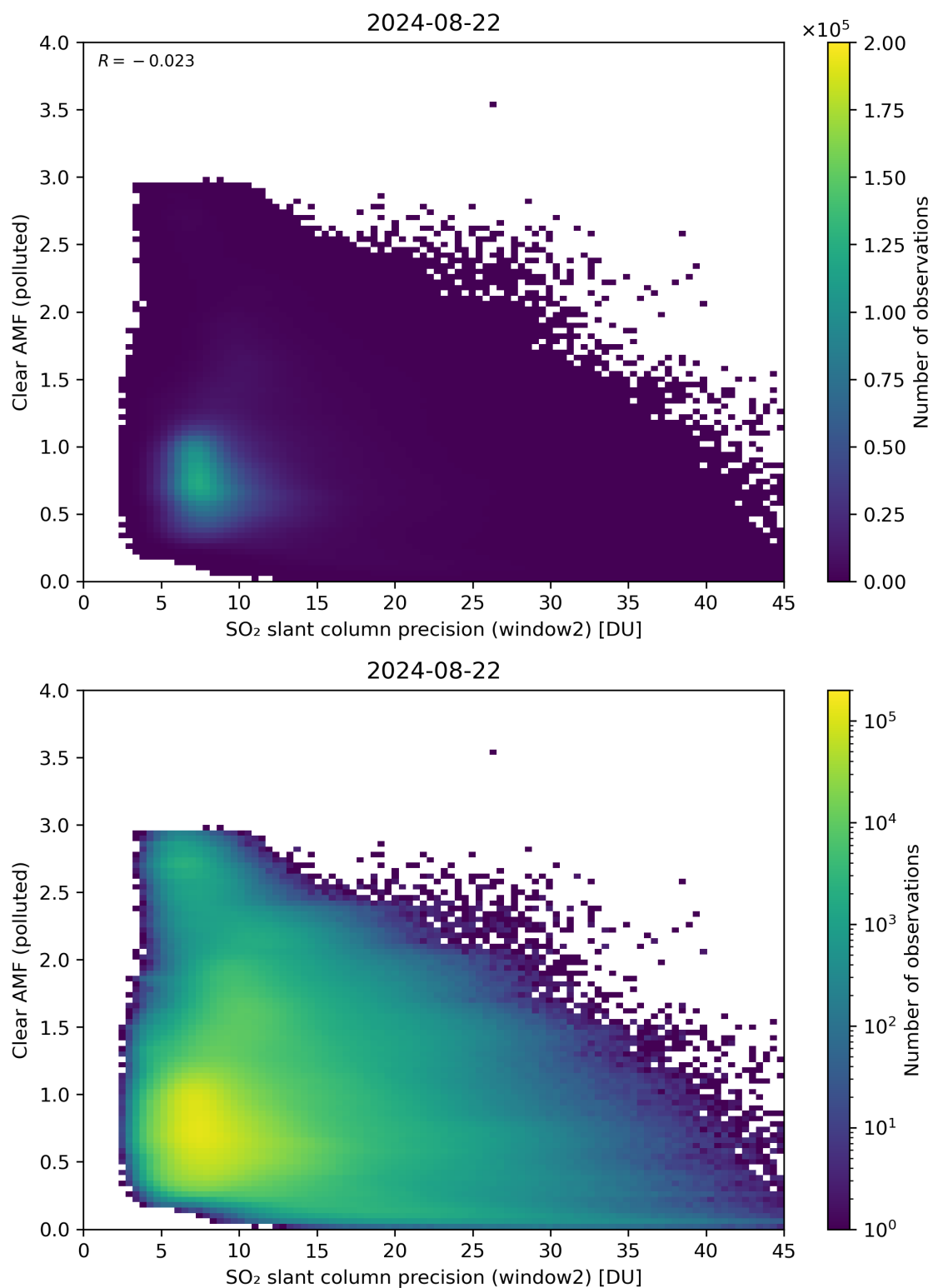
Figure 246: Scatter density plot of “SO 2 slant column precision (window2)” against “Clear AMF (polluted)” for 2024-08-22 to 2024-08-23.
