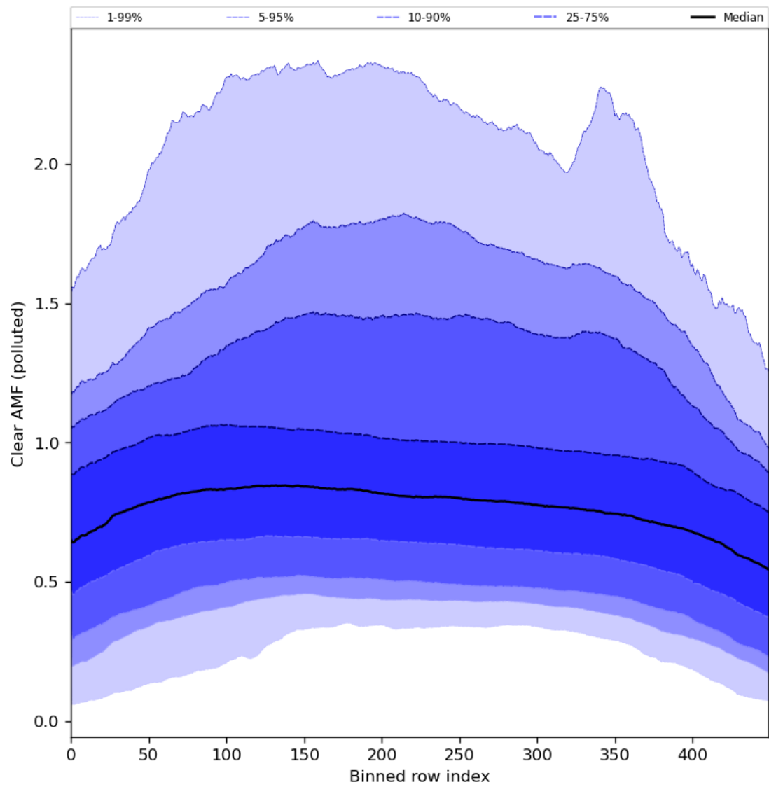
Figure 96: Along track statistics of “Clear AMF (polluted)” for 2024-08-22 to 2024-08-23
