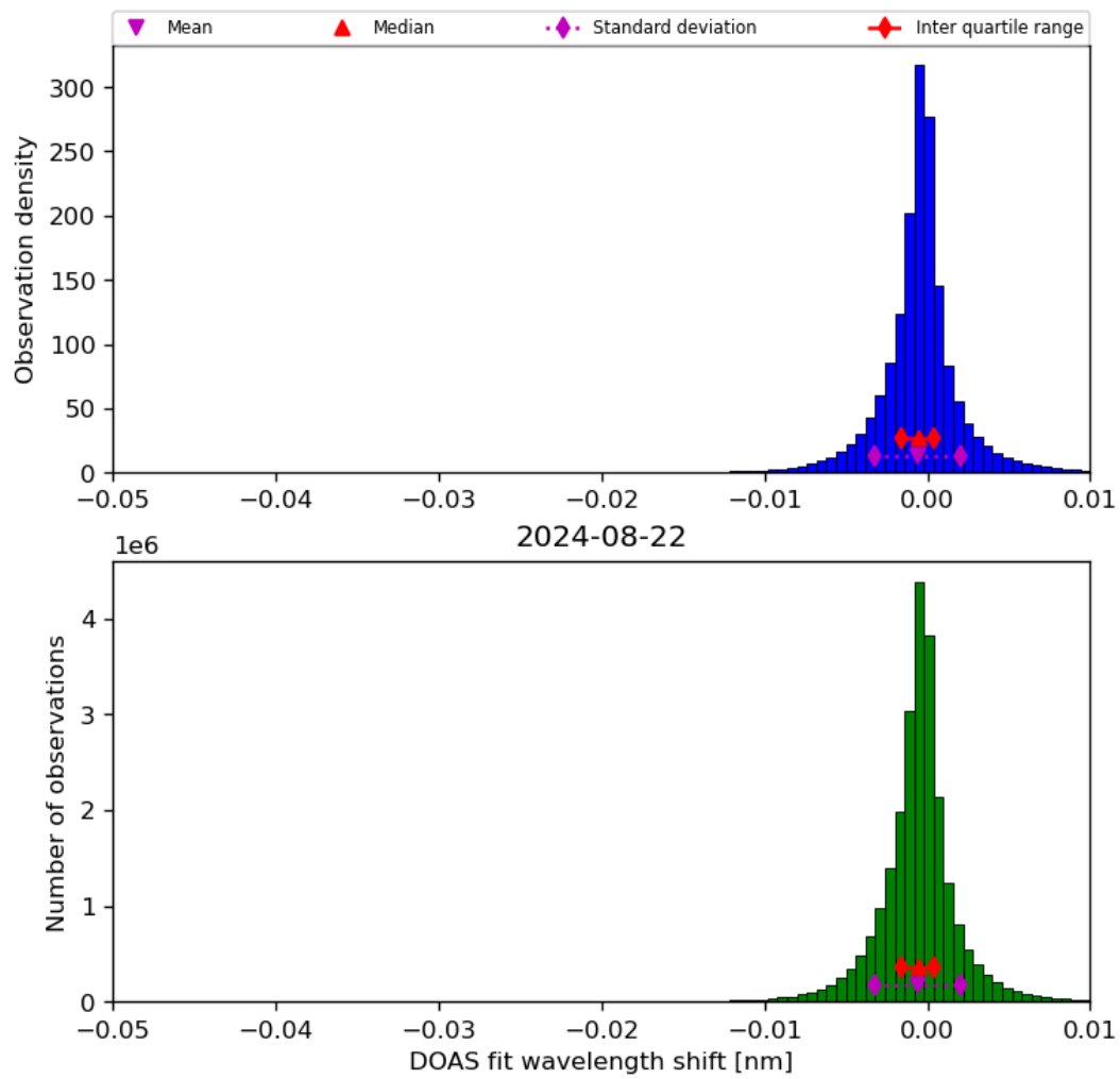
Figure 68: Histogram of “DOAS fit wavelength shift” for 2024-08-22 to 2024-08-23
