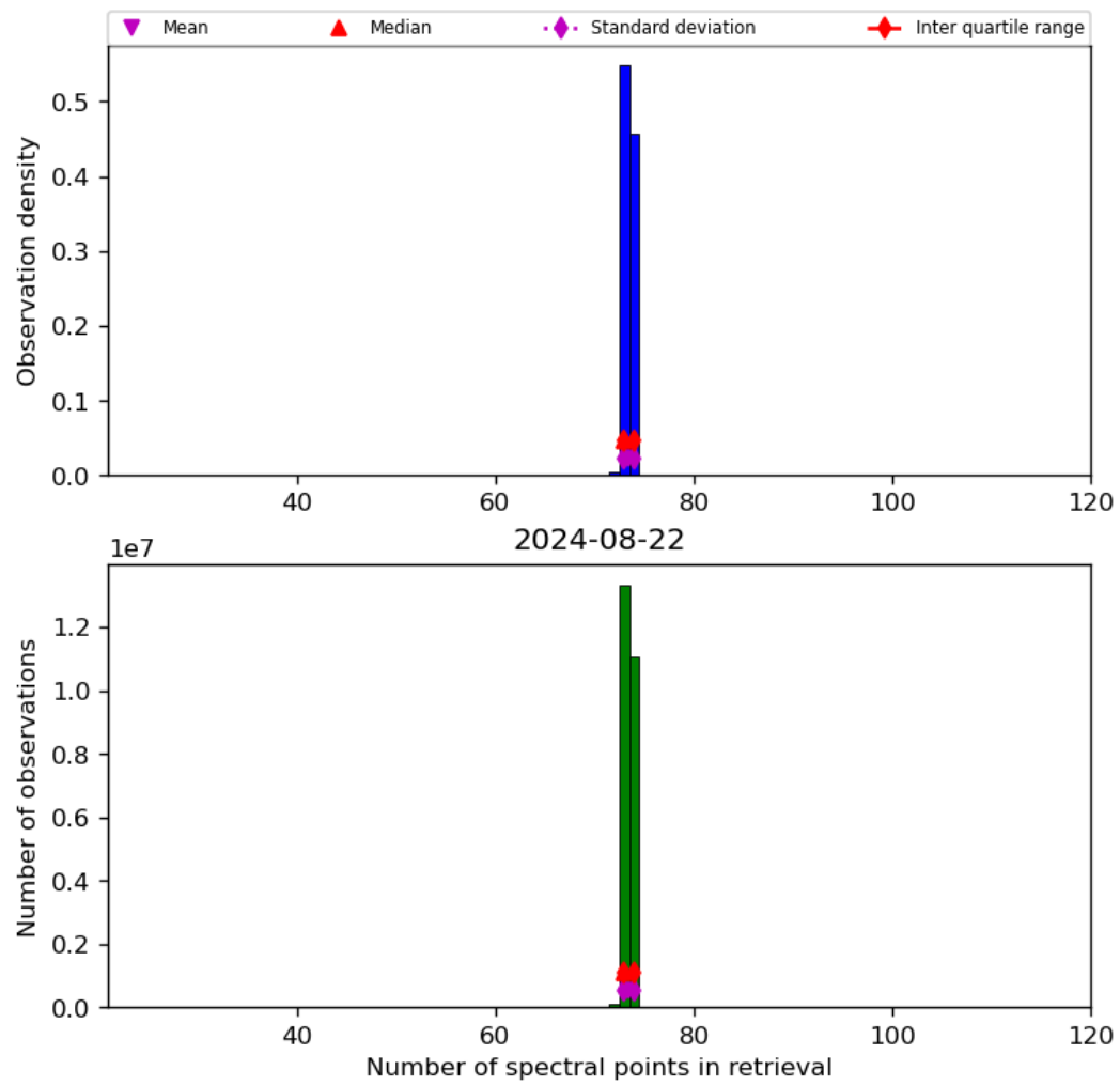
Figure 74: Histogram of “Number of spectral points in retrieval” for 2024-08-22 to 2024-08-23
