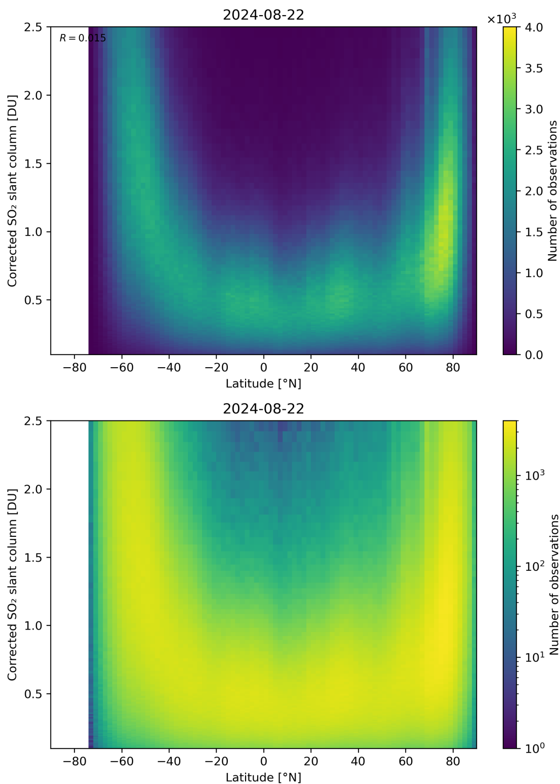
Figure 146: Scatter density plot of “Latitude” against “Corrected SO 2 slant column” for 2024-08-22 to 2024-08-23.
