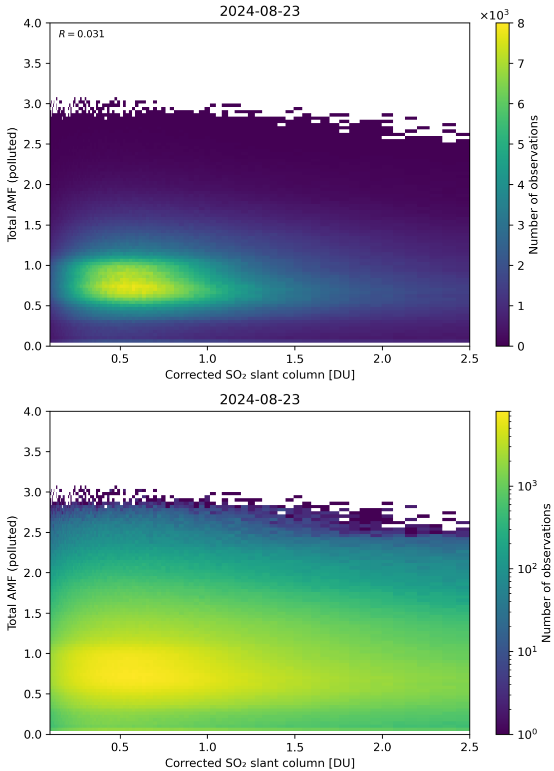
Figure 192: Scatter density plot of “Corrected SO 2 slant column” against “Total AMF (polluted)” for 2024-08-22 to 2024-08-24.
