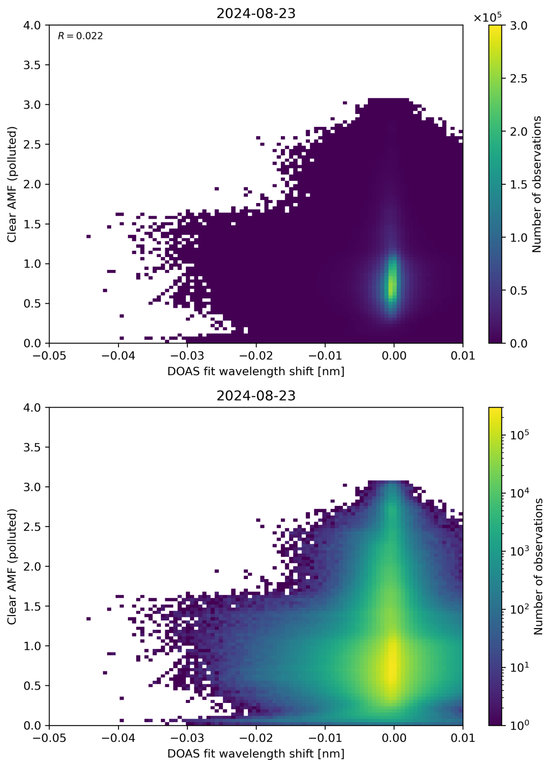
Figure 129: Scatter density plot of “DOAS fit wavelength shift” against “Clear AMF (polluted)” for 2024-08-22 to 2024-08-24.
