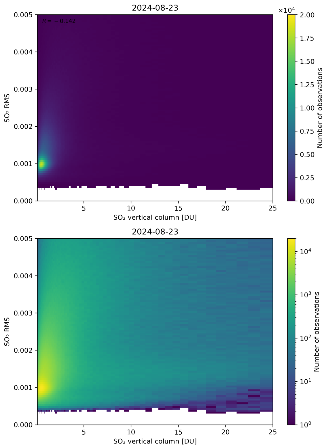
Figure 278: Scatter density plot of “SO 2 vertical column” against “SO 2 RMS” for 2024-08-22 to 2024-08-24.
