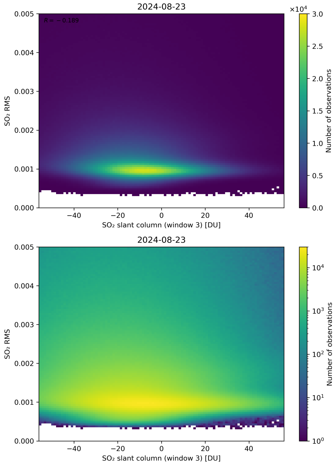
Figure 256: Scatter density plot of “SO 2 slant column (window 3)” against “SO 2 RMS” for 2024-08-22 to 2024-08-24.
