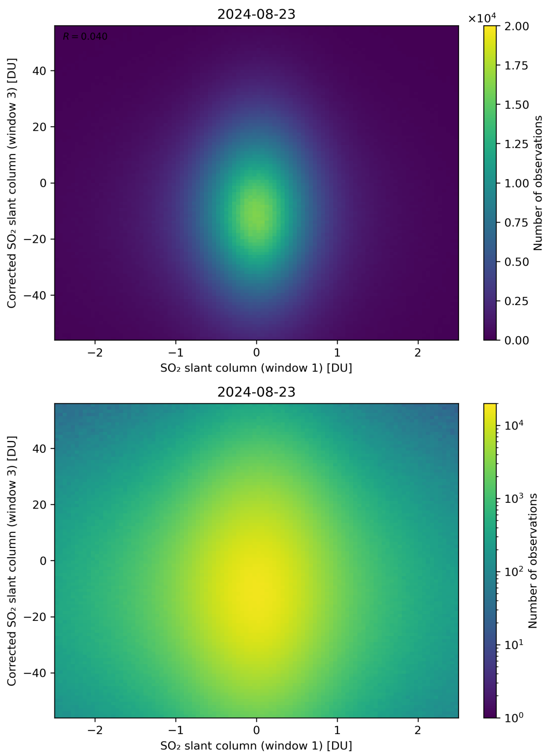
Figure 234: Scatter density plot of “SO 2 slant column (window 1)” against “Corrected SO 2 slant column (window 3)” for 2024-08-22 to 2024-08-24.
