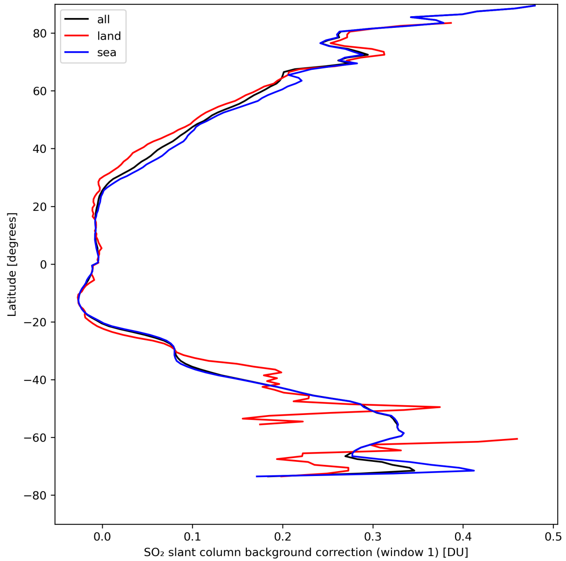
Figure 36: Zonal average of “SO 2 slant column background correction (window 1)” for 2024-08-22 to 2024-08-24.
