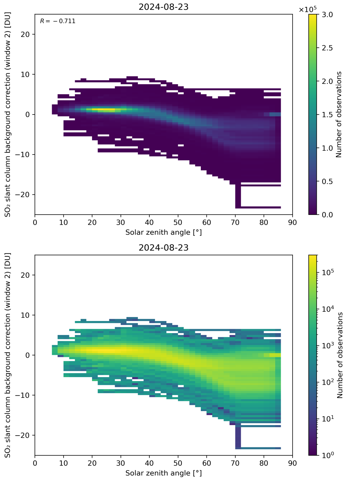
Figure 159: Scatter density plot of “Solar zenith angle” against “SO 2 slant column background correction (window 2)” for 2024-08-22 to 2024-08-24.
