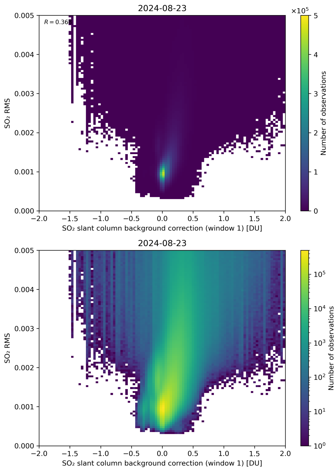
Figure 102: Scatter density plot of “SO 2 slant column background correction (window 1)” against “SO 2 RMS” for 2024-08-22 to 2024-08-24.
