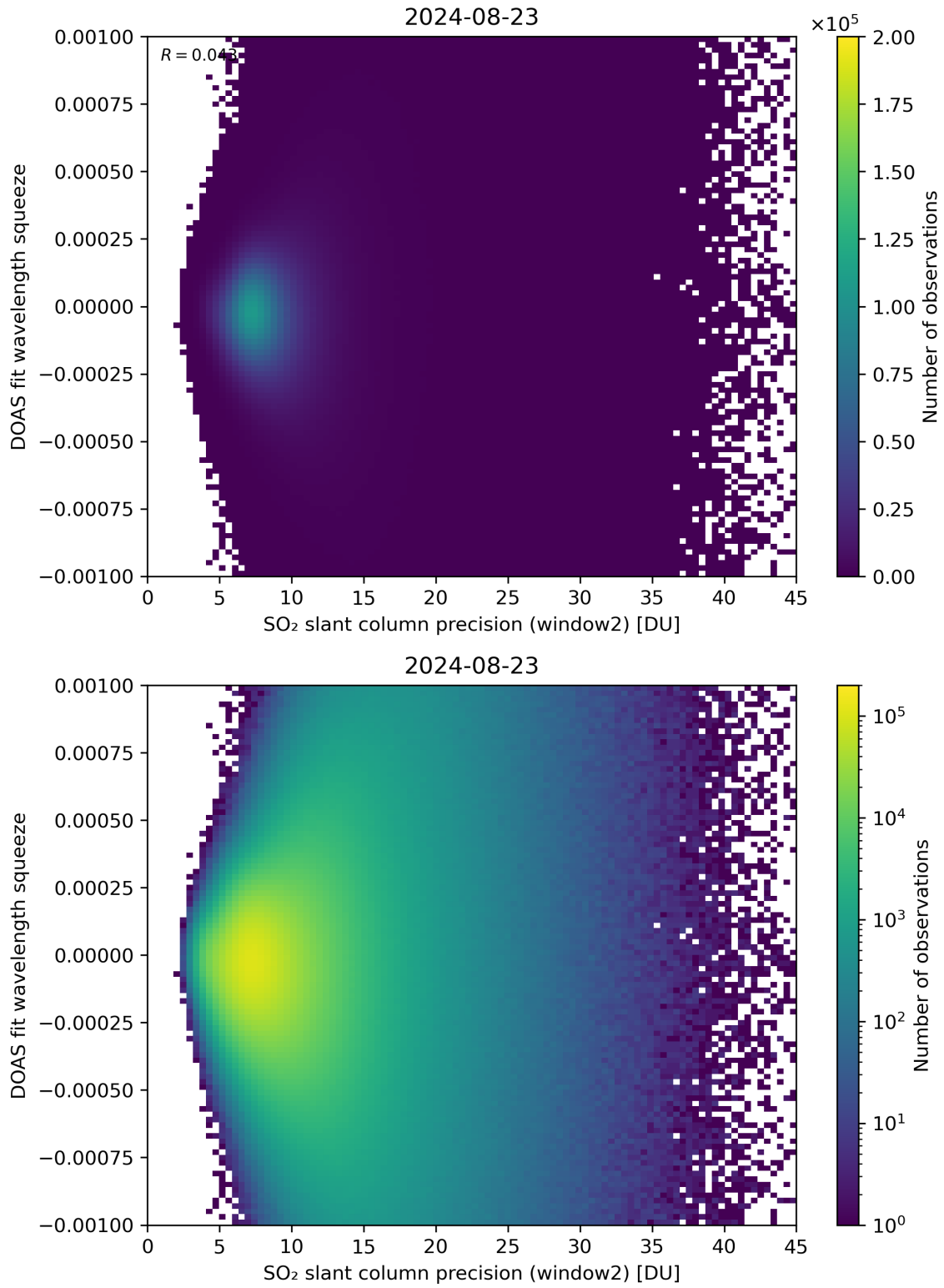
Figure 244: Scatter density plot of “SO 2 slant column precision (window2)” against “DOAS fit wavelength squeeze” for 2024-08-22 to 2024-08-24.
