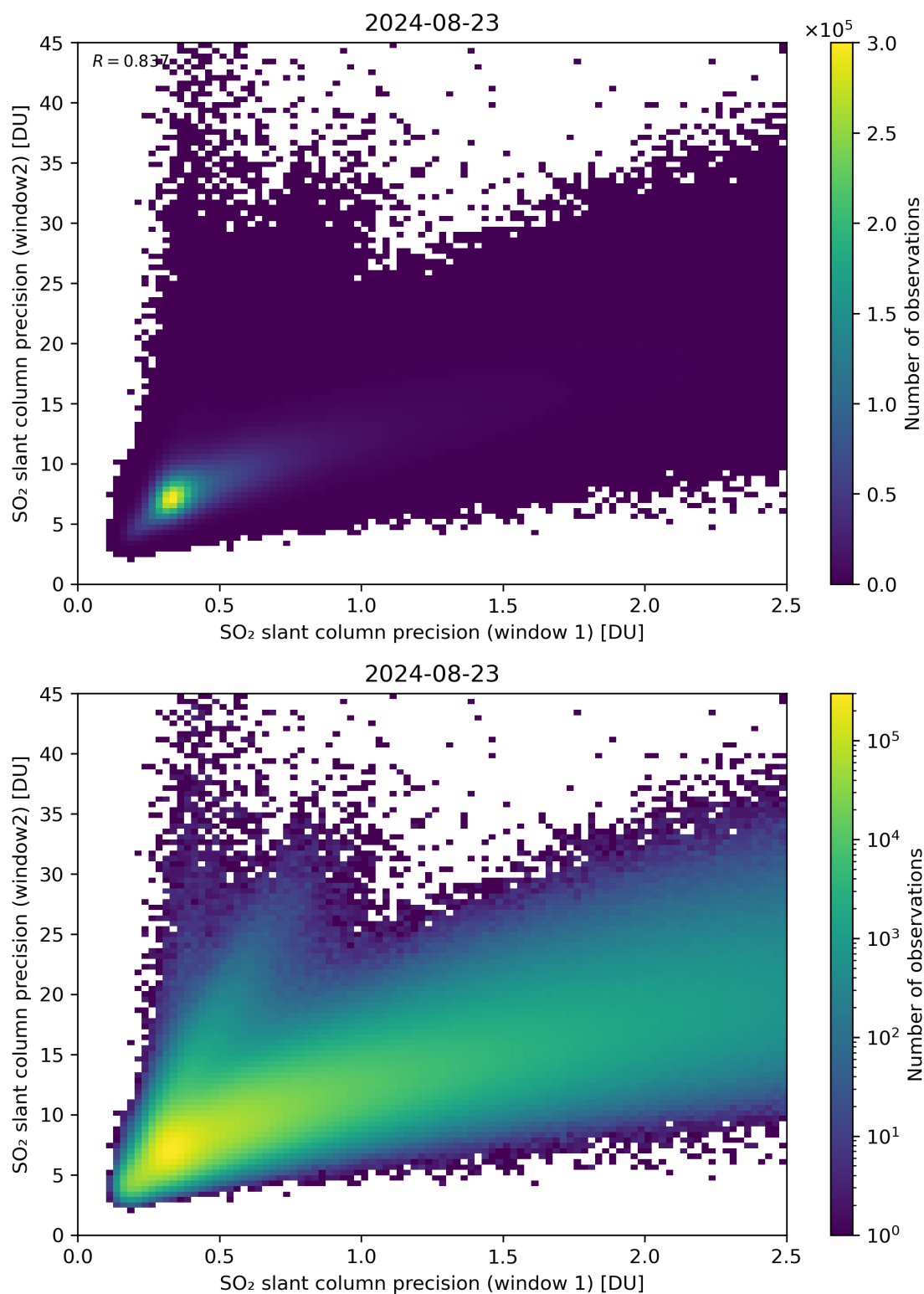
Figure 227: Scatter density plot of “SO 2 slant column precision (window 1)” against “SO 2 slant column precision (window 2)” for 2024-08-22 to 2024-08-24.
