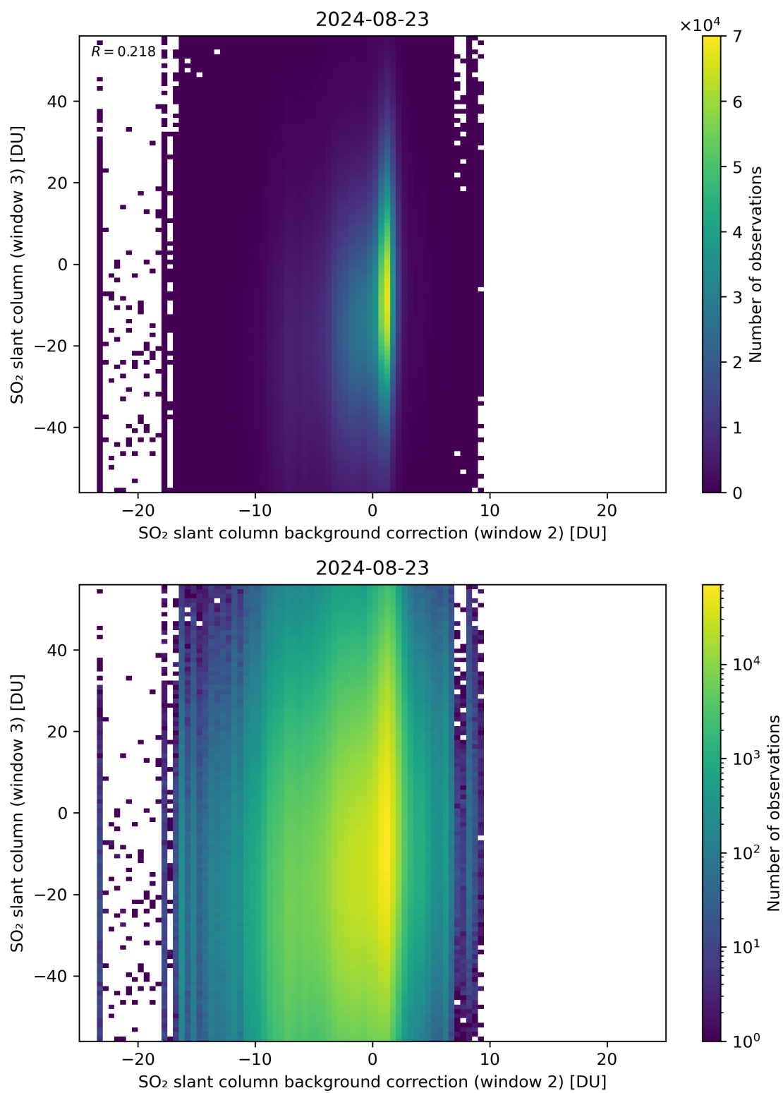
Figure 117: Scatter density plot of “SO 2 slant column background correction (window 2)” against “SO 2 slant column (window 3)” for 2024-08-22 to 2024-08-24.
