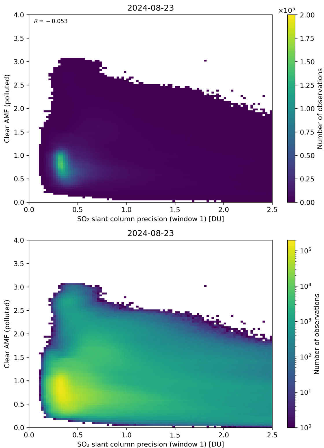
Figure 224: Scatter density plot of “SO 2 slant column precision (window 1)” against “Clear AMF (polluted)” for 2024-08-22 to 2024-08-24.
