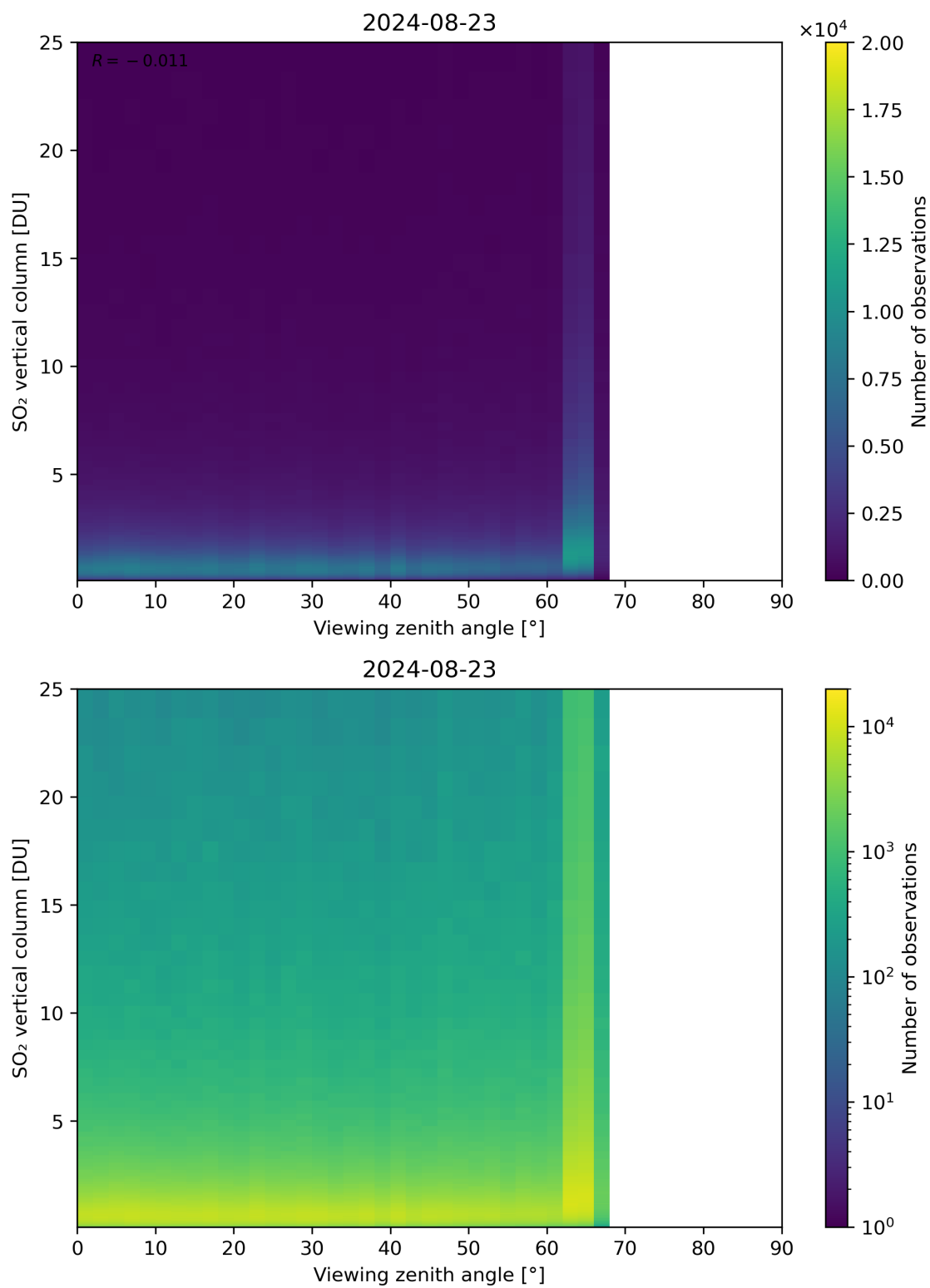
Figure 327: Scatter density plot of “Viewing zenith angle” against “SO 2 vertical column” for 2024-08-22 to 2024-08-24.
