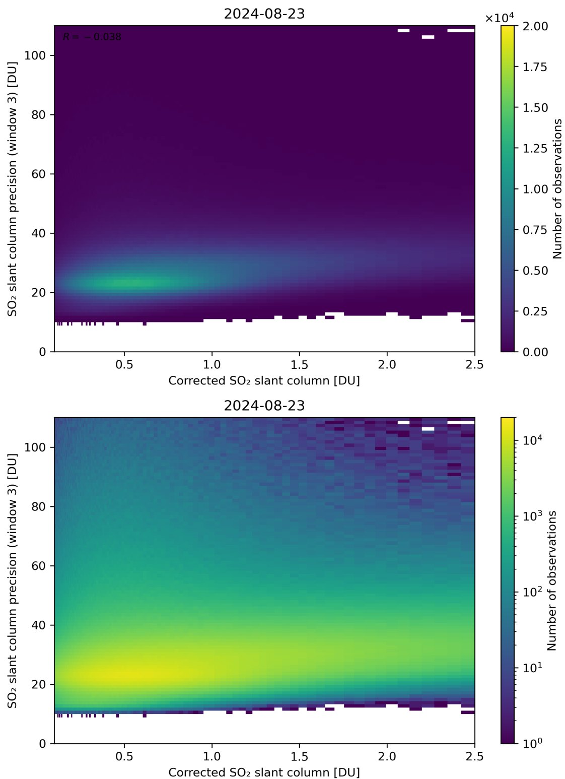
Figure 191: Scatter density plot of “Corrected SO 2 slant column” against “SO 2 slant column precision (window 3)” for 2024-08-22 to 2024-08-24.
