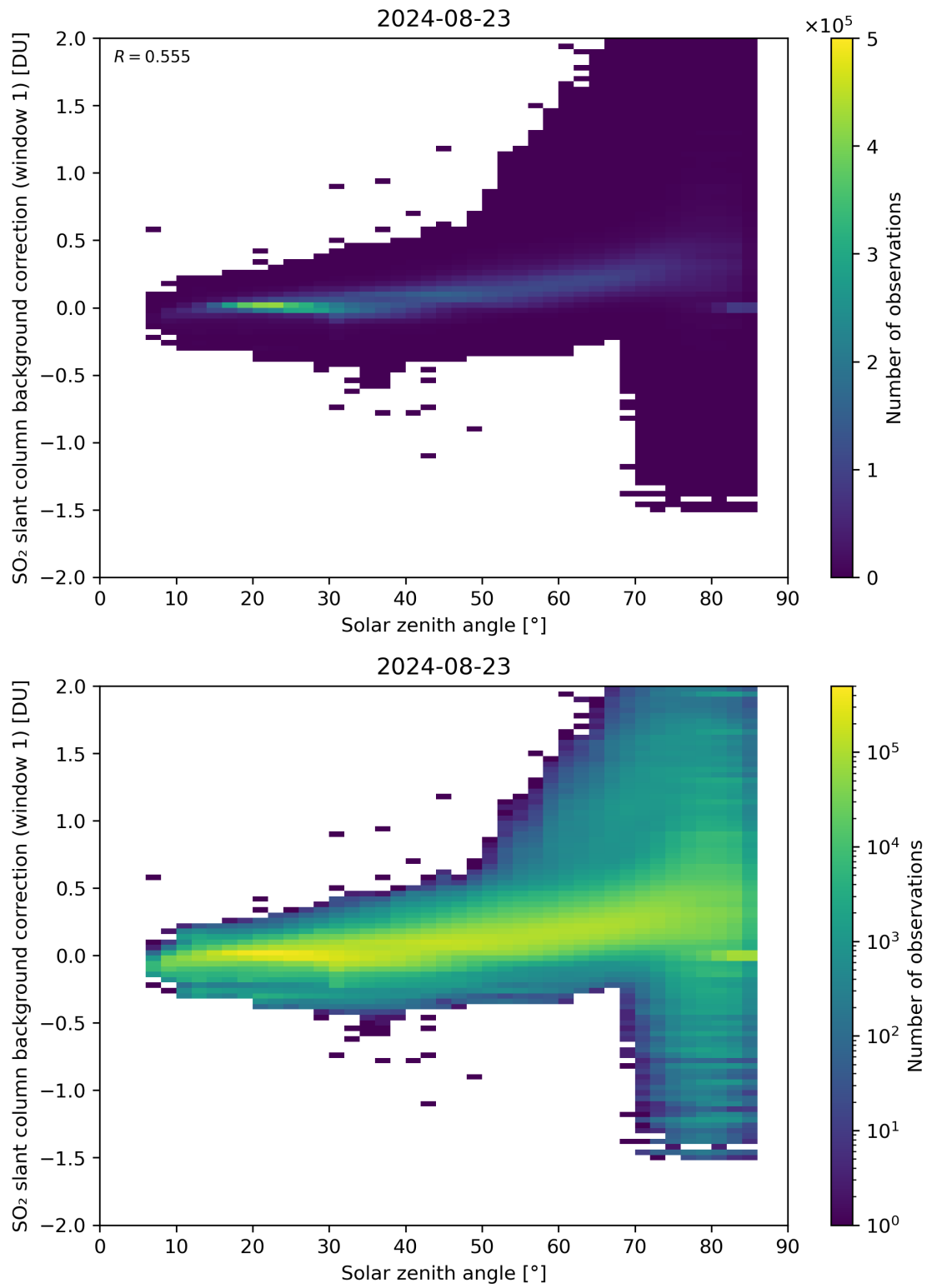
Figure 158: Scatter density plot of “Solar zenith angle” against “SO 2 slant column background correction (window 1)” for 2024-08-22 to 2024-08-24.
