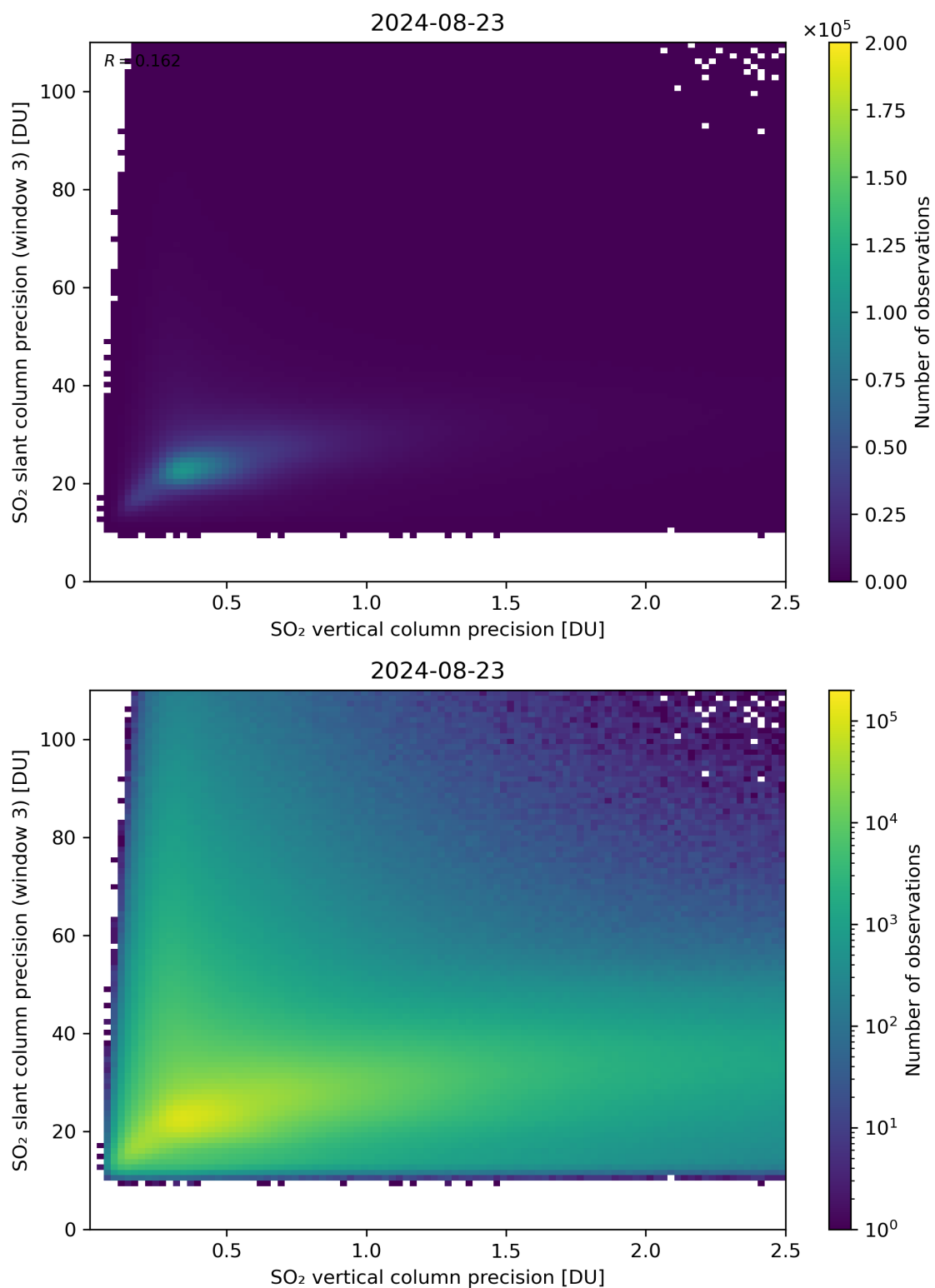
Figure 293: Scatter density plot of “SO 2 vertical column precision” against “SO 2 slant column precision (window 3)” for 2024-08-22 to 2024-08-24.
