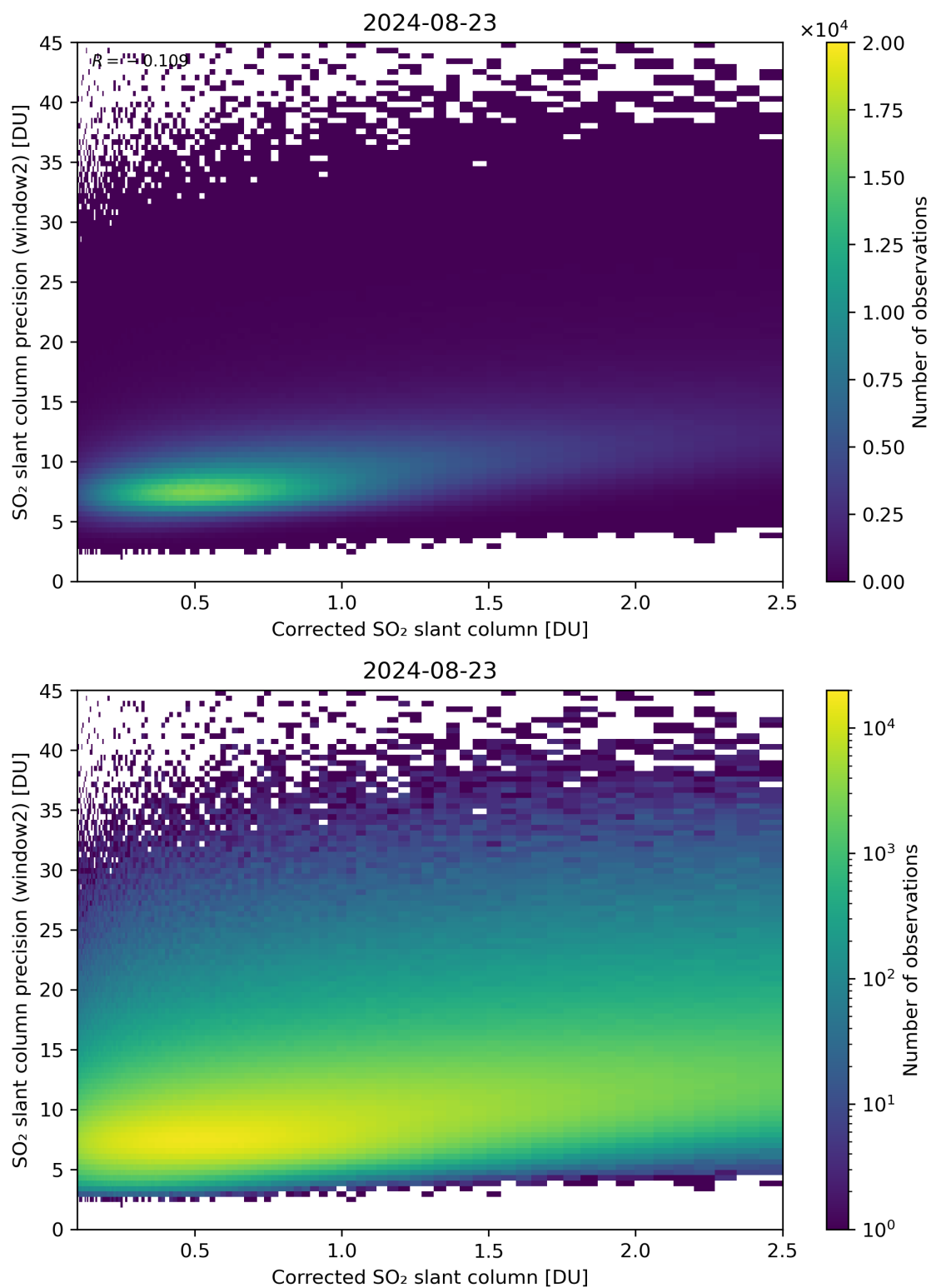
Figure 189: Scatter density plot of “Corrected SO 2 slant column” against “SO 2 slant column precision (window2)” for 2024-08-22 to 2024-08-24.
