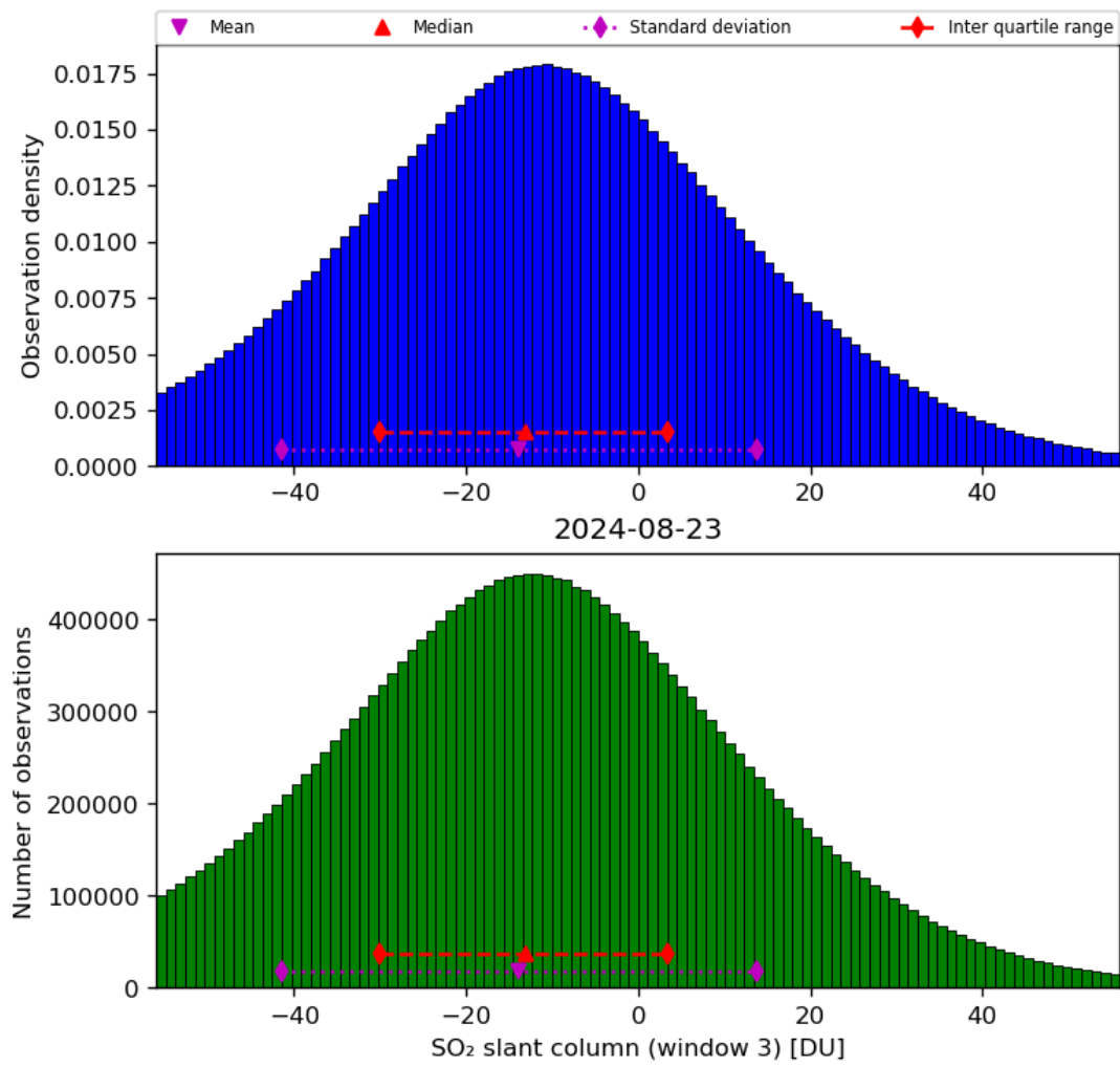
Figure 64: Histogram of “SO 2 slant column (window 3)” for 2024-08-22 to 2024-08-24
