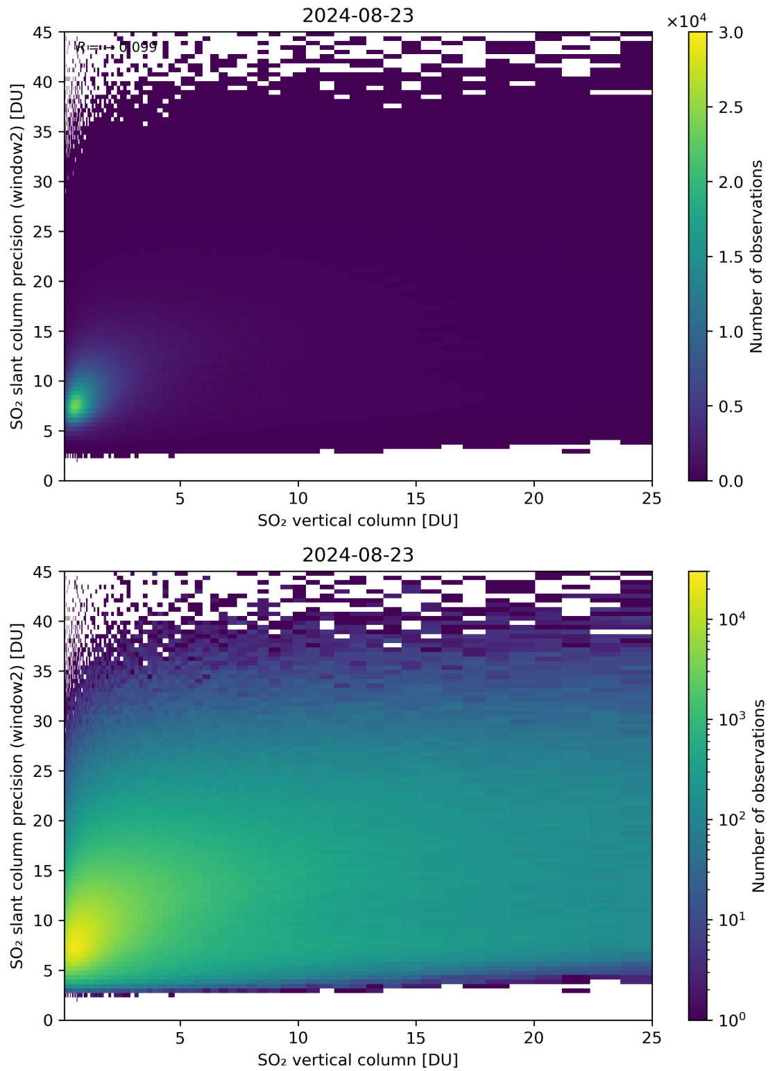
Figure 302: Scatter density plot of “SO 2 vertical column” against “SO 2 slant column precision (window2)” for 2024-08-22 to 2024-08-24.
