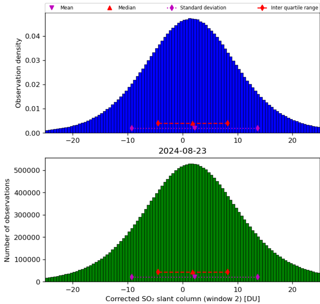
Figure 62: Histogram of “Corrected SO 2 slant column (window 2)” for 2024-08-22 to 2024-08-24
