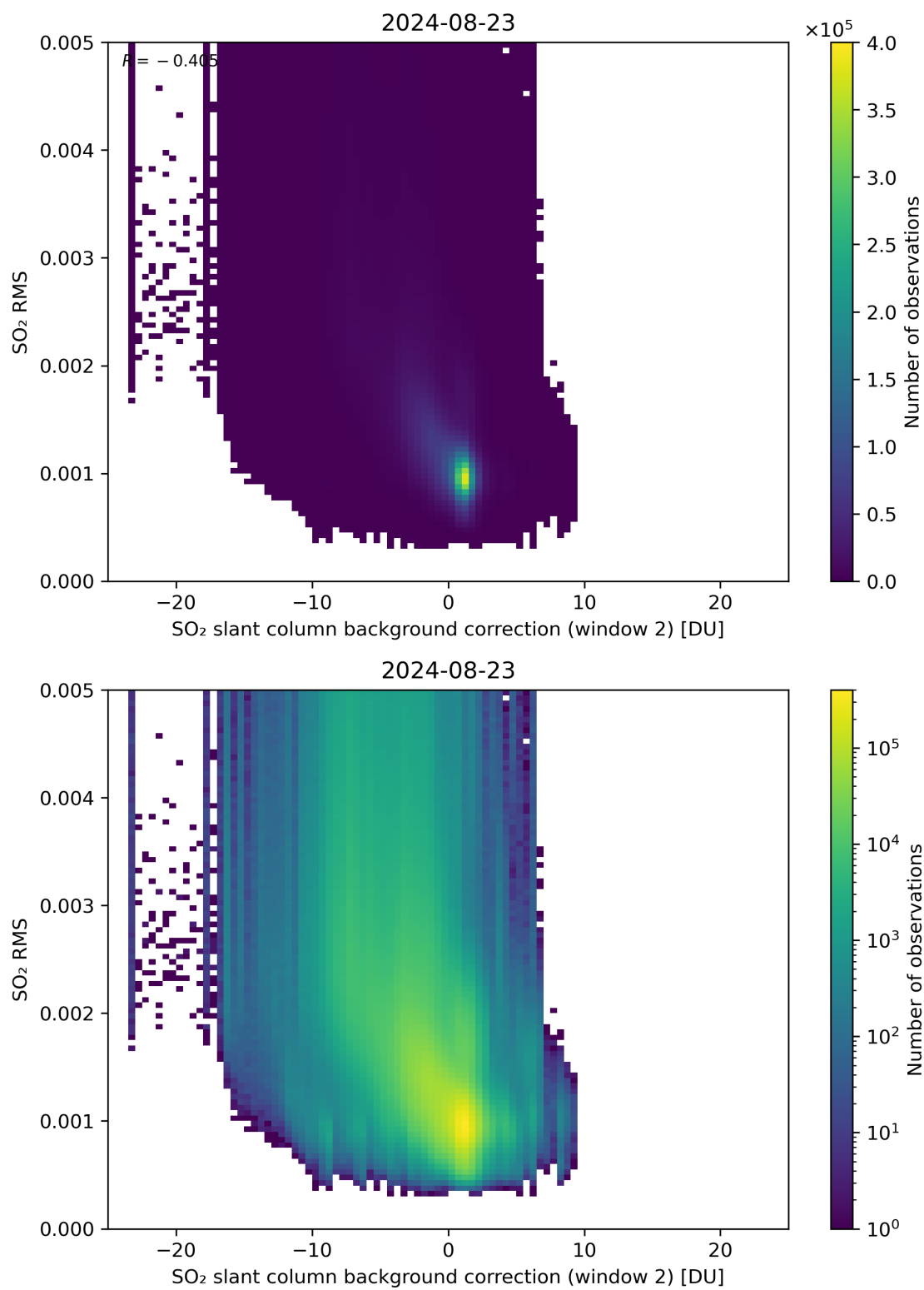
Figure 114: Scatter density plot of “SO 2 slant column background correction (window 2)” against “SO 2 RMS” for 2024-08-22 to 2024-08-24.
