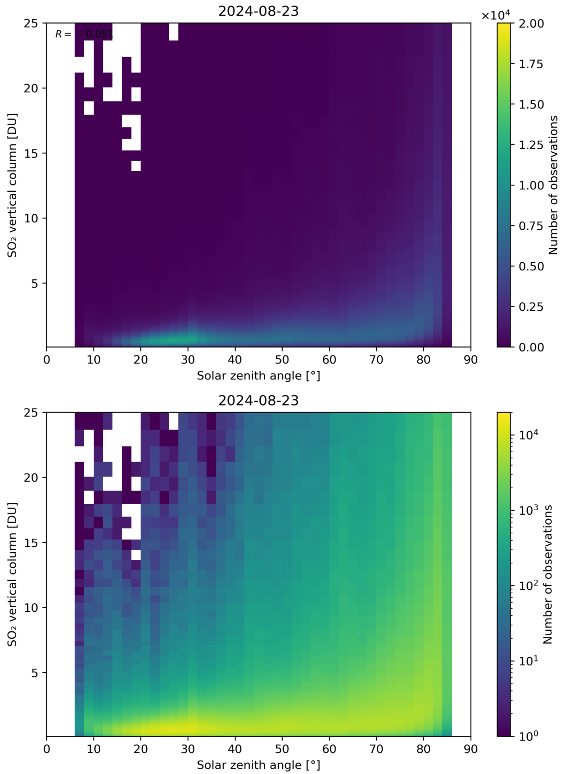
Figure 176: Scatter density plot of “Solar zenith angle” against “SO 2 vertical column” for 2024-08-22 to 2024-08-24.
