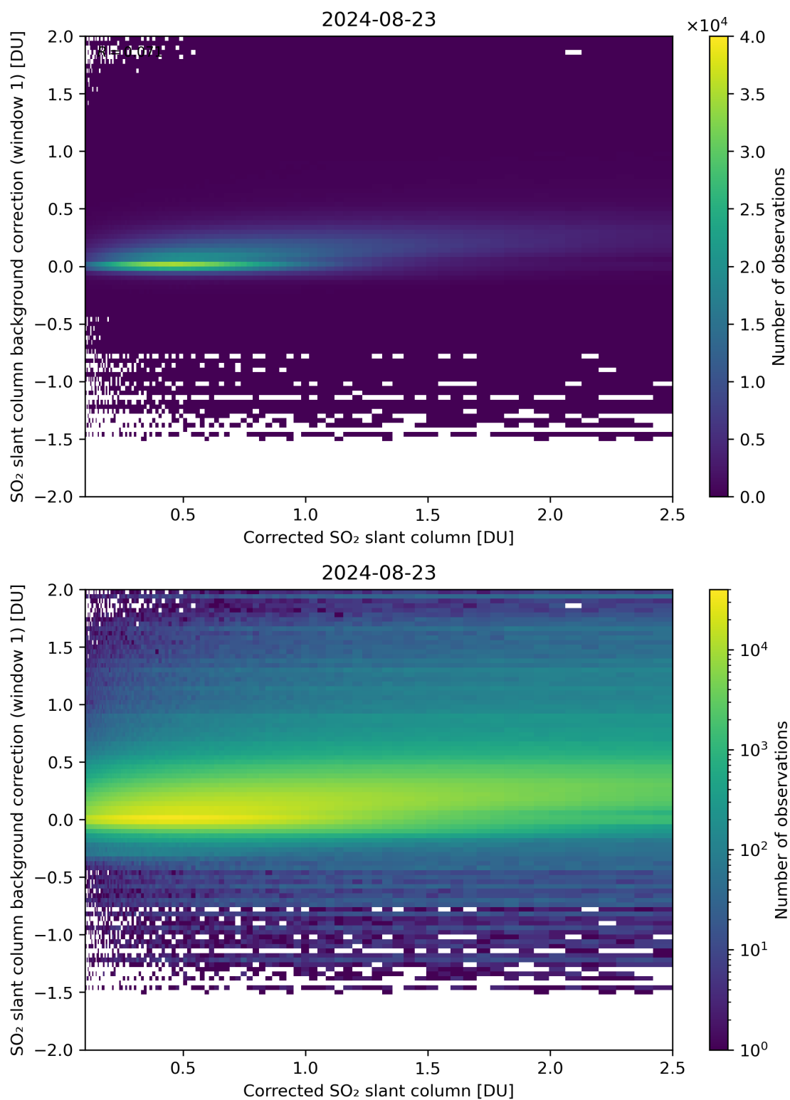
Figure 178: Scatter density plot of “Corrected SO 2 slant column” against “SO 2 slant column background correction (window 1)” for 2024-08-22 to 2024-08-24.
