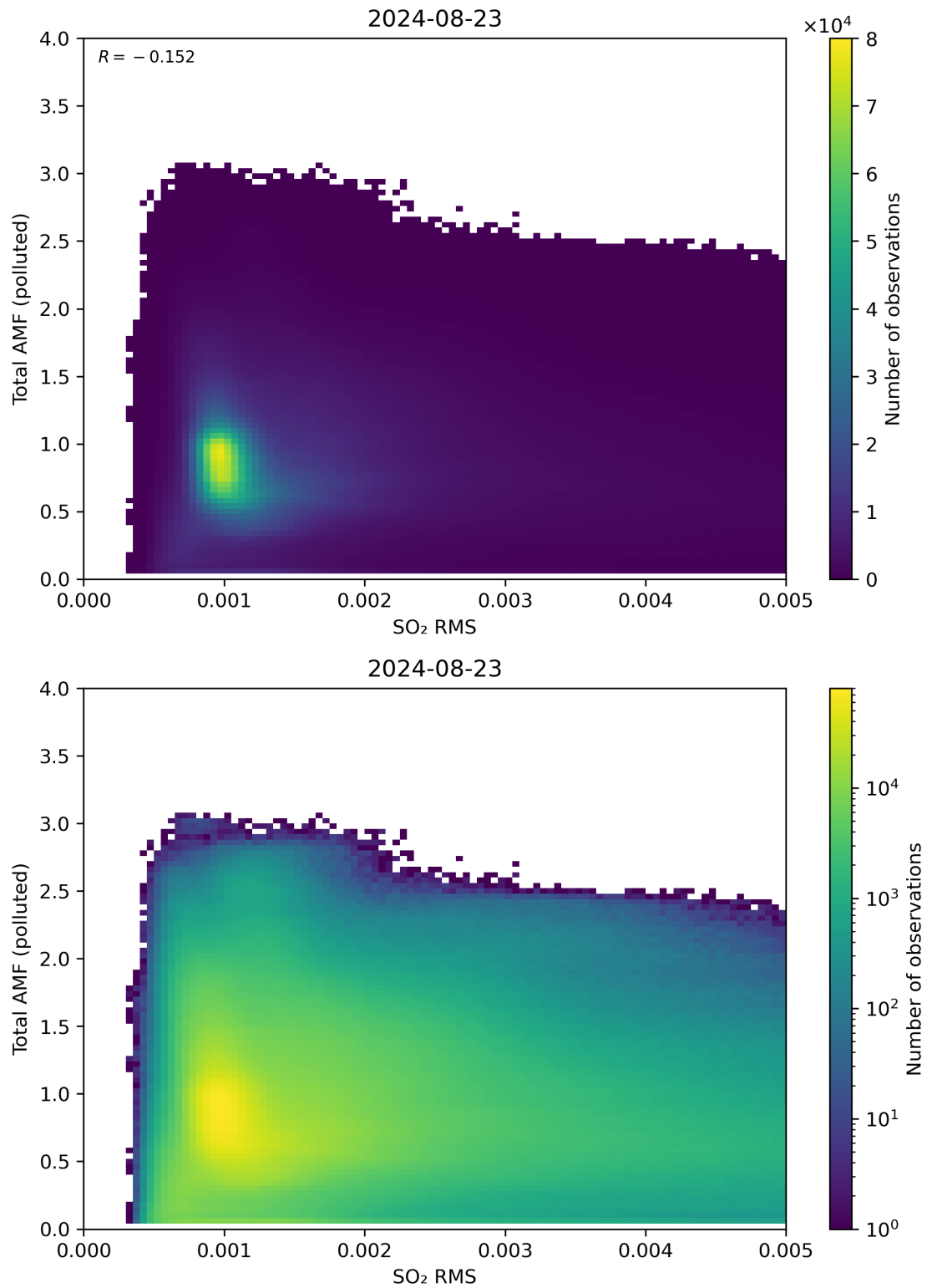
Figure 137: Scatter density plot of “SO 2 RMS” against “Total AMF (polluted)” for 2024-08-22 to 2024-08-24.
