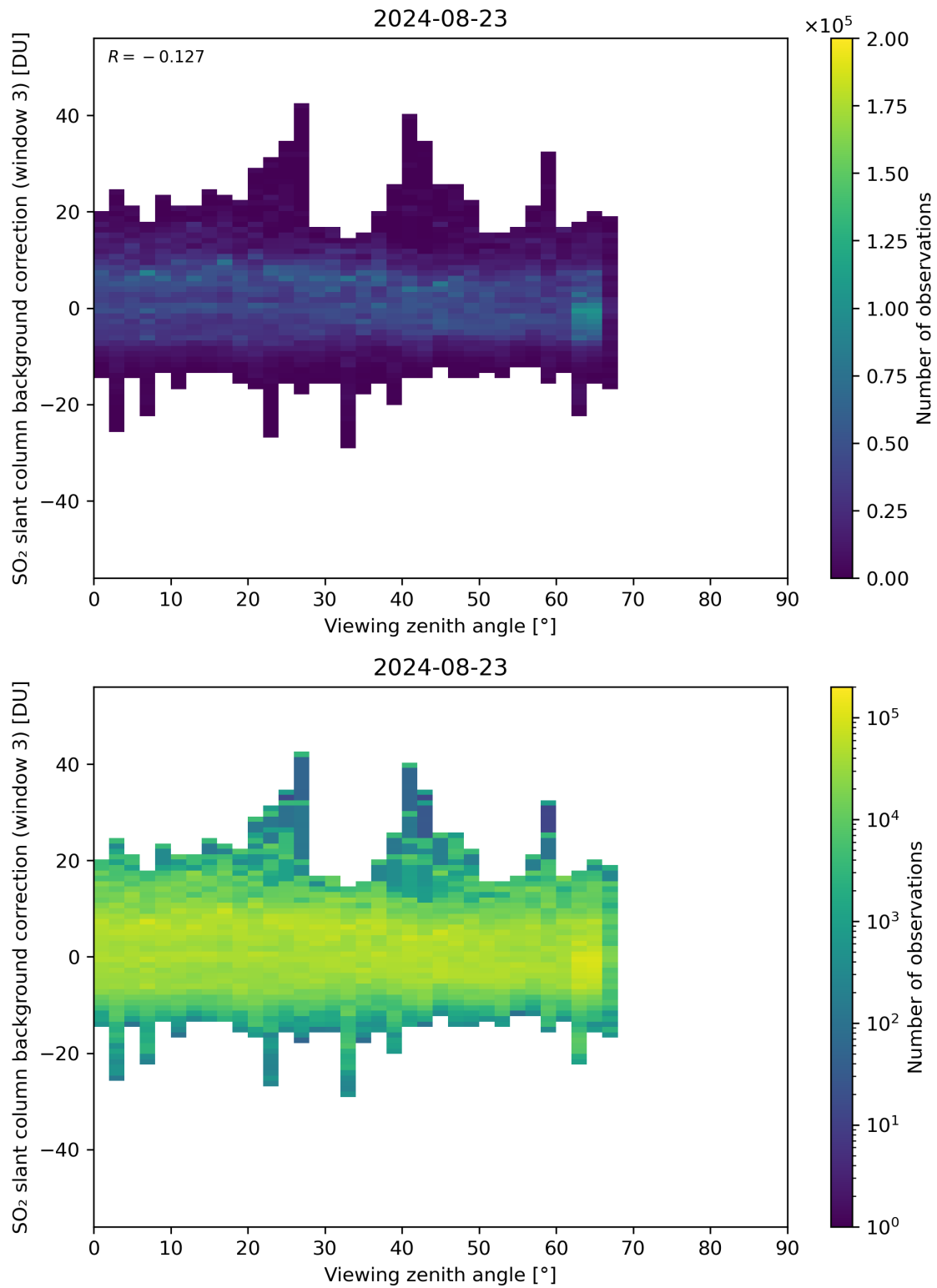
Figure 310: Scatter density plot of “Viewing zenith angle” against “SO 2 slant column background correction (window 3)” for 2024-08-22 to 2024-08-24.
