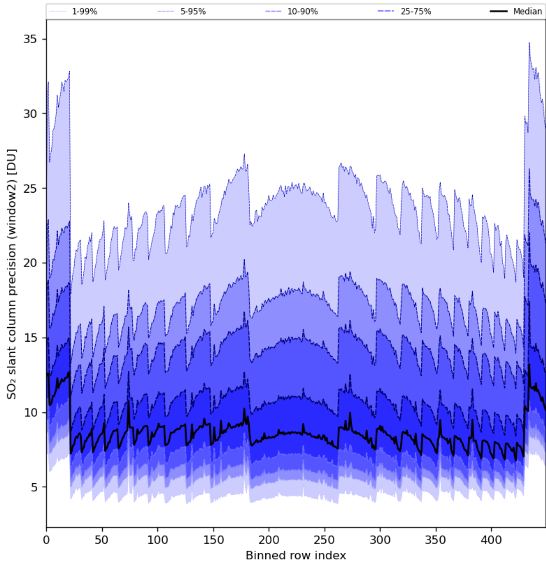
Figure 84: Along track statistics of “SO 2 slant column precision (window2)” for 2024-08-22 to 2024-08-24
