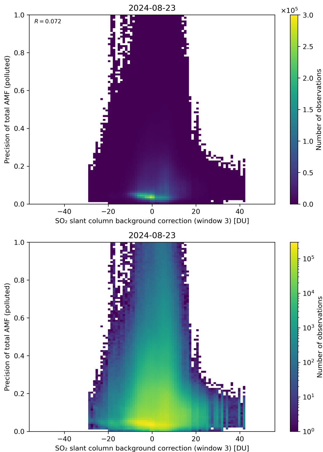
Figure 126: Scatter density plot of “SO 2 slant column background correction (window 3)” against “Precision of total AMF (polluted)” for 2024-08-22 to 2024-08-24.
