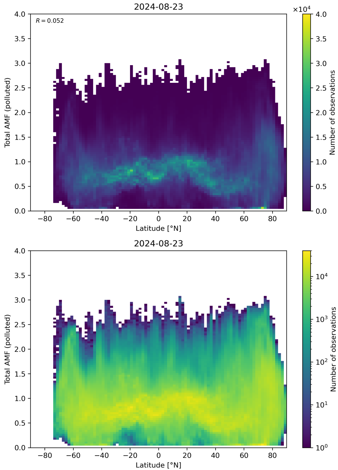
Figure 154: Scatter density plot of “Latitude” against “Total AMF (polluted)” for 2024-08-22 to 2024-08-24.
