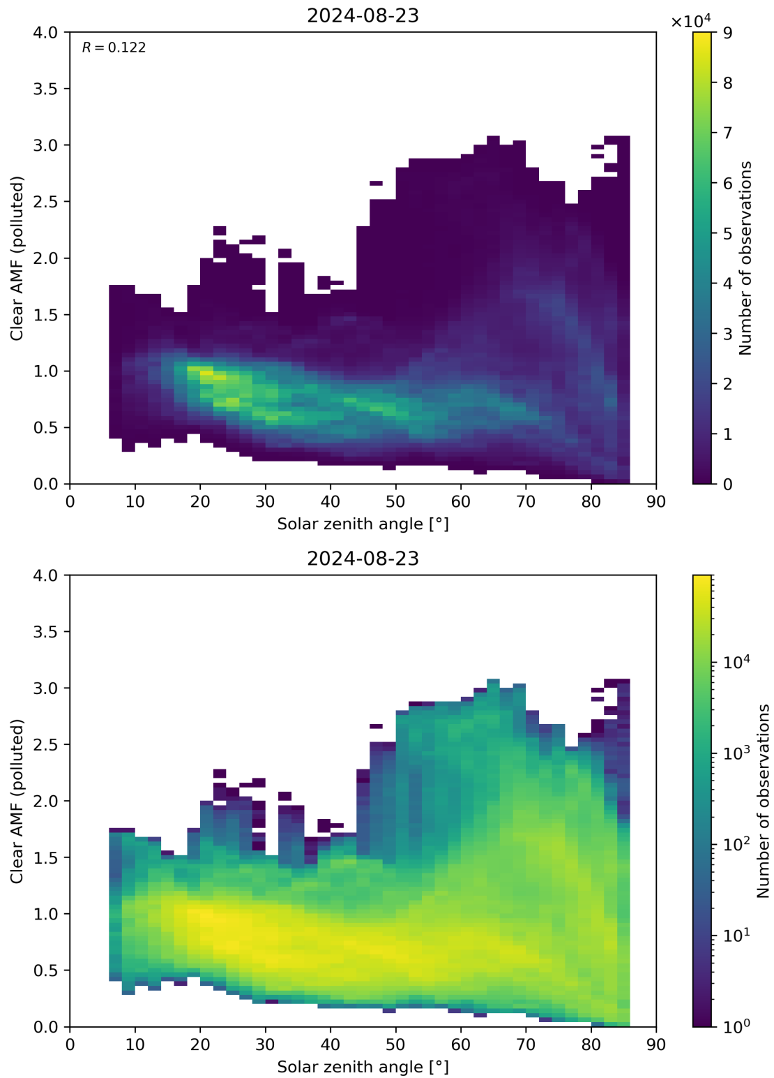
Figure 165: Scatter density plot of “Solar zenith angle” against “Clear AMF (polluted)” for 2024-08-22 to 2024-08-24.
