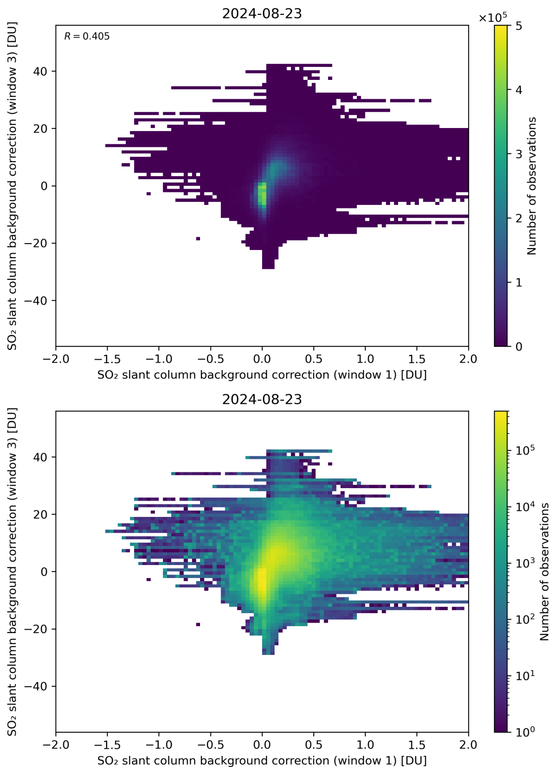
Figure 99: Scatter density plot of “SO 2 slant column background correction (window 1)” against “SO 2 slant column background correction (window 3)” for 2024-08-22 to 2024-08-24.
