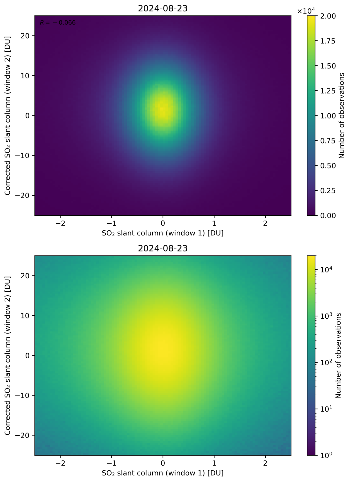
Figure 233: Scatter density plot of “SO 2 slant column (window 1)” against “Corrected SO 2 slant column (window 2)” for 2024-08-22 to 2024-08-24.
