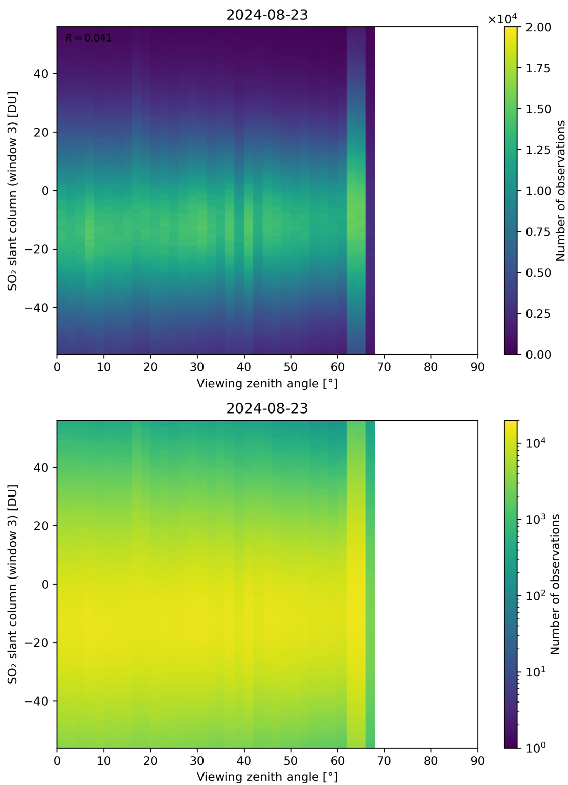
Figure 323: Scatter density plot of “Viewing zenith angle” against “SO 2 slant column (window 3)” for 2024-08-22 to 2024-08-24.
