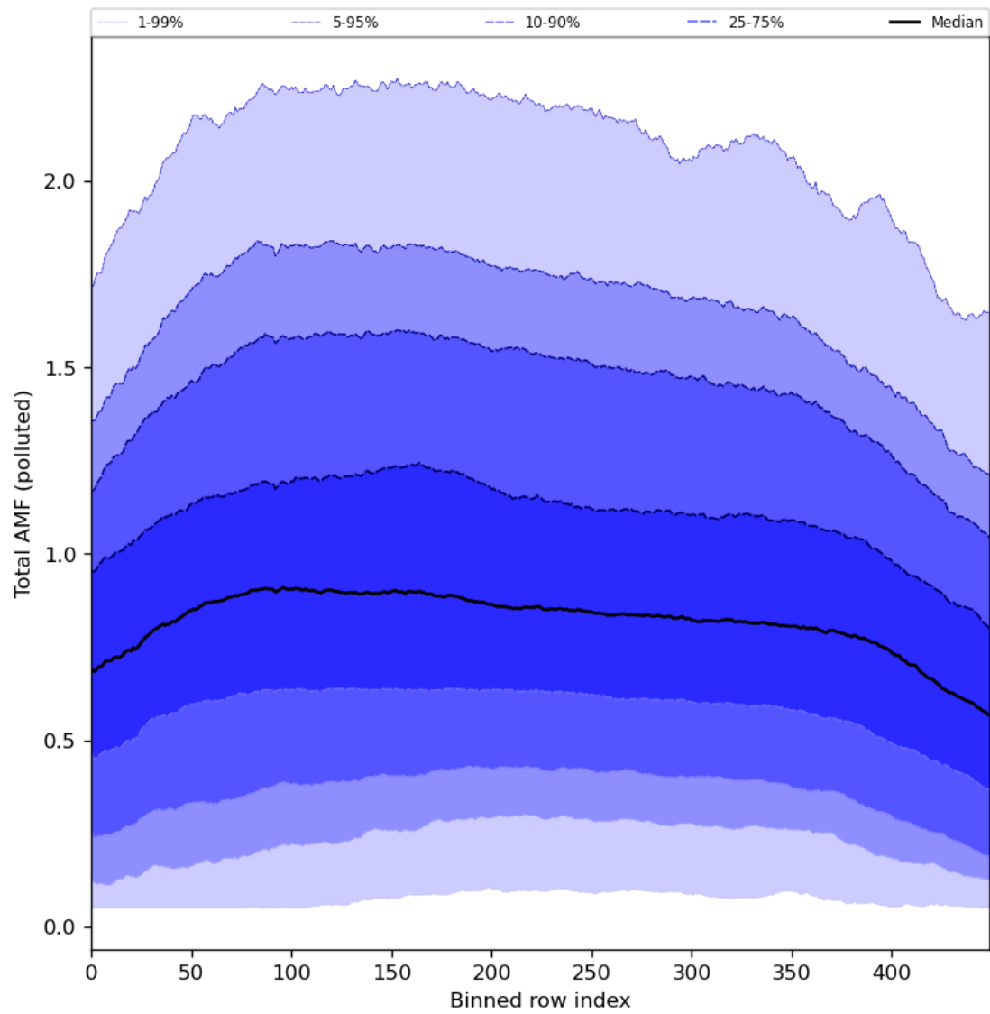
Figure 94: Along track statistics of “Total AMF (polluted)” for 2024-08-22 to 2024-08-24
