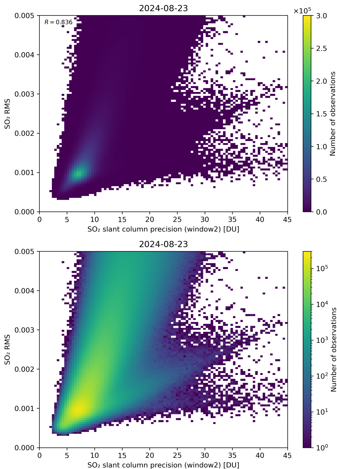
Figure 245: Scatter density plot of “SO 2 slant column precision (window2)” against “SO 2 RMS” for 2024-08-22 to 2024-08-24.
