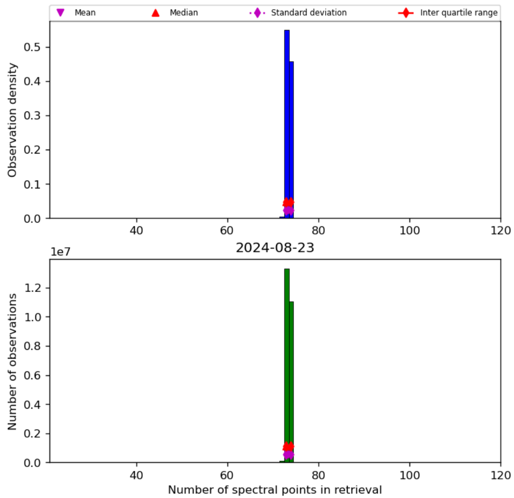
Figure 74: Histogram of “Number of spectral points in retrieval” for 2024-08-22 to 2024-08-24
