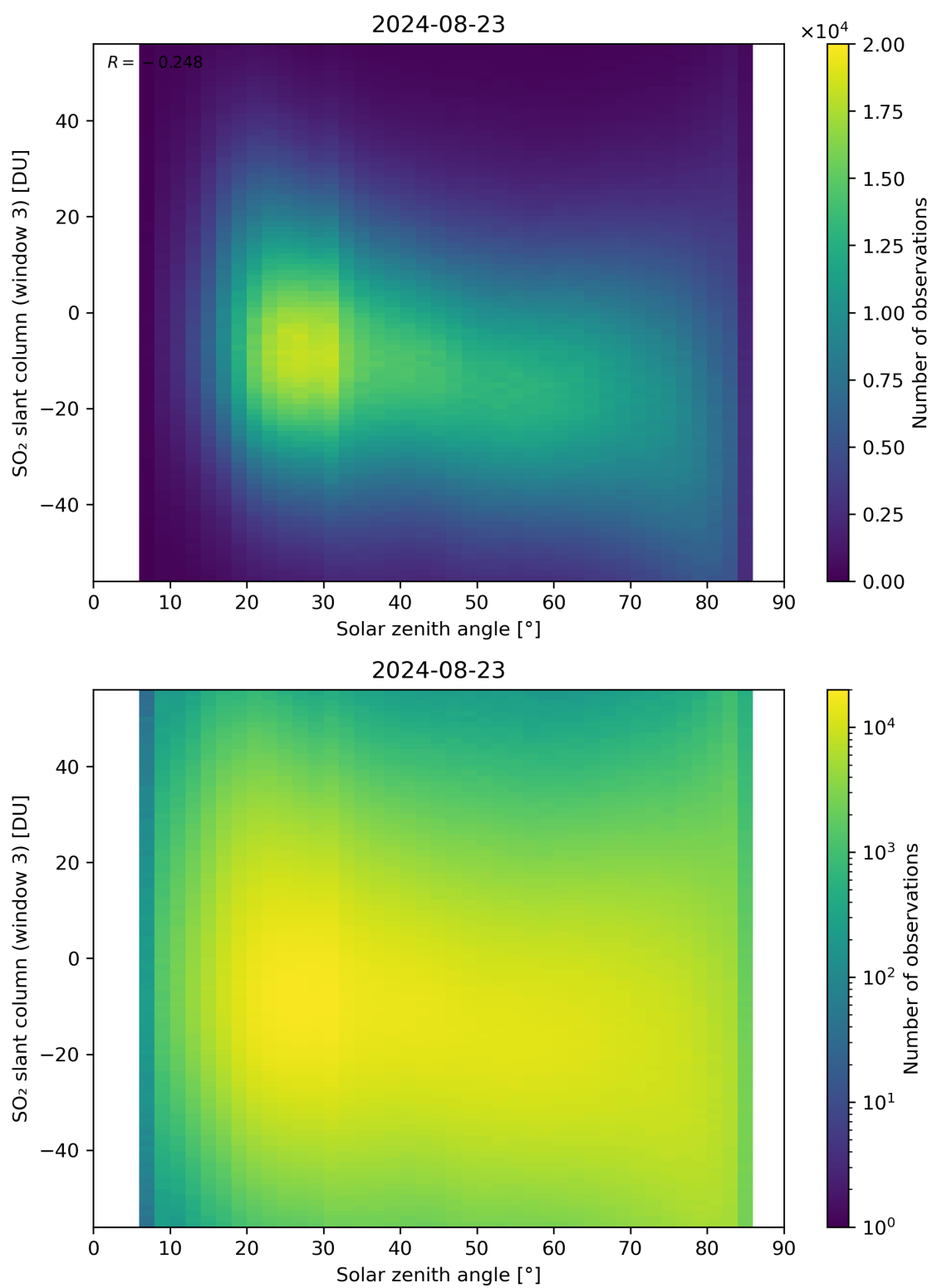
Figure 172: Scatter density plot of “Solar zenith angle” against “SO 2 slant column (window 3)” for 2024-08-22 to 2024-08-24.
