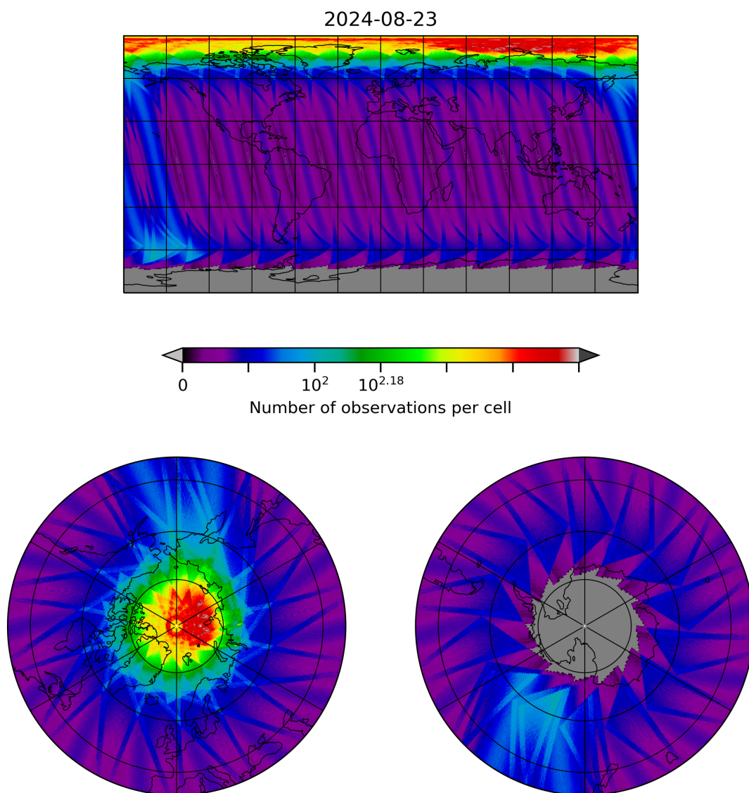
Figure 28: Map of the number of observations for 2024-08-22 to 2024-08-24
