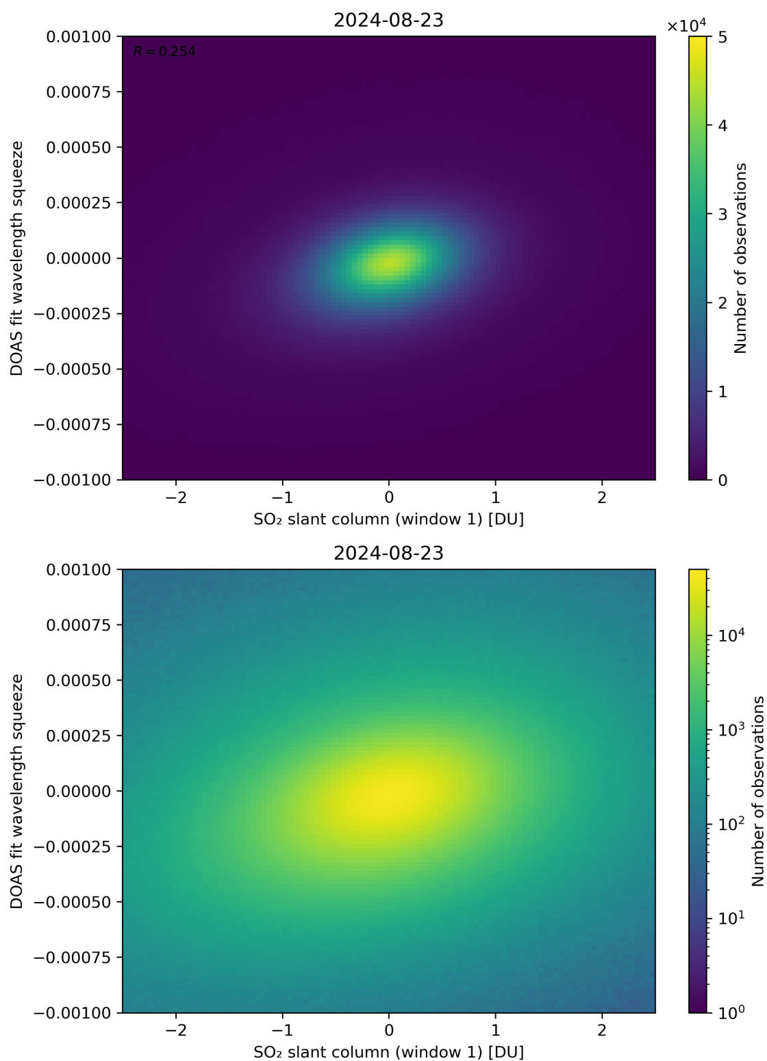
Figure 216: Scatter density plot of “SO 2 slant column (window 1)” against “DOAS fit wavelength squeeze” for 2024-08-22 to 2024-08-24.
