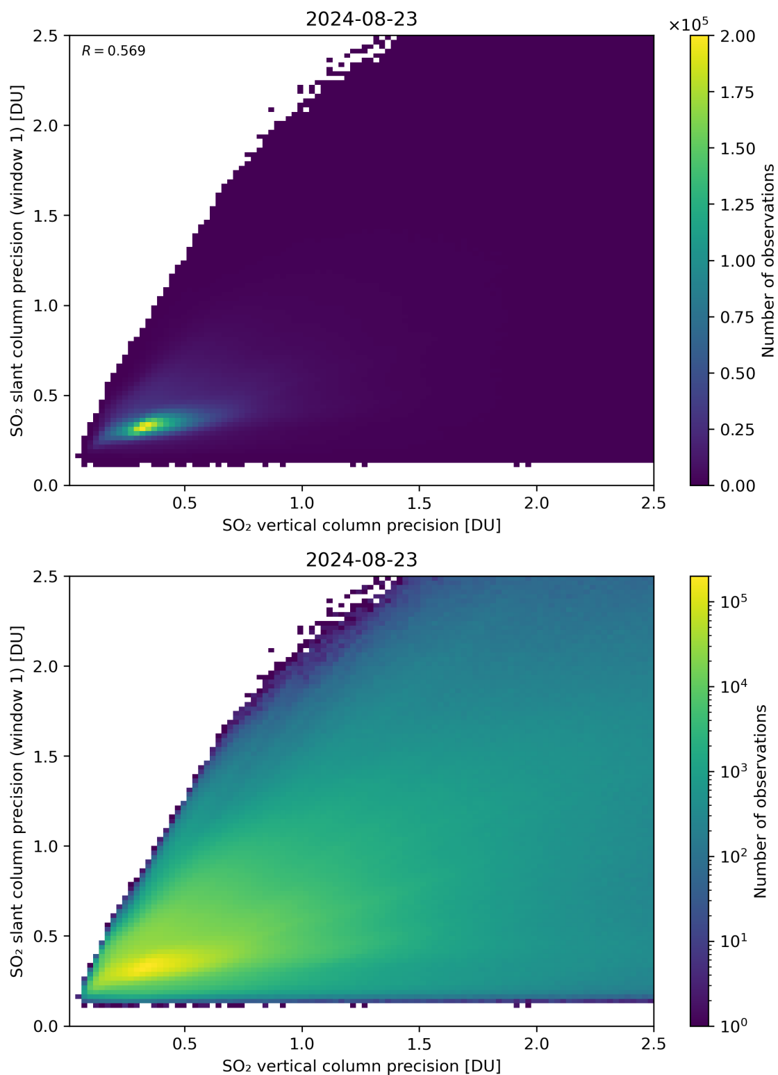
Figure 290: Scatter density plot of “SO 2 vertical column precision” against “SO 2 slant column precision (window 1)” for 2024-08-22 to 2024-08-24.
