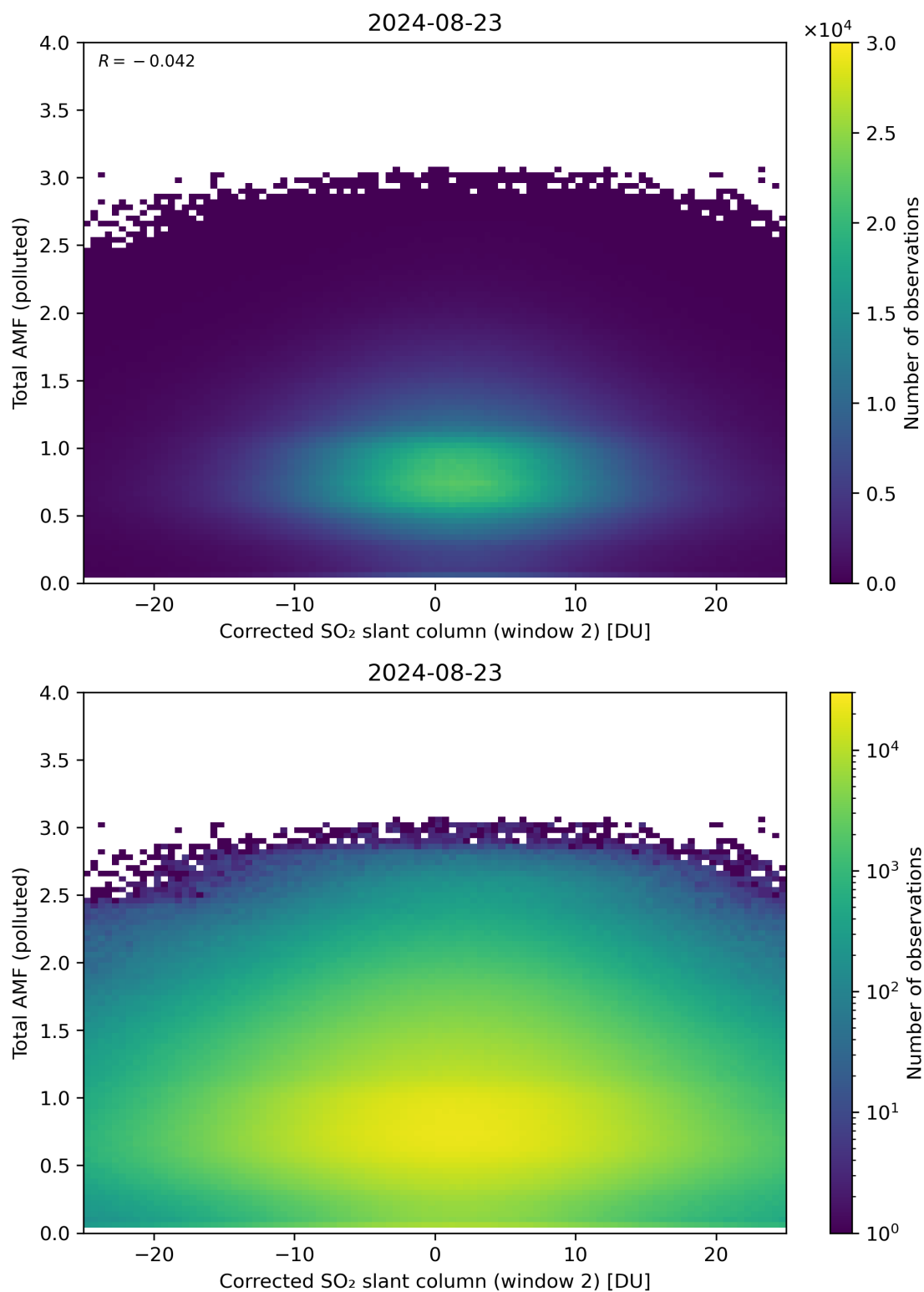
Figure 203: Scatter density plot of “Corrected SO 2 slant column (window 2)” against “Total AMF (polluted)” for 2024-08-22 to 2024-08-24.
