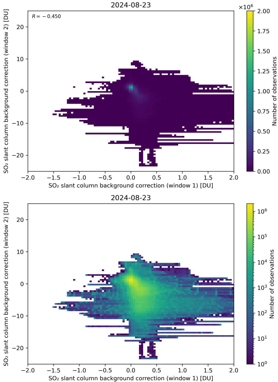
Figure 98: Scatter density plot of “SO 2 slant column background correction (window 1)” against “SO 2 slant column background correction (window 2)” for 2024-08-22 to 2024-08-24.
