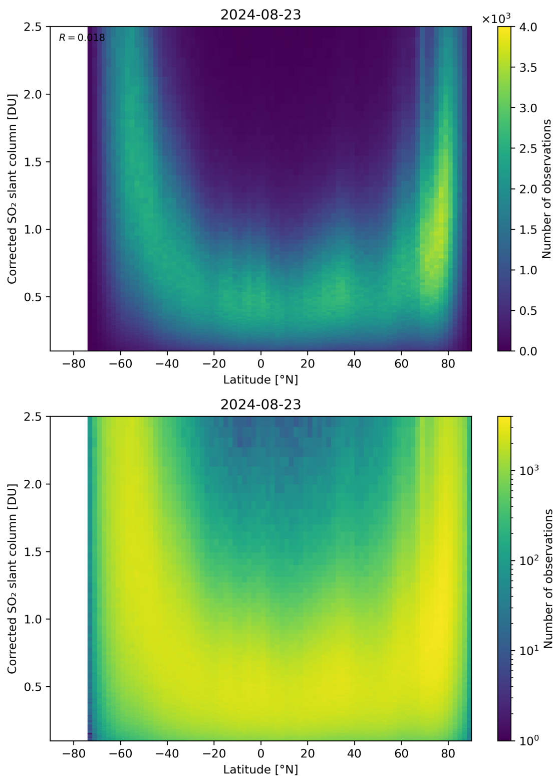
Figure 146: Scatter density plot of “Latitude” against “Corrected SO 2 slant column” for 2024-08-22 to 2024-08-24.
