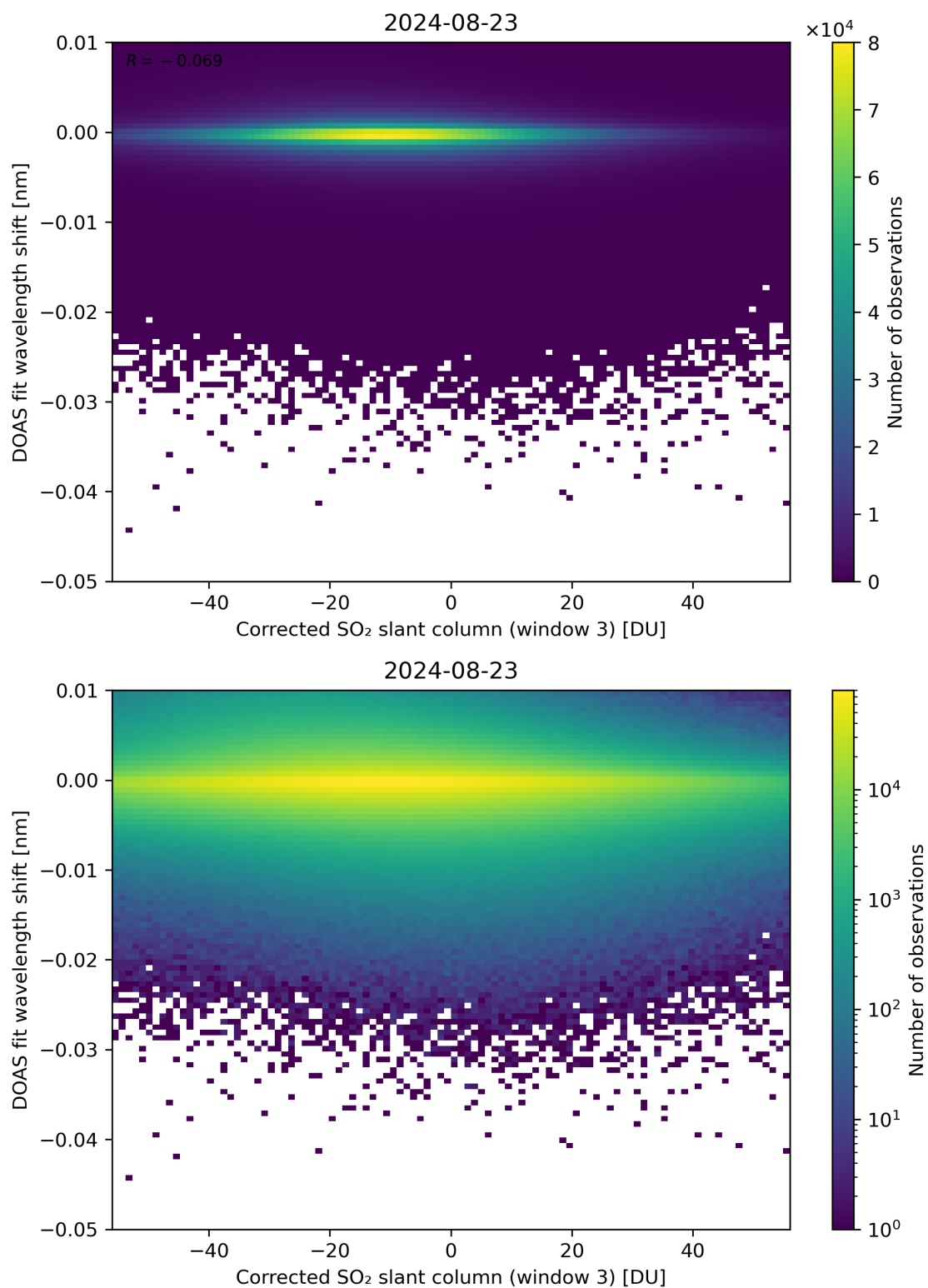
Figure 206: Scatter density plot of “Corrected SO 2 slant column (window 3)” against “DOAS fit wavelength shift” for 2024-08-22 to 2024-08-24.
