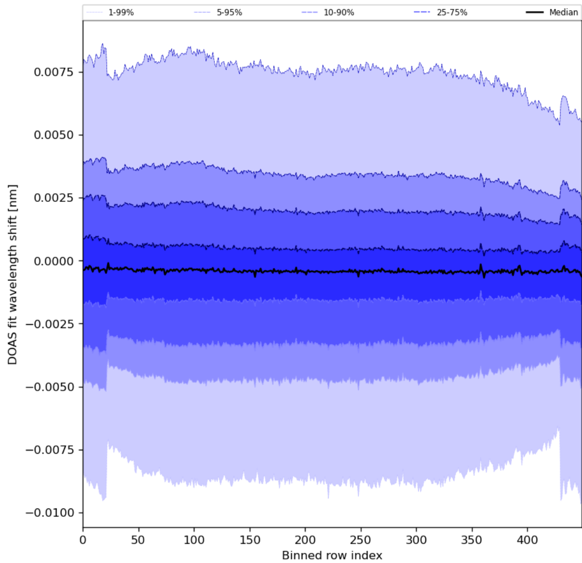
Figure 91: Along track statistics of “DOAS fit wavelength shift” for 2024-08-22 to 2024-08-24
