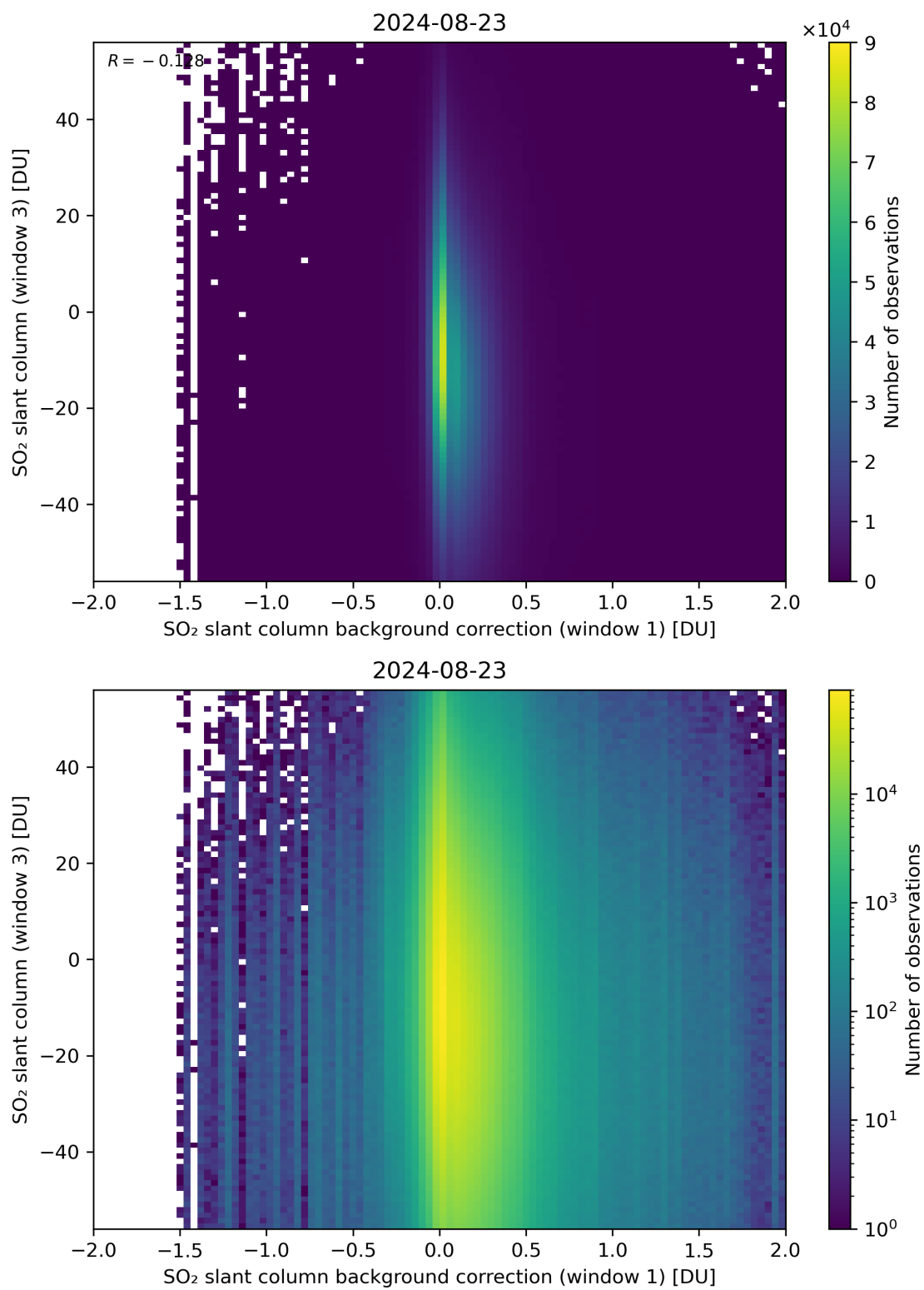
Figure 107: Scatter density plot of “SO 2 slant column background correction (window 1)” against “SO 2 slant column (window 3)” for 2024-08-22 to 2024-08-24.
