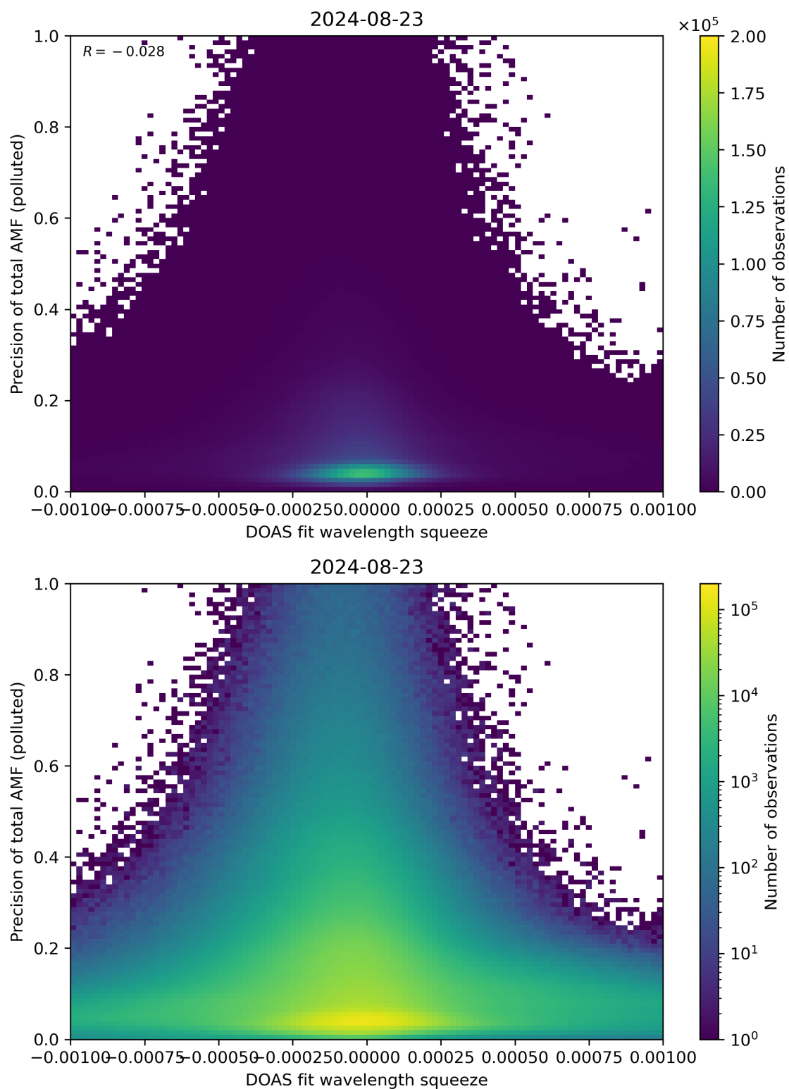
Figure 135: Scatter density plot of “DOAS fit wavelength squeeze” against “Precision of total AMF (polluted)” for 2024-08-22 to 2024-08-24.
