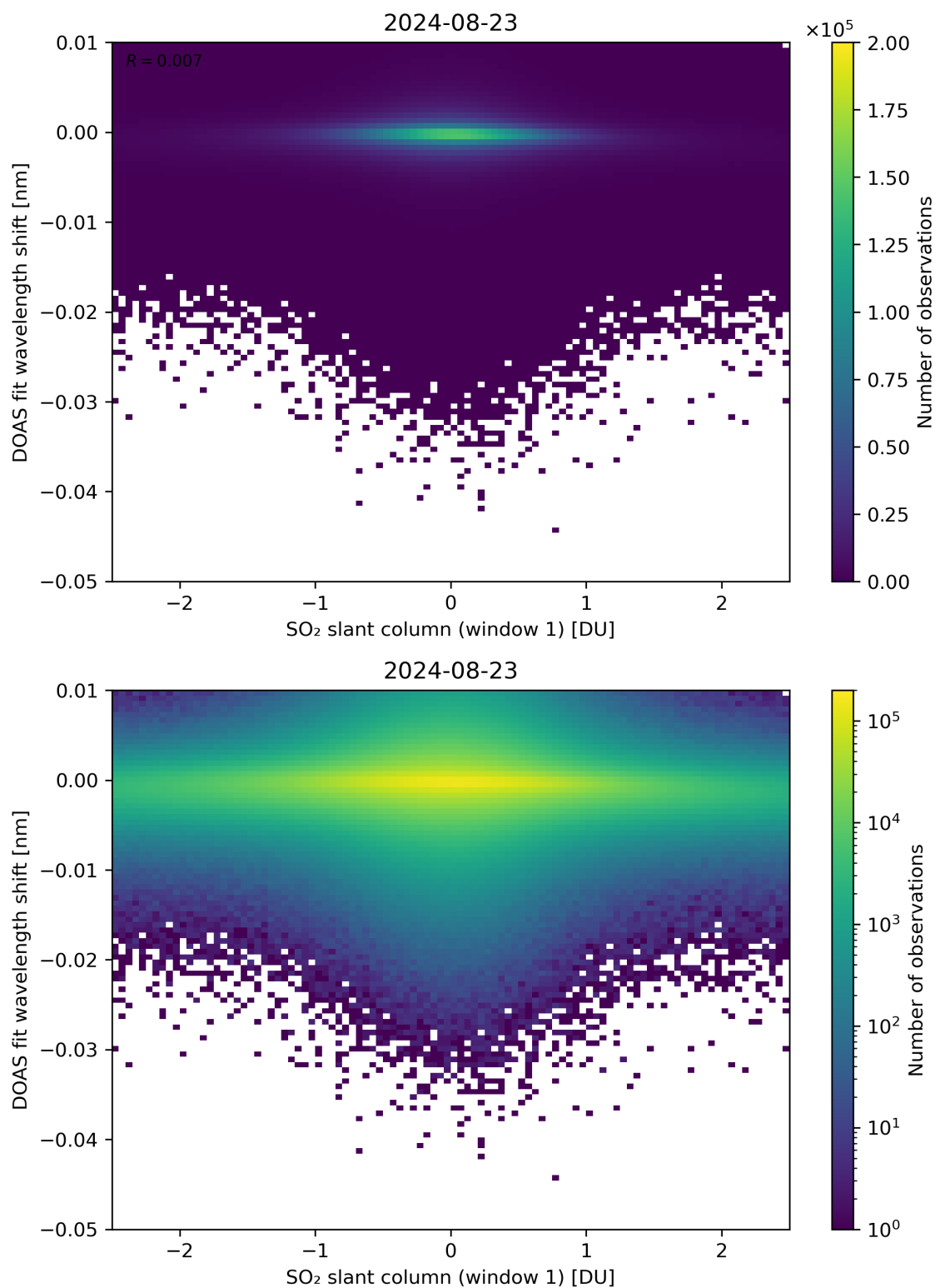
Figure 215: Scatter density plot of “SO 2 slant column (window 1)” against “DOAS fit wavelength shift” for 2024-08-22 to 2024-08-24.
