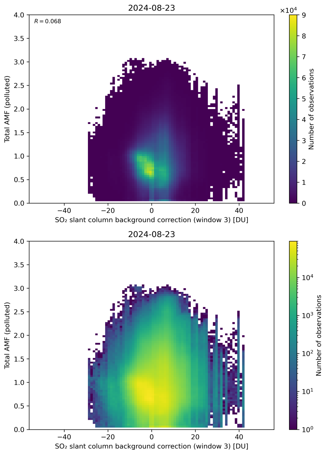
Figure 125: Scatter density plot of “SO 2 slant column background correction (window 3)” against “Total AMF (polluted)” for 2024-08-22 to 2024-08-24.
