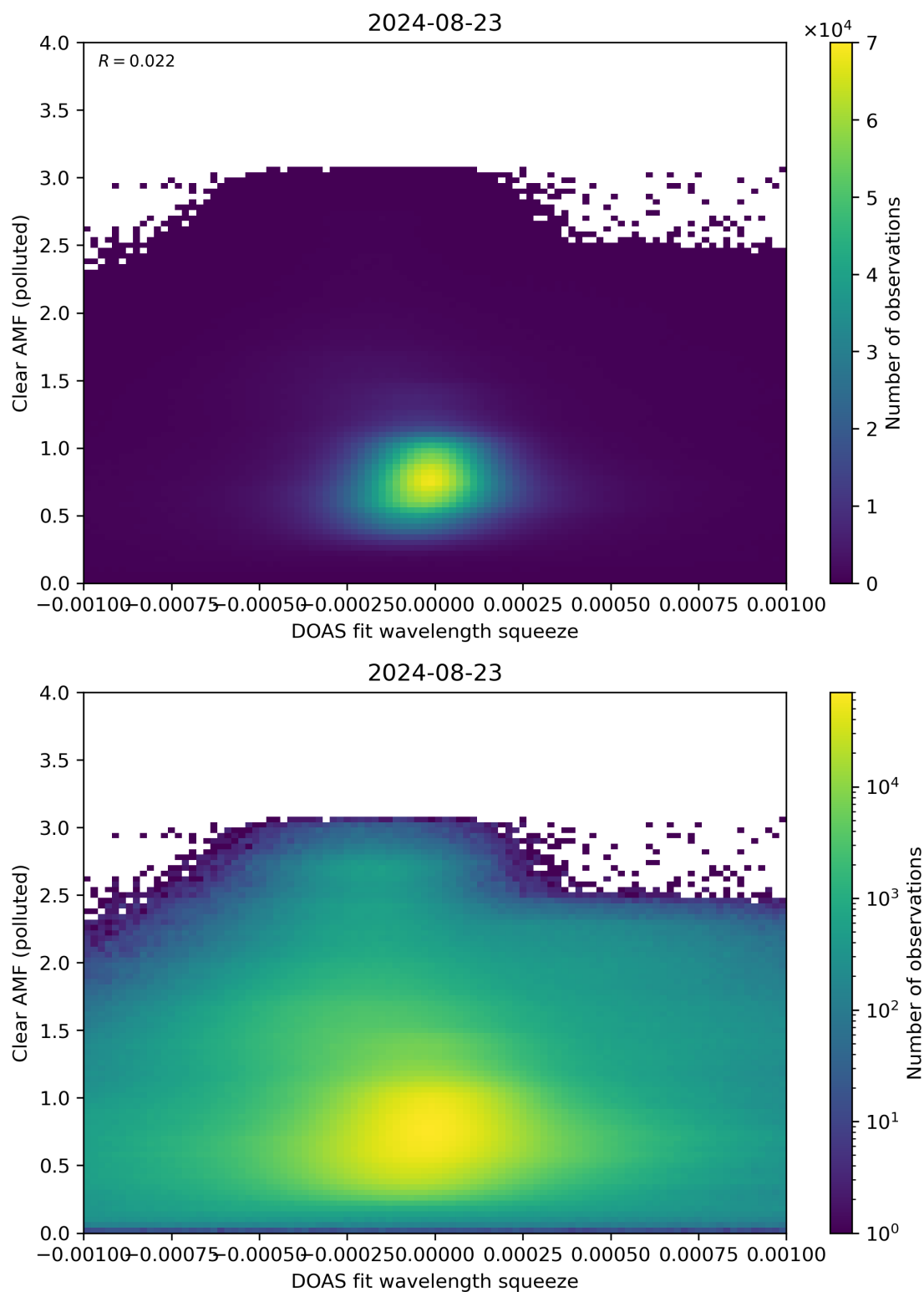
Figure 133: Scatter density plot of “DOAS fit wavelength squeeze” against “Clear AMF (polluted)” for 2024-08-22 to 2024-08-24.
