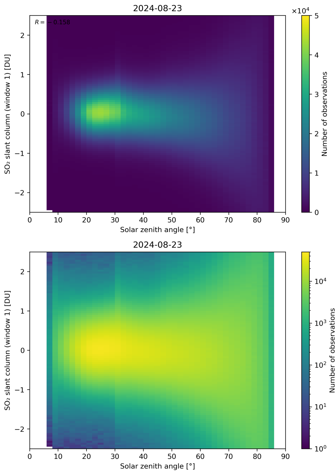
Figure 169: Scatter density plot of “Solar zenith angle” against “SO 2 slant column (window 1)” for 2024-08-22 to 2024-08-24.
