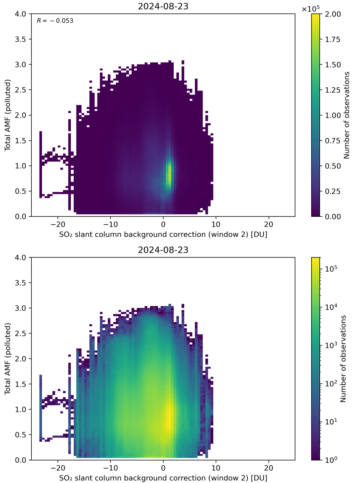
Figure 119: Scatter density plot of “SO 2 slant column background correction (window 2)” against “Total AMF (polluted)” for 2024-08-22 to 2024-08-24.
