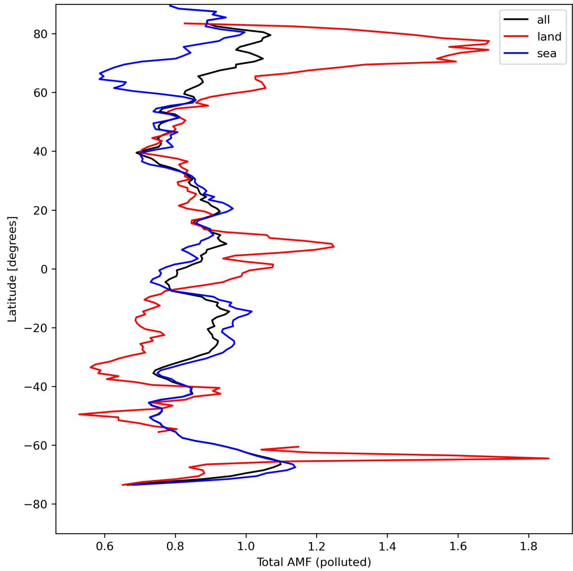
Figure 48: Zonal average of “Total AMF (polluted)” for 2024-08-22 to 2024-08-24.
