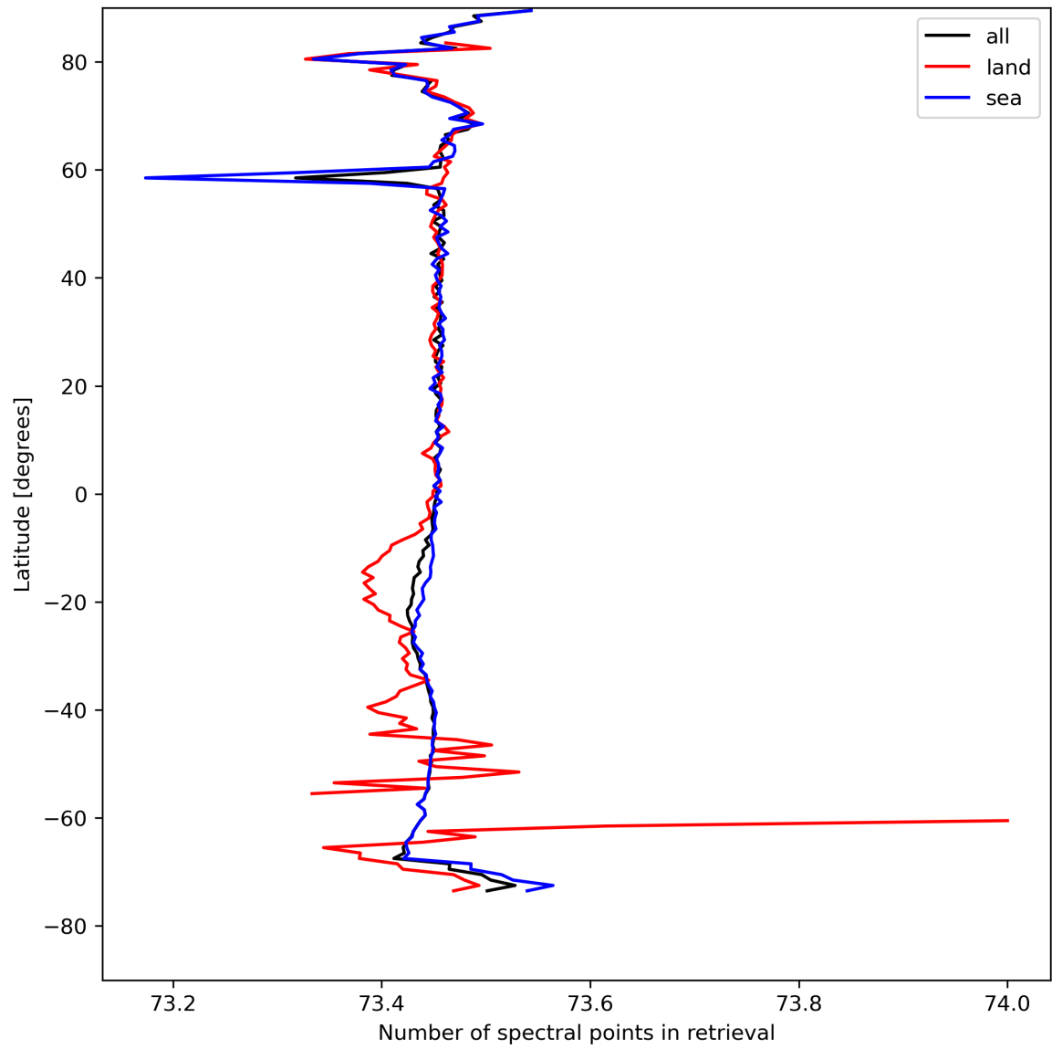
Figure 51: Zonal average of “Number of spectral points in retrieval” for 2024-08-22 to 2024-08-24.
