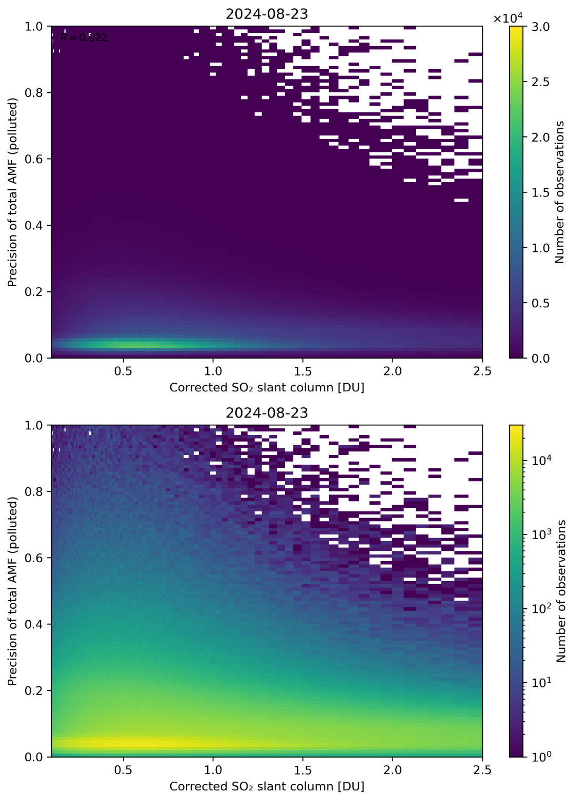
Figure 193: Scatter density plot of “Corrected SO 2 slant column” against “Precision of total AMF (polluted)” for 2024-08-22 to 2024-08-24.
