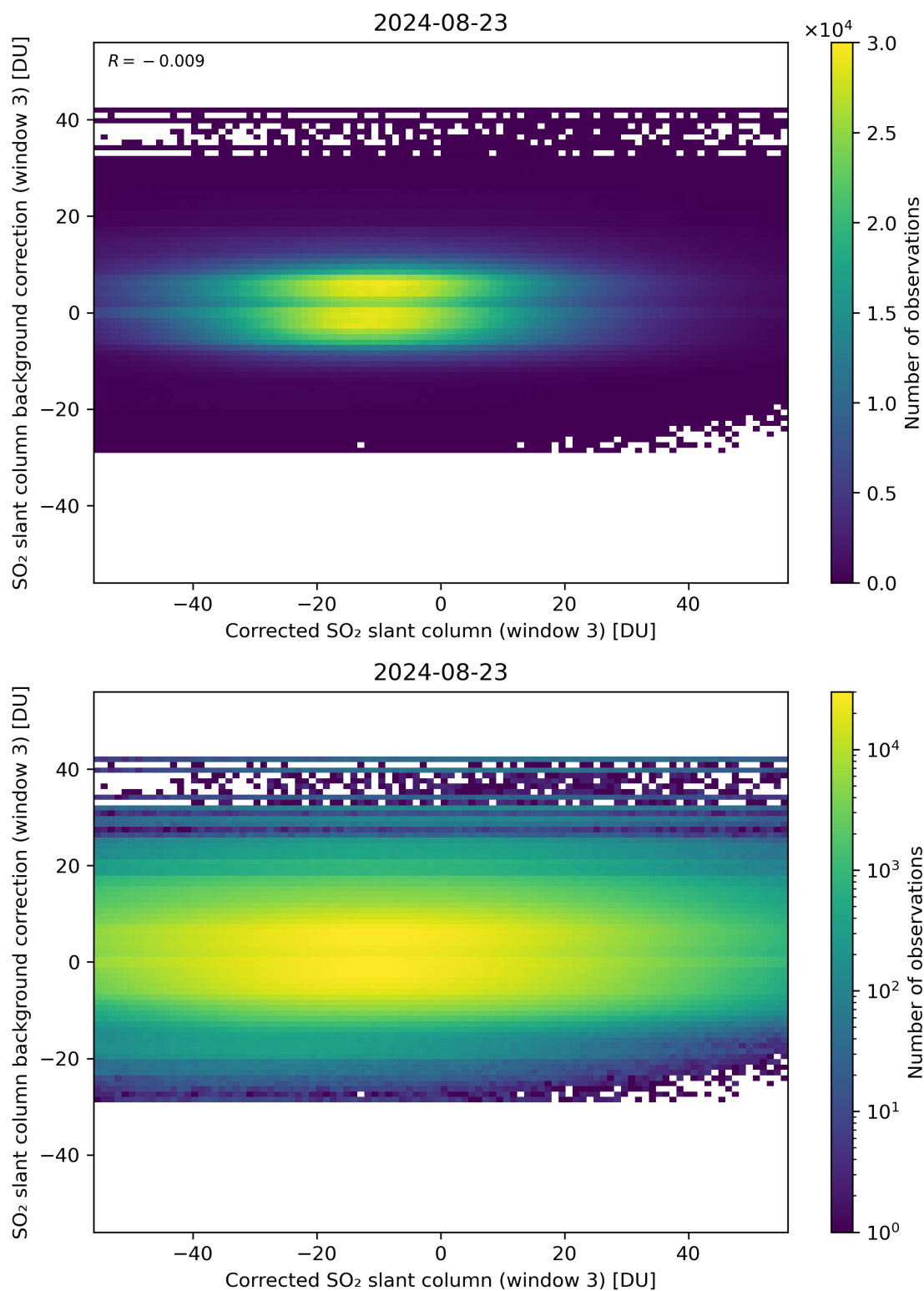
Figure 205: Scatter density plot of “Corrected SO 2 slant column (window 3)” against “SO 2 slant column background correction (window 3)” for 2024-08-22 to 2024-08-24.
