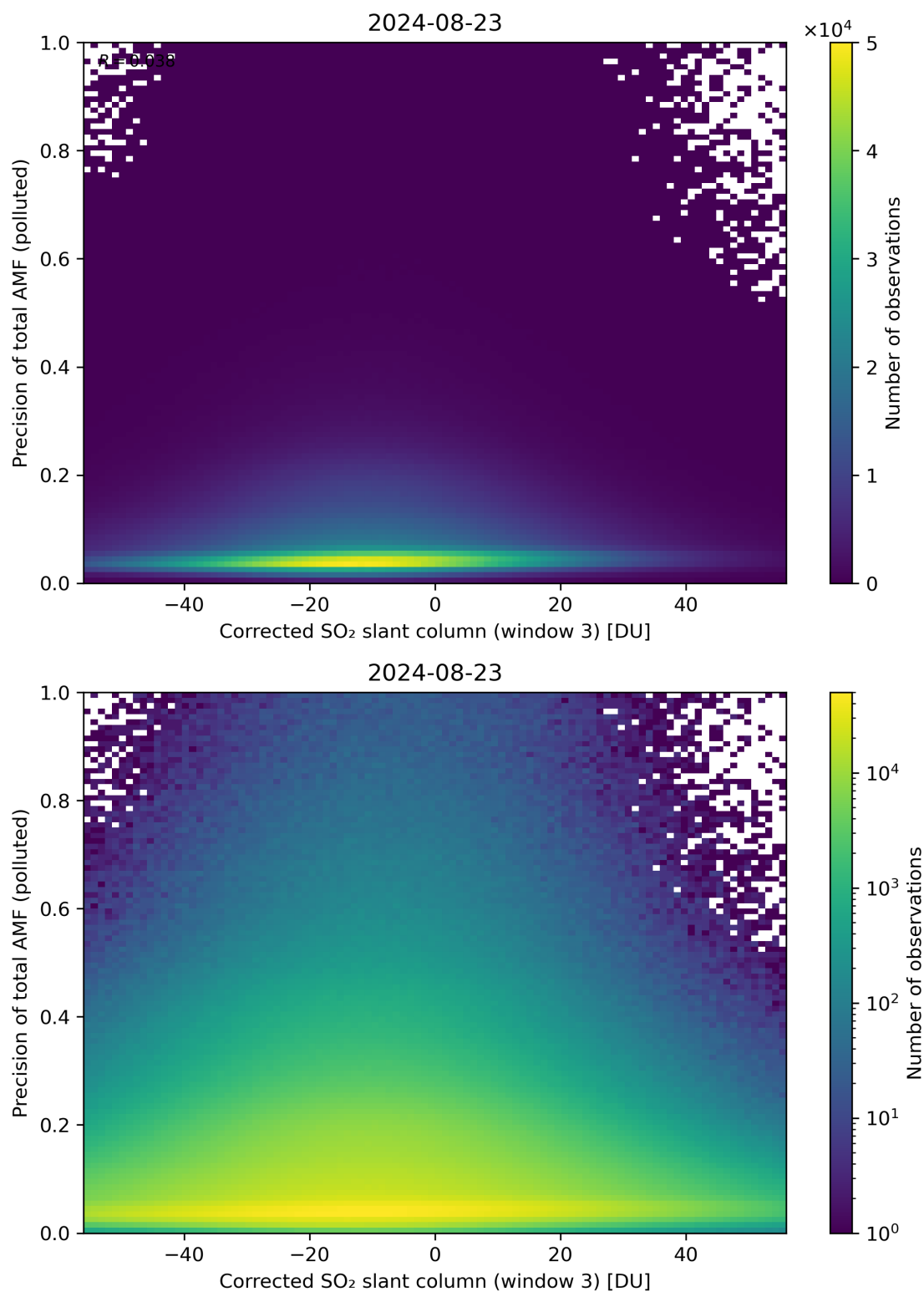
Figure 211: Scatter density plot of “Corrected SO 2 slant column (window 3)” against “Precision of total AMF (polluted)” for 2024-08-22 to 2024-08-24.
