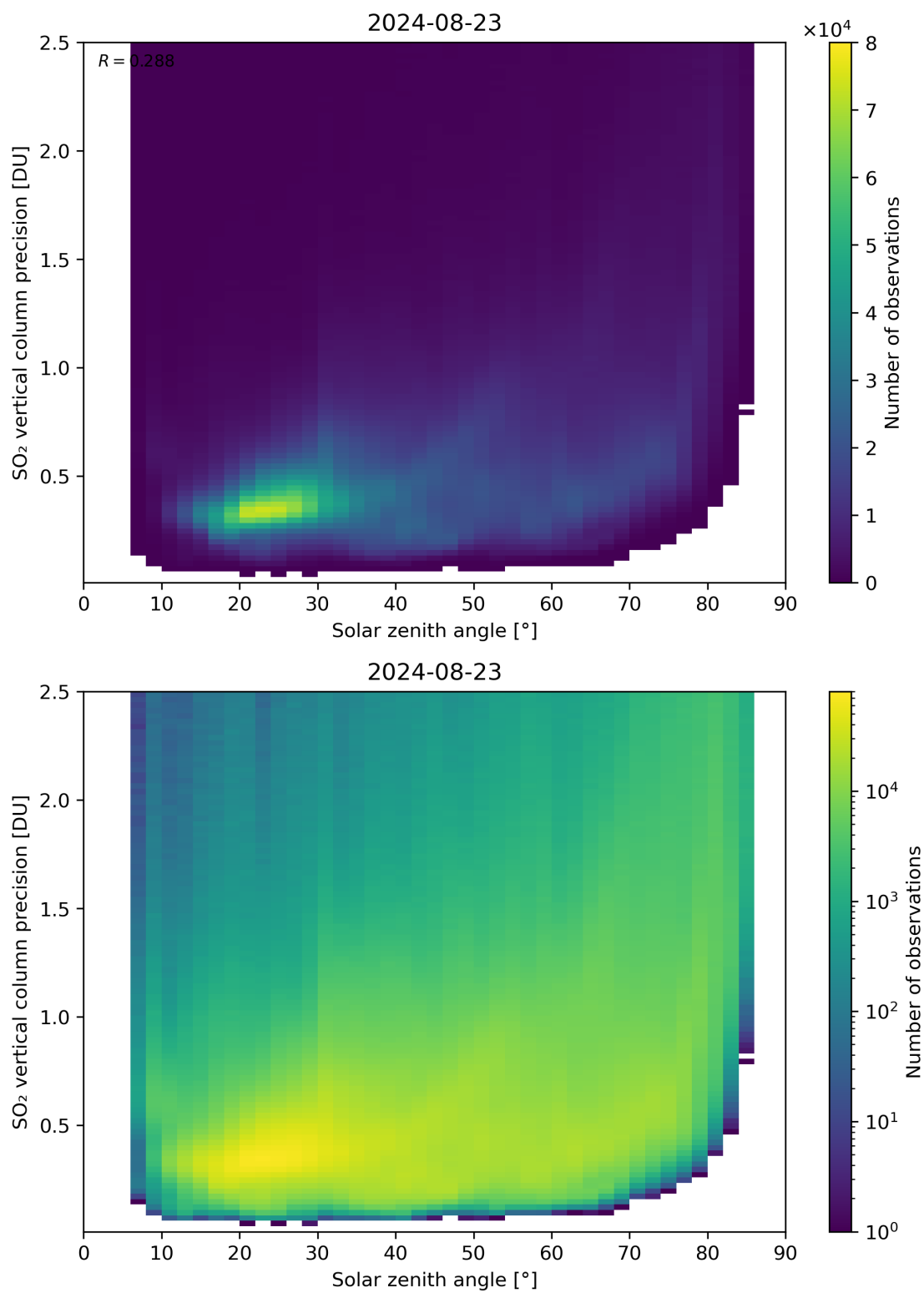
Figure 177: Scatter density plot of “Solar zenith angle” against “SO 2 vertical column precision” for 2024-08-22 to 2024-08-24.
