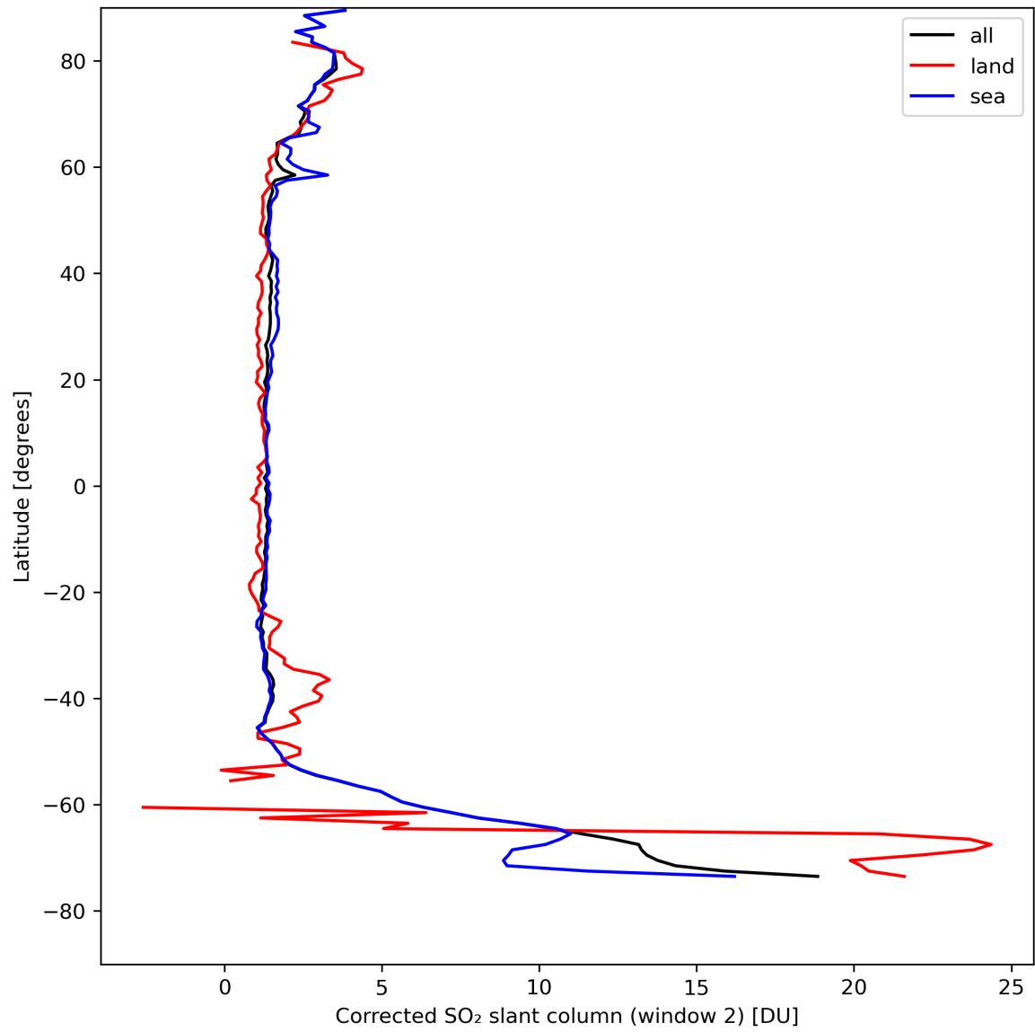
Figure 39: Zonal average of “Corrected SO 2 slant column (window 2)” for 2024-08-22 to 2024-08-24.
