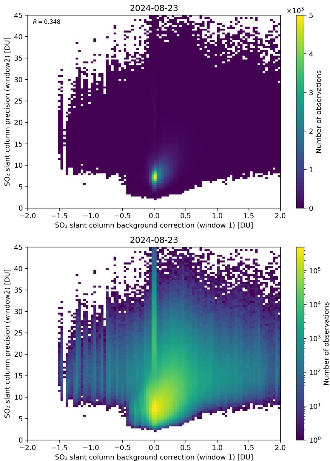
Figure 106: Scatter density plot of “SO 2 slant column background correction (window 1)” against “SO 2 slant column precision (window2)” for 2024-08-22 to 2024-08-24.
