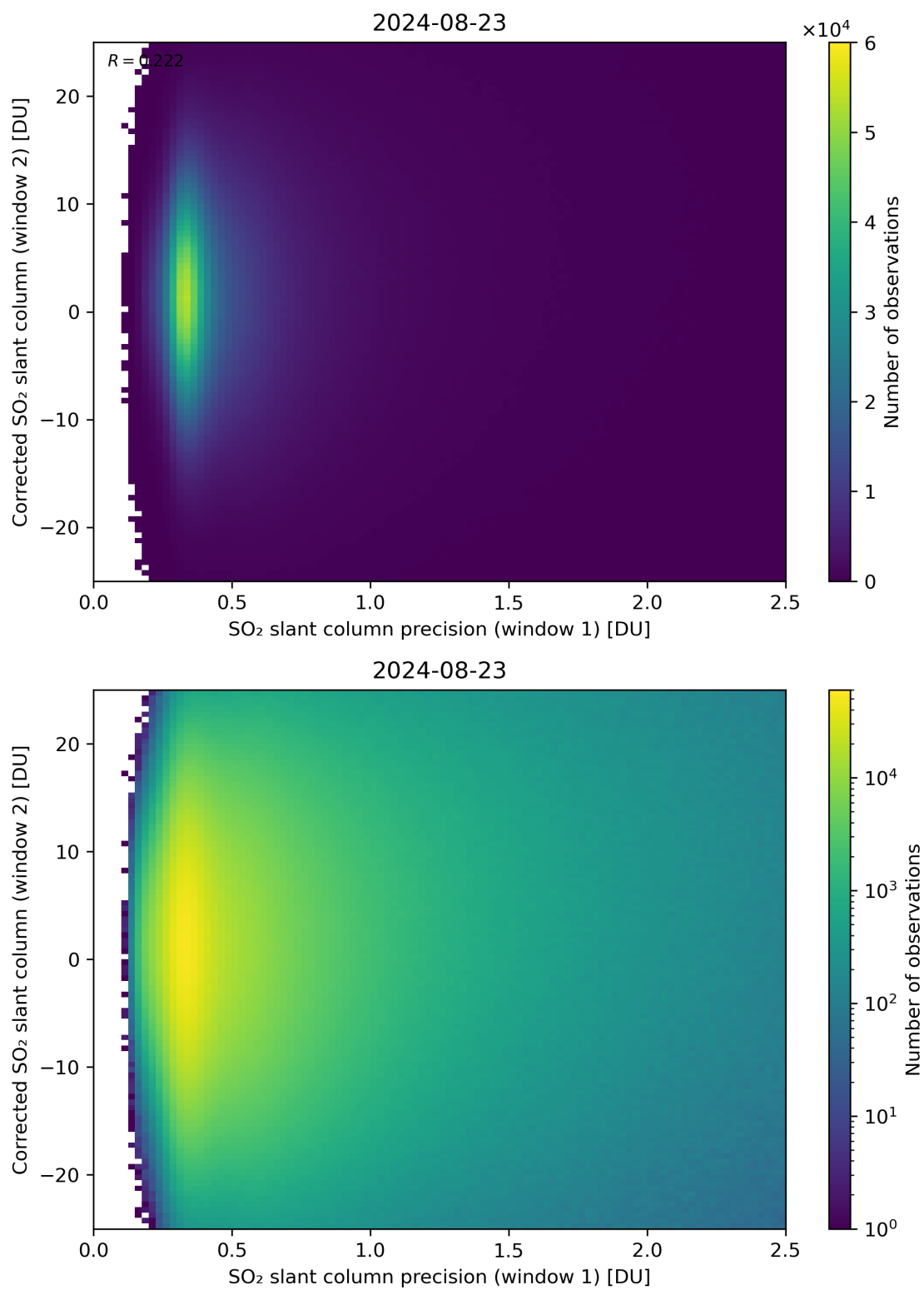
Figure 225: Scatter density plot of “SO 2 slant column precision (window 1)” against “Corrected SO 2 slant column (window 2)” for 2024-08-22 to 2024-08-24.
