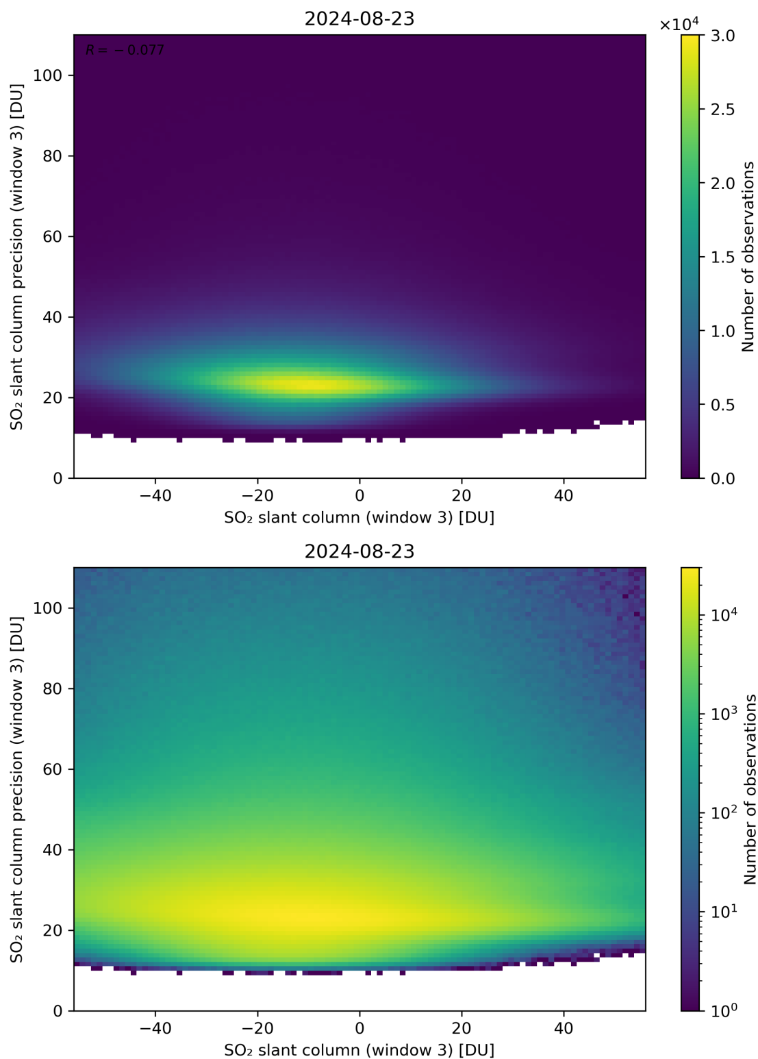
Figure 267: Scatter density plot of “SO 2 slant column (window 3)” against “SO 2 slant column precision (window 3)” for 2024-08-22 to 2024-08-24.
