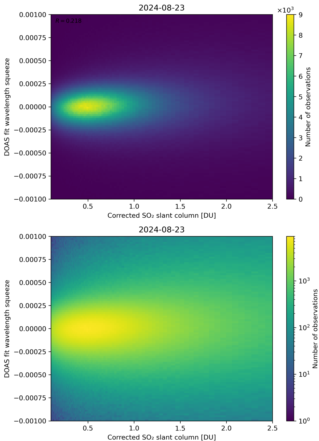
Figure 182: Scatter density plot of “Corrected SO 2 slant column” against “DOAS fit wavelength squeeze” for 2024-08-22 to 2024-08-24.
