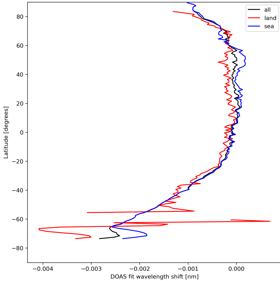
Figure 45: Zonal average of “DOAS fit wavelength shift” for 2024-08-22 to 2024-08-24.
