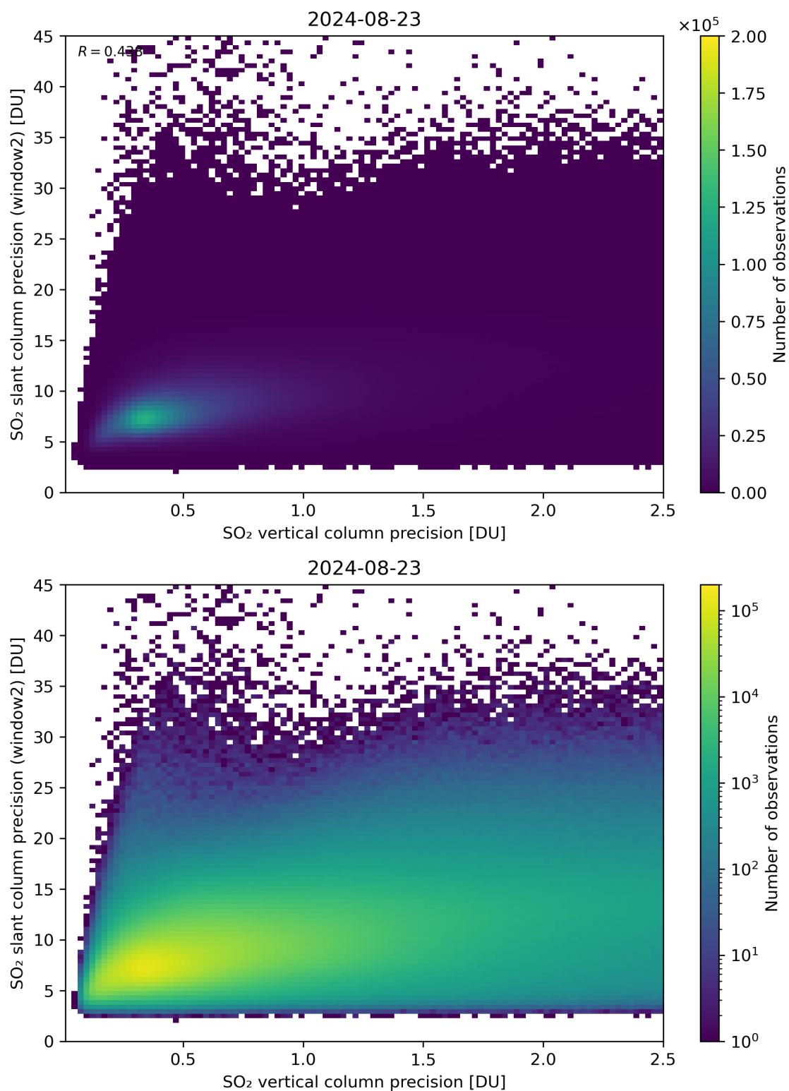
Figure 291: Scatter density plot of “SO 2 vertical column precision” against “SO 2 slant column precision (window2)” for 2024-08-22 to 2024-08-24.
