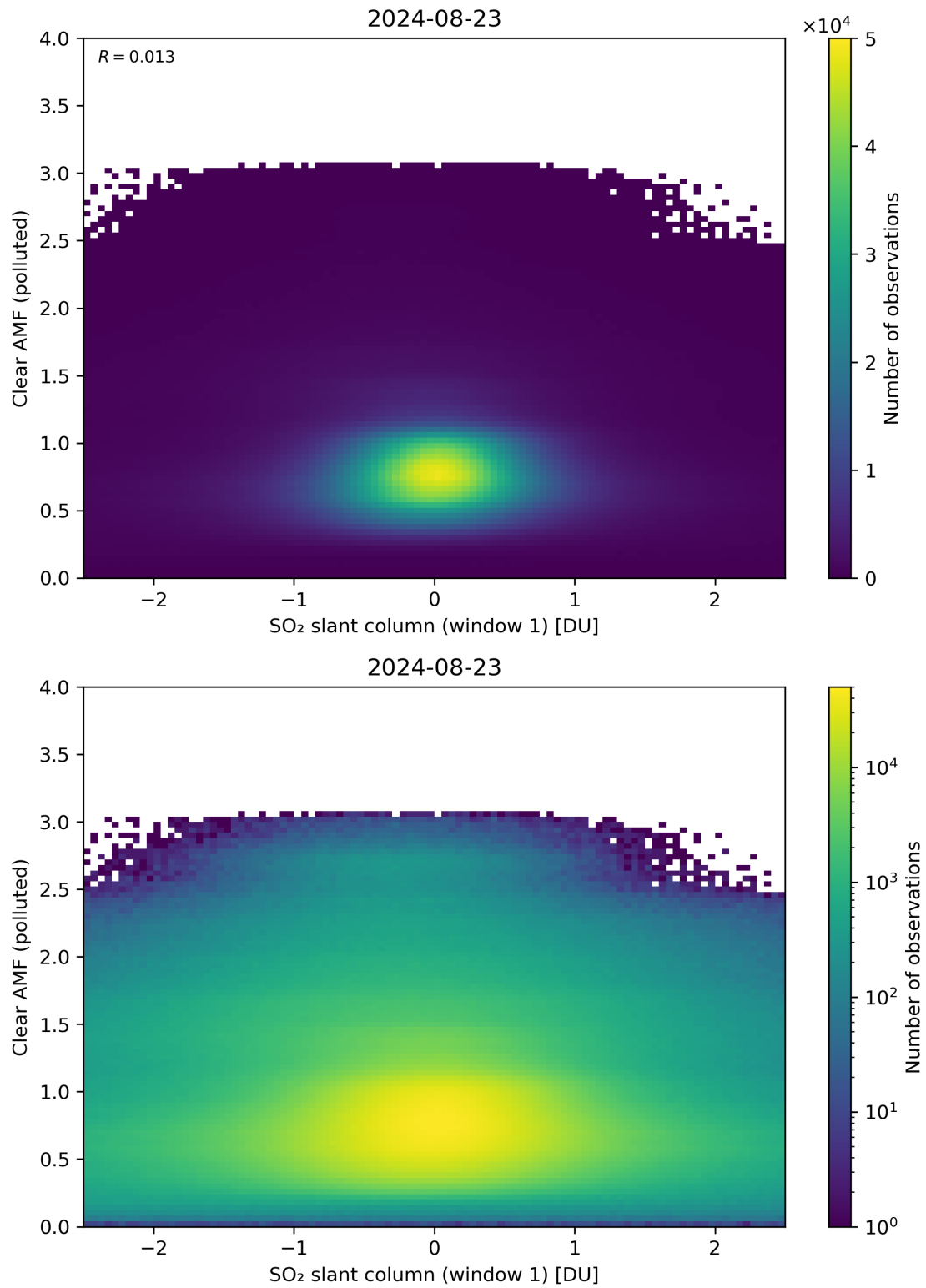
Figure 232: Scatter density plot of “SO 2 slant column (window 1)” against “Clear AMF (polluted)” for 2024-08-22 to 2024-08-24.
