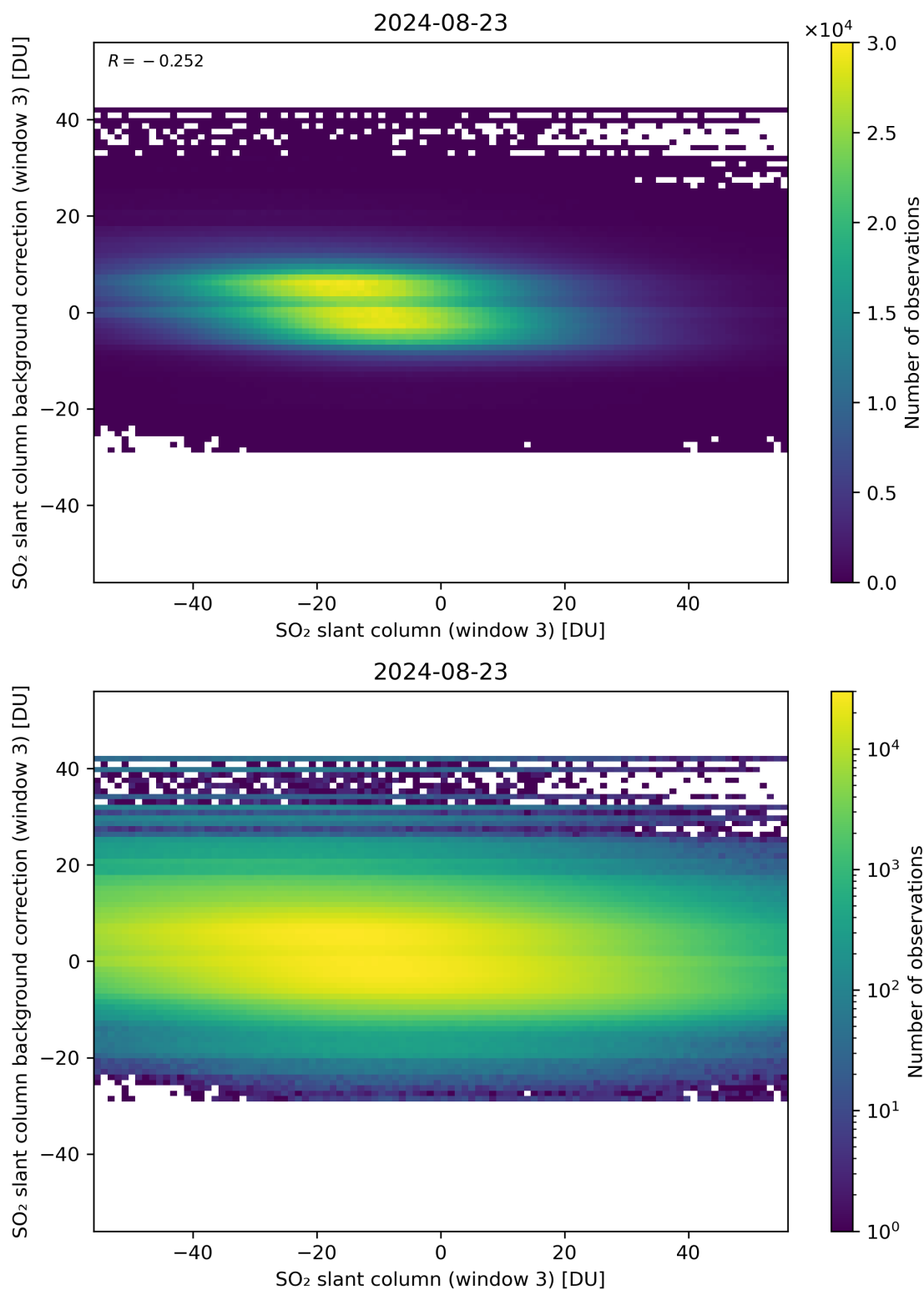
Figure 253: Scatter density plot of “SO 2 slant column (window 3)” against “SO 2 slant column background correction (window 3)” for 2024-08-22 to 2024-08-24.
