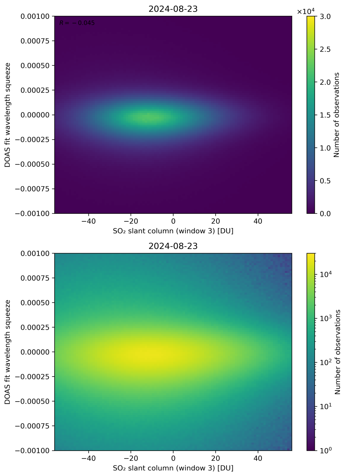
Figure 255: Scatter density plot of “SO 2 slant column (window 3)” against “DOAS fit wavelength squeeze” for 2024-08-22 to 2024-08-24.
