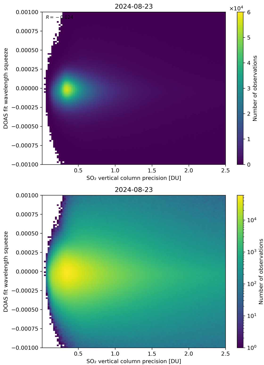
Figure 283: Scatter density plot of “SO 2 vertical column precision” against “DOAS fit wavelength squeeze” for 2024-08-22 to 2024-08-24.
