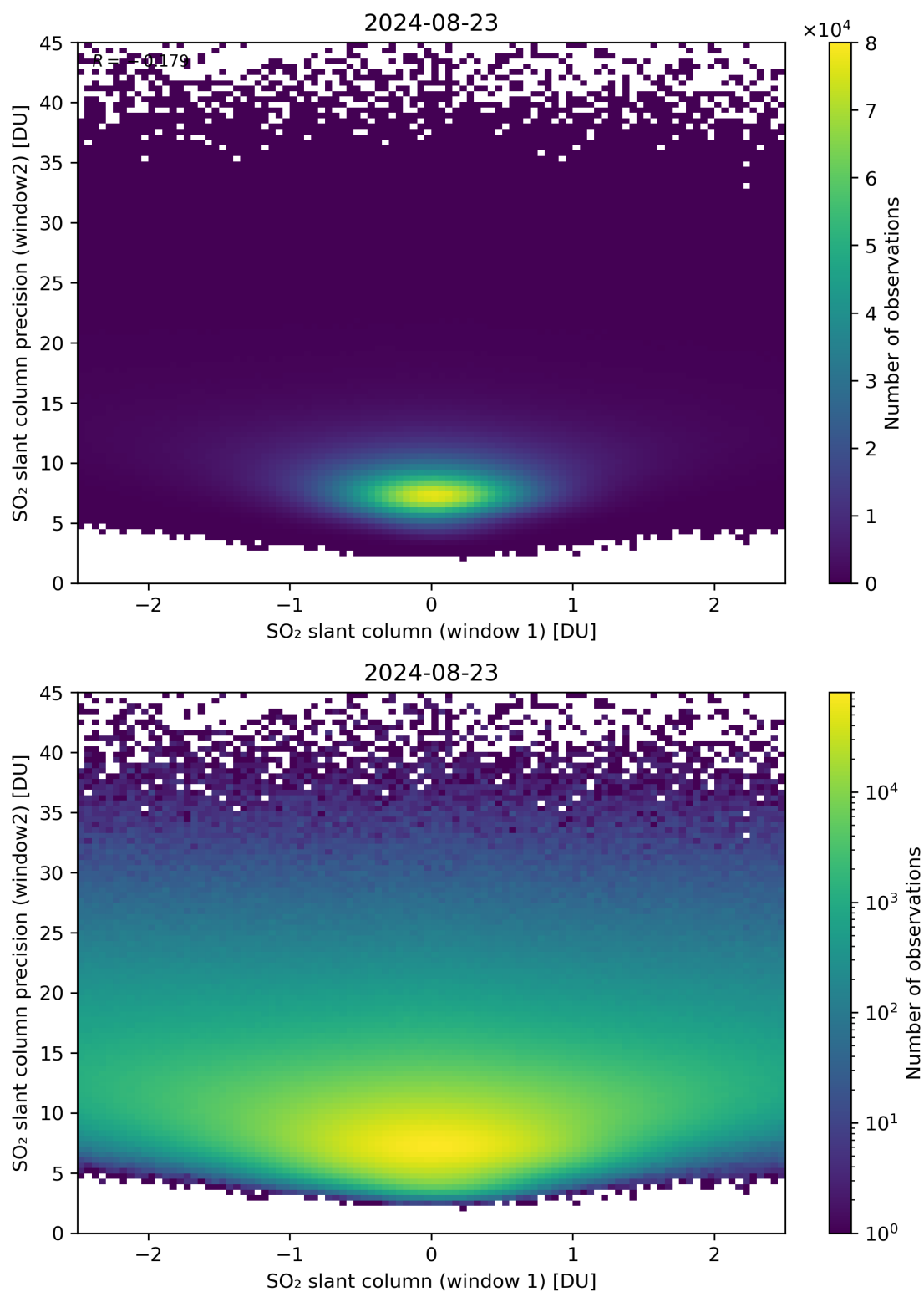
Figure 236: Scatter density plot of “SO 2 slant column (window 1)” against “SO 2 slant column precision (window2)” for 2024-08-22 to 2024-08-24.
