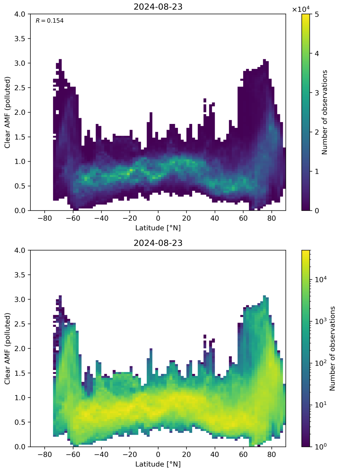
Figure 145: Scatter density plot of “Latitude” against “Clear AMF (polluted)” for 2024-08-22 to 2024-08-24.
