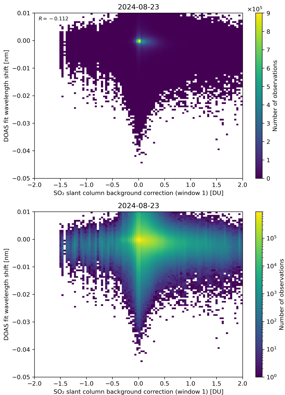
Figure 100: Scatter density plot of “SO 2 slant column background correction (window 1)” against “DOAS fit wavelength shift” for 2024-08-22 to 2024-08-24.
