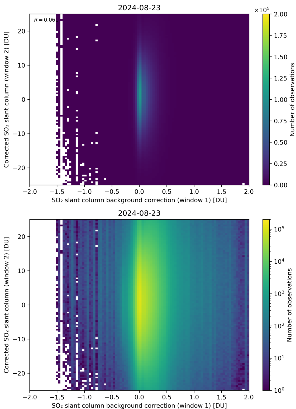
Figure 104: Scatter density plot of “SO 2 slant column background correction (window 1)” against “Corrected SO 2 slant column (window 2)” for 2024-08-22 to 2024-08-24.
