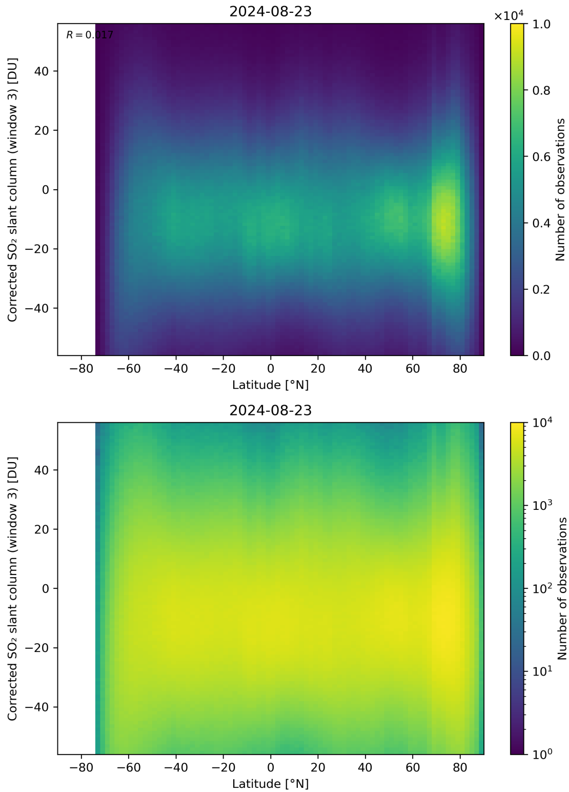
Figure 148: Scatter density plot of “Latitude” against “Corrected SO 2 slant column (window 3)” for 2024-08-22 to 2024-08-24.
