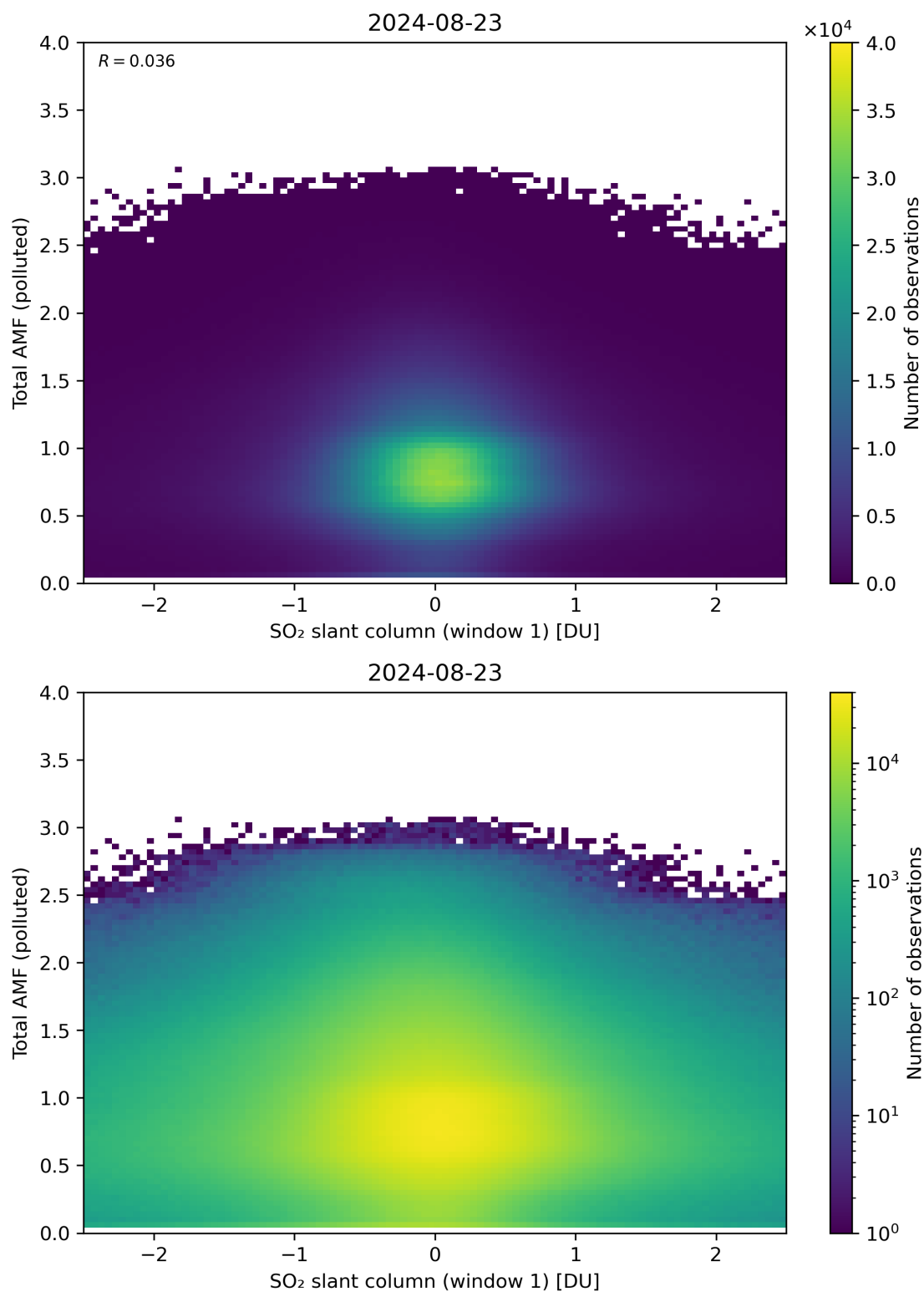
Figure 239: Scatter density plot of “SO 2 slant column (window 1)” against “Total AMF (polluted)” for 2024-08-22 to 2024-08-24.
