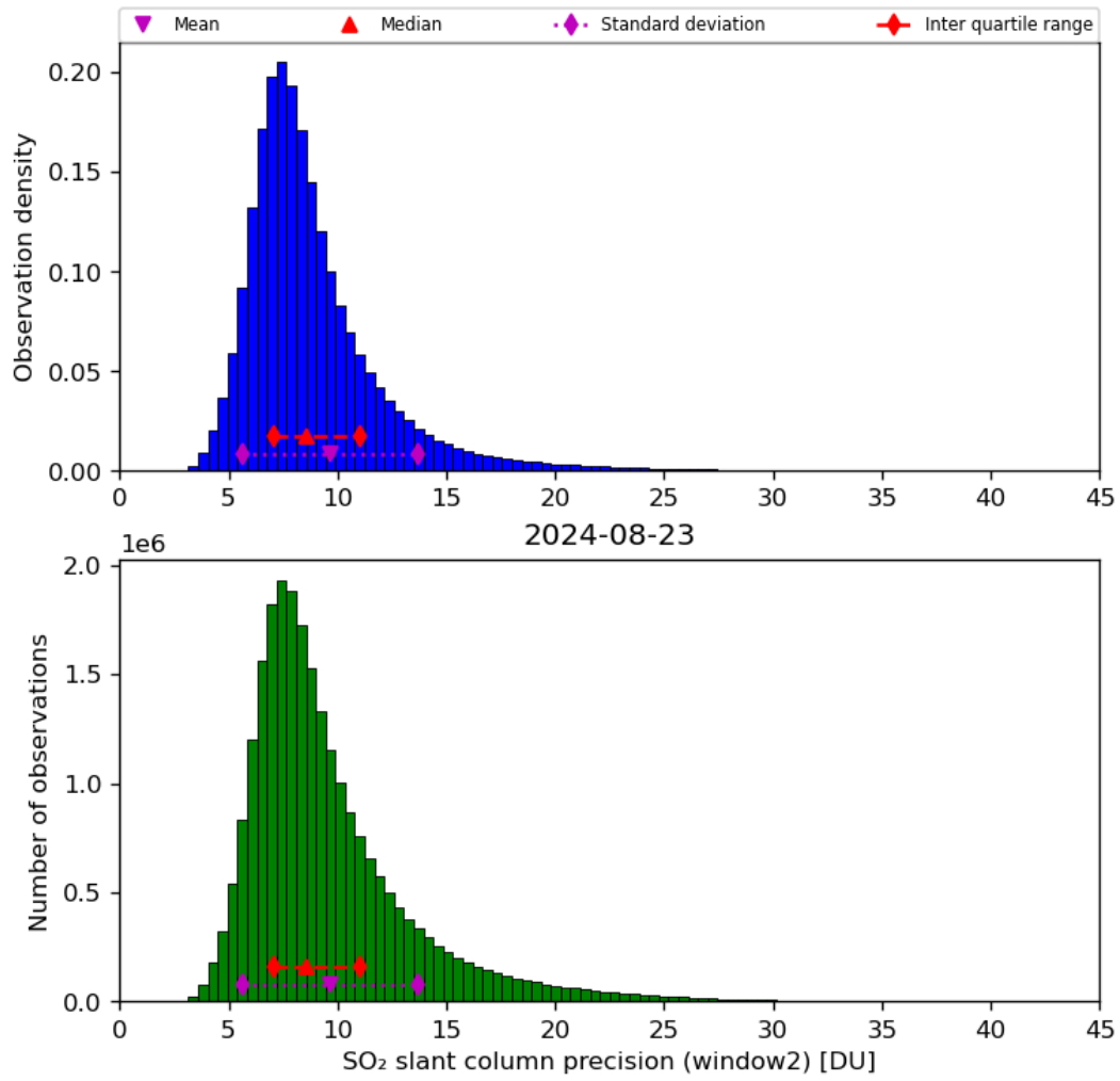
Figure 61: Histogram of “SO 2 slant column precision (window2)” for 2024-08-22 to 2024-08-24
