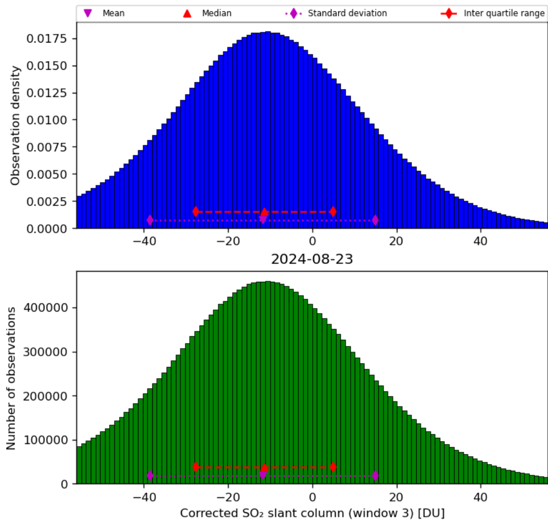
Figure 66: Histogram of “Corrected SO 2 slant column (window 3)” for 2024-08-22 to 2024-08-24
