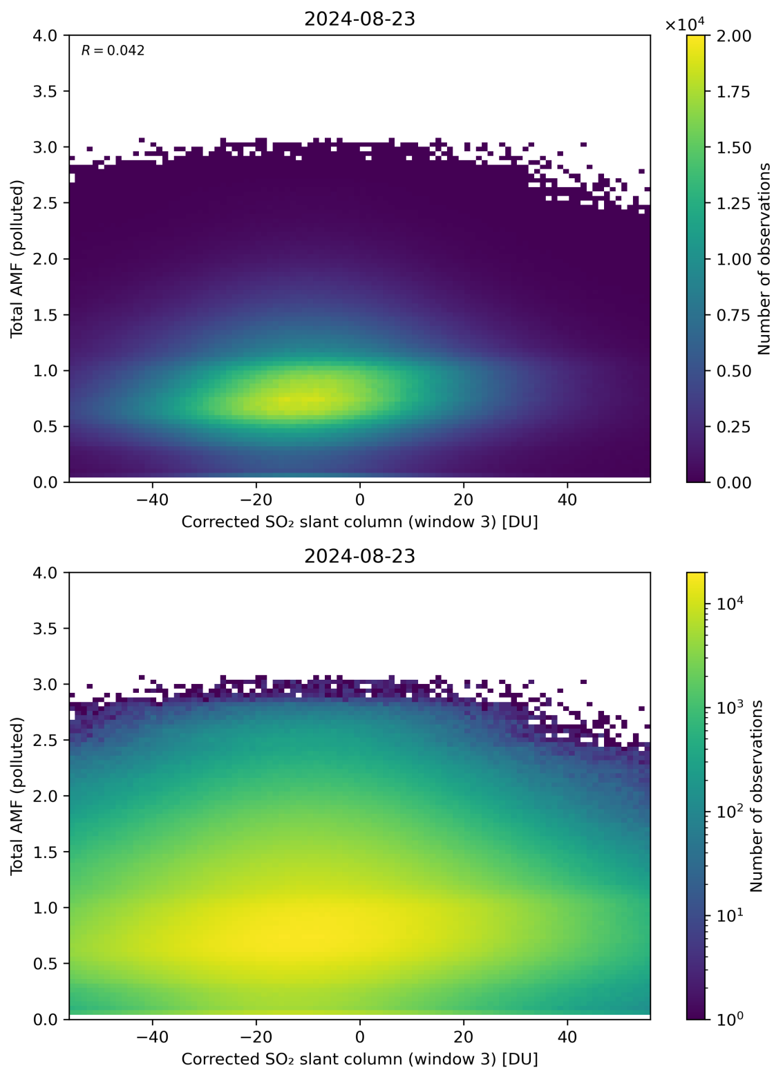
Figure 210: Scatter density plot of “Corrected SO 2 slant column (window 3)” against “Total AMF (polluted)” for 2024-08-22 to 2024-08-24.
