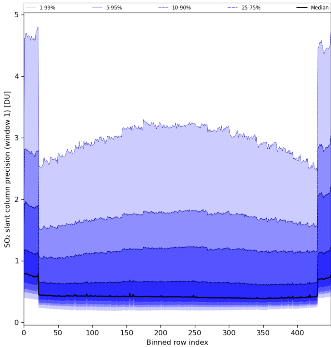
Figure 80: Along track statistics of “SO 2 slant column precision (window 1)” for 2024-08-22 to 2024-08-24
