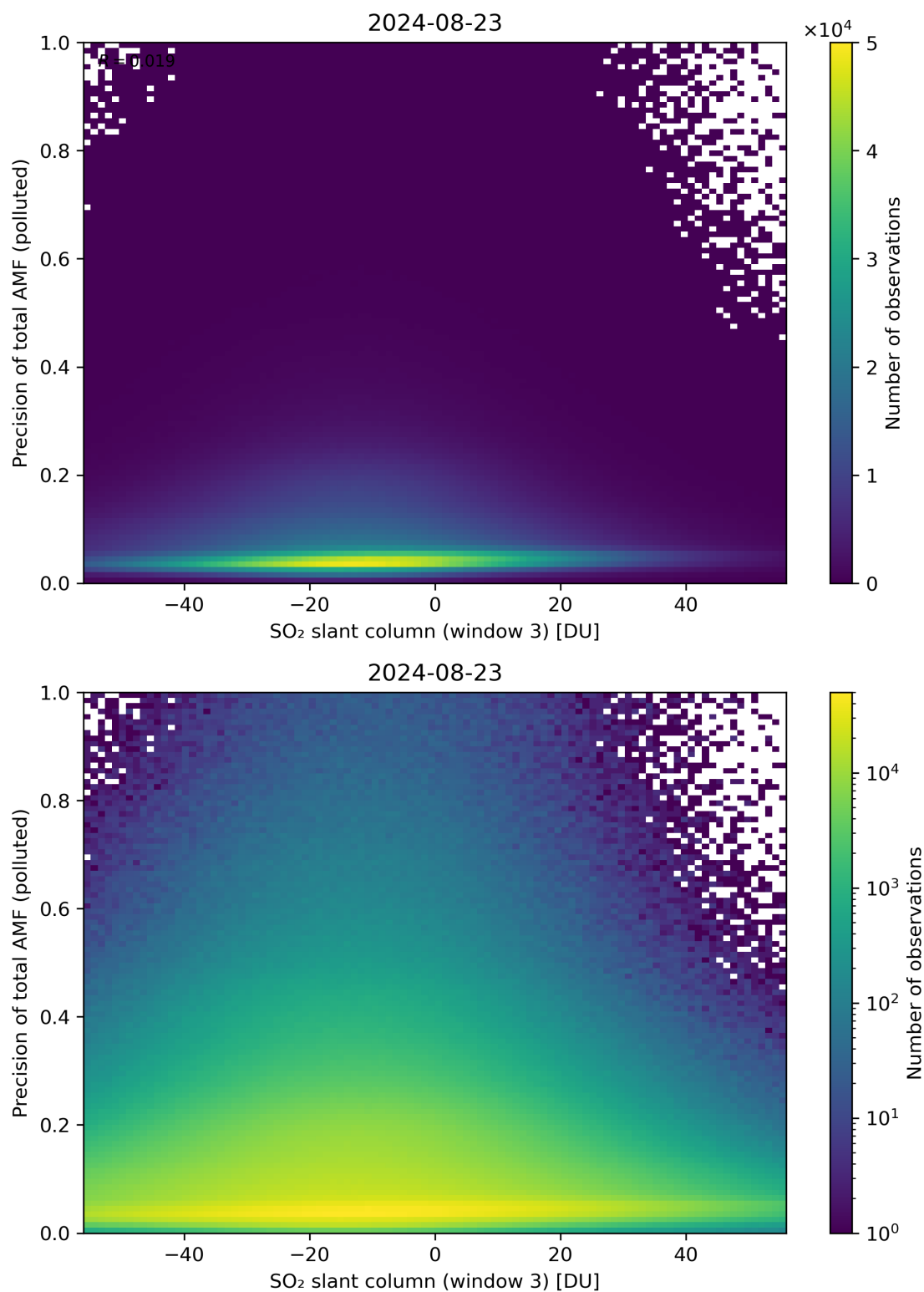
Figure 269: Scatter density plot of “SO 2 slant column (window 3)” against “Precision of total AMF (polluted)” for 2024-08-22 to 2024-08-24.
