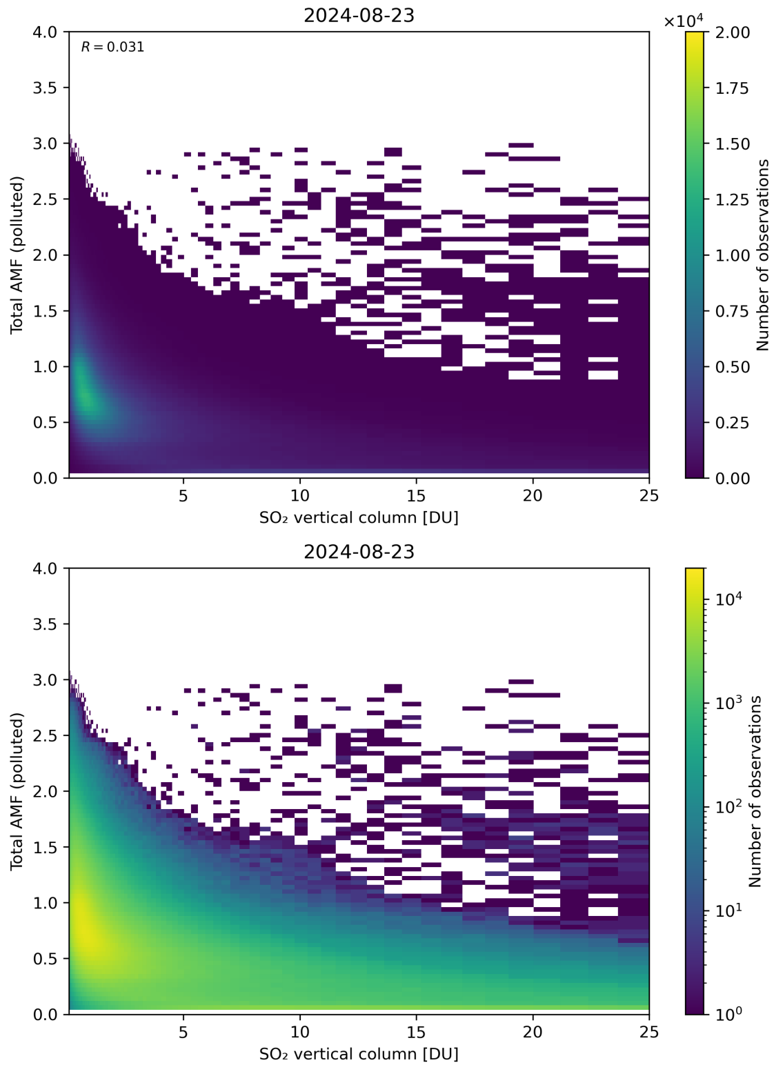
Figure 305: Scatter density plot of “SO 2 vertical column” against “Total AMF (polluted)” for 2024-08-22 to 2024-08-24.
