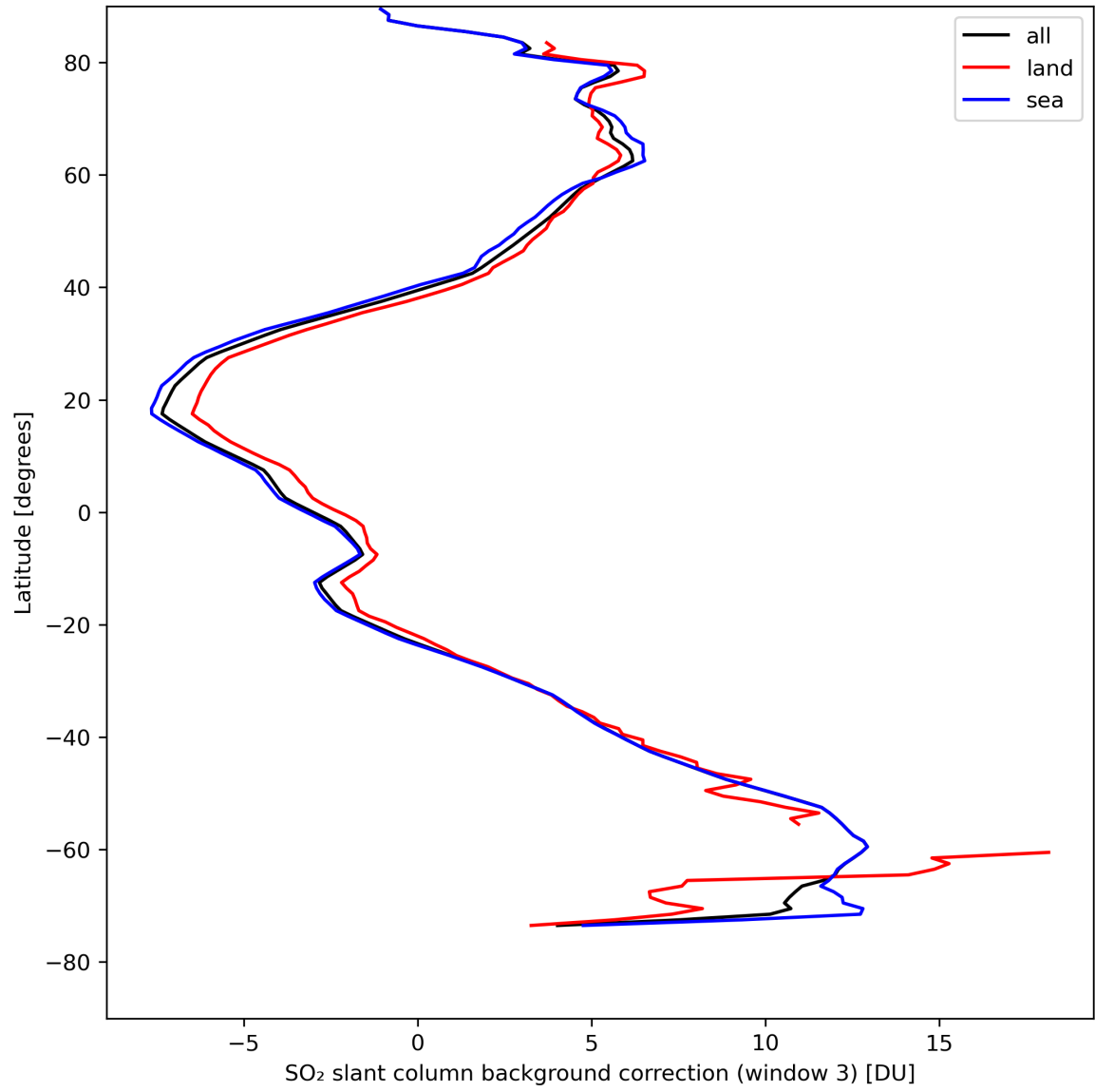
Figure 44: Zonal average of “SO 2 slant column background correction (window 3)” for 2024-08-22 to 2024-08-24.
