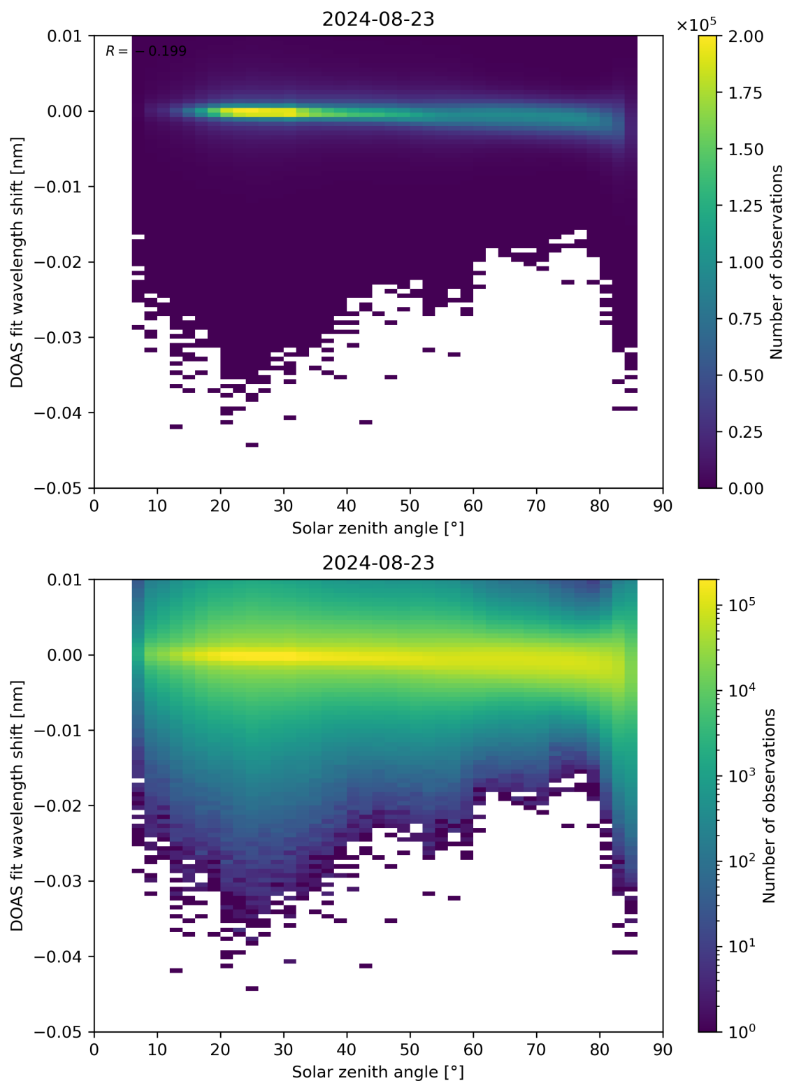
Figure 161: Scatter density plot of “Solar zenith angle” against “DOAS fit wavelength shift” for 2024-08-22 to 2024-08-24.
