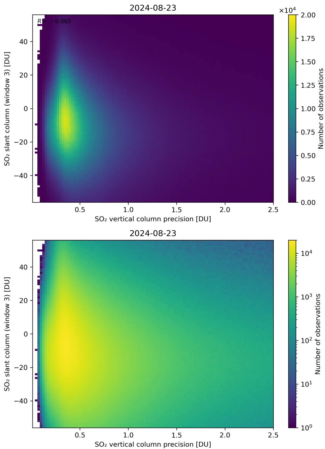
Figure 292: Scatter density plot of “SO 2 vertical column precision” against “SO 2 slant column (window 3)” for 2024-08-22 to 2024-08-24.
