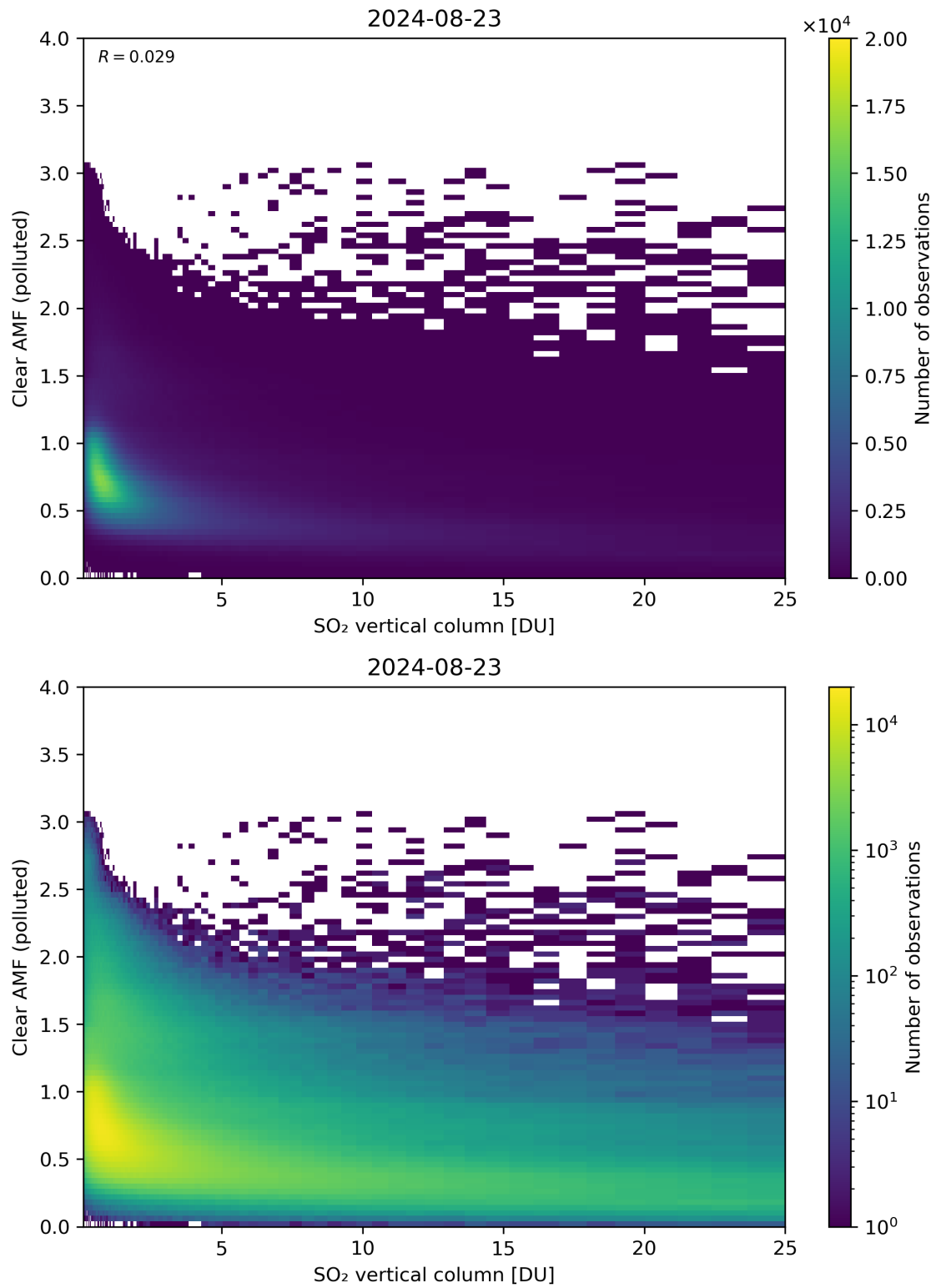
Figure 296: Scatter density plot of “SO 2 vertical column” against “Clear AMF (polluted)” for 2024-08-22 to 2024-08-24.
