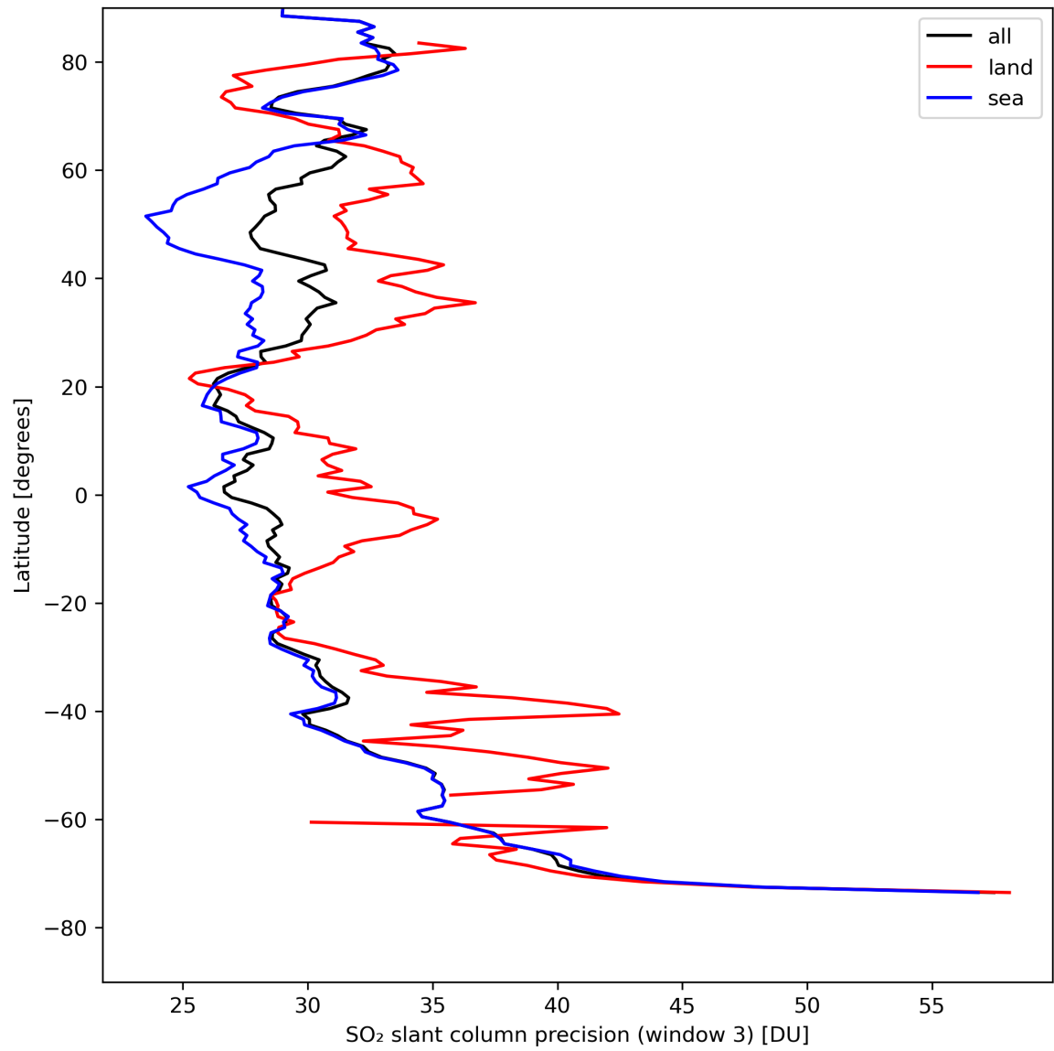
Figure 42: Zonal average of “SO 2 slant column precision (window 3)” for 2024-08-22 to 2024-08-24.
