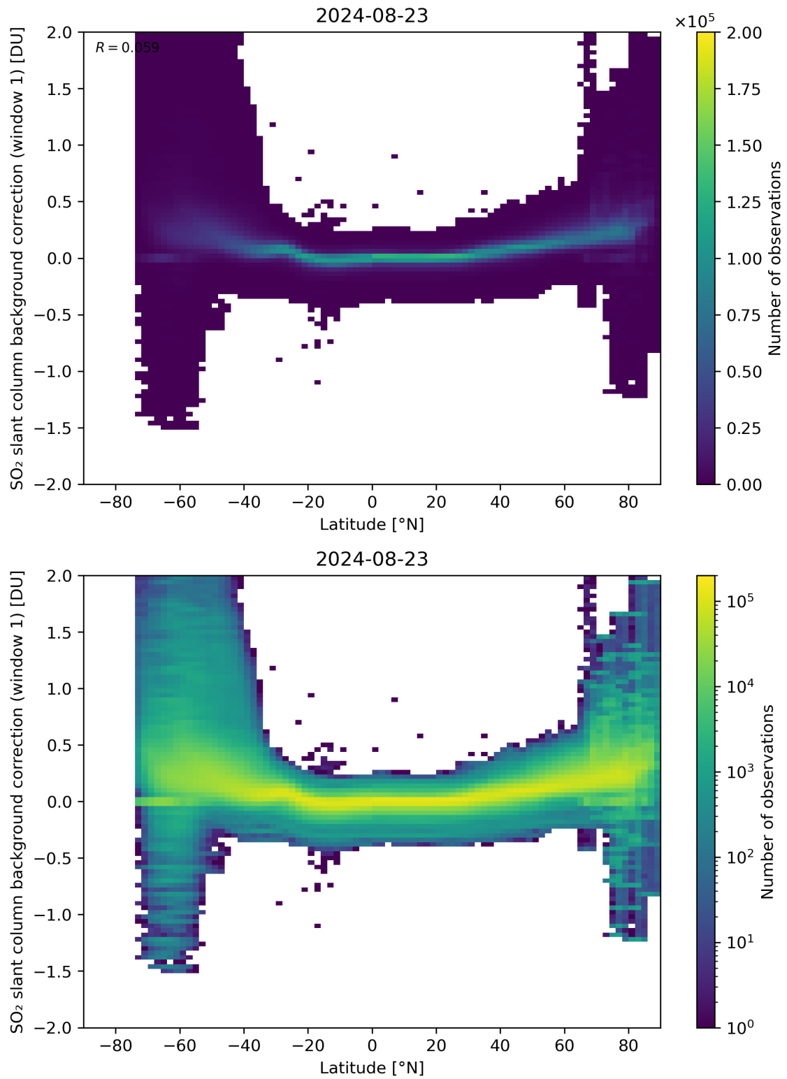
Figure 139: Scatter density plot of “Latitude” against “SO 2 slant column background correction (window 1)” for 2024-08-22 to 2024-08-24.
