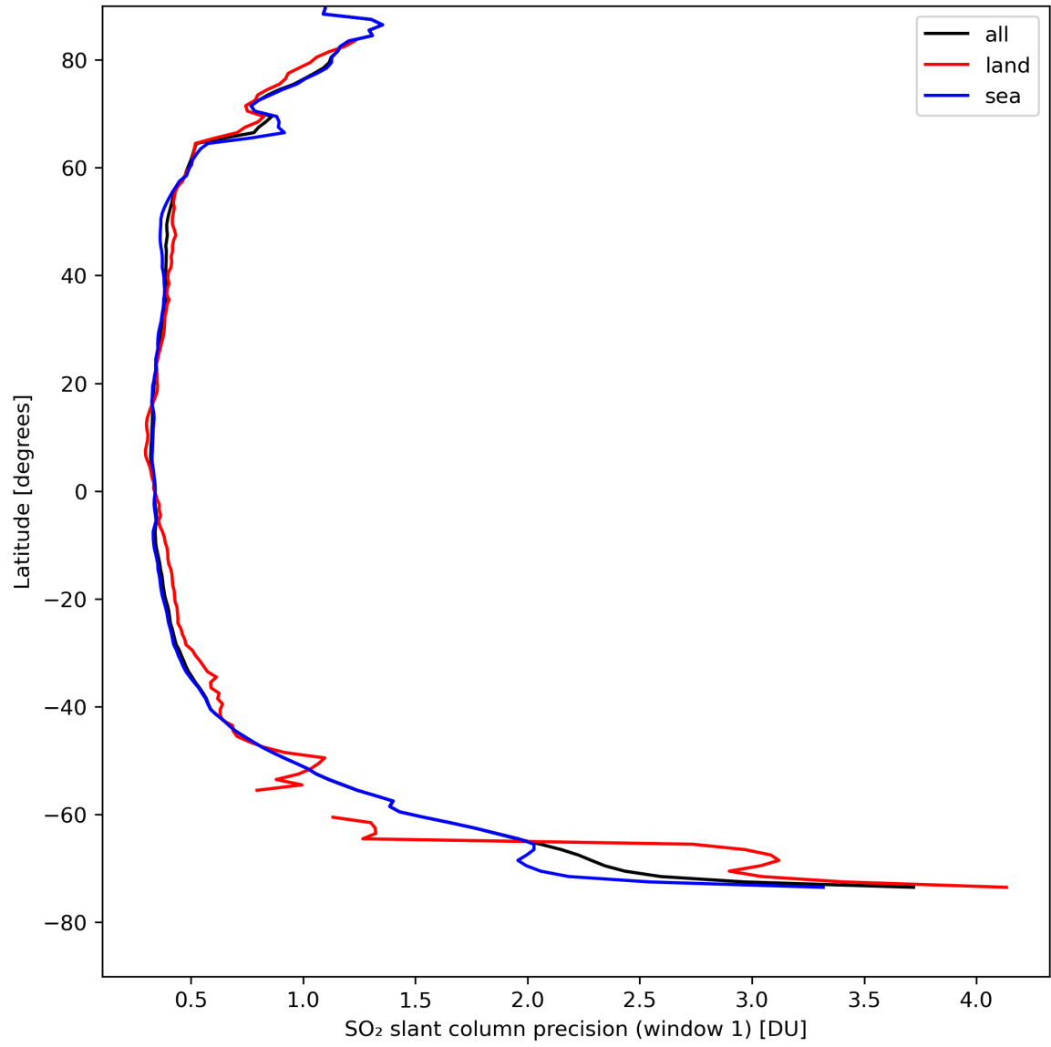
Figure 34: Zonal average of “SO 2 slant column precision (window 1)” for 2024-08-22 to 2024-08-24.
