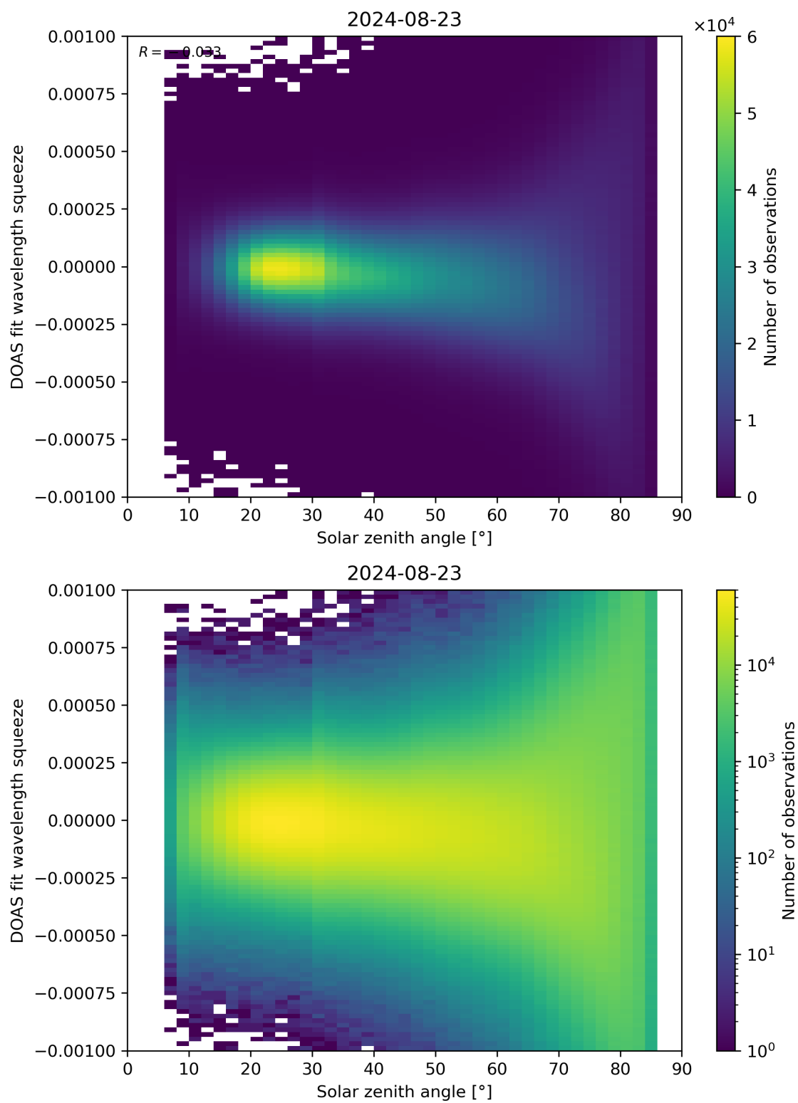
Figure 162: Scatter density plot of “Solar zenith angle” against “DOAS fit wavelength squeeze” for 2024-08-22 to 2024-08-24.
