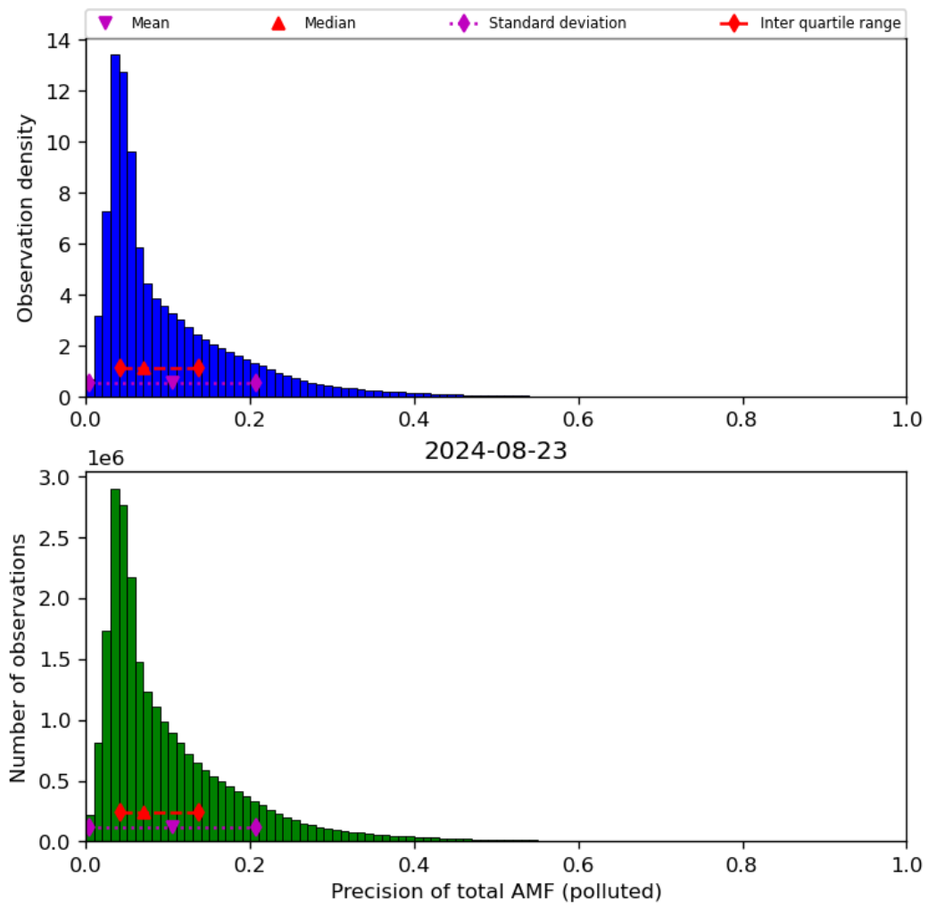
Figure 72: Histogram of “Precision of total AMF (polluted)” for 2024-08-22 to 2024-08-24
