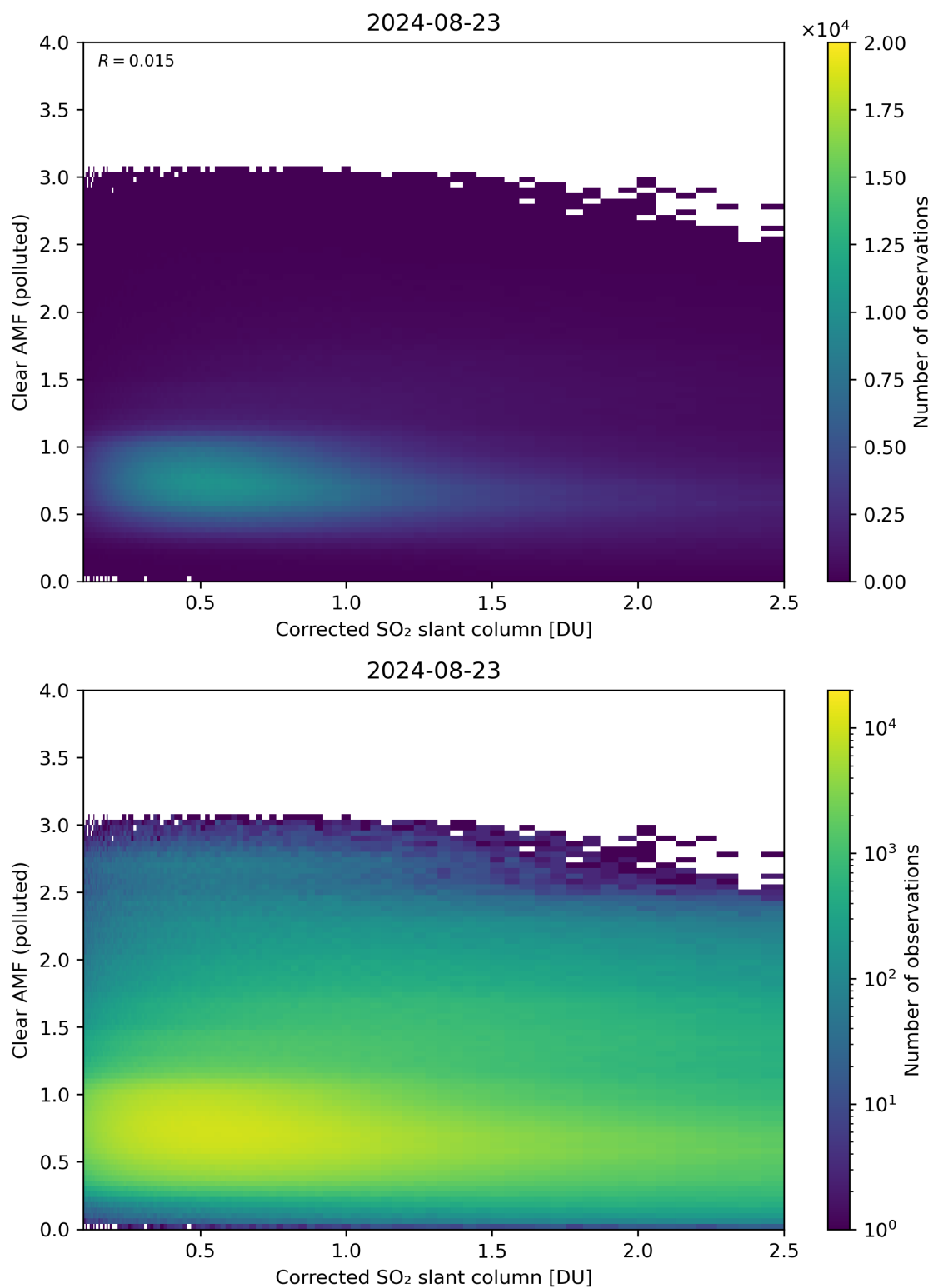
Figure 184: Scatter density plot of “Corrected SO 2 slant column” against “Clear AMF (polluted)” for 2024-08-22 to 2024-08-24.
