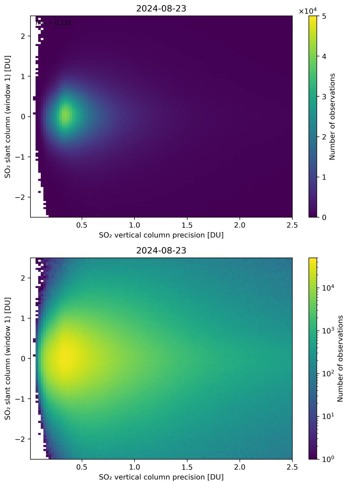
Figure 289: Scatter density plot of “SO 2 vertical column precision” against “SO 2 slant column (window 1)” for 2024-08-22 to 2024-08-24.
