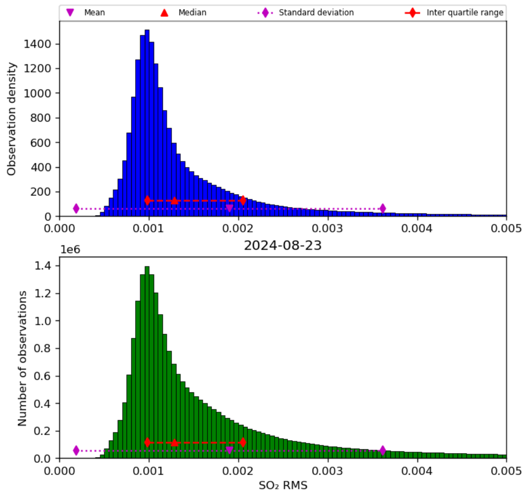
Figure 70: Histogram of “SO 2 RMS” for 2024-08-22 to 2024-08-24
