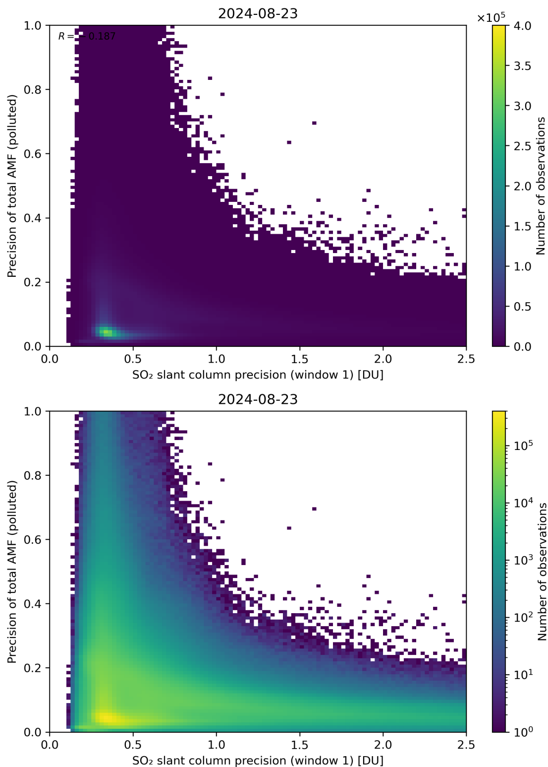
Figure 231: Scatter density plot of “SO 2 slant column precision (window 1)” against “Precision of total AMF (polluted)” for 2024-08-22 to 2024-08-24.
