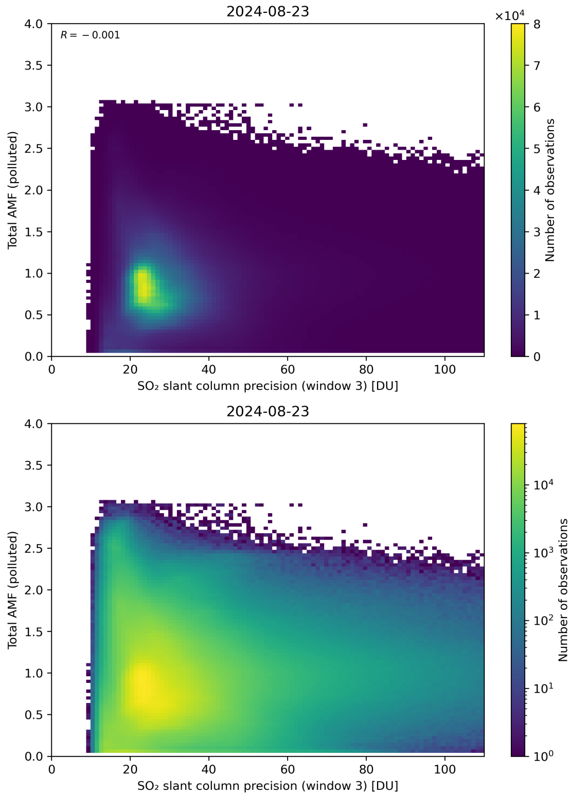
Figure 263: Scatter density plot of “SO 2 slant column precision (window 3)” against “Total AMF (polluted)” for 2024-08-22 to 2024-08-24.
