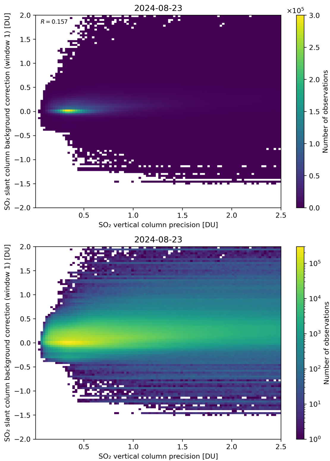
Figure 279: Scatter density plot of “SO 2 vertical column precision” against “SO 2 slant column background correction (window 1)” for 2024-08-22 to 2024-08-24.
