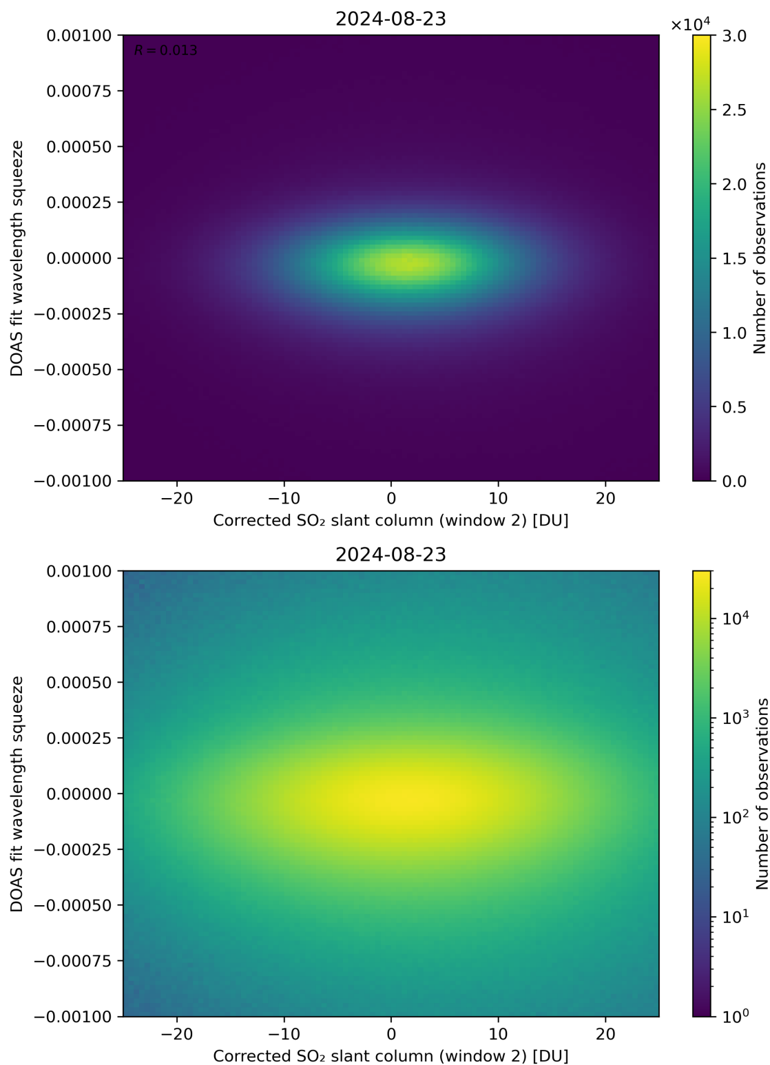
Figure 197: Scatter density plot of “Corrected SO 2 slant column (window 2)” against “DOAS fit wavelength squeeze” for 2024-08-22 to 2024-08-24.
