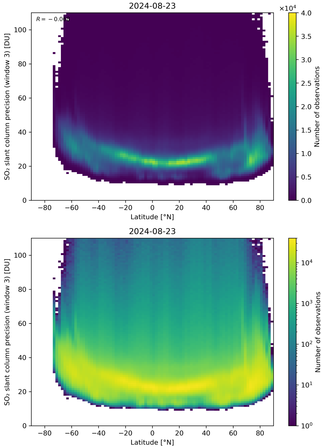
Figure 153: Scatter density plot of “Latitude” against “SO 2 slant column precision (window 3)” for 2024-08-22 to 2024-08-24.
