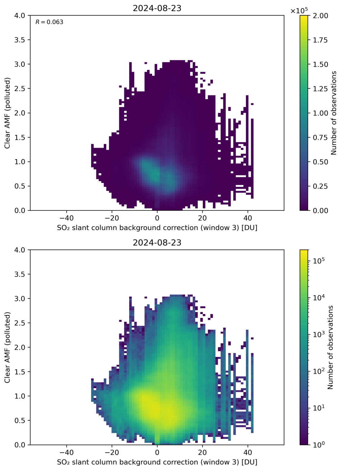
Figure 124: Scatter density plot of “SO 2 slant column background correction (window 3)” against “Clear AMF (polluted)” for 2024-08-22 to 2024-08-24.
