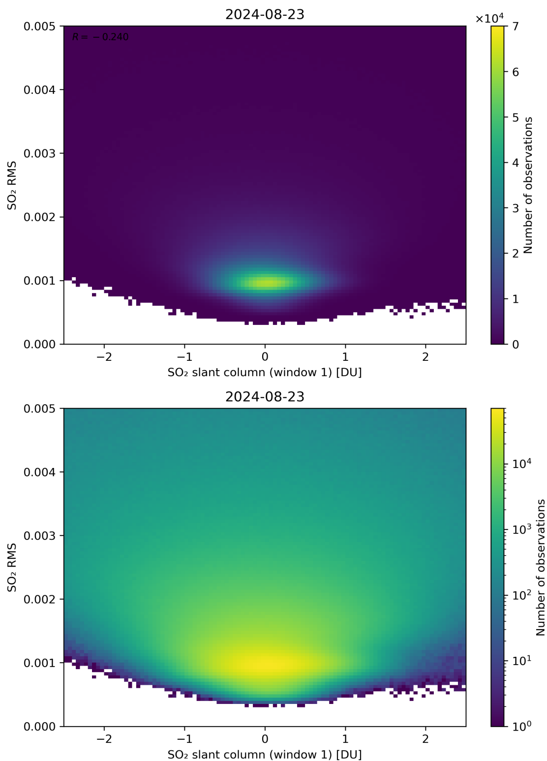
Figure 217: Scatter density plot of “SO 2 slant column (window 1)” against “SO 2 RMS” for 2024-08-22 to 2024-08-24.
