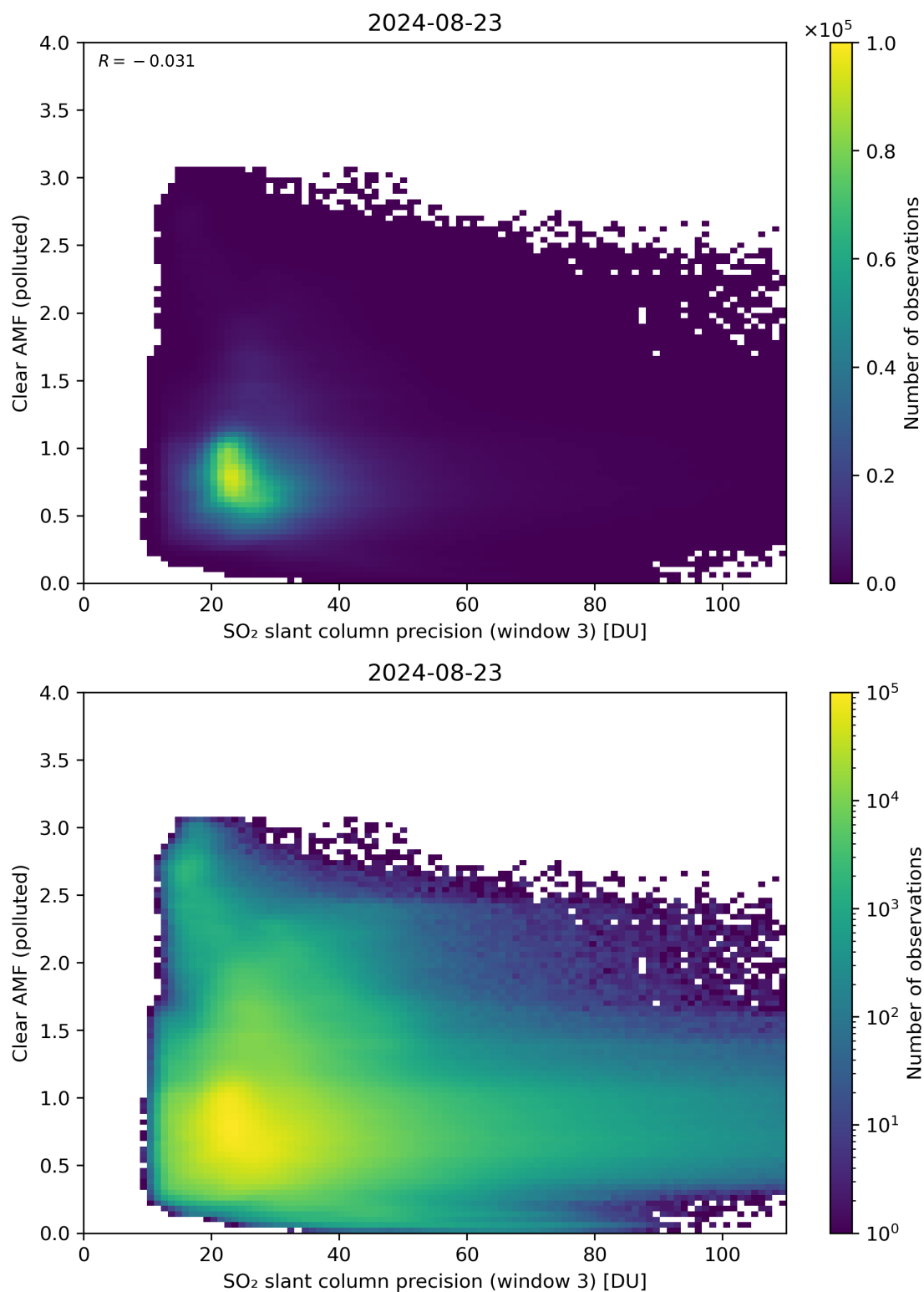
Figure 261: Scatter density plot of “SO 2 slant column precision (window 3)” against “Clear AMF (polluted)” for 2024-08-22 to 2024-08-24.
