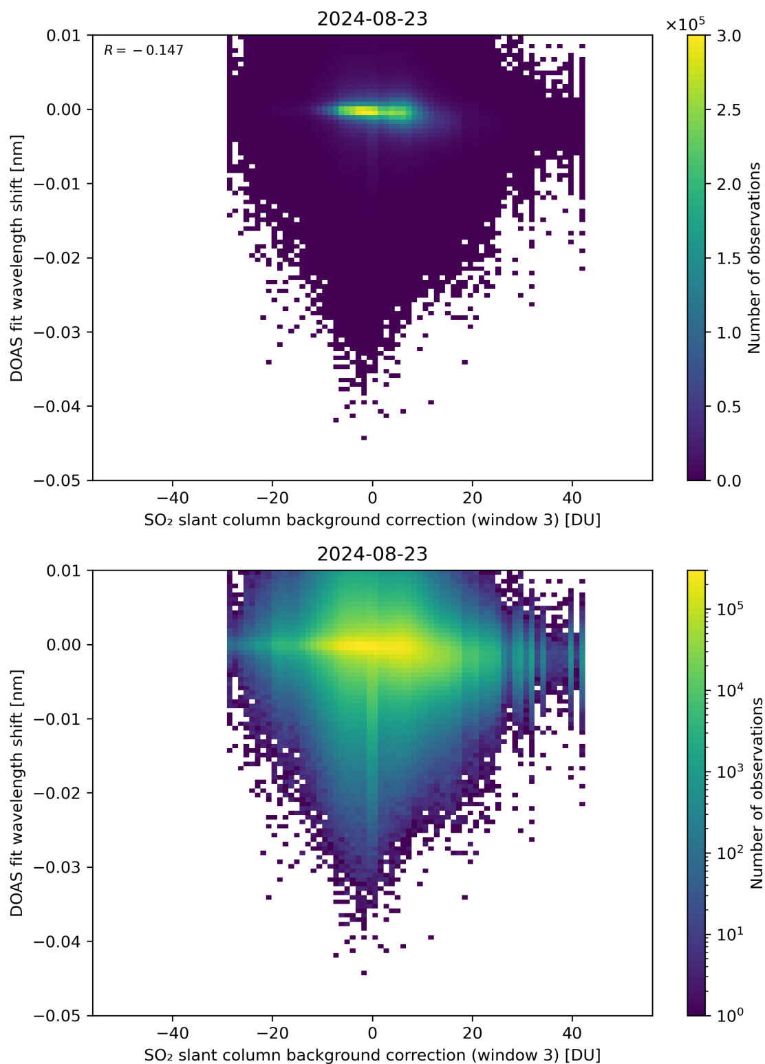
Figure 121: Scatter density plot of “SO 2 slant column background correction (window 3)” against “DOAS fit wavelength shift” for 2024-08-22 to 2024-08-24.
