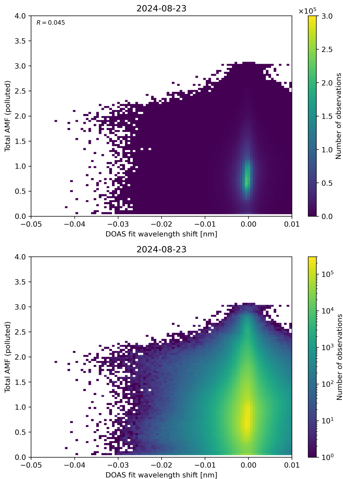
Figure 130: Scatter density plot of “DOAS fit wavelength shift” against “Total AMF (polluted)” for 2024-08-22 to 2024-08-24.
