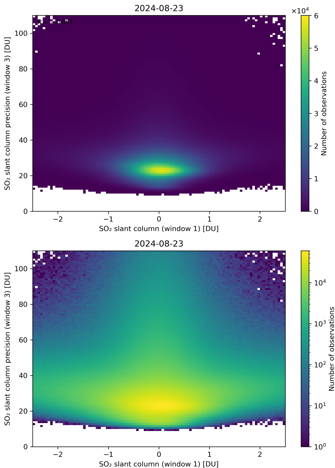
Figure 238: Scatter density plot of “SO 2 slant column (window 1)” against “SO 2 slant column precision (window 3)” for 2024-08-22 to 2024-08-24.
