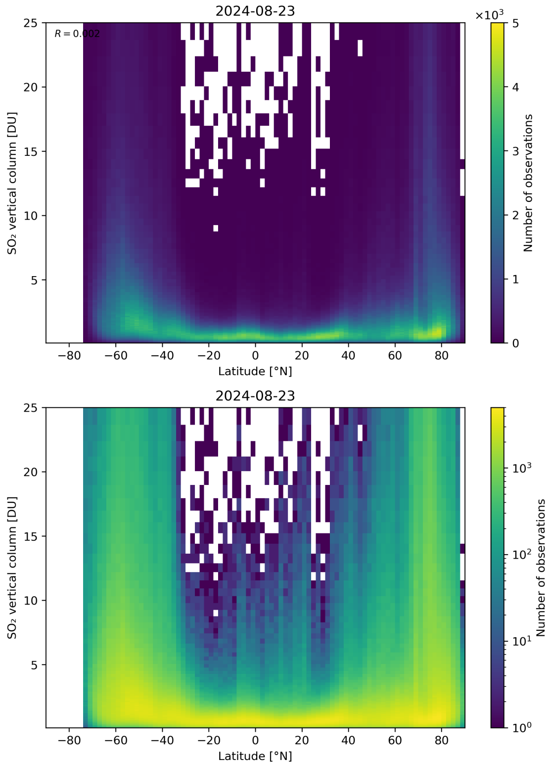
Figure 156: Scatter density plot of “Latitude” against “SO 2 vertical column” for 2024-08-22 to 2024-08-24.
