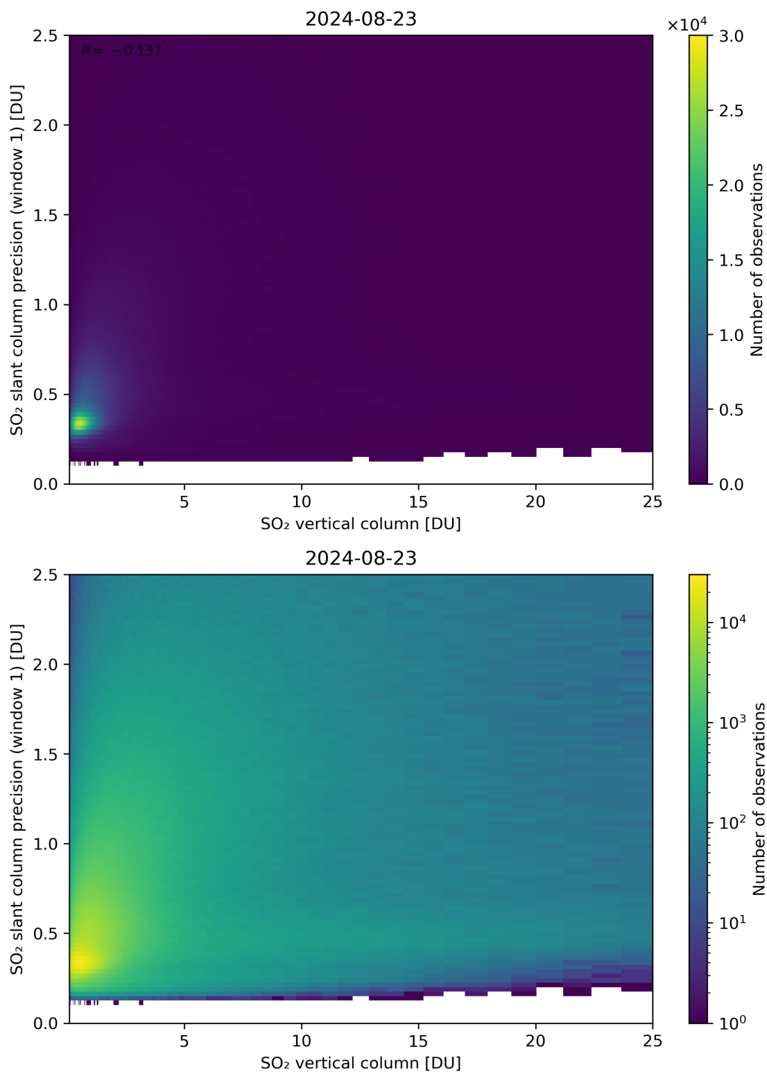
Figure 301: Scatter density plot of “SO 2 vertical column” against “SO 2 slant column precision (window 1)” for 2024-08-22 to 2024-08-24.
