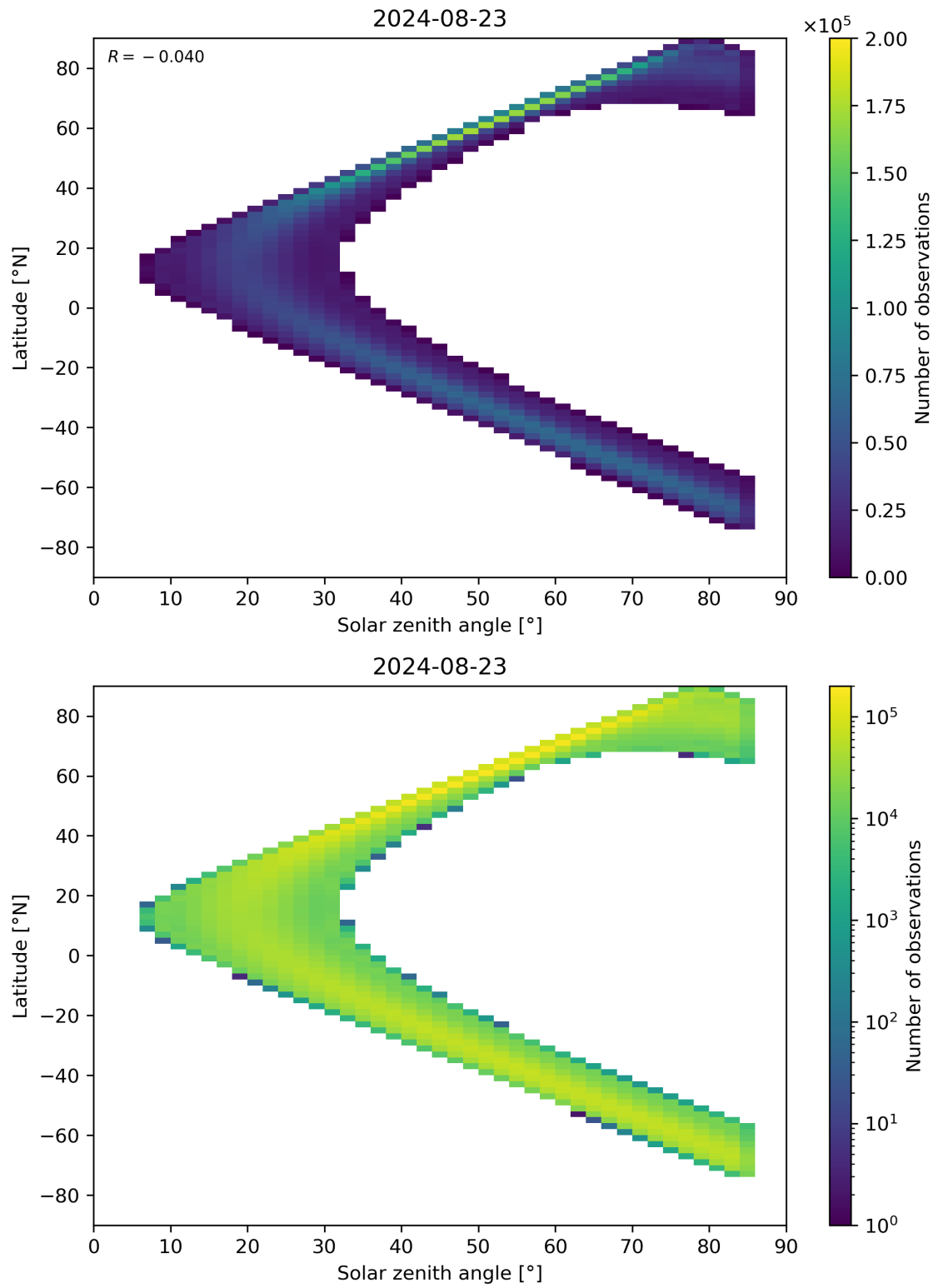
Figure 164: Scatter density plot of “Solar zenith angle” against “Latitude” for 2024-08-22 to 2024-08-24.
