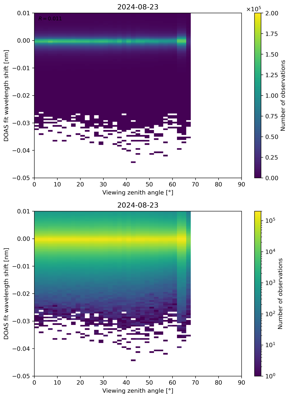
Figure 311: Scatter density plot of “Viewing zenith angle” against “DOAS fit wavelength shift” for 2024-08-22 to 2024-08-24.
