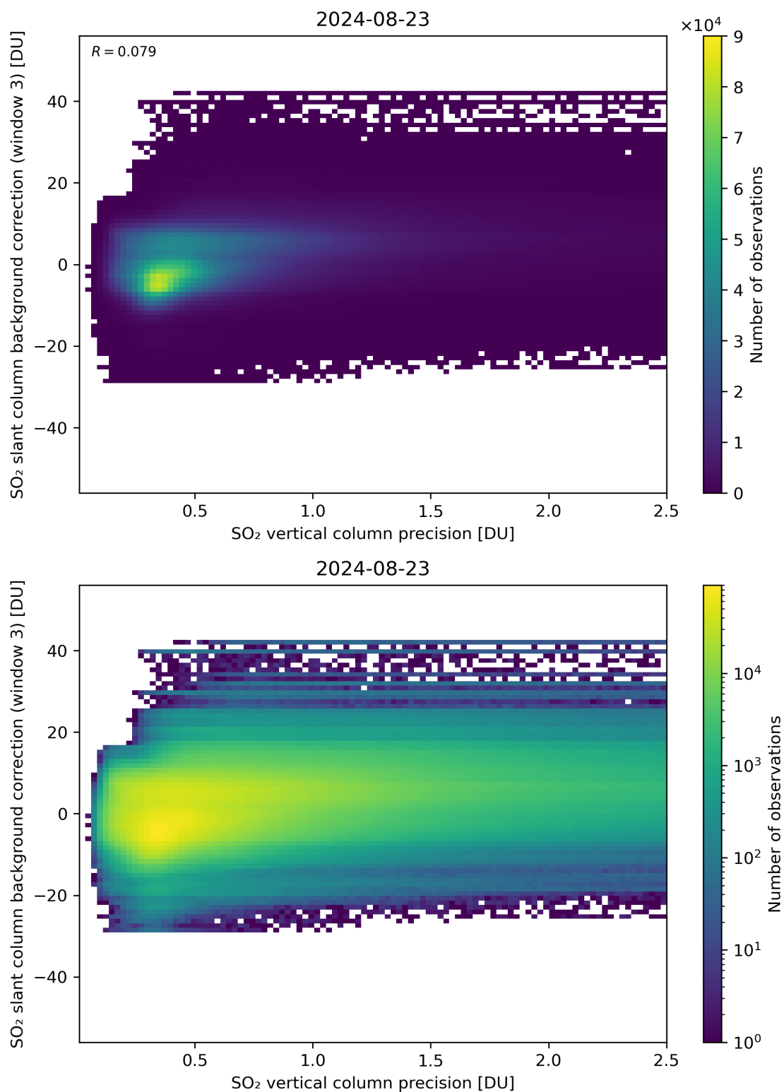
Figure 281: Scatter density plot of “SO 2 vertical column precision” against “SO 2 slant column background correction (window 3)” for 2024-08-22 to 2024-08-24.
