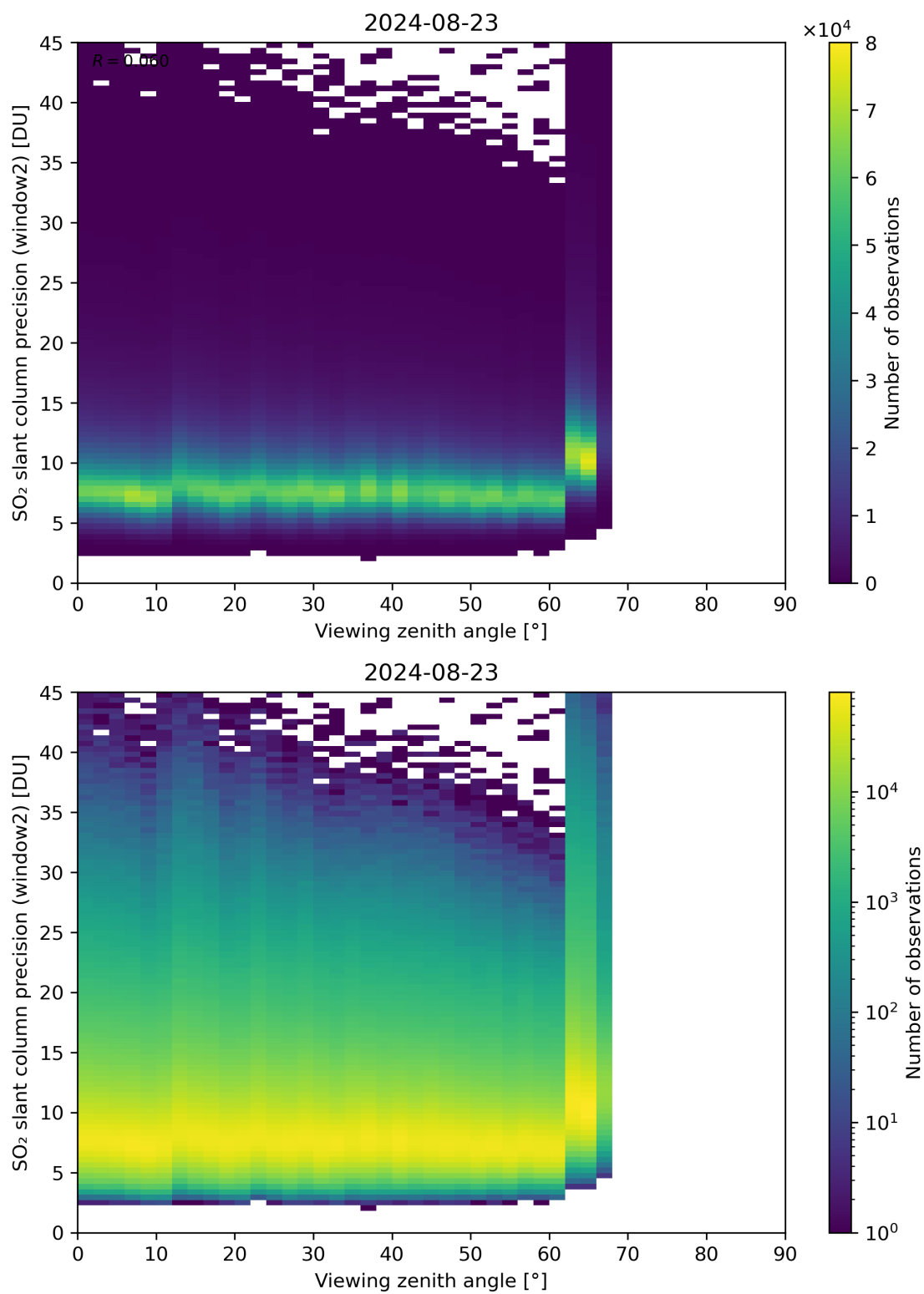
Figure 322: Scatter density plot of “Viewing zenith angle” against “SO 2 slant column precision (window2)” for 2024-08-22 to 2024-08-24.
