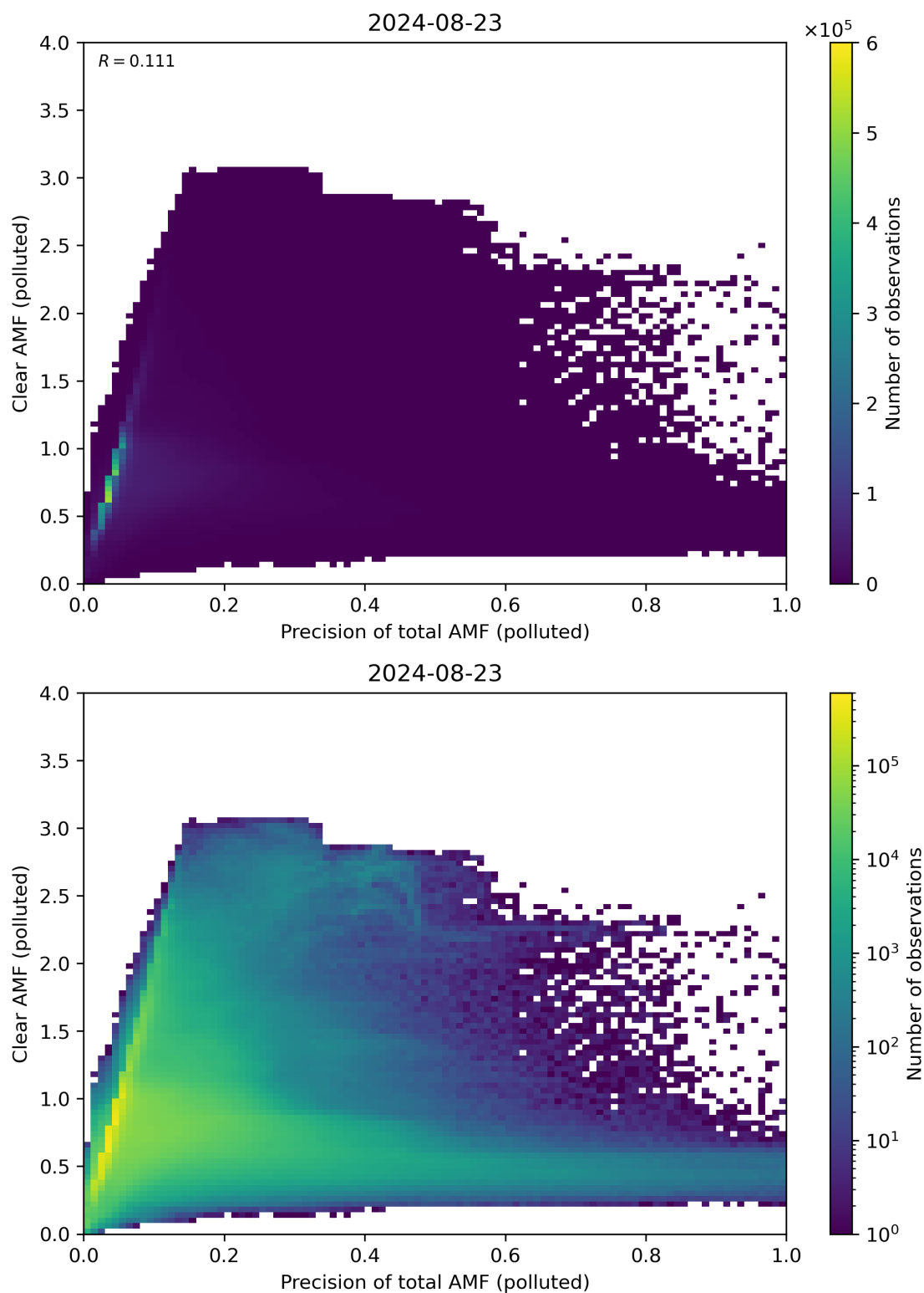
Figure 270: Scatter density plot of “Precision of total AMF (polluted)” against “Clear AMF (polluted)” for 2024-08-22 to 2024-08-24.
