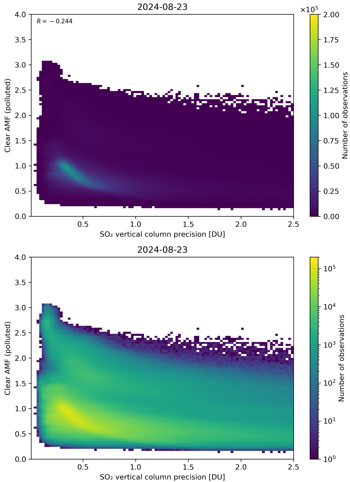
Figure 285: Scatter density plot of “SO 2 vertical column precision” against “Clear AMF (polluted)” for 2024-08-22 to 2024-08-24.
