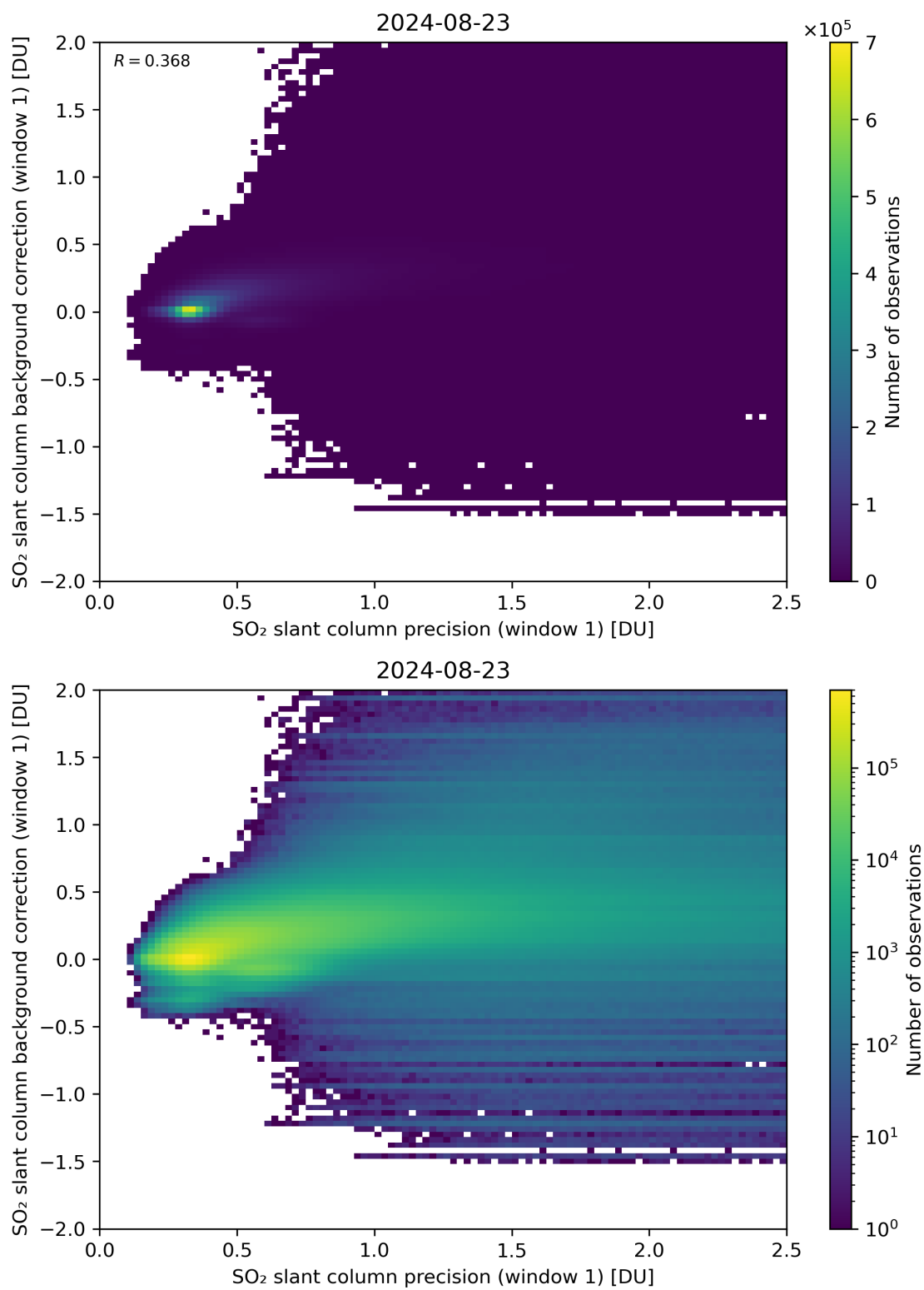
Figure 218: Scatter density plot of “SO 2 slant column precision (window 1)” against “SO 2 slant column background correction (window 1)” for 2024-08-22 to 2024-08-24.
