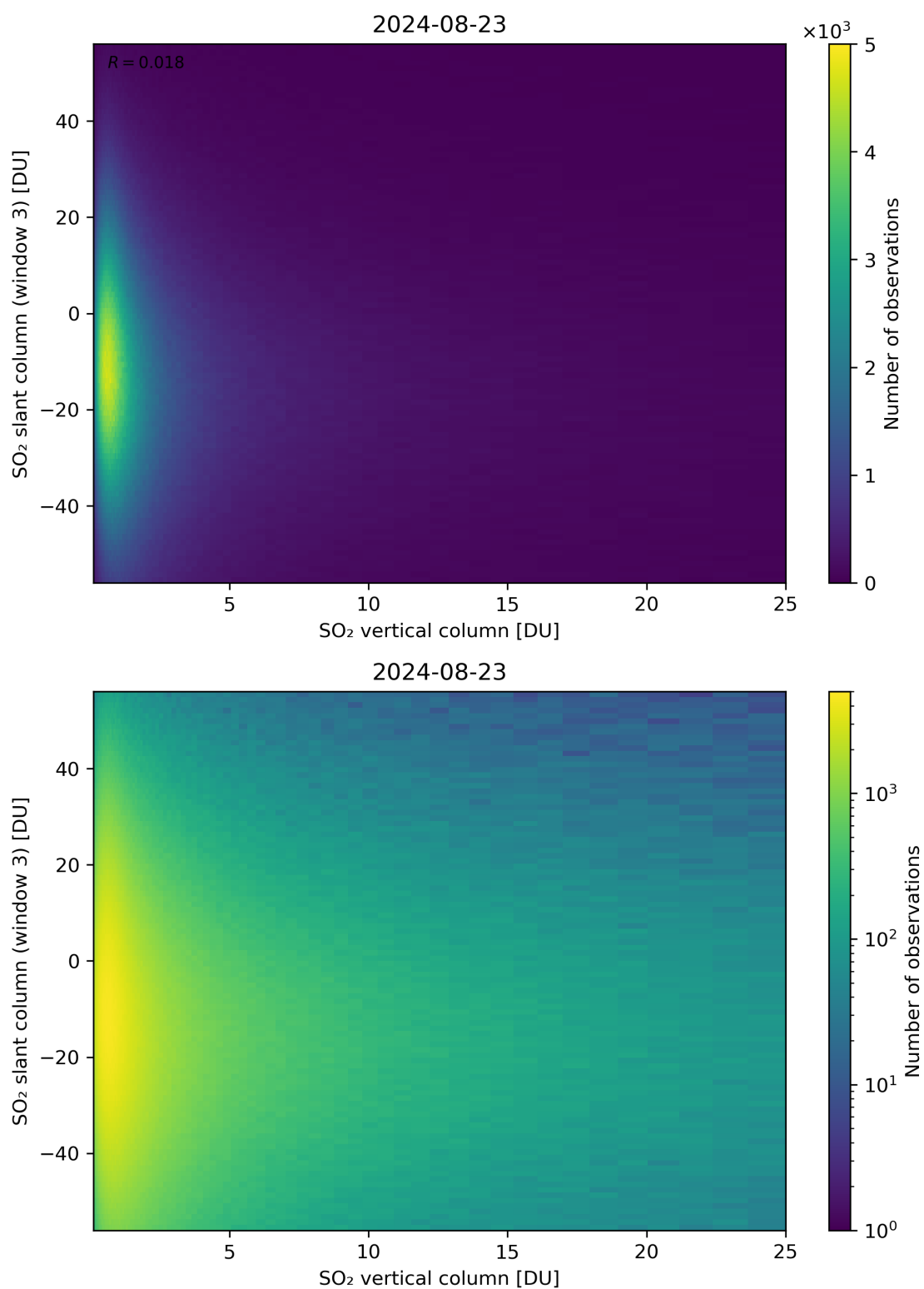
Figure 303: Scatter density plot of “SO 2 vertical column” against “SO 2 slant column (window 3)” for 2024-08-22 to 2024-08-24.
