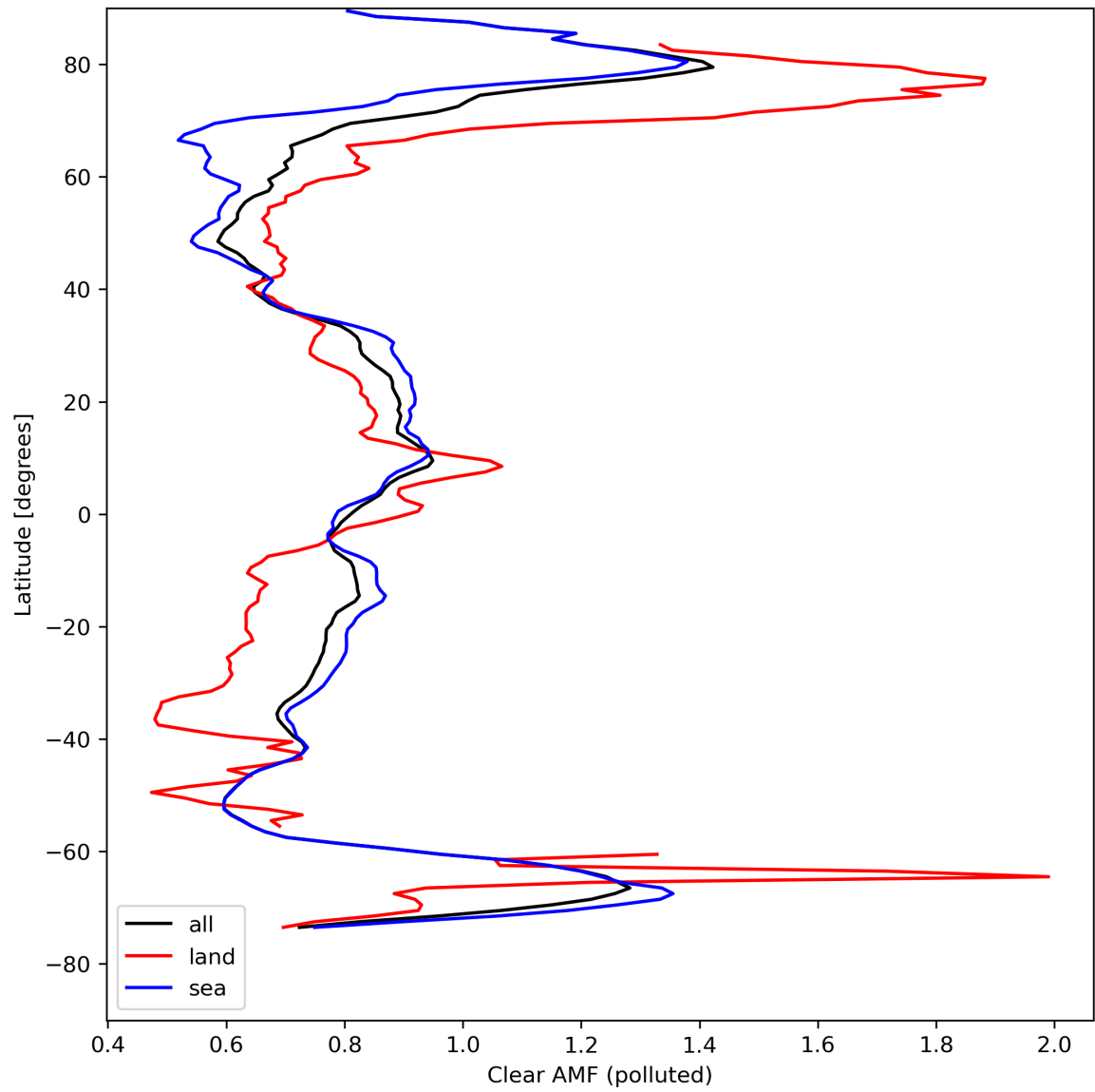
Figure 50: Zonal average of “Clear AMF (polluted)” for 2024-08-22 to 2024-08-24.
