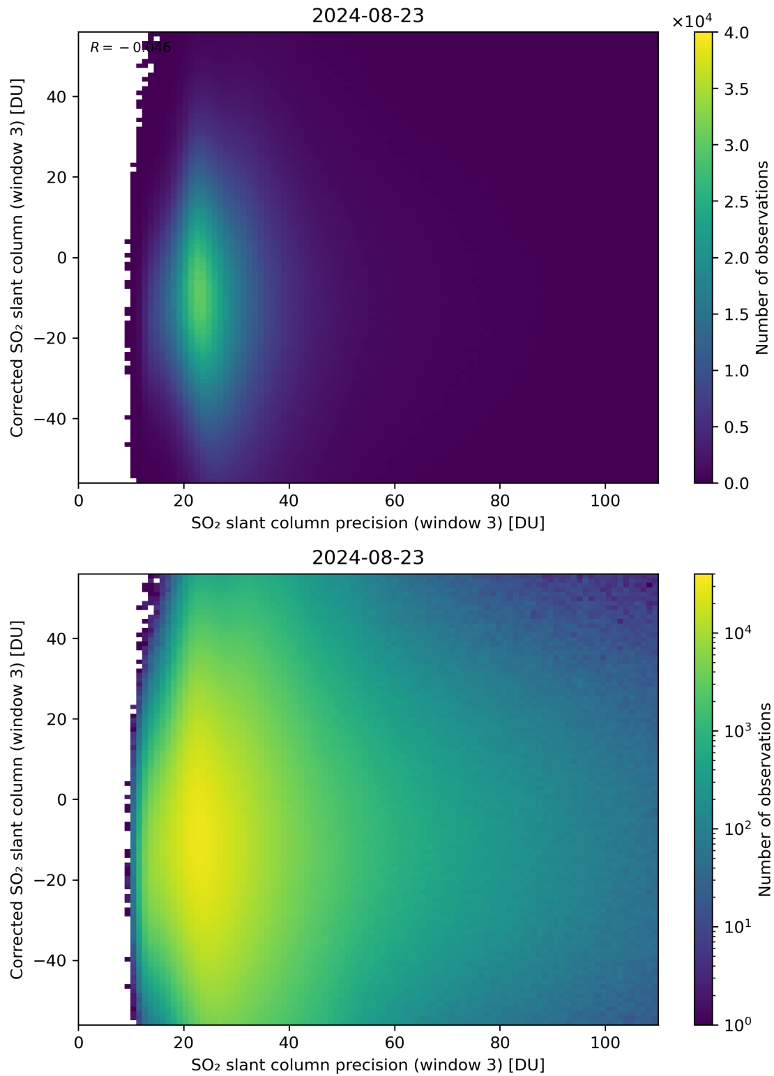
Figure 262: Scatter density plot of “SO 2 slant column precision (window 3)” against “Corrected SO 2 slant column (window 3)” for 2024-08-22 to 2024-08-24.
