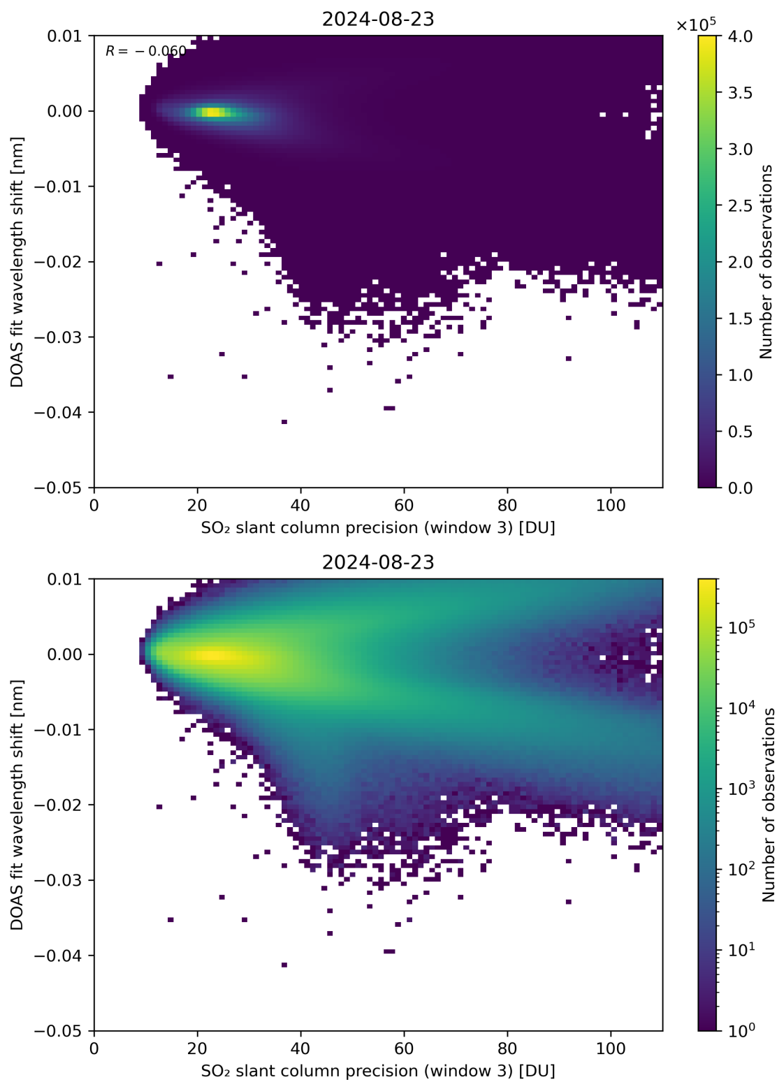
Figure 258: Scatter density plot of “SO 2 slant column precision (window 3)” against “DOAS fit wavelength shift” for 2024-08-22 to 2024-08-24.
