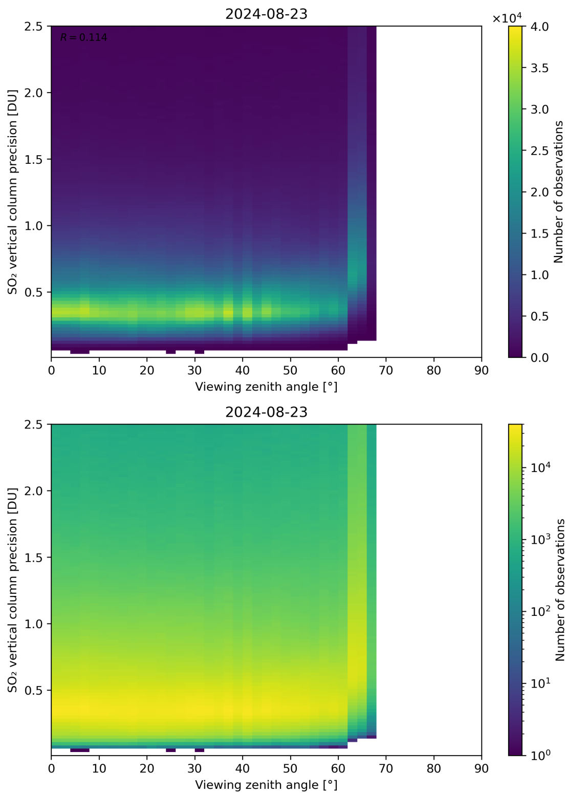
Figure 328: Scatter density plot of “Viewing zenith angle” against “SO 2 vertical column precision” for 2024-08-22 to 2024-08-24.
