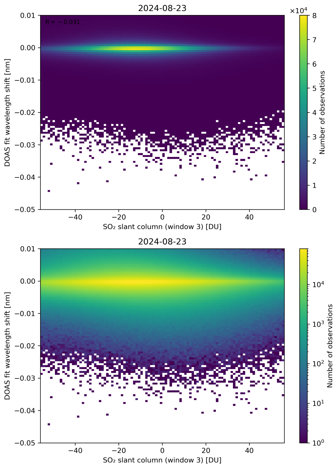
Figure 254: Scatter density plot of “SO 2 slant column (window 3)” against “DOAS fit wavelength shift” for 2024-08-22 to 2024-08-24.
