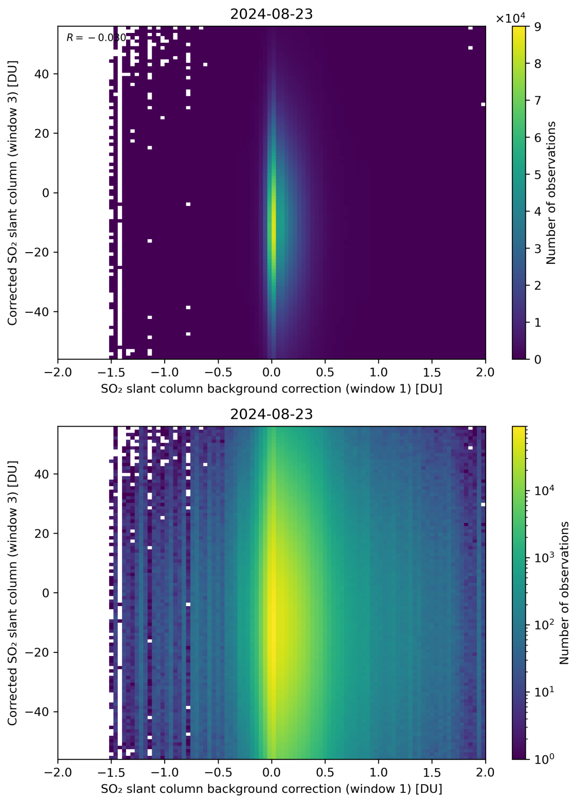
Figure 105: Scatter density plot of “SO 2 slant column background correction (window 1)” against “Corrected SO 2 slant column (window 3)” for 2024-08-22 to 2024-08-24.
