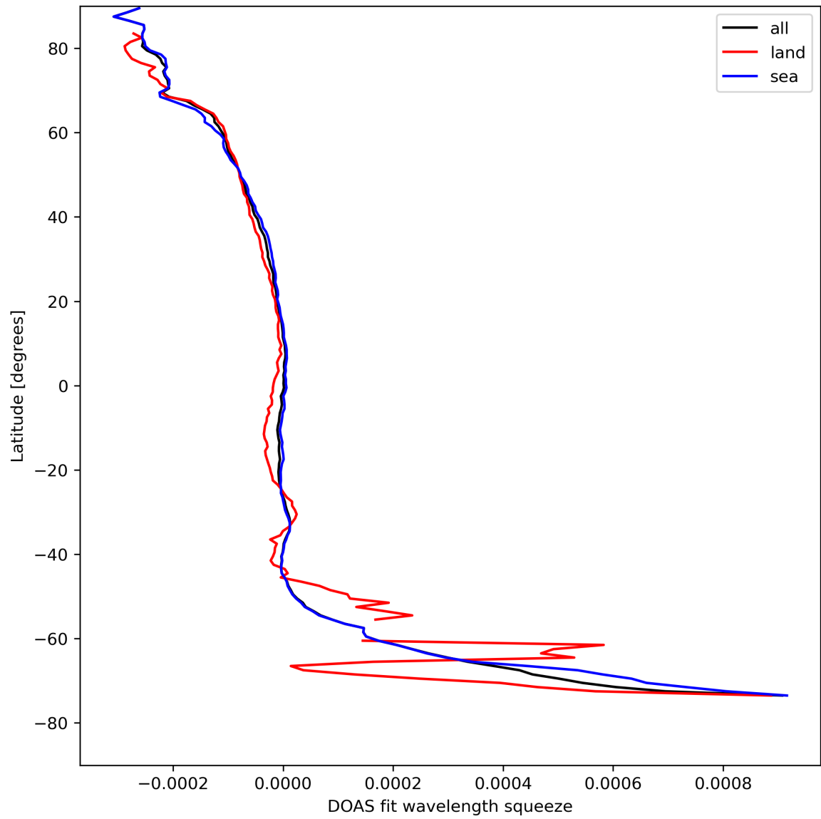
Figure 46: Zonal average of “DOAS fit wavelength squeeze” for 2024-08-22 to 2024-08-24.
