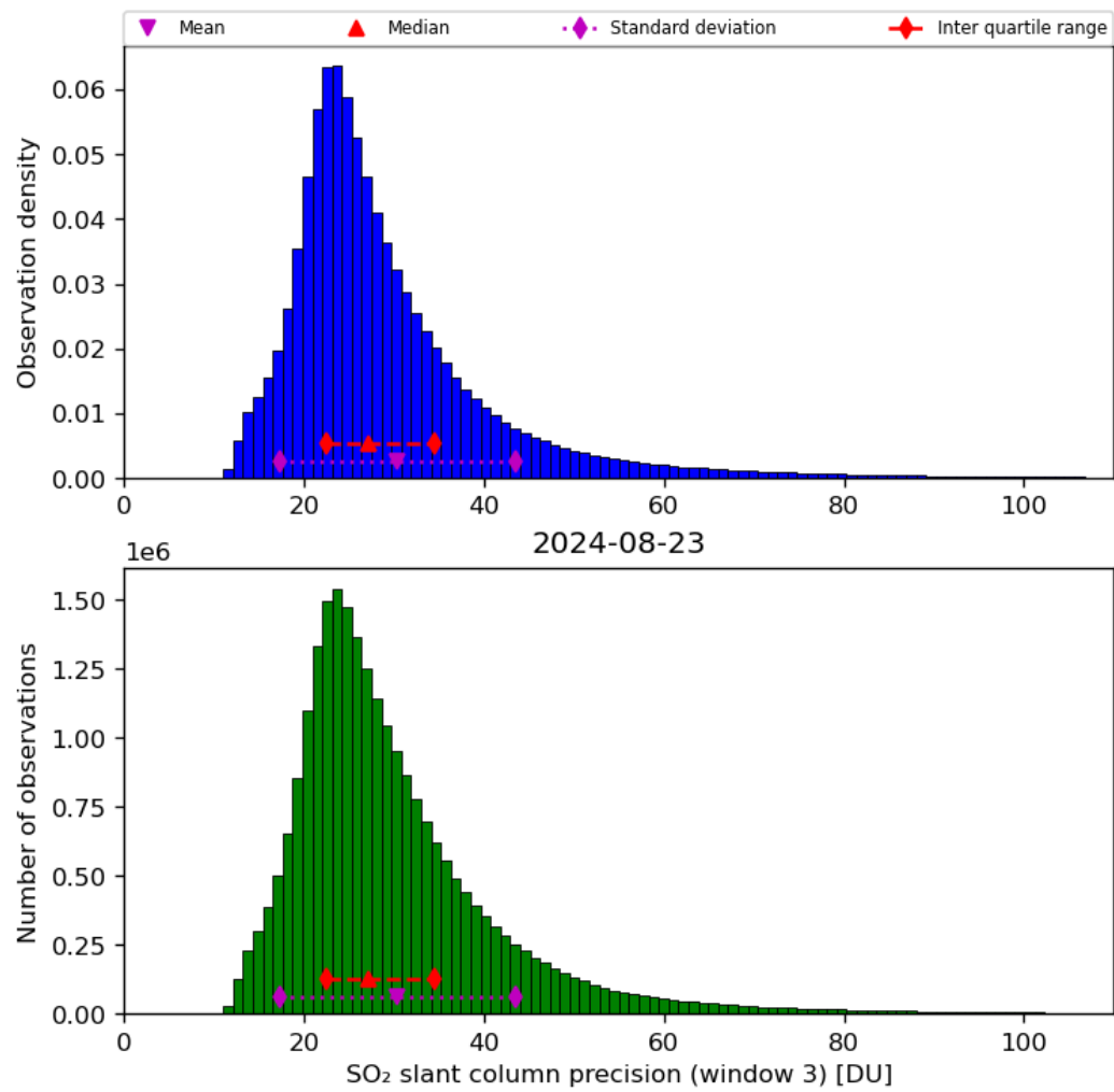
Figure 65: Histogram of “SO 2 slant column precision (window 3)” for 2024-08-22 to 2024-08-24
