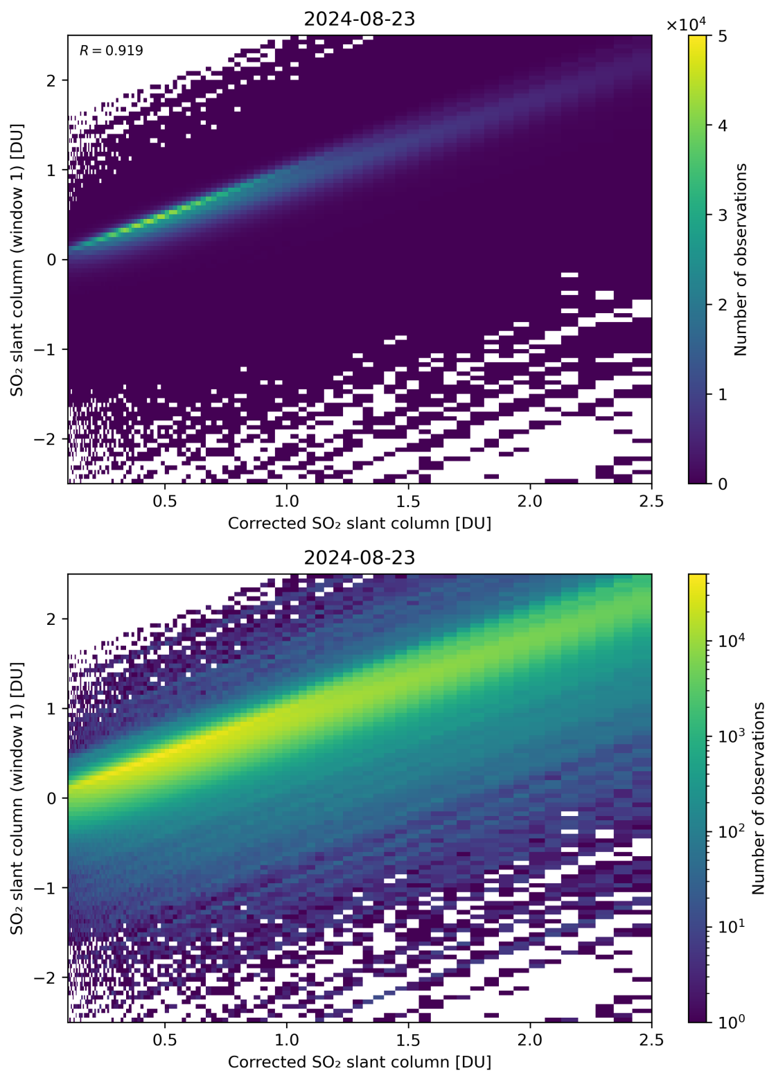
Figure 187: Scatter density plot of “Corrected SO 2 slant column” against “SO 2 slant column (window 1)” for 2024-08-22 to 2024-08-24.
