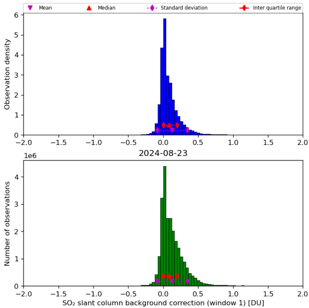
Figure 59: Histogram of “SO 2 slant column background correction (window 1)” for 2024-08-22 to 2024-08-24
