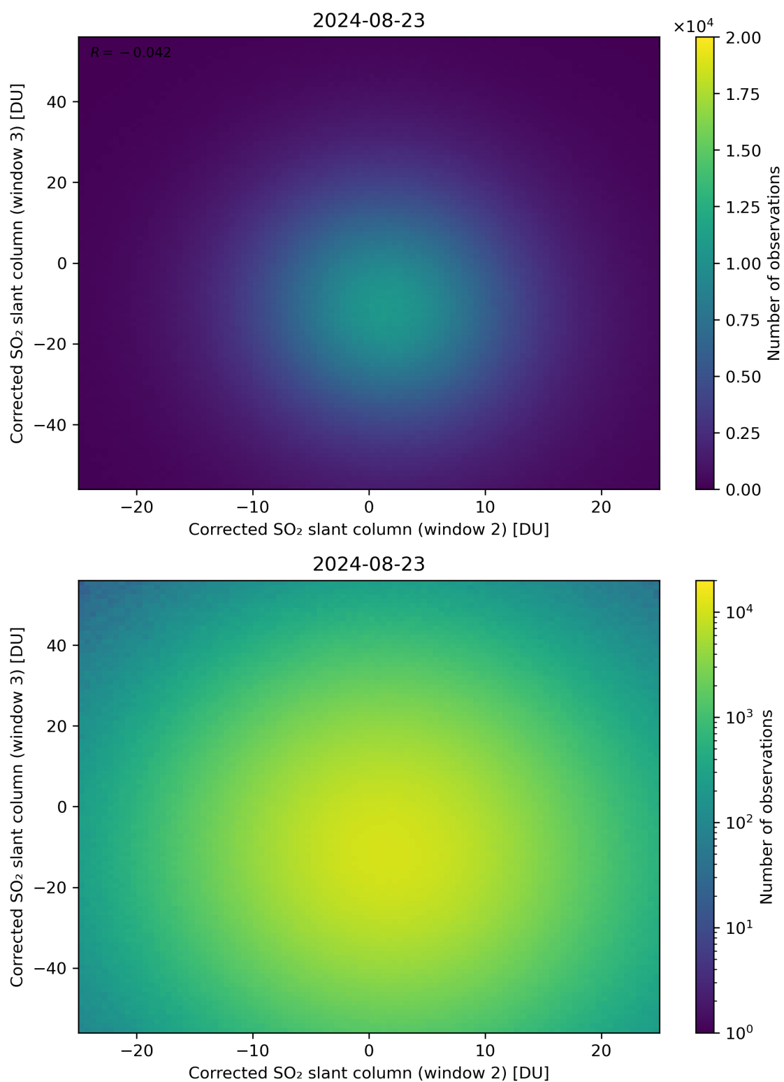
Figure 200: Scatter density plot of “Corrected SO 2 slant column (window 2)” against “Corrected SO 2 slant column (window 3)” for 2024-08-22 to 2024-08-24.
