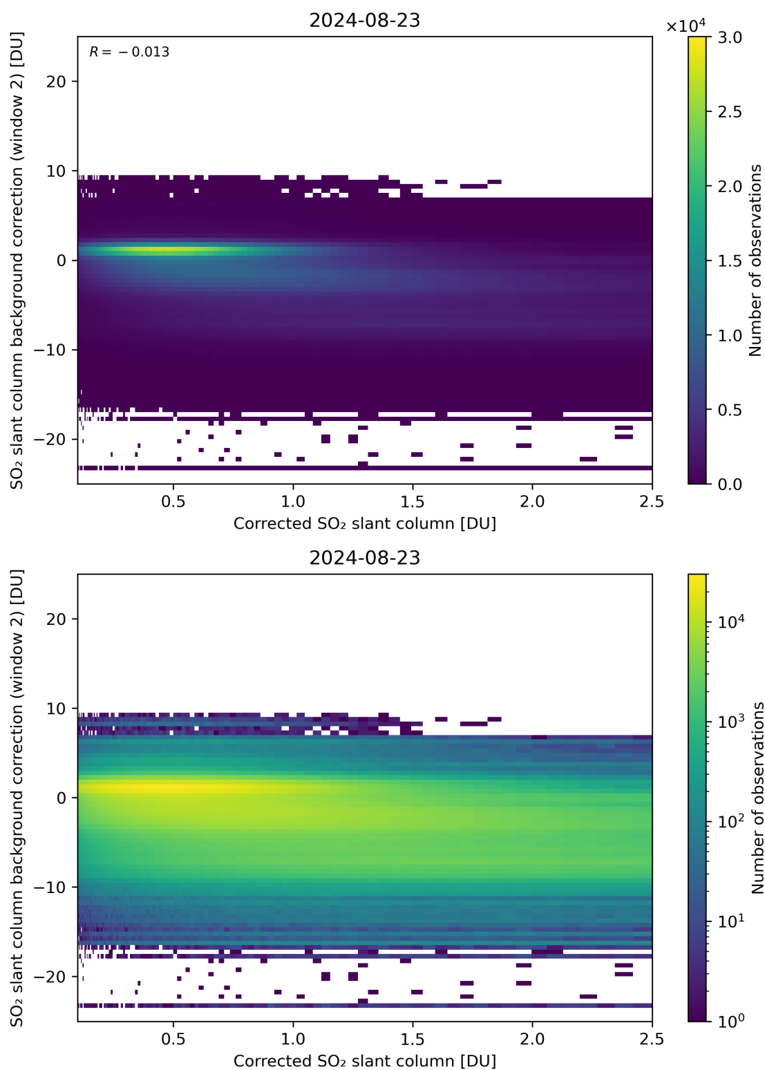
Figure 179: Scatter density plot of “Corrected SO 2 slant column” against “SO 2 slant column background correction (window 2)” for 2024-08-22 to 2024-08-24.
