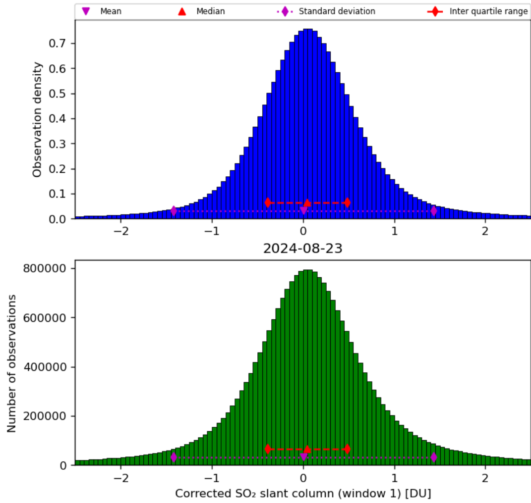
Figure 58: Histogram of “Corrected SO 2 slant column (window 1)” for 2024-08-22 to 2024-08-24
