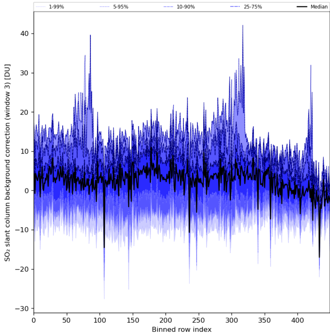
Figure 90: Along track statistics of “SO 2 slant column background correction (window 3)” for 2024-08-22 to 2024-08-24
