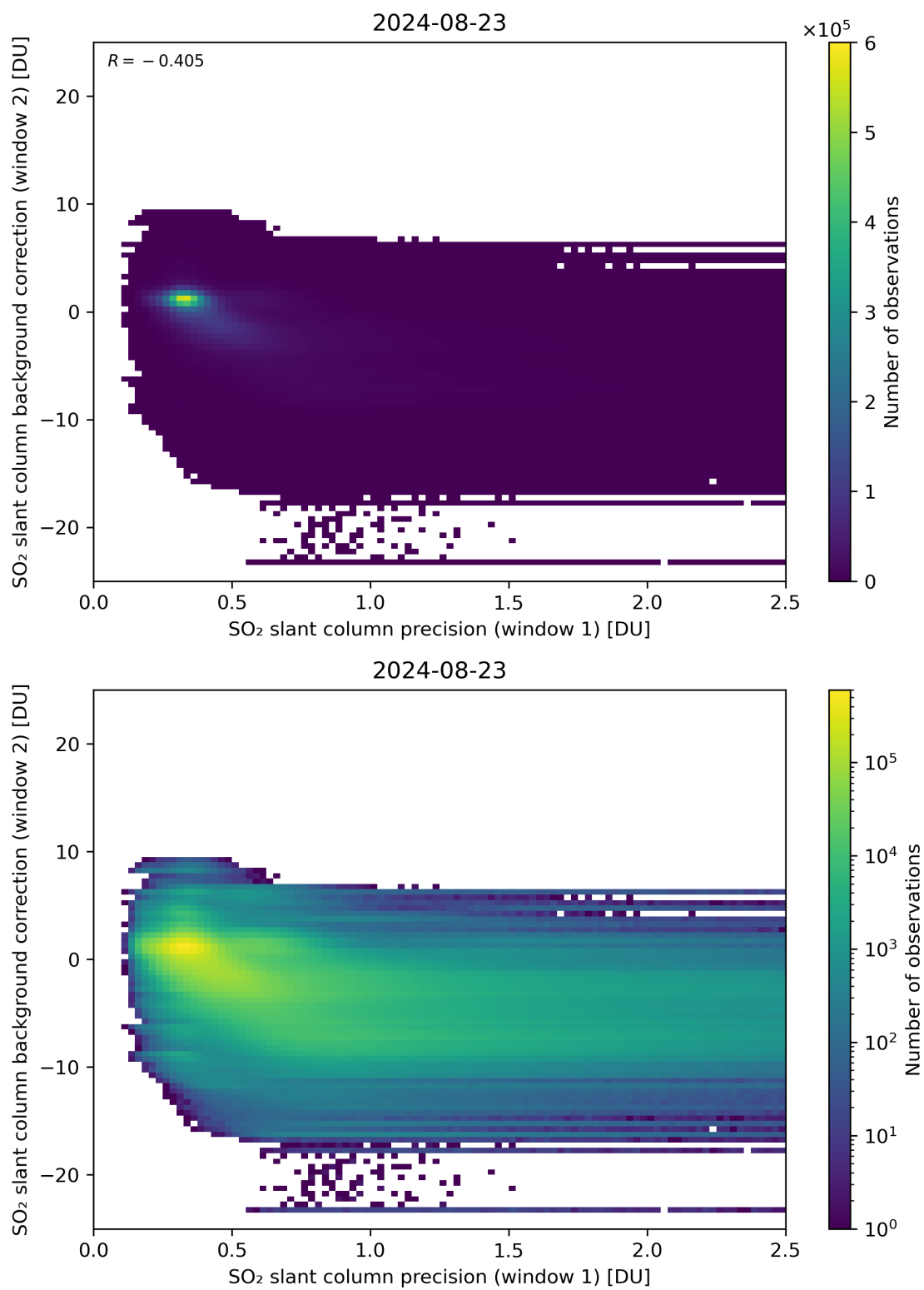
Figure 219: Scatter density plot of “SO 2 slant column precision (window 1)” against “SO 2 slant column background correction (window 2)” for 2024-08-22 to 2024-08-24.
