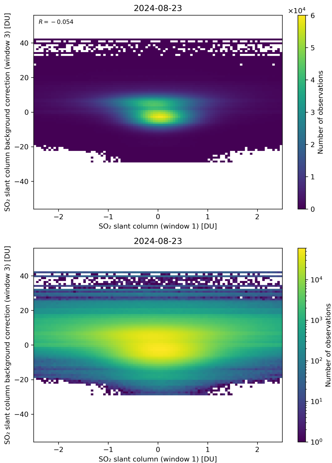
Figure 214: Scatter density plot of “SO 2 slant column (window 1)” against “SO 2 slant column background correction (window 3)” for 2024-08-22 to 2024-08-24.
