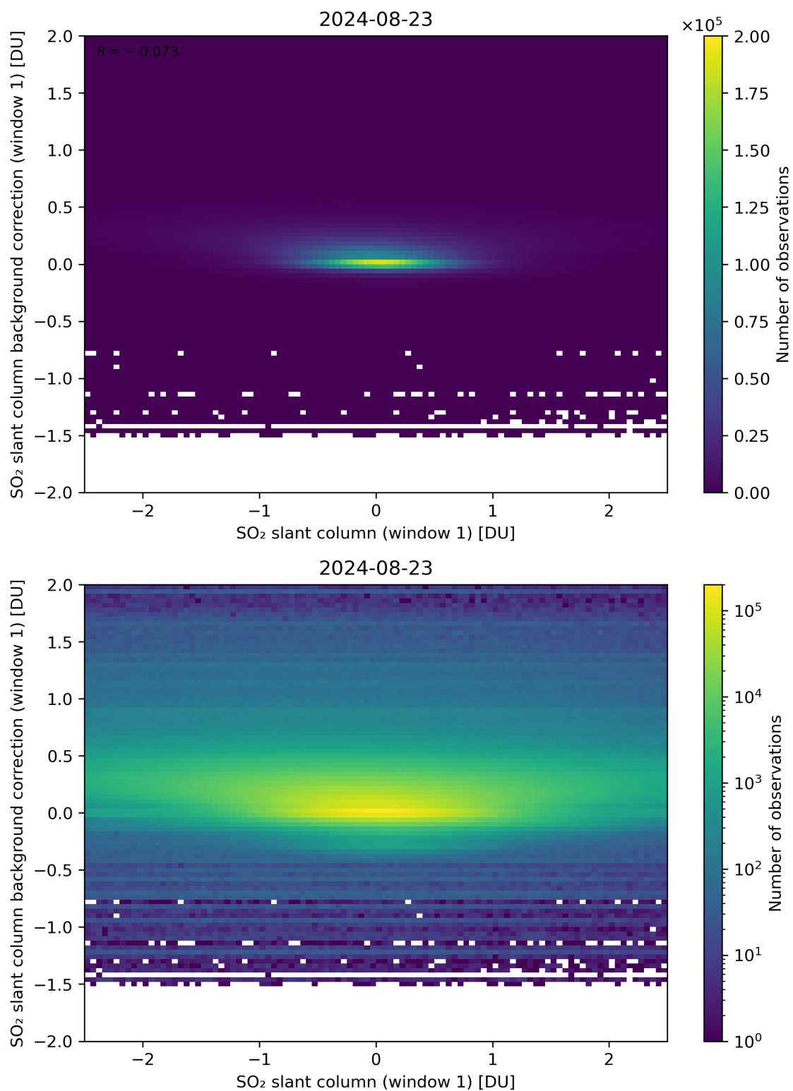
Figure 212: Scatter density plot of “SO 2 slant column (window 1)” against “SO 2 slant column background correction (window 1)” for 2024-08-22 to 2024-08-24.
