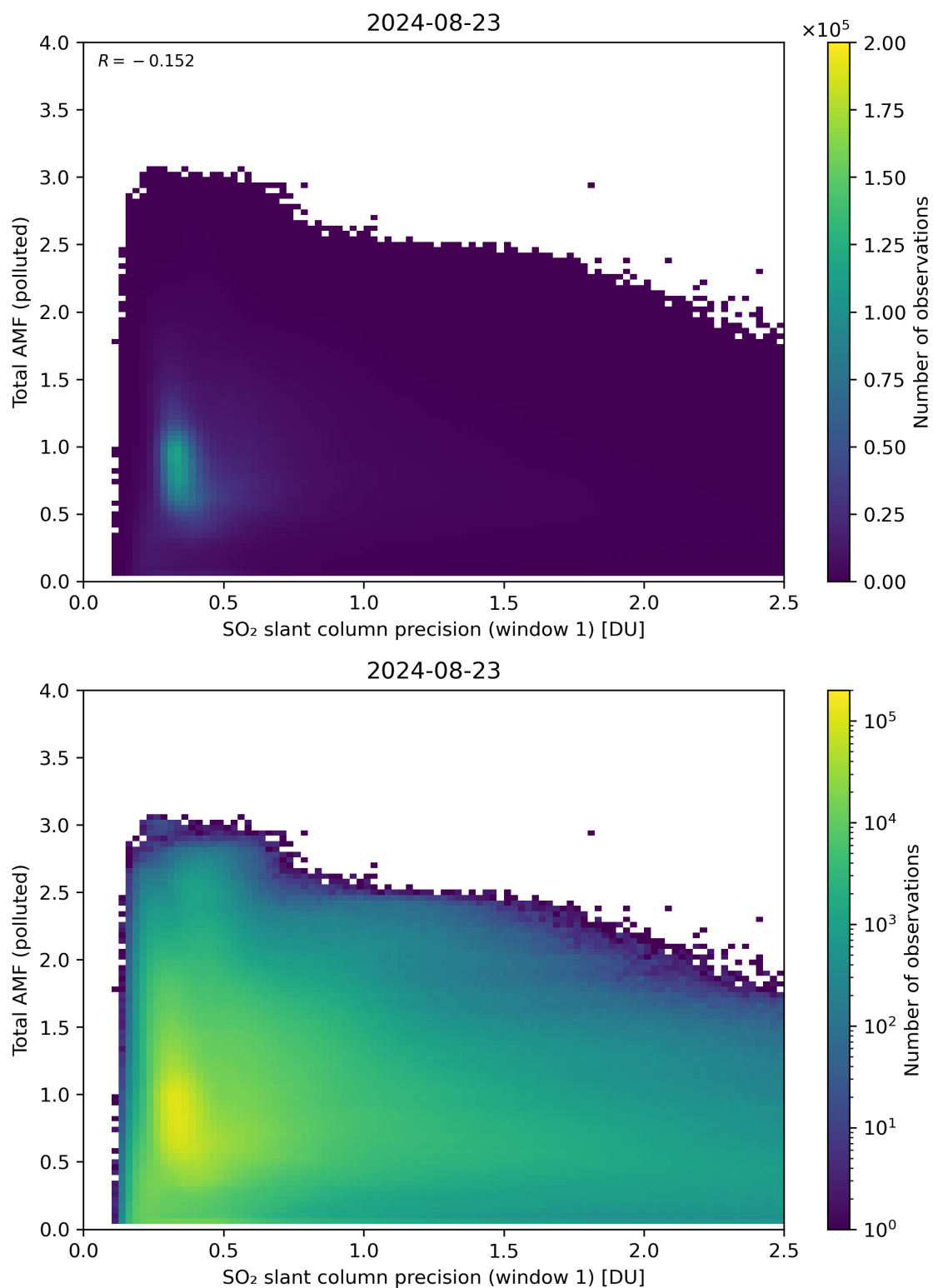
Figure 230: Scatter density plot of “SO 2 slant column precision (window 1)” against “Total AMF (polluted)” for 2024-08-22 to 2024-08-24.
