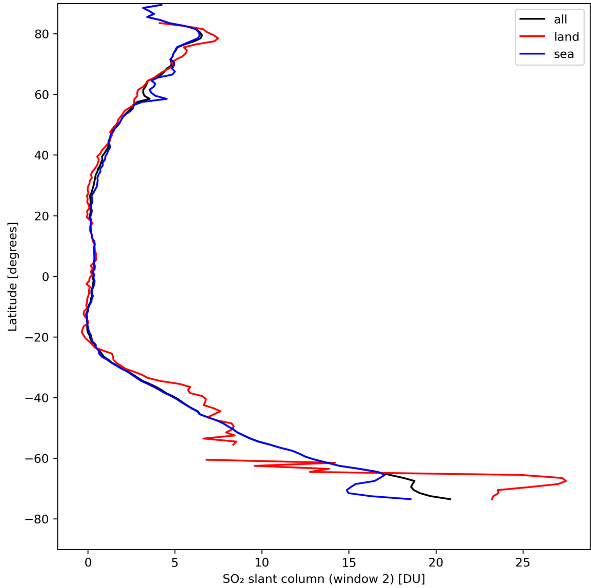
Figure 37: Zonal average of “SO 2 slant column (window 2)” for 2024-08-22 to 2024-08-24.
