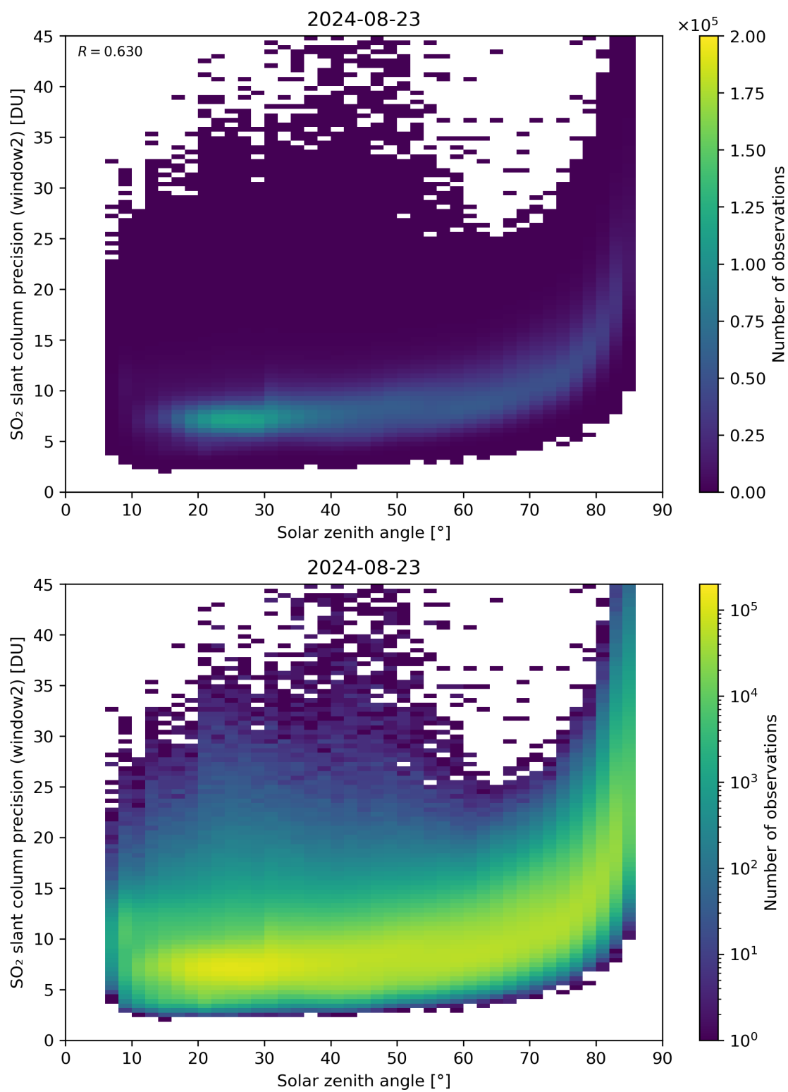
Figure 171: Scatter density plot of “Solar zenith angle” against “SO 2 slant column precision (window2)” for 2024-08-22 to 2024-08-24.
