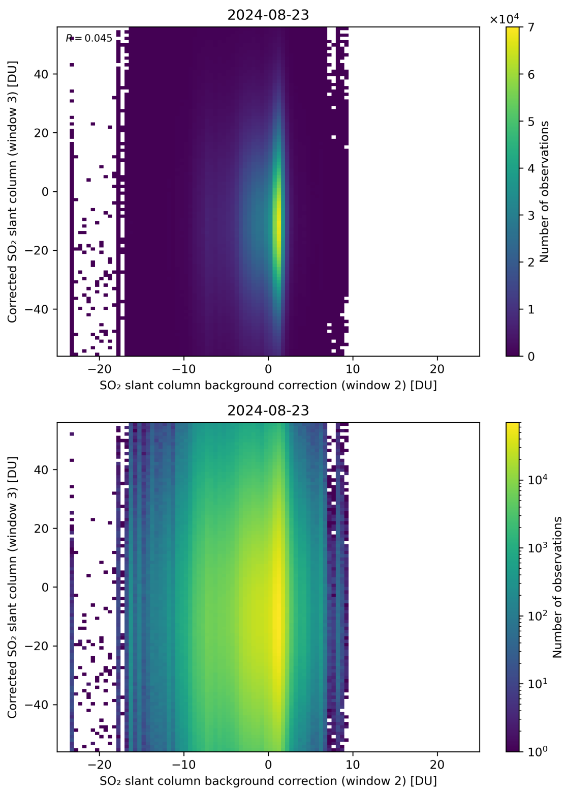
Figure 116: Scatter density plot of “SO 2 slant column background correction (window 2)” against “Corrected SO 2 slant column (window 3)” for 2024-08-22 to 2024-08-24.
