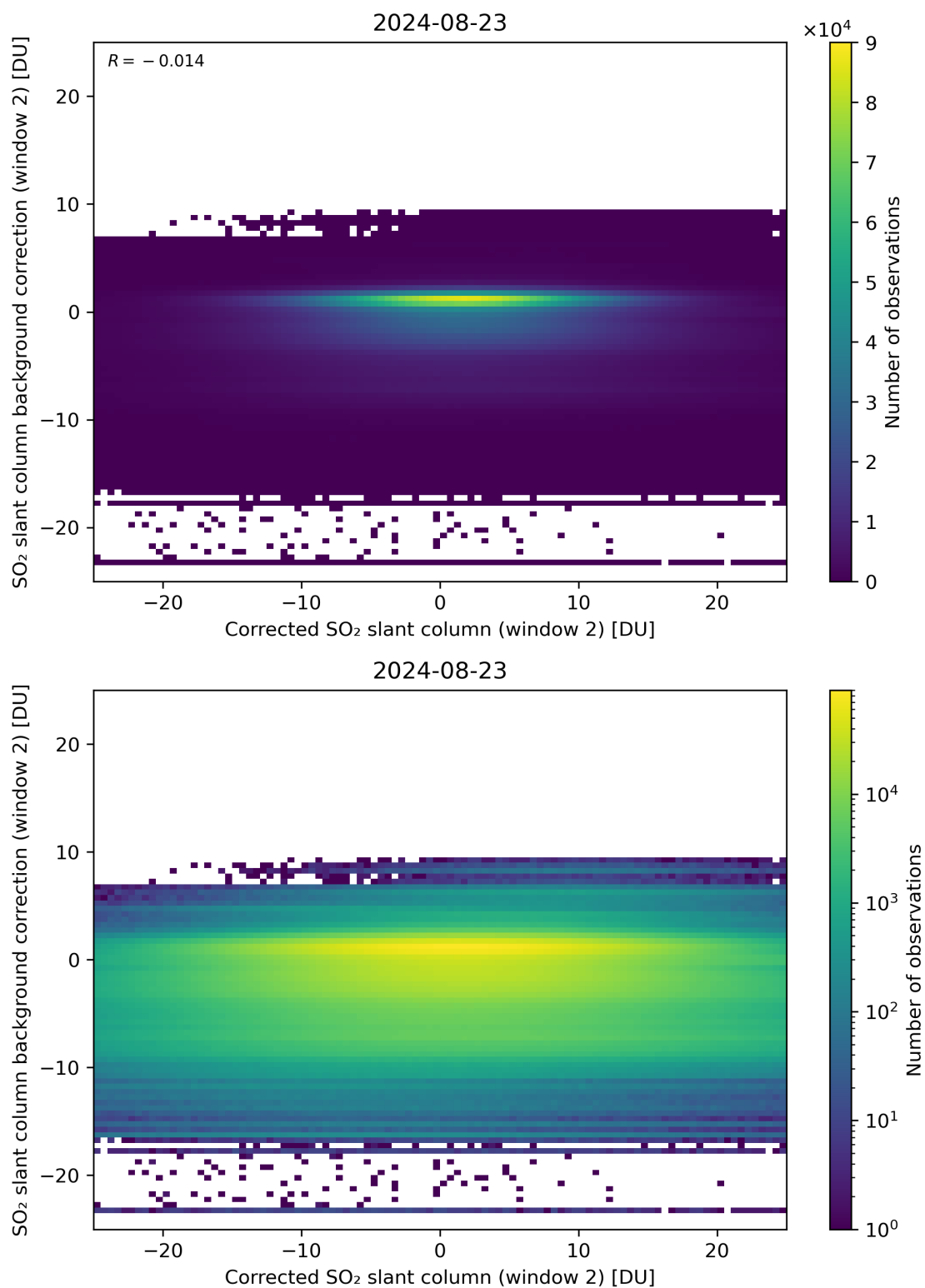
Figure 194: Scatter density plot of “Corrected SO 2 slant column (window 2)” against “SO 2 slant column background correction (window 2)” for 2024-08-22 to 2024-08-24.
