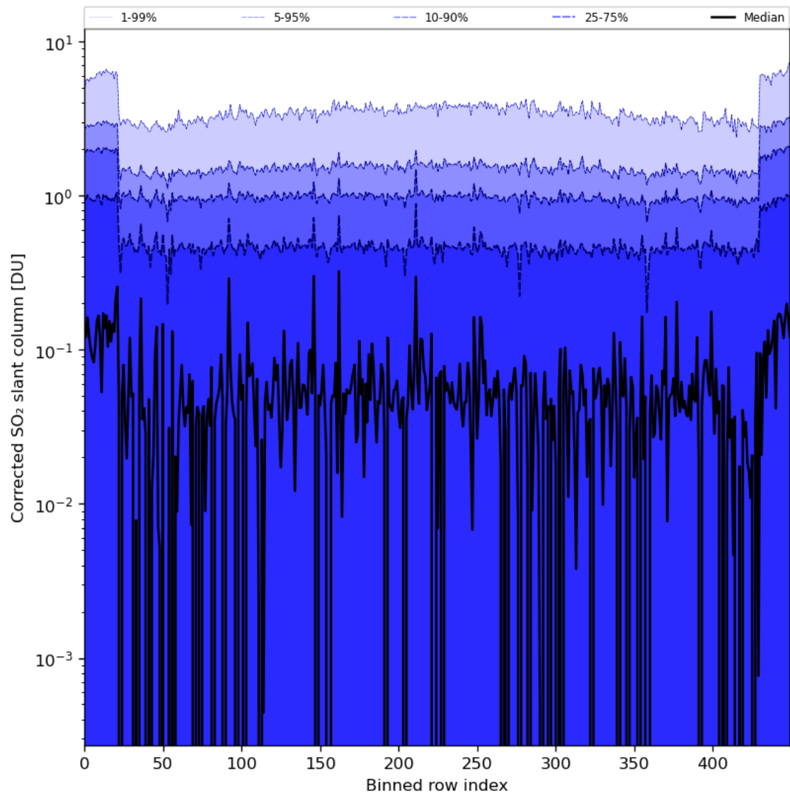
Figure 78: Along track statistics of “Corrected SO 2 slant column” for 2024-08-22 to 2024-08-24
