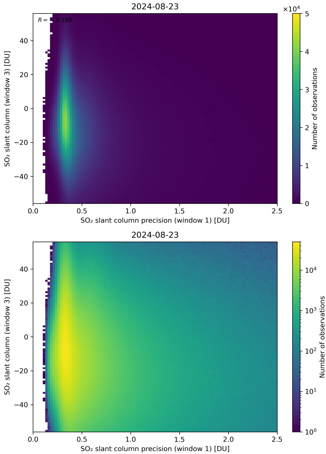
Figure 228: Scatter density plot of “SO 2 slant column precision (window 1)” against “SO 2 slant column (window 3)” for 2024-08-22 to 2024-08-24.
