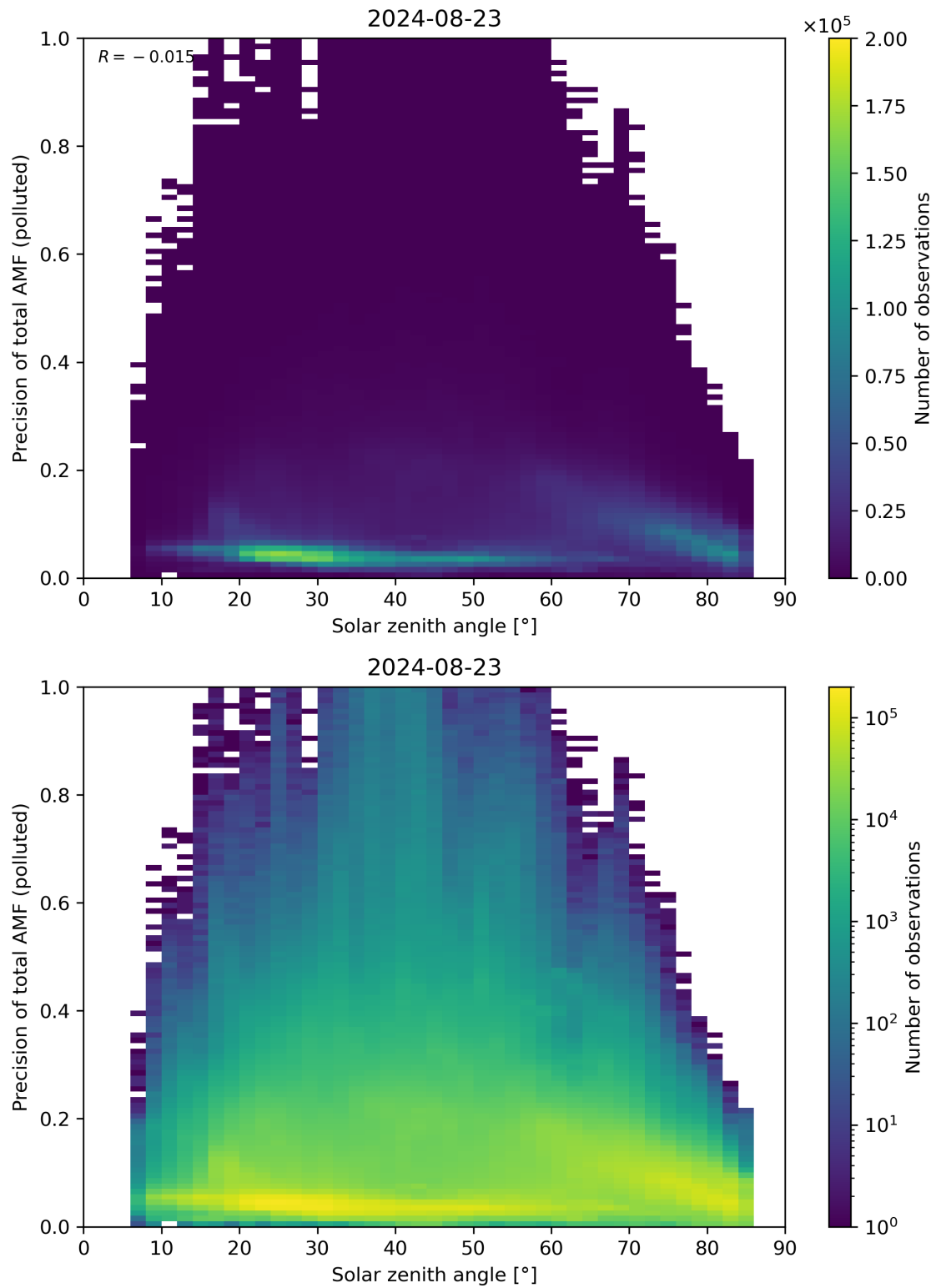
Figure 175: Scatter density plot of “Solar zenith angle” against “Precision of total AMF (polluted)” for 2024-08-22 to 2024-08-24.
