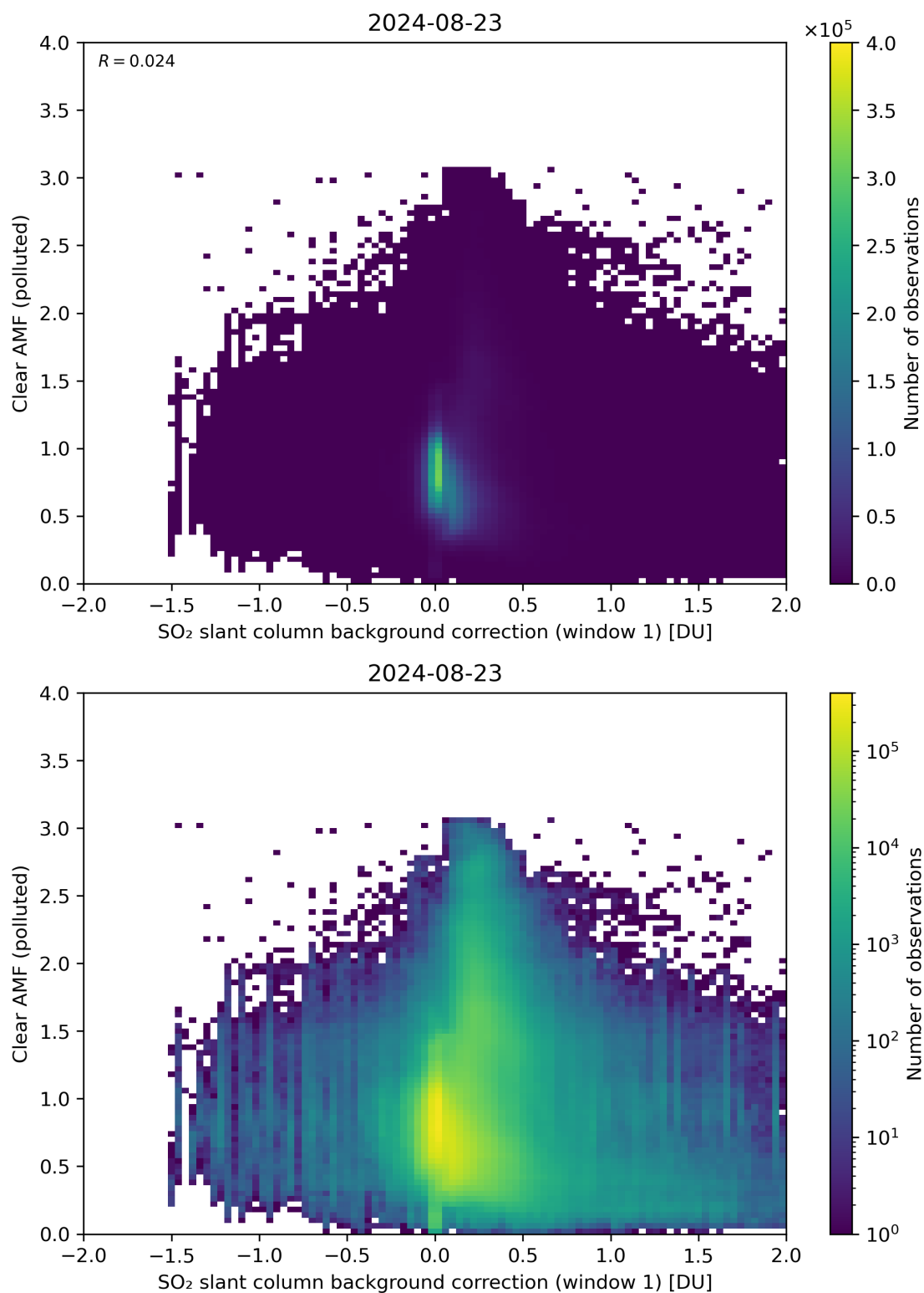
Figure 103: Scatter density plot of “SO 2 slant column background correction (window 1)” against “Clear AMF (polluted)” for 2024-08-22 to 2024-08-24.
