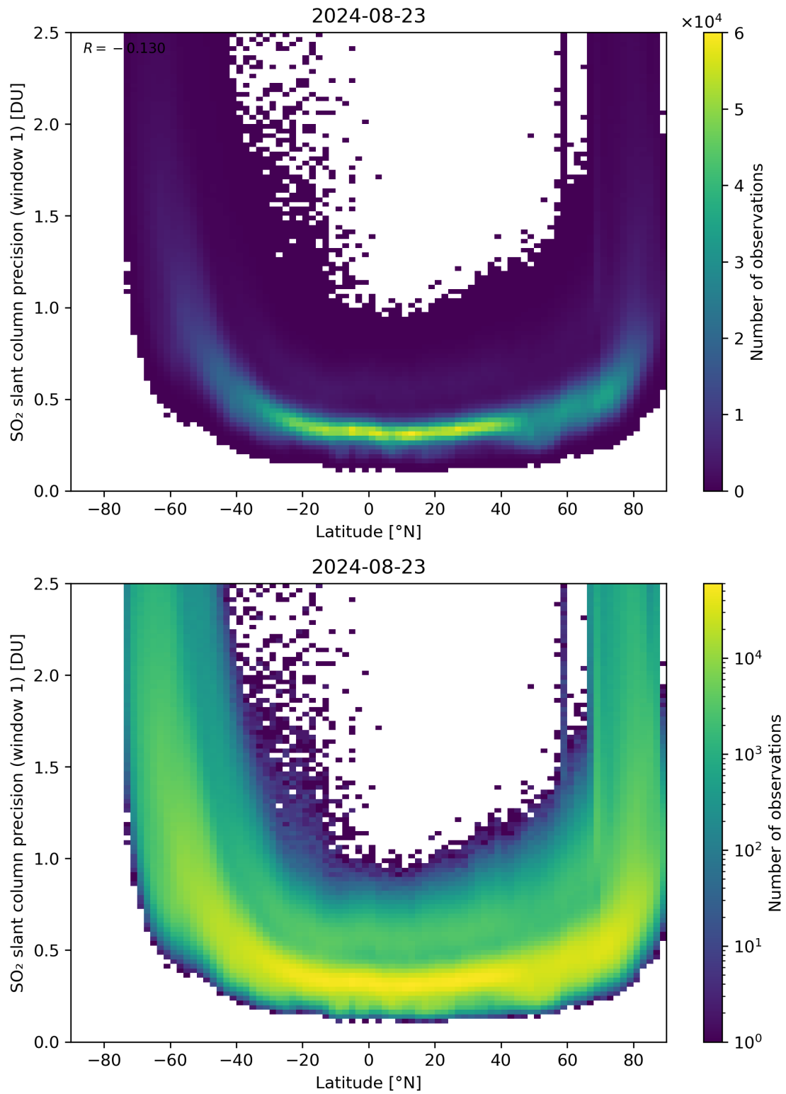
Figure 150: Scatter density plot of “Latitude” against “SO 2 slant column precision (window 1)” for 2024-08-22 to 2024-08-24.
