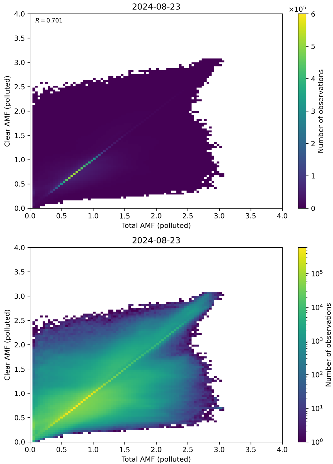
Figure 271: Scatter density plot of “Total AMF (polluted)” against “Clear AMF (polluted)” for 2024-08-22 to 2024-08-24.
