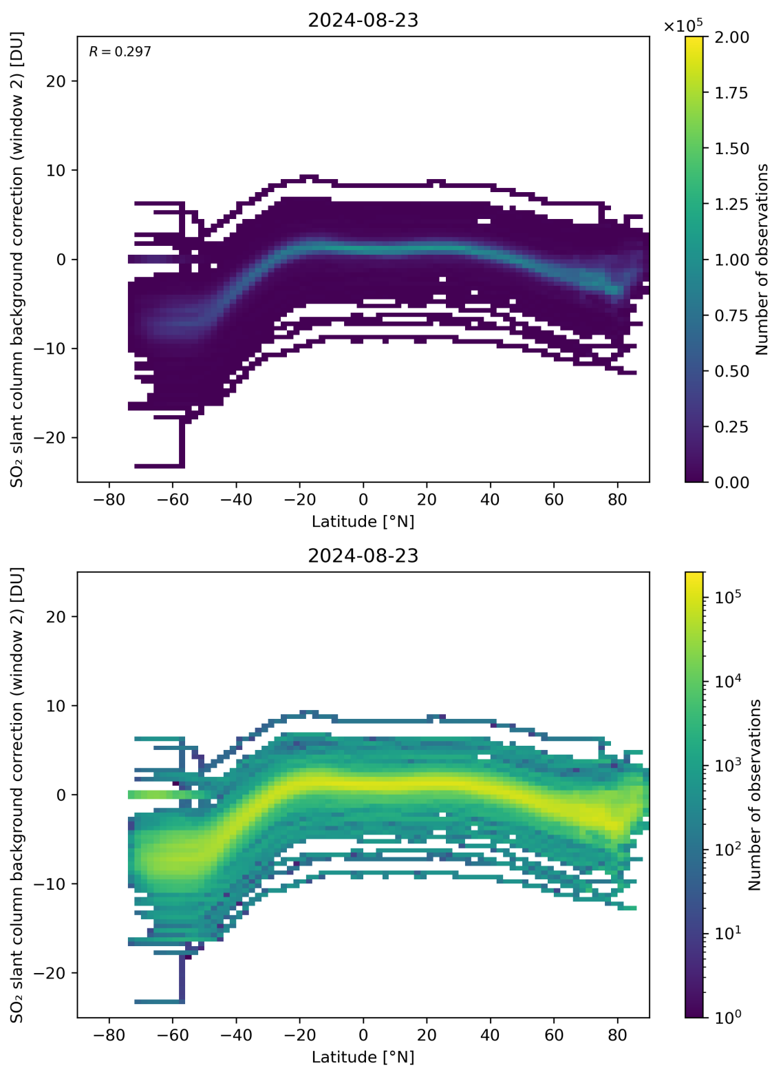
Figure 140: Scatter density plot of “Latitude” against “SO 2 slant column background correction (window 2)” for 2024-08-22 to 2024-08-24.
