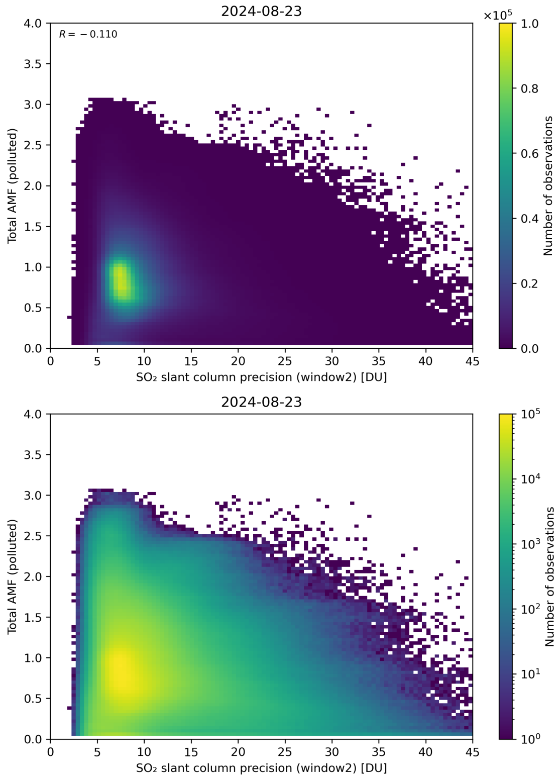
Figure 251: Scatter density plot of “SO 2 slant column precision (window2)” against “Total AMF (polluted)” for 2024-08-22 to 2024-08-24.
