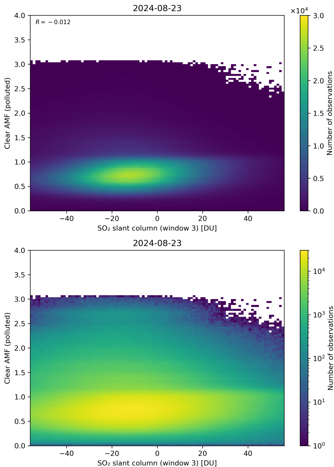
Figure 265: Scatter density plot of “SO 2 slant column (window 3)” against “Clear AMF (polluted)” for 2024-08-22 to 2024-08-24.
