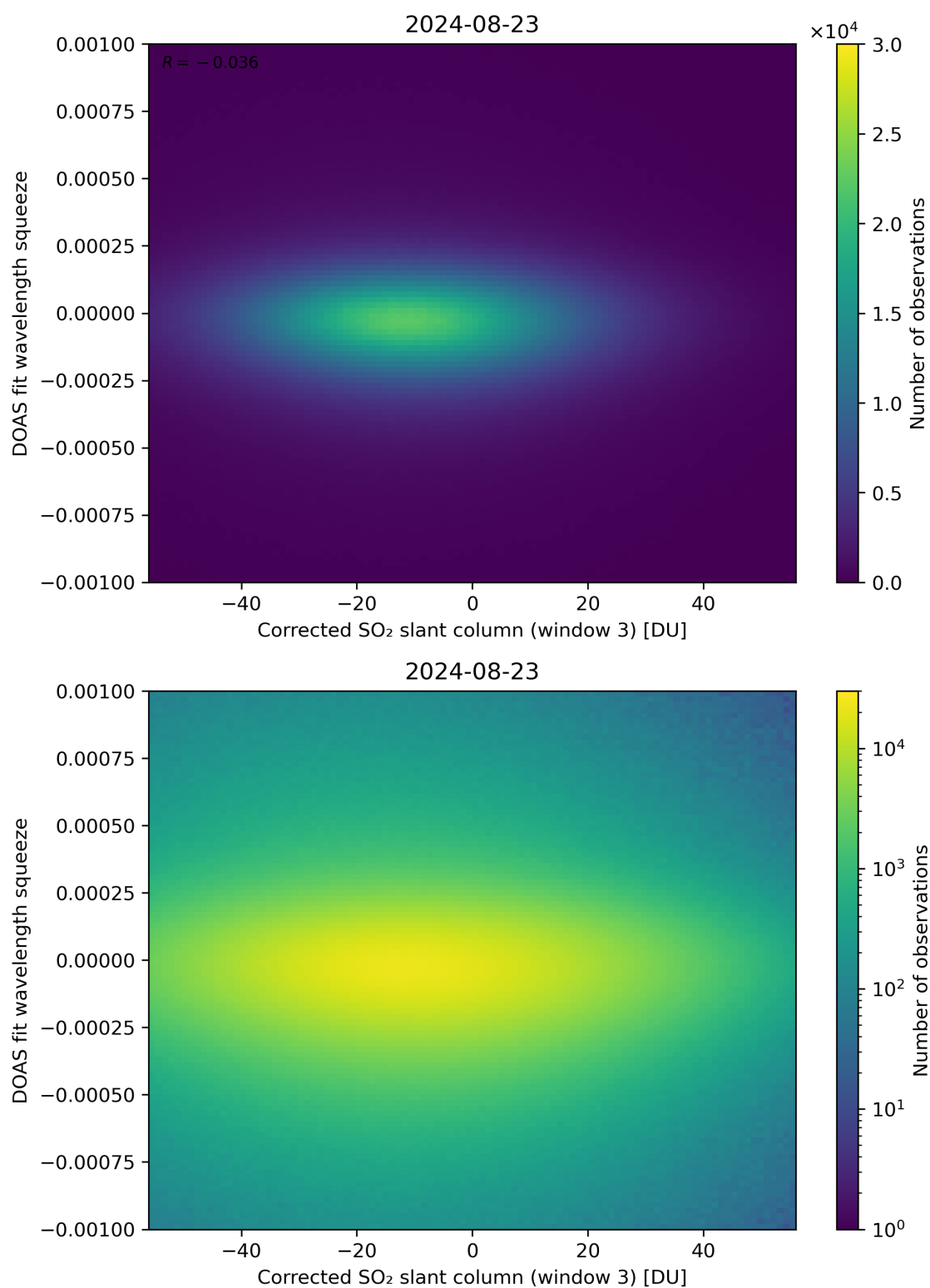
Figure 207: Scatter density plot of “Corrected SO 2 slant column (window 3)” against “DOAS fit wavelength squeeze” for 2024-08-22 to 2024-08-24.
