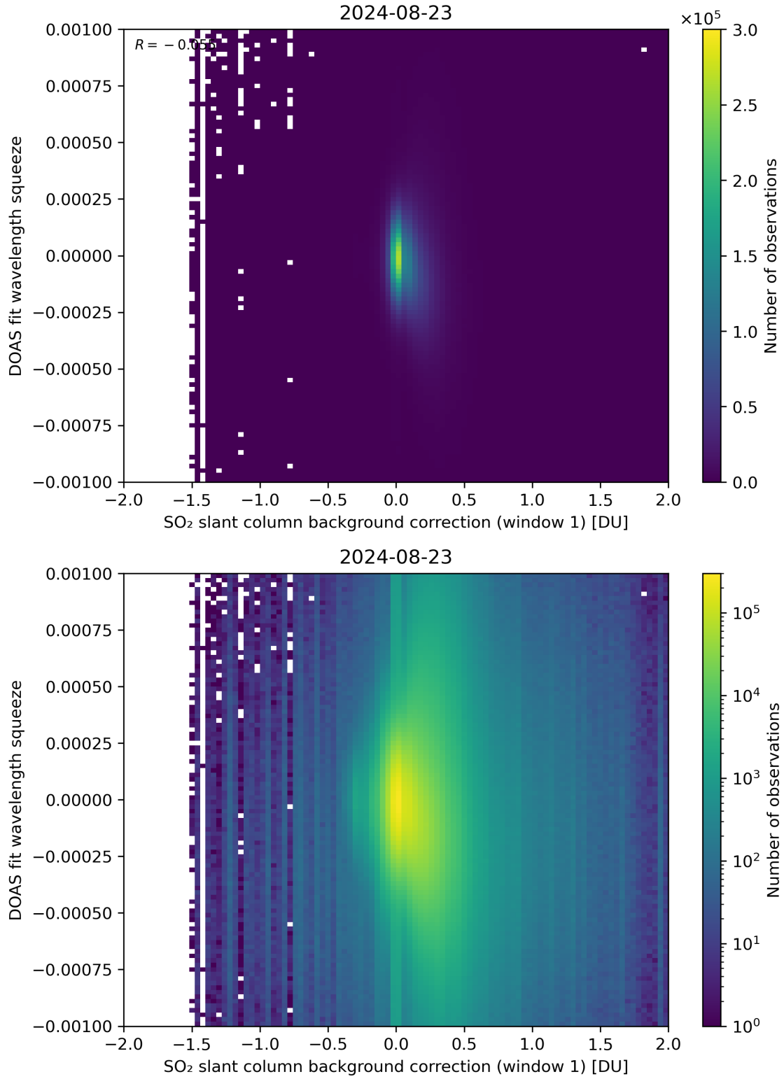
Figure 101: Scatter density plot of “SO 2 slant column background correction (window 1)” against “DOAS fit wavelength squeeze” for 2024-08-22 to 2024-08-24.
