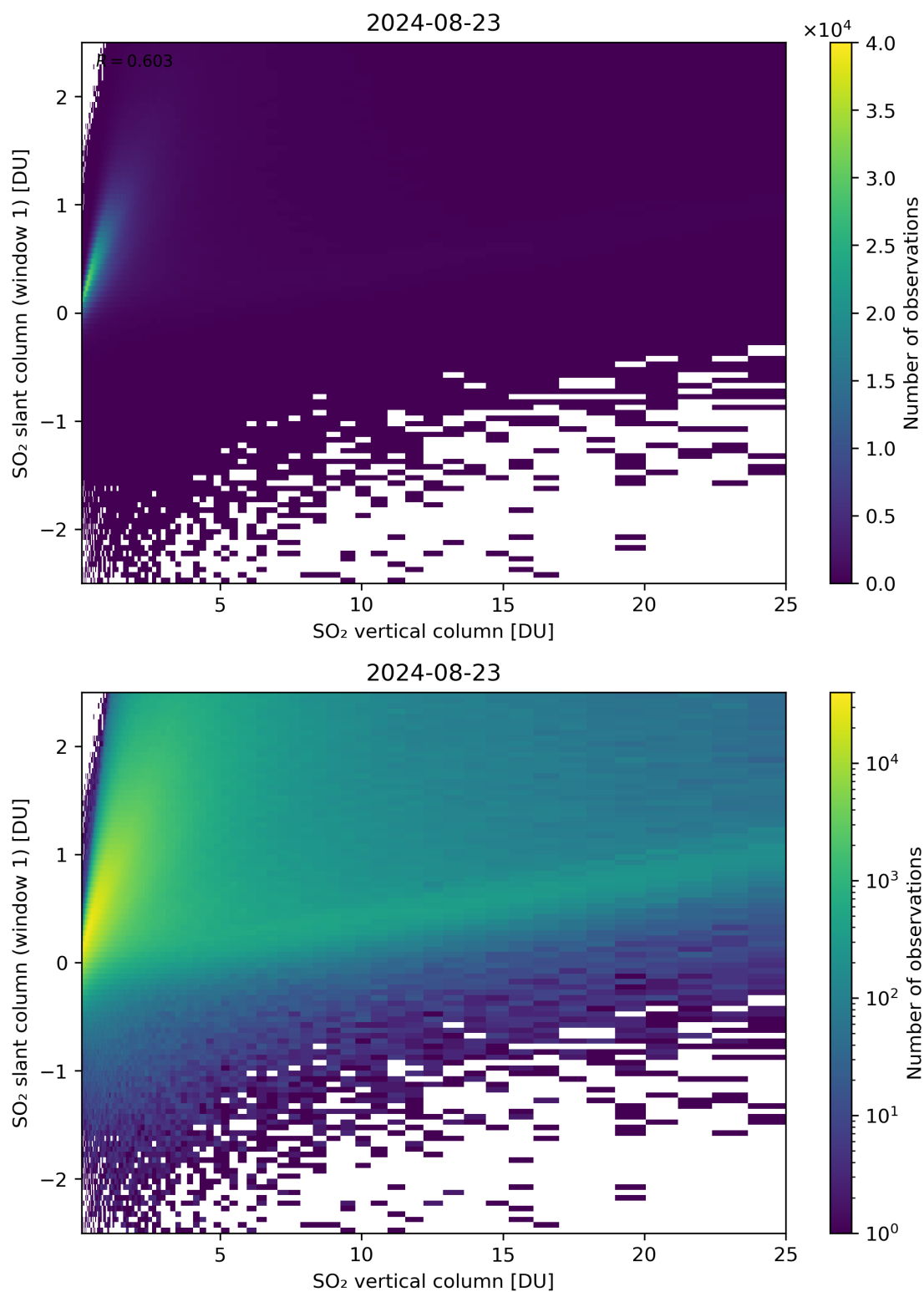
Figure 300: Scatter density plot of “SO 2 vertical column” against “SO 2 slant column (window 1)” for 2024-08-22 to 2024-08-24.
