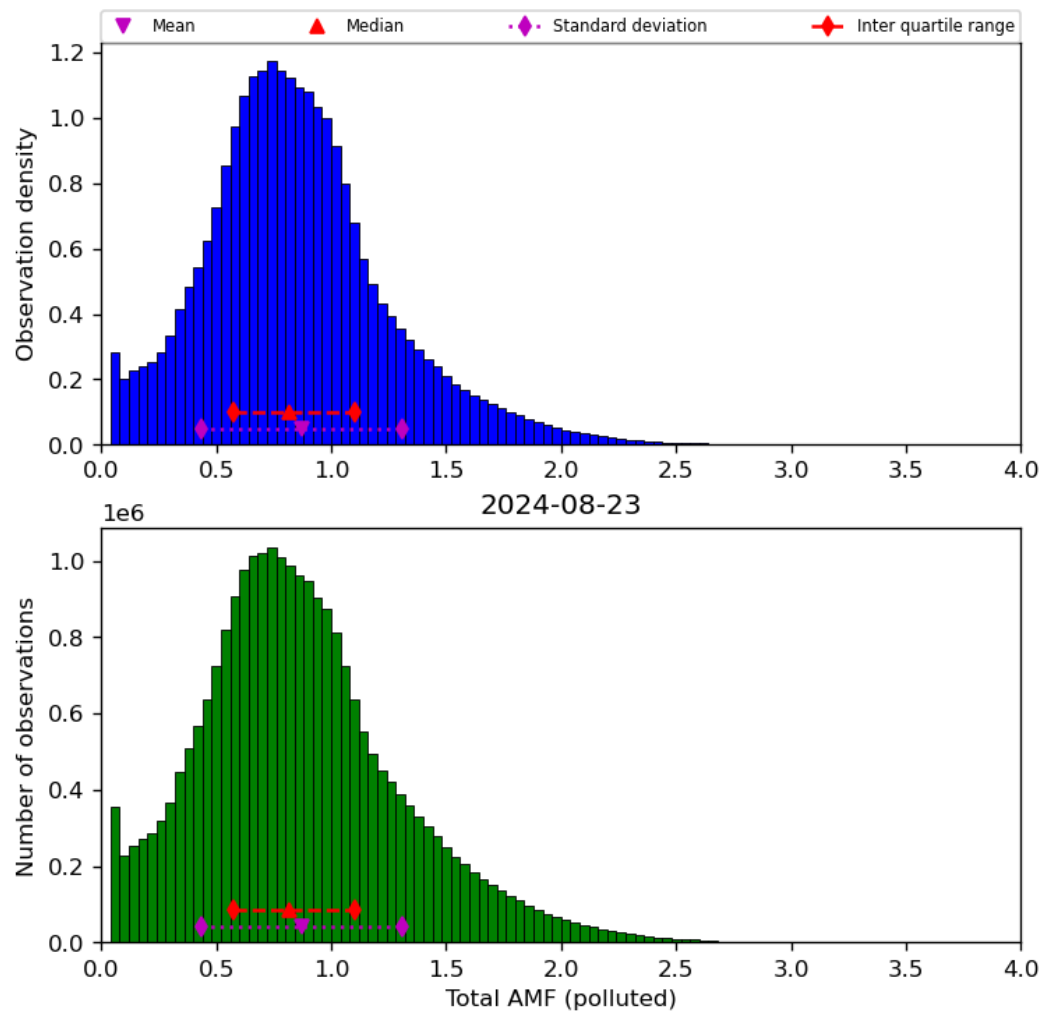
Figure 71: Histogram of “Total AMF (polluted)” for 2024-08-22 to 2024-08-24
