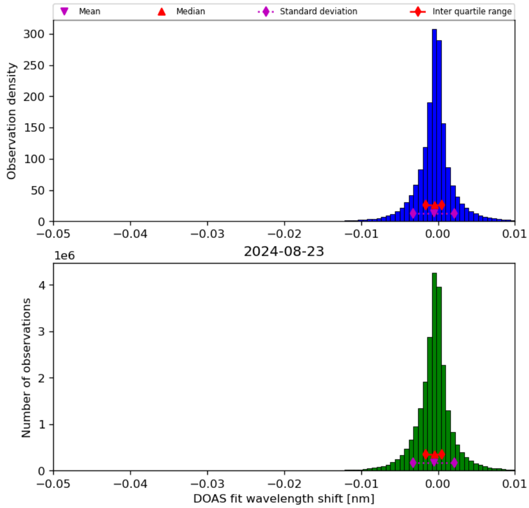
Figure 68: Histogram of “DOAS fit wavelength shift” for 2024-08-22 to 2024-08-24
