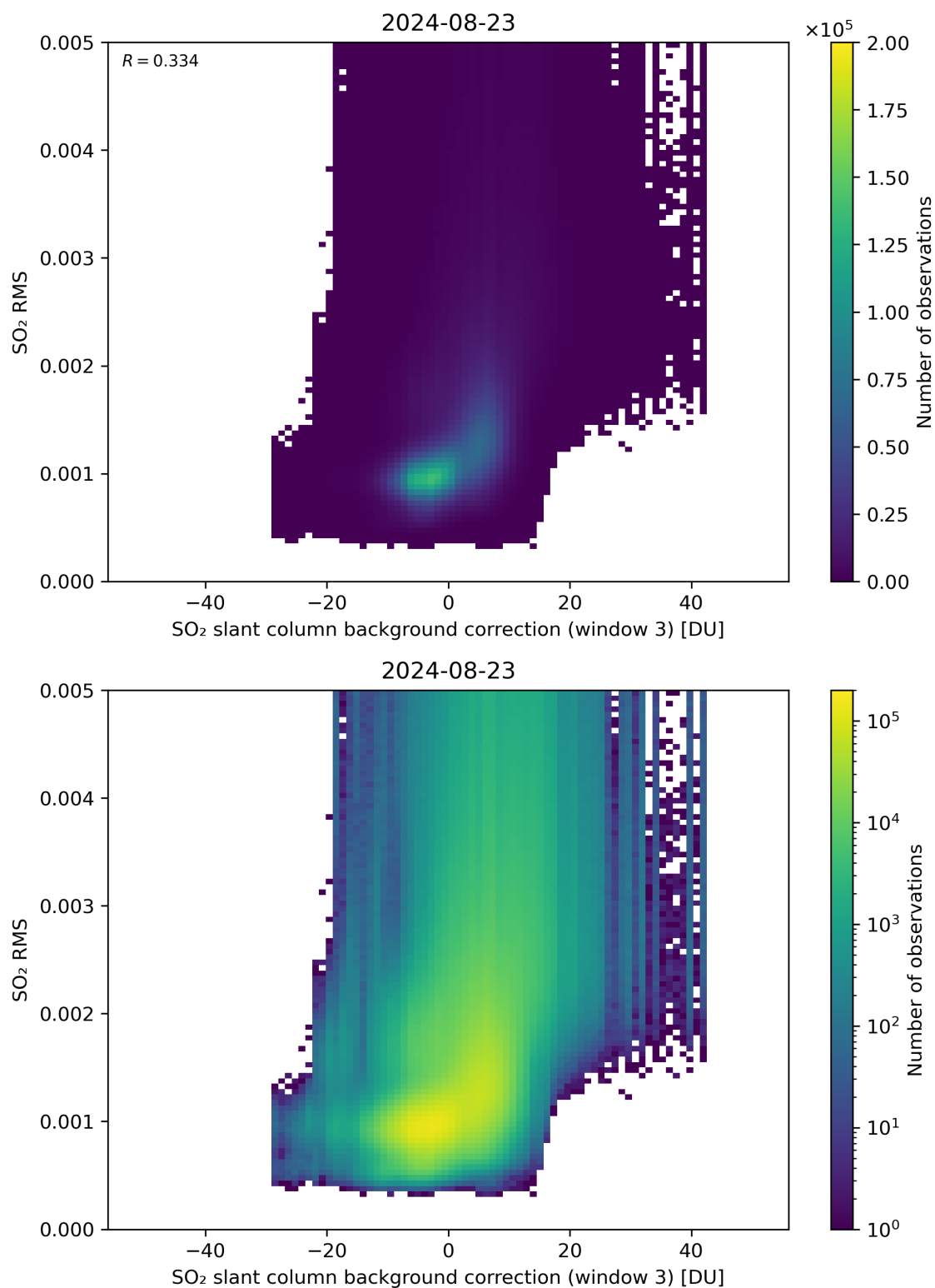
Figure 123: Scatter density plot of “SO 2 slant column background correction (window 3)” against “SO 2 RMS” for 2024-08-22 to 2024-08-24.
