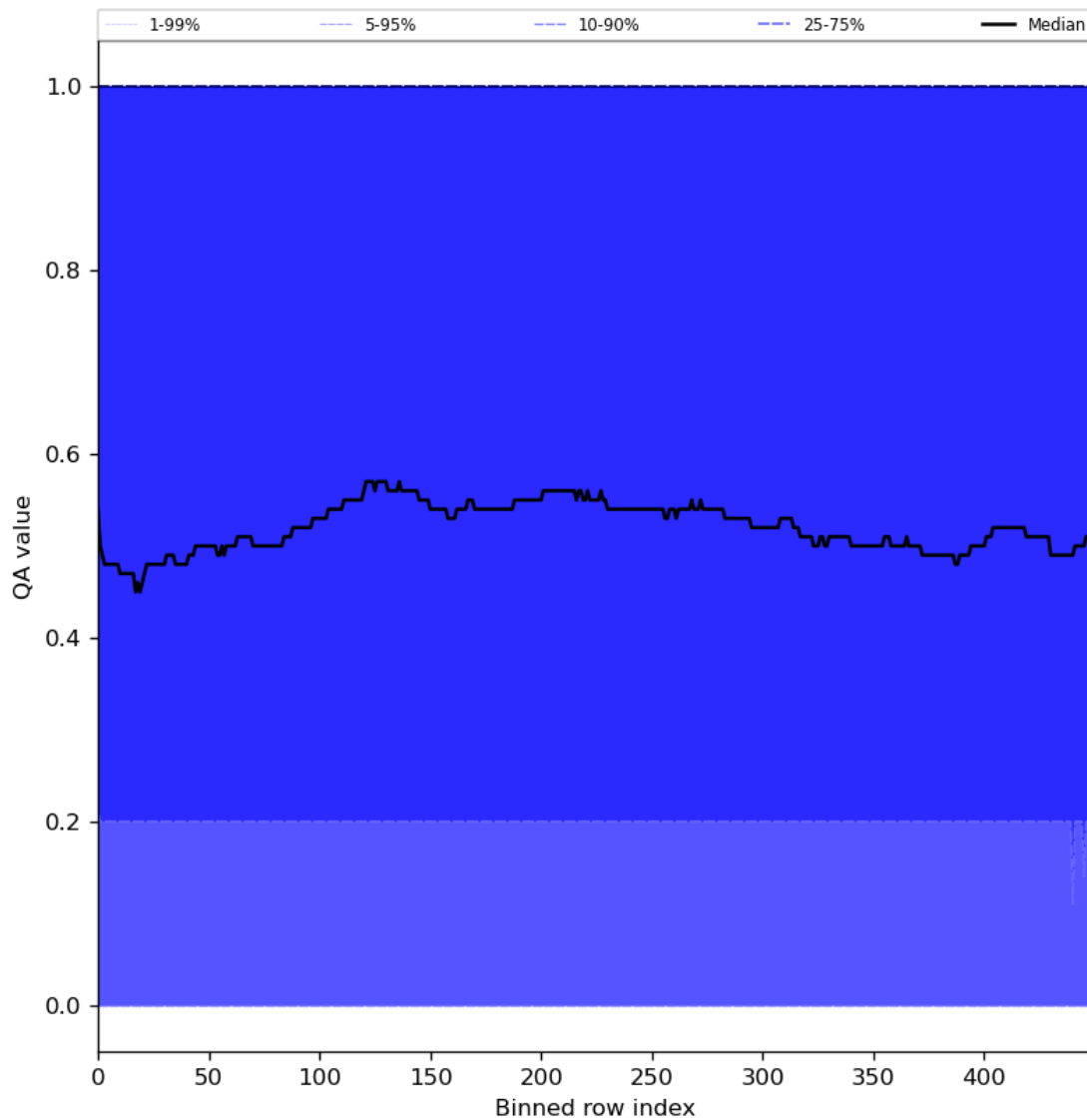
Figure 75: Along track statistics of “QA value” for 2024-08-22 to 2024-08-24
