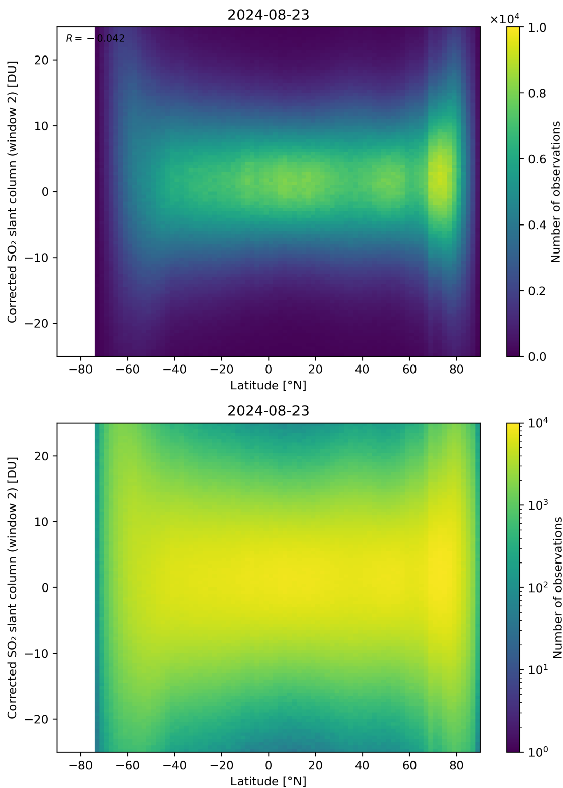
Figure 147: Scatter density plot of “Latitude” against “Corrected SO 2 slant column (window 2)” for 2024-08-22 to 2024-08-24.
