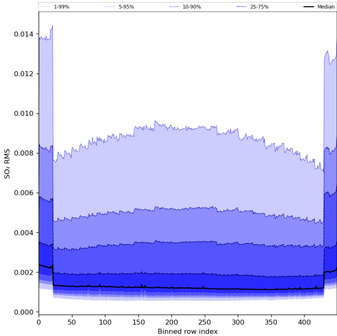
Figure 93: Along track statistics of “SO 2 RMS” for 2024-08-22 to 2024-08-24
