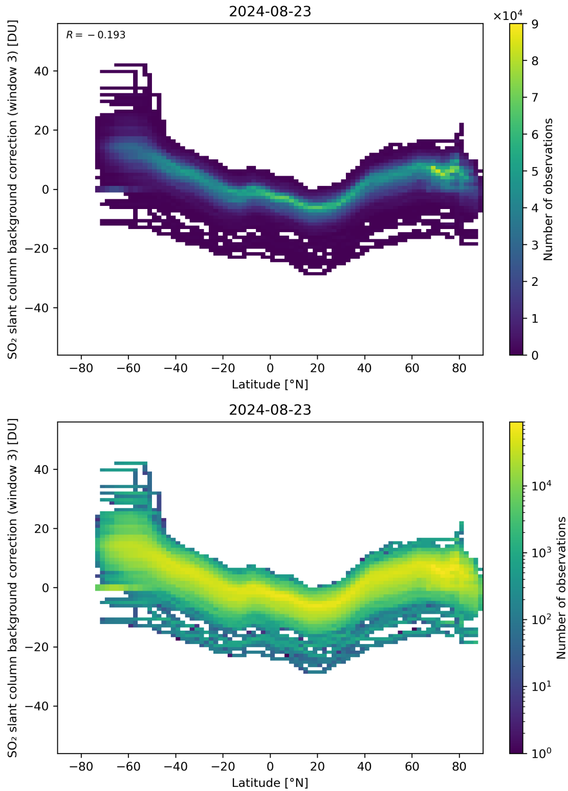
Figure 141: Scatter density plot of “Latitude” against “SO 2 slant column background correction (window 3)” for 2024-08-22 to 2024-08-24.
