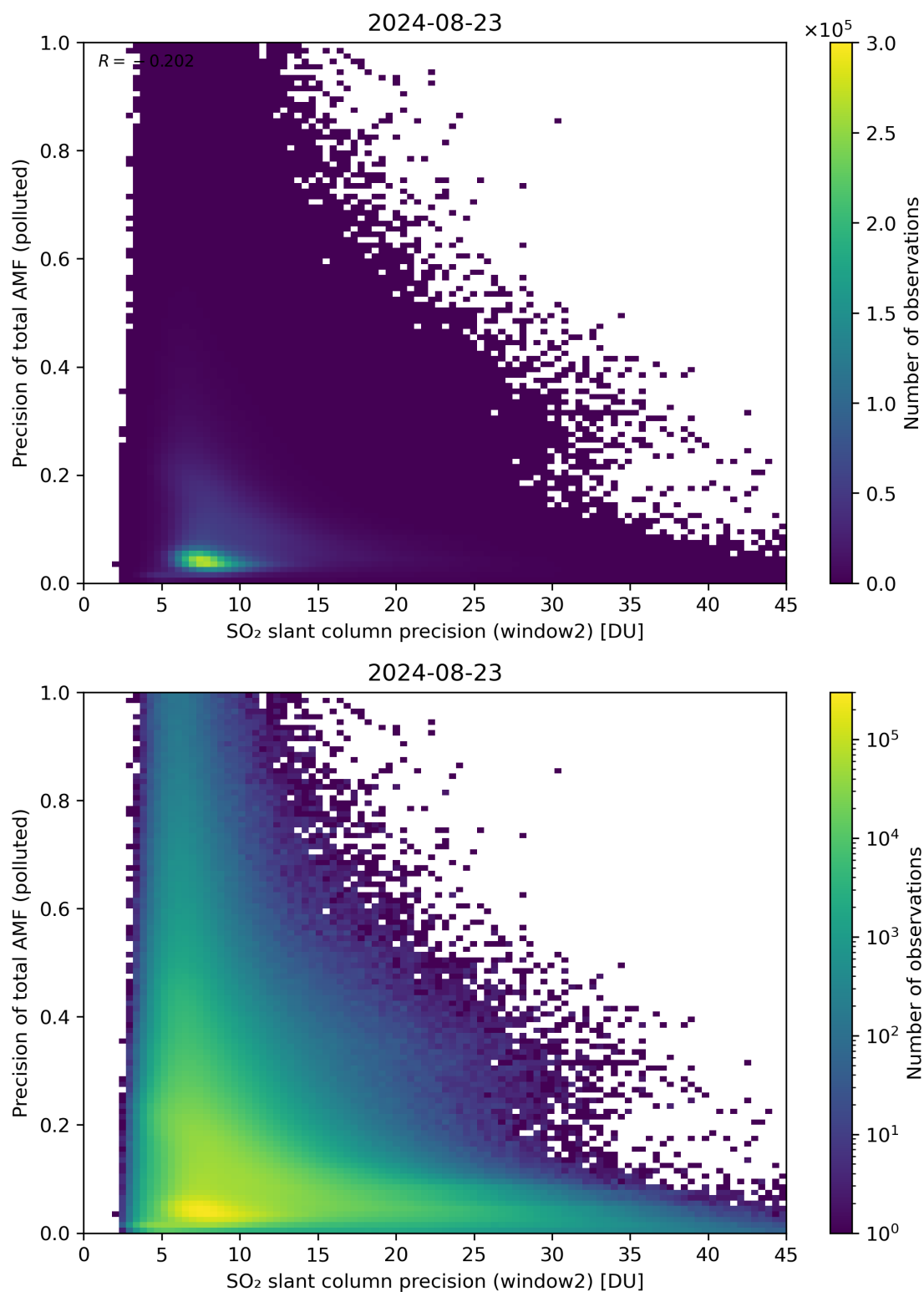
Figure 252: Scatter density plot of “SO 2 slant column precision (window2)” against “Precision of total AMF (polluted)” for 2024-08-22 to 2024-08-24.
