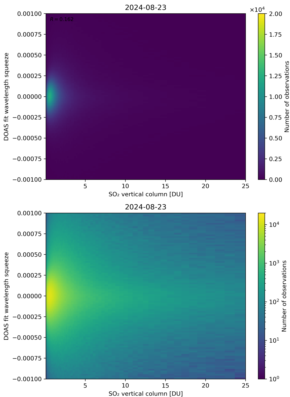
Figure 277: Scatter density plot of “SO 2 vertical column” against “DOAS fit wavelength squeeze” for 2024-08-22 to 2024-08-24.
