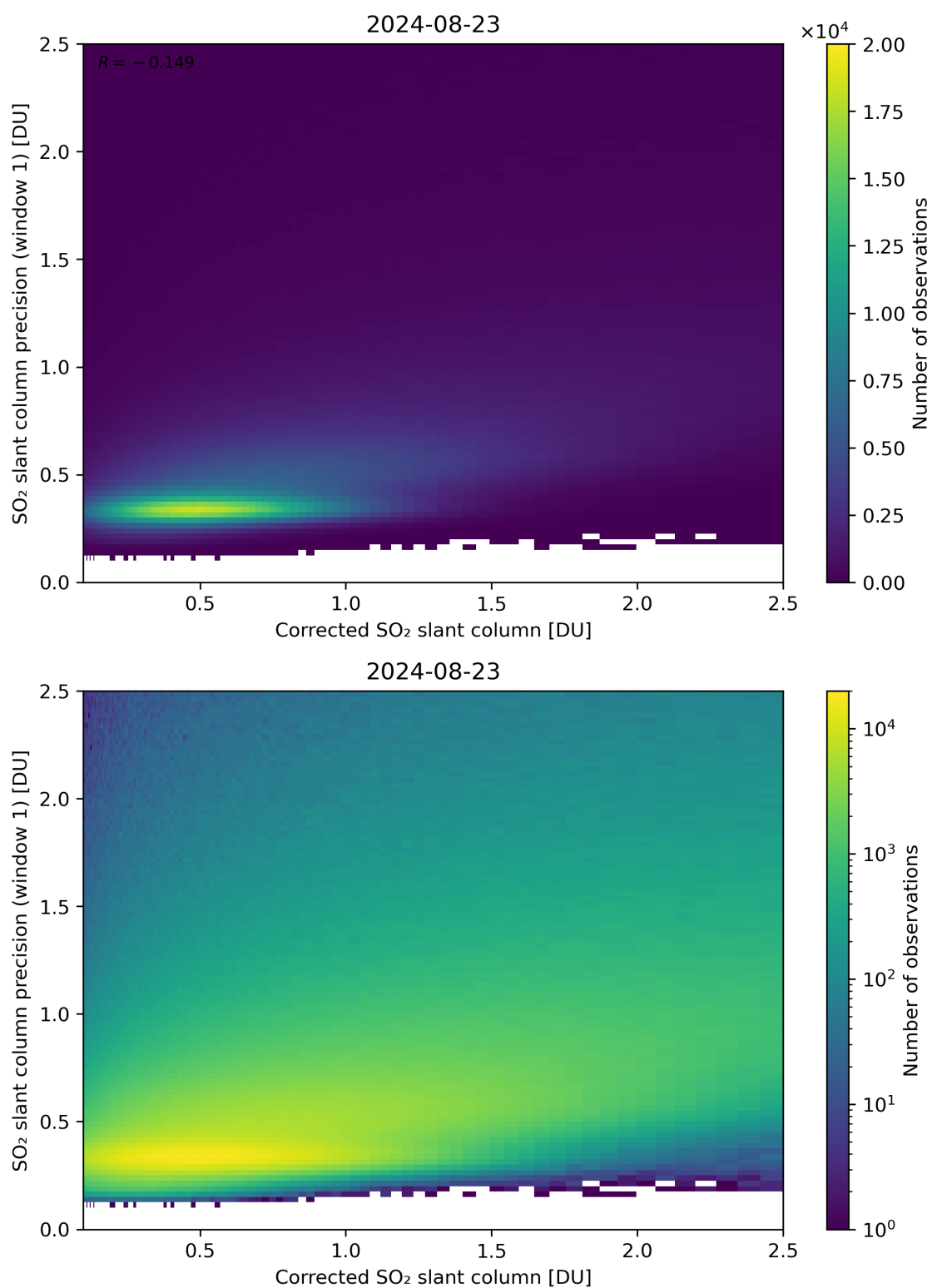
Figure 188: Scatter density plot of “Corrected SO 2 slant column” against “SO 2 slant column precision (window 1)” for 2024-08-22 to 2024-08-24.
