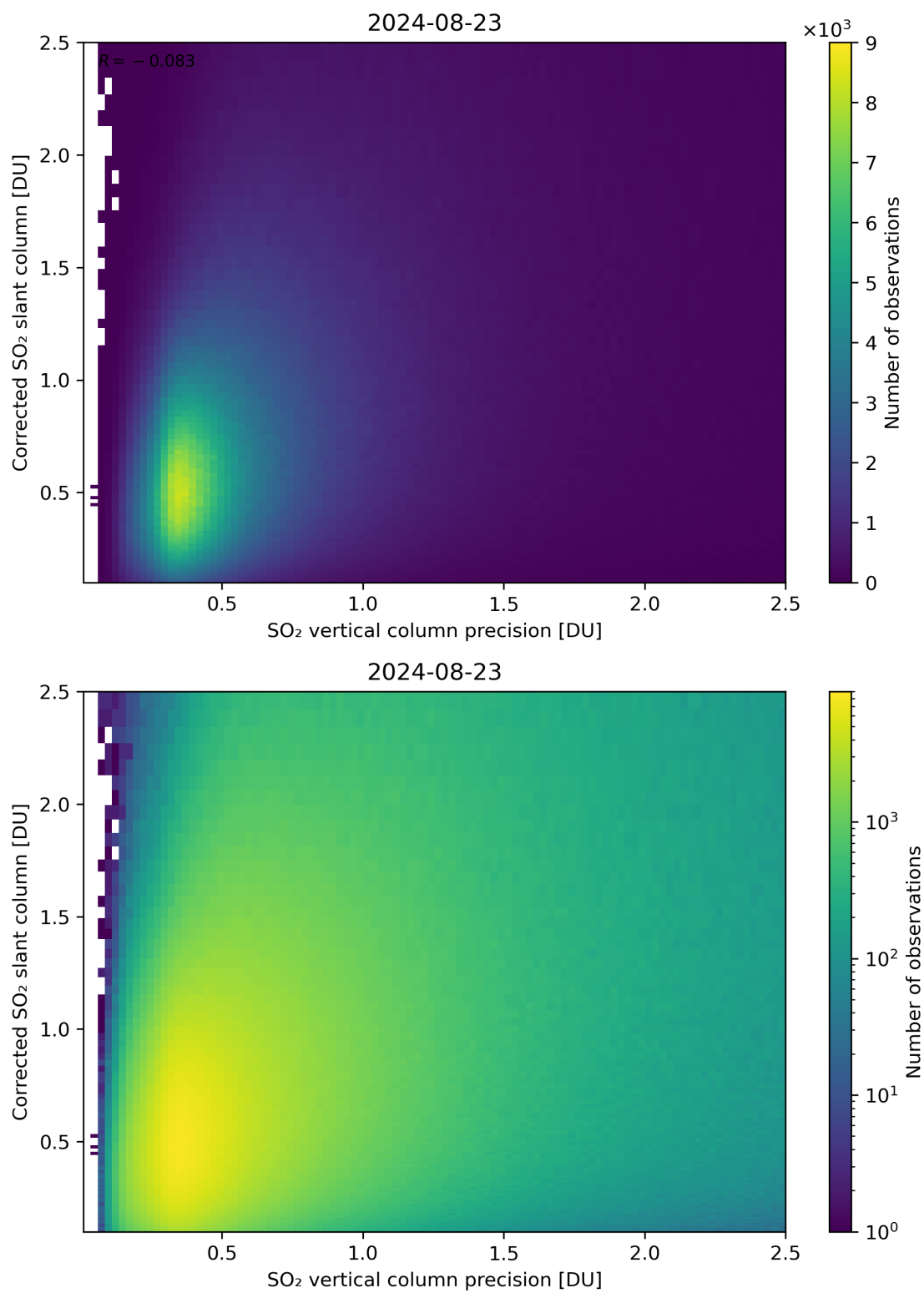
Figure 286: Scatter density plot of “SO 2 vertical column precision” against “Corrected SO 2 slant column” for 2024-08-22 to 2024-08-24.
