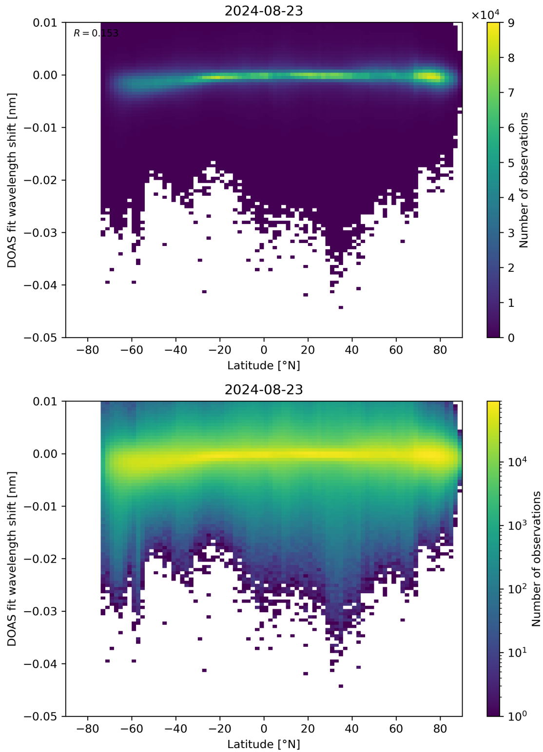
Figure 142: Scatter density plot of “Latitude” against “DOAS fit wavelength shift” for 2024-08-22 to 2024-08-24.
