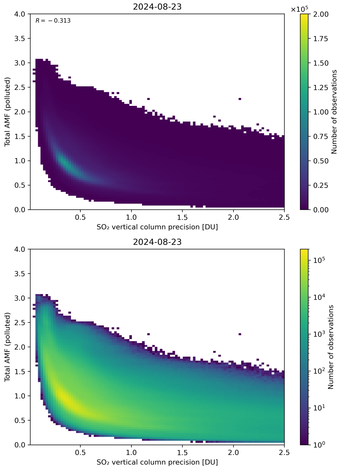
Figure 294: Scatter density plot of “SO 2 vertical column precision” against “Total AMF (polluted)” for 2024-08-22 to 2024-08-24.
