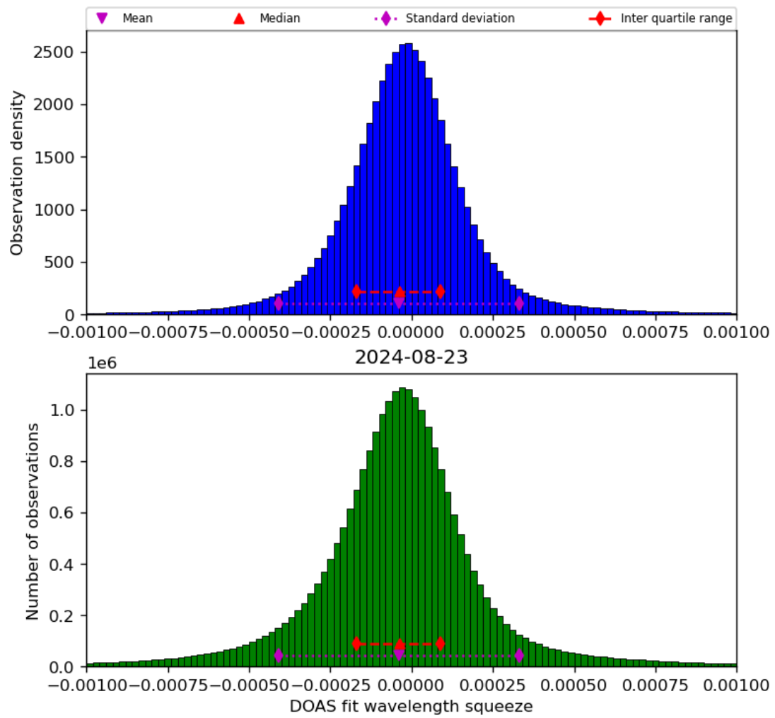
Figure 69: Histogram of “DOAS fit wavelength squeeze” for 2024-08-22 to 2024-08-24
