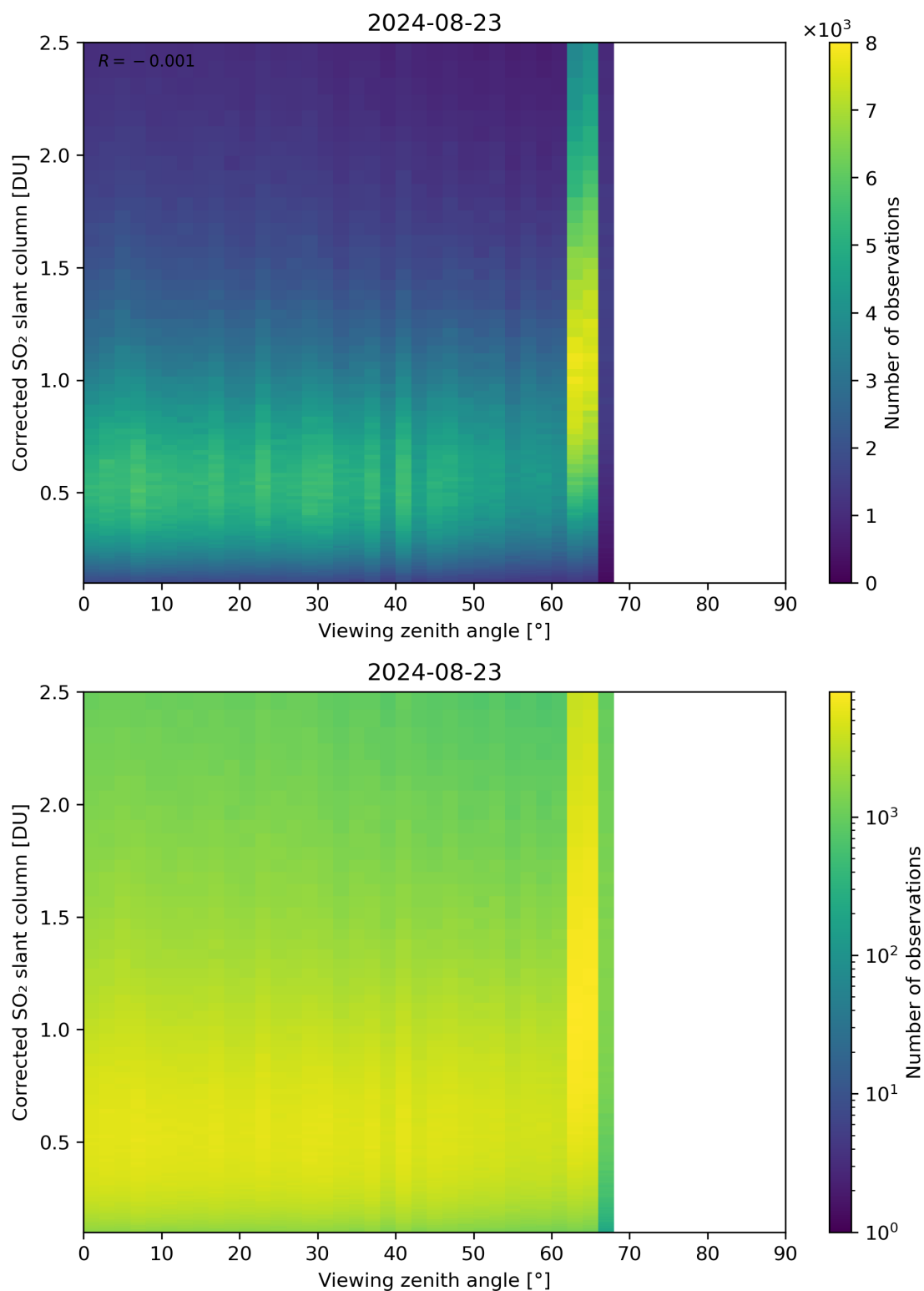
Figure 317: Scatter density plot of “Viewing zenith angle” against “Corrected SO 2 slant column” for 2024-08-22 to 2024-08-24.
