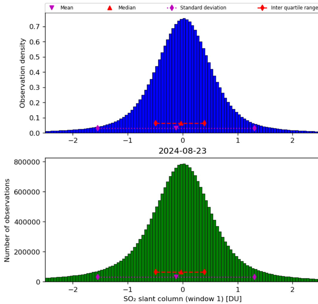
Figure 56: Histogram of “SO 2 slant column (window 1)” for 2024-08-22 to 2024-08-24
