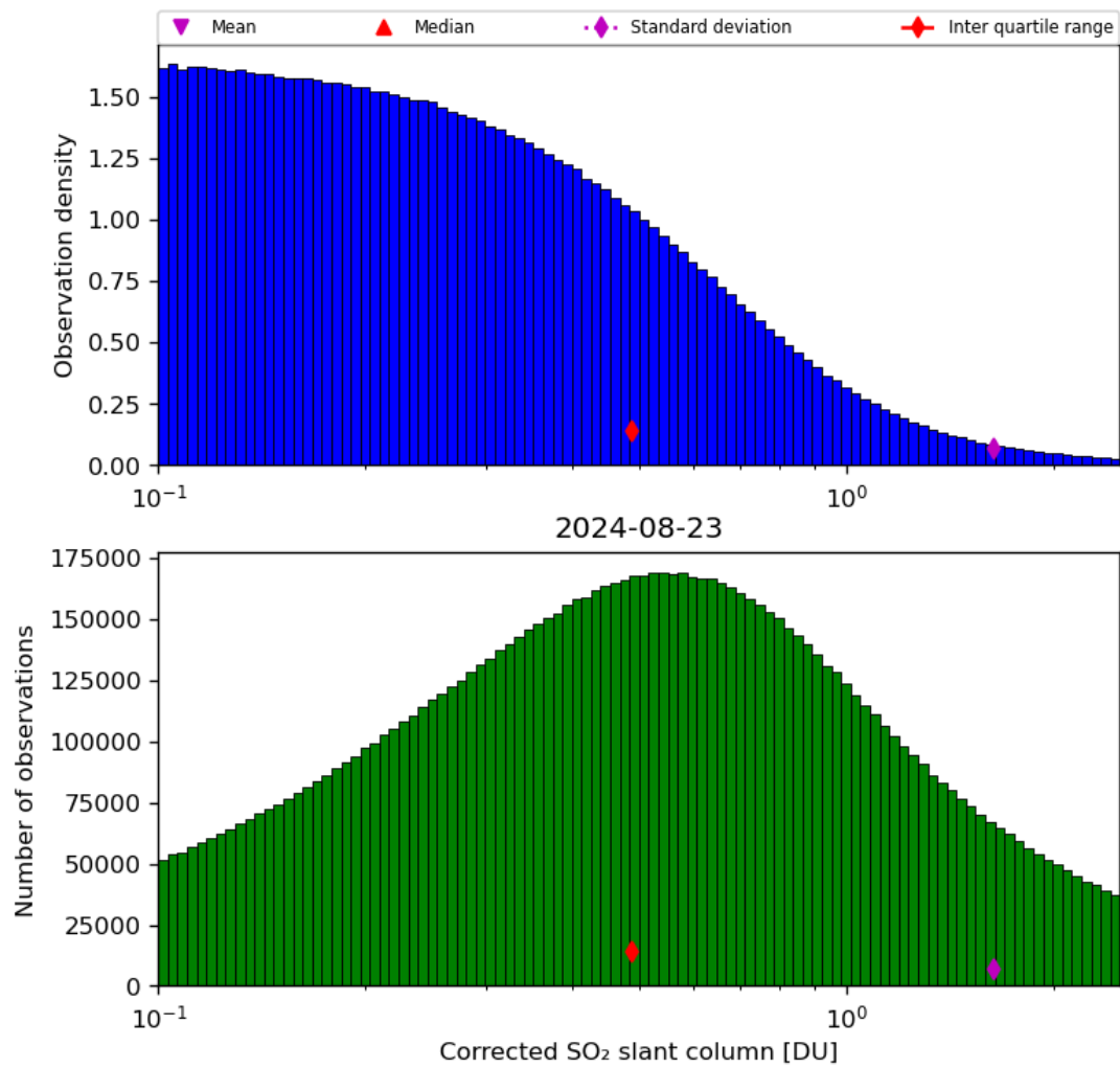
Figure 55: Histogram of “Corrected SO 2 slant column” for 2024-08-22 to 2024-08-24
