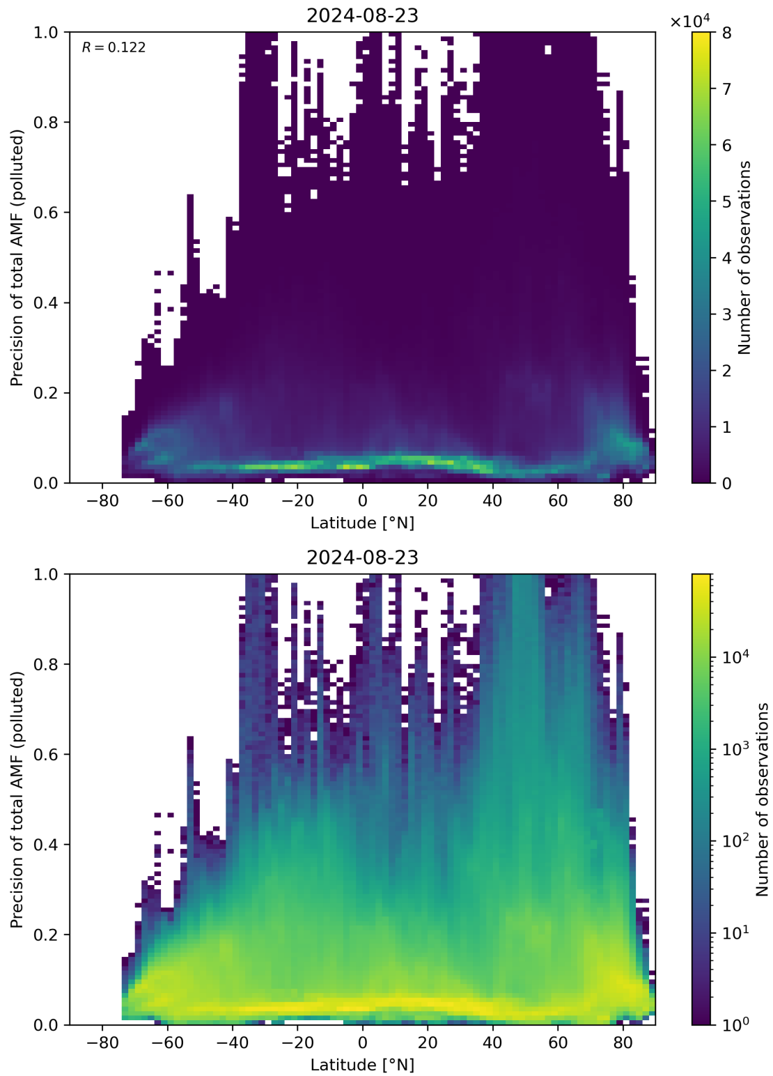
Figure 155: Scatter density plot of “Latitude” against “Precision of total AMF (polluted)” for 2024-08-22 to 2024-08-24.
