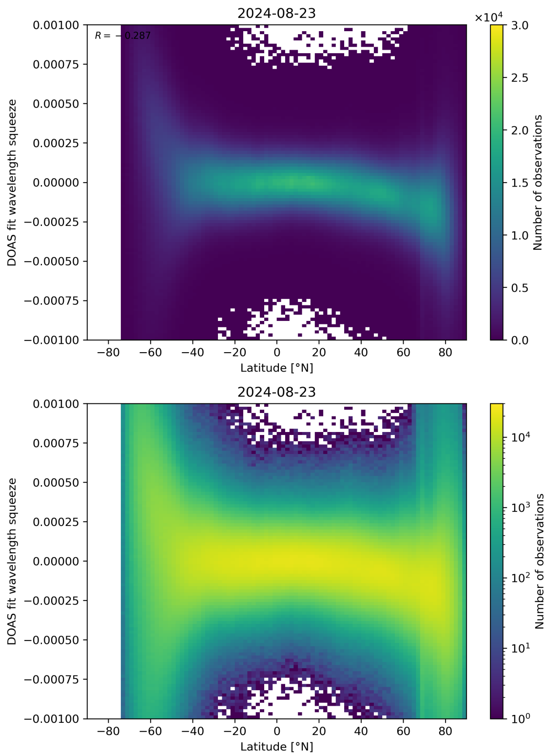
Figure 143: Scatter density plot of “Latitude” against “DOAS fit wavelength squeeze” for 2024-08-22 to 2024-08-24.
