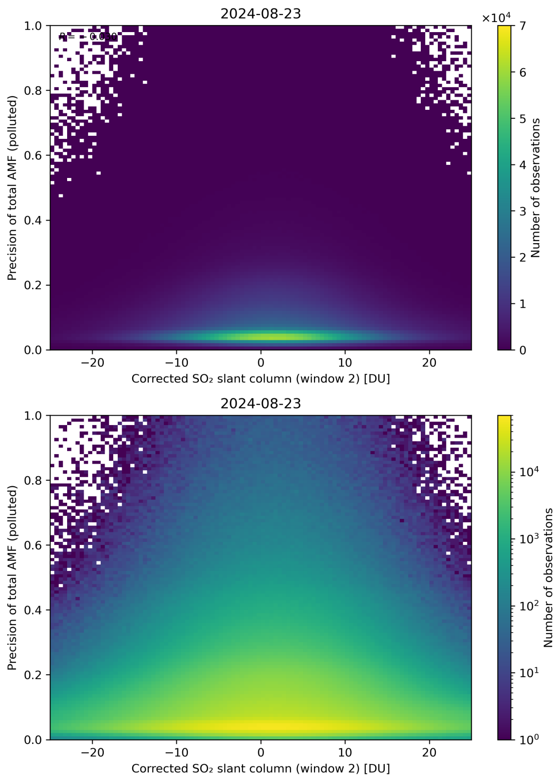
Figure 204: Scatter density plot of “Corrected SO 2 slant column (window 2)” against “Precision of total AMF (polluted)” for 2024-08-22 to 2024-08-24.
