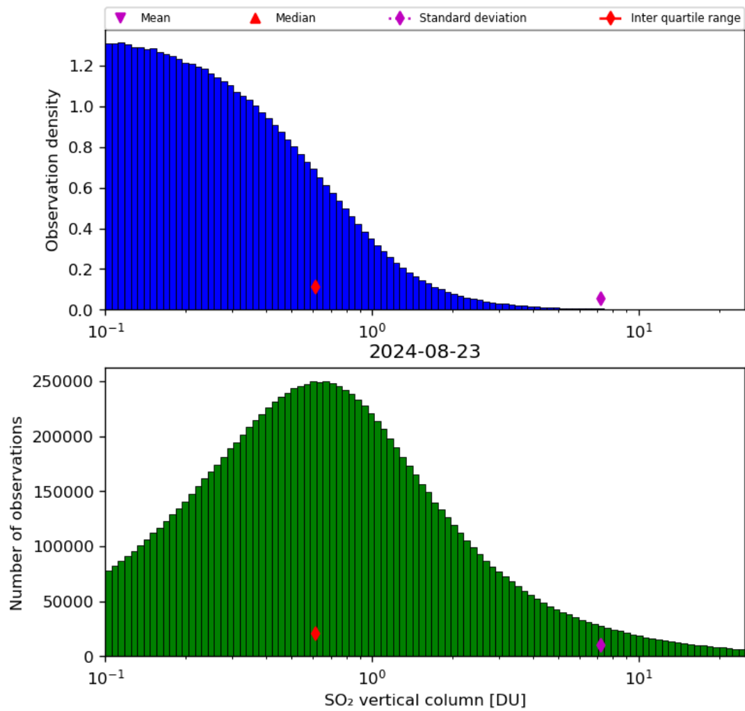
Figure 53: Histogram of “SO 2 vertical column” for 2024-08-22 to 2024-08-24
