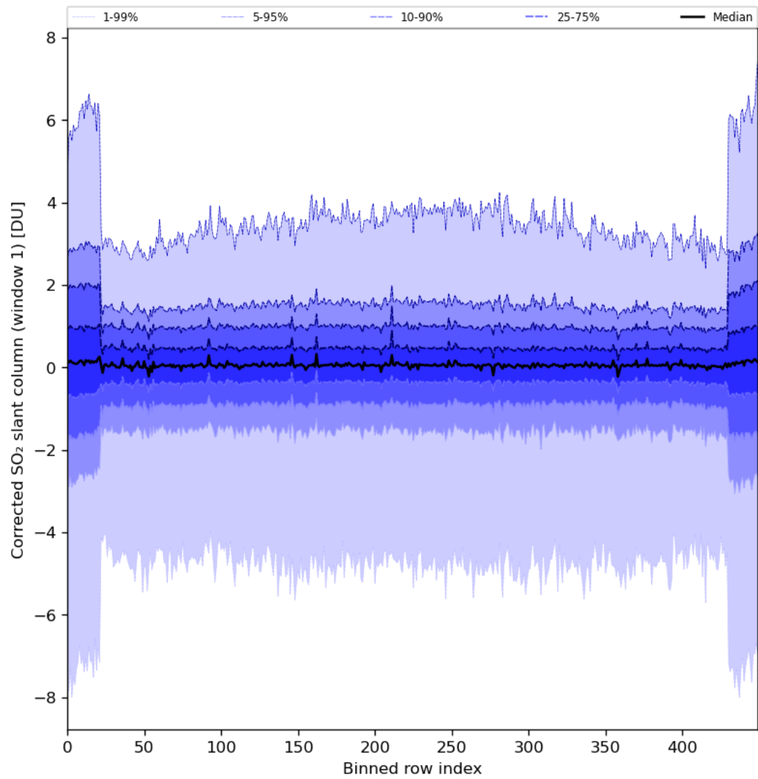
Figure 81: Along track statistics of “Corrected SO 2 slant column (window 1)” for 2024-08-22 to 2024-08-24
