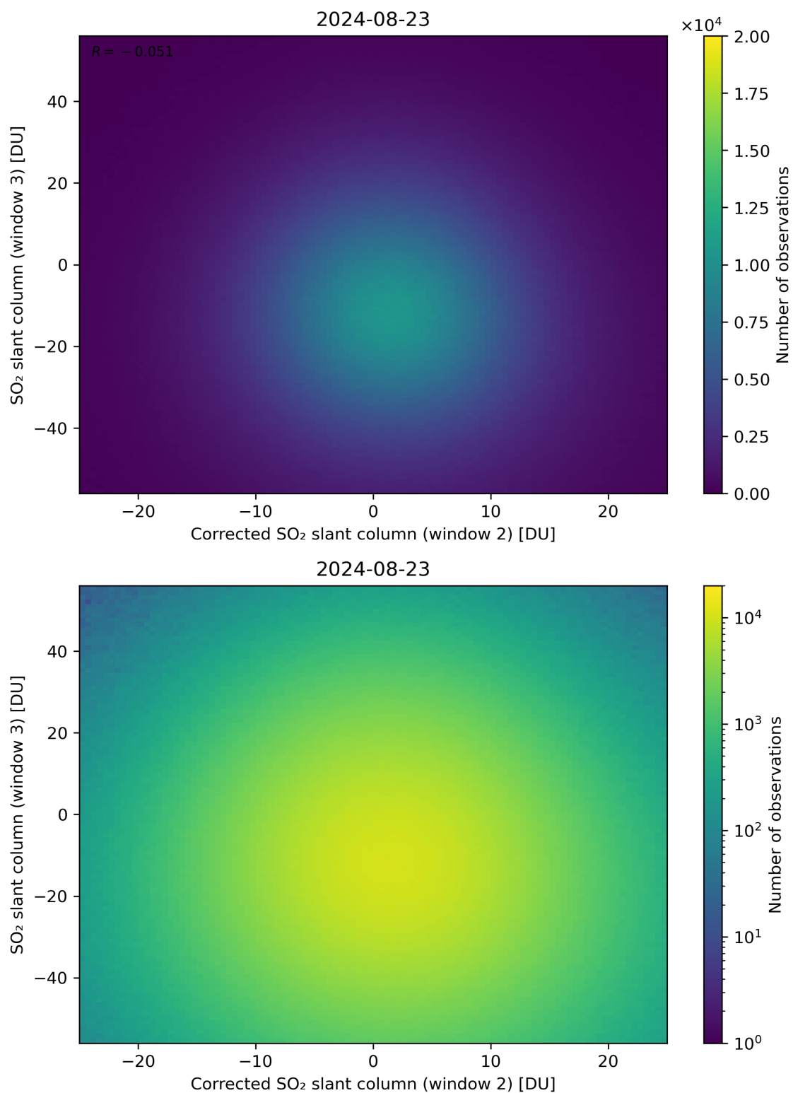
Figure 201: Scatter density plot of “Corrected SO 2 slant column (window 2)” against “SO 2 slant column (window 3)” for 2024-08-22 to 2024-08-24.
