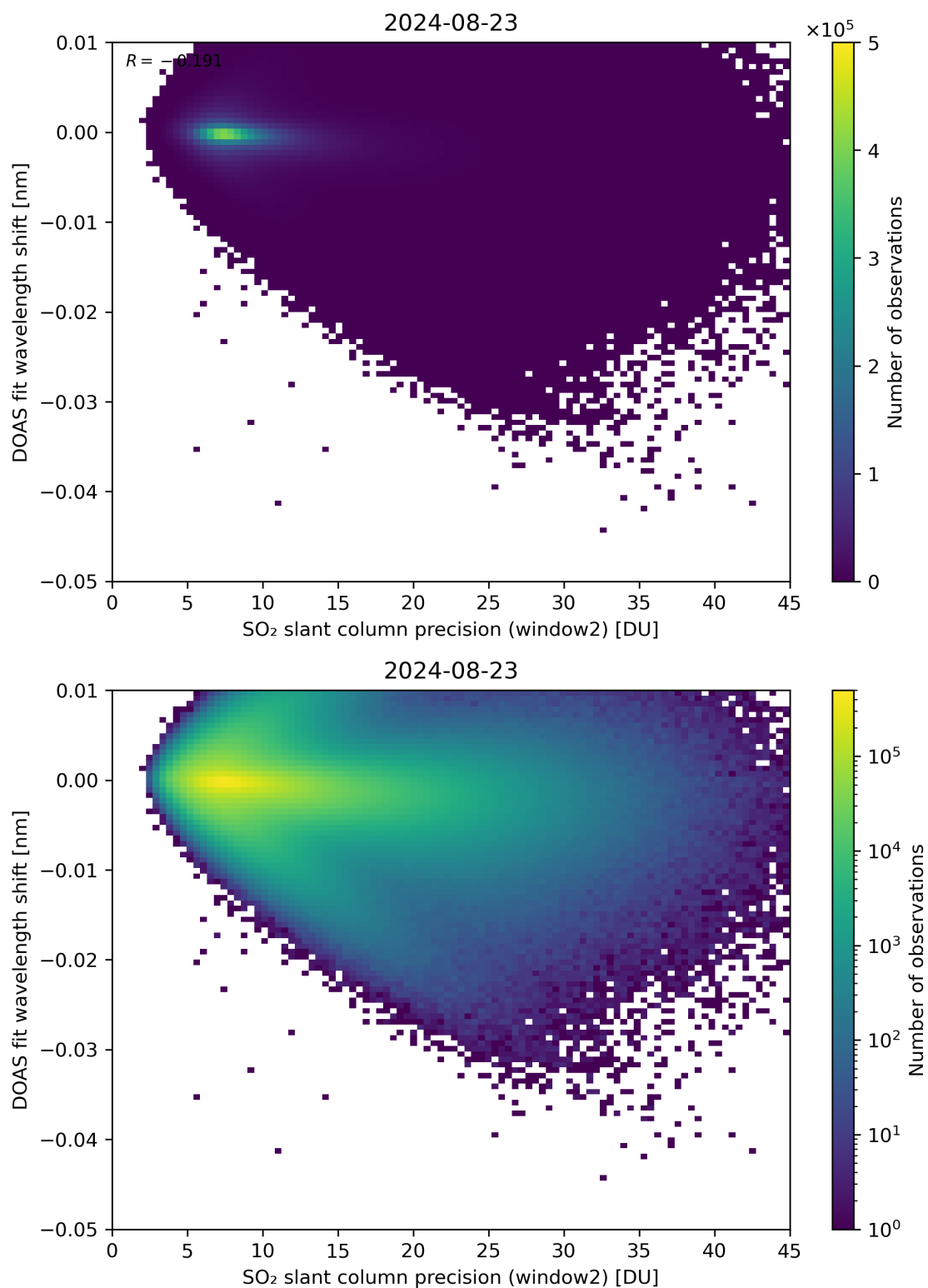
Figure 243: Scatter density plot of “SO 2 slant column precision (window2)” against “DOAS fit wavelength shift” for 2024-08-22 to 2024-08-24.
