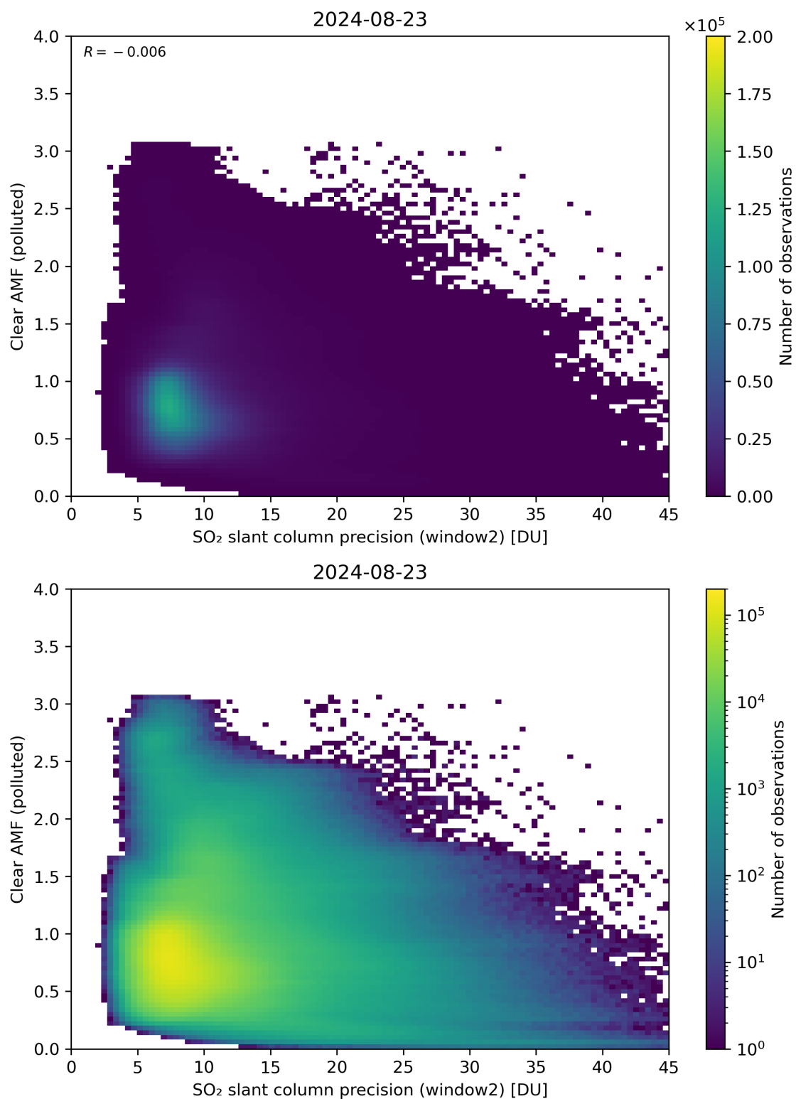
Figure 246: Scatter density plot of “SO 2 slant column precision (window2)” against “Clear AMF (polluted)” for 2024-08-22 to 2024-08-24.
