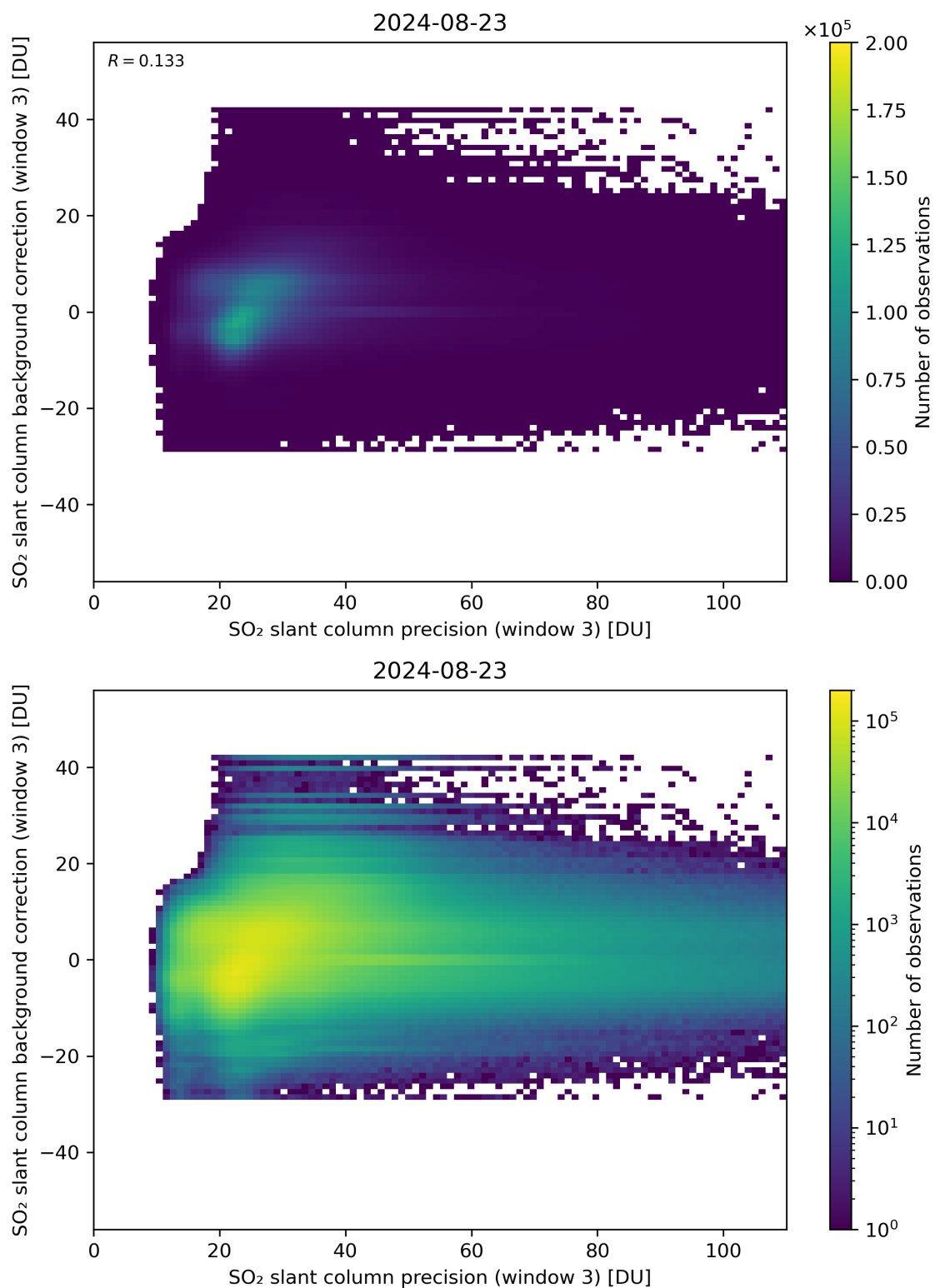
Figure 257: Scatter density plot of “SO 2 slant column precision (window 3)” against “SO 2 slant column background correction (window 3)” for 2024-08-22 to 2024-08-24.
