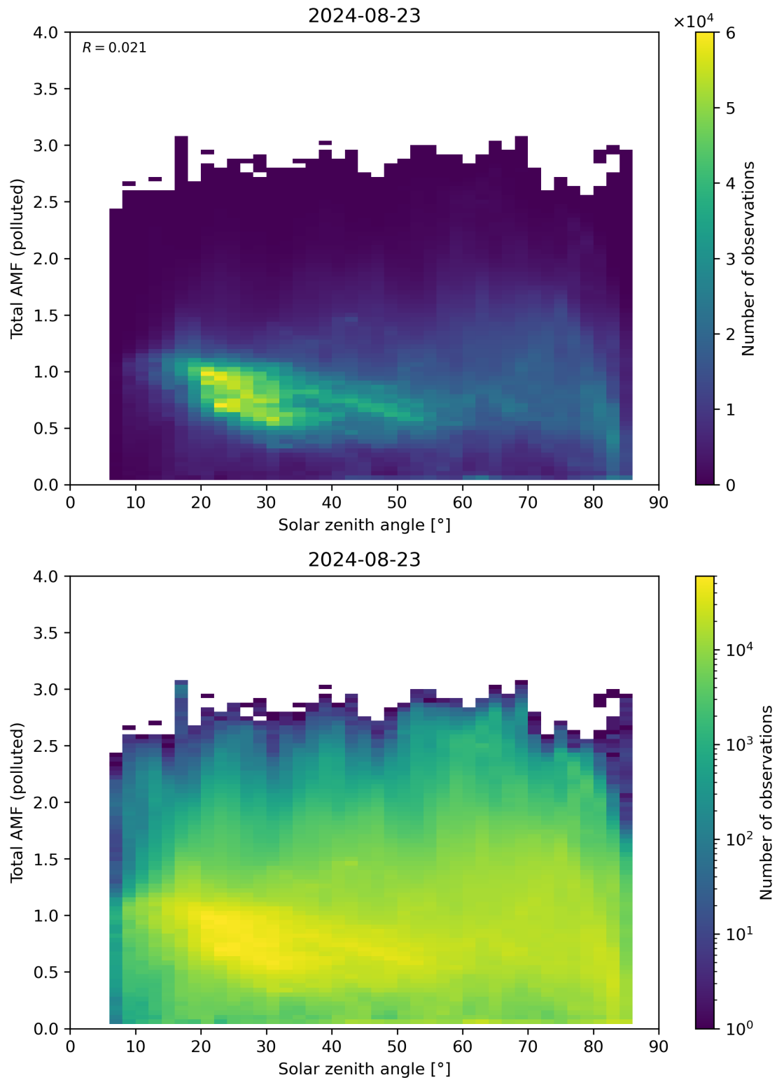
Figure 174: Scatter density plot of “Solar zenith angle” against “Total AMF (polluted)” for 2024-08-22 to 2024-08-24.
