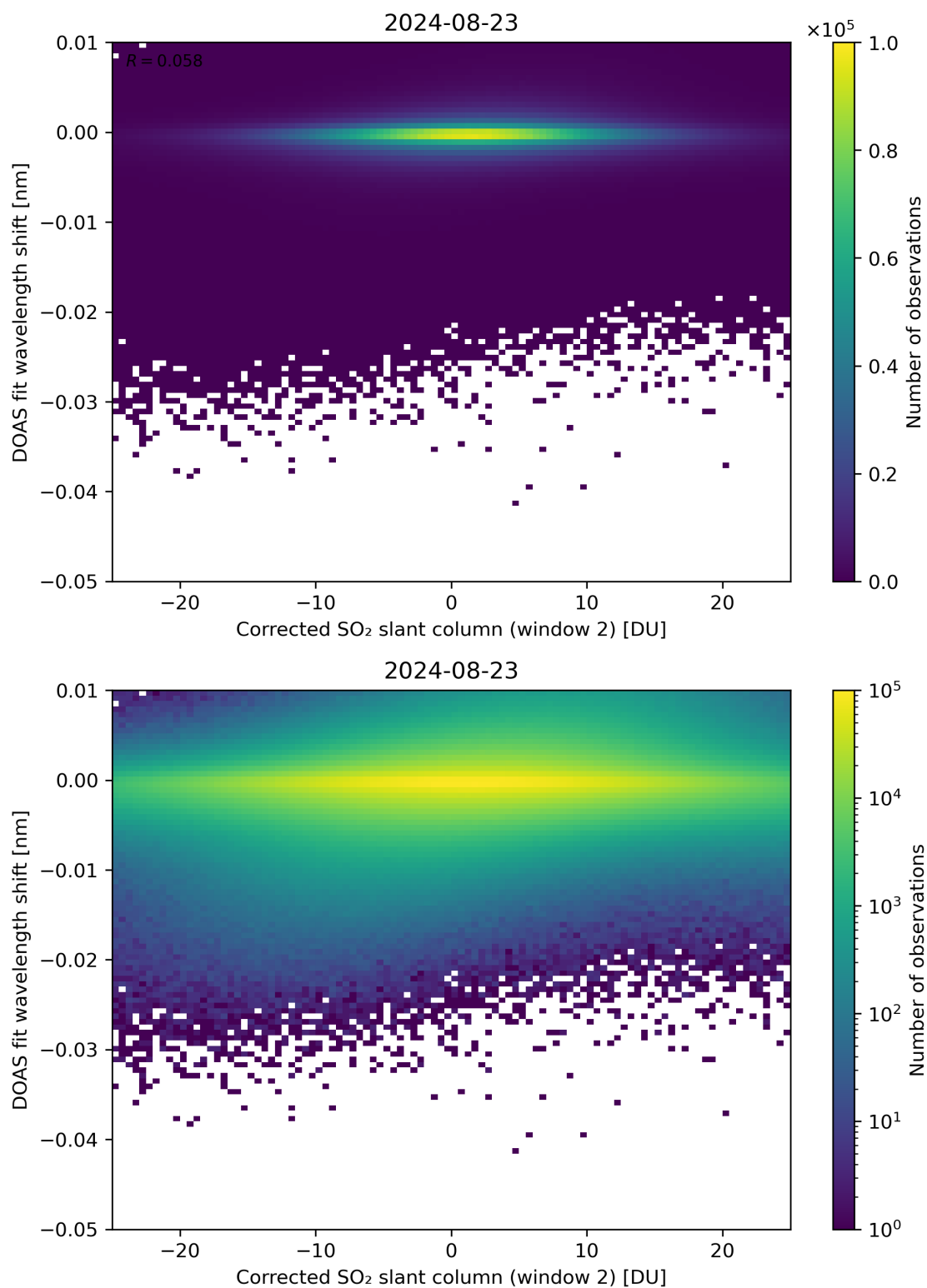
Figure 196: Scatter density plot of “Corrected SO 2 slant column (window 2)” against “DOAS fit wavelength shift” for 2024-08-22 to 2024-08-24.
