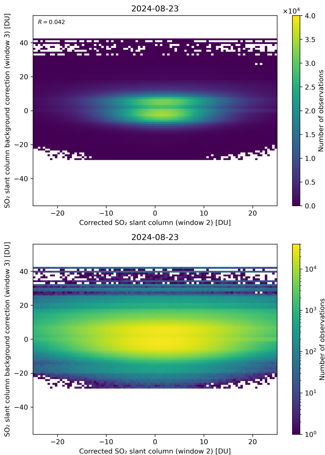
Figure 195: Scatter density plot of “Corrected SO 2 slant column (window 2)” against “SO 2 slant column background correction (window 3)” for 2024-08-22 to 2024-08-24.
