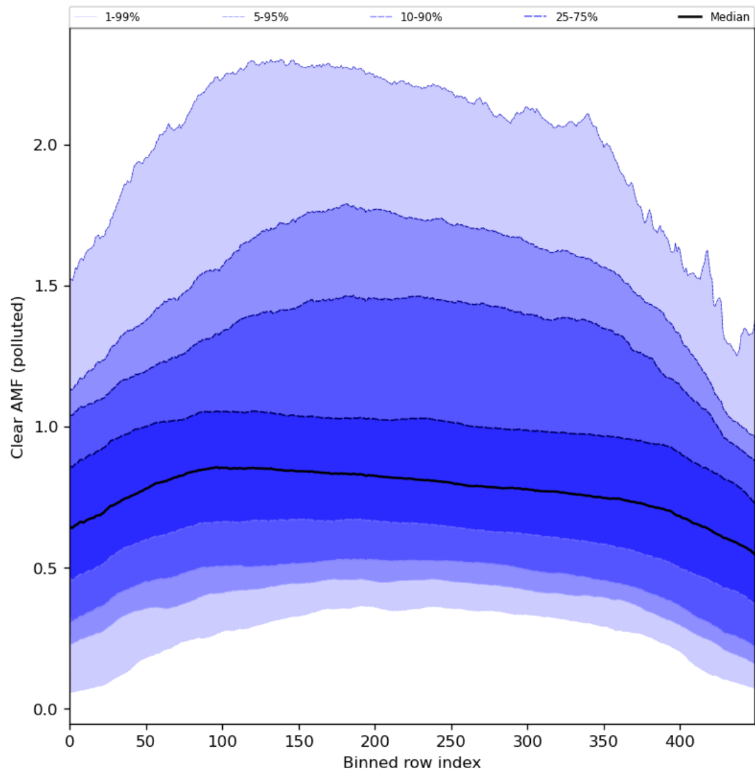
Figure 96: Along track statistics of “Clear AMF (polluted)” for 2024-08-22 to 2024-08-24
