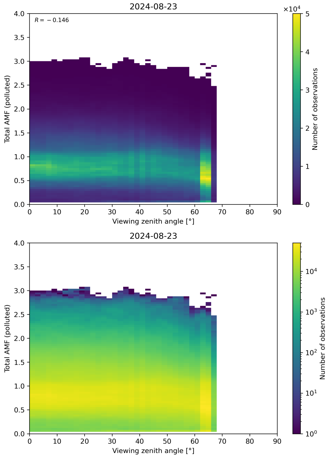
Figure 325: Scatter density plot of “Viewing zenith angle” against “Total AMF (polluted)” for 2024-08-22 to 2024-08-24.
