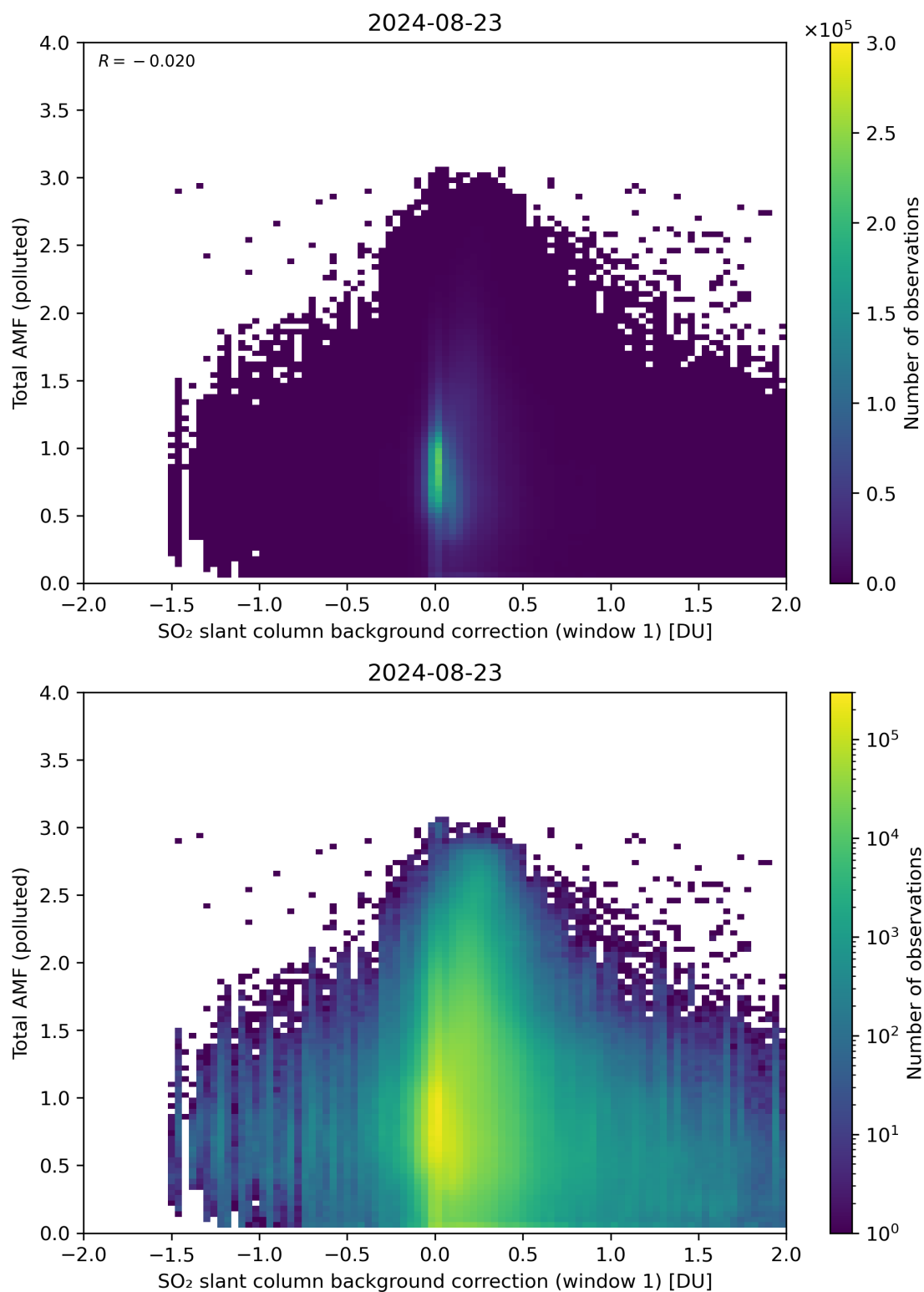
Figure 109: Scatter density plot of “SO 2 slant column background correction (window 1)” against “Total AMF (polluted)” for 2024-08-22 to 2024-08-24.
