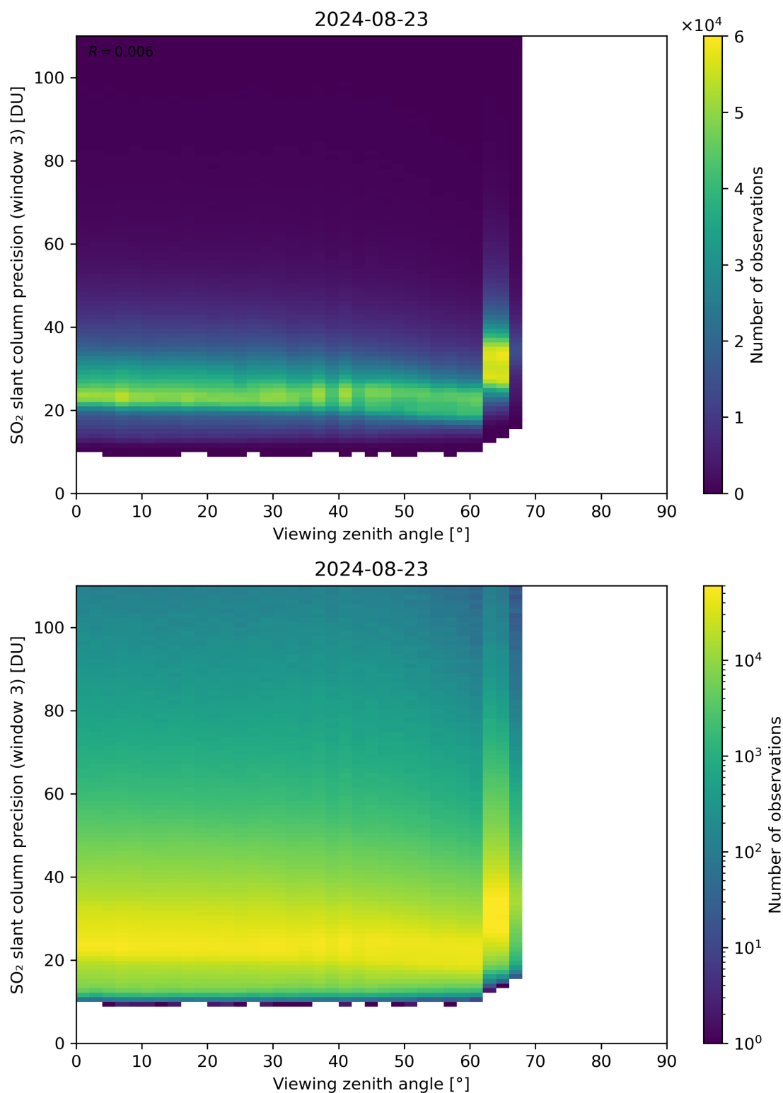
Figure 324: Scatter density plot of “Viewing zenith angle” against “SO 2 slant column precision (window 3)” for 2024-08-22 to 2024-08-24.
