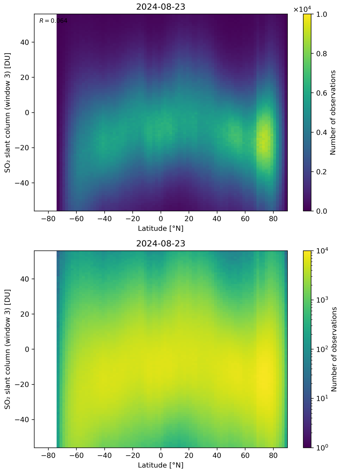
Figure 152: Scatter density plot of “Latitude” against “SO 2 slant column (window 3)” for 2024-08-22 to 2024-08-24.
