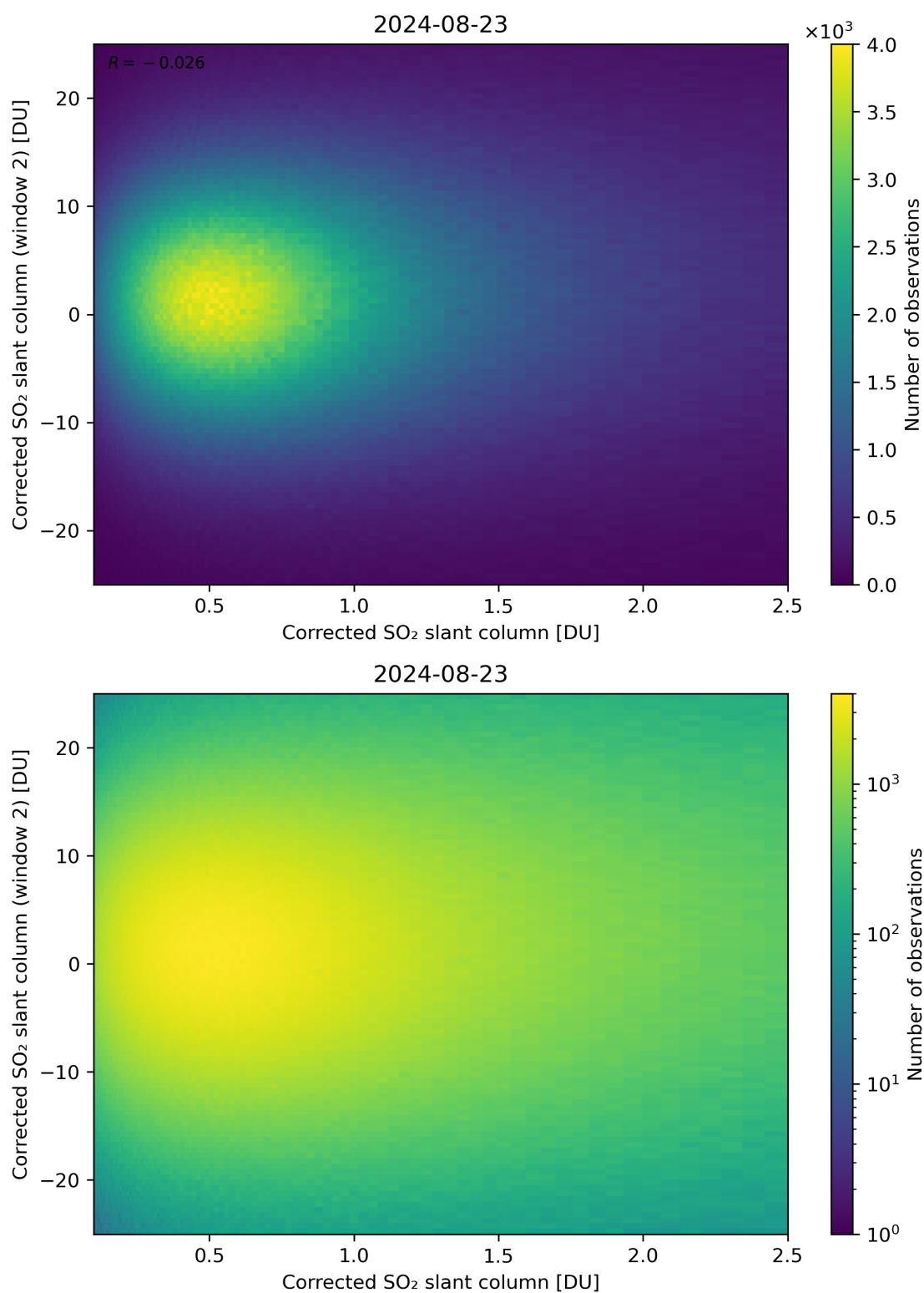
Figure 185: Scatter density plot of “Corrected SO 2 slant column” against “Corrected SO 2 slant column (window 2)” for 2024-08-22 to 2024-08-24.
