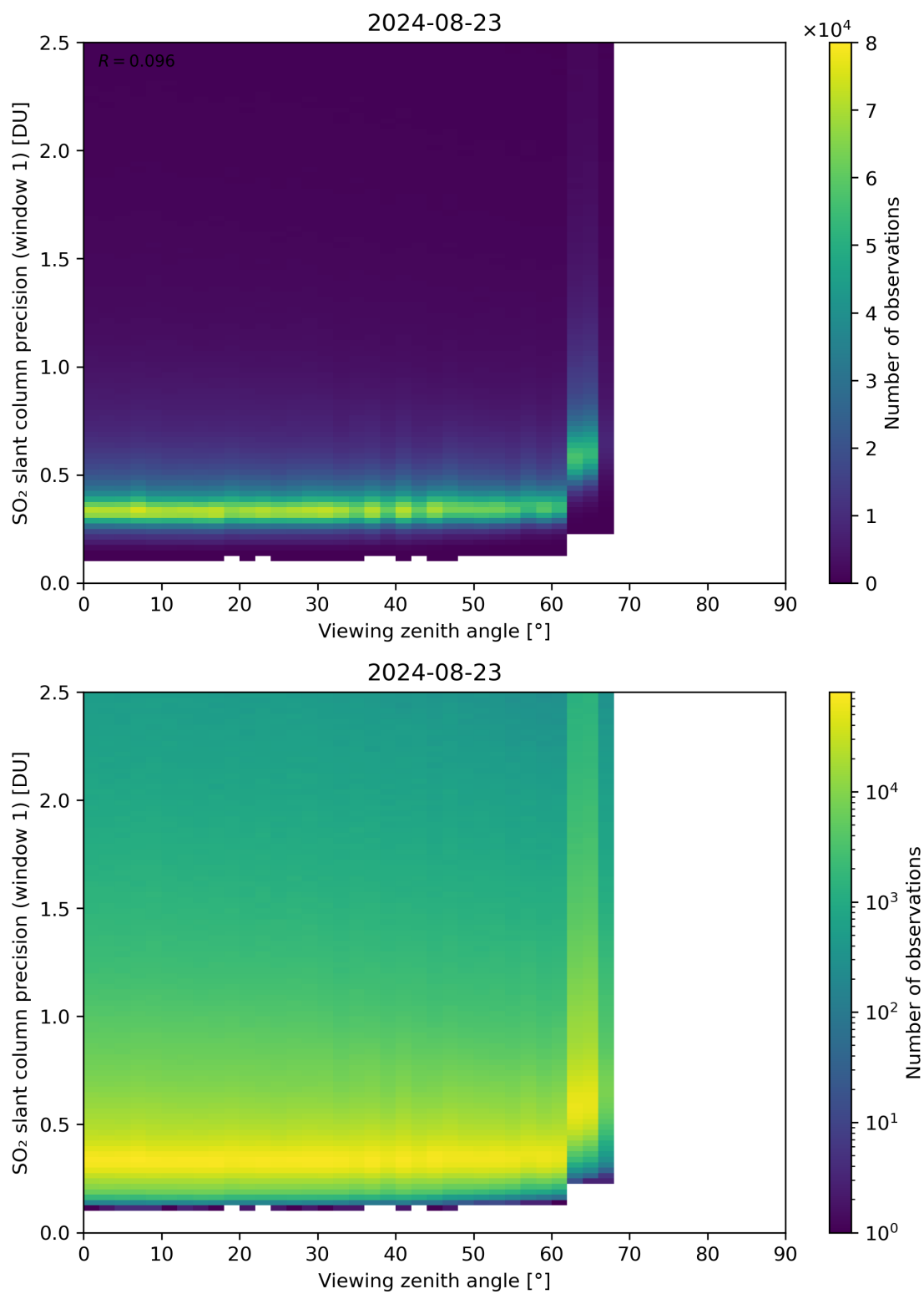
Figure 321: Scatter density plot of “Viewing zenith angle” against “SO 2 slant column precision (window 1)” for 2024-08-22 to 2024-08-24.
