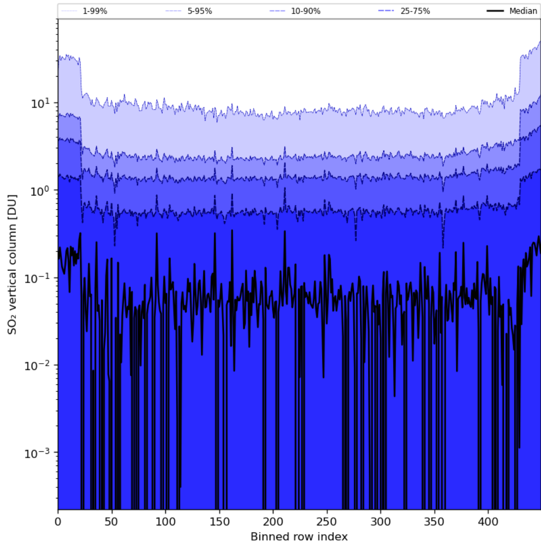
Figure 76: Along track statistics of “SO 2 vertical column” for 2024-08-22 to 2024-08-24
