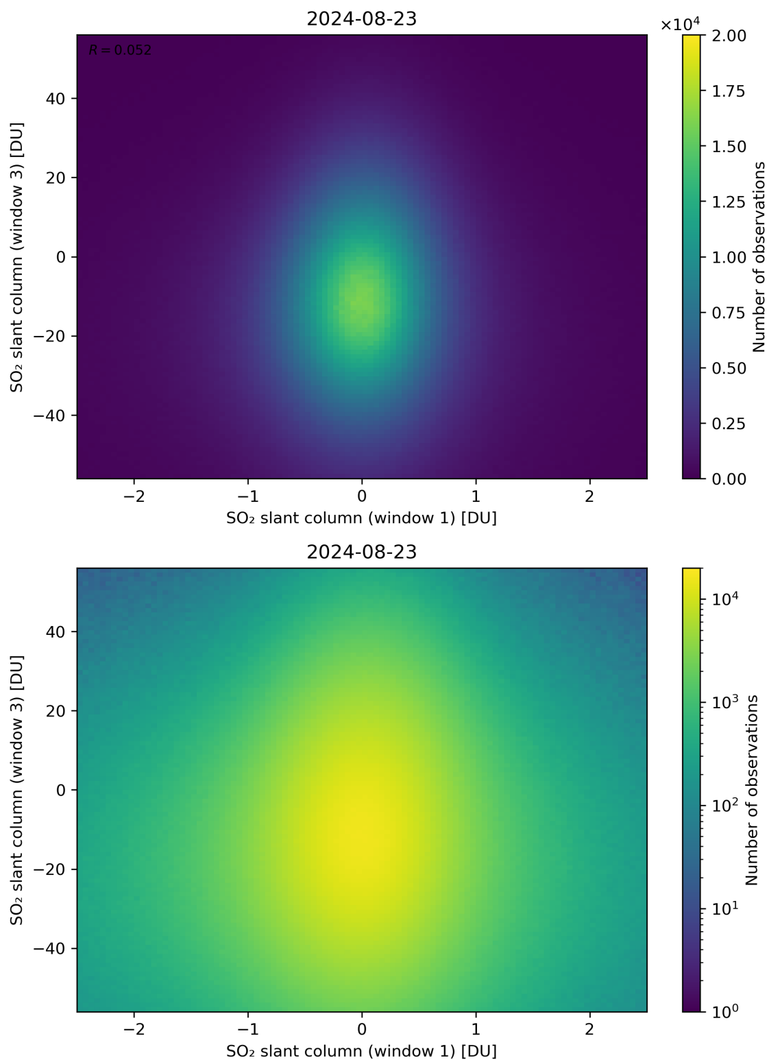
Figure 237: Scatter density plot of “SO 2 slant column (window 1)” against “SO 2 slant column (window 3)” for 2024-08-22 to 2024-08-24.
