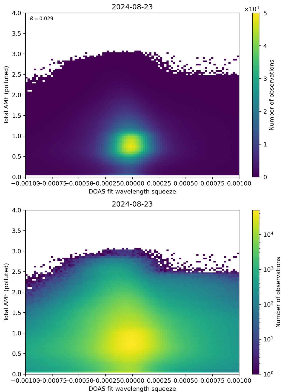
Figure 134: Scatter density plot of “DOAS fit wavelength squeeze” against “Total AMF (polluted)” for 2024-08-22 to 2024-08-24.
