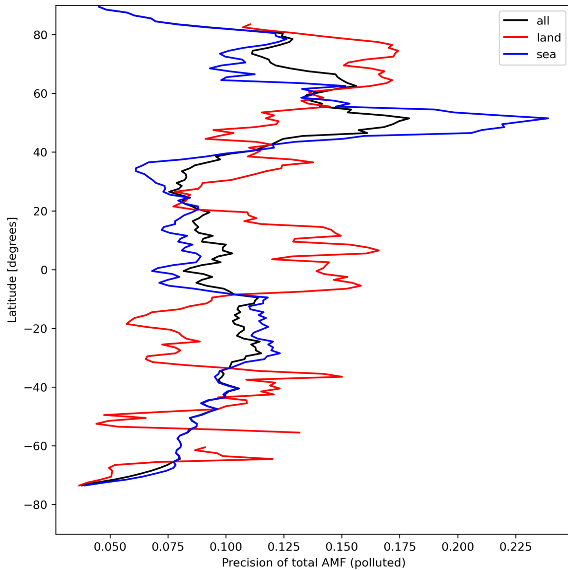
Figure 49: Zonal average of “Precision of total AMF (polluted)” for 2024-08-22 to 2024-08-24.
