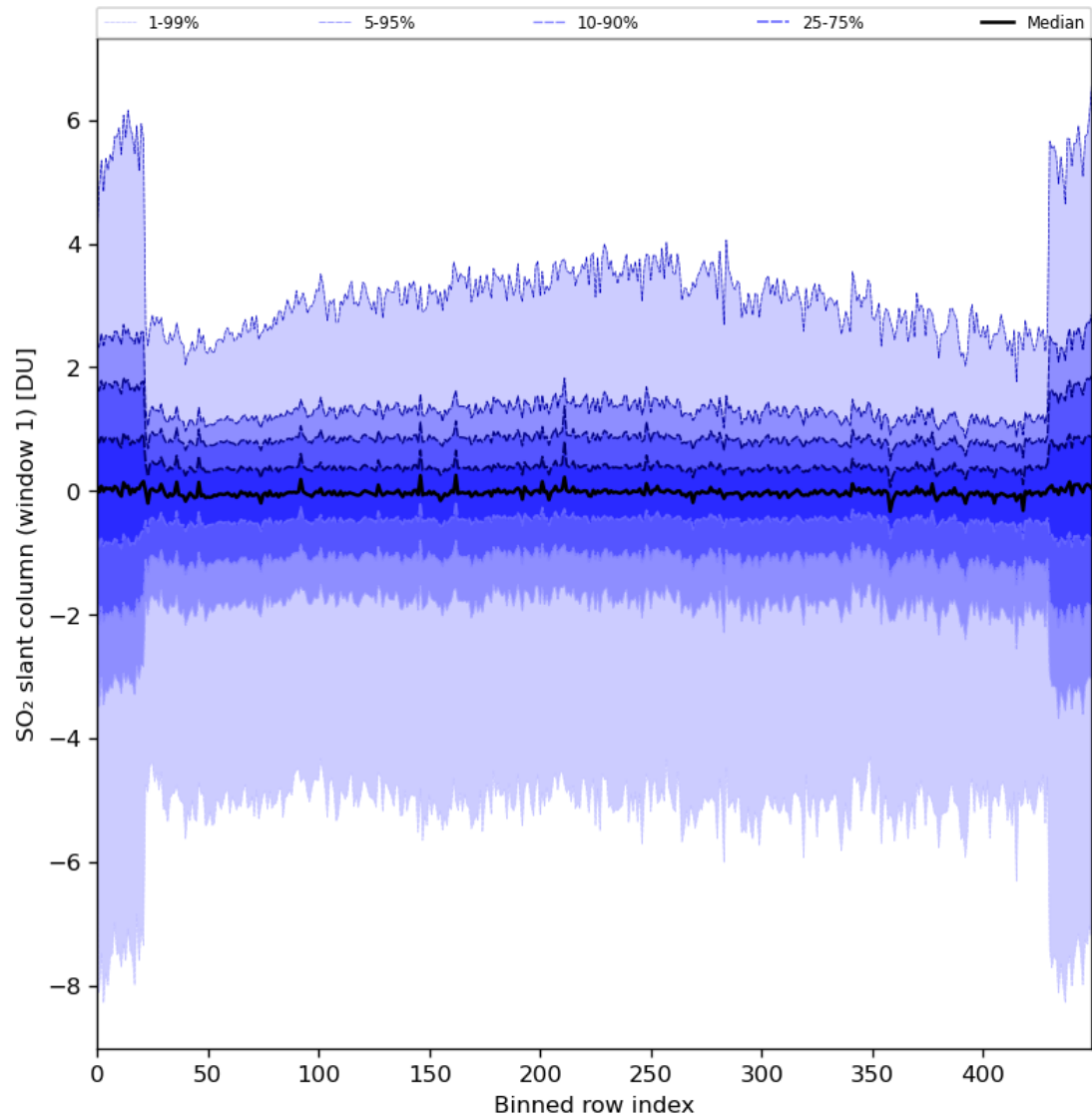
Figure 79: Along track statistics of “SO 2 slant column (window 1)” for 2024-08-22 to 2024-08-24
