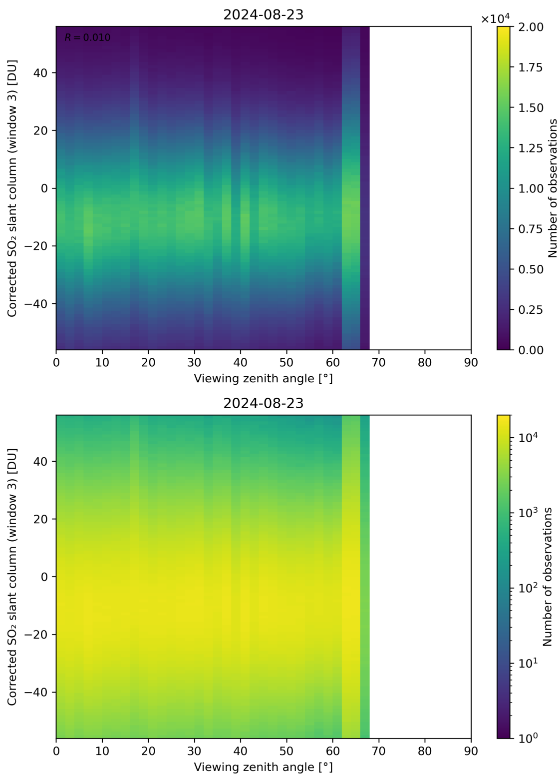
Figure 319: Scatter density plot of “Viewing zenith angle” against “Corrected SO 2 slant column (window 3)” for 2024-08-22 to 2024-08-24.
