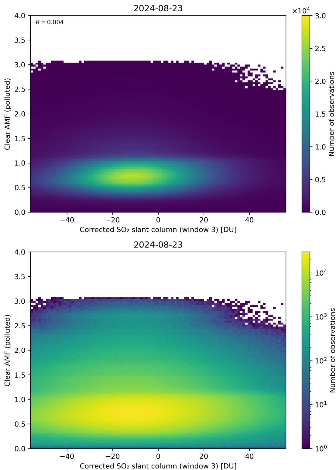
Figure 209: Scatter density plot of “Corrected SO 2 slant column (window 3)” against “Clear AMF (polluted)” for 2024-08-22 to 2024-08-24.
