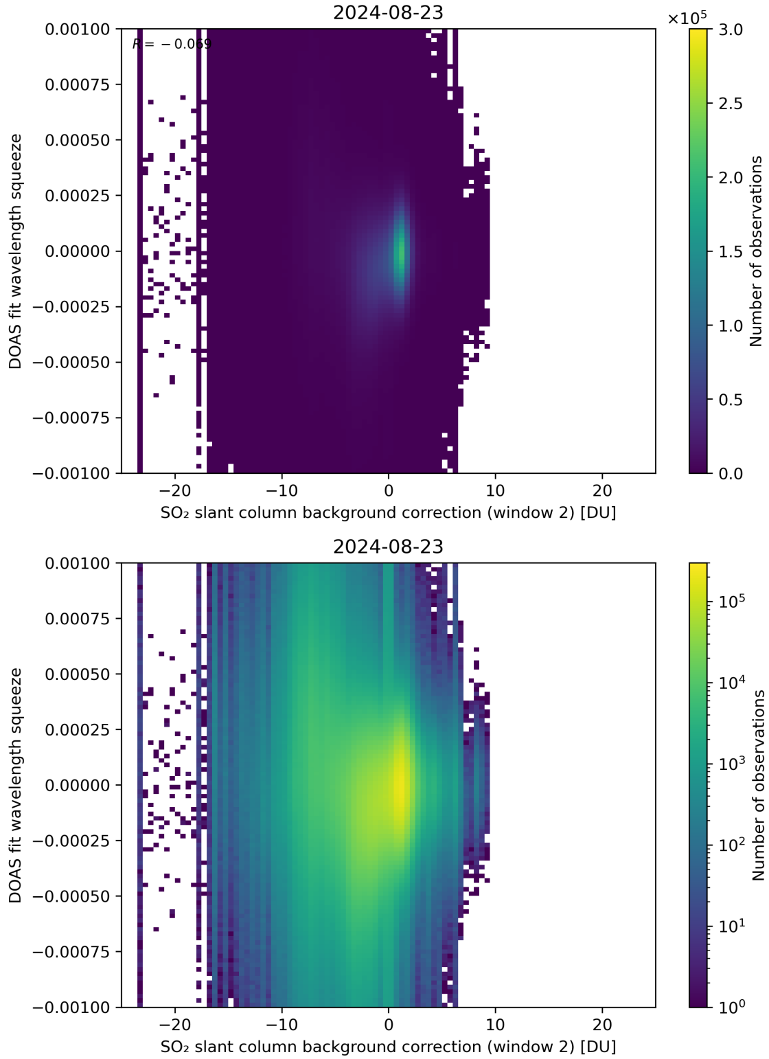
Figure 113: Scatter density plot of “SO 2 slant column background correction (window 2)” against “DOAS fit wavelength squeeze” for 2024-08-22 to 2024-08-24.
