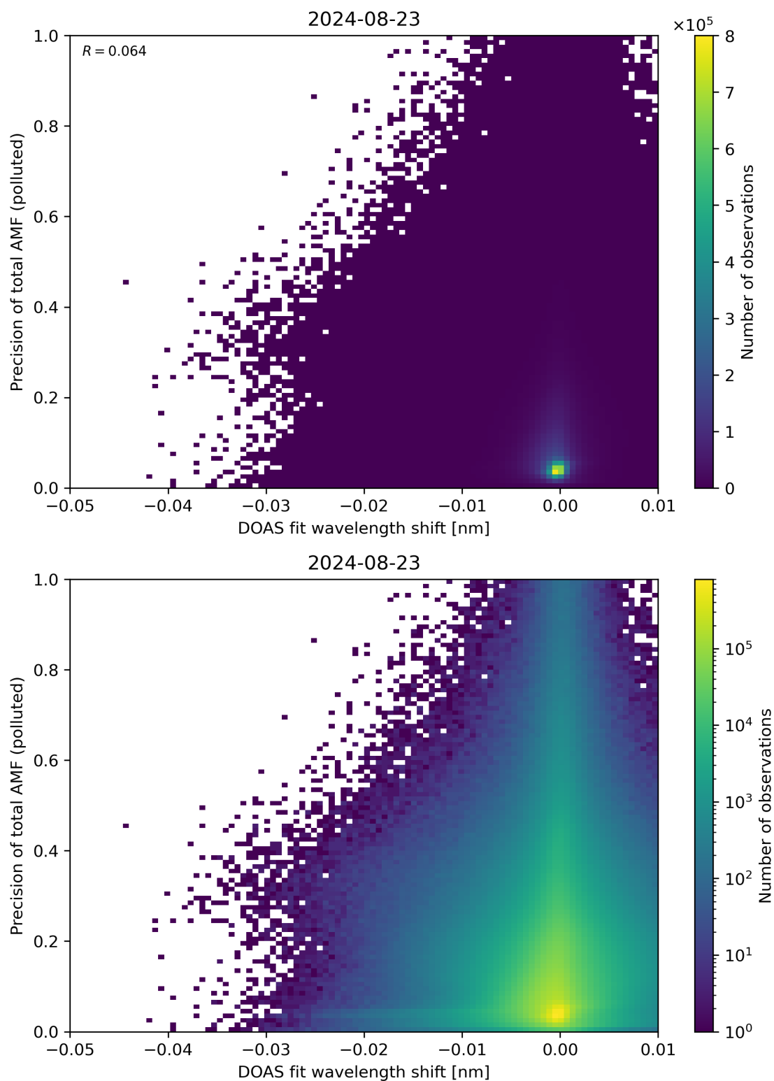
Figure 131: Scatter density plot of “DOAS fit wavelength shift” against “Precision of total AMF (polluted)” for 2024-08-22 to 2024-08-24.
