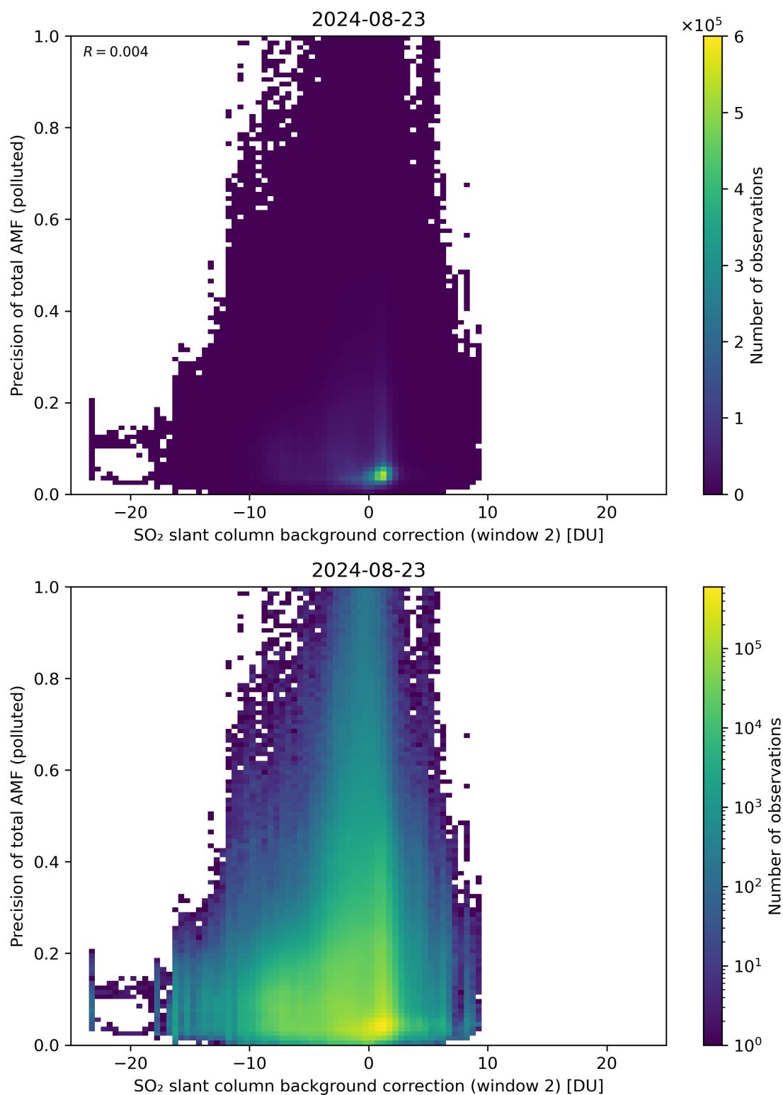
Figure 120: Scatter density plot of “SO 2 slant column background correction (window 2)” against “Precision of total AMF (polluted)” for 2024-08-22 to 2024-08-24.
