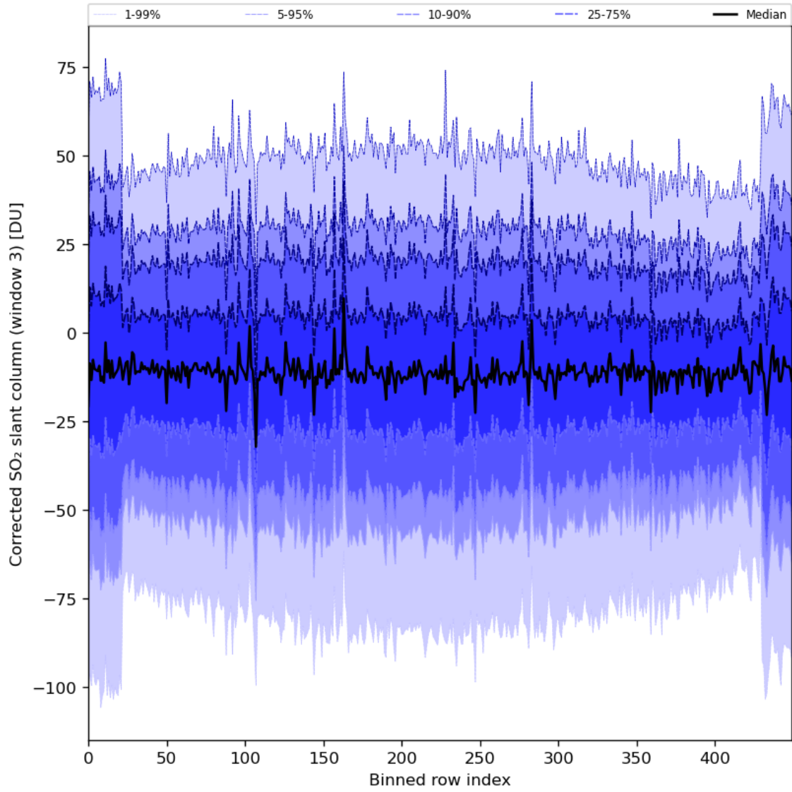
Figure 89: Along track statistics of “Corrected SO 2 slant column (window 3)” for 2024-08-22 to 2024-08-24
