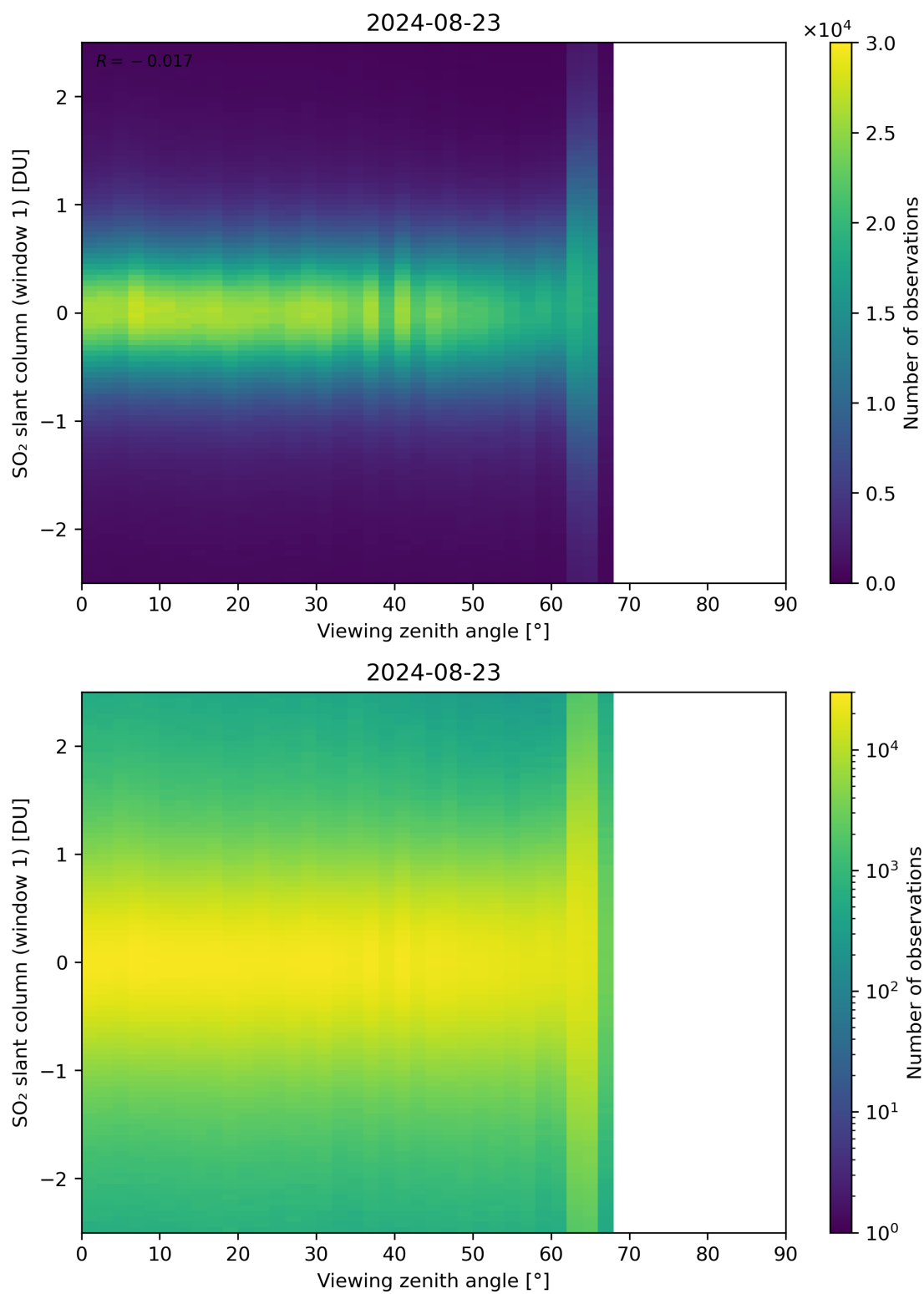
Figure 320: Scatter density plot of “Viewing zenith angle” against “SO 2 slant column (window 1)” for 2024-08-22 to 2024-08-24.
