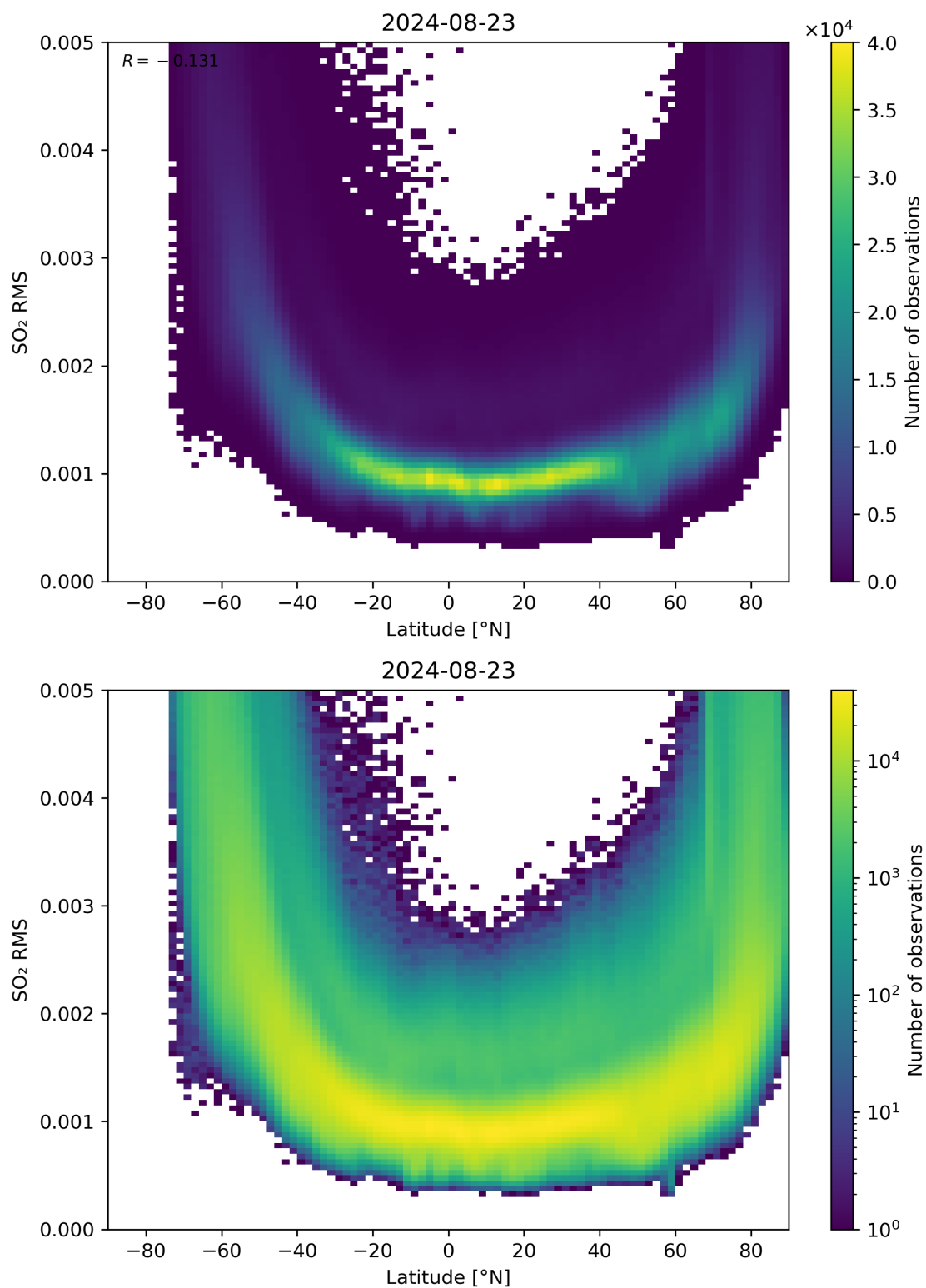
Figure 144: Scatter density plot of “Latitude” against “SO 2 RMS” for 2024-08-22 to 2024-08-24.
