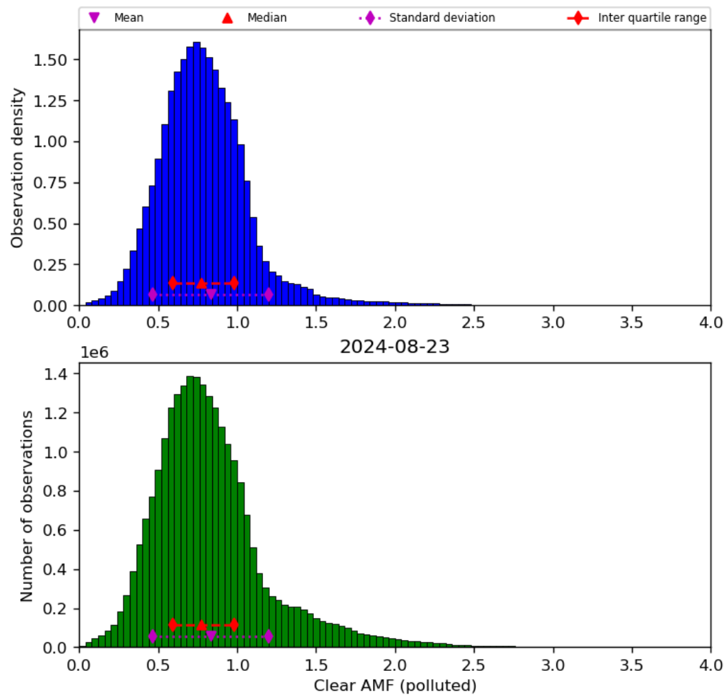
Figure 73: Histogram of “Clear AMF (polluted)” for 2024-08-22 to 2024-08-24
