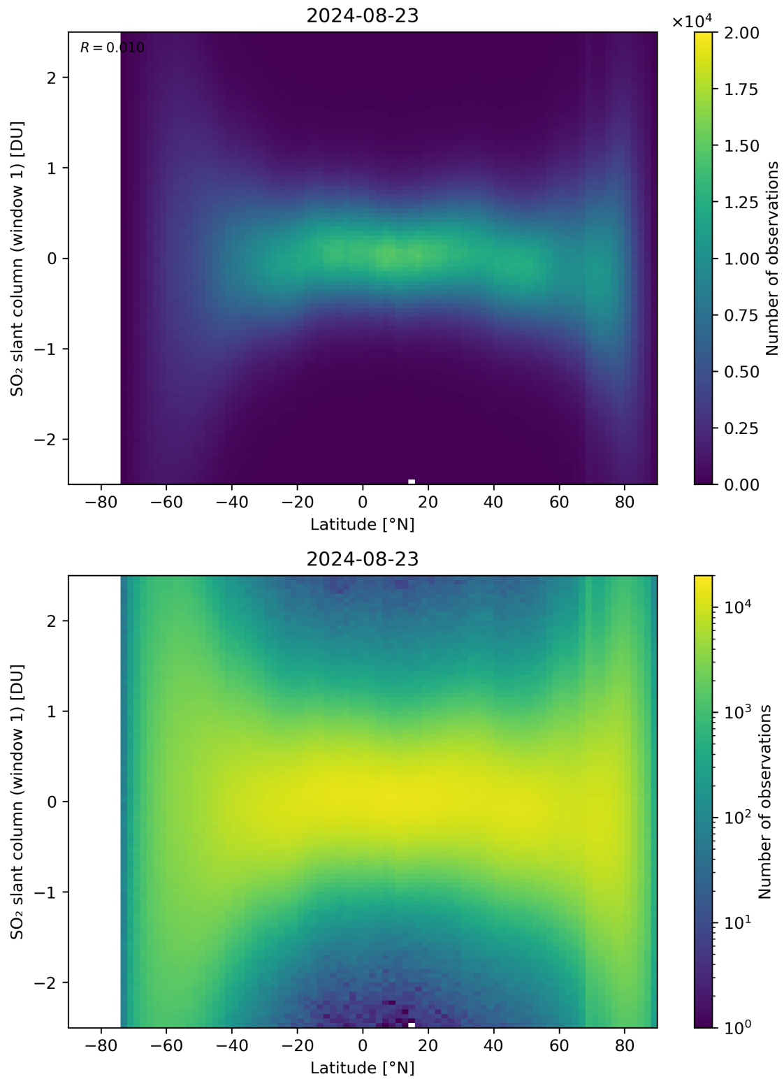
Figure 149: Scatter density plot of “Latitude” against “SO 2 slant column (window 1)” for 2024-08-22 to 2024-08-24.
