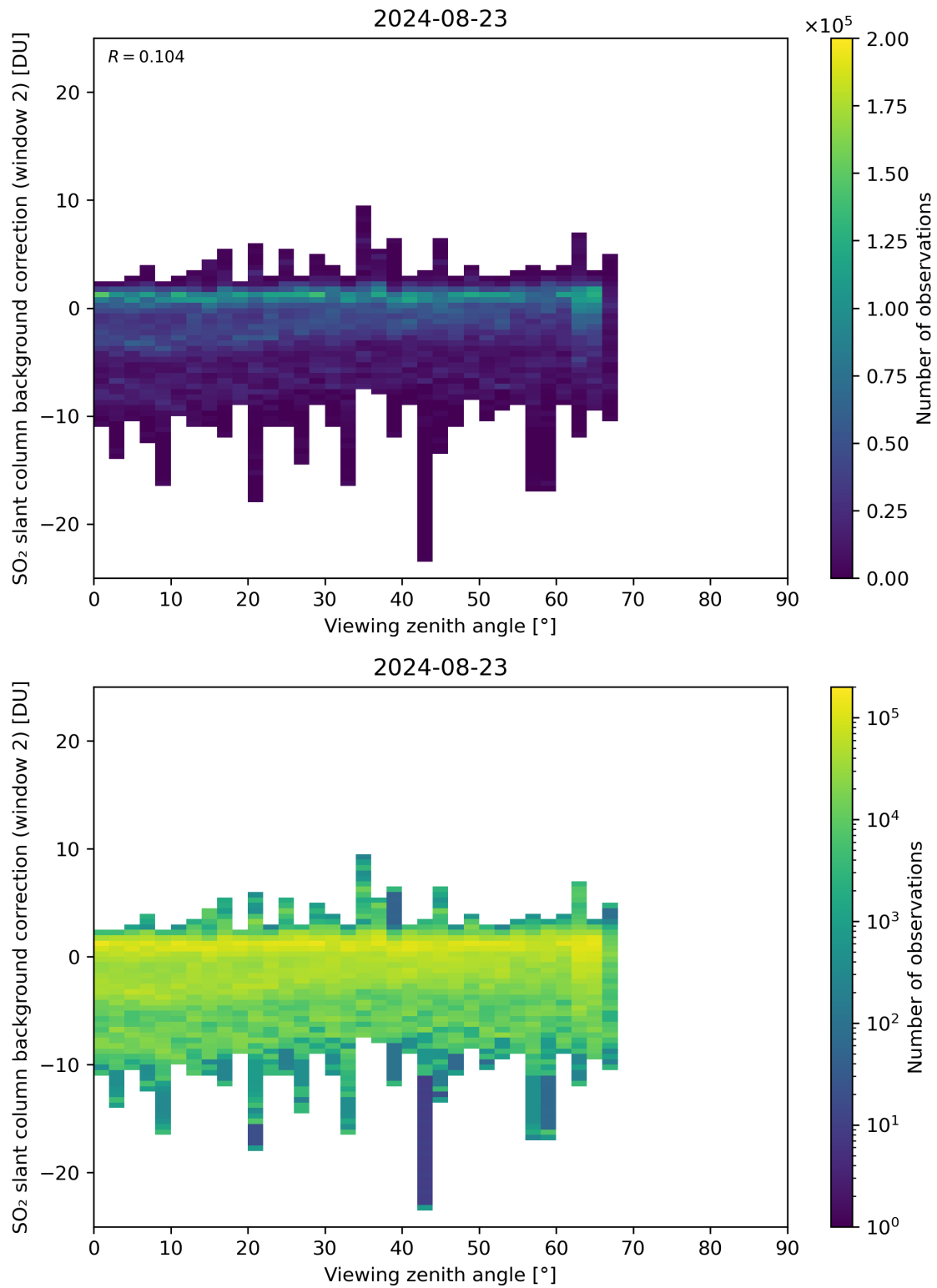
Figure 309: Scatter density plot of “Viewing zenith angle” against “SO 2 slant column background correction (window 2)” for 2024-08-22 to 2024-08-24.
