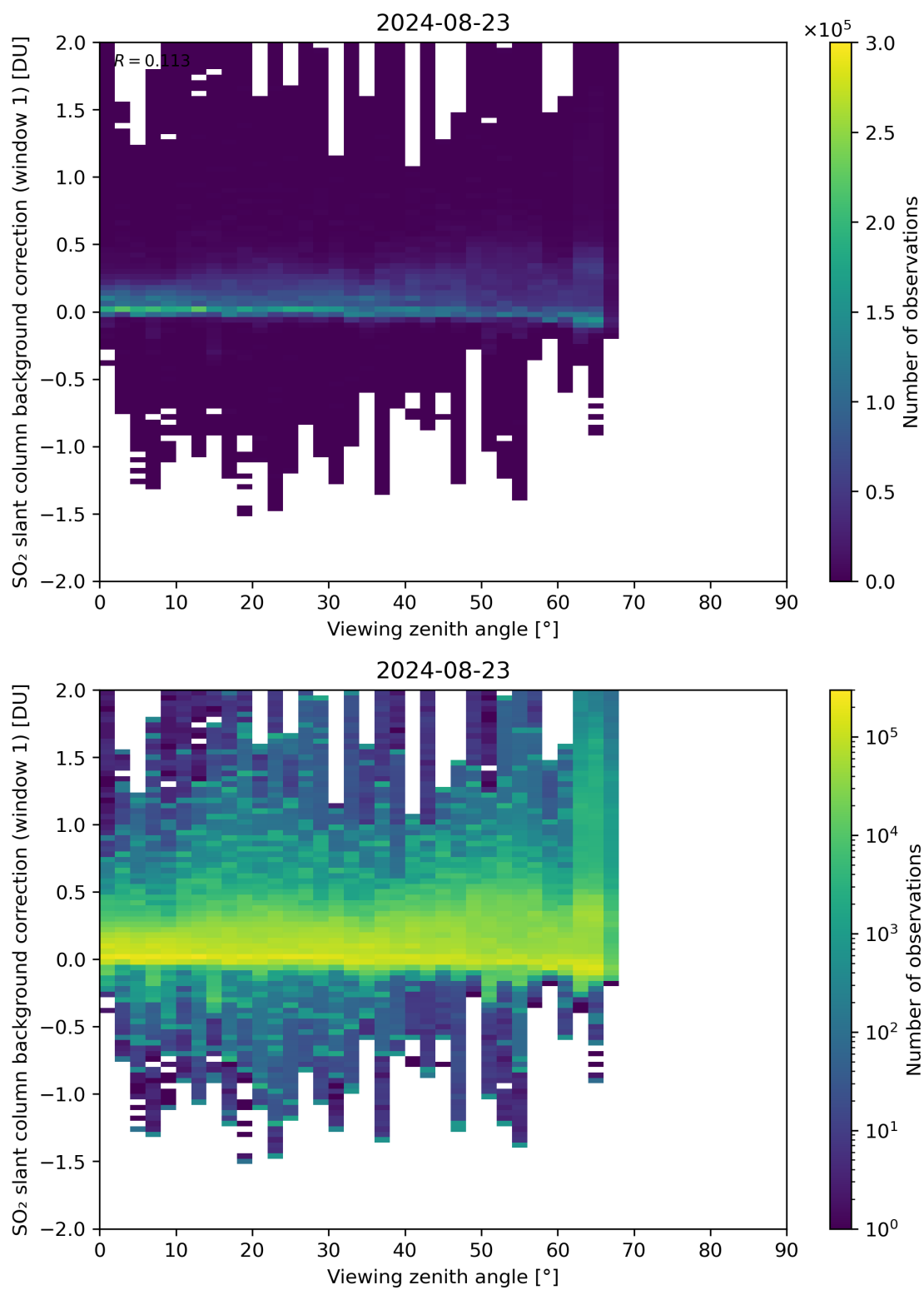
Figure 308: Scatter density plot of “Viewing zenith angle” against “SO 2 slant column background correction (window 1)” for 2024-08-22 to 2024-08-24.
