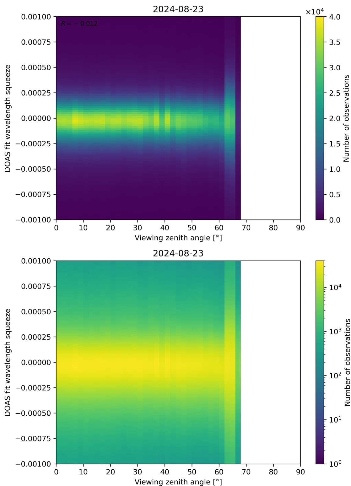
Figure 312: Scatter density plot of “Viewing zenith angle” against “DOAS fit wavelength squeeze” for 2024-08-22 to 2024-08-24.
