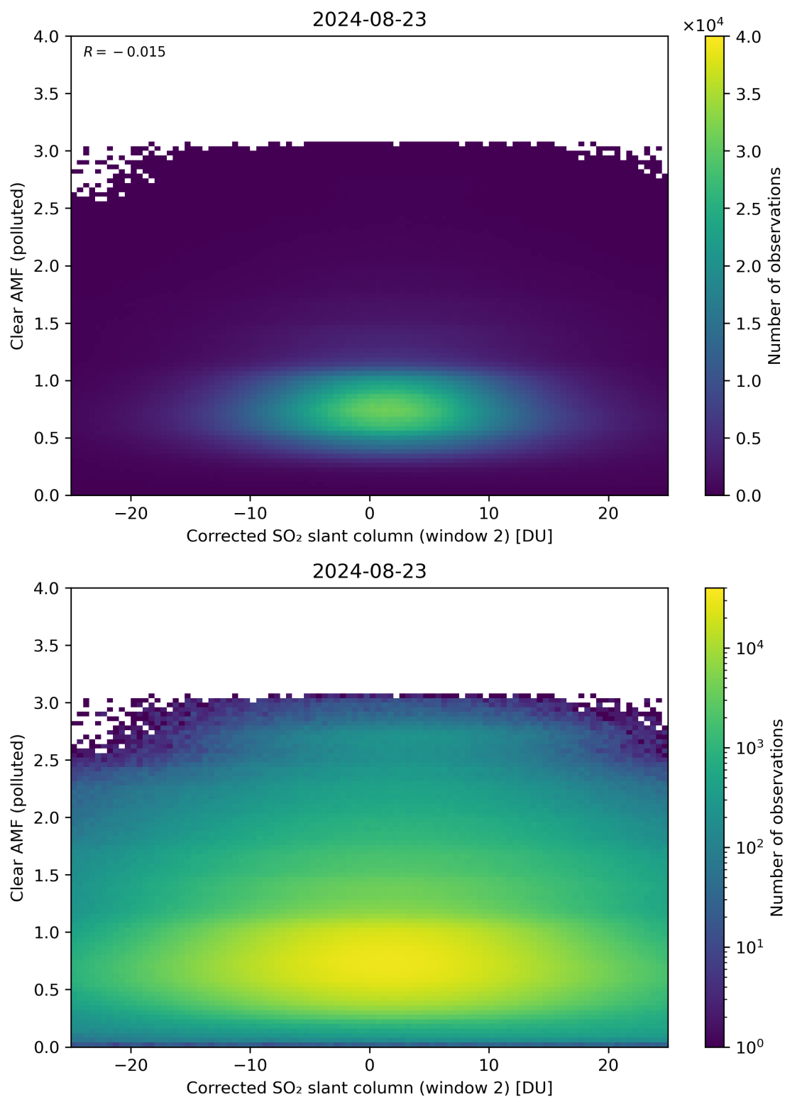
Figure 199: Scatter density plot of “Corrected SO 2 slant column (window 2)” against “Clear AMF (polluted)” for 2024-08-22 to 2024-08-24.
