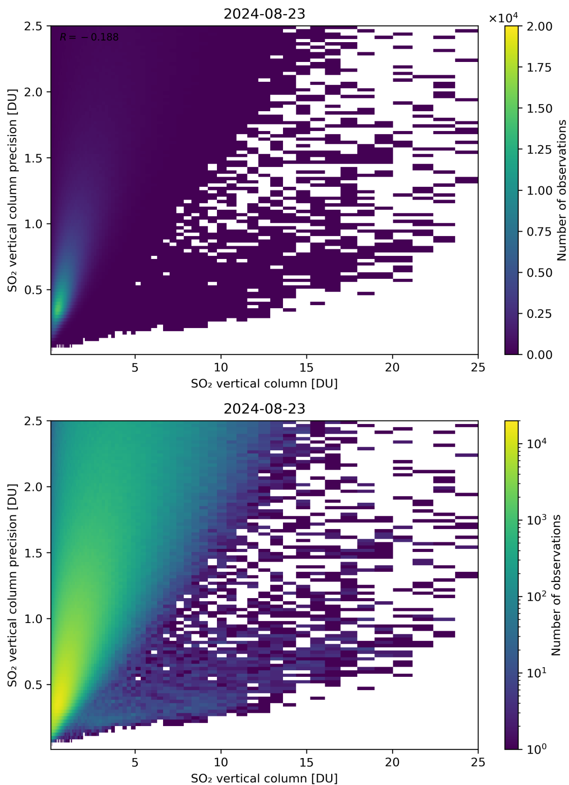
Figure 307: Scatter density plot of “SO 2 vertical column” against “SO 2 vertical column precision” for 2024-08-22 to 2024-08-24.
