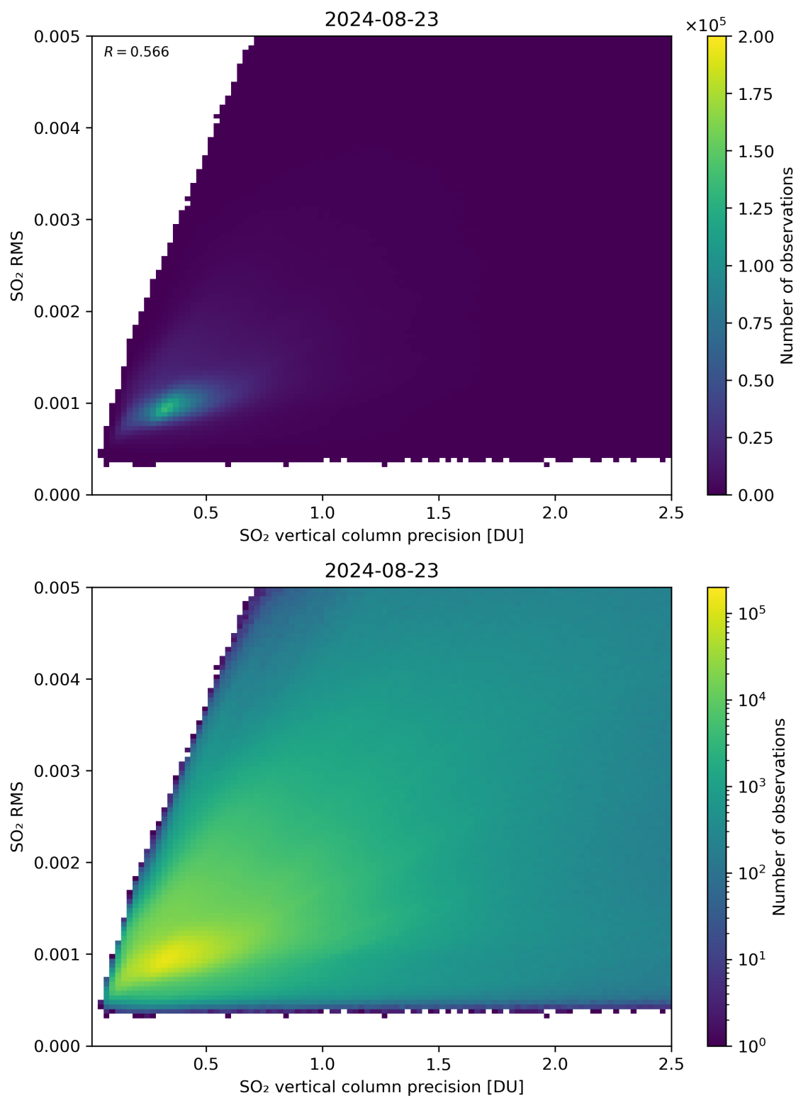
Figure 284: Scatter density plot of “SO 2 vertical column precision” against “SO 2 RMS” for 2024-08-22 to 2024-08-24.
