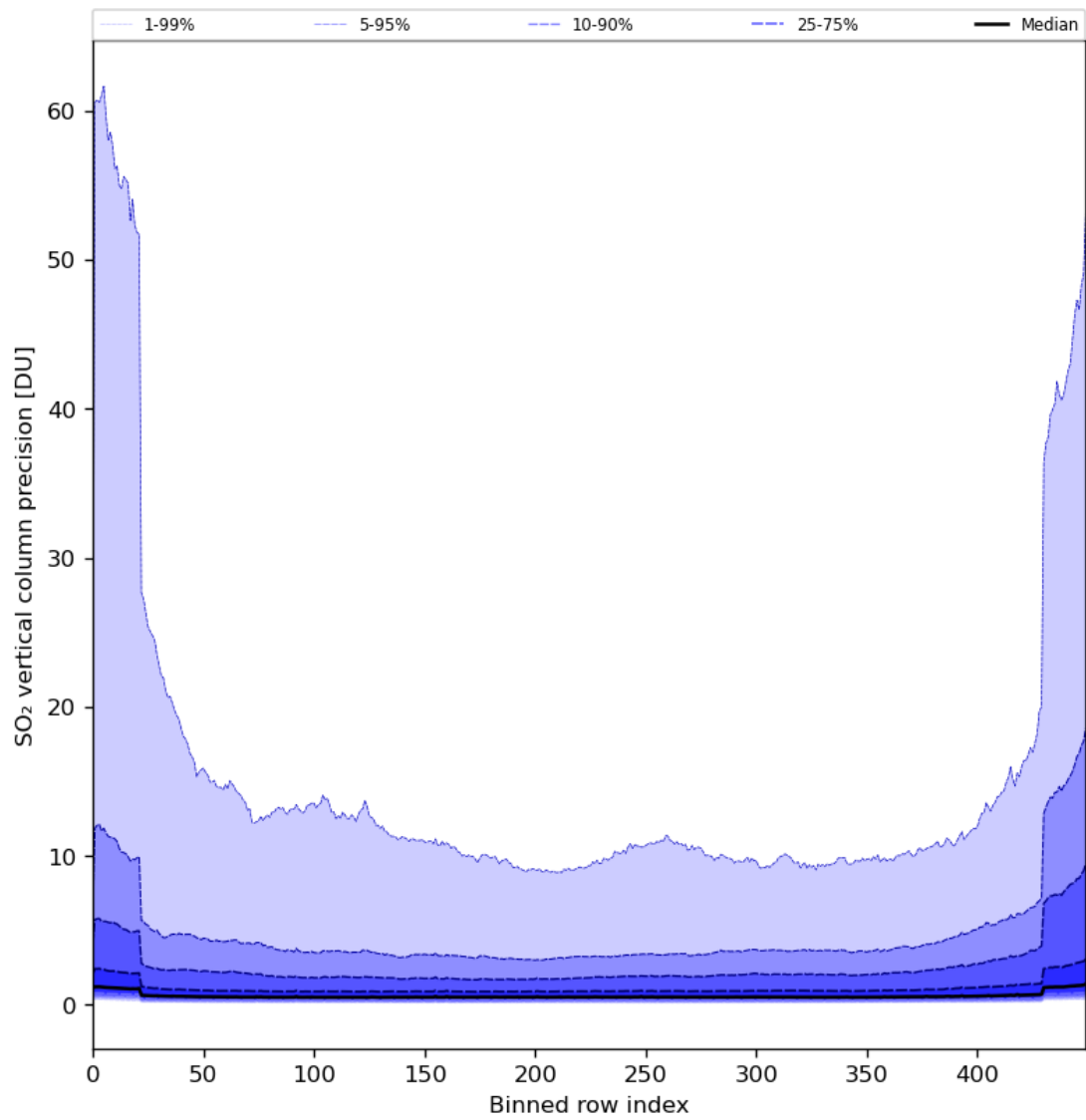
Figure 77: Along track statistics of “SO 2 vertical column precision” for 2024-08-22 to 2024-08-24
