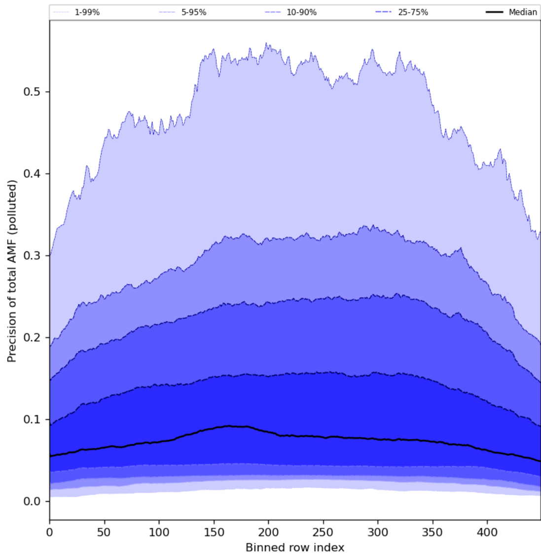
Figure 95: Along track statistics of “Precision of total AMF (polluted)” for 2024-08-22 to 2024-08-24
