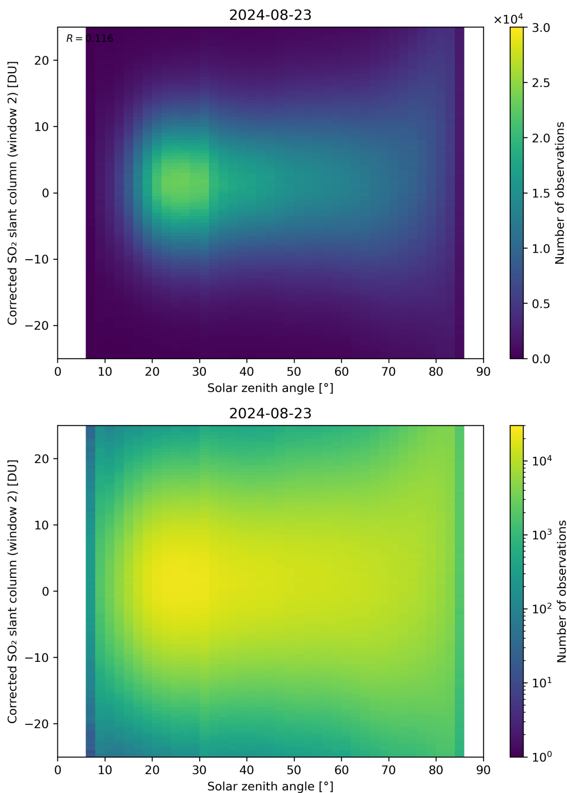
Figure 167: Scatter density plot of “Solar zenith angle” against “Corrected SO 2 slant column (window 2)” for 2024-08-22 to 2024-08-24.
