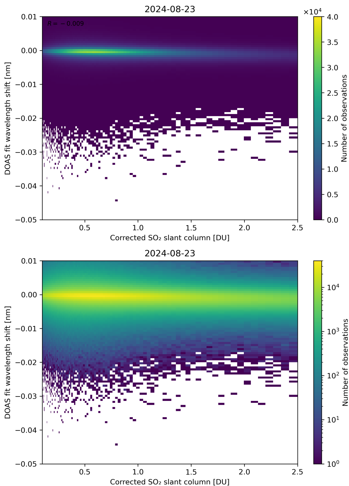
Figure 181: Scatter density plot of “Corrected SO 2 slant column” against “DOAS fit wavelength shift” for 2024-08-22 to 2024-08-24.
