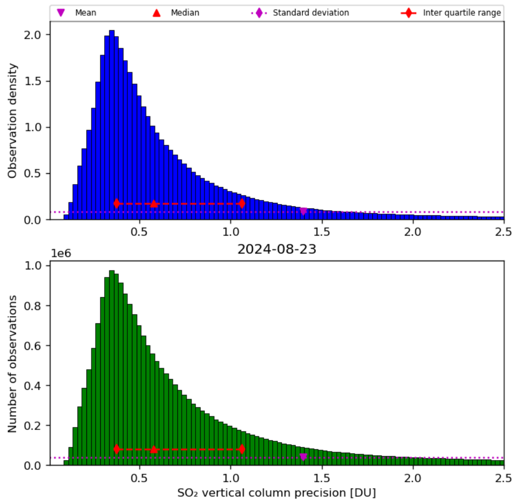
Figure 54: Histogram of “SO 2 vertical column precision” for 2024-08-22 to 2024-08-24
