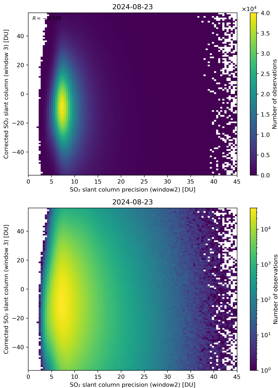
Figure 248: Scatter density plot of “SO 2 slant column precision (window2)” against “Corrected SO 2 slant column (window 3)” for 2024-08-22 to 2024-08-24.
