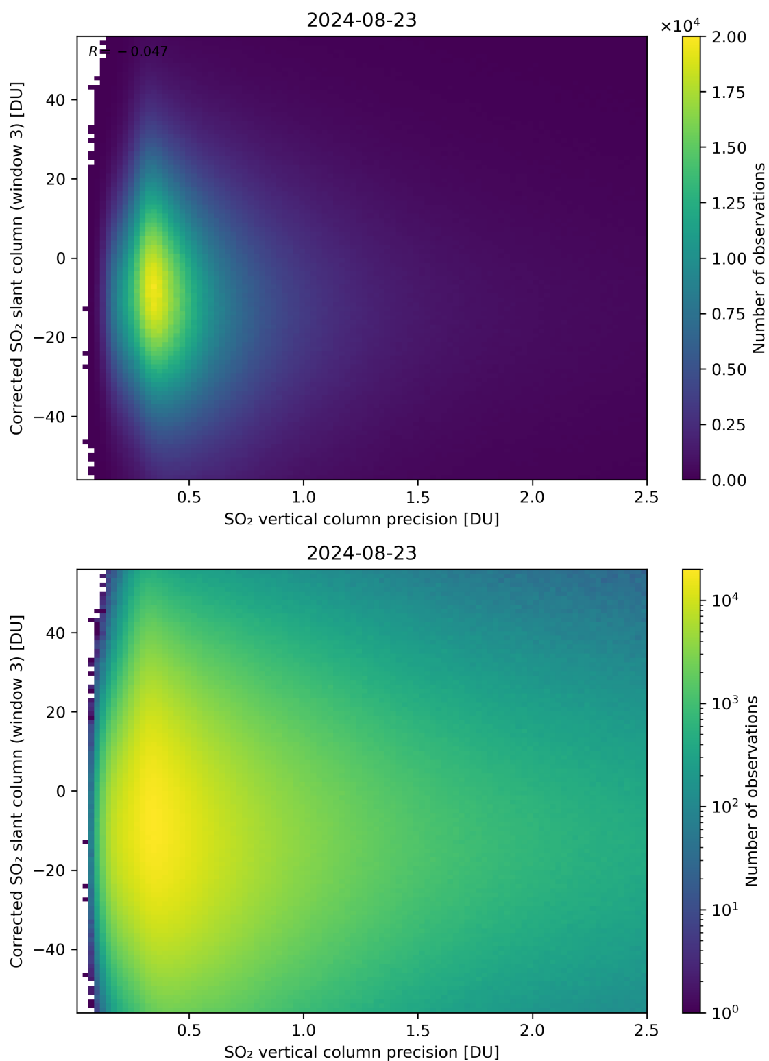
Figure 288: Scatter density plot of “SO 2 vertical column precision” against “Corrected SO 2 slant column (window 3)” for 2024-08-22 to 2024-08-24.
