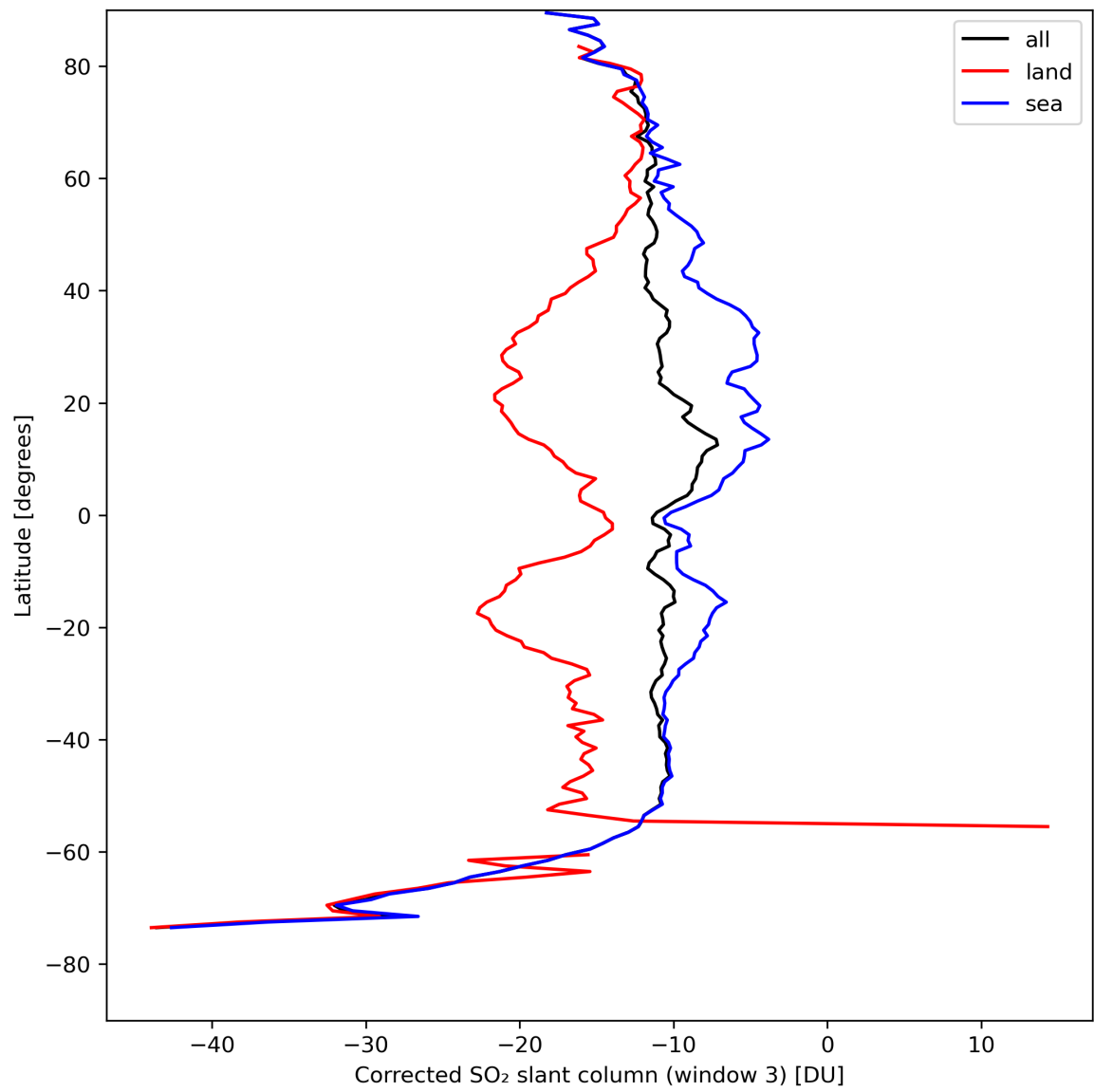
Figure 43: Zonal average of “Corrected SO 2 slant column (window 3)” for 2024-08-22 to 2024-08-24.
