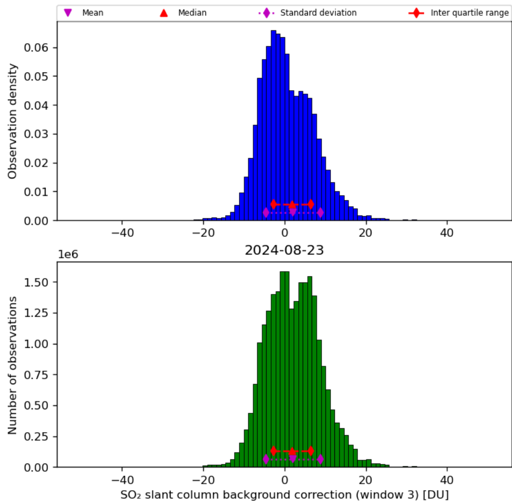
Figure 67: Histogram of “SO 2 slant column background correction (window 3)” for 2024-08-22 to 2024-08-24
