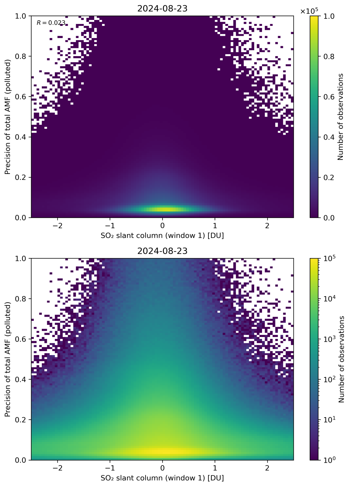
Figure 240: Scatter density plot of “SO 2 slant column (window 1)” against “Precision of total AMF (polluted)” for 2024-08-22 to 2024-08-24.
