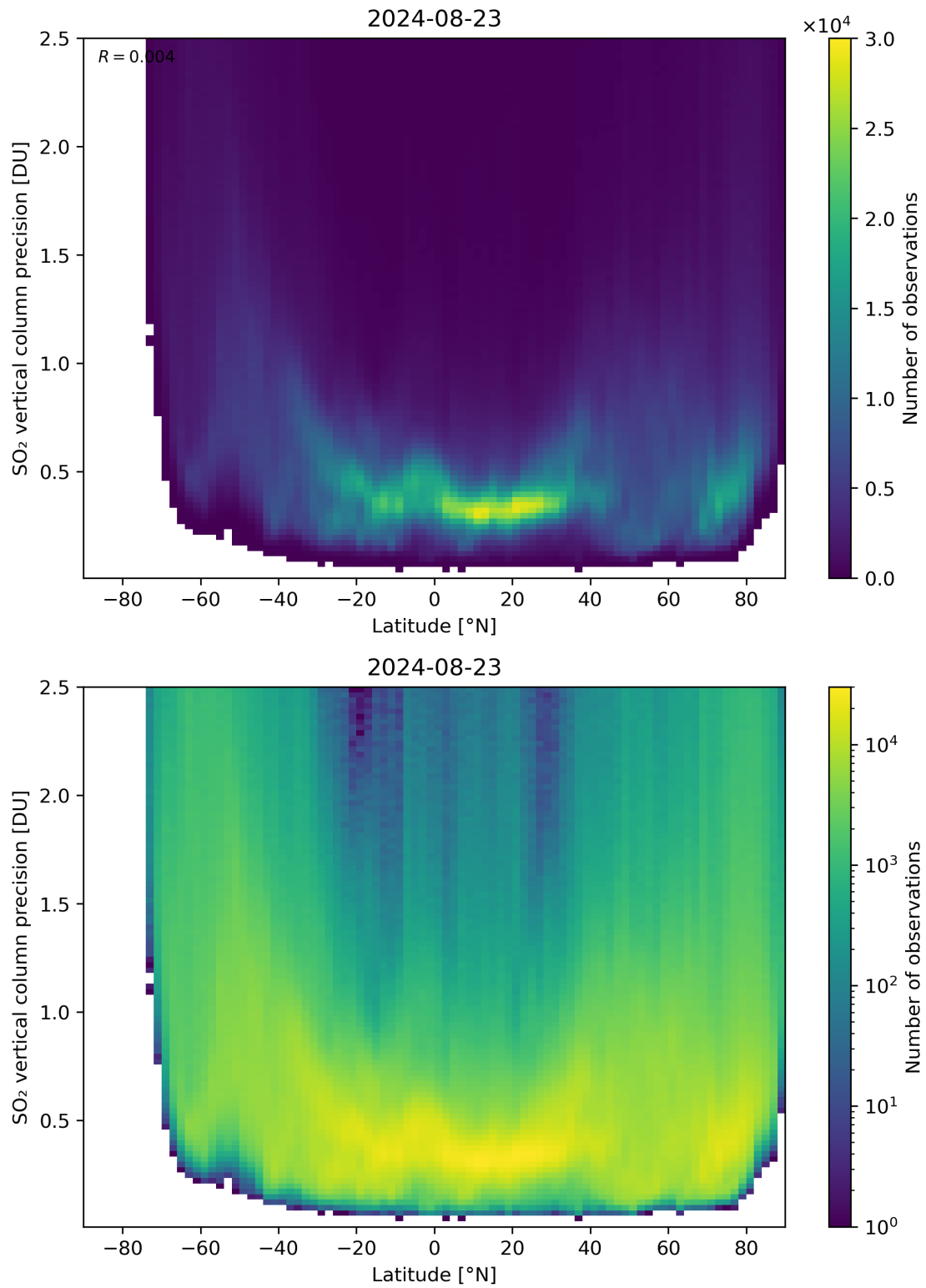
Figure 157: Scatter density plot of “Latitude” against “SO 2 vertical column precision” for 2024-08-22 to 2024-08-24.
