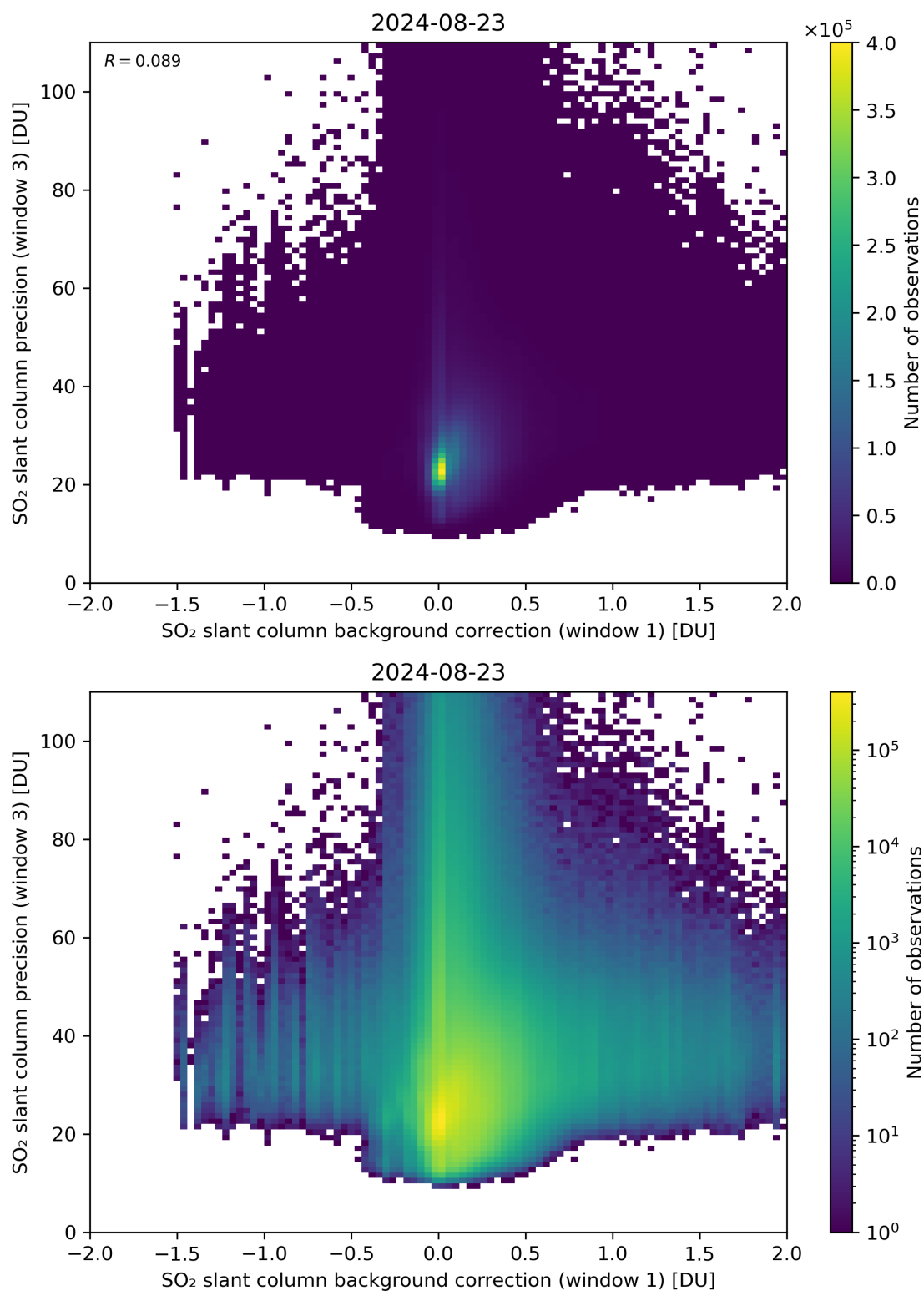
Figure 108: Scatter density plot of “SO 2 slant column background correction (window 1)” against “SO 2 slant column precision (window 3)” for 2024-08-22 to 2024-08-24.
