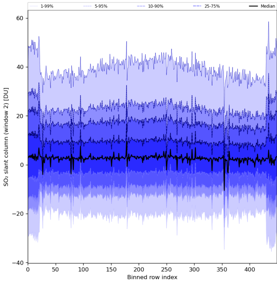
Figure 83: Along track statistics of “SO 2 slant column (window 2)” for 2024-08-22 to 2024-08-24
