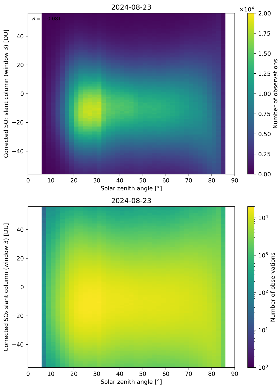
Figure 168: Scatter density plot of “Solar zenith angle” against “Corrected SO 2 slant column (window 3)” for 2024-08-22 to 2024-08-24.
