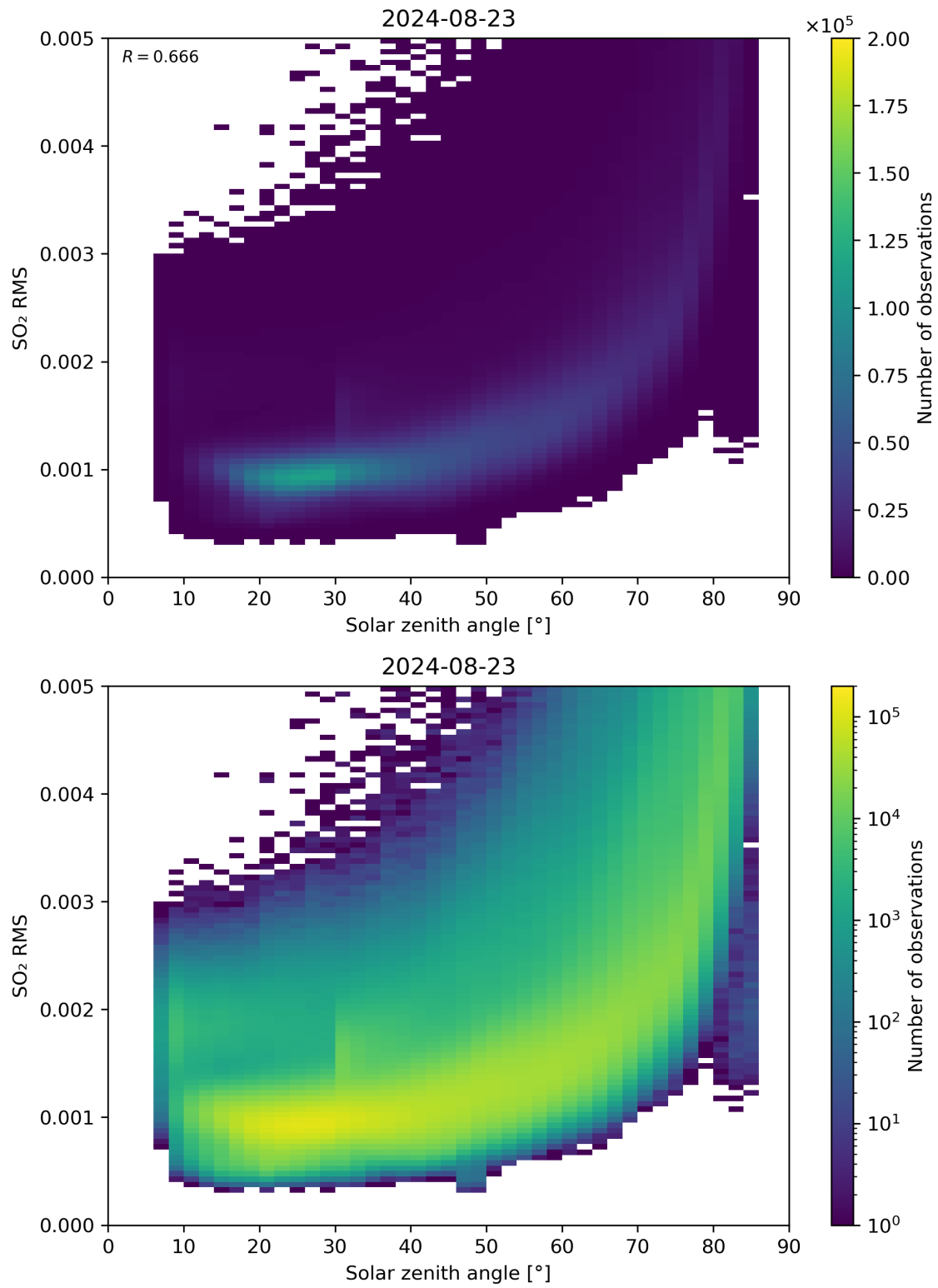
Figure 163: Scatter density plot of “Solar zenith angle” against “SO 2 RMS” for 2024-08-22 to 2024-08-24.
