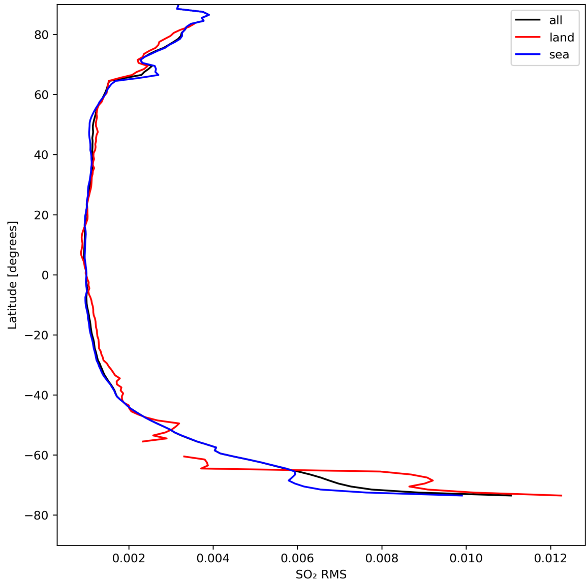
Figure 47: Zonal average of “SO 2 RMS” for 2024-08-22 to 2024-08-24.
