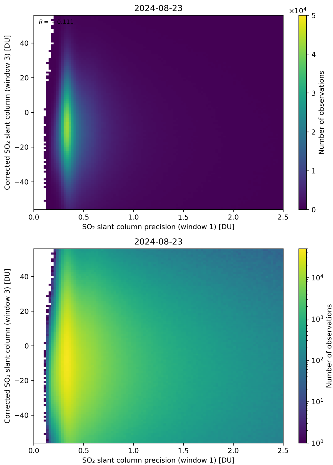
Figure 226: Scatter density plot of “SO 2 slant column precision (window 1)” against “Corrected SO 2 slant column (window 3)” for 2024-08-22 to 2024-08-24.
