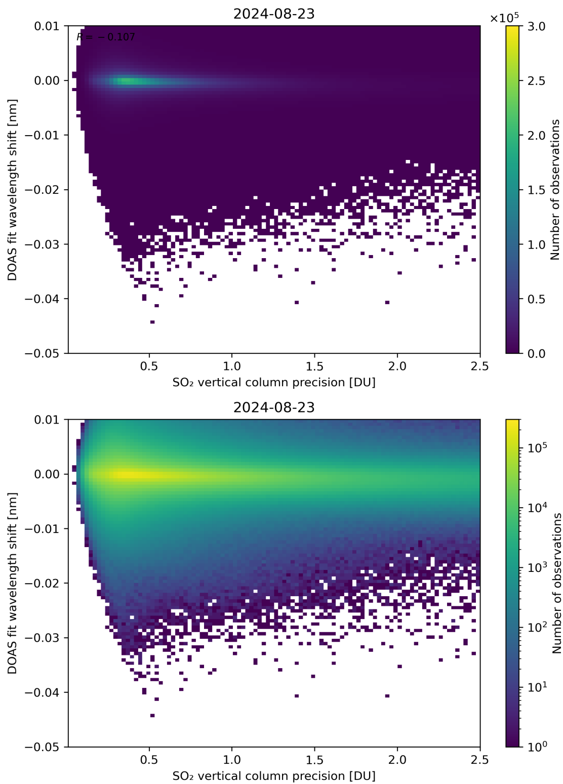
Figure 282: Scatter density plot of “SO 2 vertical column precision” against “DOAS fit wavelength shift” for 2024-08-22 to 2024-08-24.
