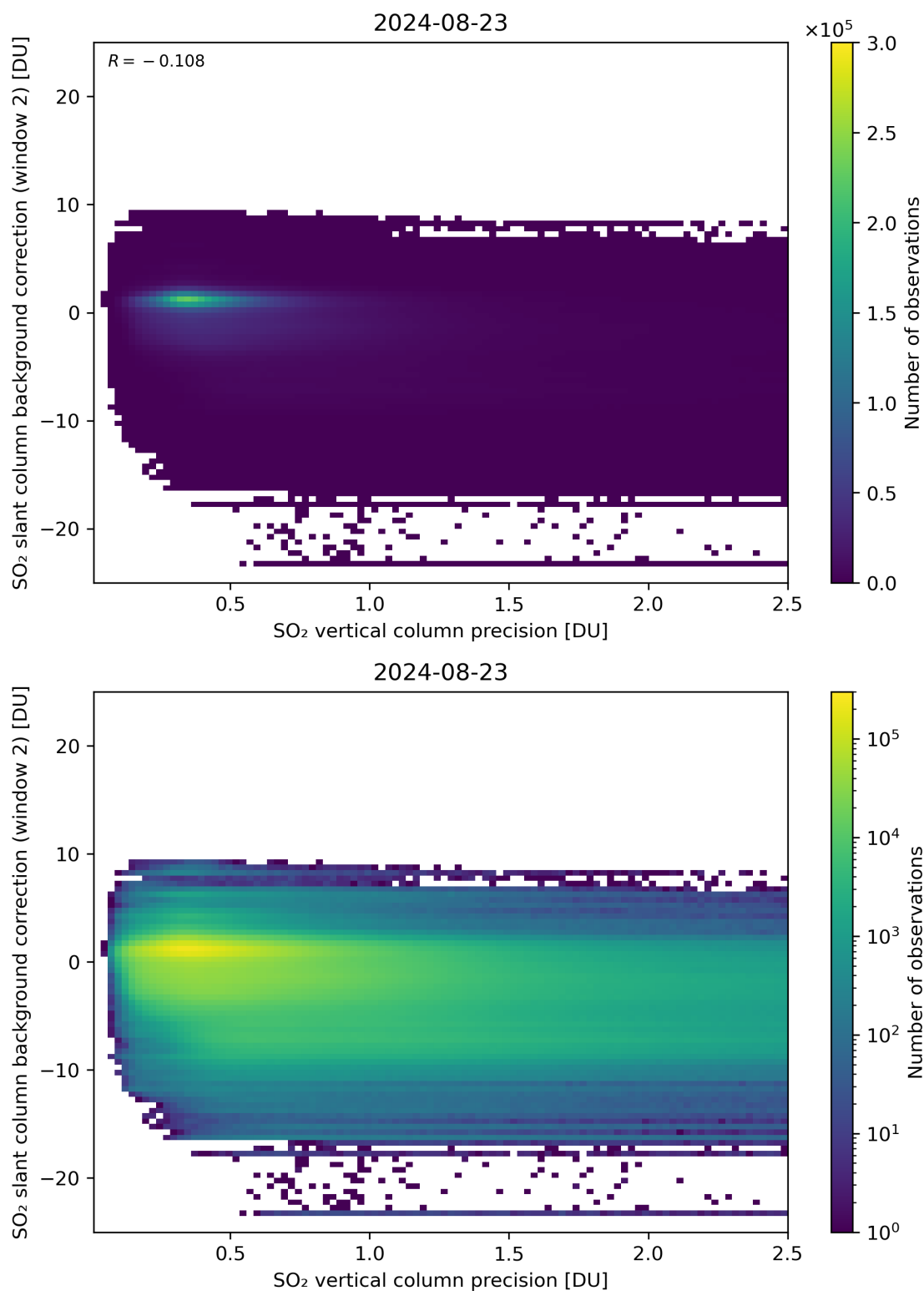
Figure 280: Scatter density plot of “SO 2 vertical column precision” against “SO 2 slant column background correction (window 2)” for 2024-08-22 to 2024-08-24.
