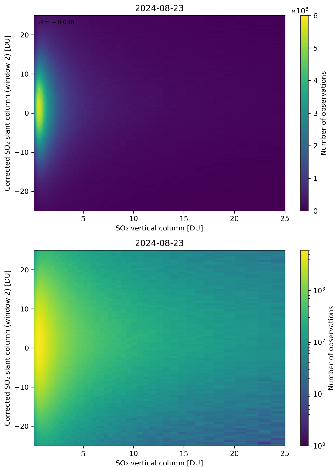
Figure 298: Scatter density plot of “SO 2 vertical column” against “Corrected SO 2 slant column (window 2)” for 2024-08-22 to 2024-08-24.
