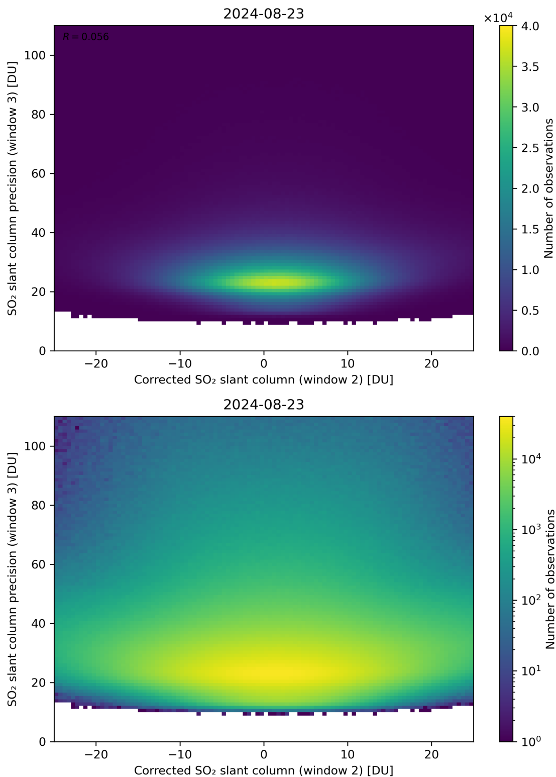
Figure 202: Scatter density plot of “Corrected SO 2 slant column (window 2)” against “SO 2 slant column precision (window 3)” for 2024-08-22 to 2024-08-24.
