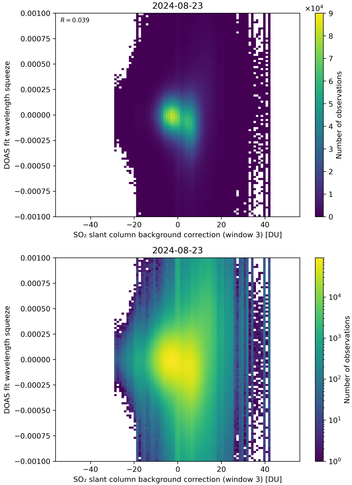
Figure 122: Scatter density plot of “SO 2 slant column background correction (window 3)” against “DOAS fit wavelength squeeze” for 2024-08-22 to 2024-08-24.
