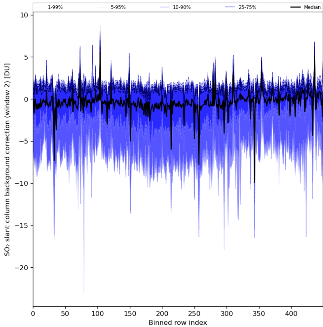
Figure 86: Along track statistics of “SO 2 slant column background correction (window 2)” for 2024-08-22 to 2024-08-24
