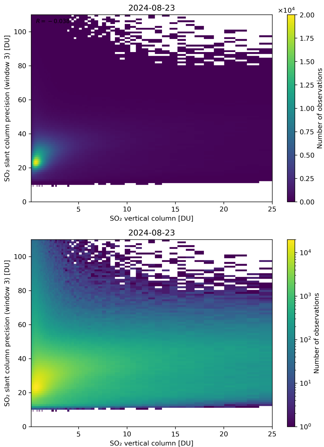
Figure 304: Scatter density plot of “SO 2 vertical column” against “SO 2 slant column precision (window 3)” for 2024-08-22 to 2024-08-24.
