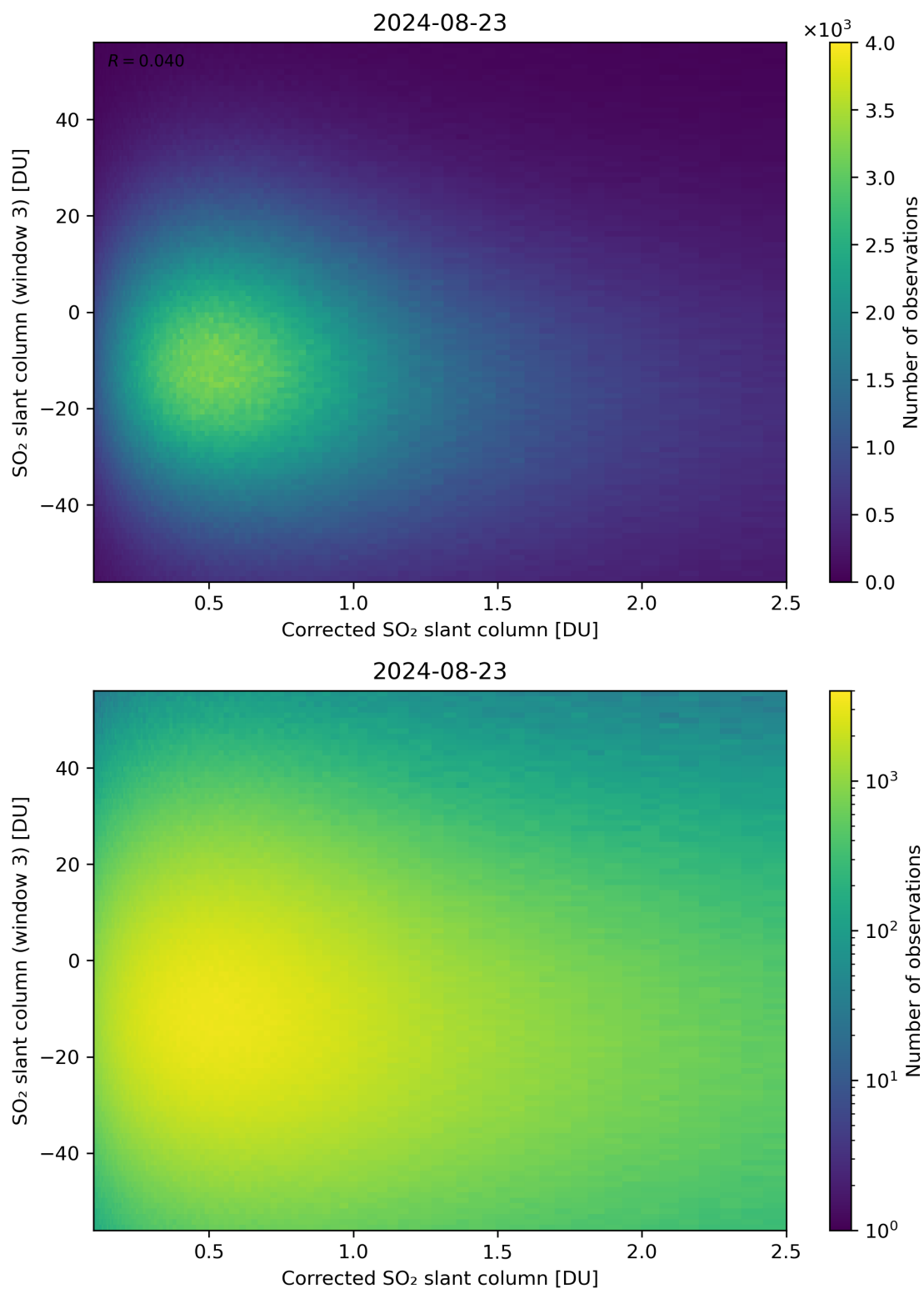
Figure 190: Scatter density plot of “Corrected SO 2 slant column” against “SO 2 slant column (window 3)” for 2024-08-22 to 2024-08-24.
