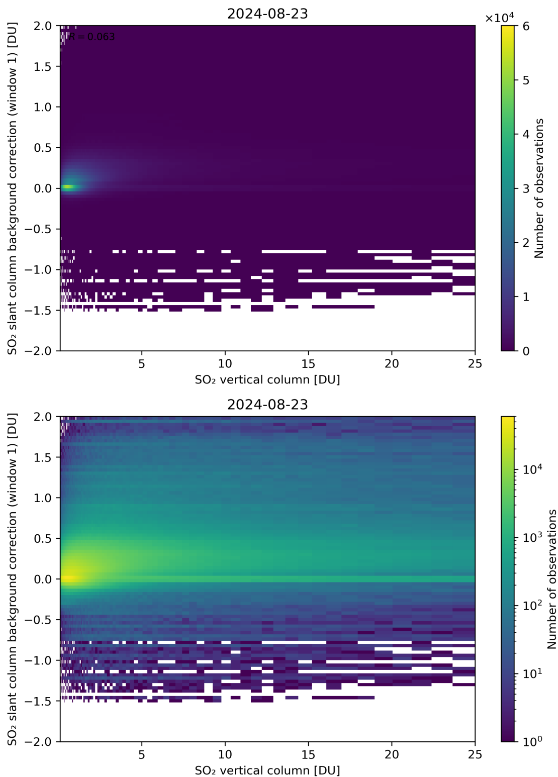
Figure 273: Scatter density plot of “SO 2 vertical column” against “SO 2 slant column background correction (window 1)” for 2024-08-22 to 2024-08-24.
