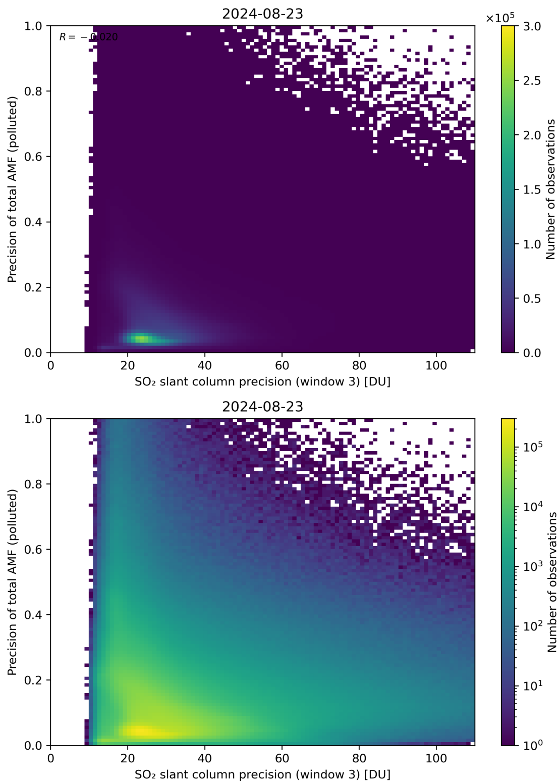
Figure 264: Scatter density plot of “SO 2 slant column precision (window 3)” against “Precision of total AMF (polluted)” for 2024-08-22 to 2024-08-24.
