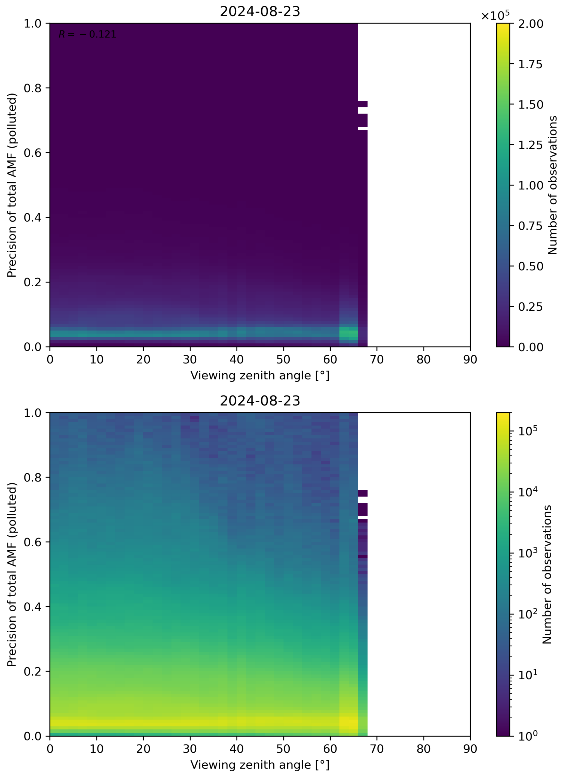
Figure 326: Scatter density plot of “Viewing zenith angle” against “Precision of total AMF (polluted)” for 2024-08-22 to 2024-08-24.
