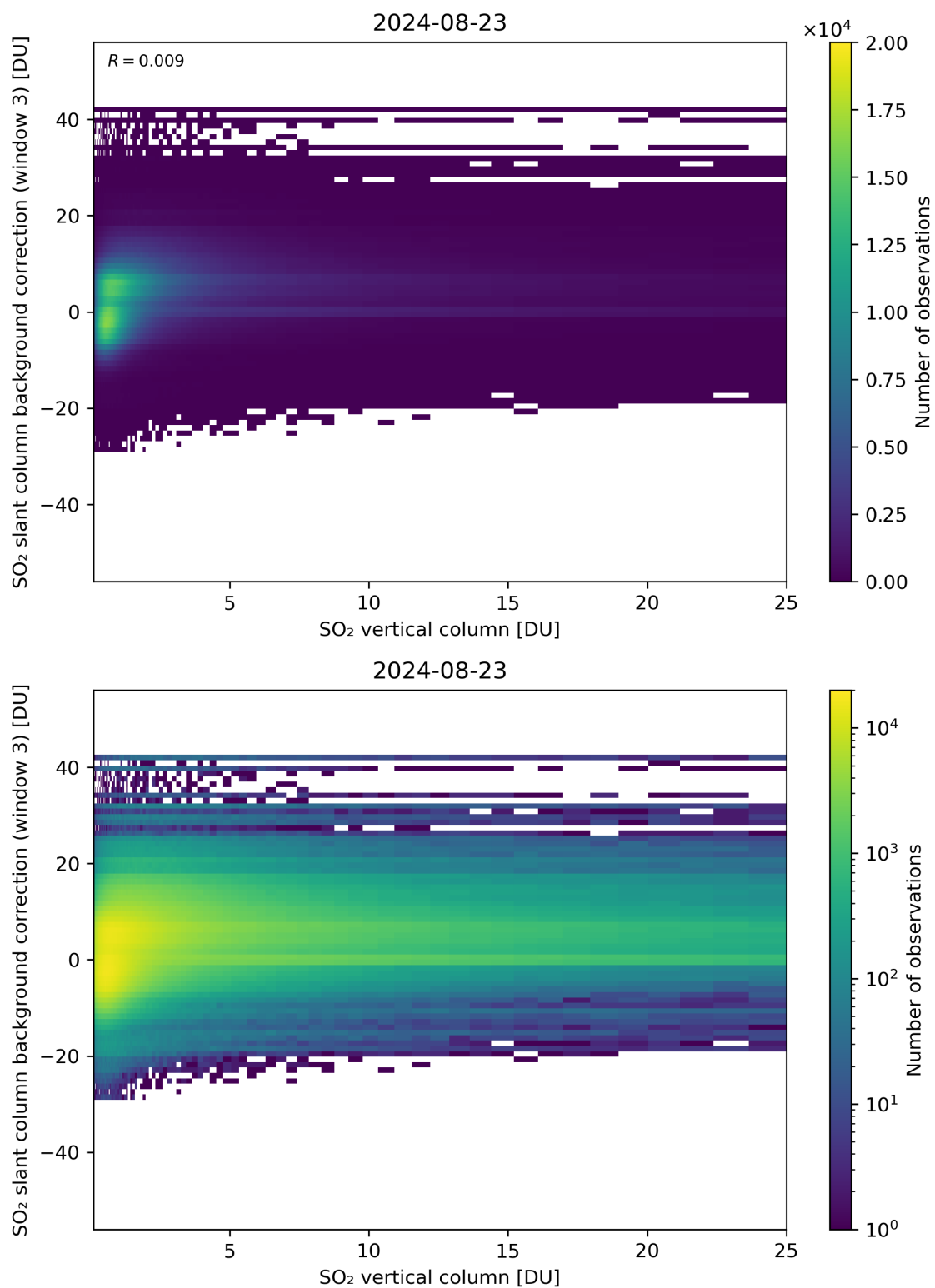
Figure 275: Scatter density plot of “SO 2 vertical column” against “SO 2 slant column background correction (window 3)” for 2024-08-22 to 2024-08-24.
