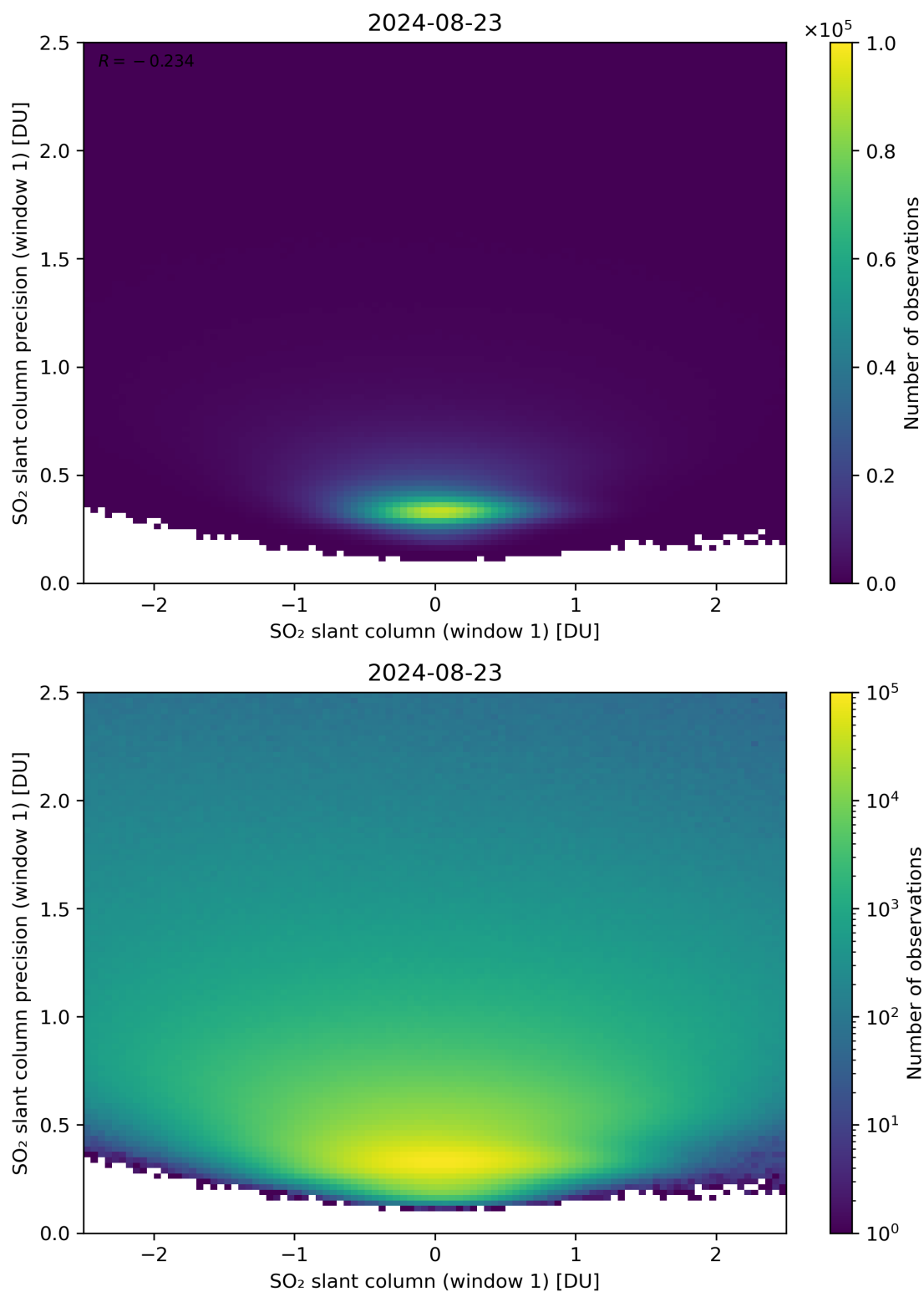
Figure 235: Scatter density plot of “SO 2 slant column (window 1)” against “SO 2 slant column precision (window 1)” for 2024-08-22 to 2024-08-24.
