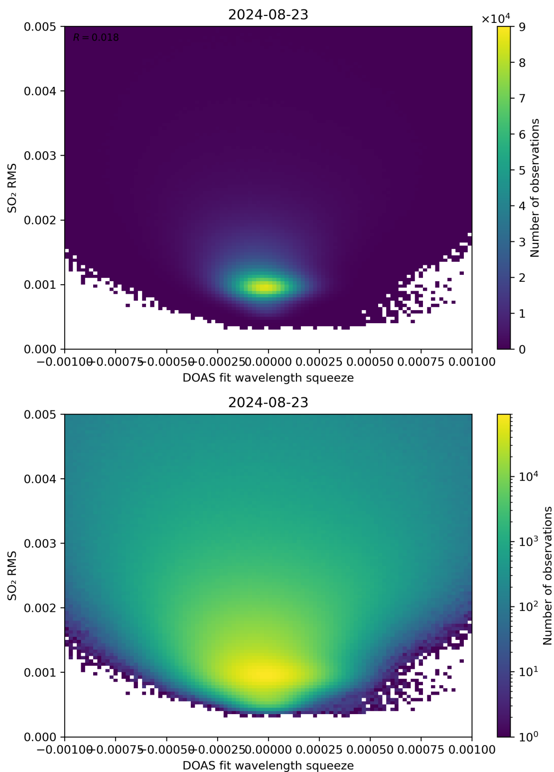
Figure 132: Scatter density plot of “DOAS fit wavelength squeeze” against “SO 2 RMS” for 2024-08-22 to 2024-08-24.
