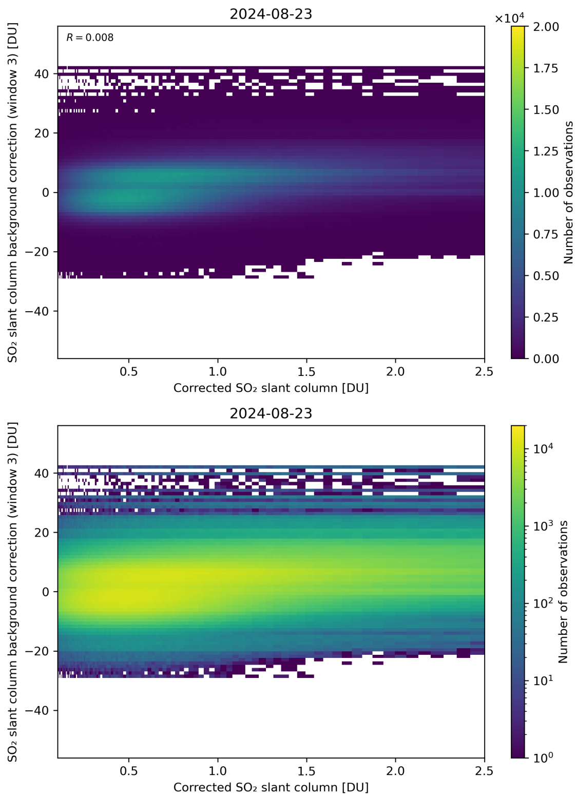
Figure 180: Scatter density plot of “Corrected SO 2 slant column” against “SO 2 slant column background correction (window 3)” for 2024-08-22 to 2024-08-24.
