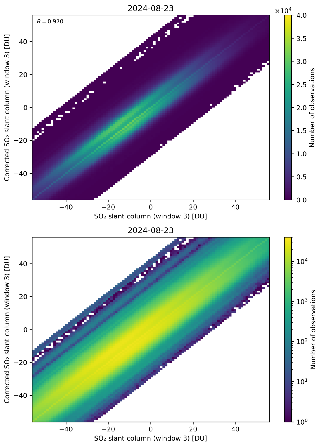
Figure 266: Scatter density plot of “SO 2 slant column (window 3)” against “Corrected SO 2 slant column (window 3)” for 2024-08-22 to 2024-08-24.
