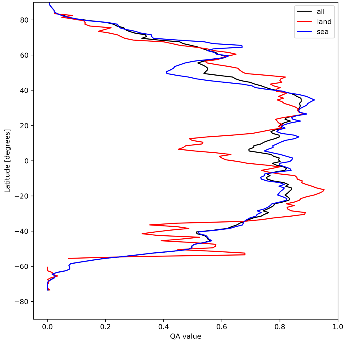
Figure 29: Zonal average of “QA value” for 2024-08-22 to 2024-08-24.
