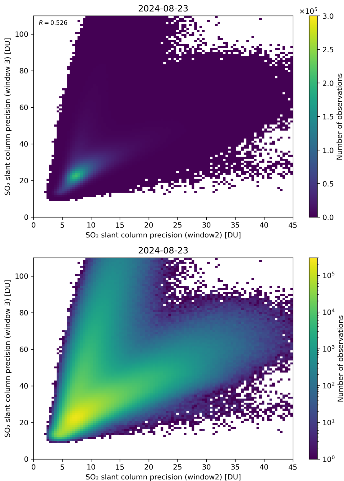
Figure 250: Scatter density plot of “SO 2 slant column precision (window2)” against “SO 2 slant column precision (window 3)” for 2024-08-22 to 2024-08-24.
