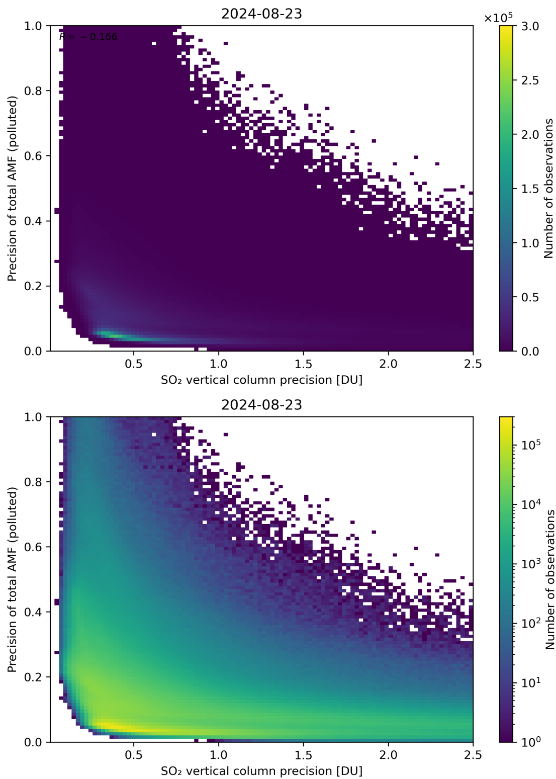
Figure 295: Scatter density plot of “SO 2 vertical column precision” against “Precision of total AMF (polluted)” for 2024-08-22 to 2024-08-24.
