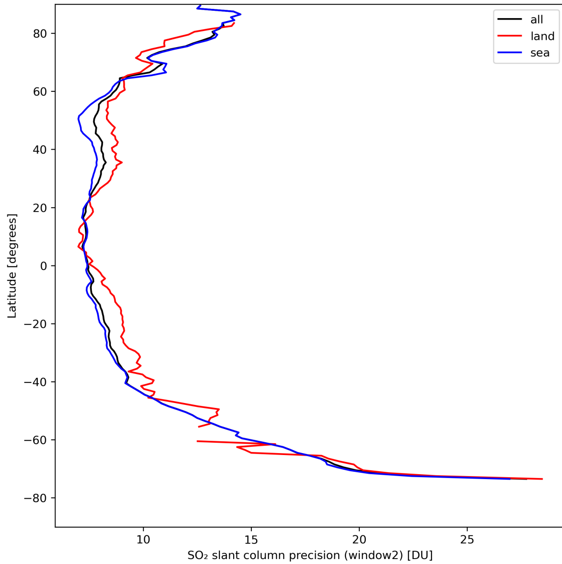
Figure 38: Zonal average of “SO 2 slant column precision (window2)” for 2024-08-22 to 2024-08-24.
