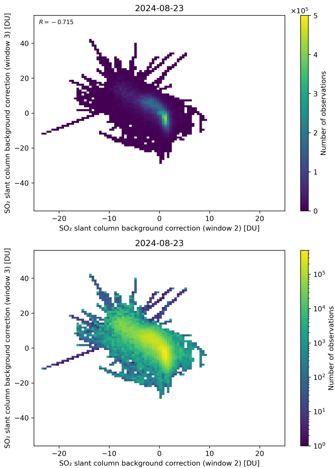
Figure 111: Scatter density plot of “SO 2 slant column background correction (window 2)” against “SO 2 slant column background correction (window 3)” for 2024-08-22 to 2024-08-24.
