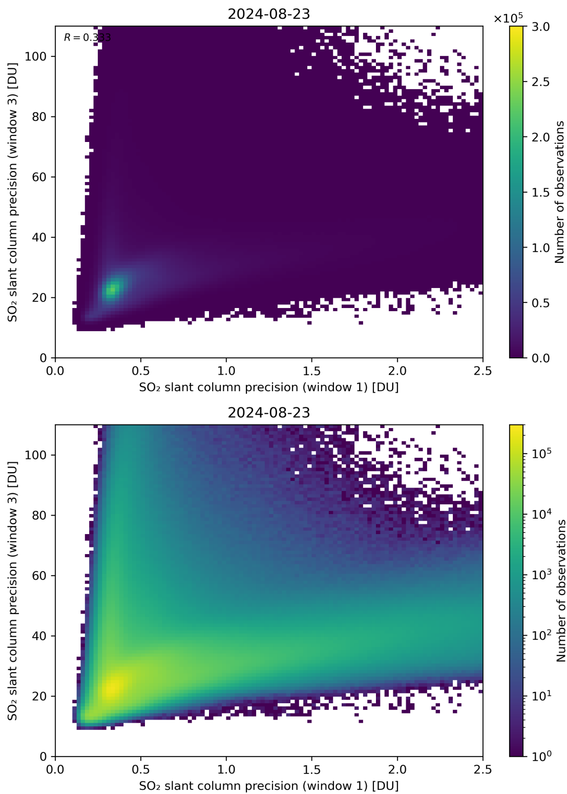
Figure 229: Scatter density plot of “SO 2 slant column precision (window 1)” against “SO 2 slant column precision (window 3)” for 2024-08-22 to 2024-08-24.
