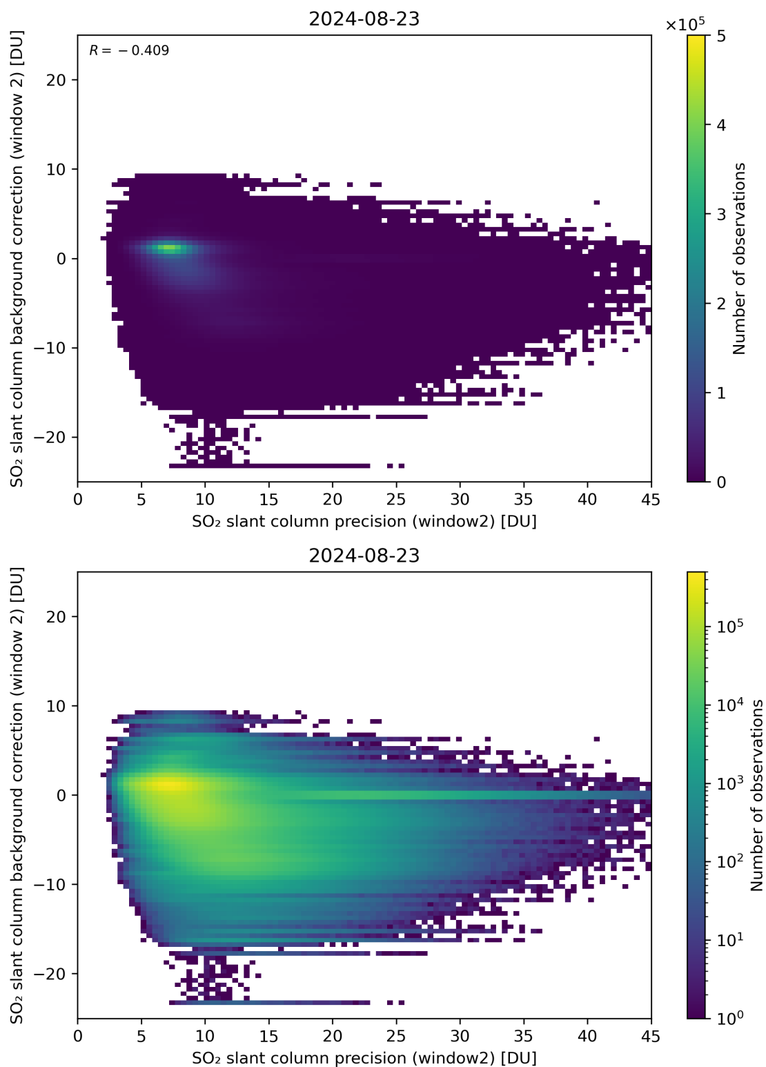
Figure 241: Scatter density plot of “SO 2 slant column precision (window2)” against “SO 2 slant column background correction (window 2)” for 2024-08-22 to 2024-08-24.
