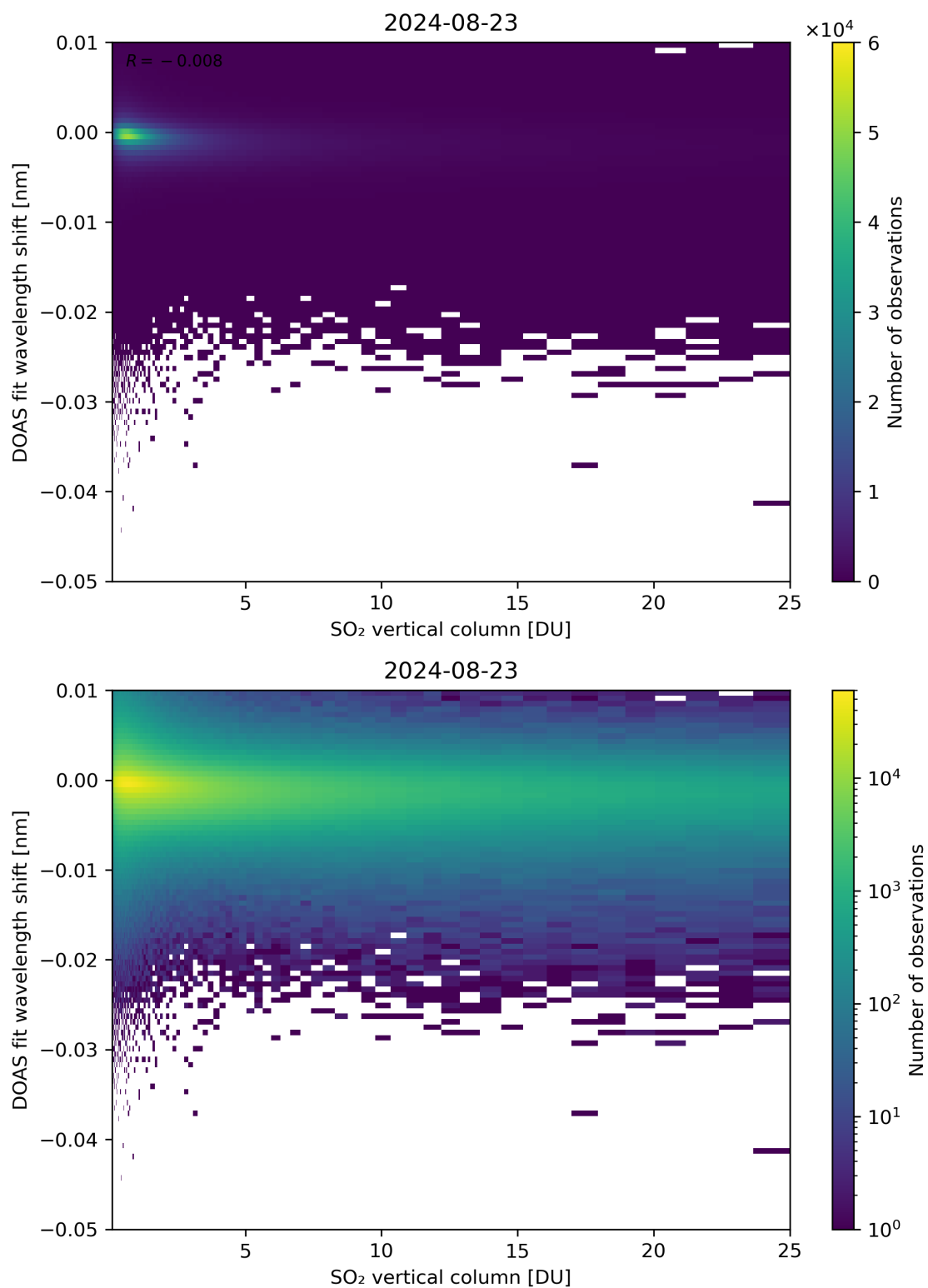
Figure 276: Scatter density plot of “SO 2 vertical column” against “DOAS fit wavelength shift” for 2024-08-22 to 2024-08-24.
