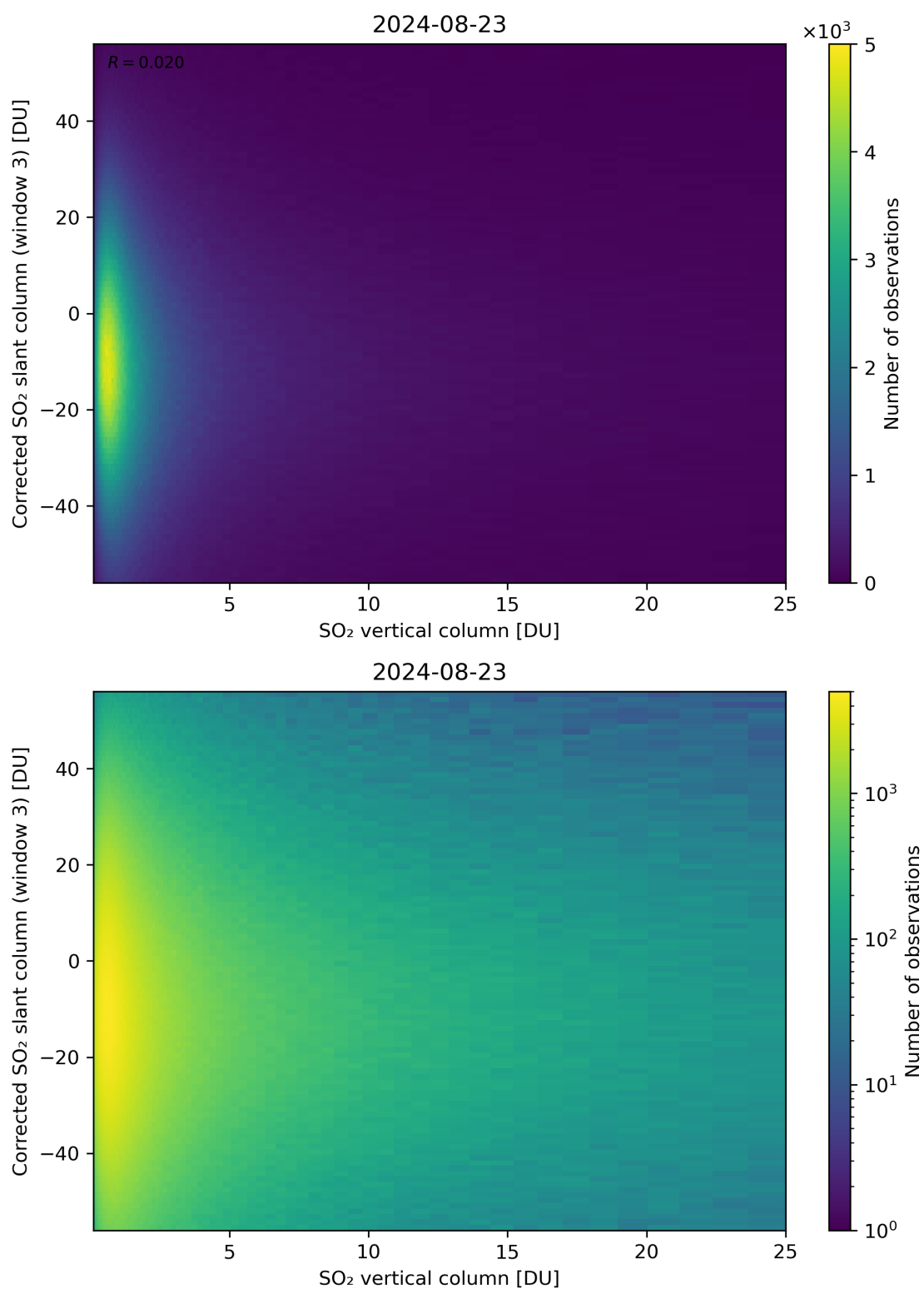
Figure 299: Scatter density plot of “SO 2 vertical column” against “Corrected SO 2 slant column (window 3)” for 2024-08-22 to 2024-08-24.
