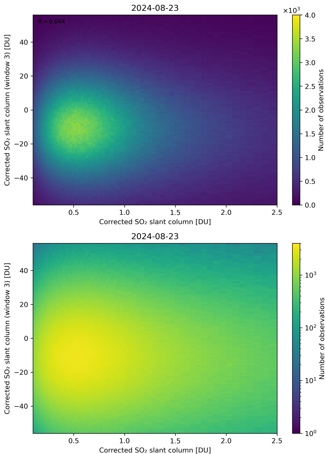
Figure 186: Scatter density plot of “Corrected SO 2 slant column” against “Corrected SO 2 slant column (window 3)” for 2024-08-22 to 2024-08-24.
