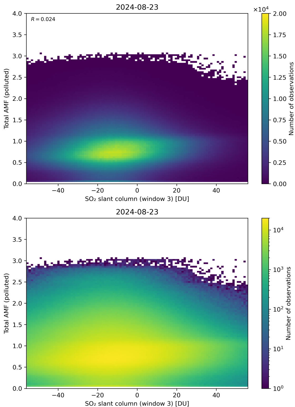
Figure 268: Scatter density plot of “SO 2 slant column (window 3)” against “Total AMF (polluted)” for 2024-08-22 to 2024-08-24.
