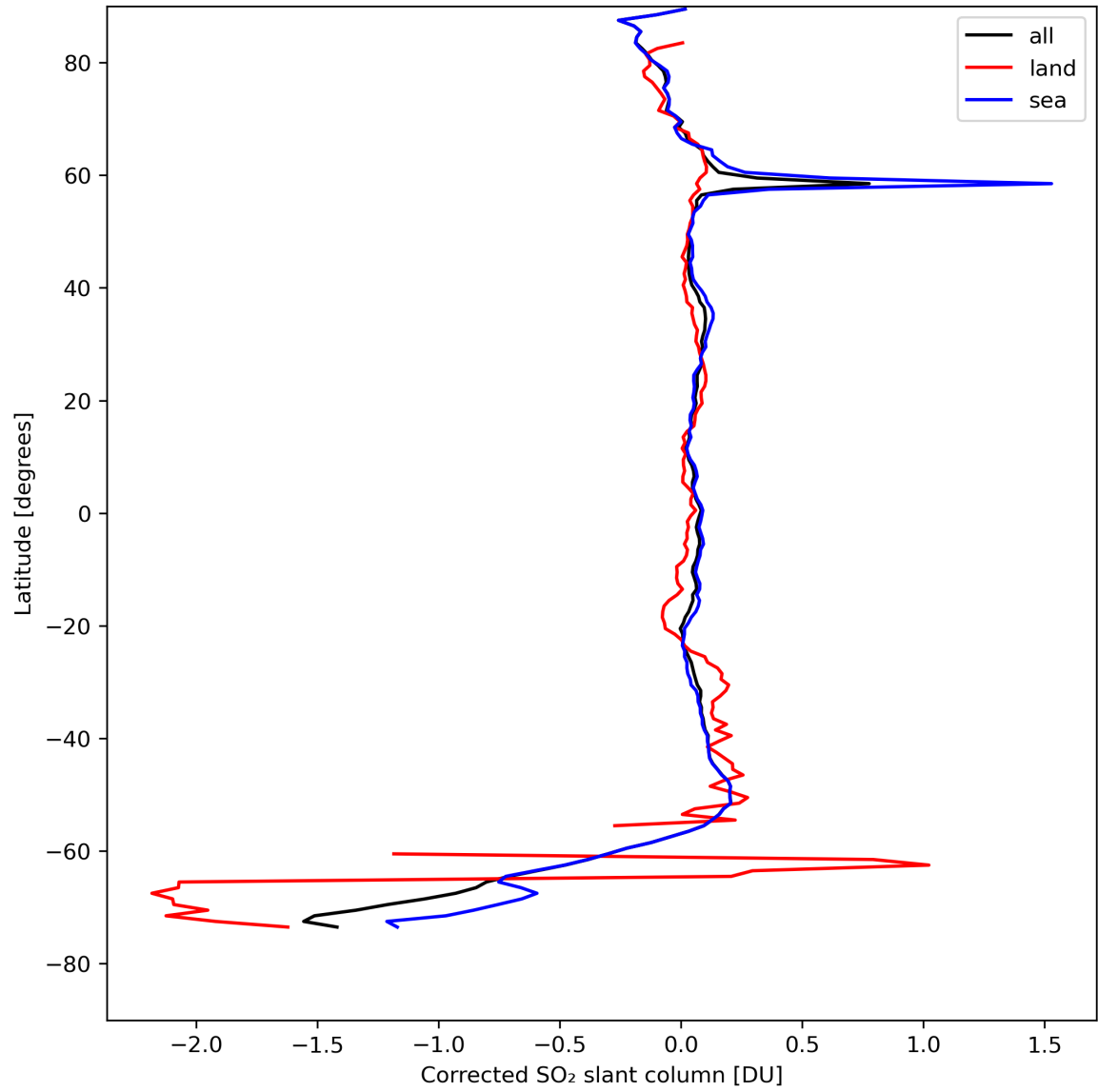
Figure 32: Zonal average of “Corrected SO 2 slant column” for 2024-08-22 to 2024-08-24.
