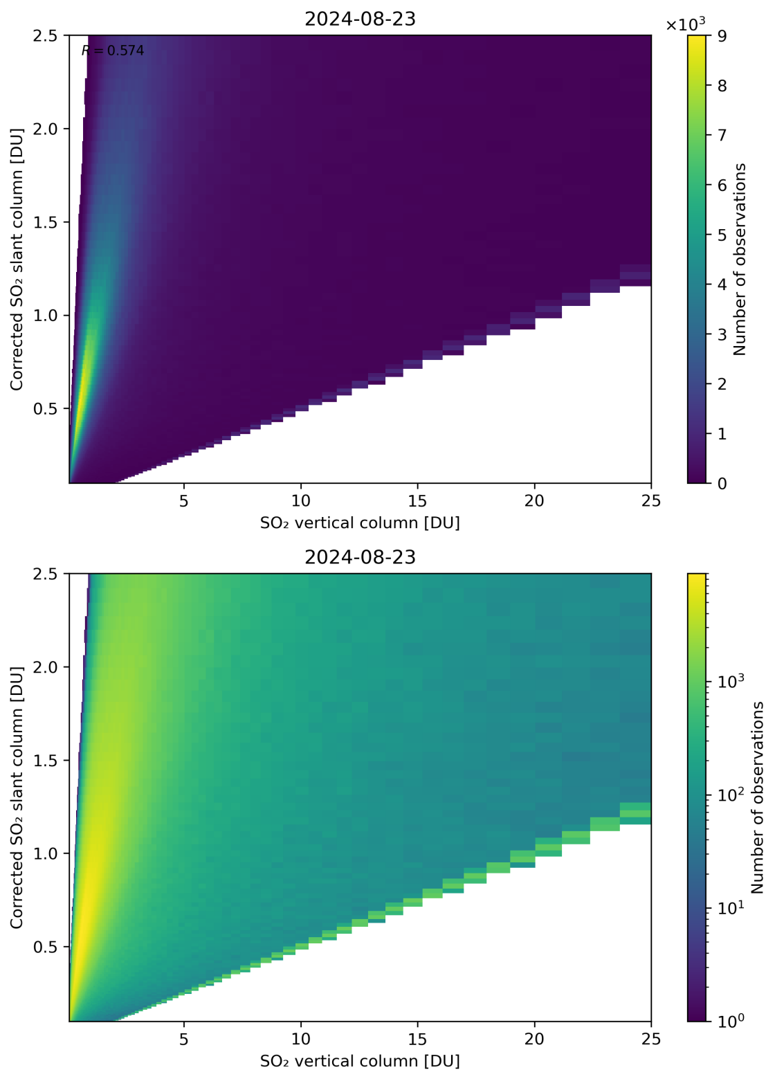
Figure 297: Scatter density plot of “SO 2 vertical column” against “Corrected SO 2 slant column” for 2024-08-22 to 2024-08-24.
