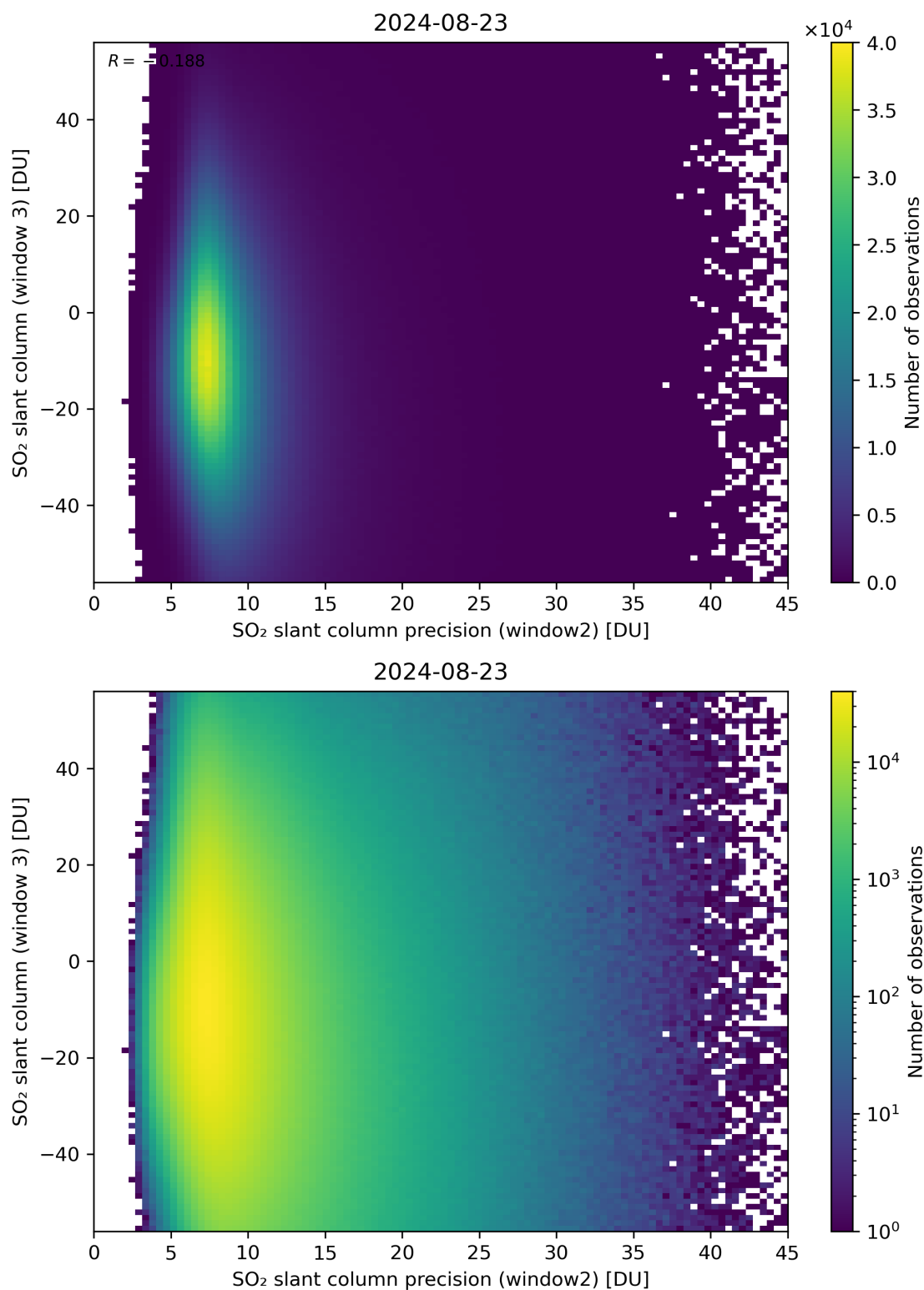
Figure 249: Scatter density plot of “SO 2 slant column precision (window2)” against “SO 2 slant column (window 3)” for 2024-08-22 to 2024-08-24.
