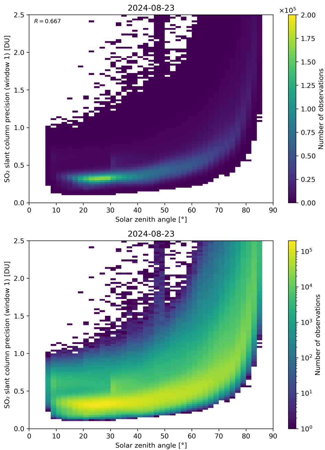
Figure 170: Scatter density plot of “Solar zenith angle” against “SO 2 slant column precision (window 1)” for 2024-08-22 to 2024-08-24.
