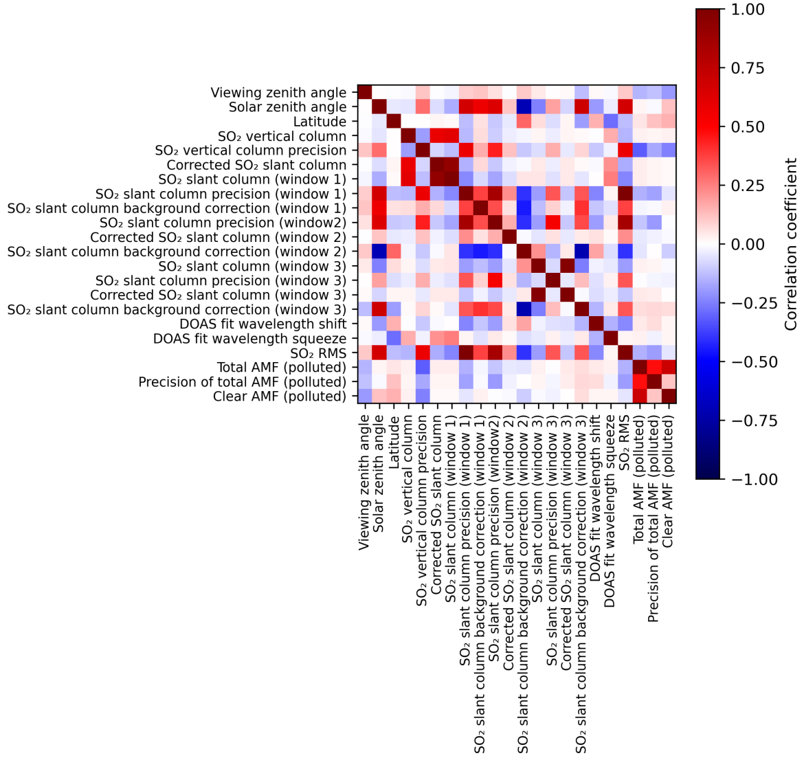
Figure 2: Map of correlation matrix for 2024-08-22 to 2024-08-24.
