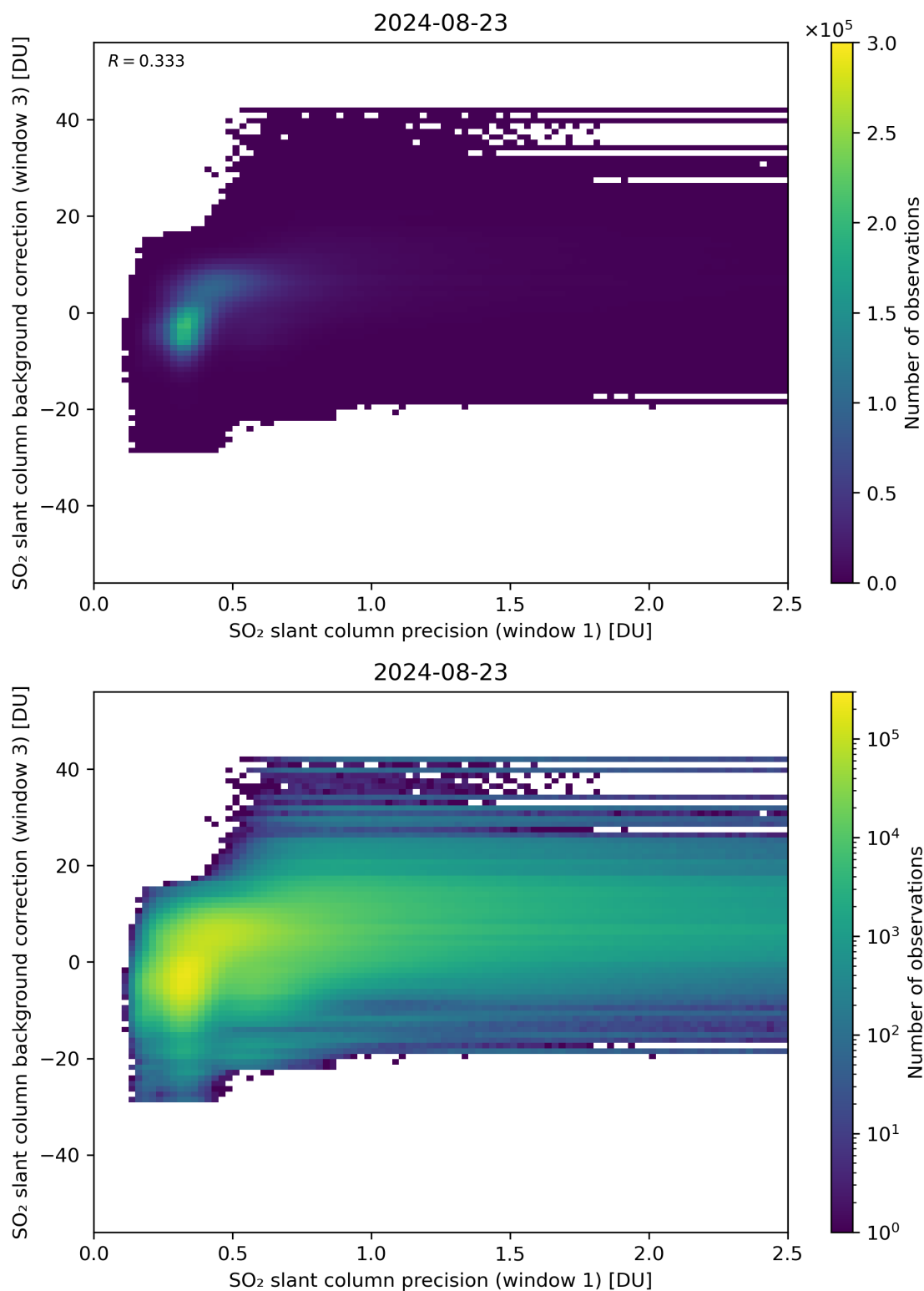
Figure 220: Scatter density plot of “SO 2 slant column precision (window 1)” against “SO 2 slant column background correction (window 3)” for 2024-08-22 to 2024-08-24.
