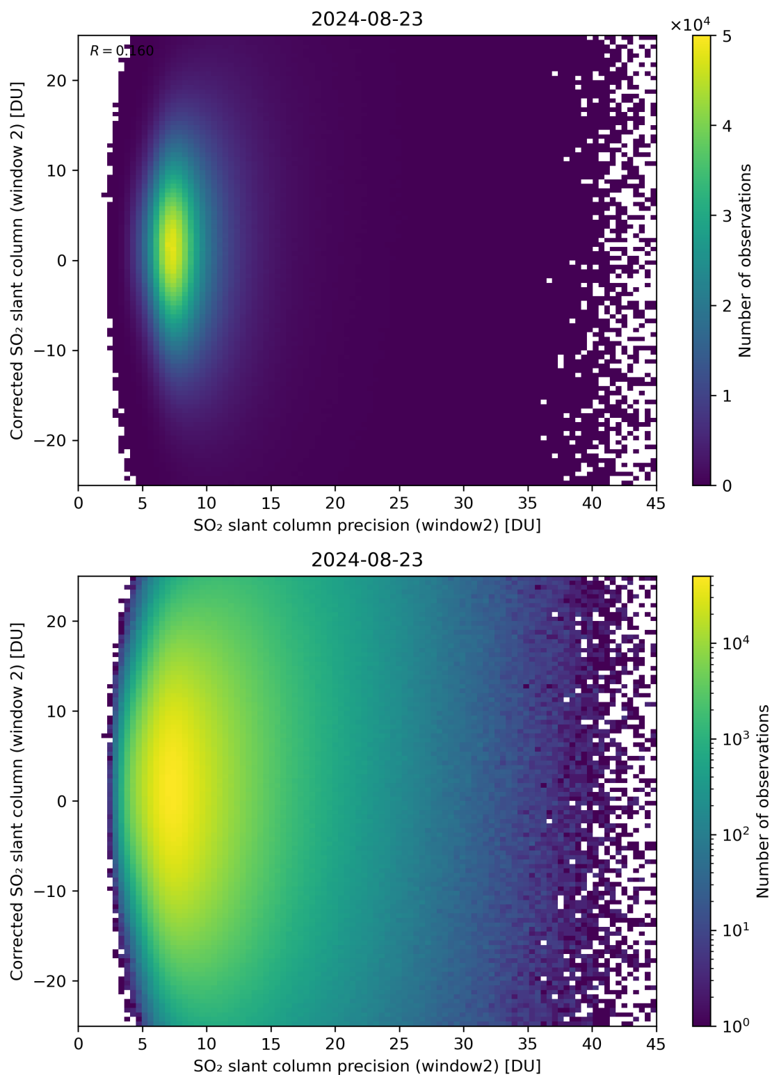
Figure 247: Scatter density plot of “SO 2 slant column precision (window2)” against “Corrected SO 2 slant column (window 2)” for 2024-08-22 to 2024-08-24.
