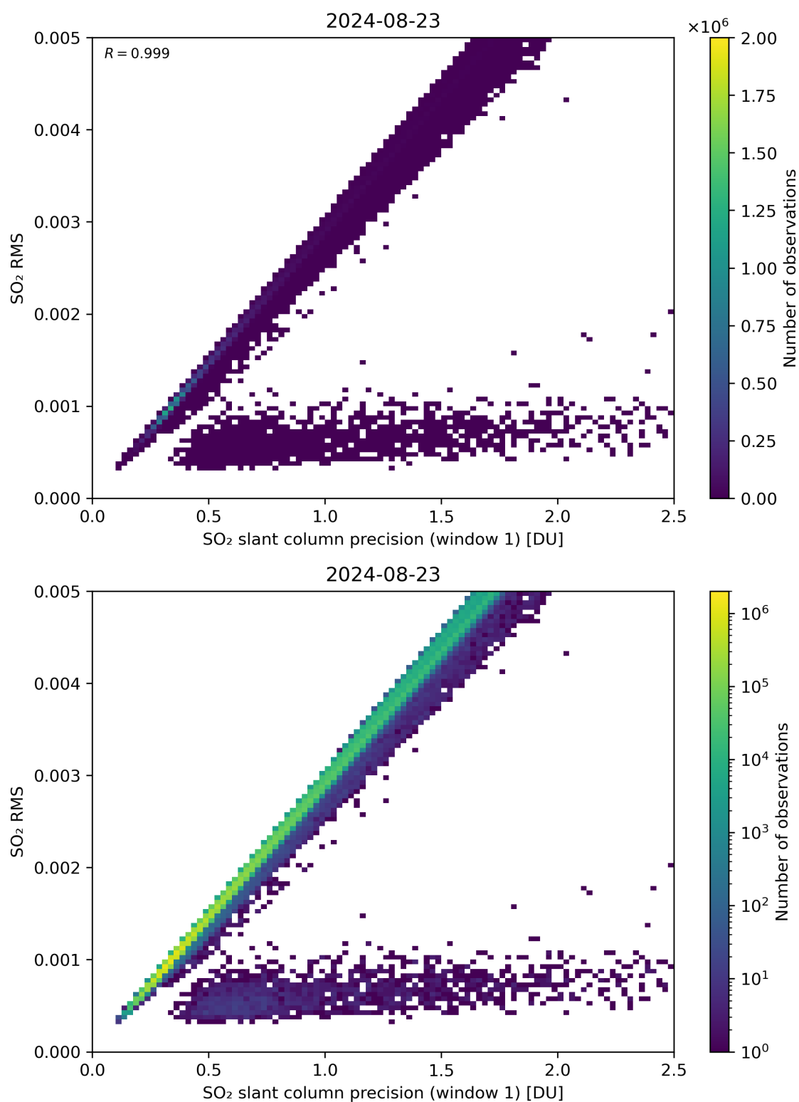
Figure 223: Scatter density plot of “SO 2 slant column precision (window 1)” against “SO 2 RMS” for 2024-08-22 to 2024-08-24.
