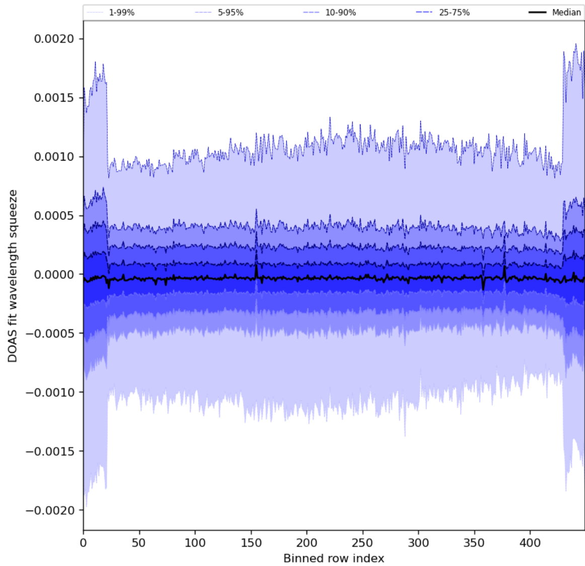
Figure 92: Along track statistics of “DOAS fit wavelength squeeze” for 2024-08-22 to 2024-08-24
