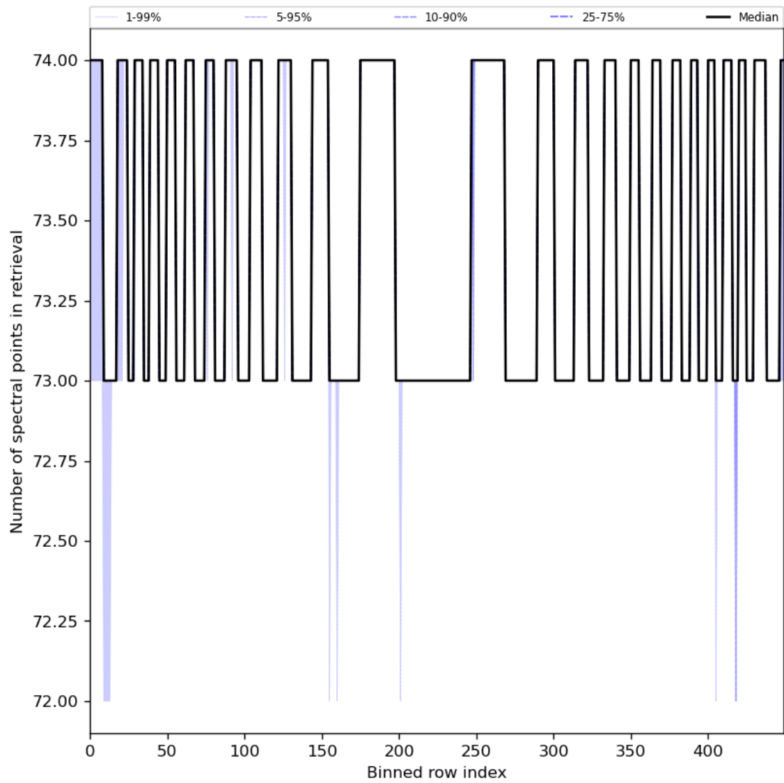
Figure 97: Along track statistics of “Number of spectral points in retrieval” for 2024-08-22 to 2024-08-24
