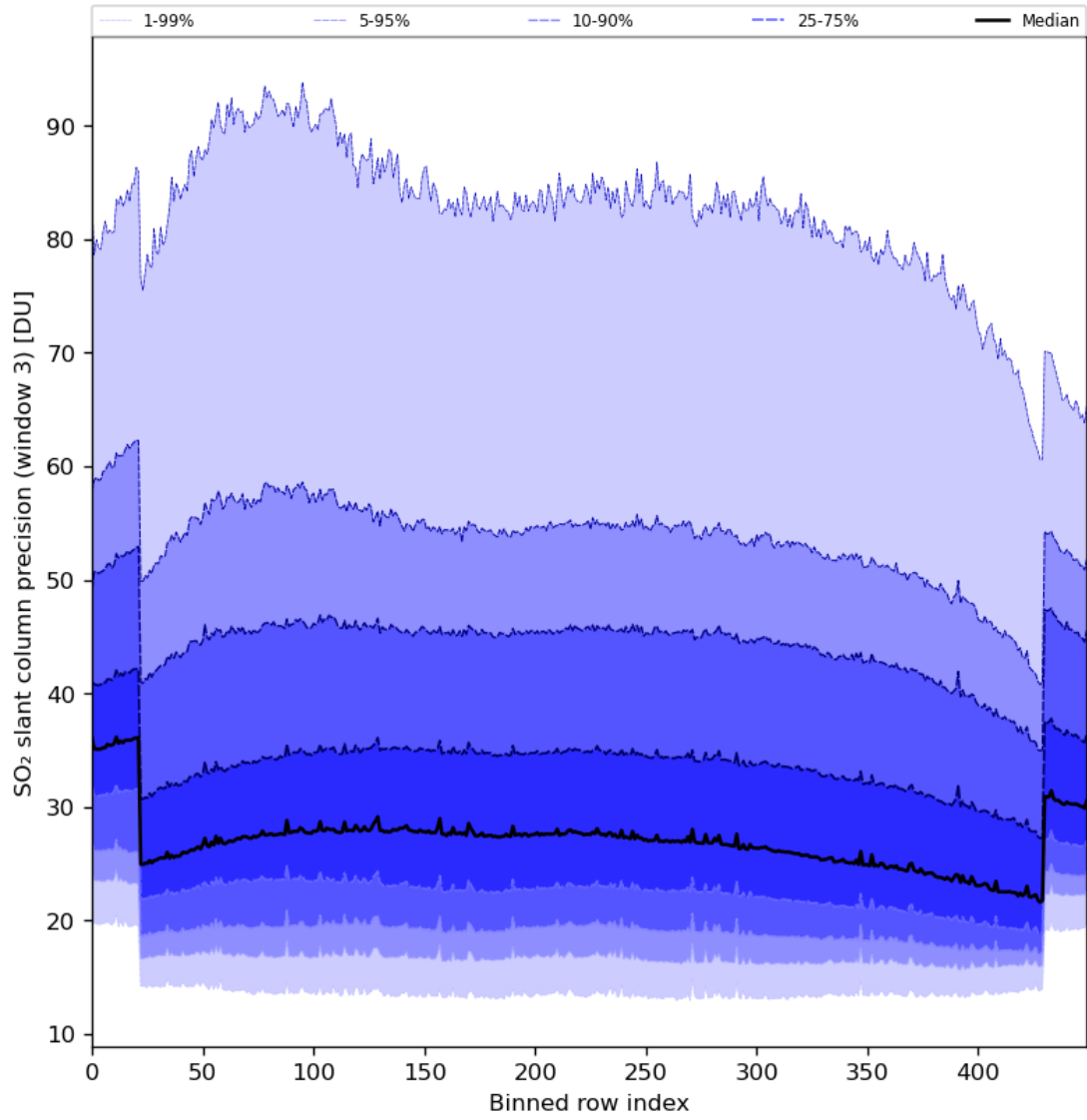
Figure 88: Along track statistics of “SO 2 slant column precision (window 3)” for 2024-08-22 to 2024-08-24
