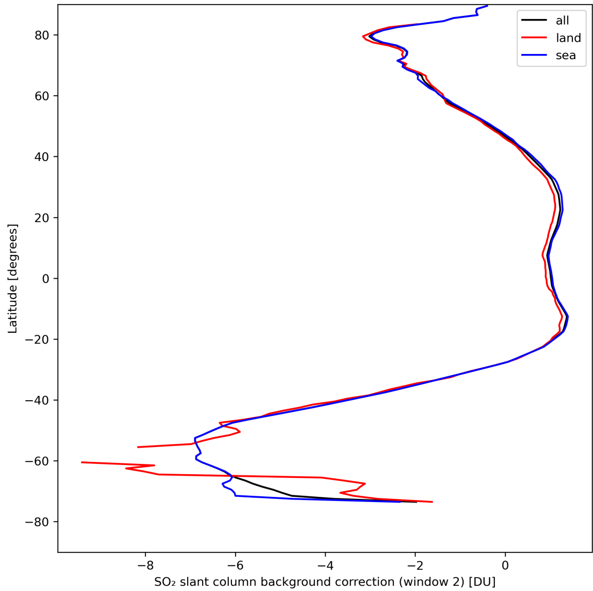
Figure 40: Zonal average of “SO 2 slant column background correction (window 2)” for 2024-08-22 to 2024-08-24.
