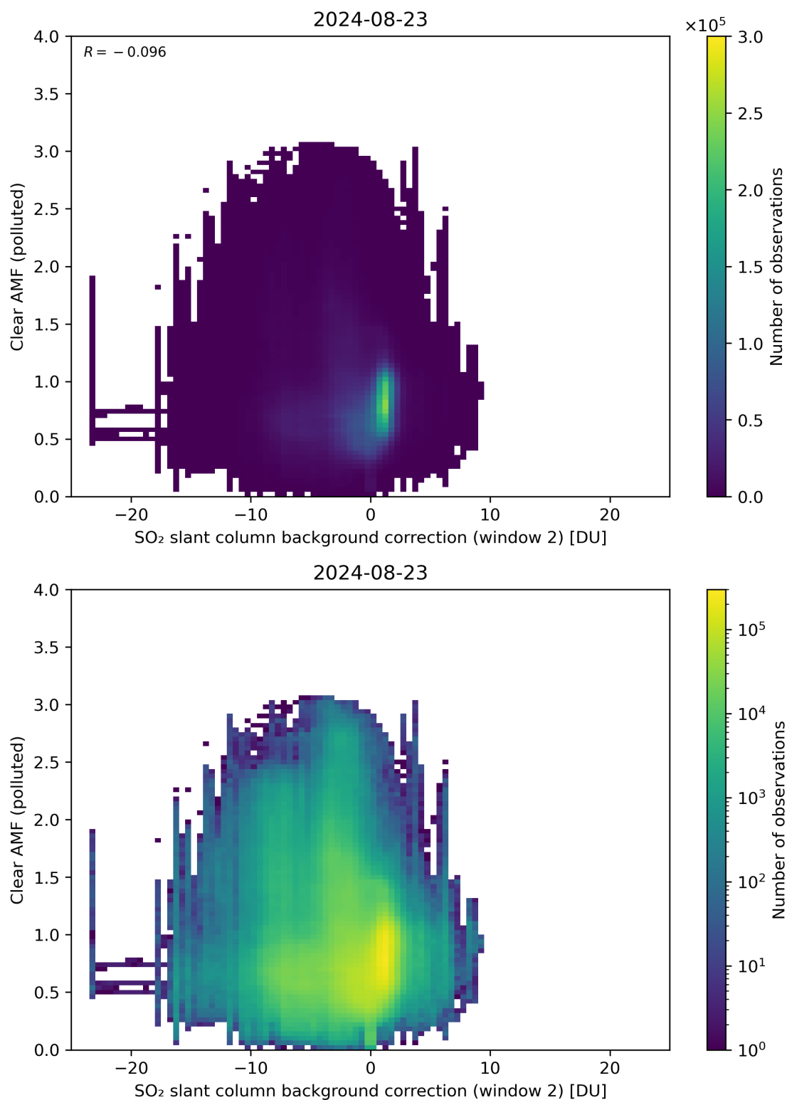
Figure 115: Scatter density plot of “SO 2 slant column background correction (window 2)” against “Clear AMF (polluted)” for 2024-08-22 to 2024-08-24.
