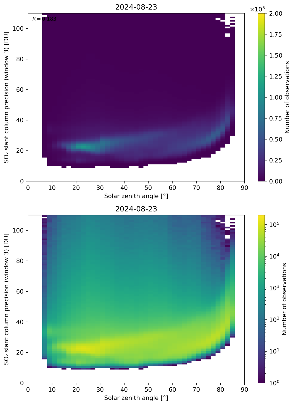
Figure 173: Scatter density plot of “Solar zenith angle” against “SO 2 slant column precision (window 3)” for 2024-08-22 to 2024-08-24.
