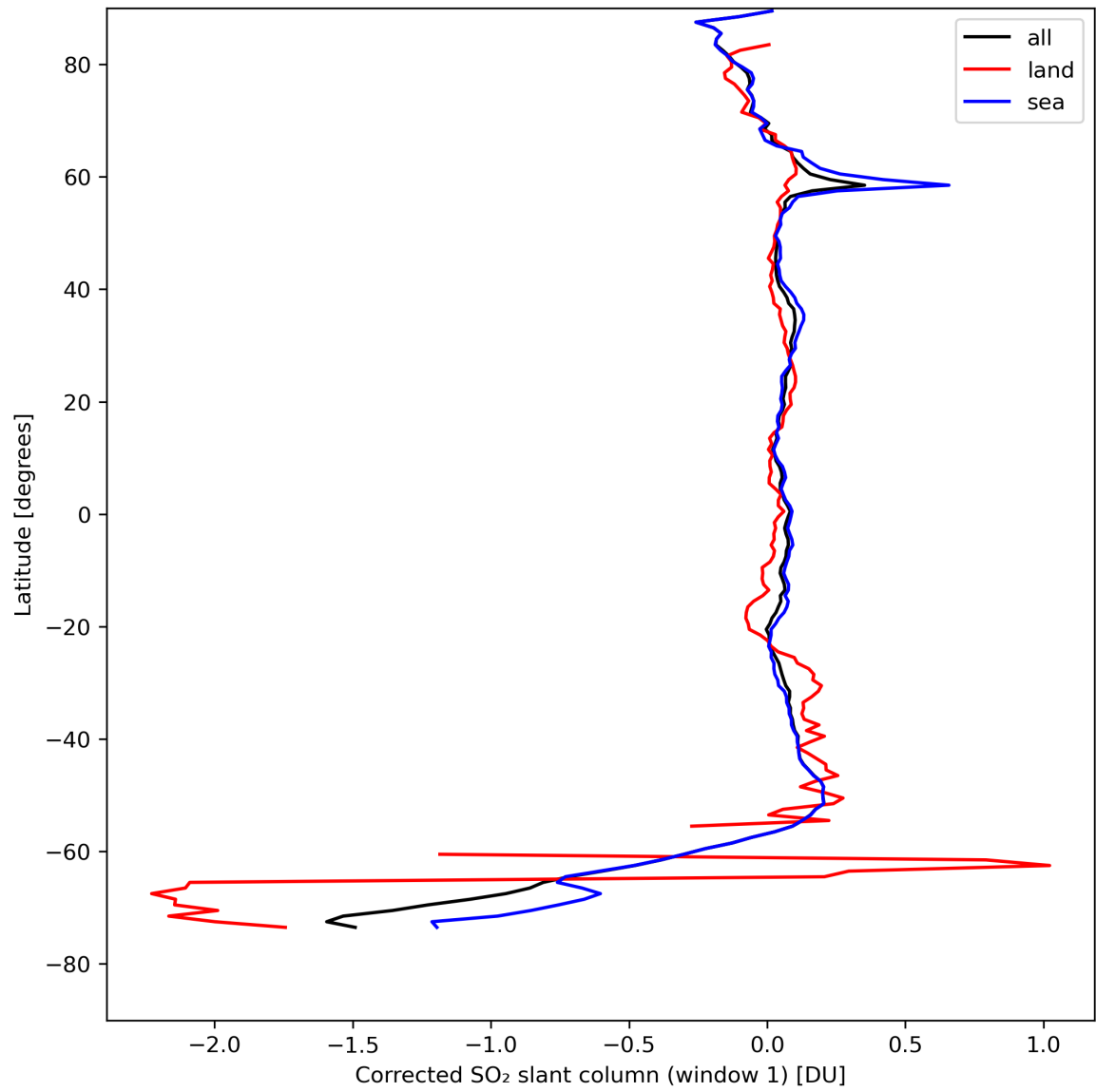
Figure 35: Zonal average of “Corrected SO 2 slant column (window 1)” for 2024-08-22 to 2024-08-24.
