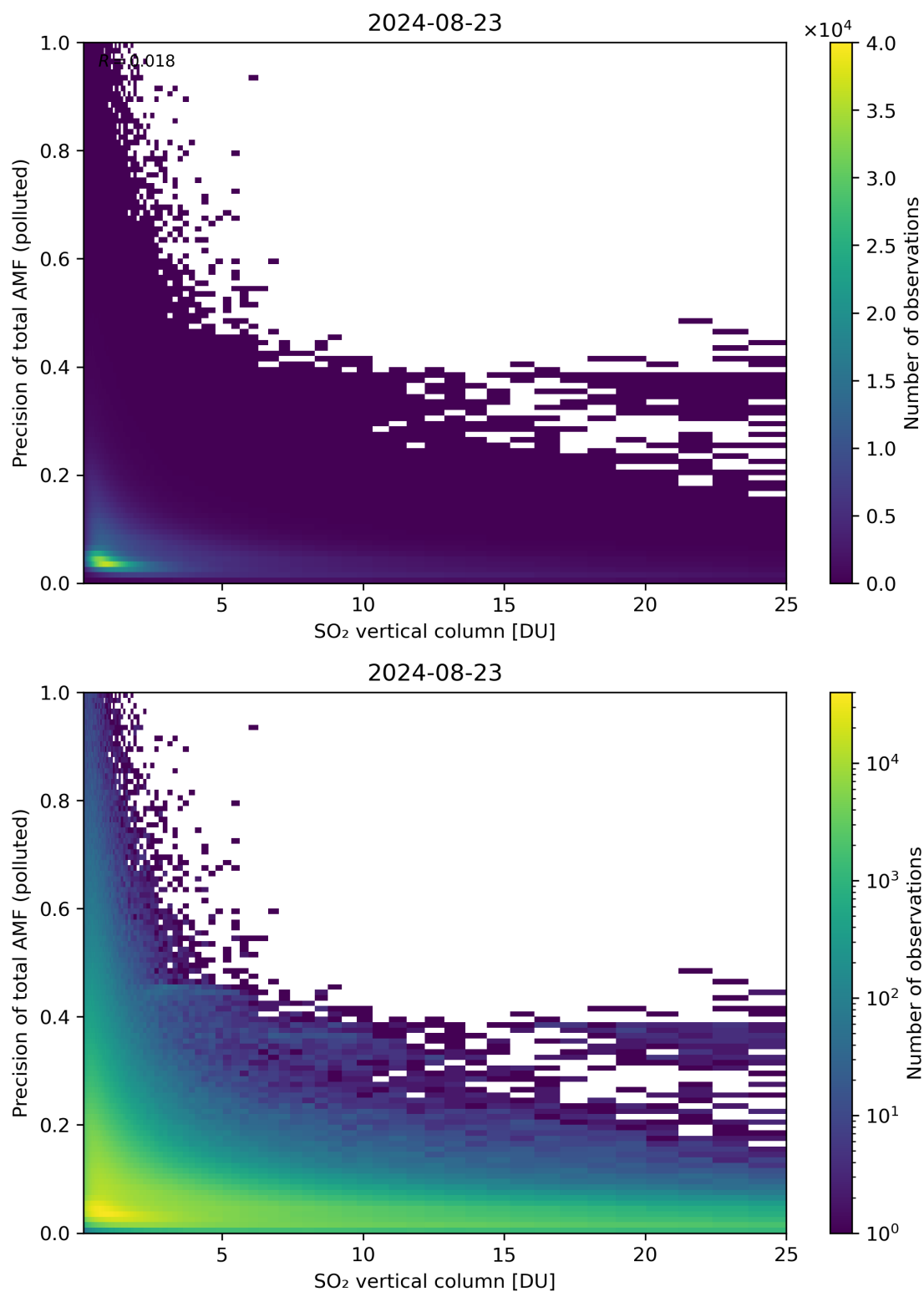
Figure 306: Scatter density plot of “SO 2 vertical column” against “Precision of total AMF (polluted)” for 2024-08-22 to 2024-08-24.
