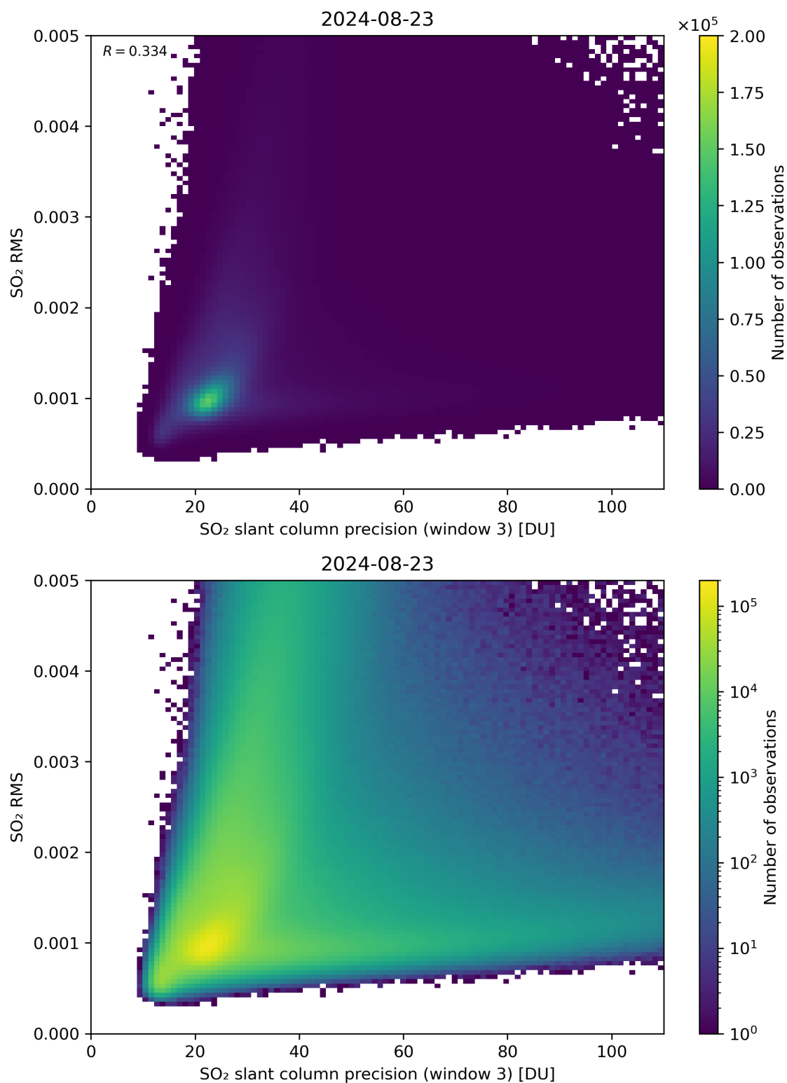
Figure 260: Scatter density plot of “SO 2 slant column precision (window 3)” against “SO 2 RMS” for 2024-08-22 to 2024-08-24.
