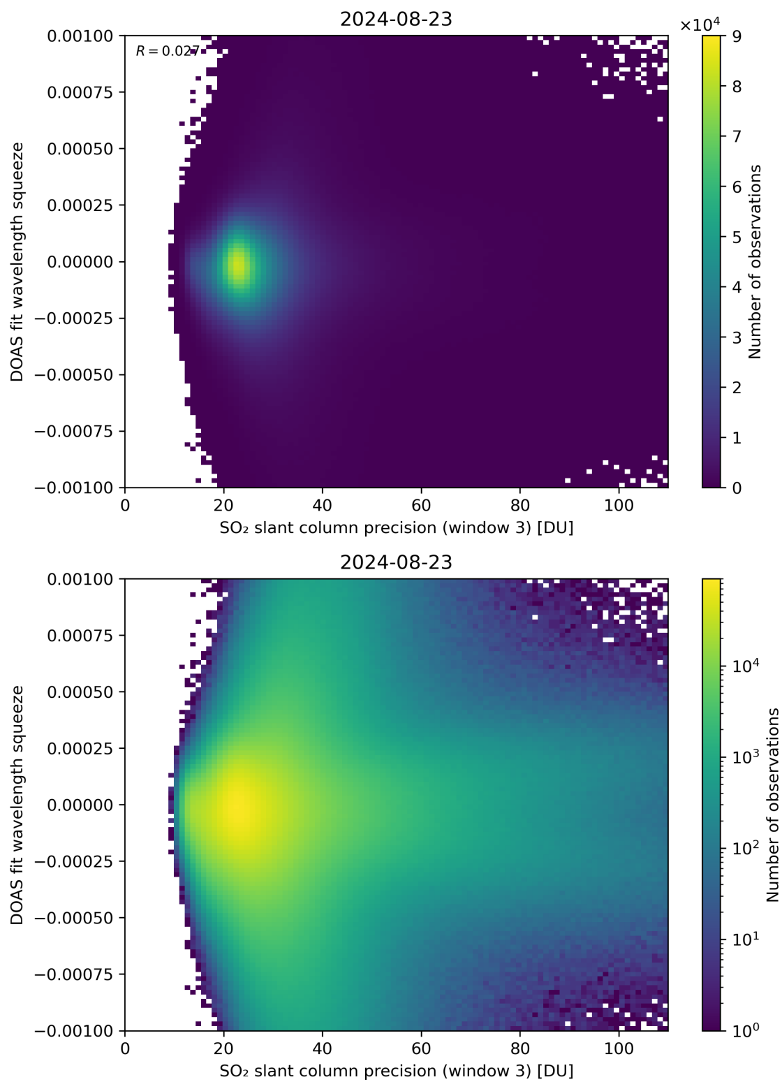
Figure 259: Scatter density plot of “SO 2 slant column precision (window 3)” against “DOAS fit wavelength squeeze” for 2024-08-22 to 2024-08-24.
