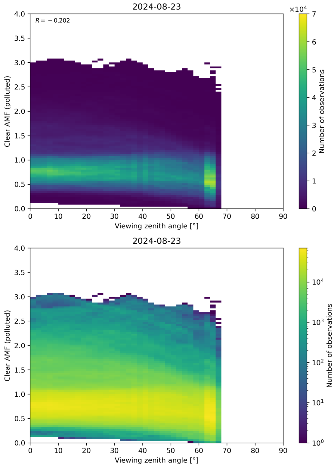
Figure 316: Scatter density plot of “Viewing zenith angle” against “Clear AMF (polluted)” for 2024-08-22 to 2024-08-24.
