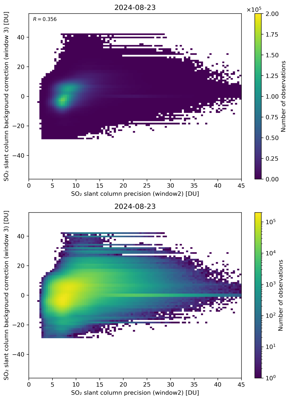
Figure 242: Scatter density plot of “SO 2 slant column precision (window2)” against “SO 2 slant column background correction (window 3)” for 2024-08-22 to 2024-08-24.
