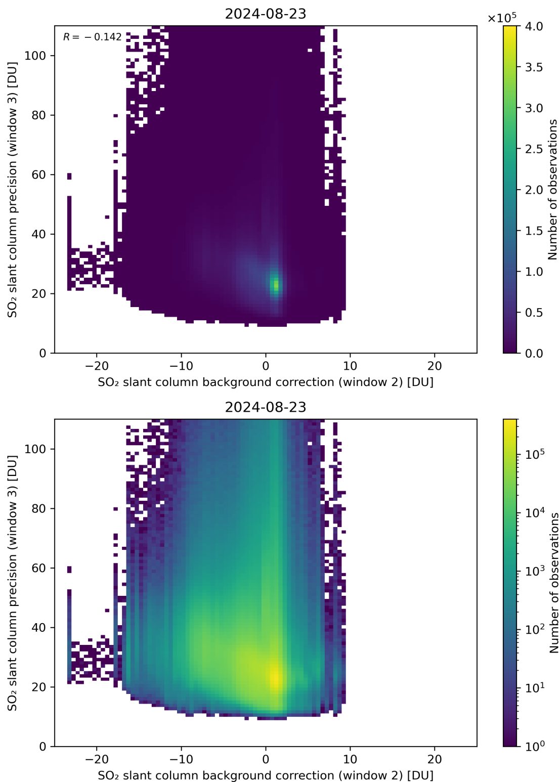
Figure 118: Scatter density plot of “SO 2 slant column background correction (window 2)” against “SO 2 slant column precision (window 3)” for 2024-08-22 to 2024-08-24.
