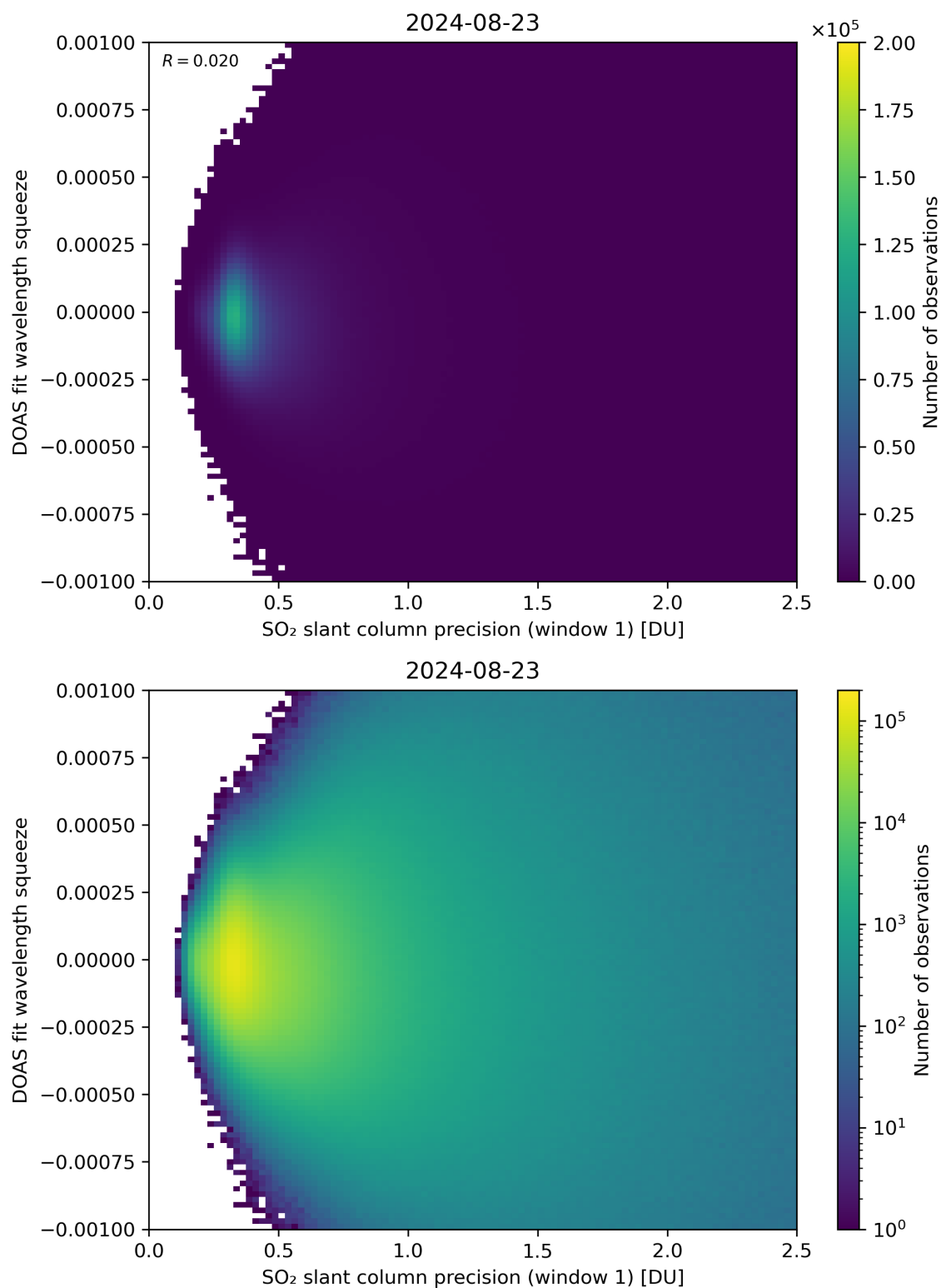
Figure 222: Scatter density plot of “SO 2 slant column precision (window 1)” against “DOAS fit wavelength squeeze” for 2024-08-22 to 2024-08-24.
