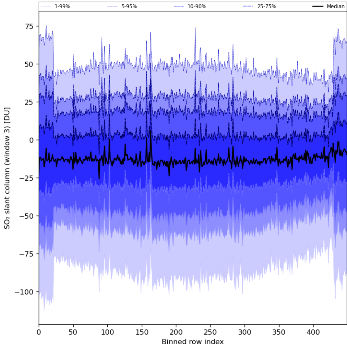
Figure 87: Along track statistics of “SO 2 slant column (window 3)” for 2024-08-22 to 2024-08-24
