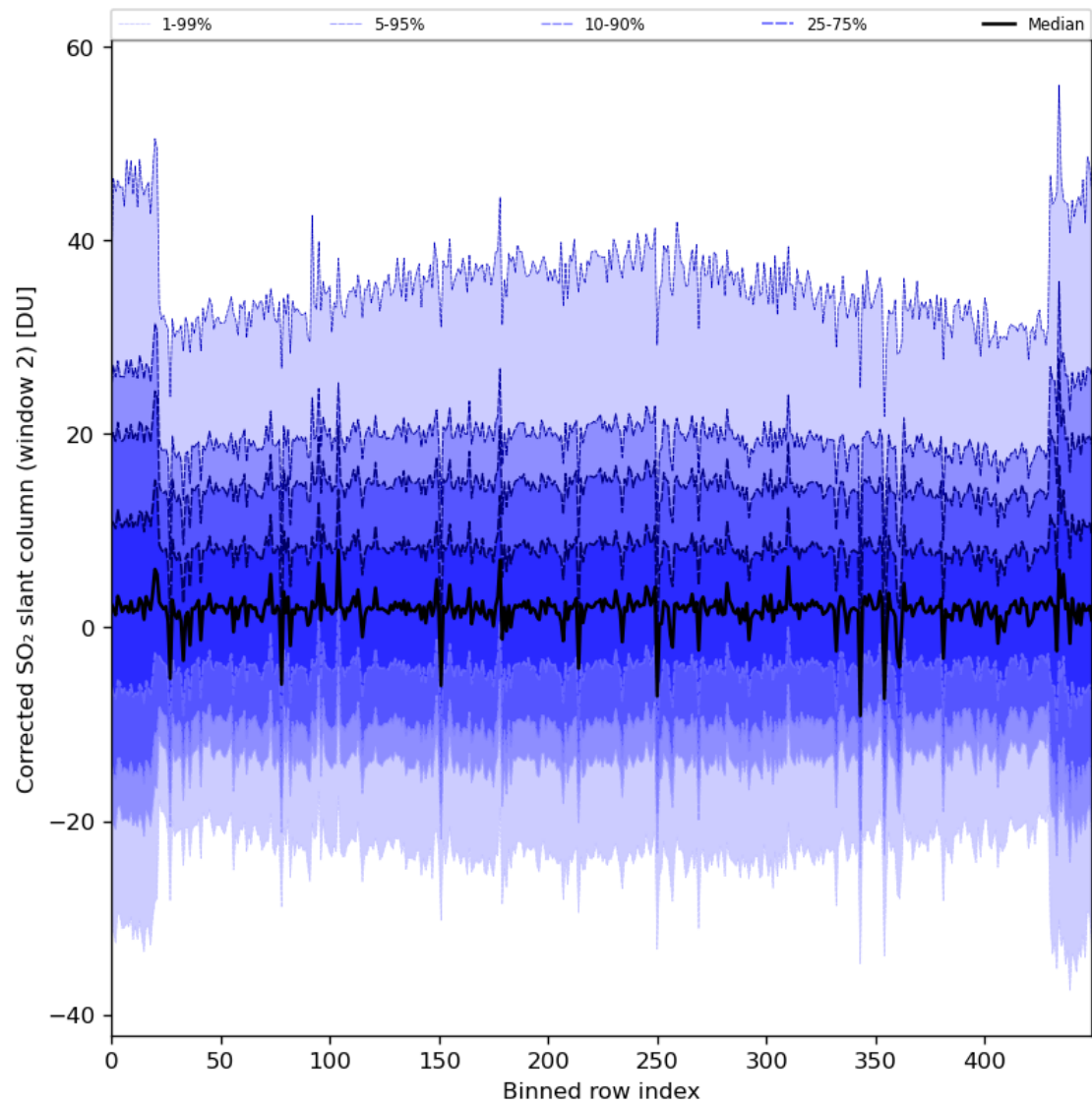
Figure 85: Along track statistics of "Corrected SO 2 slant column (window 2)" for 2024-08-22 to 2024-08-24
