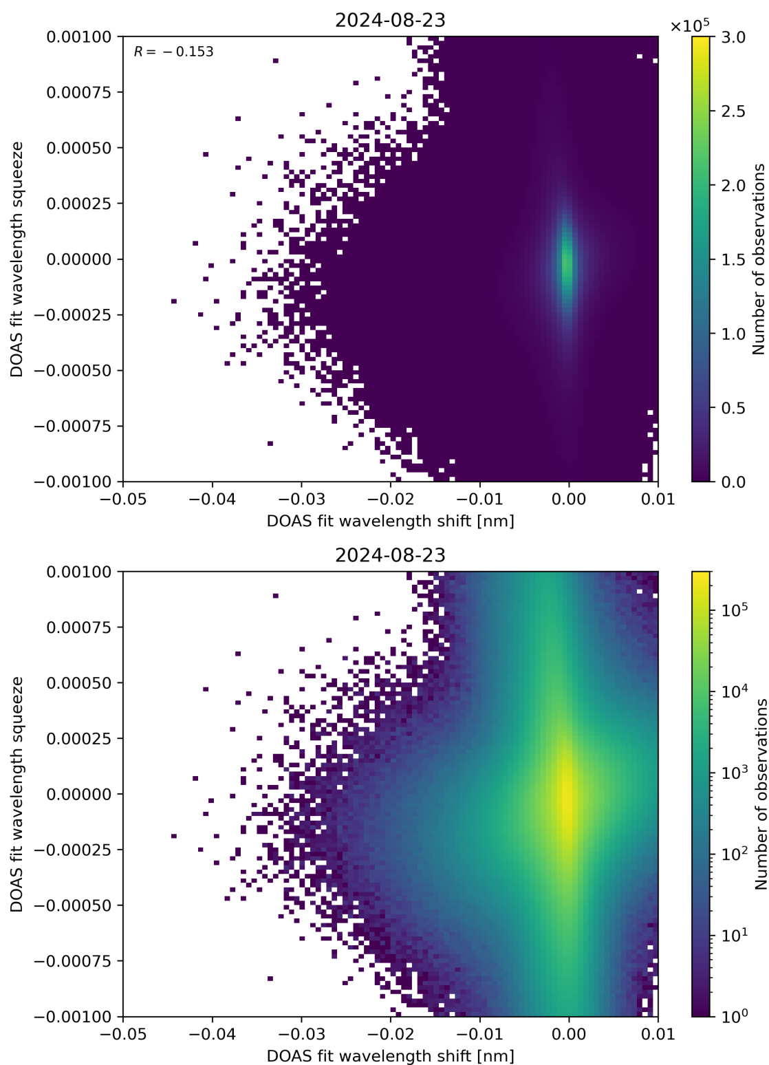
Figure 127: Scatter density plot of “DOAS fit wavelength shift” against “DOAS fit wavelength squeeze” for 2024-08-22 to 2024-08-24.
