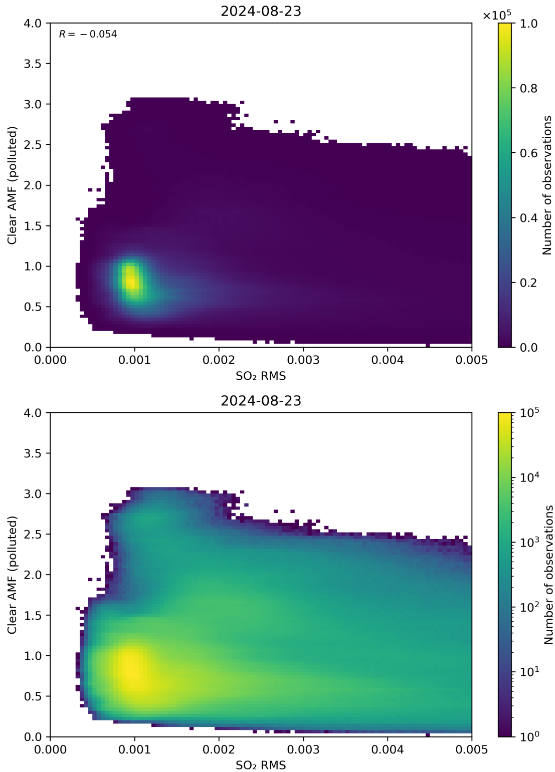
Figure 136: Scatter density plot of “SO 2 RMS” against “Clear AMF (polluted)” for 2024-08-22 to 2024-08-24.
