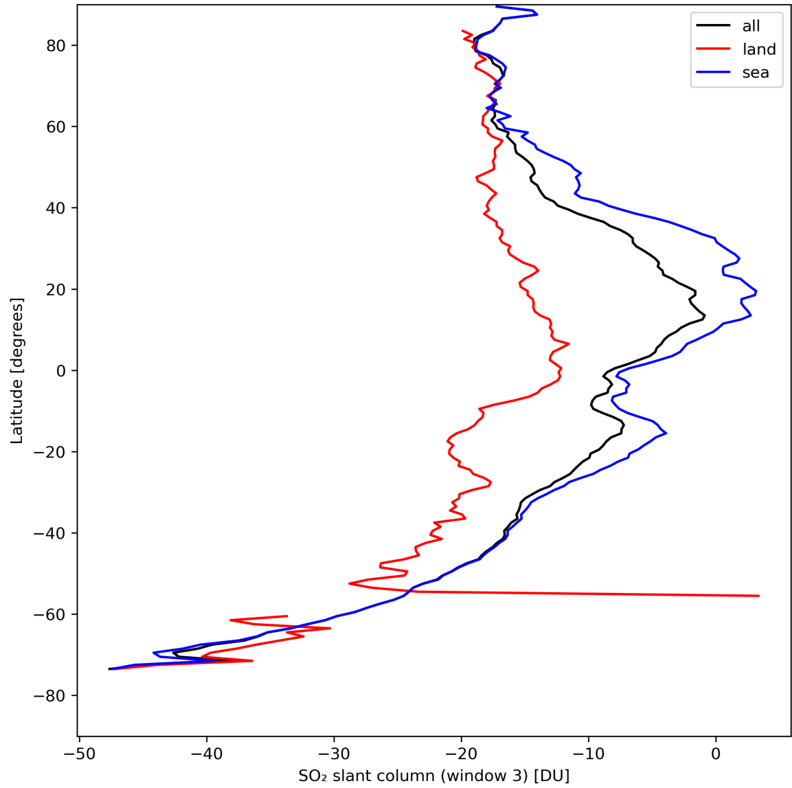
Figure 41: Zonal average of “SO 2 slant column (window 3)” for 2024-08-22 to 2024-08-24.
