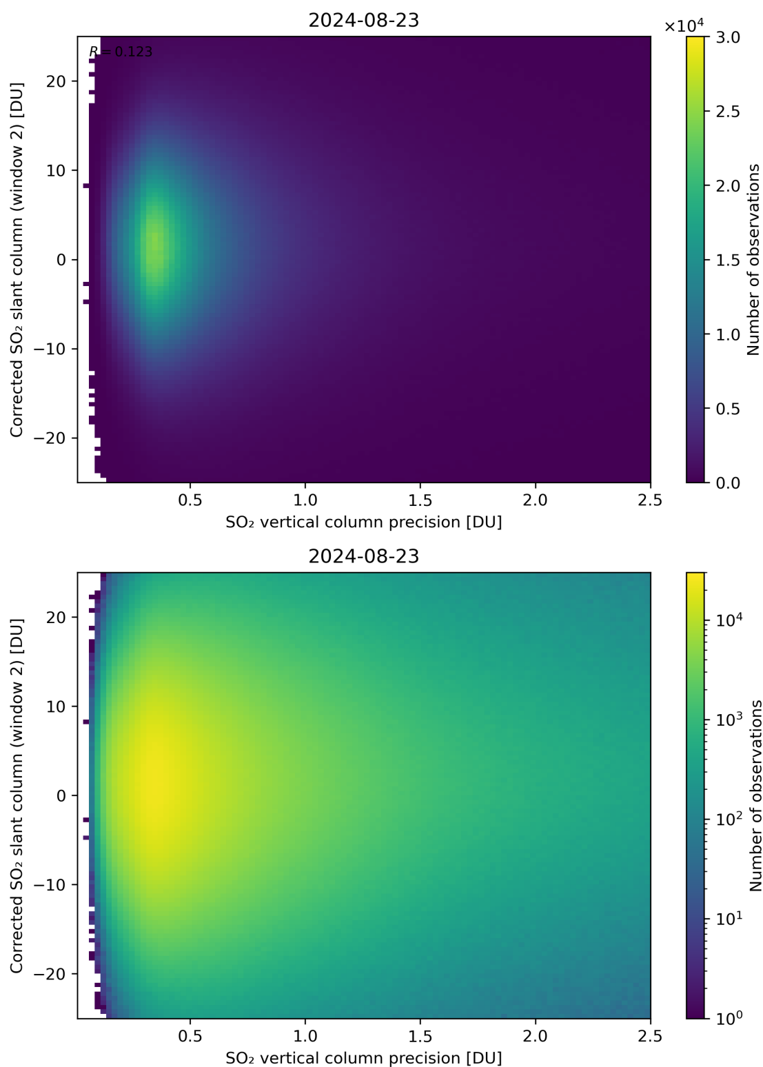
Figure 287: Scatter density plot of “SO 2 vertical column precision” against “Corrected SO 2 slant column (window 2)” for 2024-08-22 to 2024-08-24.
