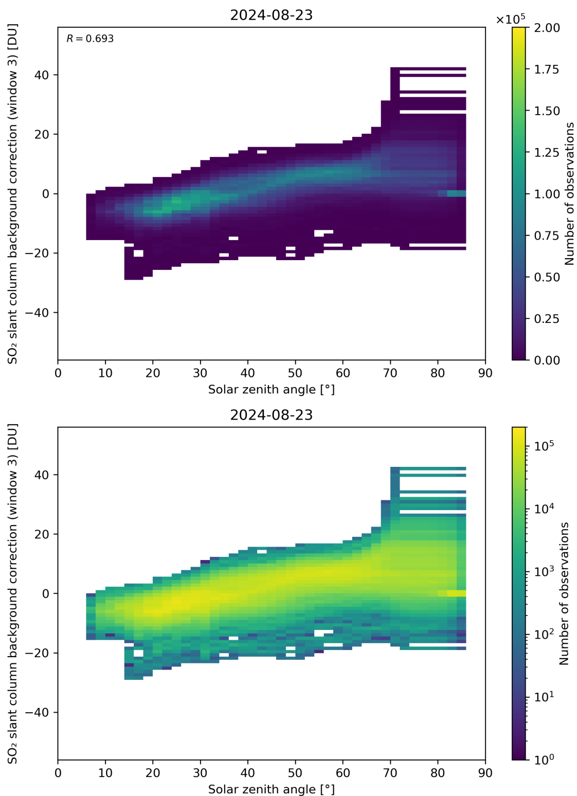
Figure 160: Scatter density plot of “Solar zenith angle” against “SO 2 slant column background correction (window 3)” for 2024-08-22 to 2024-08-24.
