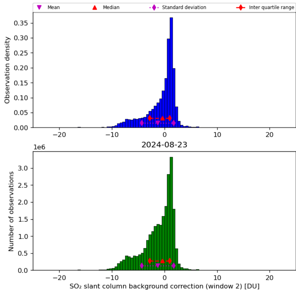
Figure 63: Histogram of “SO 2 slant column background correction (window 2)” for 2024-08-22 to 2024-08-24
