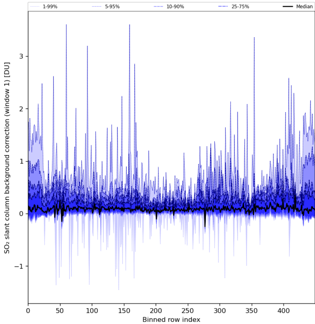
Figure 82: Along track statistics of “SO 2 slant column background correction (window 1)” for 2024-08-22 to 2024-08-24
