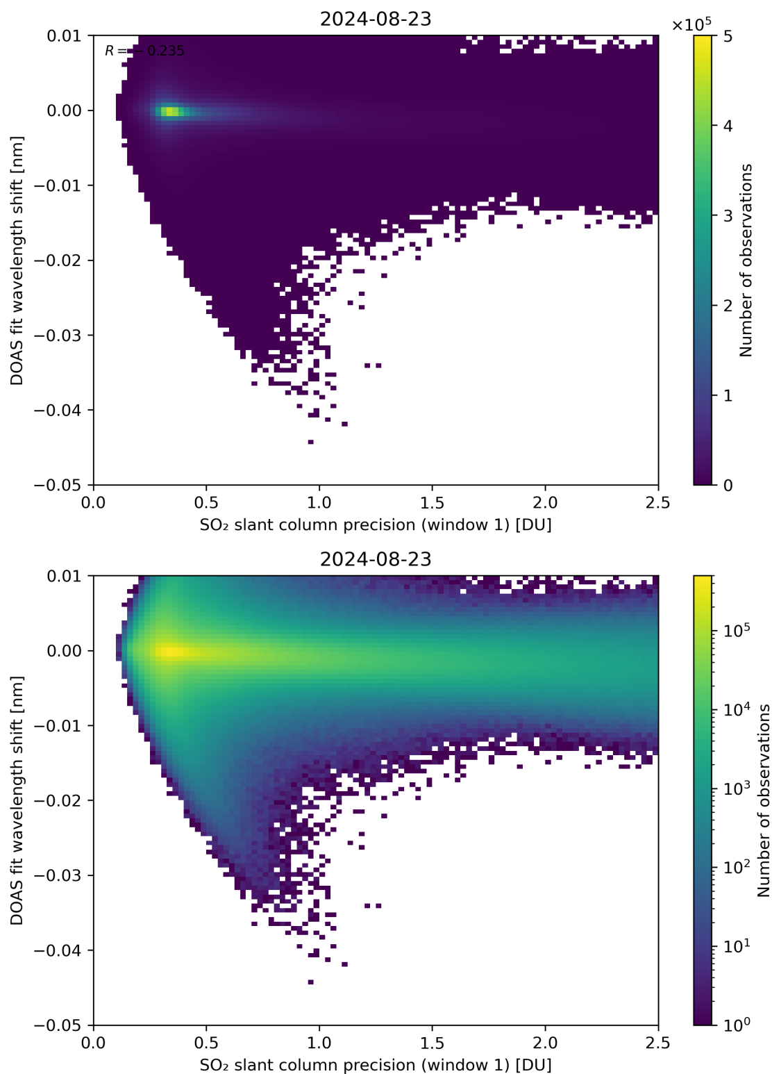
Figure 221: Scatter density plot of “SO 2 slant column precision (window 1)” against “DOAS fit wavelength shift” for 2024-08-22 to 2024-08-24.
