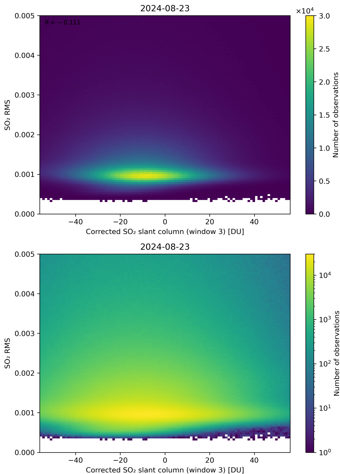
Figure 208: Scatter density plot of “Corrected SO 2 slant column (window 3)” against “SO 2 RMS” for 2024-08-22 to 2024-08-24.
