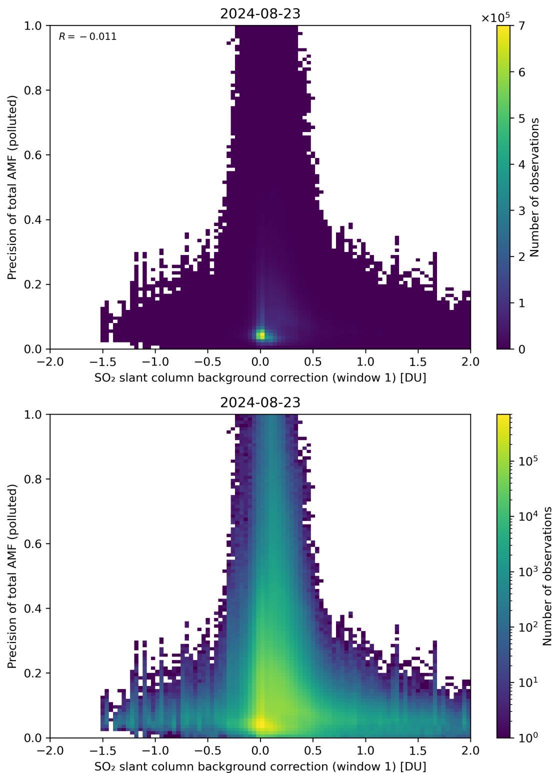
Figure 110: Scatter density plot of “SO 2 slant column background correction (window 1)” against “Precision of total AMF (polluted)” for 2024-08-22 to 2024-08-24.
