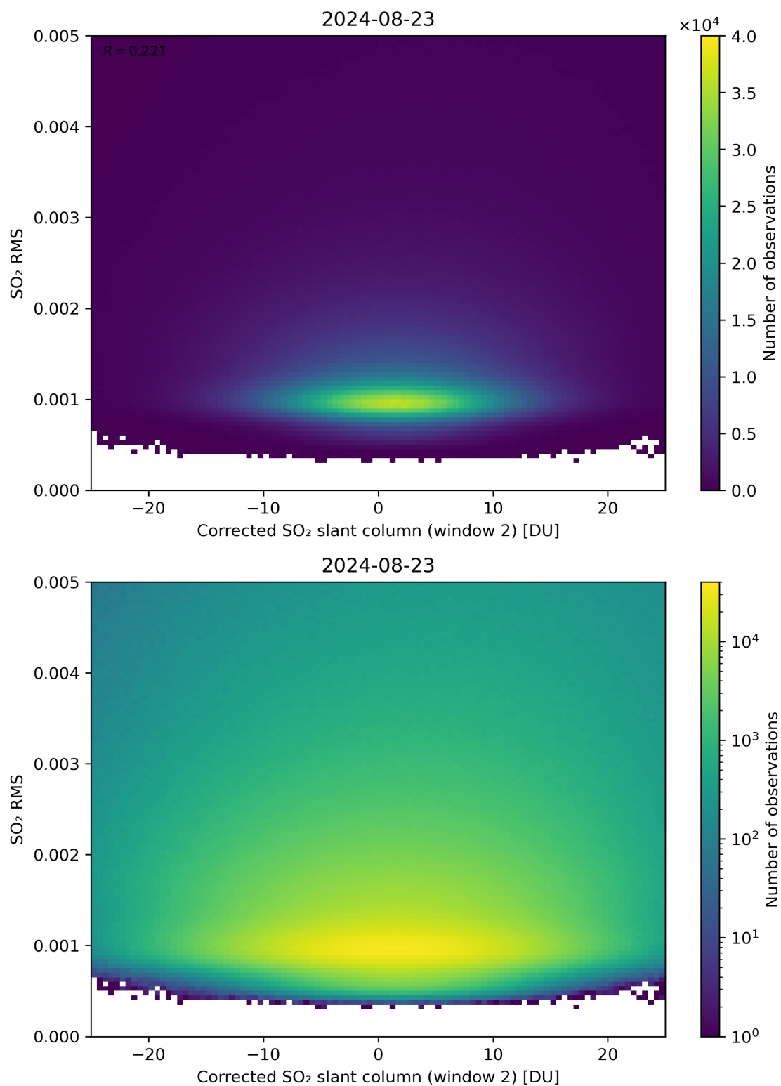
Figure 198: Scatter density plot of “Corrected SO 2 slant column (window 2)” against “SO 2 RMS” for 2024-08-22 to 2024-08-24.
