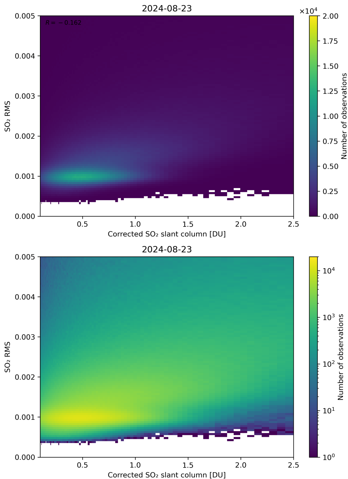
Figure 183: Scatter density plot of “Corrected SO 2 slant column” against “SO 2 RMS” for 2024-08-22 to 2024-08-24.
