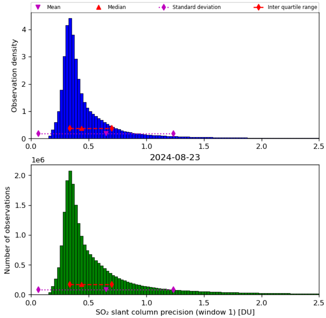
Figure 57: Histogram of “SO 2 slant column precision (window 1)” for 2024-08-22 to 2024-08-24
