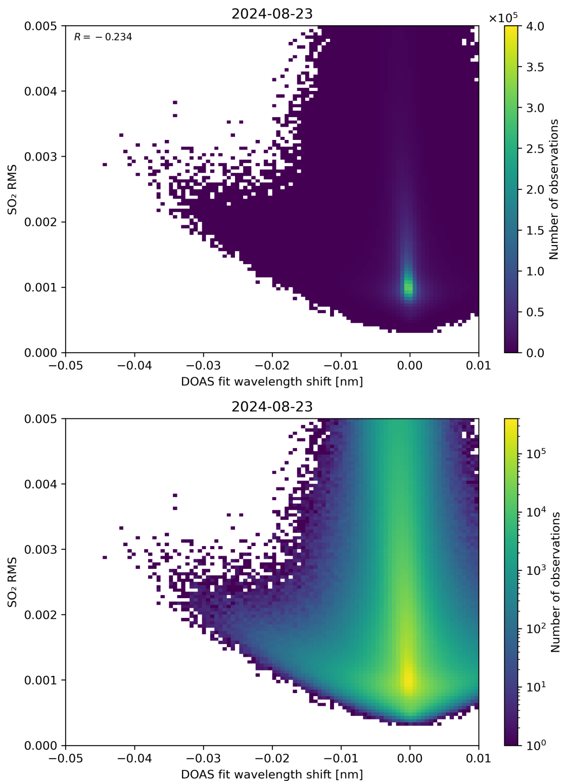
Figure 128: Scatter density plot of “DOAS fit wavelength shift” against “SO 2 RMS” for 2024-08-22 to 2024-08-24.
