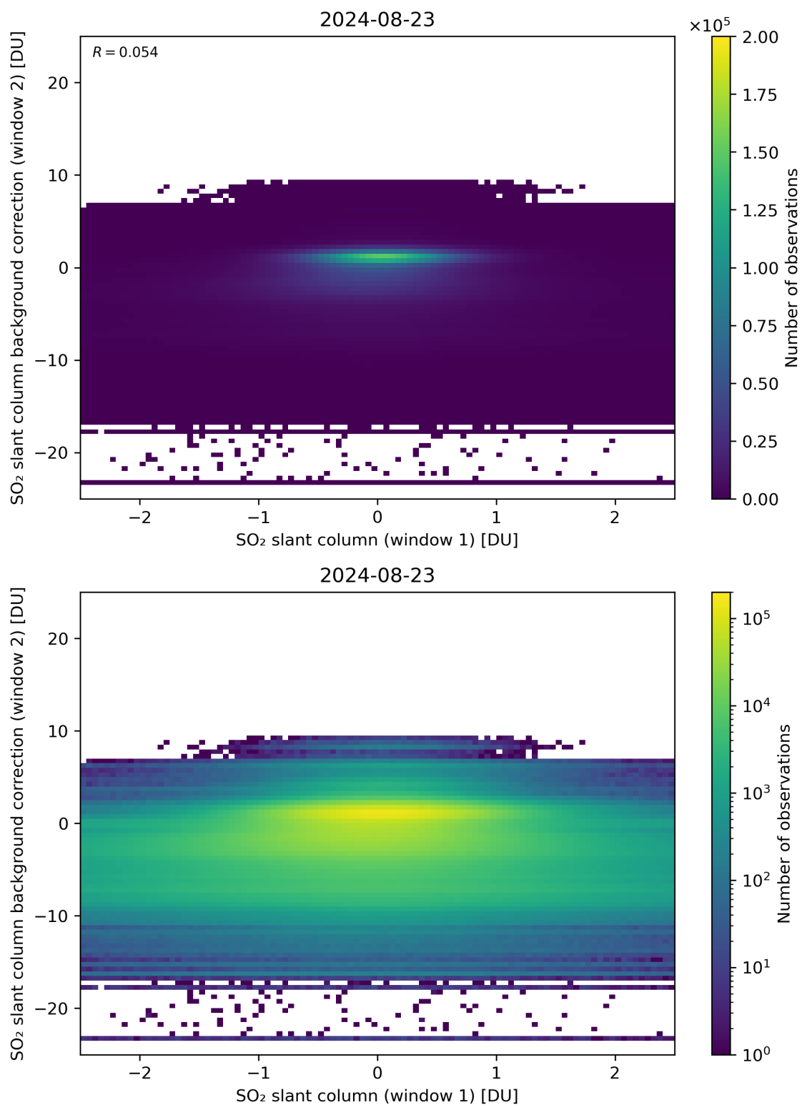
Figure 213: Scatter density plot of “SO 2 slant column (window 1)” against “SO 2 slant column background correction (window 2)” for 2024-08-22 to 2024-08-24.
