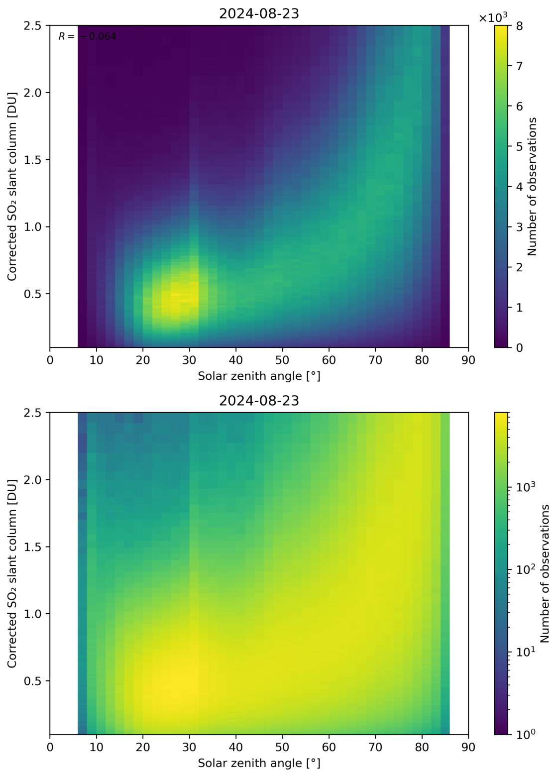
Figure 166: Scatter density plot of “Solar zenith angle” against “Corrected SO 2 slant column” for 2024-08-22 to 2024-08-24.
