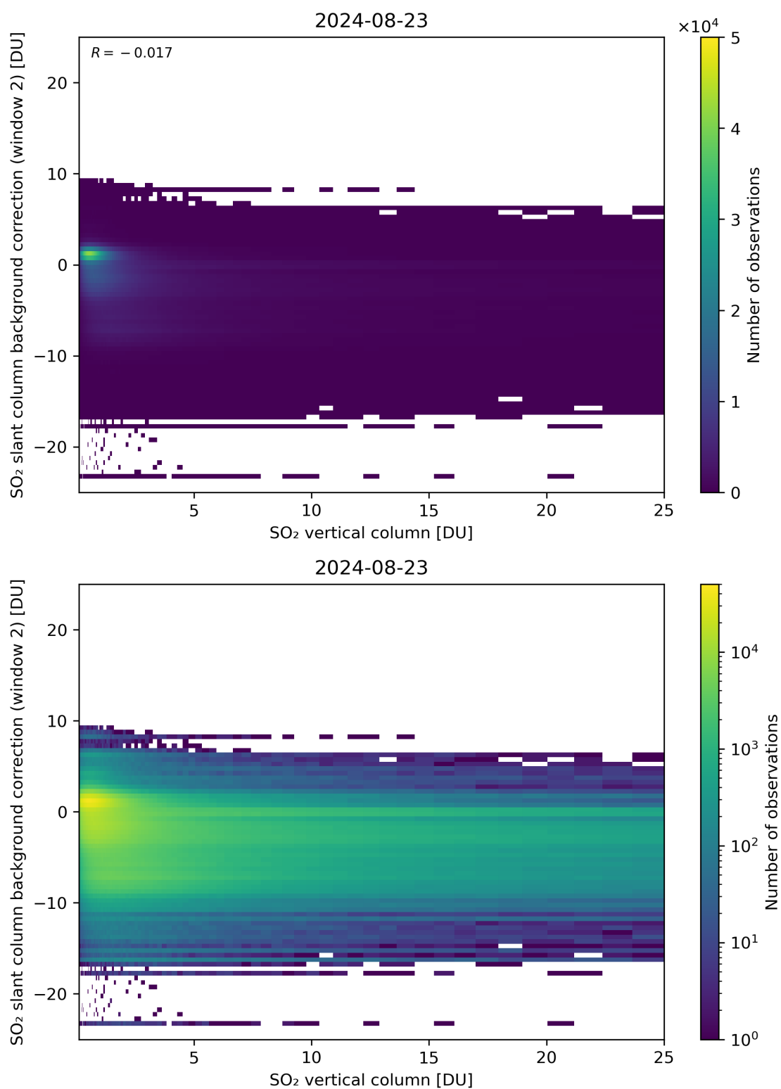
Figure 274: Scatter density plot of “SO 2 vertical column” against “SO 2 slant column background correction (window 2)” for 2024-08-22 to 2024-08-24.
