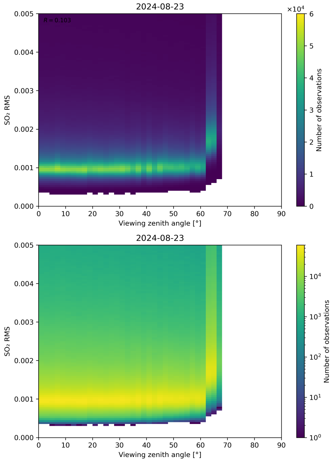
Figure 313: Scatter density plot of “Viewing zenith angle” against “SO 2 RMS” for 2024-08-22 to 2024-08-24.
