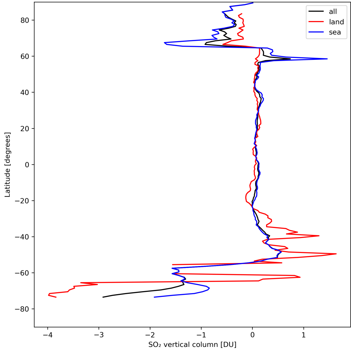
Figure 30: Zonal average of “SO 2 vertical column” for 2024-08-22 to 2024-08-24.
