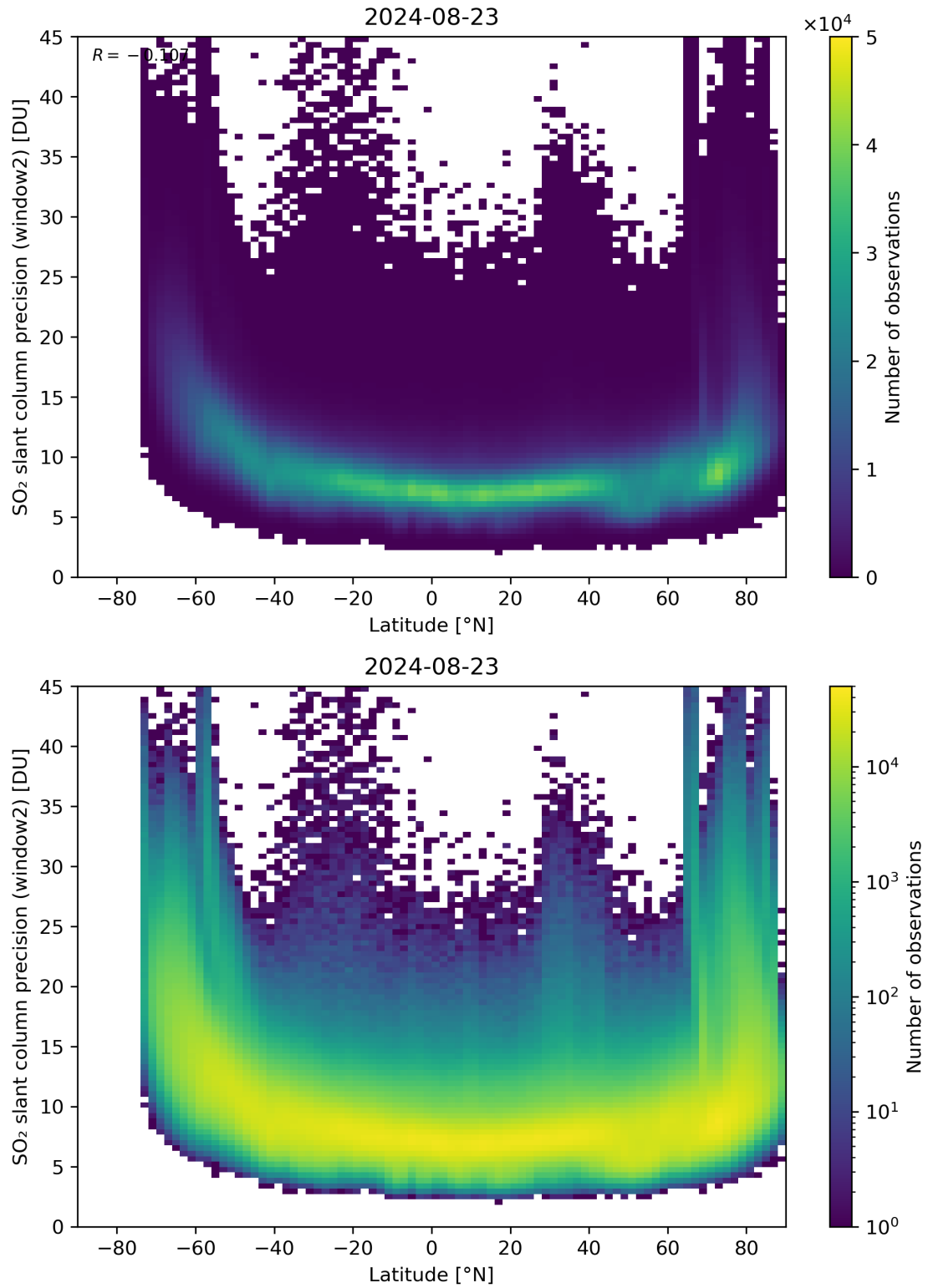
Figure 151: Scatter density plot of “Latitude” against “SO 2 slant column precision (window2)” for 2024-08-22 to 2024-08-24.
