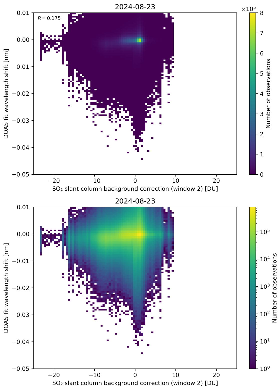
Figure 112: Scatter density plot of “SO 2 slant column background correction (window 2)” against “DOAS fit wavelength shift” for 2024-08-22 to 2024-08-24.
