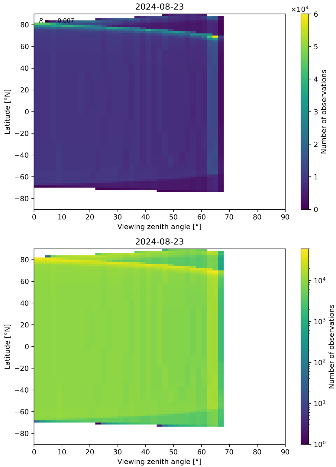
Figure 314: Scatter density plot of “Viewing zenith angle” against “Latitude” for 2024-08-22 to 2024-08-24.
