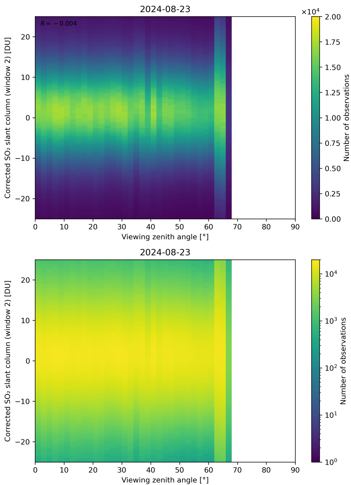
Figure 318: Scatter density plot of “Viewing zenith angle” against “Corrected SO 2 slant column (window 2)” for 2024-08-22 to 2024-08-24.
