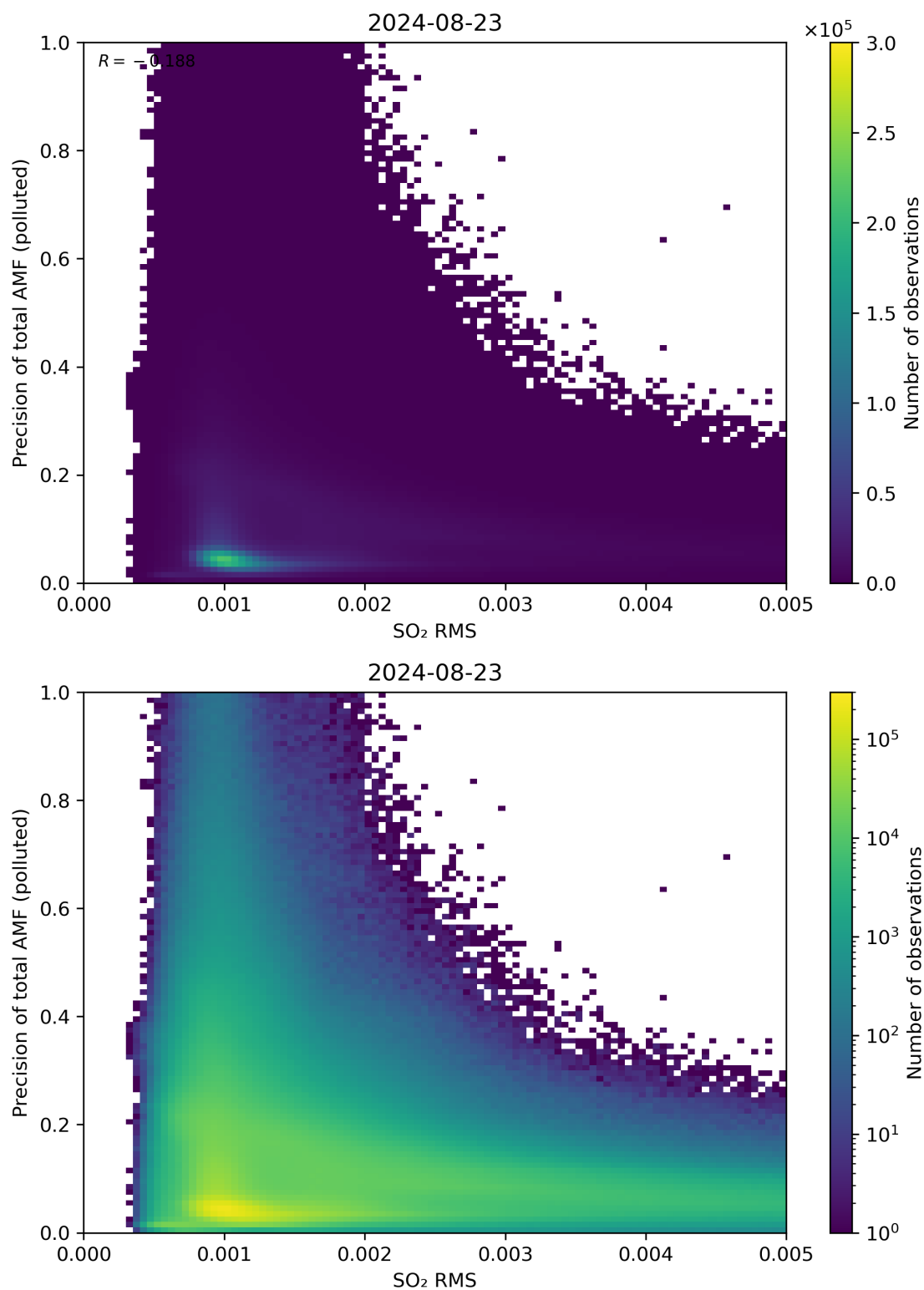
Figure 138: Scatter density plot of “SO 2 RMS” against “Precision of total AMF (polluted)” for 2024-08-22 to 2024-08-24.
