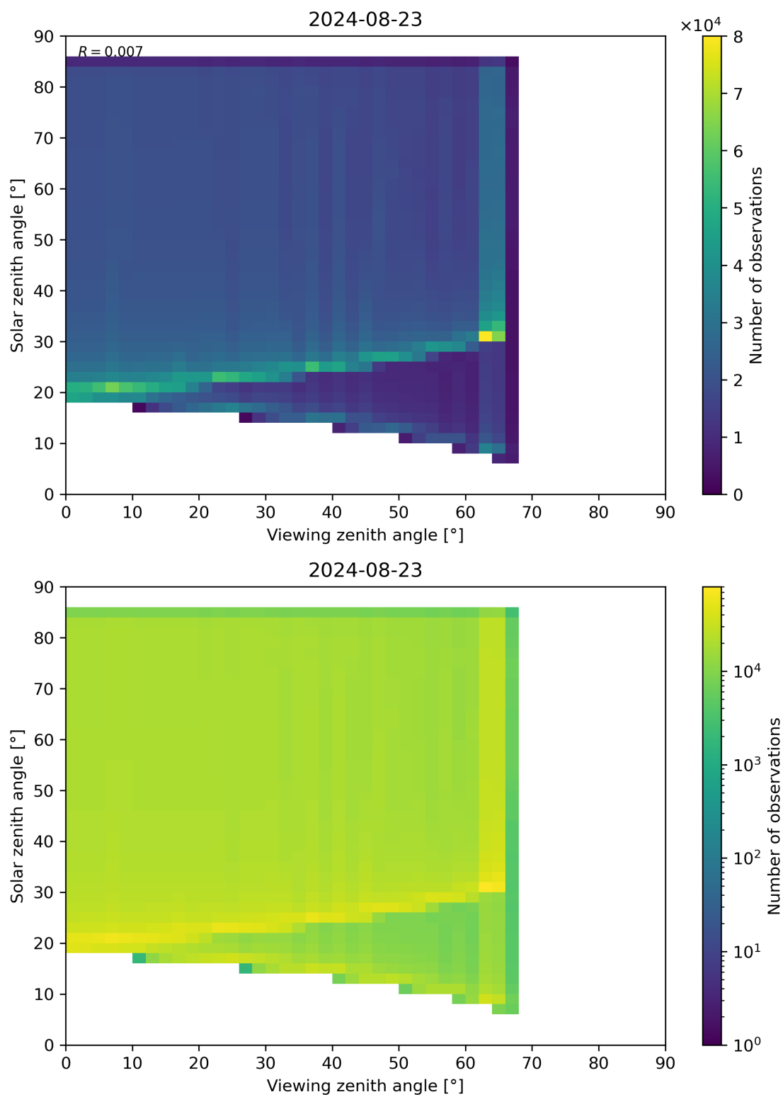
Figure 315: Scatter density plot of “Viewing zenith angle” against “Solar zenith angle” for 2024-08-22 to 2024-08-24.
