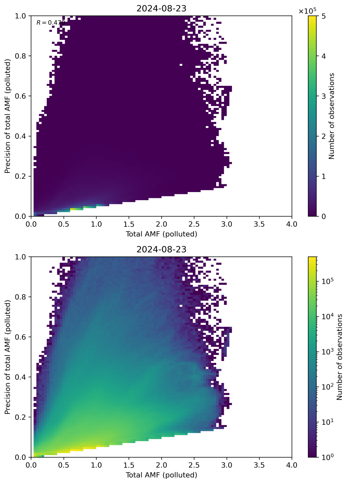
Figure 272: Scatter density plot of “Total AMF (polluted)” against “Precision of total AMF (polluted)” for 2024-08-22 to 2024-08-24.
