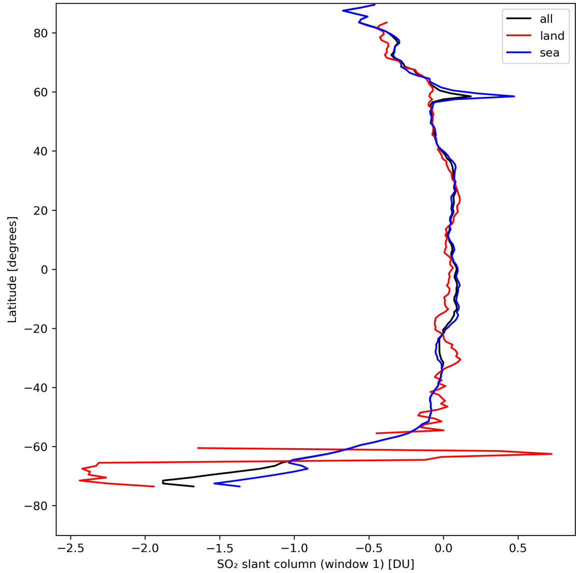
Figure 33: Zonal average of “SO 2 slant column (window 1)” for 2024-08-22 to 2024-08-24.
