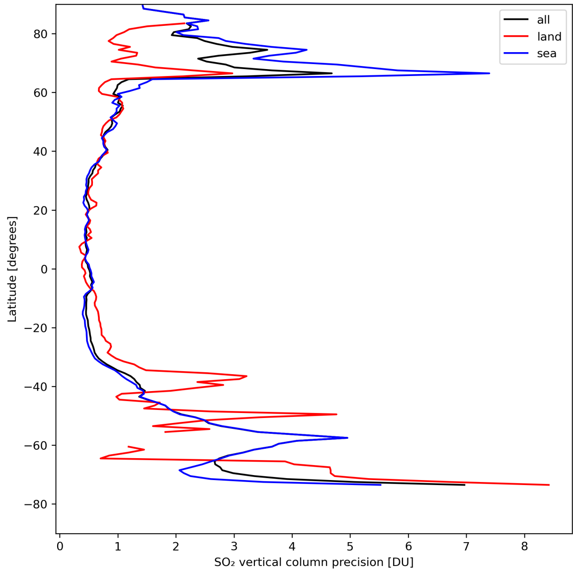
Figure 31: Zonal average of “SO 2 vertical column precision” for 2024-08-22 to 2024-08-24.
