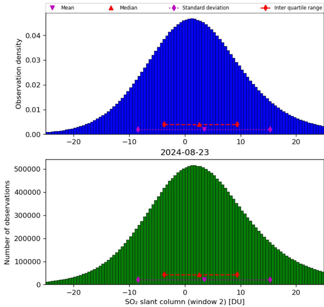
Figure 60: Histogram of “SO 2 slant column (window 2)” for 2024-08-22 to 2024-08-24
