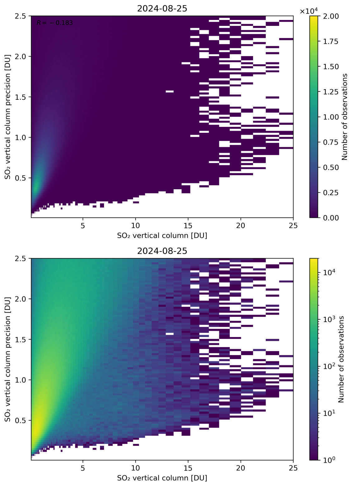
Figure 307: Scatter density plot of “SO 2 vertical column” against “SO 2 vertical column precision” for 2024-08-24 to 2024-08-26.
