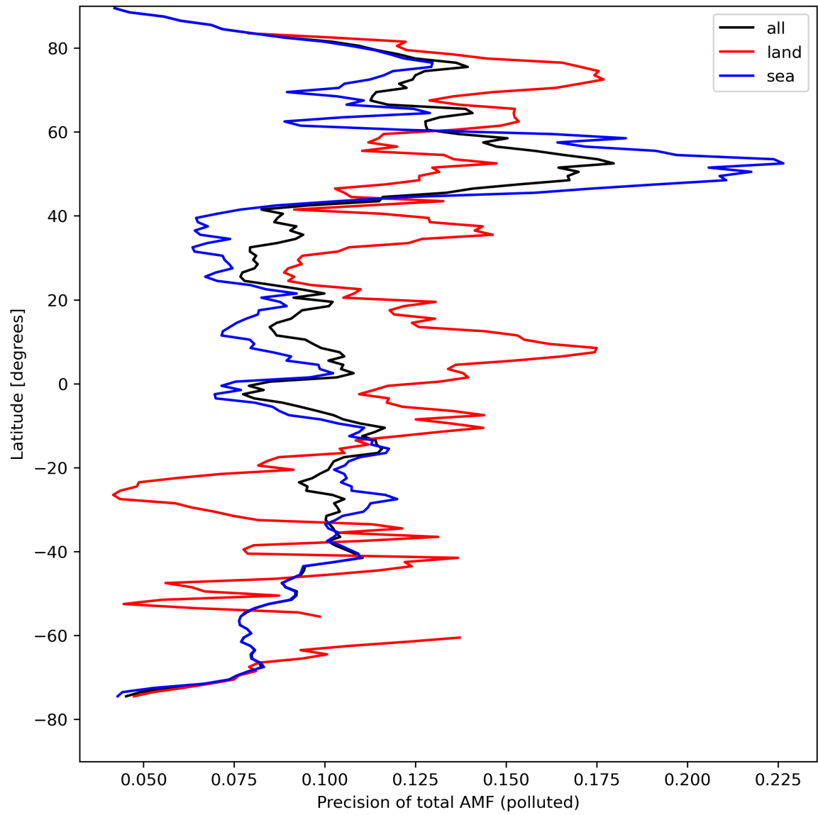
Figure 49: Zonal average of “Precision of total AMF (polluted)” for 2024-08-24 to 2024-08-26.
