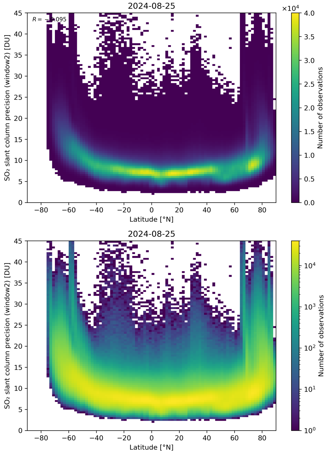
Figure 151: Scatter density plot of “Latitude” against “SO 2 slant column precision (window2)” for 2024-08-24 to 2024-08-26.
