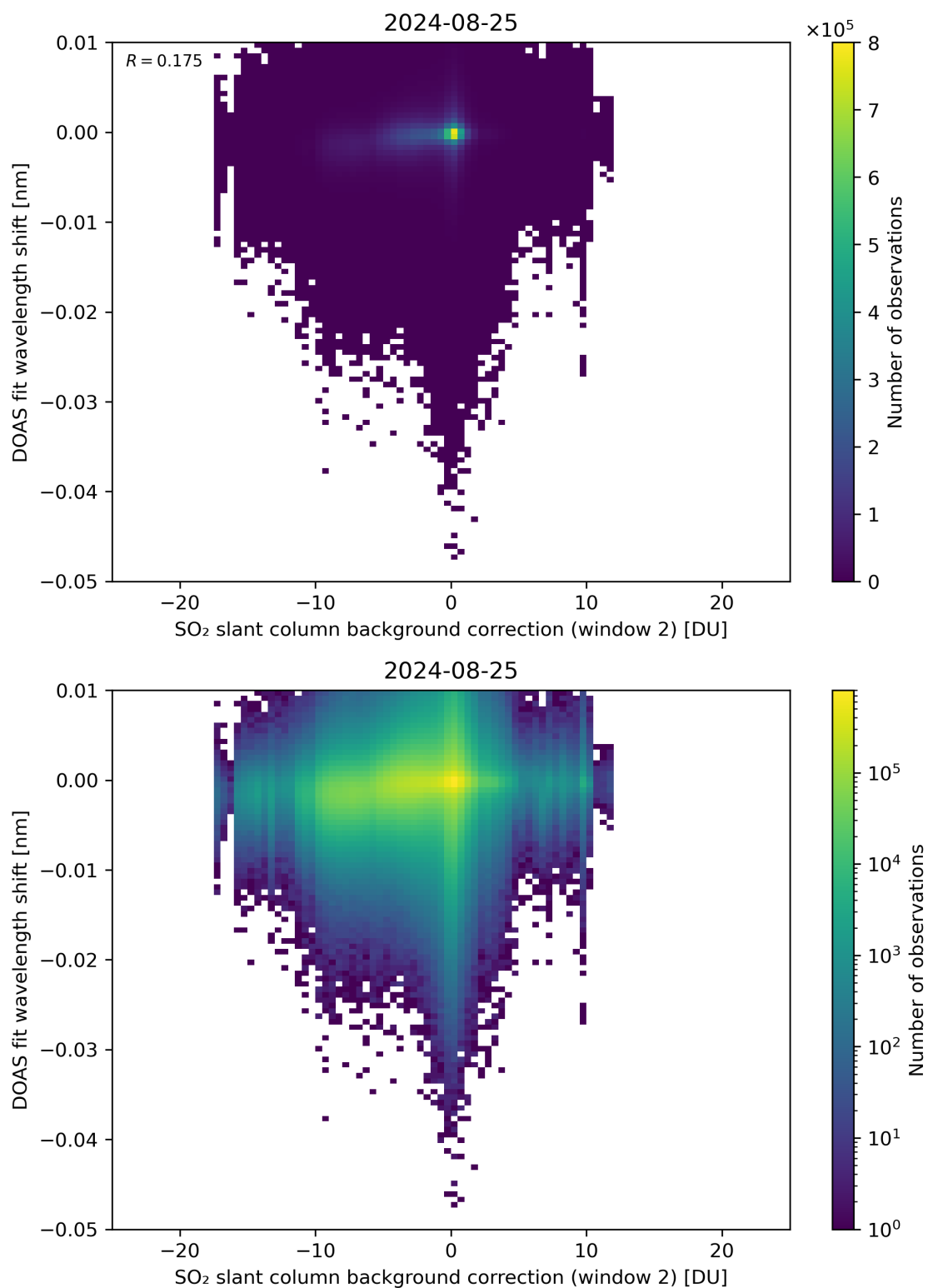
Figure 112: Scatter density plot of “SO 2 slant column background correction (window 2)” against “DOAS fit wavelength shift” for 2024-08-24 to 2024-08-26.
