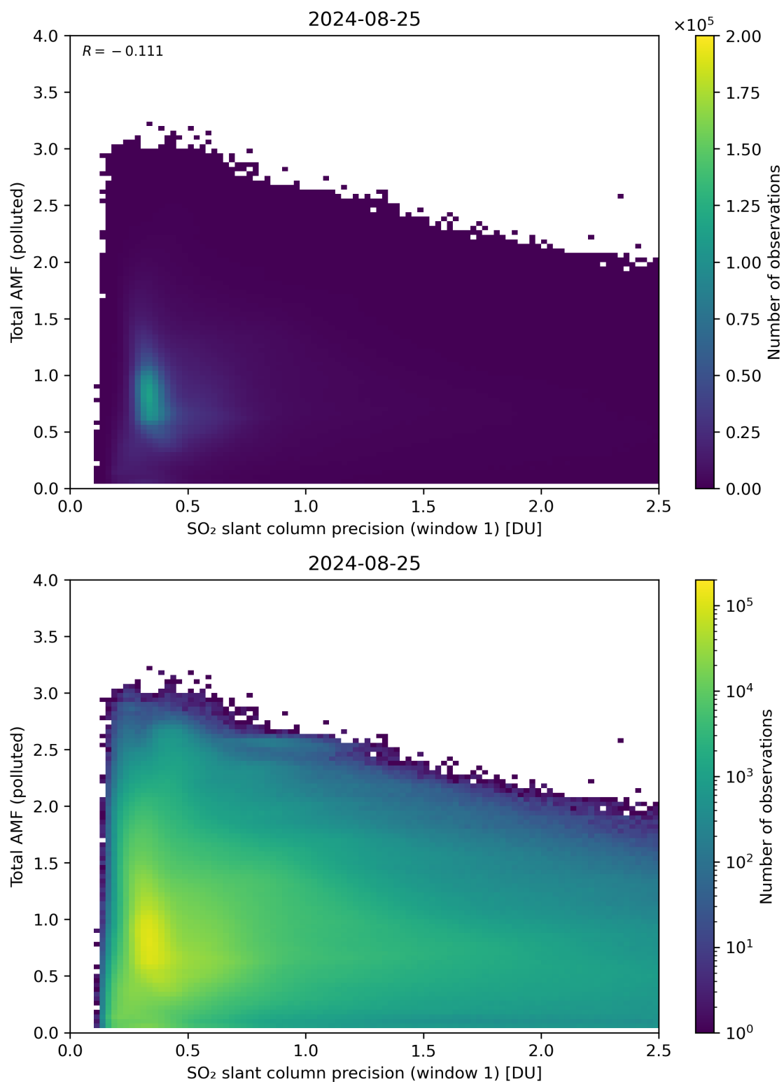
Figure 230: Scatter density plot of “SO 2 slant column precision (window 1)” against “Total AMF (polluted)” for 2024-08-24 to 2024-08-26.
