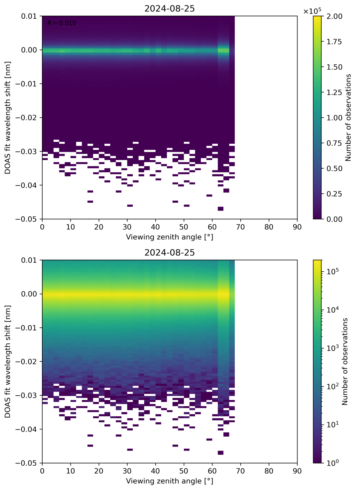
Figure 311: Scatter density plot of “Viewing zenith angle” against “DOAS fit wavelength shift” for 2024-08-24 to 2024-08-26.
