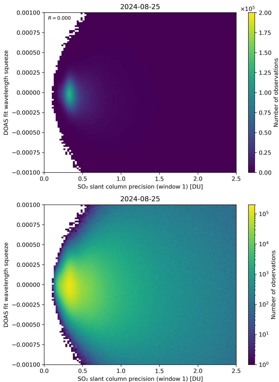
Figure 222: Scatter density plot of “SO 2 slant column precision (window 1)” against “DOAS fit wavelength squeeze” for 2024-08-24 to 2024-08-26.
