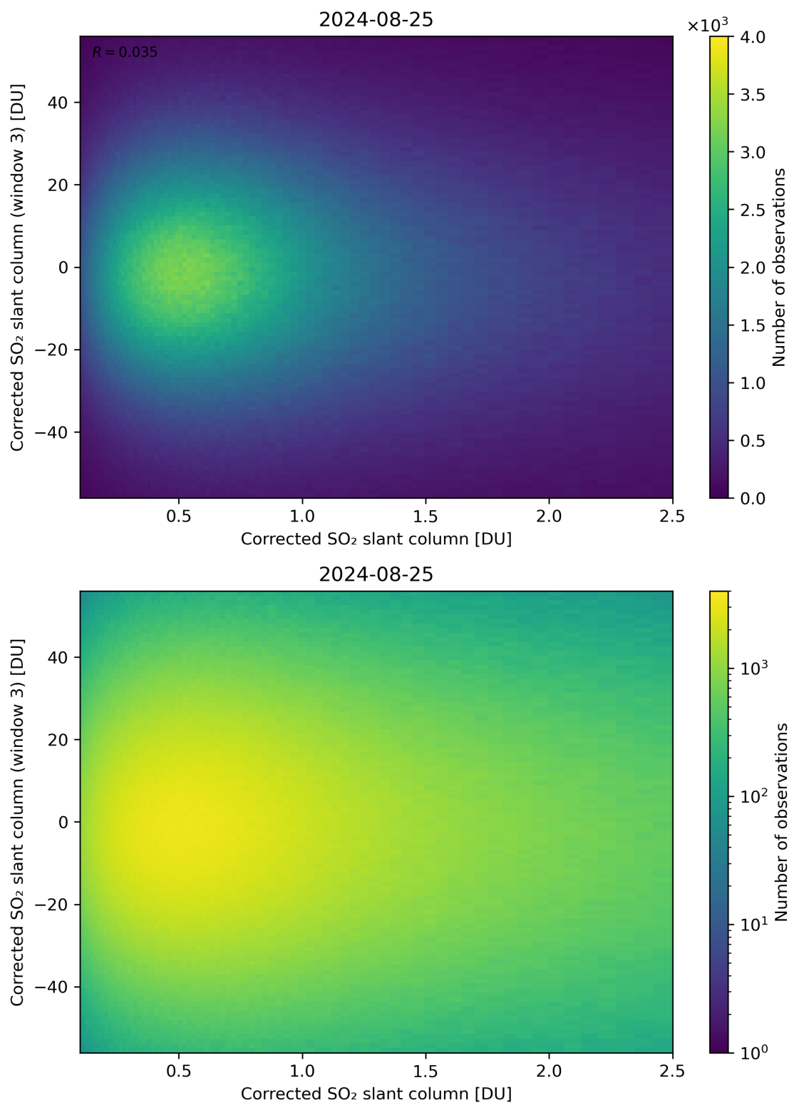
Figure 186: Scatter density plot of “Corrected SO 2 slant column” against “Corrected SO 2 slant column (window 3)” for 2024-08-24 to 2024-08-26.
