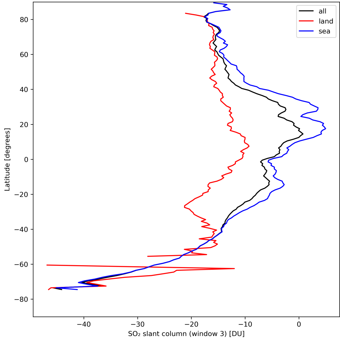
Figure 41: Zonal average of “SO 2 slant column (window 3)” for 2024-08-24 to 2024-08-26.
