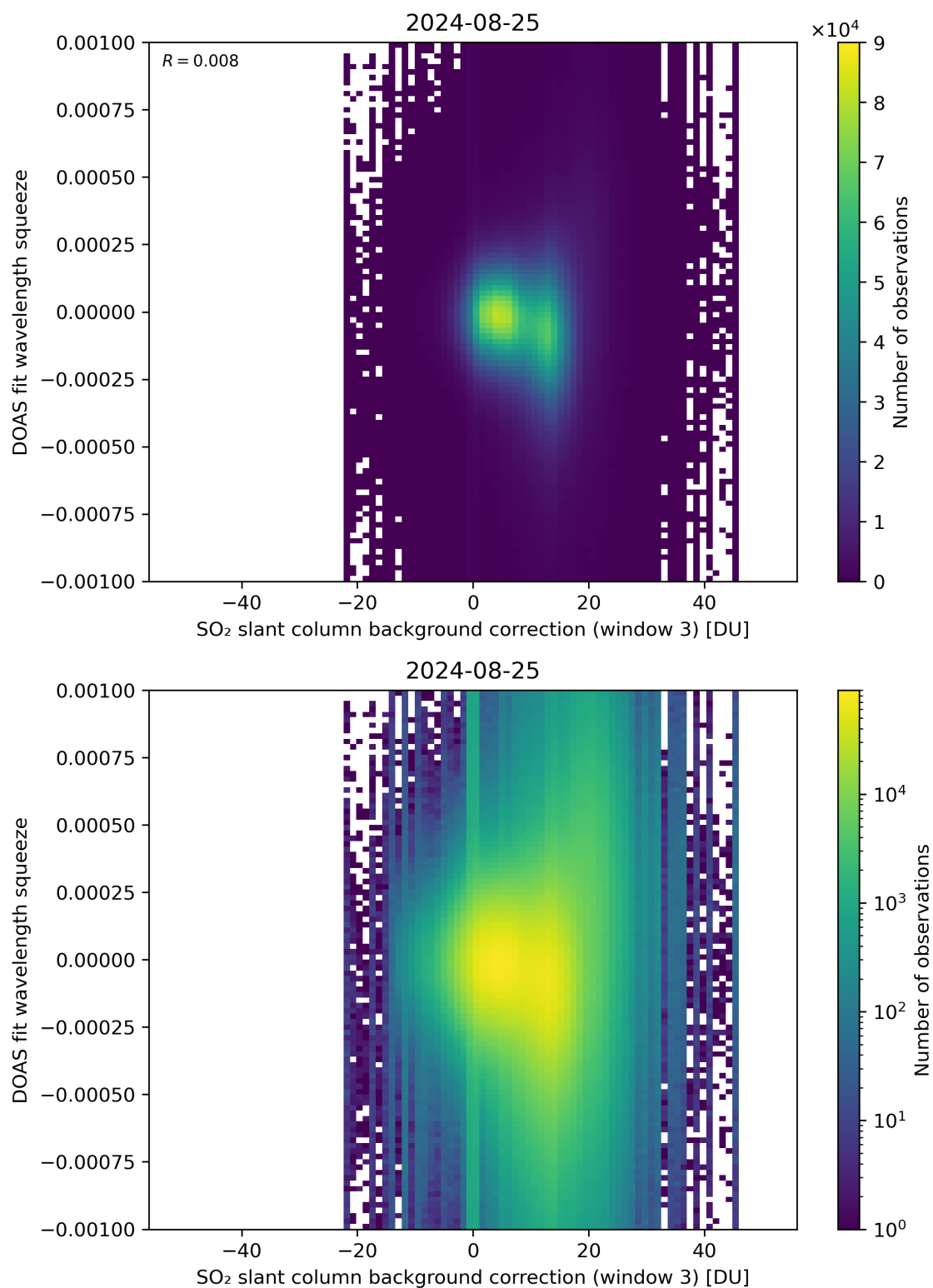
Figure 122: Scatter density plot of “SO 2 slant column background correction (window 3)” against “DOAS fit wavelength squeeze” for 2024-08-24 to 2024-08-26.
