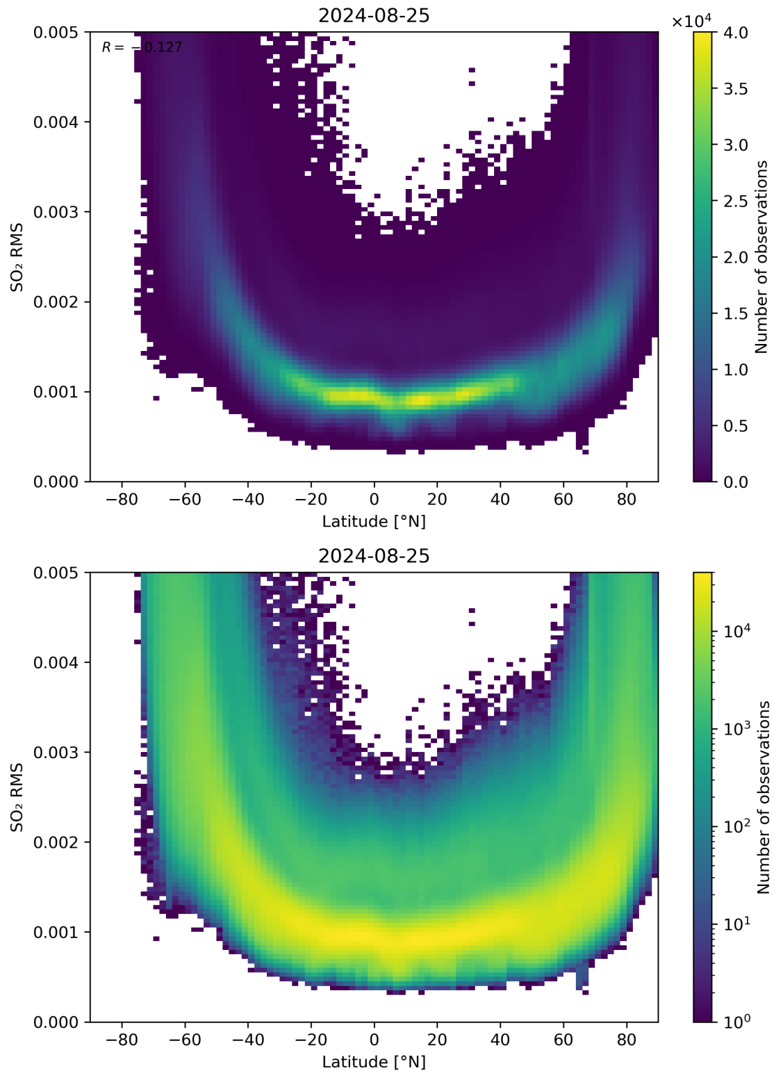
Figure 144: Scatter density plot of “Latitude” against “SO 2 RMS” for 2024-08-24 to 2024-08-26.
