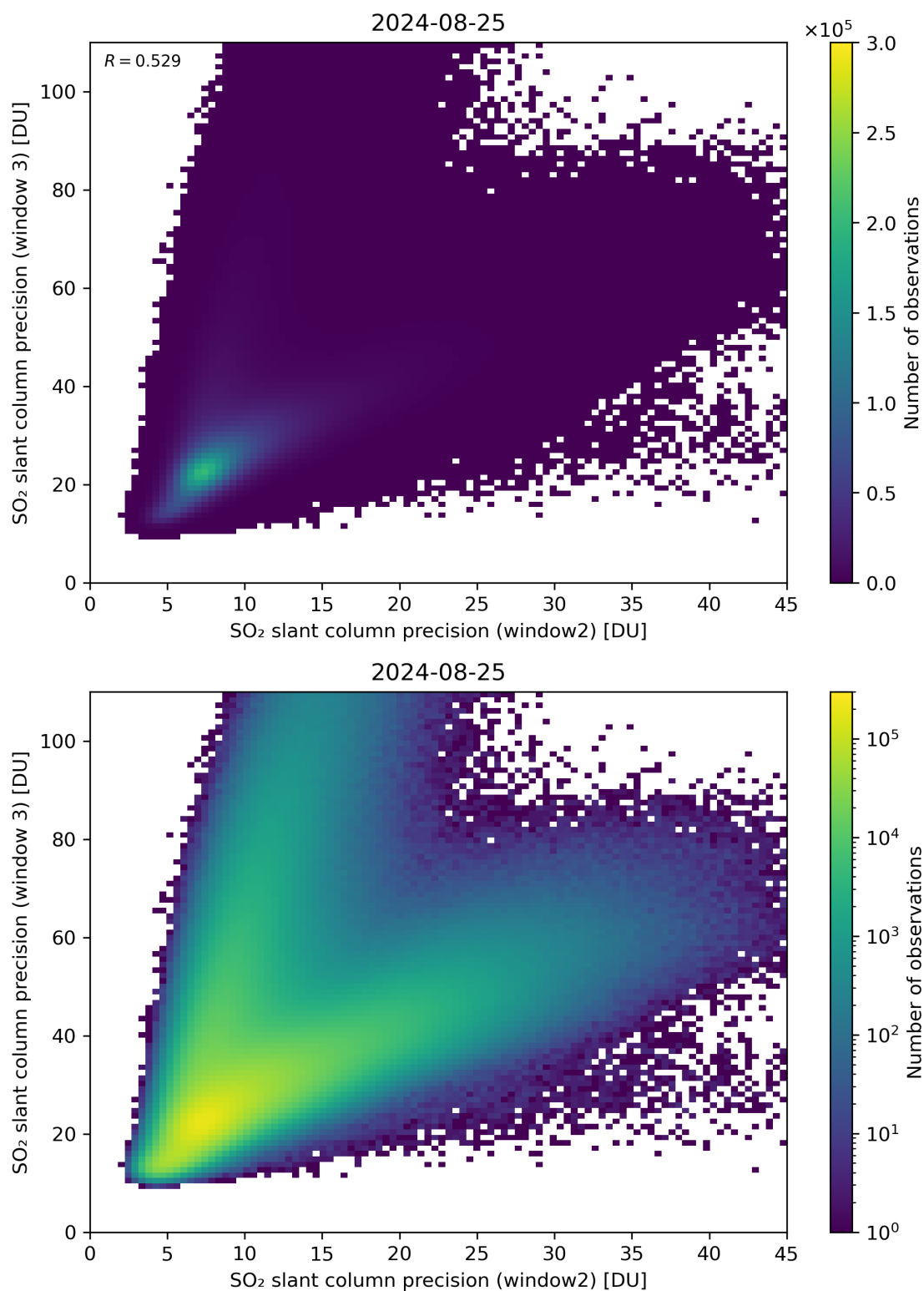
Figure 250: Scatter density plot of “SO 2 slant column precision (window2)” against “SO 2 slant column precision (window 3)” for 2024-08-24 to 2024-08-26.
