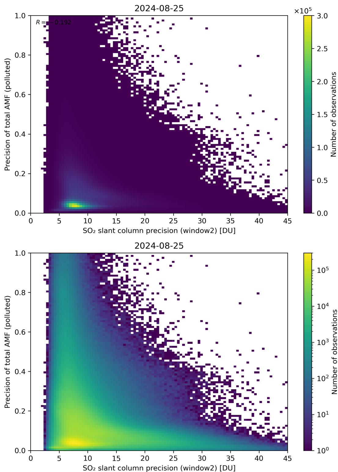
Figure 252: Scatter density plot of “SO 2 slant column precision (window2)” against “Precision of total AMF (polluted)” for 2024-08-24 to 2024-08-26.
