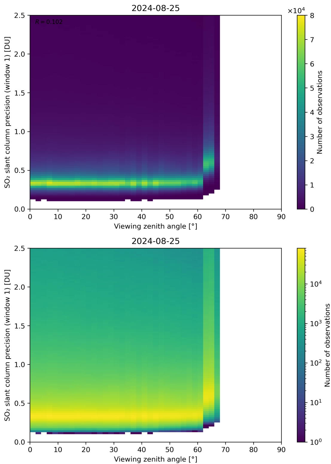
Figure 321: Scatter density plot of “Viewing zenith angle” against “SO 2 slant column precision (window 1)” for 2024-08-24 to 2024-08-26.
