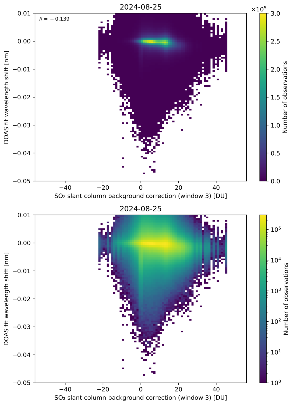
Figure 121: Scatter density plot of “SO 2 slant column background correction (window 3)” against “DOAS fit wavelength shift” for 2024-08-24 to 2024-08-26.
