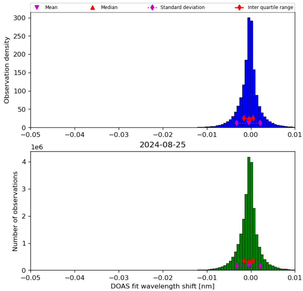
Figure 68: Histogram of “DOAS fit wavelength shift” for 2024-08-24 to 2024-08-26
