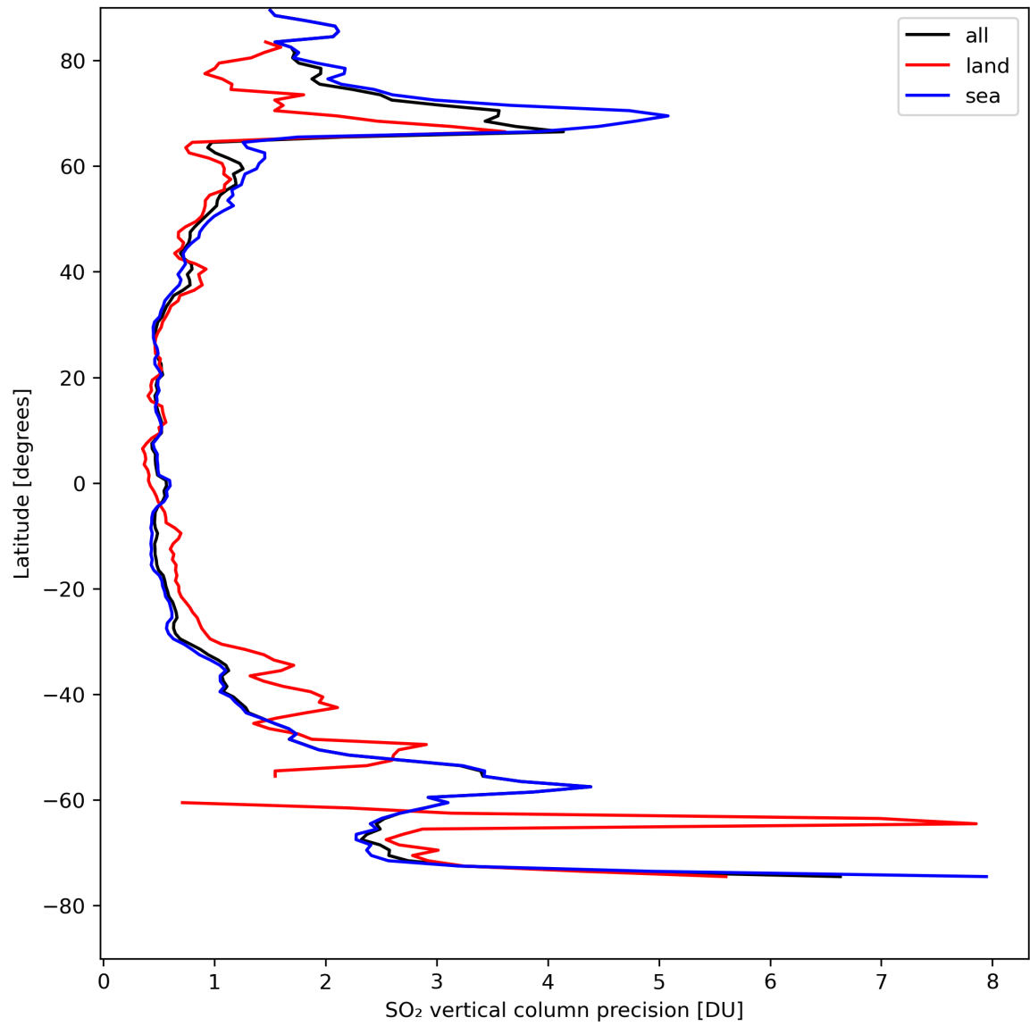
Figure 31: Zonal average of “SO 2 vertical column precision” for 2024-08-24 to 2024-08-26.
