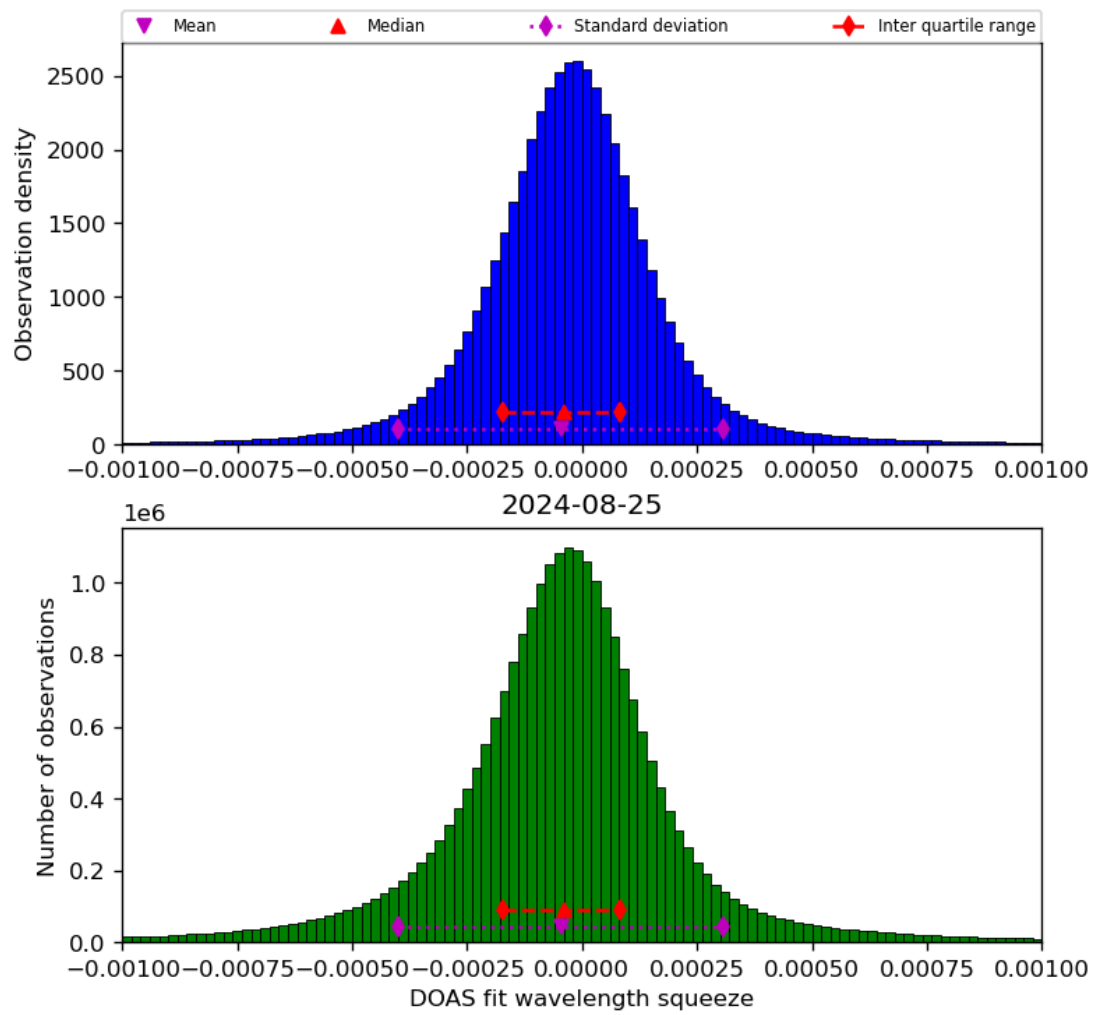
Figure 69: Histogram of “DOAS fit wavelength squeeze” for 2024-08-24 to 2024-08-26
