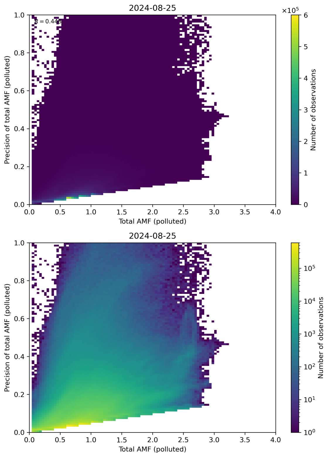
Figure 272: Scatter density plot of “Total AMF (polluted)” against “Precision of total AMF (polluted)” for 2024-08-24 to 2024-08-26.
