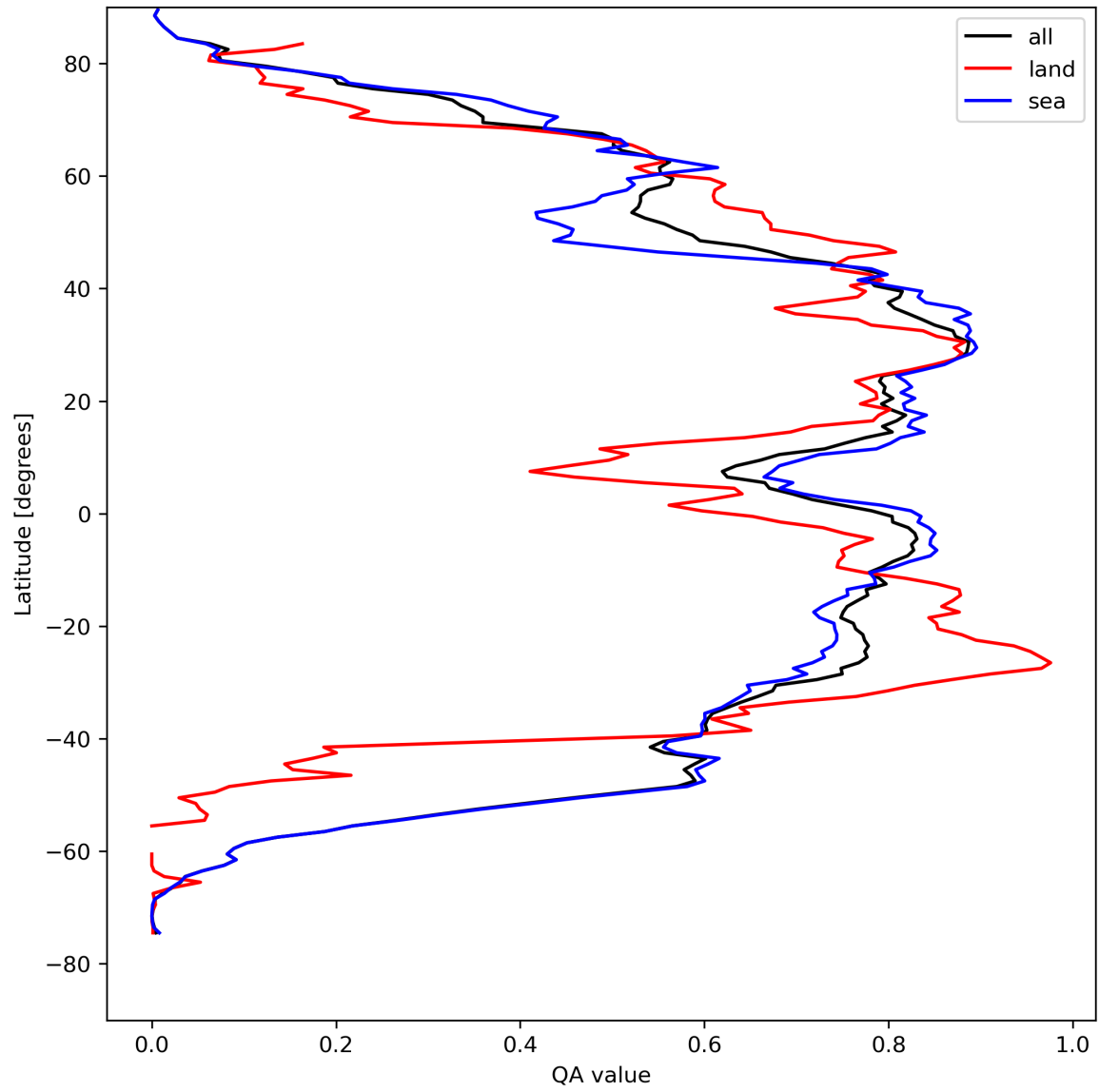
Figure 29: Zonal average of “QA value” for 2024-08-24 to 2024-08-26.
