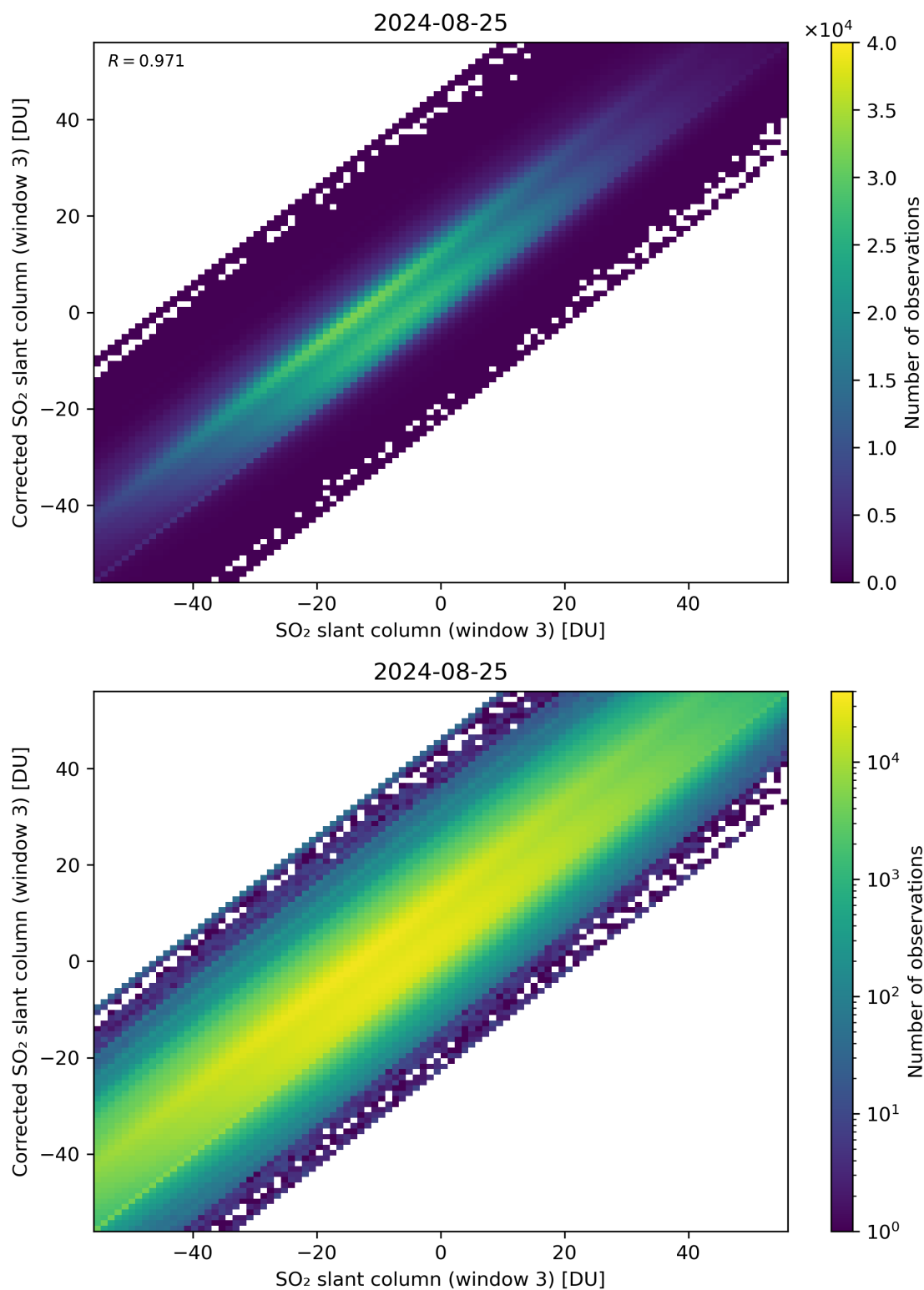
Figure 266: Scatter density plot of “SO 2 slant column (window 3)” against “Corrected SO 2 slant column (window 3)” for 2024-08-24 to 2024-08-26.
