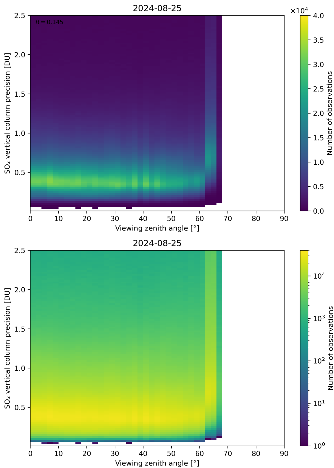
Figure 328: Scatter density plot of “Viewing zenith angle” against “SO 2 vertical column precision” for 2024-08-24 to 2024-08-26.
