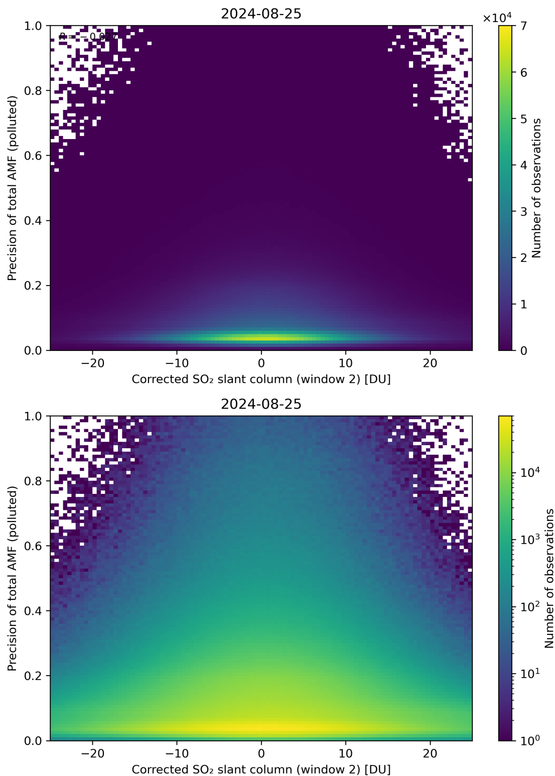
Figure 204: Scatter density plot of “Corrected SO 2 slant column (window 2)” against “Precision of total AMF (polluted)” for 2024-08-24 to 2024-08-26.
