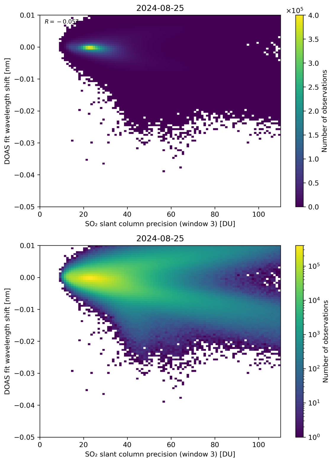
Figure 258: Scatter density plot of “SO 2 slant column precision (window 3)” against “DOAS fit wavelength shift” for 2024-08-24 to 2024-08-26.
