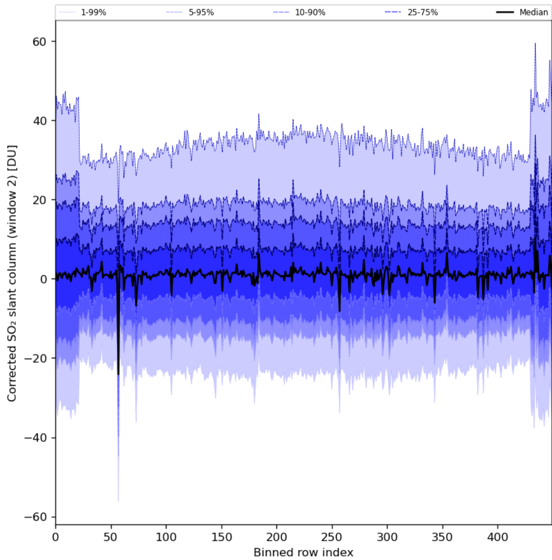
Figure 85: Along track statistics of “Corrected SO 2 slant column (window 2)” for 2024-08-24 to 2024-08-26
