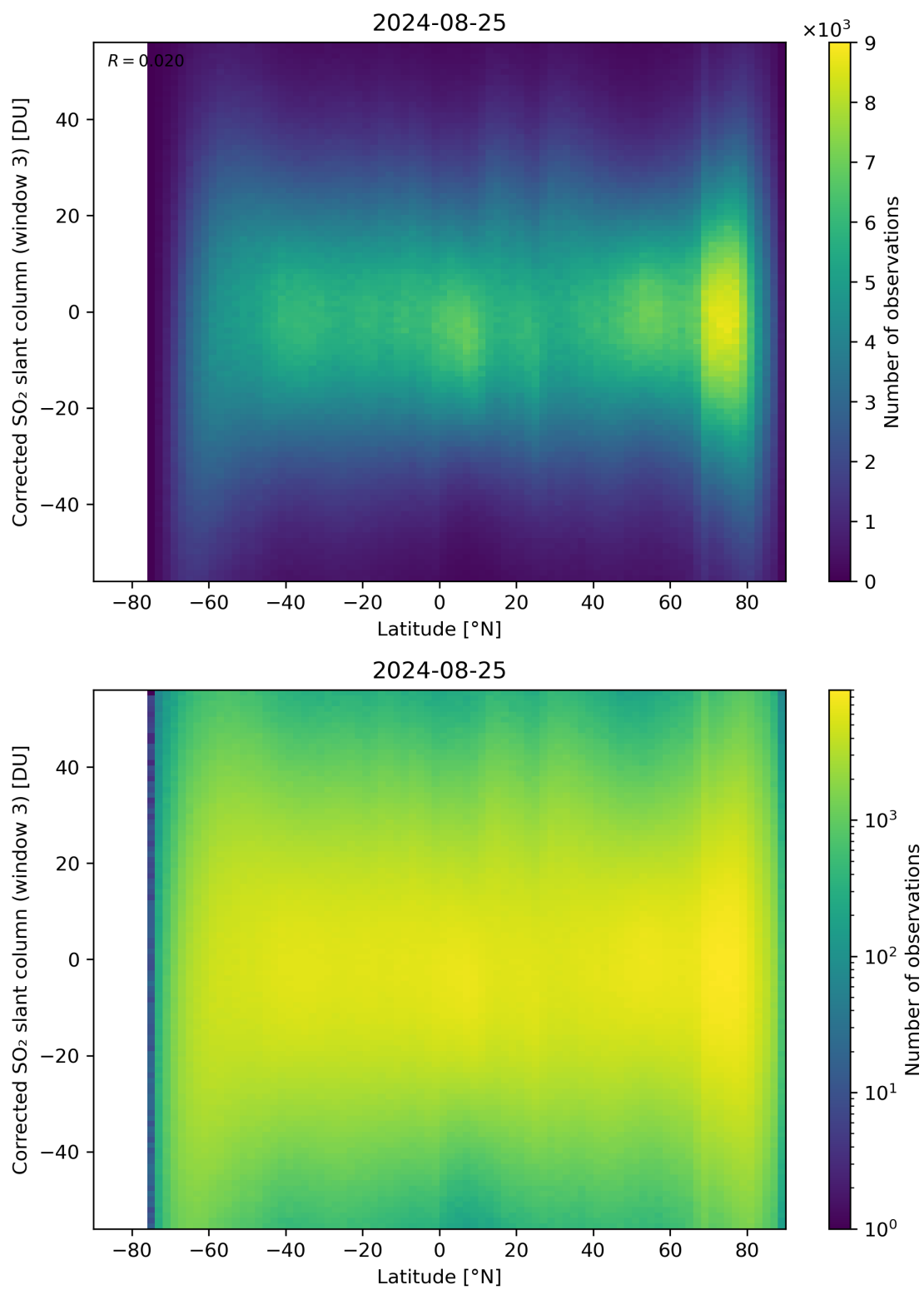
Figure 148: Scatter density plot of “Latitude” against “Corrected SO 2 slant column (window 3)” for 2024-08-24 to 2024-08-26.
