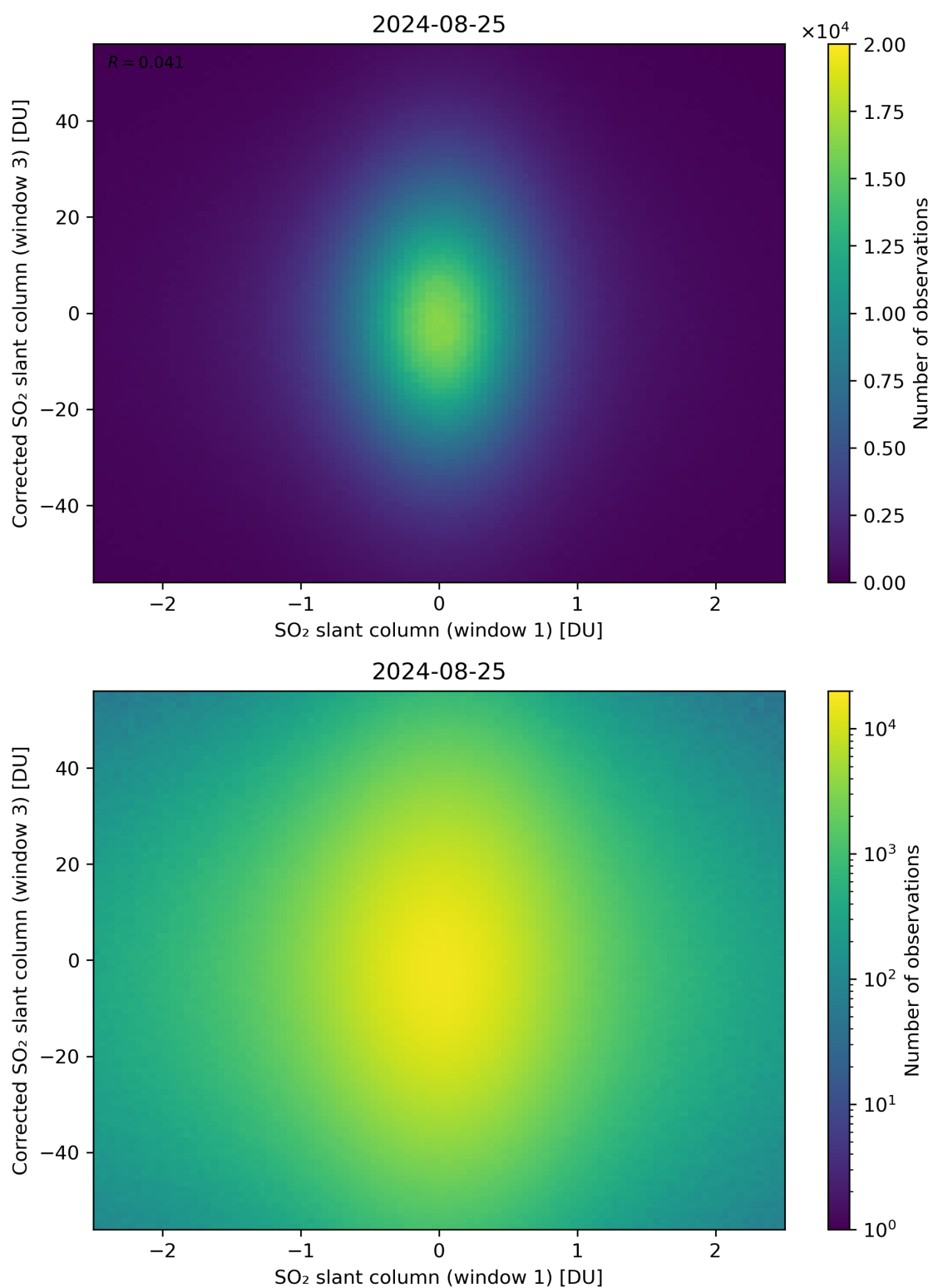
Figure 234: Scatter density plot of “SO 2 slant column (window 1)” against “Corrected SO 2 slant column (window 3)” for 2024-08-24 to 2024-08-26.
