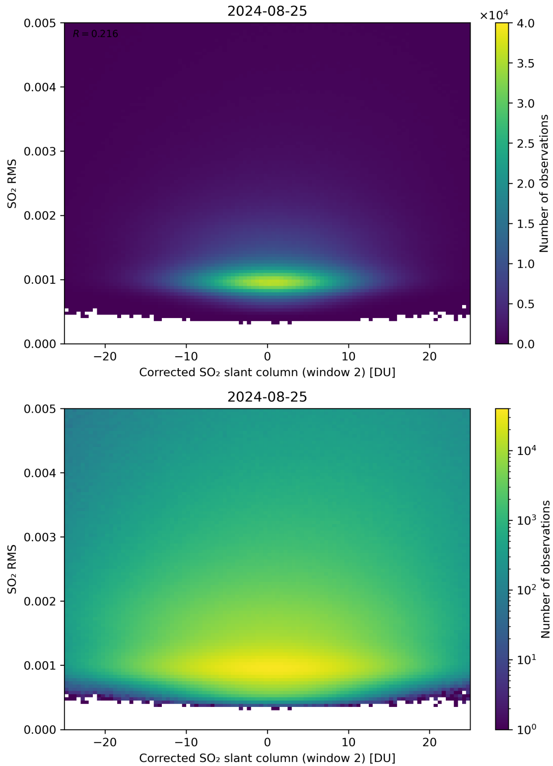
Figure 198: Scatter density plot of “Corrected SO 2 slant column (window 2)” against “SO 2 RMS” for 2024-08-24 to 2024-08-26.
