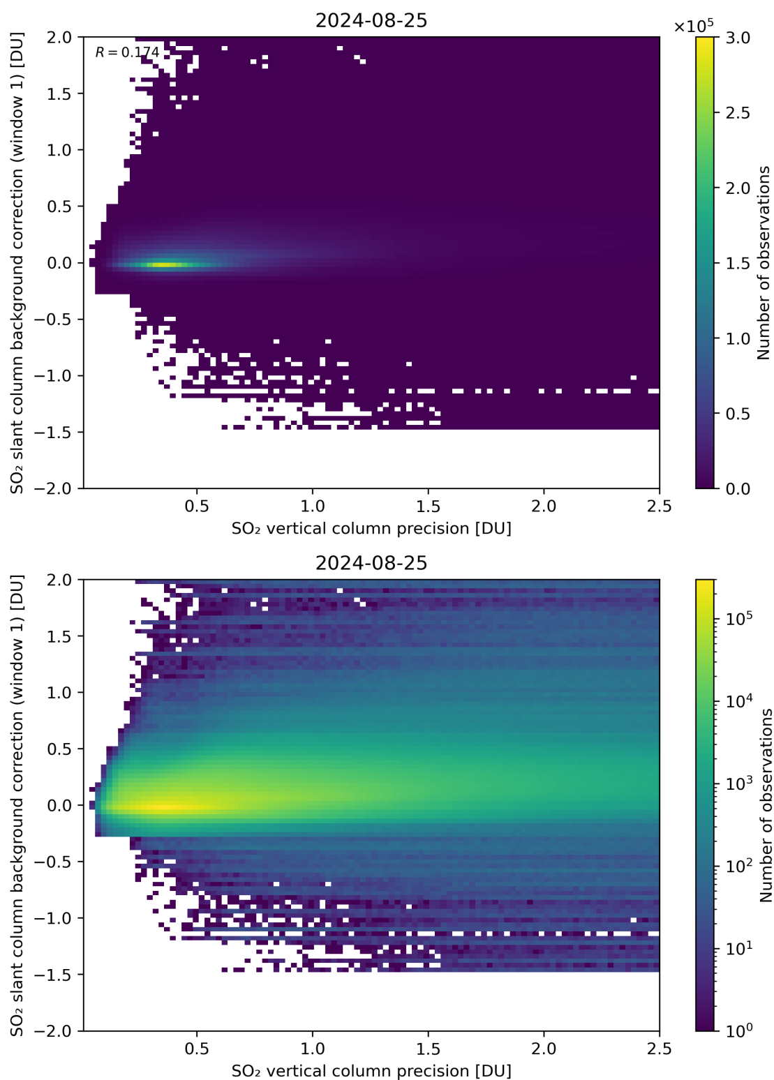
Figure 279: Scatter density plot of “SO 2 vertical column precision” against “SO 2 slant column background correction (window 1)” for 2024-08-24 to 2024-08-26.
