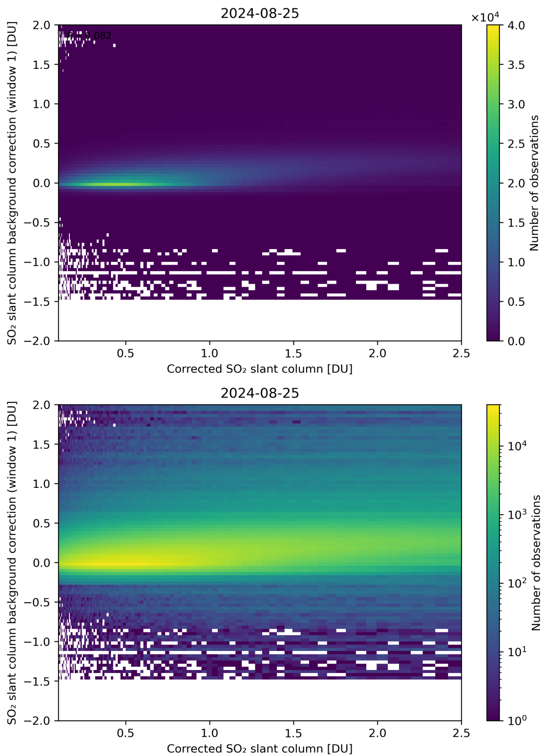
Figure 178: Scatter density plot of “Corrected SO 2 slant column” against “SO 2 slant column background correction (window 1)” for 2024-08-24 to 2024-08-26.
