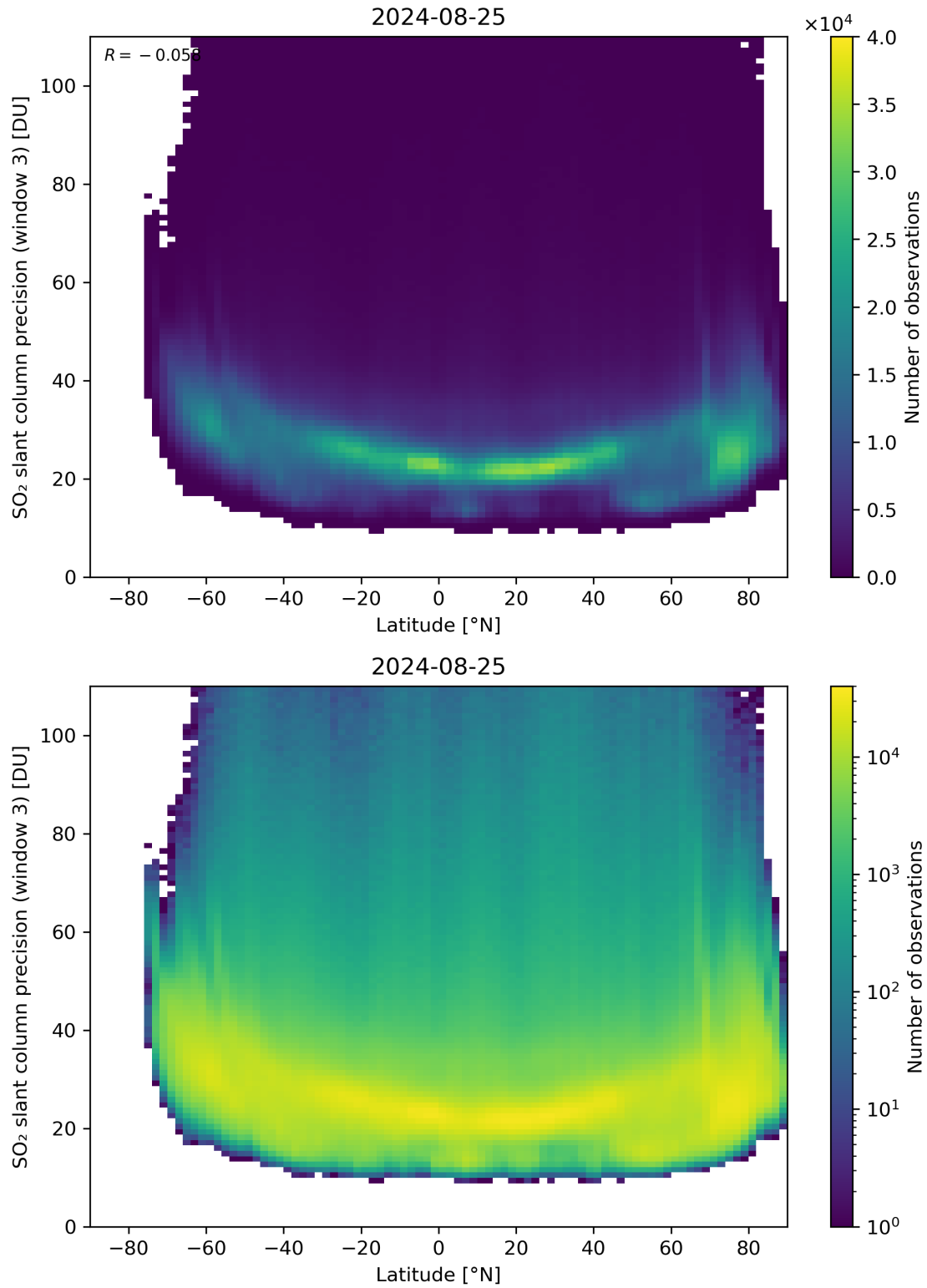
Figure 153: Scatter density plot of “Latitude” against “SO 2 slant column precision (window 3)” for 2024-08-24 to 2024-08-26.
