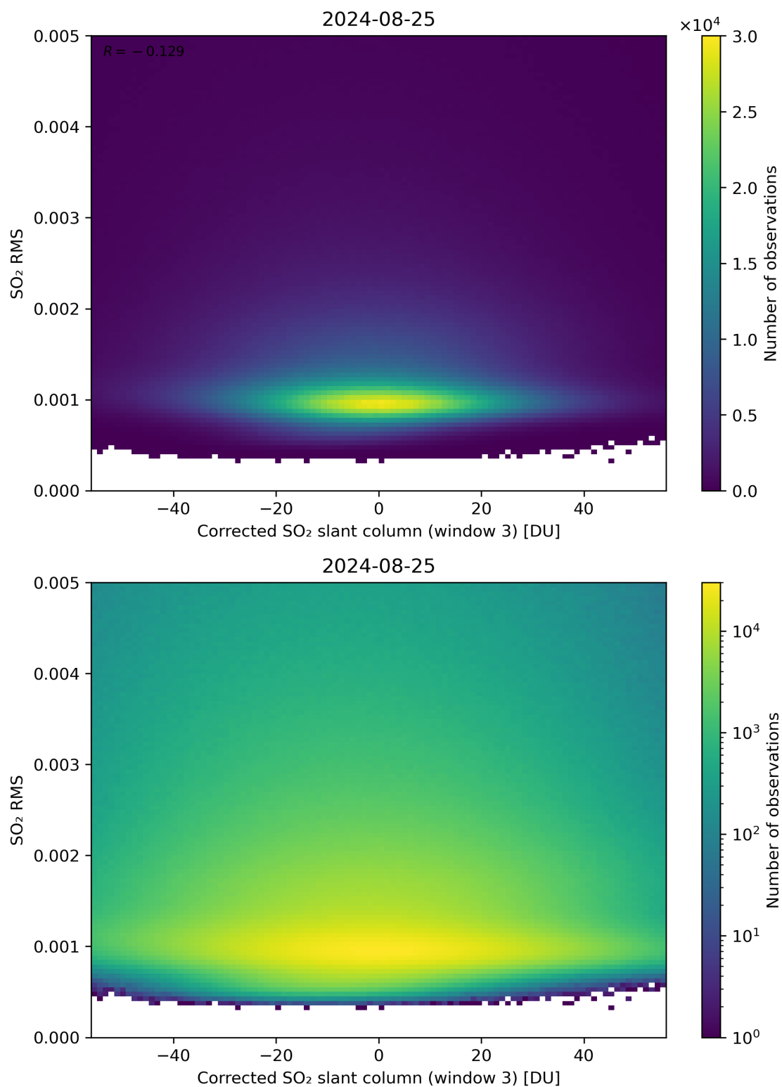
Figure 208: Scatter density plot of “Corrected SO 2 slant column (window 3)” against “SO 2 RMS” for 2024-08-24 to 2024-08-26.
