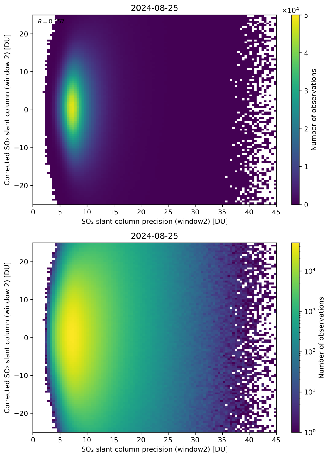
Figure 247: Scatter density plot of “SO 2 slant column precision (window2)” against “Corrected SO 2 slant column (window 2)” for 2024-08-24 to 2024-08-26.
