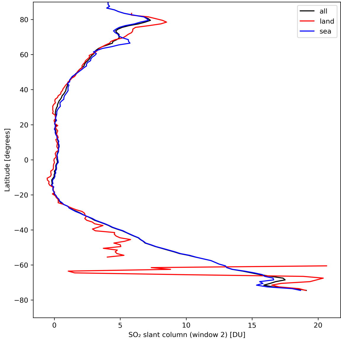
Figure 37: Zonal average of “SO 2 slant column (window 2)” for 2024-08-24 to 2024-08-26.
