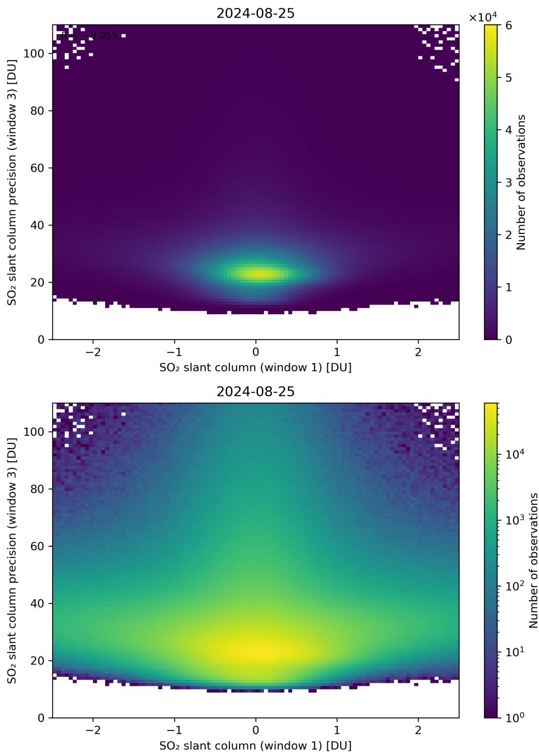
Figure 238: Scatter density plot of “SO 2 slant column (window 1)” against “SO 2 slant column precision (window 3)” for 2024-08-24 to 2024-08-26.
