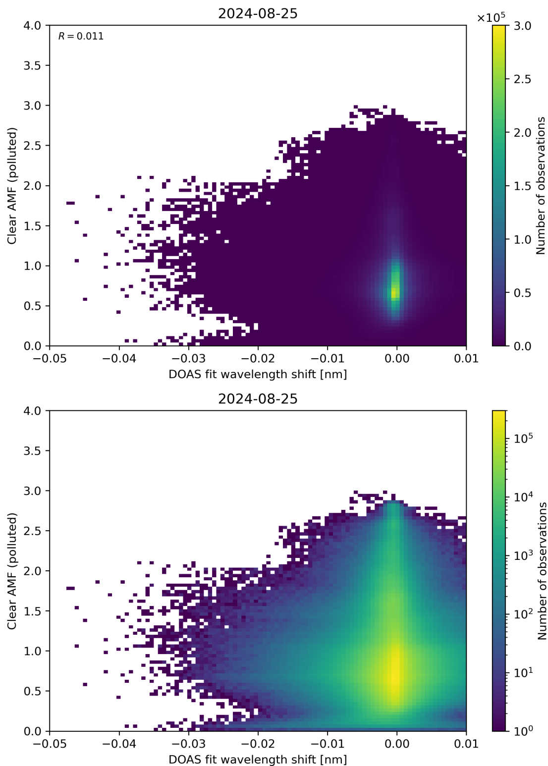
Figure 129: Scatter density plot of “DOAS fit wavelength shift” against “Clear AMF (polluted)” for 2024-08-24 to 2024-08-26.
