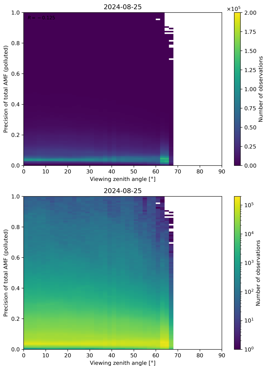
Figure 326: Scatter density plot of “Viewing zenith angle” against “Precision of total AMF (polluted)” for 2024-08-24 to 2024-08-26.
