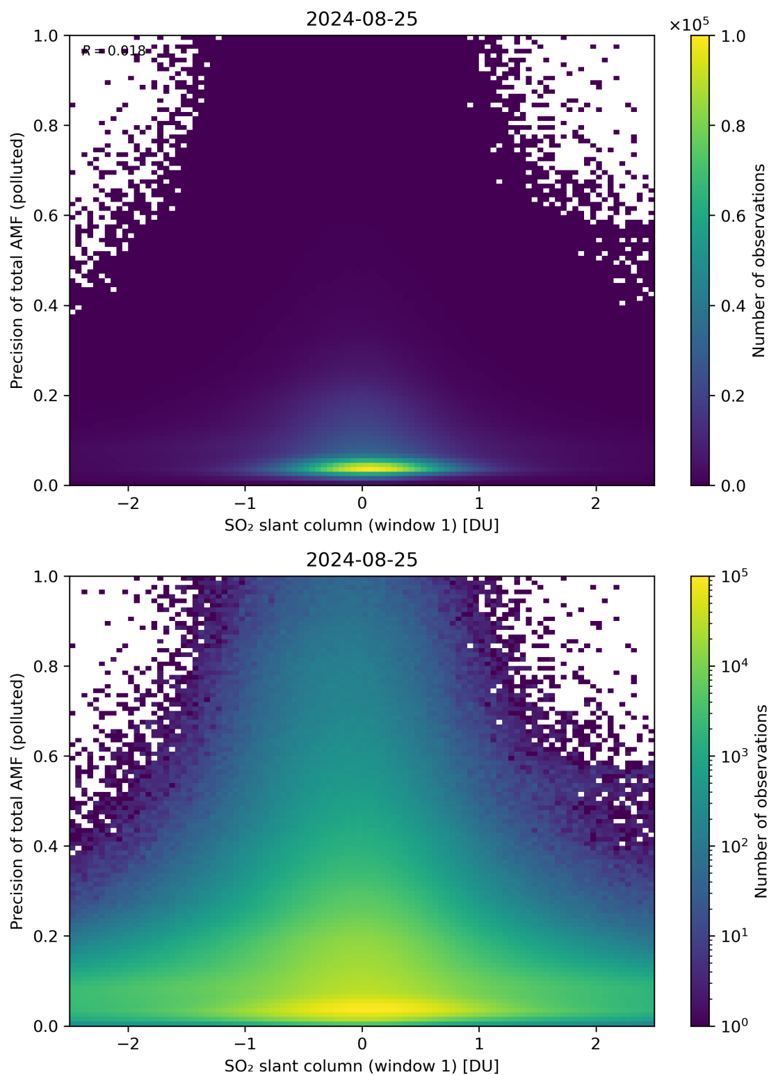
Figure 240: Scatter density plot of “SO 2 slant column (window 1)” against “Precision of total AMF (polluted)” for 2024-08-24 to 2024-08-26.
