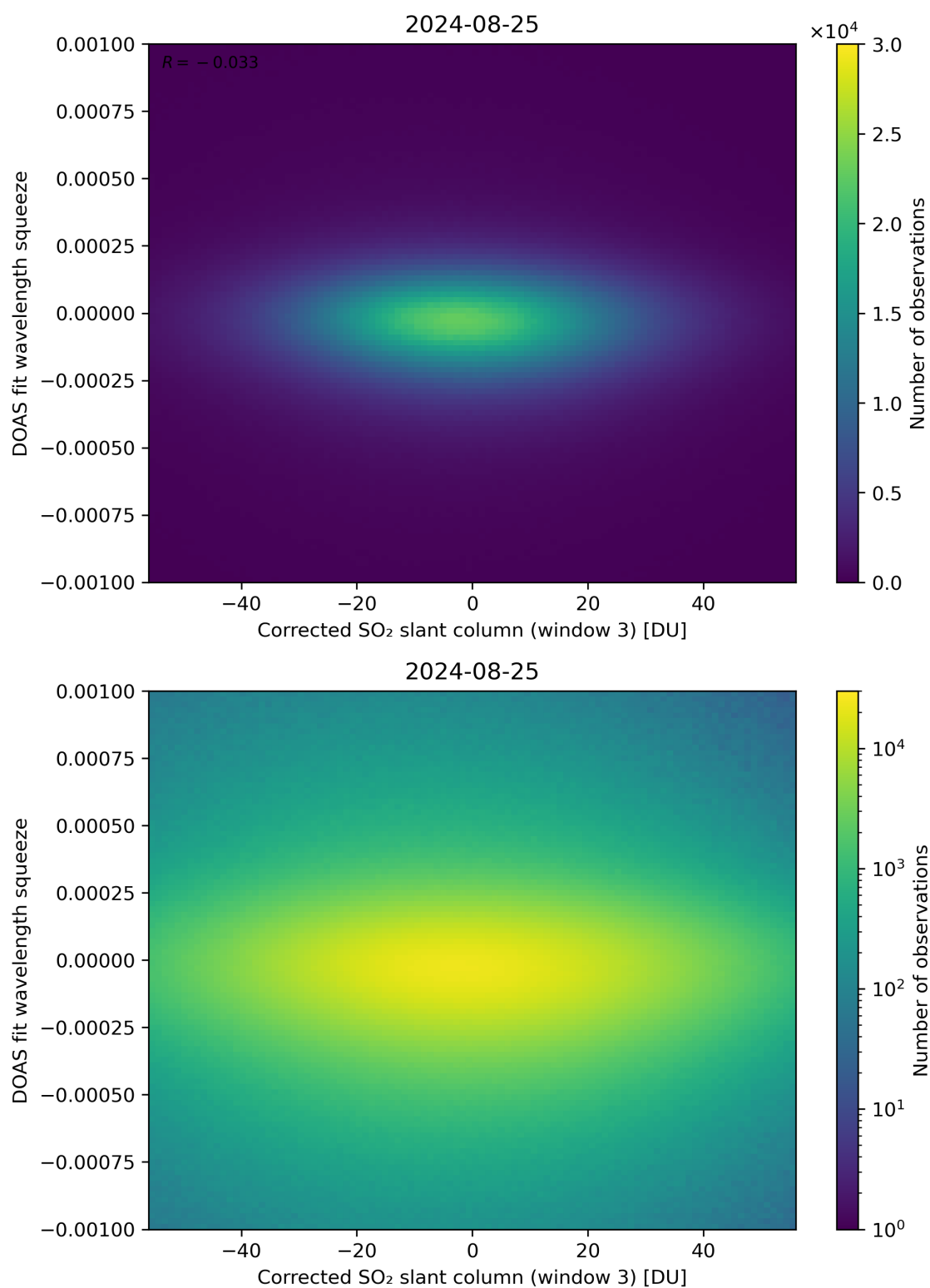
Figure 207: Scatter density plot of “Corrected SO 2 slant column (window 3)” against “DOAS fit wavelength squeeze” for 2024-08-24 to 2024-08-26.
