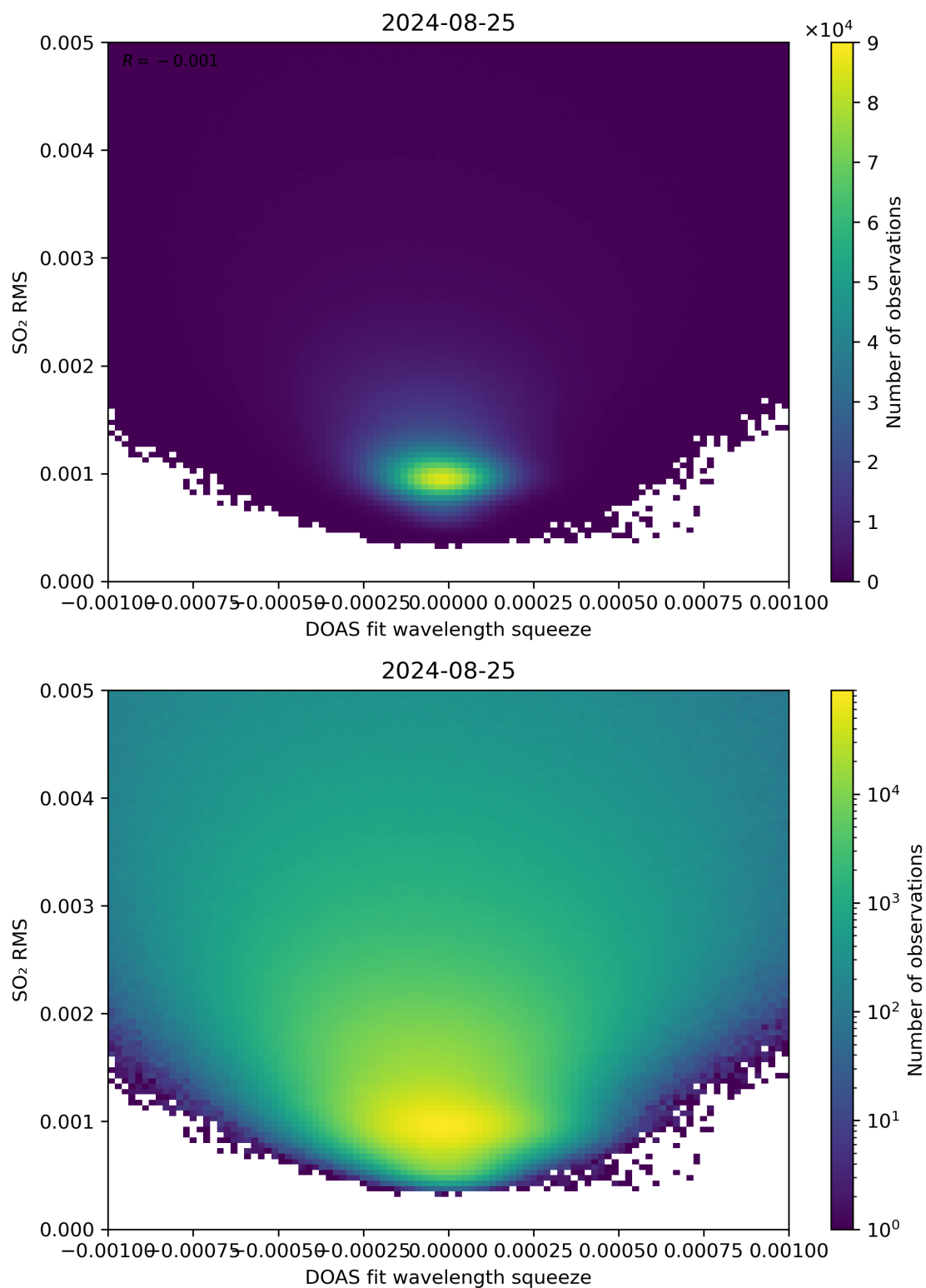
Figure 132: Scatter density plot of “DOAS fit wavelength squeeze” against “SO 2 RMS” for 2024-08-24 to 2024-08-26.
