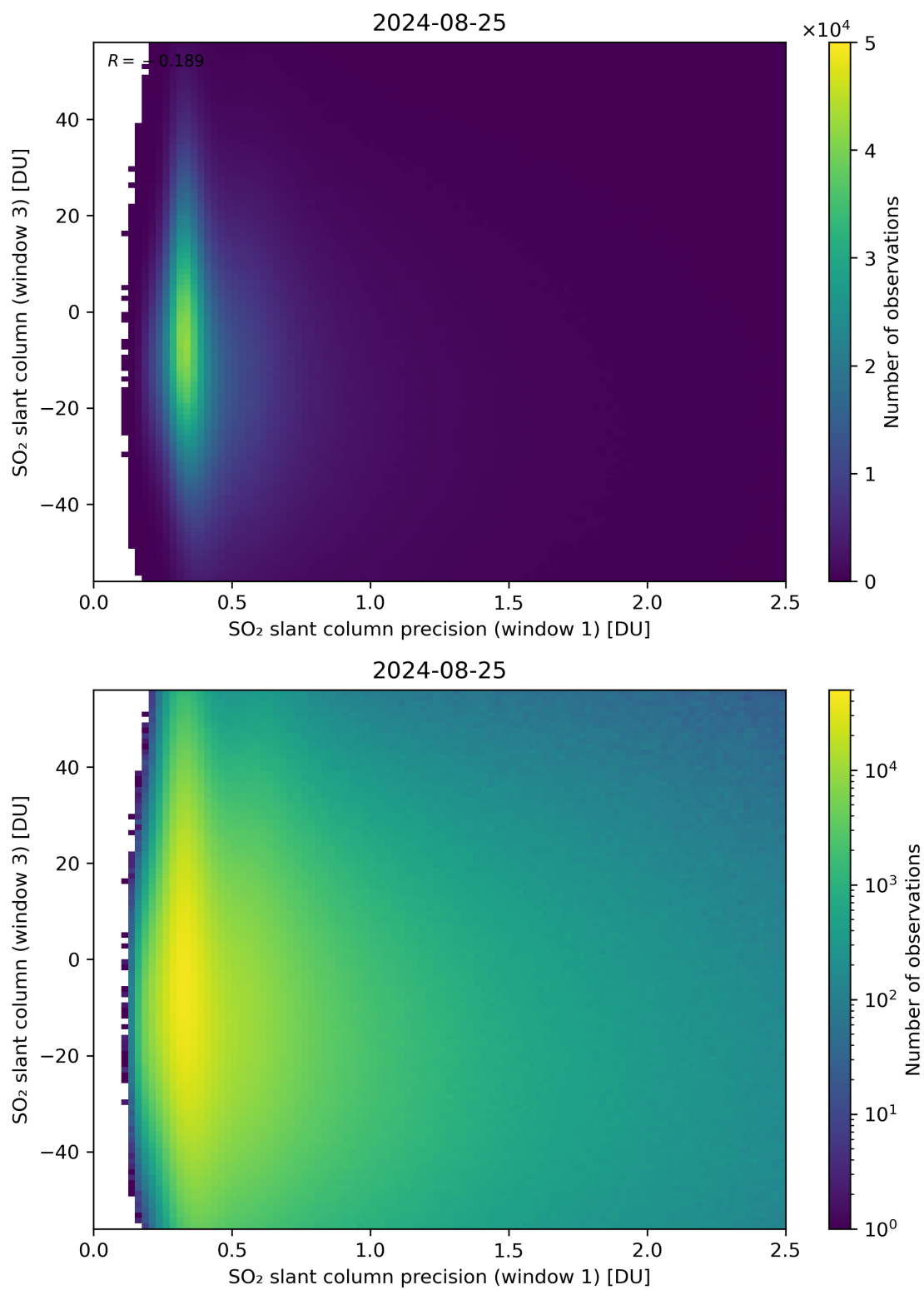
Figure 228: Scatter density plot of “SO 2 slant column precision (window 1)” against “SO 2 slant column (window 3)” for 2024-08-24 to 2024-08-26.
