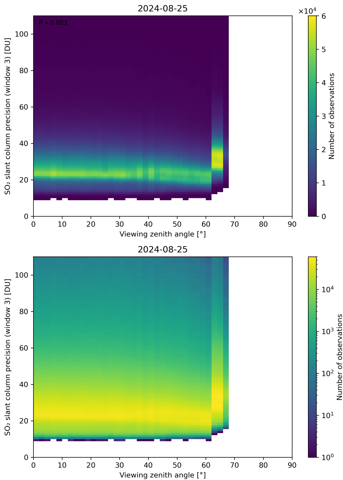
Figure 324: Scatter density plot of “Viewing zenith angle” against “SO 2 slant column precision (window 3)” for 2024-08-24 to 2024-08-26.
