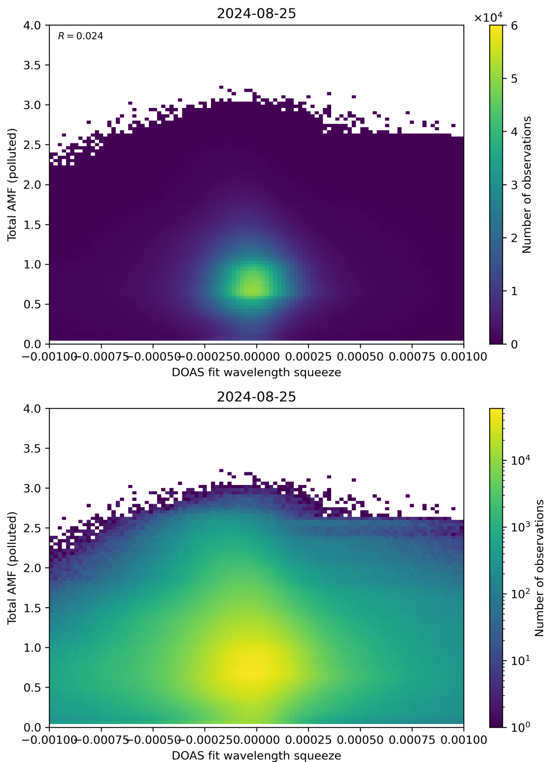
Figure 134: Scatter density plot of “DOAS fit wavelength squeeze” against “Total AMF (polluted)” for 2024-08-24 to 2024-08-26.
