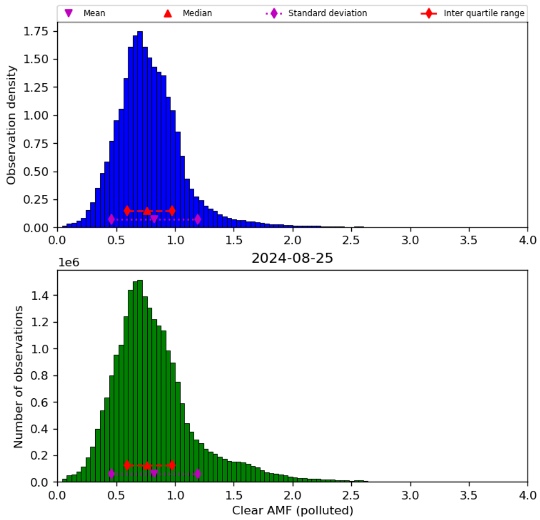
Figure 73: Histogram of “Clear AMF (polluted)” for 2024-08-24 to 2024-08-26
