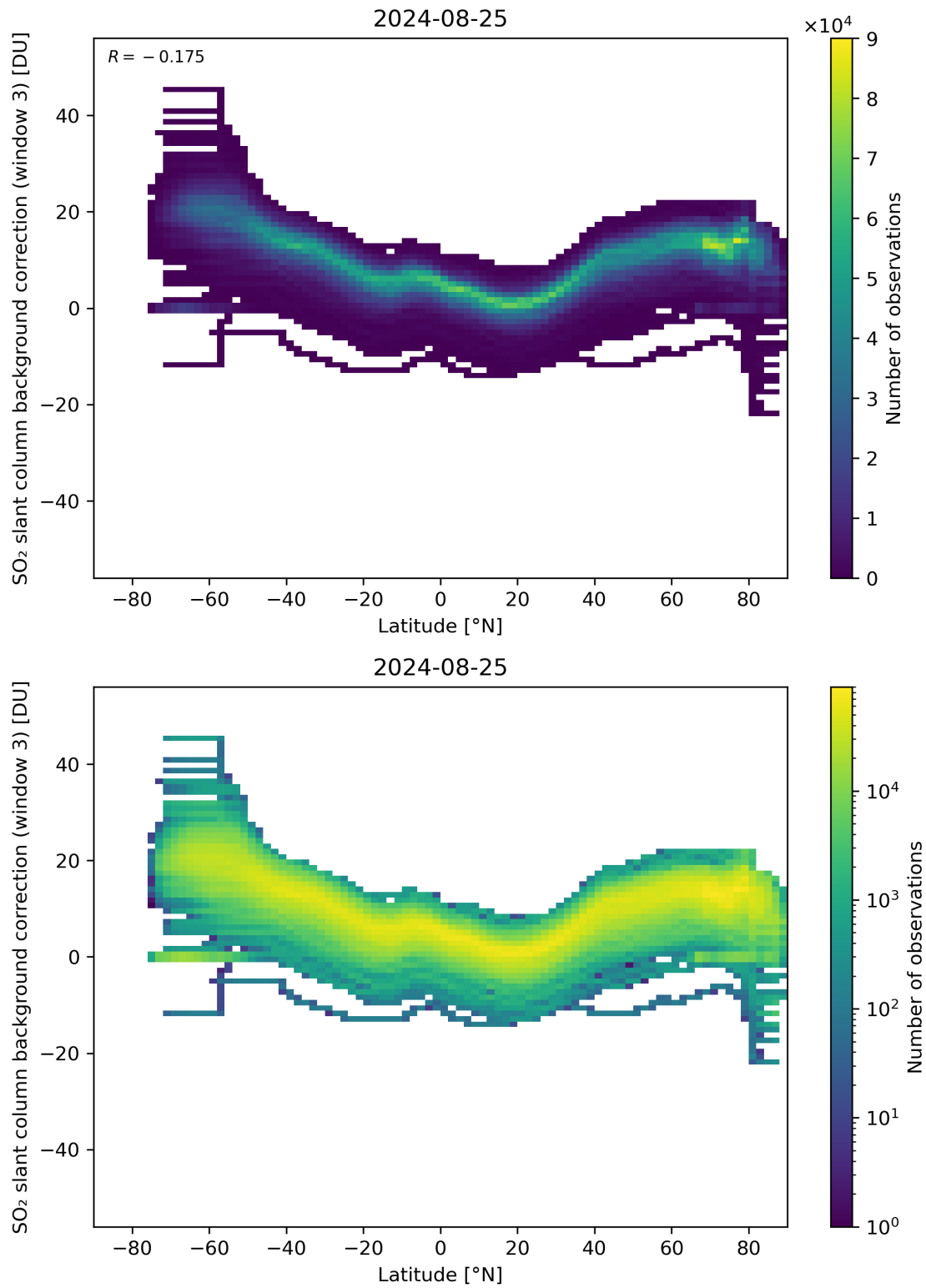
Figure 141: Scatter density plot of “Latitude” against “SO 2 slant column background correction (window 3)” for 2024-08-24 to 2024-08-26.
