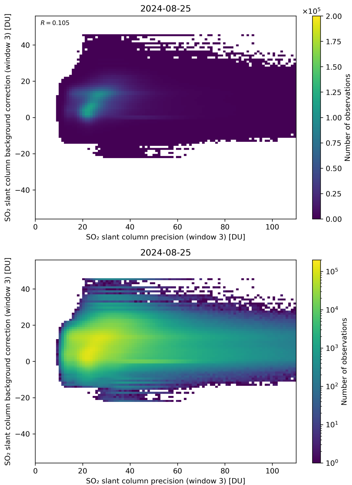
Figure 257: Scatter density plot of “SO 2 slant column precision (window 3)” against “SO 2 slant column background correction (window 3)” for 2024-08-24 to 2024-08-26.
