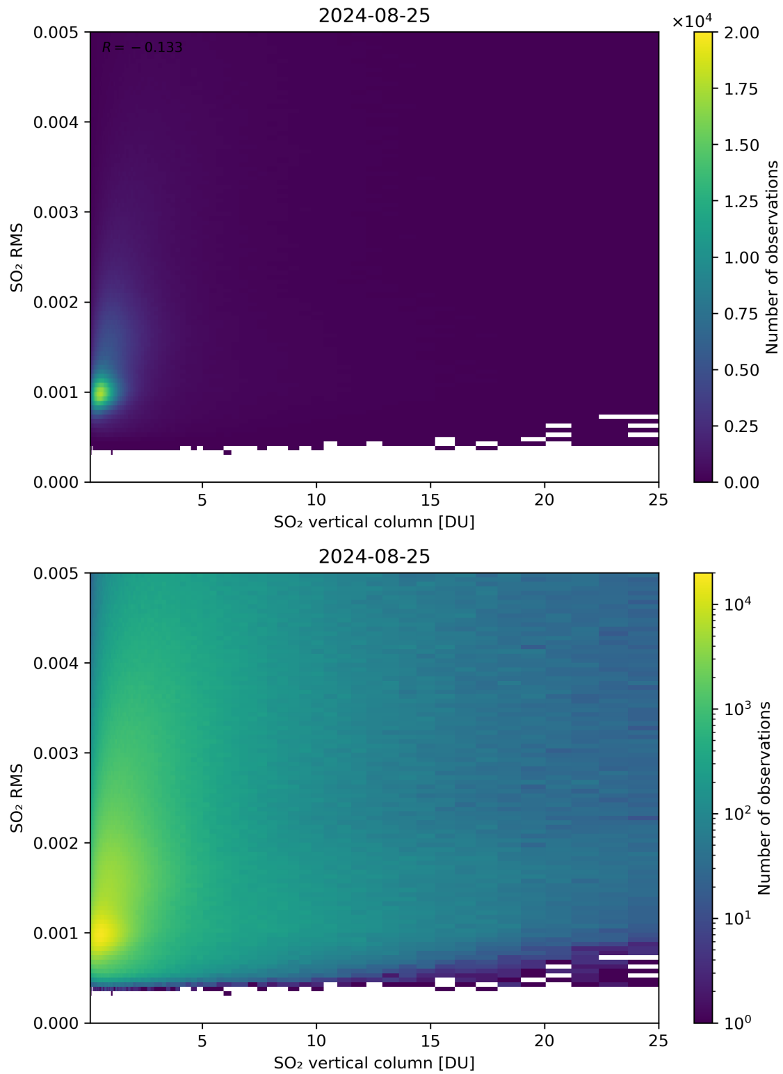
Figure 278: Scatter density plot of “SO 2 vertical column” against “SO 2 RMS” for 2024-08-24 to 2024-08-26.
