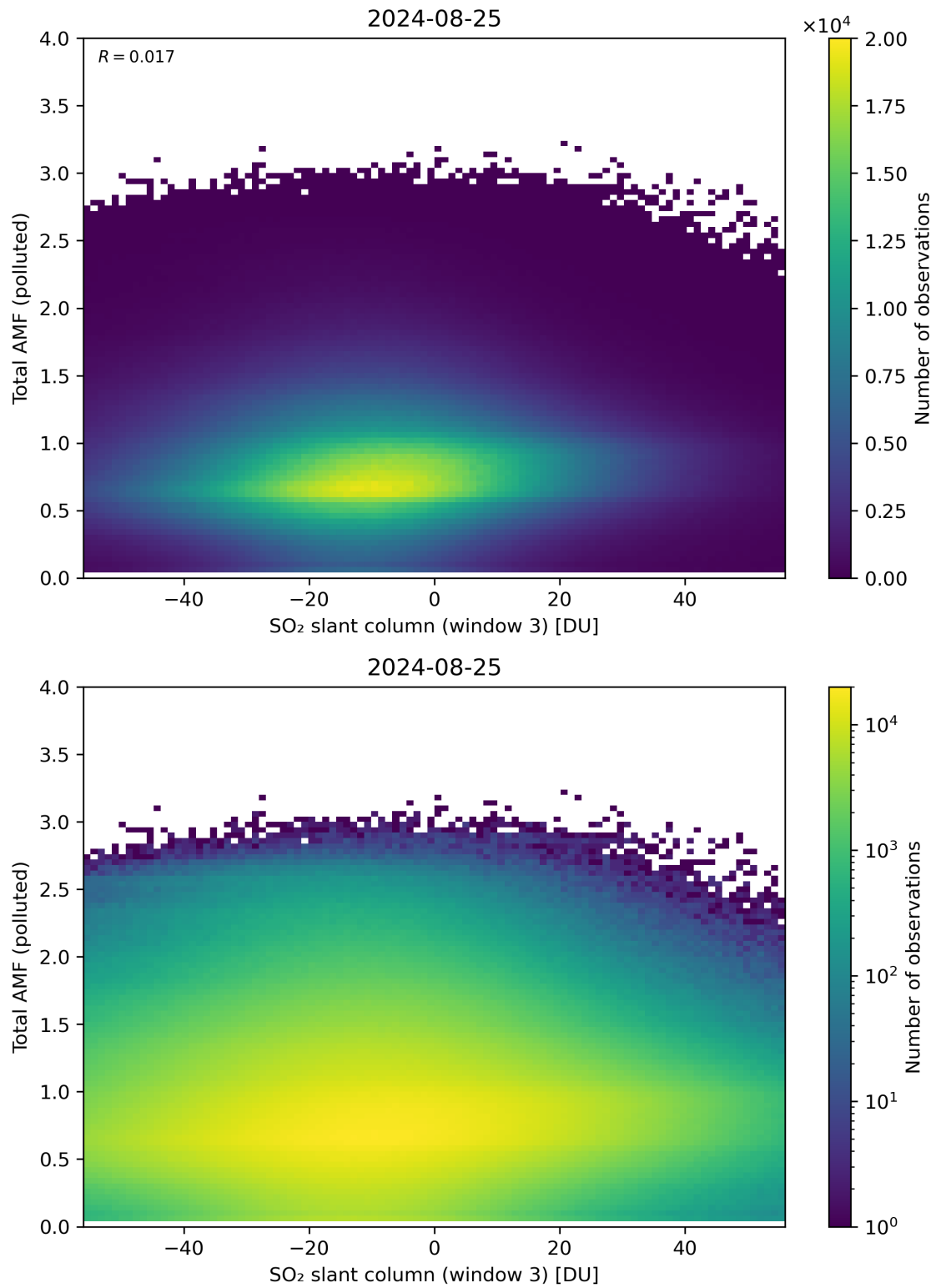
Figure 268: Scatter density plot of “SO 2 slant column (window 3)” against “Total AMF (polluted)” for 2024-08-24 to 2024-08-26.
