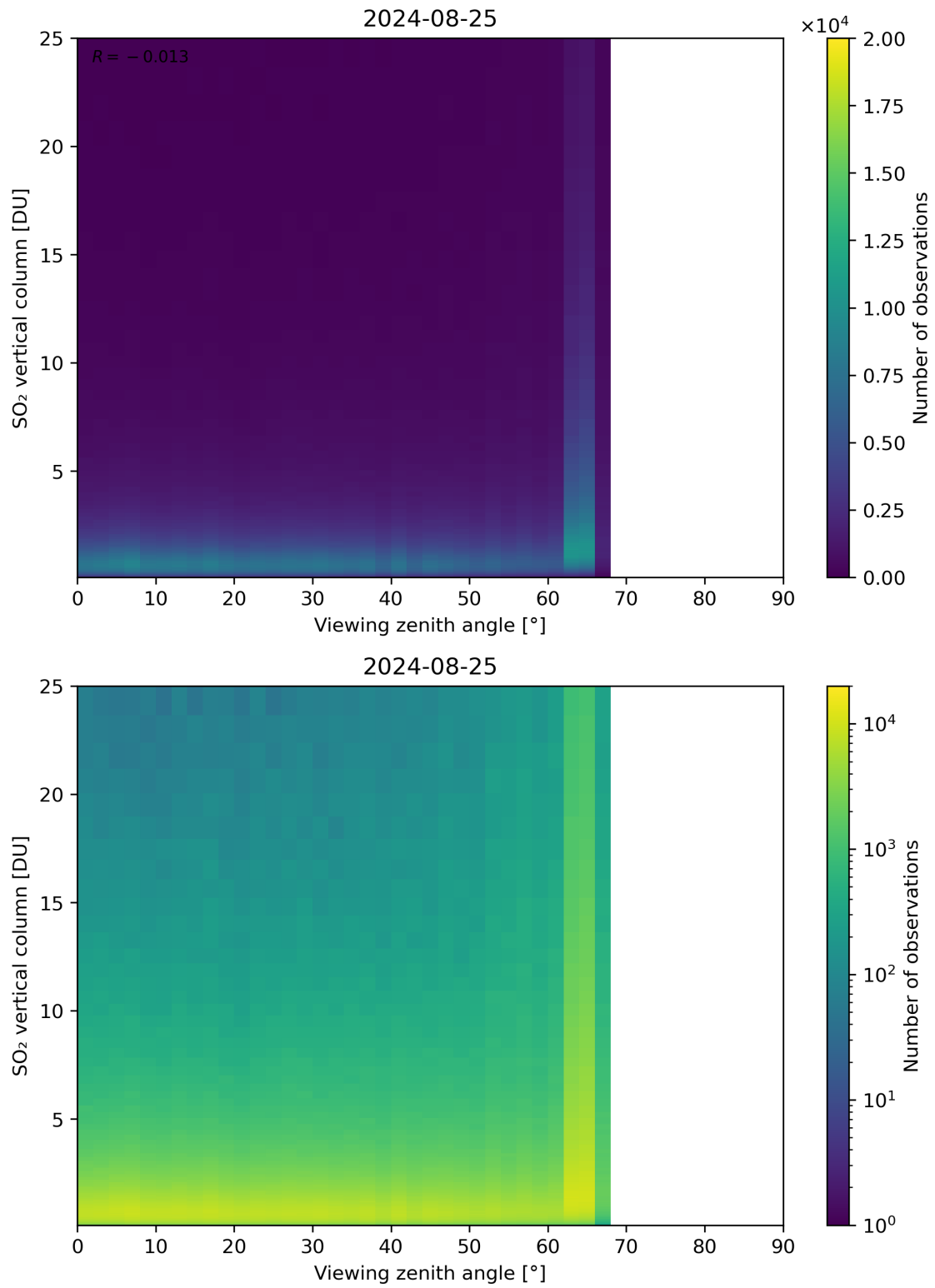
Figure 327: Scatter density plot of “Viewing zenith angle” against “SO 2 vertical column” for 2024-08-24 to 2024-08-26.
