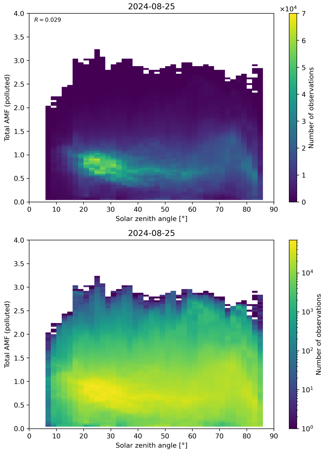
Figure 174: Scatter density plot of “Solar zenith angle” against “Total AMF (polluted)” for 2024-08-24 to 2024-08-26.
