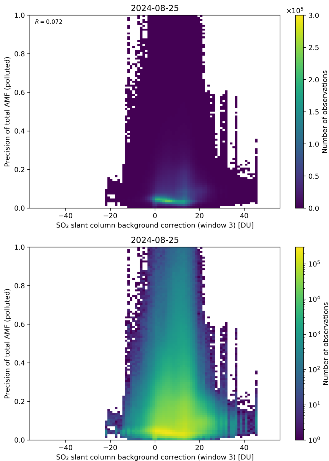
Figure 126: Scatter density plot of “SO 2 slant column background correction (window 3)” against “Precision of total AMF (polluted)” for 2024-08-24 to 2024-08-26.
