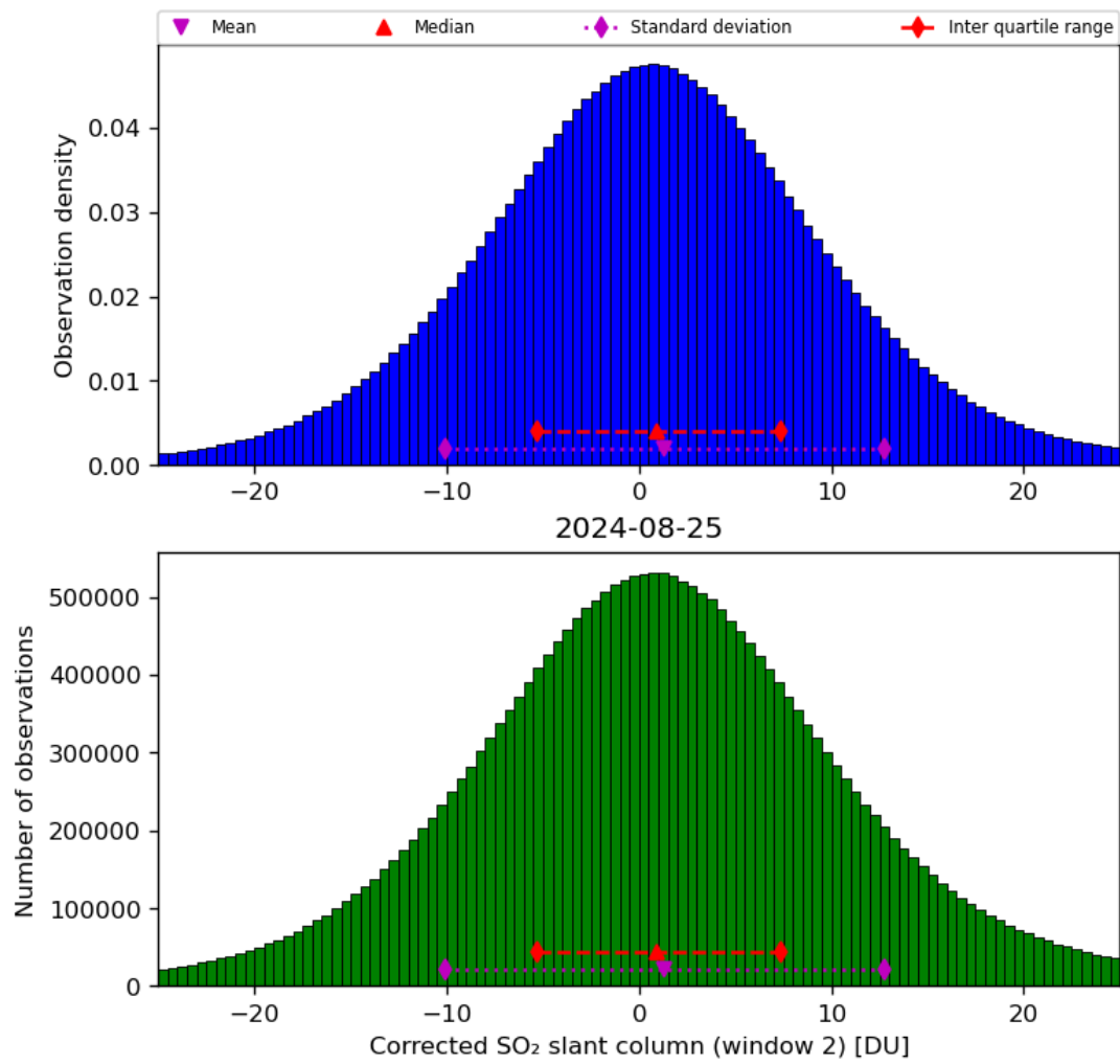
Figure 62: Histogram of “Corrected SO 2 slant column (window 2)” for 2024-08-24 to 2024-08-26
