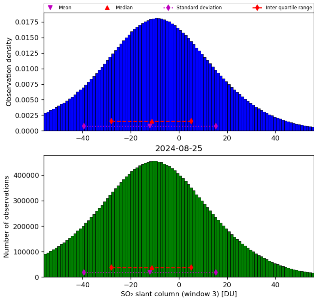
Figure 64: Histogram of “SO 2 slant column (window 3)” for 2024-08-24 to 2024-08-26
