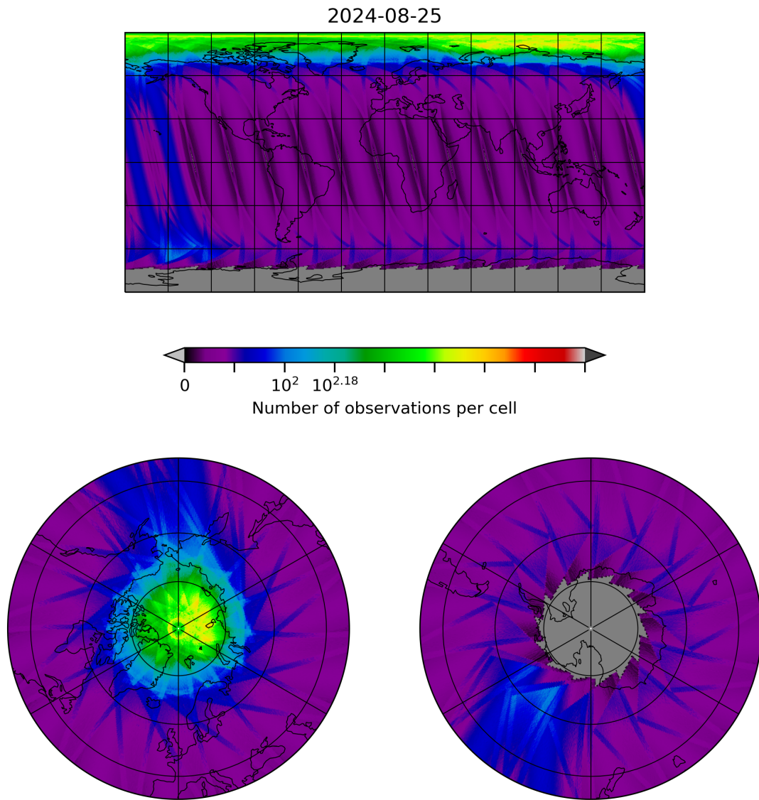
Figure 28: Map of the number of observations for 2024-08-24 to 2024-08-26
