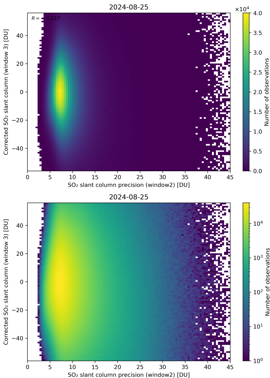
Figure 248: Scatter density plot of “SO 2 slant column precision (window2)” against “Corrected SO 2 slant column (window 3)” for 2024-08-24 to 2024-08-26.
