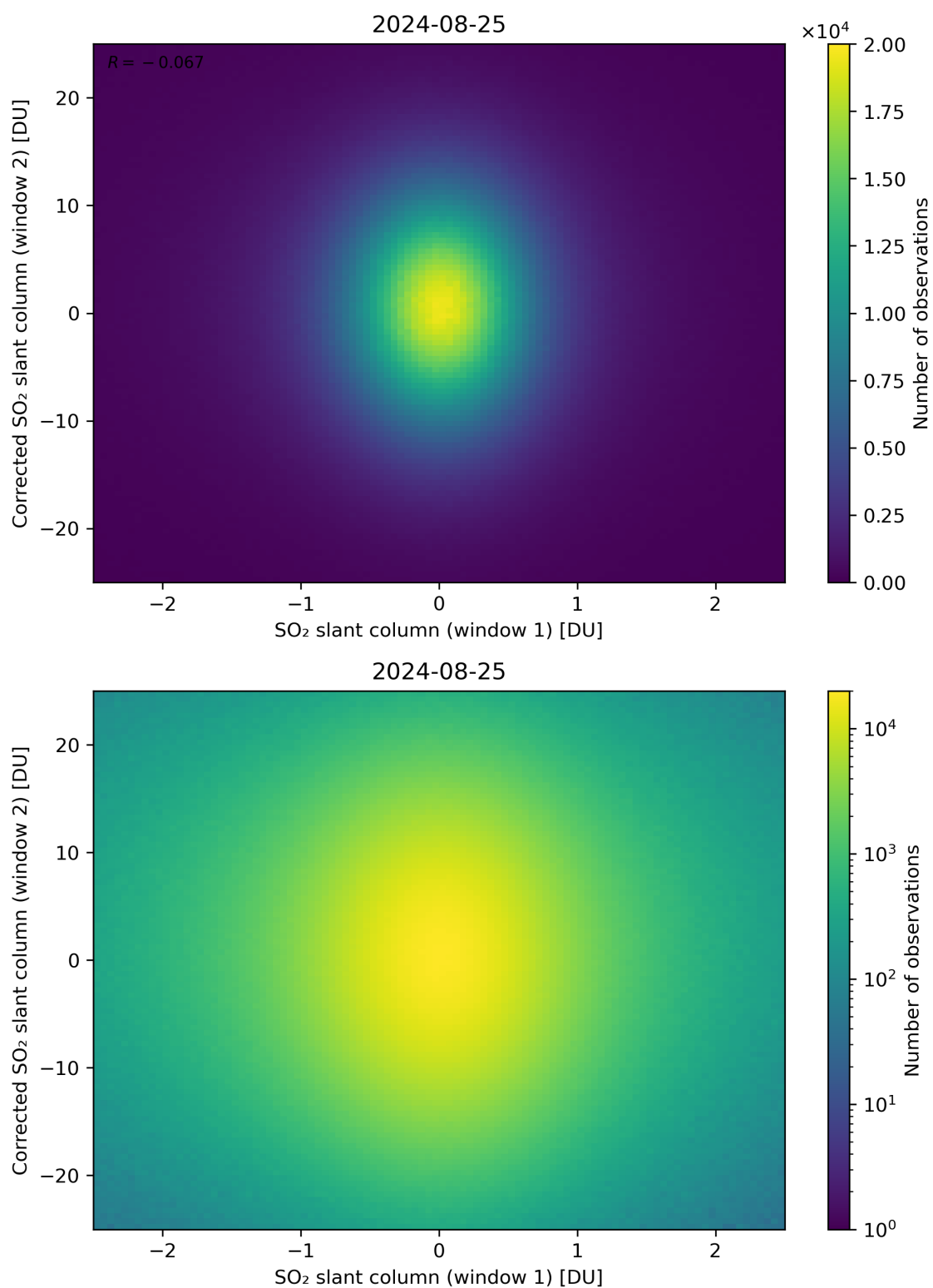
Figure 233: Scatter density plot of “SO 2 slant column (window 1)” against “Corrected SO 2 slant column (window 2)” for 2024-08-24 to 2024-08-26.
