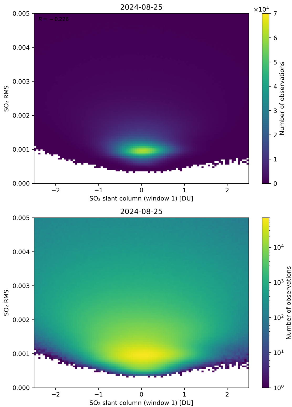
Figure 217: Scatter density plot of “SO 2 slant column (window 1)” against “SO 2 RMS” for 2024-08-24 to 2024-08-26.
