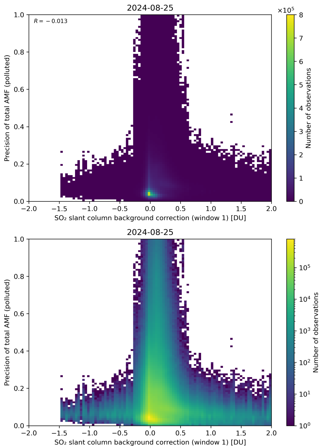
Figure 110: Scatter density plot of “SO 2 slant column background correction (window 1)” against “Precision of total AMF (polluted)” for 2024-08-24 to 2024-08-26.
