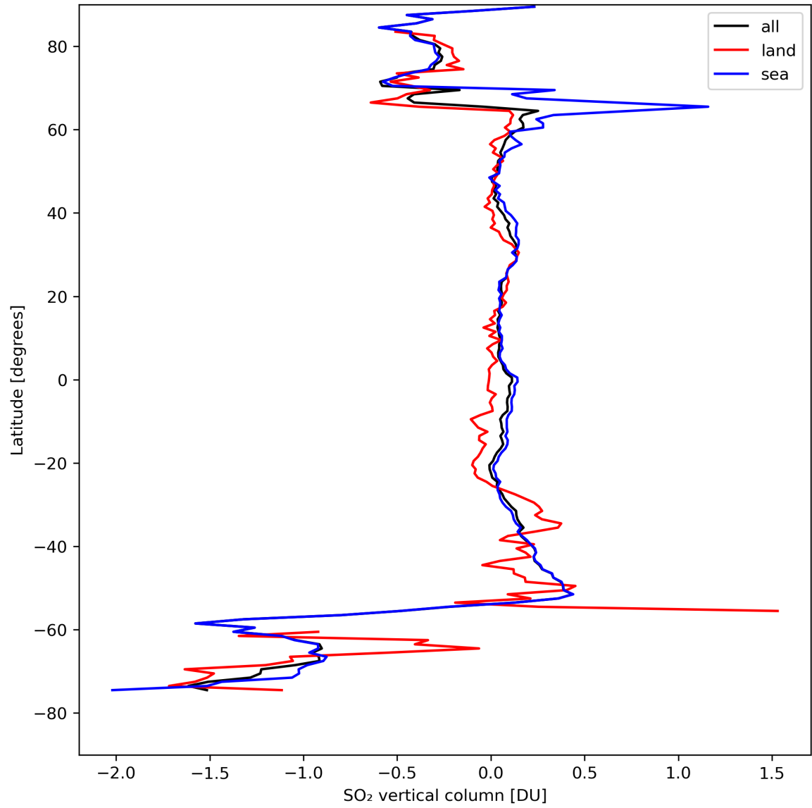
Figure 30: Zonal average of “SO 2 vertical column” for 2024-08-24 to 2024-08-26.
