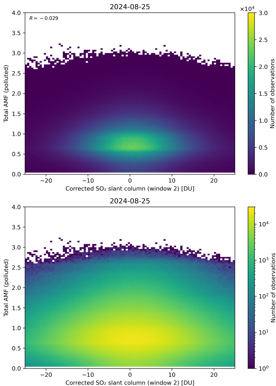
Figure 203: Scatter density plot of “Corrected SO 2 slant column (window 2)” against “Total AMF (polluted)” for 2024-08-24 to 2024-08-26.
