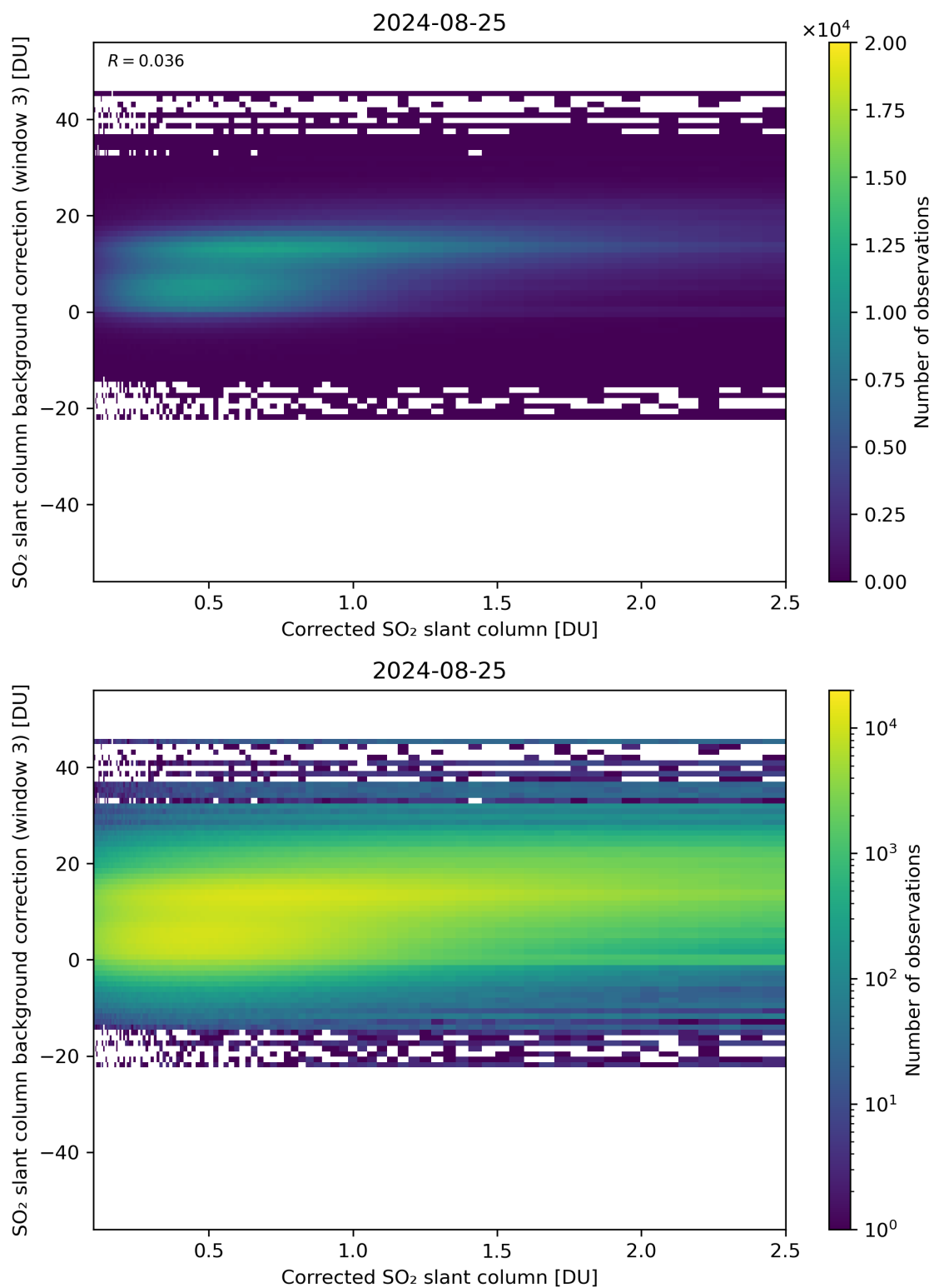
Figure 180: Scatter density plot of “Corrected SO 2 slant column” against “SO 2 slant column background correction (window 3)” for 2024-08-24 to 2024-08-26.
