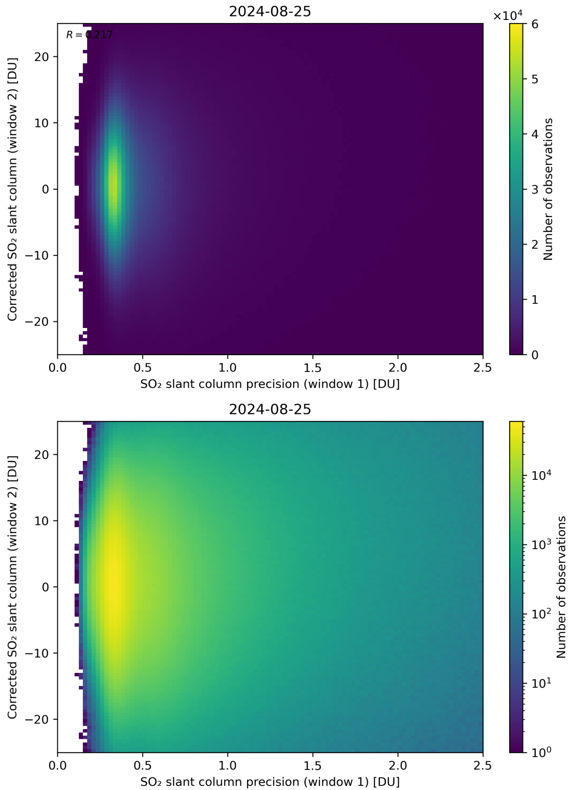
Figure 225: Scatter density plot of “SO 2 slant column precision (window 1)” against “Corrected SO 2 slant column (window 2)” for 2024-08-24 to 2024-08-26.
