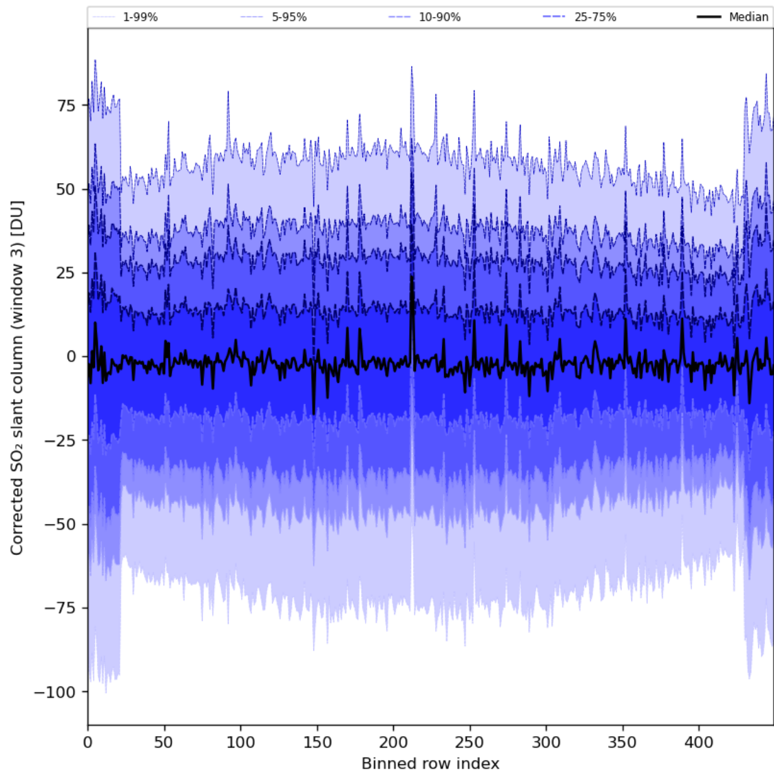
Figure 89: Along track statistics of “Corrected SO 2 slant column (window 3)” for 2024-08-24 to 2024-08-26
