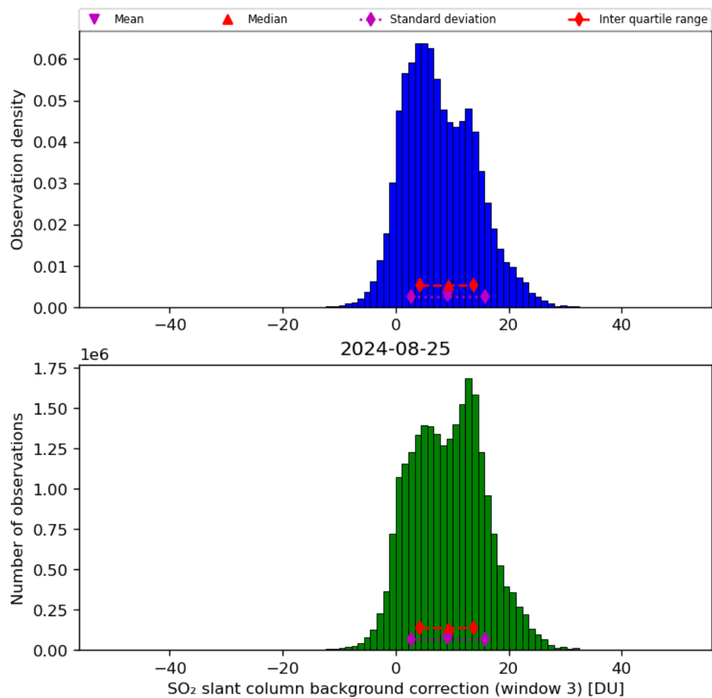
Figure 67: Histogram of “SO 2 slant column background correction (window 3)” for 2024-08-24 to 2024-08-26
