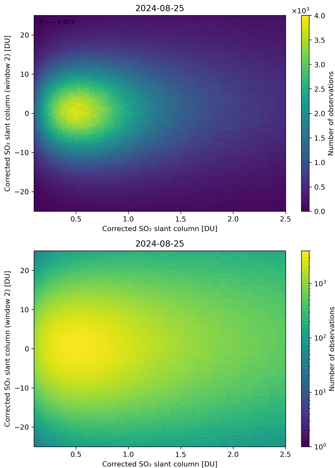
Figure 185: Scatter density plot of “Corrected SO 2 slant column” against “Corrected SO 2 slant column (window 2)” for 2024-08-24 to 2024-08-26.
