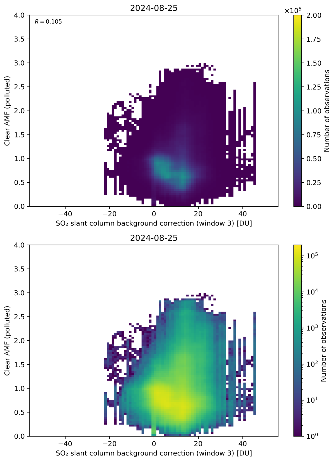
Figure 124: Scatter density plot of “SO 2 slant column background correction (window 3)” against “Clear AMF (polluted)” for 2024-08-24 to 2024-08-26.
