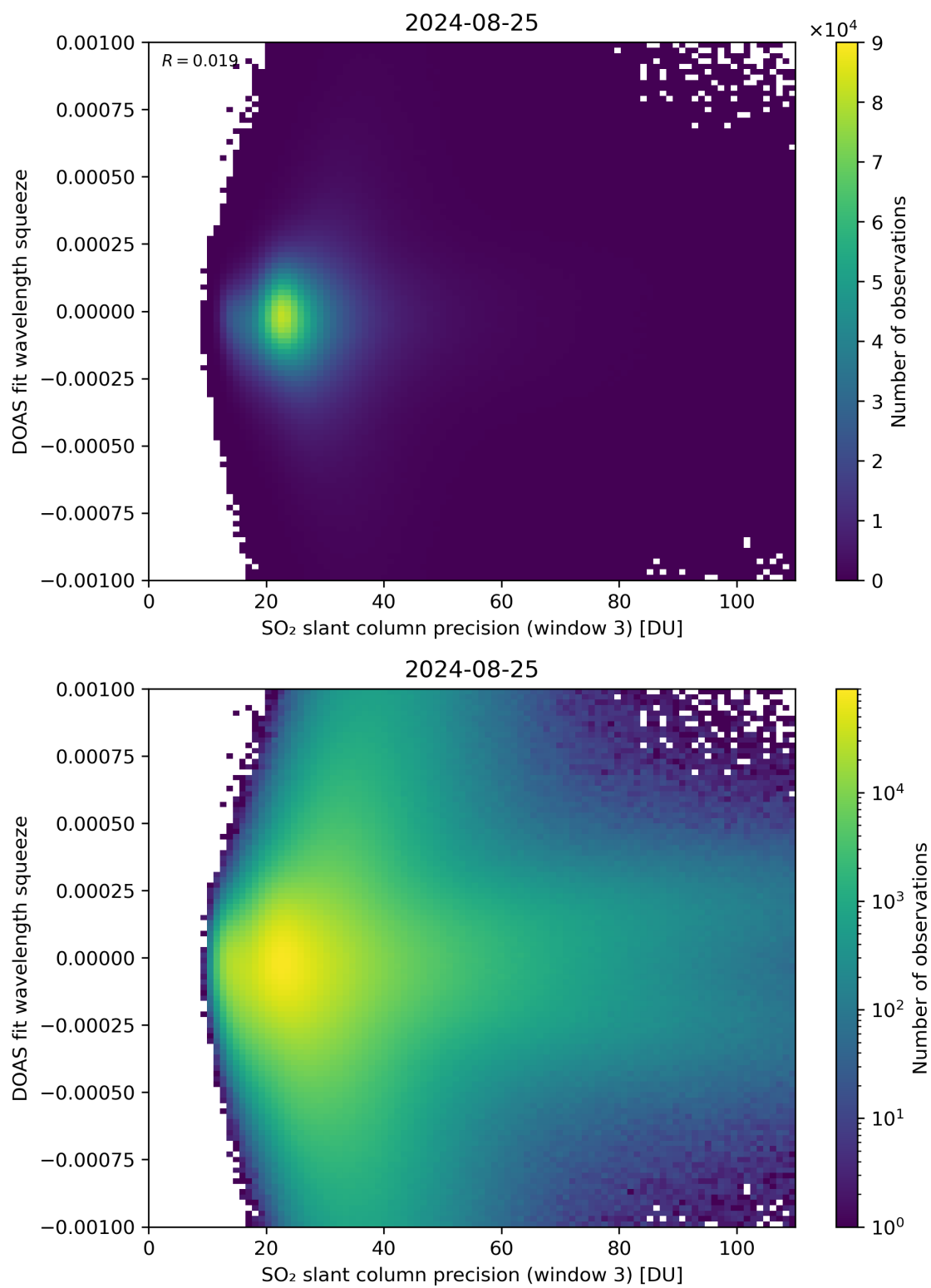
Figure 259: Scatter density plot of “SO 2 slant column precision (window 3)” against “DOAS fit wavelength squeeze” for 2024-08-24 to 2024-08-26.
