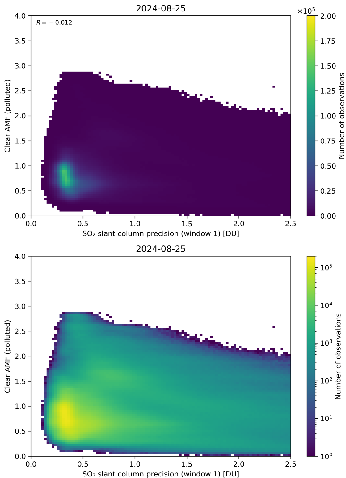
Figure 224: Scatter density plot of “SO 2 slant column precision (window 1)” against “Clear AMF (polluted)” for 2024-08-24 to 2024-08-26.
