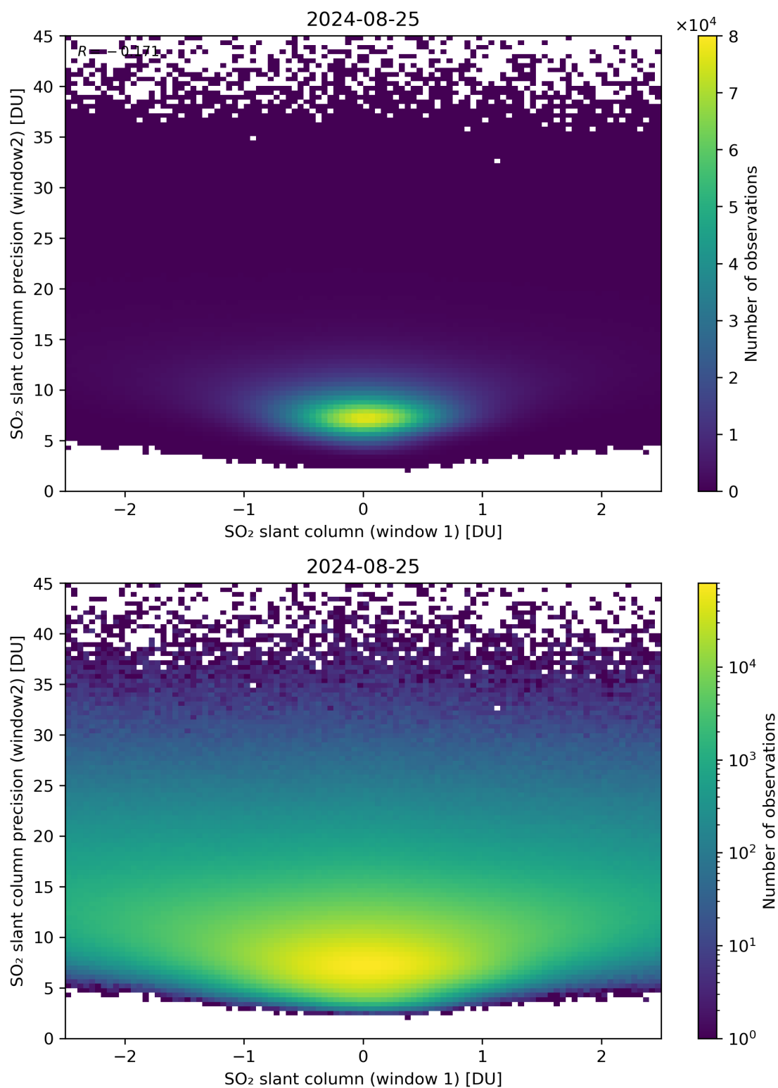
Figure 236: Scatter density plot of “SO 2 slant column (window 1)” against “SO 2 slant column precision (window2)” for 2024-08-24 to 2024-08-26.
