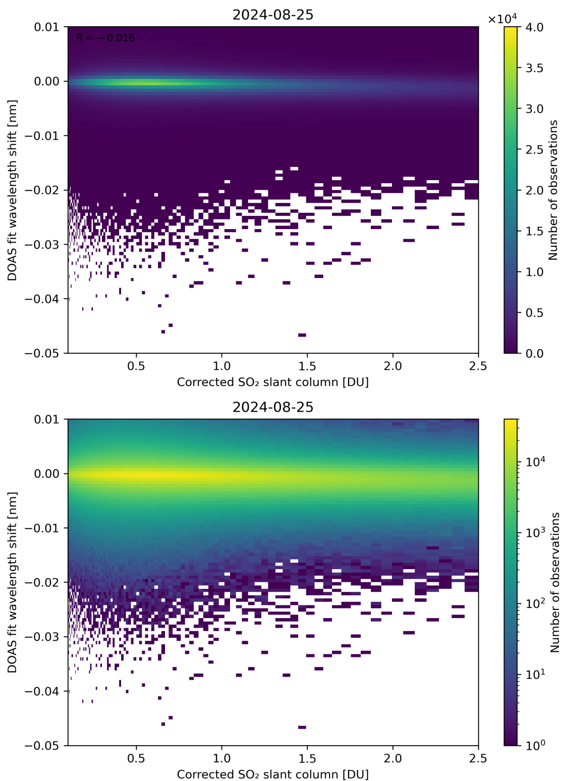
Figure 181: Scatter density plot of “Corrected SO 2 slant column” against “DOAS fit wavelength shift” for 2024-08-24 to 2024-08-26.
