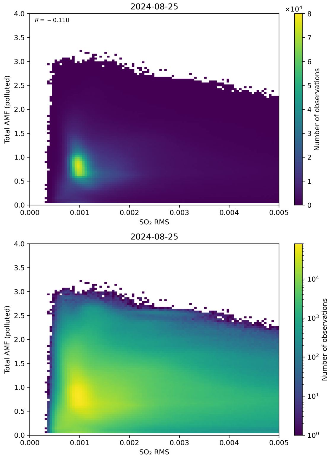
Figure 137: Scatter density plot of “SO 2 RMS” against “Total AMF (polluted)” for 2024-08-24 to 2024-08-26.
