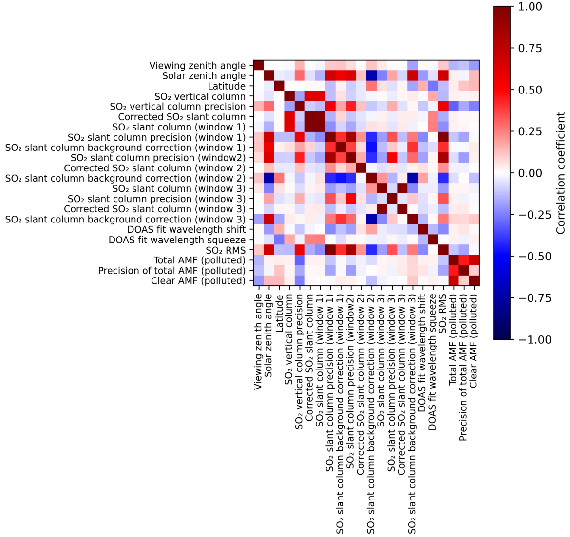
Figure 2: Map of correlation matrix for 2024-08-24 to 2024-08-26.
