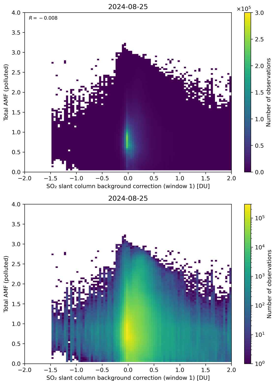
Figure 109: Scatter density plot of “SO 2 slant column background correction (window 1)” against “Total AMF (polluted)” for 2024-08-24 to 2024-08-26.
