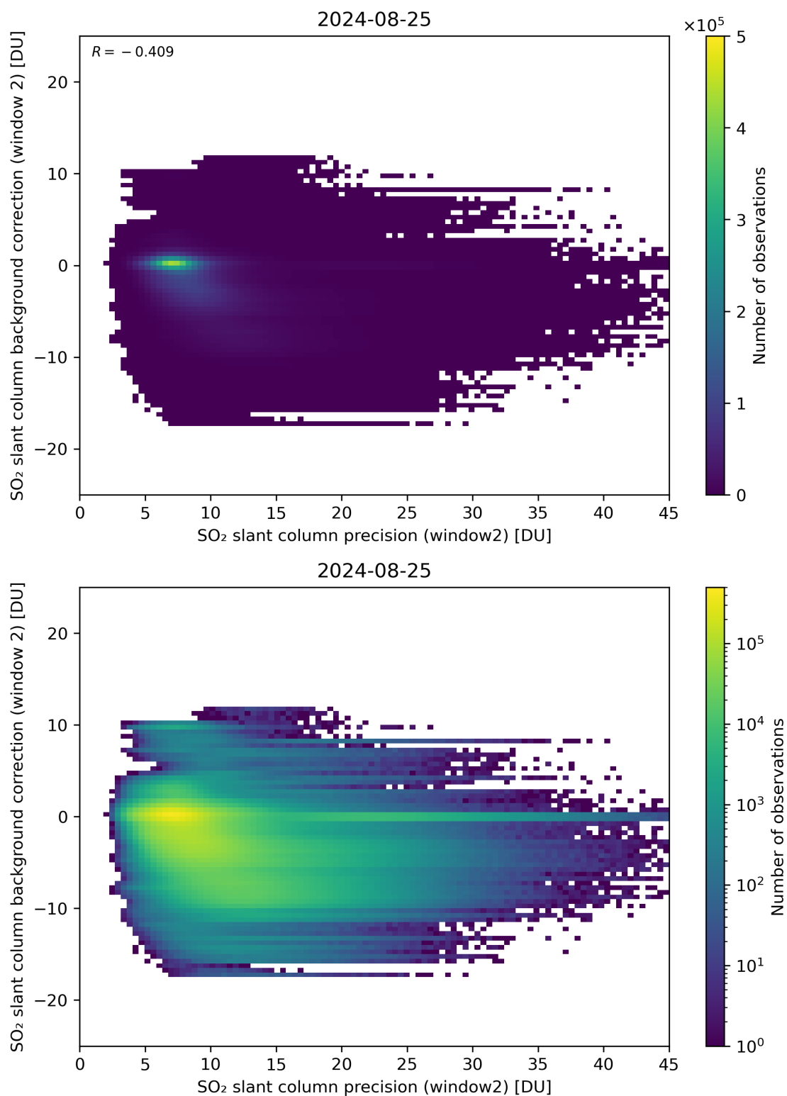
Figure 241: Scatter density plot of “SO 2 slant column precision (window2)” against “SO 2 slant column background correction (window 2)” for 2024-08-24 to 2024-08-26.
