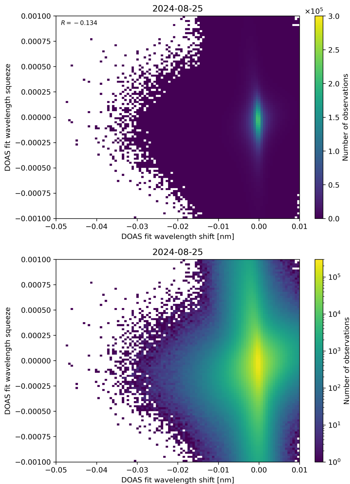
Figure 127: Scatter density plot of “DOAS fit wavelength shift” against “DOAS fit wavelength squeeze” for 2024-08-24 to 2024-08-26.
