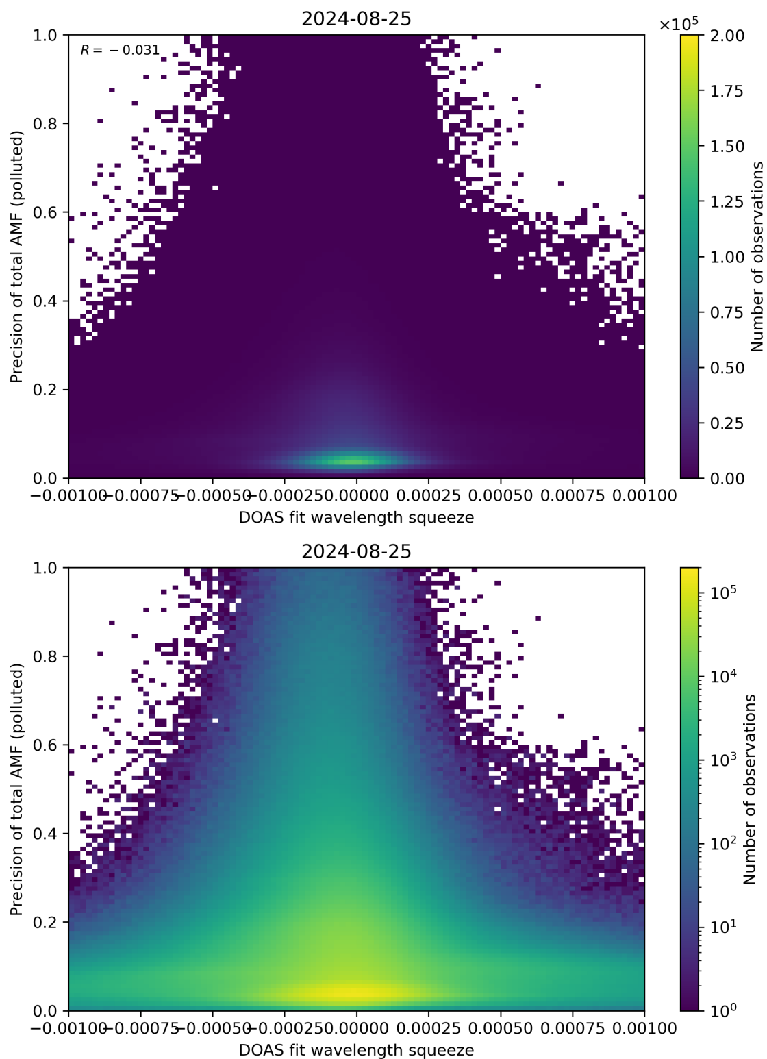
Figure 135: Scatter density plot of “DOAS fit wavelength squeeze” against “Precision of total AMF (polluted)” for 2024-08-24 to 2024-08-26.
