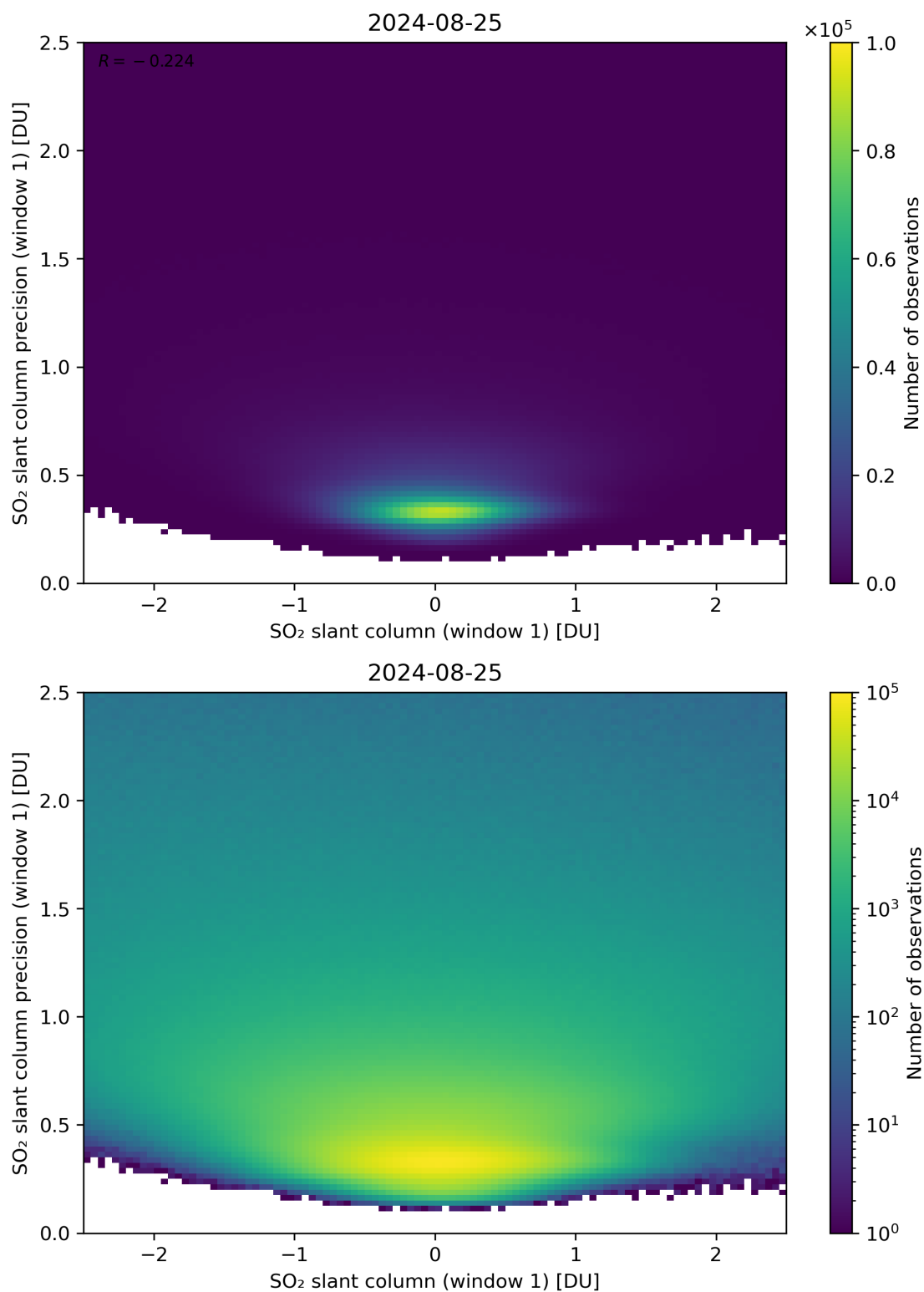
Figure 235: Scatter density plot of “SO 2 slant column (window 1)” against “SO 2 slant column precision (window 1)” for 2024-08-24 to 2024-08-26.
