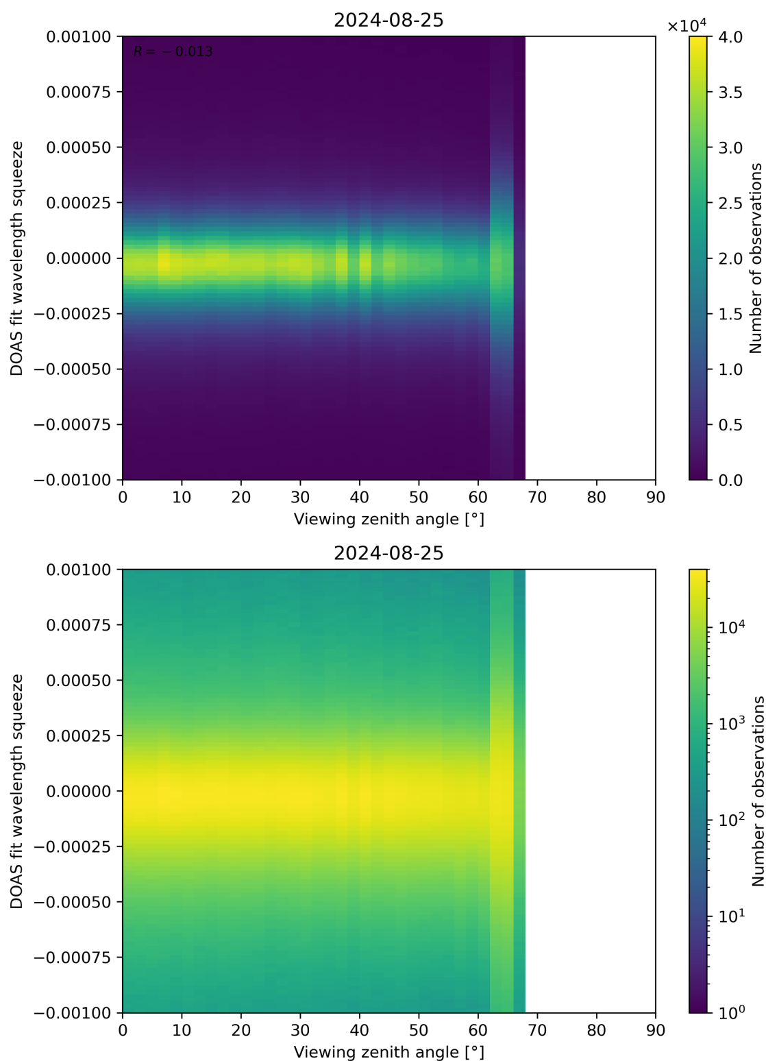
Figure 312: Scatter density plot of “Viewing zenith angle” against “DOAS fit wavelength squeeze” for 2024-08-24 to 2024-08-26.
