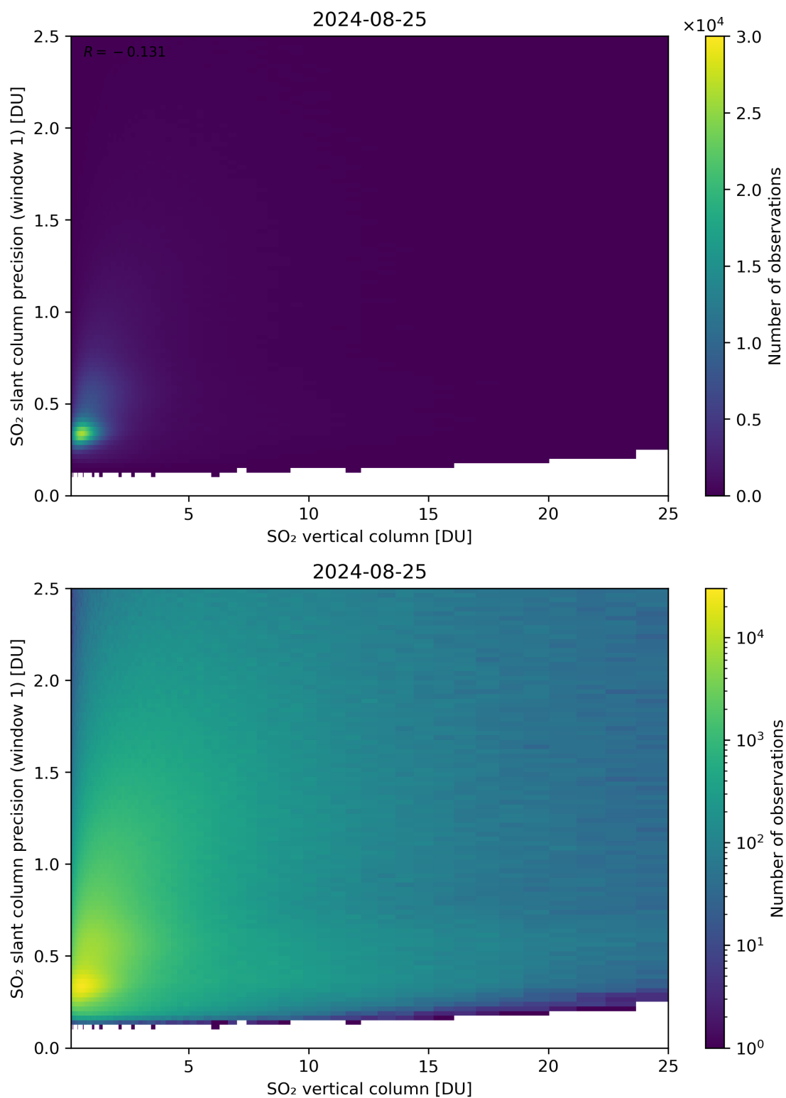
Figure 301: Scatter density plot of “SO 2 vertical column” against “SO 2 slant column precision (window 1)” for 2024-08-24 to 2024-08-26.
