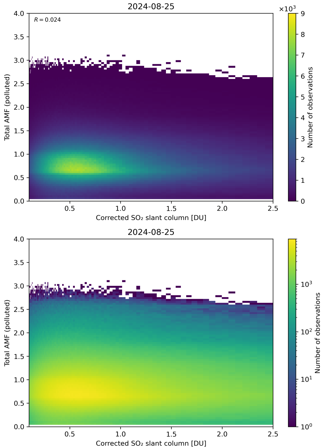
Figure 192: Scatter density plot of “Corrected SO 2 slant column” against “Total AMF (polluted)” for 2024-08-24 to 2024-08-26.
