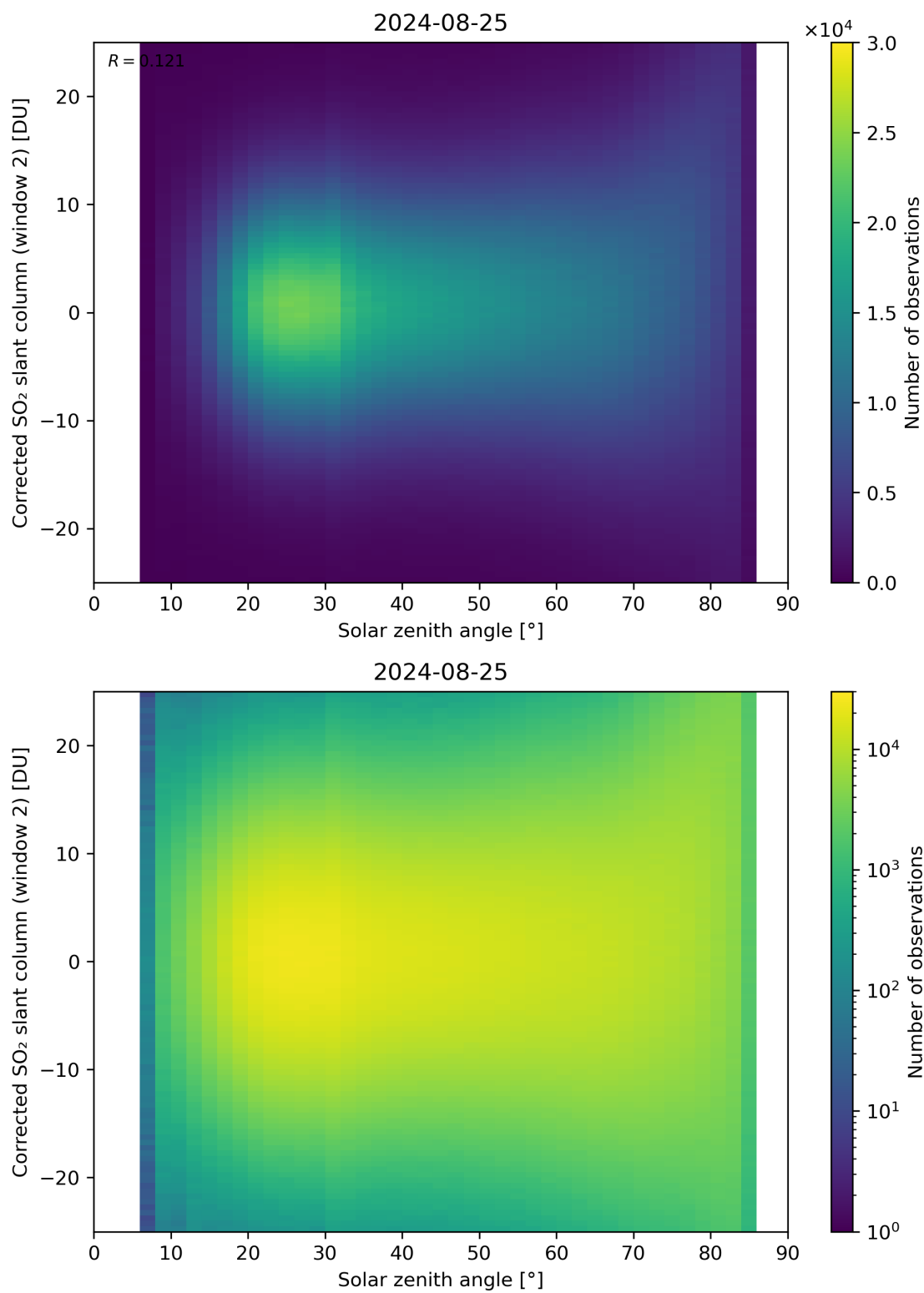
Figure 167: Scatter density plot of “Solar zenith angle” against “Corrected SO 2 slant column (window 2)” for 2024-08-24 to 2024-08-26.
