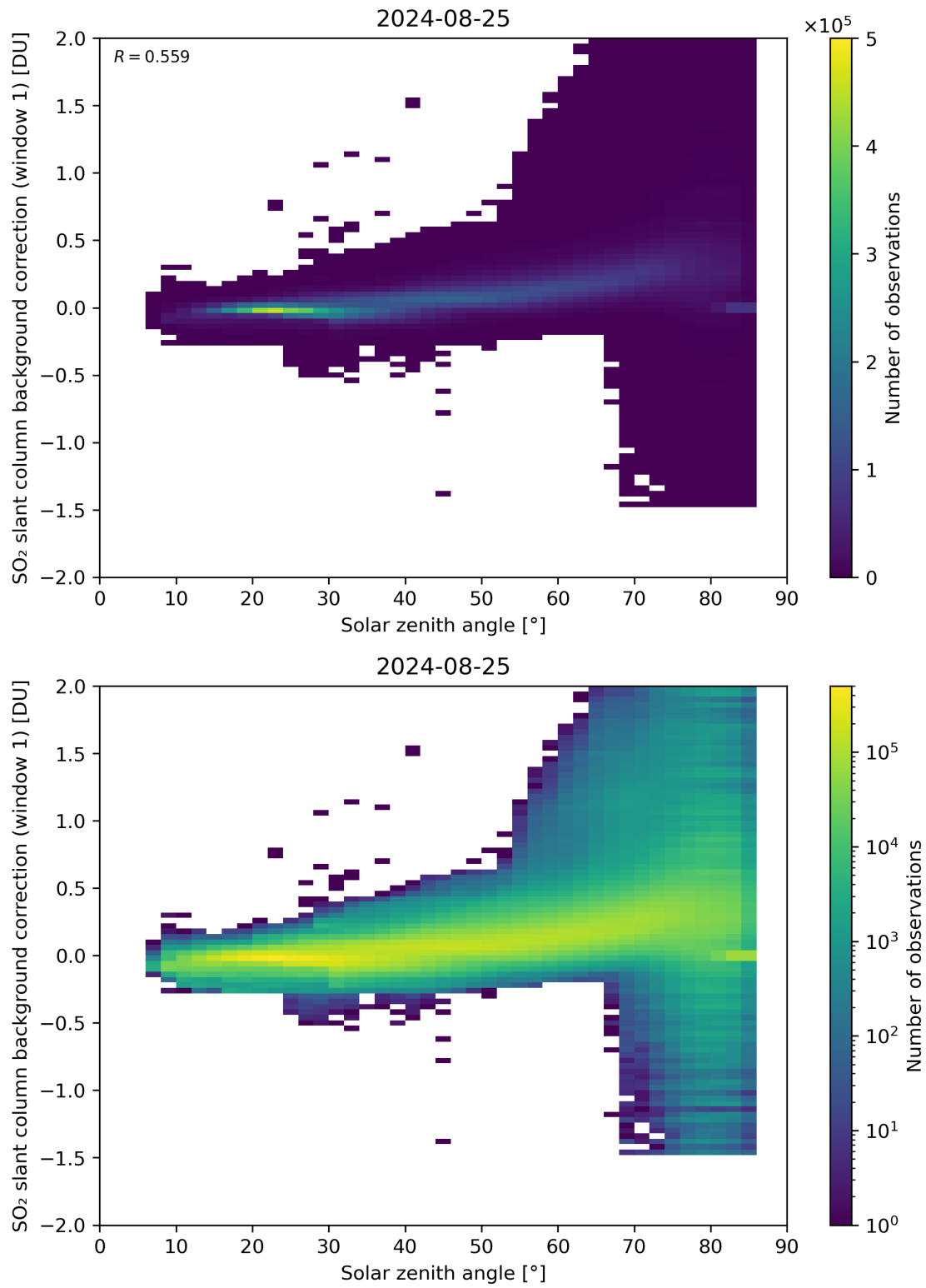
Figure 158: Scatter density plot of “Solar zenith angle” against “SO 2 slant column background correction (window 1)” for 2024-08-24 to 2024-08-26.
