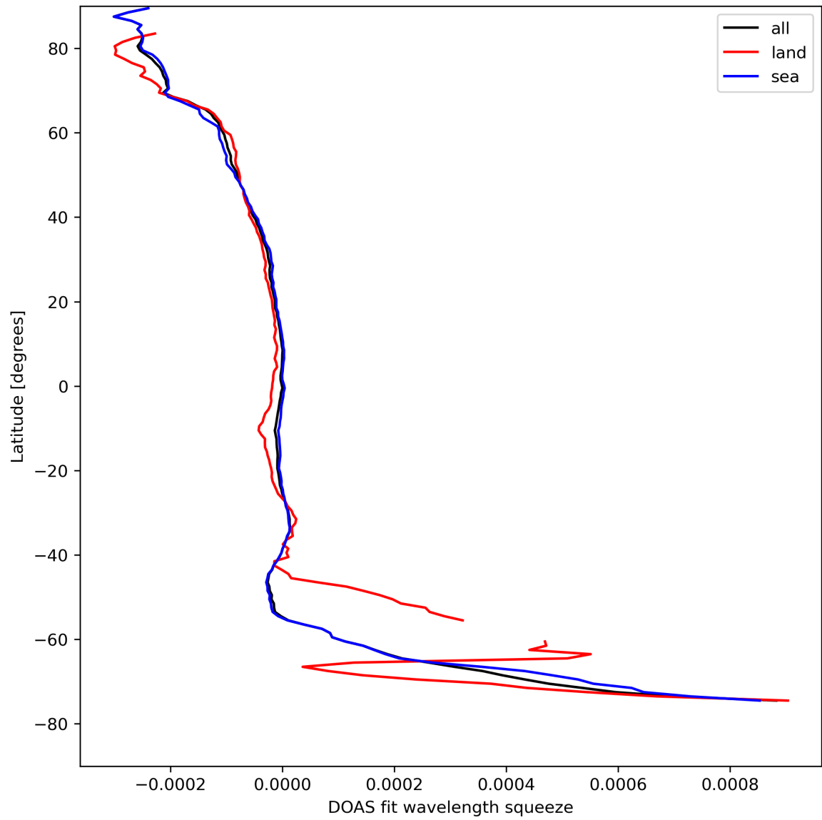
Figure 46: Zonal average of “DOAS fit wavelength squeeze” for 2024-08-24 to 2024-08-26.
