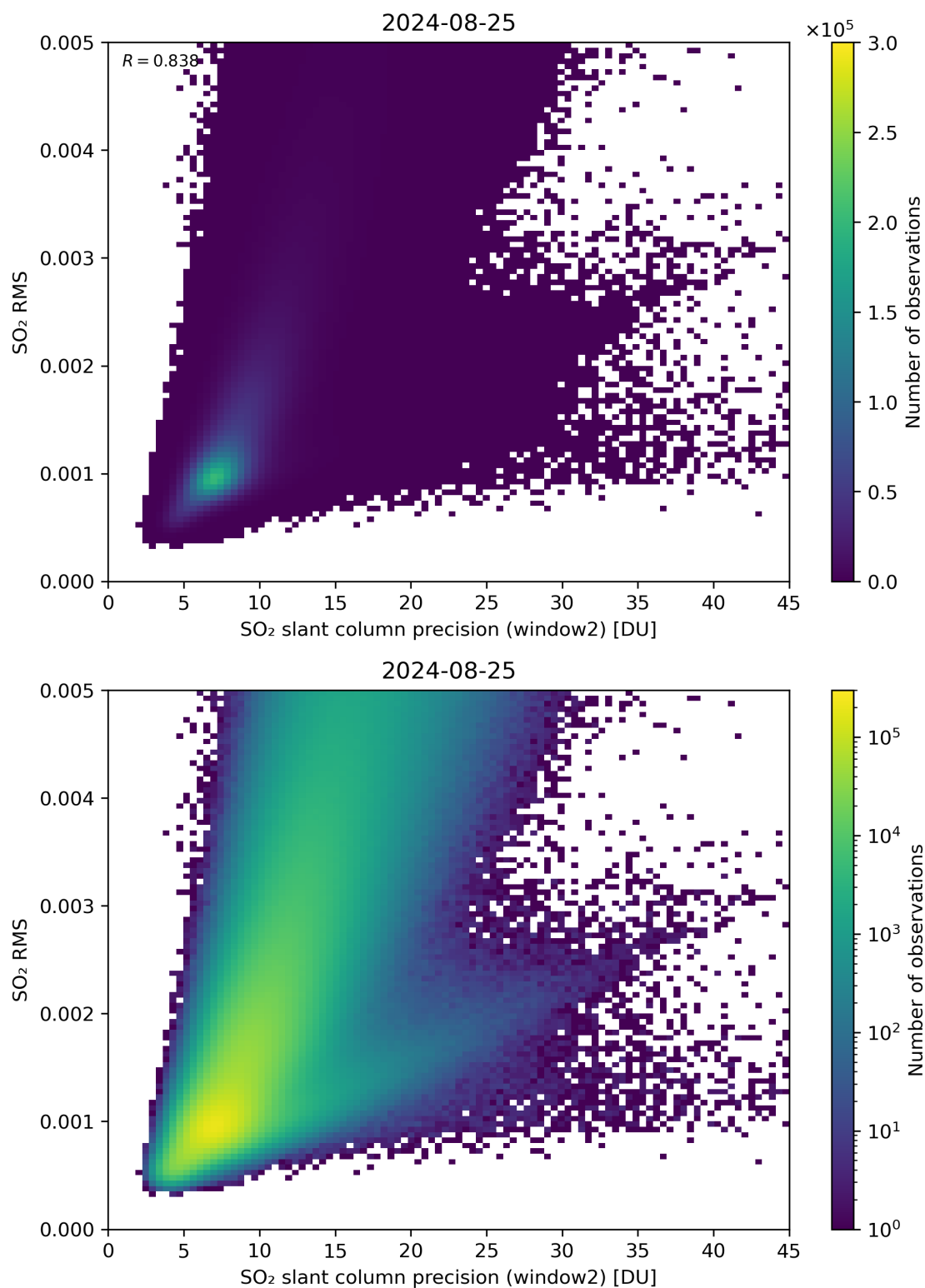
Figure 245: Scatter density plot of “SO 2 slant column precision (window2)” against “SO 2 RMS” for 2024-08-24 to 2024-08-26.
