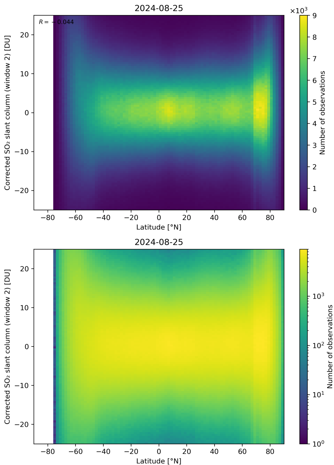
Figure 147: Scatter density plot of “Latitude” against “Corrected SO 2 slant column (window 2)” for 2024-08-24 to 2024-08-26.
