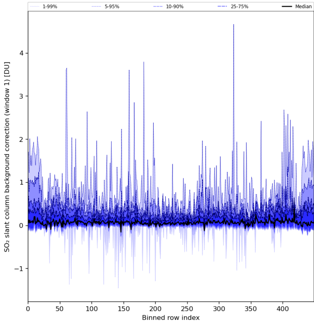
Figure 82: Along track statistics of “SO 2 slant column background correction (window 1)” for 2024-08-24 to 2024-08-26
