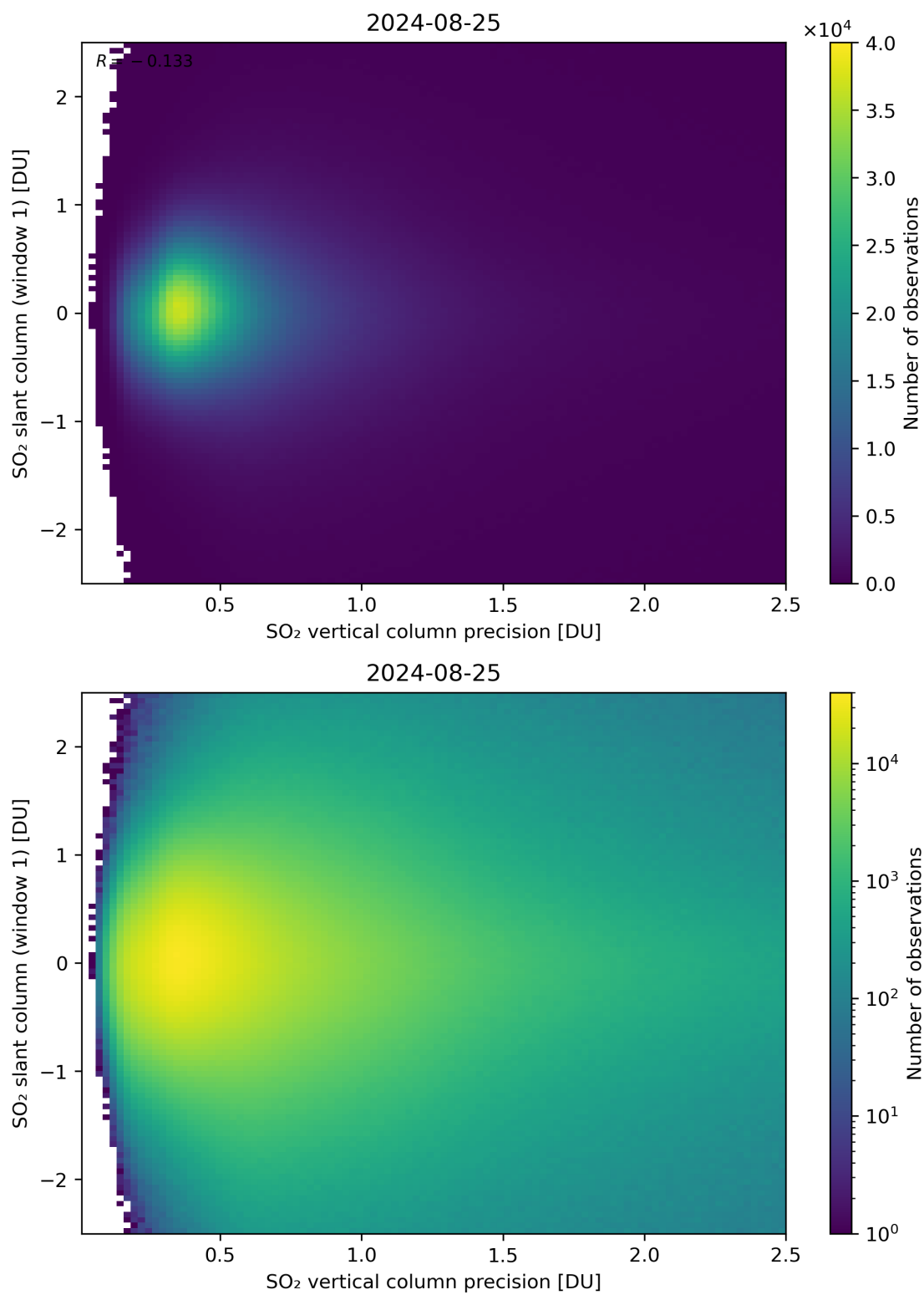
Figure 289: Scatter density plot of “SO 2 vertical column precision” against “SO 2 slant column (window 1)” for 2024-08-24 to 2024-08-26.
