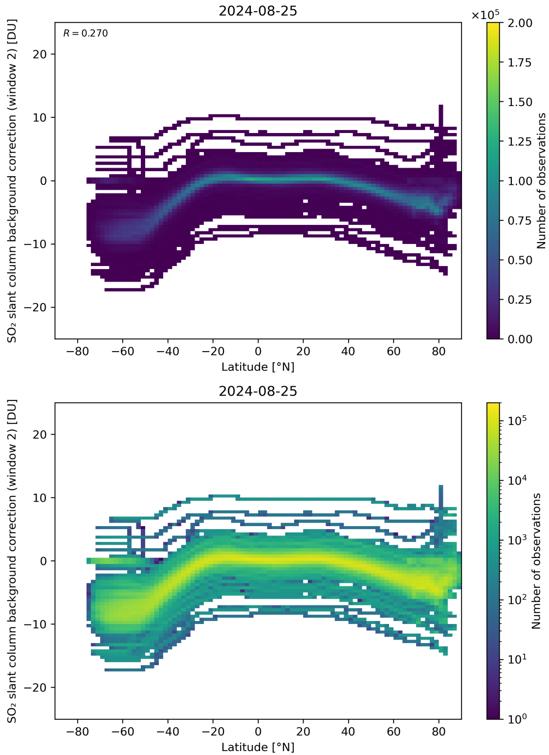
Figure 140: Scatter density plot of “Latitude” against “SO 2 slant column background correction (window 2)” for 2024-08-24 to 2024-08-26.
