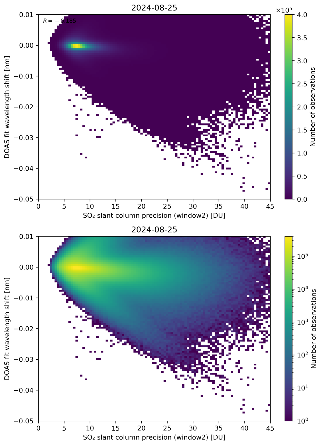
Figure 243: Scatter density plot of “SO 2 slant column precision (window2)” against “DOAS fit wavelength shift” for 2024-08-24 to 2024-08-26.
