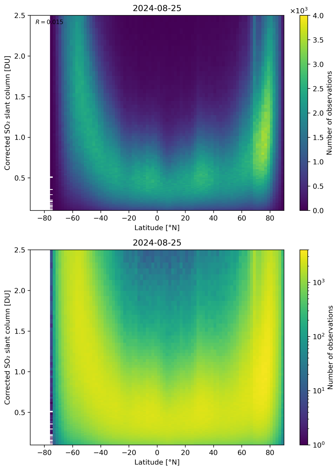
Figure 146: Scatter density plot of “Latitude” against “Corrected SO 2 slant column” for 2024-08-24 to 2024-08-26.
