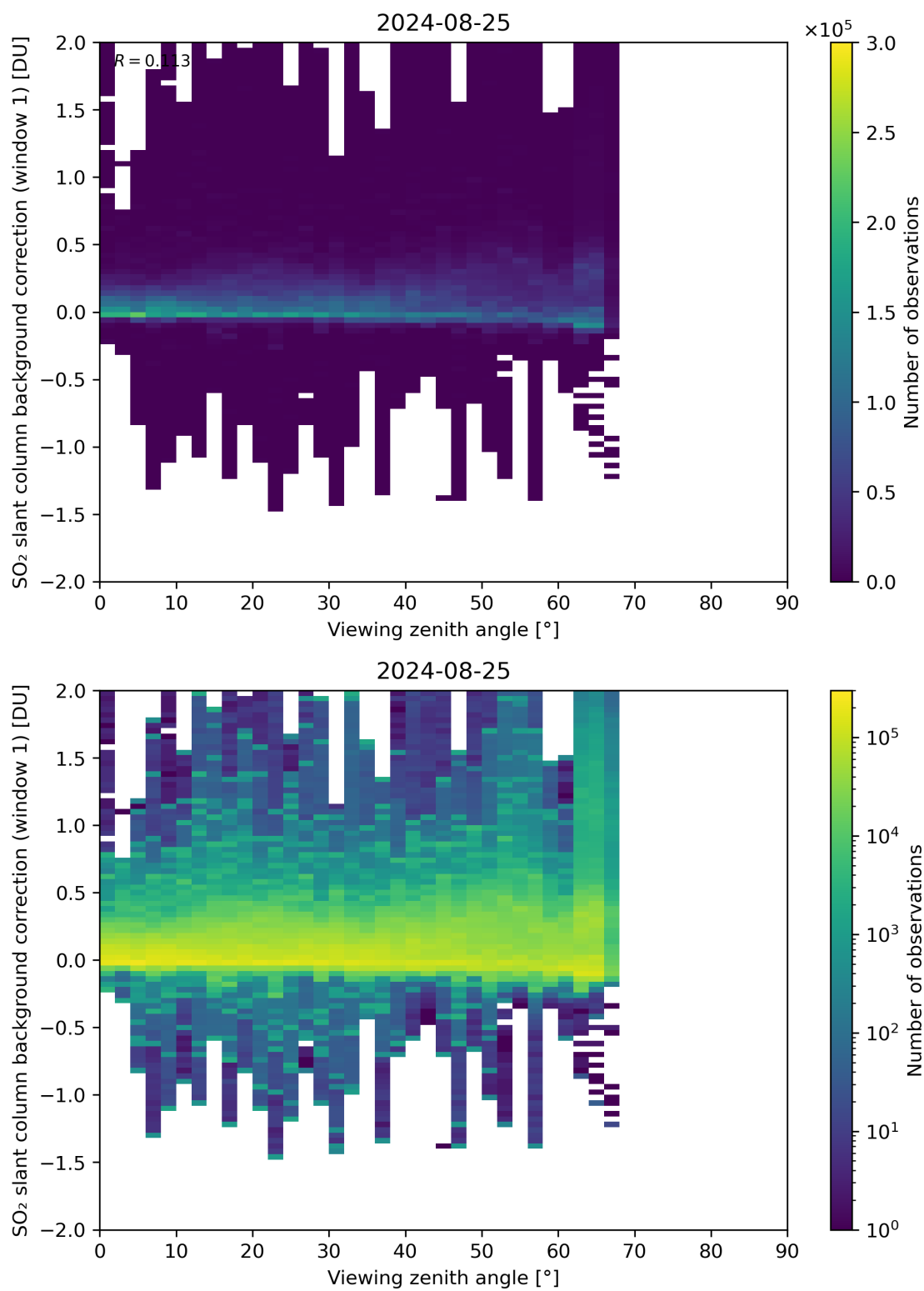
Figure 308: Scatter density plot of “Viewing zenith angle” against “SO 2 slant column background correction (window 1)” for 2024-08-24 to 2024-08-26.
