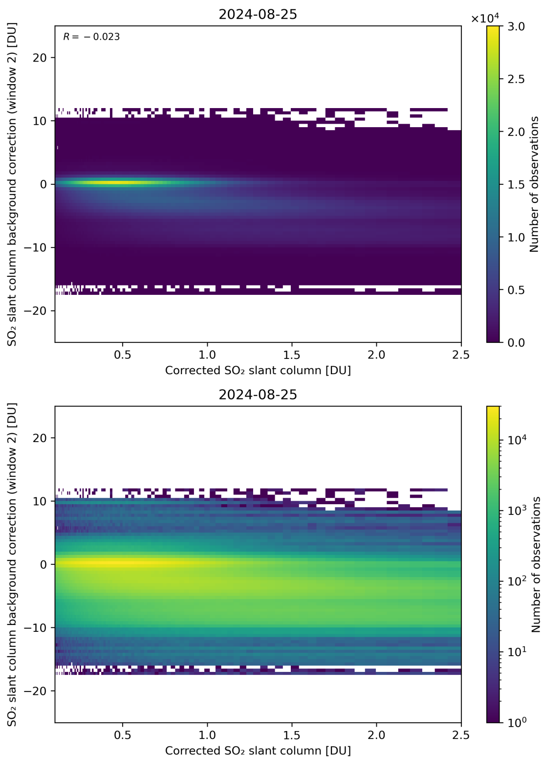
Figure 179: Scatter density plot of “Corrected SO 2 slant column” against “SO 2 slant column background correction (window 2)” for 2024-08-24 to 2024-08-26.
