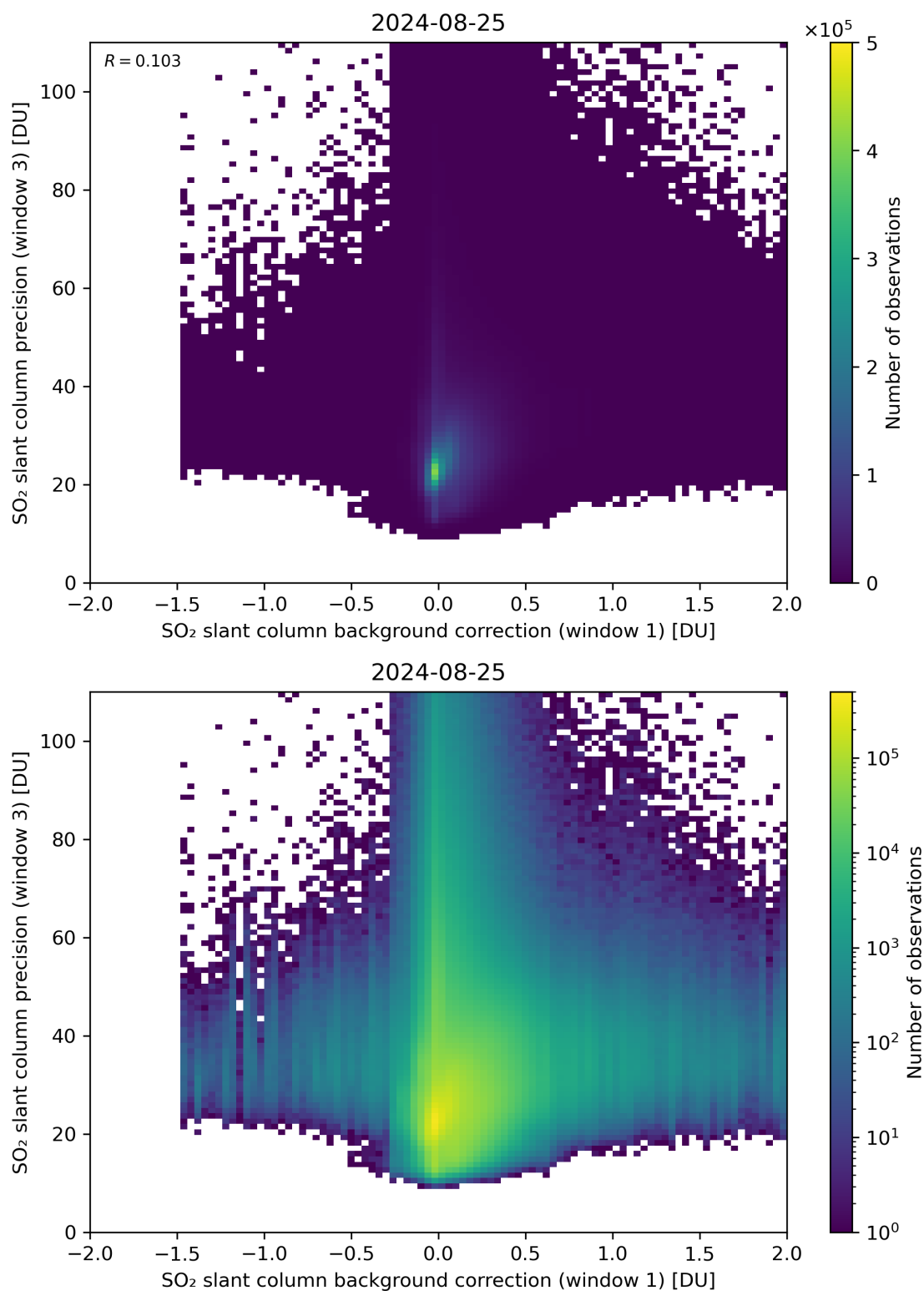
Figure 108: Scatter density plot of “SO 2 slant column background correction (window 1)” against “SO 2 slant column precision (window 3)” for 2024-08-24 to 2024-08-26.
