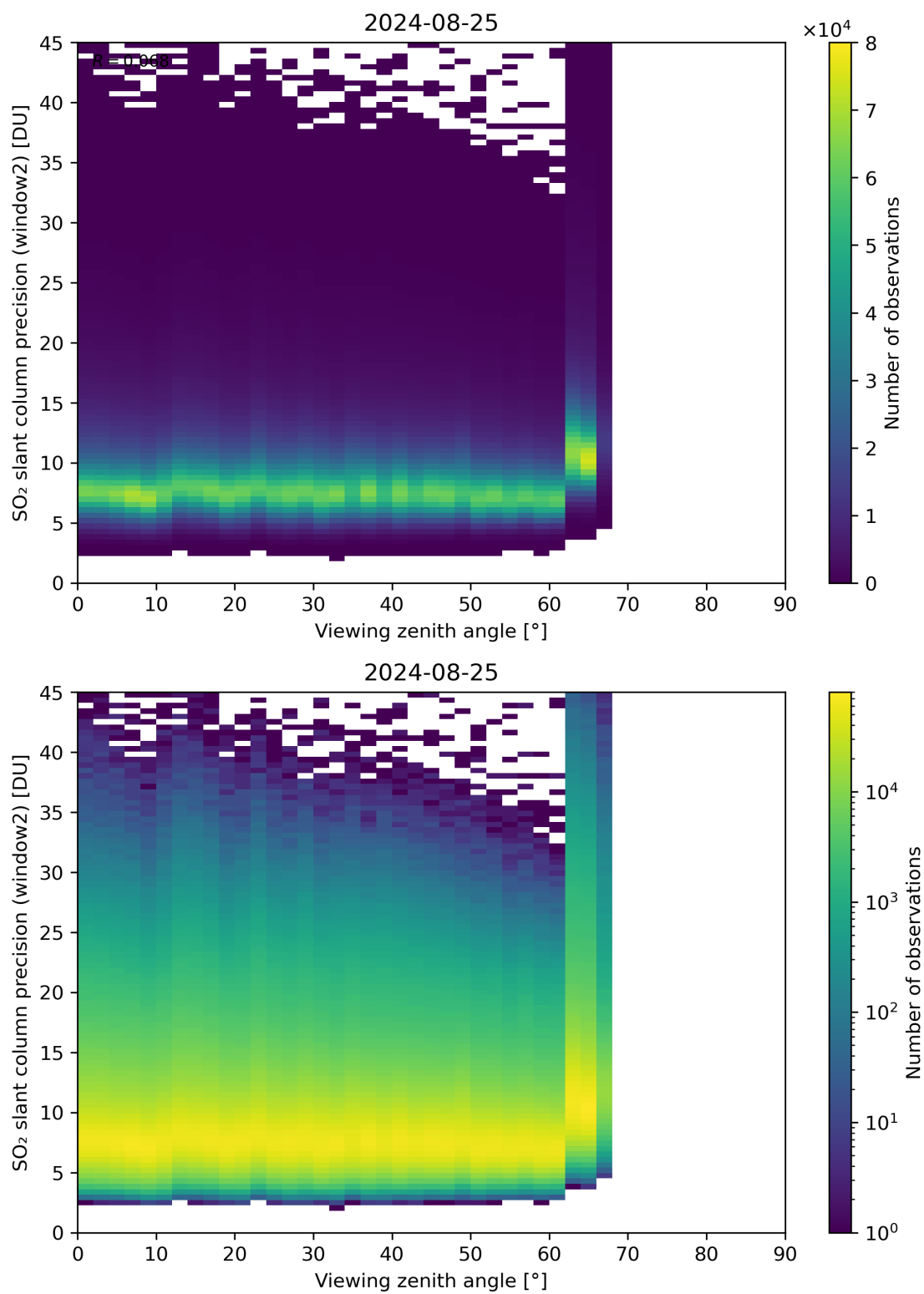
Figure 322: Scatter density plot of “Viewing zenith angle” against “SO 2 slant column precision (window2)” for 2024-08-24 to 2024-08-26.
