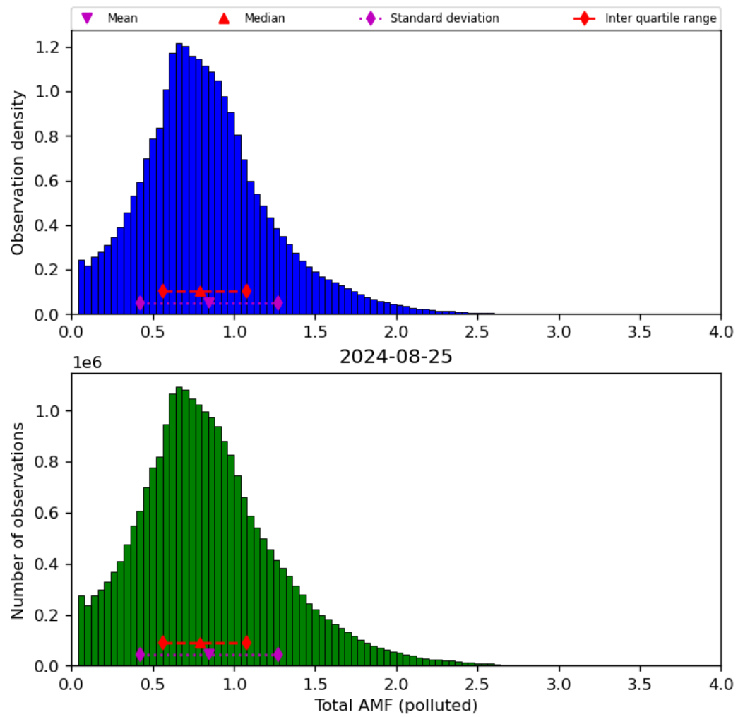
Figure 71: Histogram of “Total AMF (polluted)” for 2024-08-24 to 2024-08-26
