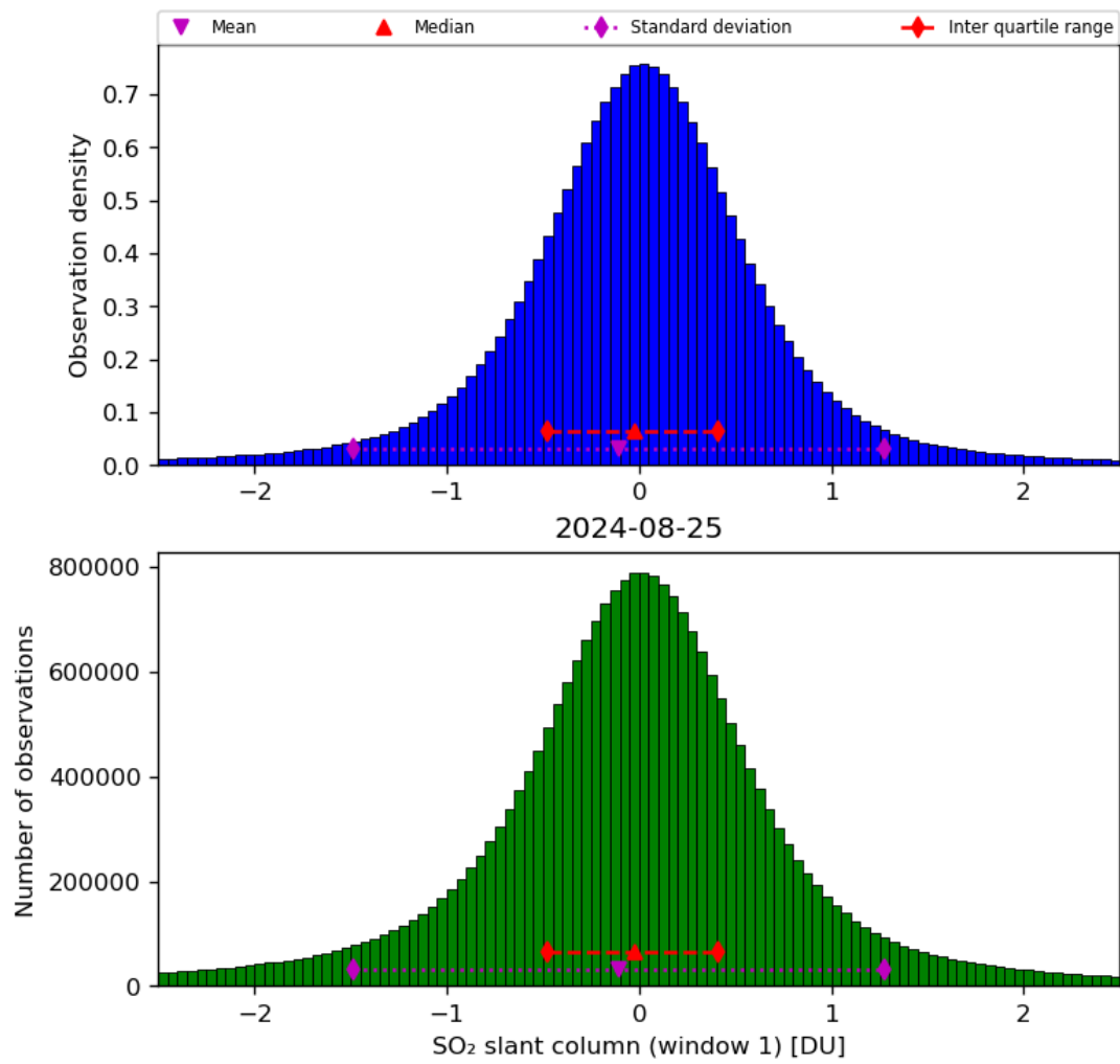
Figure 56: Histogram of “SO 2 slant column (window 1)” for 2024-08-24 to 2024-08-26
