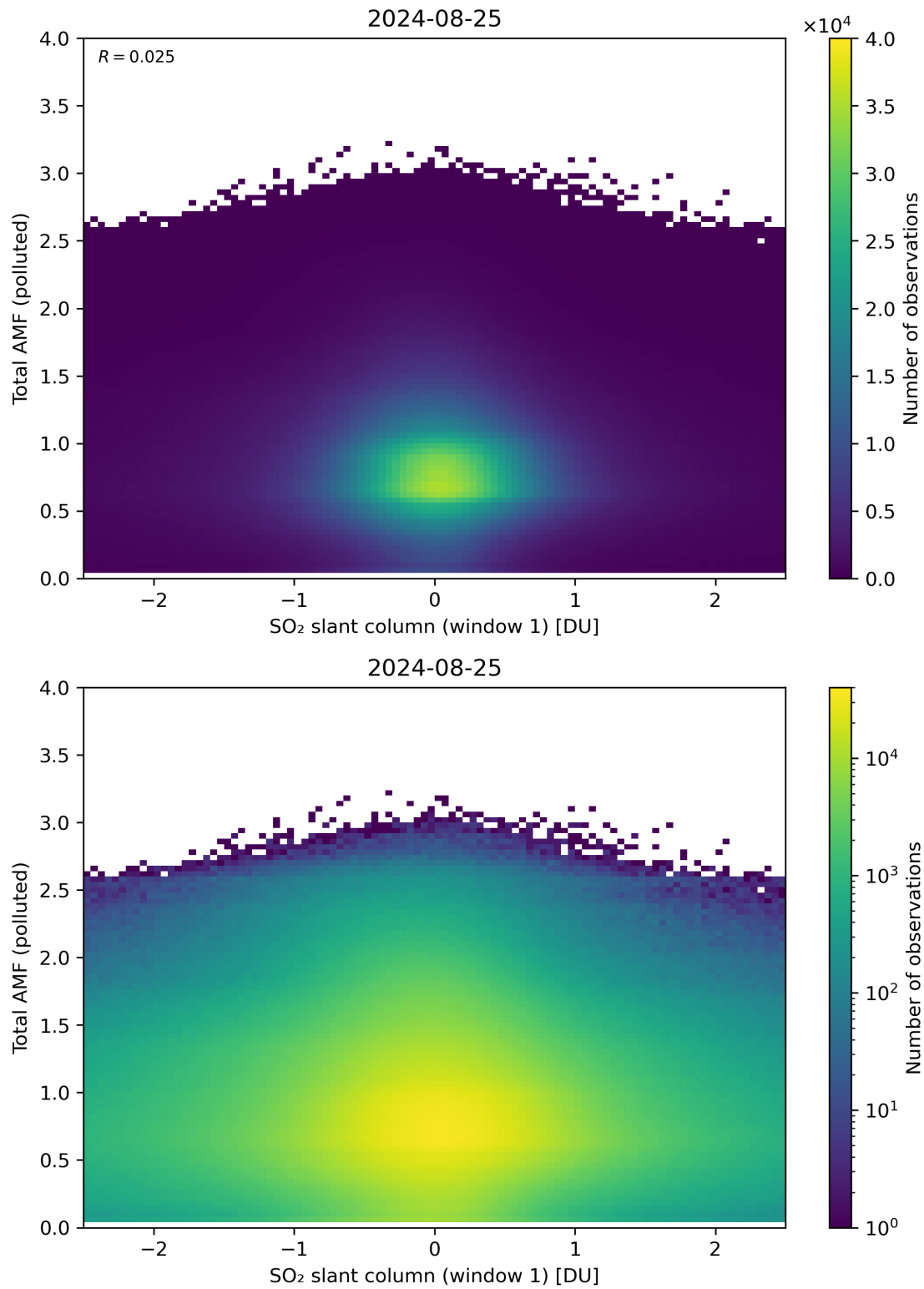
Figure 239: Scatter density plot of “SO 2 slant column (window 1)” against “Total AMF (polluted)” for 2024-08-24 to 2024-08-26.
