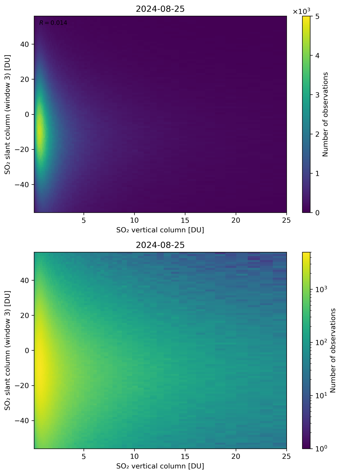
Figure 303: Scatter density plot of “SO 2 vertical column” against “SO 2 slant column (window 3)” for 2024-08-24 to 2024-08-26.
