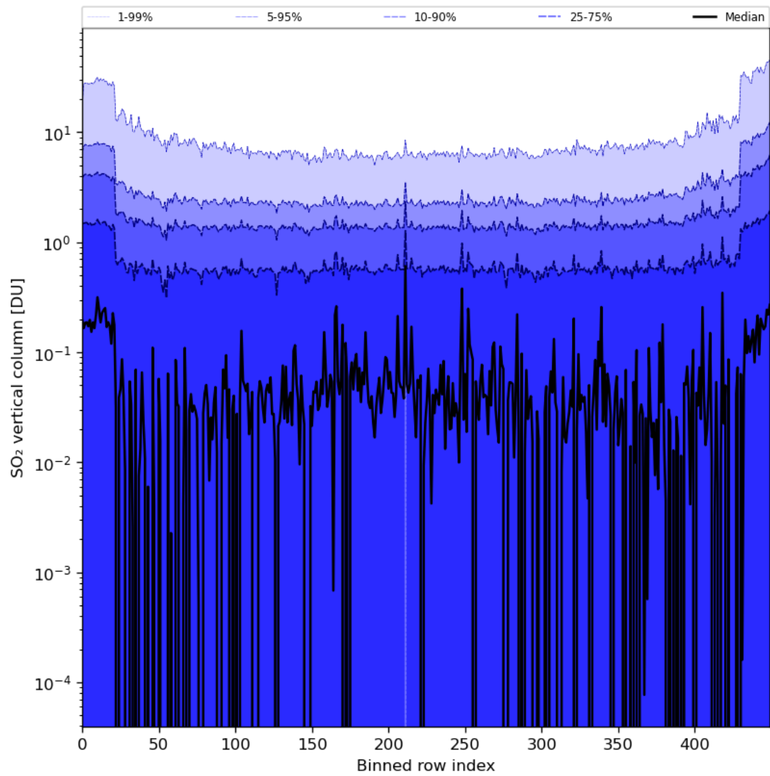
Figure 76: Along track statistics of “SO 2 vertical column” for 2024-08-24 to 2024-08-26
