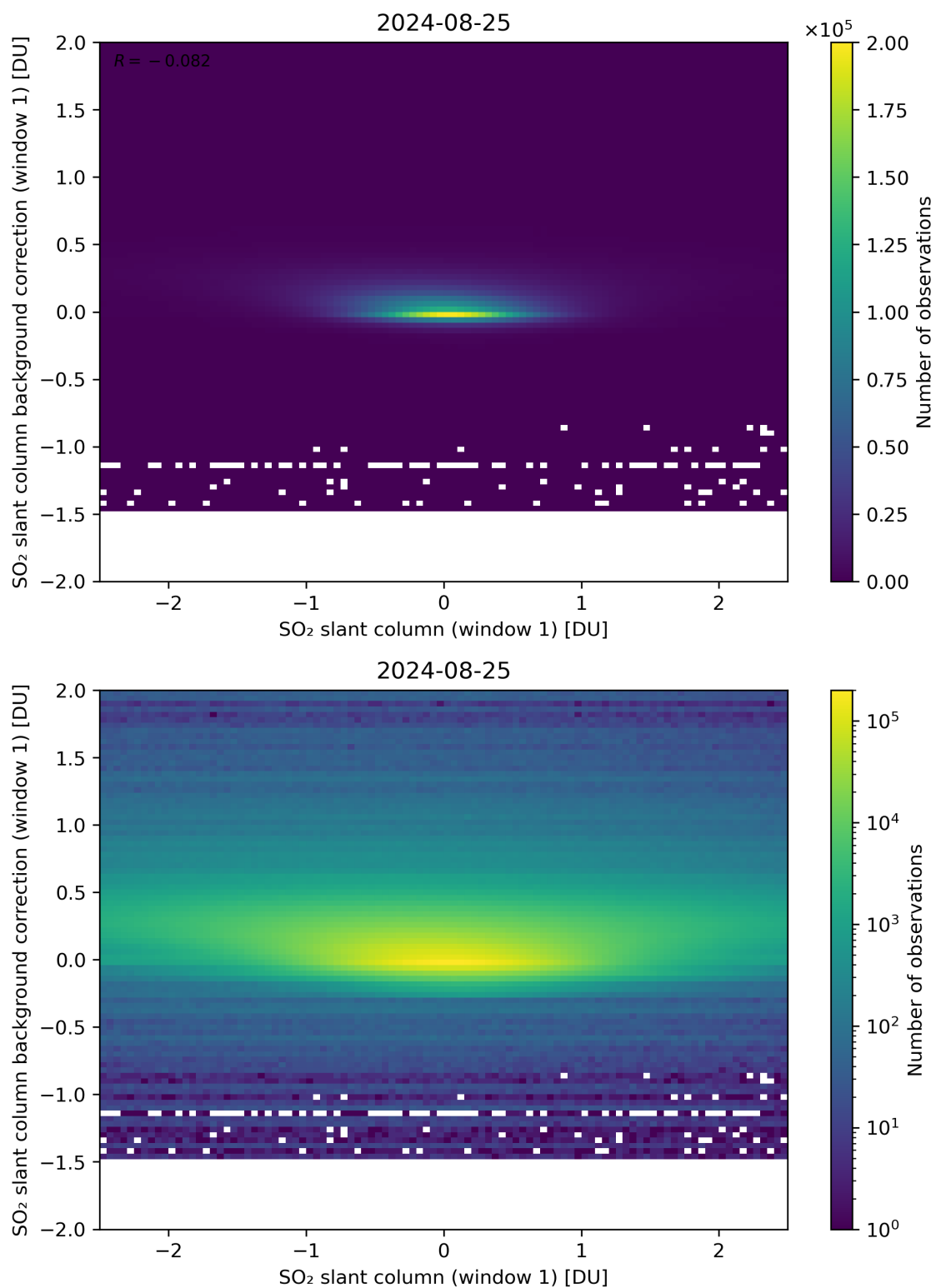
Figure 212: Scatter density plot of “SO 2 slant column (window 1)” against “SO 2 slant column background correction (window 1)” for 2024-08-24 to 2024-08-26.
