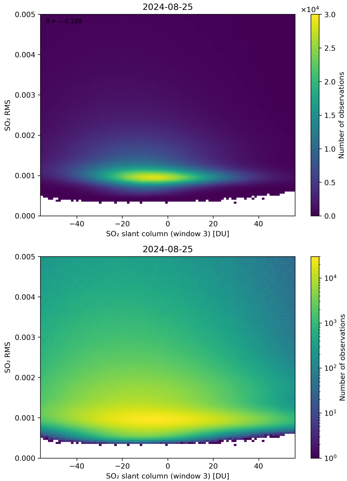
Figure 256: Scatter density plot of “SO 2 slant column (window 3)” against “SO 2 RMS” for 2024-08-24 to 2024-08-26.
