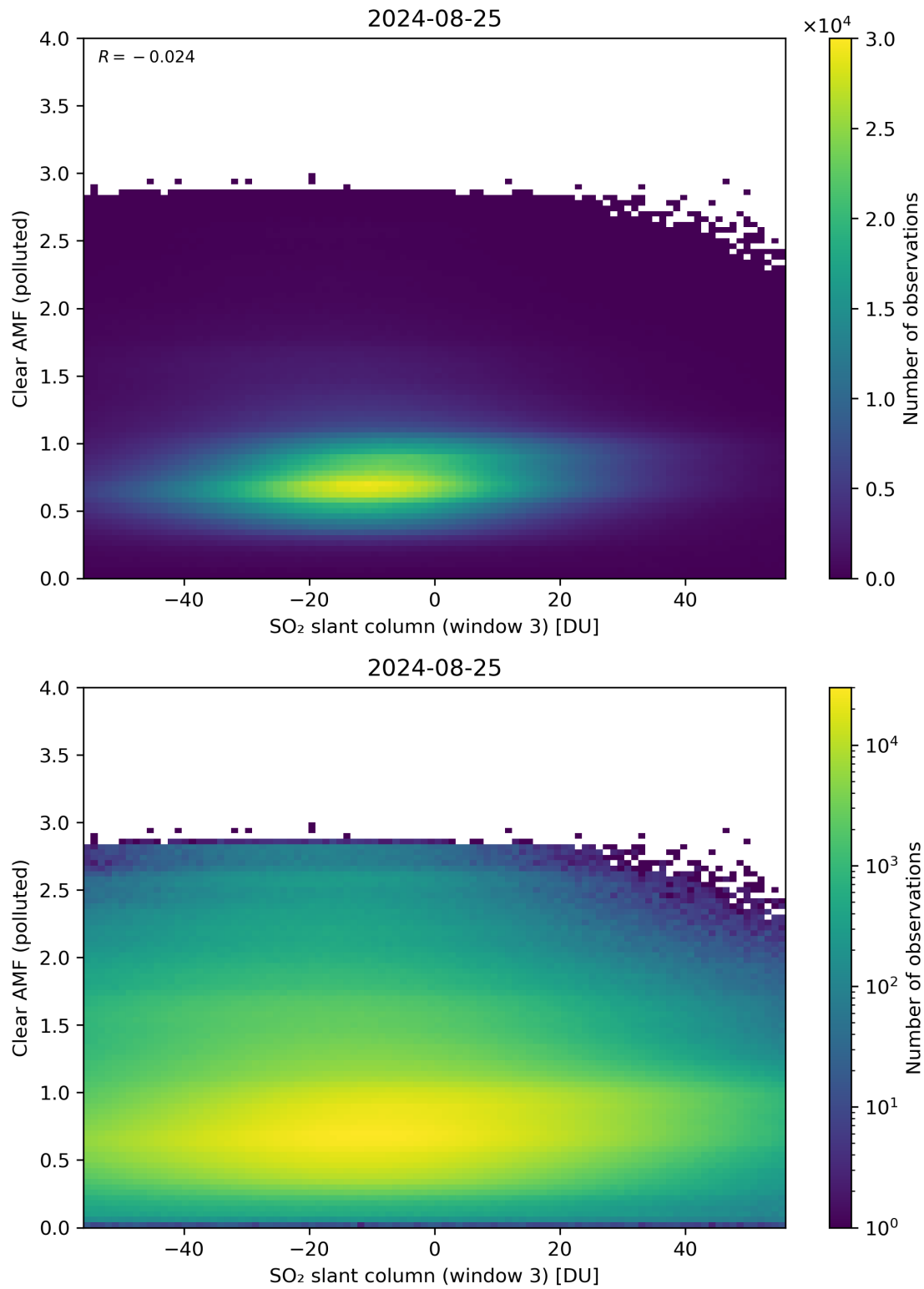
Figure 265: Scatter density plot of “SO 2 slant column (window 3)” against “Clear AMF (polluted)” for 2024-08-24 to 2024-08-26.
