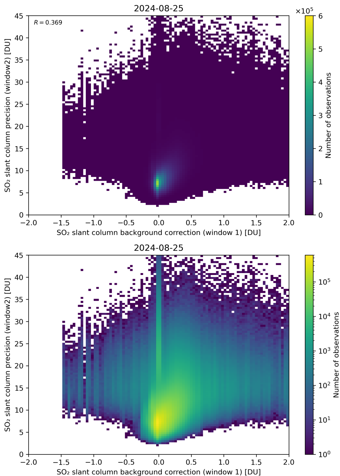
Figure 106: Scatter density plot of “SO 2 slant column background correction (window 1)” against “SO 2 slant column precision (window2)” for 2024-08-24 to 2024-08-26.
