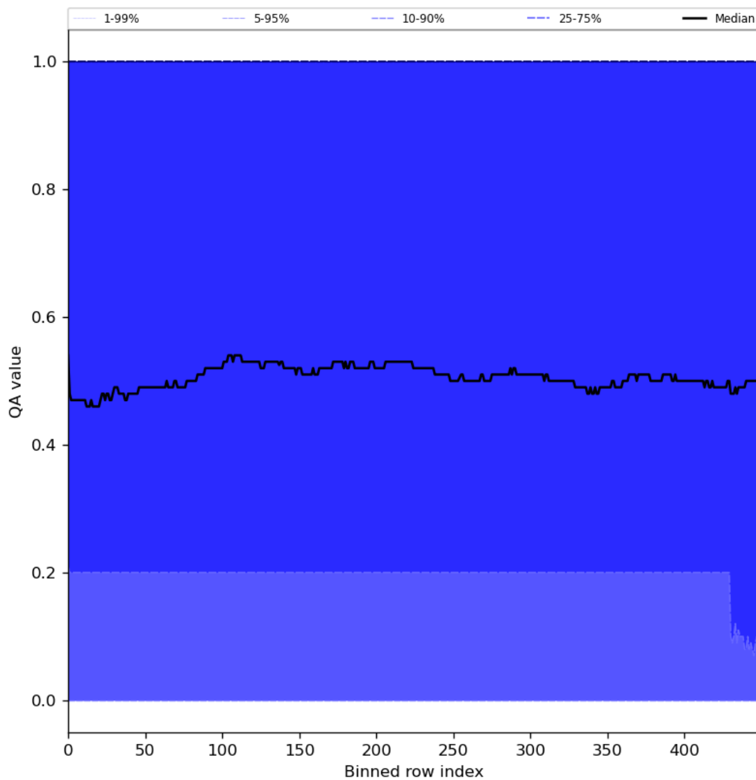
Figure 75: Along track statistics of “QA value” for 2024-08-24 to 2024-08-26
