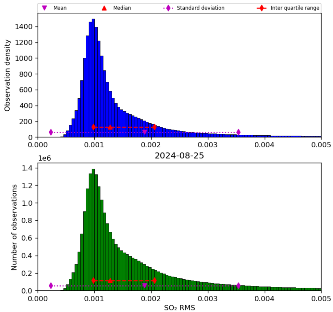
Figure 70: Histogram of “SO 2 RMS” for 2024-08-24 to 2024-08-26
