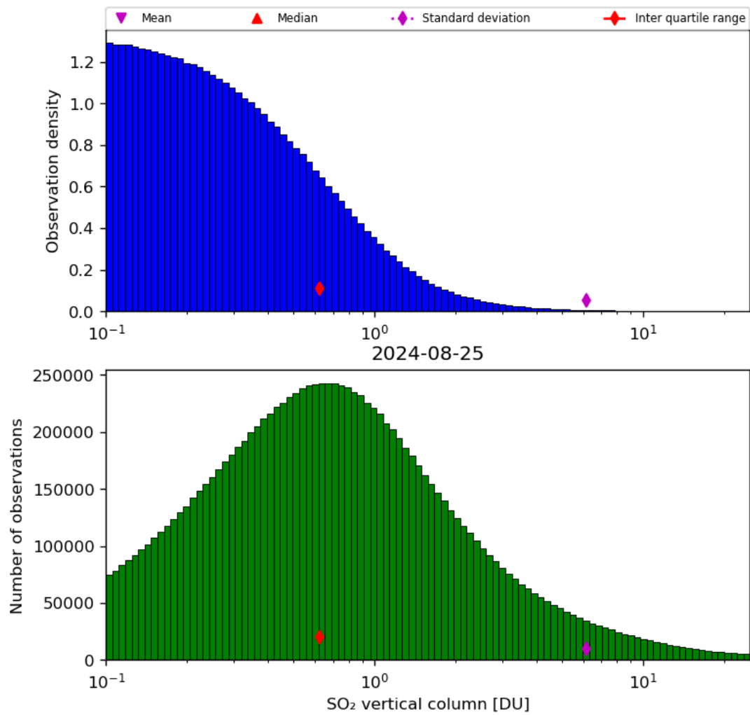
Figure 53: Histogram of “SO 2 vertical column” for 2024-08-24 to 2024-08-26
