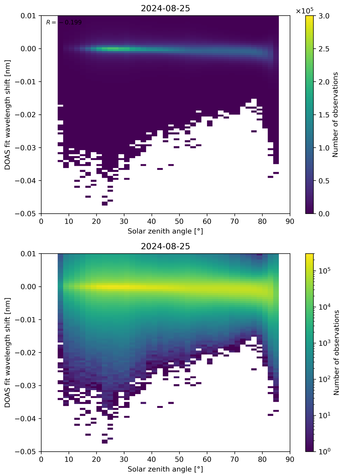
Figure 161: Scatter density plot of “Solar zenith angle” against “DOAS fit wavelength shift” for 2024-08-24 to 2024-08-26.
