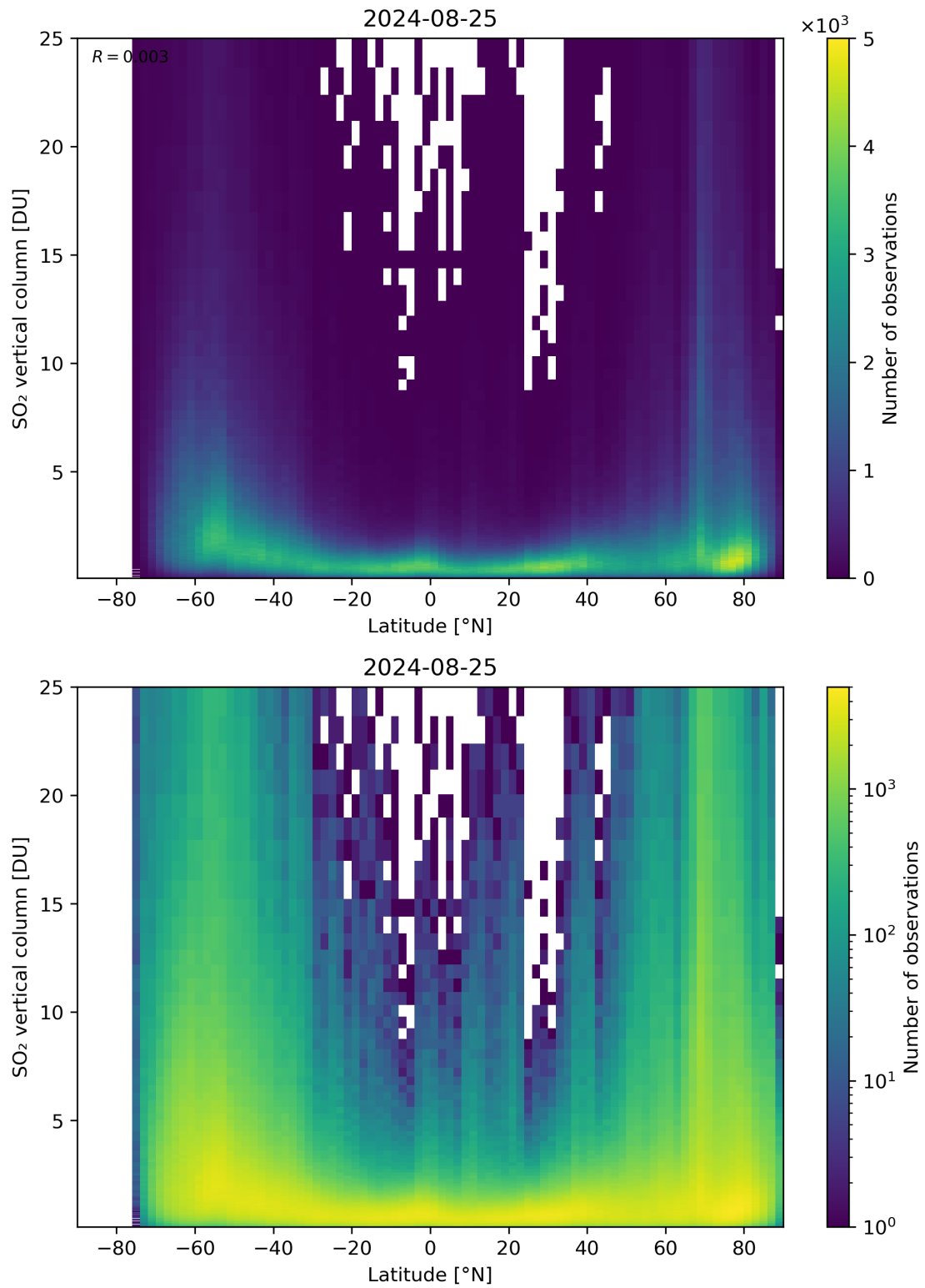
Figure 156: Scatter density plot of “Latitude” against “SO 2 vertical column” for 2024-08-24 to 2024-08-26.
