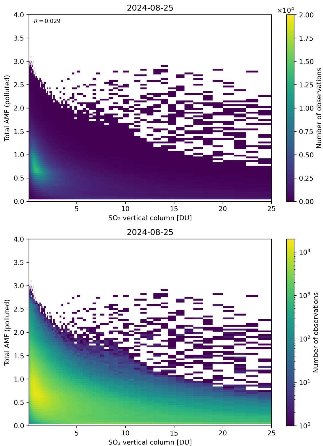
Figure 305: Scatter density plot of “SO 2 vertical column” against “Total AMF (polluted)” for 2024-08-24 to 2024-08-26.
