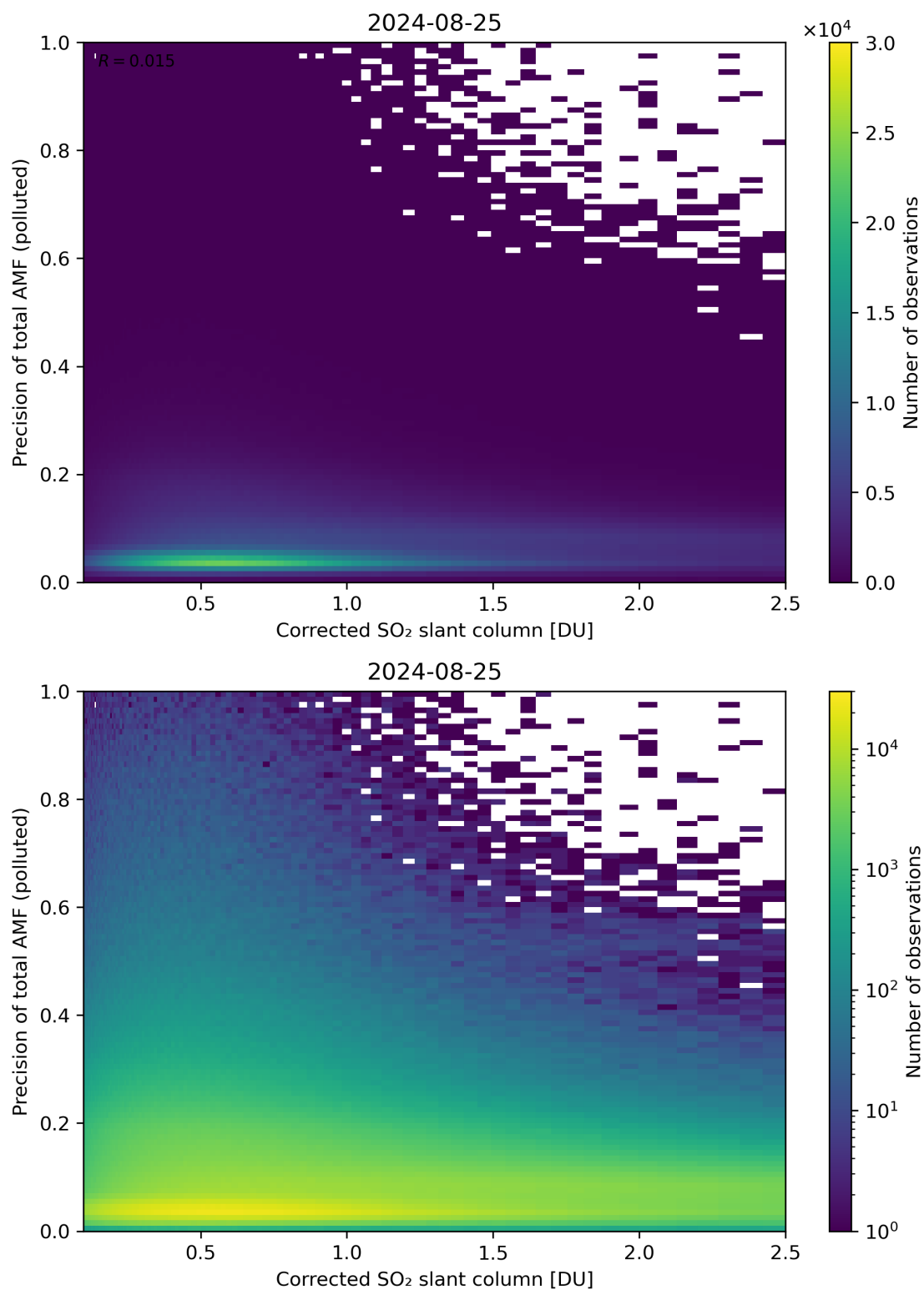
Figure 193: Scatter density plot of “Corrected SO 2 slant column” against “Precision of total AMF (polluted)” for 2024-08-24 to 2024-08-26.
