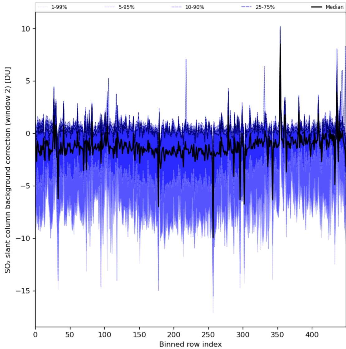
Figure 86: Along track statistics of “SO 2 slant column background correction (window 2)” for 2024-08-24 to 2024-08-26
