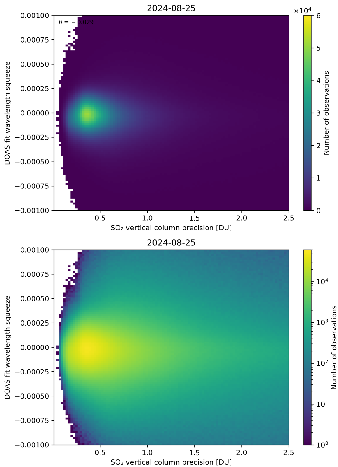
Figure 283: Scatter density plot of “SO 2 vertical column precision” against “DOAS fit wavelength squeeze” for 2024-08-24 to 2024-08-26.
