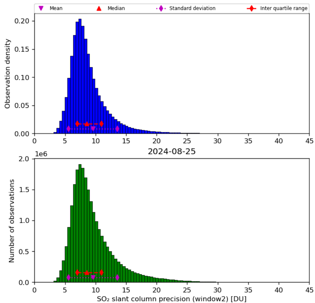
Figure 61: Histogram of “SO 2 slant column precision (window2)” for 2024-08-24 to 2024-08-26
