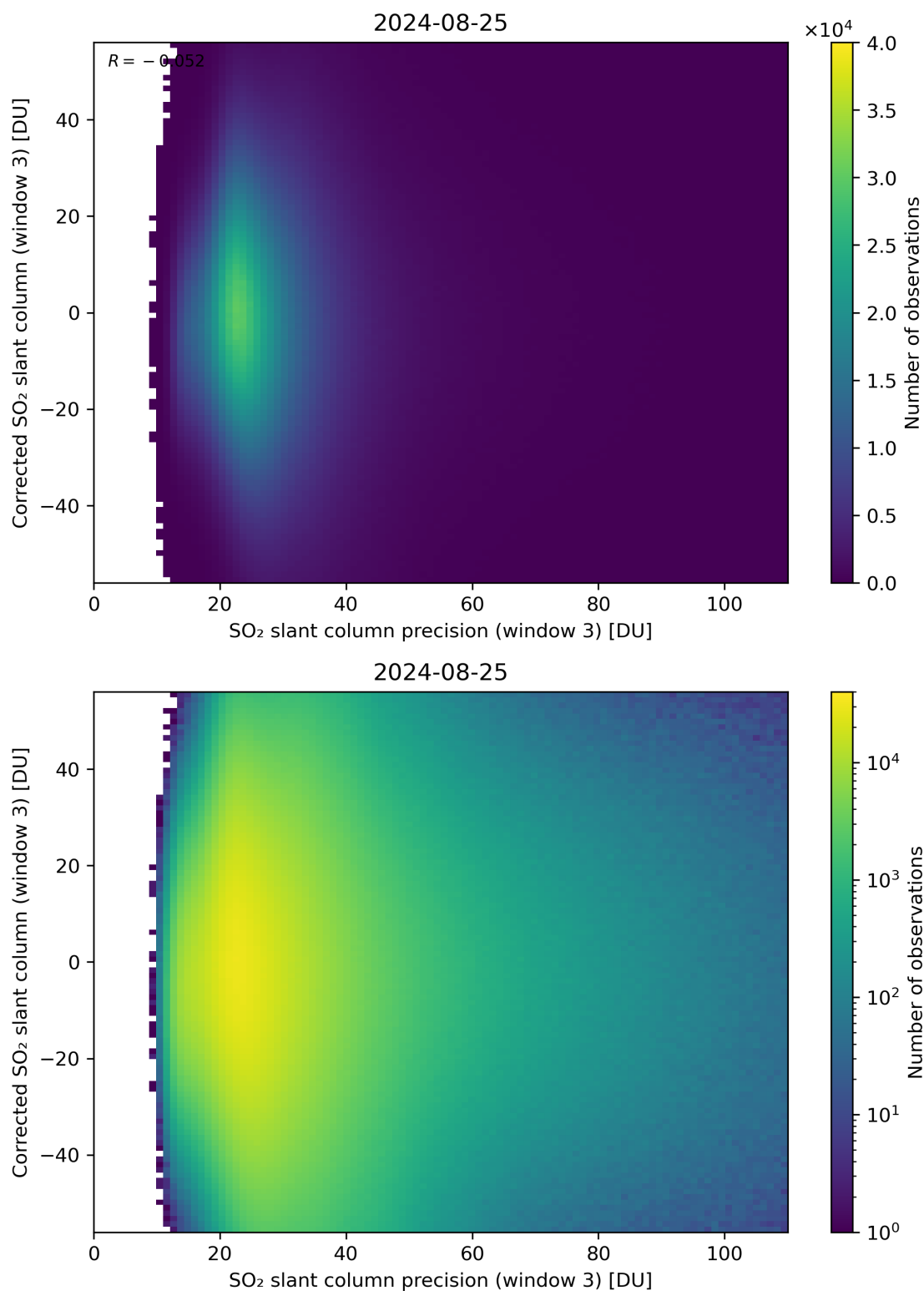
Figure 262: Scatter density plot of “SO 2 slant column precision (window 3)” against “Corrected SO 2 slant column (window 3)” for 2024-08-24 to 2024-08-26.
