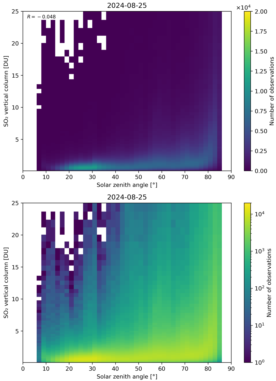
Figure 176: Scatter density plot of “Solar zenith angle” against “SO 2 vertical column” for 2024-08-24 to 2024-08-26.
