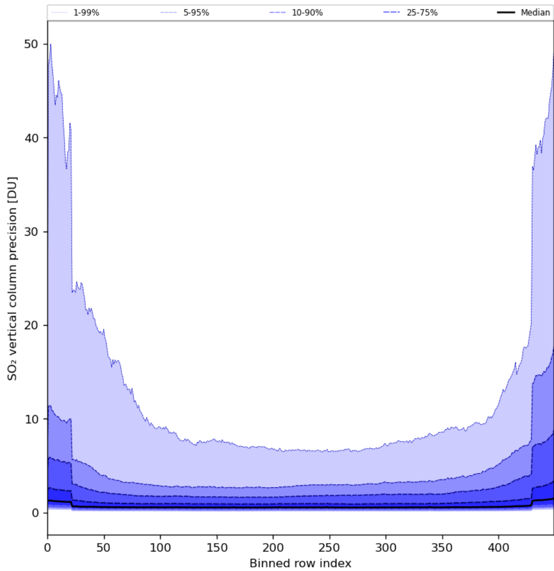
Figure 77: Along track statistics of “SO 2 vertical column precision” for 2024-08-24 to 2024-08-26
