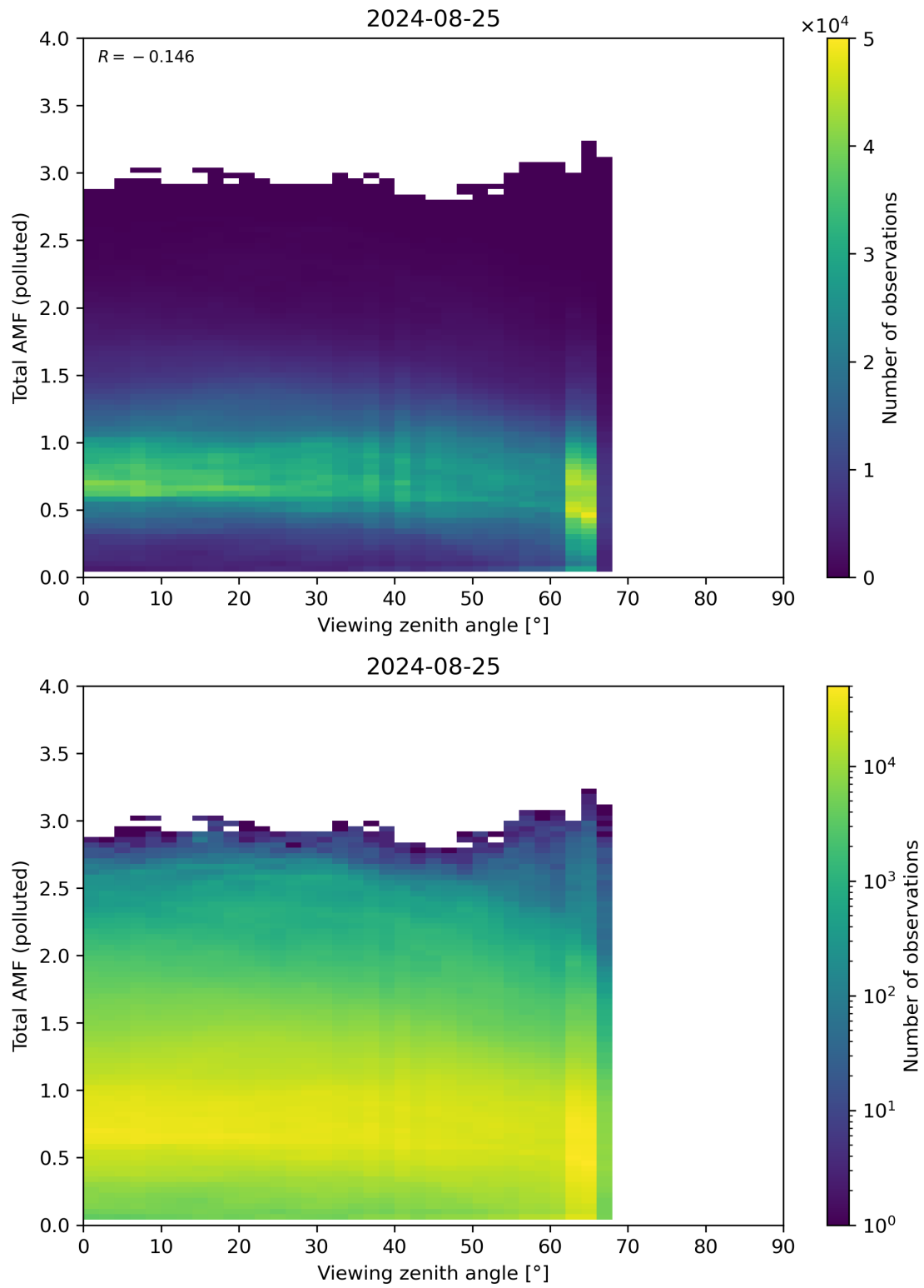
Figure 325: Scatter density plot of “Viewing zenith angle” against “Total AMF (polluted)” for 2024-08-24 to 2024-08-26.
