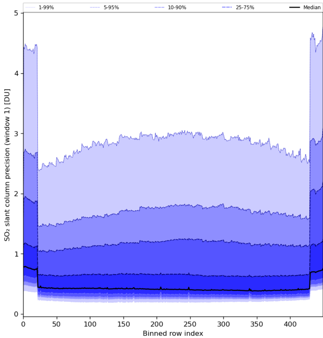
Figure 80: Along track statistics of “SO 2 slant column precision (window 1)” for 2024-08-24 to 2024-08-26
