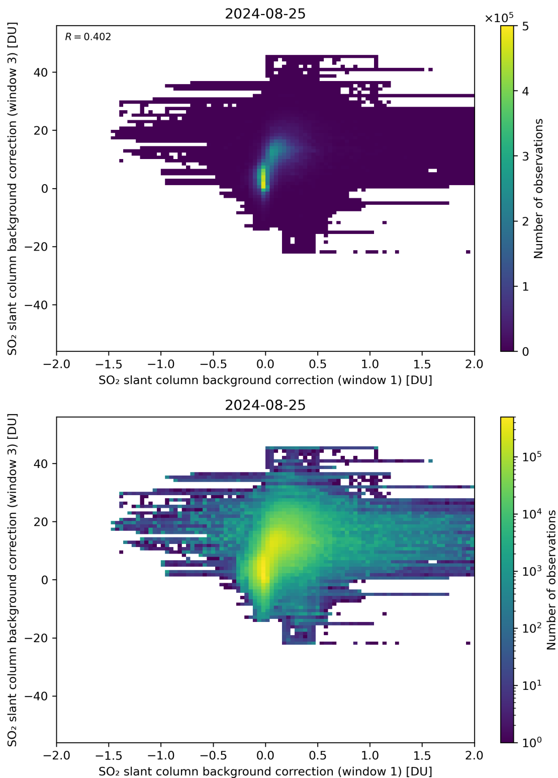
Figure 99: Scatter density plot of “SO 2 slant column background correction (window 1)” against “SO 2 slant column background correction (window 3)” for 2024-08-24 to 2024-08-26.
