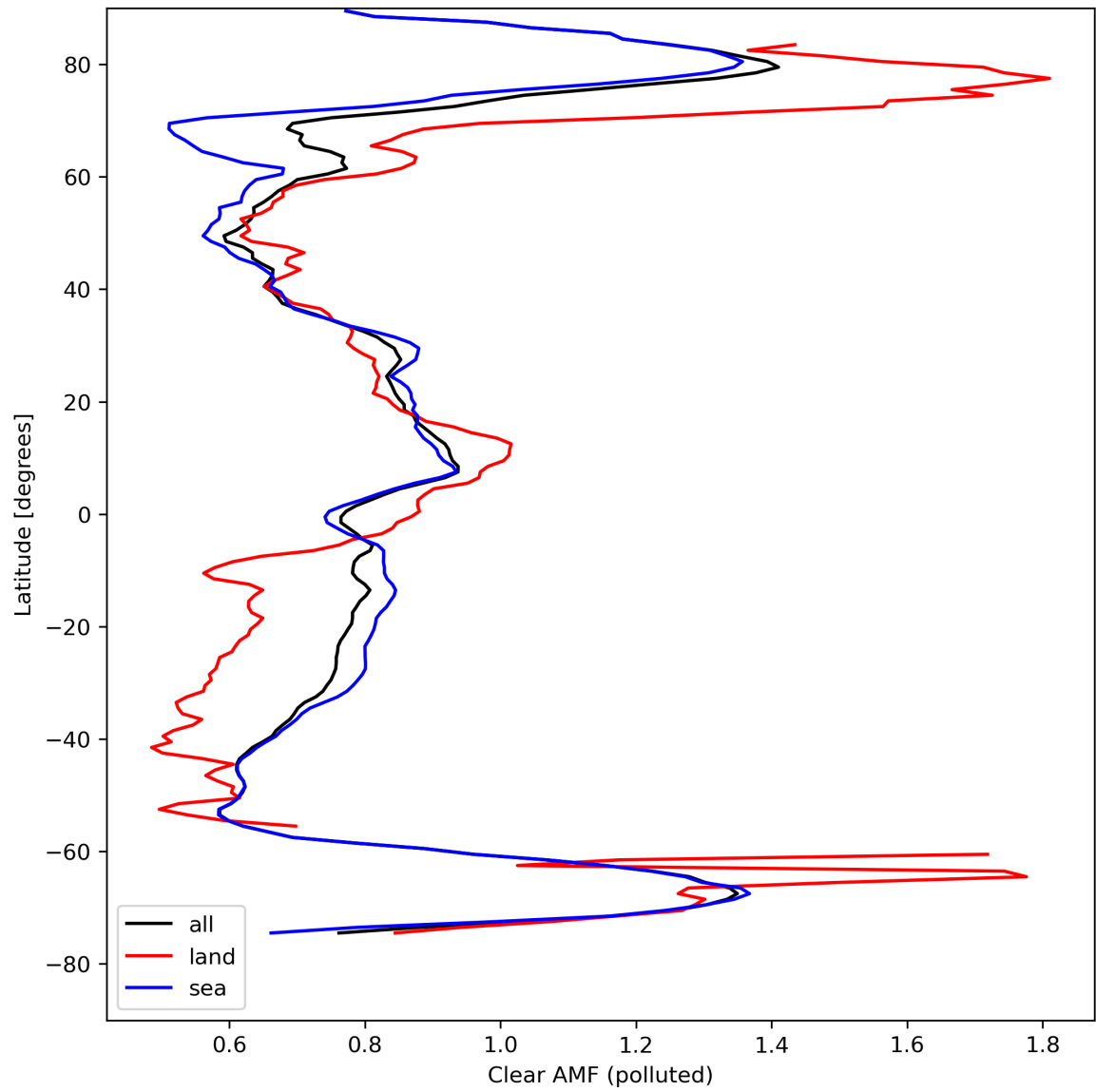
Figure 50: Zonal average of “Clear AMF (polluted)” for 2024-08-24 to 2024-08-26.
