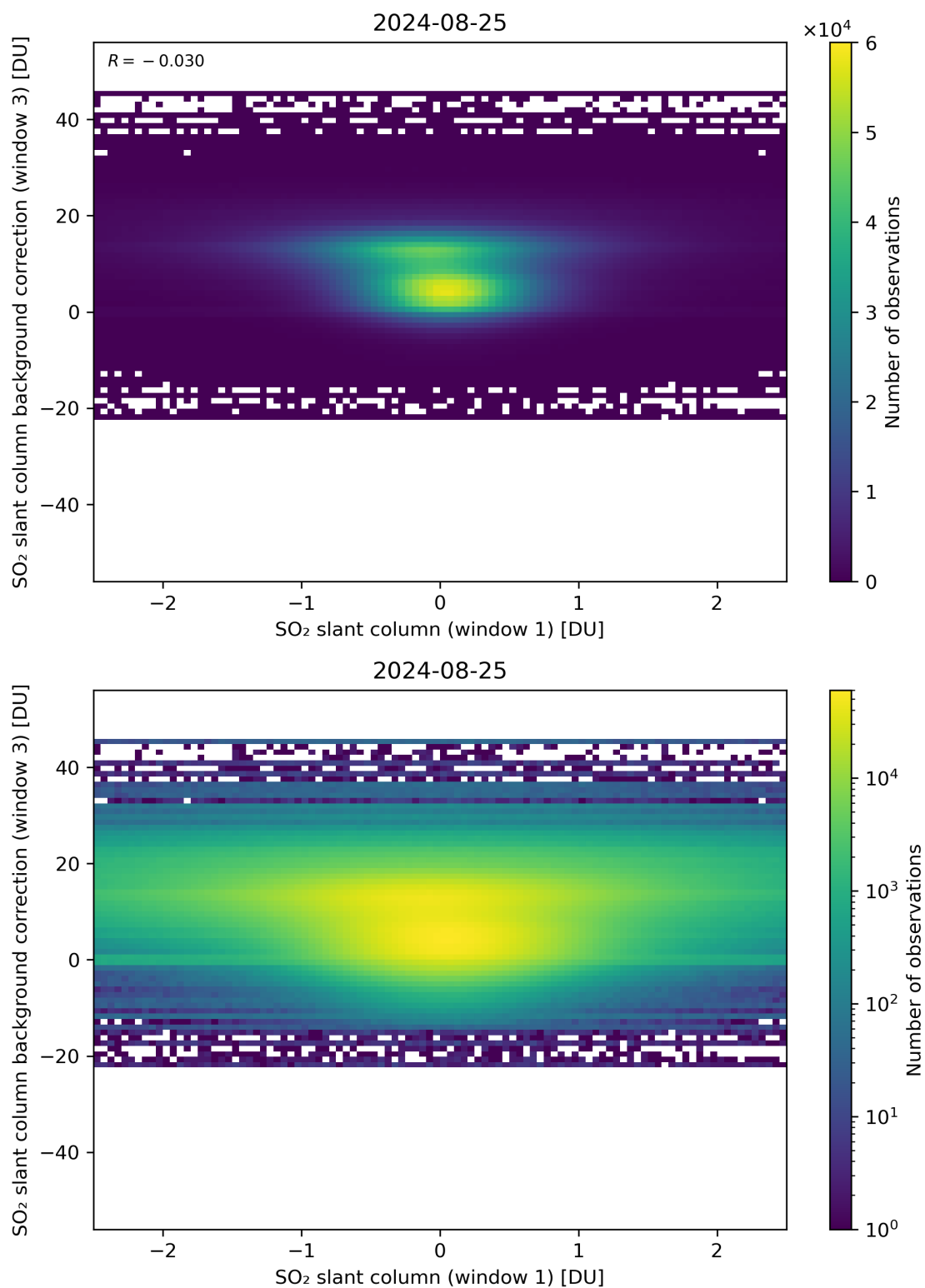
Figure 214: Scatter density plot of “SO 2 slant column (window 1)” against “SO 2 slant column background correction (window 3)” for 2024-08-24 to 2024-08-26.
