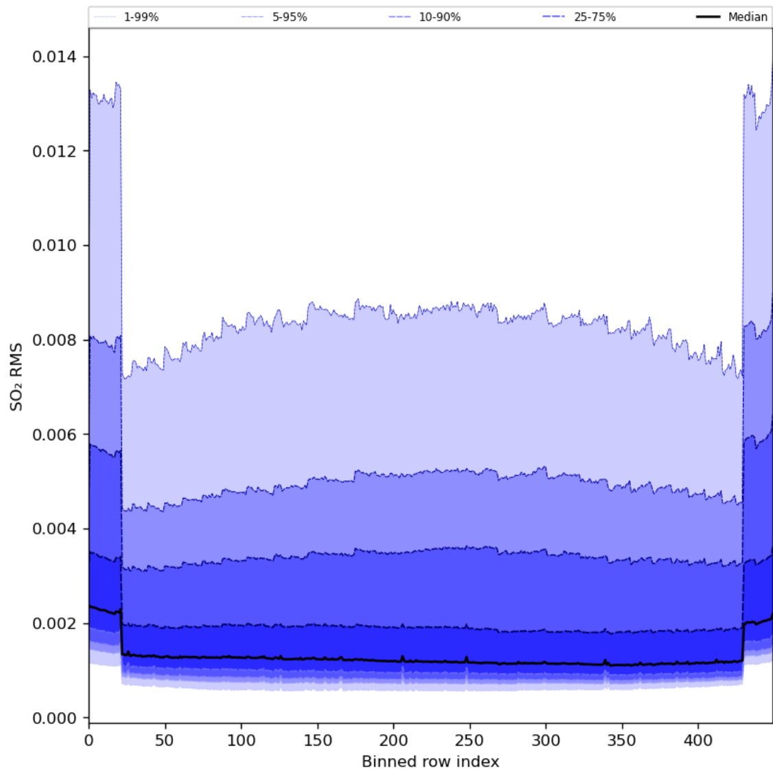
Figure 93: Along track statistics of “SO 2 RMS” for 2024-08-24 to 2024-08-26
