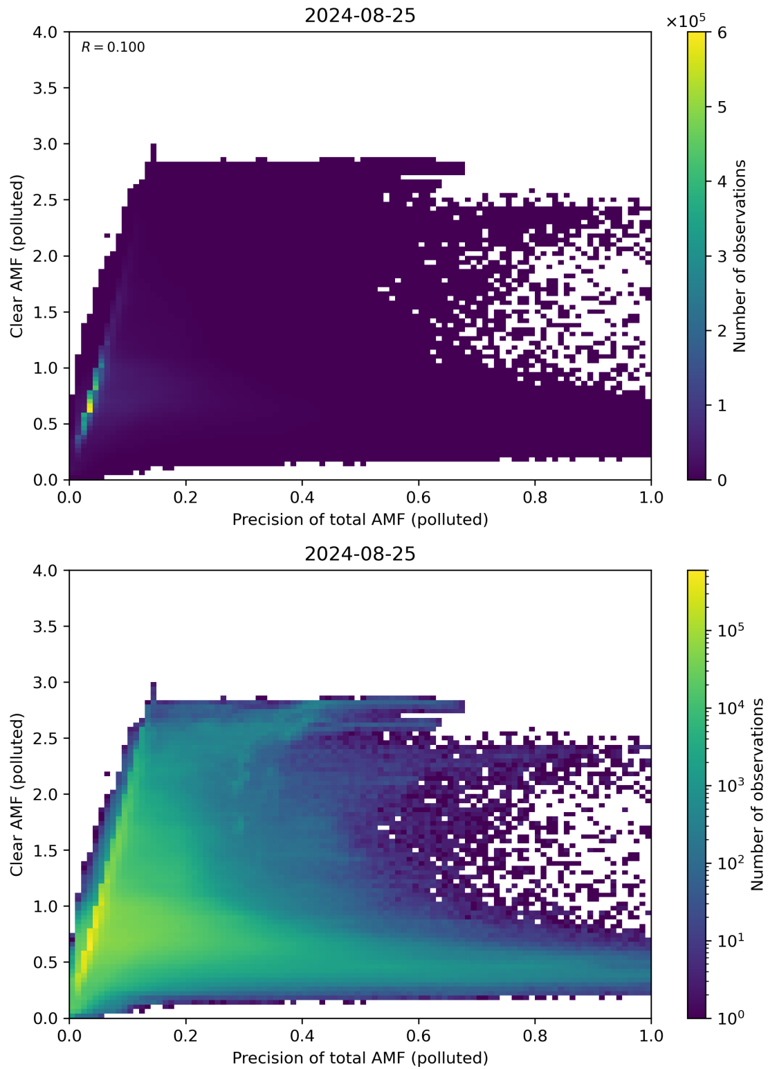
Figure 270: Scatter density plot of “Precision of total AMF (polluted)” against “Clear AMF (polluted)” for 2024-08-24 to 2024-08-26.
