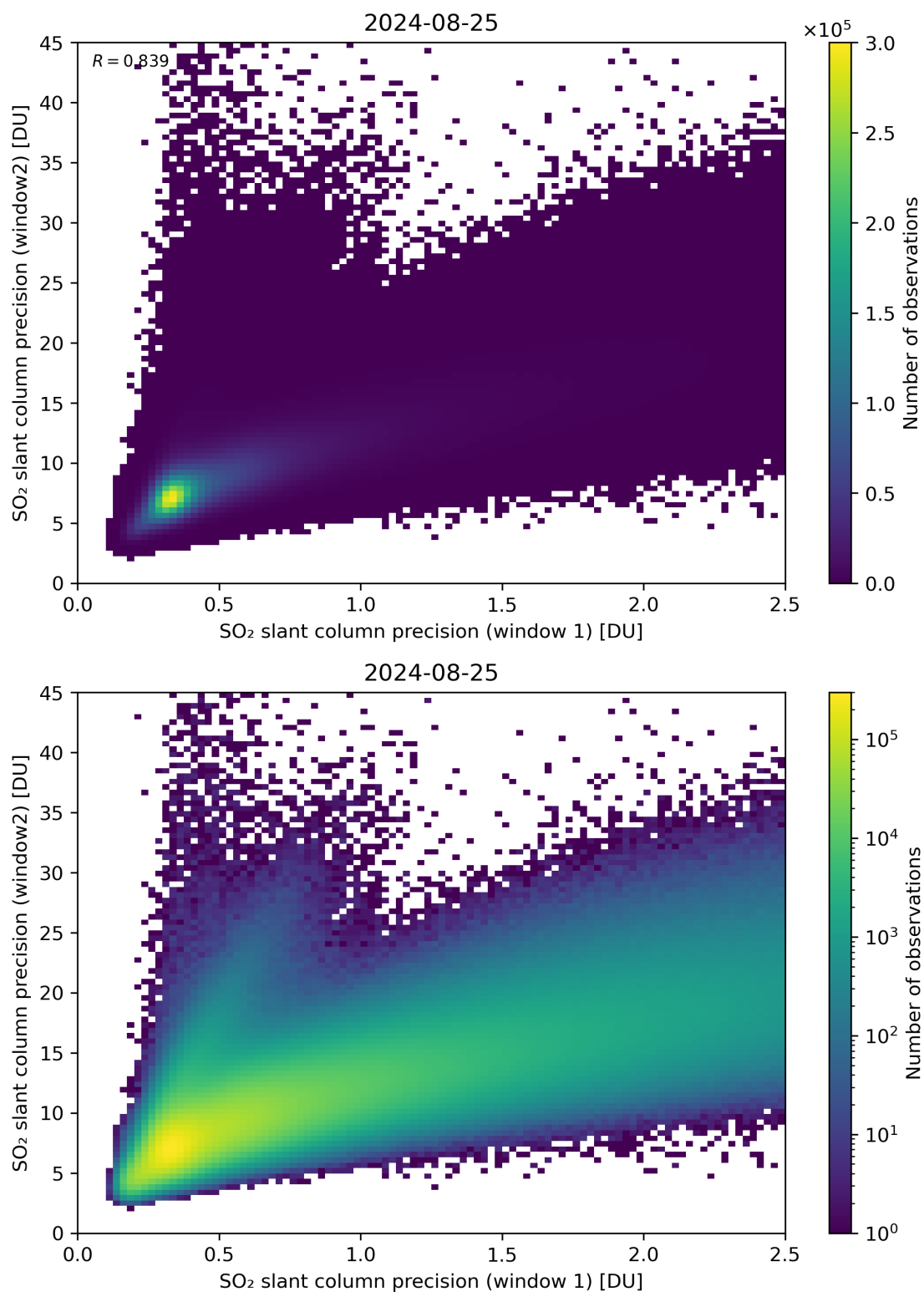
Figure 227: Scatter density plot of “SO 2 slant column precision (window 1)” against “SO 2 slant column precision (window2)” for 2024-08-24 to 2024-08-26.
