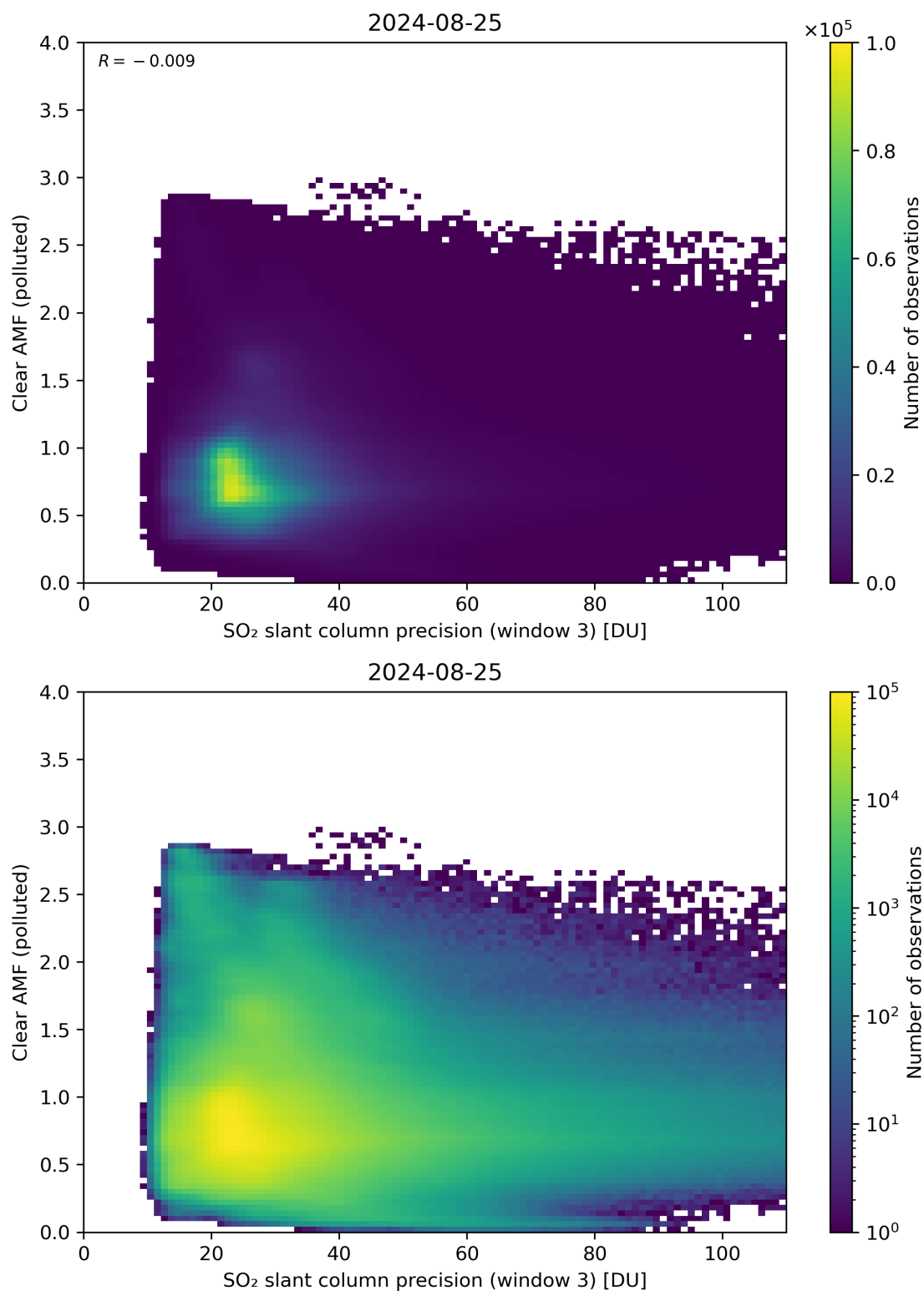
Figure 261: Scatter density plot of “SO 2 slant column precision (window 3)” against “Clear AMF (polluted)” for 2024-08-24 to 2024-08-26.
