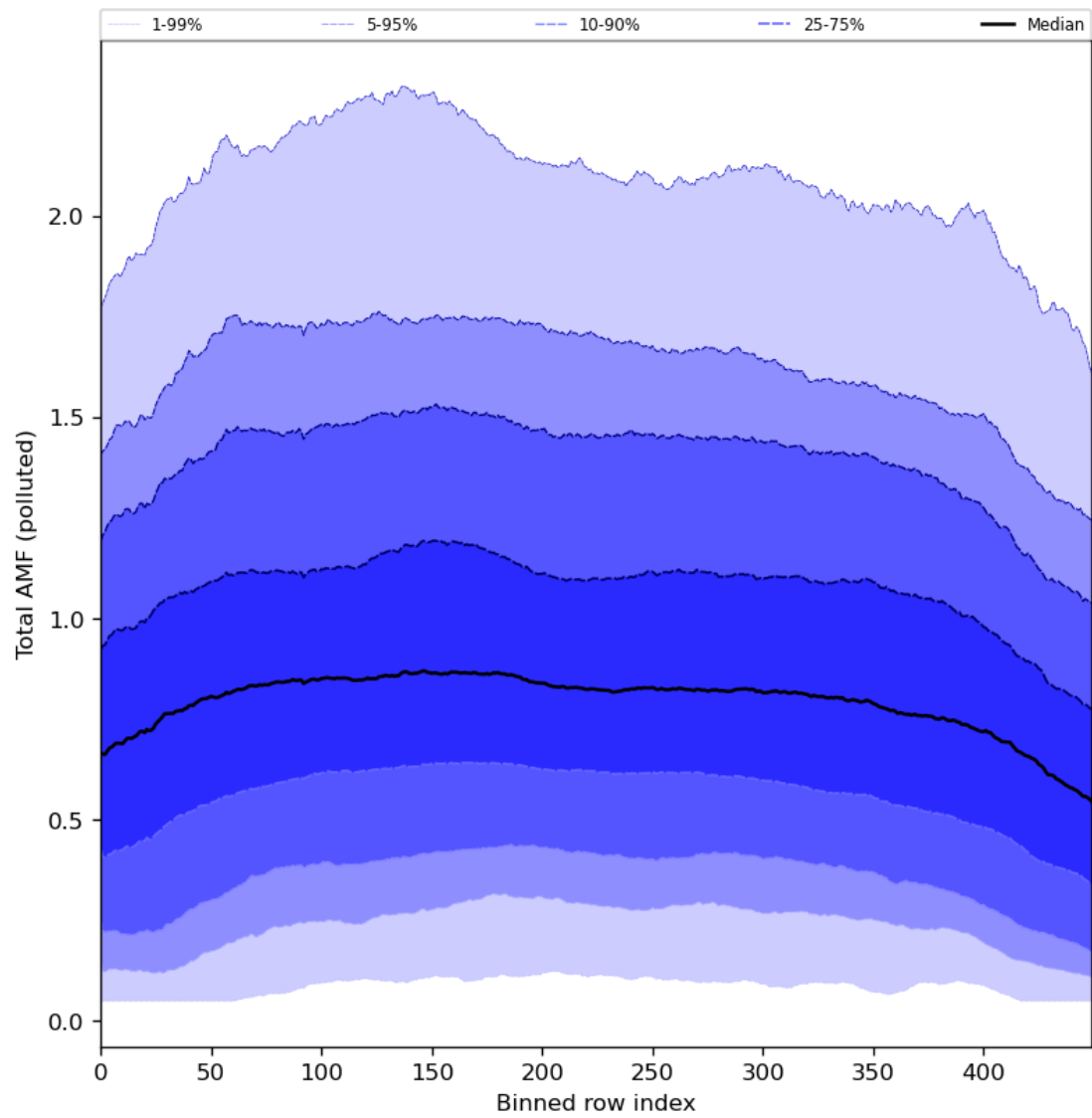
Figure 94: Along track statistics of “Total AMF (polluted)” for 2024-08-24 to 2024-08-26
