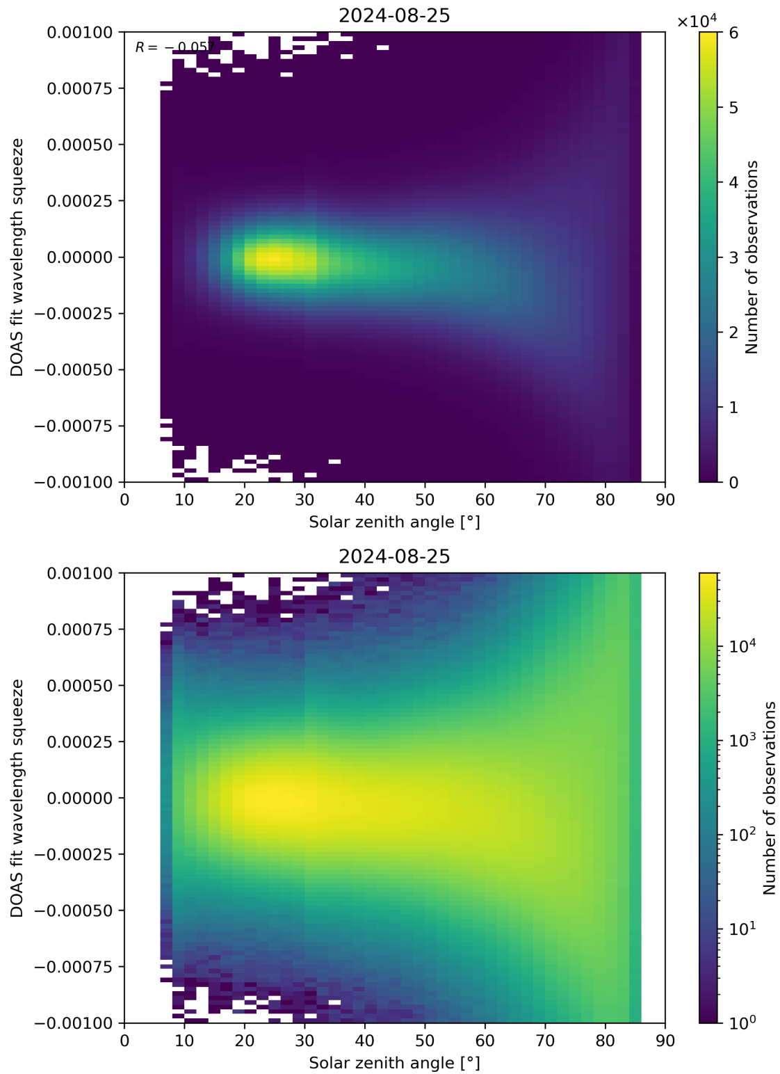
Figure 162: Scatter density plot of “Solar zenith angle” against “DOAS fit wavelength squeeze” for 2024-08-24 to 2024-08-26.
