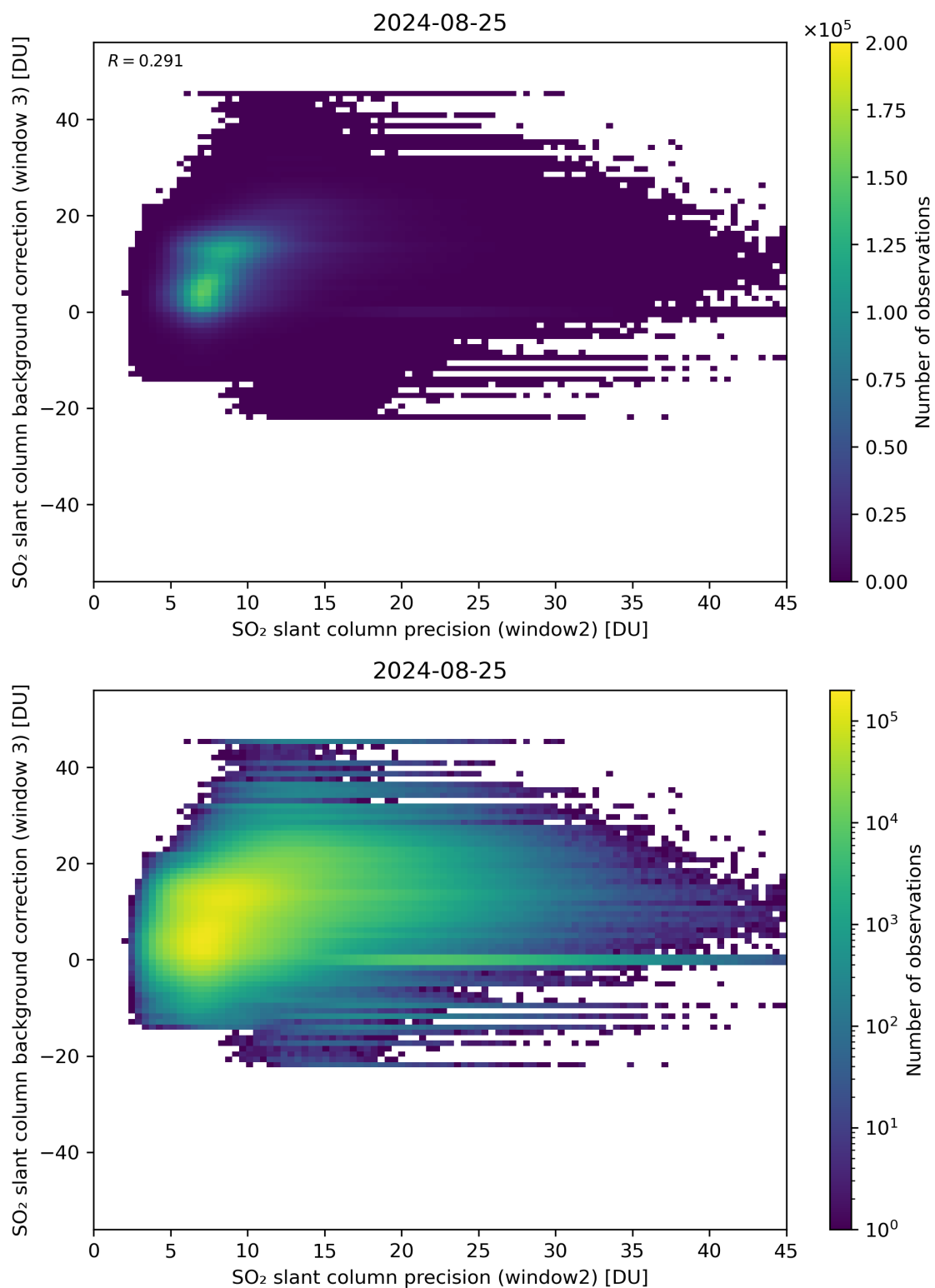
Figure 242: Scatter density plot of “SO 2 slant column precision (window2)” against “SO 2 slant column background correction (window 3)” for 2024-08-24 to 2024-08-26.
