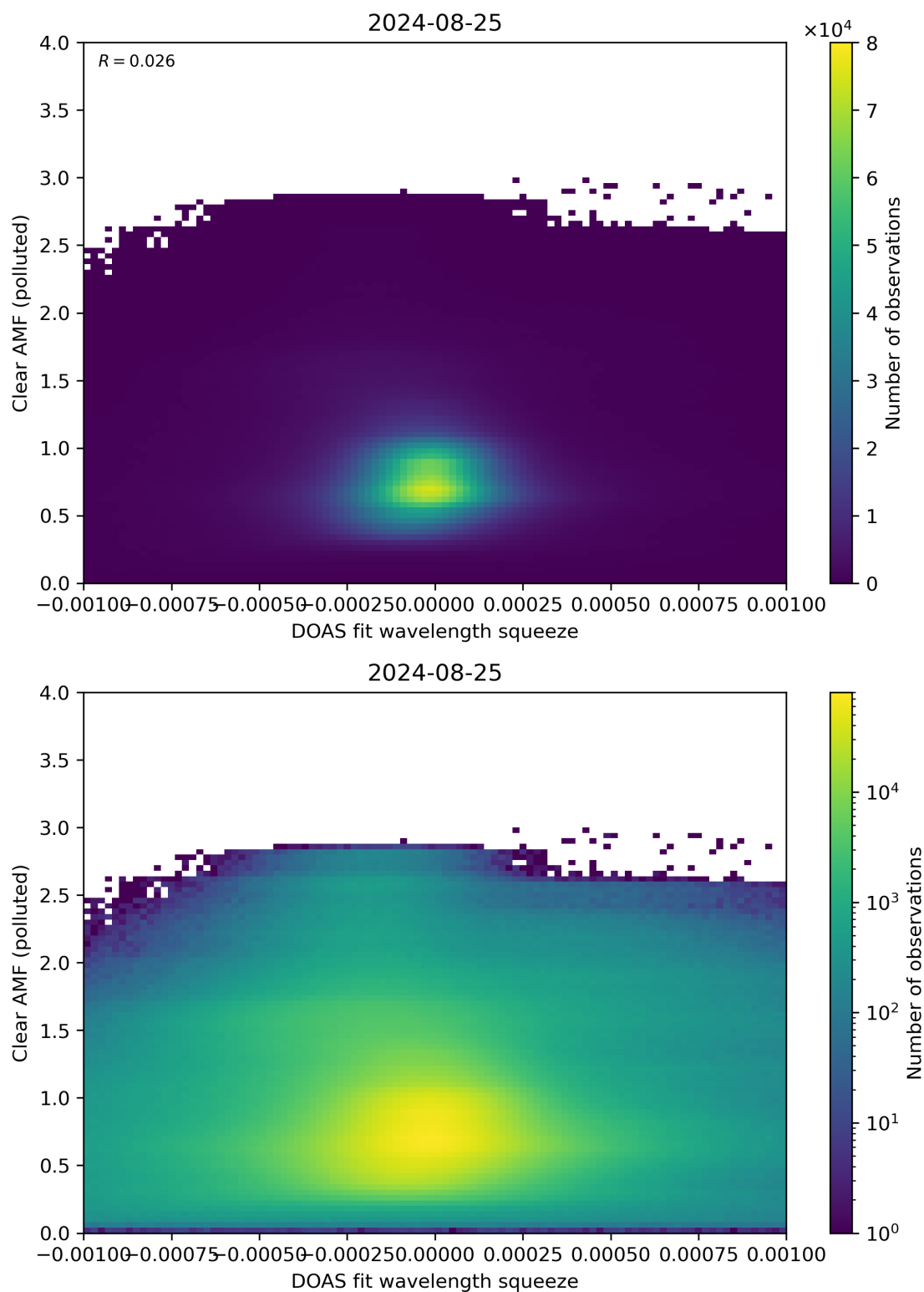
Figure 133: Scatter density plot of “DOAS fit wavelength squeeze” against “Clear AMF (polluted)” for 2024-08-24 to 2024-08-26.
