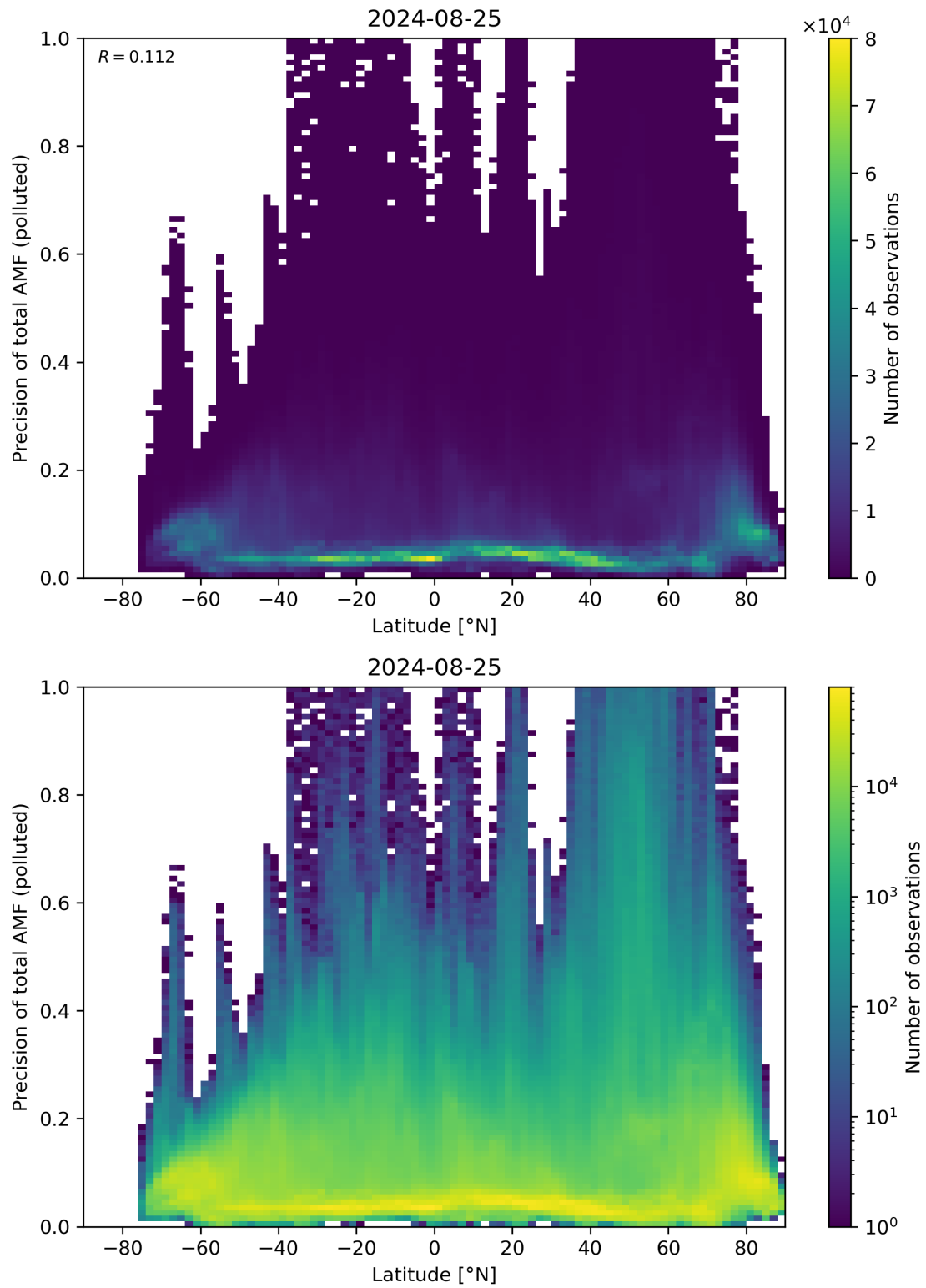
Figure 155: Scatter density plot of “Latitude” against “Precision of total AMF (polluted)” for 2024-08-24 to 2024-08-26.
