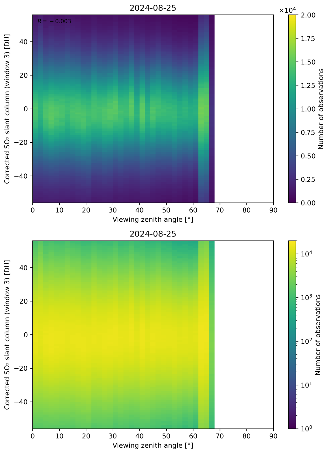
Figure 319: Scatter density plot of “Viewing zenith angle” against “Corrected SO 2 slant column (window 3)” for 2024-08-24 to 2024-08-26.
