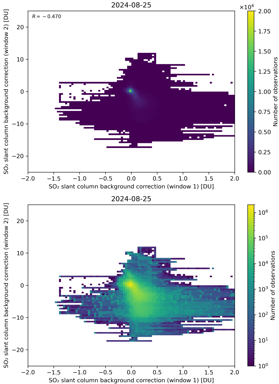
Figure 98: Scatter density plot of “SO 2 slant column background correction (window 1)” against “SO 2 slant column background correction (window 2)” for 2024-08-24 to 2024-08-26.
