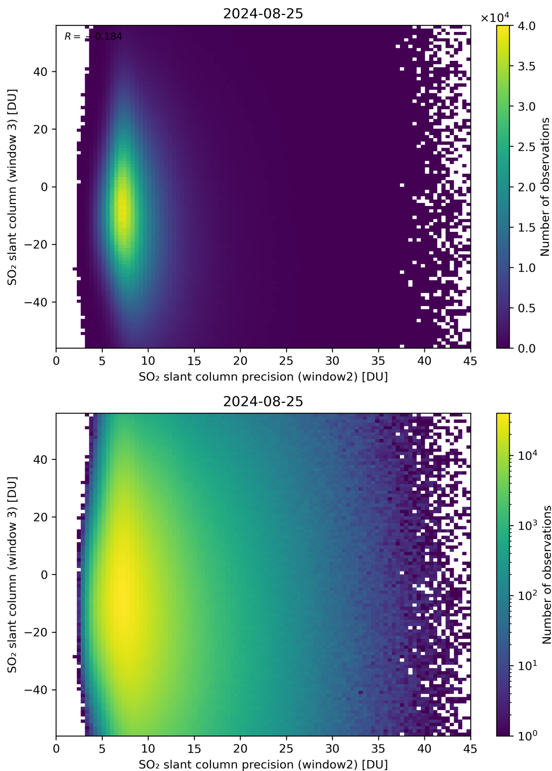
Figure 249: Scatter density plot of “SO 2 slant column precision (window2)” against “SO 2 slant column (window 3)” for 2024-08-24 to 2024-08-26.
