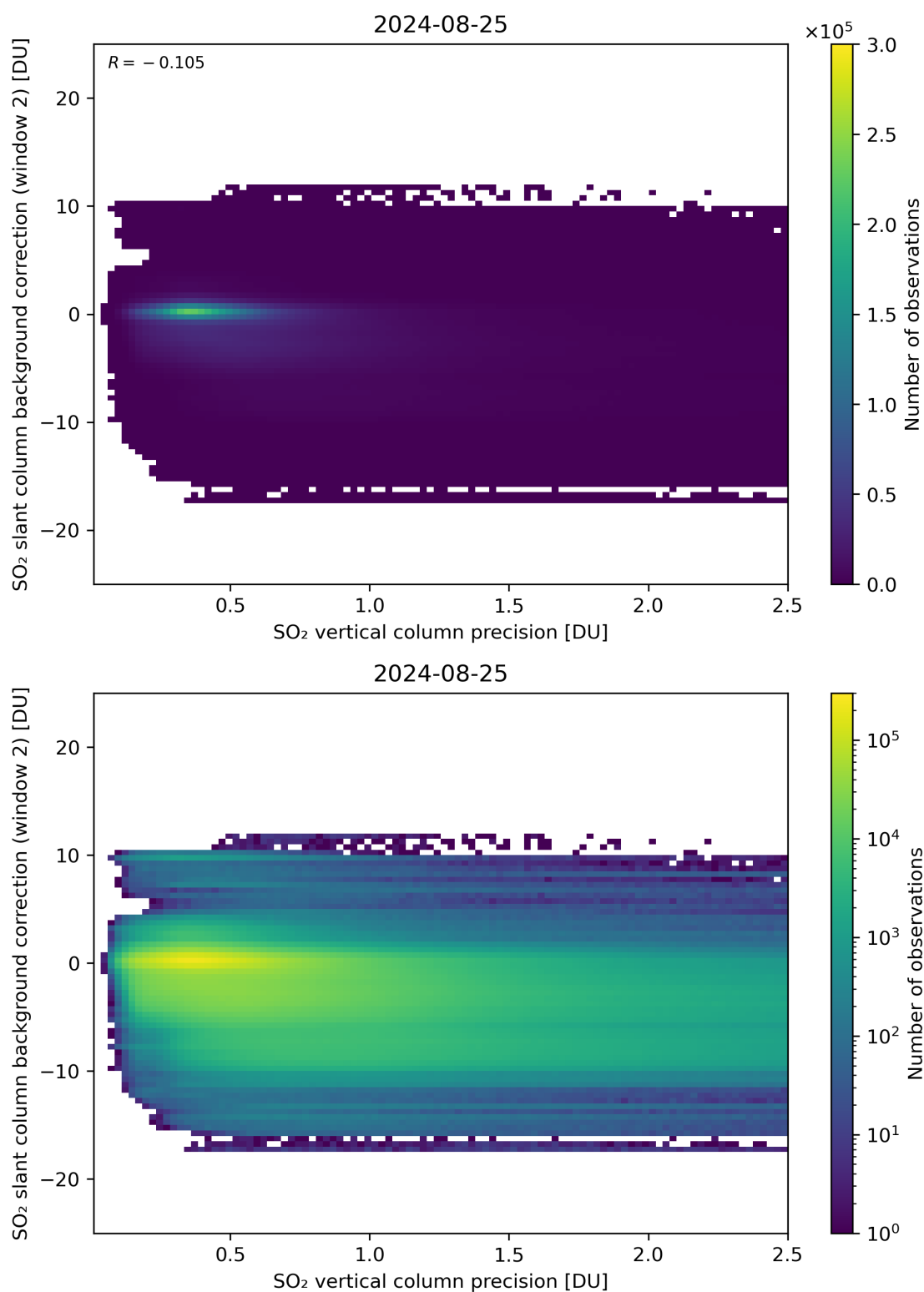
Figure 280: Scatter density plot of “SO 2 vertical column precision” against “SO 2 slant column background correction (window 2)” for 2024-08-24 to 2024-08-26.
