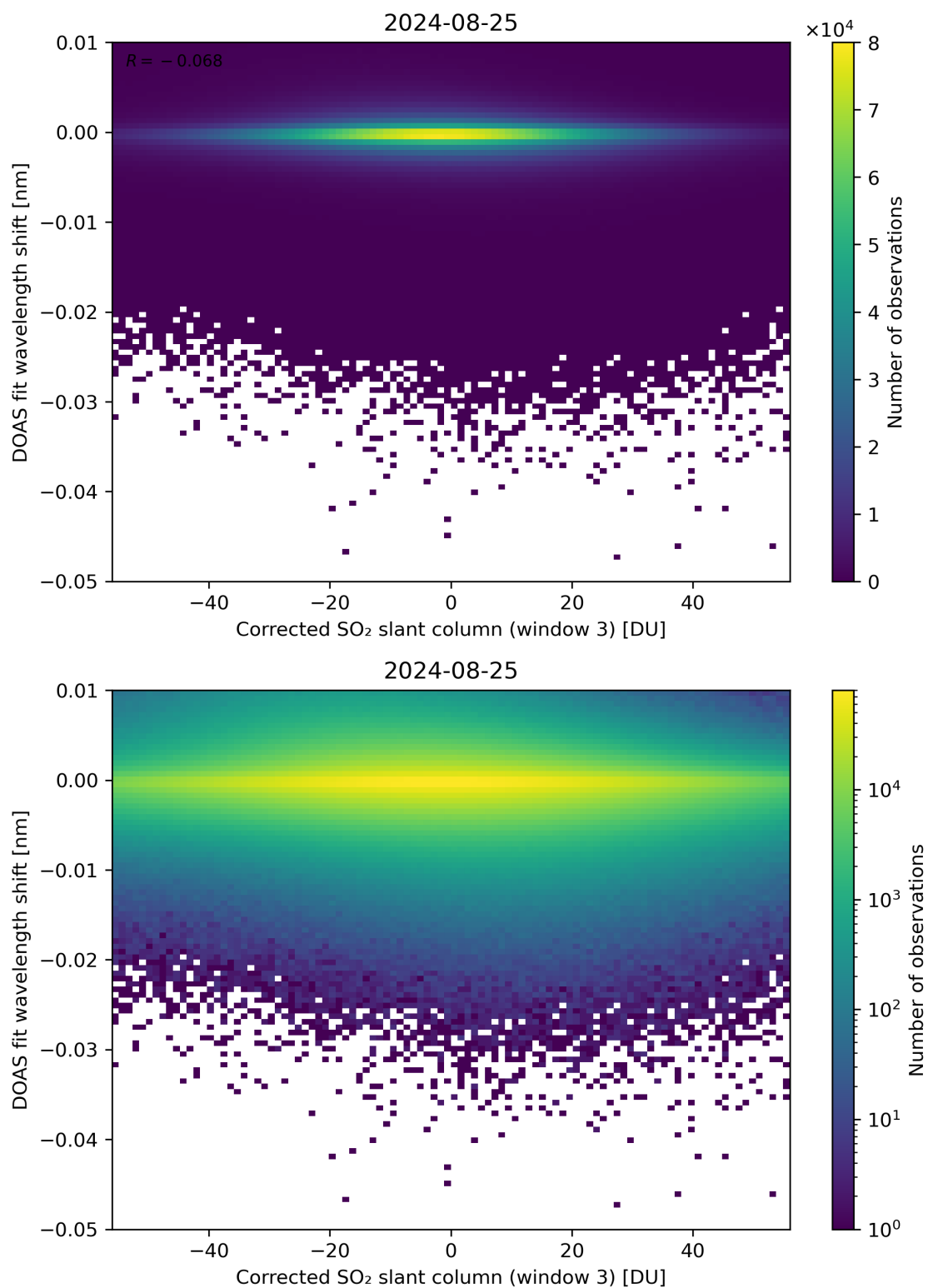
Figure 206: Scatter density plot of “Corrected SO 2 slant column (window 3)” against “DOAS fit wavelength shift” for 2024-08-24 to 2024-08-26.
