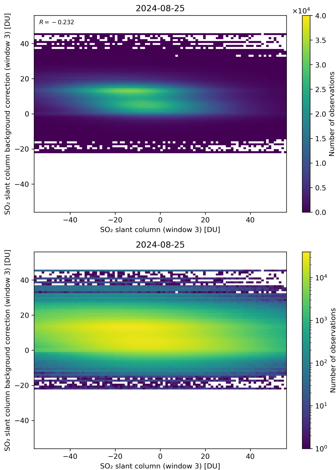
Figure 253: Scatter density plot of “SO 2 slant column (window 3)” against “SO 2 slant column background correction (window 3)” for 2024-08-24 to 2024-08-26.
