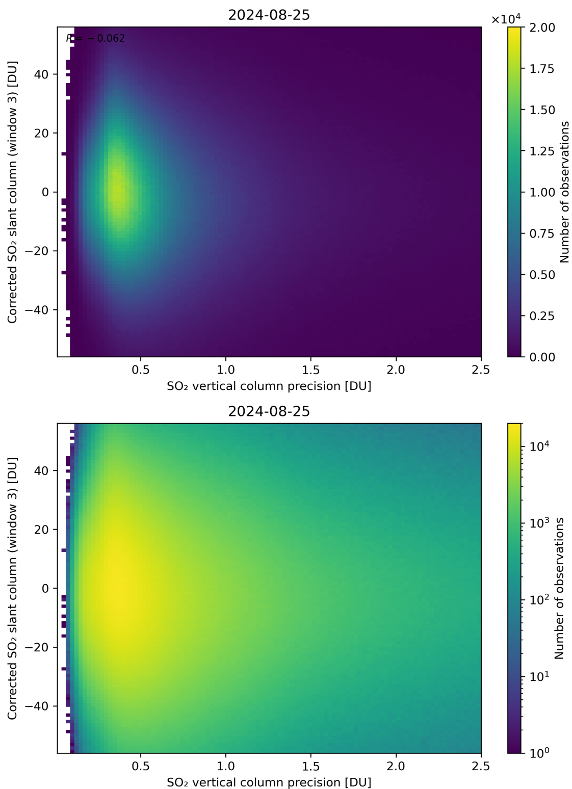
Figure 288: Scatter density plot of “SO 2 vertical column precision” against “Corrected SO 2 slant column (window 3)” for 2024-08-24 to 2024-08-26.
