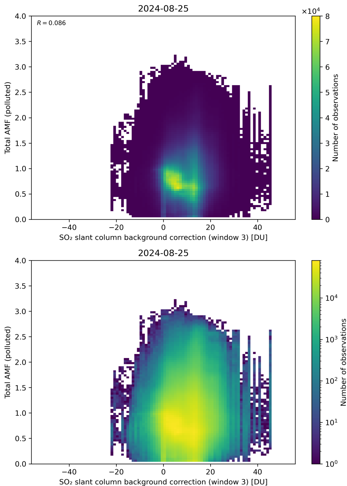
Figure 125: Scatter density plot of “SO 2 slant column background correction (window 3)” against “Total AMF (polluted)” for 2024-08-24 to 2024-08-26.
