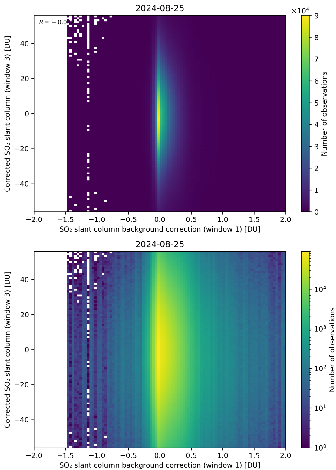
Figure 105: Scatter density plot of “SO 2 slant column background correction (window 1)” against “Corrected SO 2 slant column (window 3)” for 2024-08-24 to 2024-08-26.
