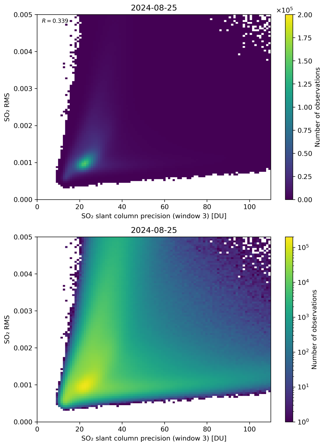
Figure 260: Scatter density plot of “SO 2 slant column precision (window 3)” against “SO 2 RMS” for 2024-08-24 to 2024-08-26.
