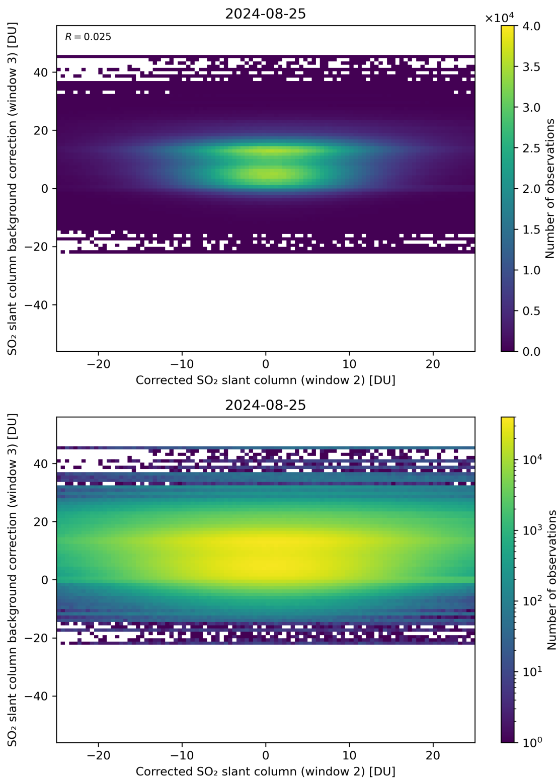
Figure 195: Scatter density plot of “Corrected SO 2 slant column (window 2)” against “SO 2 slant column background correction (window 3)” for 2024-08-24 to 2024-08-26.
