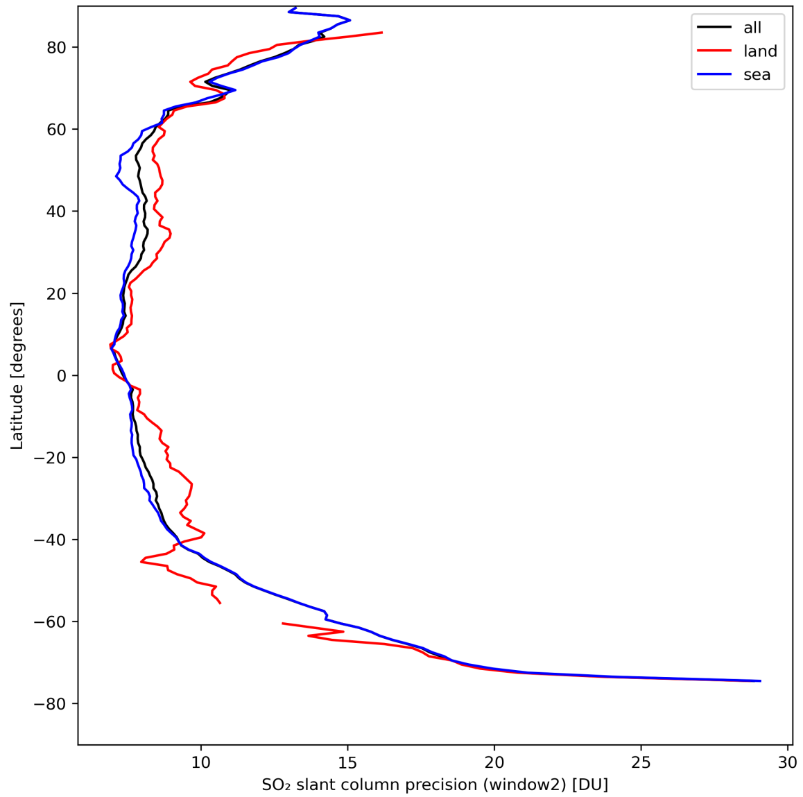
Figure 38: Zonal average of “SO 2 slant column precision (window2)” for 2024-08-24 to 2024-08-26.
