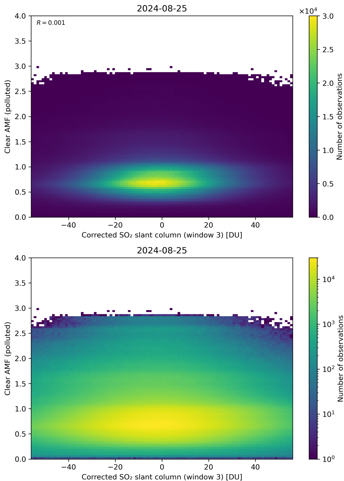
Figure 209: Scatter density plot of “Corrected SO 2 slant column (window 3)” against “Clear AMF (polluted)” for 2024-08-24 to 2024-08-26.
