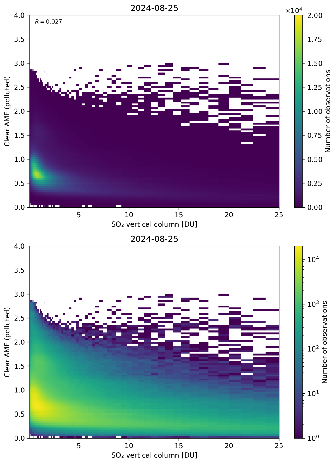
Figure 296: Scatter density plot of “SO 2 vertical column” against “Clear AMF (polluted)” for 2024-08-24 to 2024-08-26.
