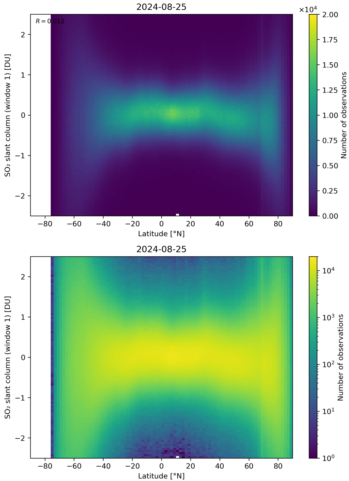
Figure 149: Scatter density plot of “Latitude” against “SO 2 slant column (window 1)” for 2024-08-24 to 2024-08-26.
