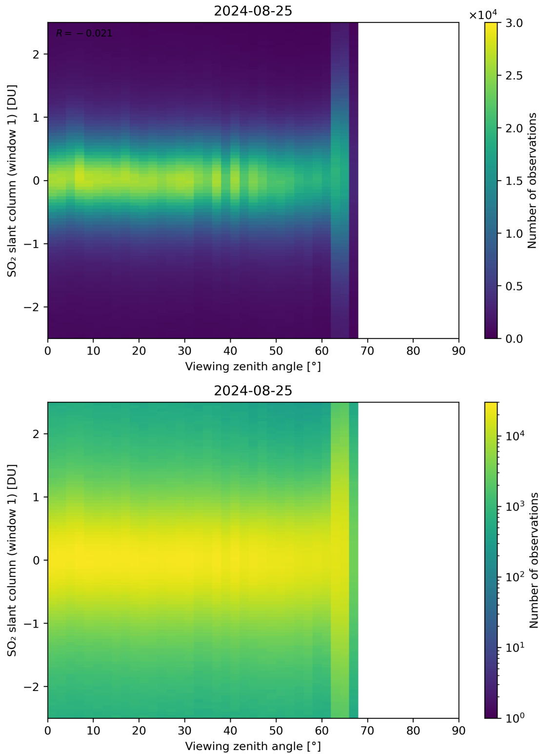
Figure 320: Scatter density plot of “Viewing zenith angle” against “SO 2 slant column (window 1)” for 2024-08-24 to 2024-08-26.
