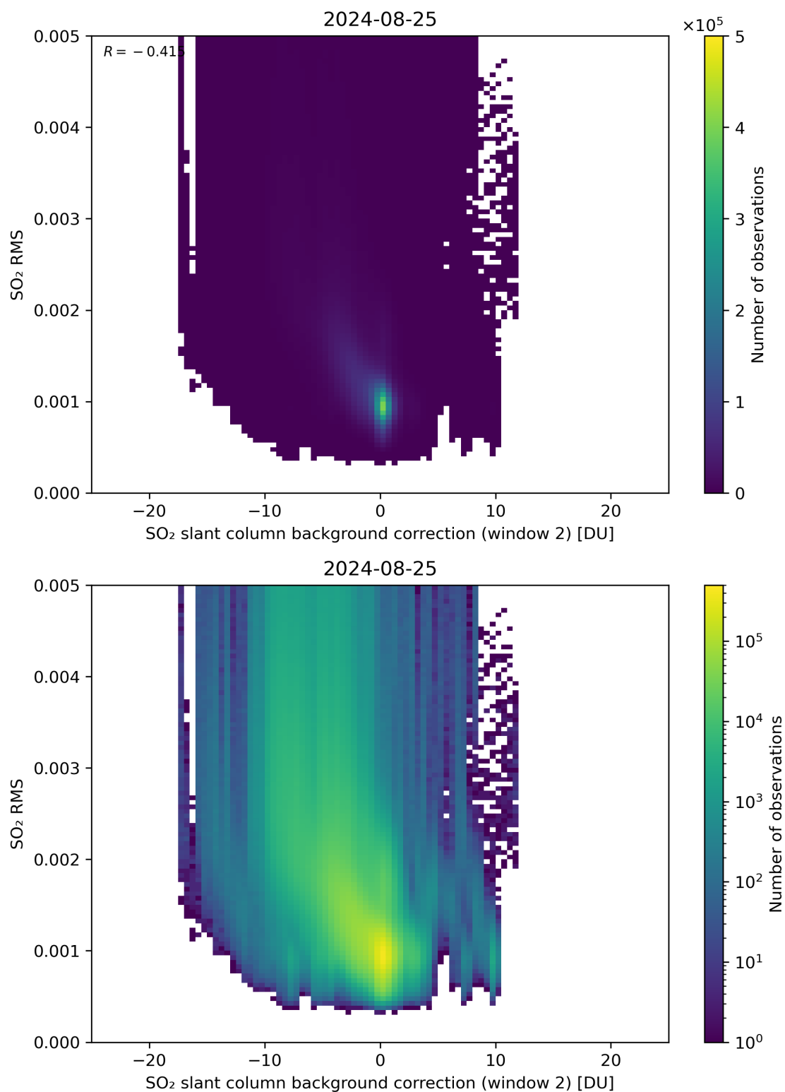
Figure 114: Scatter density plot of “SO 2 slant column background correction (window 2)” against “SO 2 RMS” for 2024-08-24 to 2024-08-26.
