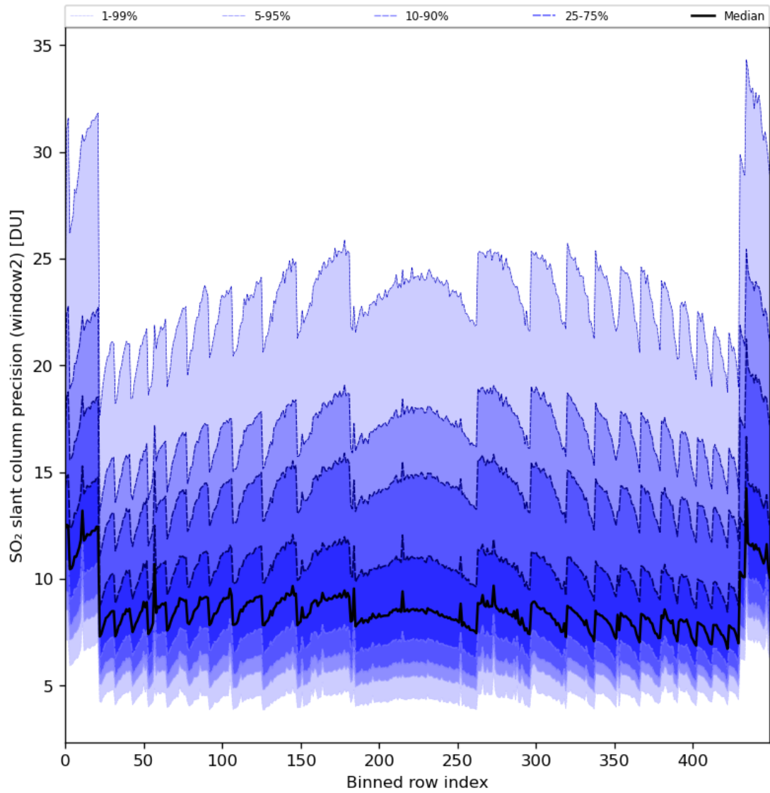
Figure 84: Along track statistics of “SO 2 slant column precision (window2)” for 2024-08-24 to 2024-08-26
