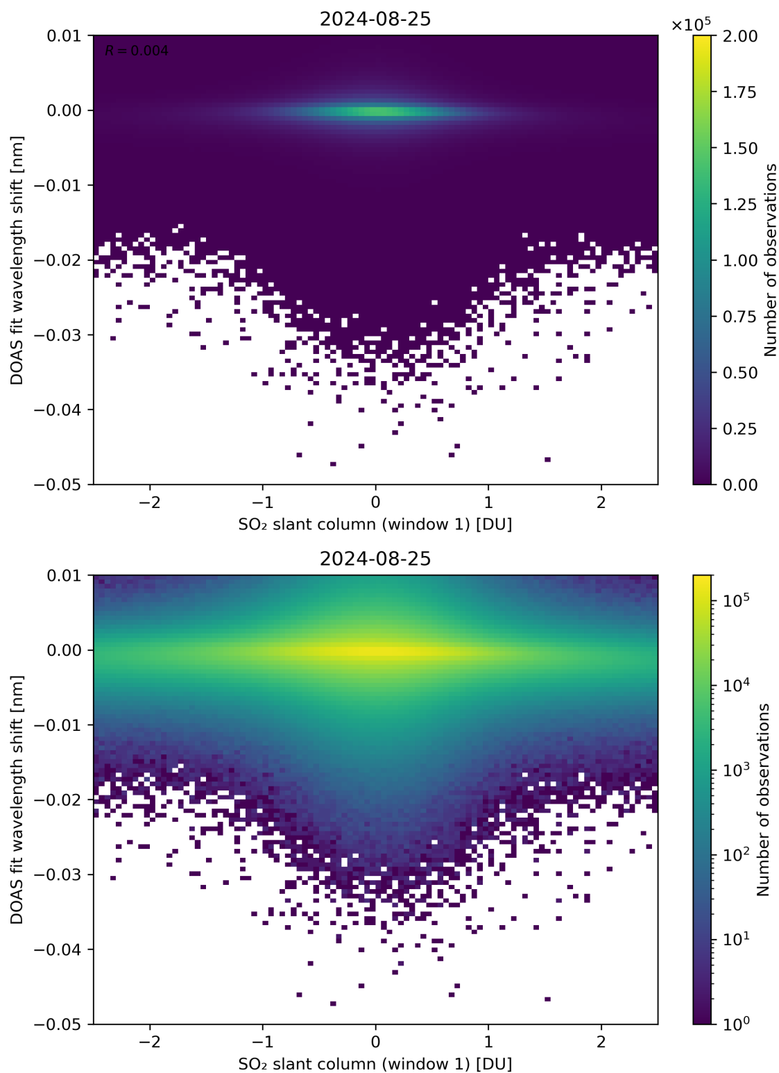
Figure 215: Scatter density plot of “SO 2 slant column (window 1)” against “DOAS fit wavelength shift” for 2024-08-24 to 2024-08-26.
