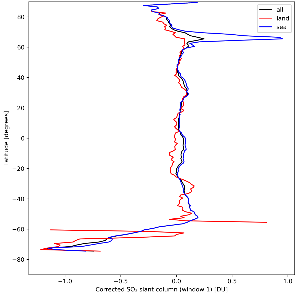
Figure 35: Zonal average of “Corrected SO 2 slant column (window 1)” for 2024-08-24 to 2024-08-26.
