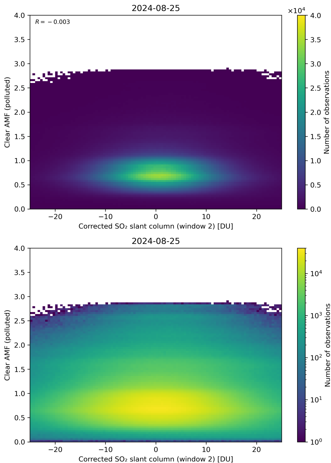
Figure 199: Scatter density plot of “Corrected SO 2 slant column (window 2)” against “Clear AMF (polluted)” for 2024-08-24 to 2024-08-26.
