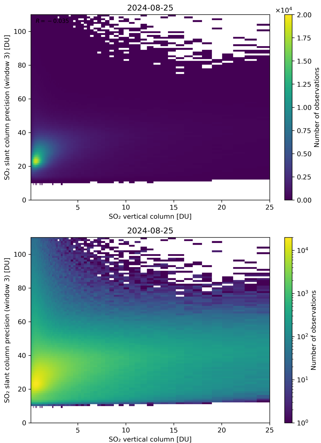
Figure 304: Scatter density plot of “SO 2 vertical column” against “SO 2 slant column precision (window 3)” for 2024-08-24 to 2024-08-26.
