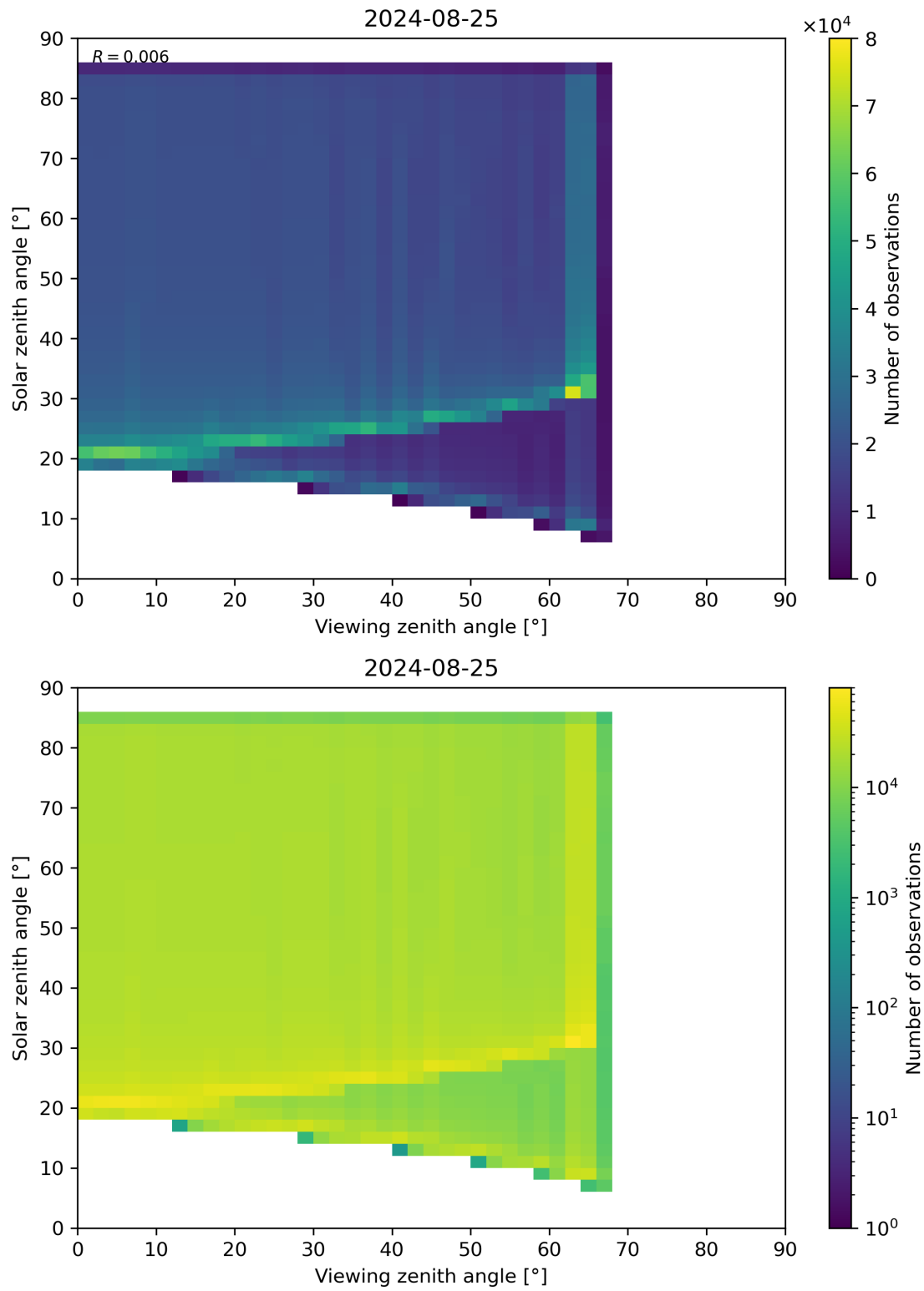
Figure 315: Scatter density plot of “Viewing zenith angle” against “Solar zenith angle” for 2024-08-24 to 2024-08-26.
