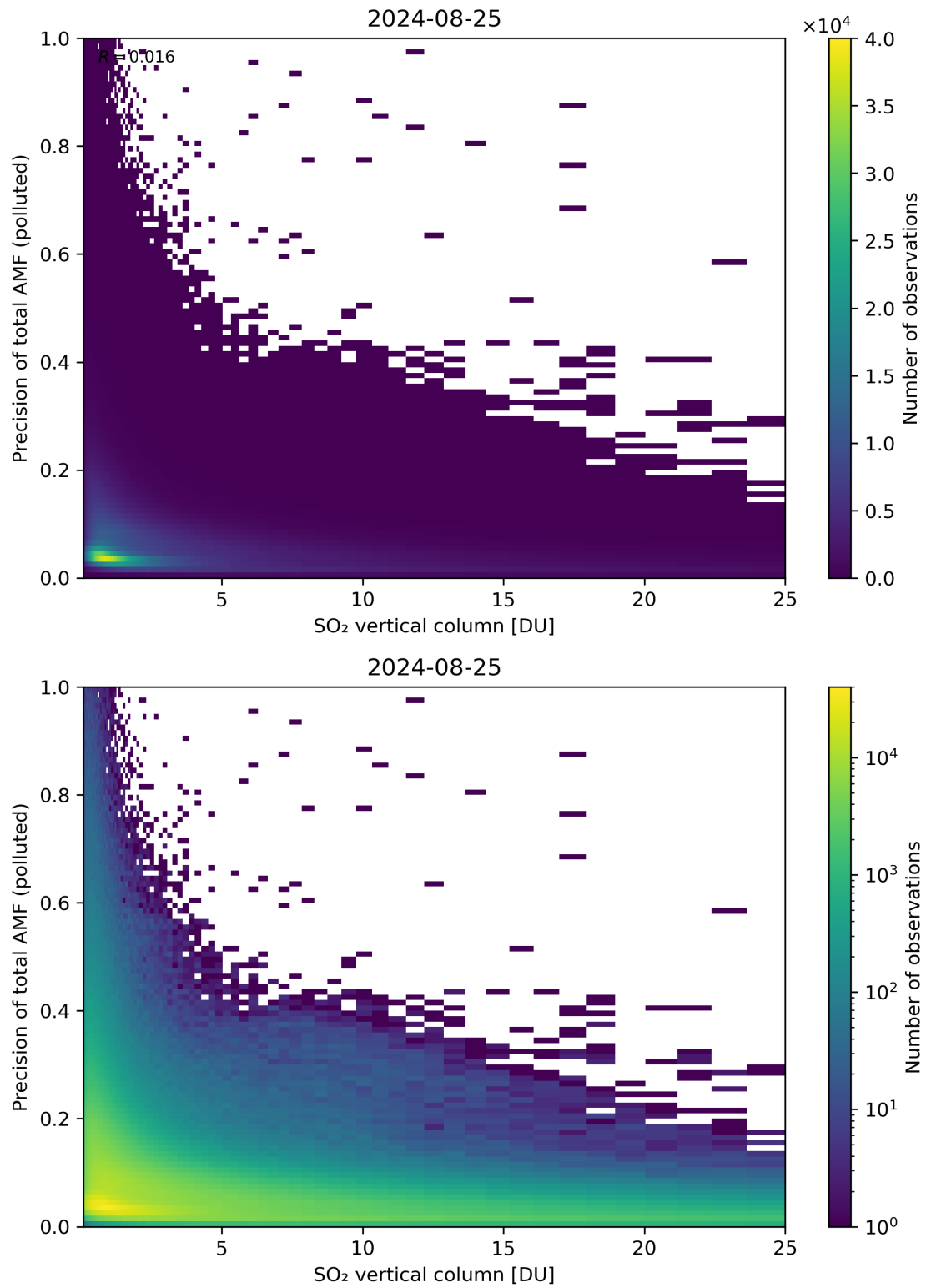
Figure 306: Scatter density plot of “SO 2 vertical column” against “Precision of total AMF (polluted)” for 2024-08-24 to 2024-08-26.
