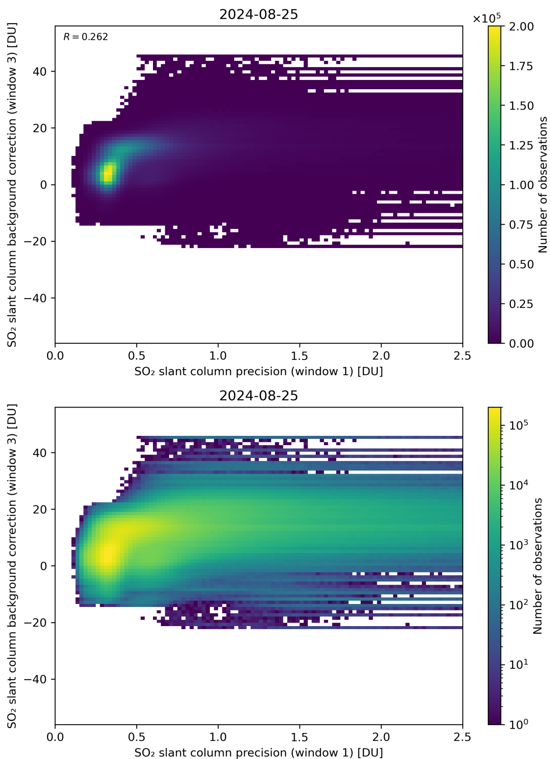
Figure 220: Scatter density plot of “SO 2 slant column precision (window 1)” against “SO 2 slant column background correction (window 3)” for 2024-08-24 to 2024-08-26.
