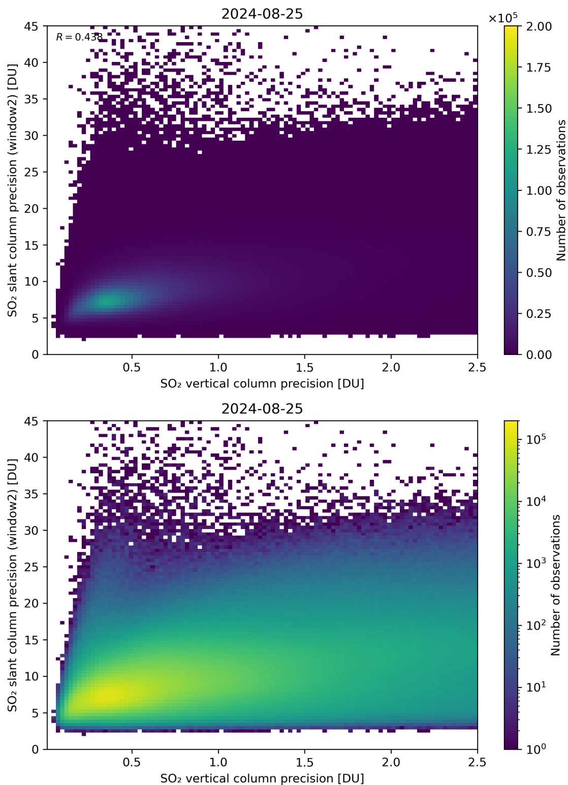
Figure 291: Scatter density plot of “SO 2 vertical column precision” against “SO 2 slant column precision (window2)” for 2024-08-24 to 2024-08-26.
