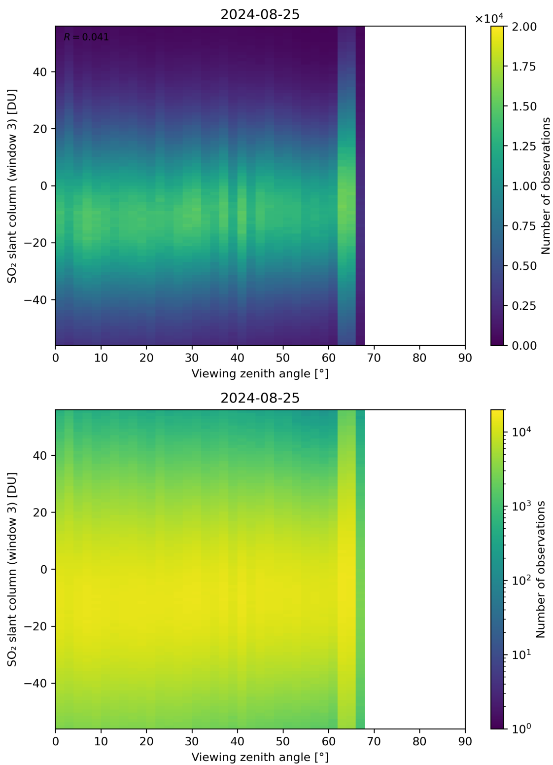
Figure 323: Scatter density plot of “Viewing zenith angle” against “SO 2 slant column (window 3)” for 2024-08-24 to 2024-08-26.
