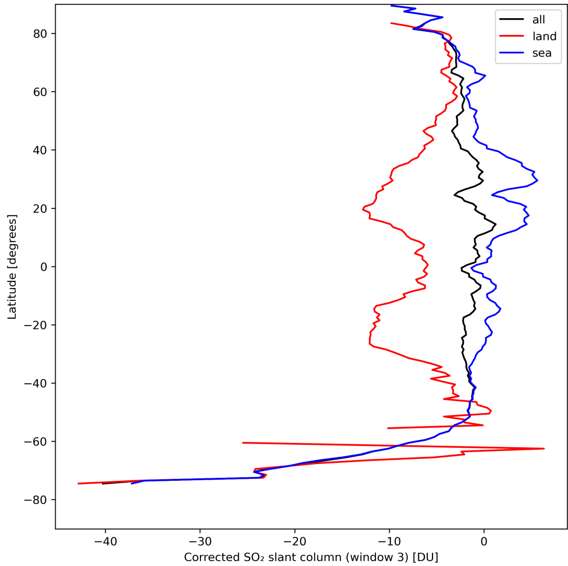
Figure 43: Zonal average of “Corrected SO 2 slant column (window 3)” for 2024-08-24 to 2024-08-26.
