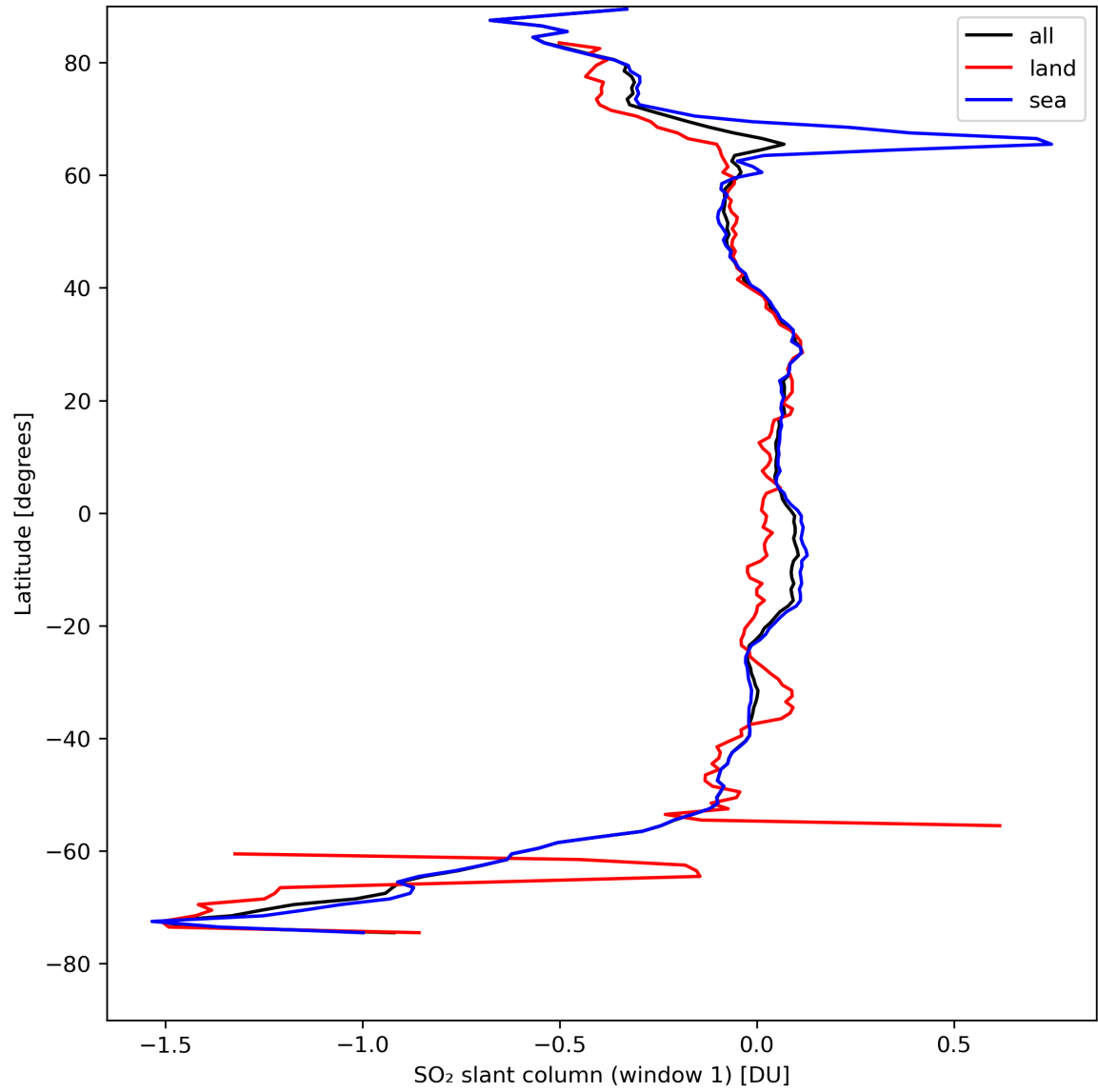
Figure 33: Zonal average of “SO 2 slant column (window 1)” for 2024-08-24 to 2024-08-26.
