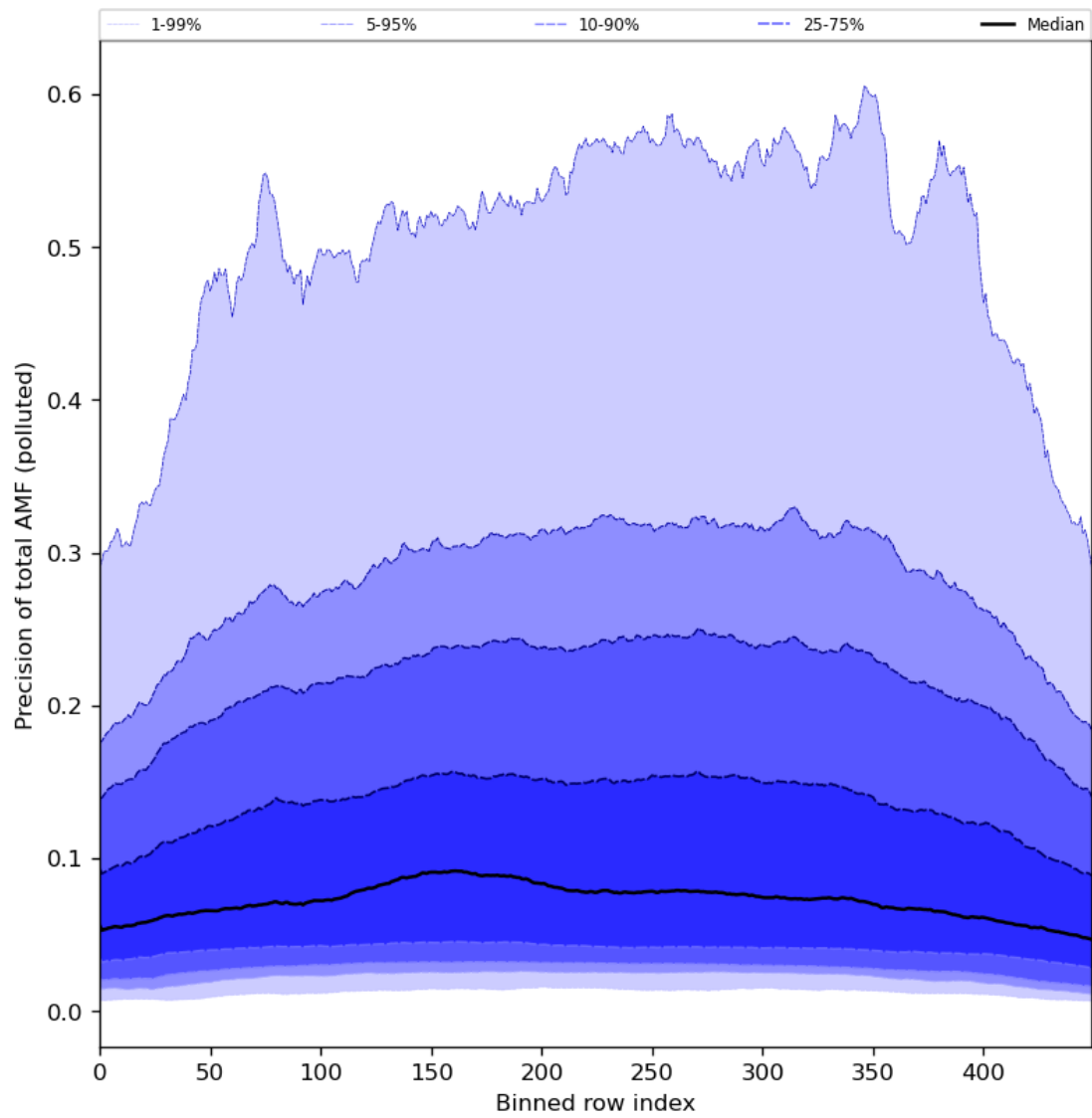
Figure 95: Along track statistics of “Precision of total AMF (polluted)” for 2024-08-24 to 2024-08-26
