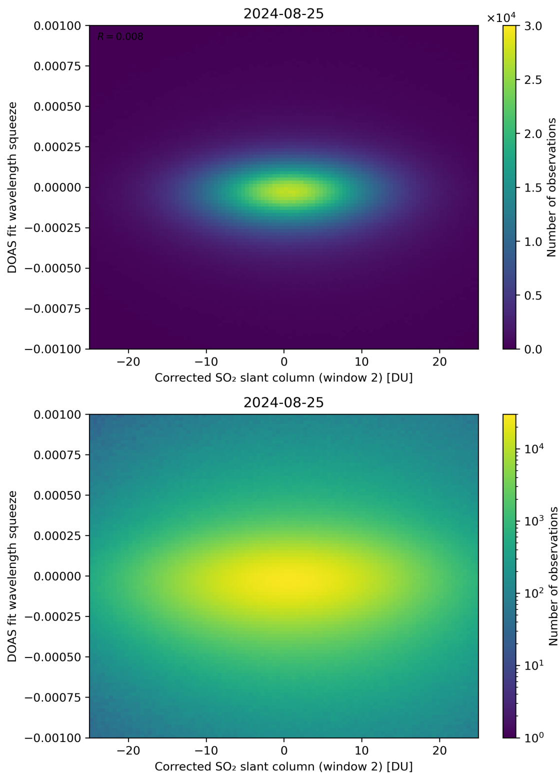
Figure 197: Scatter density plot of “Corrected SO 2 slant column (window 2)” against “DOAS fit wavelength squeeze” for 2024-08-24 to 2024-08-26.
