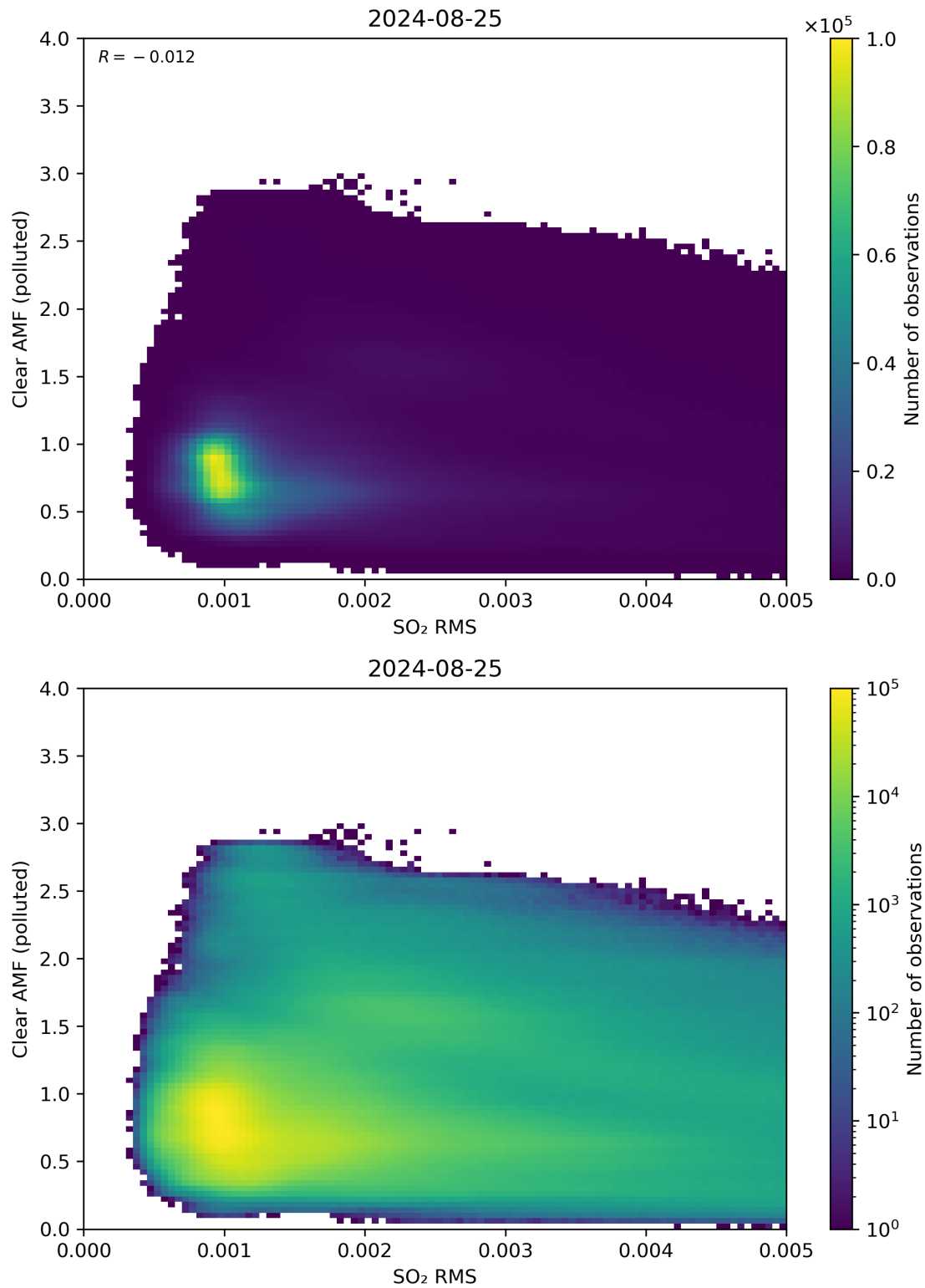
Figure 136: Scatter density plot of “SO 2 RMS” against “Clear AMF (polluted)” for 2024-08-24 to 2024-08-26.
