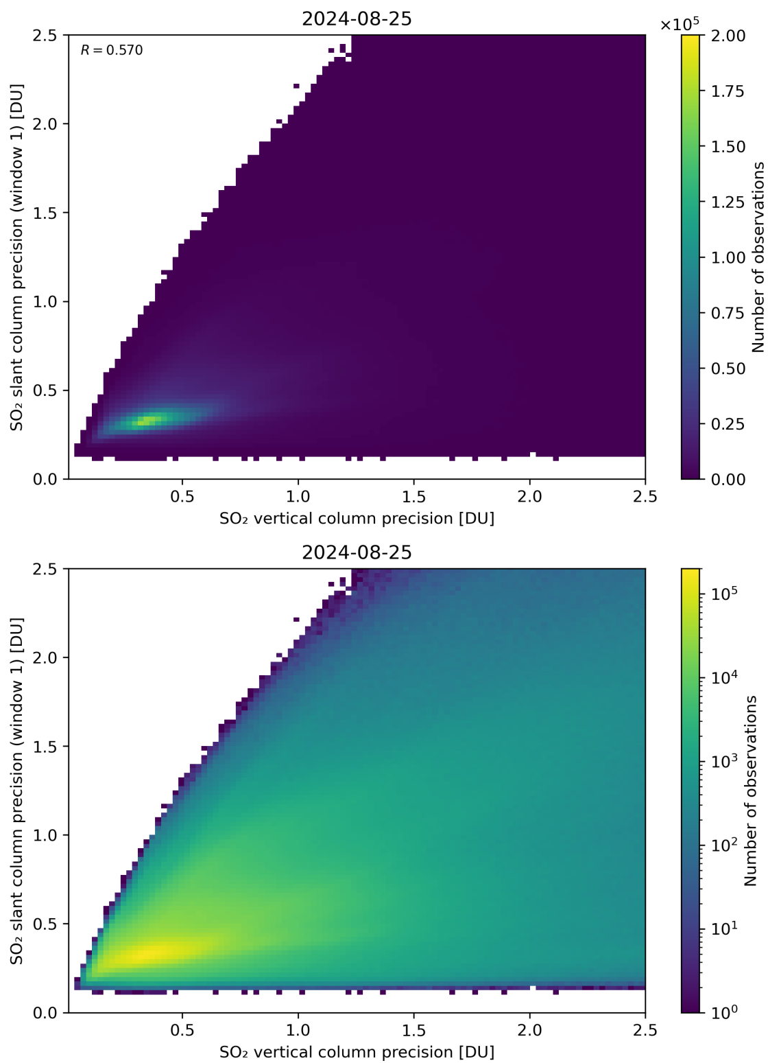
Figure 290: Scatter density plot of “SO 2 vertical column precision” against “SO 2 slant column precision (window 1)” for 2024-08-24 to 2024-08-26.
