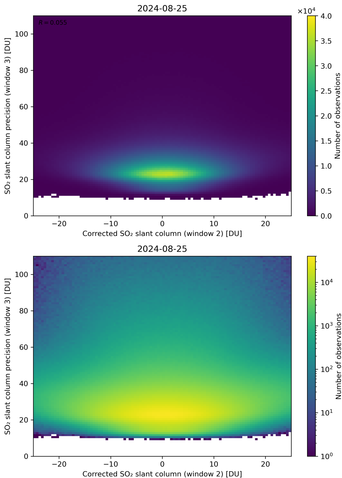
Figure 202: Scatter density plot of “Corrected SO 2 slant column (window 2)” against “SO 2 slant column precision (window 3)” for 2024-08-24 to 2024-08-26.
