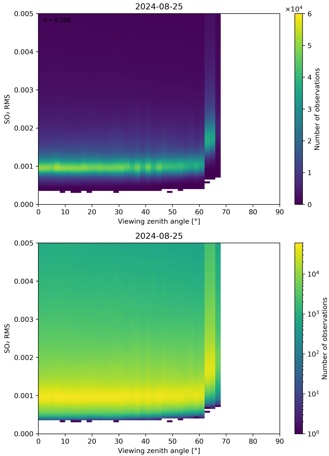
Figure 313: Scatter density plot of “Viewing zenith angle” against “SO 2 RMS” for 2024-08-24 to 2024-08-26.
