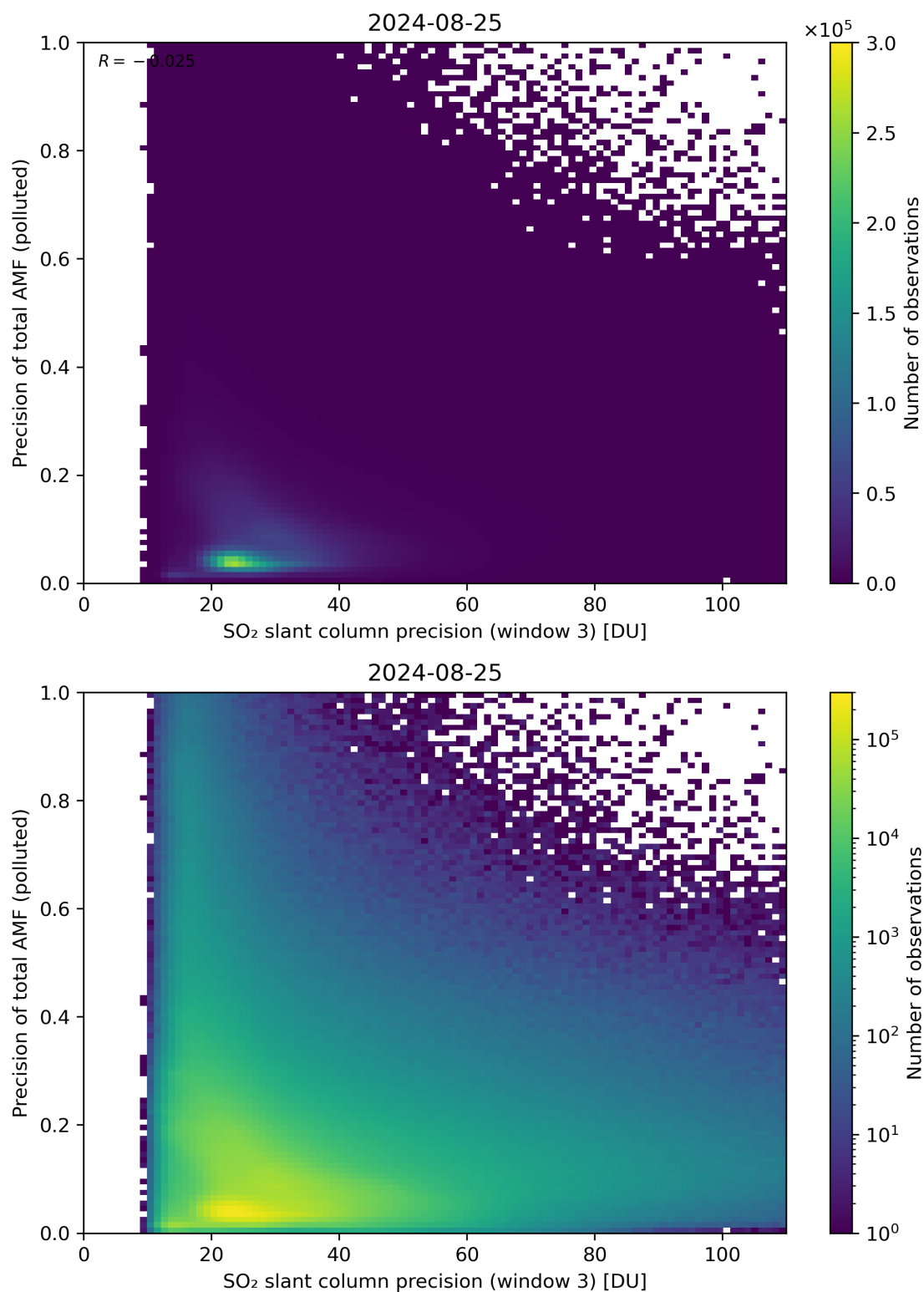
Figure 264: Scatter density plot of “SO 2 slant column precision (window 3)” against “Precision of total AMF (polluted)” for 2024-08-24 to 2024-08-26.
