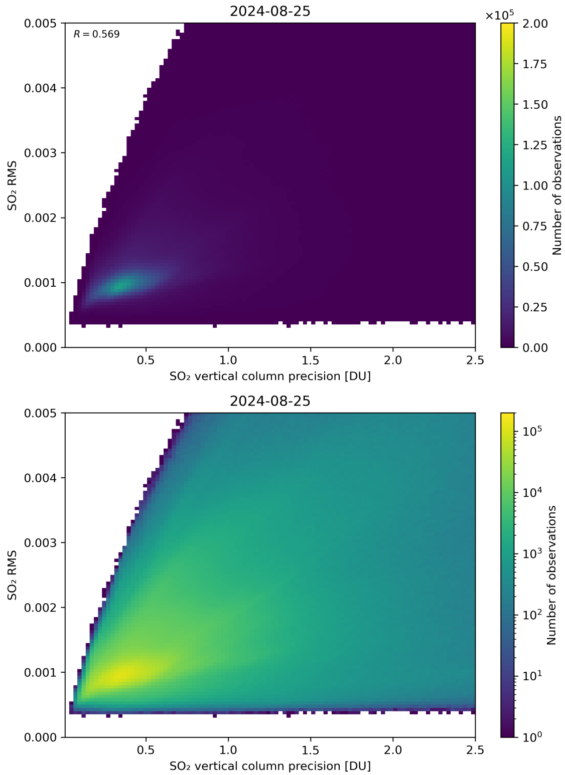
Figure 284: Scatter density plot of “SO 2 vertical column precision” against “SO 2 RMS” for 2024-08-24 to 2024-08-26.
