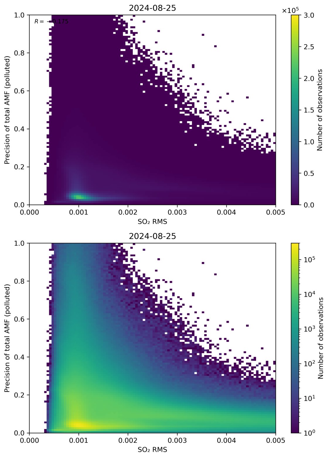
Figure 138: Scatter density plot of “SO 2 RMS” against “Precision of total AMF (polluted)” for 2024-08-24 to 2024-08-26.
