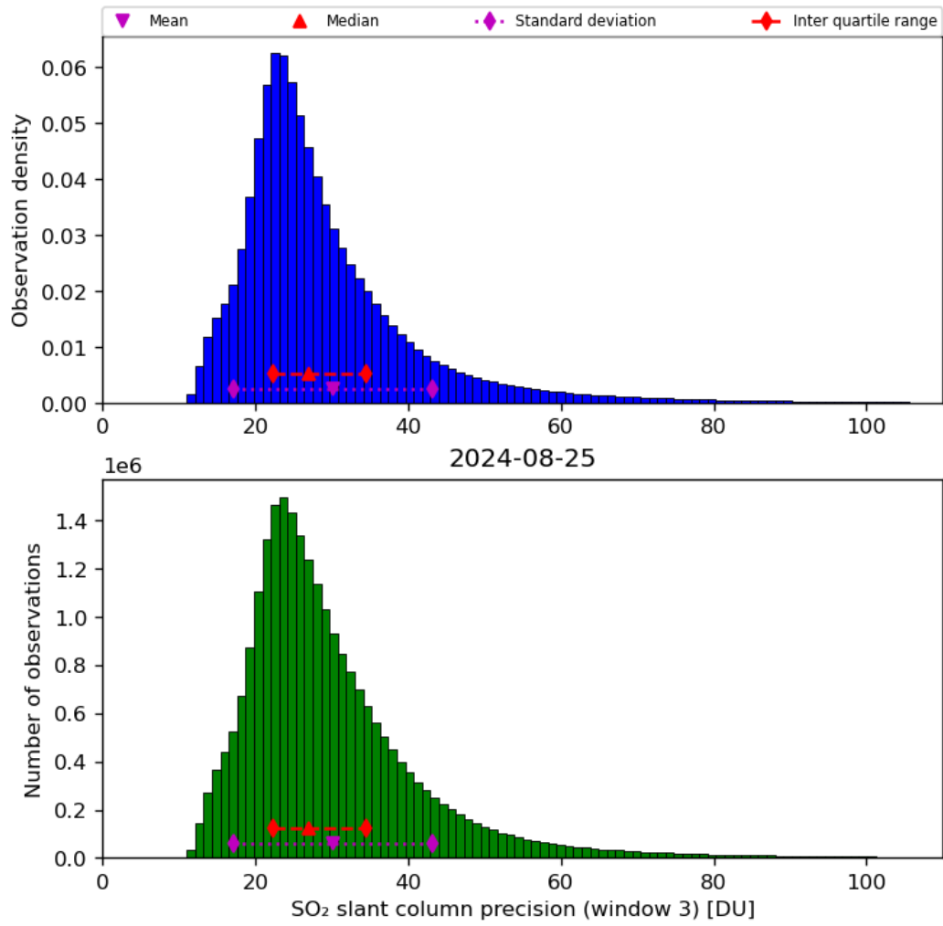
Figure 65: Histogram of “SO 2 slant column precision (window 3)” for 2024-08-24 to 2024-08-26
