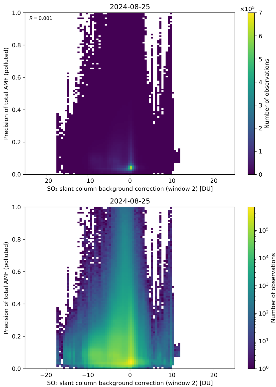
Figure 120: Scatter density plot of “SO 2 slant column background correction (window 2)” against “Precision of total AMF (polluted)” for 2024-08-24 to 2024-08-26.
