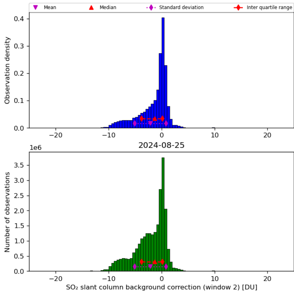
Figure 63: Histogram of “SO 2 slant column background correction (window 2)” for 2024-08-24 to 2024-08-26
