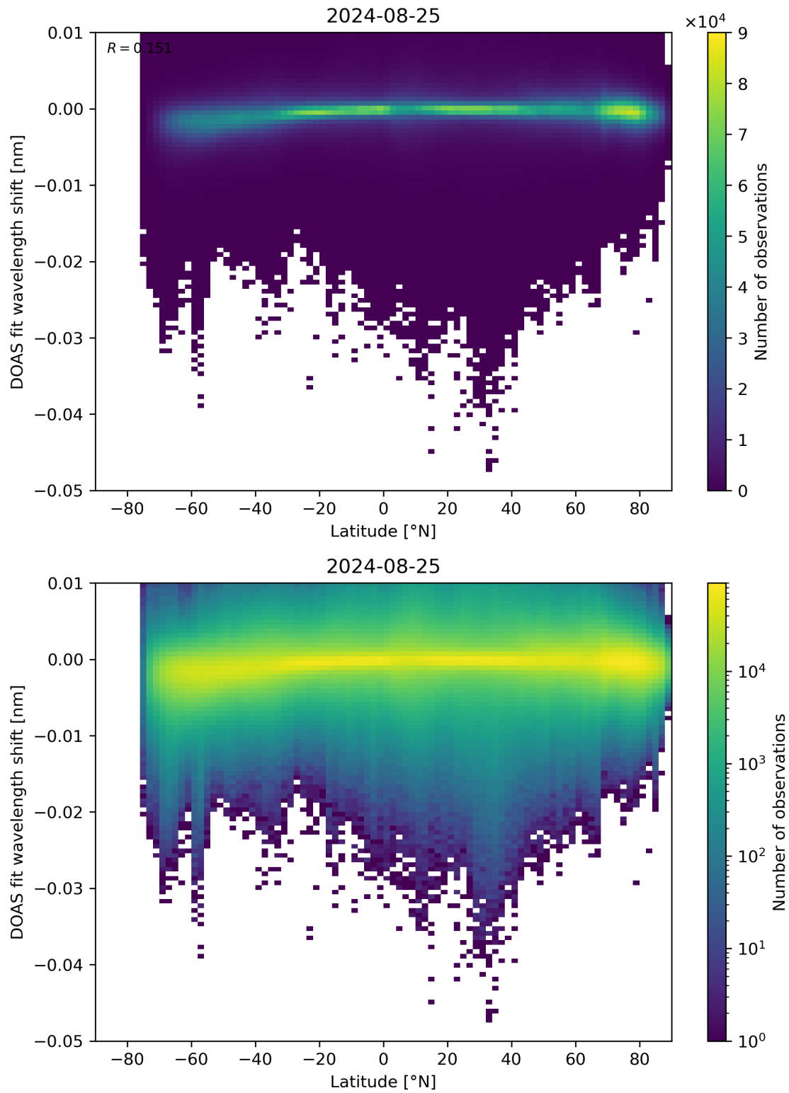
Figure 142: Scatter density plot of “Latitude” against “DOAS fit wavelength shift” for 2024-08-24 to 2024-08-26.
