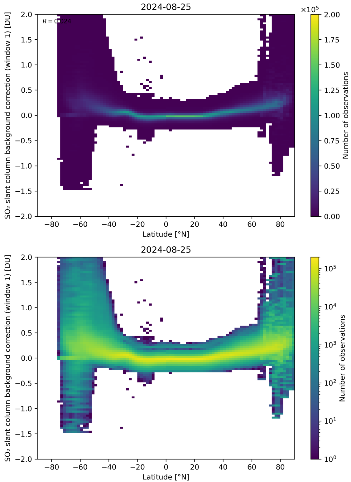
Figure 139: Scatter density plot of “Latitude” against “SO 2 slant column background correction (window 1)” for 2024-08-24 to 2024-08-26.
