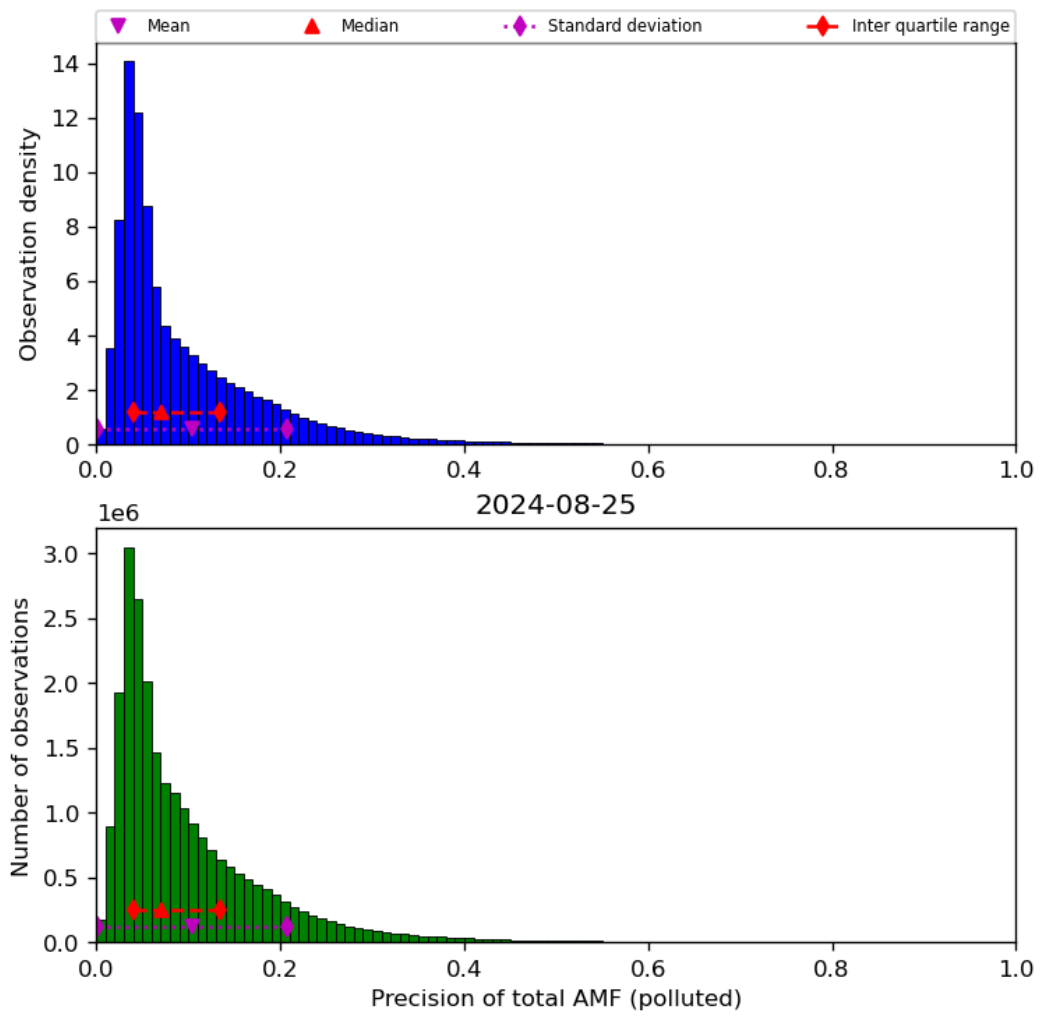
Figure 72: Histogram of “Precision of total AMF (polluted)” for 2024-08-24 to 2024-08-26
