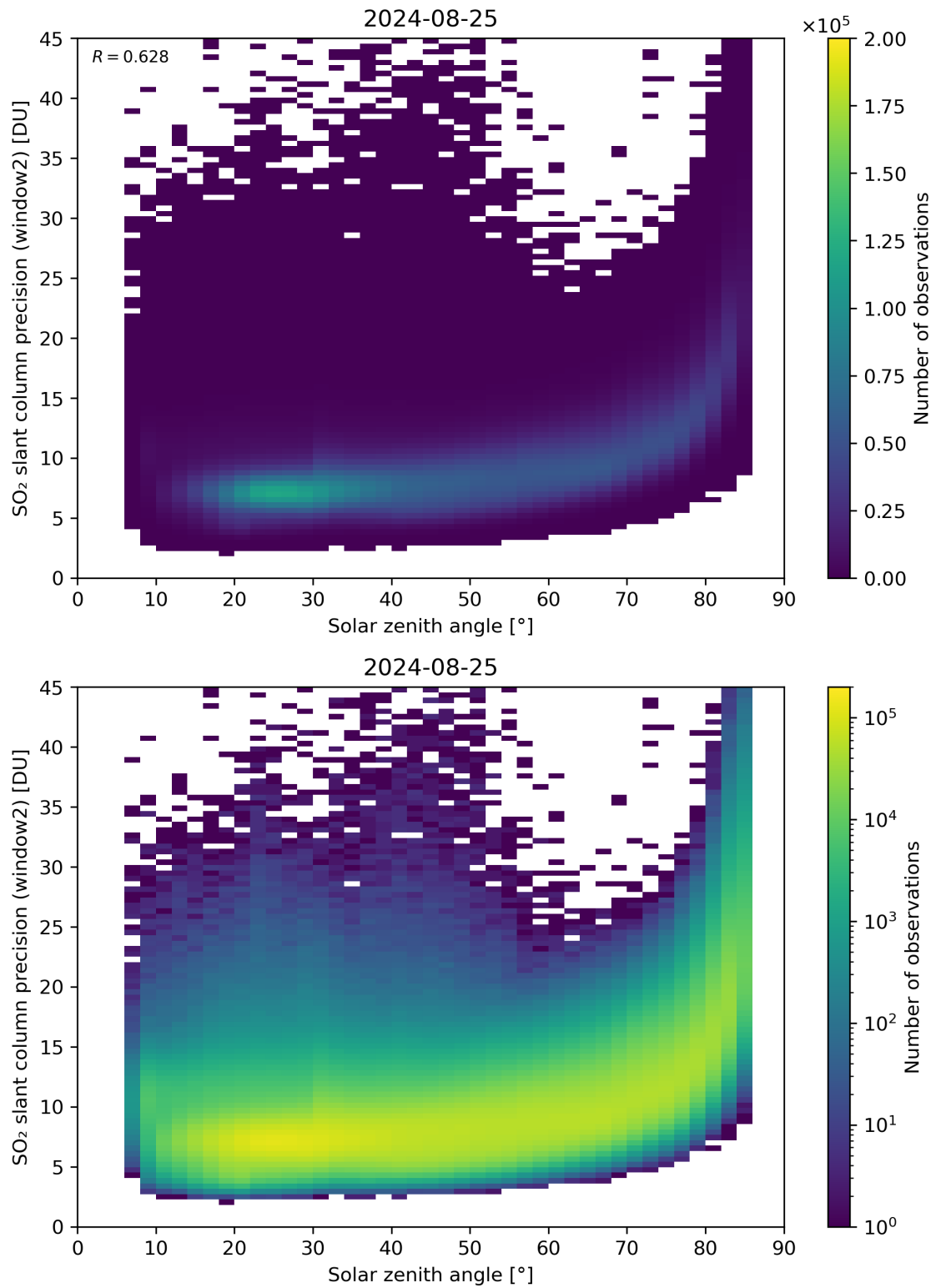
Figure 171: Scatter density plot of “Solar zenith angle” against “SO 2 slant column precision (window2)” for 2024-08-24 to 2024-08-26.
