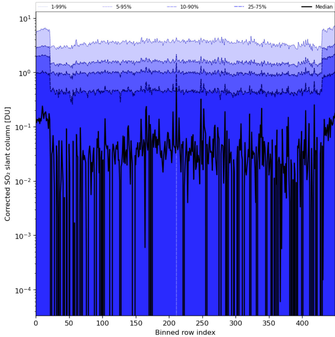
Figure 78: Along track statistics of “Corrected SO 2 slant column” for 2024-08-24 to 2024-08-26
