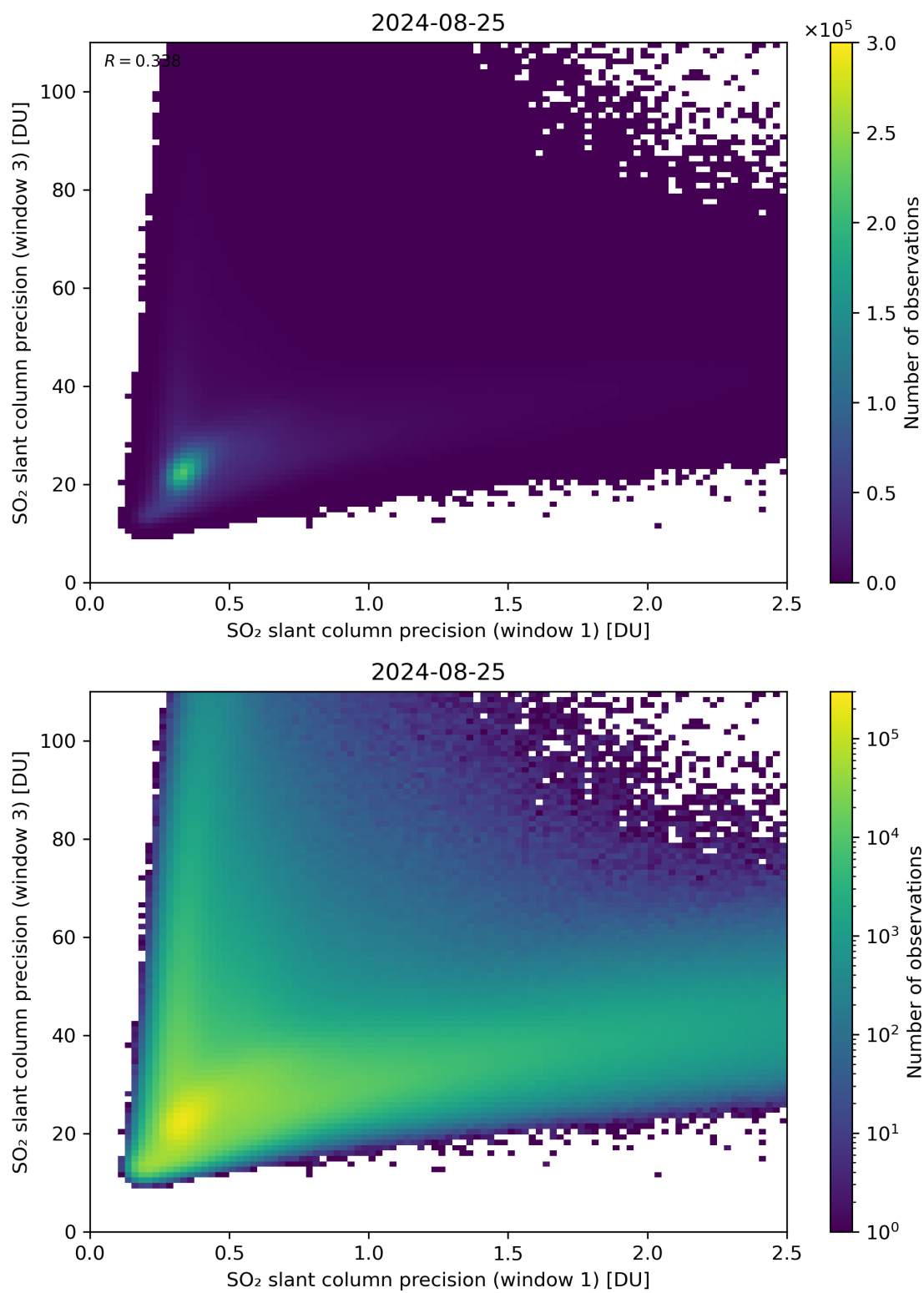
Figure 229: Scatter density plot of “SO 2 slant column precision (window 1)” against “SO 2 slant column precision (window 3)” for 2024-08-24 to 2024-08-26.
