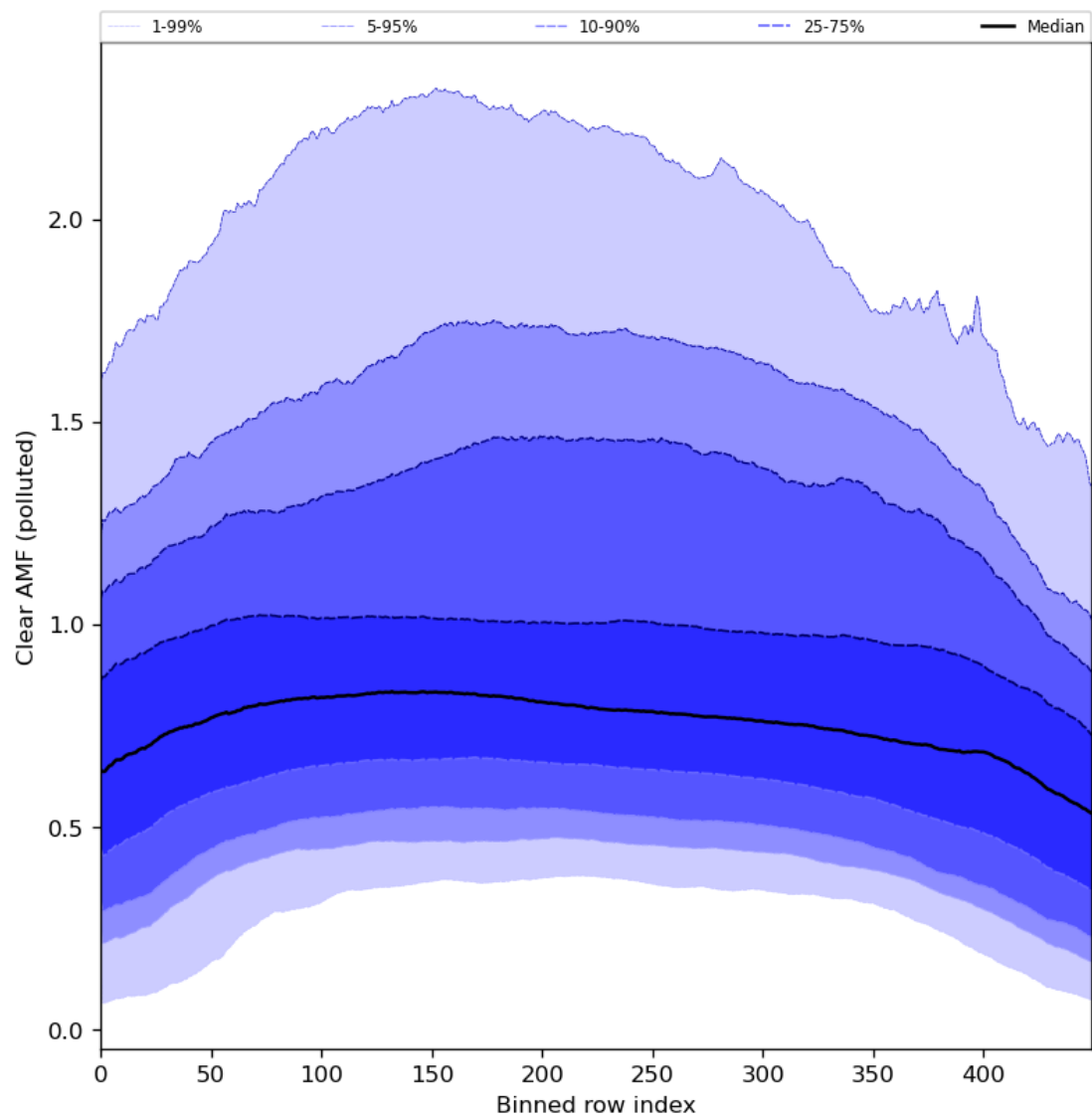
Figure 96: Along track statistics of “Clear AMF (polluted)” for 2024-08-24 to 2024-08-26
