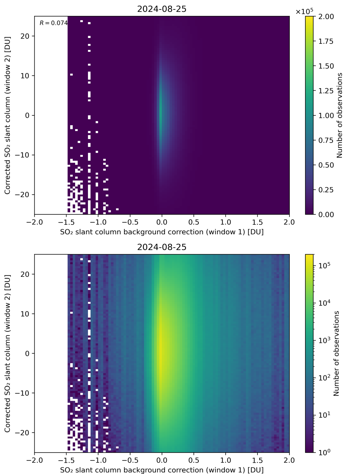
Figure 104: Scatter density plot of “SO 2 slant column background correction (window 1)” against “Corrected SO 2 slant column (window 2)” for 2024-08-24 to 2024-08-26.
