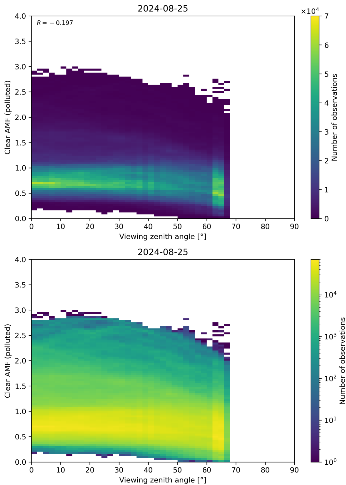
Figure 316: Scatter density plot of “Viewing zenith angle” against “Clear AMF (polluted)” for 2024-08-24 to 2024-08-26.
