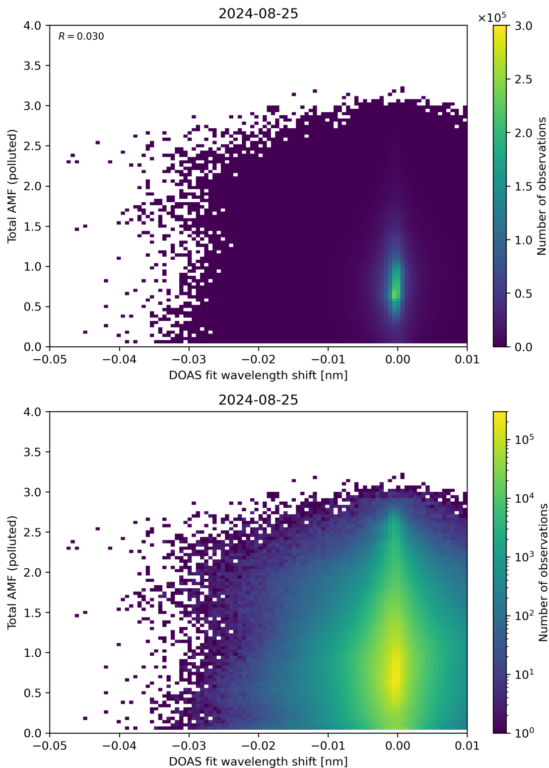
Figure 130: Scatter density plot of “DOAS fit wavelength shift” against “Total AMF (polluted)” for 2024-08-24 to 2024-08-26.
