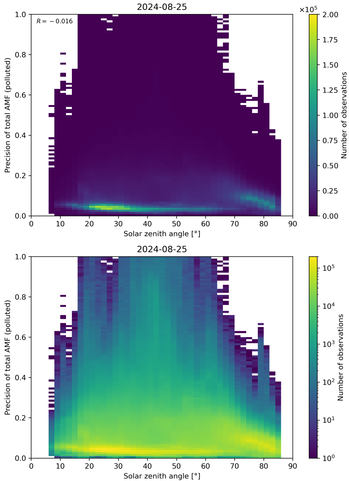
Figure 175: Scatter density plot of “Solar zenith angle” against “Precision of total AMF (polluted)” for 2024-08-24 to 2024-08-26.
