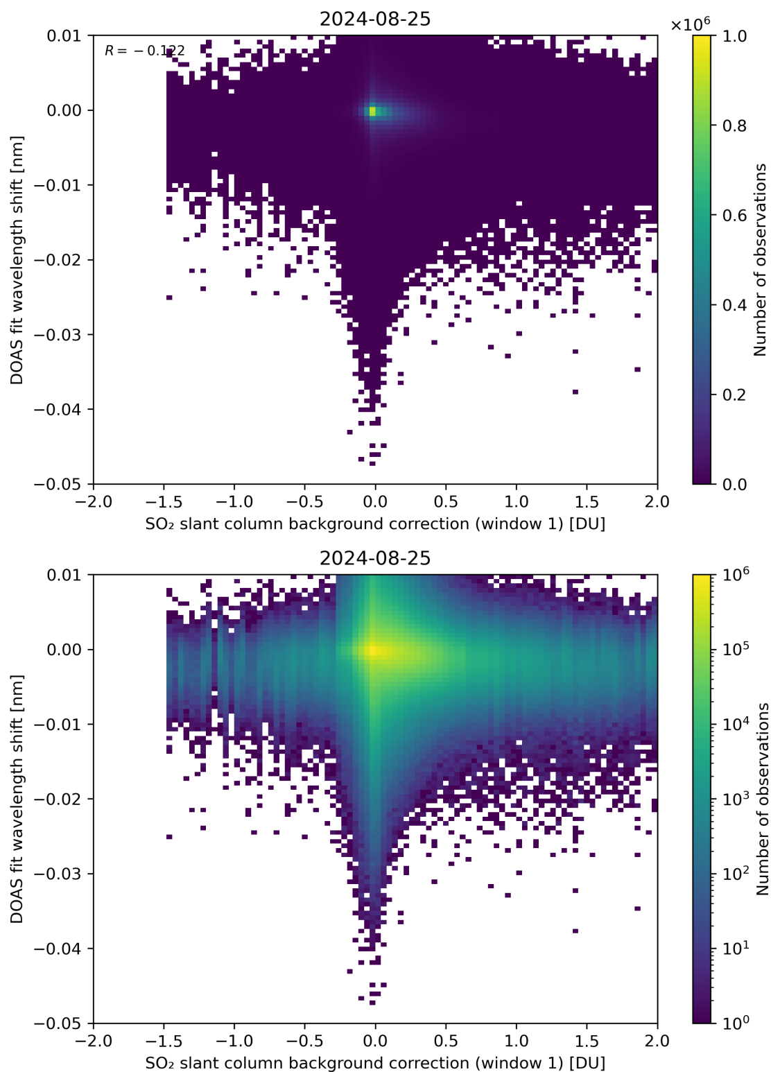
Figure 100: Scatter density plot of “SO 2 slant column background correction (window 1)” against “DOAS fit wavelength shift” for 2024-08-24 to 2024-08-26.
