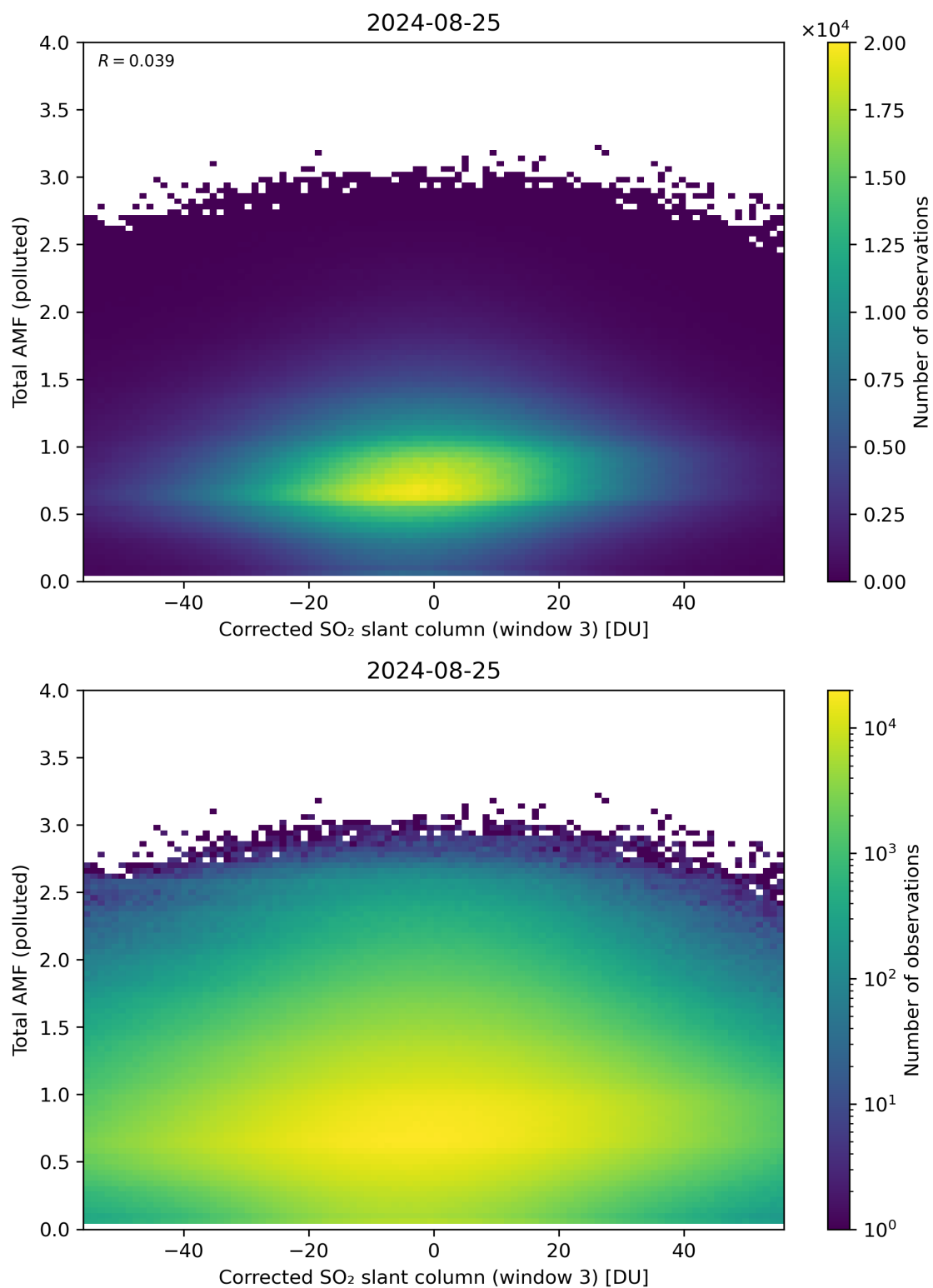
Figure 210: Scatter density plot of “Corrected SO 2 slant column (window 3)” against “Total AMF (polluted)” for 2024-08-24 to 2024-08-26.
