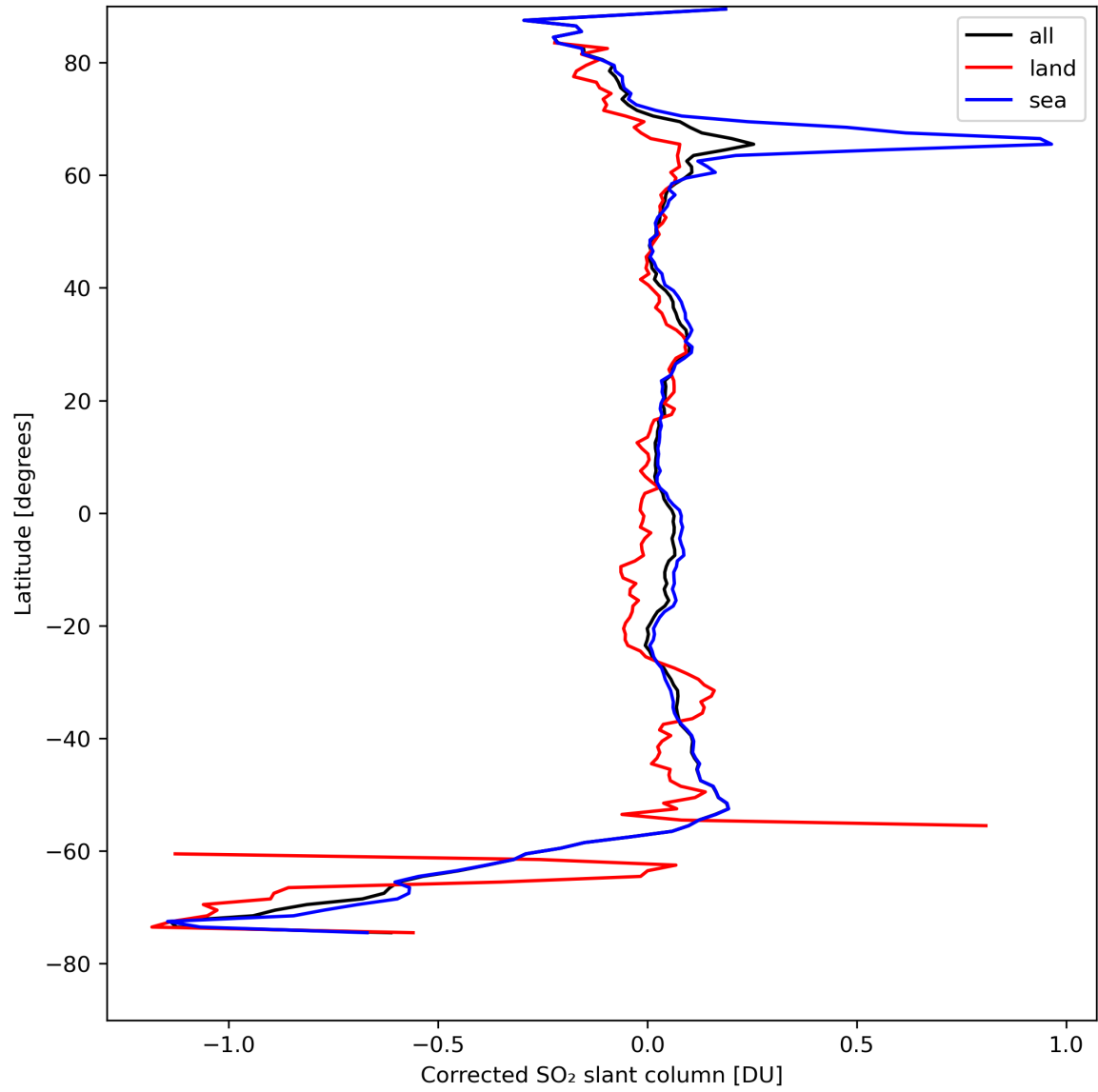
Figure 32: Zonal average of “Corrected SO 2 slant column” for 2024-08-24 to 2024-08-26.
