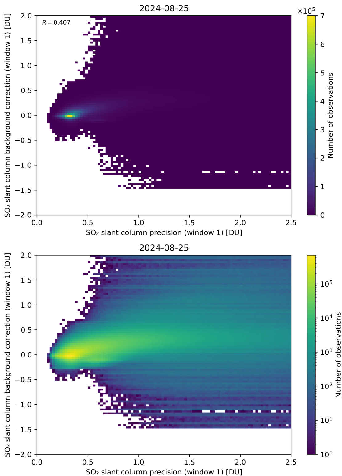
Figure 218: Scatter density plot of “SO 2 slant column precision (window 1)” against “SO 2 slant column background correction (window 1)” for 2024-08-24 to 2024-08-26.
