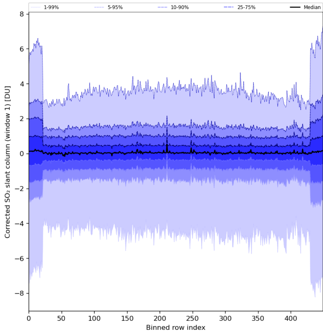
Figure 81: Along track statistics of “Corrected SO 2 slant column (window 1)” for 2024-08-24 to 2024-08-26
