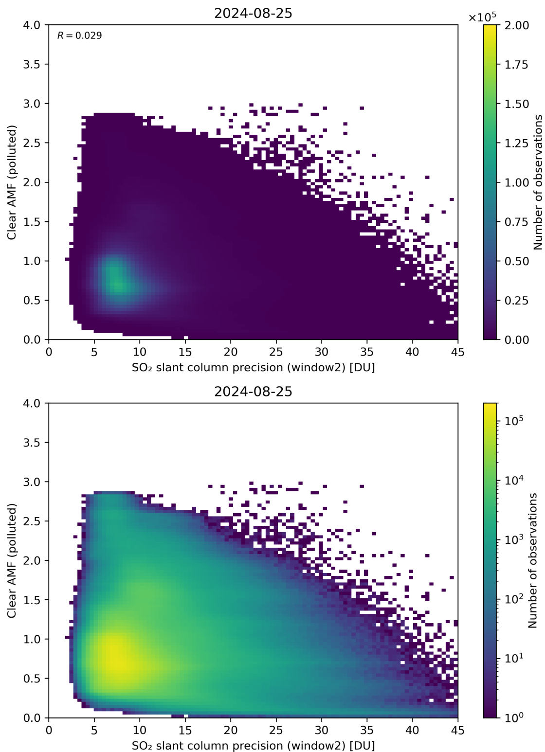
Figure 246: Scatter density plot of “SO 2 slant column precision (window2)” against “Clear AMF (polluted)” for 2024-08-24 to 2024-08-26.
