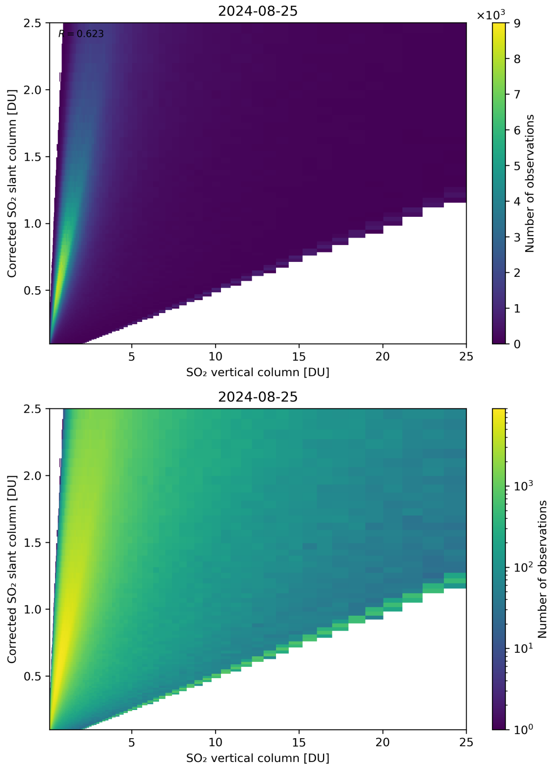
Figure 297: Scatter density plot of “SO 2 vertical column” against “Corrected SO 2 slant column” for 2024-08-24 to 2024-08-26.
