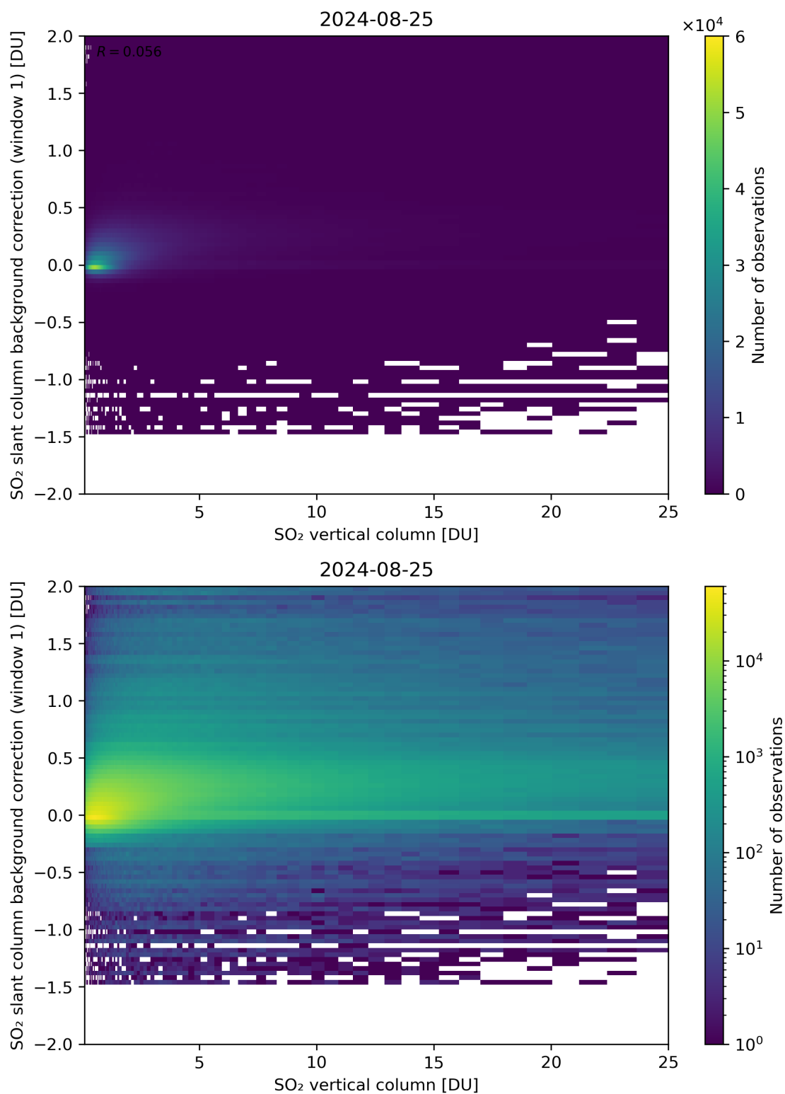
Figure 273: Scatter density plot of “SO 2 vertical column” against “SO 2 slant column background correction (window 1)” for 2024-08-24 to 2024-08-26.
