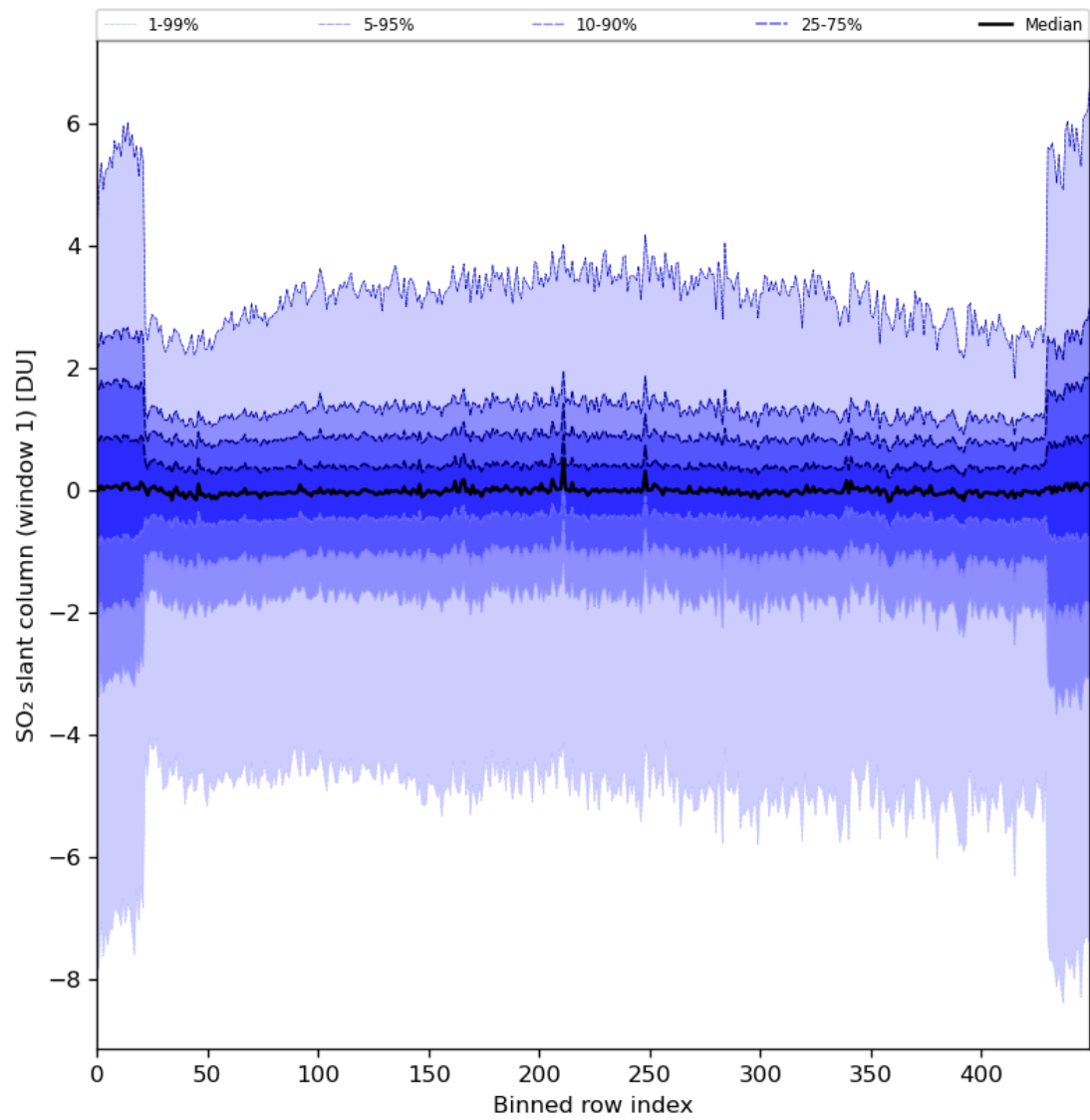
Figure 79: Along track statistics of “SO 2 slant column (window 1)” for 2024-08-24 to 2024-08-26
