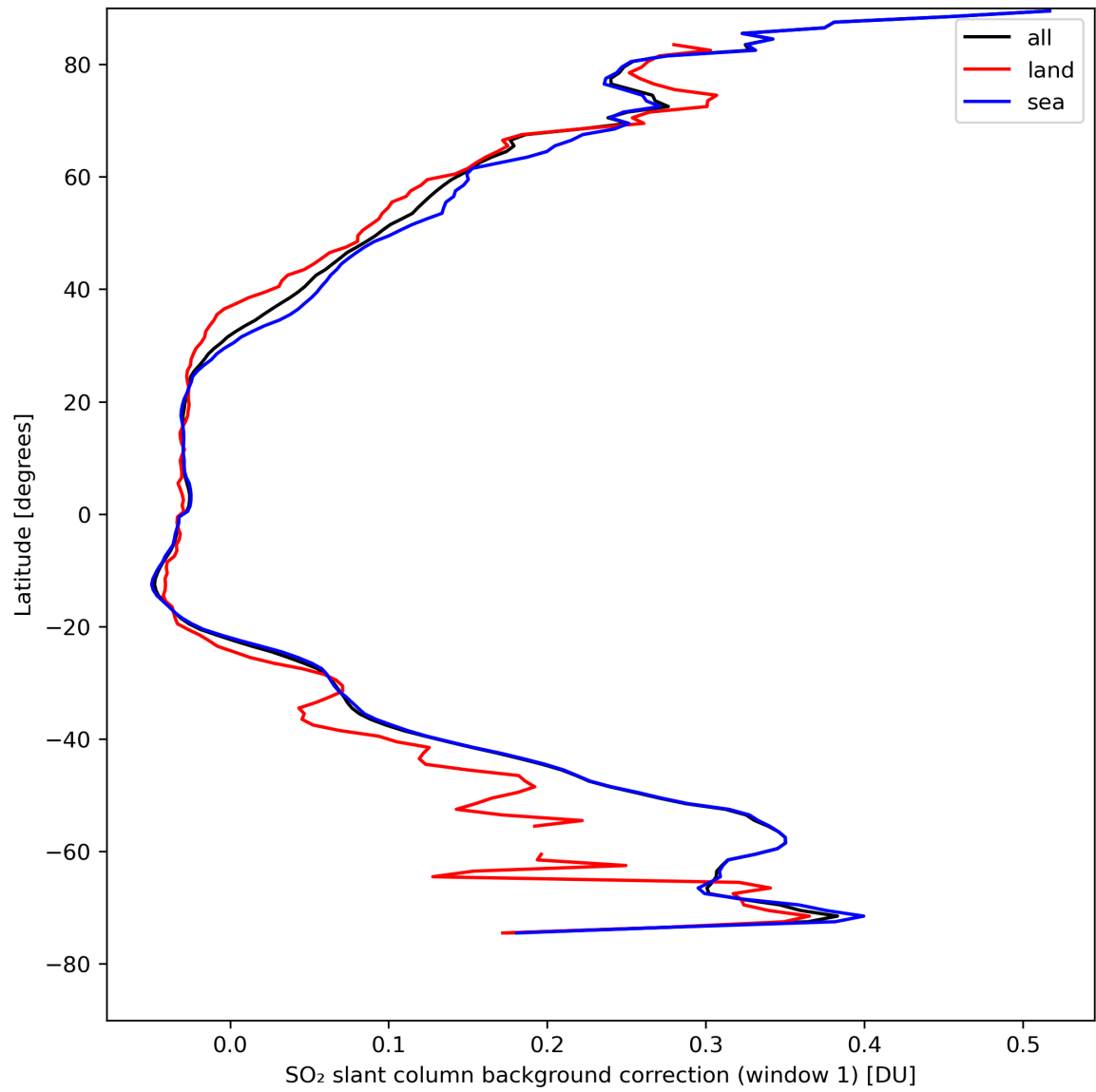
Figure 36: Zonal average of “SO 2 slant column background correction (window 1)” for 2024-08-24 to 2024-08-26.
