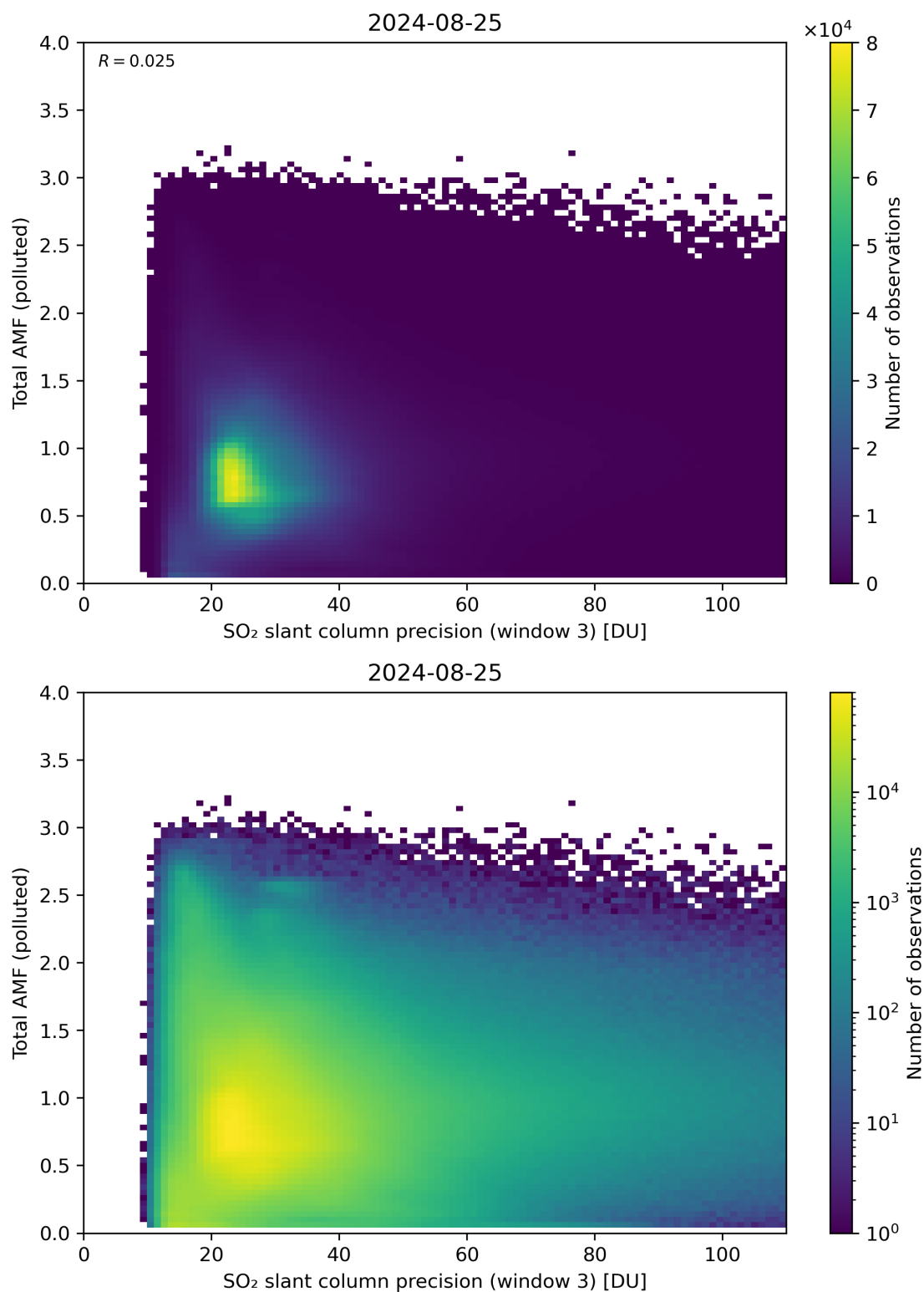
Figure 263: Scatter density plot of “SO 2 slant column precision (window 3)” against “Total AMF (polluted)” for 2024-08-24 to 2024-08-26.
