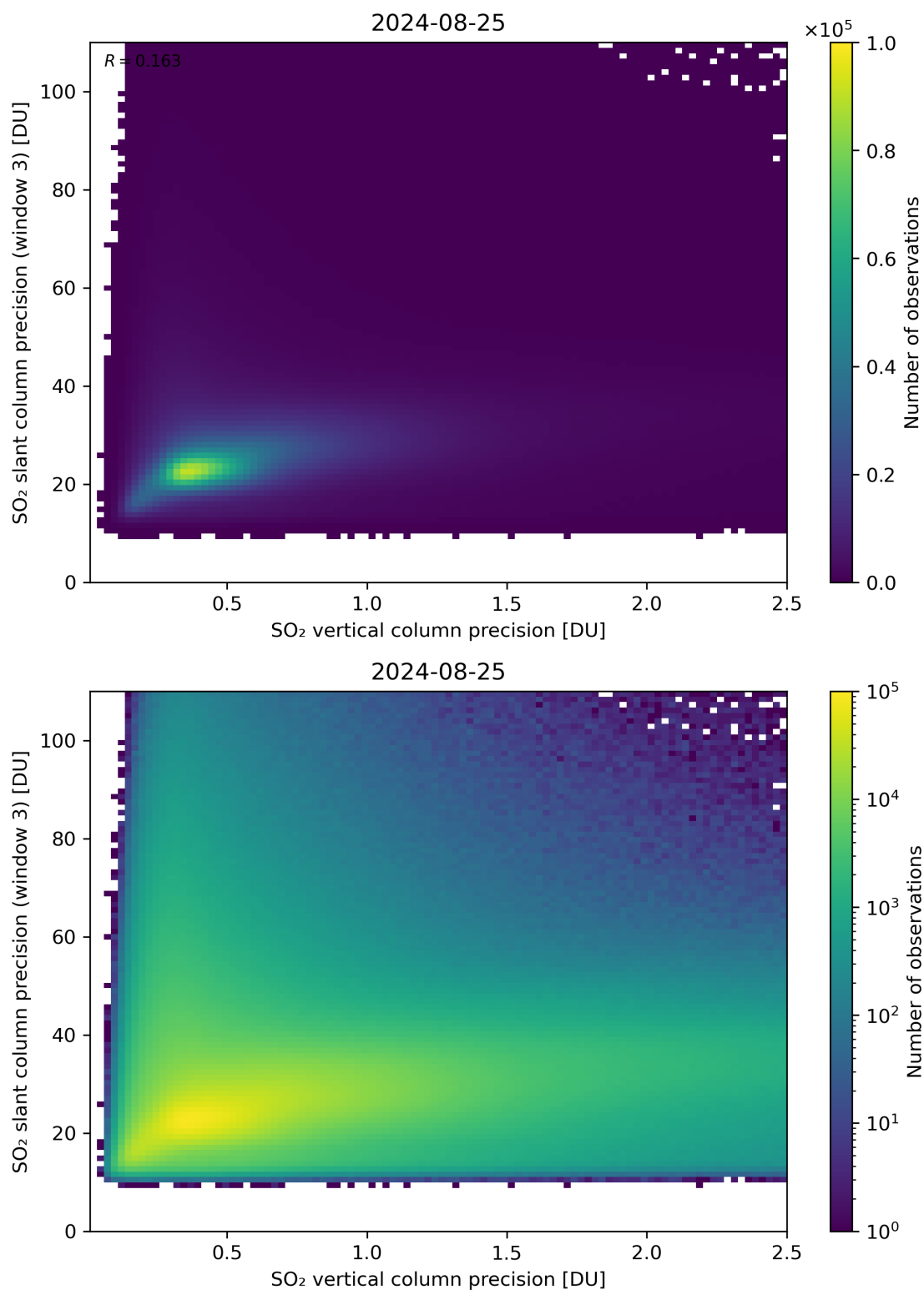
Figure 293: Scatter density plot of “SO 2 vertical column precision” against “SO 2 slant column precision (window 3)” for 2024-08-24 to 2024-08-26.
