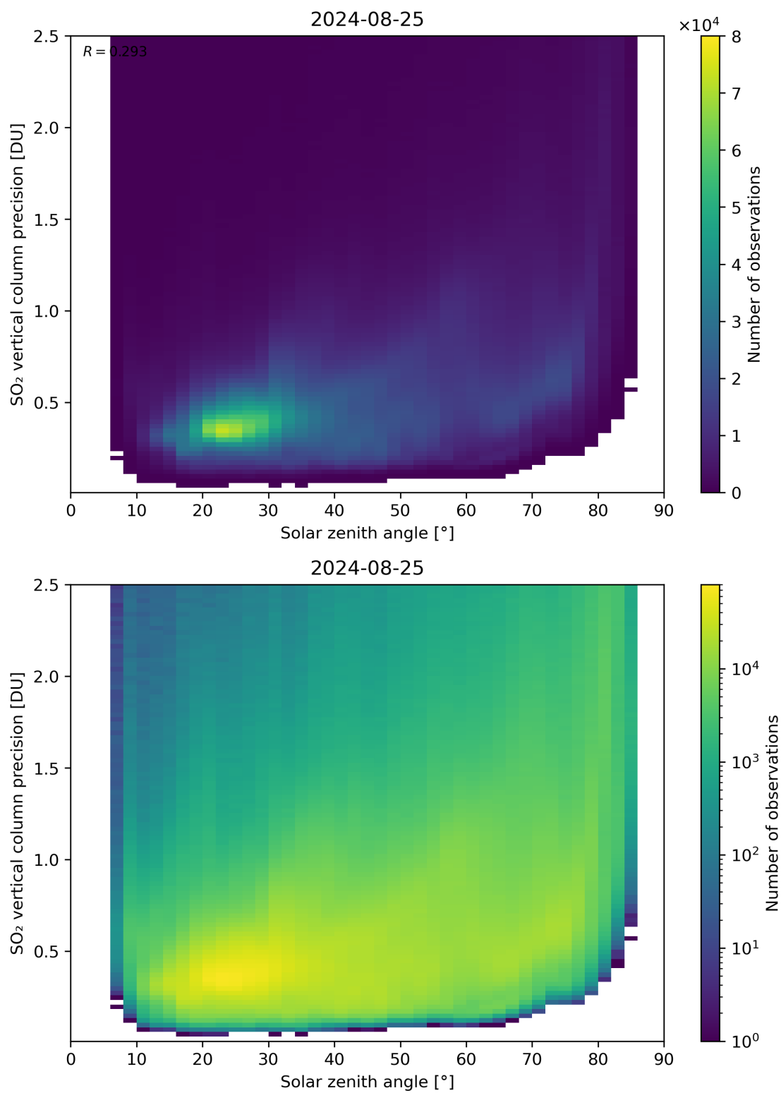
Figure 177: Scatter density plot of “Solar zenith angle” against “SO 2 vertical column precision” for 2024-08-24 to 2024-08-26.
