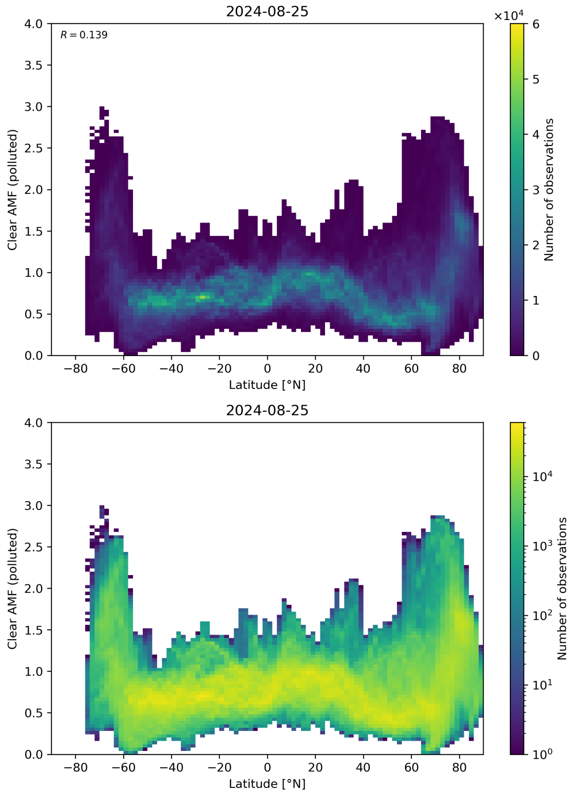
Figure 145: Scatter density plot of “Latitude” against “Clear AMF (polluted)” for 2024-08-24 to 2024-08-26.
