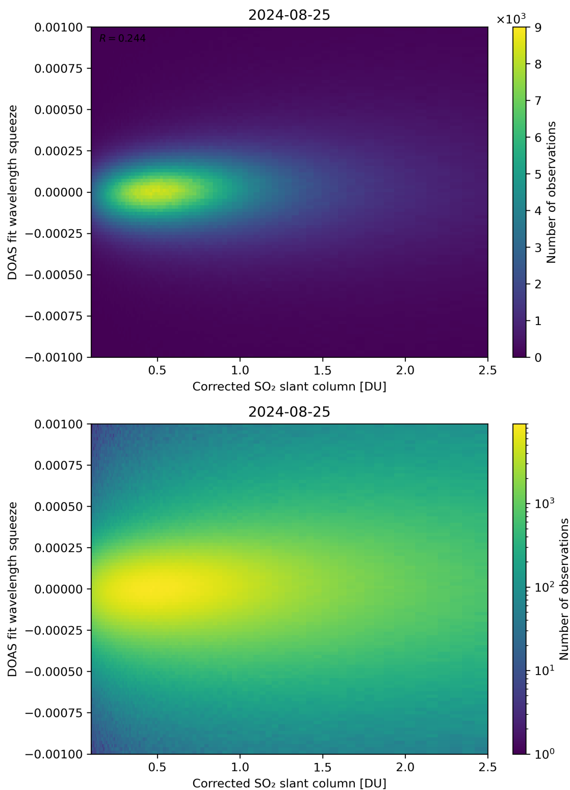
Figure 182: Scatter density plot of “Corrected SO 2 slant column” against “DOAS fit wavelength squeeze” for 2024-08-24 to 2024-08-26.
