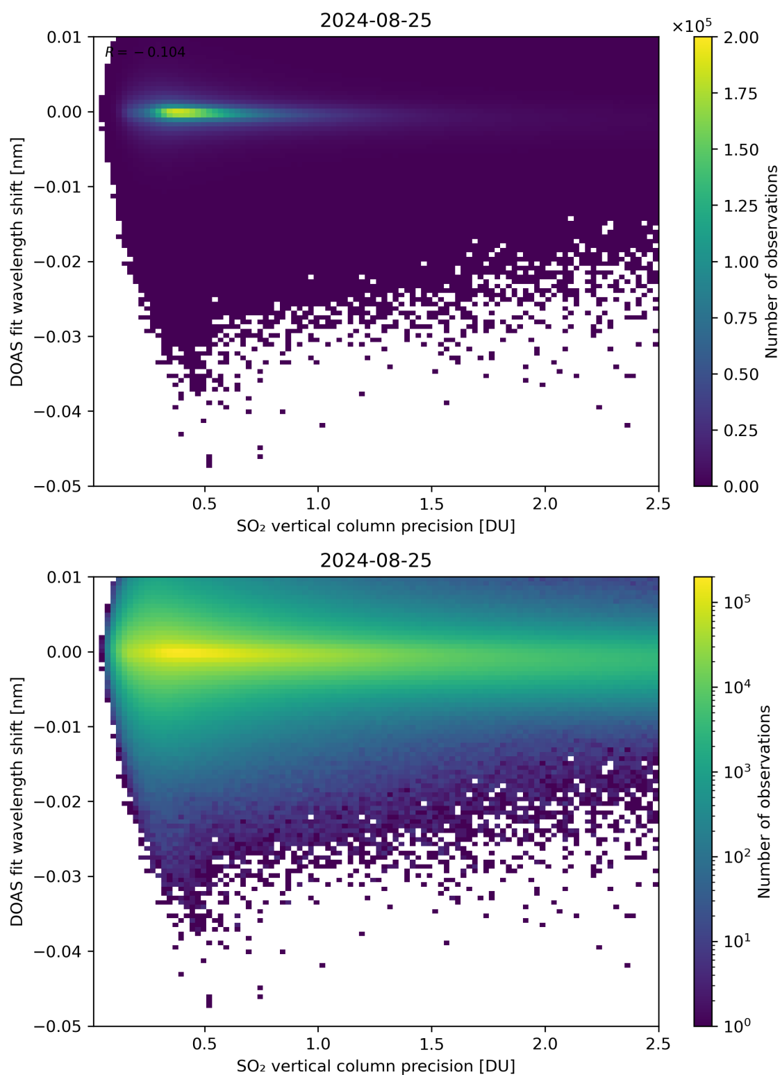
Figure 282: Scatter density plot of “SO 2 vertical column precision” against “DOAS fit wavelength shift” for 2024-08-24 to 2024-08-26.
