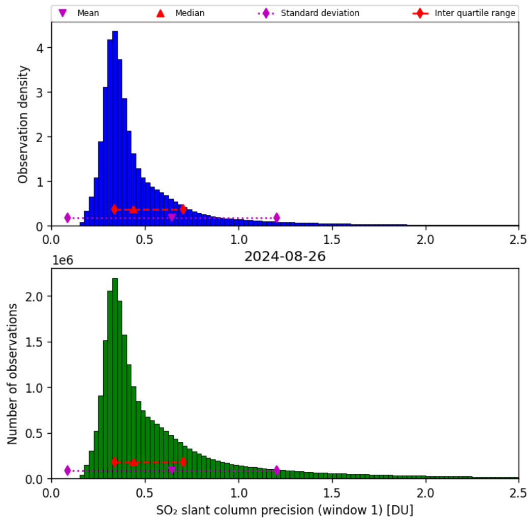
Figure 57: Histogram of “SO 2 slant column precision (window 1)” for 2024-08-25 to 2024-08-27
