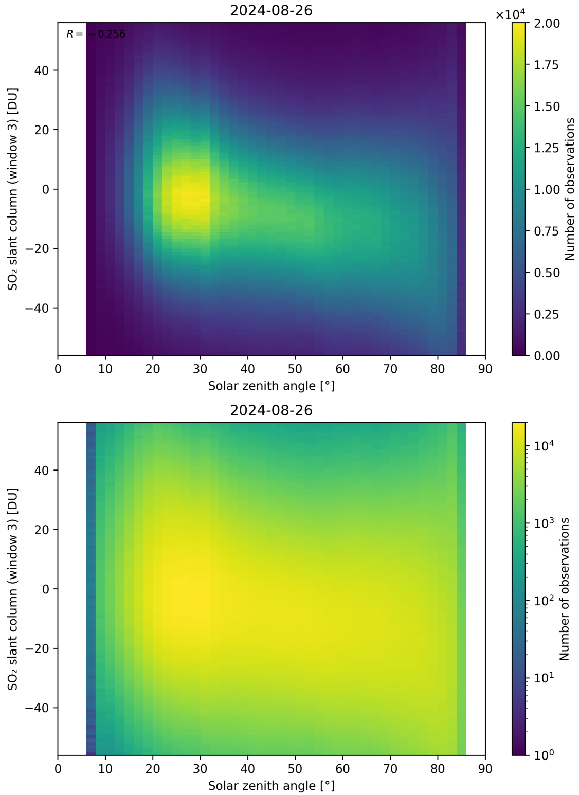
Figure 172: Scatter density plot of “Solar zenith angle” against “SO 2 slant column (window 3)” for 2024-08-25 to 2024-08-27.
