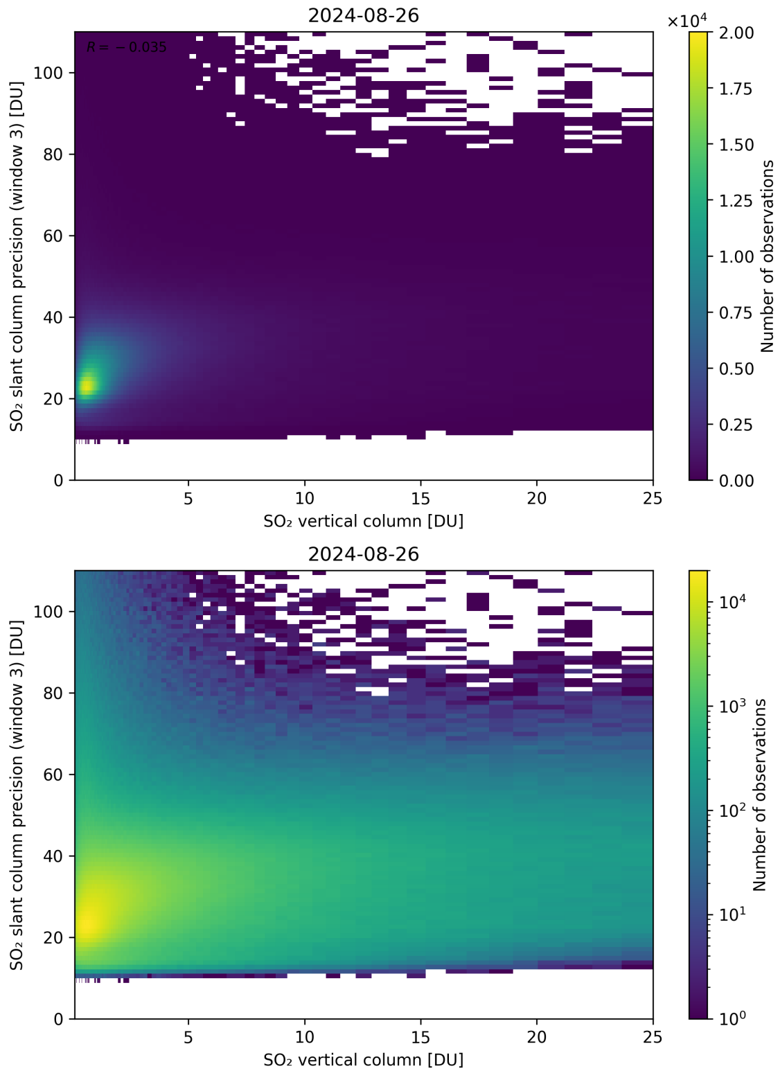
Figure 304: Scatter density plot of “SO 2 vertical column” against “SO 2 slant column precision (window 3)” for 2024-08-25 to 2024-08-27.
