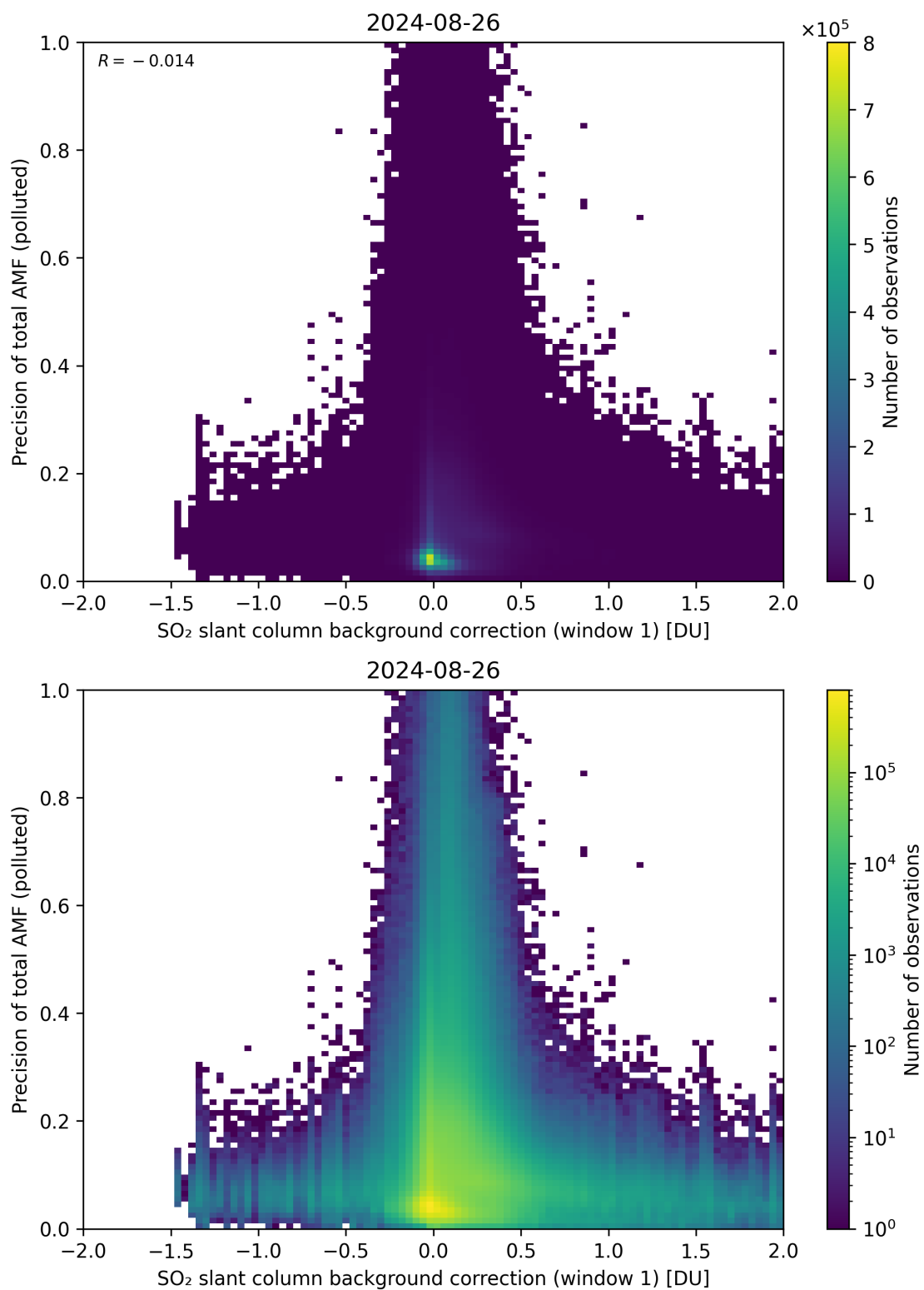
Figure 110: Scatter density plot of “SO 2 slant column background correction (window 1)” against “Precision of total AMF (polluted)” for 2024-08-25 to 2024-08-27.
