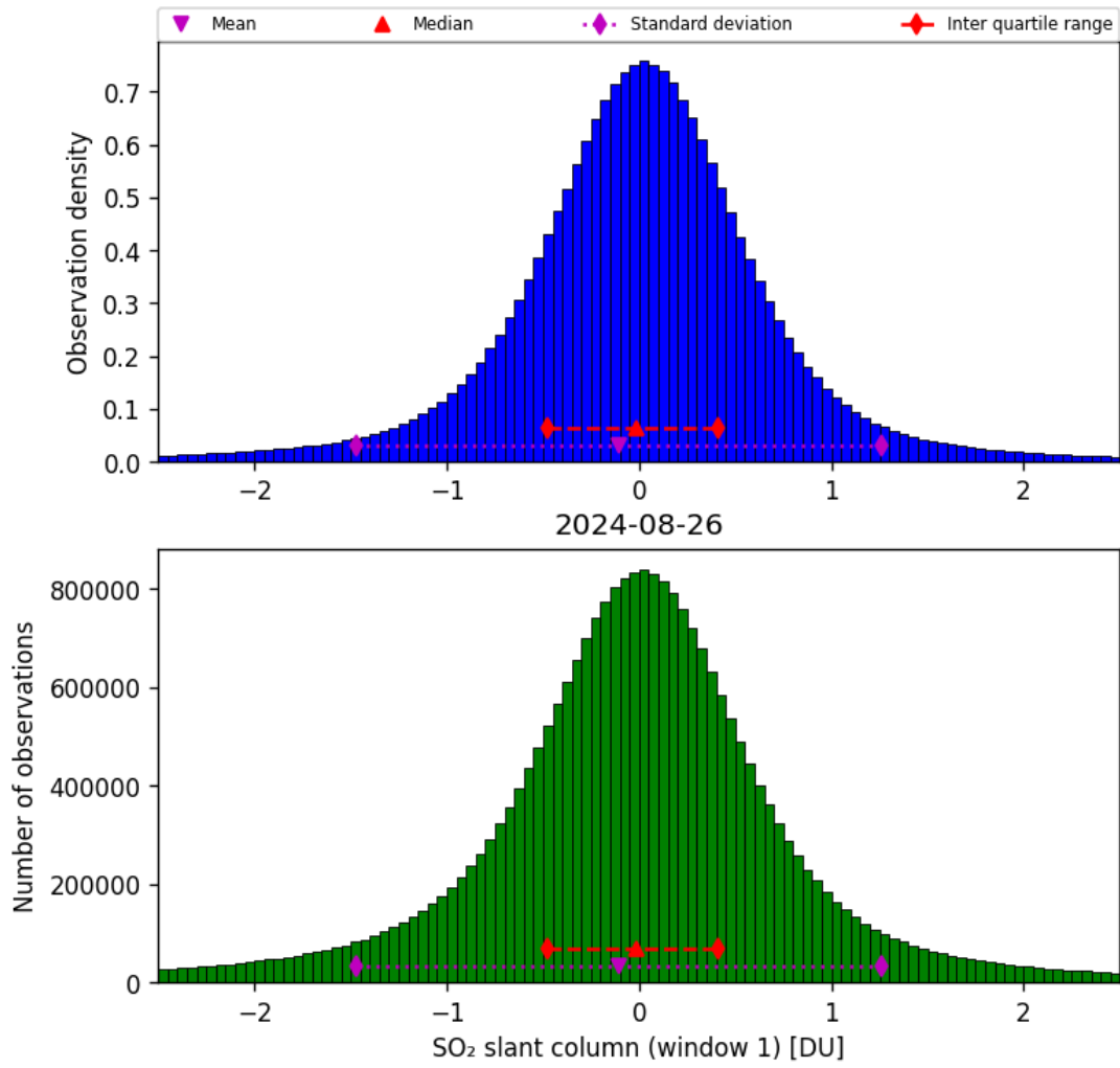
Figure 56: Histogram of “SO 2 slant column (window 1)” for 2024-08-25 to 2024-08-27
