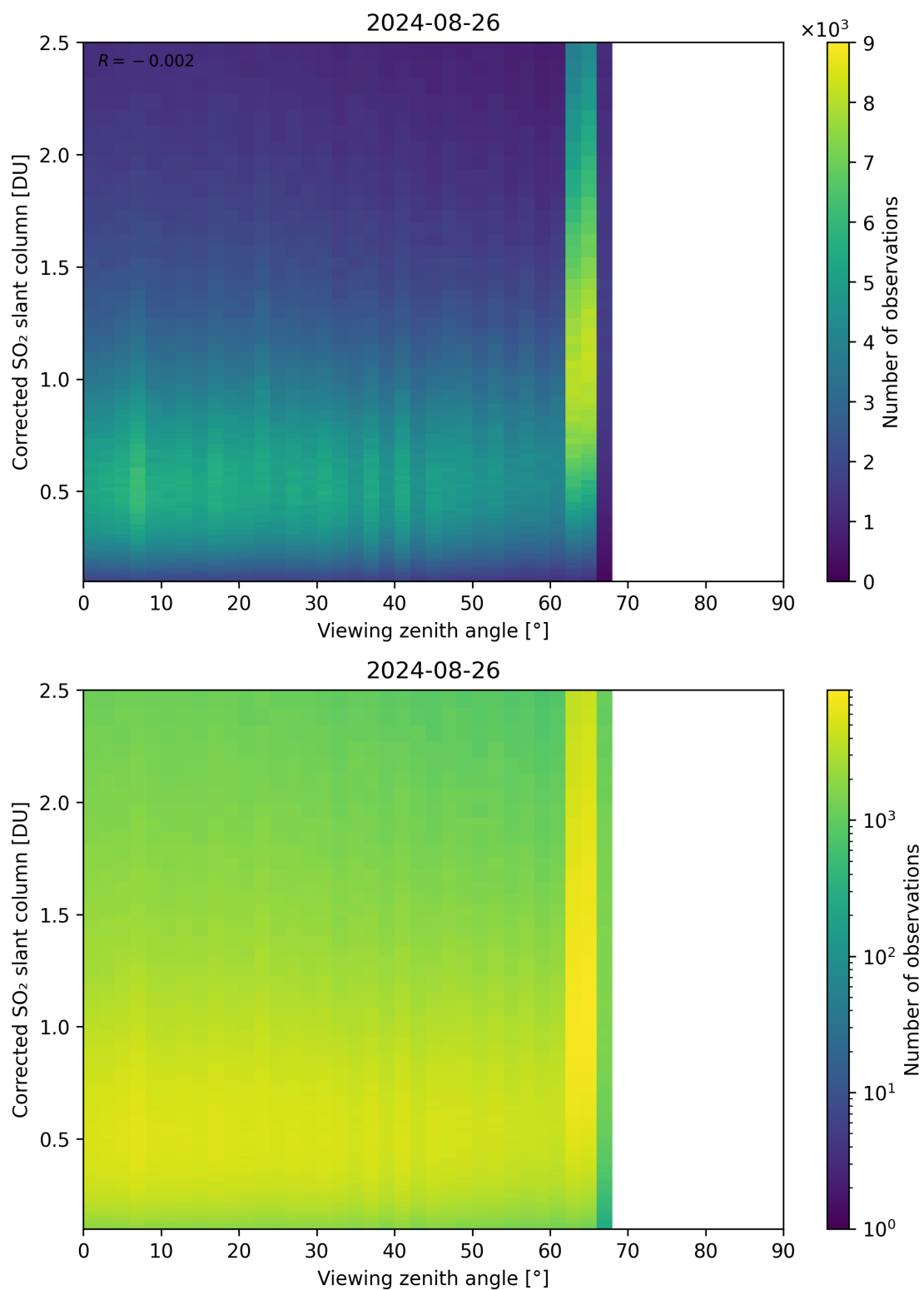
Figure 317: Scatter density plot of “Viewing zenith angle” against “Corrected SO 2 slant column” for 2024-08-25 to 2024-08-27.
