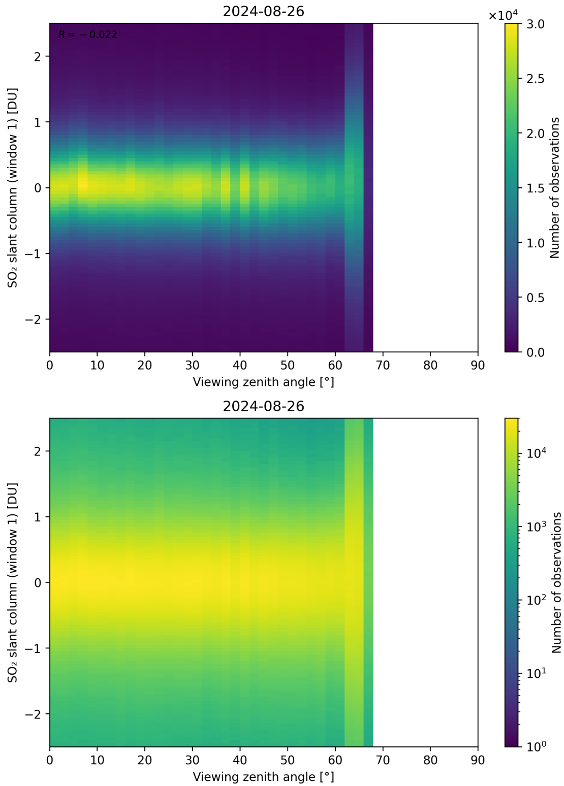
Figure 320: Scatter density plot of “Viewing zenith angle” against “SO 2 slant column (window 1)” for 2024-08-25 to 2024-08-27.
