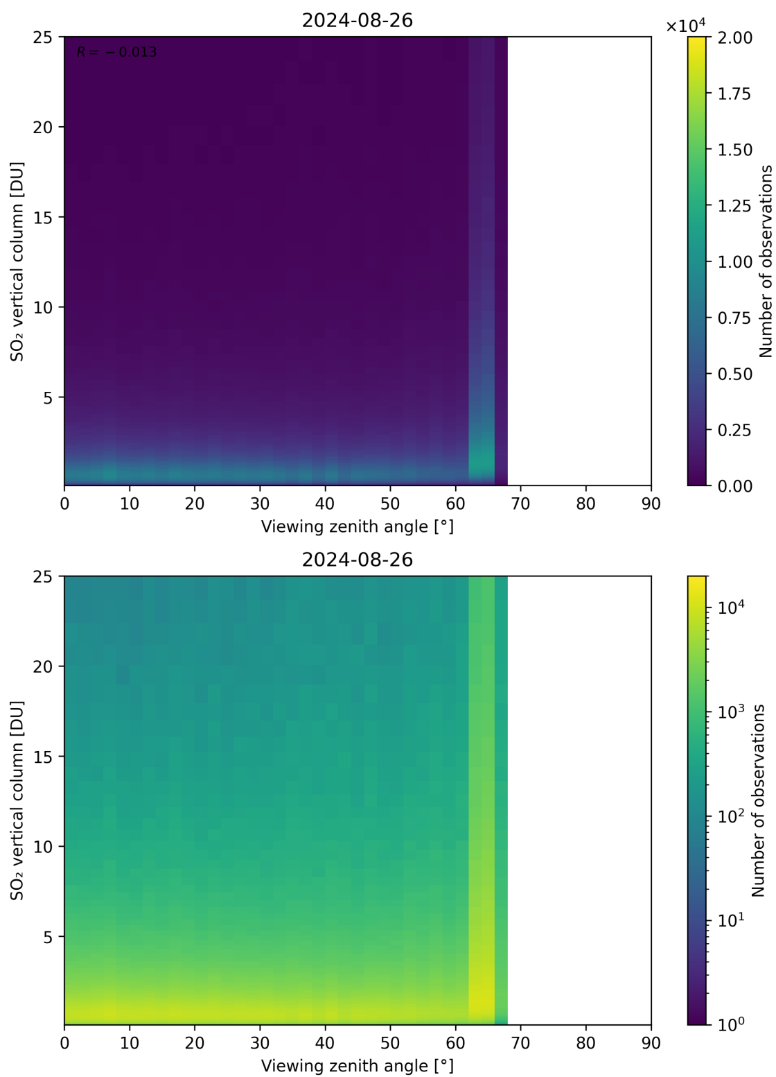
Figure 327: Scatter density plot of “Viewing zenith angle” against “SO 2 vertical column” for 2024-08-25 to 2024-08-27.
