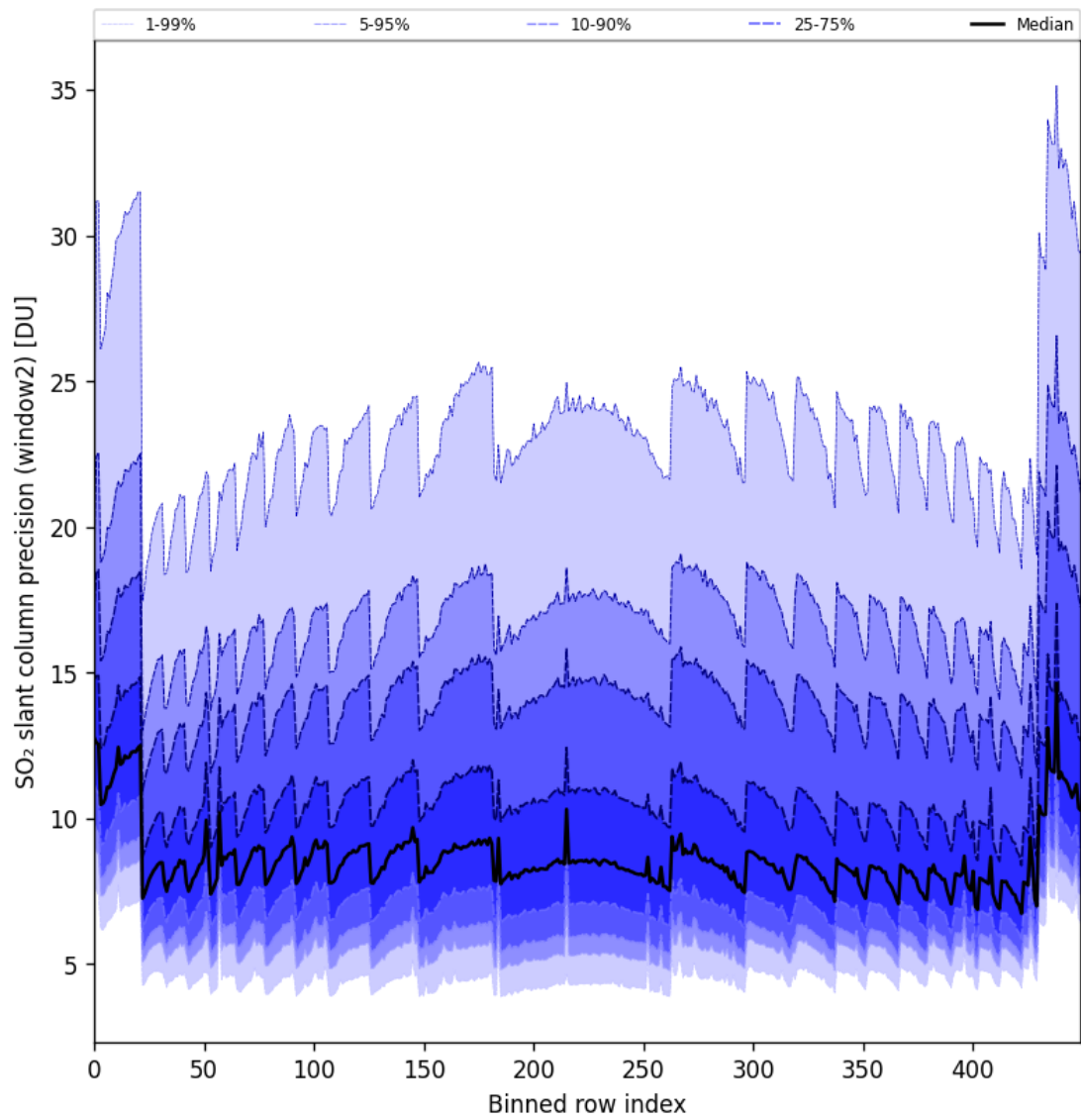
Figure 84: Along track statistics of “SO 2 slant column precision (window2)” for 2024-08-25 to 2024-08-27
