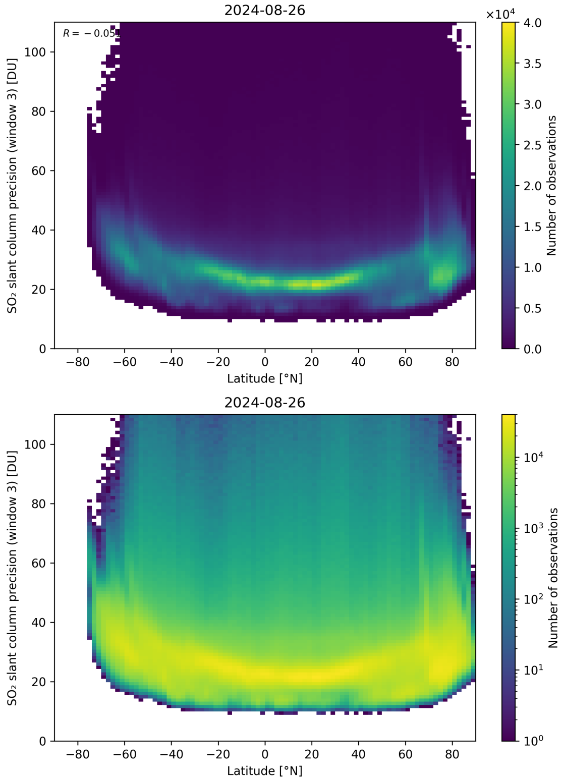
Figure 153: Scatter density plot of “Latitude” against “SO 2 slant column precision (window 3)” for 2024-08-25 to 2024-08-27.
