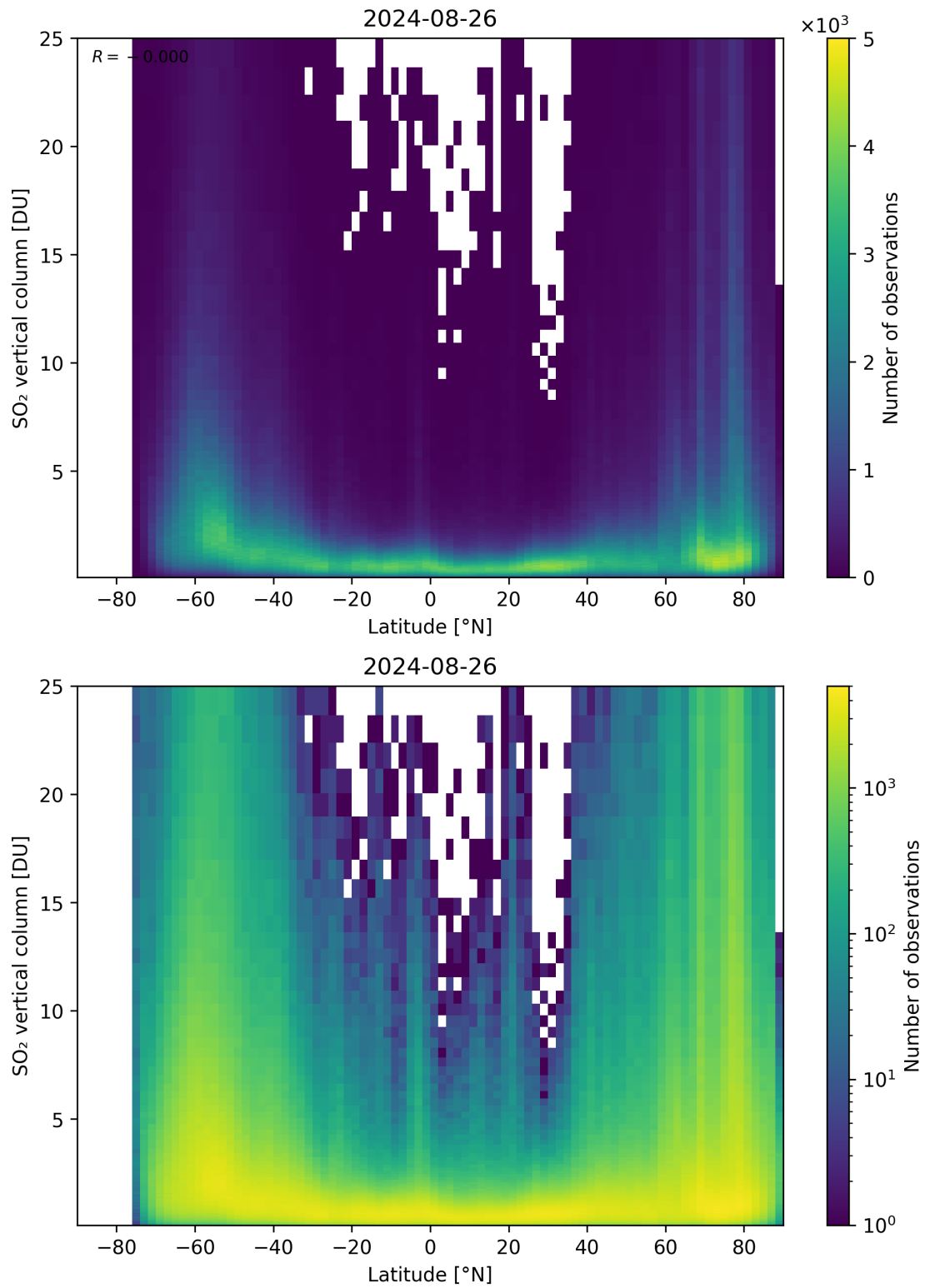
Figure 156: Scatter density plot of “Latitude” against “SO 2 vertical column” for 2024-08-25 to 2024-08-27.
