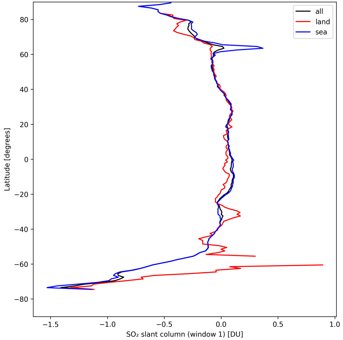
Figure 33: Zonal average of “SO 2 slant column (window 1)” for 2024-08-25 to 2024-08-27.
