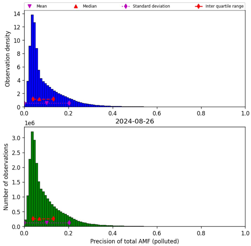
Figure 72: Histogram of “Precision of total AMF (polluted)” for 2024-08-25 to 2024-08-27
