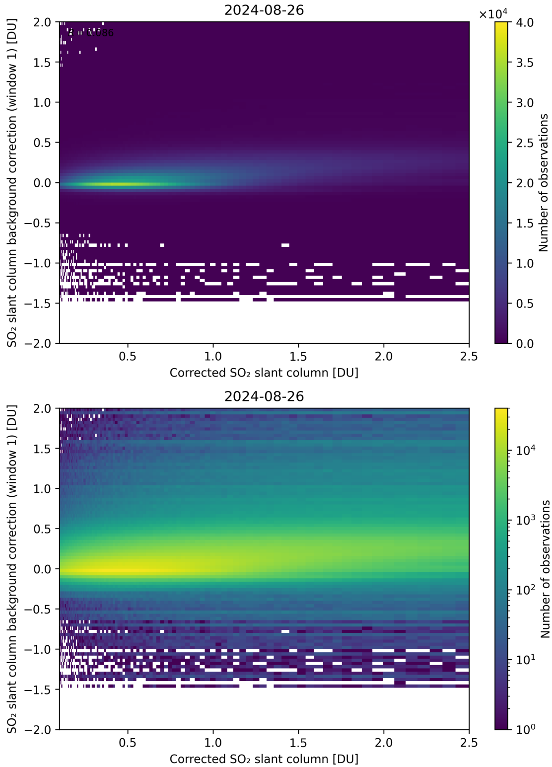
Figure 178: Scatter density plot of “Corrected SO 2 slant column” against “SO 2 slant column background correction (window 1)” for 2024-08-25 to 2024-08-27.
