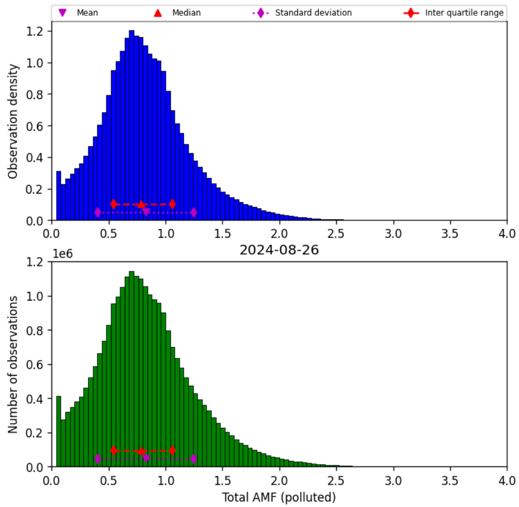
Figure 71: Histogram of “Total AMF (polluted)” for 2024-08-25 to 2024-08-27
