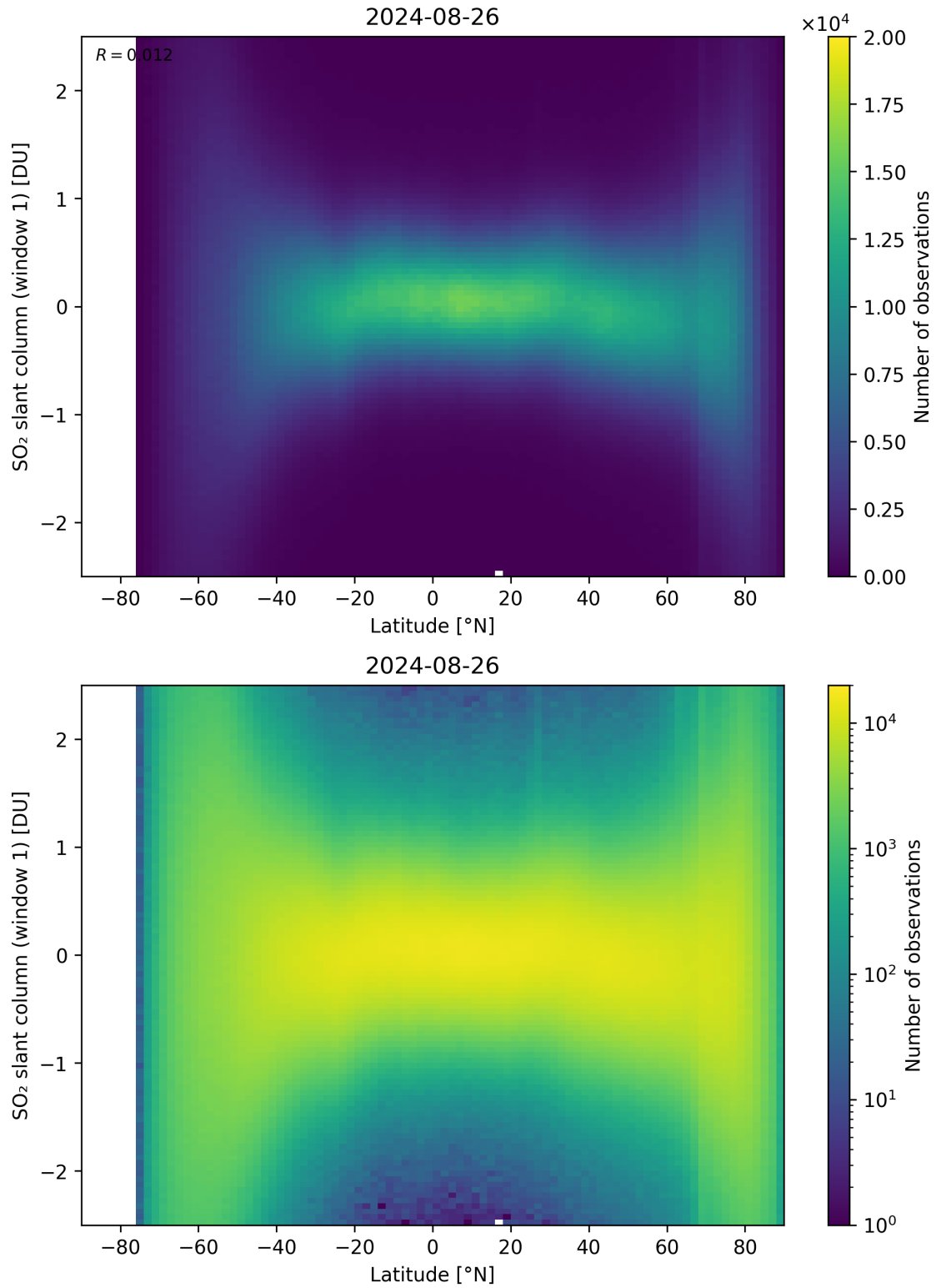
Figure 149: Scatter density plot of “Latitude” against “SO 2 slant column (window 1)” for 2024-08-25 to 2024-08-27.
