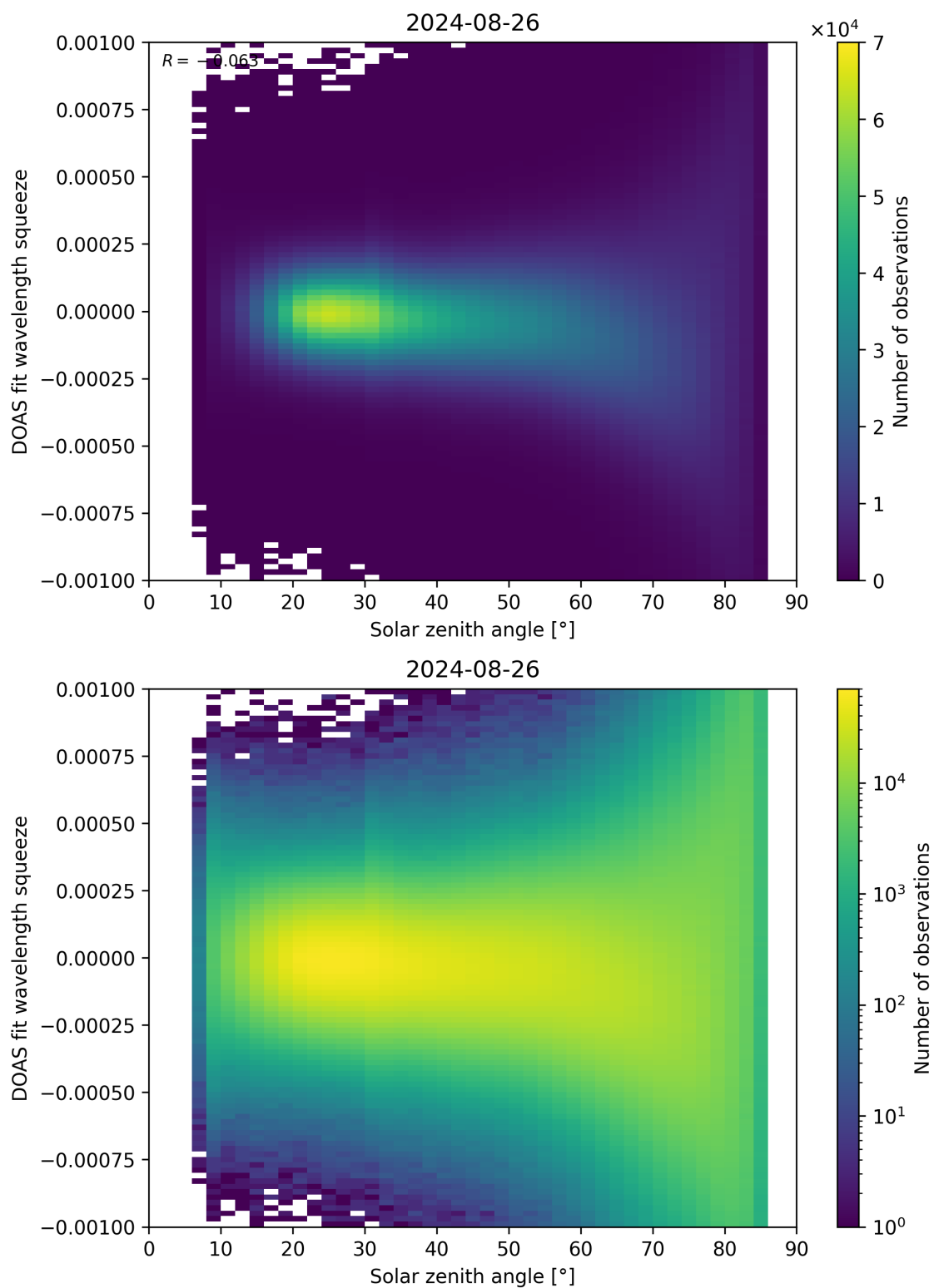
Figure 162: Scatter density plot of “Solar zenith angle” against “DOAS fit wavelength squeeze” for 2024-08-25 to 2024-08-27.
