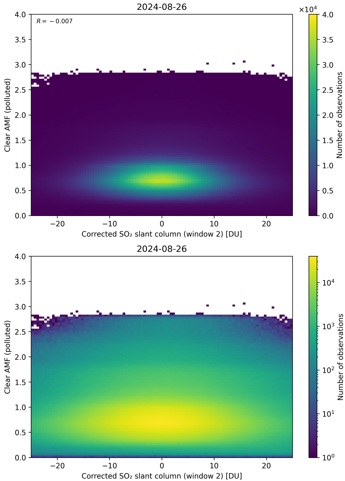
Figure 199: Scatter density plot of “Corrected SO 2 slant column (window 2)” against “Clear AMF (polluted)” for 2024-08-25 to 2024-08-27.
