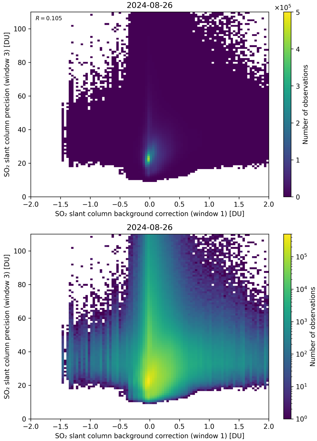
Figure 108: Scatter density plot of “SO 2 slant column background correction (window 1)” against “SO 2 slant column precision (window 3)” for 2024-08-25 to 2024-08-27.
