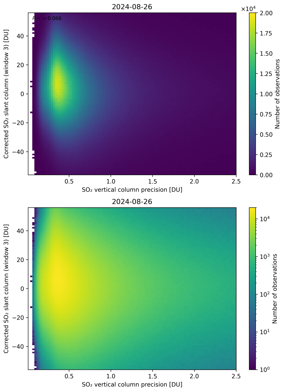
Figure 288: Scatter density plot of “SO 2 vertical column precision” against “Corrected SO 2 slant column (window 3)” for 2024-08-25 to 2024-08-27.
