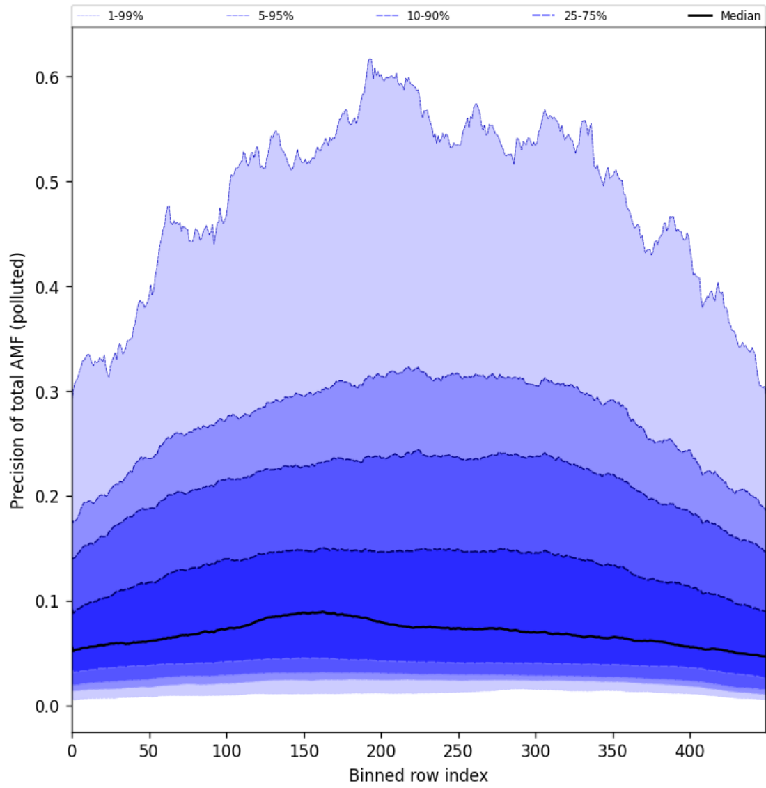
Figure 95: Along track statistics of “Precision of total AMF (polluted)” for 2024-08-25 to 2024-08-27
