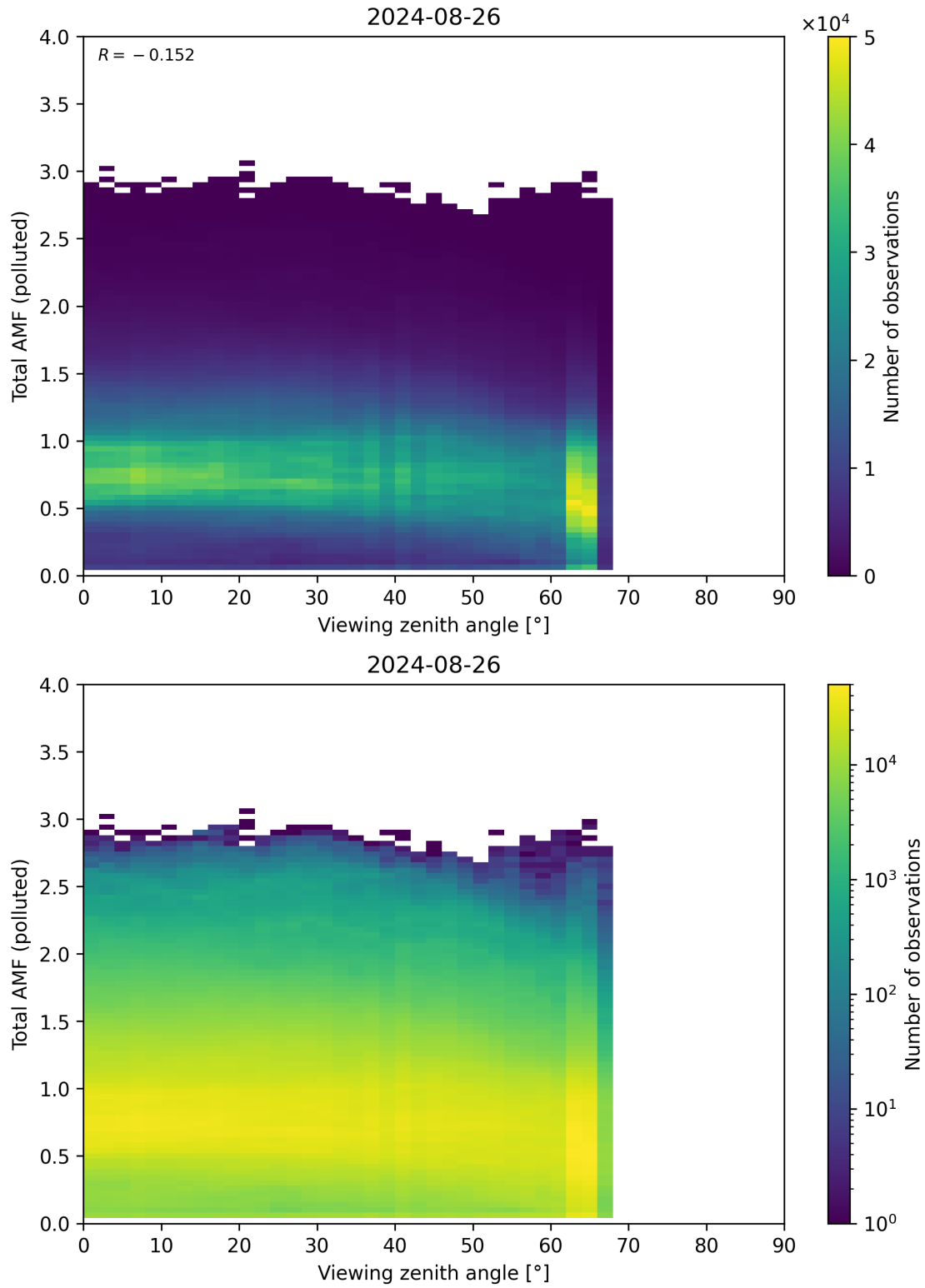
Figure 325: Scatter density plot of “Viewing zenith angle” against “Total AMF (polluted)” for 2024-08-25 to 2024-08-27.
