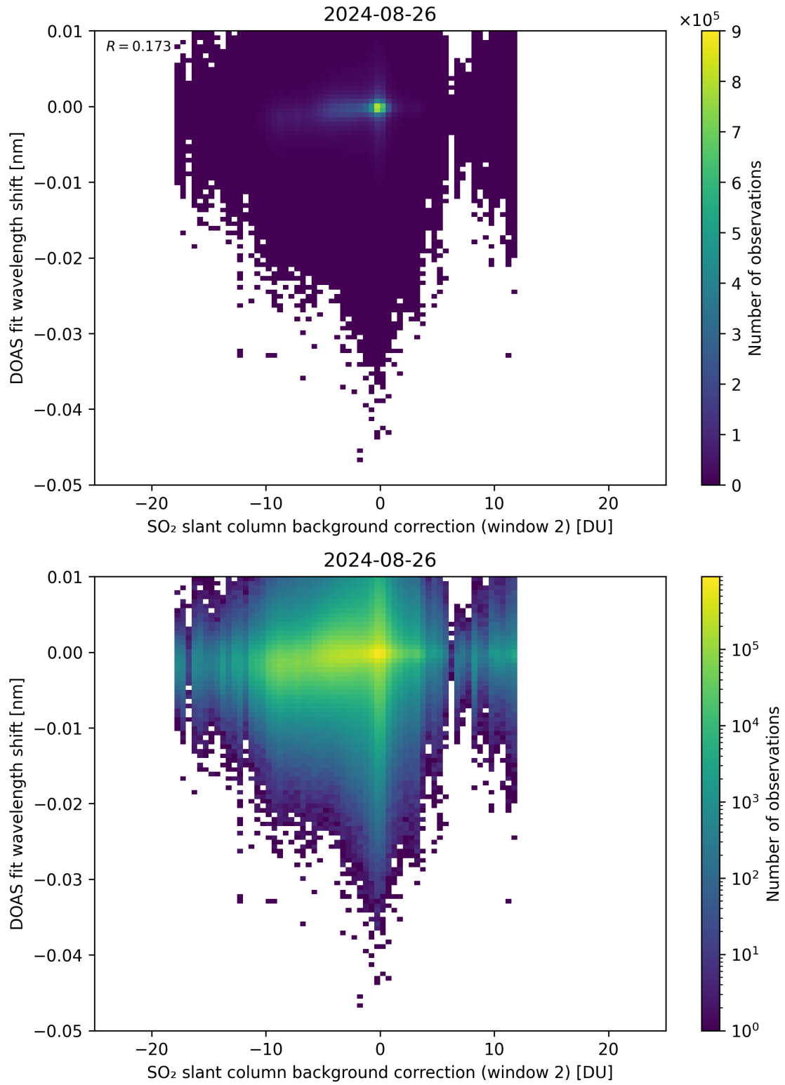
Figure 112: Scatter density plot of “SO 2 slant column background correction (window 2)” against “DOAS fit wavelength shift” for 2024-08-25 to 2024-08-27.
