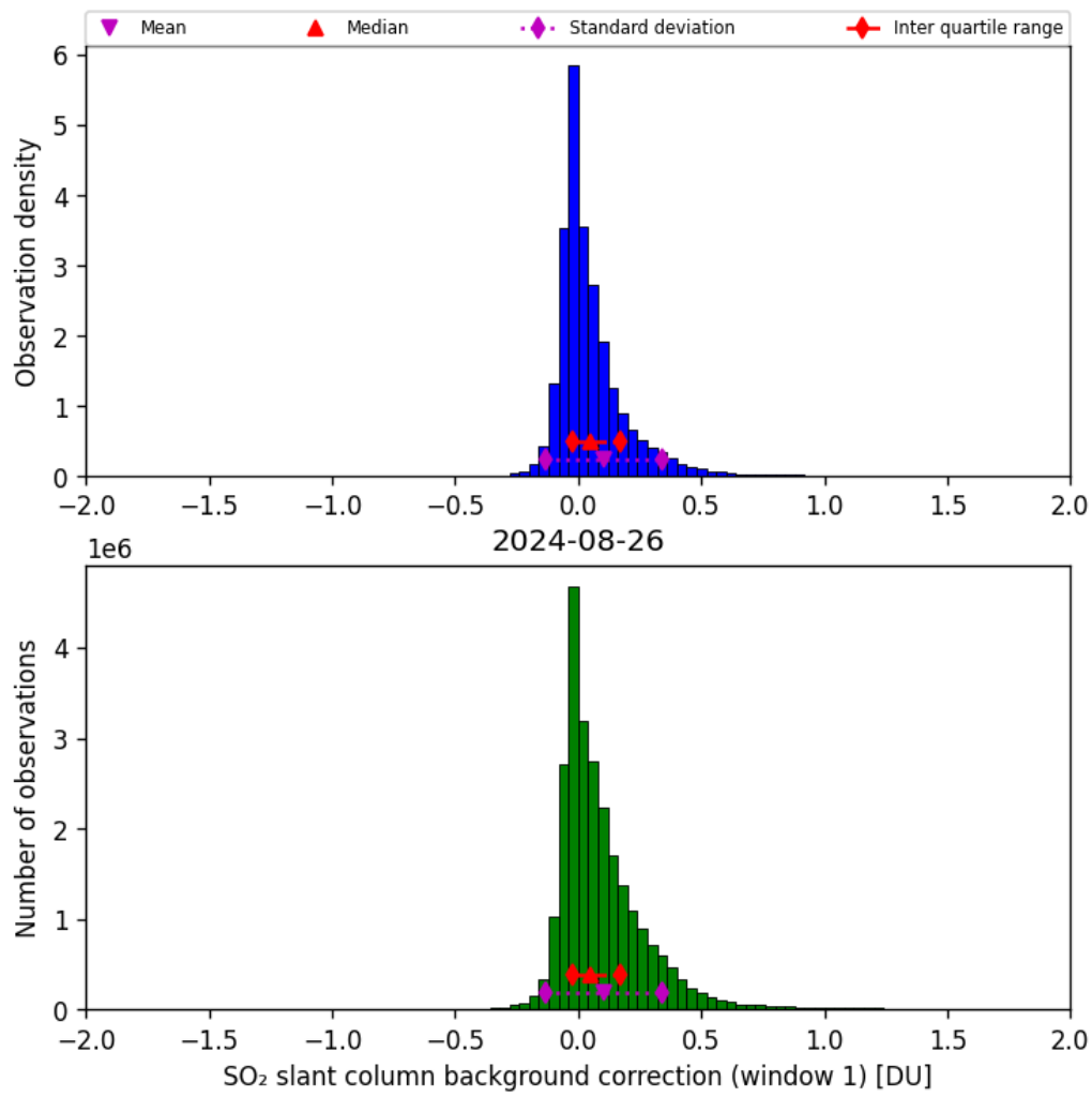
Figure 59: Histogram of “SO 2 slant column background correction (window 1)” for 2024-08-25 to 2024-08-27
