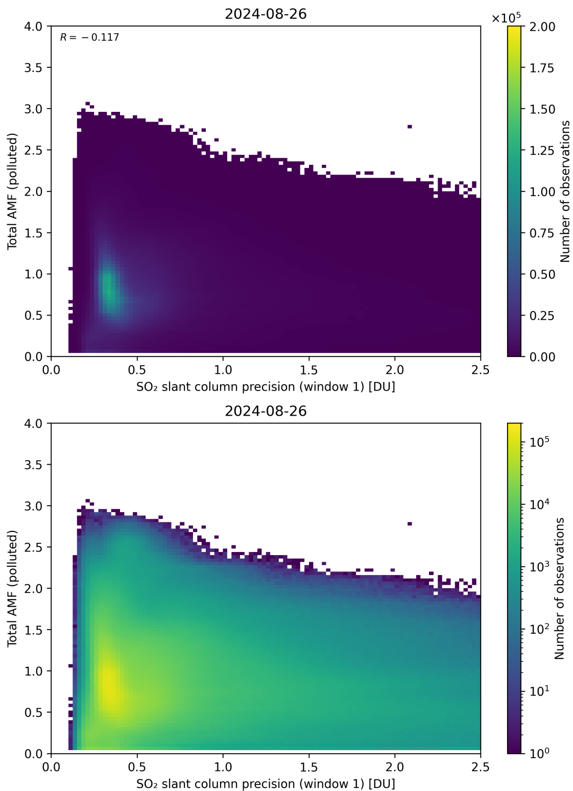
Figure 230: Scatter density plot of “SO 2 slant column precision (window 1)” against “Total AMF (polluted)” for 2024-08-25 to 2024-08-27.
