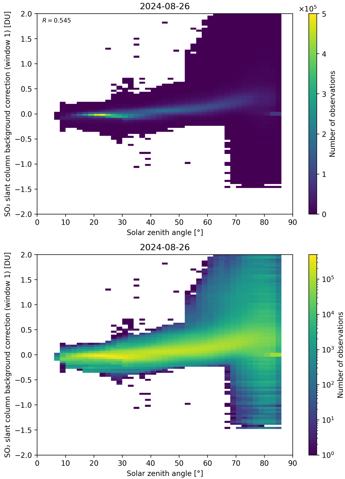
Figure 158: Scatter density plot of “Solar zenith angle” against “SO 2 slant column background correction (window 1)” for 2024-08-25 to 2024-08-27.
