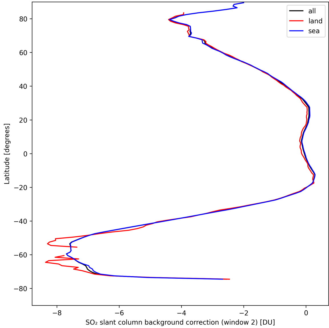
Figure 40: Zonal average of “SO 2 slant column background correction (window 2)” for 2024-08-25 to 2024-08-27.
