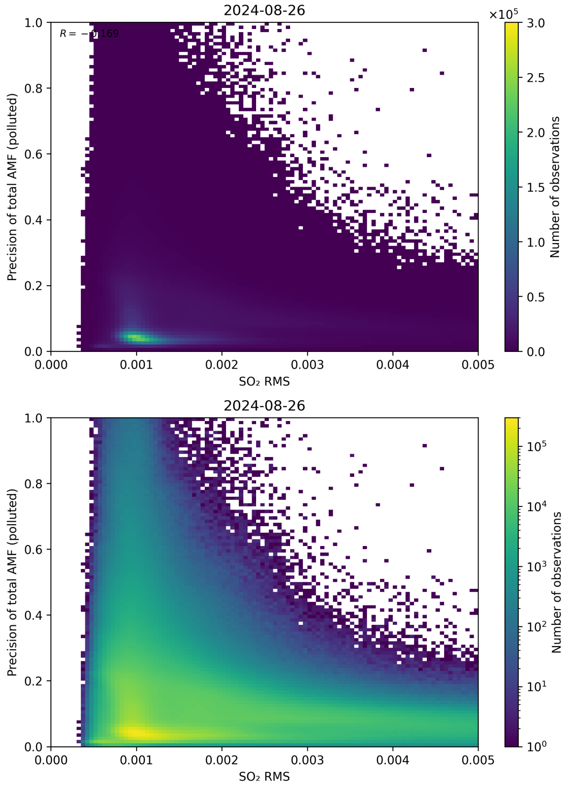
Figure 138: Scatter density plot of “SO 2 RMS” against “Precision of total AMF (polluted)” for 2024-08-25 to 2024-08-27.
