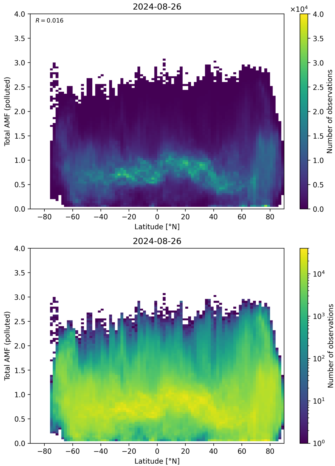
Figure 154: Scatter density plot of “Latitude” against “Total AMF (polluted)” for 2024-08-25 to 2024-08-27.
