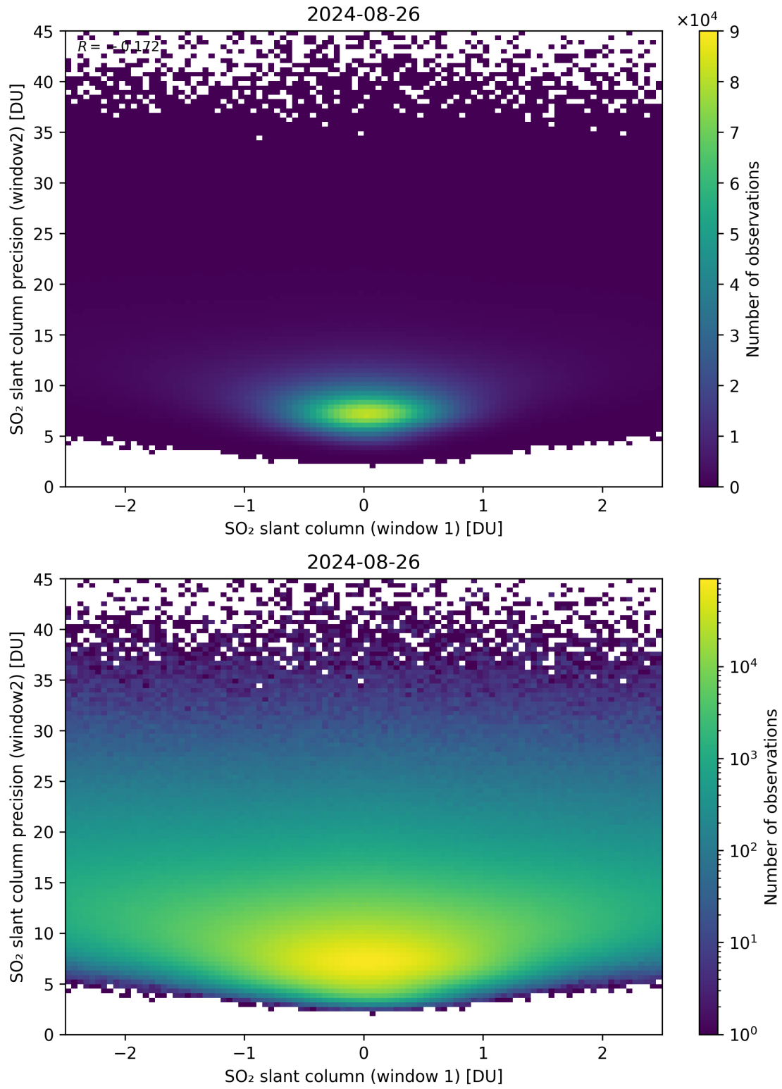
Figure 236: Scatter density plot of “SO 2 slant column (window 1)” against “SO 2 slant column precision (window2)” for 2024-08-25 to 2024-08-27.
