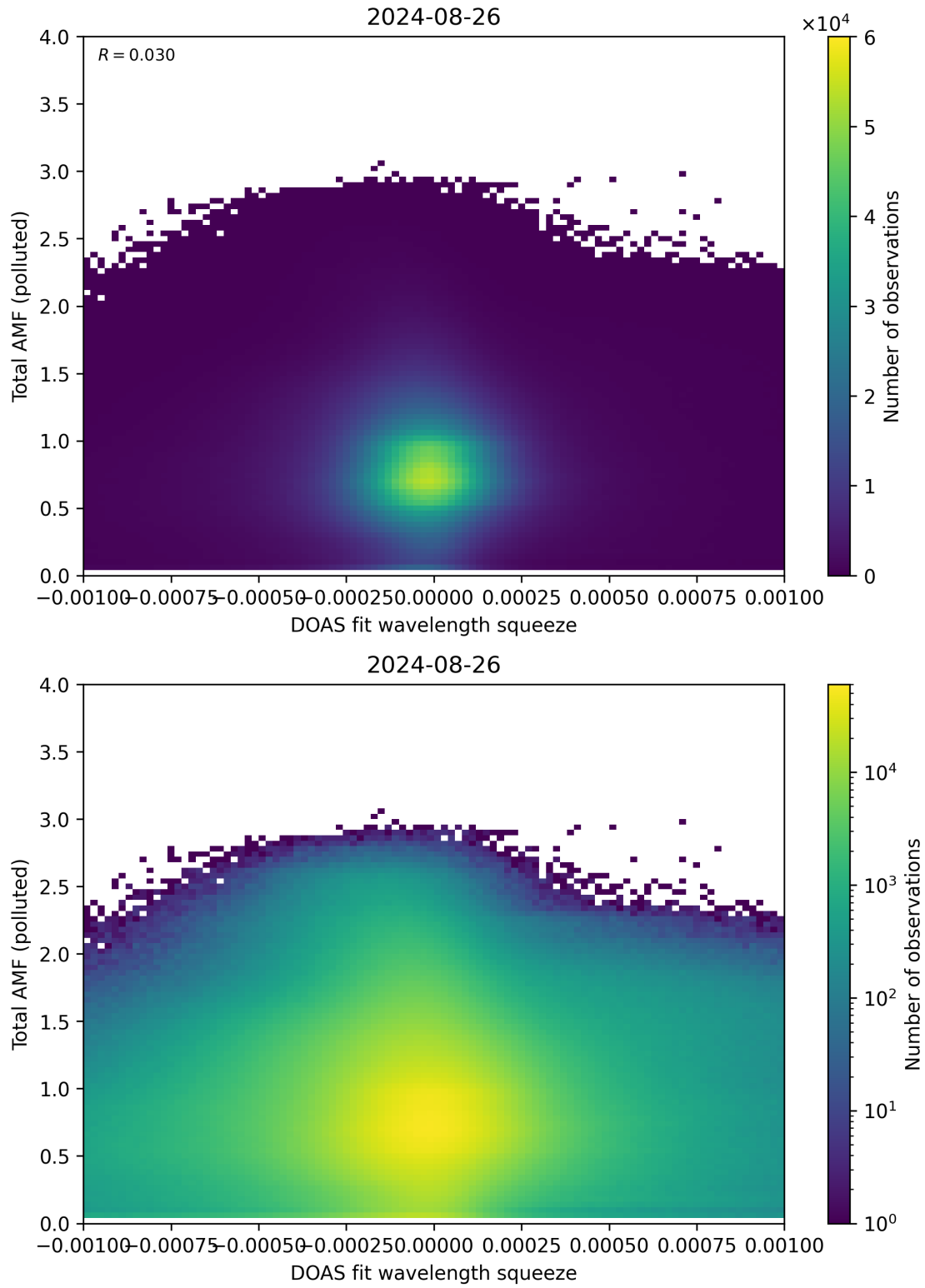
Figure 134: Scatter density plot of “DOAS fit wavelength squeeze” against “Total AMF (polluted)” for 2024-08-25 to 2024-08-27.
