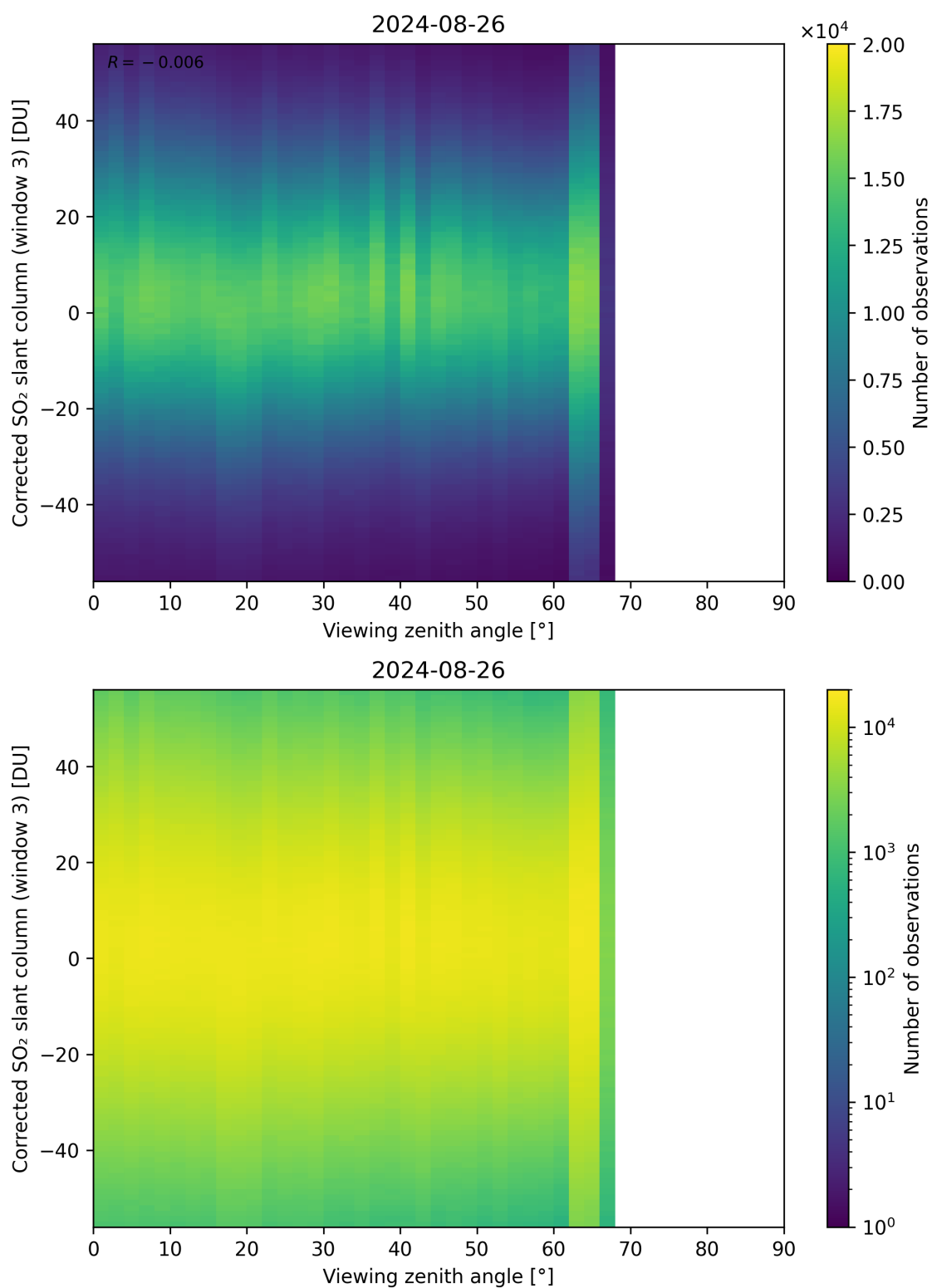
Figure 319: Scatter density plot of “Viewing zenith angle” against “Corrected SO 2 slant column (window 3)” for 2024-08-25 to 2024-08-27.
