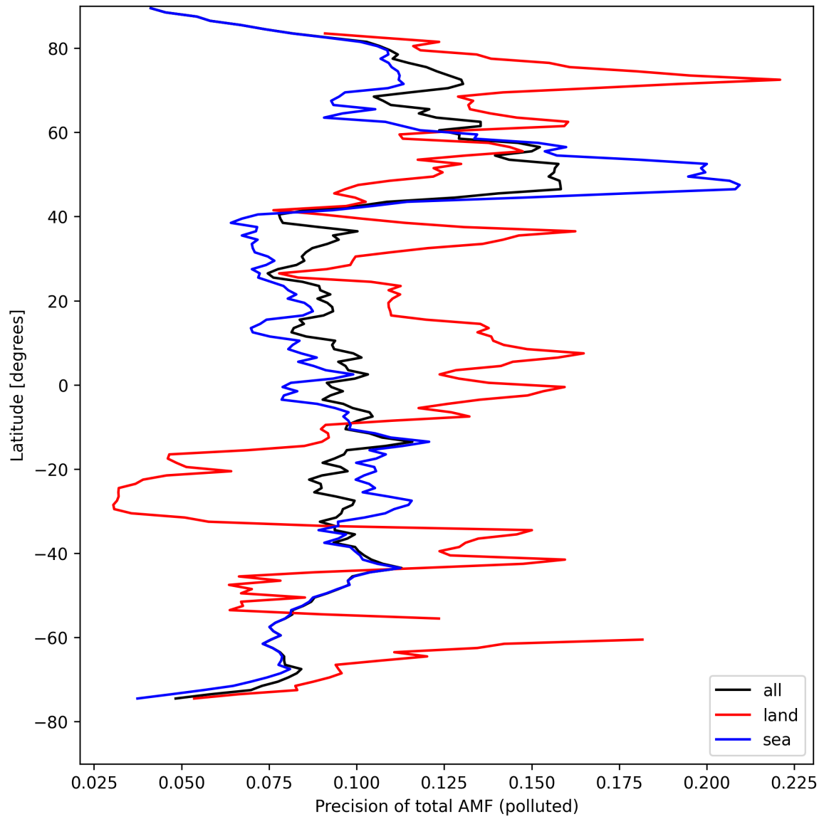
Figure 49: Zonal average of “Precision of total AMF (polluted)” for 2024-08-25 to 2024-08-27.
