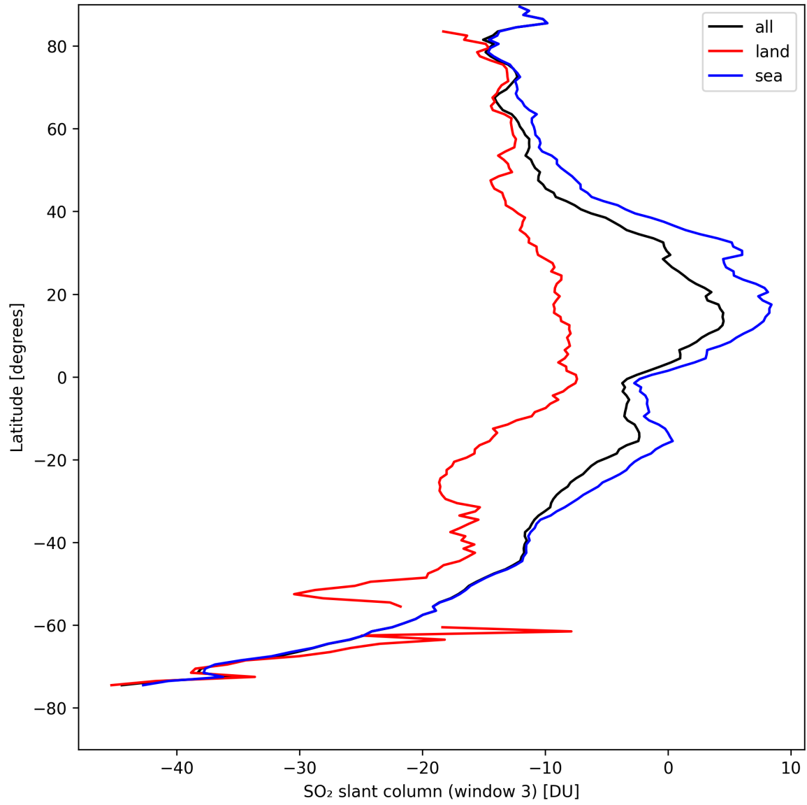
Figure 41: Zonal average of “SO 2 slant column (window 3)” for 2024-08-25 to 2024-08-27.
