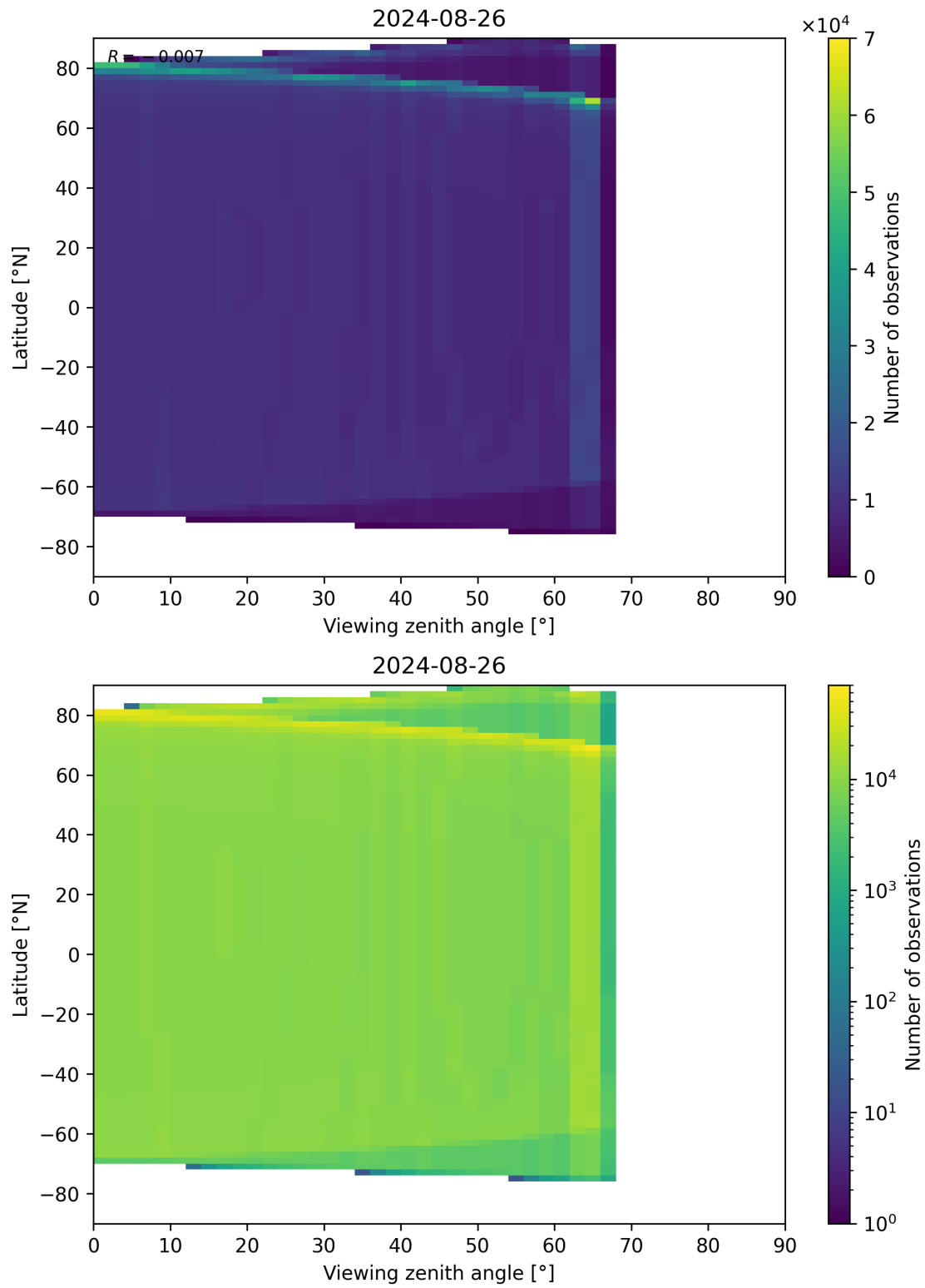
Figure 314: Scatter density plot of “Viewing zenith angle” against “Latitude” for 2024-08-25 to 2024-08-27.
