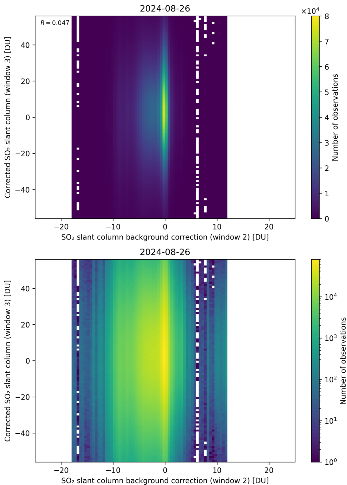
Figure 116: Scatter density plot of “SO 2 slant column background correction (window 2)” against “Corrected SO 2 slant column (window 3)” for 2024-08-25 to 2024-08-27.
