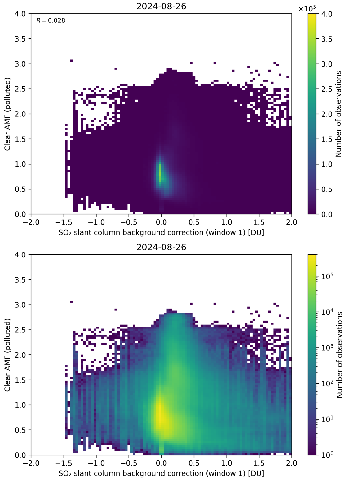
Figure 103: Scatter density plot of “SO 2 slant column background correction (window 1)” against “Clear AMF (polluted)” for 2024-08-25 to 2024-08-27.
