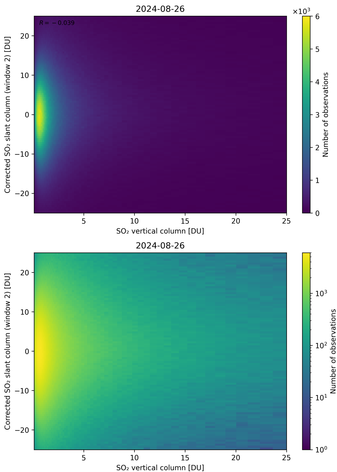
Figure 298: Scatter density plot of “SO 2 vertical column” against “Corrected SO 2 slant column (window 2)” for 2024-08-25 to 2024-08-27.
