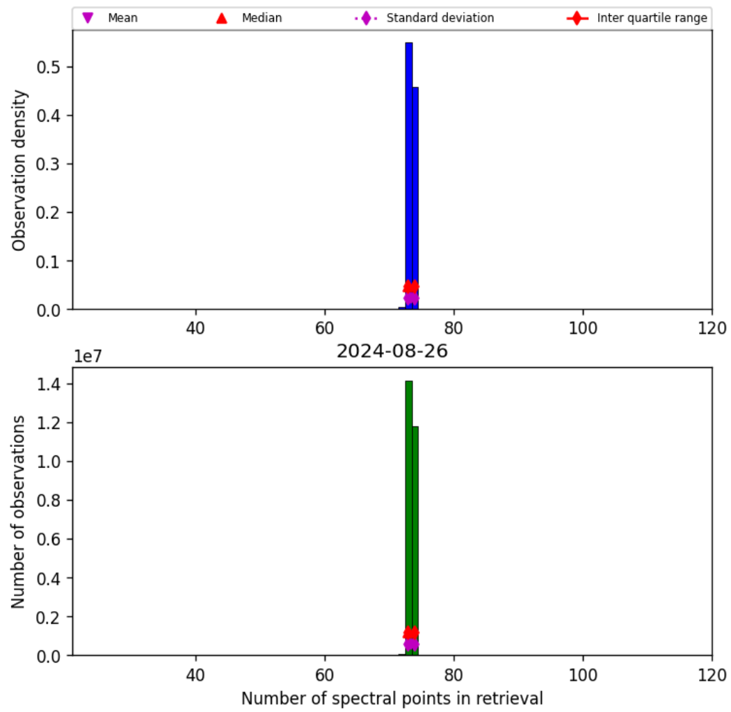
Figure 74: Histogram of “Number of spectral points in retrieval” for 2024-08-25 to 2024-08-27
