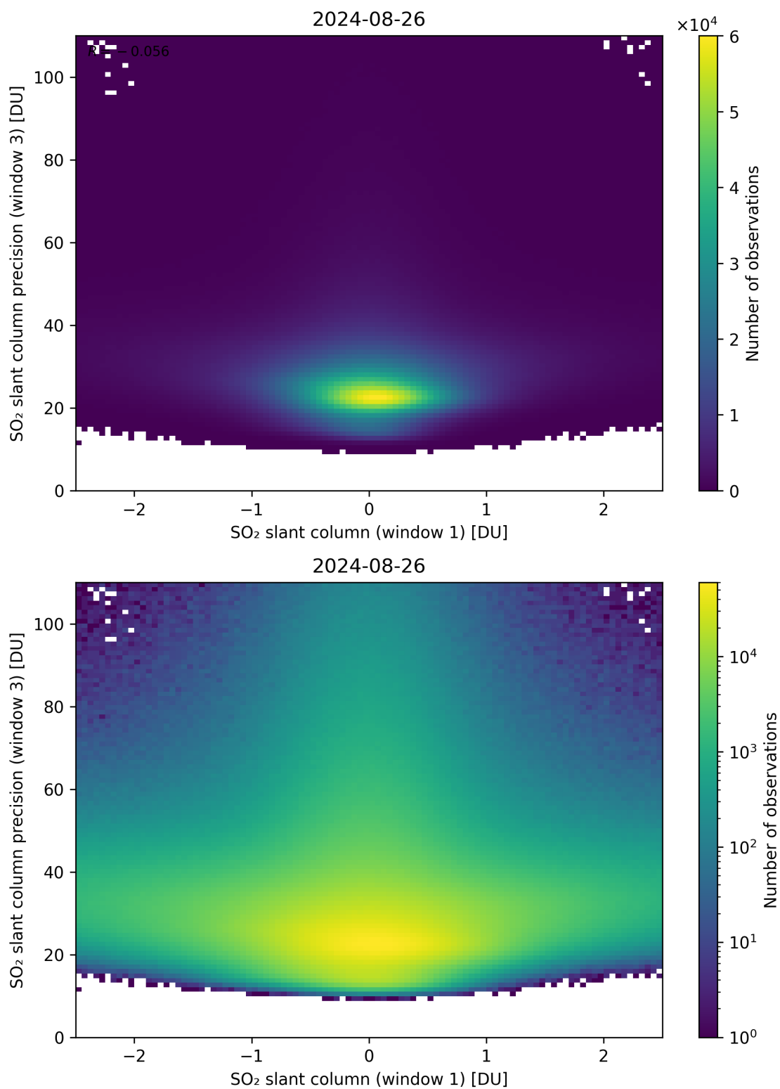
Figure 238: Scatter density plot of “SO 2 slant column (window 1)” against “SO 2 slant column precision (window 3)” for 2024-08-25 to 2024-08-27.
