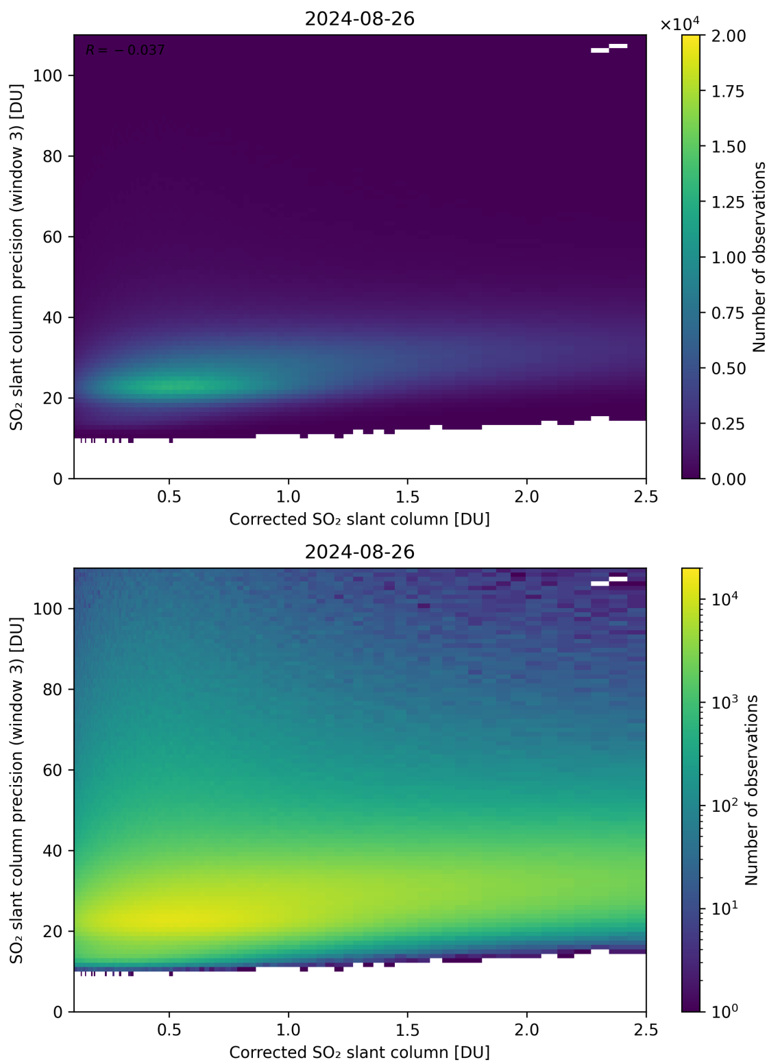
Figure 191: Scatter density plot of “Corrected SO 2 slant column” against “SO 2 slant column precision (window 3)” for 2024-08-25 to 2024-08-27.
