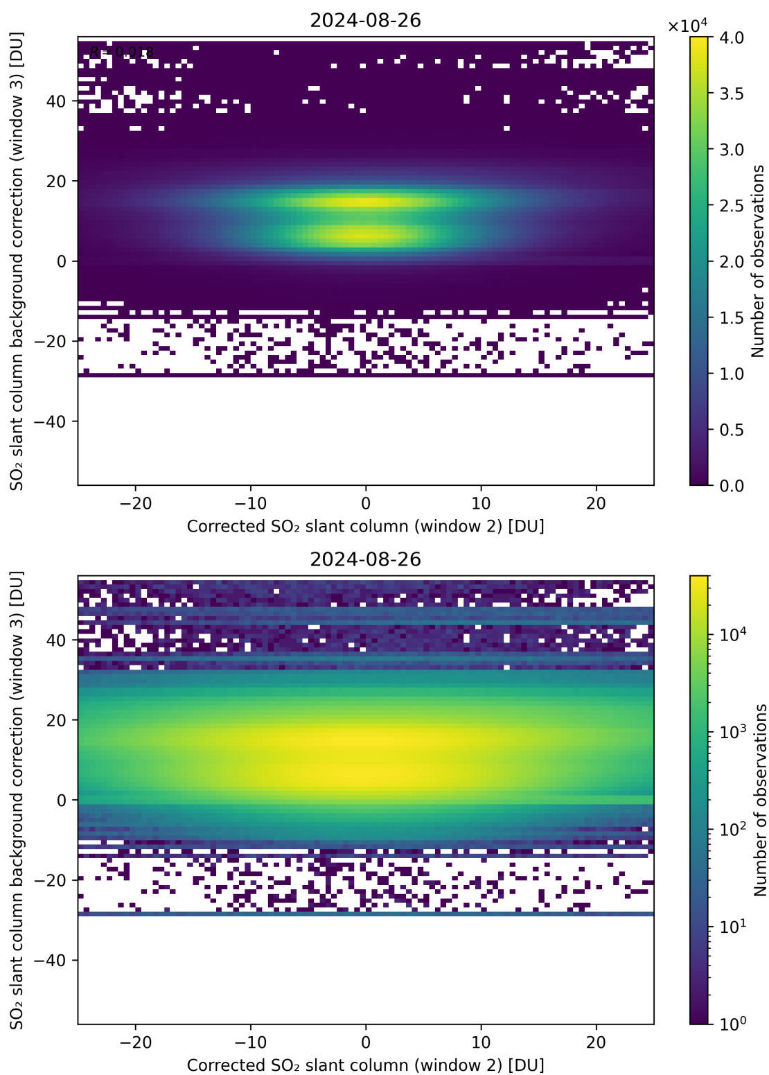
Figure 195: Scatter density plot of “Corrected SO 2 slant column (window 2)” against “SO 2 slant column background correction (window 3)” for 2024-08-25 to 2024-08-27.
