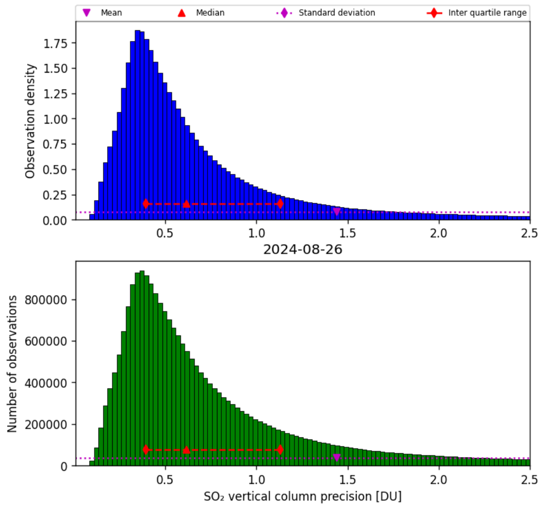
Figure 54: Histogram of “SO 2 vertical column precision” for 2024-08-25 to 2024-08-27
