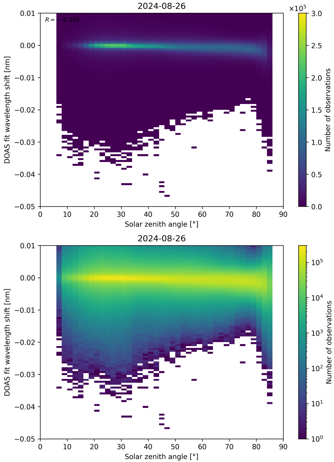
Figure 161: Scatter density plot of “Solar zenith angle” against “DOAS fit wavelength shift” for 2024-08-25 to 2024-08-27.
