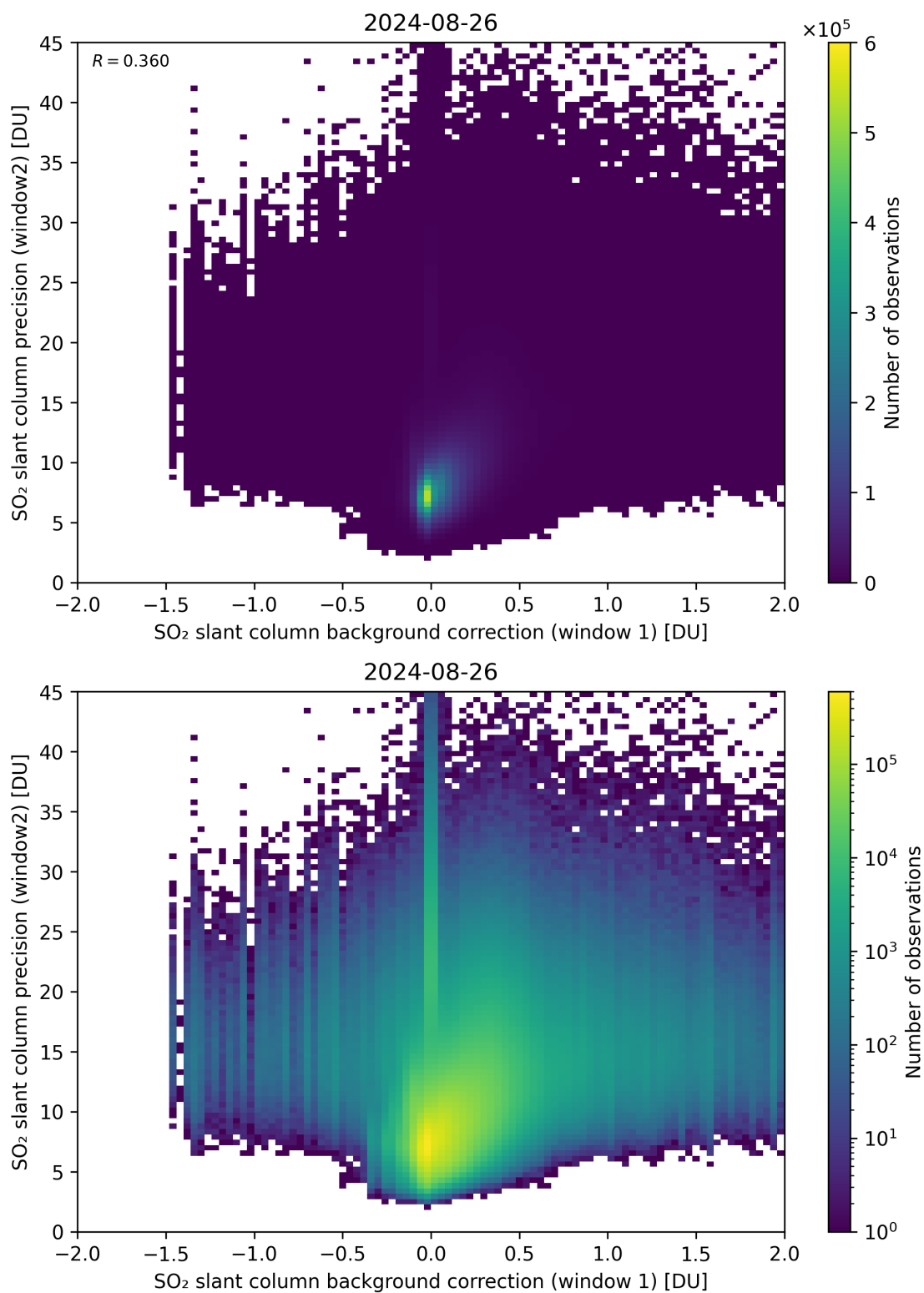
Figure 106: Scatter density plot of “SO 2 slant column background correction (window 1)” against “SO 2 slant column precision (window2)” for 2024-08-25 to 2024-08-27.
