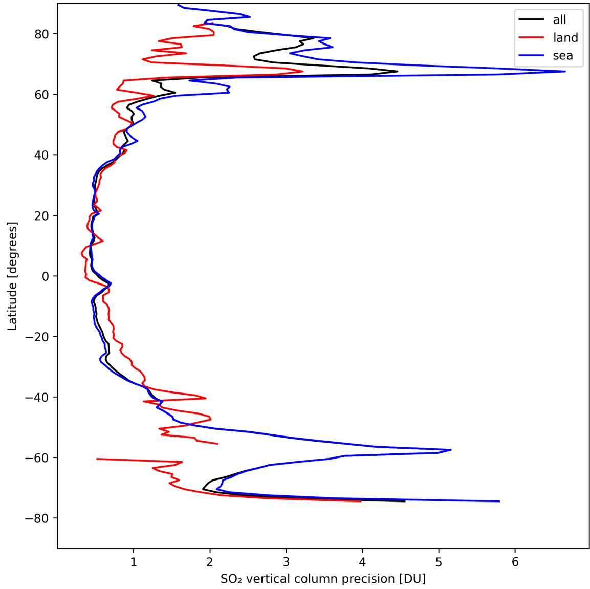
Figure 31: Zonal average of “SO 2 vertical column precision” for 2024-08-25 to 2024-08-27.
