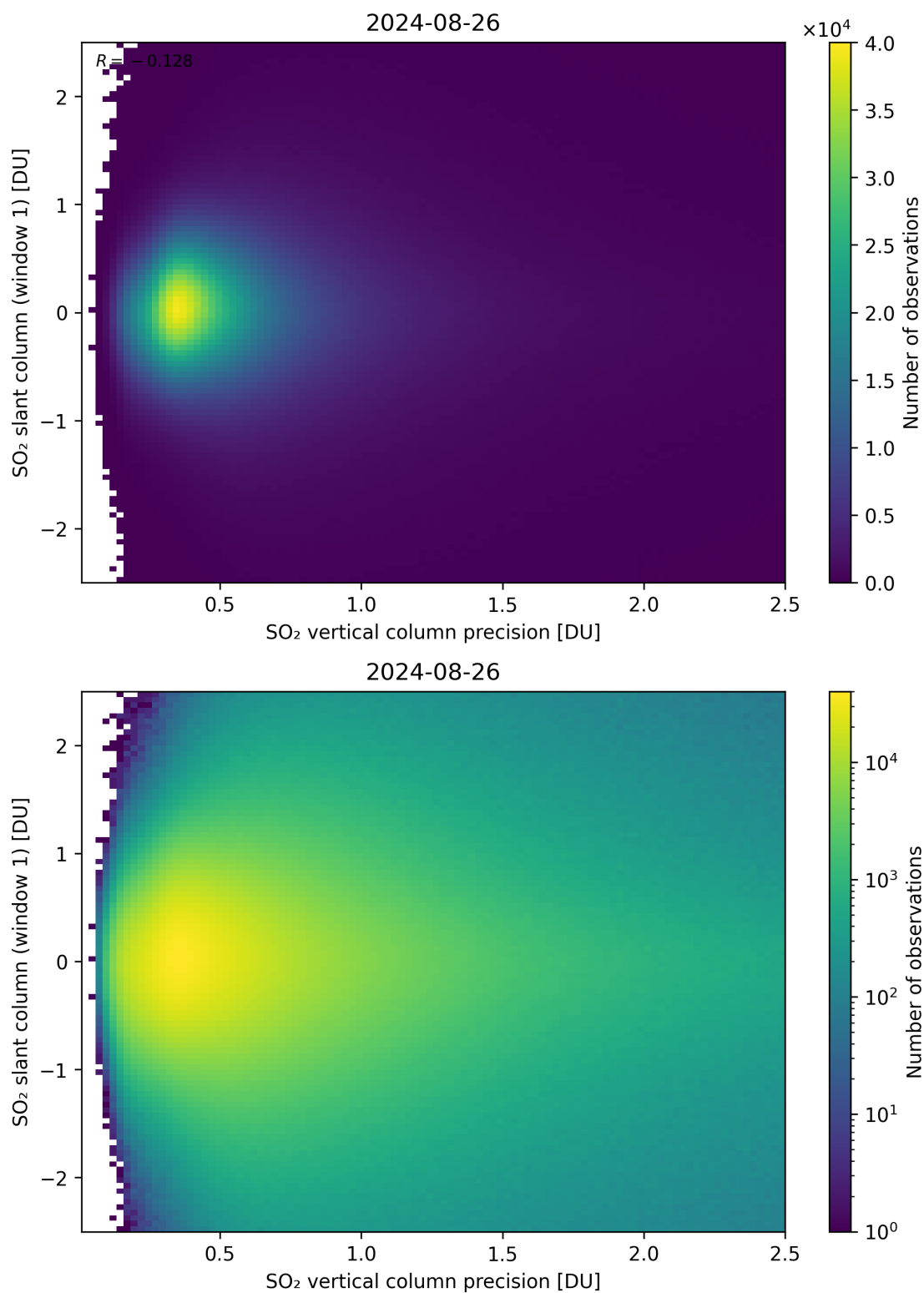
Figure 289: Scatter density plot of “SO 2 vertical column precision” against “SO 2 slant column (window 1)” for 2024-08-25 to 2024-08-27.
