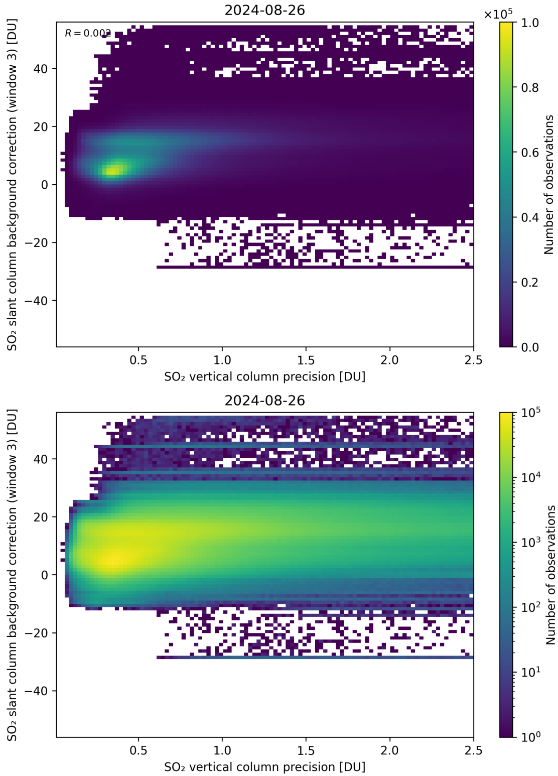
Figure 281: Scatter density plot of “SO 2 vertical column precision” against “SO 2 slant column background correction (window 3)” for 2024-08-25 to 2024-08-27.
