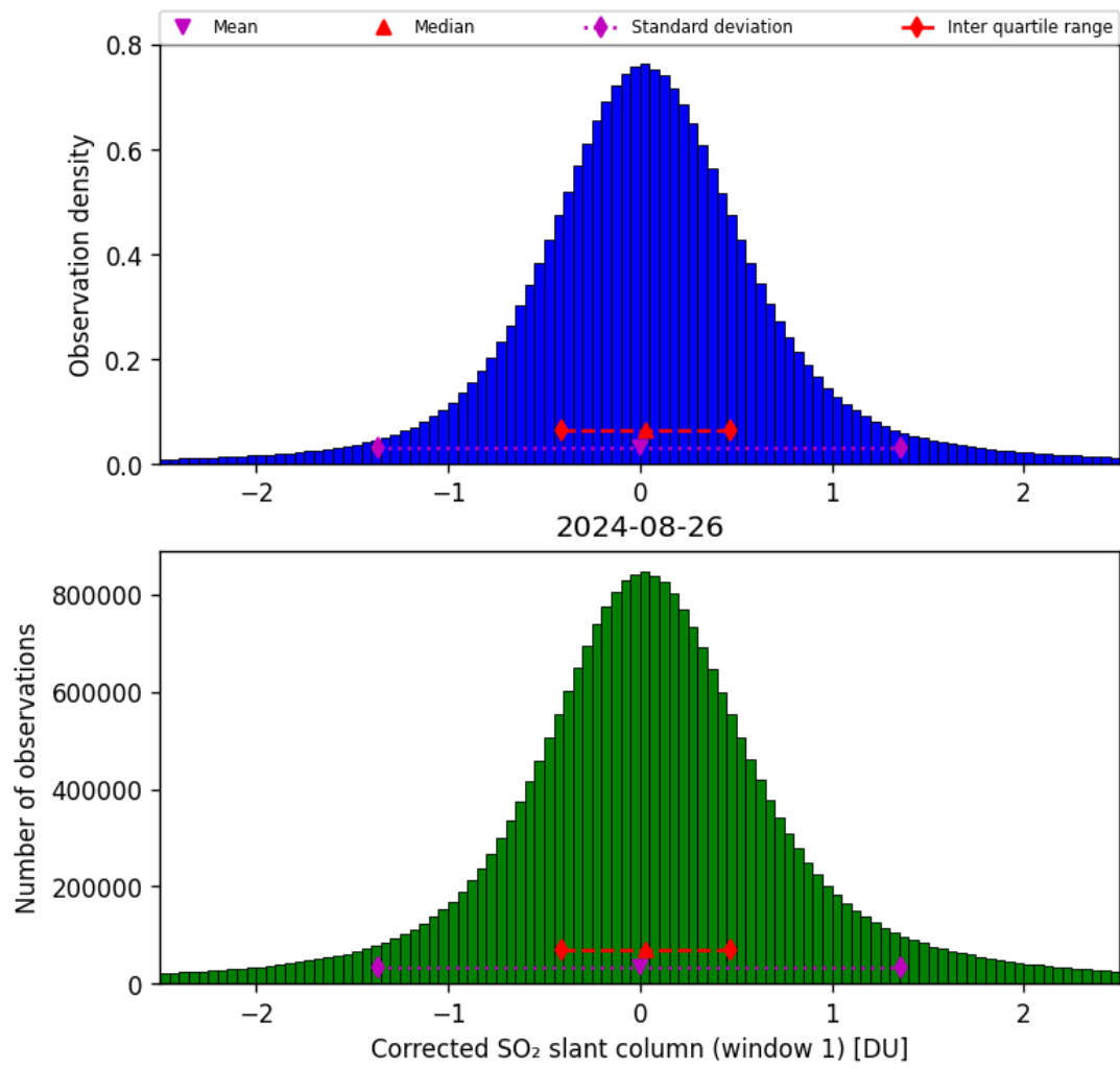
Figure 58: Histogram of “Corrected SO 2 slant column (window 1)” for 2024-08-25 to 2024-08-27
