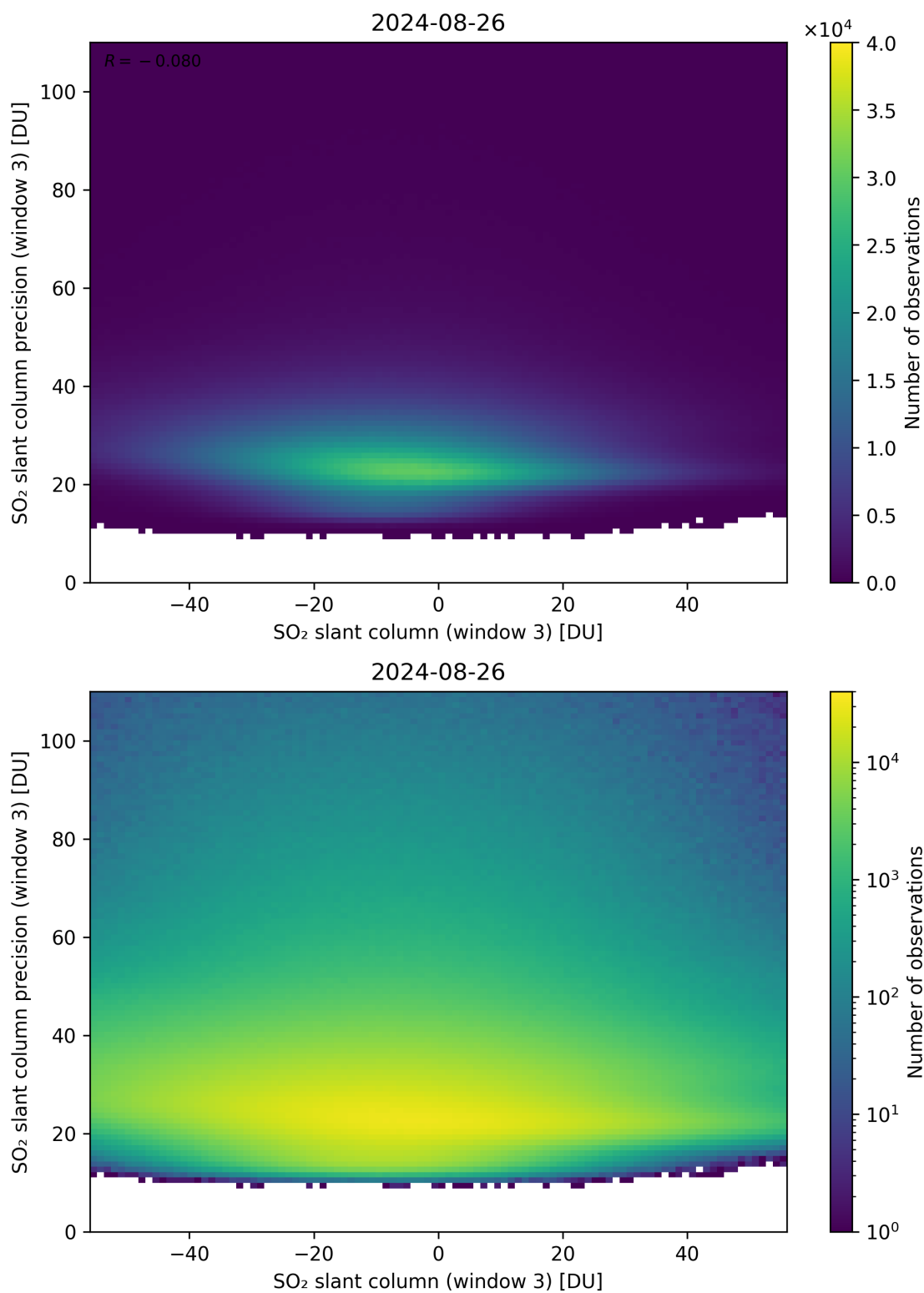
Figure 267: Scatter density plot of “SO 2 slant column (window 3)” against “SO 2 slant column precision (window 3)” for 2024-08-25 to 2024-08-27.
