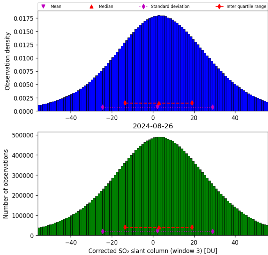
Figure 66: Histogram of “Corrected SO 2 slant column (window 3)” for 2024-08-25 to 2024-08-27
