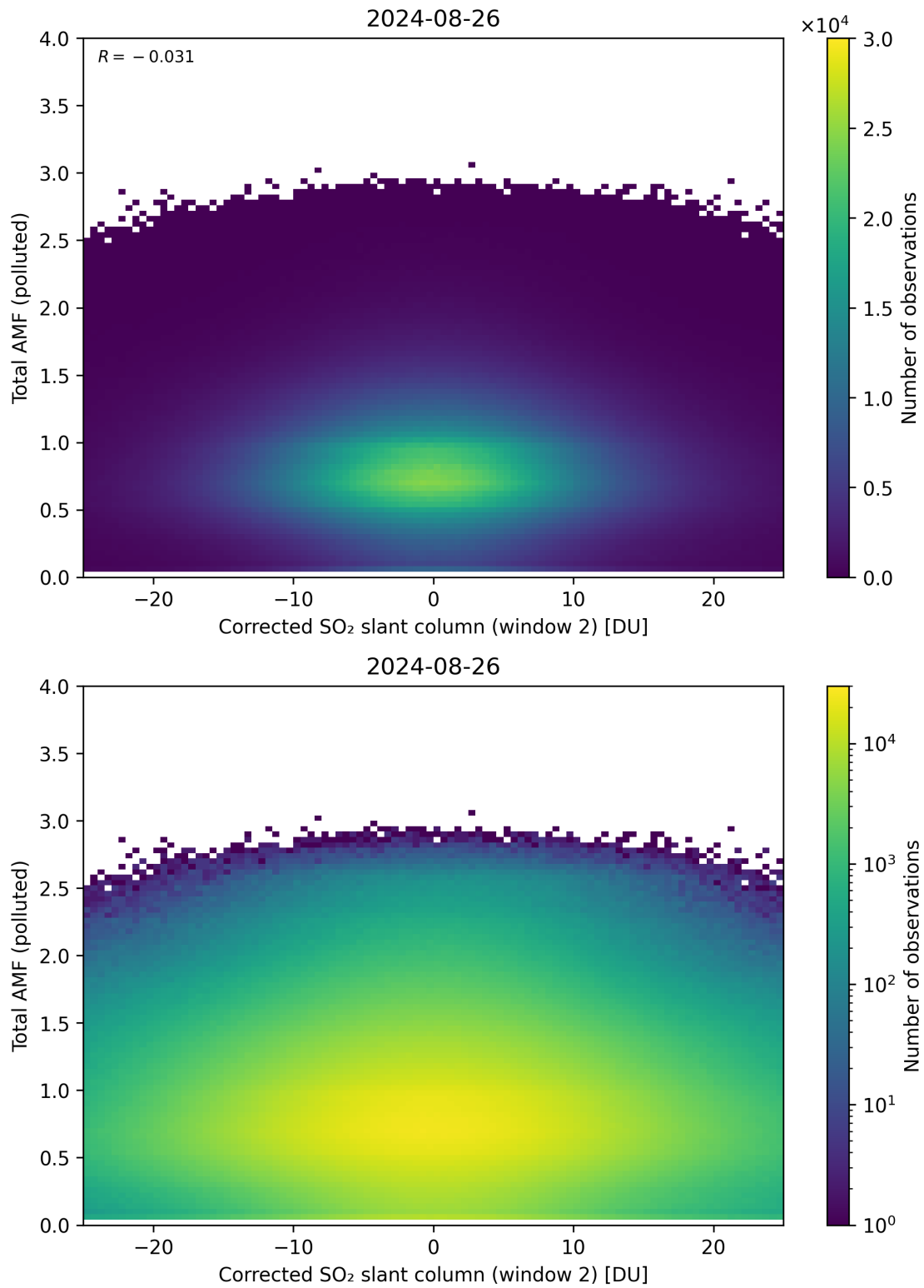
Figure 203: Scatter density plot of “Corrected SO 2 slant column (window 2)” against “Total AMF (polluted)” for 2024-08-25 to 2024-08-27.
