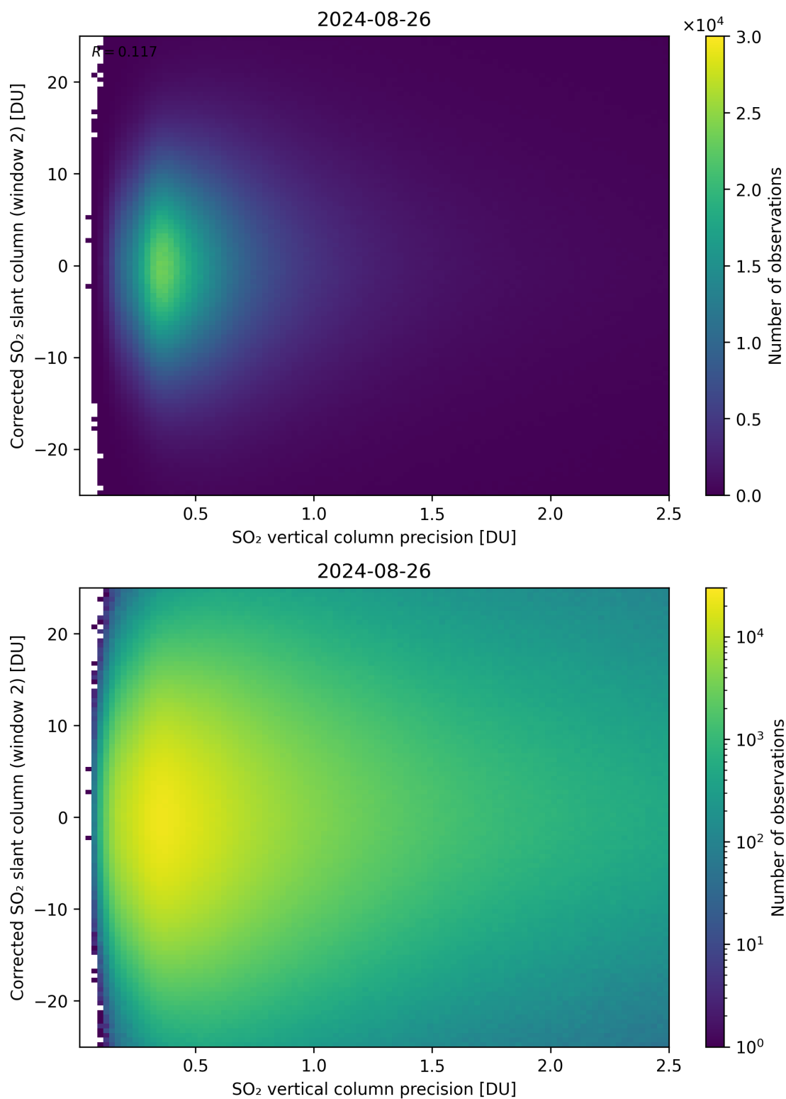
Figure 287: Scatter density plot of “SO 2 vertical column precision” against “Corrected SO 2 slant column (window 2)” for 2024-08-25 to 2024-08-27.
