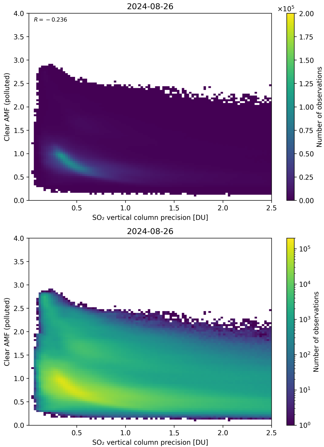
Figure 285: Scatter density plot of “SO 2 vertical column precision” against “Clear AMF (polluted)” for 2024-08-25 to 2024-08-27.
