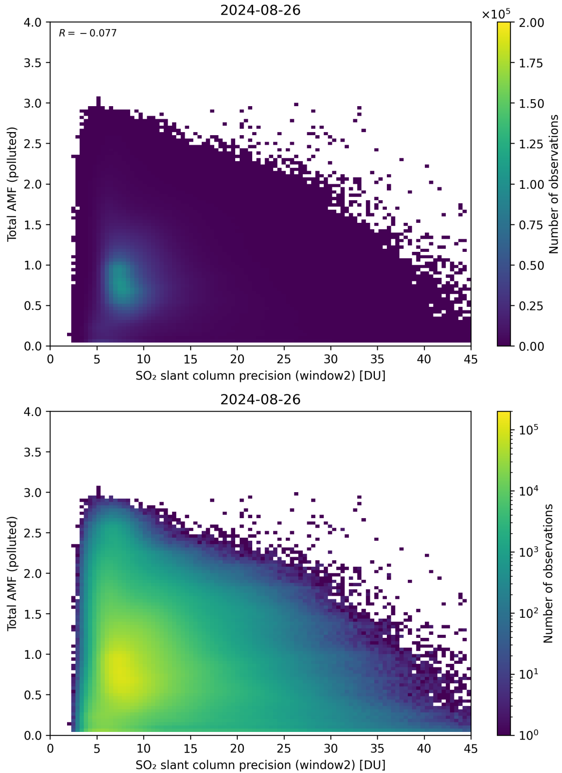
Figure 251: Scatter density plot of “SO 2 slant column precision (window2)” against “Total AMF (polluted)” for 2024-08-25 to 2024-08-27.
