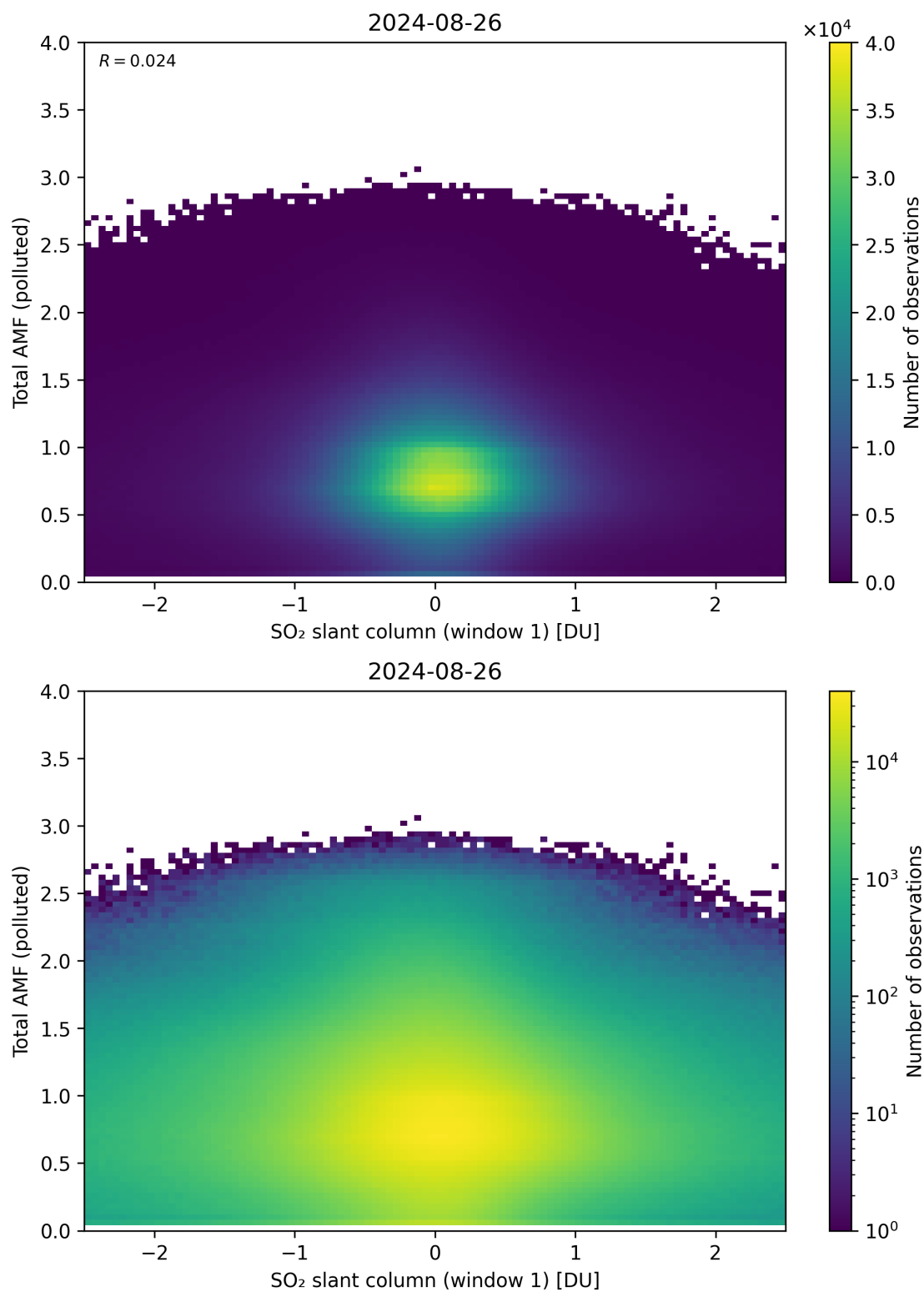
Figure 239: Scatter density plot of “SO 2 slant column (window 1)” against “Total AMF (polluted)” for 2024-08-25 to 2024-08-27.
