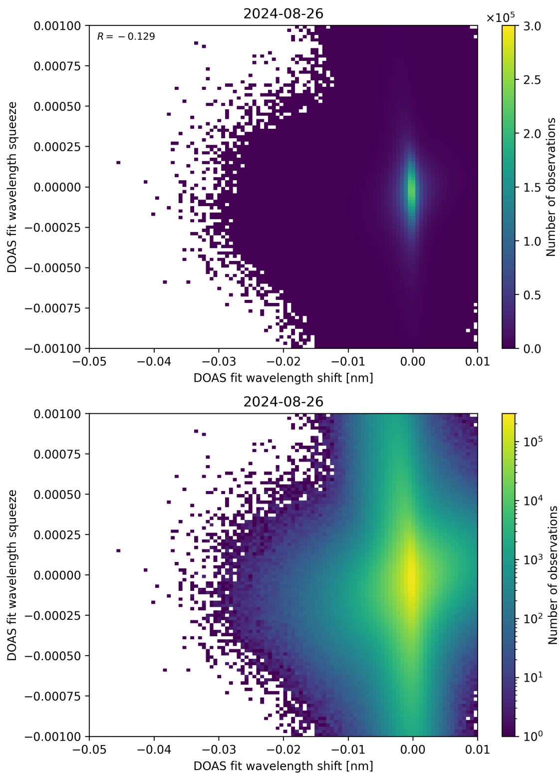
Figure 127: Scatter density plot of “DOAS fit wavelength shift” against “DOAS fit wavelength squeeze” for 2024-08-25 to 2024-08-27.
