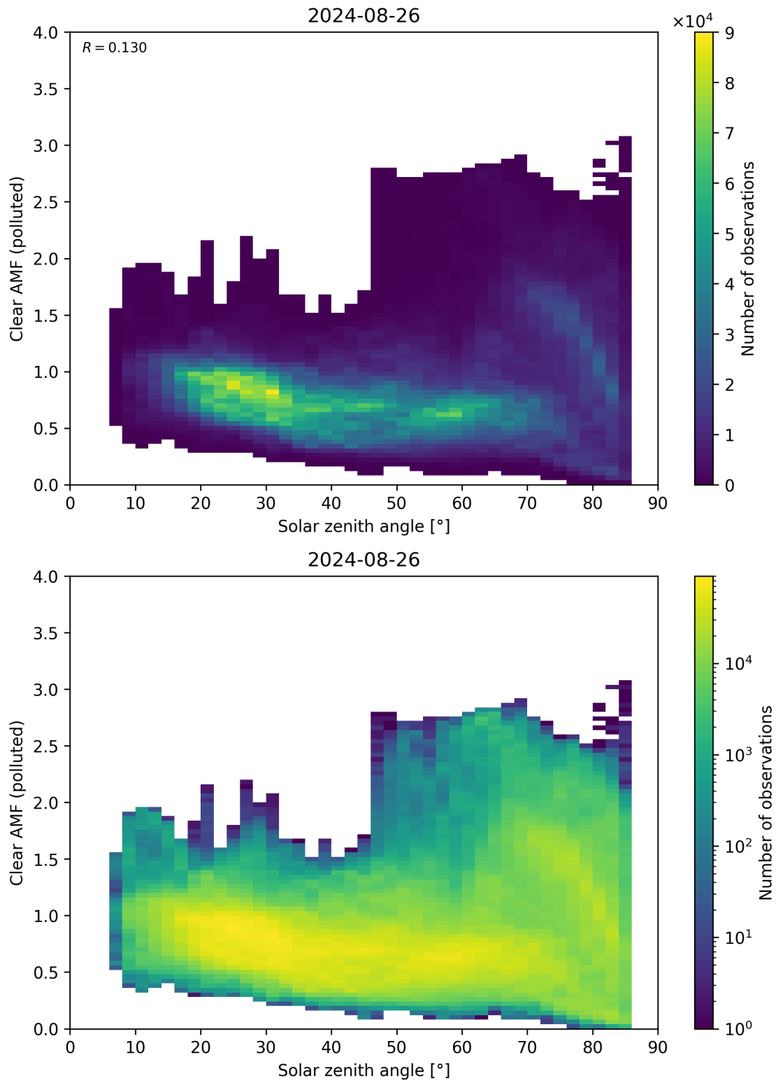
Figure 165: Scatter density plot of “Solar zenith angle” against “Clear AMF (polluted)” for 2024-08-25 to 2024-08-27.
