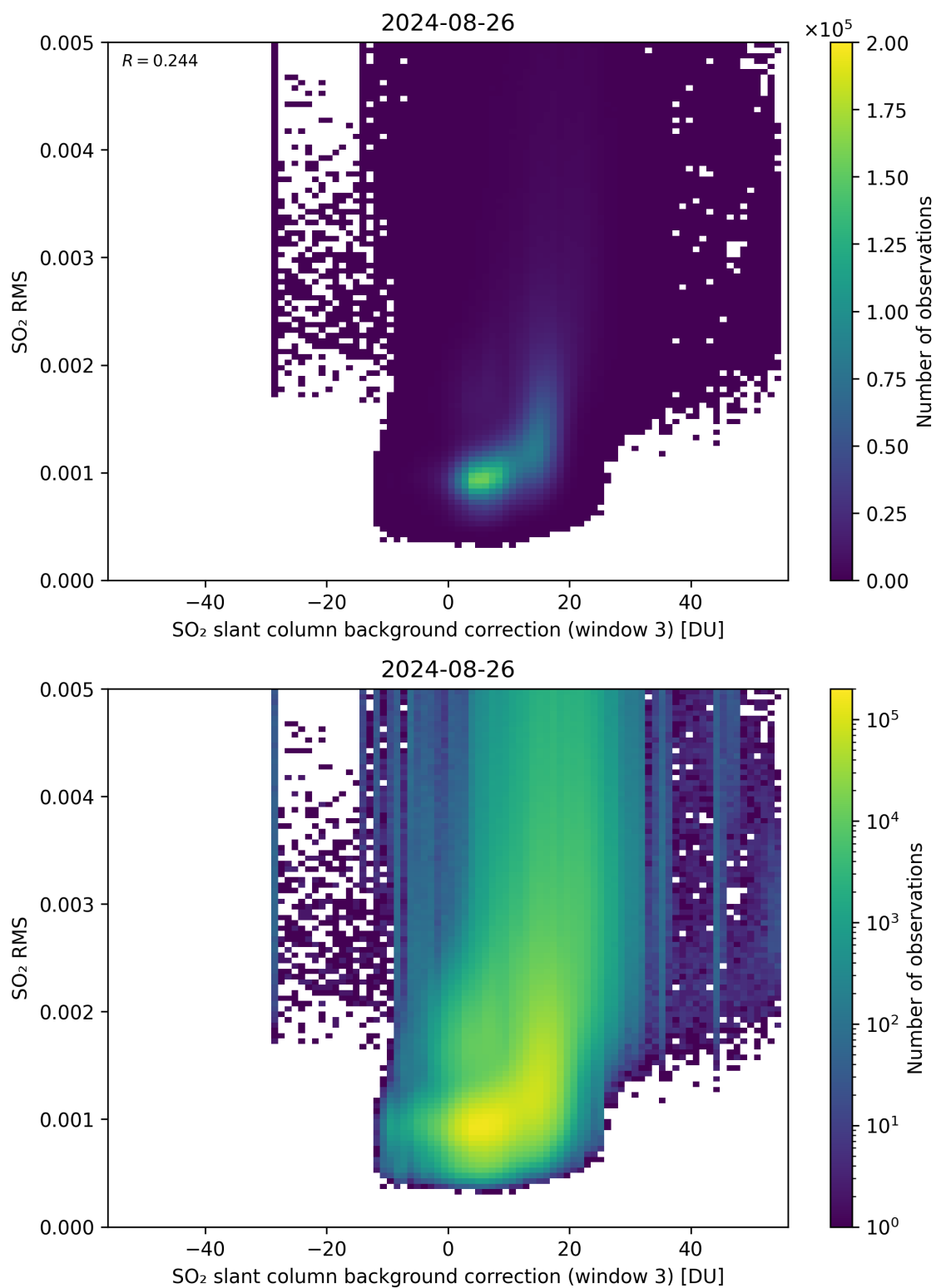
Figure 123: Scatter density plot of “SO 2 slant column background correction (window 3)” against “SO 2 RMS” for 2024-08-25 to 2024-08-27.
