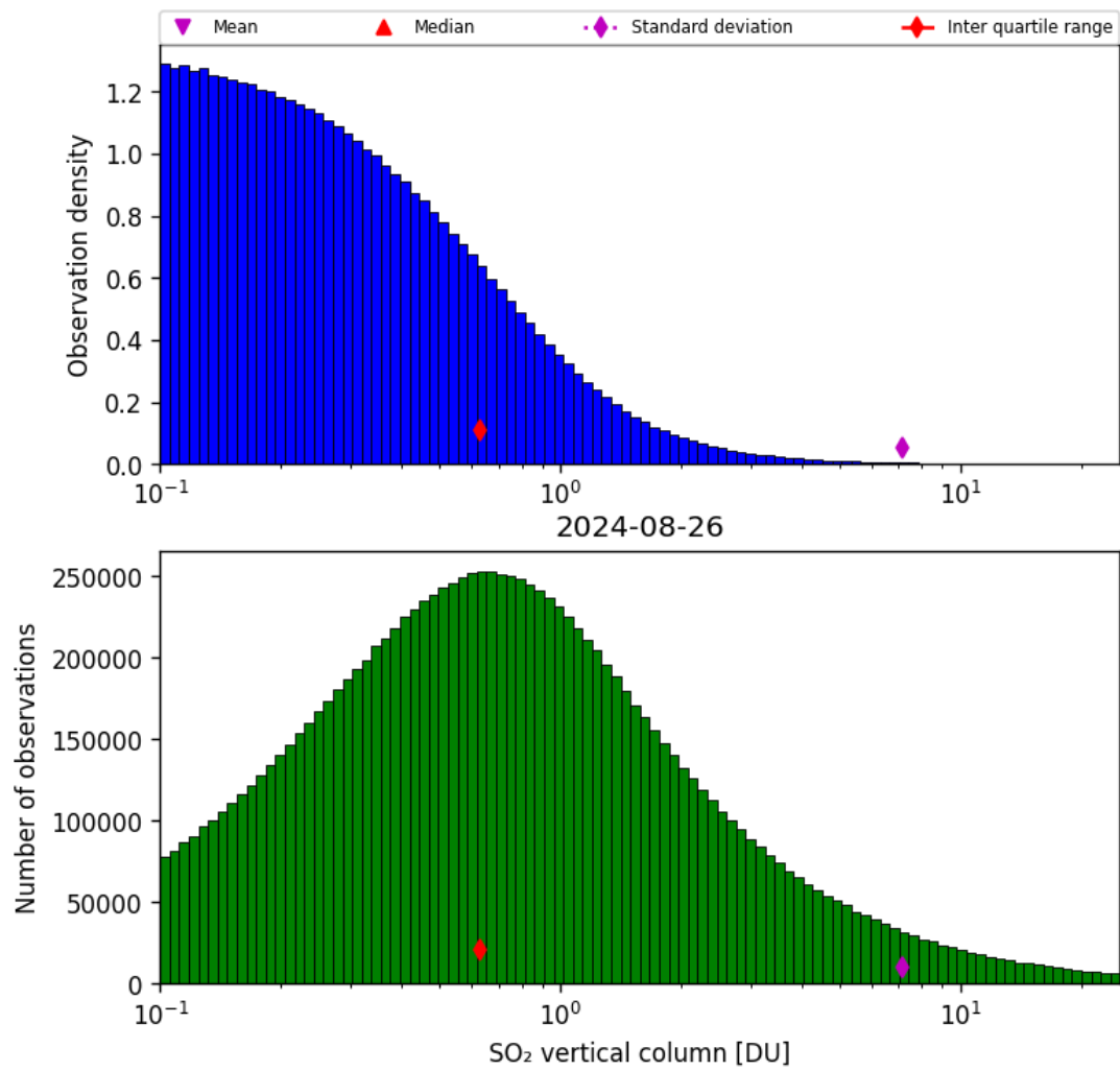
Figure 53: Histogram of “SO 2 vertical column” for 2024-08-25 to 2024-08-27
