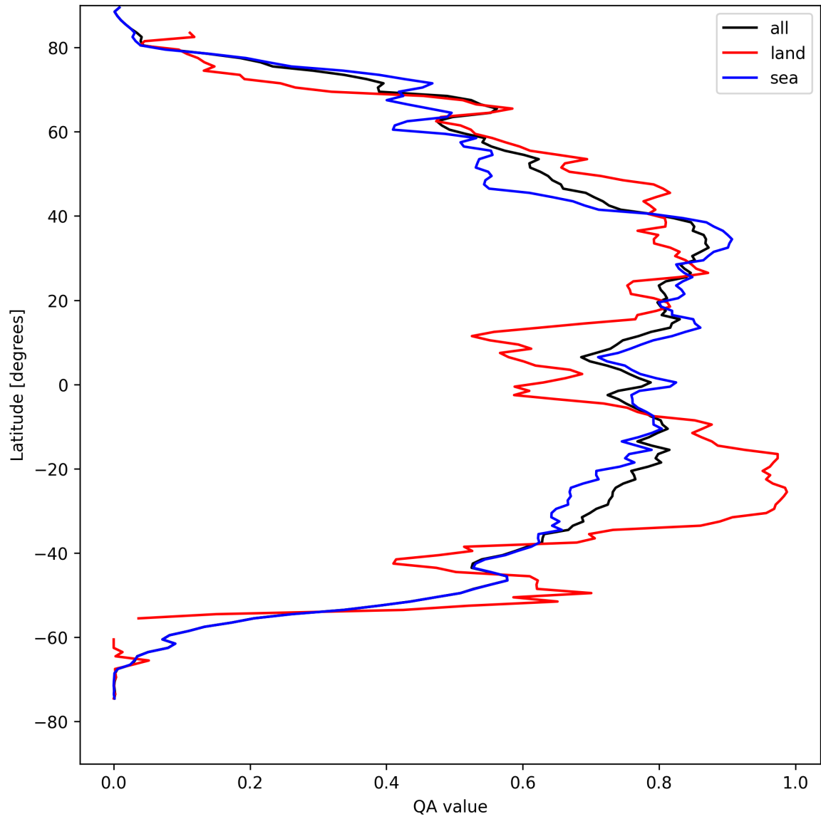
Figure 29: Zonal average of “QA value” for 2024-08-25 to 2024-08-27.
