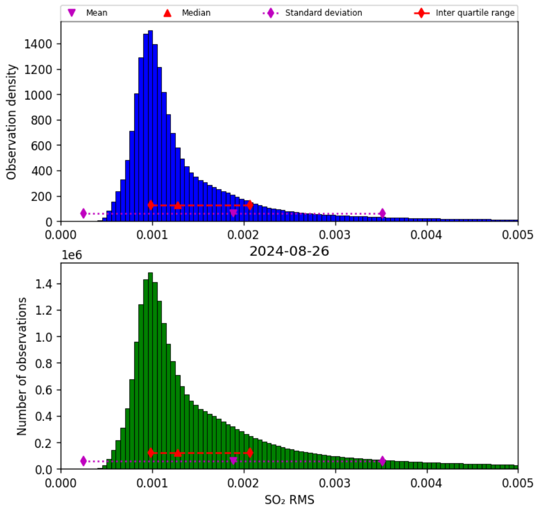
Figure 70: Histogram of “SO 2 RMS” for 2024-08-25 to 2024-08-27
