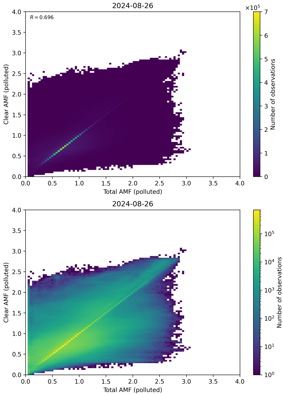
Figure 271: Scatter density plot of “Total AMF (polluted)” against “Clear AMF (polluted)” for 2024-08-25 to 2024-08-27.
