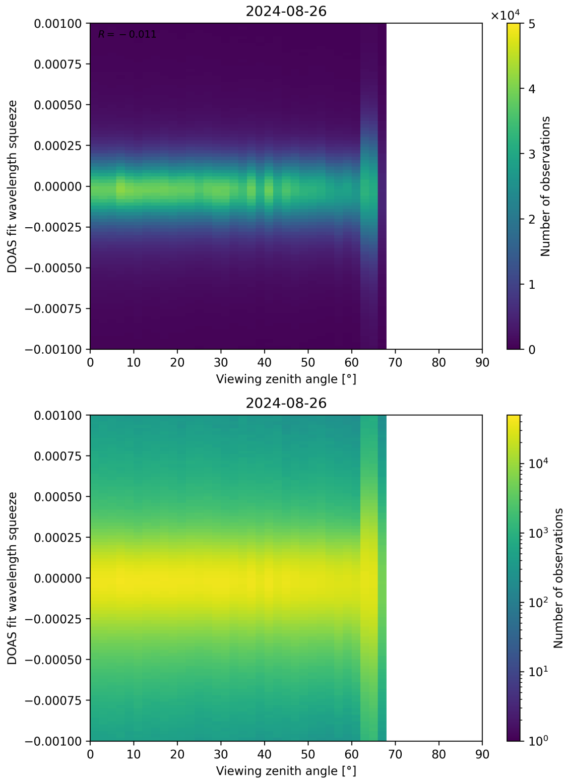
Figure 312: Scatter density plot of “Viewing zenith angle” against “DOAS fit wavelength squeeze” for 2024-08-25 to 2024-08-27.
