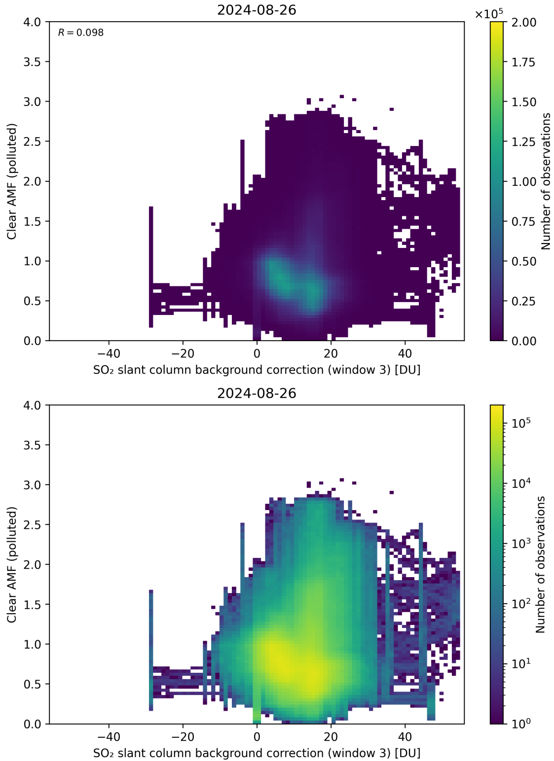
Figure 124: Scatter density plot of “SO 2 slant column background correction (window 3)” against “Clear AMF (polluted)” for 2024-08-25 to 2024-08-27.
