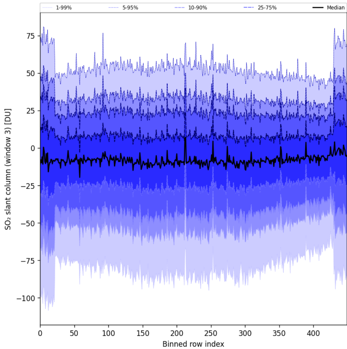
Figure 87: Along track statistics of “SO 2 slant column (window 3)” for 2024-08-25 to 2024-08-27
