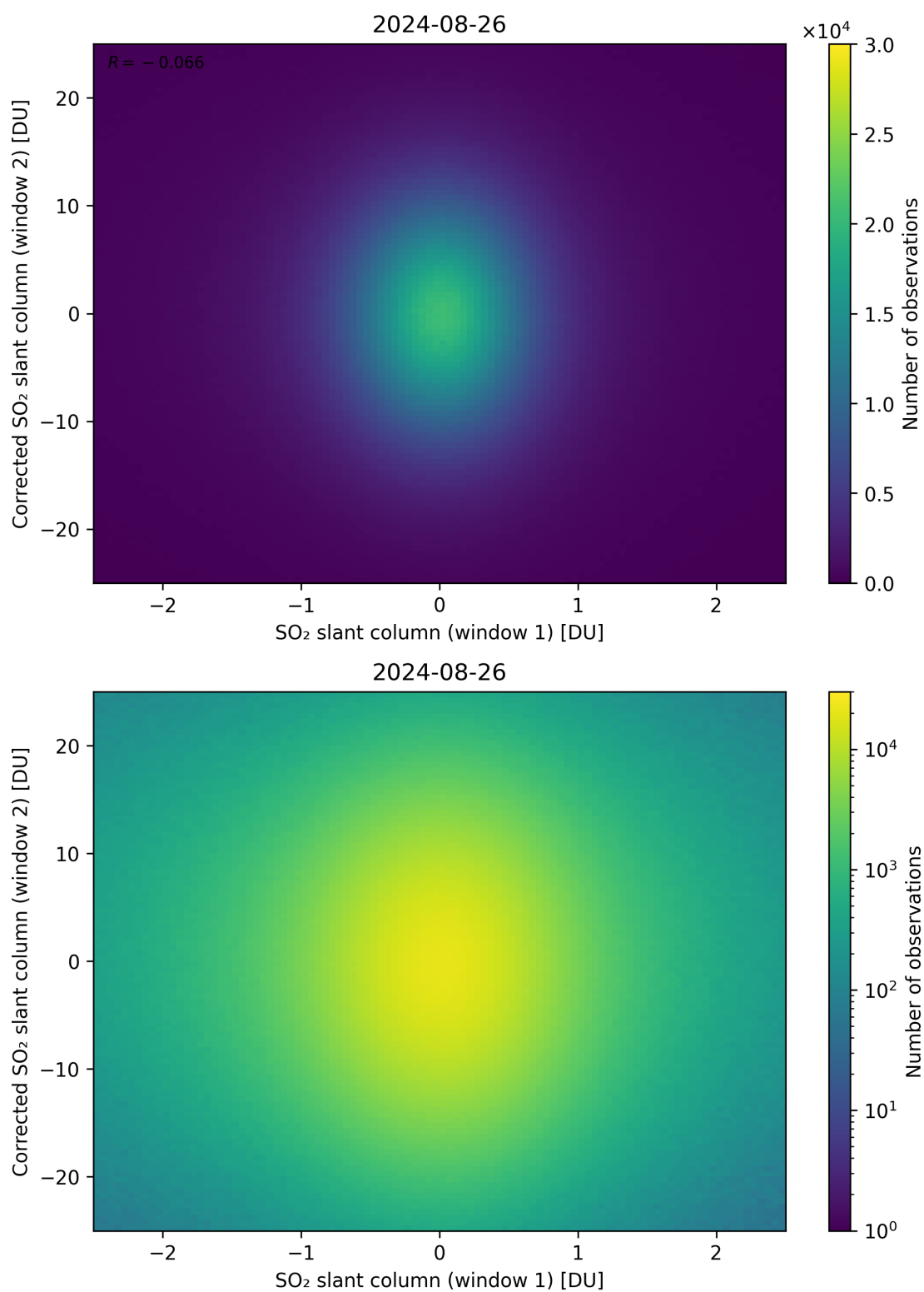
Figure 233: Scatter density plot of “SO 2 slant column (window 1)” against “Corrected SO 2 slant column (window 2)” for 2024-08-25 to 2024-08-27.
