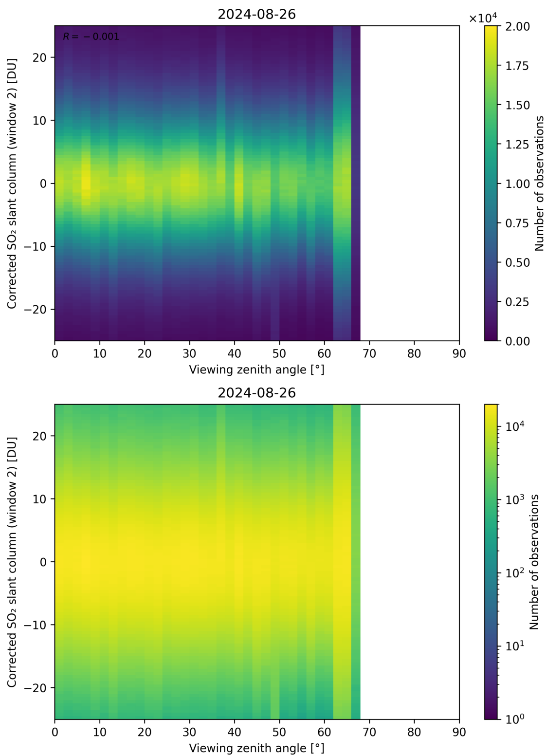
Figure 318: Scatter density plot of “Viewing zenith angle” against “Corrected SO 2 slant column (window 2)” for 2024-08-25 to 2024-08-27.
