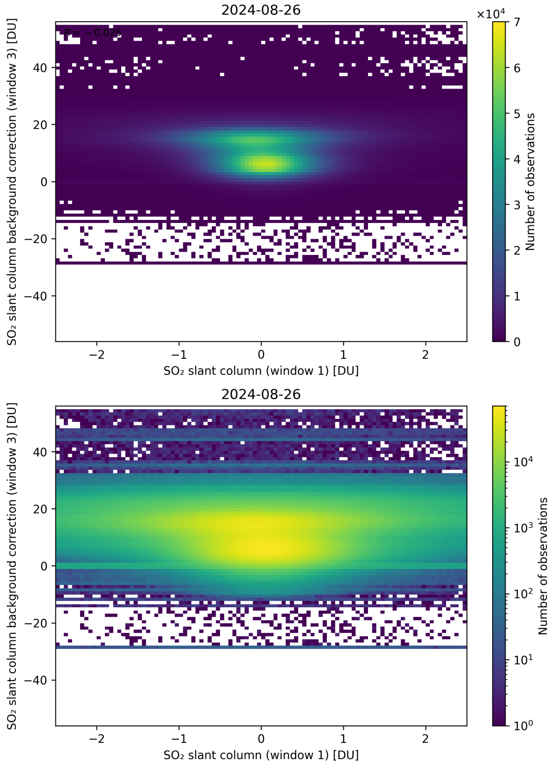
Figure 214: Scatter density plot of “SO 2 slant column (window 1)” against “SO 2 slant column background correction (window 3)” for 2024-08-25 to 2024-08-27.
