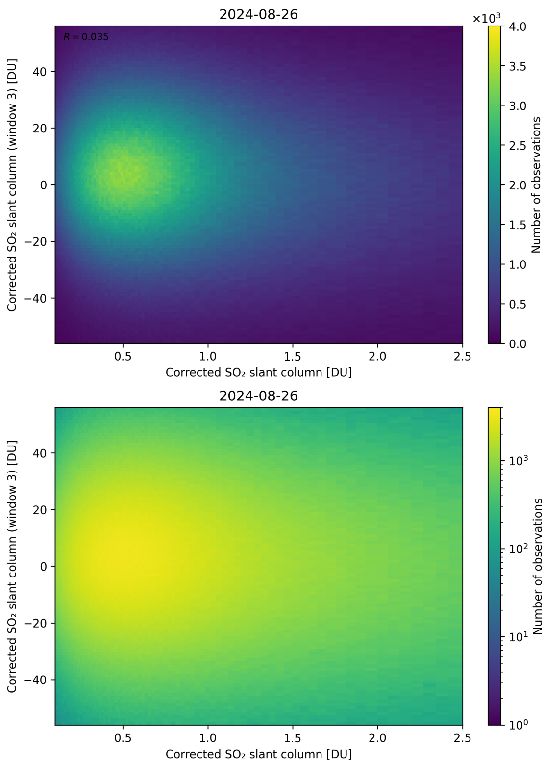
Figure 186: Scatter density plot of “Corrected SO 2 slant column” against “Corrected SO 2 slant column (window 3)” for 2024-08-25 to 2024-08-27.
