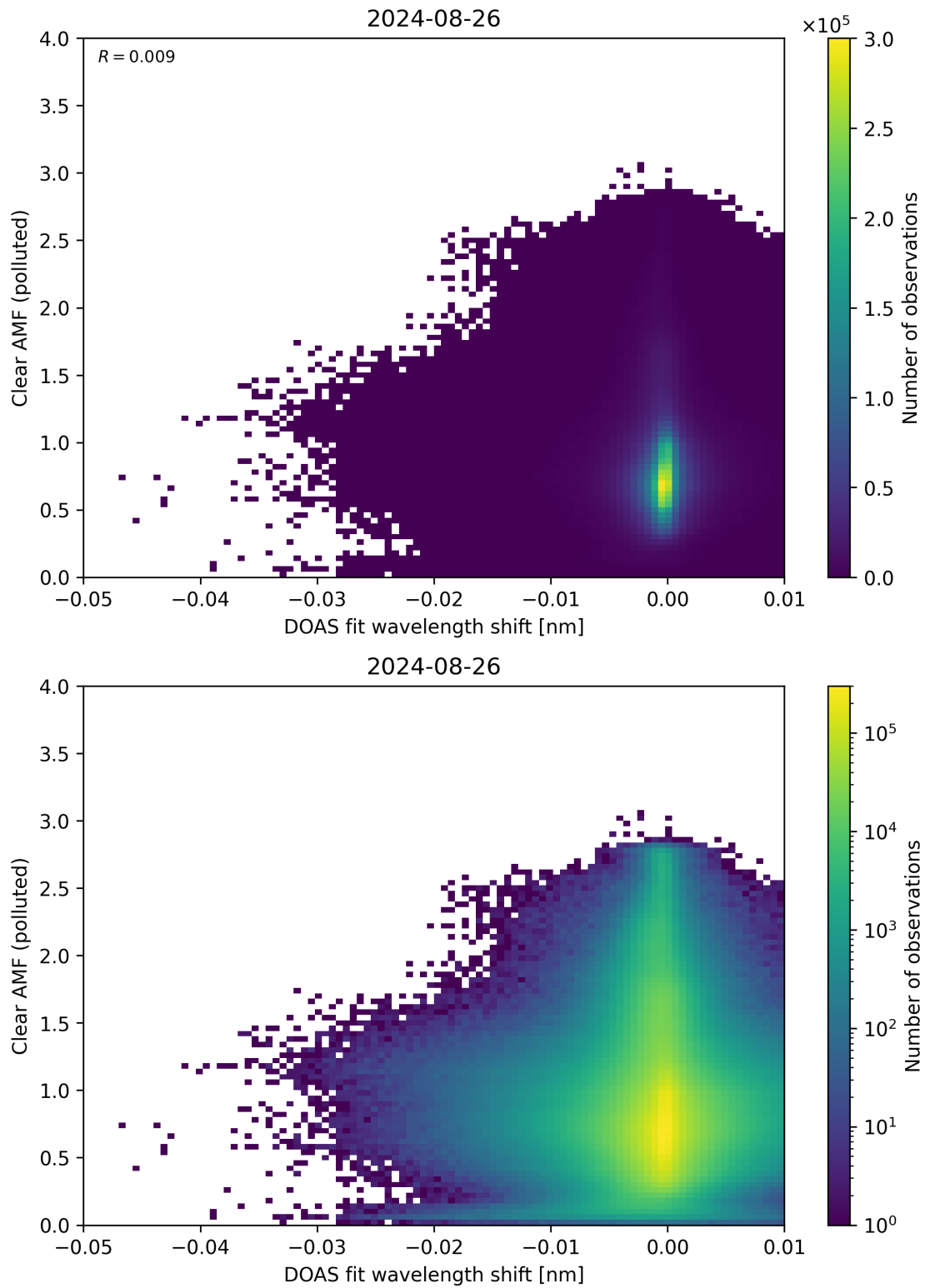
Figure 129: Scatter density plot of “DOAS fit wavelength shift” against “Clear AMF (polluted)” for 2024-08-25 to 2024-08-27.
