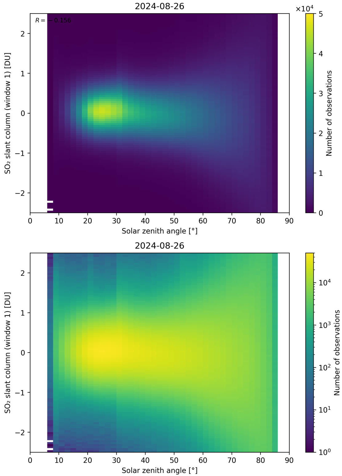
Figure 169: Scatter density plot of “Solar zenith angle” against “SO 2 slant column (window 1)” for 2024-08-25 to 2024-08-27.
