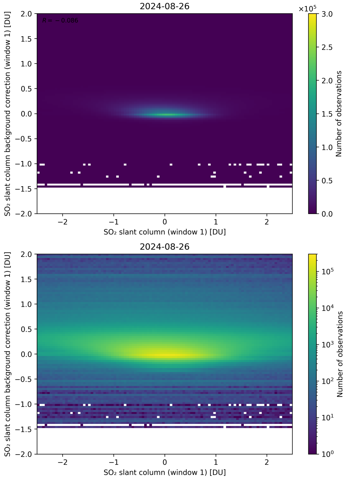
Figure 212: Scatter density plot of “SO 2 slant column (window 1)” against “SO 2 slant column background correction (window 1)” for 2024-08-25 to 2024-08-27.
