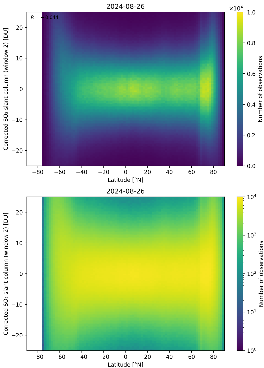
Figure 147: Scatter density plot of “Latitude” against “Corrected SO 2 slant column (window 2)” for 2024-08-25 to 2024-08-27.
