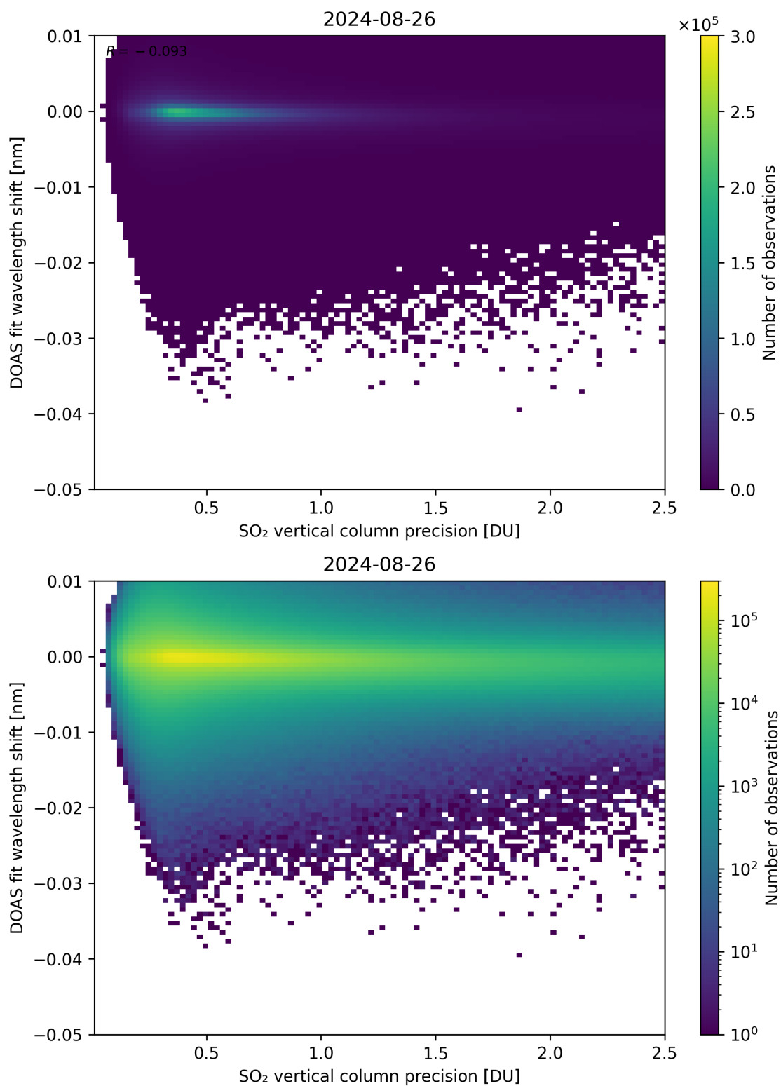
Figure 282: Scatter density plot of “SO 2 vertical column precision” against “DOAS fit wavelength shift” for 2024-08-25 to 2024-08-27.
