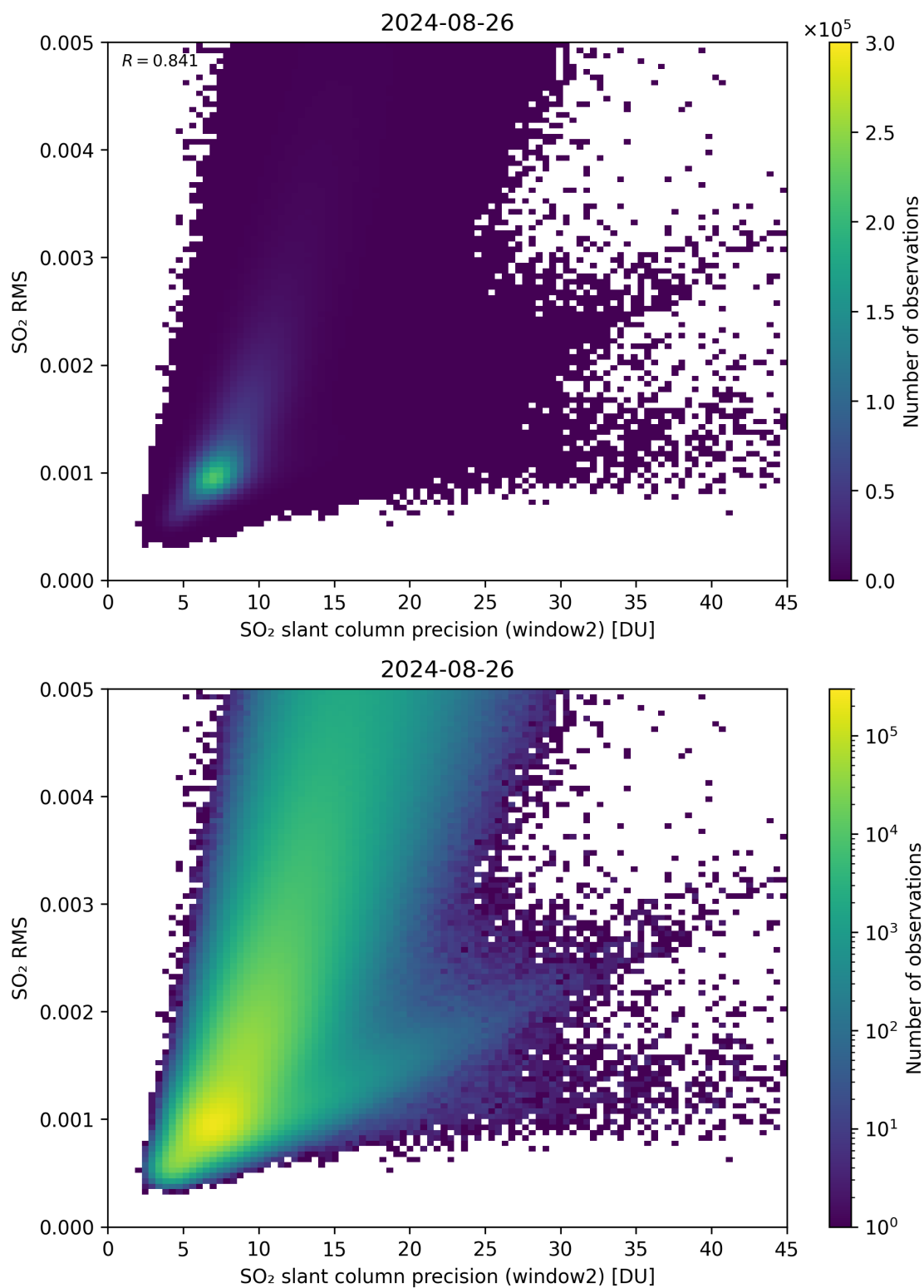
Figure 245: Scatter density plot of “SO 2 slant column precision (window2)” against “SO 2 RMS” for 2024-08-25 to 2024-08-27.
