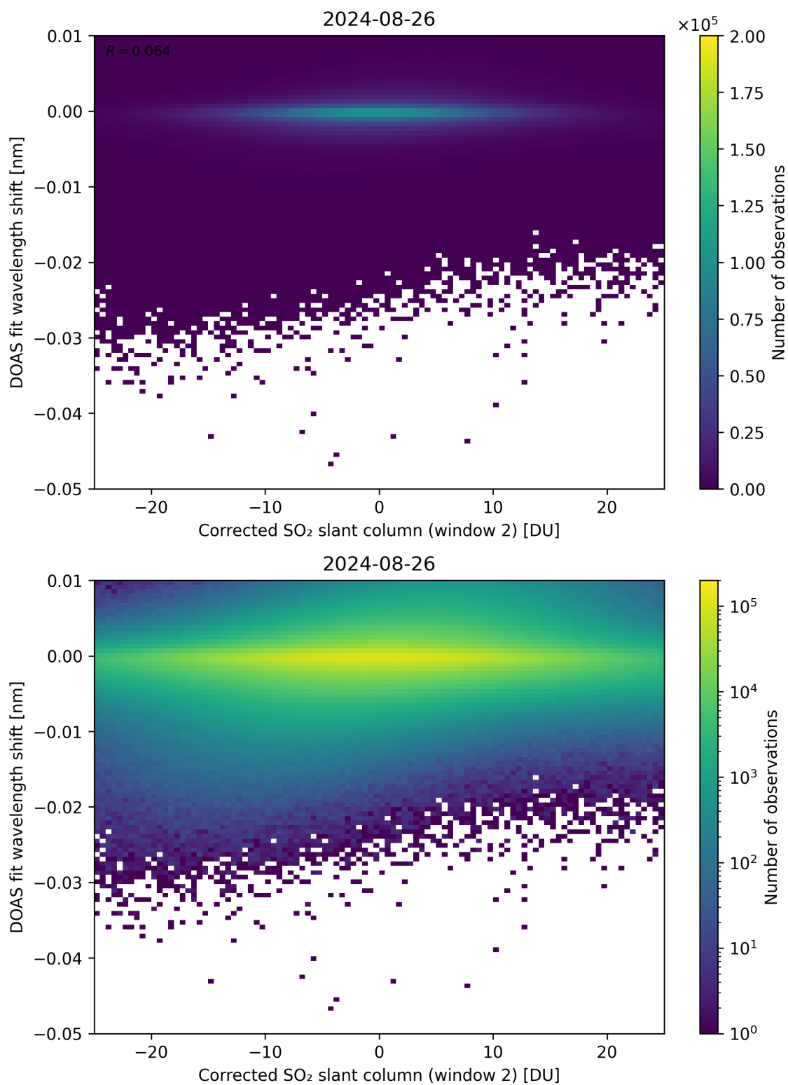
Figure 196: Scatter density plot of “Corrected SO 2 slant column (window 2)” against “DOAS fit wavelength shift” for 2024-08-25 to 2024-08-27.
