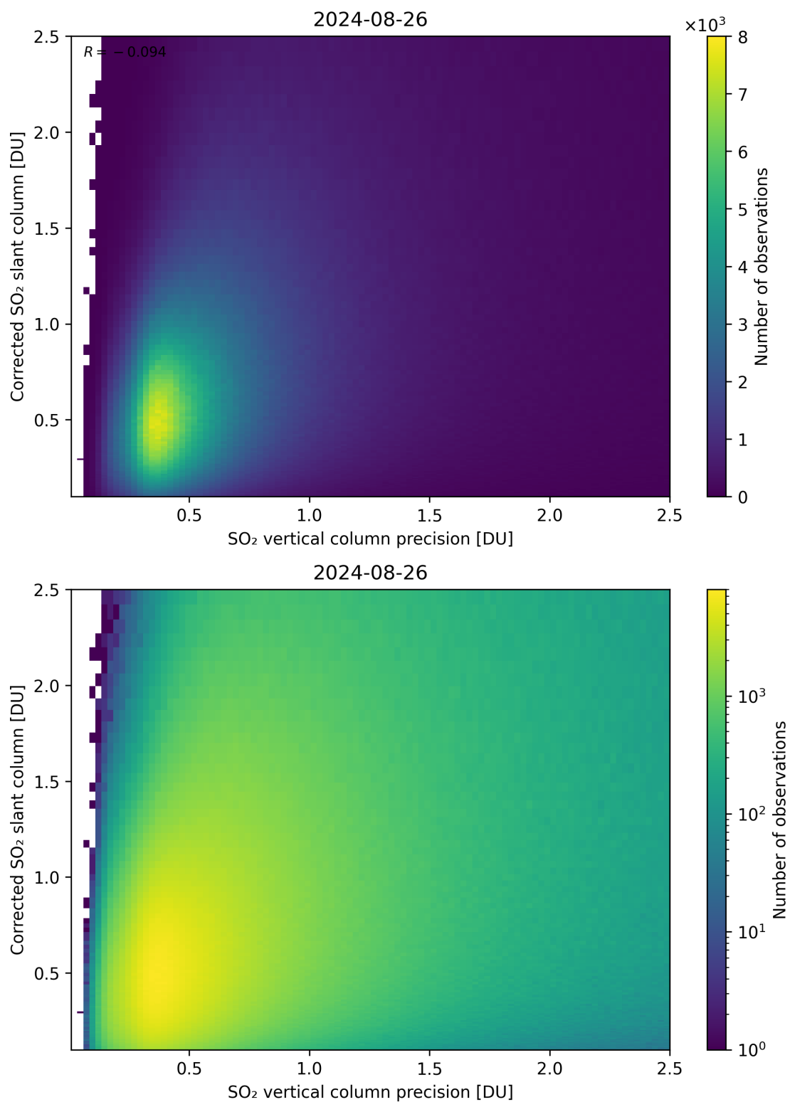
Figure 286: Scatter density plot of “SO 2 vertical column precision” against “Corrected SO 2 slant column” for 2024-08-25 to 2024-08-27.
