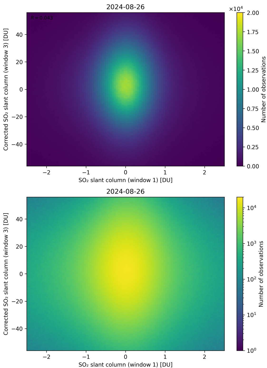
Figure 234: Scatter density plot of “SO 2 slant column (window 1)” against “Corrected SO 2 slant column (window 3)” for 2024-08-25 to 2024-08-27.
