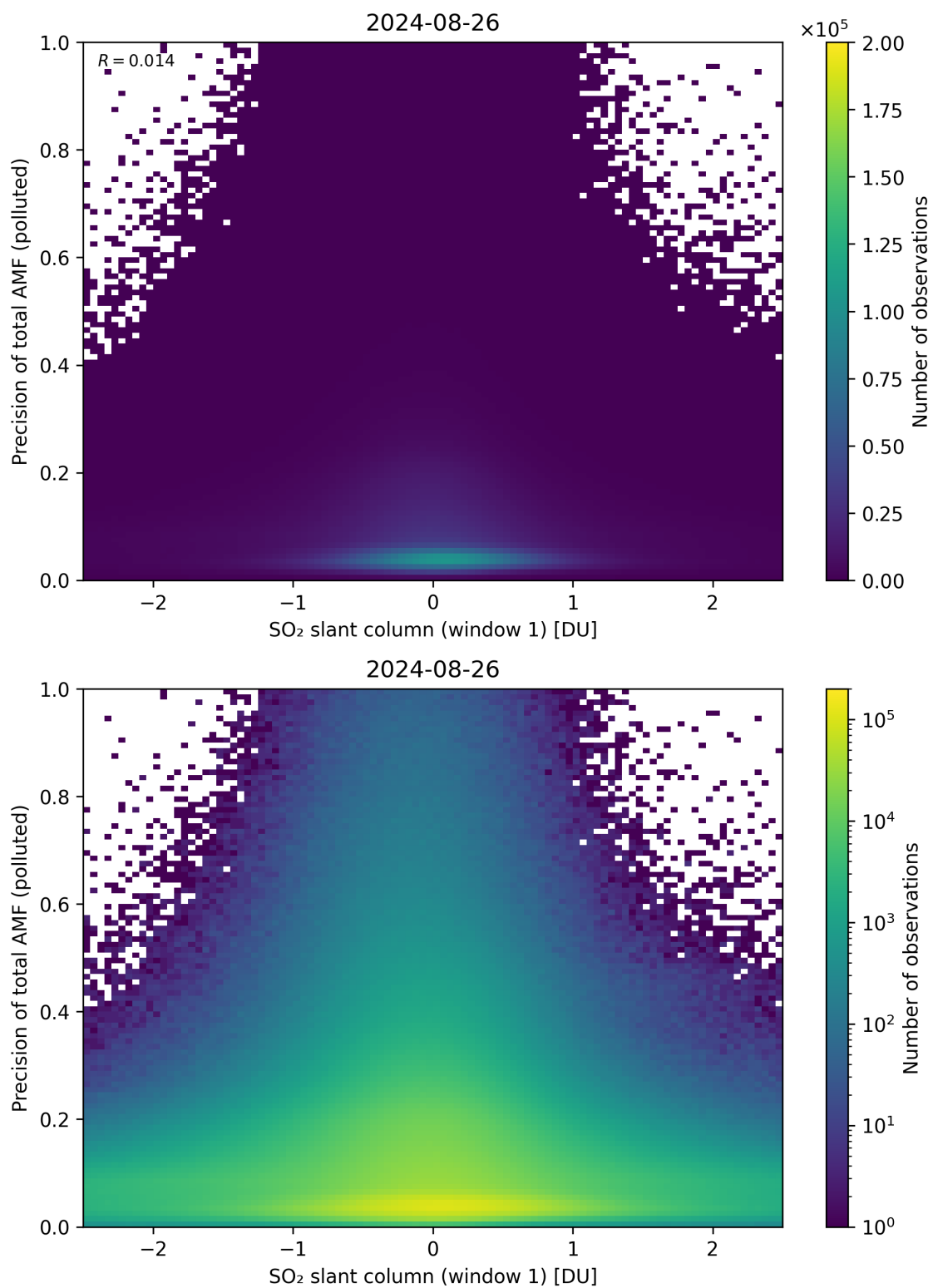
Figure 240: Scatter density plot of “SO 2 slant column (window 1)” against “Precision of total AMF (polluted)” for 2024-08-25 to 2024-08-27.
