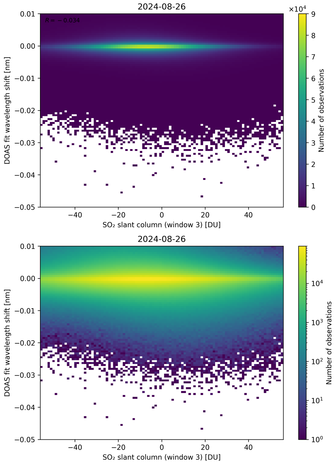
Figure 254: Scatter density plot of “SO 2 slant column (window 3)” against “DOAS fit wavelength shift” for 2024-08-25 to 2024-08-27.
