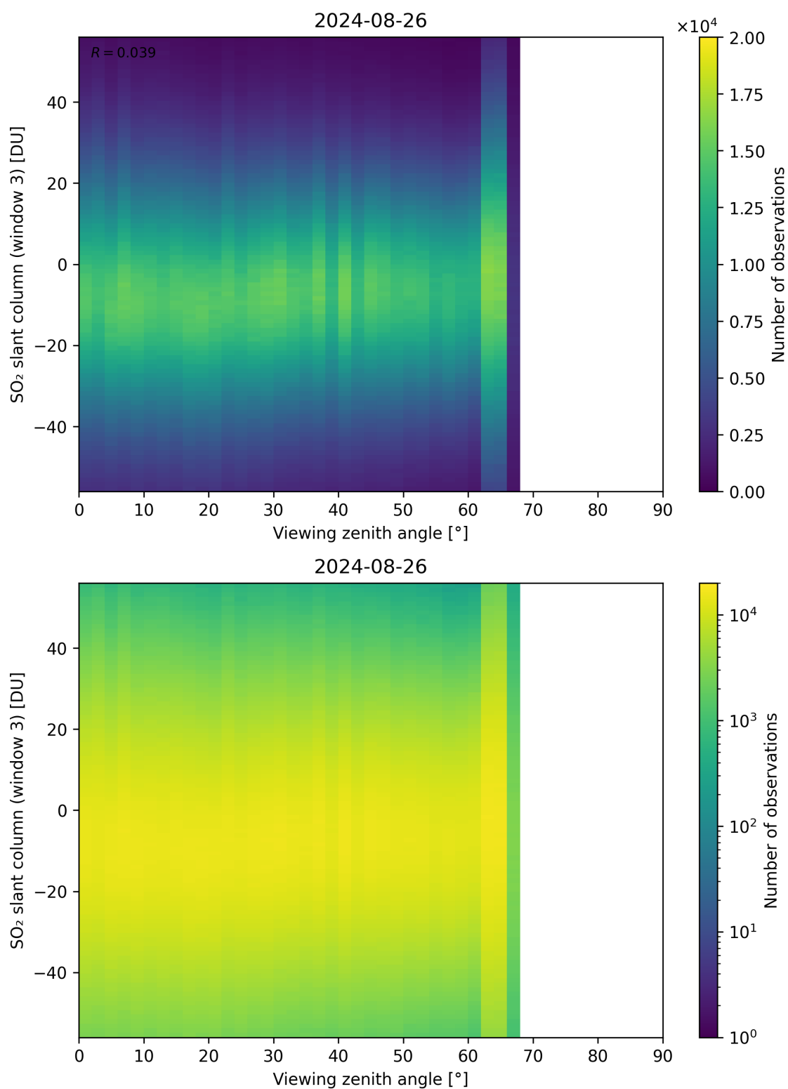
Figure 323: Scatter density plot of “Viewing zenith angle” against “SO 2 slant column (window 3)” for 2024-08-25 to 2024-08-27.
