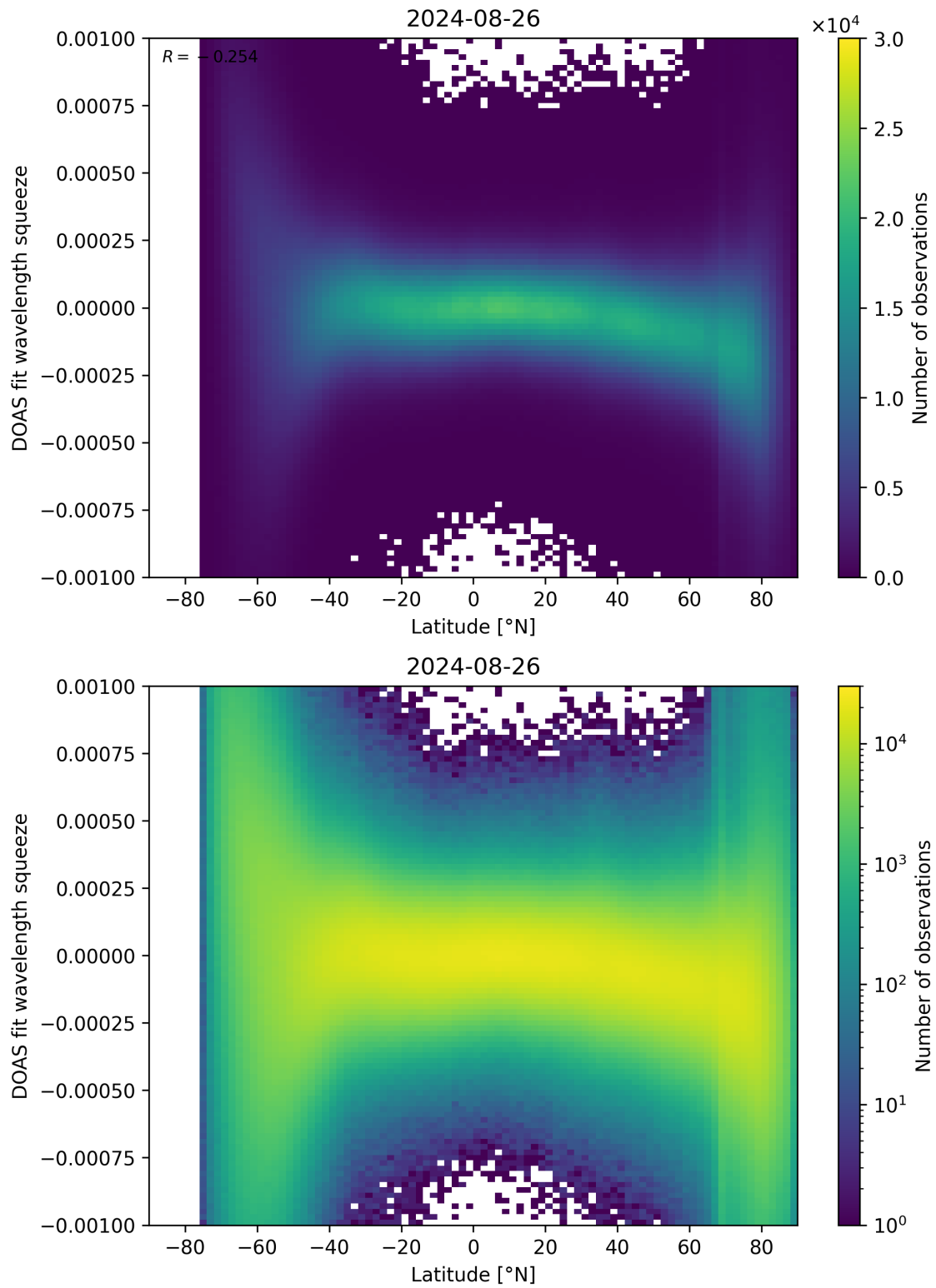
Figure 143: Scatter density plot of “Latitude” against “DOAS fit wavelength squeeze” for 2024-08-25 to 2024-08-27.
