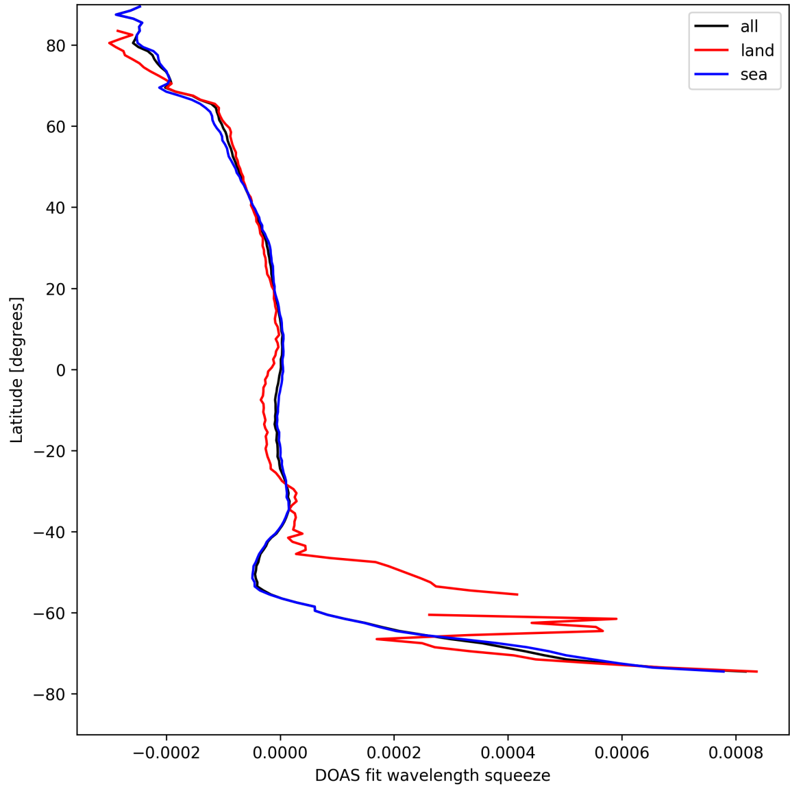
Figure 46: Zonal average of “DOAS fit wavelength squeeze” for 2024-08-25 to 2024-08-27.
