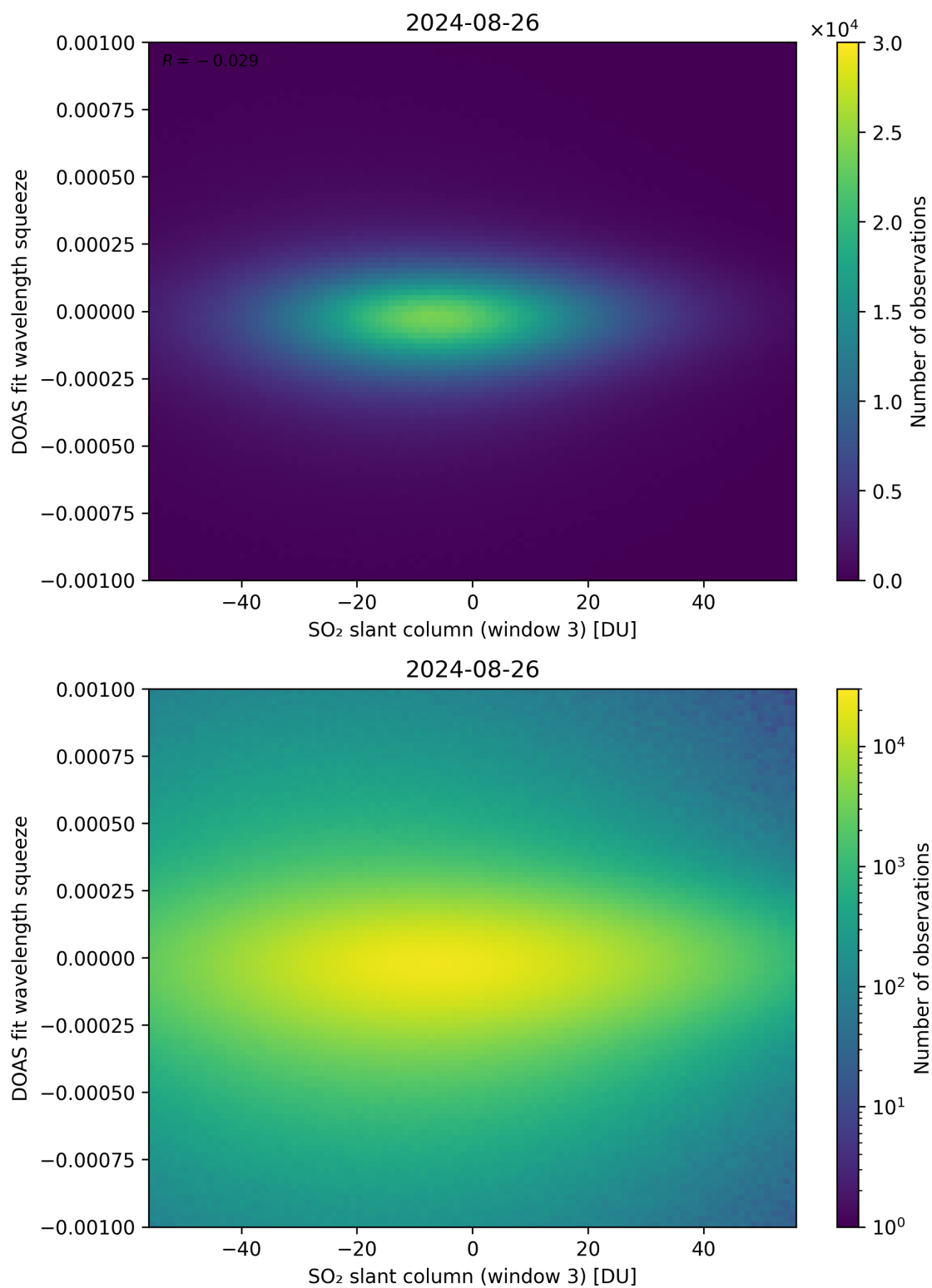
Figure 255: Scatter density plot of “SO 2 slant column (window 3)” against “DOAS fit wavelength squeeze” for 2024-08-25 to 2024-08-27.
