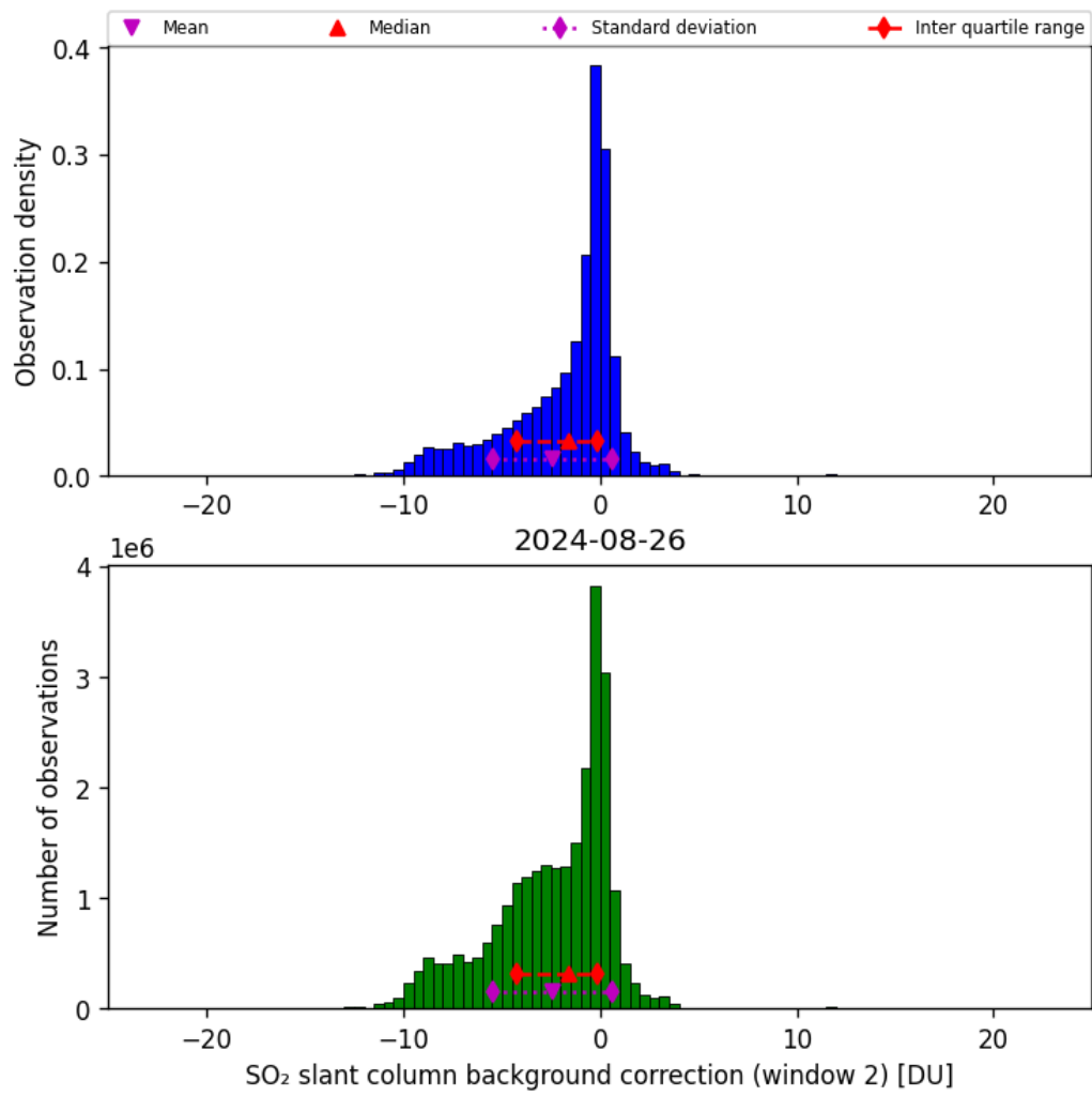
Figure 63: Histogram of “SO 2 slant column background correction (window 2)” for 2024-08-25 to 2024-08-27
