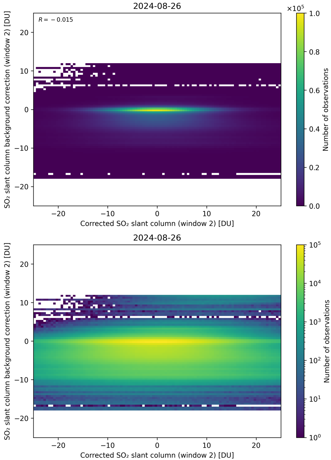
Figure 194: Scatter density plot of “Corrected SO 2 slant column (window 2)” against “SO 2 slant column background correction (window 2)” for 2024-08-25 to 2024-08-27.
