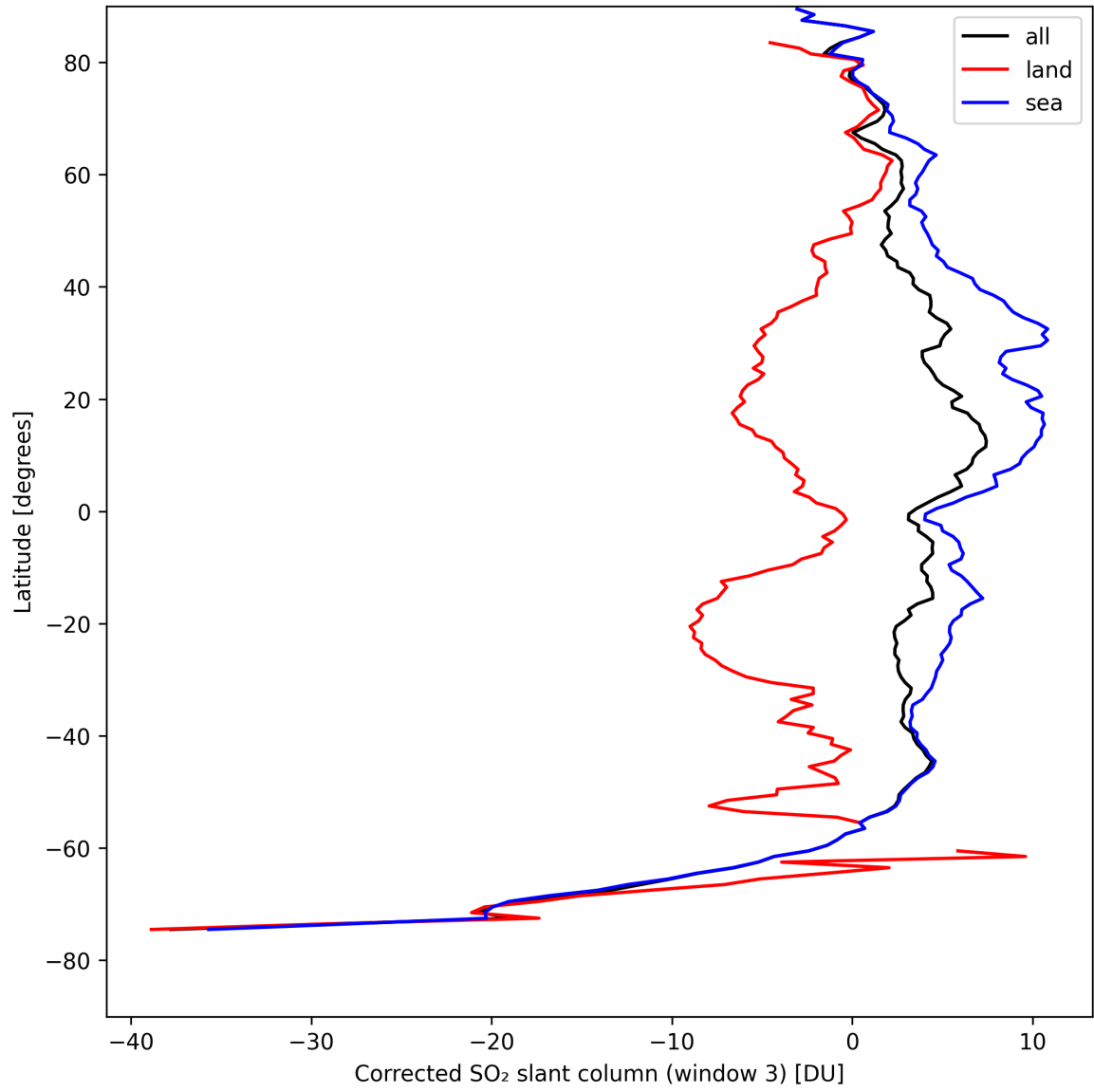
Figure 43: Zonal average of “Corrected SO 2 slant column (window 3)” for 2024-08-25 to 2024-08-27.
