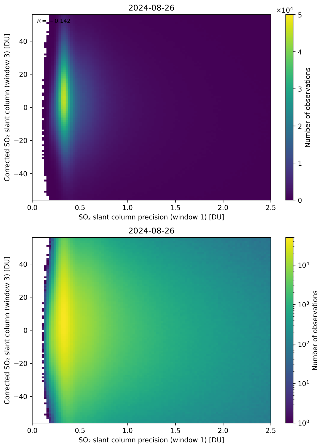
Figure 226: Scatter density plot of “SO 2 slant column precision (window 1)” against “Corrected SO 2 slant column (window 3)” for 2024-08-25 to 2024-08-27.
