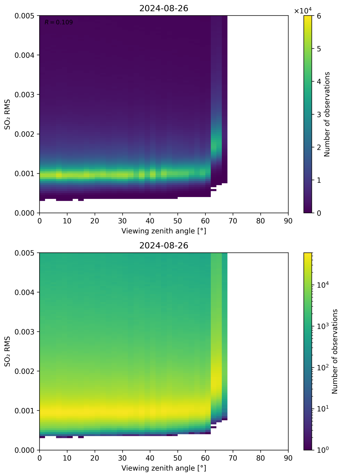
Figure 313: Scatter density plot of “Viewing zenith angle” against “SO 2 RMS” for 2024-08-25 to 2024-08-27.
