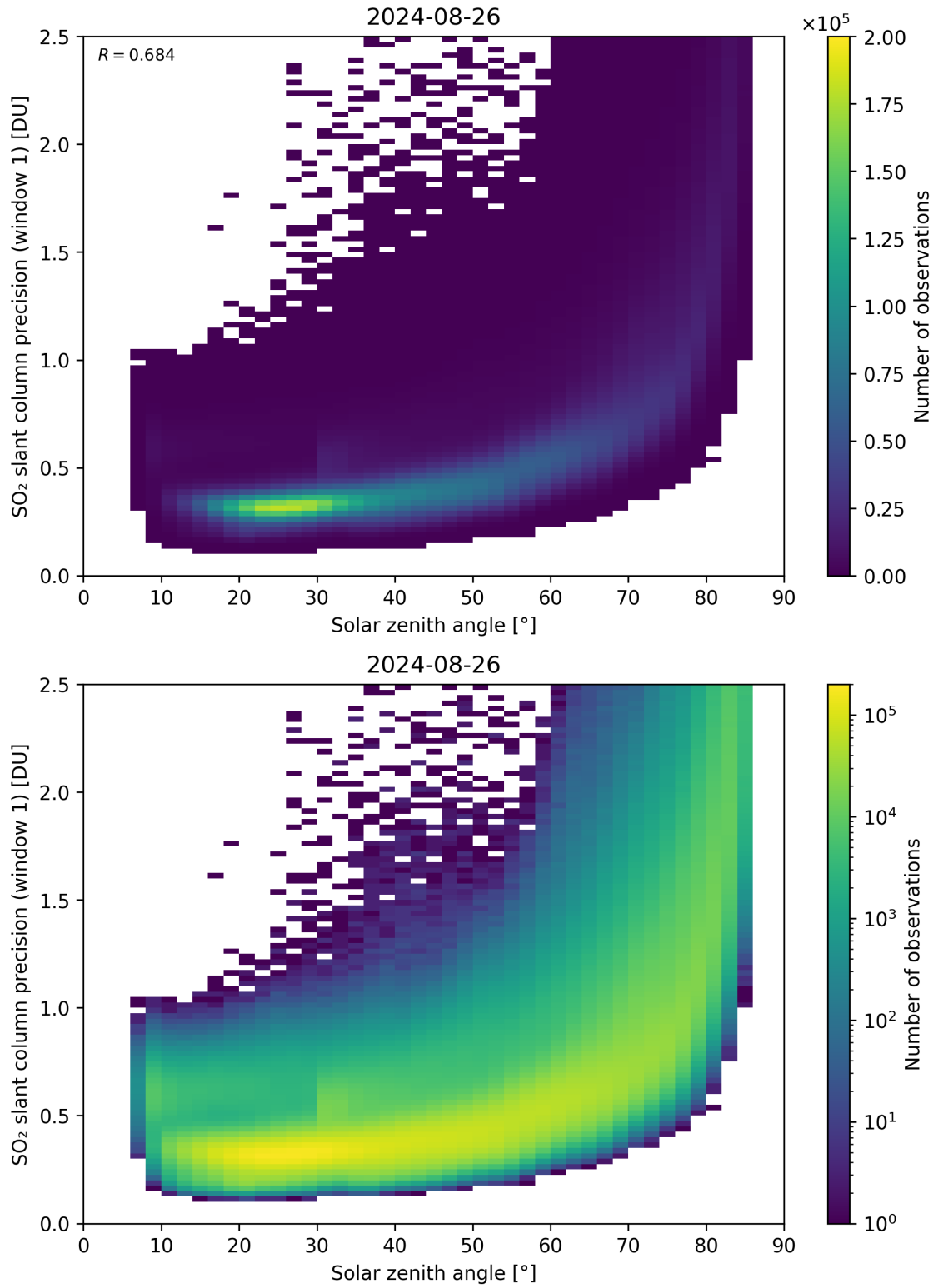
Figure 170: Scatter density plot of “Solar zenith angle” against “SO 2 slant column precision (window 1)” for 2024-08-25 to 2024-08-27.
