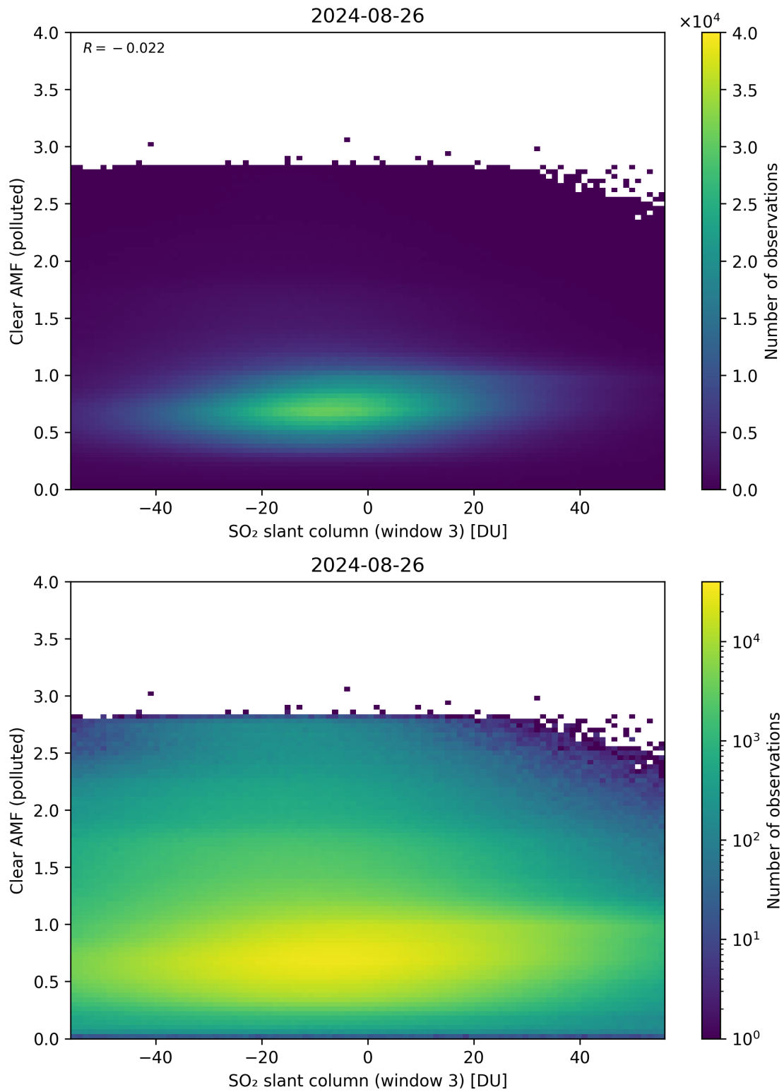
Figure 265: Scatter density plot of “SO 2 slant column (window 3)” against “Clear AMF (polluted)” for 2024-08-25 to 2024-08-27.
