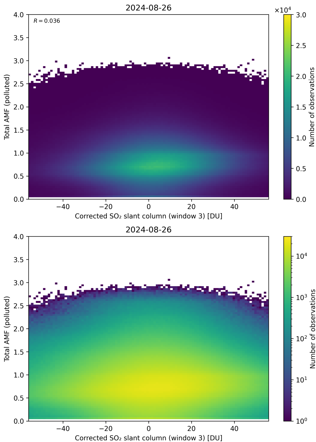
Figure 210: Scatter density plot of “Corrected SO 2 slant column (window 3)” against “Total AMF (polluted)” for 2024-08-25 to 2024-08-27.
