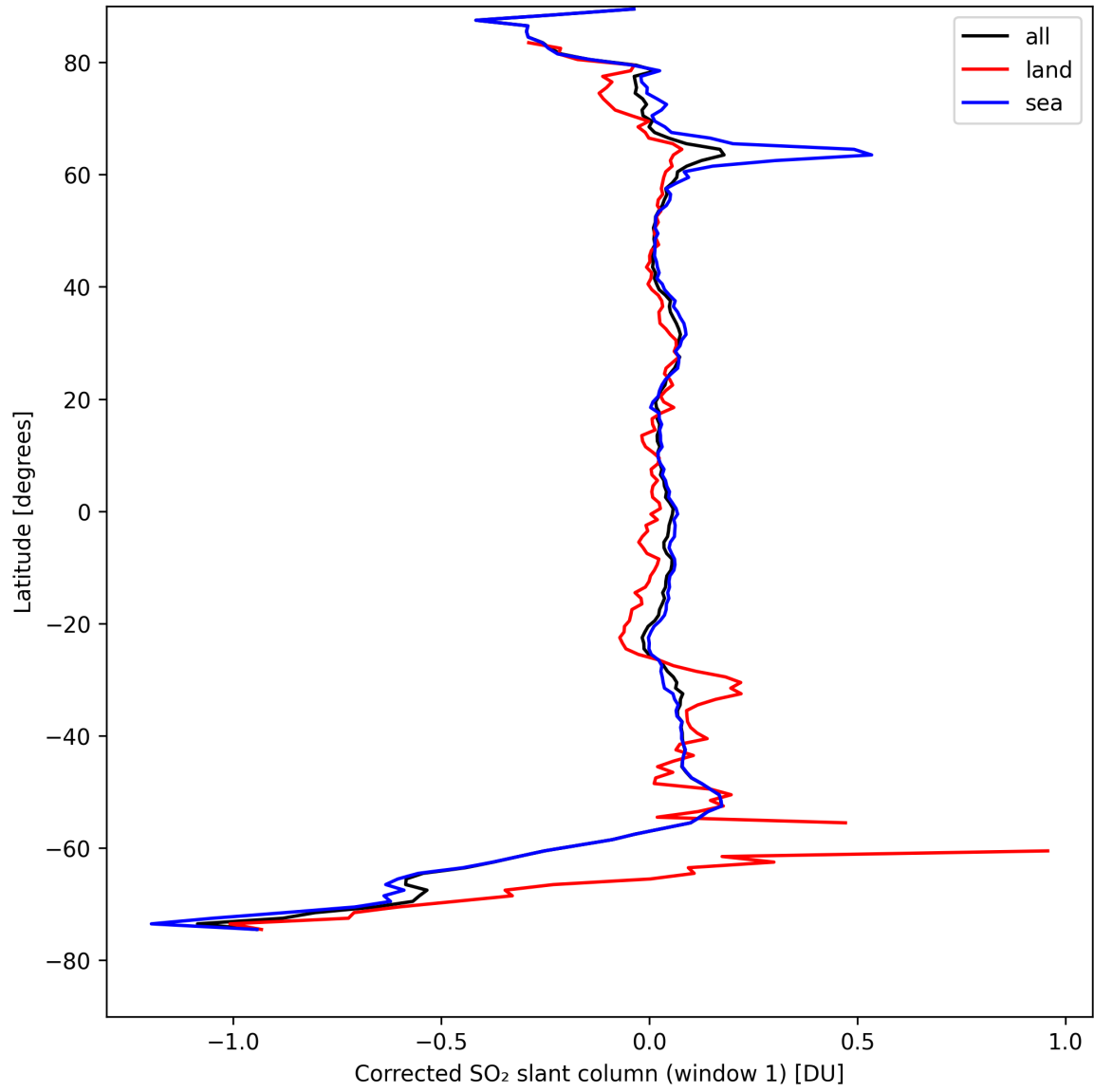
Figure 35: Zonal average of “Corrected SO 2 slant column (window 1)” for 2024-08-25 to 2024-08-27.
