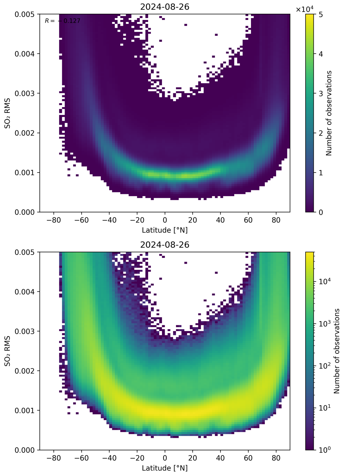
Figure 144: Scatter density plot of “Latitude” against “SO 2 RMS” for 2024-08-25 to 2024-08-27.
