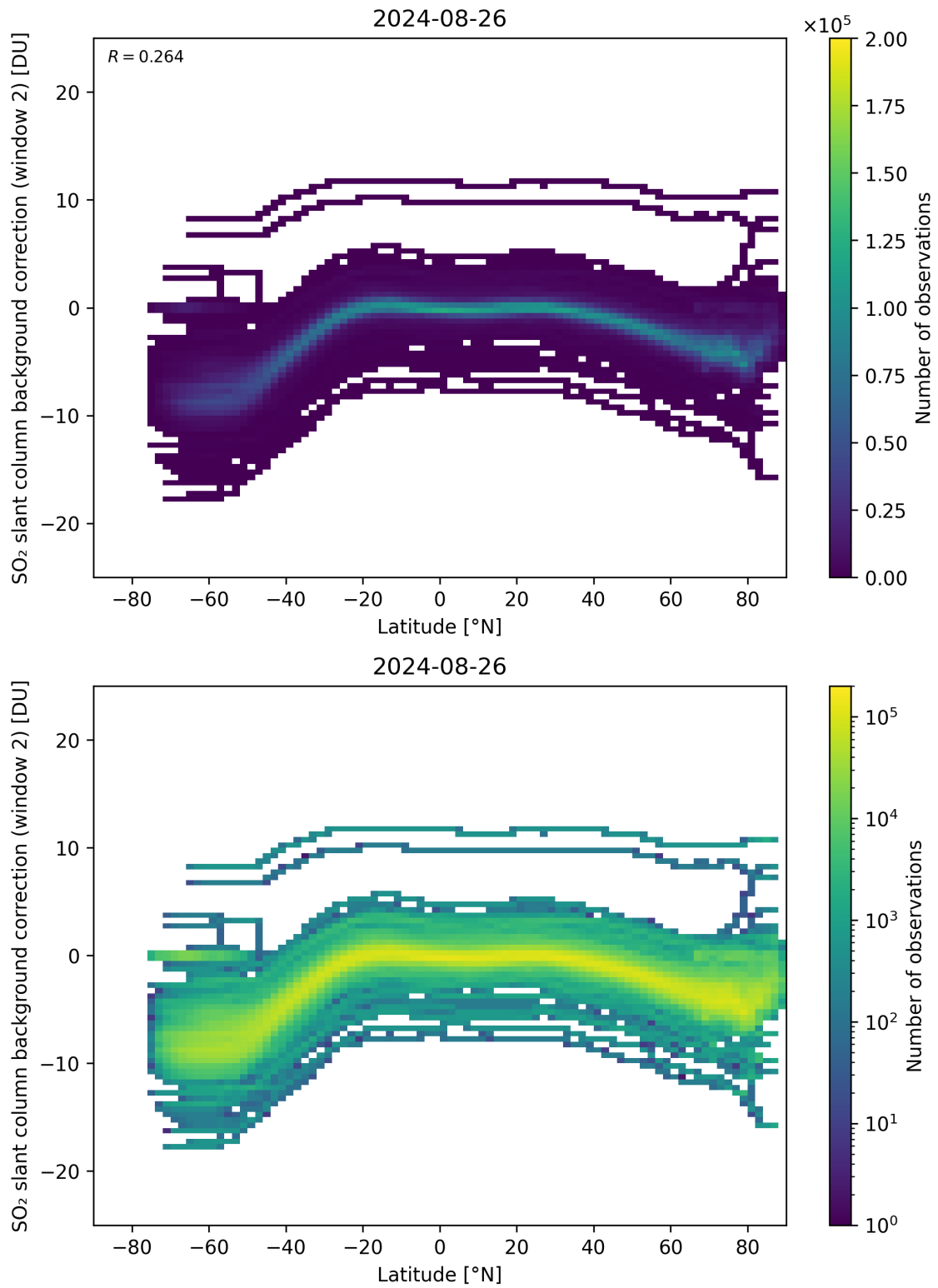
Figure 140: Scatter density plot of “Latitude” against “SO 2 slant column background correction (window 2)” for 2024-08-25 to 2024-08-27.
