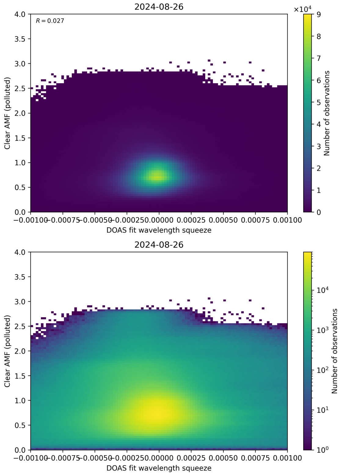
Figure 133: Scatter density plot of “DOAS fit wavelength squeeze” against “Clear AMF (polluted)” for 2024-08-25 to 2024-08-27.
