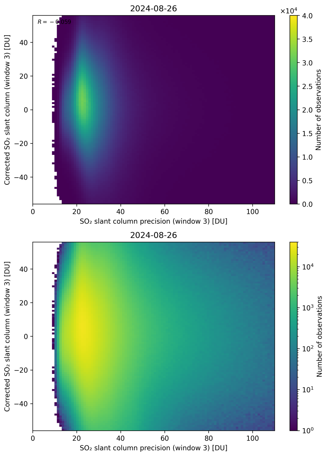
Figure 262: Scatter density plot of “SO 2 slant column precision (window 3)” against “Corrected SO 2 slant column (window 3)” for 2024-08-25 to 2024-08-27.
