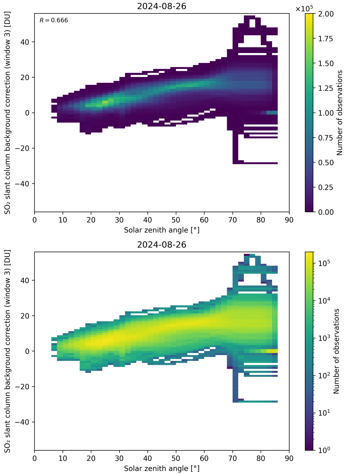
Figure 160: Scatter density plot of “Solar zenith angle” against “SO 2 slant column background correction (window 3)” for 2024-08-25 to 2024-08-27.
