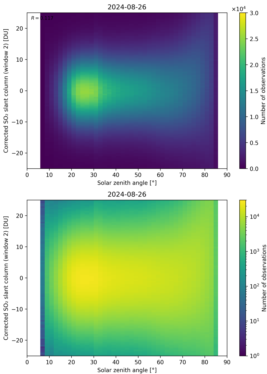
Figure 167: Scatter density plot of “Solar zenith angle” against “Corrected SO 2 slant column (window 2)” for 2024-08-25 to 2024-08-27.
