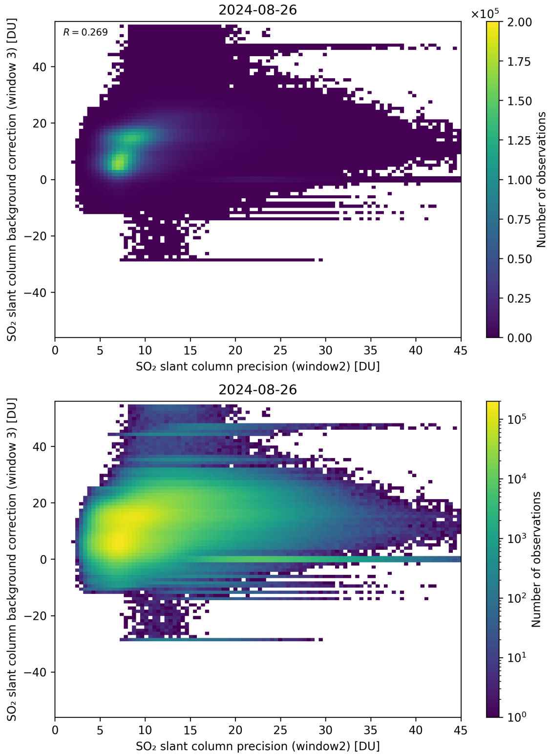
Figure 242: Scatter density plot of “SO 2 slant column precision (window2)” against “SO 2 slant column background correction (window 3)” for 2024-08-25 to 2024-08-27.
