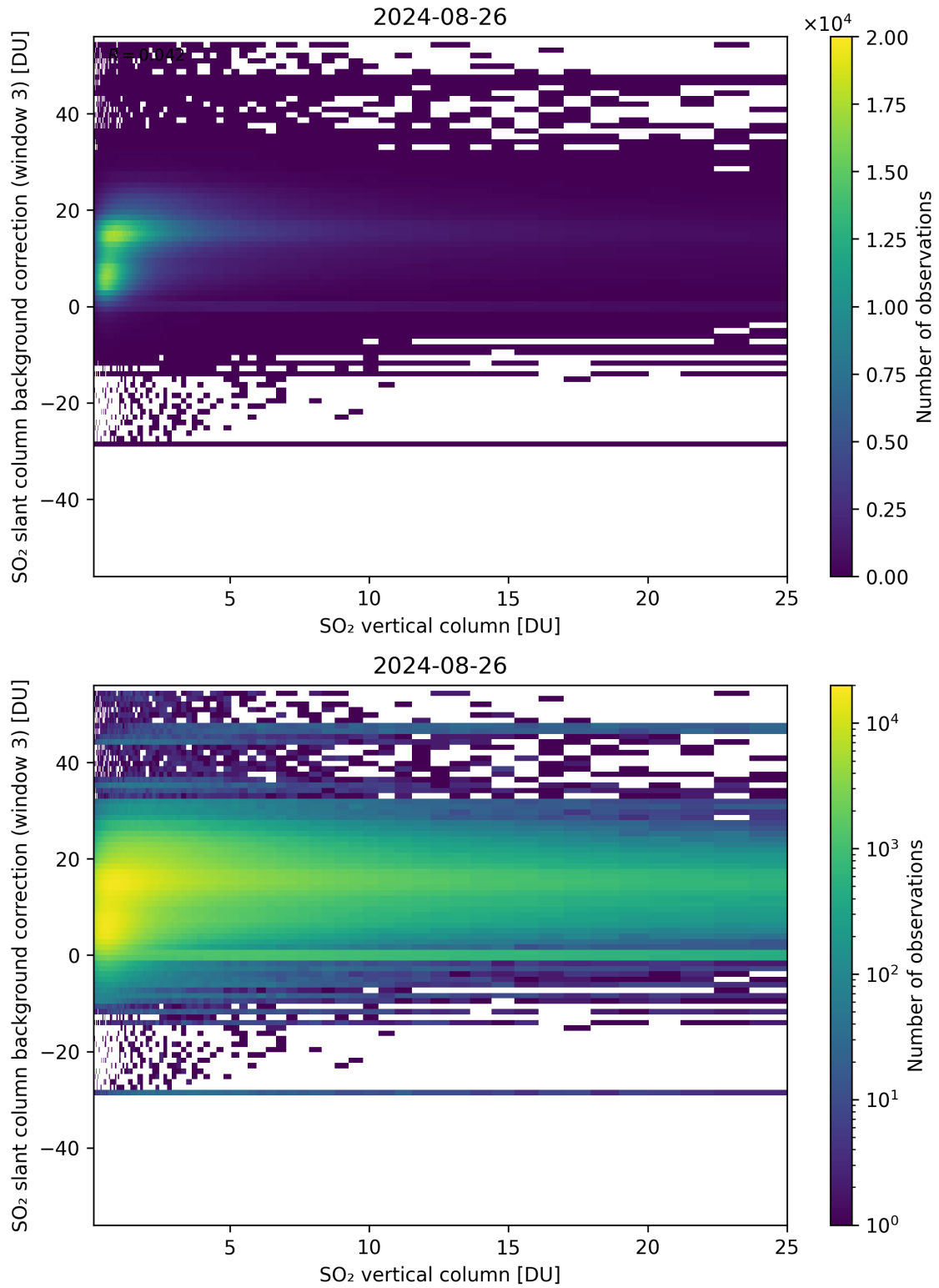
Figure 275: Scatter density plot of “SO 2 vertical column” against “SO 2 slant column background correction (window 3)” for 2024-08-25 to 2024-08-27.
