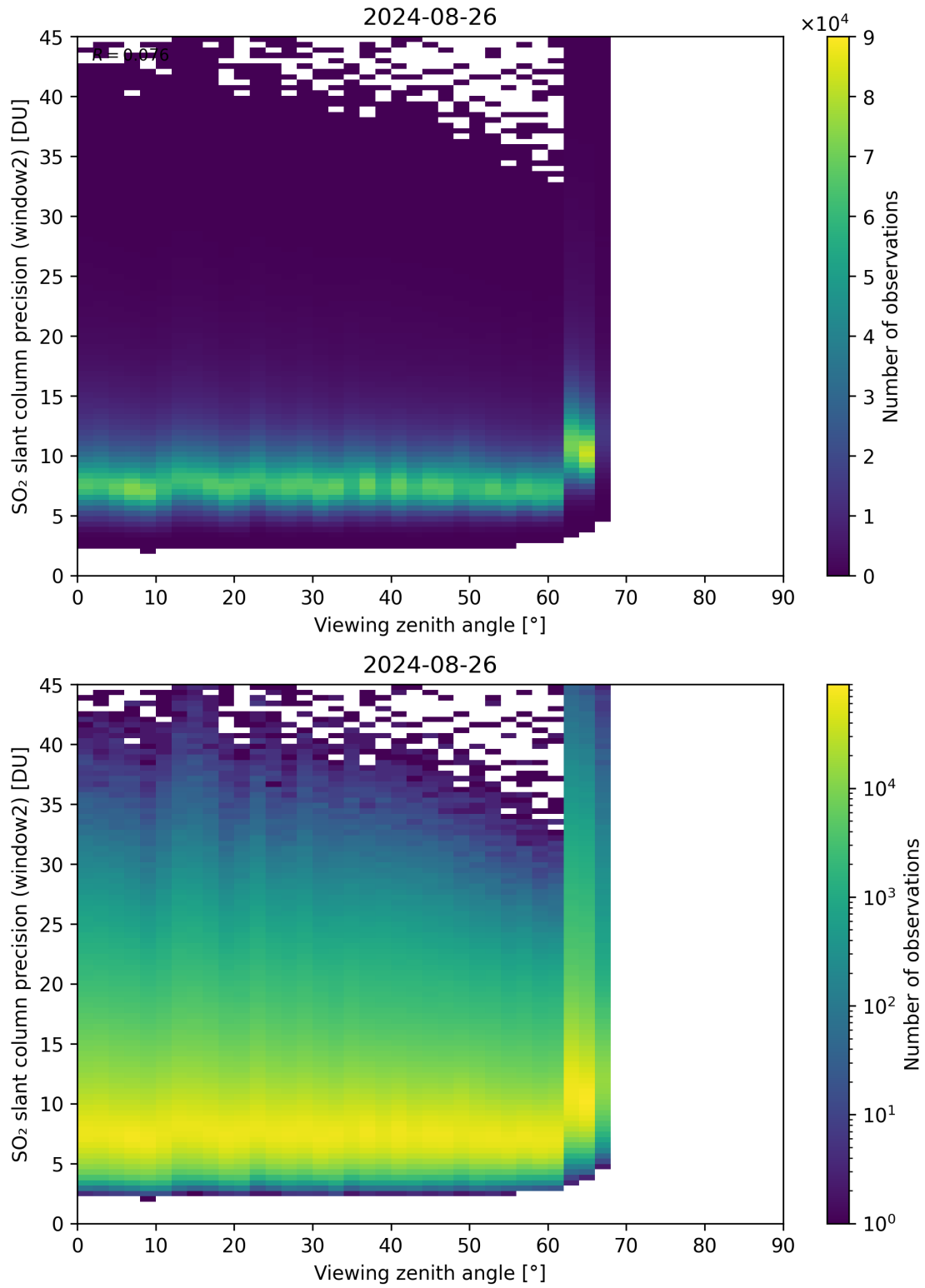
Figure 322: Scatter density plot of “Viewing zenith angle” against “SO 2 slant column precision (window2)” for 2024-08-25 to 2024-08-27.
