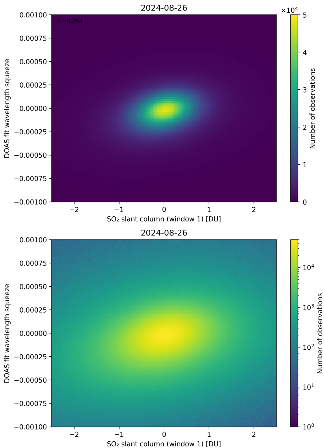
Figure 216: Scatter density plot of “SO 2 slant column (window 1)” against “DOAS fit wavelength squeeze” for 2024-08-25 to 2024-08-27.
