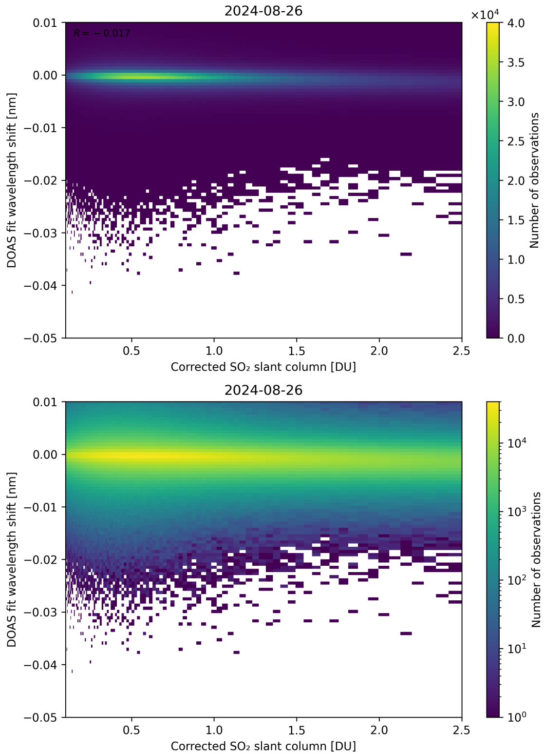
Figure 181: Scatter density plot of “Corrected SO 2 slant column” against “DOAS fit wavelength shift” for 2024-08-25 to 2024-08-27.
