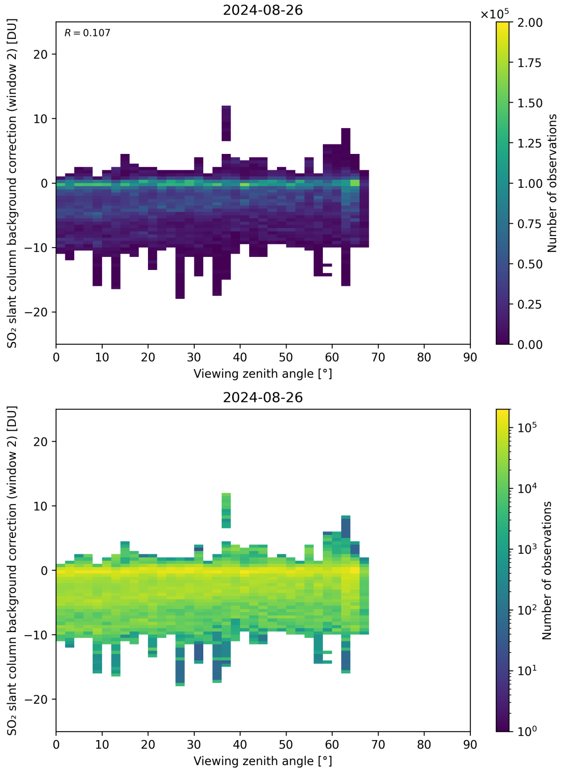
Figure 309: Scatter density plot of “Viewing zenith angle” against “SO 2 slant column background correction (window 2)” for 2024-08-25 to 2024-08-27.
