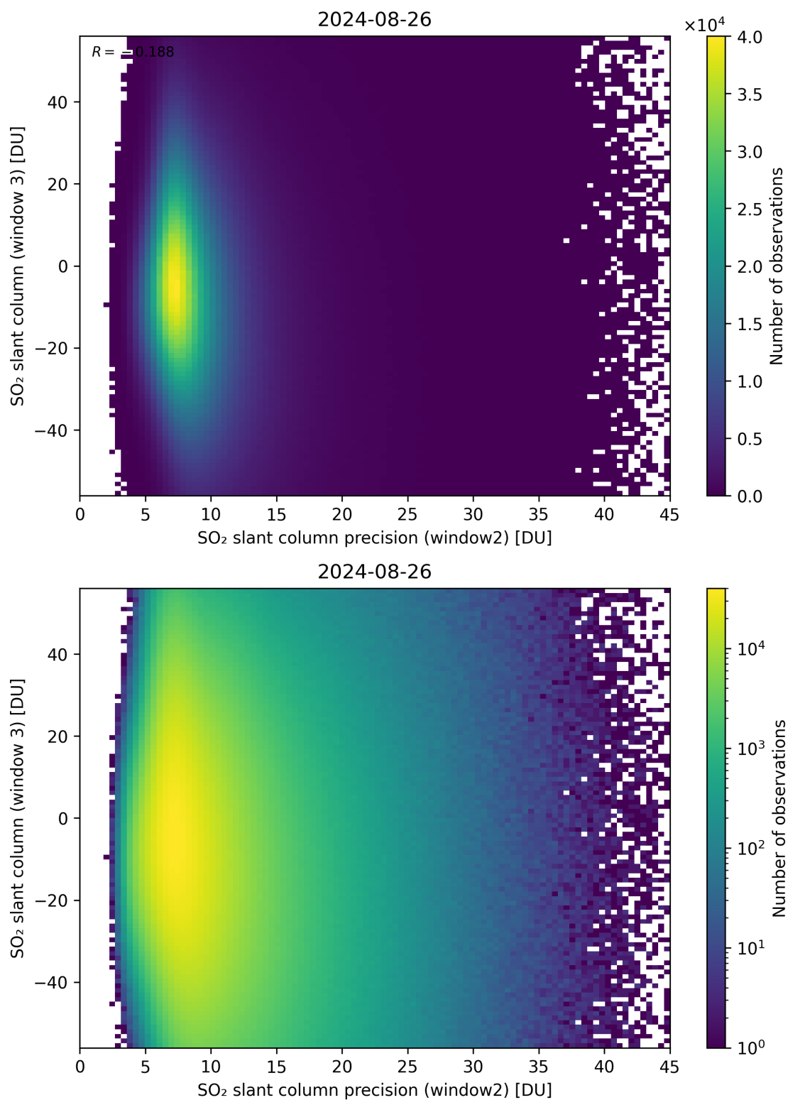
Figure 249: Scatter density plot of “SO 2 slant column precision (window2)” against “SO 2 slant column (window 3)” for 2024-08-25 to 2024-08-27.
