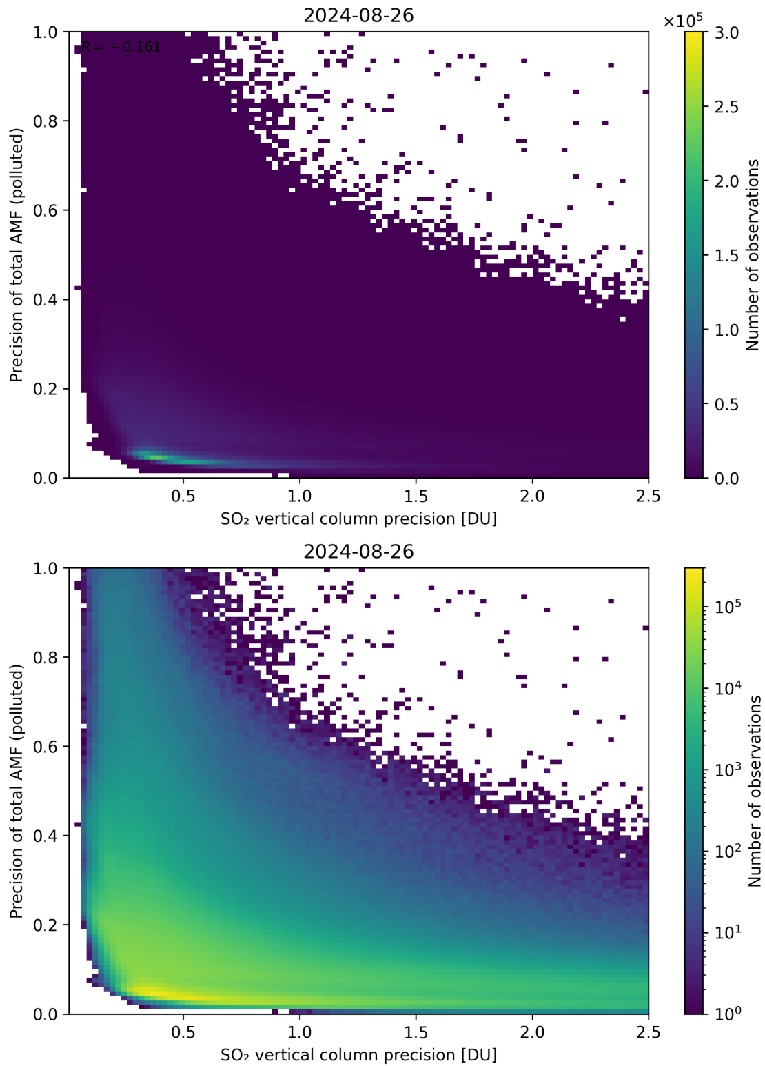
Figure 295: Scatter density plot of “SO 2 vertical column precision” against “Precision of total AMF (polluted)” for 2024-08-25 to 2024-08-27.
