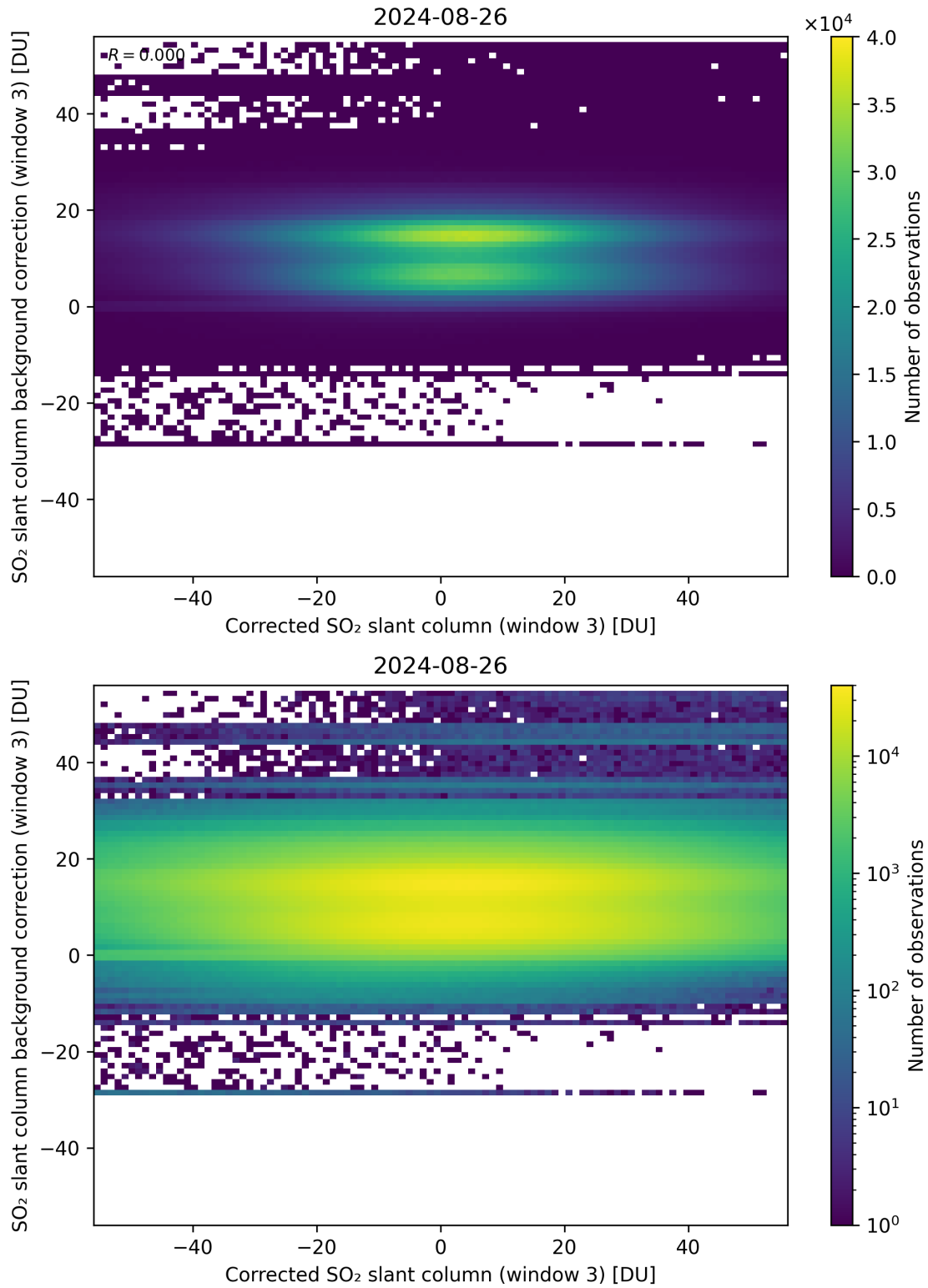
Figure 205: Scatter density plot of “Corrected SO 2 slant column (window 3)” against “SO 2 slant column background correction (window 3)” for 2024-08-25 to 2024-08-27.
