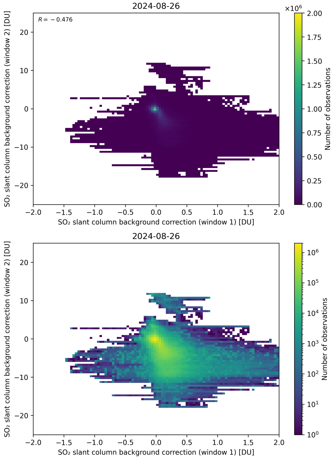
Figure 98: Scatter density plot of “SO 2 slant column background correction (window 1)” against “SO 2 slant column background correction (window 2)” for 2024-08-25 to 2024-08-27.
