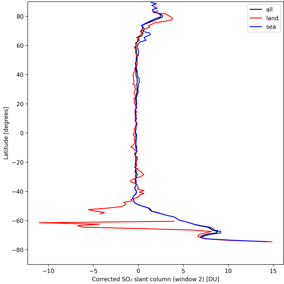
Figure 39: Zonal average of “Corrected SO 2 slant column (window 2)” for 2024-08-25 to 2024-08-27.
