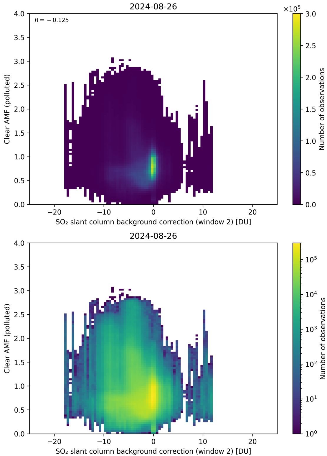
Figure 115: Scatter density plot of “SO 2 slant column background correction (window 2)” against “Clear AMF (polluted)” for 2024-08-25 to 2024-08-27.
