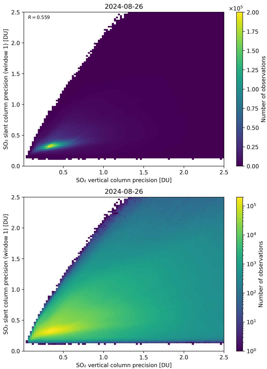
Figure 290: Scatter density plot of “SO 2 vertical column precision” against “SO 2 slant column precision (window 1)” for 2024-08-25 to 2024-08-27.
