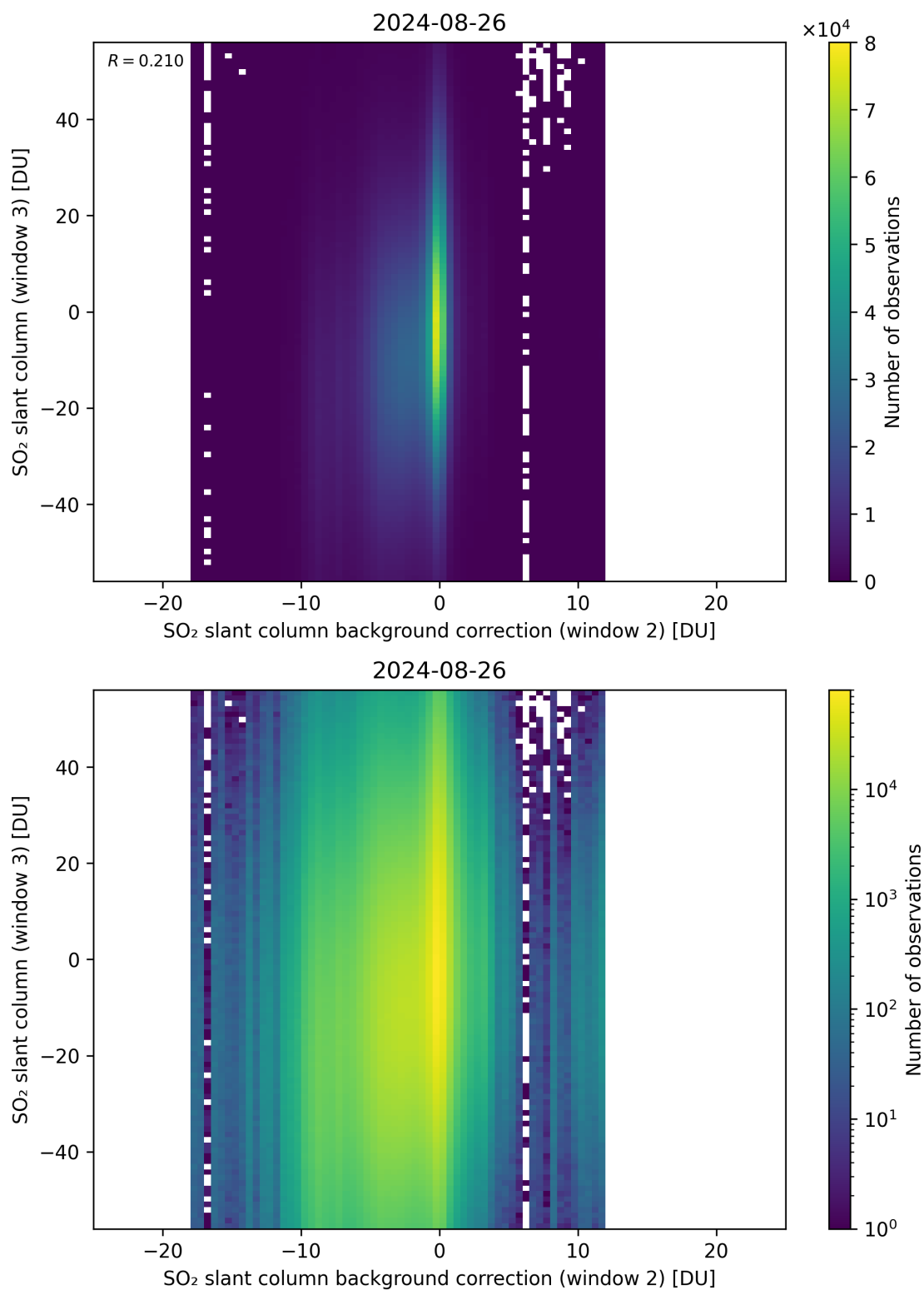
Figure 117: Scatter density plot of “SO 2 slant column background correction (window 2)” against “SO 2 slant column (window 3)” for 2024-08-25 to 2024-08-27.
