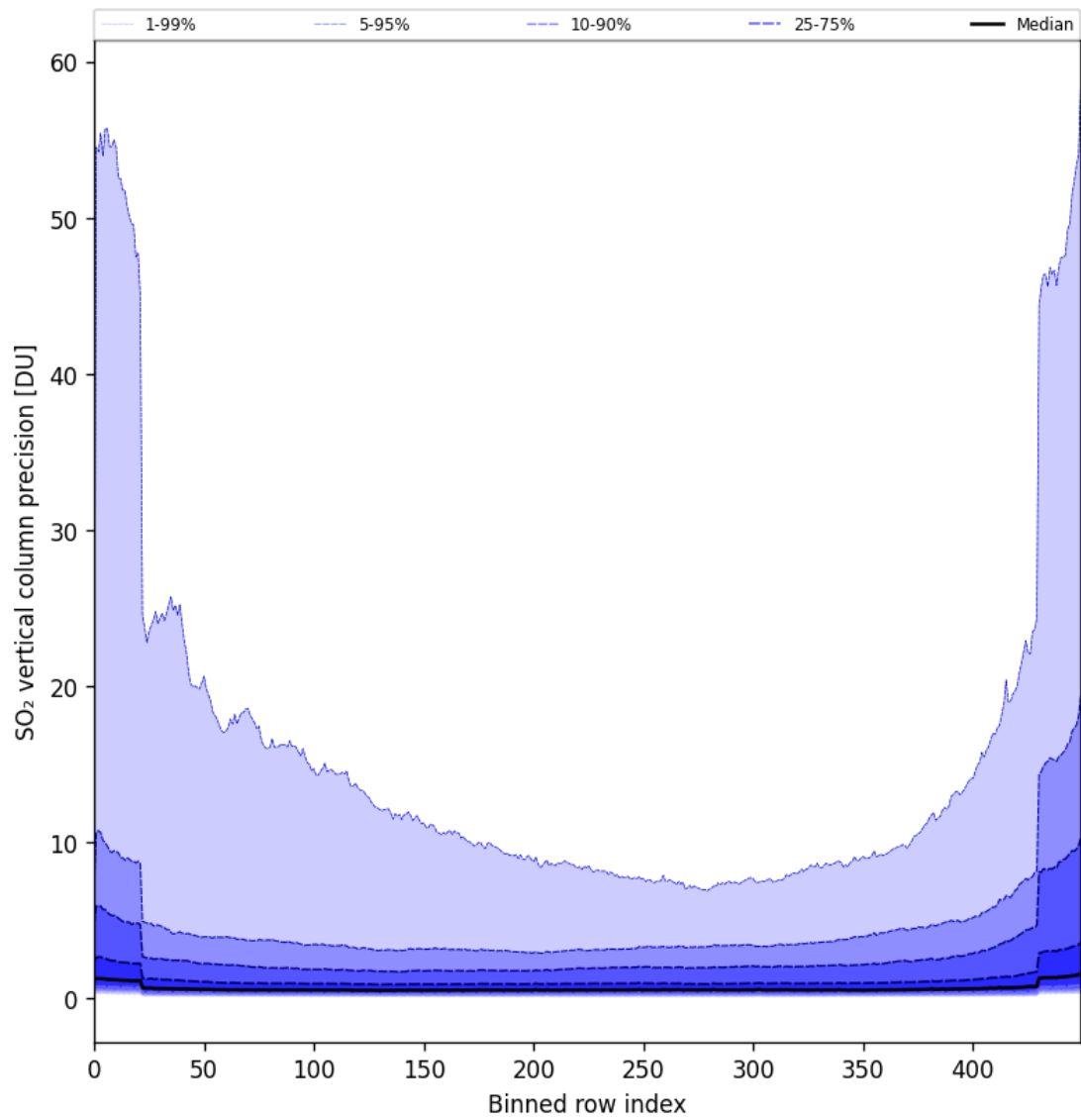
Figure 77: Along track statistics of “SO 2 vertical column precision” for 2024-08-25 to 2024-08-27
