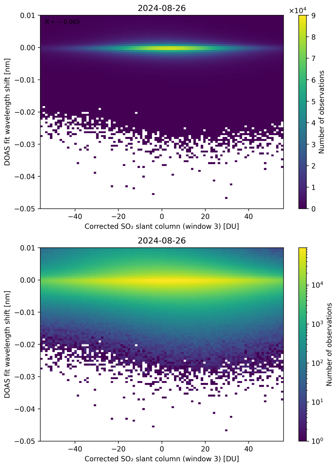
Figure 206: Scatter density plot of “Corrected SO 2 slant column (window 3)” against “DOAS fit wavelength shift” for 2024-08-25 to 2024-08-27.
