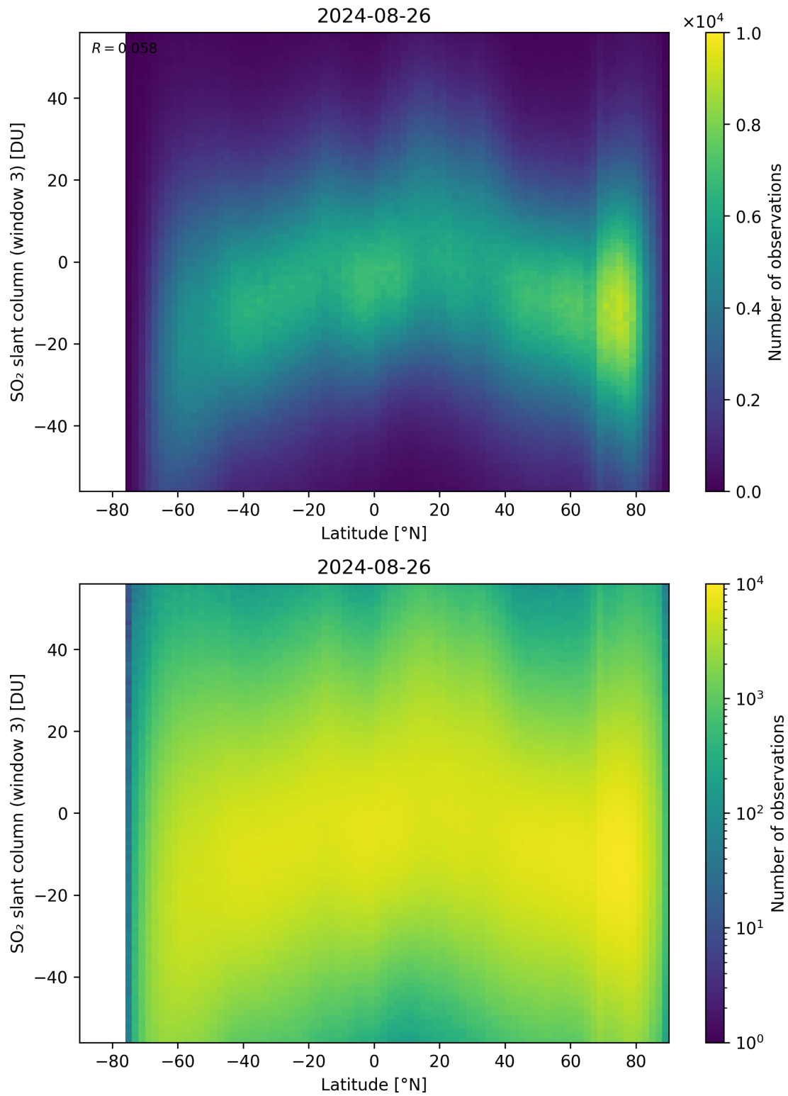
Figure 152: Scatter density plot of “Latitude” against “SO 2 slant column (window 3)” for 2024-08-25 to 2024-08-27.
