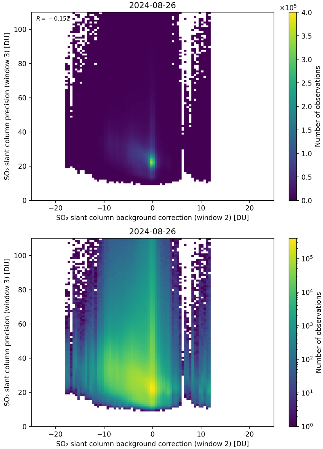
Figure 118: Scatter density plot of “SO 2 slant column background correction (window 2)” against “SO 2 slant column precision (window 3)” for 2024-08-25 to 2024-08-27.
