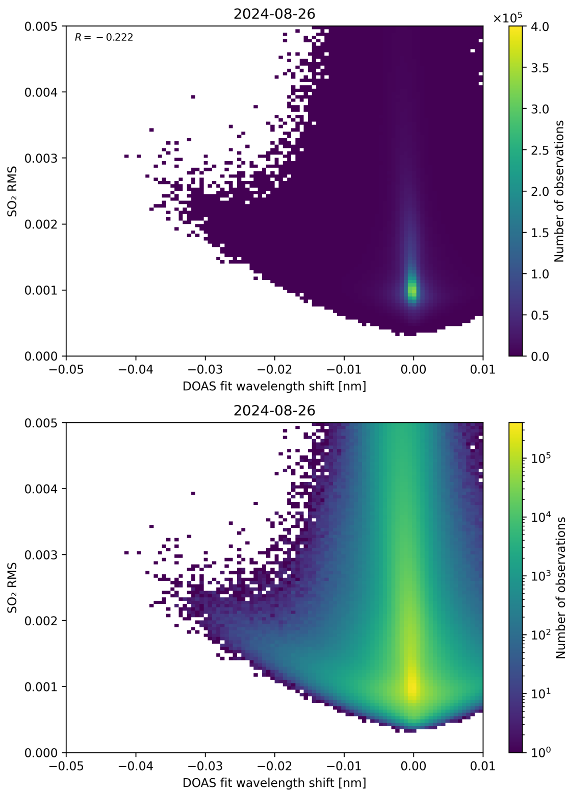
Figure 128: Scatter density plot of “DOAS fit wavelength shift” against “SO 2 RMS” for 2024-08-25 to 2024-08-27.
