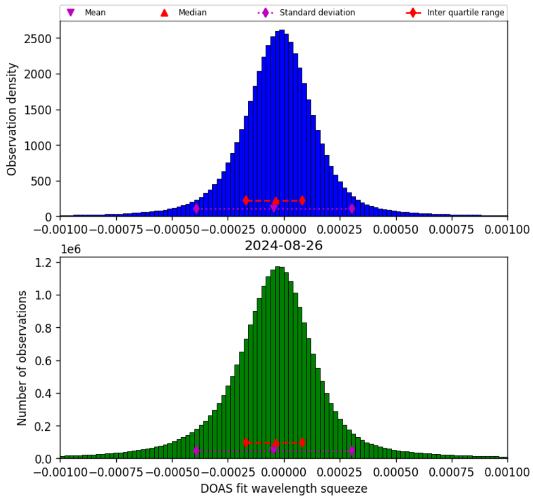
Figure 69: Histogram of “DOAS fit wavelength squeeze” for 2024-08-25 to 2024-08-27
