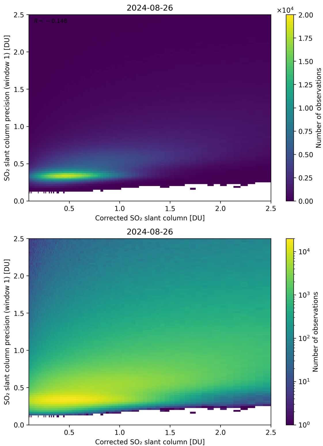
Figure 188: Scatter density plot of “Corrected SO 2 slant column” against “SO 2 slant column precision (window 1)” for 2024-08-25 to 2024-08-27.
