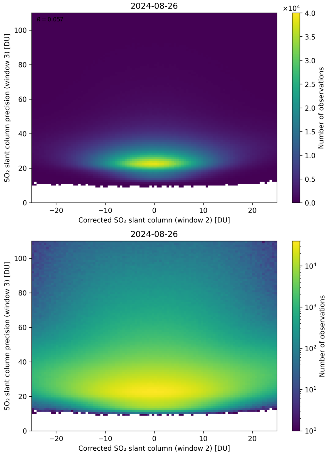
Figure 202: Scatter density plot of “Corrected SO 2 slant column (window 2)” against “SO 2 slant column precision (window 3)” for 2024-08-25 to 2024-08-27.
