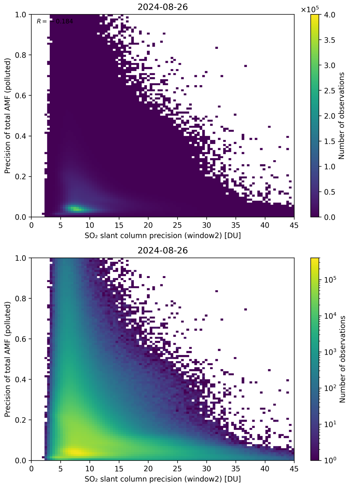
Figure 252: Scatter density plot of “SO 2 slant column precision (window2)” against “Precision of total AMF (polluted)” for 2024-08-25 to 2024-08-27.
