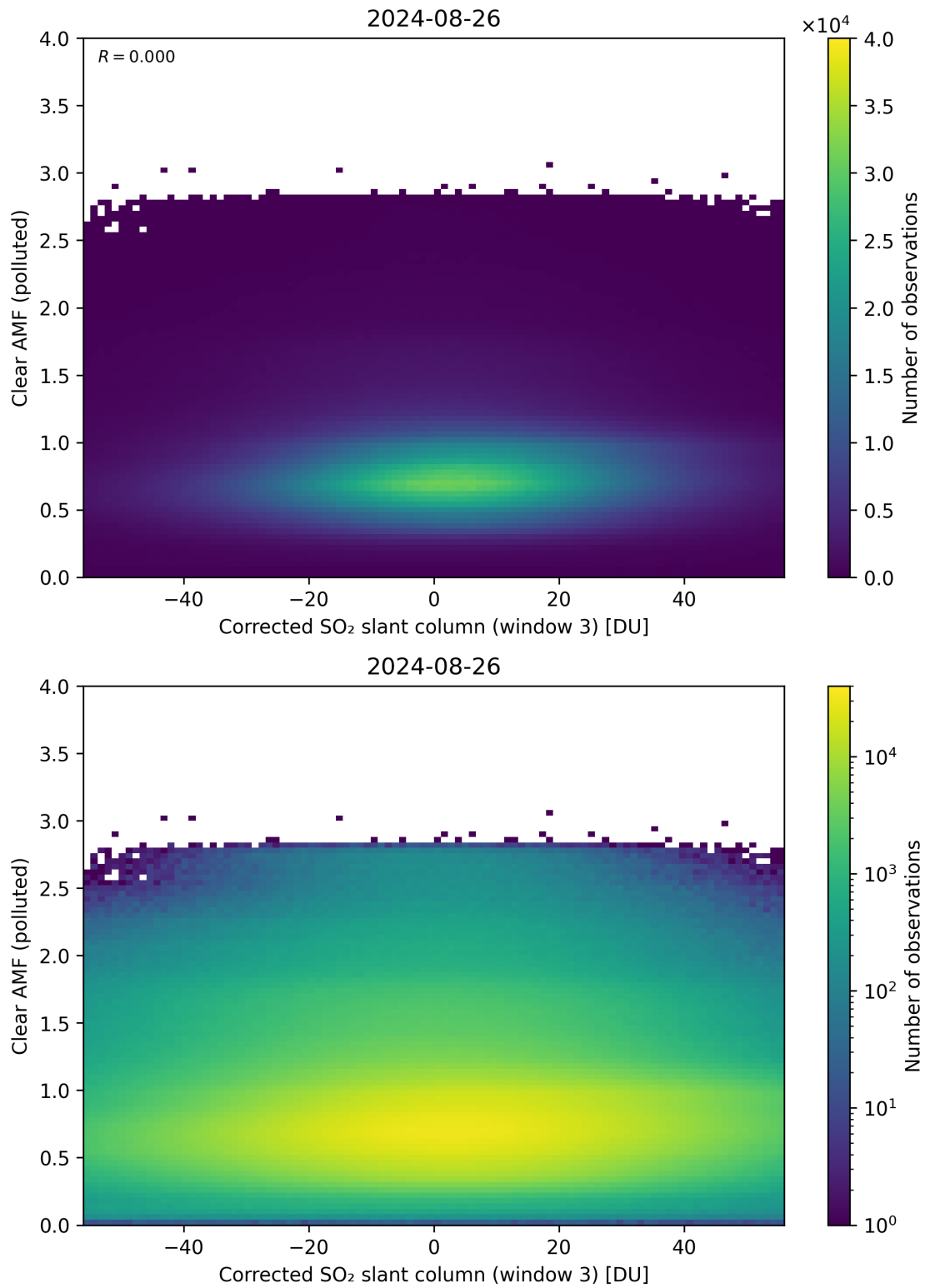
Figure 209: Scatter density plot of “Corrected SO 2 slant column (window 3)” against “Clear AMF (polluted)” for 2024-08-25 to 2024-08-27.
