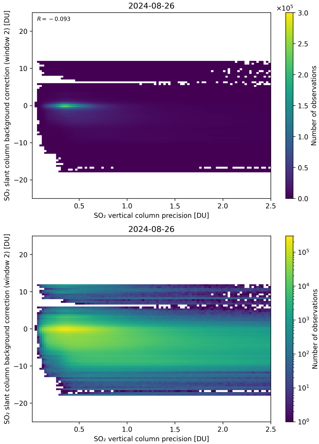
Figure 280: Scatter density plot of “SO 2 vertical column precision” against “SO 2 slant column background correction (window 2)” for 2024-08-25 to 2024-08-27.
