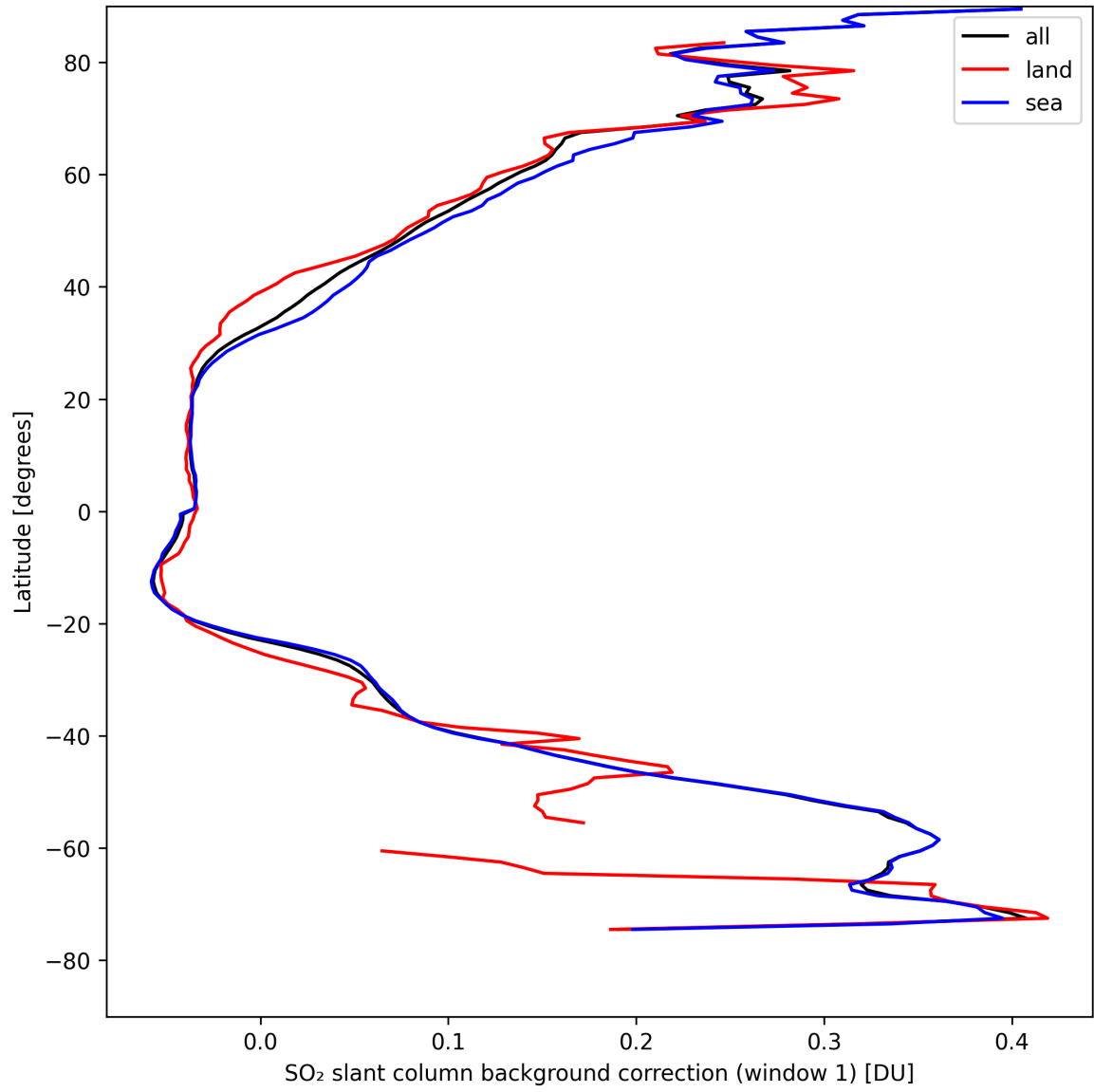
Figure 36: Zonal average of “SO 2 slant column background correction (window 1)” for 2024-08-25 to 2024-08-27.
