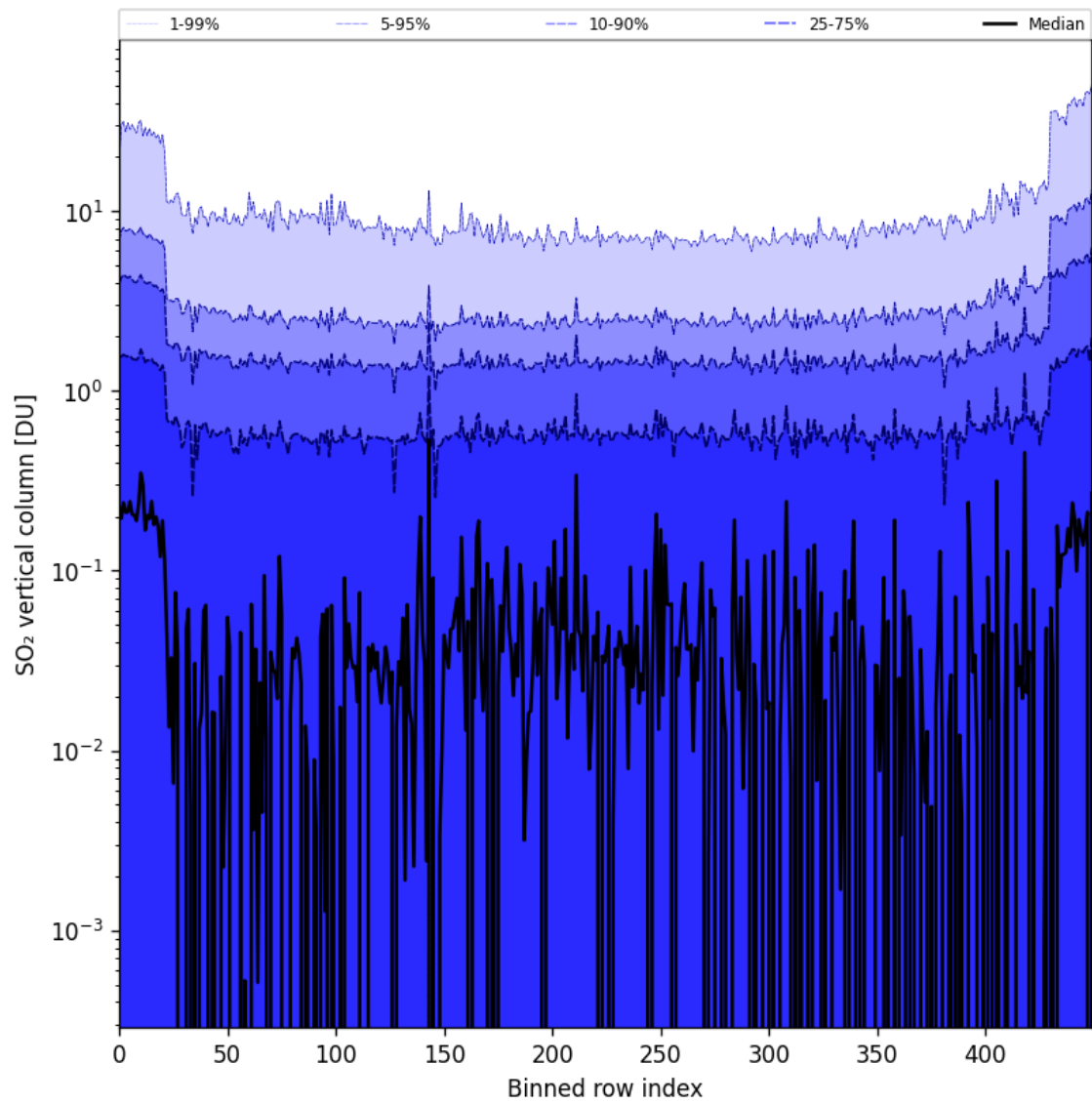
Figure 76: Along track statistics of “SO 2 vertical column” for 2024-08-25 to 2024-08-27
