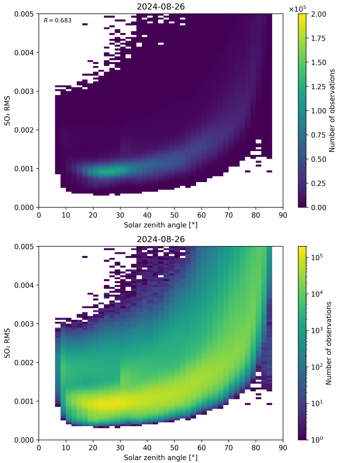
Figure 163: Scatter density plot of “Solar zenith angle” against “SO 2 RMS” for 2024-08-25 to 2024-08-27.
