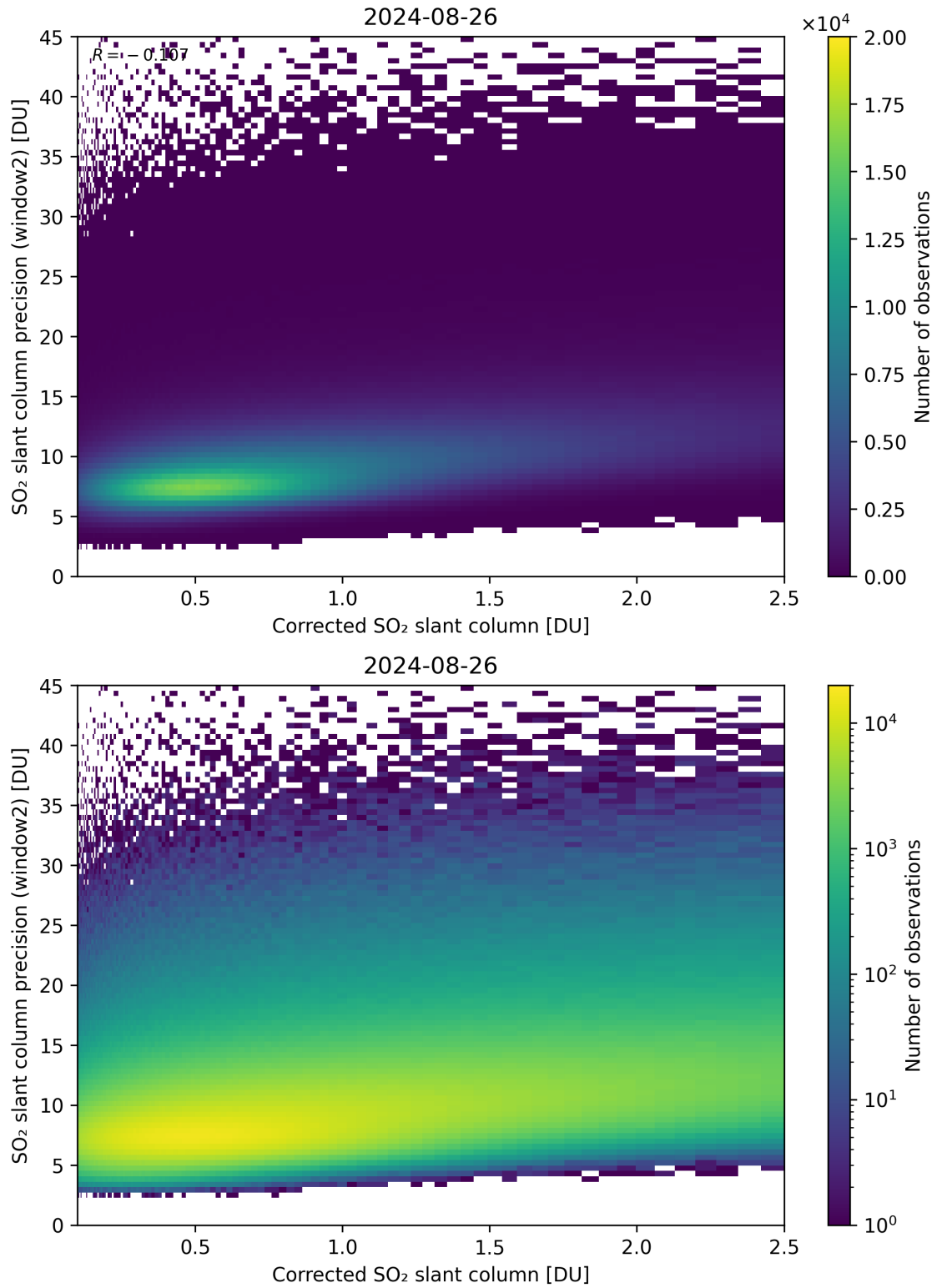
Figure 189: Scatter density plot of “Corrected SO 2 slant column” against “SO 2 slant column precision (window2)” for 2024-08-25 to 2024-08-27.
