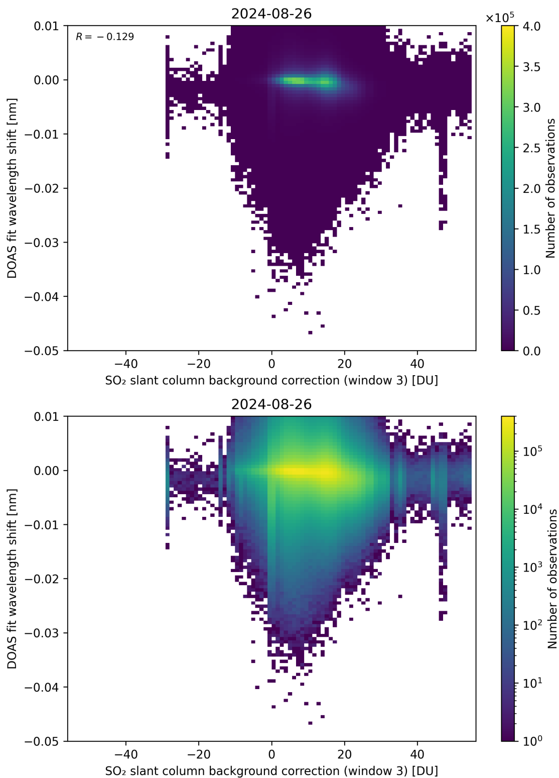
Figure 121: Scatter density plot of “SO 2 slant column background correction (window 3)” against “DOAS fit wavelength shift” for 2024-08-25 to 2024-08-27.
