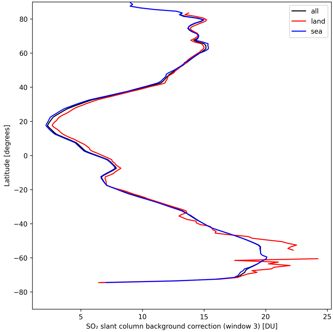
Figure 44: Zonal average of “SO 2 slant column background correction (window 3)” for 2024-08-25 to 2024-08-27.
