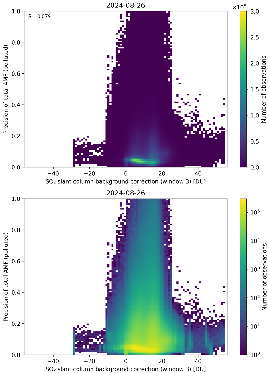
Figure 126: Scatter density plot of “SO 2 slant column background correction (window 3)” against “Precision of total AMF (polluted)” for 2024-08-25 to 2024-08-27.
