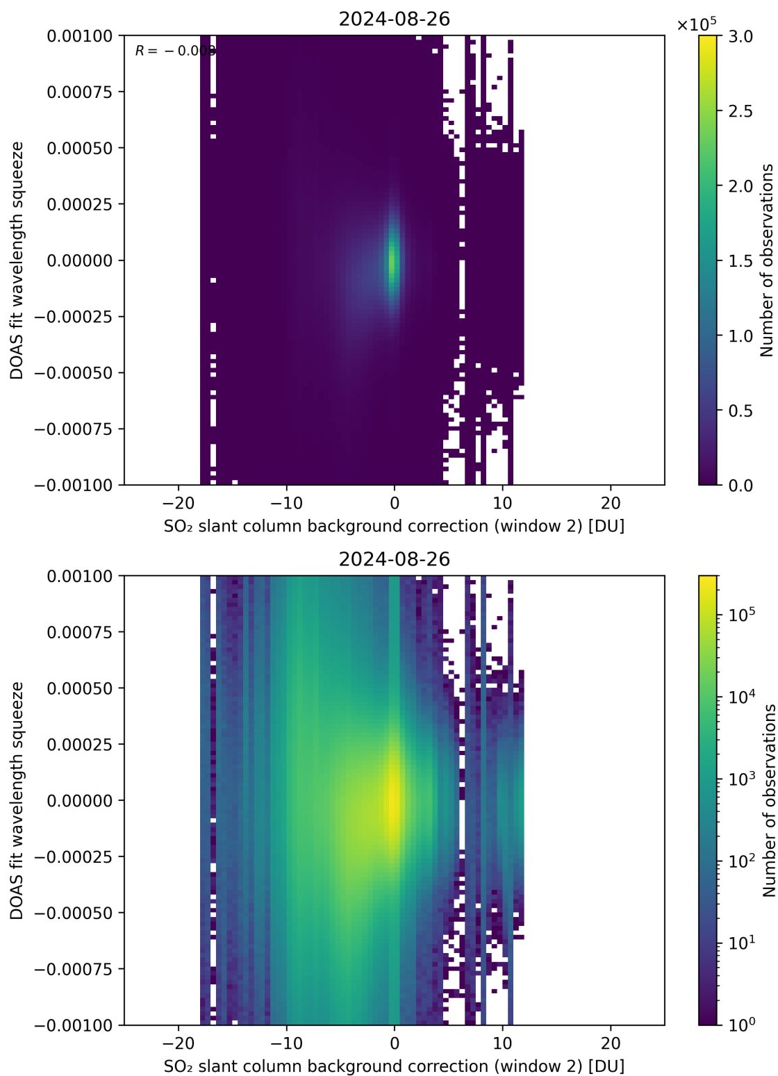
Figure 113: Scatter density plot of “SO 2 slant column background correction (window 2)” against “DOAS fit wavelength squeeze” for 2024-08-25 to 2024-08-27.
