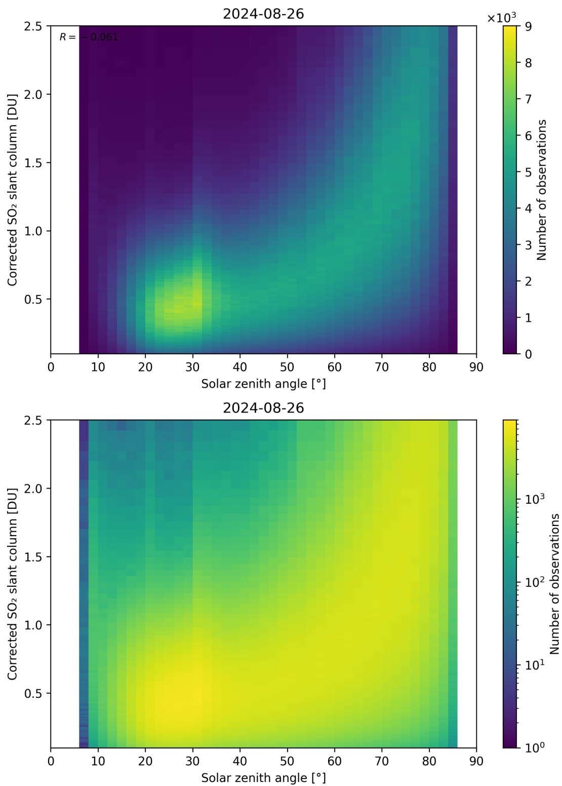
Figure 166: Scatter density plot of “Solar zenith angle” against “Corrected SO 2 slant column” for 2024-08-25 to 2024-08-27.
