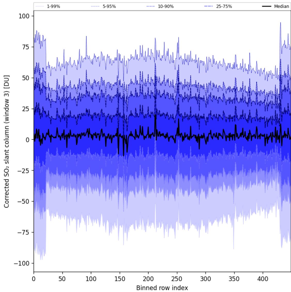
Figure 89: Along track statistics of “Corrected SO 2 slant column (window 3)” for 2024-08-25 to 2024-08-27
