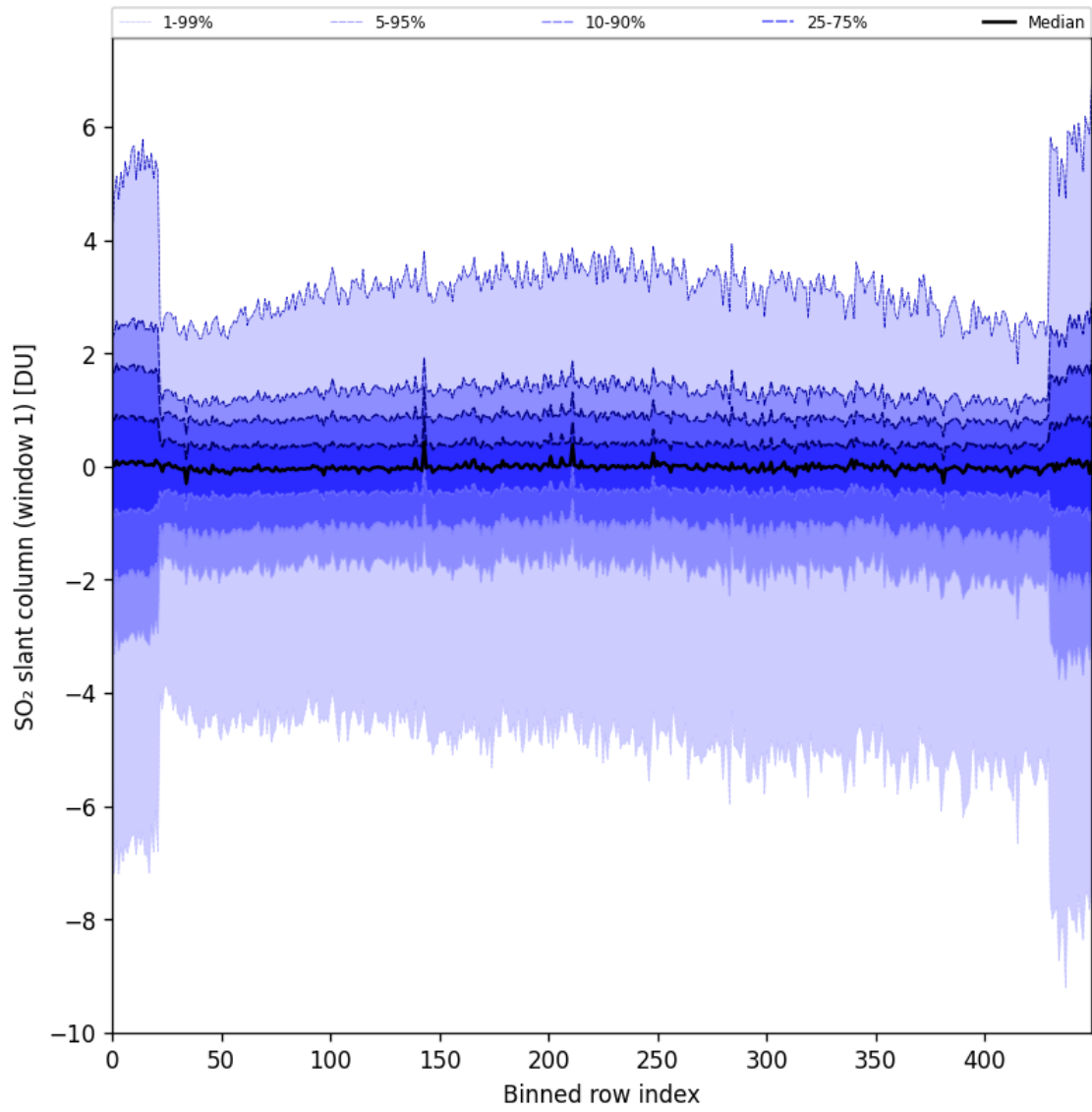
Figure 79: Along track statistics of “SO 2 slant column (window 1)” for 2024-08-25 to 2024-08-27
