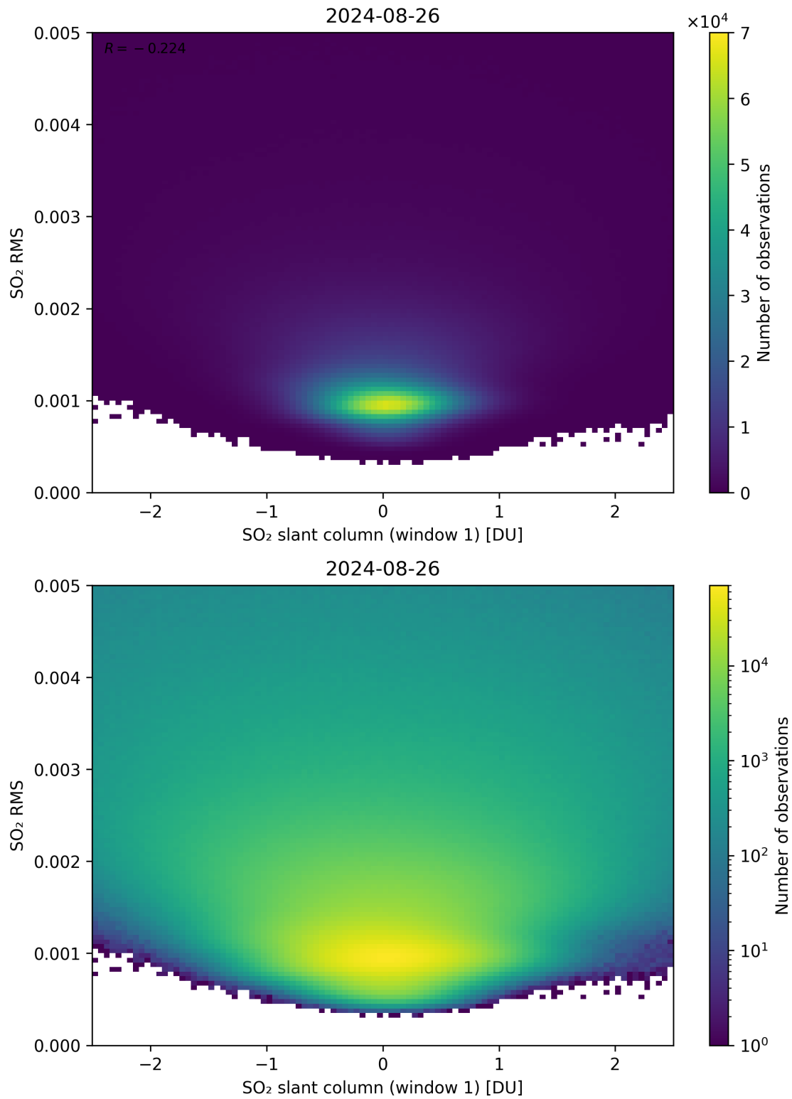
Figure 217: Scatter density plot of “SO 2 slant column (window 1)” against “SO 2 RMS” for 2024-08-25 to 2024-08-27.
