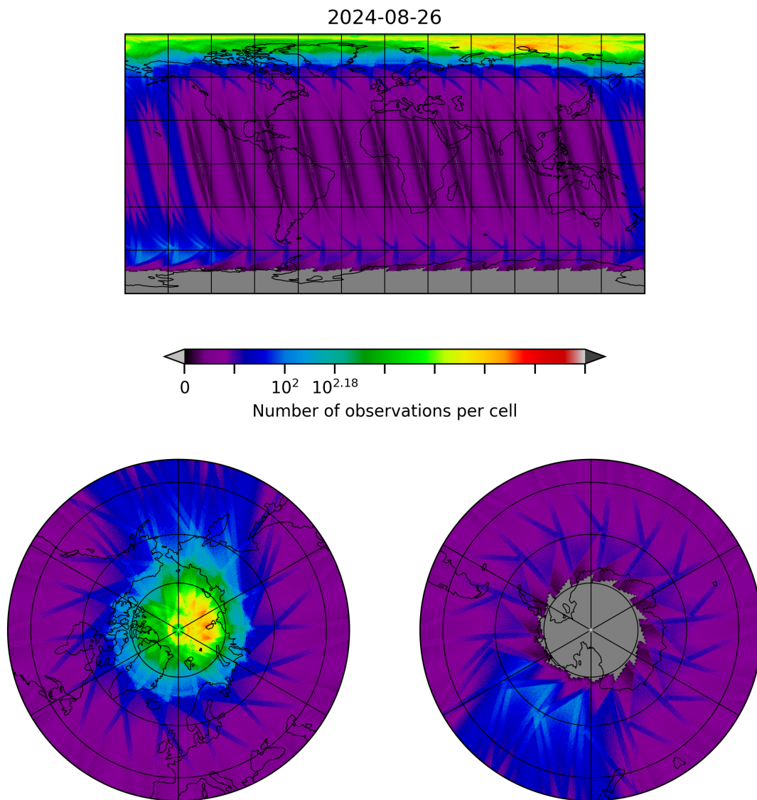
Figure 28: Map of the number of observations for 2024-08-25 to 2024-08-27
