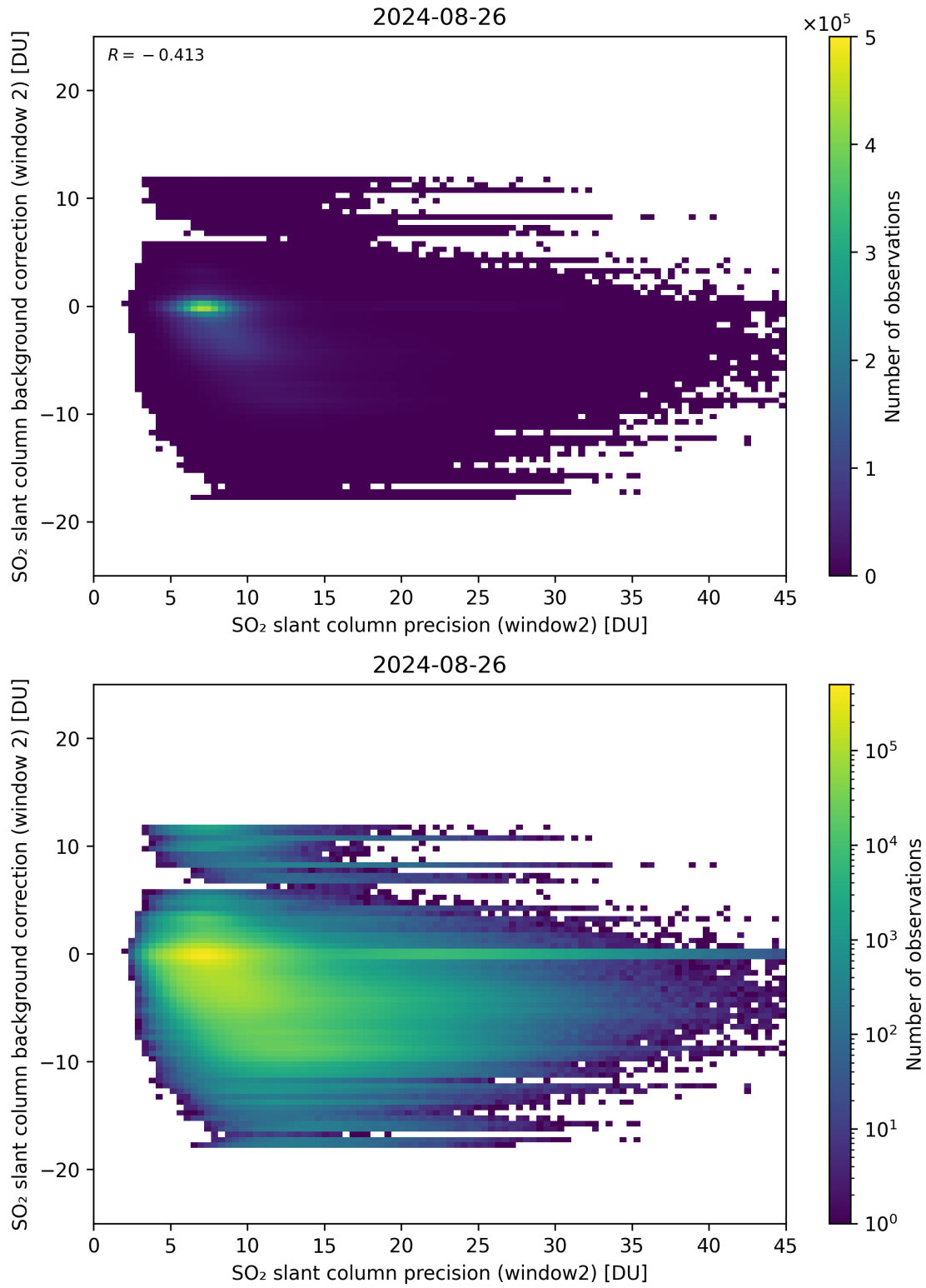
Figure 241: Scatter density plot of “SO 2 slant column precision (window2)” against “SO 2 slant column background correction (window 2)” for 2024-08-25 to 2024-08-27.
