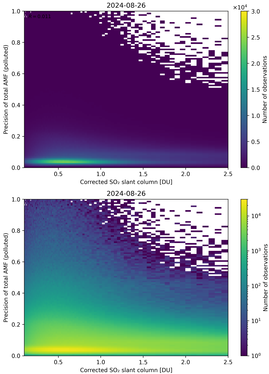
Figure 193: Scatter density plot of “Corrected SO 2 slant column” against “Precision of total AMF (polluted)” for 2024-08-25 to 2024-08-27.
