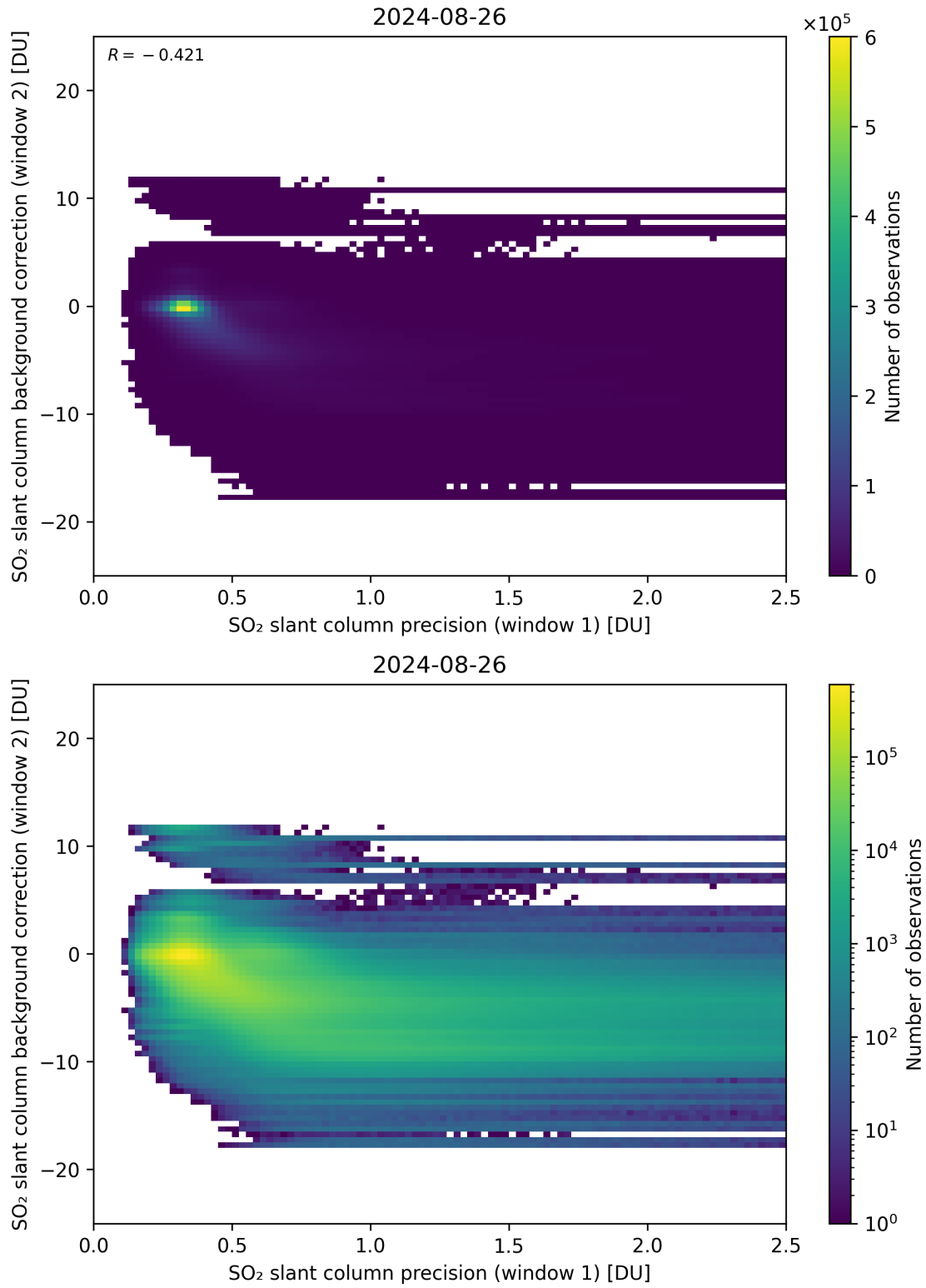
Figure 219: Scatter density plot of “SO 2 slant column precision (window 1)” against “SO 2 slant column background correction (window 2)” for 2024-08-25 to 2024-08-27.
