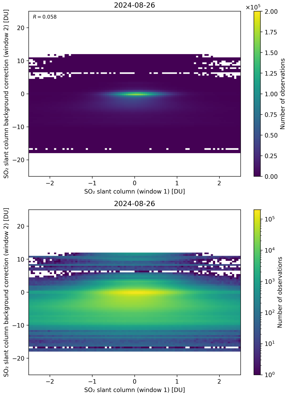
Figure 213: Scatter density plot of “SO 2 slant column (window 1)” against “SO 2 slant column background correction (window 2)” for 2024-08-25 to 2024-08-27.
