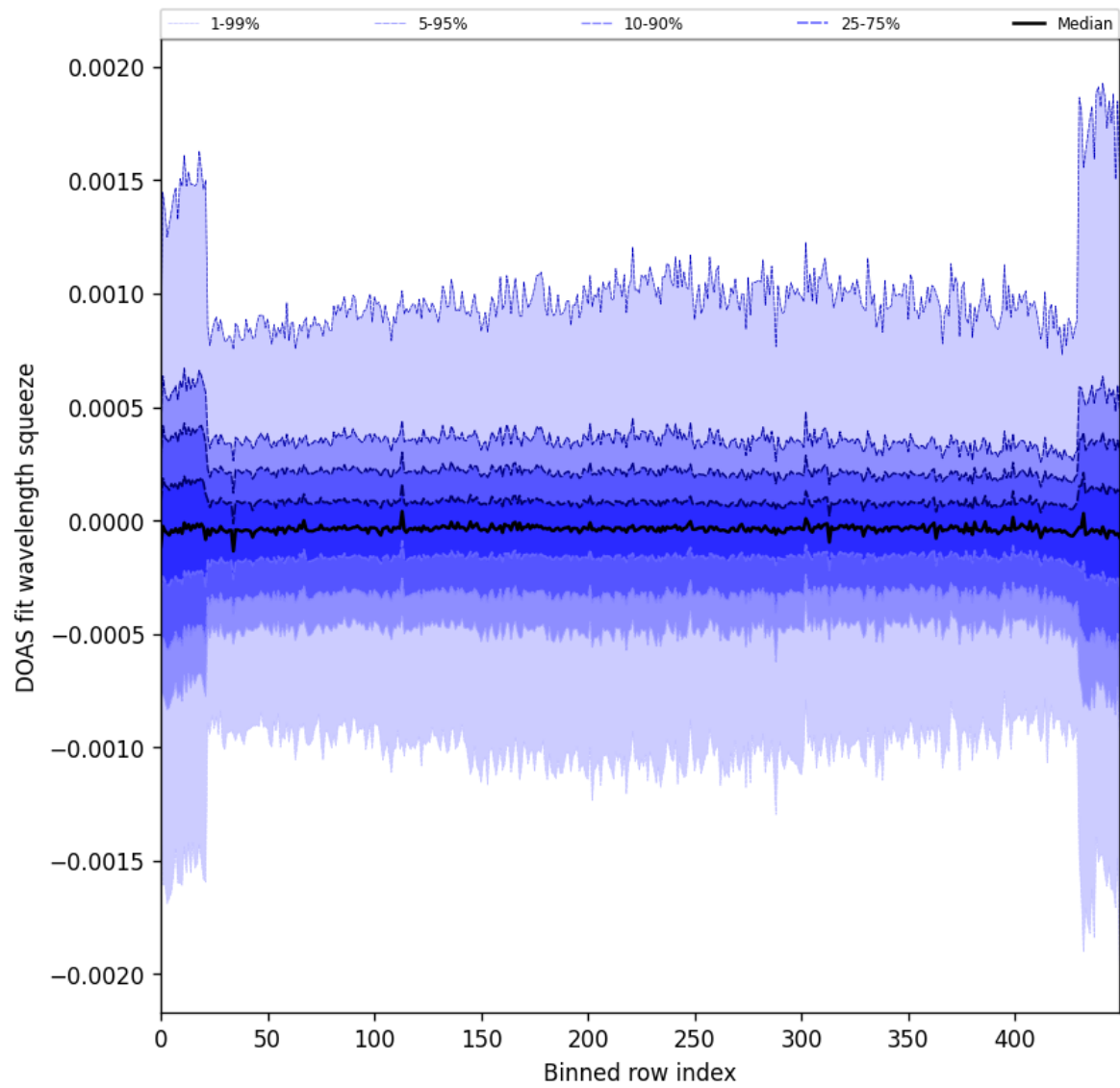
Figure 92: Along track statistics of “DOAS fit wavelength squeeze” for 2024-08-25 to 2024-08-27
