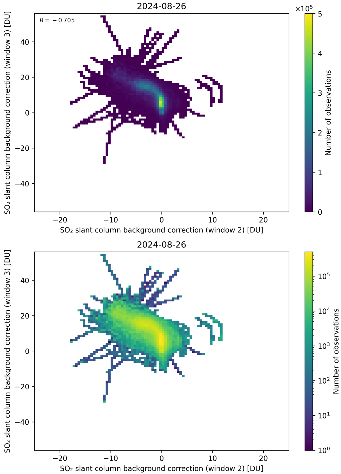
Figure 111: Scatter density plot of “SO 2 slant column background correction (window 2)” against “SO 2 slant column background correction (window 3)” for 2024-08-25 to 2024-08-27.
