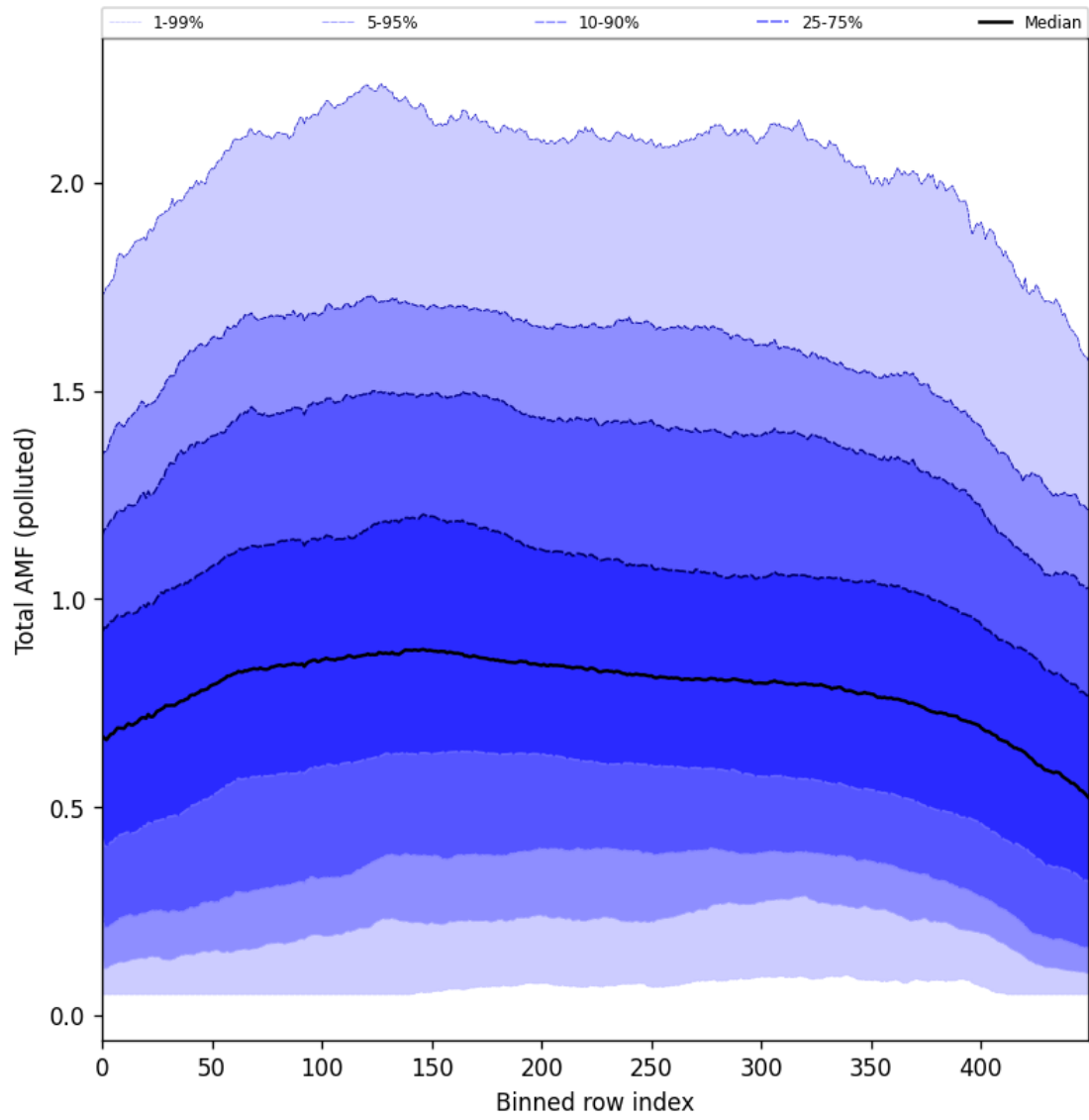
Figure 94: Along track statistics of “Total AMF (polluted)” for 2024-08-25 to 2024-08-27
