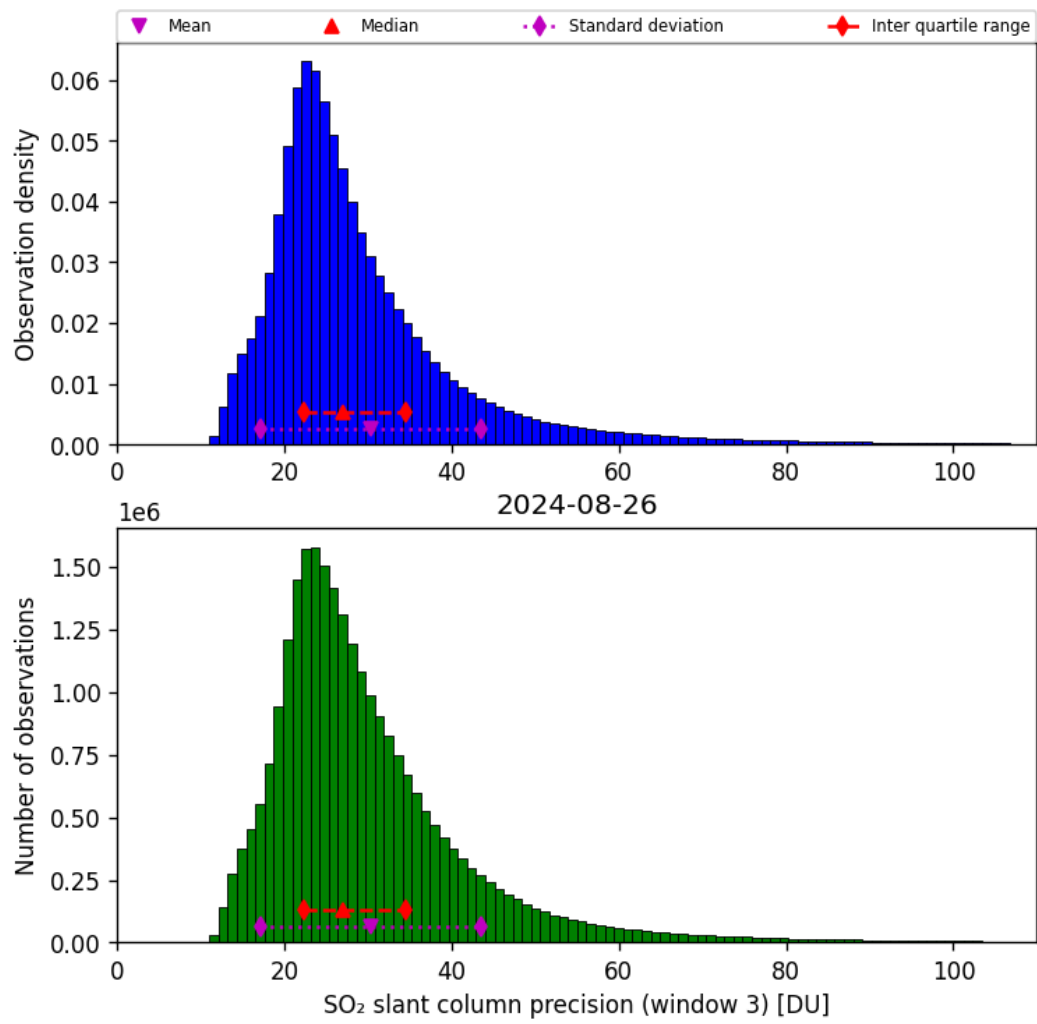
Figure 65: Histogram of “SO 2 slant column precision (window 3)” for 2024-08-25 to 2024-08-27
