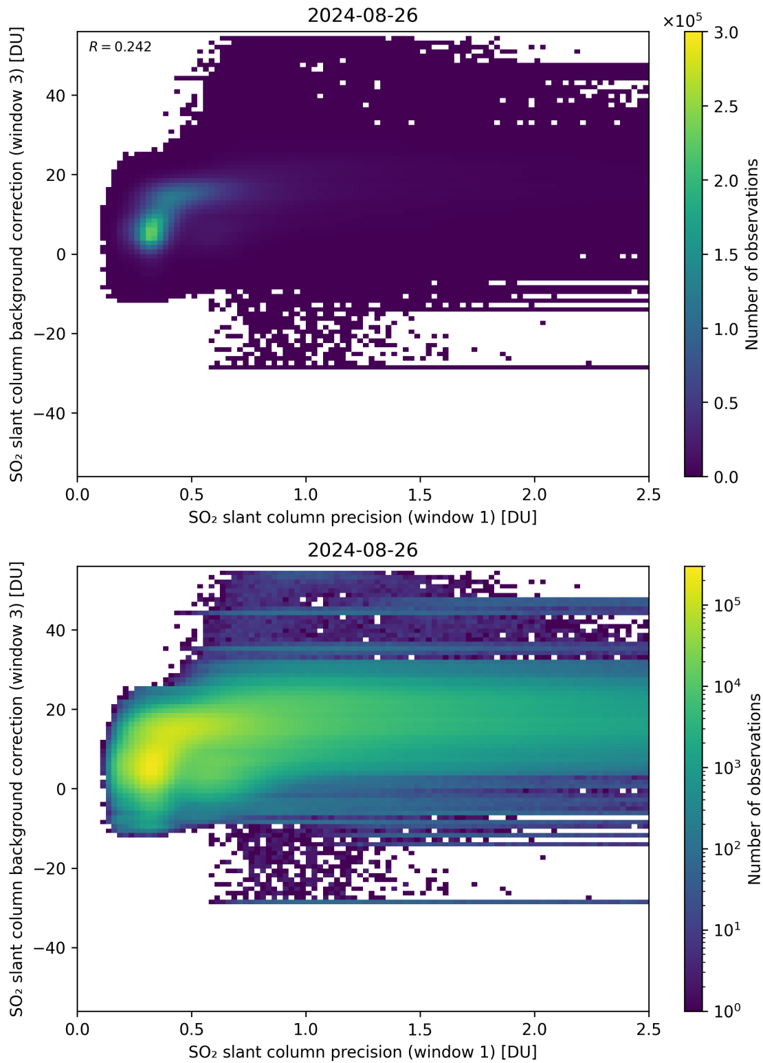
Figure 220: Scatter density plot of “SO 2 slant column precision (window 1)” against “SO 2 slant column background correction (window 3)” for 2024-08-25 to 2024-08-27.
