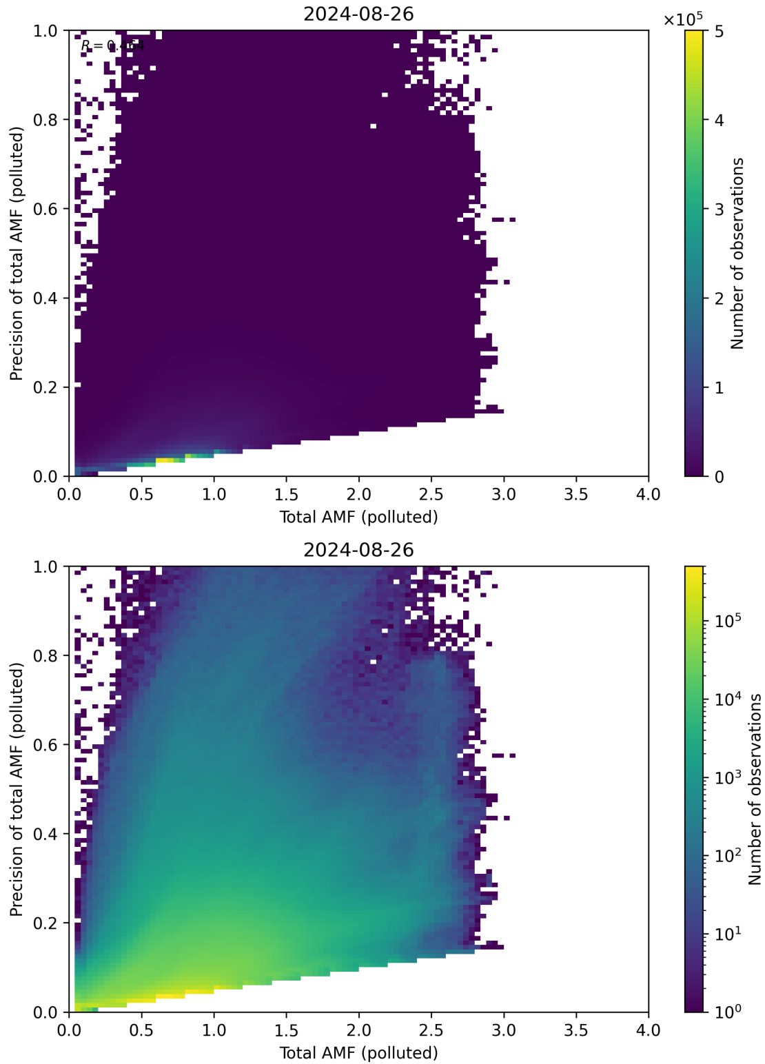
Figure 272: Scatter density plot of “Total AMF (polluted)” against “Precision of total AMF (polluted)” for 2024-08-25 to 2024-08-27.
