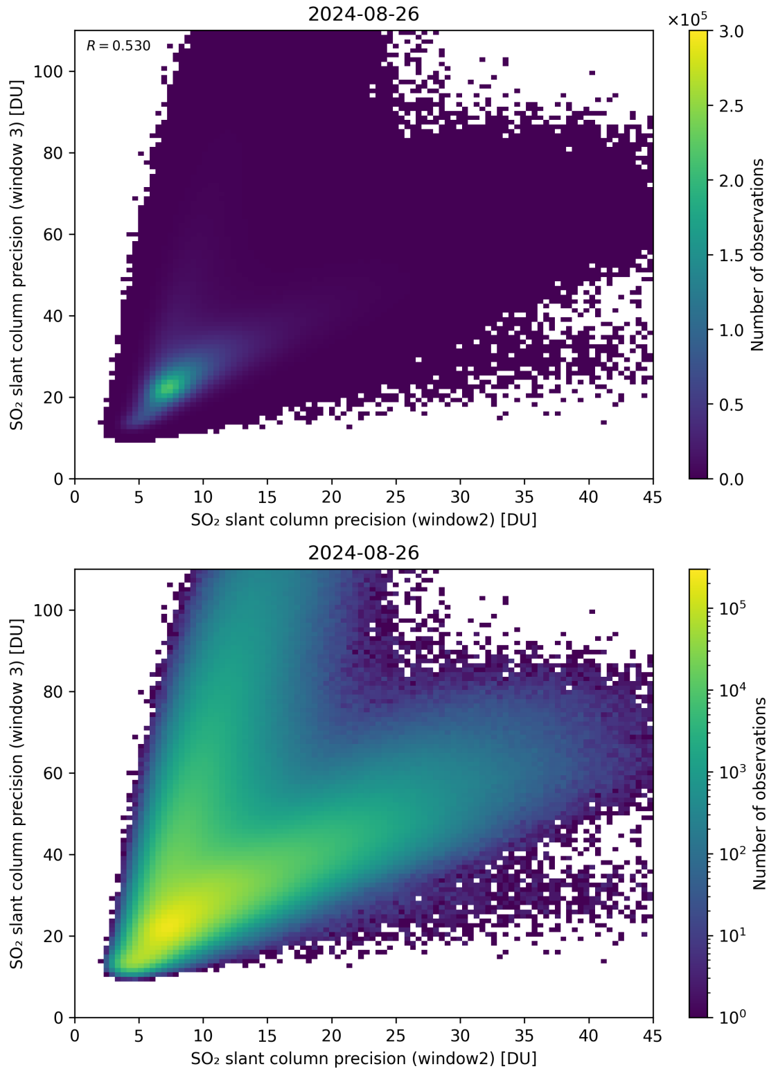
Figure 250: Scatter density plot of “SO 2 slant column precision (window2)” against “SO 2 slant column precision (window 3)” for 2024-08-25 to 2024-08-27.
