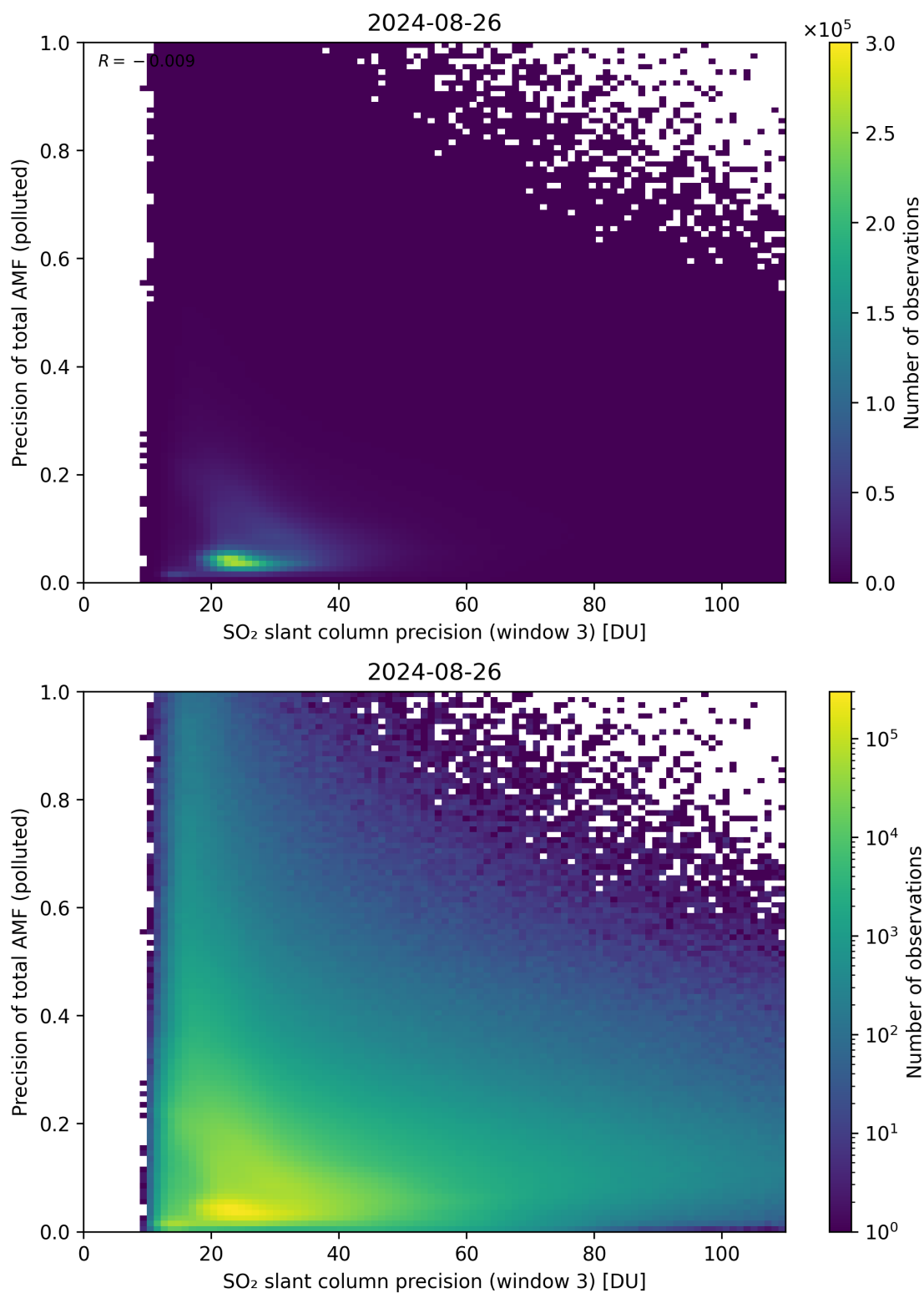
Figure 264: Scatter density plot of “SO 2 slant column precision (window 3)” against “Precision of total AMF (polluted)” for 2024-08-25 to 2024-08-27.
