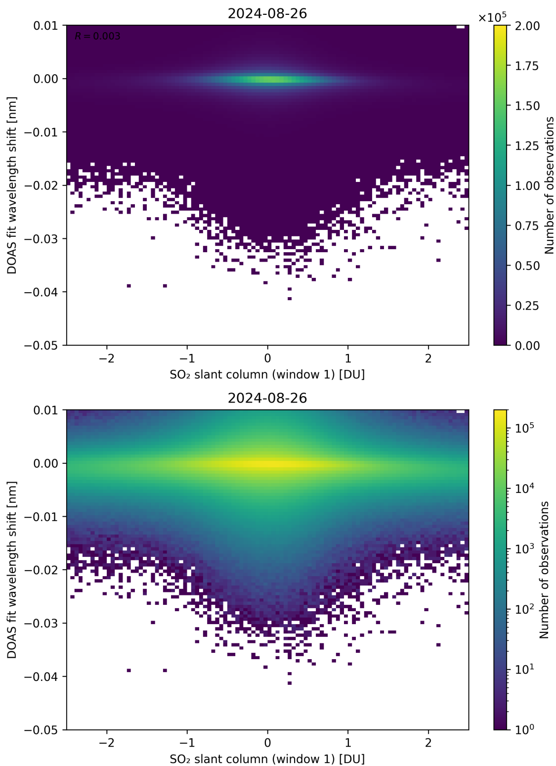
Figure 215: Scatter density plot of “SO 2 slant column (window 1)” against “DOAS fit wavelength shift” for 2024-08-25 to 2024-08-27.
