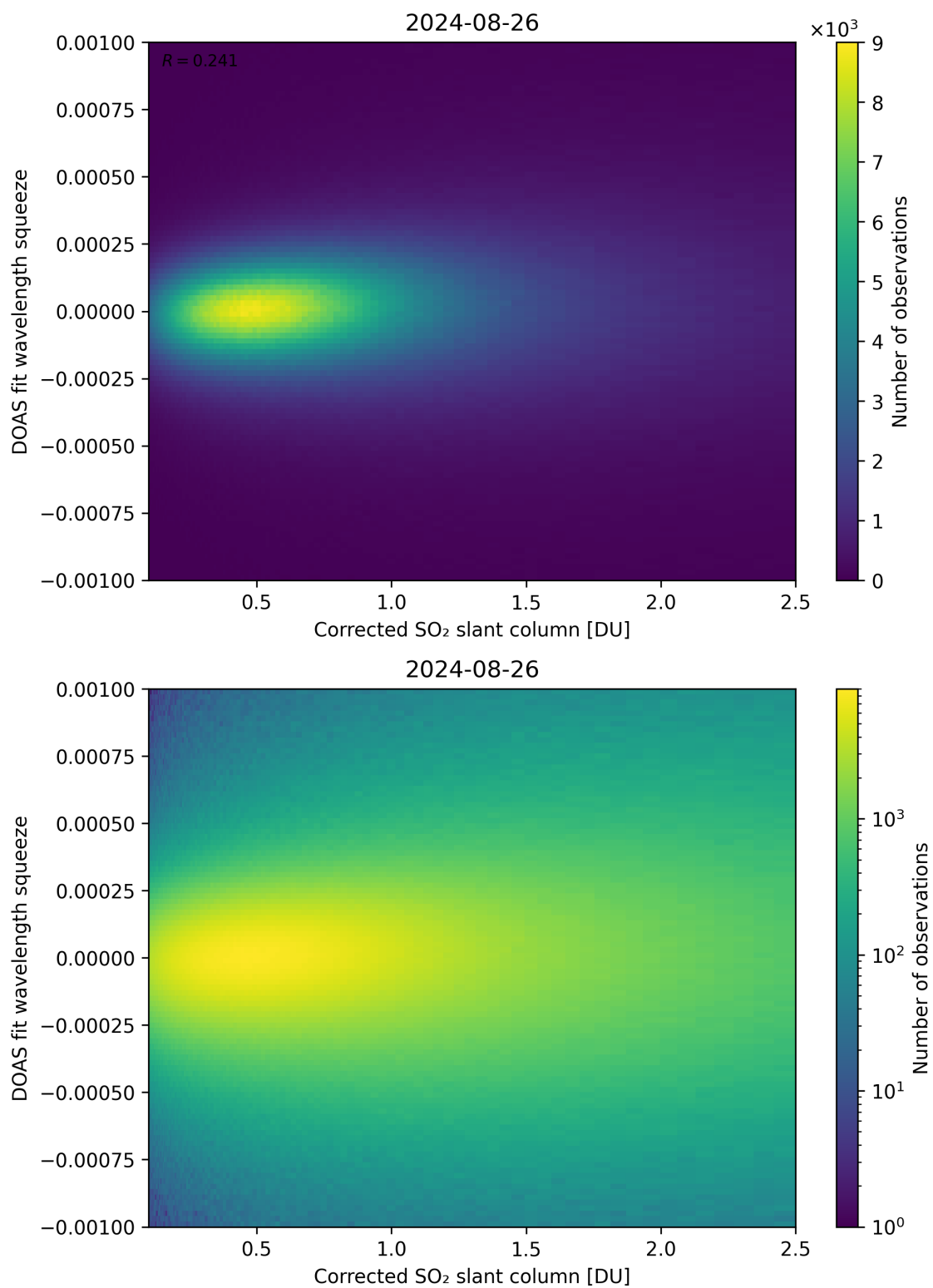
Figure 182: Scatter density plot of “Corrected SO 2 slant column” against “DOAS fit wavelength squeeze” for 2024-08-25 to 2024-08-27.
