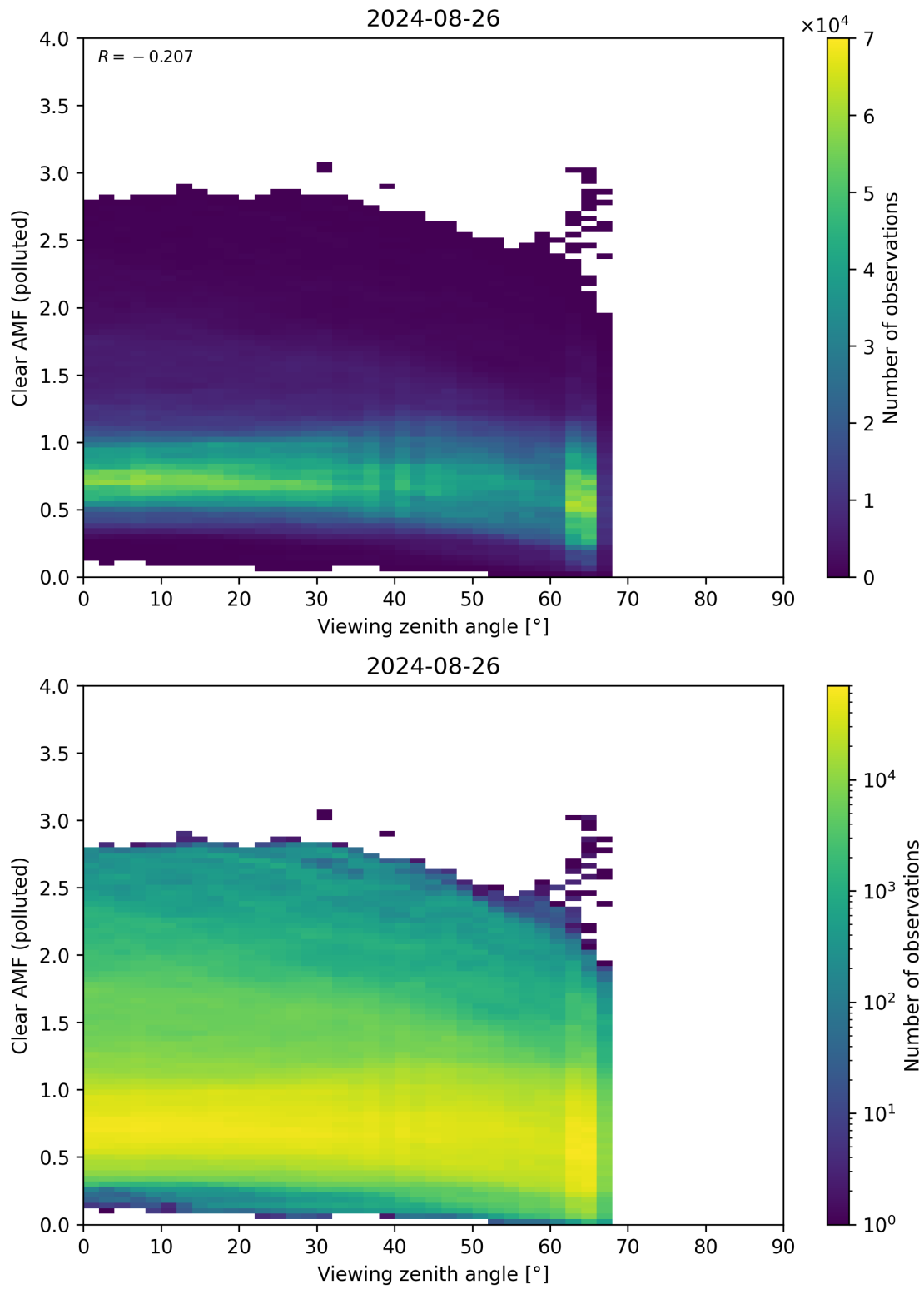
Figure 316: Scatter density plot of “Viewing zenith angle” against “Clear AMF (polluted)” for 2024-08-25 to 2024-08-27.
