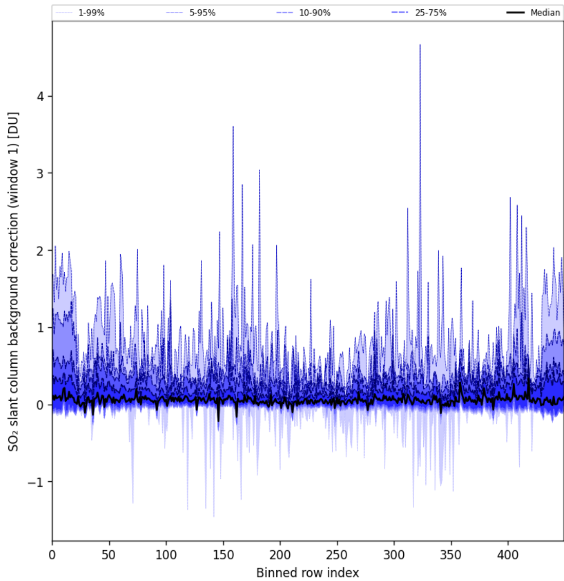
Figure 82: Along track statistics of “SO 2 slant column background correction (window 1)” for 2024-08-25 to 2024-08-27
