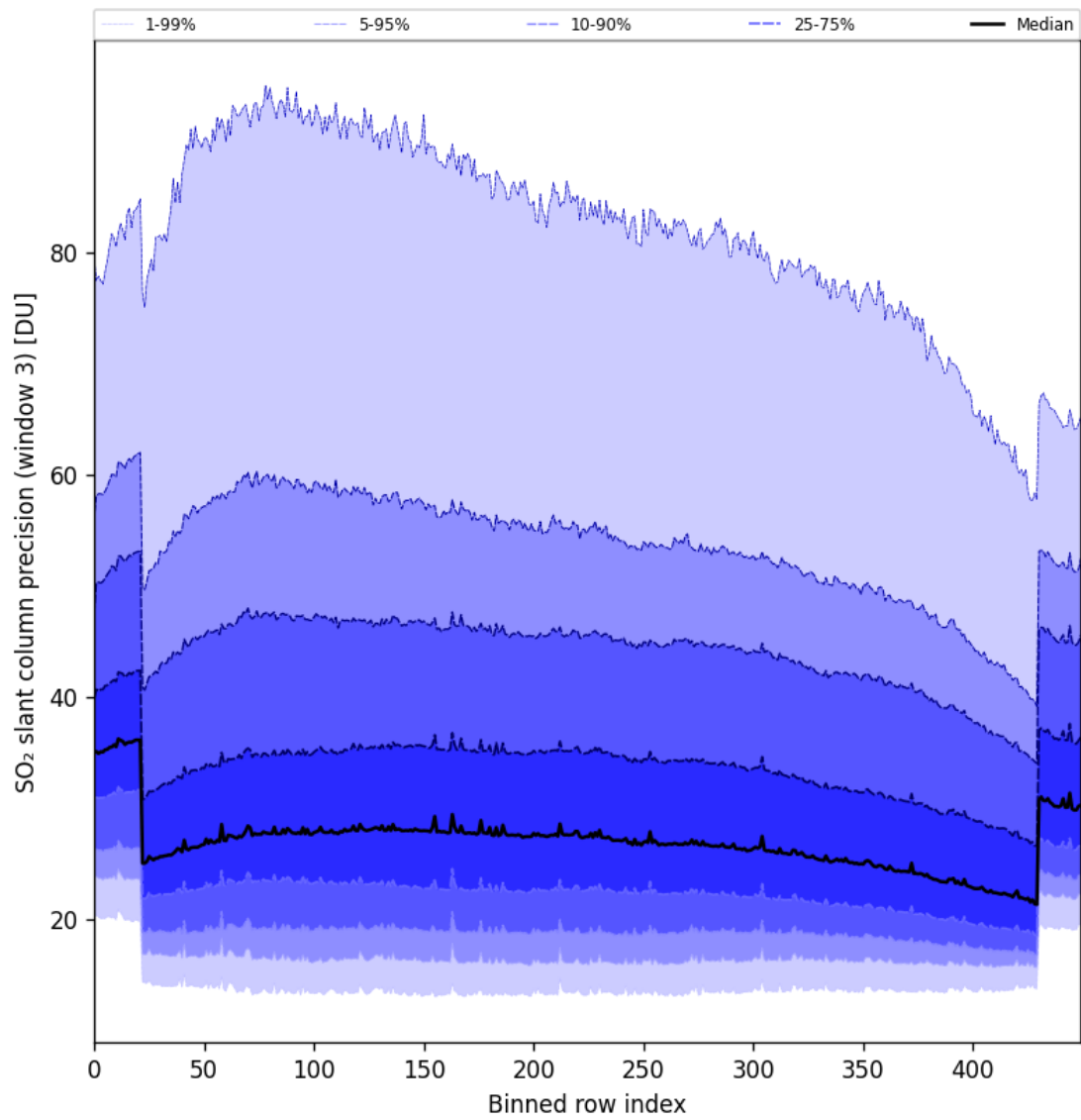
Figure 88: Along track statistics of “SO 2 slant column precision (window 3)” for 2024-08-25 to 2024-08-27
