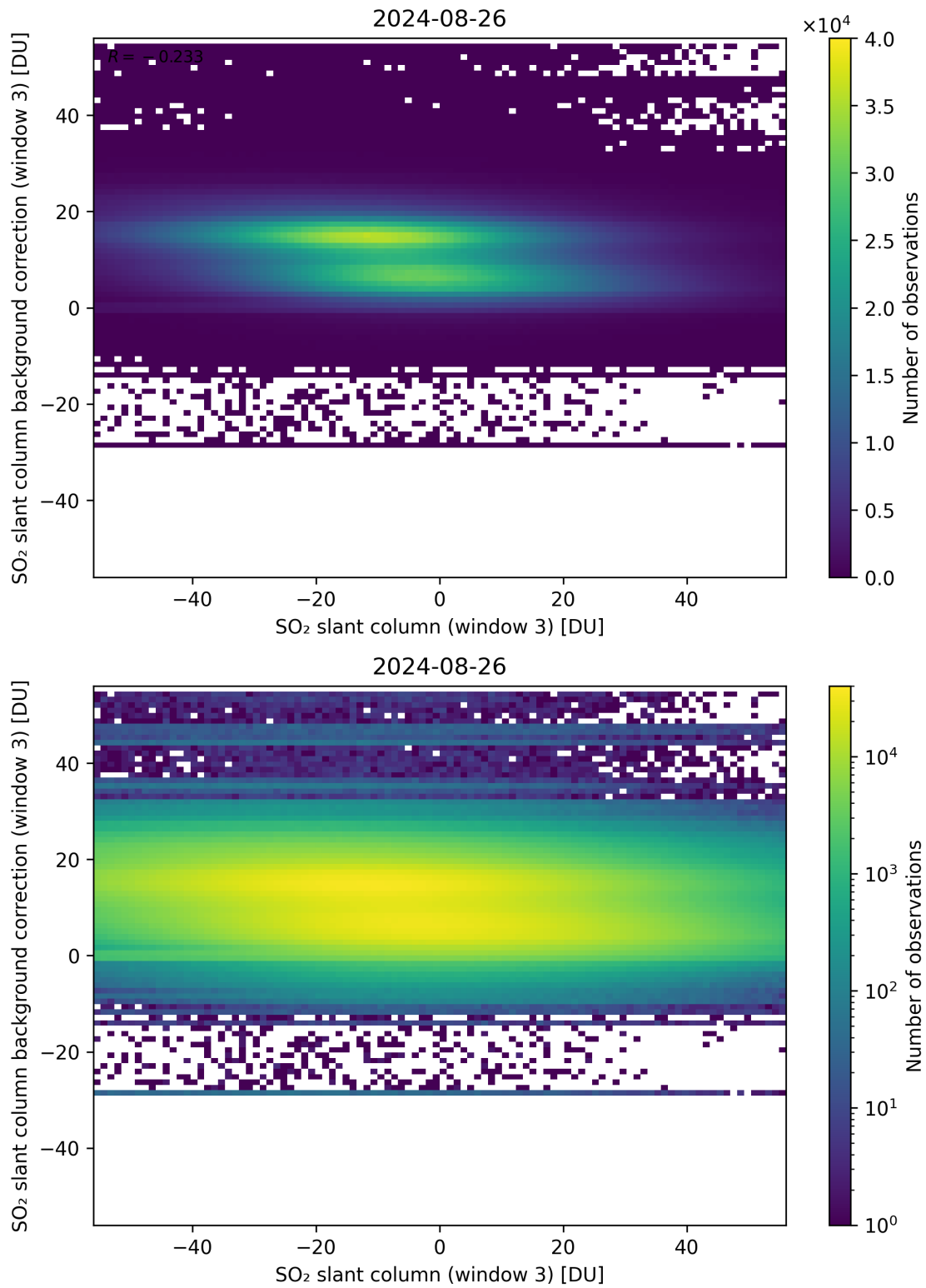
Figure 253: Scatter density plot of “SO 2 slant column (window 3)” against “SO 2 slant column background correction (window 3)” for 2024-08-25 to 2024-08-27.
