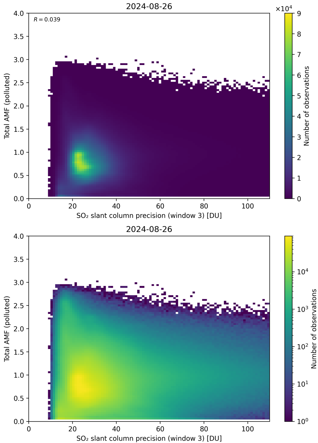
Figure 263: Scatter density plot of “SO 2 slant column precision (window 3)” against “Total AMF (polluted)” for 2024-08-25 to 2024-08-27.
