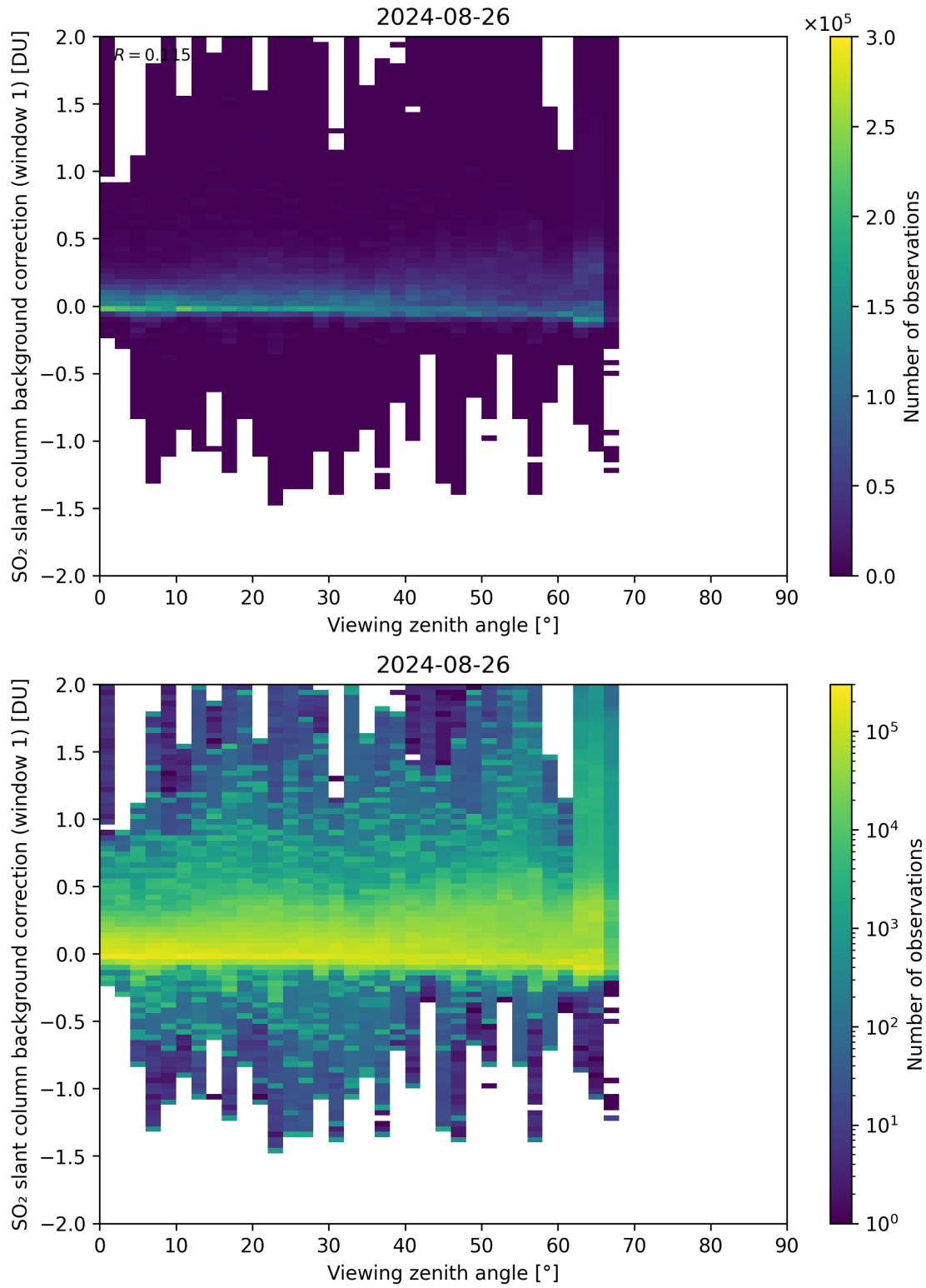
Figure 308: Scatter density plot of “Viewing zenith angle” against “SO 2 slant column background correction (window 1)” for 2024-08-25 to 2024-08-27.
