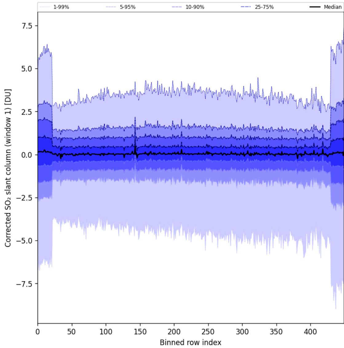
Figure 81: Along track statistics of “Corrected SO 2 slant column (window 1)” for 2024-08-25 to 2024-08-27
