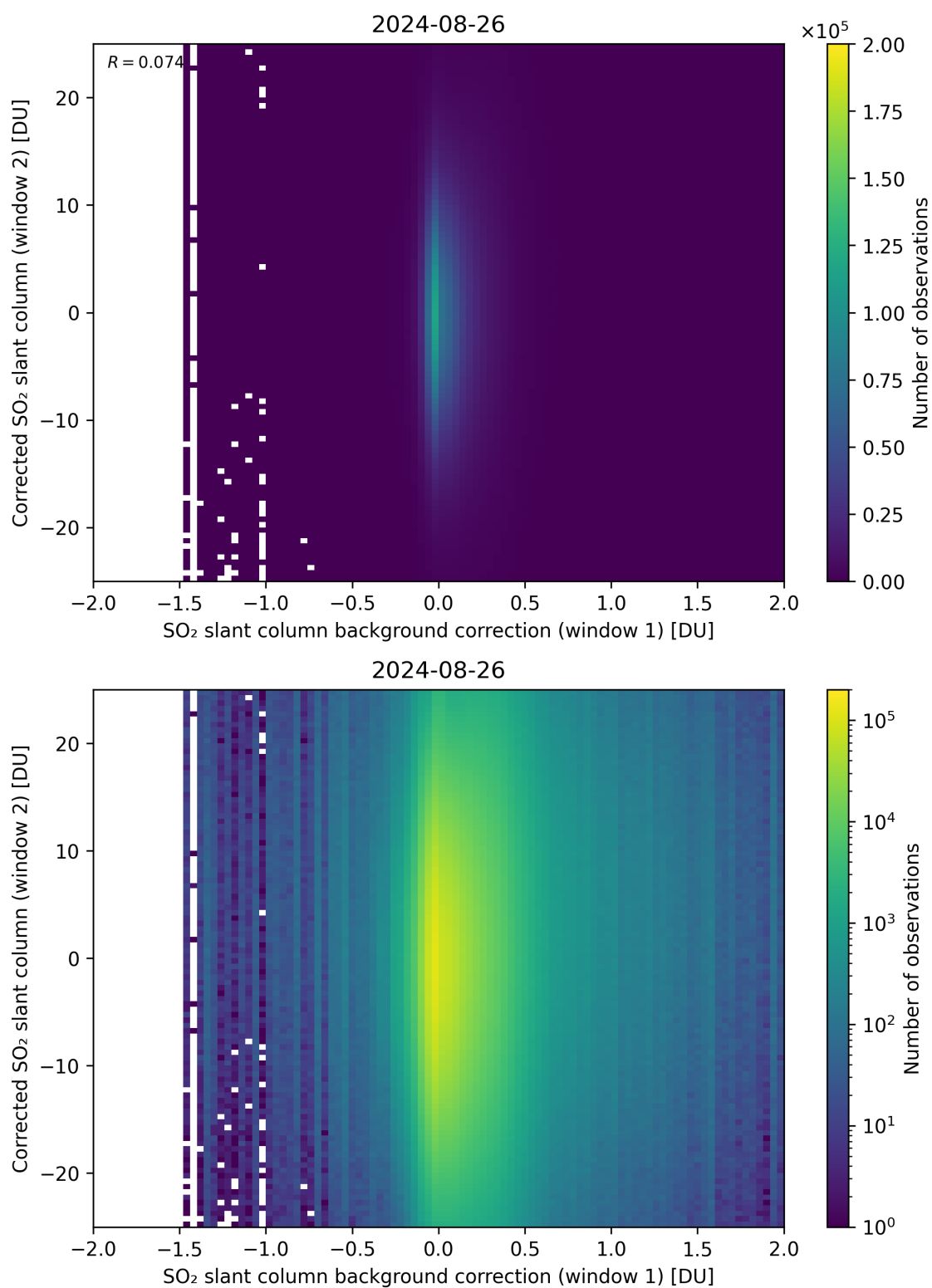
Figure 104: Scatter density plot of “SO 2 slant column background correction (window 1)” against “Corrected SO 2 slant column (window 2)” for 2024-08-25 to 2024-08-27.
