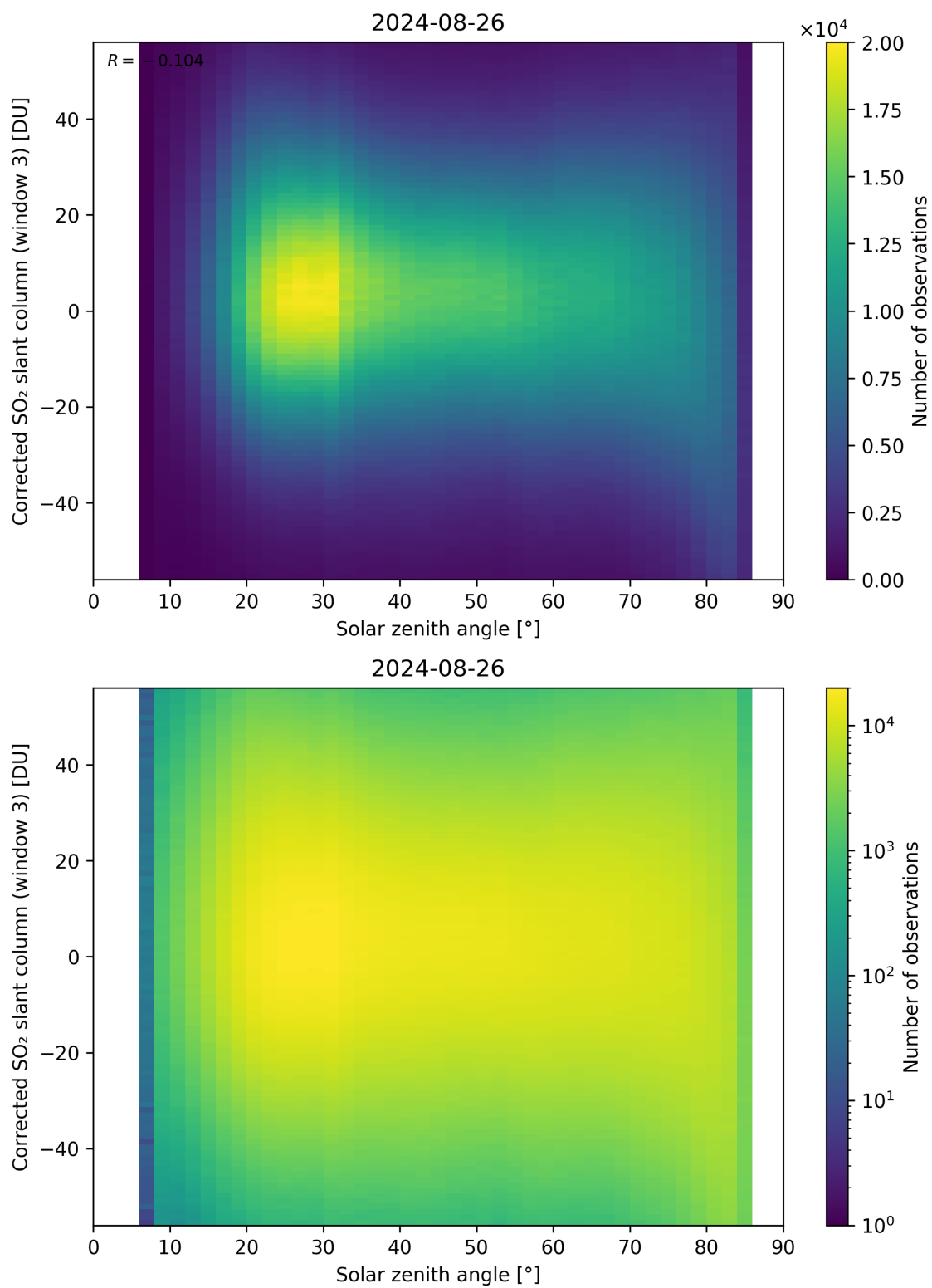
Figure 168: Scatter density plot of “Solar zenith angle” against “Corrected SO 2 slant column (window 3)” for 2024-08-25 to 2024-08-27.
