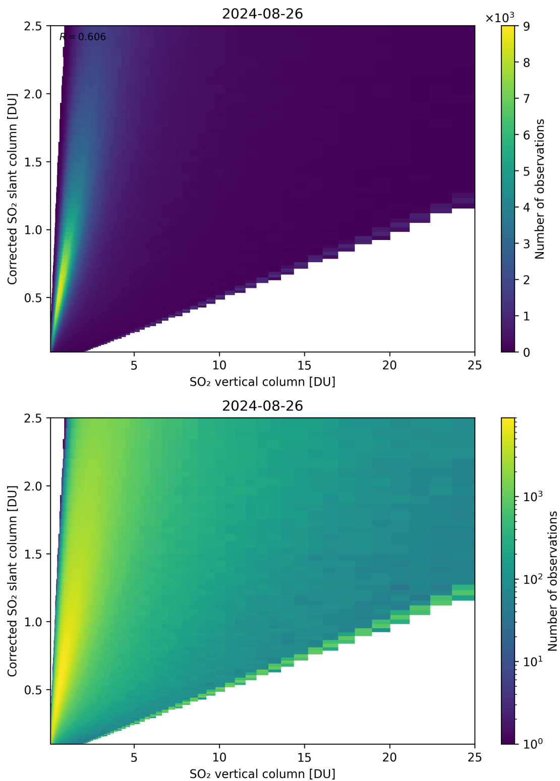
Figure 297: Scatter density plot of “SO 2 vertical column” against “Corrected SO 2 slant column” for 2024-08-25 to 2024-08-27.
