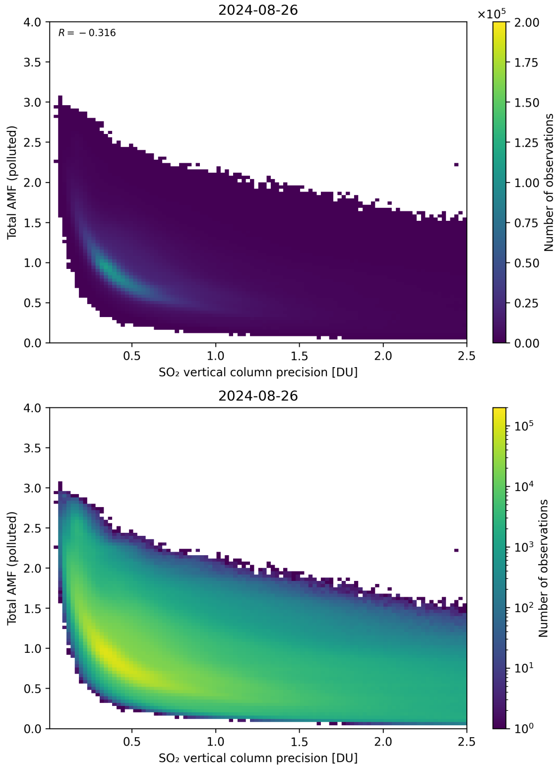
Figure 294: Scatter density plot of “SO 2 vertical column precision” against “Total AMF (polluted)” for 2024-08-25 to 2024-08-27.
