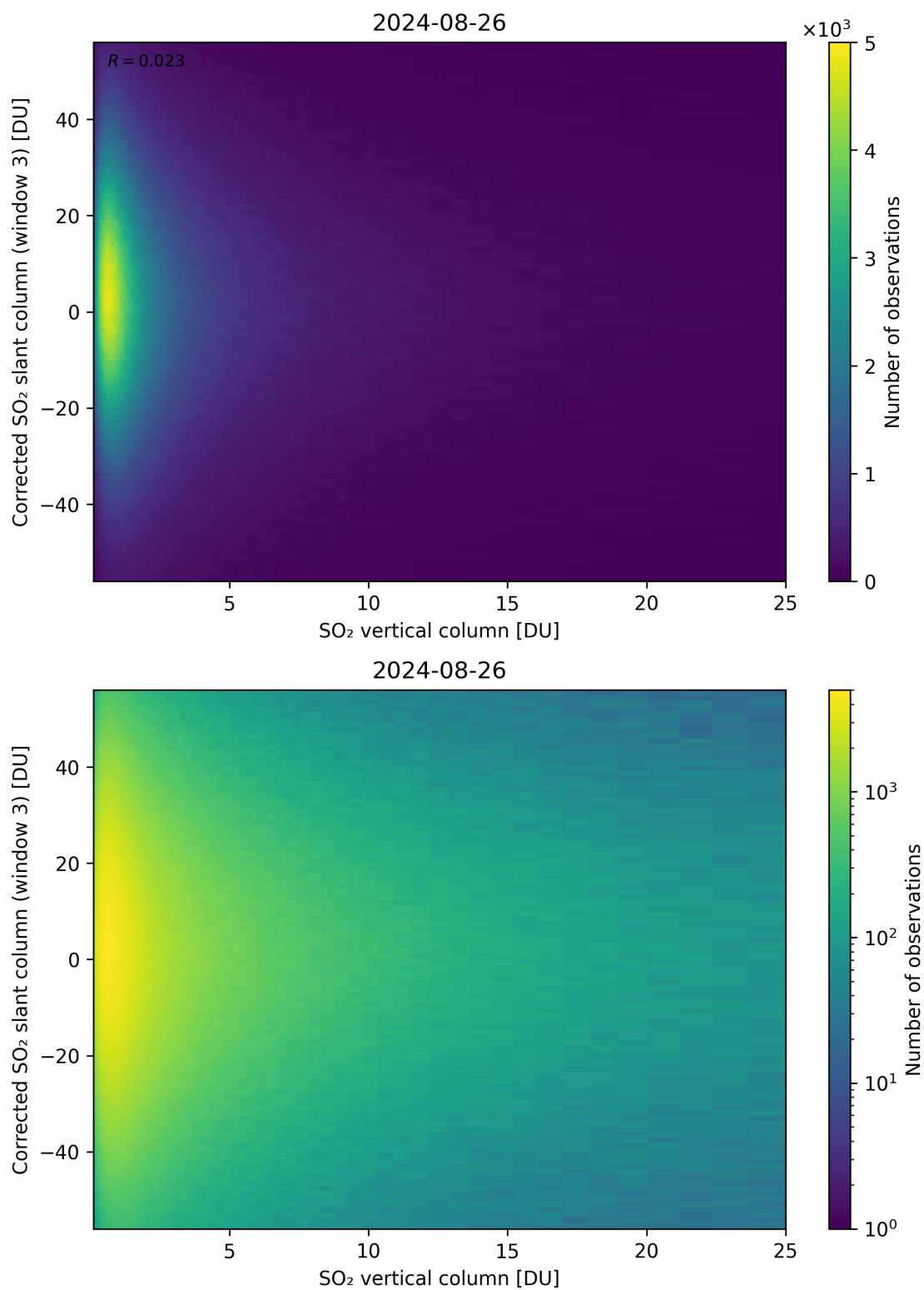
Figure 299: Scatter density plot of “SO 2 vertical column” against “Corrected SO 2 slant column (window 3)” for 2024-08-25 to 2024-08-27.
