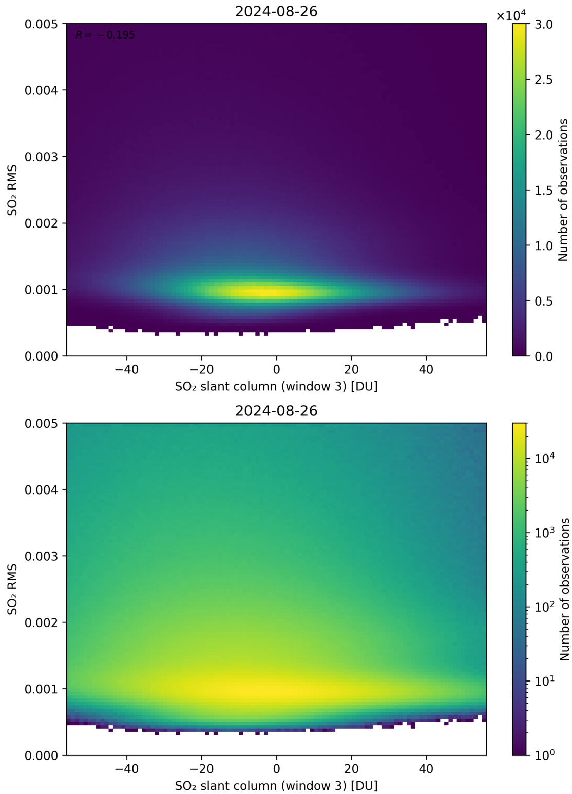
Figure 256: Scatter density plot of “SO 2 slant column (window 3)” against “SO 2 RMS” for 2024-08-25 to 2024-08-27.
