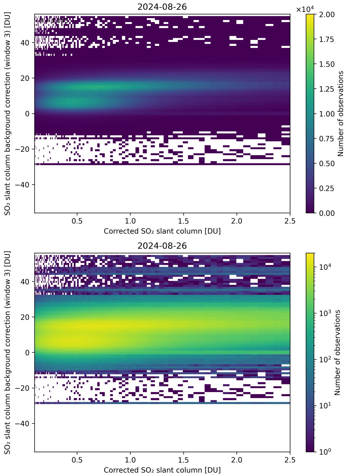
Figure 180: Scatter density plot of “Corrected SO 2 slant column” against “SO 2 slant column background correction (window 3)” for 2024-08-25 to 2024-08-27.
