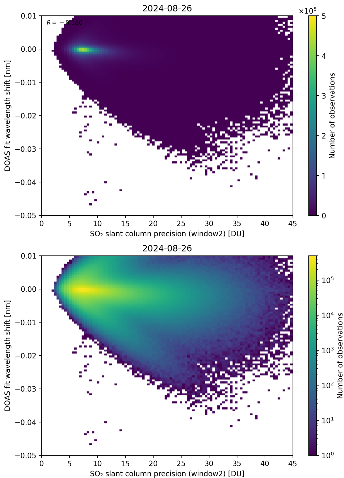
Figure 243: Scatter density plot of “SO 2 slant column precision (window2)” against “DOAS fit wavelength shift” for 2024-08-25 to 2024-08-27.
