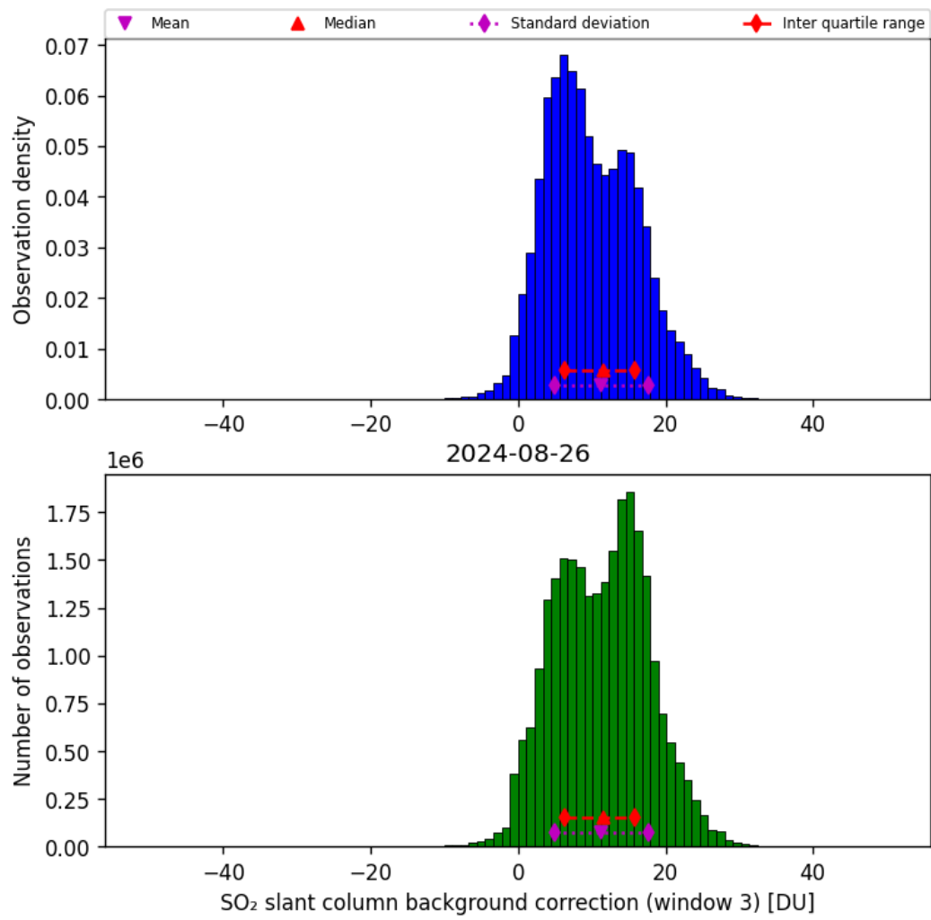
Figure 67: Histogram of “SO 2 slant column background correction (window 3)” for 2024-08-25 to 2024-08-27
