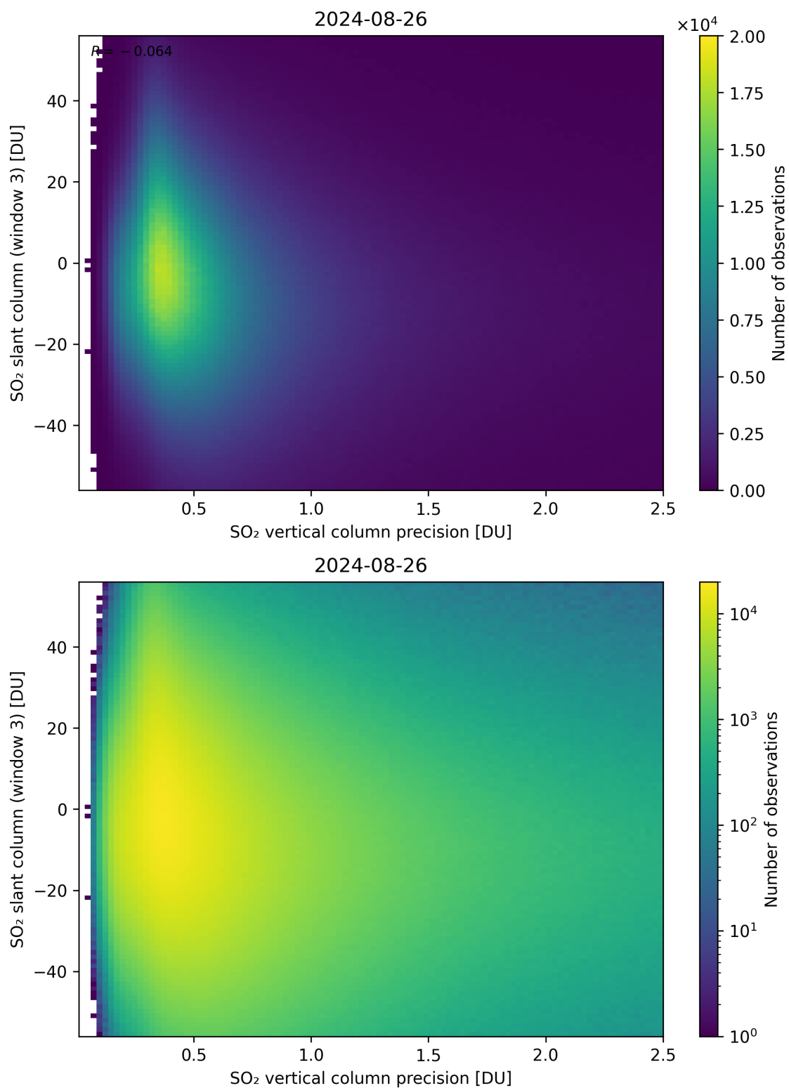
Figure 292: Scatter density plot of “SO 2 vertical column precision” against “SO 2 slant column (window 3)” for 2024-08-25 to 2024-08-27.
