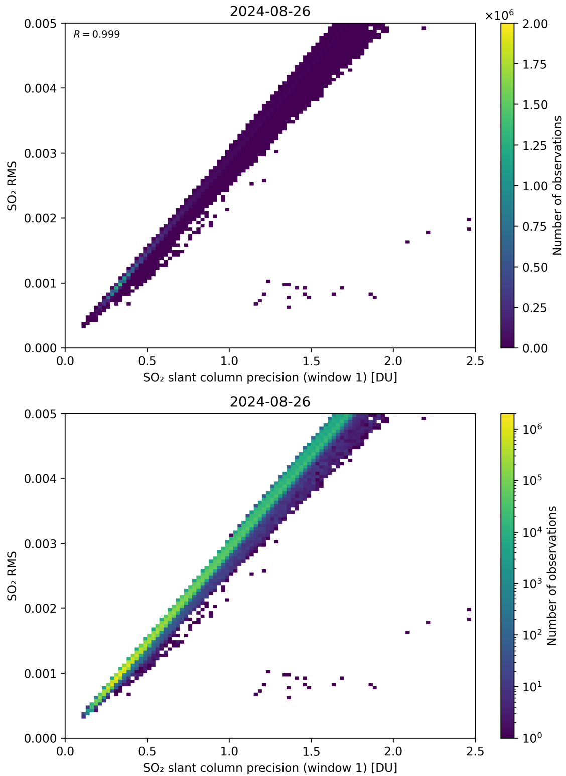
Figure 223: Scatter density plot of “SO 2 slant column precision (window 1)” against “SO 2 RMS” for 2024-08-25 to 2024-08-27.
