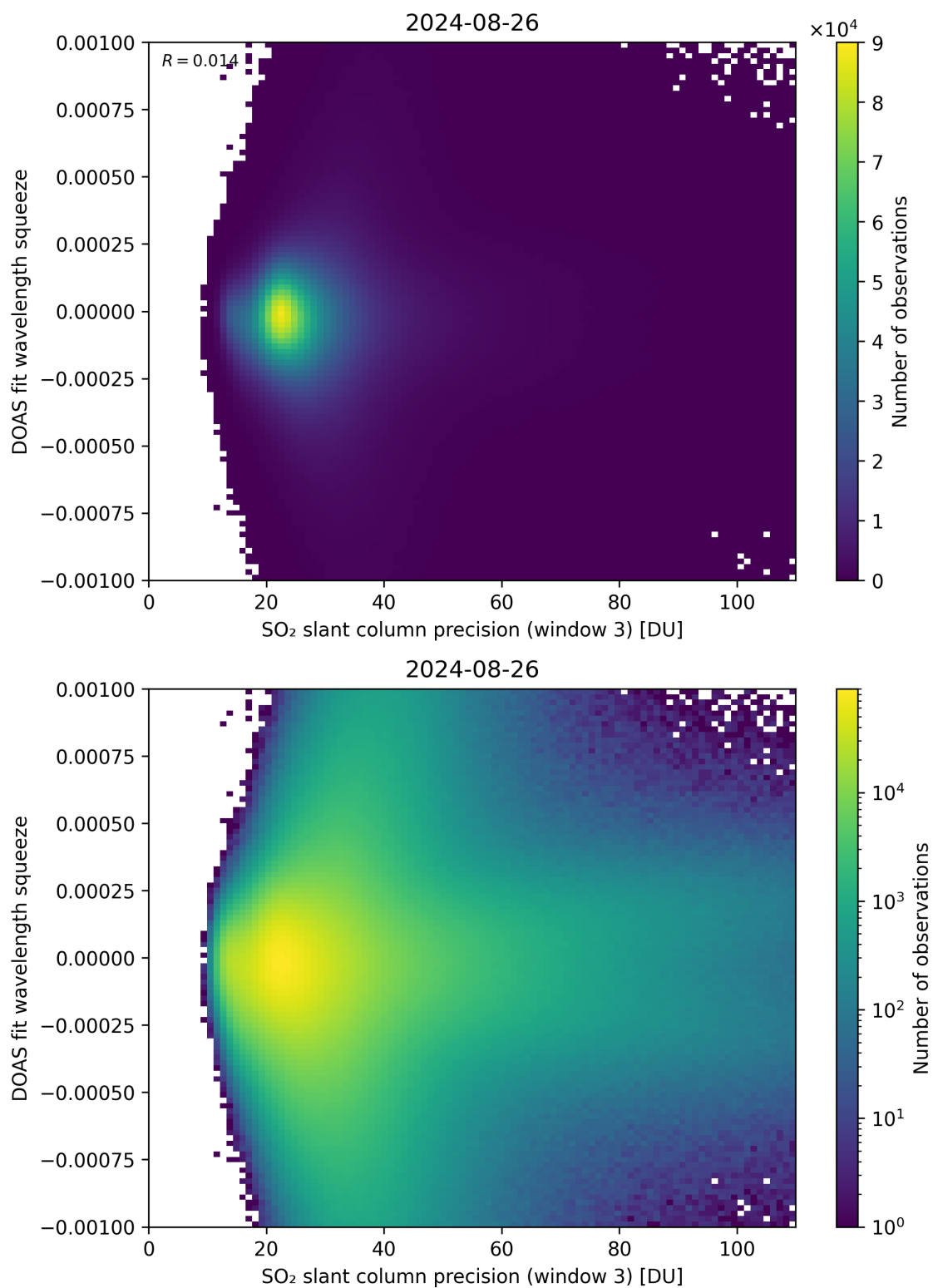
Figure 259: Scatter density plot of “SO 2 slant column precision (window 3)” against “DOAS fit wavelength squeeze” for 2024-08-25 to 2024-08-27.
