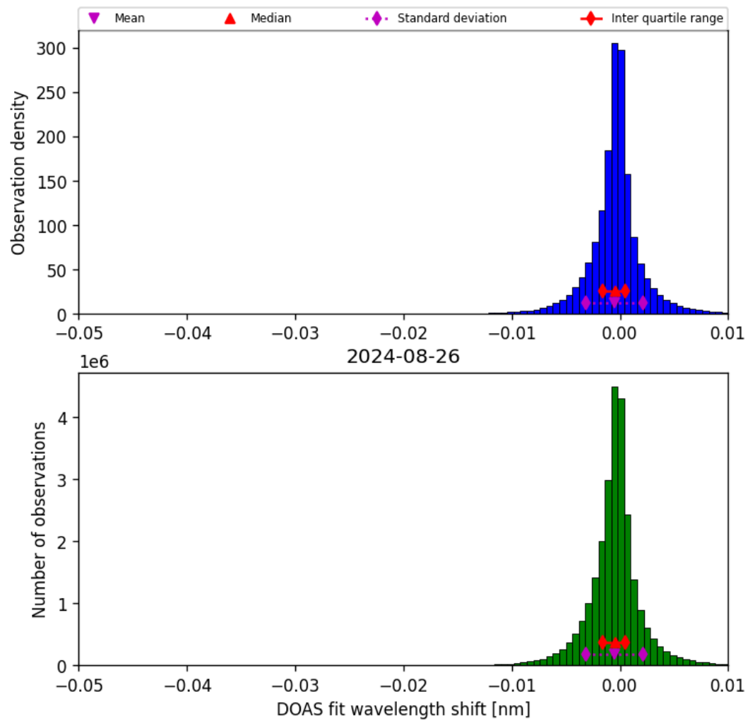
Figure 68: Histogram of “DOAS fit wavelength shift” for 2024-08-25 to 2024-08-27
