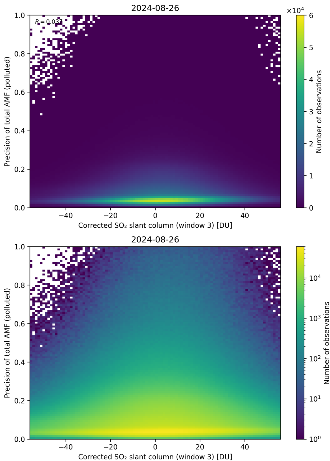
Figure 211: Scatter density plot of “Corrected SO 2 slant column (window 3)” against “Precision of total AMF (polluted)” for 2024-08-25 to 2024-08-27.
