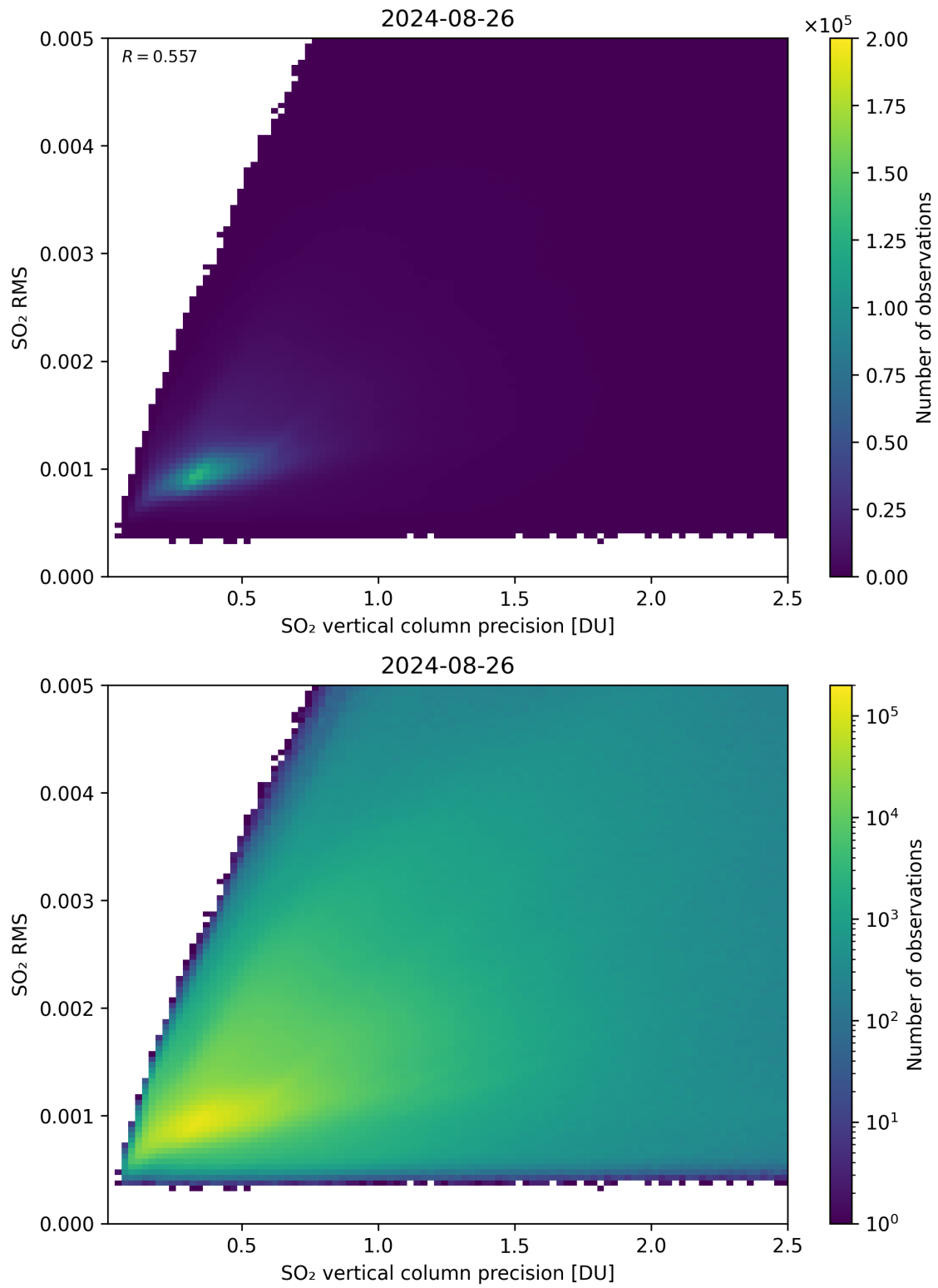
Figure 284: Scatter density plot of “SO 2 vertical column precision” against “SO 2 RMS” for 2024-08-25 to 2024-08-27.
