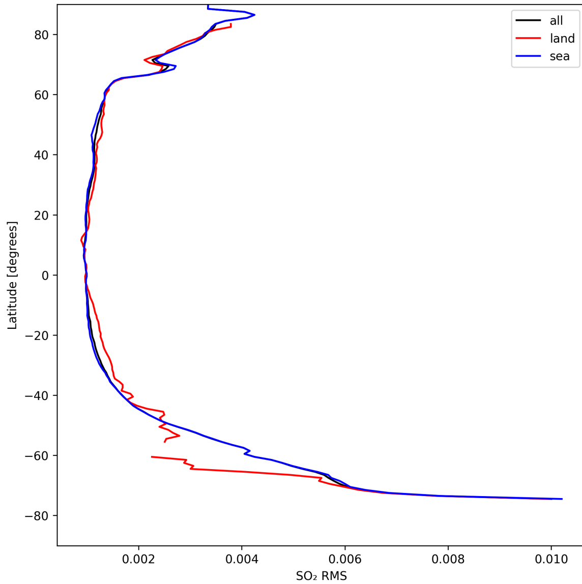
Figure 47: Zonal average of “SO 2 RMS” for 2024-08-25 to 2024-08-27.
