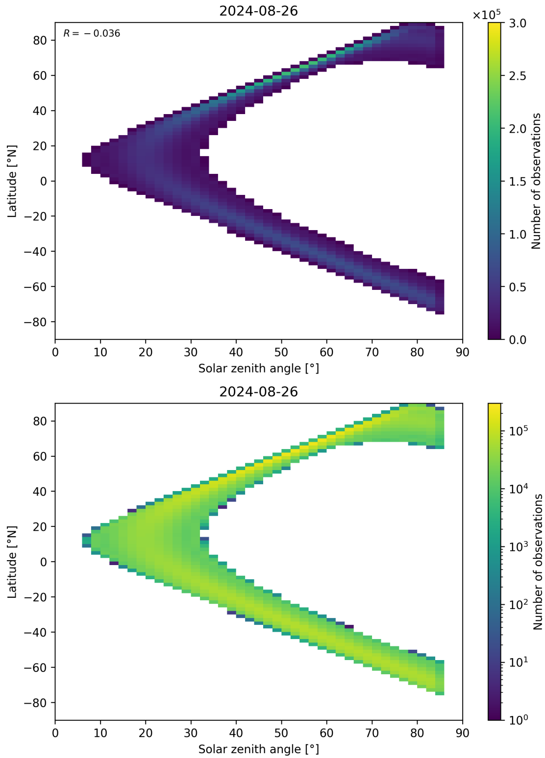
Figure 164: Scatter density plot of “Solar zenith angle” against “Latitude” for 2024-08-25 to 2024-08-27.
