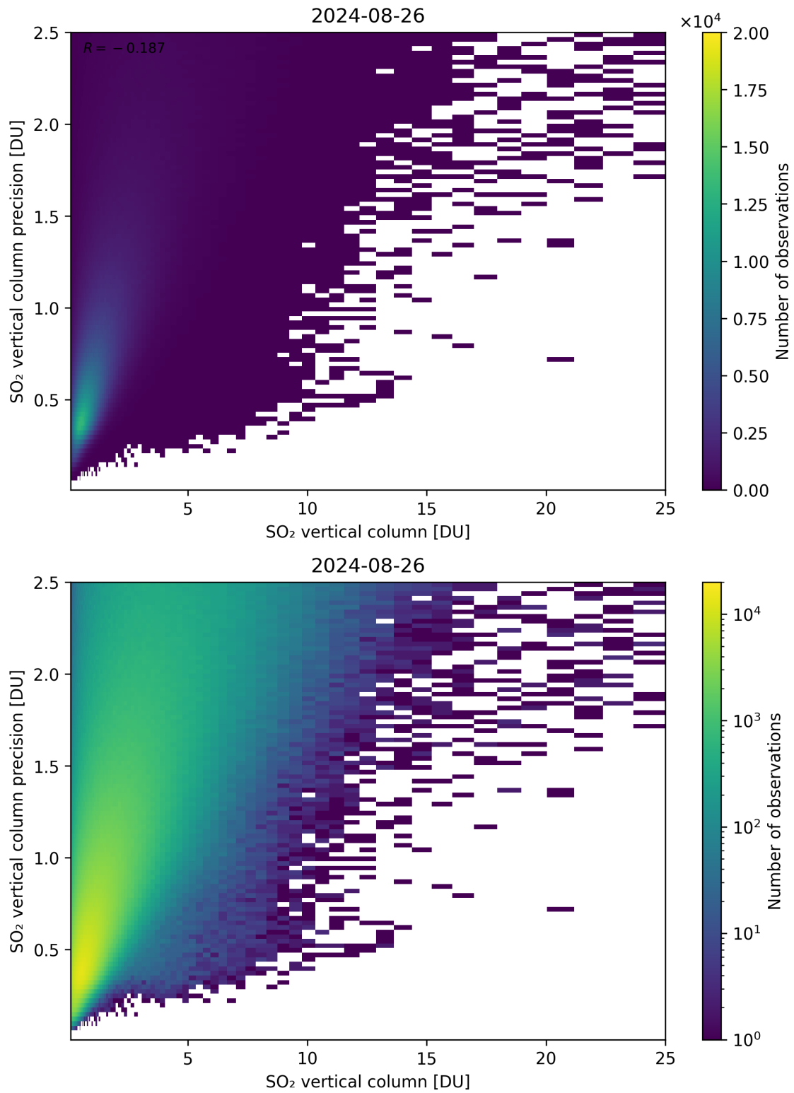
Figure 307: Scatter density plot of “SO 2 vertical column” against “SO 2 vertical column precision” for 2024-08-25 to 2024-08-27.
