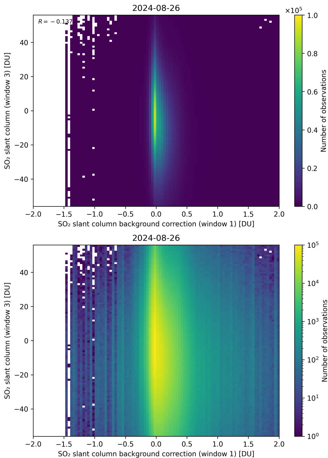
Figure 107: Scatter density plot of “SO 2 slant column background correction (window 1)” against “SO 2 slant column (window 3)” for 2024-08-25 to 2024-08-27.
