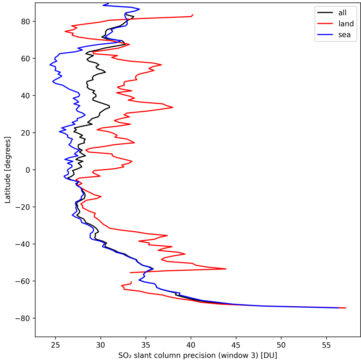
Figure 42: Zonal average of “SO 2 slant column precision (window 3)” for 2024-08-25 to 2024-08-27.
