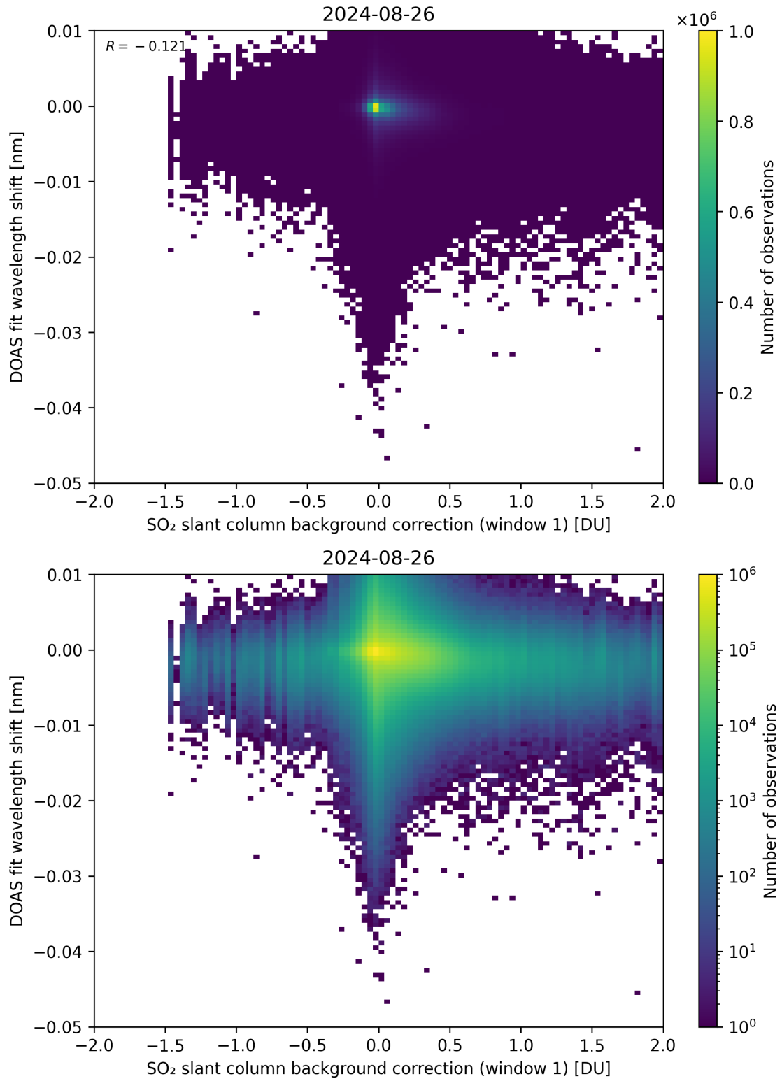
Figure 100: Scatter density plot of “SO 2 slant column background correction (window 1)” against “DOAS fit wavelength shift” for 2024-08-25 to 2024-08-27.
