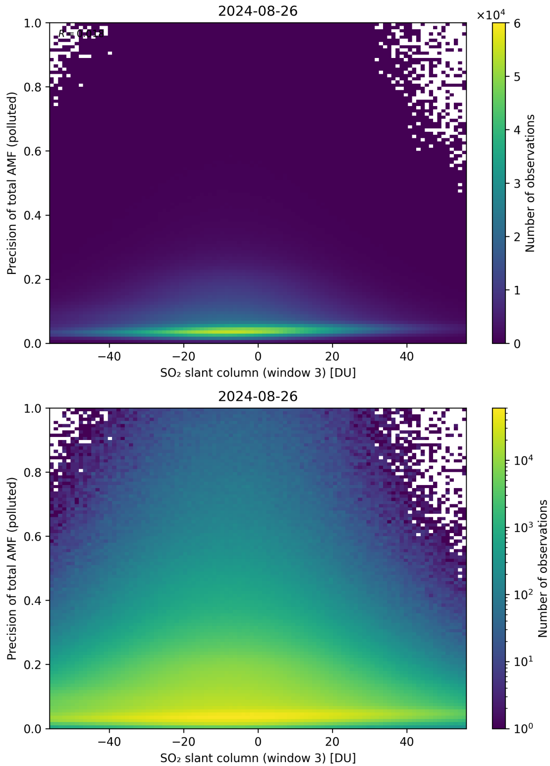
Figure 269: Scatter density plot of “SO 2 slant column (window 3)” against “Precision of total AMF (polluted)” for 2024-08-25 to 2024-08-27.
