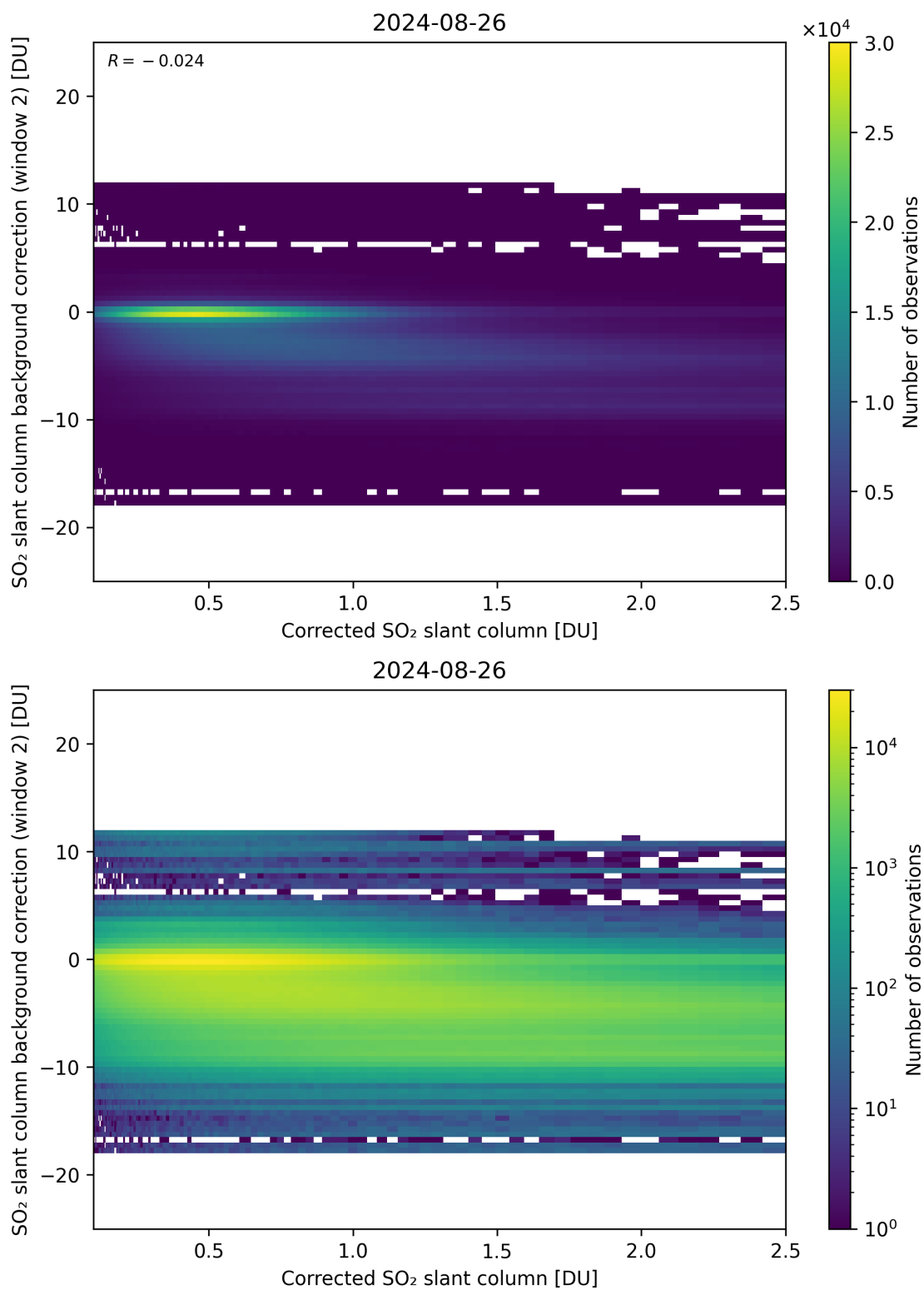
Figure 179: Scatter density plot of “Corrected SO 2 slant column” against “SO 2 slant column background correction (window 2)” for 2024-08-25 to 2024-08-27.
