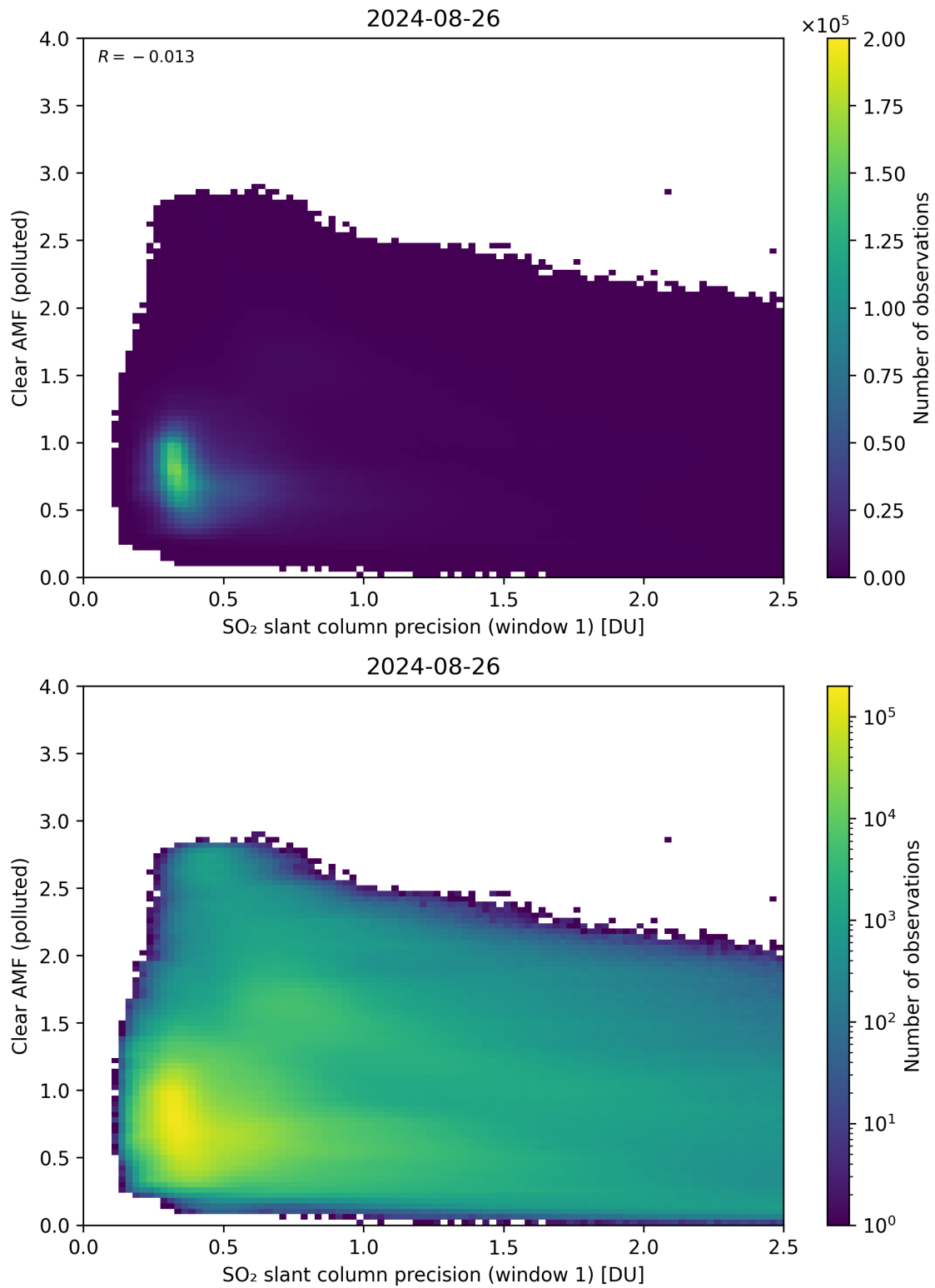
Figure 224: Scatter density plot of “SO 2 slant column precision (window 1)” against “Clear AMF (polluted)” for 2024-08-25 to 2024-08-27.
