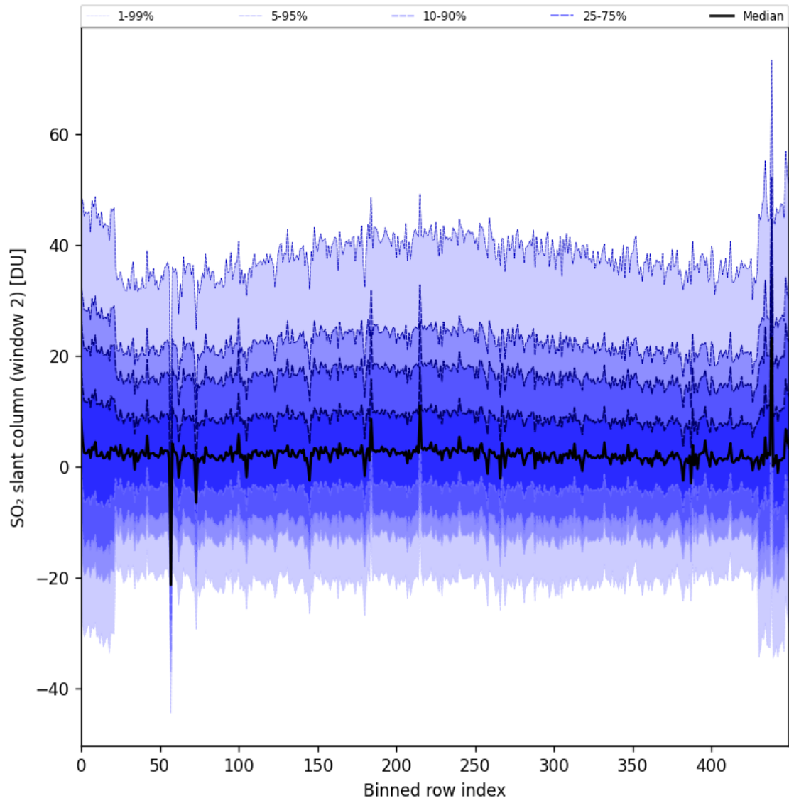
Figure 83: Along track statistics of “SO 2 slant column (window 2)” for 2024-08-25 to 2024-08-27
