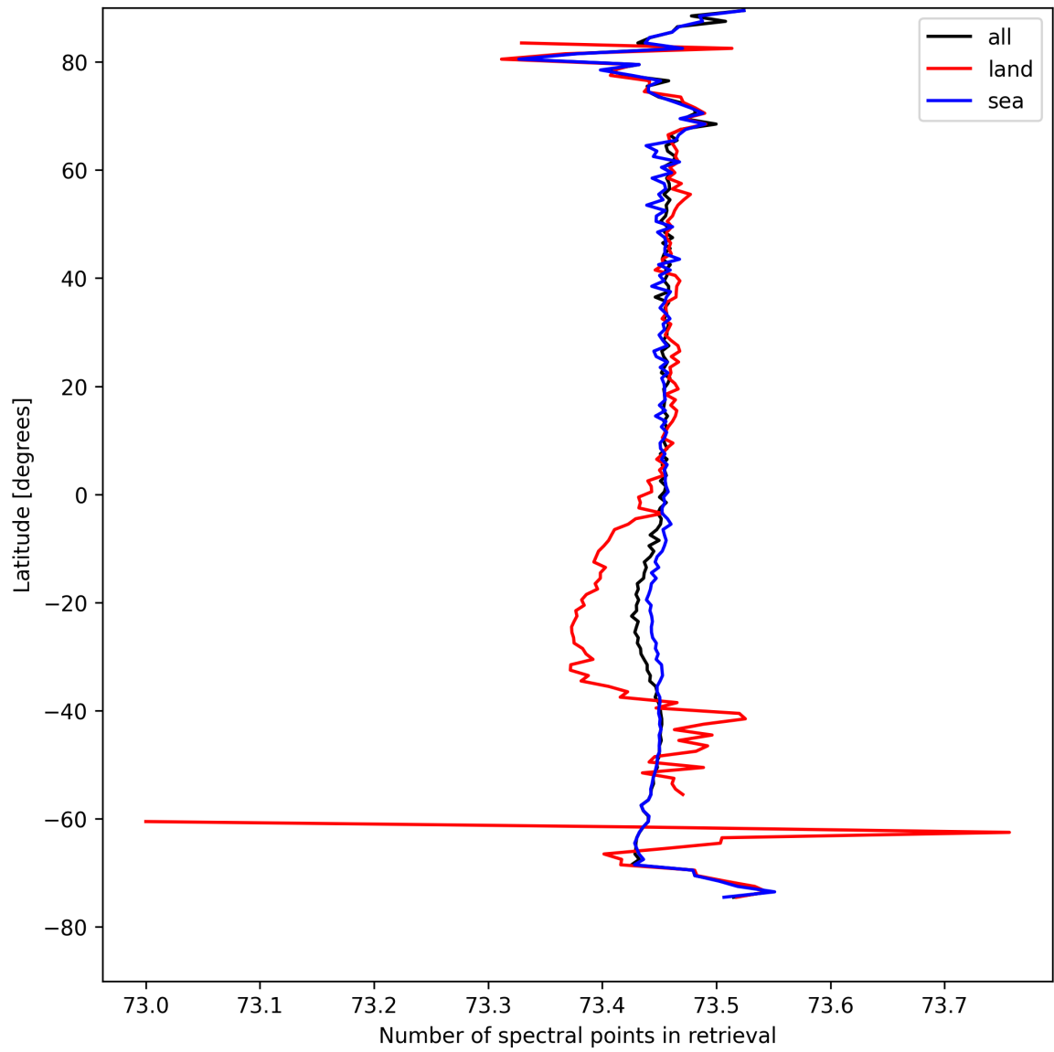
Figure 51: Zonal average of “Number of spectral points in retrieval” for 2024-08-25 to 2024-08-27.
