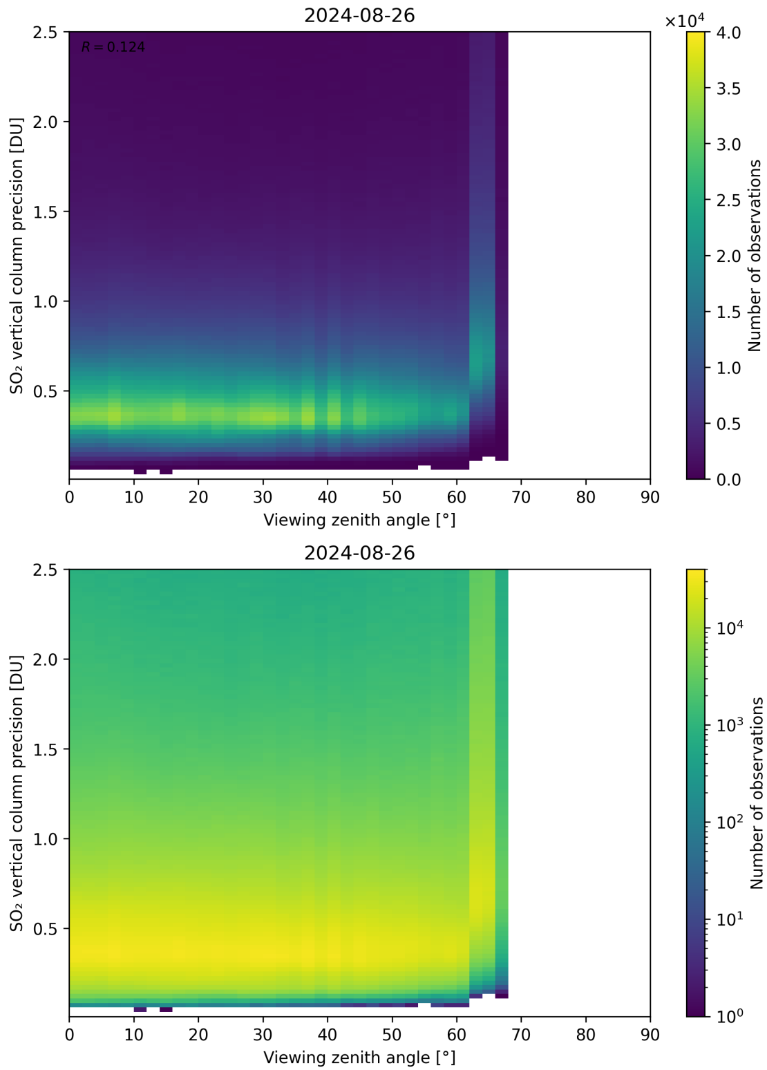
Figure 328: Scatter density plot of “Viewing zenith angle” against “SO 2 vertical column precision” for 2024-08-25 to 2024-08-27.
