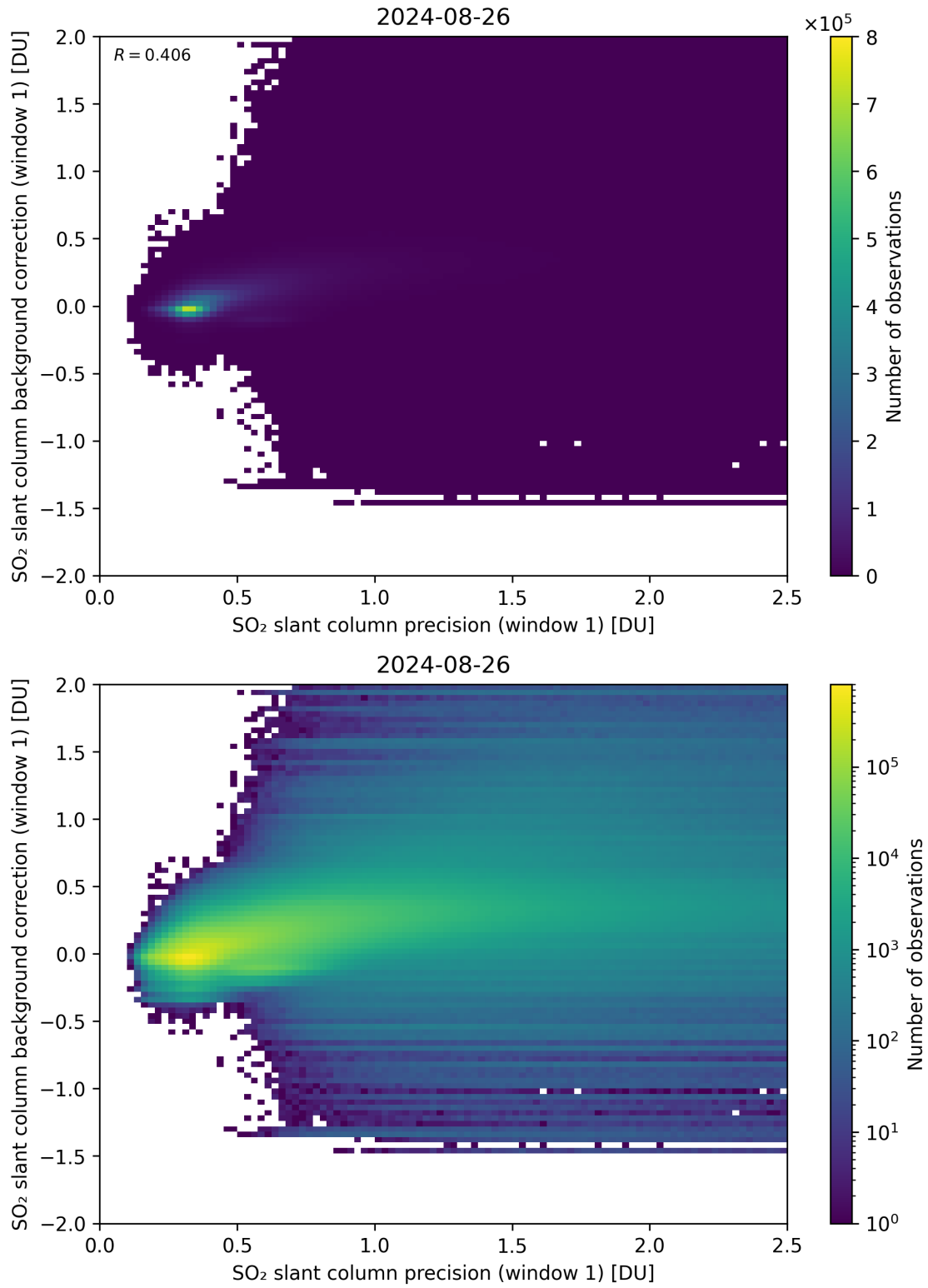
Figure 218: Scatter density plot of “SO 2 slant column precision (window 1)” against “SO 2 slant column background correction (window 1)” for 2024-08-25 to 2024-08-27.
