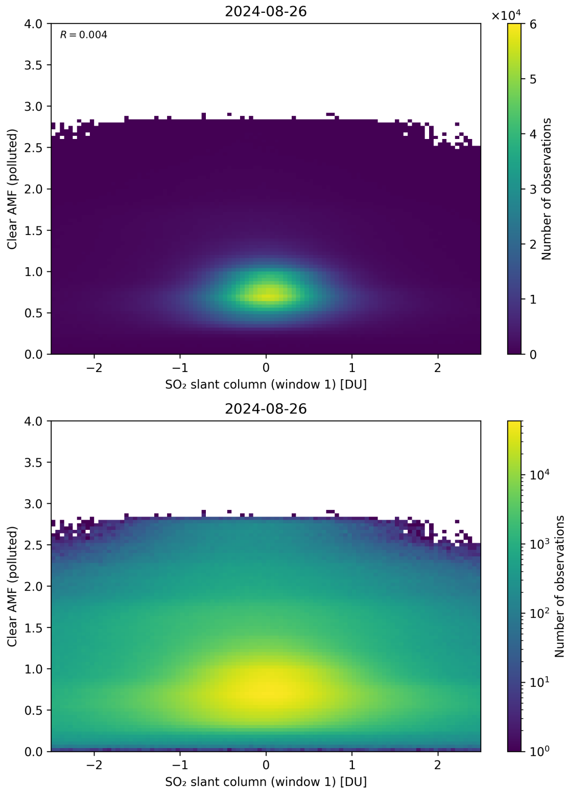
Figure 232: Scatter density plot of “SO 2 slant column (window 1)” against “Clear AMF (polluted)” for 2024-08-25 to 2024-08-27.
