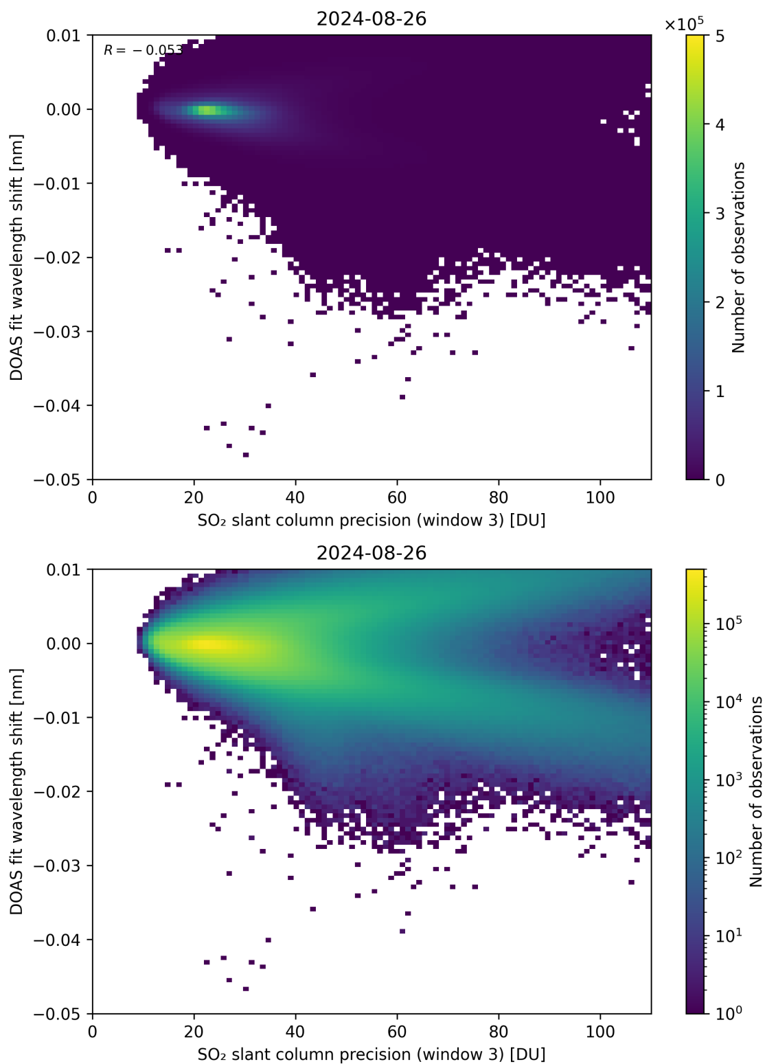
Figure 258: Scatter density plot of “SO 2 slant column precision (window 3)” against “DOAS fit wavelength shift” for 2024-08-25 to 2024-08-27.
