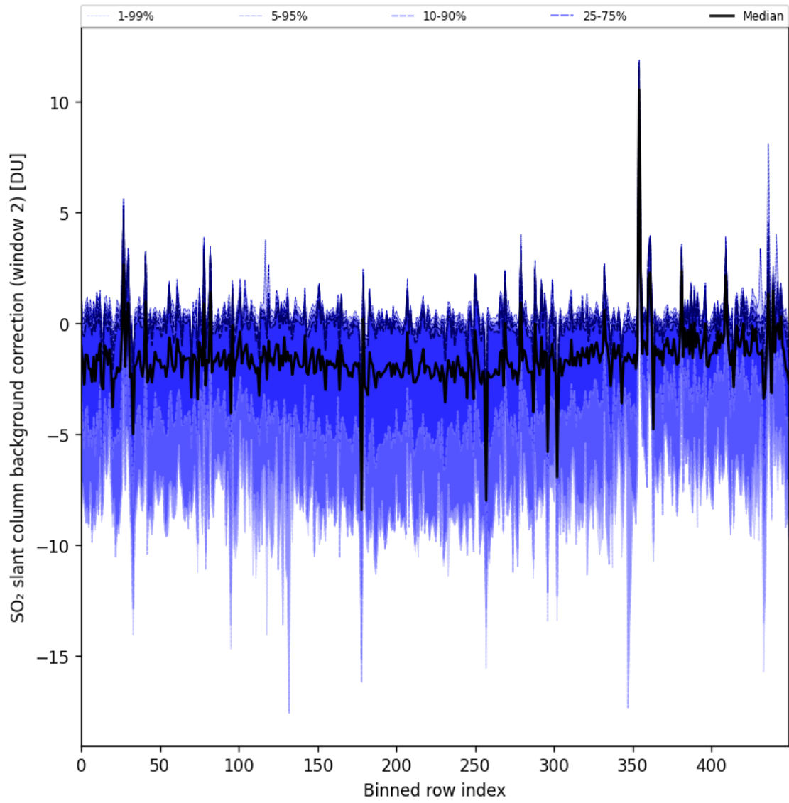
Figure 86: Along track statistics of “SO 2 slant column background correction (window 2)” for 2024-08-25 to 2024-08-27
