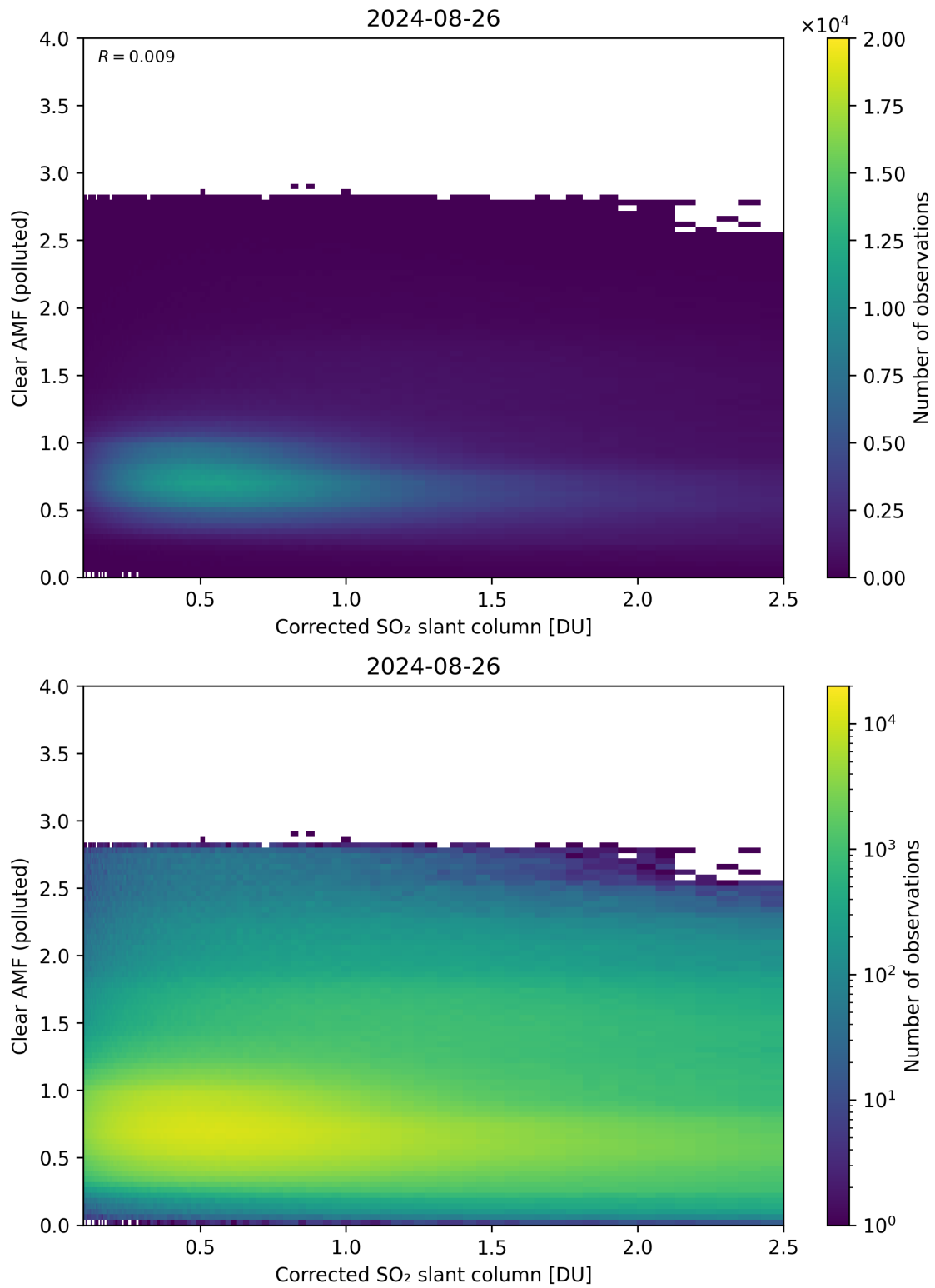
Figure 184: Scatter density plot of “Corrected SO 2 slant column” against “Clear AMF (polluted)” for 2024-08-25 to 2024-08-27.
