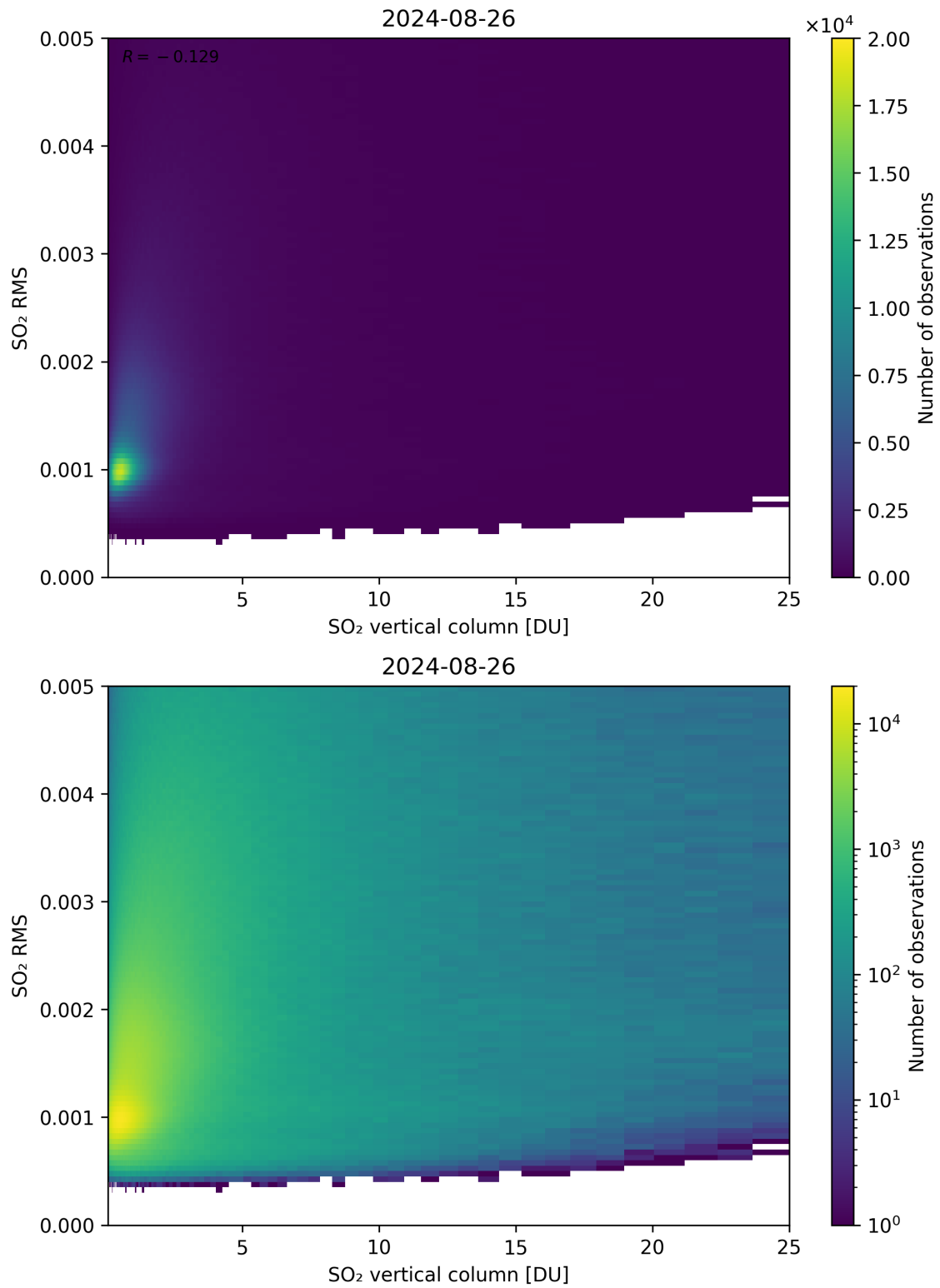
Figure 278: Scatter density plot of “SO 2 vertical column” against “SO 2 RMS” for 2024-08-25 to 2024-08-27.
