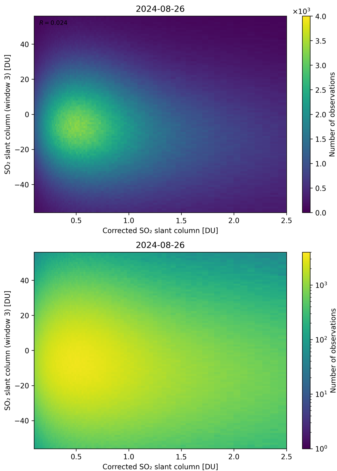
Figure 190: Scatter density plot of “Corrected SO 2 slant column” against “SO 2 slant column (window 3)” for 2024-08-25 to 2024-08-27.
