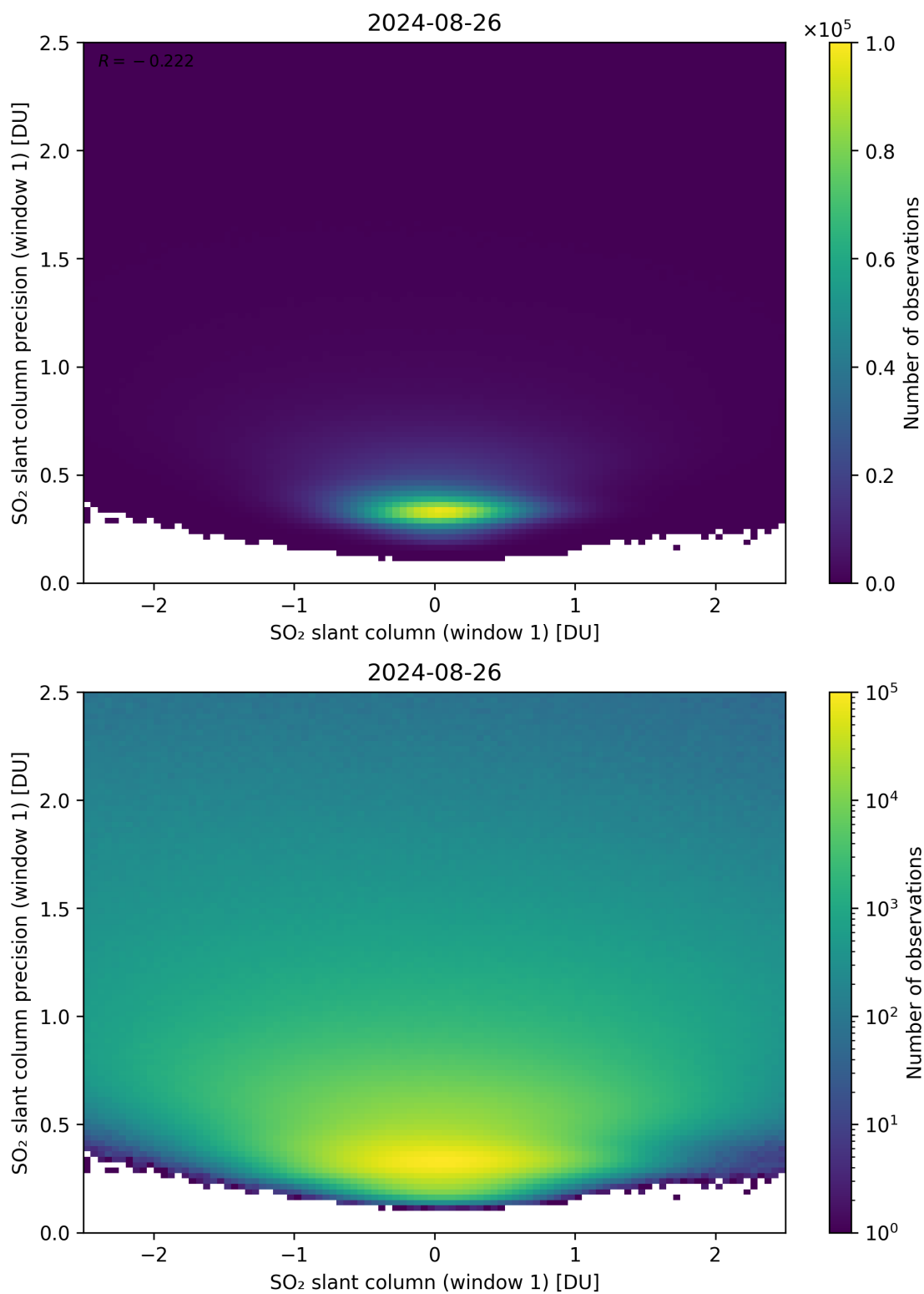
Figure 235: Scatter density plot of “SO 2 slant column (window 1)” against “SO 2 slant column precision (window 1)” for 2024-08-25 to 2024-08-27.
