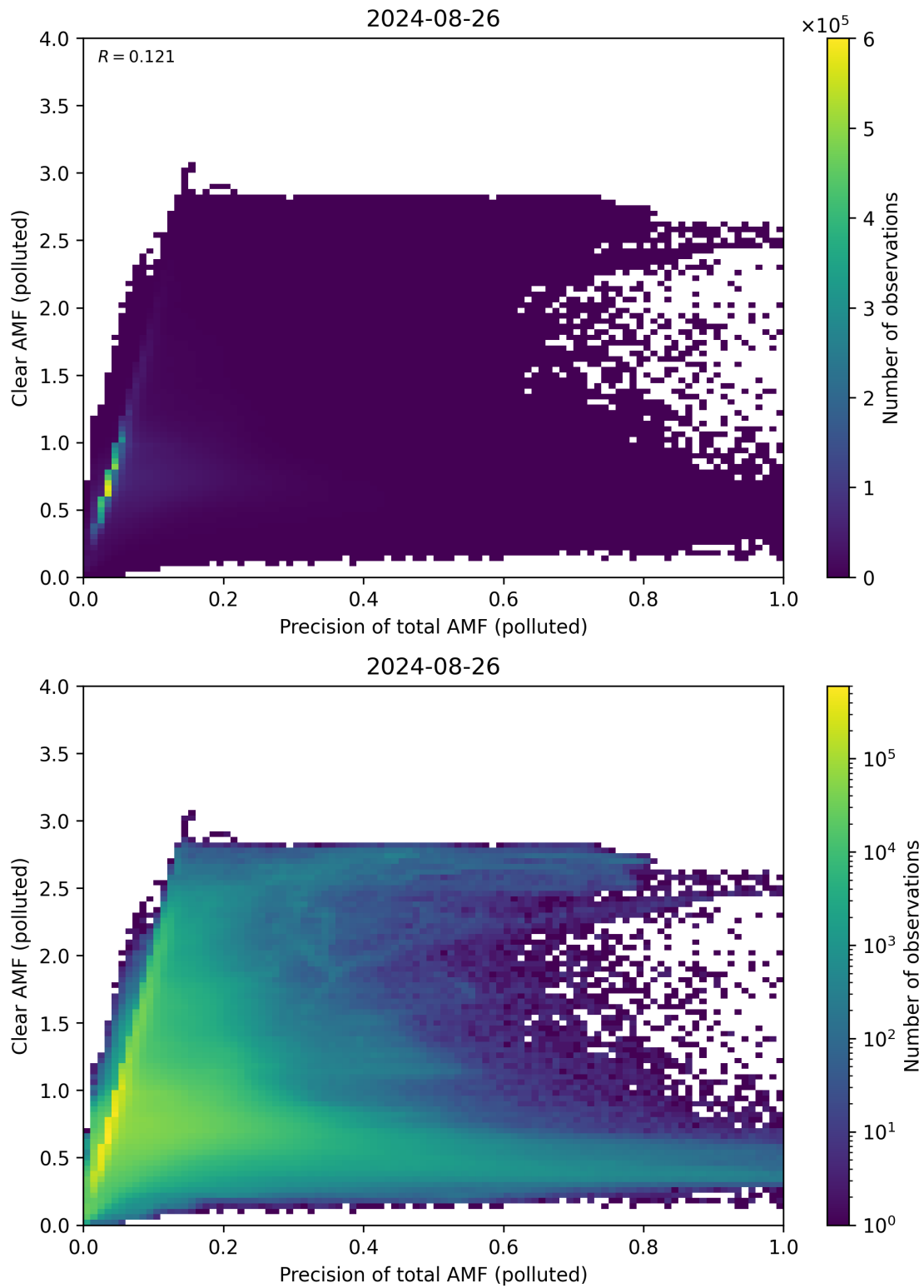
Figure 270: Scatter density plot of “Precision of total AMF (polluted)” against “Clear AMF (polluted)” for 2024-08-25 to 2024-08-27.
