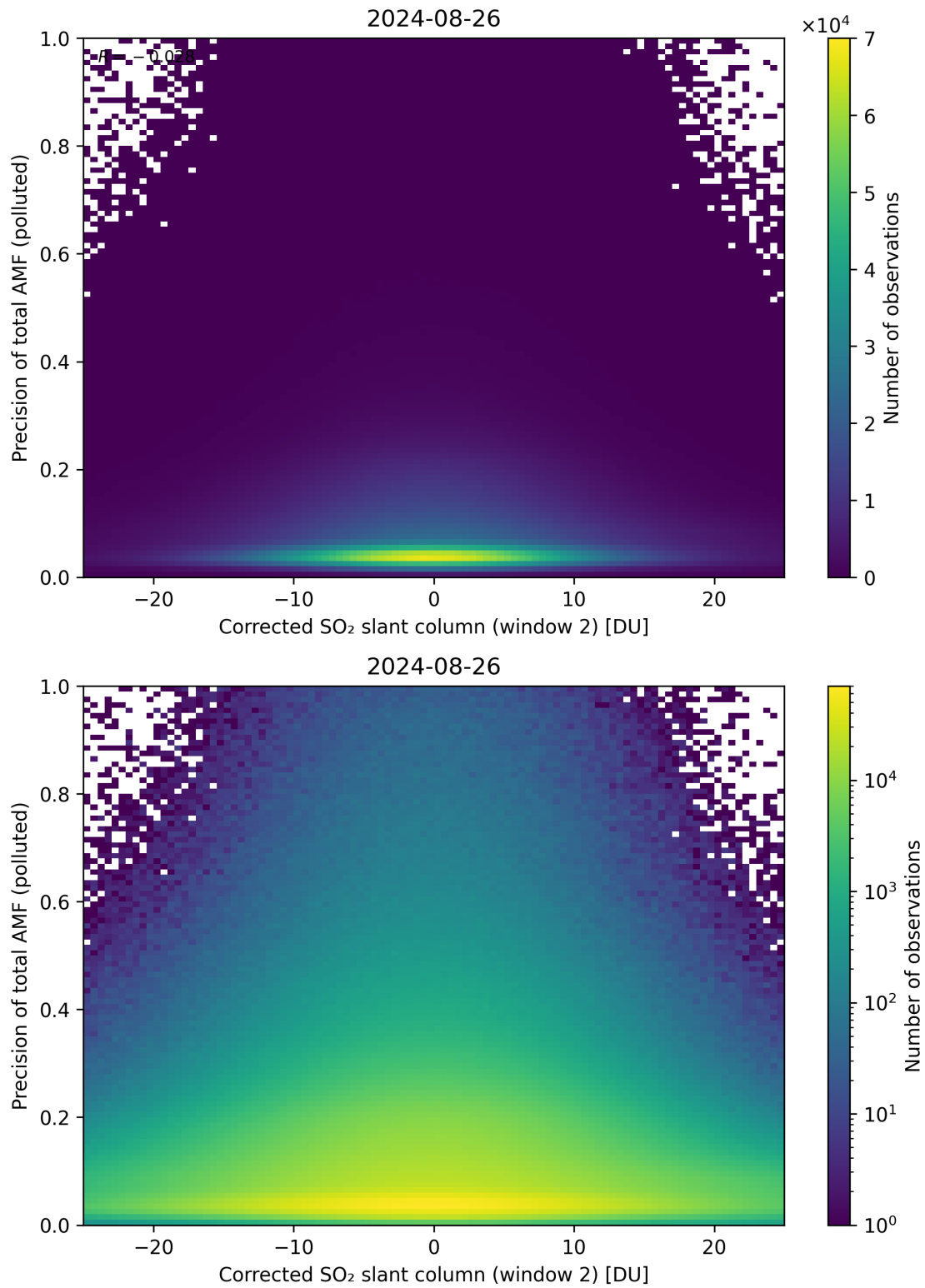
Figure 204: Scatter density plot of “Corrected SO 2 slant column (window 2)” against “Precision of total AMF (polluted)” for 2024-08-25 to 2024-08-27.
