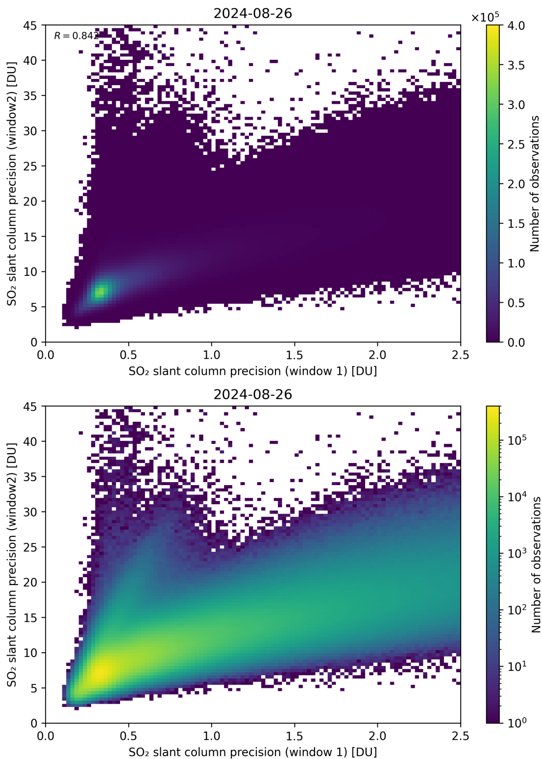
Figure 227: Scatter density plot of “SO 2 slant column precision (window 1)” against “SO 2 slant column precision (window2)” for 2024-08-25 to 2024-08-27.
