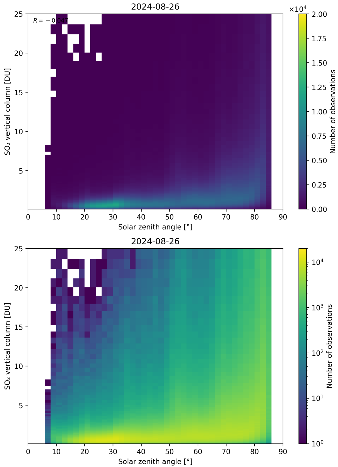
Figure 176: Scatter density plot of “Solar zenith angle” against “SO 2 vertical column” for 2024-08-25 to 2024-08-27.
