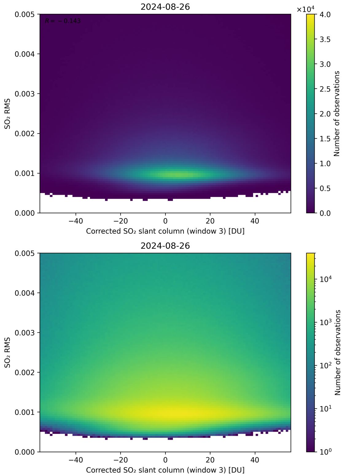
Figure 208: Scatter density plot of “Corrected SO 2 slant column (window 3)” against “SO 2 RMS” for 2024-08-25 to 2024-08-27.
