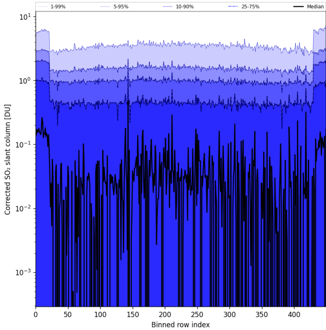
Figure 78: Along track statistics of “Corrected SO 2 slant column” for 2024-08-25 to 2024-08-27
