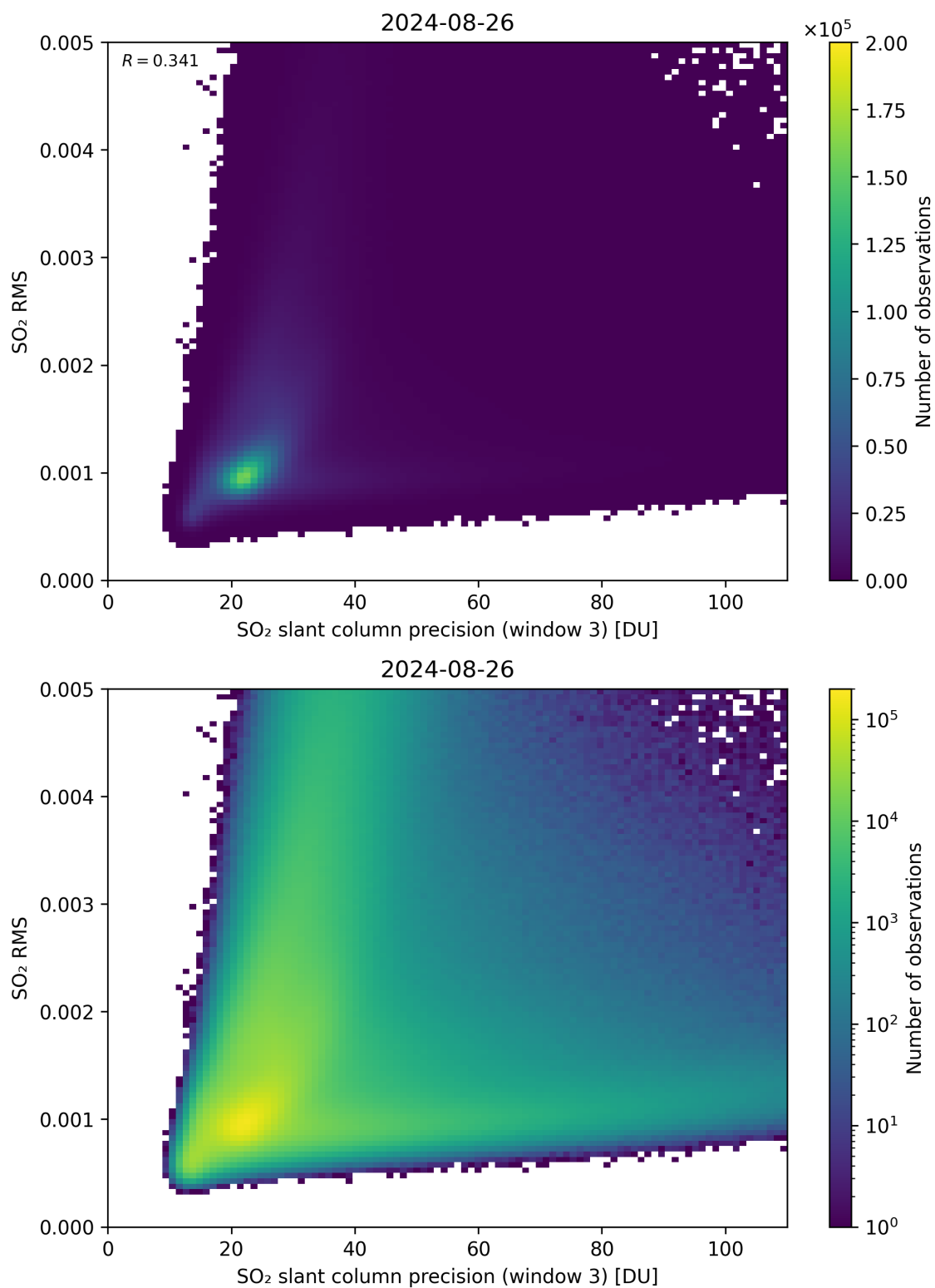
Figure 260: Scatter density plot of “SO 2 slant column precision (window 3)” against “SO 2 RMS” for 2024-08-25 to 2024-08-27.
