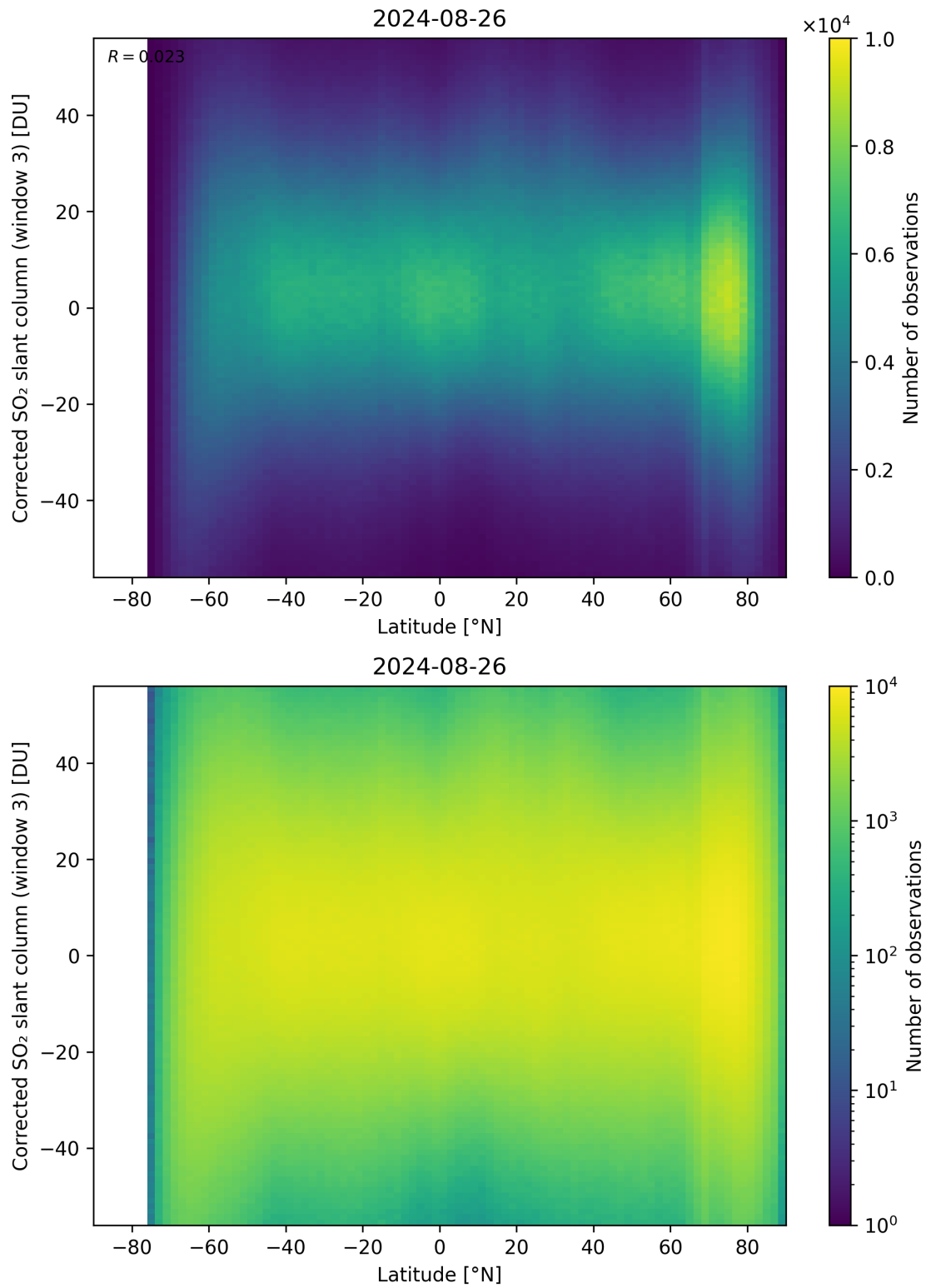
Figure 148: Scatter density plot of “Latitude” against “Corrected SO 2 slant column (window 3)” for 2024-08-25 to 2024-08-27.
