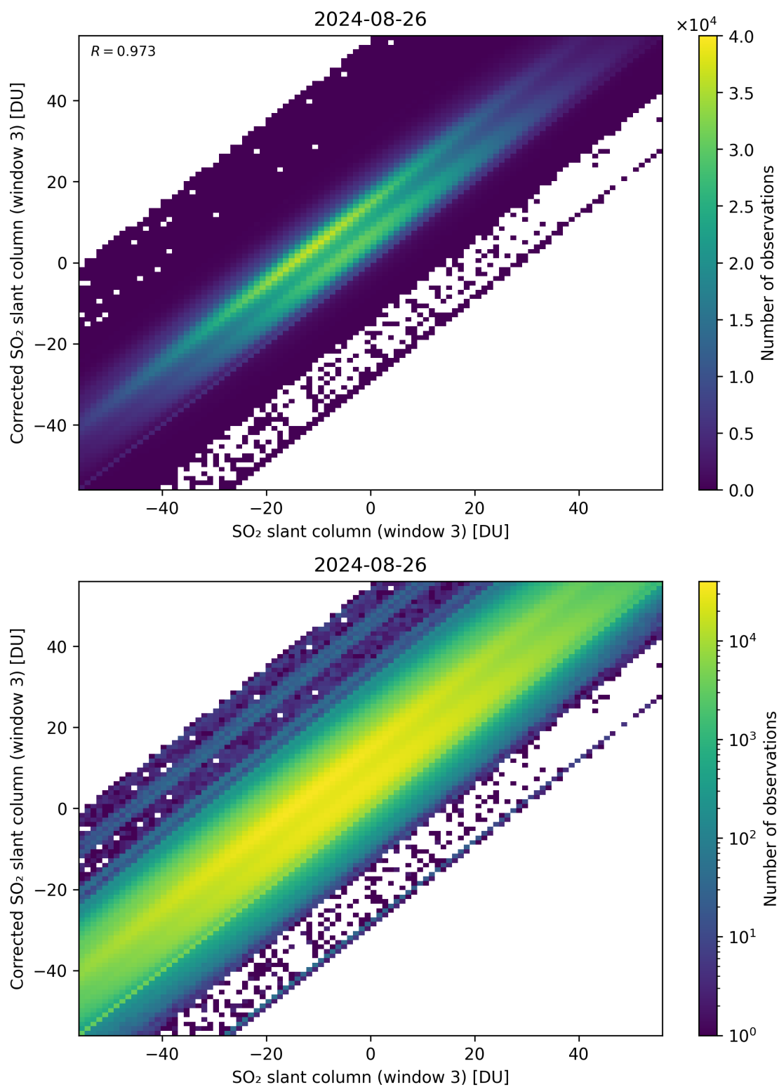
Figure 266: Scatter density plot of “SO 2 slant column (window 3)” against “Corrected SO 2 slant column (window 3)” for 2024-08-25 to 2024-08-27.
