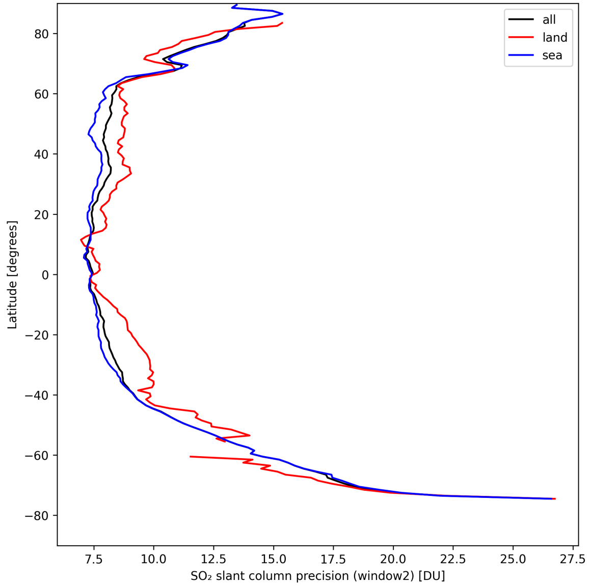
Figure 38: Zonal average of “SO 2 slant column precision (window2)” for 2024-08-25 to 2024-08-27.
