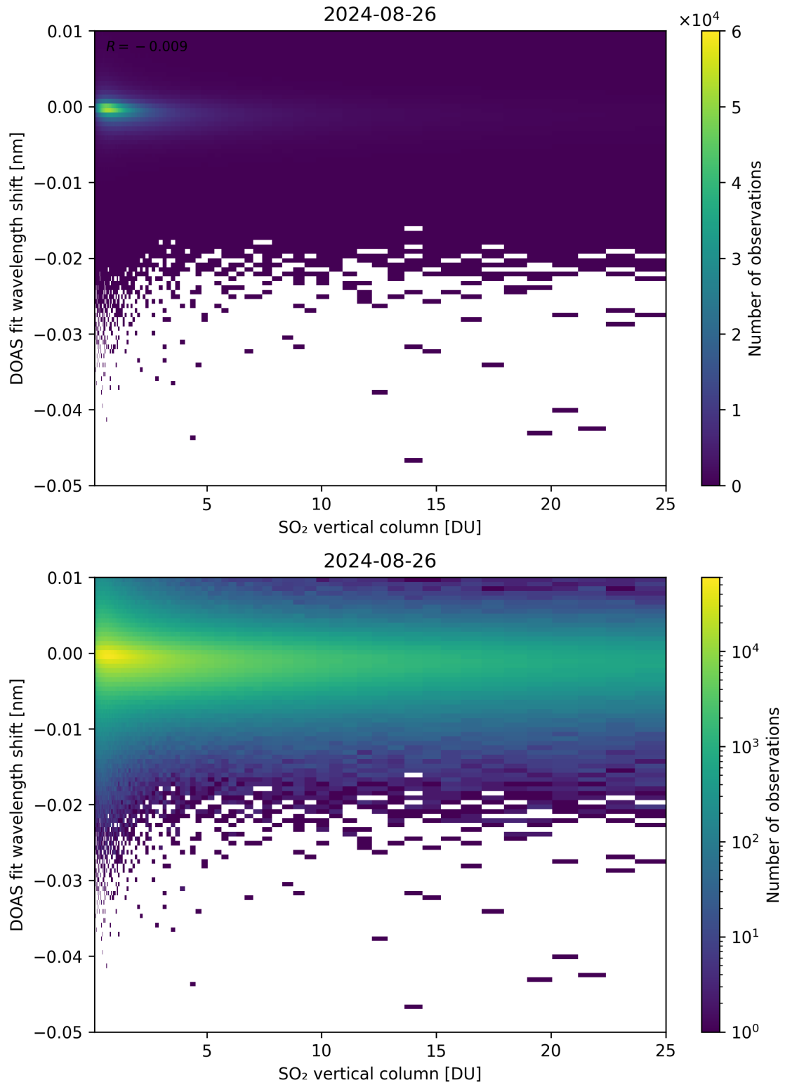
Figure 276: Scatter density plot of “SO 2 vertical column” against “DOAS fit wavelength shift” for 2024-08-25 to 2024-08-27.
