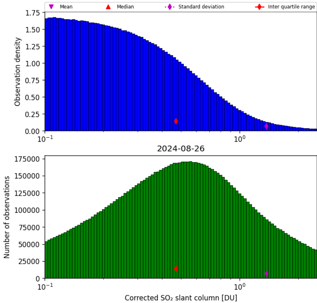
Figure 55: Histogram of “Corrected SO 2 slant column” for 2024-08-25 to 2024-08-27
