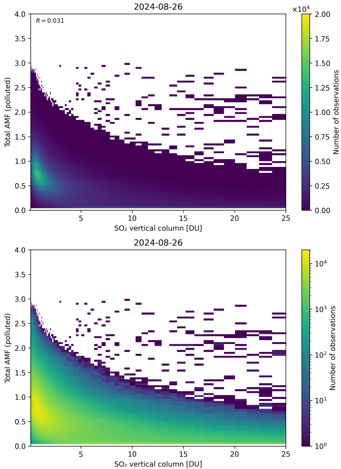
Figure 305: Scatter density plot of “SO 2 vertical column” against “Total AMF (polluted)” for 2024-08-25 to 2024-08-27.
