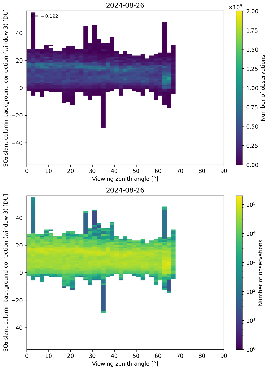
Figure 310: Scatter density plot of “Viewing zenith angle” against “SO 2 slant column background correction (window 3)” for 2024-08-25 to 2024-08-27.
