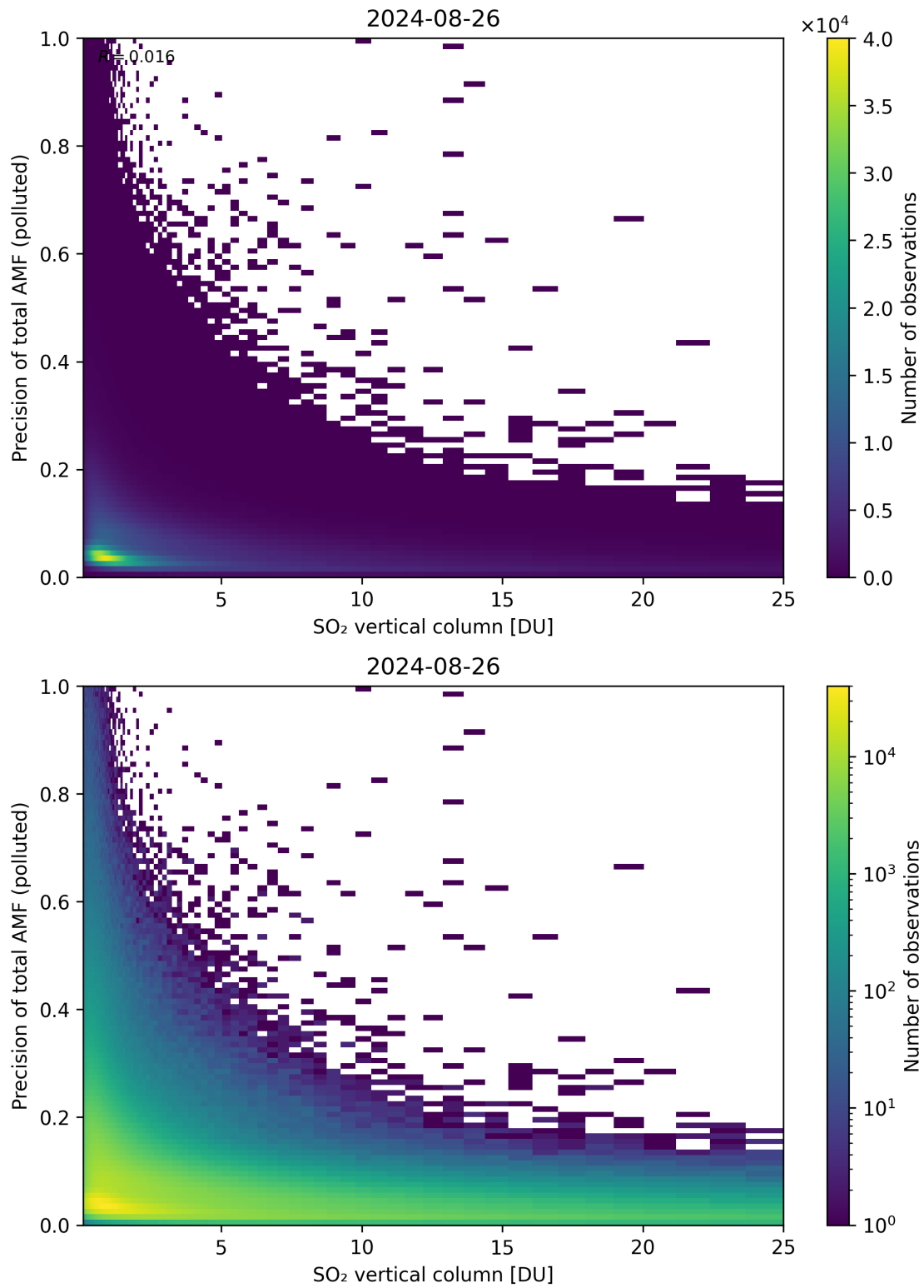
Figure 306: Scatter density plot of “SO 2 vertical column” against “Precision of total AMF (polluted)” for 2024-08-25 to 2024-08-27.
