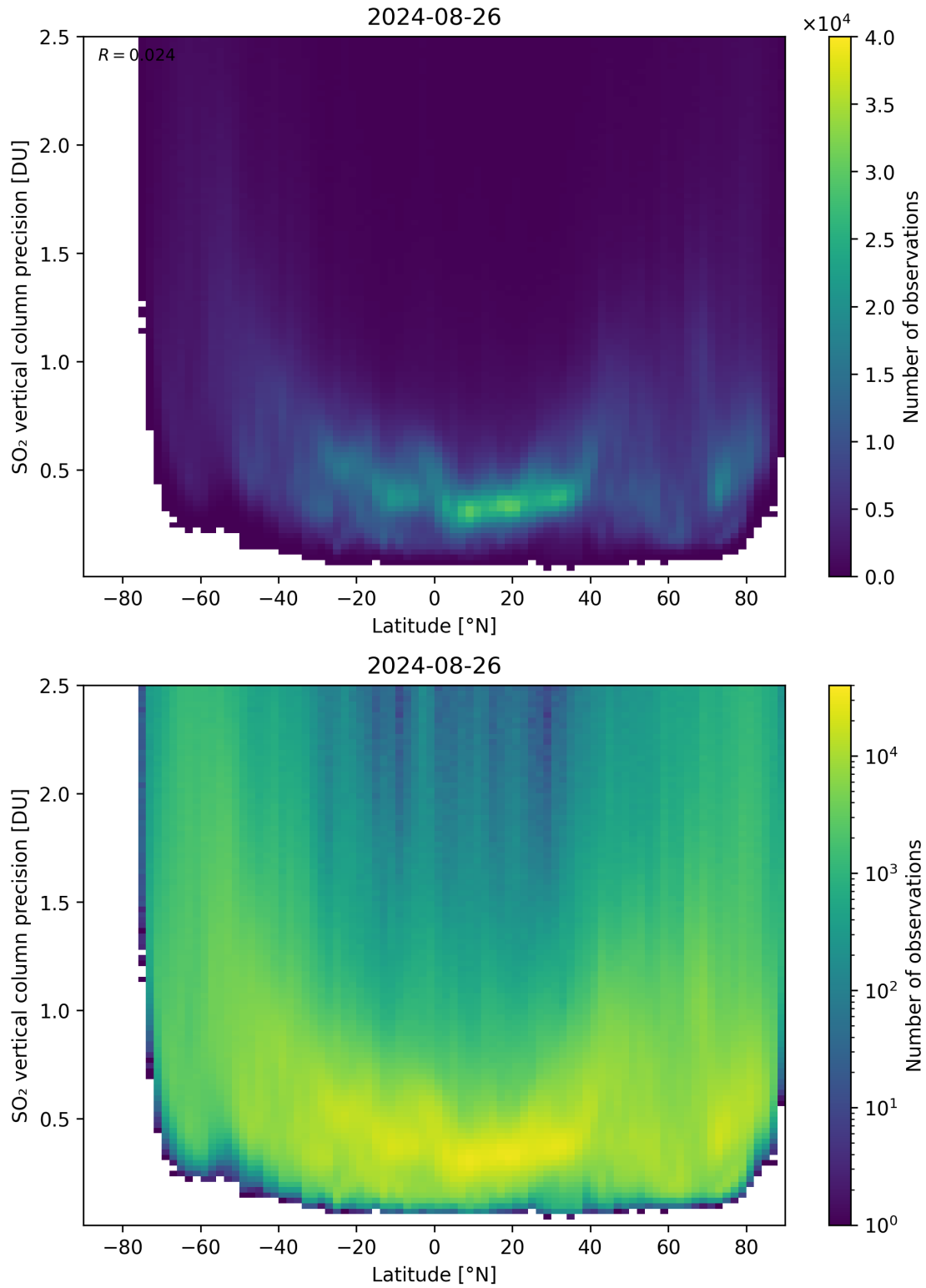
Figure 157: Scatter density plot of “Latitude” against “SO 2 vertical column precision” for 2024-08-25 to 2024-08-27.
