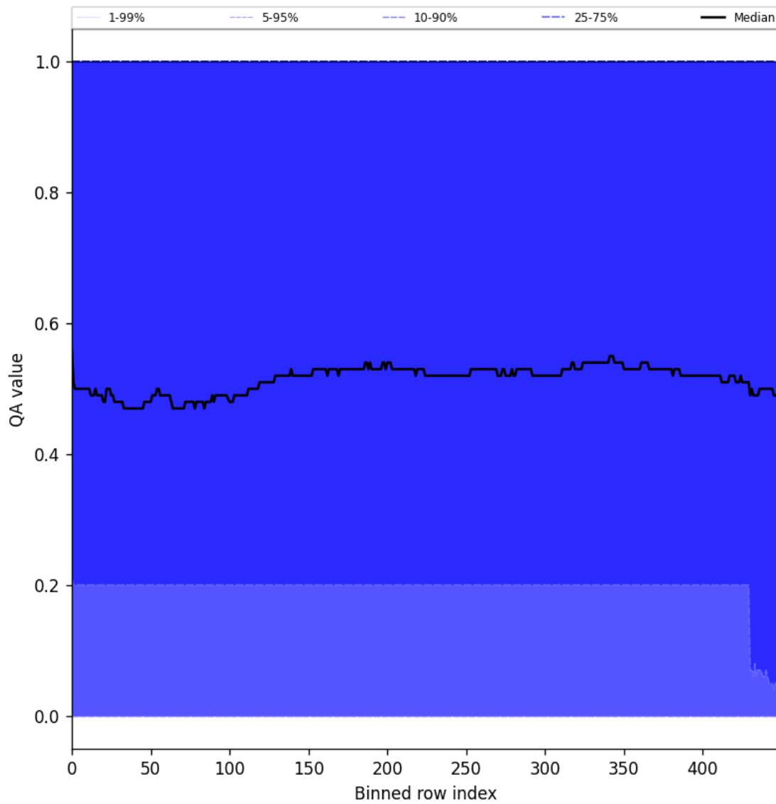
Figure 75: Along track statistics of “QA value” for 2024-08-25 to 2024-08-27
