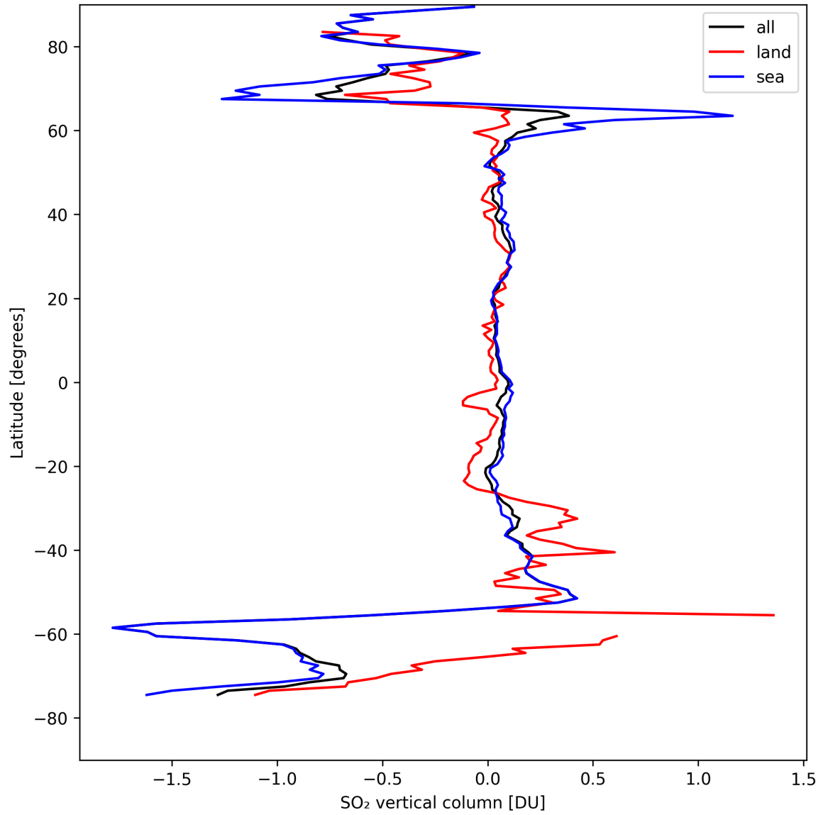
Figure 30: Zonal average of “SO 2 vertical column” for 2024-08-25 to 2024-08-27.
