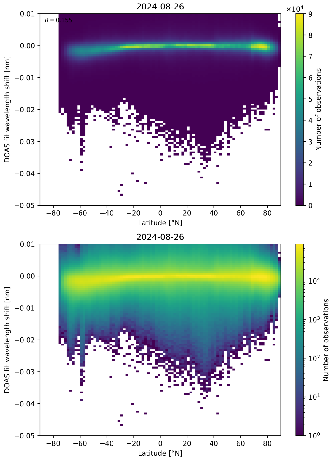
Figure 142: Scatter density plot of “Latitude” against “DOAS fit wavelength shift” for 2024-08-25 to 2024-08-27.
