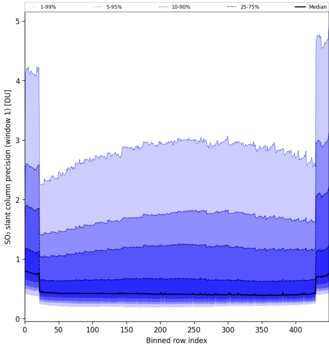
Figure 80: Along track statistics of “SO 2 slant column precision (window 1)” for 2024-08-25 to 2024-08-27
