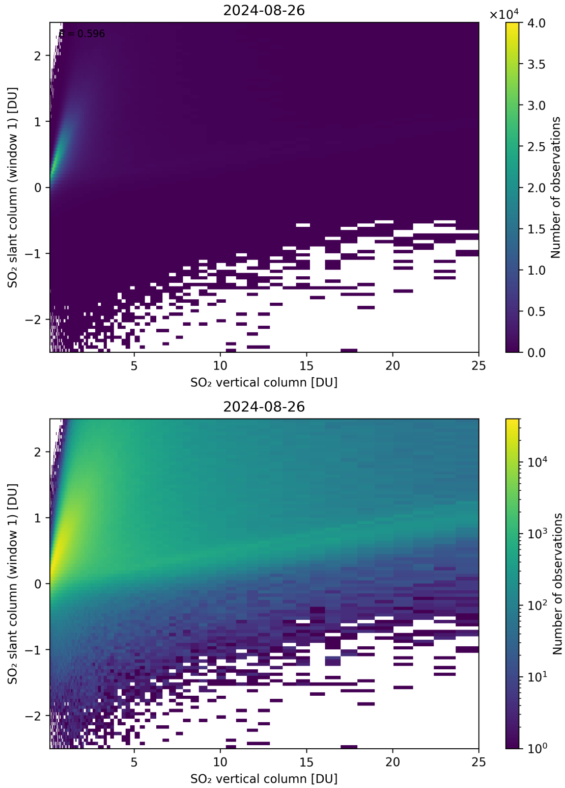
Figure 300: Scatter density plot of “SO 2 vertical column” against “SO 2 slant column (window 1)” for 2024-08-25 to 2024-08-27.
