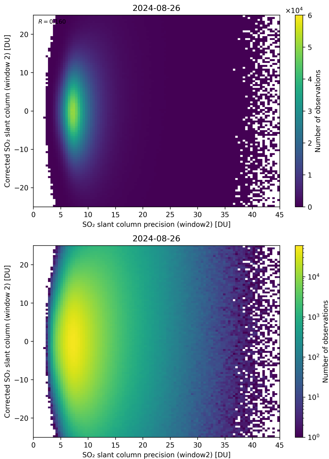
Figure 247: Scatter density plot of “SO 2 slant column precision (window2)” against “Corrected SO 2 slant column (window 2)” for 2024-08-25 to 2024-08-27.
