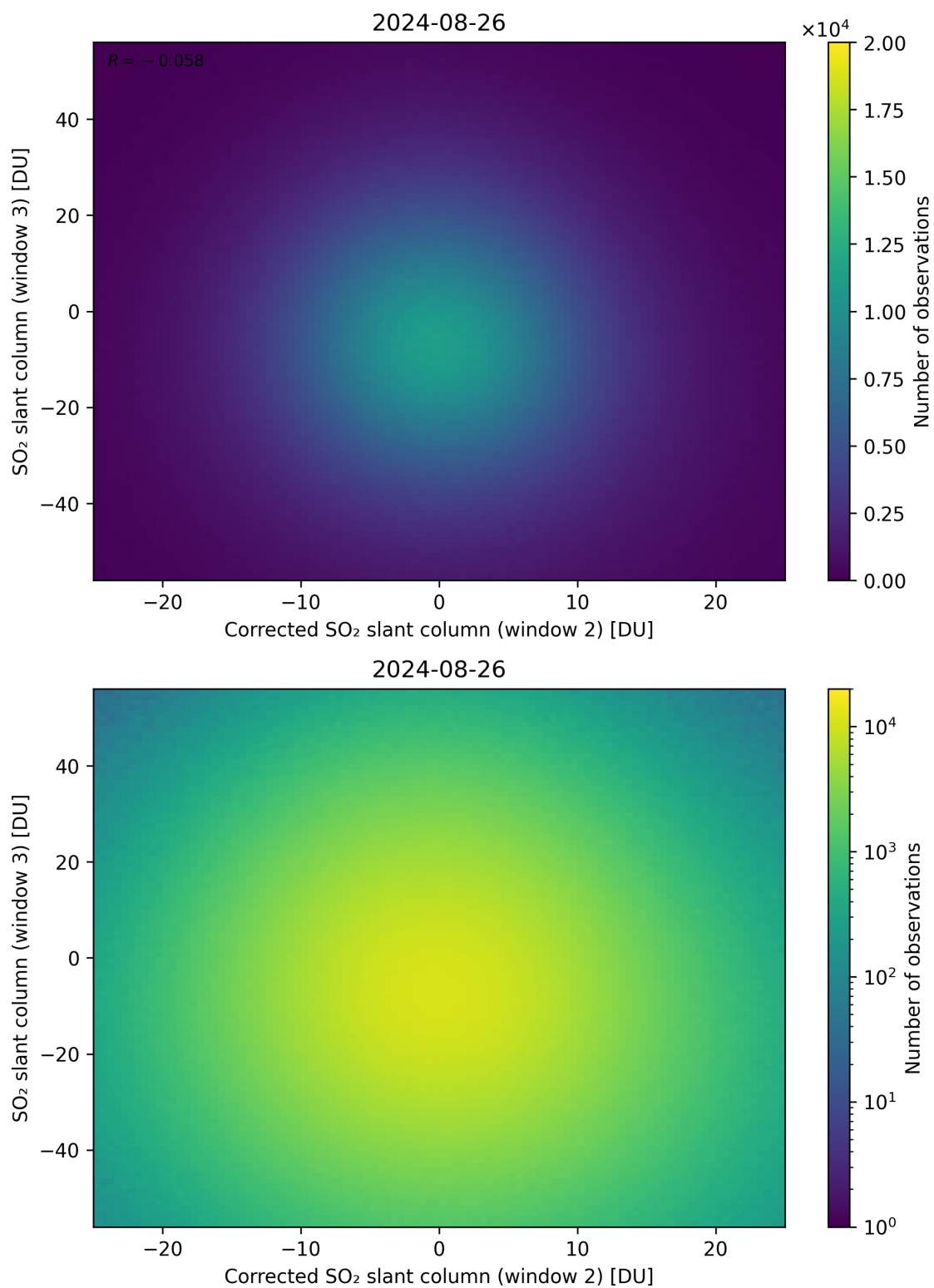
Figure 201: Scatter density plot of “Corrected SO 2 slant column (window 2)” against “SO 2 slant column (window 3)” for 2024-08-25 to 2024-08-27.
