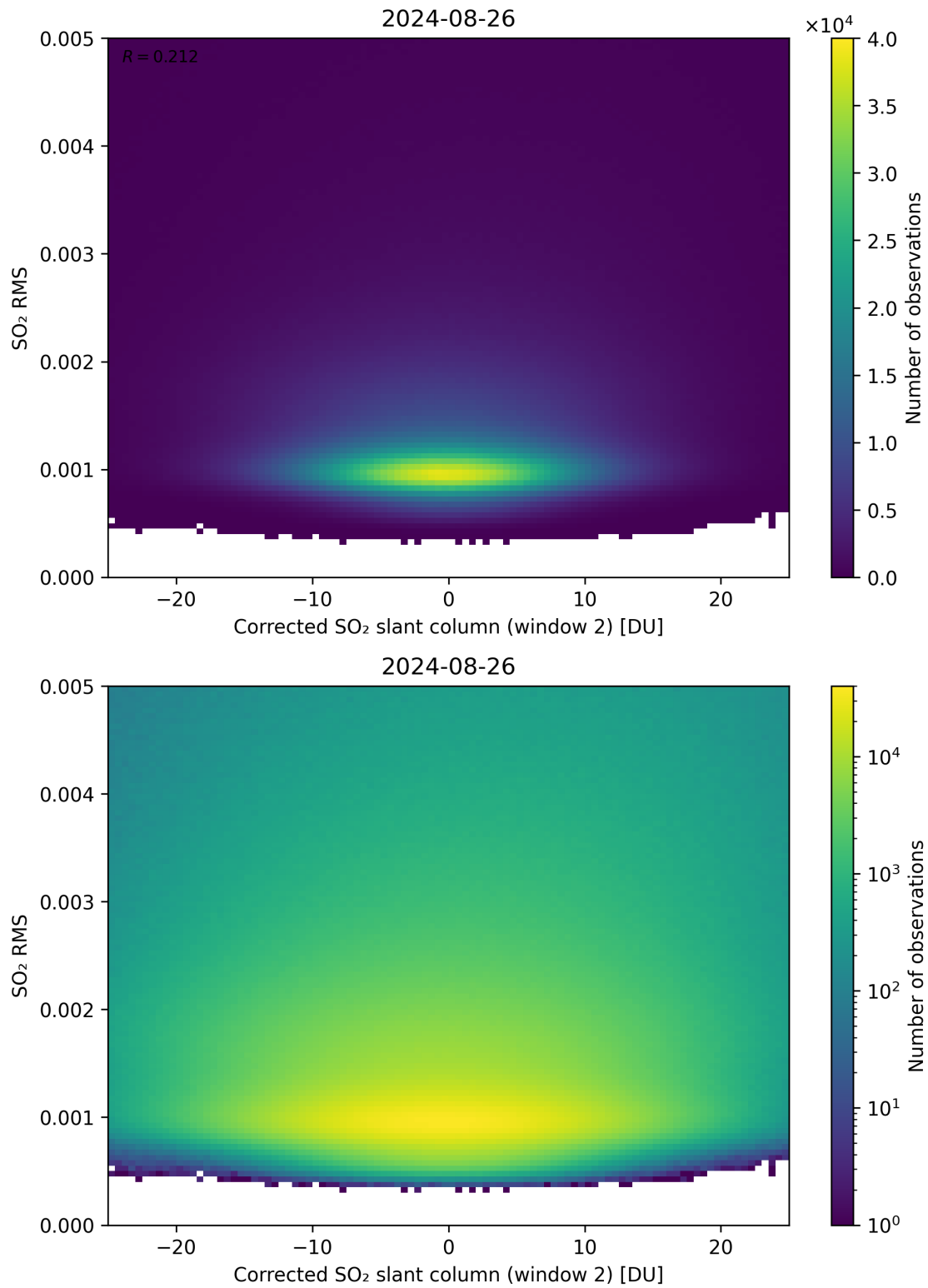
Figure 198: Scatter density plot of “Corrected SO 2 slant column (window 2)” against “SO 2 RMS” for 2024-08-25 to 2024-08-27.
