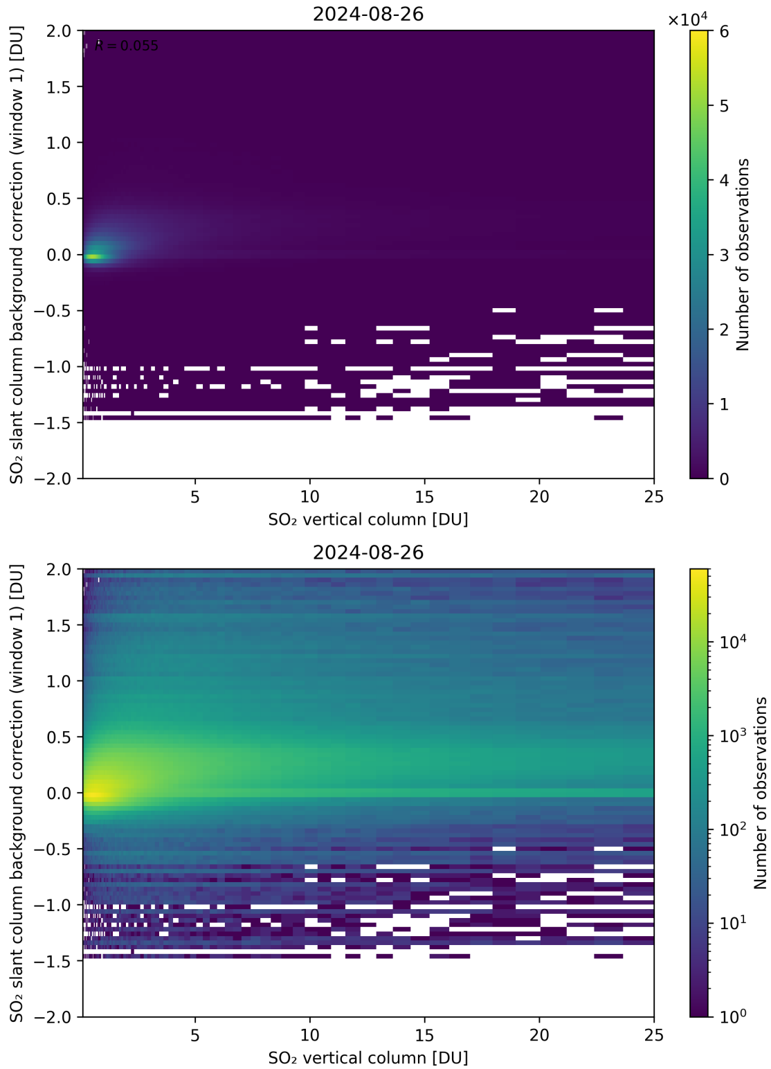
Figure 273: Scatter density plot of “SO 2 vertical column” against “SO 2 slant column background correction (window 1)” for 2024-08-25 to 2024-08-27.
