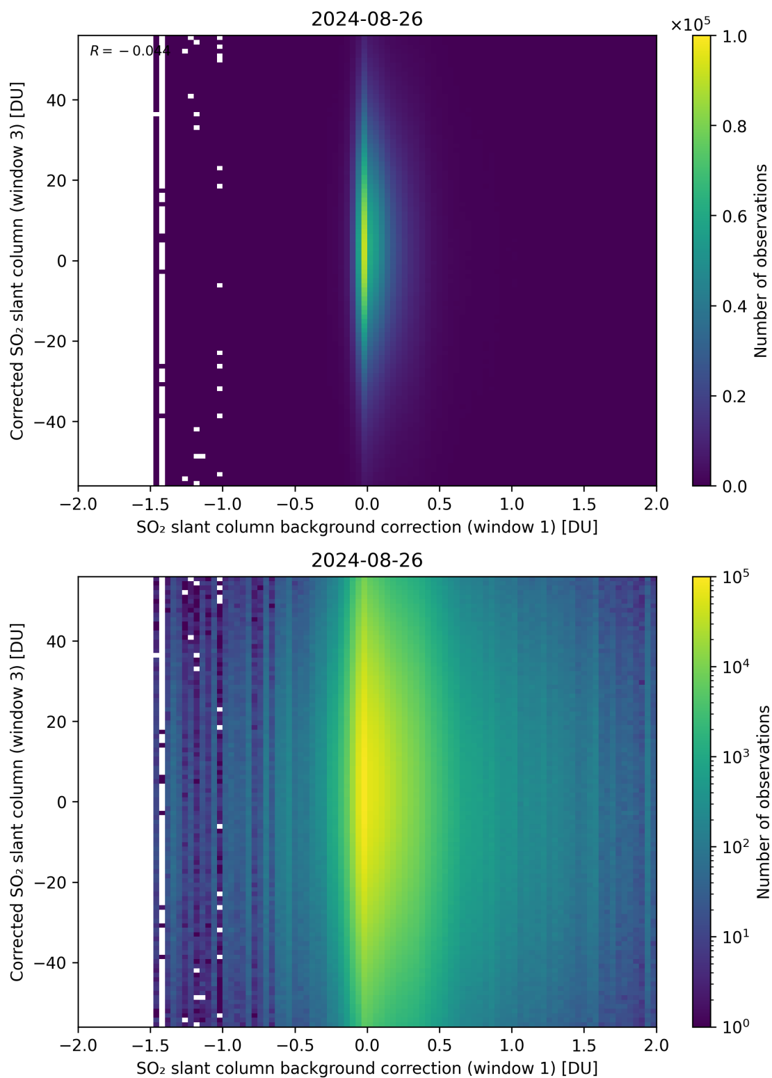
Figure 105: Scatter density plot of “SO 2 slant column background correction (window 1)” against “Corrected SO 2 slant column (window 3)” for 2024-08-25 to 2024-08-27.
