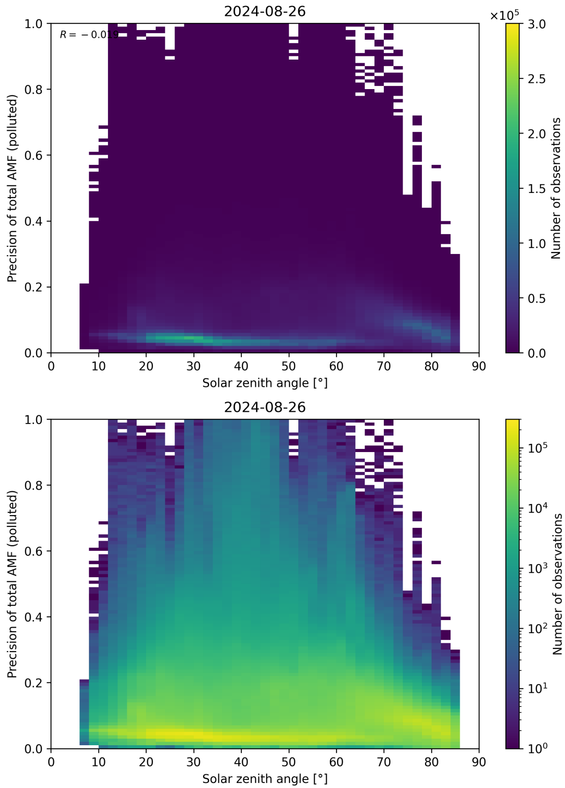
Figure 175: Scatter density plot of “Solar zenith angle” against “Precision of total AMF (polluted)” for 2024-08-25 to 2024-08-27.
