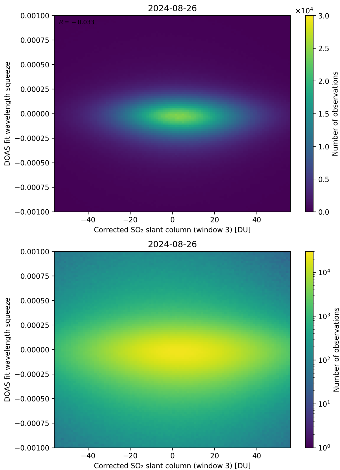
Figure 207: Scatter density plot of “Corrected SO 2 slant column (window 3)” against “DOAS fit wavelength squeeze” for 2024-08-25 to 2024-08-27.
