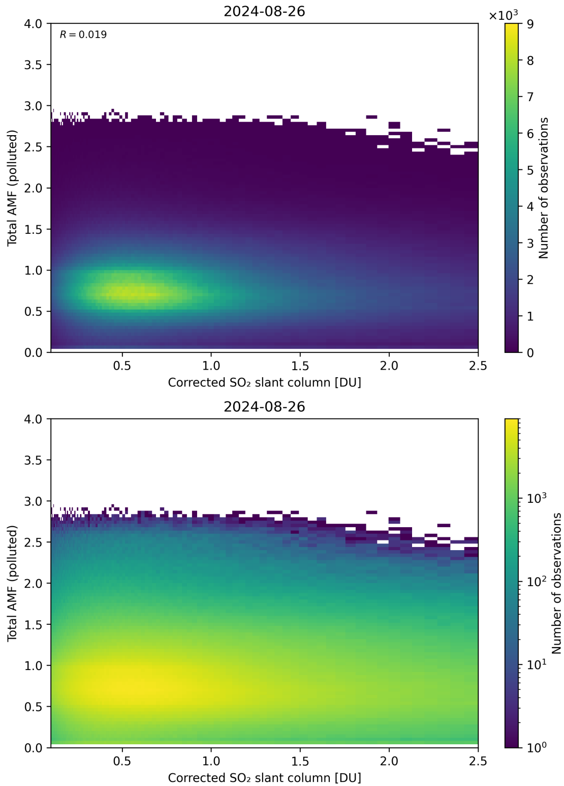
Figure 192: Scatter density plot of “Corrected SO 2 slant column” against “Total AMF (polluted)” for 2024-08-25 to 2024-08-27.
