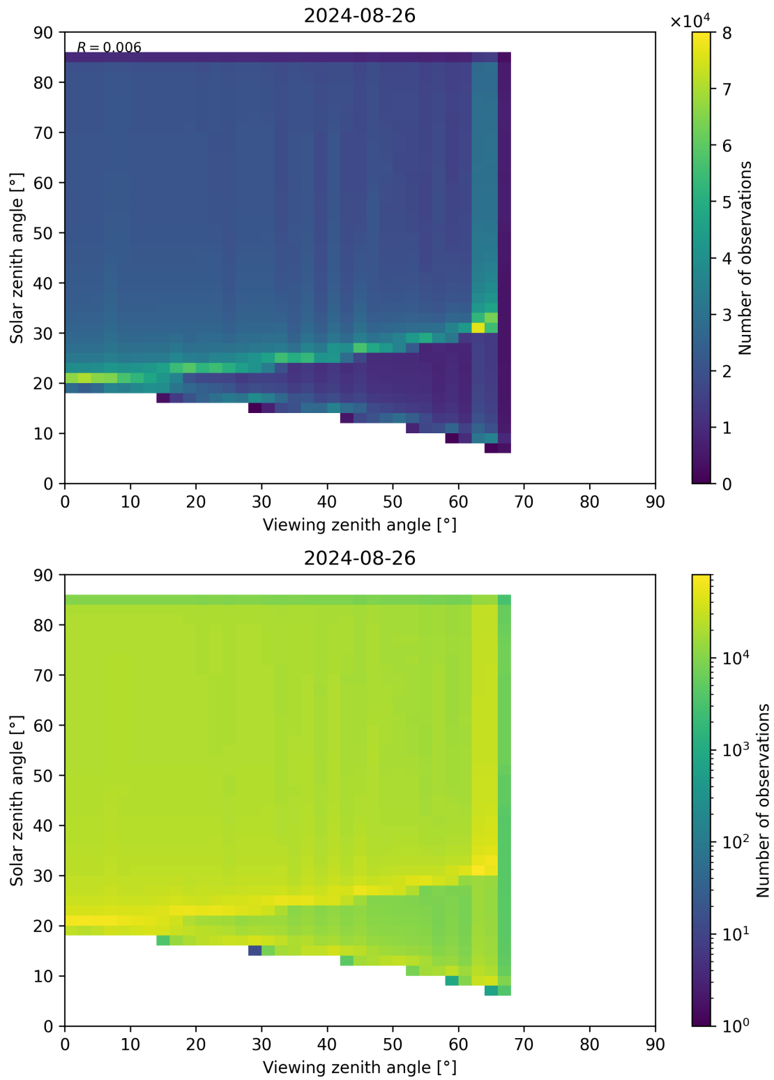
Figure 315: Scatter density plot of “Viewing zenith angle” against “Solar zenith angle” for 2024-08-25 to 2024-08-27.
