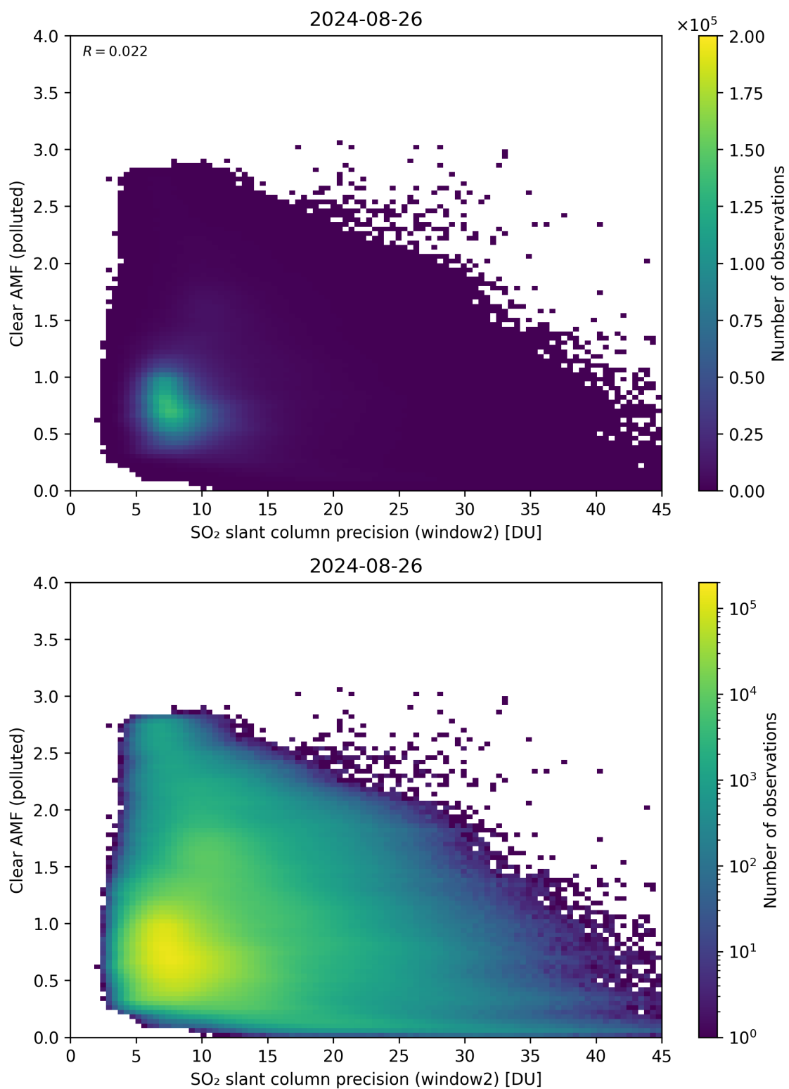
Figure 246: Scatter density plot of “SO 2 slant column precision (window2)” against “Clear AMF (polluted)” for 2024-08-25 to 2024-08-27.
