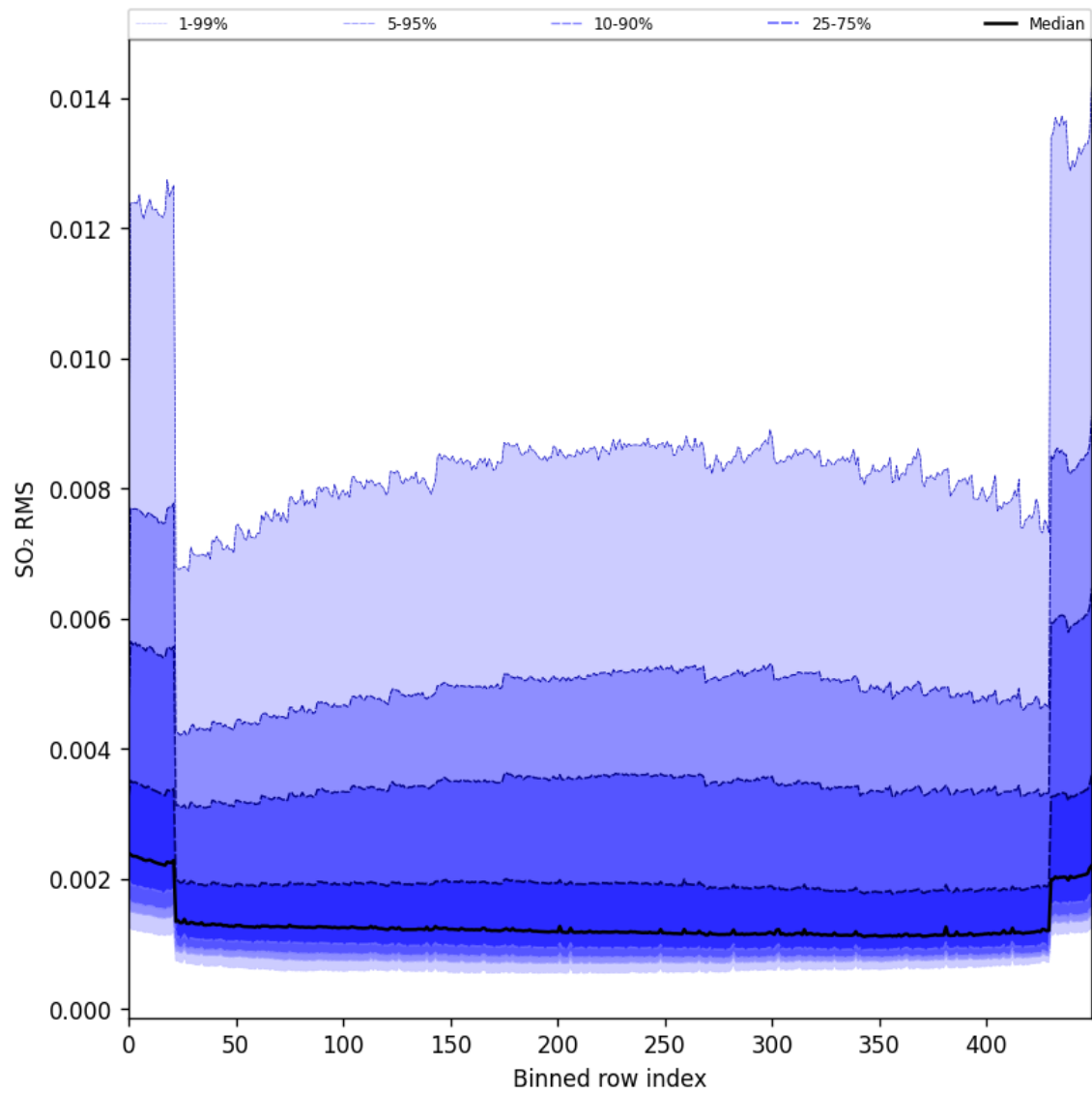
Figure 93: Along track statistics of “SO 2 RMS” for 2024-08-25 to 2024-08-27
