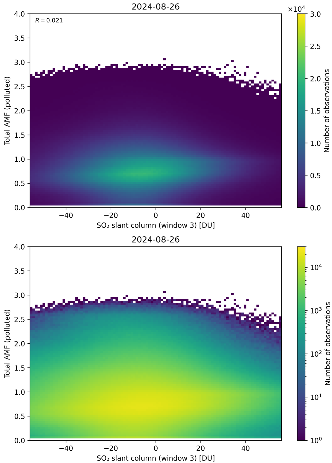
Figure 268: Scatter density plot of “SO 2 slant column (window 3)” against “Total AMF (polluted)” for 2024-08-25 to 2024-08-27.
