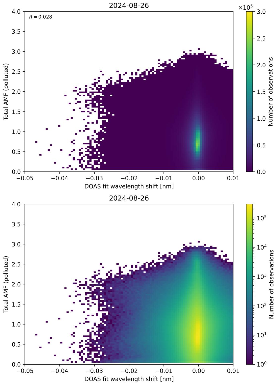
Figure 130: Scatter density plot of “DOAS fit wavelength shift” against “Total AMF (polluted)” for 2024-08-25 to 2024-08-27.
