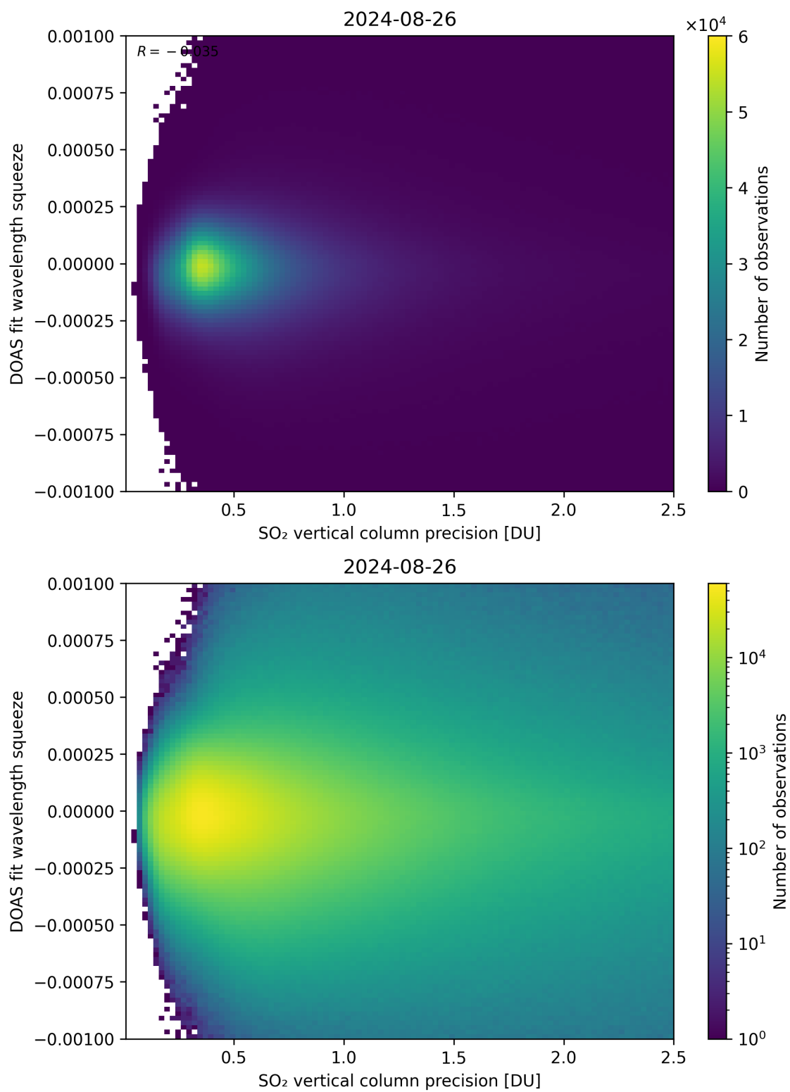
Figure 283: Scatter density plot of “SO 2 vertical column precision” against “DOAS fit wavelength squeeze” for 2024-08-25 to 2024-08-27.
