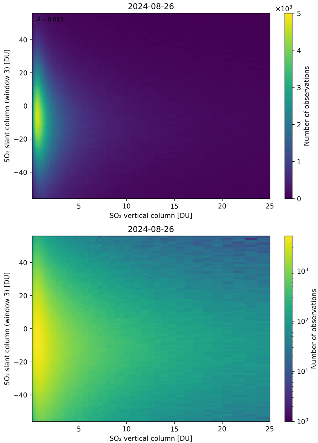
Figure 303: Scatter density plot of “SO 2 vertical column” against “SO 2 slant column (window 3)” for 2024-08-25 to 2024-08-27.
