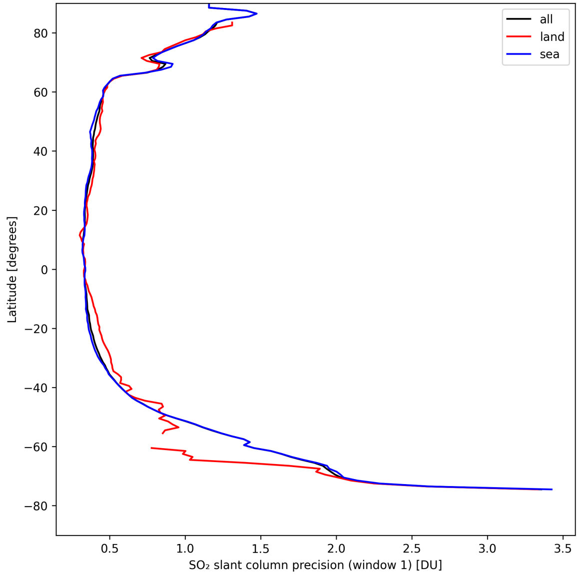
Figure 34: Zonal average of “SO 2 slant column precision (window 1)” for 2024-08-25 to 2024-08-27.
