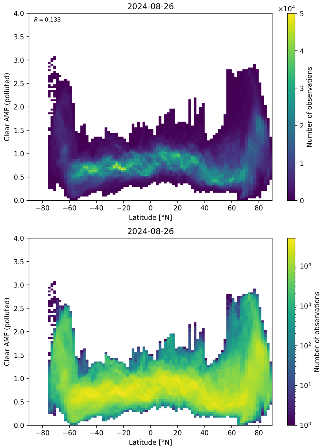
Figure 145: Scatter density plot of “Latitude” against “Clear AMF (polluted)” for 2024-08-25 to 2024-08-27.
