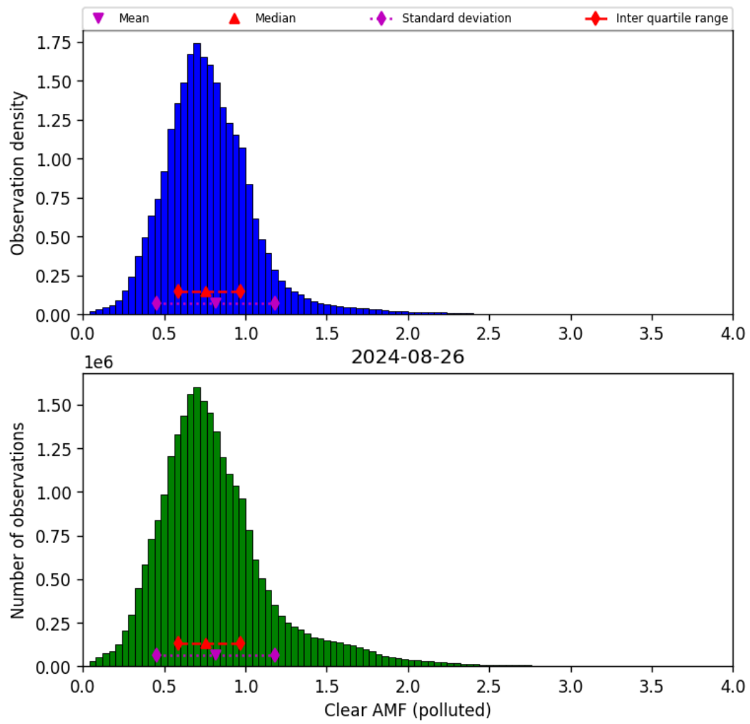
Figure 73: Histogram of “Clear AMF (polluted)” for 2024-08-25 to 2024-08-27
