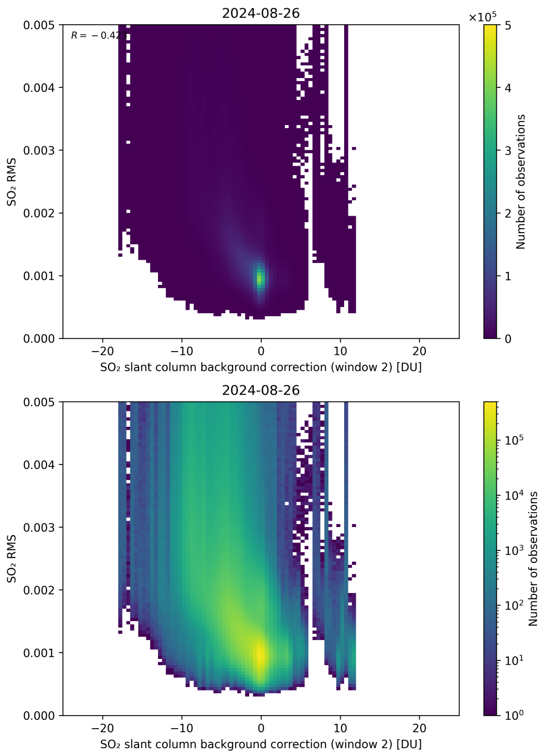
Figure 114: Scatter density plot of “SO 2 slant column background correction (window 2)” against “SO 2 RMS” for 2024-08-25 to 2024-08-27.
