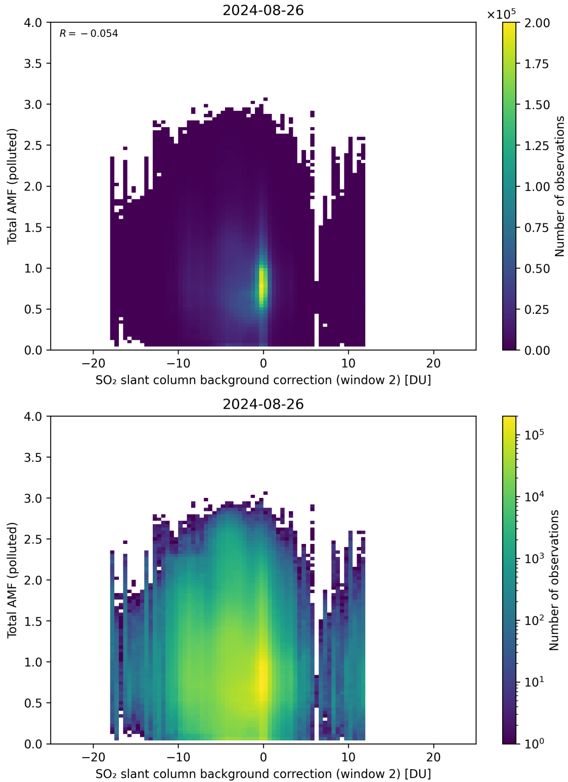
Figure 119: Scatter density plot of “SO 2 slant column background correction (window 2)” against “Total AMF (polluted)” for 2024-08-25 to 2024-08-27.
