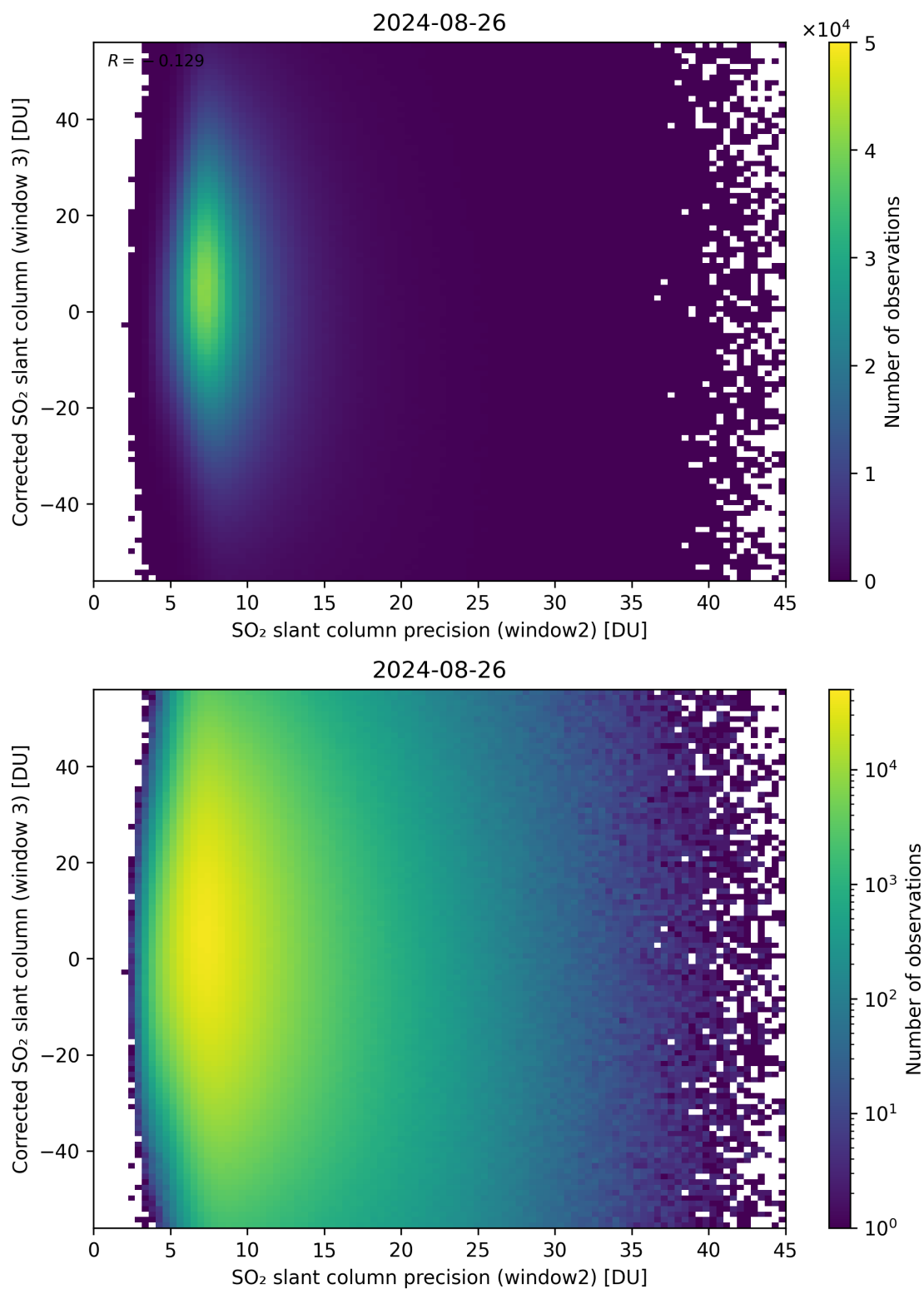
Figure 248: Scatter density plot of “SO 2 slant column precision (window2)” against “Corrected SO 2 slant column (window 3)” for 2024-08-25 to 2024-08-27.
