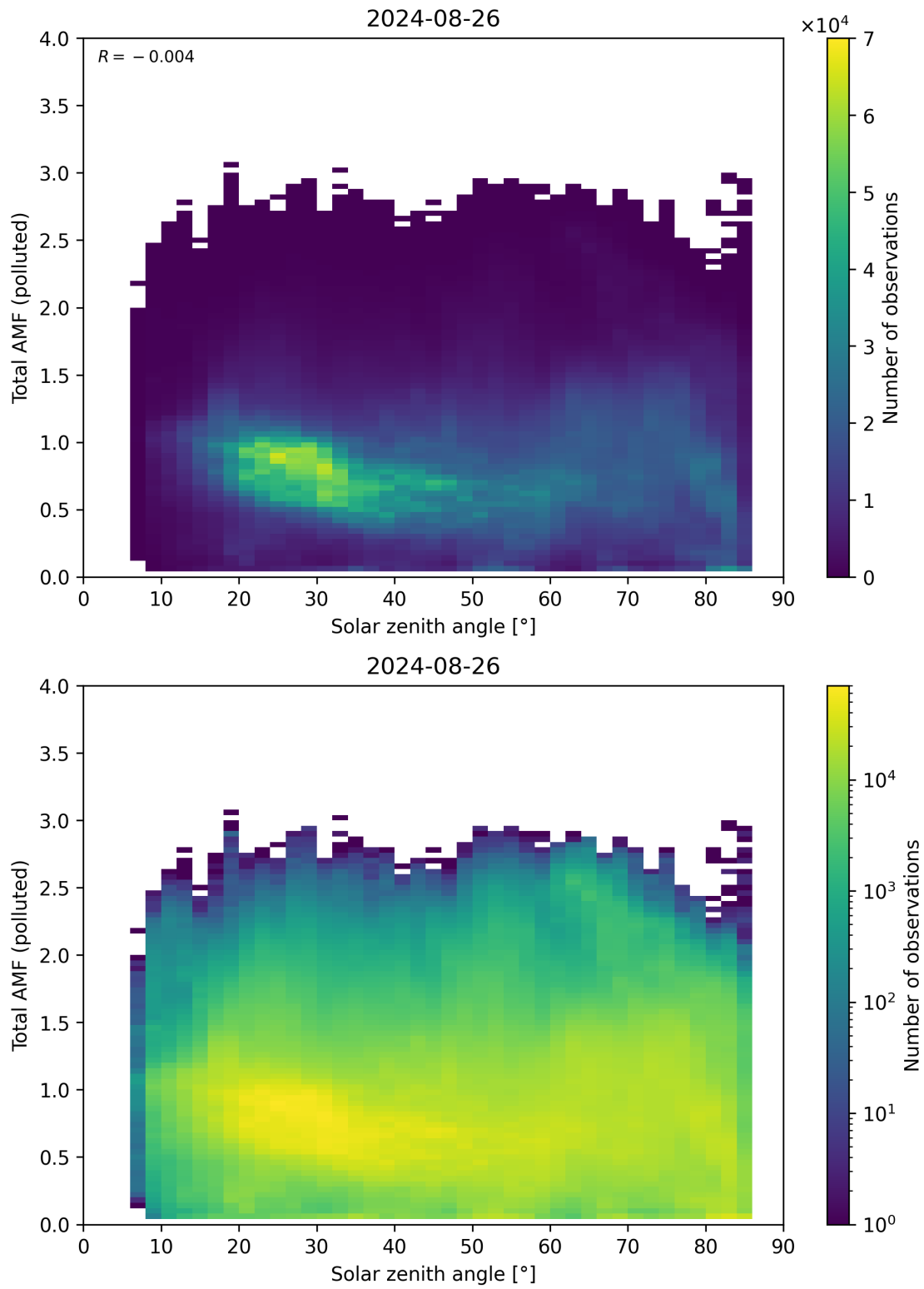
Figure 174: Scatter density plot of “Solar zenith angle” against “Total AMF (polluted)” for 2024-08-25 to 2024-08-27.
