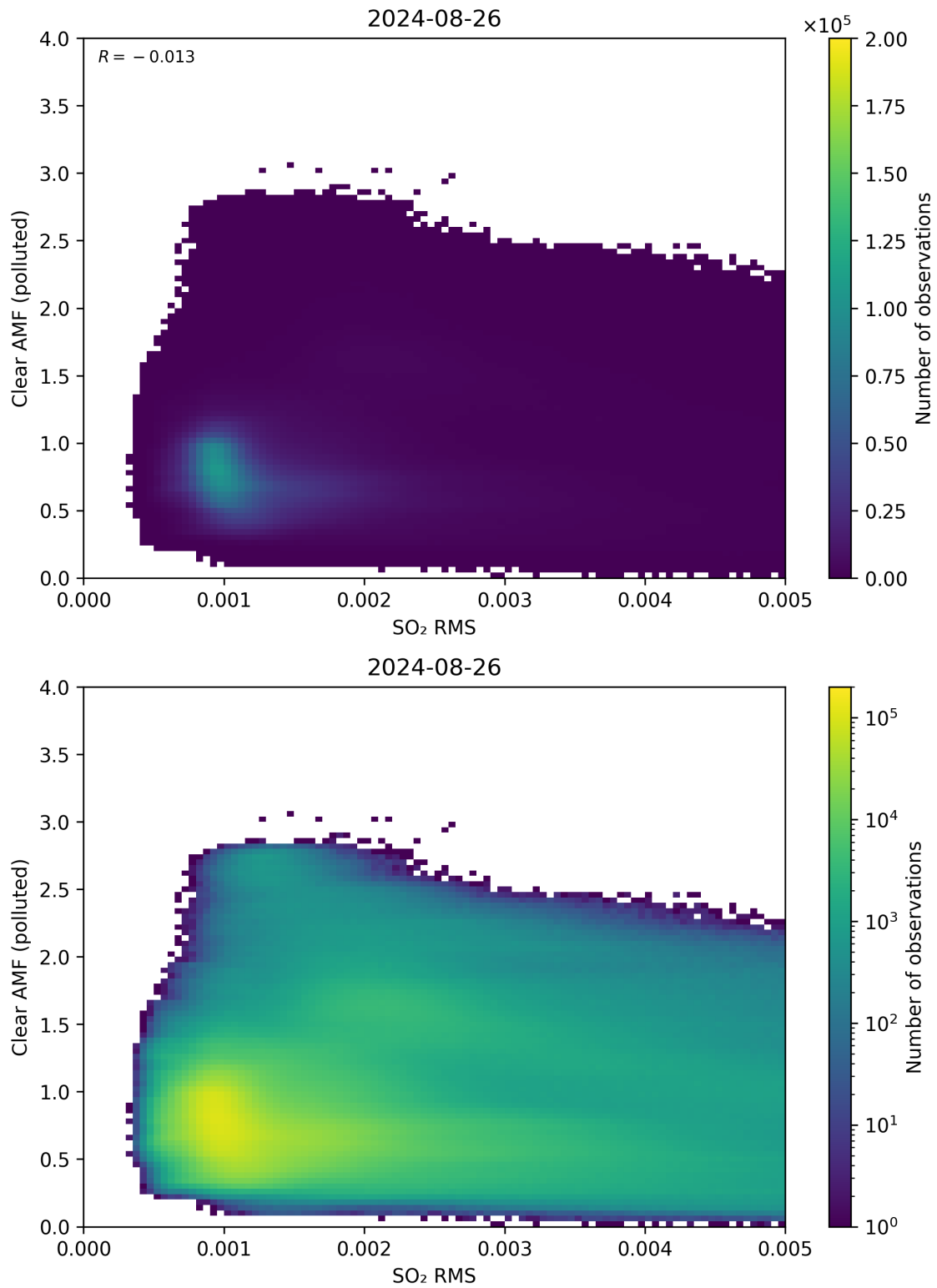
Figure 136: Scatter density plot of “SO 2 RMS” against “Clear AMF (polluted)” for 2024-08-25 to 2024-08-27.
