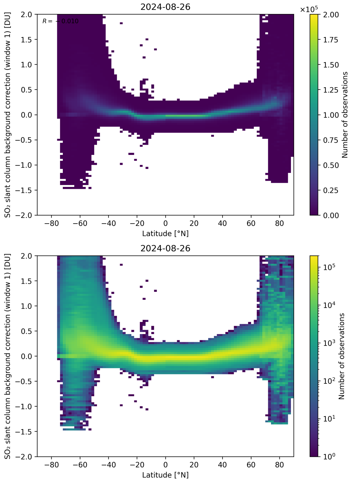
Figure 139: Scatter density plot of “Latitude” against “SO 2 slant column background correction (window 1)” for 2024-08-25 to 2024-08-27.
