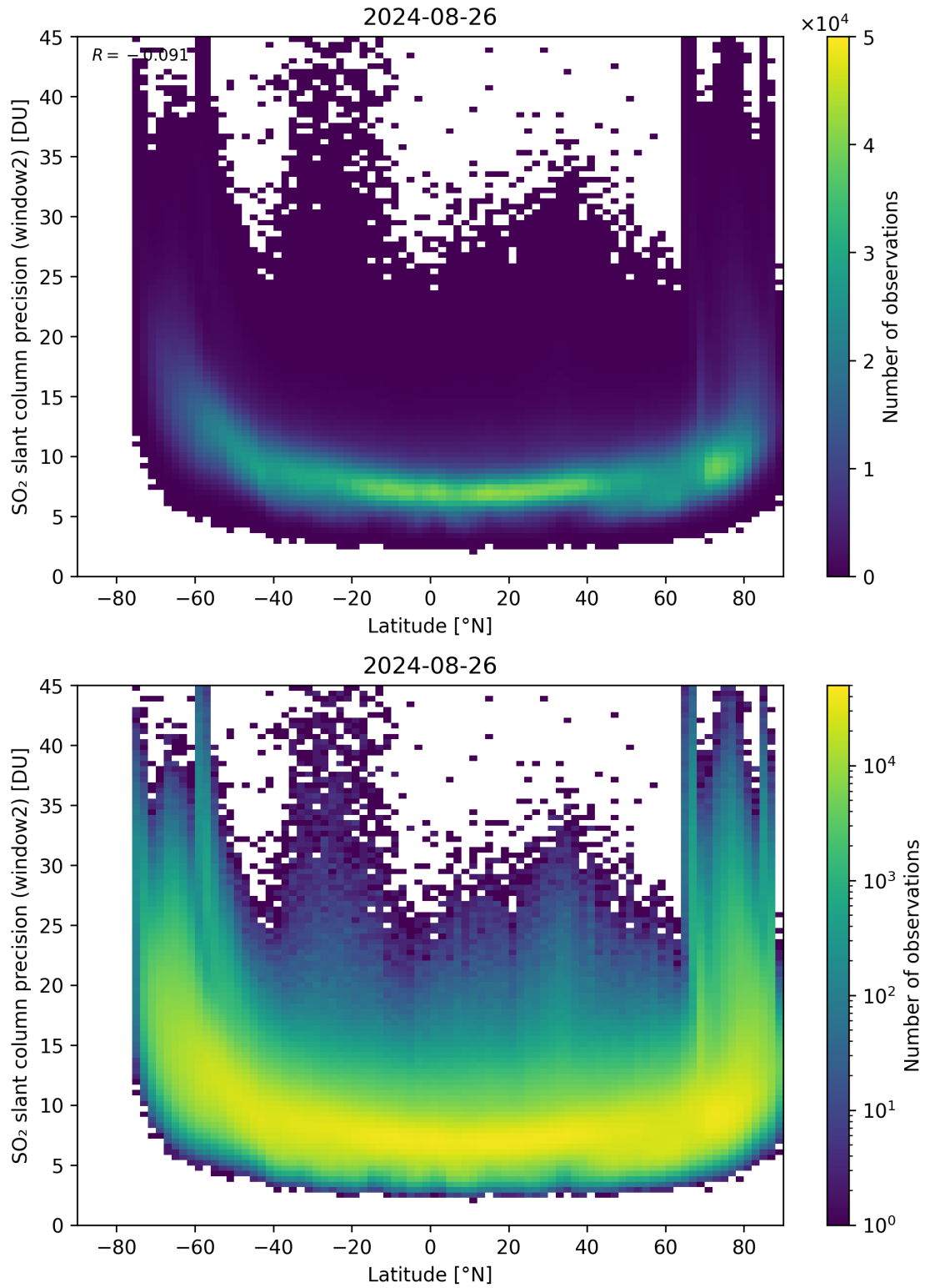
Figure 151: Scatter density plot of “Latitude” against “SO 2 slant column precision (window2)” for 2024-08-25 to 2024-08-27.
