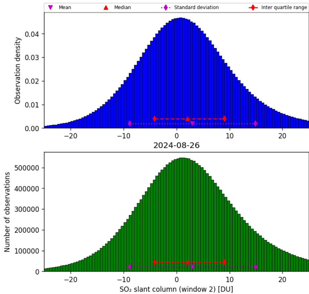
Figure 60: Histogram of “SO 2 slant column (window 2)” for 2024-08-25 to 2024-08-27
