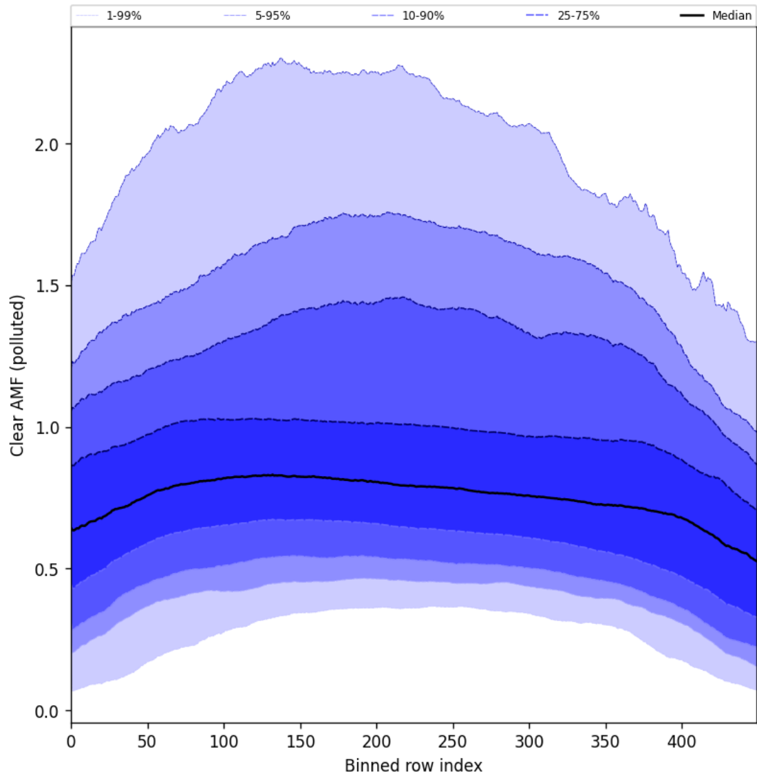
Figure 96: Along track statistics of “Clear AMF (polluted)” for 2024-08-25 to 2024-08-27
