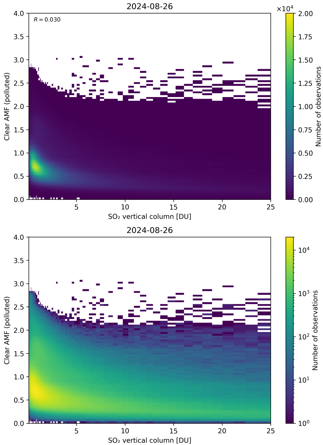
Figure 296: Scatter density plot of “SO 2 vertical column” against “Clear AMF (polluted)” for 2024-08-25 to 2024-08-27.
