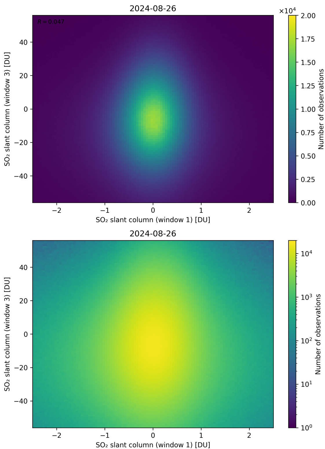
Figure 237: Scatter density plot of “SO 2 slant column (window 1)” against “SO 2 slant column (window 3)” for 2024-08-25 to 2024-08-27.
