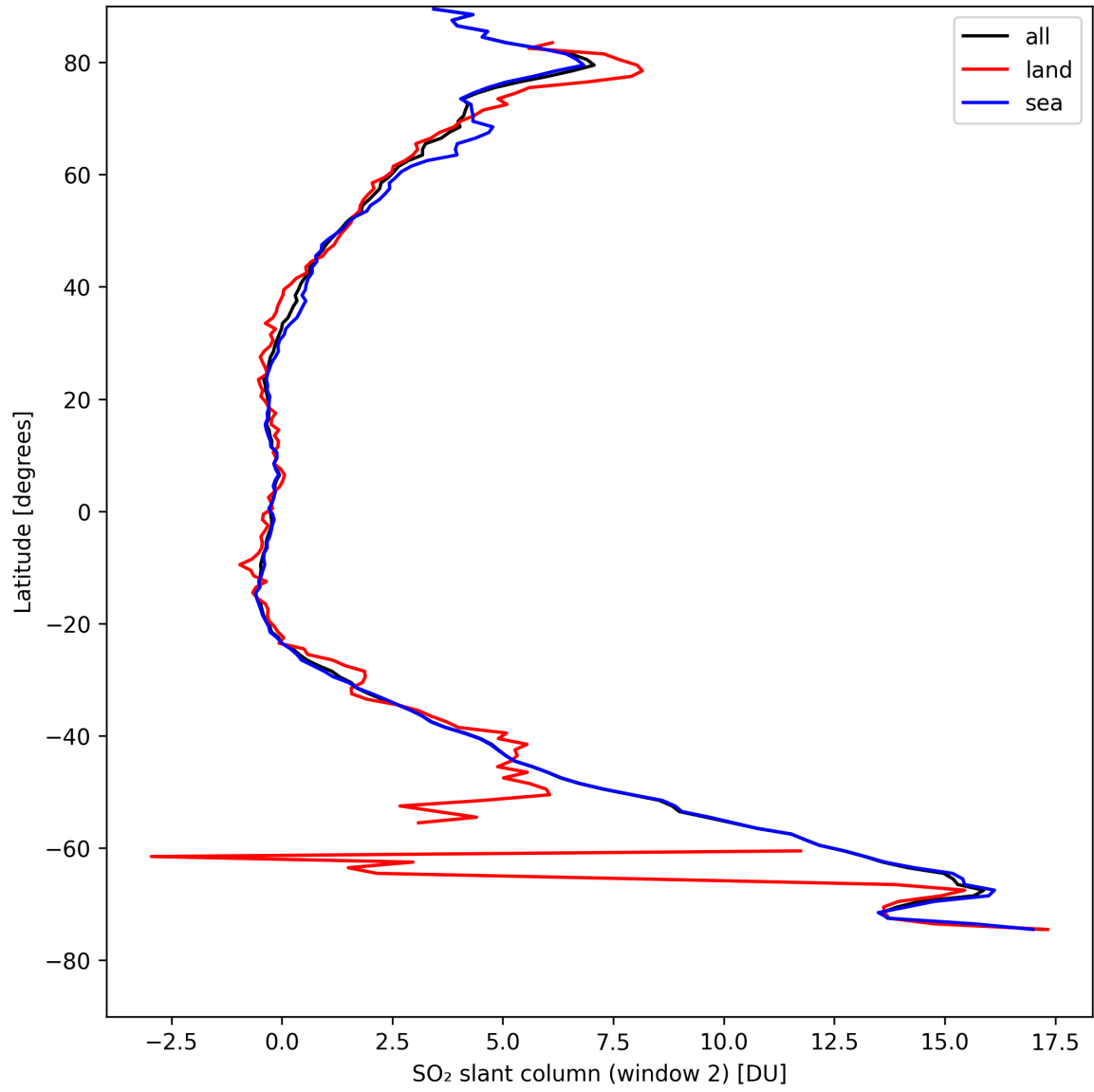
Figure 37: Zonal average of “SO 2 slant column (window 2)” for 2024-08-25 to 2024-08-27.
