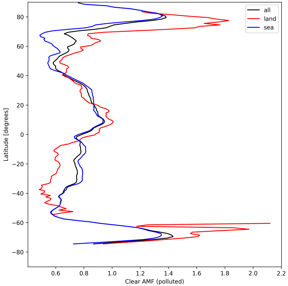
Figure 50: Zonal average of “Clear AMF (polluted)” for 2024-08-25 to 2024-08-27.
