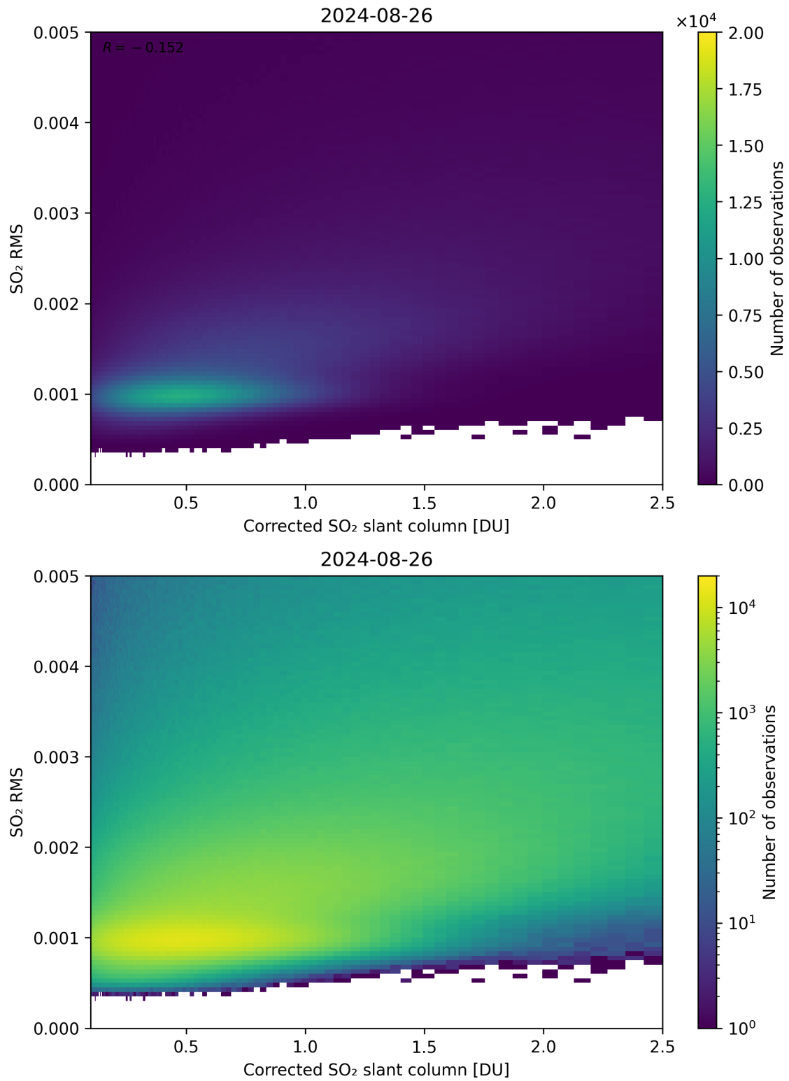
Figure 183: Scatter density plot of “Corrected SO 2 slant column” against “SO 2 RMS” for 2024-08-25 to 2024-08-27.
