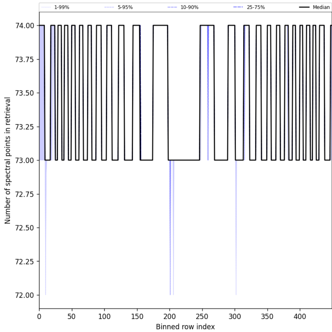
Figure 97: Along track statistics of “Number of spectral points in retrieval” for 2024-08-25 to 2024-08-27
