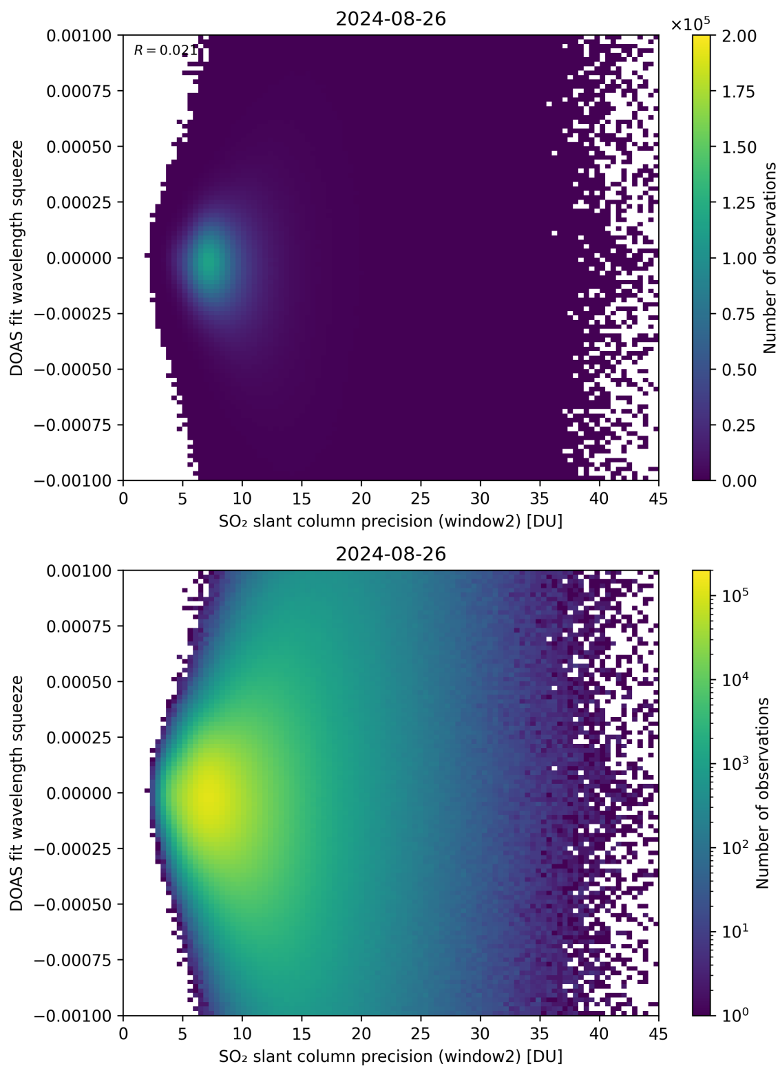
Figure 244: Scatter density plot of “SO 2 slant column precision (window2)” against “DOAS fit wavelength squeeze” for 2024-08-25 to 2024-08-27.
