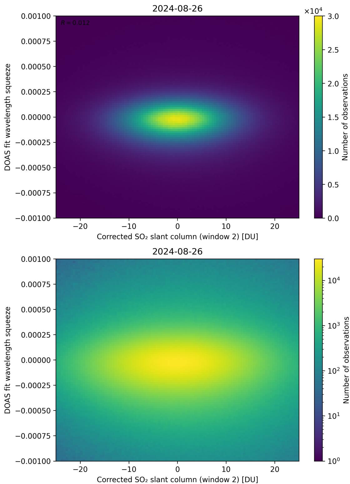
Figure 197: Scatter density plot of “Corrected SO 2 slant column (window 2)” against “DOAS fit wavelength squeeze” for 2024-08-25 to 2024-08-27.
