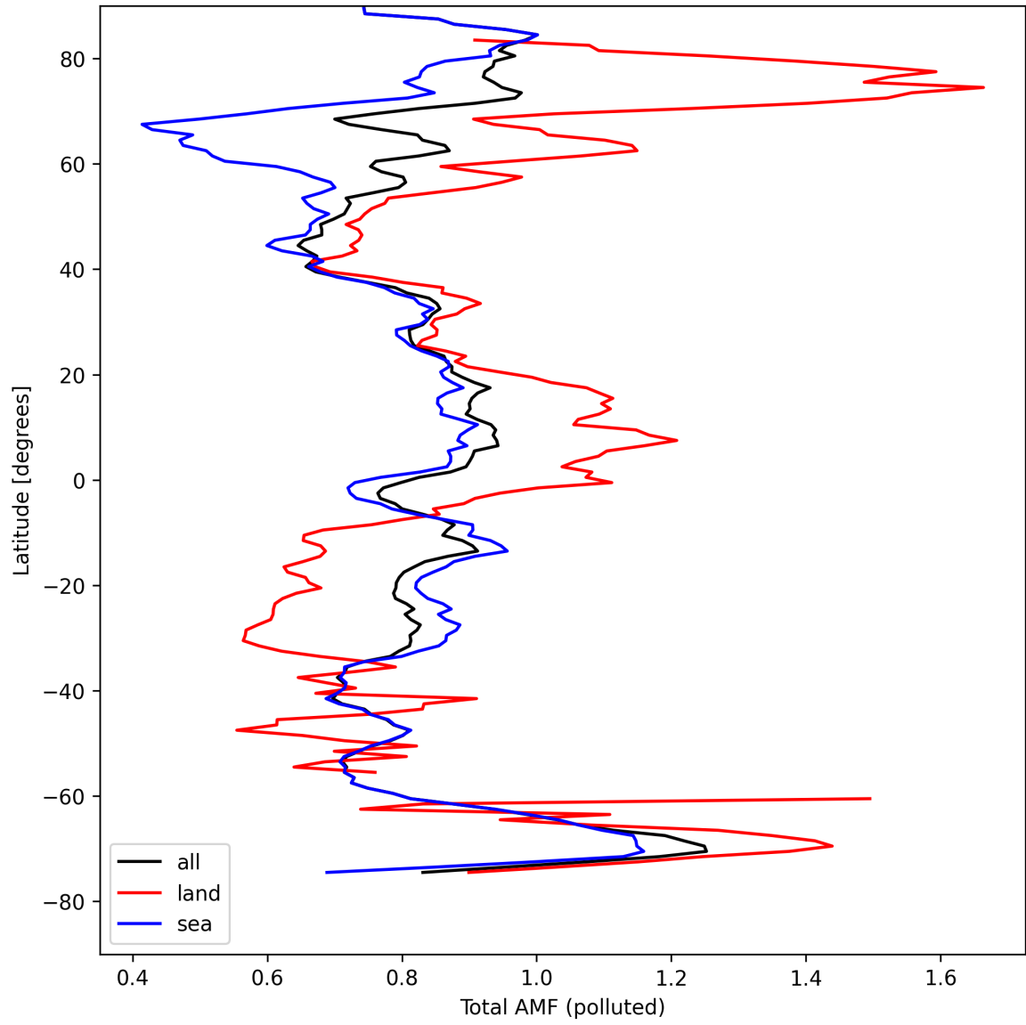
Figure 48: Zonal average of “Total AMF (polluted)” for 2024-08-25 to 2024-08-27.
