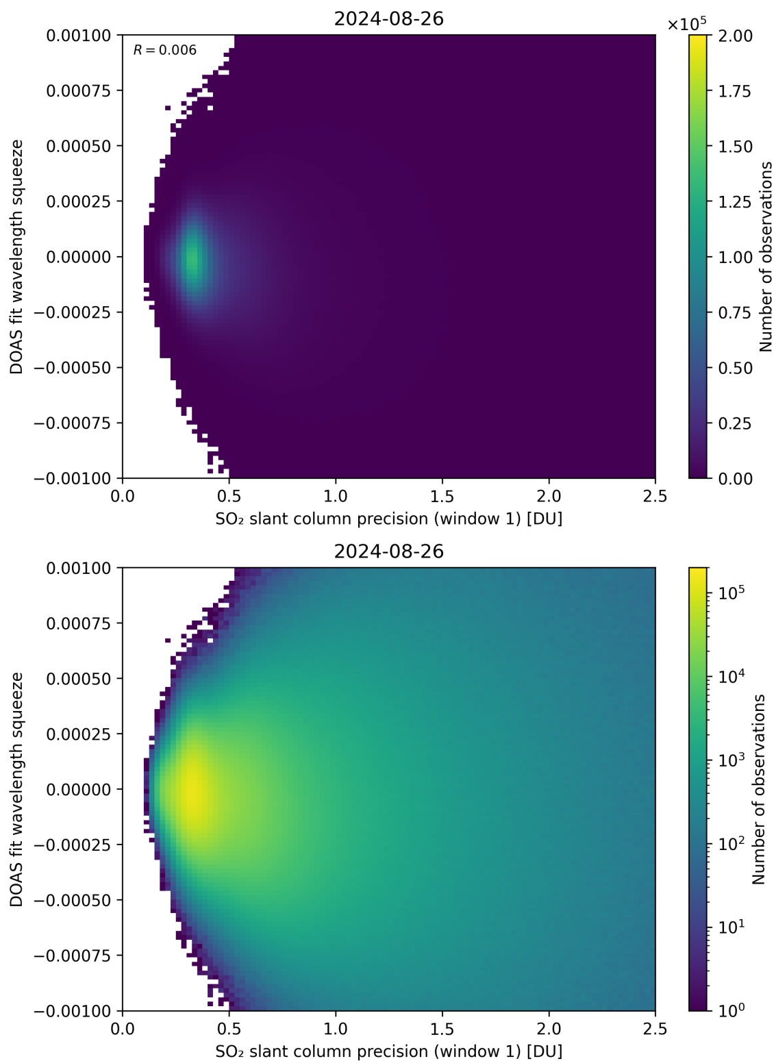
Figure 222: Scatter density plot of “SO 2 slant column precision (window 1)” against “DOAS fit wavelength squeeze” for 2024-08-25 to 2024-08-27.
