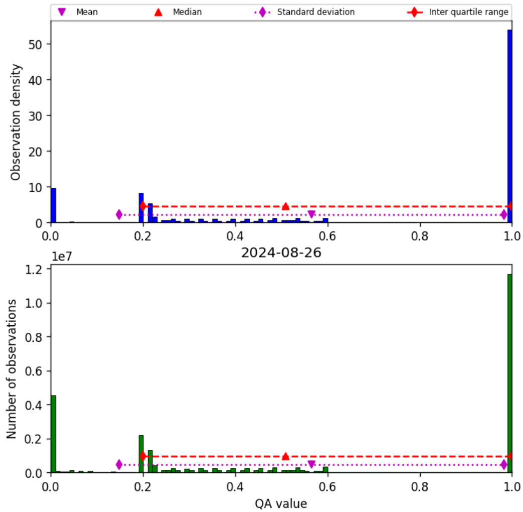
Figure 52: Histogram of “QA value” for 2024-08-25 to 2024-08-27
