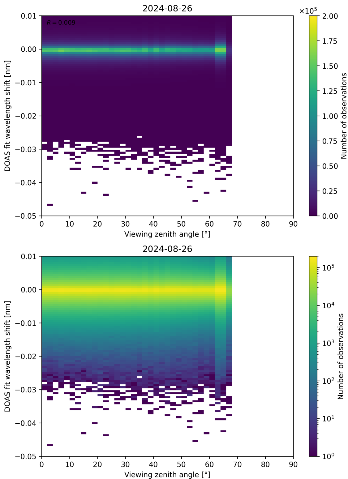
Figure 311: Scatter density plot of “Viewing zenith angle” against “DOAS fit wavelength shift” for 2024-08-25 to 2024-08-27.
