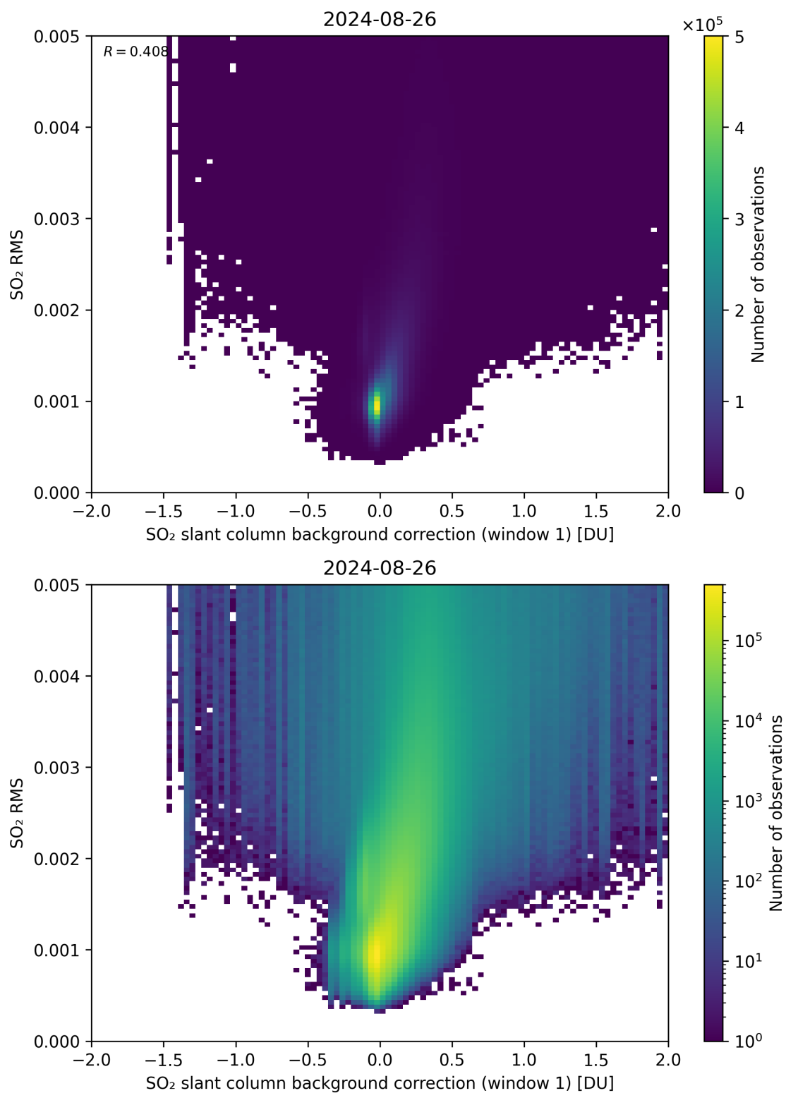
Figure 102: Scatter density plot of “SO 2 slant column background correction (window 1)” against “SO 2 RMS” for 2024-08-25 to 2024-08-27.
