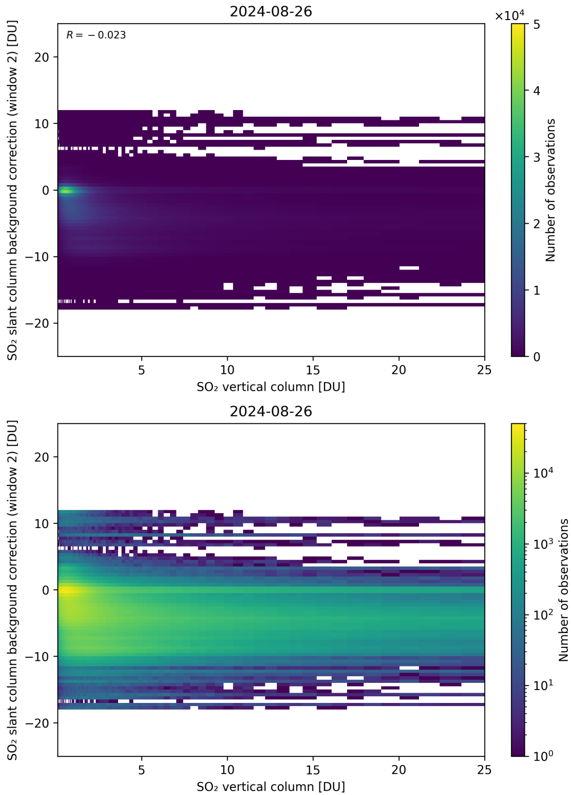
Figure 274: Scatter density plot of “SO 2 vertical column” against “SO 2 slant column background correction (window 2)” for 2024-08-25 to 2024-08-27.
