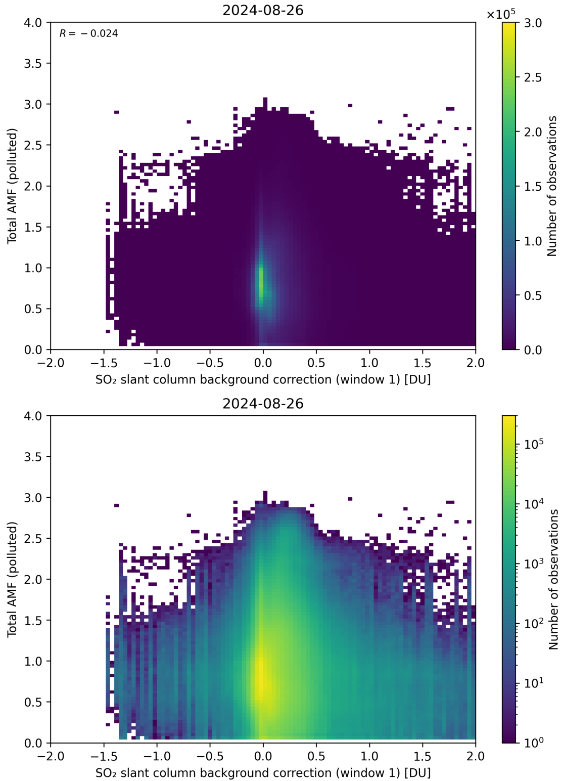
Figure 109: Scatter density plot of “SO 2 slant column background correction (window 1)” against “Total AMF (polluted)” for 2024-08-25 to 2024-08-27.
