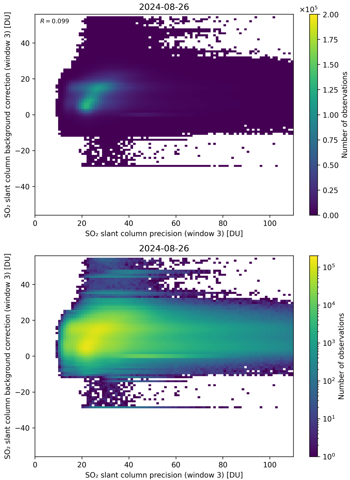
Figure 257: Scatter density plot of “SO 2 slant column precision (window 3)” against “SO 2 slant column background correction (window 3)” for 2024-08-25 to 2024-08-27.
