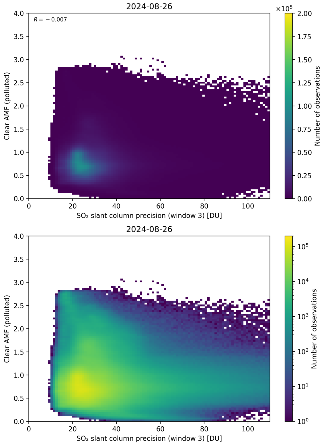
Figure 261: Scatter density plot of “SO 2 slant column precision (window 3)” against “Clear AMF (polluted)” for 2024-08-25 to 2024-08-27.
