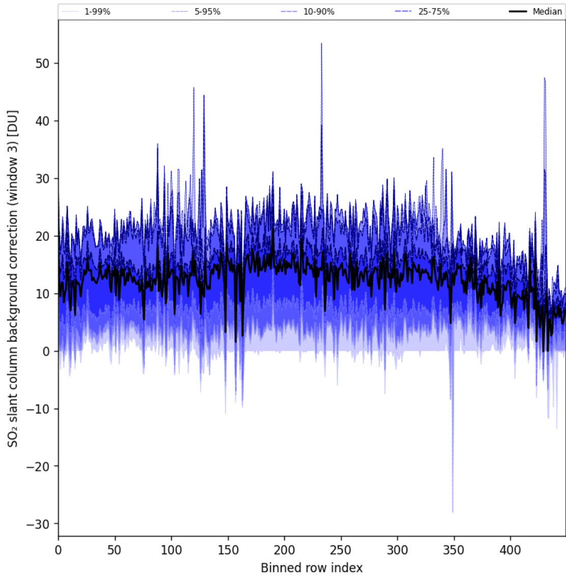
Figure 90: Along track statistics of “SO 2 slant column background correction (window 3)” for 2024-08-25 to 2024-08-27
