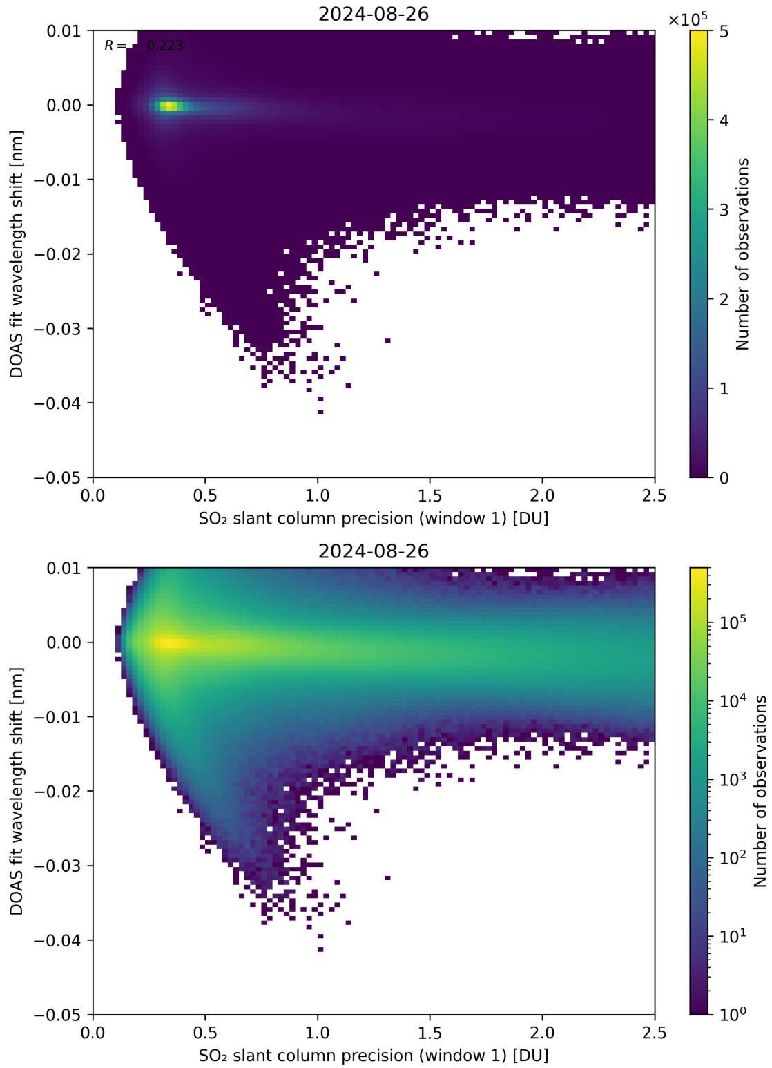
Figure 221: Scatter density plot of “SO 2 slant column precision (window 1)” against “DOAS fit wavelength shift” for 2024-08-25 to 2024-08-27.
