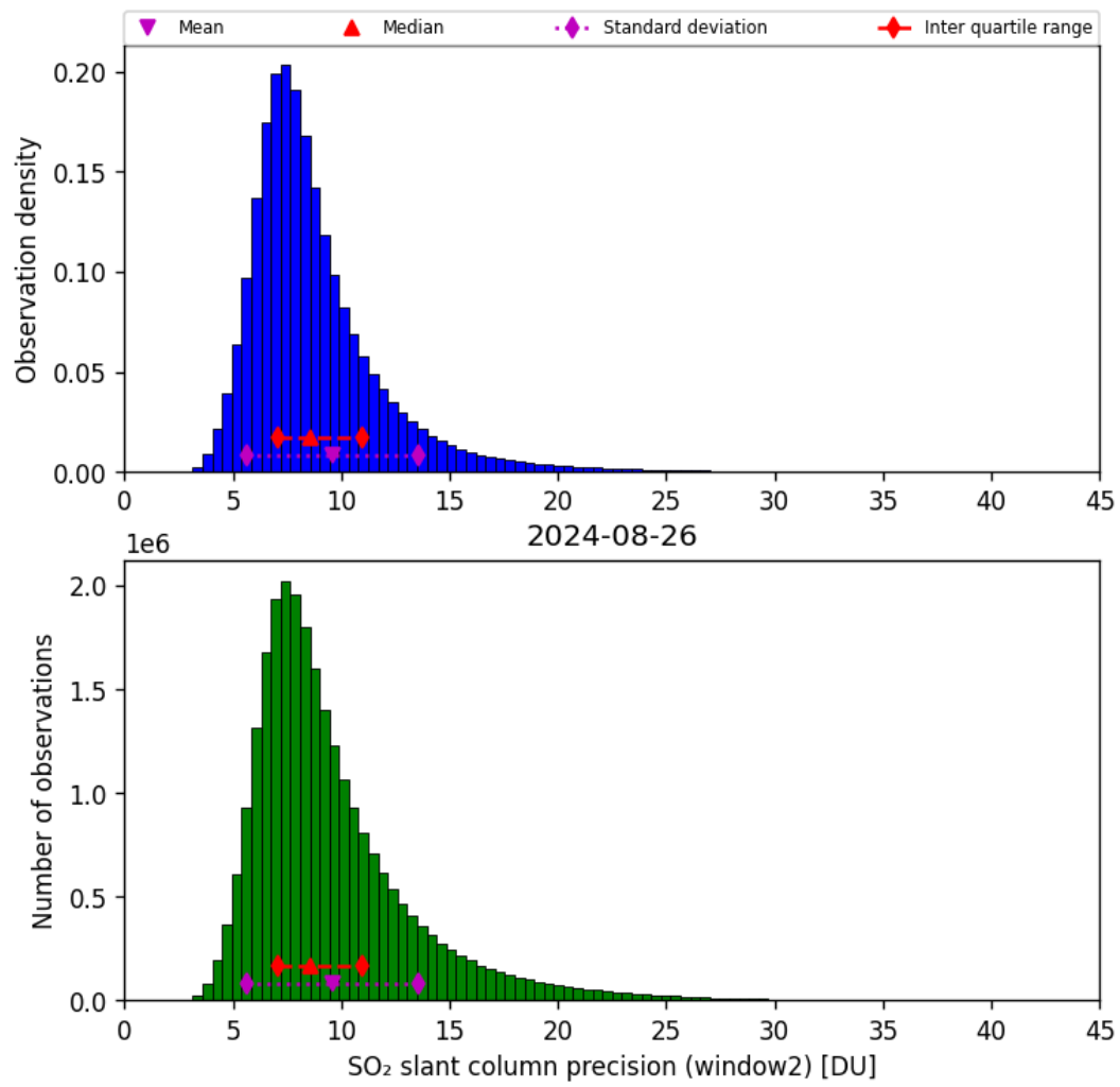
Figure 61: Histogram of “SO 2 slant column precision (window2)” for 2024-08-25 to 2024-08-27
