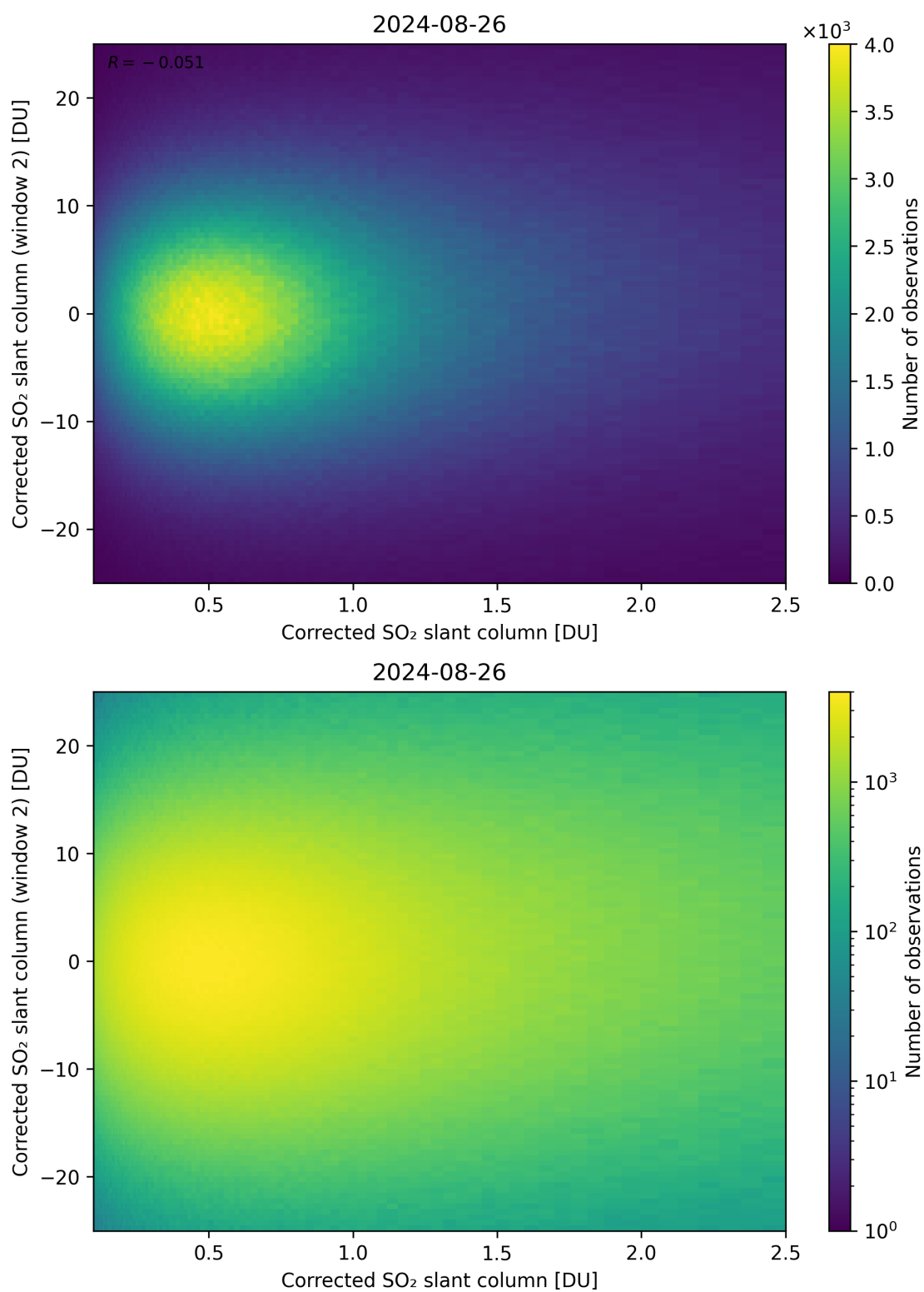
Figure 185: Scatter density plot of “Corrected SO 2 slant column” against “Corrected SO 2 slant column (window 2)” for 2024-08-25 to 2024-08-27.
