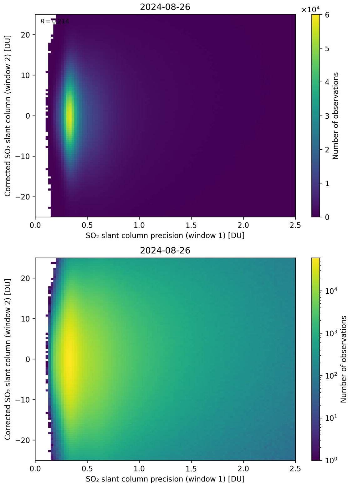
Figure 225: Scatter density plot of “SO 2 slant column precision (window 1)” against “Corrected SO 2 slant column (window 2)” for 2024-08-25 to 2024-08-27.
