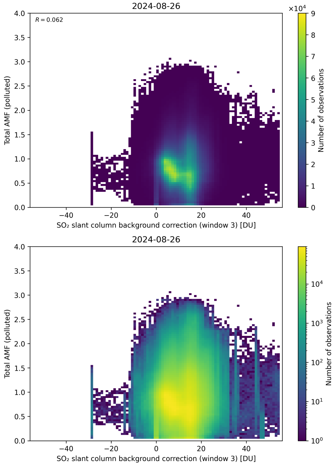
Figure 125: Scatter density plot of “SO 2 slant column background correction (window 3)” against “Total AMF (polluted)” for 2024-08-25 to 2024-08-27.
