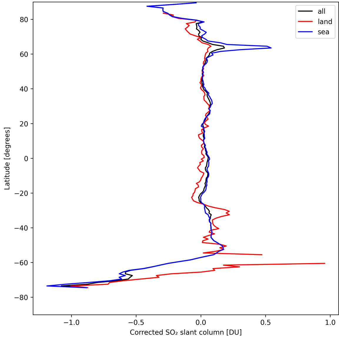
Figure 32: Zonal average of “Corrected SO 2 slant column” for 2024-08-25 to 2024-08-27.
