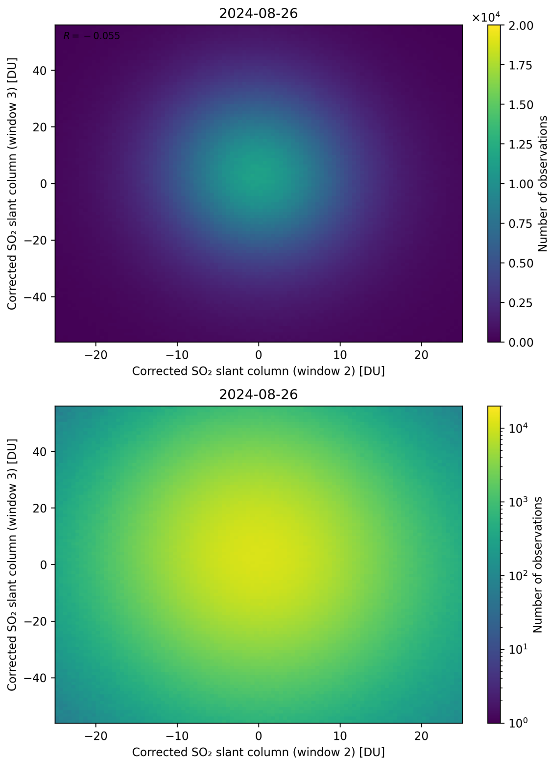
Figure 200: Scatter density plot of “Corrected SO 2 slant column (window 2)” against “Corrected SO 2 slant column (window 3)” for 2024-08-25 to 2024-08-27.
