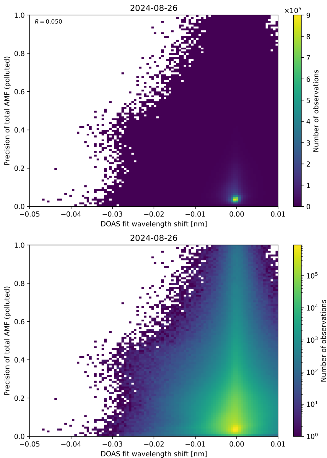
Figure 131: Scatter density plot of “DOAS fit wavelength shift” against “Precision of total AMF (polluted)” for 2024-08-25 to 2024-08-27.
