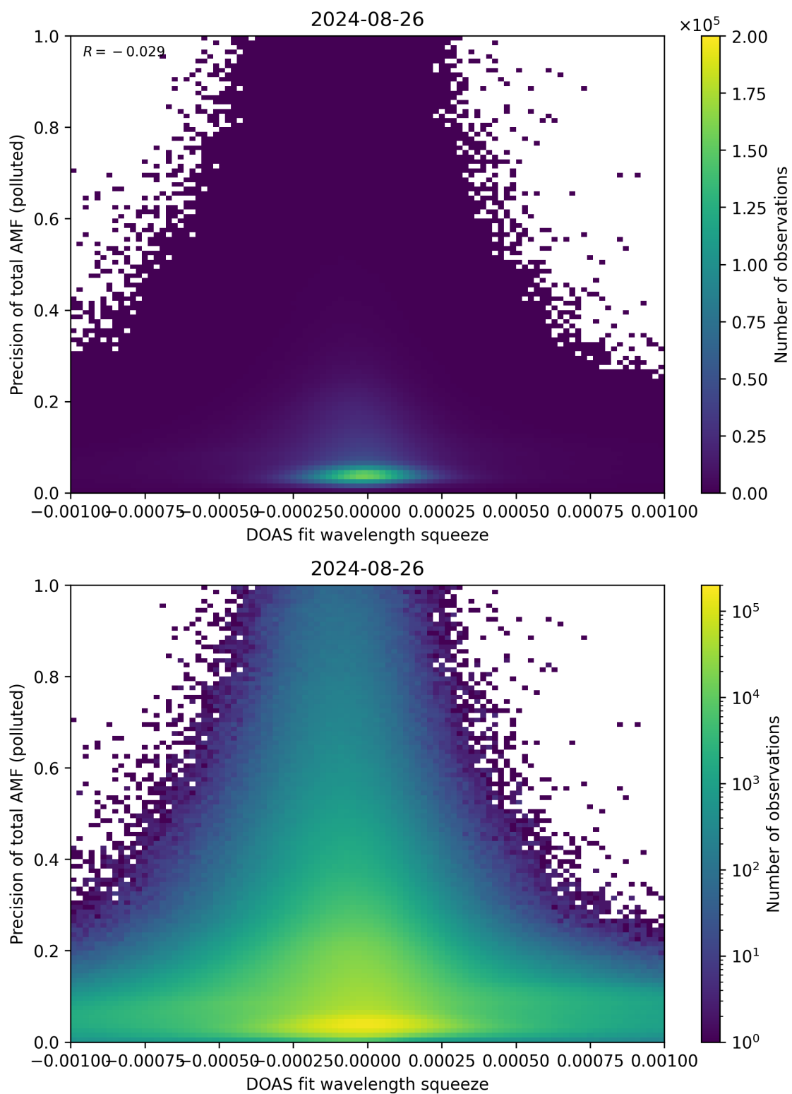
Figure 135: Scatter density plot of “DOAS fit wavelength squeeze” against “Precision of total AMF (polluted)” for 2024-08-25 to 2024-08-27.
