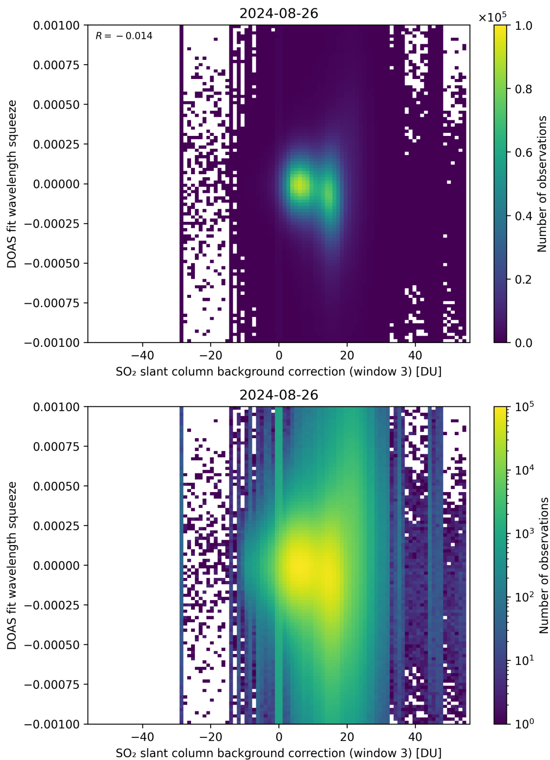
Figure 122: Scatter density plot of “SO 2 slant column background correction (window 3)” against “DOAS fit wavelength squeeze” for 2024-08-25 to 2024-08-27.
