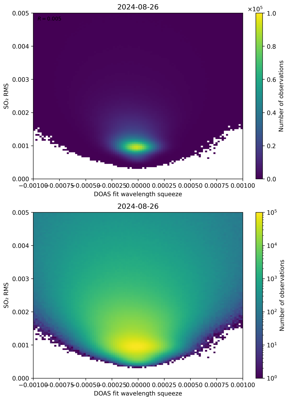
Figure 132: Scatter density plot of “DOAS fit wavelength squeeze” against “SO 2 RMS” for 2024-08-25 to 2024-08-27.
