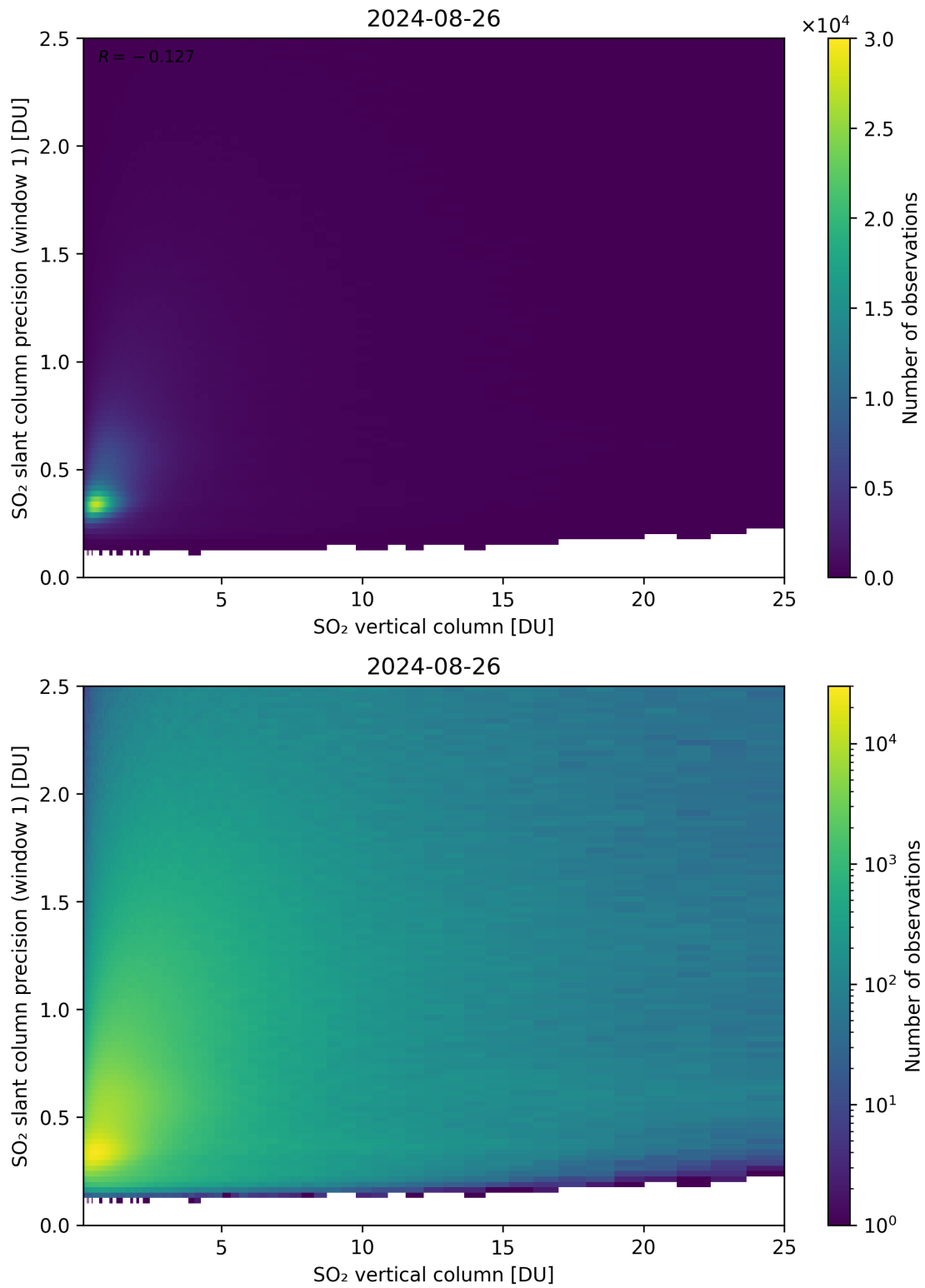
Figure 301: Scatter density plot of “SO 2 vertical column” against “SO 2 slant column precision (window 1)” for 2024-08-25 to 2024-08-27.
