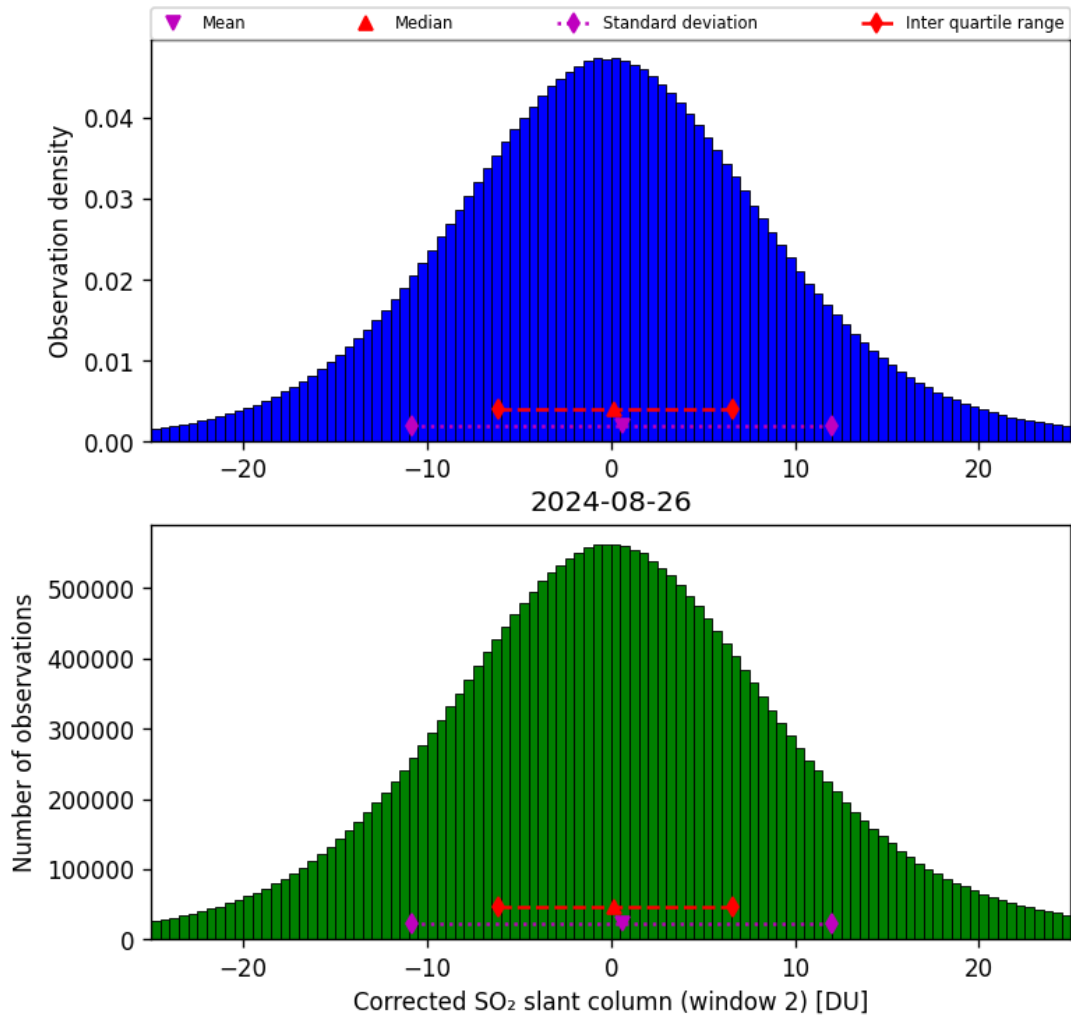
Figure 62: Histogram of “Corrected SO 2 slant column (window 2)” for 2024-08-25 to 2024-08-27
