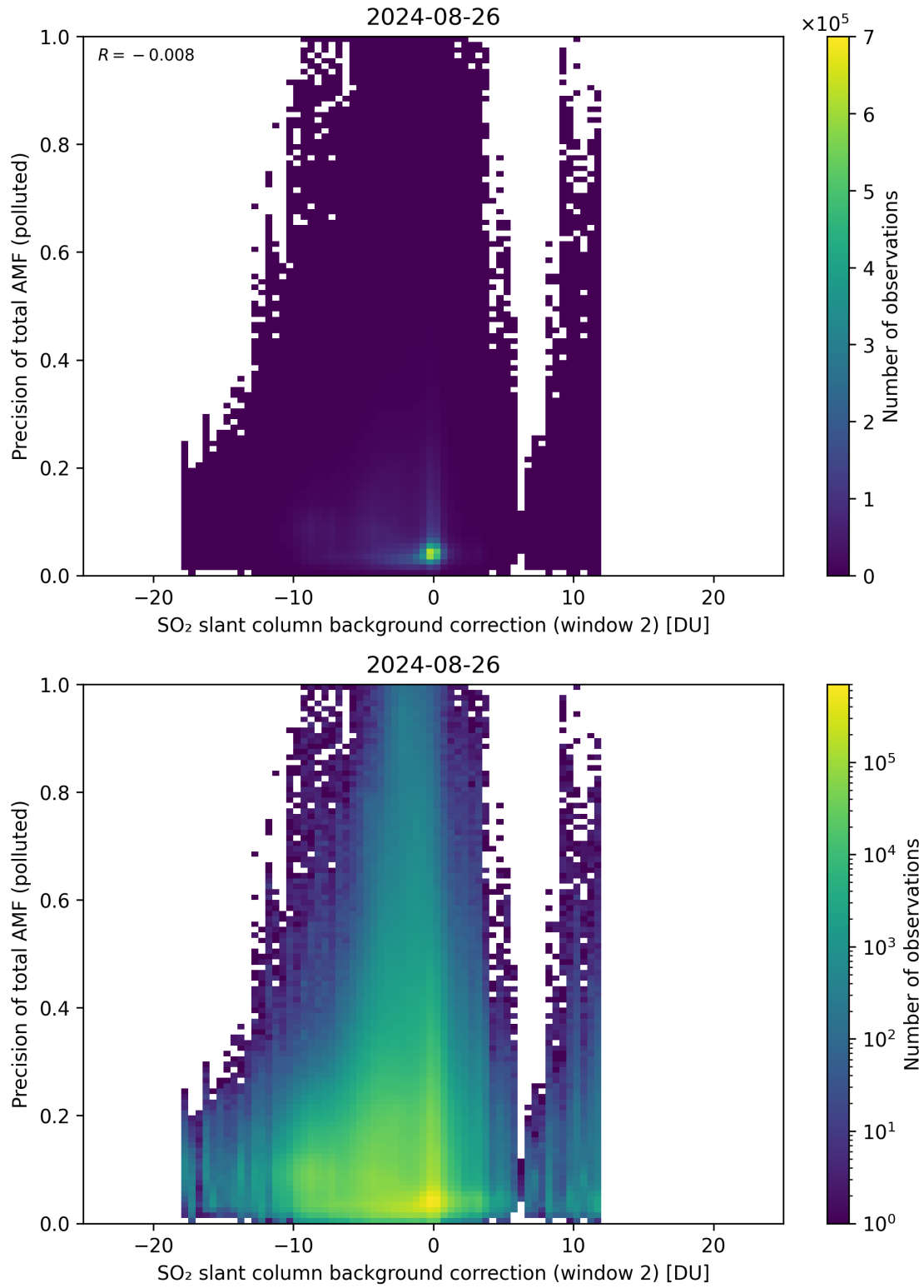
Figure 120: Scatter density plot of “SO 2 slant column background correction (window 2)” against “Precision of total AMF (polluted)” for 2024-08-25 to 2024-08-27.
