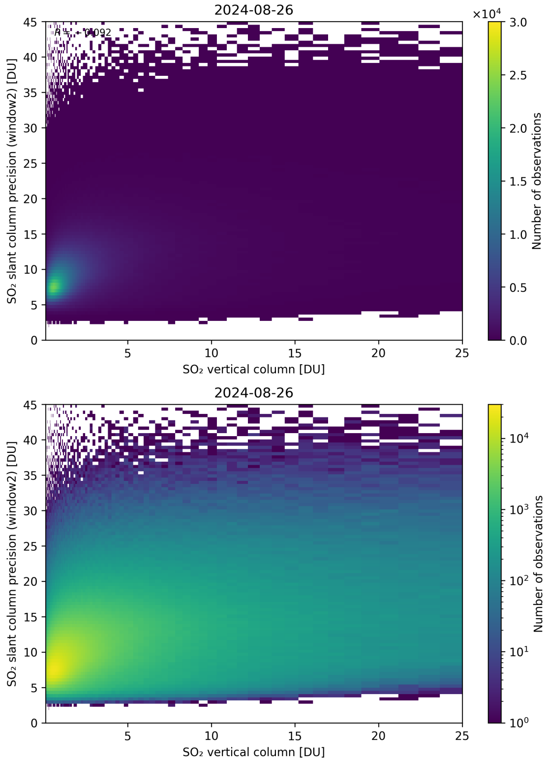
Figure 302: Scatter density plot of “SO 2 vertical column” against “SO 2 slant column precision (window2)” for 2024-08-25 to 2024-08-27.
