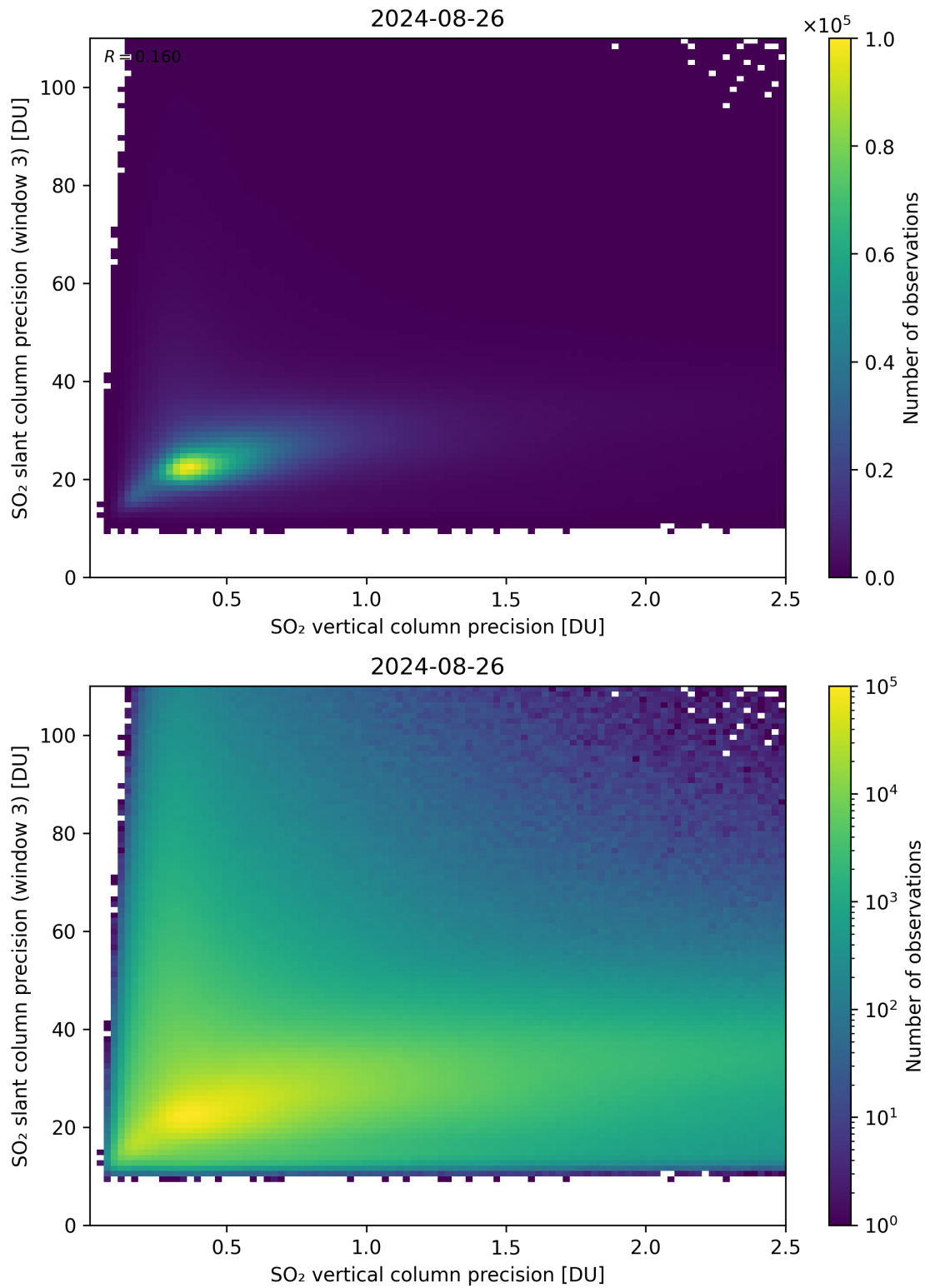
Figure 293: Scatter density plot of “SO 2 vertical column precision” against “SO 2 slant column precision (window 3)” for 2024-08-25 to 2024-08-27.
