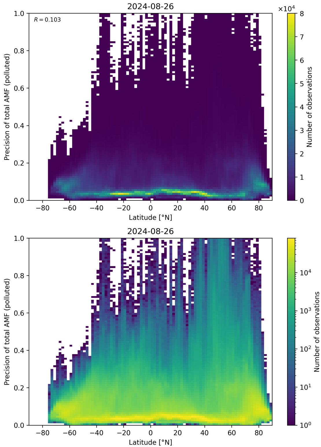
Figure 155: Scatter density plot of “Latitude” against “Precision of total AMF (polluted)” for 2024-08-25 to 2024-08-27.
