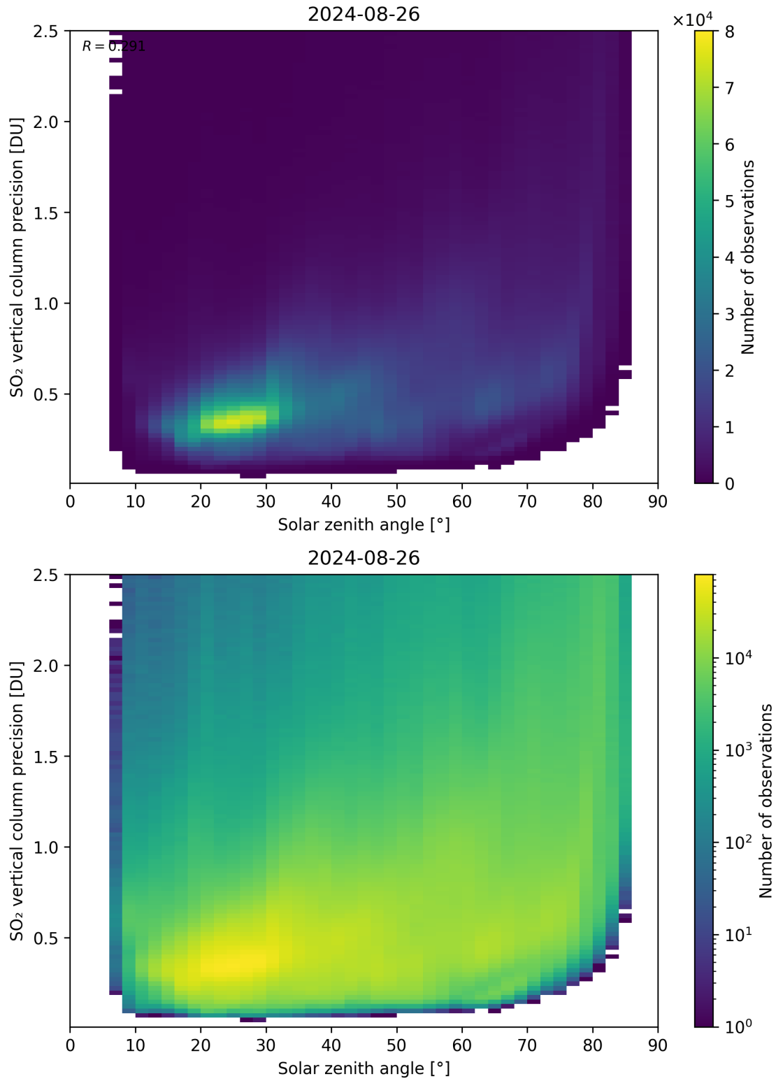
Figure 177: Scatter density plot of “Solar zenith angle” against “SO 2 vertical column precision” for 2024-08-25 to 2024-08-27.
