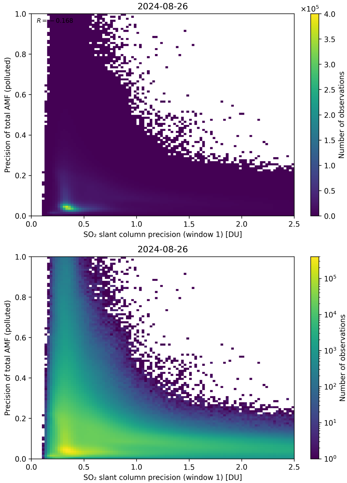
Figure 231: Scatter density plot of “SO 2 slant column precision (window 1)” against “Precision of total AMF (polluted)” for 2024-08-25 to 2024-08-27.
