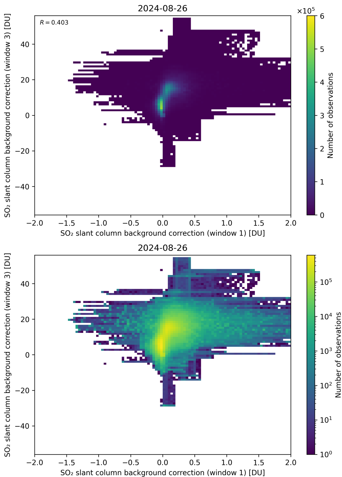
Figure 99: Scatter density plot of “SO 2 slant column background correction (window 1)” against “SO 2 slant column background correction (window 3)” for 2024-08-25 to 2024-08-27.
