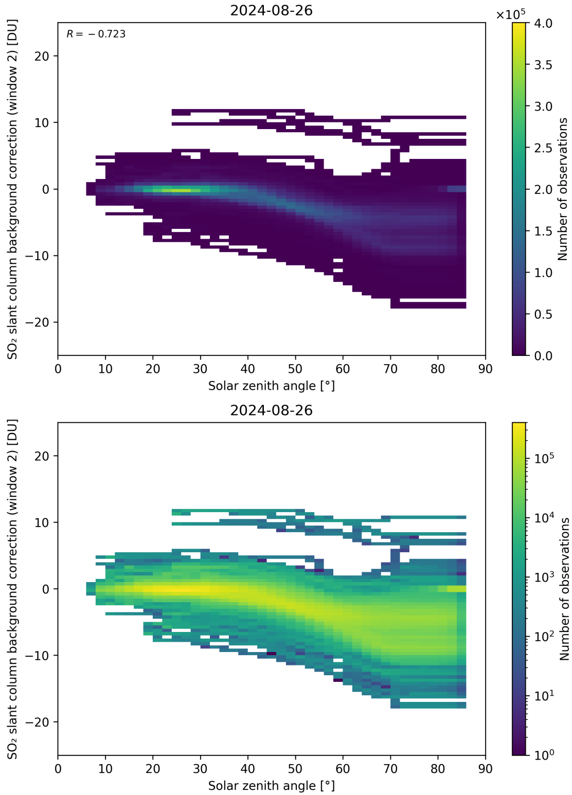
Figure 159: Scatter density plot of “Solar zenith angle” against “SO 2 slant column background correction (window 2)” for 2024-08-25 to 2024-08-27.
