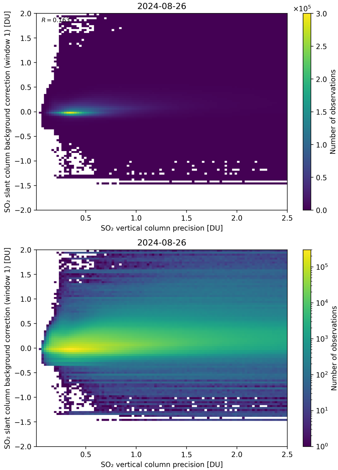
Figure 279: Scatter density plot of “SO 2 vertical column precision” against “SO 2 slant column background correction (window 1)” for 2024-08-25 to 2024-08-27.
