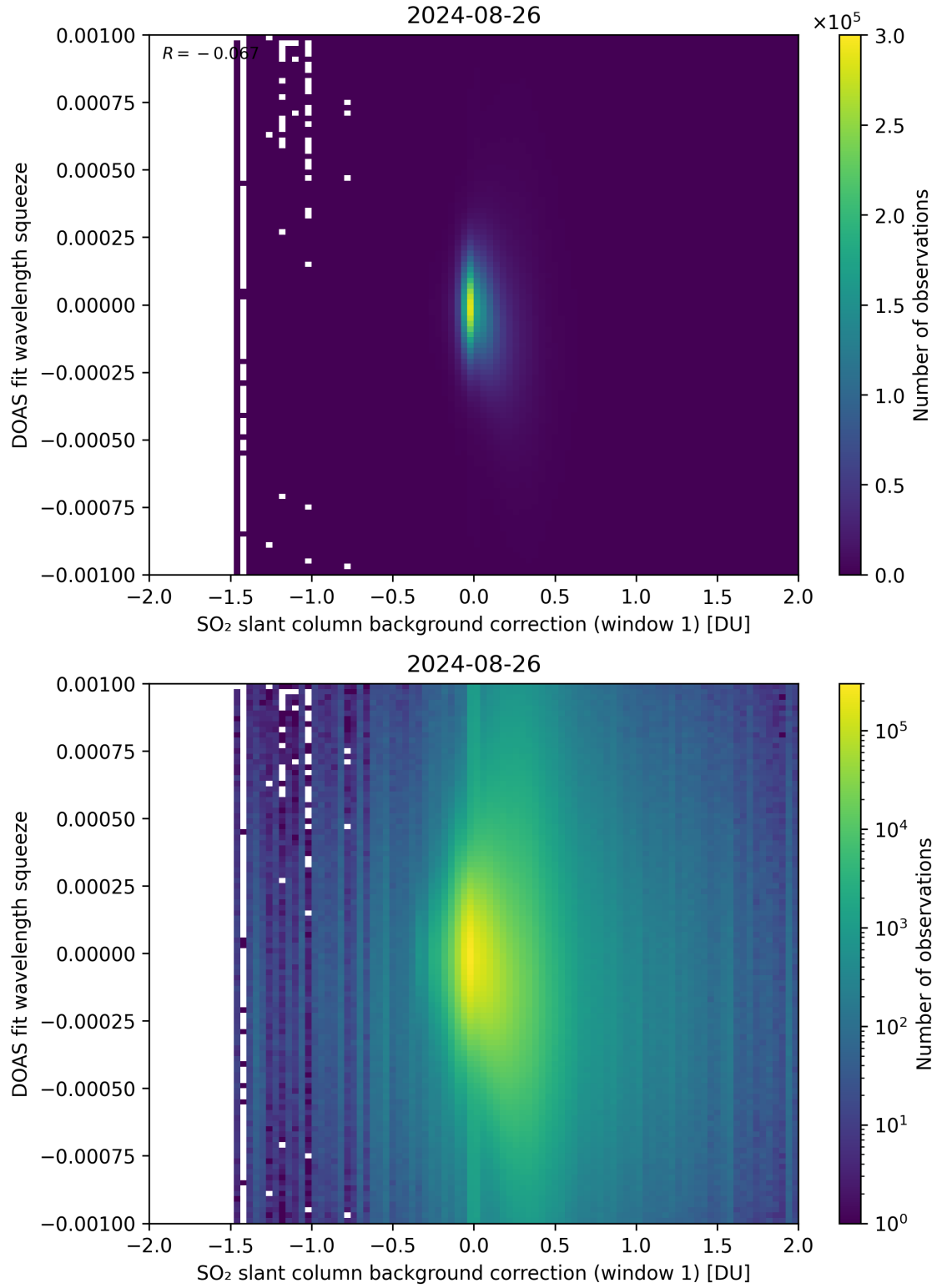
Figure 101: Scatter density plot of “SO 2 slant column background correction (window 1)” against “DOAS fit wavelength squeeze” for 2024-08-25 to 2024-08-27.
