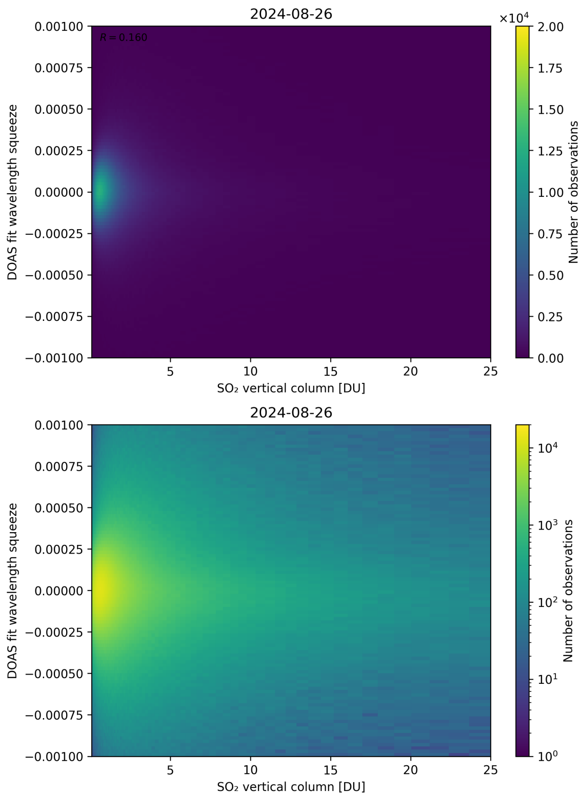
Figure 277: Scatter density plot of “SO 2 vertical column” against “DOAS fit wavelength squeeze” for 2024-08-25 to 2024-08-27.
