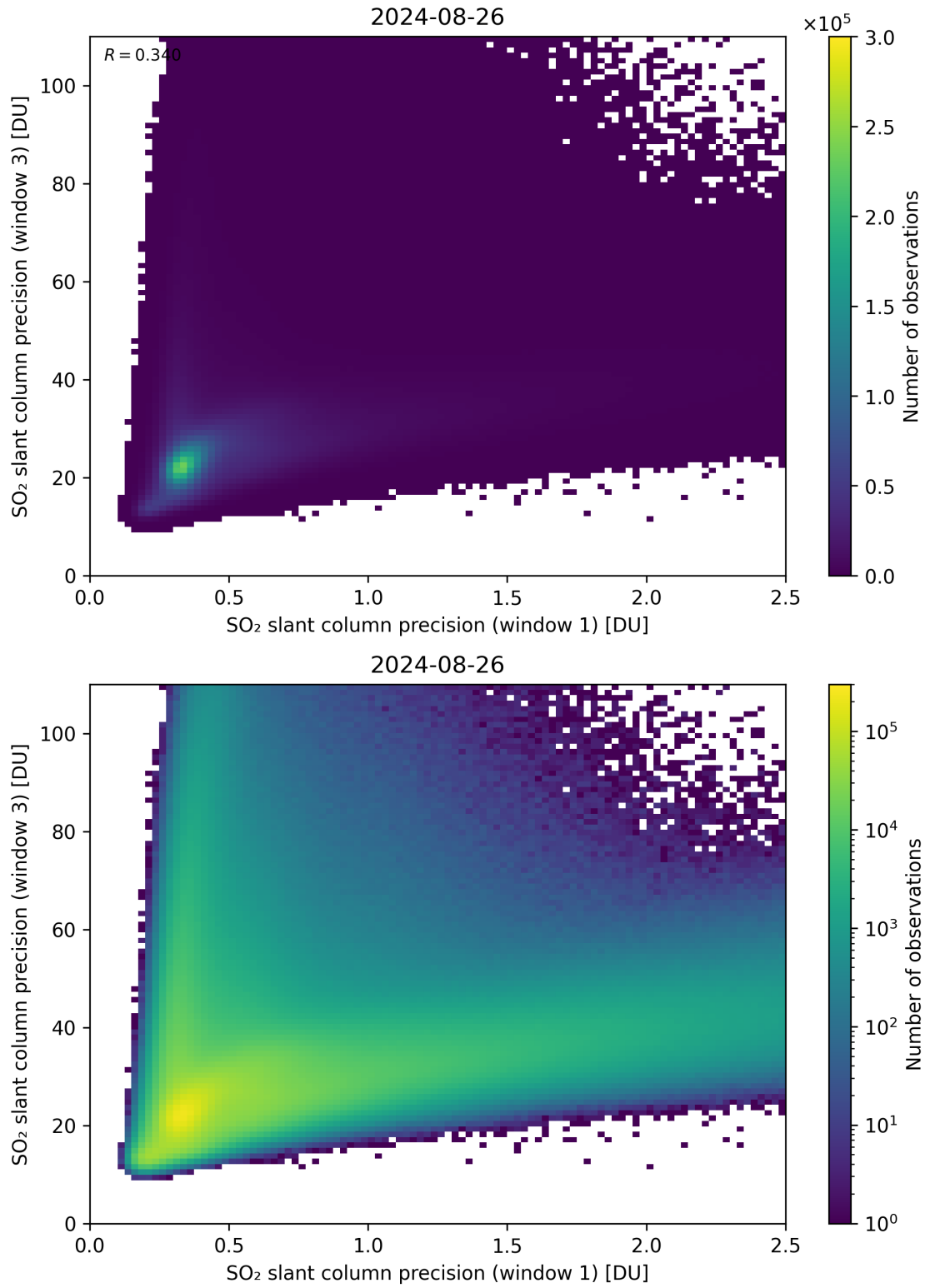
Figure 229: Scatter density plot of “SO 2 slant column precision (window 1)” against “SO 2 slant column precision (window 3)” for 2024-08-25 to 2024-08-27.
