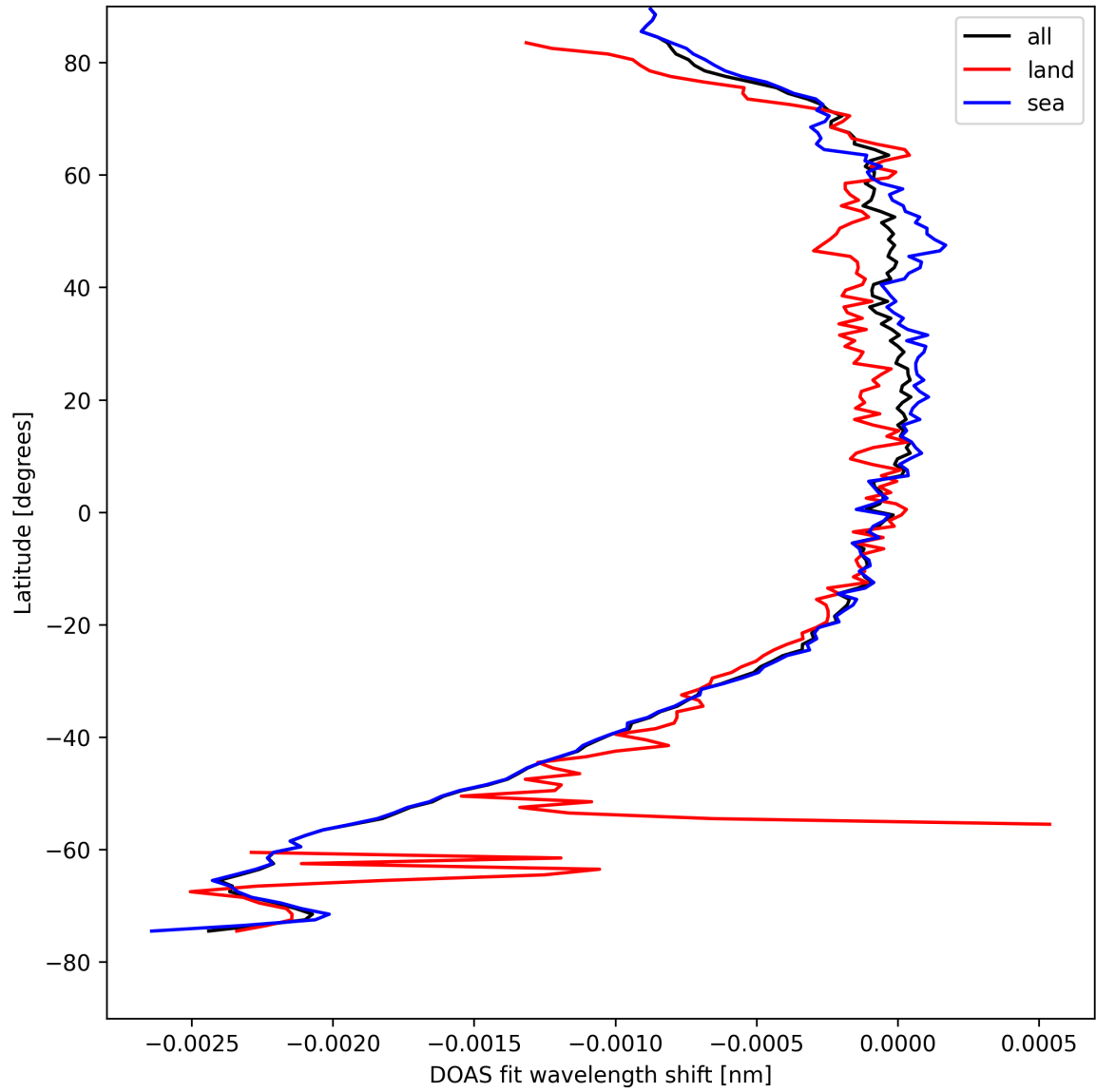
Figure 45: Zonal average of “DOAS fit wavelength shift” for 2024-08-25 to 2024-08-27.
