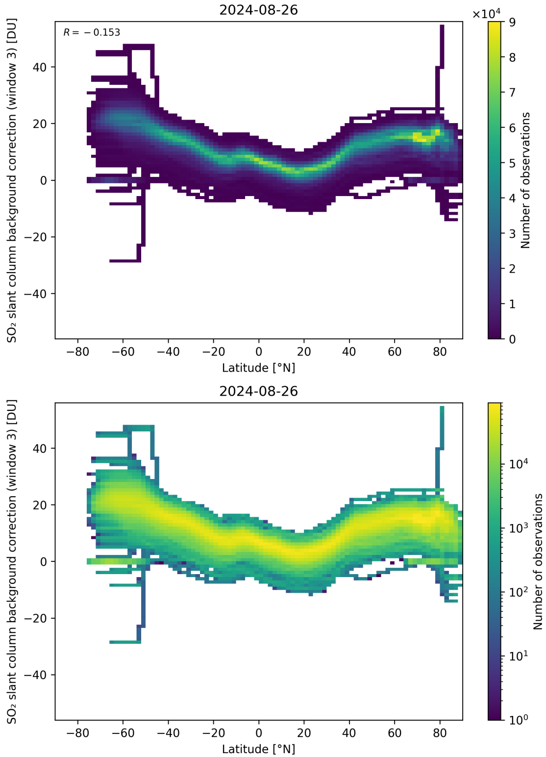
Figure 141: Scatter density plot of “Latitude” against “SO 2 slant column background correction (window 3)” for 2024-08-25 to 2024-08-27.
