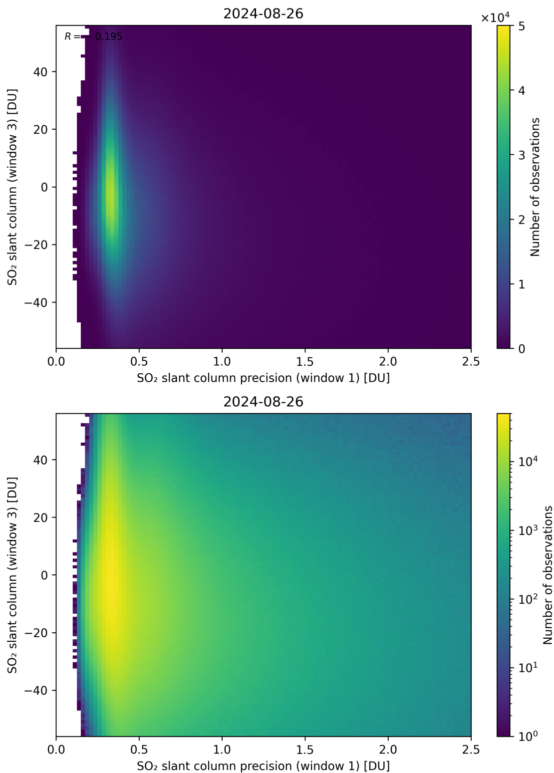
Figure 228: Scatter density plot of “SO 2 slant column precision (window 1)” against “SO 2 slant column (window 3)” for 2024-08-25 to 2024-08-27.
