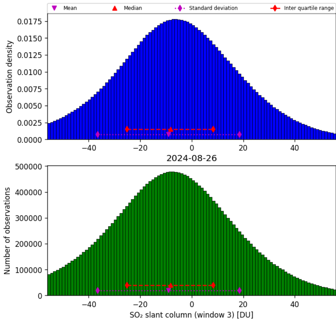
Figure 64: Histogram of “SO 2 slant column (window 3)” for 2024-08-25 to 2024-08-27
