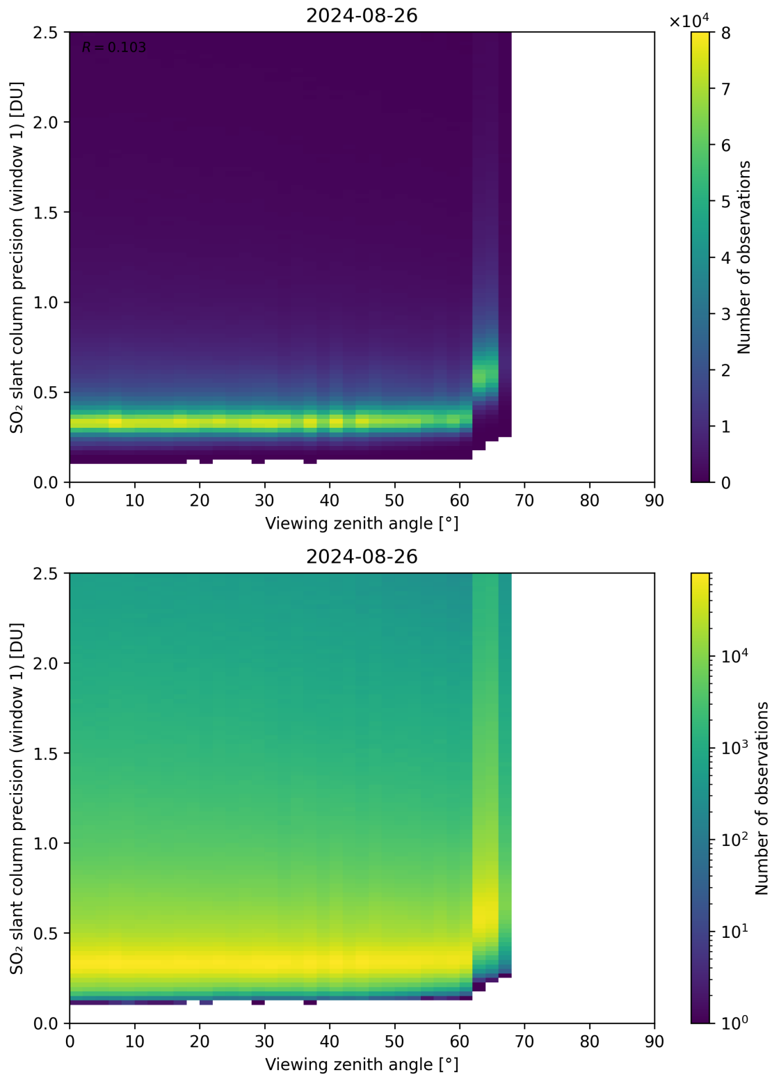
Figure 321: Scatter density plot of “Viewing zenith angle” against “SO 2 slant column precision (window 1)” for 2024-08-25 to 2024-08-27.
