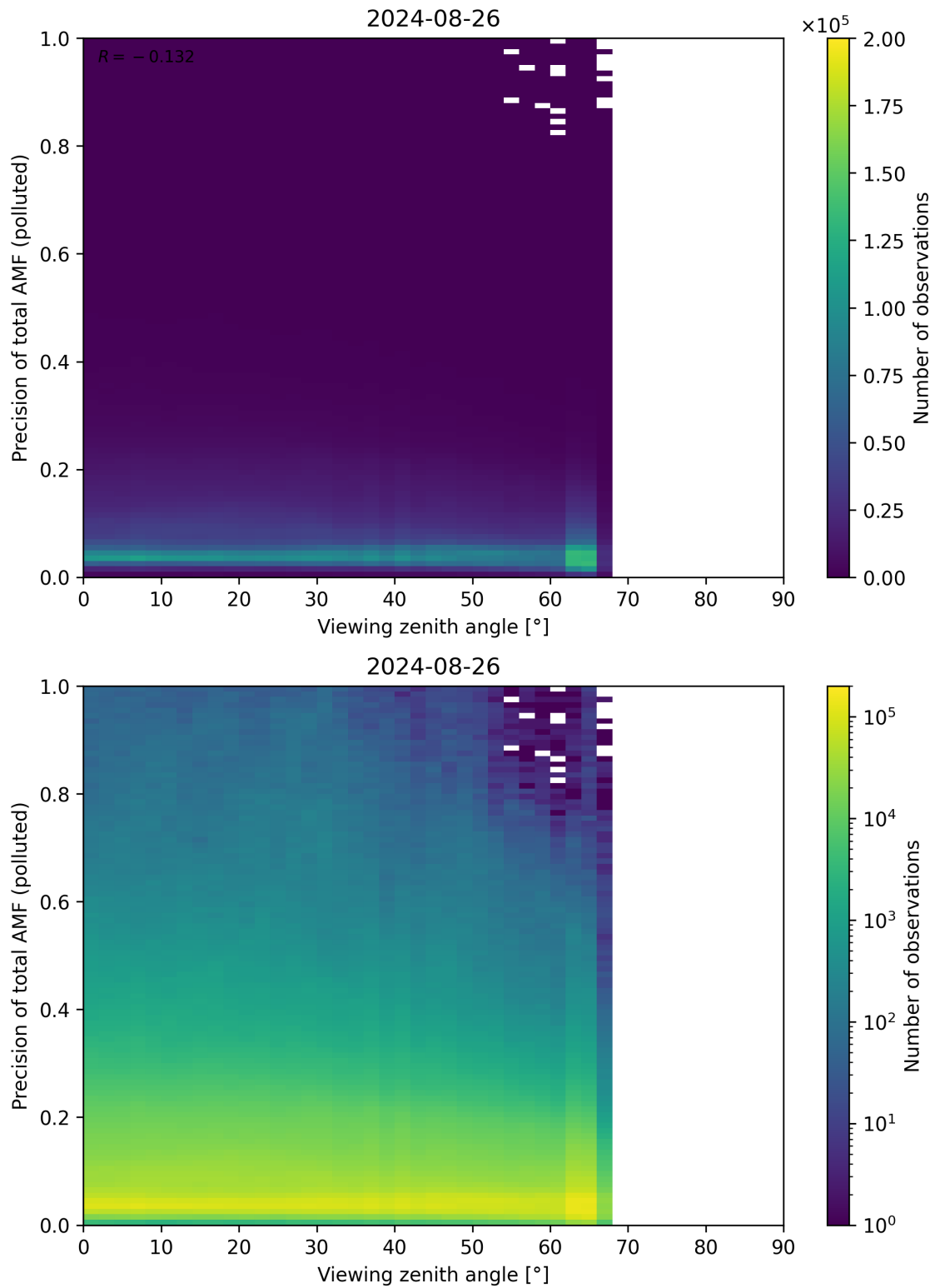
Figure 326: Scatter density plot of “Viewing zenith angle” against “Precision of total AMF (polluted)” for 2024-08-25 to 2024-08-27.
