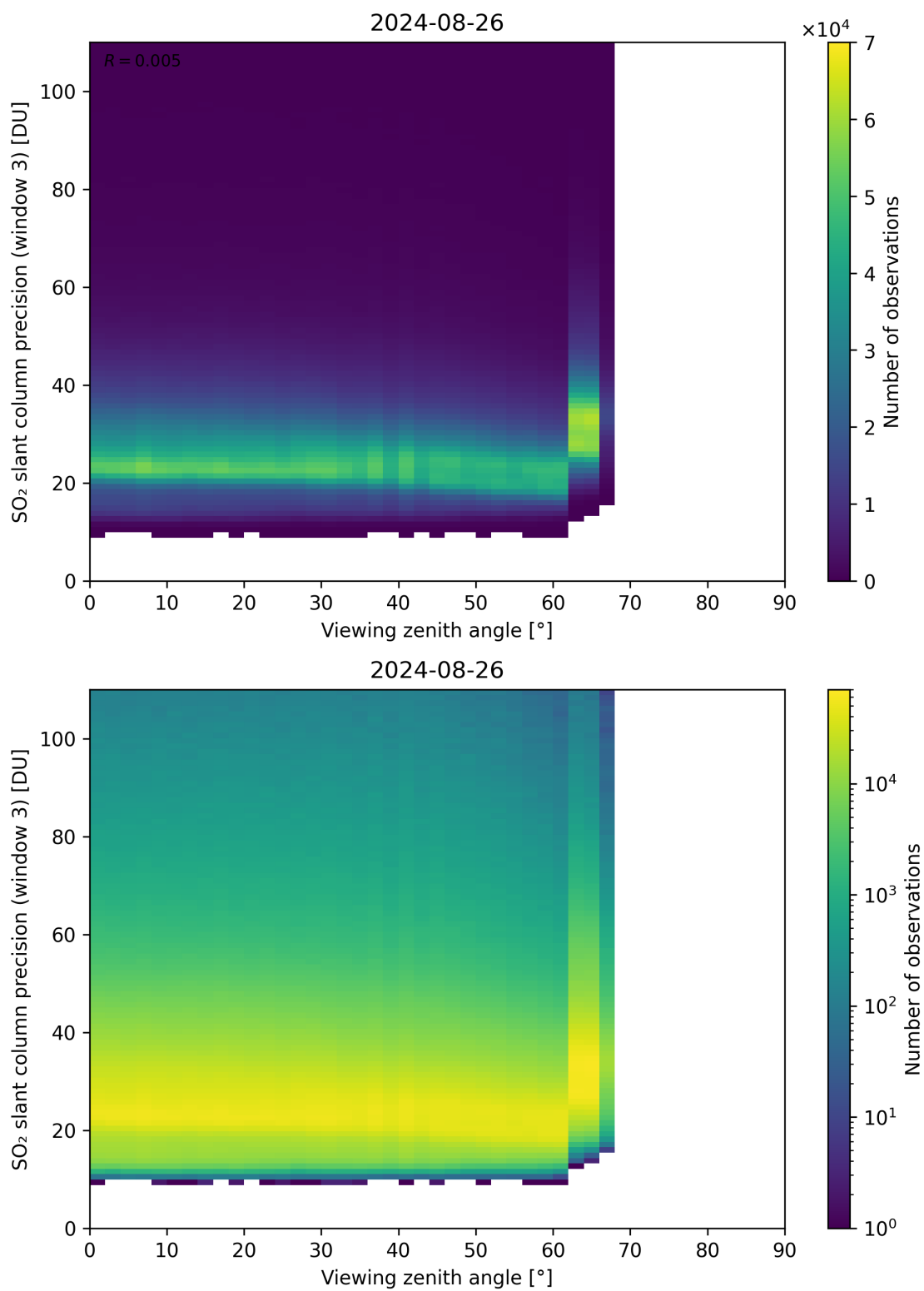
Figure 324: Scatter density plot of “Viewing zenith angle” against “SO 2 slant column precision (window 3)” for 2024-08-25 to 2024-08-27.
