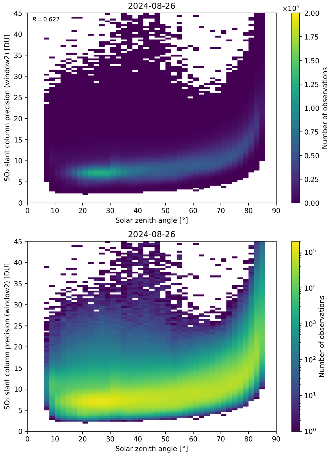
Figure 171: Scatter density plot of “Solar zenith angle” against “SO 2 slant column precision (window2)” for 2024-08-25 to 2024-08-27.
