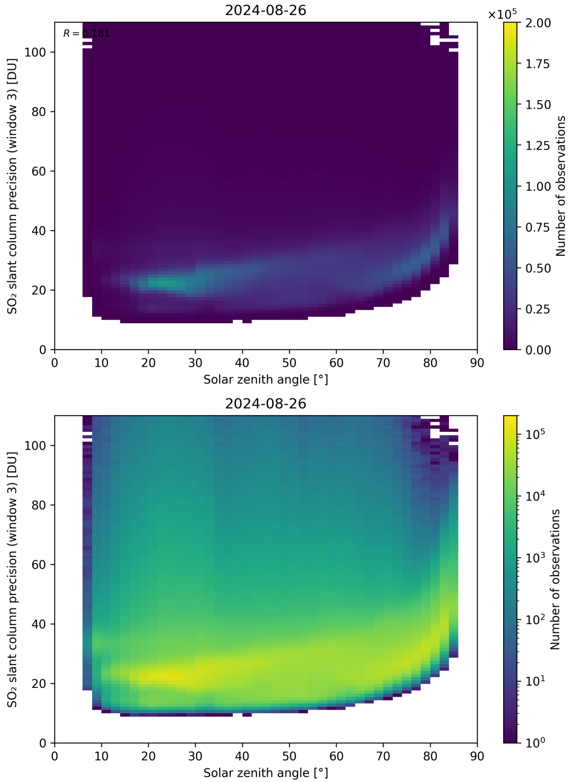
Figure 173: Scatter density plot of “Solar zenith angle” against “SO 2 slant column precision (window 3)” for 2024-08-25 to 2024-08-27.
