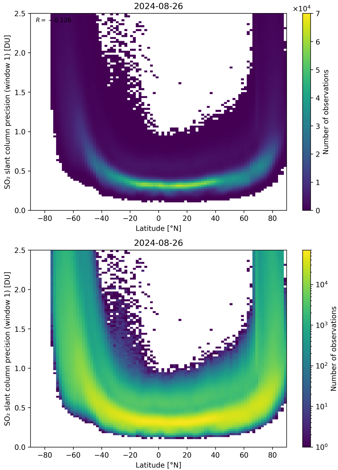
Figure 150: Scatter density plot of “Latitude” against “SO 2 slant column precision (window 1)” for 2024-08-25 to 2024-08-27.
