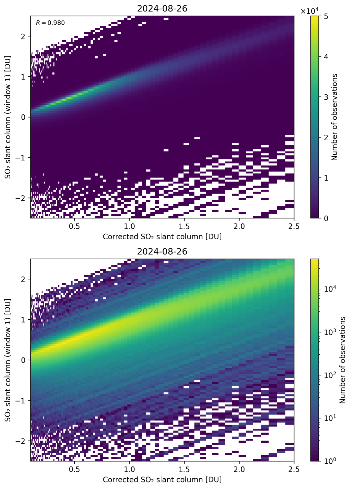
Figure 187: Scatter density plot of “Corrected SO 2 slant column” against “SO 2 slant column (window 1)” for 2024-08-25 to 2024-08-27.
