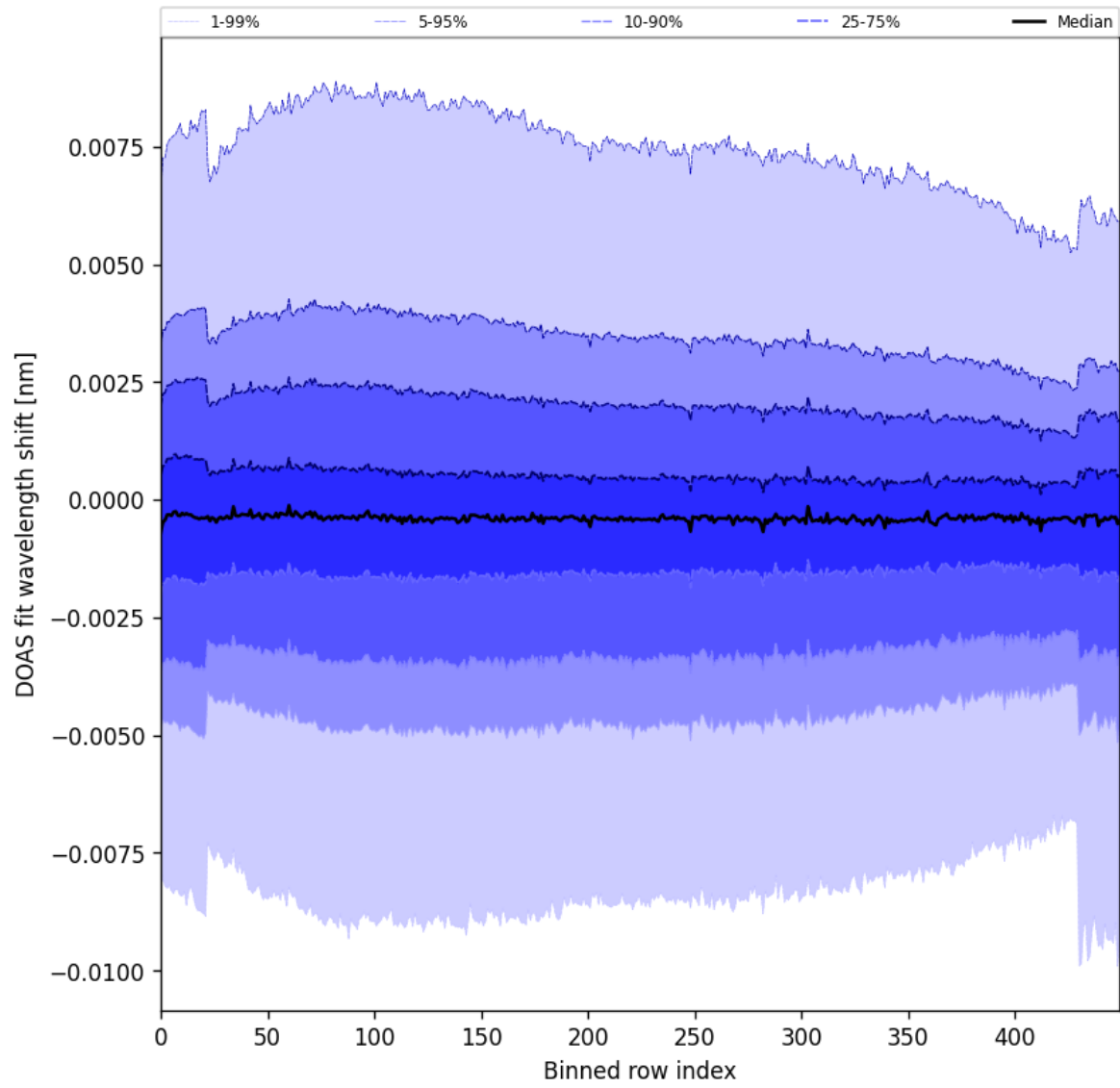
Figure 91: Along track statistics of “DOAS fit wavelength shift” for 2024-08-25 to 2024-08-27
