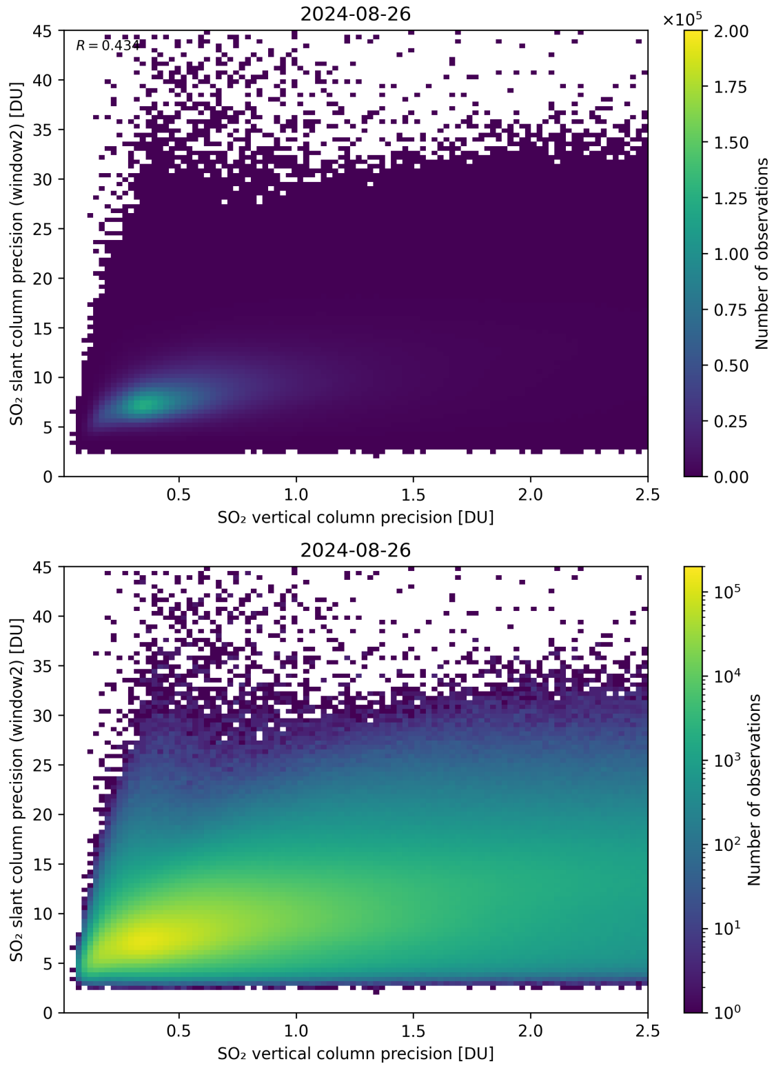
Figure 291: Scatter density plot of “SO 2 vertical column precision” against “SO 2 slant column precision (window2)” for 2024-08-25 to 2024-08-27.
