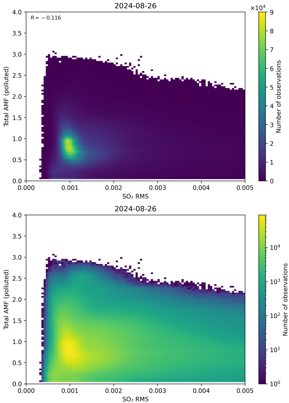
Figure 137: Scatter density plot of “SO 2 RMS” against “Total AMF (polluted)” for 2024-08-25 to 2024-08-27.
