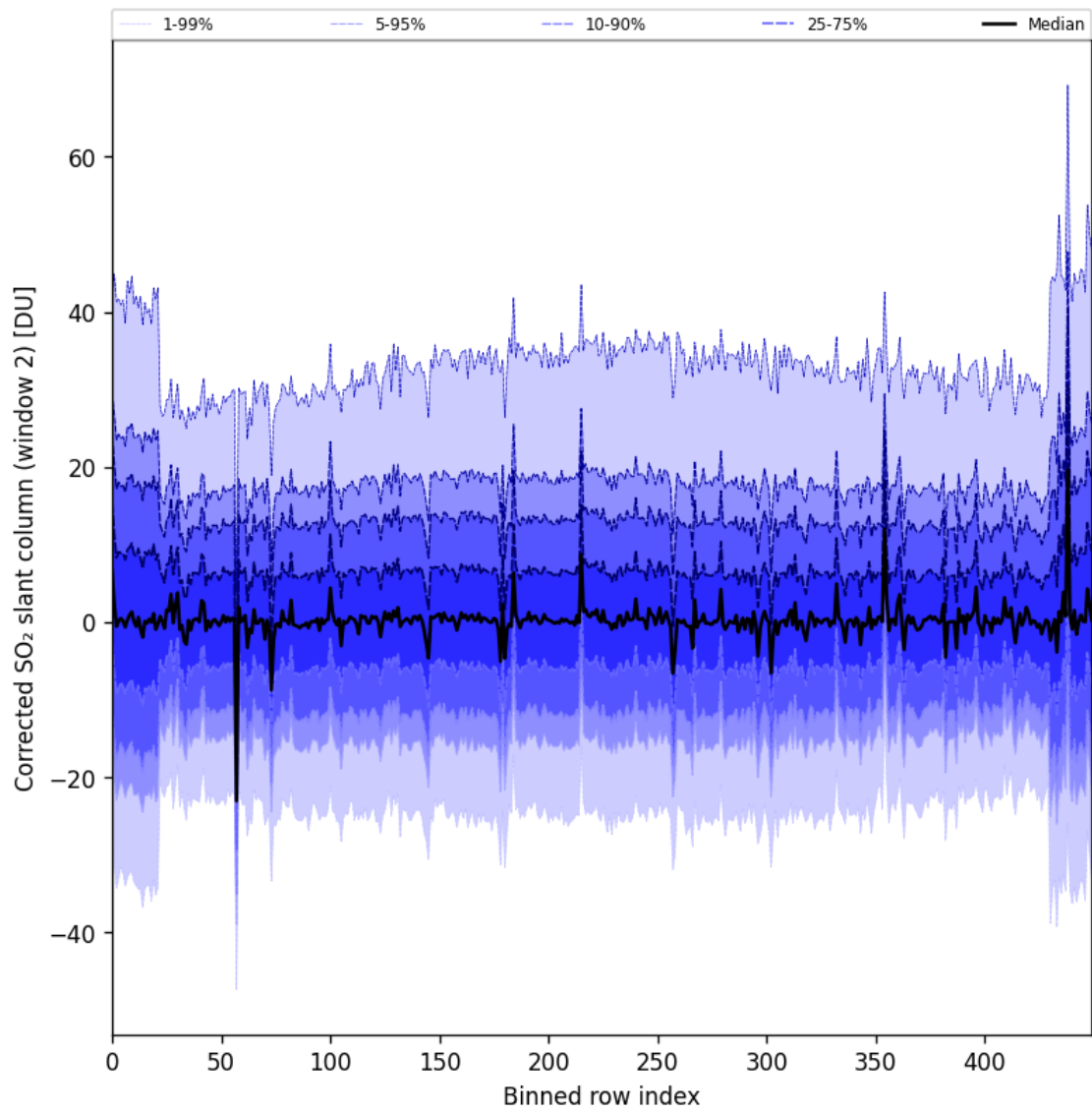
Figure 85: Along track statistics of “Corrected SO 2 slant column (window 2)” for 2024-08-25 to 2024-08-27
