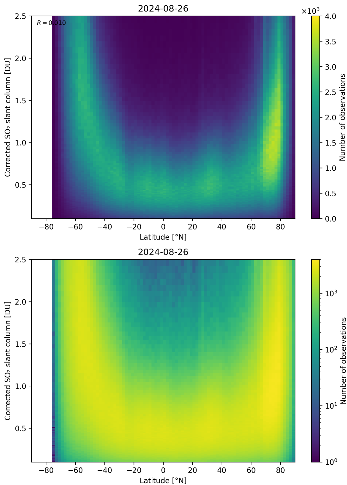
Figure 146: Scatter density plot of “Latitude” against “Corrected SO 2 slant column” for 2024-08-25 to 2024-08-27.
