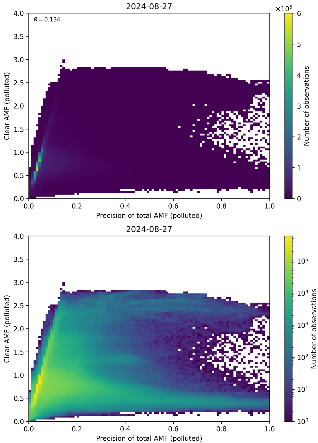
Figure 270: Scatter density plot of “Precision of total AMF (polluted)” against “Clear AMF (polluted)” for 2024-08-27 to 2024-08-28.
