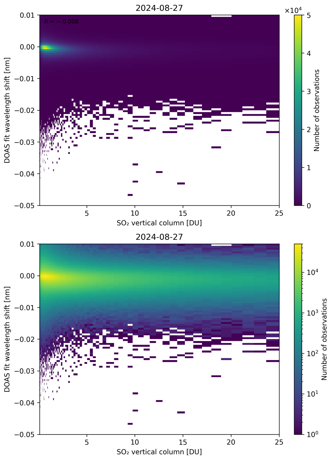
Figure 276: Scatter density plot of “SO 2 vertical column” against “DOAS fit wavelength shift” for 2024-08-27 to 2024-08-28.
