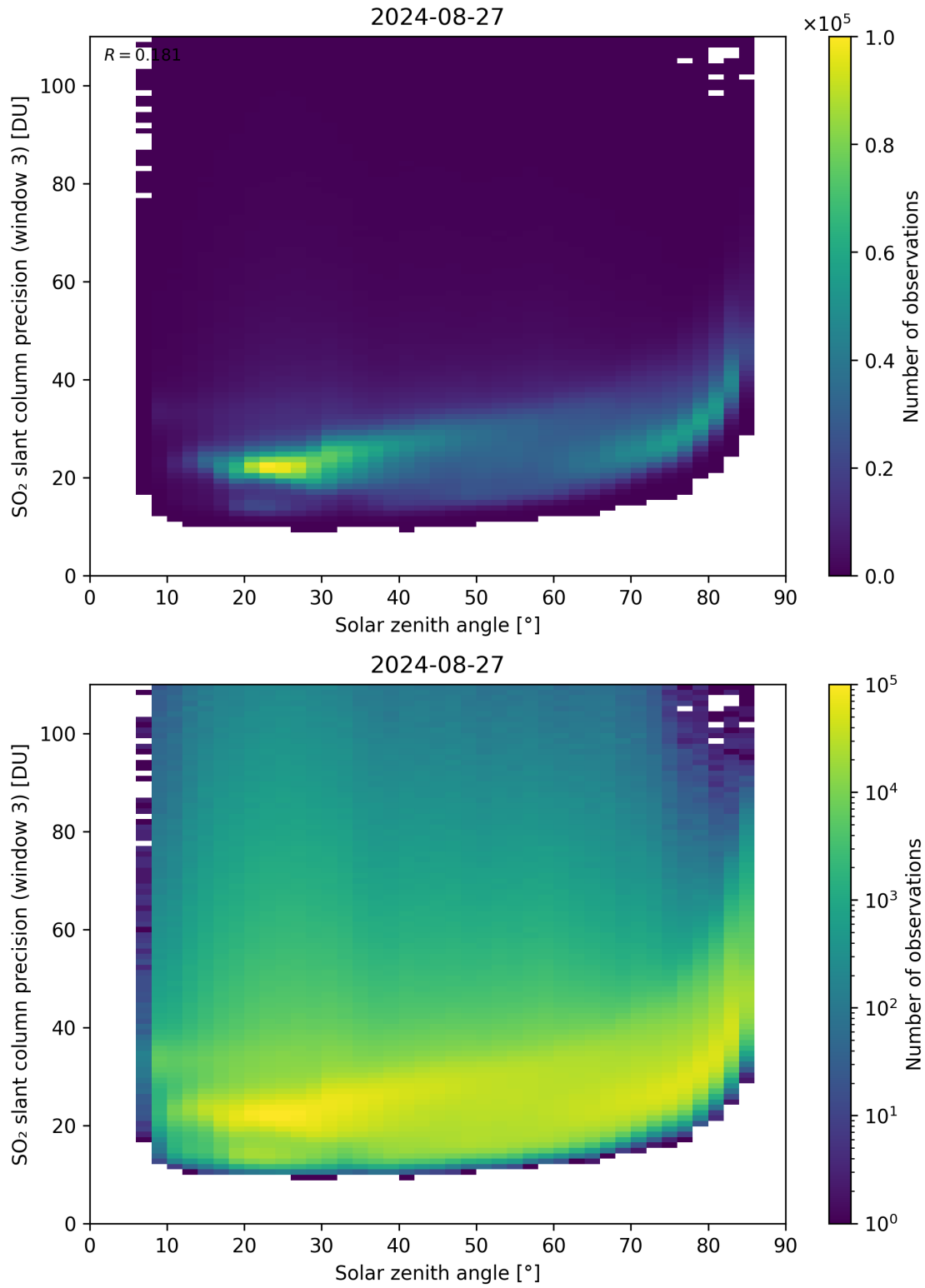
Figure 173: Scatter density plot of “Solar zenith angle” against “SO 2 slant column precision (window 3)” for 2024-08-27 to 2024-08-28.
