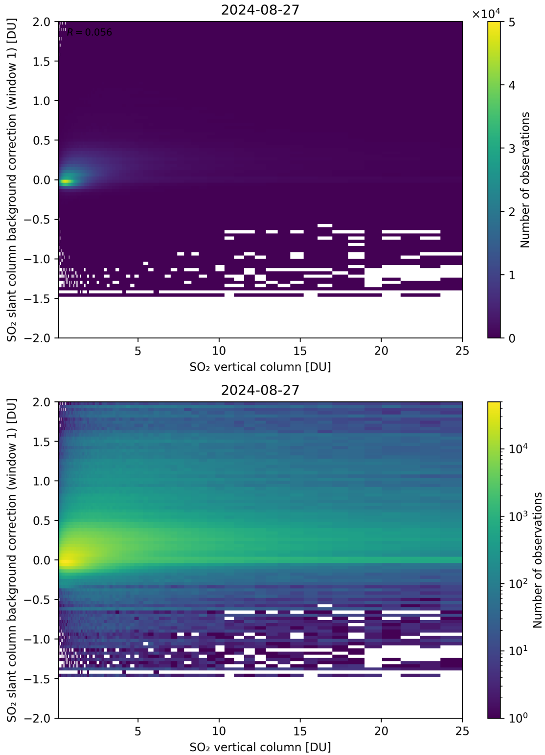
Figure 273: Scatter density plot of “SO 2 vertical column” against “SO 2 slant column background correction (window 1)” for 2024-08-27 to 2024-08-28.
