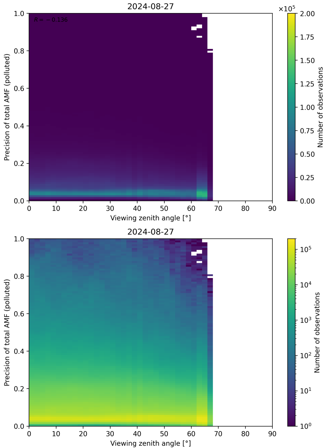
Figure 326: Scatter density plot of “Viewing zenith angle” against “Precision of total AMF (polluted)” for 2024-08-27 to 2024-08-28.
