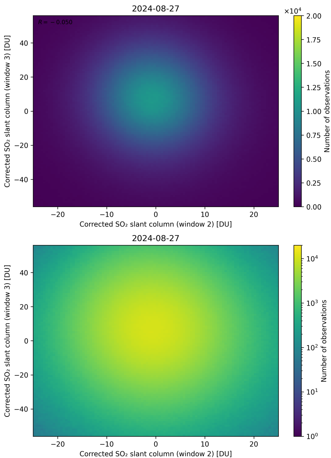
Figure 200: Scatter density plot of “Corrected SO 2 slant column (window 2)” against “Corrected SO 2 slant column (window 3)” for 2024-08-27 to 2024-08-28.
