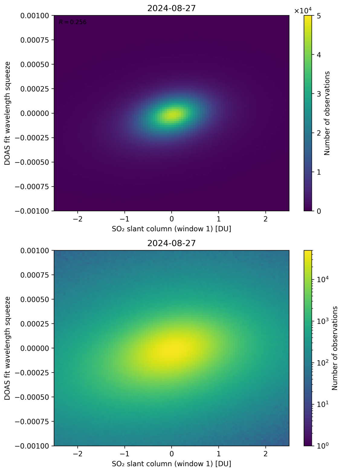
Figure 216: Scatter density plot of “SO 2 slant column (window 1)” against “DOAS fit wavelength squeeze” for 2024-08-27 to 2024-08-28.
