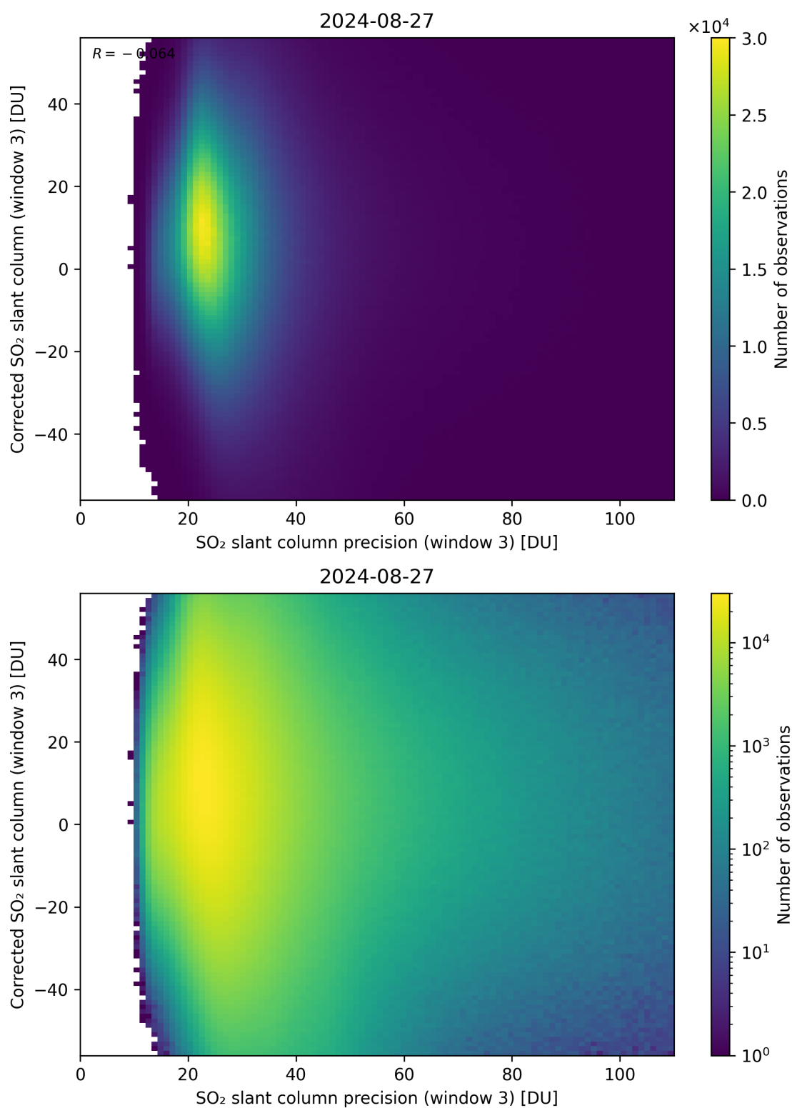
Figure 262: Scatter density plot of “SO 2 slant column precision (window 3)” against “Corrected SO 2 slant column (window 3)” for 2024-08-27 to 2024-08-28.
