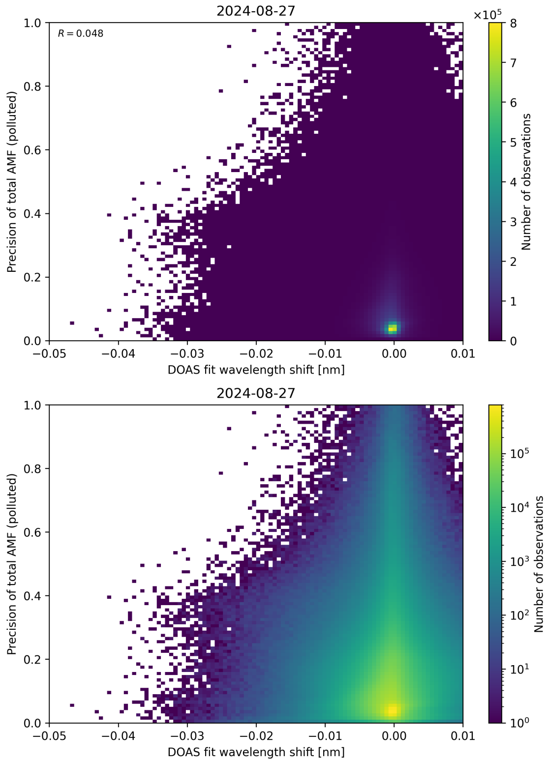
Figure 131: Scatter density plot of “DOAS fit wavelength shift” against “Precision of total AMF (polluted)” for 2024-08-27 to 2024-08-28.
