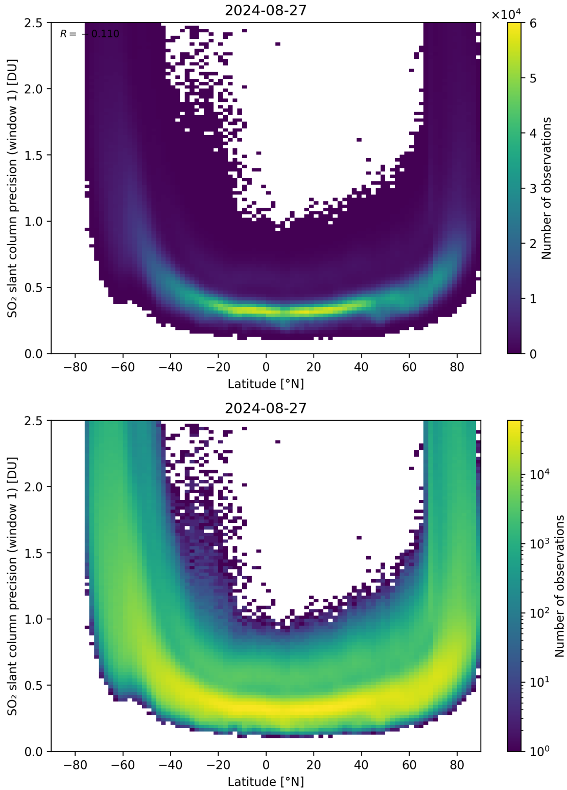
Figure 150: Scatter density plot of “Latitude” against “SO 2 slant column precision (window 1)” for 2024-08-27 to 2024-08-28.
