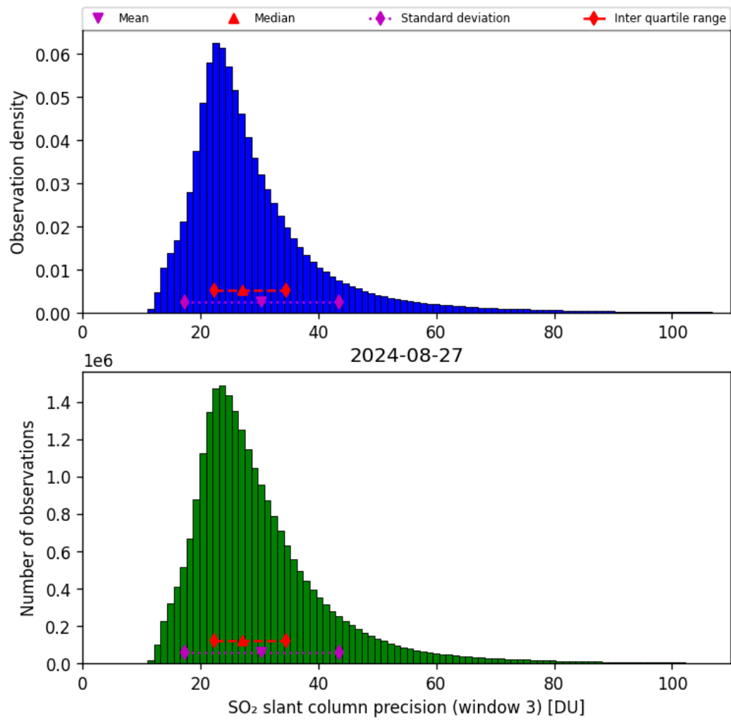
Figure 65: Histogram of “SO 2 slant column precision (window 3)” for 2024-08-27 to 2024-08-28
