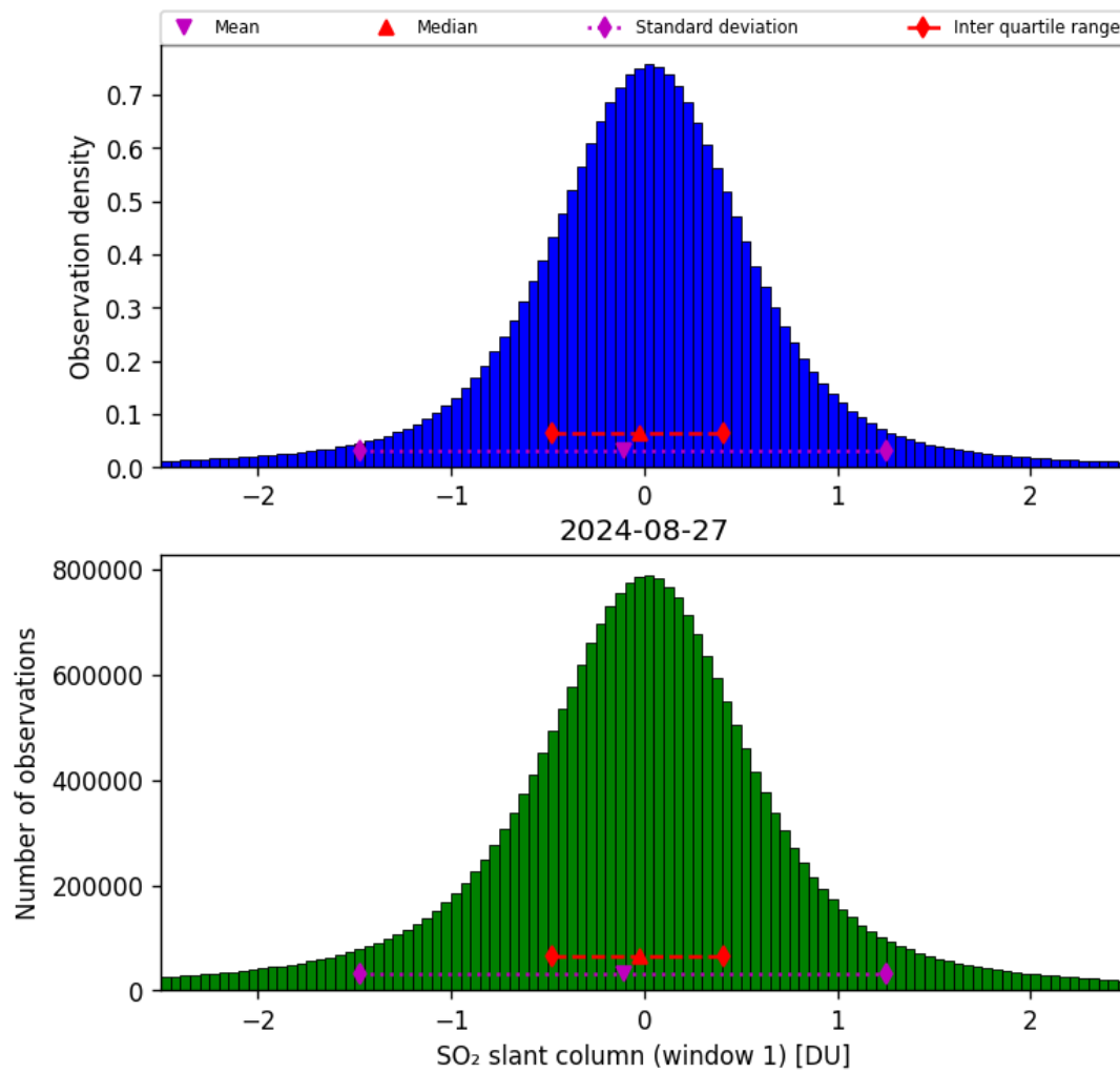
Figure 56: Histogram of “SO 2 slant column (window 1)” for 2024-08-27 to 2024-08-28
