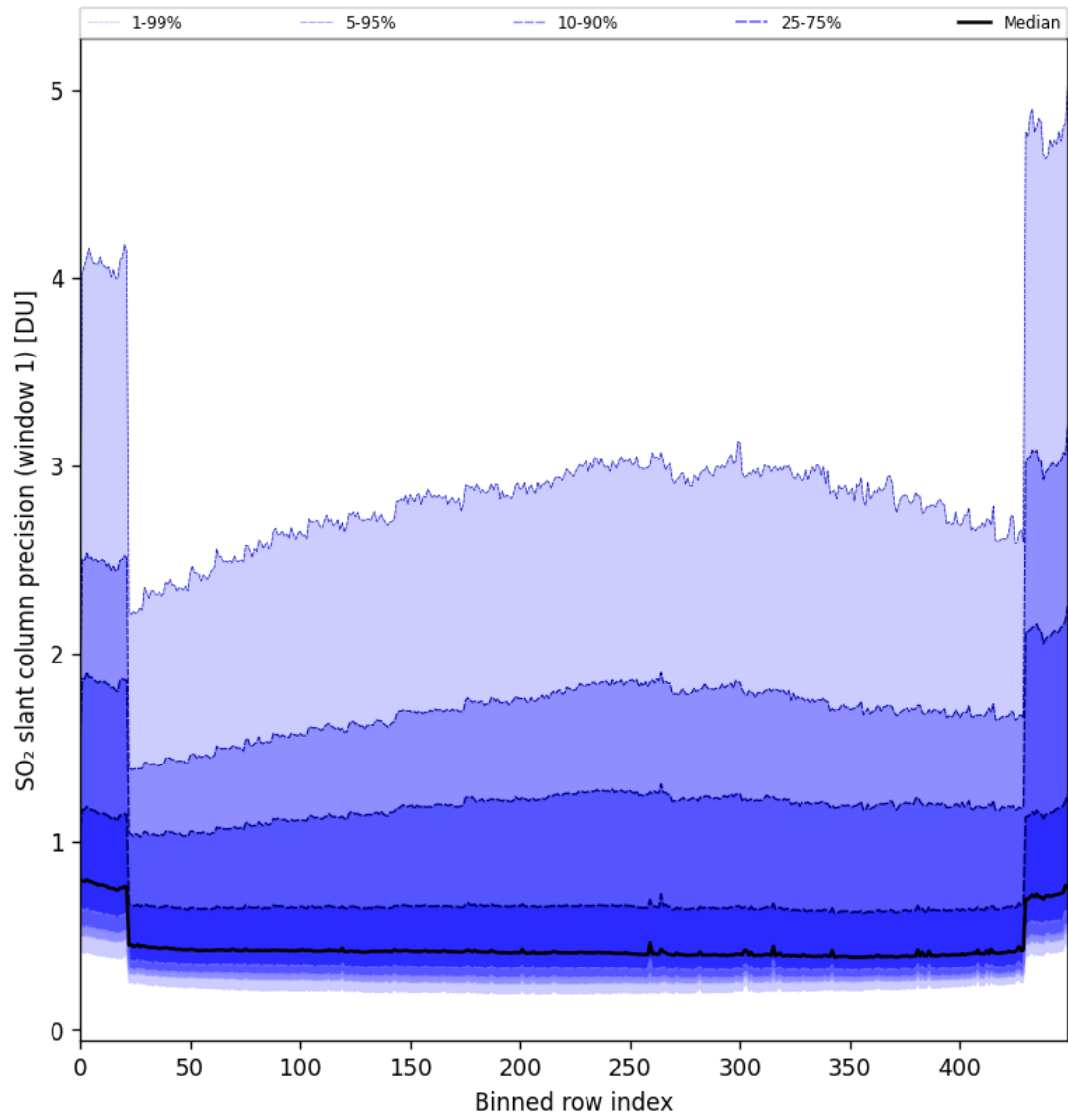
Figure 80: Along track statistics of “SO 2 slant column precision (window 1)” for 2024-08-27 to 2024-08-28
