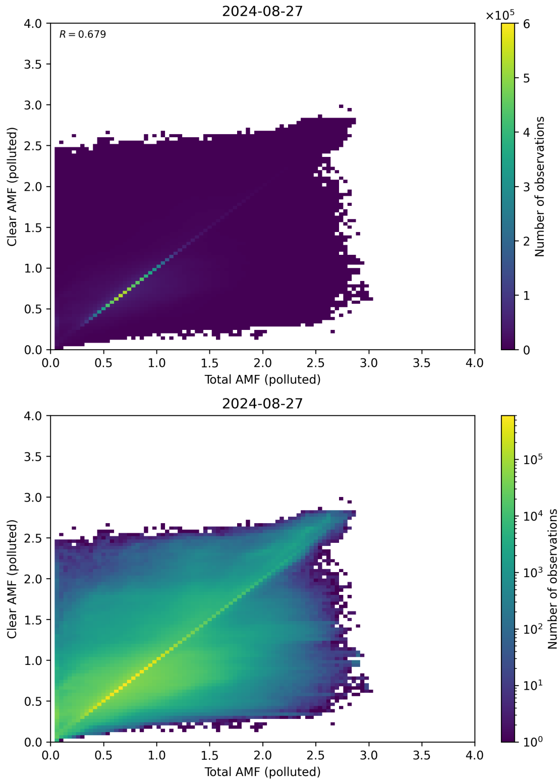
Figure 271: Scatter density plot of “Total AMF (polluted)” against “Clear AMF (polluted)” for 2024-08-27 to 2024-08-28.
