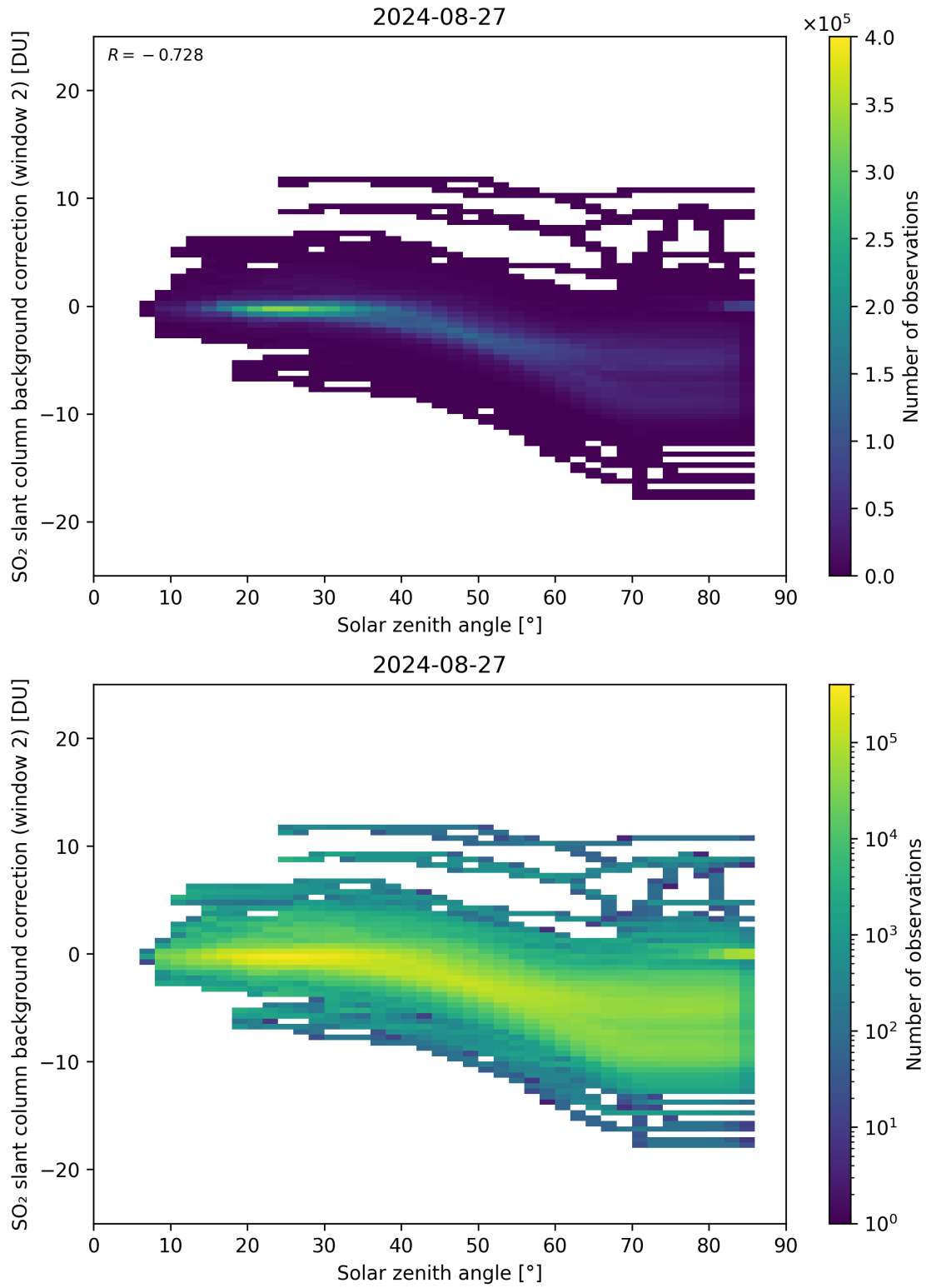
Figure 159: Scatter density plot of “Solar zenith angle” against “SO 2 slant column background correction (window 2)” for 2024-08-27 to 2024-08-28.
