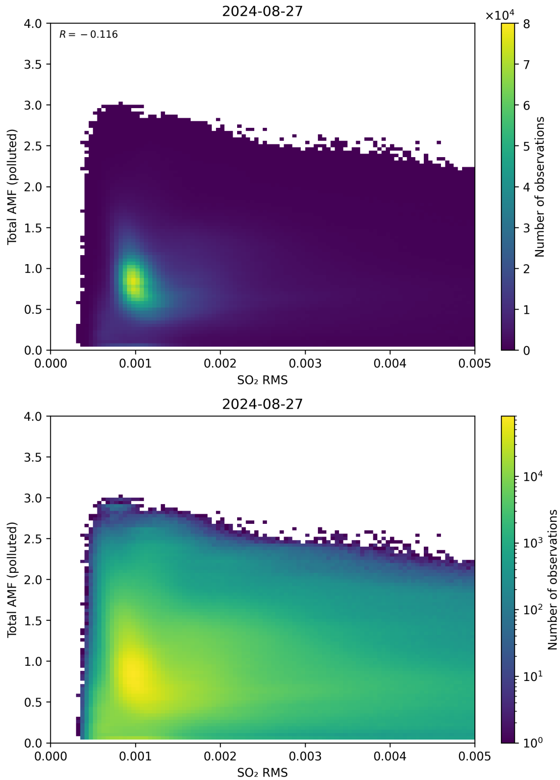
Figure 137: Scatter density plot of “SO 2 RMS” against “Total AMF (polluted)” for 2024-08-27 to 2024-08-28.
