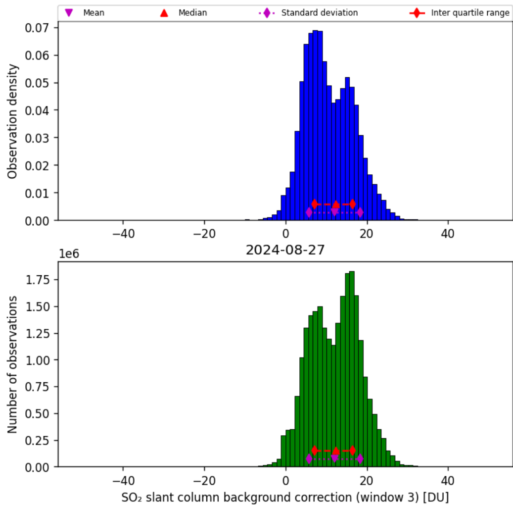
Figure 67: Histogram of “SO 2 slant column background correction (window 3)” for 2024-08-27 to 2024-08-28
