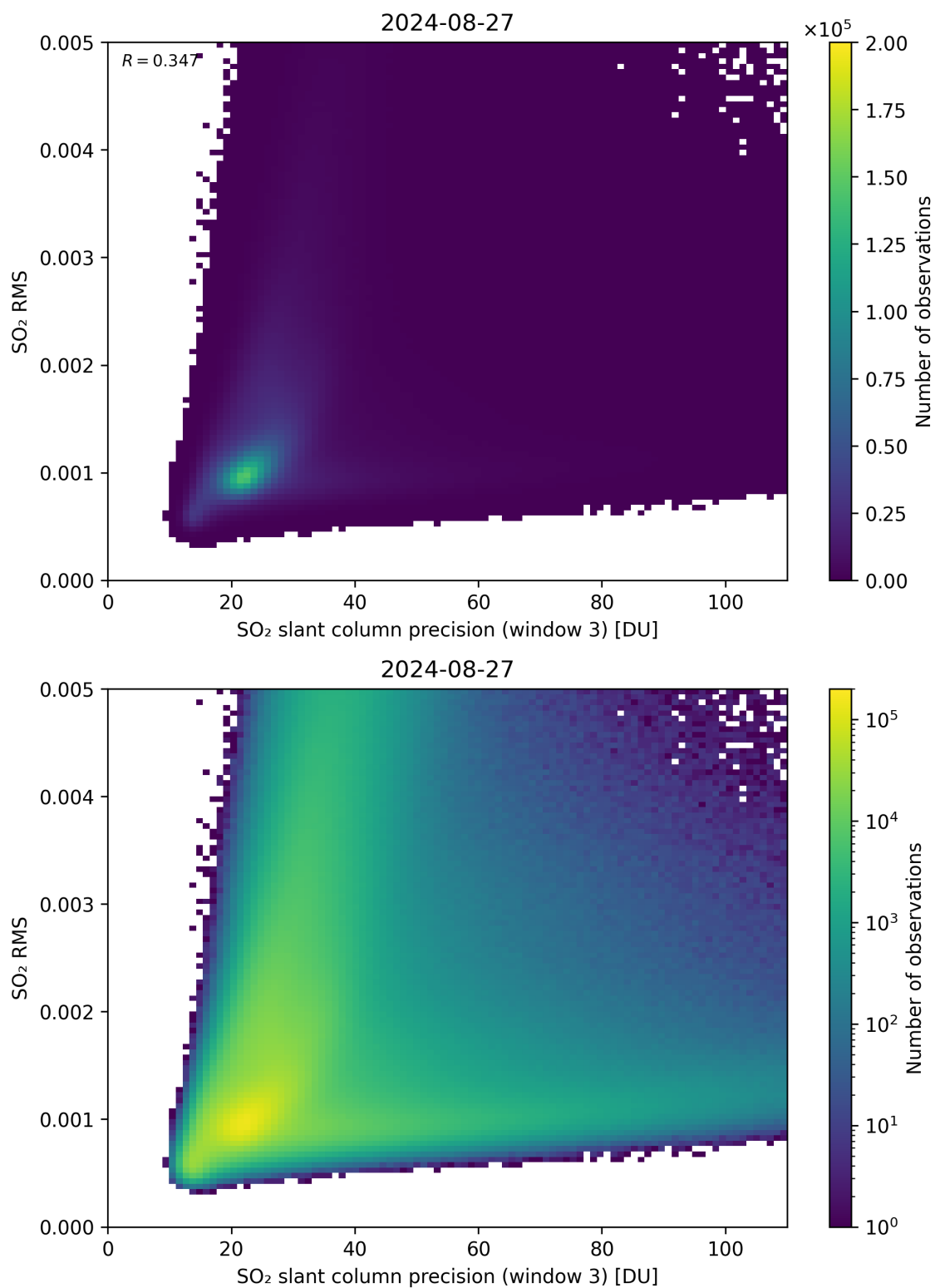
Figure 260: Scatter density plot of “SO 2 slant column precision (window 3)” against “SO 2 RMS” for 2024-08-27 to 2024-08-28.
