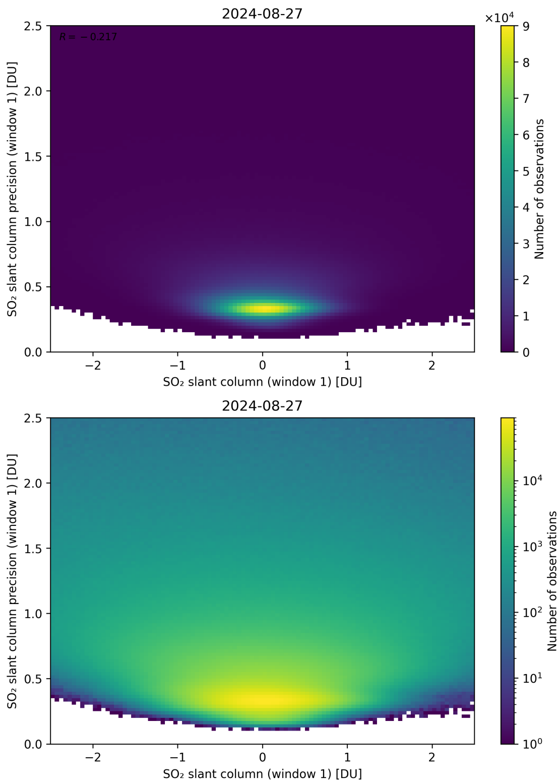
Figure 235: Scatter density plot of “SO 2 slant column (window 1)” against “SO 2 slant column precision (window 1)” for 2024-08-27 to 2024-08-28.
