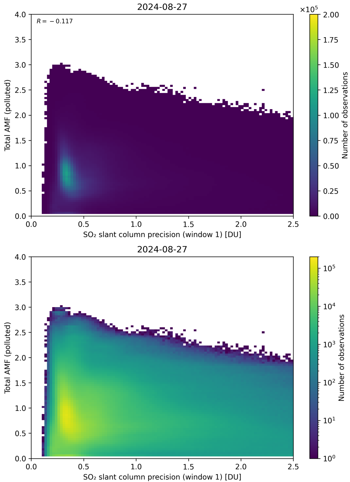
Figure 230: Scatter density plot of “SO 2 slant column precision (window 1)” against “Total AMF (polluted)” for 2024-08-27 to 2024-08-28.
