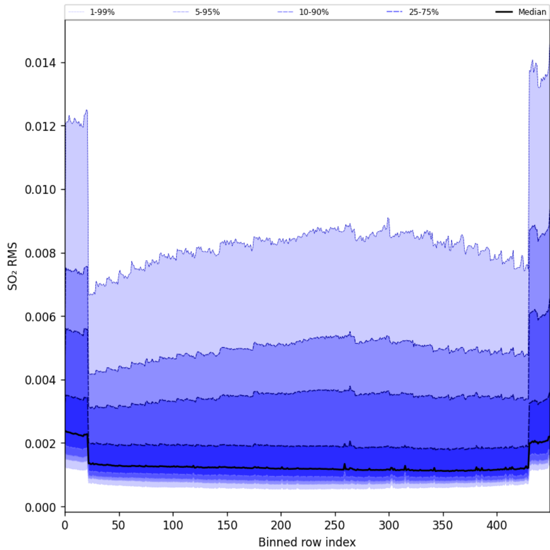
Figure 93: Along track statistics of “SO 2 RMS” for 2024-08-27 to 2024-08-28
