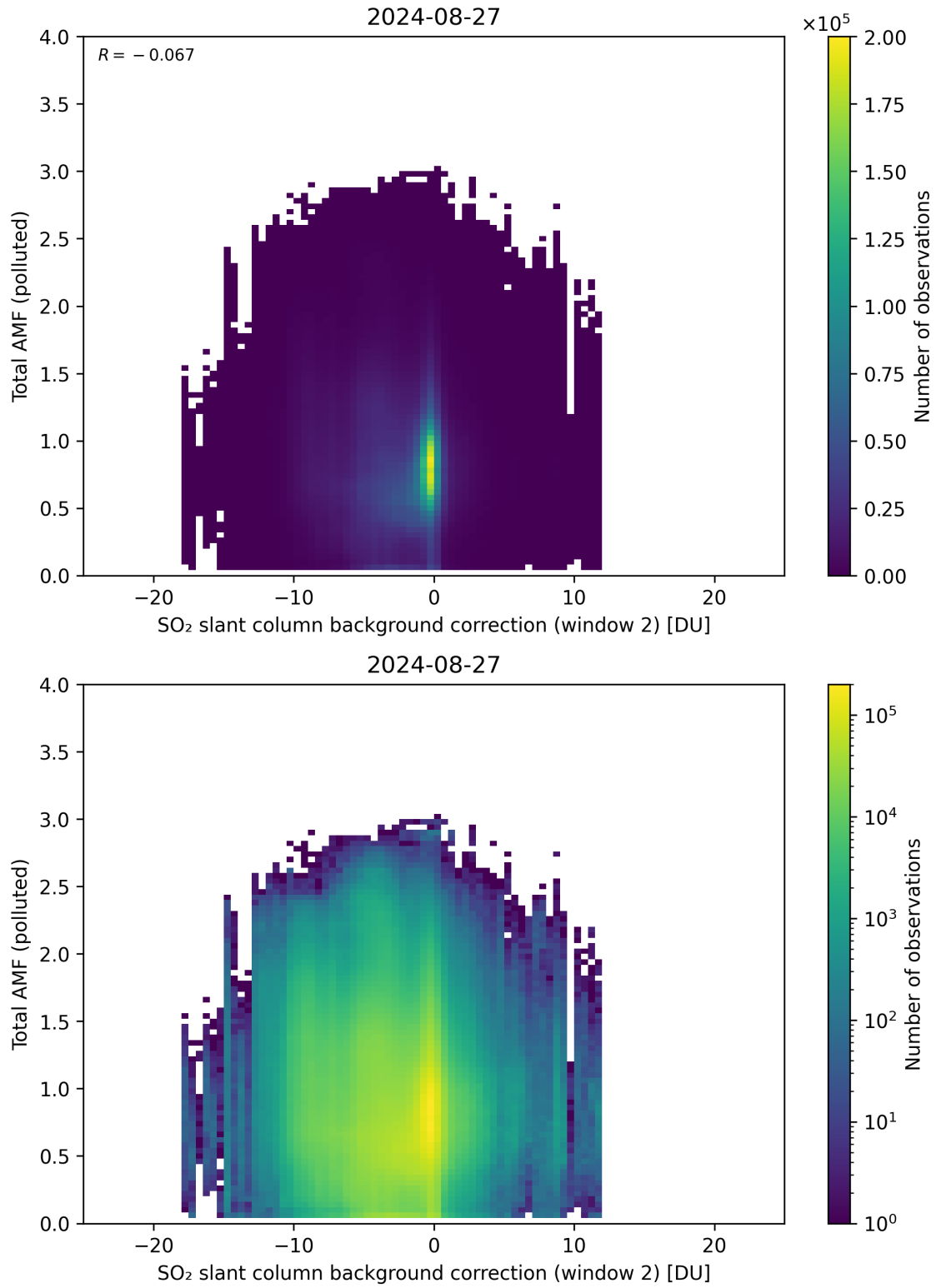
Figure 119: Scatter density plot of “SO 2 slant column background correction (window 2)” against “Total AMF (polluted)” for 2024-08-27 to 2024-08-28.
