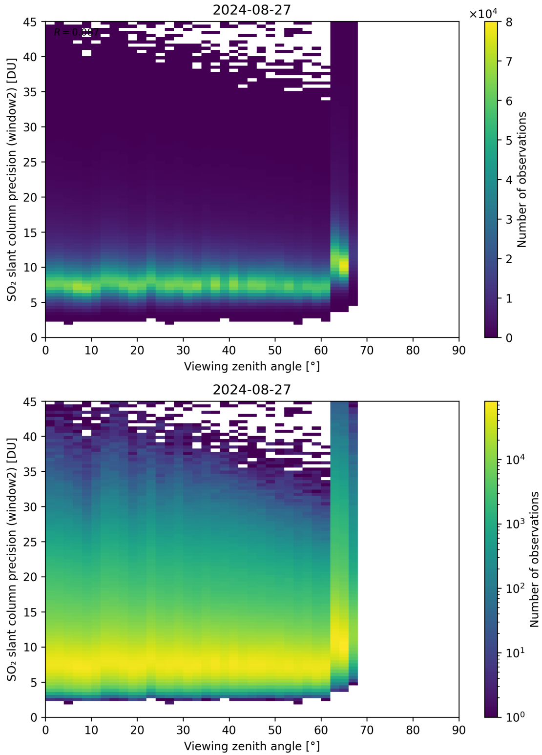
Figure 322: Scatter density plot of “Viewing zenith angle” against “SO 2 slant column precision (window2)” for 2024-08-27 to 2024-08-28.
