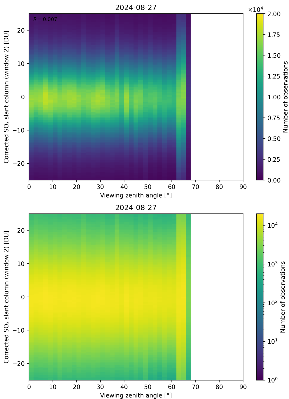
Figure 318: Scatter density plot of “Viewing zenith angle” against “Corrected SO 2 slant column (window 2)” for 2024-08-27 to 2024-08-28.
