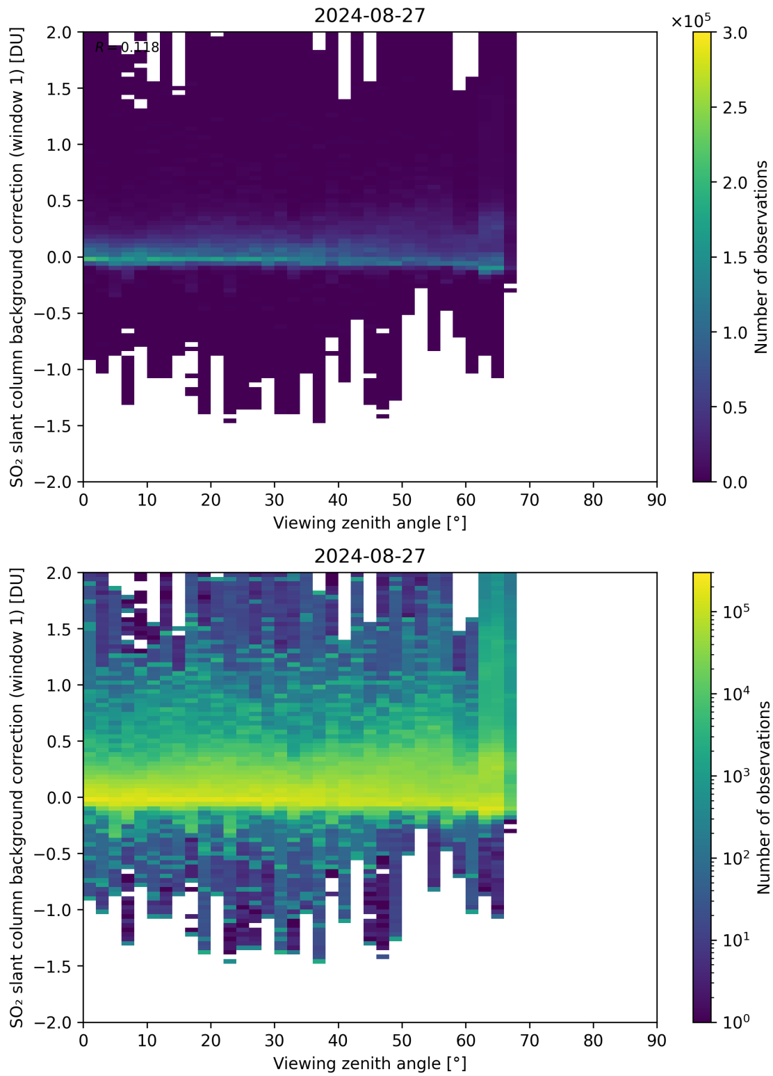
Figure 308: Scatter density plot of “Viewing zenith angle” against “SO 2 slant column background correction (window 1)” for 2024-08-27 to 2024-08-28.
