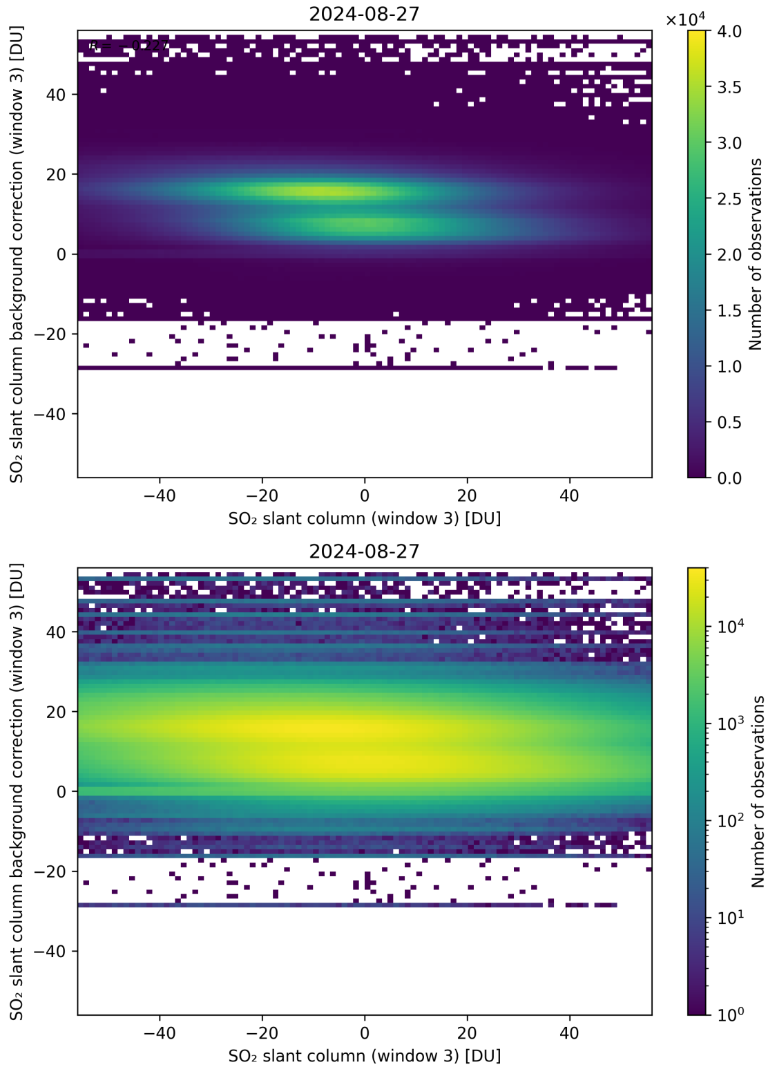
Figure 253: Scatter density plot of “SO 2 slant column (window 3)” against “SO 2 slant column background correction (window 3)” for 2024-08-27 to 2024-08-28.
