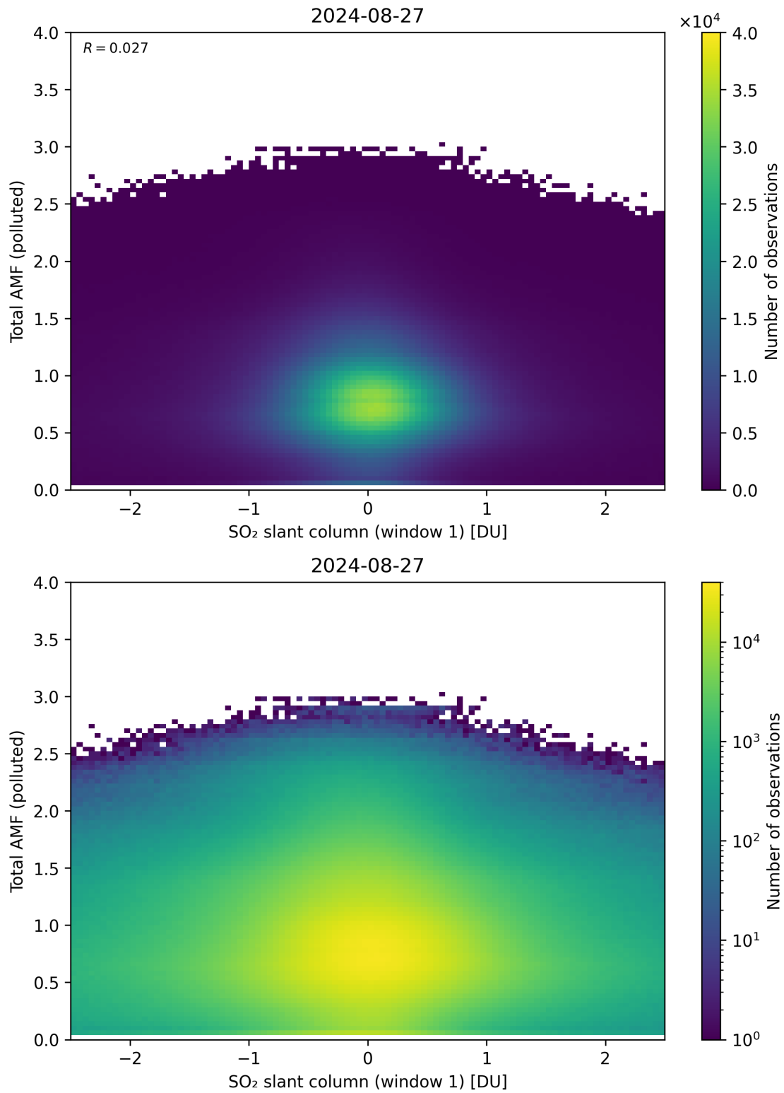
Figure 239: Scatter density plot of “SO 2 slant column (window 1)” against “Total AMF (polluted)” for 2024-08-27 to 2024-08-28.
