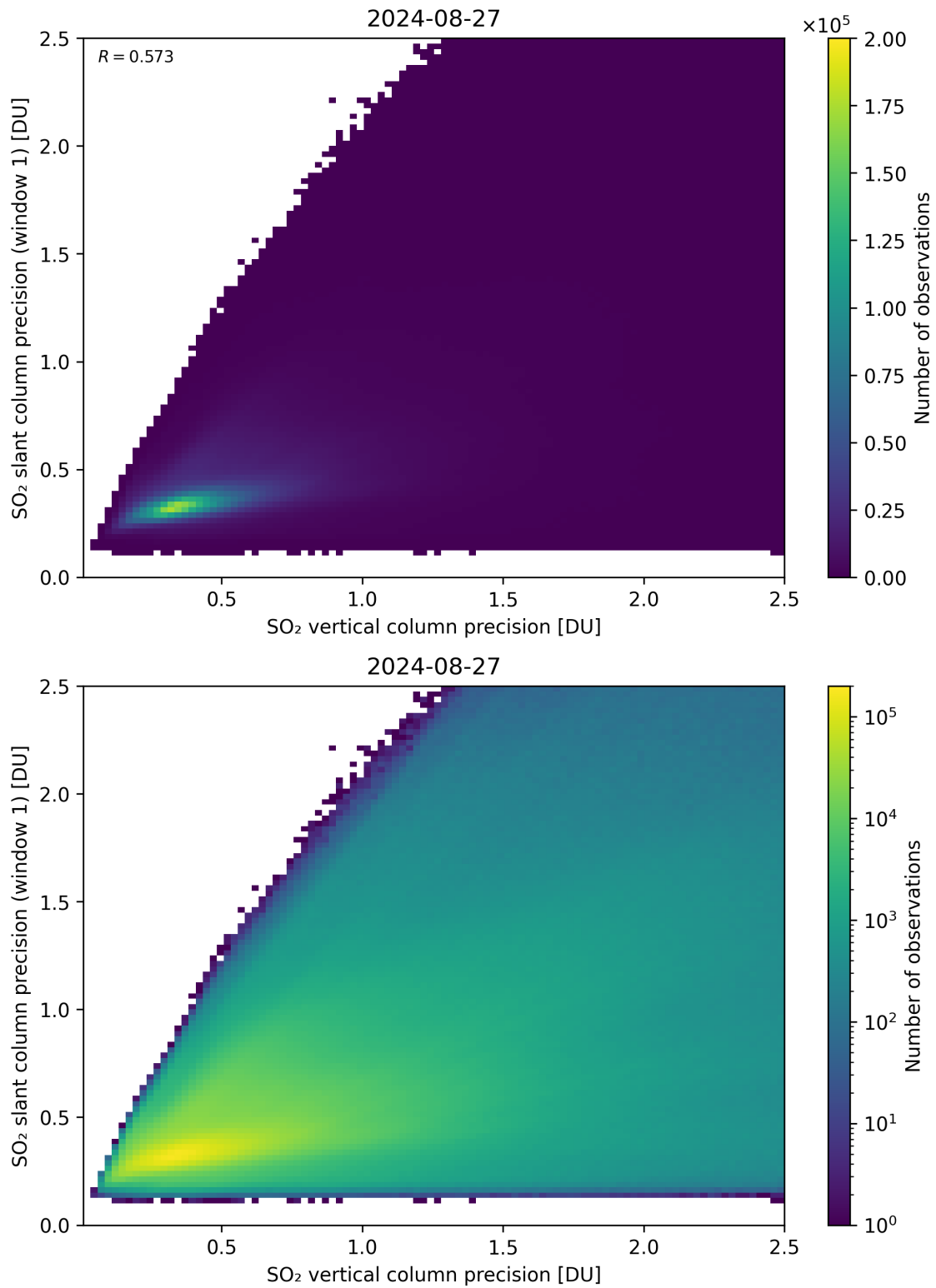
Figure 290: Scatter density plot of “SO 2 vertical column precision” against “SO 2 slant column precision (window 1)” for 2024-08-27 to 2024-08-28.
