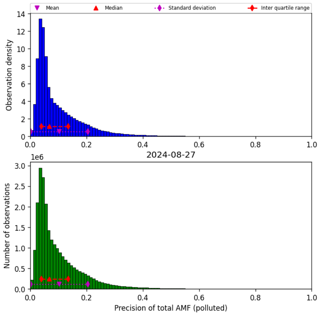
Figure 72: Histogram of “Precision of total AMF (polluted)” for 2024-08-27 to 2024-08-28
