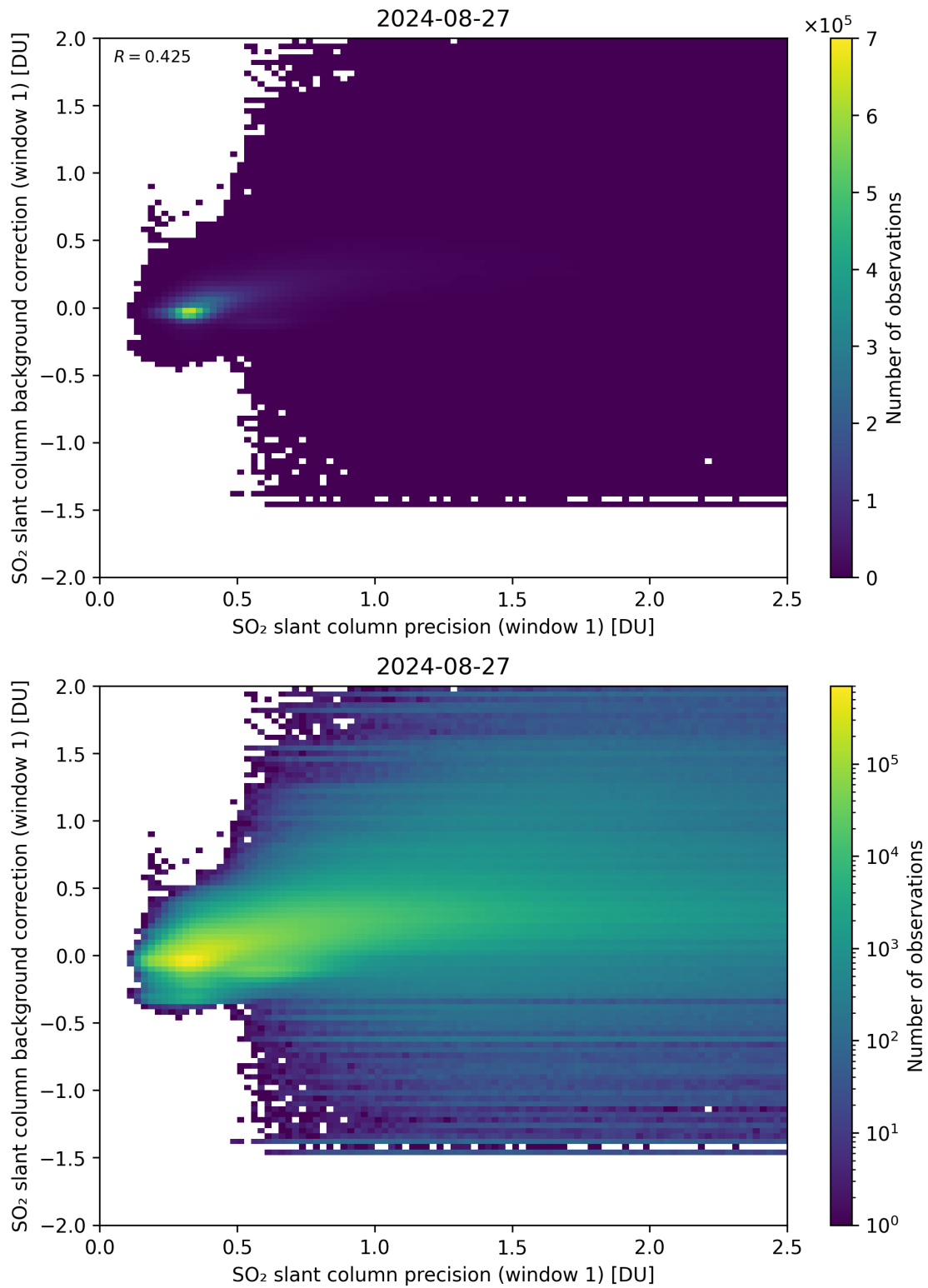
Figure 218: Scatter density plot of “SO 2 slant column precision (window 1)” against “SO 2 slant column background correction (window 1)” for 2024-08-27 to 2024-08-28.
