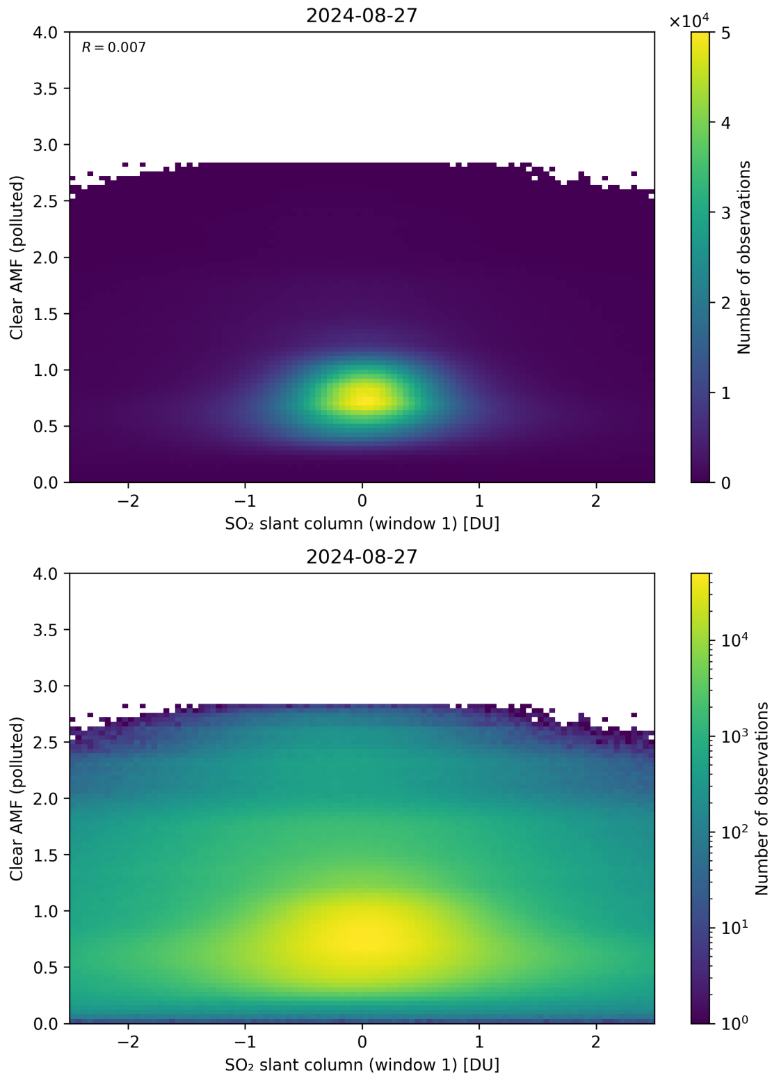
Figure 232: Scatter density plot of “SO 2 slant column (window 1)” against “Clear AMF (polluted)” for 2024-08-27 to 2024-08-28.
