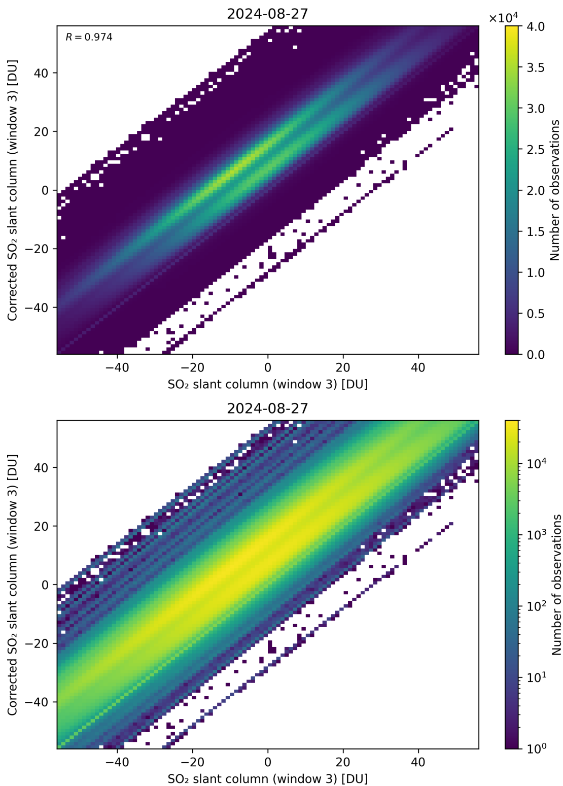
Figure 266: Scatter density plot of “SO 2 slant column (window 3)” against “Corrected SO 2 slant column (window 3)” for 2024-08-27 to 2024-08-28.
