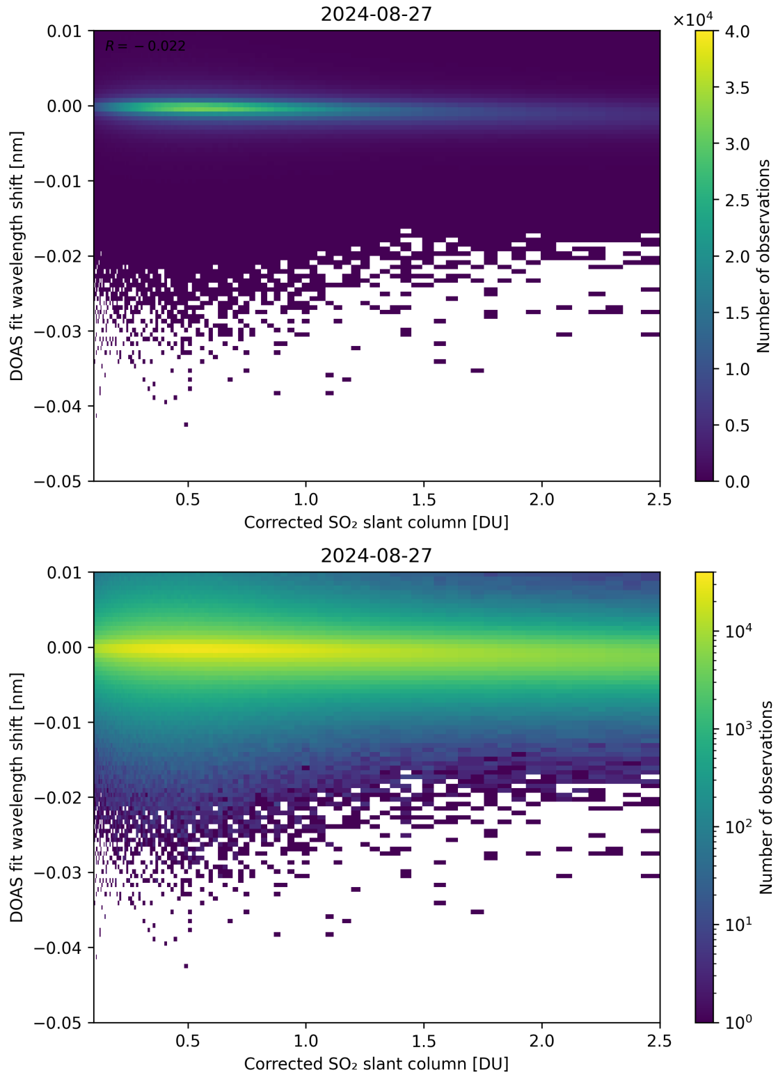
Figure 181: Scatter density plot of “Corrected SO 2 slant column” against “DOAS fit wavelength shift” for 2024-08-27 to 2024-08-28.
