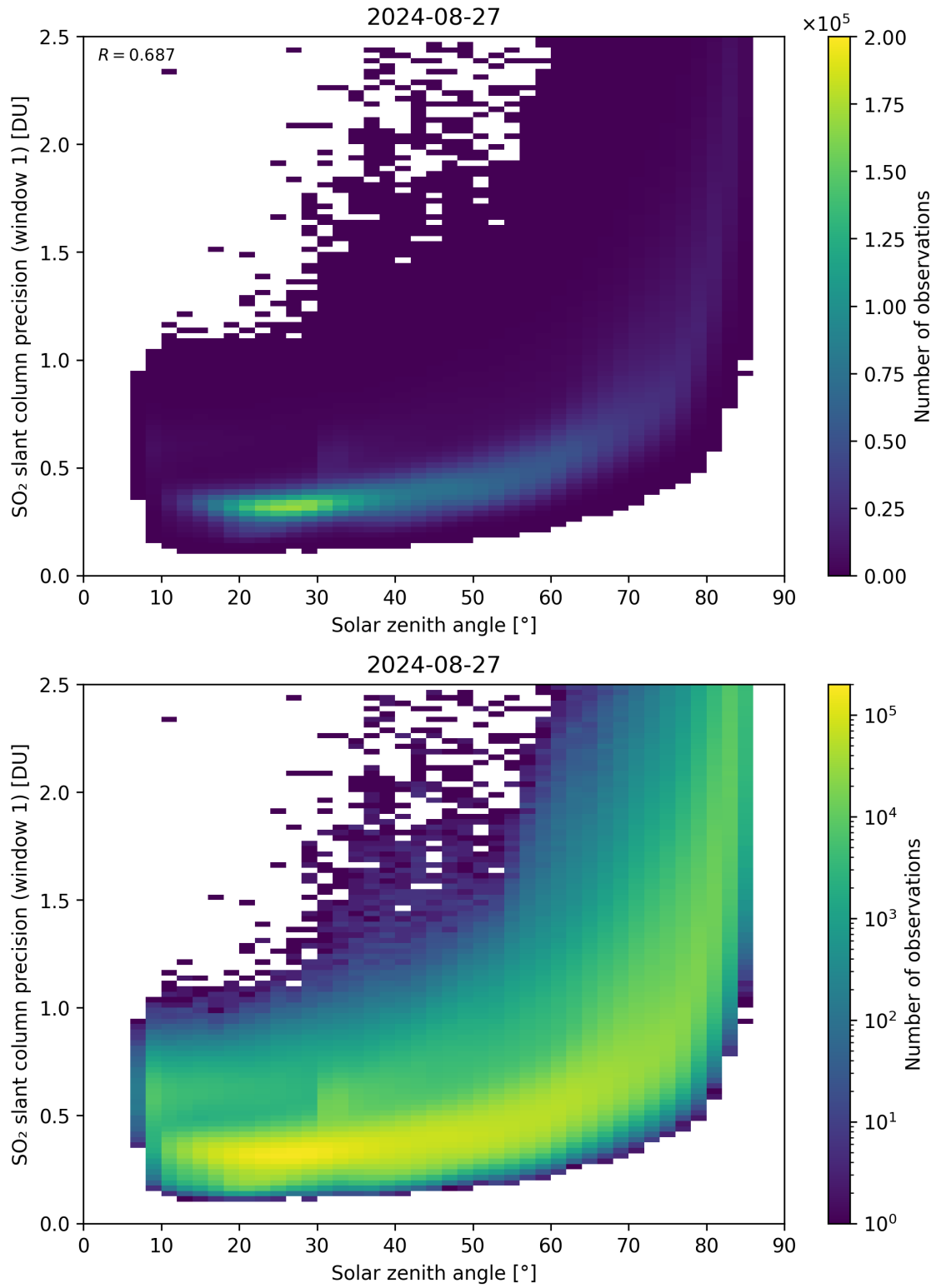
Figure 170: Scatter density plot of “Solar zenith angle” against “SO 2 slant column precision (window 1)” for 2024-08-27 to 2024-08-28.
