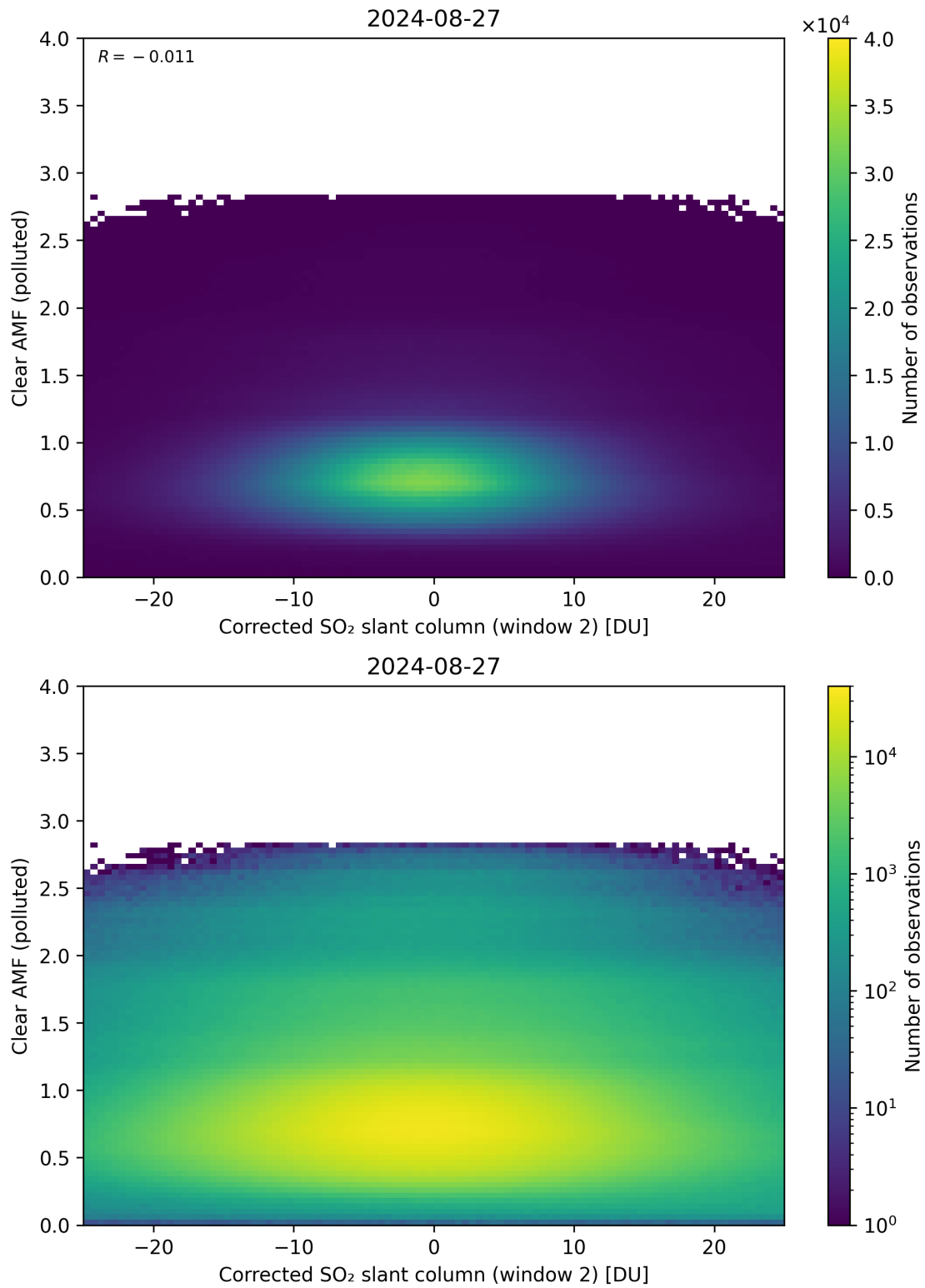
Figure 199: Scatter density plot of “Corrected SO 2 slant column (window 2)” against “Clear AMF (polluted)” for 2024-08-27 to 2024-08-28.
