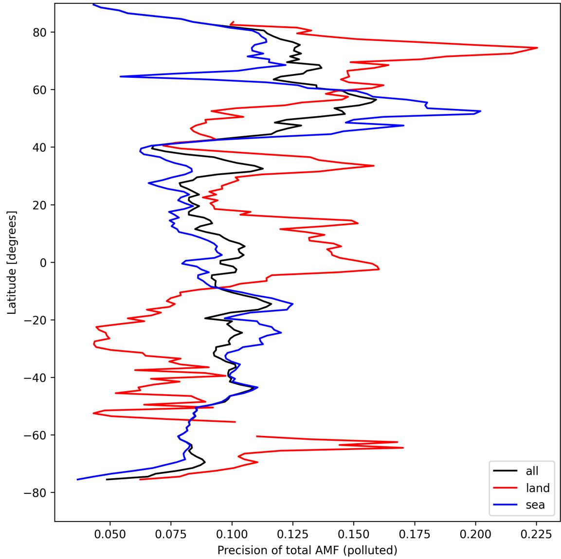
Figure 49: Zonal average of “Precision of total AMF (polluted)” for 2024-08-27 to 2024-08-28.
