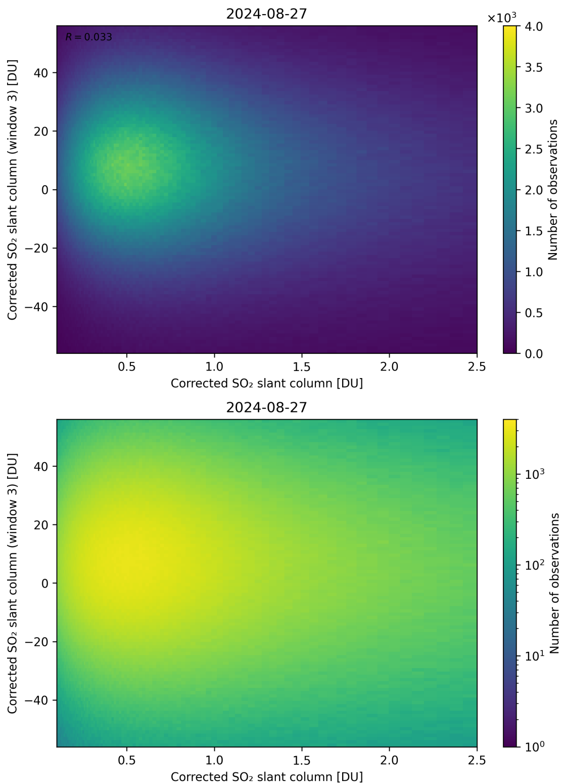
Figure 186: Scatter density plot of “Corrected SO 2 slant column” against “Corrected SO 2 slant column (window 3)” for 2024-08-27 to 2024-08-28.
