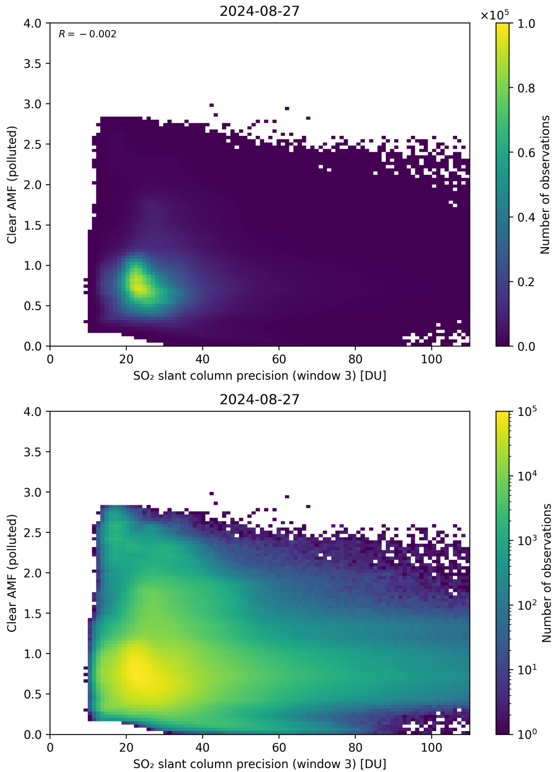
Figure 261: Scatter density plot of “SO 2 slant column precision (window 3)” against “Clear AMF (polluted)” for 2024-08-27 to 2024-08-28.
