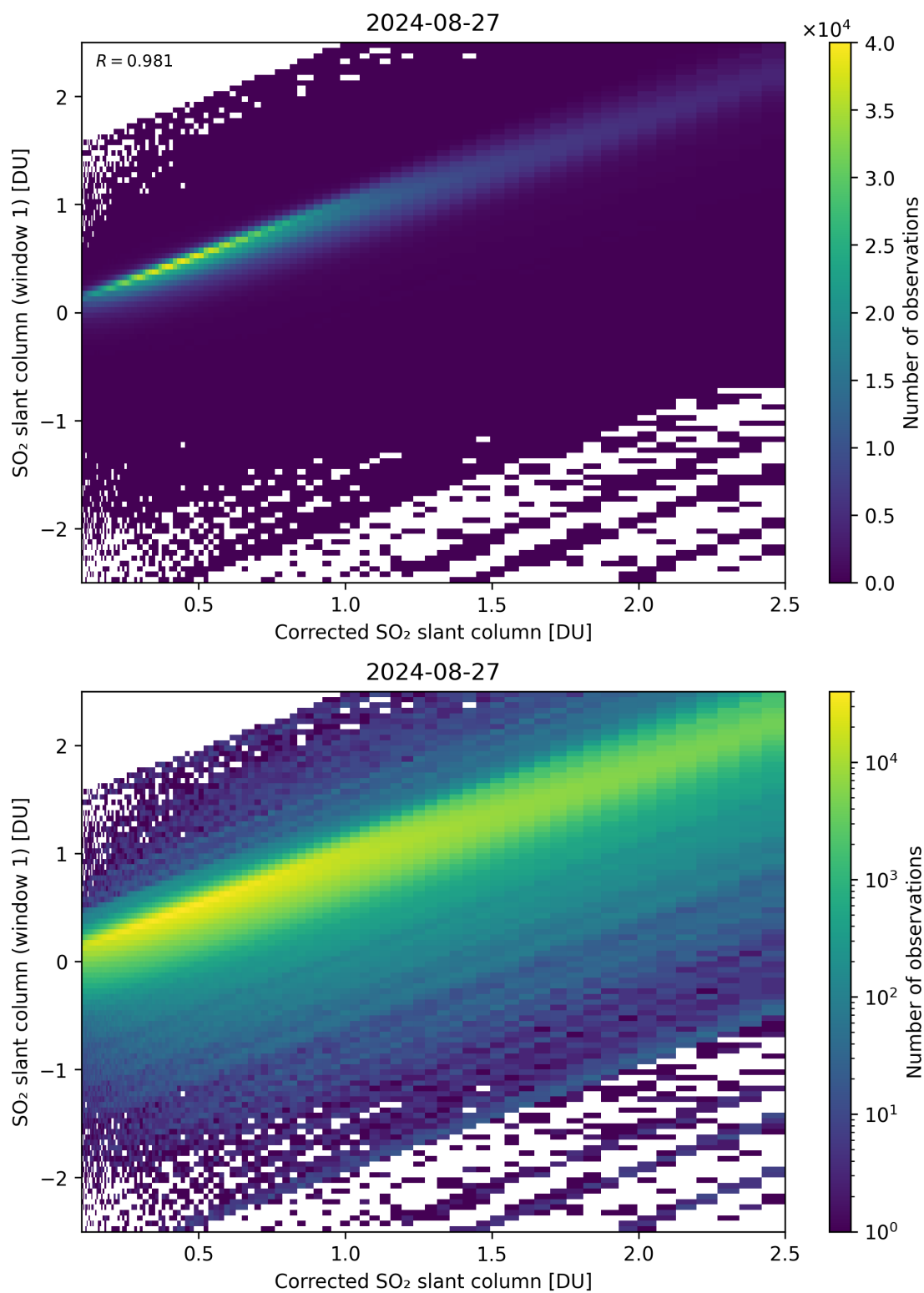
Figure 187: Scatter density plot of “Corrected SO 2 slant column” against “SO 2 slant column (window 1)” for 2024-08-27 to 2024-08-28.
