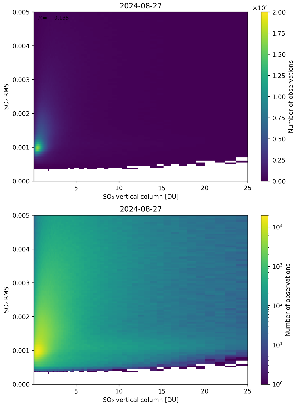
Figure 278: Scatter density plot of “SO 2 vertical column” against “SO 2 RMS” for 2024-08-27 to 2024-08-28.
