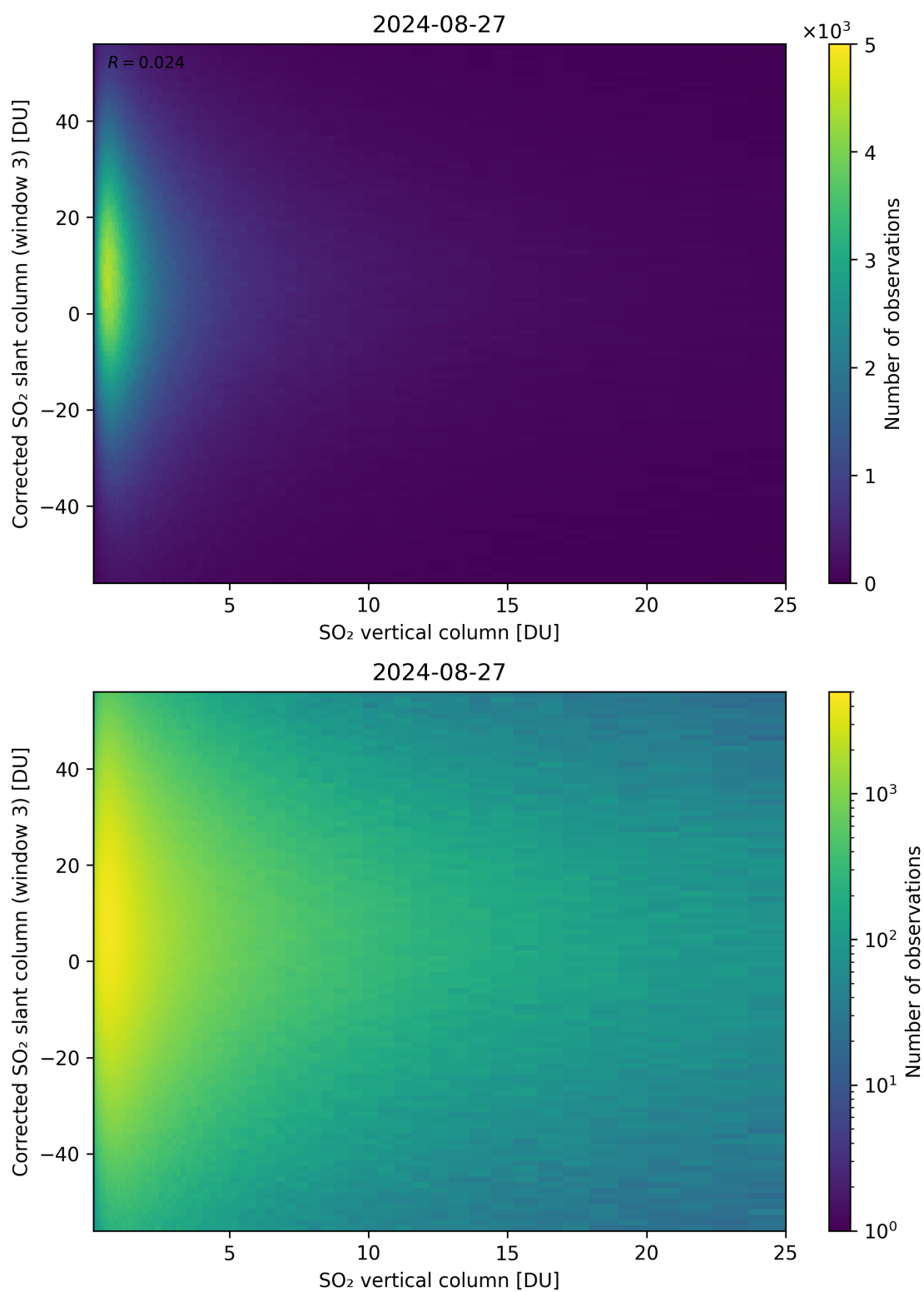
Figure 299: Scatter density plot of “SO 2 vertical column” against “Corrected SO 2 slant column (window 3)” for 2024-08-27 to 2024-08-28.
