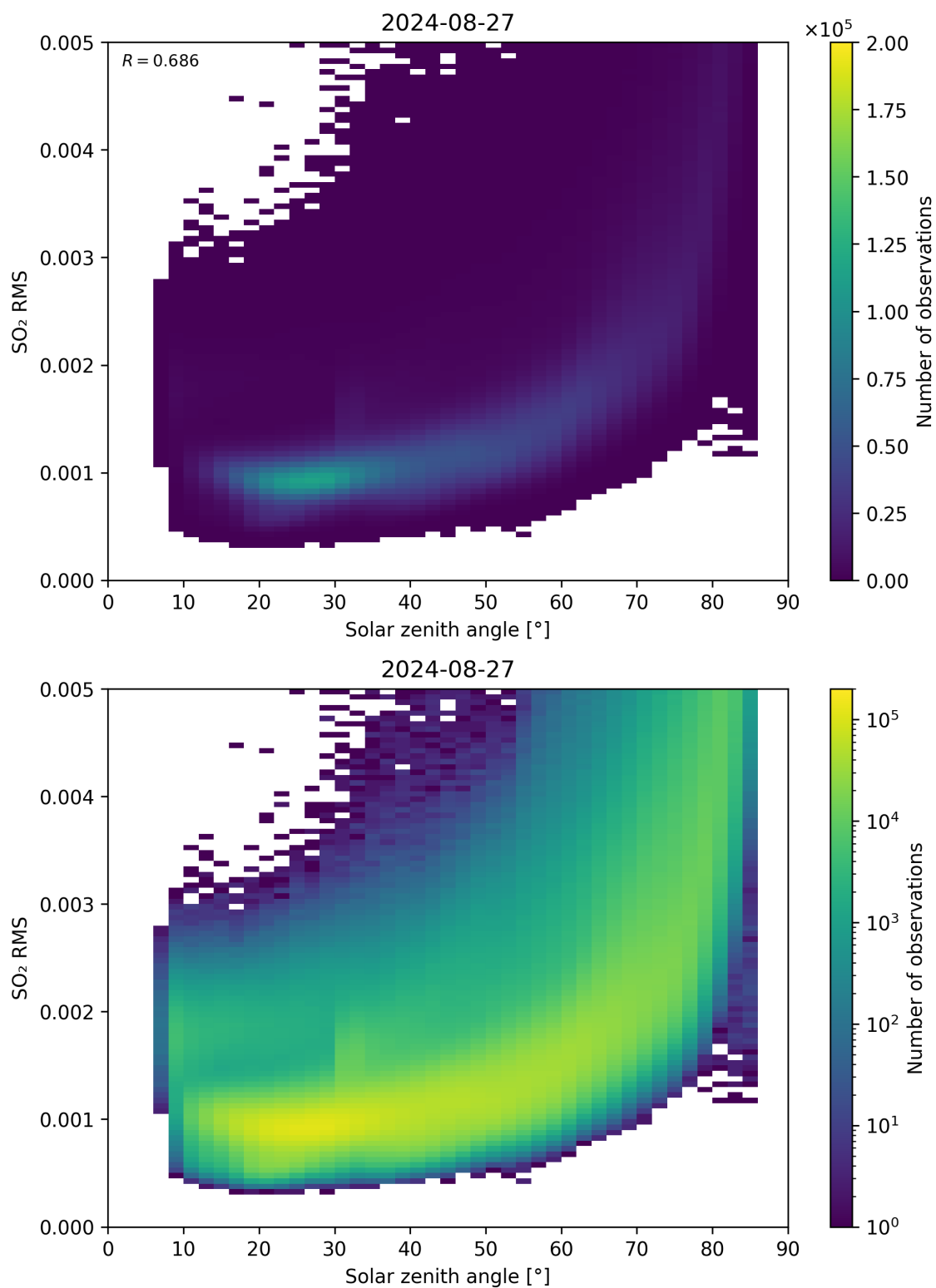
Figure 163: Scatter density plot of “Solar zenith angle” against “SO 2 RMS” for 2024-08-27 to 2024-08-28.
