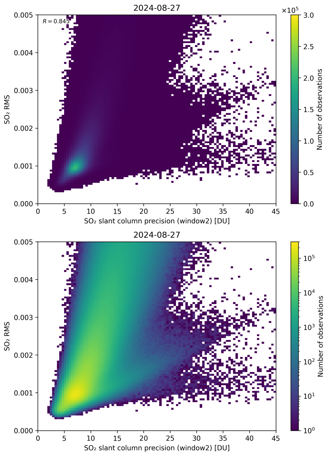
Figure 245: Scatter density plot of “SO 2 slant column precision (window2)” against “SO 2 RMS” for 2024-08-27 to 2024-08-28.
