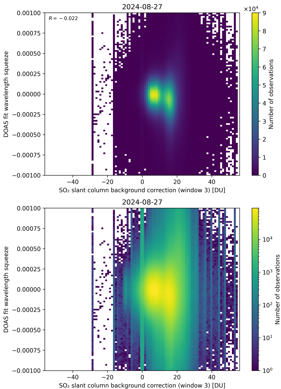
Figure 122: Scatter density plot of “SO 2 slant column background correction (window 3)” against “DOAS fit wavelength squeeze” for 2024-08-27 to 2024-08-28.
