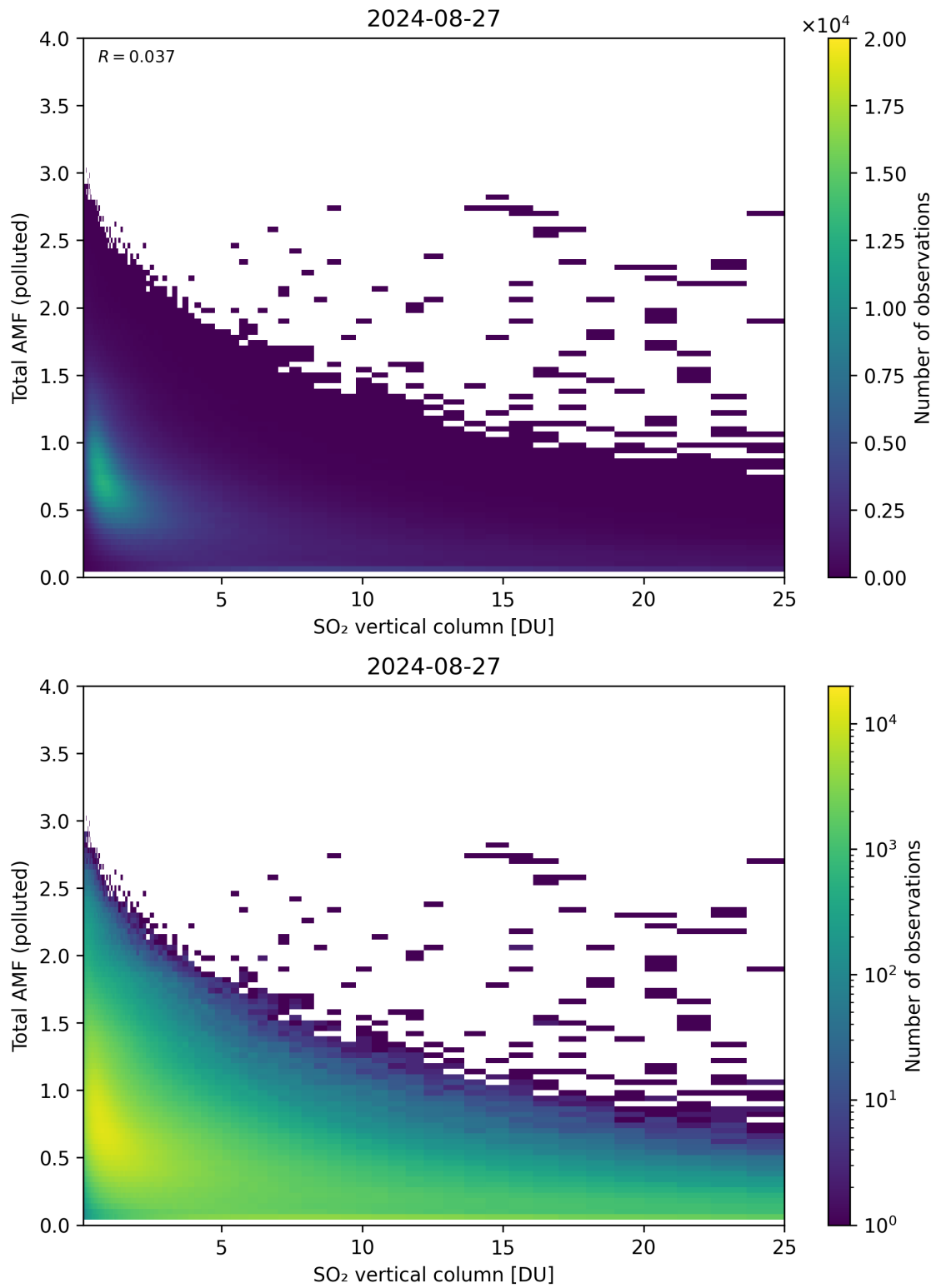
Figure 305: Scatter density plot of “SO 2 vertical column” against “Total AMF (polluted)” for 2024-08-27 to 2024-08-28.
