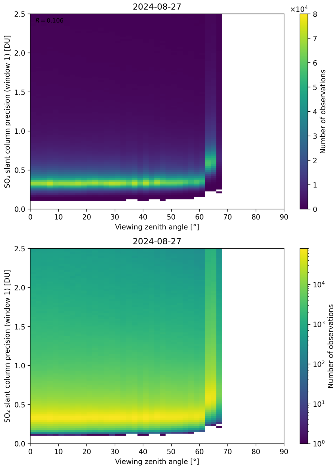
Figure 321: Scatter density plot of “Viewing zenith angle” against “SO 2 slant column precision (window 1)” for 2024-08-27 to 2024-08-28.
