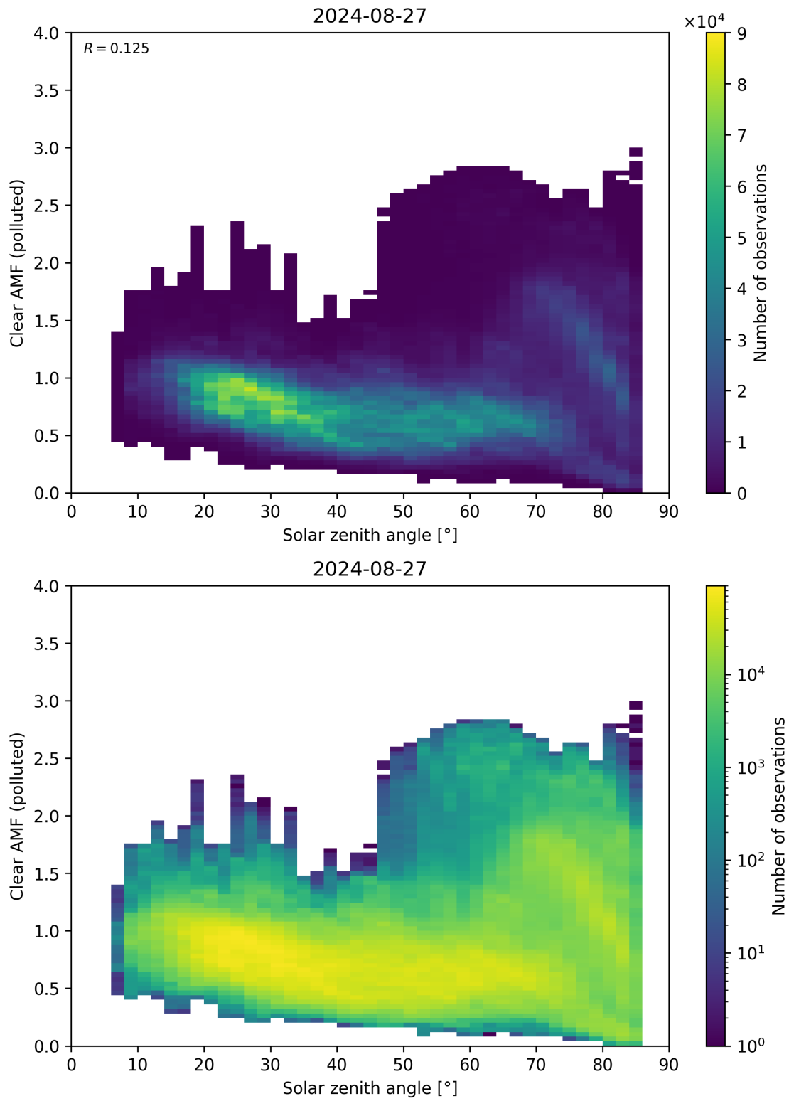
Figure 165: Scatter density plot of “Solar zenith angle” against “Clear AMF (polluted)” for 2024-08-27 to 2024-08-28.
