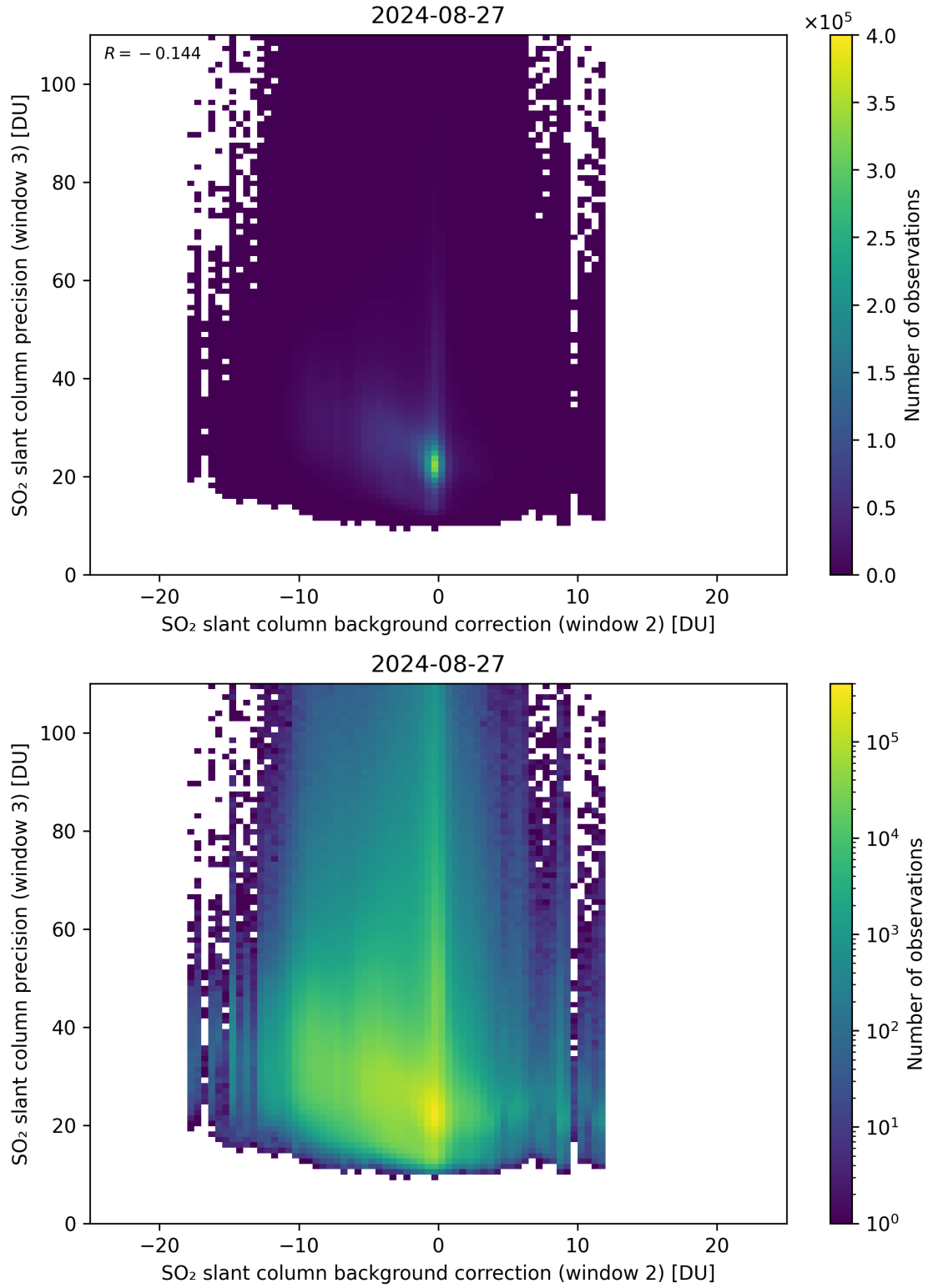
Figure 118: Scatter density plot of “SO 2 slant column background correction (window 2)” against “SO 2 slant column precision (window 3)” for 2024-08-27 to 2024-08-28.
