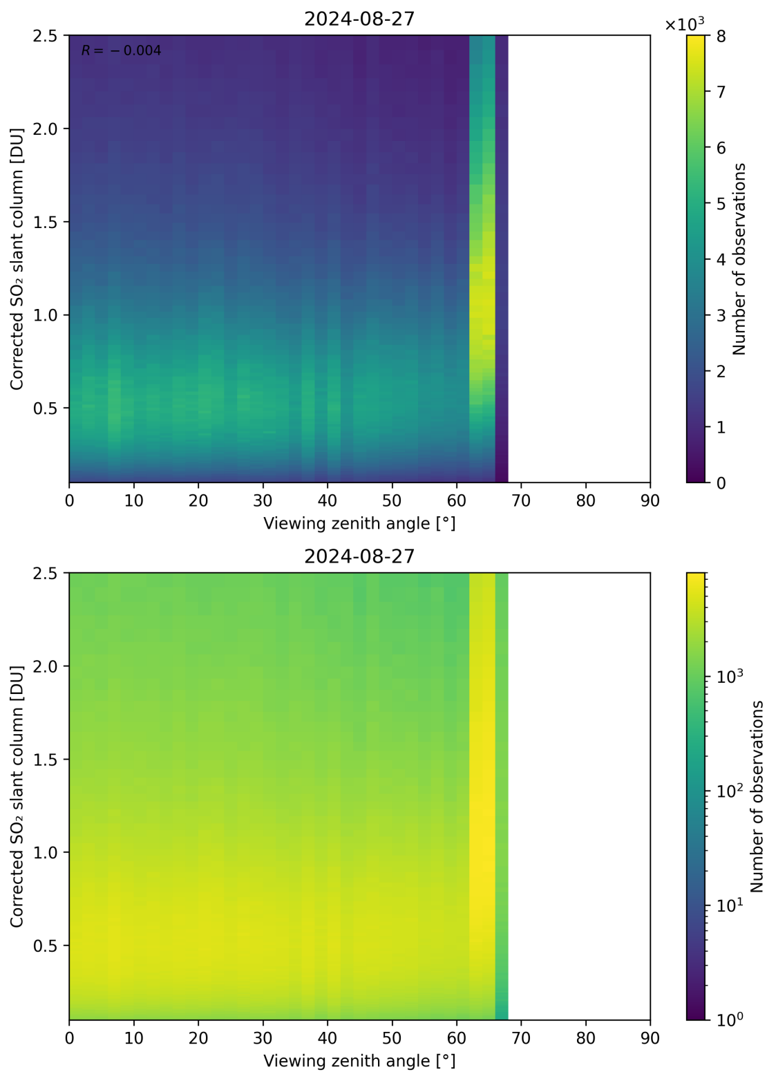
Figure 317: Scatter density plot of “Viewing zenith angle” against “Corrected SO 2 slant column” for 2024-08-27 to 2024-08-28.
