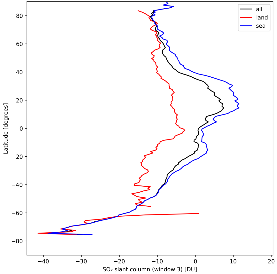
Figure 41: Zonal average of “SO 2 slant column (window 3)” for 2024-08-27 to 2024-08-28.
