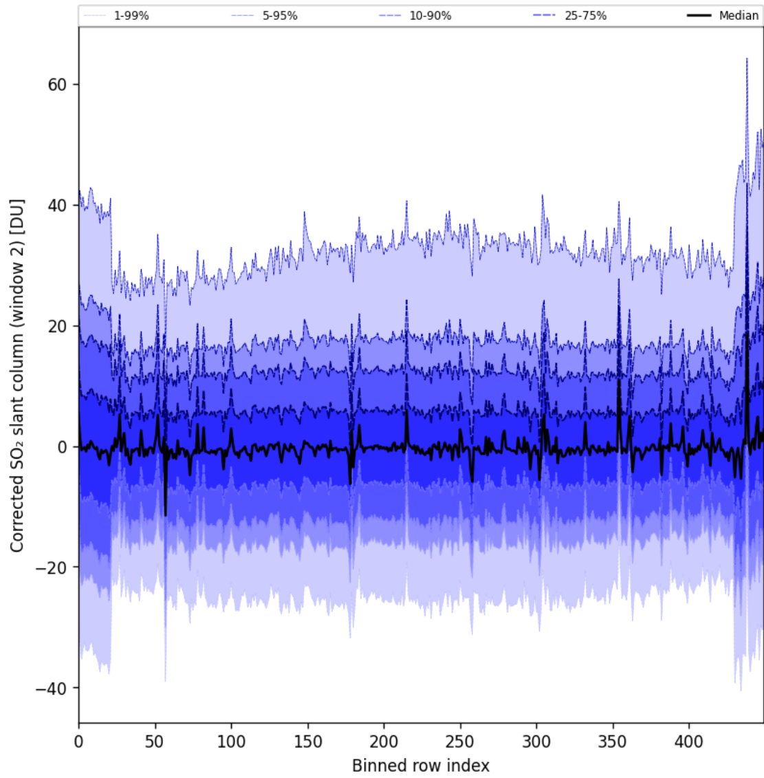
Figure 85: Along track statistics of “Corrected SO 2 slant column (window 2)” for 2024-08-27 to 2024-08-28
