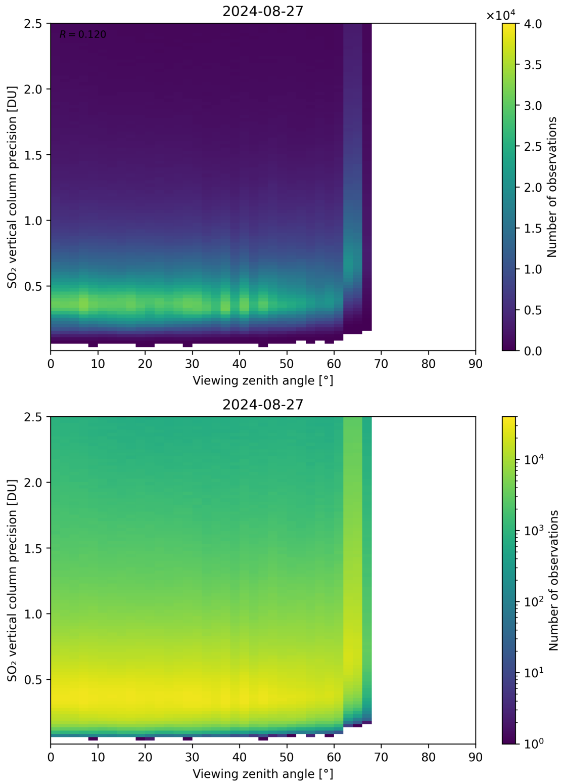
Figure 328: Scatter density plot of “Viewing zenith angle” against “SO 2 vertical column precision” for 2024-08-27 to 2024-08-28.
