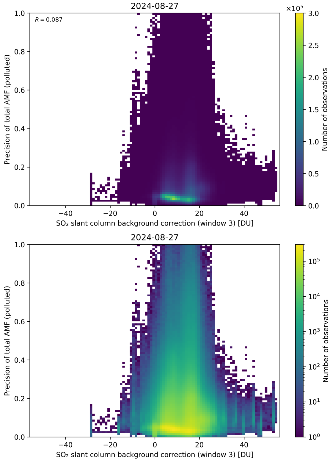
Figure 126: Scatter density plot of “SO 2 slant column background correction (window 3)” against “Precision of total AMF (polluted)” for 2024-08-27 to 2024-08-28.
