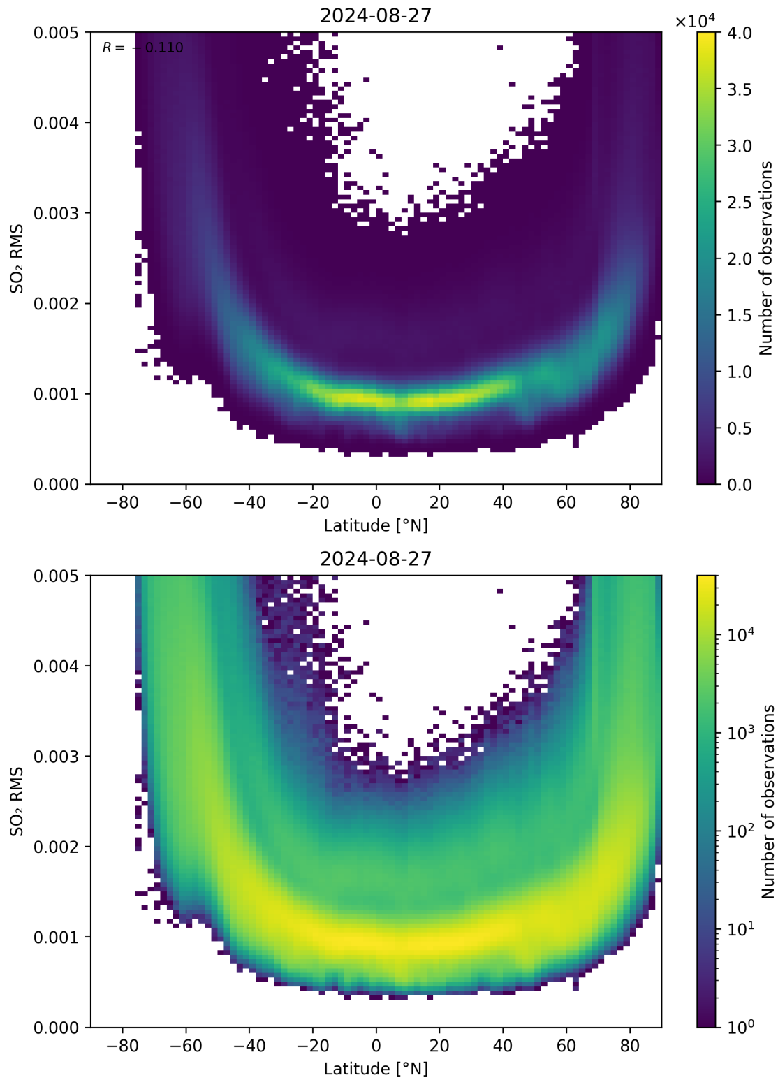
Figure 144: Scatter density plot of “Latitude” against “SO 2 RMS” for 2024-08-27 to 2024-08-28.
