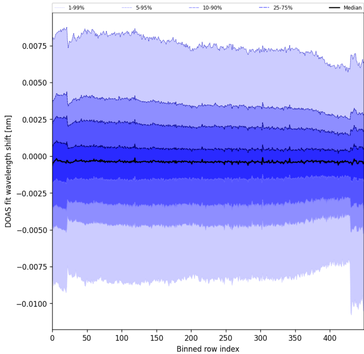
Figure 91: Along track statistics of “DOAS fit wavelength shift” for 2024-08-27 to 2024-08-28
