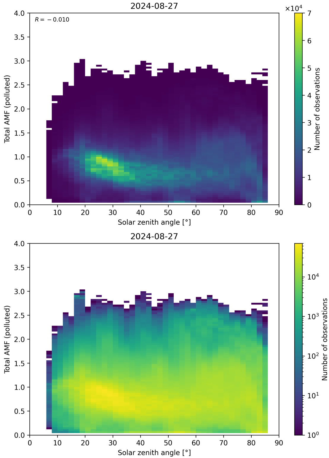
Figure 174: Scatter density plot of “Solar zenith angle” against “Total AMF (polluted)” for 2024-08-27 to 2024-08-28.
