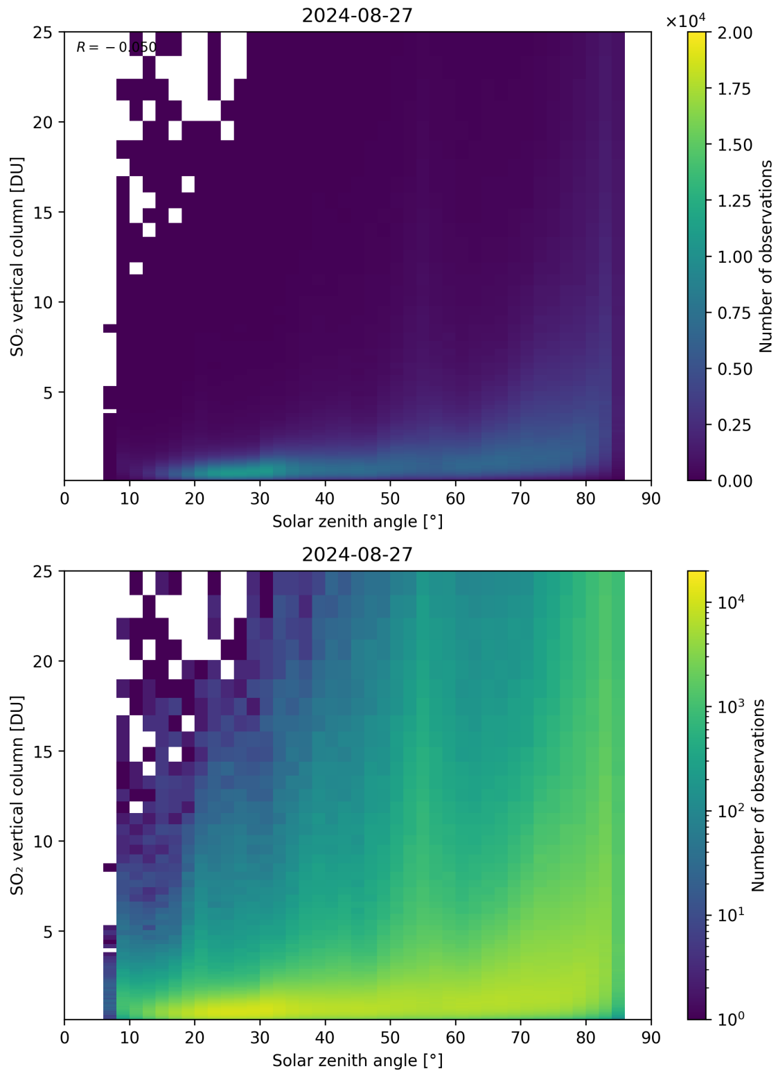
Figure 176: Scatter density plot of “Solar zenith angle” against “SO 2 vertical column” for 2024-08-27 to 2024-08-28.
