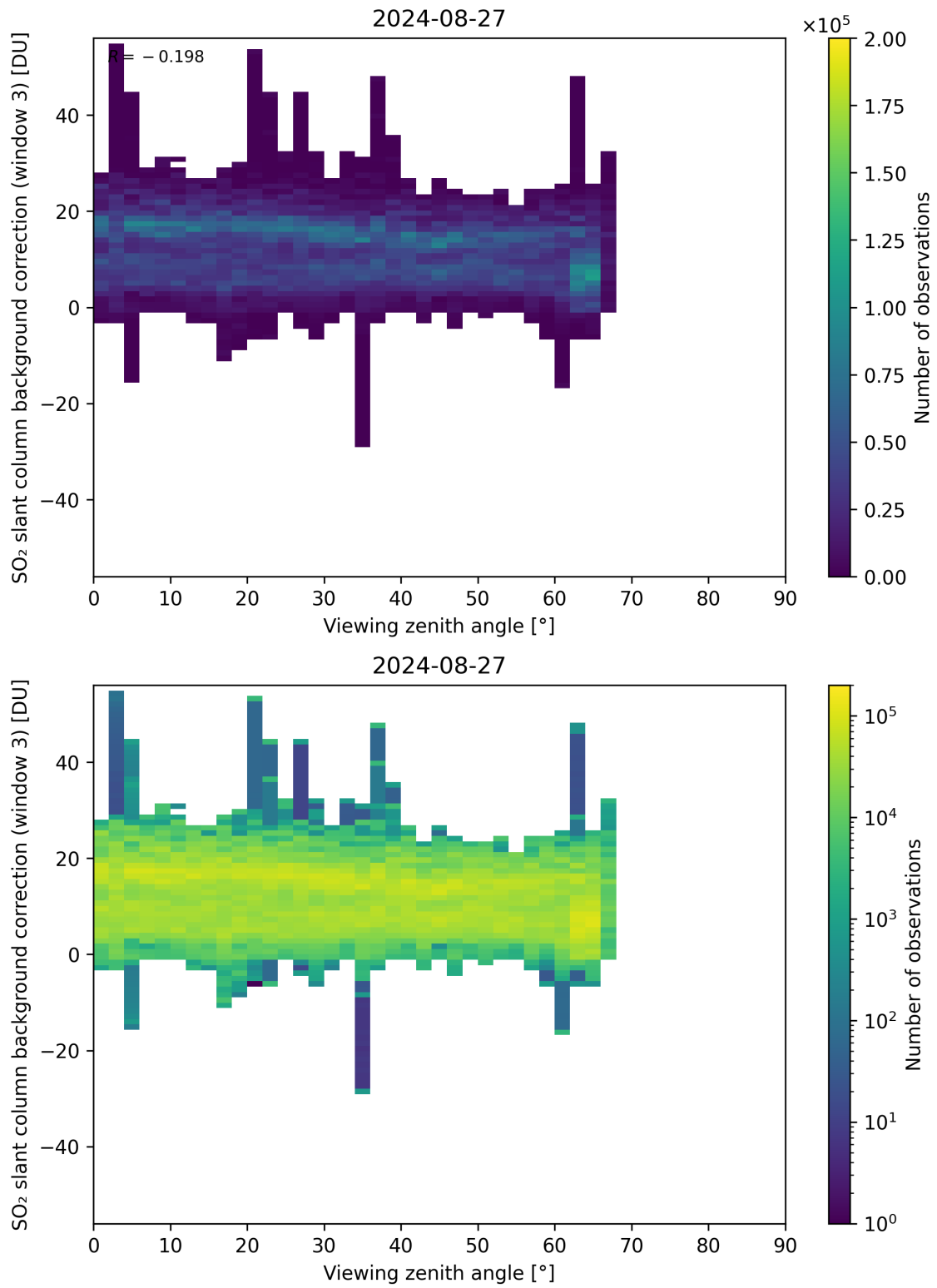
Figure 310: Scatter density plot of “Viewing zenith angle” against “SO 2 slant column background correction (window 3)” for 2024-08-27 to 2024-08-28.
