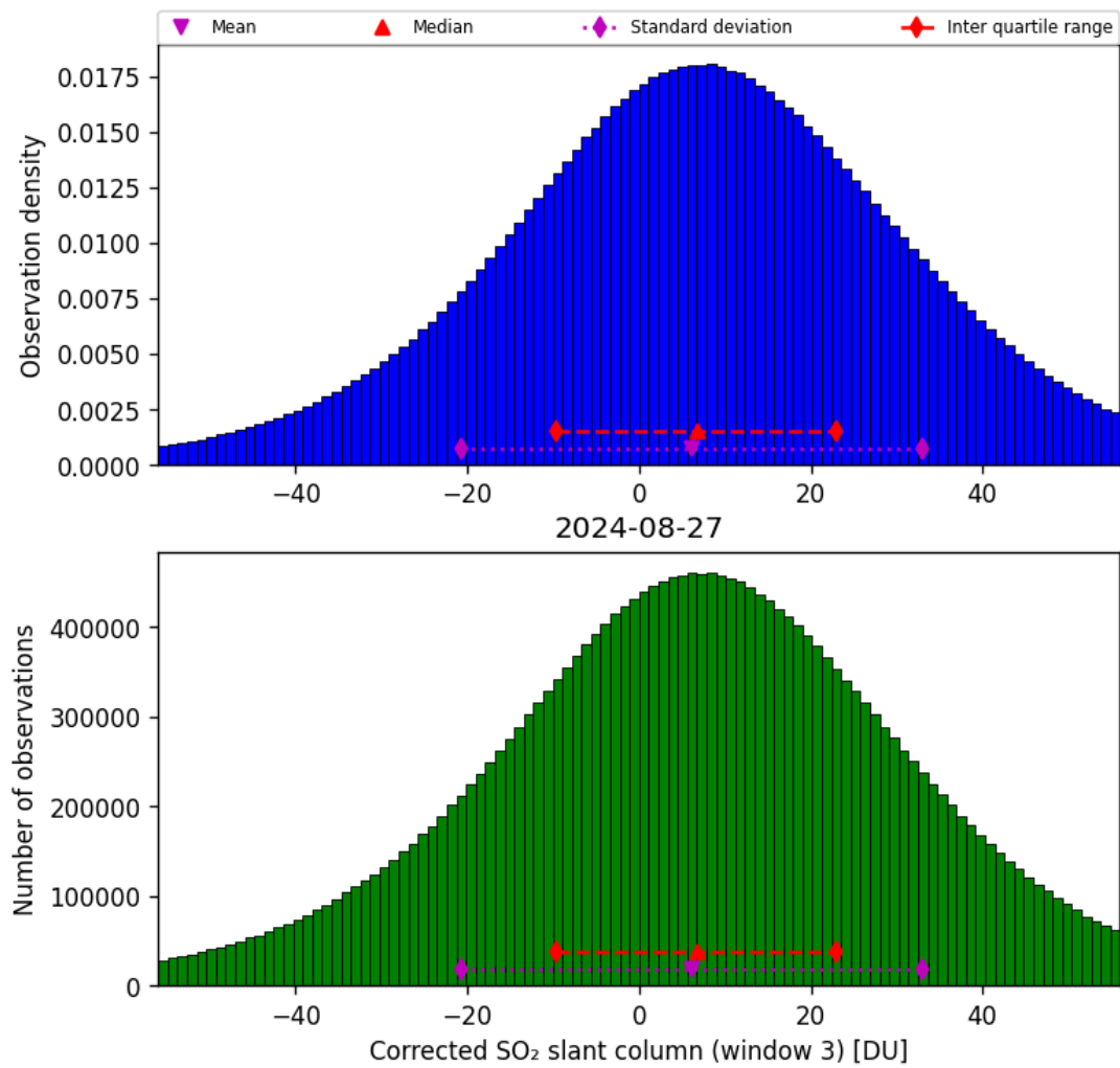
Figure 66: Histogram of “Corrected SO 2 slant column (window 3)” for 2024-08-27 to 2024-08-28
