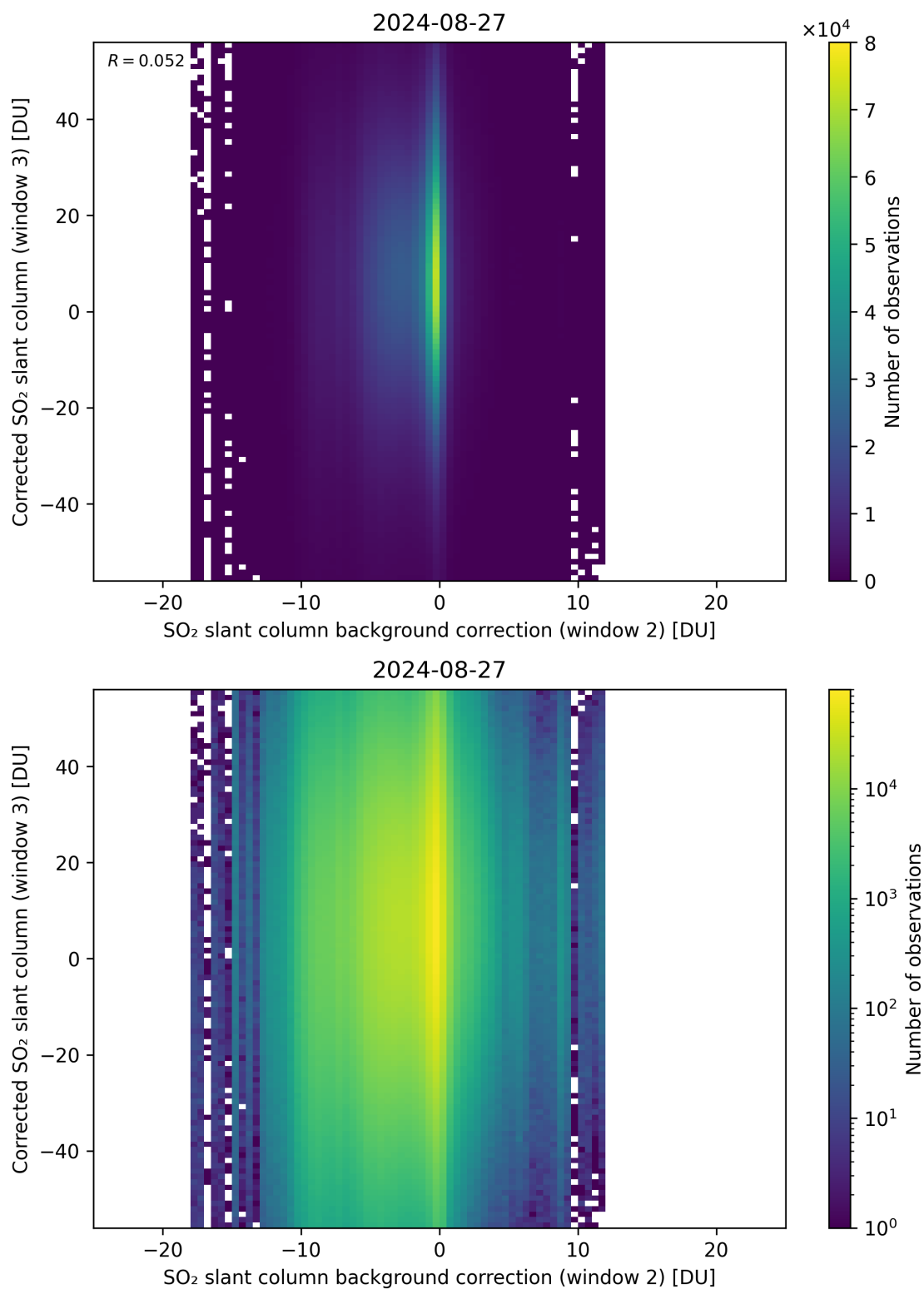
Figure 116: Scatter density plot of “SO 2 slant column background correction (window 2)” against “Corrected SO 2 slant column (window 3)” for 2024-08-27 to 2024-08-28.
