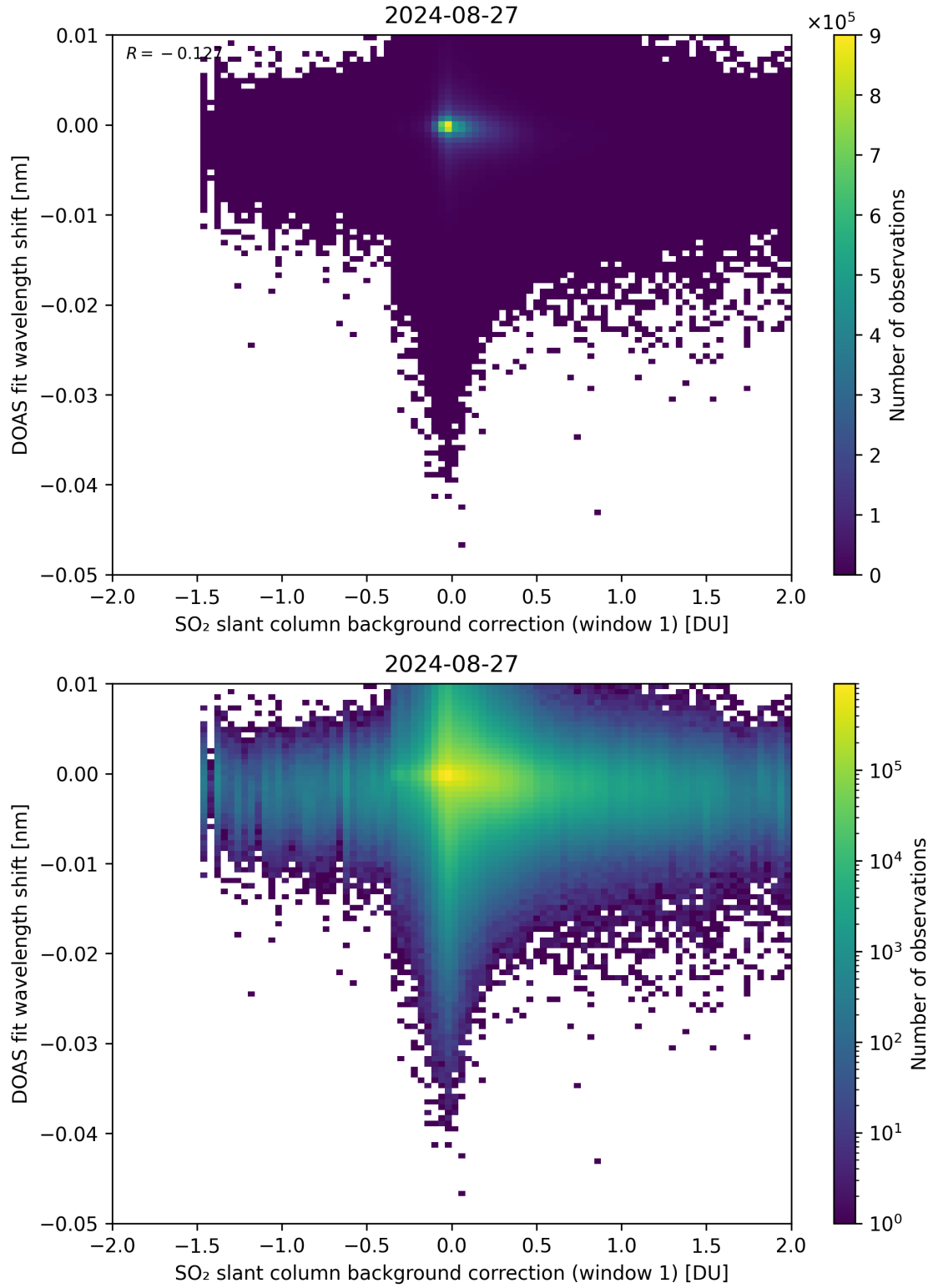
Figure 100: Scatter density plot of “SO 2 slant column background correction (window 1)” against “DOAS fit wavelength shift” for 2024-08-27 to 2024-08-28.
