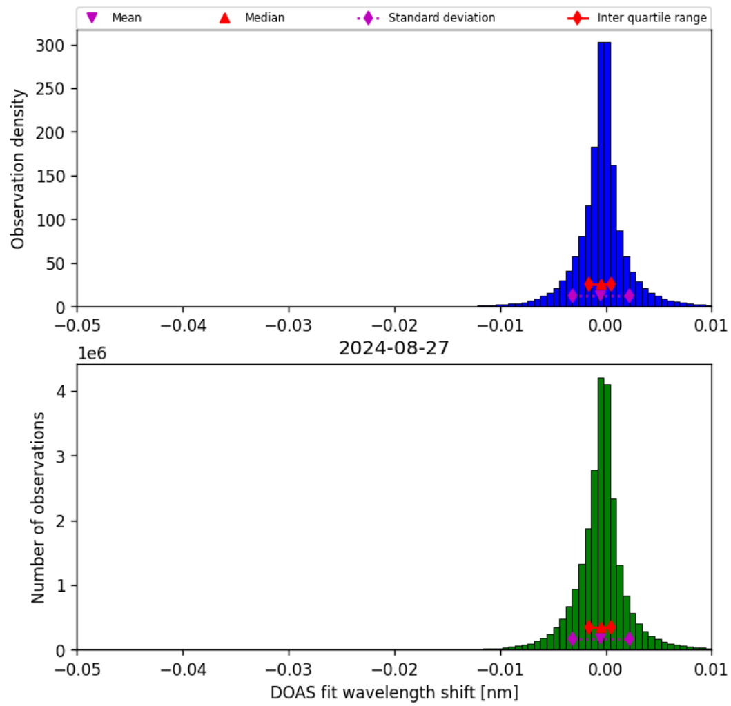
Figure 68: Histogram of “DOAS fit wavelength shift” for 2024-08-27 to 2024-08-28
