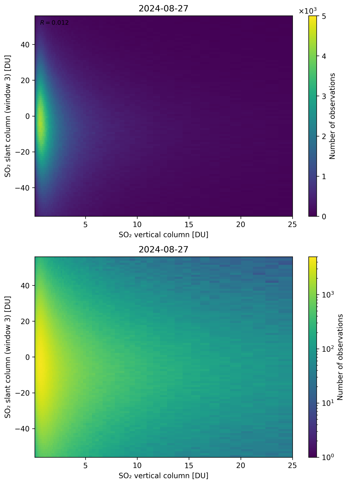
Figure 303: Scatter density plot of “SO 2 vertical column” against “SO 2 slant column (window 3)” for 2024-08-27 to 2024-08-28.
