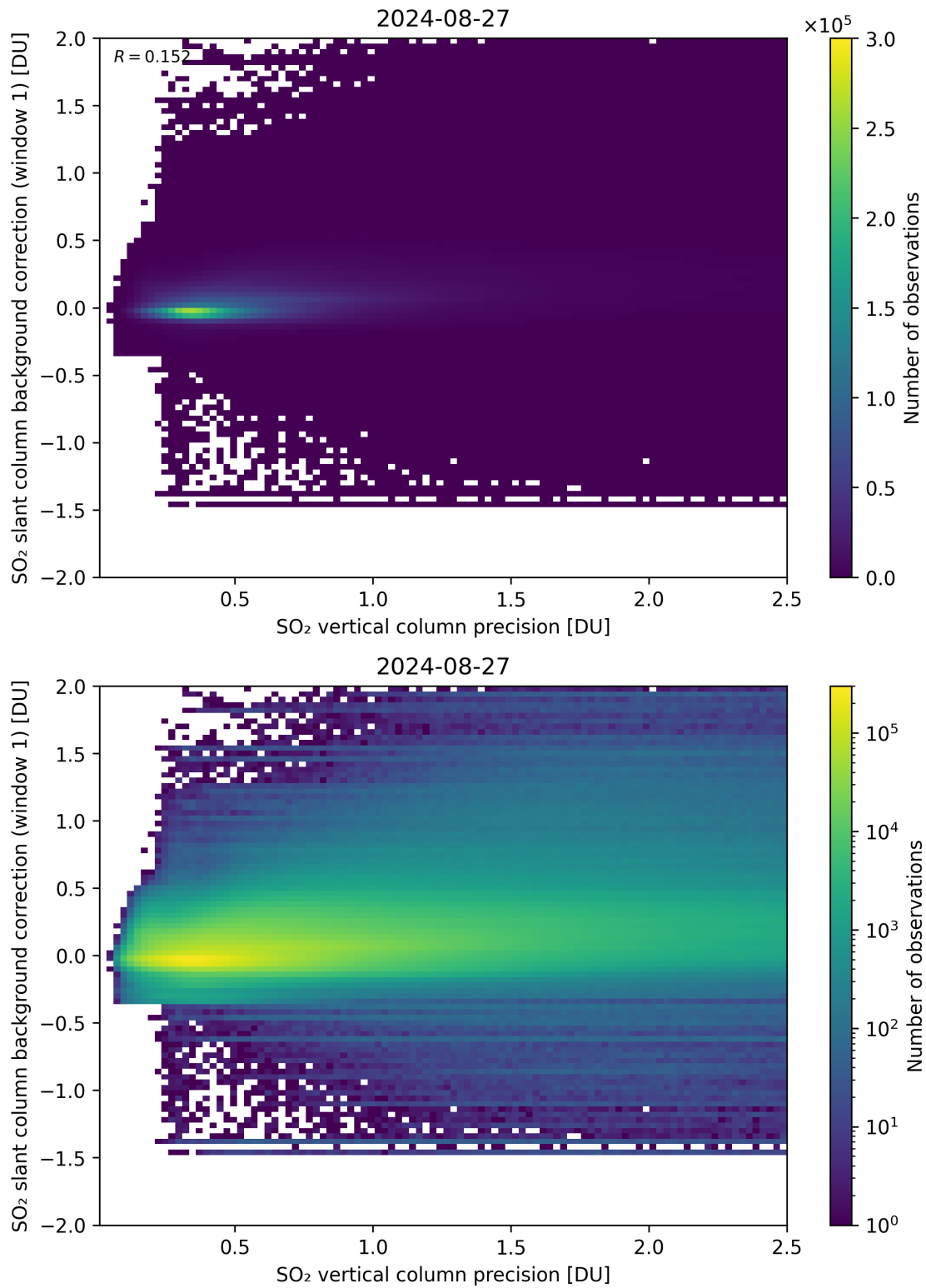
Figure 279: Scatter density plot of “SO 2 vertical column precision” against “SO 2 slant column background correction (window 1)” for 2024-08-27 to 2024-08-28.
