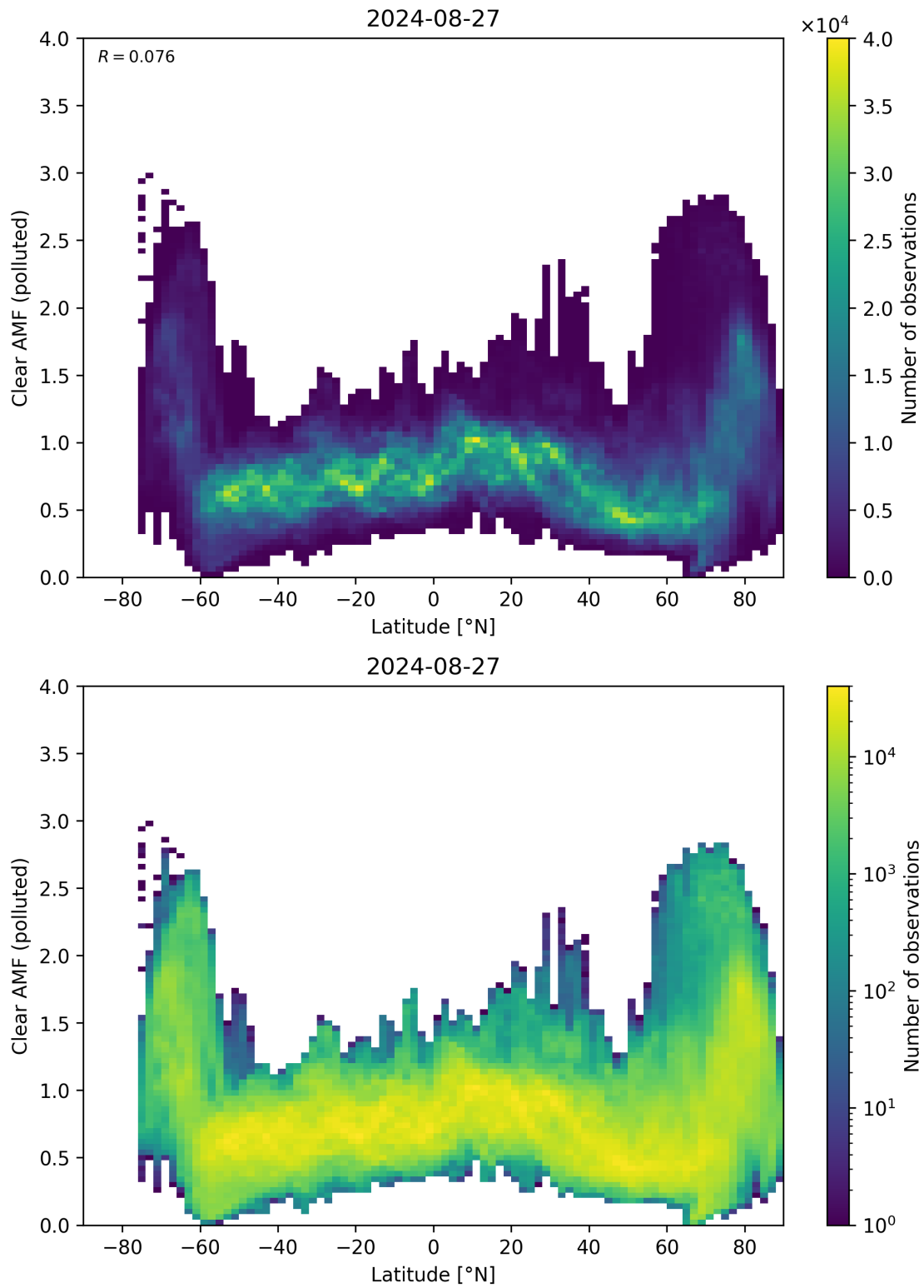
Figure 145: Scatter density plot of “Latitude” against “Clear AMF (polluted)” for 2024-08-27 to 2024-08-28.
