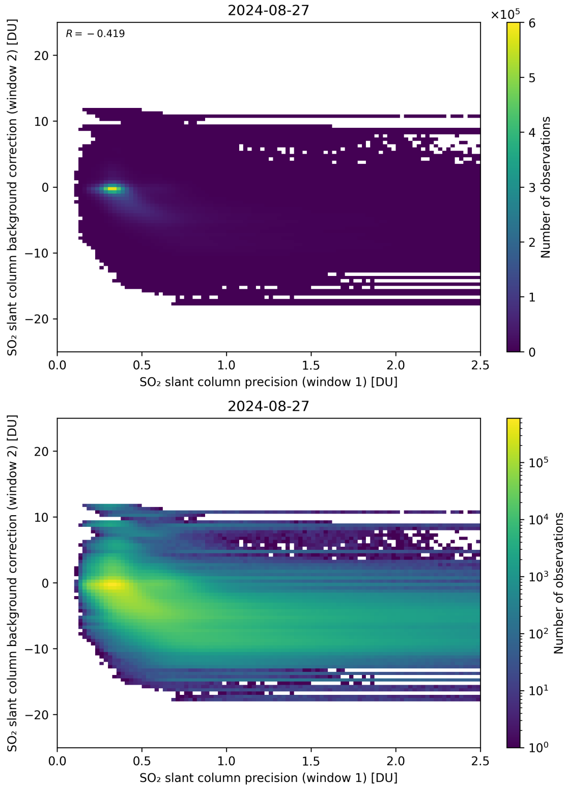
Figure 219: Scatter density plot of “SO 2 slant column precision (window 1)” against “SO 2 slant column background correction (window 2)” for 2024-08-27 to 2024-08-28.
