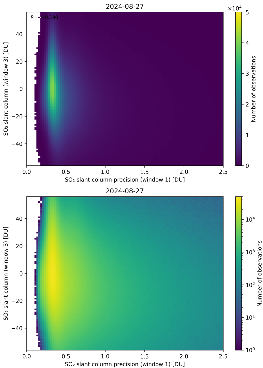
Figure 228: Scatter density plot of “SO 2 slant column precision (window 1)” against “SO 2 slant column (window 3)” for 2024-08-27 to 2024-08-28.
