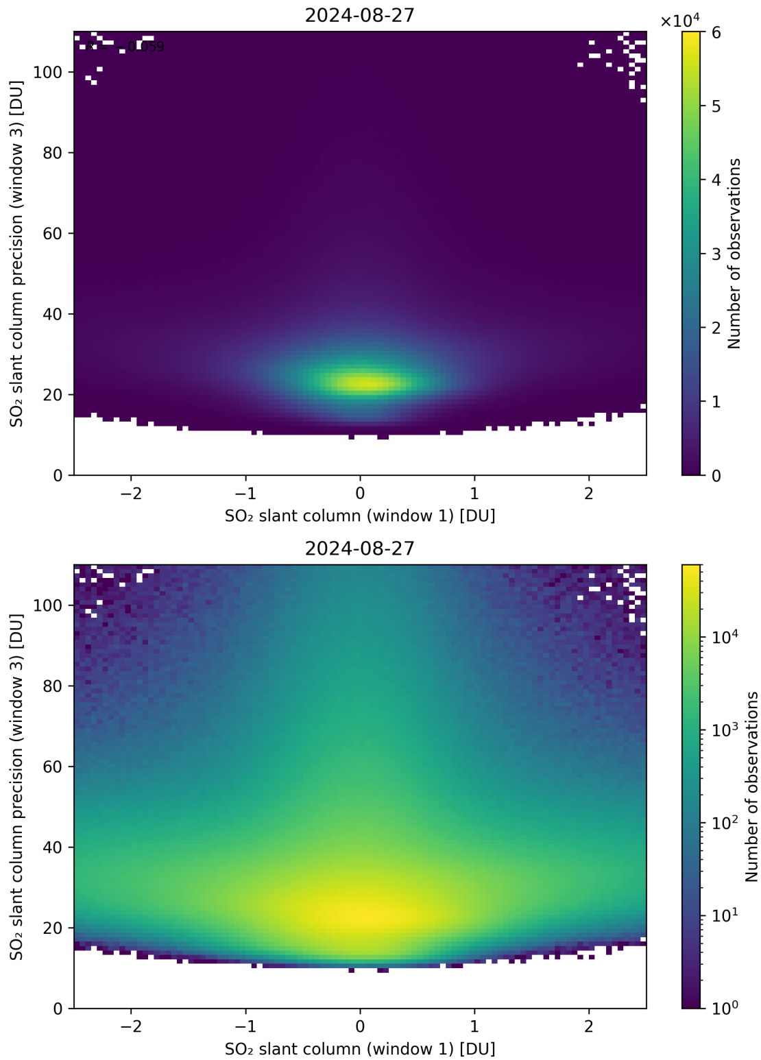
Figure 238: Scatter density plot of “SO 2 slant column (window 1)” against “SO 2 slant column precision (window 3)” for 2024-08-27 to 2024-08-28.
