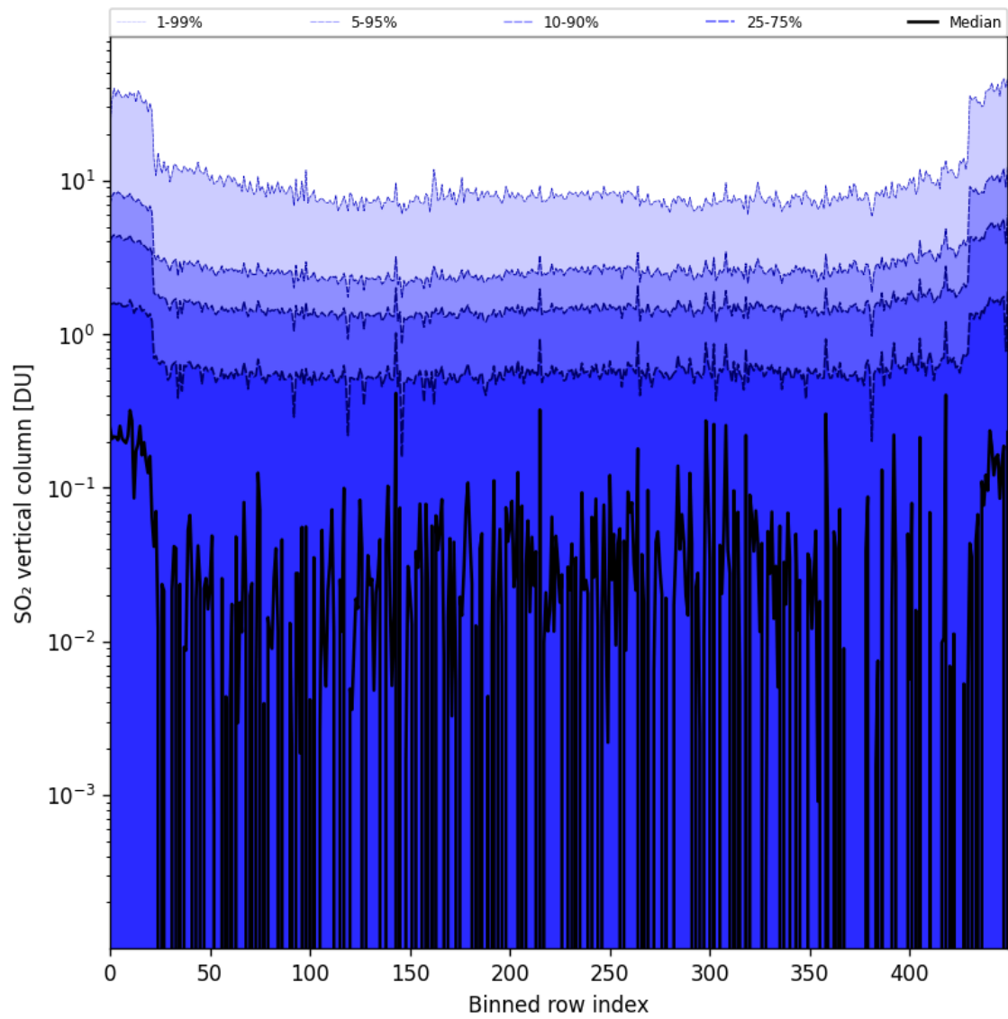
Figure 76: Along track statistics of “SO 2 vertical column” for 2024-08-27 to 2024-08-28
