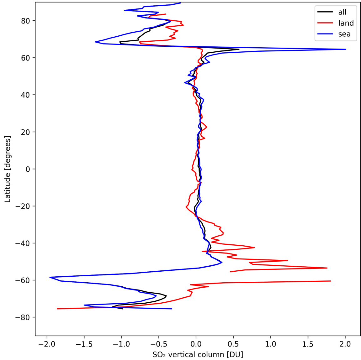
Figure 30: Zonal average of “SO 2 vertical column” for 2024-08-27 to 2024-08-28.
