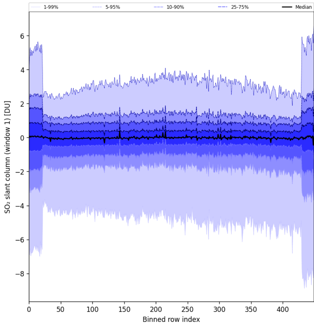
Figure 79: Along track statistics of “SO 2 slant column (window 1)” for 2024-08-27 to 2024-08-28
