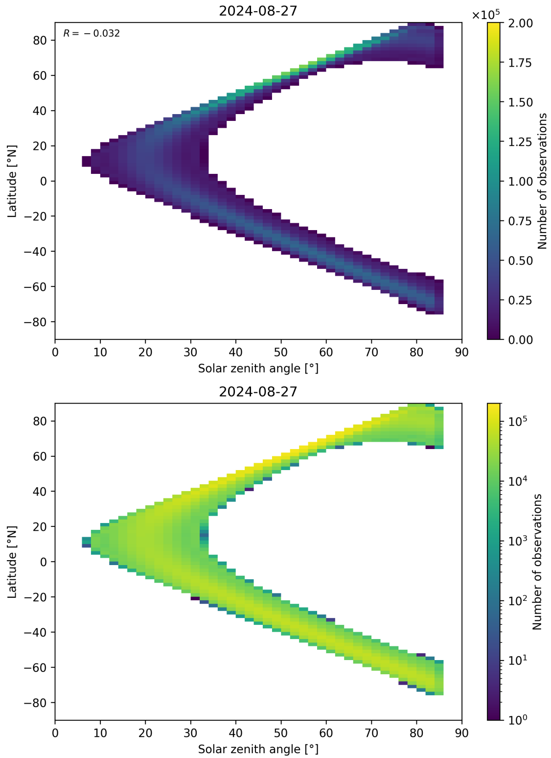
Figure 164: Scatter density plot of “Solar zenith angle” against “Latitude” for 2024-08-27 to 2024-08-28.
