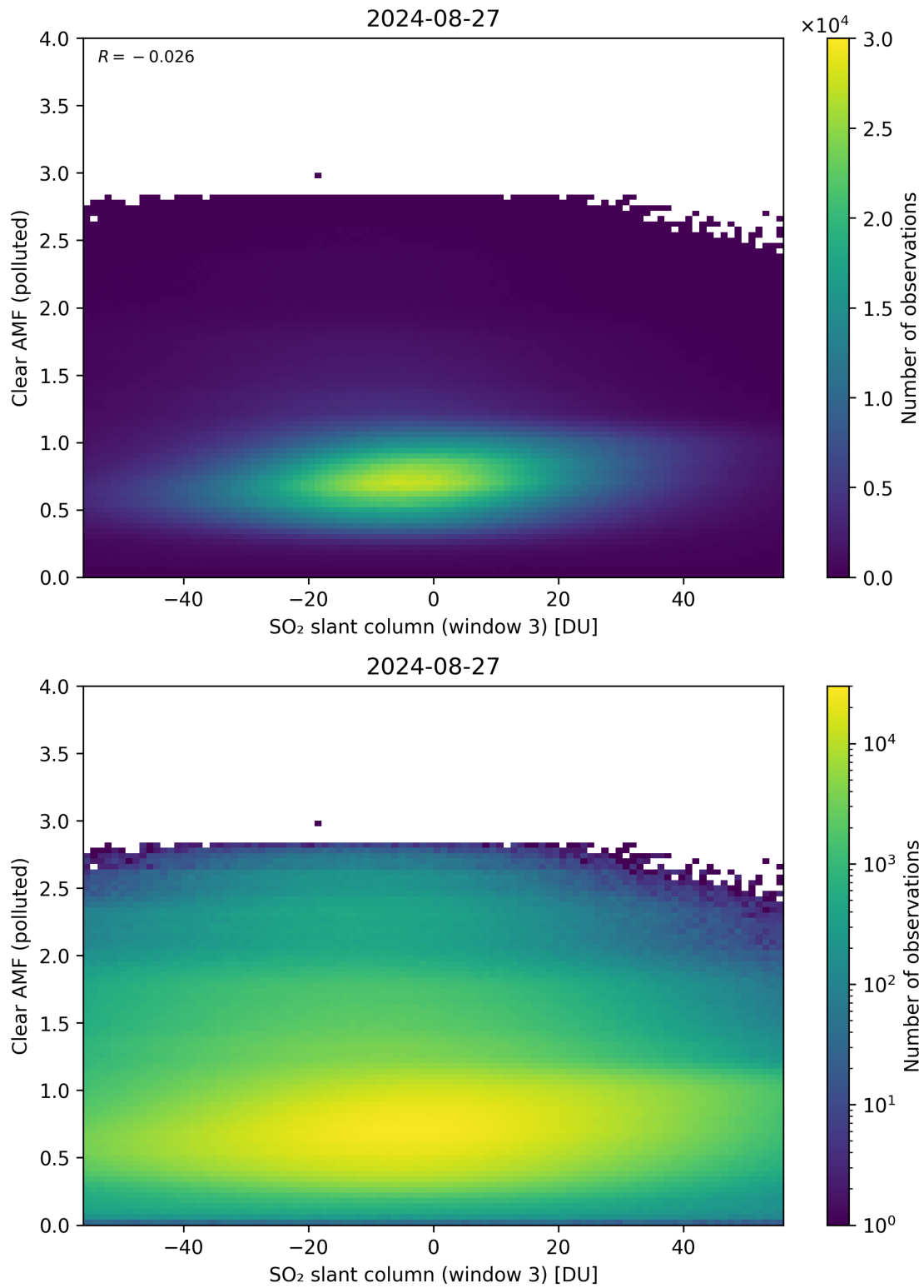
Figure 265: Scatter density plot of “SO 2 slant column (window 3)” against “Clear AMF (polluted)” for 2024-08-27 to 2024-08-28.
