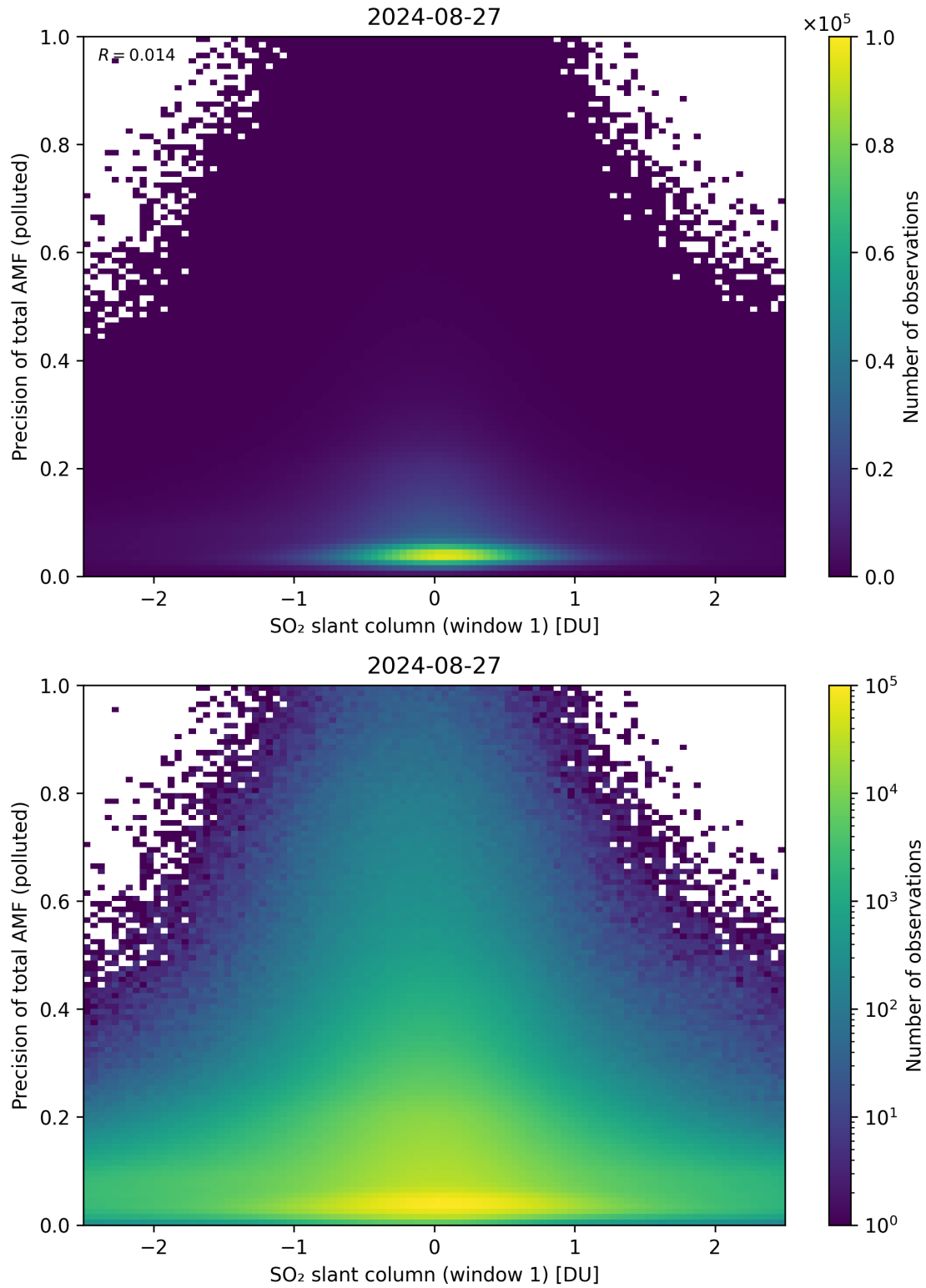
Figure 240: Scatter density plot of “SO 2 slant column (window 1)” against “Precision of total AMF (polluted)” for 2024-08-27 to 2024-08-28.
