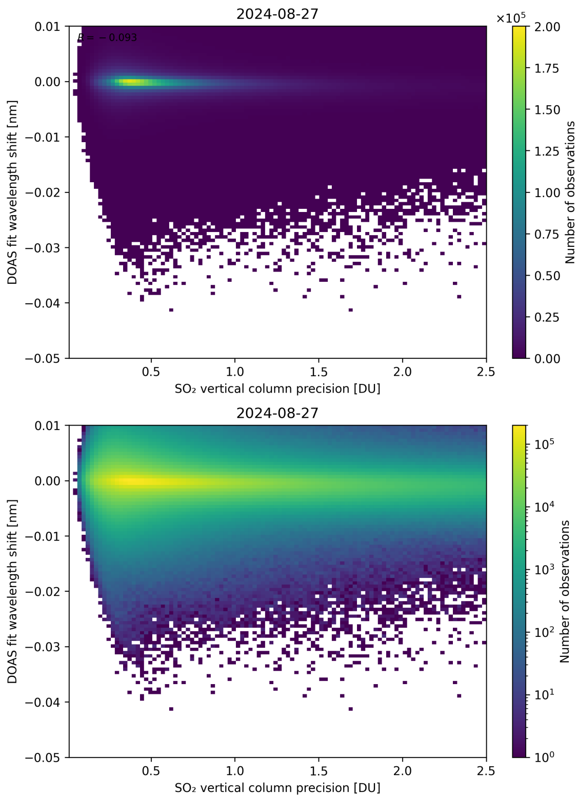
Figure 282: Scatter density plot of “SO 2 vertical column precision” against “DOAS fit wavelength shift” for 2024-08-27 to 2024-08-28.
