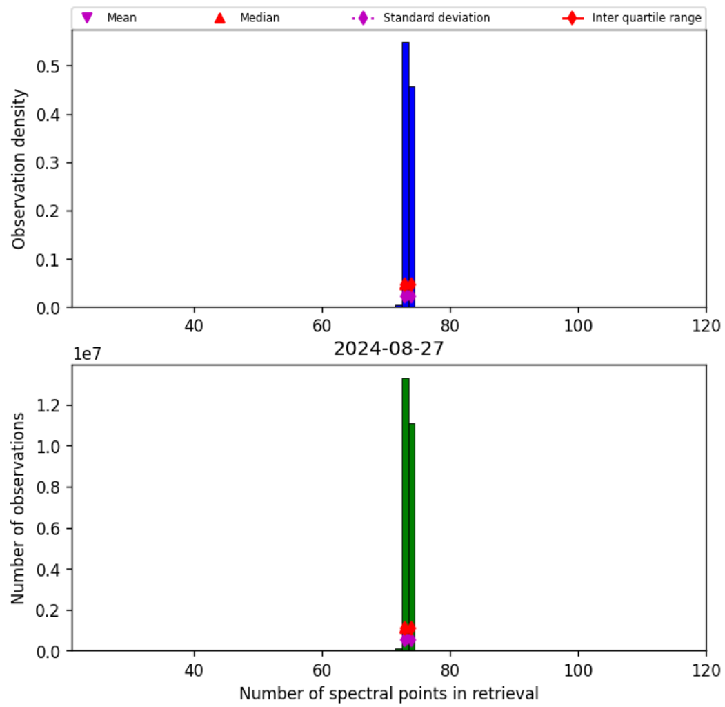
Figure 74: Histogram of “Number of spectral points in retrieval” for 2024-08-27 to 2024-08-28
