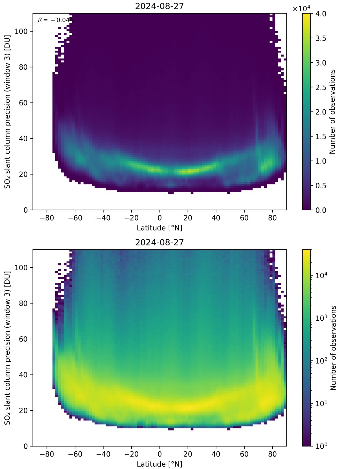
Figure 153: Scatter density plot of “Latitude” against “SO 2 slant column precision (window 3)” for 2024-08-27 to 2024-08-28.
