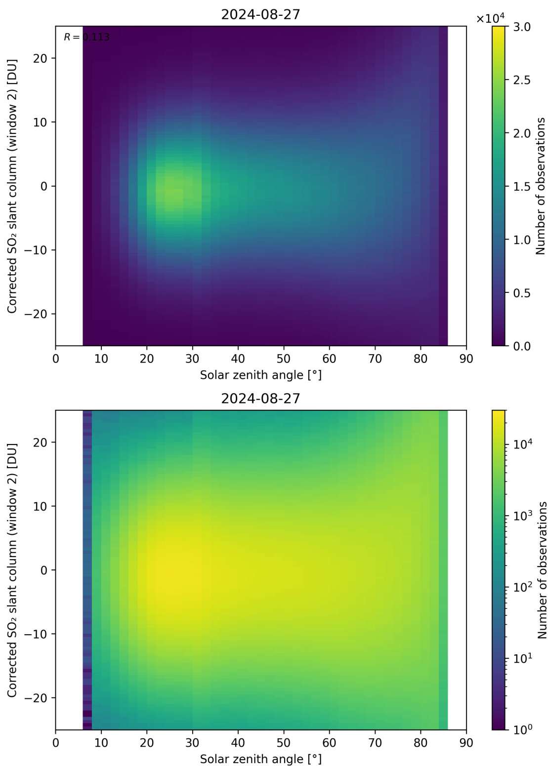
Figure 167: Scatter density plot of “Solar zenith angle” against “Corrected SO 2 slant column (window 2)” for 2024-08-27 to 2024-08-28.
