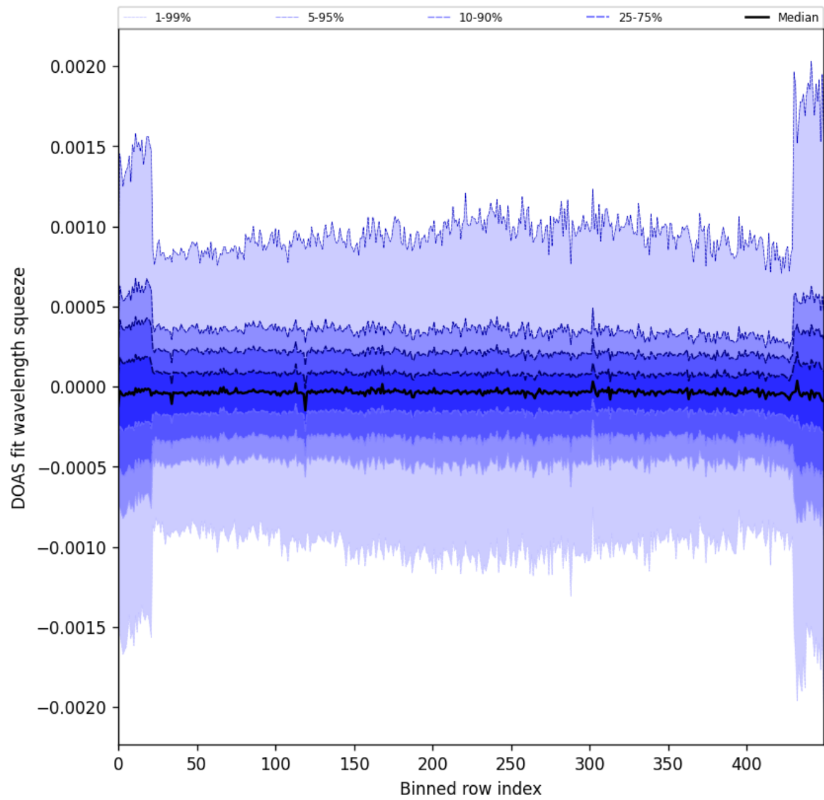
Figure 92: Along track statistics of “DOAS fit wavelength squeeze” for 2024-08-27 to 2024-08-28
