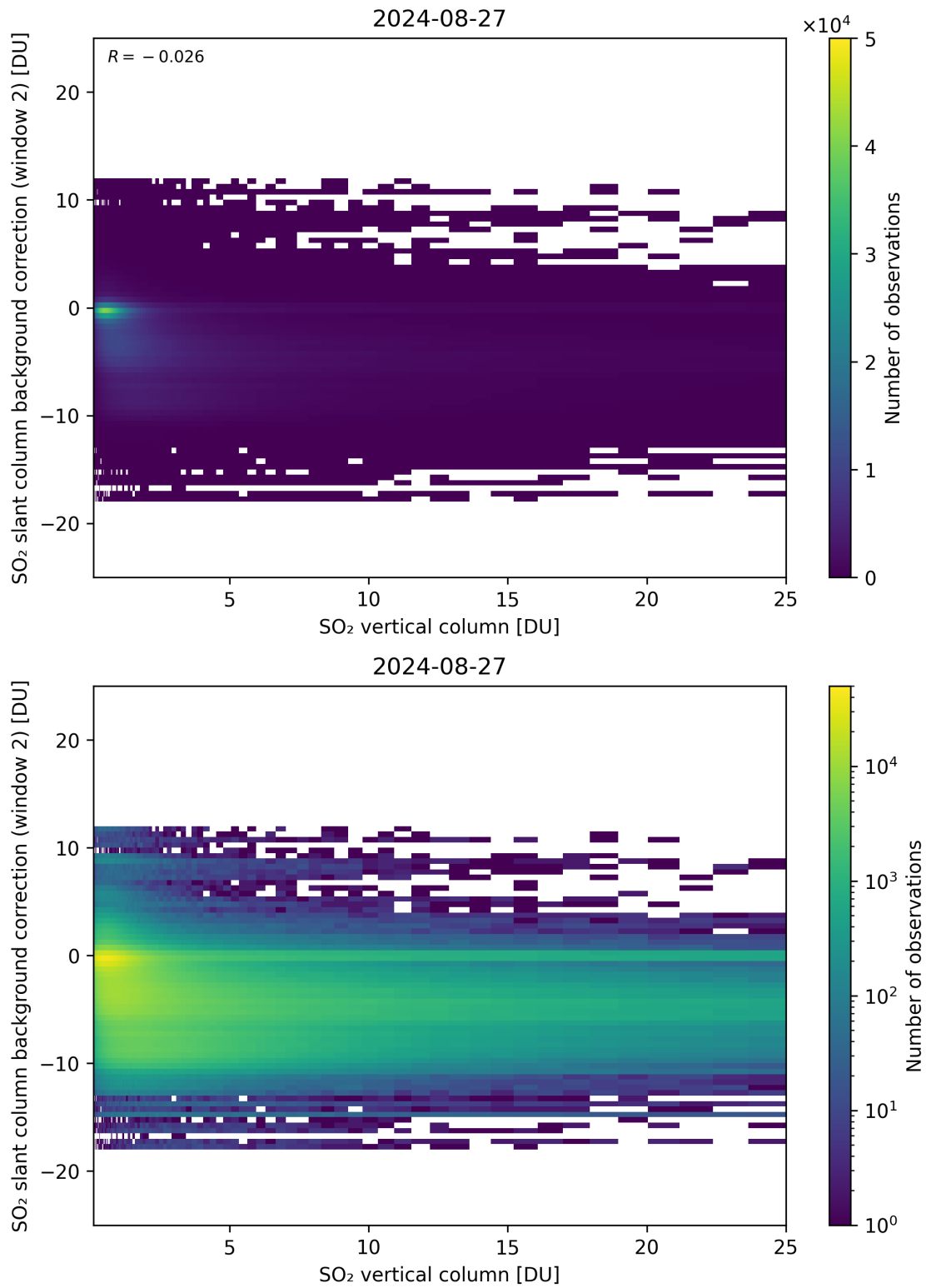
Figure 274: Scatter density plot of “SO 2 vertical column” against “SO 2 slant column background correction (window 2)” for 2024-08-27 to 2024-08-28.
