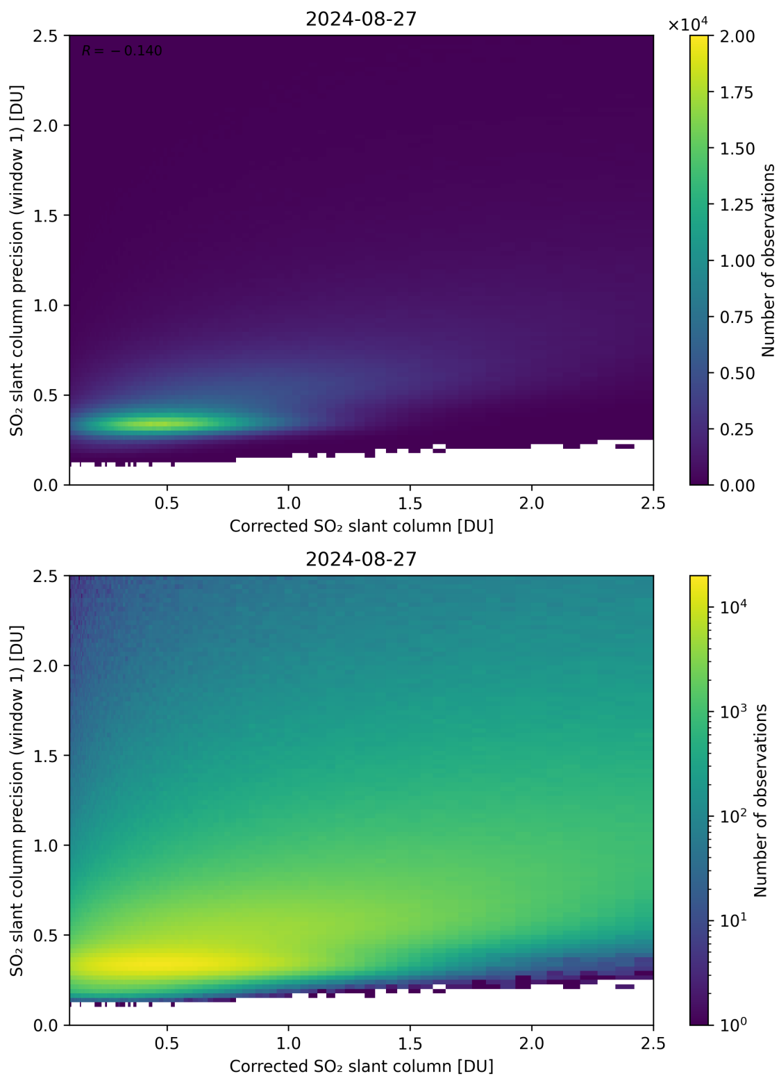
Figure 188: Scatter density plot of “Corrected SO 2 slant column” against “SO 2 slant column precision (window 1)” for 2024-08-27 to 2024-08-28.
