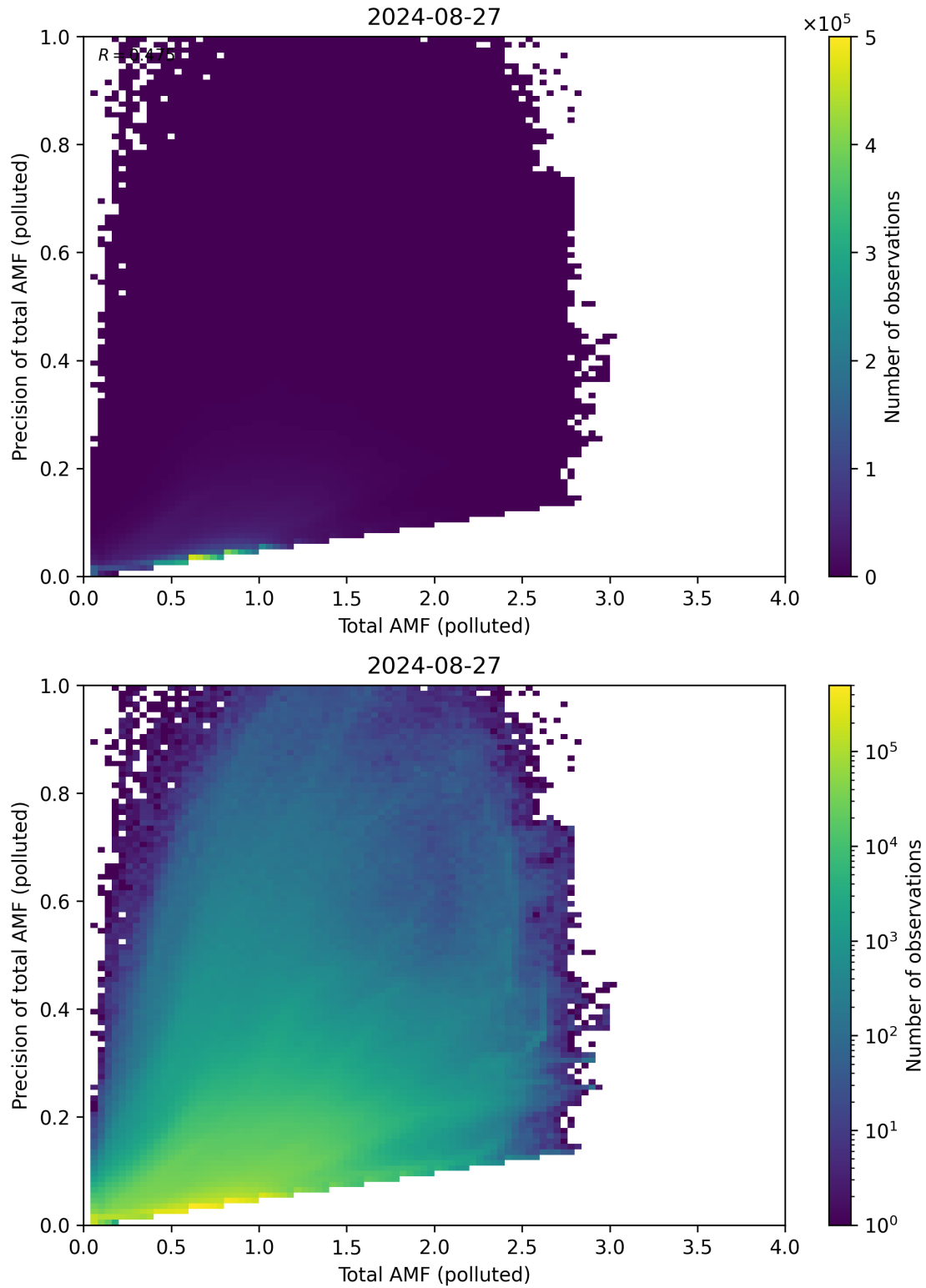
Figure 272: Scatter density plot of “Total AMF (polluted)” against “Precision of total AMF (polluted)” for 2024-08-27 to 2024-08-28.
