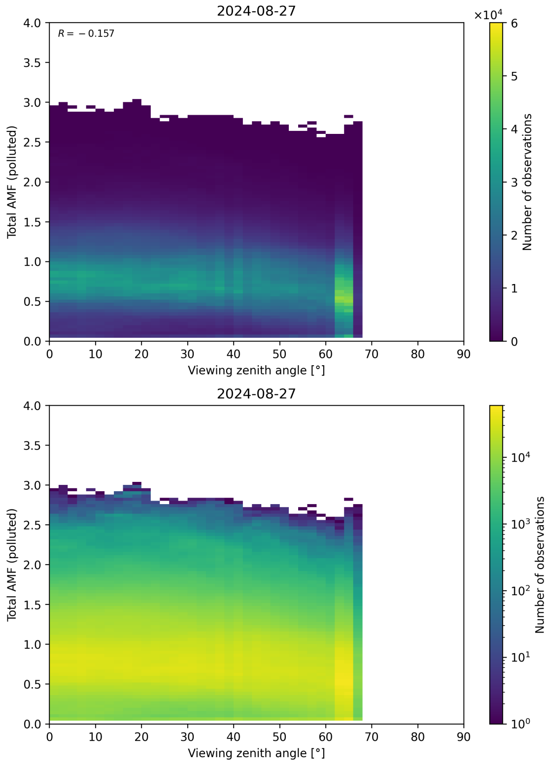
Figure 325: Scatter density plot of “Viewing zenith angle” against “Total AMF (polluted)” for 2024-08-27 to 2024-08-28.
