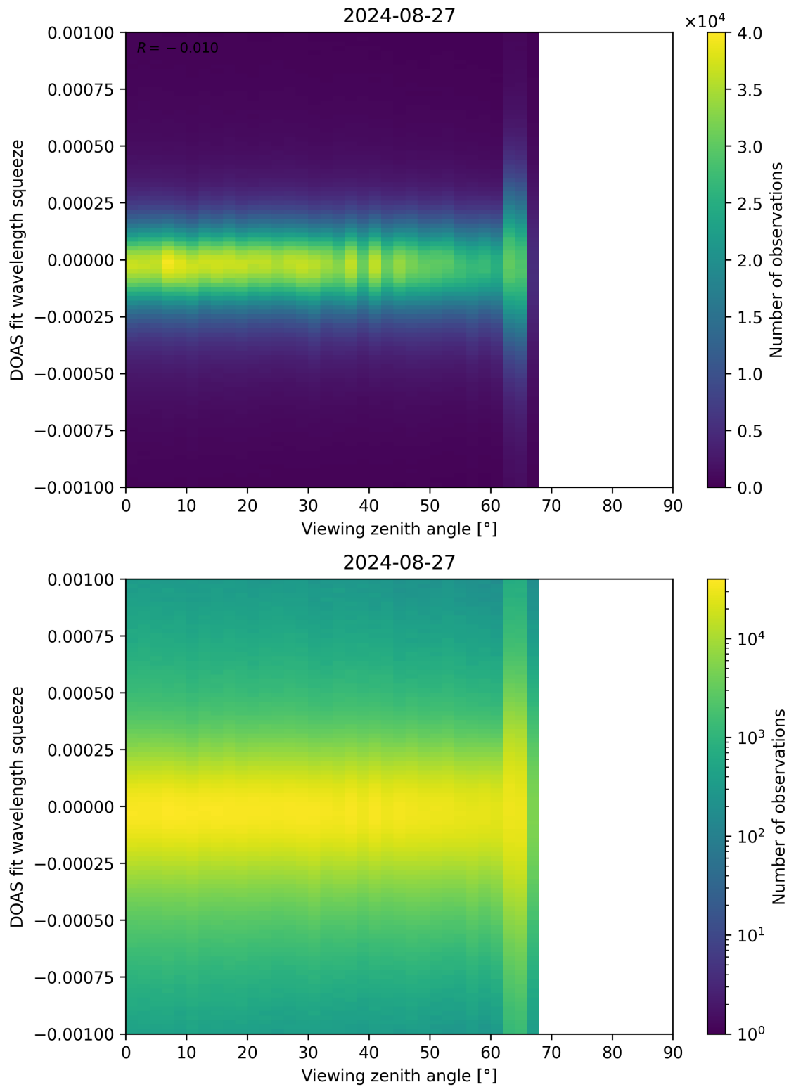
Figure 312: Scatter density plot of “Viewing zenith angle” against “DOAS fit wavelength squeeze” for 2024-08-27 to 2024-08-28.
