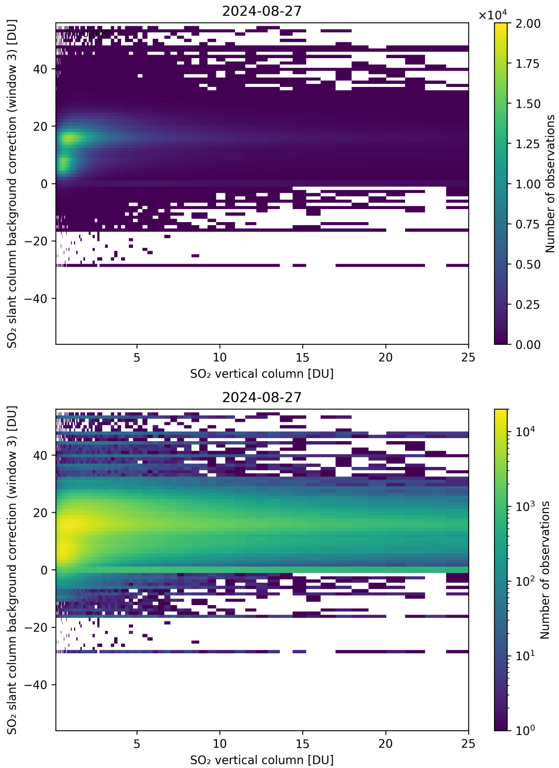
Figure 275: Scatter density plot of “SO 2 vertical column” against “SO 2 slant column background correction (window 3)” for 2024-08-27 to 2024-08-28.
