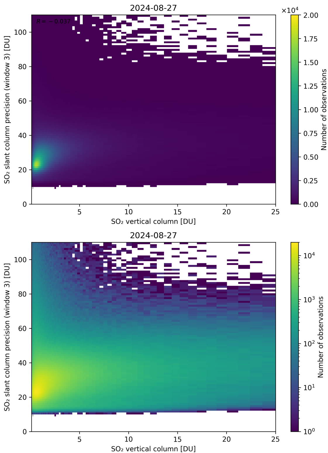
Figure 304: Scatter density plot of “SO 2 vertical column” against “SO 2 slant column precision (window 3)” for 2024-08-27 to 2024-08-28.
