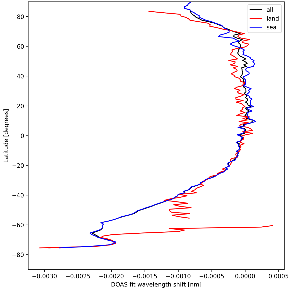
Figure 45: Zonal average of “DOAS fit wavelength shift” for 2024-08-27 to 2024-08-28.
