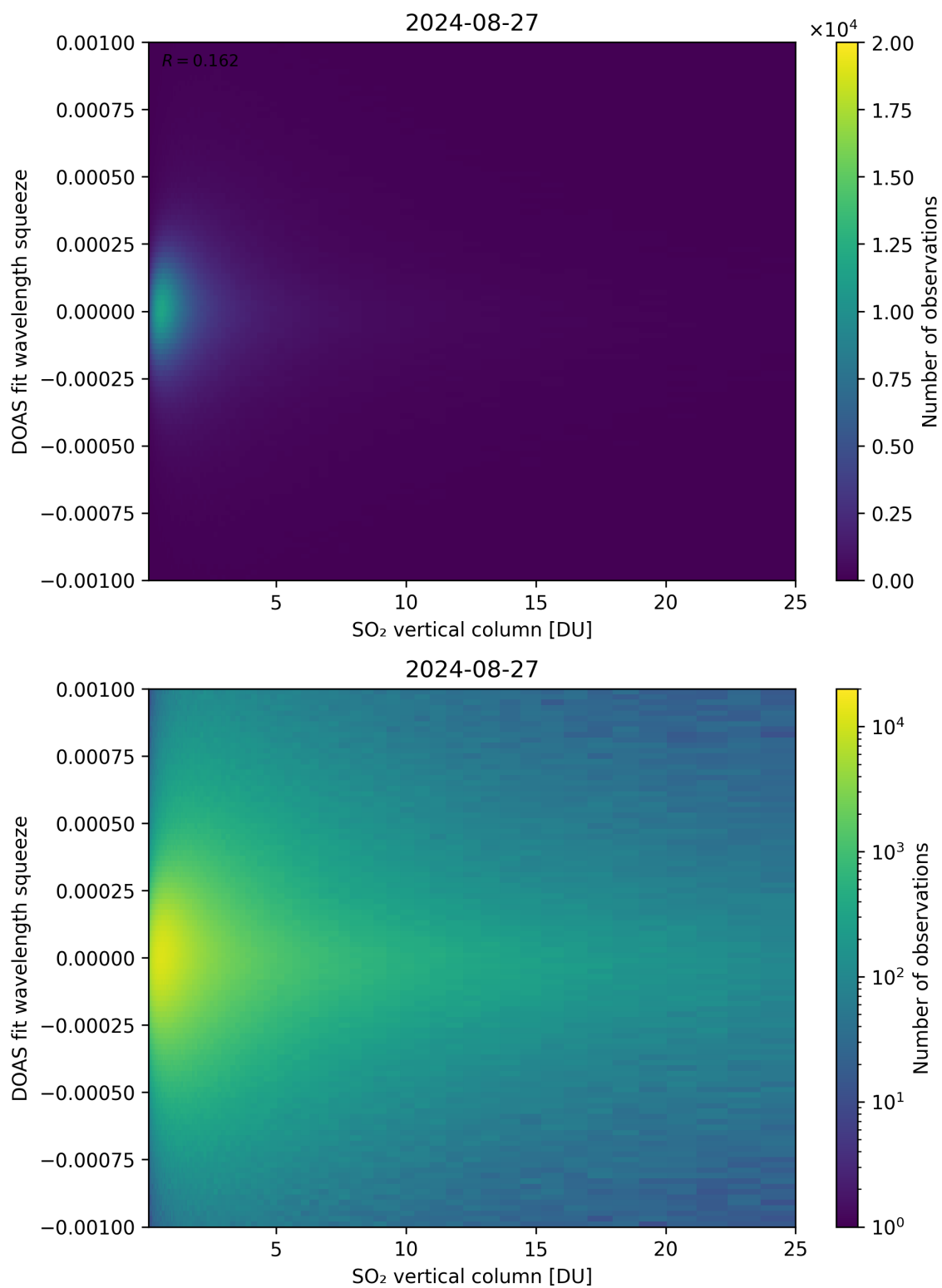
Figure 277: Scatter density plot of “SO 2 vertical column” against “DOAS fit wavelength squeeze” for 2024-08-27 to 2024-08-28.
