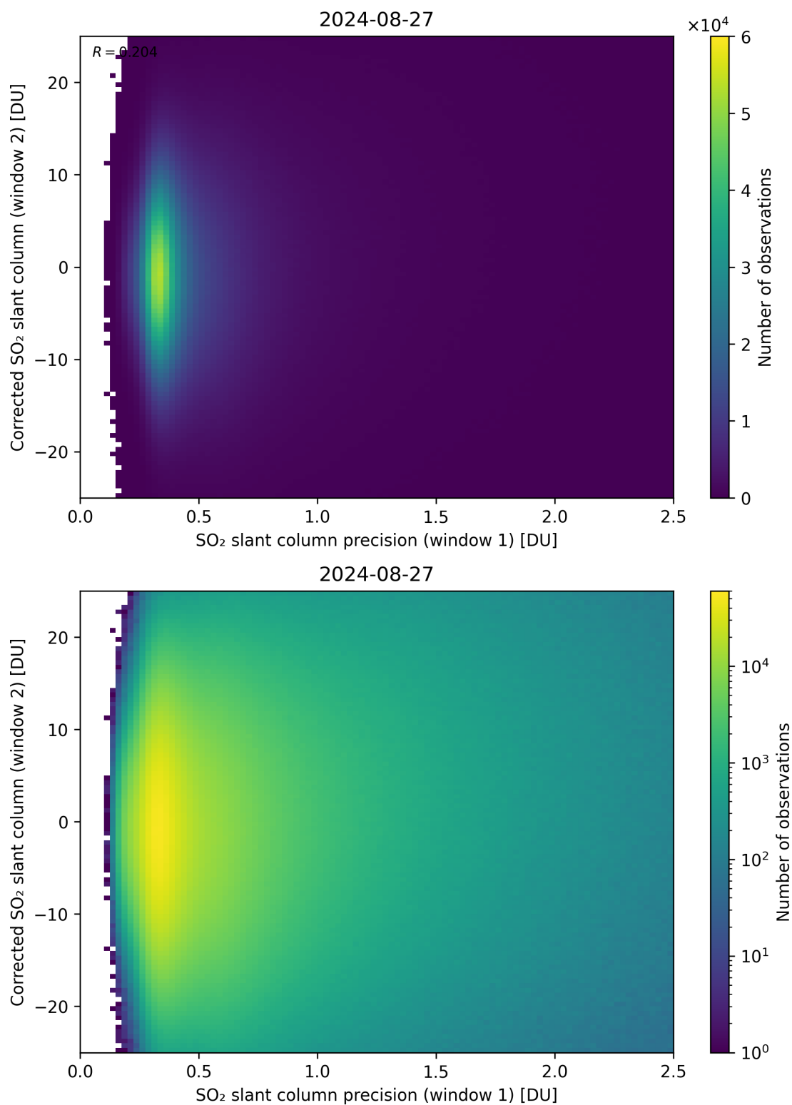
Figure 225: Scatter density plot of “SO 2 slant column precision (window 1)” against “Corrected SO 2 slant column (window 2)” for 2024-08-27 to 2024-08-28.
