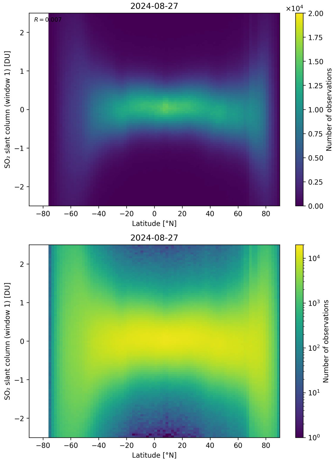
Figure 149: Scatter density plot of “Latitude” against “SO 2 slant column (window 1)” for 2024-08-27 to 2024-08-28.
