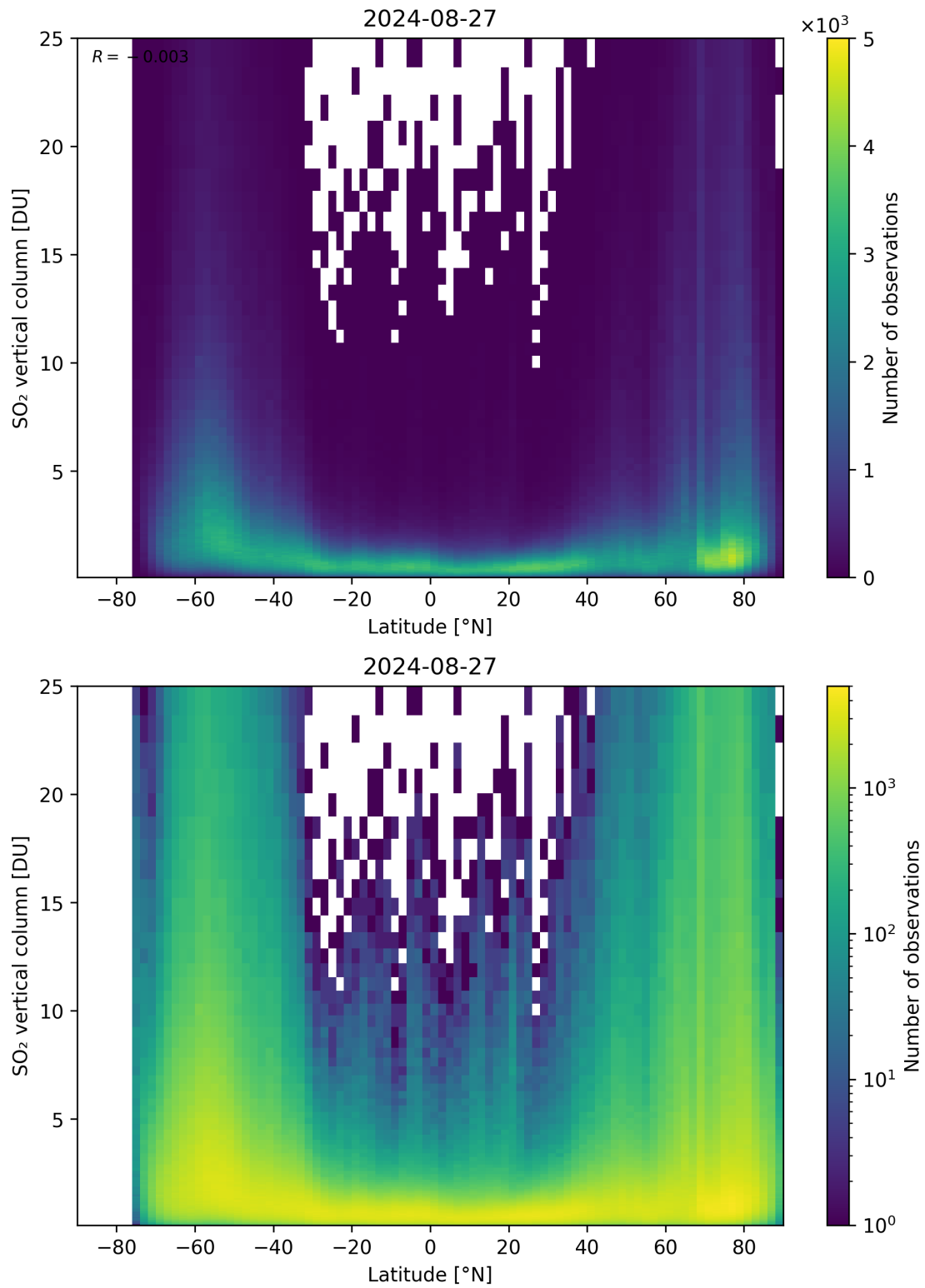
Figure 156: Scatter density plot of “Latitude” against “SO 2 vertical column” for 2024-08-27 to 2024-08-28.
