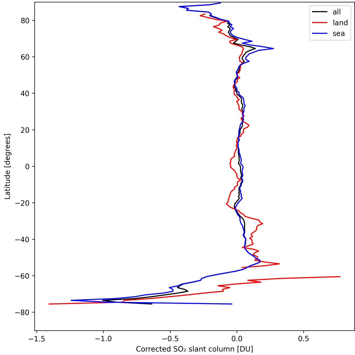
Figure 32: Zonal average of “Corrected SO 2 slant column” for 2024-08-27 to 2024-08-28.
