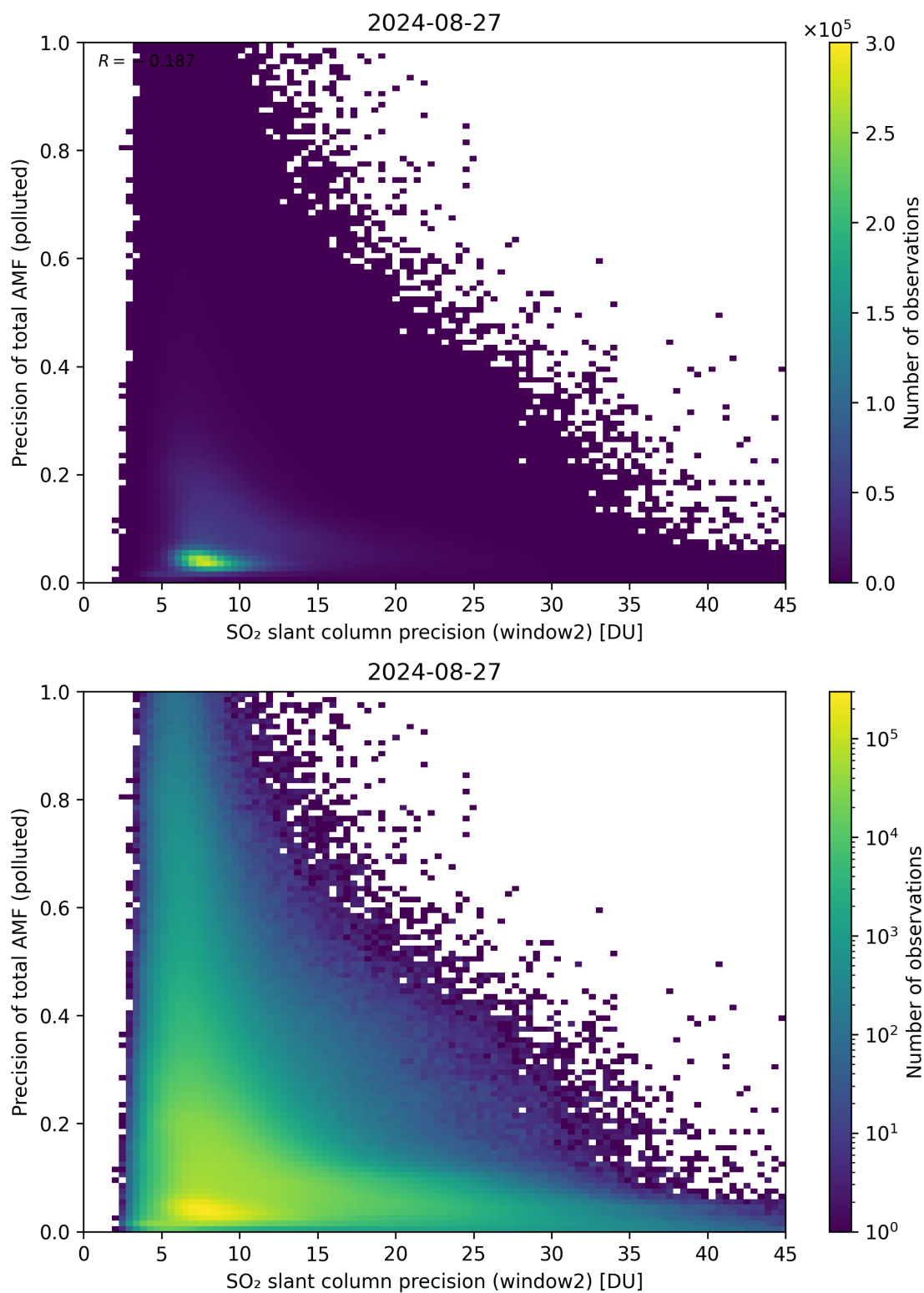
Figure 252: Scatter density plot of “SO 2 slant column precision (window2)” against “Precision of total AMF (polluted)” for 2024-08-27 to 2024-08-28.
