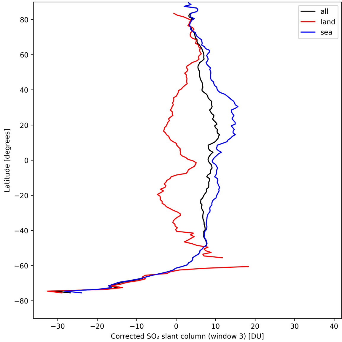
Figure 43: Zonal average of “Corrected SO 2 slant column (window 3)” for 2024-08-27 to 2024-08-28.
