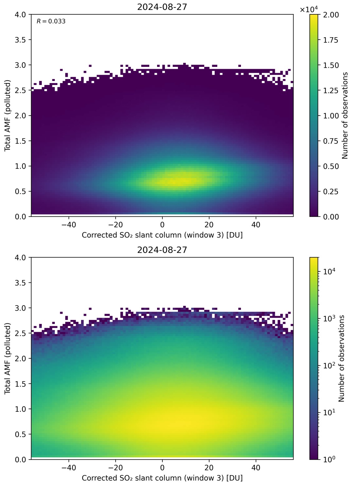
Figure 210: Scatter density plot of “Corrected SO 2 slant column (window 3)” against “Total AMF (polluted)” for 2024-08-27 to 2024-08-28.
