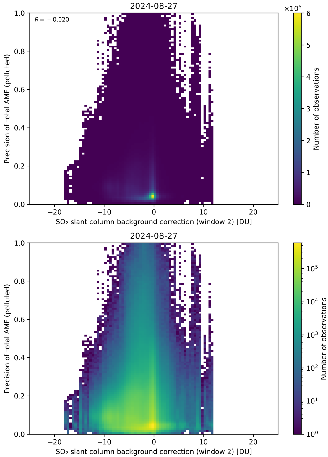
Figure 120: Scatter density plot of “SO 2 slant column background correction (window 2)” against “Precision of total AMF (polluted)” for 2024-08-27 to 2024-08-28.
