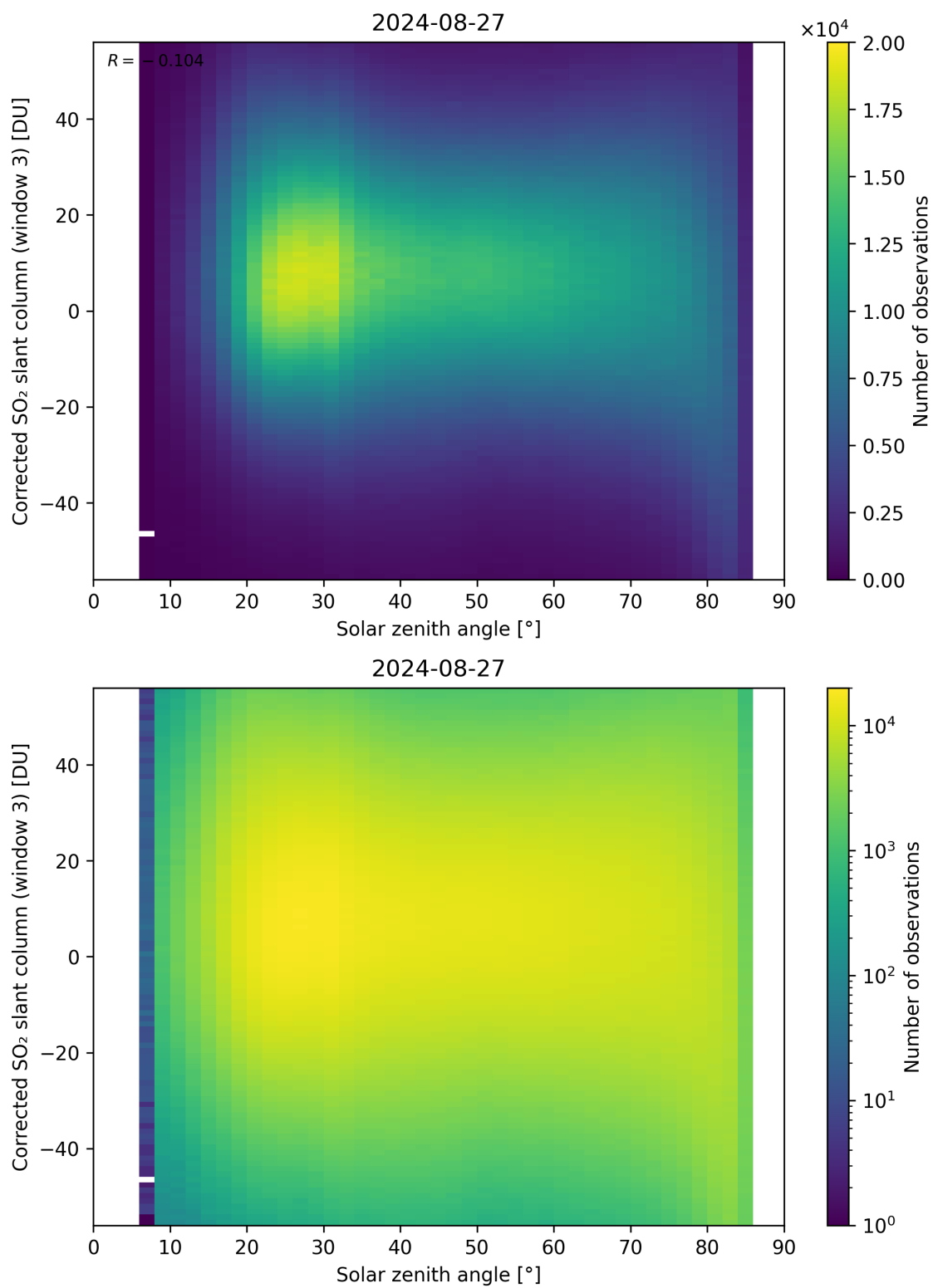
Figure 168: Scatter density plot of “Solar zenith angle” against “Corrected SO 2 slant column (window 3)” for 2024-08-27 to 2024-08-28.
