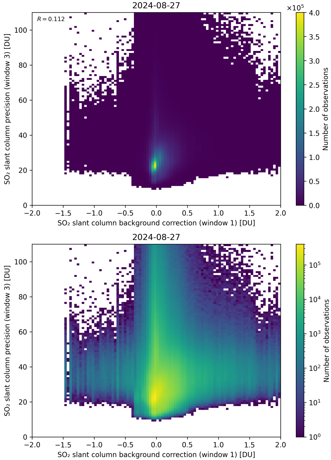
Figure 108: Scatter density plot of “SO 2 slant column background correction (window 1)” against “SO 2 slant column precision (window 3)” for 2024-08-27 to 2024-08-28.
