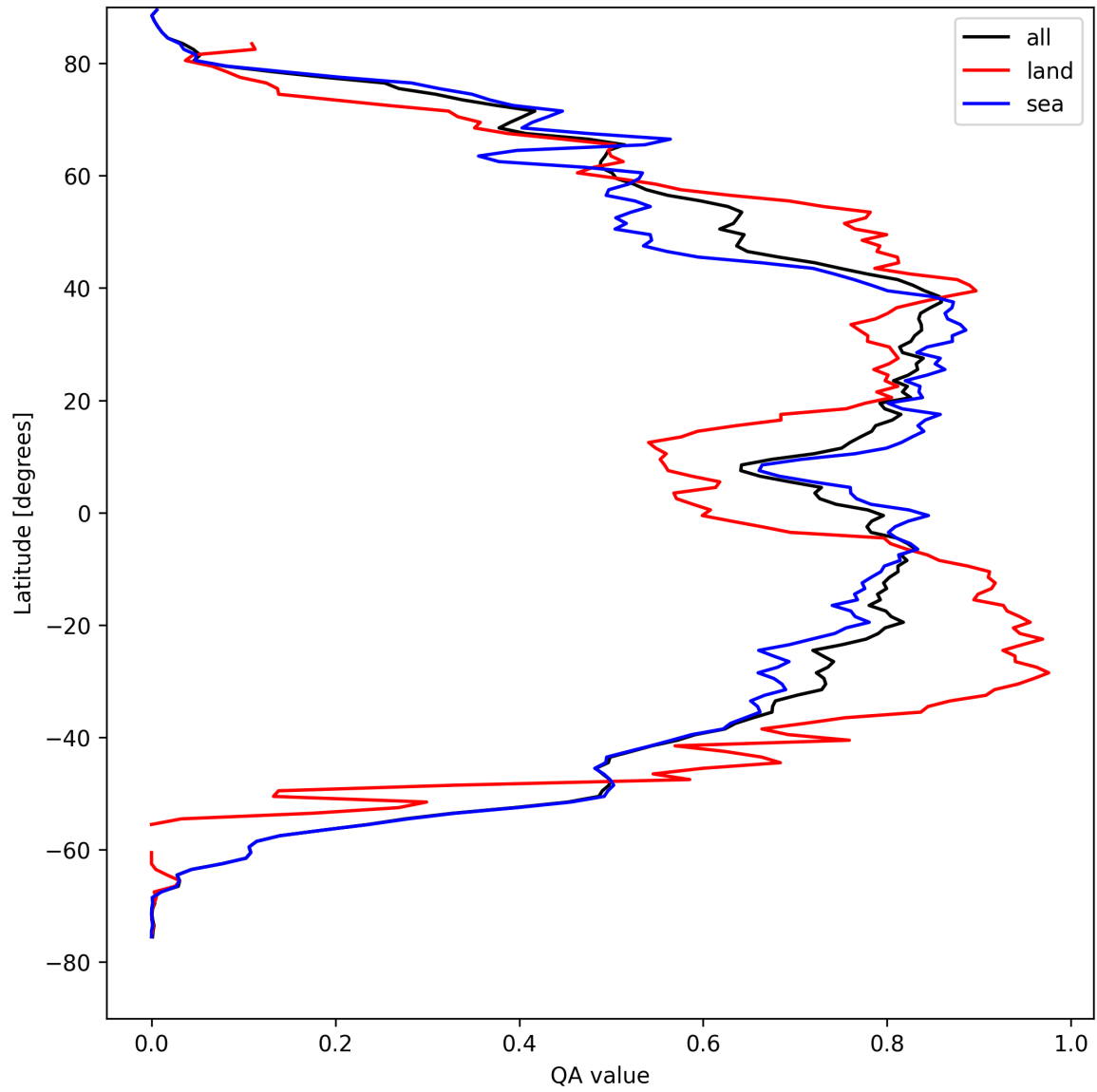
Figure 29: Zonal average of “QA value” for 2024-08-27 to 2024-08-28.
