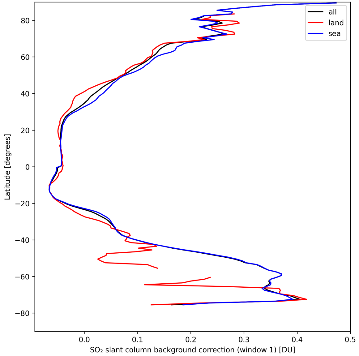
Figure 36: Zonal average of “SO 2 slant column background correction (window 1)” for 2024-08-27 to 2024-08-28.
