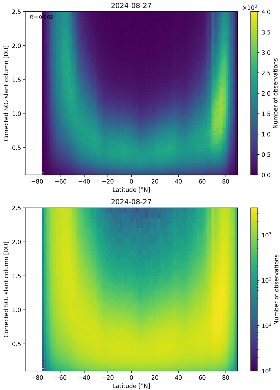
Figure 146: Scatter density plot of “Latitude” against “Corrected SO 2 slant column” for 2024-08-27 to 2024-08-28.
