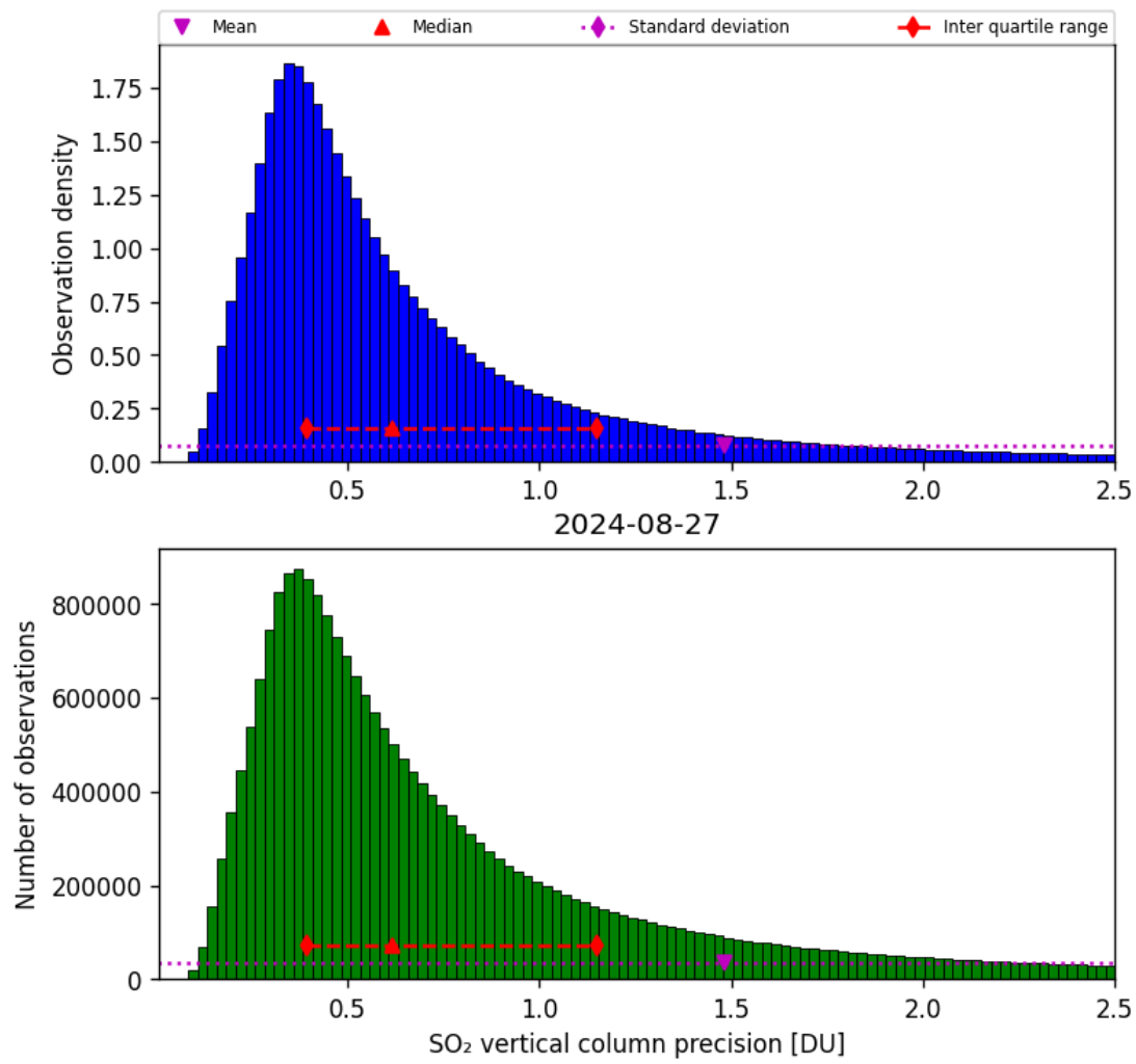
Figure 54: Histogram of “SO 2 vertical column precision” for 2024-08-27 to 2024-08-28
