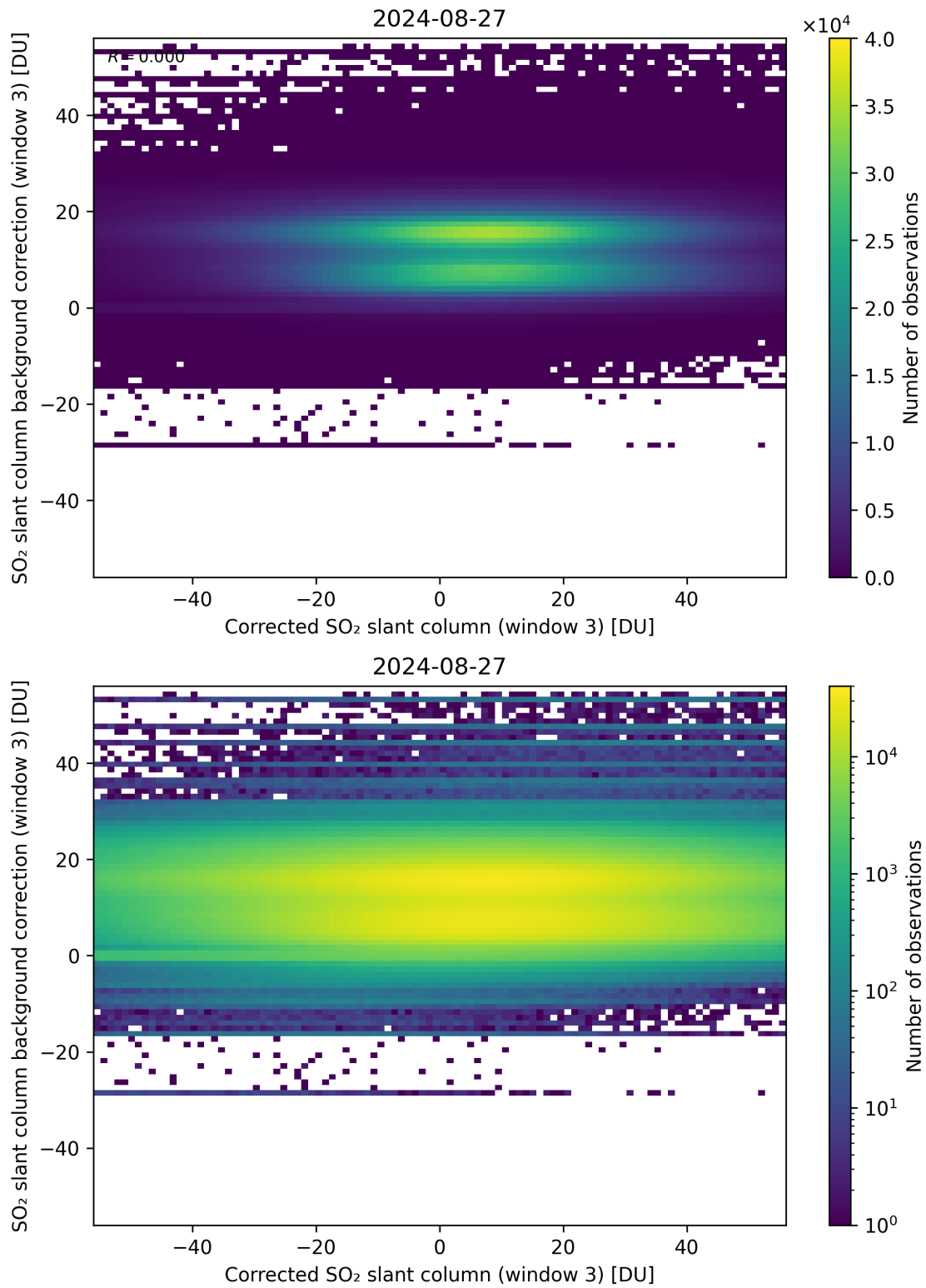
Figure 205: Scatter density plot of “Corrected SO 2 slant column (window 3)” against “SO 2 slant column background correction (window 3)” for 2024-08-27 to 2024-08-28.
