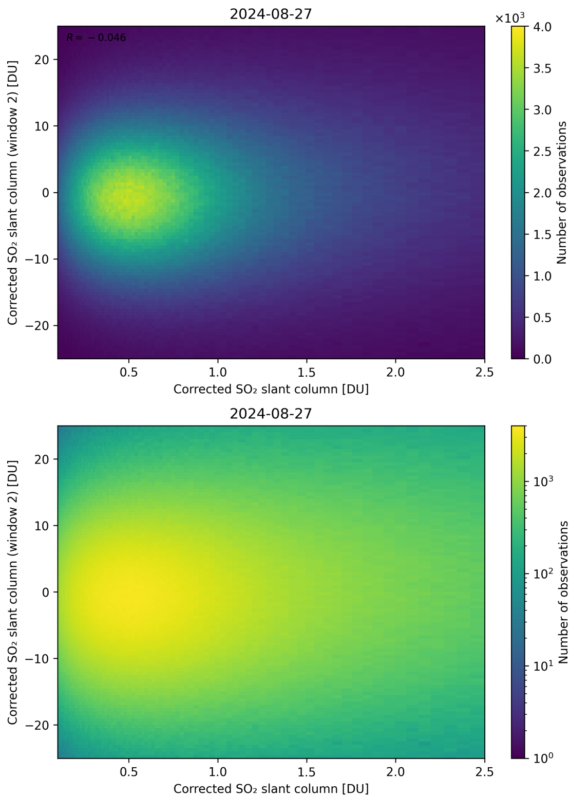
Figure 185: Scatter density plot of “Corrected SO 2 slant column” against “Corrected SO 2 slant column (window 2)” for 2024-08-27 to 2024-08-28.
