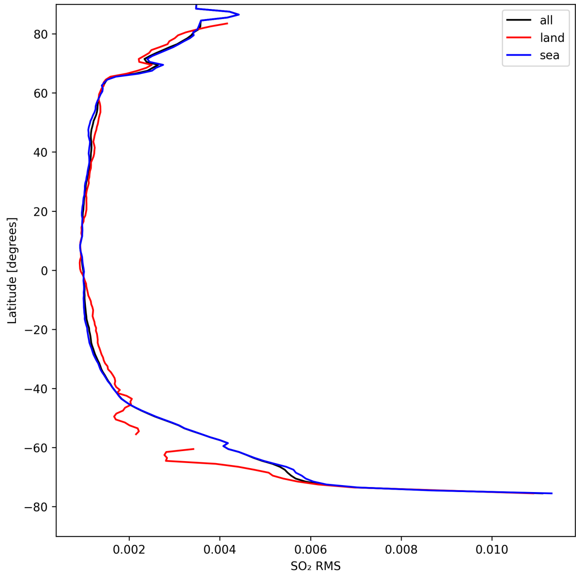
Figure 47: Zonal average of “SO 2 RMS” for 2024-08-27 to 2024-08-28.
