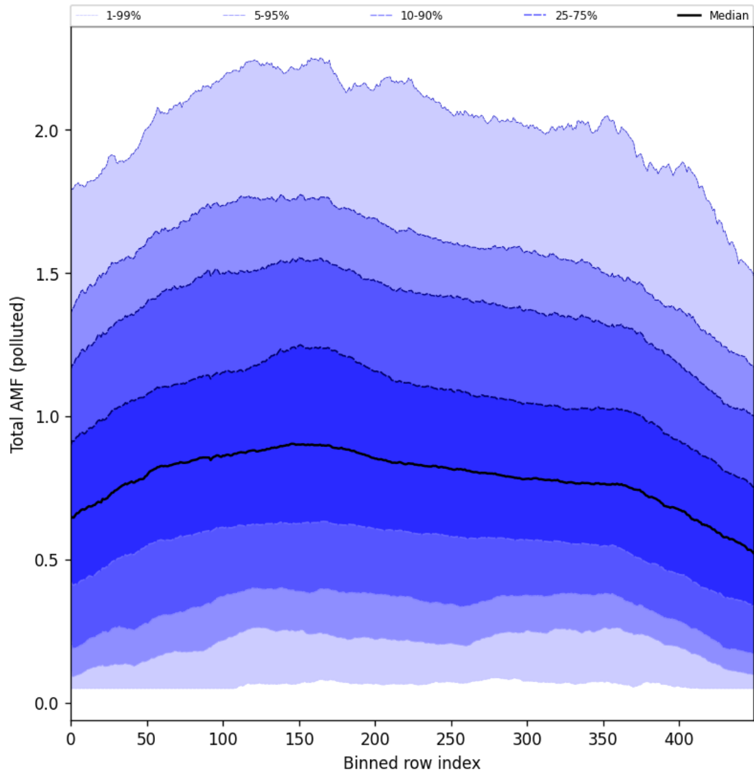
Figure 94: Along track statistics of “Total AMF (polluted)” for 2024-08-27 to 2024-08-28
