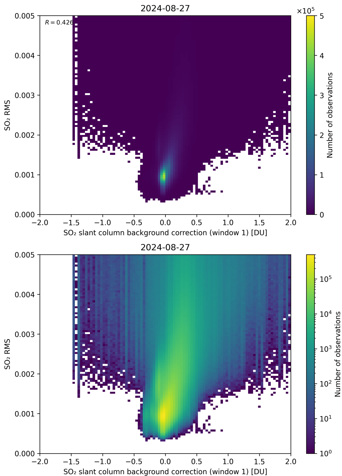
Figure 102: Scatter density plot of “SO 2 slant column background correction (window 1)” against “SO 2 RMS” for 2024-08-27 to 2024-08-28.
