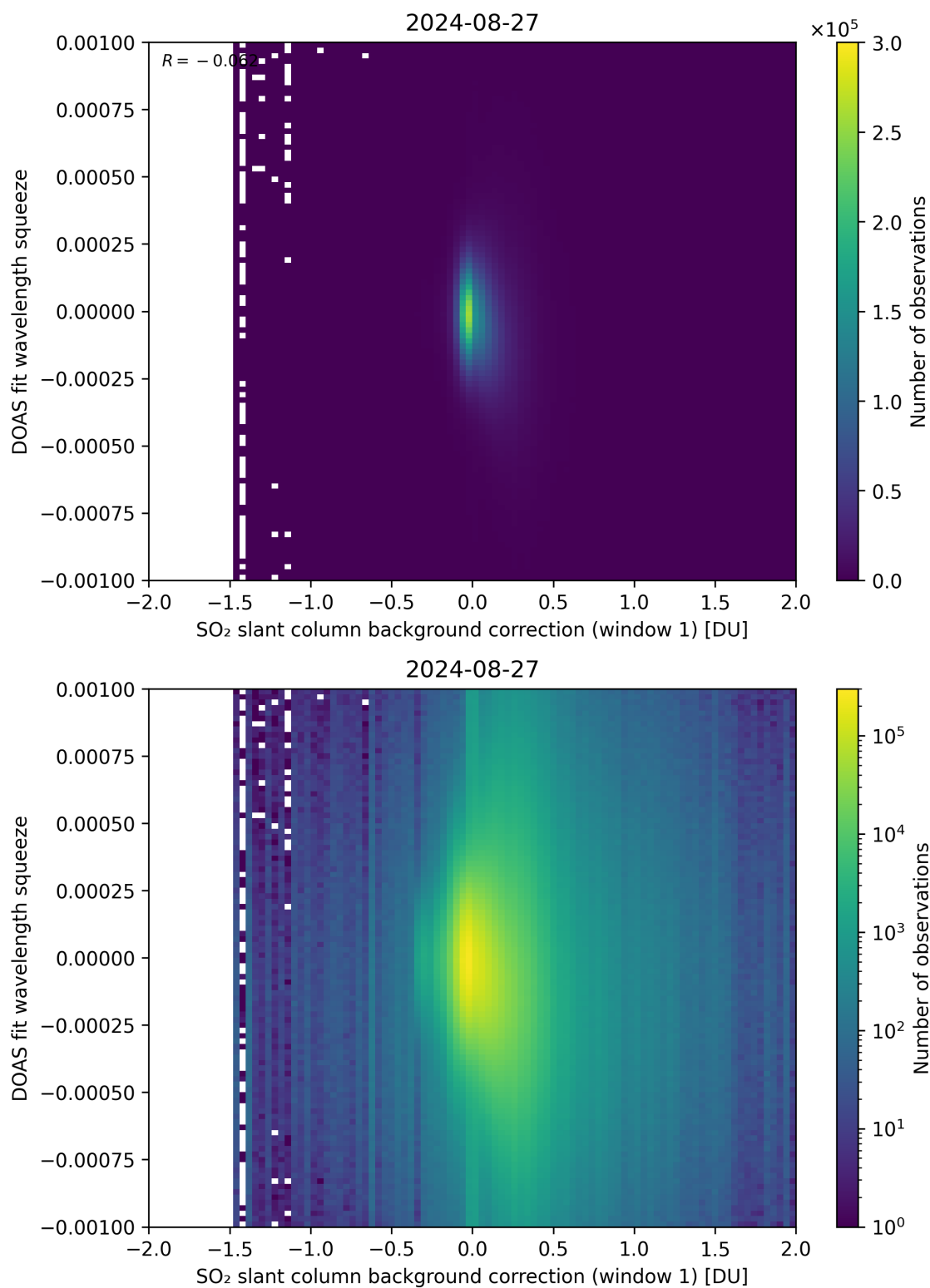
Figure 101: Scatter density plot of “SO 2 slant column background correction (window 1)” against “DOAS fit wavelength squeeze” for 2024-08-27 to 2024-08-28.
