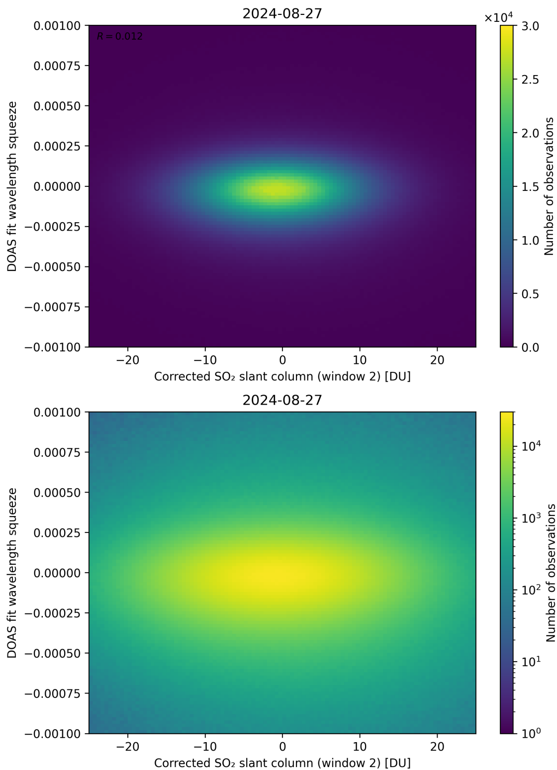
Figure 197: Scatter density plot of “Corrected SO 2 slant column (window 2)” against “DOAS fit wavelength squeeze” for 2024-08-27 to 2024-08-28.
