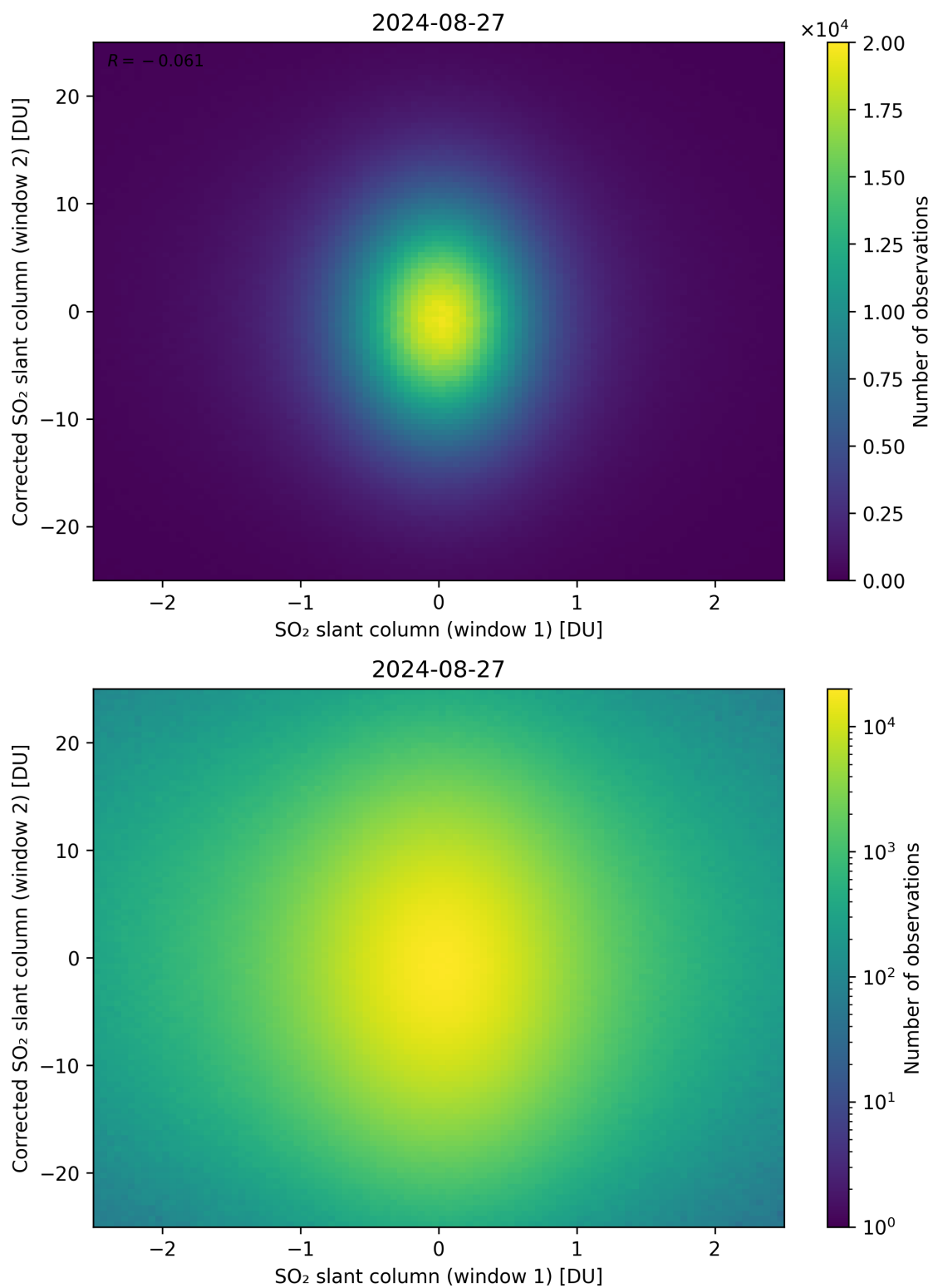
Figure 233: Scatter density plot of “SO 2 slant column (window 1)” against “Corrected SO 2 slant column (window 2)” for 2024-08-27 to 2024-08-28.
