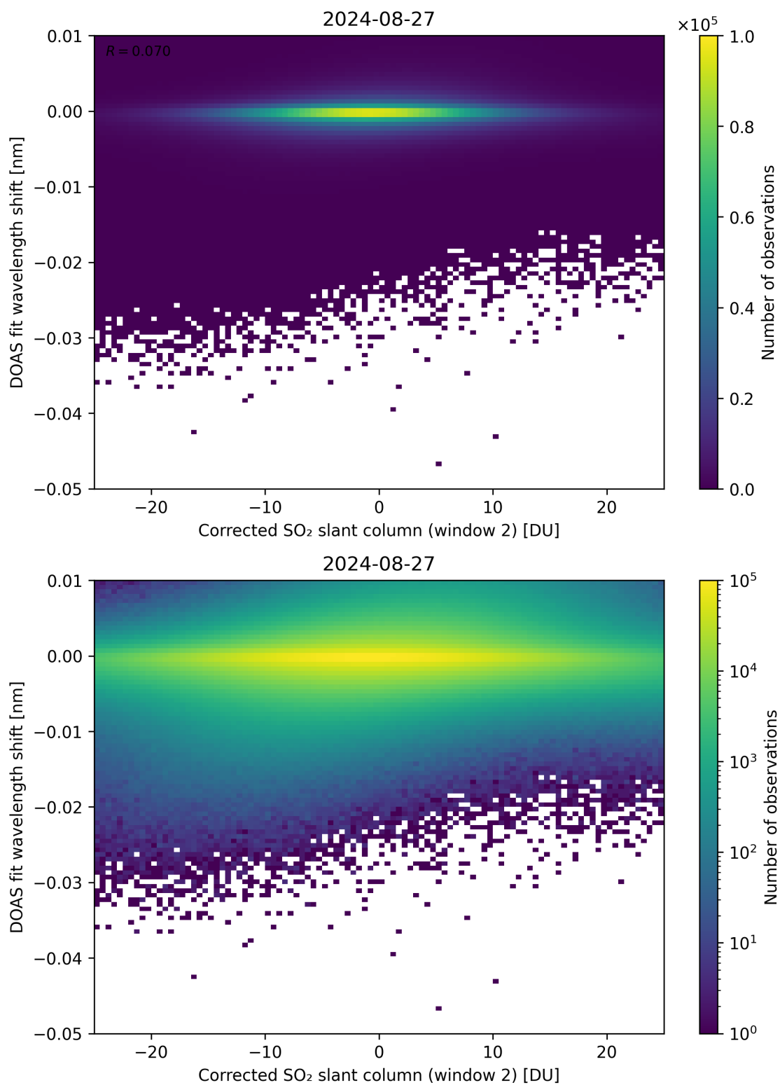
Figure 196: Scatter density plot of “Corrected SO 2 slant column (window 2)” against “DOAS fit wavelength shift” for 2024-08-27 to 2024-08-28.
