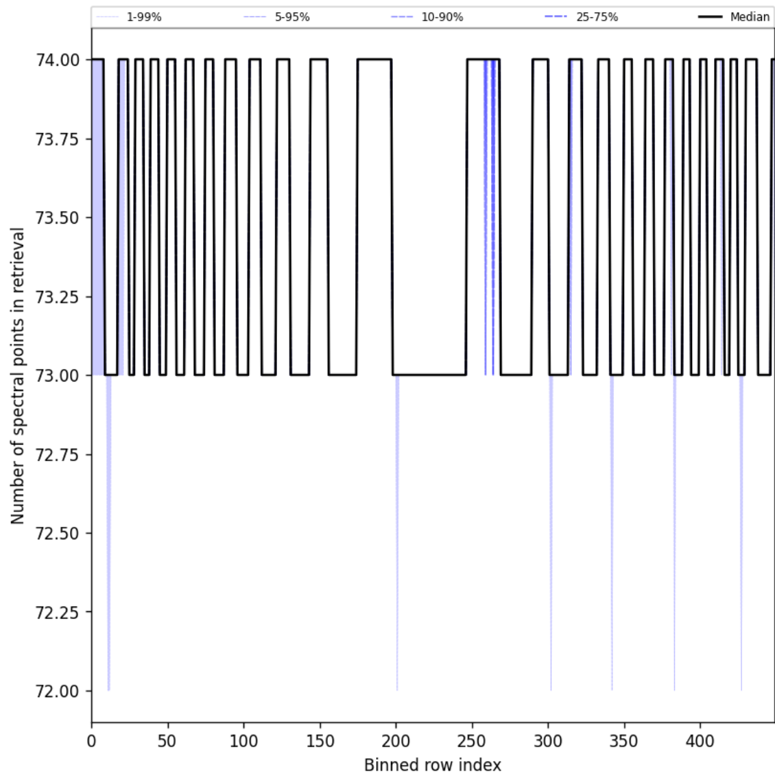
Figure 97: Along track statistics of “Number of spectral points in retrieval” for 2024-08-27 to 2024-08-28
