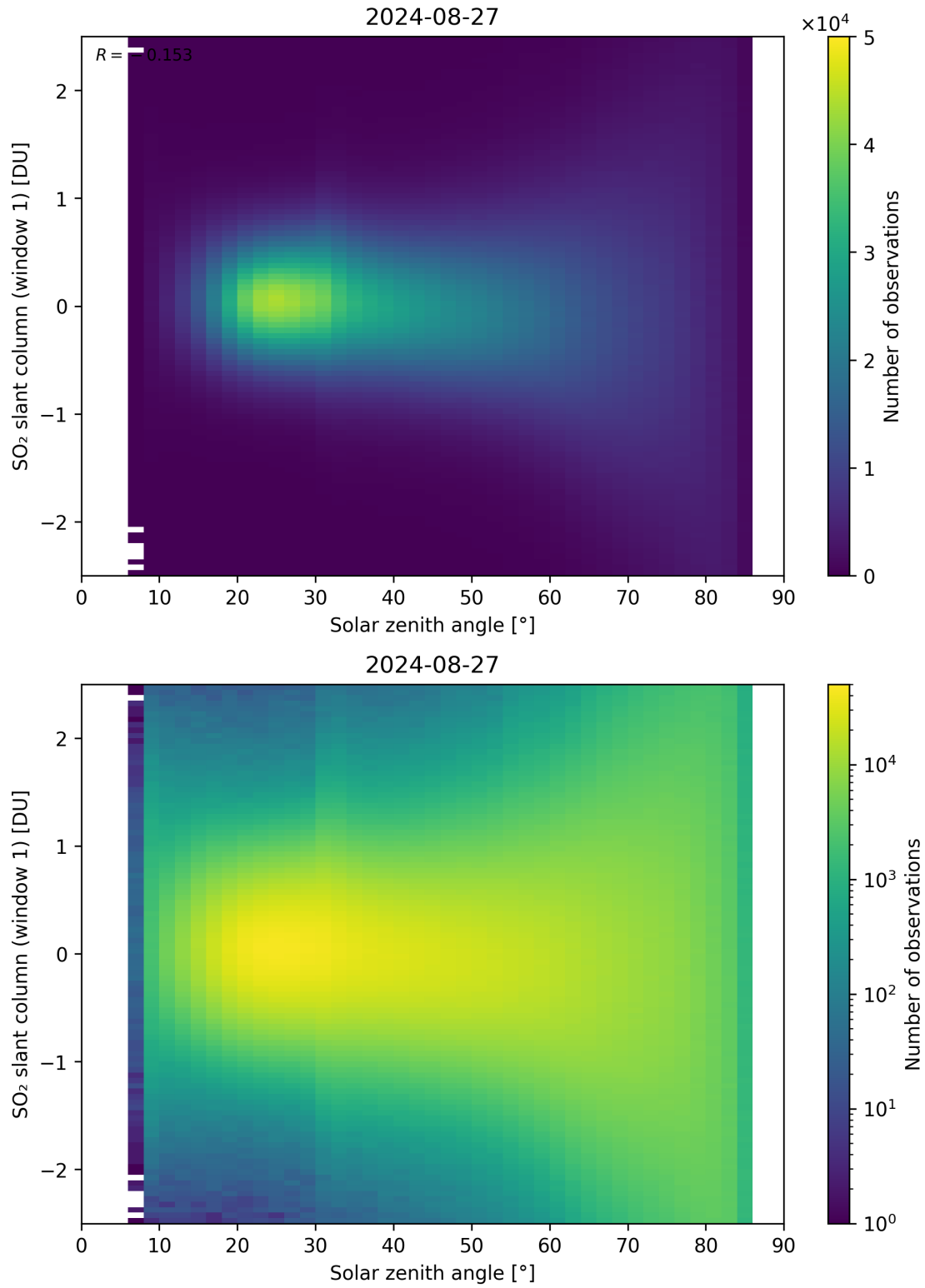
Figure 169: Scatter density plot of “Solar zenith angle” against “SO 2 slant column (window 1)” for 2024-08-27 to 2024-08-28.
