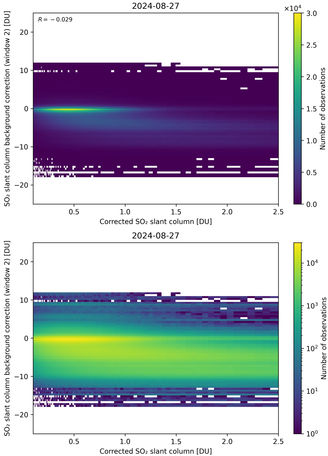
Figure 179: Scatter density plot of “Corrected SO 2 slant column” against “SO 2 slant column background correction (window 2)” for 2024-08-27 to 2024-08-28.
