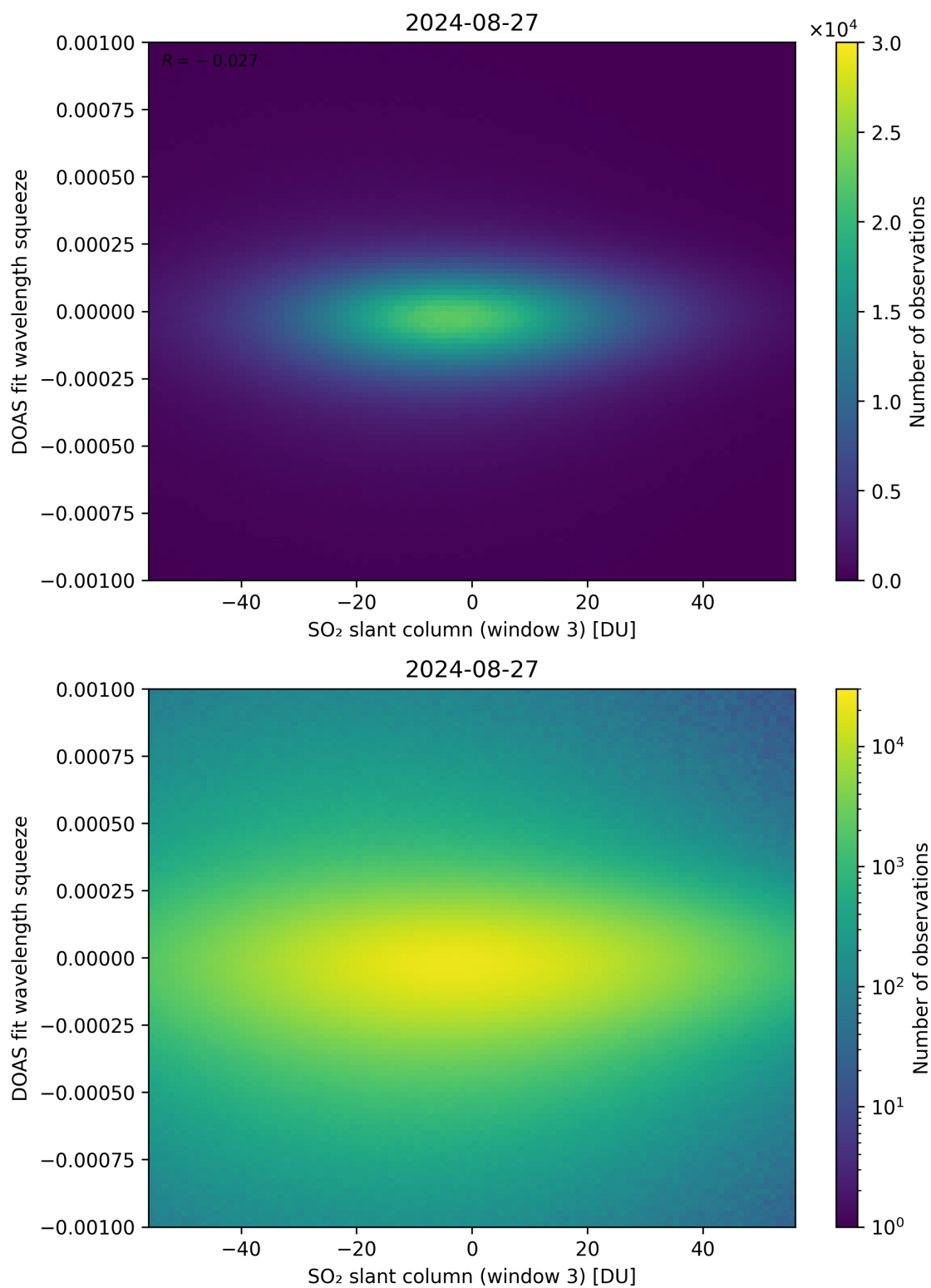
Figure 255: Scatter density plot of “SO 2 slant column (window 3)” against “DOAS fit wavelength squeeze” for 2024-08-27 to 2024-08-28.
