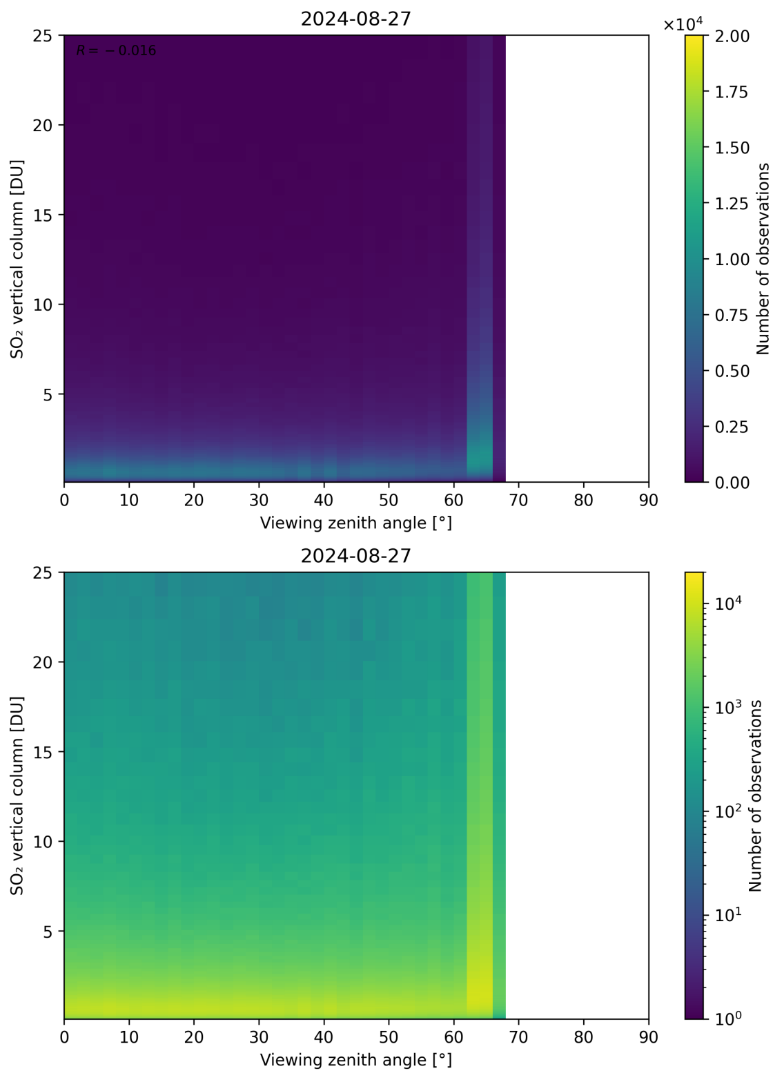
Figure 327: Scatter density plot of “Viewing zenith angle” against “SO 2 vertical column” for 2024-08-27 to 2024-08-28.
