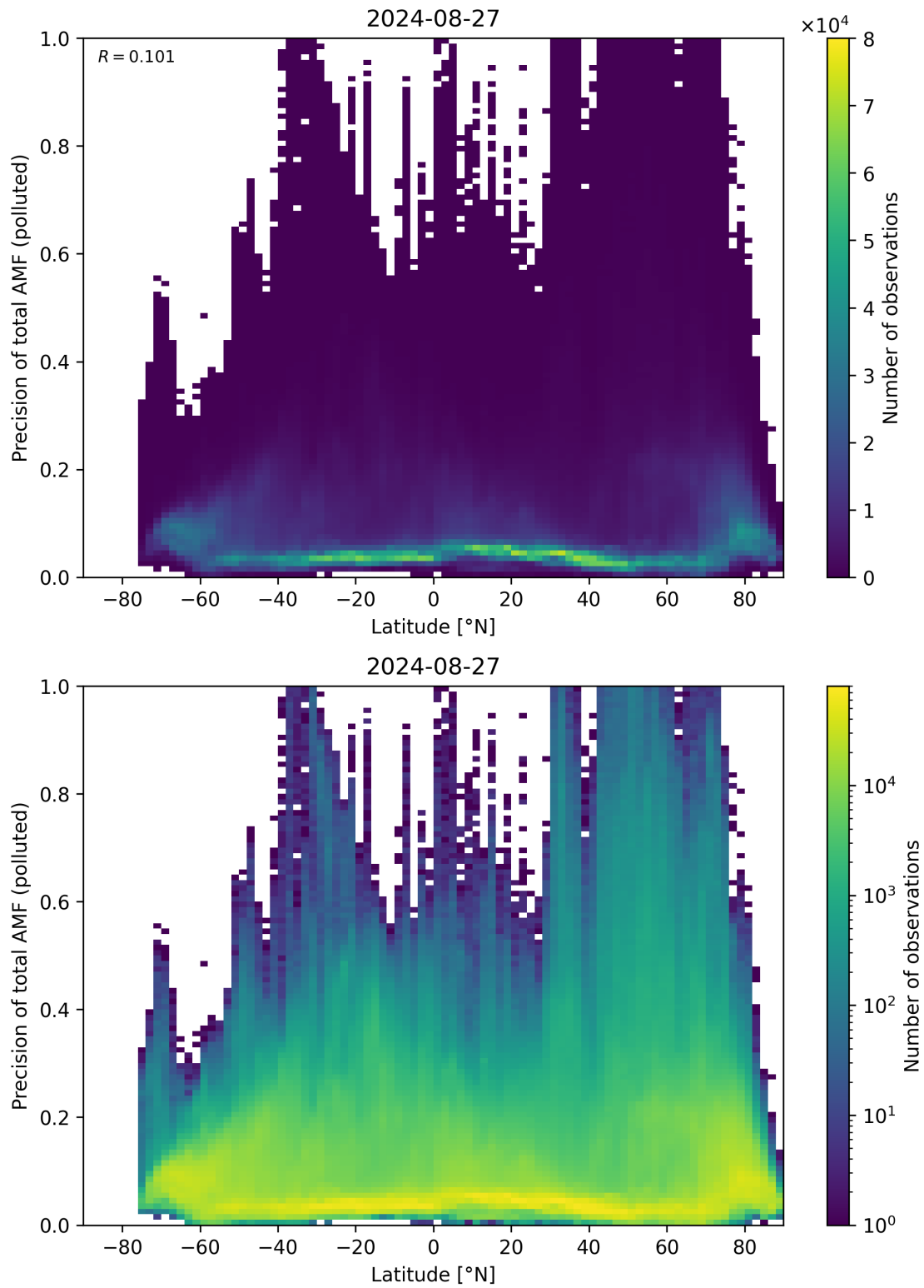
Figure 155: Scatter density plot of “Latitude” against “Precision of total AMF (polluted)” for 2024-08-27 to 2024-08-28.
