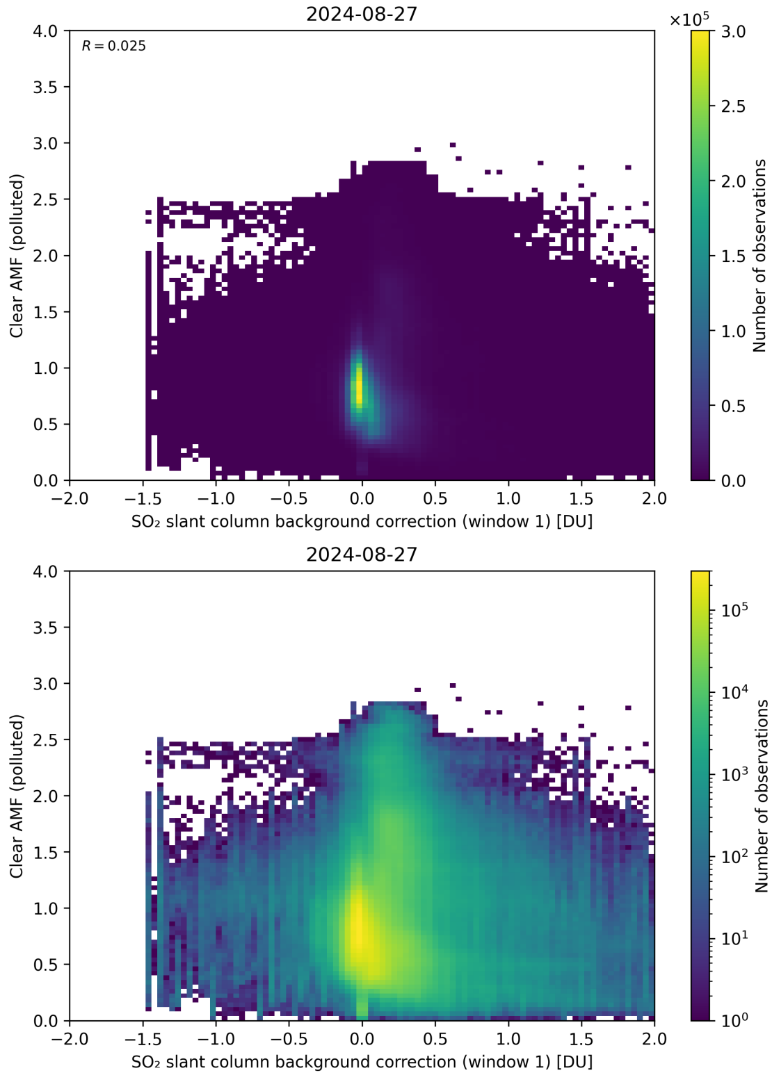
Figure 103: Scatter density plot of “SO 2 slant column background correction (window 1)” against “Clear AMF (polluted)” for 2024-08-27 to 2024-08-28.
