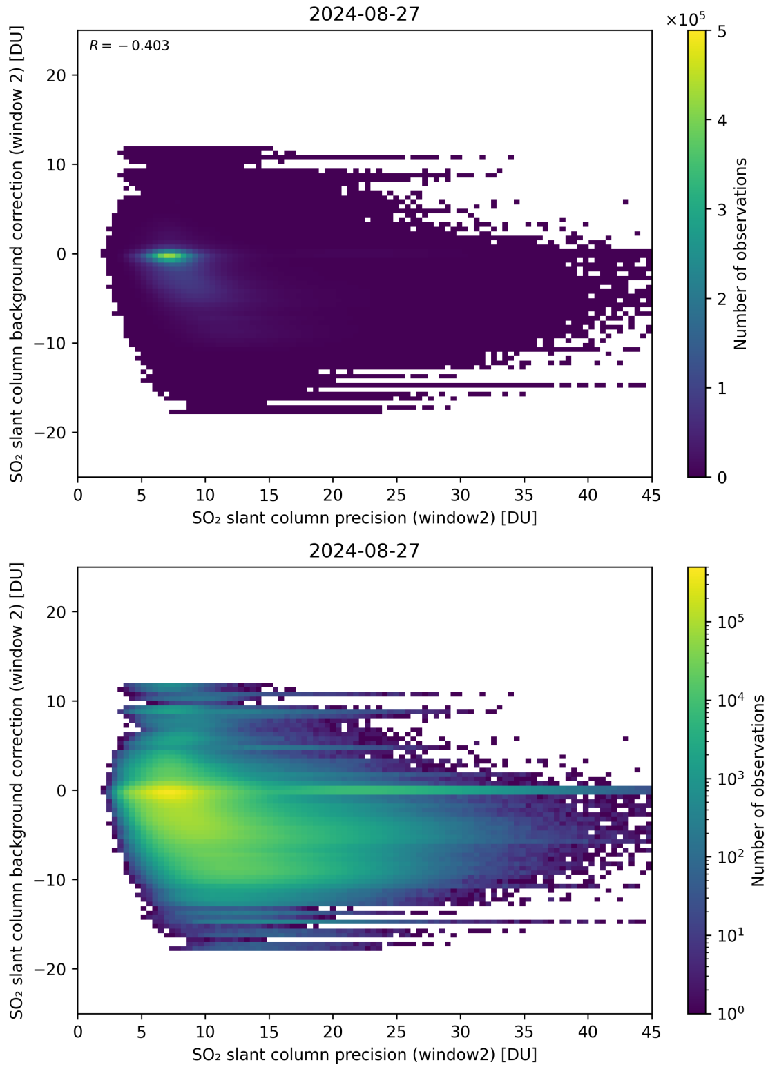
Figure 241: Scatter density plot of “SO 2 slant column precision (window2)” against “SO 2 slant column background correction (window 2)” for 2024-08-27 to 2024-08-28.
