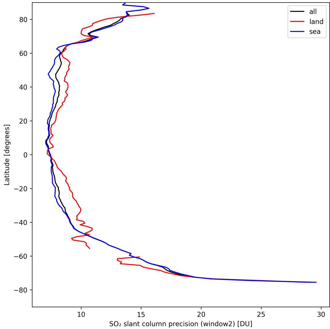
Figure 38: Zonal average of “SO 2 slant column precision (window2)” for 2024-08-27 to 2024-08-28.
