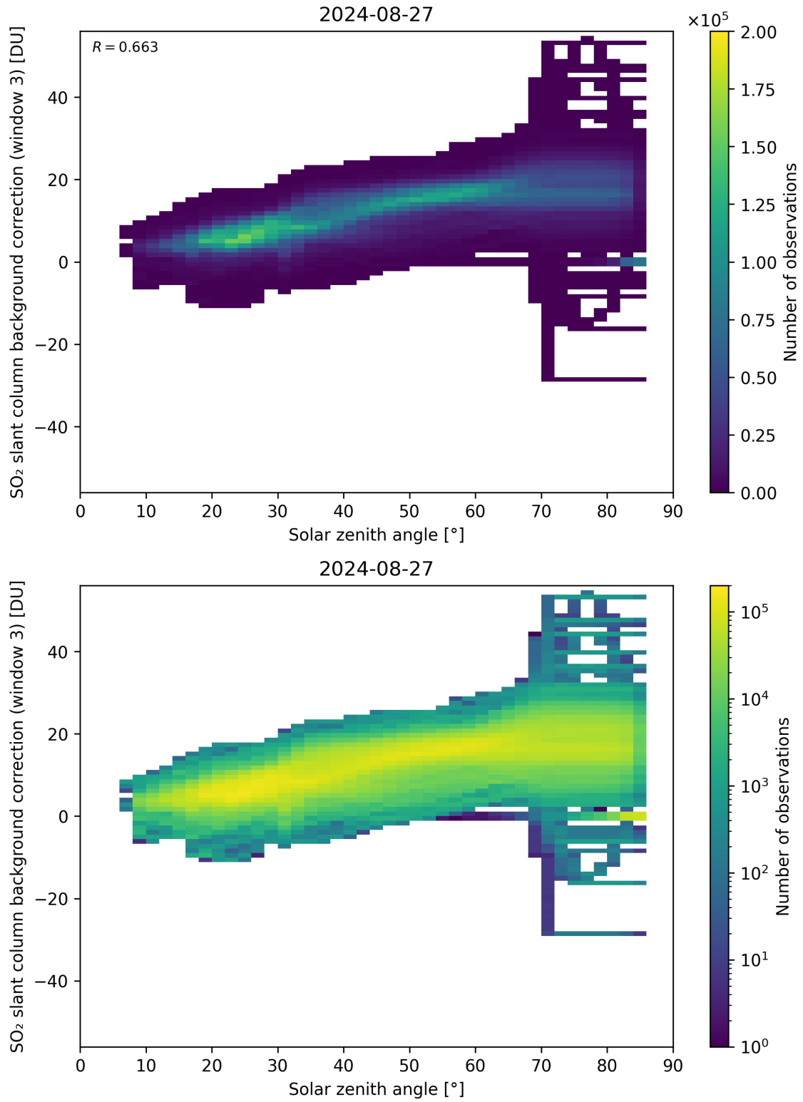
Figure 160: Scatter density plot of “Solar zenith angle” against “SO 2 slant column background correction (window 3)” for 2024-08-27 to 2024-08-28.
