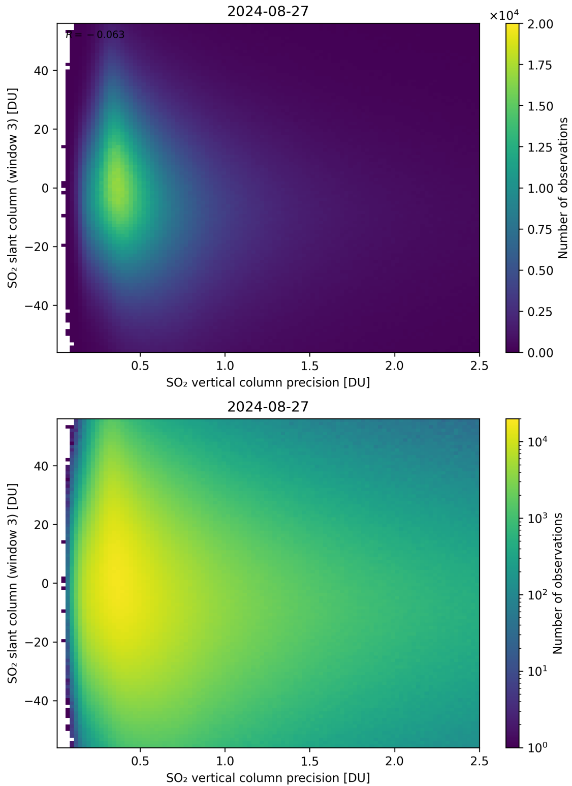
Figure 292: Scatter density plot of “SO 2 vertical column precision” against “SO 2 slant column (window 3)” for 2024-08-27 to 2024-08-28.
