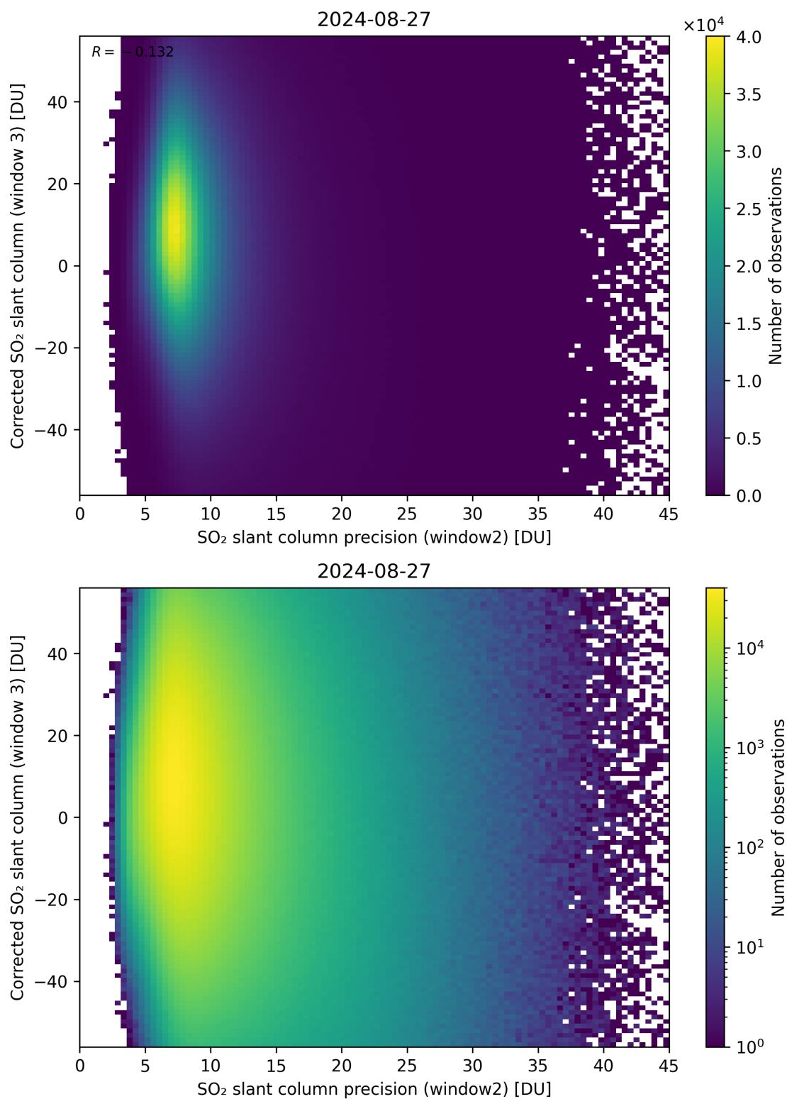
Figure 248: Scatter density plot of “SO 2 slant column precision (window2)” against “Corrected SO 2 slant column (window 3)” for 2024-08-27 to 2024-08-28.
