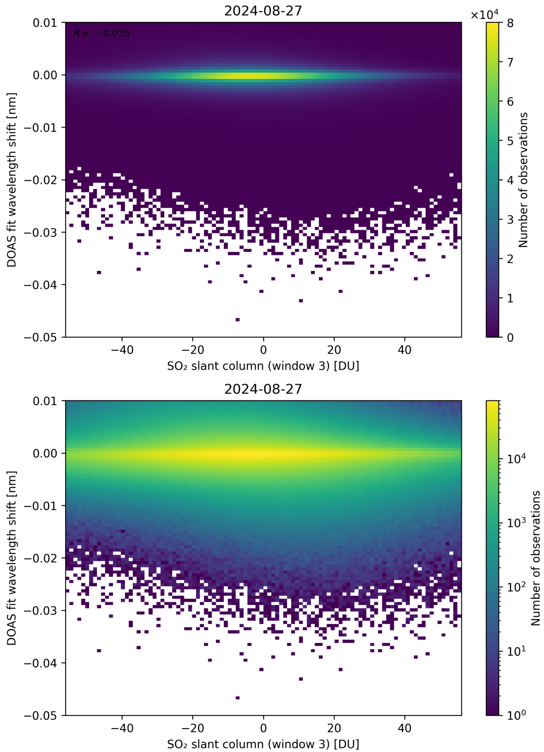
Figure 254: Scatter density plot of “SO 2 slant column (window 3)” against “DOAS fit wavelength shift” for 2024-08-27 to 2024-08-28.
