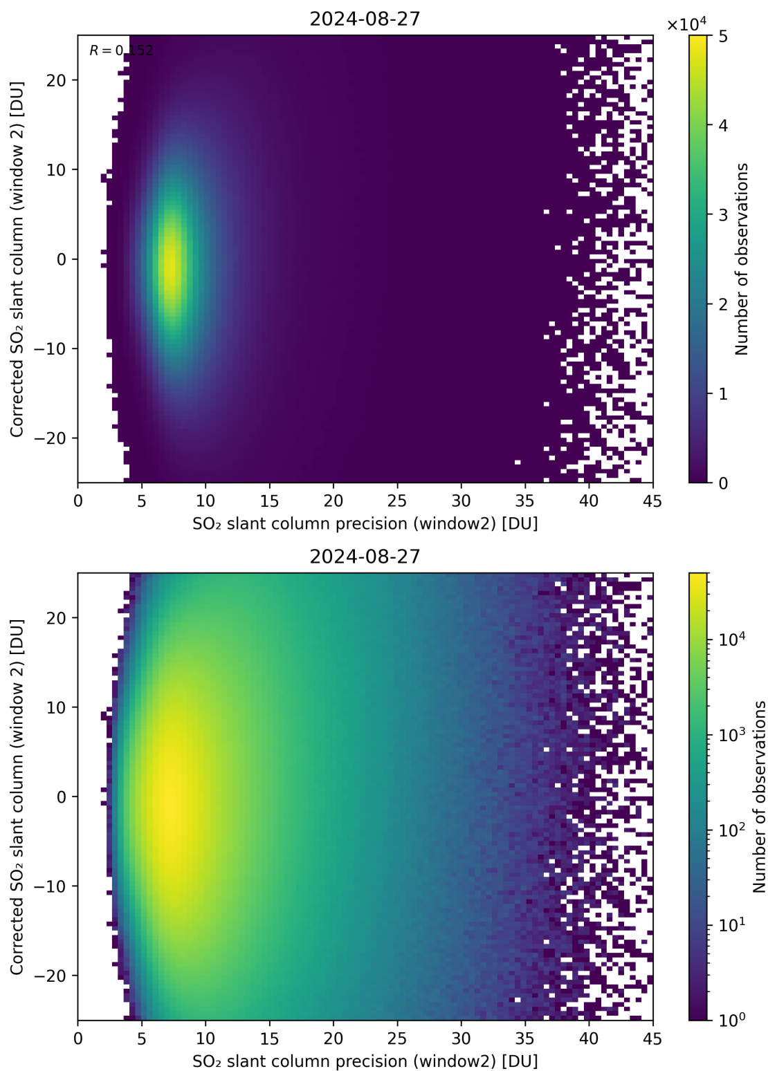
Figure 247: Scatter density plot of “SO 2 slant column precision (window2)” against “Corrected SO 2 slant column (window 2)” for 2024-08-27 to 2024-08-28.
