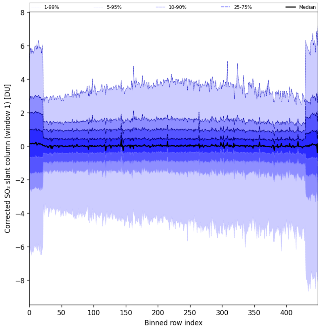
Figure 81: Along track statistics of “Corrected SO 2 slant column (window 1)” for 2024-08-27 to 2024-08-28
