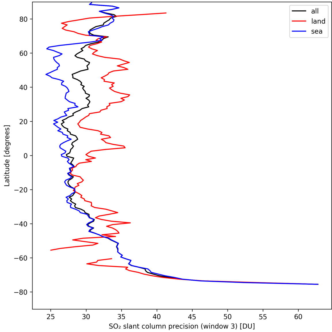
Figure 42: Zonal average of “SO 2 slant column precision (window 3)” for 2024-08-27 to 2024-08-28.
