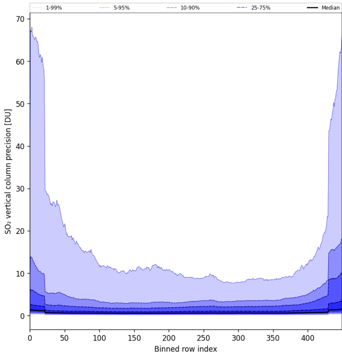
Figure 77: Along track statistics of “SO 2 vertical column precision” for 2024-08-27 to 2024-08-28
