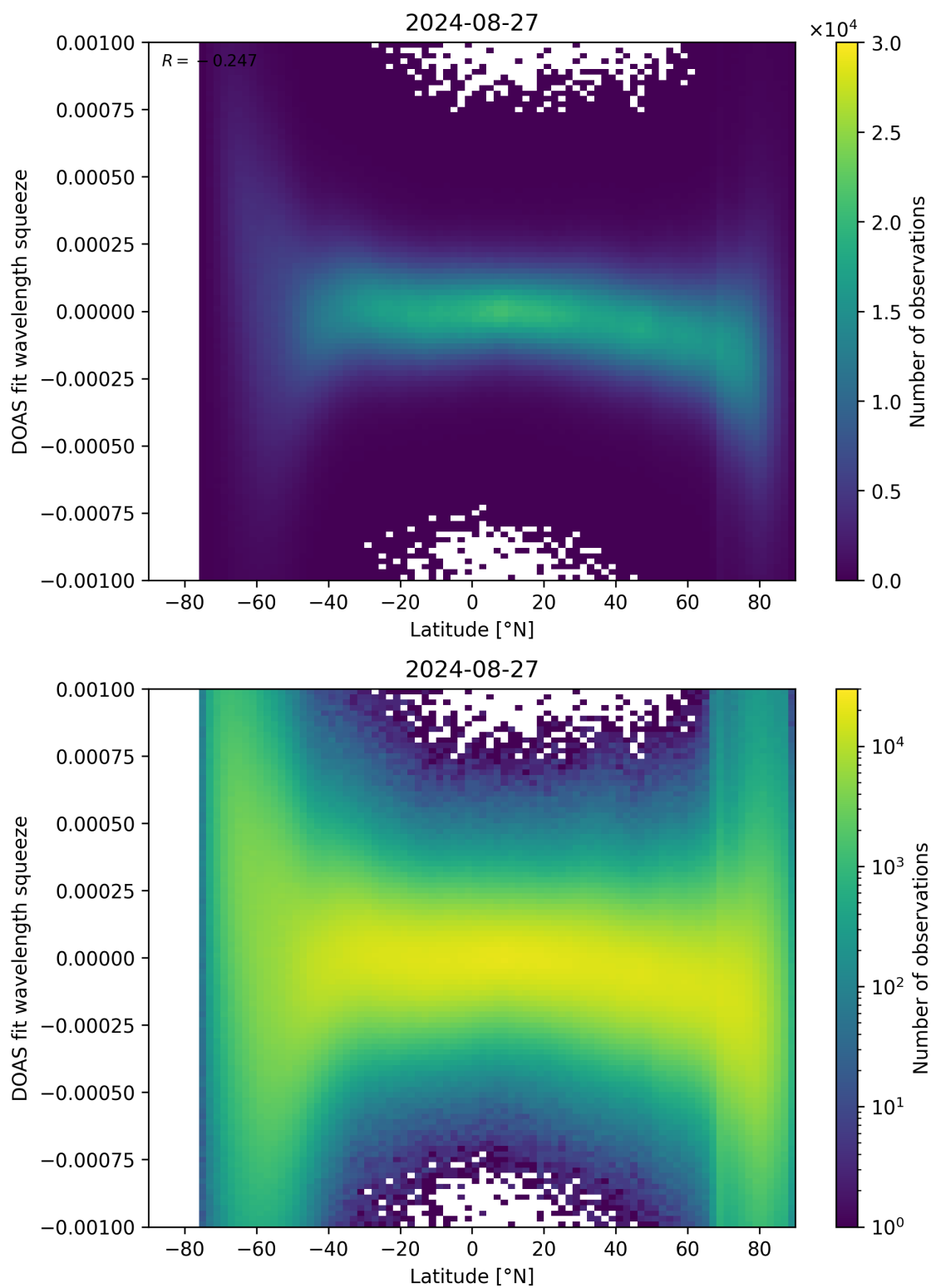
Figure 143: Scatter density plot of “Latitude” against “DOAS fit wavelength squeeze” for 2024-08-27 to 2024-08-28.
