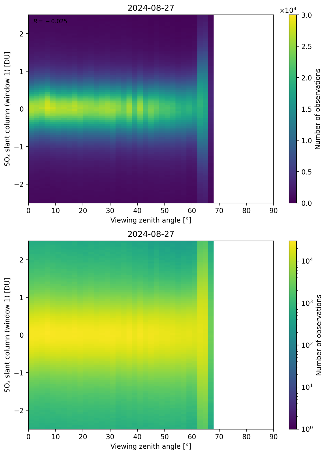
Figure 320: Scatter density plot of “Viewing zenith angle” against “SO 2 slant column (window 1)” for 2024-08-27 to 2024-08-28.
