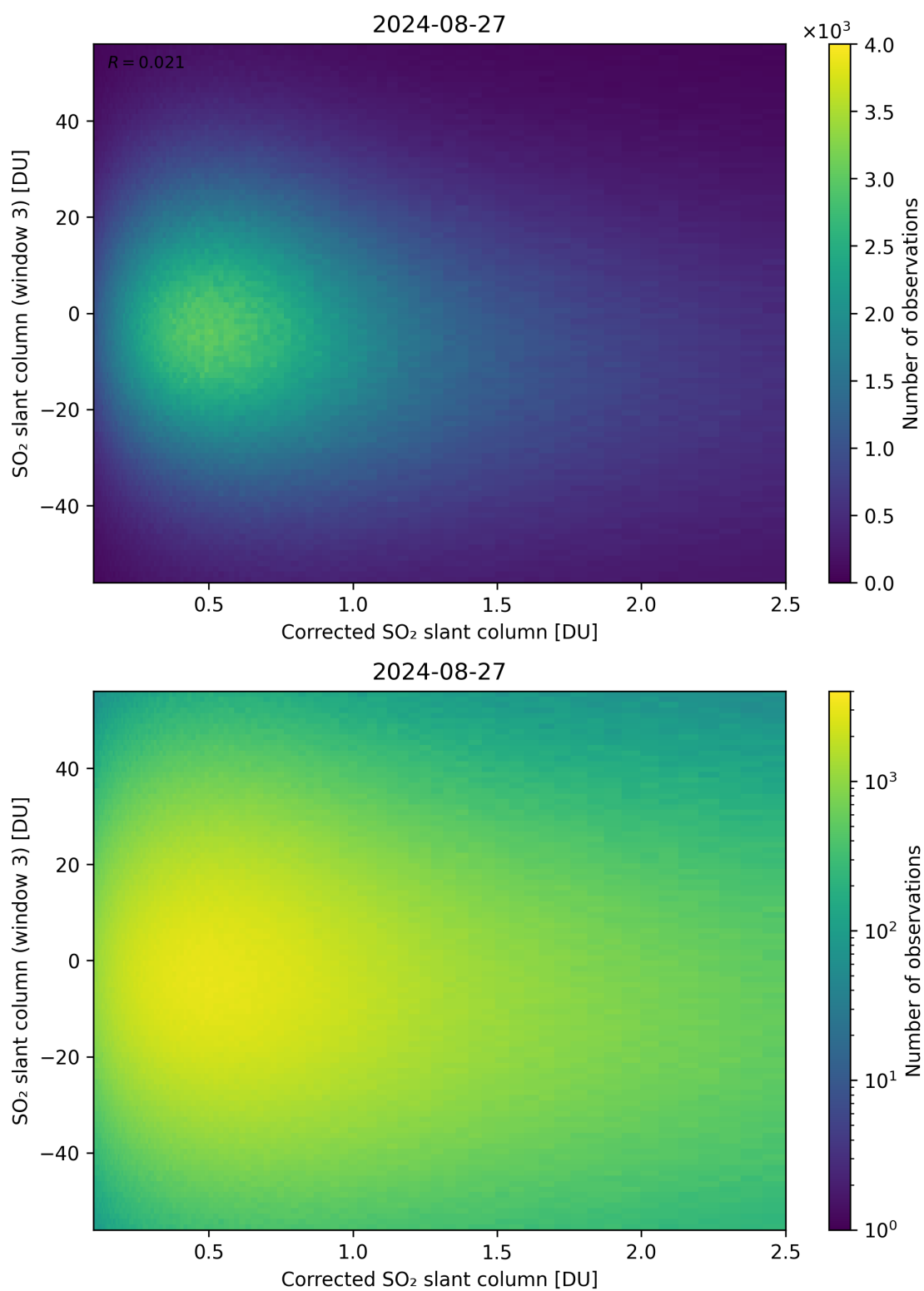
Figure 190: Scatter density plot of “Corrected SO 2 slant column” against “SO 2 slant column (window 3)” for 2024-08-27 to 2024-08-28.
