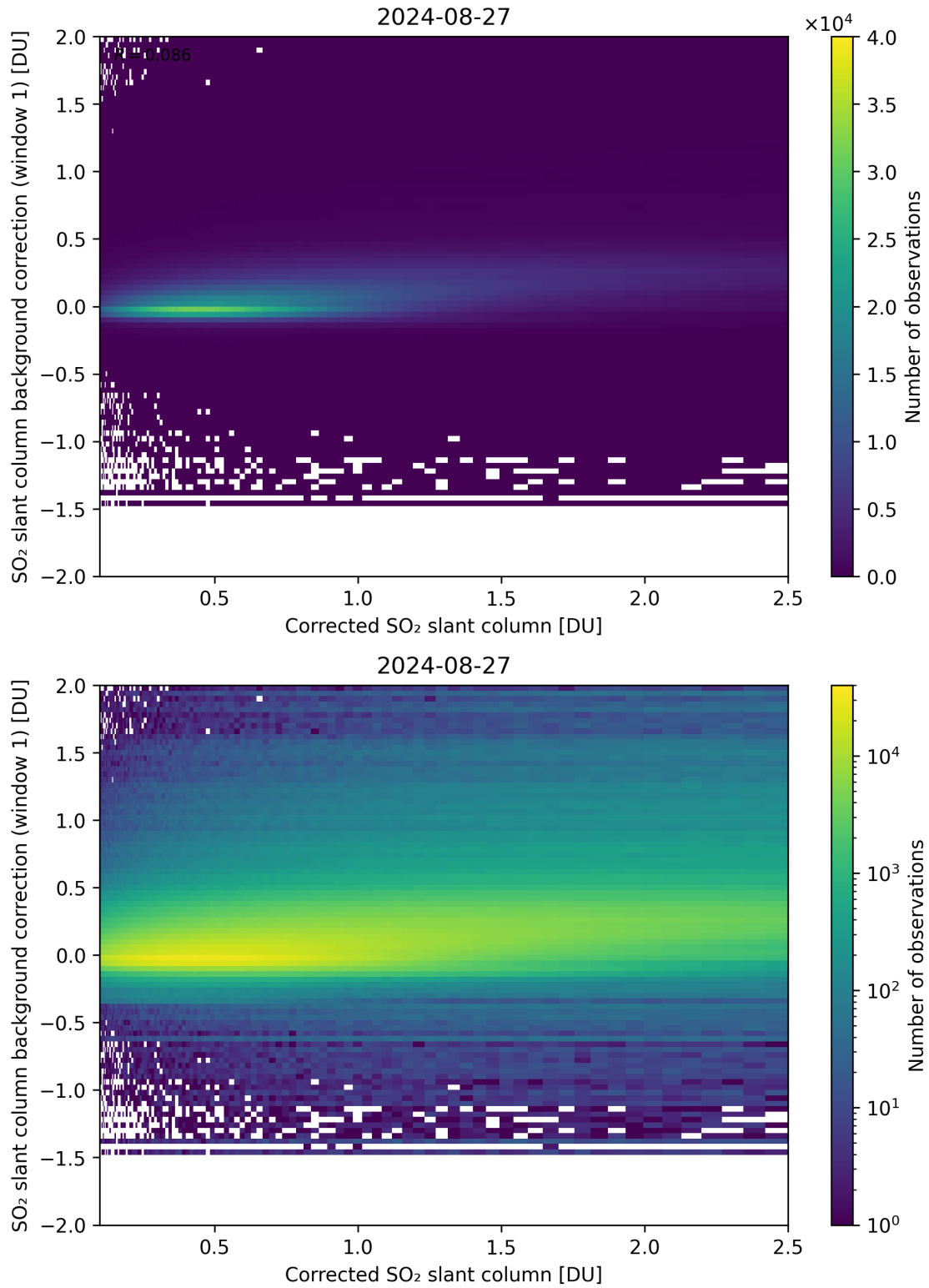
Figure 178: Scatter density plot of “Corrected SO 2 slant column” against “SO 2 slant column background correction (window 1)” for 2024-08-27 to 2024-08-28.
