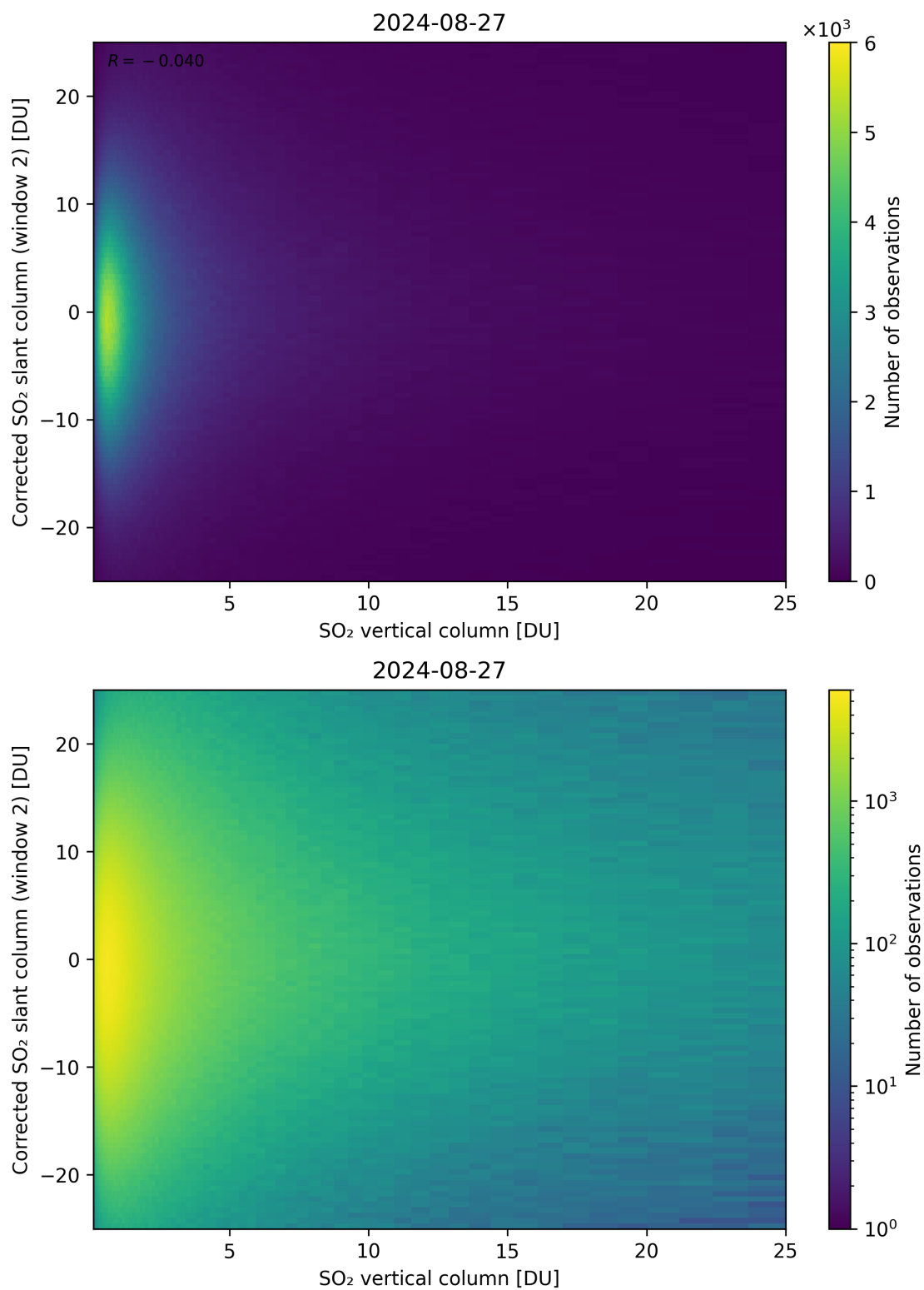
Figure 298: Scatter density plot of “SO 2 vertical column” against “Corrected SO 2 slant column (window 2)” for 2024-08-27 to 2024-08-28.
