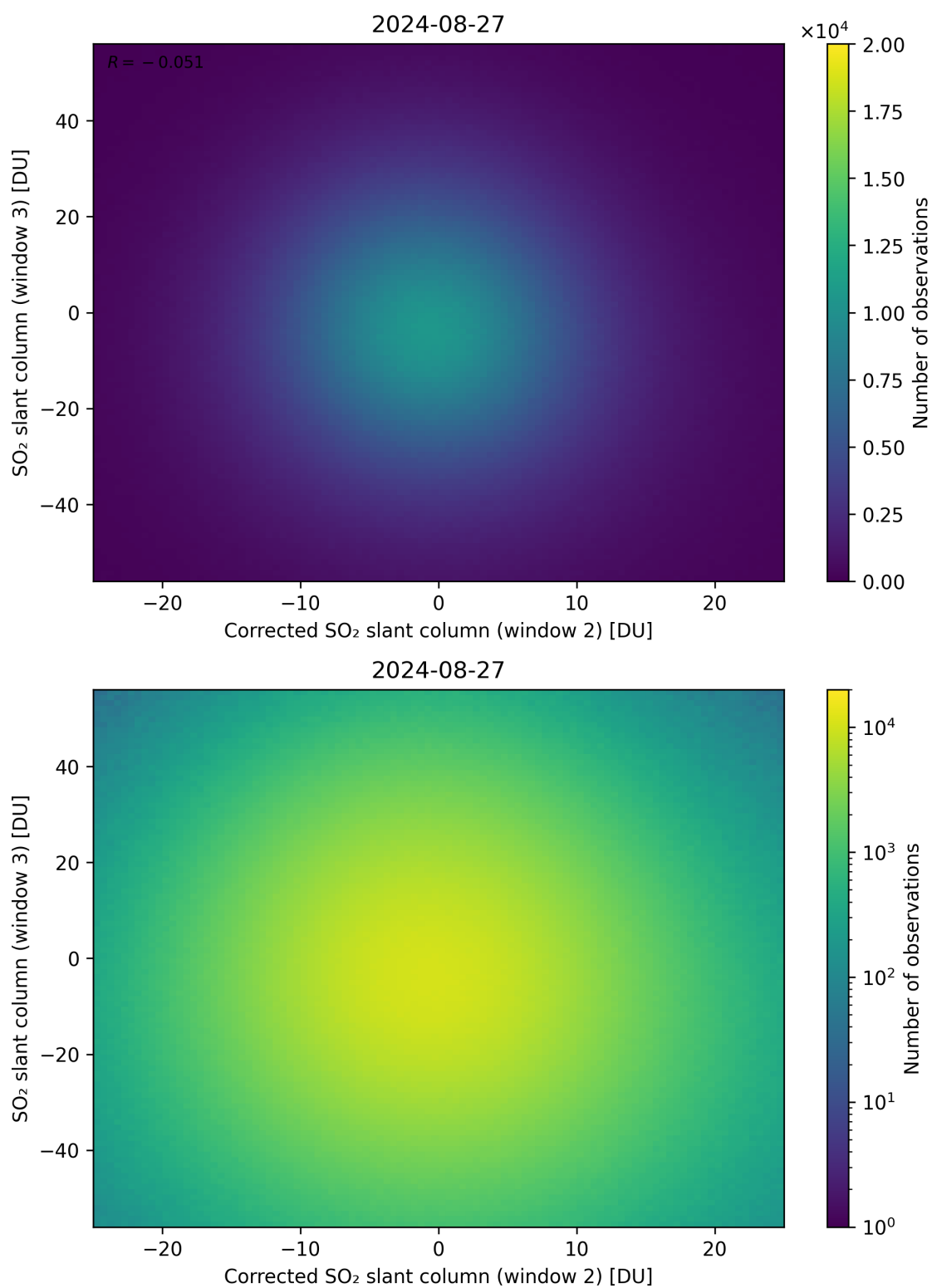
Figure 201: Scatter density plot of “Corrected SO 2 slant column (window 2)” against “SO 2 slant column (window 3)” for 2024-08-27 to 2024-08-28.
