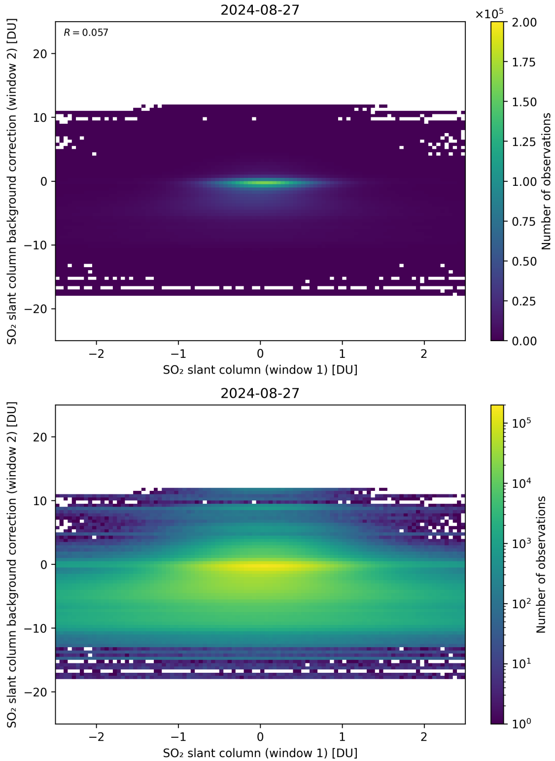
Figure 213: Scatter density plot of “SO 2 slant column (window 1)” against “SO 2 slant column background correction (window 2)” for 2024-08-27 to 2024-08-28.
