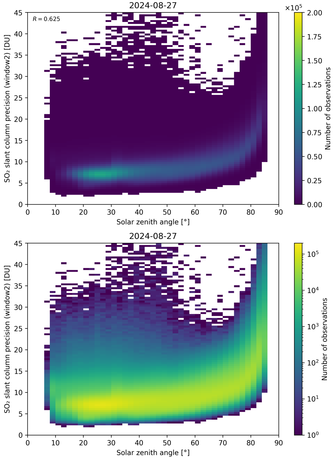
Figure 171: Scatter density plot of “Solar zenith angle” against “SO 2 slant column precision (window2)” for 2024-08-27 to 2024-08-28.
