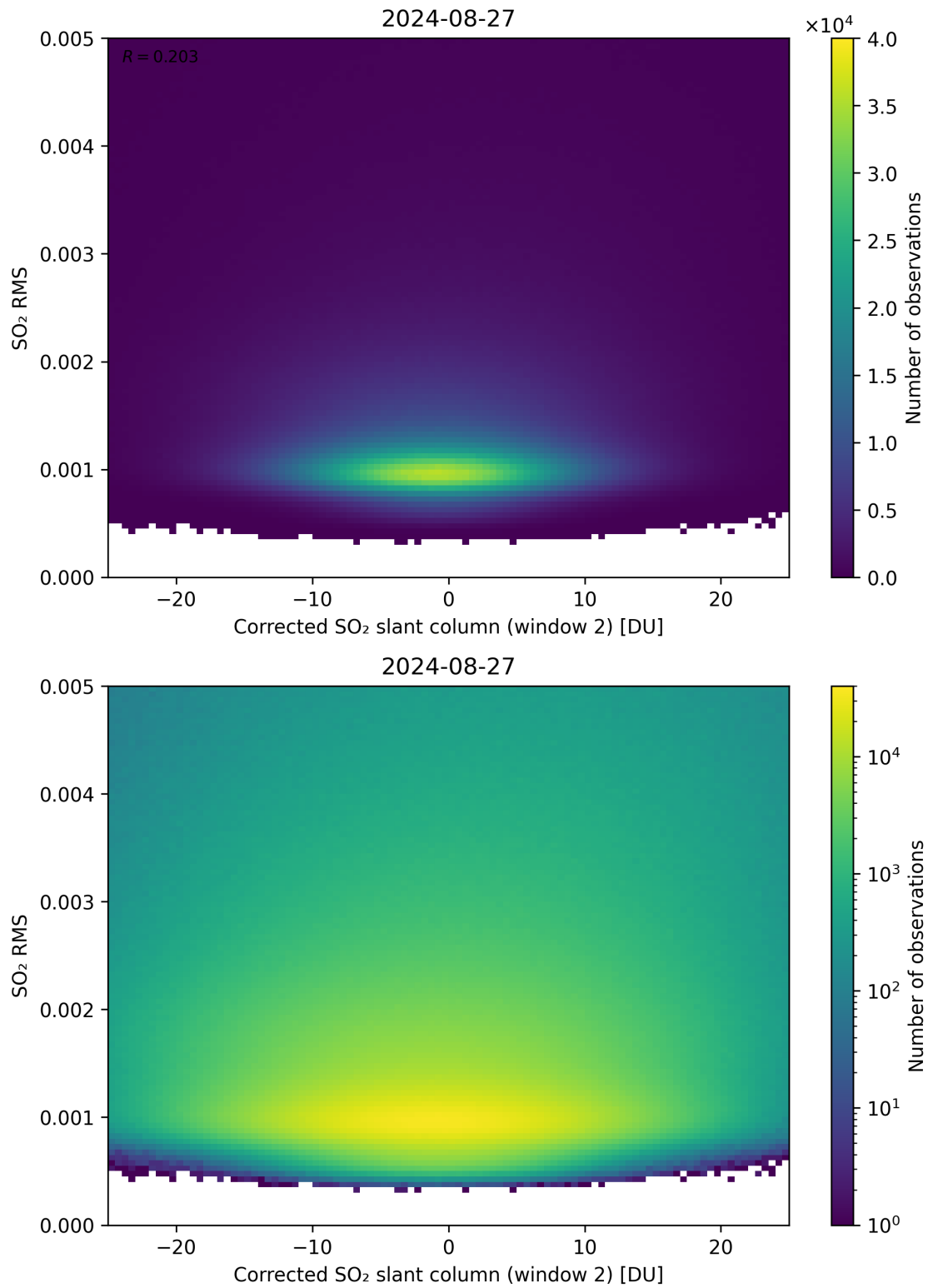
Figure 198: Scatter density plot of “Corrected SO 2 slant column (window 2)” against “SO 2 RMS” for 2024-08-27 to 2024-08-28.
