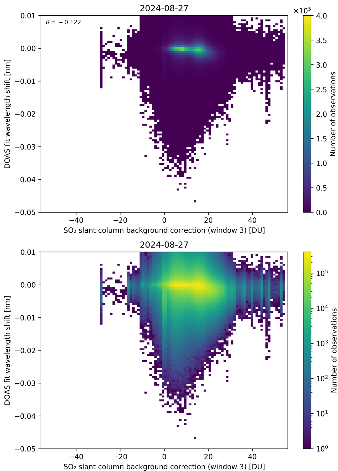
Figure 121: Scatter density plot of “SO 2 slant column background correction (window 3)” against “DOAS fit wavelength shift” for 2024-08-27 to 2024-08-28.
