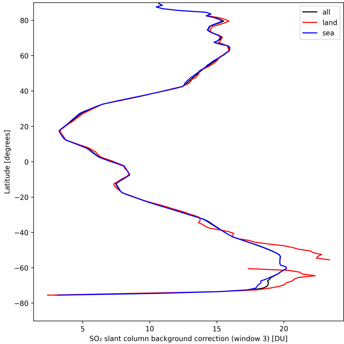
Figure 44: Zonal average of “SO 2 slant column background correction (window 3)” for 2024-08-27 to 2024-08-28.
