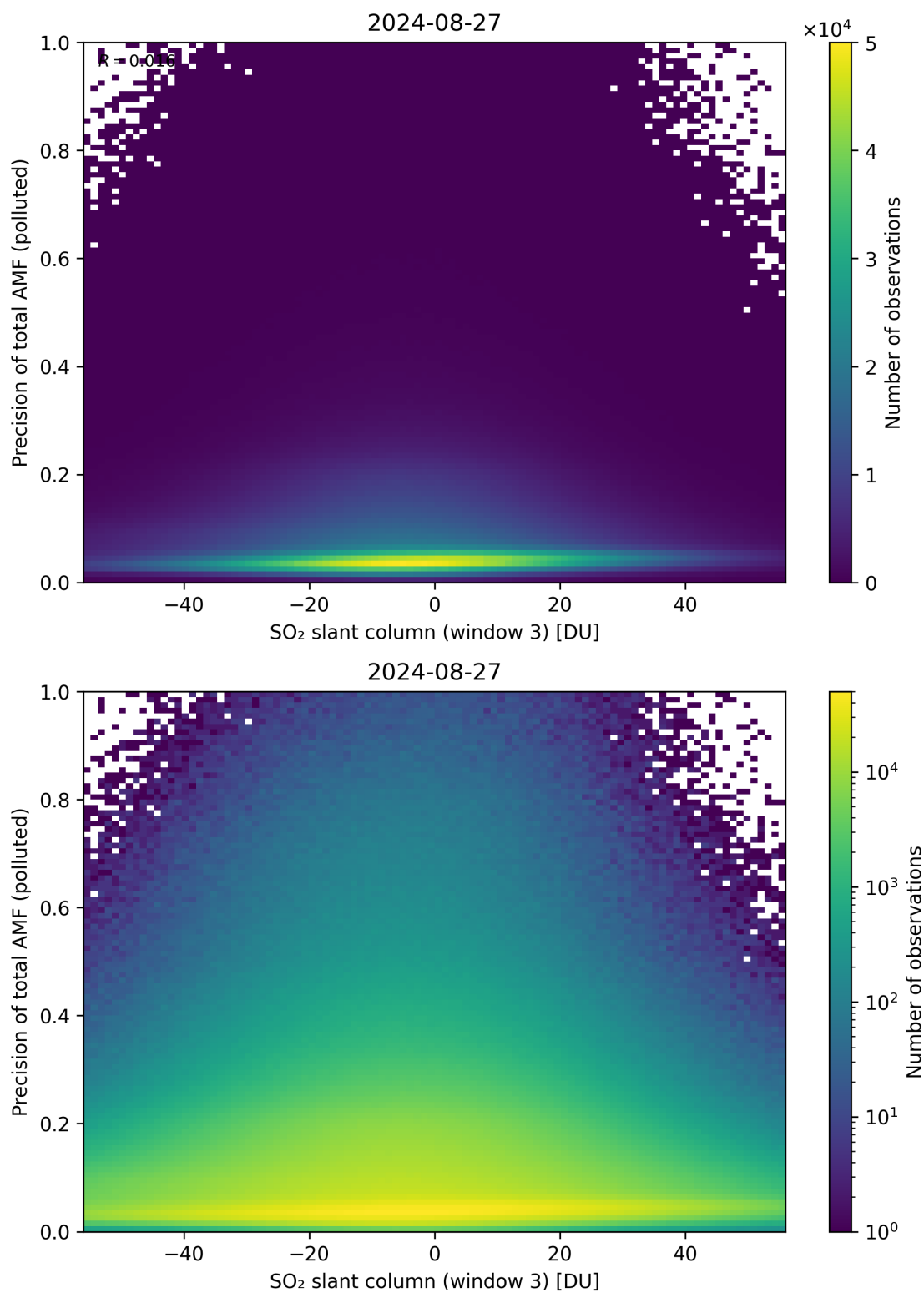
Figure 269: Scatter density plot of “SO 2 slant column (window 3)” against “Precision of total AMF (polluted)” for 2024-08-27 to 2024-08-28.
