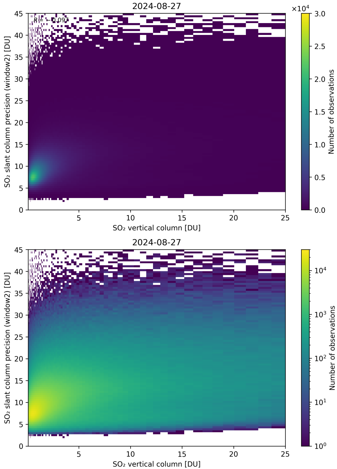
Figure 302: Scatter density plot of “SO 2 vertical column” against “SO 2 slant column precision (window2)” for 2024-08-27 to 2024-08-28.
