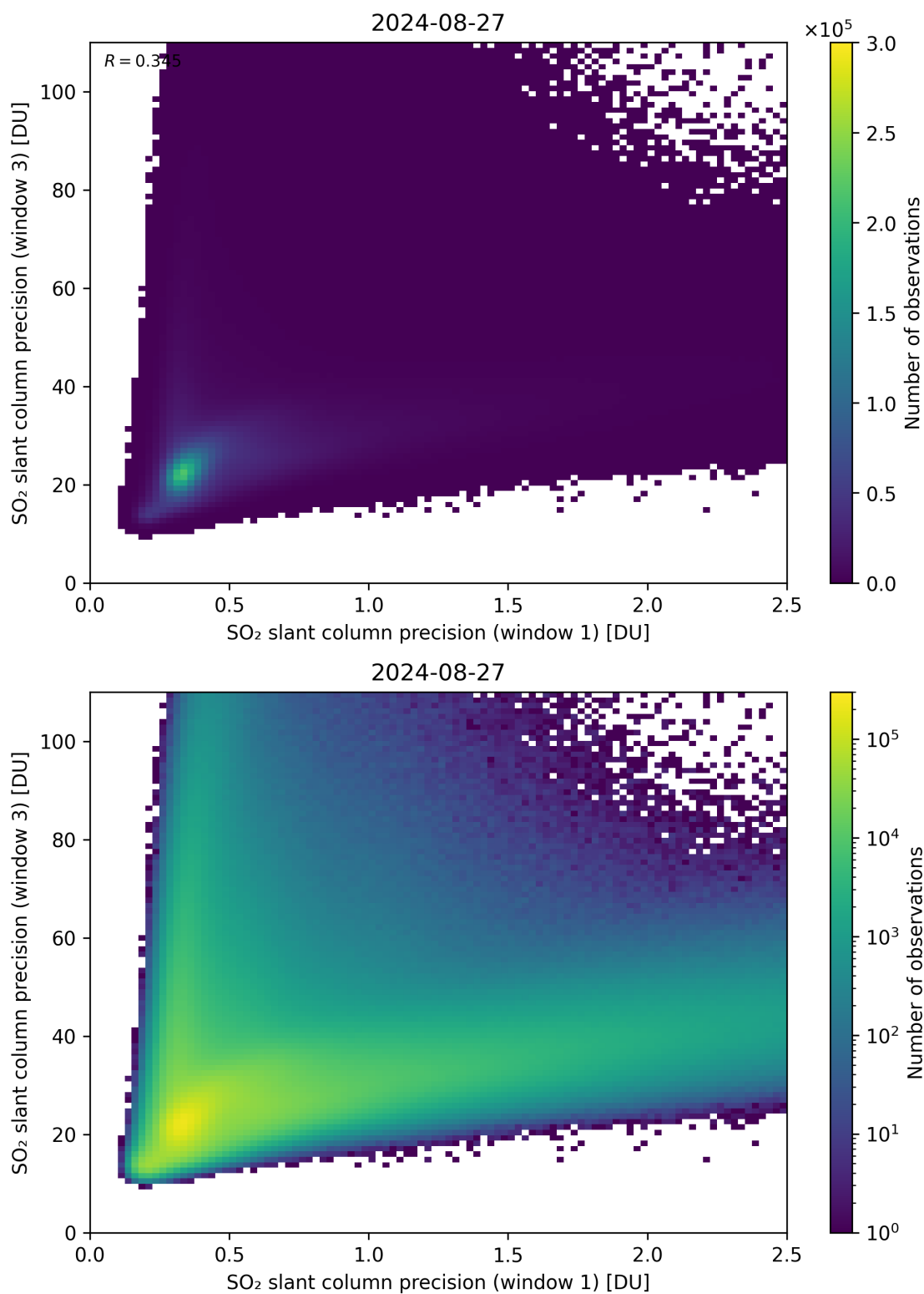
Figure 229: Scatter density plot of “SO 2 slant column precision (window 1)” against “SO 2 slant column precision (window 3)” for 2024-08-27 to 2024-08-28.
