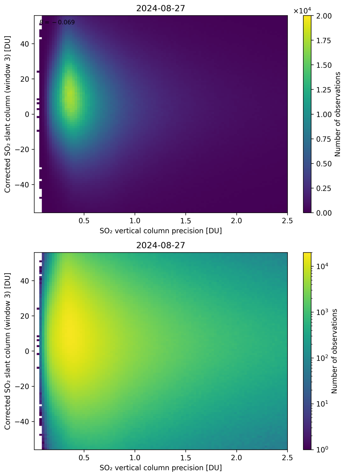
Figure 288: Scatter density plot of “SO 2 vertical column precision” against “Corrected SO 2 slant column (window 3)” for 2024-08-27 to 2024-08-28.
