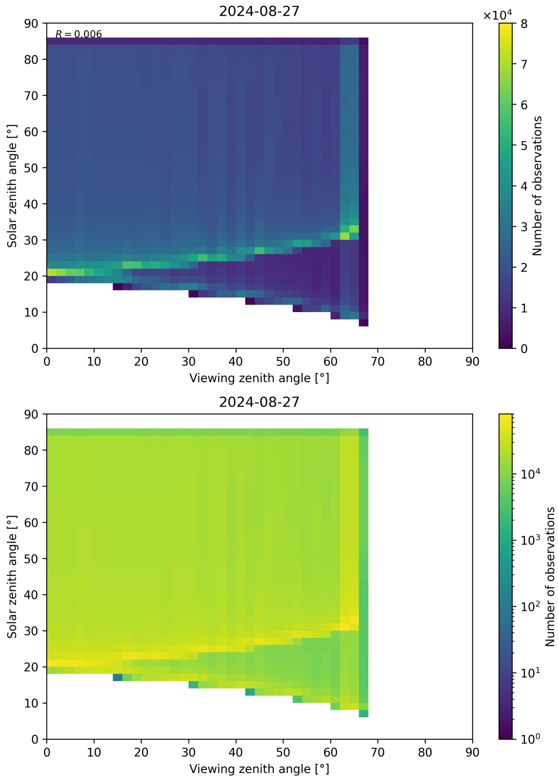
Figure 315: Scatter density plot of “Viewing zenith angle” against “Solar zenith angle” for 2024-08-27 to 2024-08-28.
