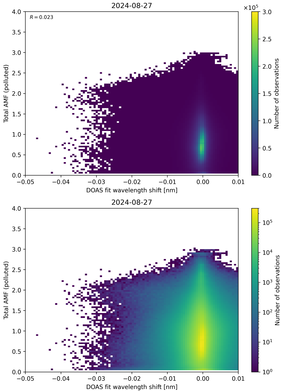
Figure 130: Scatter density plot of “DOAS fit wavelength shift” against “Total AMF (polluted)” for 2024-08-27 to 2024-08-28.
