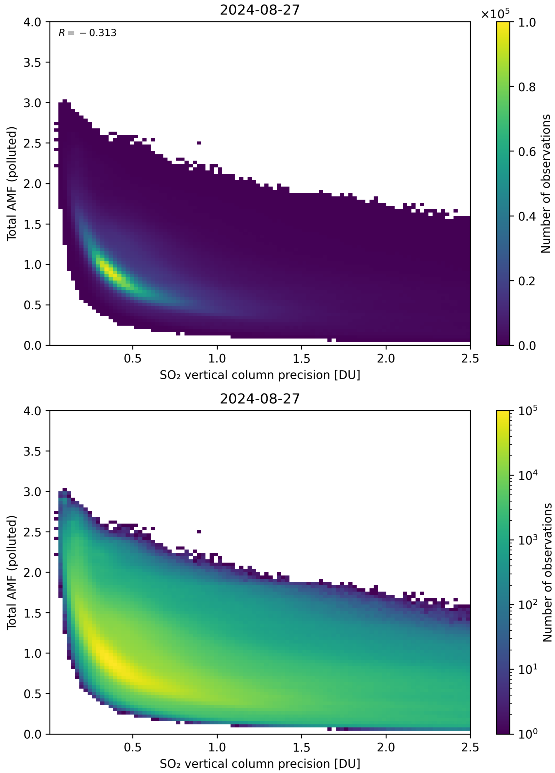
Figure 294: Scatter density plot of “SO 2 vertical column precision” against “Total AMF (polluted)” for 2024-08-27 to 2024-08-28.
