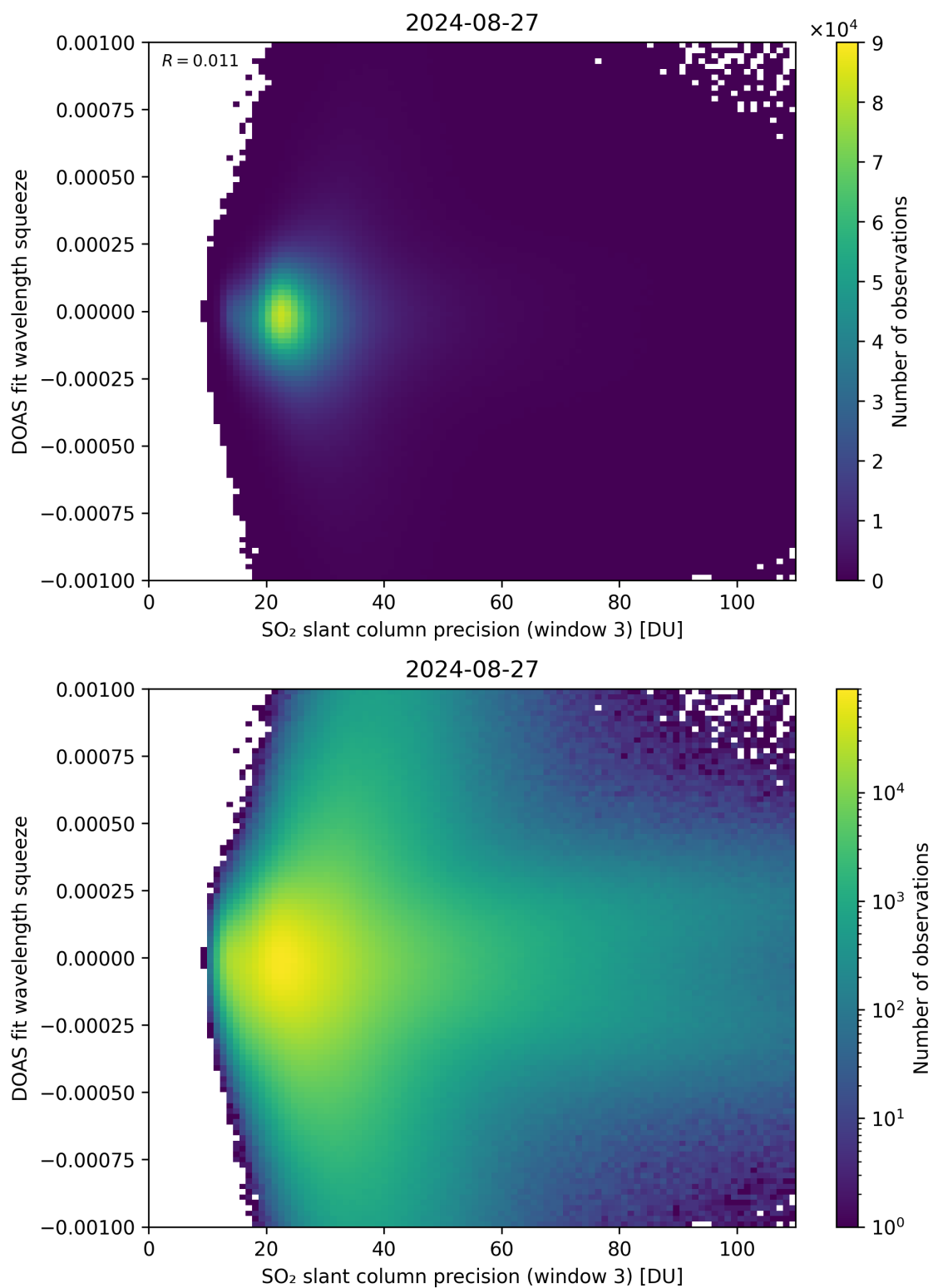
Figure 259: Scatter density plot of “SO 2 slant column precision (window 3)” against “DOAS fit wavelength squeeze” for 2024-08-27 to 2024-08-28.
