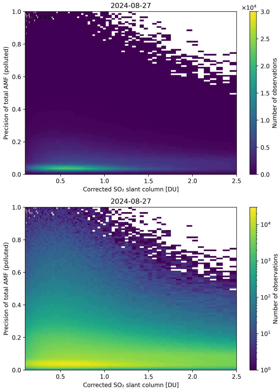
Figure 193: Scatter density plot of “Corrected SO 2 slant column” against “Precision of total AMF (polluted)” for 2024-08-27 to 2024-08-28.
