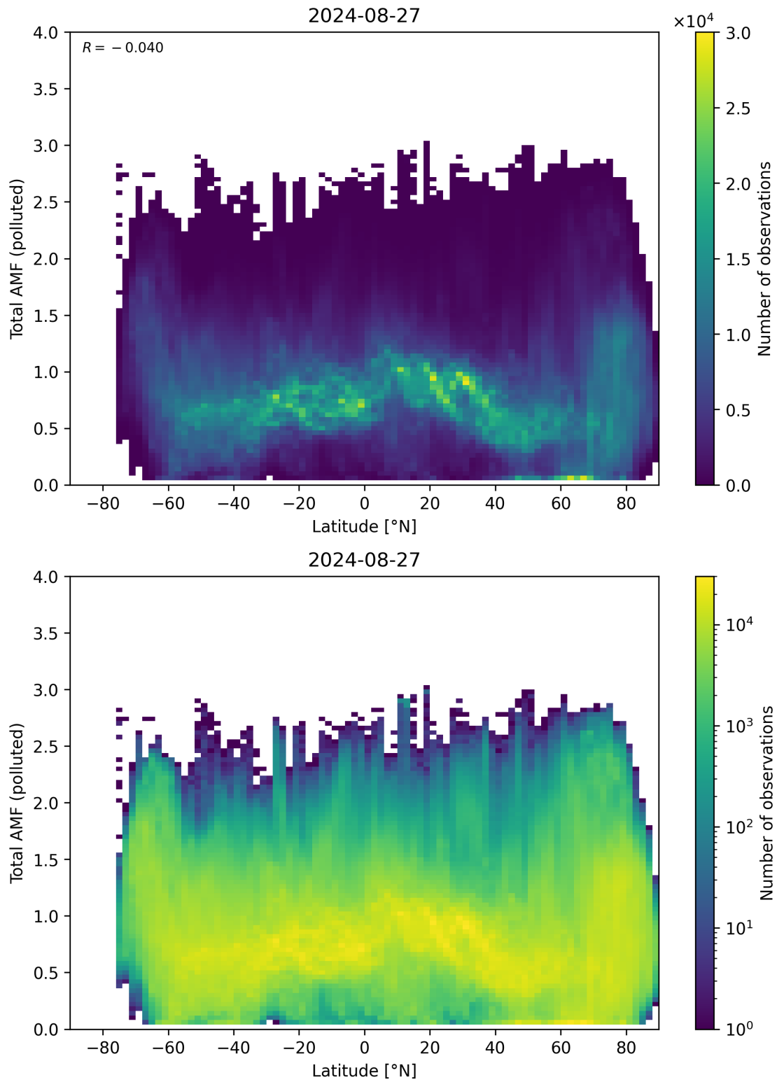
Figure 154: Scatter density plot of “Latitude” against “Total AMF (polluted)” for 2024-08-27 to 2024-08-28.
