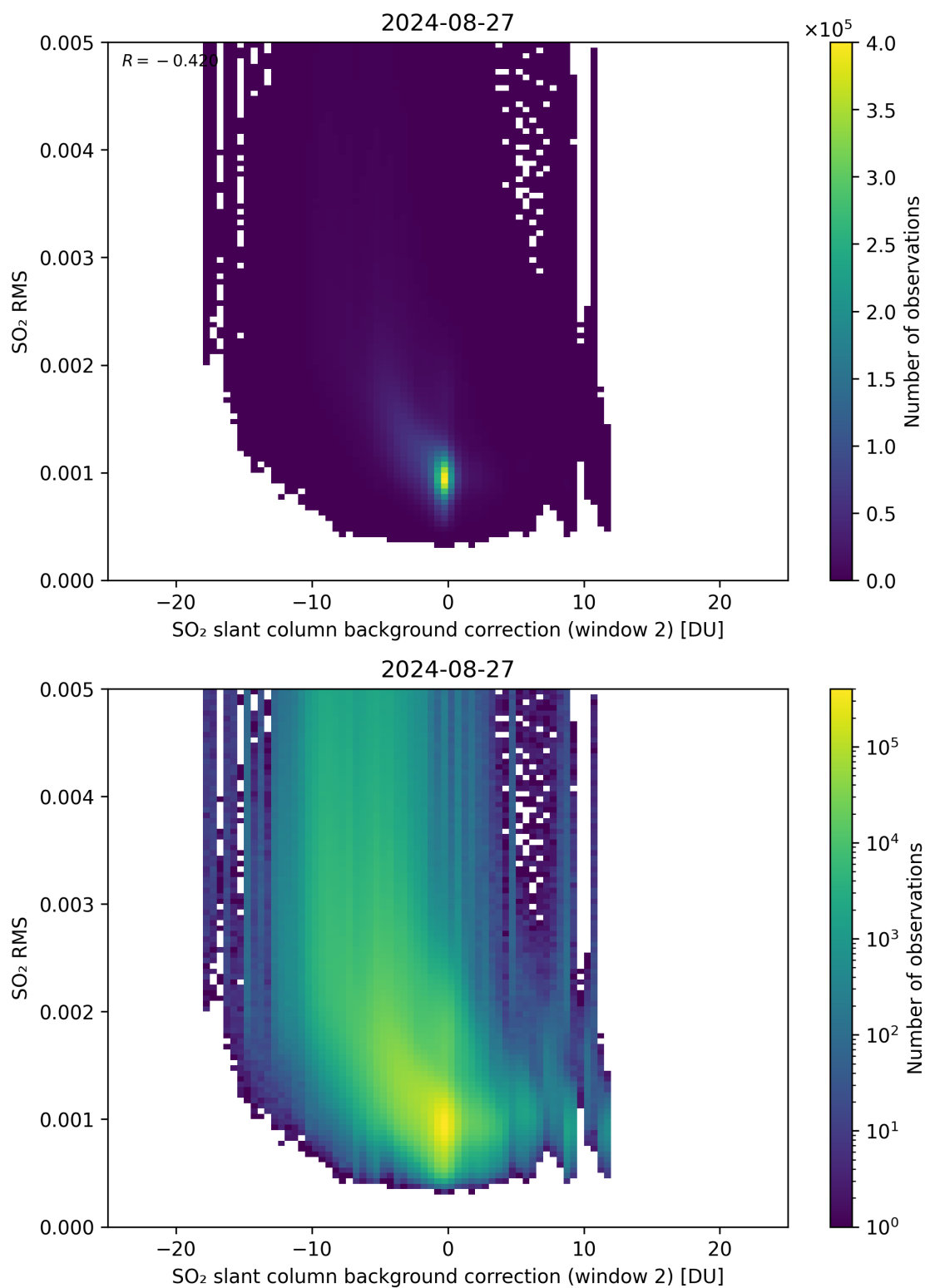
Figure 114: Scatter density plot of “SO 2 slant column background correction (window 2)” against “SO 2 RMS” for 2024-08-27 to 2024-08-28.
