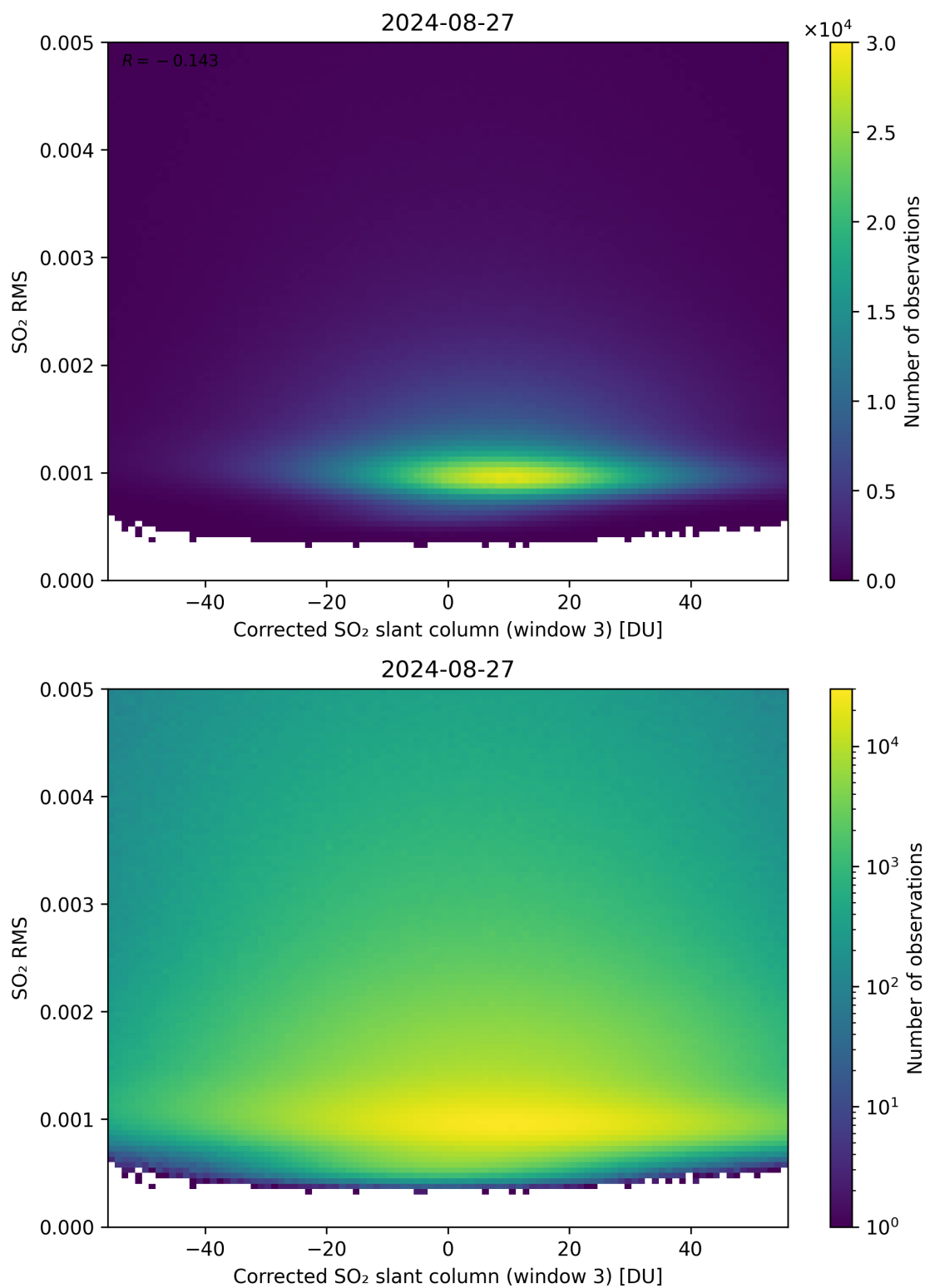
Figure 208: Scatter density plot of “Corrected SO 2 slant column (window 3)” against “SO 2 RMS” for 2024-08-27 to 2024-08-28.
