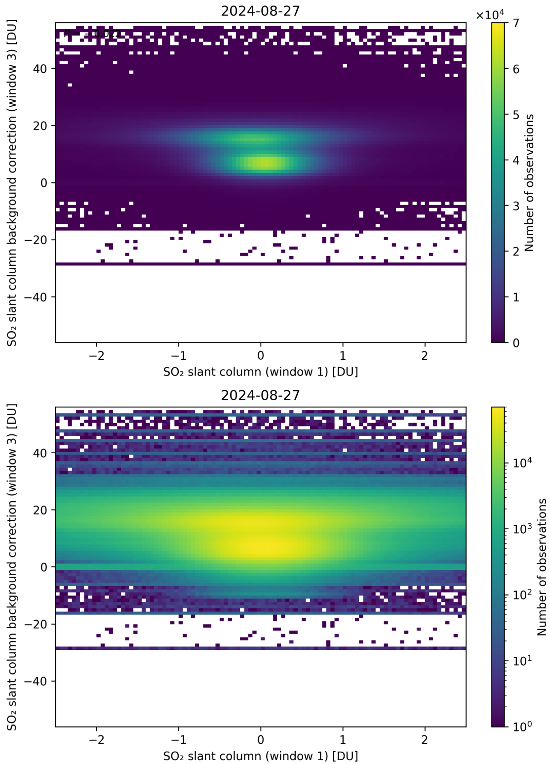
Figure 214: Scatter density plot of “SO 2 slant column (window 1)” against “SO 2 slant column background correction (window 3)” for 2024-08-27 to 2024-08-28.
