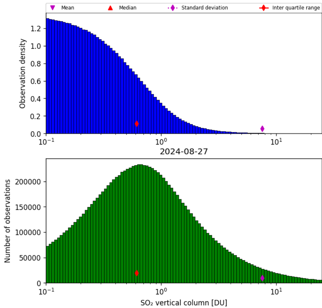
Figure 53: Histogram of “SO 2 vertical column” for 2024-08-27 to 2024-08-28
