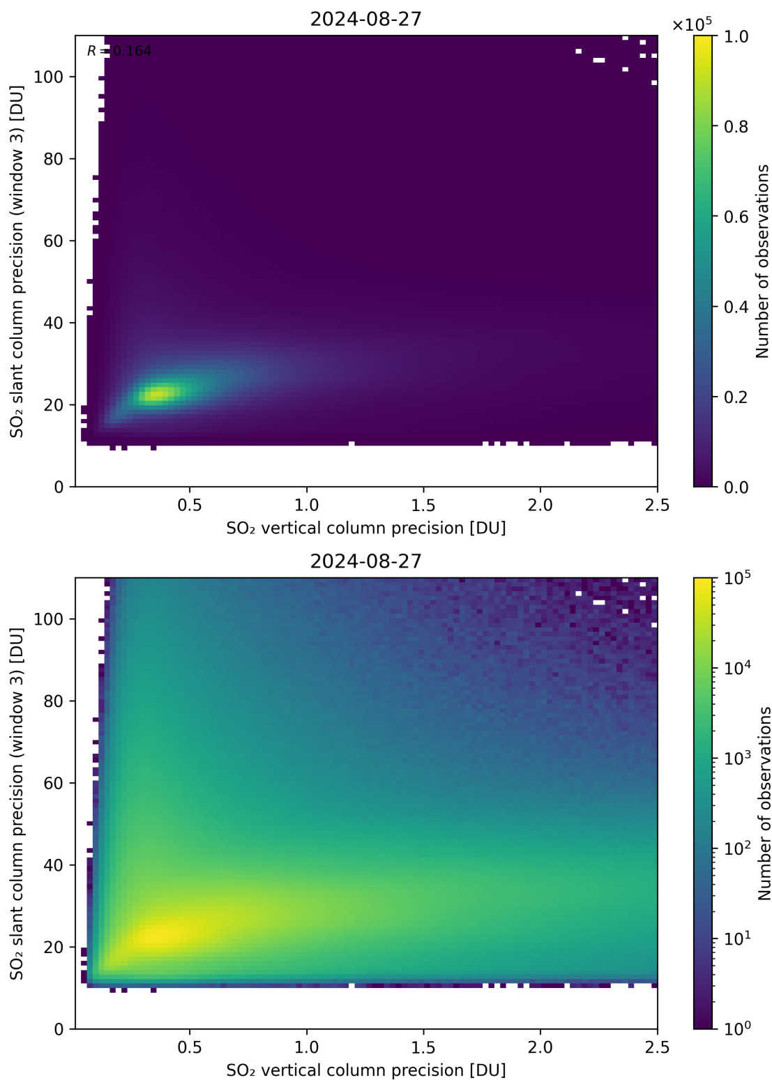
Figure 293: Scatter density plot of “SO 2 vertical column precision” against “SO 2 slant column precision (window 3)” for 2024-08-27 to 2024-08-28.
