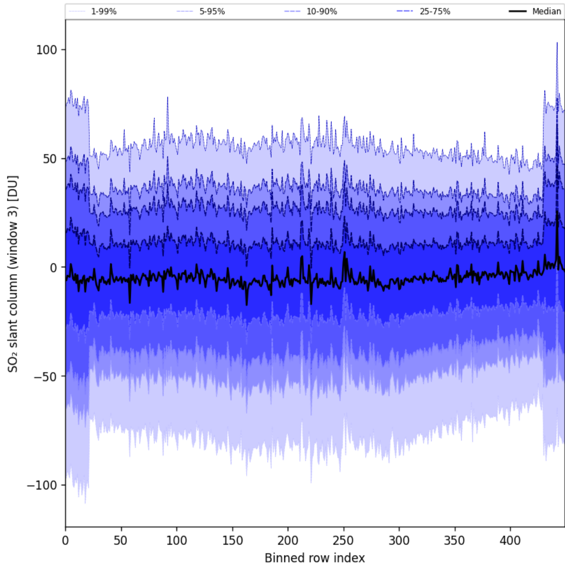
Figure 87: Along track statistics of “SO 2 slant column (window 3)” for 2024-08-27 to 2024-08-28
