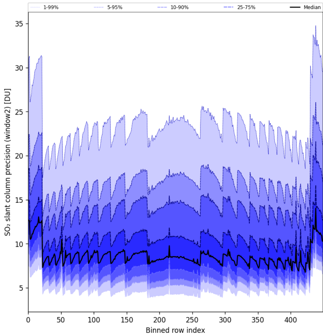
Figure 84: Along track statistics of “SO 2 slant column precision (window2)” for 2024-08-27 to 2024-08-28
