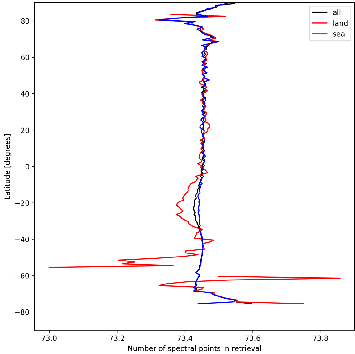
Figure 51: Zonal average of “Number of spectral points in retrieval” for 2024-08-27 to 2024-08-28.
