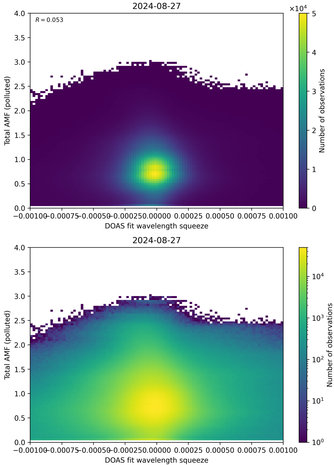
Figure 134: Scatter density plot of “DOAS fit wavelength squeeze” against “Total AMF (polluted)” for 2024-08-27 to 2024-08-28.
