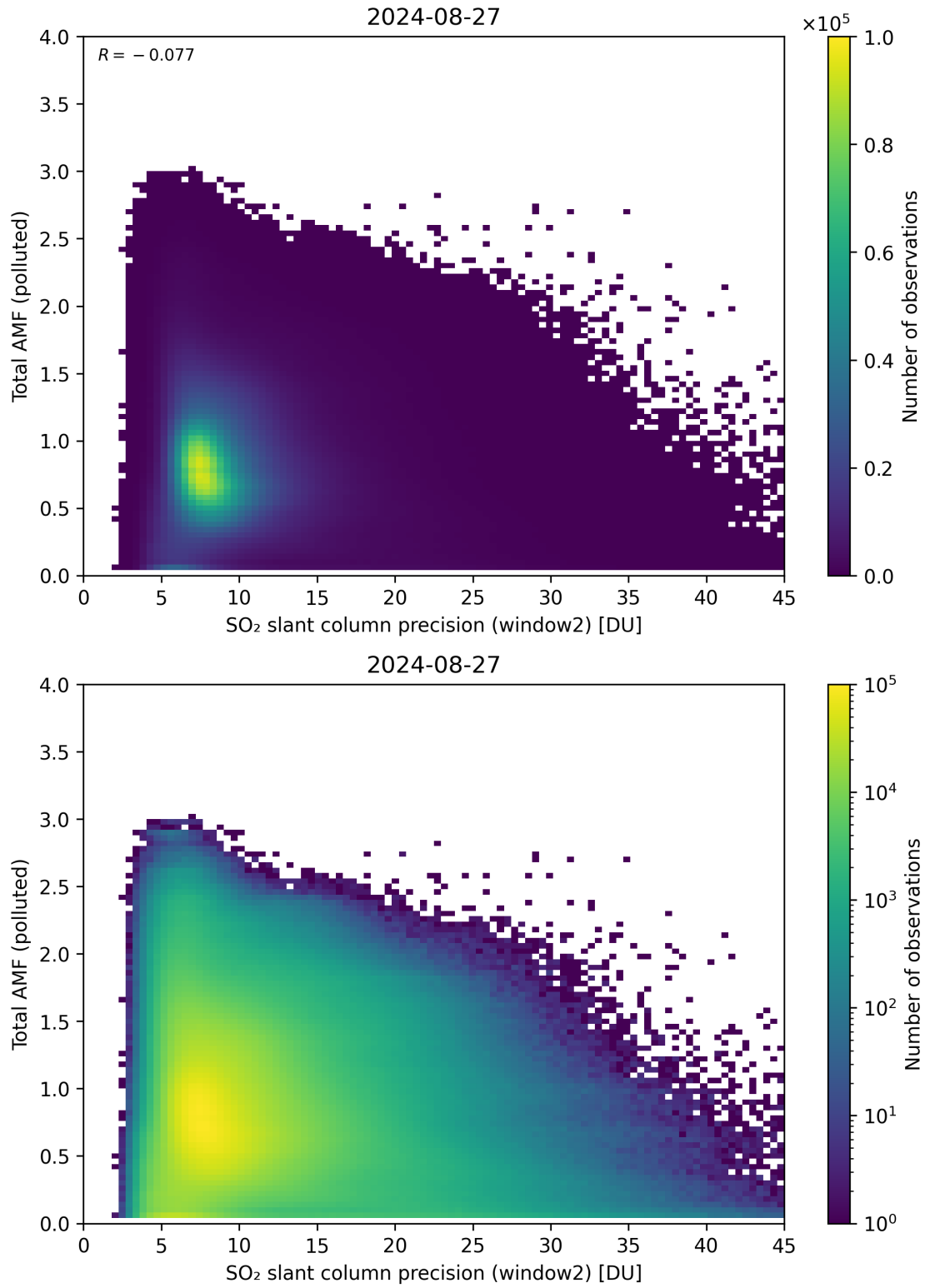
Figure 251: Scatter density plot of “SO 2 slant column precision (window2)” against “Total AMF (polluted)” for 2024-08-27 to 2024-08-28.
