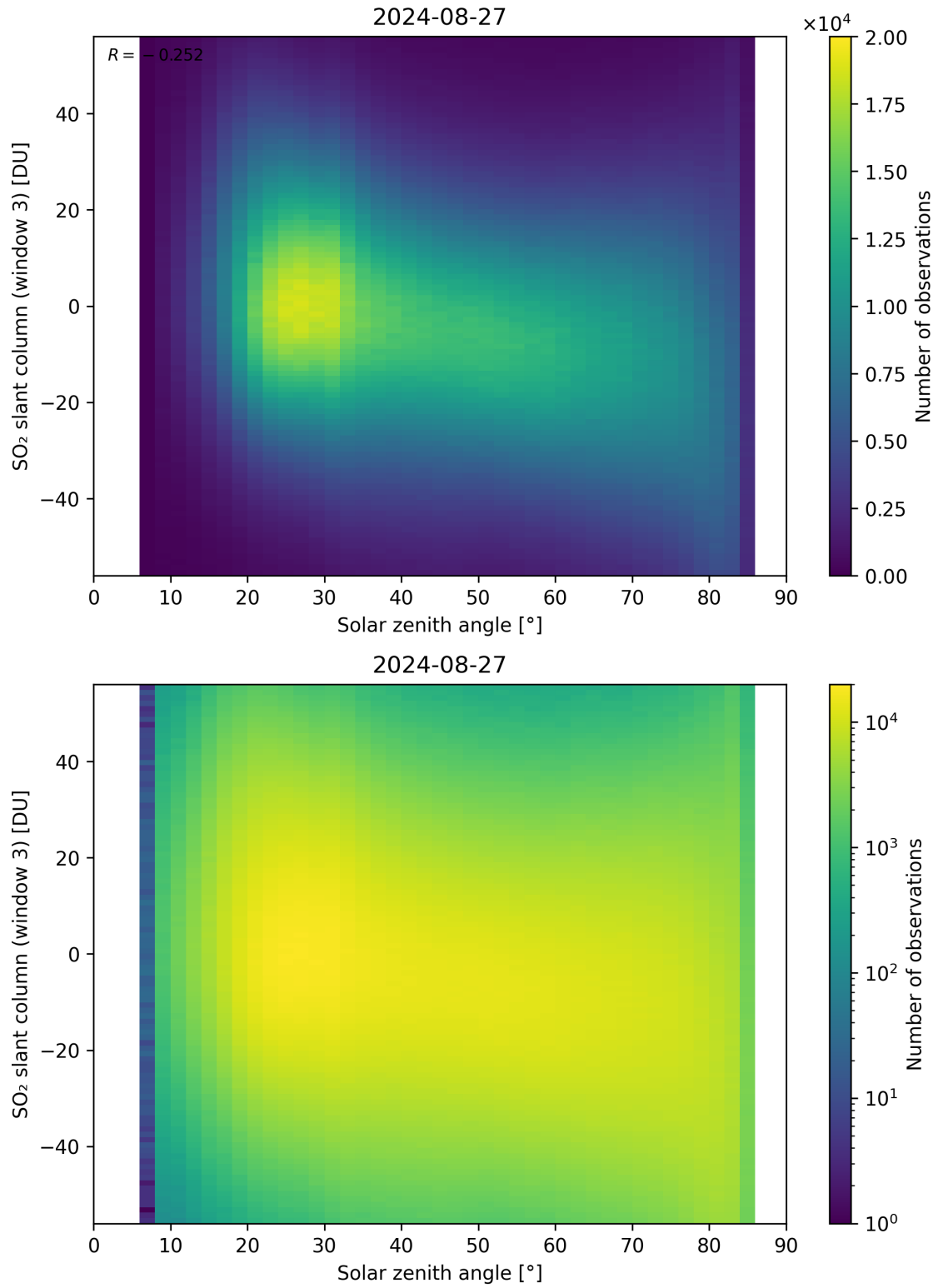
Figure 172: Scatter density plot of “Solar zenith angle” against “SO 2 slant column (window 3)” for 2024-08-27 to 2024-08-28.
