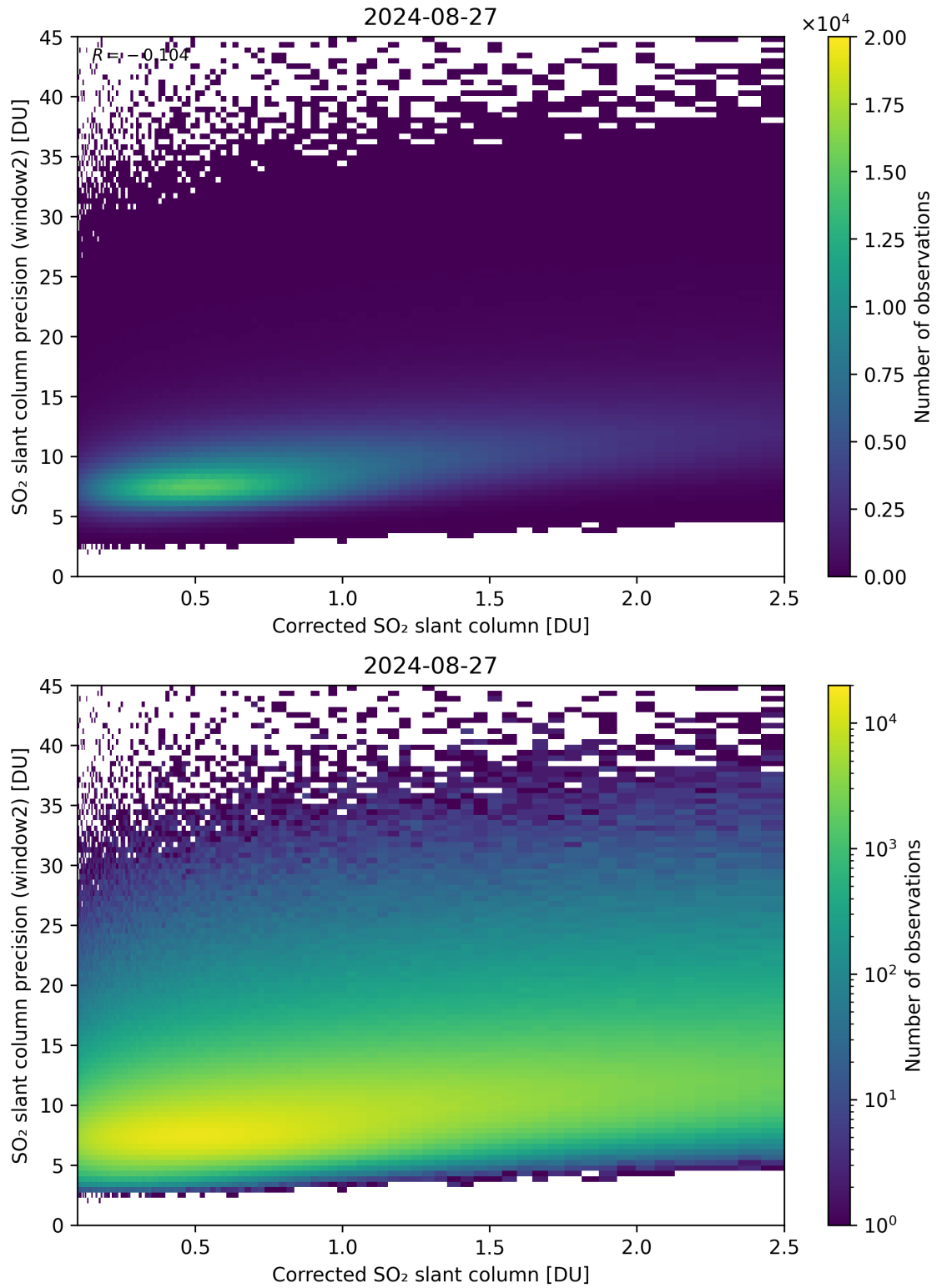
Figure 189: Scatter density plot of “Corrected SO 2 slant column” against “SO 2 slant column precision (window2)” for 2024-08-27 to 2024-08-28.
