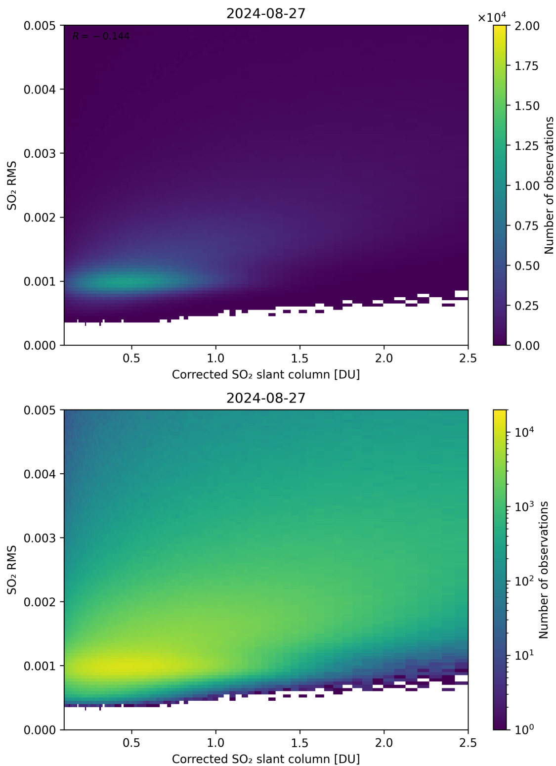
Figure 183: Scatter density plot of “Corrected SO 2 slant column” against “SO 2 RMS” for 2024-08-27 to 2024-08-28.
