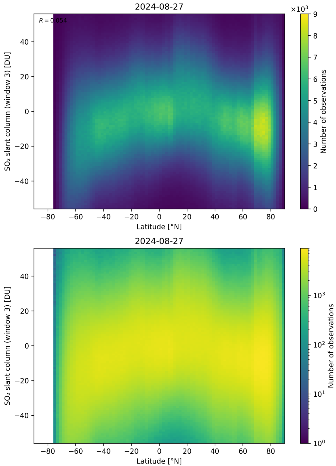
Figure 152: Scatter density plot of “Latitude” against “SO 2 slant column (window 3)” for 2024-08-27 to 2024-08-28.
