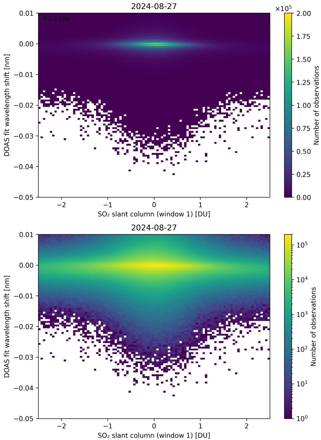
Figure 215: Scatter density plot of “SO 2 slant column (window 1)” against “DOAS fit wavelength shift” for 2024-08-27 to 2024-08-28.
