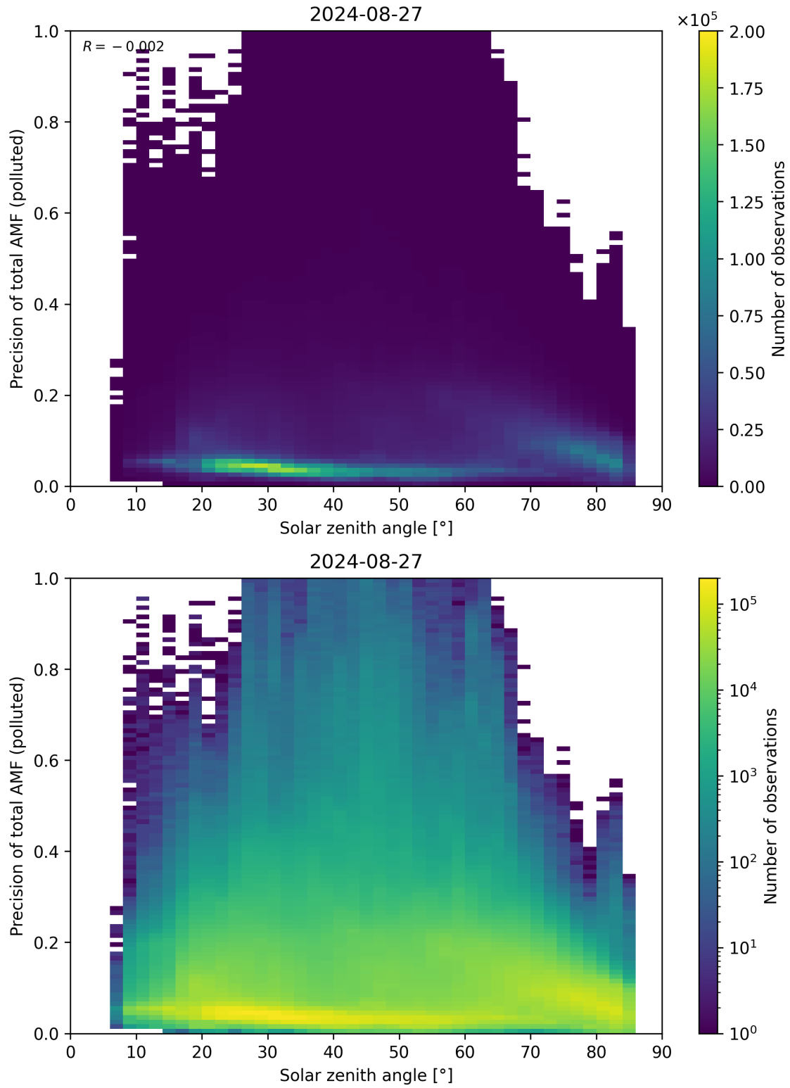
Figure 175: Scatter density plot of “Solar zenith angle” against “Precision of total AMF (polluted)” for 2024-08-27 to 2024-08-28.
