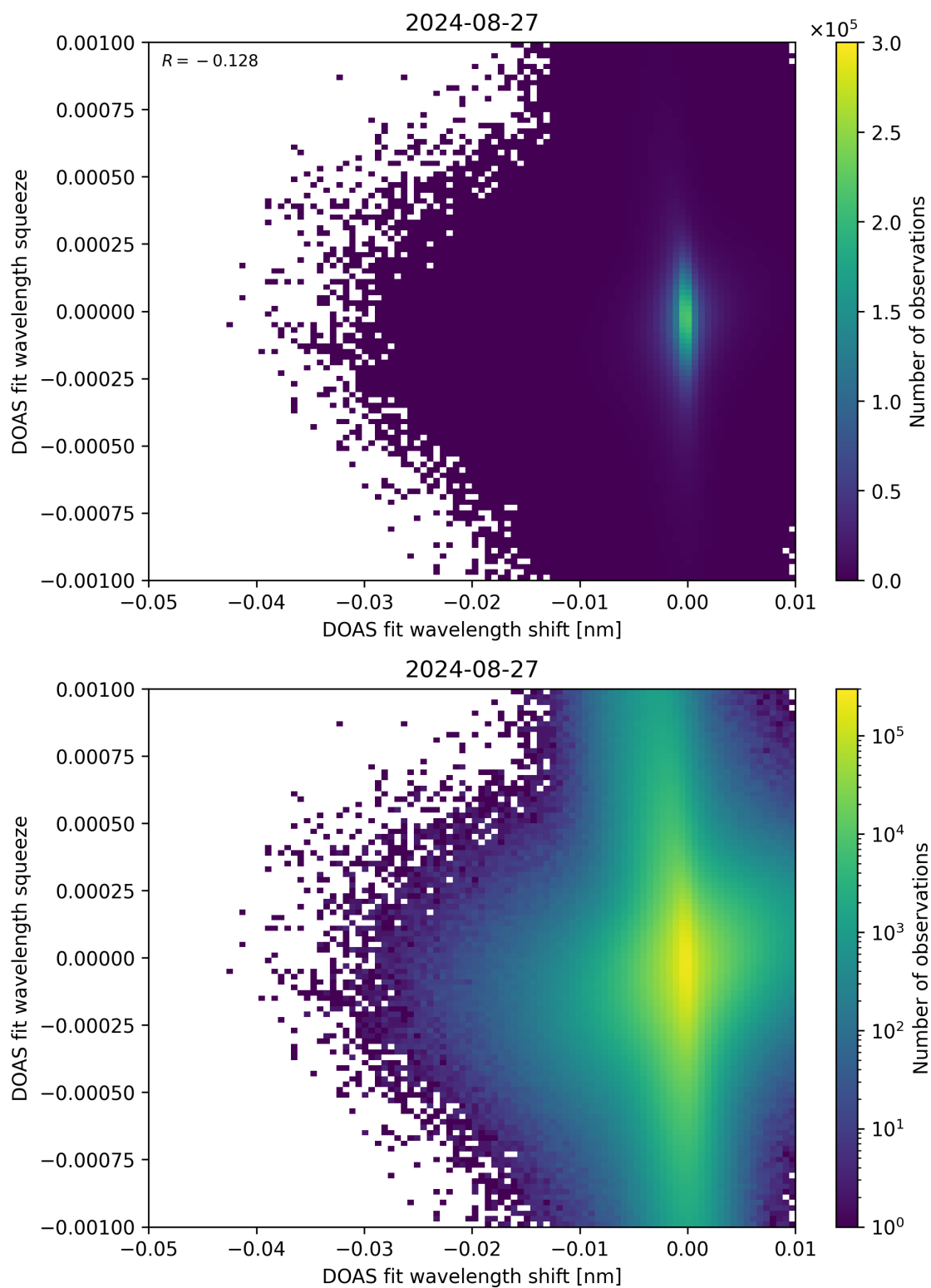
Figure 127: Scatter density plot of “DOAS fit wavelength shift” against “DOAS fit wavelength squeeze” for 2024-08-27 to 2024-08-28.
