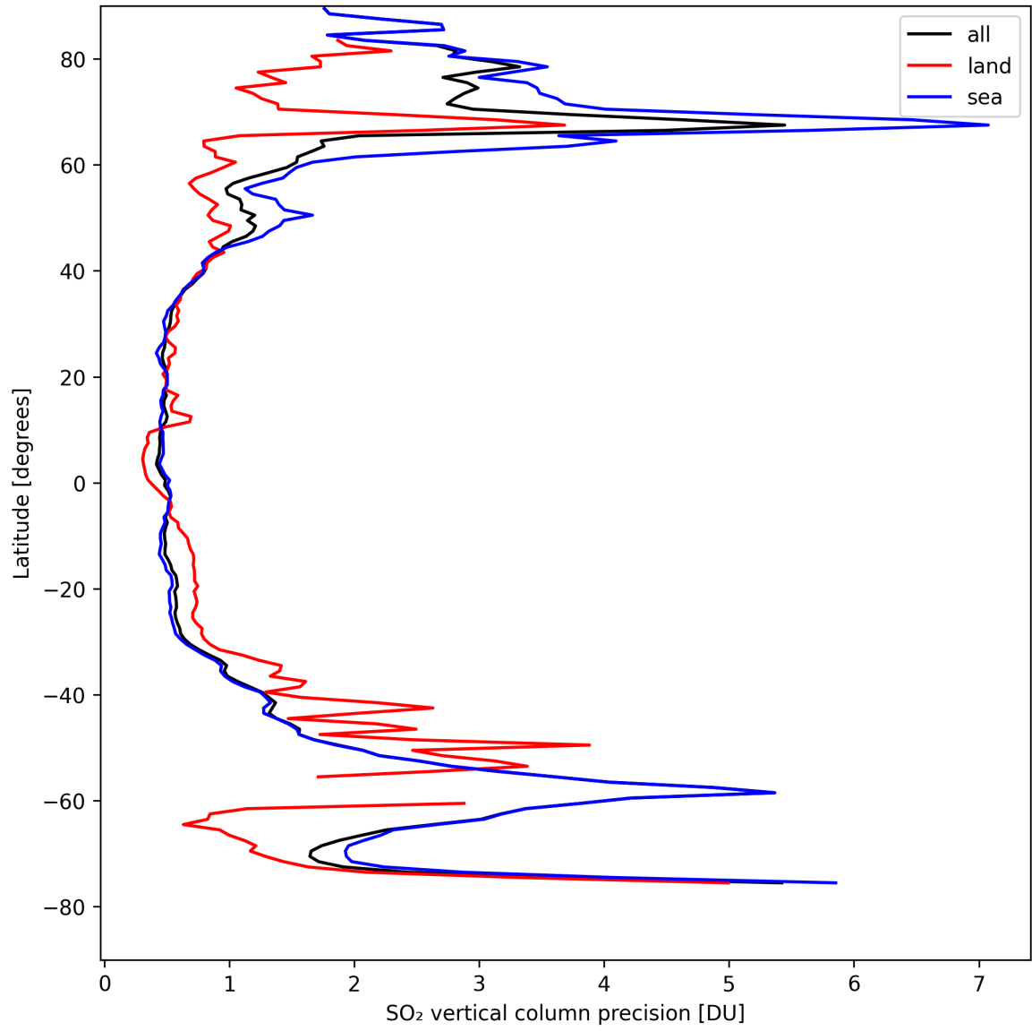
Figure 31: Zonal average of “SO 2 vertical column precision” for 2024-08-27 to 2024-08-28.
