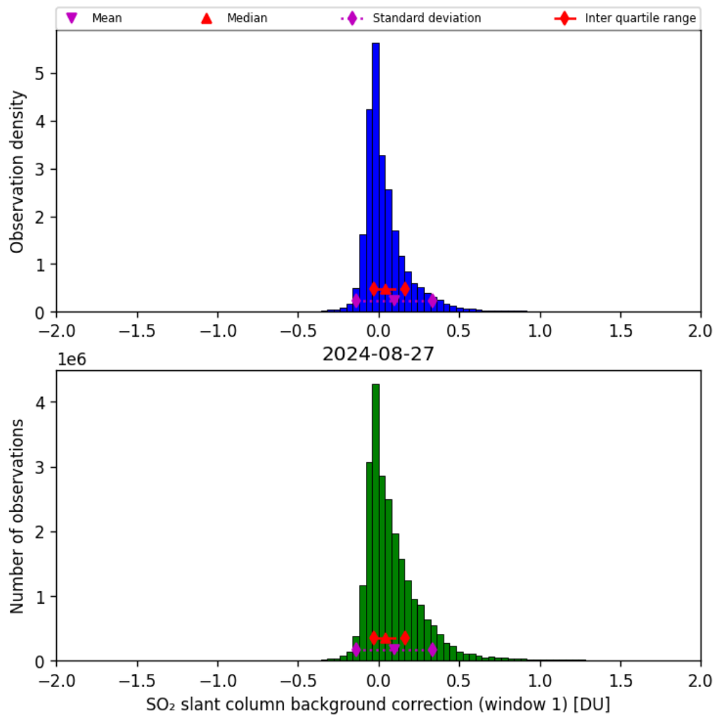
Figure 59: Histogram of “SO 2 slant column background correction (window 1)” for 2024-08-27 to 2024-08-28
