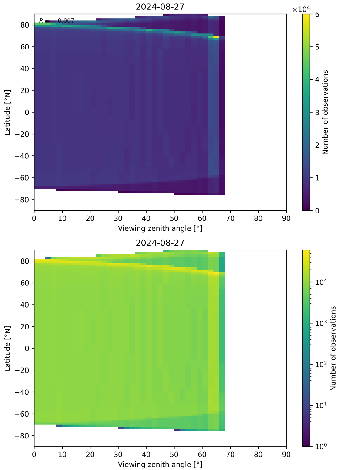
Figure 314: Scatter density plot of “Viewing zenith angle” against “Latitude” for 2024-08-27 to 2024-08-28.
