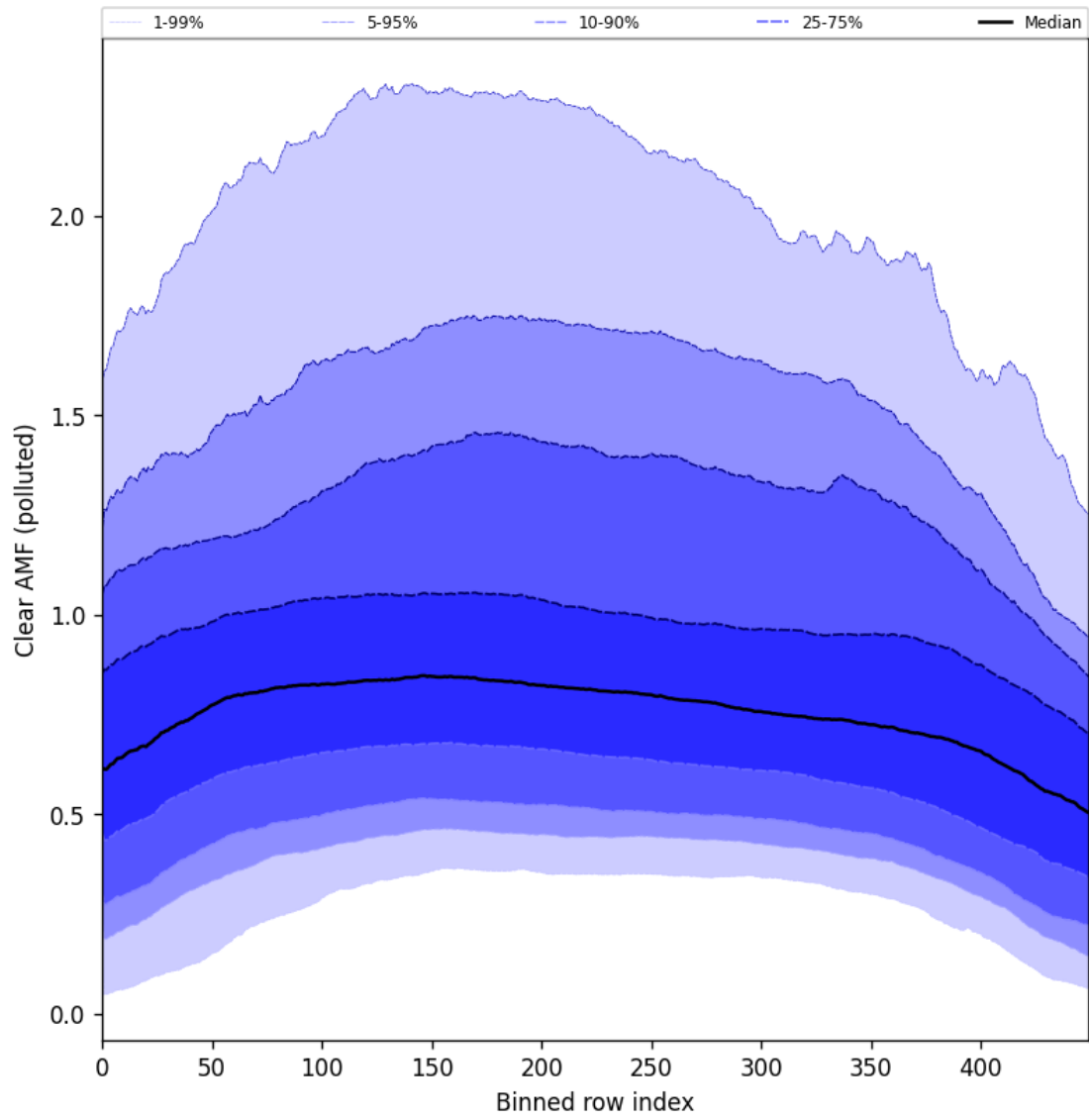
Figure 96: Along track statistics of “Clear AMF (polluted)” for 2024-08-27 to 2024-08-28
