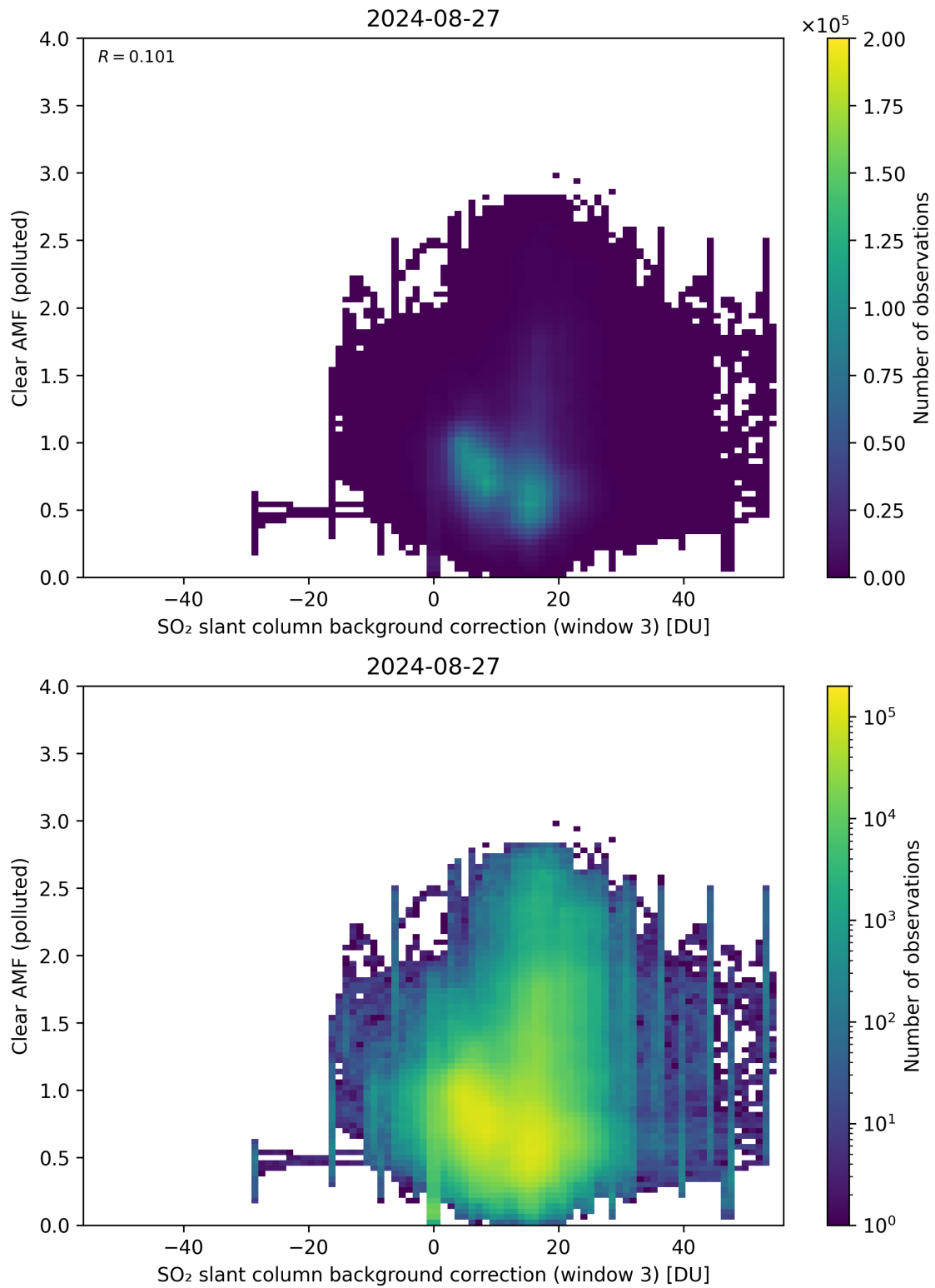
Figure 124: Scatter density plot of “SO 2 slant column background correction (window 3)” against “Clear AMF (polluted)” for 2024-08-27 to 2024-08-28.
