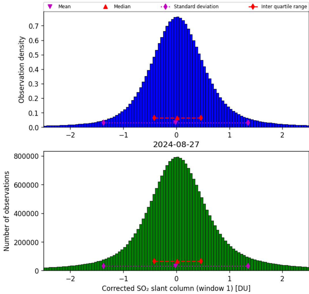
Figure 58: Histogram of “Corrected SO 2 slant column (window 1)” for 2024-08-27 to 2024-08-28
