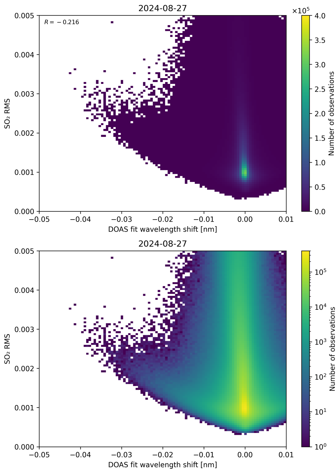
Figure 128: Scatter density plot of “DOAS fit wavelength shift” against “SO 2 RMS” for 2024-08-27 to 2024-08-28.
