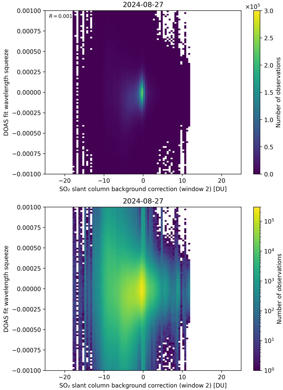
Figure 113: Scatter density plot of “SO 2 slant column background correction (window 2)” against “DOAS fit wavelength squeeze” for 2024-08-27 to 2024-08-28.
