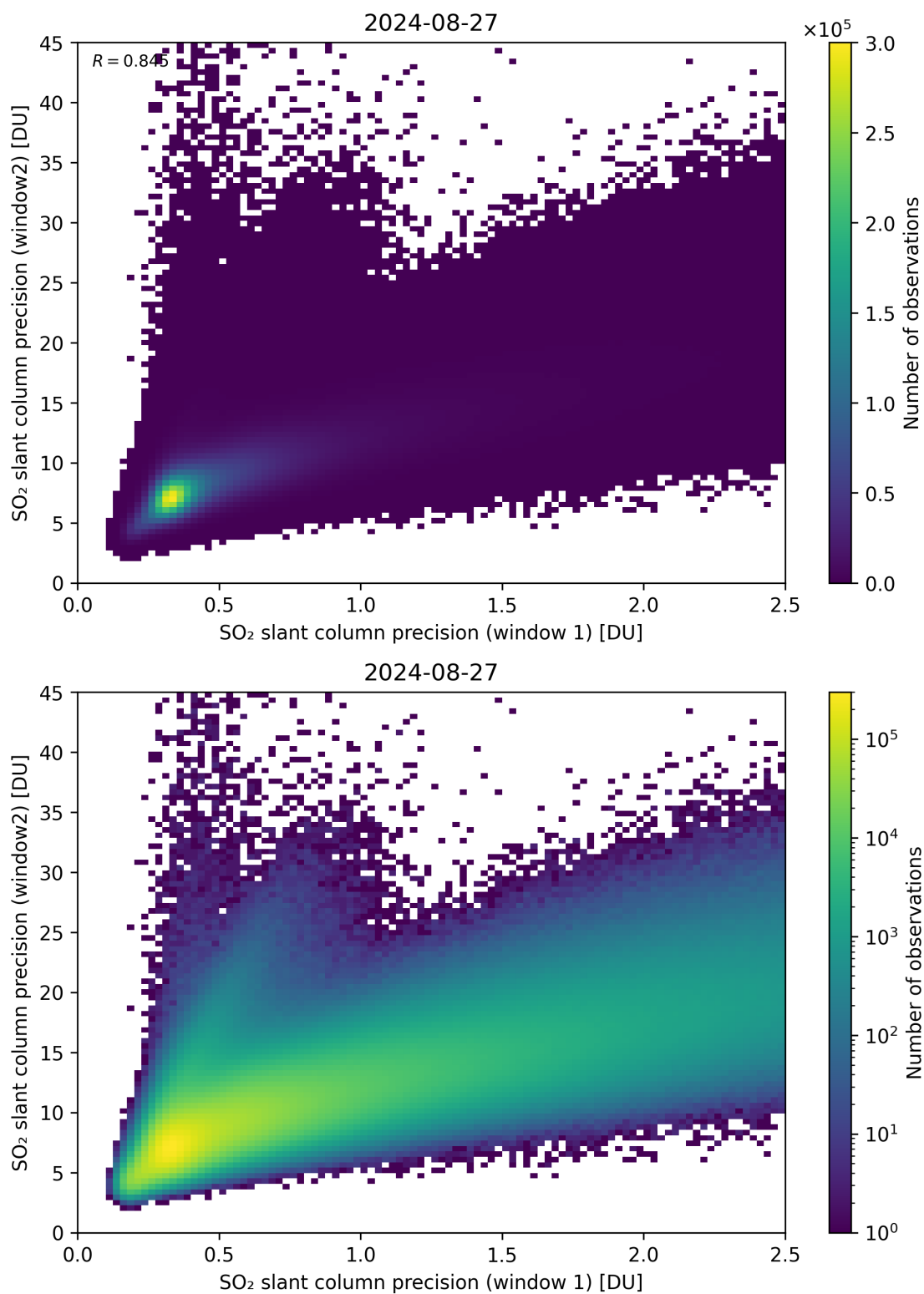
Figure 227: Scatter density plot of “SO 2 slant column precision (window 1)” against “SO 2 slant column precision (window2)” for 2024-08-27 to 2024-08-28.
