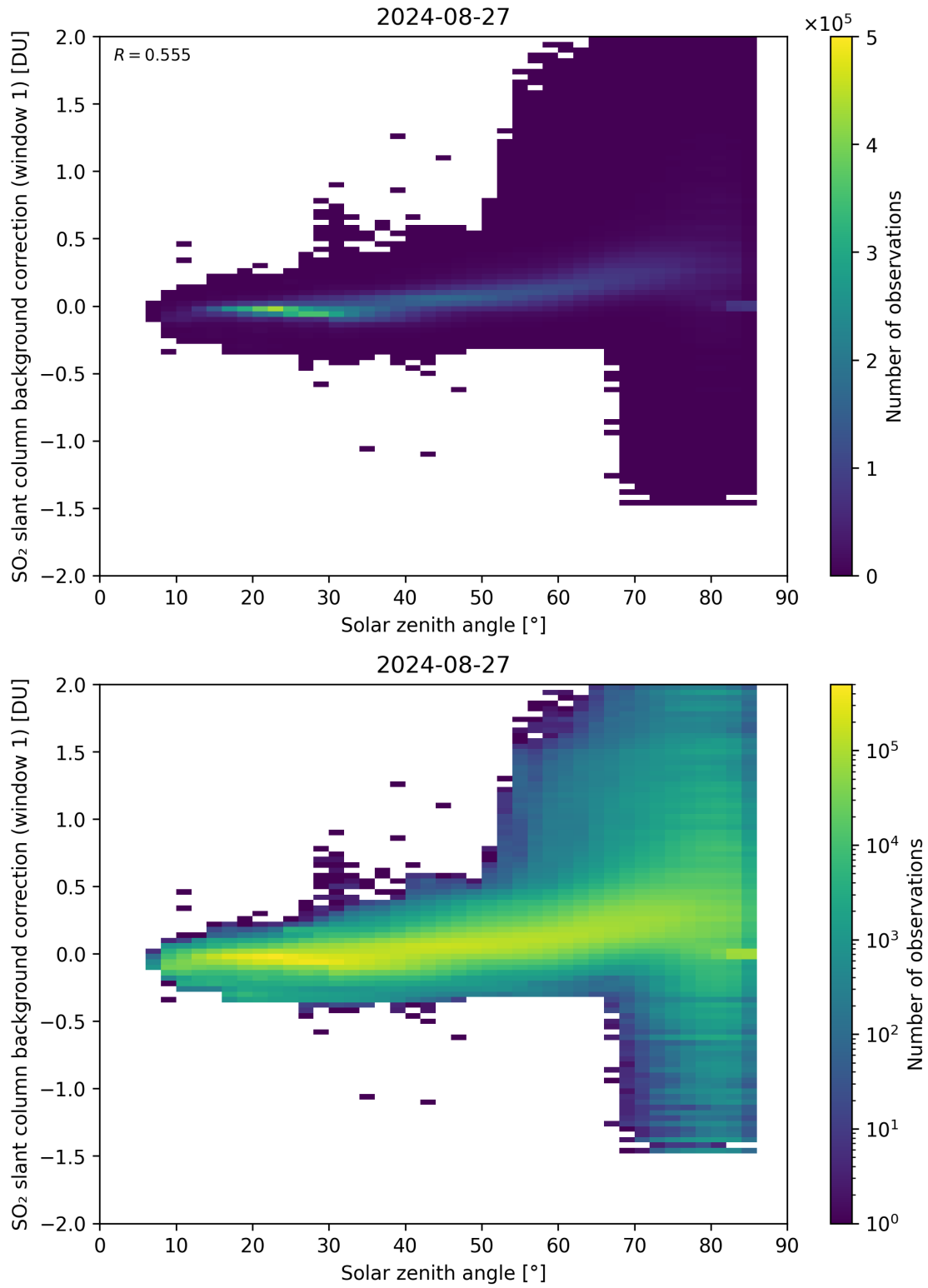
Figure 158: Scatter density plot of “Solar zenith angle” against “SO 2 slant column background correction (window 1)” for 2024-08-27 to 2024-08-28.
