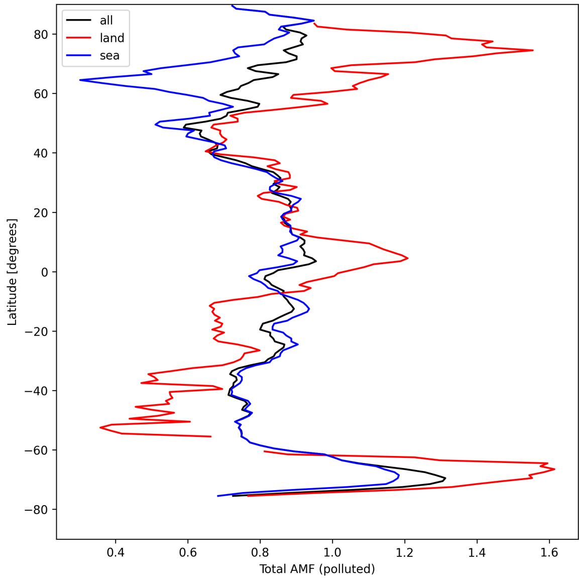
Figure 48: Zonal average of “Total AMF (polluted)” for 2024-08-27 to 2024-08-28.
