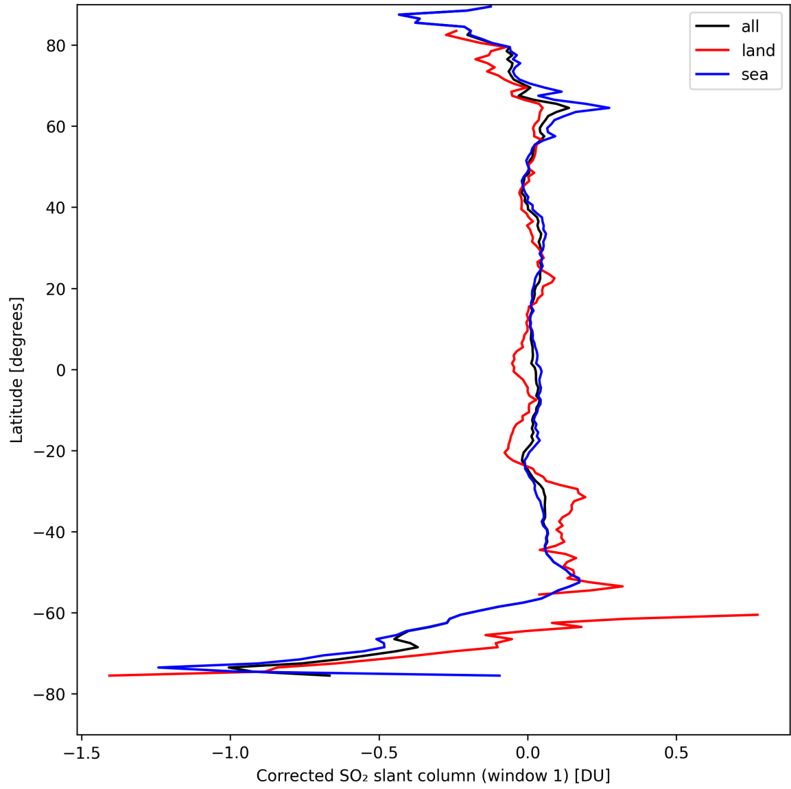
Figure 35: Zonal average of “Corrected SO 2 slant column (window 1)” for 2024-08-27 to 2024-08-28.
