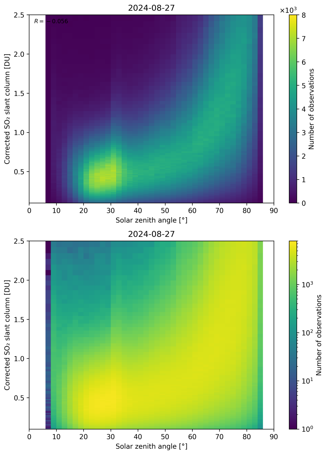
Figure 166: Scatter density plot of “Solar zenith angle” against “Corrected SO 2 slant column” for 2024-08-27 to 2024-08-28.
