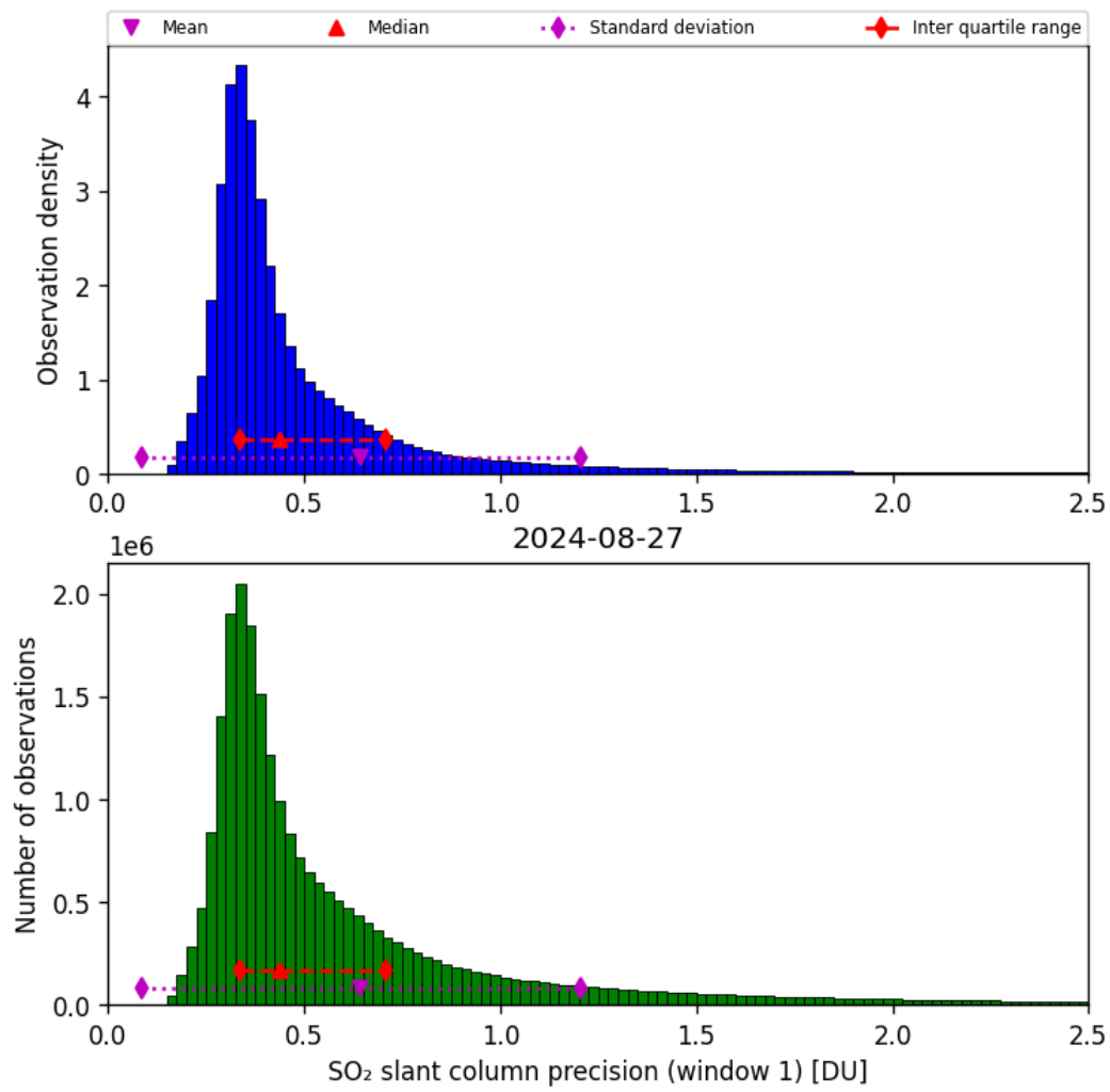
Figure 57: Histogram of “SO 2 slant column precision (window 1)” for 2024-08-27 to 2024-08-28
