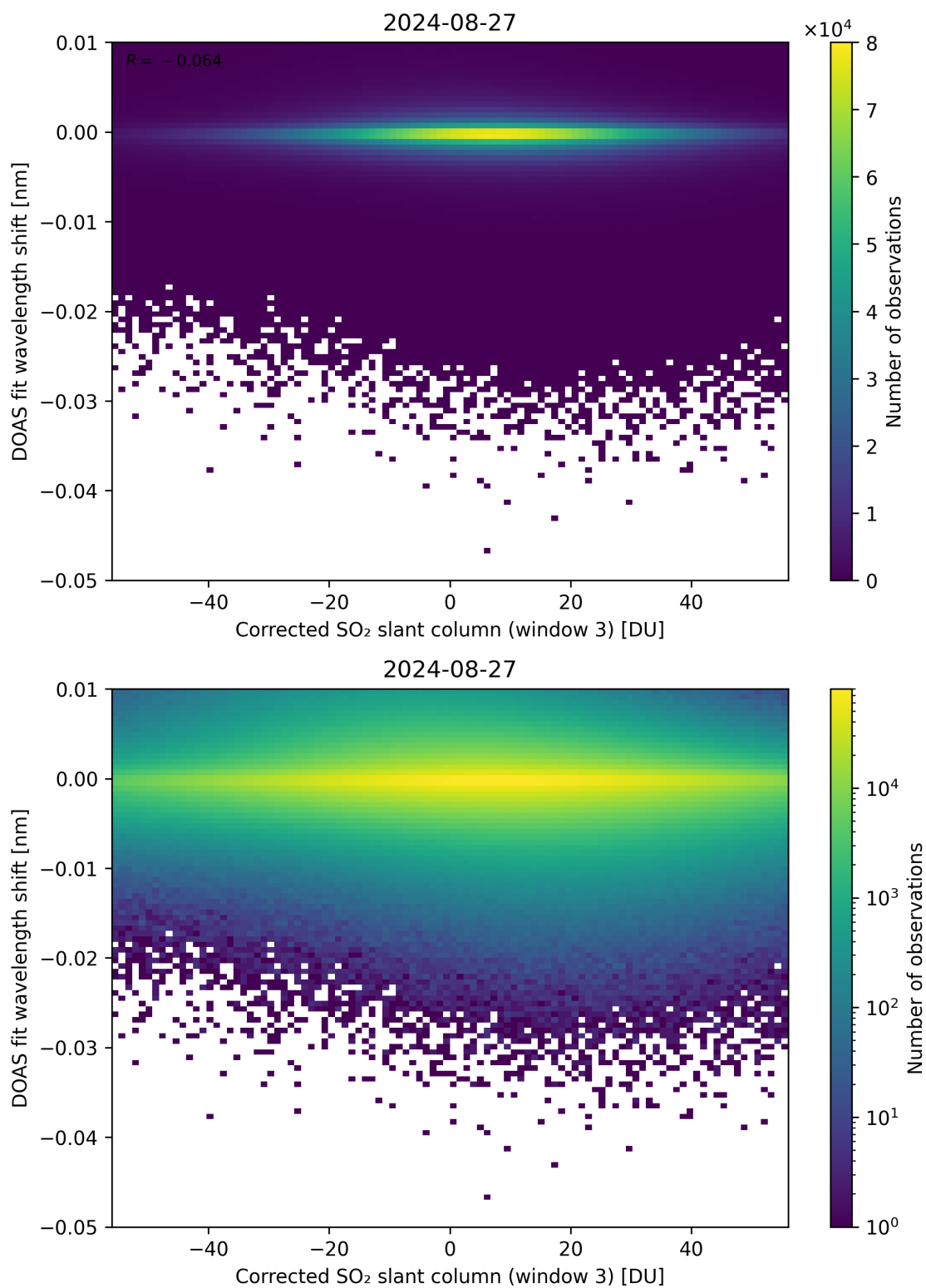
Figure 206: Scatter density plot of “Corrected SO 2 slant column (window 3)” against “DOAS fit wavelength shift” for 2024-08-27 to 2024-08-28.
