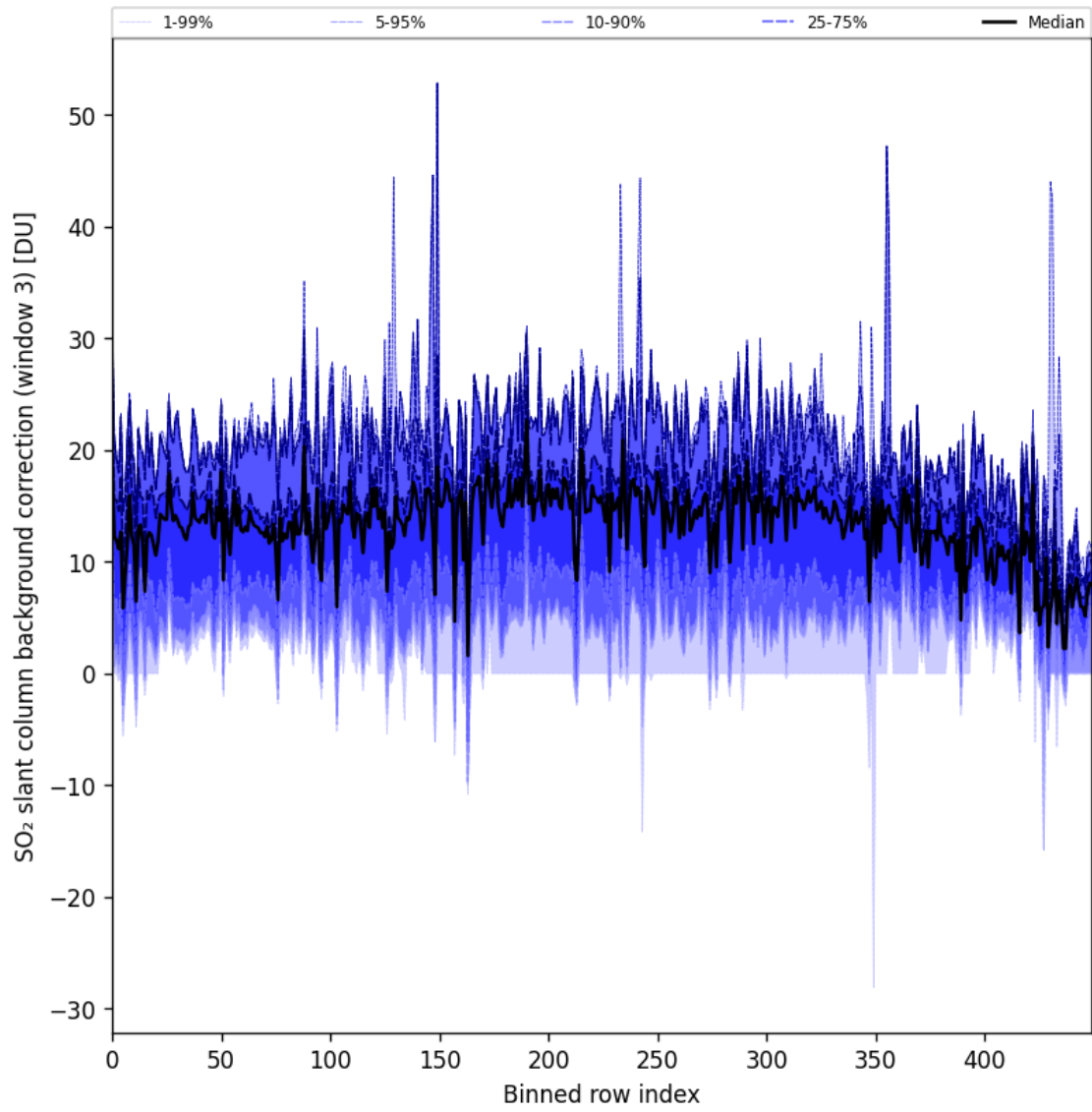
Figure 90: Along track statistics of “SO 2 slant column background correction (window 3)” for 2024-08-27 to 2024-08-28
