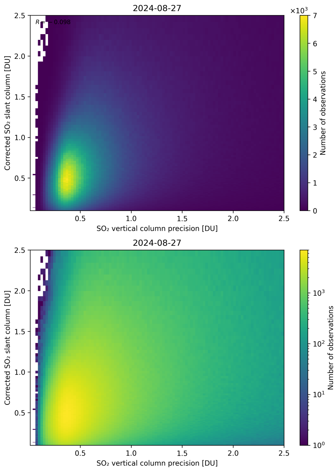
Figure 286: Scatter density plot of “SO 2 vertical column precision” against “Corrected SO 2 slant column” for 2024-08-27 to 2024-08-28.
