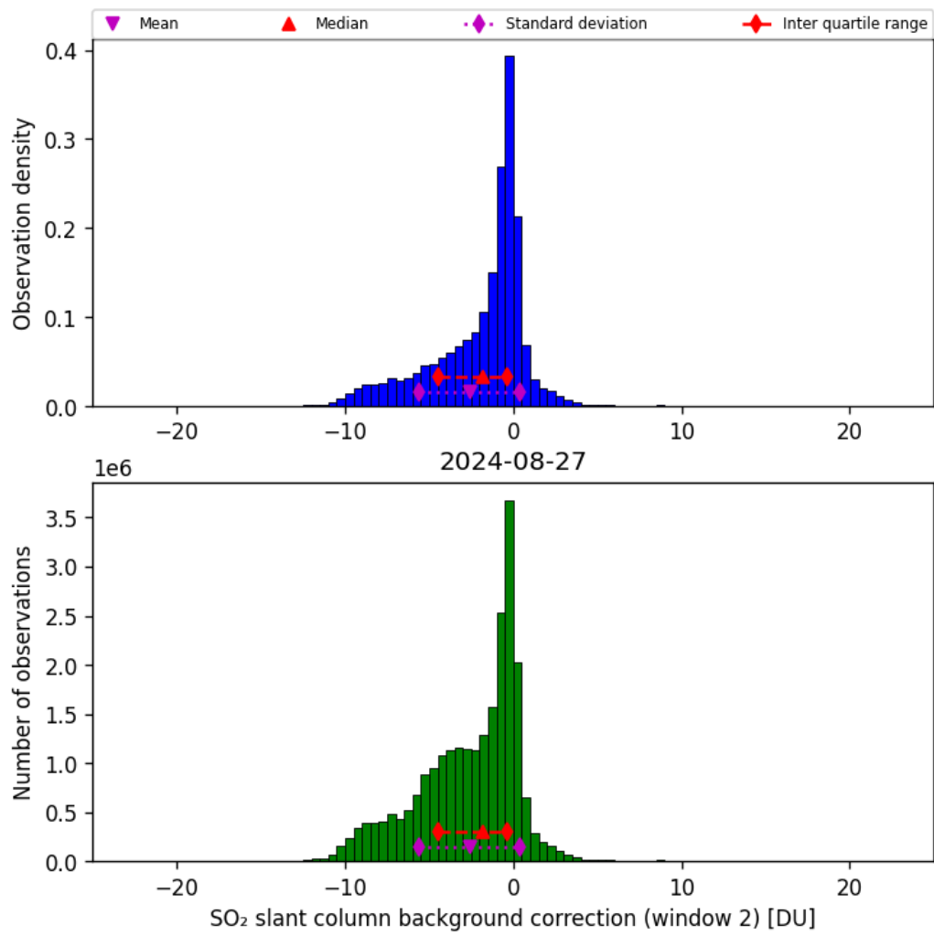
Figure 63: Histogram of “SO 2 slant column background correction (window 2)” for 2024-08-27 to 2024-08-28
