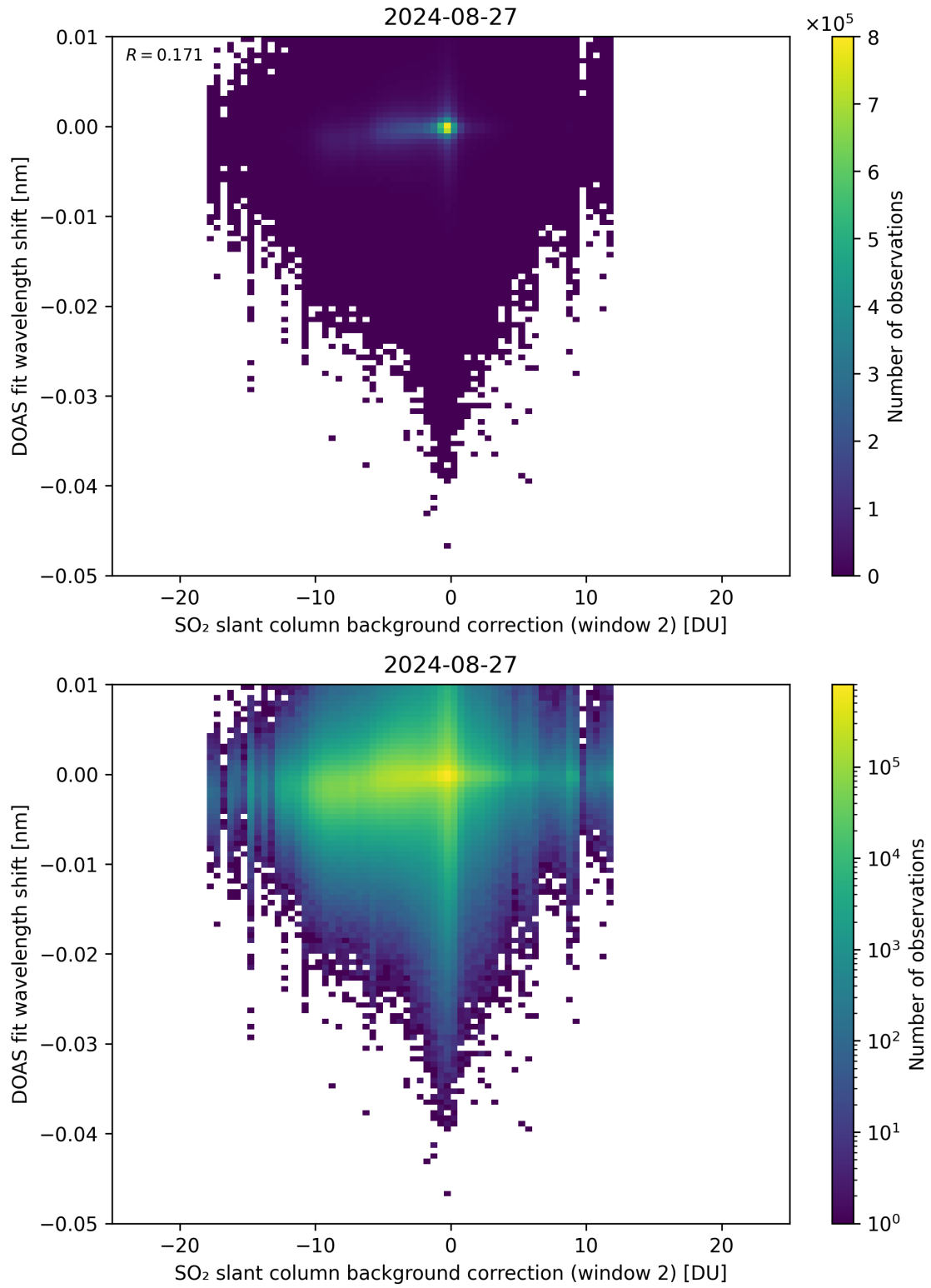
Figure 112: Scatter density plot of “SO 2 slant column background correction (window 2)” against “DOAS fit wavelength shift” for 2024-08-27 to 2024-08-28.
