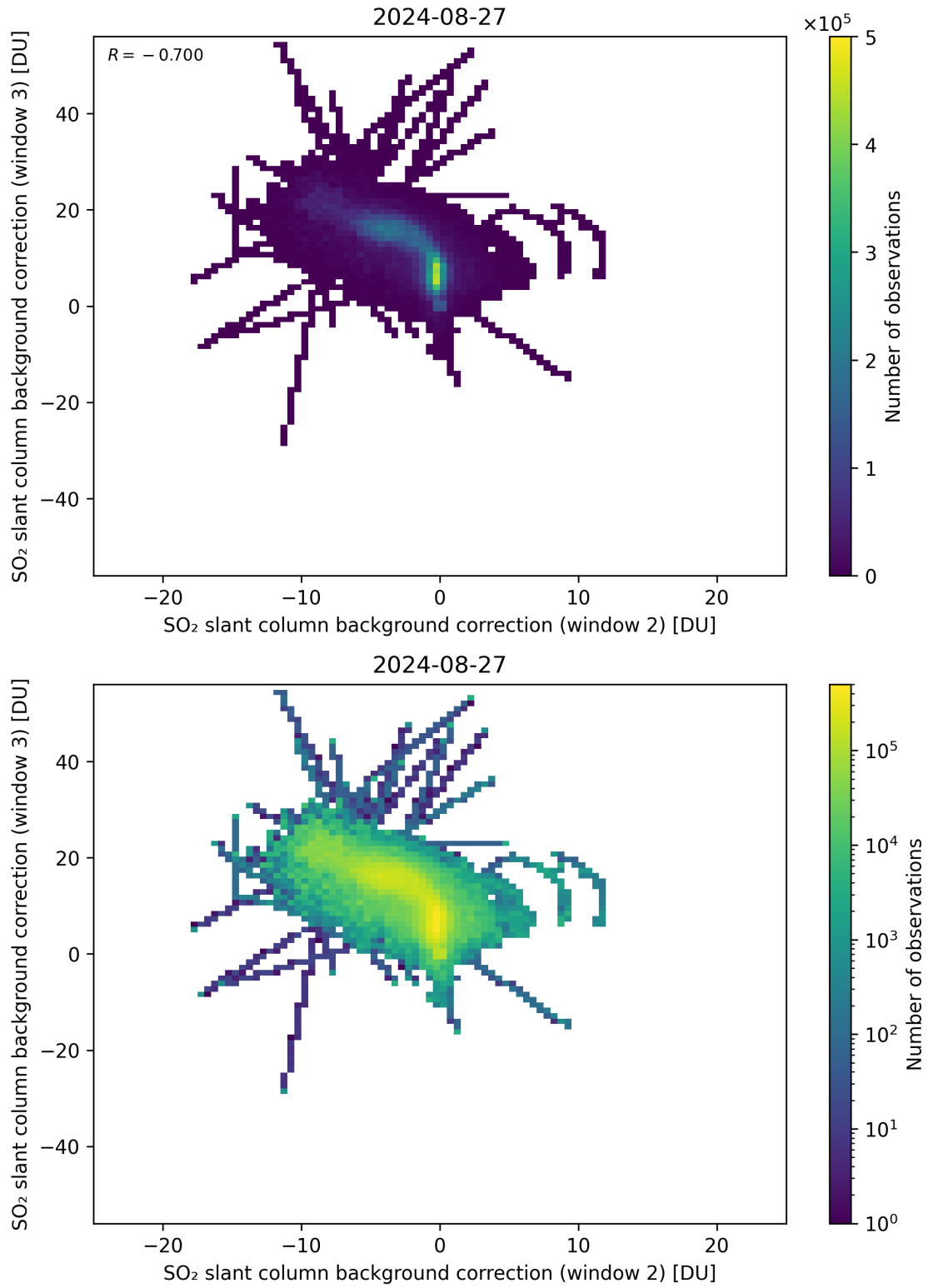
Figure 111: Scatter density plot of “SO 2 slant column background correction (window 2)” against “SO 2 slant column background correction (window 3)” for 2024-08-27 to 2024-08-28.
