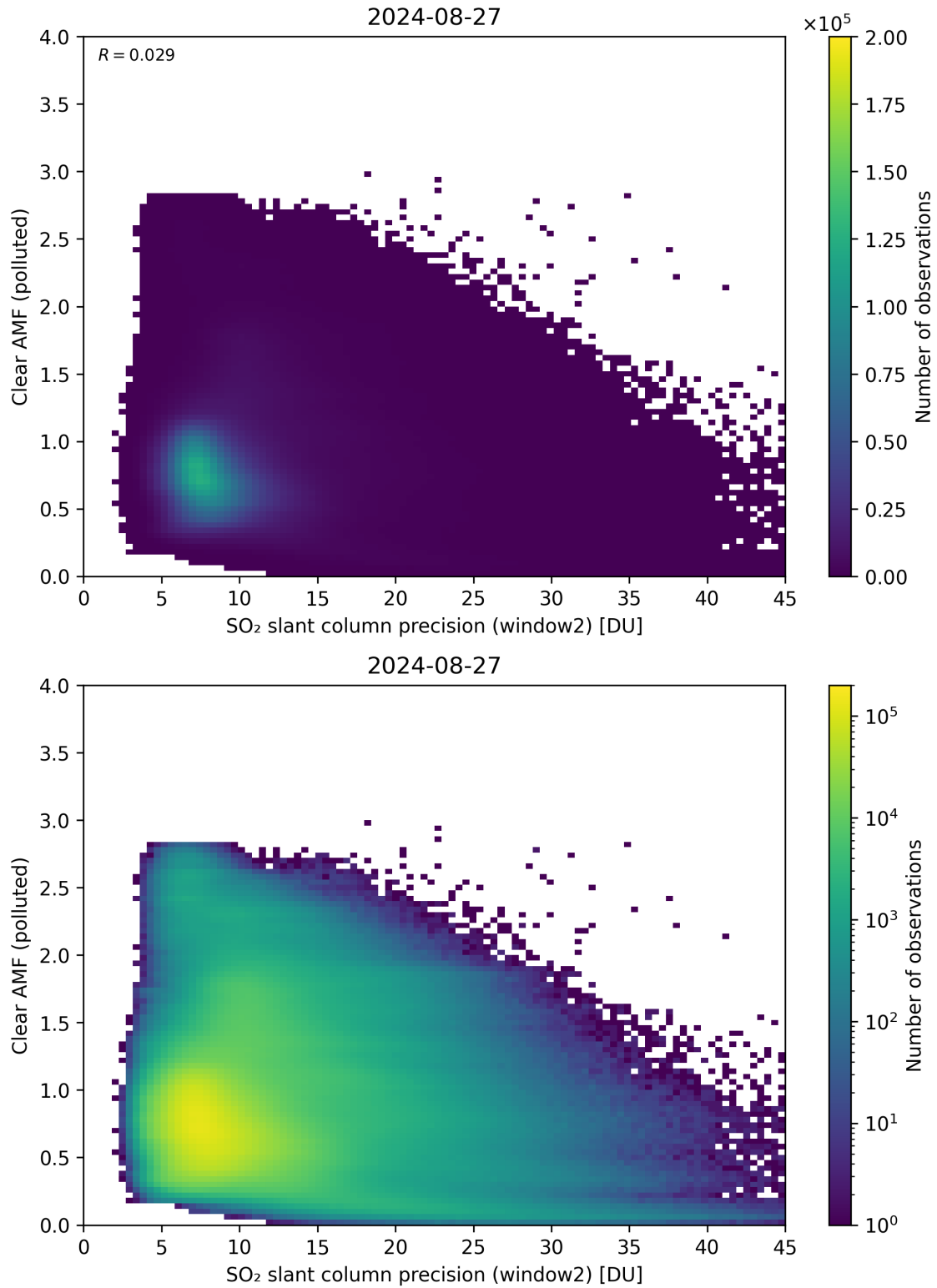
Figure 246: Scatter density plot of “SO 2 slant column precision (window2)” against “Clear AMF (polluted)” for 2024-08-27 to 2024-08-28.
