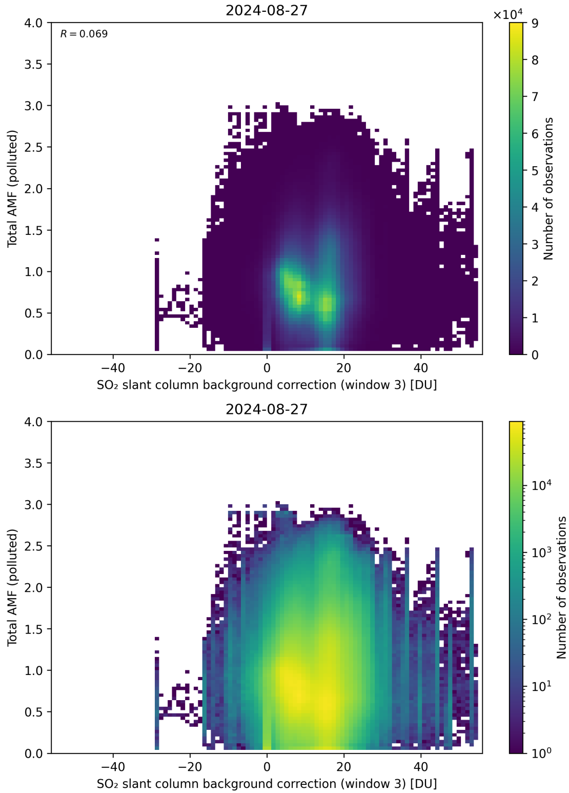
Figure 125: Scatter density plot of “SO 2 slant column background correction (window 3)” against “Total AMF (polluted)” for 2024-08-27 to 2024-08-28.
