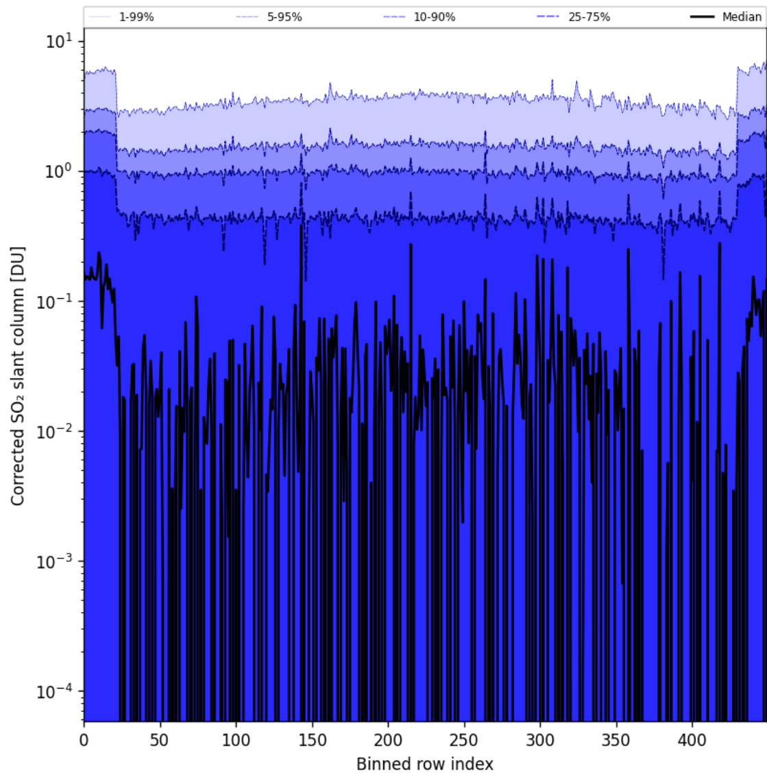
Figure 78: Along track statistics of “Corrected SO 2 slant column” for 2024-08-27 to 2024-08-28
