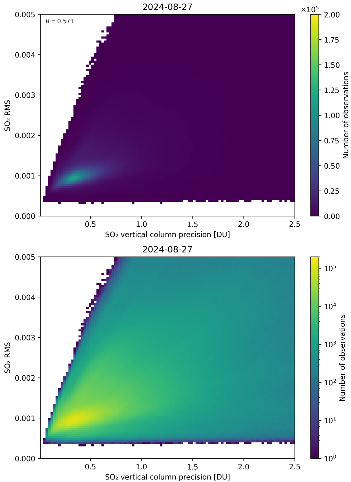
Figure 284: Scatter density plot of “SO 2 vertical column precision” against “SO 2 RMS” for 2024-08-27 to 2024-08-28.
