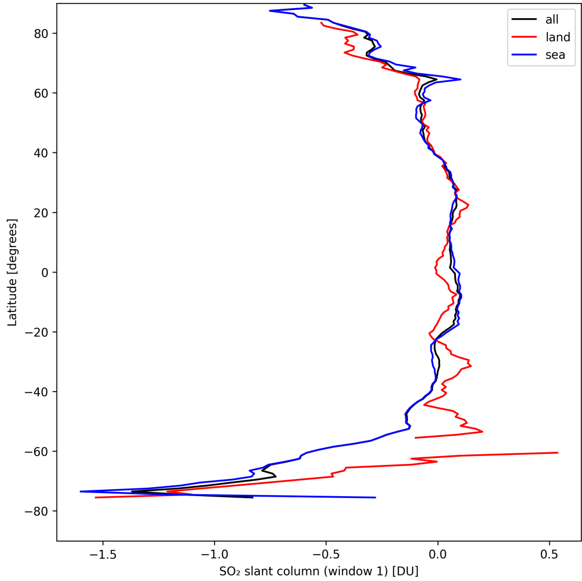
Figure 33: Zonal average of “SO 2 slant column (window 1)” for 2024-08-27 to 2024-08-28.
