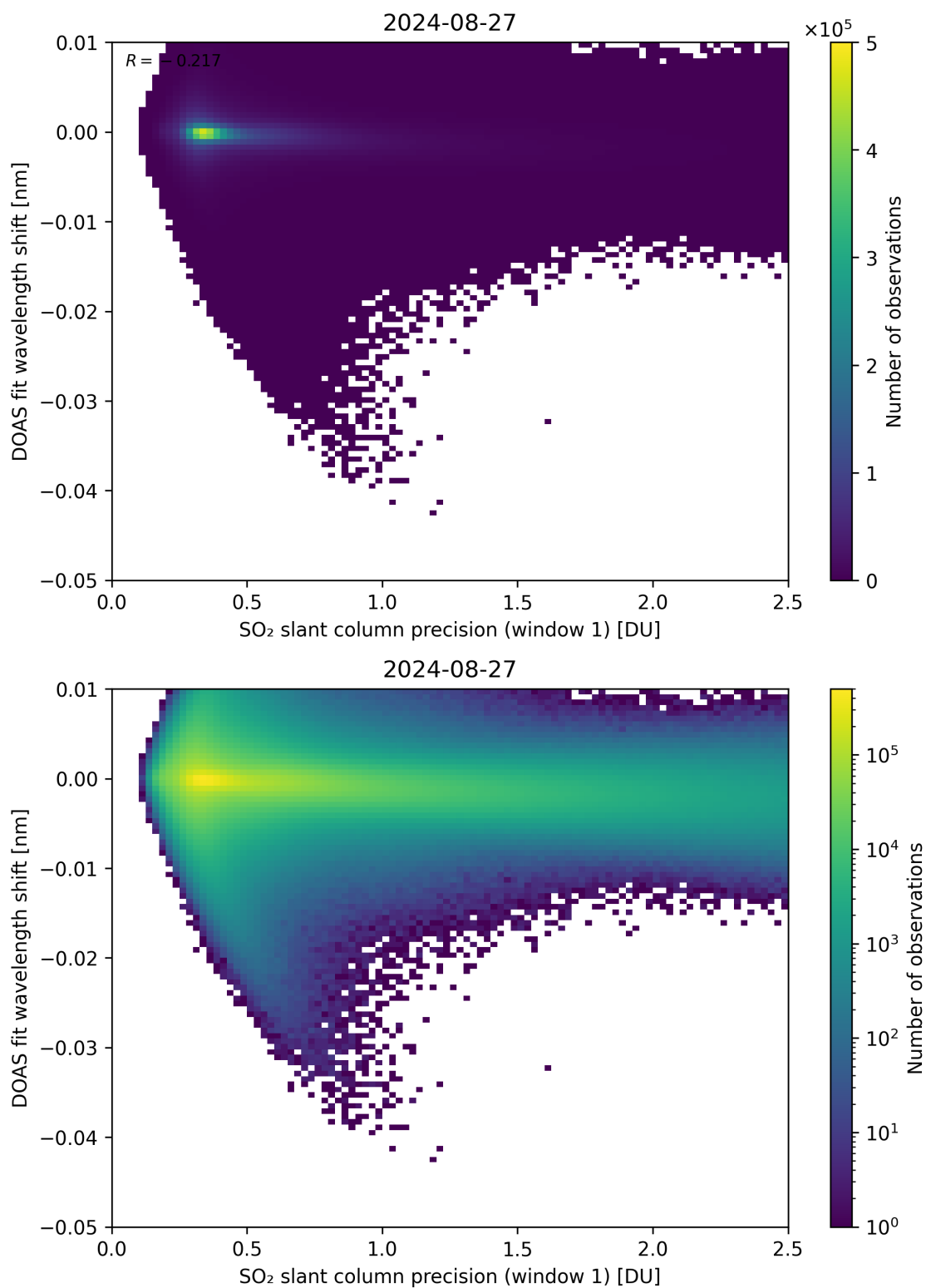
Figure 221: Scatter density plot of “SO 2 slant column precision (window 1)” against “DOAS fit wavelength shift” for 2024-08-27 to 2024-08-28.
