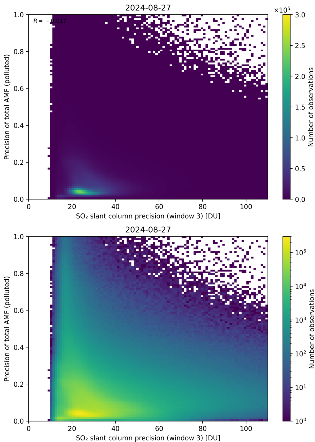
Figure 264: Scatter density plot of “SO 2 slant column precision (window 3)” against “Precision of total AMF (polluted)” for 2024-08-27 to 2024-08-28.
