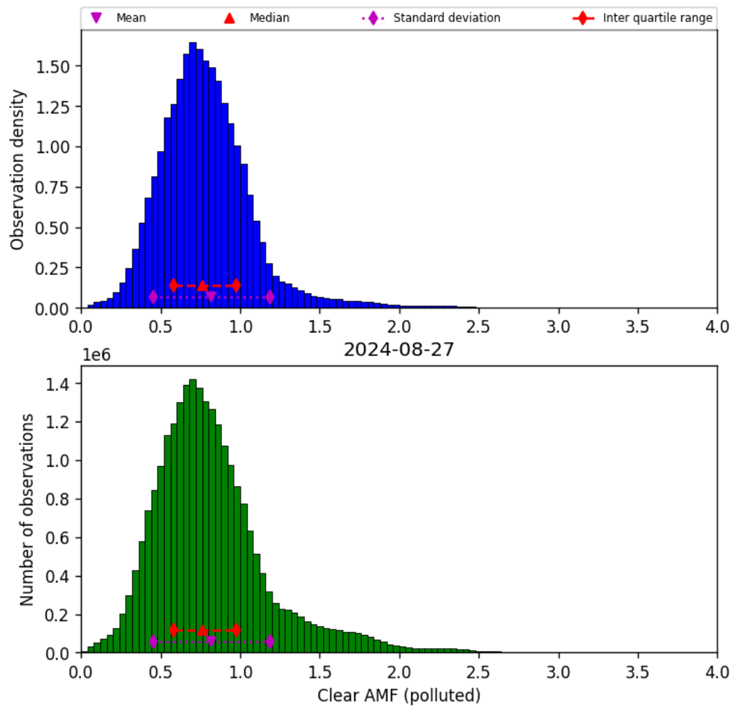
Figure 73: Histogram of “Clear AMF (polluted)” for 2024-08-27 to 2024-08-28
