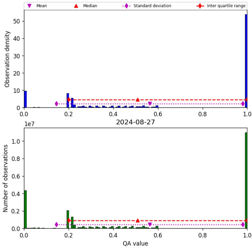
Figure 52: Histogram of “QA value” for 2024-08-27 to 2024-08-28
