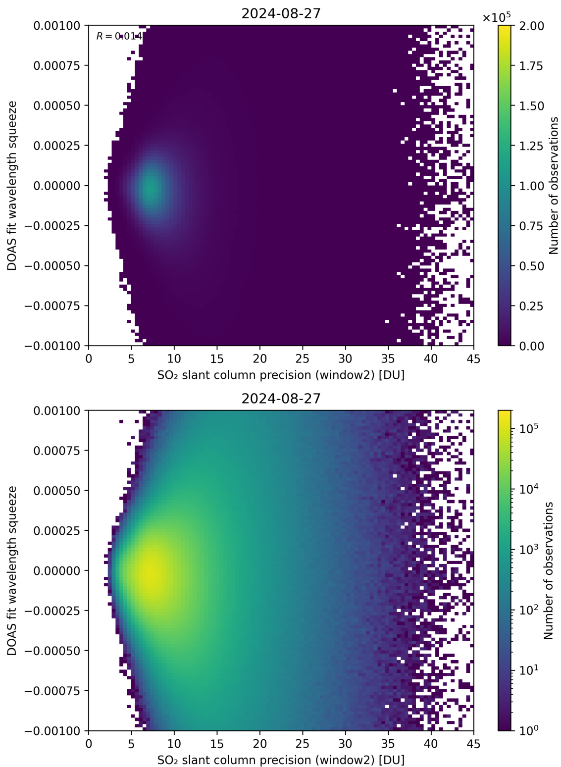
Figure 244: Scatter density plot of “SO 2 slant column precision (window2)” against “DOAS fit wavelength squeeze” for 2024-08-27 to 2024-08-28.
