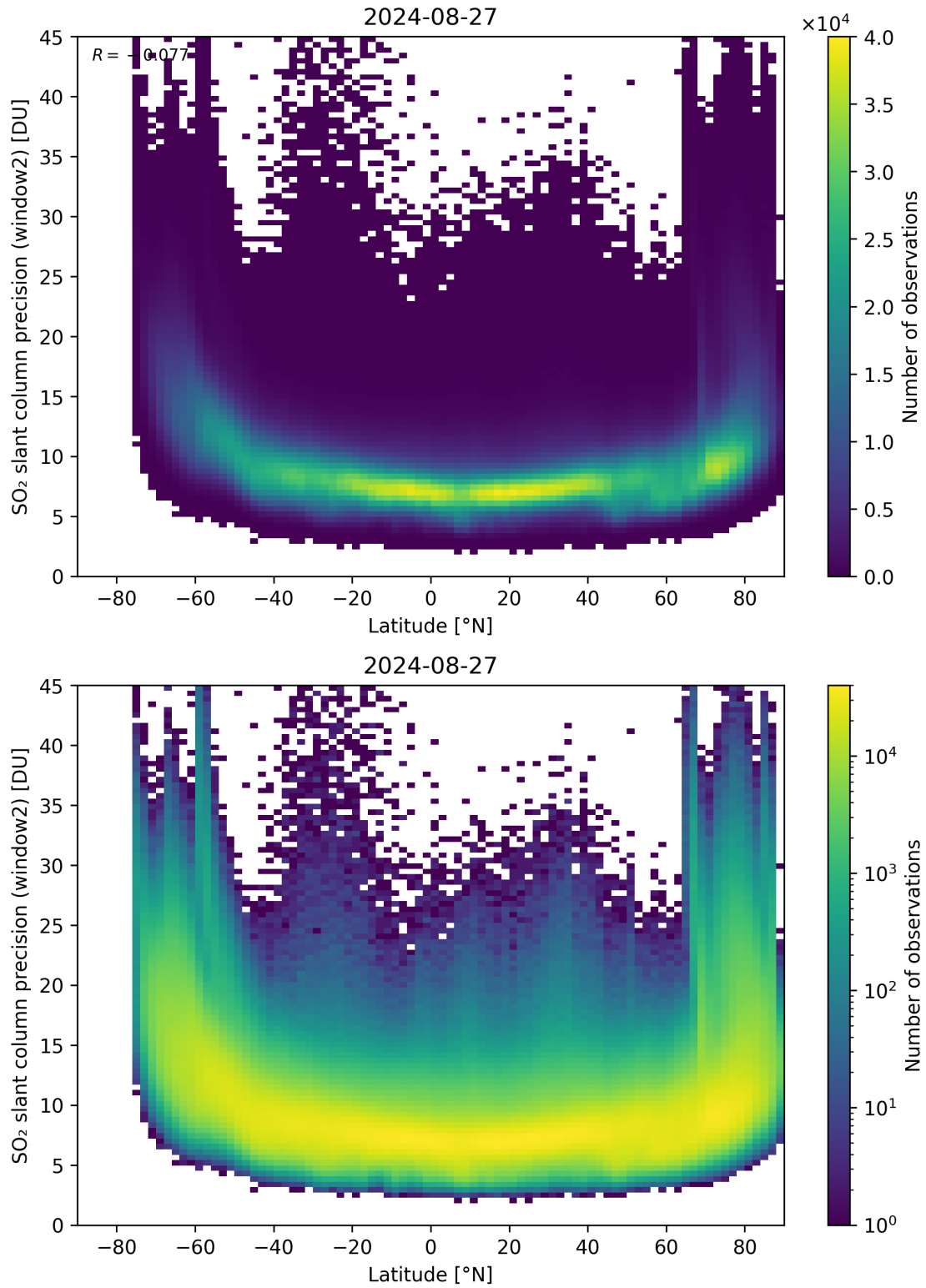
Figure 151: Scatter density plot of “Latitude” against “SO 2 slant column precision (window2)” for 2024-08-27 to 2024-08-28.
