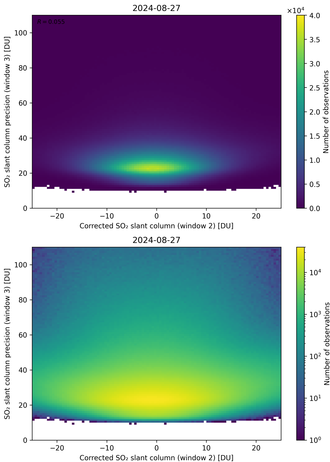
Figure 202: Scatter density plot of “Corrected SO 2 slant column (window 2)” against “SO 2 slant column precision (window 3)” for 2024-08-27 to 2024-08-28.
