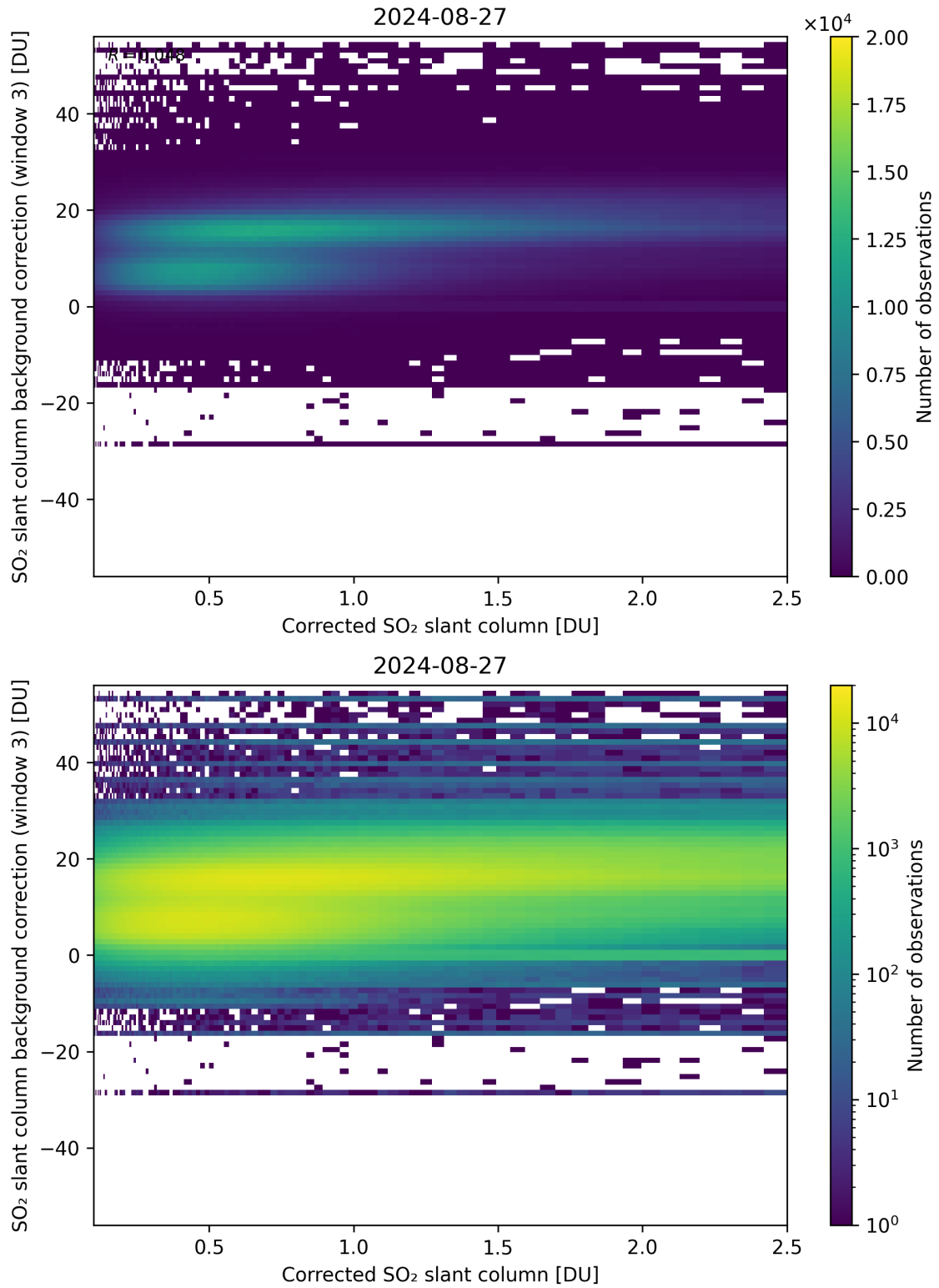
Figure 180: Scatter density plot of “Corrected SO 2 slant column” against “SO 2 slant column background correction (window 3)” for 2024-08-27 to 2024-08-28.
