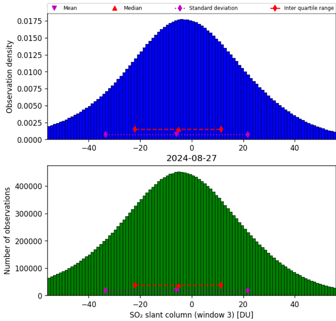
Figure 64: Histogram of “SO 2 slant column (window 3)” for 2024-08-27 to 2024-08-28
