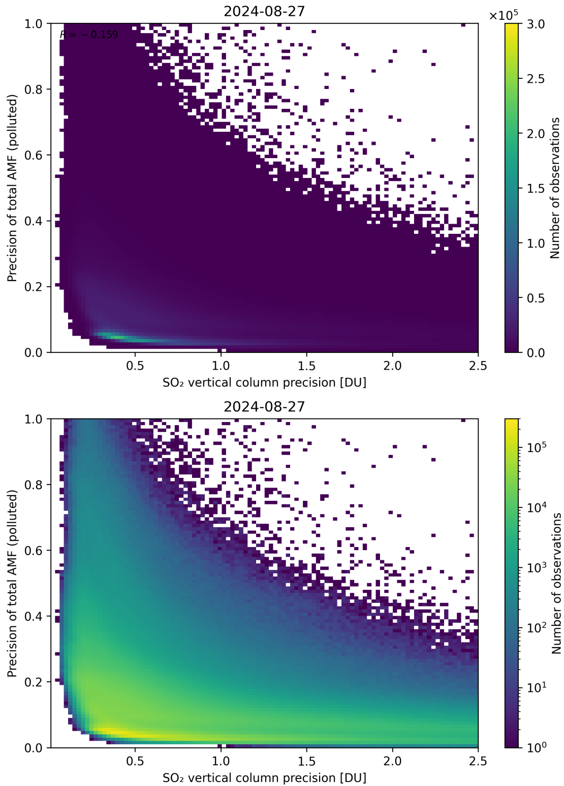
Figure 295: Scatter density plot of “SO 2 vertical column precision” against “Precision of total AMF (polluted)” for 2024-08-27 to 2024-08-28.
