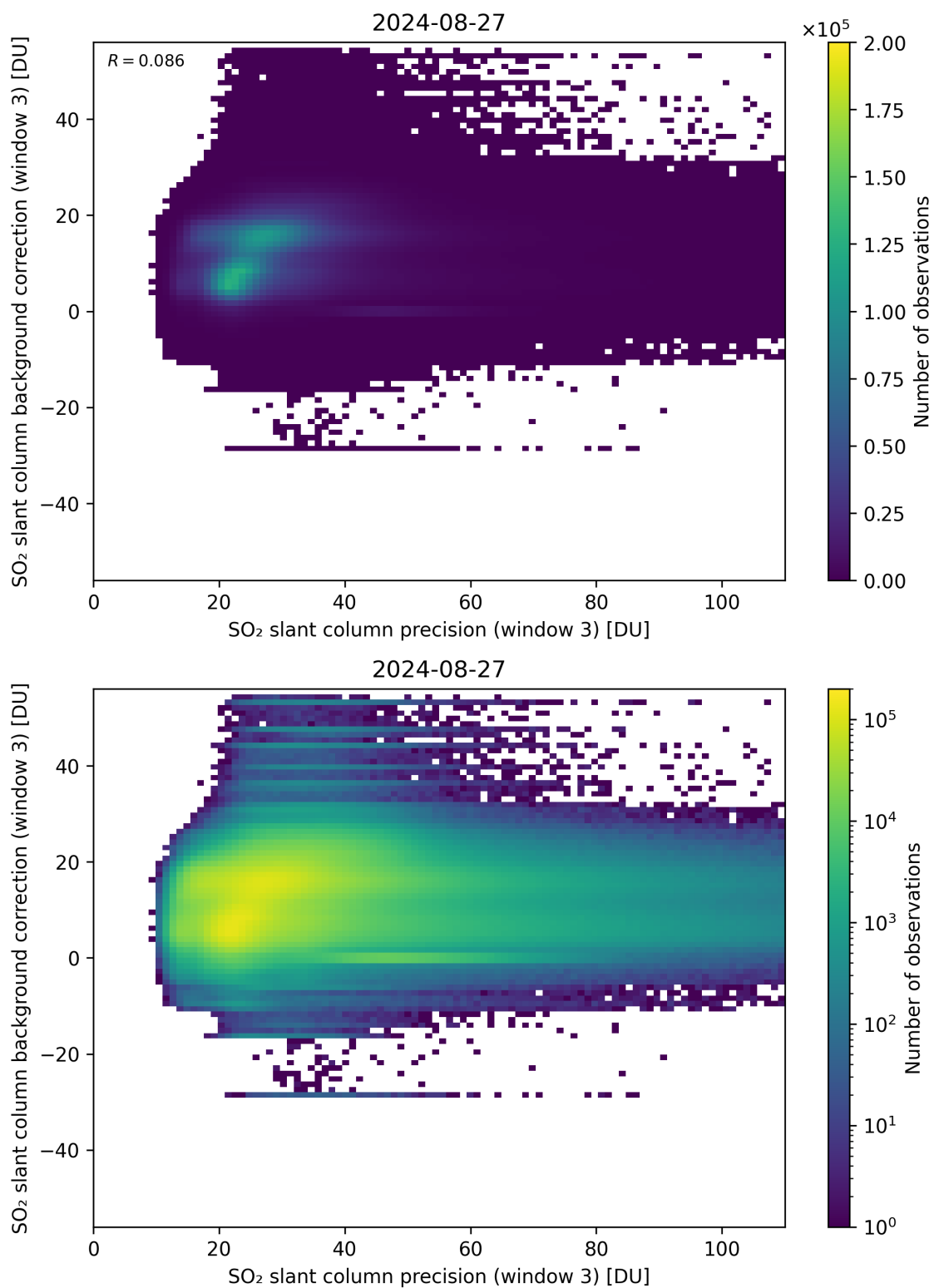
Figure 257: Scatter density plot of “SO 2 slant column precision (window 3)” against “SO 2 slant column background correction (window 3)” for 2024-08-27 to 2024-08-28.
