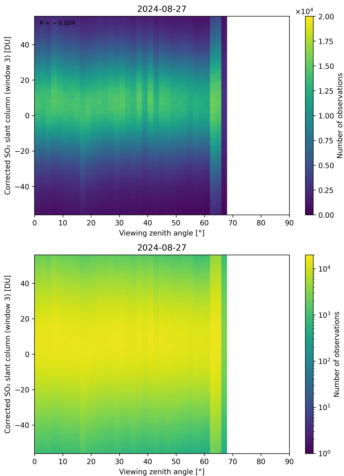
Figure 319: Scatter density plot of “Viewing zenith angle” against “Corrected SO 2 slant column (window 3)” for 2024-08-27 to 2024-08-28.
