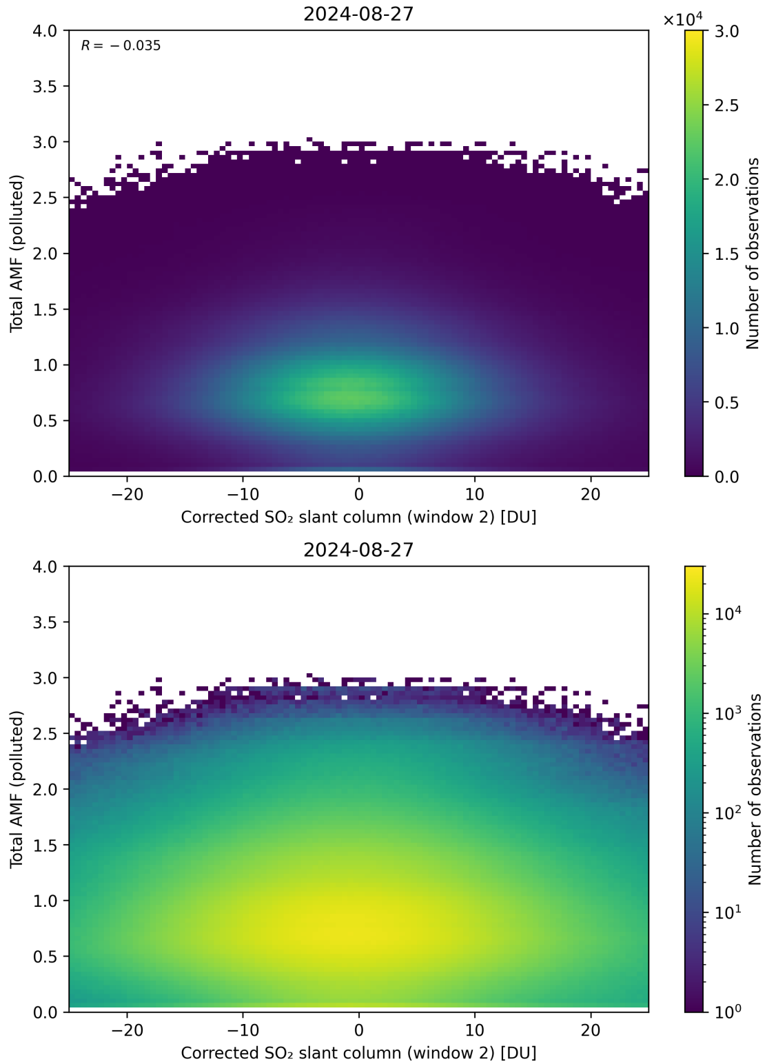
Figure 203: Scatter density plot of “Corrected SO 2 slant column (window 2)” against “Total AMF (polluted)” for 2024-08-27 to 2024-08-28.
