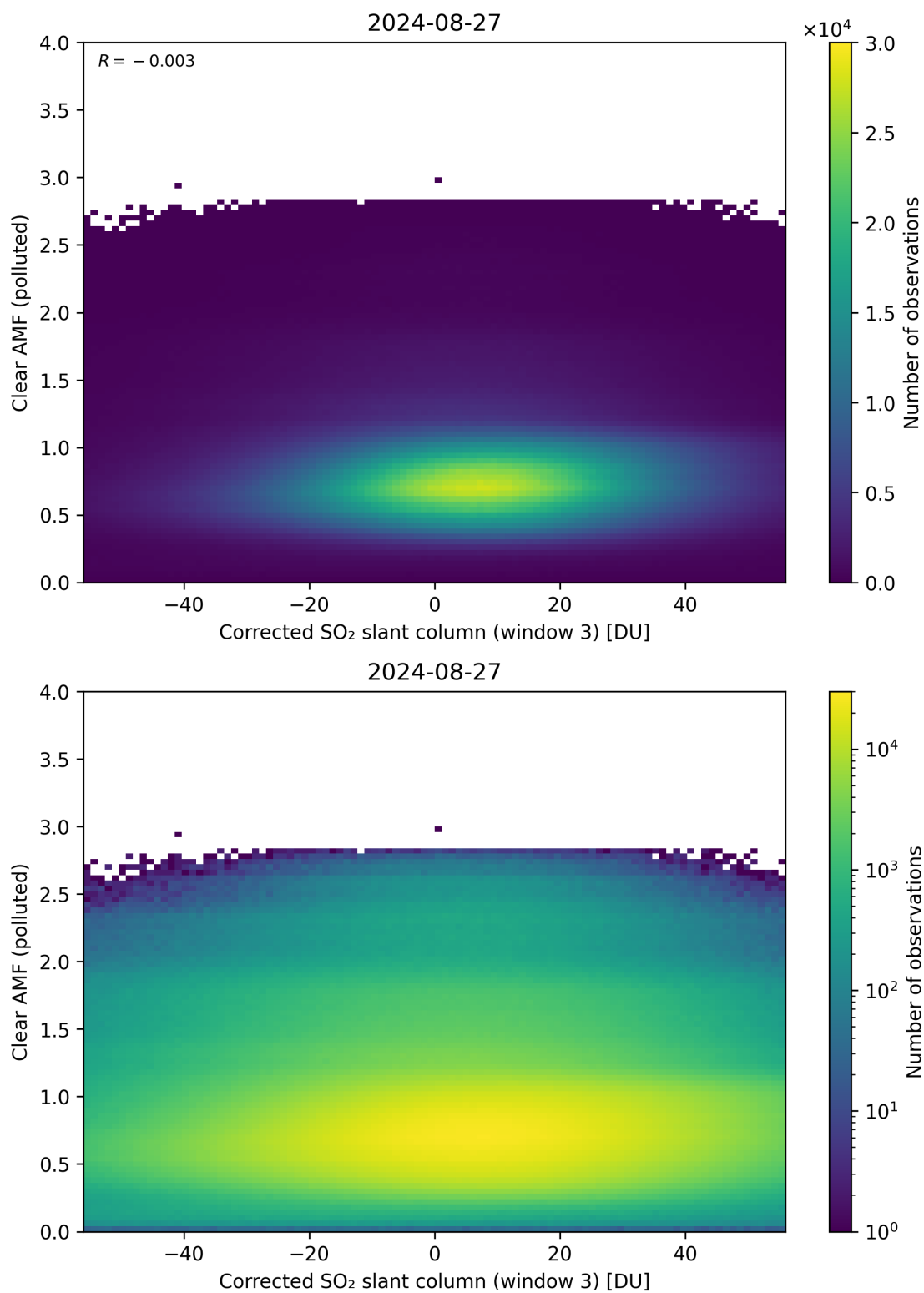
Figure 209: Scatter density plot of “Corrected SO 2 slant column (window 3)” against “Clear AMF (polluted)” for 2024-08-27 to 2024-08-28.
