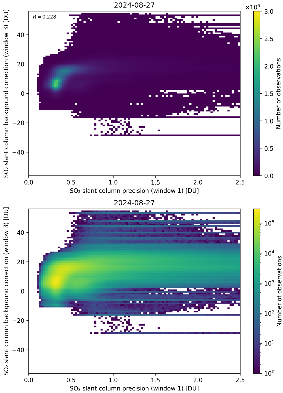
Figure 220: Scatter density plot of “SO 2 slant column precision (window 1)” against “SO 2 slant column background correction (window 3)” for 2024-08-27 to 2024-08-28.
