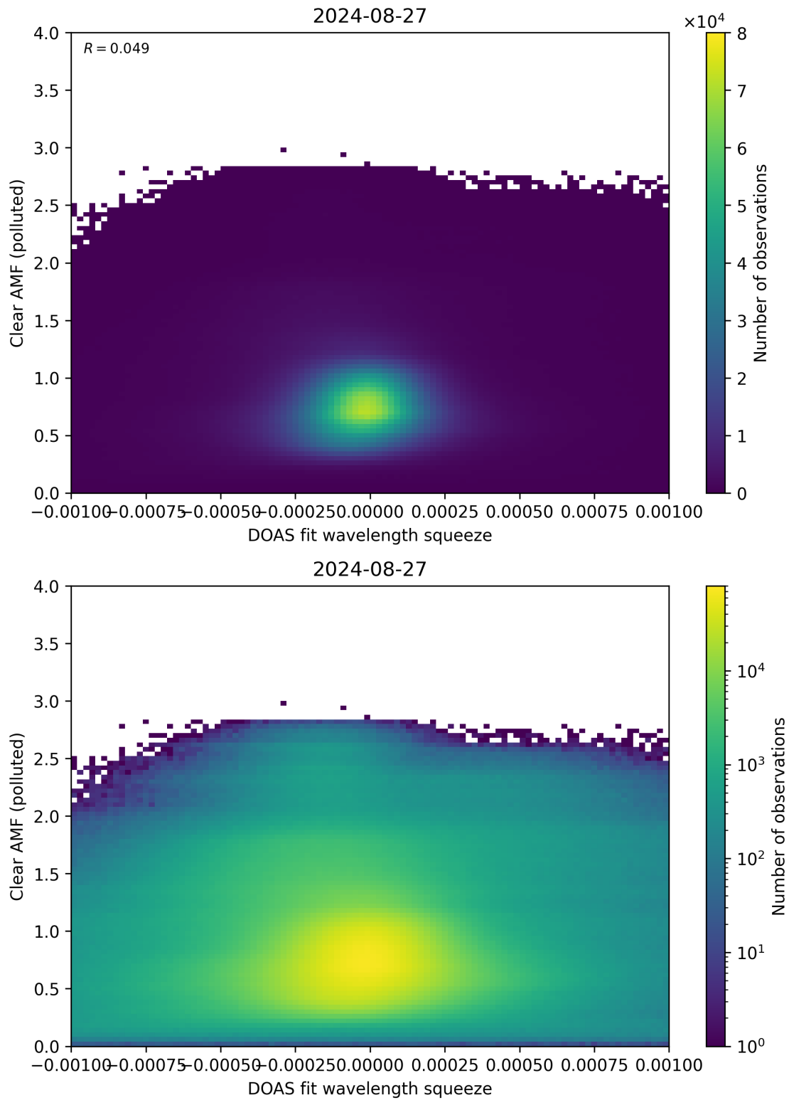
Figure 133: Scatter density plot of “DOAS fit wavelength squeeze” against “Clear AMF (polluted)” for 2024-08-27 to 2024-08-28.
