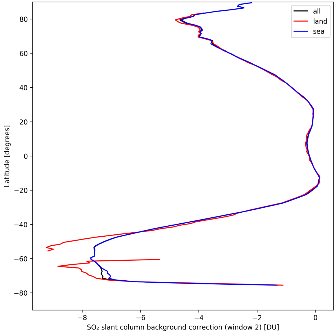
Figure 40: Zonal average of "SO 2 slant column background correction (window 2)" for 2024-08-27 to 2024-08-28.
