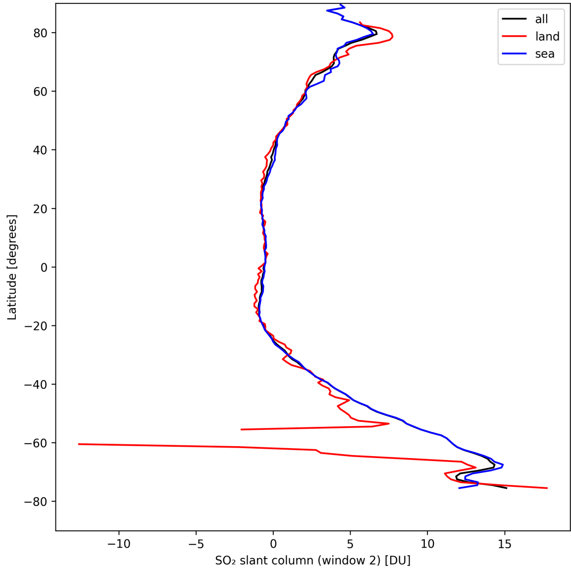
Figure 37: Zonal average of “SO 2 slant column (window 2)” for 2024-08-27 to 2024-08-28.
