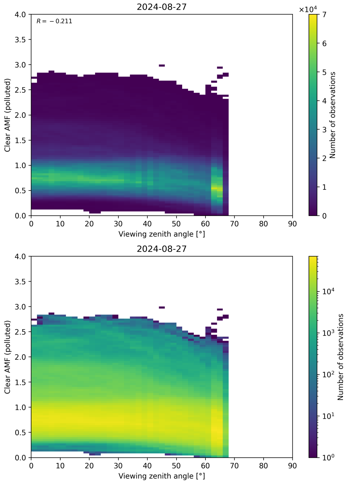
Figure 316: Scatter density plot of “Viewing zenith angle” against “Clear AMF (polluted)” for 2024-08-27 to 2024-08-28.
