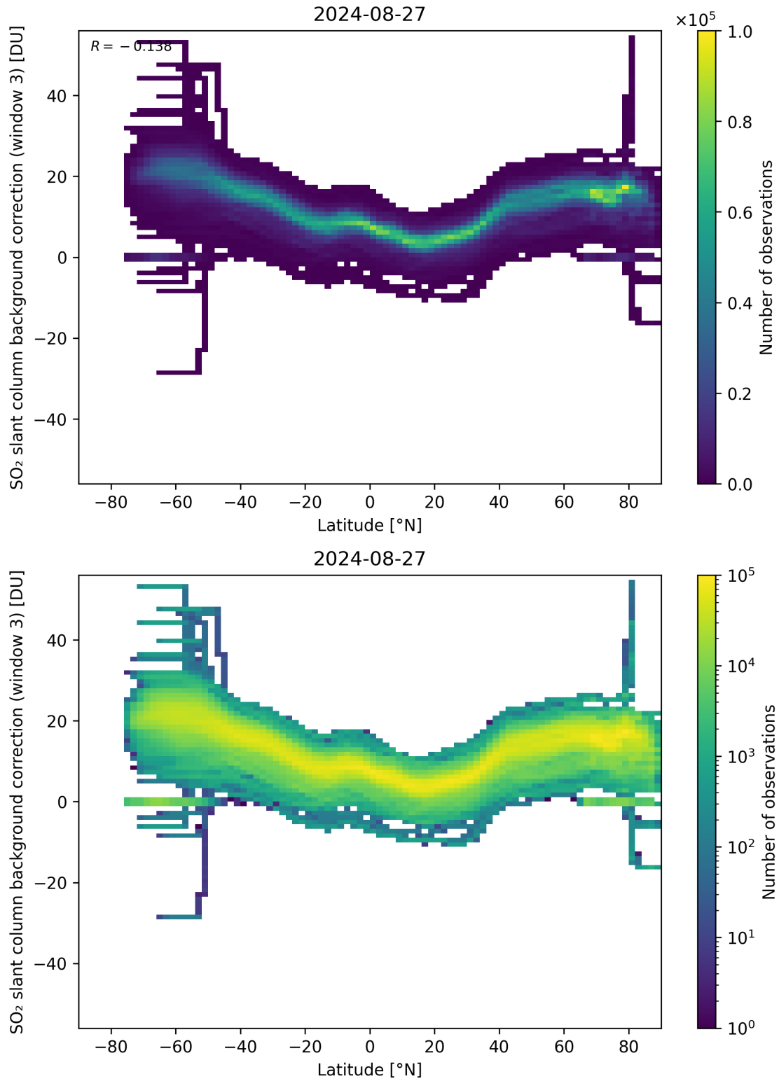
Figure 141: Scatter density plot of “Latitude” against “SO 2 slant column background correction (window 3)” for 2024-08-27 to 2024-08-28.
