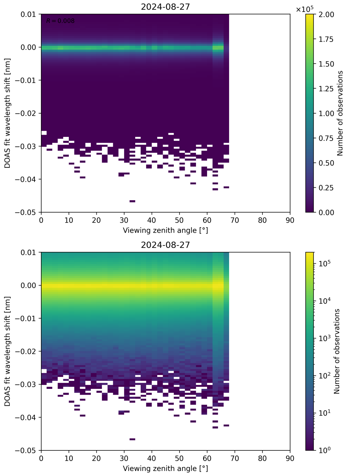
Figure 311: Scatter density plot of “Viewing zenith angle” against “DOAS fit wavelength shift” for 2024-08-27 to 2024-08-28.
