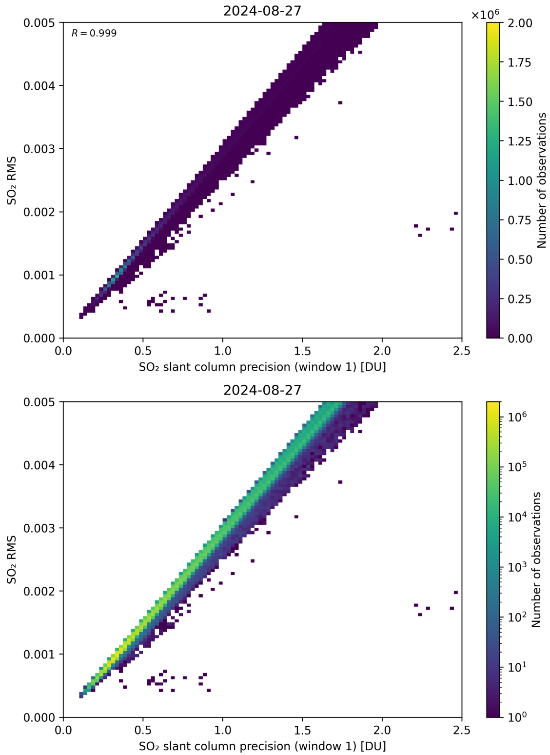
Figure 223: Scatter density plot of “SO 2 slant column precision (window 1)” against “SO 2 RMS” for 2024-08-27 to 2024-08-28.
