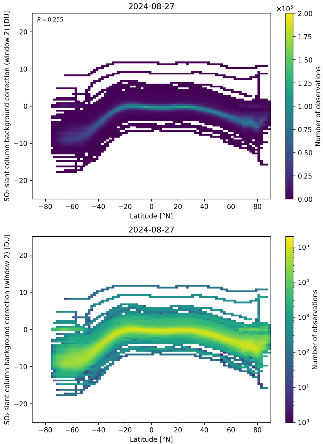
Figure 140: Scatter density plot of “Latitude” against “SO 2 slant column background correction (window 2)” for 2024-08-27 to 2024-08-28.
