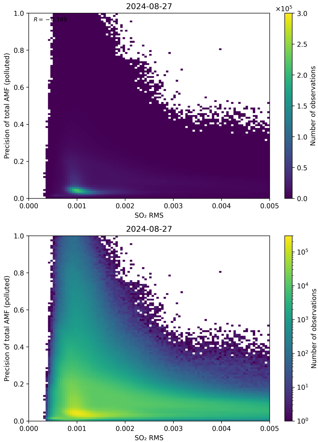
Figure 138: Scatter density plot of “SO 2 RMS” against “Precision of total AMF (polluted)” for 2024-08-27 to 2024-08-28.
