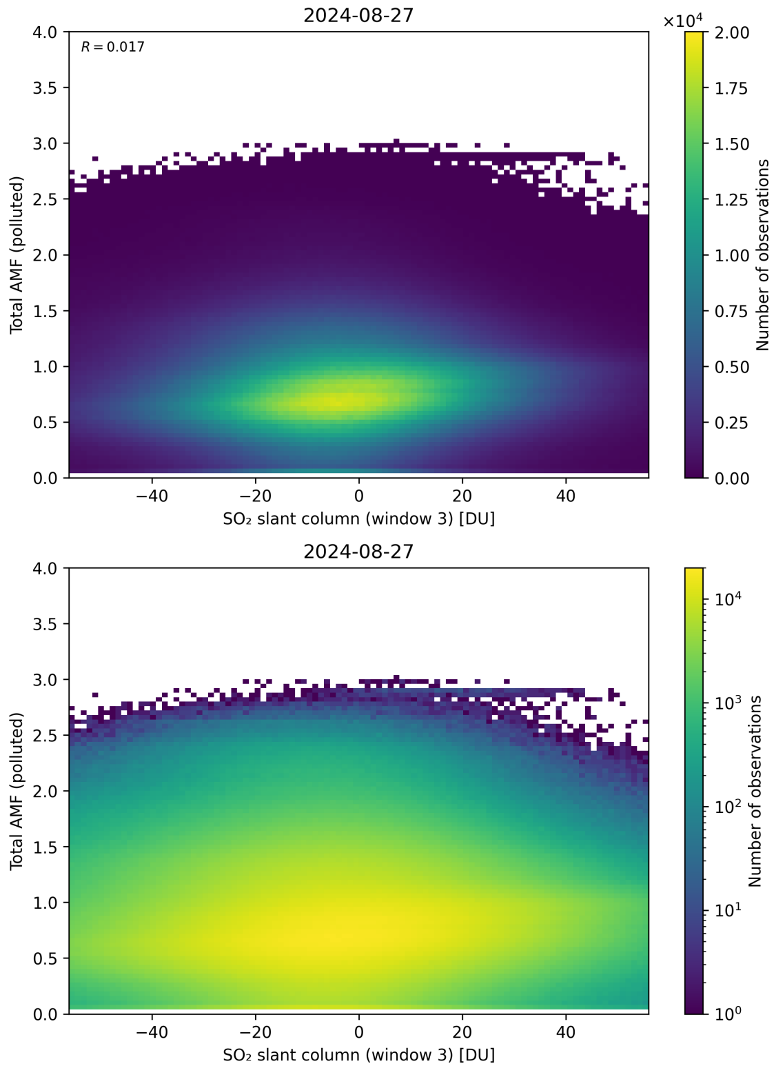
Figure 268: Scatter density plot of “SO 2 slant column (window 3)” against “Total AMF (polluted)” for 2024-08-27 to 2024-08-28.
