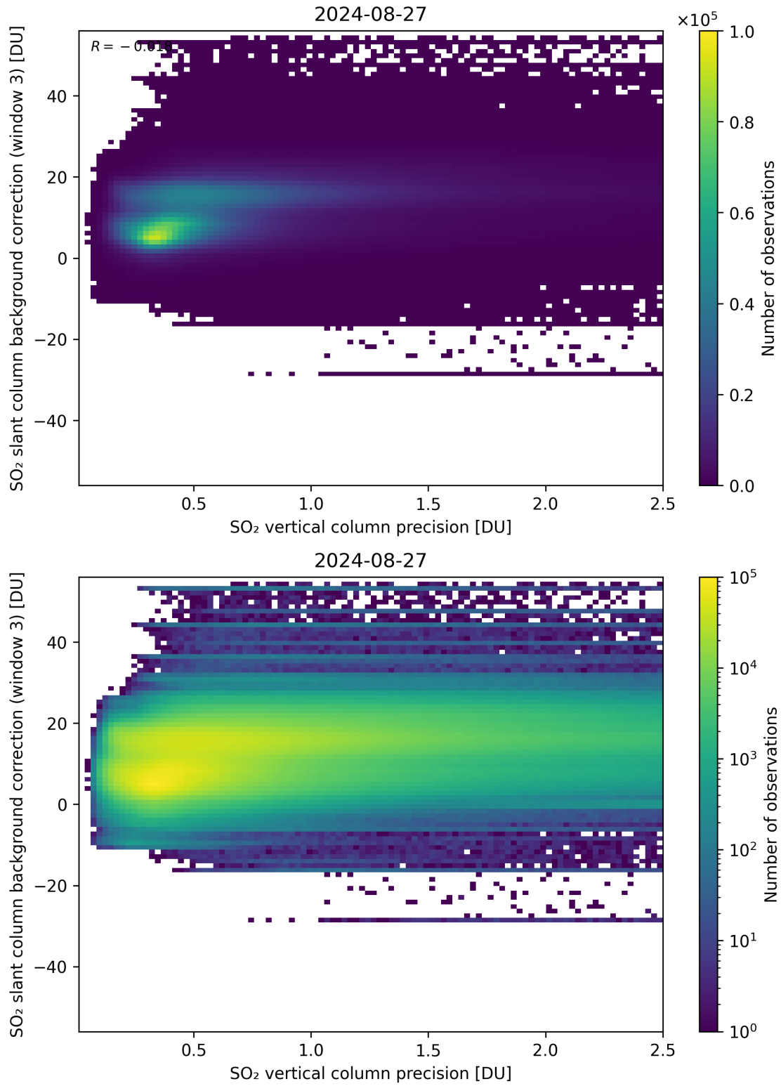
Figure 281: Scatter density plot of “SO 2 vertical column precision” against “SO 2 slant column background correction (window 3)” for 2024-08-27 to 2024-08-28.
