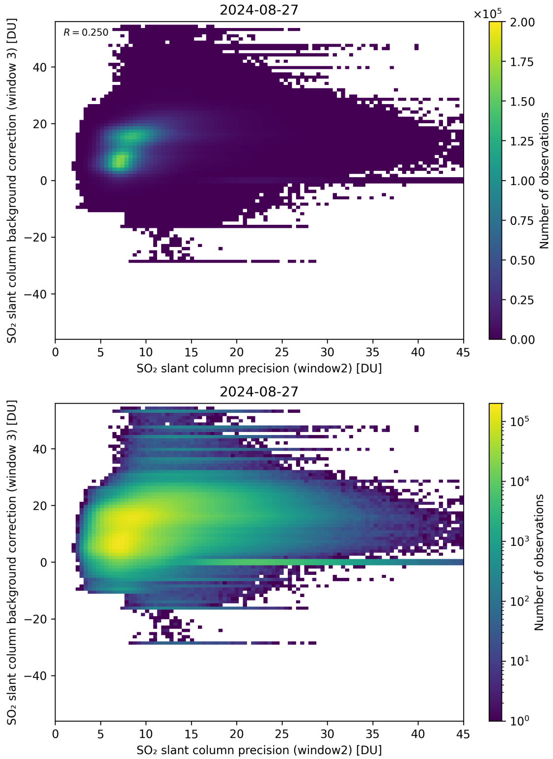
Figure 242: Scatter density plot of “SO 2 slant column precision (window2)” against “SO 2 slant column background correction (window 3)” for 2024-08-27 to 2024-08-28.
