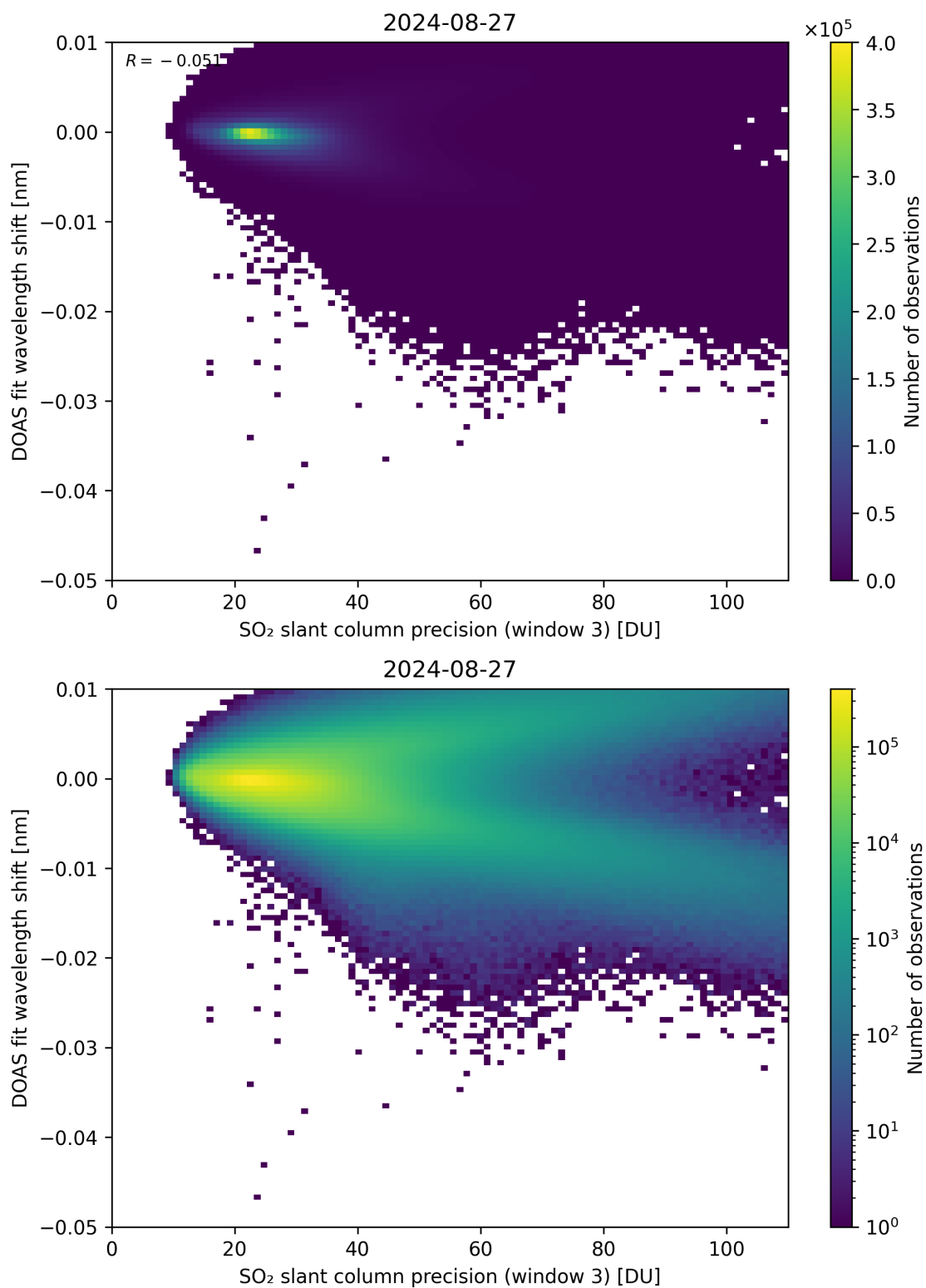
Figure 258: Scatter density plot of “SO 2 slant column precision (window 3)” against “DOAS fit wavelength shift” for 2024-08-27 to 2024-08-28.
