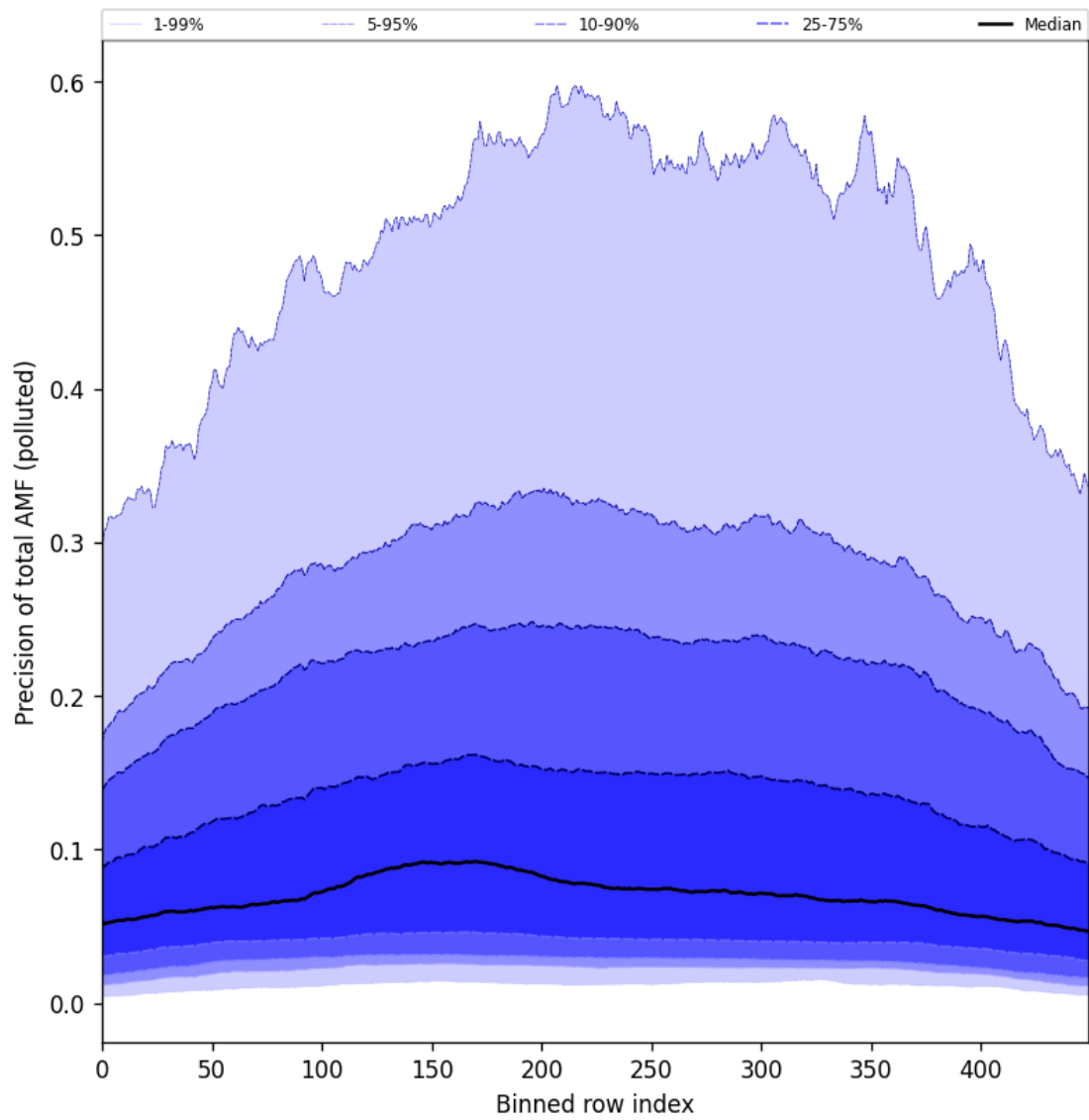
Figure 95: Along track statistics of “Precision of total AMF (polluted)” for 2024-08-27 to 2024-08-28
