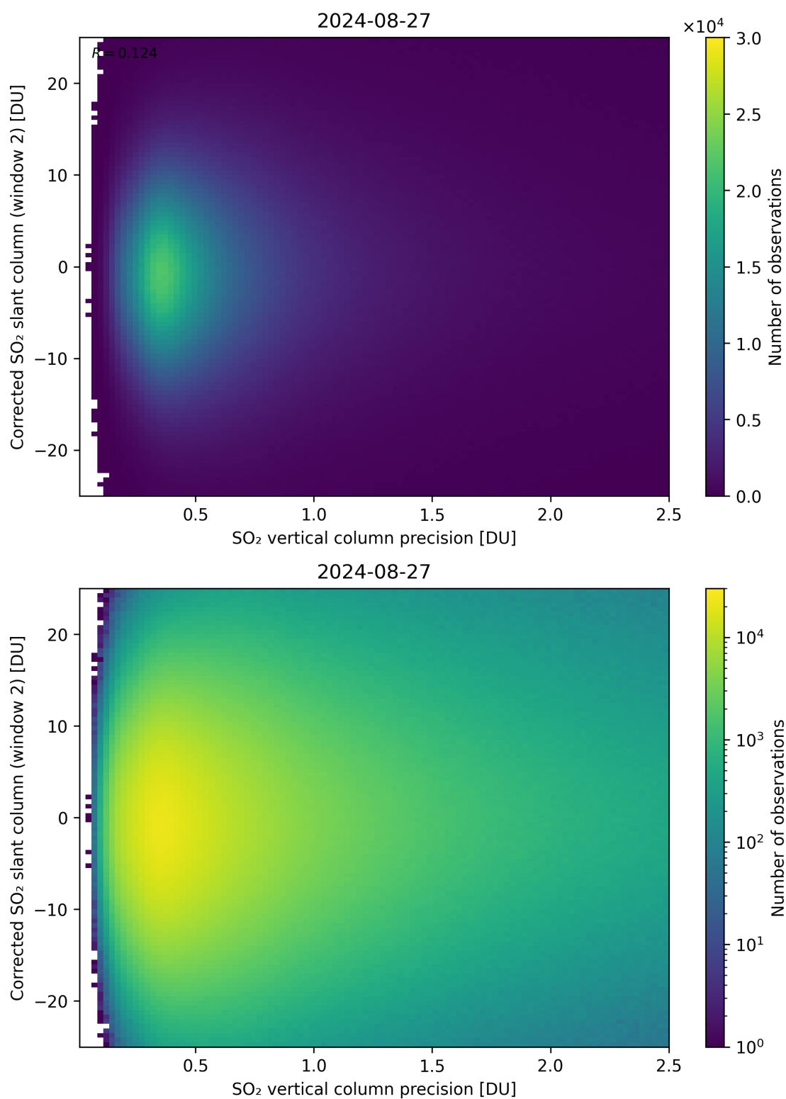
Figure 287: Scatter density plot of “SO 2 vertical column precision” against “Corrected SO 2 slant column (window 2)” for 2024-08-27 to 2024-08-28.
