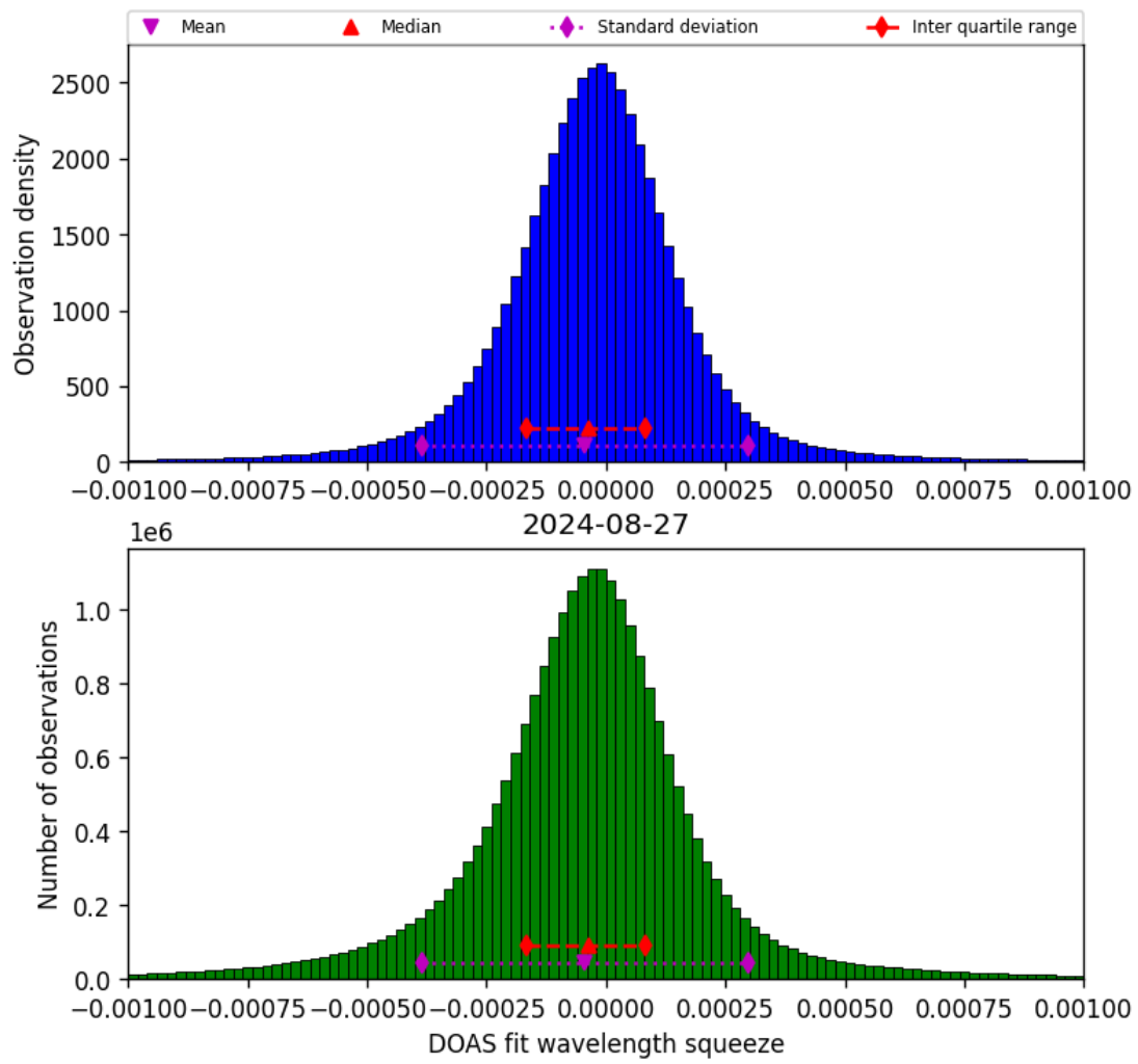
Figure 69: Histogram of “DOAS fit wavelength squeeze” for 2024-08-27 to 2024-08-28
