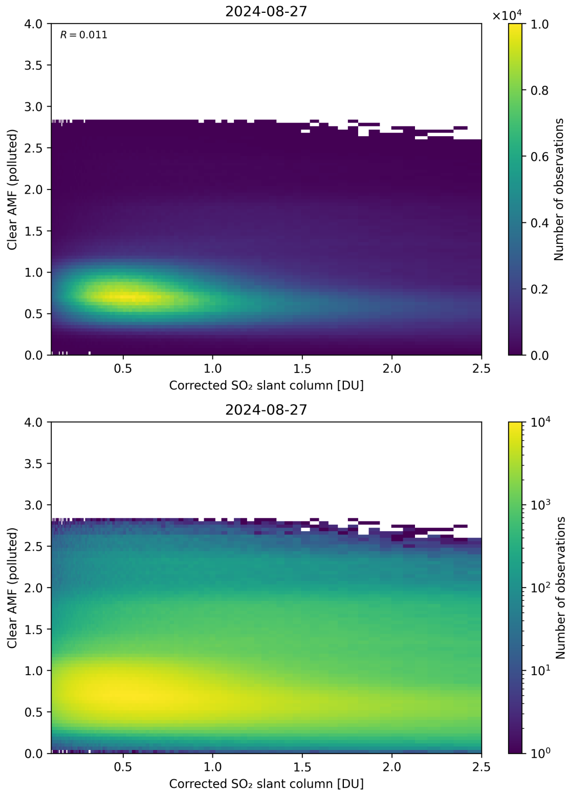
Figure 184: Scatter density plot of “Corrected SO 2 slant column” against “Clear AMF (polluted)” for 2024-08-27 to 2024-08-28.
