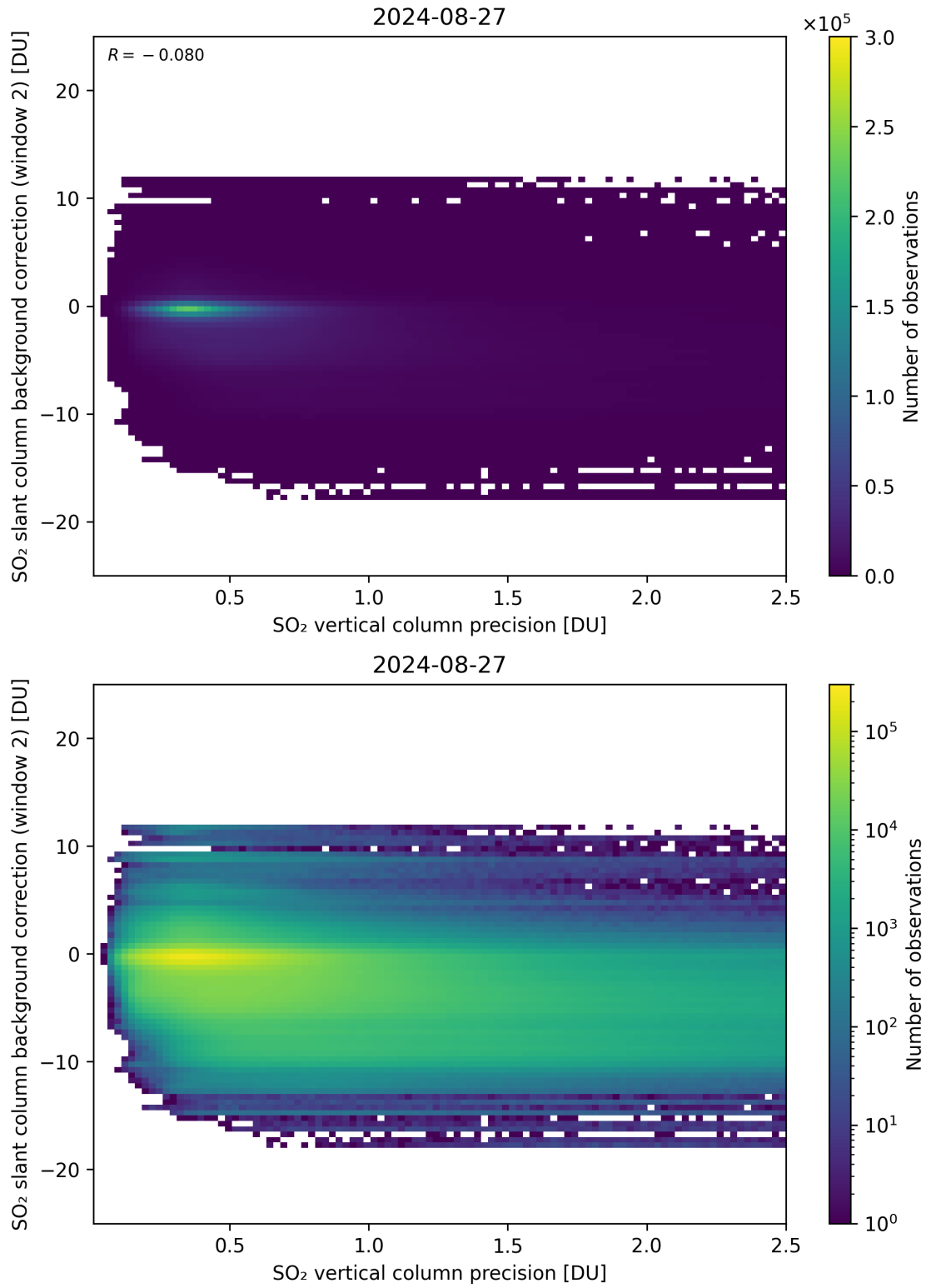
Figure 280: Scatter density plot of “SO 2 vertical column precision” against “SO 2 slant column background correction (window 2)” for 2024-08-27 to 2024-08-28.
