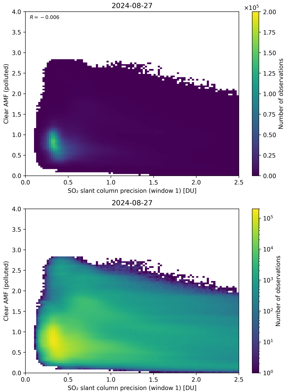
Figure 224: Scatter density plot of “SO 2 slant column precision (window 1)” against “Clear AMF (polluted)” for 2024-08-27 to 2024-08-28.
