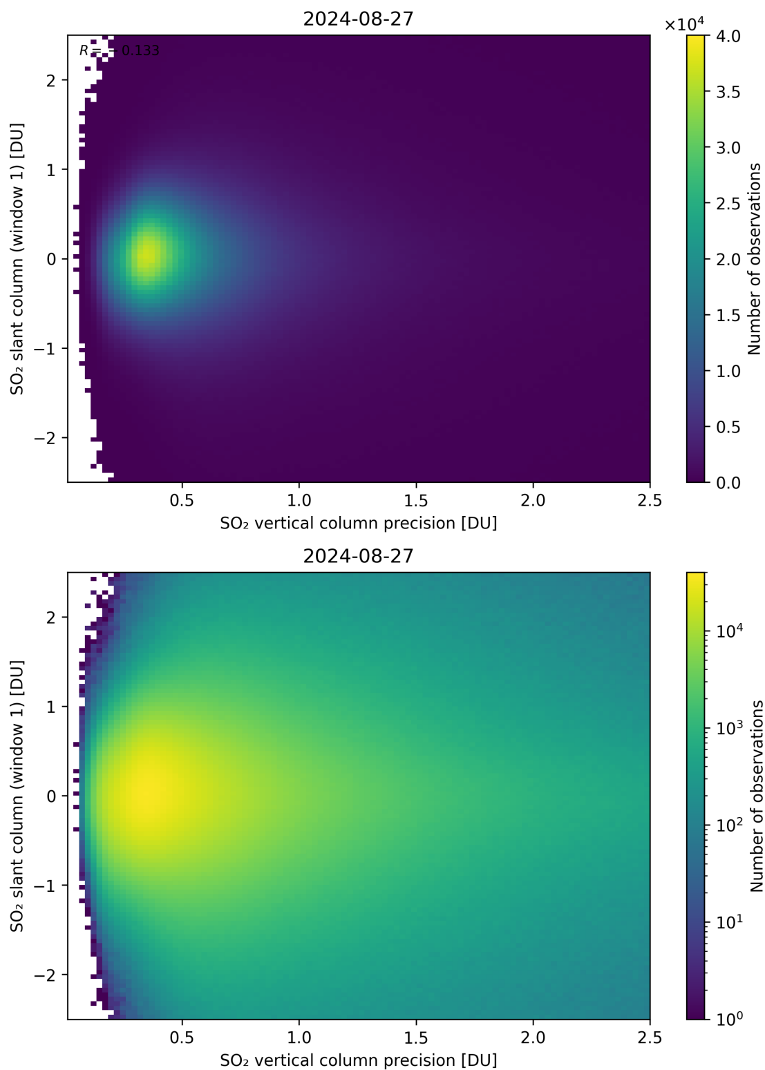
Figure 289: Scatter density plot of “SO 2 vertical column precision” against “SO 2 slant column (window 1)” for 2024-08-27 to 2024-08-28.
