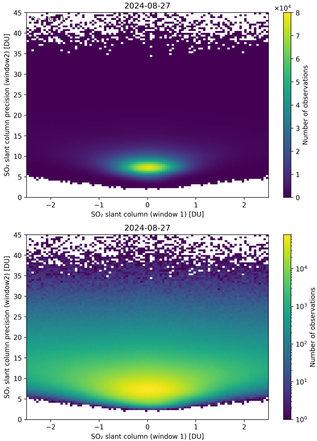
Figure 236: Scatter density plot of “SO 2 slant column (window 1)” against “SO 2 slant column precision (window2)” for 2024-08-27 to 2024-08-28.
