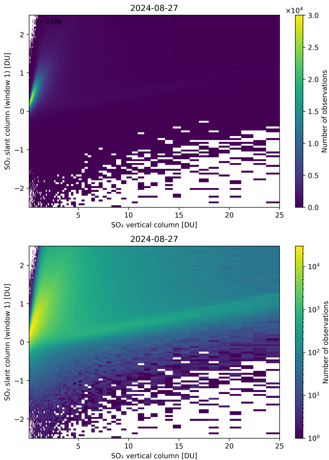
Figure 300: Scatter density plot of “SO 2 vertical column” against “SO 2 slant column (window 1)” for 2024-08-27 to 2024-08-28.
