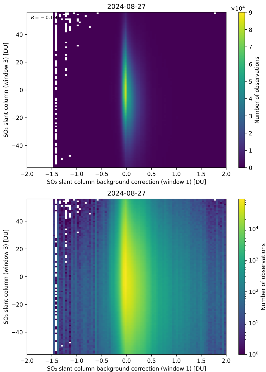
Figure 107: Scatter density plot of “SO 2 slant column background correction (window 1)” against “SO 2 slant column (window 3)” for 2024-08-27 to 2024-08-28.
