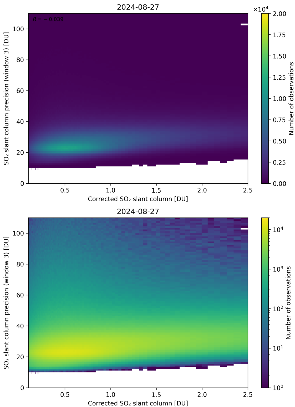
Figure 191: Scatter density plot of “Corrected SO 2 slant column” against “SO 2 slant column precision (window 3)” for 2024-08-27 to 2024-08-28.
