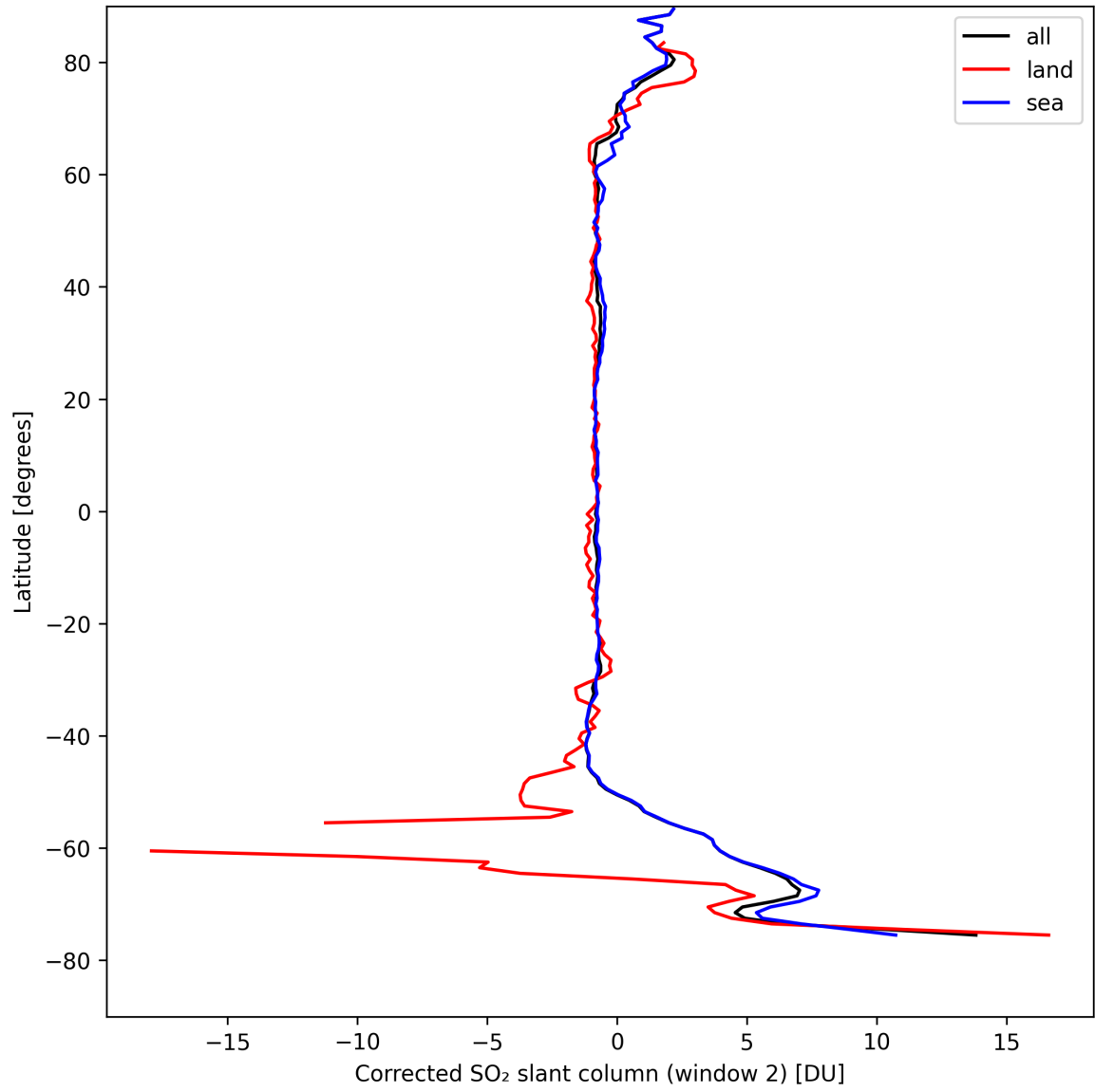
Figure 39: Zonal average of “Corrected SO 2 slant column (window 2)” for 2024-08-27 to 2024-08-28.
