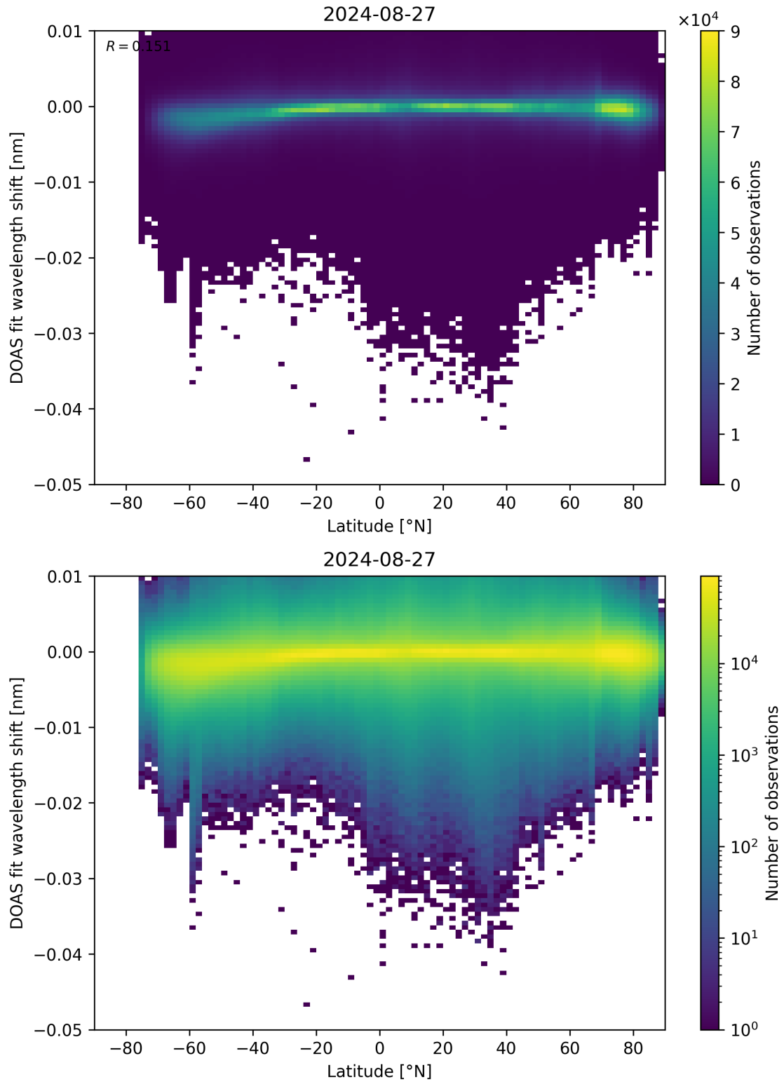
Figure 142: Scatter density plot of “Latitude” against “DOAS fit wavelength shift” for 2024-08-27 to 2024-08-28.
