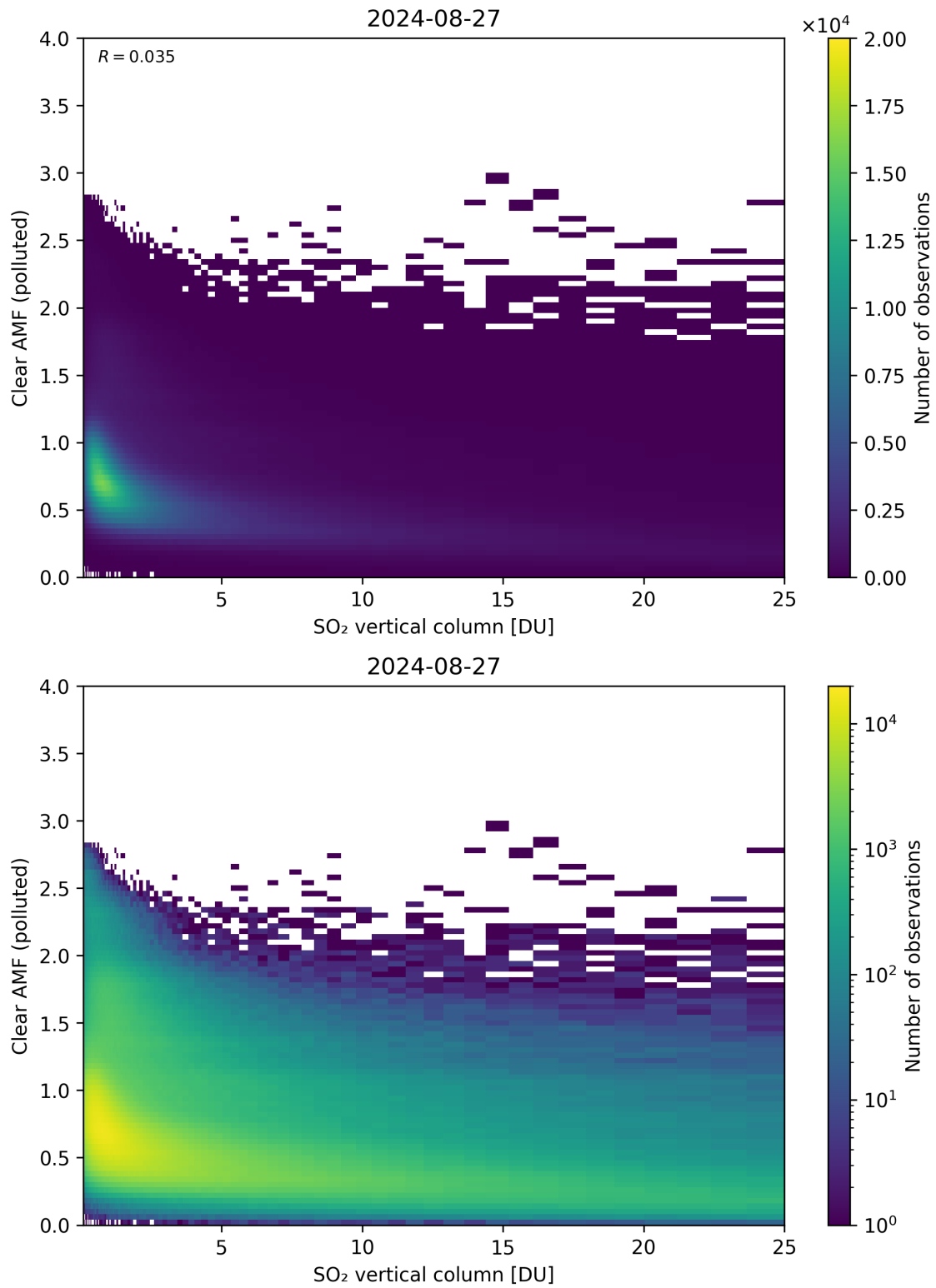
Figure 296: Scatter density plot of “SO 2 vertical column” against “Clear AMF (polluted)” for 2024-08-27 to 2024-08-28.
