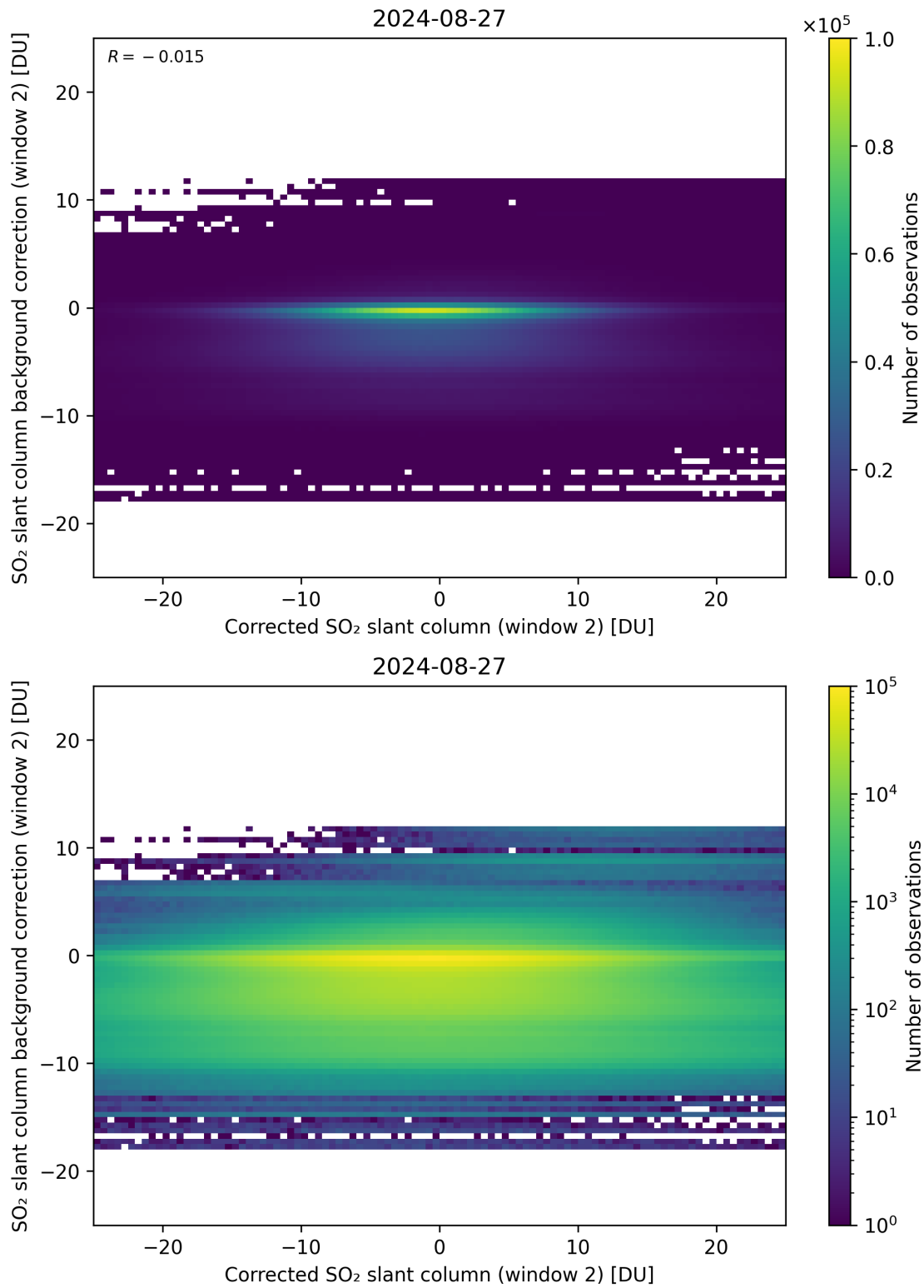
Figure 194: Scatter density plot of “Corrected SO 2 slant column (window 2)” against “SO 2 slant column background correction (window 2)” for 2024-08-27 to 2024-08-28.
