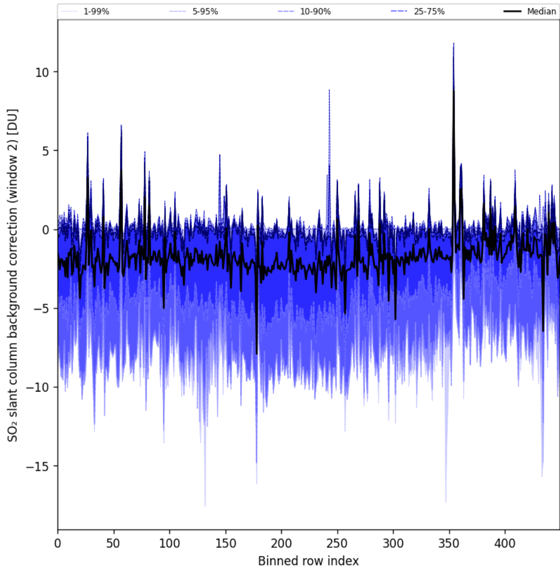
Figure 86: Along track statistics of “SO 2 slant column background correction (window 2)” for 2024-08-27 to 2024-08-28
