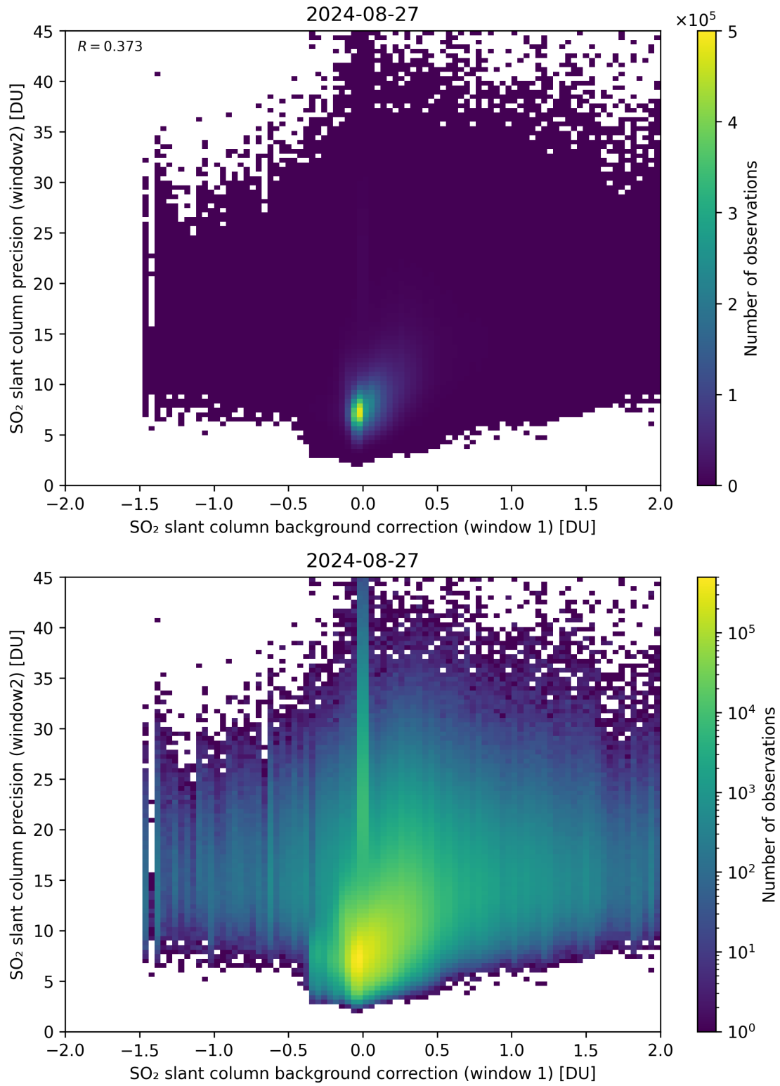
Figure 106: Scatter density plot of “SO 2 slant column background correction (window 1)” against “SO 2 slant column precision (window2)” for 2024-08-27 to 2024-08-28.
