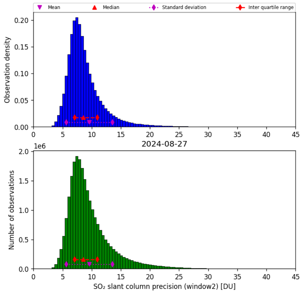
Figure 61: Histogram of “SO 2 slant column precision (window2)” for 2024-08-27 to 2024-08-28
