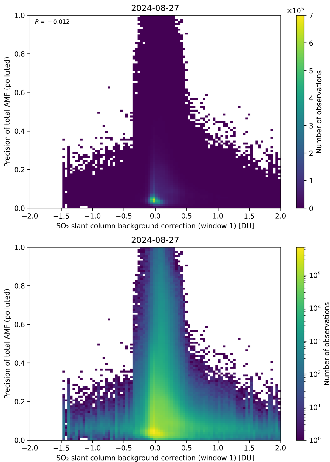
Figure 110: Scatter density plot of “SO 2 slant column background correction (window 1)” against “Precision of total AMF (polluted)” for 2024-08-27 to 2024-08-28.
