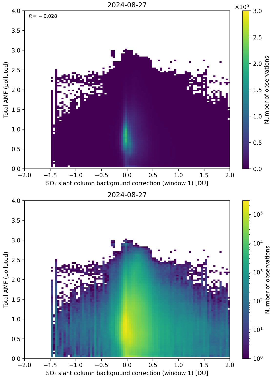
Figure 109: Scatter density plot of “SO 2 slant column background correction (window 1)” against “Total AMF (polluted)” for 2024-08-27 to 2024-08-28.
