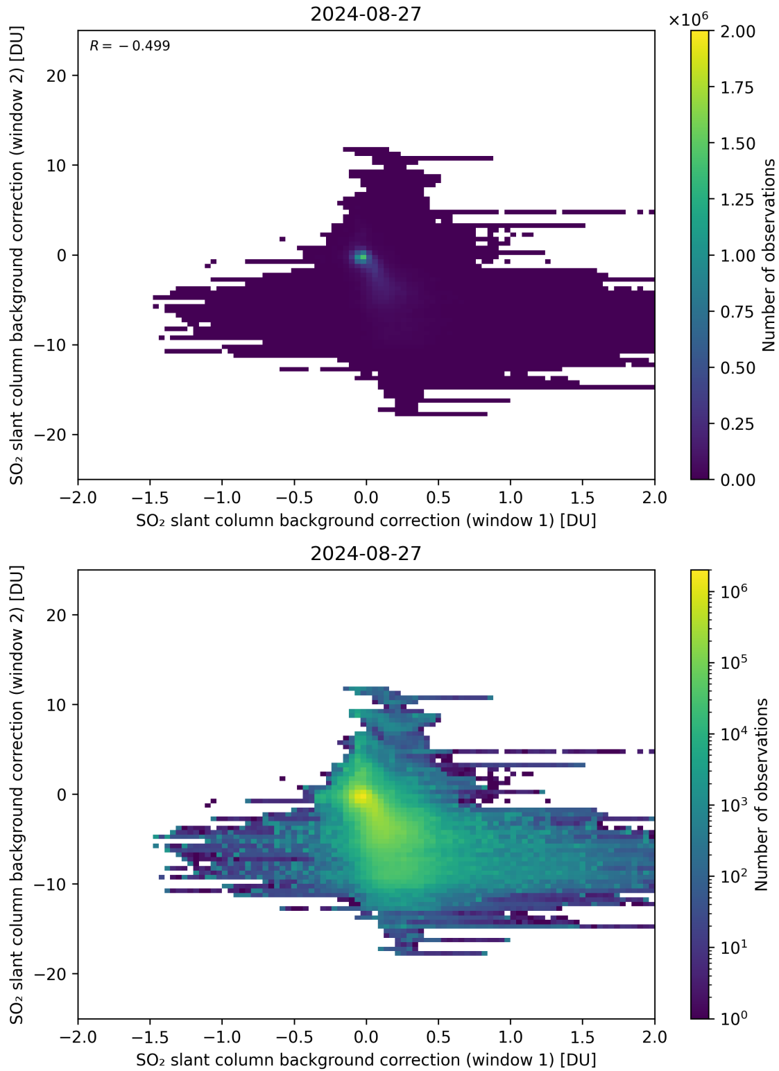
Figure 98: Scatter density plot of “SO 2 slant column background correction (window 1)” against “SO 2 slant column background correction (window 2)” for 2024-08-27 to 2024-08-28.
