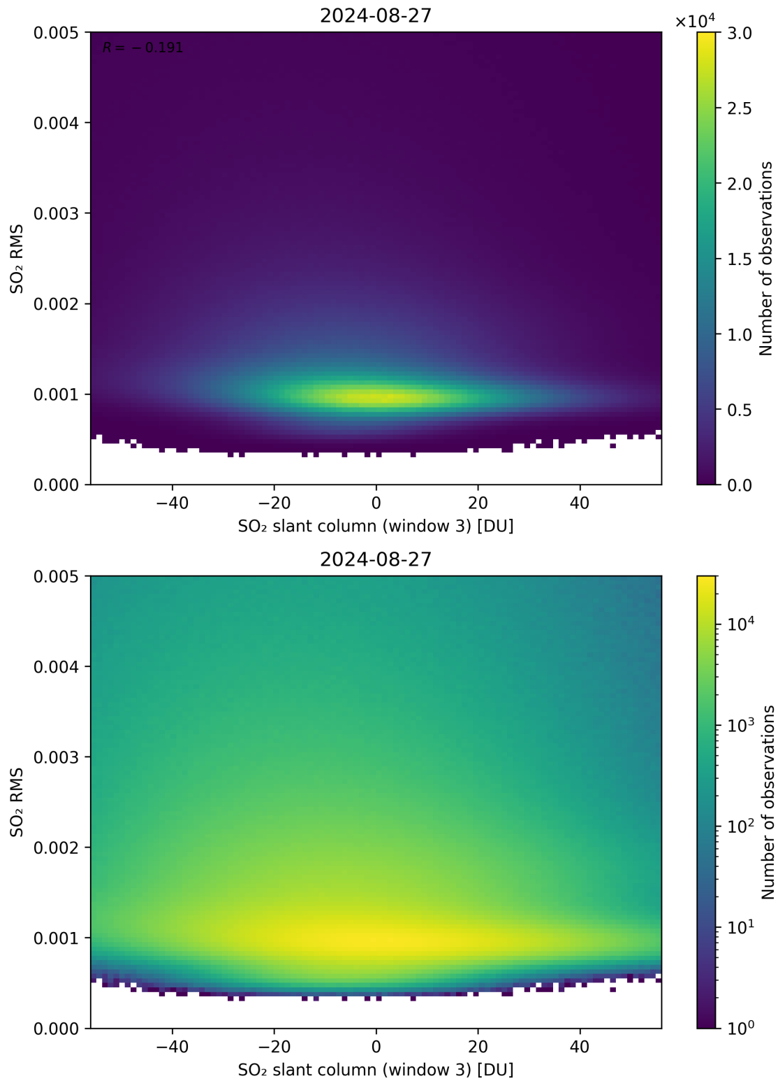
Figure 256: Scatter density plot of “SO 2 slant column (window 3)” against “SO 2 RMS” for 2024-08-27 to 2024-08-28.
