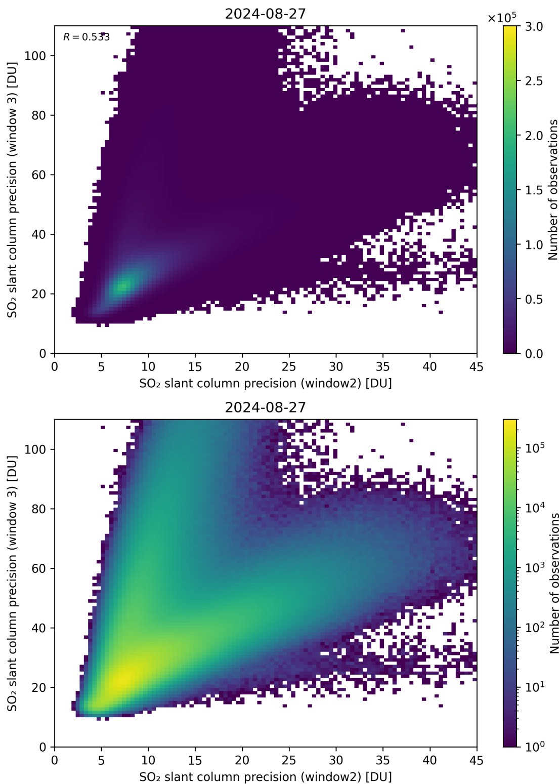
Figure 250: Scatter density plot of “SO 2 slant column precision (window2)” against “SO 2 slant column precision (window 3)” for 2024-08-27 to 2024-08-28.
