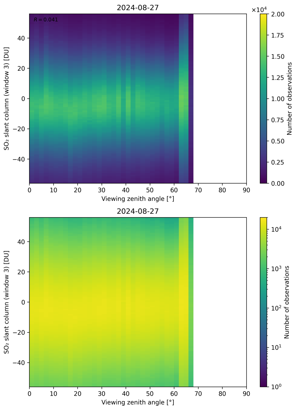
Figure 323: Scatter density plot of “Viewing zenith angle” against “SO 2 slant column (window 3)” for 2024-08-27 to 2024-08-28.
