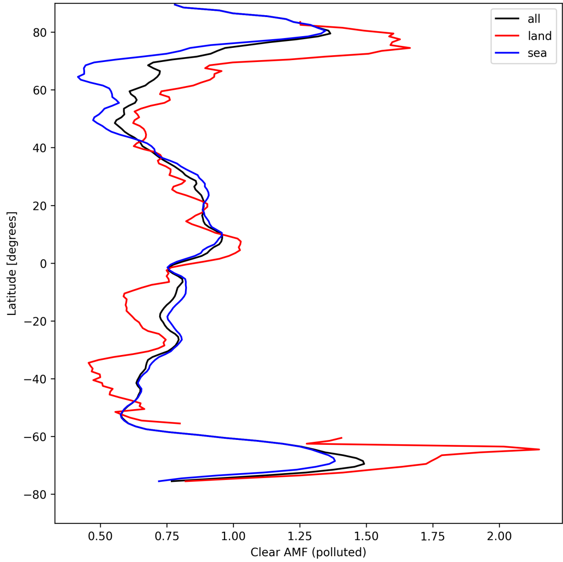
Figure 50: Zonal average of “Clear AMF (polluted)” for 2024-08-27 to 2024-08-28.
