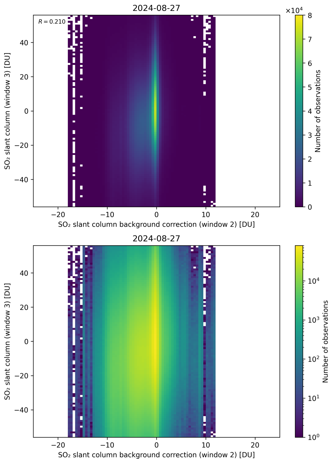
Figure 117: Scatter density plot of “SO 2 slant column background correction (window 2)” against “SO 2 slant column (window 3)” for 2024-08-27 to 2024-08-28.
