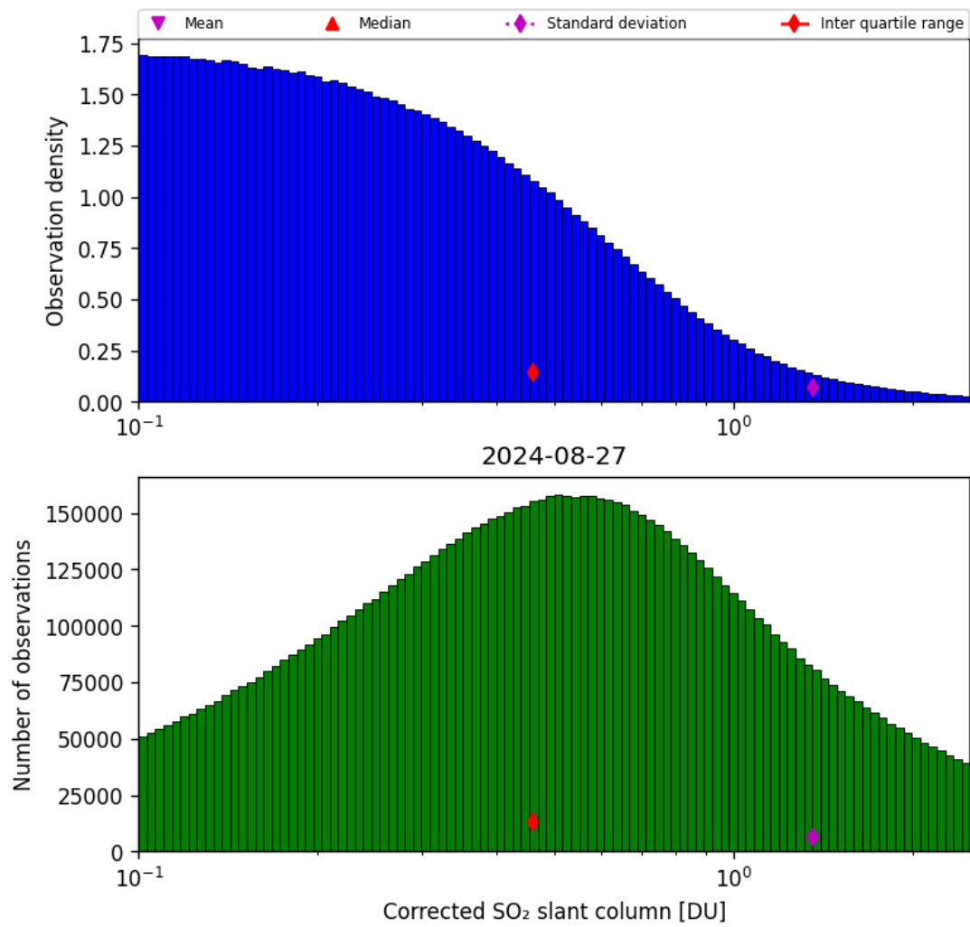
Figure 55: Histogram of “Corrected SO 2 slant column” for 2024-08-27 to 2024-08-28
