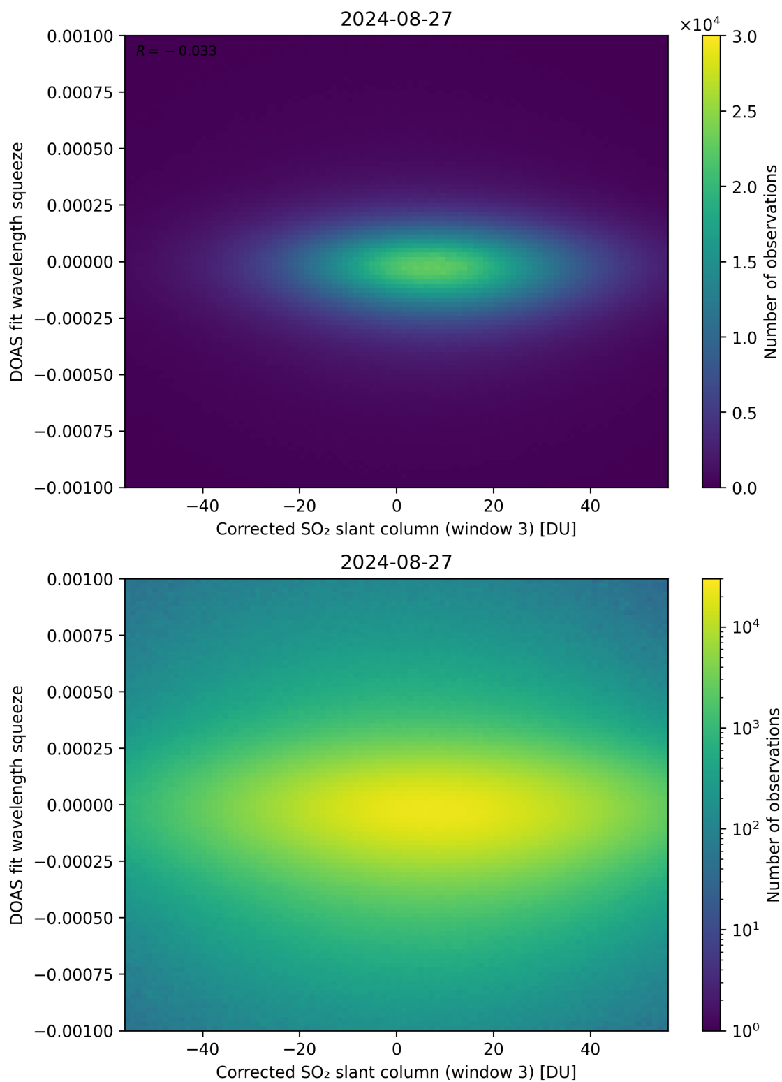
Figure 207: Scatter density plot of “Corrected SO 2 slant column (window 3)” against “DOAS fit wavelength squeeze” for 2024-08-27 to 2024-08-28.
