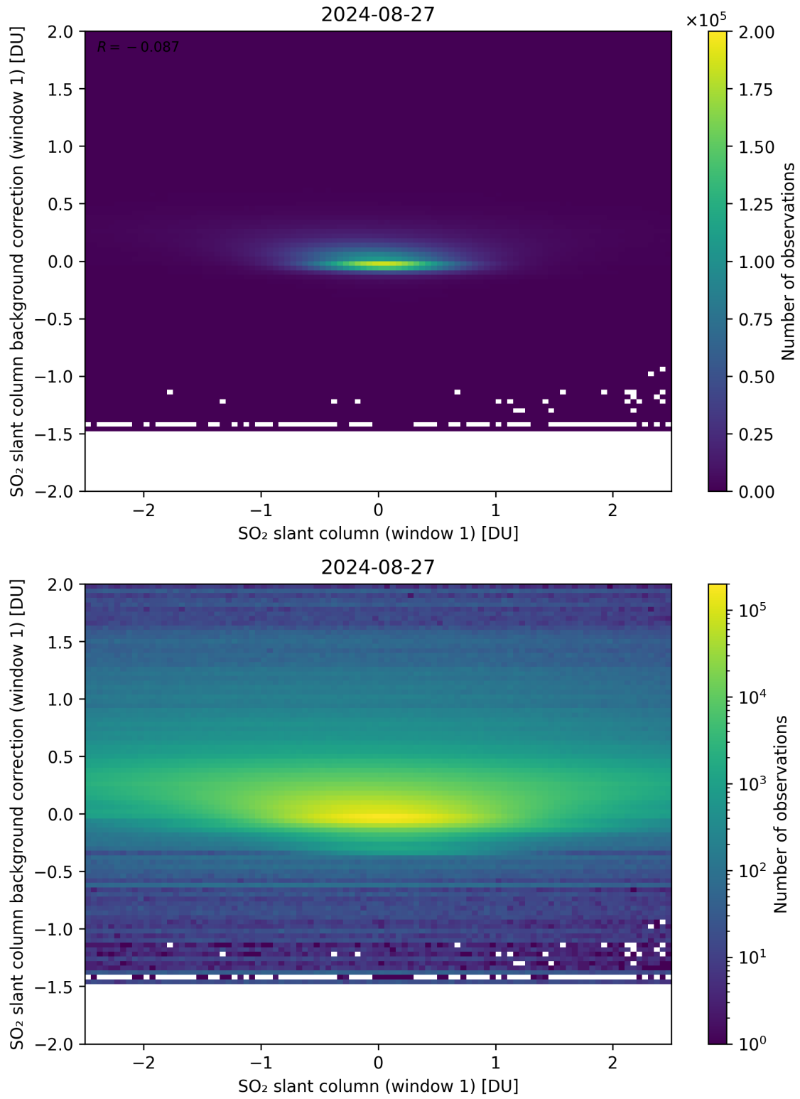
Figure 212: Scatter density plot of “SO 2 slant column (window 1)” against “SO 2 slant column background correction (window 1)” for 2024-08-27 to 2024-08-28.
