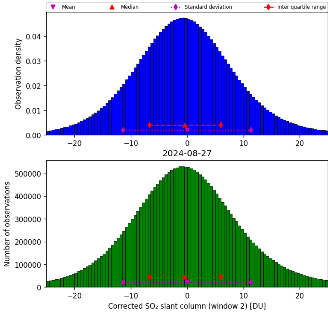
Figure 62: Histogram of “Corrected SO 2 slant column (window 2)” for 2024-08-27 to 2024-08-28
