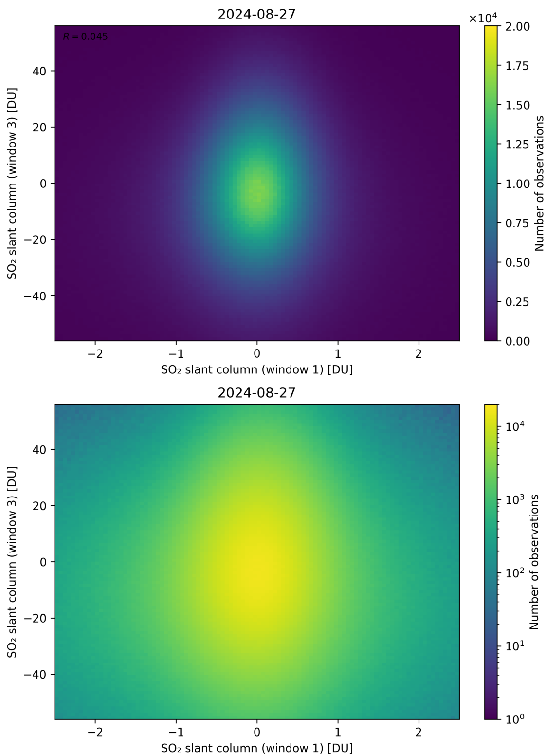
Figure 237: Scatter density plot of “SO 2 slant column (window 1)” against “SO 2 slant column (window 3)” for 2024-08-27 to 2024-08-28.
