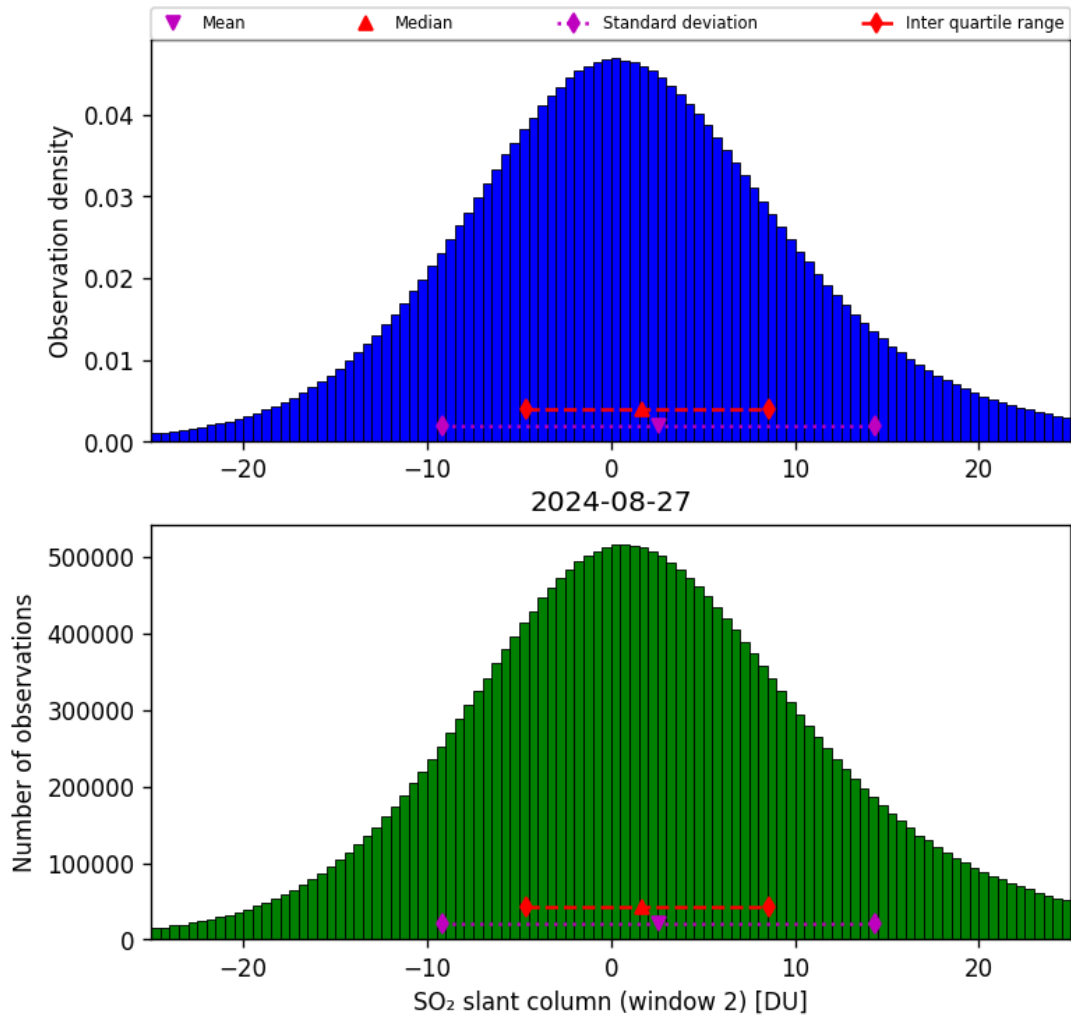
Figure 60: Histogram of “SO 2 slant column (window 2)” for 2024-08-27 to 2024-08-28
