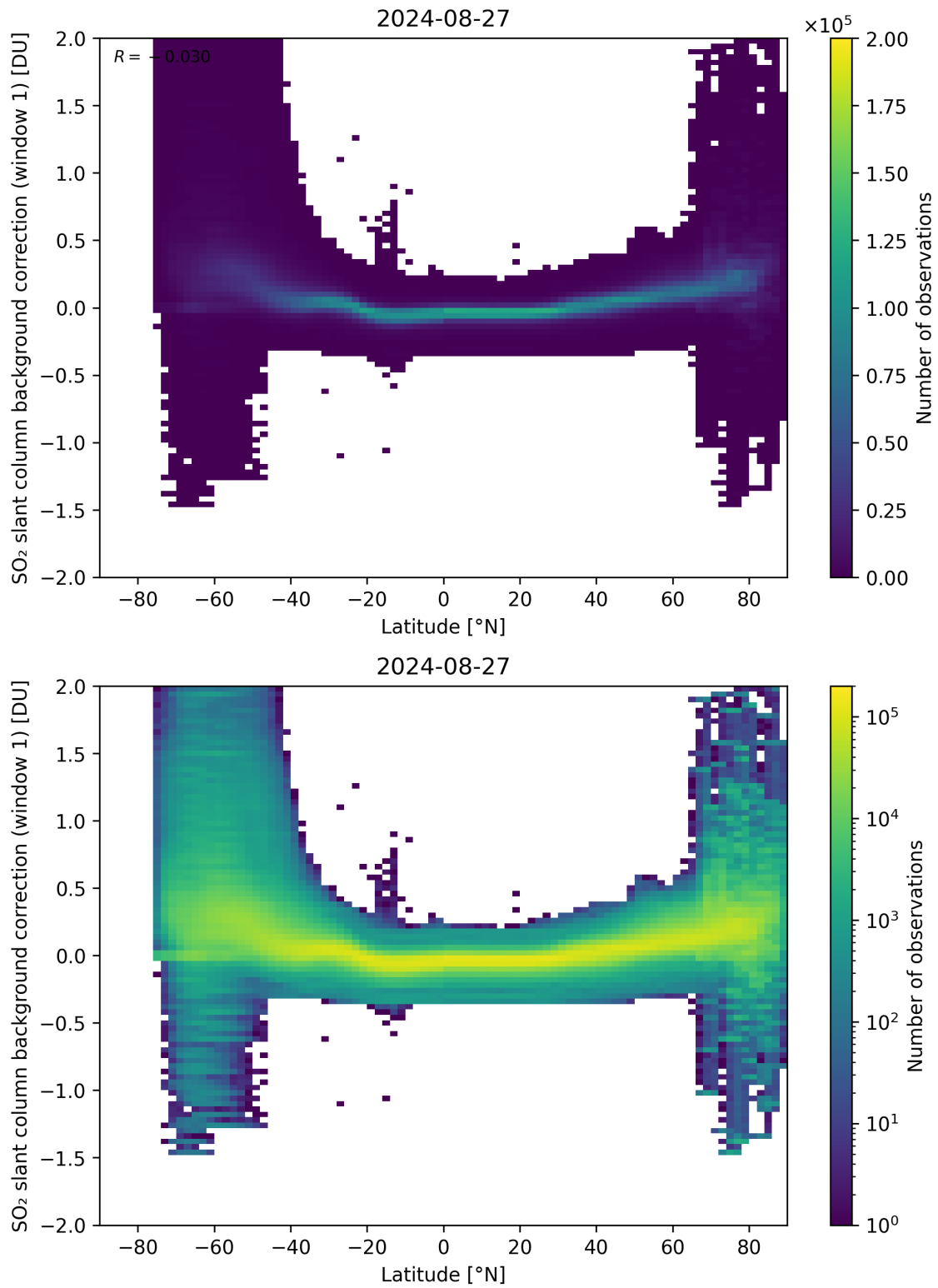
Figure 139: Scatter density plot of “Latitude” against “SO 2 slant column background correction (window 1)” for 2024-08-27 to 2024-08-28.
