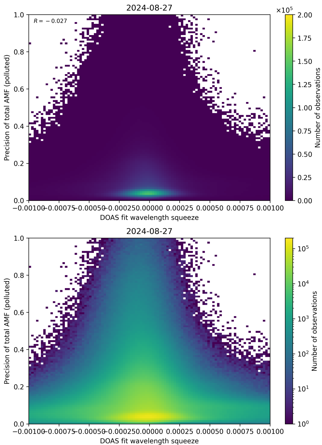
Figure 135: Scatter density plot of “DOAS fit wavelength squeeze” against “Precision of total AMF (polluted)” for 2024-08-27 to 2024-08-28.
