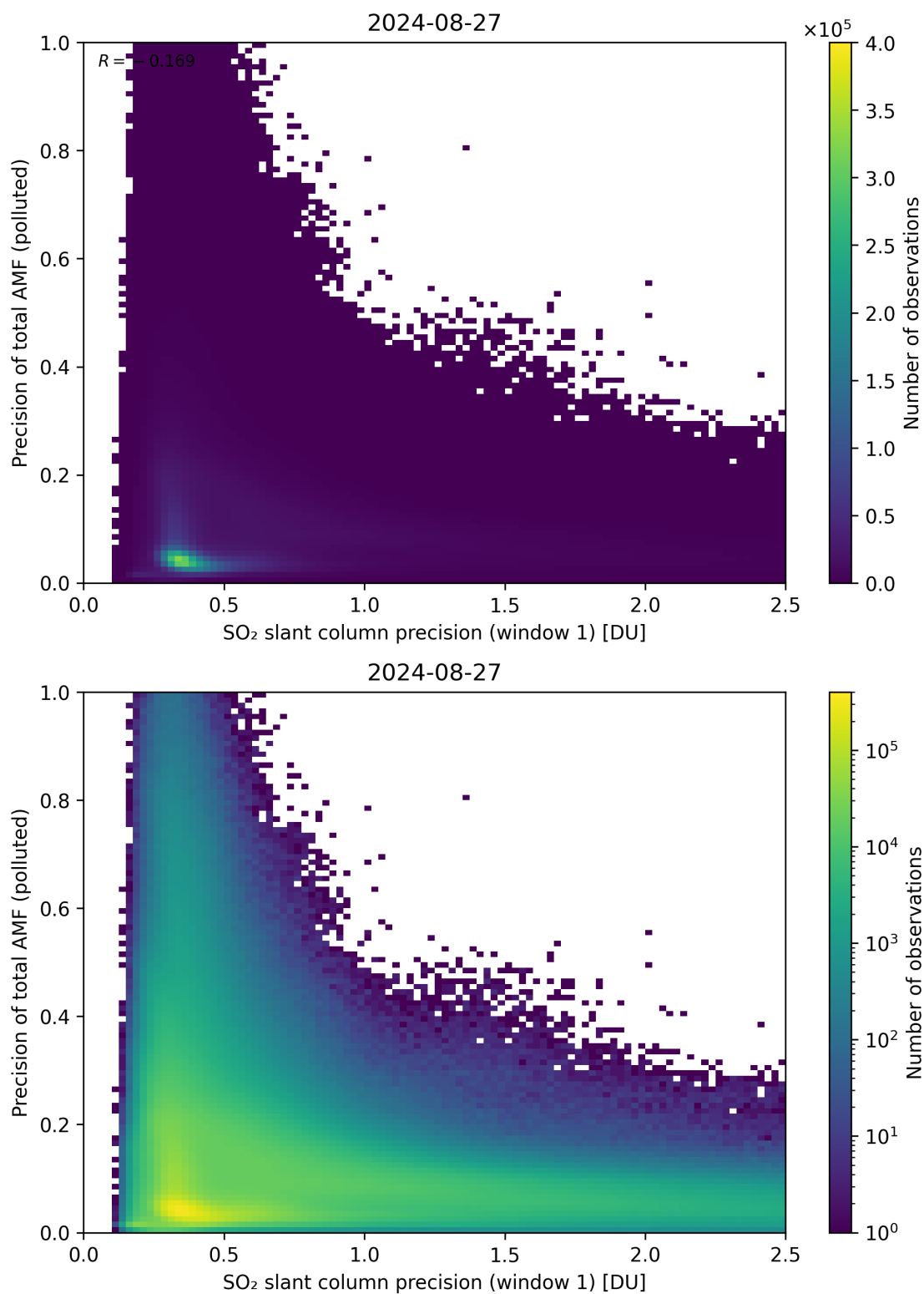
Figure 231: Scatter density plot of “SO 2 slant column precision (window 1)” against “Precision of total AMF (polluted)” for 2024-08-27 to 2024-08-28.
