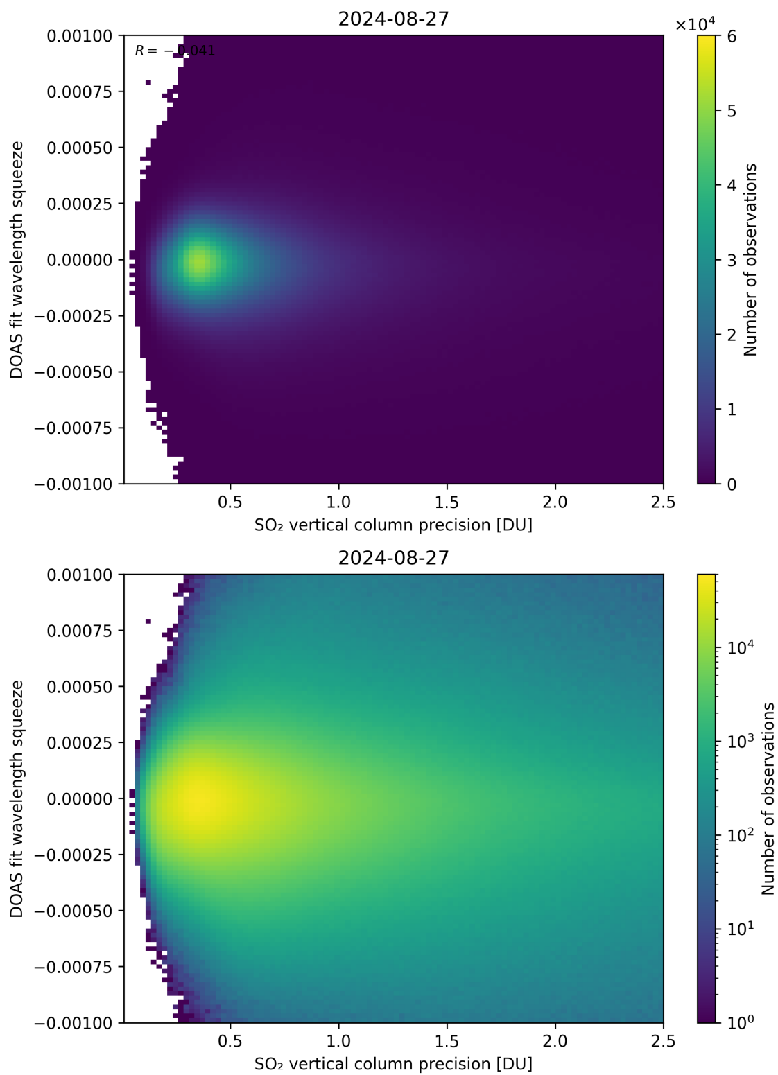
Figure 283: Scatter density plot of “SO 2 vertical column precision” against “DOAS fit wavelength squeeze” for 2024-08-27 to 2024-08-28.
