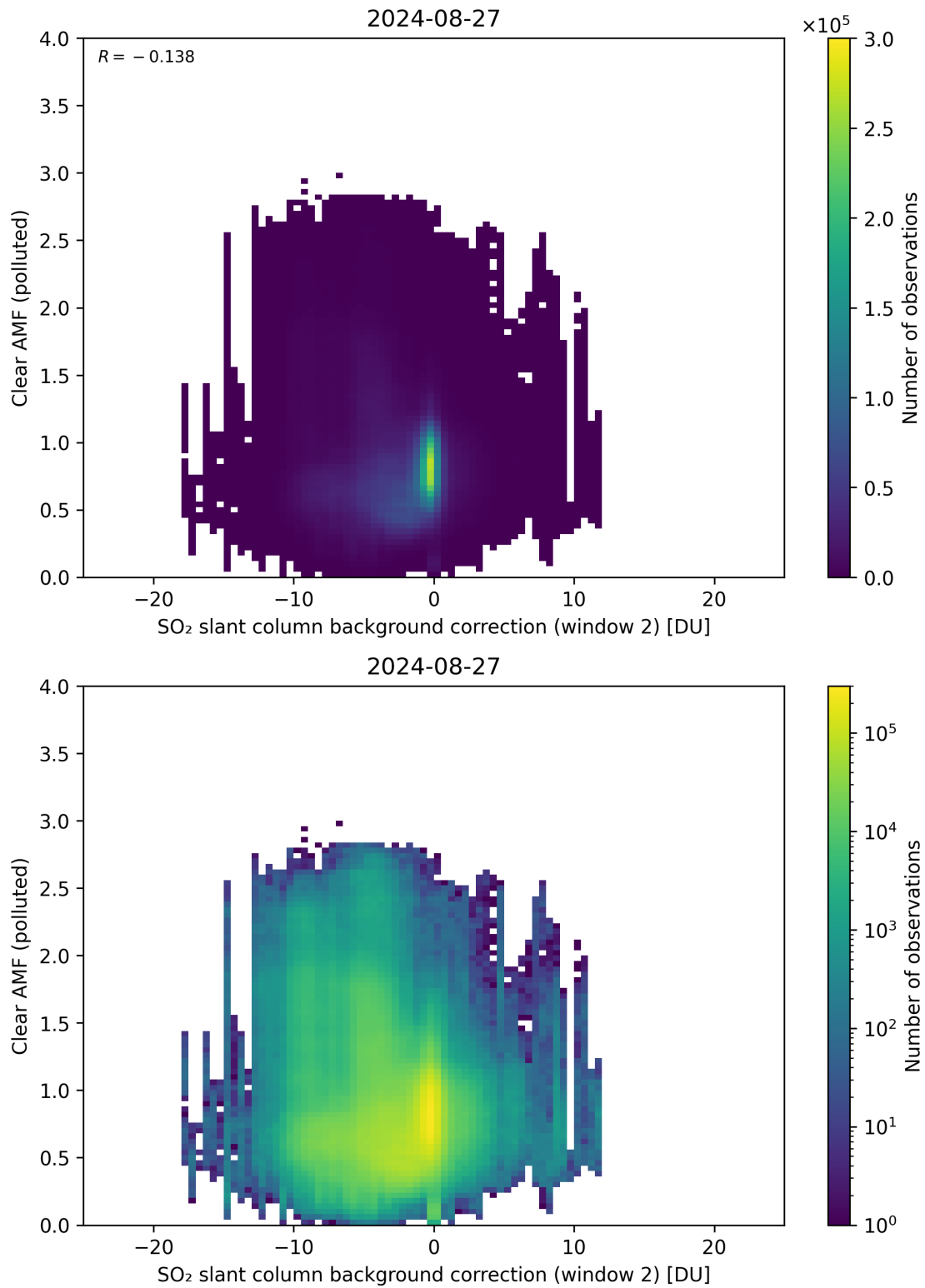
Figure 115: Scatter density plot of “SO 2 slant column background correction (window 2)” against “Clear AMF (polluted)” for 2024-08-27 to 2024-08-28.
