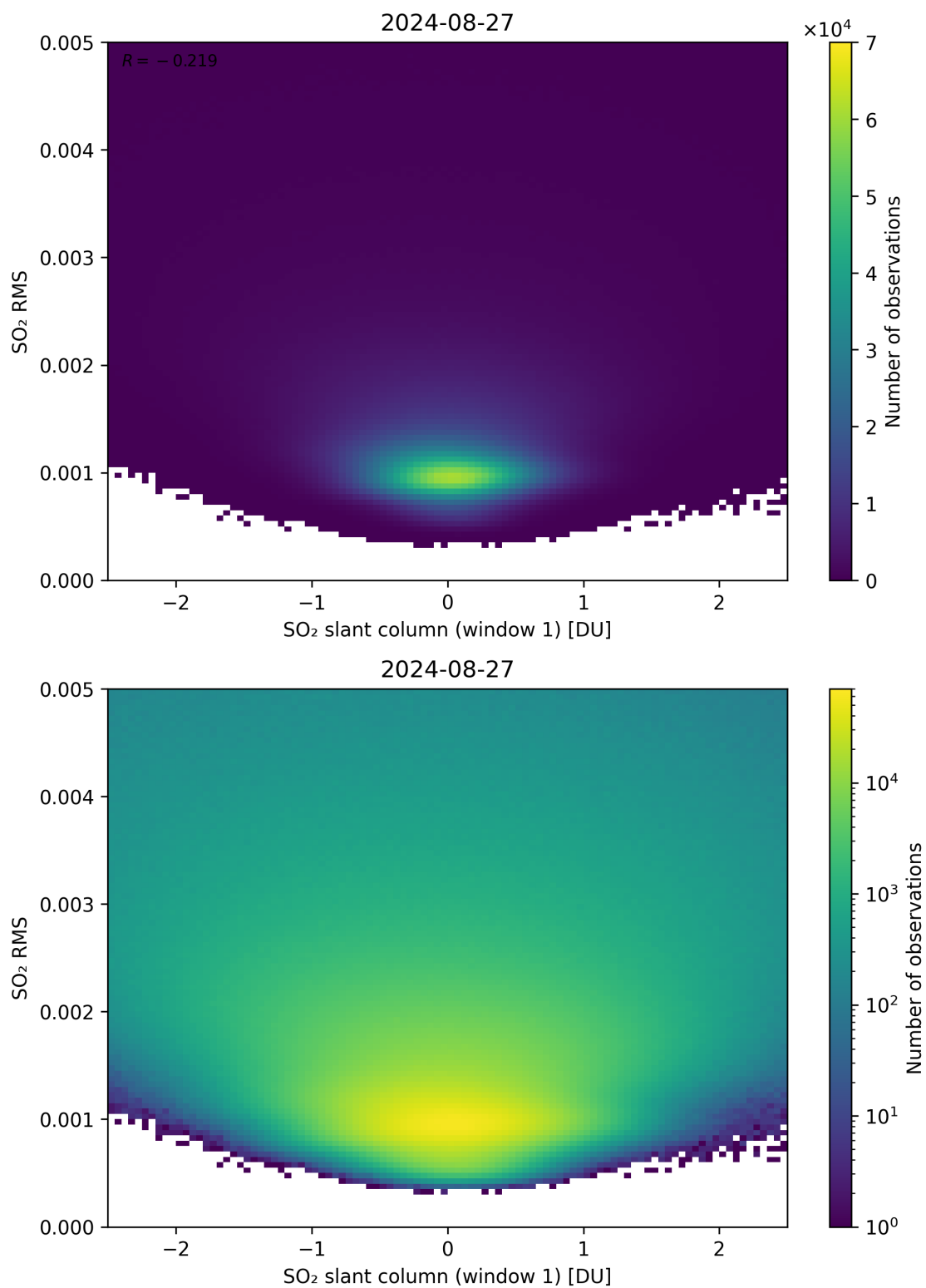
Figure 217: Scatter density plot of “SO 2 slant column (window 1)” against “SO 2 RMS” for 2024-08-27 to 2024-08-28.
