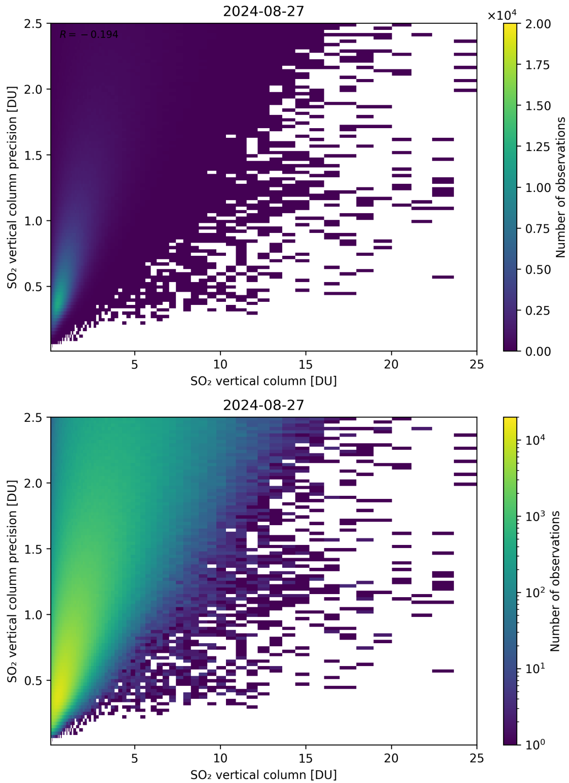
Figure 307: Scatter density plot of “SO 2 vertical column” against “SO 2 vertical column precision” for 2024-08-27 to 2024-08-28.
