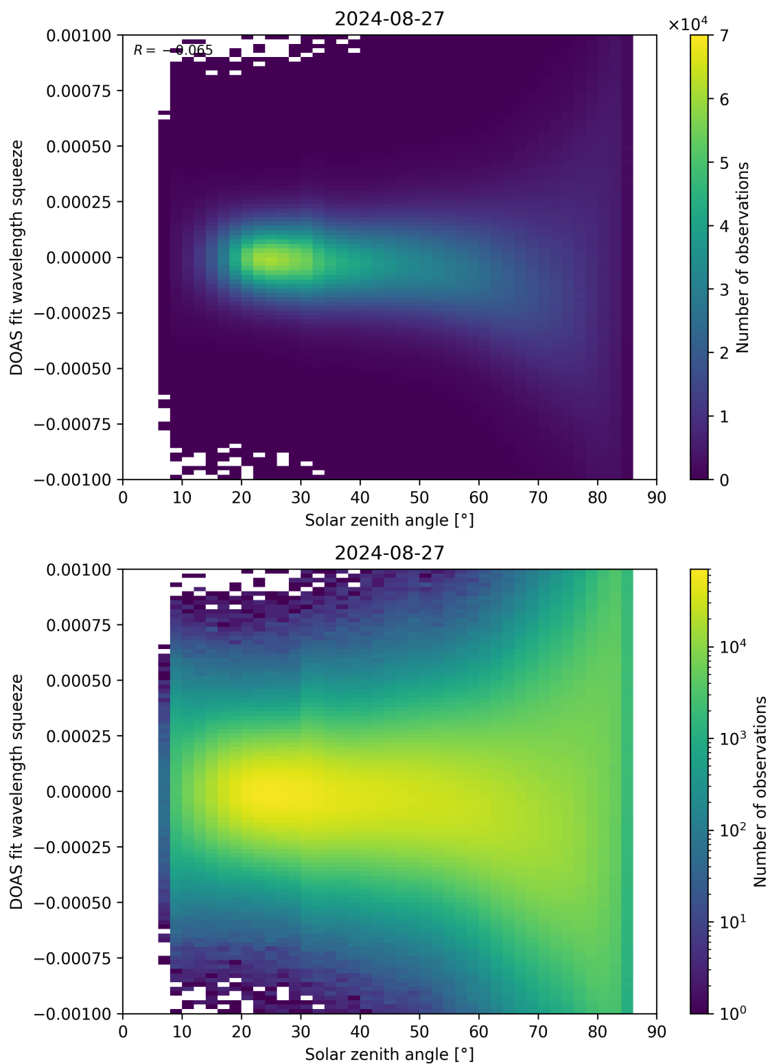
Figure 162: Scatter density plot of “Solar zenith angle” against “DOAS fit wavelength squeeze” for 2024-08-27 to 2024-08-28.
