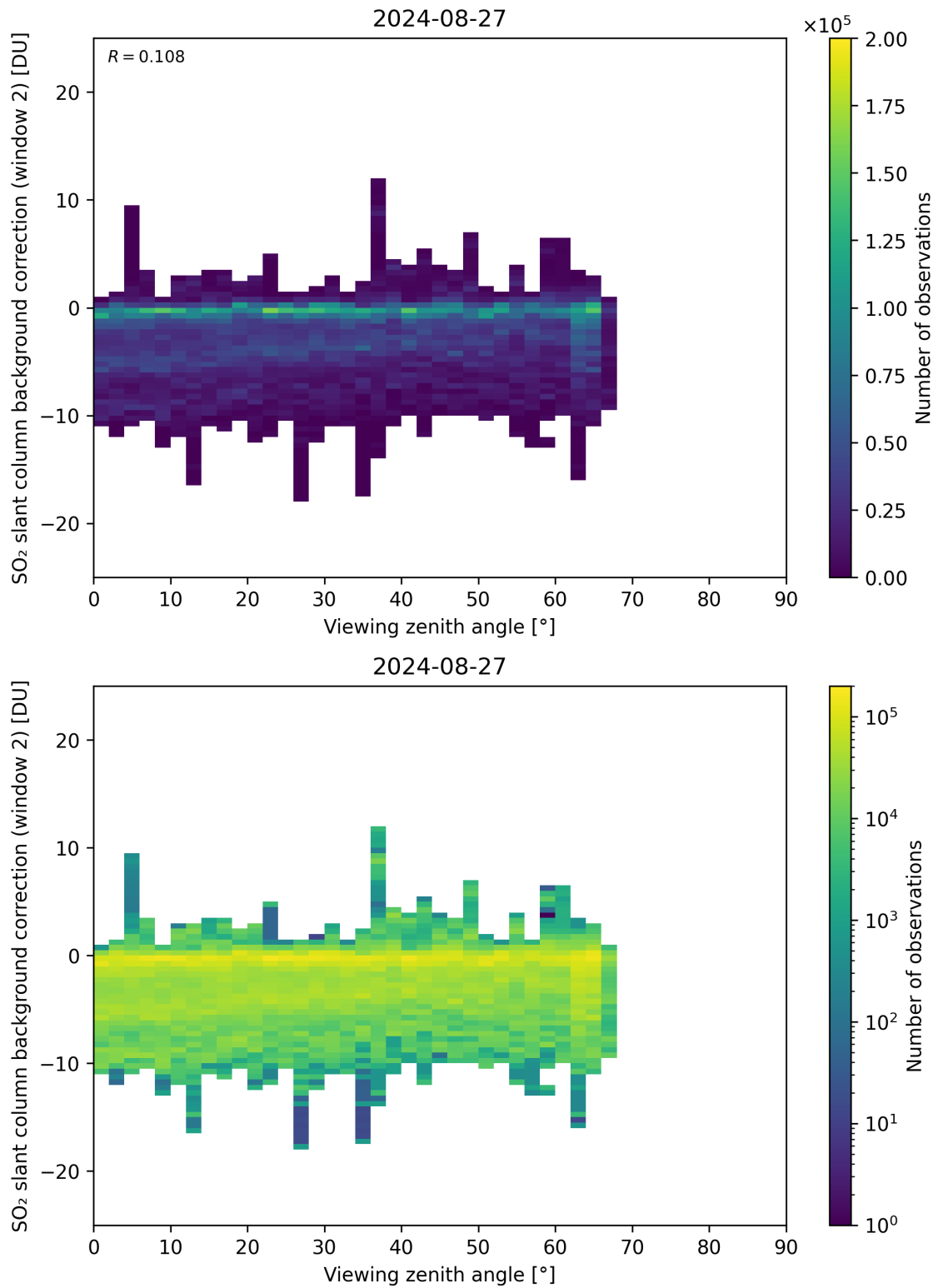
Figure 309: Scatter density plot of “Viewing zenith angle” against “SO 2 slant column background correction (window 2)” for 2024-08-27 to 2024-08-28.
