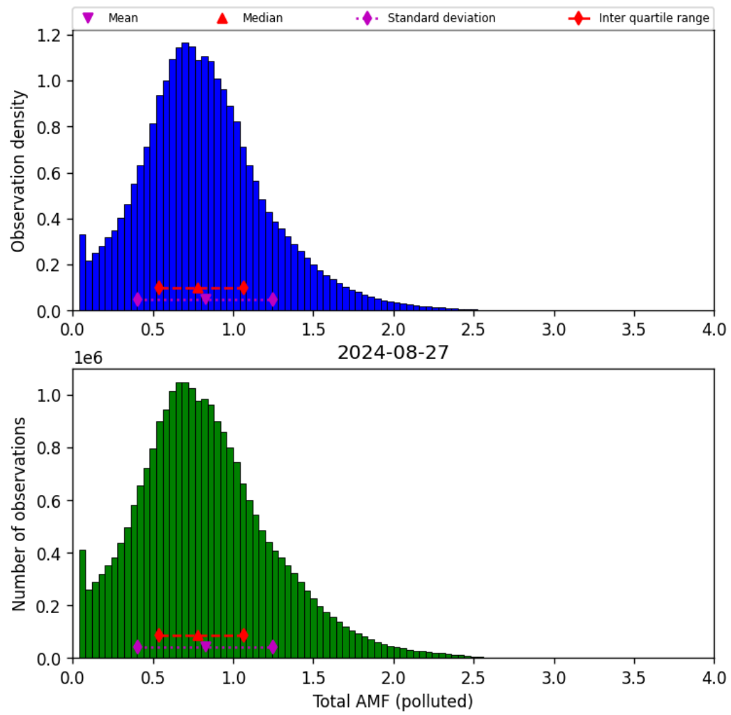
Figure 71: Histogram of “Total AMF (polluted)” for 2024-08-27 to 2024-08-28
