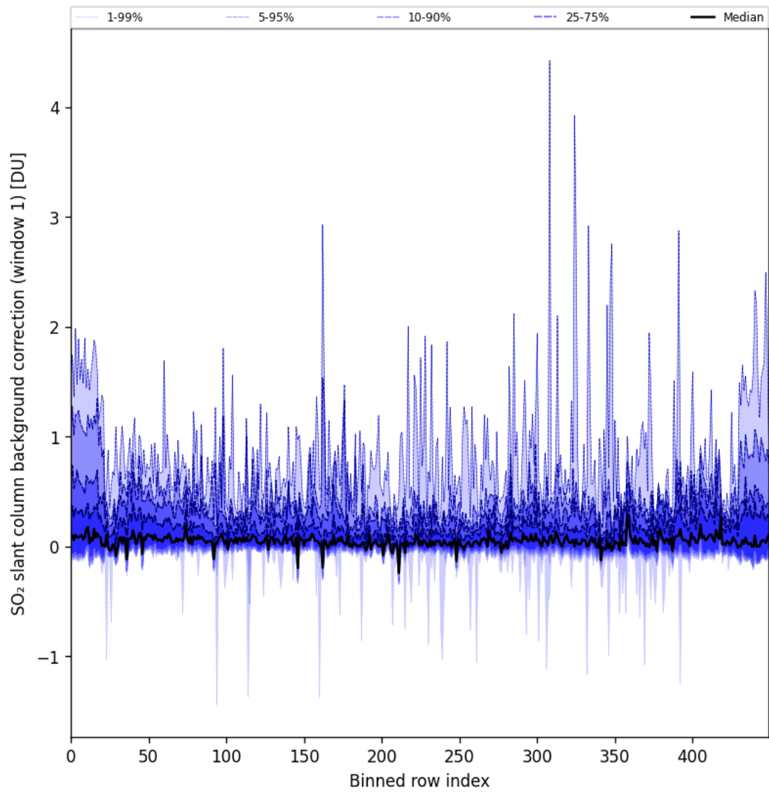
Figure 82: Along track statistics of “SO 2 slant column background correction (window 1)” for 2024-08-27 to 2024-08-28
