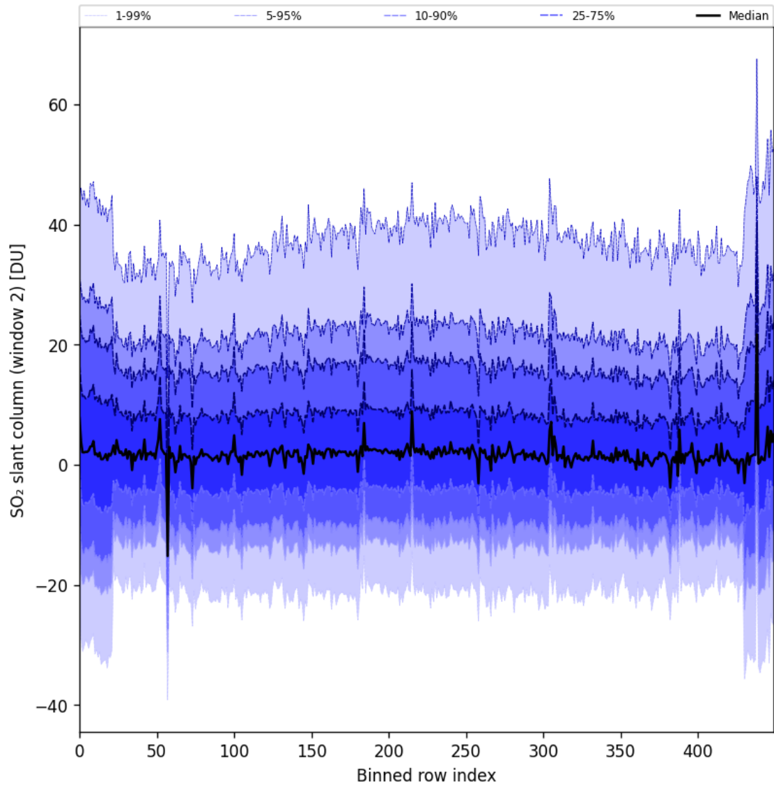
Figure 83: Along track statistics of “SO 2 slant column (window 2)” for 2024-08-27 to 2024-08-28
