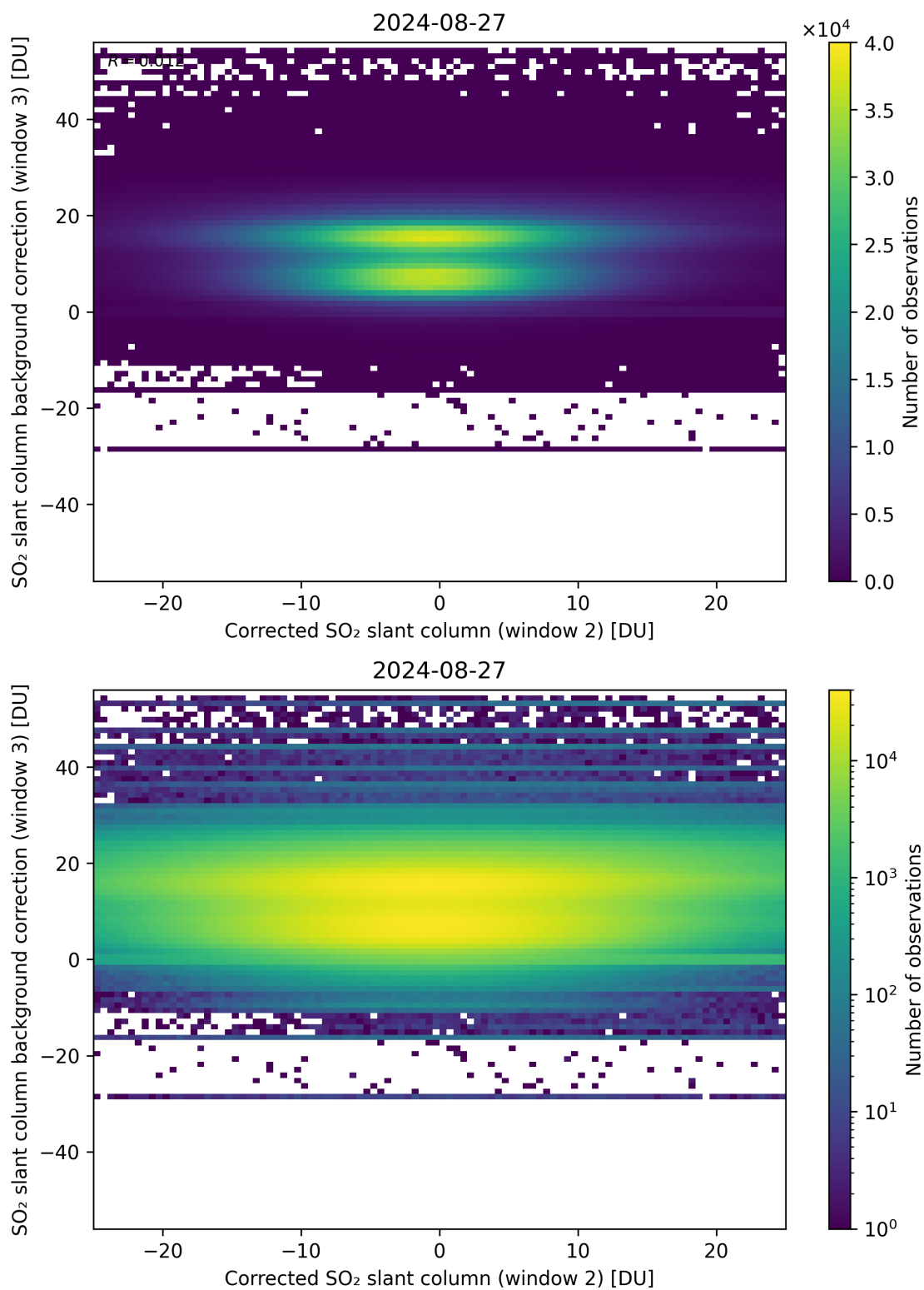
Figure 195: Scatter density plot of “Corrected SO 2 slant column (window 2)” against “SO 2 slant column background correction (window 3)” for 2024-08-27 to 2024-08-28.
