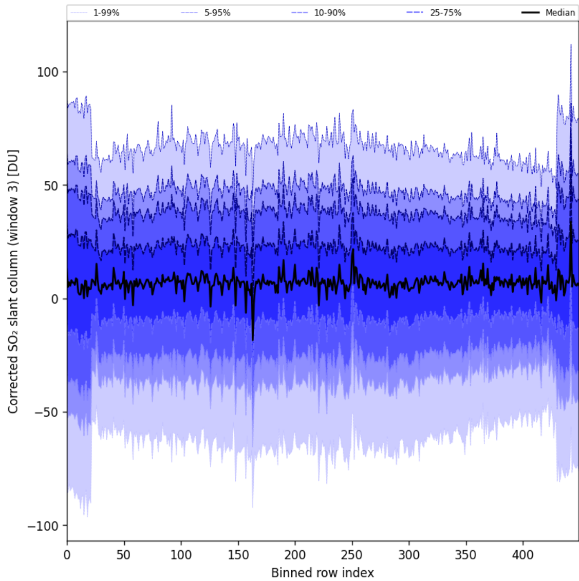
Figure 89: Along track statistics of “Corrected SO 2 slant column (window 3)” for 2024-08-27 to 2024-08-28
