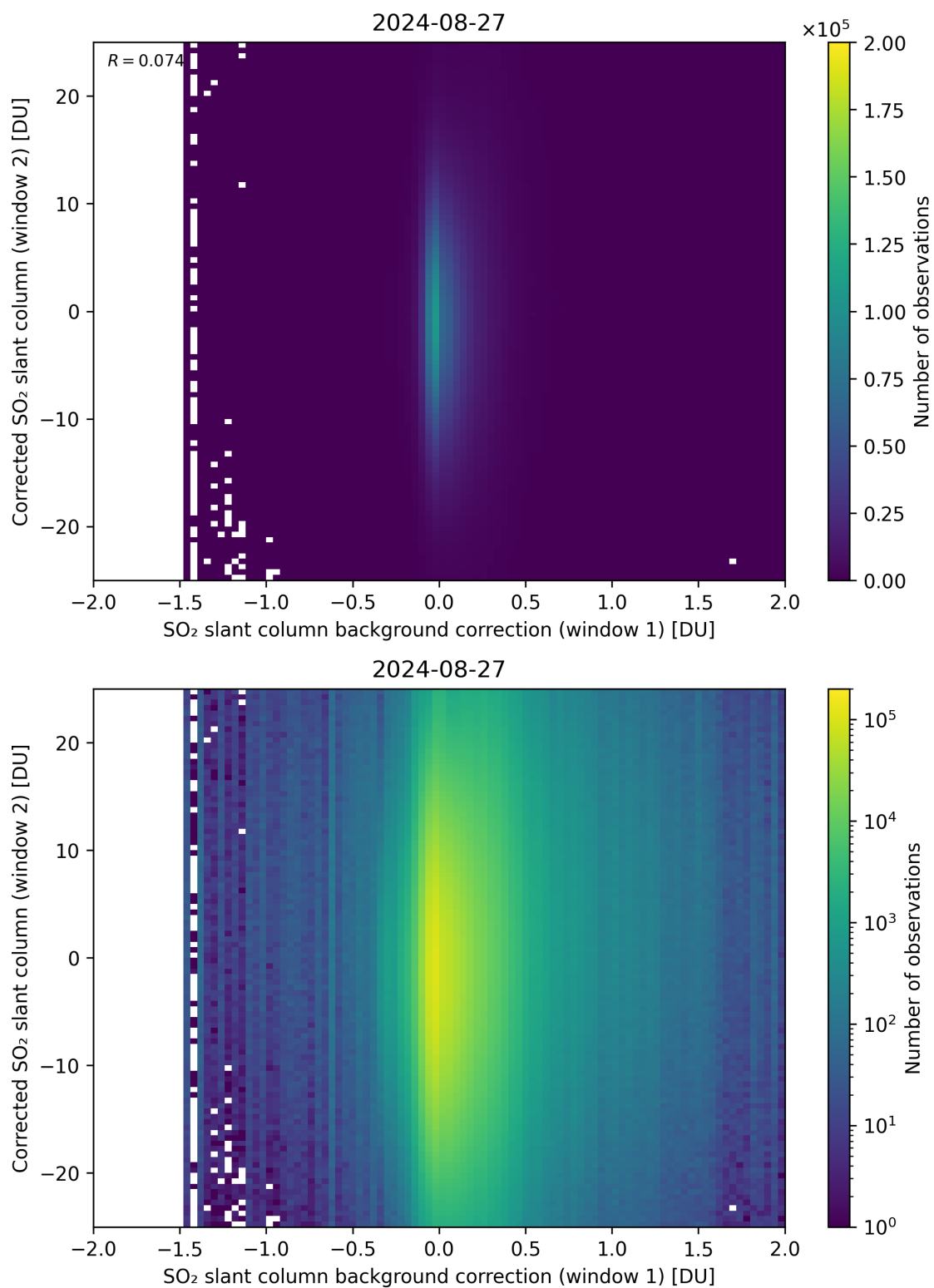
Figure 104: Scatter density plot of “SO 2 slant column background correction (window 1)” against “Corrected SO 2 slant column (window 2)” for 2024-08-27 to 2024-08-28.
