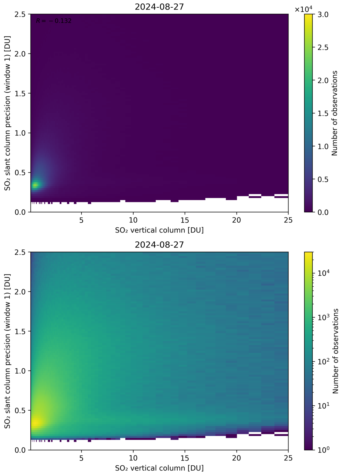
Figure 301: Scatter density plot of “SO 2 vertical column” against “SO 2 slant column precision (window 1)” for 2024-08-27 to 2024-08-28.
