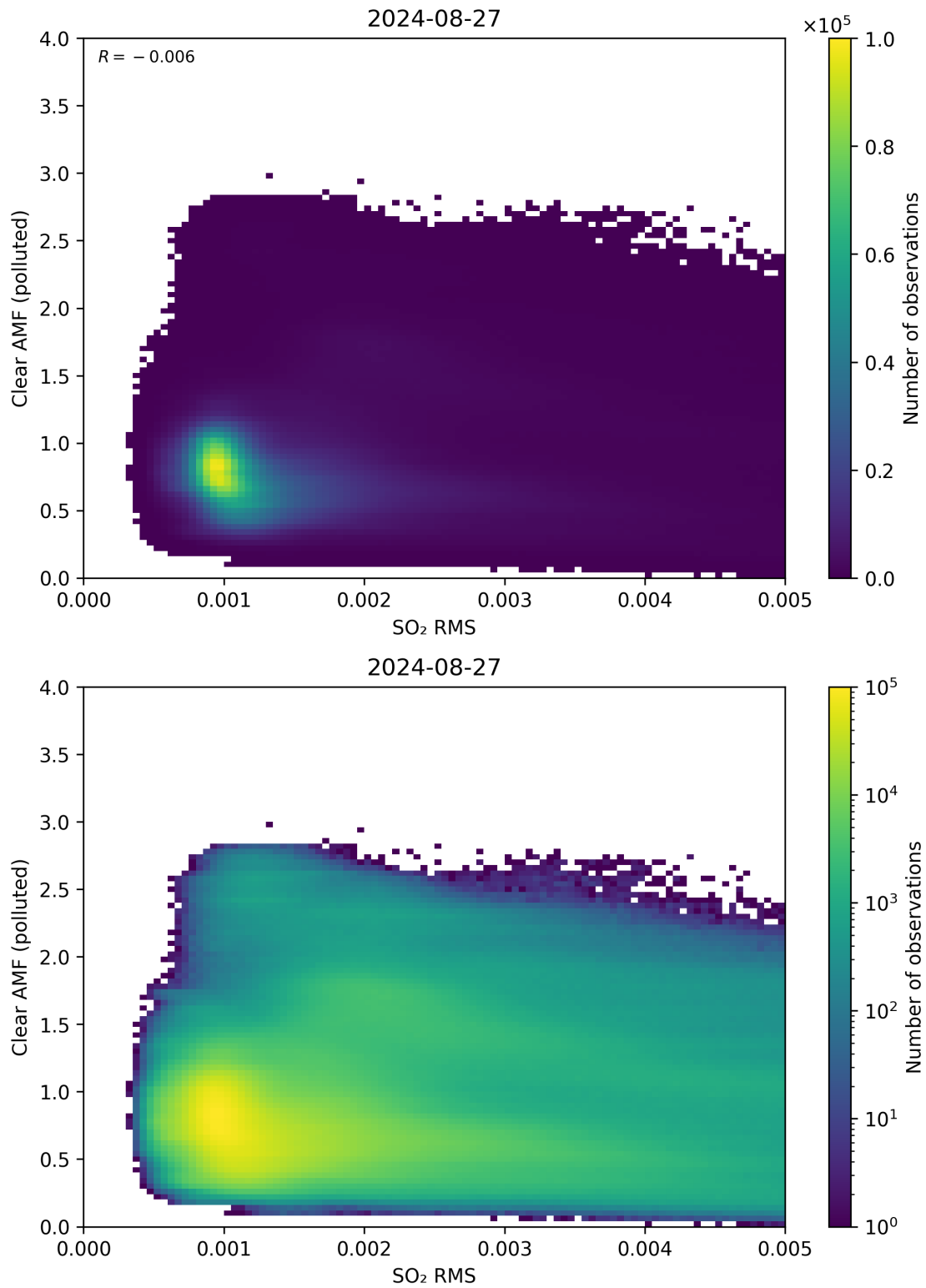
Figure 136: Scatter density plot of “SO 2 RMS” against “Clear AMF (polluted)” for 2024-08-27 to 2024-08-28.
