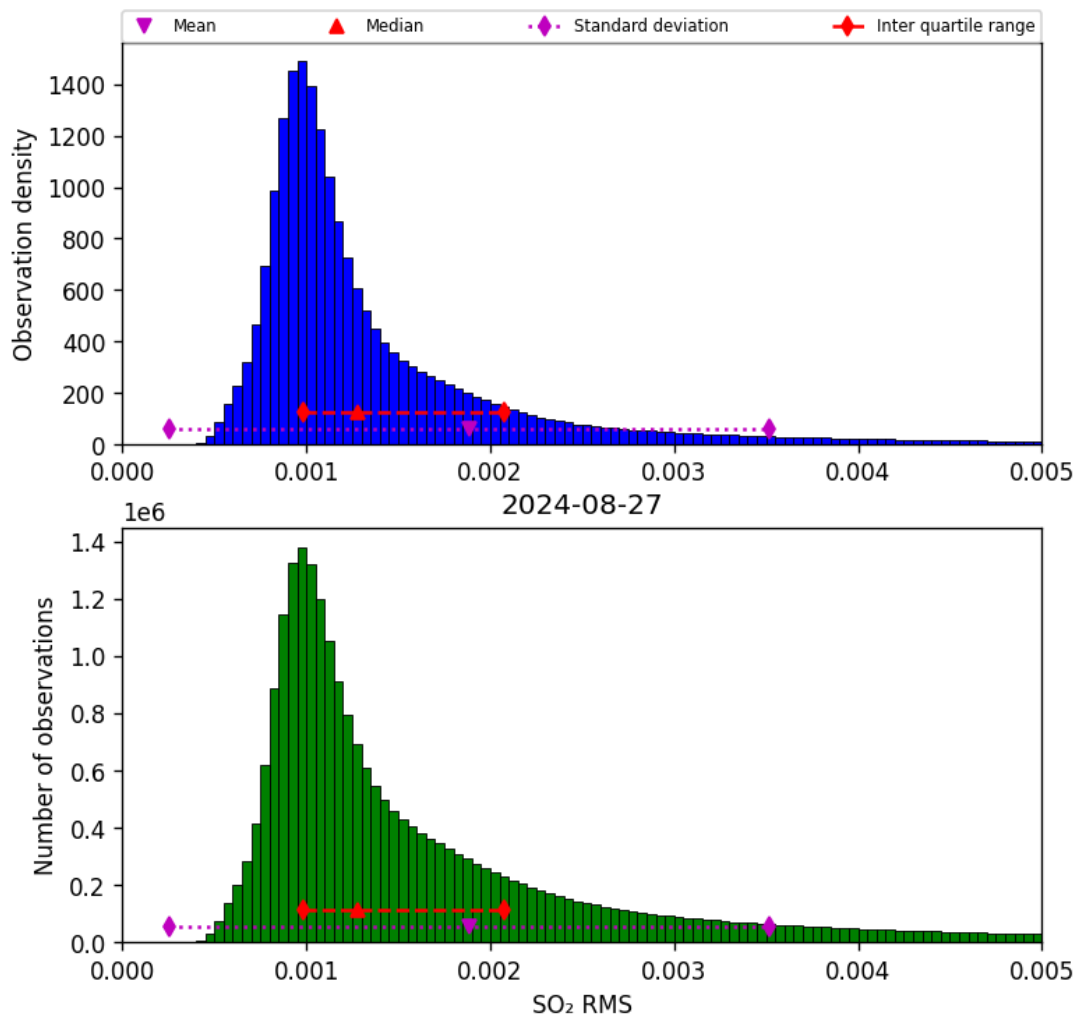
Figure 70: Histogram of “SO 2 RMS” for 2024-08-27 to 2024-08-28
