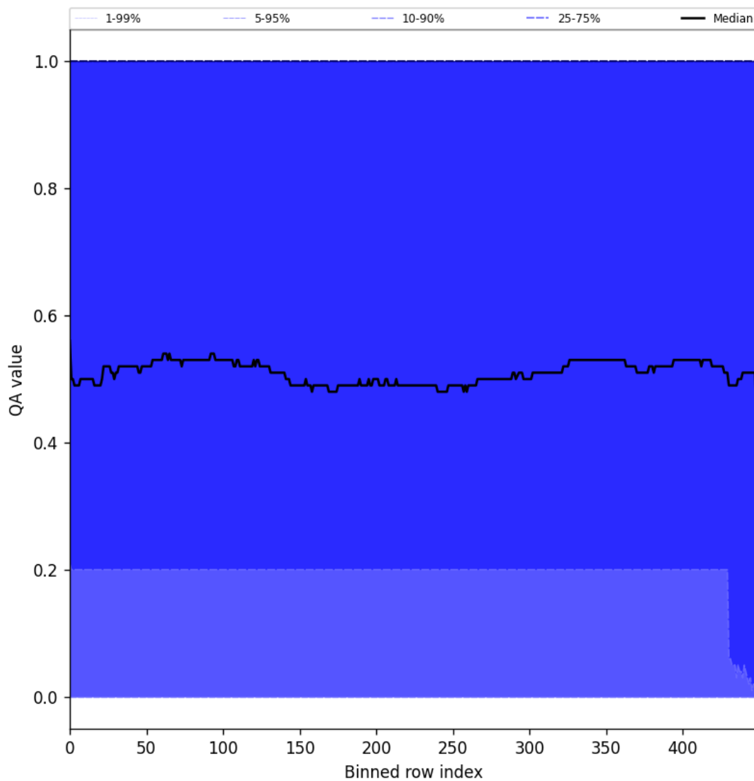
Figure 75: Along track statistics of “QA value” for 2024-08-27 to 2024-08-28
