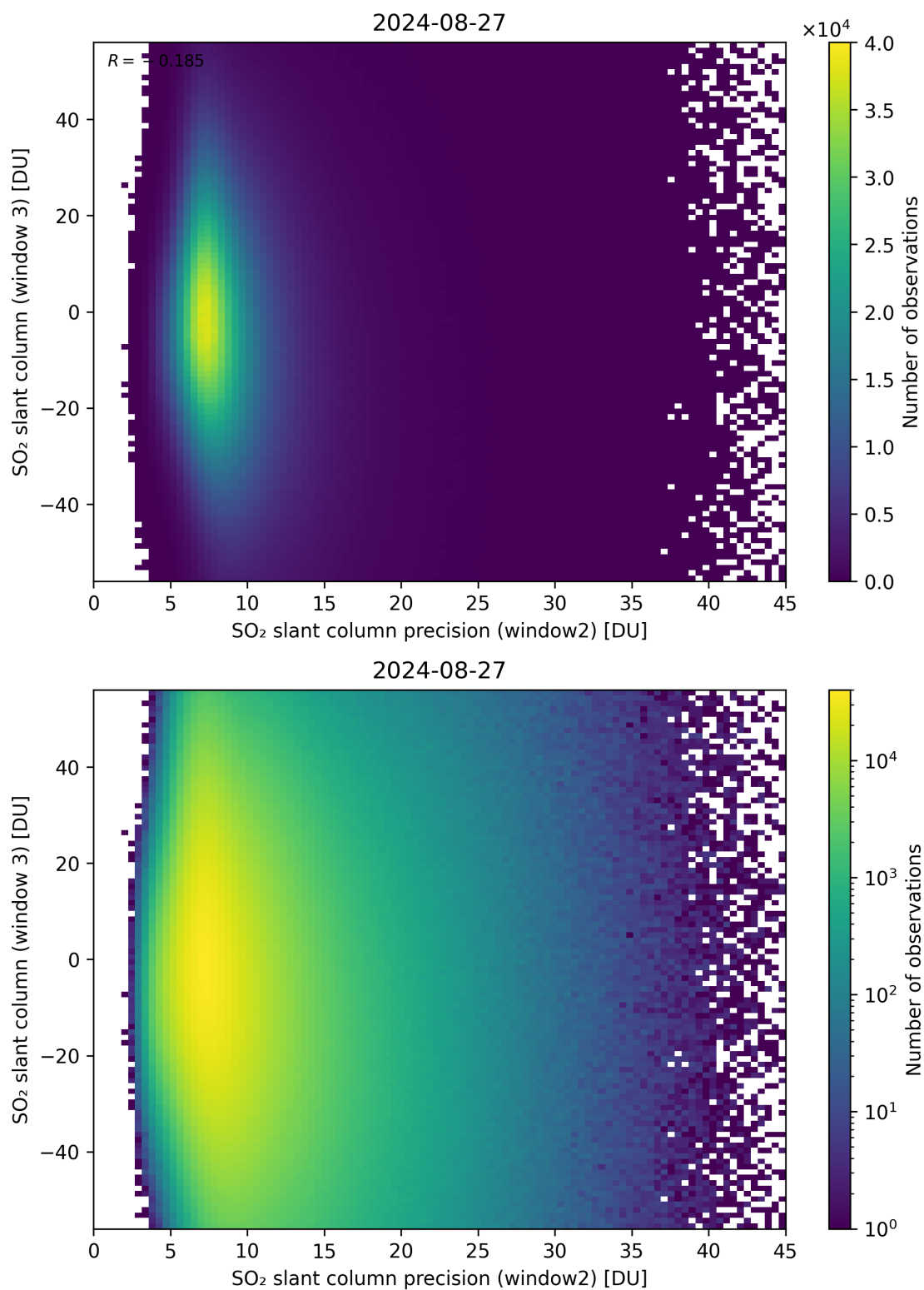
Figure 249: Scatter density plot of “SO 2 slant column precision (window2)” against “SO 2 slant column (window 3)” for 2024-08-27 to 2024-08-28.
