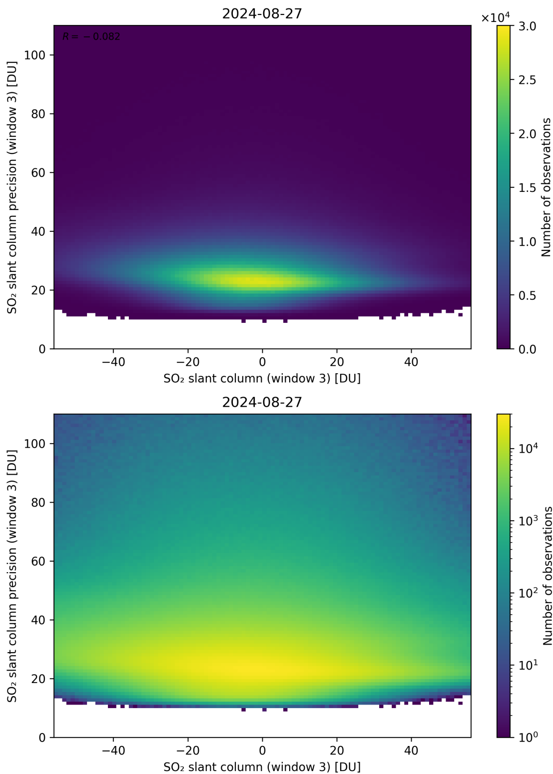
Figure 267: Scatter density plot of “SO 2 slant column (window 3)” against “SO 2 slant column precision (window 3)” for 2024-08-27 to 2024-08-28.
