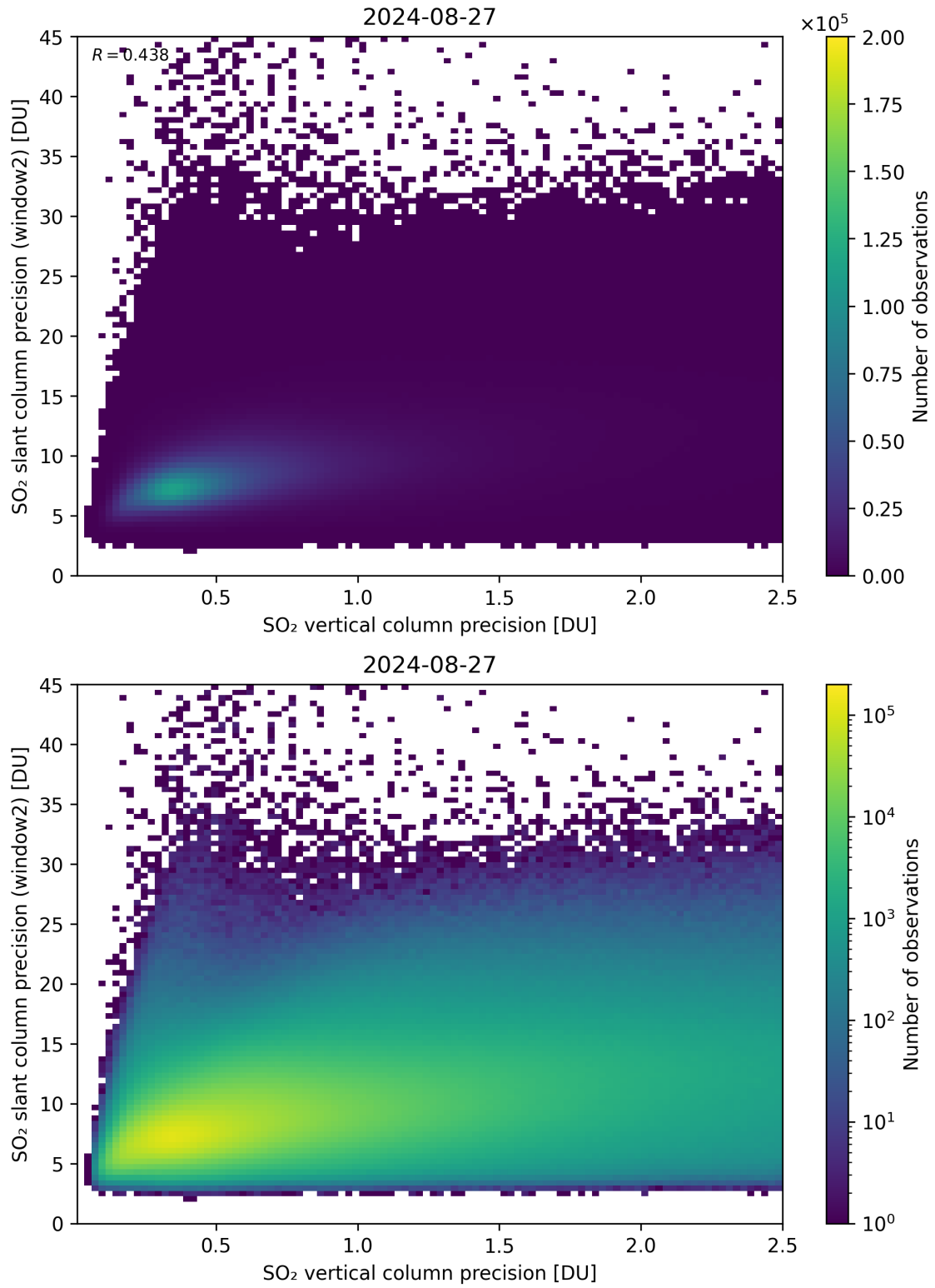
Figure 291: Scatter density plot of “SO 2 vertical column precision” against “SO 2 slant column precision (window2)” for 2024-08-27 to 2024-08-28.
