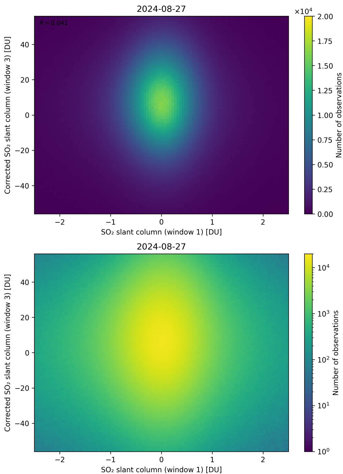
Figure 234: Scatter density plot of “SO 2 slant column (window 1)” against “Corrected SO 2 slant column (window 3)” for 2024-08-27 to 2024-08-28.
