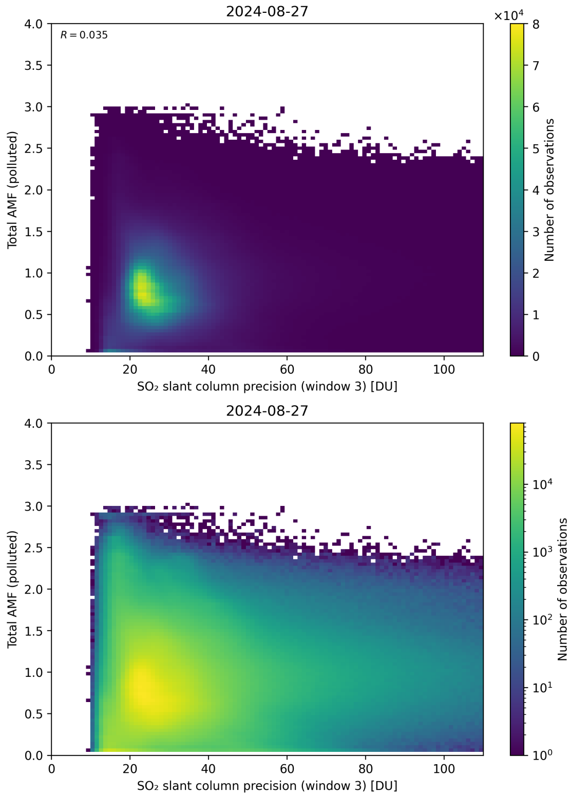
Figure 263: Scatter density plot of “SO 2 slant column precision (window 3)” against “Total AMF (polluted)” for 2024-08-27 to 2024-08-28.
