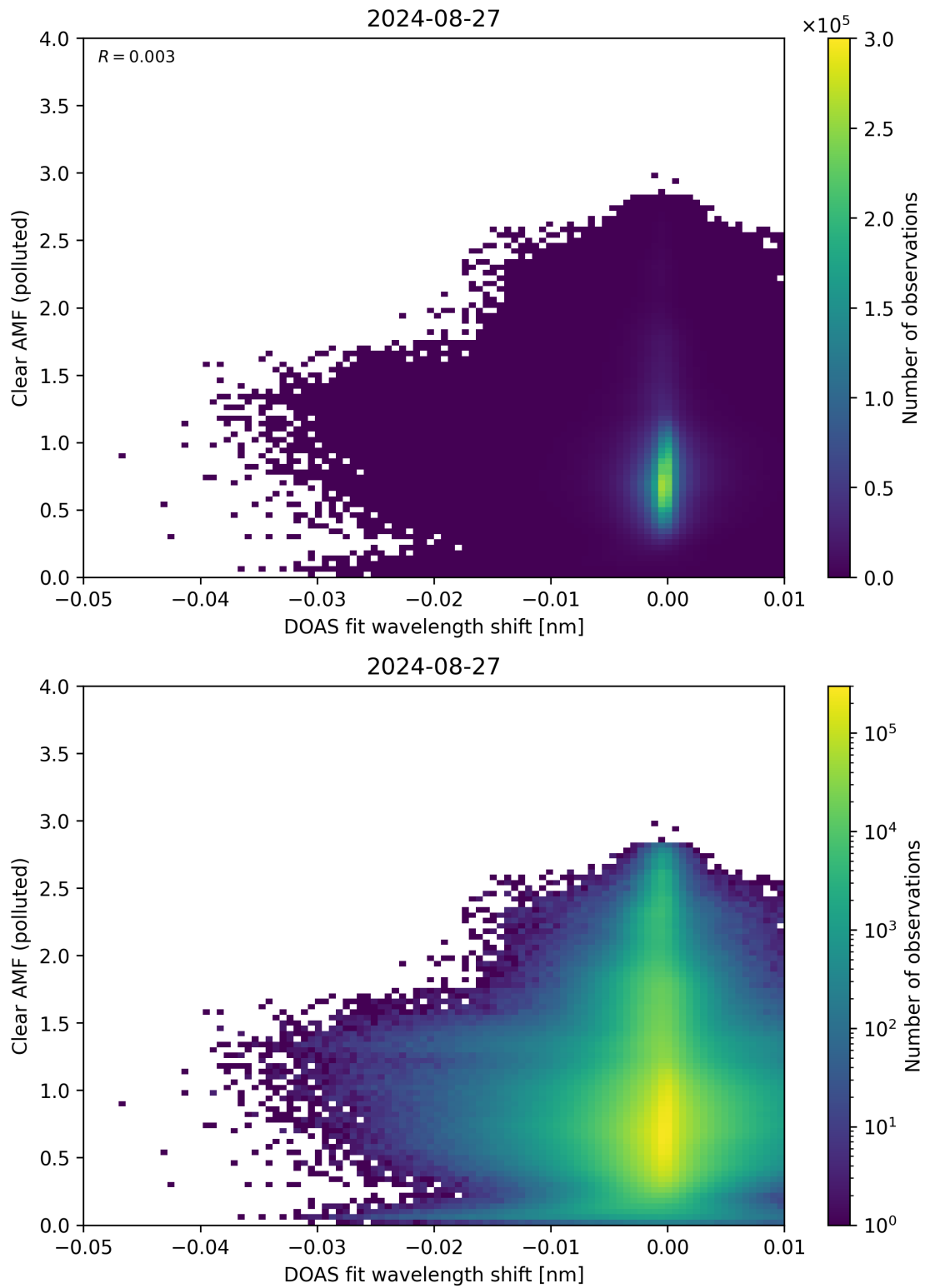
Figure 129: Scatter density plot of “DOAS fit wavelength shift” against “Clear AMF (polluted)” for 2024-08-27 to 2024-08-28.
