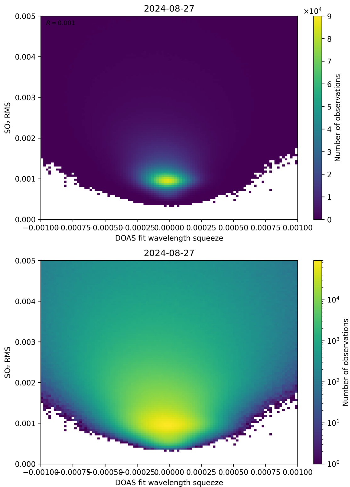
Figure 132: Scatter density plot of “DOAS fit wavelength squeeze” against “SO 2 RMS” for 2024-08-27 to 2024-08-28.
