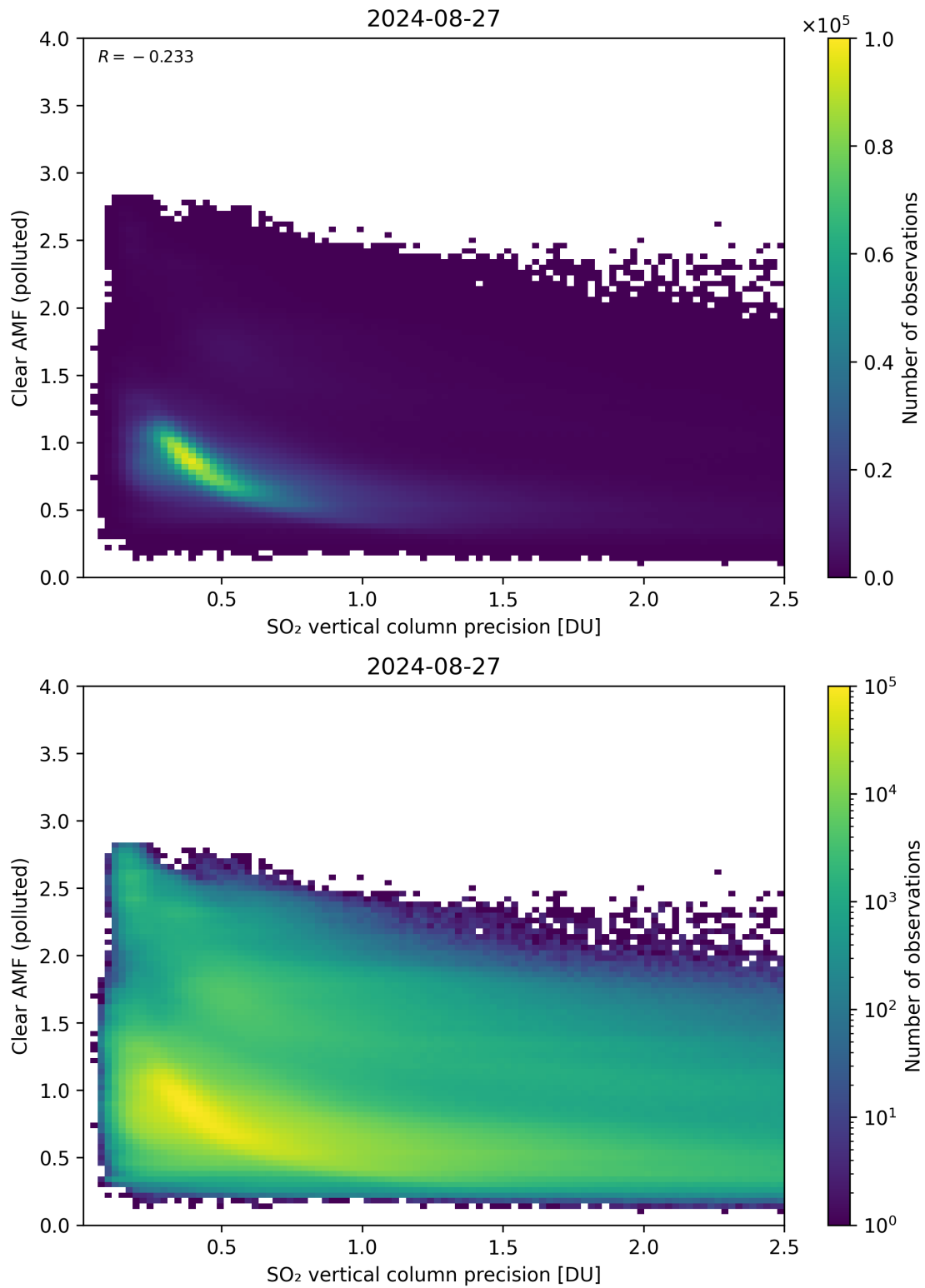
Figure 285: Scatter density plot of “SO 2 vertical column precision” against “Clear AMF (polluted)” for 2024-08-27 to 2024-08-28.
