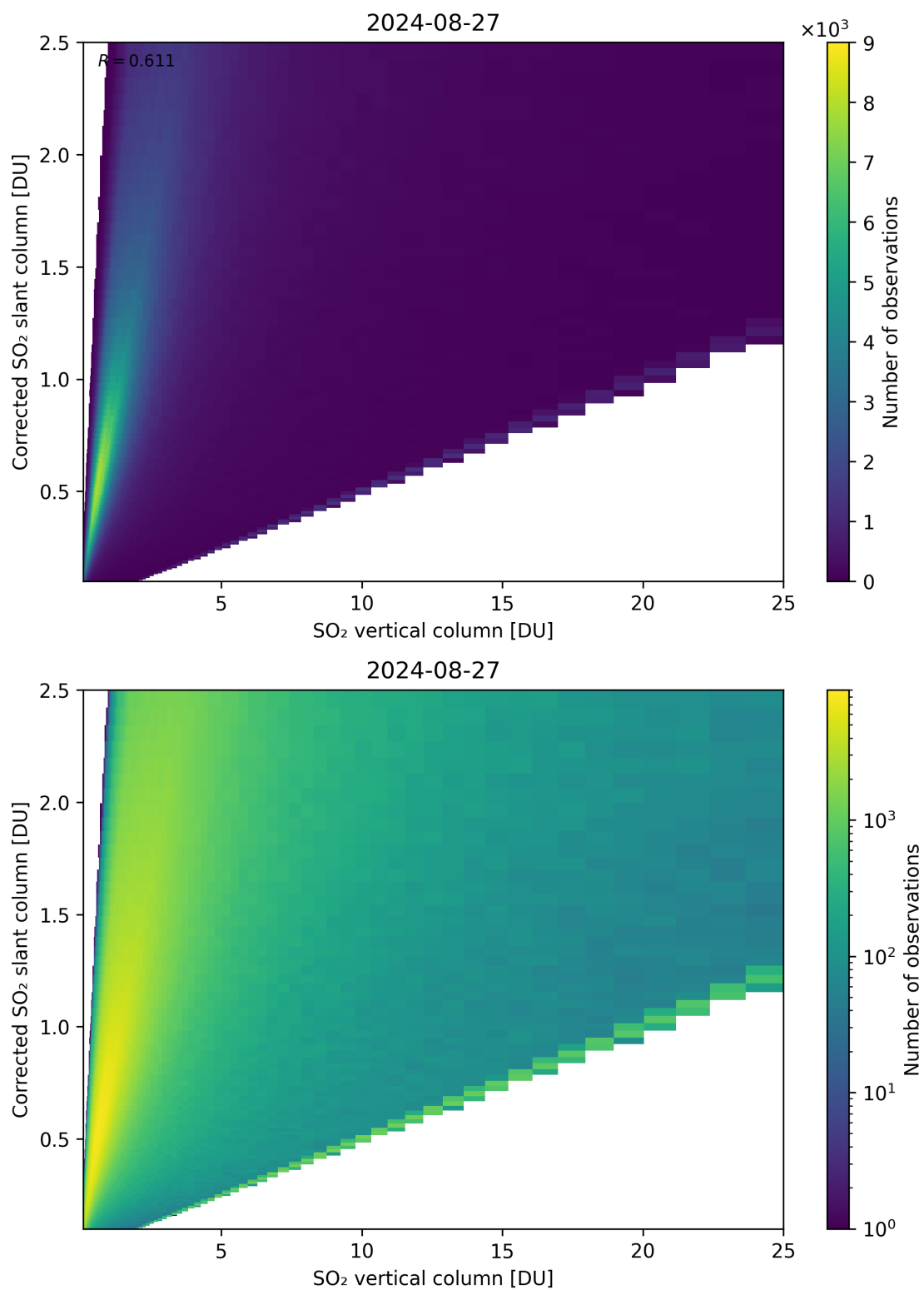
Figure 297: Scatter density plot of “SO 2 vertical column” against “Corrected SO 2 slant column” for 2024-08-27 to 2024-08-28.
