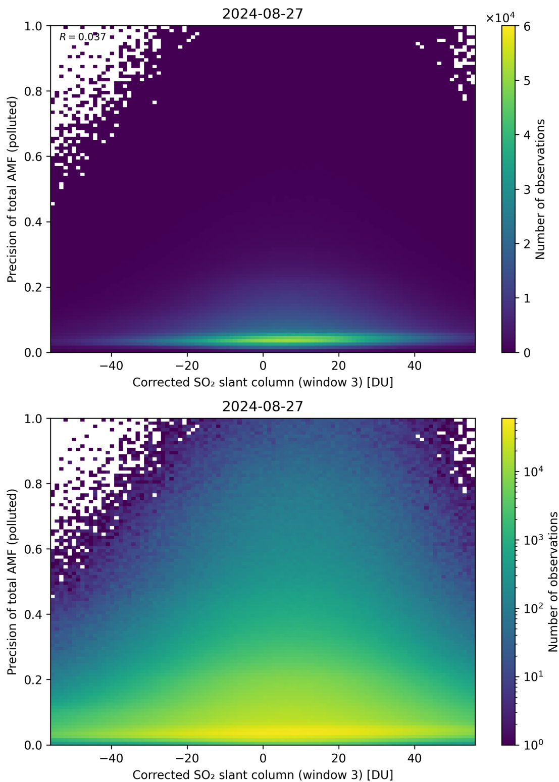
Figure 211: Scatter density plot of “Corrected SO 2 slant column (window 3)” against “Precision of total AMF (polluted)” for 2024-08-27 to 2024-08-28.
