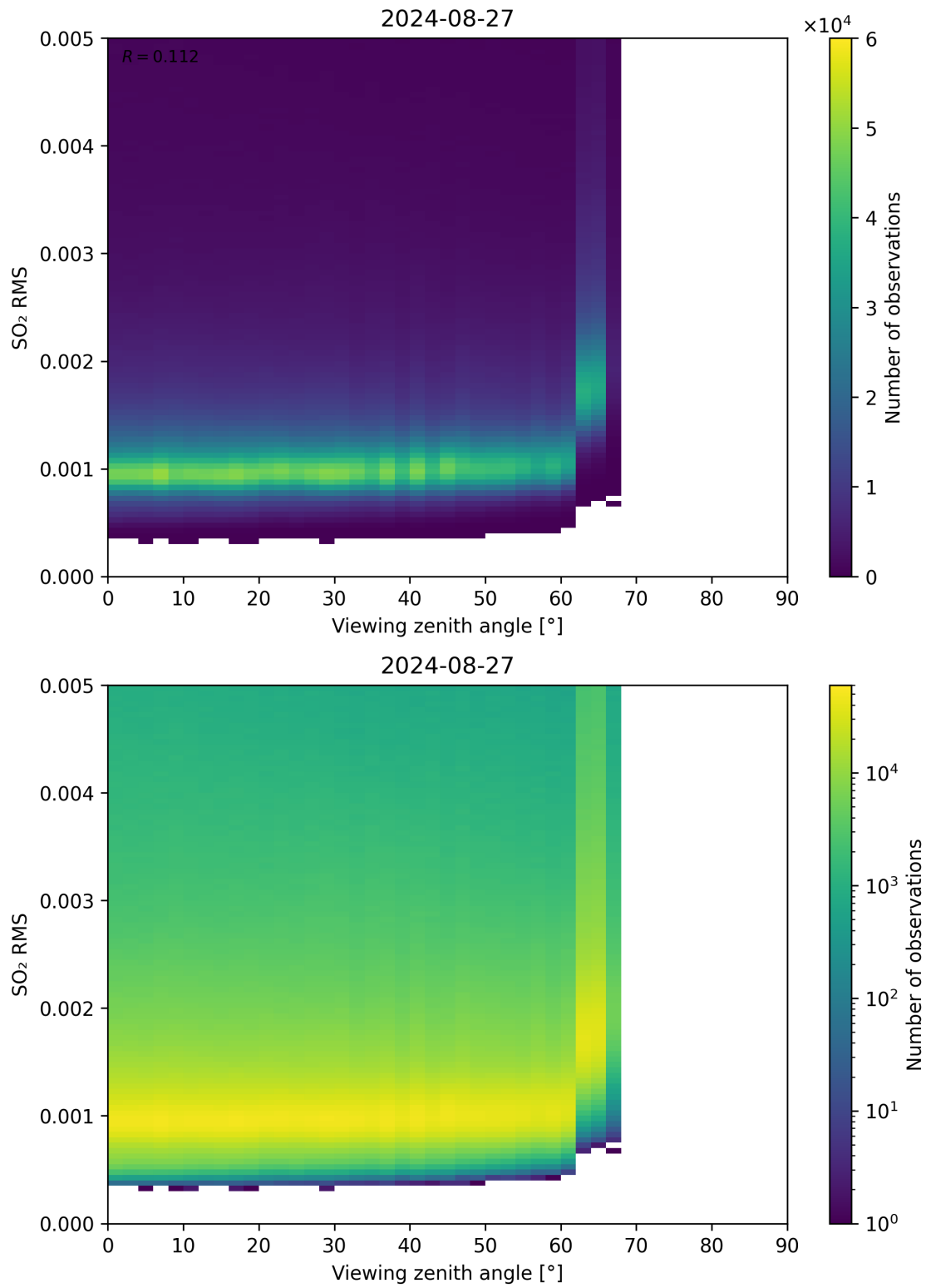
Figure 313: Scatter density plot of “Viewing zenith angle” against “SO 2 RMS” for 2024-08-27 to 2024-08-28.
