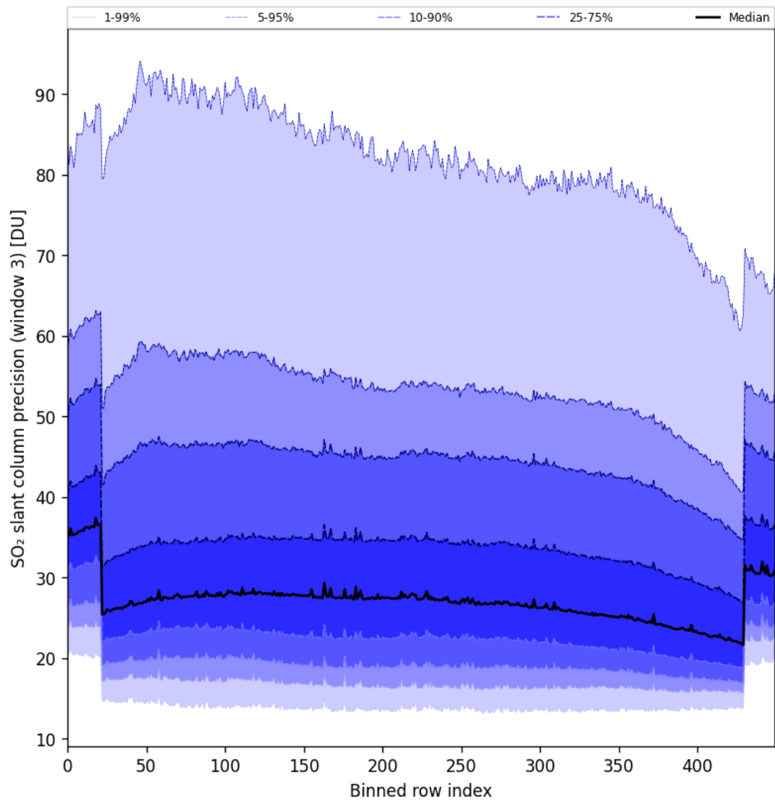
Figure 88: Along track statistics of “SO 2 slant column precision (window 3)” for 2024-08-27 to 2024-08-28
