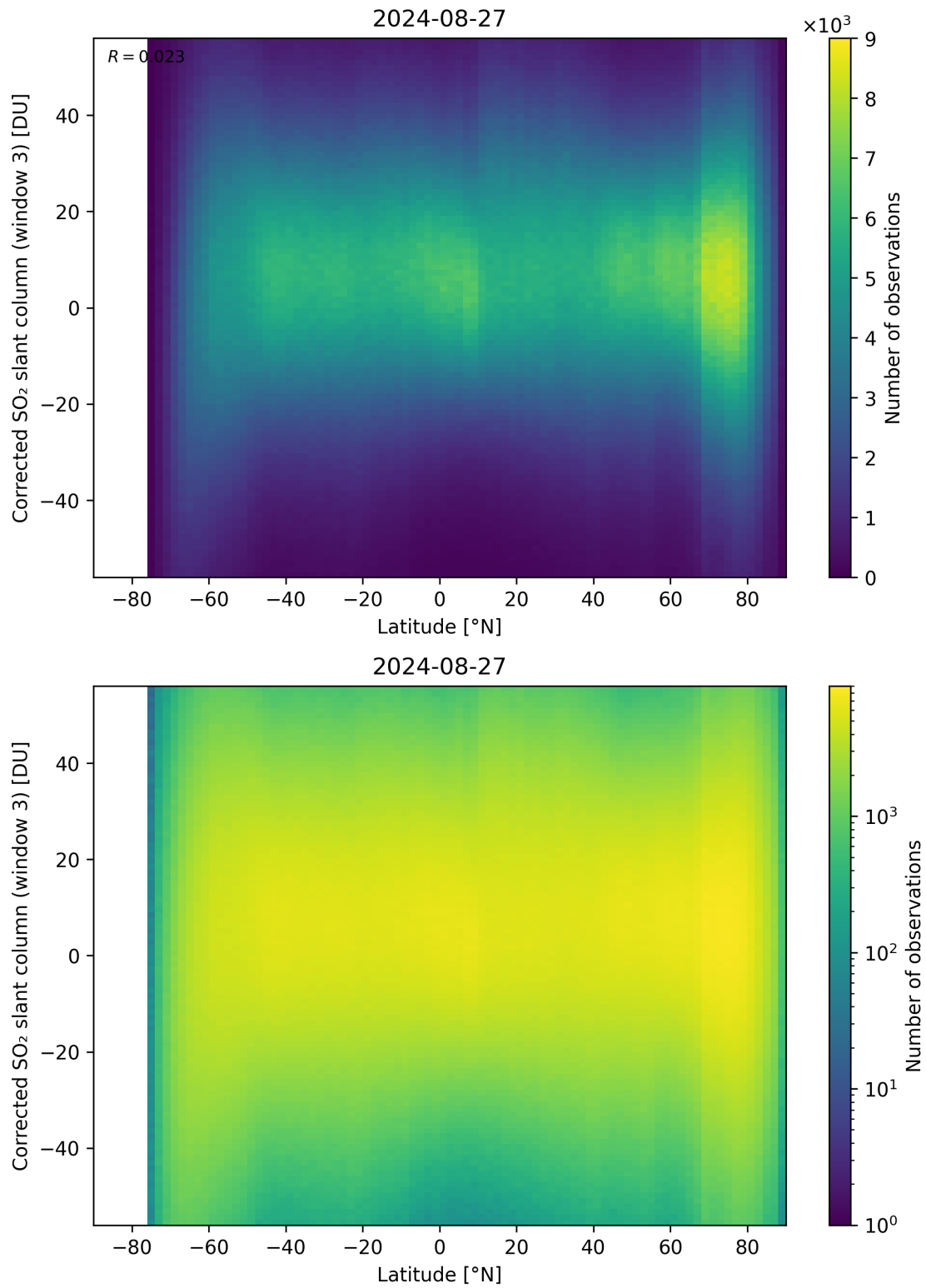
Figure 148: Scatter density plot of “Latitude” against “Corrected SO 2 slant column (window 3)” for 2024-08-27 to 2024-08-28.
