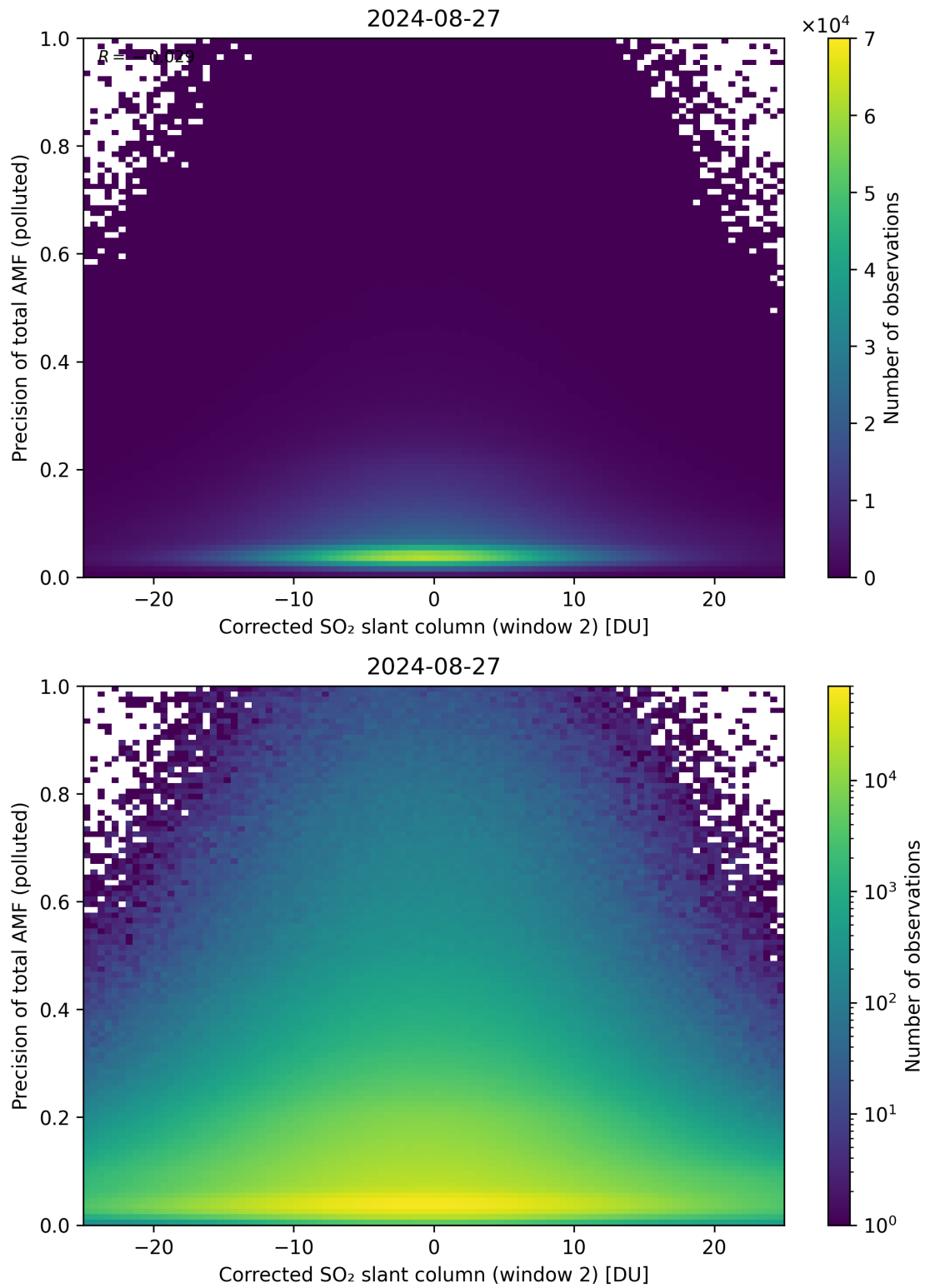
Figure 204: Scatter density plot of “Corrected SO 2 slant column (window 2)” against “Precision of total AMF (polluted)” for 2024-08-27 to 2024-08-28.
