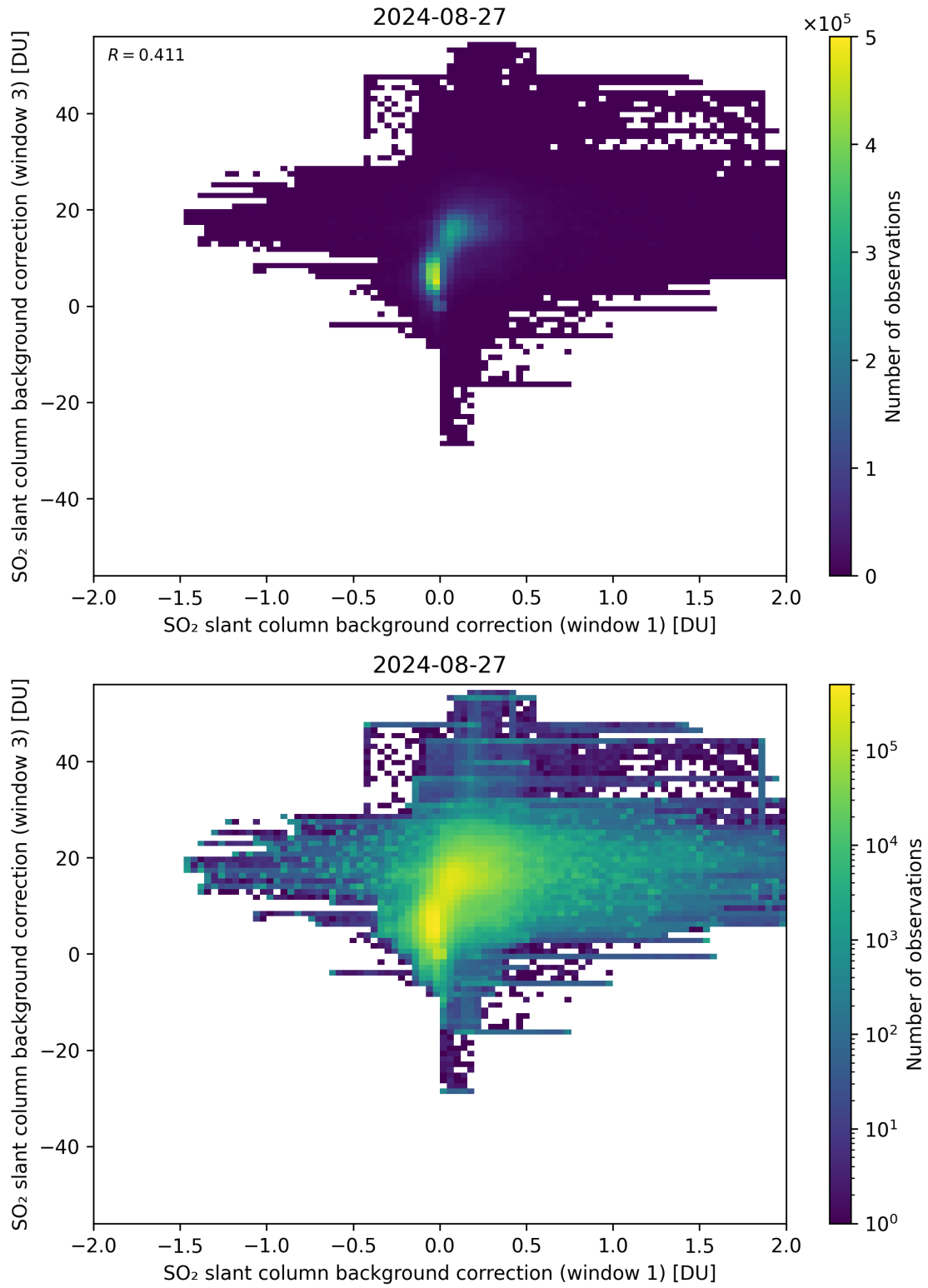
Figure 99: Scatter density plot of “SO 2 slant column background correction (window 1)” against “SO 2 slant column background correction (window 3)” for 2024-08-27 to 2024-08-28.
