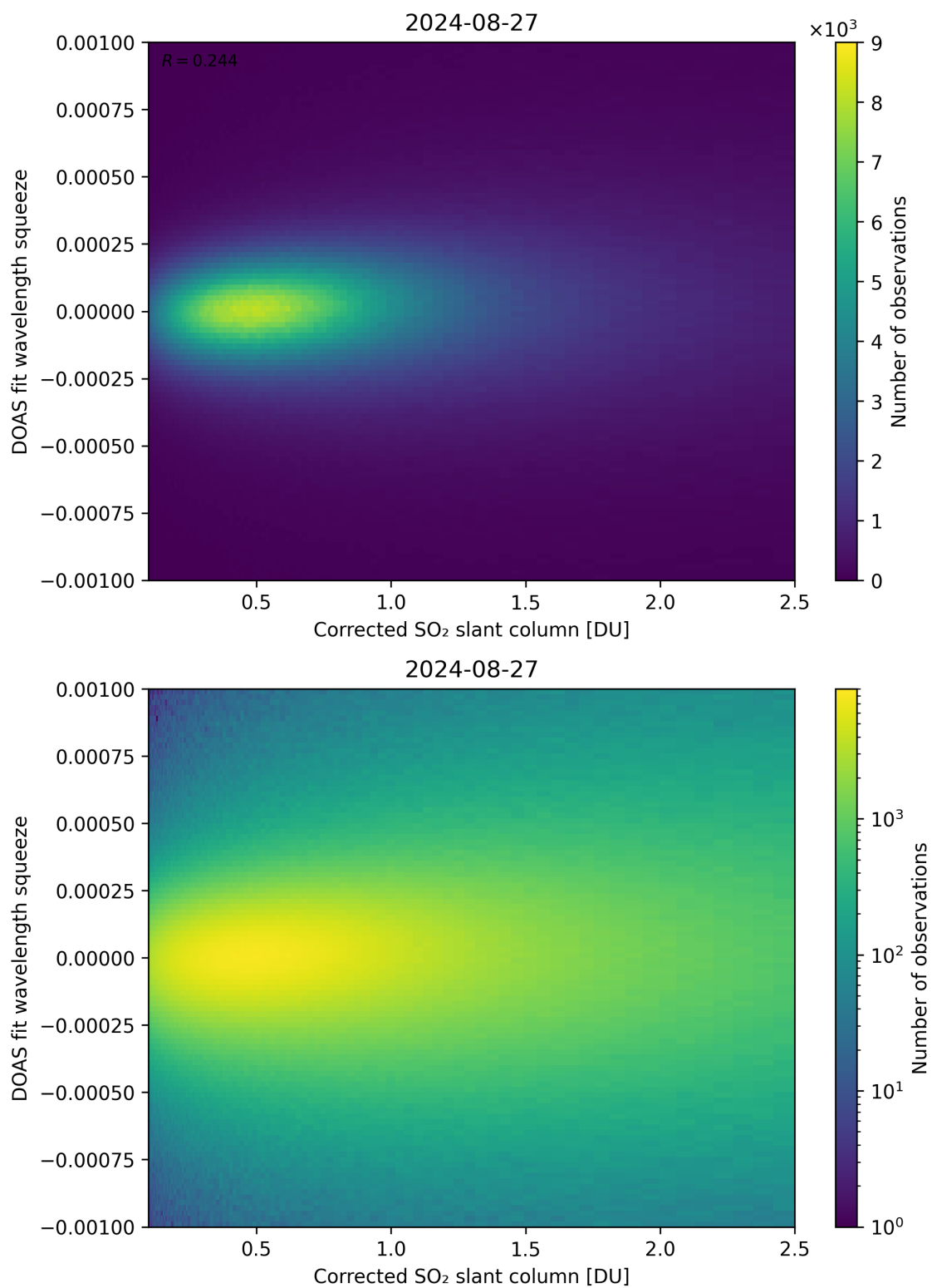
Figure 182: Scatter density plot of “Corrected SO 2 slant column” against “DOAS fit wavelength squeeze” for 2024-08-27 to 2024-08-28.
