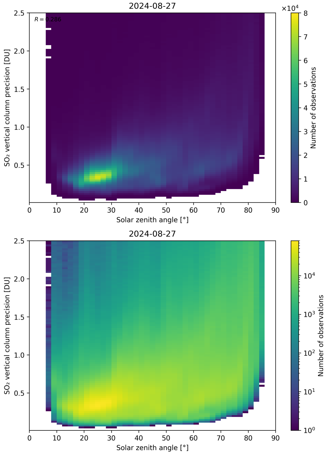
Figure 177: Scatter density plot of “Solar zenith angle” against “SO 2 vertical column precision” for 2024-08-27 to 2024-08-28.
