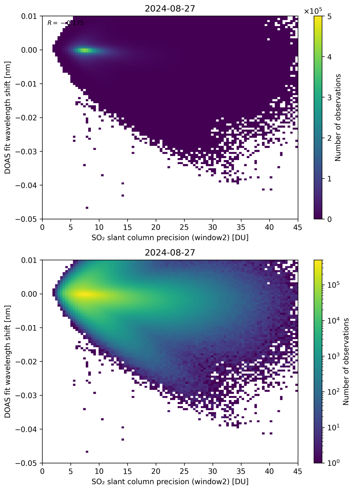
Figure 243: Scatter density plot of “SO 2 slant column precision (window2)” against “DOAS fit wavelength shift” for 2024-08-27 to 2024-08-28.
