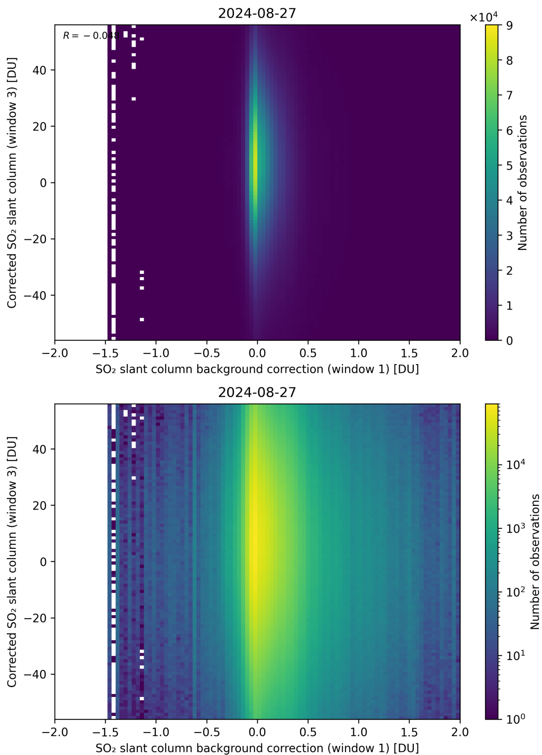
Figure 105: Scatter density plot of “SO 2 slant column background correction (window 1)” against “Corrected SO 2 slant column (window 3)” for 2024-08-27 to 2024-08-28.
