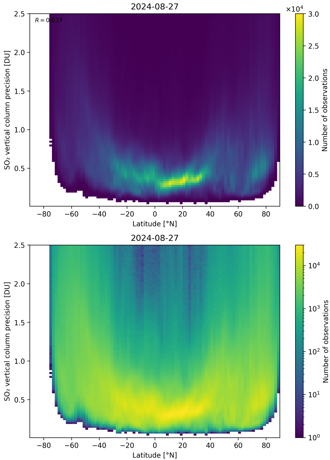
Figure 157: Scatter density plot of “Latitude” against “SO 2 vertical column precision” for 2024-08-27 to 2024-08-28.
