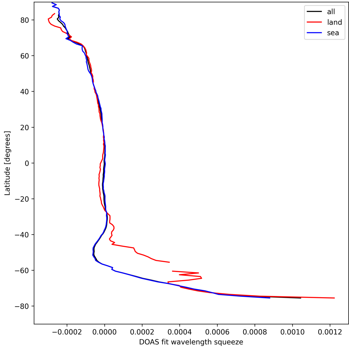
Figure 46: Zonal average of “DOAS fit wavelength squeeze” for 2024-08-27 to 2024-08-28.
