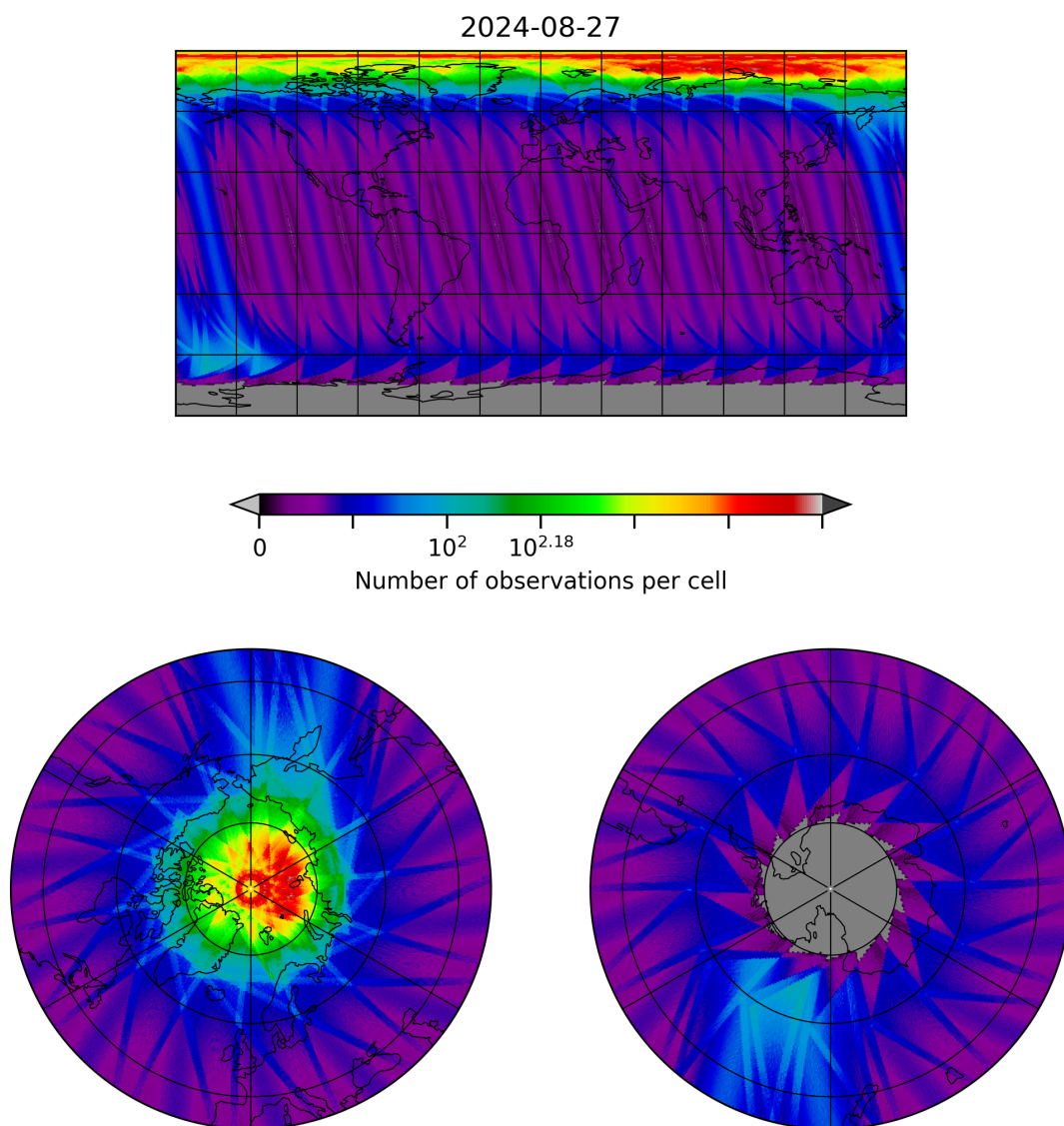
Figure 28: Map of the number of observations for 2024-08-27 to 2024-08-28
