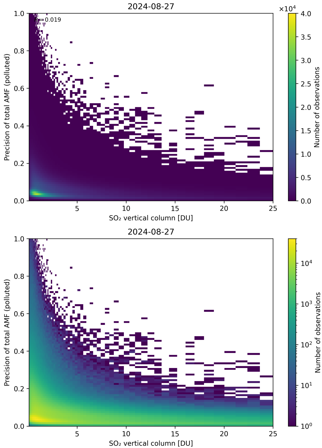
Figure 306: Scatter density plot of “SO 2 vertical column” against “Precision of total AMF (polluted)” for 2024-08-27 to 2024-08-28.
