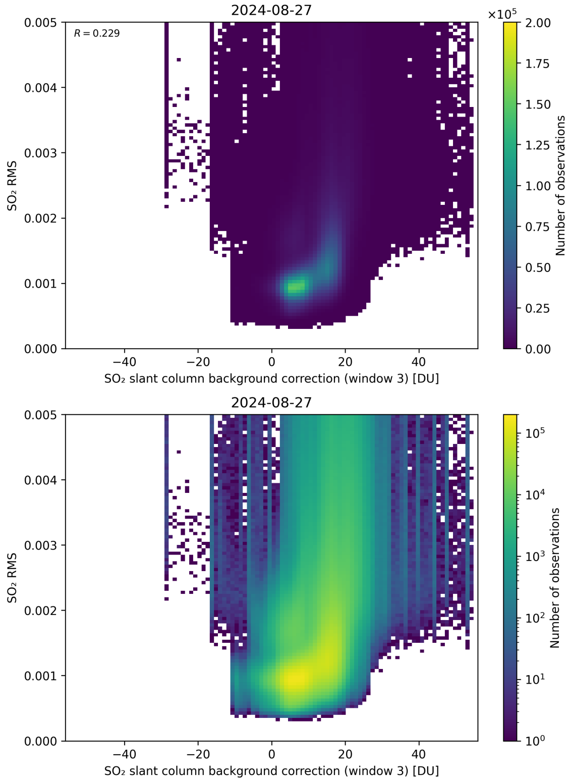
Figure 123: Scatter density plot of “SO 2 slant column background correction (window 3)” against “SO 2 RMS” for 2024-08-27 to 2024-08-28.
