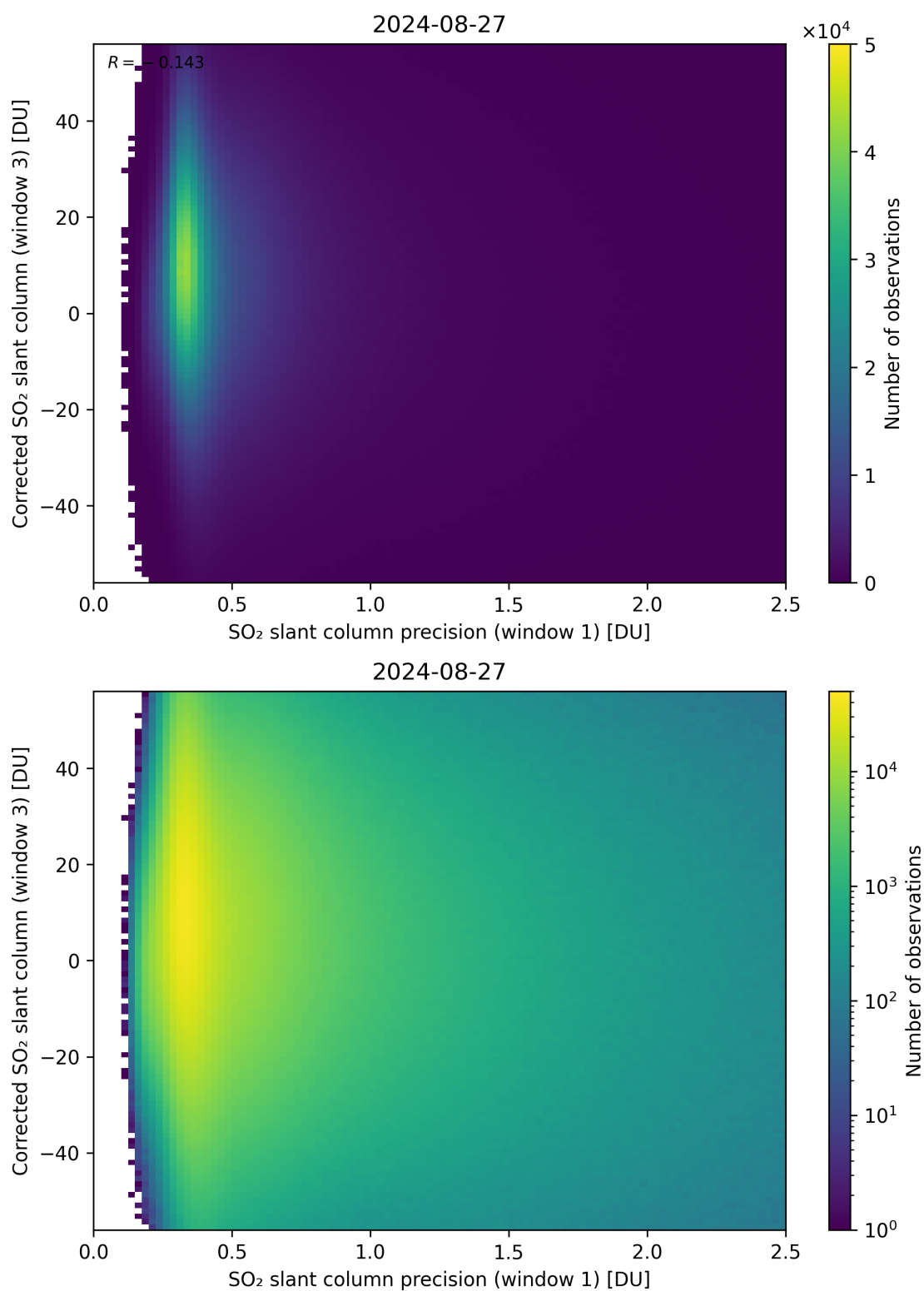
Figure 226: Scatter density plot of “SO 2 slant column precision (window 1)” against “Corrected SO 2 slant column (window 3)” for 2024-08-27 to 2024-08-28.
