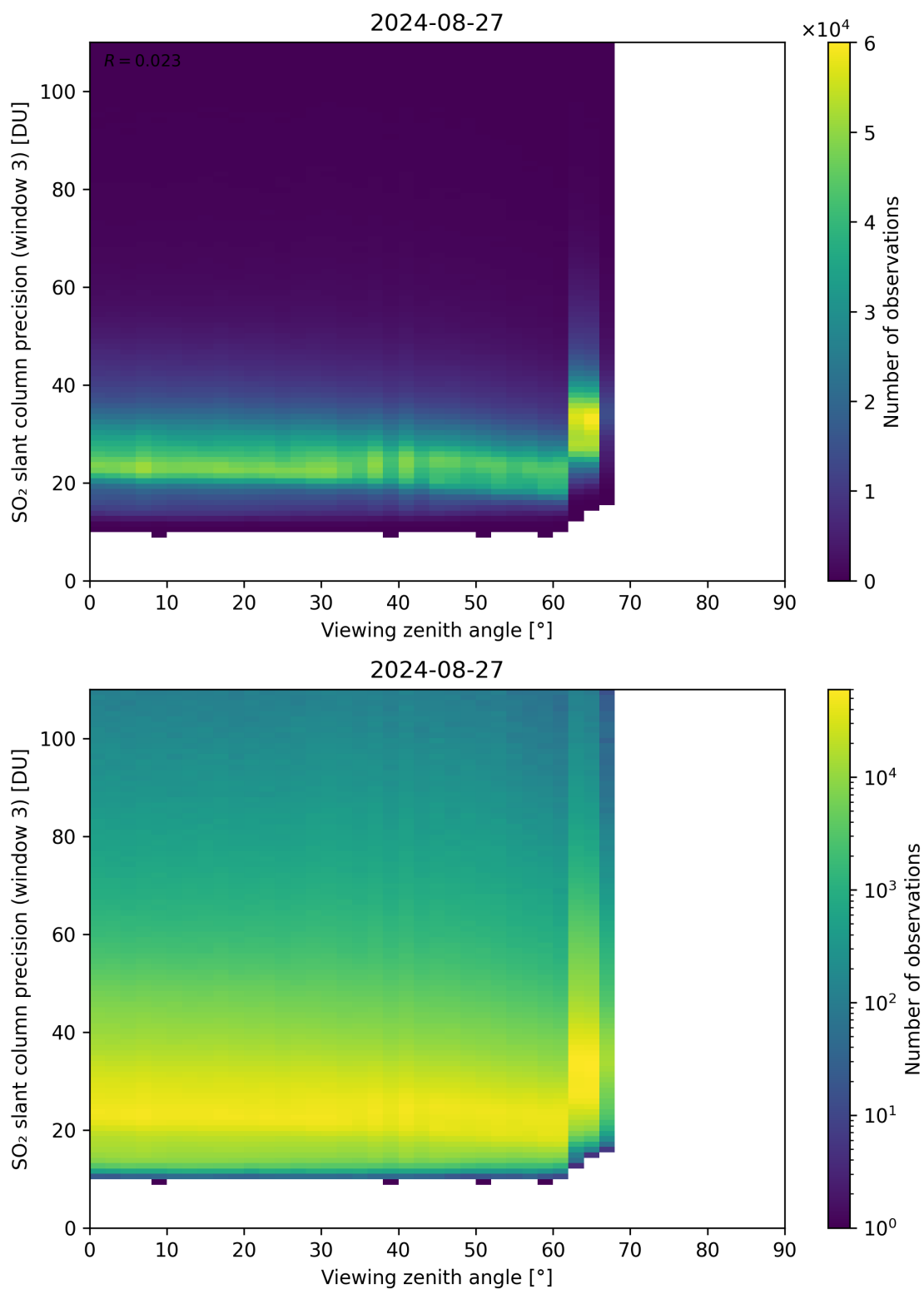
Figure 324: Scatter density plot of “Viewing zenith angle” against “SO 2 slant column precision (window 3)” for 2024-08-27 to 2024-08-28.
