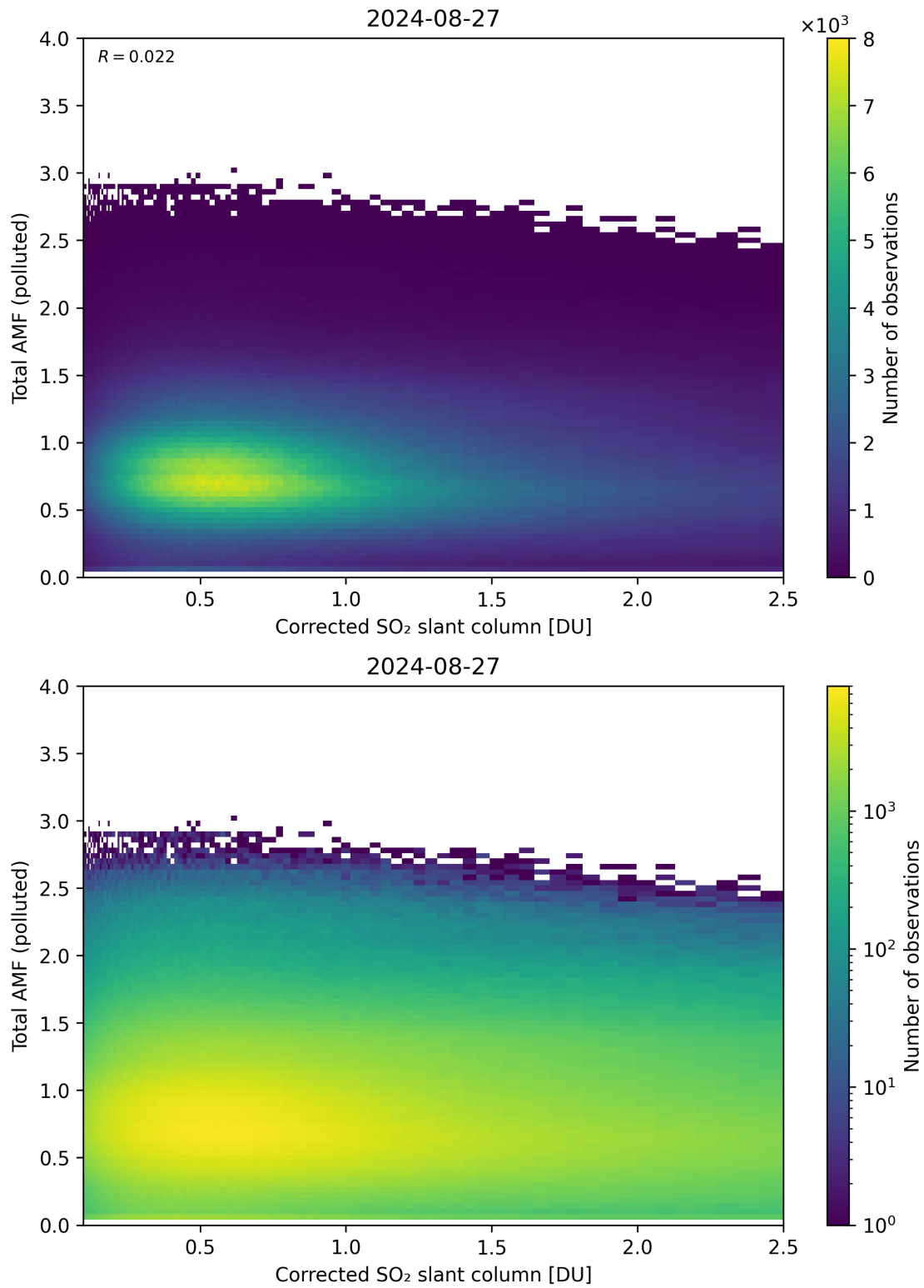
Figure 192: Scatter density plot of “Corrected SO 2 slant column” against “Total AMF (polluted)” for 2024-08-27 to 2024-08-28.
