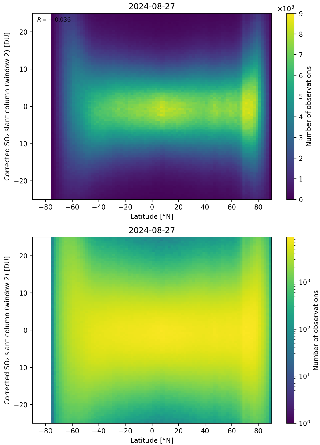
Figure 147: Scatter density plot of “Latitude” against “Corrected SO 2 slant column (window 2)” for 2024-08-27 to 2024-08-28.
