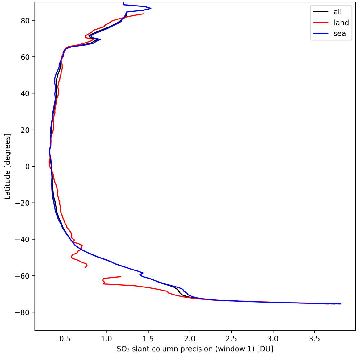
Figure 34: Zonal average of “SO 2 slant column precision (window 1)” for 2024-08-27 to 2024-08-28.
