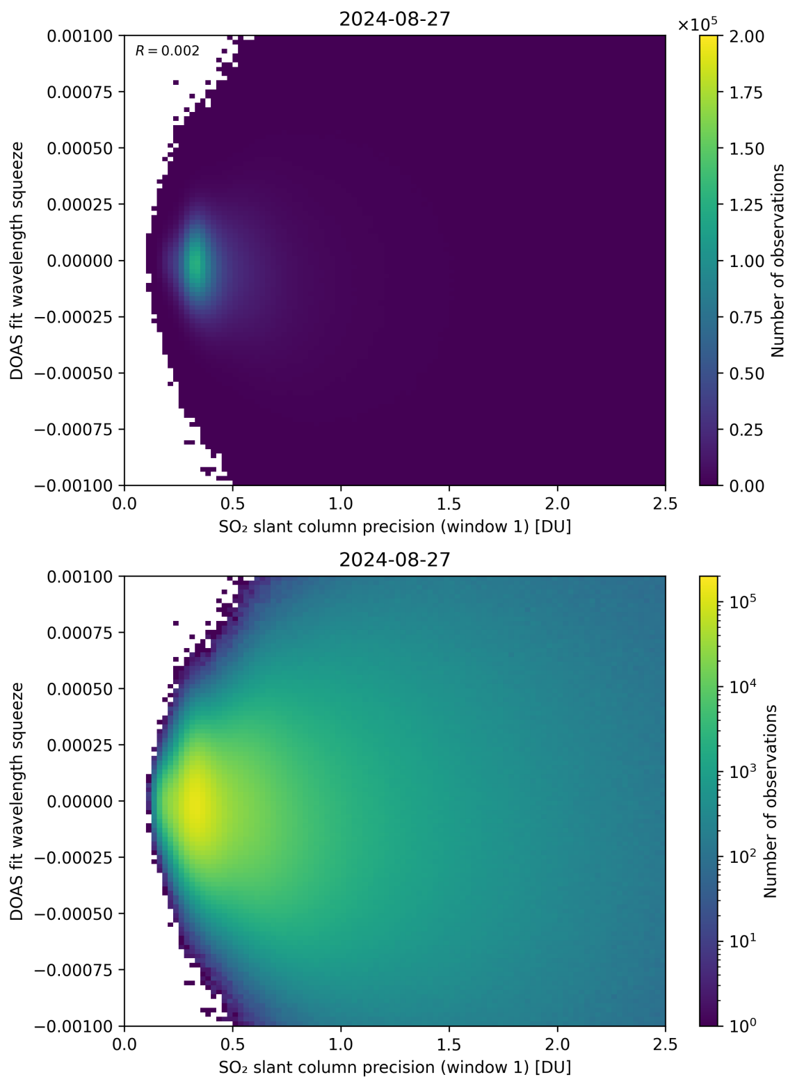
Figure 222: Scatter density plot of “SO 2 slant column precision (window 1)” against “DOAS fit wavelength squeeze” for 2024-08-27 to 2024-08-28.
