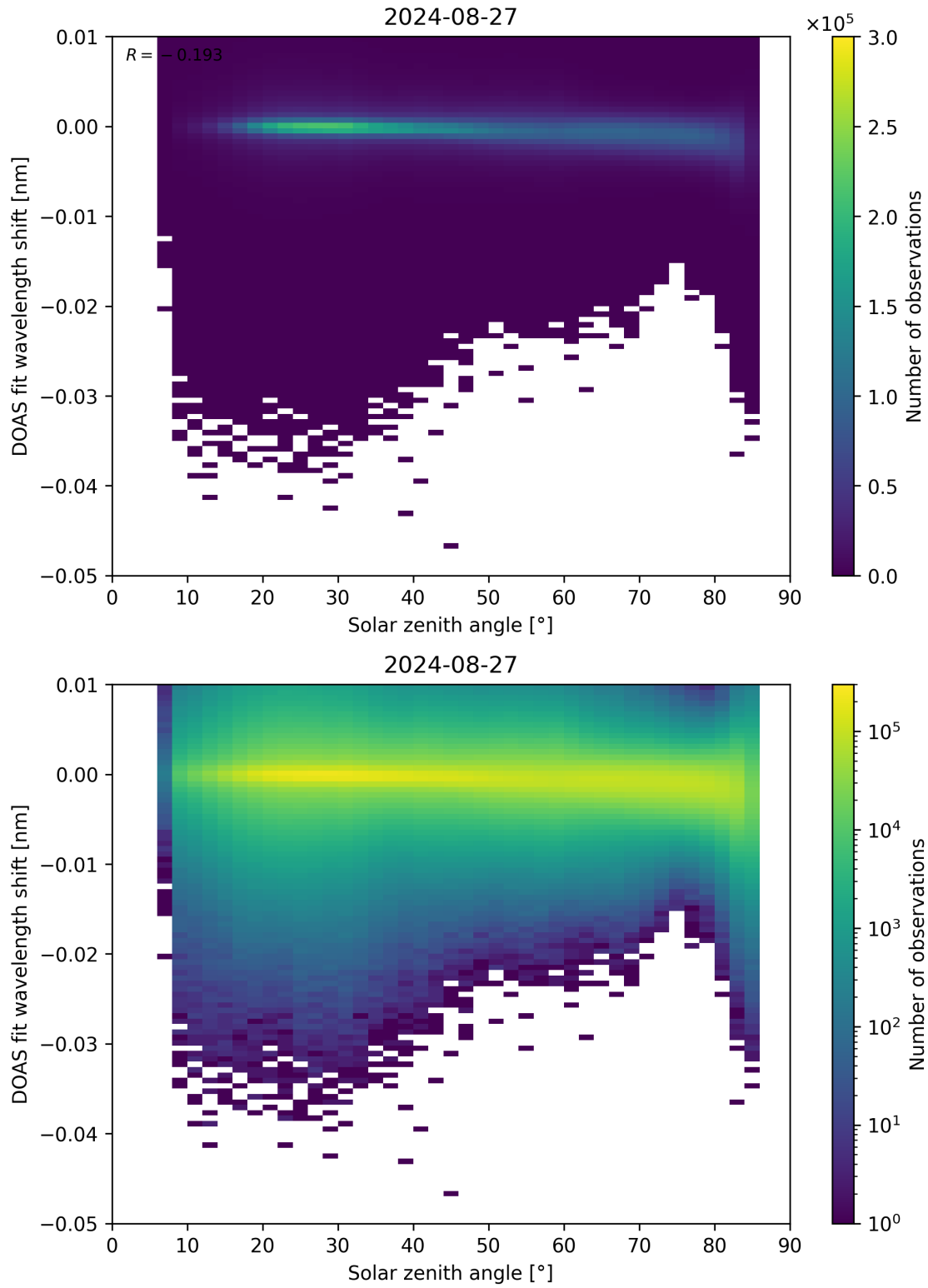
Figure 161: Scatter density plot of “Solar zenith angle” against “DOAS fit wavelength shift” for 2024-08-27 to 2024-08-28.
