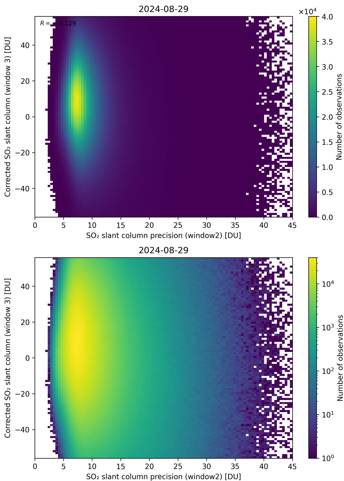
Figure 248: Scatter density plot of “SO 2 slant column precision (window2)” against “Corrected SO 2 slant column (window 3)” for 2024-08-28 to 2024-08-30.
