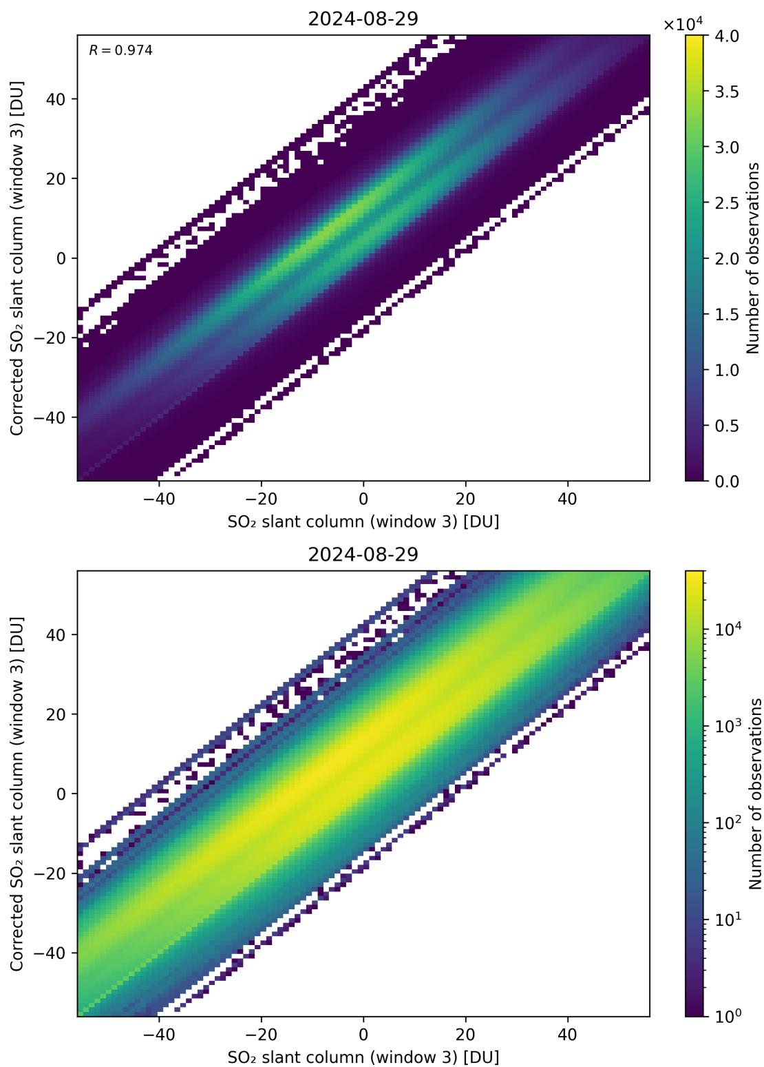
Figure 266: Scatter density plot of “SO 2 slant column (window 3)” against “Corrected SO 2 slant column (window 3)” for 2024-08-28 to 2024-08-30.
