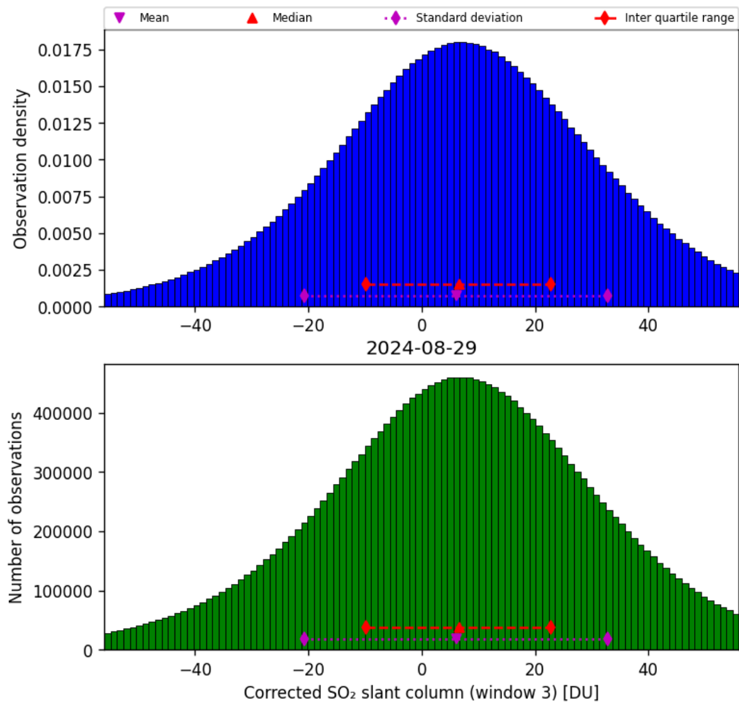
Figure 66: Histogram of “Corrected SO 2 slant column (window 3)” for 2024-08-28 to 2024-08-30
