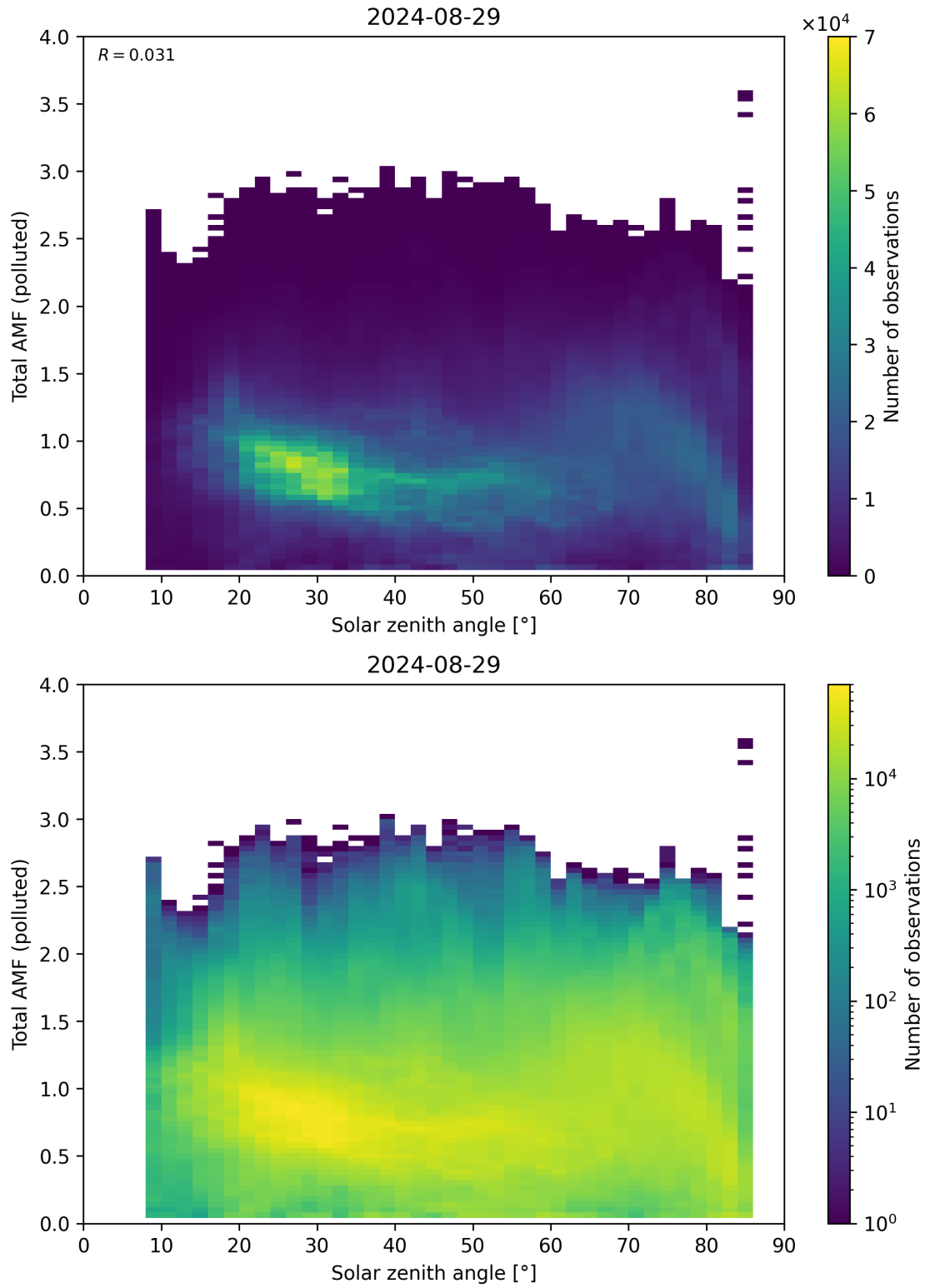
Figure 174: Scatter density plot of “Solar zenith angle” against “Total AMF (polluted)” for 2024-08-28 to 2024-08-30.
