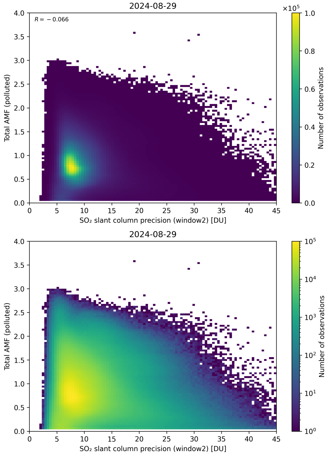
Figure 251: Scatter density plot of “SO 2 slant column precision (window2)” against “Total AMF (polluted)” for 2024-08-28 to 2024-08-30.
