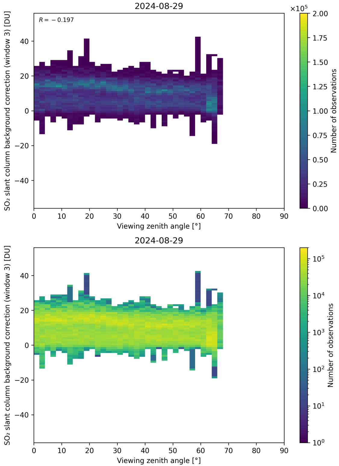
Figure 310: Scatter density plot of “Viewing zenith angle” against “SO 2 slant column background correction (window 3)” for 2024-08-28 to 2024-08-30.
