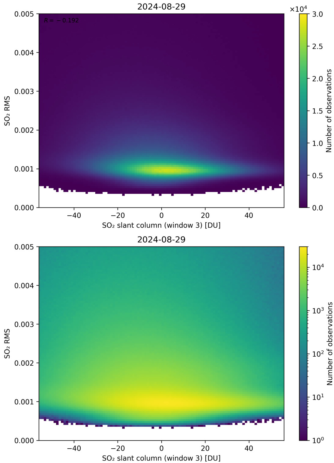
Figure 256: Scatter density plot of “SO 2 slant column (window 3)” against “SO 2 RMS” for 2024-08-28 to 2024-08-30.
