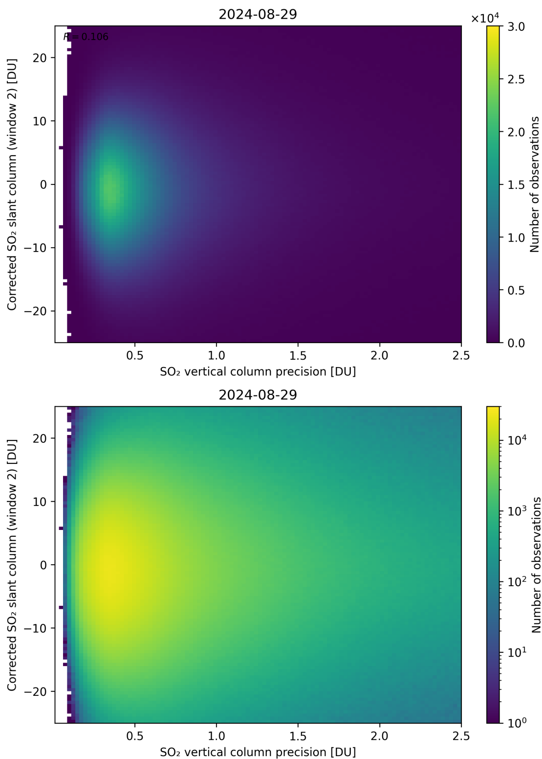
Figure 287: Scatter density plot of “SO 2 vertical column precision” against “Corrected SO 2 slant column (window 2)” for 2024-08-28 to 2024-08-30.
