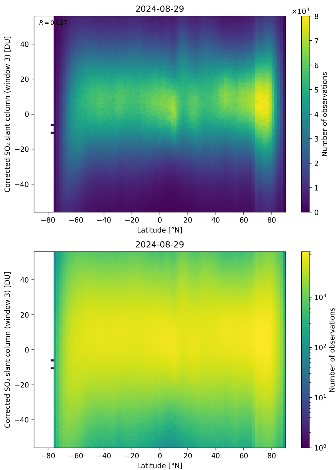
Figure 148: Scatter density plot of “Latitude” against “Corrected SO 2 slant column (window 3)” for 2024-08-28 to 2024-08-30.
