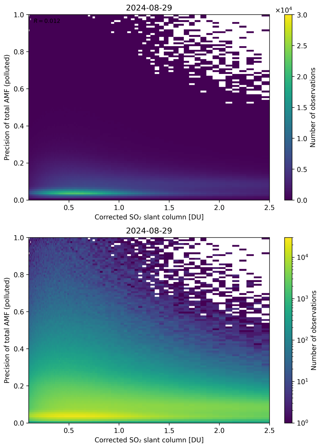
Figure 193: Scatter density plot of “Corrected SO 2 slant column” against “Precision of total AMF (polluted)” for 2024-08-28 to 2024-08-30.
