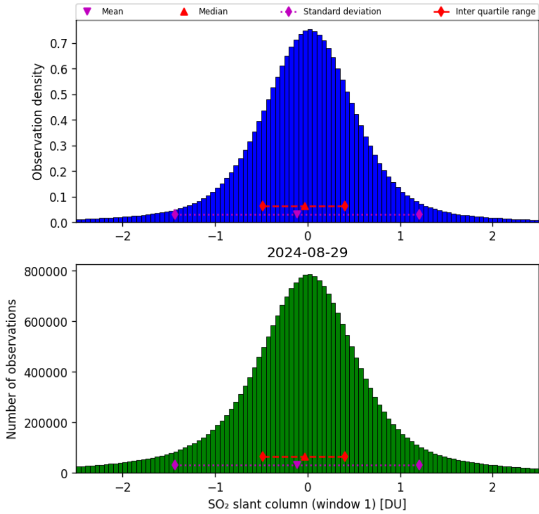
Figure 56: Histogram of “SO 2 slant column (window 1)” for 2024-08-28 to 2024-08-30
