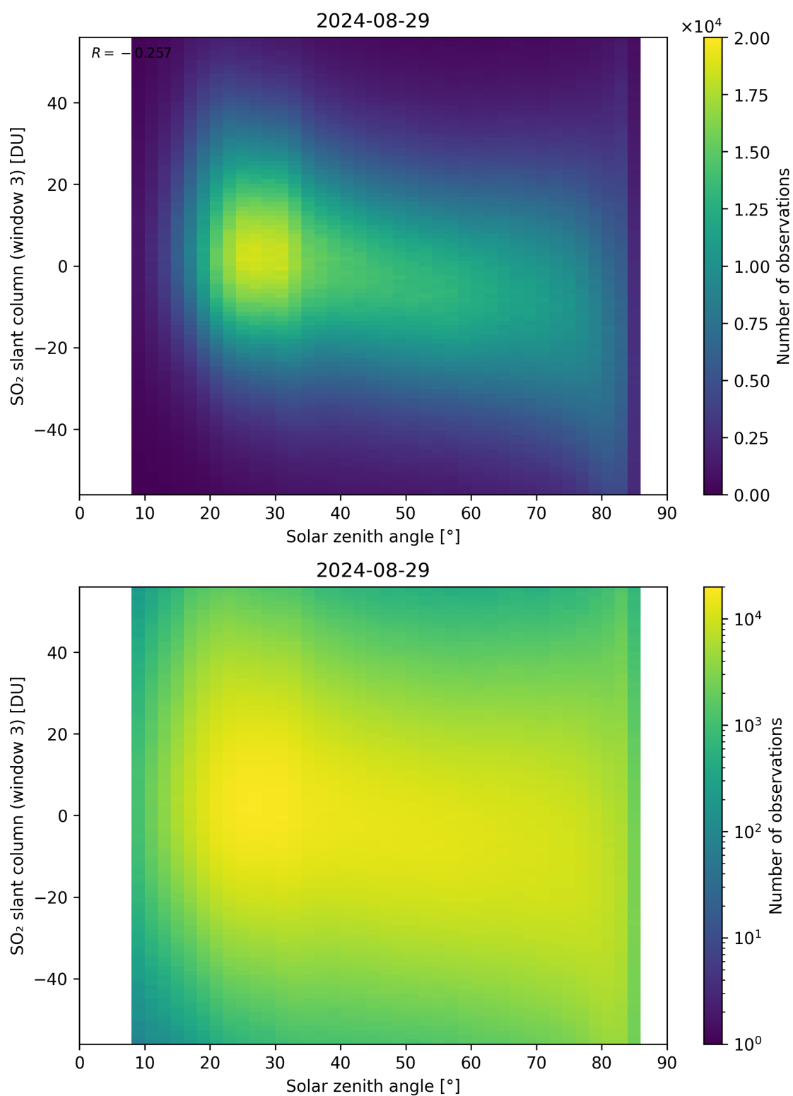
Figure 172: Scatter density plot of “Solar zenith angle” against “SO 2 slant column (window 3)” for 2024-08-28 to 2024-08-30.
