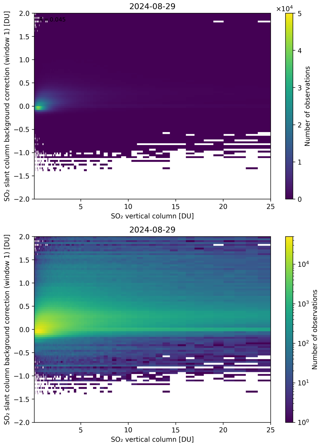
Figure 273: Scatter density plot of “SO 2 vertical column” against “SO 2 slant column background correction (window 1)” for 2024-08-28 to 2024-08-30.
