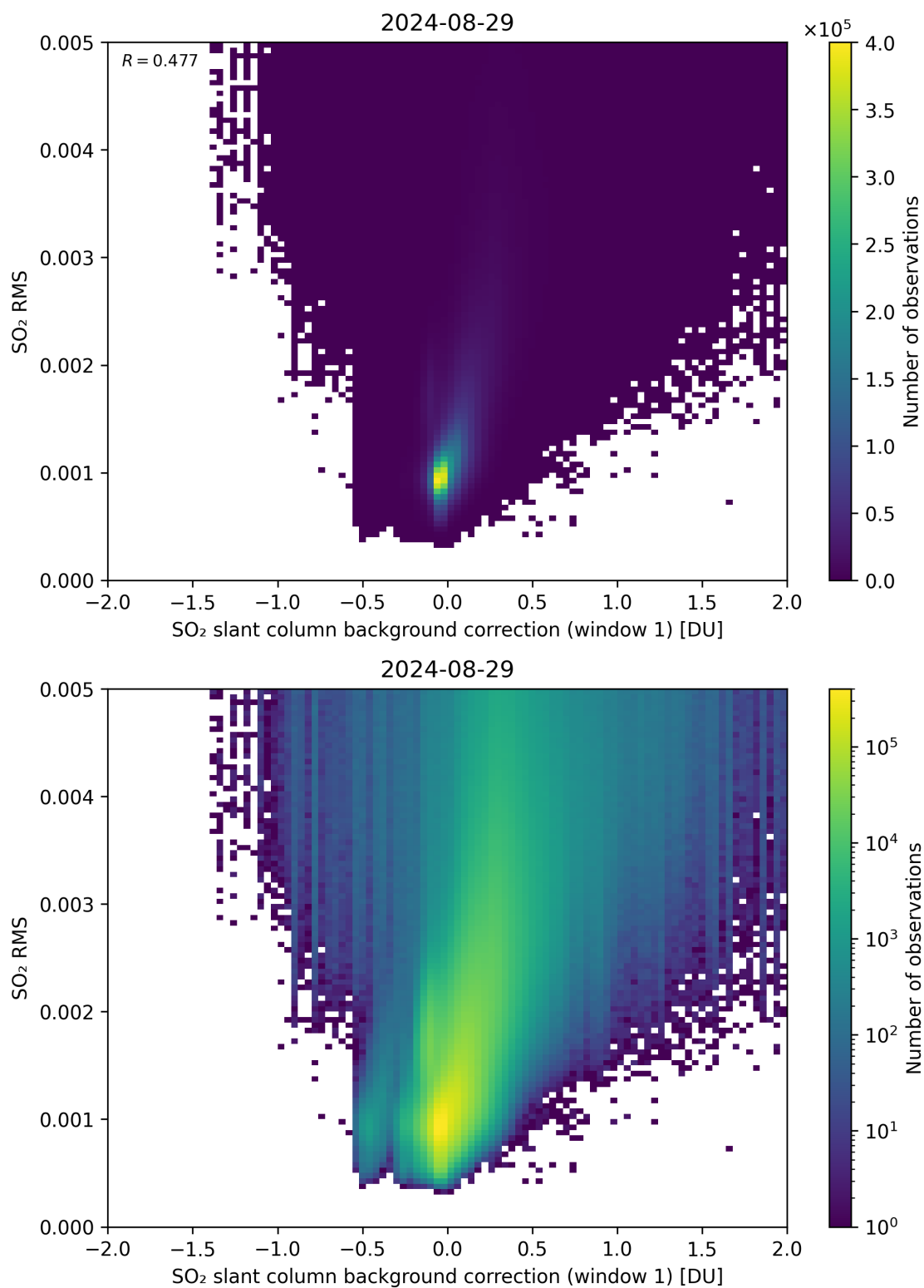
Figure 102: Scatter density plot of “SO 2 slant column background correction (window 1)” against “SO 2 RMS” for 2024-08-28 to 2024-08-30.
