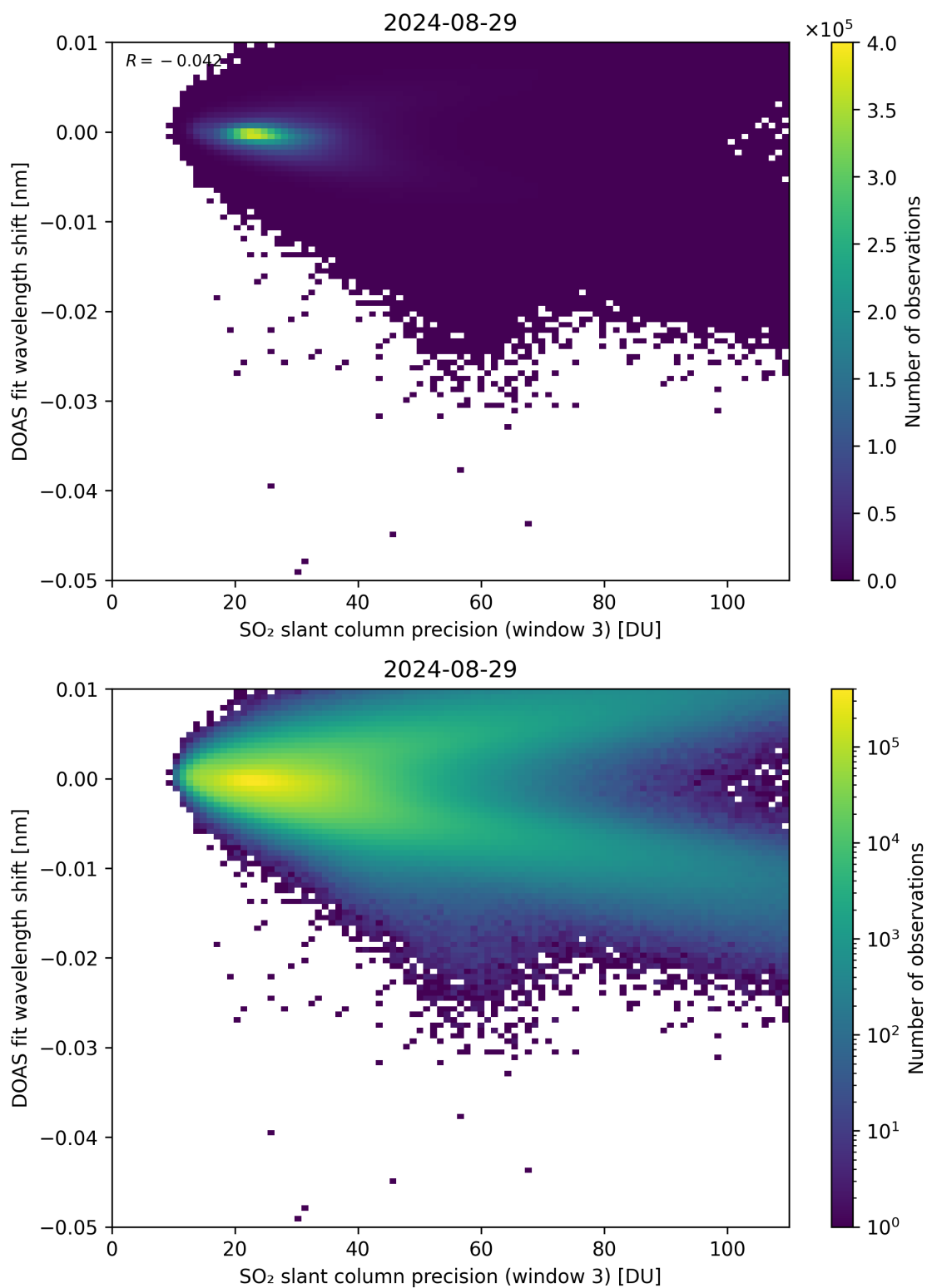
Figure 258: Scatter density plot of “SO 2 slant column precision (window 3)” against “DOAS fit wavelength shift” for 2024-08-28 to 2024-08-30.
