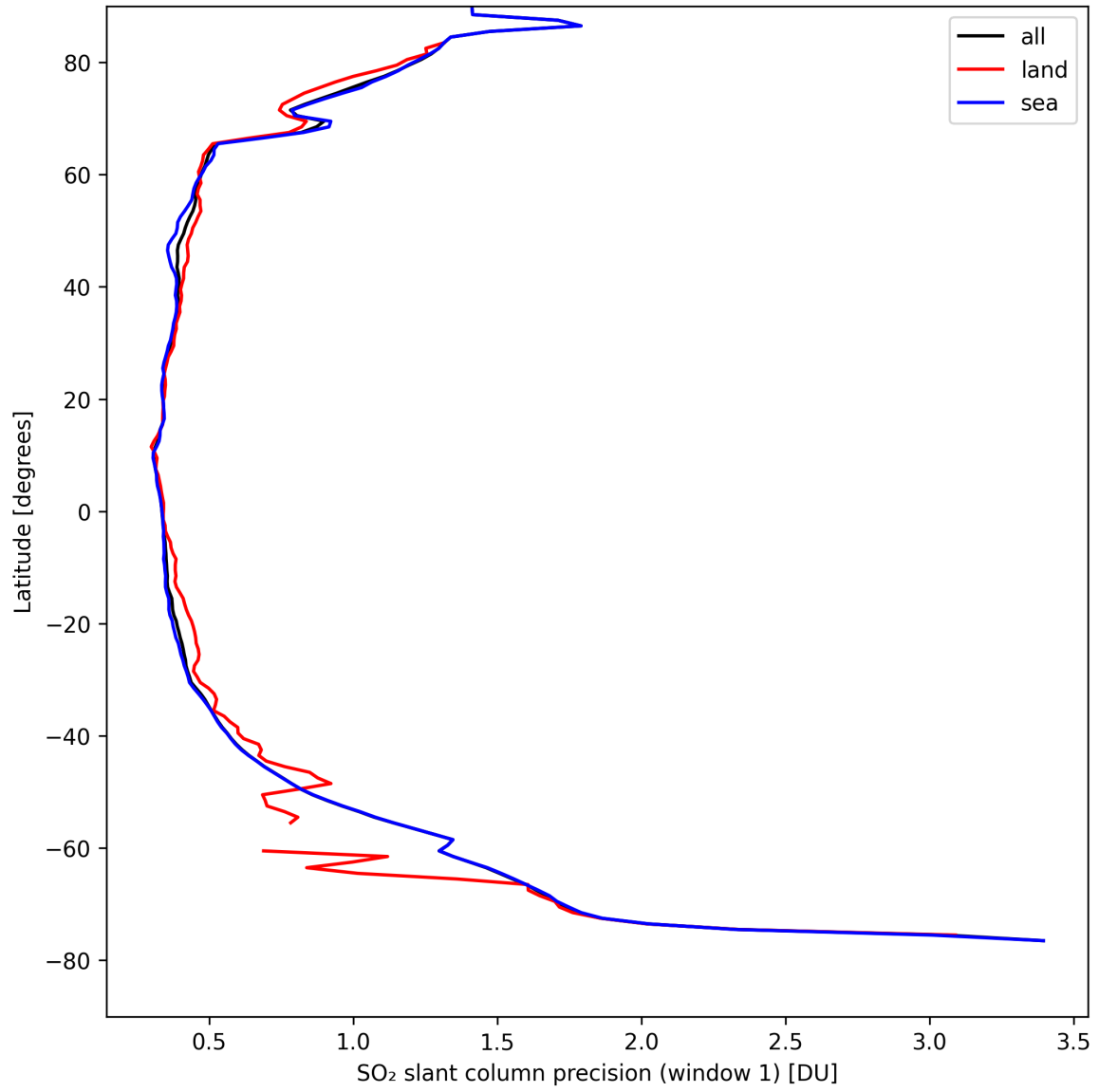
Figure 34: Zonal average of “SO 2 slant column precision (window 1)” for 2024-08-28 to 2024-08-30.
