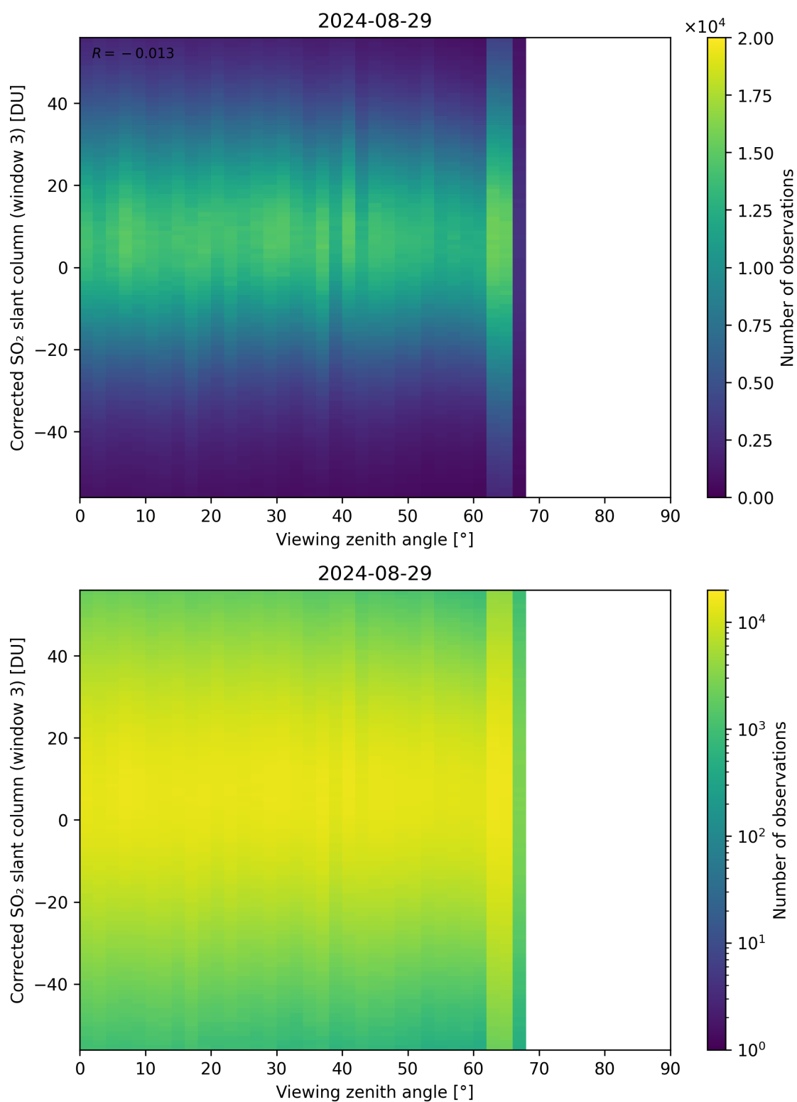
Figure 319: Scatter density plot of “Viewing zenith angle” against “Corrected SO 2 slant column (window 3)” for 2024-08-28 to 2024-08-30.
