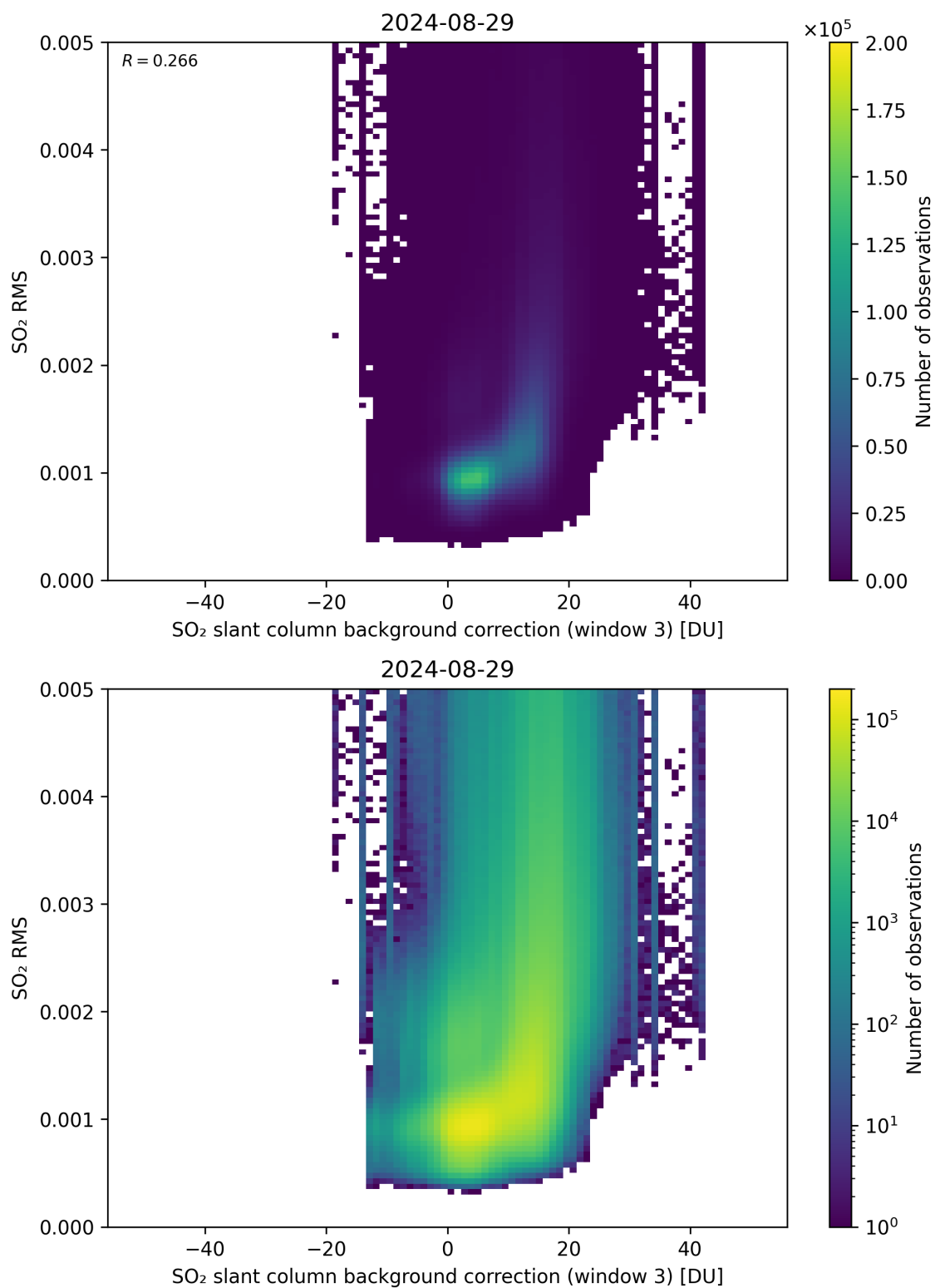
Figure 123: Scatter density plot of “SO 2 slant column background correction (window 3)” against “SO 2 RMS” for 2024-08-28 to 2024-08-30.
