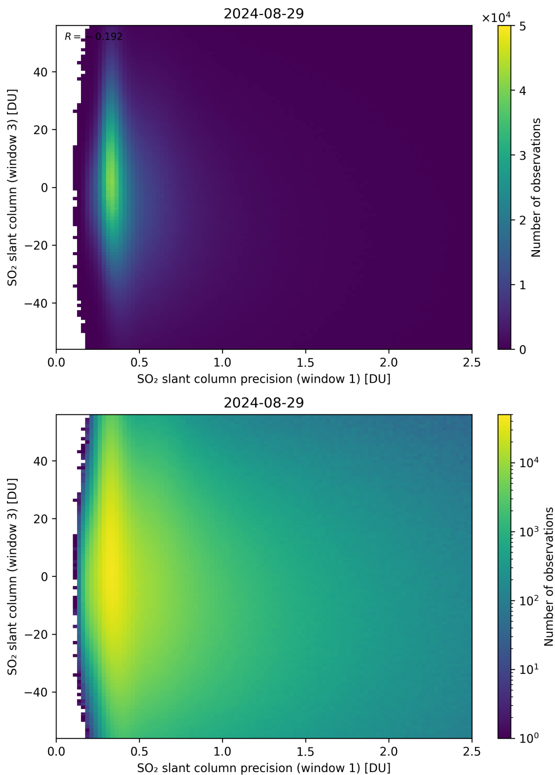
Figure 228: Scatter density plot of “SO 2 slant column precision (window 1)” against “SO 2 slant column (window 3)” for 2024-08-28 to 2024-08-30.
