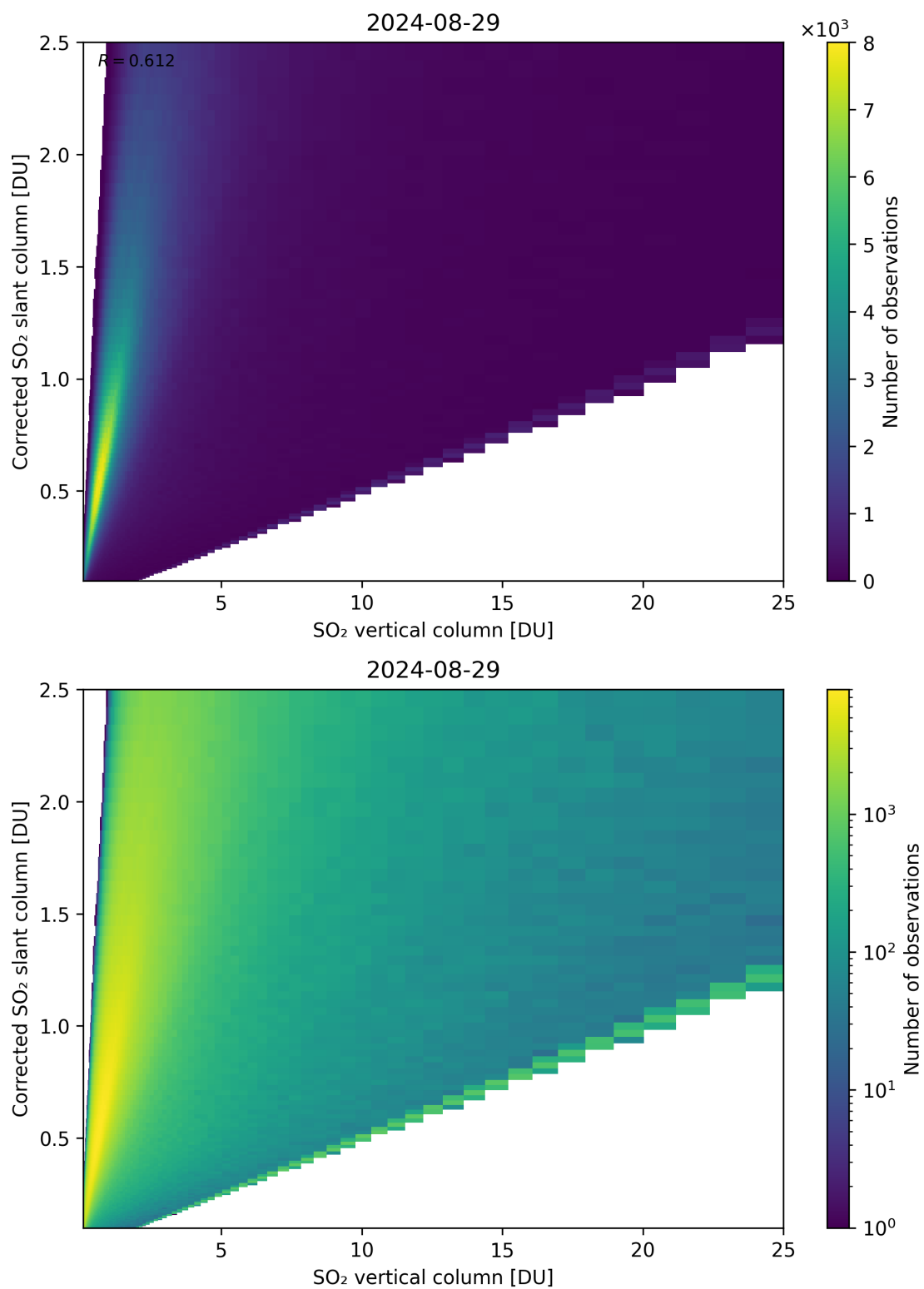
Figure 297: Scatter density plot of “SO 2 vertical column” against “Corrected SO 2 slant column” for 2024-08-28 to 2024-08-30.
