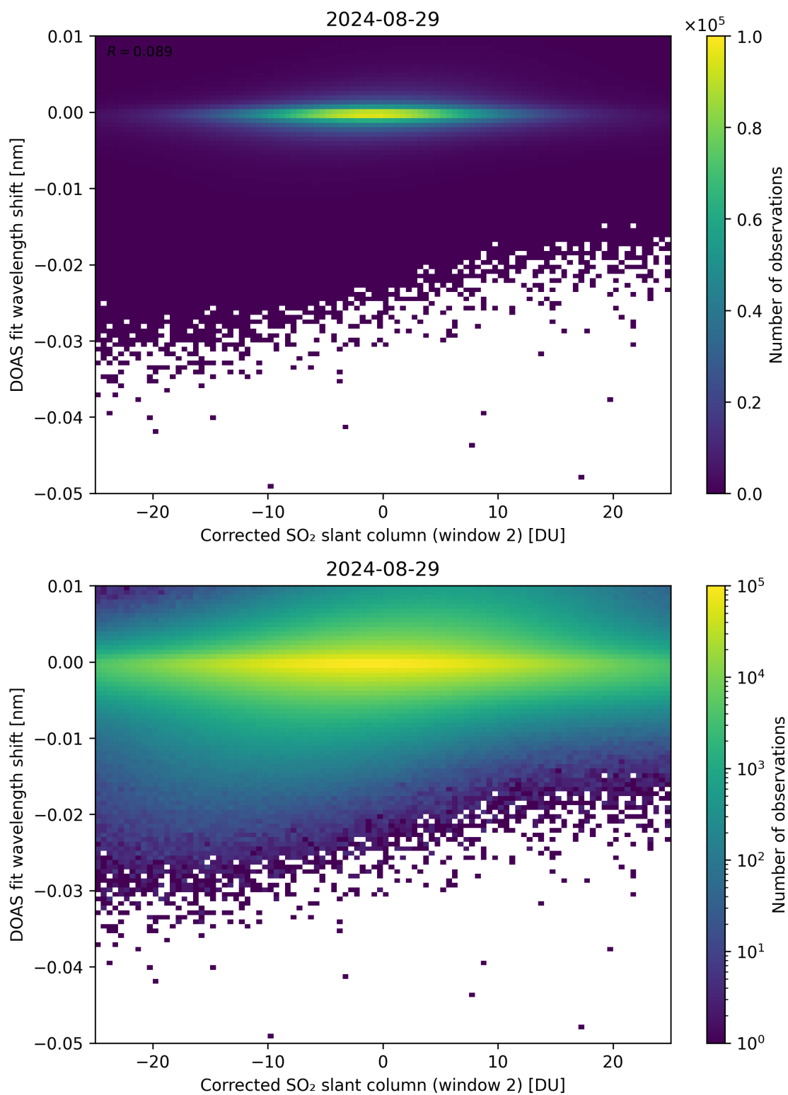
Figure 196: Scatter density plot of “Corrected SO 2 slant column (window 2)” against “DOAS fit wavelength shift” for 2024-08-28 to 2024-08-30.
