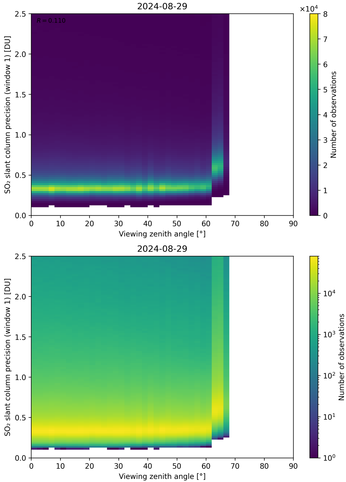
Figure 321: Scatter density plot of “Viewing zenith angle” against “SO 2 slant column precision (window 1)” for 2024-08-28 to 2024-08-30.
