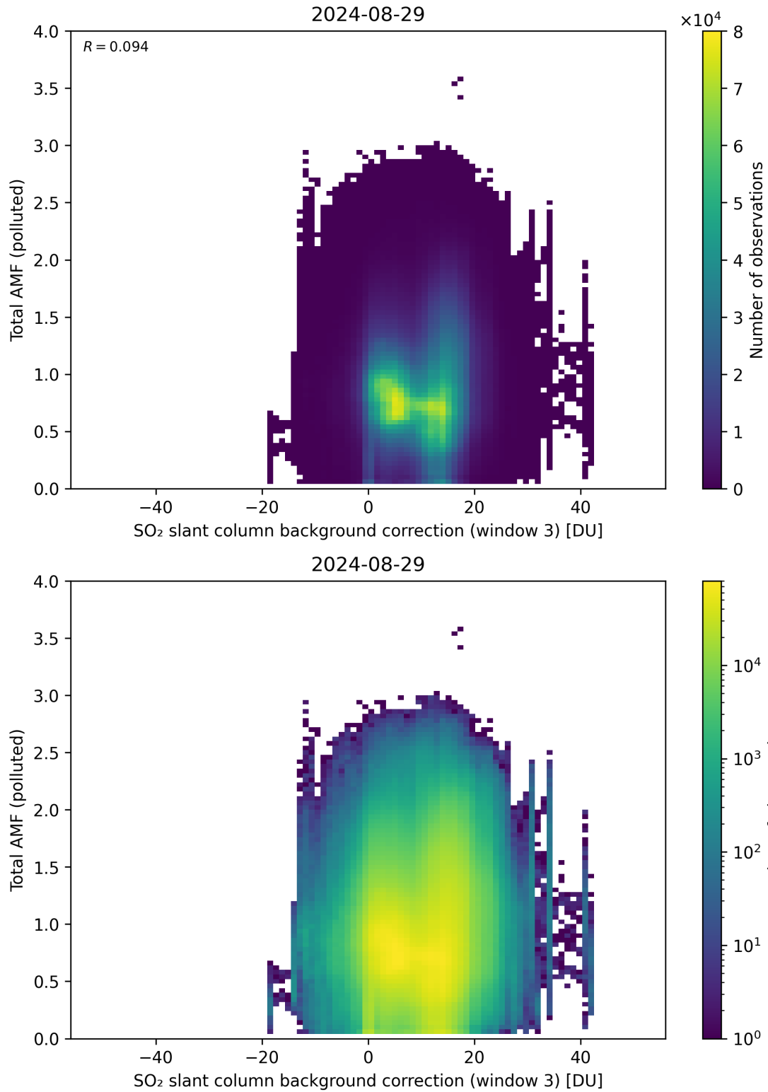
Figure 125: Scatter density plot of “SO 2 slant column background correction (window 3)” against “Total AMF (polluted)” for 2024-08-28 to 2024-08-30.
