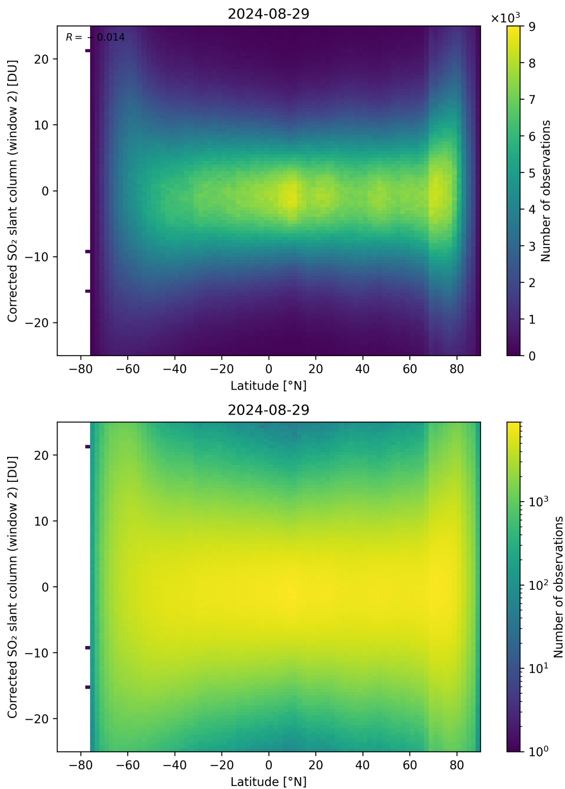
Figure 147: Scatter density plot of “Latitude” against “Corrected SO 2 slant column (window 2)” for 2024-08-28 to 2024-08-30.
