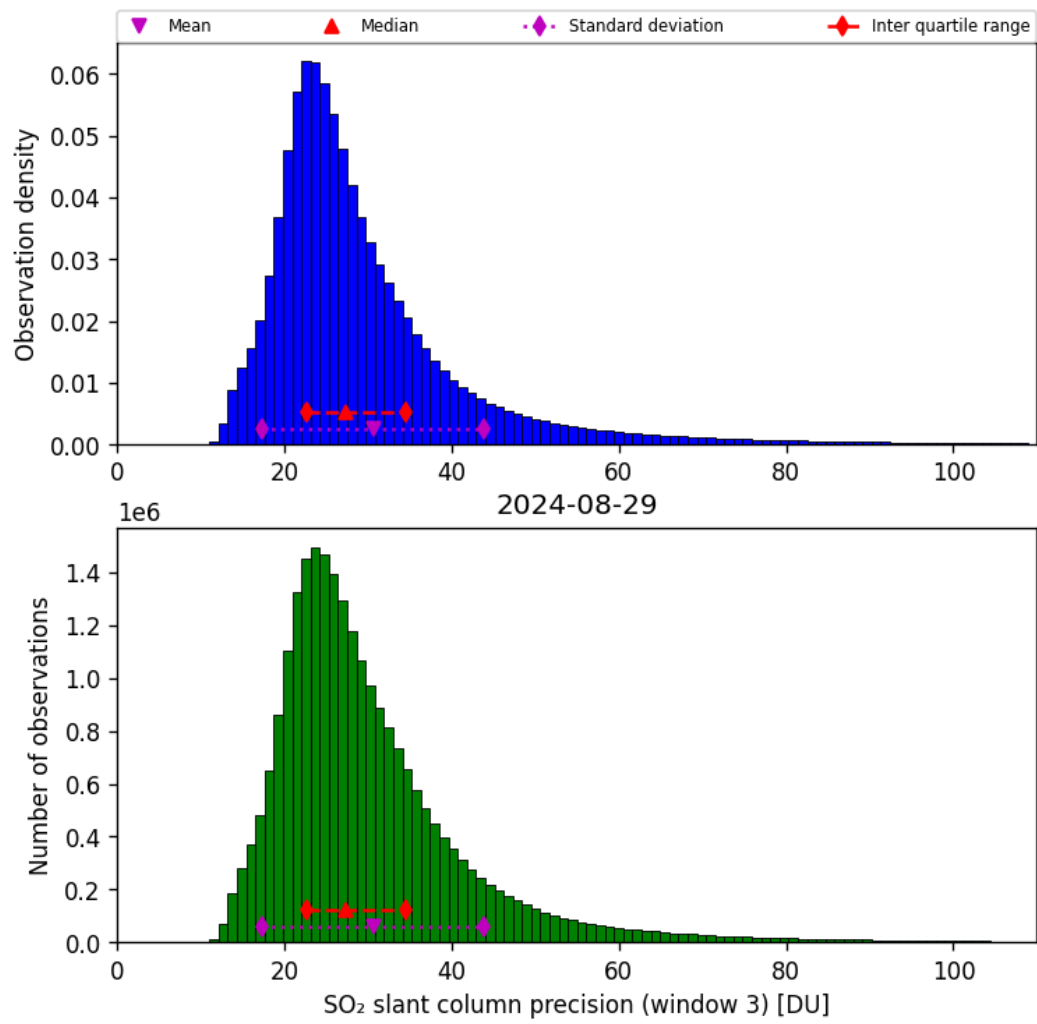
Figure 65: Histogram of “SO 2 slant column precision (window 3)” for 2024-08-28 to 2024-08-30
