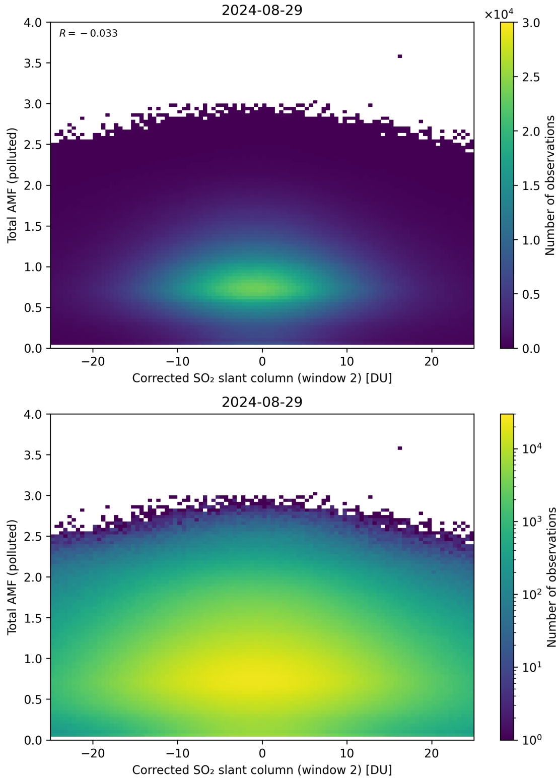
Figure 203: Scatter density plot of “Corrected SO 2 slant column (window 2)” against “Total AMF (polluted)” for 2024-08-28 to 2024-08-30.
