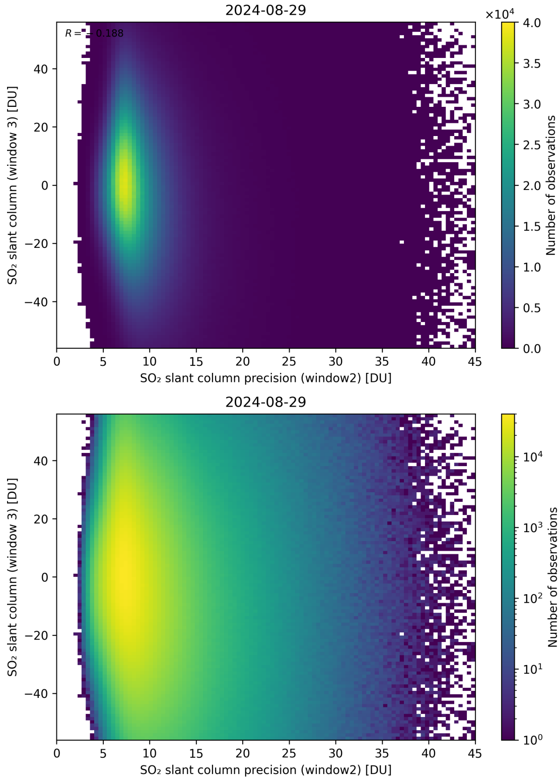
Figure 249: Scatter density plot of “SO 2 slant column precision (window2)” against “SO 2 slant column (window 3)” for 2024-08-28 to 2024-08-30.
