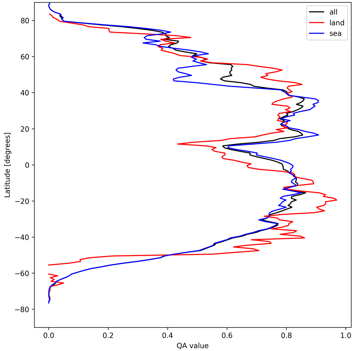
Figure 29: Zonal average of “QA value” for 2024-08-28 to 2024-08-30.
