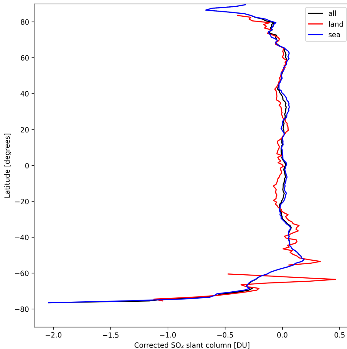
Figure 32: Zonal average of “Corrected SO 2 slant column” for 2024-08-28 to 2024-08-30.
