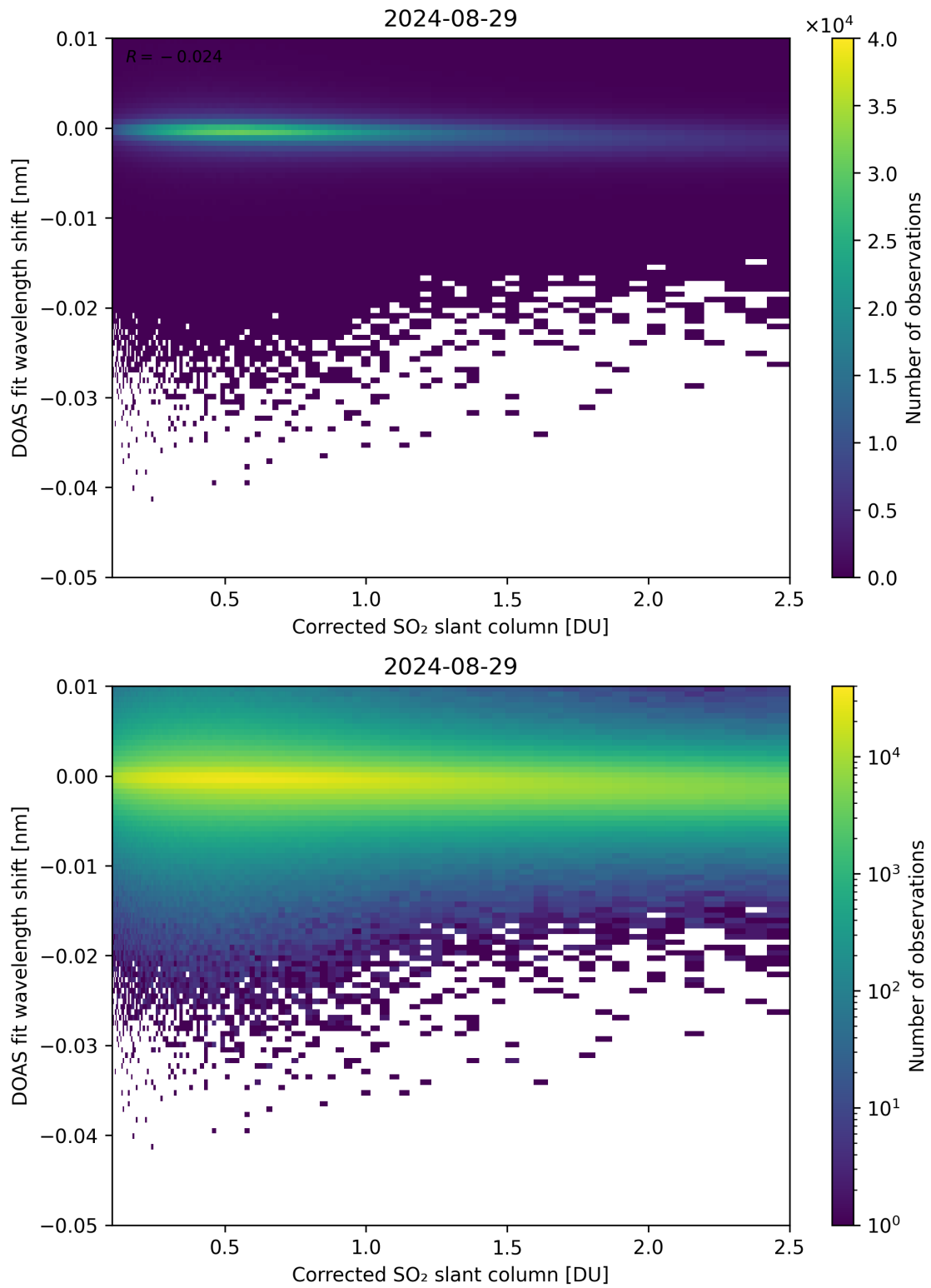
Figure 181: Scatter density plot of “Corrected SO 2 slant column” against “DOAS fit wavelength shift” for 2024-08-28 to 2024-08-30.
