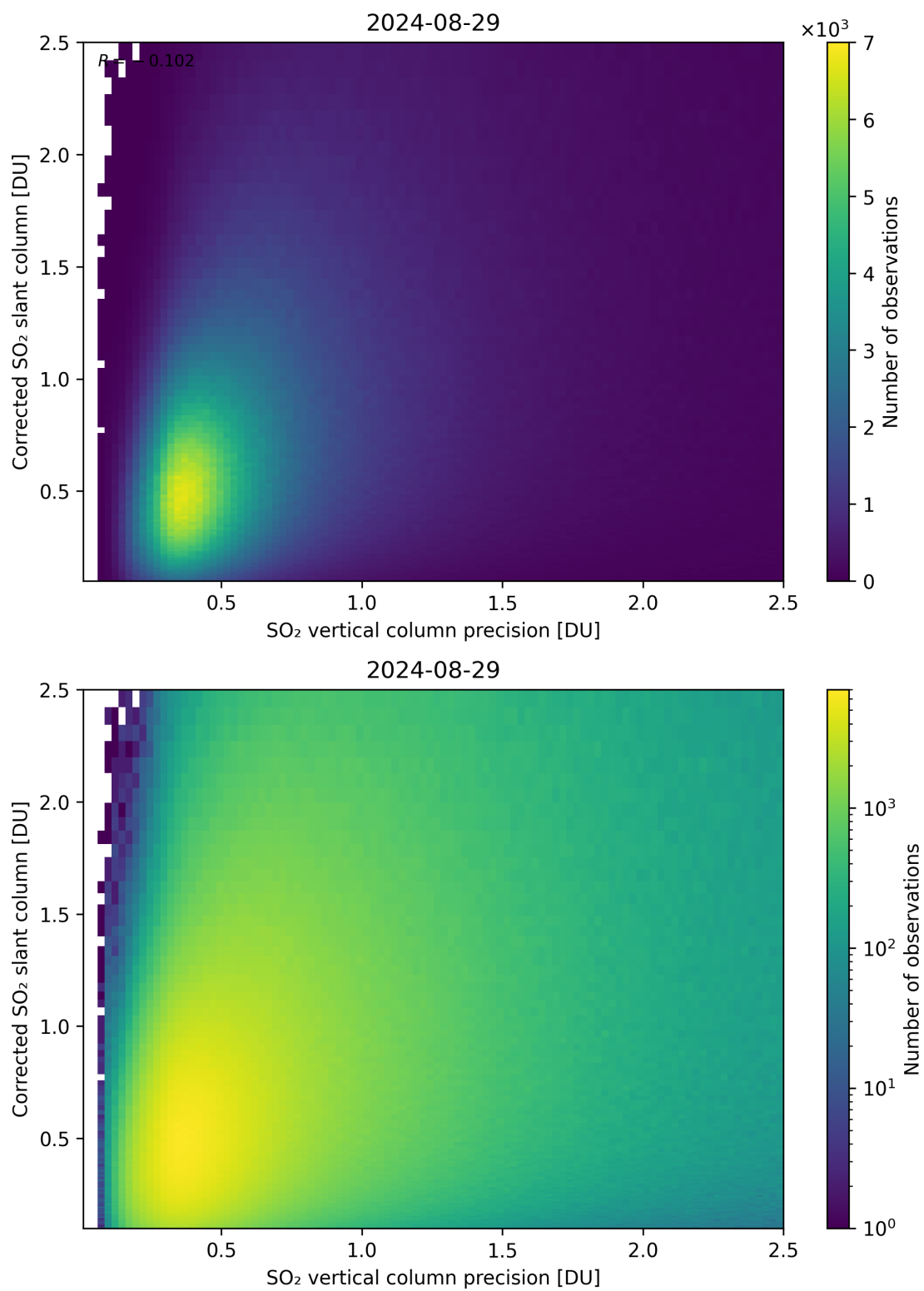
Figure 286: Scatter density plot of “SO 2 vertical column precision” against “Corrected SO 2 slant column” for 2024-08-28 to 2024-08-30.
