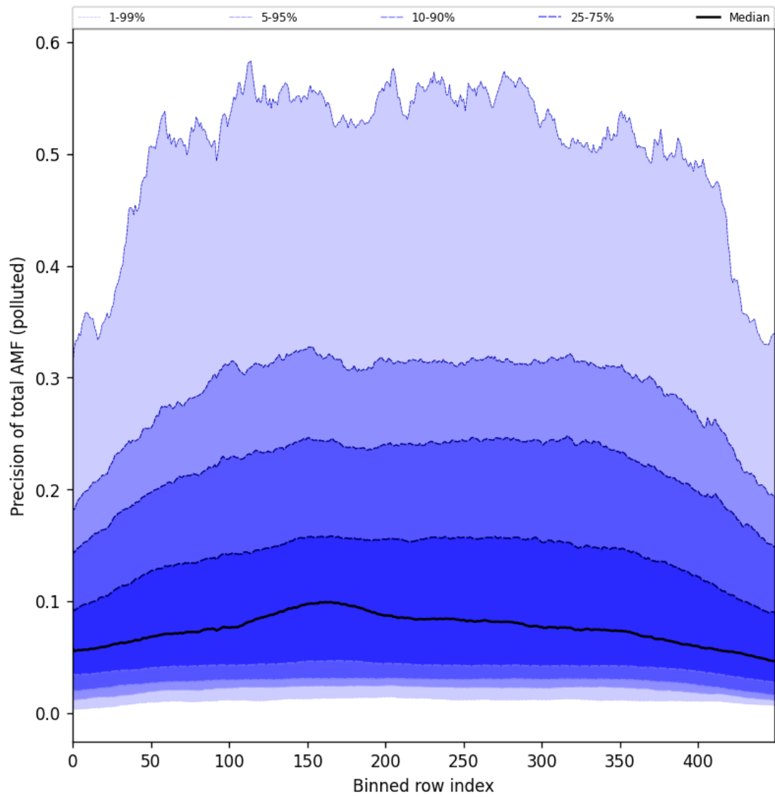
Figure 95: Along track statistics of “Precision of total AMF (polluted)” for 2024-08-28 to 2024-08-30
