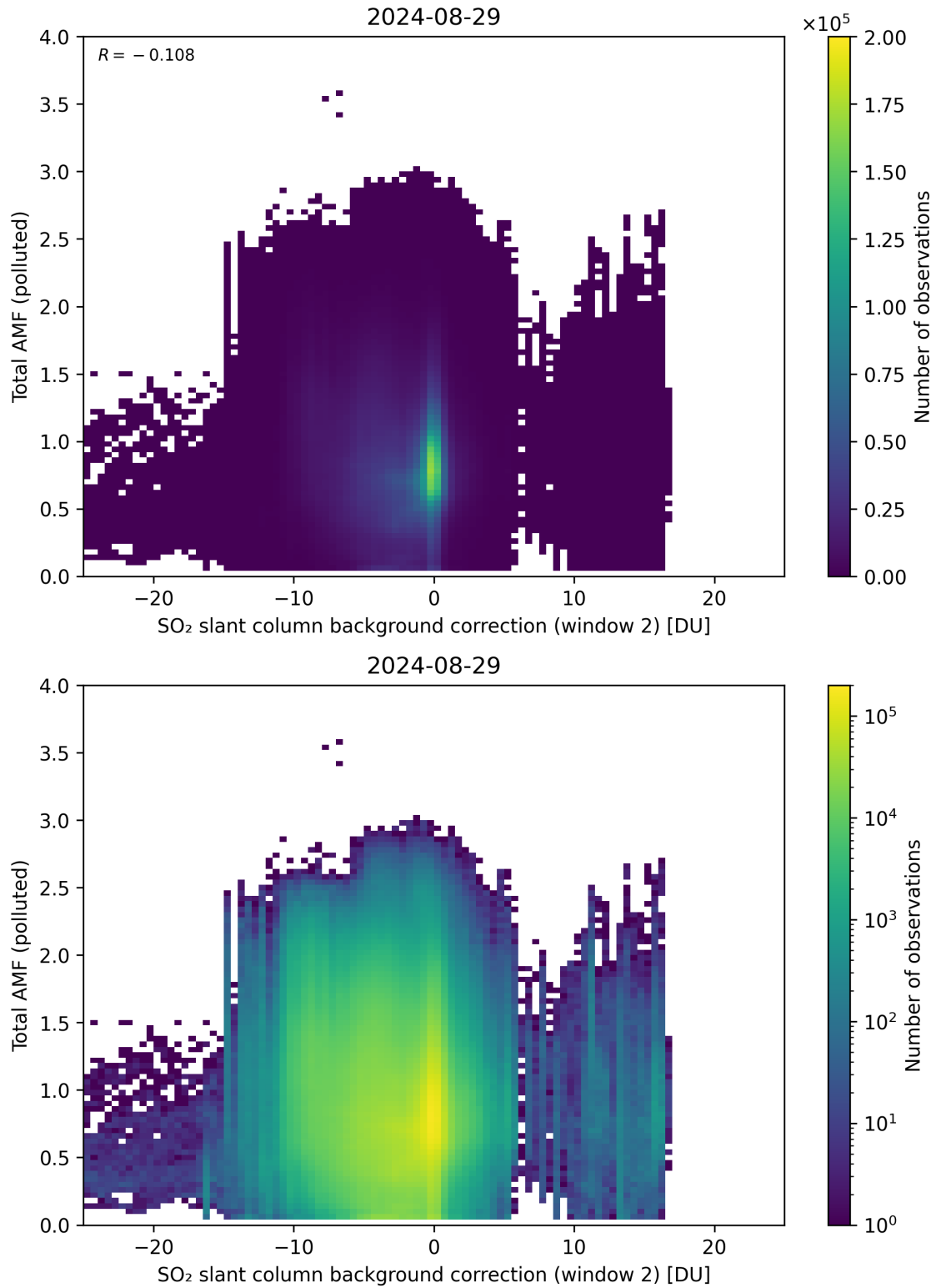
Figure 119: Scatter density plot of “SO 2 slant column background correction (window 2)” against “Total AMF (polluted)” for 2024-08-28 to 2024-08-30.
