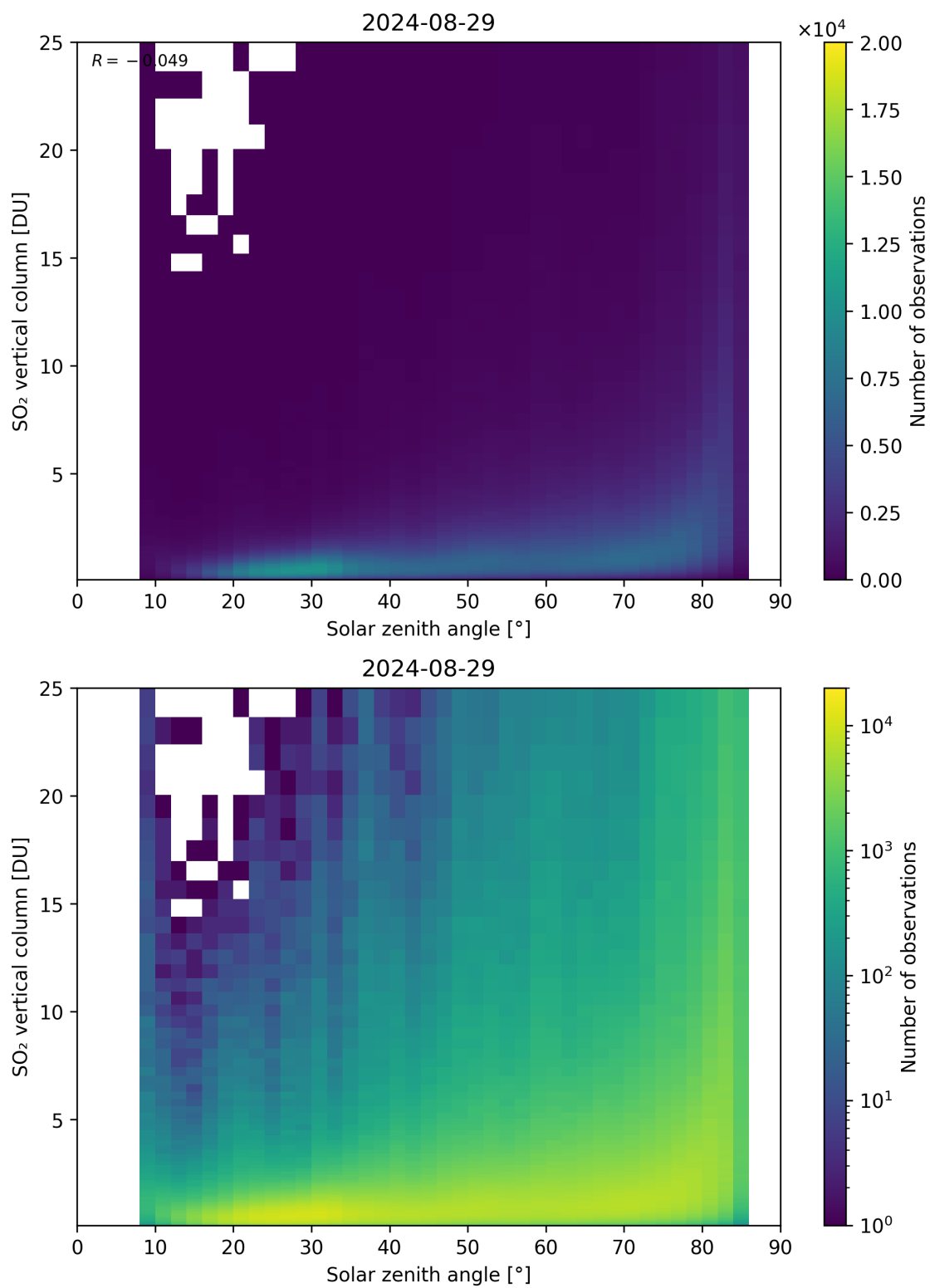
Figure 176: Scatter density plot of “Solar zenith angle” against “SO 2 vertical column” for 2024-08-28 to 2024-08-30.
