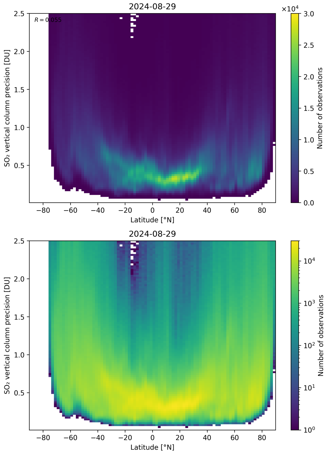
Figure 157: Scatter density plot of “Latitude” against “SO 2 vertical column precision” for 2024-08-28 to 2024-08-30.
