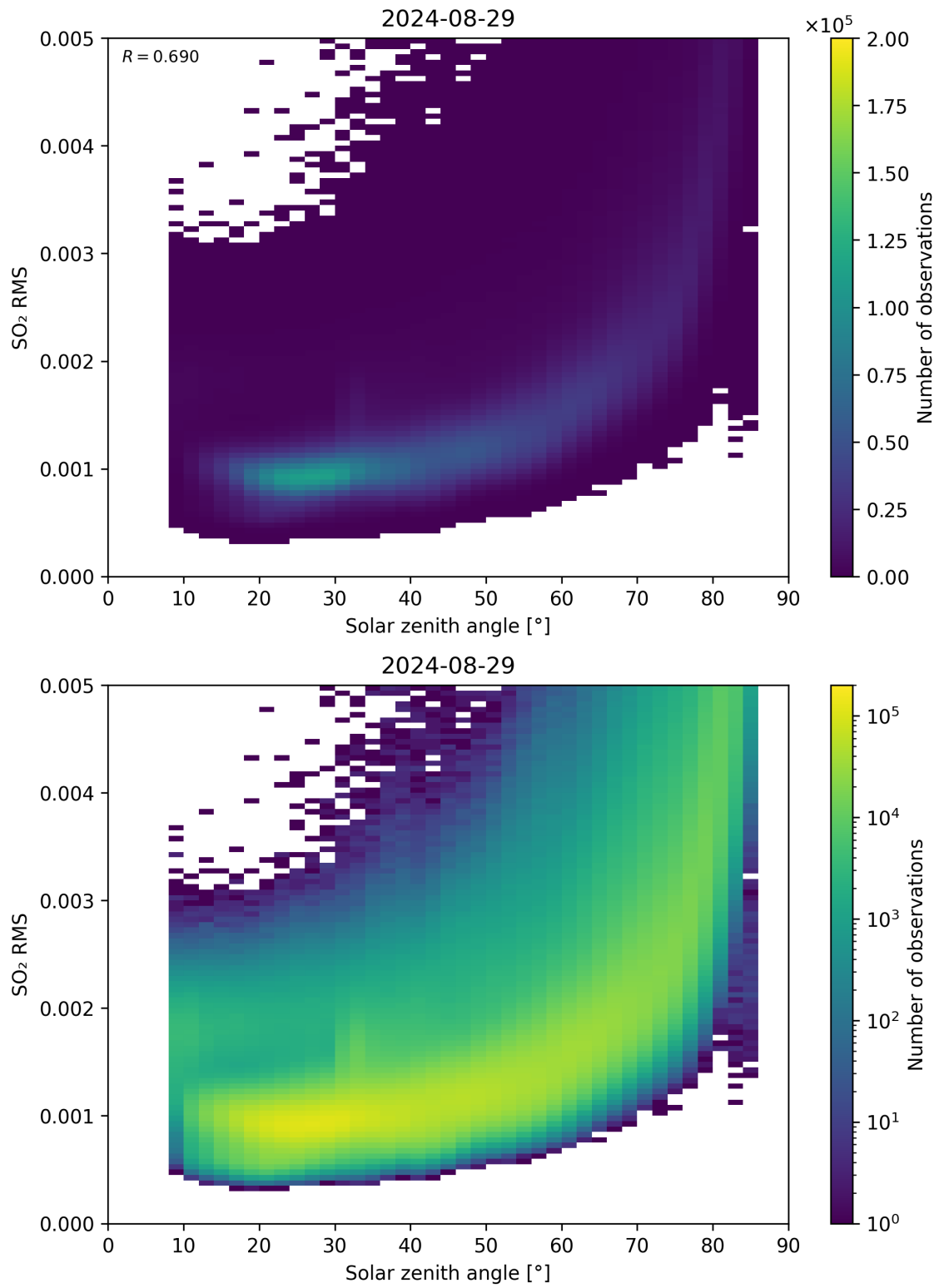
Figure 163: Scatter density plot of “Solar zenith angle” against “SO 2 RMS” for 2024-08-28 to 2024-08-30.
