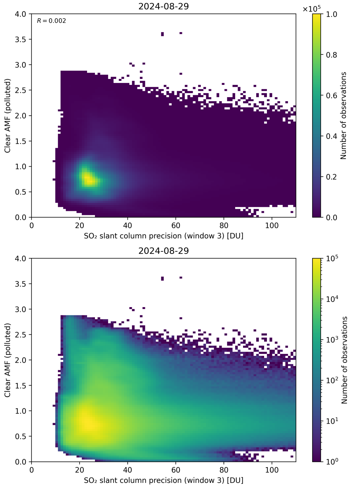
Figure 261: Scatter density plot of “SO 2 slant column precision (window 3)” against “Clear AMF (polluted)” for 2024-08-28 to 2024-08-30.
