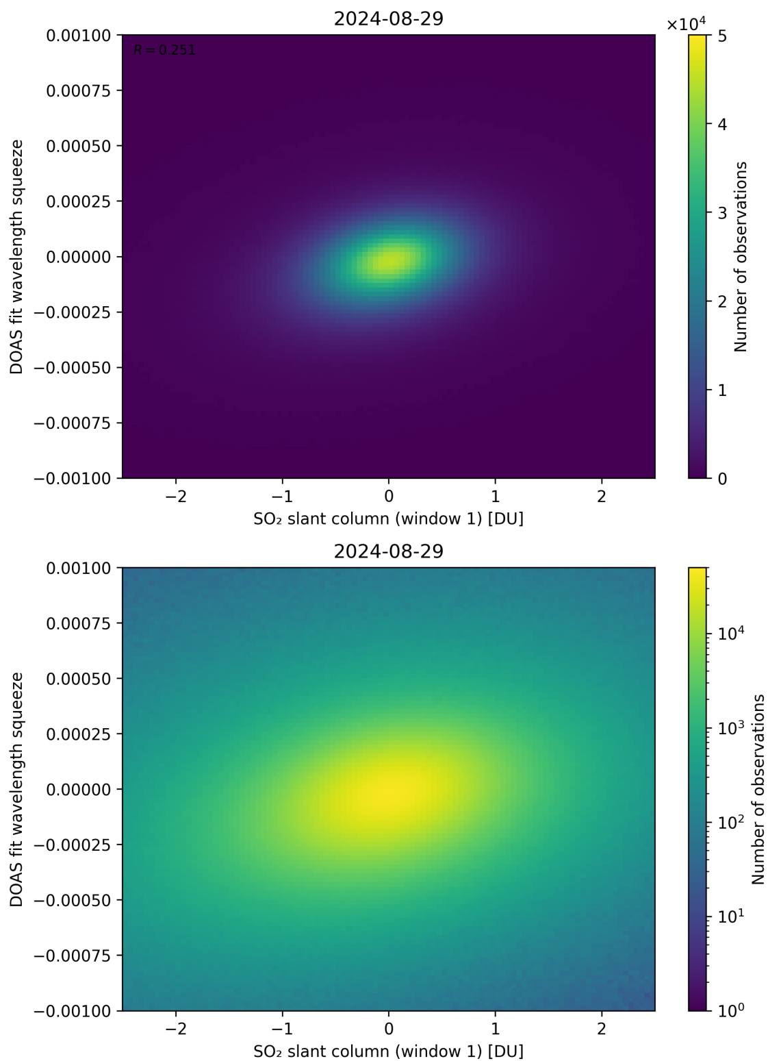
Figure 216: Scatter density plot of “SO 2 slant column (window 1)” against “DOAS fit wavelength squeeze” for 2024-08-28 to 2024-08-30.
