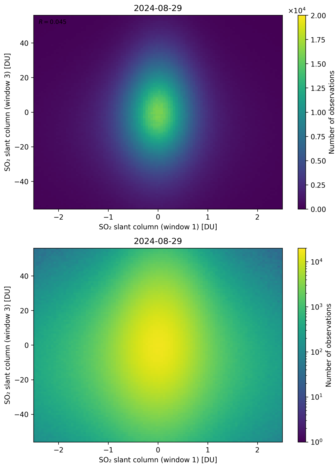
Figure 237: Scatter density plot of “SO 2 slant column (window 1)” against “SO 2 slant column (window 3)” for 2024-08-28 to 2024-08-30.
