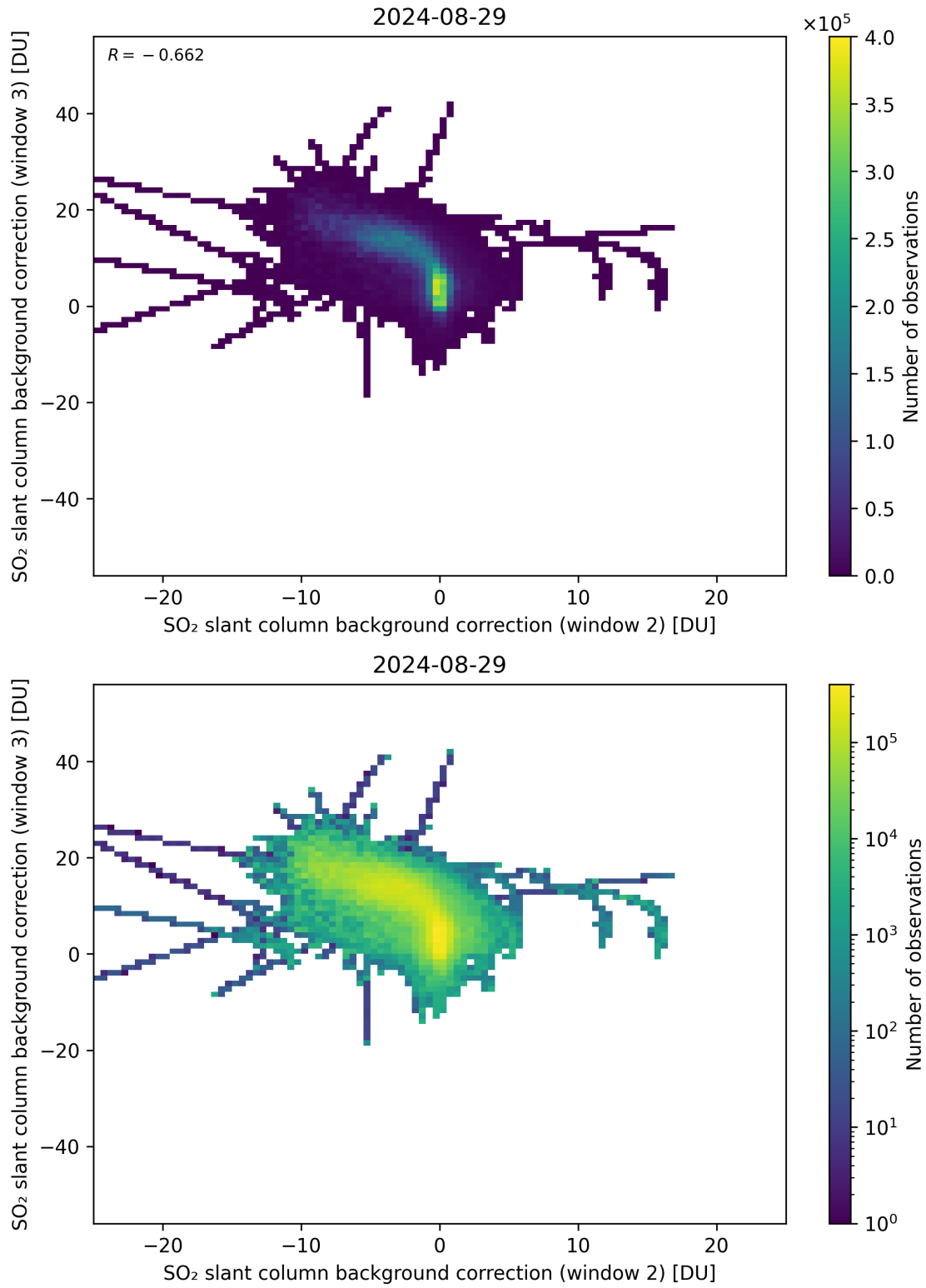
Figure 111: Scatter density plot of “SO 2 slant column background correction (window 2)” against “SO 2 slant column background correction (window 3)” for 2024-08-28 to 2024-08-30.
