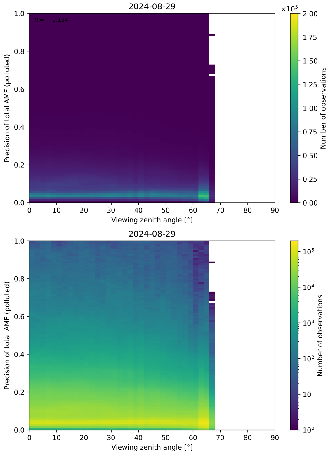
Figure 326: Scatter density plot of “Viewing zenith angle” against “Precision of total AMF (polluted)” for 2024-08-28 to 2024-08-30.
