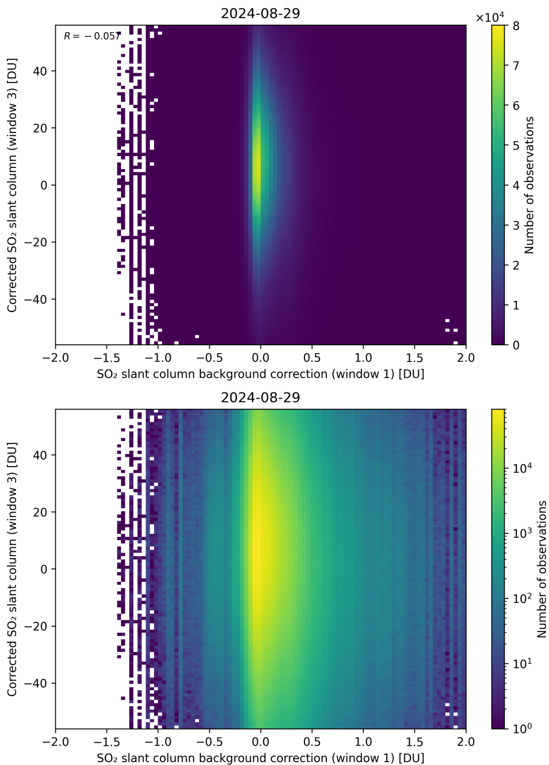
Figure 105: Scatter density plot of “SO 2 slant column background correction (window 1)” against “Corrected SO 2 slant column (window 3)” for 2024-08-28 to 2024-08-30.
