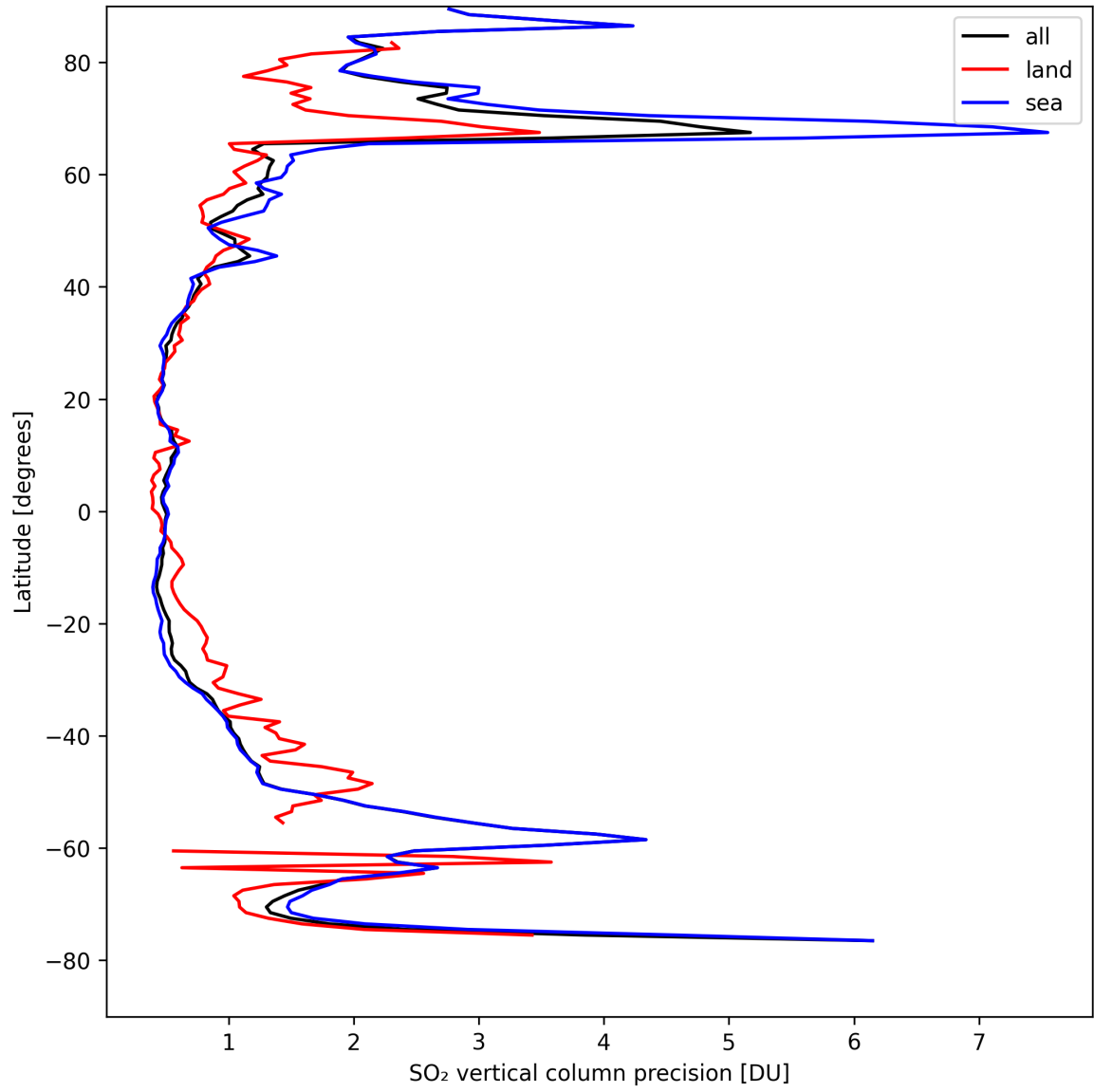
Figure 31: Zonal average of “SO 2 vertical column precision” for 2024-08-28 to 2024-08-30.
