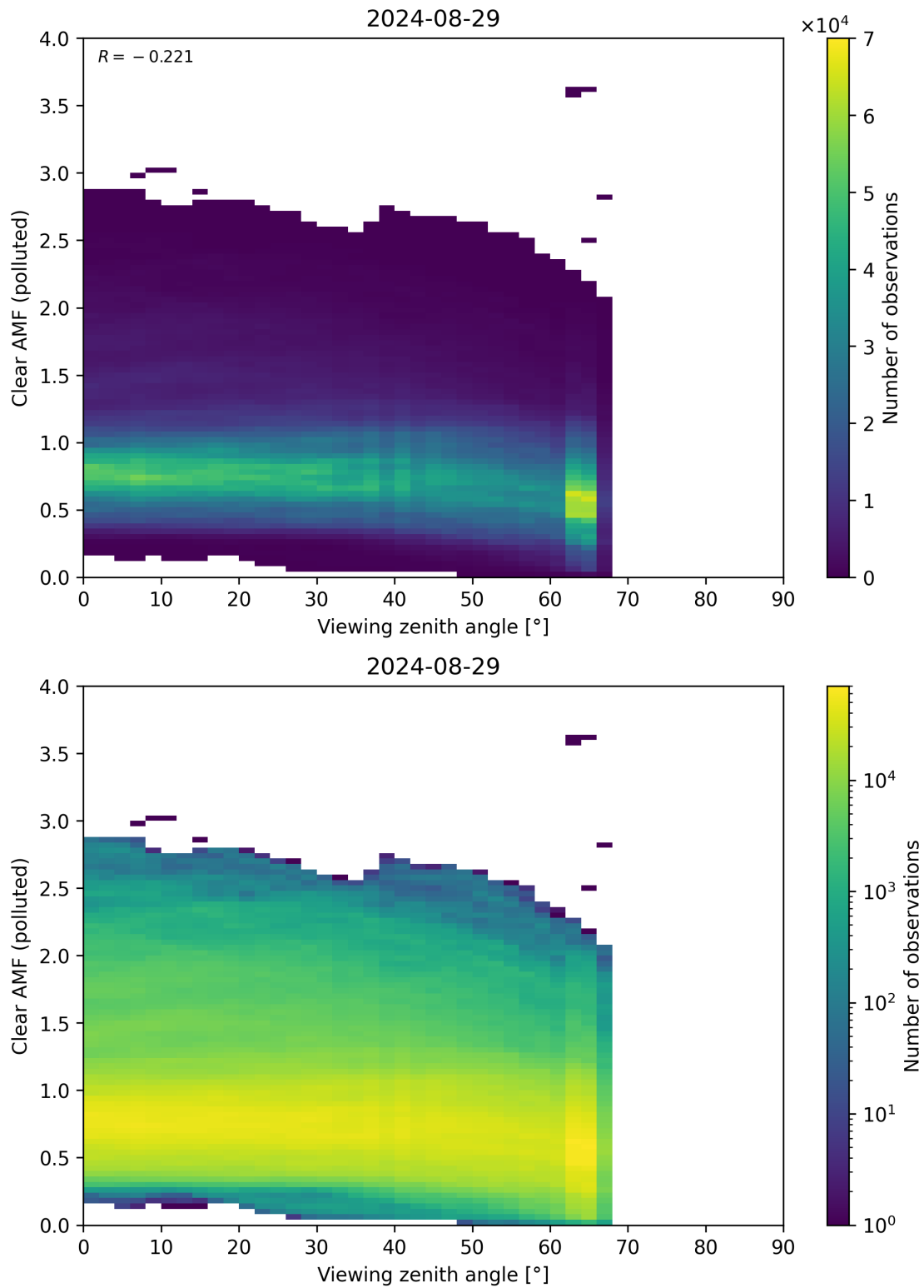
Figure 316: Scatter density plot of “Viewing zenith angle” against “Clear AMF (polluted)” for 2024-08-28 to 2024-08-30.
