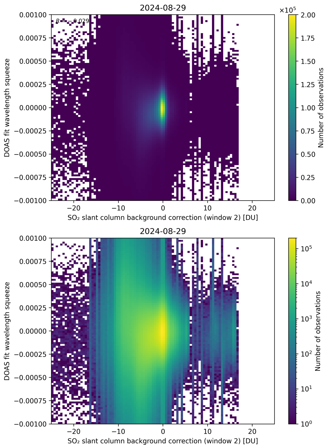
Figure 113: Scatter density plot of “SO 2 slant column background correction (window 2)” against “DOAS fit wavelength squeeze” for 2024-08-28 to 2024-08-30.
