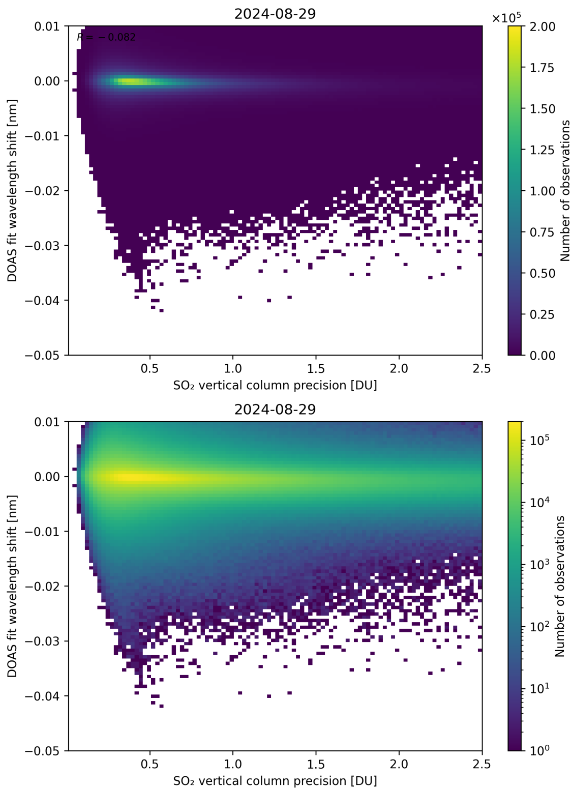
Figure 282: Scatter density plot of “SO 2 vertical column precision” against “DOAS fit wavelength shift” for 2024-08-28 to 2024-08-30.
