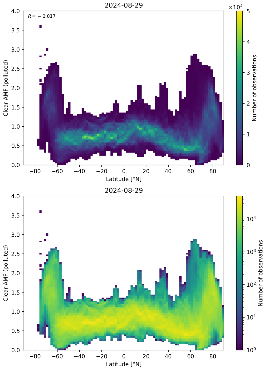
Figure 145: Scatter density plot of “Latitude” against “Clear AMF (polluted)” for 2024-08-28 to 2024-08-30.
