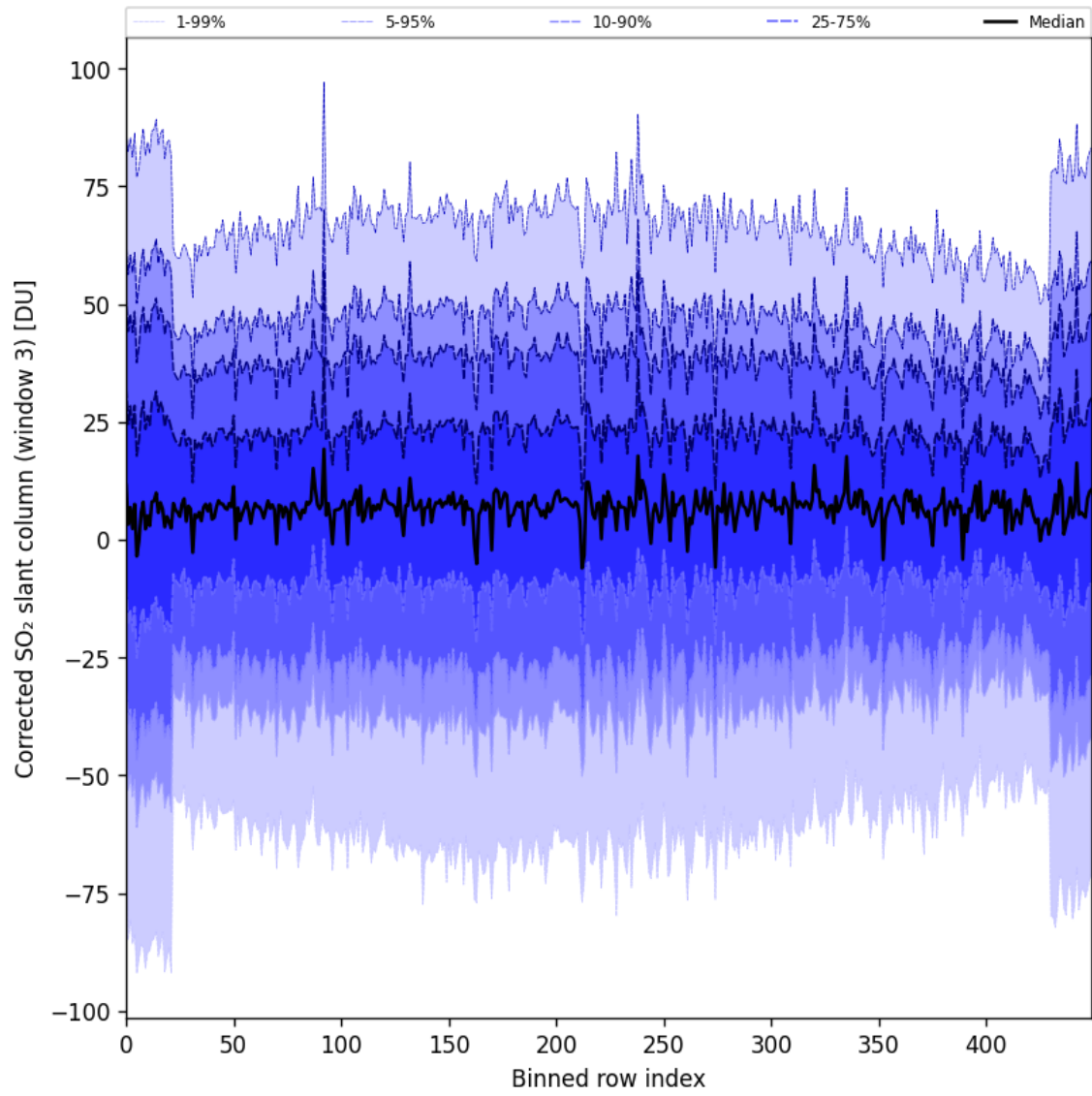
Figure 89: Along track statistics of “Corrected SO 2 slant column (window 3)” for 2024-08-28 to 2024-08-30
