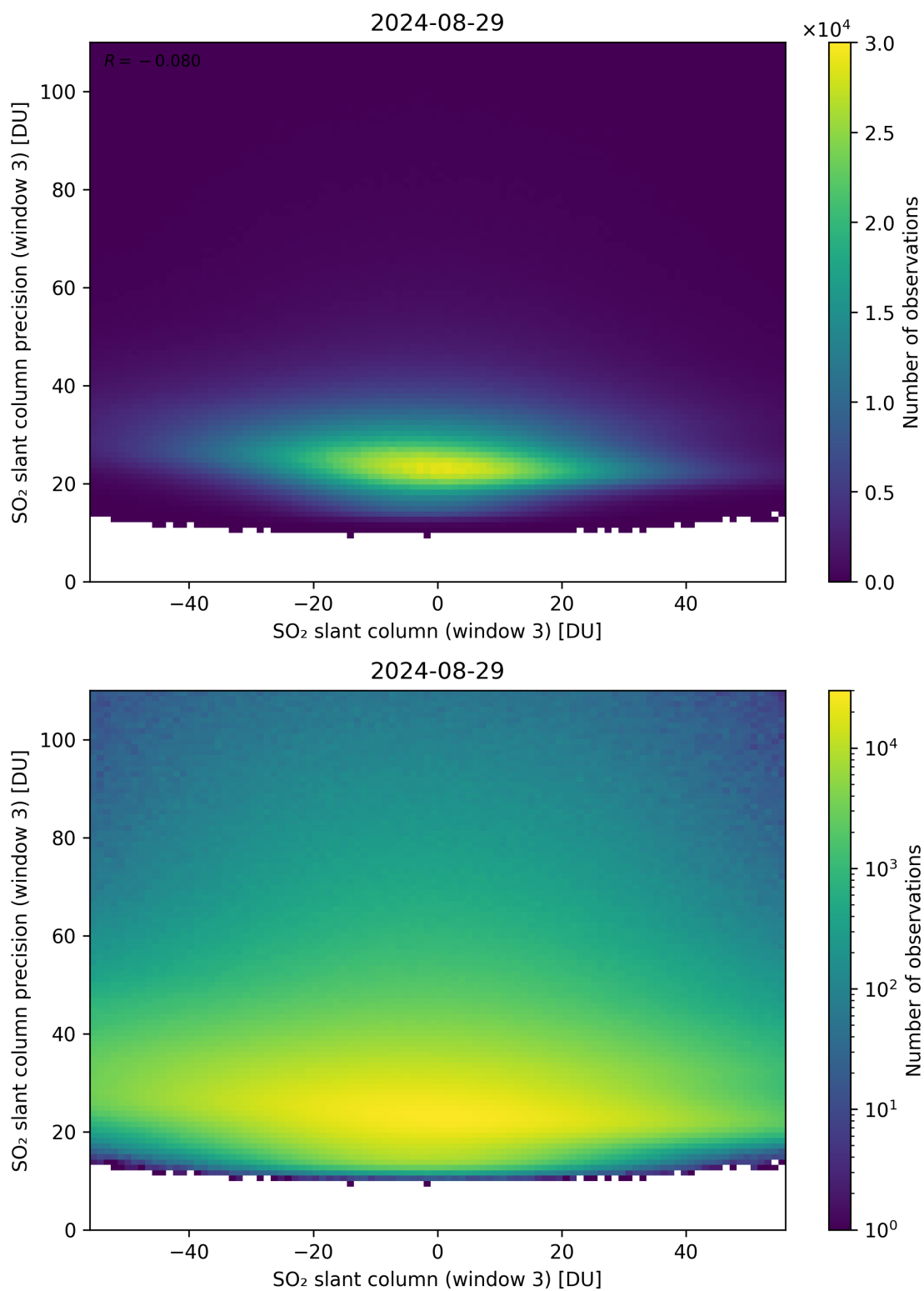
Figure 267: Scatter density plot of “SO 2 slant column (window 3)” against “SO 2 slant column precision (window 3)” for 2024-08-28 to 2024-08-30.
