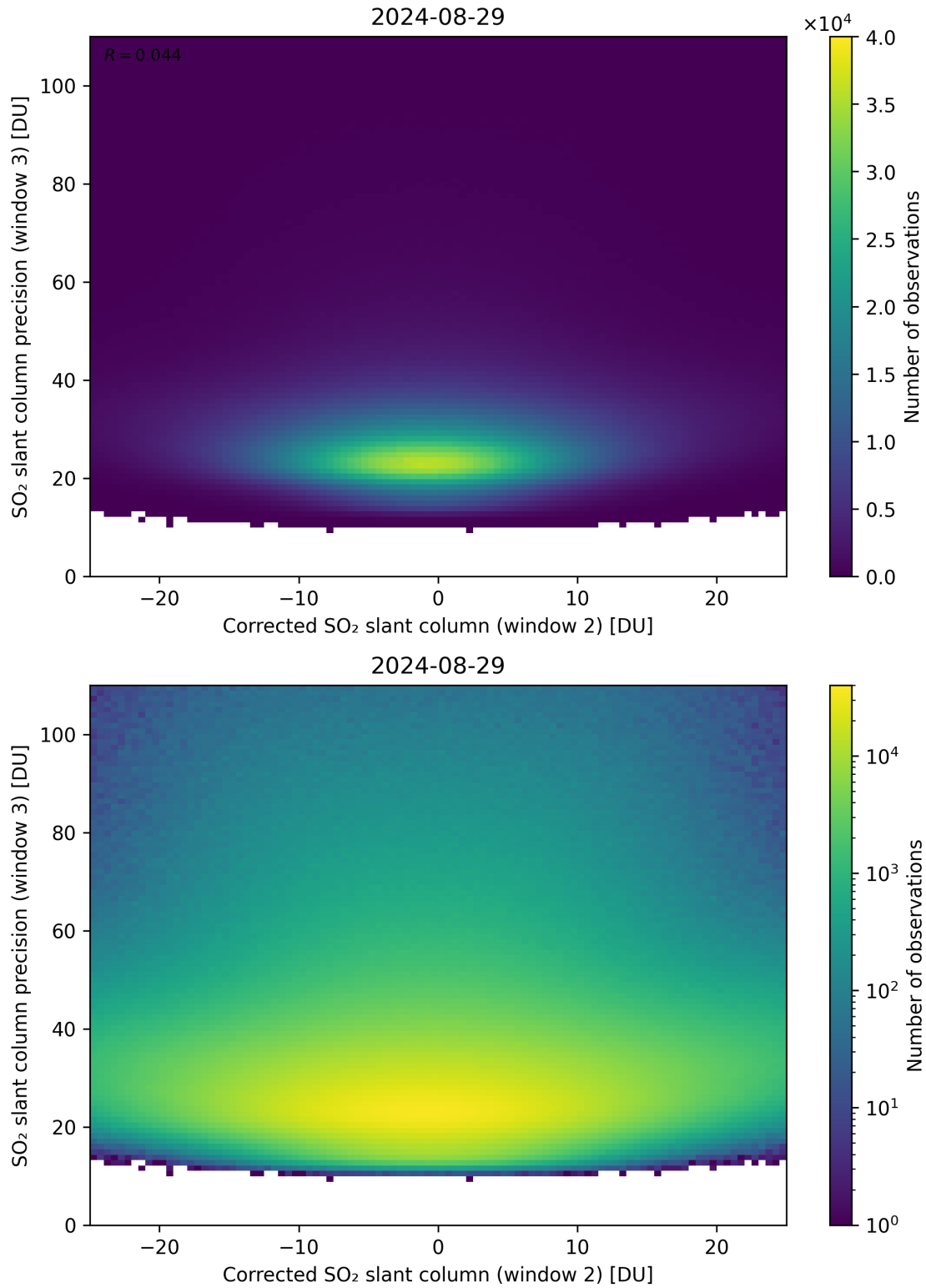
Figure 202: Scatter density plot of “Corrected SO 2 slant column (window 2)” against “SO 2 slant column precision (window 3)” for 2024-08-28 to 2024-08-30.
