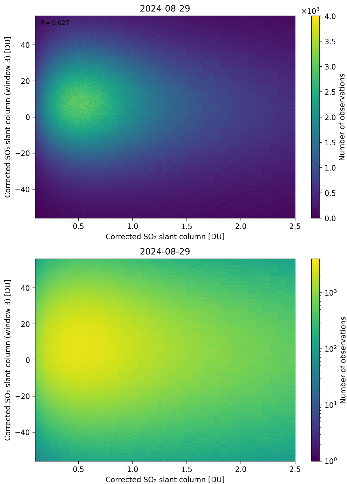
Figure 186: Scatter density plot of “Corrected SO 2 slant column” against “Corrected SO 2 slant column (window 3)” for 2024-08-28 to 2024-08-30.
