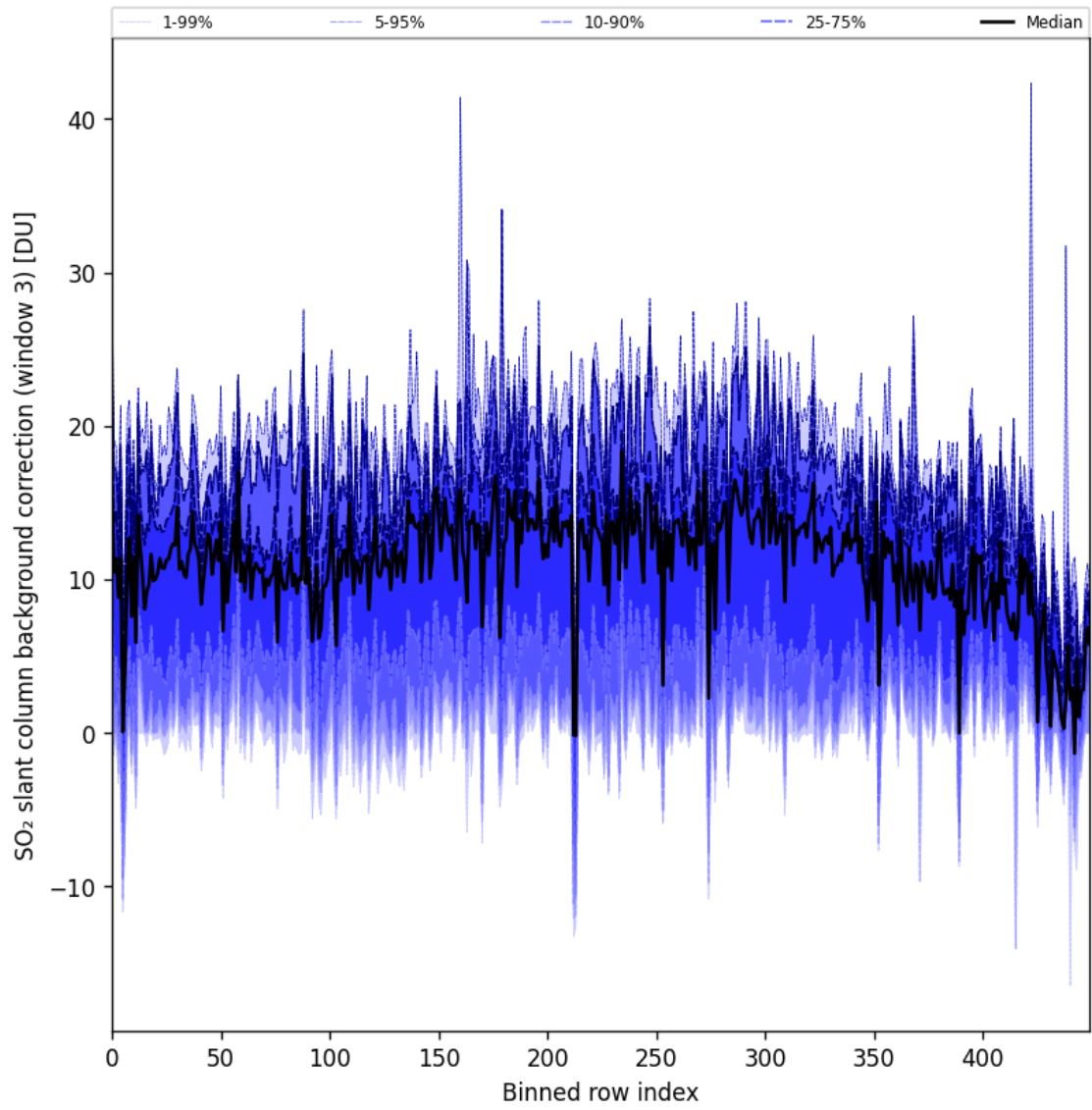
Figure 90: Along track statistics of “SO 2 slant column background correction (window 3)” for 2024-08-28 to 2024-08-30
