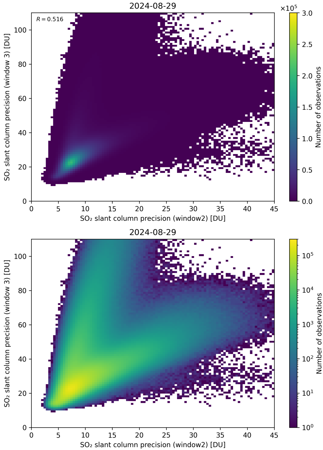
Figure 250: Scatter density plot of “SO 2 slant column precision (window2)” against “SO 2 slant column precision (window 3)” for 2024-08-28 to 2024-08-30.
