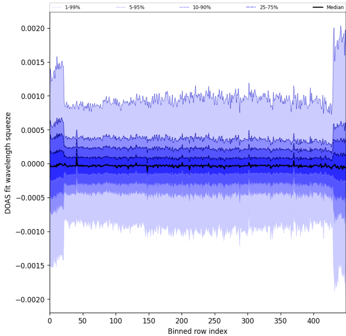
Figure 92: Along track statistics of “DOAS fit wavelength squeeze” for 2024-08-28 to 2024-08-30
