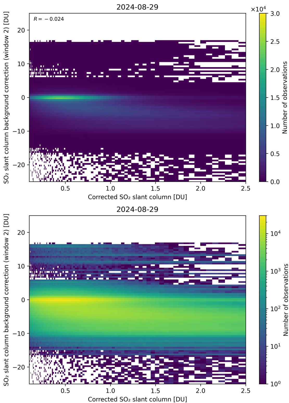
Figure 179: Scatter density plot of “Corrected SO 2 slant column” against “SO 2 slant column background correction (window 2)” for 2024-08-28 to 2024-08-30.
