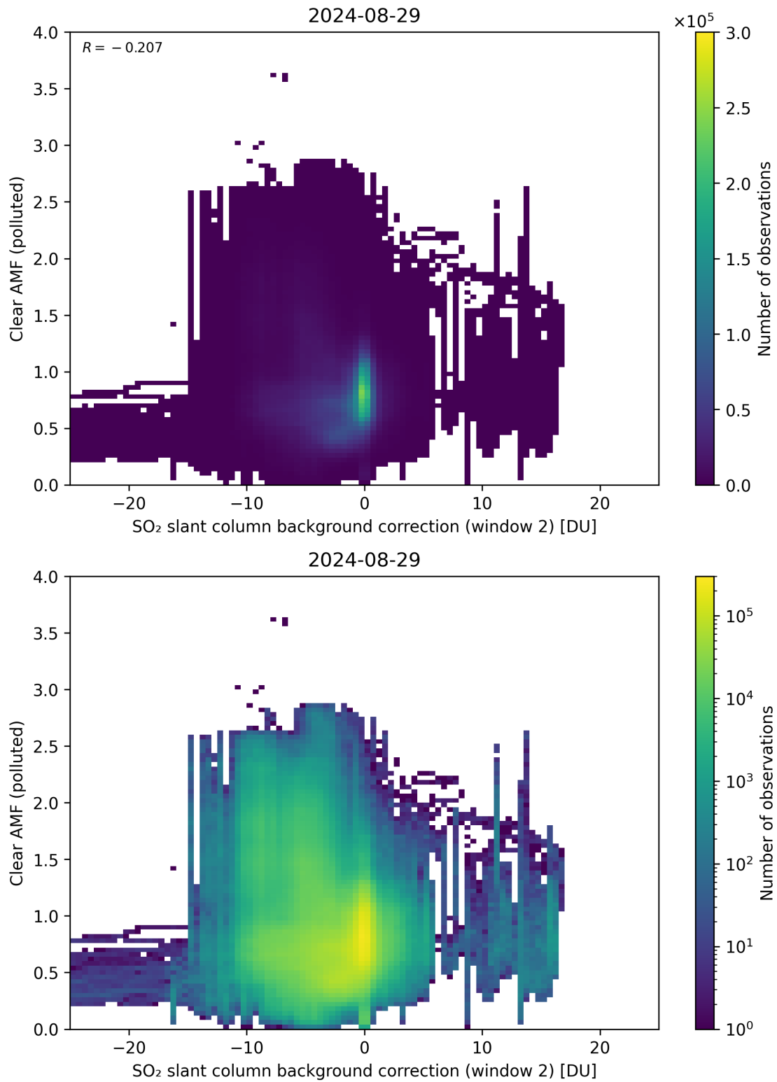
Figure 115: Scatter density plot of “SO 2 slant column background correction (window 2)” against “Clear AMF (polluted)” for 2024-08-28 to 2024-08-30.
