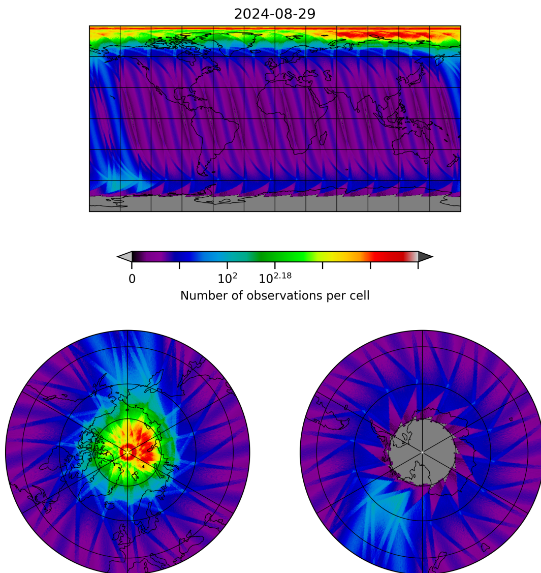
Figure 28: Map of the number of observations for 2024-08-28 to 2024-08-30
