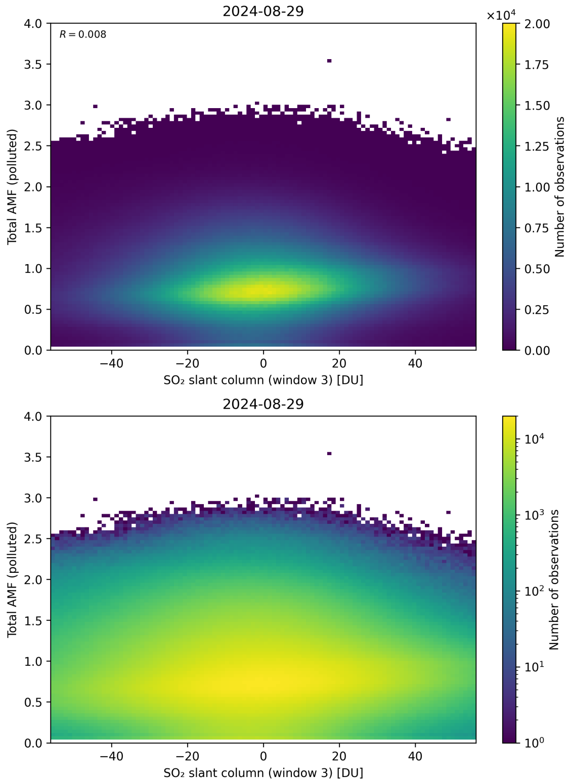
Figure 268: Scatter density plot of “SO 2 slant column (window 3)” against “Total AMF (polluted)” for 2024-08-28 to 2024-08-30.
