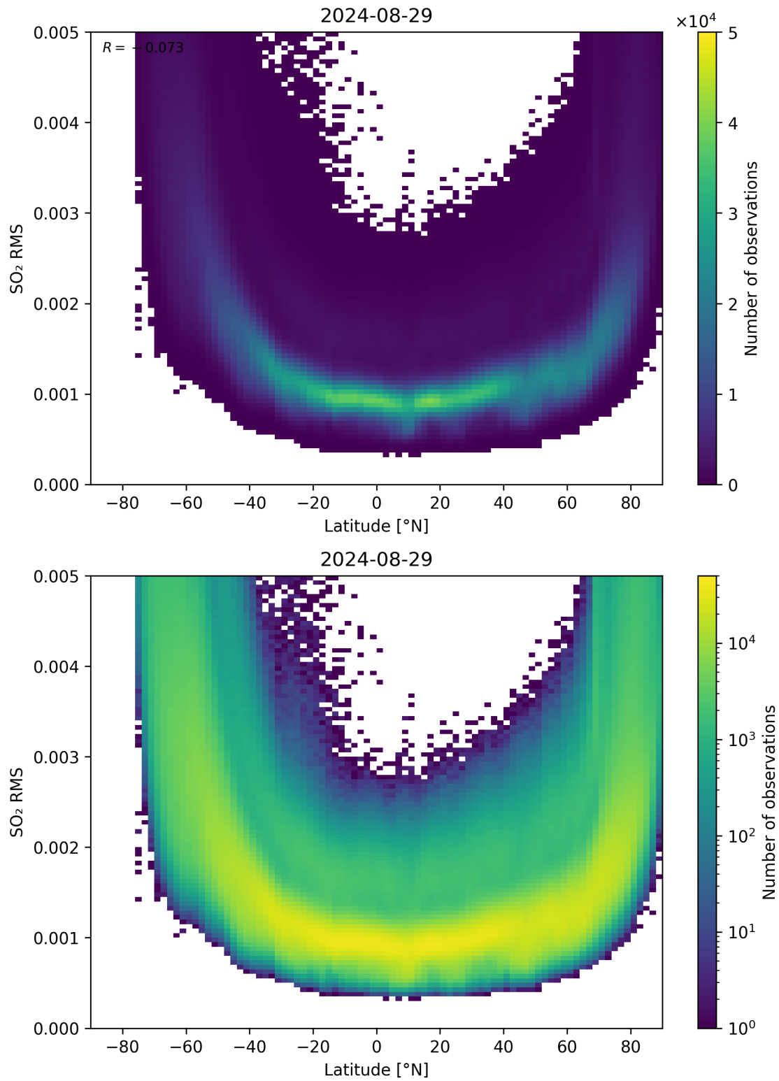
Figure 144: Scatter density plot of “Latitude” against “SO 2 RMS” for 2024-08-28 to 2024-08-30.
