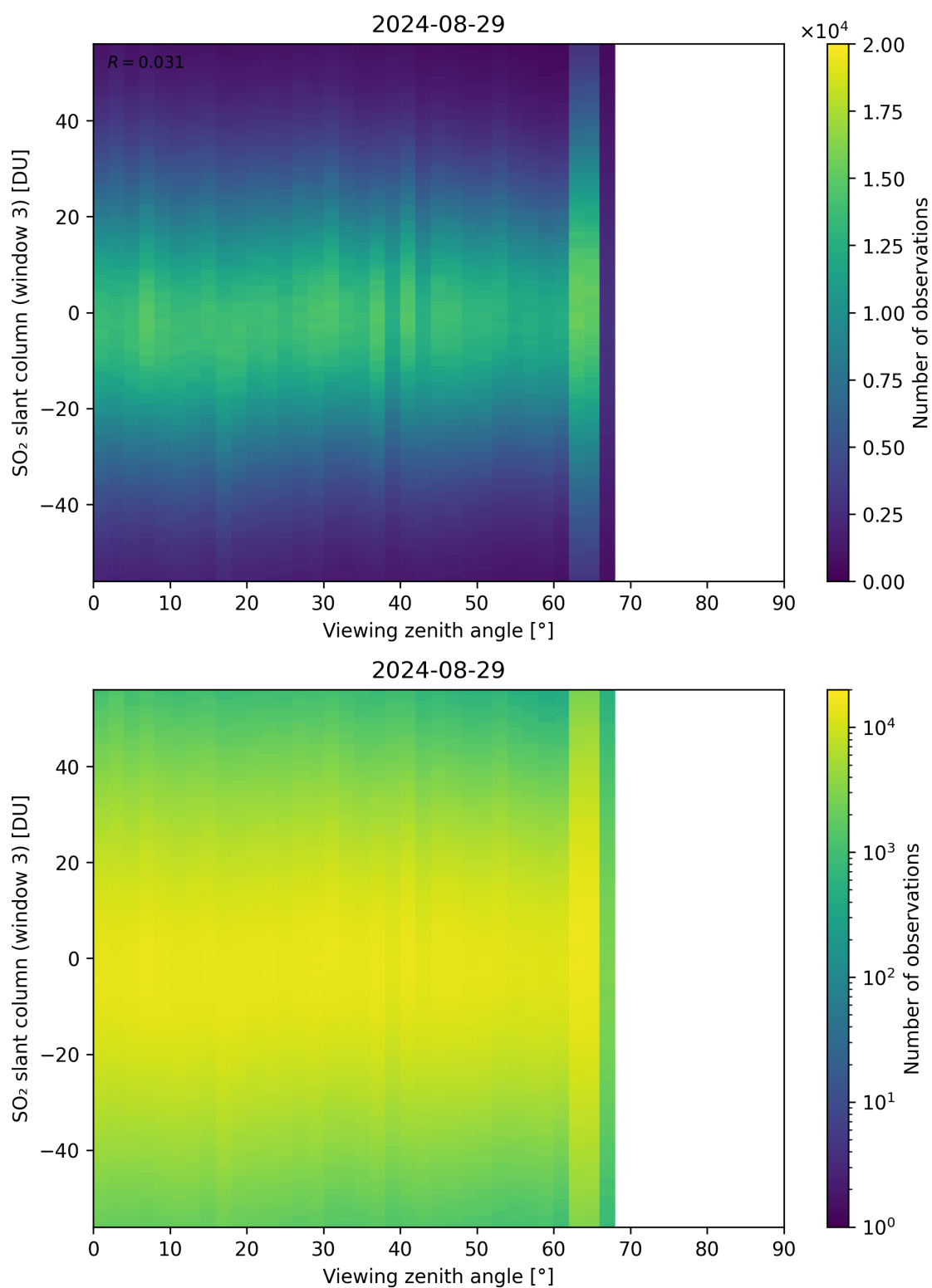
Figure 323: Scatter density plot of “Viewing zenith angle” against “SO 2 slant column (window 3)” for 2024-08-28 to 2024-08-30.
