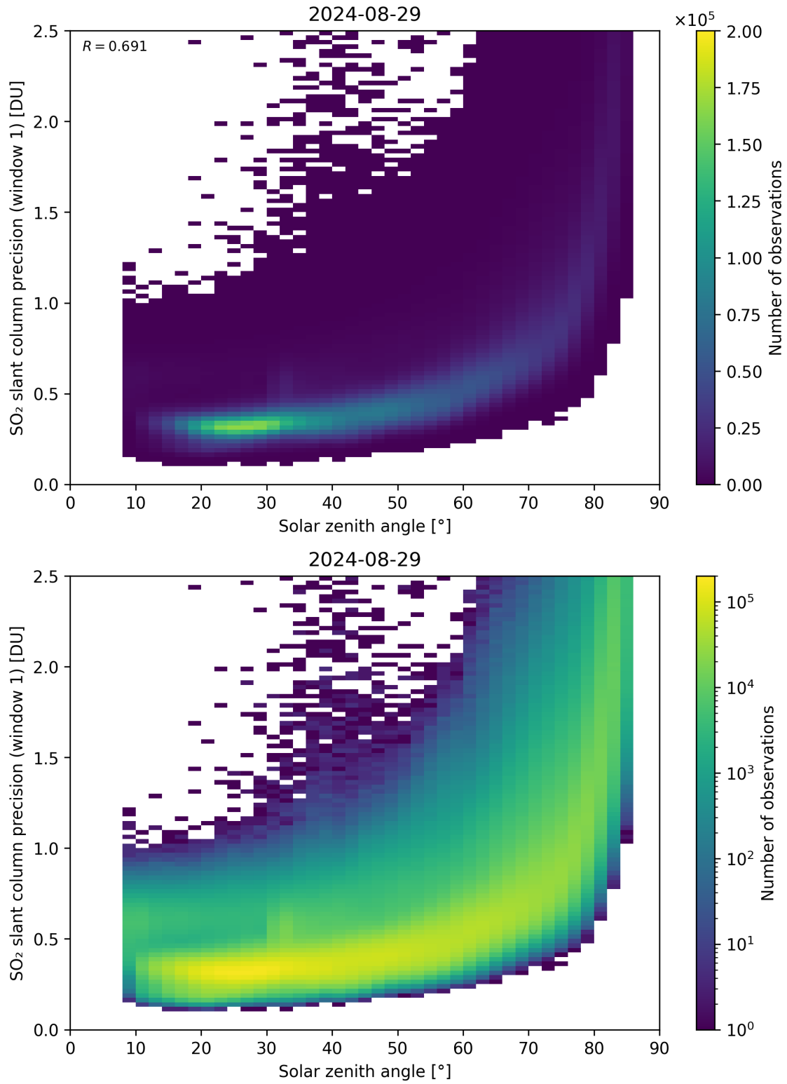
Figure 170: Scatter density plot of “Solar zenith angle” against “SO 2 slant column precision (window 1)” for 2024-08-28 to 2024-08-30.
