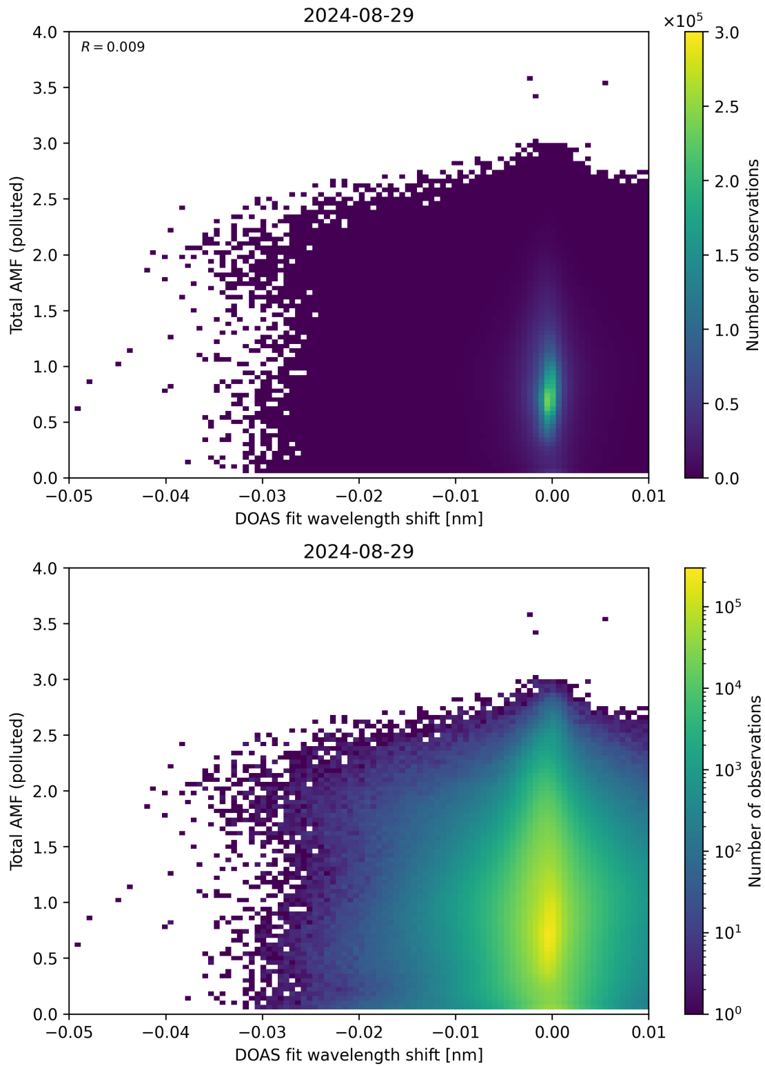
Figure 130: Scatter density plot of “DOAS fit wavelength shift” against “Total AMF (polluted)” for 2024-08-28 to 2024-08-30.
