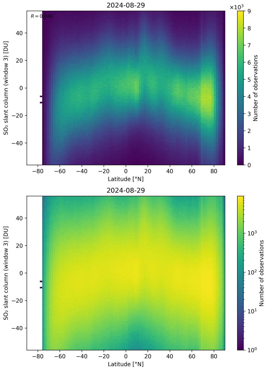
Figure 152: Scatter density plot of “Latitude” against “SO 2 slant column (window 3)” for 2024-08-28 to 2024-08-30.
