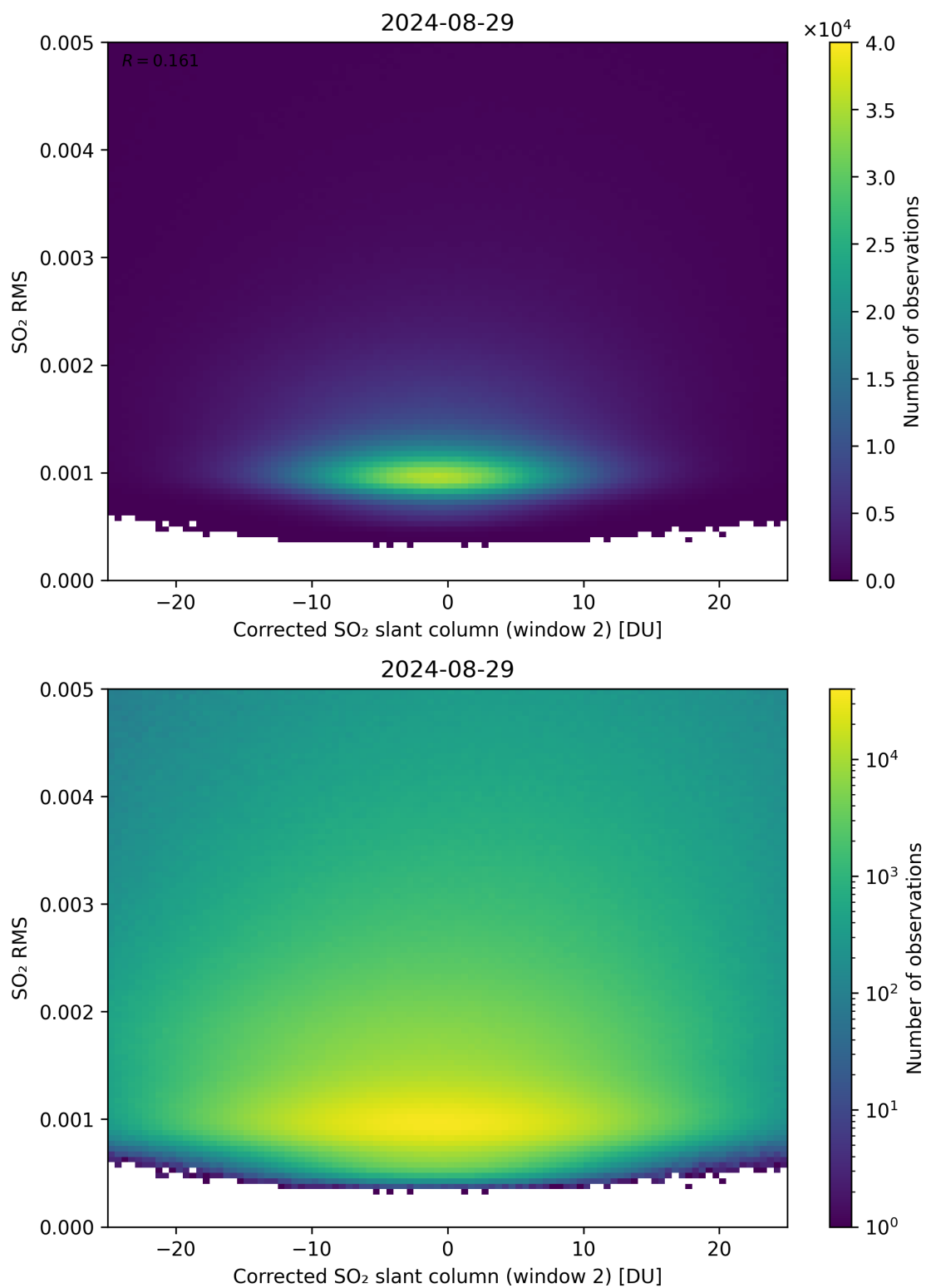
Figure 198: Scatter density plot of “Corrected SO 2 slant column (window 2)” against “SO 2 RMS” for 2024-08-28 to 2024-08-30.
