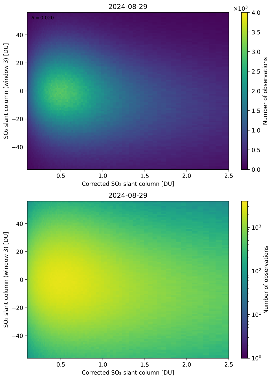
Figure 190: Scatter density plot of “Corrected SO 2 slant column” against “SO 2 slant column (window 3)” for 2024-08-28 to 2024-08-30.
