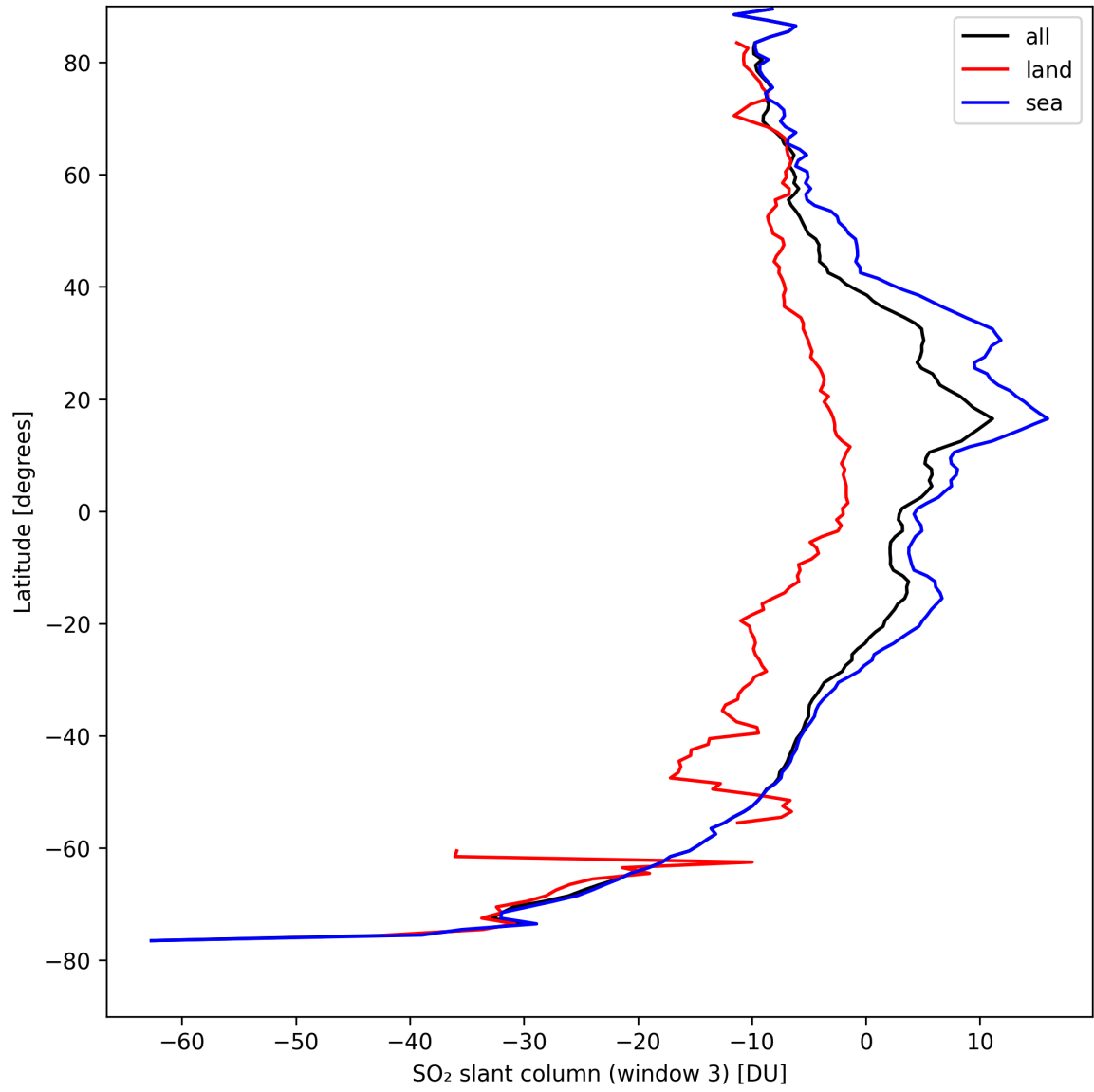
Figure 41: Zonal average of “SO 2 slant column (window 3)” for 2024-08-28 to 2024-08-30.
