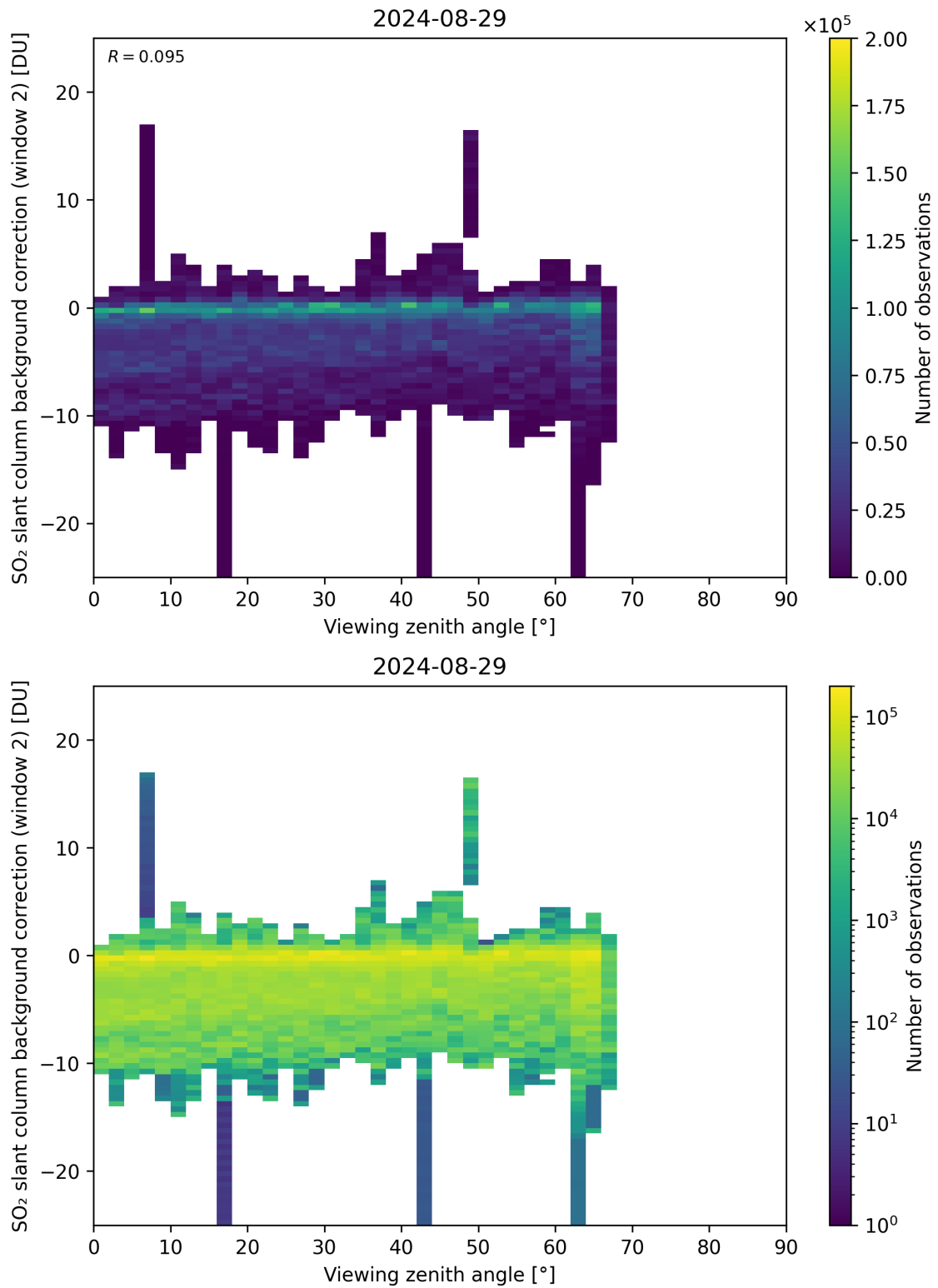
Figure 309: Scatter density plot of “Viewing zenith angle” against “SO 2 slant column background correction (window 2)” for 2024-08-28 to 2024-08-30.
