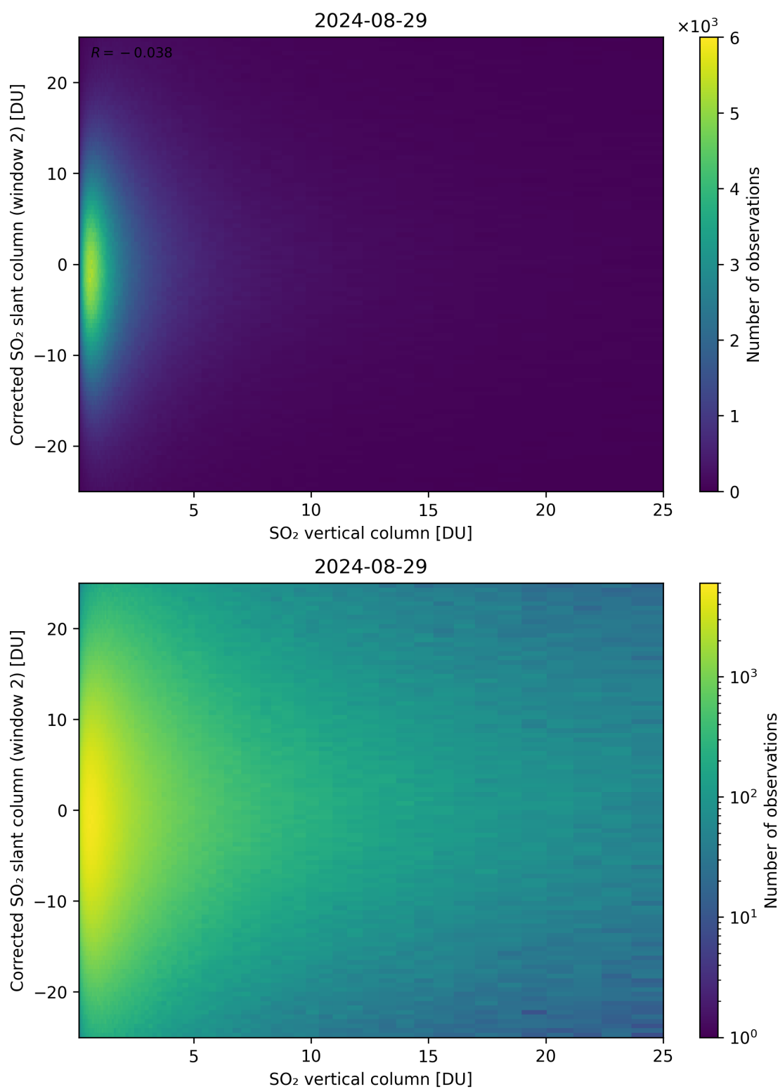
Figure 298: Scatter density plot of “SO 2 vertical column” against “Corrected SO 2 slant column (window 2)” for 2024-08-28 to 2024-08-30.
