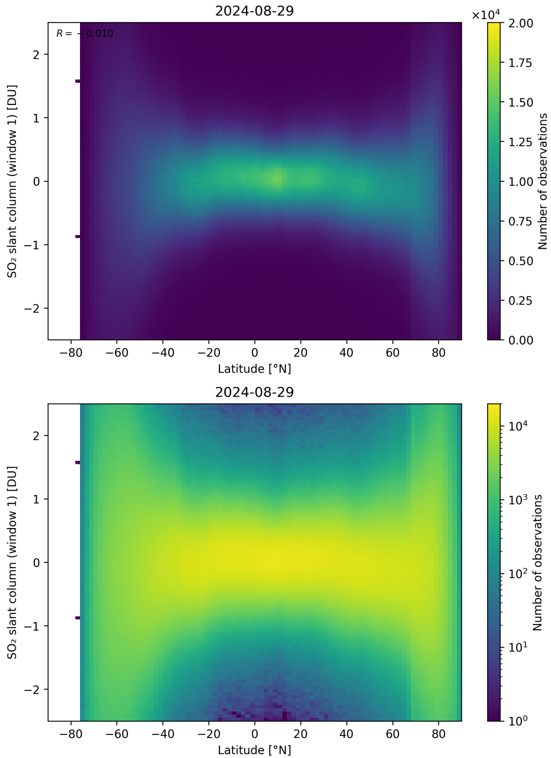
Figure 149: Scatter density plot of “Latitude” against “SO 2 slant column (window 1)” for 2024-08-28 to 2024-08-30.
