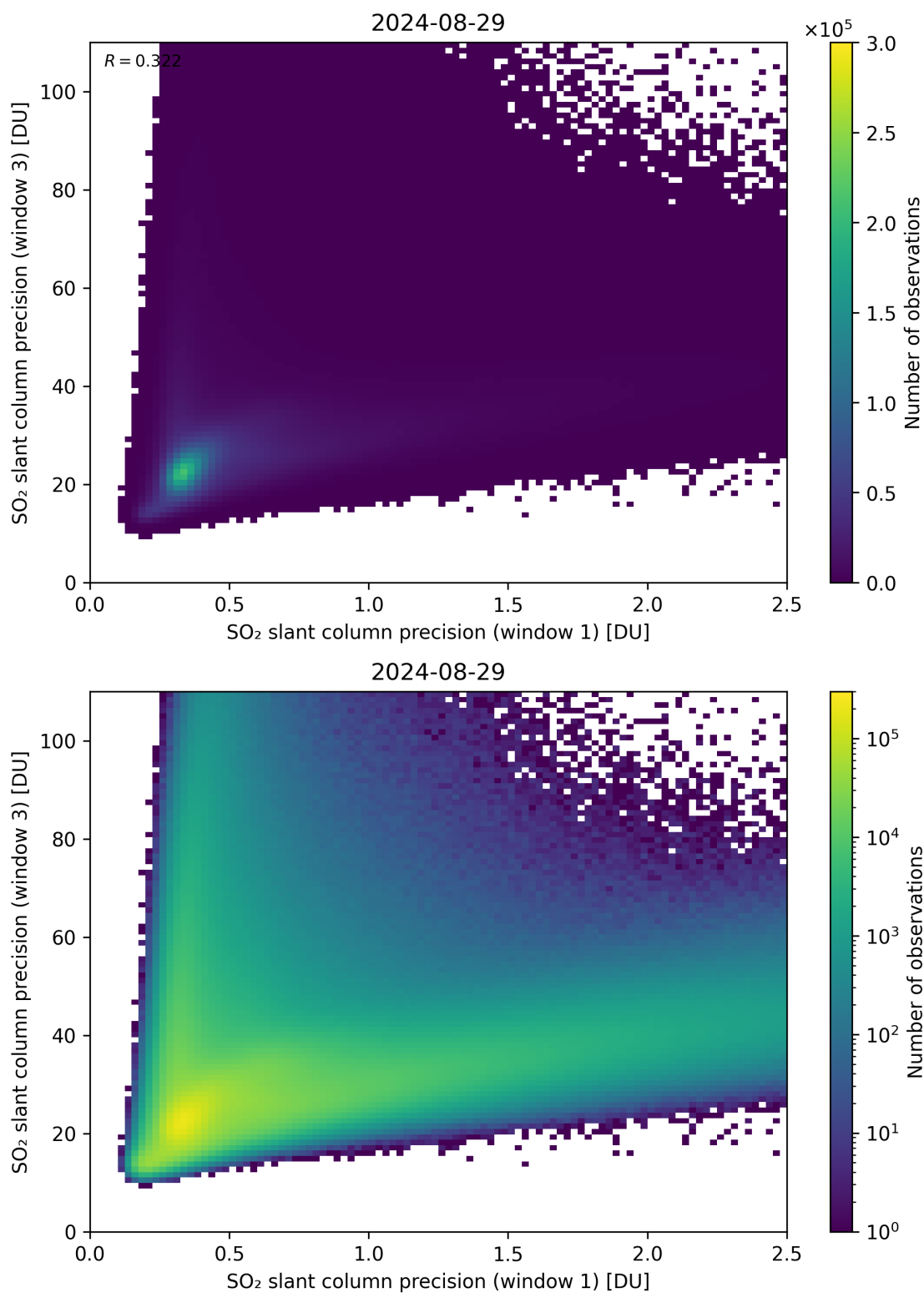
Figure 229: Scatter density plot of “SO 2 slant column precision (window 1)” against “SO 2 slant column precision (window 3)” for 2024-08-28 to 2024-08-30.
