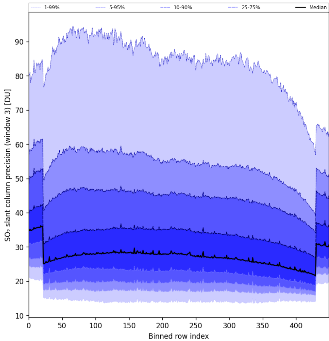
Figure 88: Along track statistics of “SO 2 slant column precision (window 3)” for 2024-08-28 to 2024-08-30
