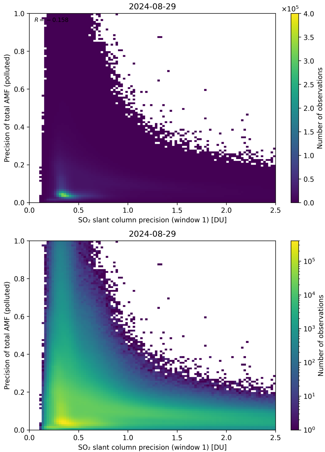
Figure 231: Scatter density plot of “SO 2 slant column precision (window 1)” against “Precision of total AMF (polluted)” for 2024-08-28 to 2024-08-30.
