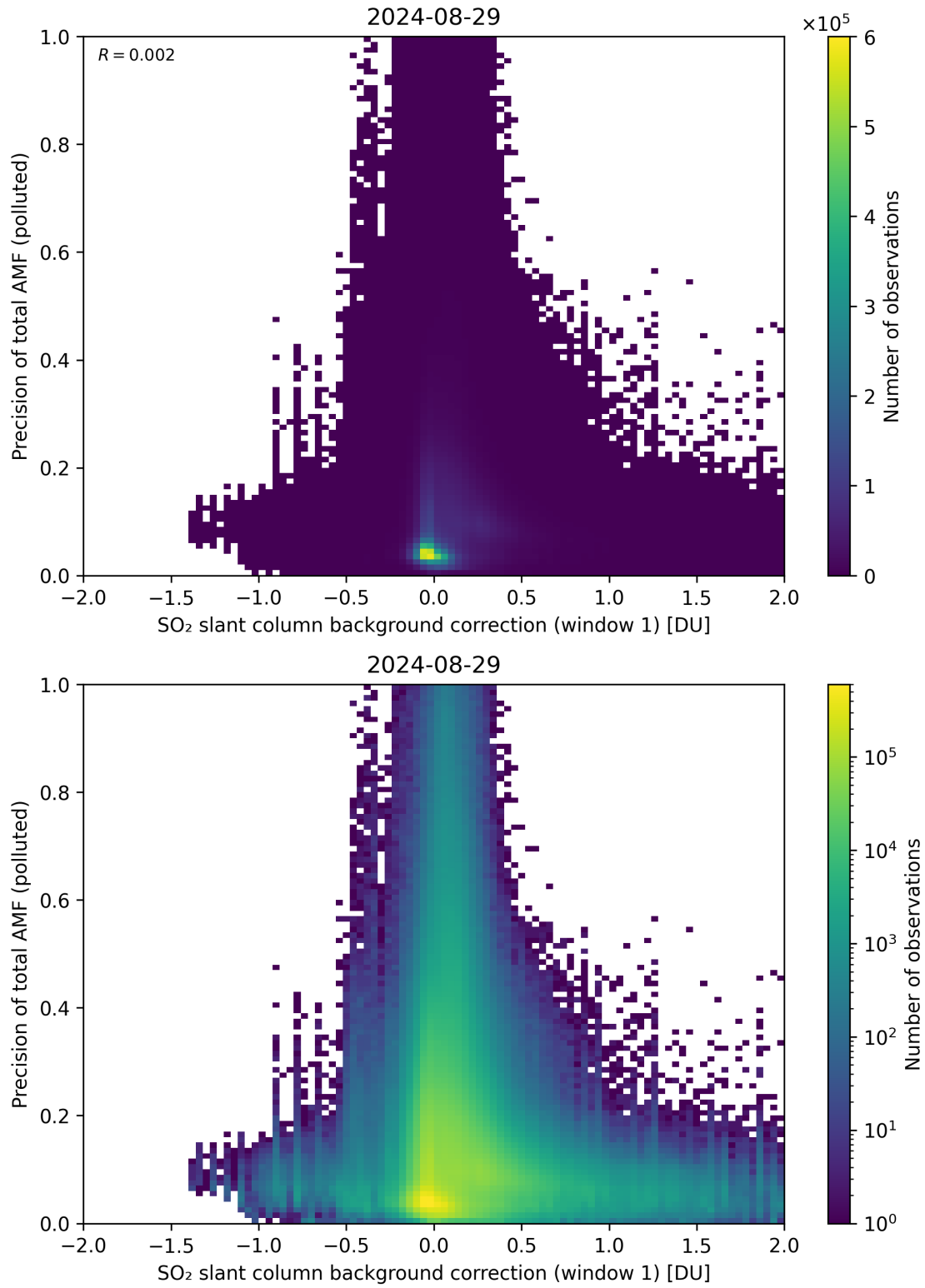
Figure 110: Scatter density plot of “SO 2 slant column background correction (window 1)” against “Precision of total AMF (polluted)” for 2024-08-28 to 2024-08-30.
