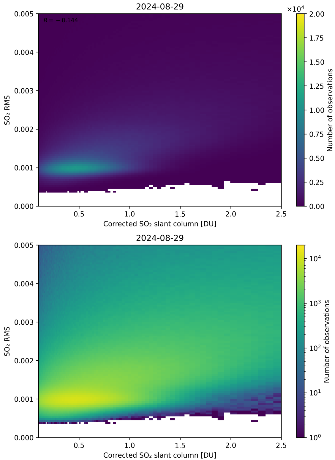
Figure 183: Scatter density plot of “Corrected SO 2 slant column” against “SO 2 RMS” for 2024-08-28 to 2024-08-30.
