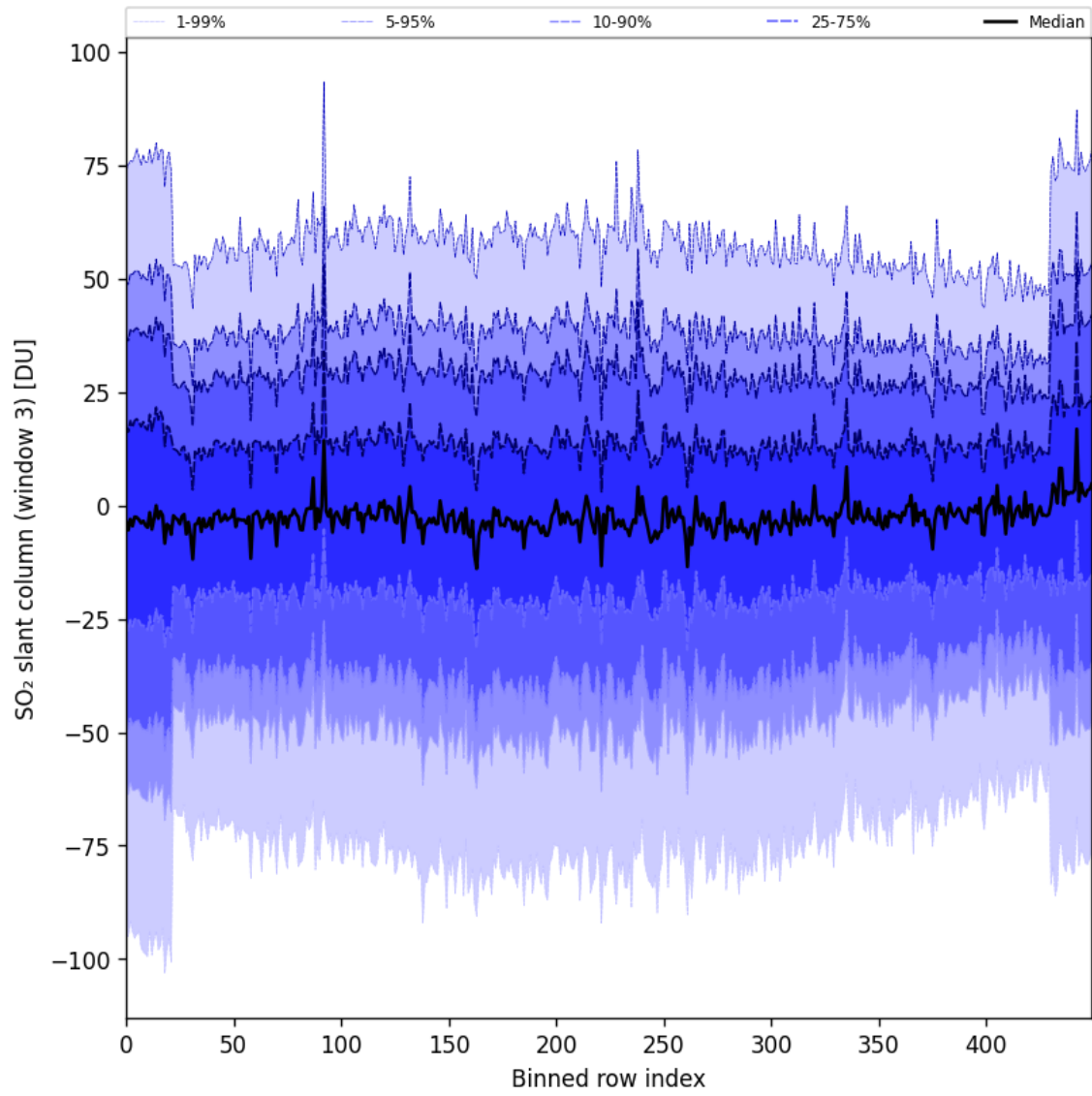
Figure 87: Along track statistics of “SO 2 slant column (window 3)” for 2024-08-28 to 2024-08-30
