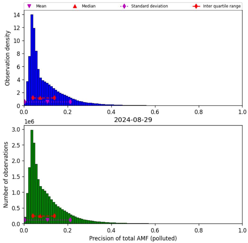
Figure 72: Histogram of “Precision of total AMF (polluted)” for 2024-08-28 to 2024-08-30
