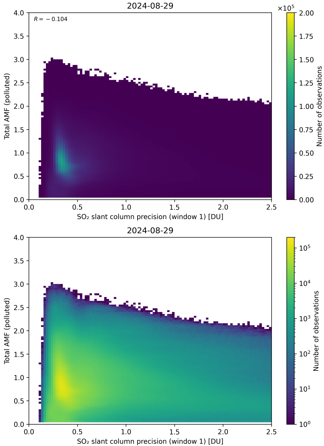
Figure 230: Scatter density plot of “SO 2 slant column precision (window 1)” against “Total AMF (polluted)” for 2024-08-28 to 2024-08-30.
