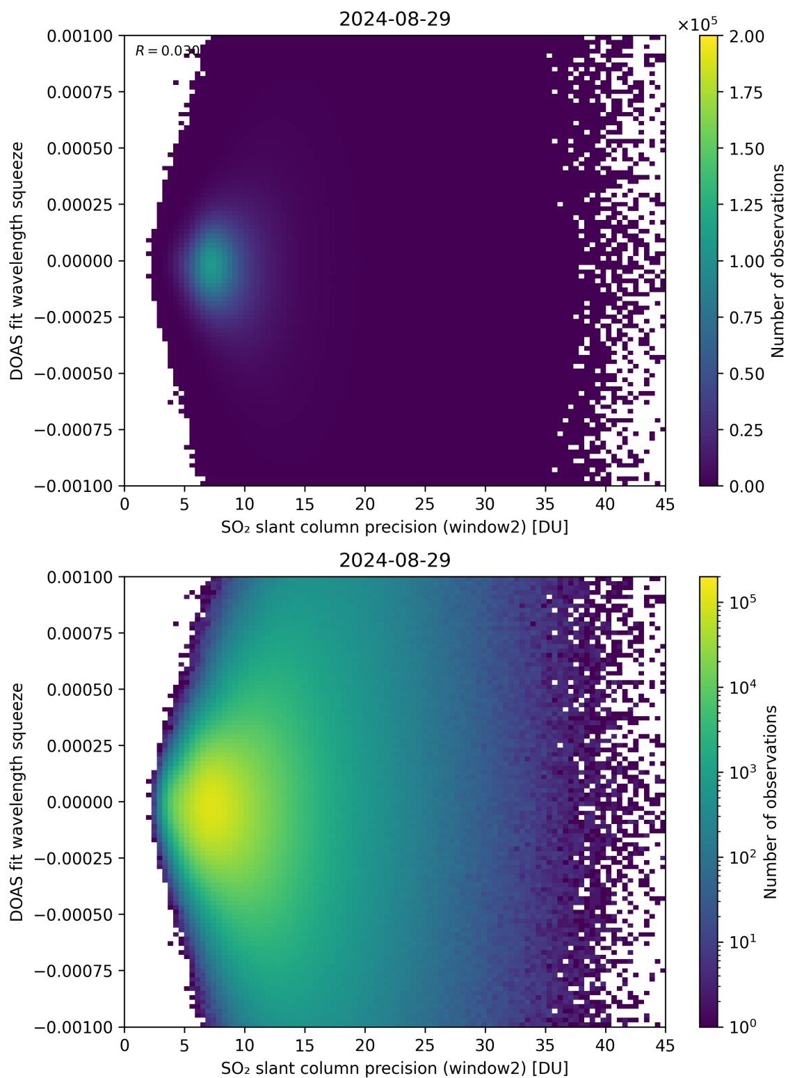
Figure 244: Scatter density plot of “SO 2 slant column precision (window2)” against “DOAS fit wavelength squeeze” for 2024-08-28 to 2024-08-30.
