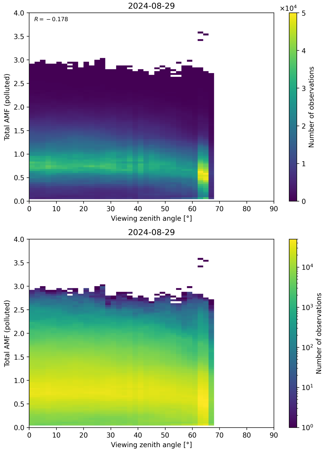
Figure 325: Scatter density plot of “Viewing zenith angle” against “Total AMF (polluted)” for 2024-08-28 to 2024-08-30.
