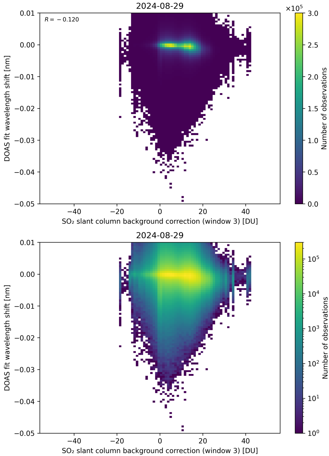
Figure 121: Scatter density plot of “SO 2 slant column background correction (window 3)” against “DOAS fit wavelength shift” for 2024-08-28 to 2024-08-30.
