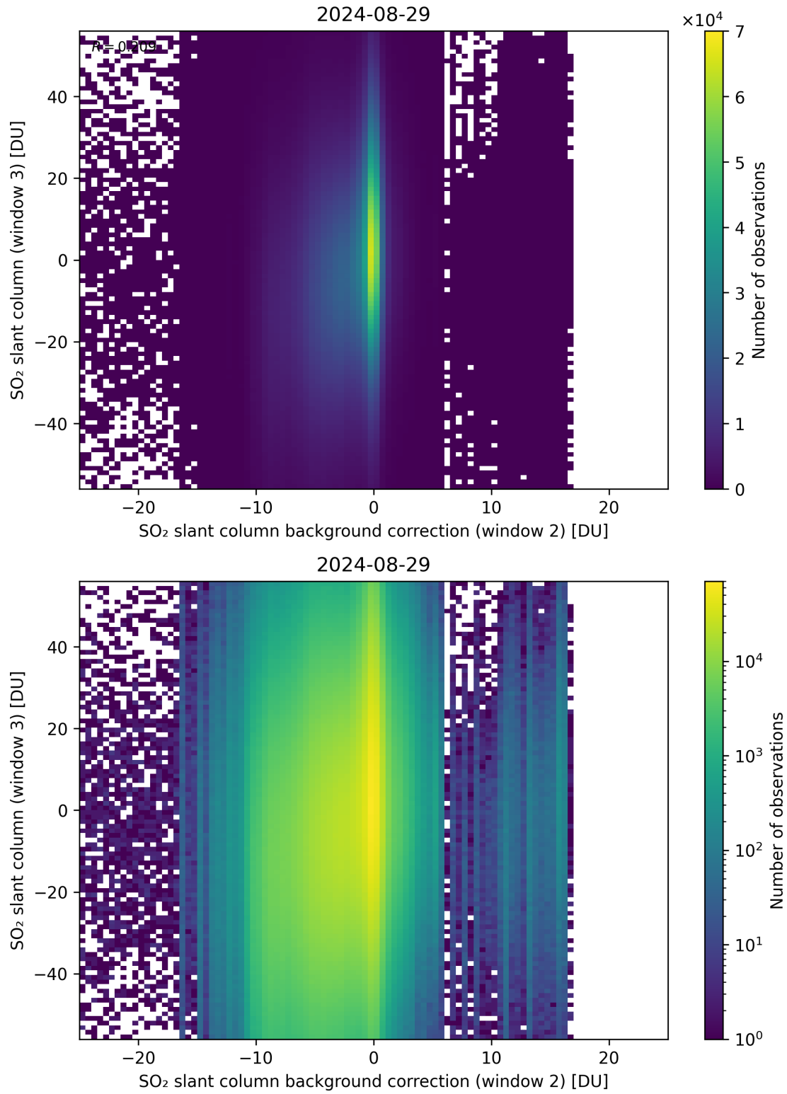
Figure 117: Scatter density plot of “SO 2 slant column background correction (window 2)” against “SO 2 slant column (window 3)” for 2024-08-28 to 2024-08-30.
