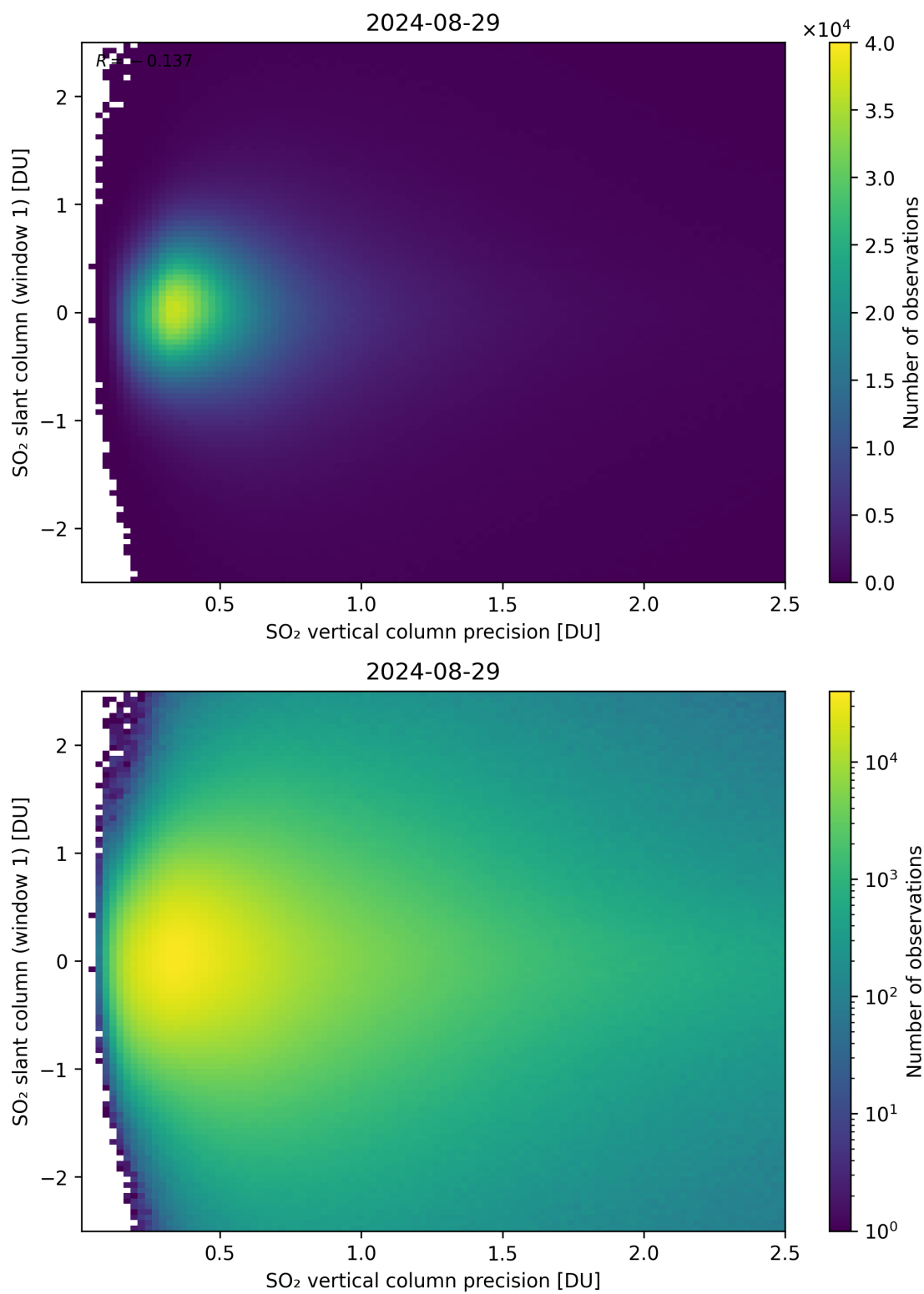
Figure 289: Scatter density plot of “SO 2 vertical column precision” against “SO 2 slant column (window 1)” for 2024-08-28 to 2024-08-30.
