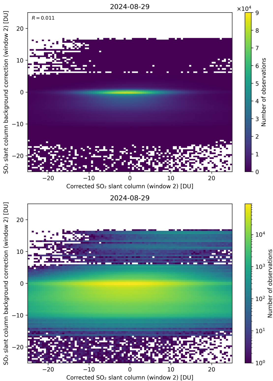
Figure 194: Scatter density plot of “Corrected SO 2 slant column (window 2)” against “SO 2 slant column background correction (window 2)” for 2024-08-28 to 2024-08-30.
