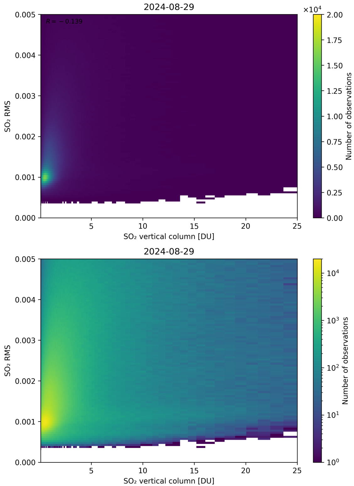
Figure 278: Scatter density plot of “SO 2 vertical column” against “SO 2 RMS” for 2024-08-28 to 2024-08-30.
