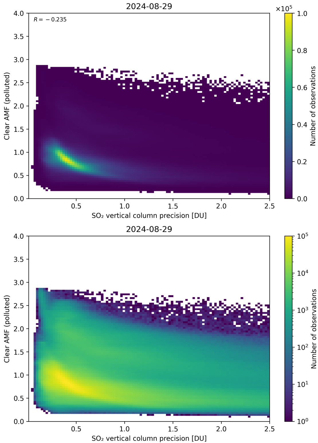
Figure 285: Scatter density plot of “SO 2 vertical column precision” against “Clear AMF (polluted)” for 2024-08-28 to 2024-08-30.
