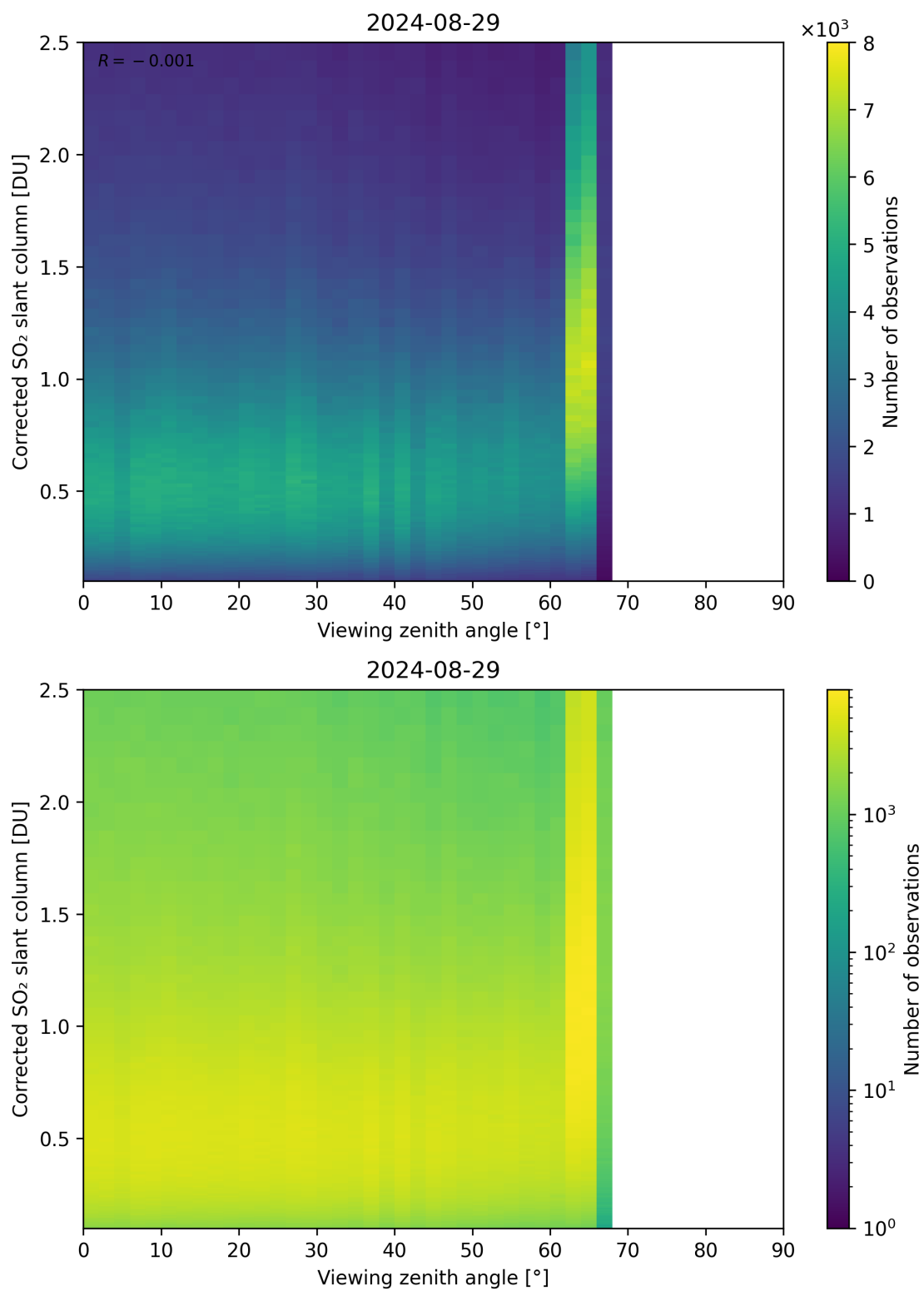
Figure 317: Scatter density plot of “Viewing zenith angle” against “Corrected SO 2 slant column” for 2024-08-28 to 2024-08-30.
