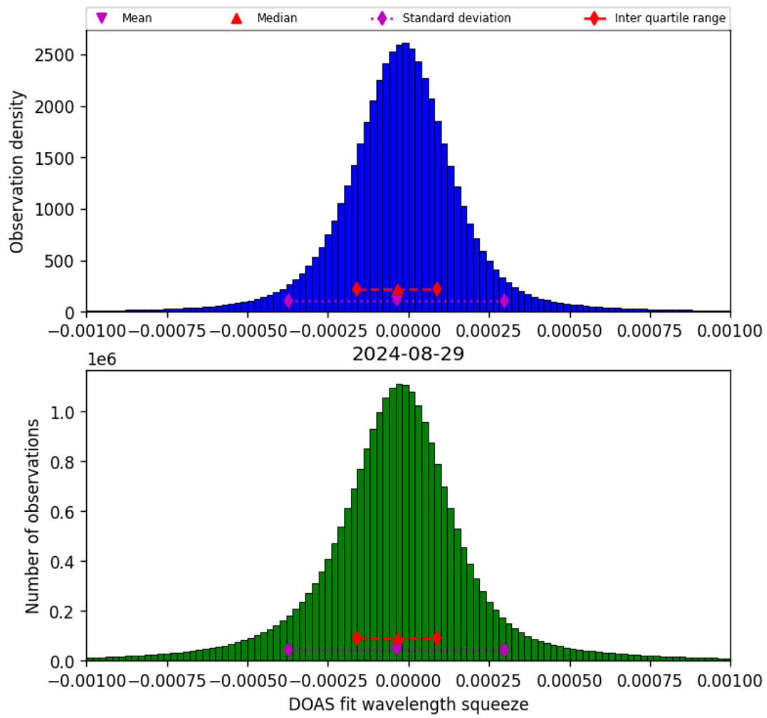
Figure 69: Histogram of “DOAS fit wavelength squeeze” for 2024-08-28 to 2024-08-30
