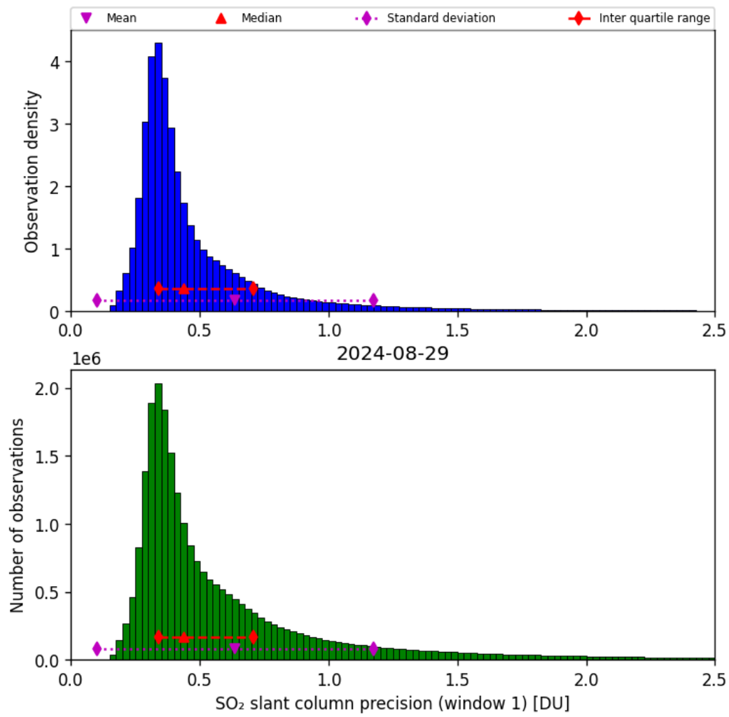
Figure 57: Histogram of “SO 2 slant column precision (window 1)” for 2024-08-28 to 2024-08-30
