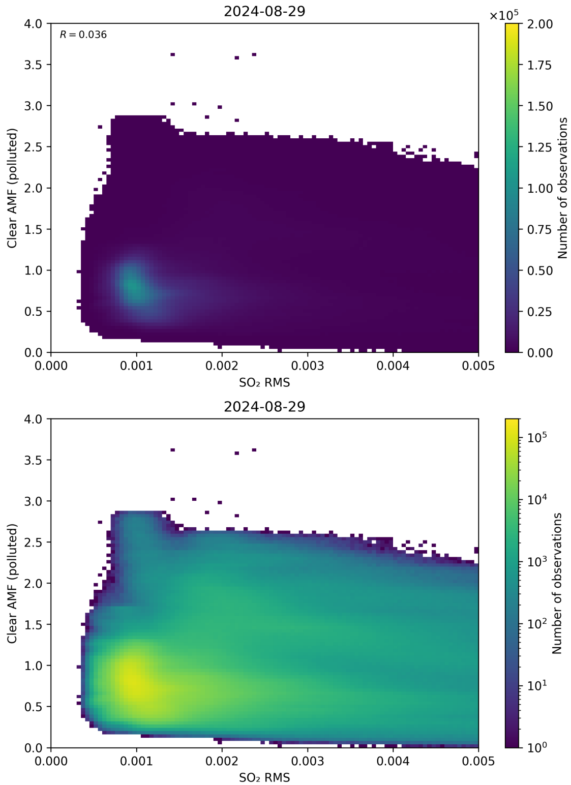
Figure 136: Scatter density plot of “SO 2 RMS” against “Clear AMF (polluted)” for 2024-08-28 to 2024-08-30.
