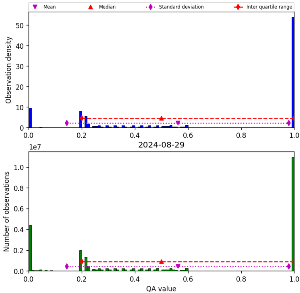
Figure 52: Histogram of “QA value” for 2024-08-28 to 2024-08-30
