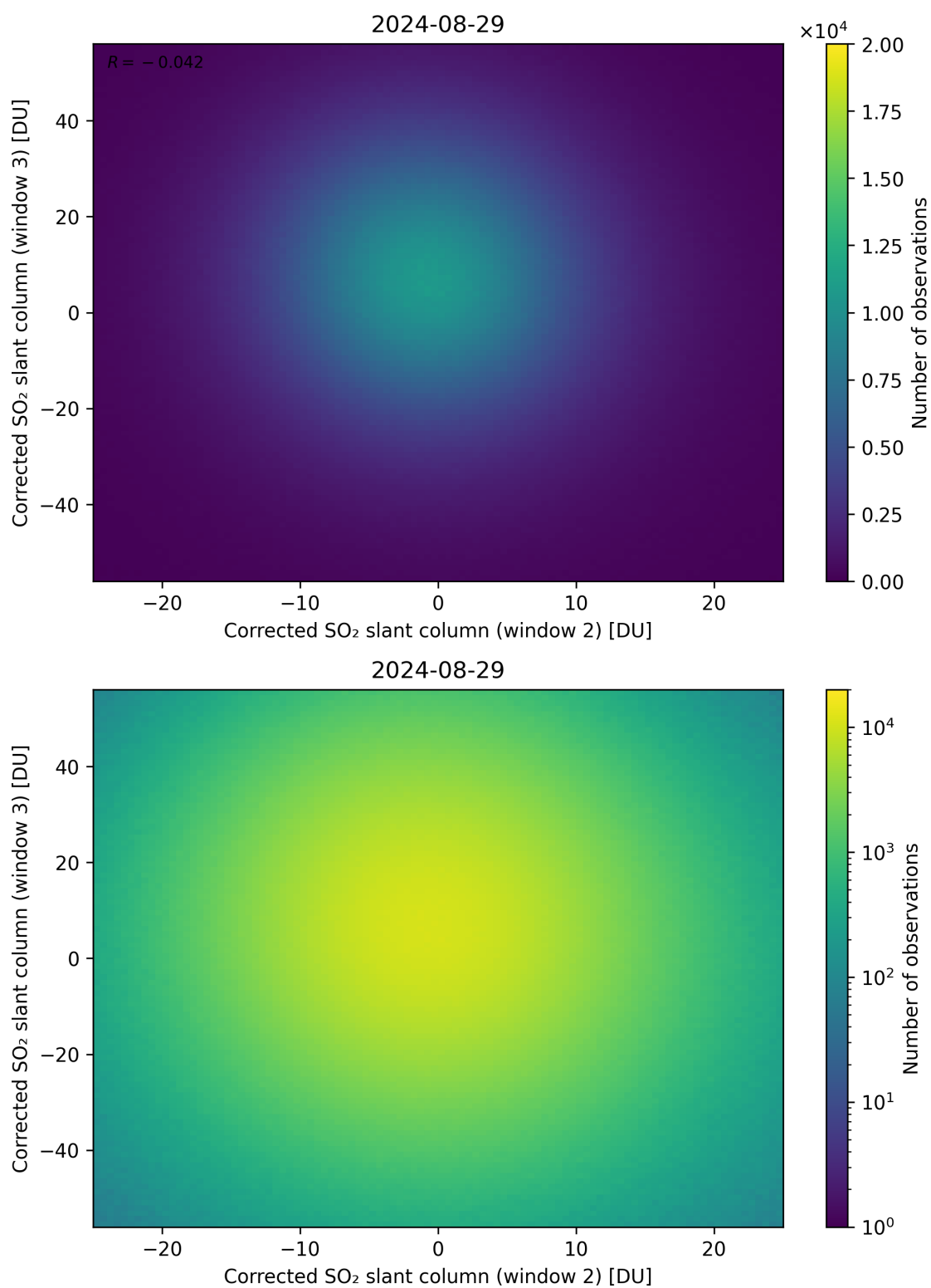
Figure 200: Scatter density plot of “Corrected SO 2 slant column (window 2)” against “Corrected SO 2 slant column (window 3)” for 2024-08-28 to 2024-08-30.
