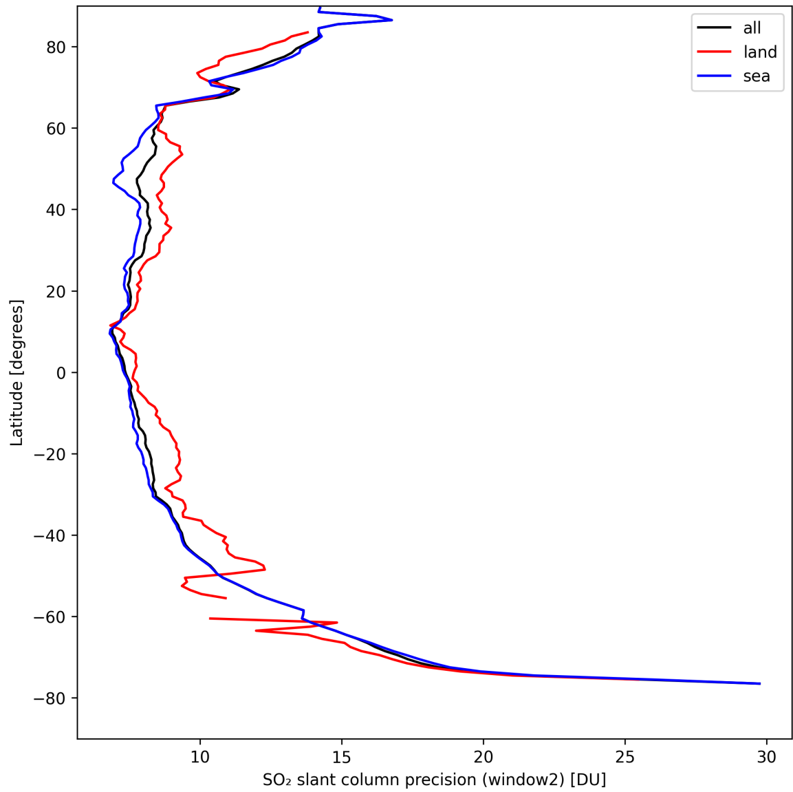
Figure 38: Zonal average of “SO 2 slant column precision (window2)” for 2024-08-28 to 2024-08-30.
