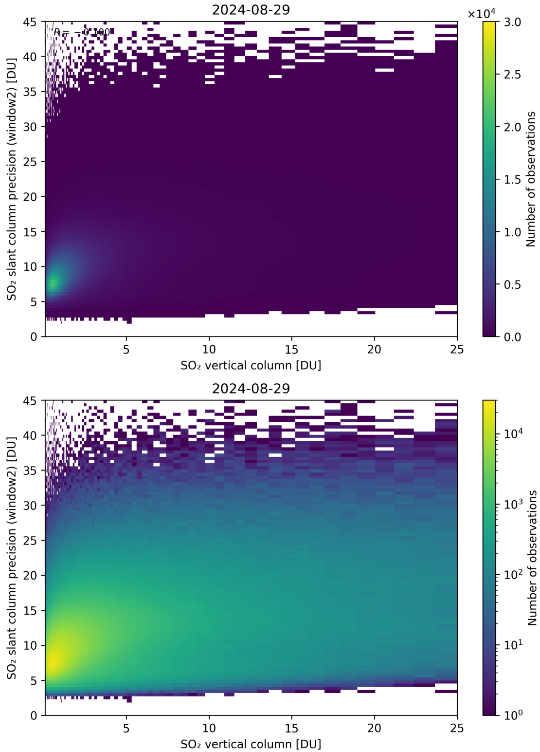
Figure 302: Scatter density plot of “SO 2 vertical column” against “SO 2 slant column precision (window2)” for 2024-08-28 to 2024-08-30.
