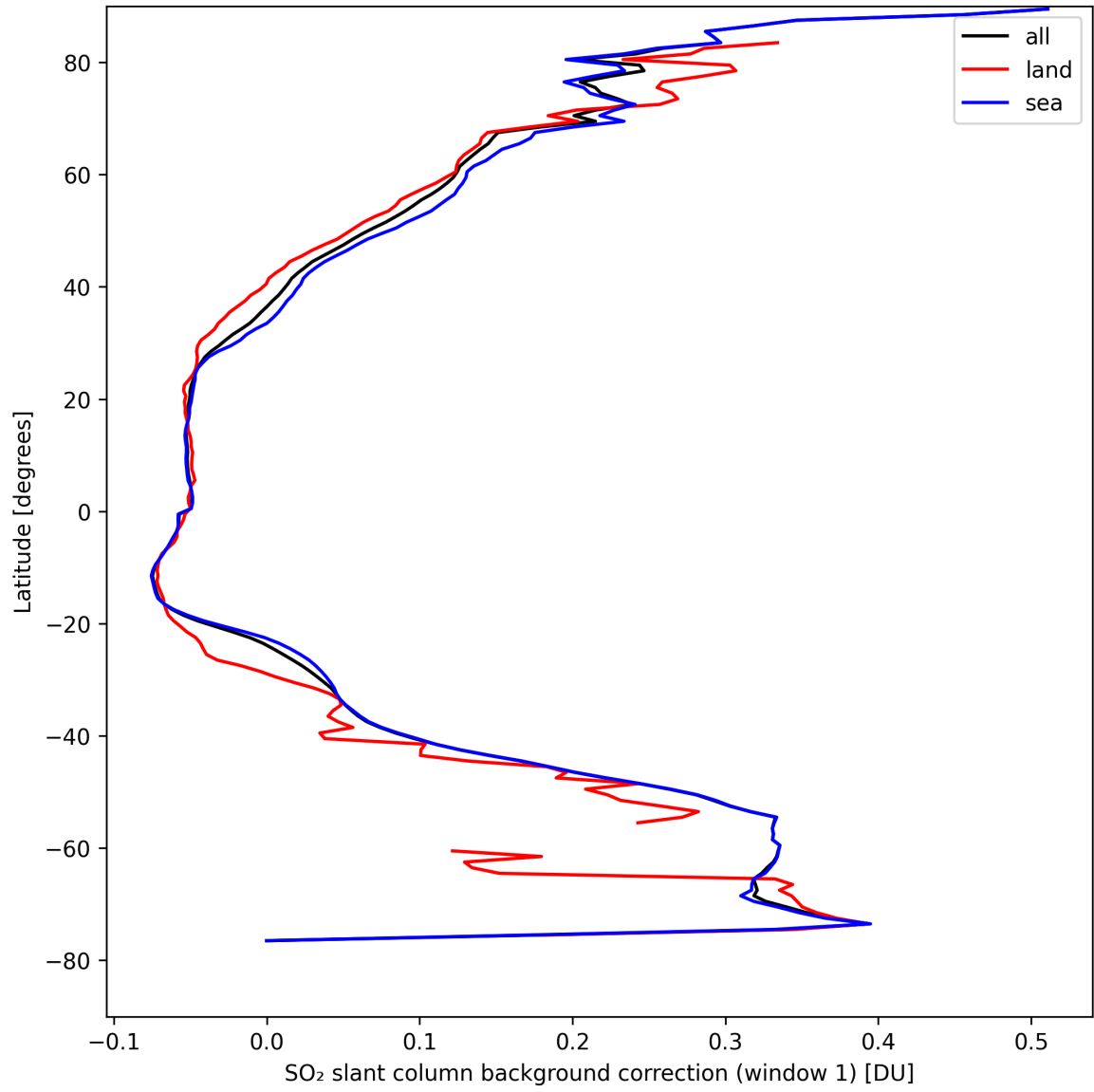
Figure 36: Zonal average of “SO 2 slant column background correction (window 1)” for 2024-08-28 to 2024-08-30.
