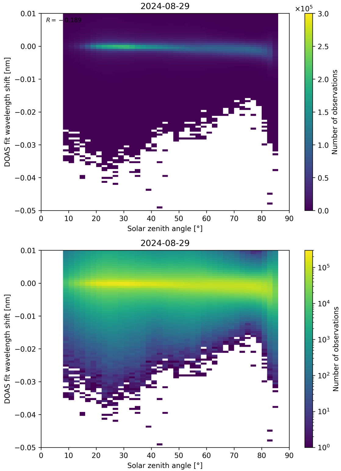
Figure 161: Scatter density plot of “Solar zenith angle” against “DOAS fit wavelength shift” for 2024-08-28 to 2024-08-30.
