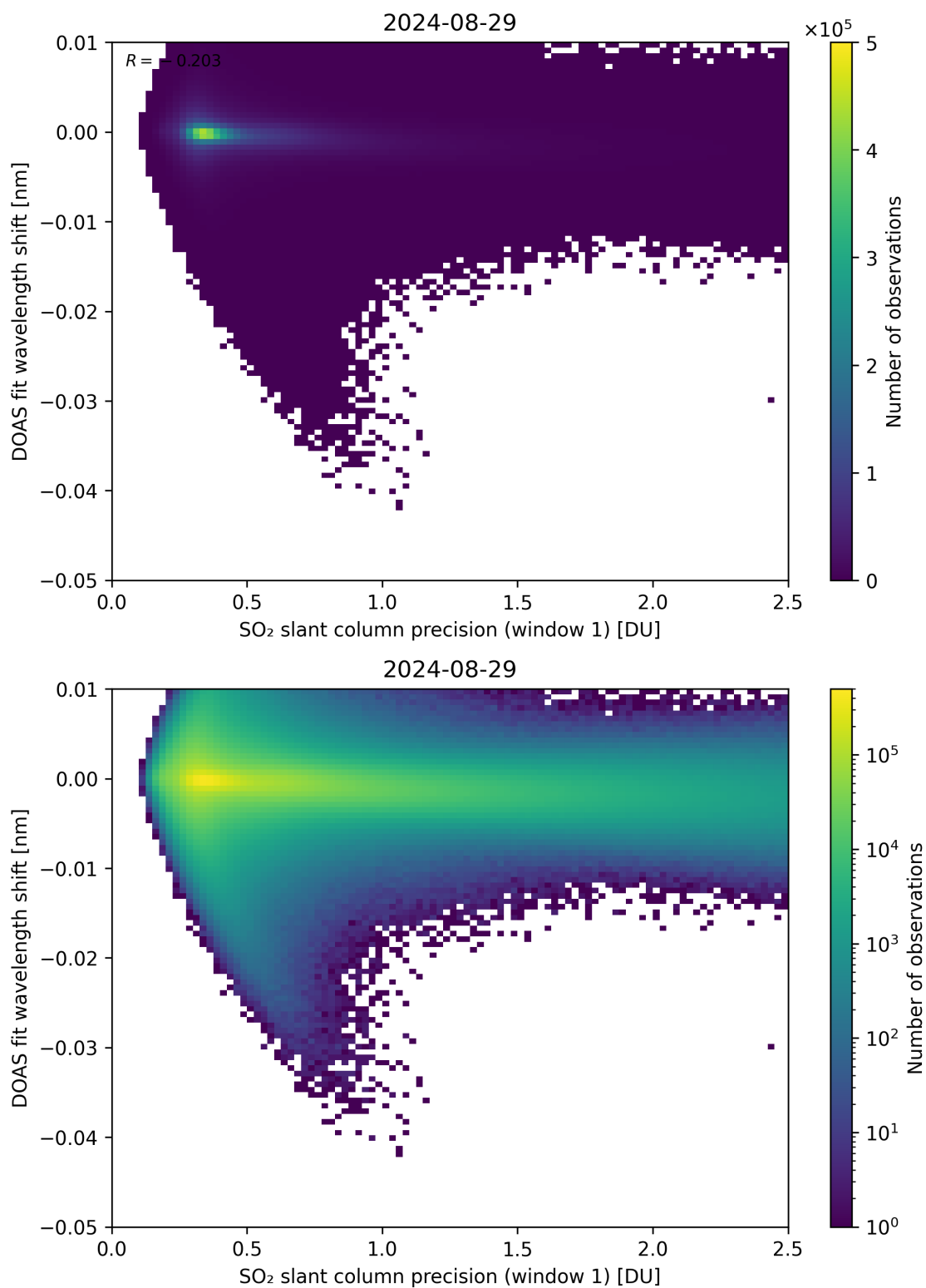
Figure 221: Scatter density plot of “SO 2 slant column precision (window 1)” against “DOAS fit wavelength shift” for 2024-08-28 to 2024-08-30.
