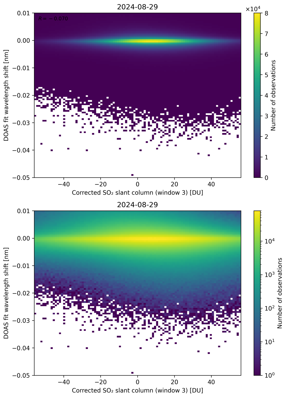
Figure 206: Scatter density plot of “Corrected SO 2 slant column (window 3)” against “DOAS fit wavelength shift” for 2024-08-28 to 2024-08-30.
