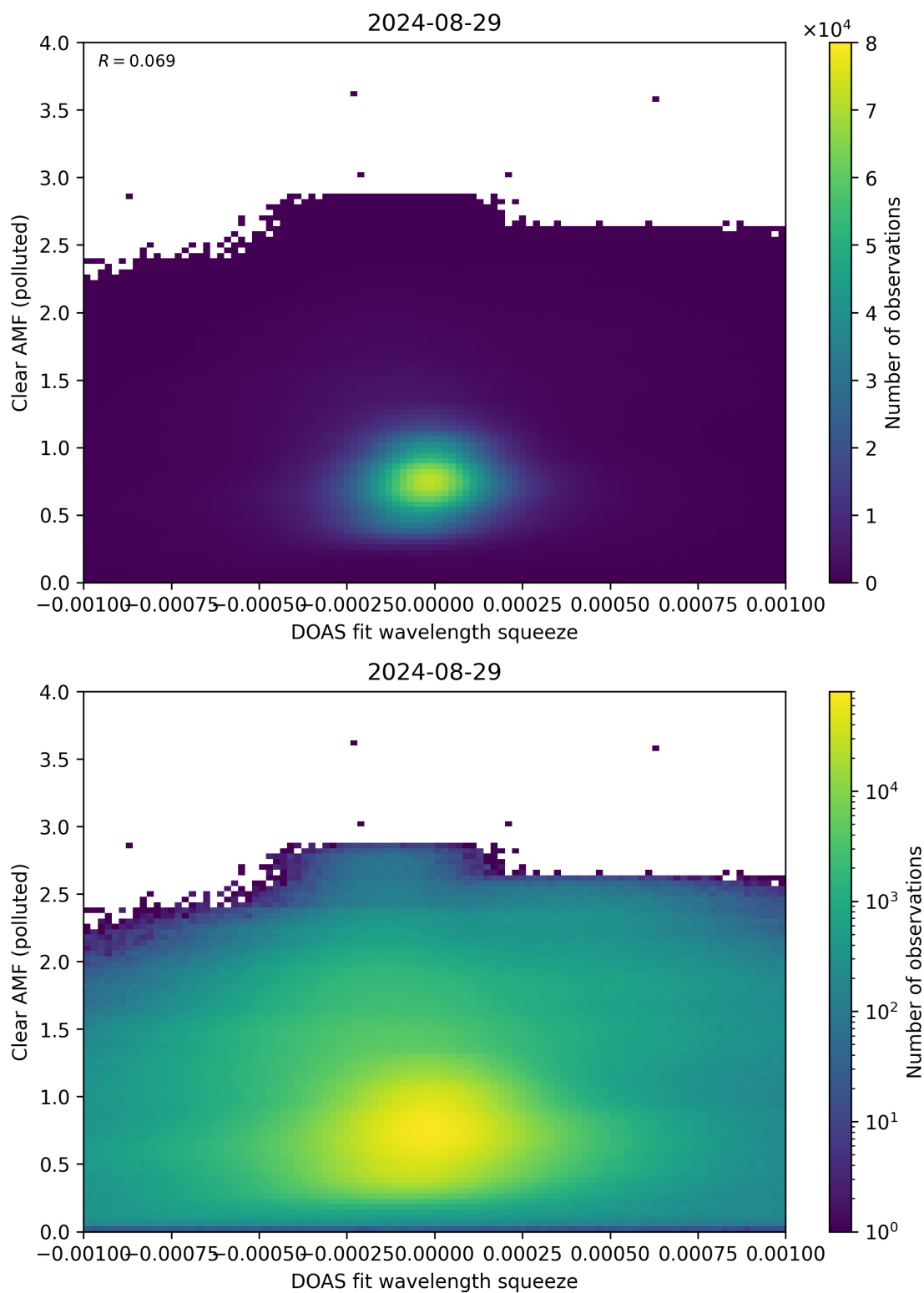
Figure 133: Scatter density plot of “DOAS fit wavelength squeeze” against “Clear AMF (polluted)” for 2024-08-28 to 2024-08-30.
