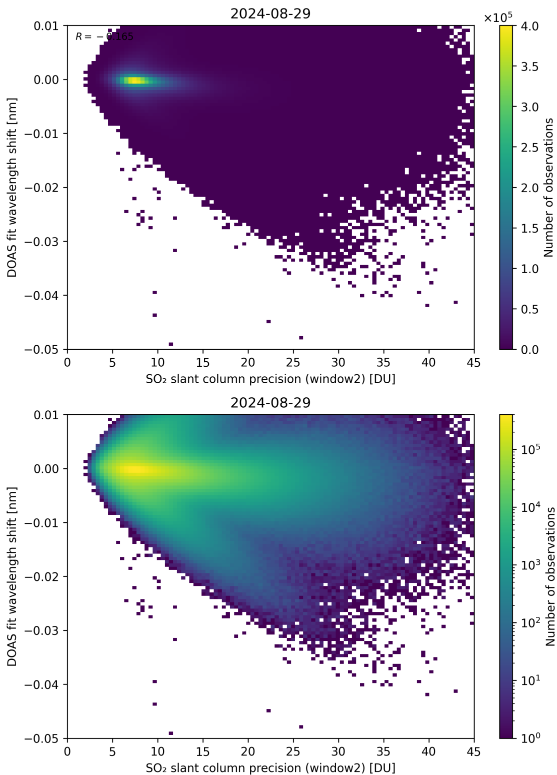
Figure 243: Scatter density plot of “SO 2 slant column precision (window2)” against “DOAS fit wavelength shift” for 2024-08-28 to 2024-08-30.
