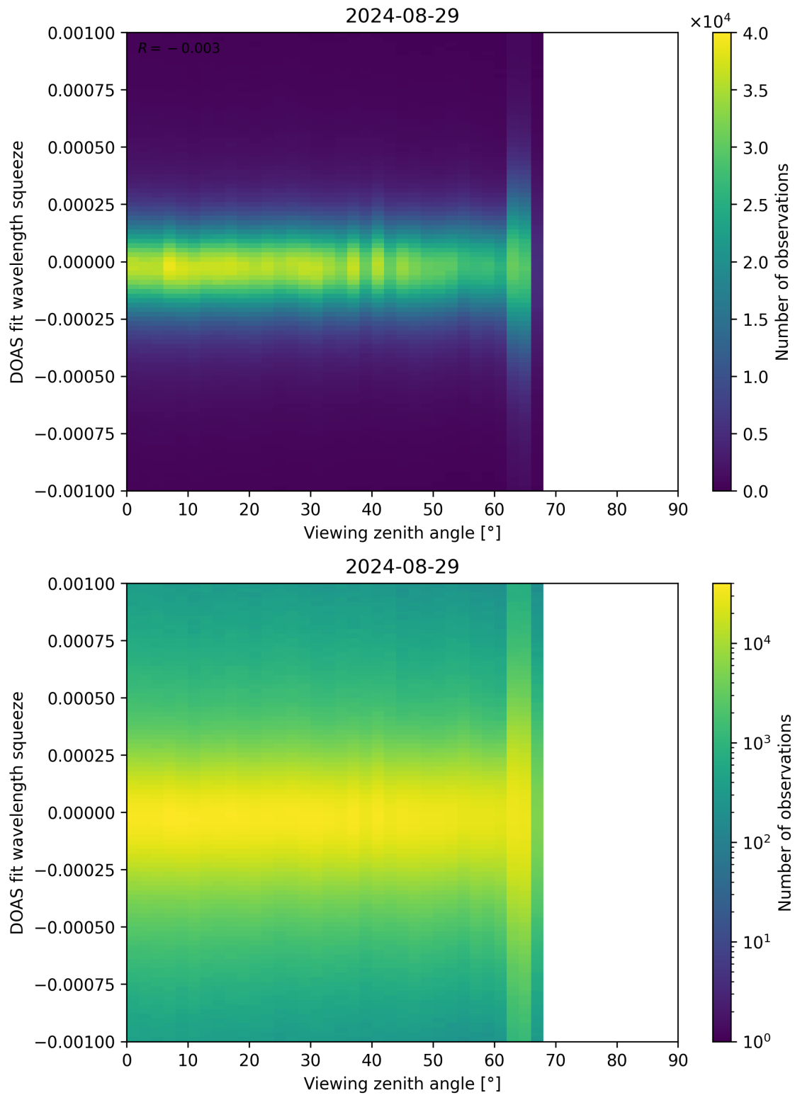
Figure 312: Scatter density plot of “Viewing zenith angle” against “DOAS fit wavelength squeeze” for 2024-08-28 to 2024-08-30.
