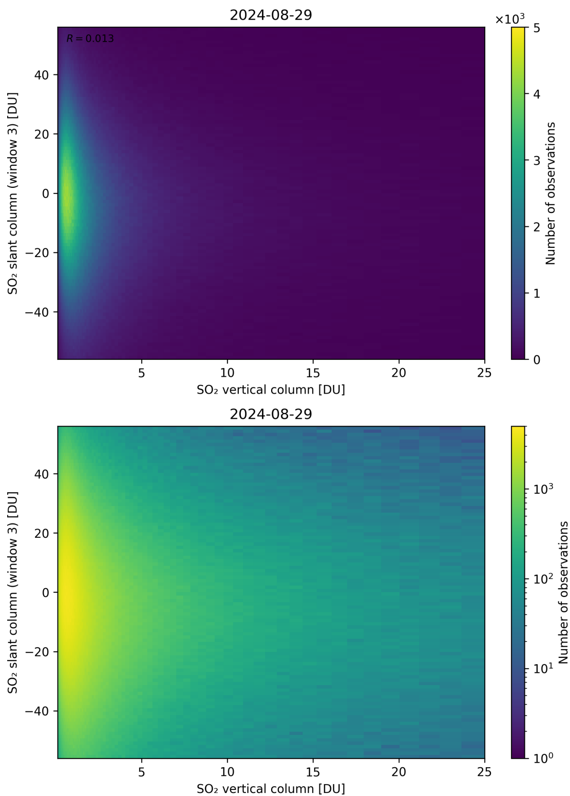
Figure 303: Scatter density plot of “SO 2 vertical column” against “SO 2 slant column (window 3)” for 2024-08-28 to 2024-08-30.
