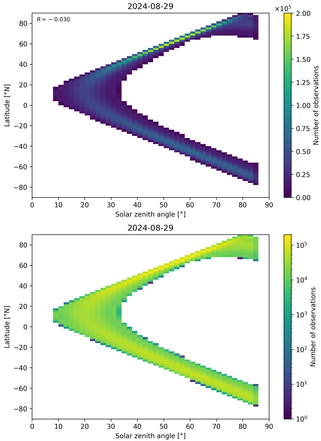
Figure 164: Scatter density plot of “Solar zenith angle” against “Latitude” for 2024-08-28 to 2024-08-30.
