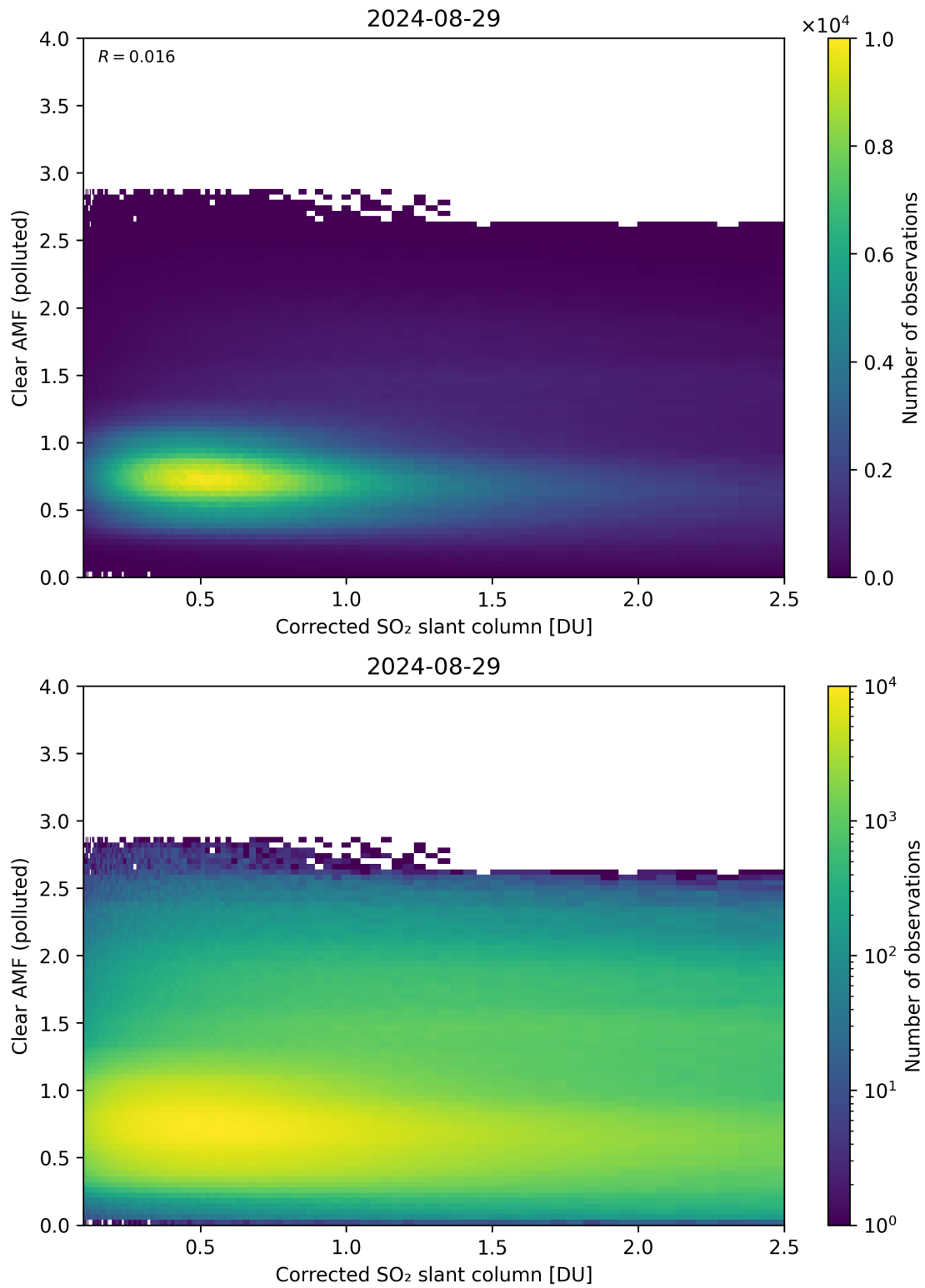
Figure 184: Scatter density plot of “Corrected SO 2 slant column” against “Clear AMF (polluted)” for 2024-08-28 to 2024-08-30.
