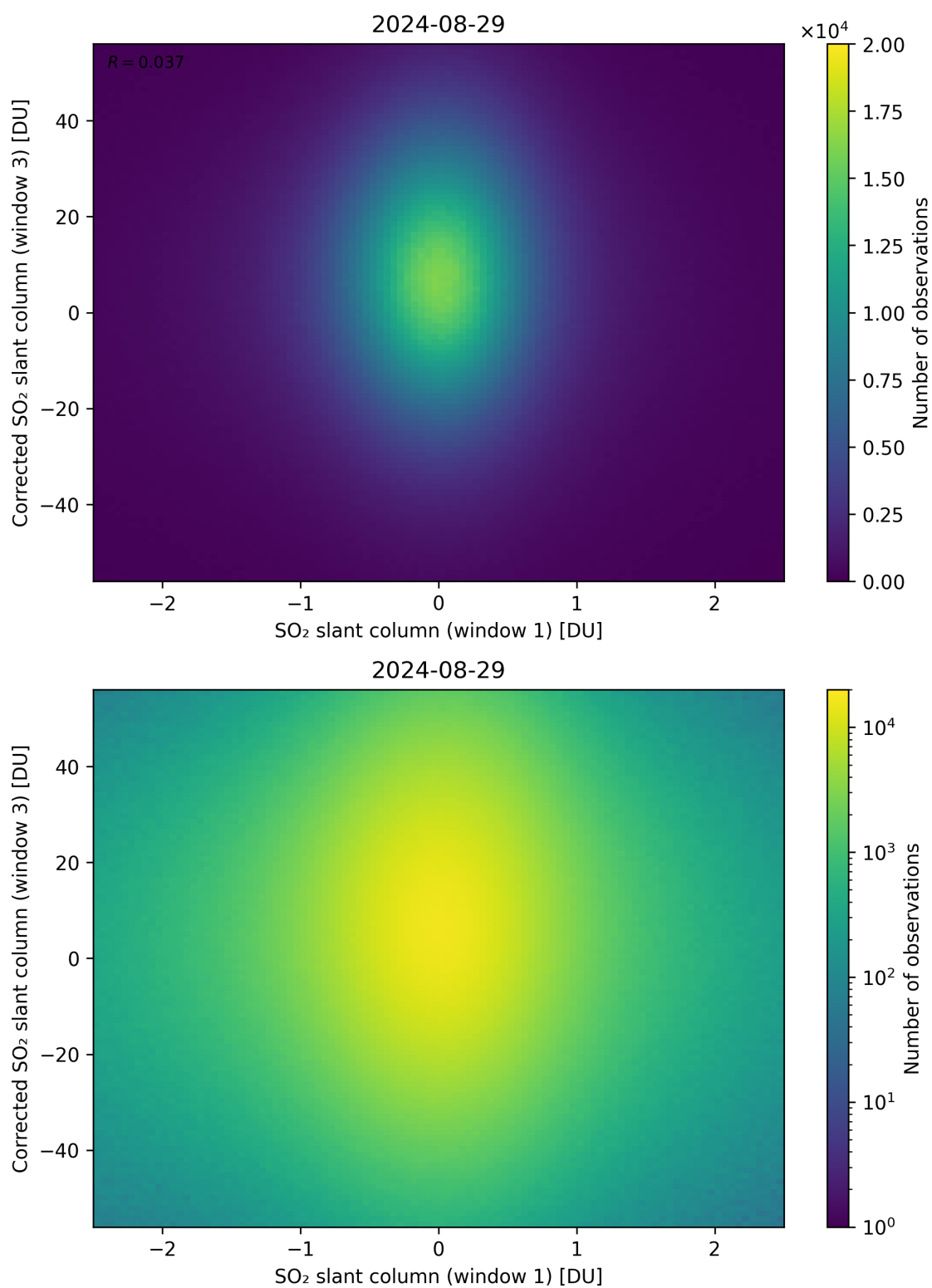
Figure 234: Scatter density plot of “SO 2 slant column (window 1)” against “Corrected SO 2 slant column (window 3)” for 2024-08-28 to 2024-08-30.
