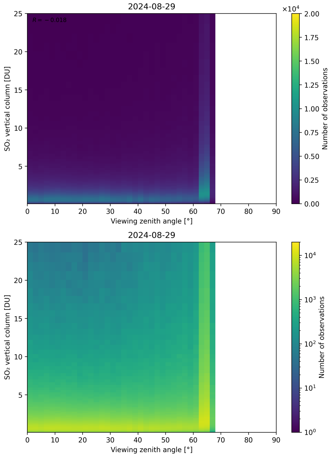
Figure 327: Scatter density plot of “Viewing zenith angle” against “SO 2 vertical column” for 2024-08-28 to 2024-08-30.
