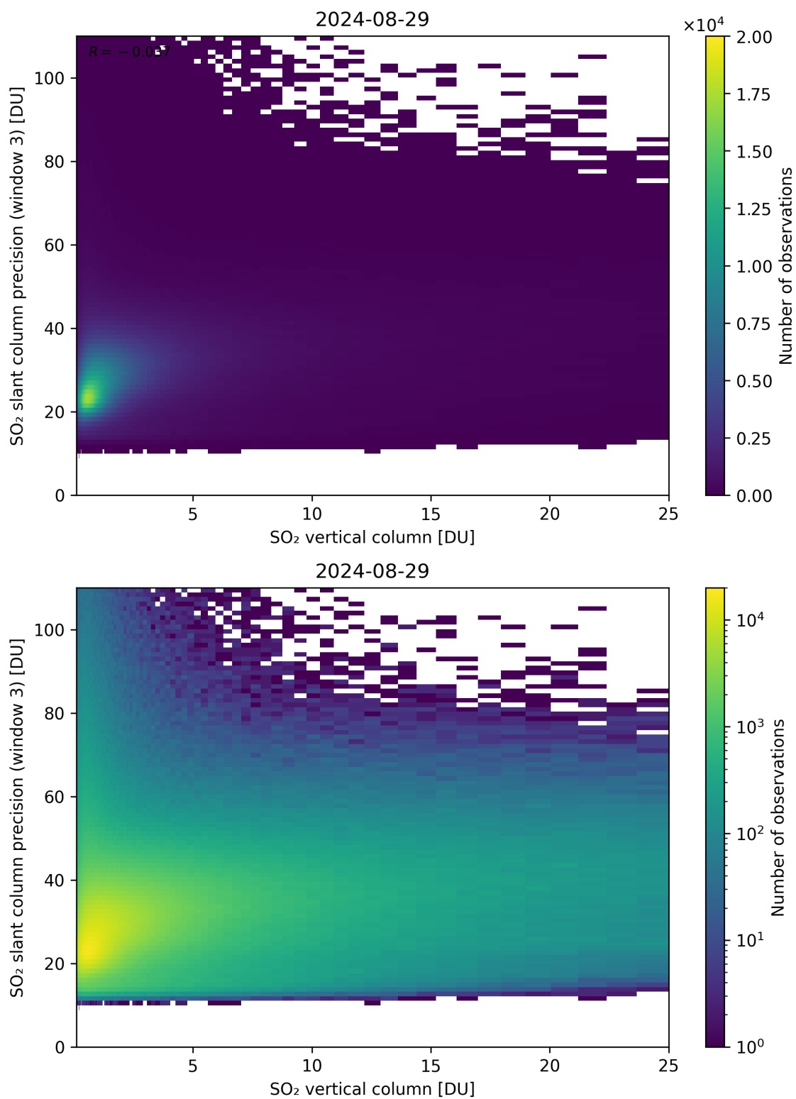
Figure 304: Scatter density plot of “SO 2 vertical column” against “SO 2 slant column precision (window 3)” for 2024-08-28 to 2024-08-30.
