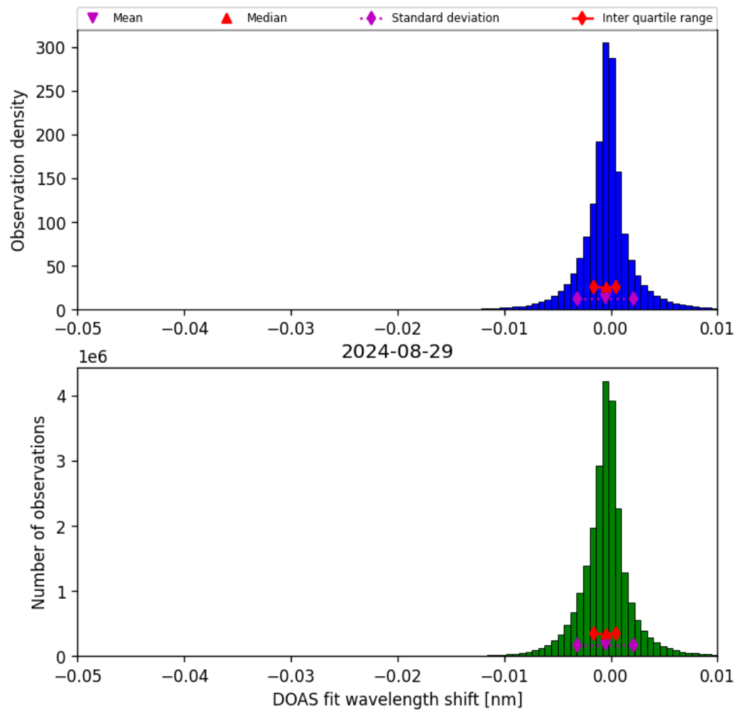
Figure 68: Histogram of “DOAS fit wavelength shift” for 2024-08-28 to 2024-08-30
