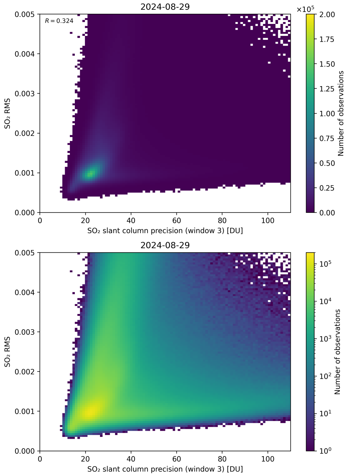
Figure 260: Scatter density plot of “SO 2 slant column precision (window 3)” against “SO 2 RMS” for 2024-08-28 to 2024-08-30.
