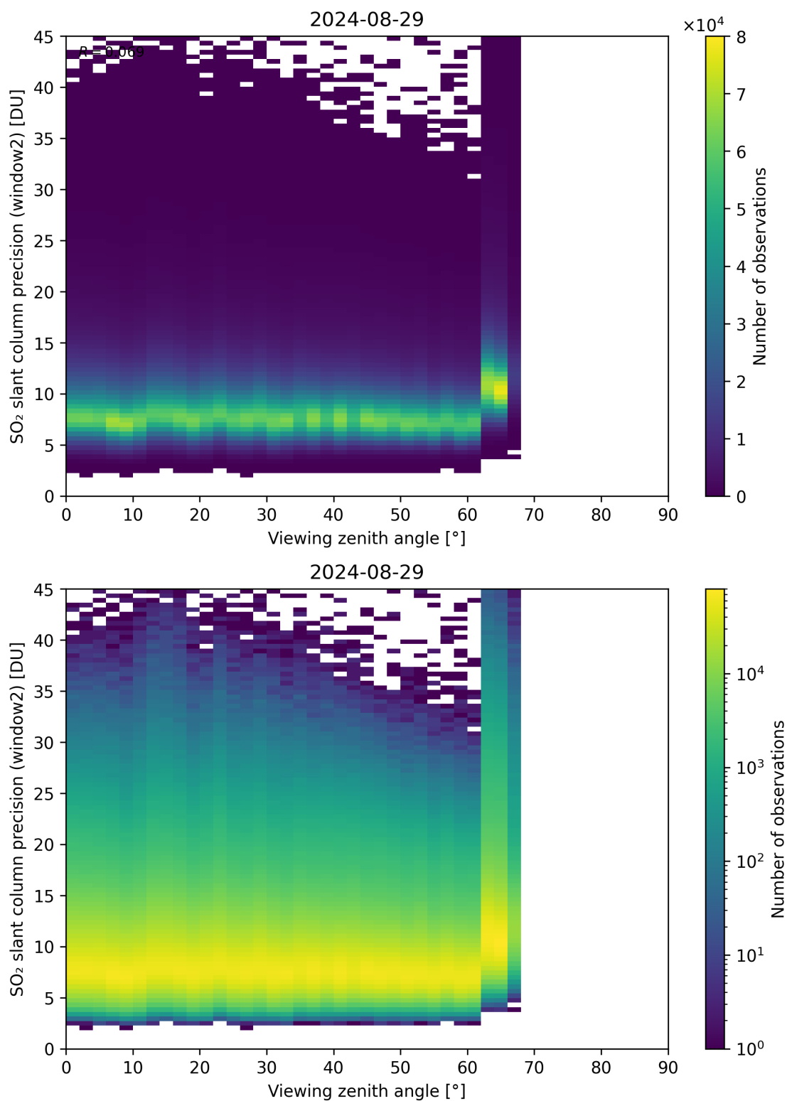
Figure 322: Scatter density plot of “Viewing zenith angle” against “SO 2 slant column precision (window2)” for 2024-08-28 to 2024-08-30.
