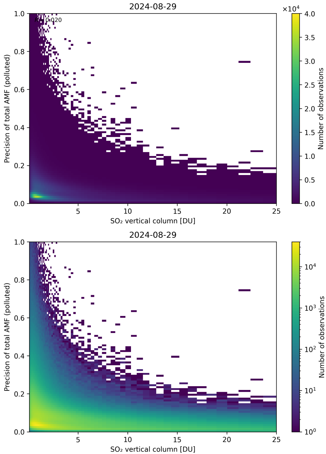
Figure 306: Scatter density plot of “SO 2 vertical column” against “Precision of total AMF (polluted)” for 2024-08-28 to 2024-08-30.
