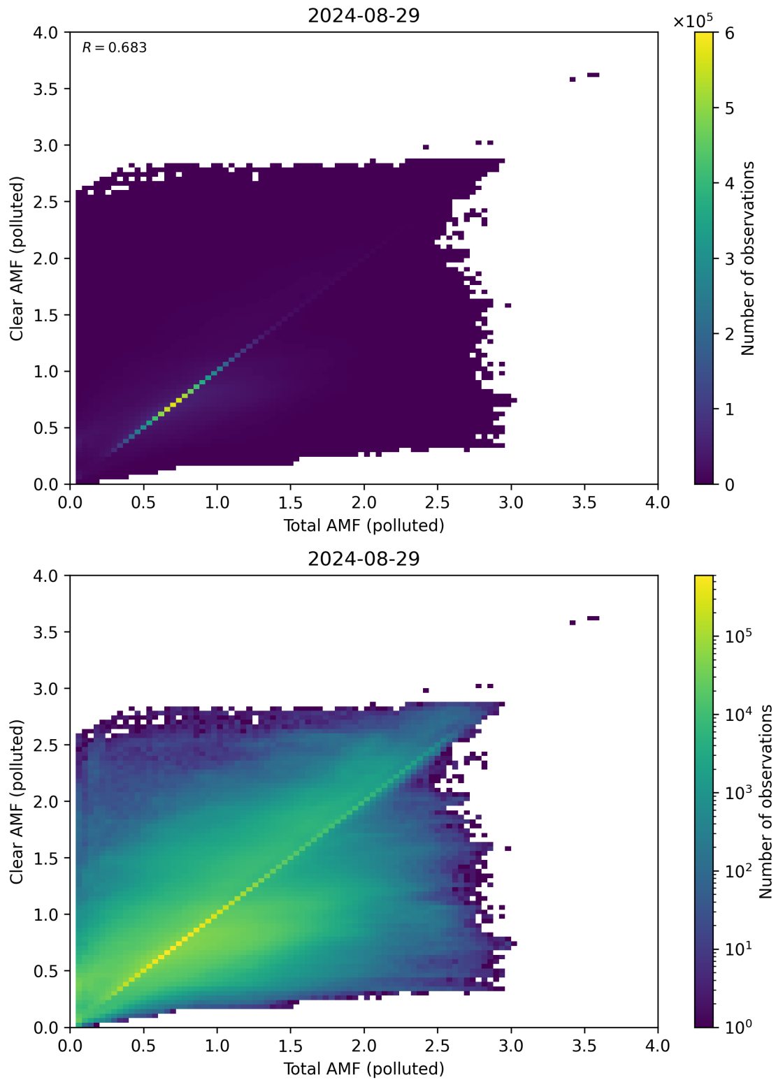
Figure 271: Scatter density plot of “Total AMF (polluted)” against “Clear AMF (polluted)” for 2024-08-28 to 2024-08-30.
