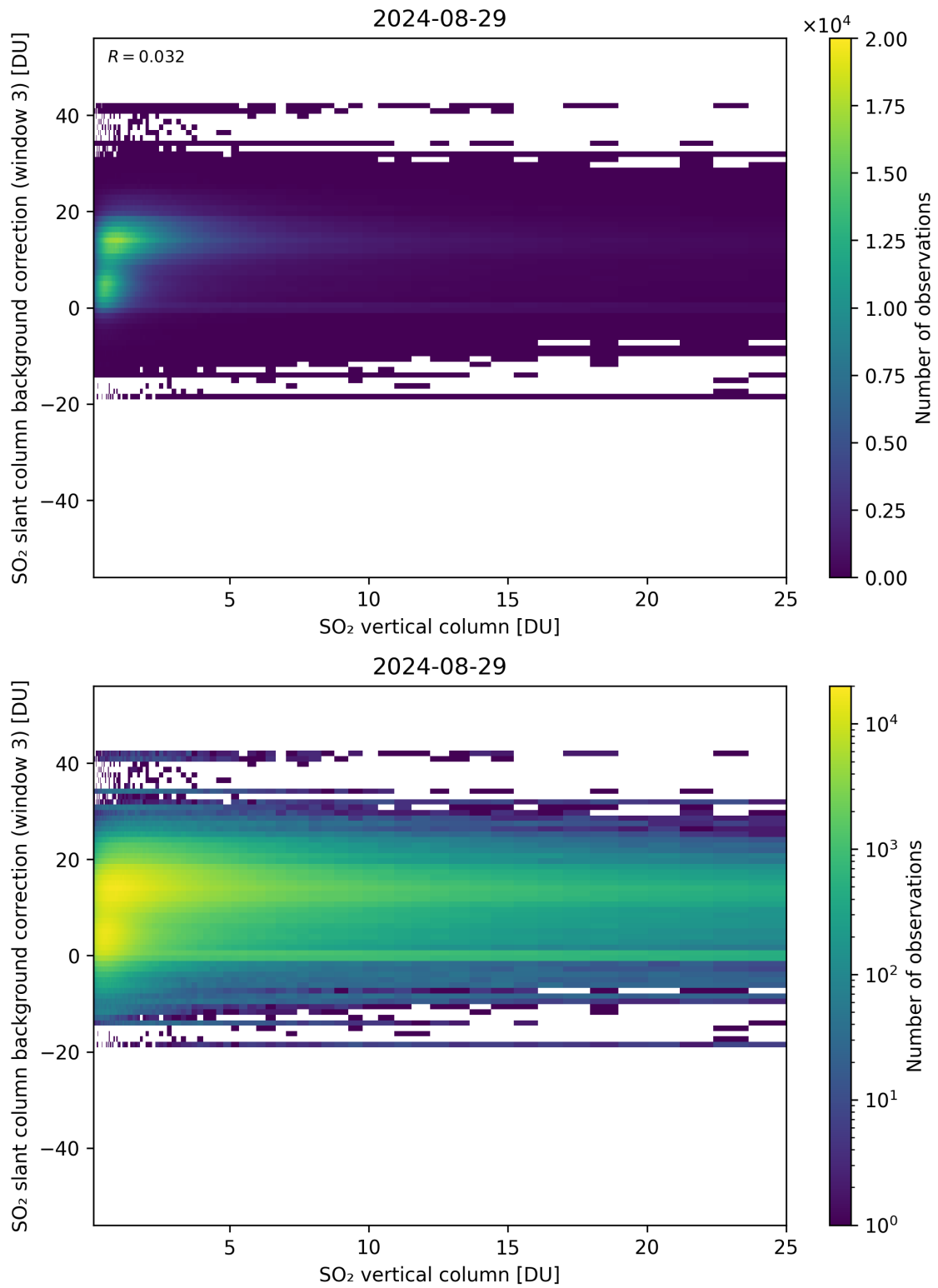
Figure 275: Scatter density plot of “SO 2 vertical column” against “SO 2 slant column background correction (window 3)” for 2024-08-28 to 2024-08-30.
