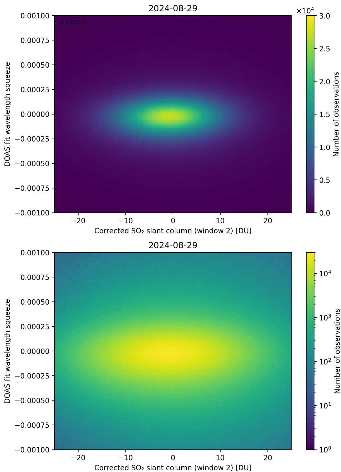
Figure 197: Scatter density plot of “Corrected SO 2 slant column (window 2)” against “DOAS fit wavelength squeeze” for 2024-08-28 to 2024-08-30.
