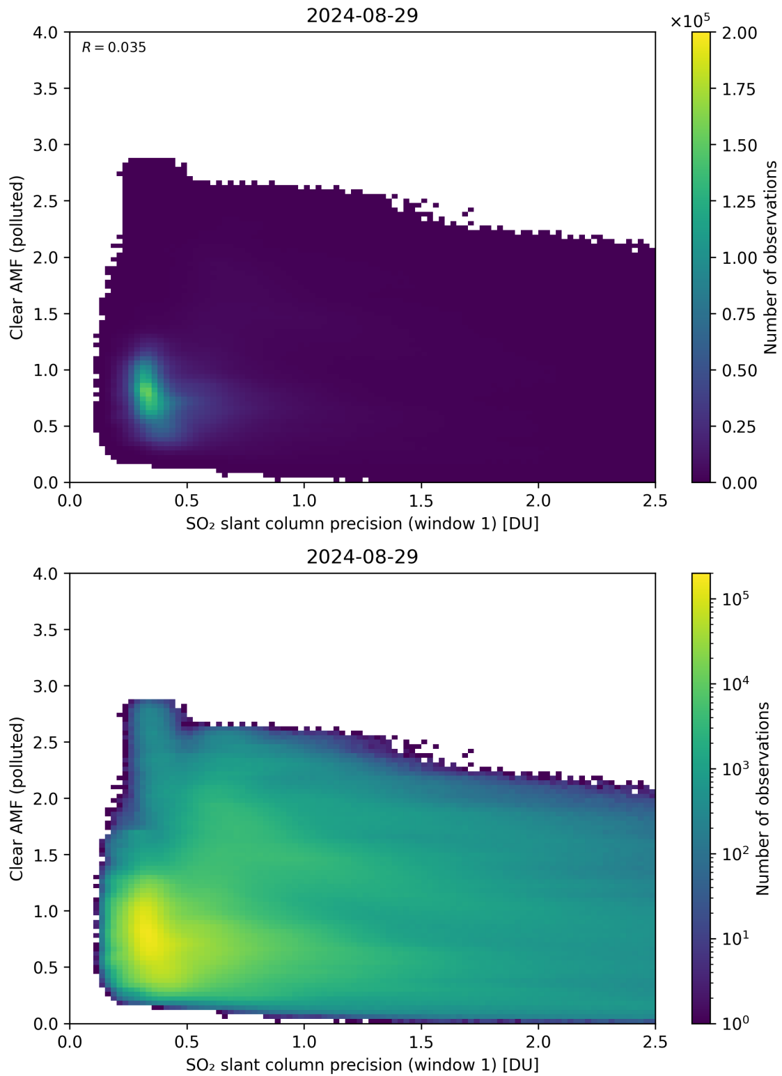
Figure 224: Scatter density plot of “SO 2 slant column precision (window 1)” against “Clear AMF (polluted)” for 2024-08-28 to 2024-08-30.
