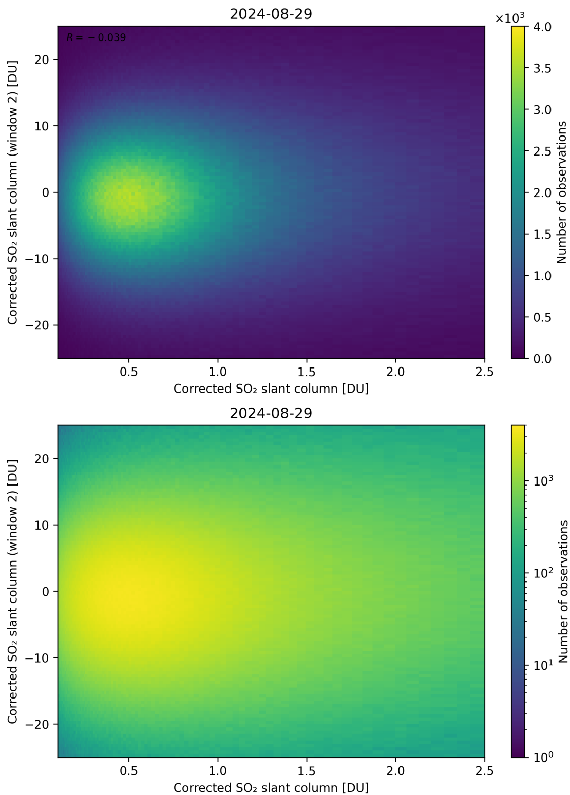
Figure 185: Scatter density plot of “Corrected SO 2 slant column” against “Corrected SO 2 slant column (window 2)” for 2024-08-28 to 2024-08-30.
