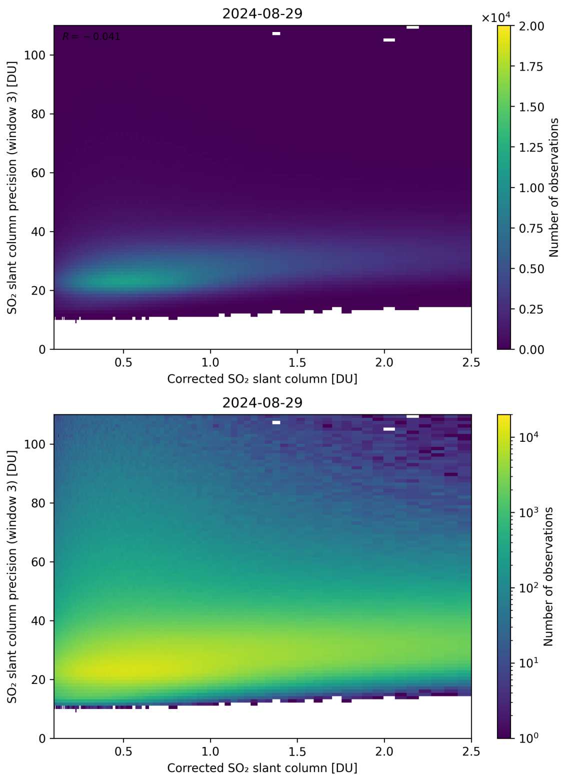
Figure 191: Scatter density plot of “Corrected SO 2 slant column” against “SO 2 slant column precision (window 3)” for 2024-08-28 to 2024-08-30.
