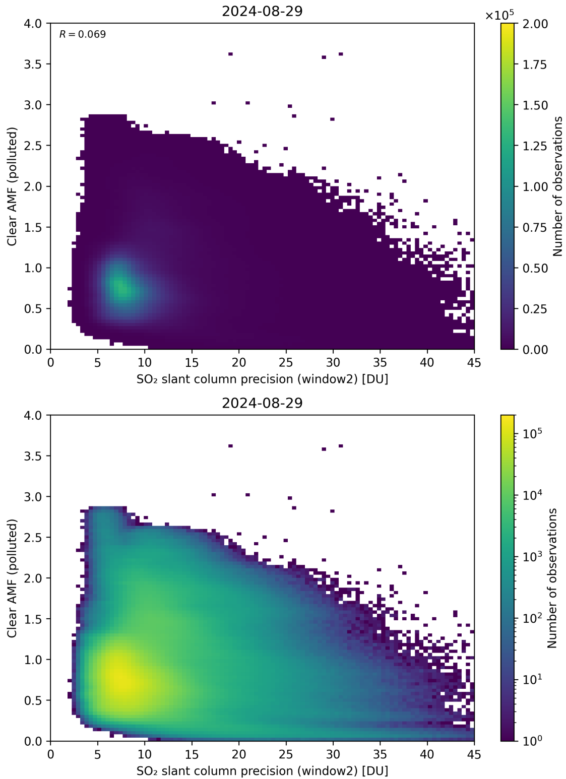
Figure 246: Scatter density plot of “SO 2 slant column precision (window2)” against “Clear AMF (polluted)” for 2024-08-28 to 2024-08-30.
