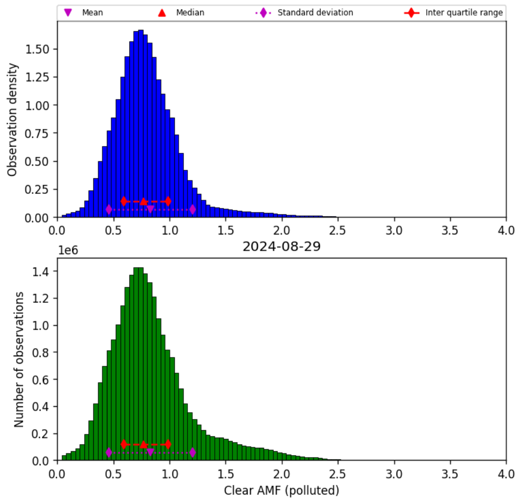
Figure 73: Histogram of “Clear AMF (polluted)” for 2024-08-28 to 2024-08-30
