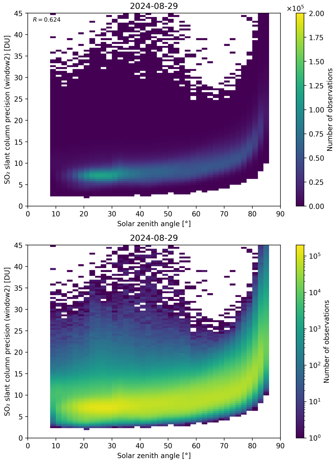
Figure 171: Scatter density plot of “Solar zenith angle” against “SO 2 slant column precision (window2)” for 2024-08-28 to 2024-08-30.
