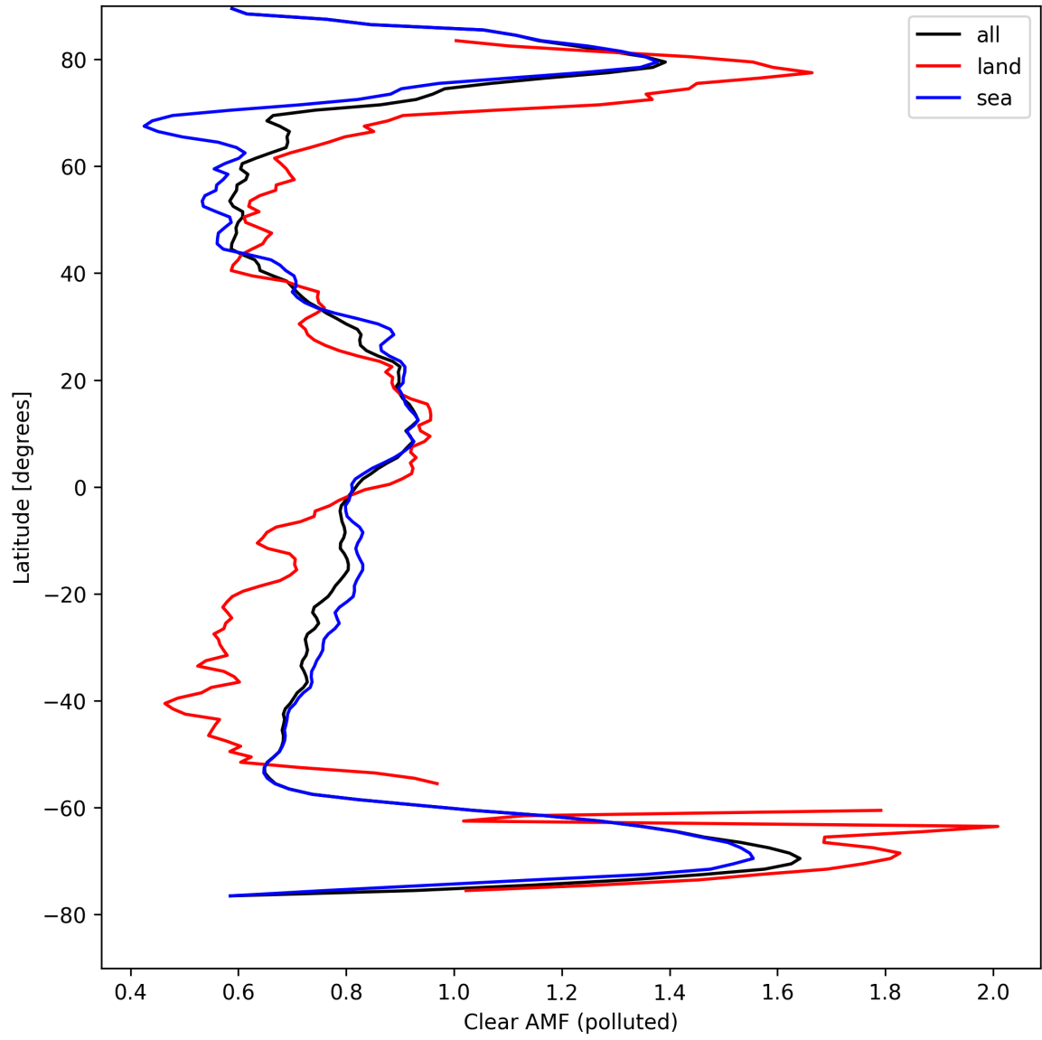
Figure 50: Zonal average of “Clear AMF (polluted)” for 2024-08-28 to 2024-08-30.
