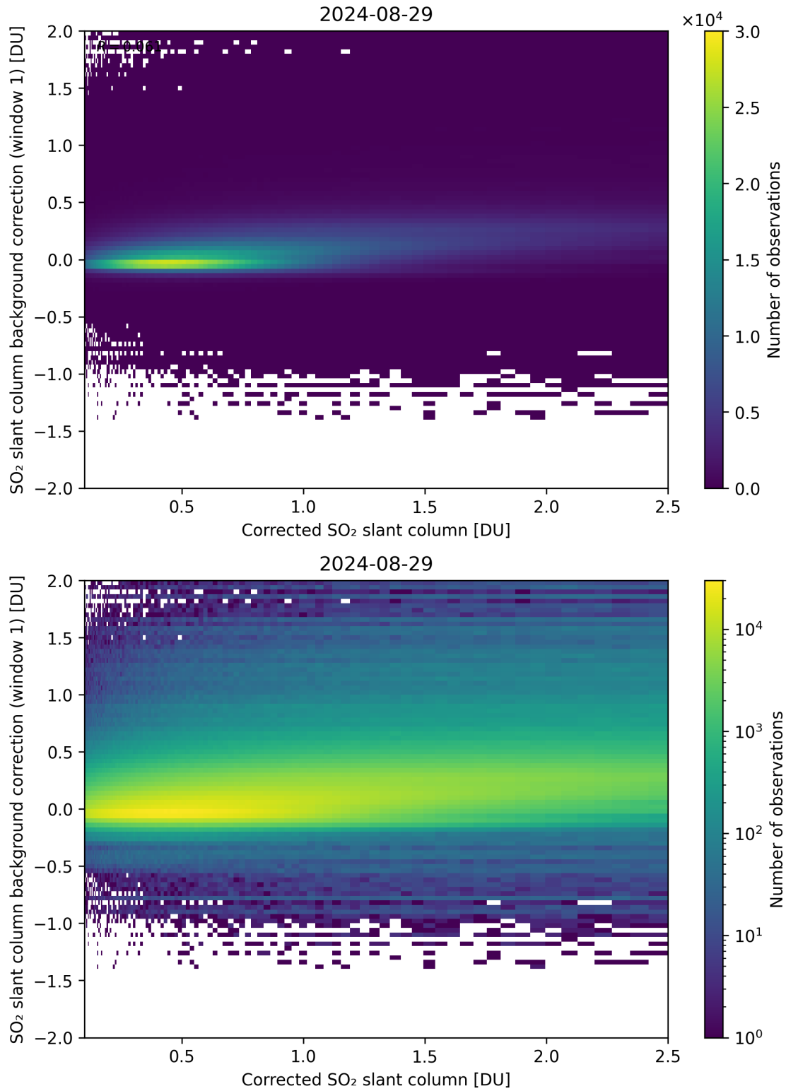
Figure 178: Scatter density plot of “Corrected SO 2 slant column” against “SO 2 slant column background correction (window 1)” for 2024-08-28 to 2024-08-30.
