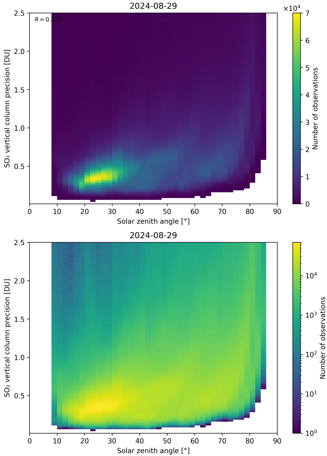
Figure 177: Scatter density plot of “Solar zenith angle” against “SO 2 vertical column precision” for 2024-08-28 to 2024-08-30.
