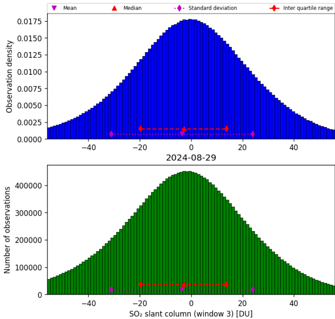
Figure 64: Histogram of “SO 2 slant column (window 3)” for 2024-08-28 to 2024-08-30
