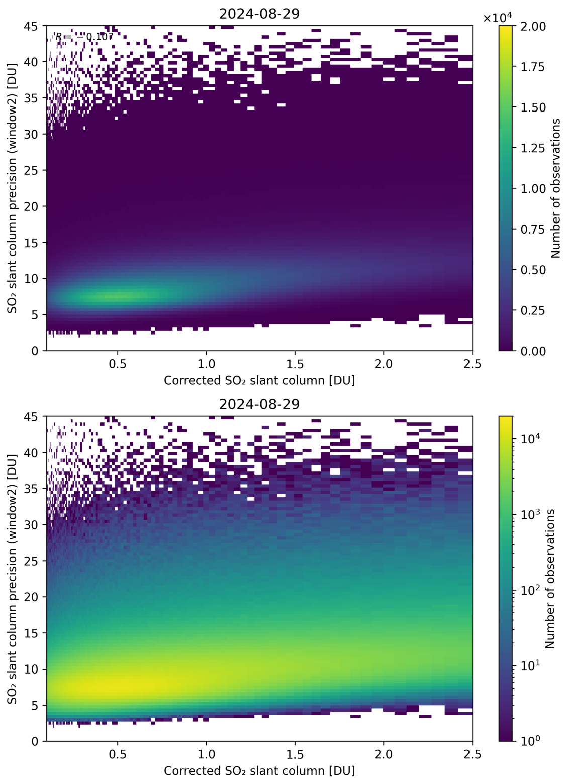
Figure 189: Scatter density plot of “Corrected SO 2 slant column” against “SO 2 slant column precision (window2)” for 2024-08-28 to 2024-08-30.
