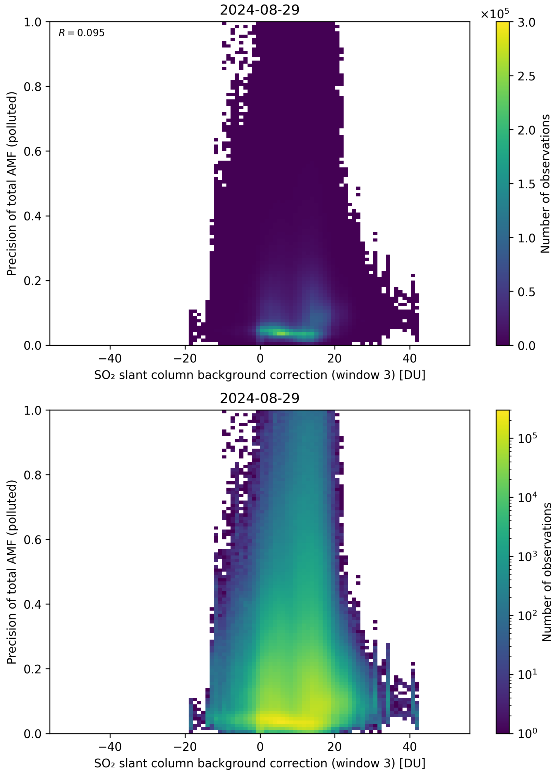
Figure 126: Scatter density plot of “SO 2 slant column background correction (window 3)” against “Precision of total AMF (polluted)” for 2024-08-28 to 2024-08-30.
