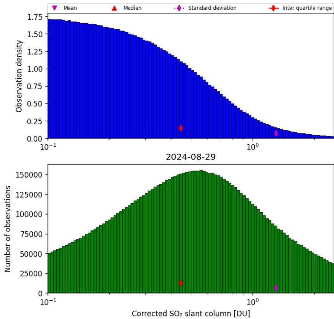
Figure 55: Histogram of “Corrected SO 2 slant column” for 2024-08-28 to 2024-08-30
