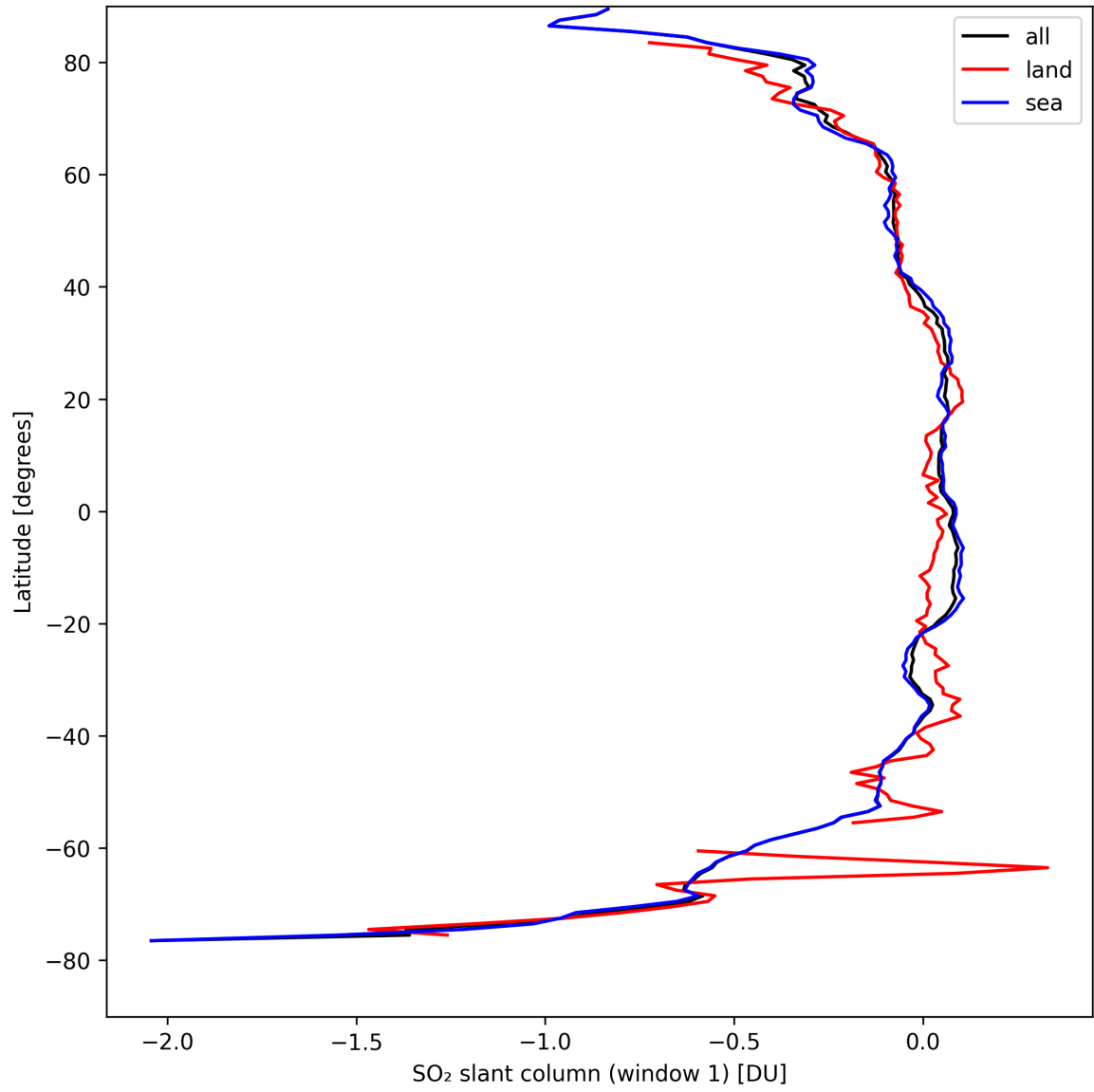
Figure 33: Zonal average of “SO 2 slant column (window 1)” for 2024-08-28 to 2024-08-30.
