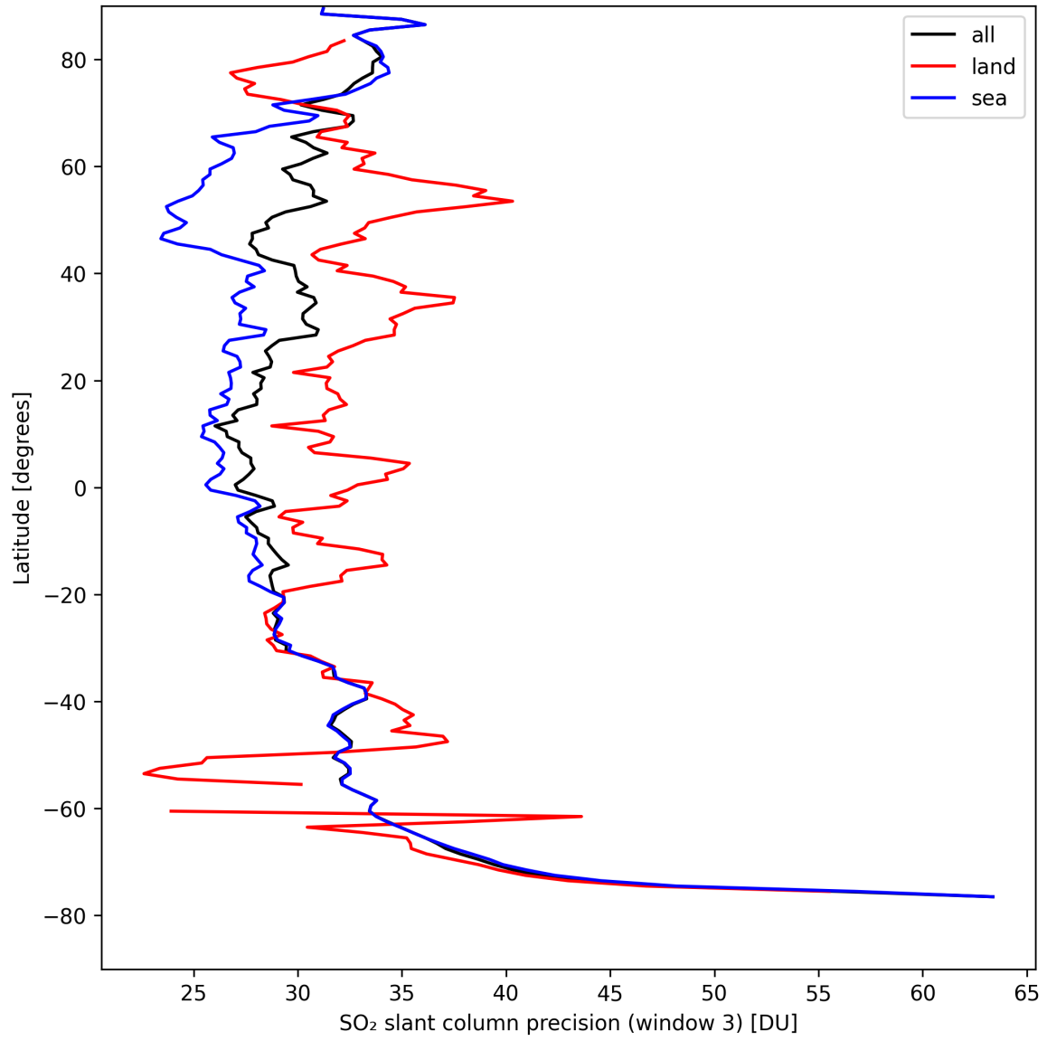
Figure 42: Zonal average of “SO 2 slant column precision (window 3)” for 2024-08-28 to 2024-08-30.
