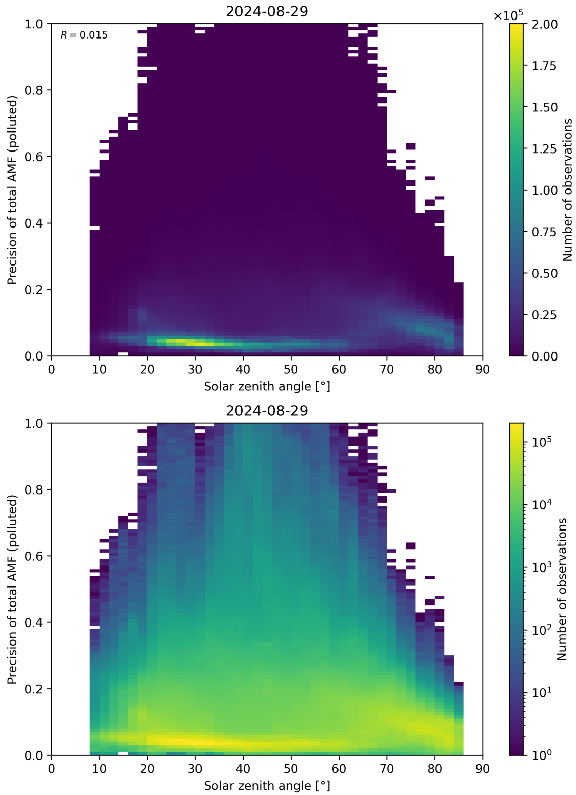
Figure 175: Scatter density plot of “Solar zenith angle” against “Precision of total AMF (polluted)” for 2024-08-28 to 2024-08-30.
