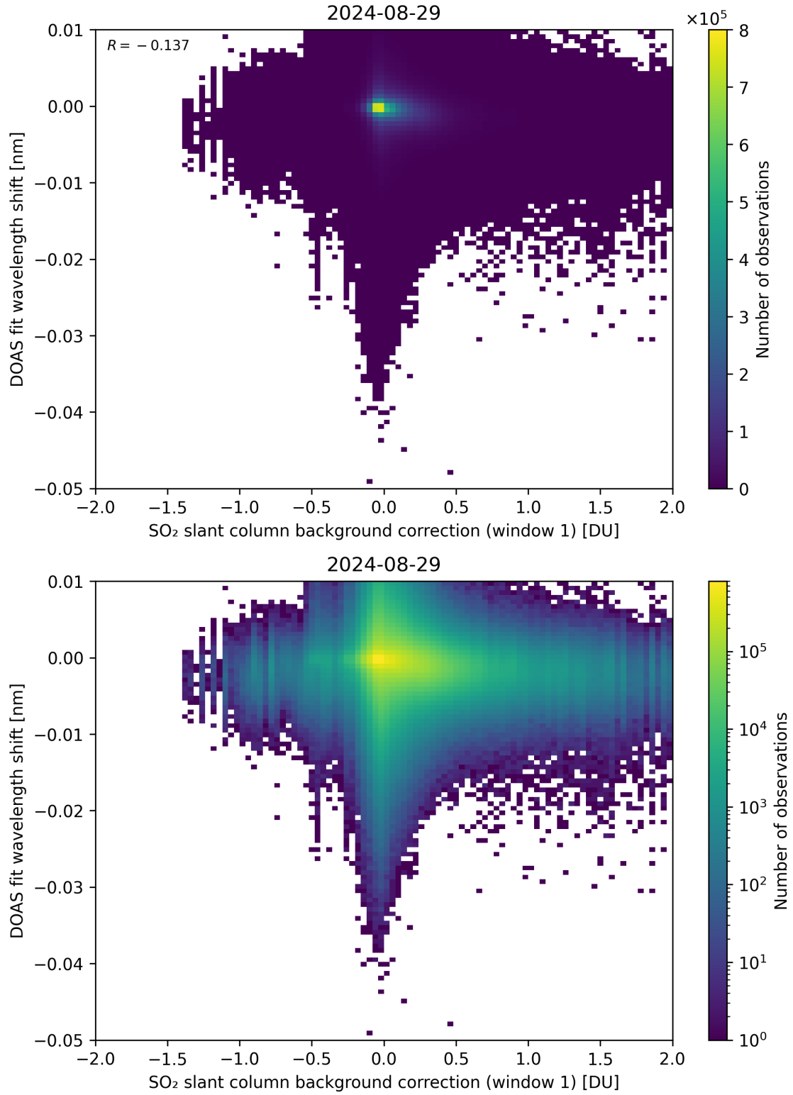
Figure 100: Scatter density plot of “SO 2 slant column background correction (window 1)” against “DOAS fit wavelength shift” for 2024-08-28 to 2024-08-30.
