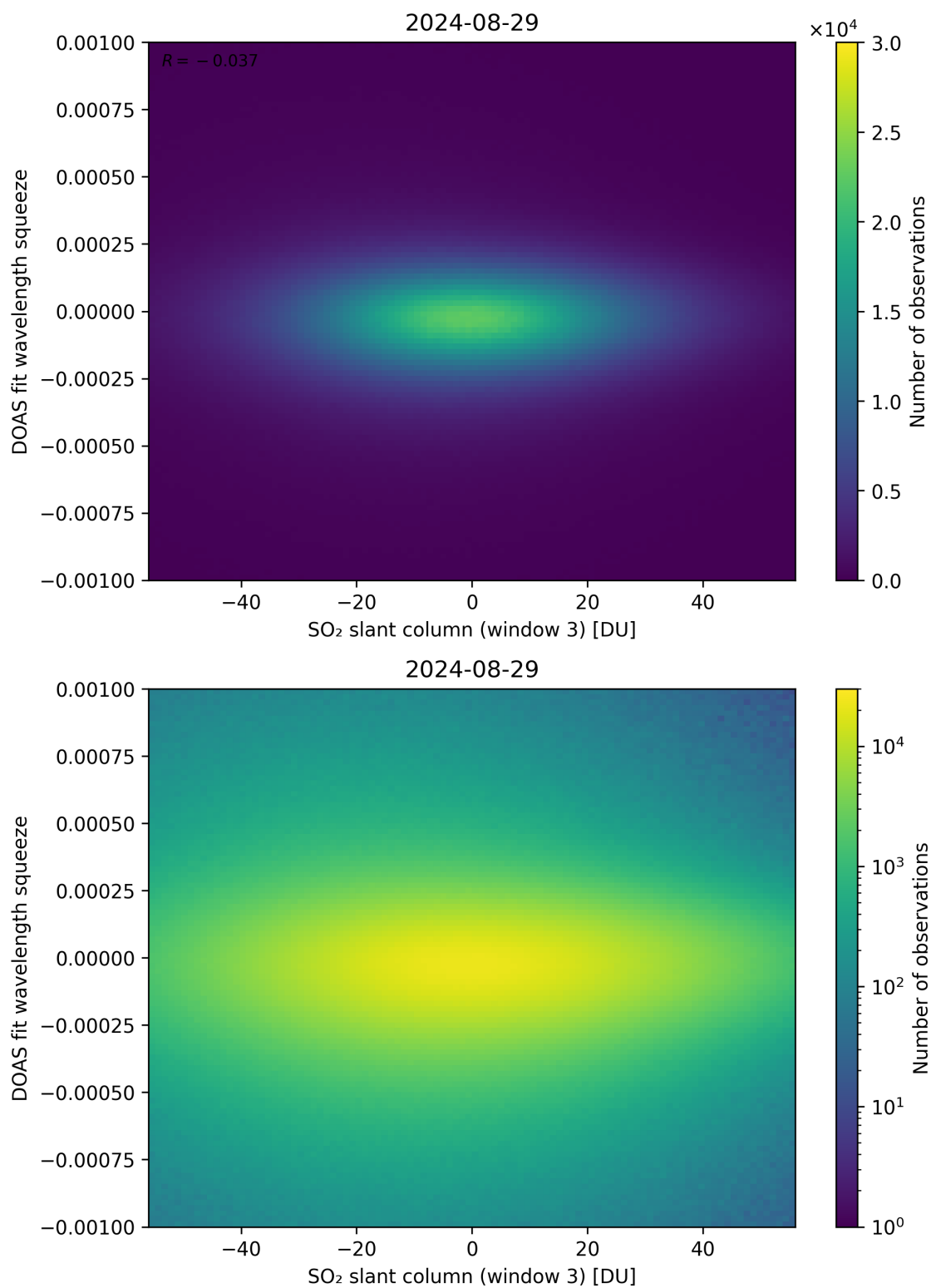
Figure 255: Scatter density plot of “SO 2 slant column (window 3)” against “DOAS fit wavelength squeeze” for 2024-08-28 to 2024-08-30.
