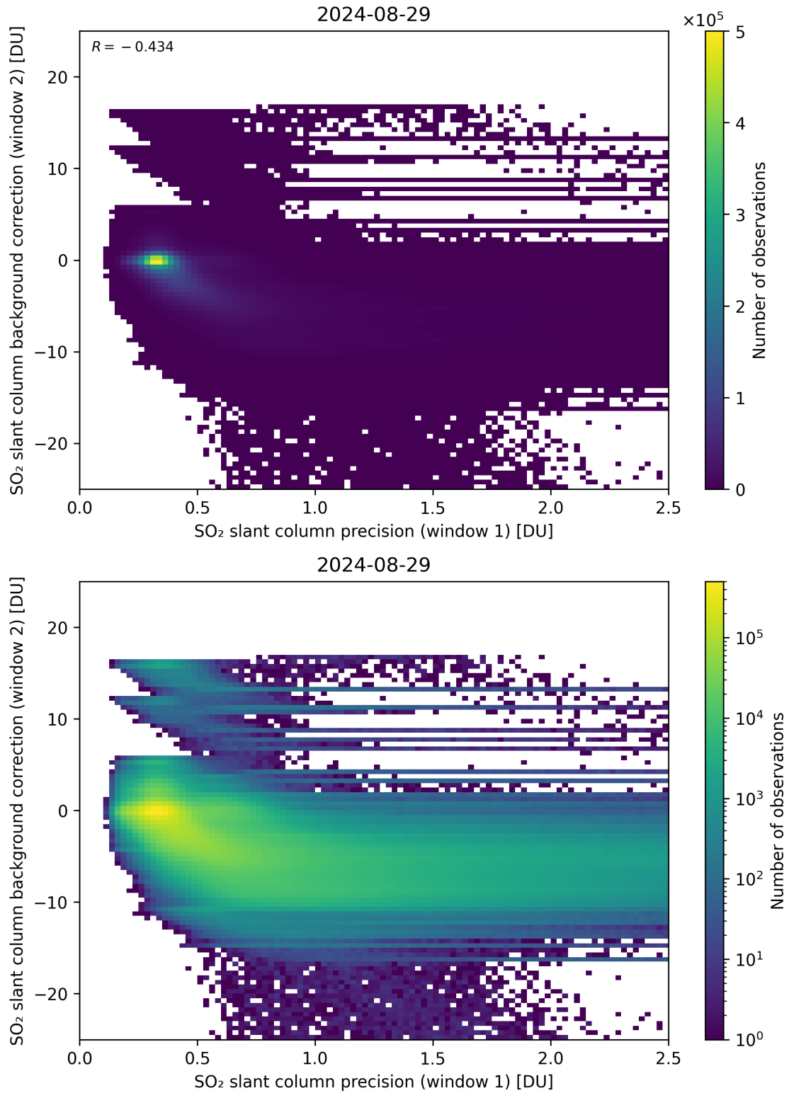
Figure 219: Scatter density plot of “SO 2 slant column precision (window 1)” against “SO 2 slant column background correction (window 2)” for 2024-08-28 to 2024-08-30.
