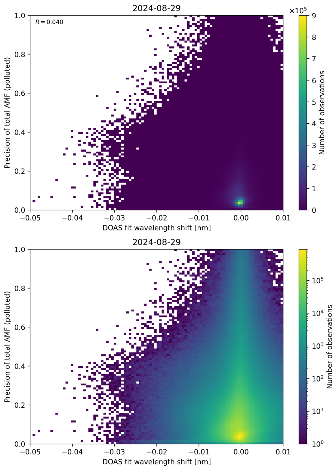
Figure 131: Scatter density plot of “DOAS fit wavelength shift” against “Precision of total AMF (polluted)” for 2024-08-28 to 2024-08-30.
