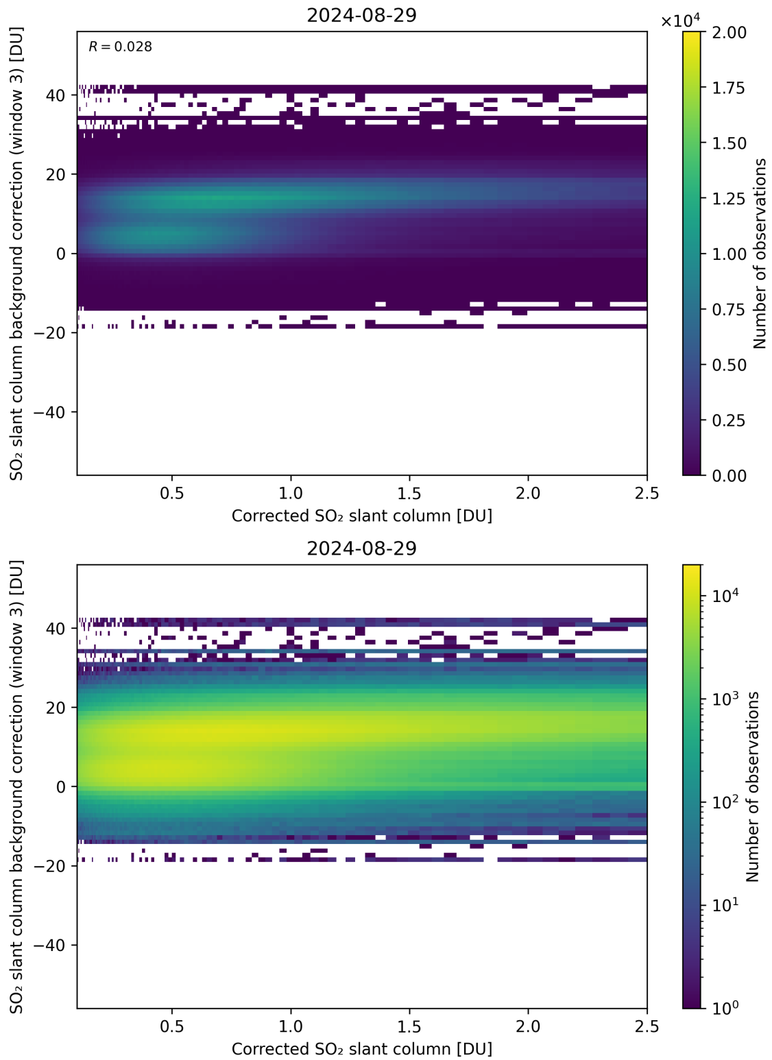
Figure 180: Scatter density plot of “Corrected SO 2 slant column” against “SO 2 slant column background correction (window 3)” for 2024-08-28 to 2024-08-30.
