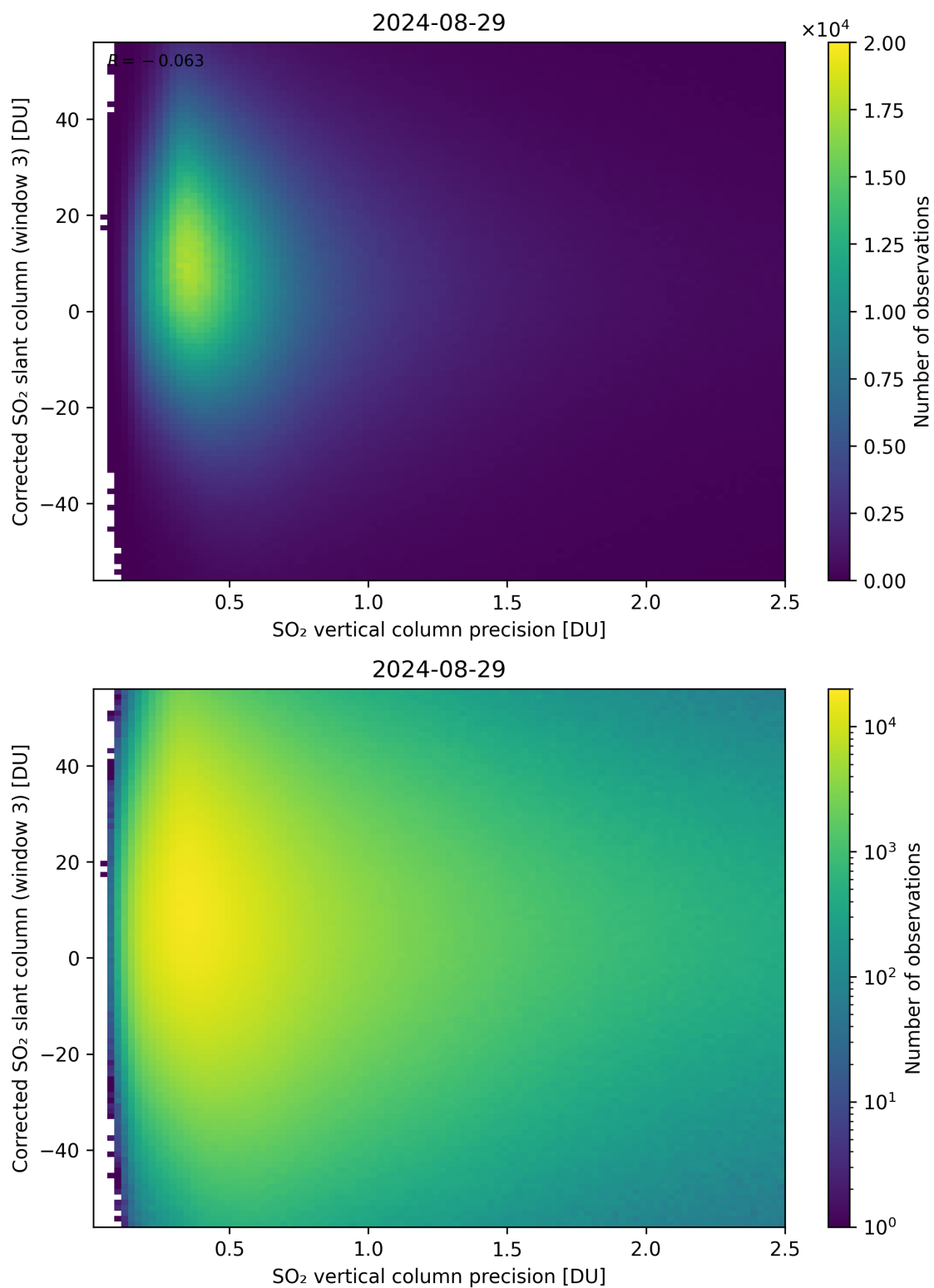
Figure 288: Scatter density plot of “SO 2 vertical column precision” against “Corrected SO 2 slant column (window 3)” for 2024-08-28 to 2024-08-30.
