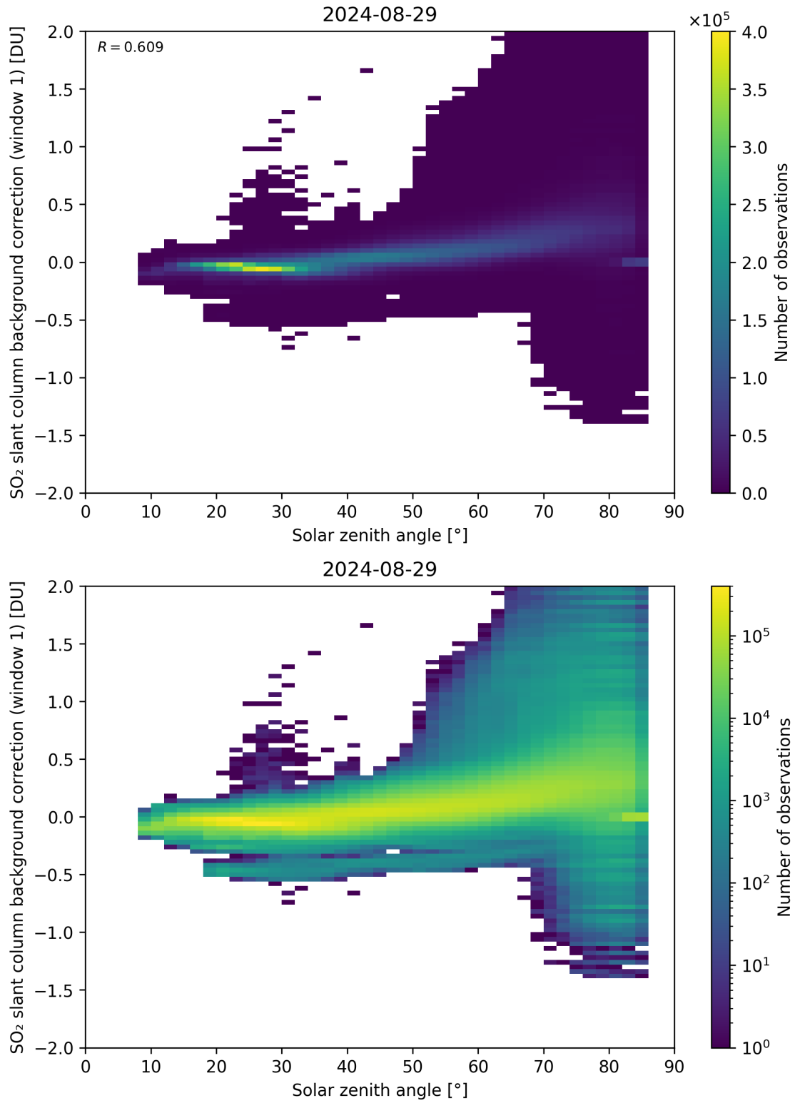
Figure 158: Scatter density plot of “Solar zenith angle” against “SO 2 slant column background correction (window 1)” for 2024-08-28 to 2024-08-30.
