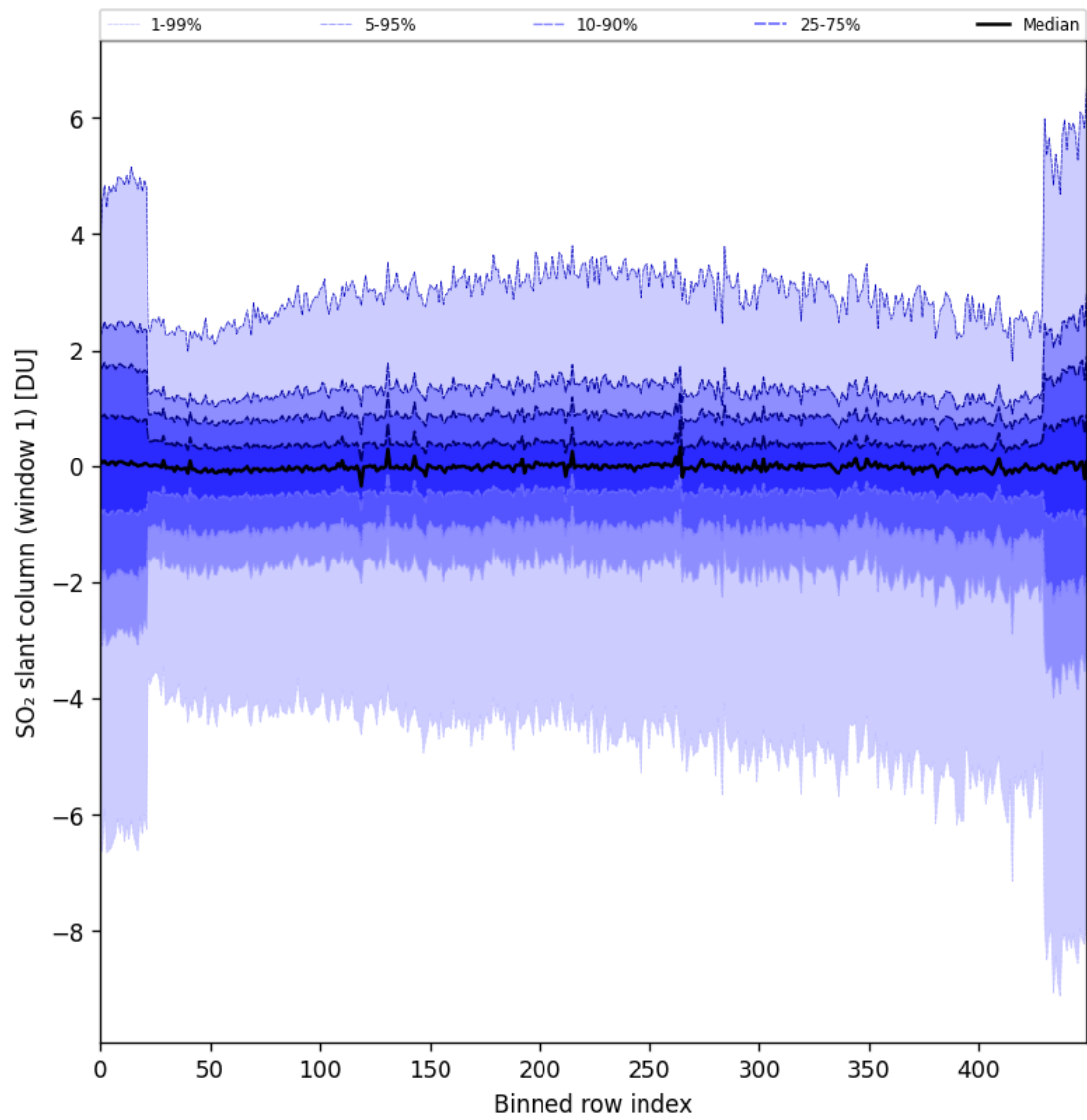
Figure 79: Along track statistics of “SO 2 slant column (window 1)” for 2024-08-28 to 2024-08-30
