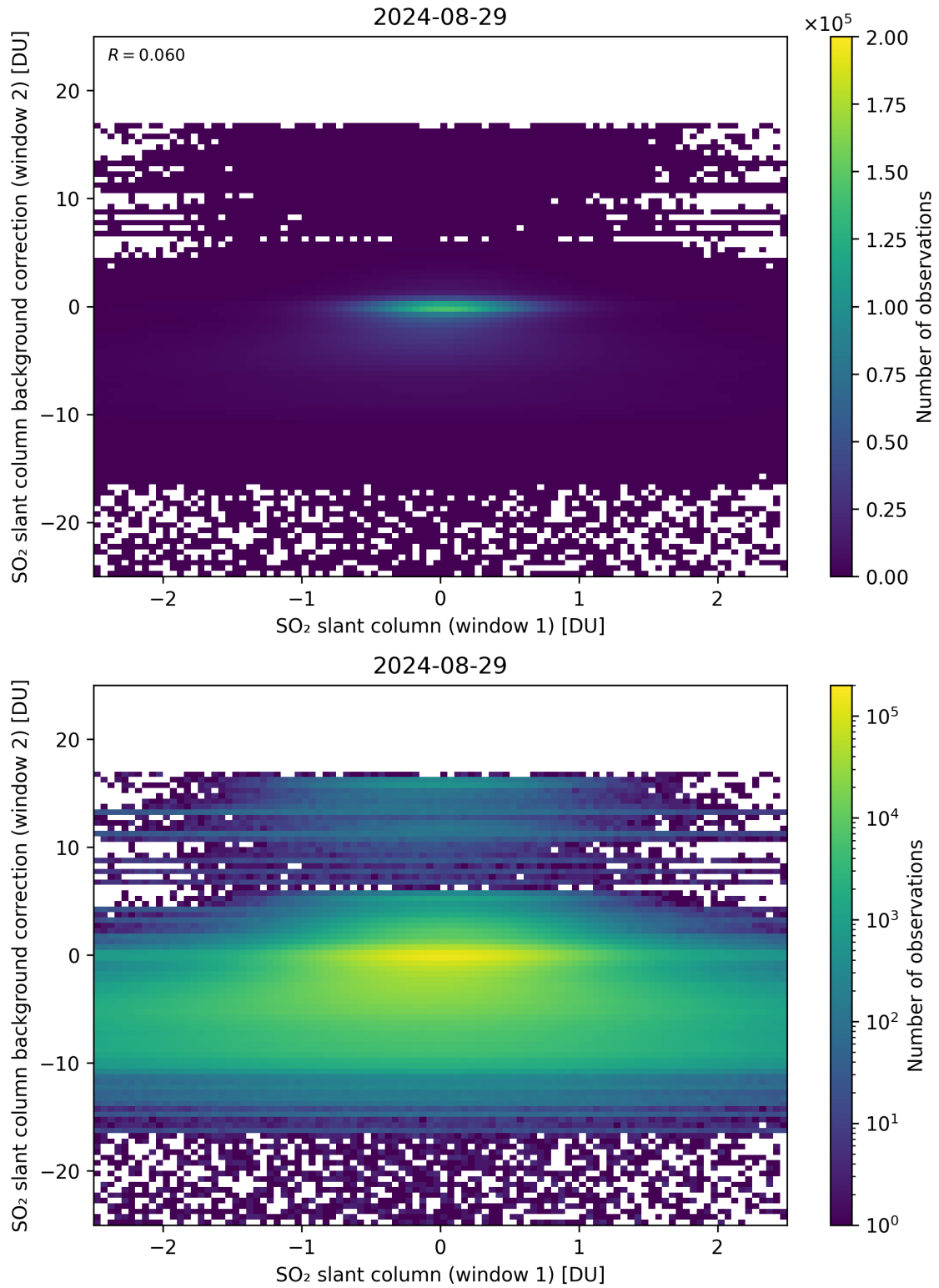
Figure 213: Scatter density plot of “SO 2 slant column (window 1)” against “SO 2 slant column background correction (window 2)” for 2024-08-28 to 2024-08-30.
