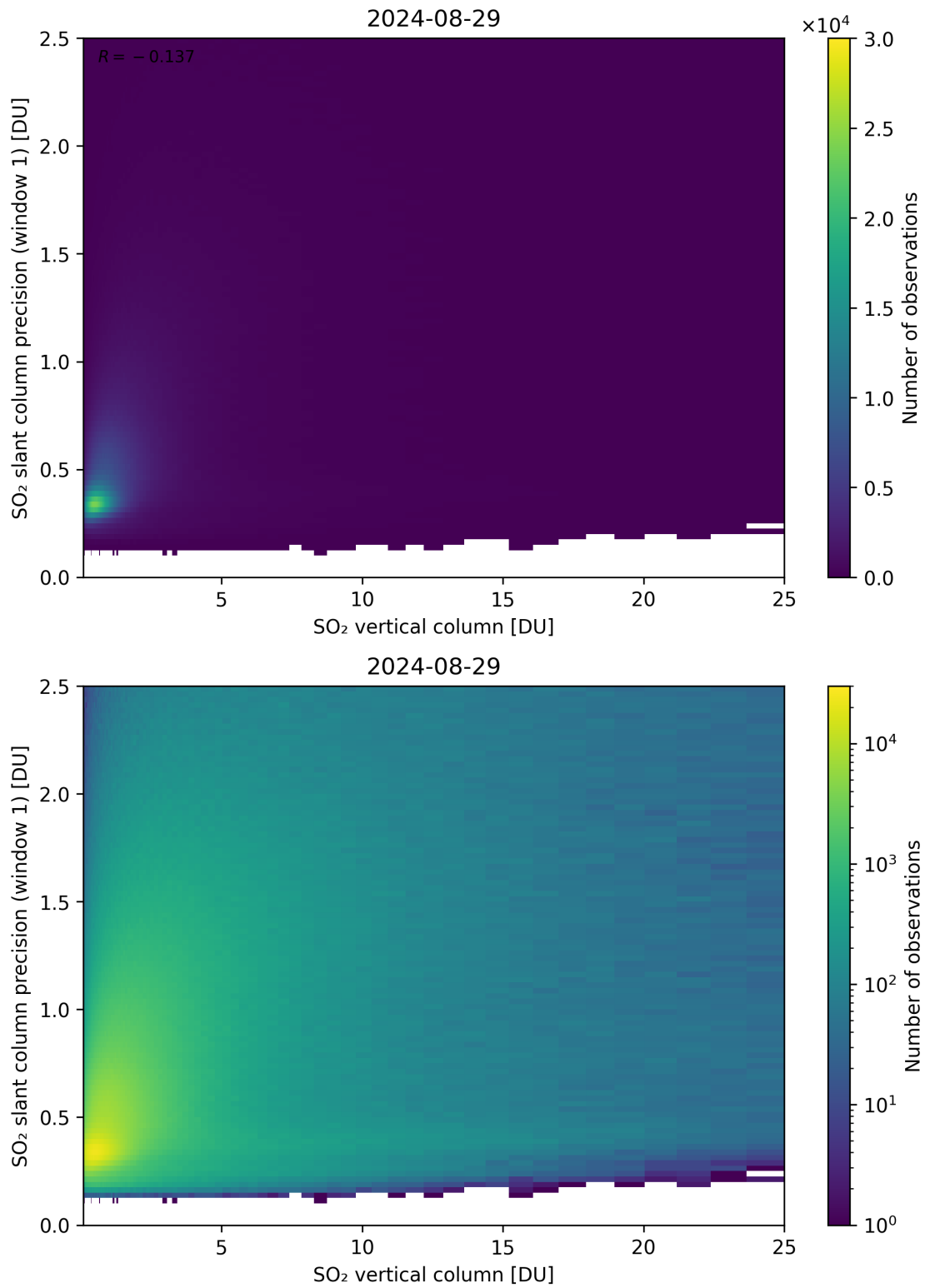
Figure 301: Scatter density plot of “SO 2 vertical column” against “SO 2 slant column precision (window 1)” for 2024-08-28 to 2024-08-30.
