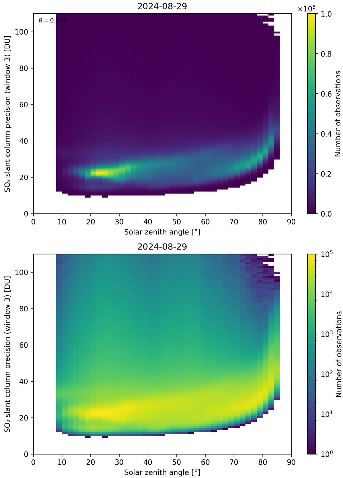
Figure 173: Scatter density plot of “Solar zenith angle” against “SO 2 slant column precision (window 3)” for 2024-08-28 to 2024-08-30.
