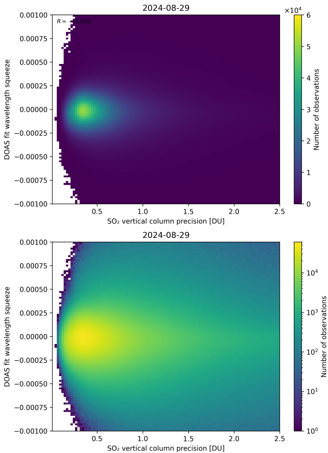
Figure 283: Scatter density plot of “SO 2 vertical column precision” against “DOAS fit wavelength squeeze” for 2024-08-28 to 2024-08-30.
