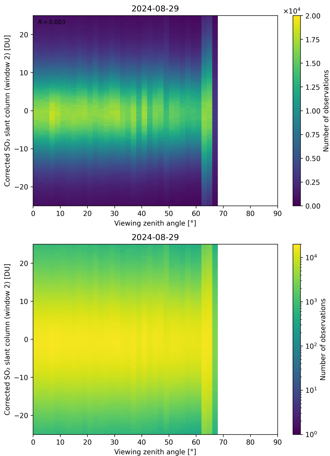
Figure 318: Scatter density plot of “Viewing zenith angle” against “Corrected SO 2 slant column (window 2)” for 2024-08-28 to 2024-08-30.
