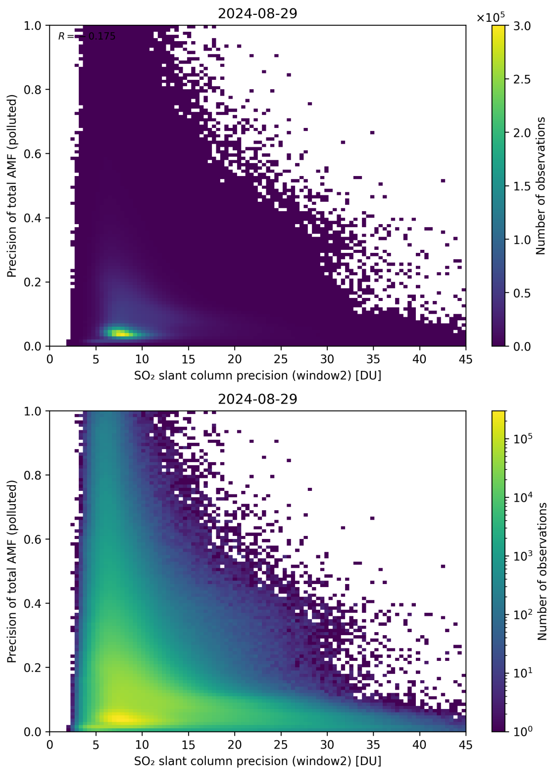
Figure 252: Scatter density plot of “SO 2 slant column precision (window2)” against “Precision of total AMF (polluted)” for 2024-08-28 to 2024-08-30.
