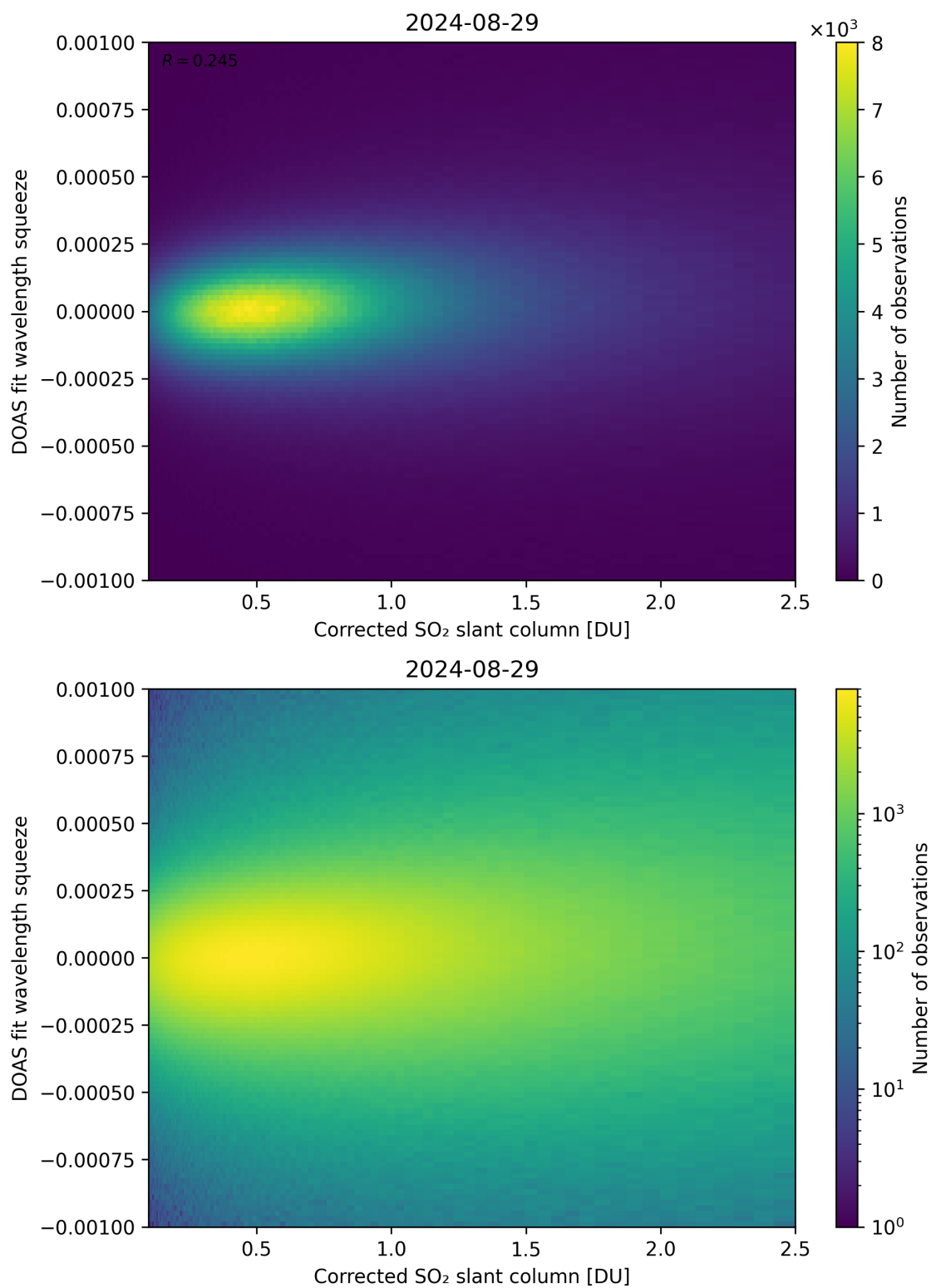
Figure 182: Scatter density plot of “Corrected SO 2 slant column” against “DOAS fit wavelength squeeze” for 2024-08-28 to 2024-08-30.
