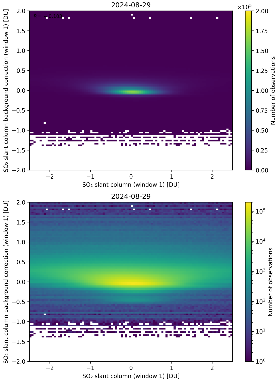
Figure 212: Scatter density plot of “SO 2 slant column (window 1)” against “SO 2 slant column background correction (window 1)” for 2024-08-28 to 2024-08-30.
