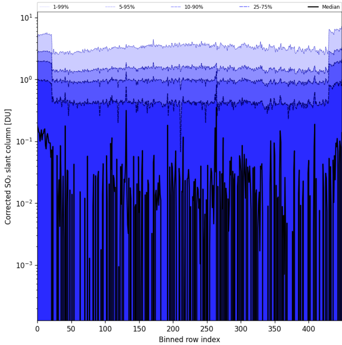
Figure 78: Along track statistics of “Corrected SO 2 slant column” for 2024-08-28 to 2024-08-30
