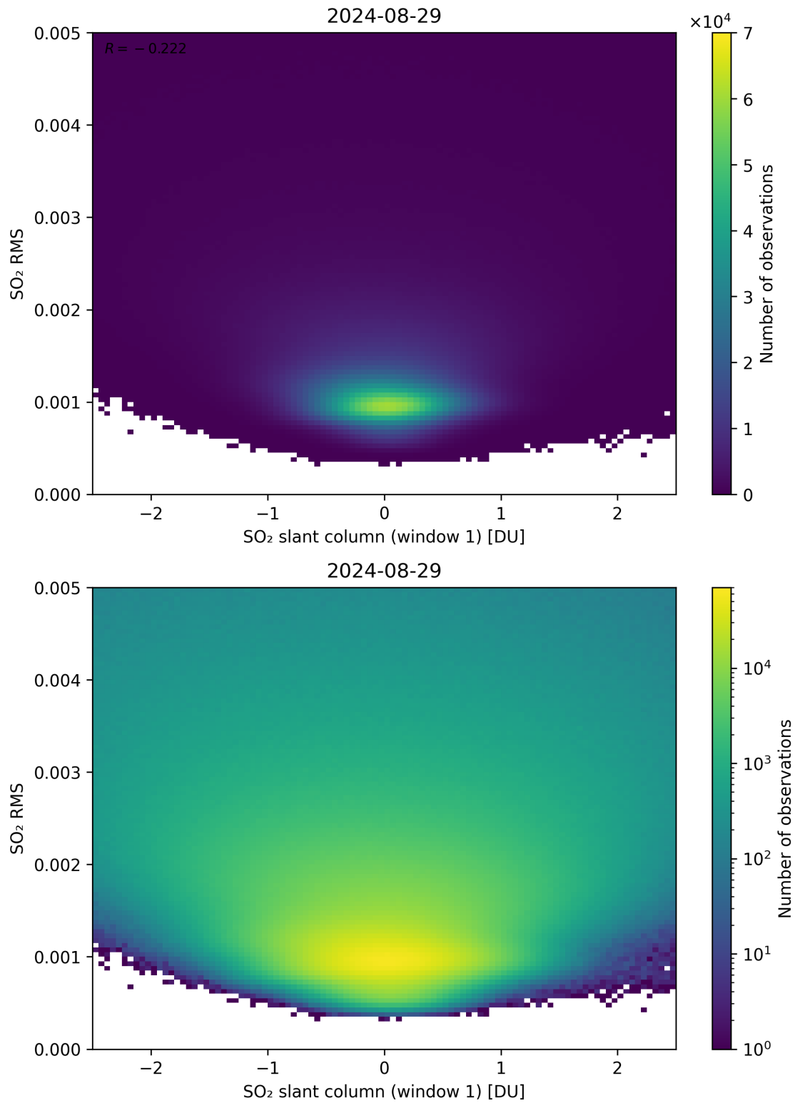
Figure 217: Scatter density plot of “SO 2 slant column (window 1)” against “SO 2 RMS” for 2024-08-28 to 2024-08-30.
