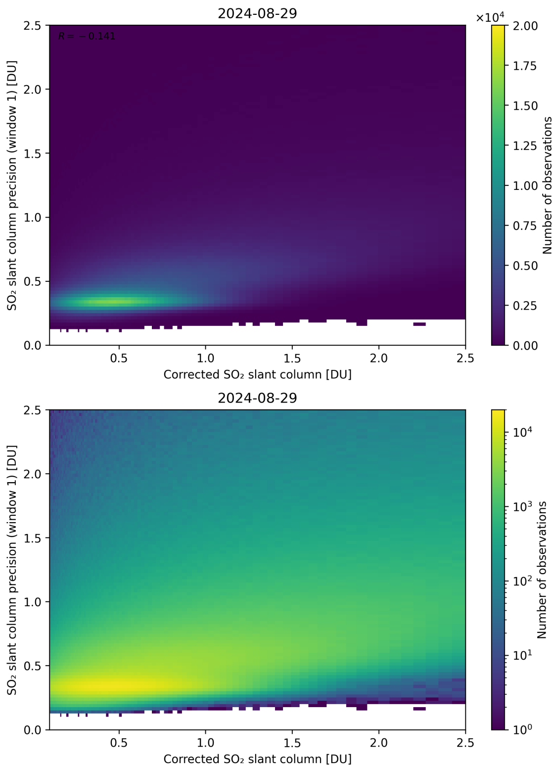
Figure 188: Scatter density plot of “Corrected SO 2 slant column” against “SO 2 slant column precision (window 1)” for 2024-08-28 to 2024-08-30.
