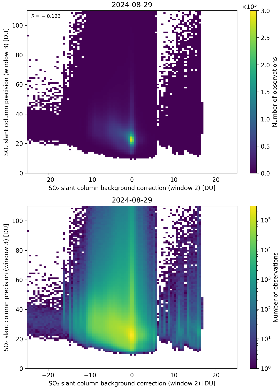
Figure 118: Scatter density plot of “SO 2 slant column background correction (window 2)” against “SO 2 slant column precision (window 3)” for 2024-08-28 to 2024-08-30.
