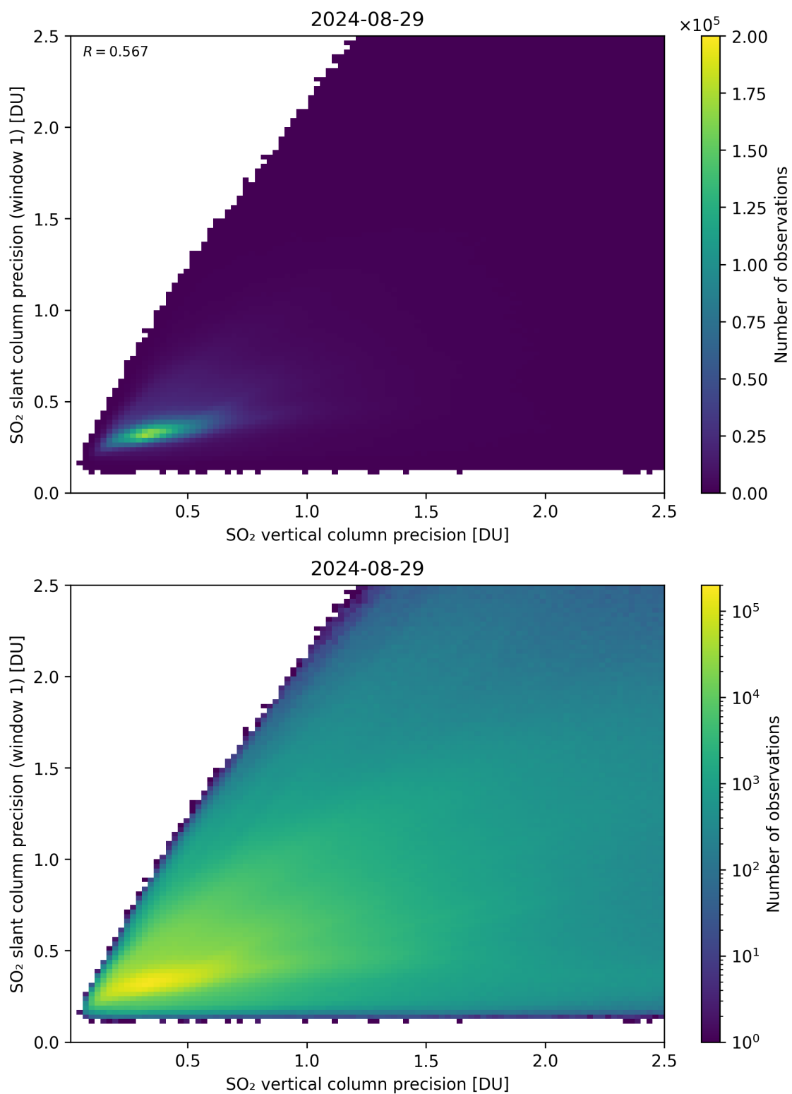
Figure 290: Scatter density plot of “SO 2 vertical column precision” against “SO 2 slant column precision (window 1)” for 2024-08-28 to 2024-08-30.
