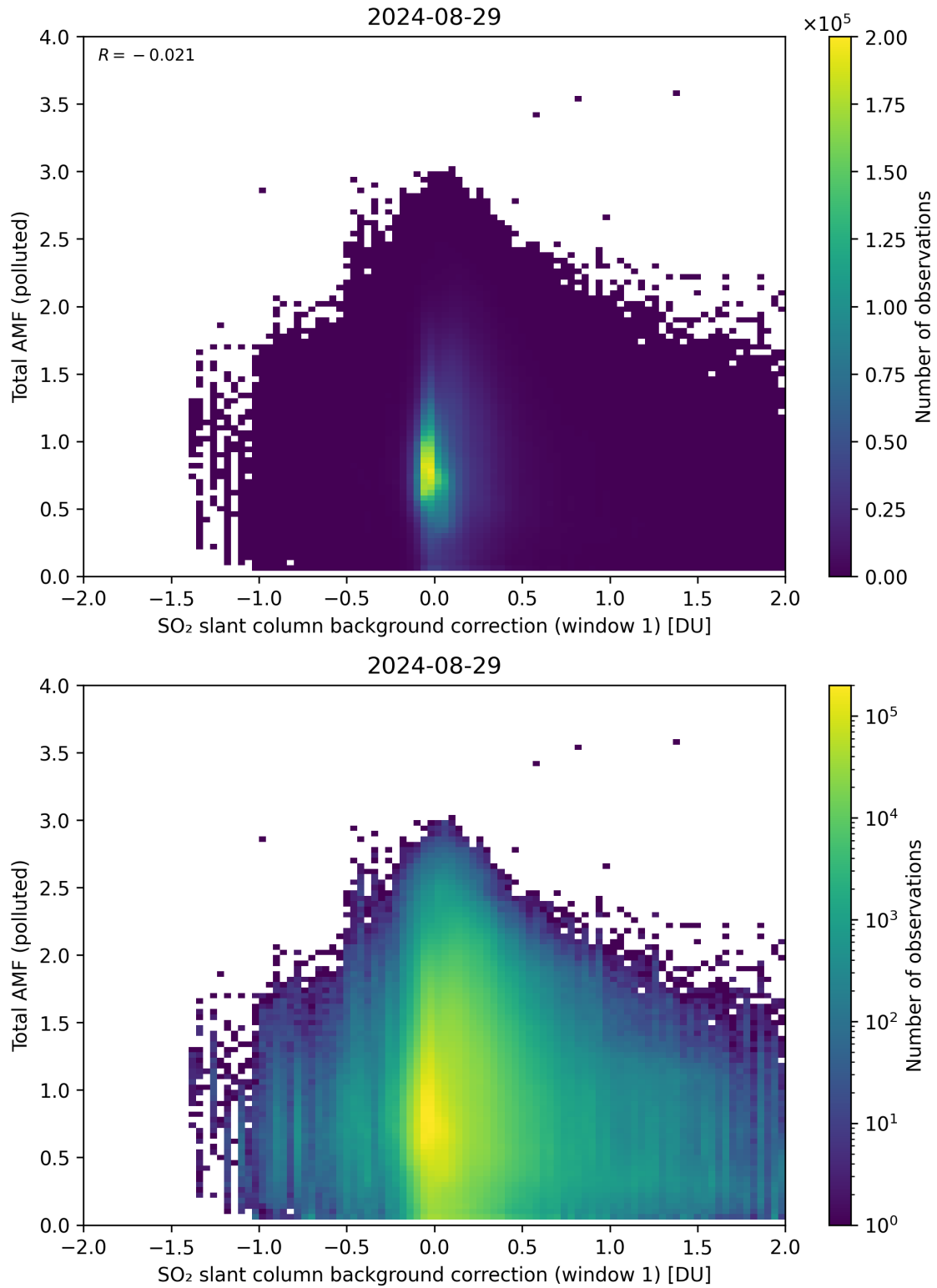
Figure 109: Scatter density plot of “SO 2 slant column background correction (window 1)” against “Total AMF (polluted)” for 2024-08-28 to 2024-08-30.
