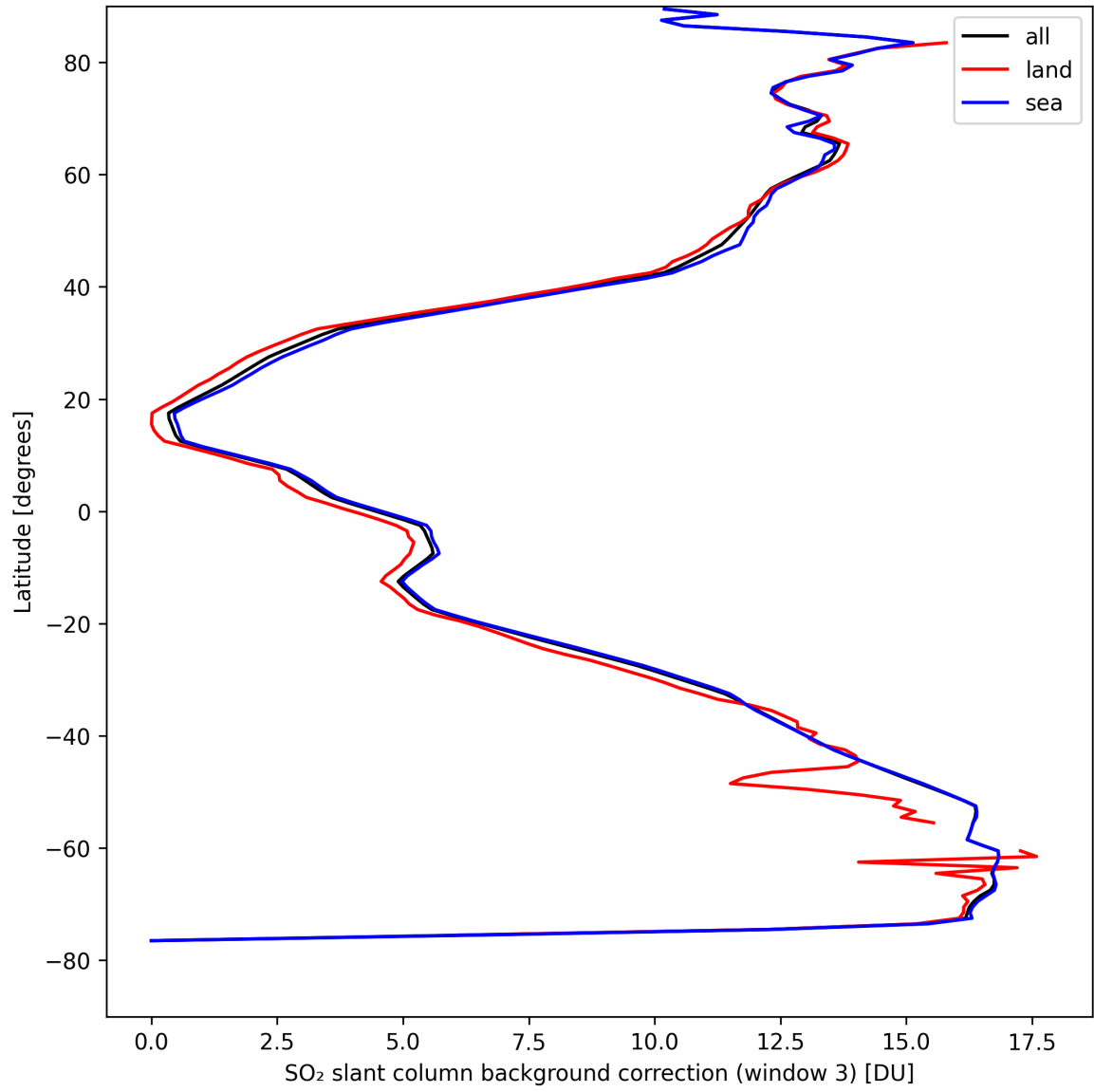
Figure 44: Zonal average of “SO 2 slant column background correction (window 3)” for 2024-08-28 to 2024-08-30.
