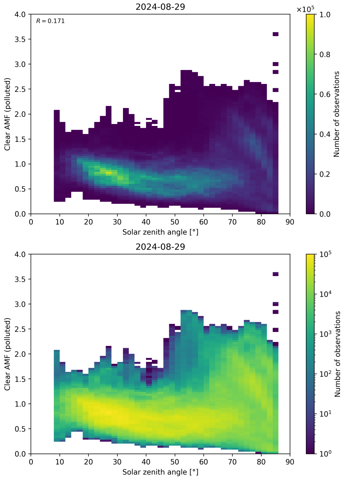
Figure 165: Scatter density plot of “Solar zenith angle” against “Clear AMF (polluted)” for 2024-08-28 to 2024-08-30.
