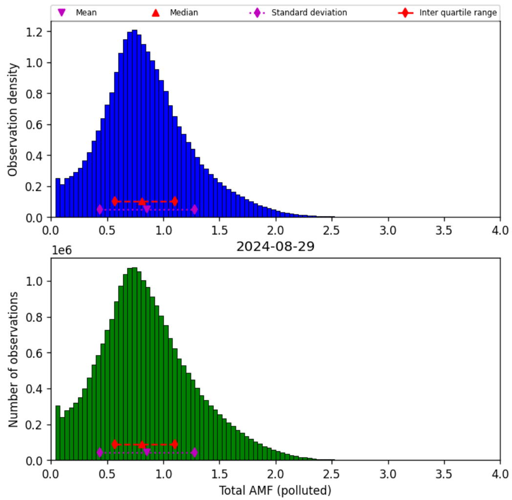
Figure 71: Histogram of “Total AMF (polluted)” for 2024-08-28 to 2024-08-30
