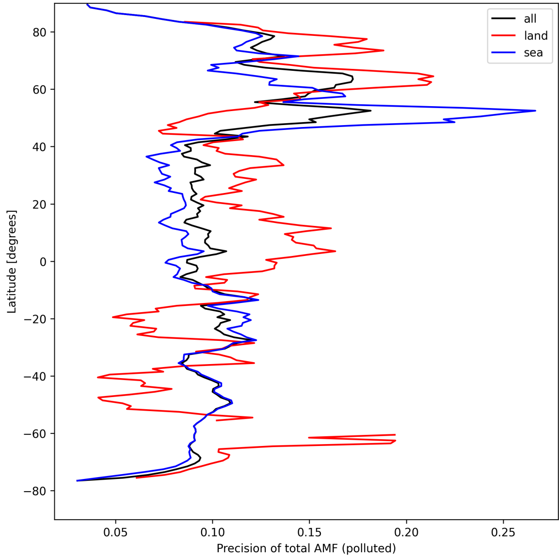
Figure 49: Zonal average of “Precision of total AMF (polluted)” for 2024-08-28 to 2024-08-30.
