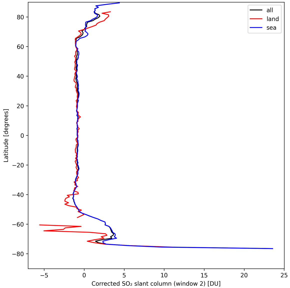
Figure 39: Zonal average of “Corrected SO 2 slant column (window 2)” for 2024-08-28 to 2024-08-30.
