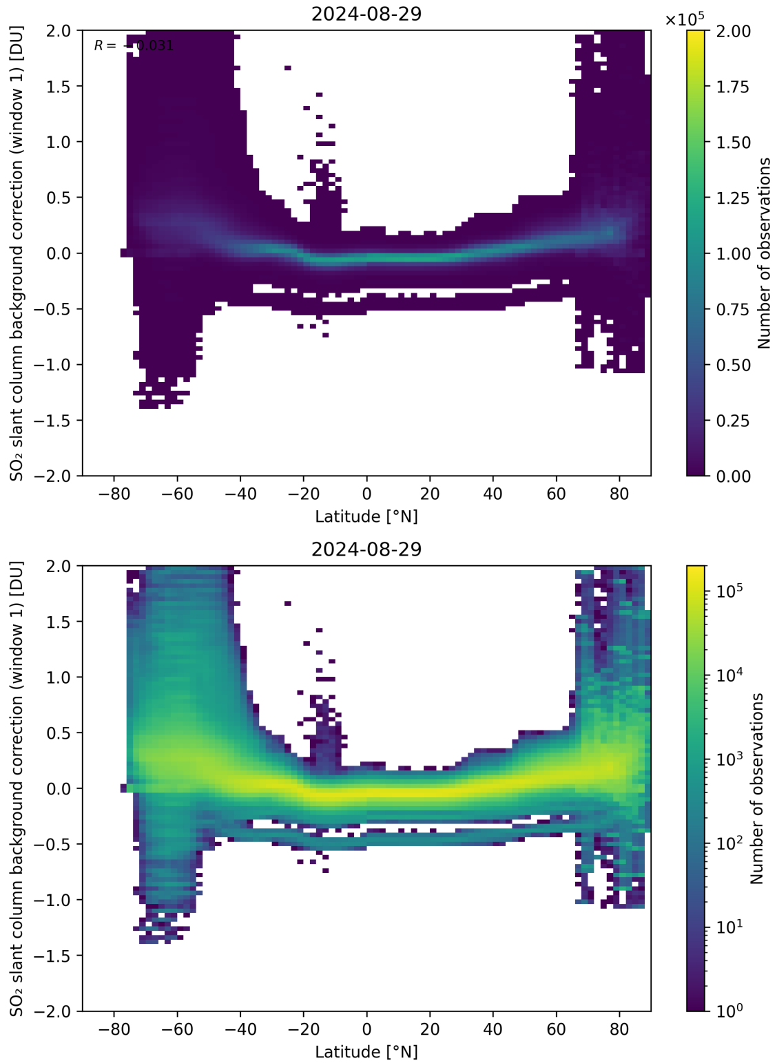
Figure 139: Scatter density plot of “Latitude” against “SO 2 slant column background correction (window 1)” for 2024-08-28 to 2024-08-30.
