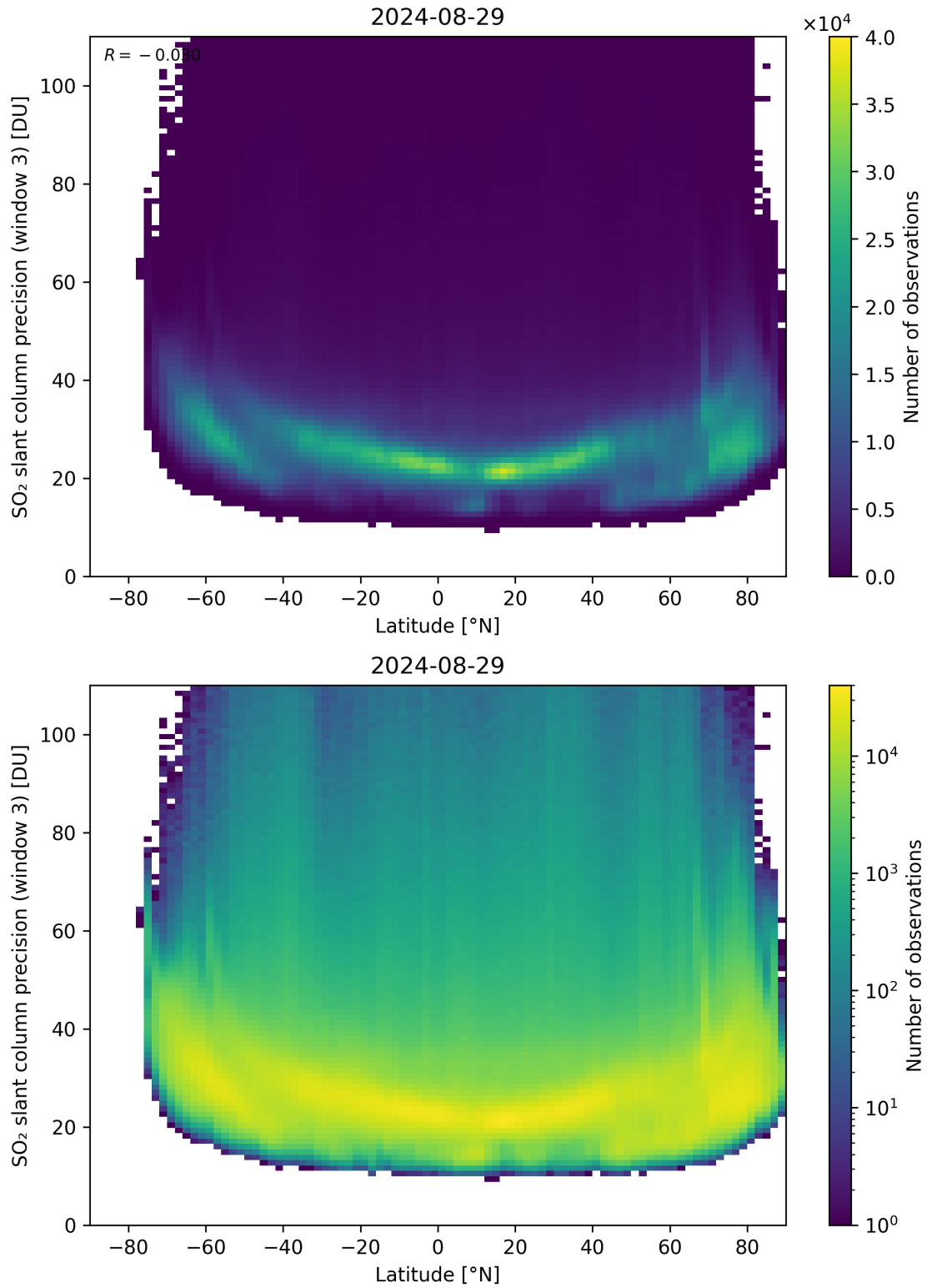
Figure 153: Scatter density plot of “Latitude” against “SO 2 slant column precision (window 3)” for 2024-08-28 to 2024-08-30.
