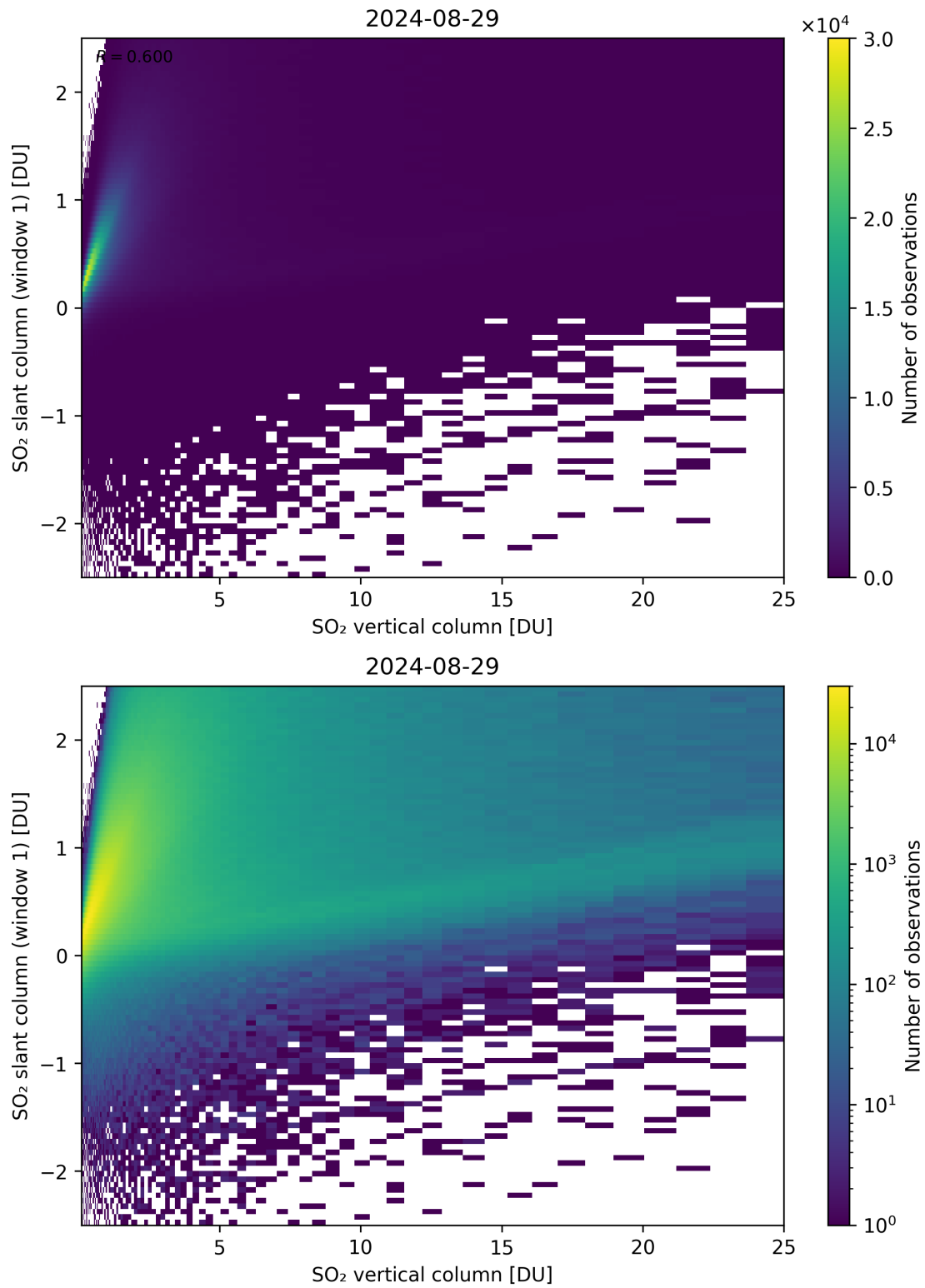
Figure 300: Scatter density plot of “SO 2 vertical column” against “SO 2 slant column (window 1)” for 2024-08-28 to 2024-08-30.
