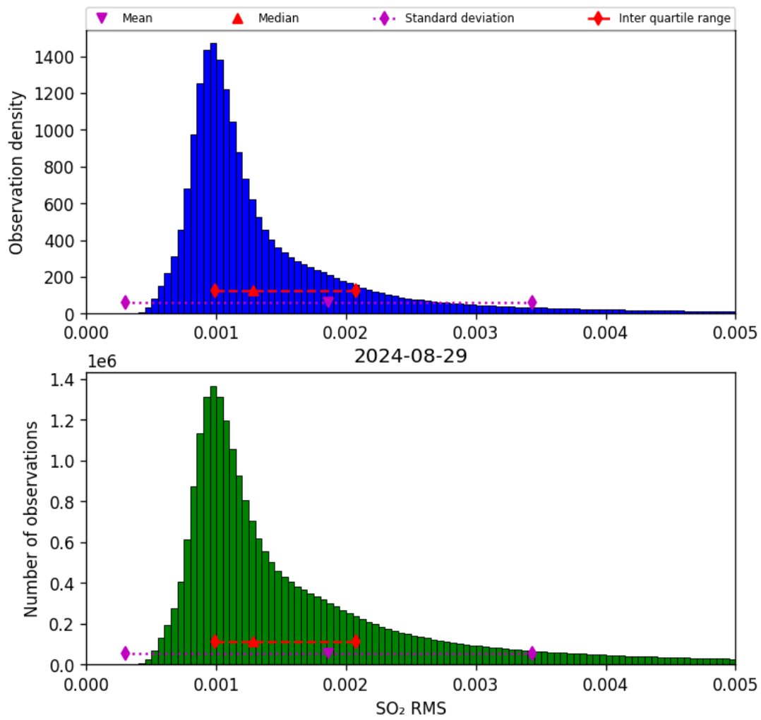
Figure 70: Histogram of “SO 2 RMS” for 2024-08-28 to 2024-08-30
