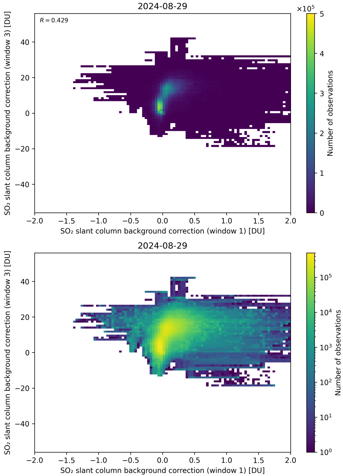
Figure 99: Scatter density plot of “SO 2 slant column background correction (window 1)” against “SO 2 slant column background correction (window 3)” for 2024-08-28 to 2024-08-30.
