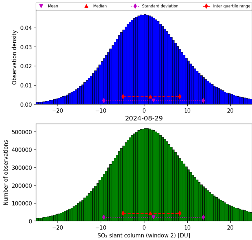
Figure 60: Histogram of “SO 2 slant column (window 2)” for 2024-08-28 to 2024-08-30
