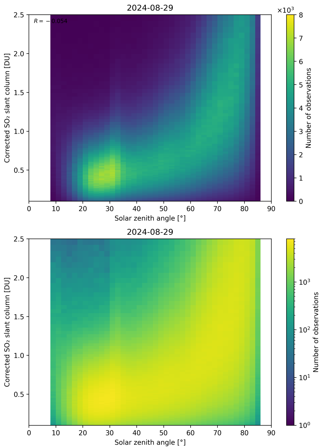
Figure 166: Scatter density plot of “Solar zenith angle” against “Corrected SO 2 slant column” for 2024-08-28 to 2024-08-30.
