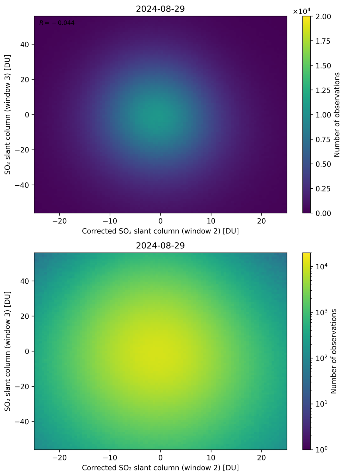
Figure 201: Scatter density plot of “Corrected SO 2 slant column (window 2)” against “SO 2 slant column (window 3)” for 2024-08-28 to 2024-08-30.
