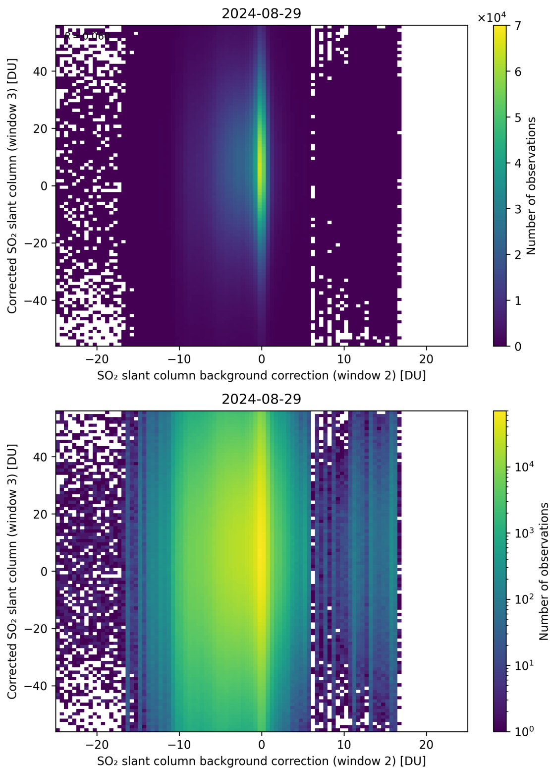
Figure 116: Scatter density plot of “SO 2 slant column background correction (window 2)” against “Corrected SO 2 slant column (window 3)” for 2024-08-28 to 2024-08-30.
