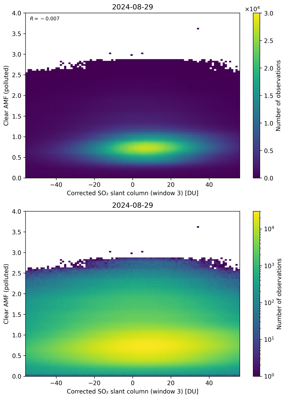
Figure 209: Scatter density plot of “Corrected SO 2 slant column (window 3)” against “Clear AMF (polluted)” for 2024-08-28 to 2024-08-30.
