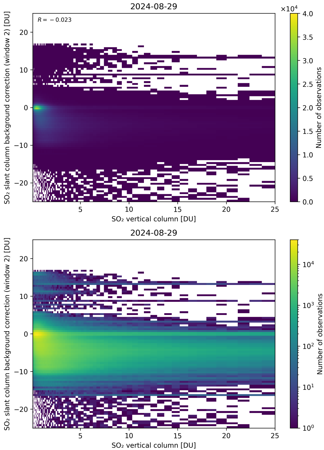
Figure 274: Scatter density plot of “SO 2 vertical column” against “SO 2 slant column background correction (window 2)” for 2024-08-28 to 2024-08-30.
