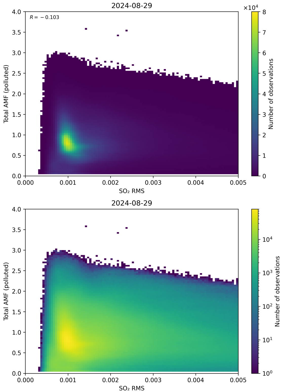
Figure 137: Scatter density plot of “SO 2 RMS” against “Total AMF (polluted)” for 2024-08-28 to 2024-08-30.
