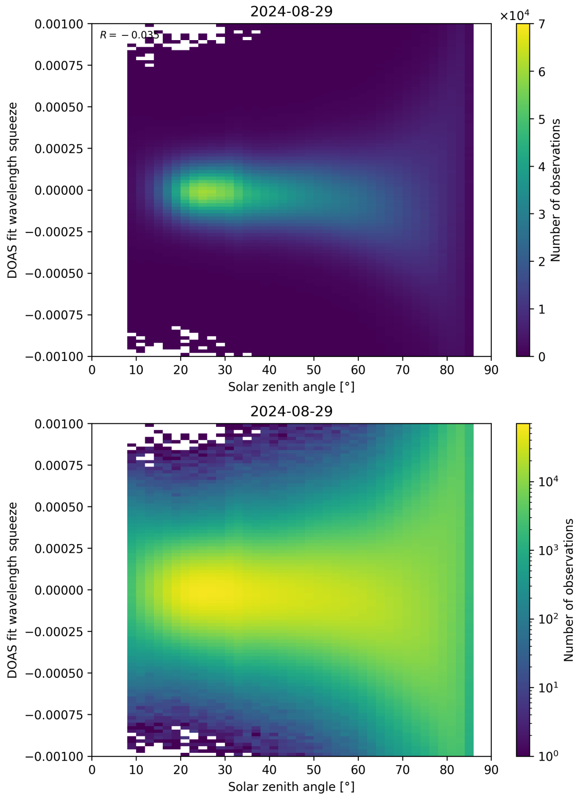
Figure 162: Scatter density plot of “Solar zenith angle” against “DOAS fit wavelength squeeze” for 2024-08-28 to 2024-08-30.
