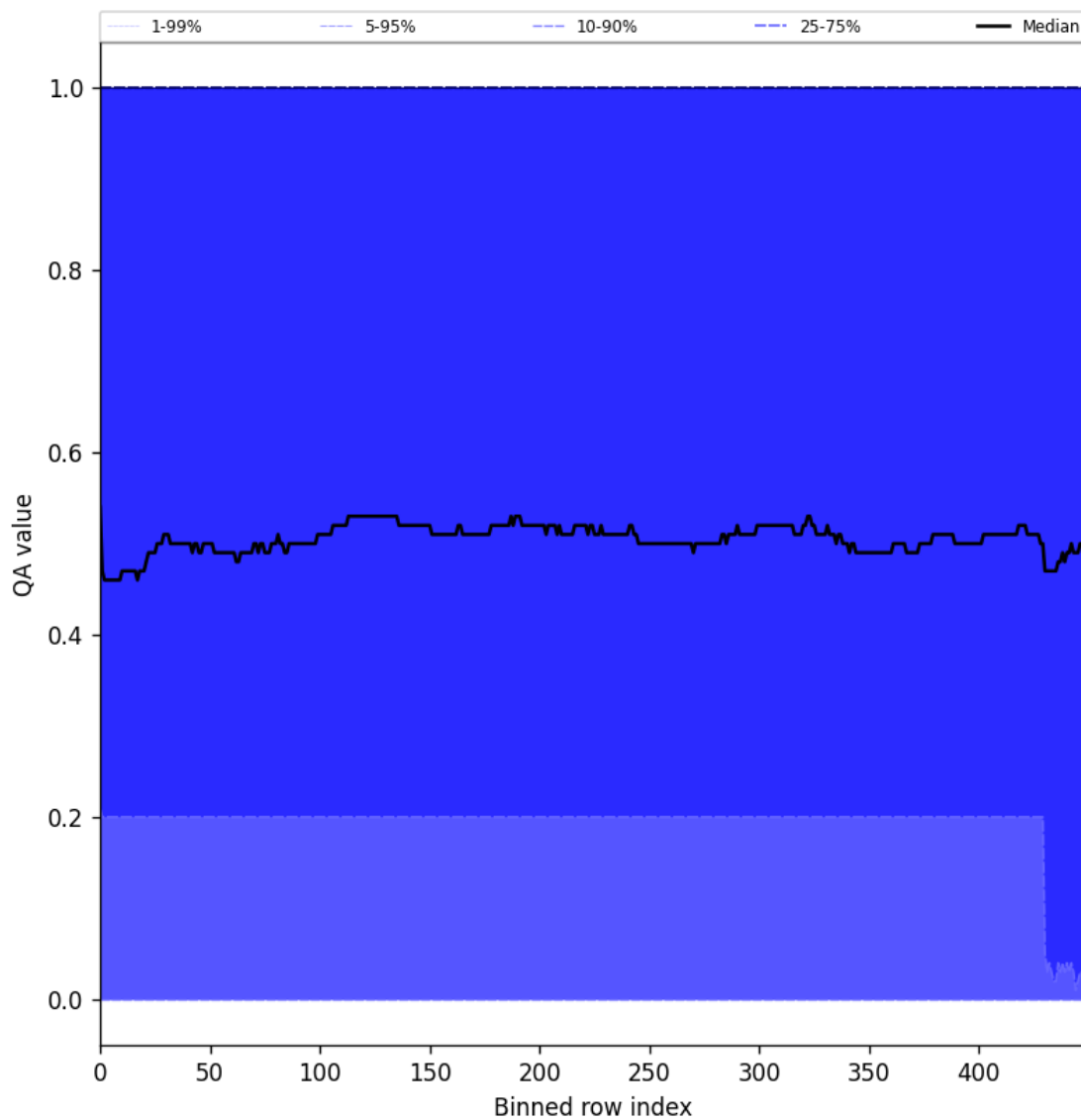
Figure 75: Along track statistics of “QA value” for 2024-08-28 to 2024-08-30
