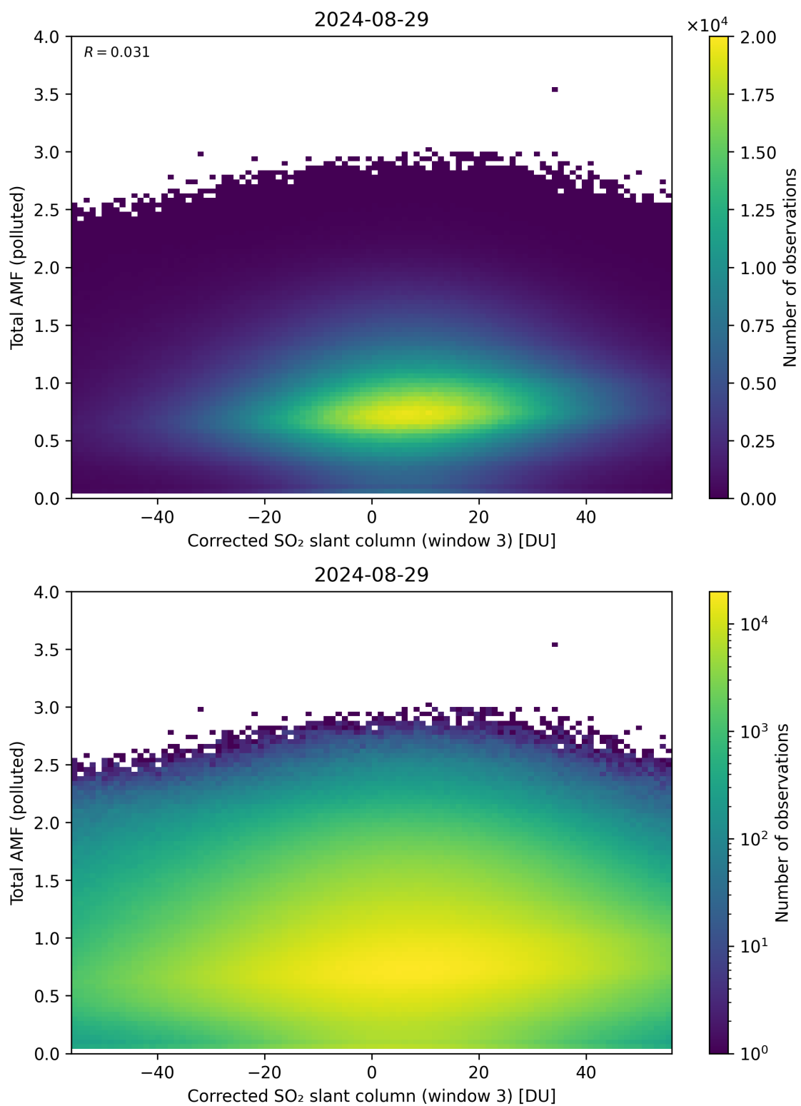
Figure 210: Scatter density plot of “Corrected SO 2 slant column (window 3)” against “Total AMF (polluted)” for 2024-08-28 to 2024-08-30.
