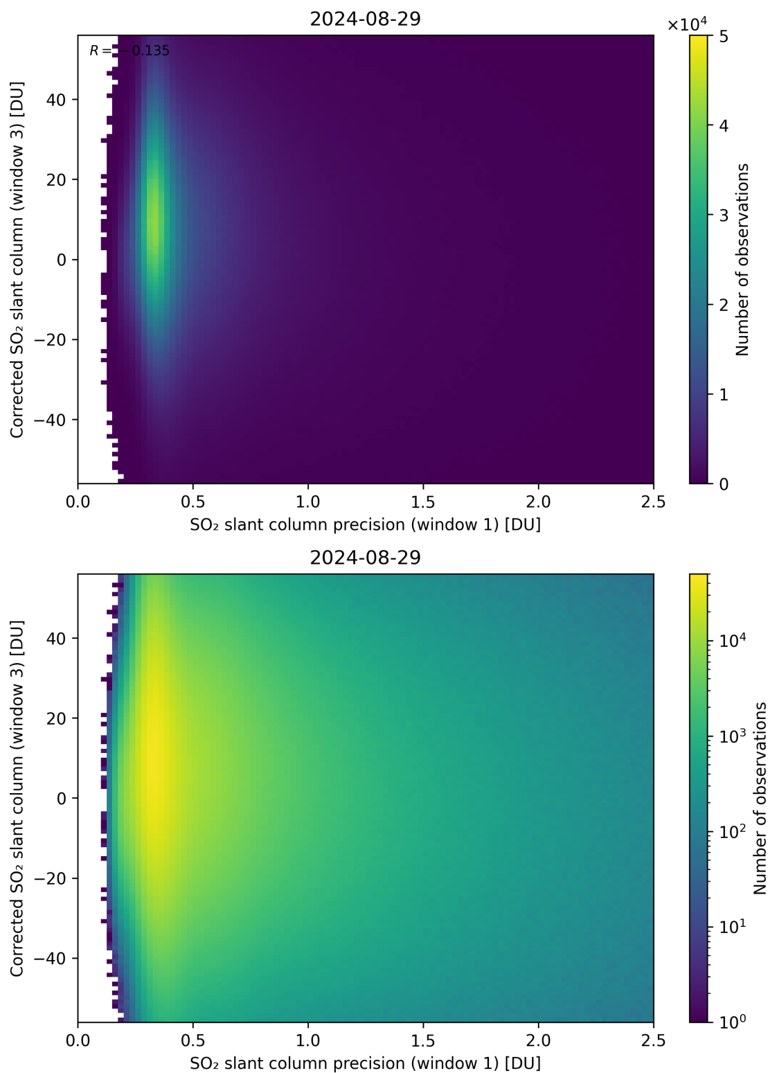
Figure 226: Scatter density plot of “SO 2 slant column precision (window 1)” against “Corrected SO 2 slant column (window 3)” for 2024-08-28 to 2024-08-30.
