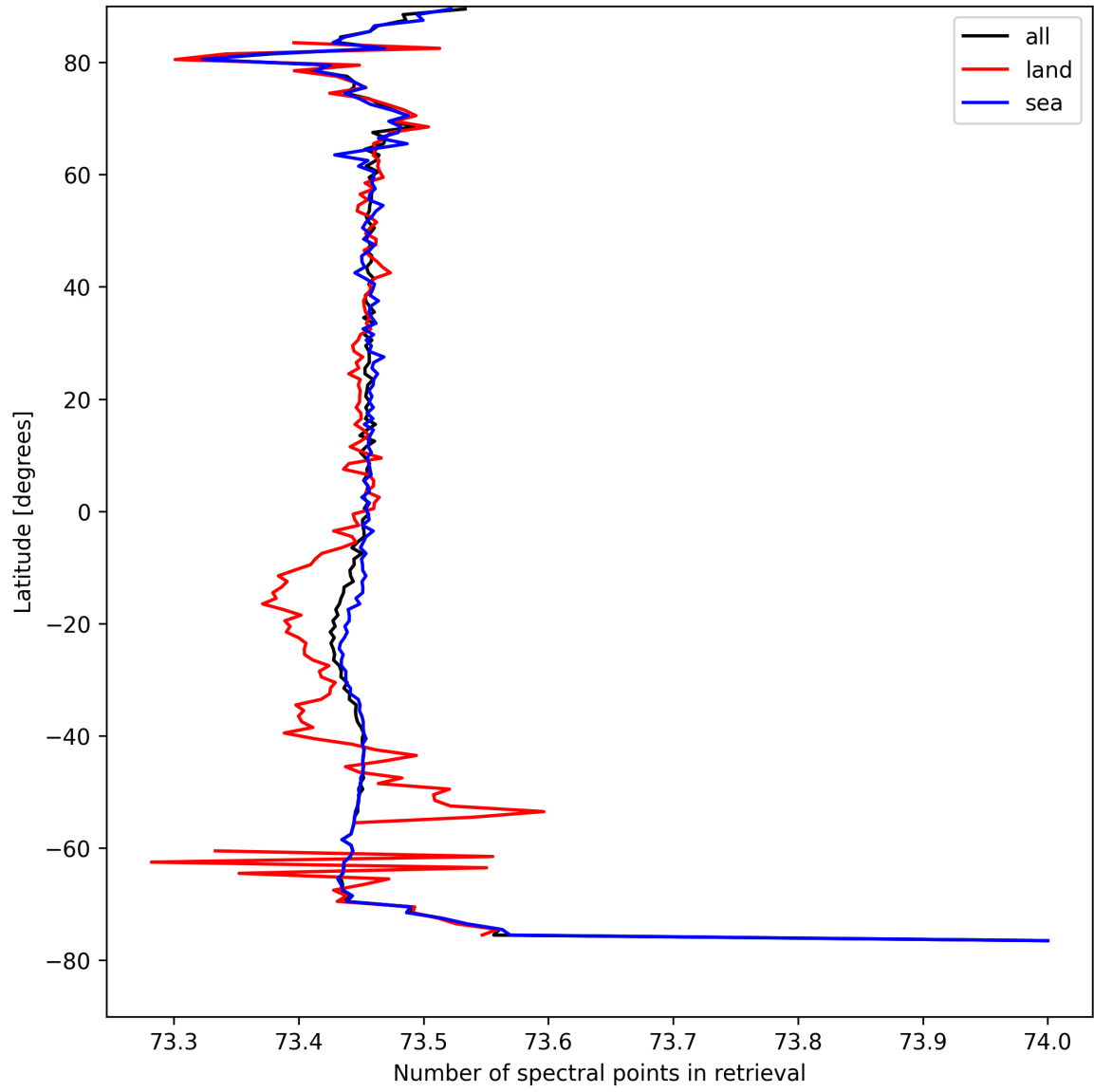
Figure 51: Zonal average of “Number of spectral points in retrieval” for 2024-08-28 to 2024-08-30.
