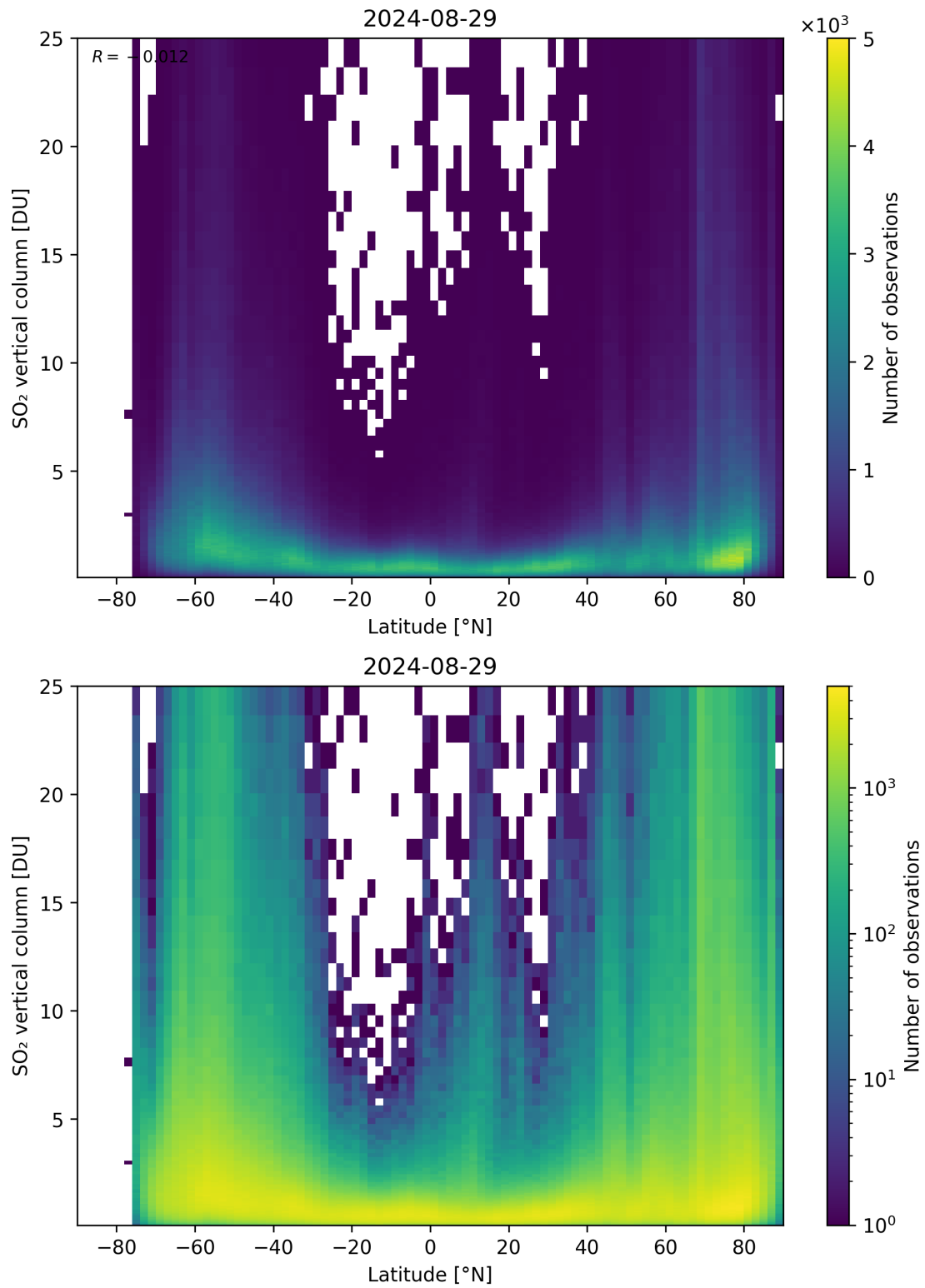
Figure 156: Scatter density plot of “Latitude” against “SO 2 vertical column” for 2024-08-28 to 2024-08-30.
