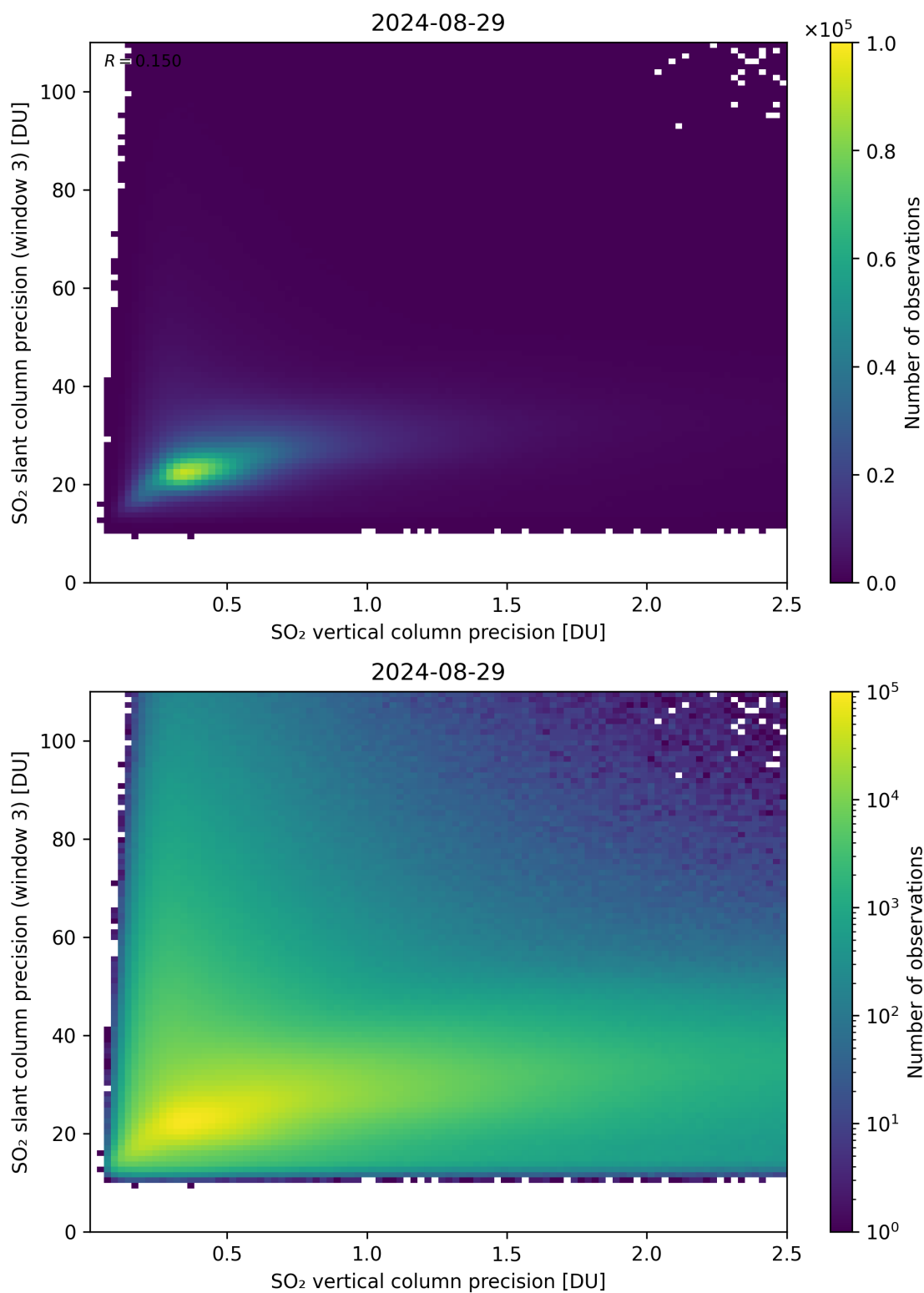
Figure 293: Scatter density plot of “SO 2 vertical column precision” against “SO 2 slant column precision (window 3)” for 2024-08-28 to 2024-08-30.
