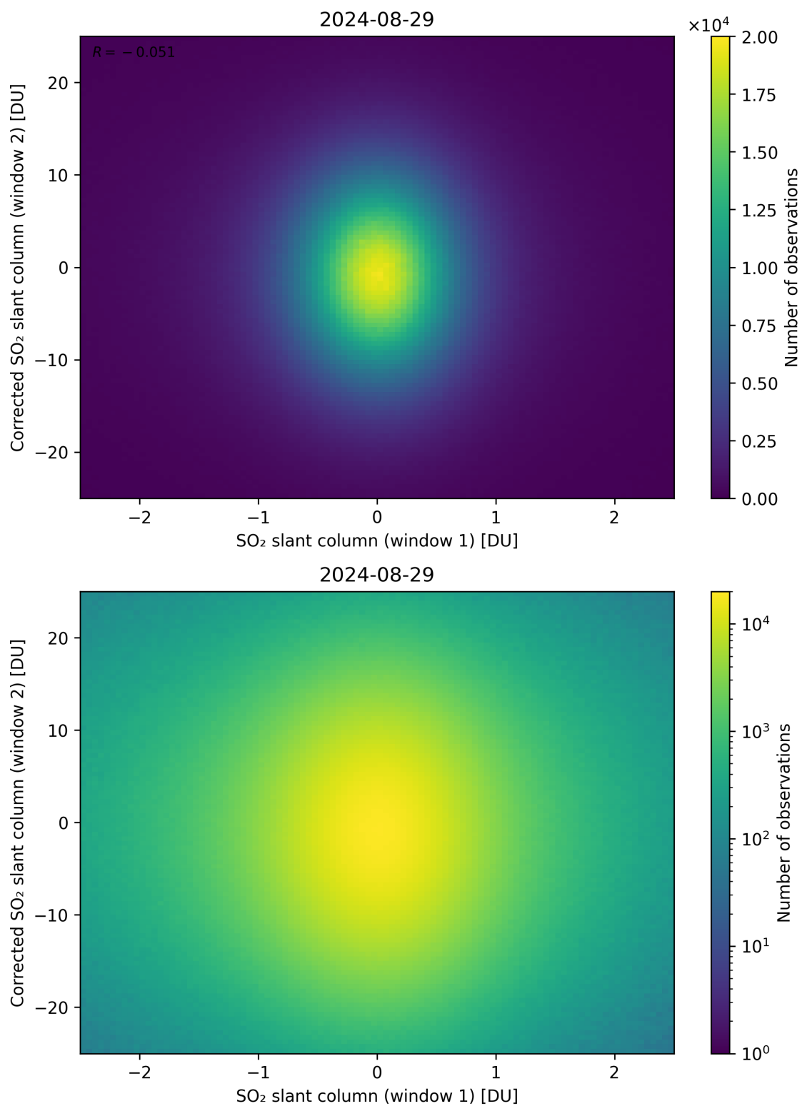
Figure 233: Scatter density plot of “SO 2 slant column (window 1)” against “Corrected SO 2 slant column (window 2)” for 2024-08-28 to 2024-08-30.
