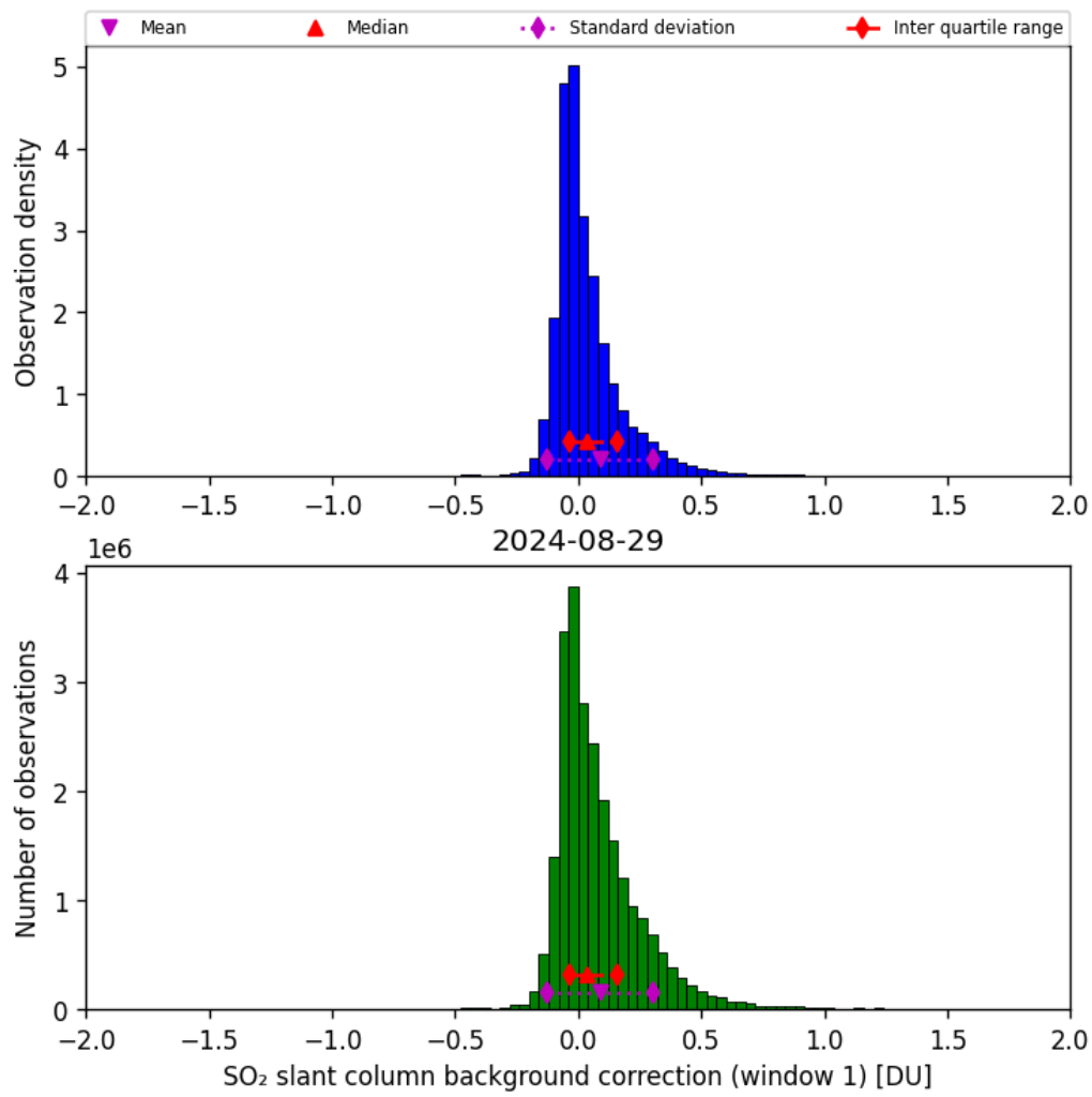
Figure 59: Histogram of “SO 2 slant column background correction (window 1)” for 2024-08-28 to 2024-08-30
