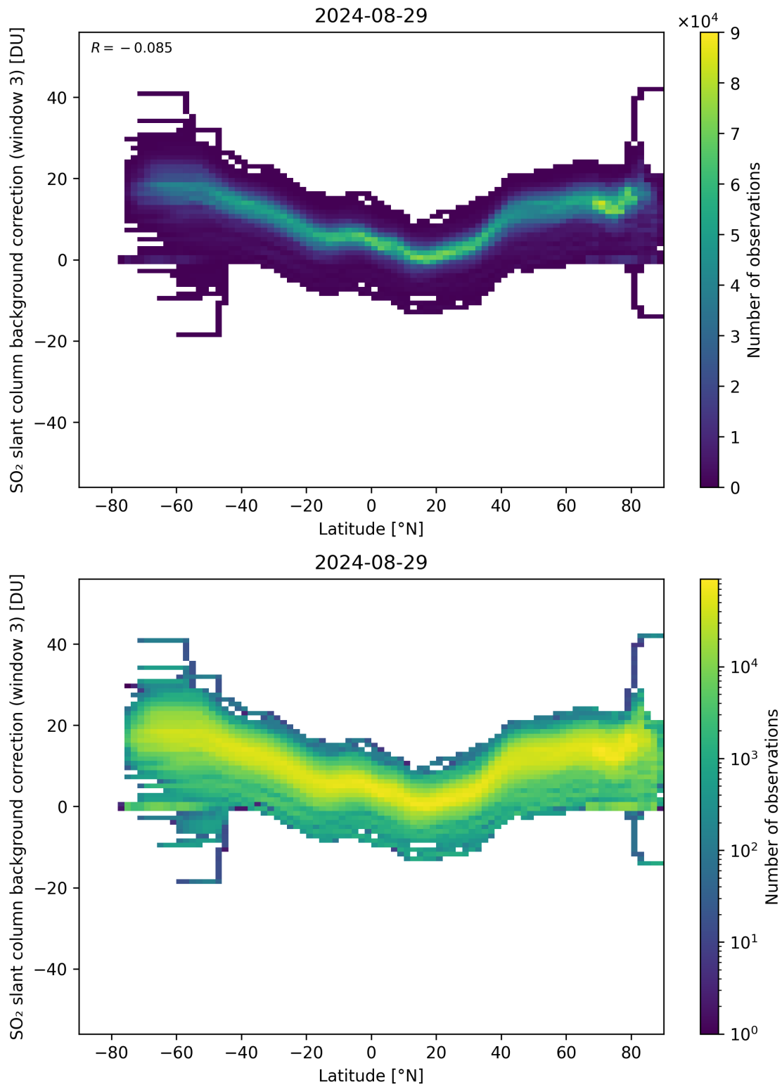
Figure 141: Scatter density plot of “Latitude” against “SO 2 slant column background correction (window 3)” for 2024-08-28 to 2024-08-30.
