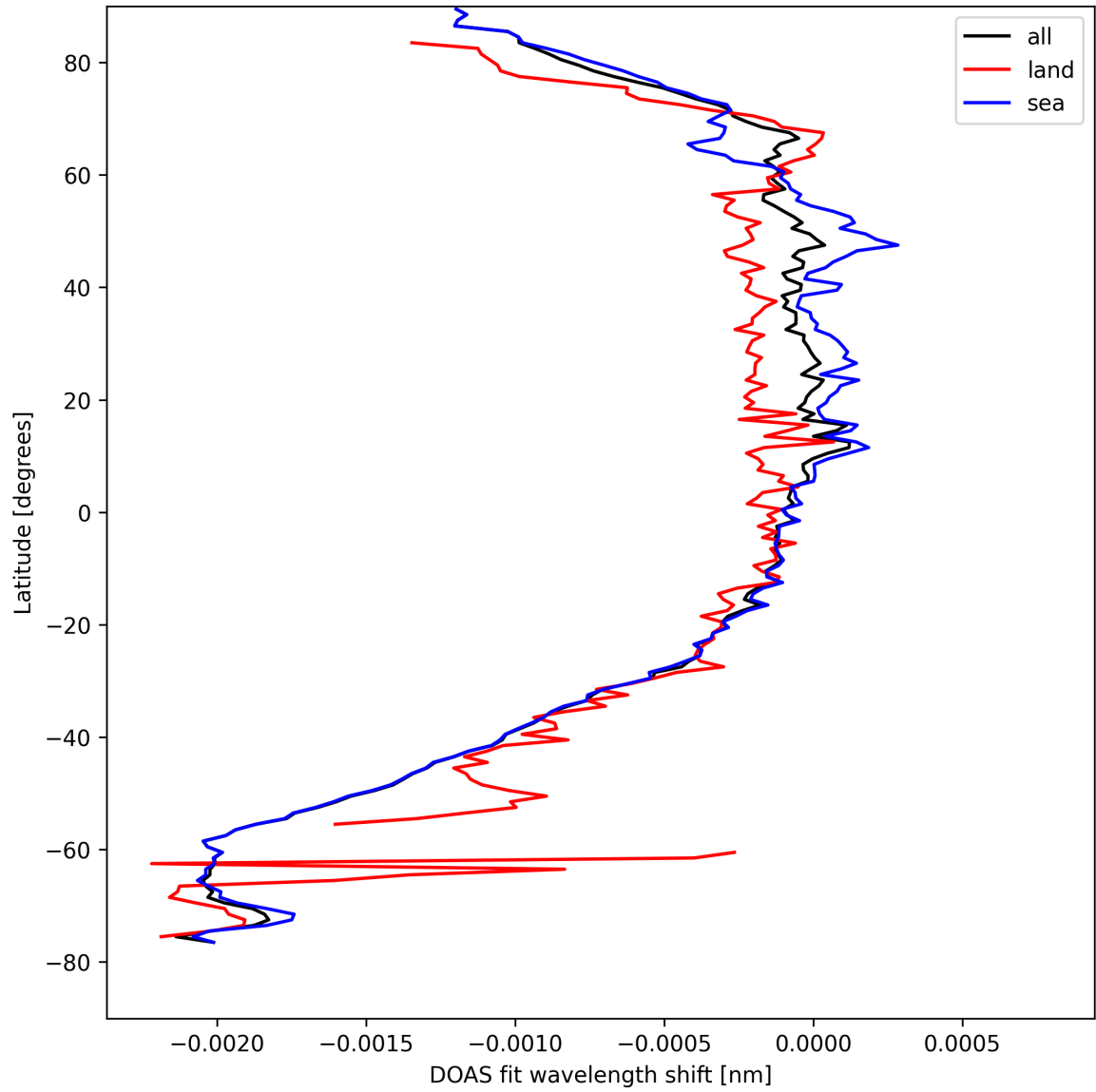
Figure 45: Zonal average of “DOAS fit wavelength shift” for 2024-08-28 to 2024-08-30.
