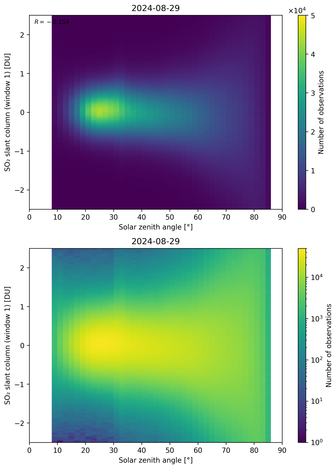
Figure 169: Scatter density plot of “Solar zenith angle” against “SO 2 slant column (window 1)” for 2024-08-28 to 2024-08-30.
