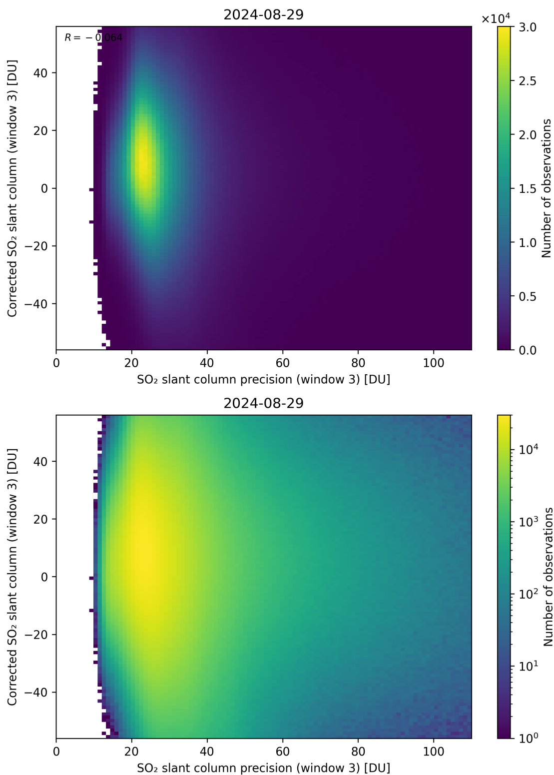
Figure 262: Scatter density plot of “SO 2 slant column precision (window 3)” against “Corrected SO 2 slant column (window 3)” for 2024-08-28 to 2024-08-30.
