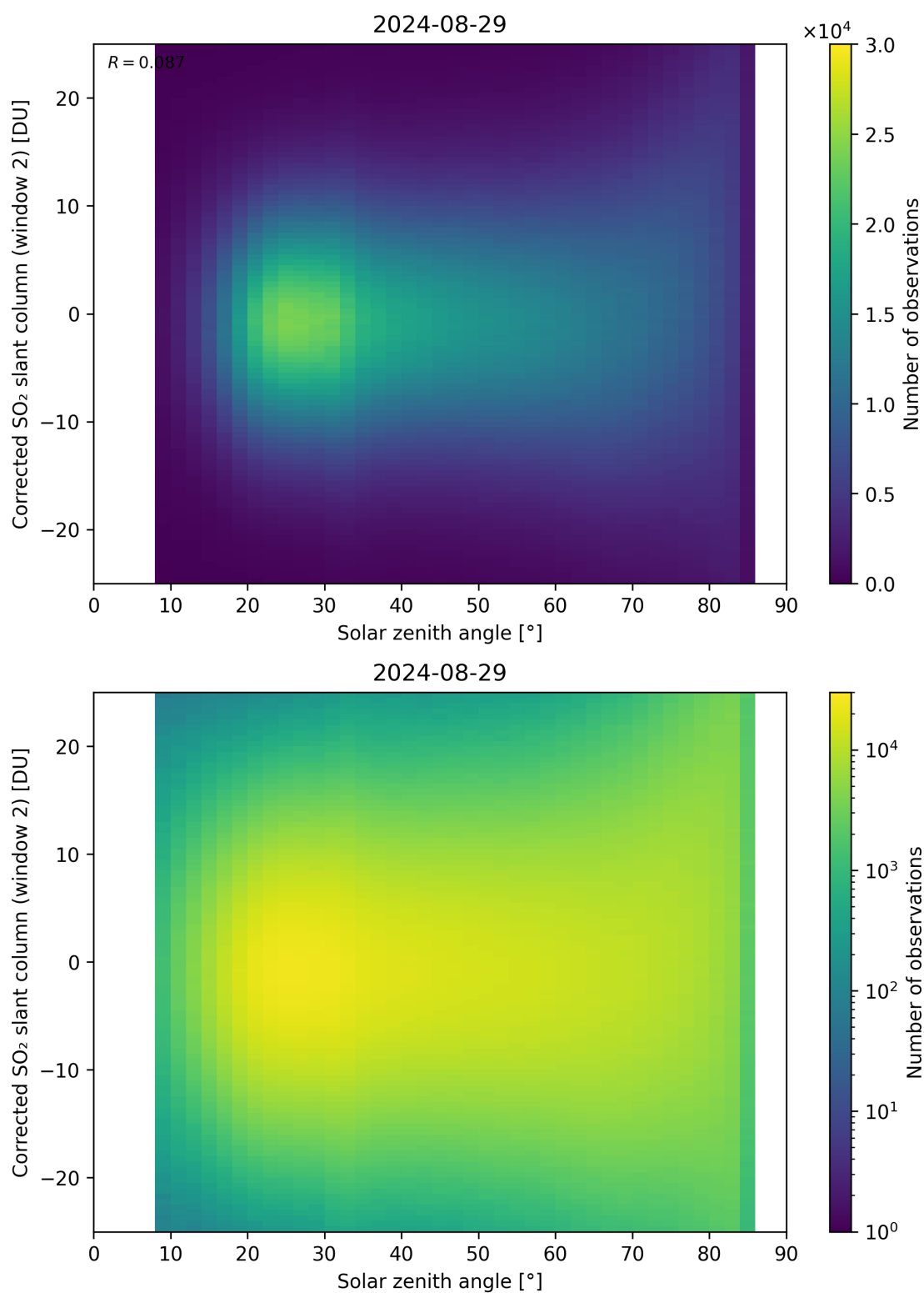
Figure 167: Scatter density plot of “Solar zenith angle” against “Corrected SO 2 slant column (window 2)” for 2024-08-28 to 2024-08-30.
