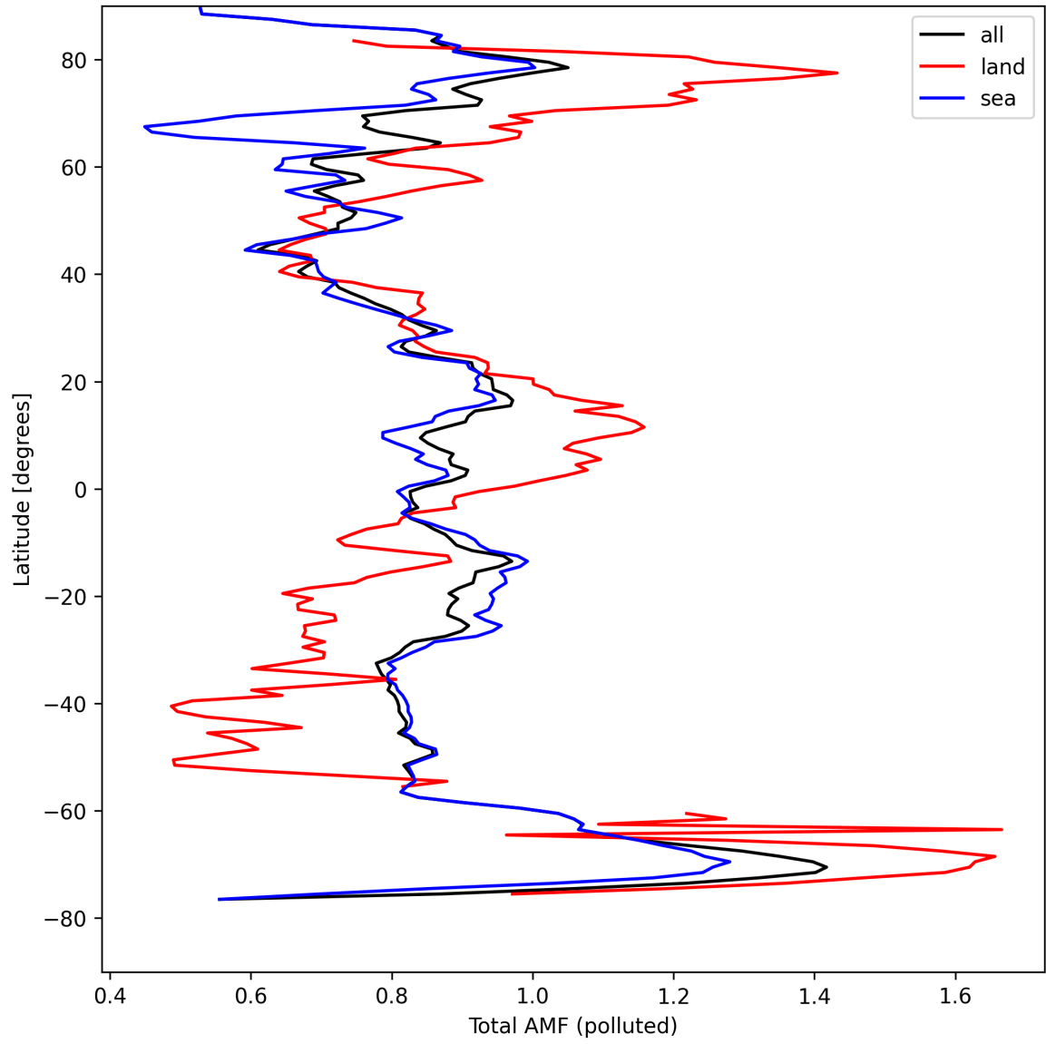
Figure 48: Zonal average of “Total AMF (polluted)” for 2024-08-28 to 2024-08-30.
