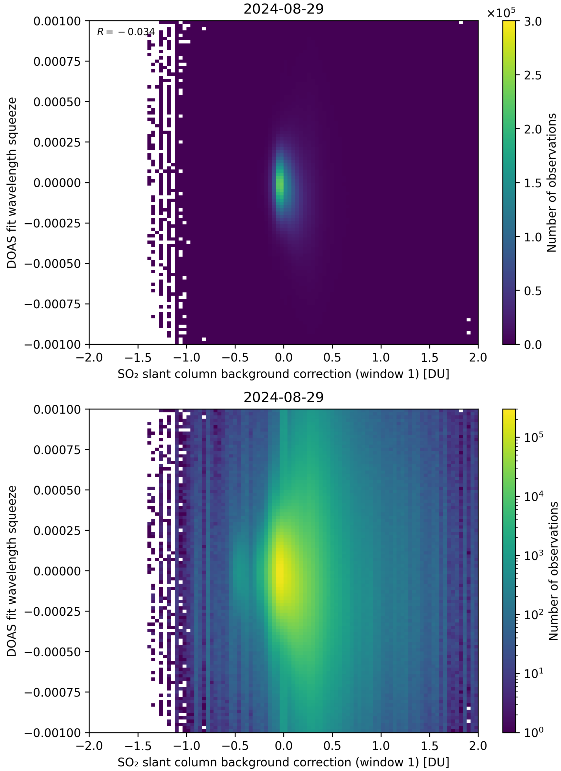
Figure 101: Scatter density plot of “SO 2 slant column background correction (window 1)” against “DOAS fit wavelength squeeze” for 2024-08-28 to 2024-08-30.
