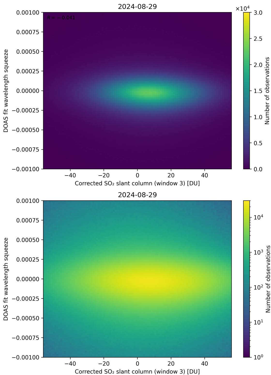
Figure 207: Scatter density plot of “Corrected SO 2 slant column (window 3)” against “DOAS fit wavelength squeeze” for 2024-08-28 to 2024-08-30.
