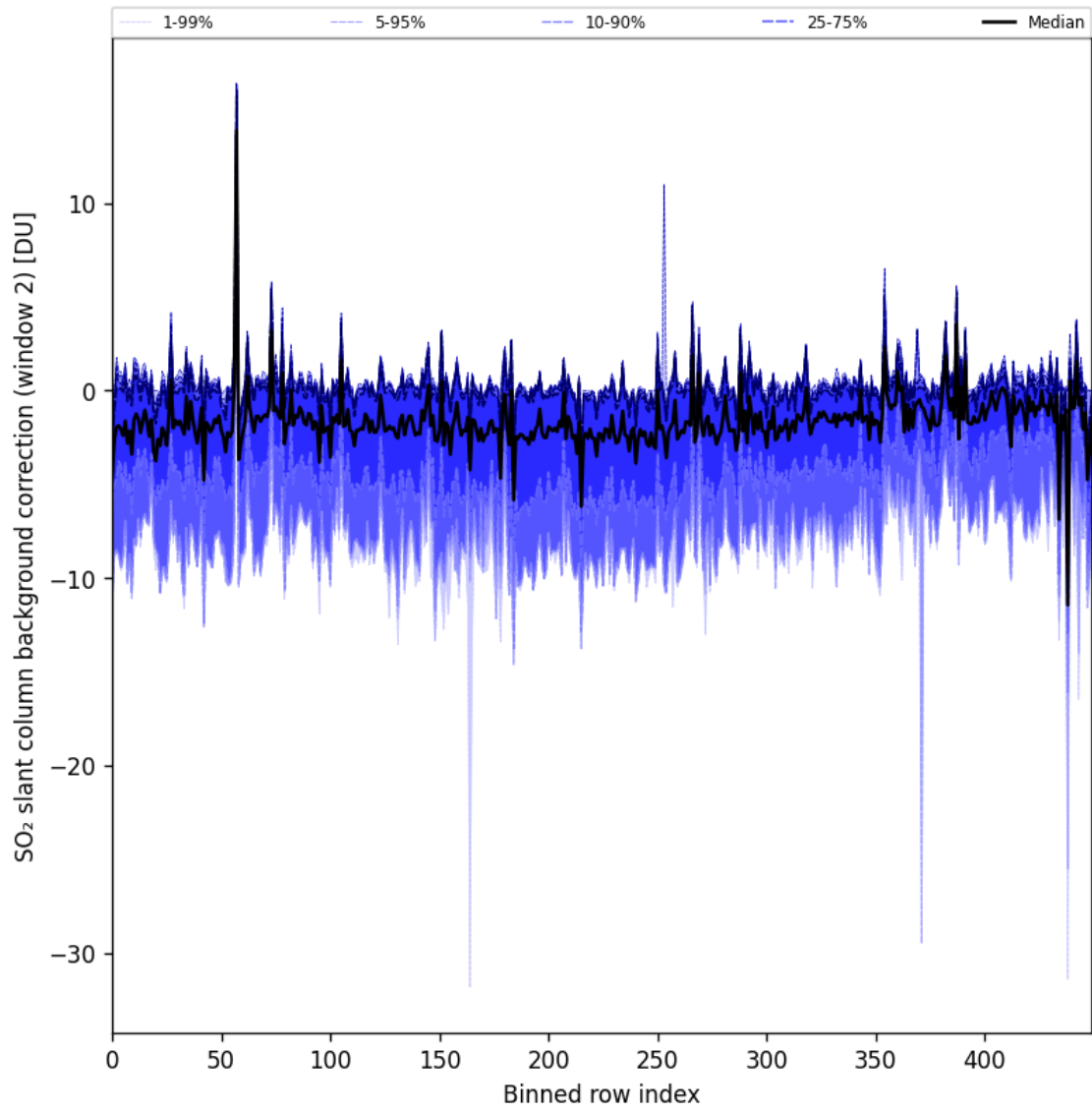
Figure 86: Along track statistics of “SO 2 slant column background correction (window 2)” for 2024-08-28 to 2024-08-30
