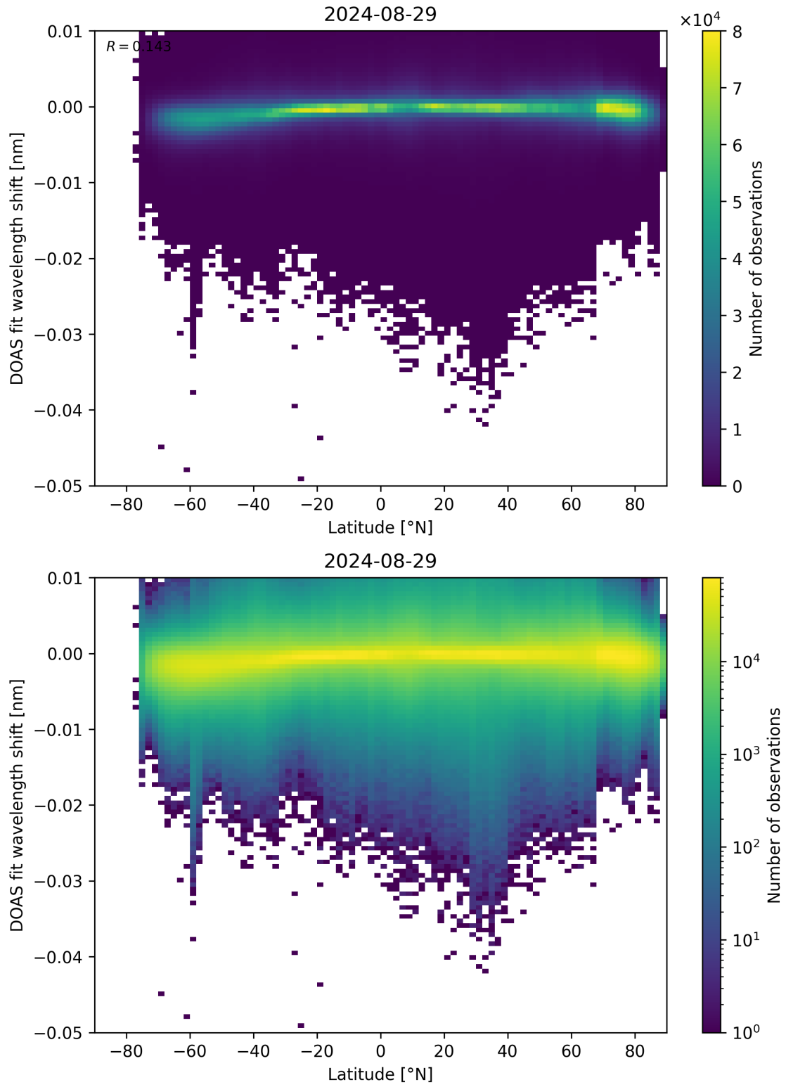
Figure 142: Scatter density plot of “Latitude” against “DOAS fit wavelength shift” for 2024-08-28 to 2024-08-30.
