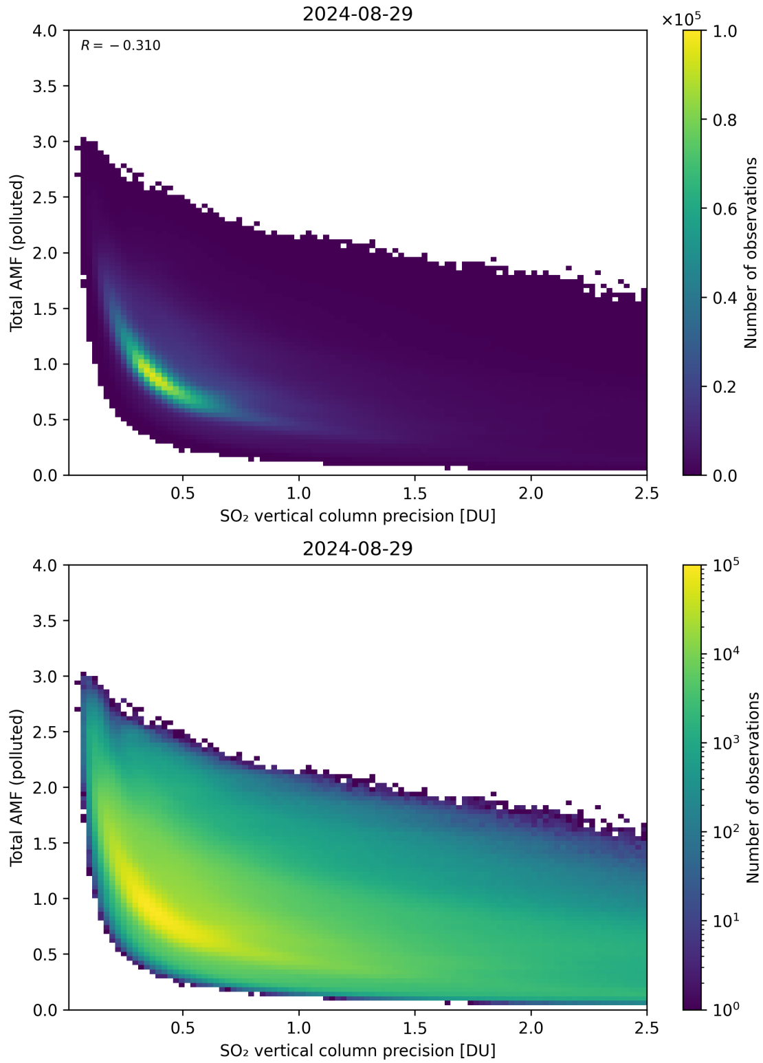
Figure 294: Scatter density plot of “SO 2 vertical column precision” against “Total AMF (polluted)” for 2024-08-28 to 2024-08-30.
