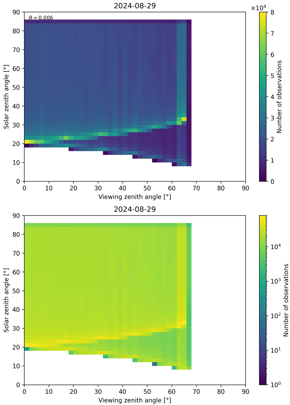
Figure 315: Scatter density plot of “Viewing zenith angle” against “Solar zenith angle” for 2024-08-28 to 2024-08-30.
