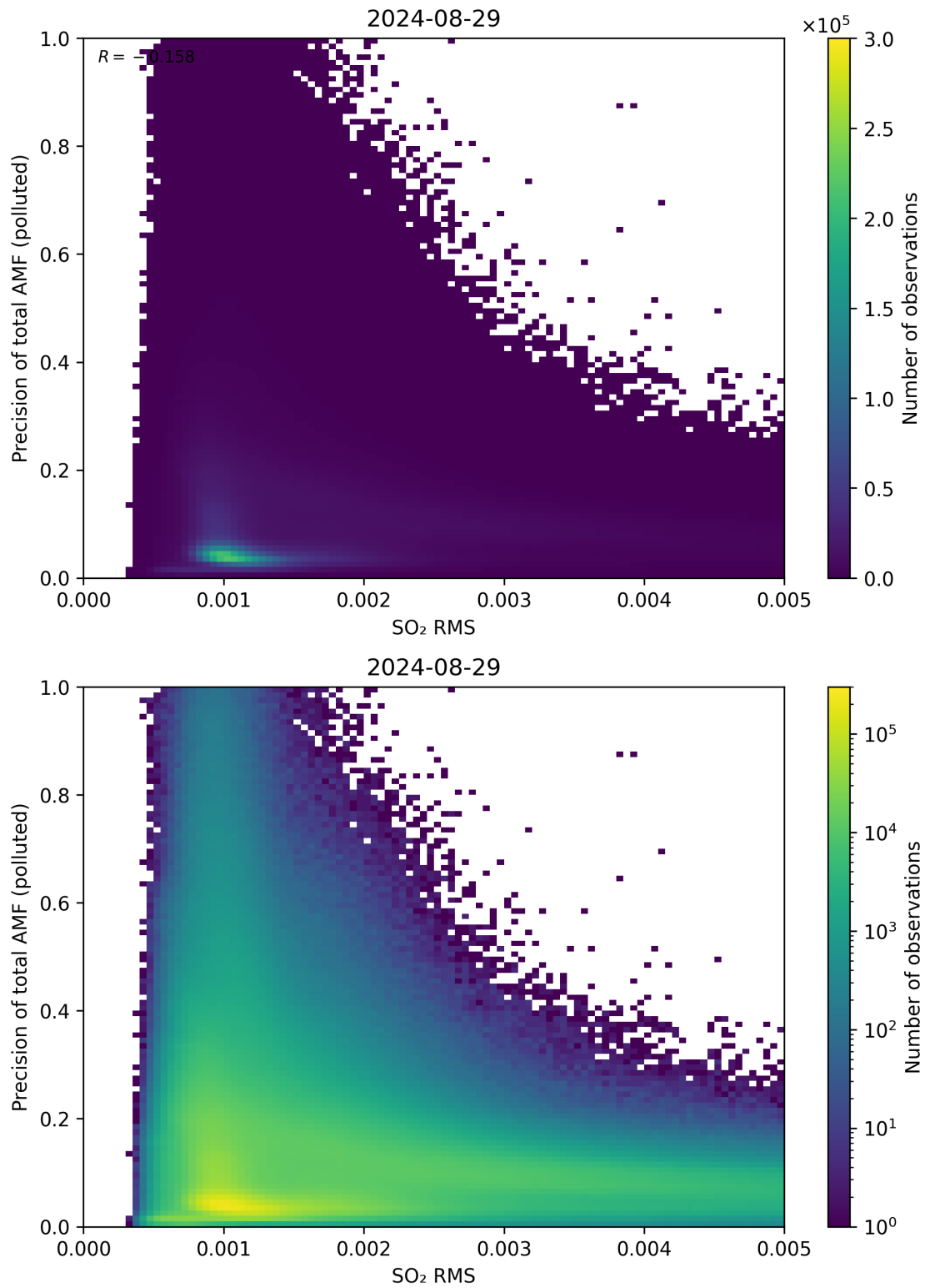
Figure 138: Scatter density plot of “SO 2 RMS” against “Precision of total AMF (polluted)” for 2024-08-28 to 2024-08-30.
