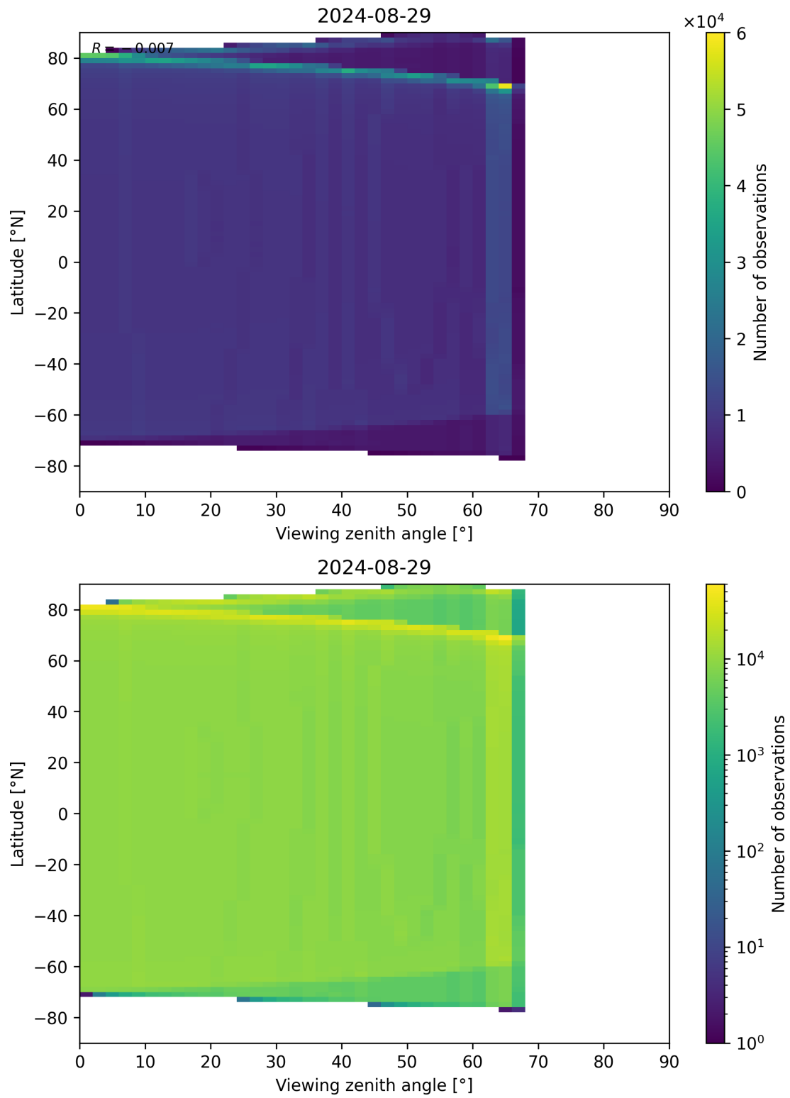
Figure 314: Scatter density plot of “Viewing zenith angle” against “Latitude” for 2024-08-28 to 2024-08-30.
