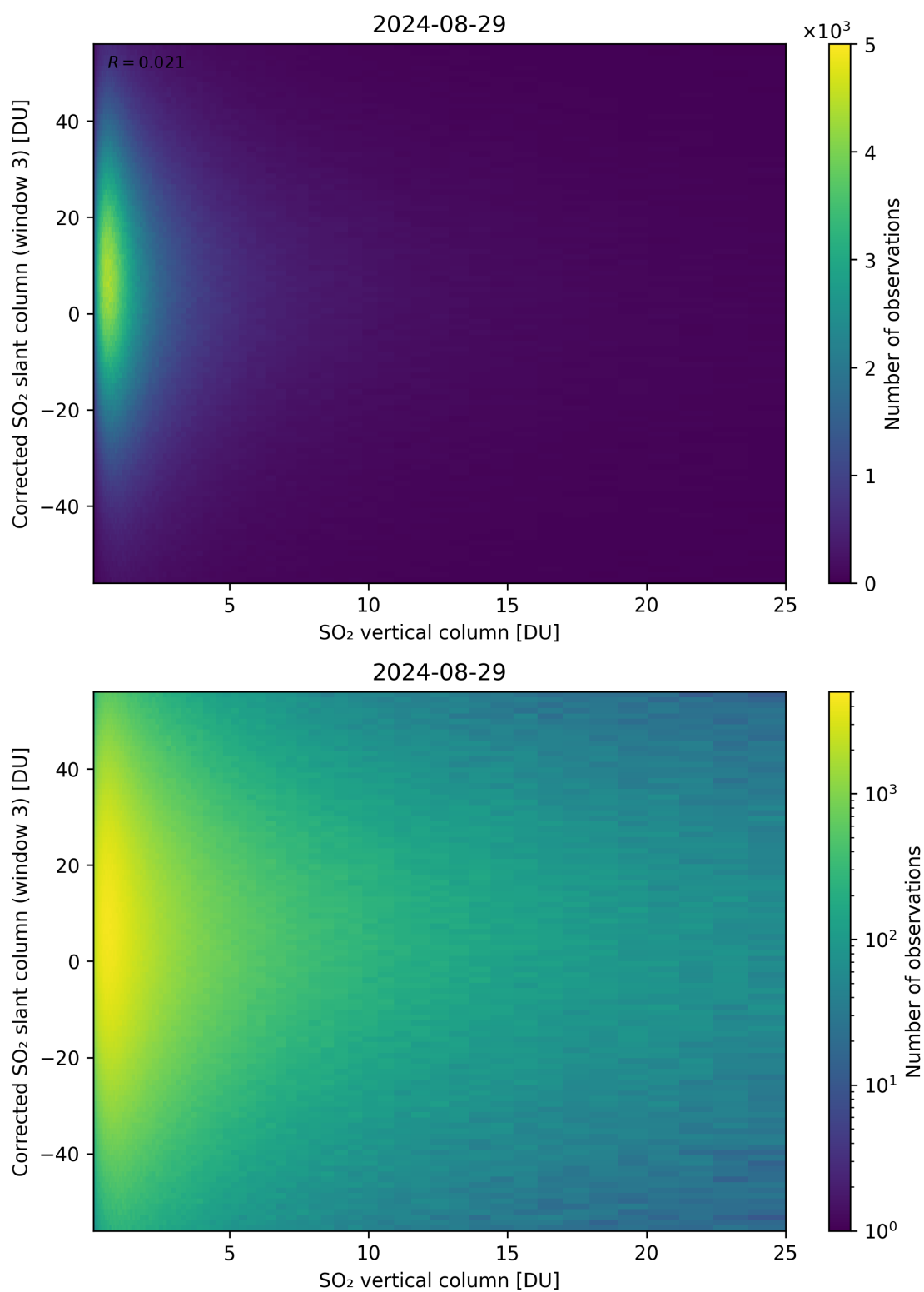
Figure 299: Scatter density plot of “SO 2 vertical column” against “Corrected SO 2 slant column (window 3)” for 2024-08-28 to 2024-08-30.
