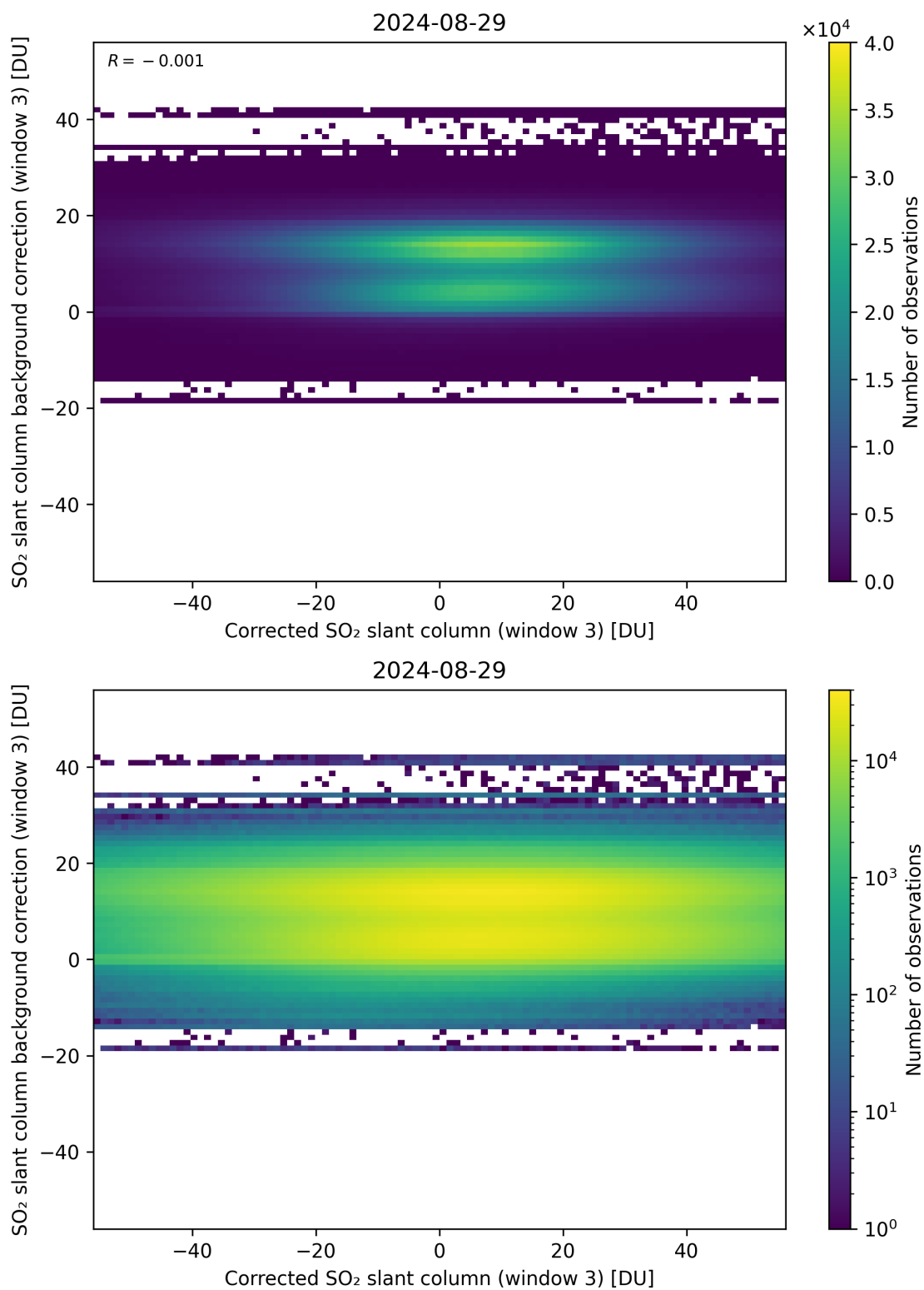
Figure 205: Scatter density plot of “Corrected SO 2 slant column (window 3)” against “SO 2 slant column background correction (window 3)” for 2024-08-28 to 2024-08-30.
