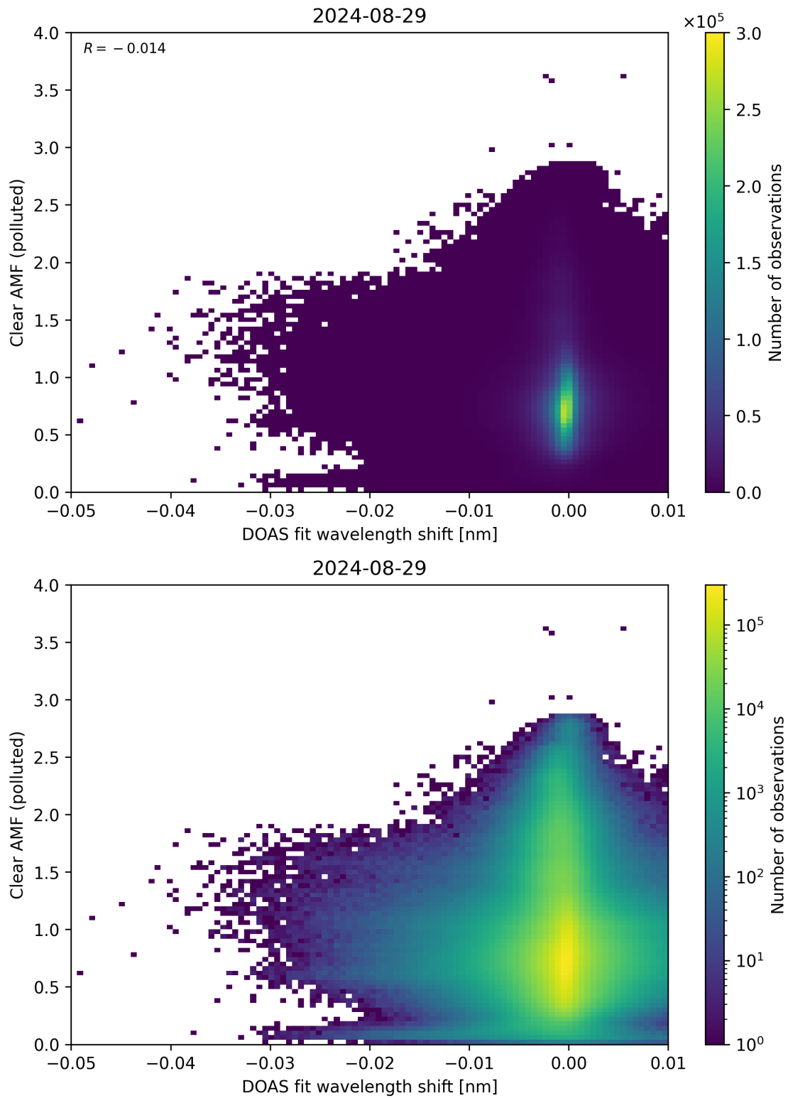
Figure 129: Scatter density plot of “DOAS fit wavelength shift” against “Clear AMF (polluted)” for 2024-08-28 to 2024-08-30.
