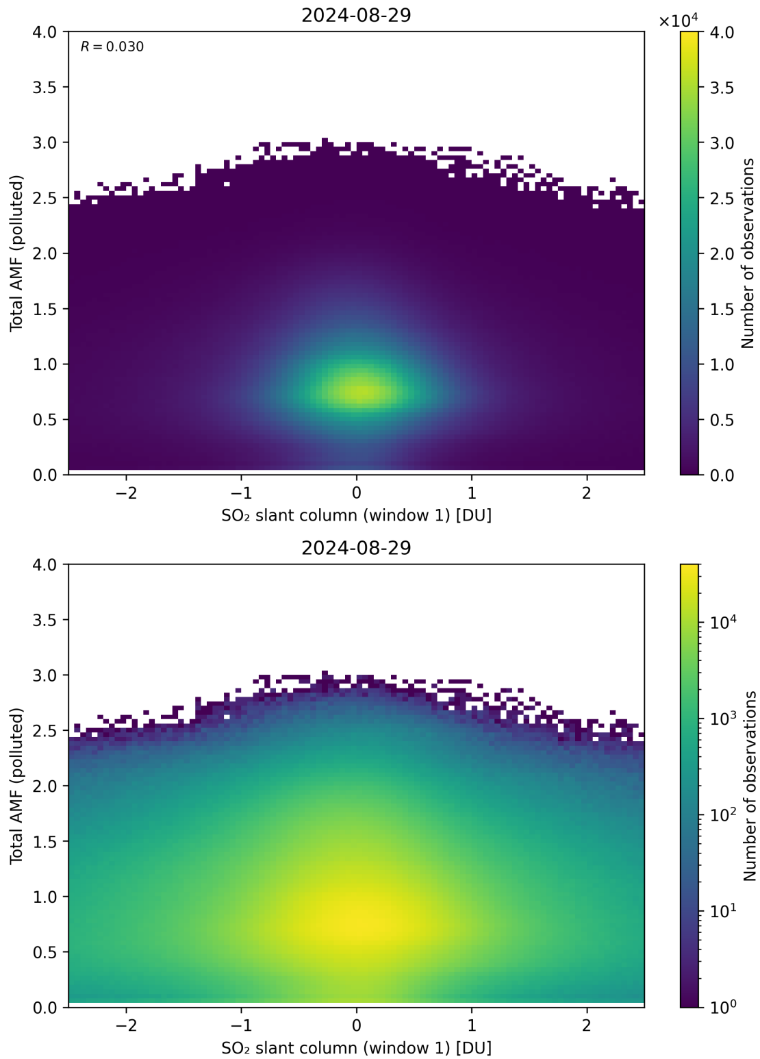
Figure 239: Scatter density plot of “SO 2 slant column (window 1)” against “Total AMF (polluted)” for 2024-08-28 to 2024-08-30.
