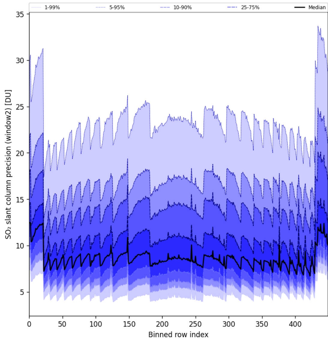
Figure 84: Along track statistics of “SO 2 slant column precision (window2)” for 2024-08-28 to 2024-08-30
