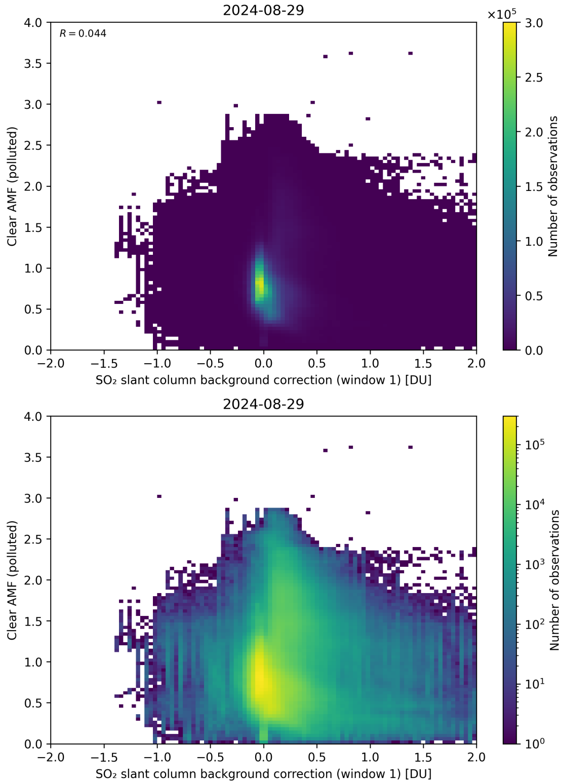
Figure 103: Scatter density plot of “SO 2 slant column background correction (window 1)” against “Clear AMF (polluted)” for 2024-08-28 to 2024-08-30.
