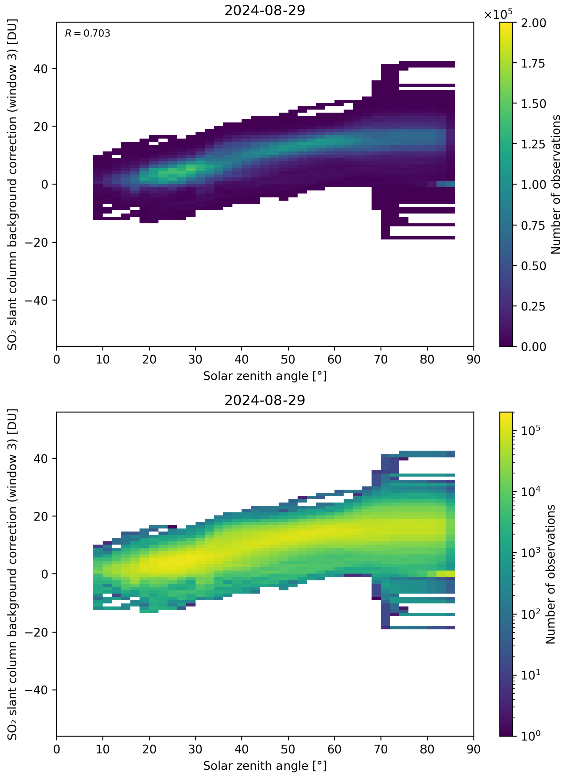
Figure 160: Scatter density plot of “Solar zenith angle” against “SO 2 slant column background correction (window 3)” for 2024-08-28 to 2024-08-30.
