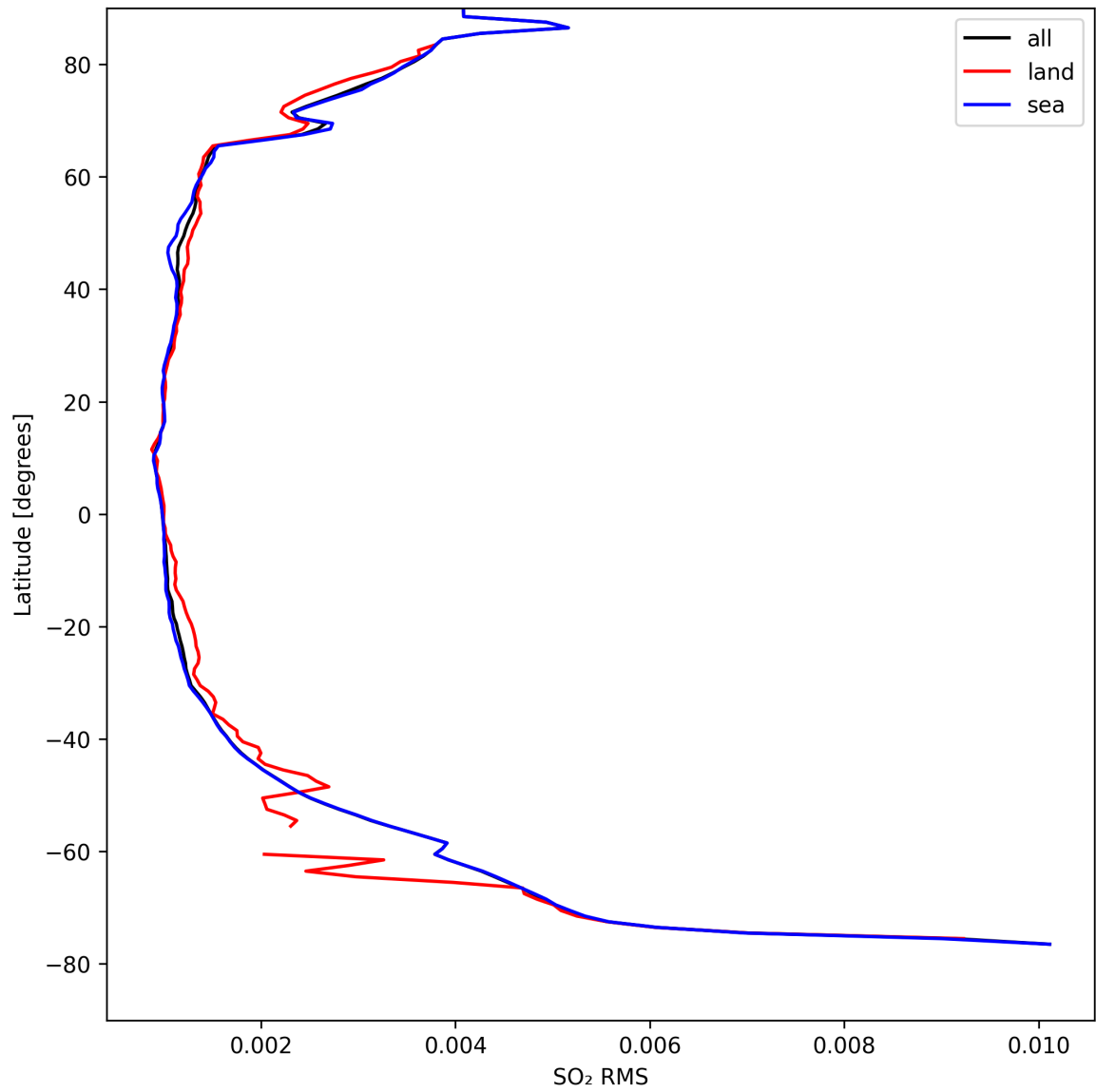
Figure 47: Zonal average of “SO 2 RMS” for 2024-08-28 to 2024-08-30.
