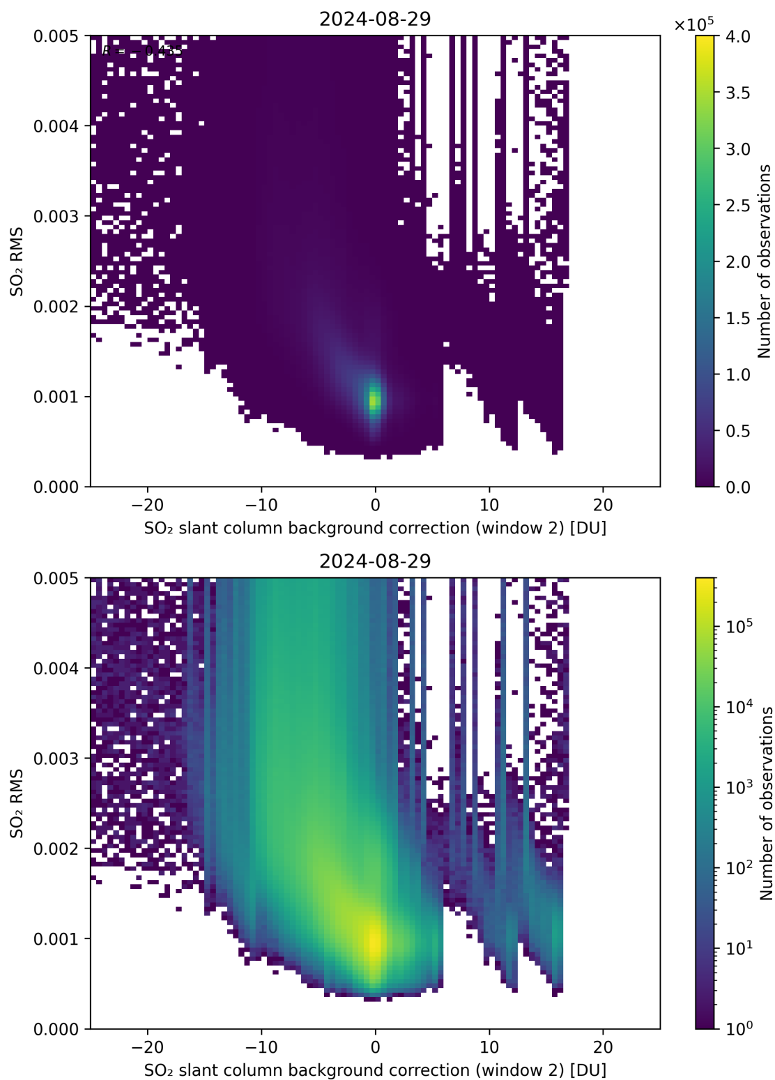
Figure 114: Scatter density plot of “SO 2 slant column background correction (window 2)” against “SO 2 RMS” for 2024-08-28 to 2024-08-30.
