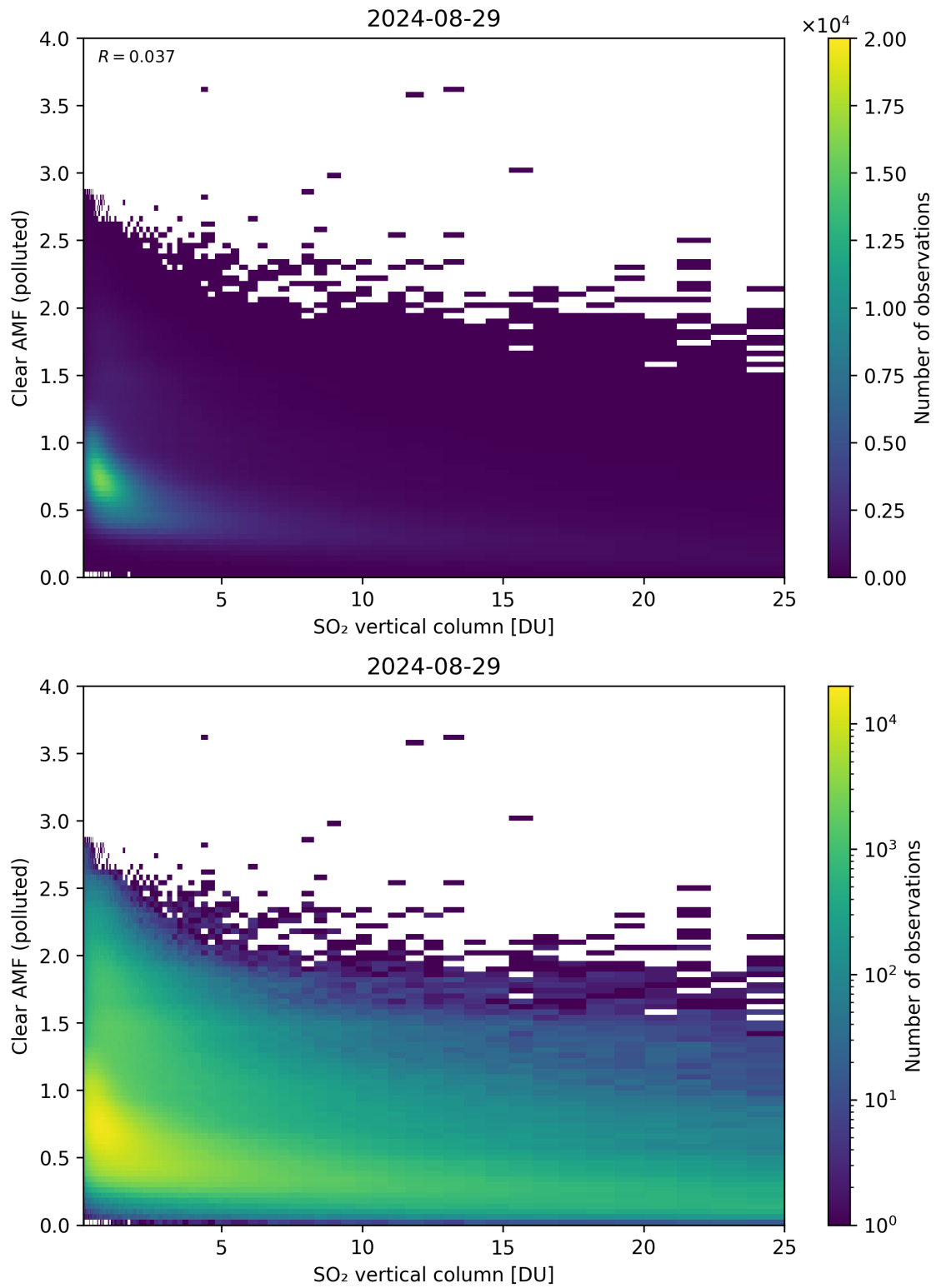
Figure 296: Scatter density plot of “SO 2 vertical column” against “Clear AMF (polluted)” for 2024-08-28 to 2024-08-30.
