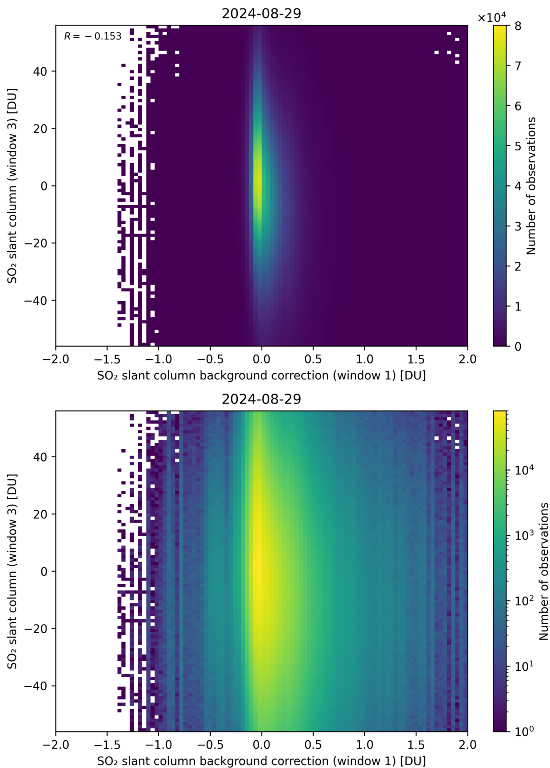
Figure 107: Scatter density plot of “SO 2 slant column background correction (window 1)” against “SO 2 slant column (window 3)” for 2024-08-28 to 2024-08-30.
