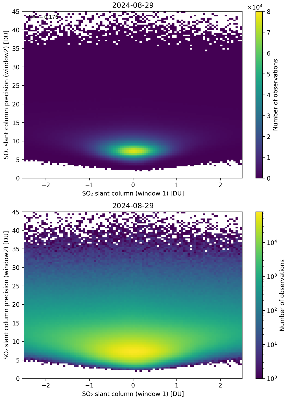
Figure 236: Scatter density plot of “SO 2 slant column (window 1)” against “SO 2 slant column precision (window2)” for 2024-08-28 to 2024-08-30.
