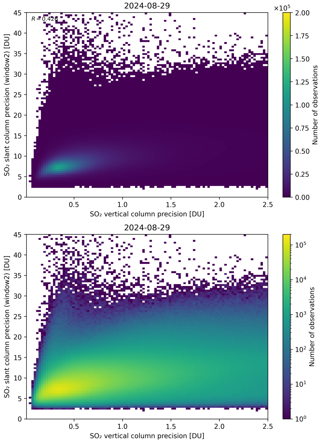
Figure 291: Scatter density plot of “SO 2 vertical column precision” against “SO 2 slant column precision (window2)” for 2024-08-28 to 2024-08-30.
