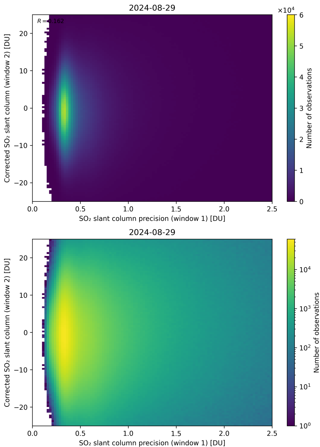
Figure 225: Scatter density plot of “SO 2 slant column precision (window 1)” against “Corrected SO 2 slant column (window 2)” for 2024-08-28 to 2024-08-30.
