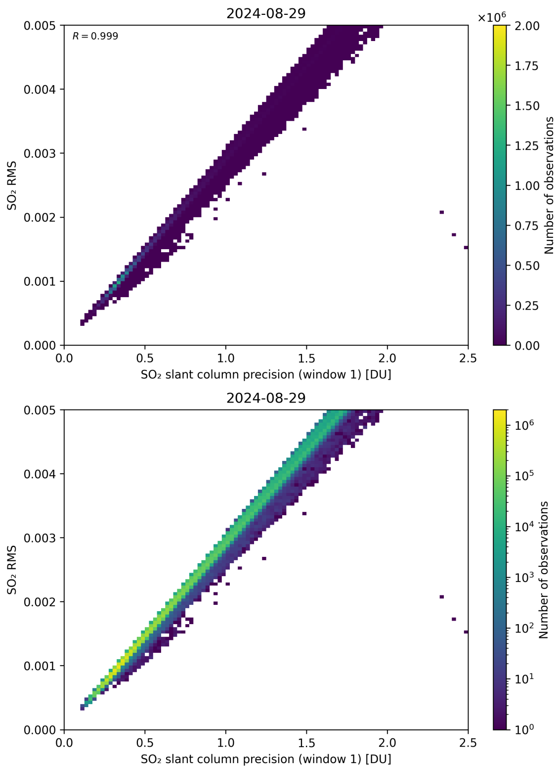
Figure 223: Scatter density plot of “SO 2 slant column precision (window 1)” against “SO 2 RMS” for 2024-08-28 to 2024-08-30.
