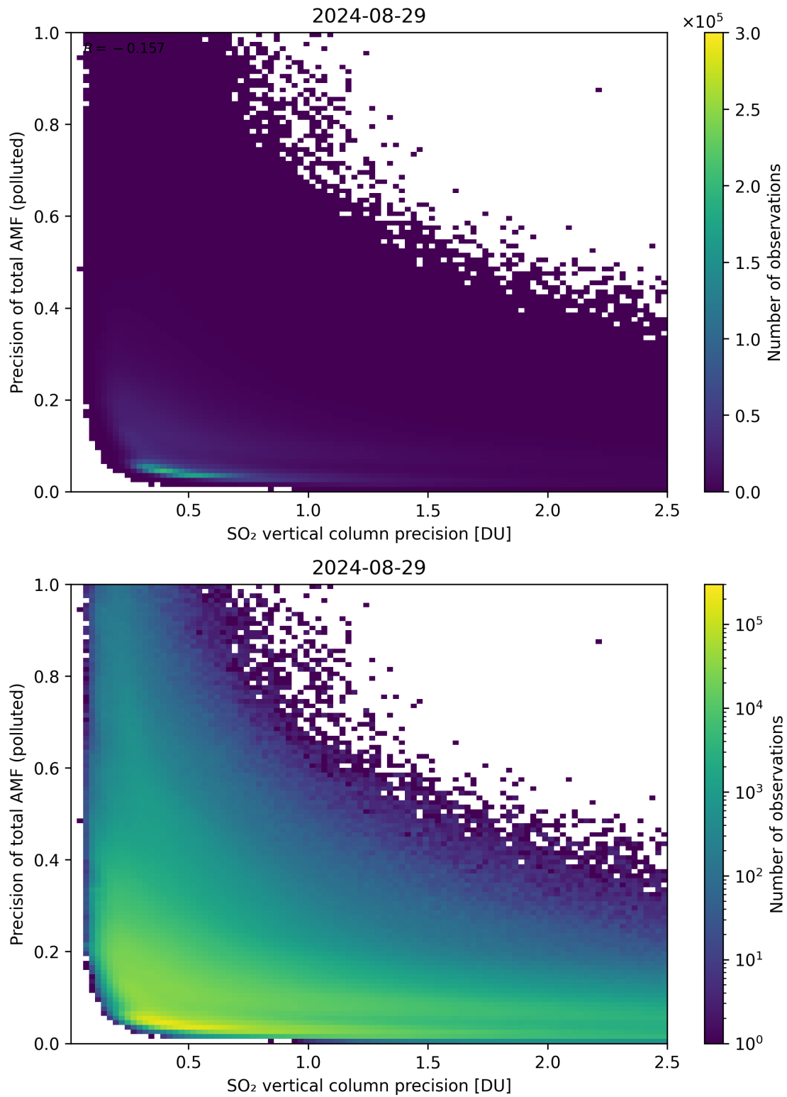
Figure 295: Scatter density plot of “SO 2 vertical column precision” against “Precision of total AMF (polluted)” for 2024-08-28 to 2024-08-30.
