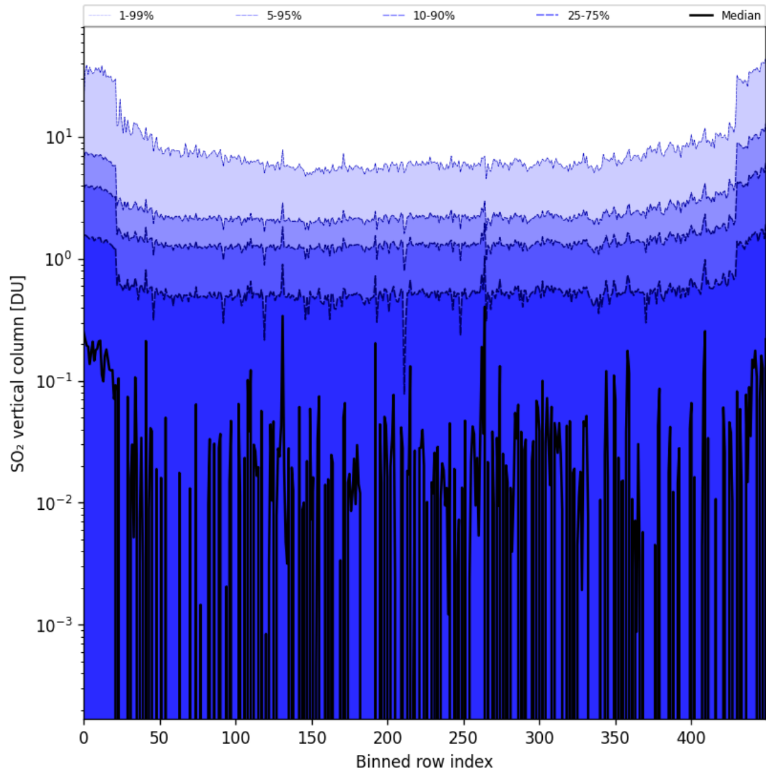
Figure 76: Along track statistics of “SO 2 vertical column” for 2024-08-28 to 2024-08-30
