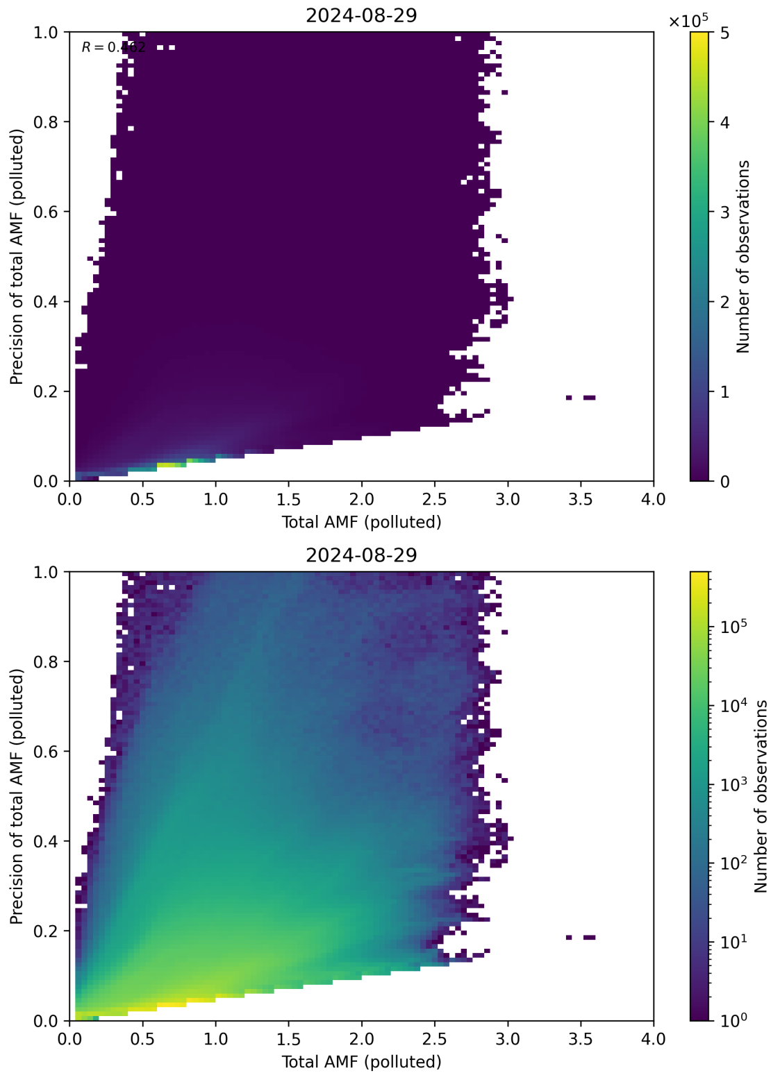
Figure 272: Scatter density plot of “Total AMF (polluted)” against “Precision of total AMF (polluted)” for 2024-08-28 to 2024-08-30.
