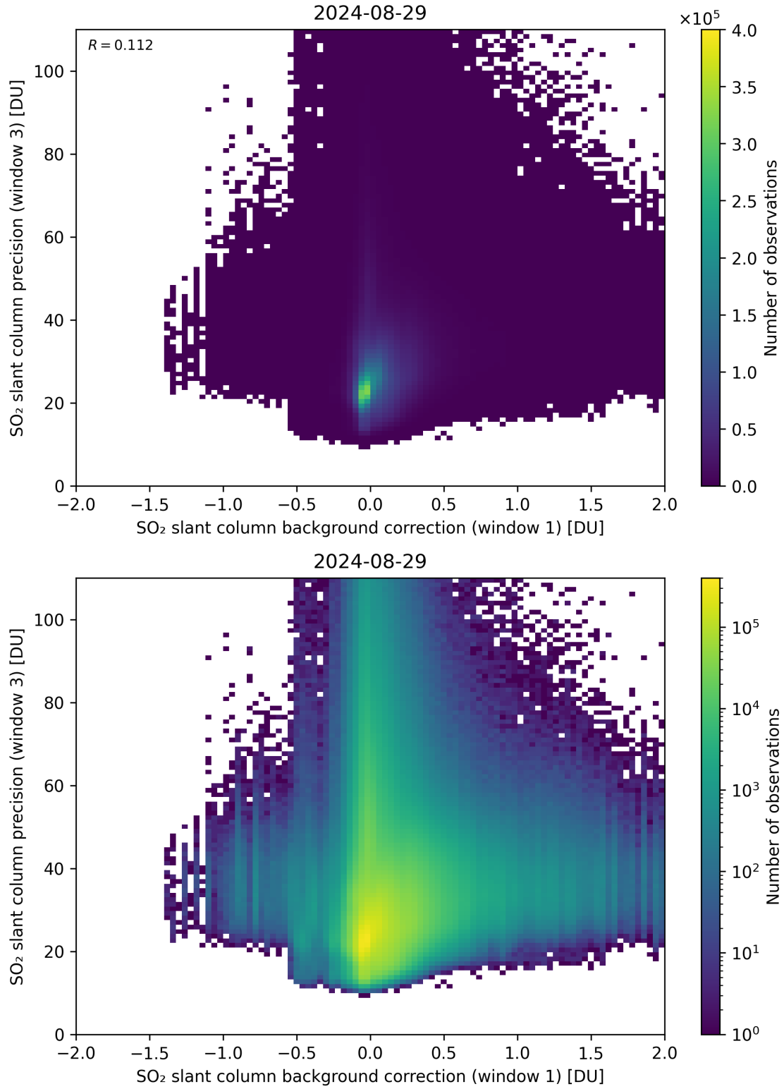
Figure 108: Scatter density plot of “SO 2 slant column background correction (window 1)” against “SO 2 slant column precision (window 3)” for 2024-08-28 to 2024-08-30.
