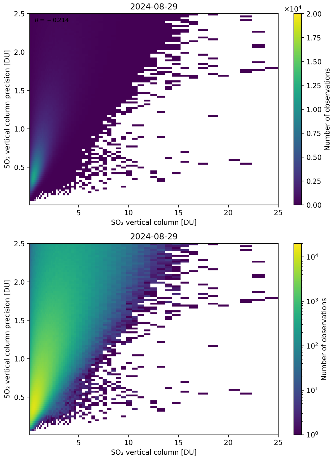
Figure 307: Scatter density plot of “SO 2 vertical column” against “SO 2 vertical column precision” for 2024-08-28 to 2024-08-30.
