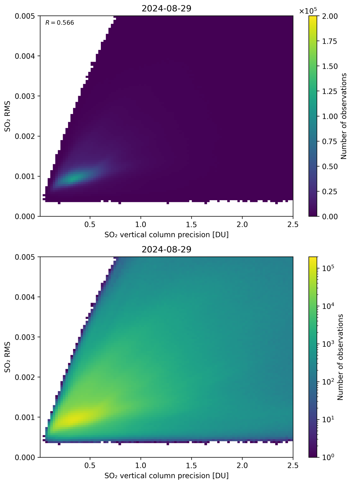
Figure 284: Scatter density plot of “SO 2 vertical column precision” against “SO 2 RMS” for 2024-08-28 to 2024-08-30.
