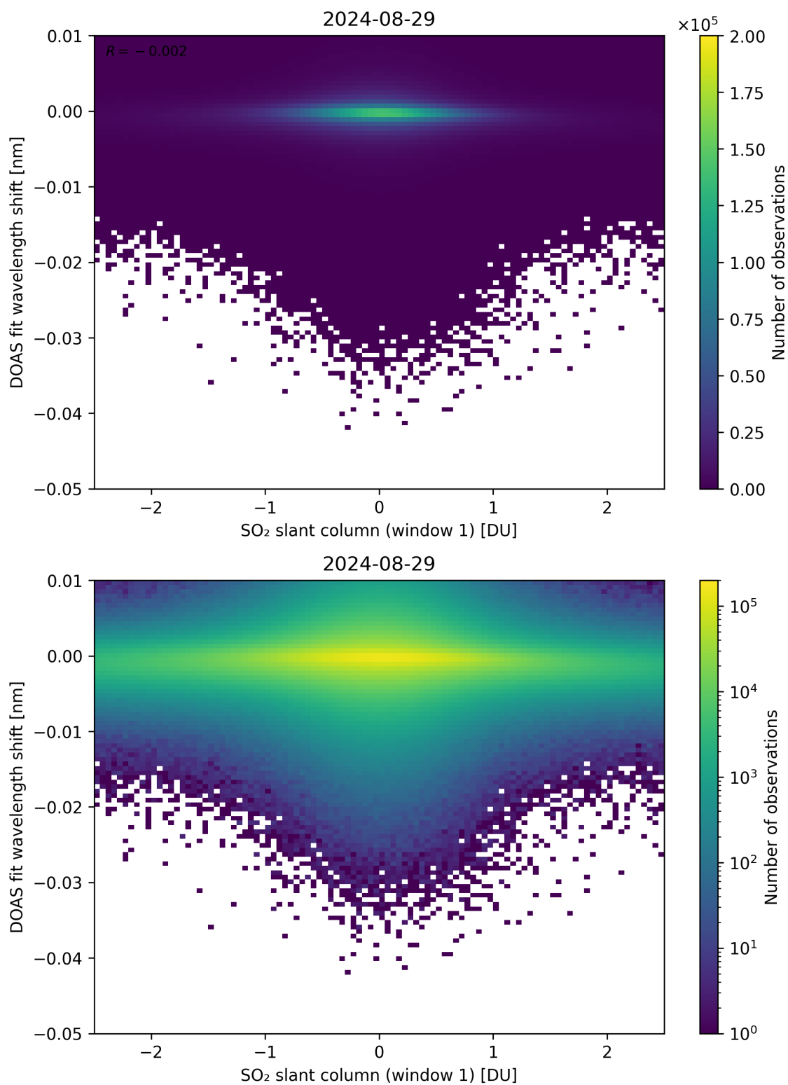
Figure 215: Scatter density plot of “SO 2 slant column (window 1)” against “DOAS fit wavelength shift” for 2024-08-28 to 2024-08-30.
