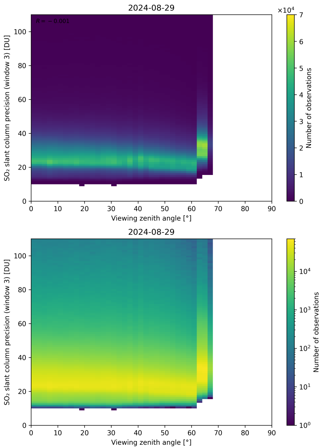
Figure 324: Scatter density plot of “Viewing zenith angle” against “SO 2 slant column precision (window 3)” for 2024-08-28 to 2024-08-30.
