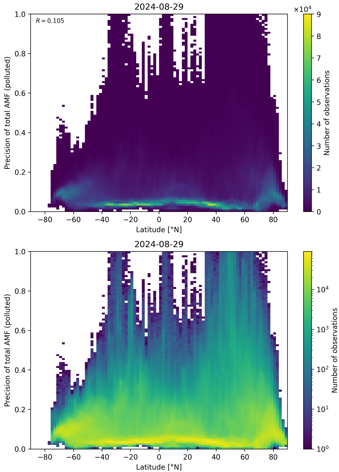
Figure 155: Scatter density plot of “Latitude” against “Precision of total AMF (polluted)” for 2024-08-28 to 2024-08-30.
