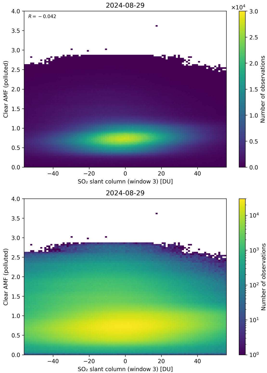
Figure 265: Scatter density plot of “SO 2 slant column (window 3)” against “Clear AMF (polluted)” for 2024-08-28 to 2024-08-30.
