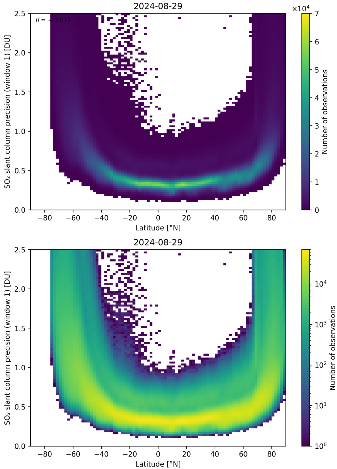
Figure 150: Scatter density plot of “Latitude” against “SO 2 slant column precision (window 1)” for 2024-08-28 to 2024-08-30.
