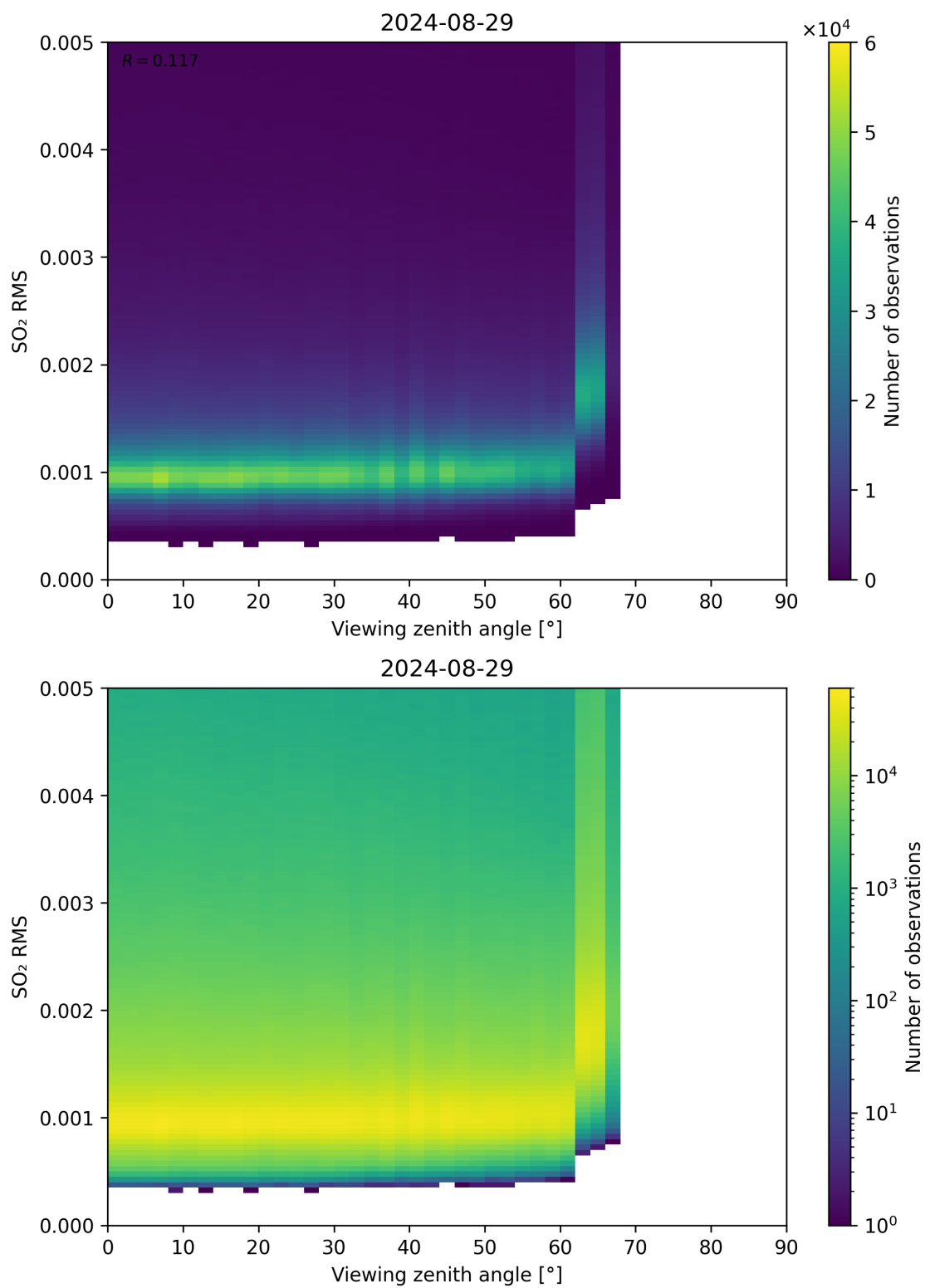
Figure 313: Scatter density plot of “Viewing zenith angle” against “SO 2 RMS” for 2024-08-28 to 2024-08-30.
