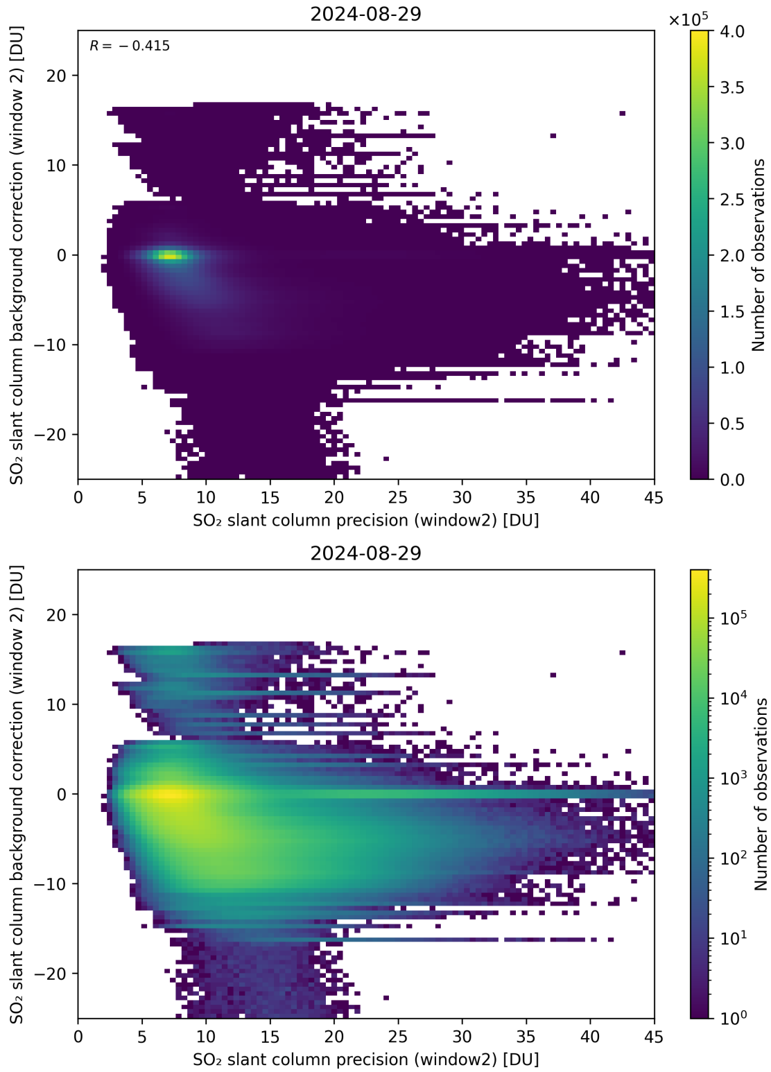
Figure 241: Scatter density plot of “SO 2 slant column precision (window2)” against “SO 2 slant column background correction (window 2)” for 2024-08-28 to 2024-08-30.
