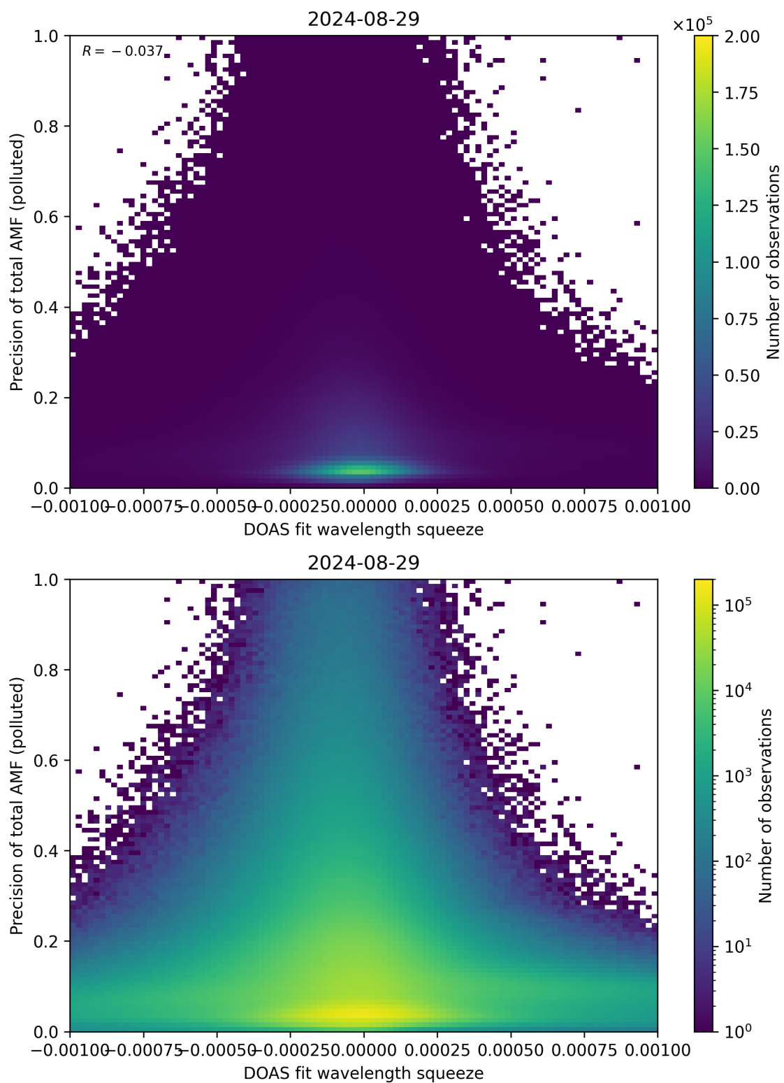
Figure 135: Scatter density plot of “DOAS fit wavelength squeeze” against “Precision of total AMF (polluted)” for 2024-08-28 to 2024-08-30.
