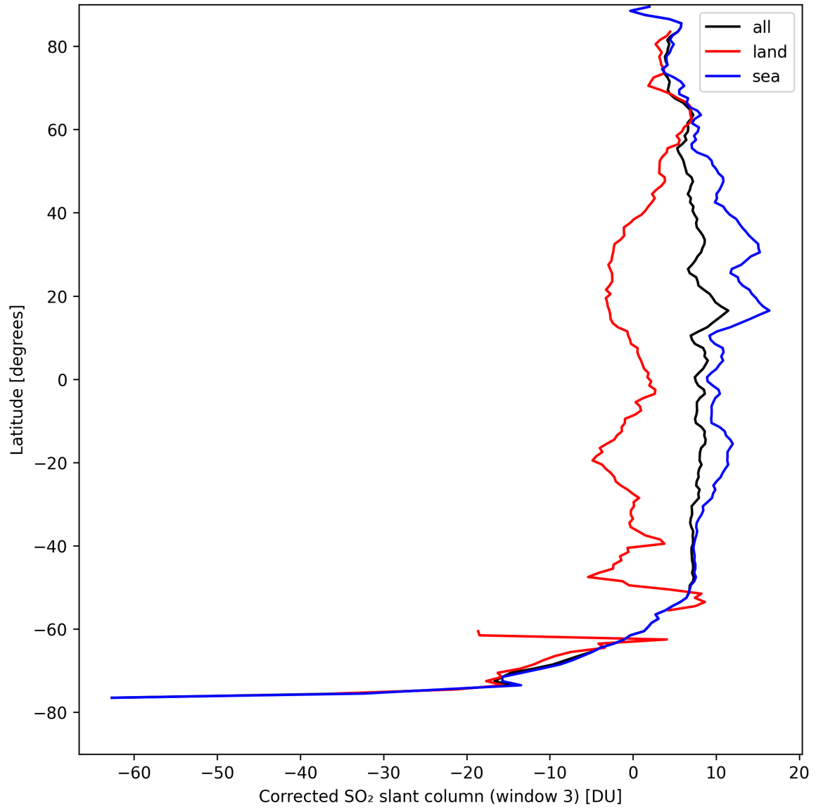
Figure 43: Zonal average of “Corrected SO 2 slant column (window 3)” for 2024-08-28 to 2024-08-30.
