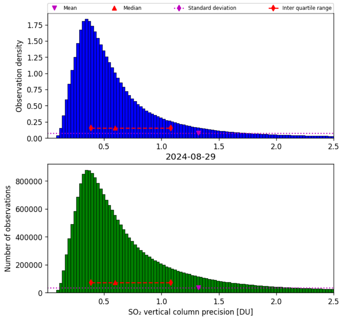
Figure 54: Histogram of “SO 2 vertical column precision” for 2024-08-28 to 2024-08-30
