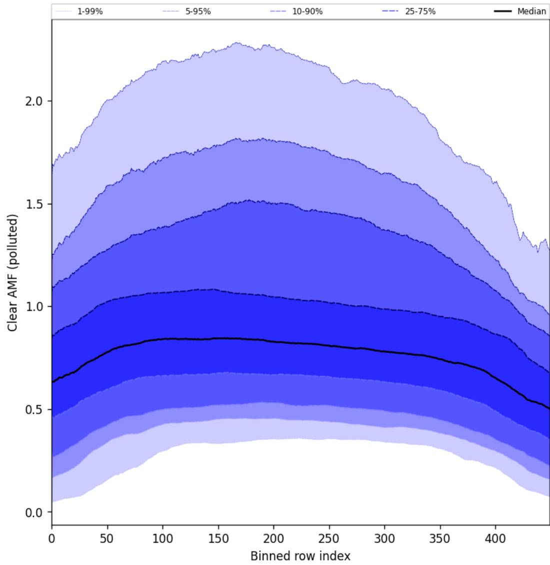
Figure 96: Along track statistics of “Clear AMF (polluted)” for 2024-08-28 to 2024-08-30
