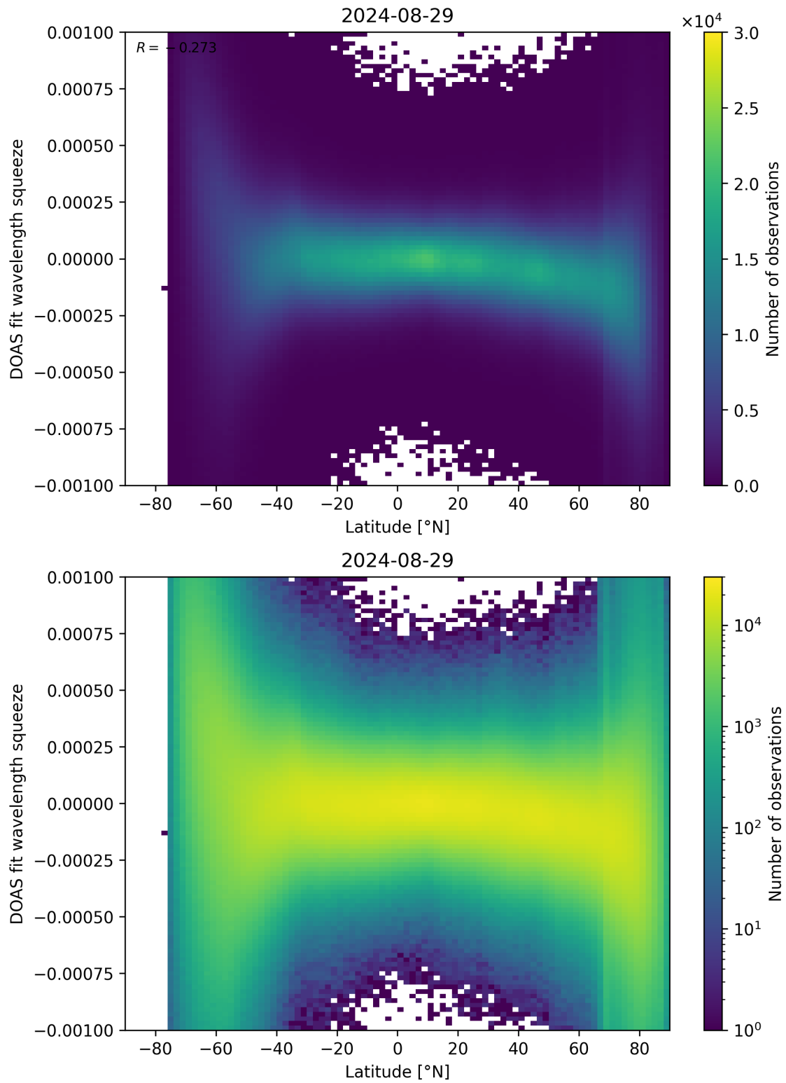
Figure 143: Scatter density plot of “Latitude” against “DOAS fit wavelength squeeze” for 2024-08-28 to 2024-08-30.
