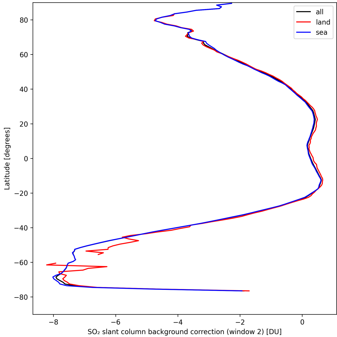
Figure 40: Zonal average of "SO 2 slant column background correction (window 2)" for 2024-08-29 to 2024-08-31.
