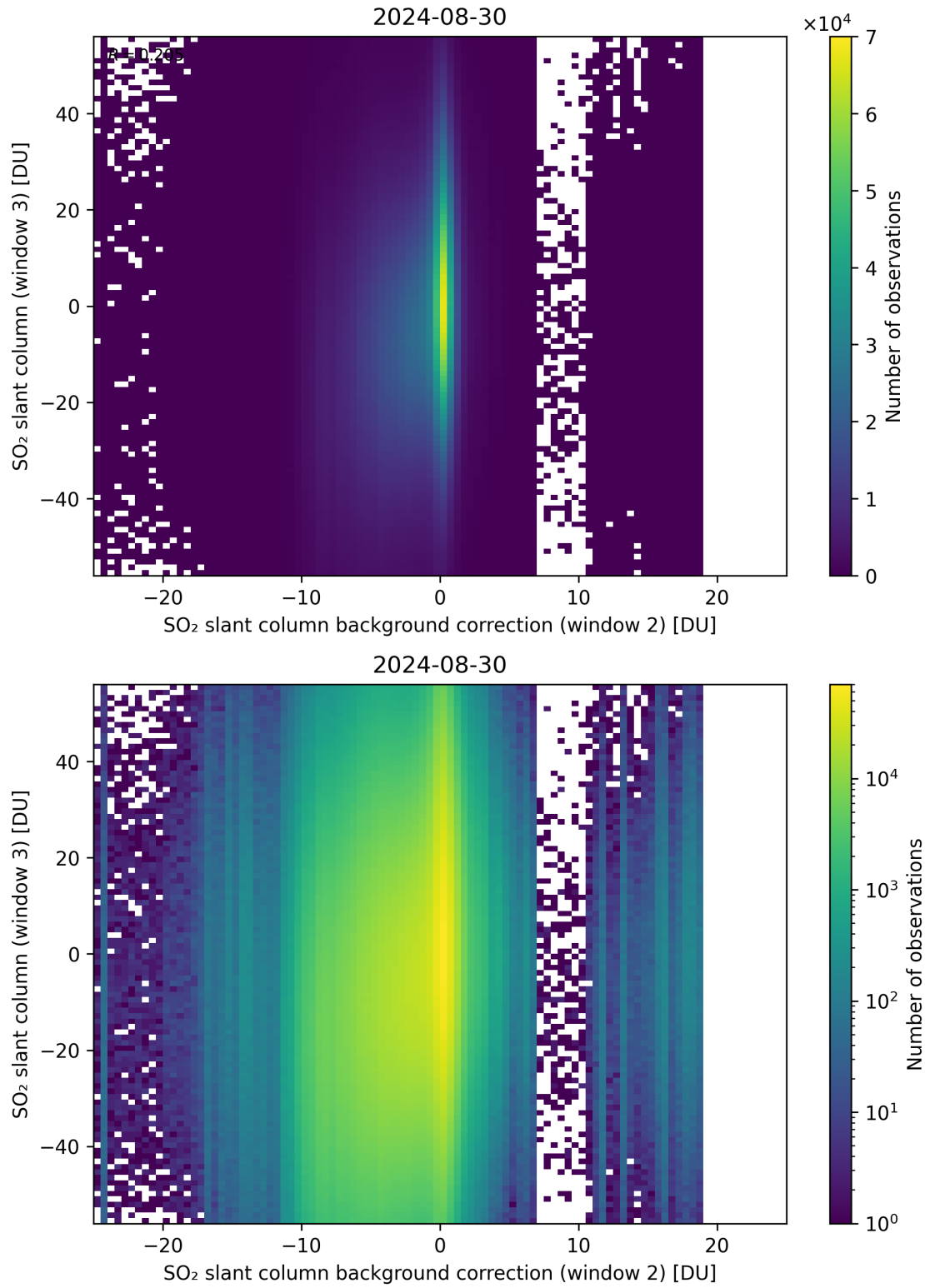
Figure 117: Scatter density plot of “SO 2 slant column background correction (window 2)” against “SO 2 slant column (window 3)” for 2024-08-29 to 2024-08-31.
