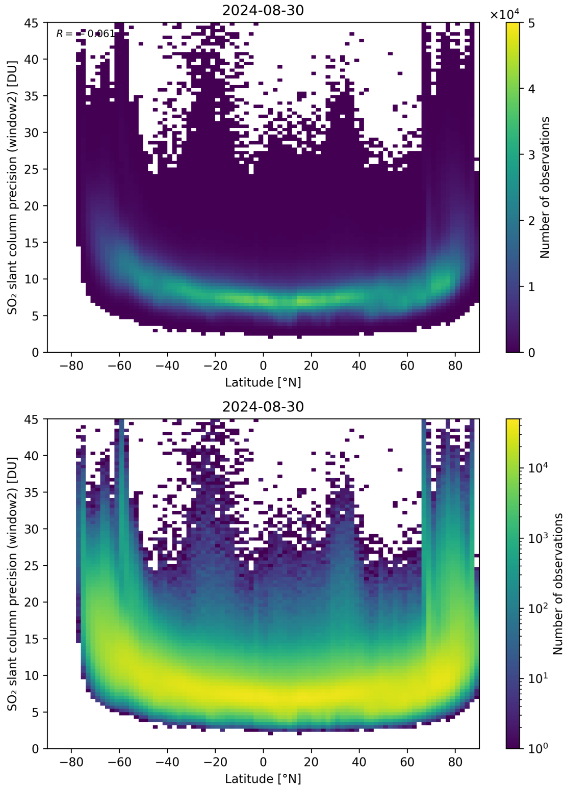
Figure 151: Scatter density plot of “Latitude” against “SO 2 slant column precision (window2)” for 2024-08-29 to 2024-08-31.
