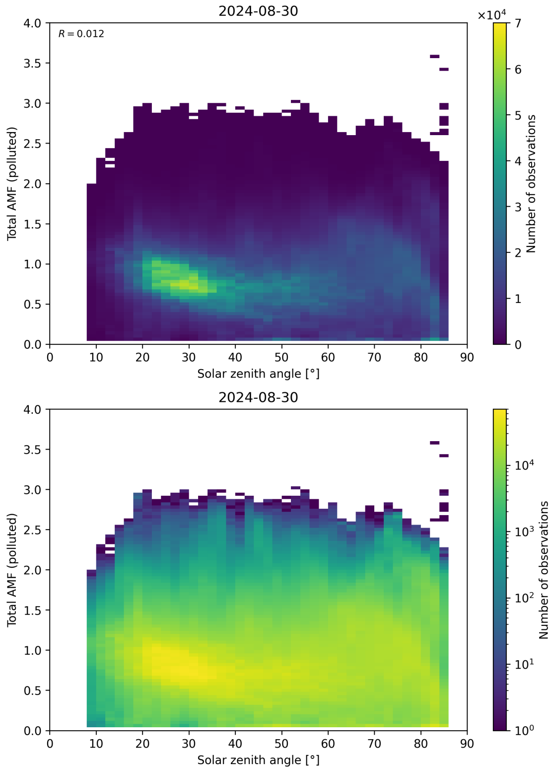
Figure 174: Scatter density plot of “Solar zenith angle” against “Total AMF (polluted)” for 2024-08-29 to 2024-08-31.
