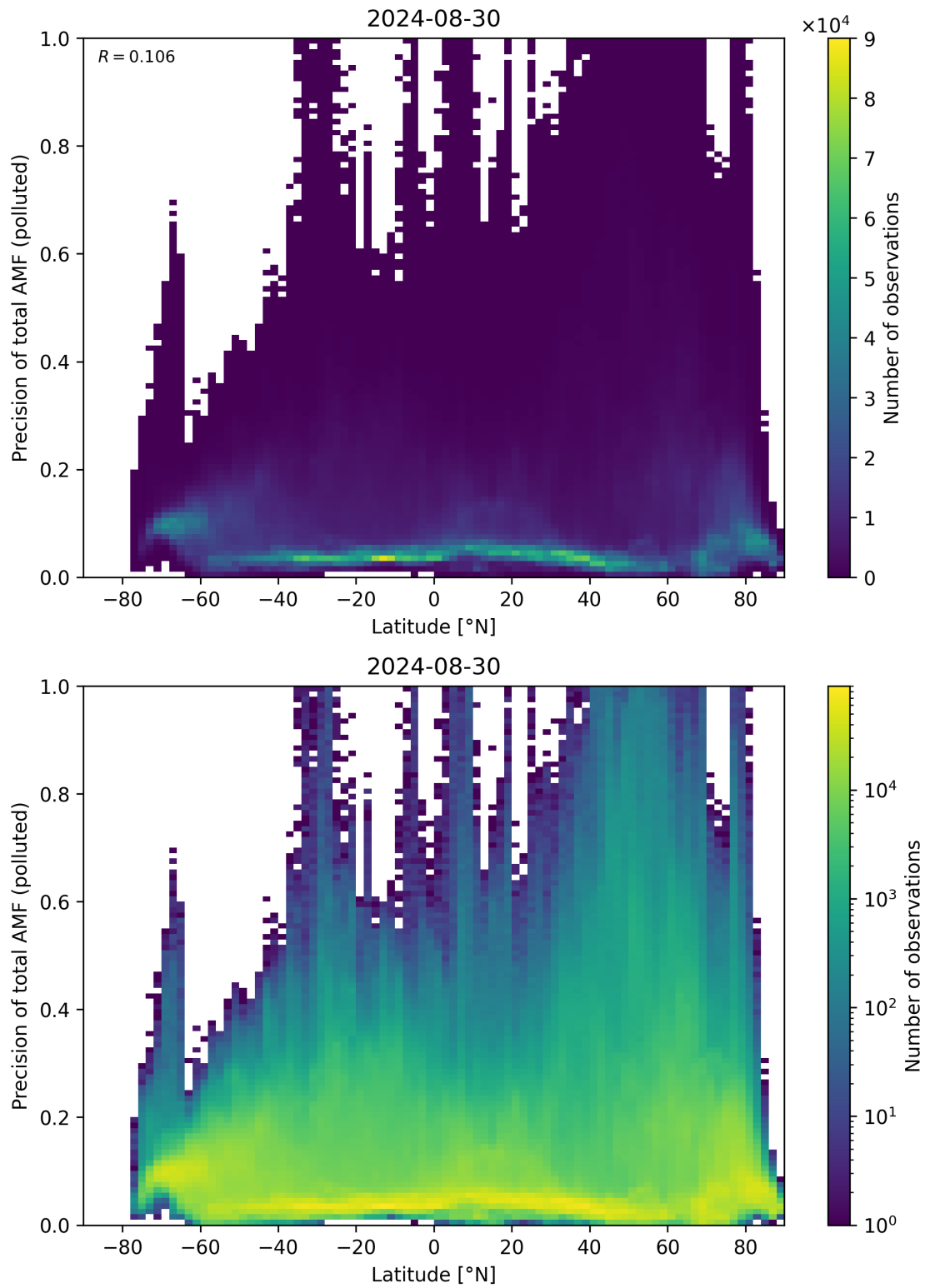
Figure 155: Scatter density plot of “Latitude” against “Precision of total AMF (polluted)” for 2024-08-29 to 2024-08-31.
