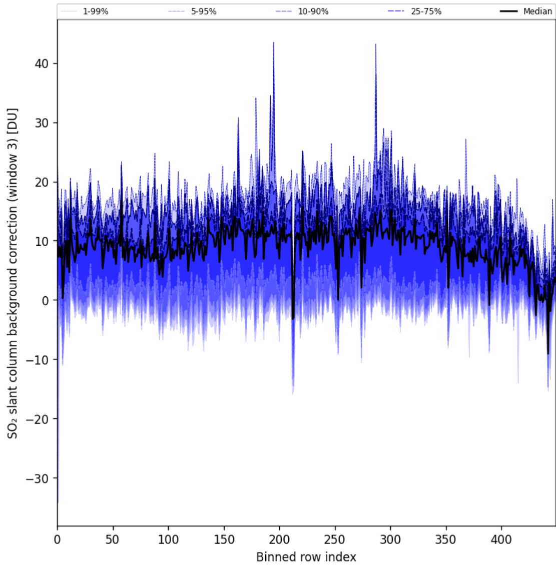
Figure 90: Along track statistics of “SO 2 slant column background correction (window 3)” for 2024-08-29 to 2024-08-31
