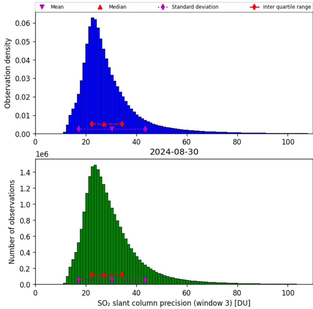
Figure 65: Histogram of “SO 2 slant column precision (window 3)” for 2024-08-29 to 2024-08-31
