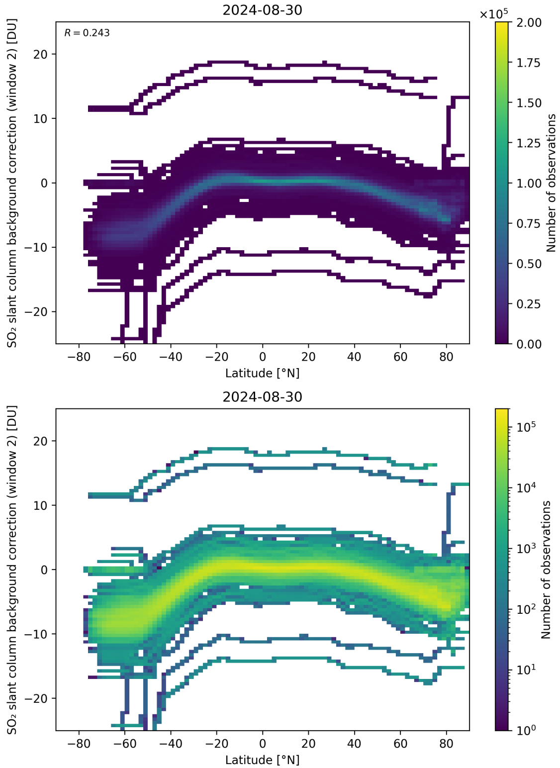
Figure 140: Scatter density plot of “Latitude” against “SO 2 slant column background correction (window 2)” for 2024-08-29 to 2024-08-31.
