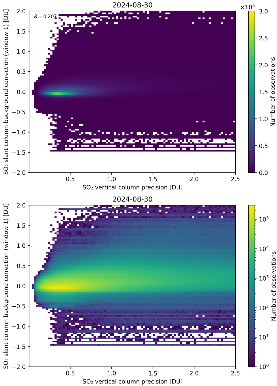
Figure 279: Scatter density plot of “SO 2 vertical column precision” against “SO 2 slant column background correction (window 1)” for 2024-08-29 to 2024-08-31.
