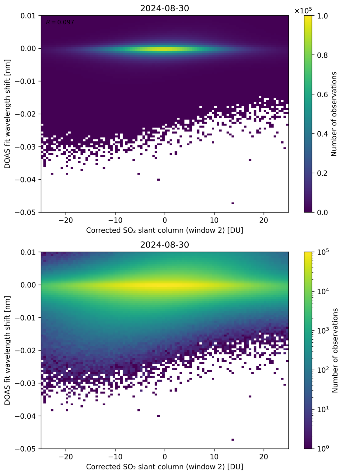
Figure 196: Scatter density plot of “Corrected SO 2 slant column (window 2)” against “DOAS fit wavelength shift” for 2024-08-29 to 2024-08-31.
