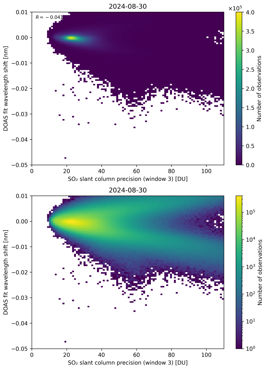
Figure 258: Scatter density plot of “SO 2 slant column precision (window 3)” against “DOAS fit wavelength shift” for 2024-08-29 to 2024-08-31.
