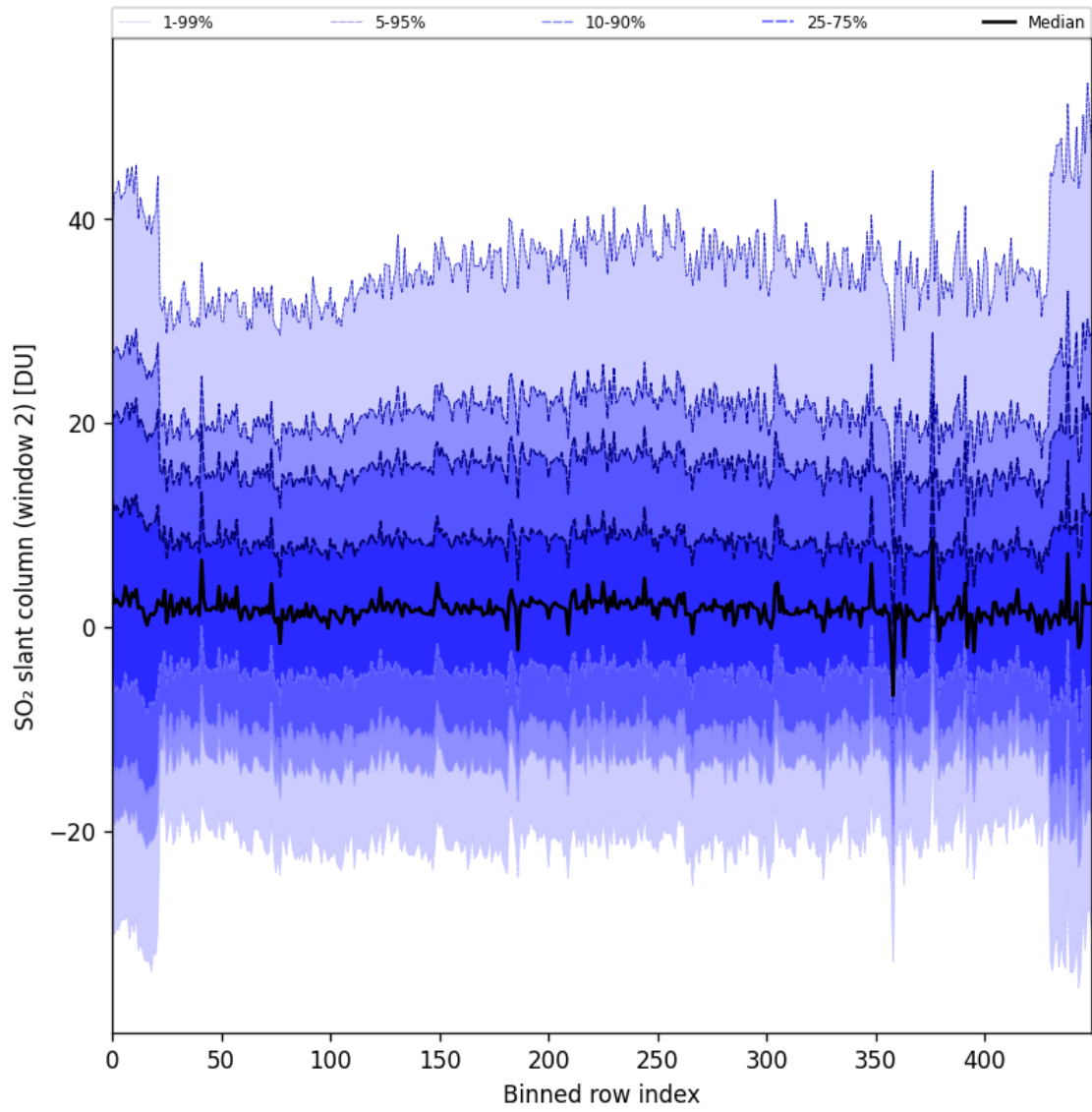
Figure 83: Along track statistics of “SO 2 slant column (window 2)” for 2024-08-29 to 2024-08-31
