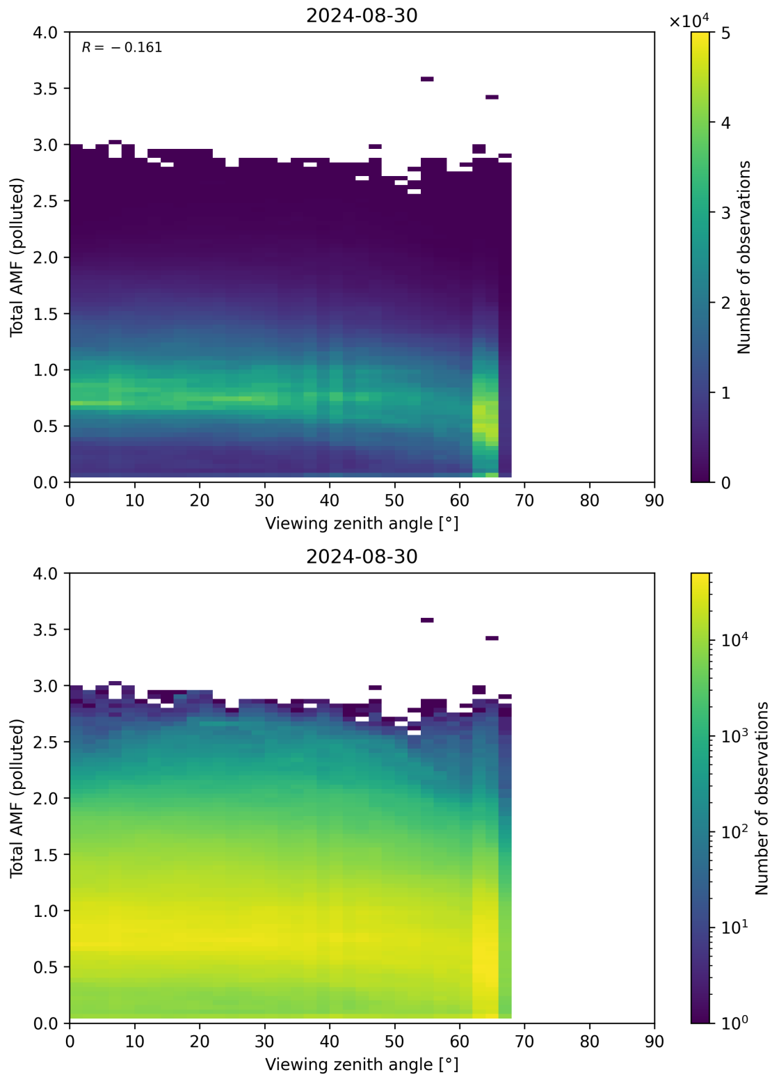
Figure 325: Scatter density plot of “Viewing zenith angle” against “Total AMF (polluted)” for 2024-08-29 to 2024-08-31.
