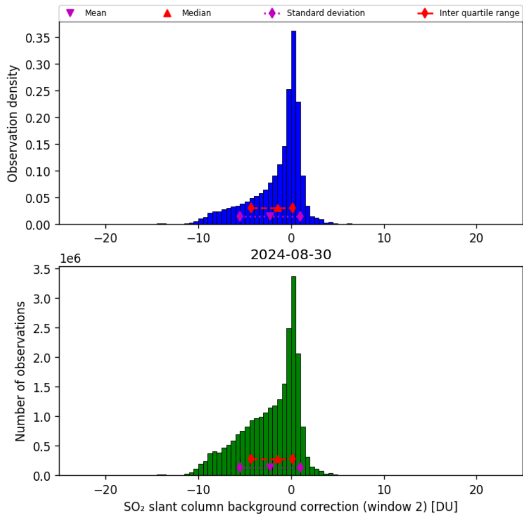
Figure 63: Histogram of “SO 2 slant column background correction (window 2)” for 2024-08-29 to 2024-08-31
