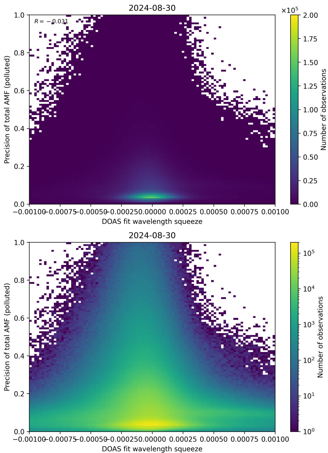
Figure 135: Scatter density plot of “DOAS fit wavelength squeeze” against “Precision of total AMF (polluted)” for 2024-08-29 to 2024-08-31.
