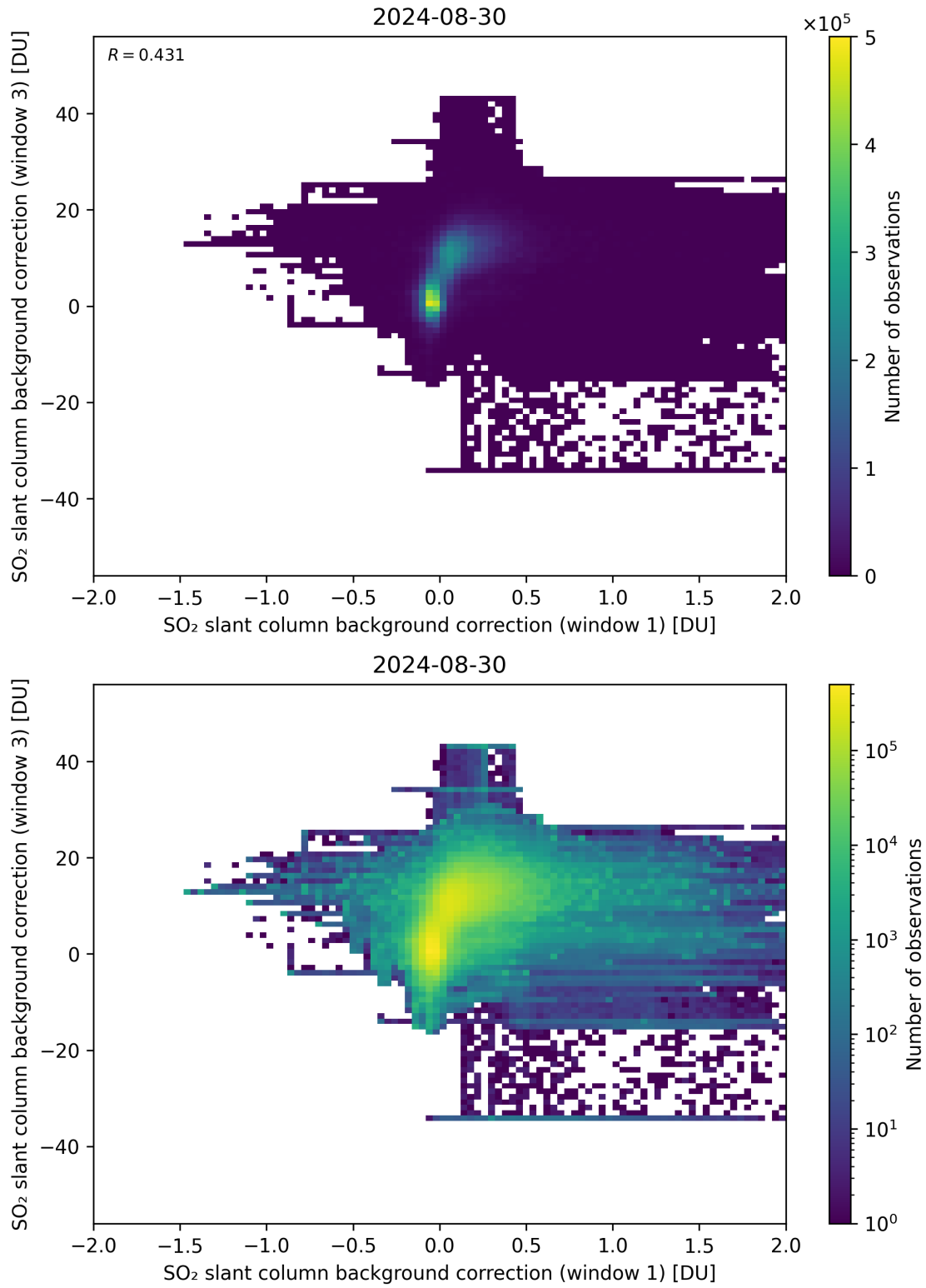
Figure 99: Scatter density plot of “SO 2 slant column background correction (window 1)” against “SO 2 slant column background correction (window 3)” for 2024-08-29 to 2024-08-31.
