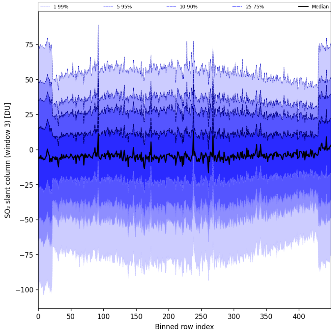
Figure 87: Along track statistics of “SO 2 slant column (window 3)” for 2024-08-29 to 2024-08-31
