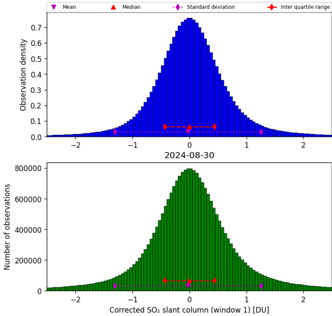
Figure 58: Histogram of “Corrected SO 2 slant column (window 1)” for 2024-08-29 to 2024-08-31
