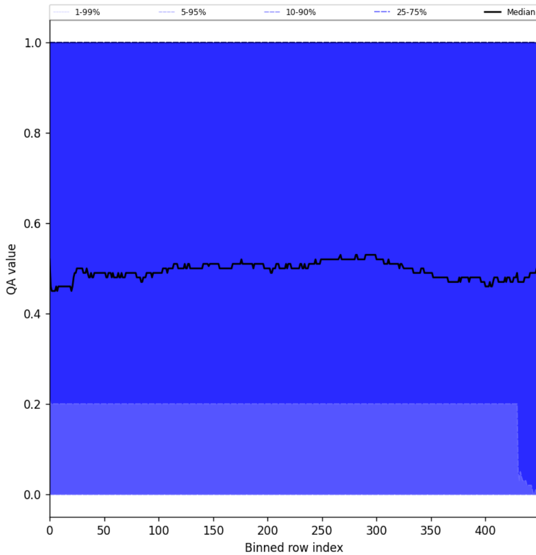
Figure 75: Along track statistics of “QA value” for 2024-08-29 to 2024-08-31
