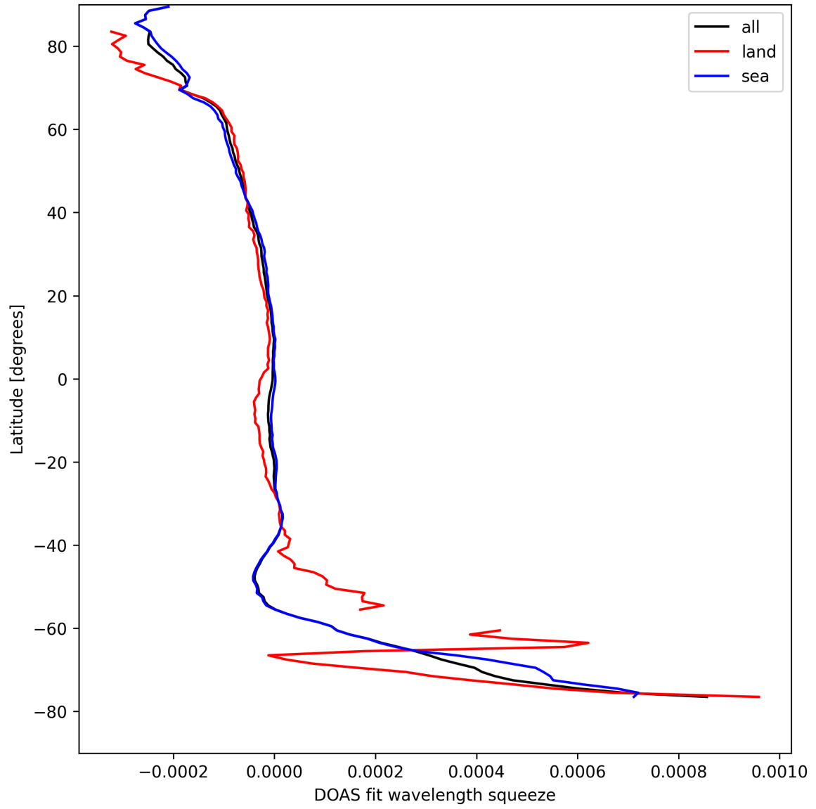
Figure 46: Zonal average of “DOAS fit wavelength squeeze” for 2024-08-29 to 2024-08-31.
