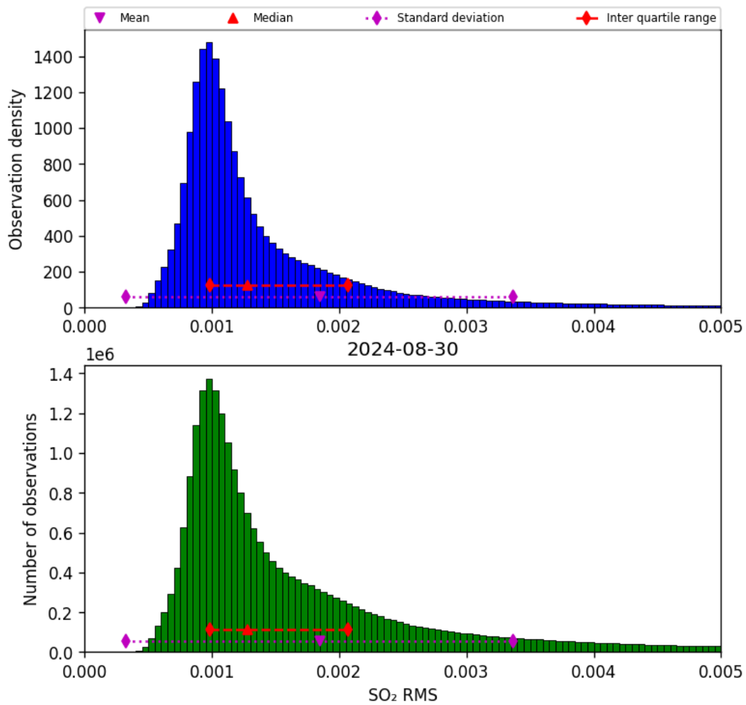
Figure 70: Histogram of “SO 2 RMS” for 2024-08-29 to 2024-08-31
