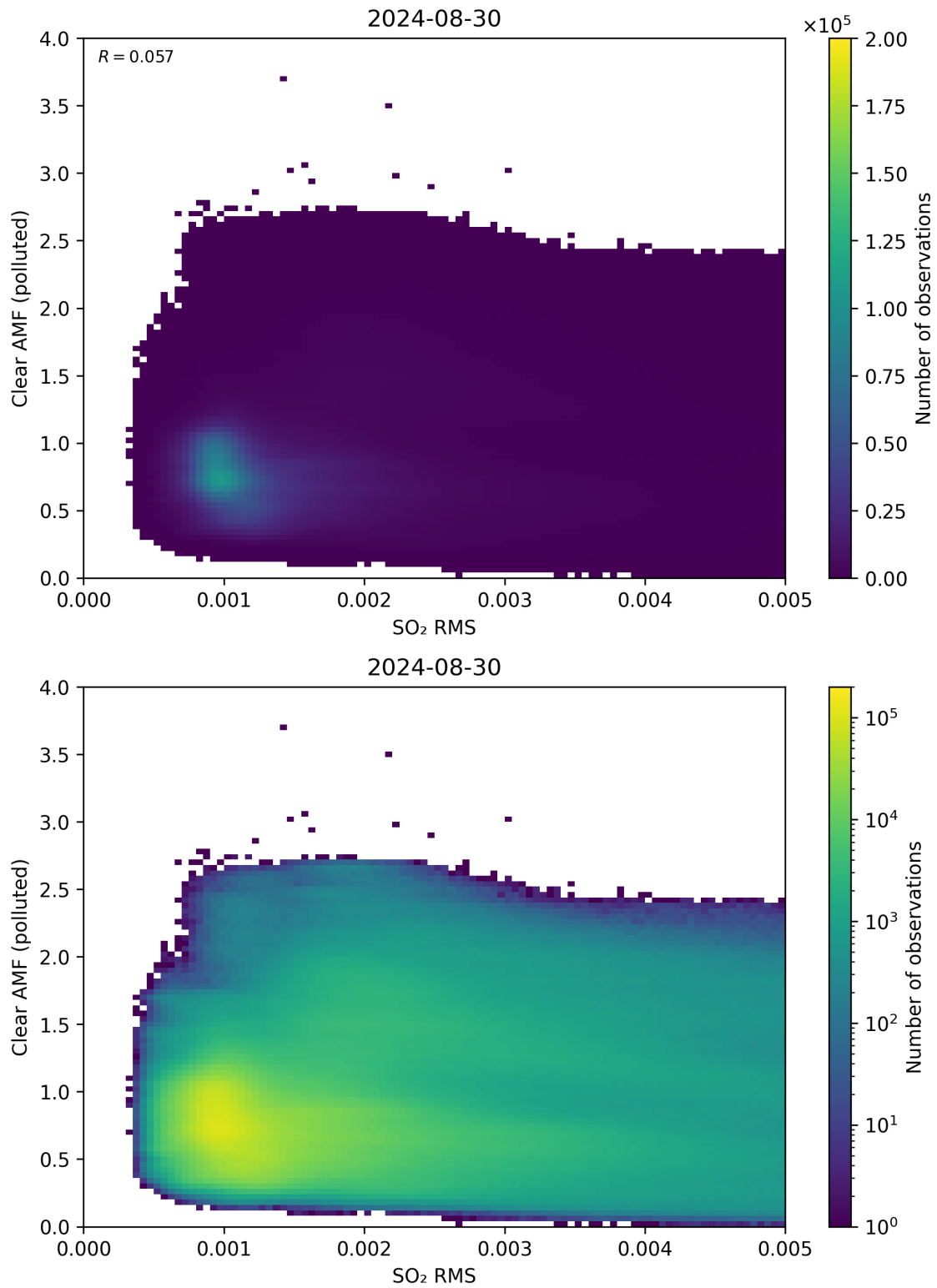
Figure 136: Scatter density plot of “SO 2 RMS” against “Clear AMF (polluted)” for 2024-08-29 to 2024-08-31.
