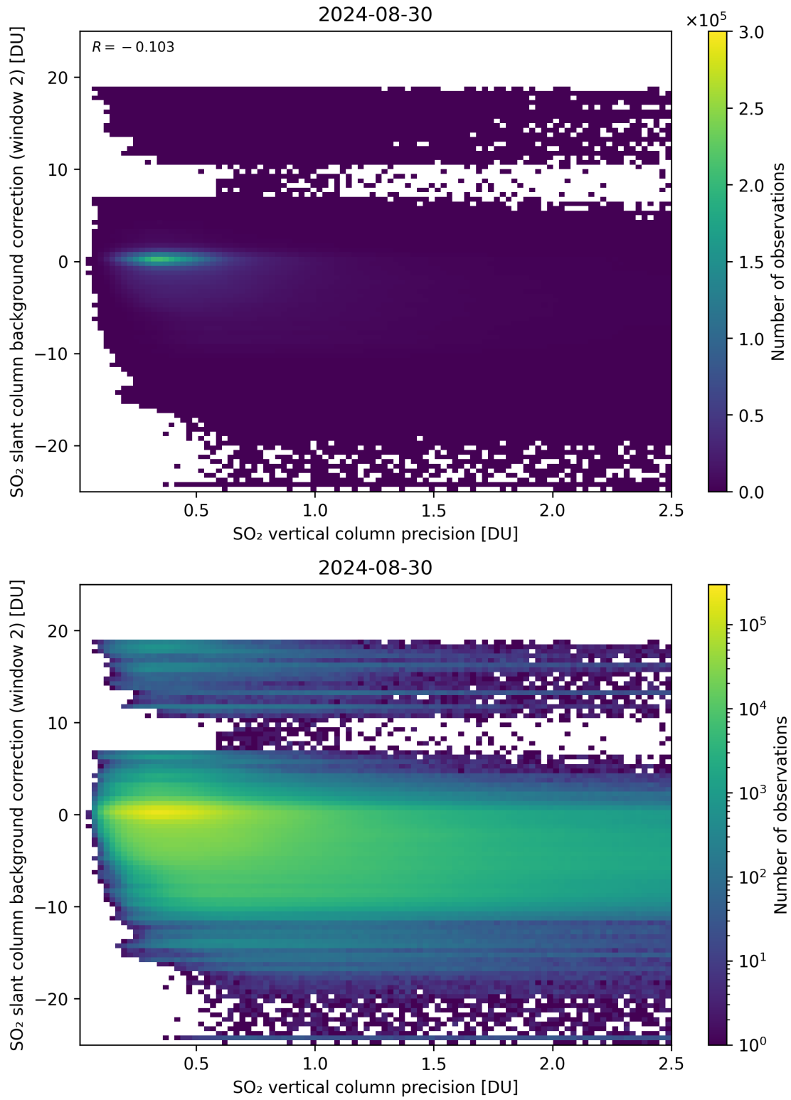
Figure 280: Scatter density plot of “SO 2 vertical column precision” against “SO 2 slant column background correction (window 2)” for 2024-08-29 to 2024-08-31.
