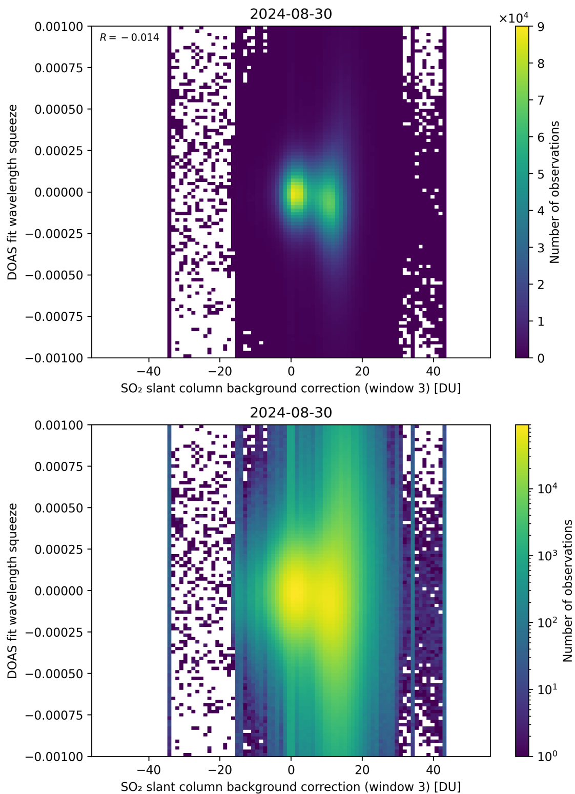
Figure 122: Scatter density plot of “SO 2 slant column background correction (window 3)” against “DOAS fit wavelength squeeze” for 2024-08-29 to 2024-08-31.
