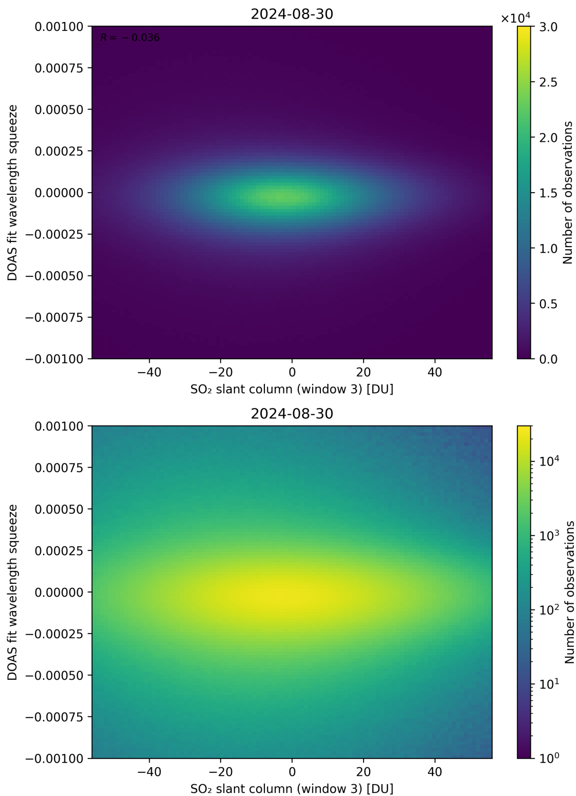
Figure 255: Scatter density plot of “SO 2 slant column (window 3)” against “DOAS fit wavelength squeeze” for 2024-08-29 to 2024-08-31.
