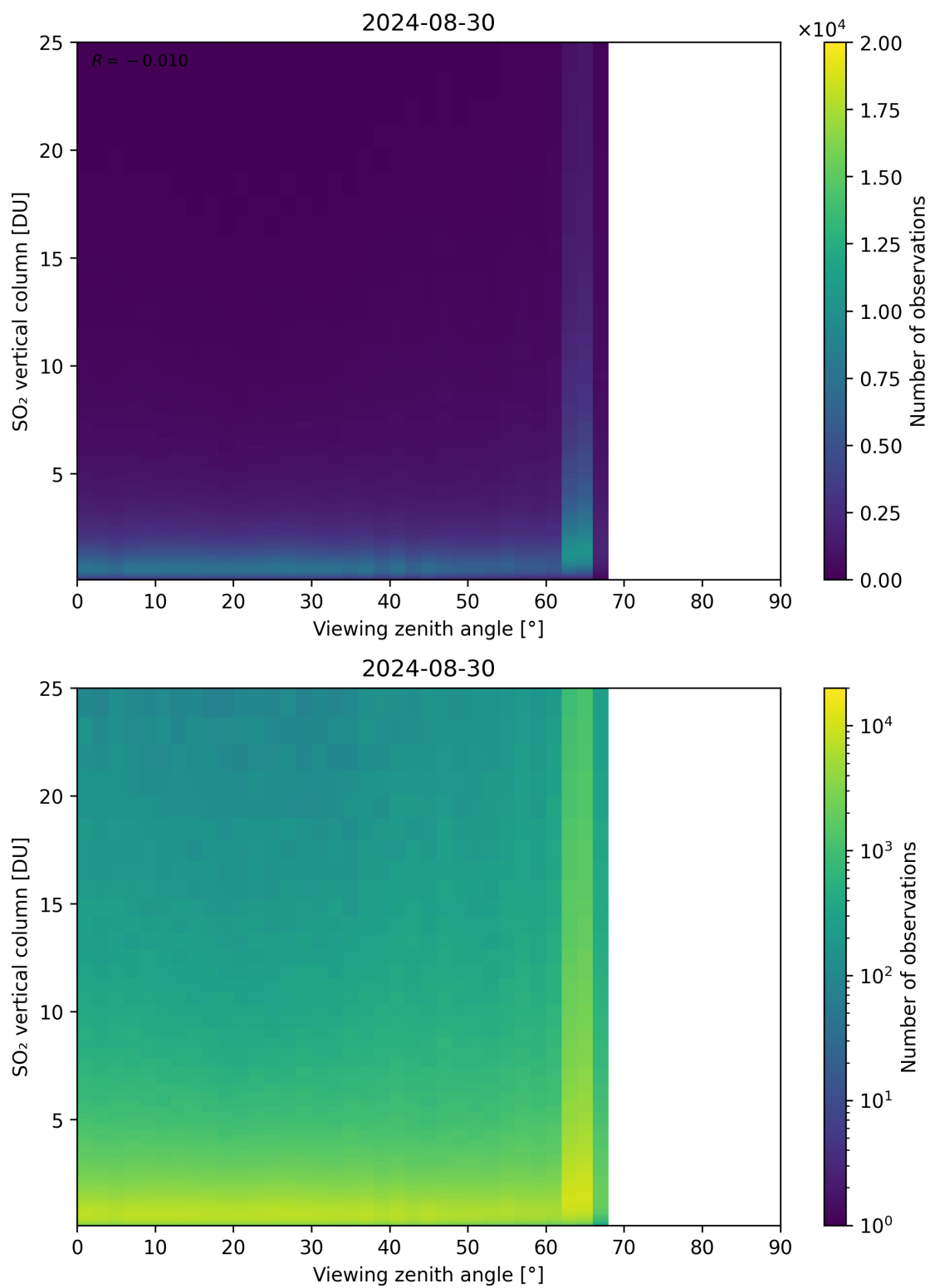
Figure 327: Scatter density plot of “Viewing zenith angle” against “SO 2 vertical column” for 2024-08-29 to 2024-08-31.
