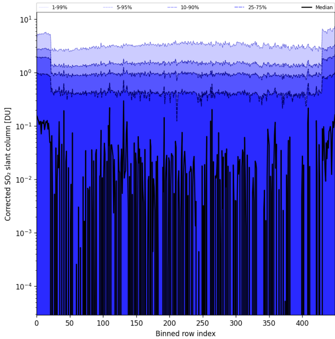
Figure 78: Along track statistics of “Corrected SO 2 slant column” for 2024-08-29 to 2024-08-31
