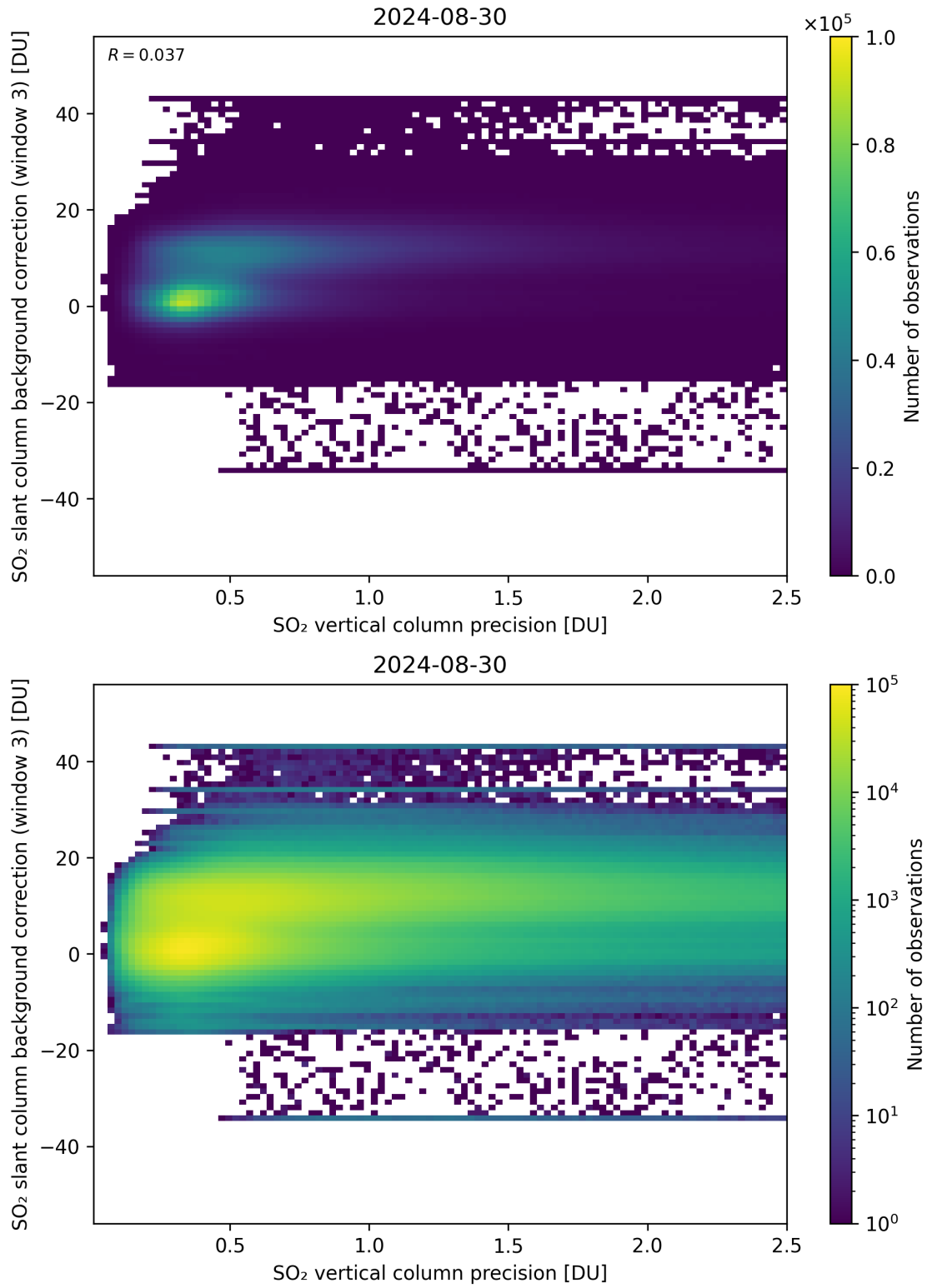
Figure 281: Scatter density plot of “SO 2 vertical column precision” against “SO 2 slant column background correction (window 3)” for 2024-08-29 to 2024-08-31.
