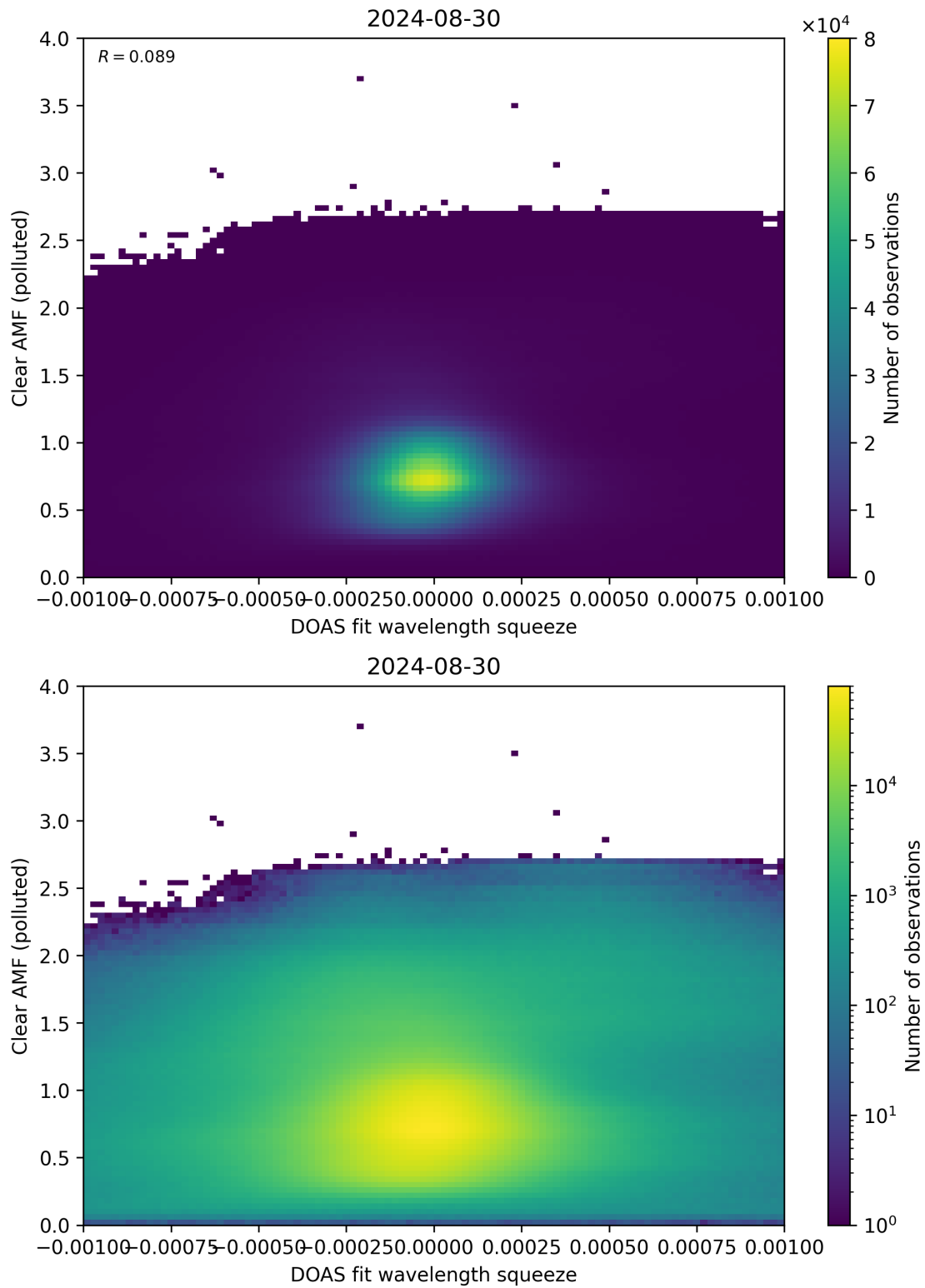
Figure 133: Scatter density plot of “DOAS fit wavelength squeeze” against “Clear AMF (polluted)” for 2024-08-29 to 2024-08-31.
