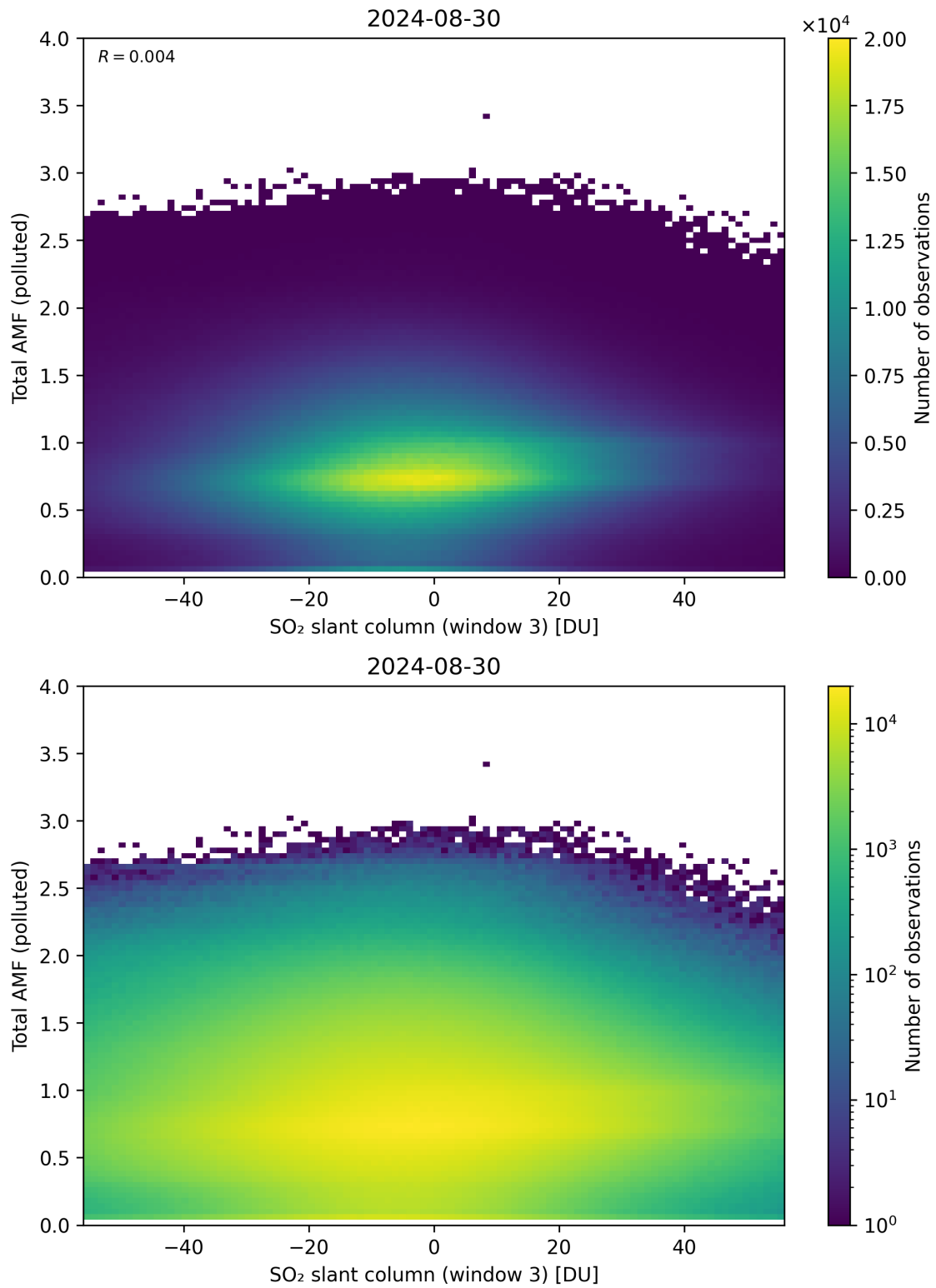
Figure 268: Scatter density plot of “SO 2 slant column (window 3)” against “Total AMF (polluted)” for 2024-08-29 to 2024-08-31.
