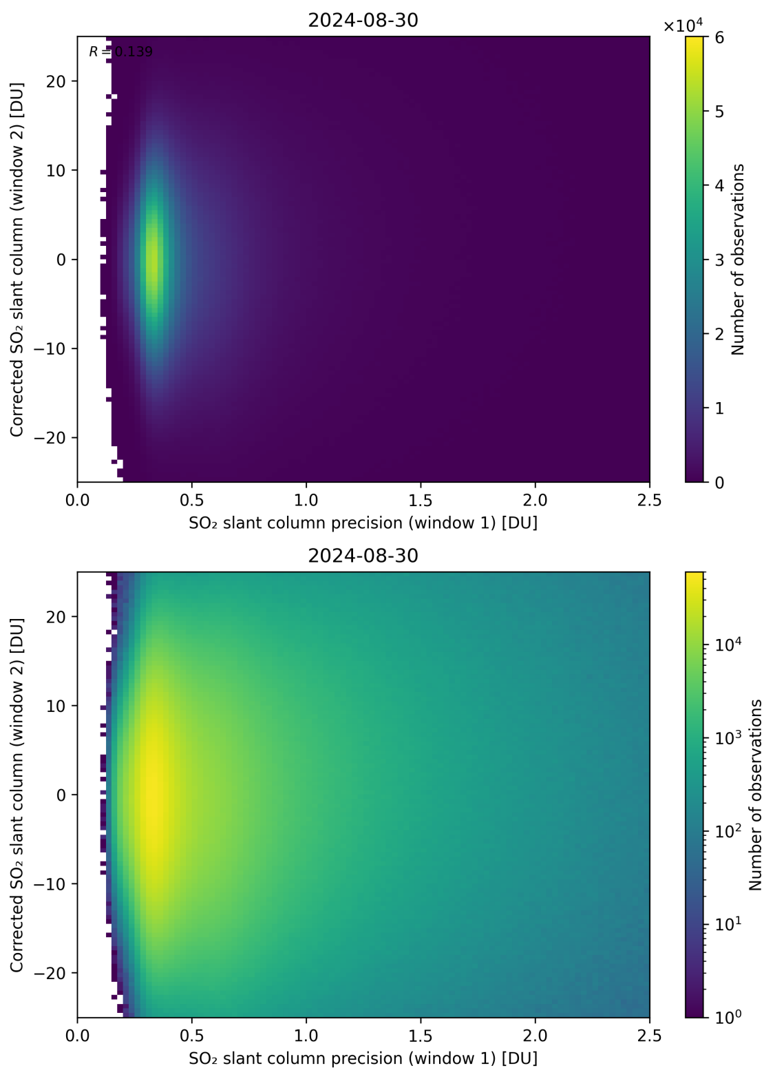
Figure 225: Scatter density plot of “SO 2 slant column precision (window 1)” against “Corrected SO 2 slant column (window 2)” for 2024-08-29 to 2024-08-31.
