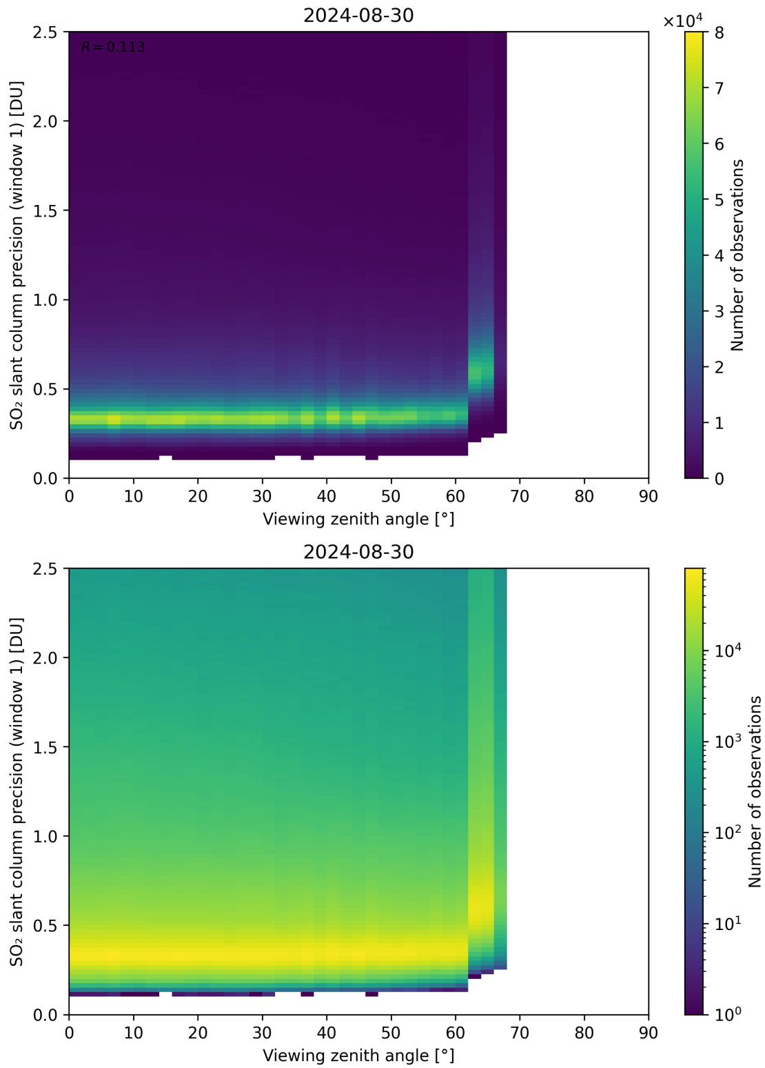
Figure 321: Scatter density plot of “Viewing zenith angle” against “SO 2 slant column precision (window 1)” for 2024-08-29 to 2024-08-31.
