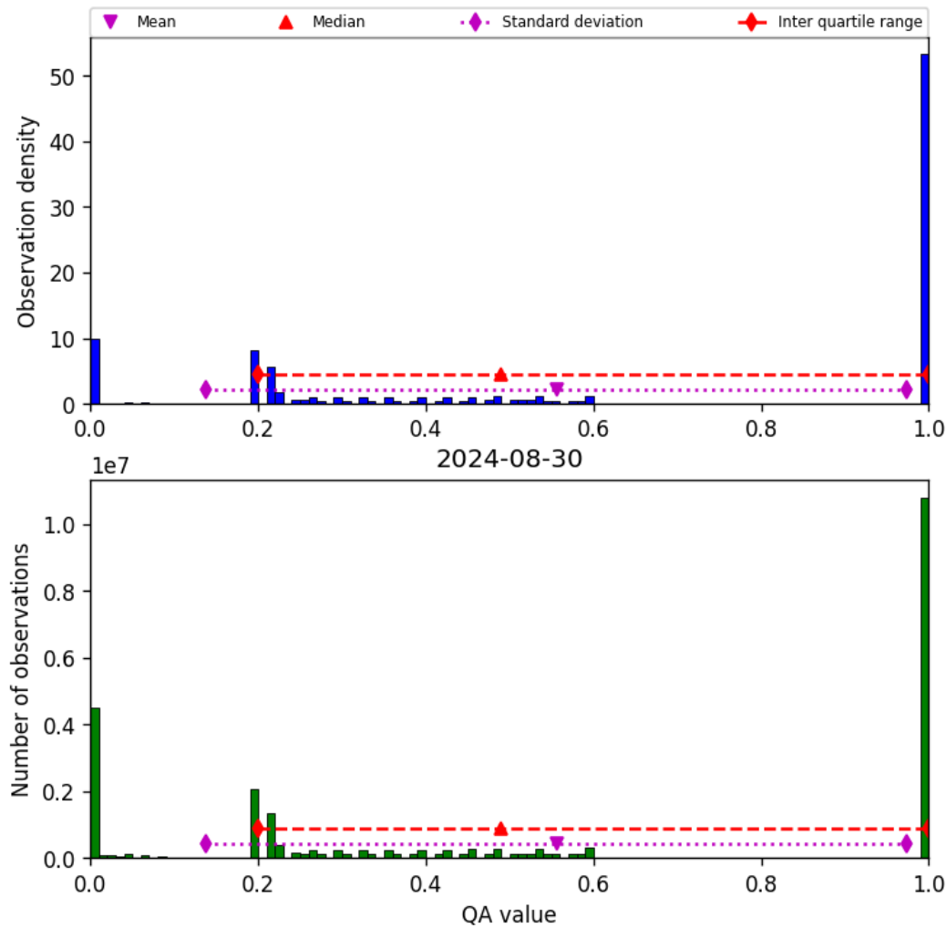
Figure 52: Histogram of “QA value” for 2024-08-29 to 2024-08-31
