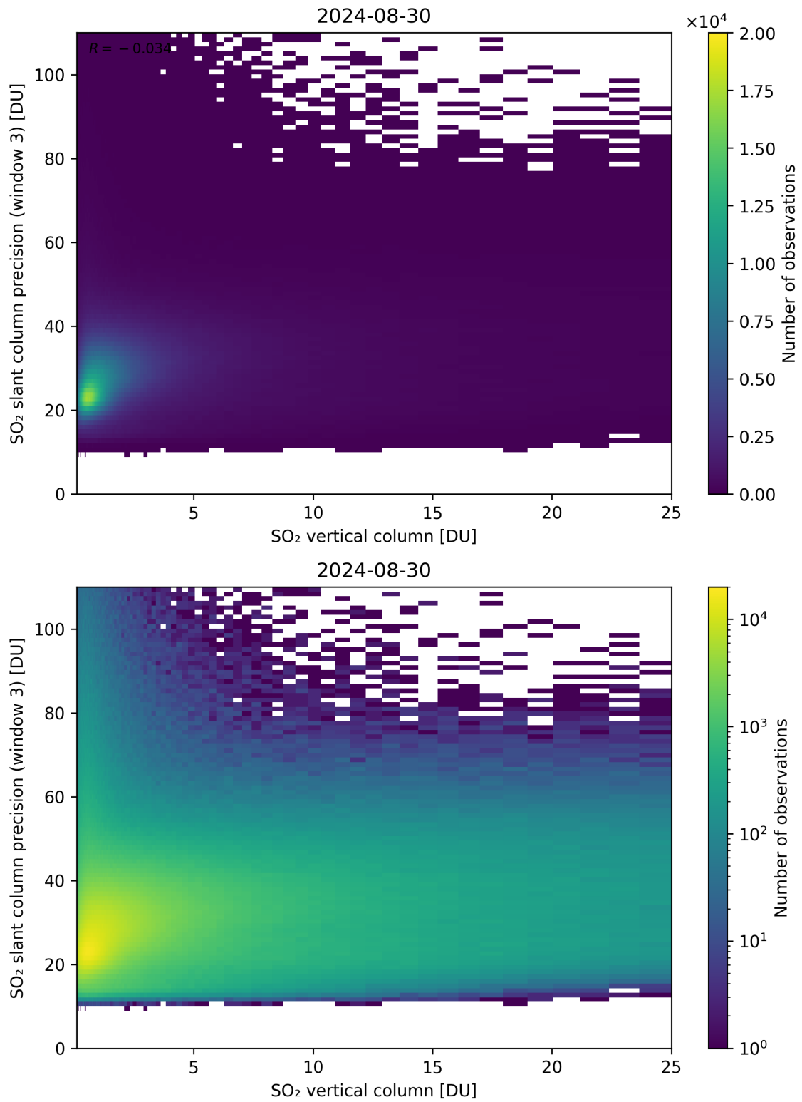
Figure 304: Scatter density plot of “SO 2 vertical column” against “SO 2 slant column precision (window 3)” for 2024-08-29 to 2024-08-31.
