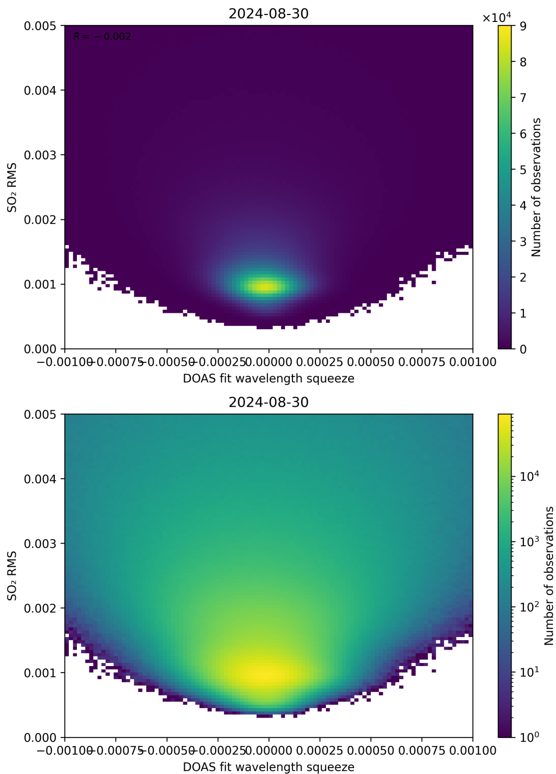
Figure 132: Scatter density plot of “DOAS fit wavelength squeeze” against “SO 2 RMS” for 2024-08-29 to 2024-08-31.
