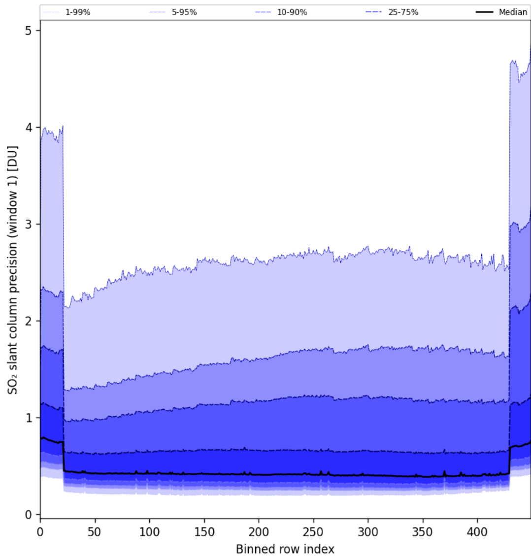
Figure 80: Along track statistics of “SO 2 slant column precision (window 1)” for 2024-08-29 to 2024-08-31
