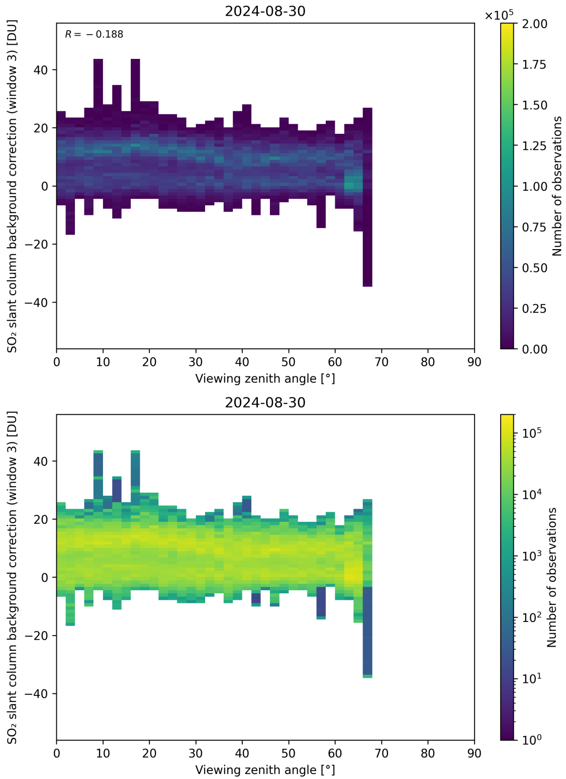
Figure 310: Scatter density plot of “Viewing zenith angle” against “SO 2 slant column background correction (window 3)” for 2024-08-29 to 2024-08-31.
