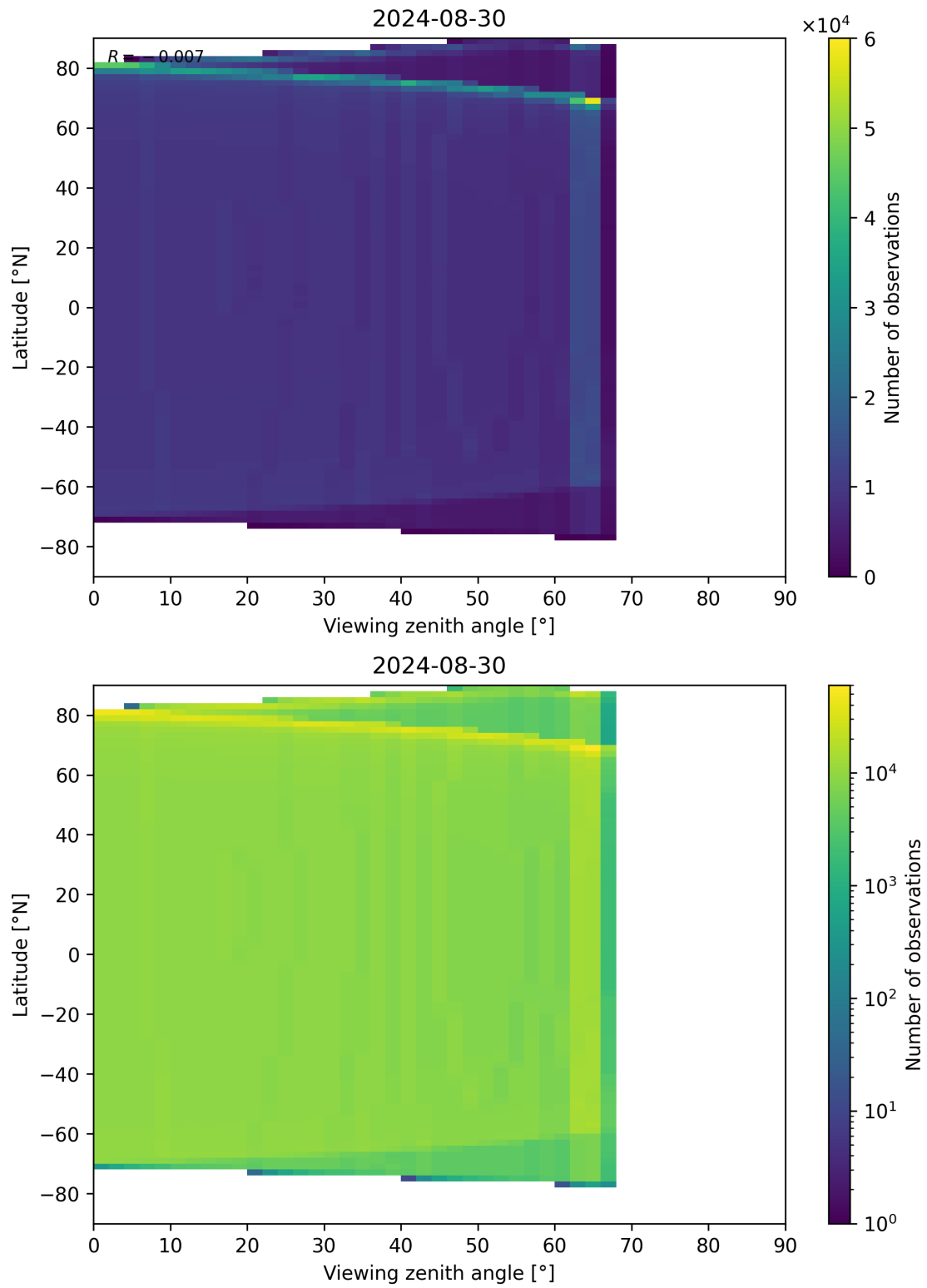
Figure 314: Scatter density plot of “Viewing zenith angle” against “Latitude” for 2024-08-29 to 2024-08-31.
