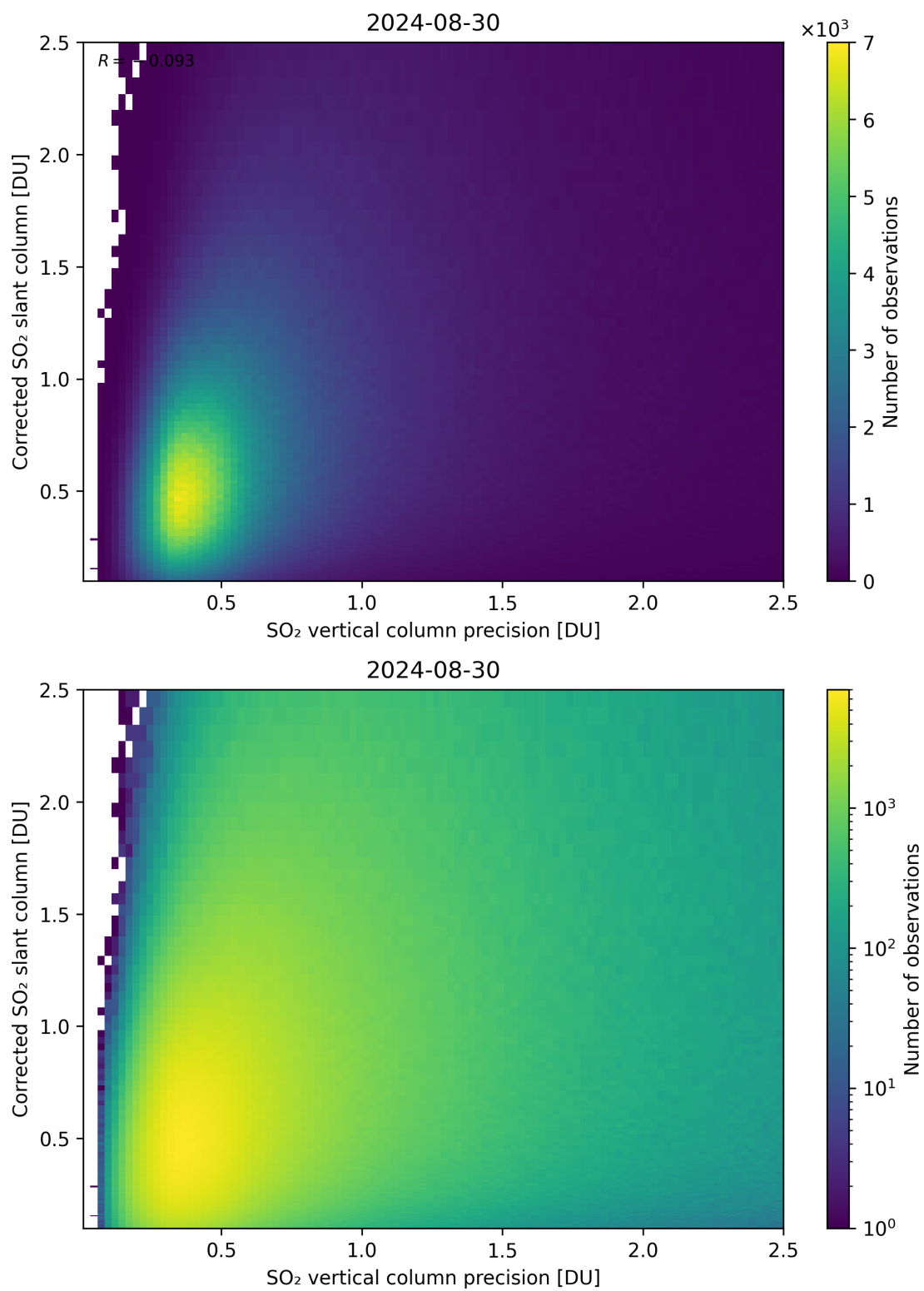
Figure 286: Scatter density plot of “SO 2 vertical column precision” against “Corrected SO 2 slant column” for 2024-08-29 to 2024-08-31.
