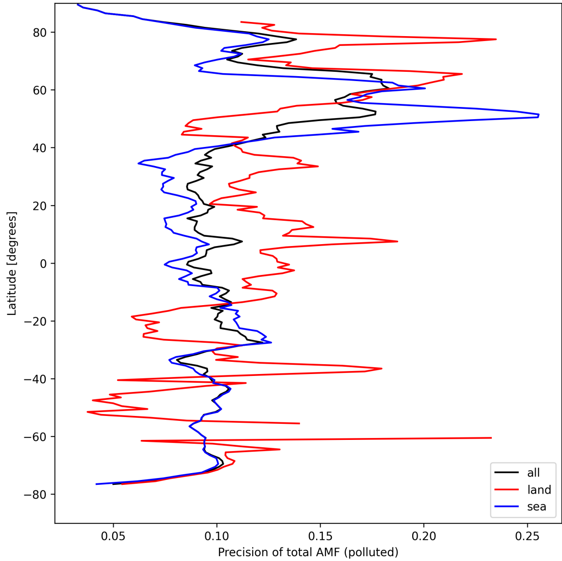
Figure 49: Zonal average of “Precision of total AMF (polluted)” for 2024-08-29 to 2024-08-31.
