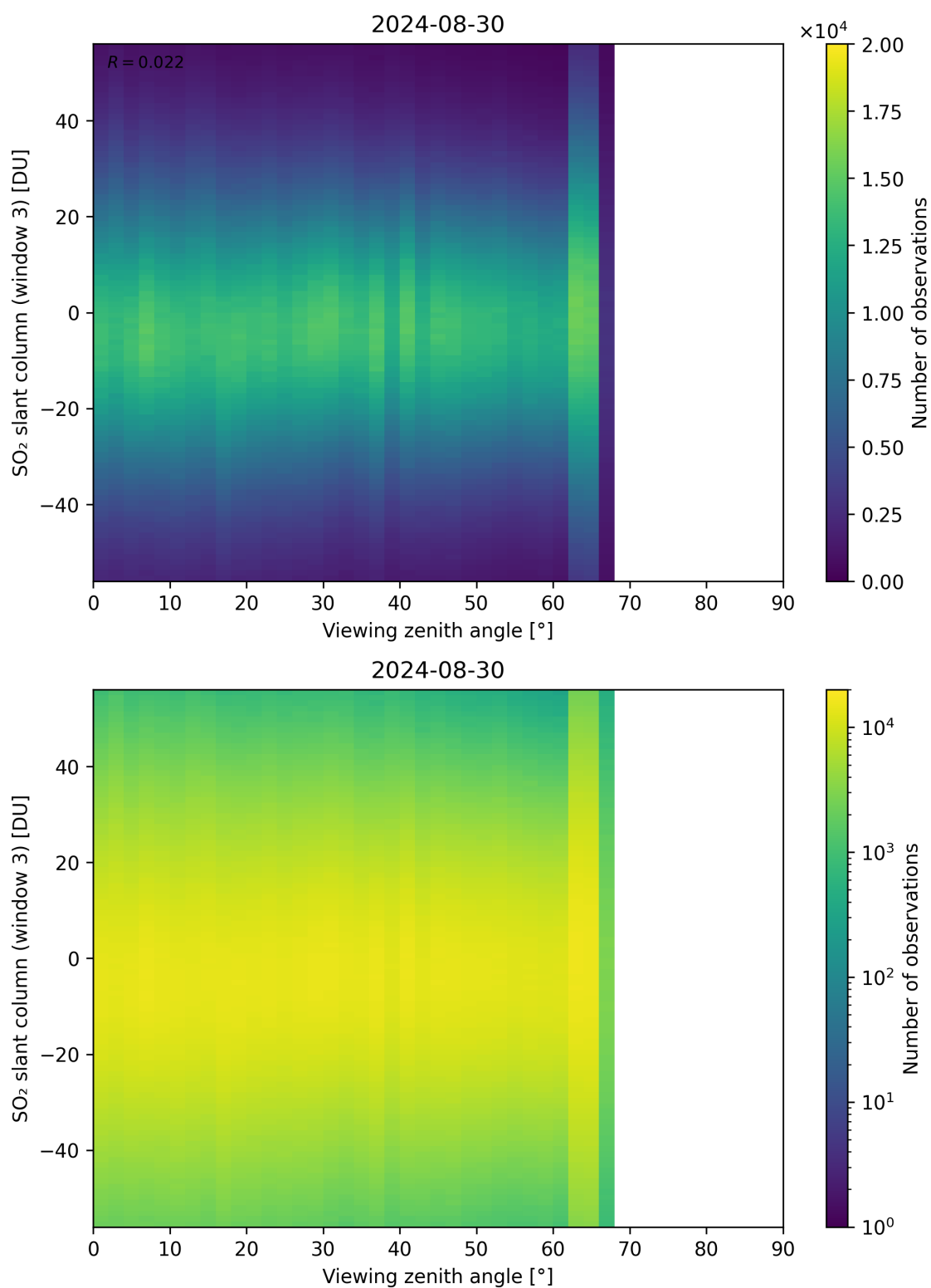
Figure 323: Scatter density plot of “Viewing zenith angle” against “SO 2 slant column (window 3)” for 2024-08-29 to 2024-08-31.
