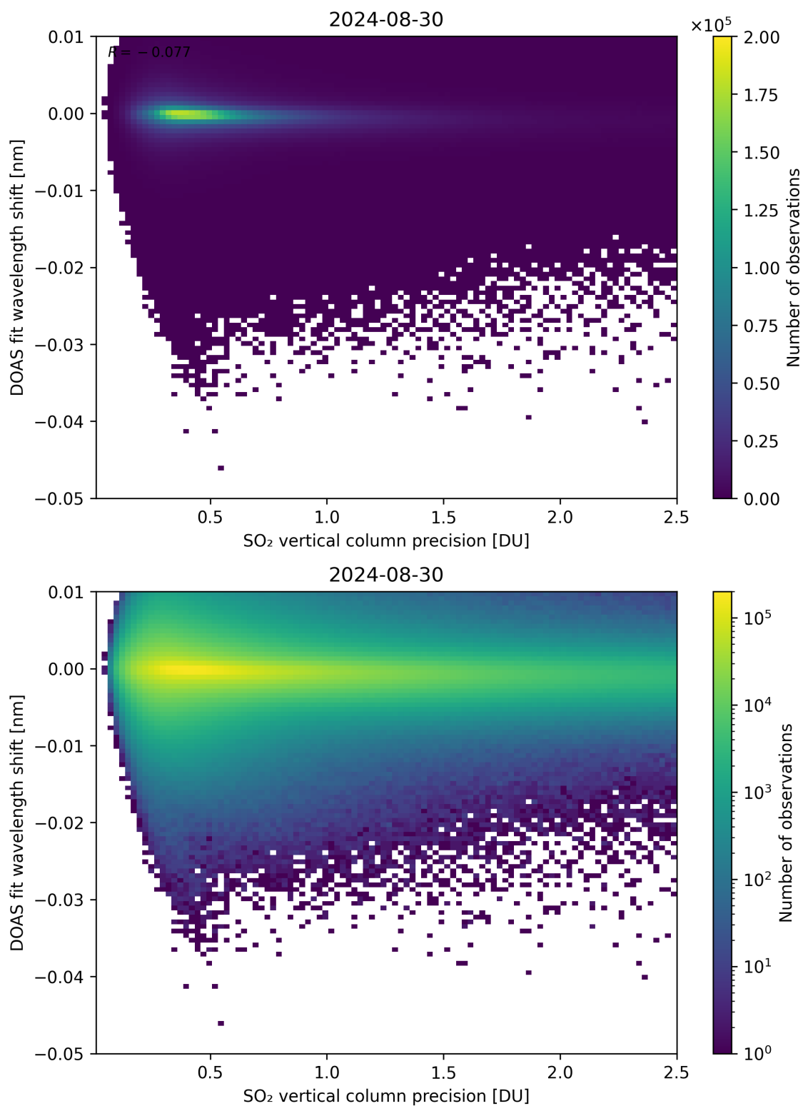
Figure 282: Scatter density plot of “SO 2 vertical column precision” against “DOAS fit wavelength shift” for 2024-08-29 to 2024-08-31.
