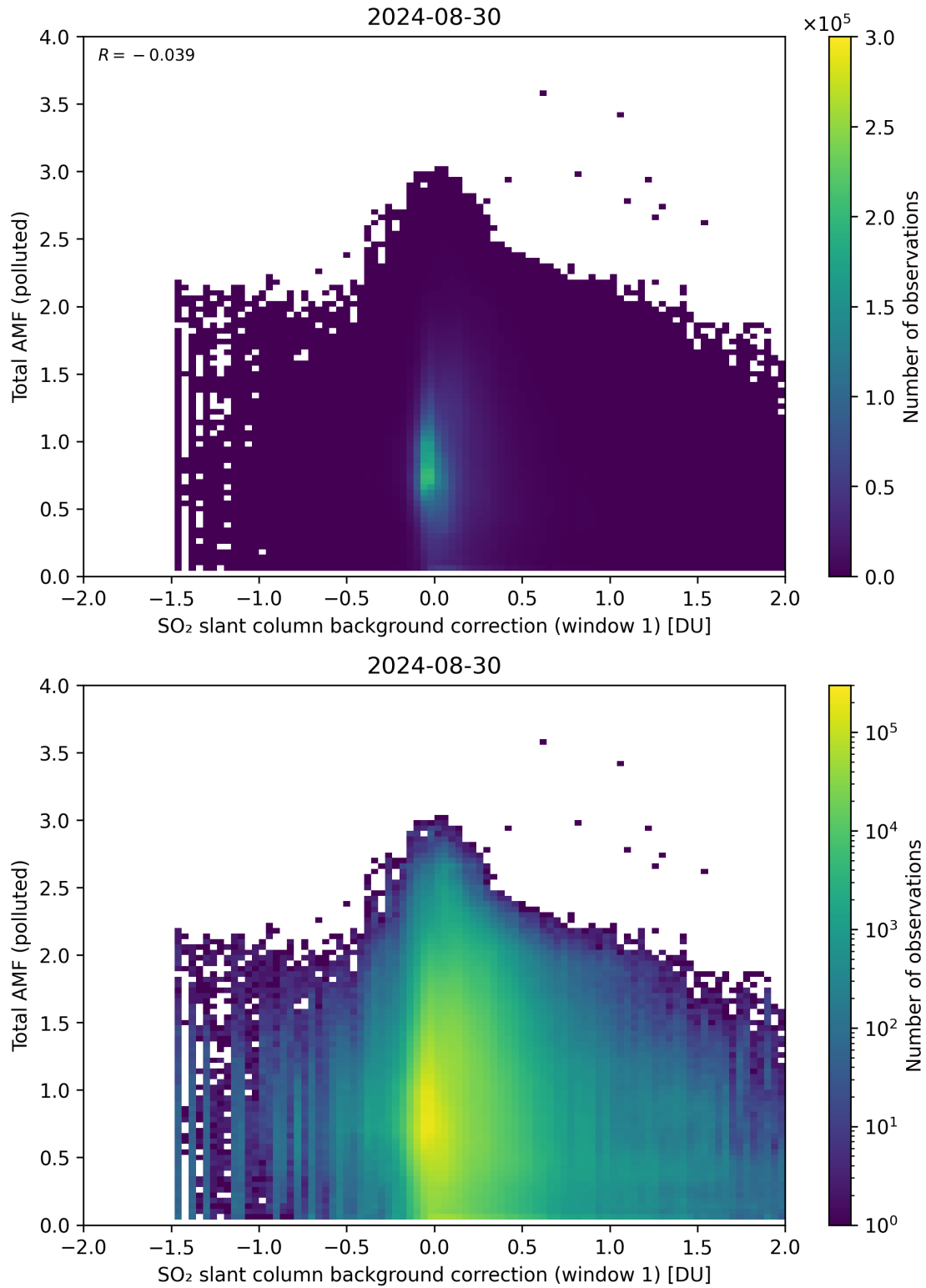
Figure 109: Scatter density plot of “SO 2 slant column background correction (window 1)” against “Total AMF (polluted)” for 2024-08-29 to 2024-08-31.
