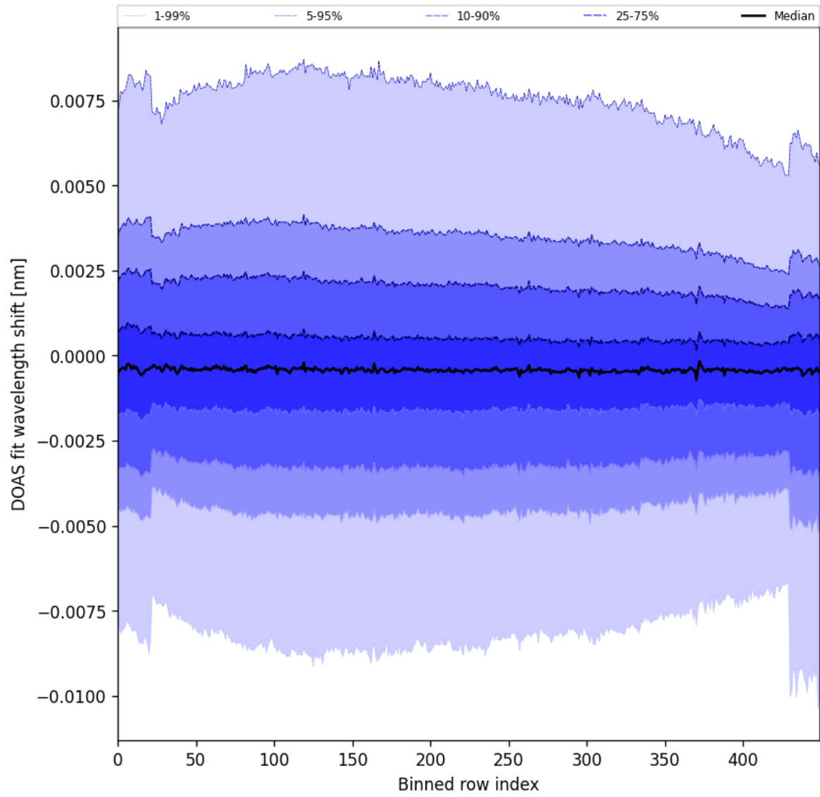
Figure 91: Along track statistics of “DOAS fit wavelength shift” for 2024-08-29 to 2024-08-31
