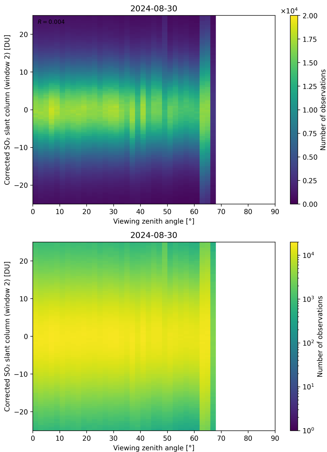
Figure 318: Scatter density plot of “Viewing zenith angle” against “Corrected SO 2 slant column (window 2)” for 2024-08-29 to 2024-08-31.
