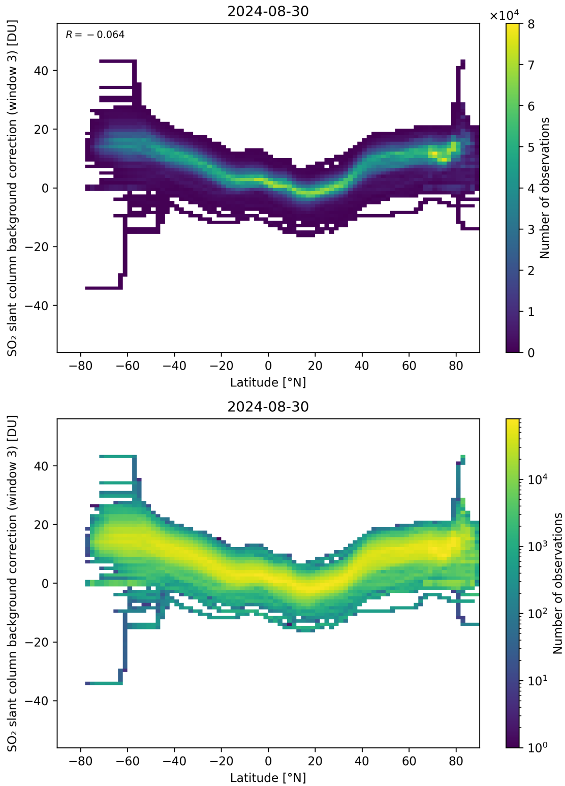
Figure 141: Scatter density plot of “Latitude” against “SO 2 slant column background correction (window 3)” for 2024-08-29 to 2024-08-31.
