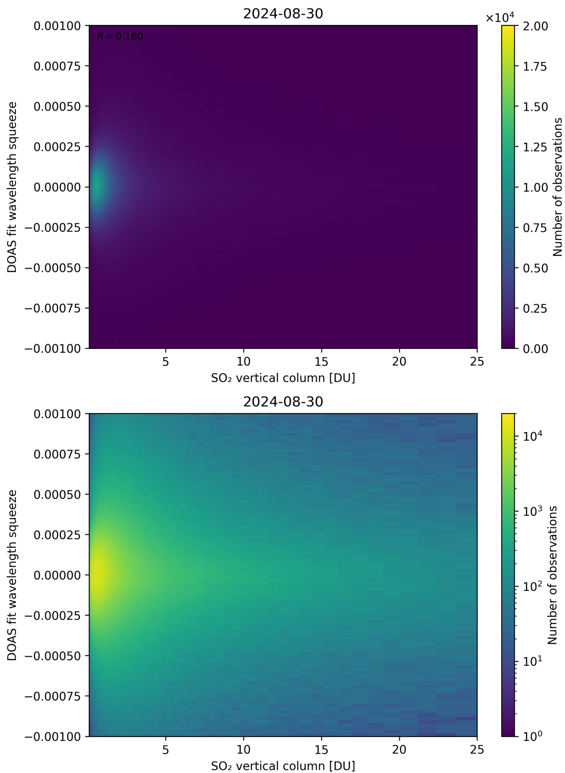
Figure 277: Scatter density plot of “SO 2 vertical column” against “DOAS fit wavelength squeeze” for 2024-08-29 to 2024-08-31.
