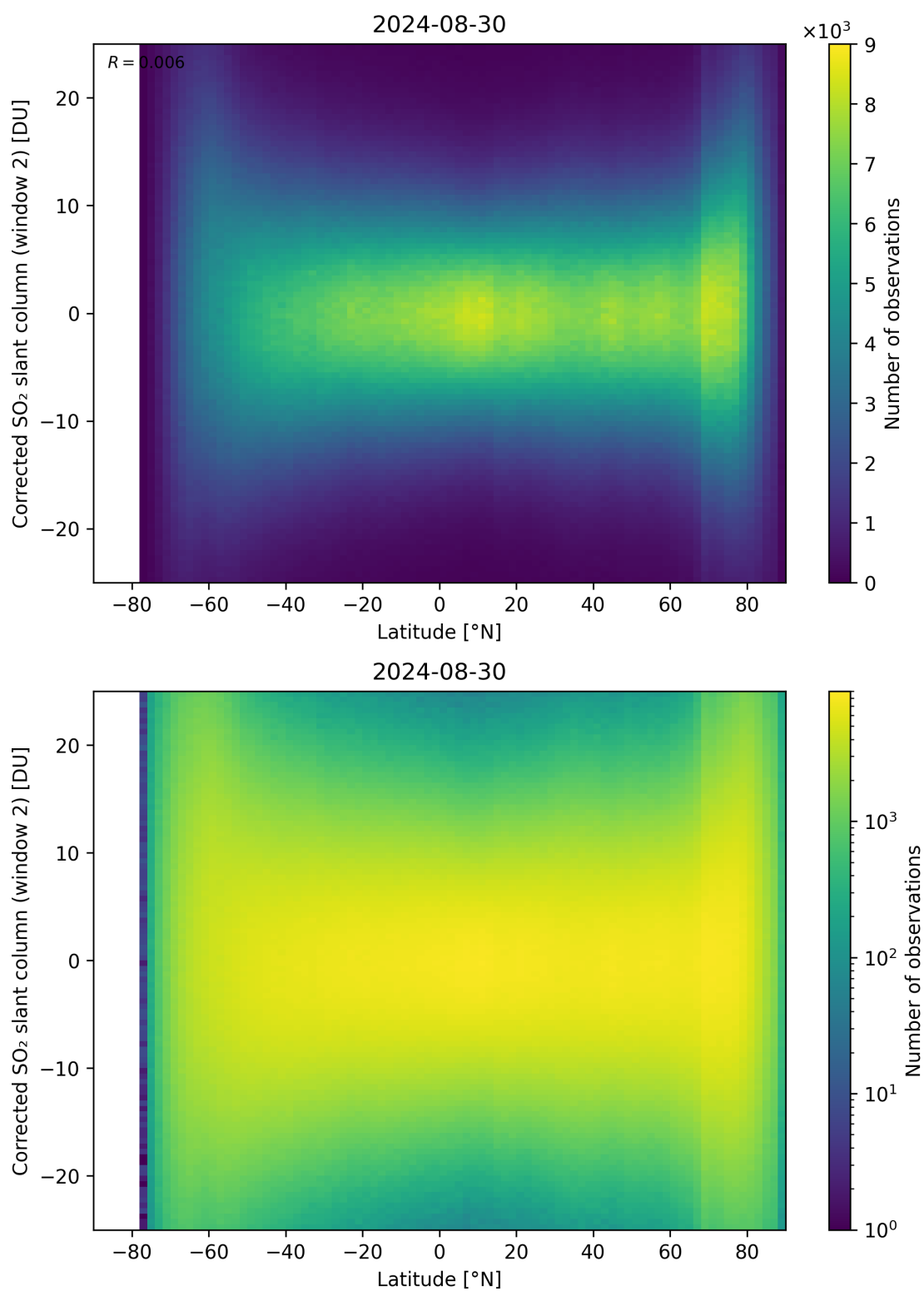
Figure 147: Scatter density plot of “Latitude” against “Corrected SO 2 slant column (window 2)” for 2024-08-29 to 2024-08-31.
