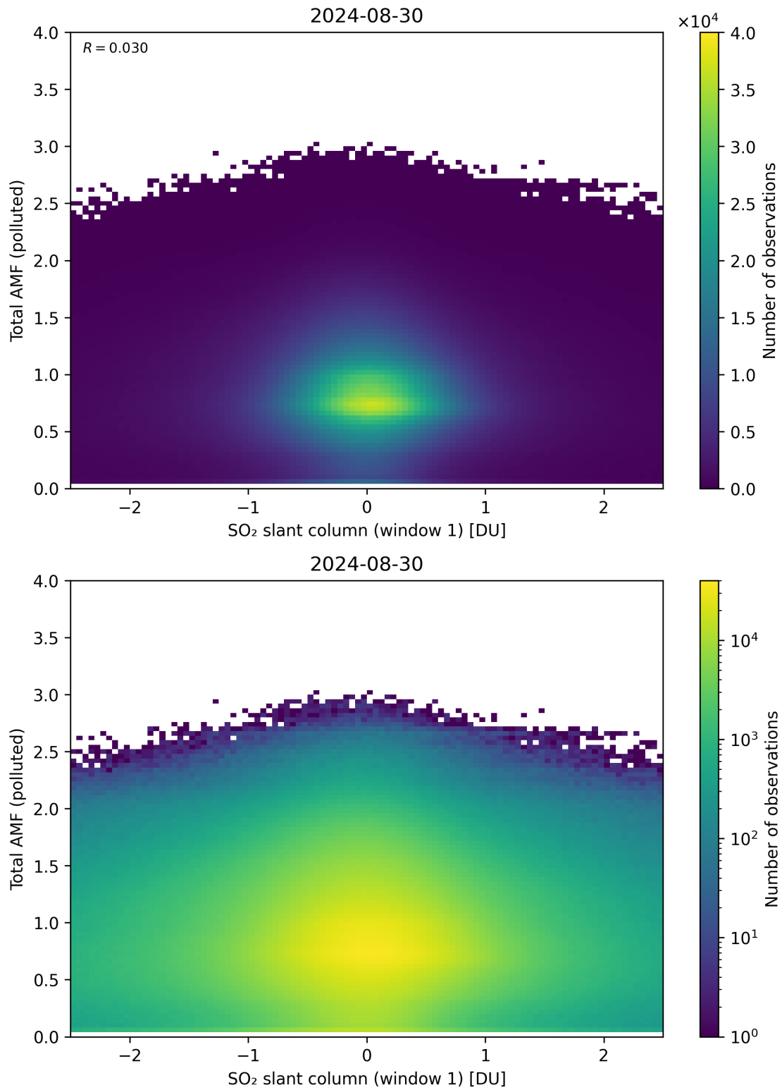
Figure 239: Scatter density plot of “SO 2 slant column (window 1)” against “Total AMF (polluted)” for 2024-08-29 to 2024-08-31.
