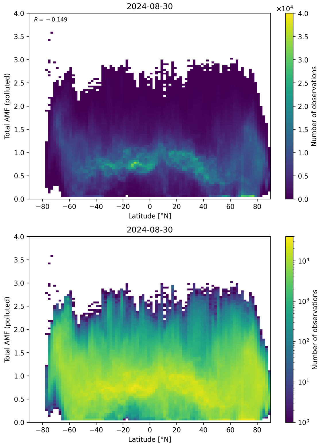
Figure 154: Scatter density plot of “Latitude” against “Total AMF (polluted)” for 2024-08-29 to 2024-08-31.
