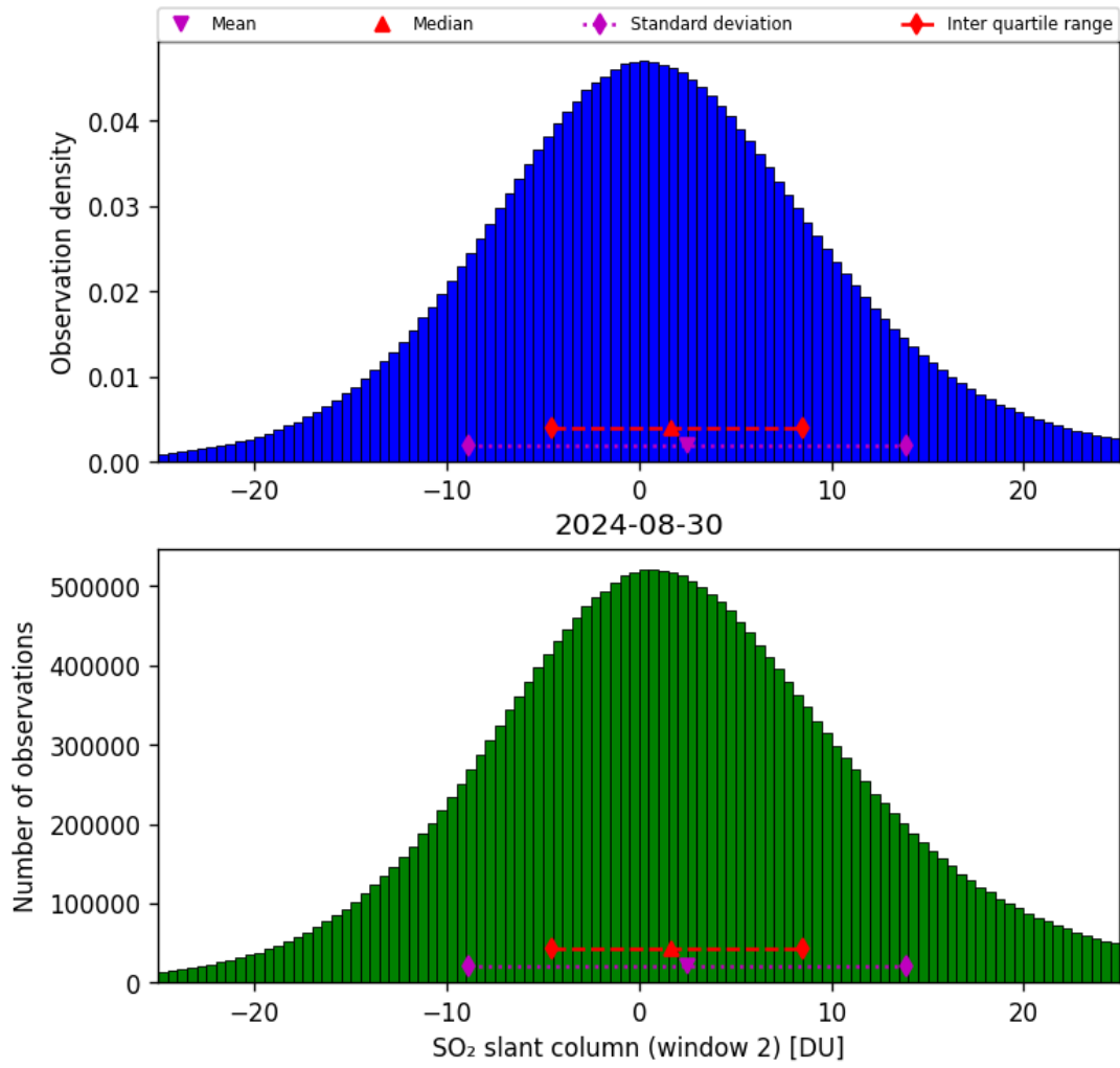
Figure 60: Histogram of “SO 2 slant column (window 2)” for 2024-08-29 to 2024-08-31
