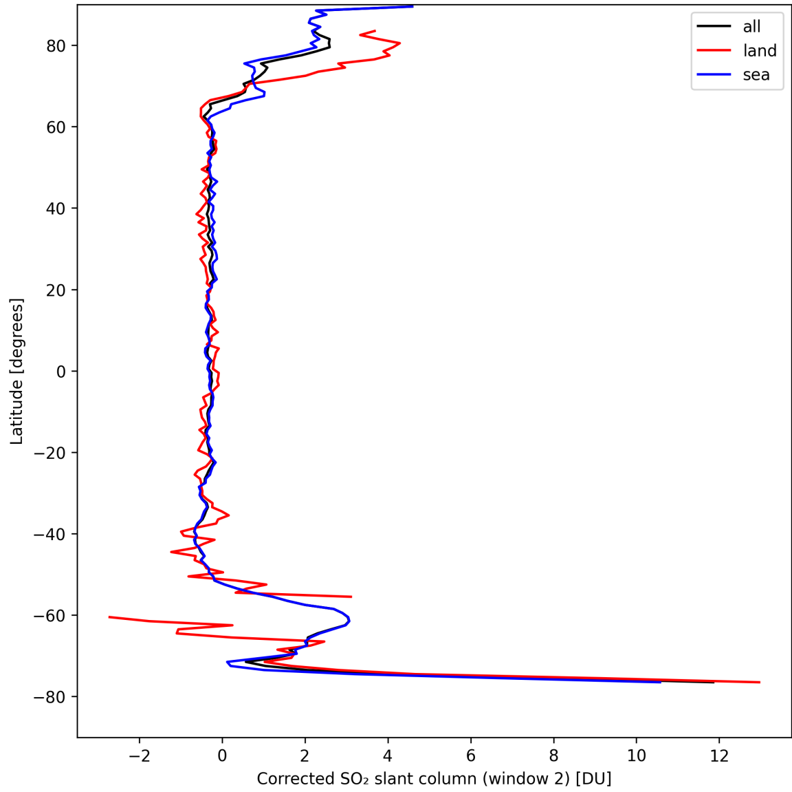
Figure 39: Zonal average of “Corrected SO 2 slant column (window 2)” for 2024-08-29 to 2024-08-31.
