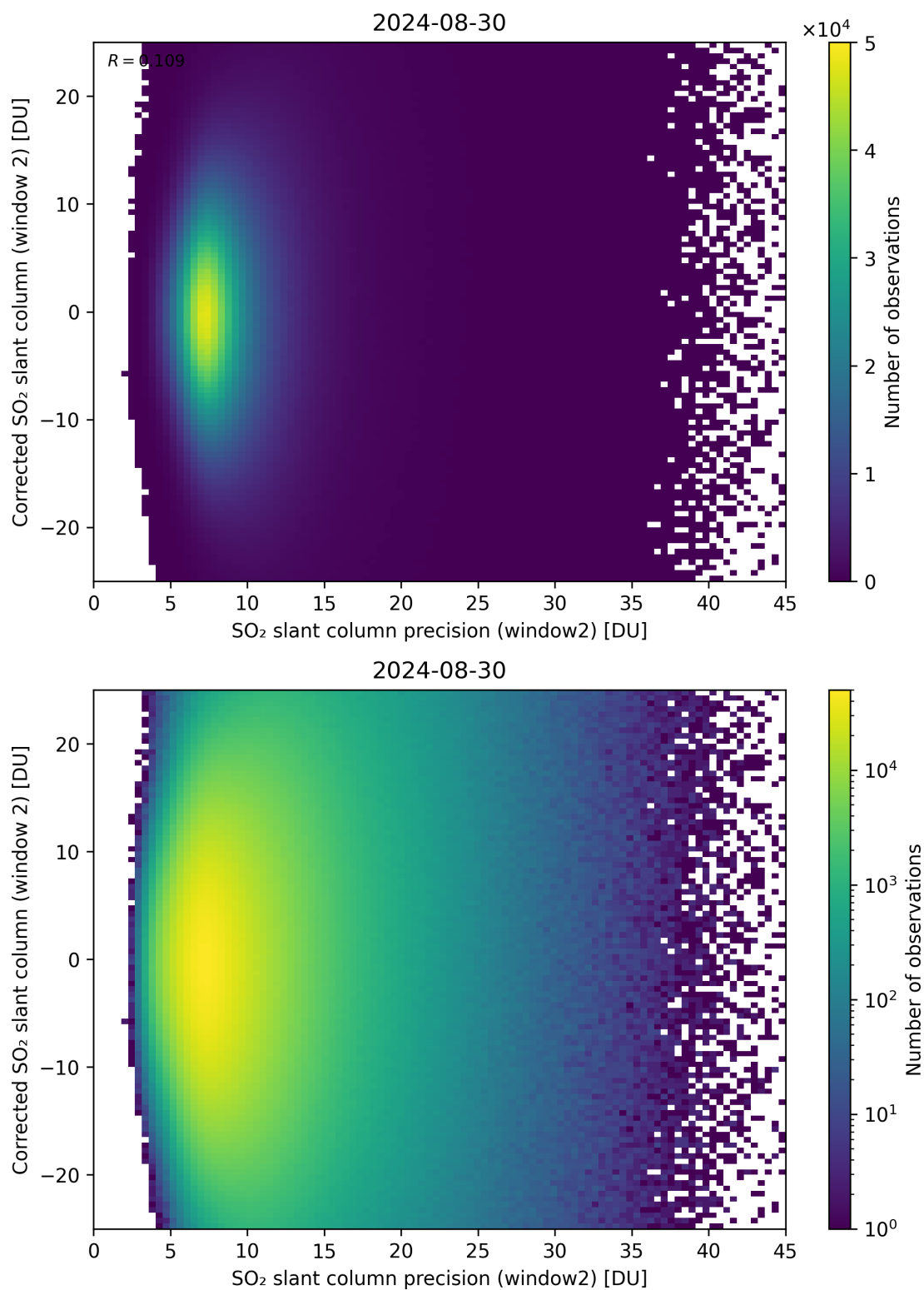
Figure 247: Scatter density plot of “SO 2 slant column precision (window2)” against “Corrected SO 2 slant column (window 2)” for 2024-08-29 to 2024-08-31.
