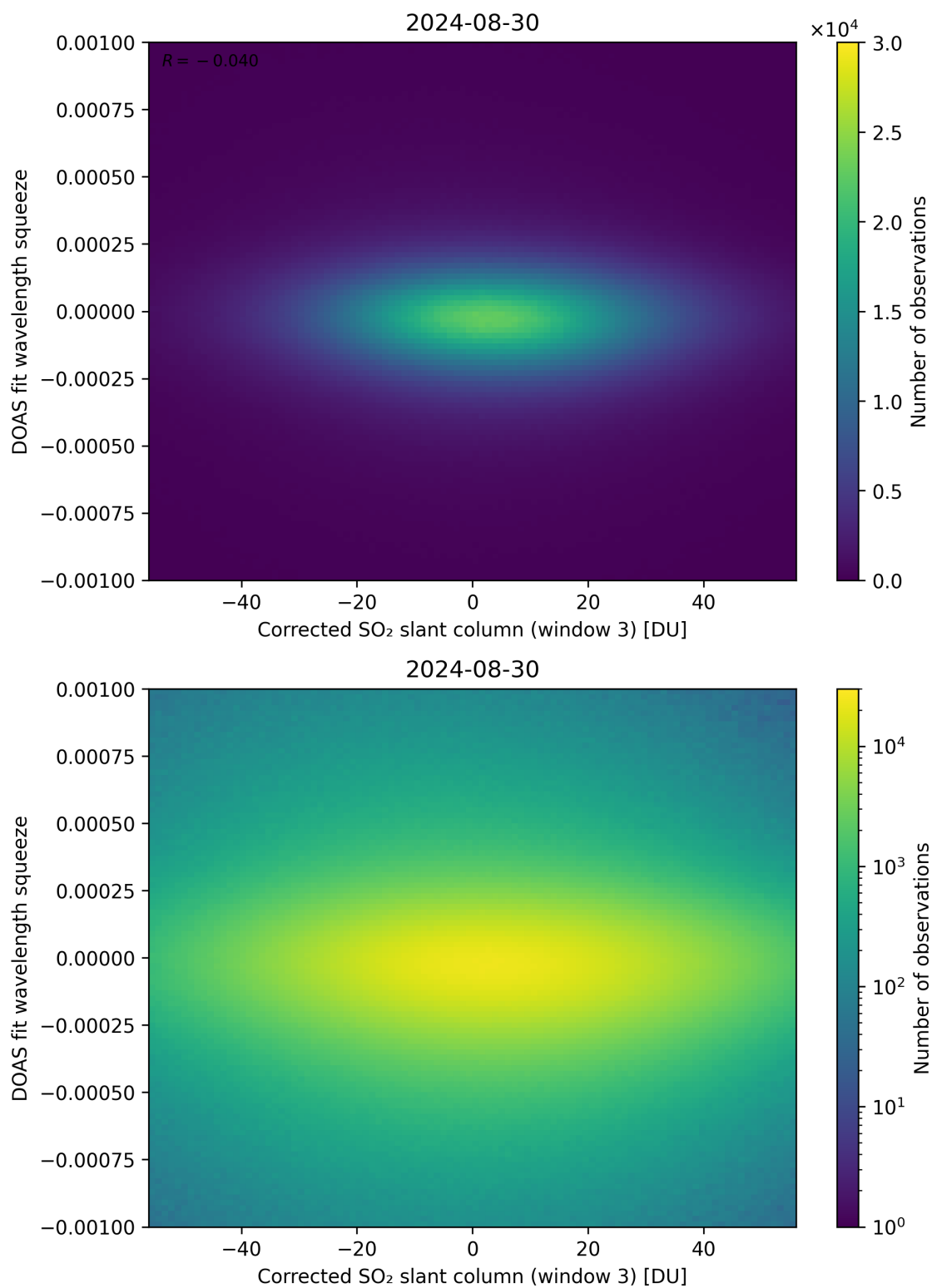
Figure 207: Scatter density plot of “Corrected SO 2 slant column (window 3)” against “DOAS fit wavelength squeeze” for 2024-08-29 to 2024-08-31.
