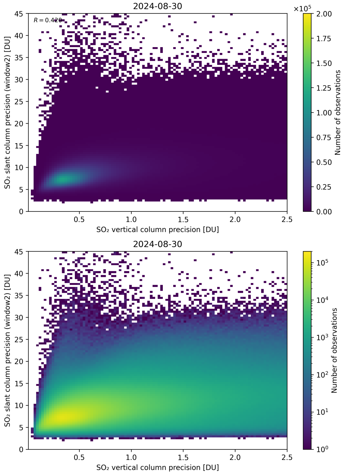
Figure 291: Scatter density plot of “SO 2 vertical column precision” against “SO 2 slant column precision (window2)” for 2024-08-29 to 2024-08-31.
