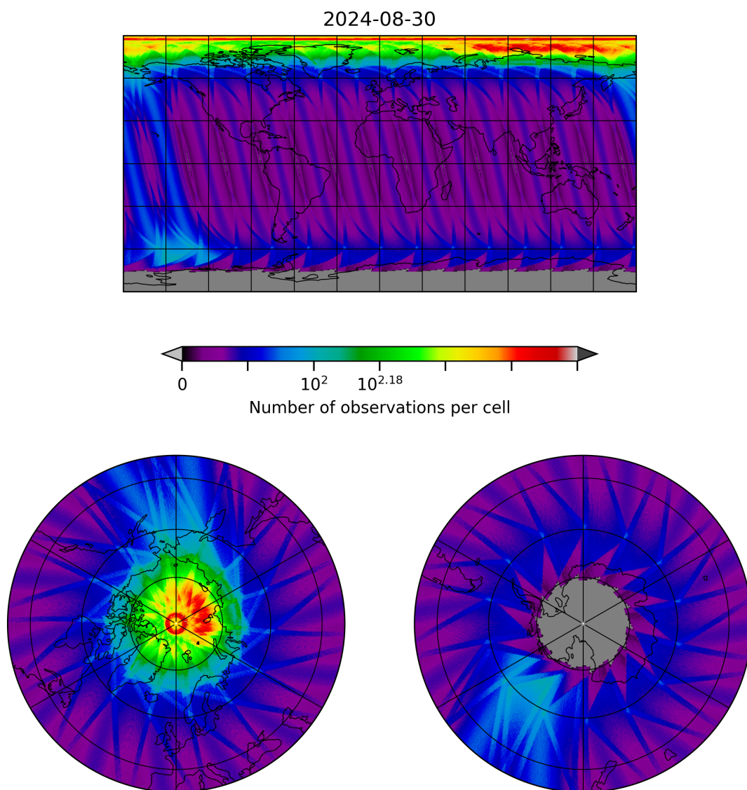
Figure 28: Map of the number of observations for 2024-08-29 to 2024-08-31
