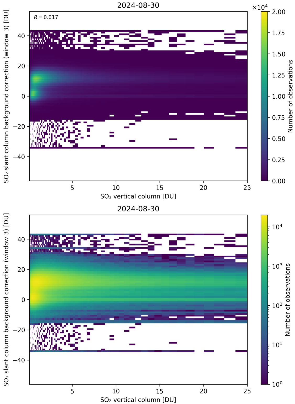
Figure 275: Scatter density plot of “SO 2 vertical column” against “SO 2 slant column background correction (window 3)” for 2024-08-29 to 2024-08-31.
