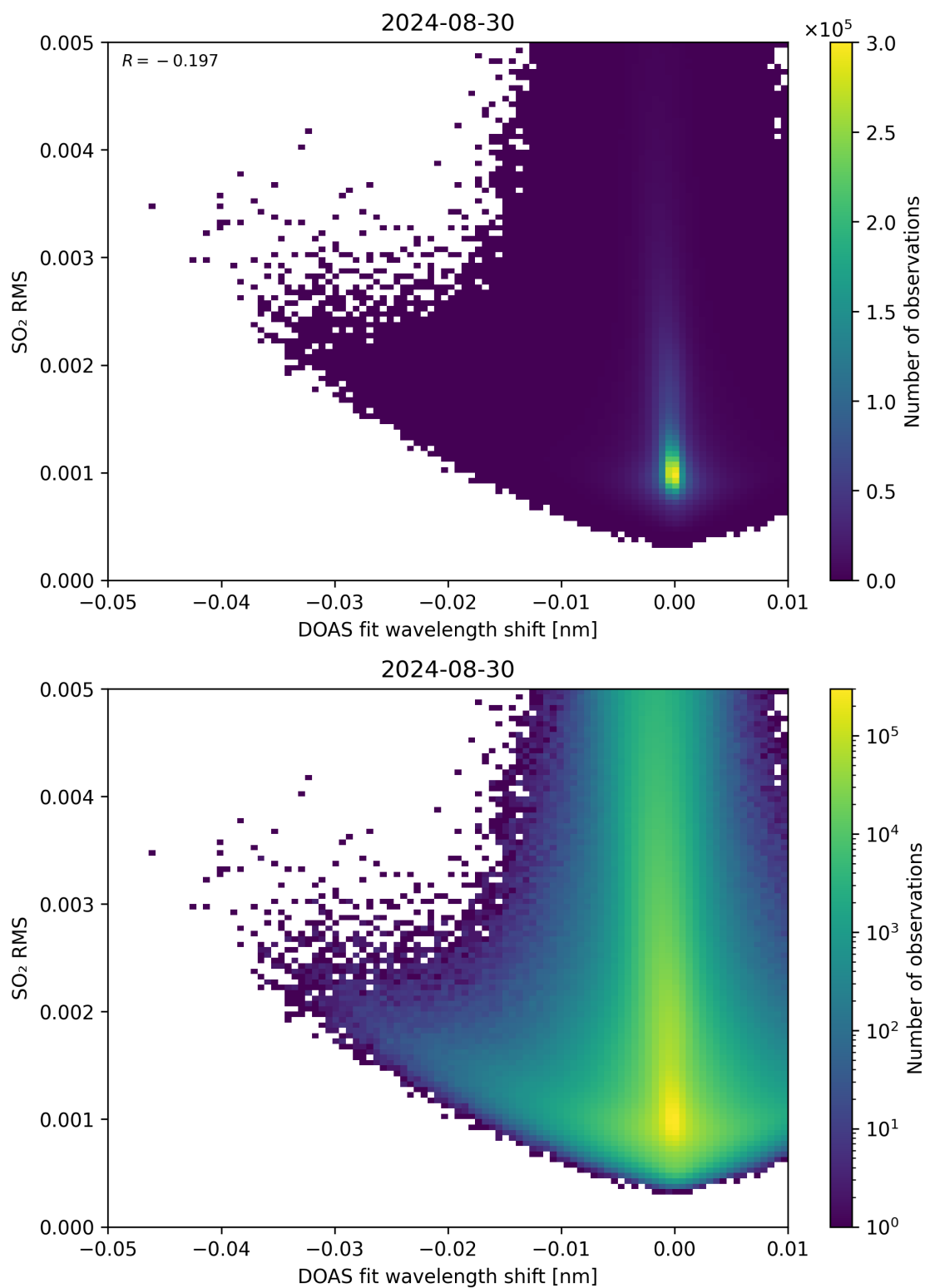
Figure 128: Scatter density plot of “DOAS fit wavelength shift” against “SO 2 RMS” for 2024-08-29 to 2024-08-31.
