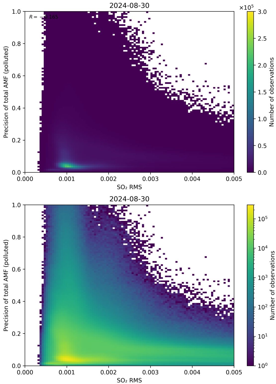
Figure 138: Scatter density plot of “SO 2 RMS” against “Precision of total AMF (polluted)” for 2024-08-29 to 2024-08-31.
