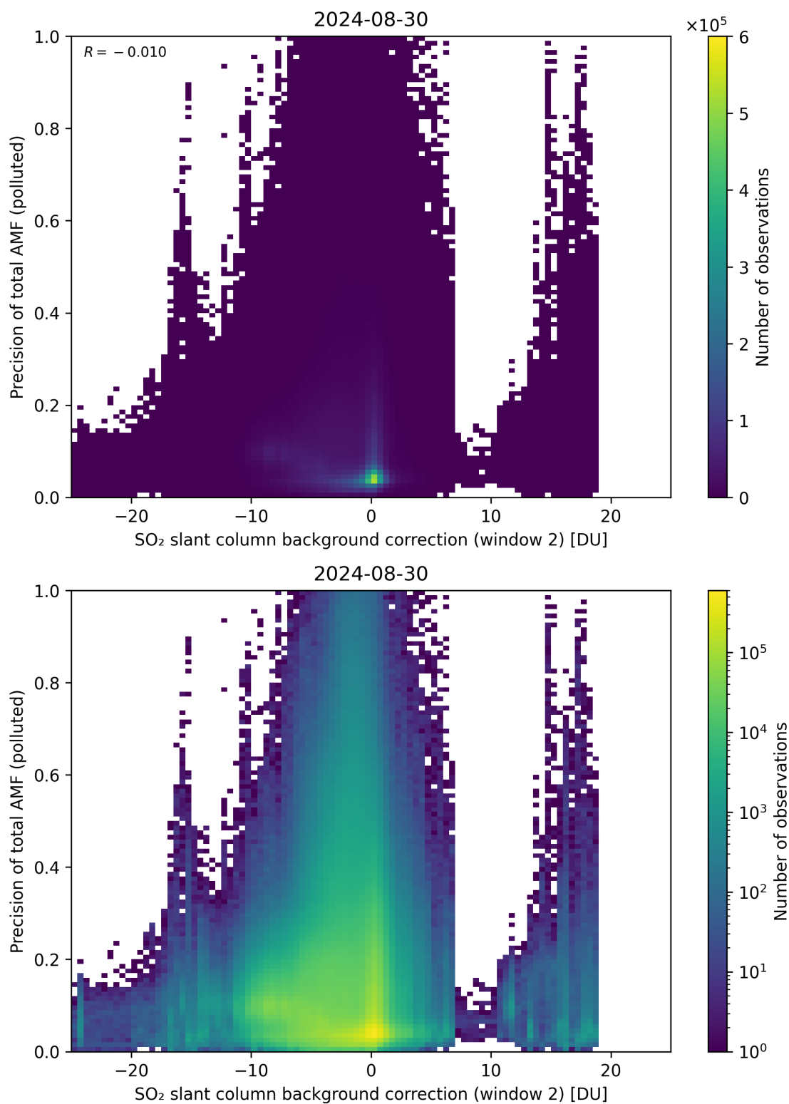
Figure 120: Scatter density plot of “SO 2 slant column background correction (window 2)” against “Precision of total AMF (polluted)” for 2024-08-29 to 2024-08-31.
