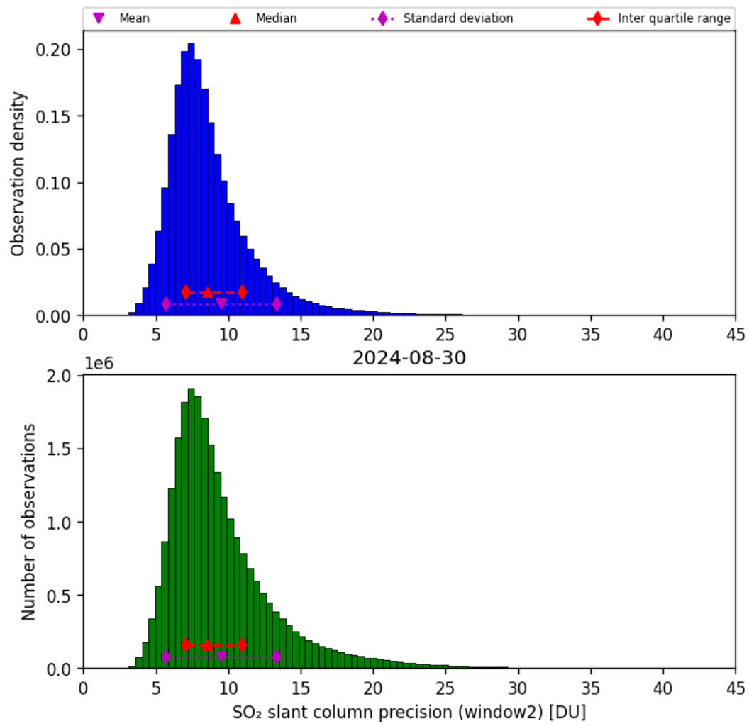
Figure 61: Histogram of “SO 2 slant column precision (window2)” for 2024-08-29 to 2024-08-31
