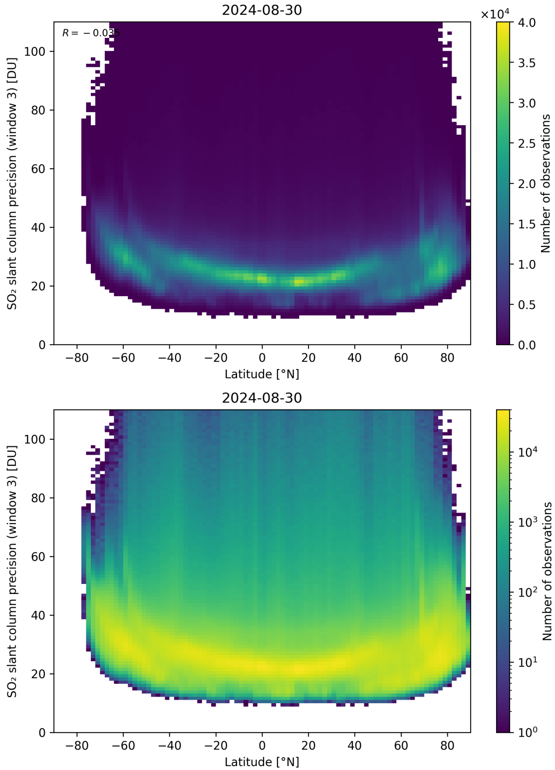
Figure 153: Scatter density plot of “Latitude” against “SO 2 slant column precision (window 3)” for 2024-08-29 to 2024-08-31.
