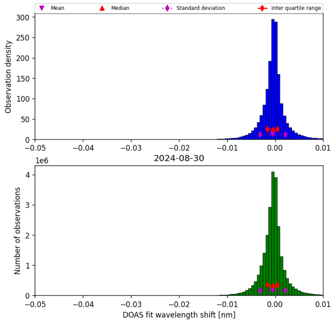
Figure 68: Histogram of “DOAS fit wavelength shift” for 2024-08-29 to 2024-08-31
