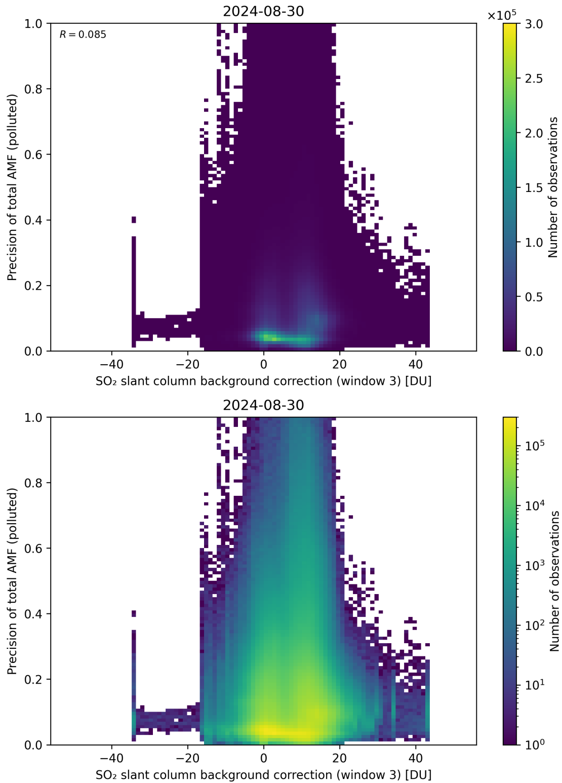
Figure 126: Scatter density plot of “SO 2 slant column background correction (window 3)” against “Precision of total AMF (polluted)” for 2024-08-29 to 2024-08-31.
