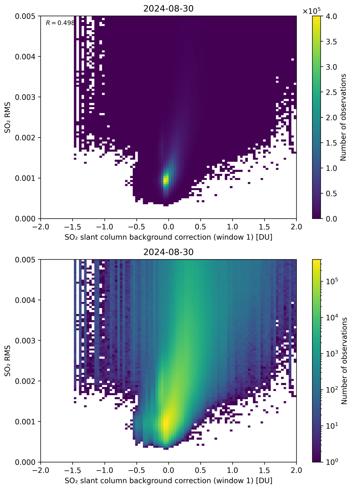
Figure 102: Scatter density plot of “SO 2 slant column background correction (window 1)” against “SO 2 RMS” for 2024-08-29 to 2024-08-31.
