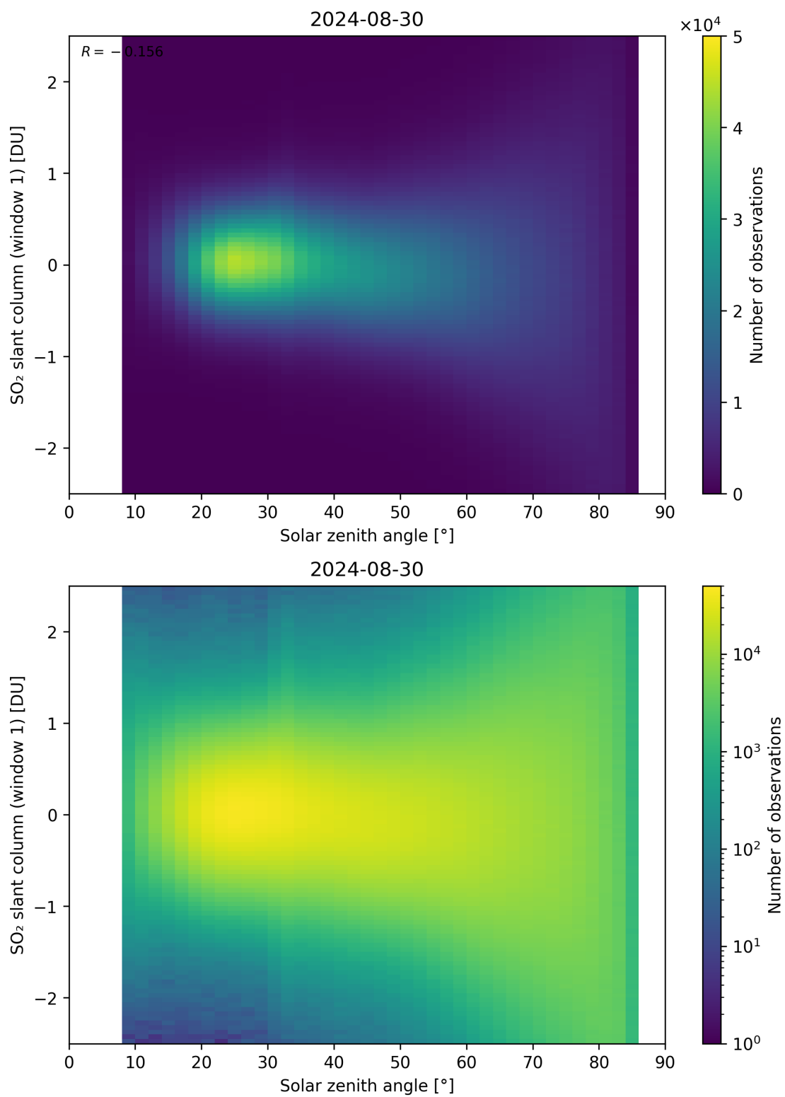
Figure 169: Scatter density plot of “Solar zenith angle” against “SO 2 slant column (window 1)” for 2024-08-29 to 2024-08-31.
