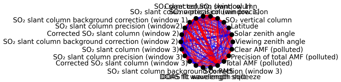
Figure 1: Map of correlation graph for 2024-08-29 to 2024-08-31.
