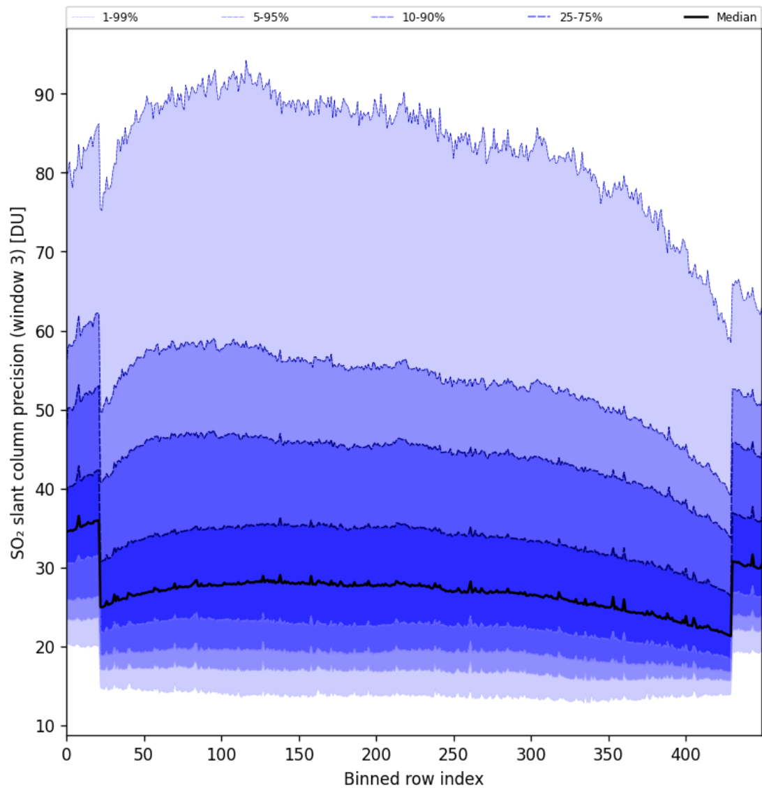
Figure 88: Along track statistics of “SO 2 slant column precision (window 3)” for 2024-08-29 to 2024-08-31
