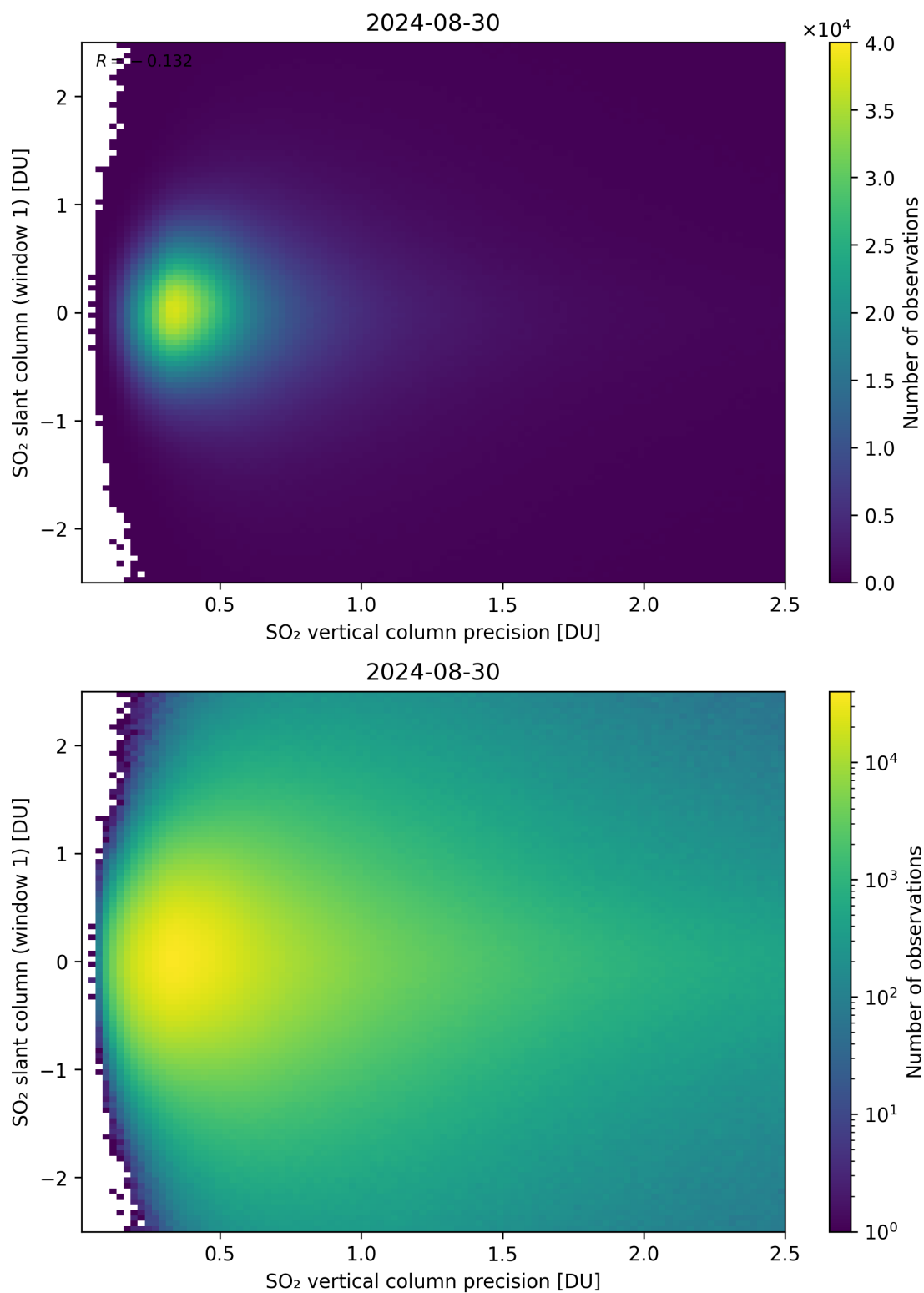
Figure 289: Scatter density plot of “SO 2 vertical column precision” against “SO 2 slant column (window 1)” for 2024-08-29 to 2024-08-31.
