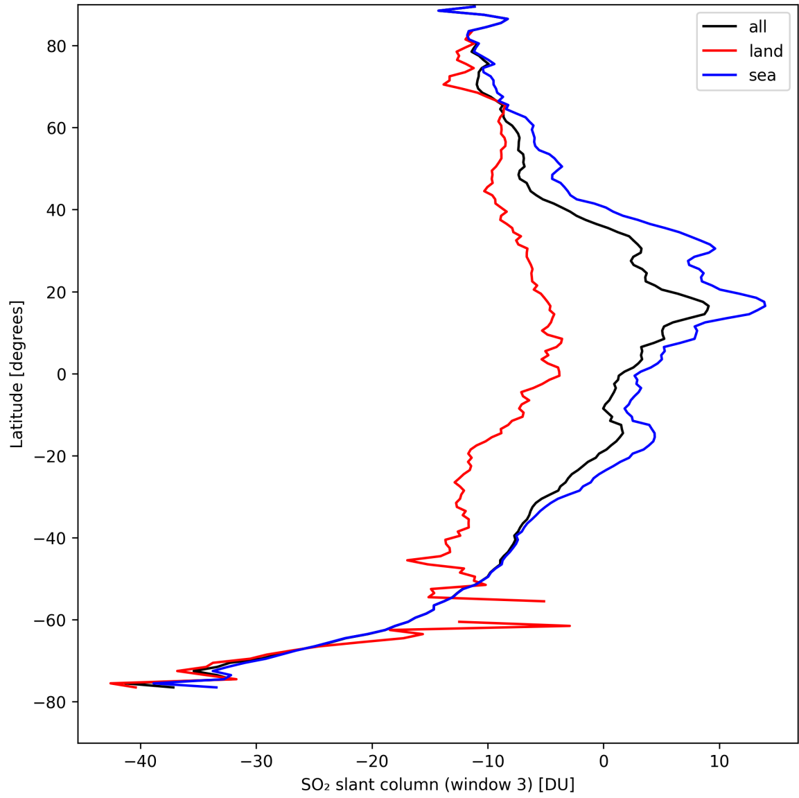
Figure 41: Zonal average of “SO 2 slant column (window 3)” for 2024-08-29 to 2024-08-31.
