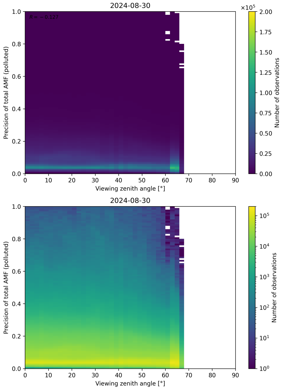
Figure 326: Scatter density plot of “Viewing zenith angle” against “Precision of total AMF (polluted)” for 2024-08-29 to 2024-08-31.
