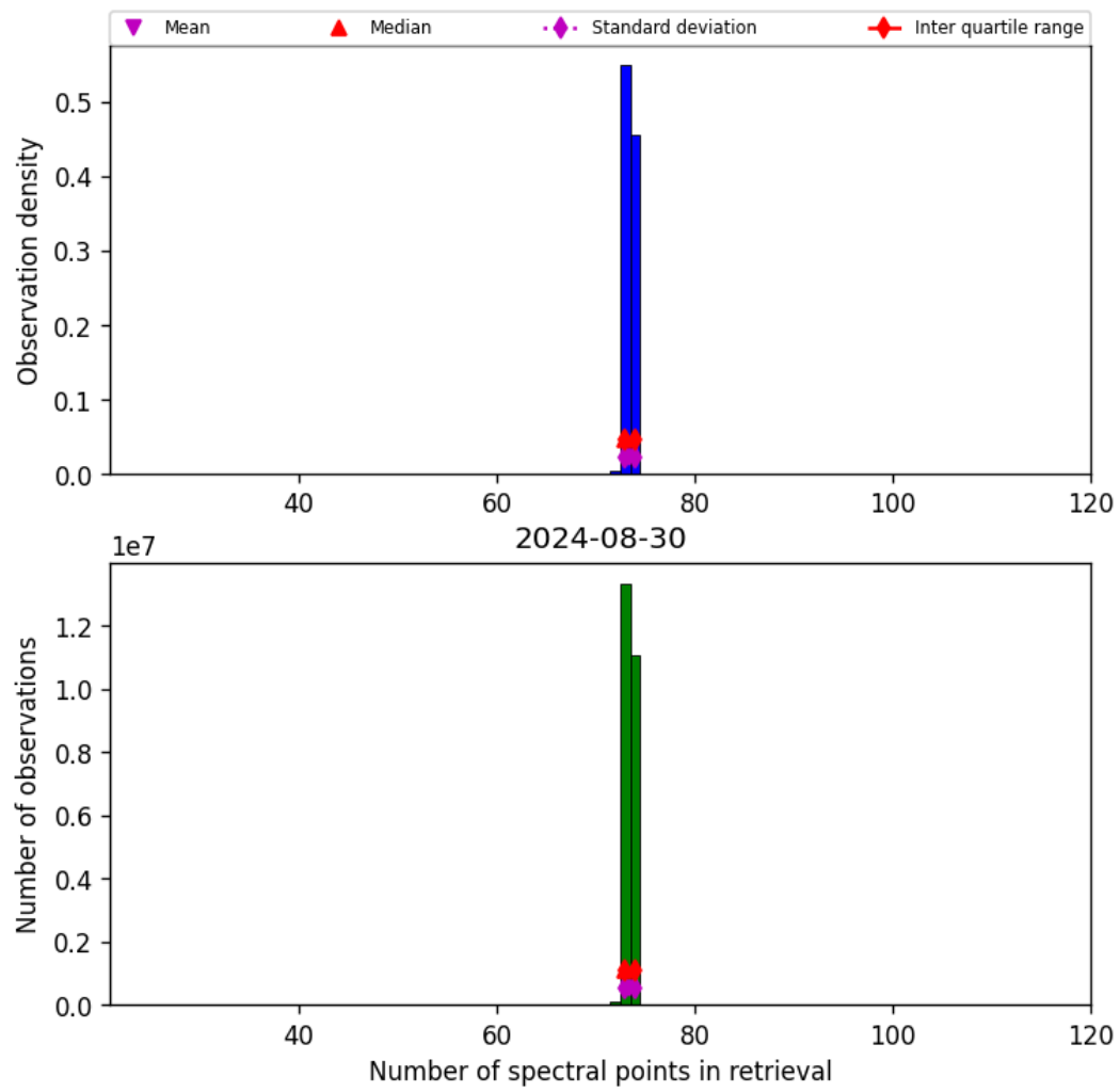
Figure 74: Histogram of “Number of spectral points in retrieval” for 2024-08-29 to 2024-08-31
