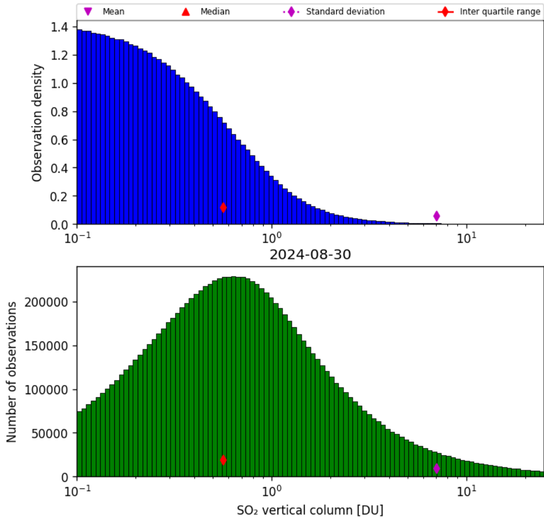
Figure 53: Histogram of “SO 2 vertical column” for 2024-08-29 to 2024-08-31
