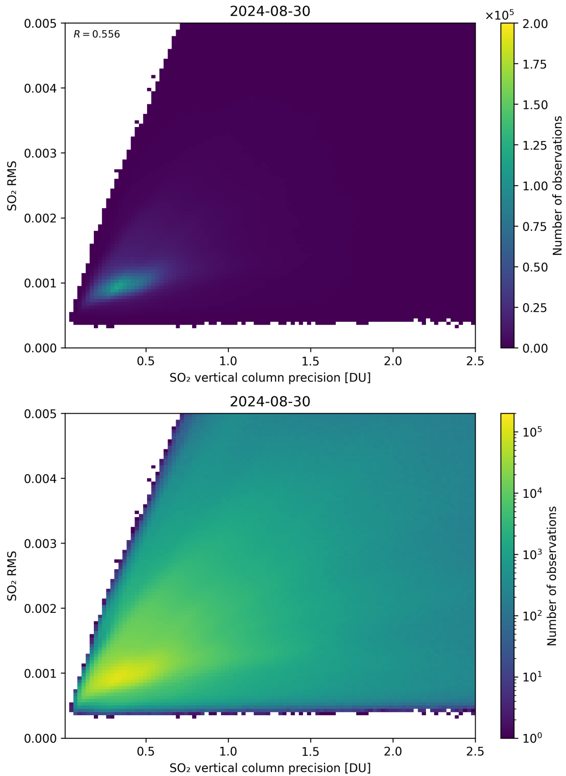
Figure 284: Scatter density plot of “SO 2 vertical column precision” against “SO 2 RMS” for 2024-08-29 to 2024-08-31.
