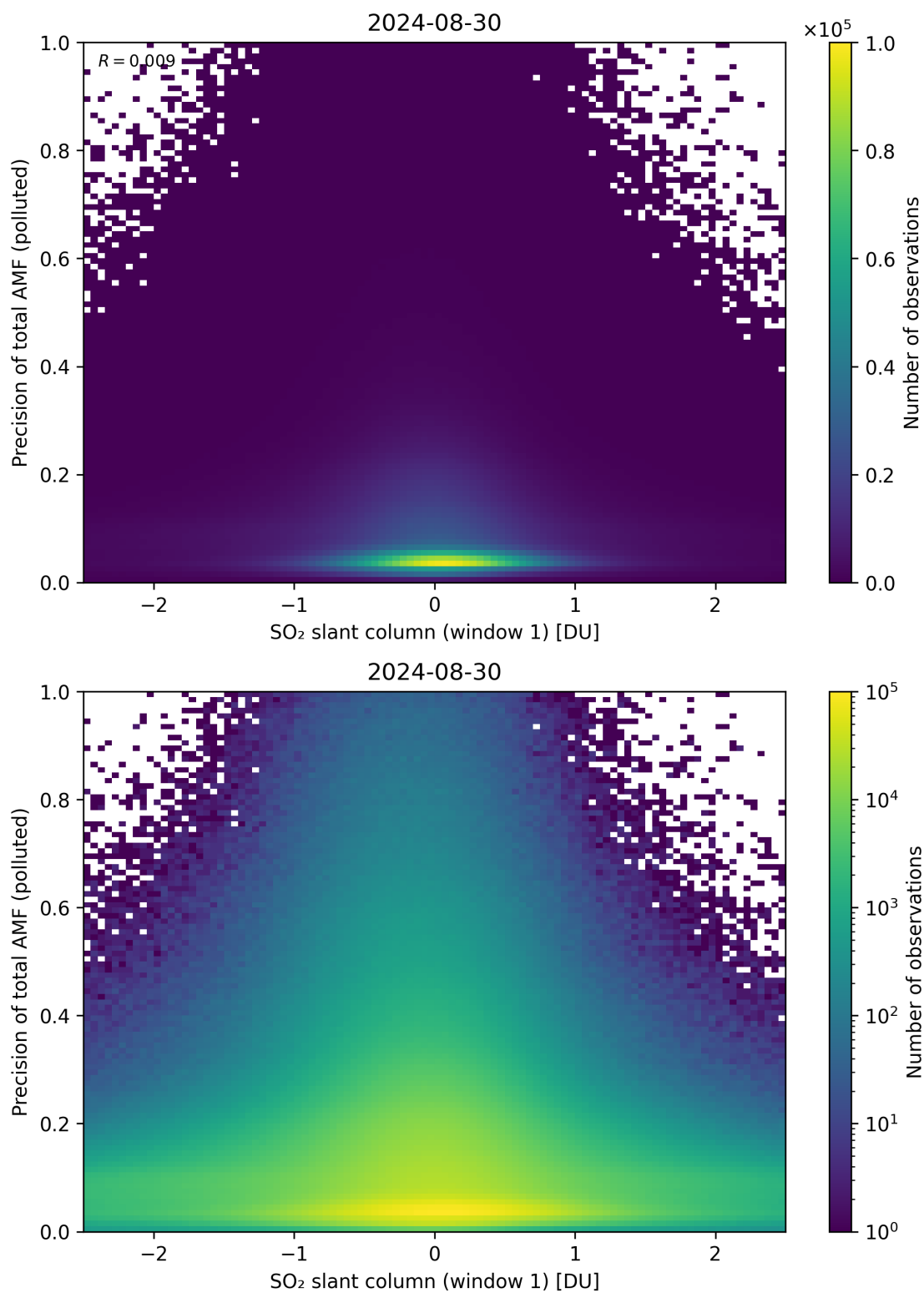
Figure 240: Scatter density plot of “SO 2 slant column (window 1)” against “Precision of total AMF (polluted)” for 2024-08-29 to 2024-08-31.
