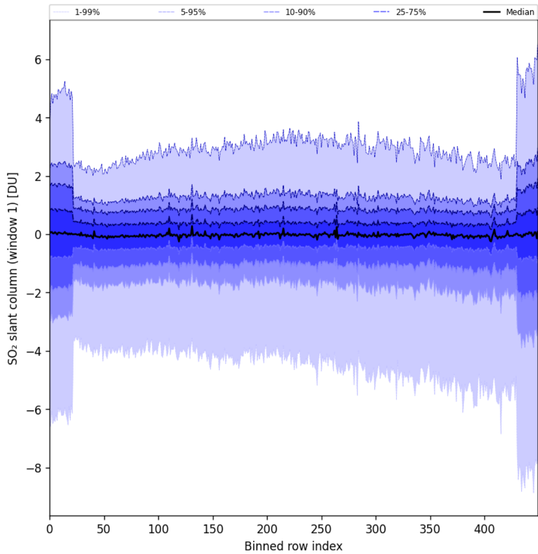
Figure 79: Along track statistics of “SO 2 slant column (window 1)” for 2024-08-29 to 2024-08-31
