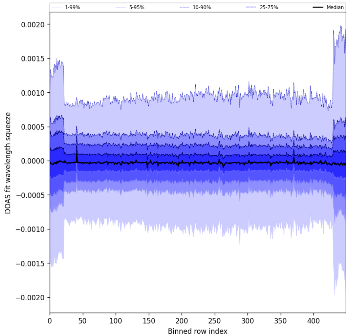
Figure 92: Along track statistics of “DOAS fit wavelength squeeze” for 2024-08-29 to 2024-08-31
