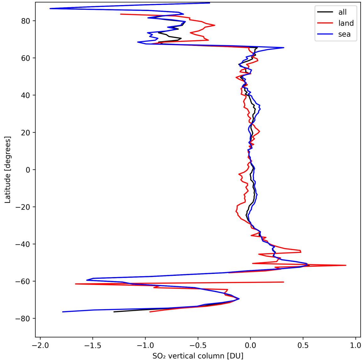
Figure 30: Zonal average of “SO 2 vertical column” for 2024-08-29 to 2024-08-31.
