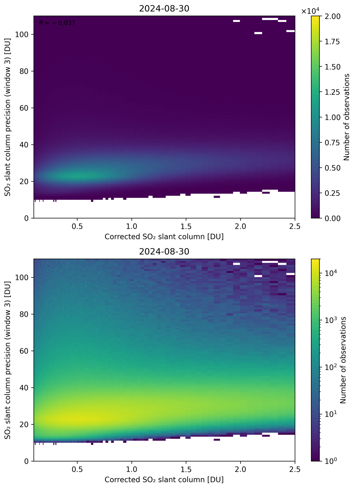
Figure 191: Scatter density plot of “Corrected SO 2 slant column” against “SO 2 slant column precision (window 3)” for 2024-08-29 to 2024-08-31.
