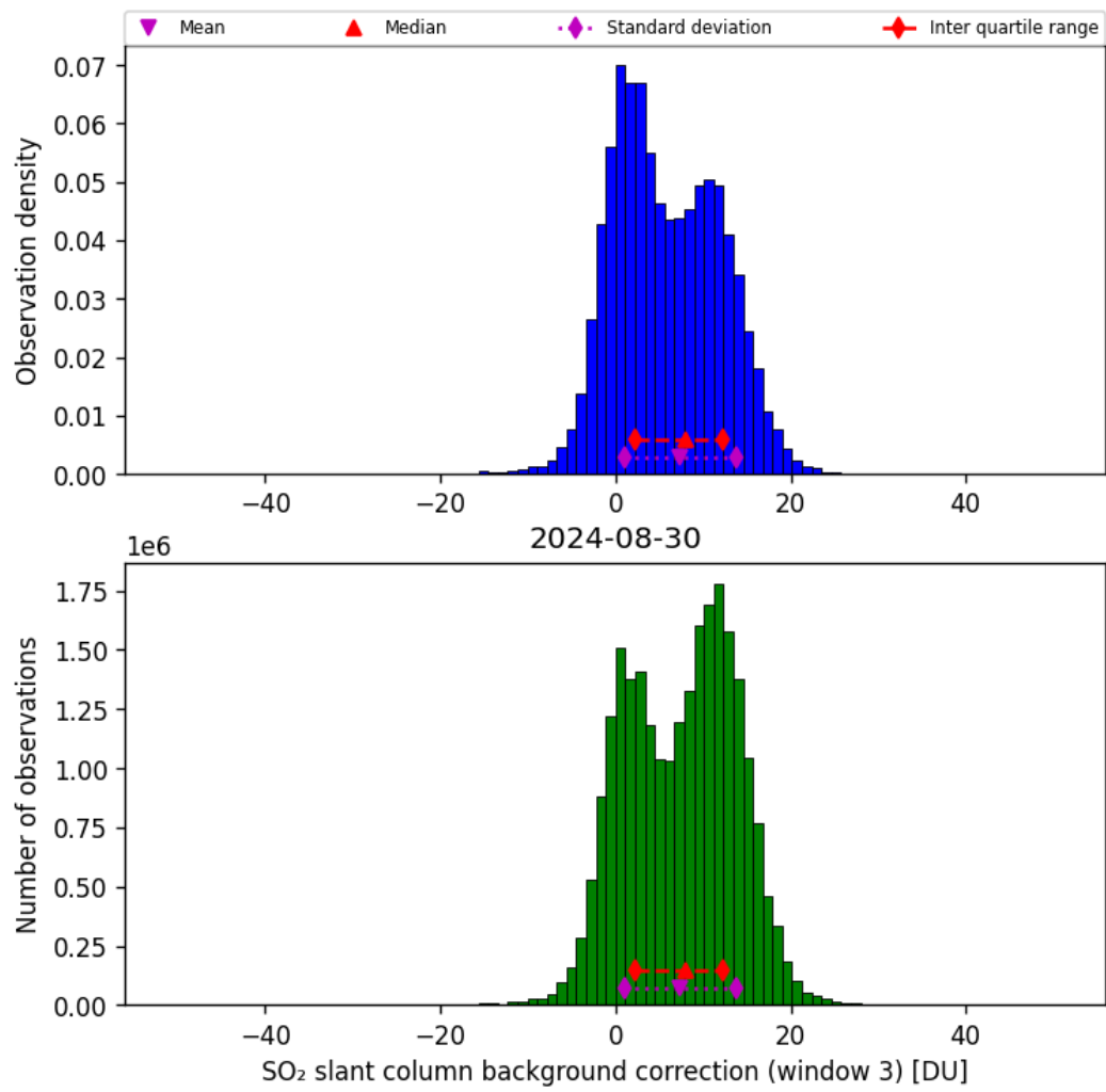
Figure 67: Histogram of “SO 2 slant column background correction (window 3)” for 2024-08-29 to 2024-08-31
