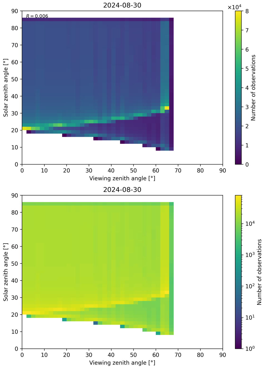
Figure 315: Scatter density plot of “Viewing zenith angle” against “Solar zenith angle” for 2024-08-29 to 2024-08-31.
