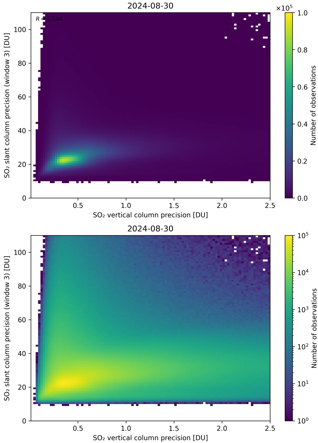
Figure 293: Scatter density plot of “SO 2 vertical column precision” against “SO 2 slant column precision (window 3)” for 2024-08-29 to 2024-08-31.
