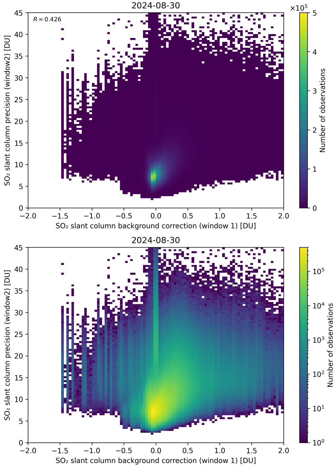
Figure 106: Scatter density plot of “SO 2 slant column background correction (window 1)” against “SO 2 slant column precision (window2)” for 2024-08-29 to 2024-08-31.
