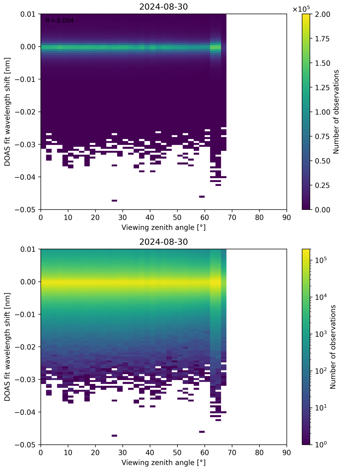
Figure 311: Scatter density plot of “Viewing zenith angle” against “DOAS fit wavelength shift” for 2024-08-29 to 2024-08-31.
