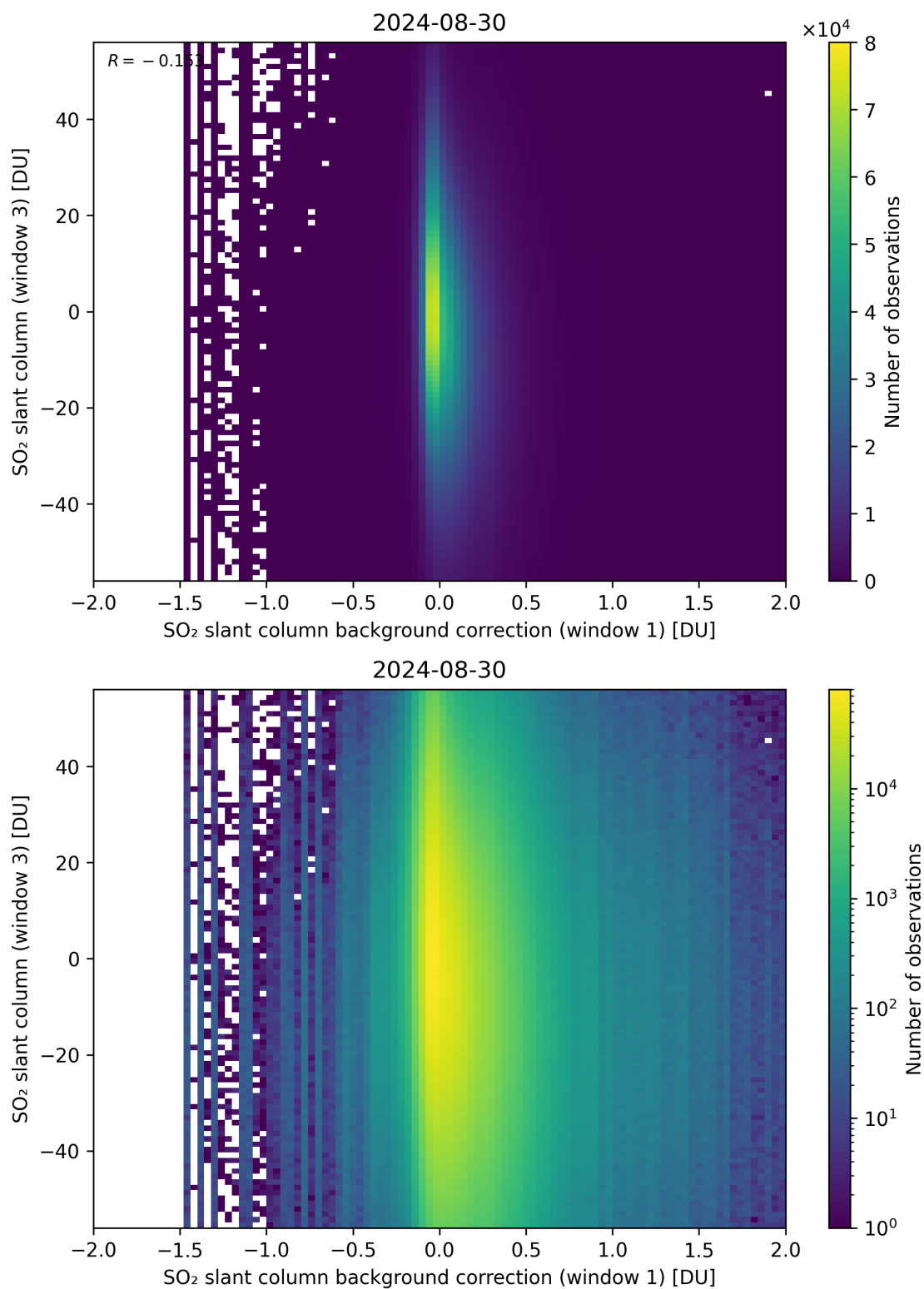
Figure 107: Scatter density plot of “SO 2 slant column background correction (window 1)” against “SO 2 slant column (window 3)” for 2024-08-29 to 2024-08-31.
