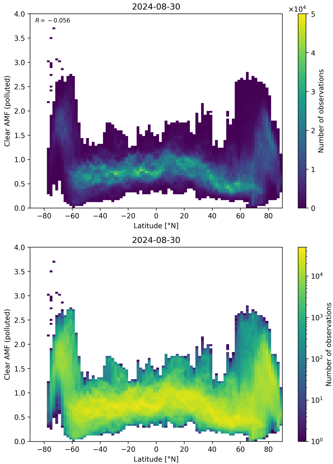
Figure 145: Scatter density plot of “Latitude” against “Clear AMF (polluted)” for 2024-08-29 to 2024-08-31.
