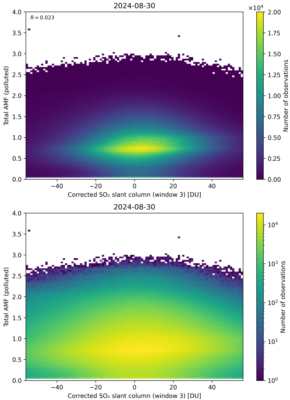
Figure 210: Scatter density plot of “Corrected SO 2 slant column (window 3)” against “Total AMF (polluted)” for 2024-08-29 to 2024-08-31.
