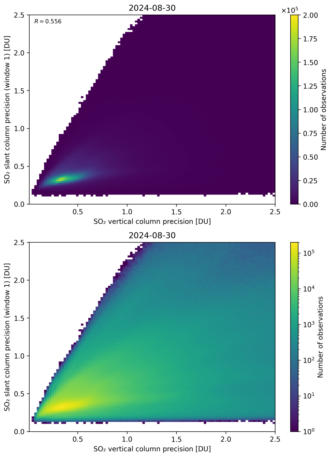
Figure 290: Scatter density plot of “SO 2 vertical column precision” against “SO 2 slant column precision (window 1)” for 2024-08-29 to 2024-08-31.
