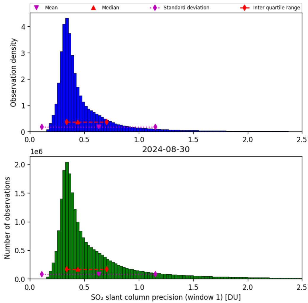
Figure 57: Histogram of “SO 2 slant column precision (window 1)” for 2024-08-29 to 2024-08-31
