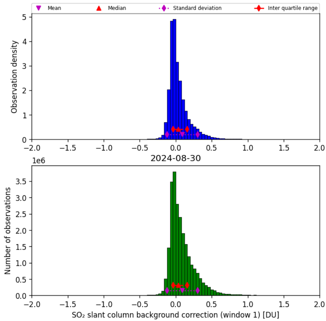
Figure 59: Histogram of “SO 2 slant column background correction (window 1)” for 2024-08-29 to 2024-08-31
