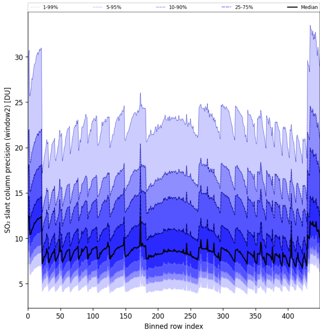
Figure 84: Along track statistics of “SO 2 slant column precision (window2)” for 2024-08-29 to 2024-08-31
