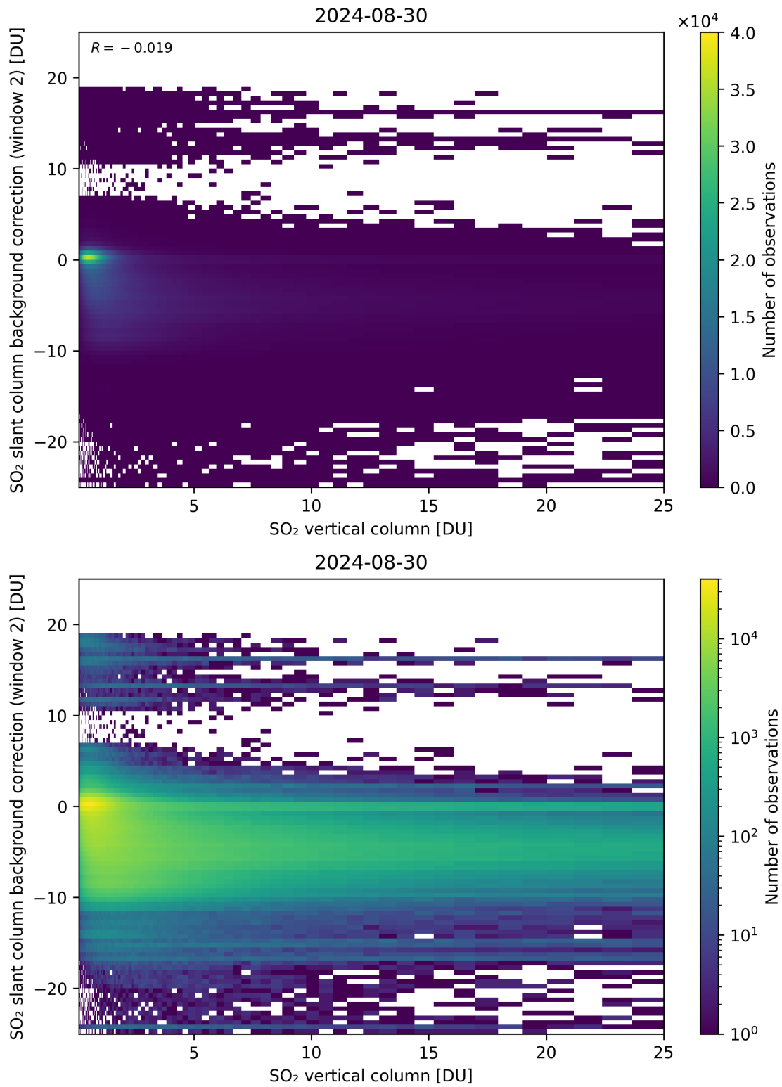
Figure 274: Scatter density plot of “SO 2 vertical column” against “SO 2 slant column background correction (window 2)” for 2024-08-29 to 2024-08-31.
