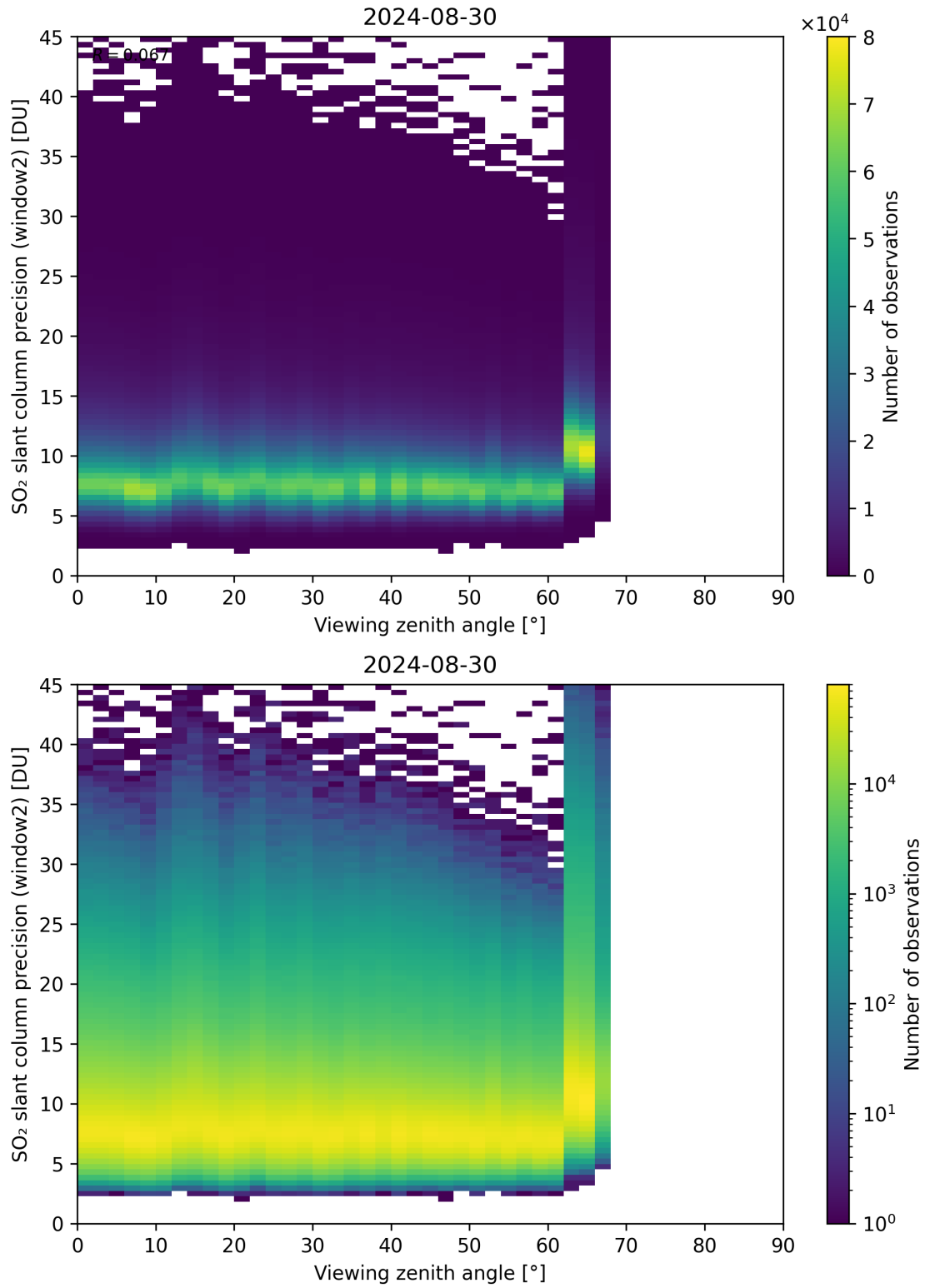
Figure 322: Scatter density plot of “Viewing zenith angle” against “SO 2 slant column precision (window2)” for 2024-08-29 to 2024-08-31.
