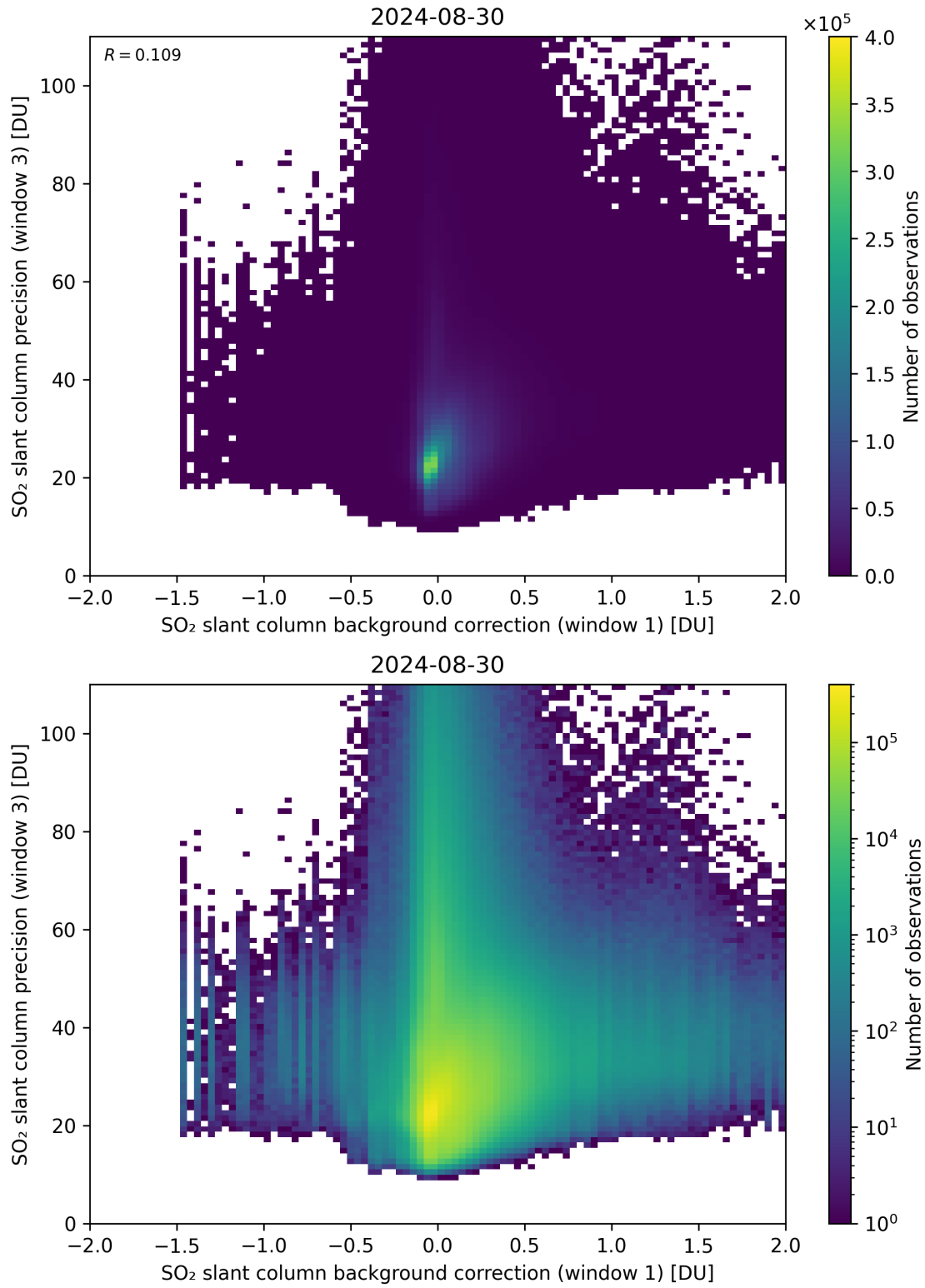
Figure 108: Scatter density plot of “SO 2 slant column background correction (window 1)” against “SO 2 slant column precision (window 3)” for 2024-08-29 to 2024-08-31.
