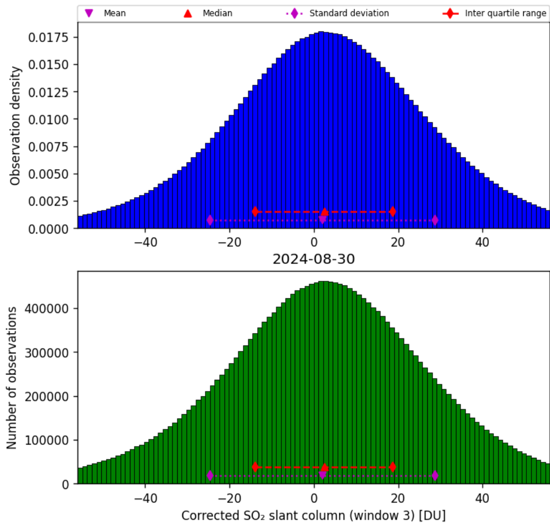
Figure 66: Histogram of “Corrected SO 2 slant column (window 3)” for 2024-08-29 to 2024-08-31
