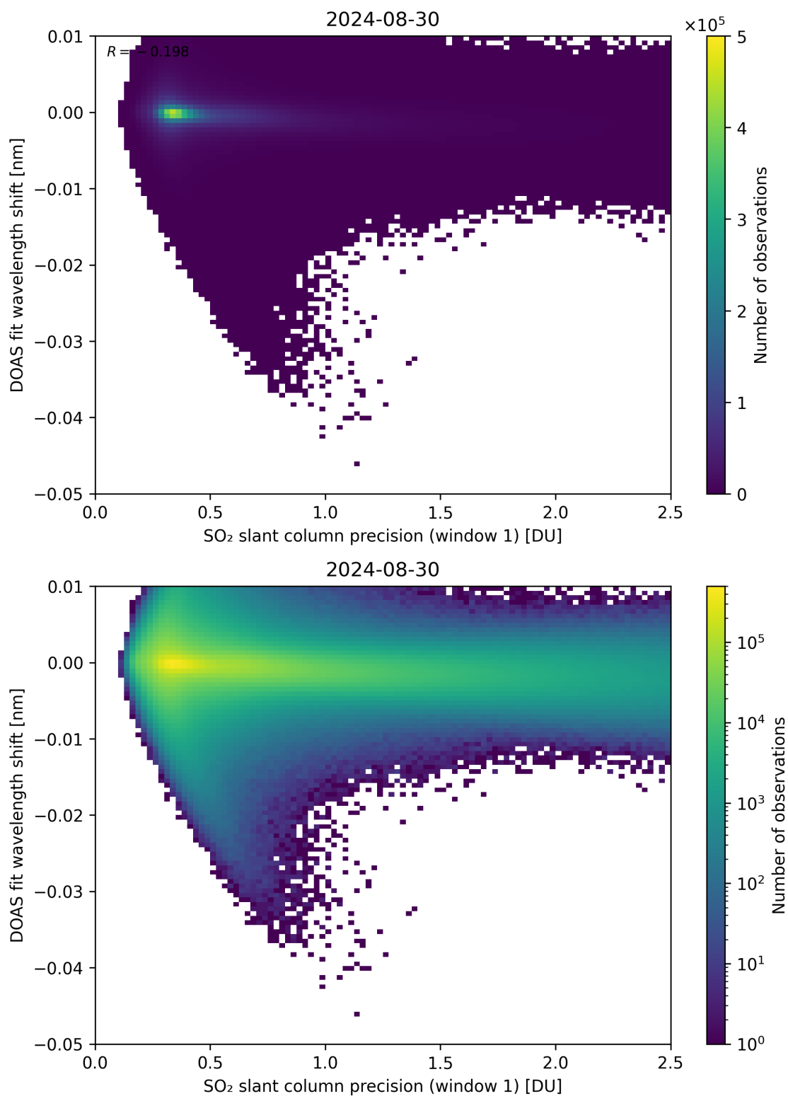
Figure 221: Scatter density plot of “SO 2 slant column precision (window 1)” against “DOAS fit wavelength shift” for 2024-08-29 to 2024-08-31.
