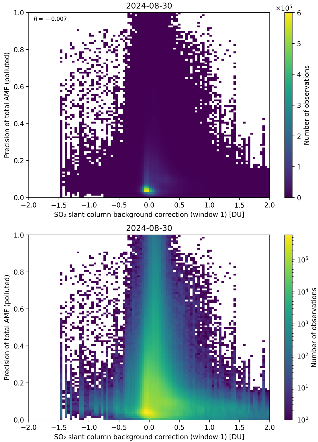
Figure 110: Scatter density plot of “SO 2 slant column background correction (window 1)” against “Precision of total AMF (polluted)” for 2024-08-29 to 2024-08-31.
