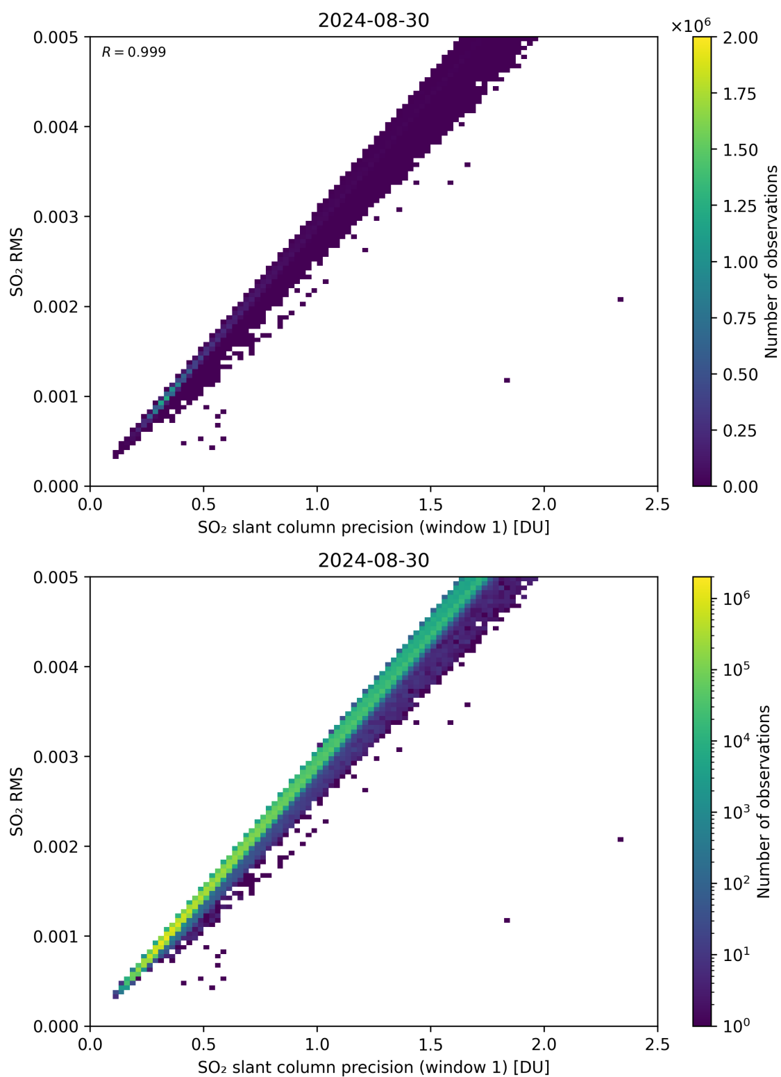
Figure 223: Scatter density plot of “SO 2 slant column precision (window 1)” against “SO 2 RMS” for 2024-08-29 to 2024-08-31.
