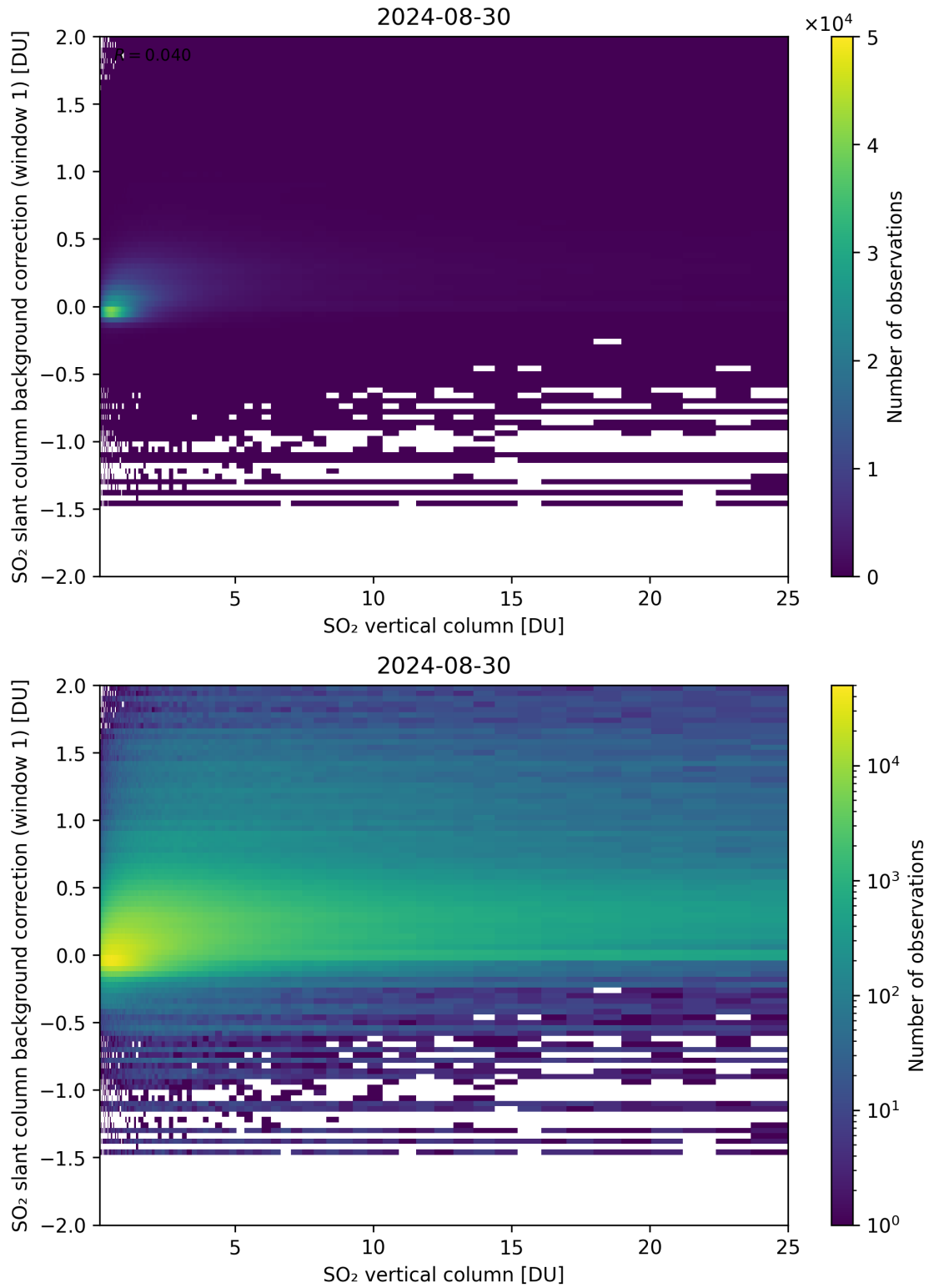
Figure 273: Scatter density plot of “SO 2 vertical column” against “SO 2 slant column background correction (window 1)” for 2024-08-29 to 2024-08-31.
