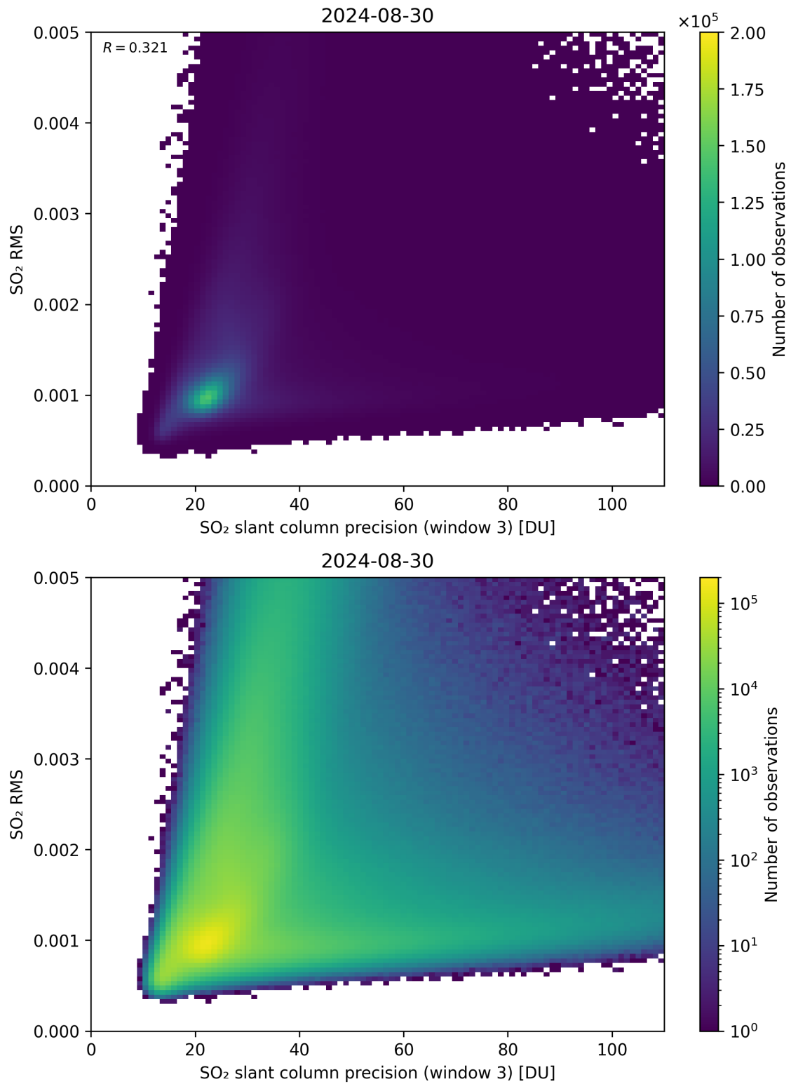
Figure 260: Scatter density plot of “SO 2 slant column precision (window 3)” against “SO 2 RMS” for 2024-08-29 to 2024-08-31.
