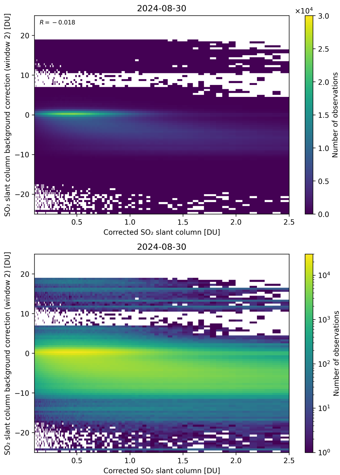
Figure 179: Scatter density plot of “Corrected SO 2 slant column” against “SO 2 slant column background correction (window 2)” for 2024-08-29 to 2024-08-31.
