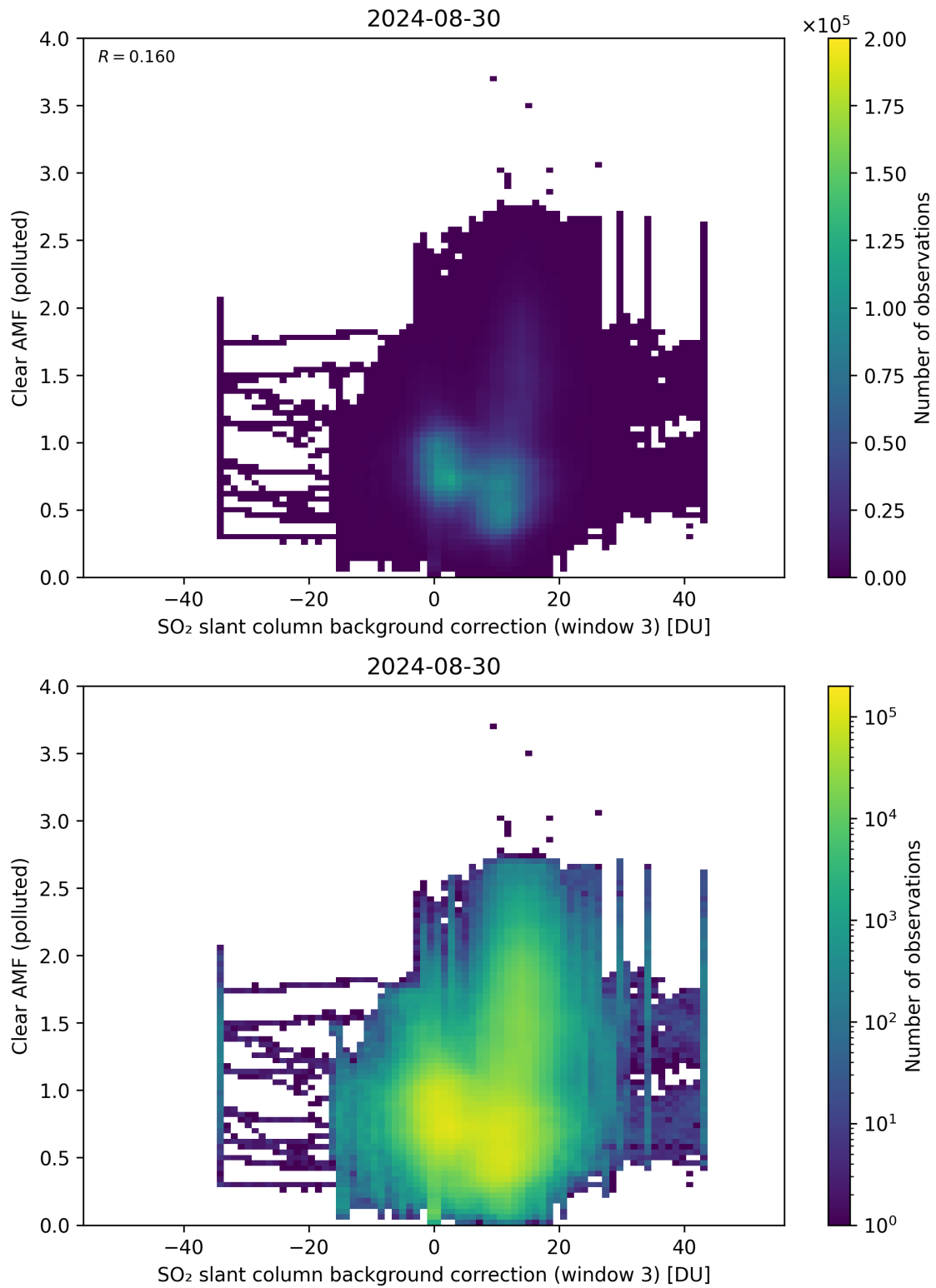
Figure 124: Scatter density plot of “SO 2 slant column background correction (window 3)” against “Clear AMF (polluted)” for 2024-08-29 to 2024-08-31.
