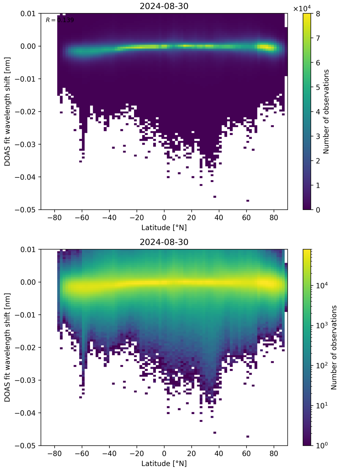
Figure 142: Scatter density plot of “Latitude” against “DOAS fit wavelength shift” for 2024-08-29 to 2024-08-31.
