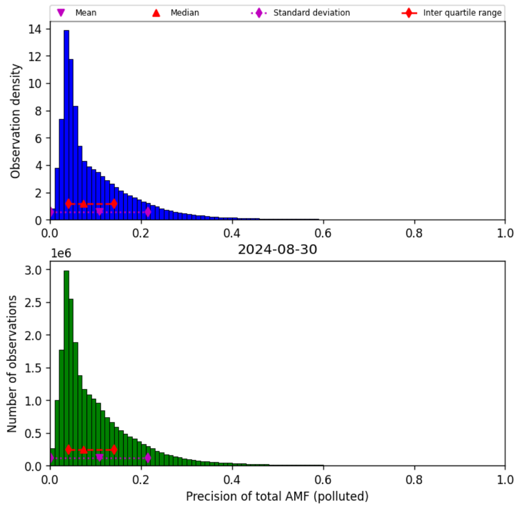
Figure 72: Histogram of “Precision of total AMF (polluted)” for 2024-08-29 to 2024-08-31
