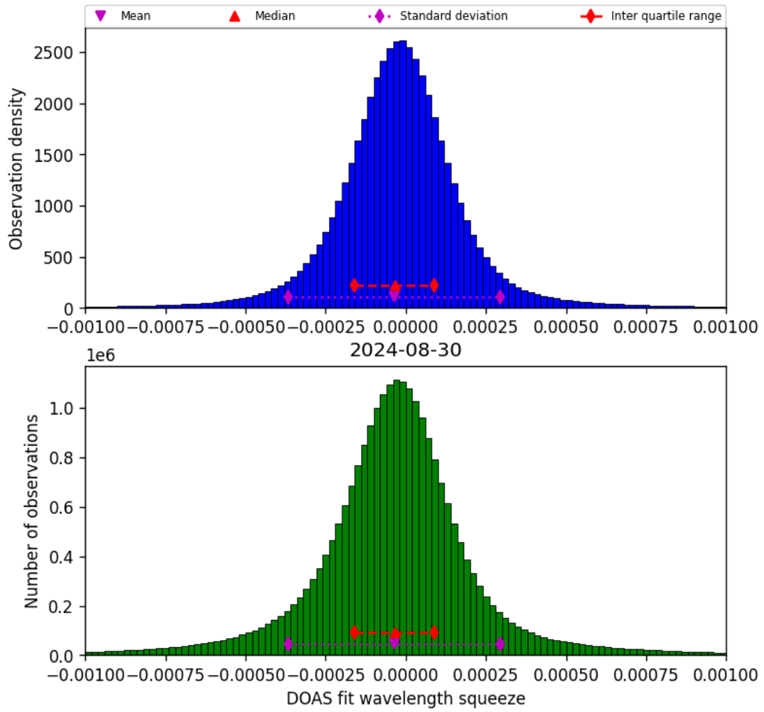
Figure 69: Histogram of “DOAS fit wavelength squeeze” for 2024-08-29 to 2024-08-31
