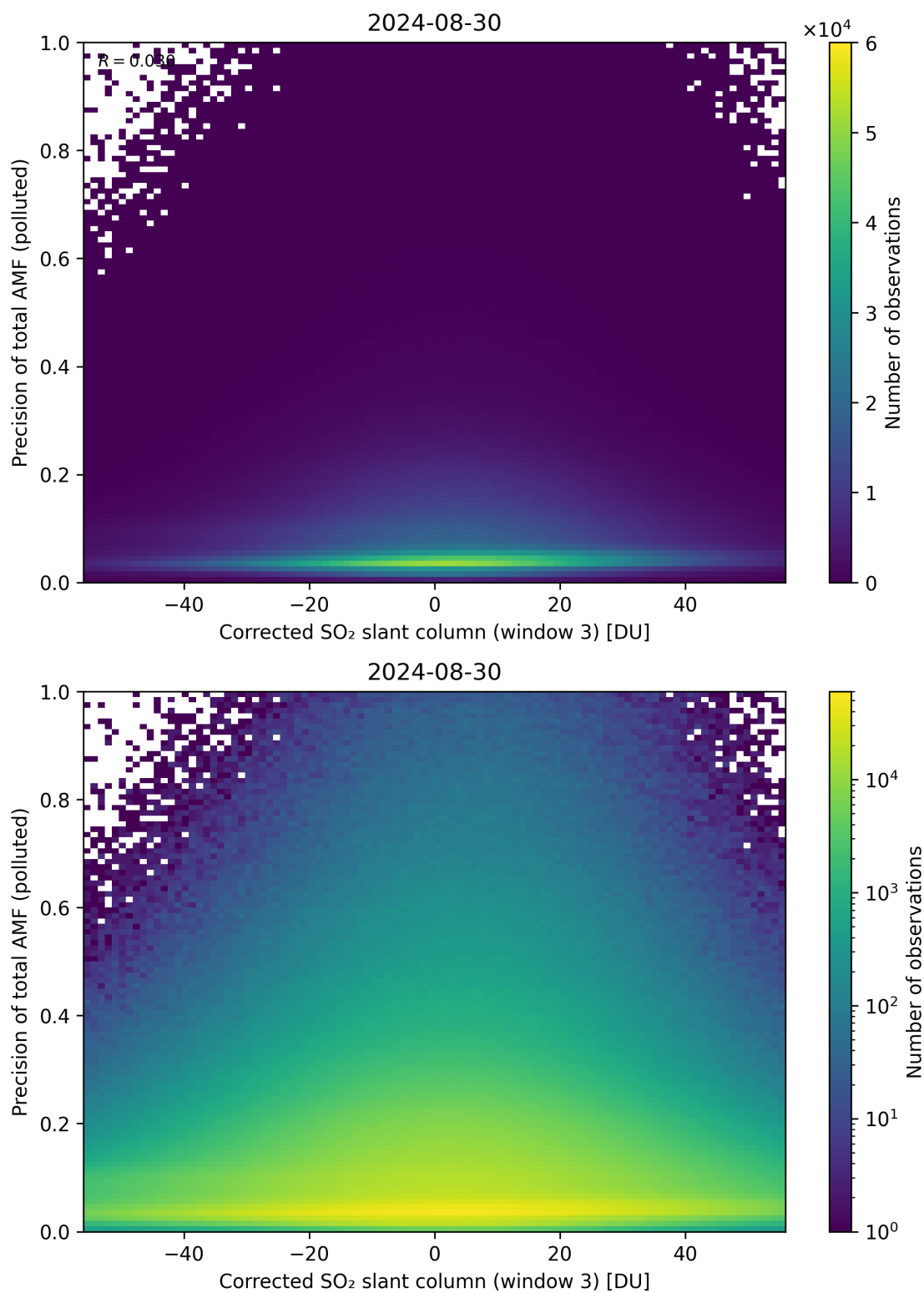
Figure 211: Scatter density plot of “Corrected SO 2 slant column (window 3)” against “Precision of total AMF (polluted)” for 2024-08-29 to 2024-08-31.
