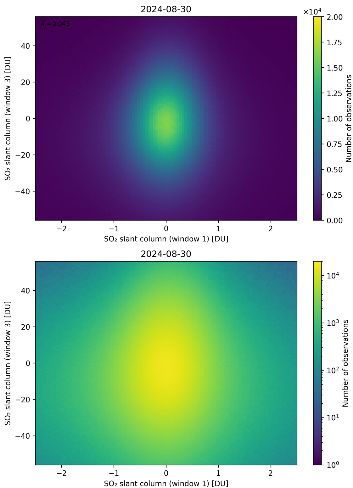
Figure 237: Scatter density plot of “SO 2 slant column (window 1)” against “SO 2 slant column (window 3)” for 2024-08-29 to 2024-08-31.
