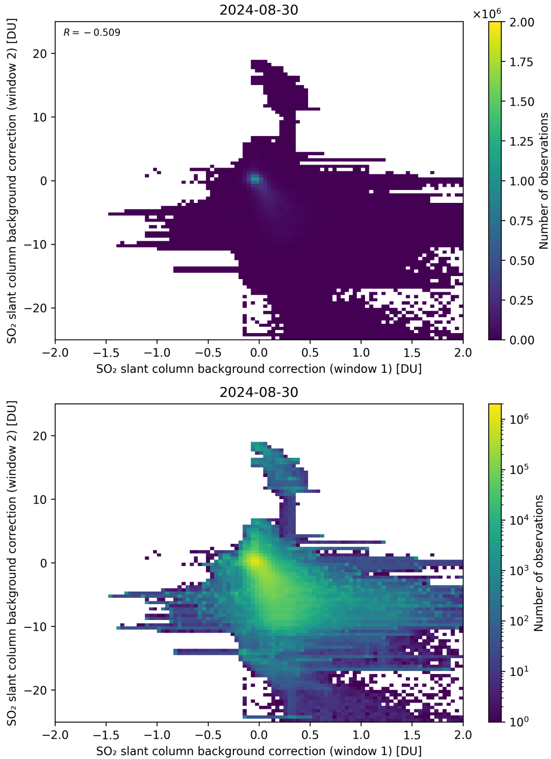
Figure 98: Scatter density plot of “SO 2 slant column background correction (window 1)” against “SO 2 slant column background correction (window 2)” for 2024-08-29 to 2024-08-31.
