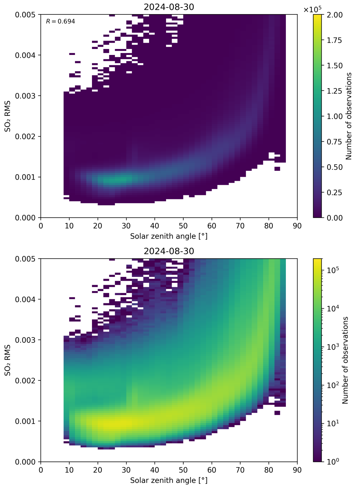
Figure 163: Scatter density plot of “Solar zenith angle” against “SO 2 RMS” for 2024-08-29 to 2024-08-31.
