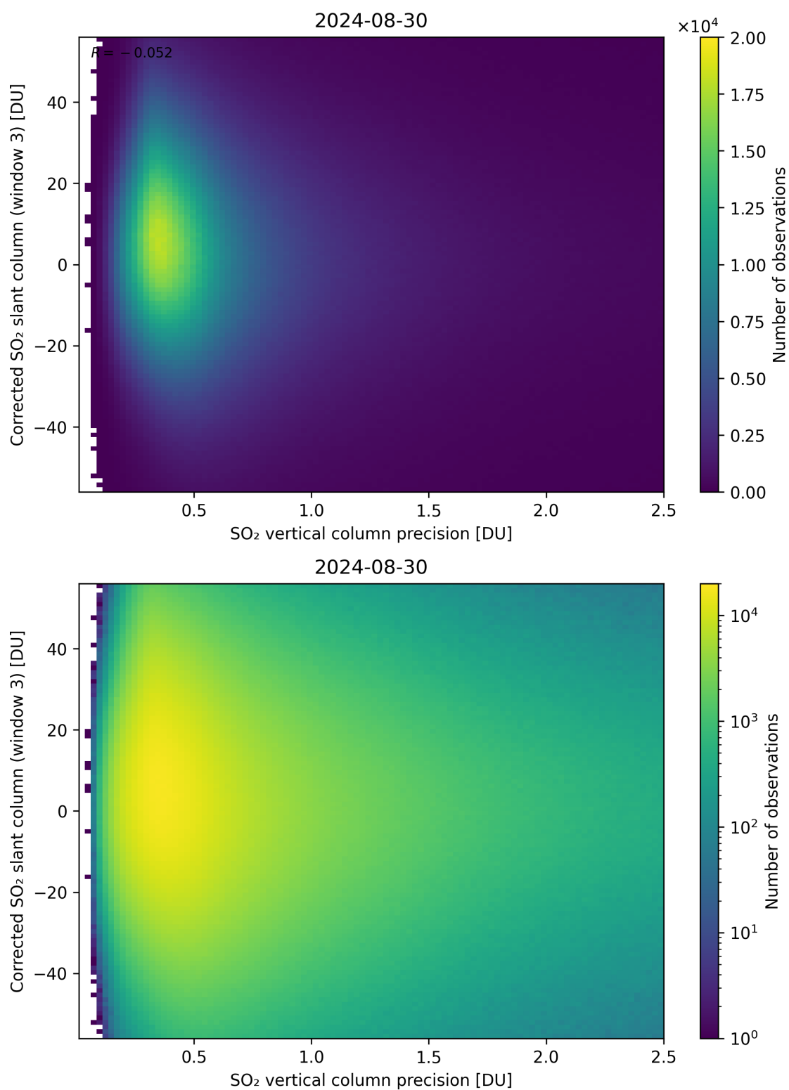
Figure 288: Scatter density plot of “SO 2 vertical column precision” against “Corrected SO 2 slant column (window 3)” for 2024-08-29 to 2024-08-31.
