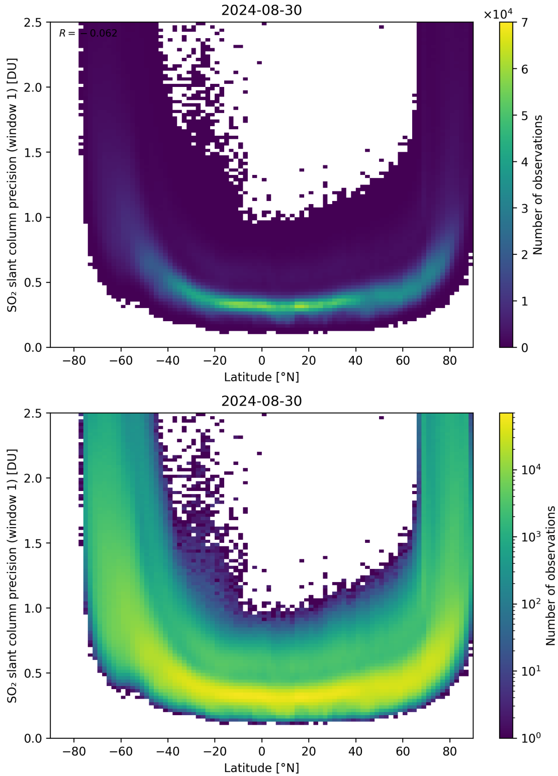
Figure 150: Scatter density plot of “Latitude” against “SO 2 slant column precision (window 1)” for 2024-08-29 to 2024-08-31.
