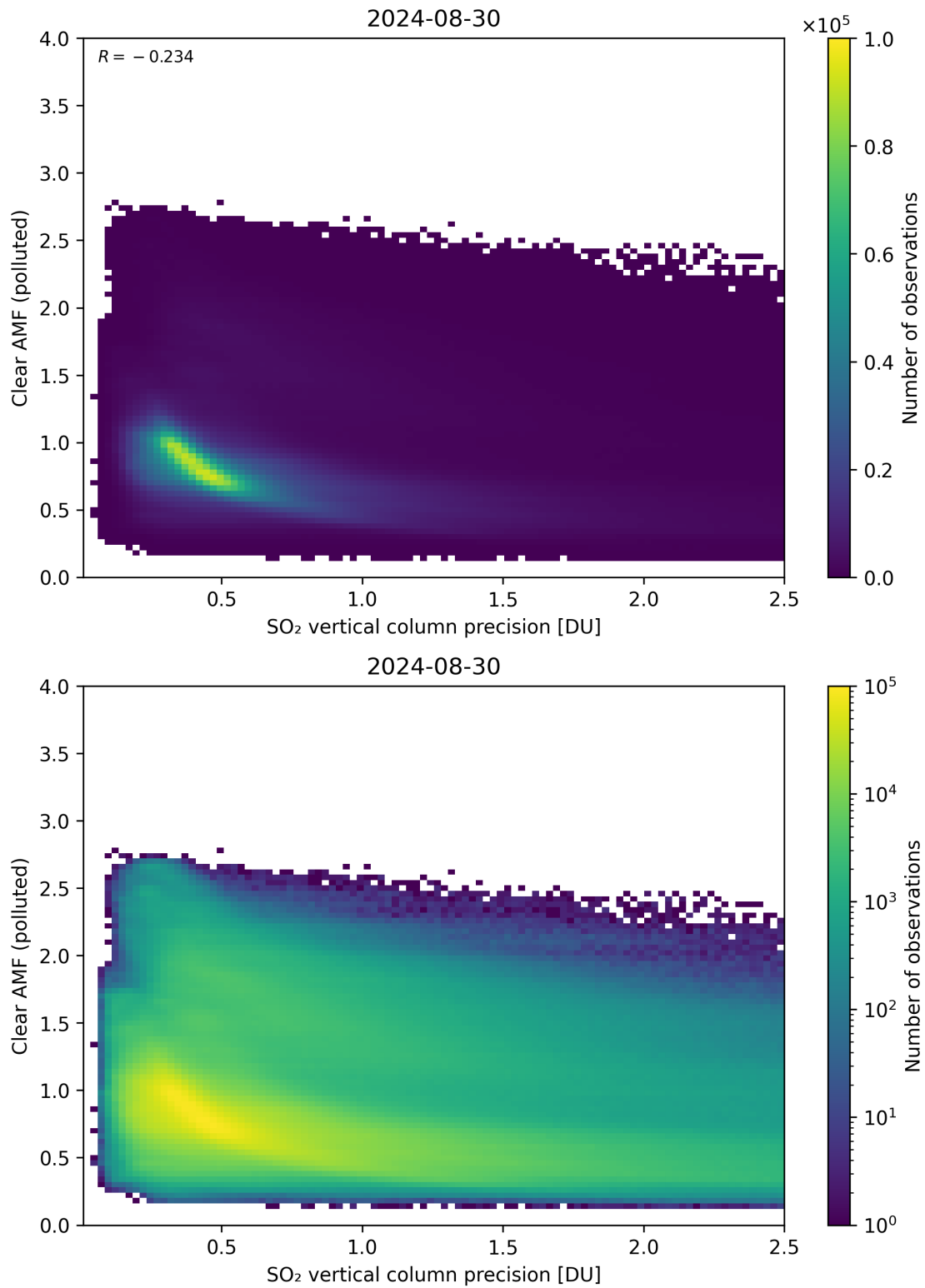
Figure 285: Scatter density plot of “SO 2 vertical column precision” against “Clear AMF (polluted)” for 2024-08-29 to 2024-08-31.
