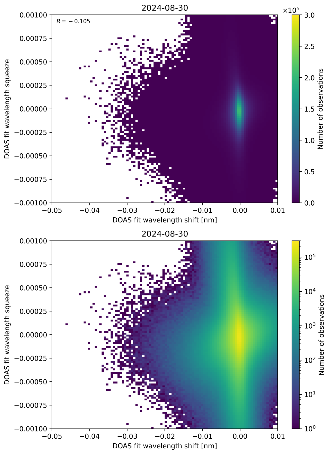
Figure 127: Scatter density plot of “DOAS fit wavelength shift” against “DOAS fit wavelength squeeze” for 2024-08-29 to 2024-08-31.
