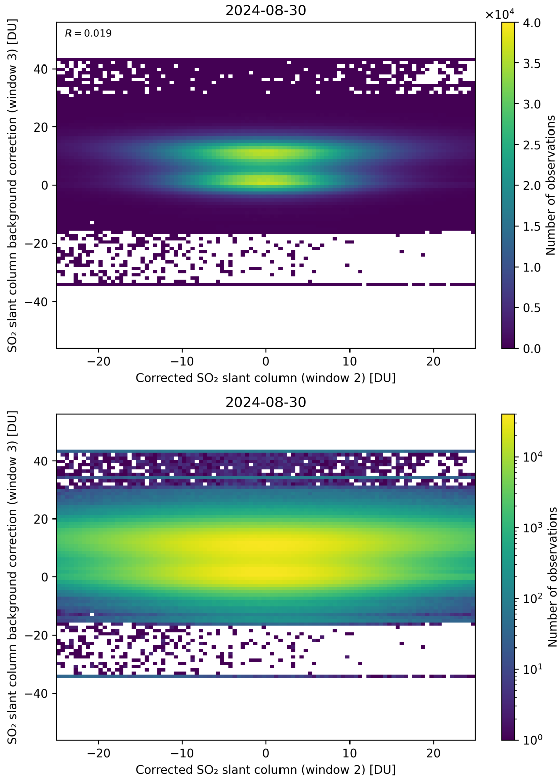
Figure 195: Scatter density plot of “Corrected SO 2 slant column (window 2)” against “SO 2 slant column background correction (window 3)” for 2024-08-29 to 2024-08-31.
