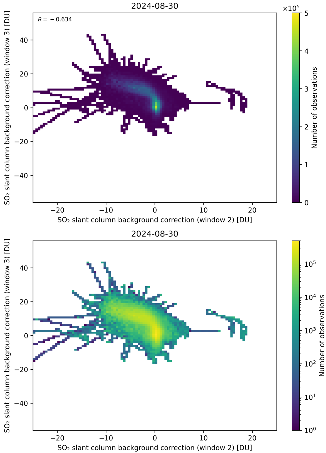
Figure 111: Scatter density plot of “SO 2 slant column background correction (window 2)” against “SO 2 slant column background correction (window 3)” for 2024-08-29 to 2024-08-31.
