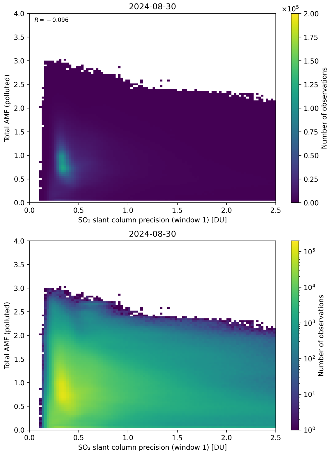
Figure 230: Scatter density plot of “SO 2 slant column precision (window 1)” against “Total AMF (polluted)” for 2024-08-29 to 2024-08-31.
