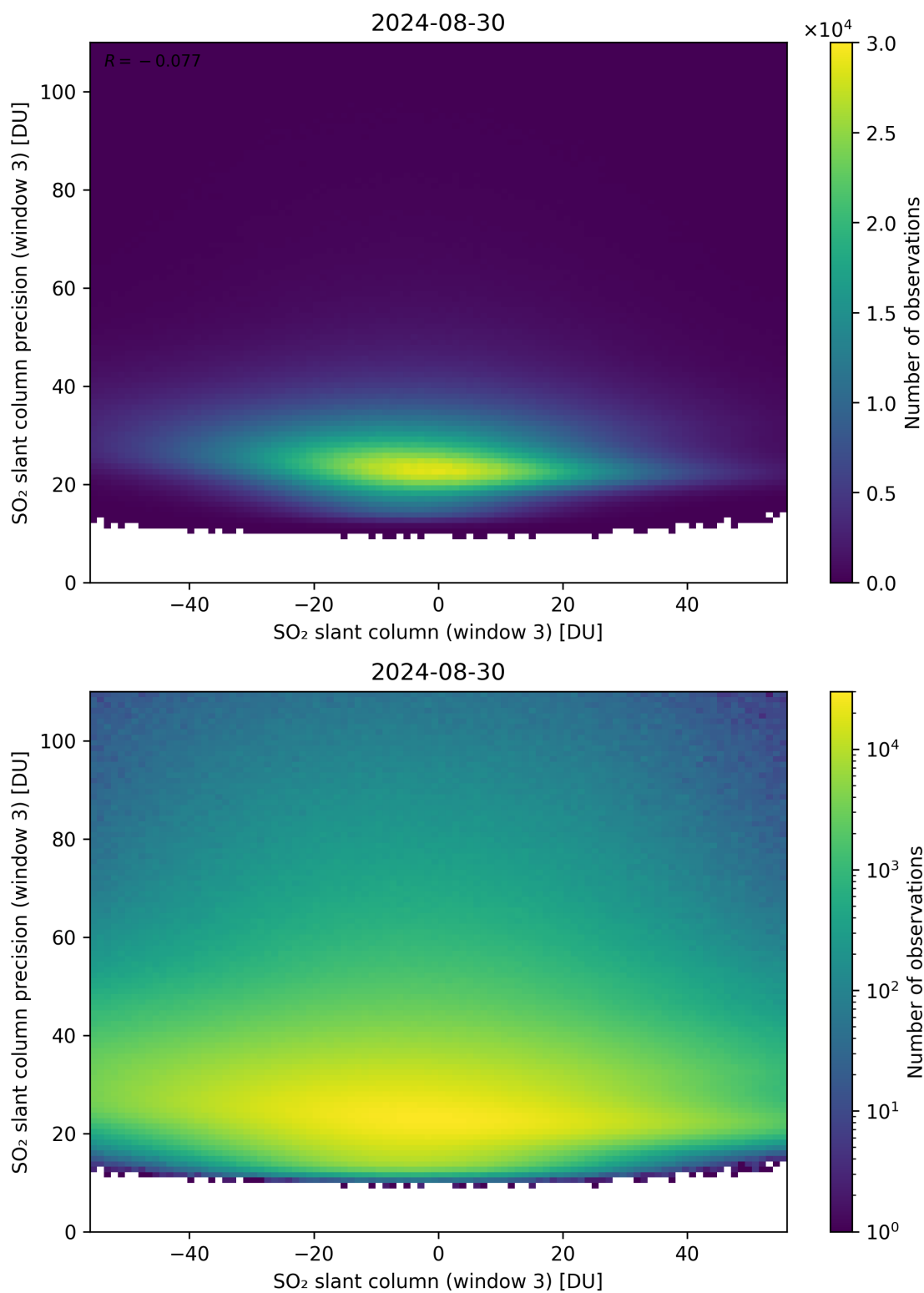
Figure 267: Scatter density plot of “SO 2 slant column (window 3)” against “SO 2 slant column precision (window 3)” for 2024-08-29 to 2024-08-31.
