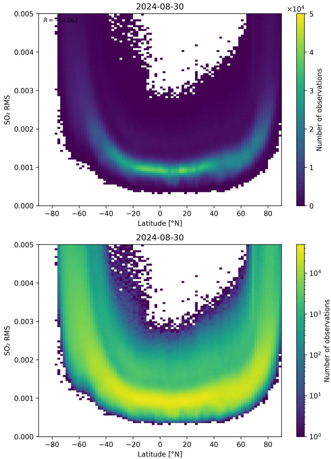
Figure 144: Scatter density plot of “Latitude” against “SO 2 RMS” for 2024-08-29 to 2024-08-31.
