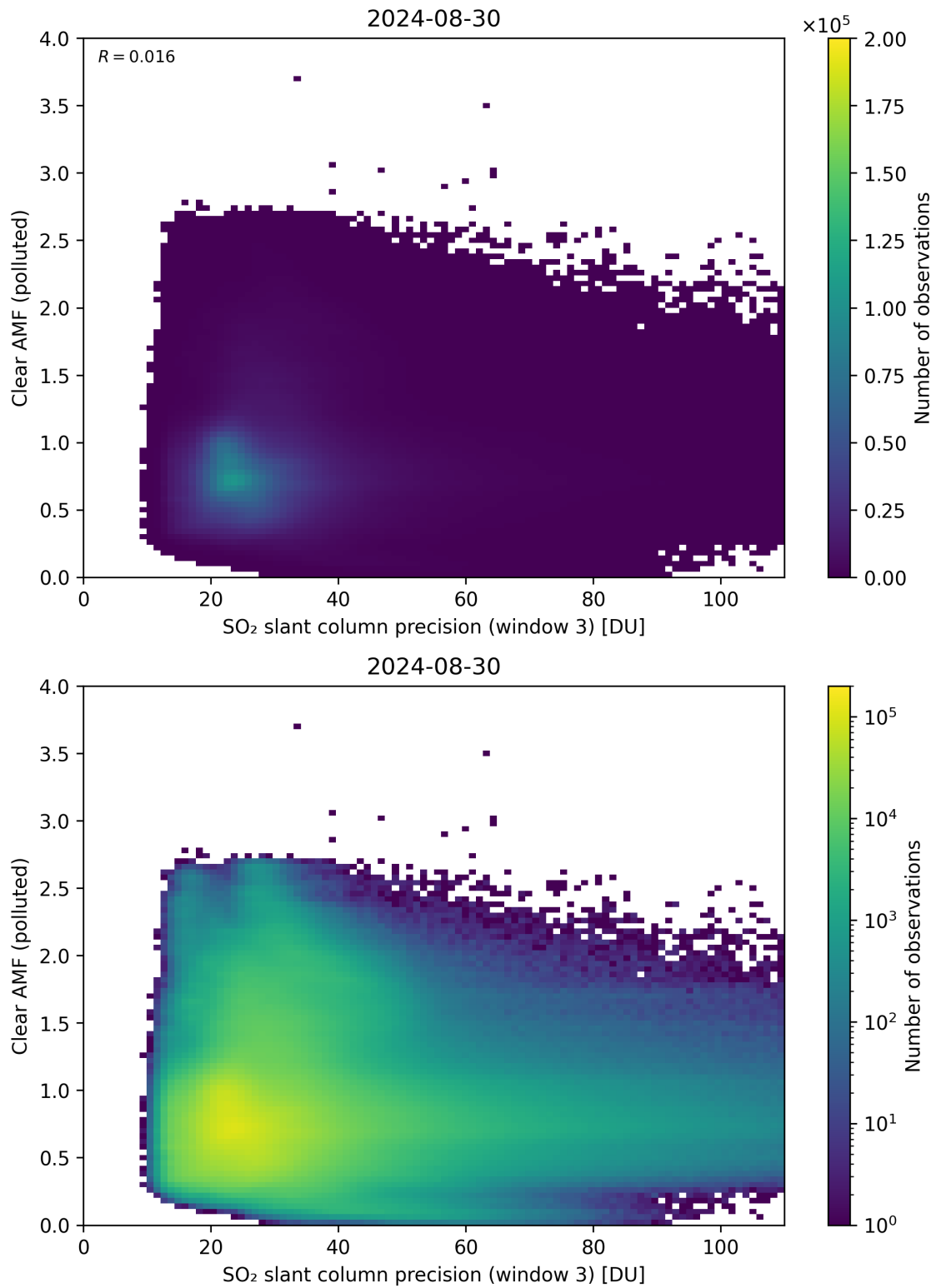
Figure 261: Scatter density plot of “SO 2 slant column precision (window 3)” against “Clear AMF (polluted)” for 2024-08-29 to 2024-08-31.
