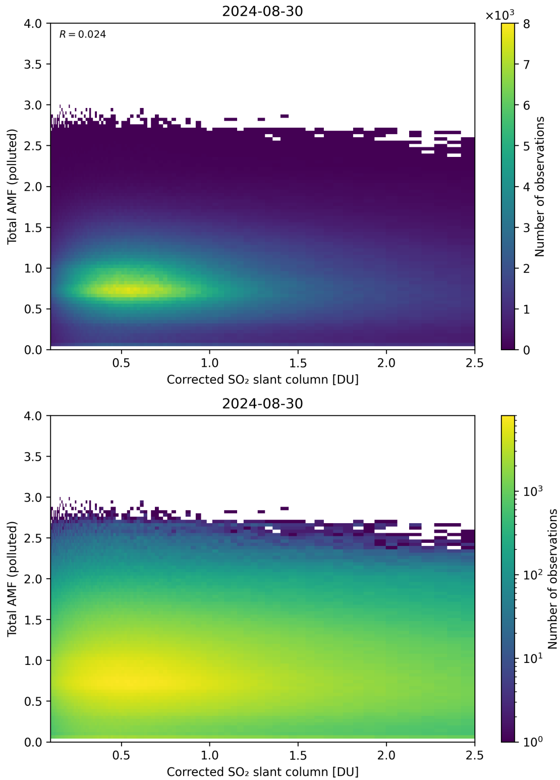
Figure 192: Scatter density plot of “Corrected SO 2 slant column” against “Total AMF (polluted)” for 2024-08-29 to 2024-08-31.
