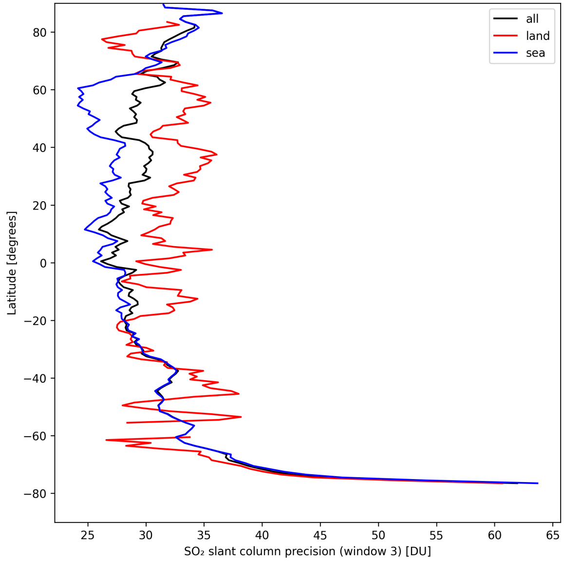
Figure 42: Zonal average of “SO 2 slant column precision (window 3)” for 2024-08-29 to 2024-08-31.
