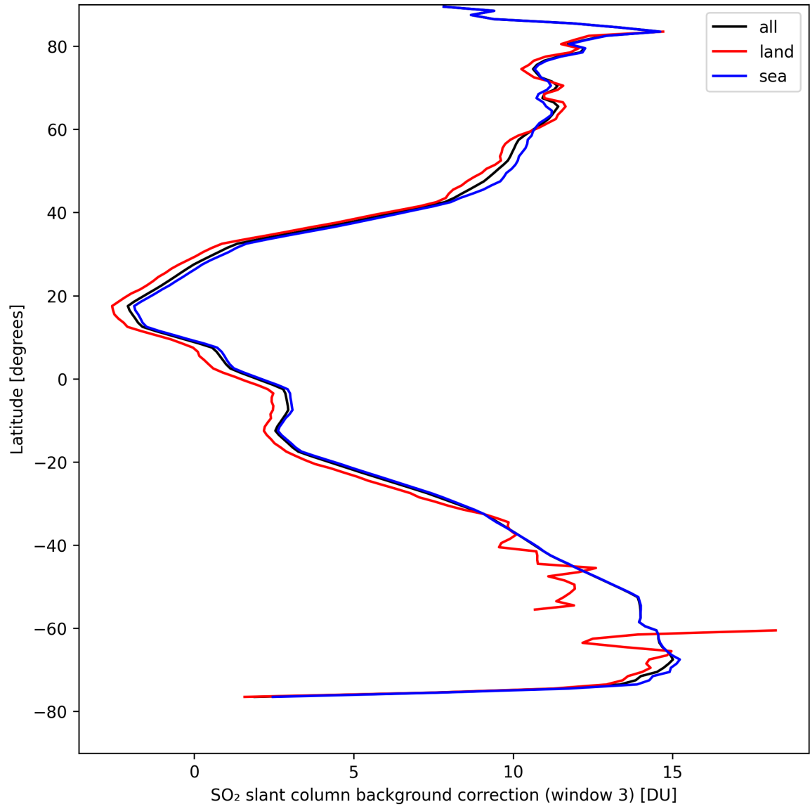
Figure 44: Zonal average of "SO 2 slant column background correction (window 3)" for 2024-08-29 to 2024-08-31.
