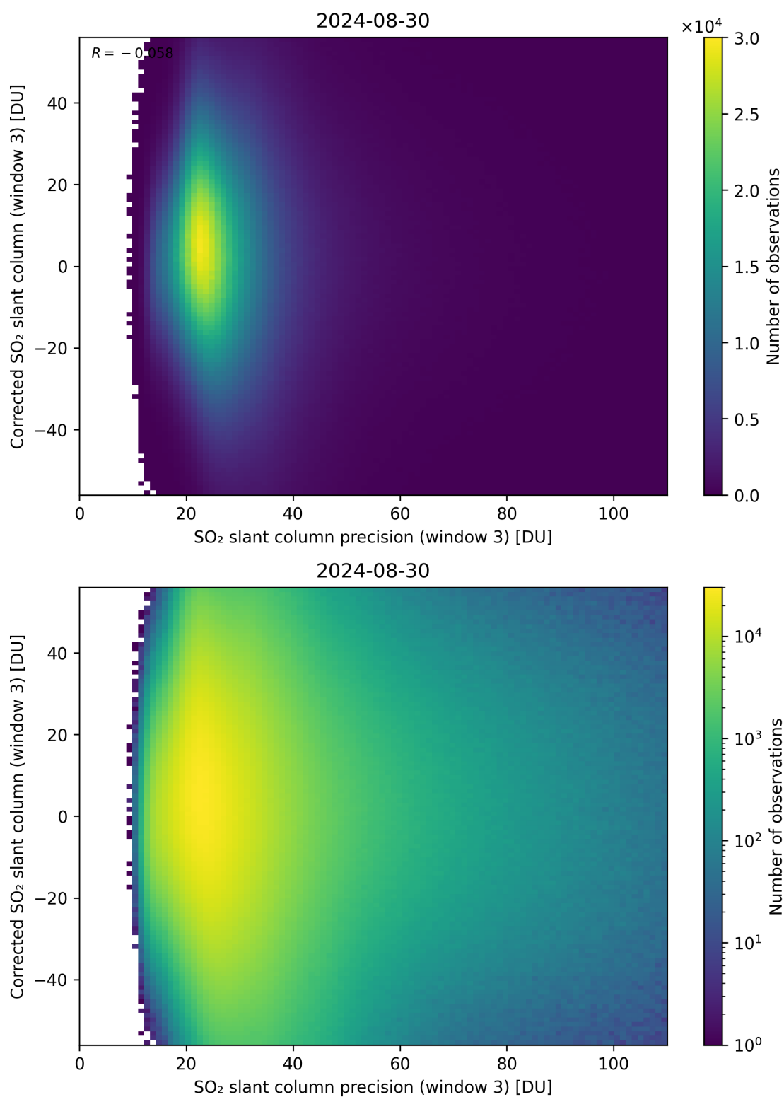
Figure 262: Scatter density plot of “SO 2 slant column precision (window 3)” against “Corrected SO 2 slant column (window 3)” for 2024-08-29 to 2024-08-31.
