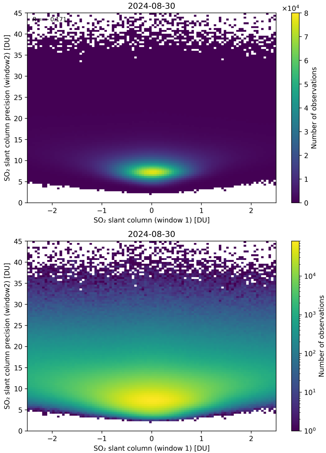
Figure 236: Scatter density plot of “SO 2 slant column (window 1)” against “SO 2 slant column precision (window2)” for 2024-08-29 to 2024-08-31.
