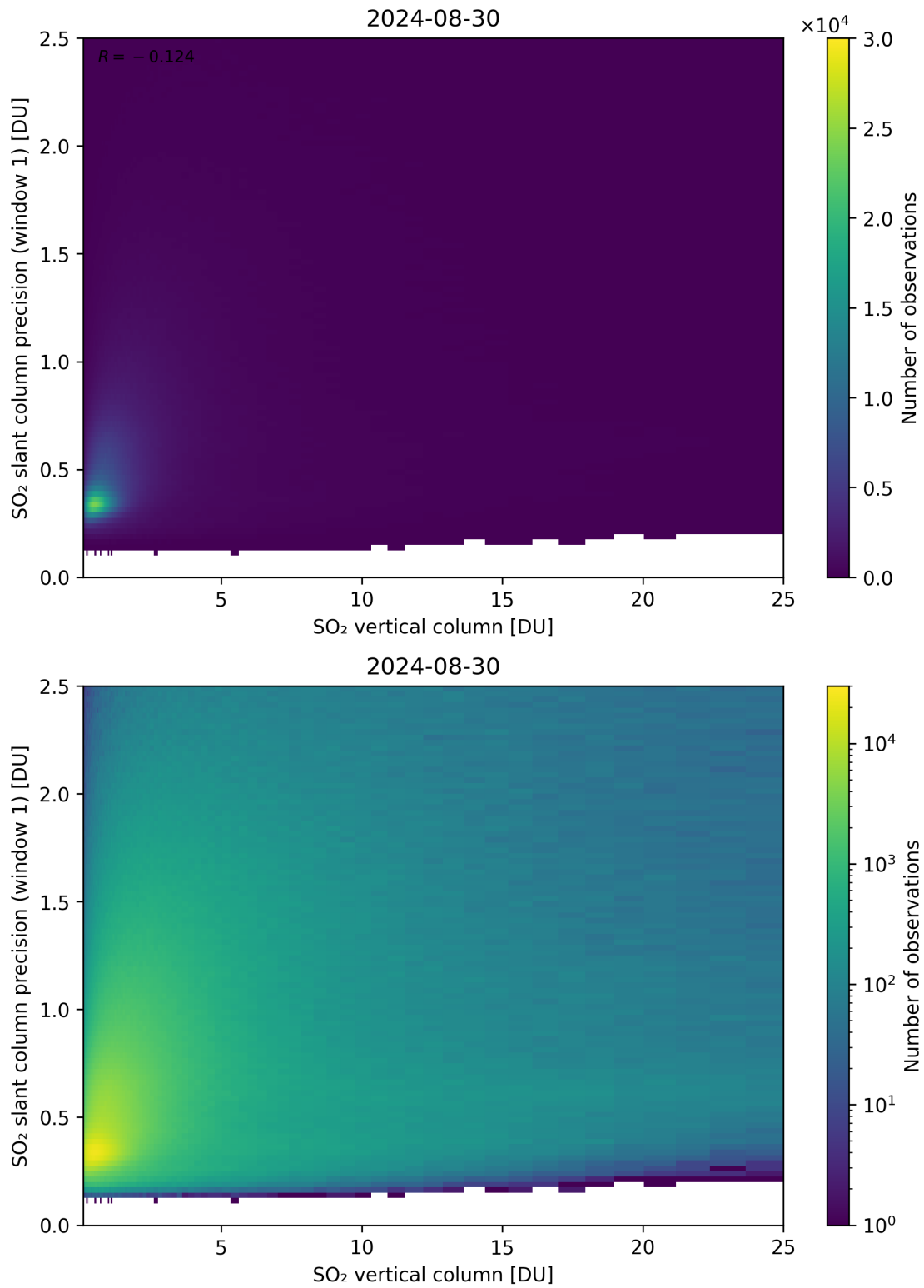
Figure 301: Scatter density plot of “SO 2 vertical column” against “SO 2 slant column precision (window 1)” for 2024-08-29 to 2024-08-31.
