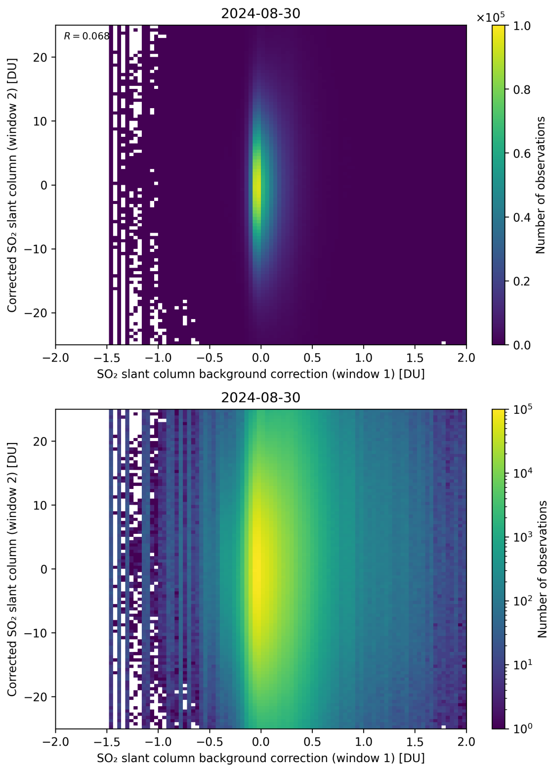
Figure 104: Scatter density plot of “SO 2 slant column background correction (window 1)” against “Corrected SO 2 slant column (window 2)” for 2024-08-29 to 2024-08-31.
