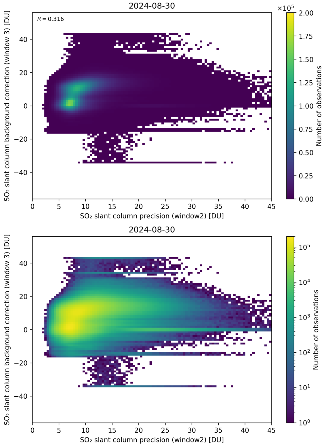
Figure 242: Scatter density plot of “SO 2 slant column precision (window2)” against “SO 2 slant column background correction (window 3)” for 2024-08-29 to 2024-08-31.
