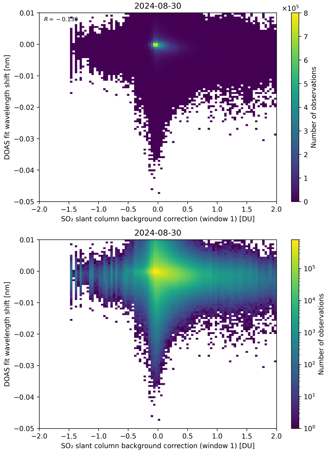
Figure 100: Scatter density plot of “SO 2 slant column background correction (window 1)” against “DOAS fit wavelength shift” for 2024-08-29 to 2024-08-31.
