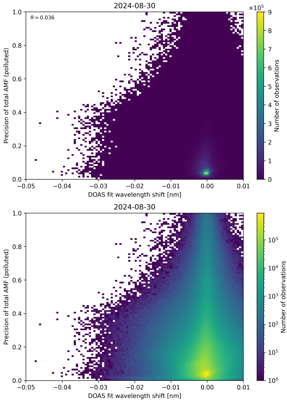
Figure 131: Scatter density plot of “DOAS fit wavelength shift” against “Precision of total AMF (polluted)” for 2024-08-29 to 2024-08-31.
