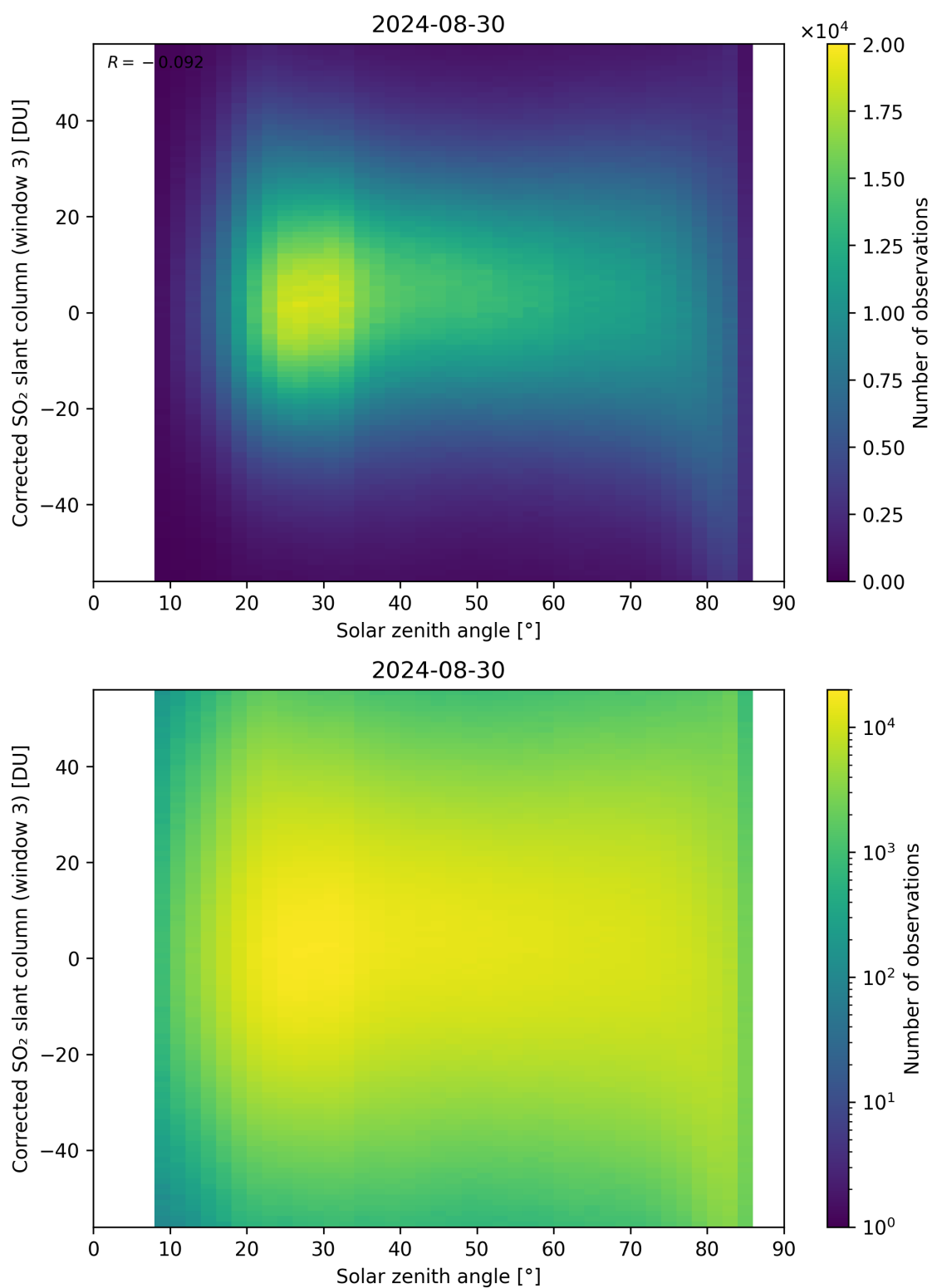
Figure 168: Scatter density plot of “Solar zenith angle” against “Corrected SO 2 slant column (window 3)” for 2024-08-29 to 2024-08-31.
