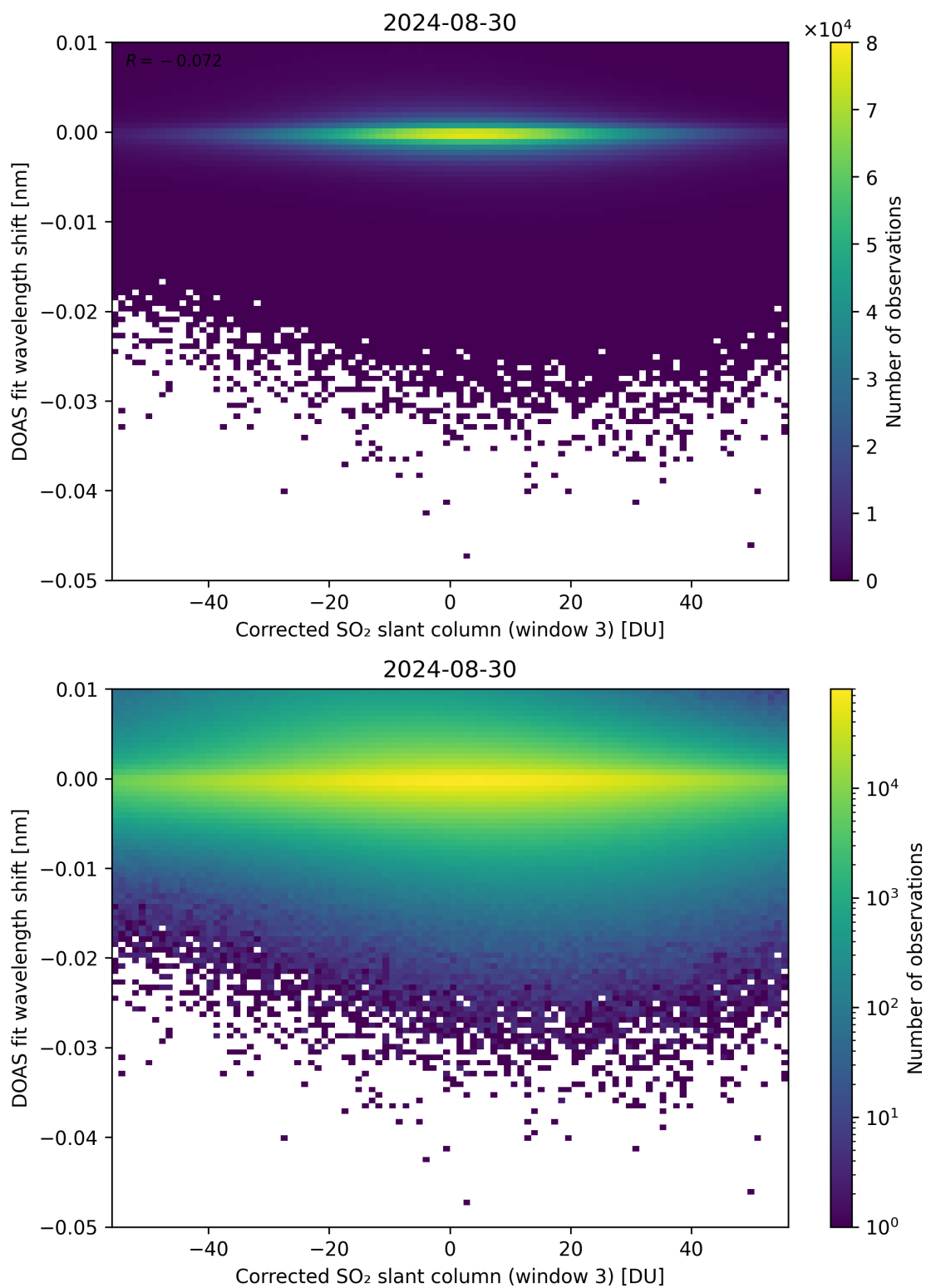
Figure 206: Scatter density plot of “Corrected SO 2 slant column (window 3)” against “DOAS fit wavelength shift” for 2024-08-29 to 2024-08-31.
