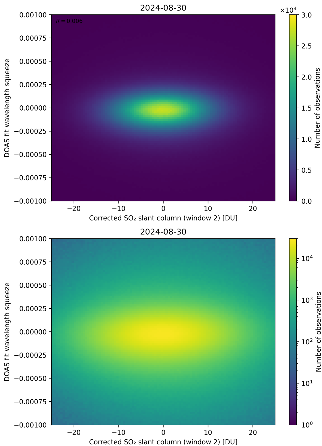
Figure 197: Scatter density plot of “Corrected SO 2 slant column (window 2)” against “DOAS fit wavelength squeeze” for 2024-08-29 to 2024-08-31.
