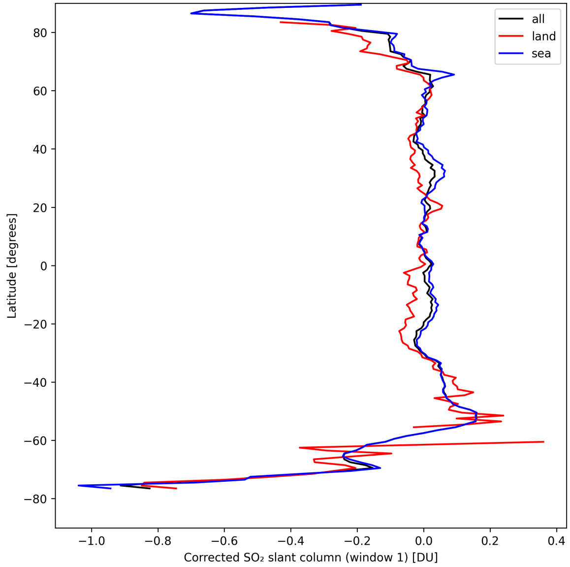
Figure 35: Zonal average of “Corrected SO 2 slant column (window 1)” for 2024-08-29 to 2024-08-31.
