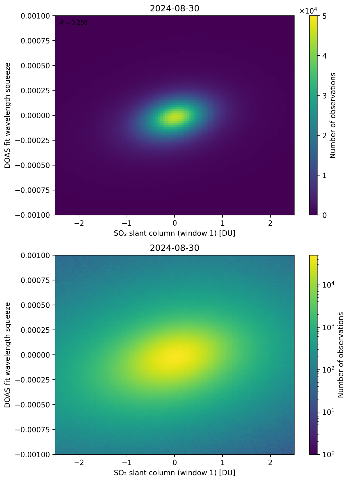
Figure 216: Scatter density plot of “SO 2 slant column (window 1)” against “DOAS fit wavelength squeeze” for 2024-08-29 to 2024-08-31.
