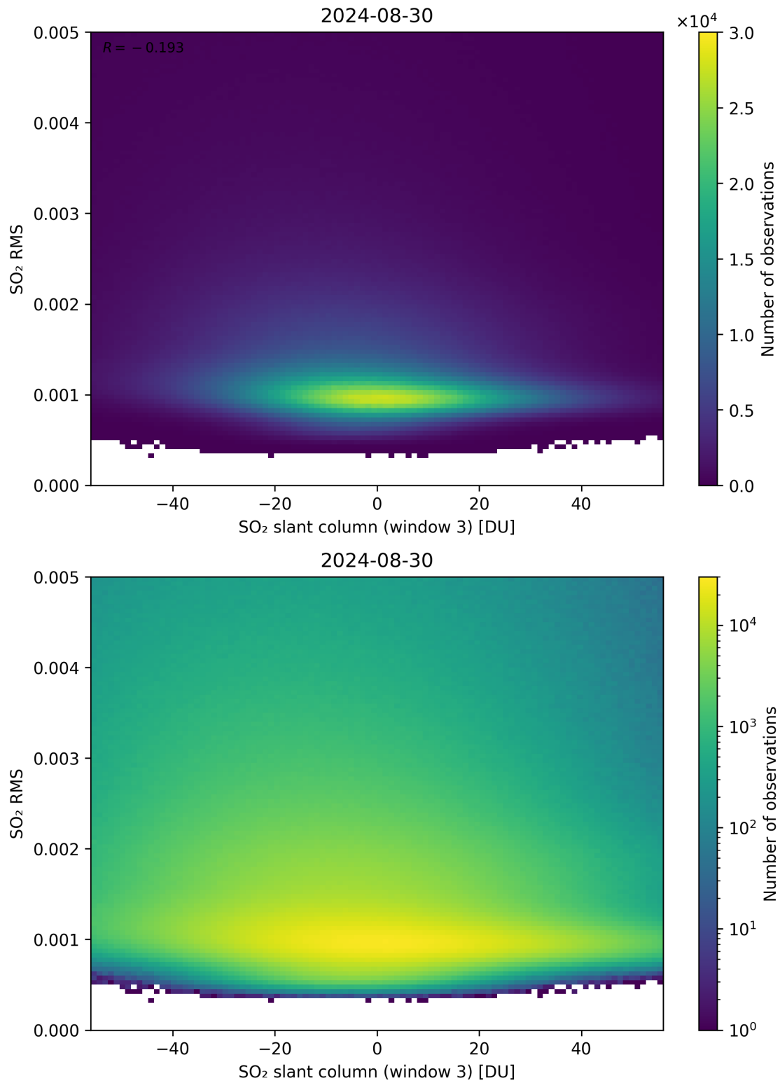
Figure 256: Scatter density plot of “SO 2 slant column (window 3)” against “SO 2 RMS” for 2024-08-29 to 2024-08-31.
