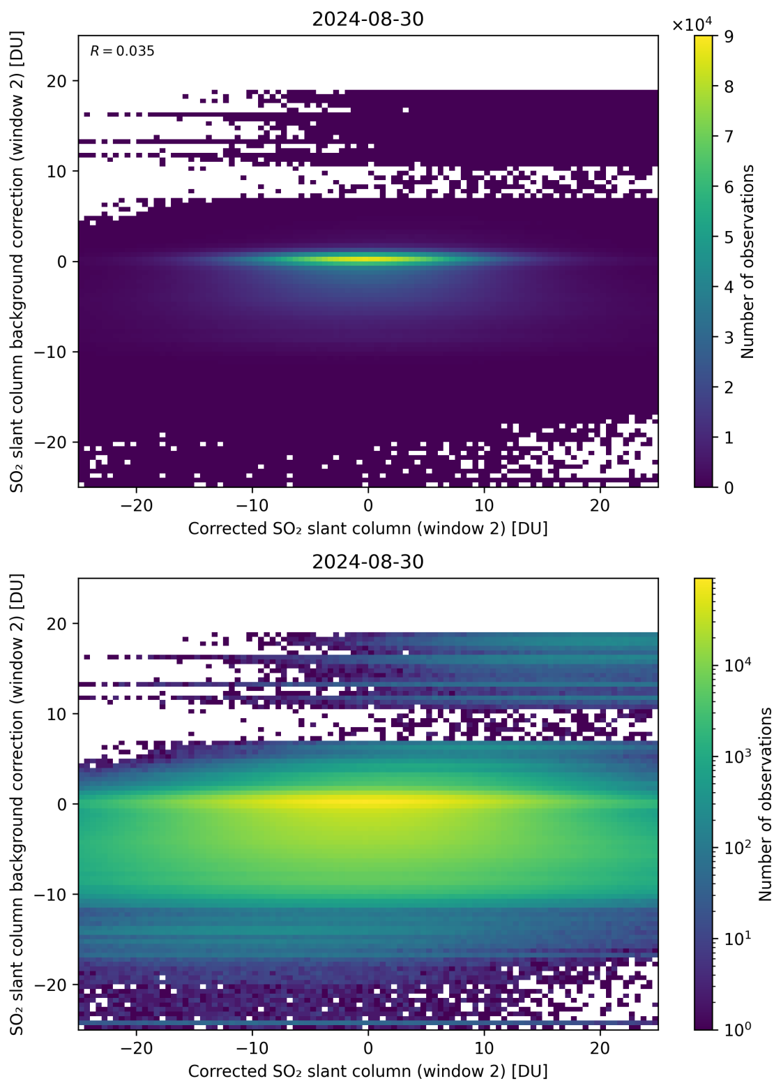
Figure 194: Scatter density plot of “Corrected SO 2 slant column (window 2)” against “SO 2 slant column background correction (window 2)” for 2024-08-29 to 2024-08-31.
