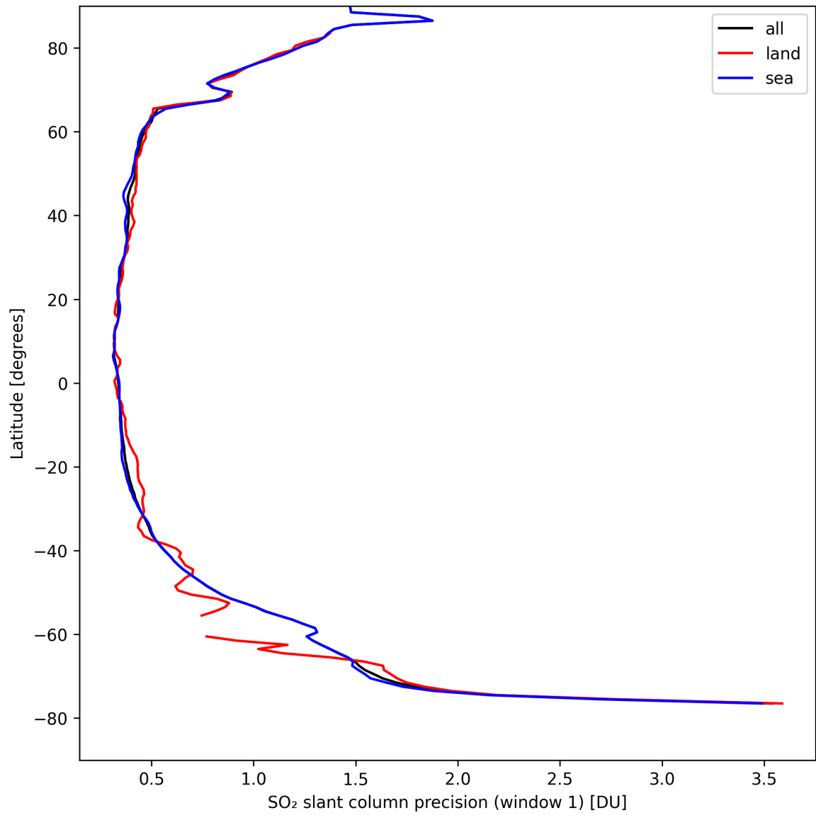
Figure 34: Zonal average of “SO 2 slant column precision (window 1)” for 2024-08-29 to 2024-08-31.
