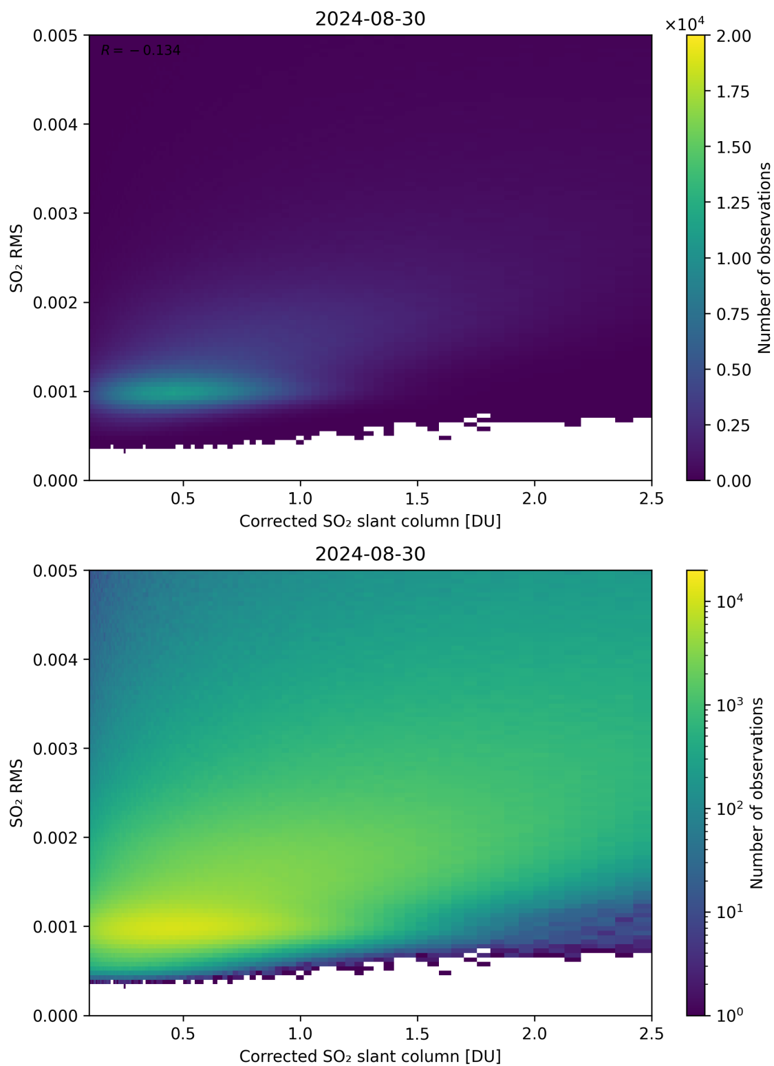
Figure 183: Scatter density plot of “Corrected SO 2 slant column” against “SO 2 RMS” for 2024-08-29 to 2024-08-31.
