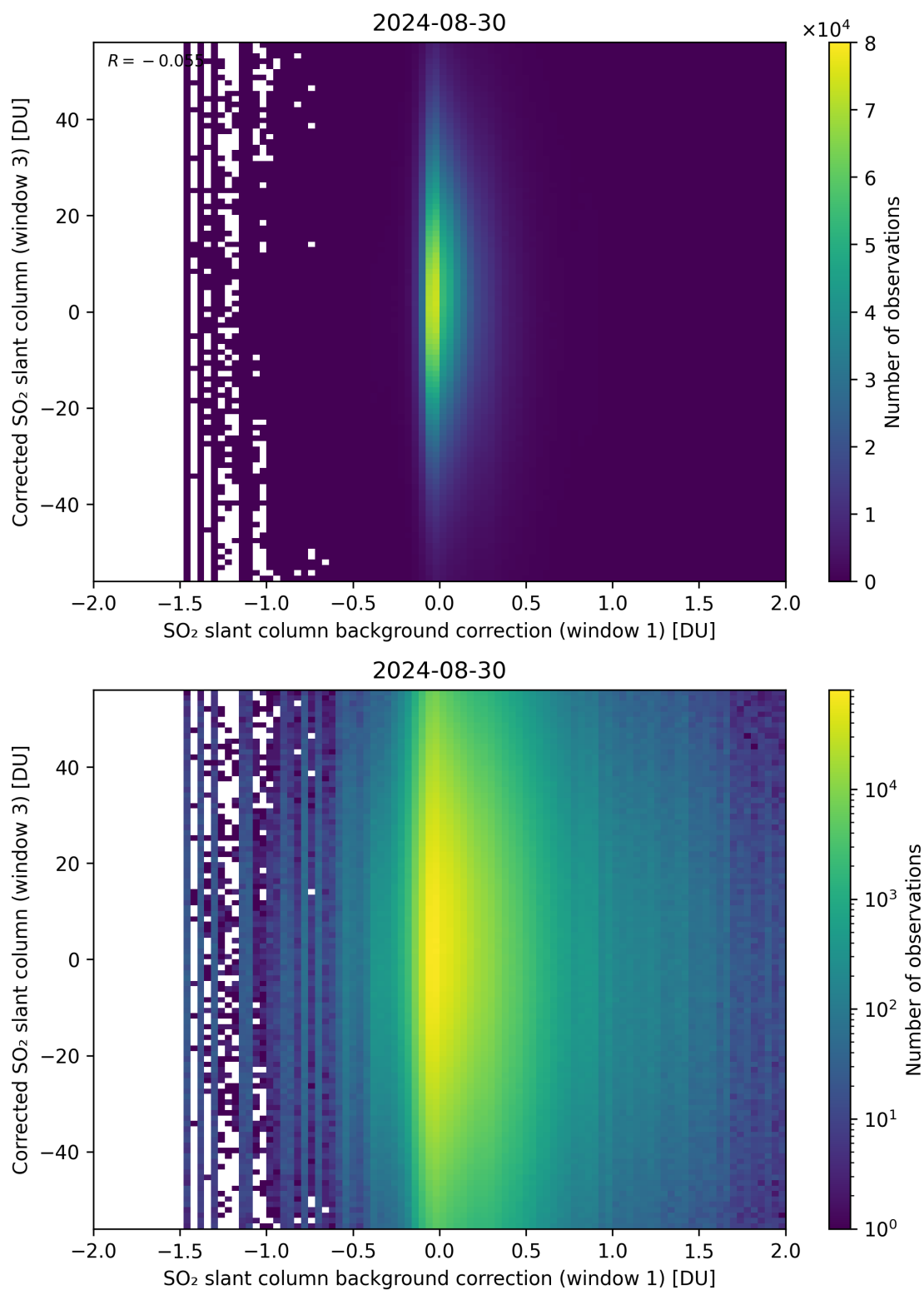
Figure 105: Scatter density plot of “SO 2 slant column background correction (window 1)” against “Corrected SO 2 slant column (window 3)” for 2024-08-29 to 2024-08-31.
