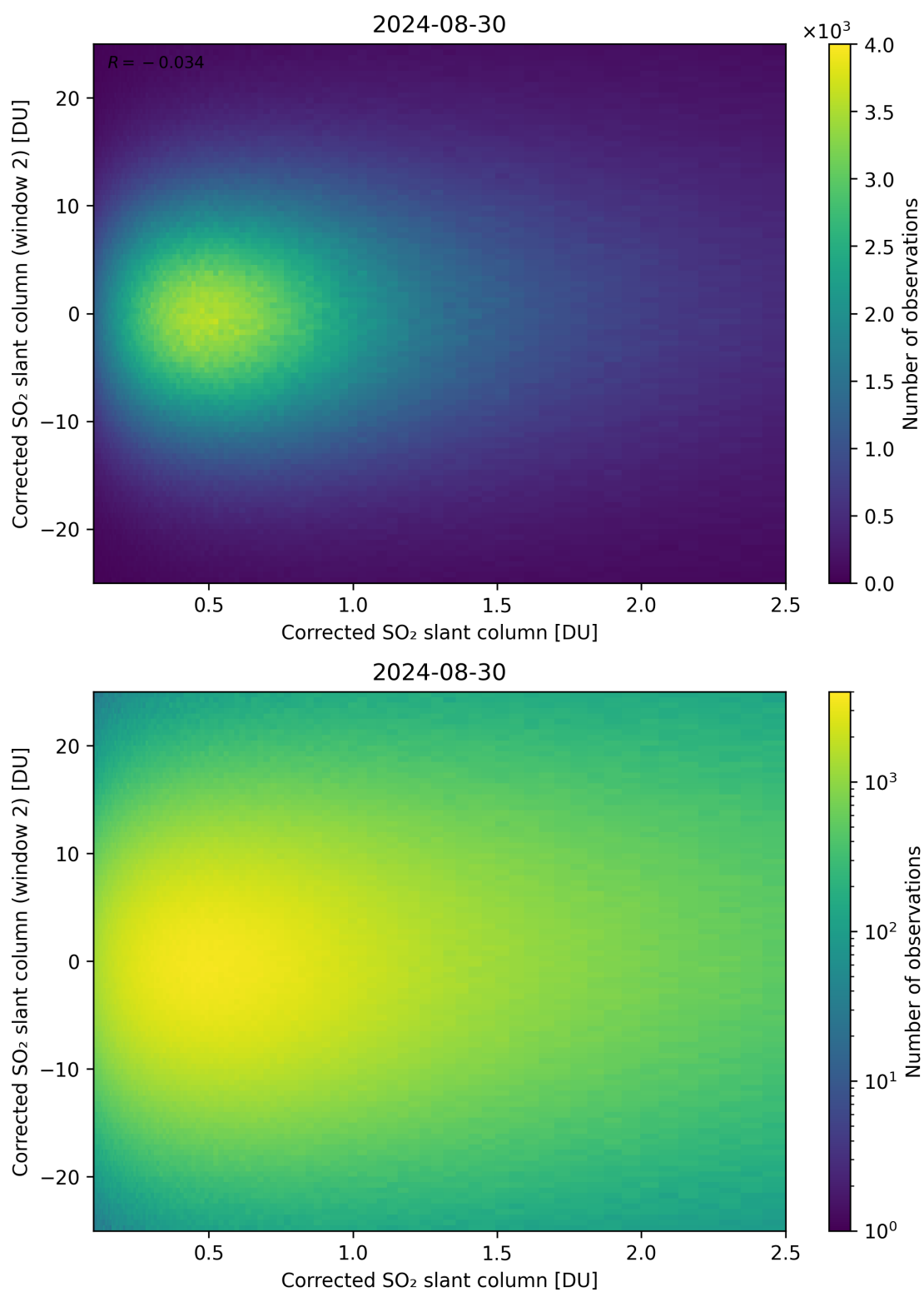
Figure 185: Scatter density plot of “Corrected SO 2 slant column” against “Corrected SO 2 slant column (window 2)” for 2024-08-29 to 2024-08-31.
