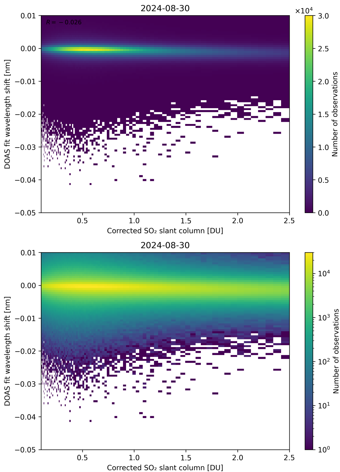
Figure 181: Scatter density plot of “Corrected SO 2 slant column” against “DOAS fit wavelength shift” for 2024-08-29 to 2024-08-31.
