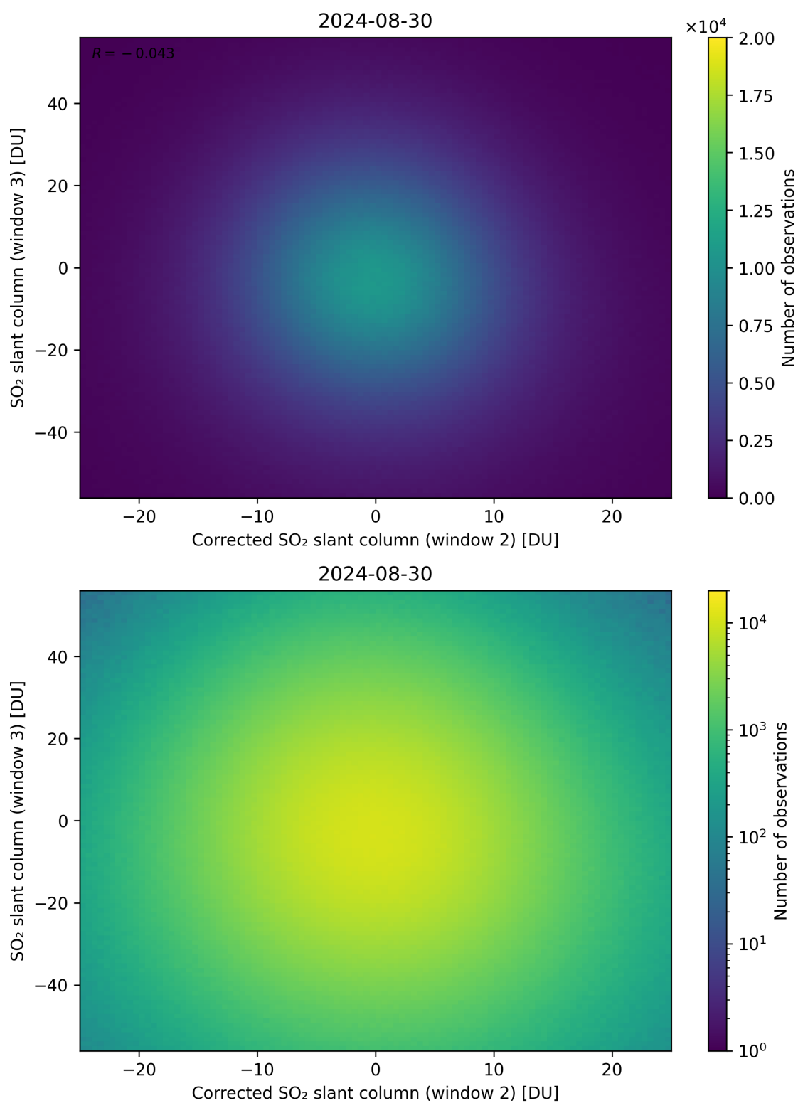
Figure 201: Scatter density plot of “Corrected SO 2 slant column (window 2)” against “SO 2 slant column (window 3)” for 2024-08-29 to 2024-08-31.
