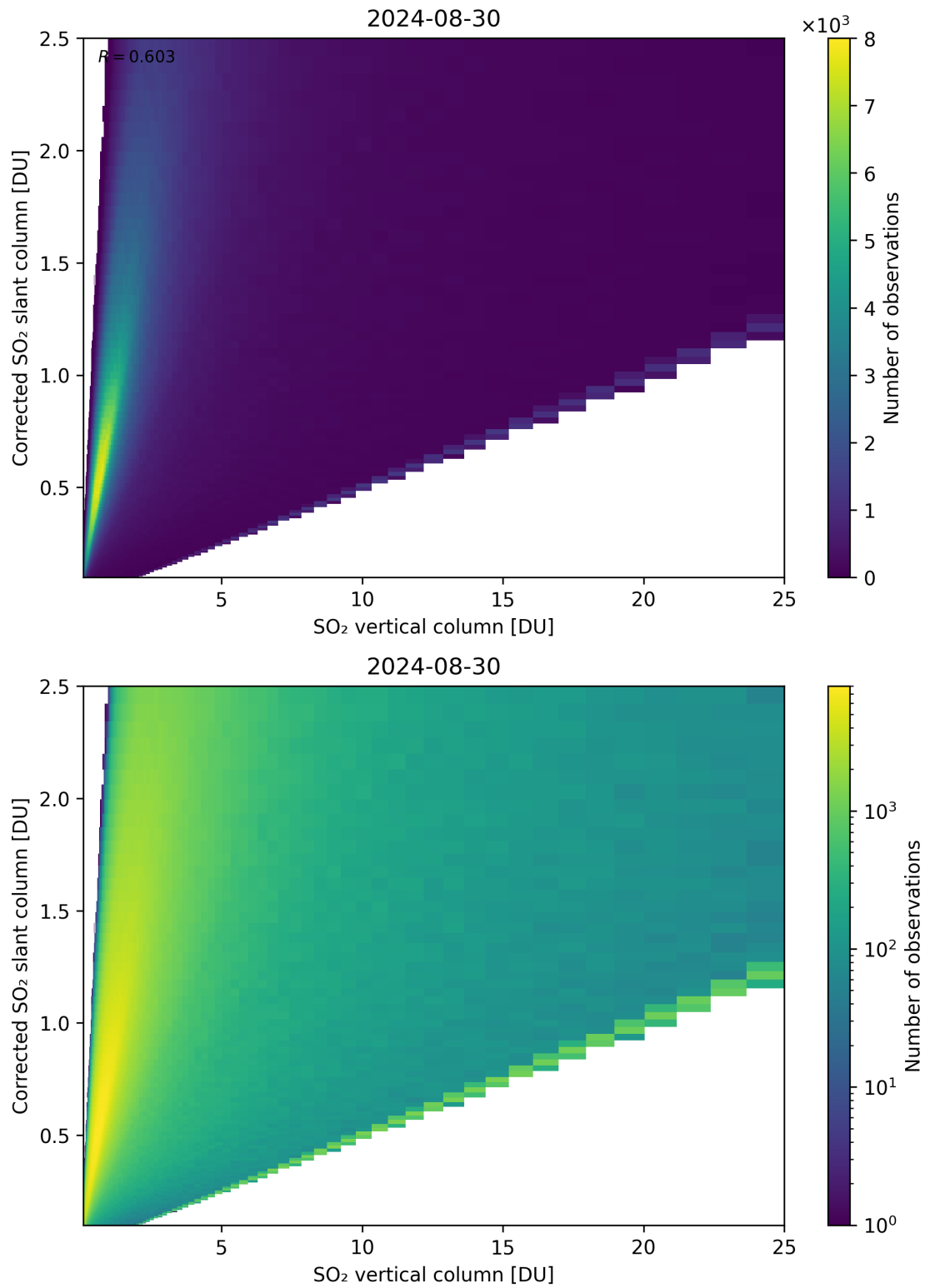
Figure 297: Scatter density plot of “SO 2 vertical column” against “Corrected SO 2 slant column” for 2024-08-29 to 2024-08-31.
