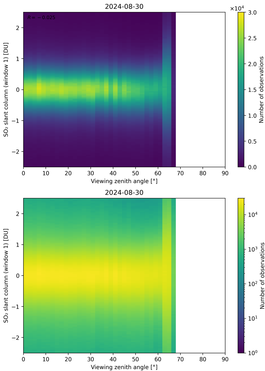
Figure 320: Scatter density plot of “Viewing zenith angle” against “SO 2 slant column (window 1)” for 2024-08-29 to 2024-08-31.
