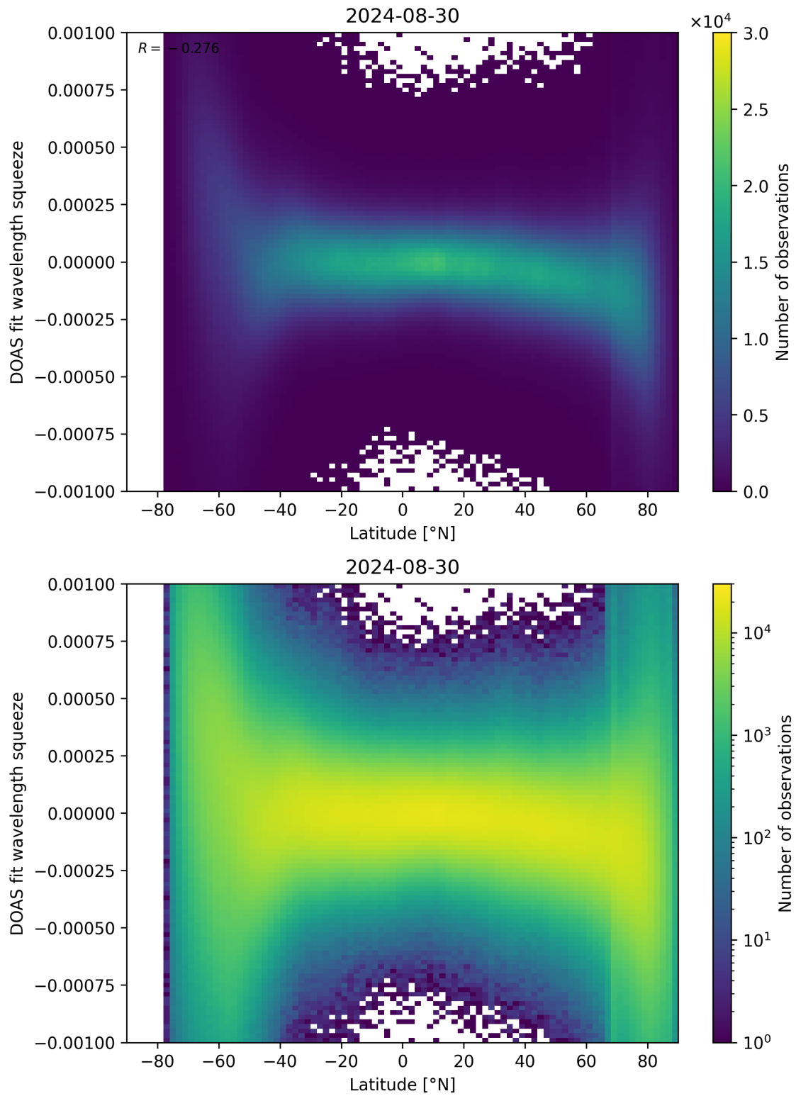
Figure 143: Scatter density plot of “Latitude” against “DOAS fit wavelength squeeze” for 2024-08-29 to 2024-08-31.
