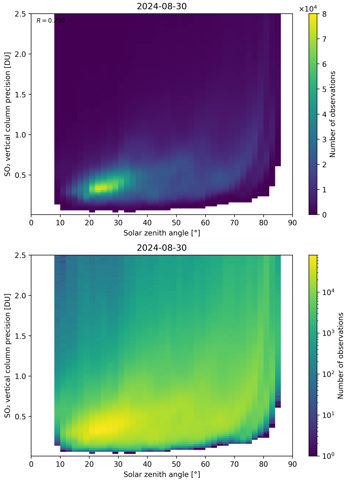
Figure 177: Scatter density plot of “Solar zenith angle” against “SO 2 vertical column precision” for 2024-08-29 to 2024-08-31.
