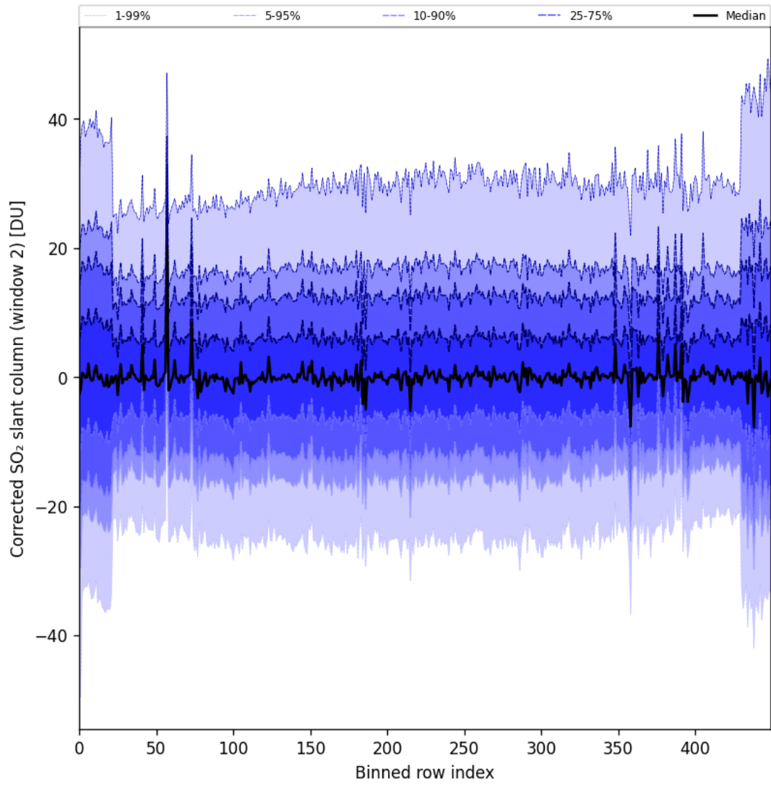
Figure 85: Along track statistics of “Corrected SO 2 slant column (window 2)” for 2024-08-29 to 2024-08-31
