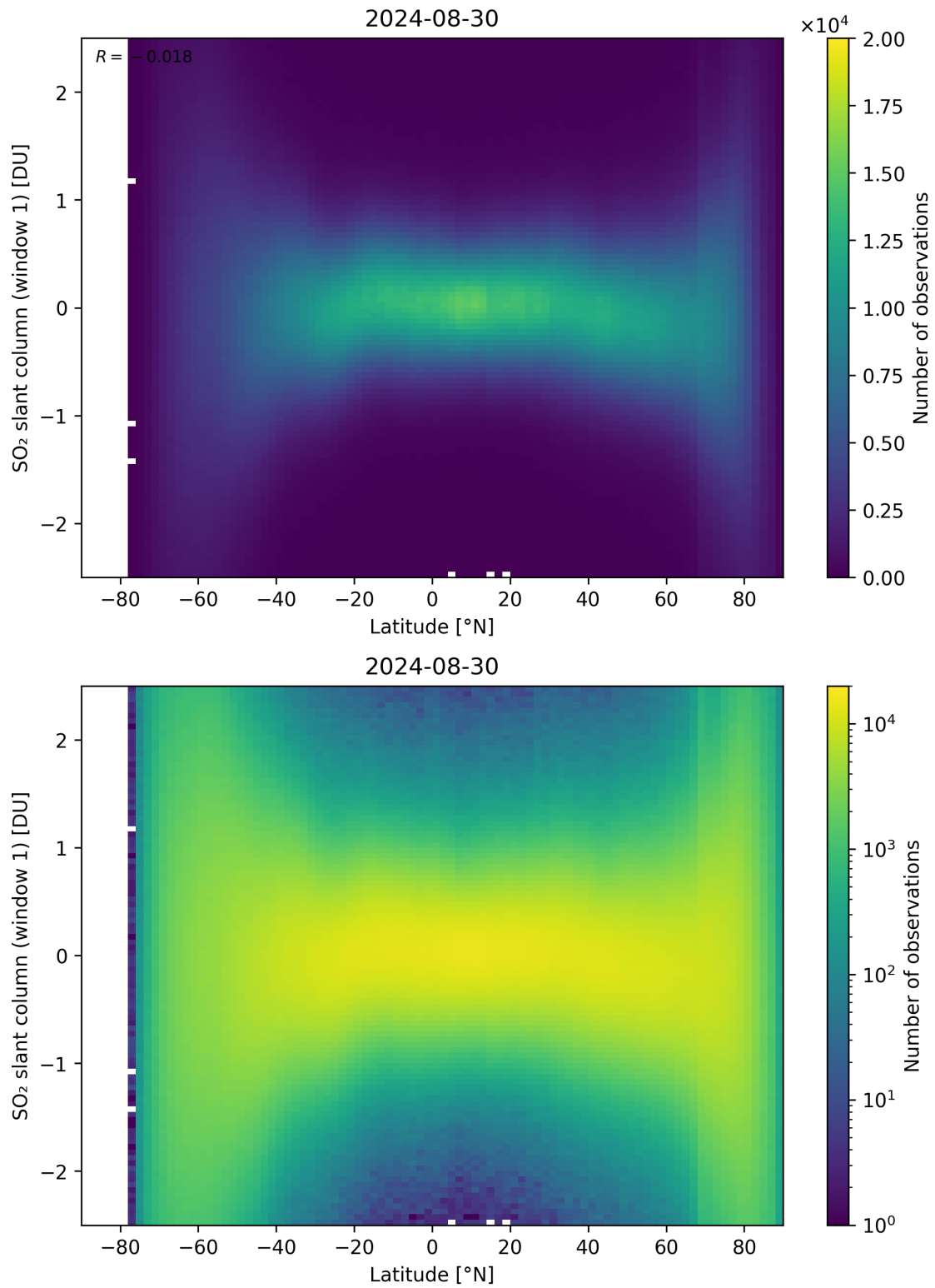
Figure 149: Scatter density plot of “Latitude” against “SO 2 slant column (window 1)” for 2024-08-29 to 2024-08-31.
