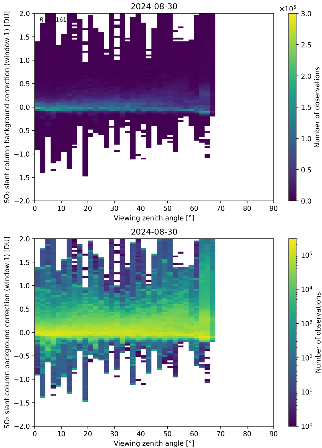
Figure 308: Scatter density plot of “Viewing zenith angle” against “SO 2 slant column background correction (window 1)” for 2024-08-29 to 2024-08-31.
