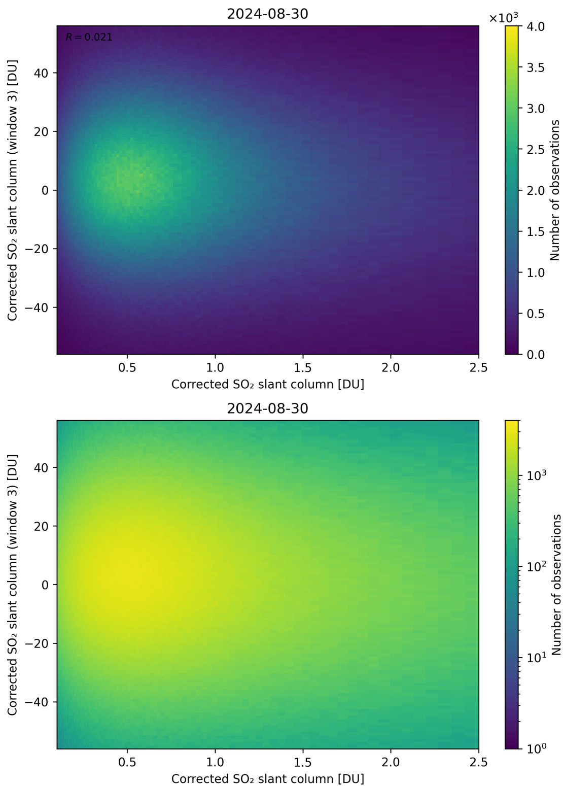
Figure 186: Scatter density plot of “Corrected SO 2 slant column” against “Corrected SO 2 slant column (window 3)” for 2024-08-29 to 2024-08-31.
