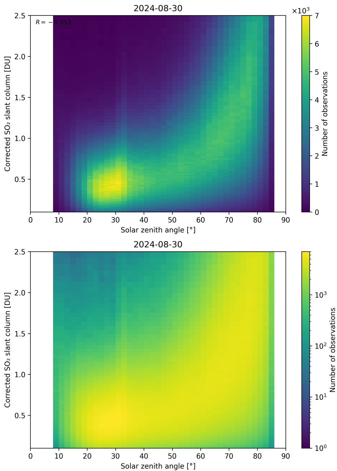
Figure 166: Scatter density plot of “Solar zenith angle” against “Corrected SO 2 slant column” for 2024-08-29 to 2024-08-31.
