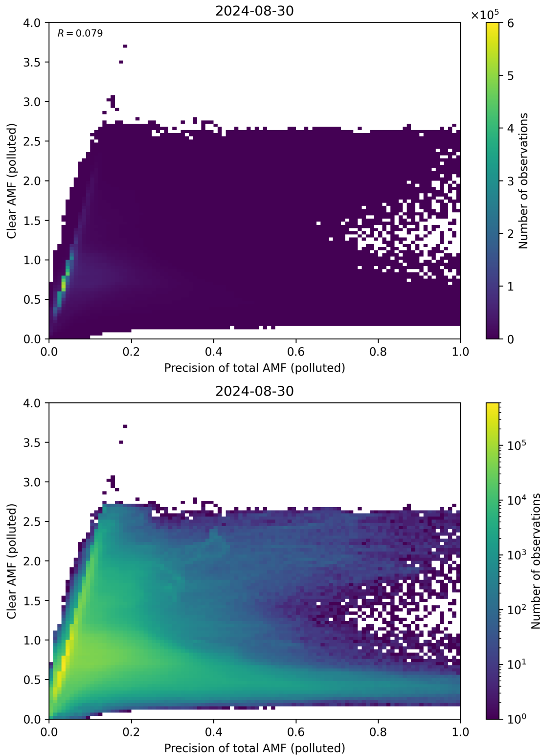
Figure 270: Scatter density plot of “Precision of total AMF (polluted)” against “Clear AMF (polluted)” for 2024-08-29 to 2024-08-31.
