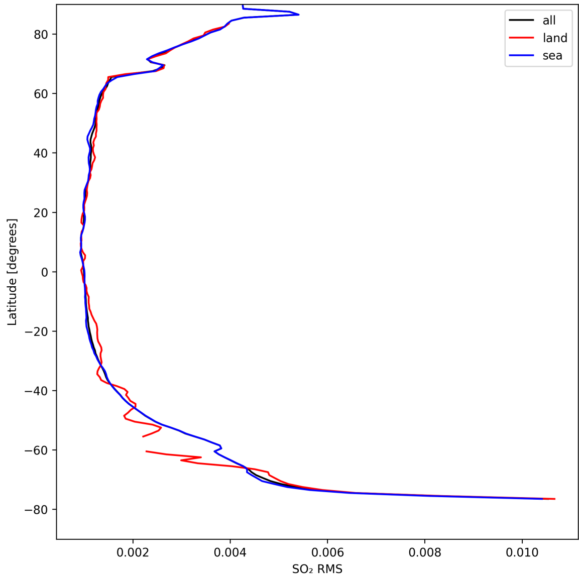
Figure 47: Zonal average of “SO 2 RMS” for 2024-08-29 to 2024-08-31.
