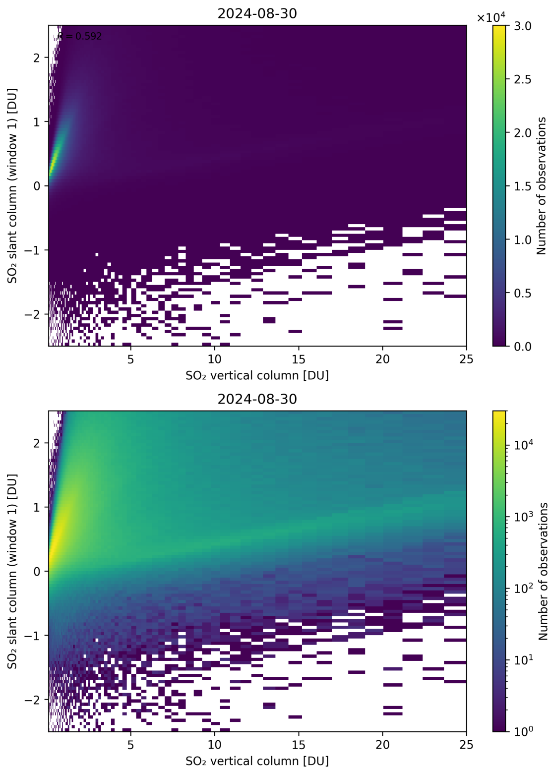
Figure 300: Scatter density plot of “SO 2 vertical column” against “SO 2 slant column (window 1)” for 2024-08-29 to 2024-08-31.
