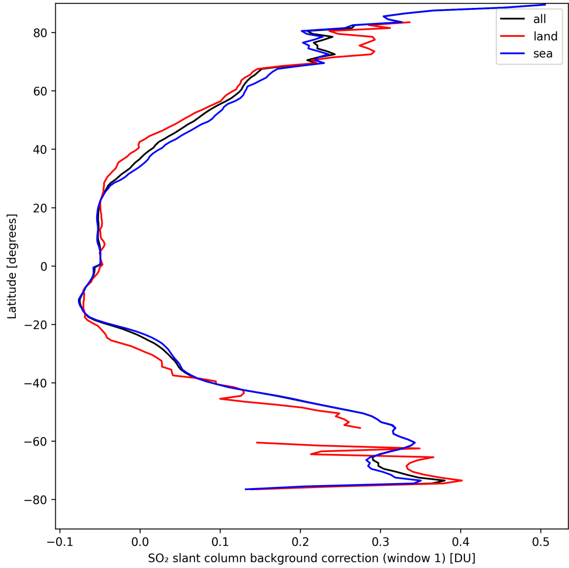
Figure 36: Zonal average of “SO 2 slant column background correction (window 1)” for 2024-08-29 to 2024-08-31.
