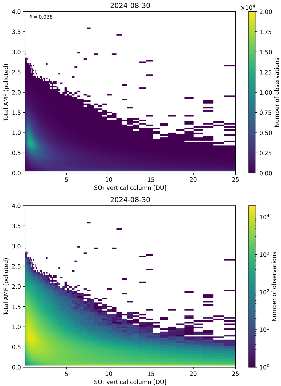
Figure 305: Scatter density plot of “SO 2 vertical column” against “Total AMF (polluted)” for 2024-08-29 to 2024-08-31.
