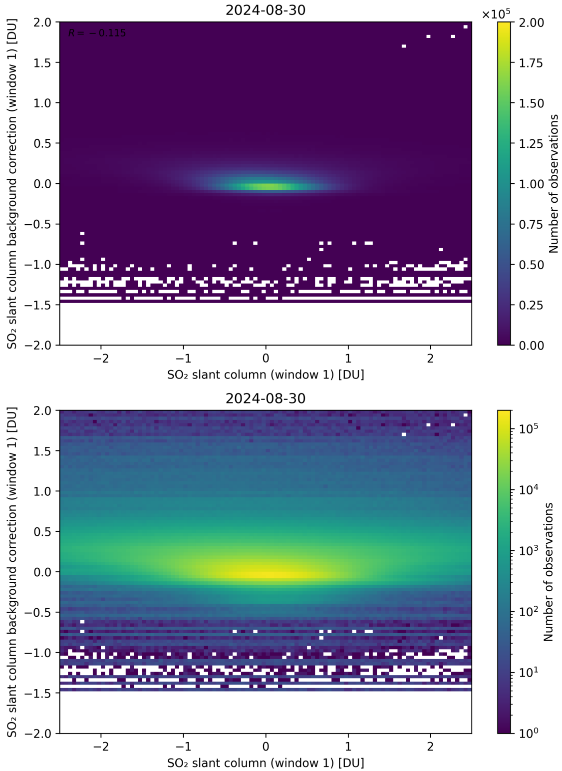
Figure 212: Scatter density plot of “SO 2 slant column (window 1)” against “SO 2 slant column background correction (window 1)” for 2024-08-29 to 2024-08-31.
