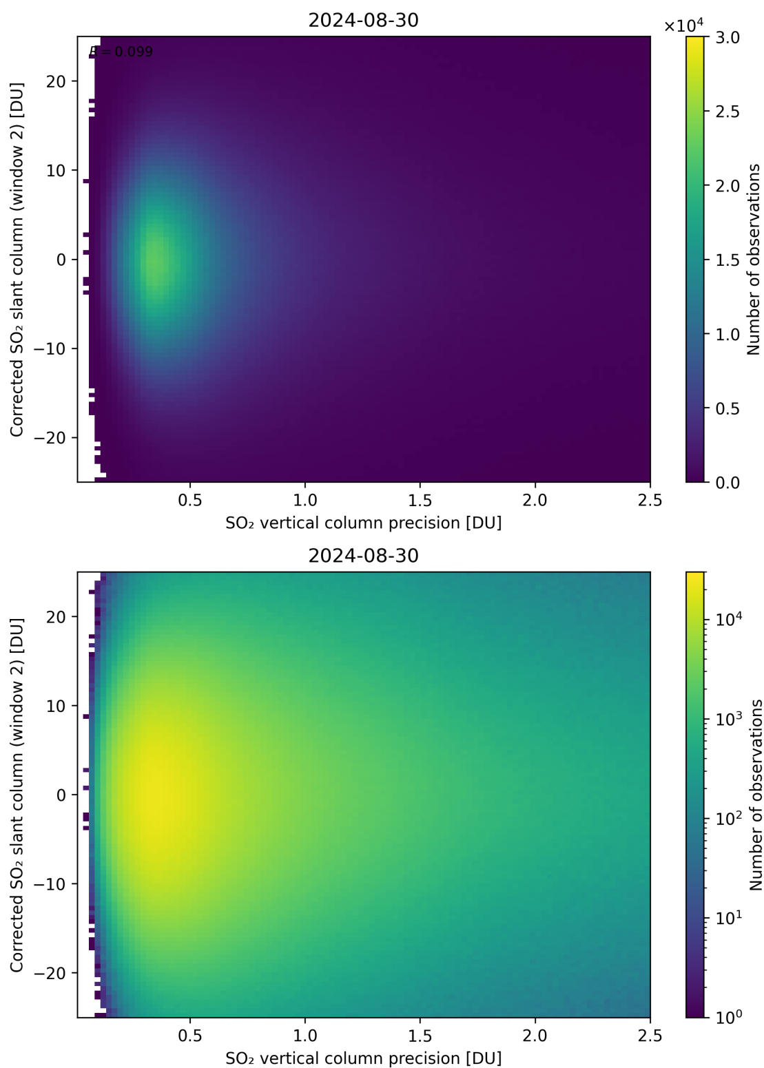
Figure 287: Scatter density plot of “SO 2 vertical column precision” against “Corrected SO 2 slant column (window 2)” for 2024-08-29 to 2024-08-31.
