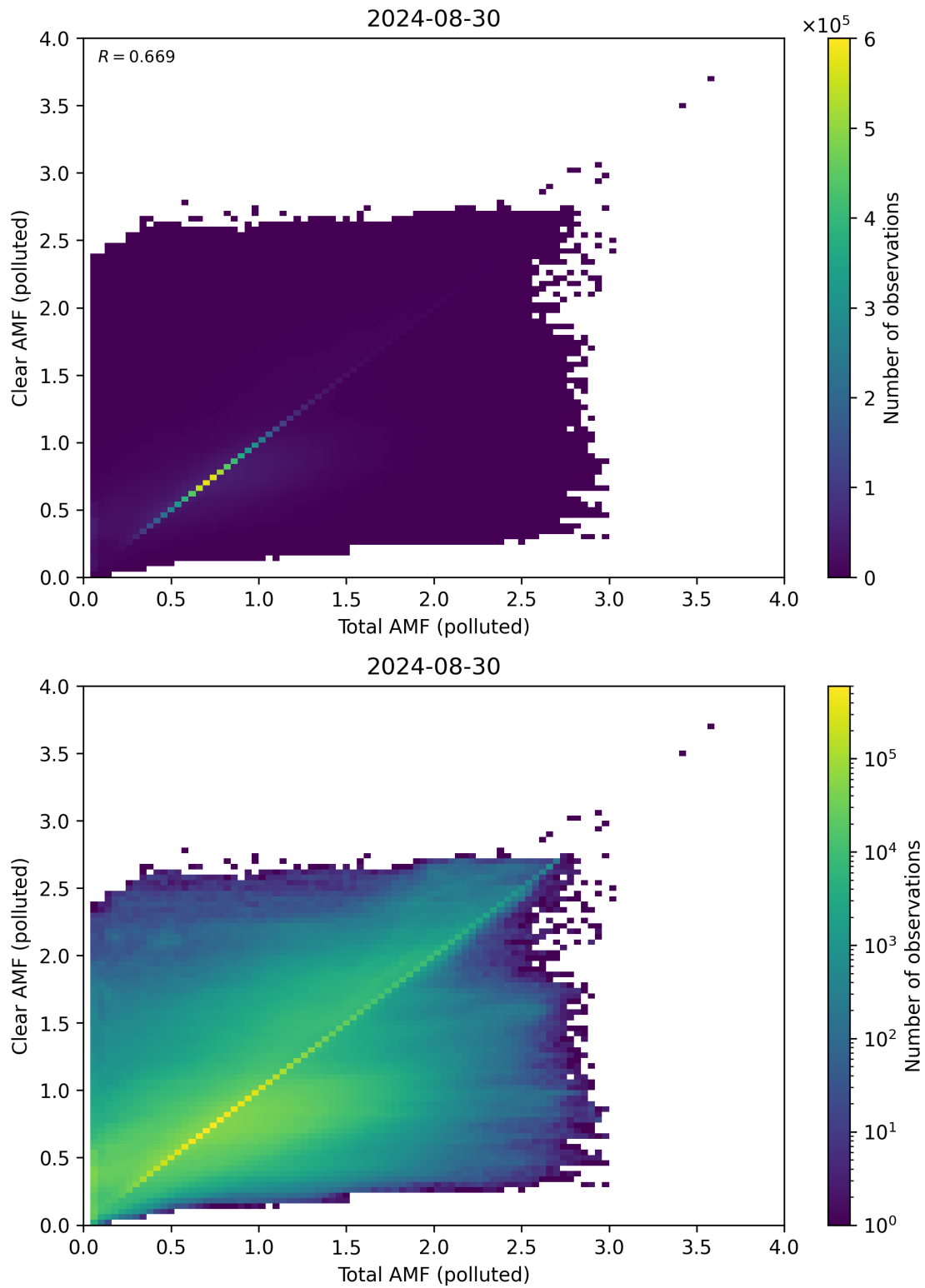
Figure 271: Scatter density plot of “Total AMF (polluted)” against “Clear AMF (polluted)” for 2024-08-29 to 2024-08-31.
