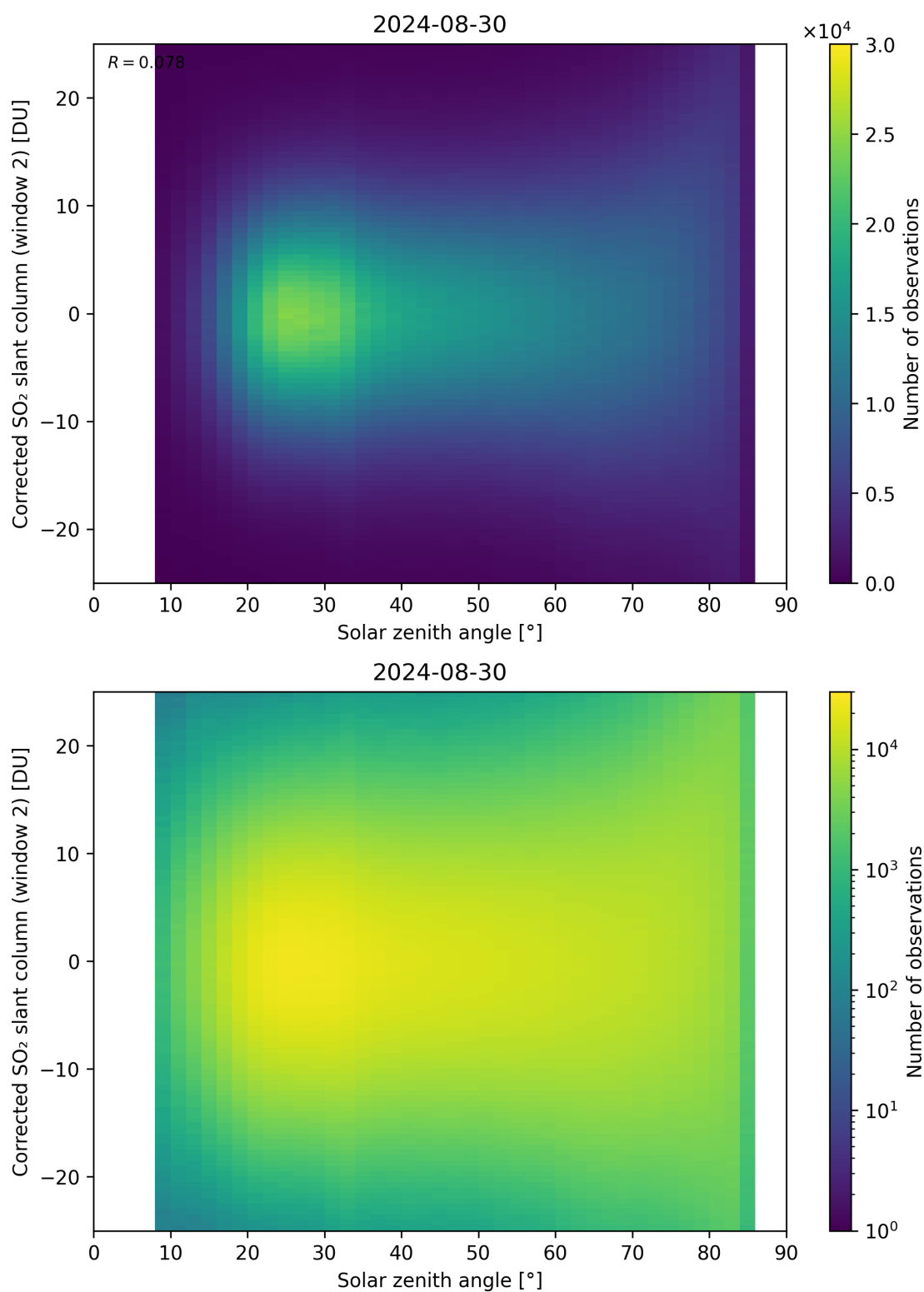
Figure 167: Scatter density plot of “Solar zenith angle” against “Corrected SO 2 slant column (window 2)” for 2024-08-29 to 2024-08-31.
