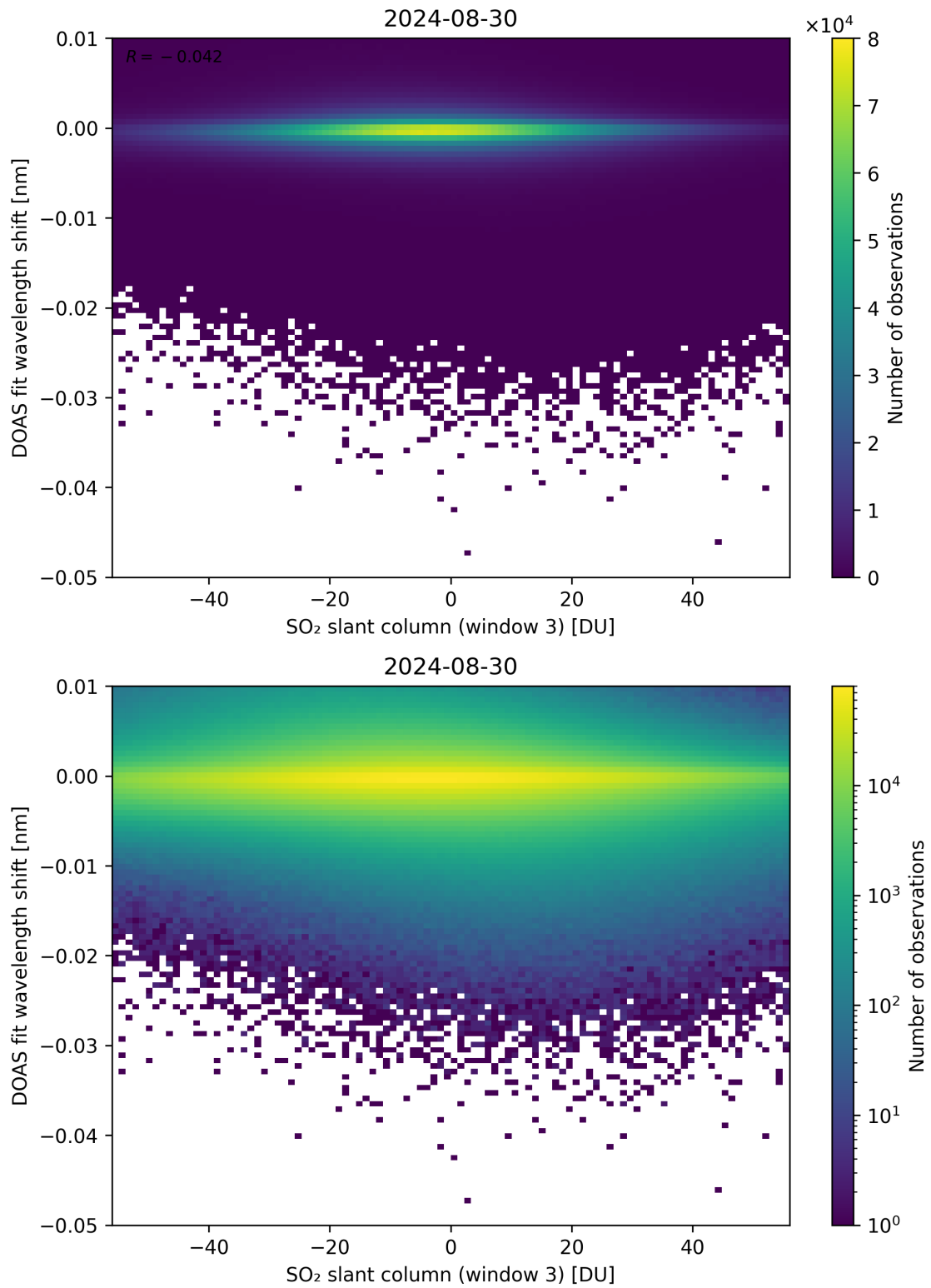
Figure 254: Scatter density plot of “SO 2 slant column (window 3)” against “DOAS fit wavelength shift” for 2024-08-29 to 2024-08-31.
