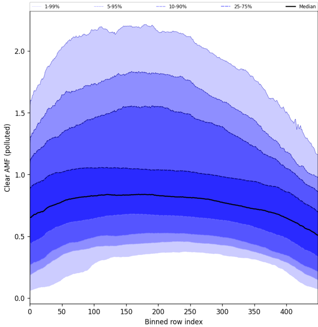
Figure 96: Along track statistics of “Clear AMF (polluted)” for 2024-08-29 to 2024-08-31
