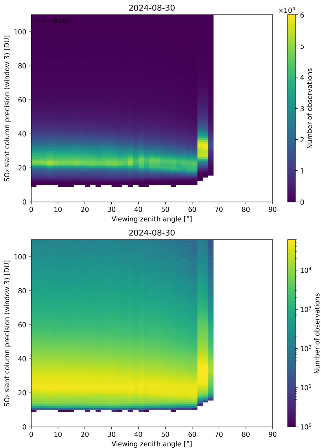
Figure 324: Scatter density plot of “Viewing zenith angle” against “SO 2 slant column precision (window 3)” for 2024-08-29 to 2024-08-31.
