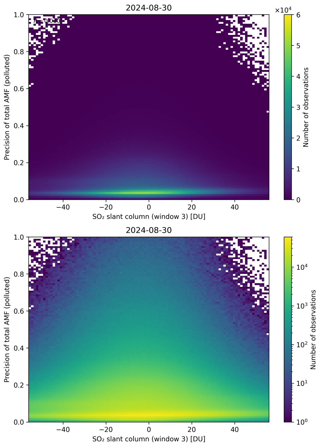
Figure 269: Scatter density plot of “SO 2 slant column (window 3)” against “Precision of total AMF (polluted)” for 2024-08-29 to 2024-08-31.
