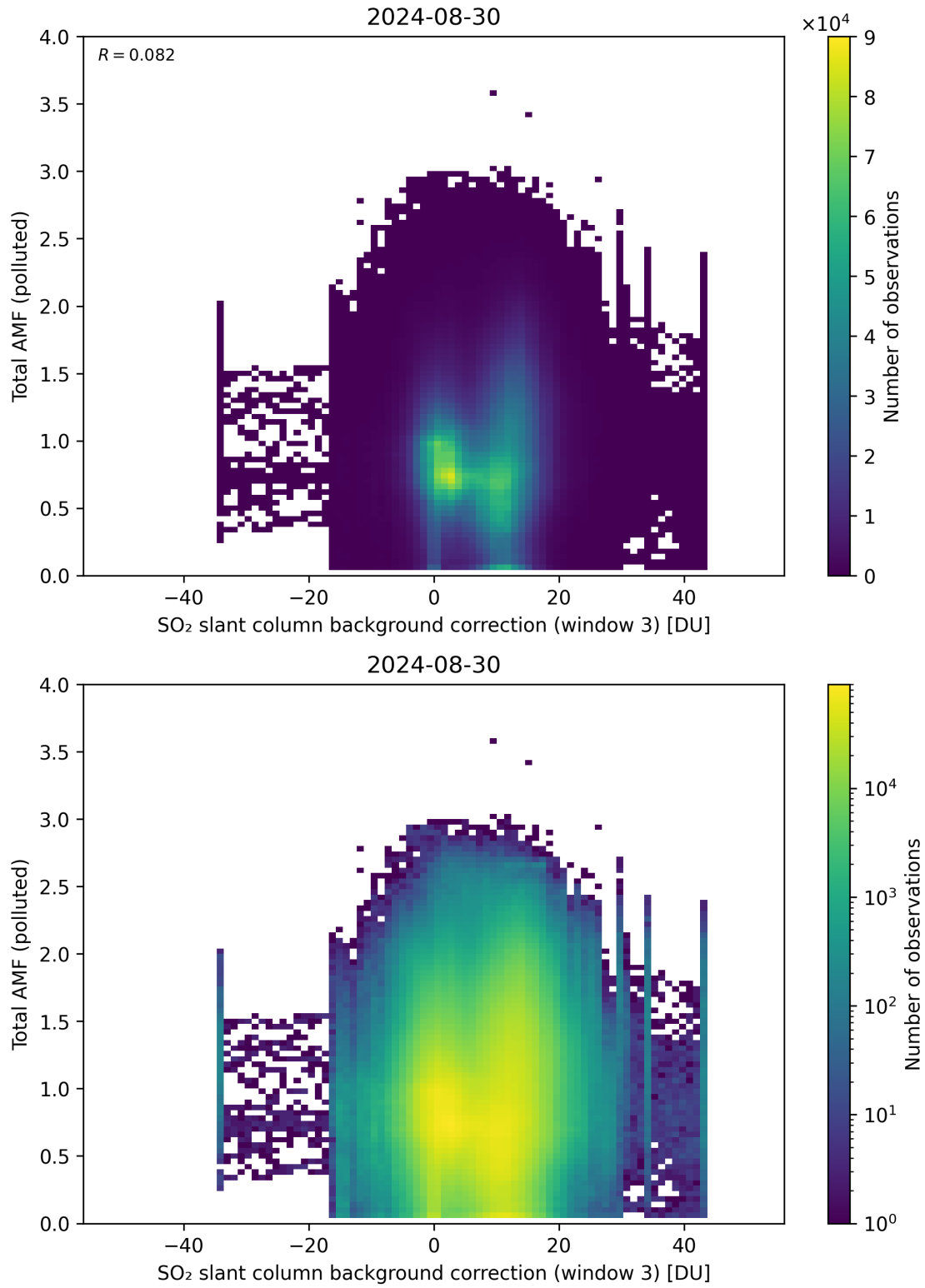
Figure 125: Scatter density plot of “SO 2 slant column background correction (window 3)” against “Total AMF (polluted)” for 2024-08-29 to 2024-08-31.
