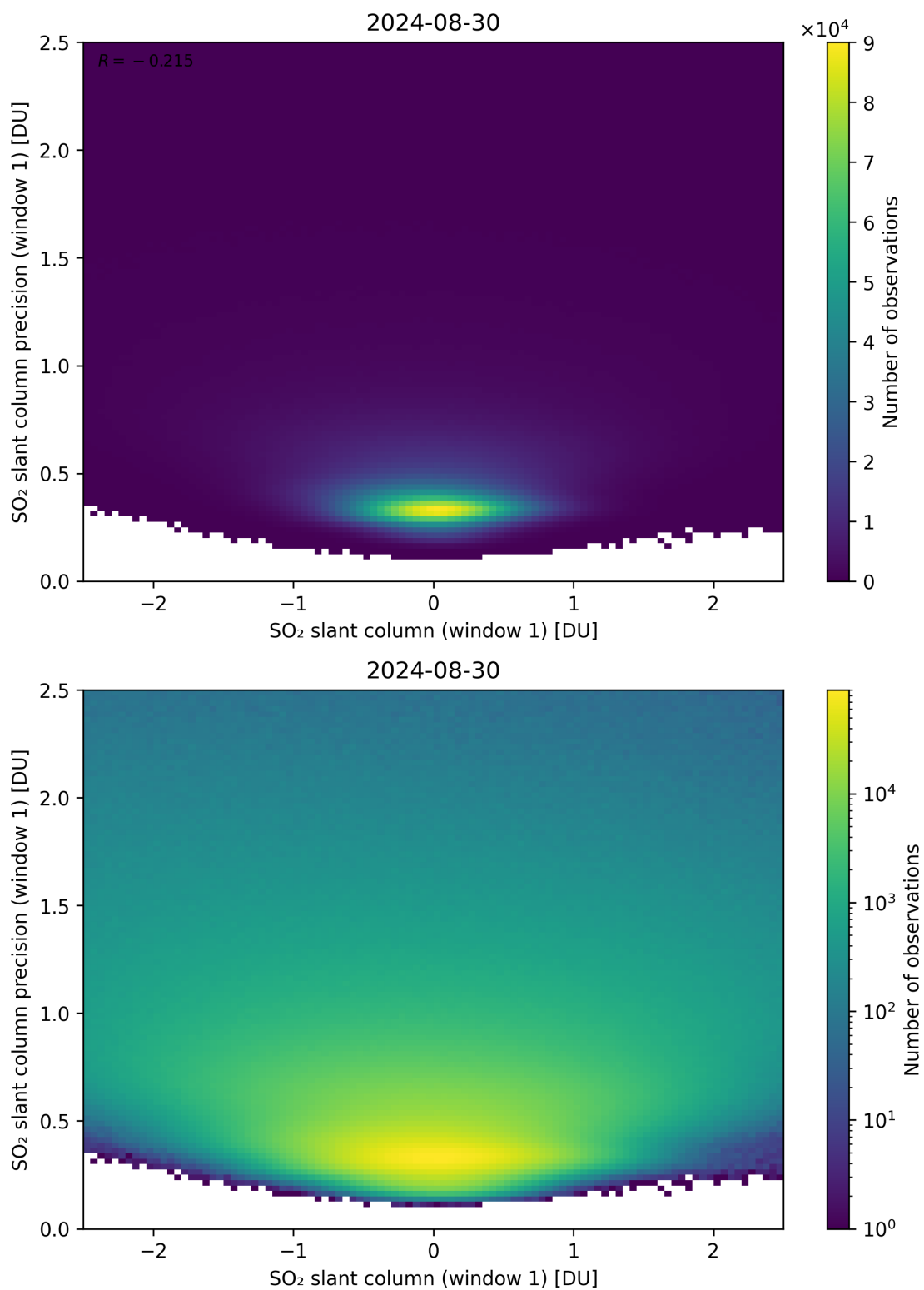
Figure 235: Scatter density plot of “SO 2 slant column (window 1)” against “SO 2 slant column precision (window 1)” for 2024-08-29 to 2024-08-31.
