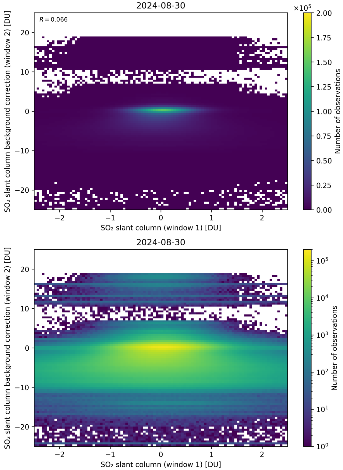
Figure 213: Scatter density plot of “SO 2 slant column (window 1)” against “SO 2 slant column background correction (window 2)” for 2024-08-29 to 2024-08-31.
