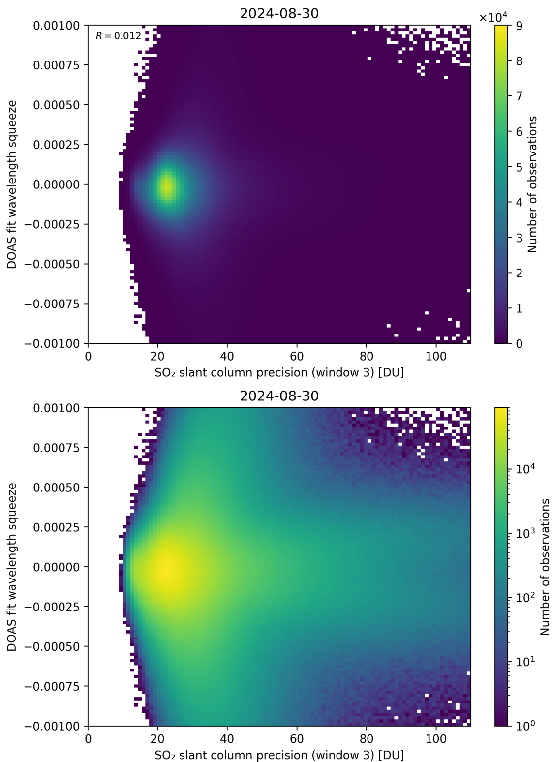
Figure 259: Scatter density plot of “SO 2 slant column precision (window 3)” against “DOAS fit wavelength squeeze” for 2024-08-29 to 2024-08-31.
