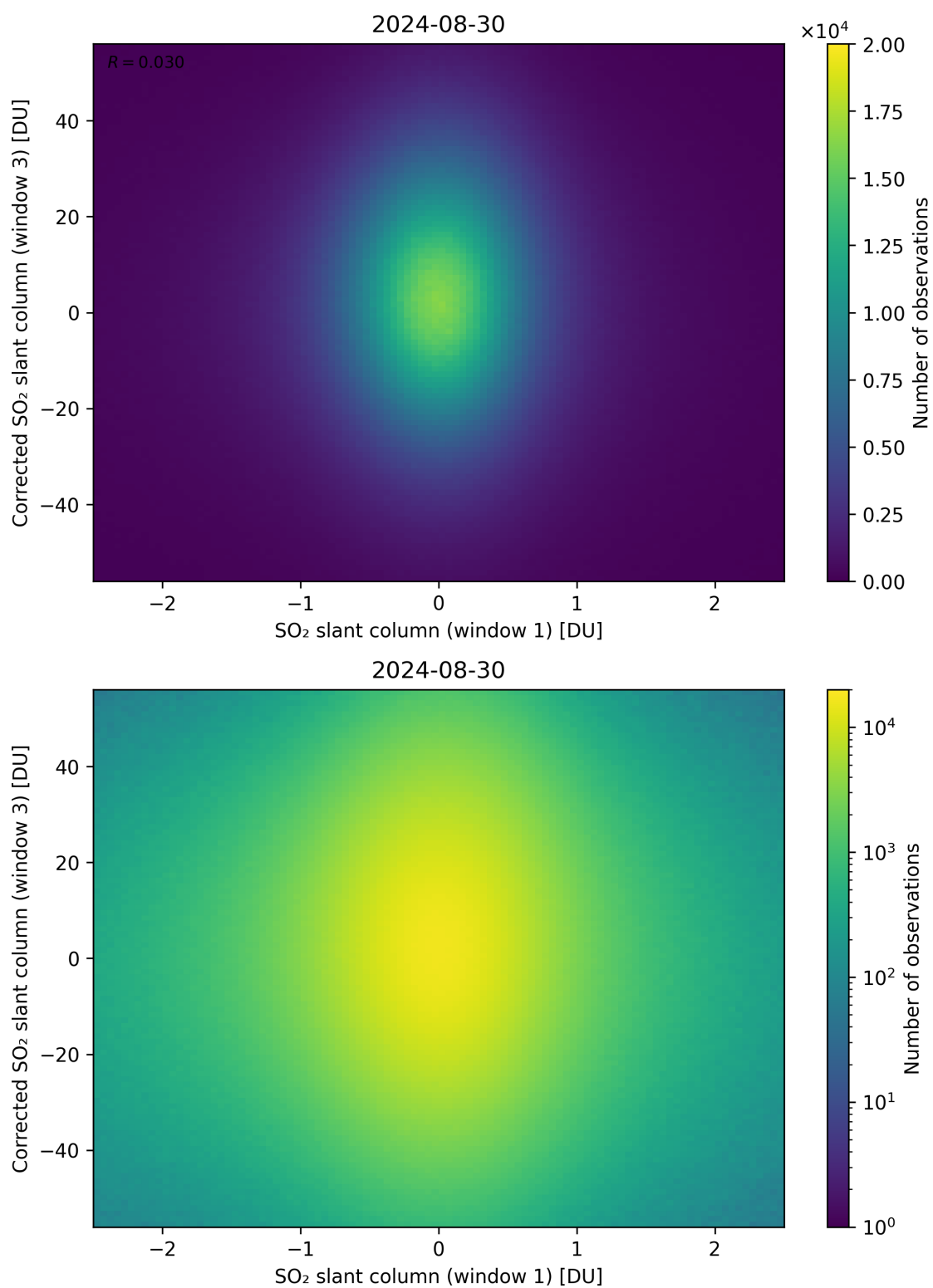
Figure 234: Scatter density plot of “SO 2 slant column (window 1)” against “Corrected SO 2 slant column (window 3)” for 2024-08-29 to 2024-08-31.
