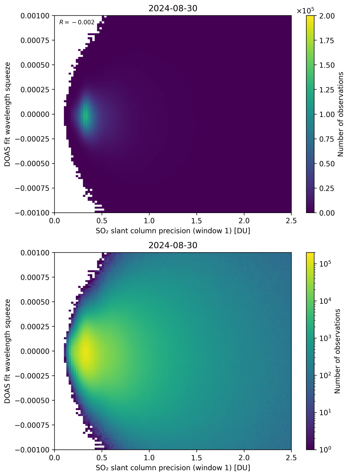
Figure 222: Scatter density plot of “SO 2 slant column precision (window 1)” against “DOAS fit wavelength squeeze” for 2024-08-29 to 2024-08-31.
