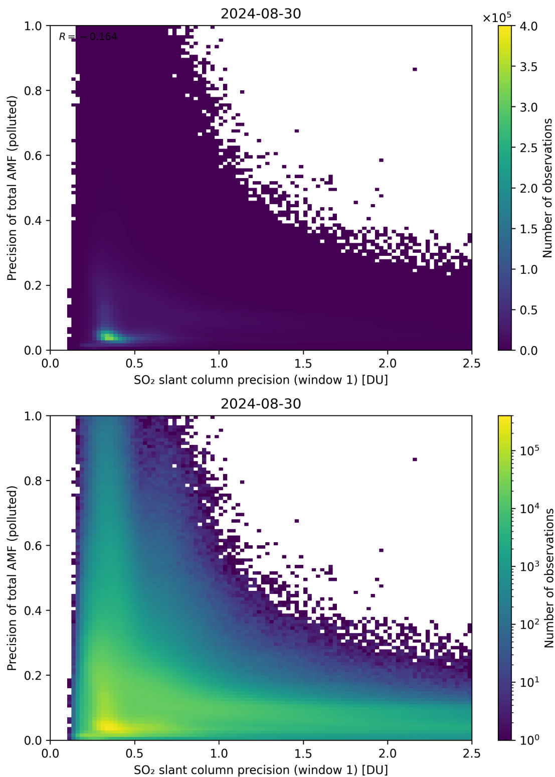
Figure 231: Scatter density plot of “SO 2 slant column precision (window 1)” against “Precision of total AMF (polluted)” for 2024-08-29 to 2024-08-31.
