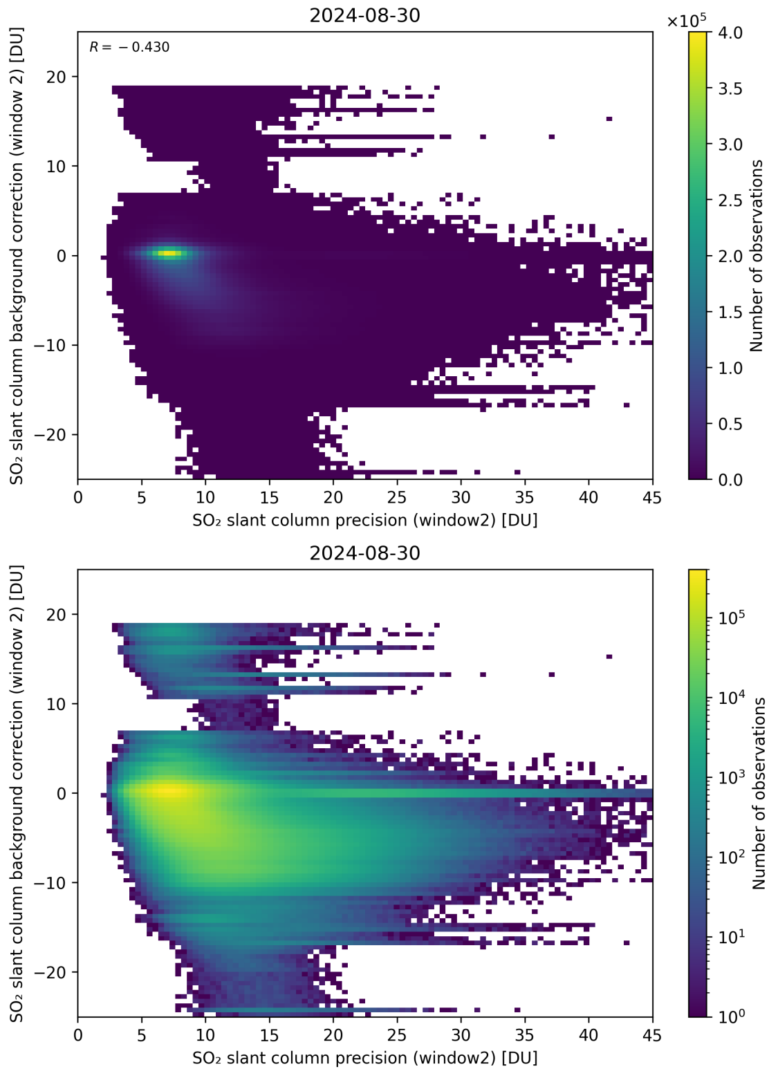
Figure 241: Scatter density plot of “SO 2 slant column precision (window2)” against “SO 2 slant column background correction (window 2)” for 2024-08-29 to 2024-08-31.
