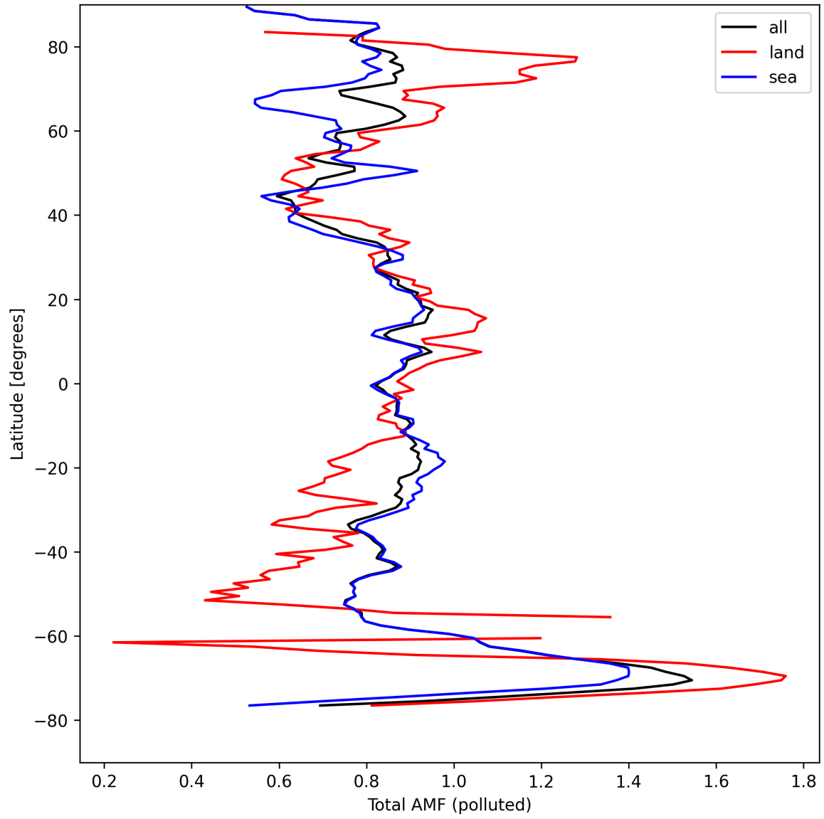
Figure 48: Zonal average of “Total AMF (polluted)” for 2024-08-29 to 2024-08-31.
