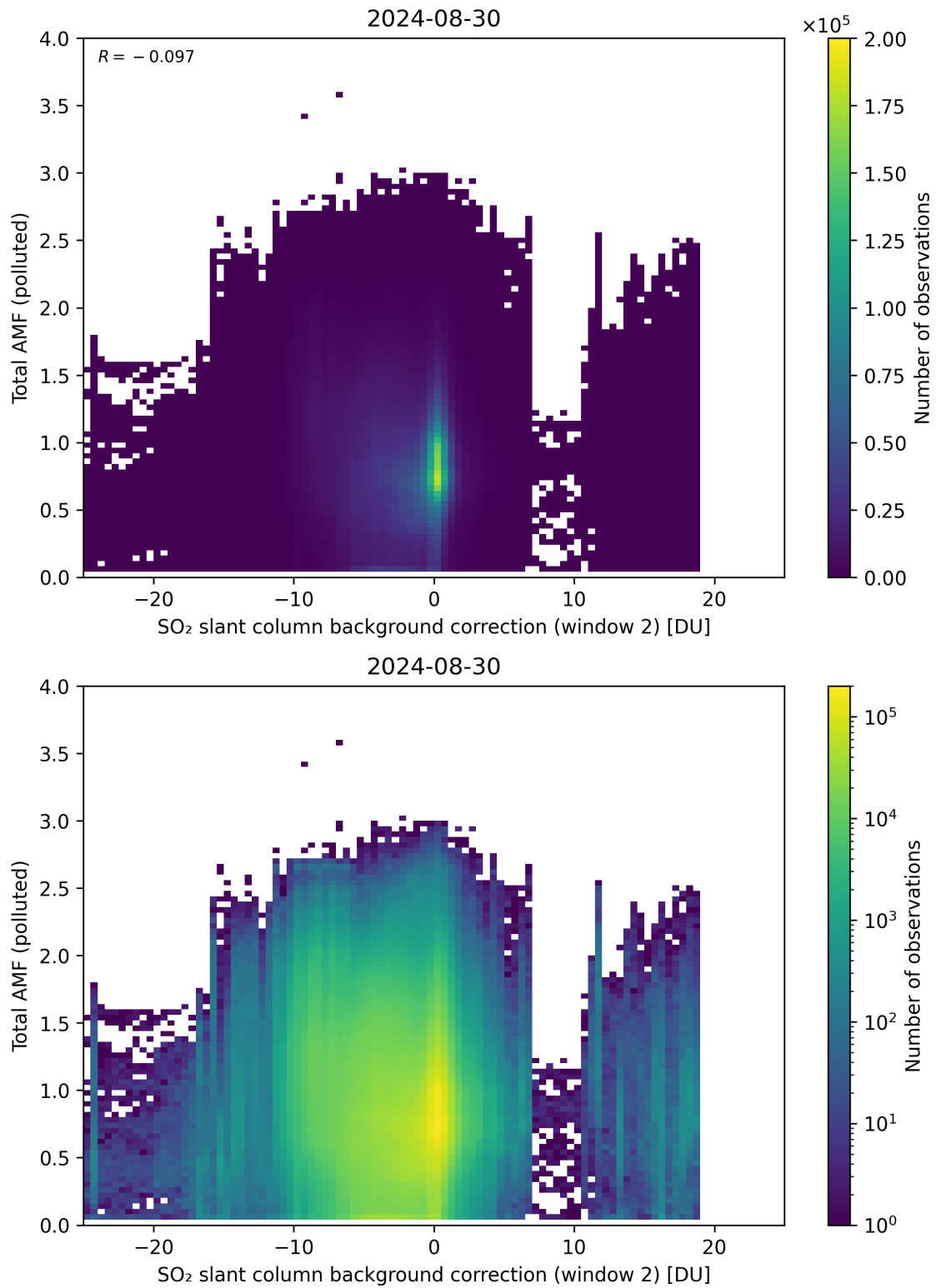
Figure 119: Scatter density plot of “SO 2 slant column background correction (window 2)” against “Total AMF (polluted)” for 2024-08-29 to 2024-08-31.
