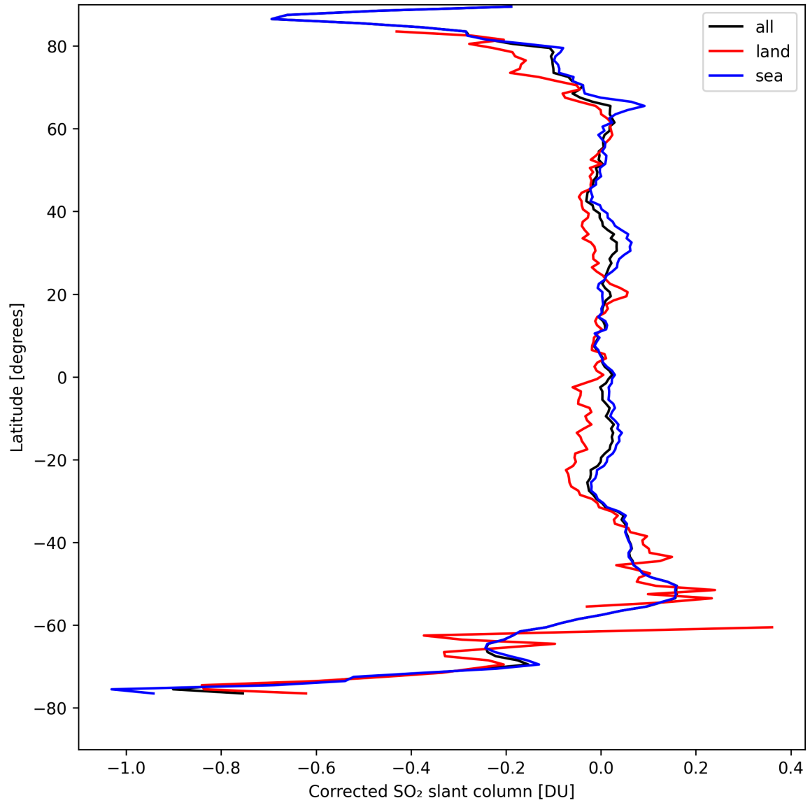
Figure 32: Zonal average of “Corrected SO 2 slant column” for 2024-08-29 to 2024-08-31.
