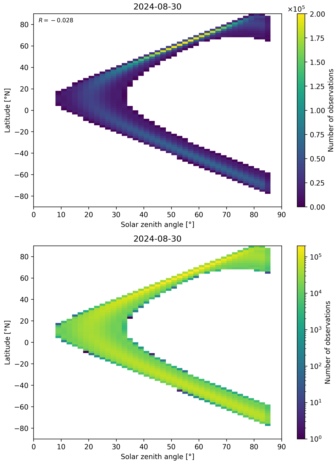
Figure 164: Scatter density plot of “Solar zenith angle” against “Latitude” for 2024-08-29 to 2024-08-31.
