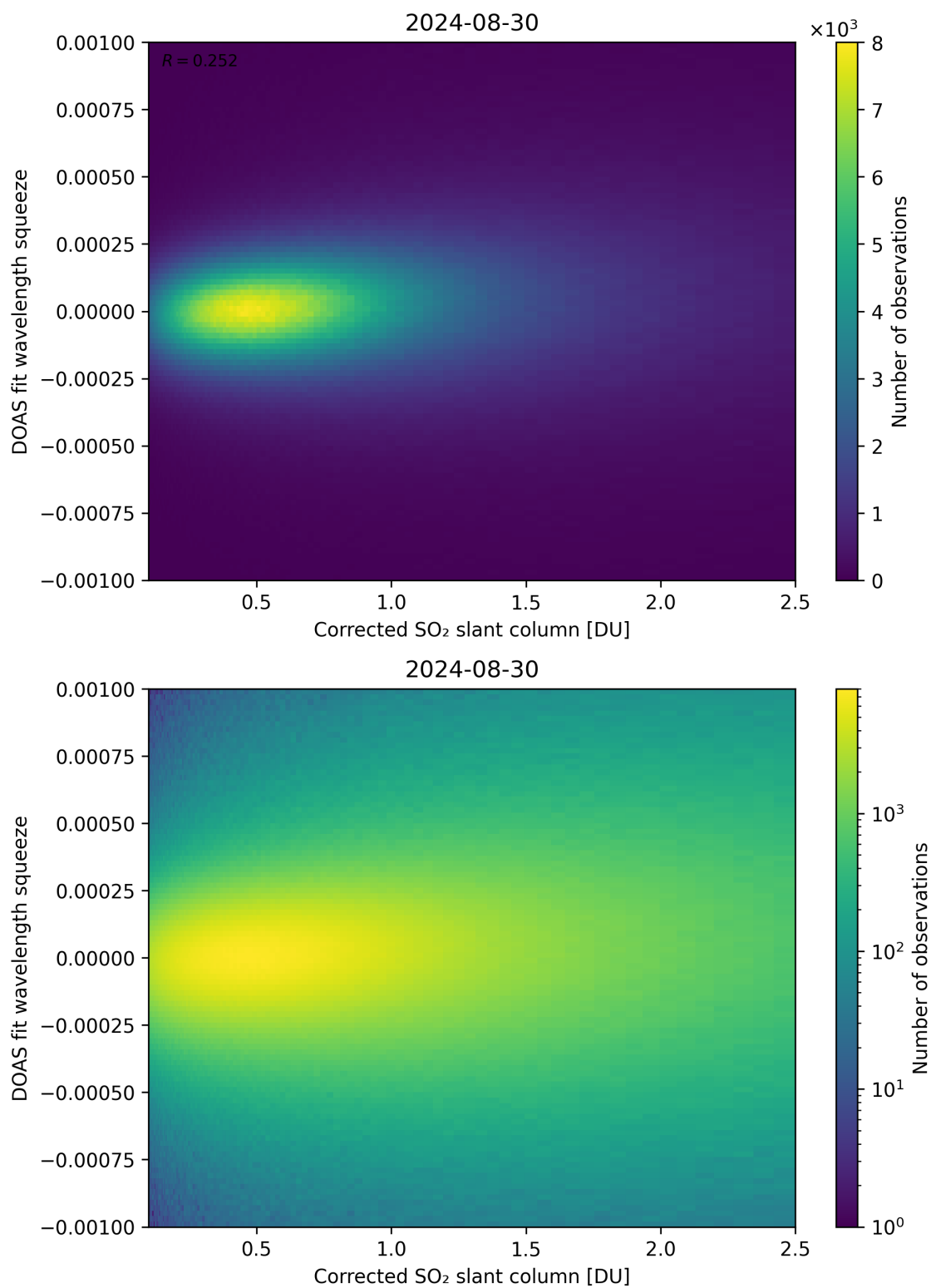
Figure 182: Scatter density plot of “Corrected SO 2 slant column” against “DOAS fit wavelength squeeze” for 2024-08-29 to 2024-08-31.
