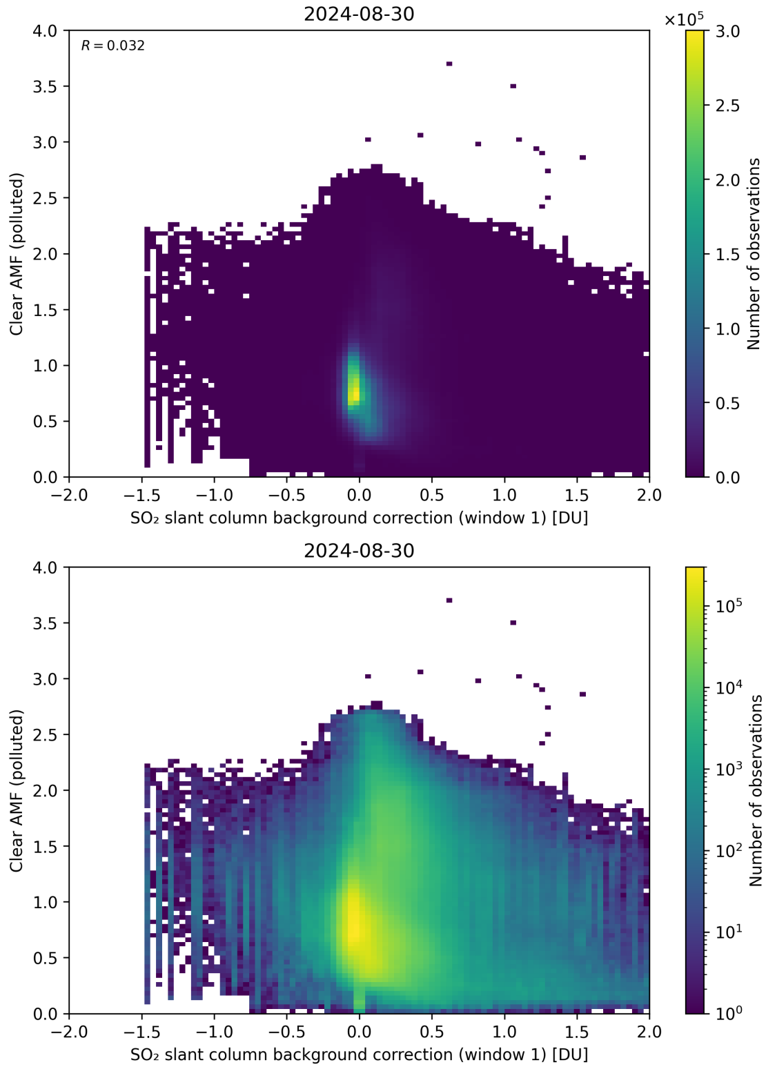
Figure 103: Scatter density plot of “SO 2 slant column background correction (window 1)” against “Clear AMF (polluted)” for 2024-08-29 to 2024-08-31.
