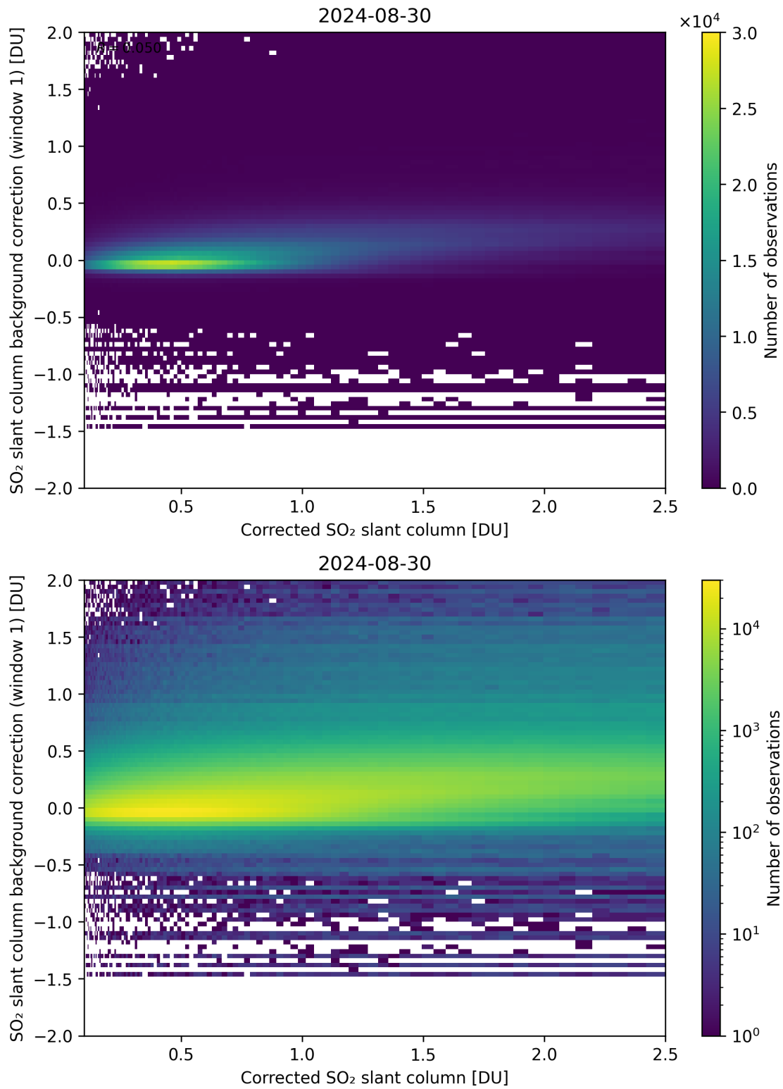
Figure 178: Scatter density plot of “Corrected SO 2 slant column” against “SO 2 slant column background correction (window 1)” for 2024-08-29 to 2024-08-31.
