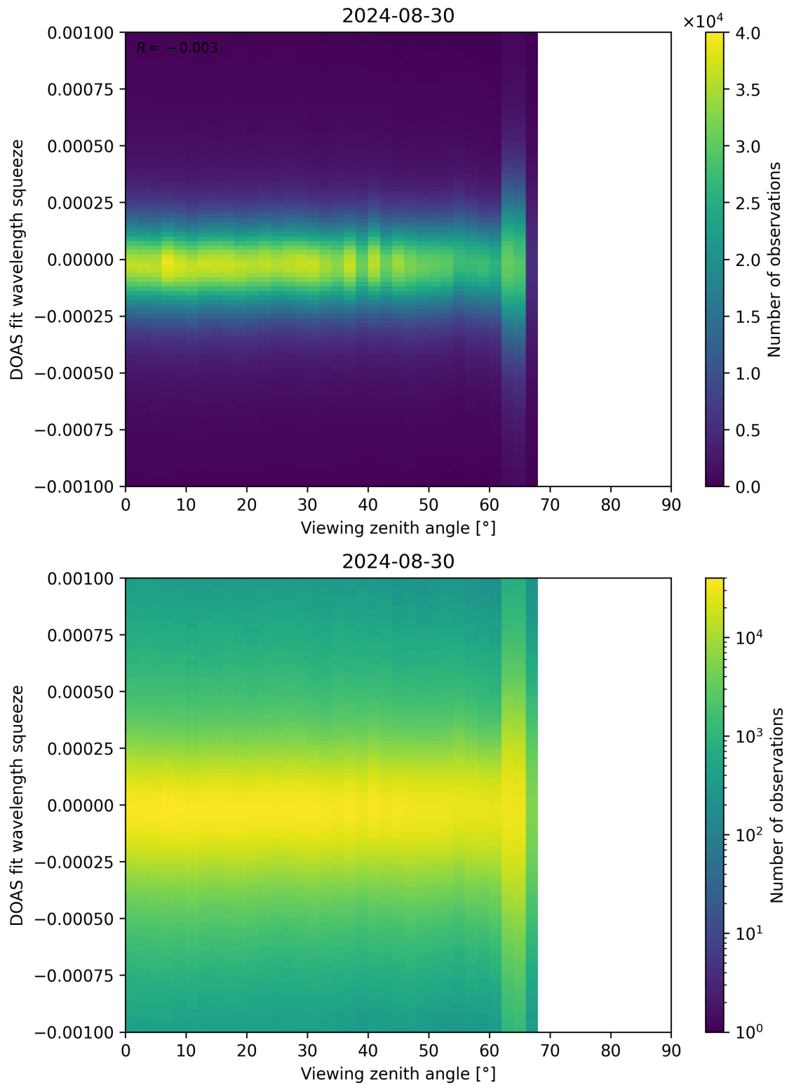
Figure 312: Scatter density plot of “Viewing zenith angle” against “DOAS fit wavelength squeeze” for 2024-08-29 to 2024-08-31.
