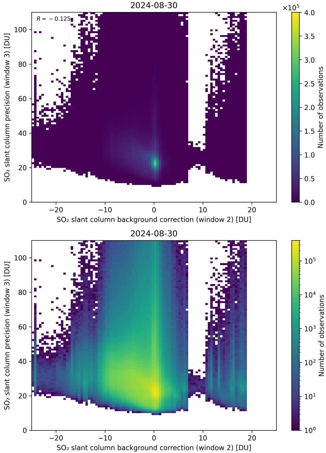
Figure 118: Scatter density plot of “SO 2 slant column background correction (window 2)” against “SO 2 slant column precision (window 3)” for 2024-08-29 to 2024-08-31.
