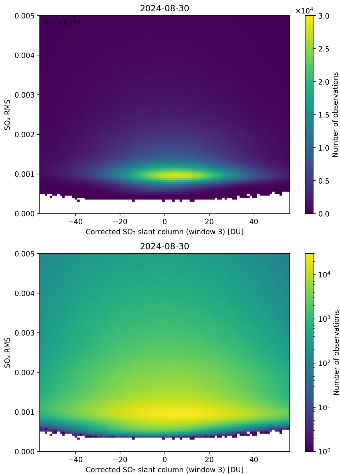
Figure 208: Scatter density plot of “Corrected SO 2 slant column (window 3)” against “SO 2 RMS” for 2024-08-29 to 2024-08-31.
