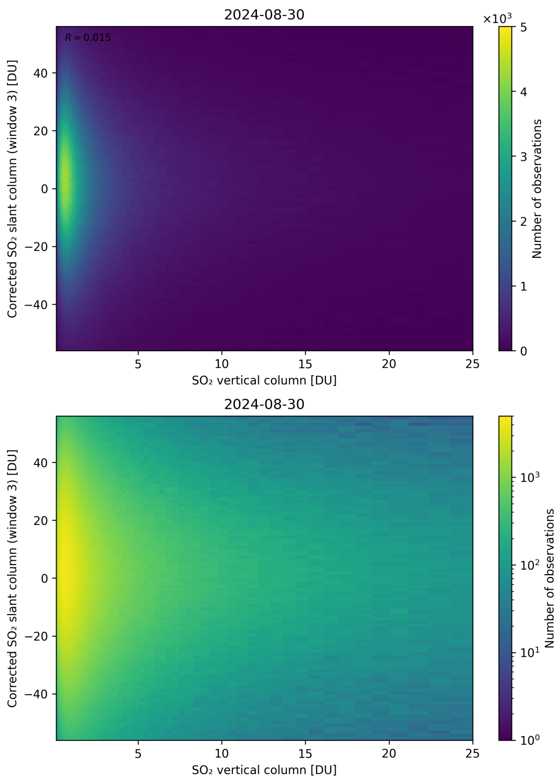
Figure 299: Scatter density plot of “SO 2 vertical column” against “Corrected SO 2 slant column (window 3)” for 2024-08-29 to 2024-08-31.
