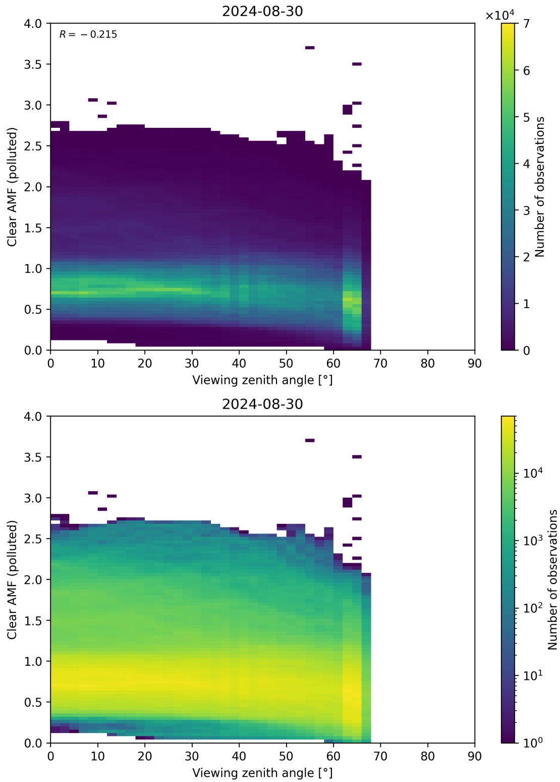
Figure 316: Scatter density plot of “Viewing zenith angle” against “Clear AMF (polluted)” for 2024-08-29 to 2024-08-31.
