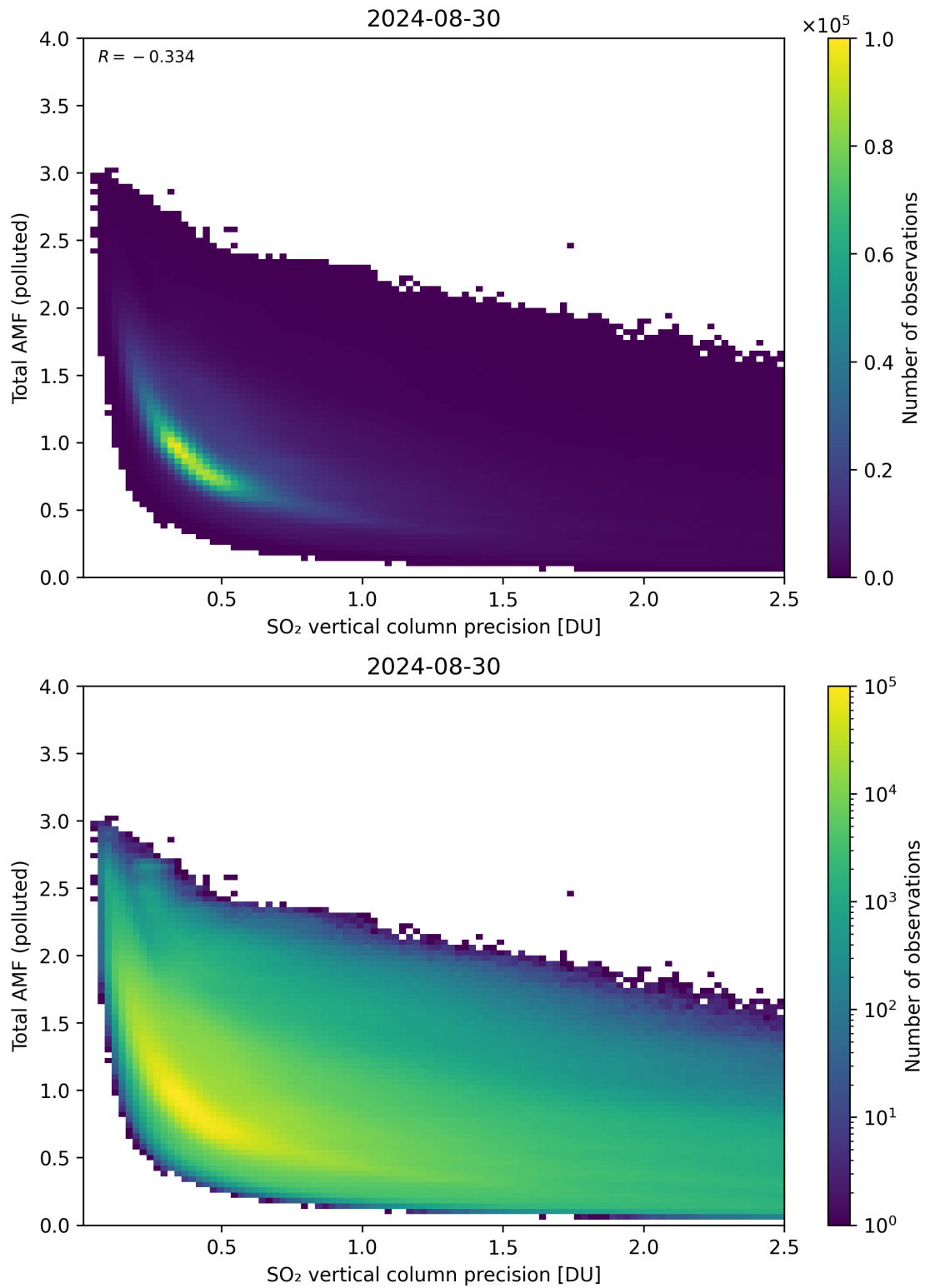
Figure 294: Scatter density plot of “SO 2 vertical column precision” against “Total AMF (polluted)” for 2024-08-29 to 2024-08-31.
