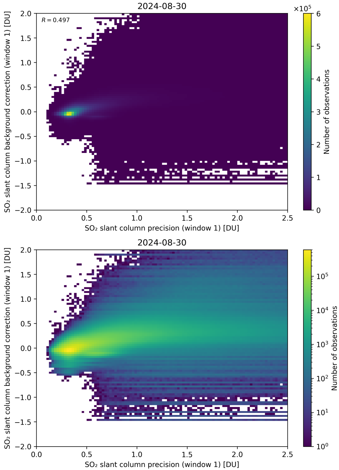
Figure 218: Scatter density plot of “SO 2 slant column precision (window 1)” against “SO 2 slant column background correction (window 1)” for 2024-08-29 to 2024-08-31.
