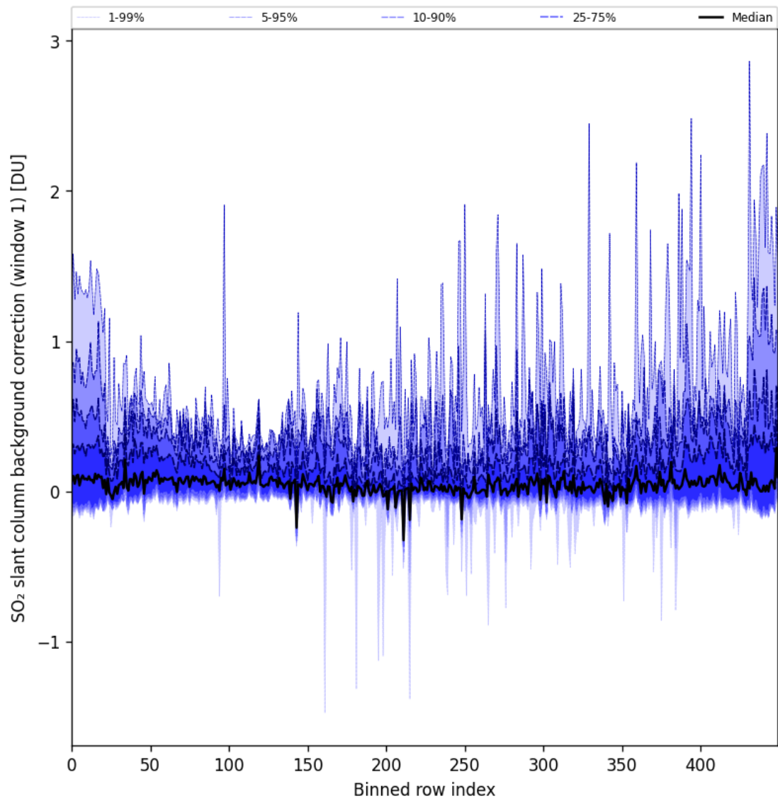
Figure 82: Along track statistics of “SO 2 slant column background correction (window 1)” for 2024-08-29 to 2024-08-31
