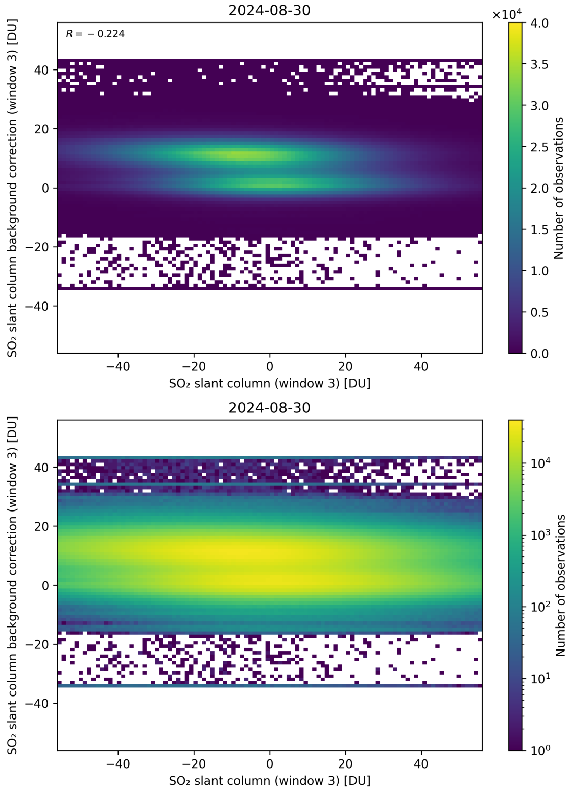
Figure 253: Scatter density plot of “SO 2 slant column (window 3)” against “SO 2 slant column background correction (window 3)” for 2024-08-29 to 2024-08-31.
