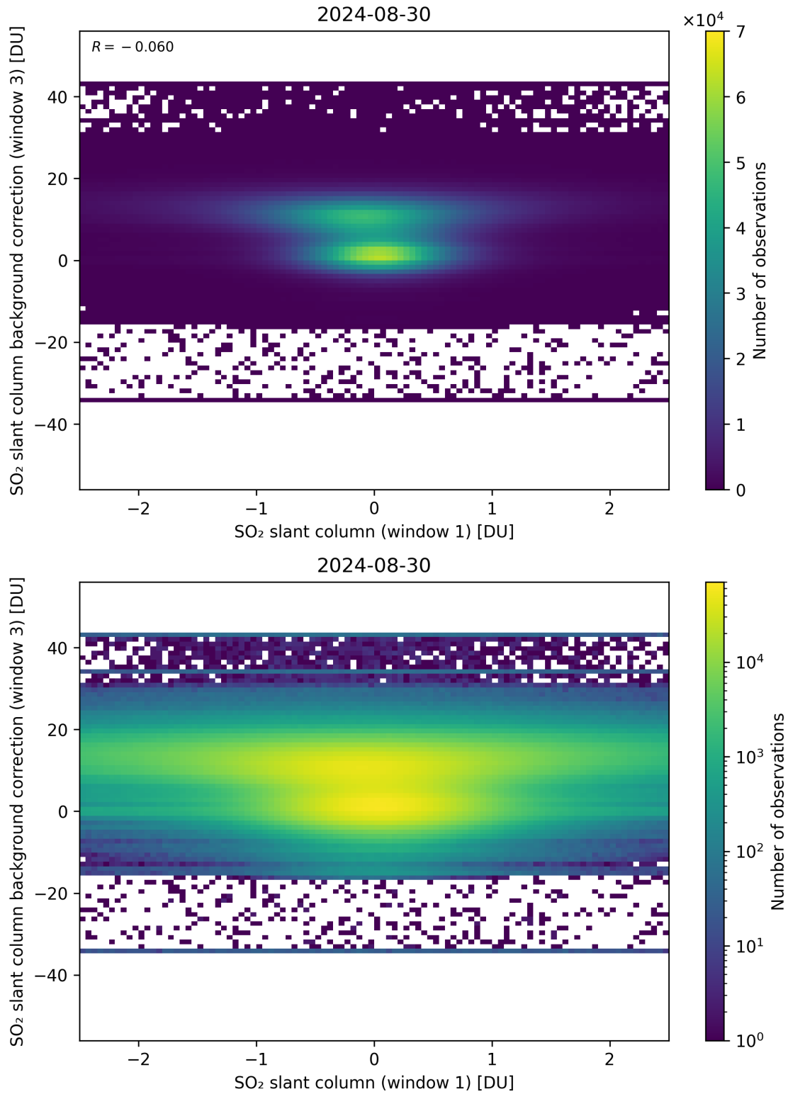
Figure 214: Scatter density plot of “SO 2 slant column (window 1)” against “SO 2 slant column background correction (window 3)” for 2024-08-29 to 2024-08-31.
