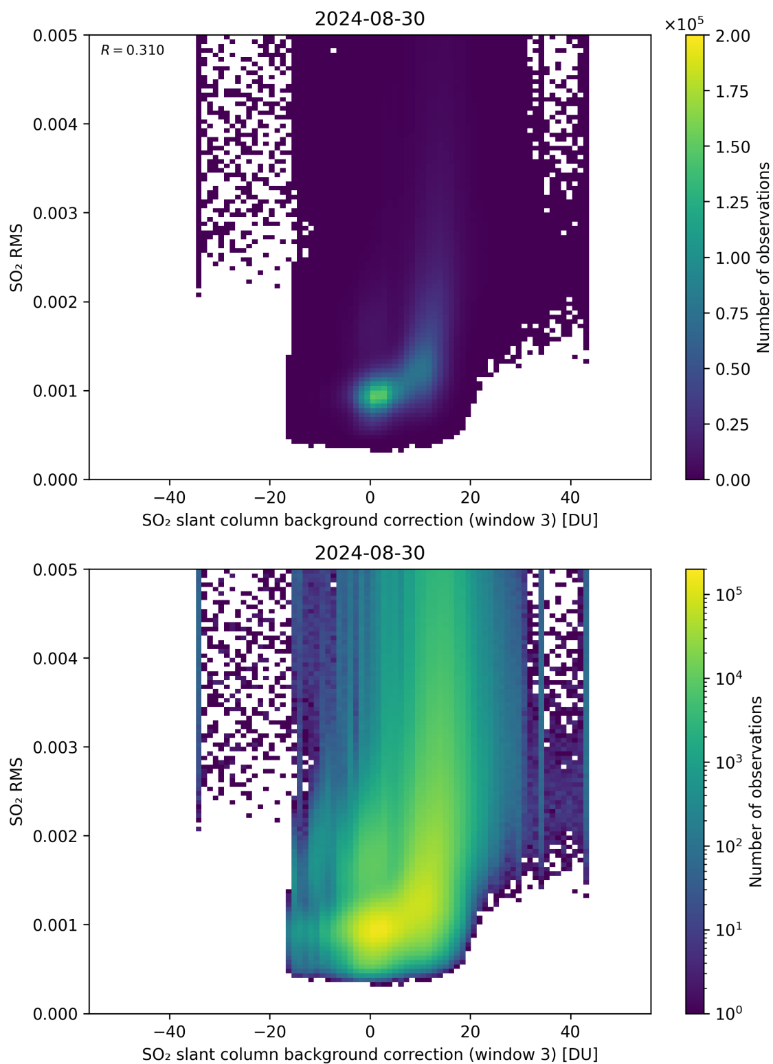
Figure 123: Scatter density plot of “SO 2 slant column background correction (window 3)” against “SO 2 RMS” for 2024-08-29 to 2024-08-31.
