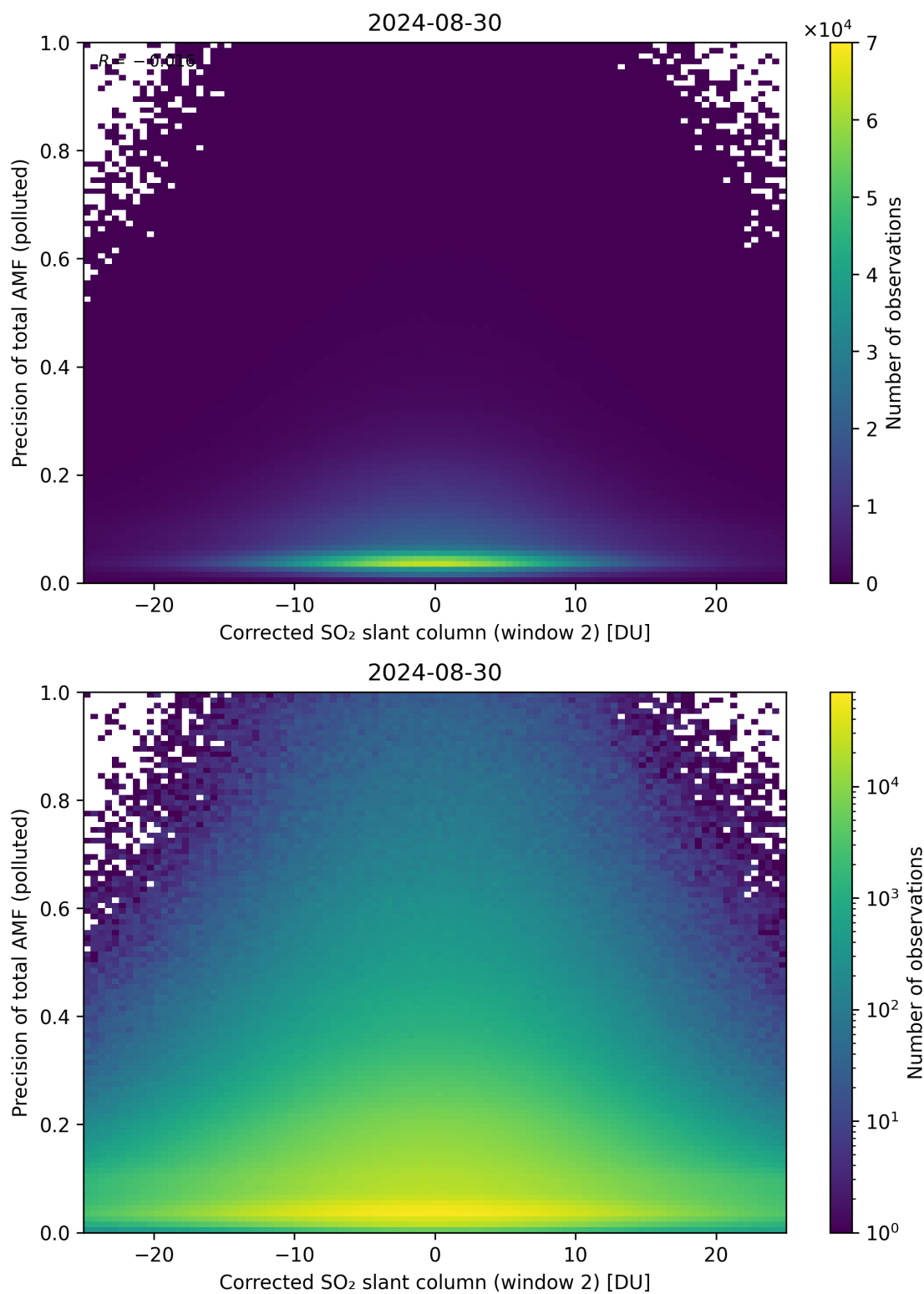
Figure 204: Scatter density plot of “Corrected SO 2 slant column (window 2)” against “Precision of total AMF (polluted)” for 2024-08-29 to 2024-08-31.
