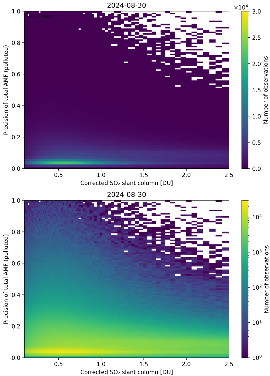
Figure 193: Scatter density plot of “Corrected SO 2 slant column” against “Precision of total AMF (polluted)” for 2024-08-29 to 2024-08-31.
