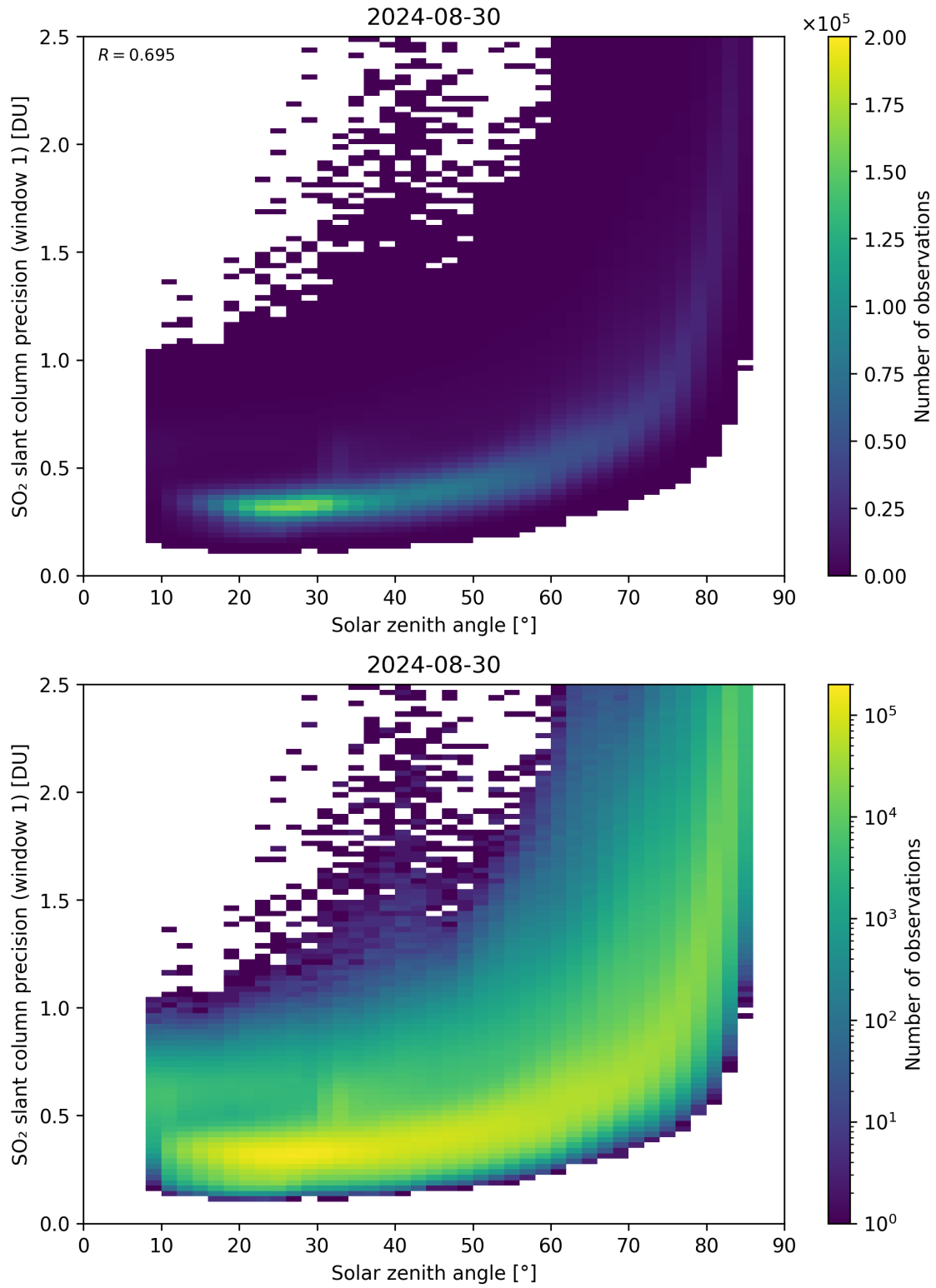
Figure 170: Scatter density plot of “Solar zenith angle” against “SO 2 slant column precision (window 1)” for 2024-08-29 to 2024-08-31.
