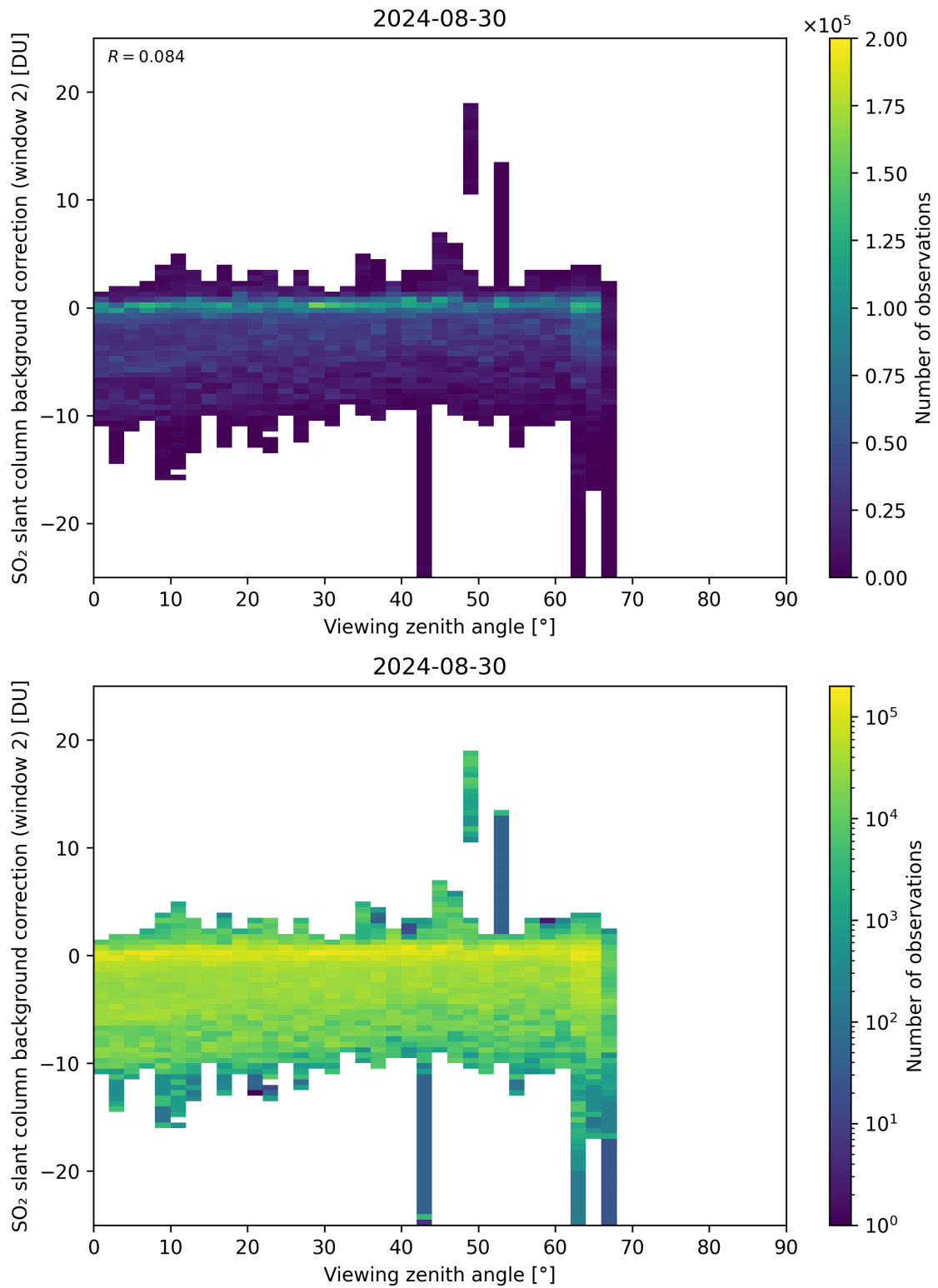
Figure 309: Scatter density plot of “Viewing zenith angle” against “SO 2 slant column background correction (window 2)” for 2024-08-29 to 2024-08-31.
