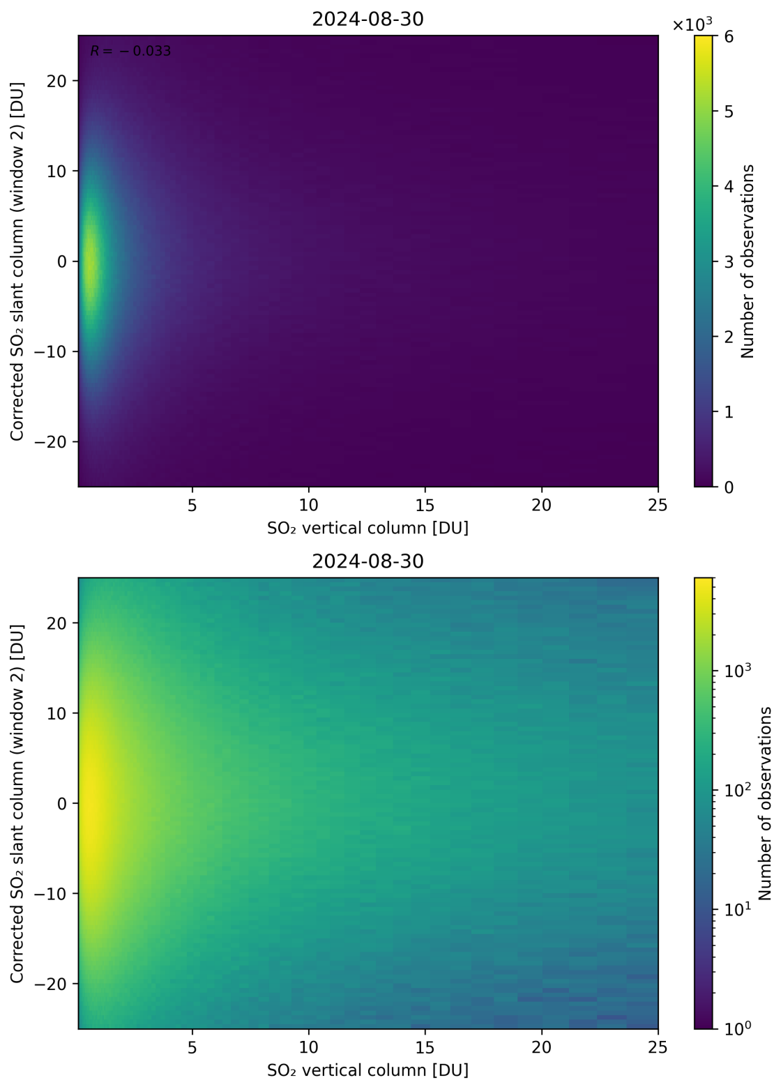
Figure 298: Scatter density plot of “SO 2 vertical column” against “Corrected SO 2 slant column (window 2)” for 2024-08-29 to 2024-08-31.
