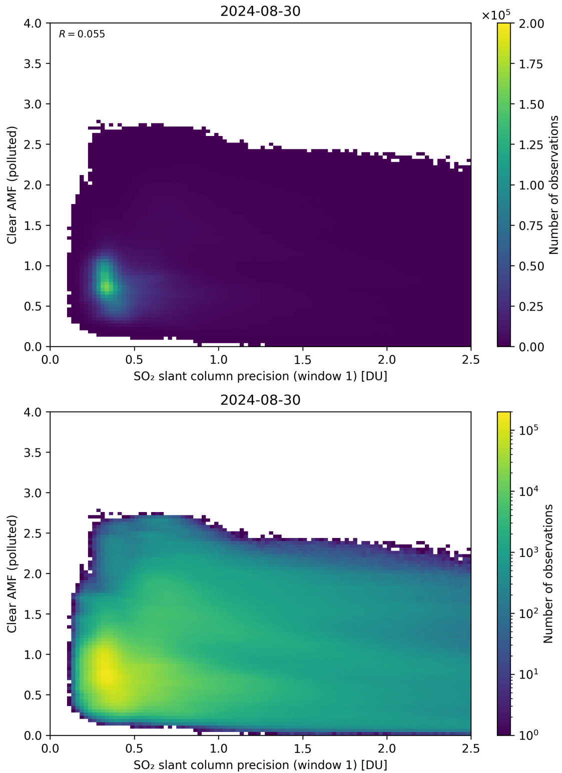
Figure 224: Scatter density plot of “SO 2 slant column precision (window 1)” against “Clear AMF (polluted)” for 2024-08-29 to 2024-08-31.
