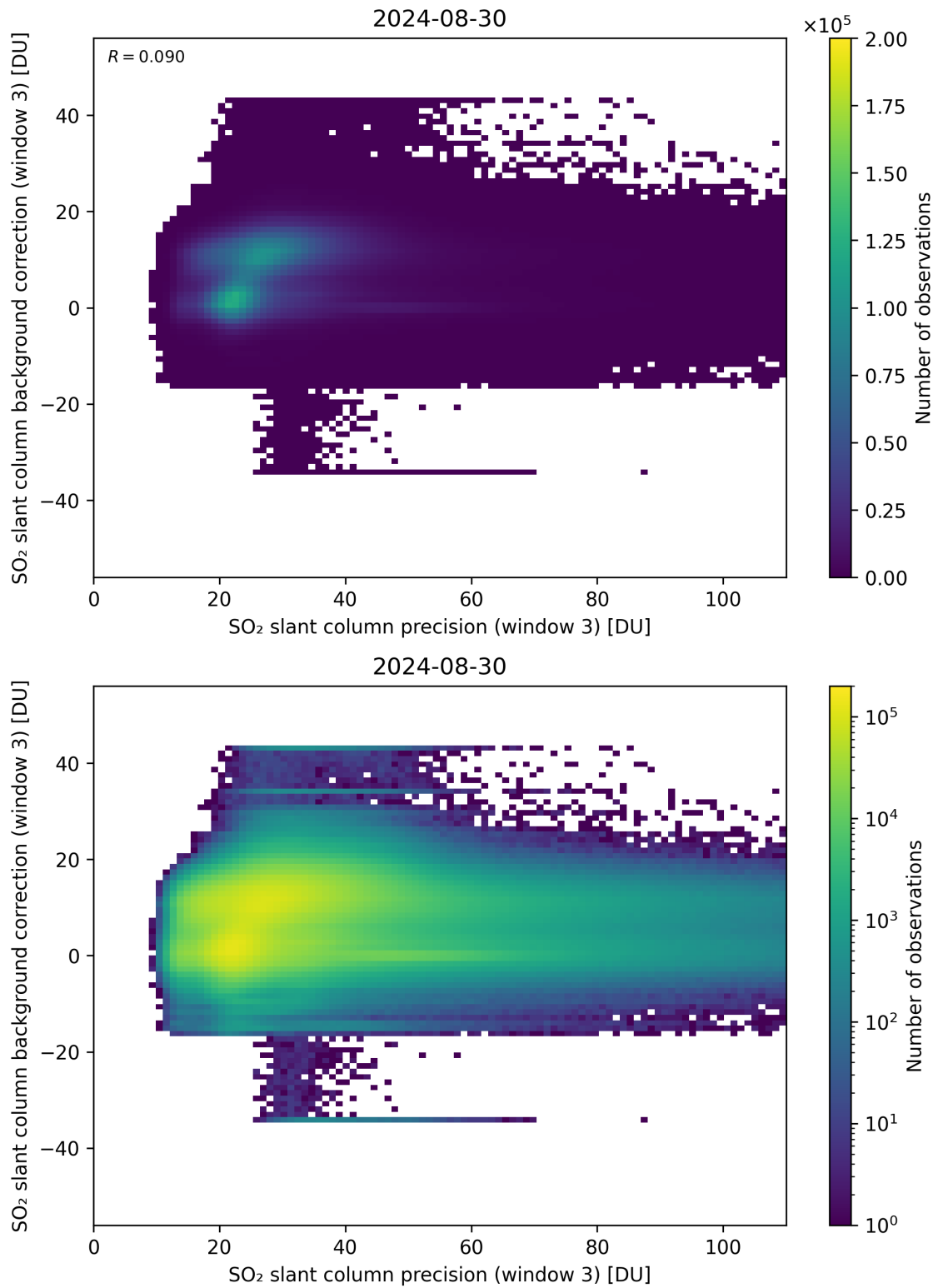
Figure 257: Scatter density plot of “SO 2 slant column precision (window 3)” against “SO 2 slant column background correction (window 3)” for 2024-08-29 to 2024-08-31.
