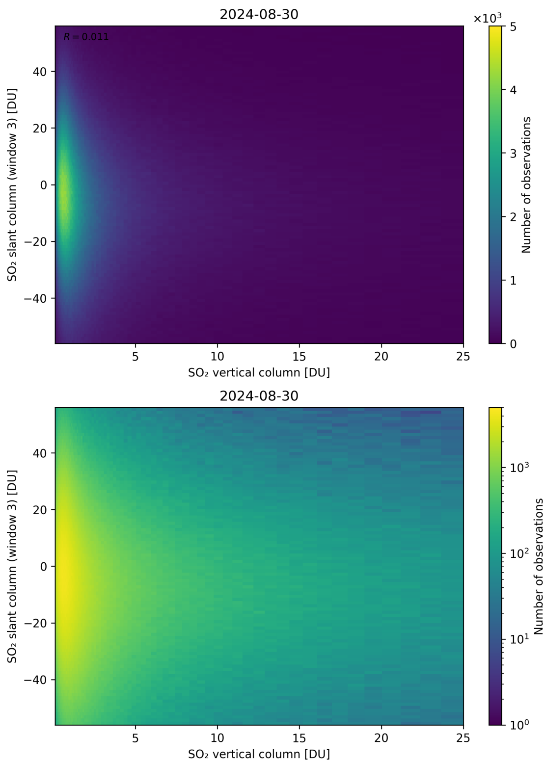
Figure 303: Scatter density plot of “SO 2 vertical column” against “SO 2 slant column (window 3)” for 2024-08-29 to 2024-08-31.
