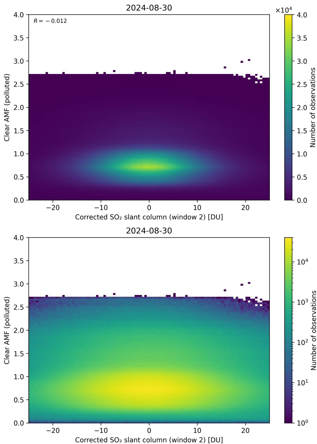
Figure 199: Scatter density plot of “Corrected SO 2 slant column (window 2)” against “Clear AMF (polluted)” for 2024-08-29 to 2024-08-31.
