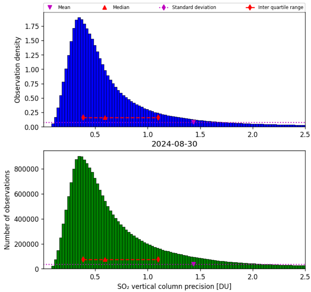
Figure 54: Histogram of “SO 2 vertical column precision” for 2024-08-29 to 2024-08-31
