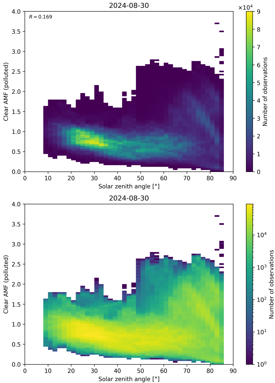
Figure 165: Scatter density plot of “Solar zenith angle” against “Clear AMF (polluted)” for 2024-08-29 to 2024-08-31.
