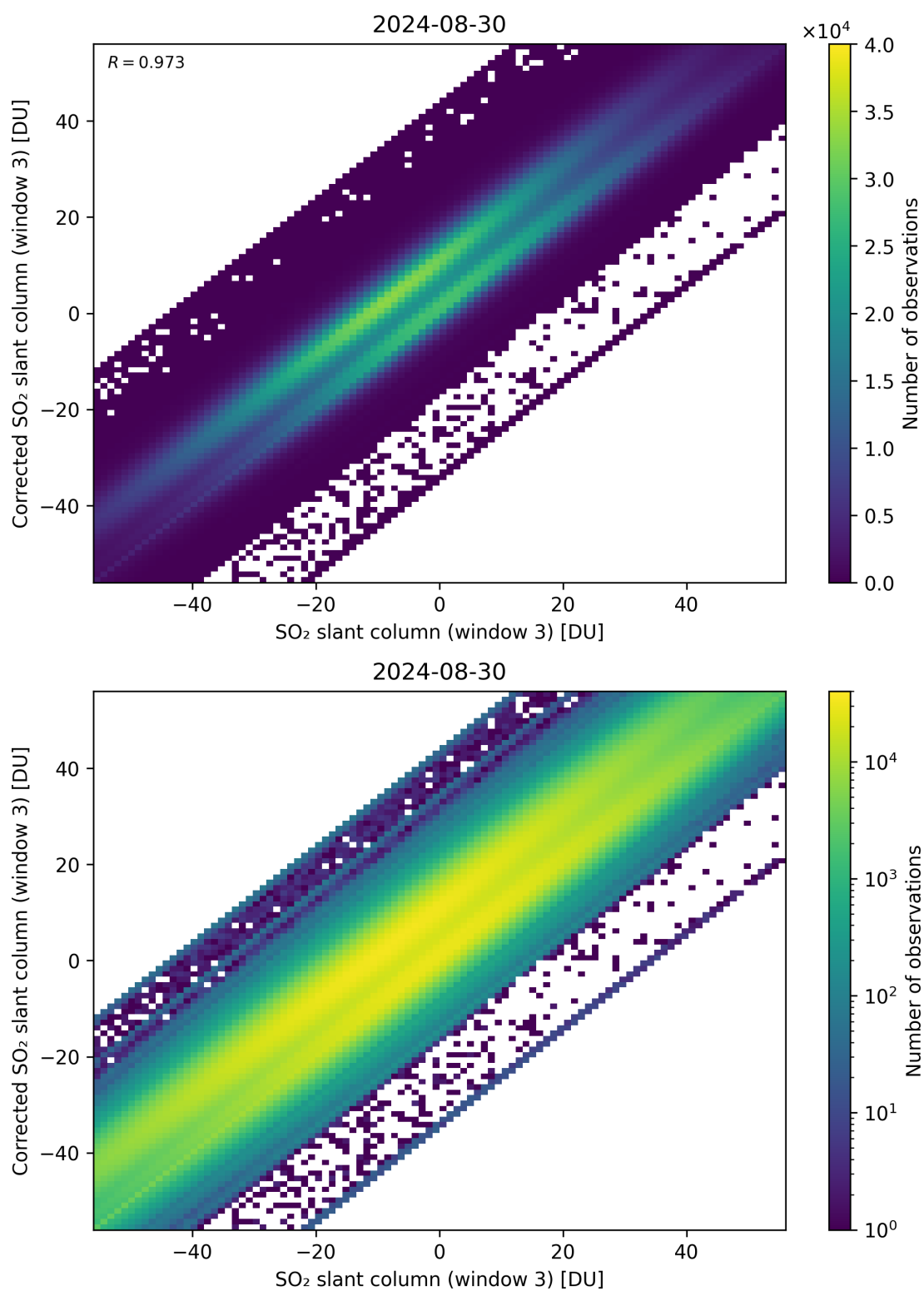
Figure 266: Scatter density plot of “SO 2 slant column (window 3)” against “Corrected SO 2 slant column (window 3)” for 2024-08-29 to 2024-08-31.
