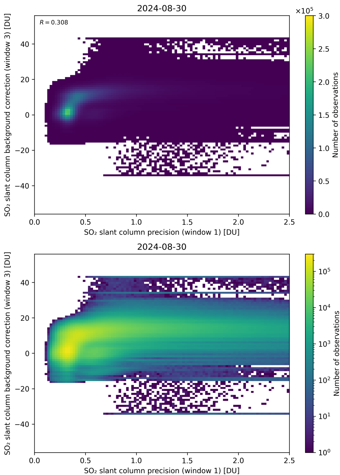
Figure 220: Scatter density plot of “SO 2 slant column precision (window 1)” against “SO 2 slant column background correction (window 3)” for 2024-08-29 to 2024-08-31.
