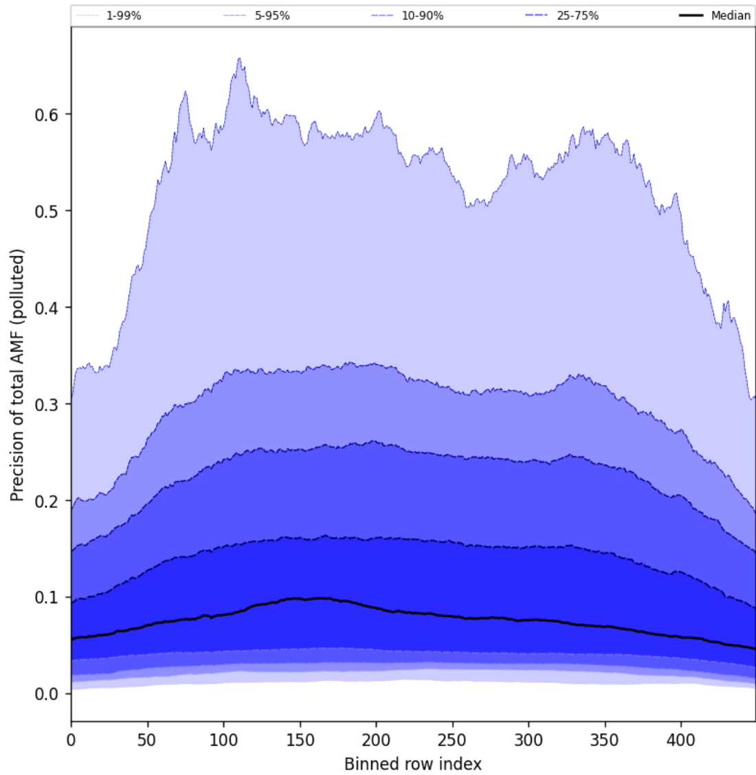
Figure 95: Along track statistics of “Precision of total AMF (polluted)” for 2024-08-29 to 2024-08-31
