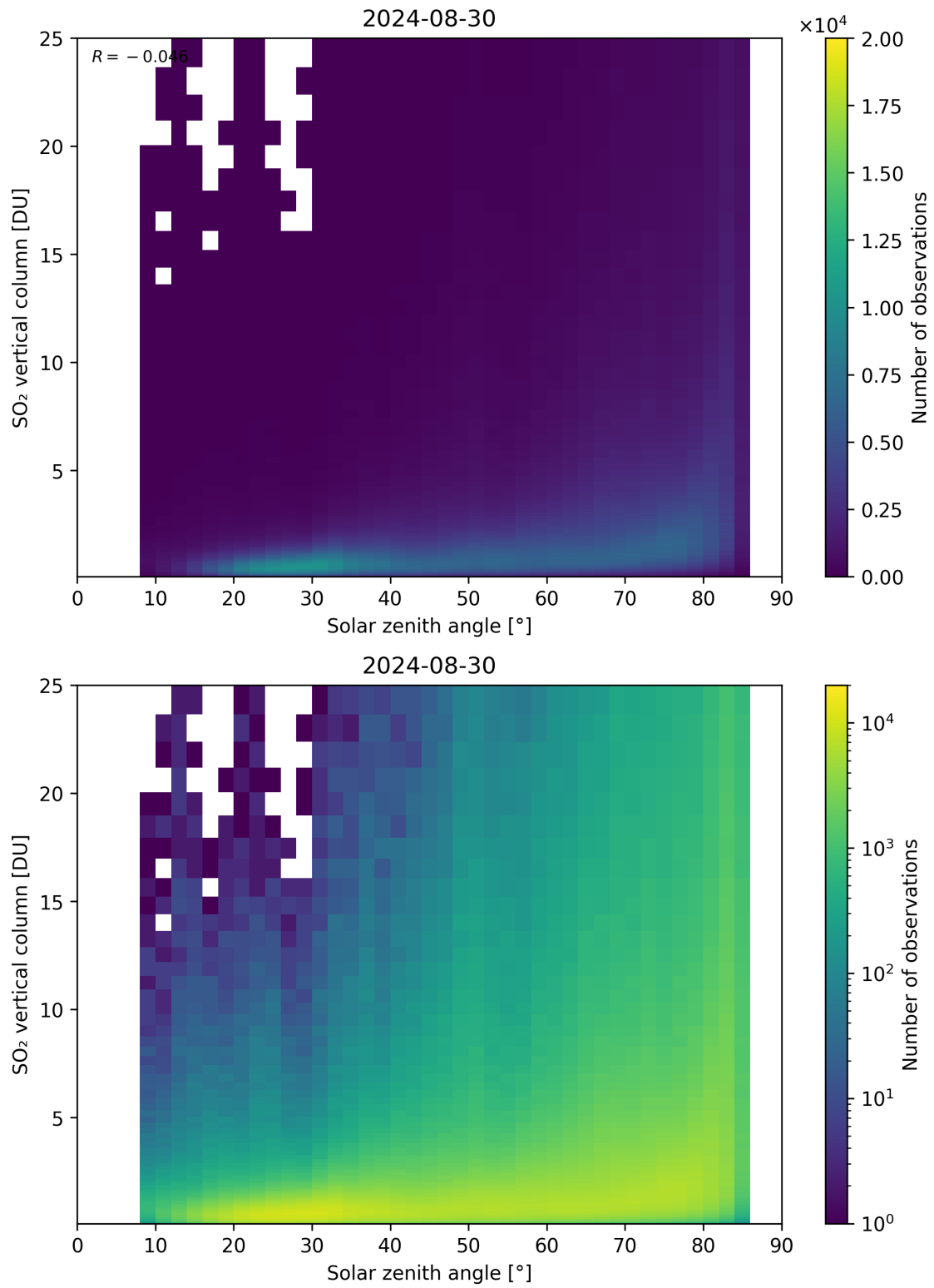
Figure 176: Scatter density plot of “Solar zenith angle” against “SO 2 vertical column” for 2024-08-29 to 2024-08-31.
