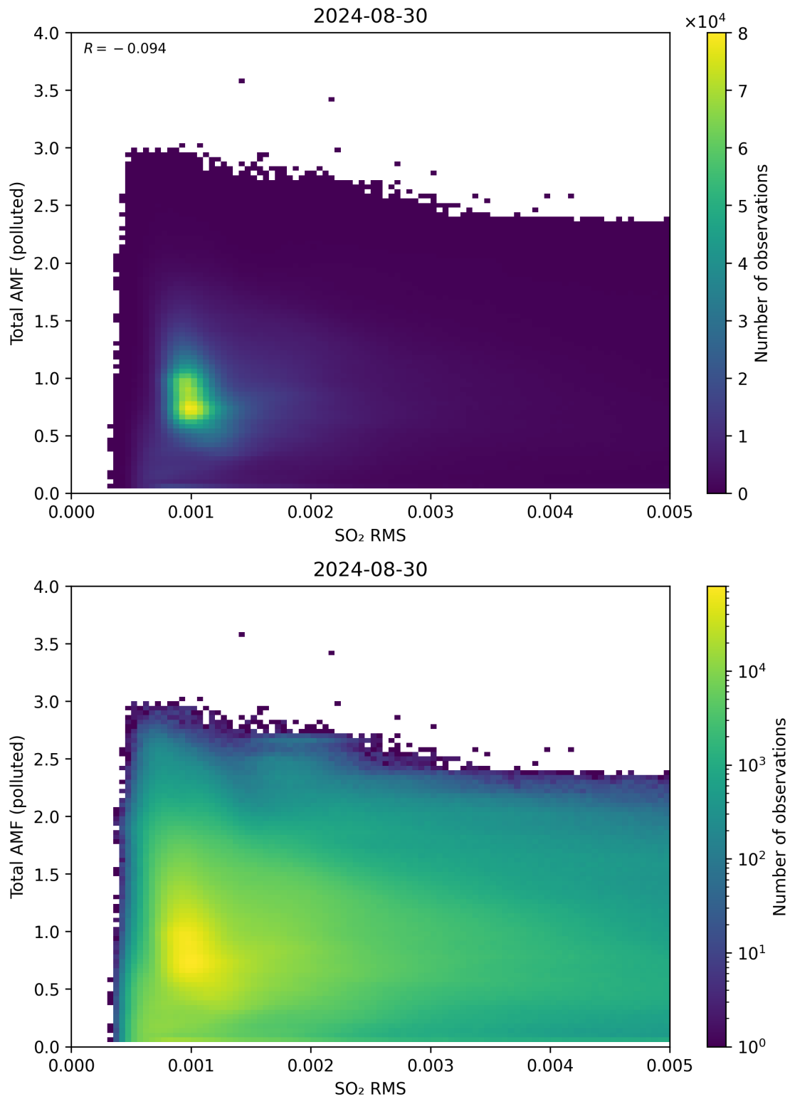
Figure 137: Scatter density plot of “SO 2 RMS” against “Total AMF (polluted)” for 2024-08-29 to 2024-08-31.
