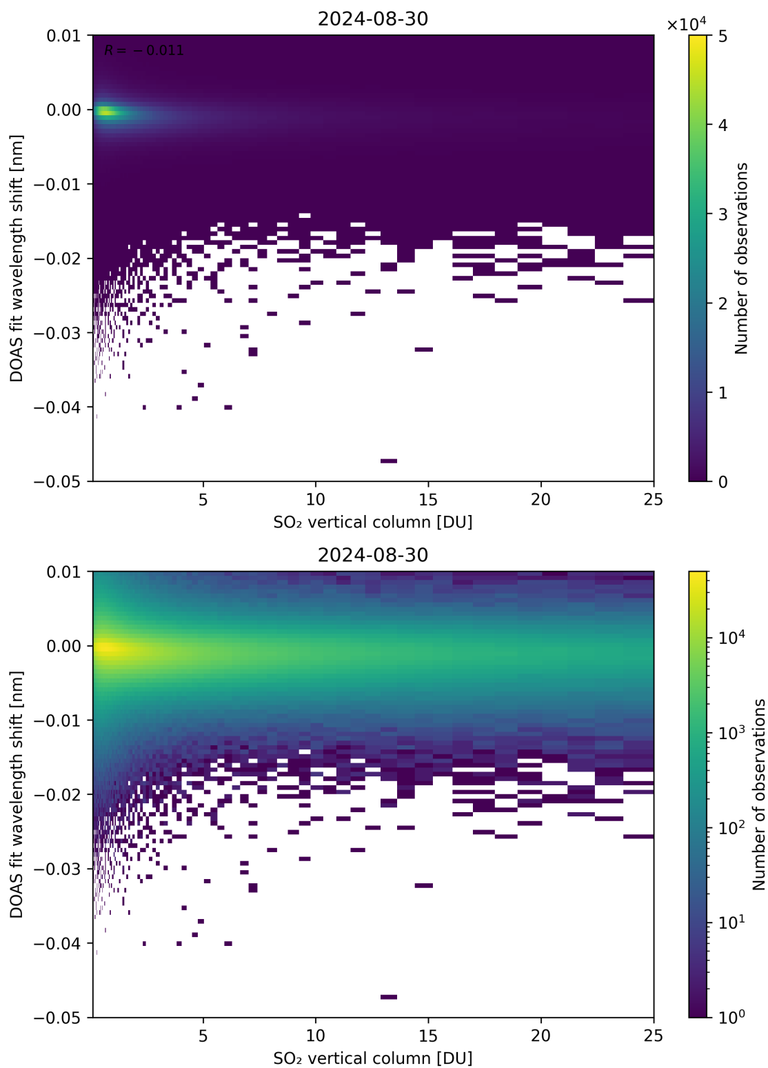
Figure 276: Scatter density plot of “SO 2 vertical column” against “DOAS fit wavelength shift” for 2024-08-29 to 2024-08-31.
