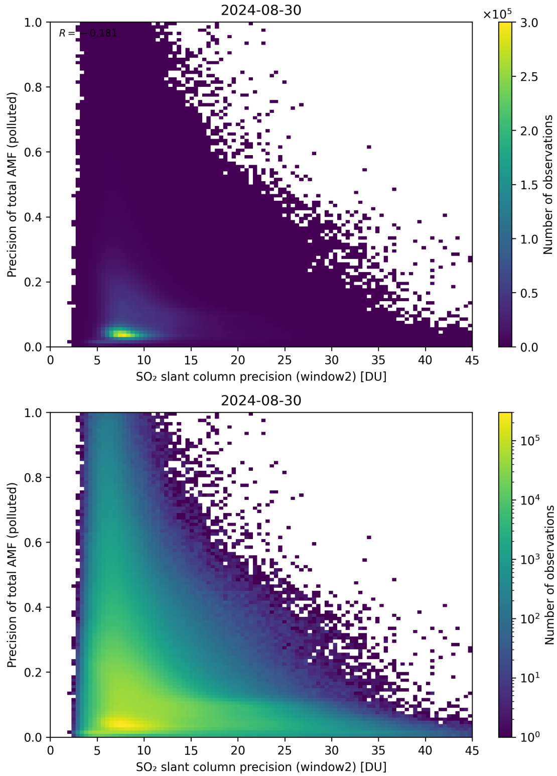
Figure 252: Scatter density plot of “SO 2 slant column precision (window2)” against “Precision of total AMF (polluted)” for 2024-08-29 to 2024-08-31.
