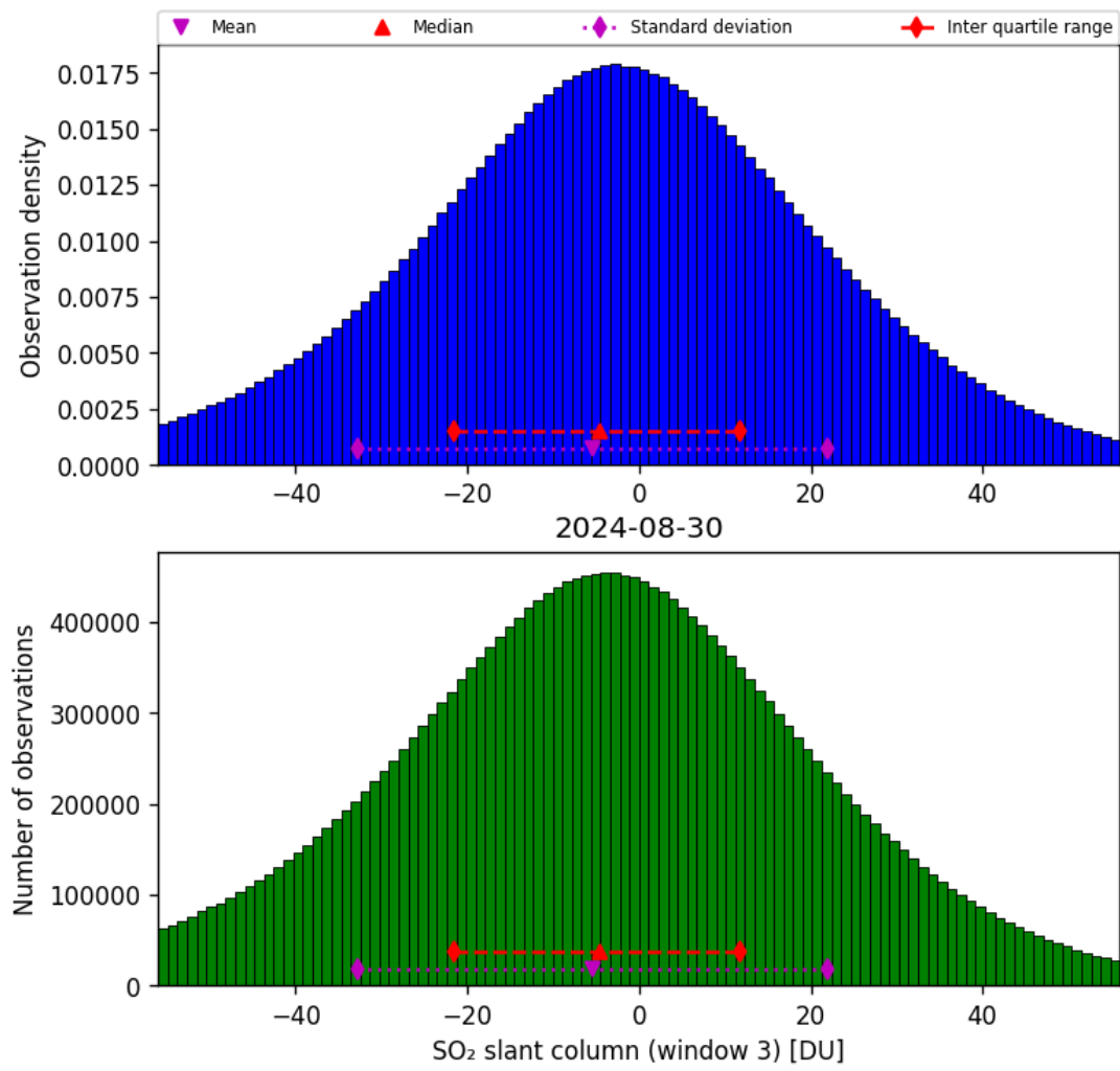
Figure 64: Histogram of “SO 2 slant column (window 3)” for 2024-08-29 to 2024-08-31
