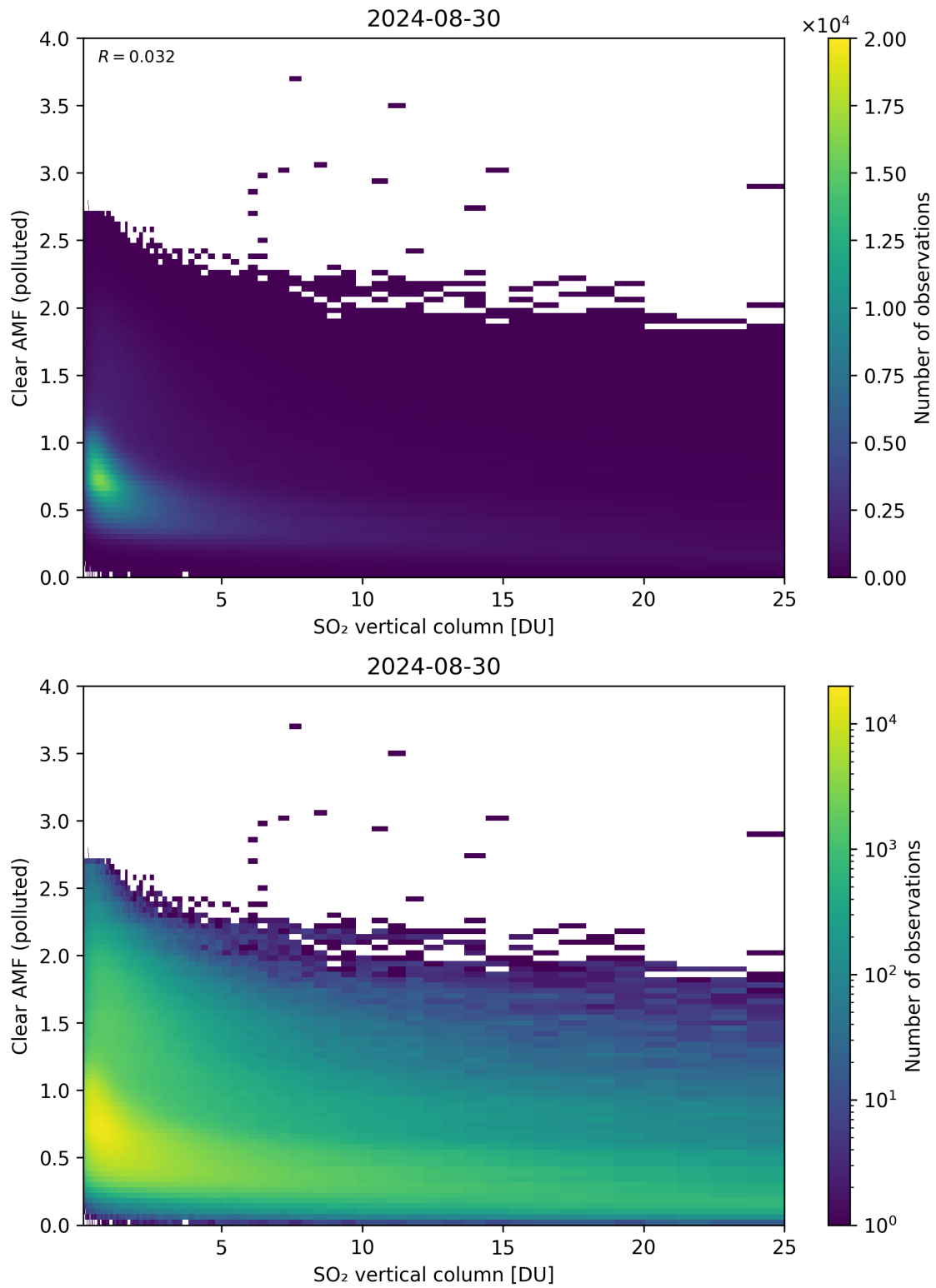
Figure 296: Scatter density plot of “SO 2 vertical column” against “Clear AMF (polluted)” for 2024-08-29 to 2024-08-31.
