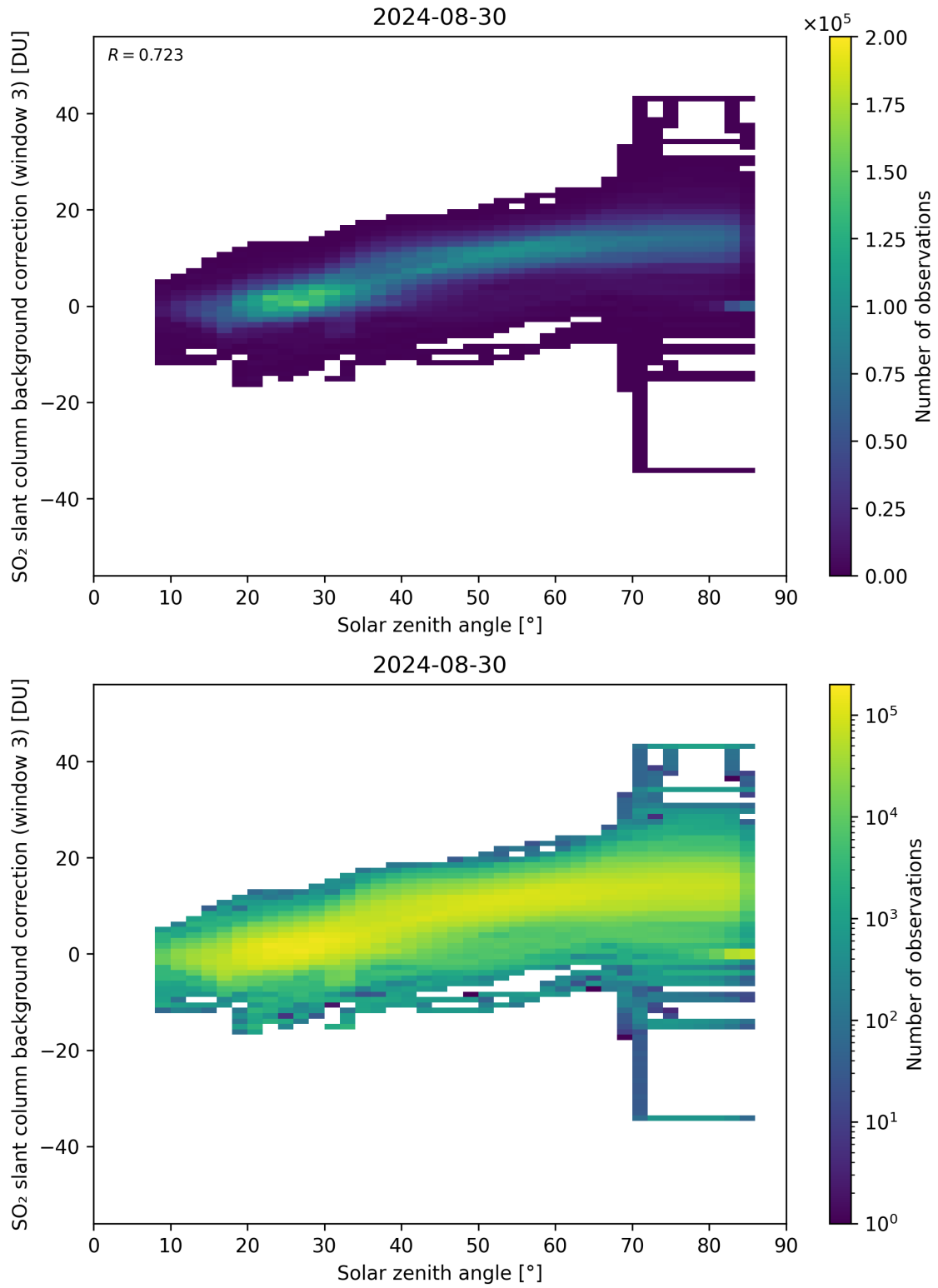
Figure 160: Scatter density plot of “Solar zenith angle” against “SO 2 slant column background correction (window 3)” for 2024-08-29 to 2024-08-31.
