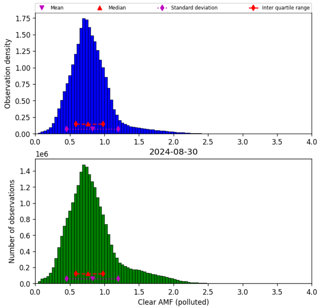
Figure 73: Histogram of “Clear AMF (polluted)” for 2024-08-29 to 2024-08-31
