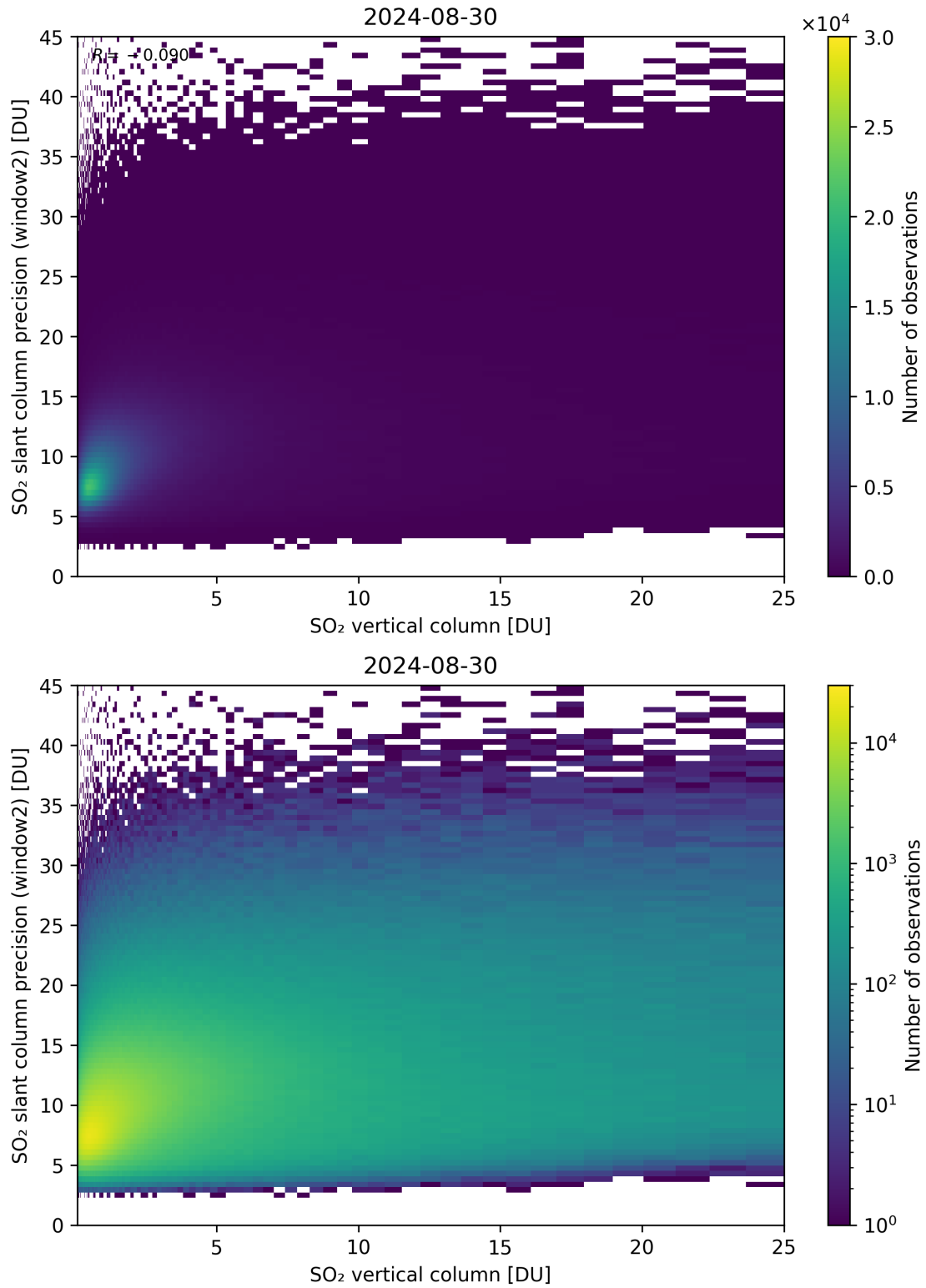
Figure 302: Scatter density plot of “SO 2 vertical column” against “SO 2 slant column precision (window2)” for 2024-08-29 to 2024-08-31.
