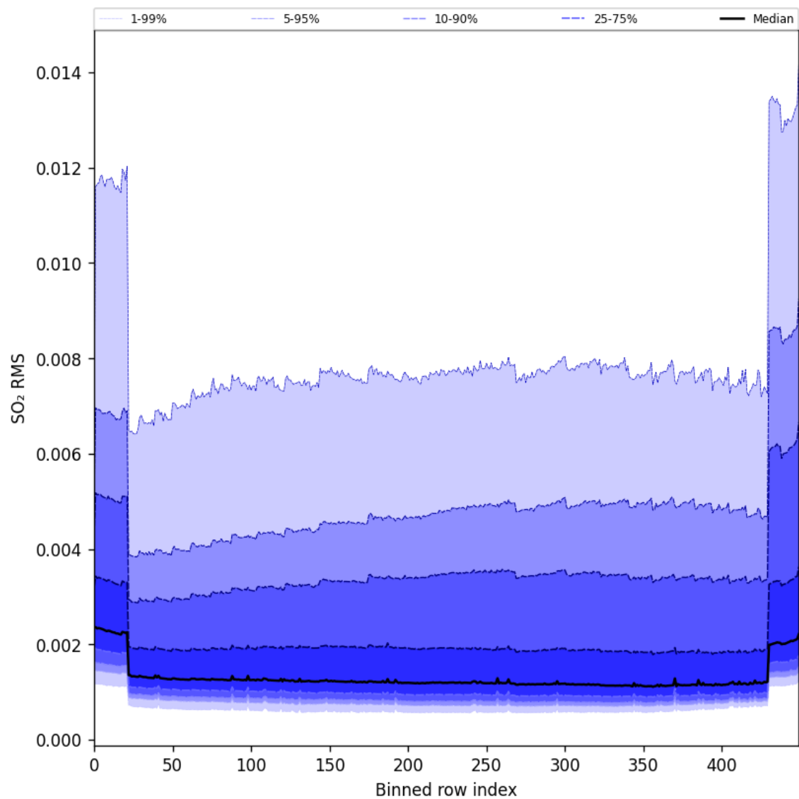
Figure 93: Along track statistics of “SO 2 RMS” for 2024-08-29 to 2024-08-31
