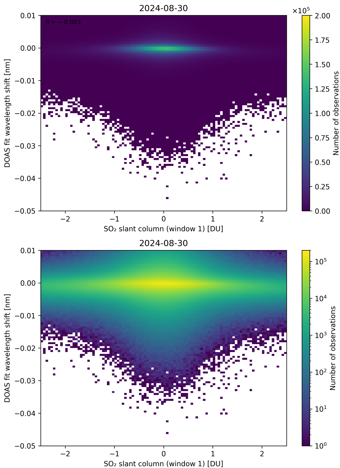
Figure 215: Scatter density plot of “SO 2 slant column (window 1)” against “DOAS fit wavelength shift” for 2024-08-29 to 2024-08-31.
