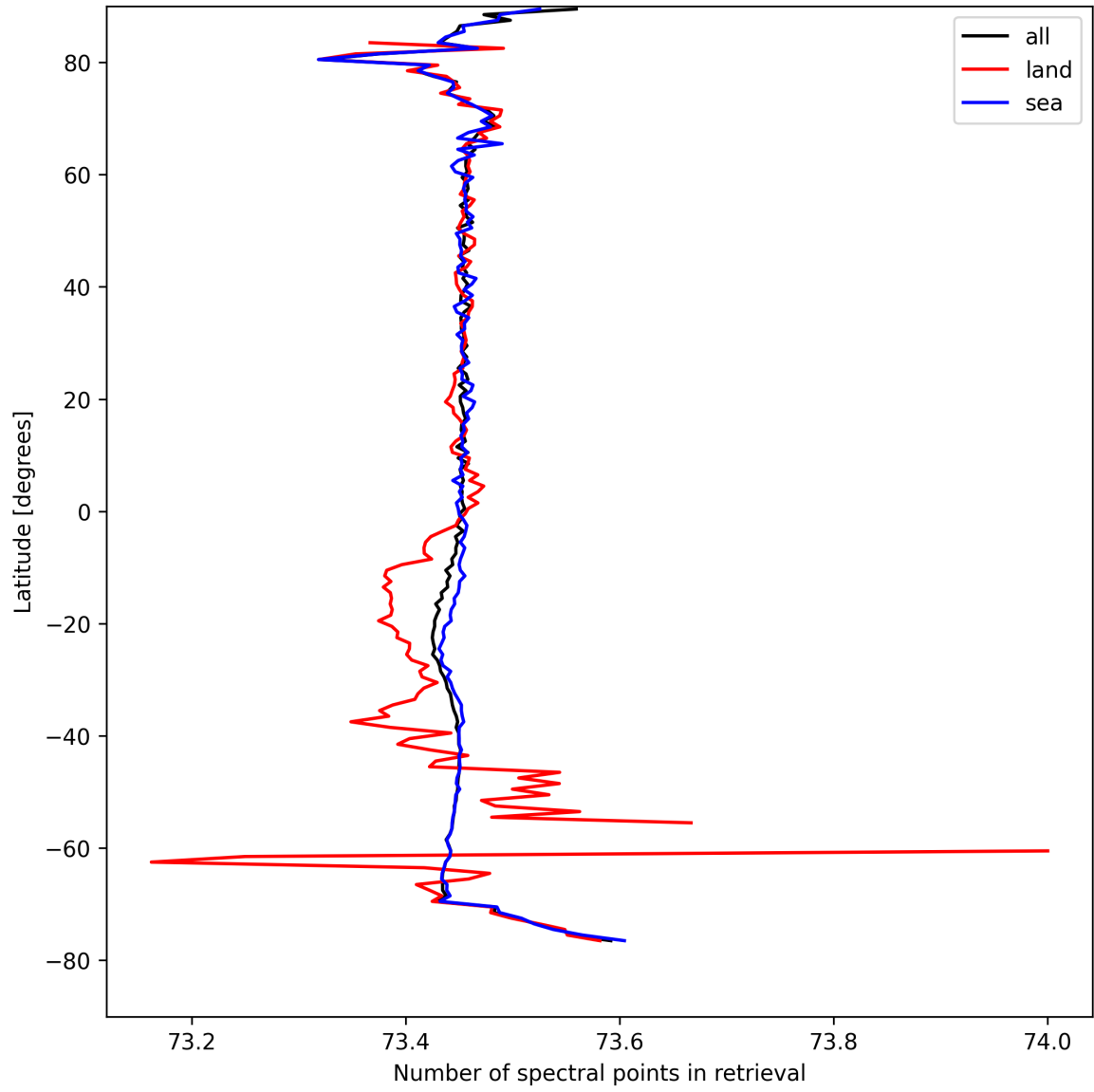
Figure 51: Zonal average of “Number of spectral points in retrieval” for 2024-08-29 to 2024-08-31.
