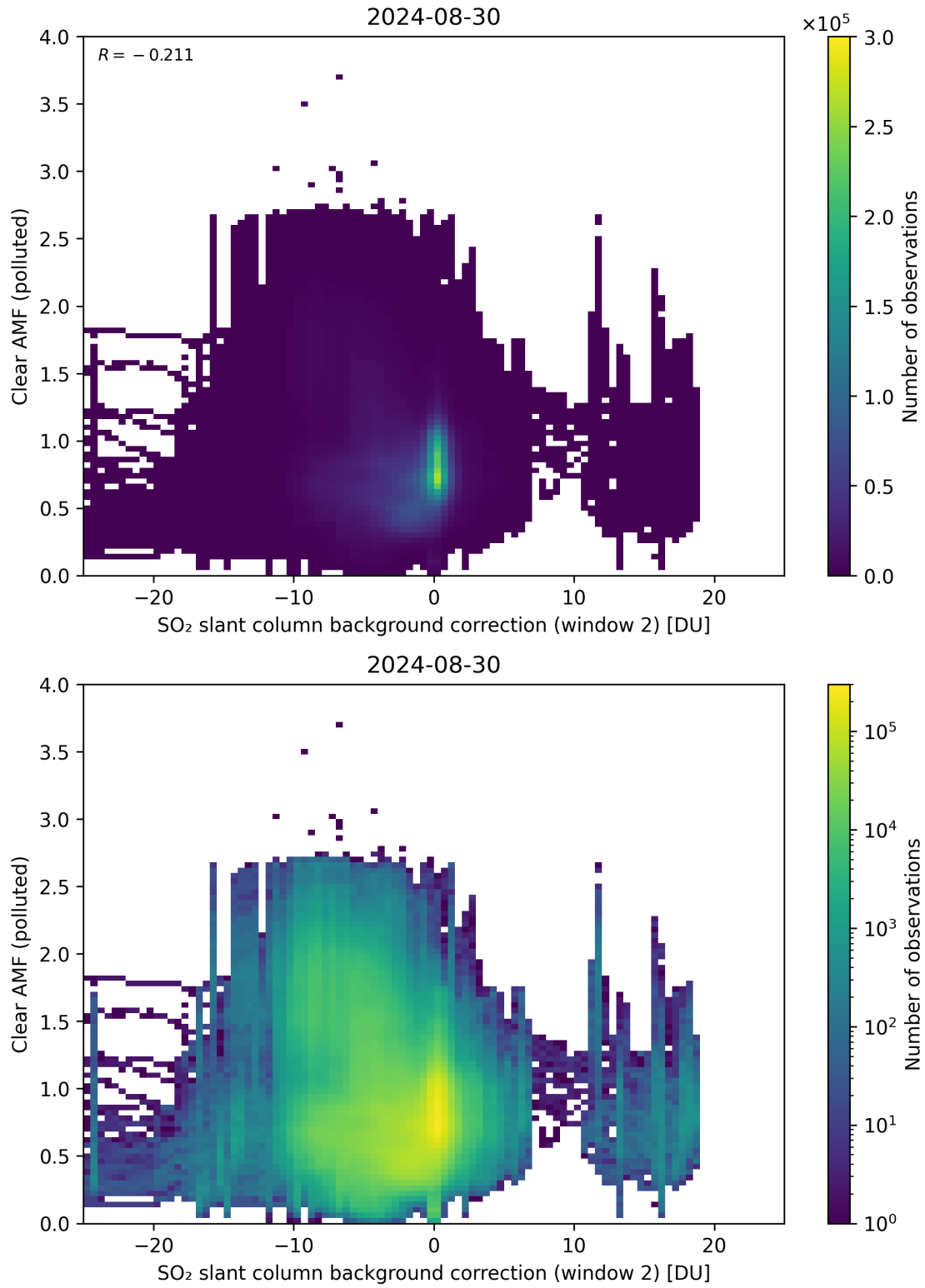
Figure 115: Scatter density plot of “SO 2 slant column background correction (window 2)” against “Clear AMF (polluted)” for 2024-08-29 to 2024-08-31.
