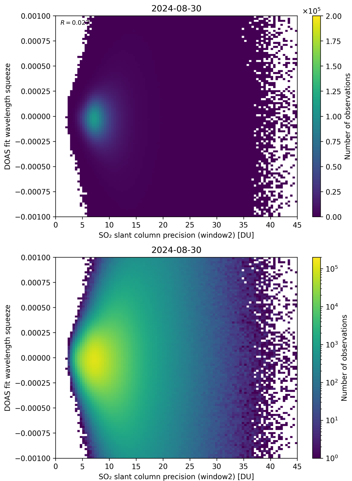
Figure 244: Scatter density plot of “SO 2 slant column precision (window2)” against “DOAS fit wavelength squeeze” for 2024-08-29 to 2024-08-31.
