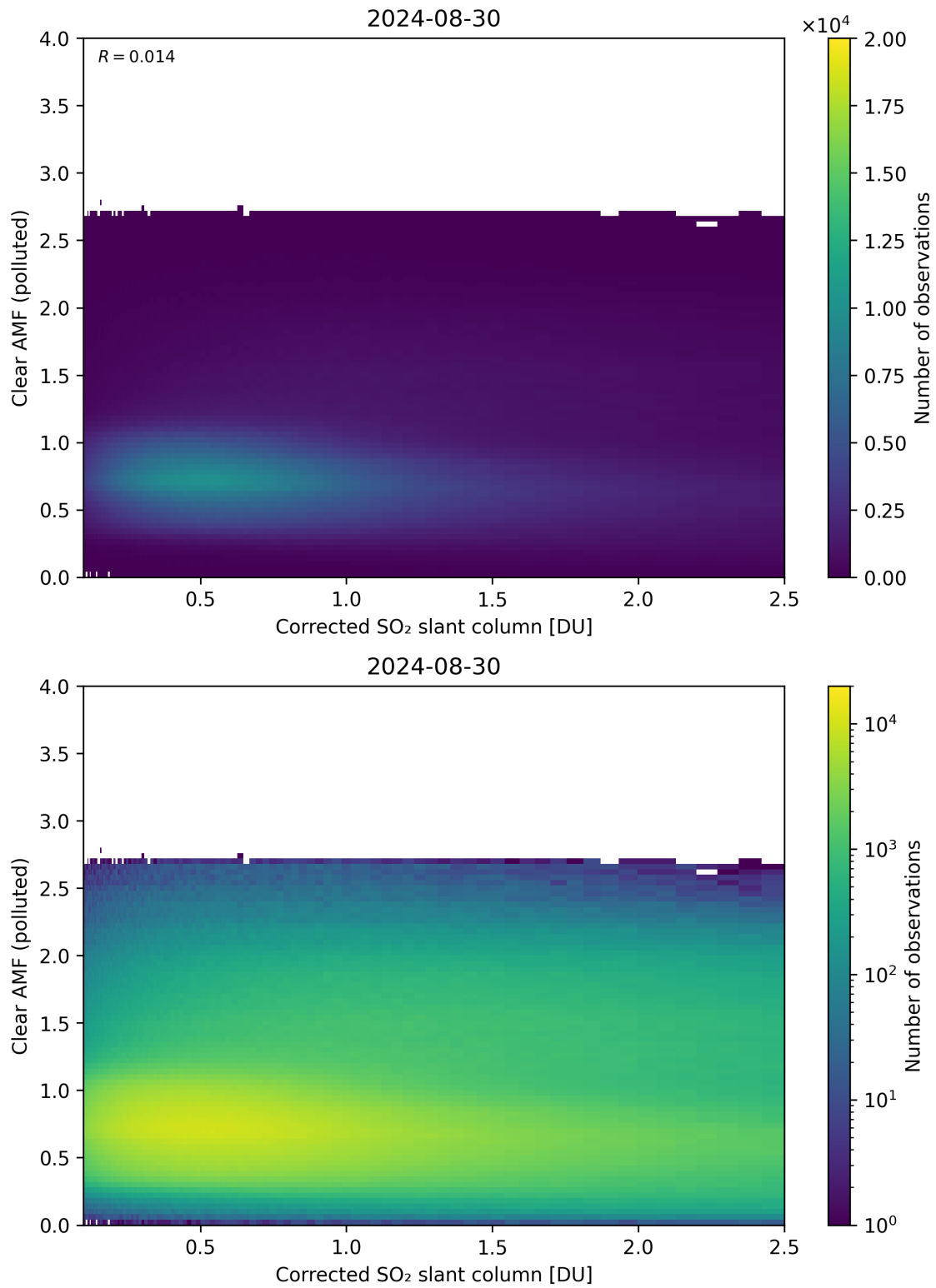
Figure 184: Scatter density plot of “Corrected SO 2 slant column” against “Clear AMF (polluted)” for 2024-08-29 to 2024-08-31.
