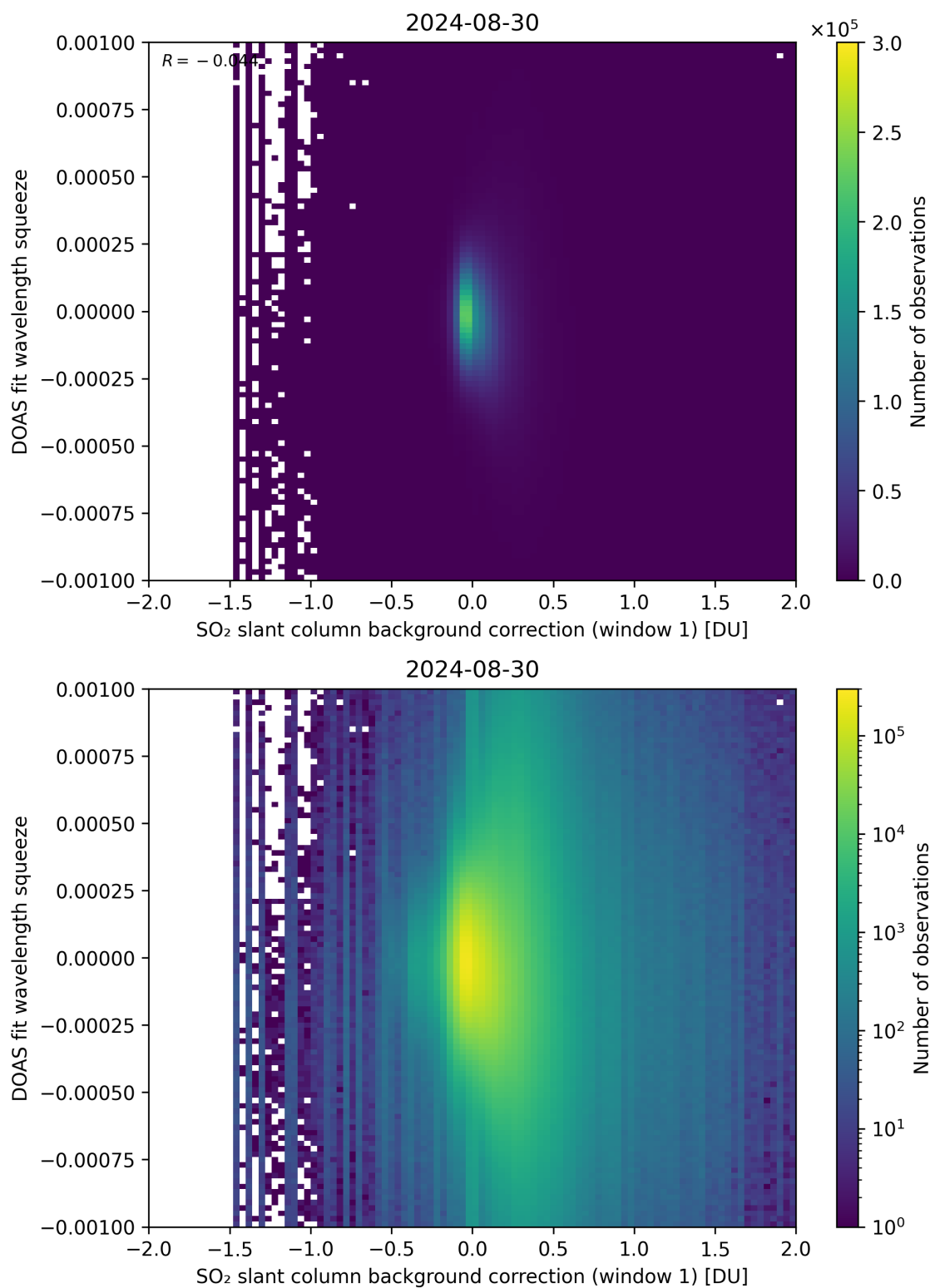
Figure 101: Scatter density plot of “SO 2 slant column background correction (window 1)” against “DOAS fit wavelength squeeze” for 2024-08-29 to 2024-08-31.
