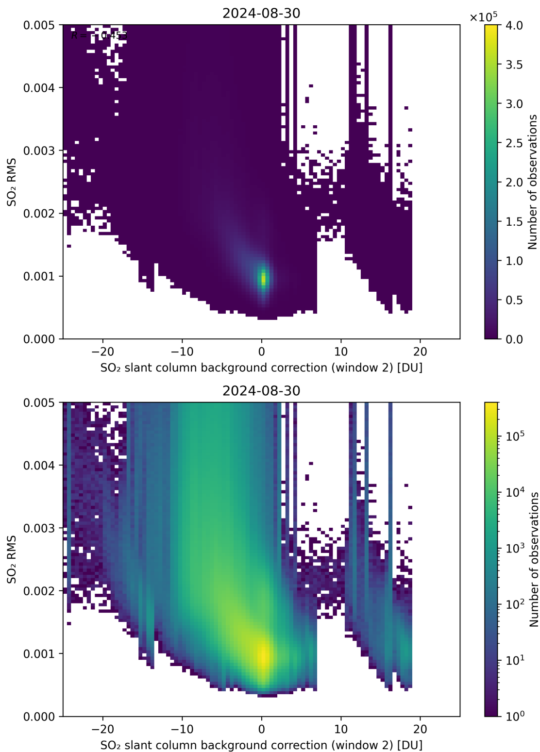
Figure 114: Scatter density plot of “SO 2 slant column background correction (window 2)” against “SO 2 RMS” for 2024-08-29 to 2024-08-31.
