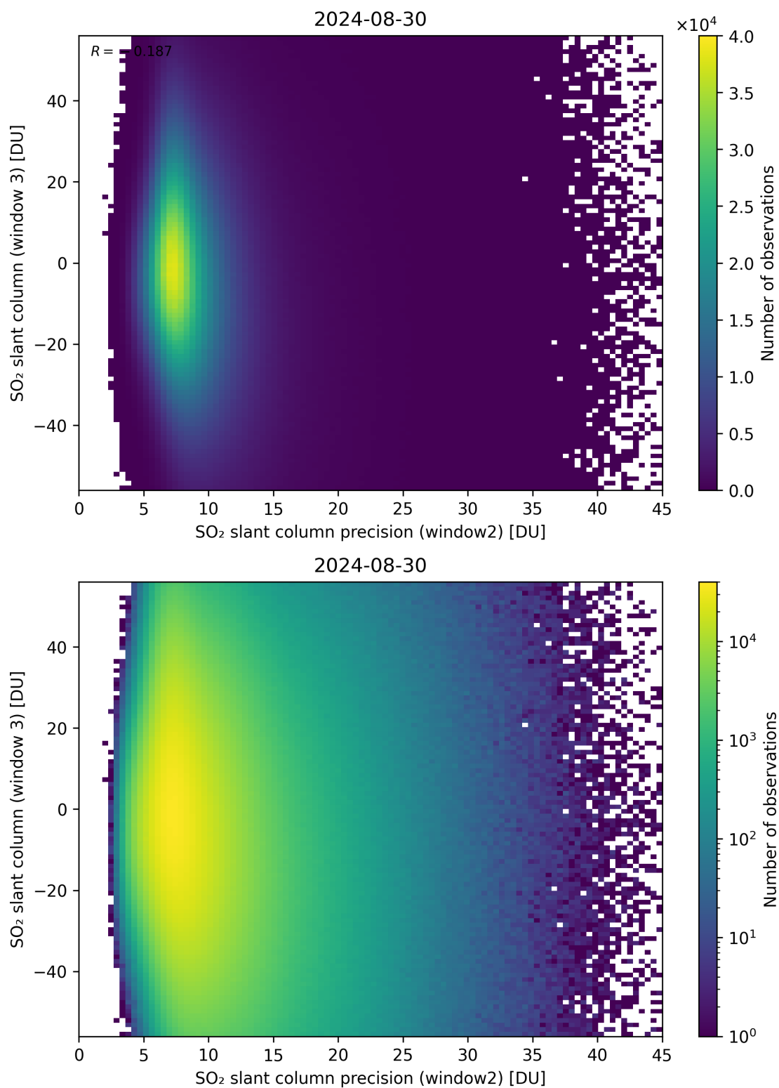
Figure 249: Scatter density plot of “SO 2 slant column precision (window2)” against “SO 2 slant column (window 3)” for 2024-08-29 to 2024-08-31.
