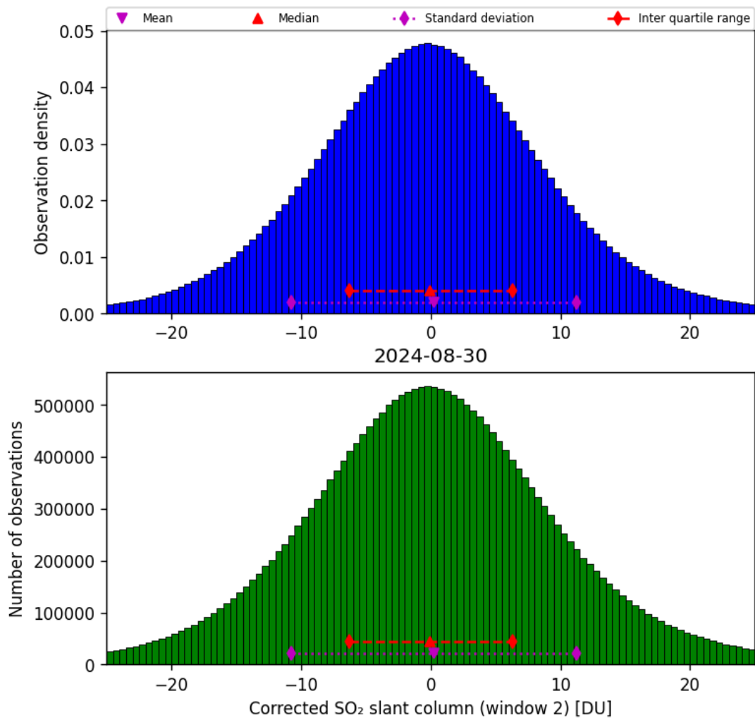
Figure 62: Histogram of “Corrected SO 2 slant column (window 2)” for 2024-08-29 to 2024-08-31
