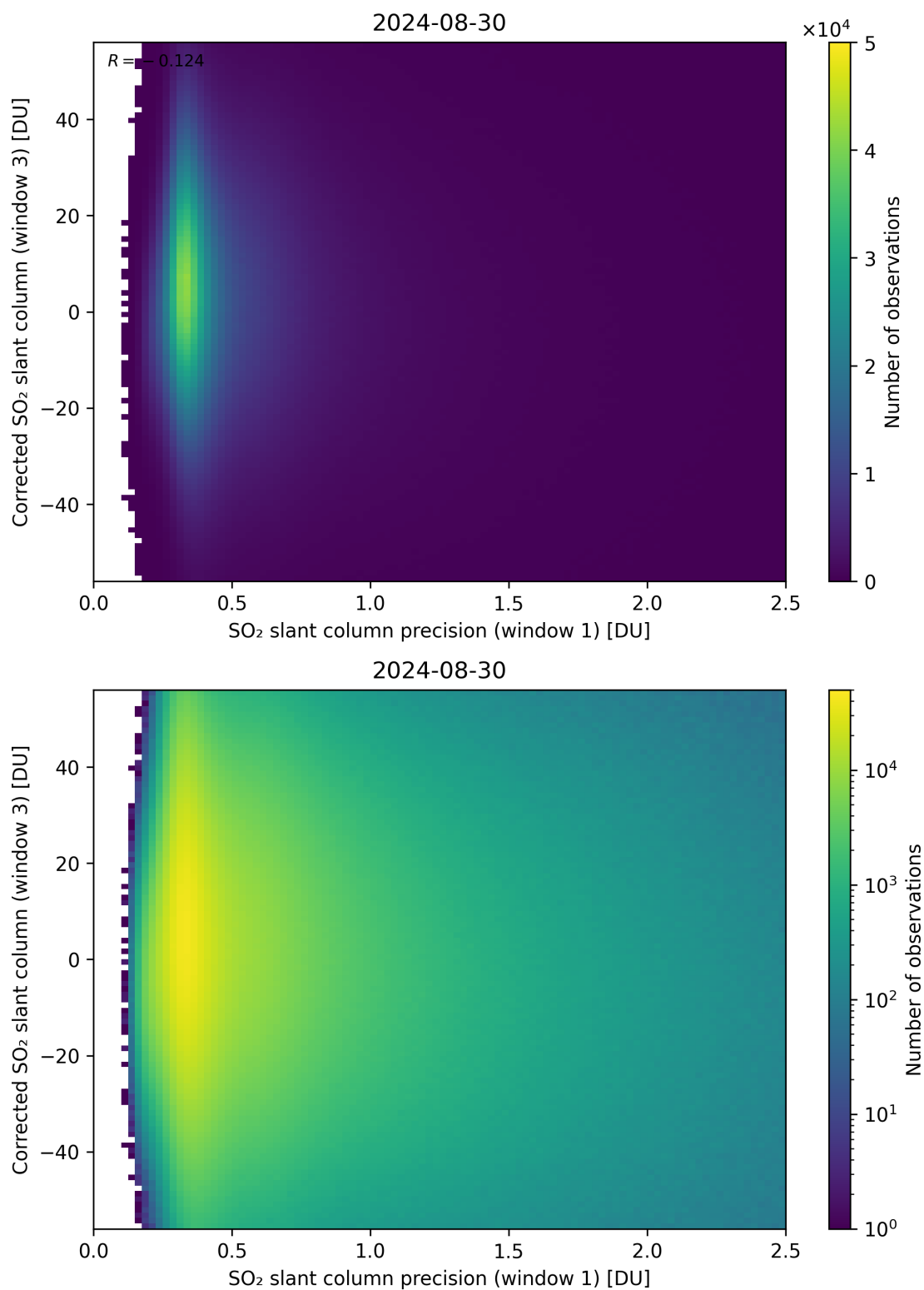
Figure 226: Scatter density plot of “SO 2 slant column precision (window 1)” against “Corrected SO 2 slant column (window 3)” for 2024-08-29 to 2024-08-31.
