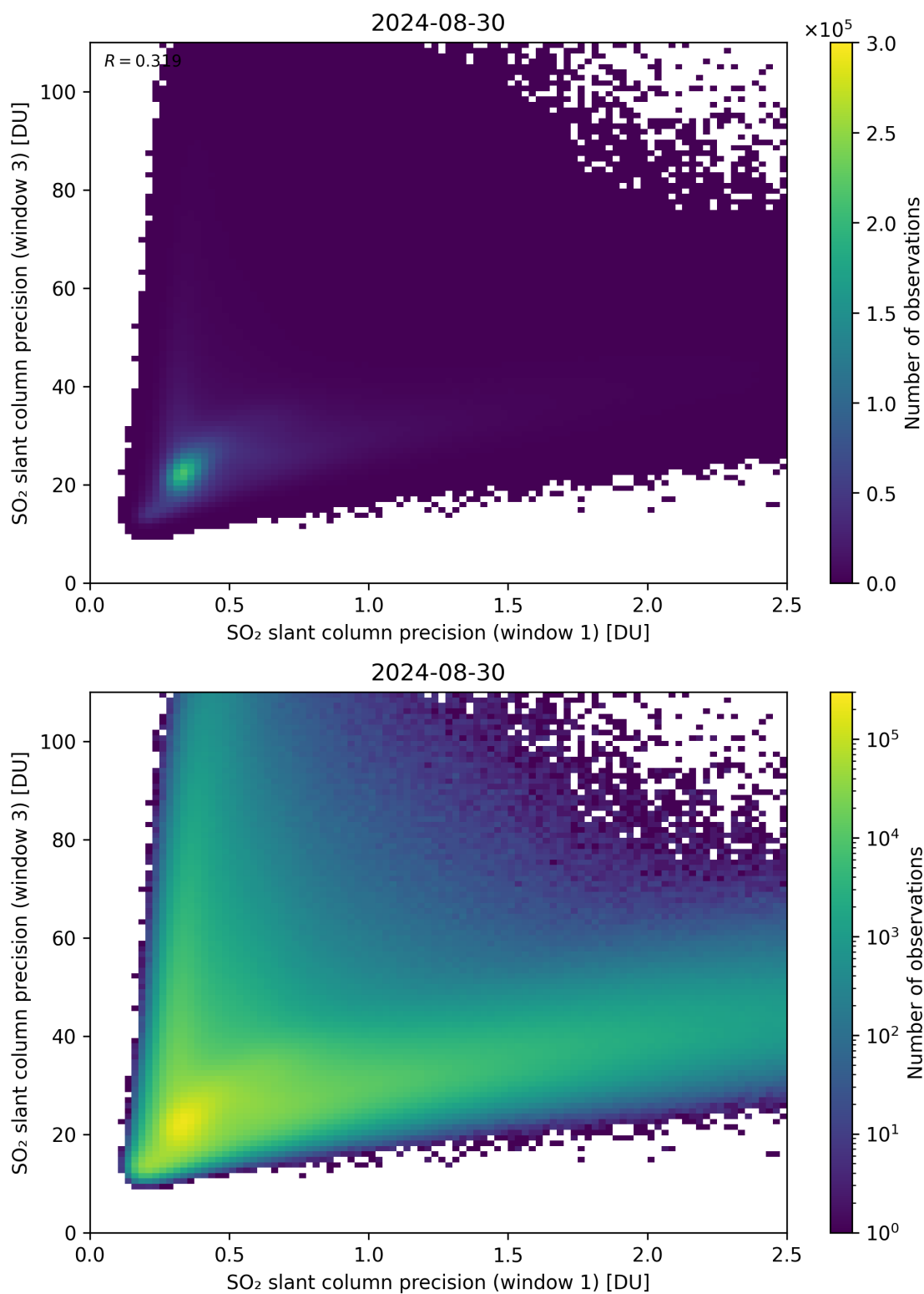
Figure 229: Scatter density plot of “SO 2 slant column precision (window 1)” against “SO 2 slant column precision (window 3)” for 2024-08-29 to 2024-08-31.
