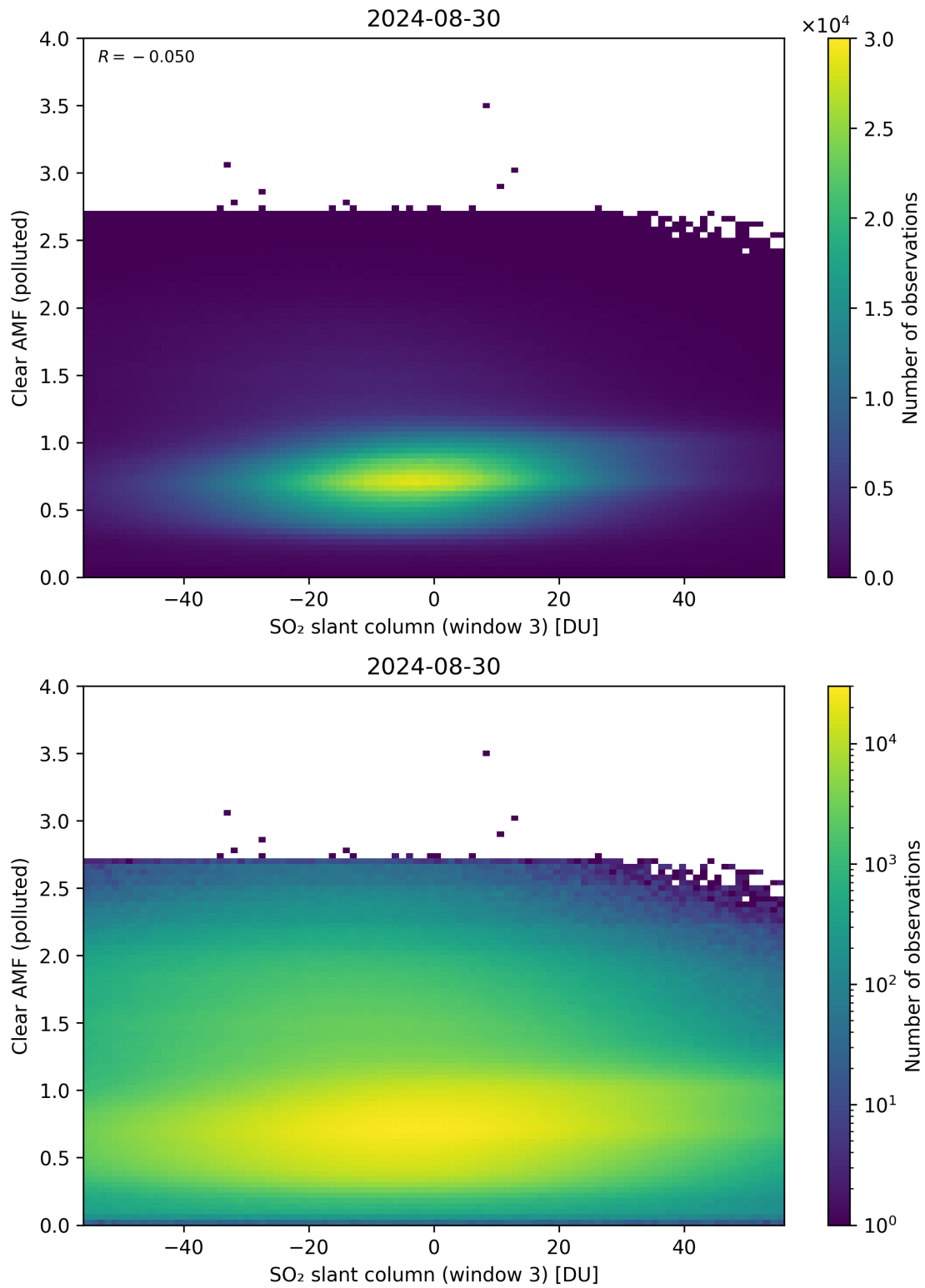
Figure 265: Scatter density plot of “SO 2 slant column (window 3)” against “Clear AMF (polluted)” for 2024-08-29 to 2024-08-31.
