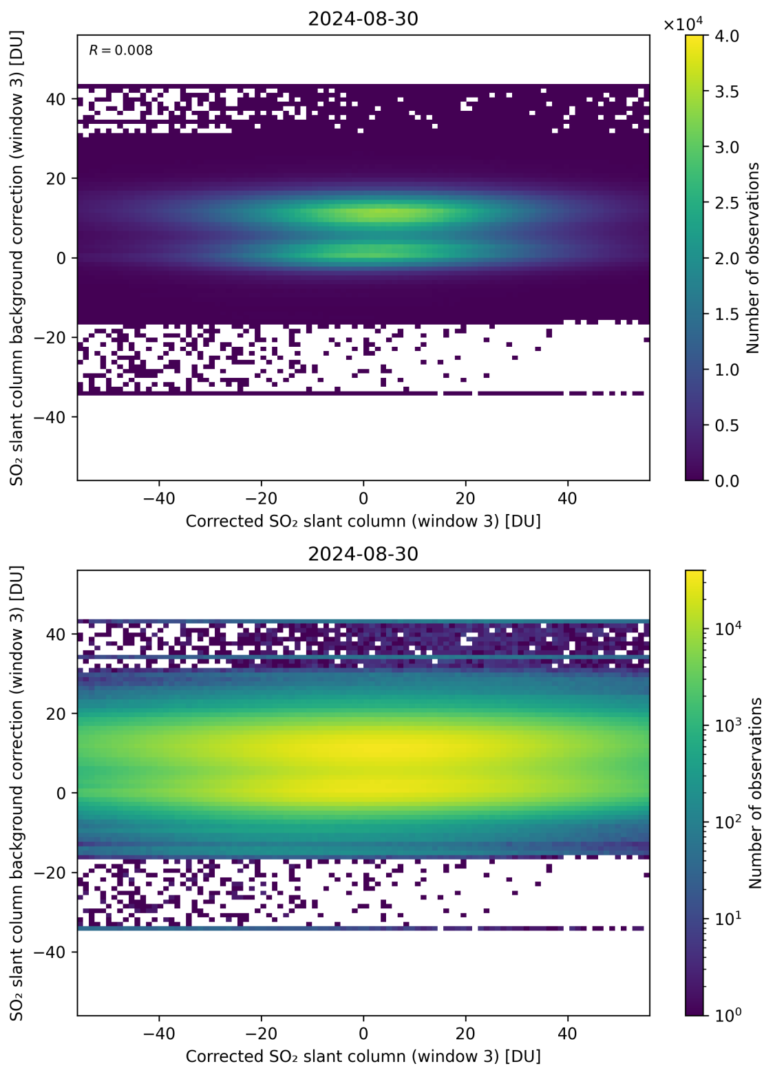
Figure 205: Scatter density plot of “Corrected SO 2 slant column (window 3)” against “SO 2 slant column background correction (window 3)” for 2024-08-29 to 2024-08-31.
