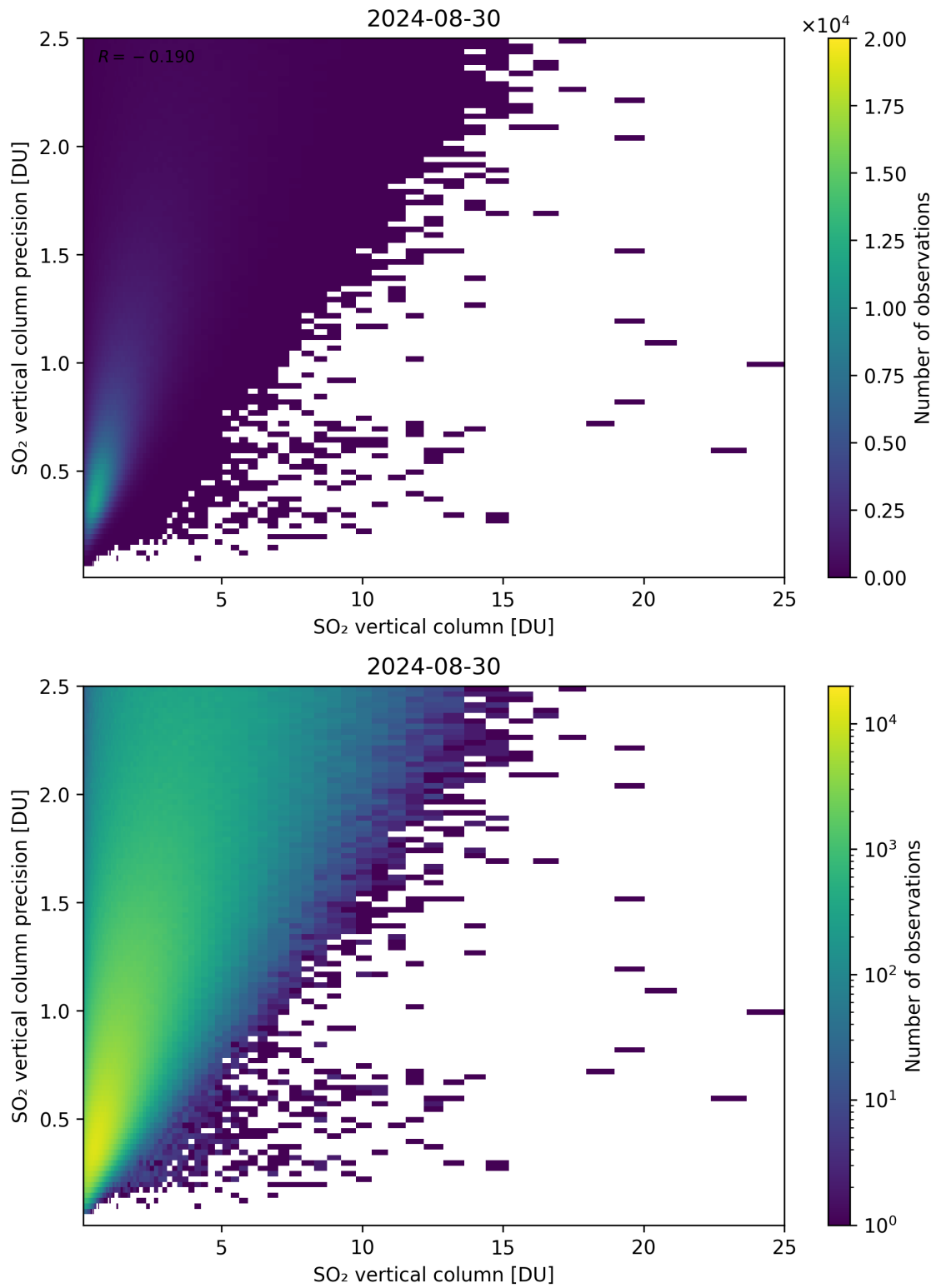
Figure 307: Scatter density plot of “SO 2 vertical column” against “SO 2 vertical column precision” for 2024-08-29 to 2024-08-31.
