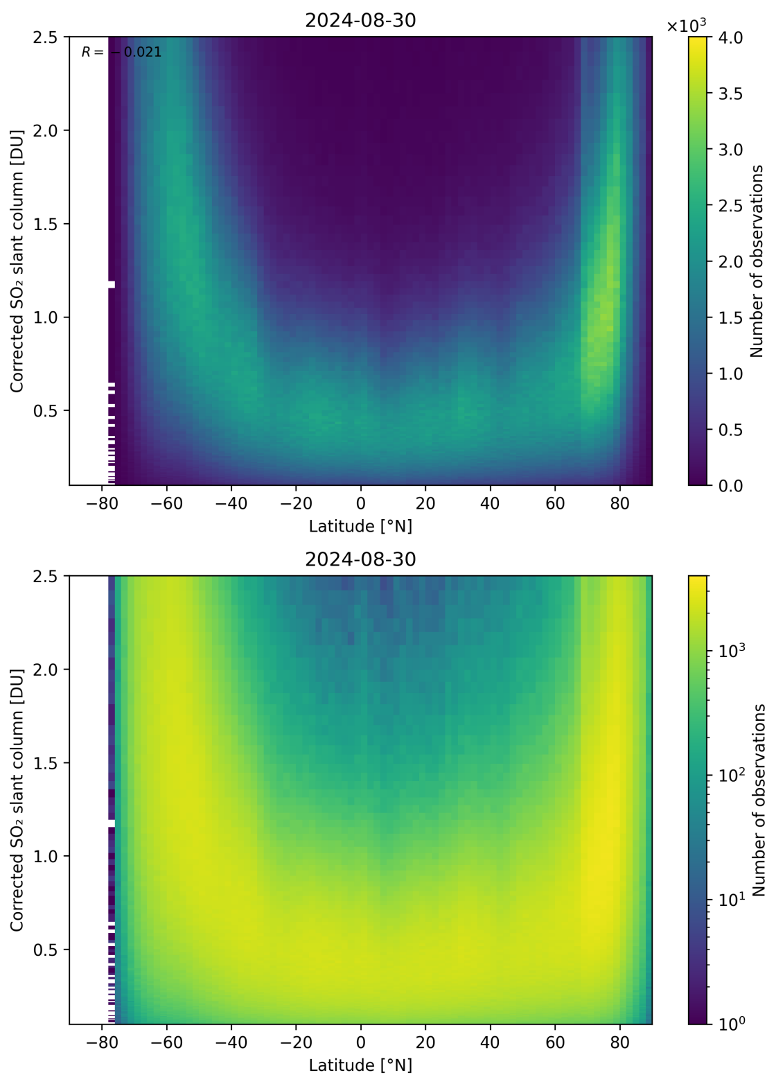
Figure 146: Scatter density plot of “Latitude” against “Corrected SO 2 slant column” for 2024-08-29 to 2024-08-31.
