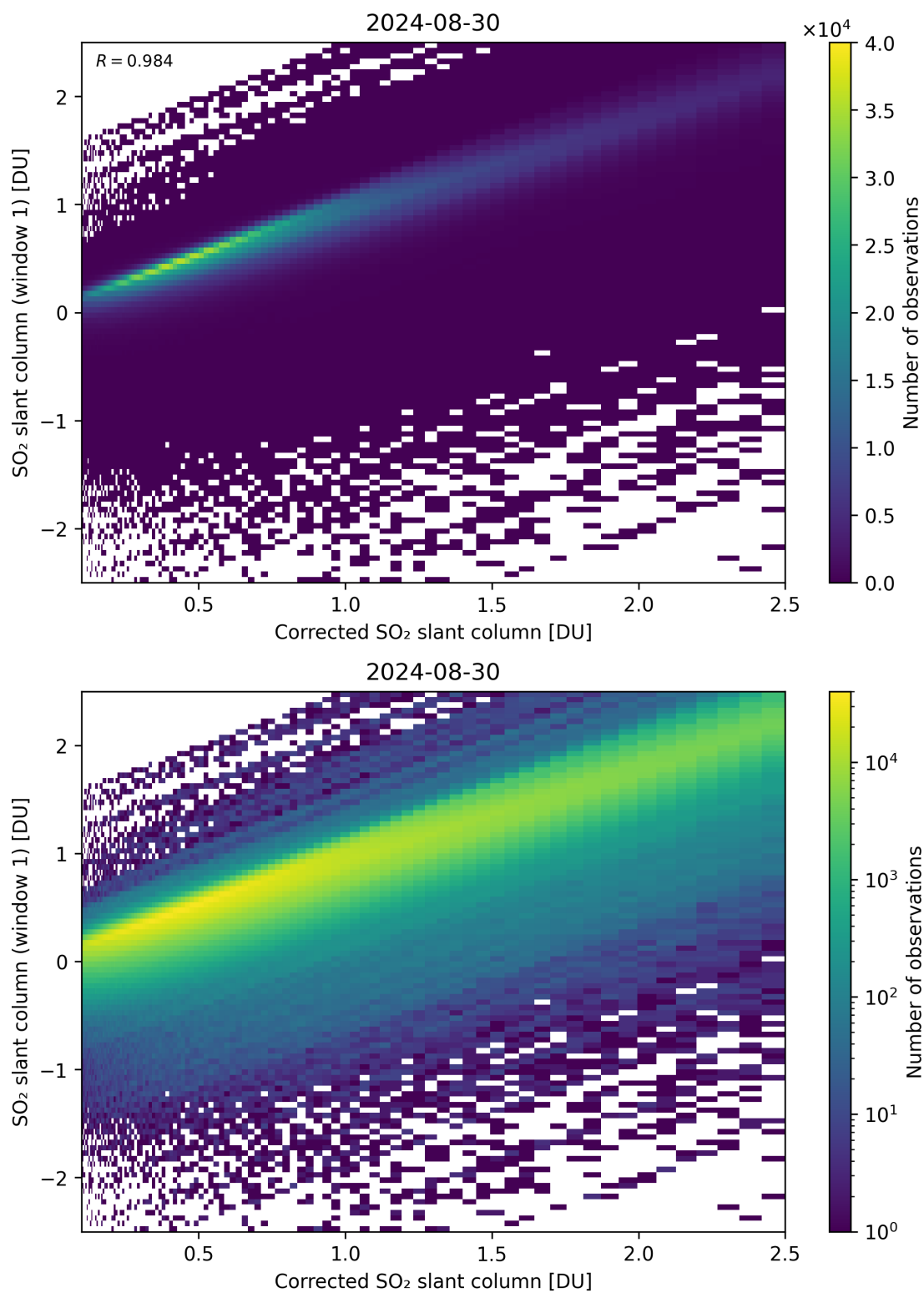
Figure 187: Scatter density plot of “Corrected SO 2 slant column” against “SO 2 slant column (window 1)” for 2024-08-29 to 2024-08-31.
