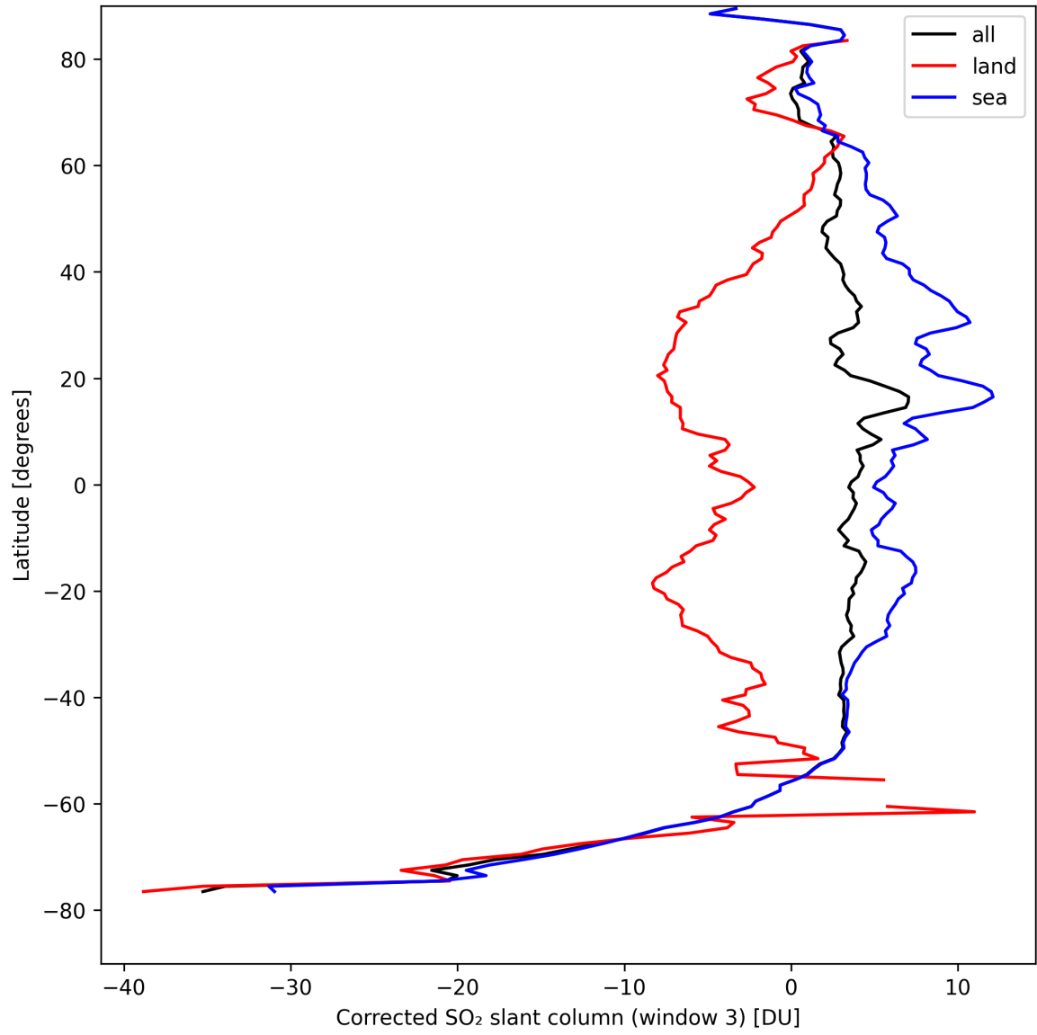
Figure 43: Zonal average of “Corrected SO 2 slant column (window 3)” for 2024-08-29 to 2024-08-31.
