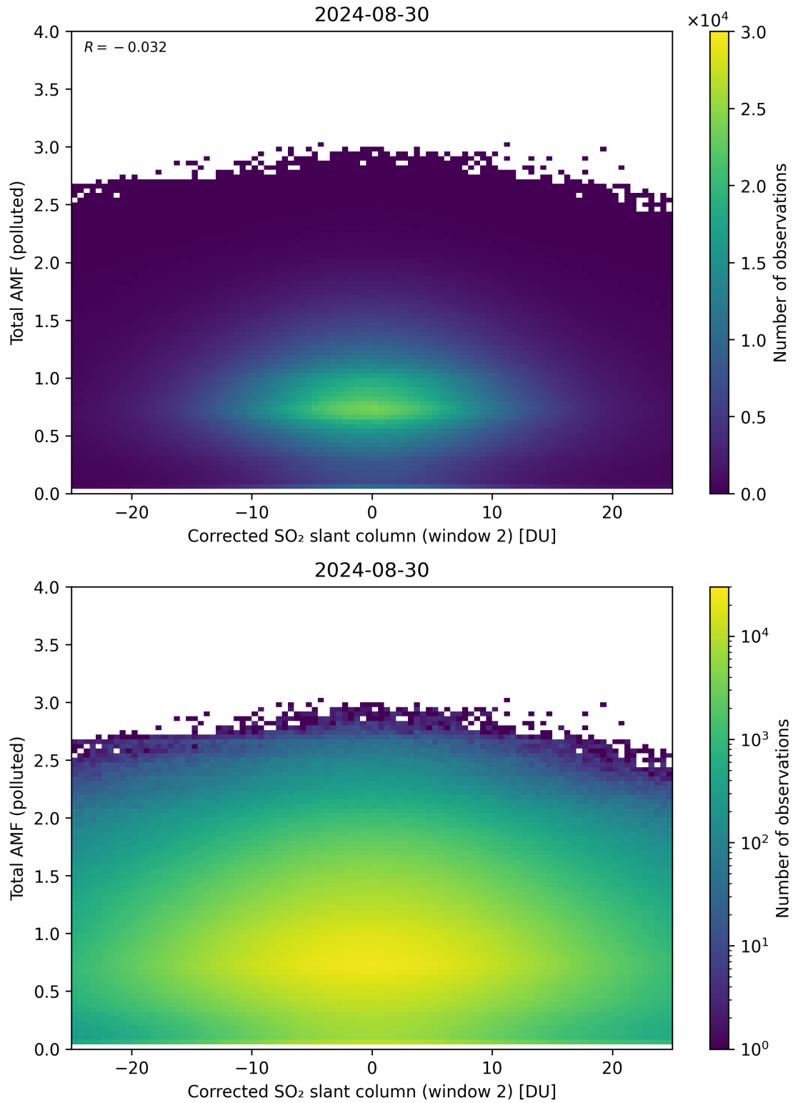
Figure 203: Scatter density plot of “Corrected SO 2 slant column (window 2)” against “Total AMF (polluted)” for 2024-08-29 to 2024-08-31.
