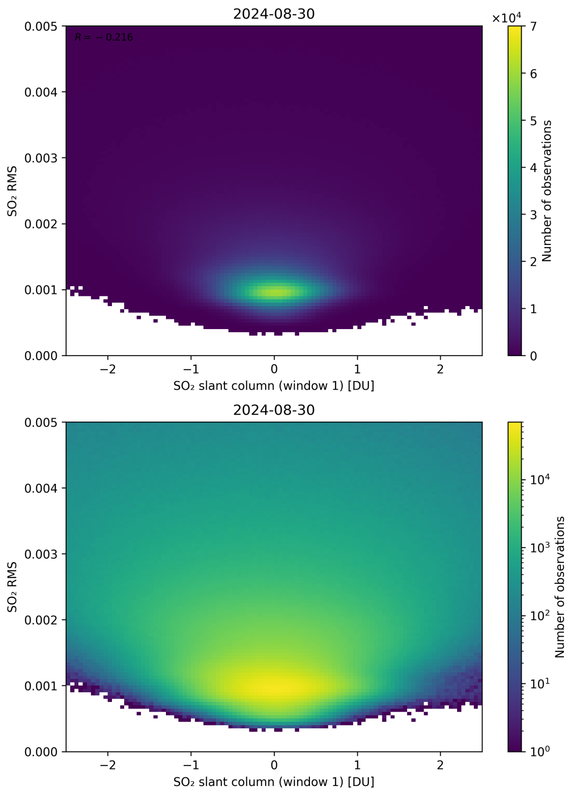
Figure 217: Scatter density plot of “SO 2 slant column (window 1)” against “SO 2 RMS” for 2024-08-29 to 2024-08-31.
