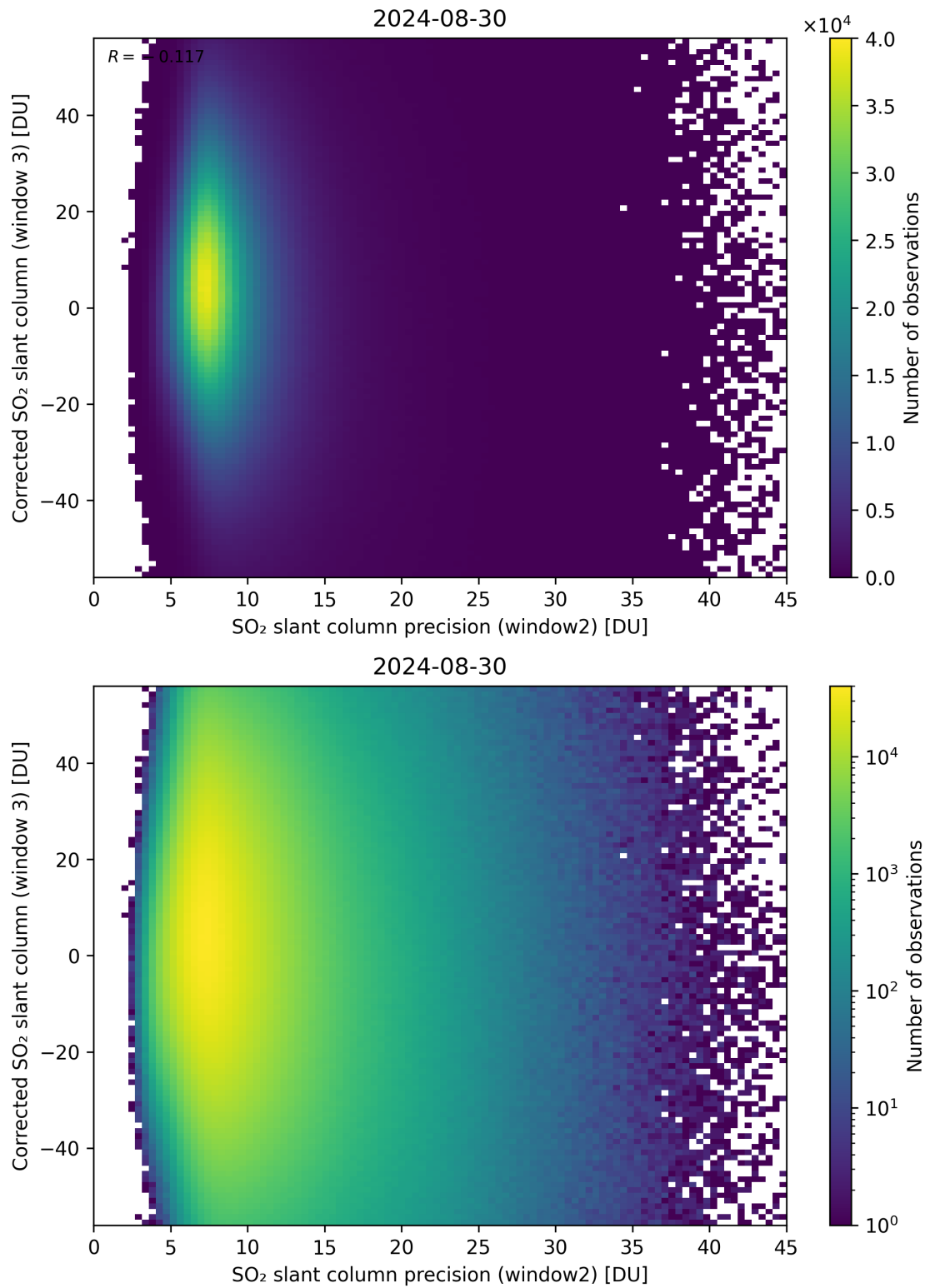
Figure 248: Scatter density plot of “SO 2 slant column precision (window2)” against “Corrected SO 2 slant column (window 3)” for 2024-08-29 to 2024-08-31.
