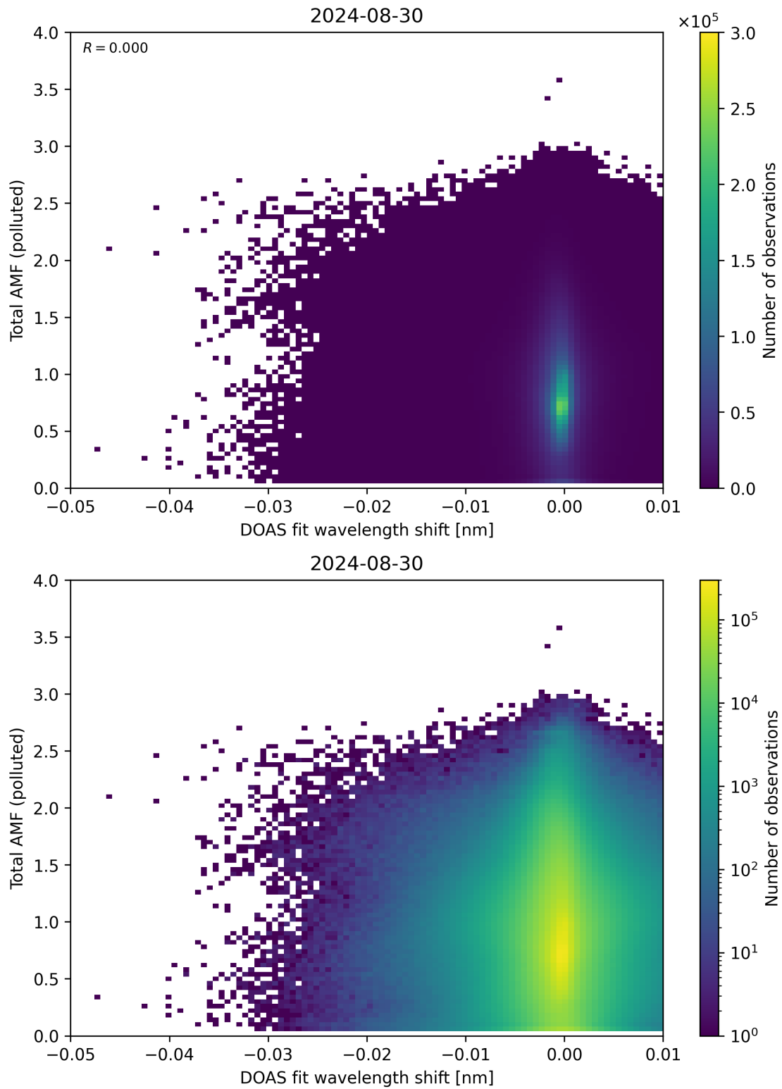
Figure 130: Scatter density plot of “DOAS fit wavelength shift” against “Total AMF (polluted)” for 2024-08-29 to 2024-08-31.
