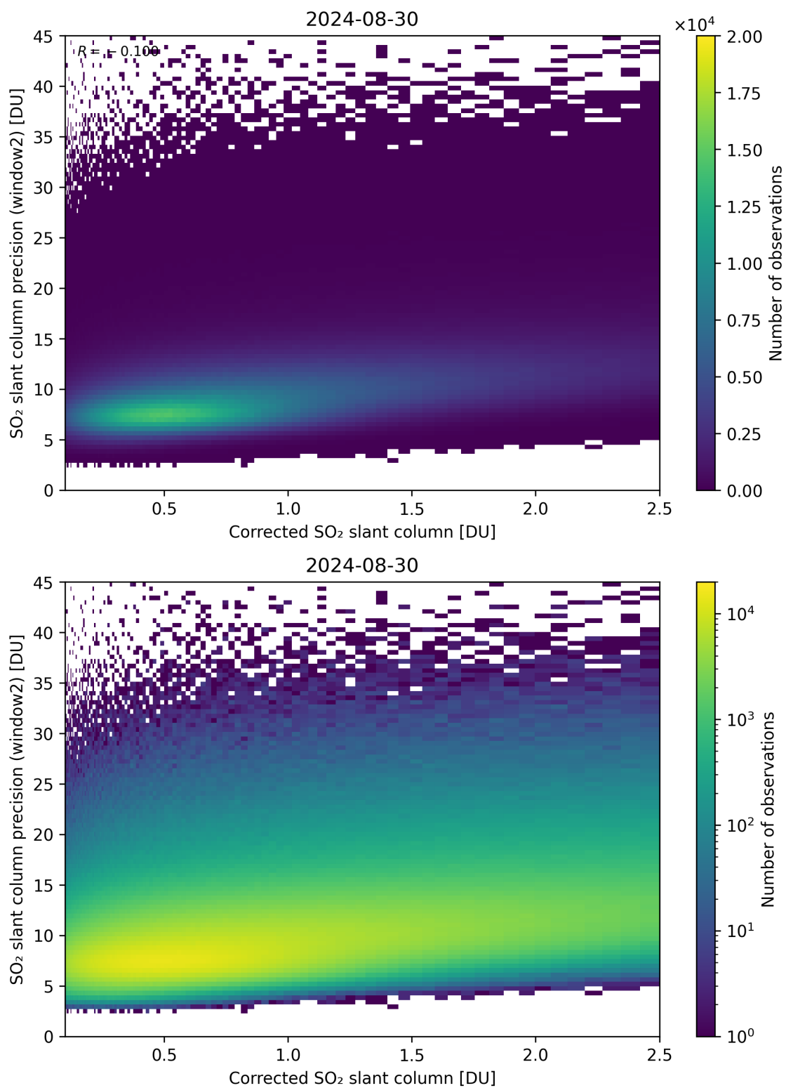
Figure 189: Scatter density plot of “Corrected SO 2 slant column” against “SO 2 slant column precision (window2)” for 2024-08-29 to 2024-08-31.
