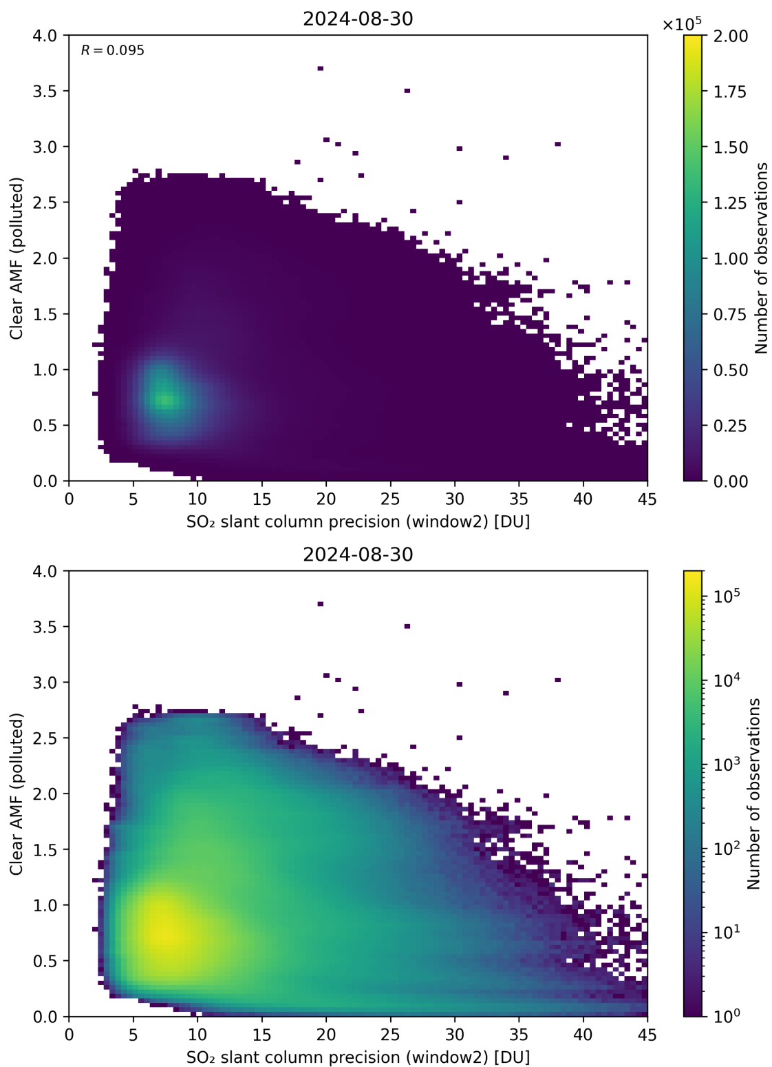
Figure 246: Scatter density plot of “SO 2 slant column precision (window2)” against “Clear AMF (polluted)” for 2024-08-29 to 2024-08-31.
