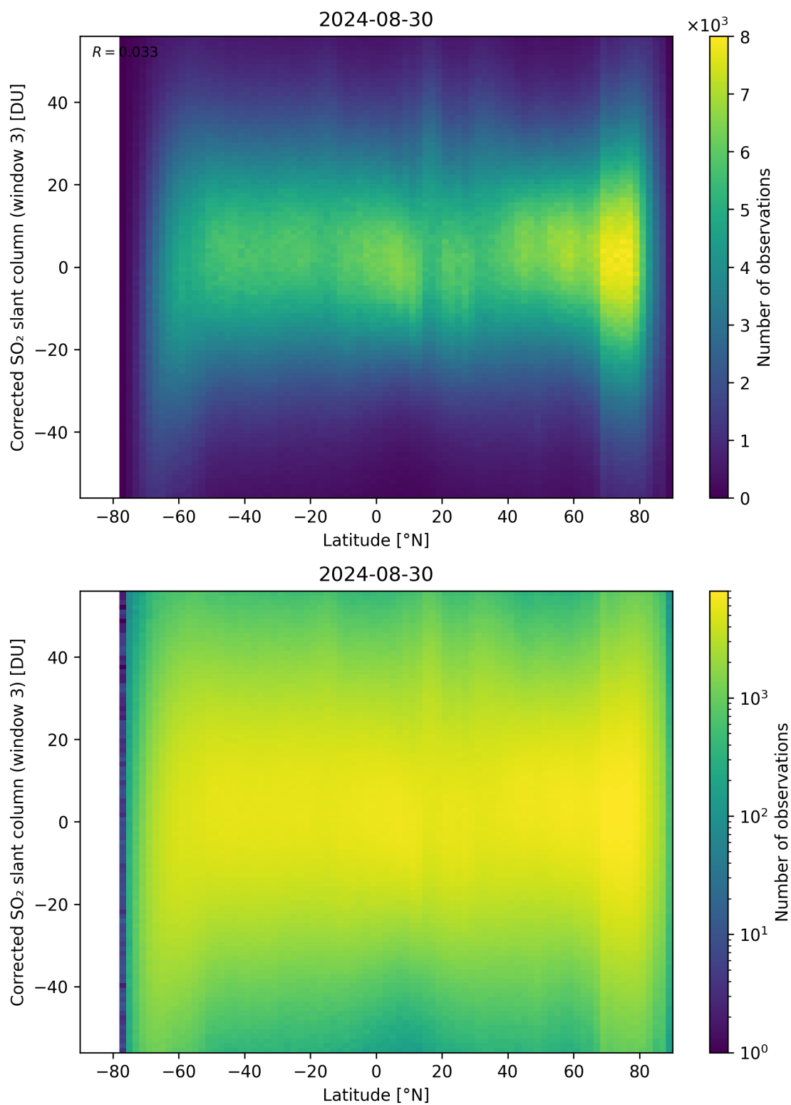
Figure 148: Scatter density plot of “Latitude” against “Corrected SO 2 slant column (window 3)” for 2024-08-29 to 2024-08-31.
