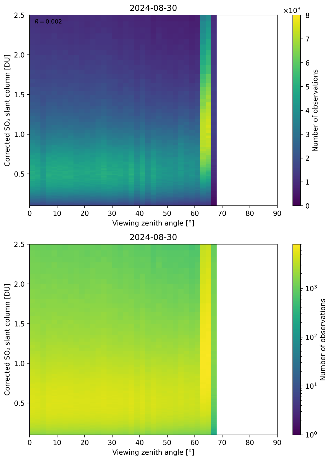
Figure 317: Scatter density plot of “Viewing zenith angle” against “Corrected SO 2 slant column” for 2024-08-29 to 2024-08-31.
