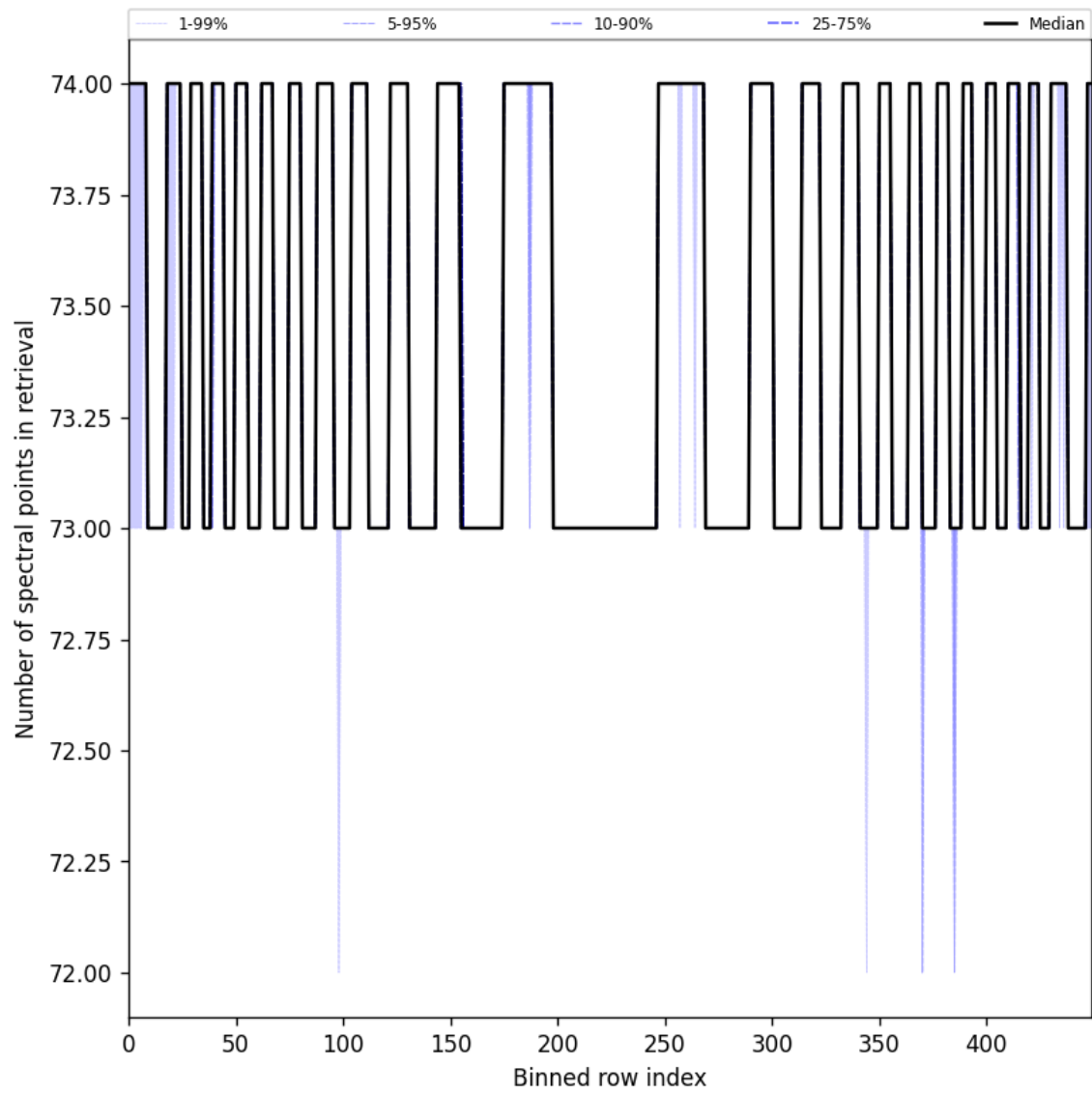
Figure 97: Along track statistics of “Number of spectral points in retrieval” for 2024-08-29 to 2024-08-31
