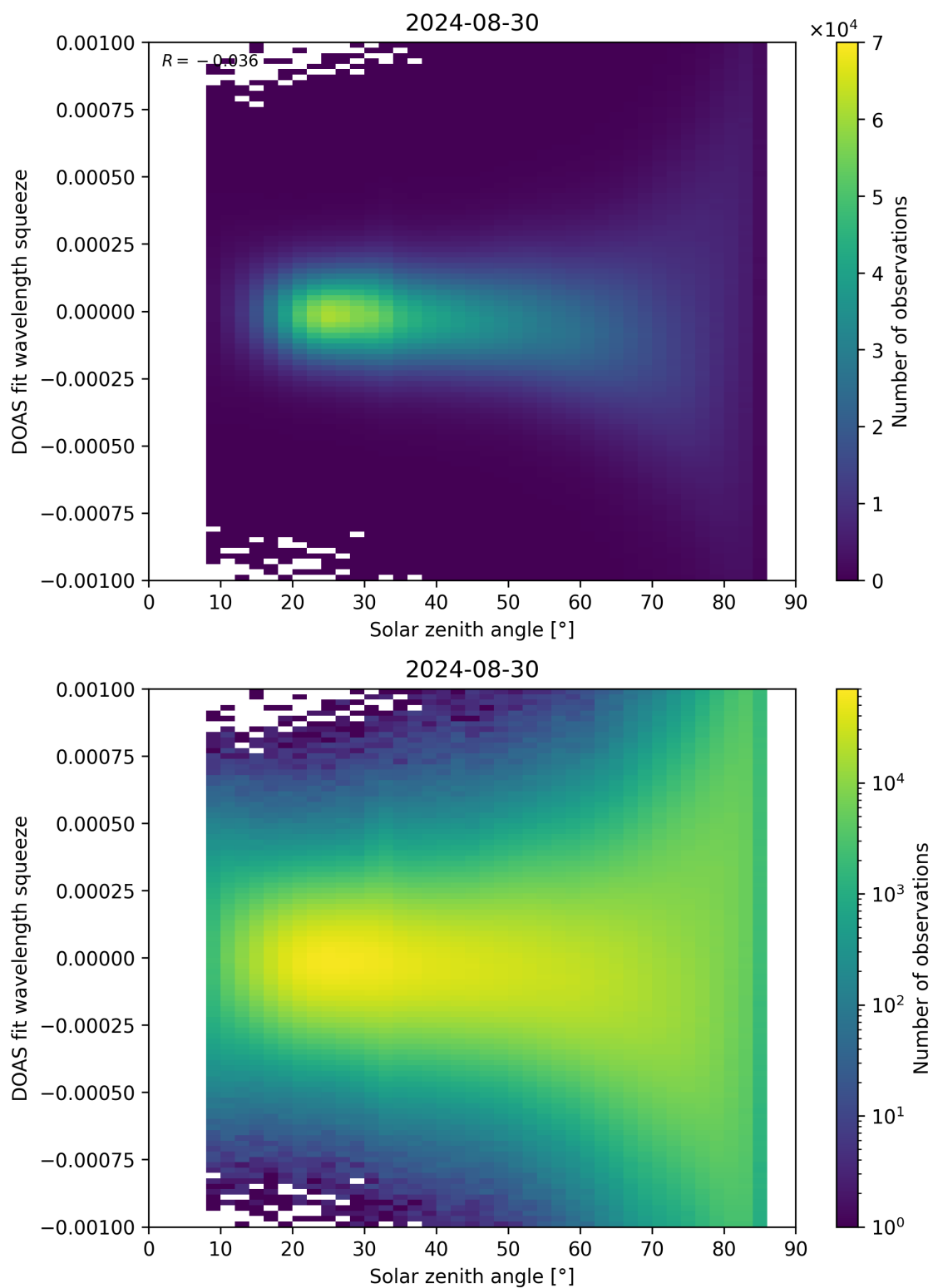
Figure 162: Scatter density plot of “Solar zenith angle” against “DOAS fit wavelength squeeze” for 2024-08-29 to 2024-08-31.
