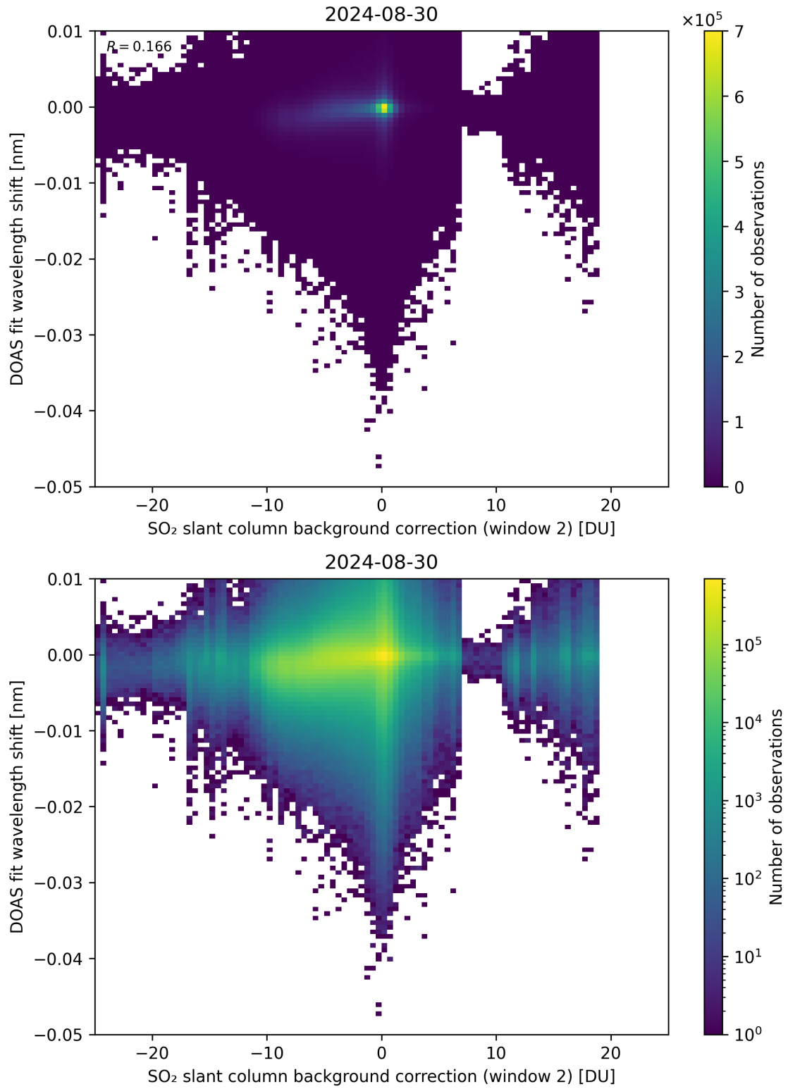
Figure 112: Scatter density plot of “SO 2 slant column background correction (window 2)” against “DOAS fit wavelength shift” for 2024-08-29 to 2024-08-31.
