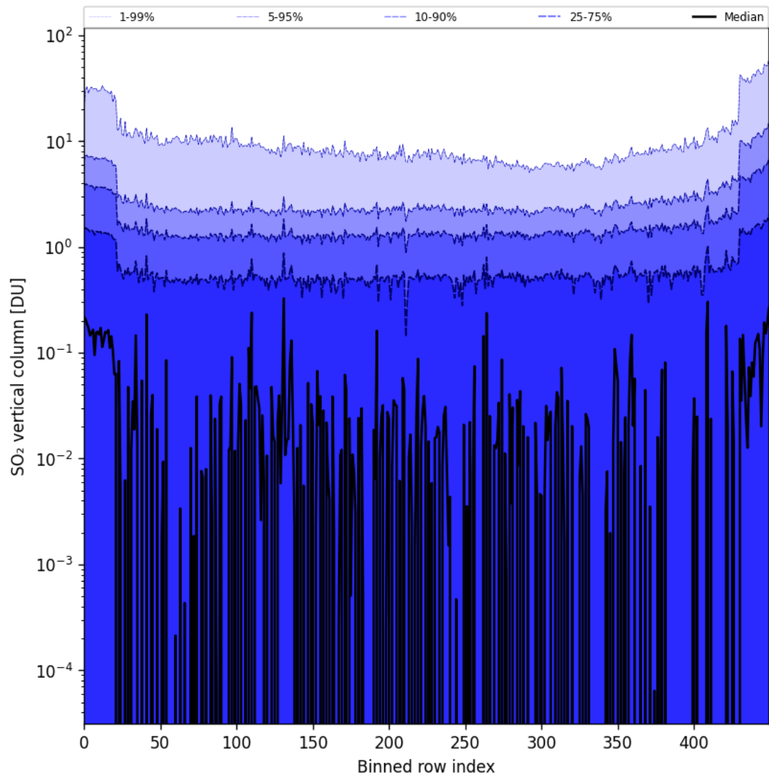
Figure 76: Along track statistics of “SO 2 vertical column” for 2024-08-29 to 2024-08-31
