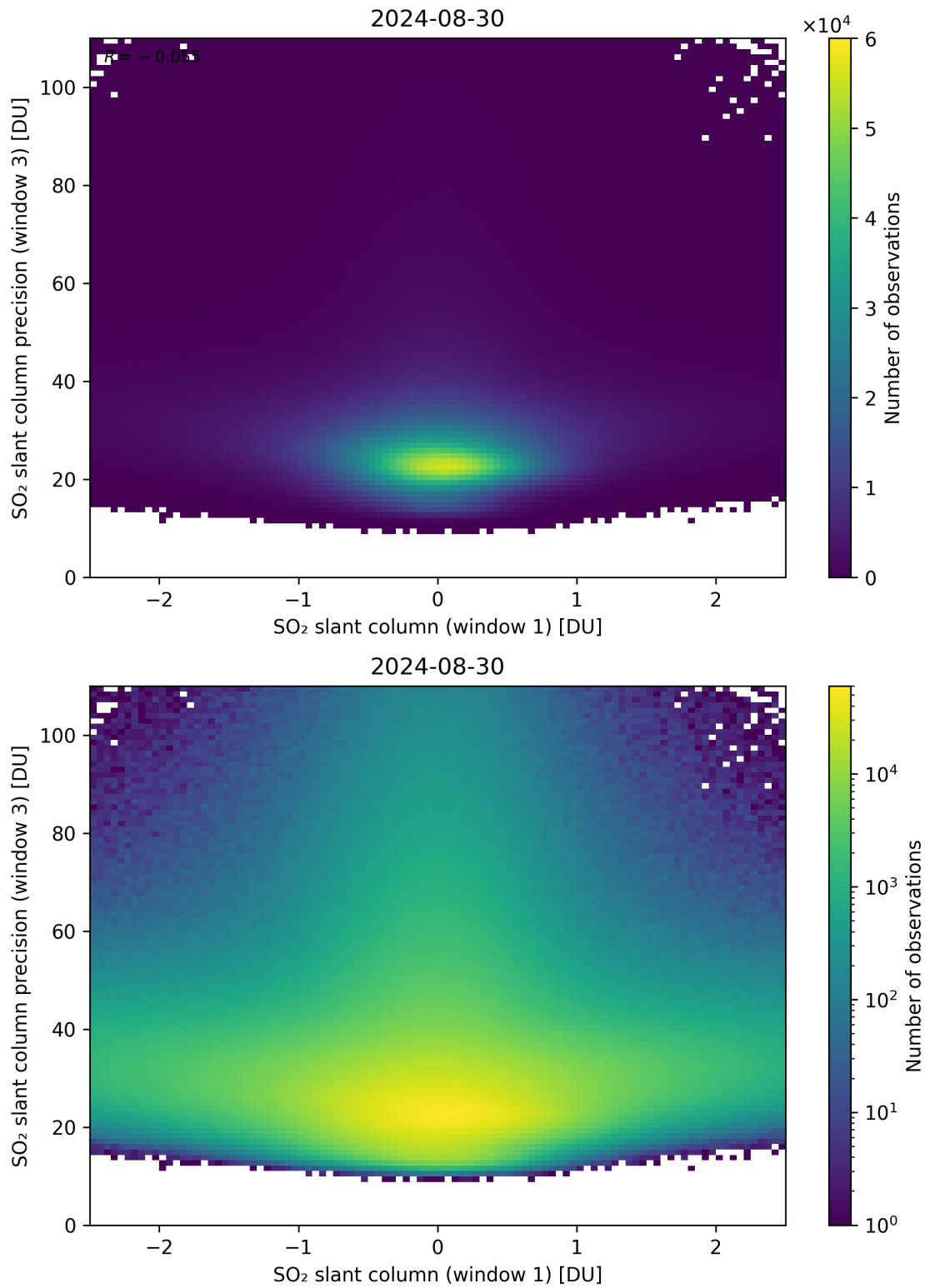
Figure 238: Scatter density plot of “SO 2 slant column (window 1)” against “SO 2 slant column precision (window 3)” for 2024-08-29 to 2024-08-31.
