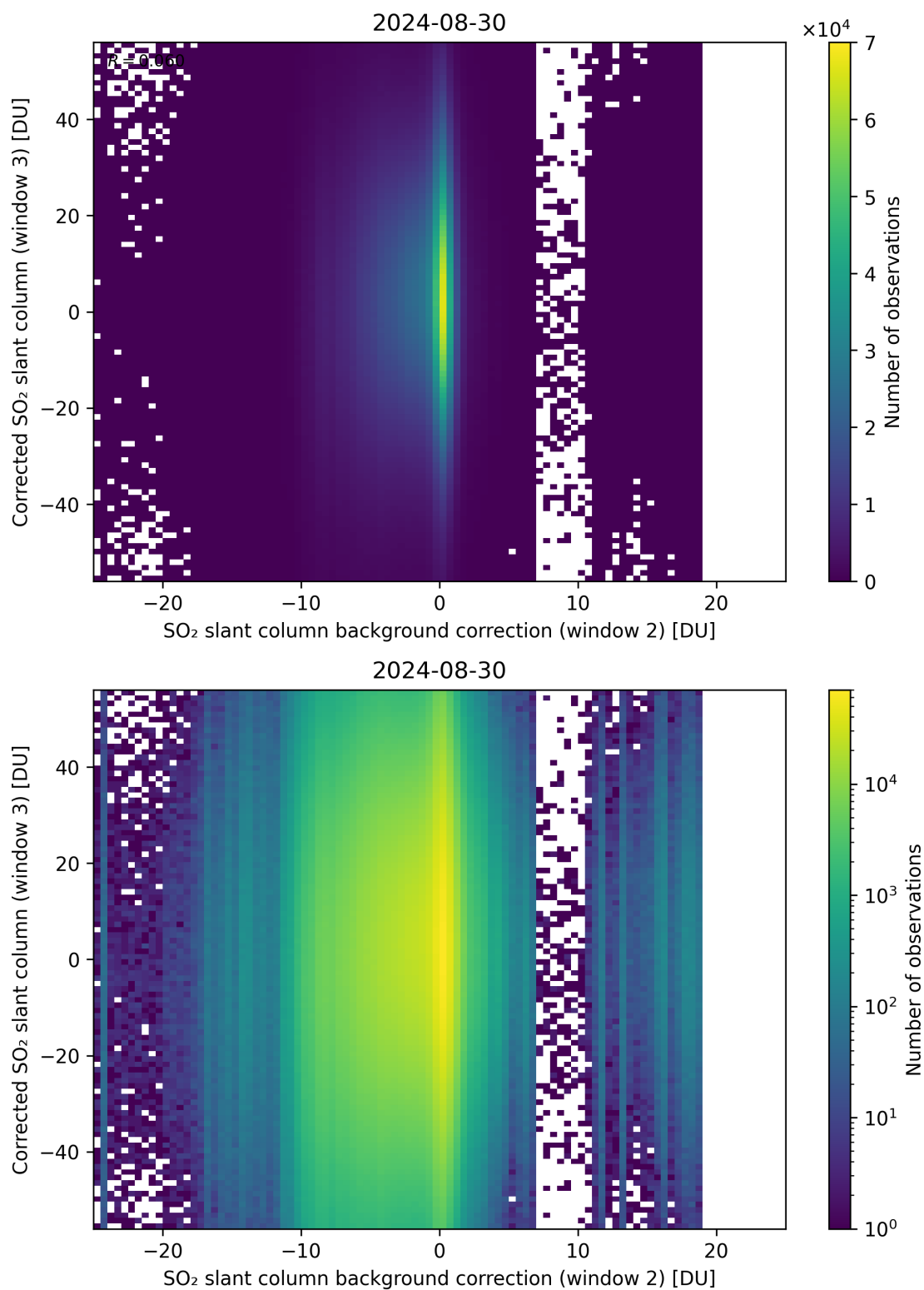
Figure 116: Scatter density plot of “SO 2 slant column background correction (window 2)” against “Corrected SO 2 slant column (window 3)” for 2024-08-29 to 2024-08-31.
