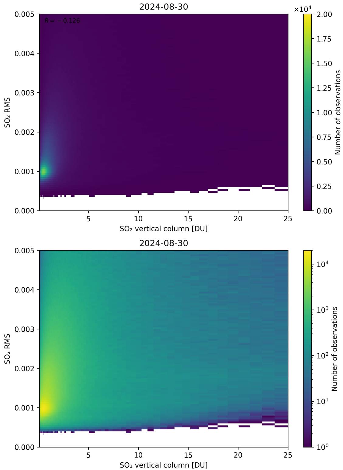
Figure 278: Scatter density plot of “SO 2 vertical column” against “SO 2 RMS” for 2024-08-29 to 2024-08-31.
