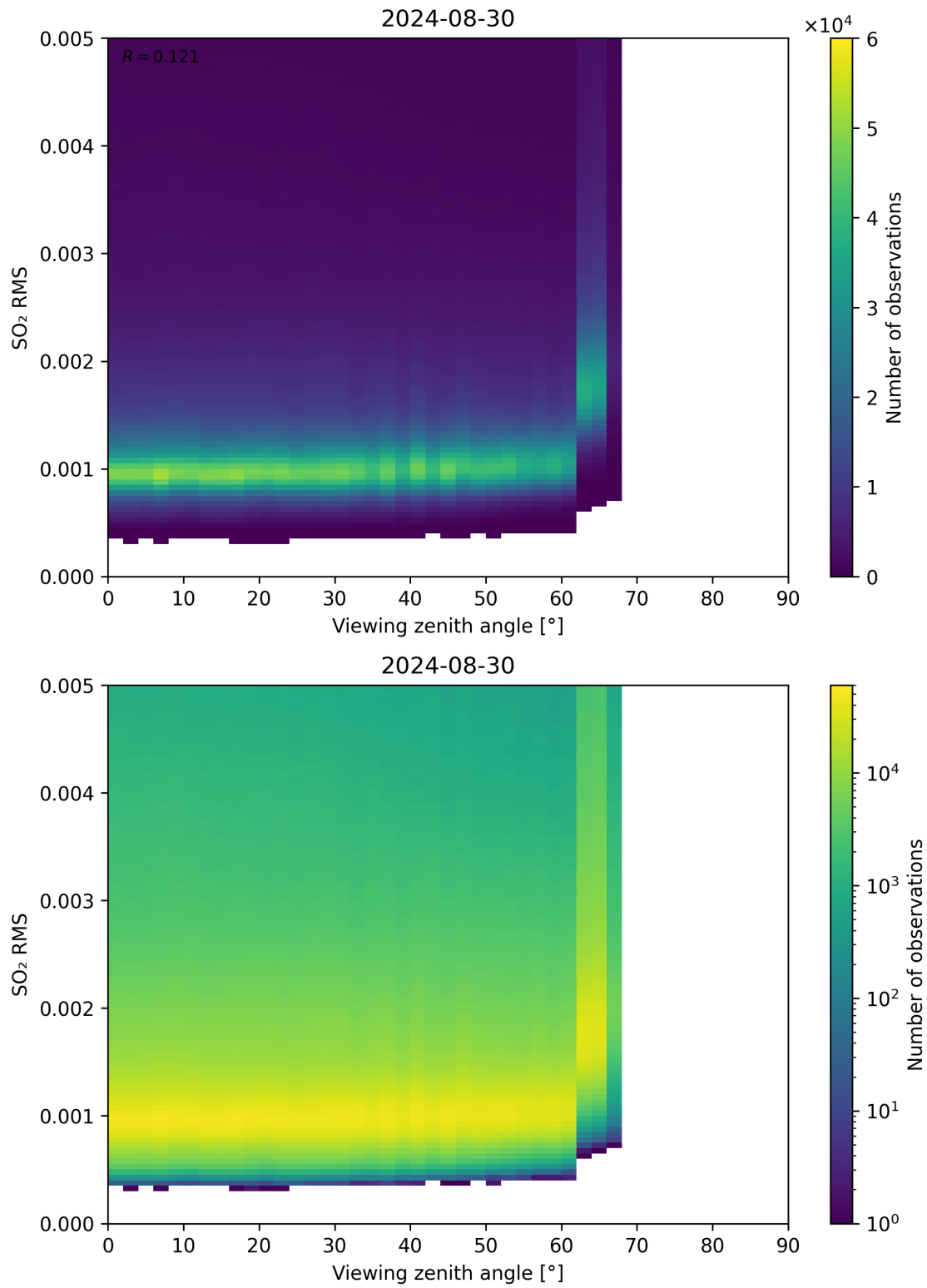
Figure 313: Scatter density plot of “Viewing zenith angle” against “SO 2 RMS” for 2024-08-29 to 2024-08-31.
