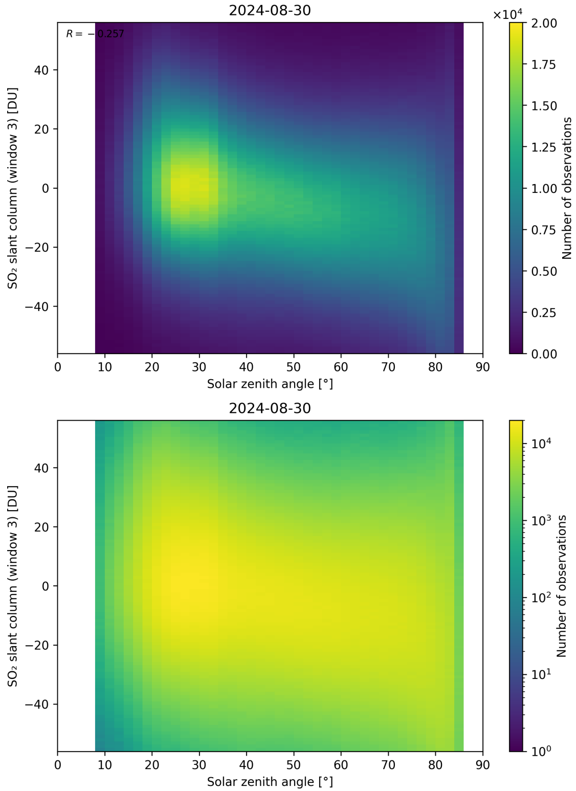
Figure 172: Scatter density plot of “Solar zenith angle” against “SO 2 slant column (window 3)” for 2024-08-29 to 2024-08-31.
