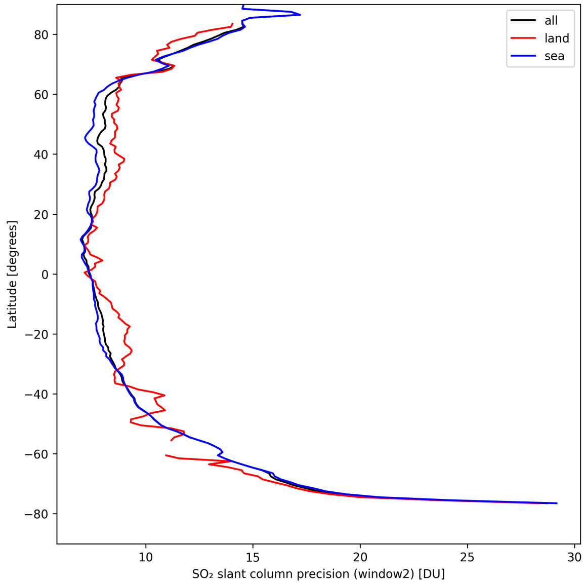
Figure 38: Zonal average of “SO 2 slant column precision (window2)” for 2024-08-29 to 2024-08-31.
