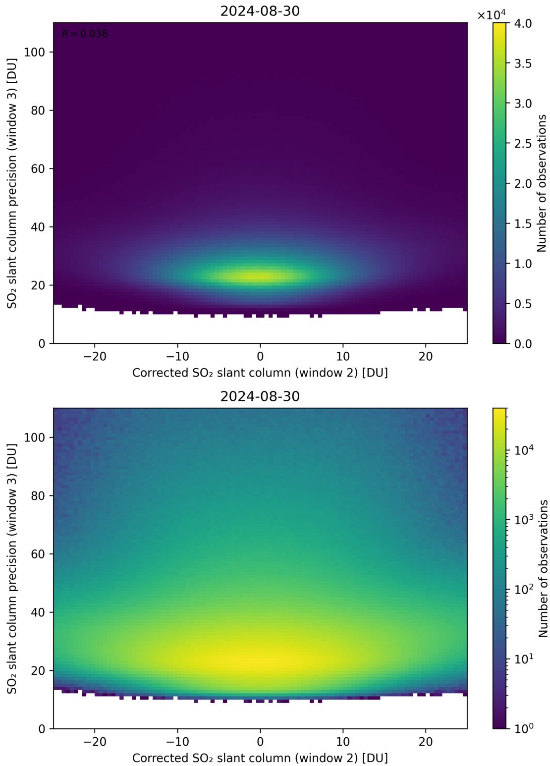
Figure 202: Scatter density plot of “Corrected SO 2 slant column (window 2)” against “SO 2 slant column precision (window 3)” for 2024-08-29 to 2024-08-31.
