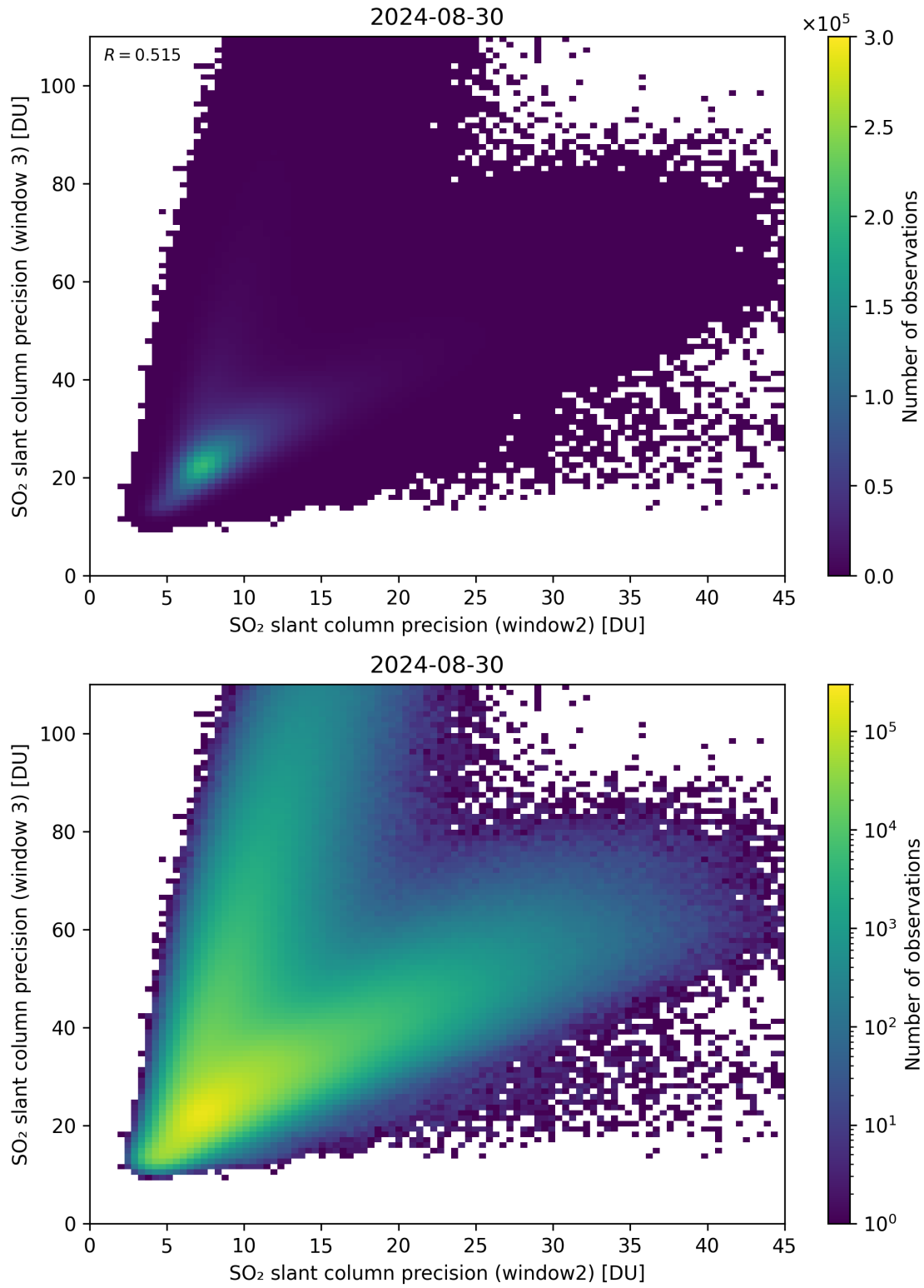
Figure 250: Scatter density plot of “SO 2 slant column precision (window2)” against “SO 2 slant column precision (window 3)” for 2024-08-29 to 2024-08-31.
