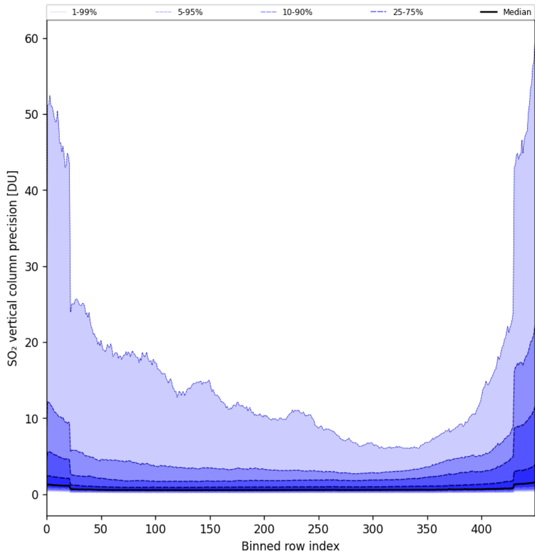
Figure 77: Along track statistics of “SO 2 vertical column precision” for 2024-08-29 to 2024-08-31
