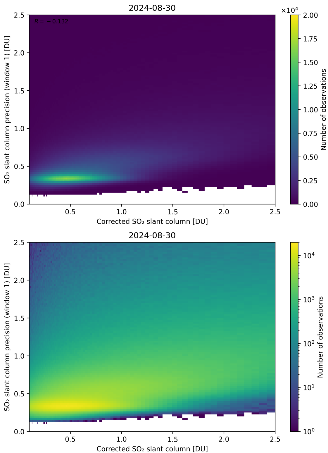
Figure 188: Scatter density plot of “Corrected SO 2 slant column” against “SO 2 slant column precision (window 1)” for 2024-08-29 to 2024-08-31.
