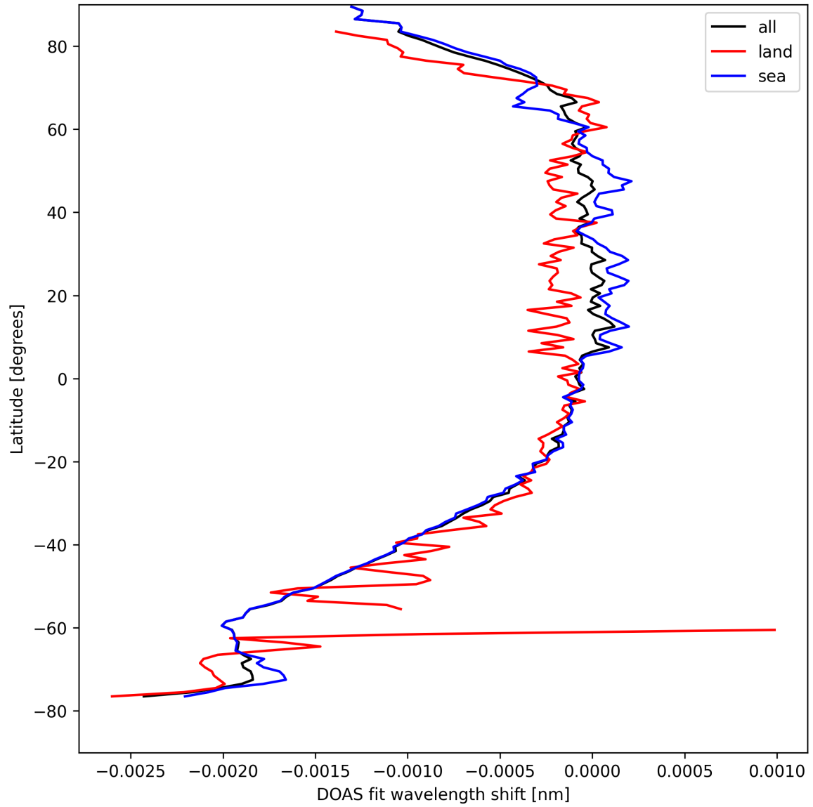
Figure 45: Zonal average of “DOAS fit wavelength shift” for 2024-08-29 to 2024-08-31.
