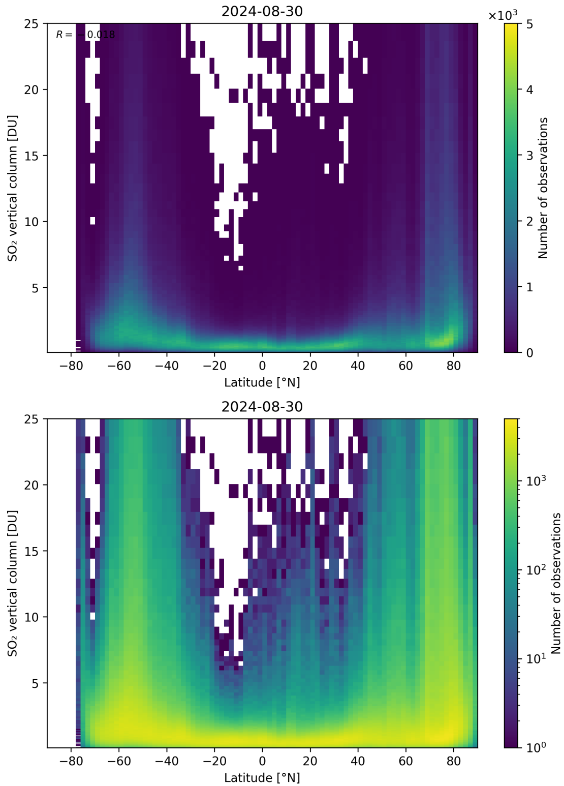
Figure 156: Scatter density plot of “Latitude” against “SO 2 vertical column” for 2024-08-29 to 2024-08-31.
