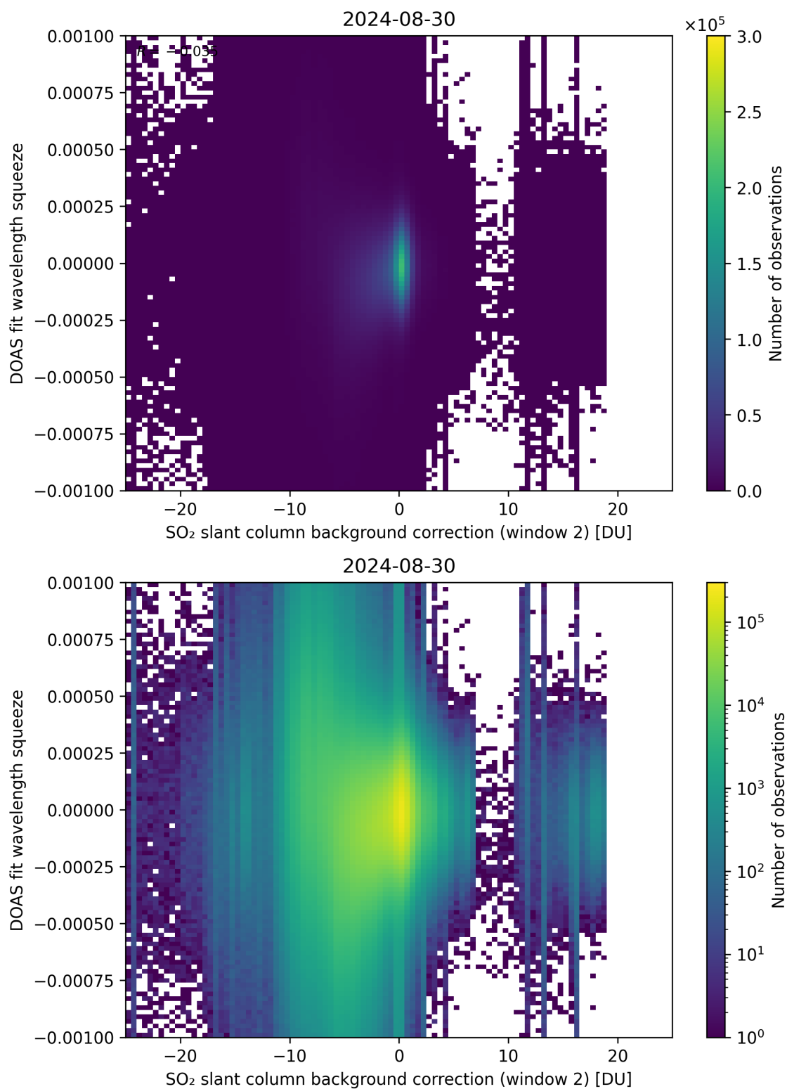
Figure 113: Scatter density plot of “SO 2 slant column background correction (window 2)” against “DOAS fit wavelength squeeze” for 2024-08-29 to 2024-08-31.
