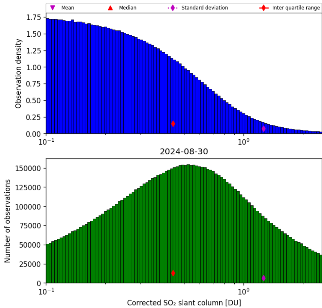
Figure 55: Histogram of “Corrected SO 2 slant column” for 2024-08-29 to 2024-08-31
