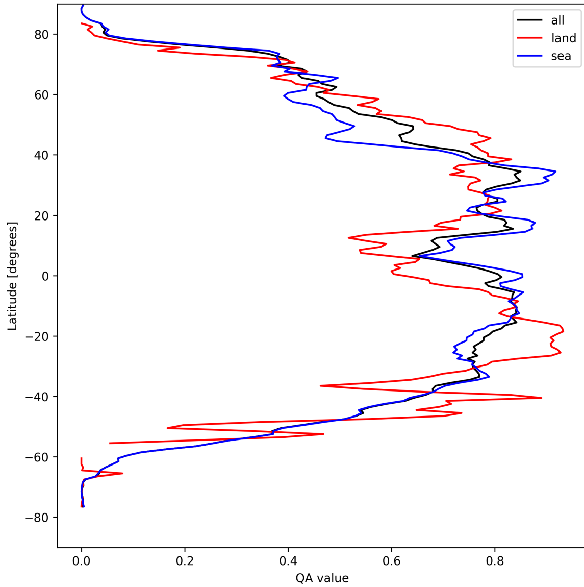
Figure 29: Zonal average of “QA value” for 2024-08-29 to 2024-08-31.
