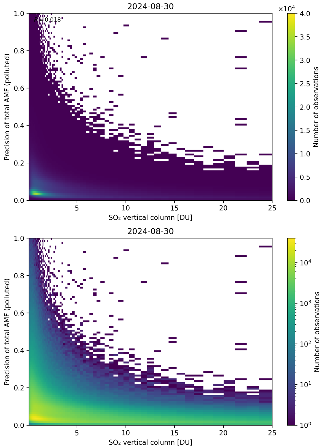
Figure 306: Scatter density plot of “SO 2 vertical column” against “Precision of total AMF (polluted)” for 2024-08-29 to 2024-08-31.
