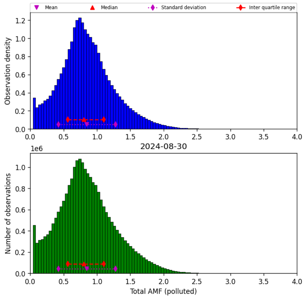
Figure 71: Histogram of “Total AMF (polluted)” for 2024-08-29 to 2024-08-31
