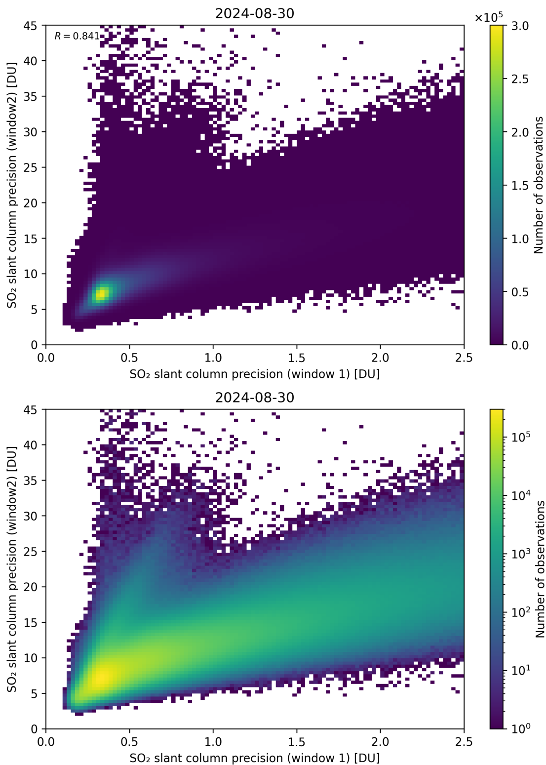
Figure 227: Scatter density plot of “SO 2 slant column precision (window 1)” against “SO 2 slant column precision (window 2)” for 2024-08-29 to 2024-08-31.
