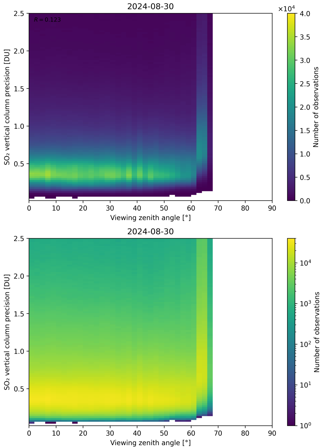
Figure 328: Scatter density plot of “Viewing zenith angle” against “SO 2 vertical column precision” for 2024-08-29 to 2024-08-31.
