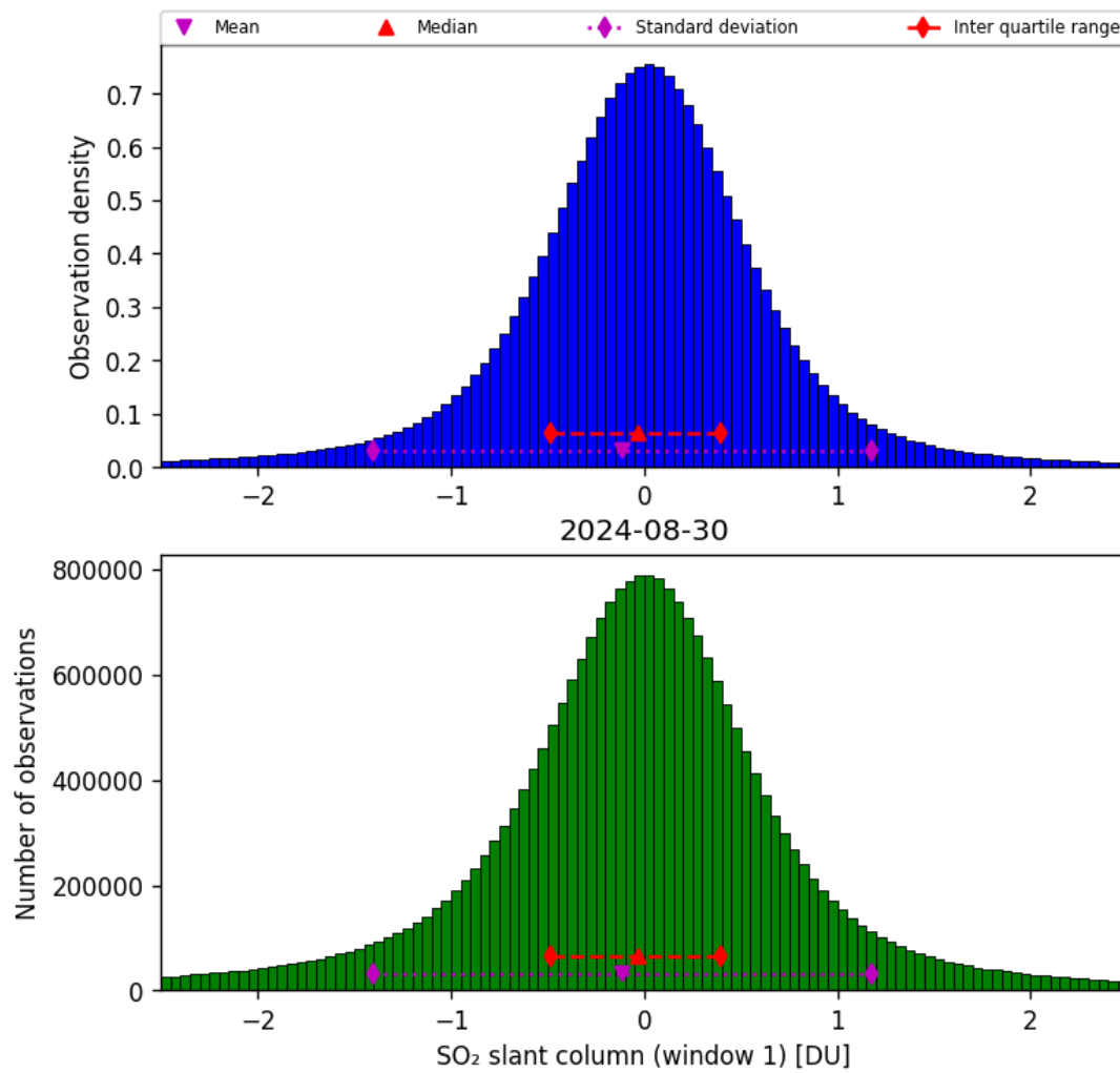
Figure 56: Histogram of “SO 2 slant column (window 1)” for 2024-08-29 to 2024-08-31
