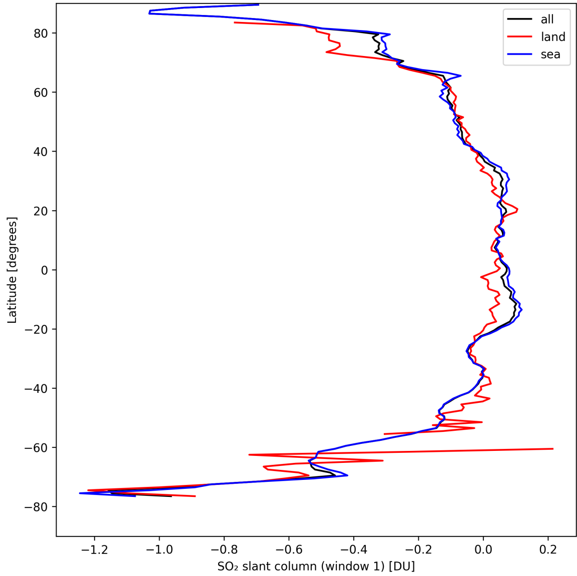
Figure 33: Zonal average of “SO 2 slant column (window 1)” for 2024-08-29 to 2024-08-31.
