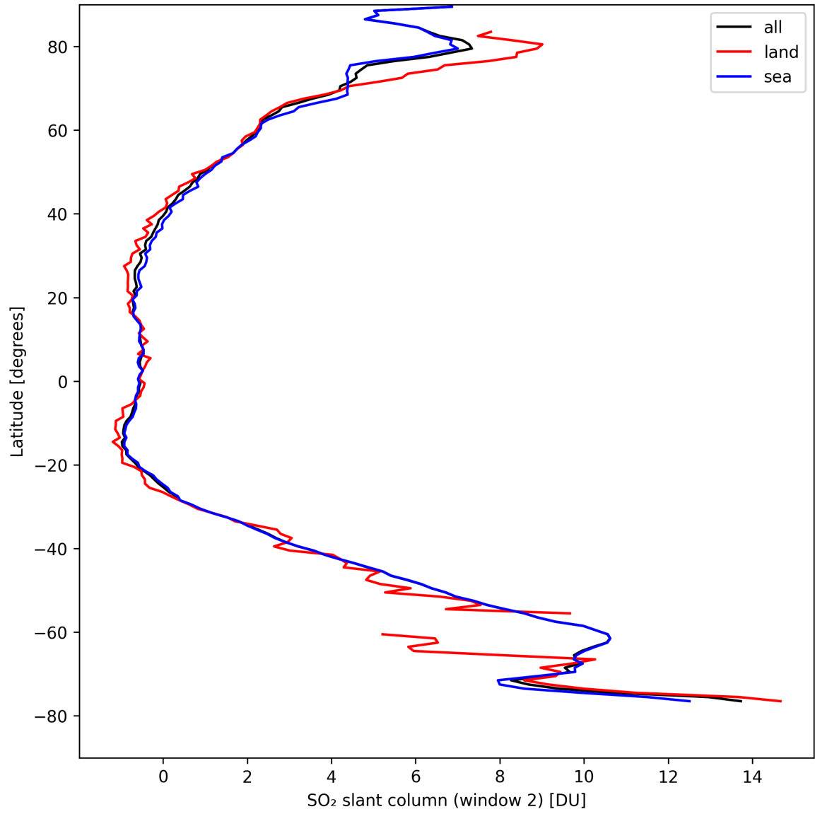
Figure 37: Zonal average of “SO 2 slant column (window 2)” for 2024-08-29 to 2024-08-31.
