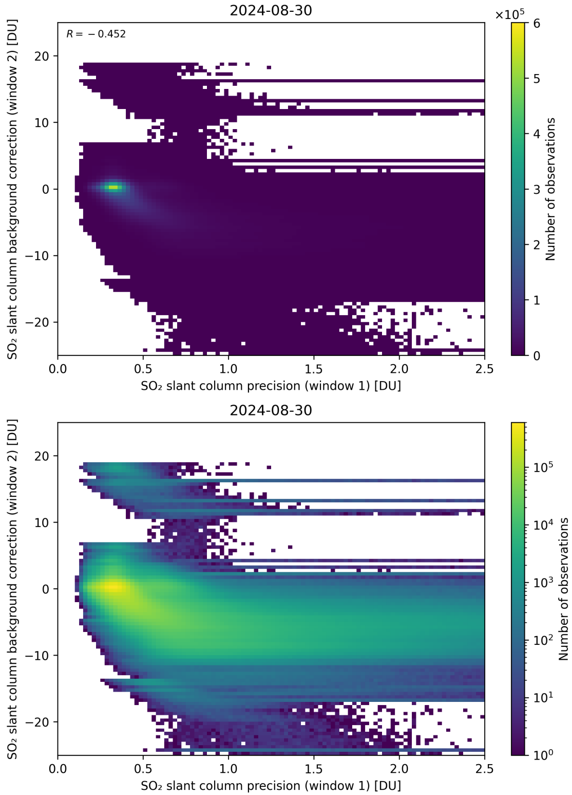
Figure 219: Scatter density plot of “SO 2 slant column precision (window 1)” against “SO 2 slant column background correction (window 2)” for 2024-08-29 to 2024-08-31.
