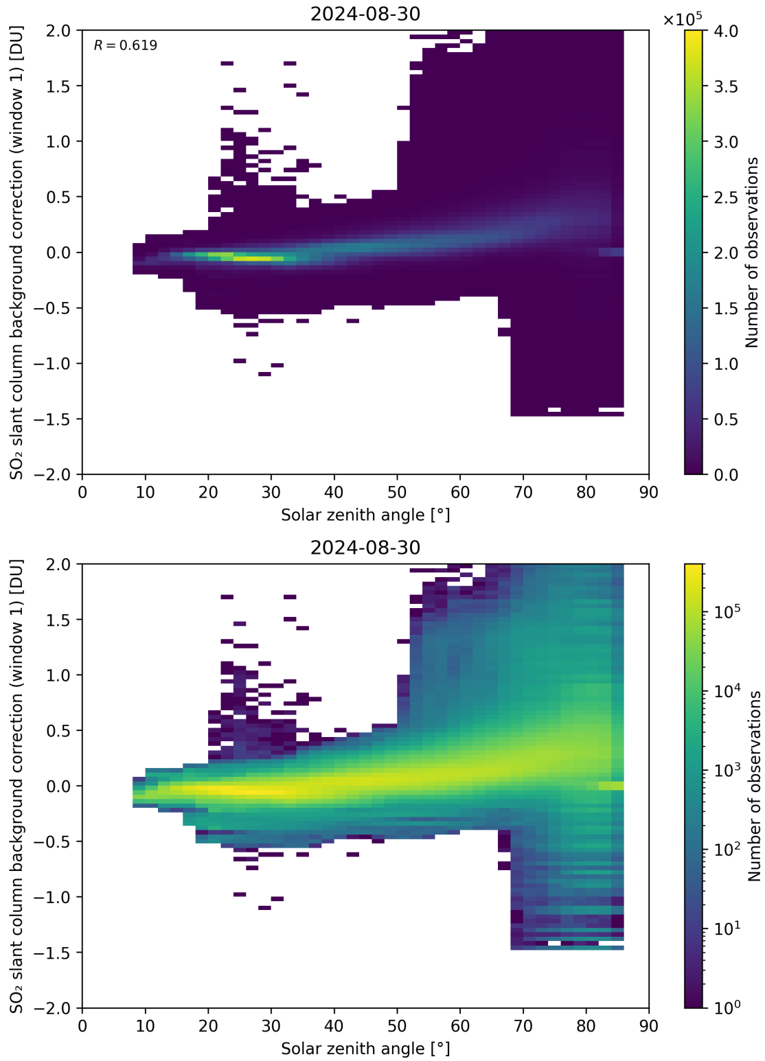
Figure 158: Scatter density plot of “Solar zenith angle” against “SO 2 slant column background correction (window 1)” for 2024-08-29 to 2024-08-31.
