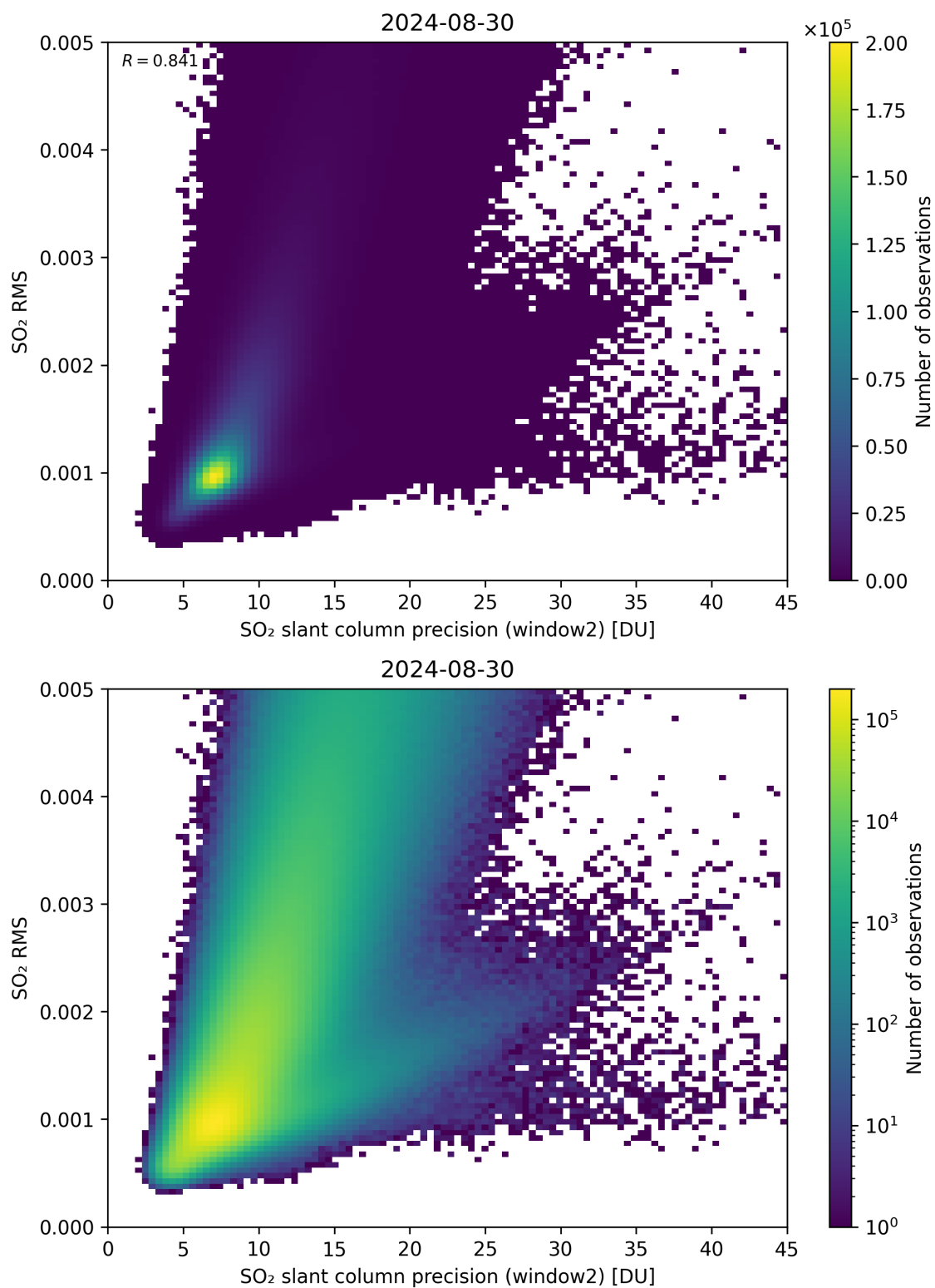
Figure 245: Scatter density plot of “SO 2 slant column precision (window2)” against “SO 2 RMS” for 2024-08-29 to 2024-08-31.
