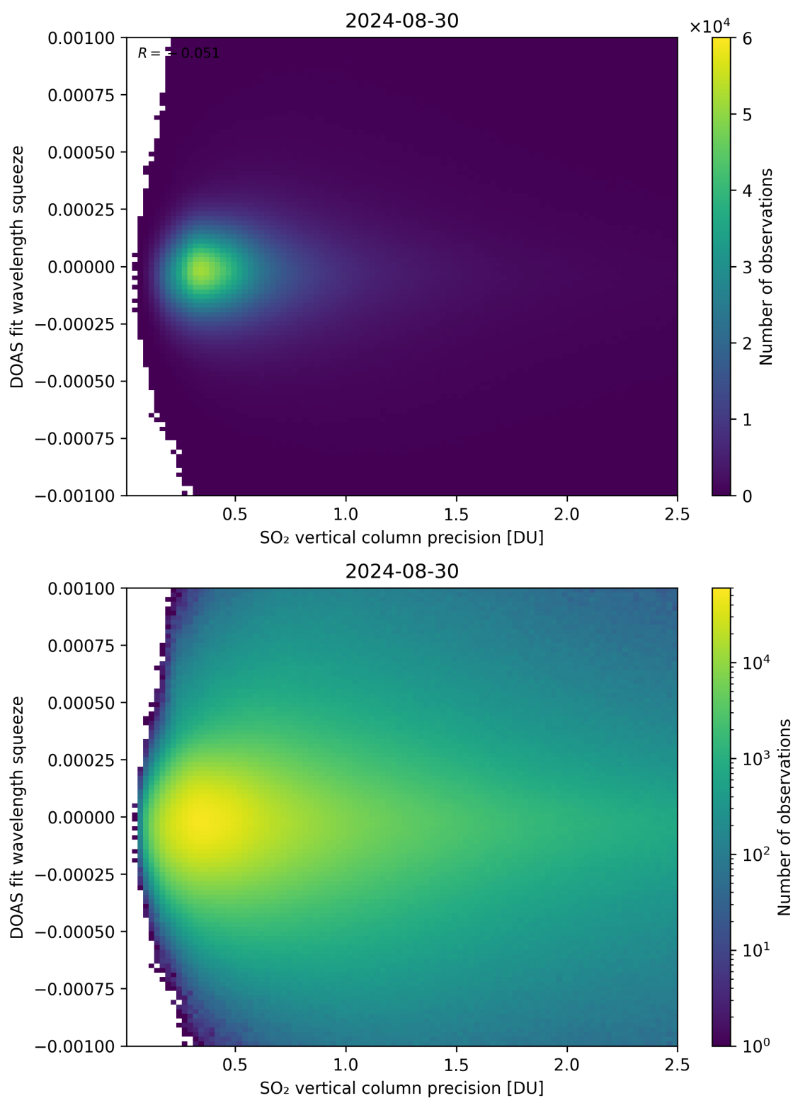
Figure 283: Scatter density plot of “SO 2 vertical column precision” against “DOAS fit wavelength squeeze” for 2024-08-29 to 2024-08-31.
