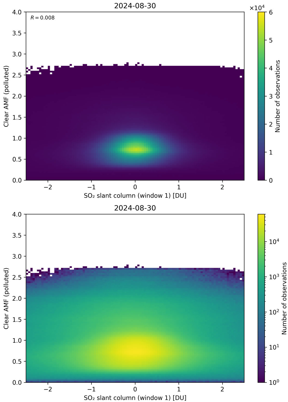
Figure 232: Scatter density plot of “SO 2 slant column (window 1)” against “Clear AMF (polluted)” for 2024-08-29 to 2024-08-31.
