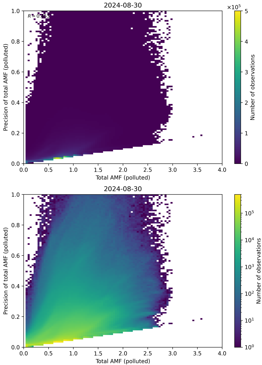
Figure 272: Scatter density plot of “Total AMF (polluted)” against “Precision of total AMF (polluted)” for 2024-08-29 to 2024-08-31.
