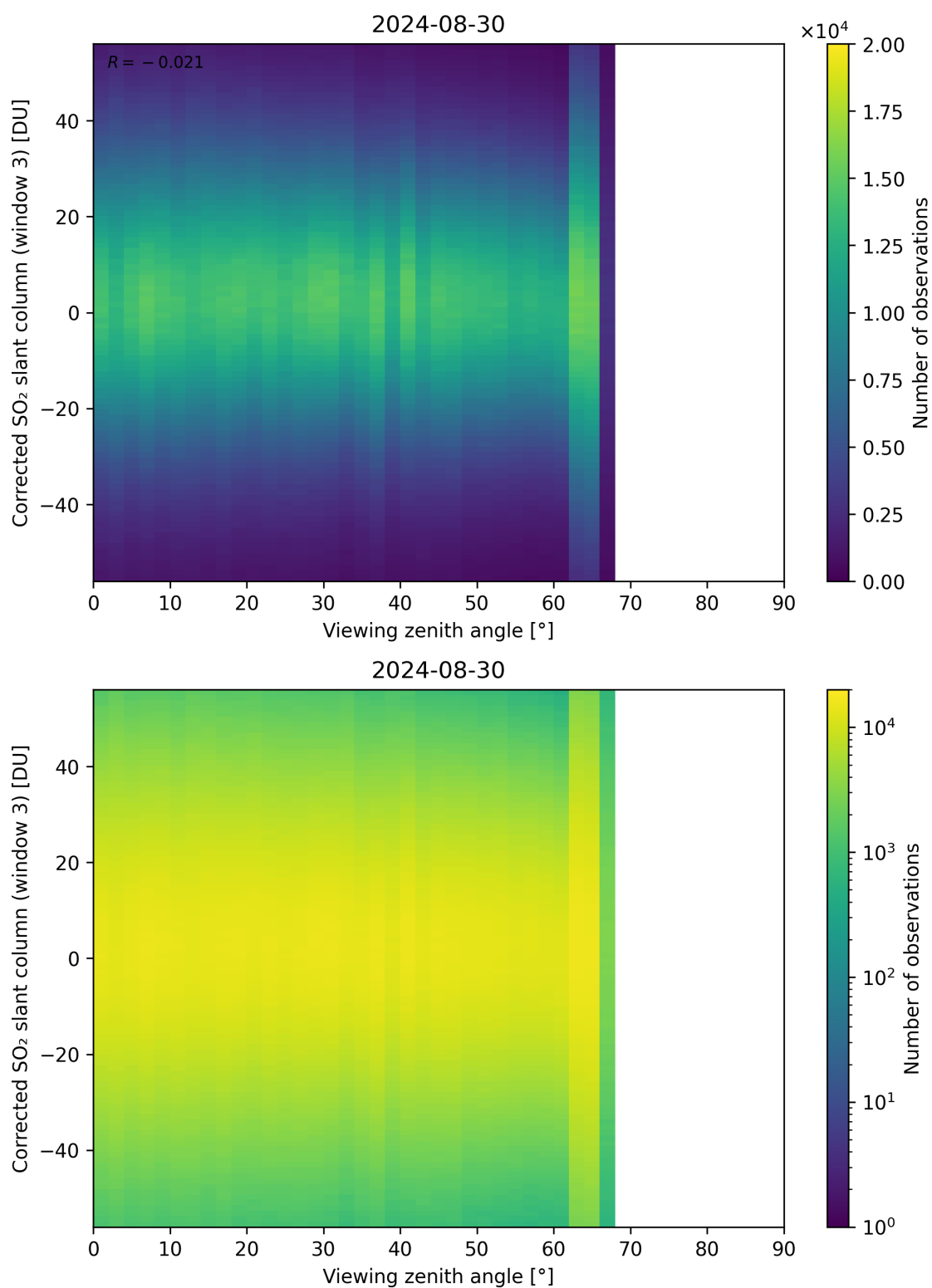
Figure 319: Scatter density plot of “Viewing zenith angle” against “Corrected SO 2 slant column (window 3)” for 2024-08-29 to 2024-08-31.
