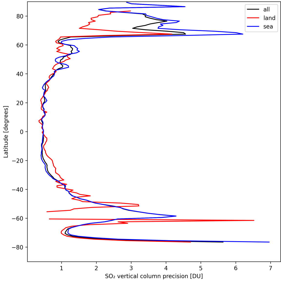
Figure 31: Zonal average of “SO 2 vertical column precision” for 2024-08-29 to 2024-08-31.
