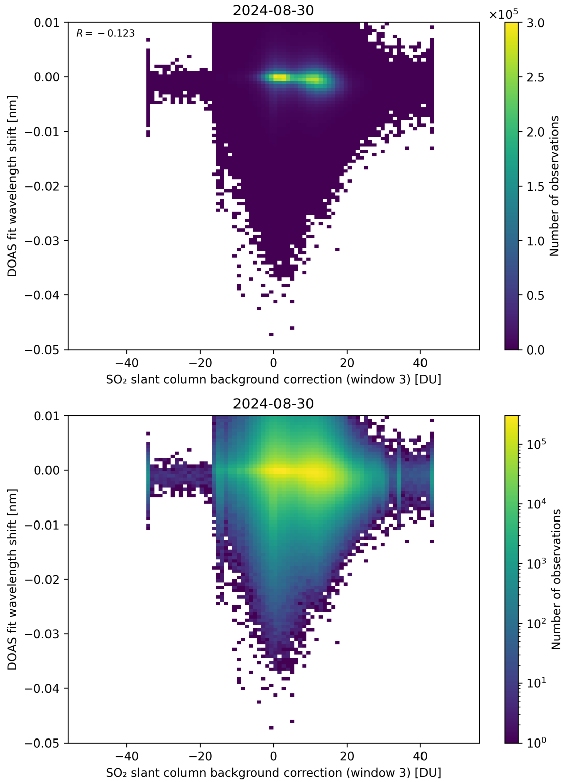
Figure 121: Scatter density plot of “SO 2 slant column background correction (window 3)” against “DOAS fit wavelength shift” for 2024-08-29 to 2024-08-31.
