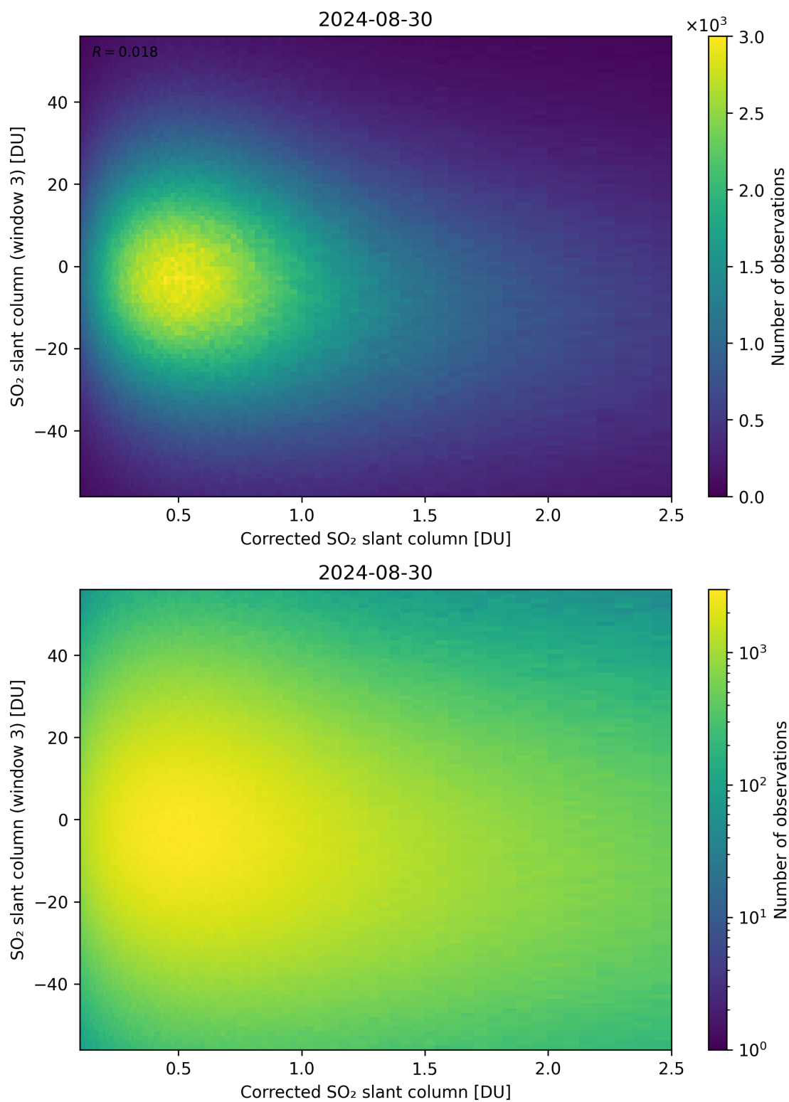
Figure 190: Scatter density plot of “Corrected SO 2 slant column” against “SO 2 slant column (window 3)” for 2024-08-29 to 2024-08-31.
