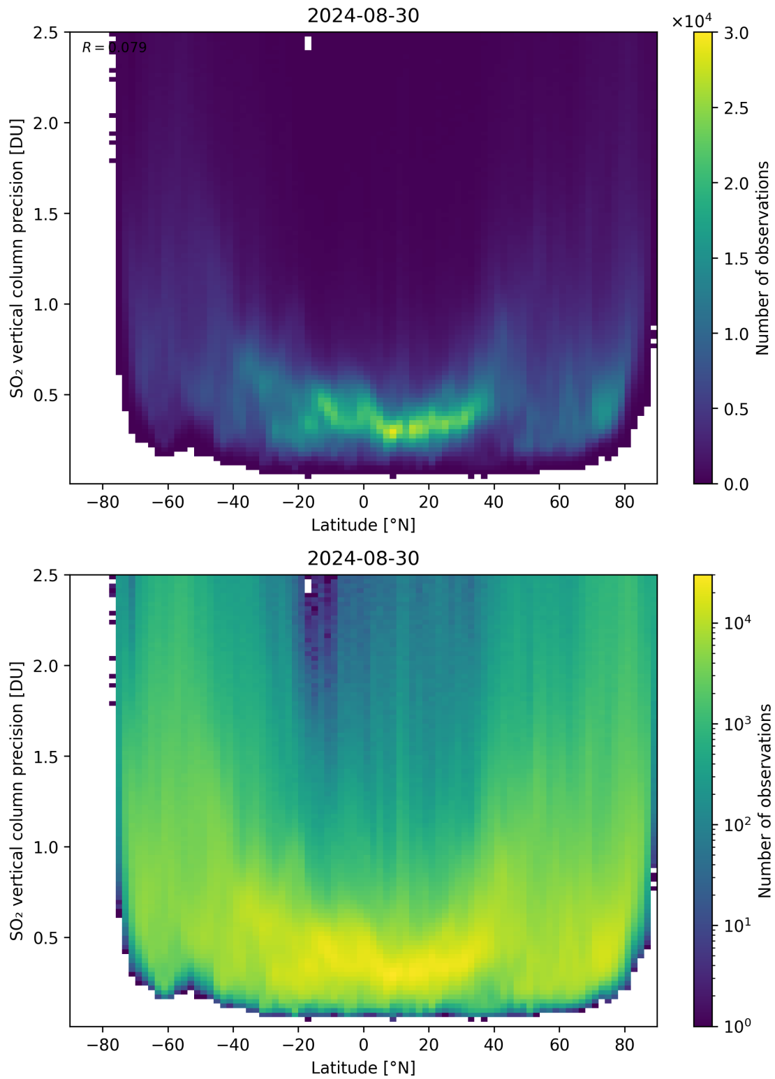
Figure 157: Scatter density plot of “Latitude” against “SO 2 vertical column precision” for 2024-08-29 to 2024-08-31.
