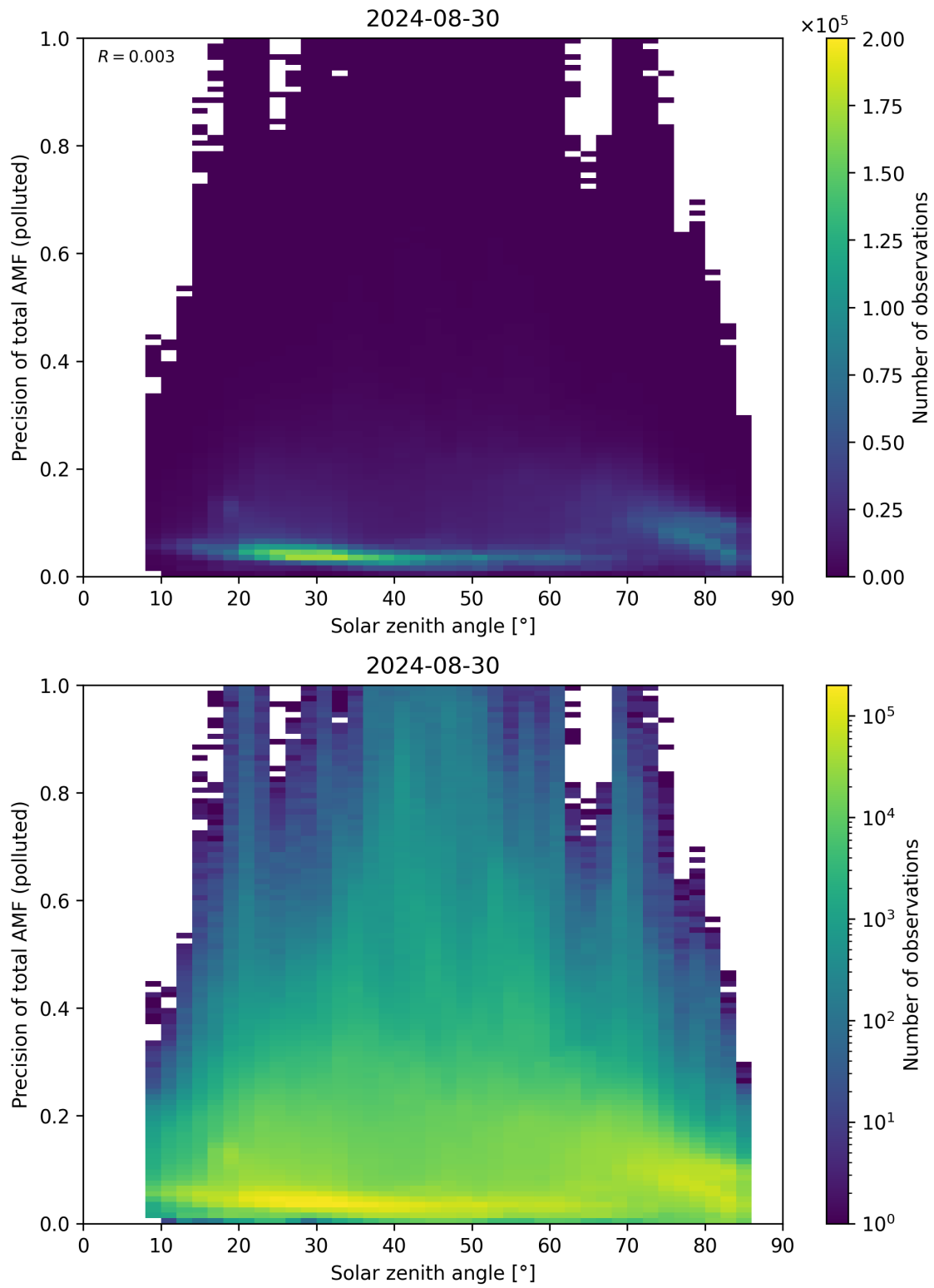
Figure 175: Scatter density plot of “Solar zenith angle” against “Precision of total AMF (polluted)” for 2024-08-29 to 2024-08-31.
