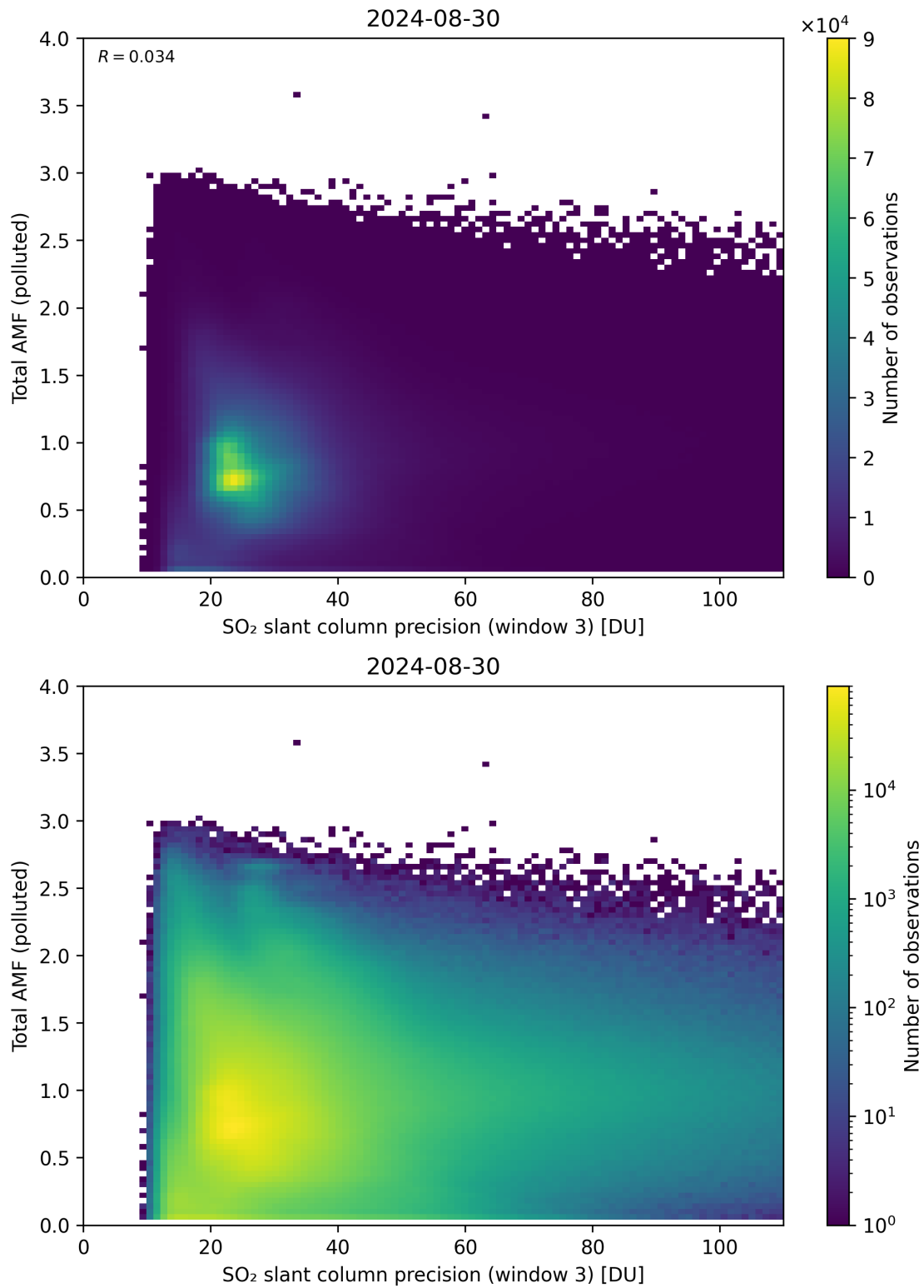
Figure 263: Scatter density plot of “SO 2 slant column precision (window 3)” against “Total AMF (polluted)” for 2024-08-29 to 2024-08-31.
