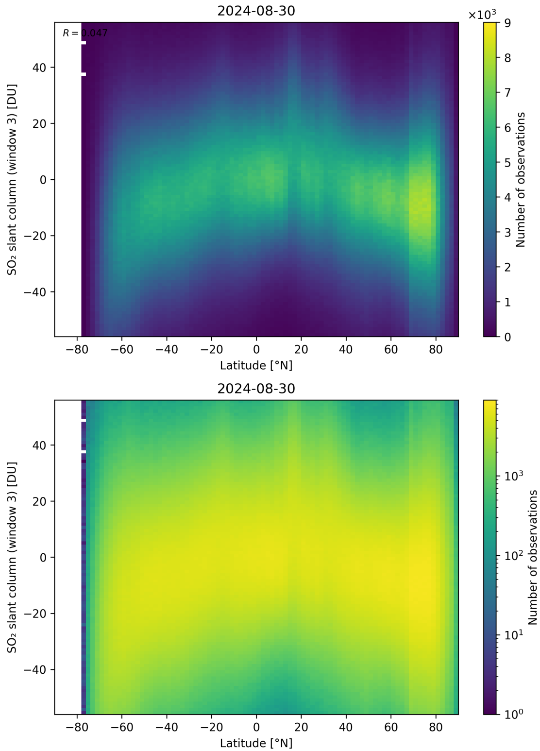
Figure 152: Scatter density plot of “Latitude” against “SO 2 slant column (window 3)” for 2024-08-29 to 2024-08-31.
