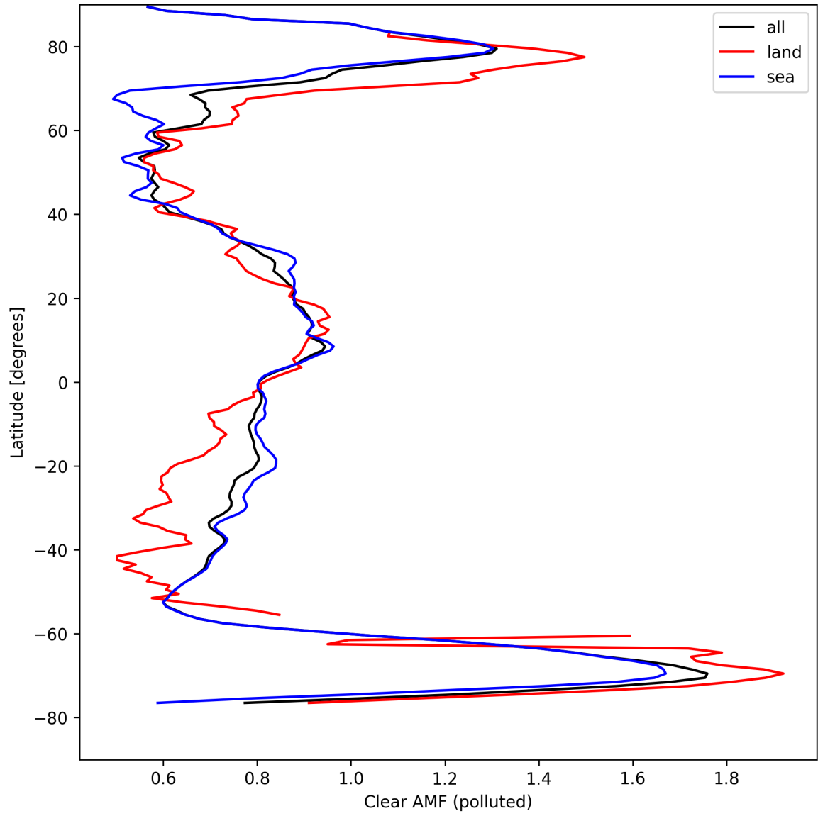
Figure 50: Zonal average of “Clear AMF (polluted)” for 2024-08-29 to 2024-08-31.
