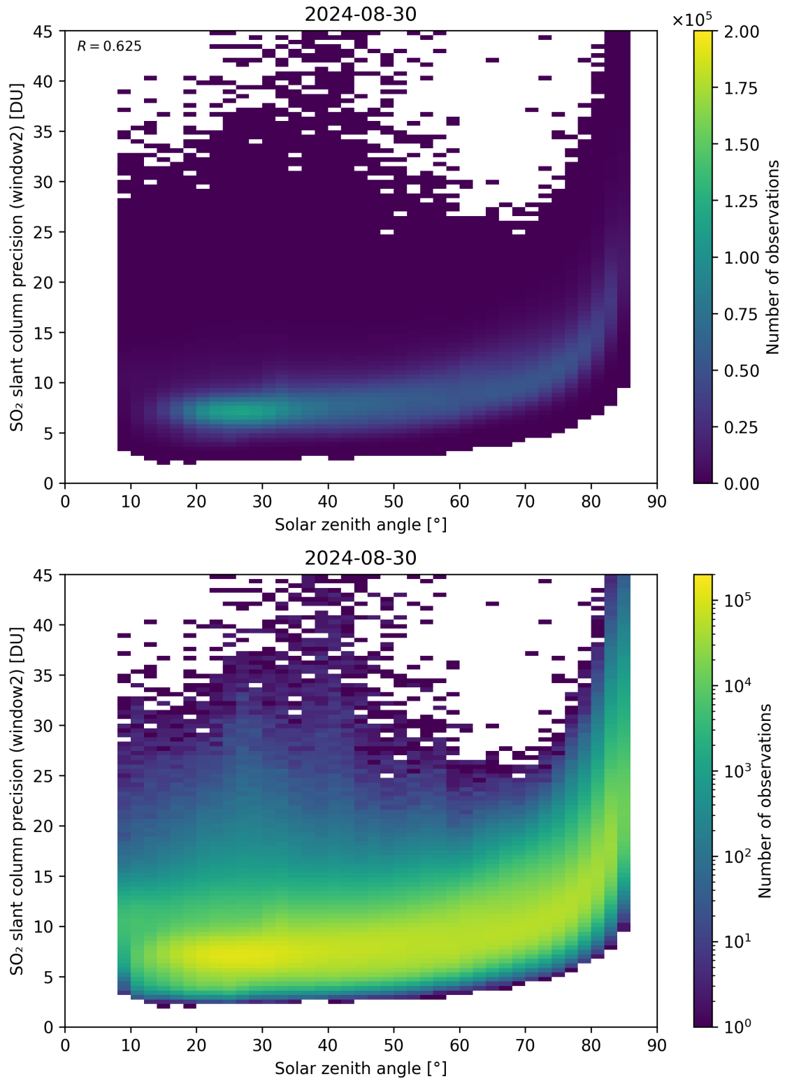
Figure 171: Scatter density plot of “Solar zenith angle” against “SO 2 slant column precision (window2)” for 2024-08-29 to 2024-08-31.
