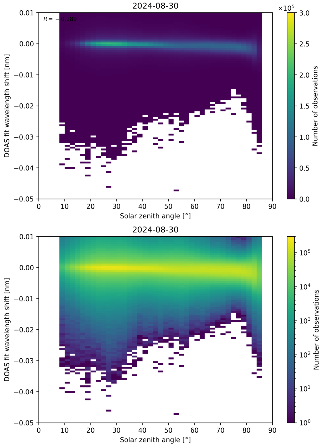
Figure 161: Scatter density plot of “Solar zenith angle” against “DOAS fit wavelength shift” for 2024-08-29 to 2024-08-31.
