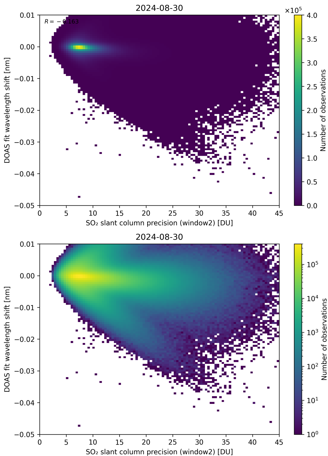
Figure 243: Scatter density plot of “SO 2 slant column precision (window2)” against “DOAS fit wavelength shift” for 2024-08-29 to 2024-08-31.
