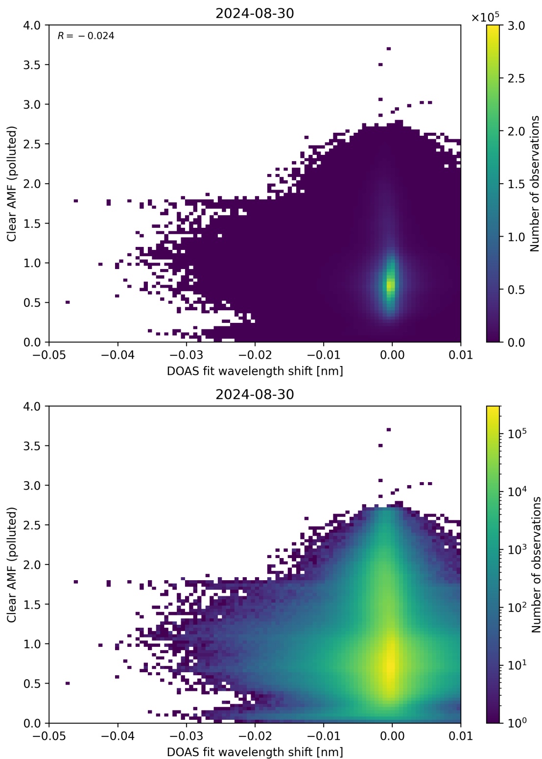
Figure 129: Scatter density plot of “DOAS fit wavelength shift” against “Clear AMF (polluted)” for 2024-08-29 to 2024-08-31.
