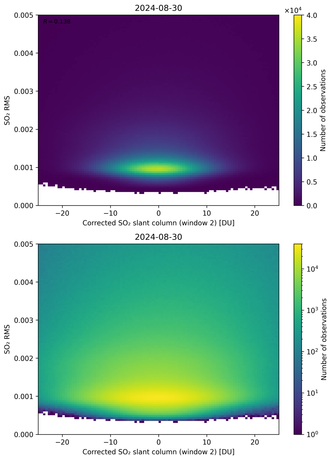
Figure 198: Scatter density plot of “Corrected SO 2 slant column (window 2)” against “SO 2 RMS” for 2024-08-29 to 2024-08-31.
