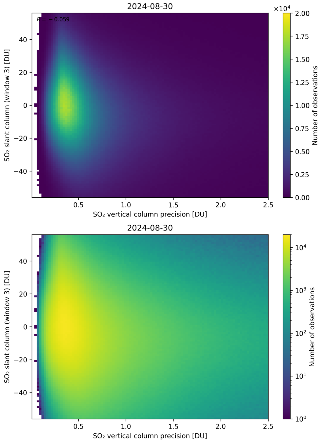
Figure 292: Scatter density plot of “SO 2 vertical column precision” against “SO 2 slant column (window 3)” for 2024-08-29 to 2024-08-31.
