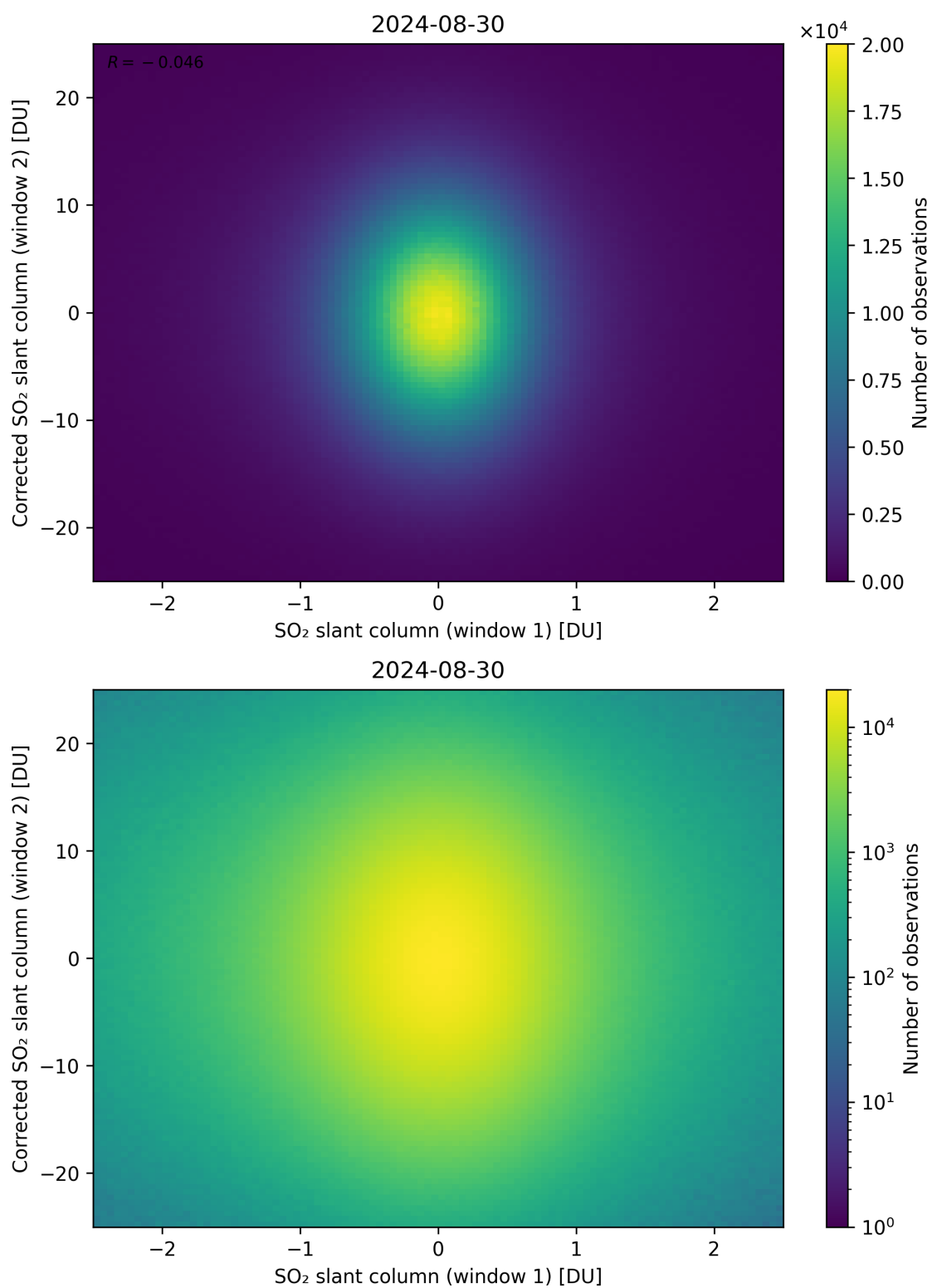
Figure 233: Scatter density plot of “SO 2 slant column (window 1)” against “Corrected SO 2 slant column (window 2)” for 2024-08-29 to 2024-08-31.
