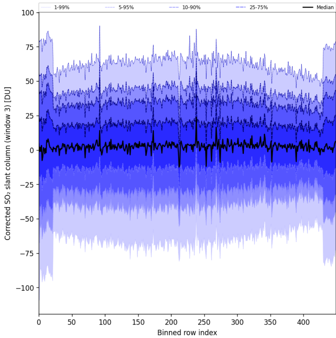
Figure 89: Along track statistics of “Corrected SO 2 slant column (window 3)” for 2024-08-29 to 2024-08-31
