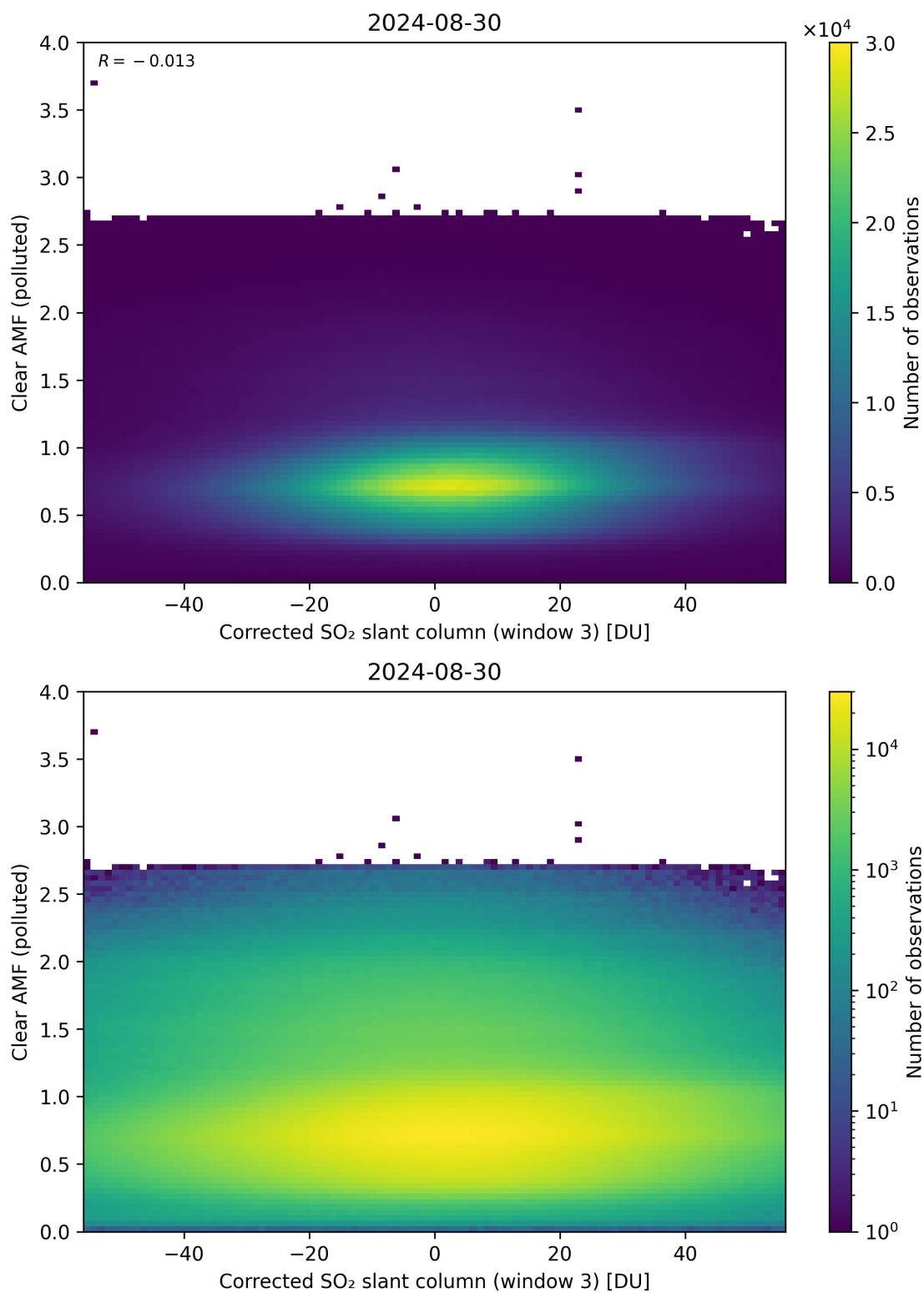
Figure 209: Scatter density plot of “Corrected SO 2 slant column (window 3)” against “Clear AMF (polluted)” for 2024-08-29 to 2024-08-31.
