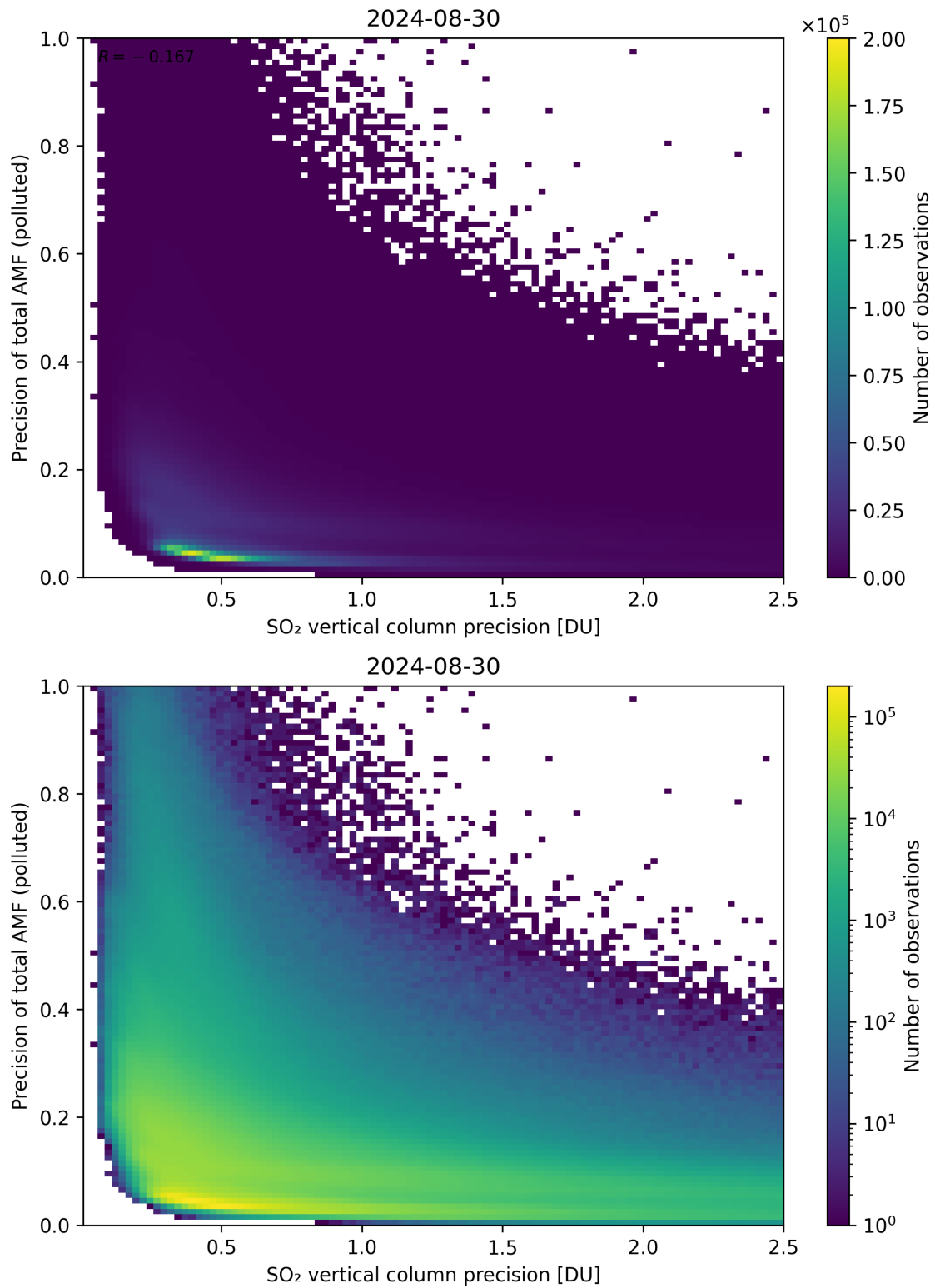
Figure 295: Scatter density plot of “SO 2 vertical column precision” against “Precision of total AMF (polluted)” for 2024-08-29 to 2024-08-31.
