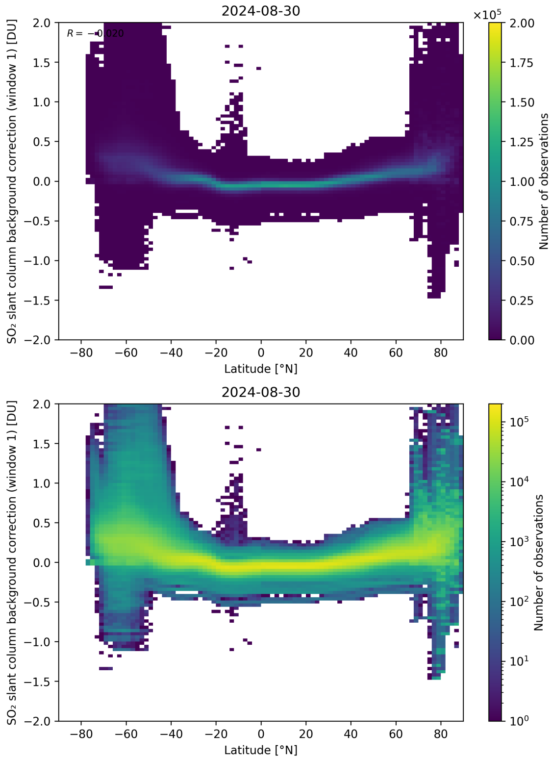
Figure 139: Scatter density plot of “Latitude” against “SO 2 slant column background correction (window 1)” for 2024-08-29 to 2024-08-31.
