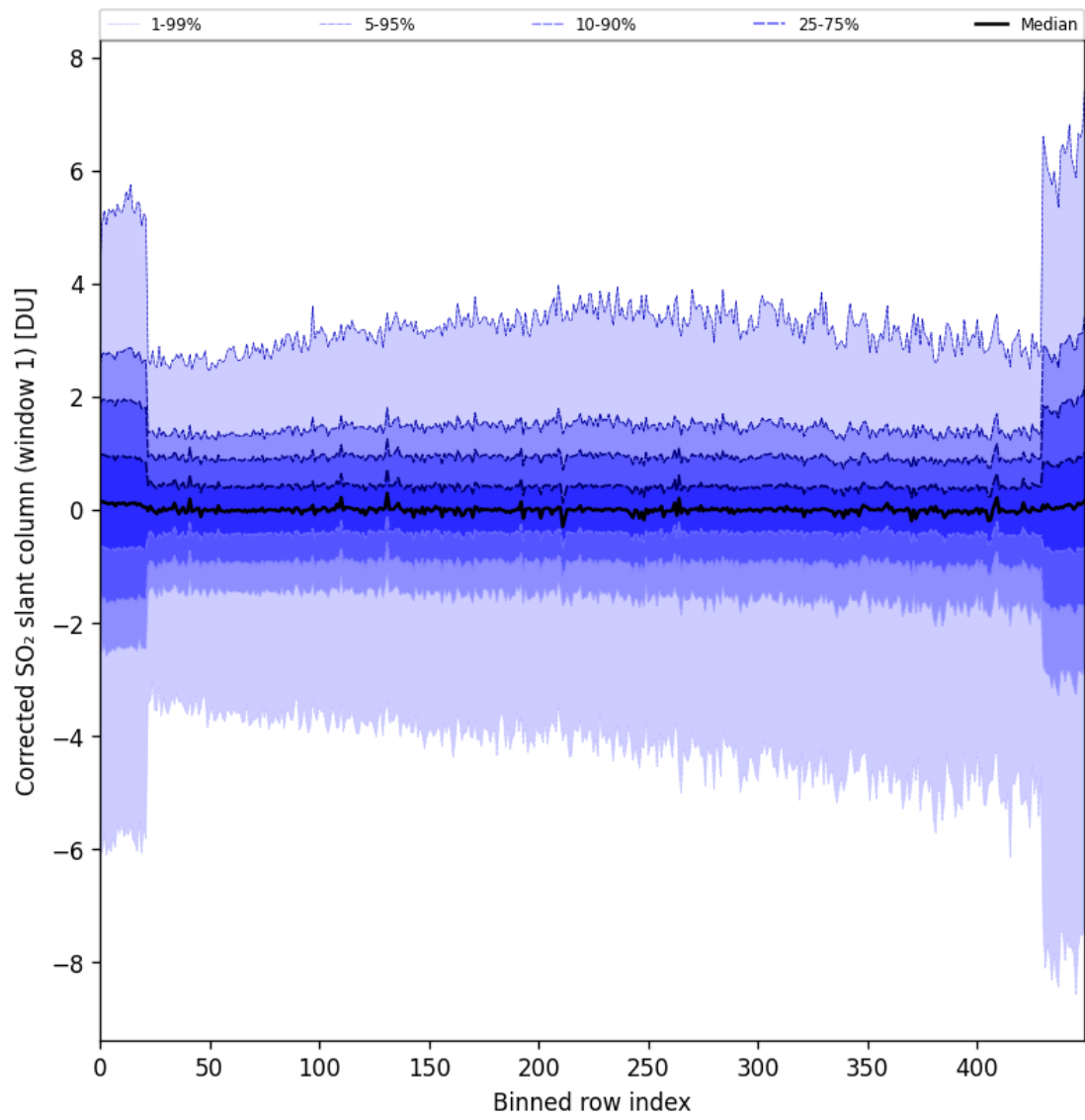
Figure 81: Along track statistics of “Corrected SO 2 slant column (window 1)” for 2024-08-29 to 2024-08-31
