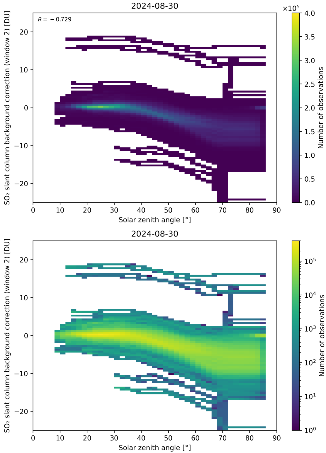
Figure 159: Scatter density plot of “Solar zenith angle” against “SO 2 slant column background correction (window 2)” for 2024-08-29 to 2024-08-31.
