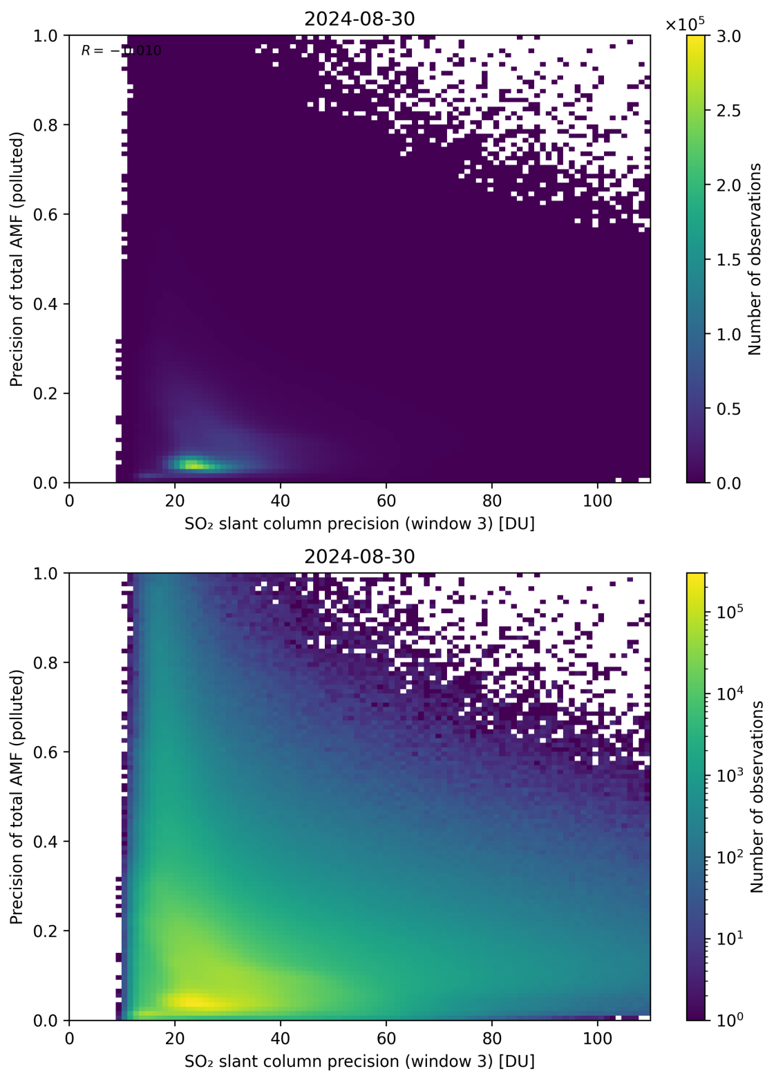
Figure 264: Scatter density plot of “SO 2 slant column precision (window 3)” against “Precision of total AMF (polluted)” for 2024-08-29 to 2024-08-31.
