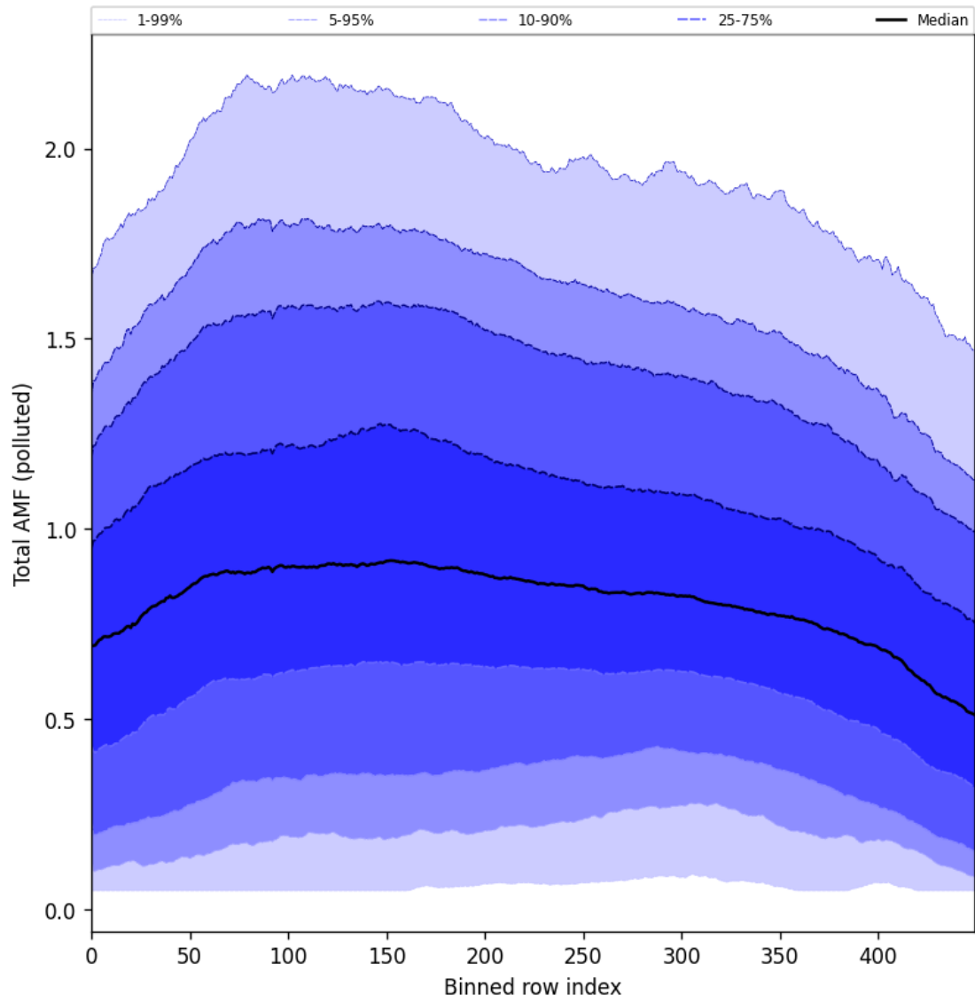
Figure 94: Along track statistics of “Total AMF (polluted)” for 2024-08-29 to 2024-08-31
