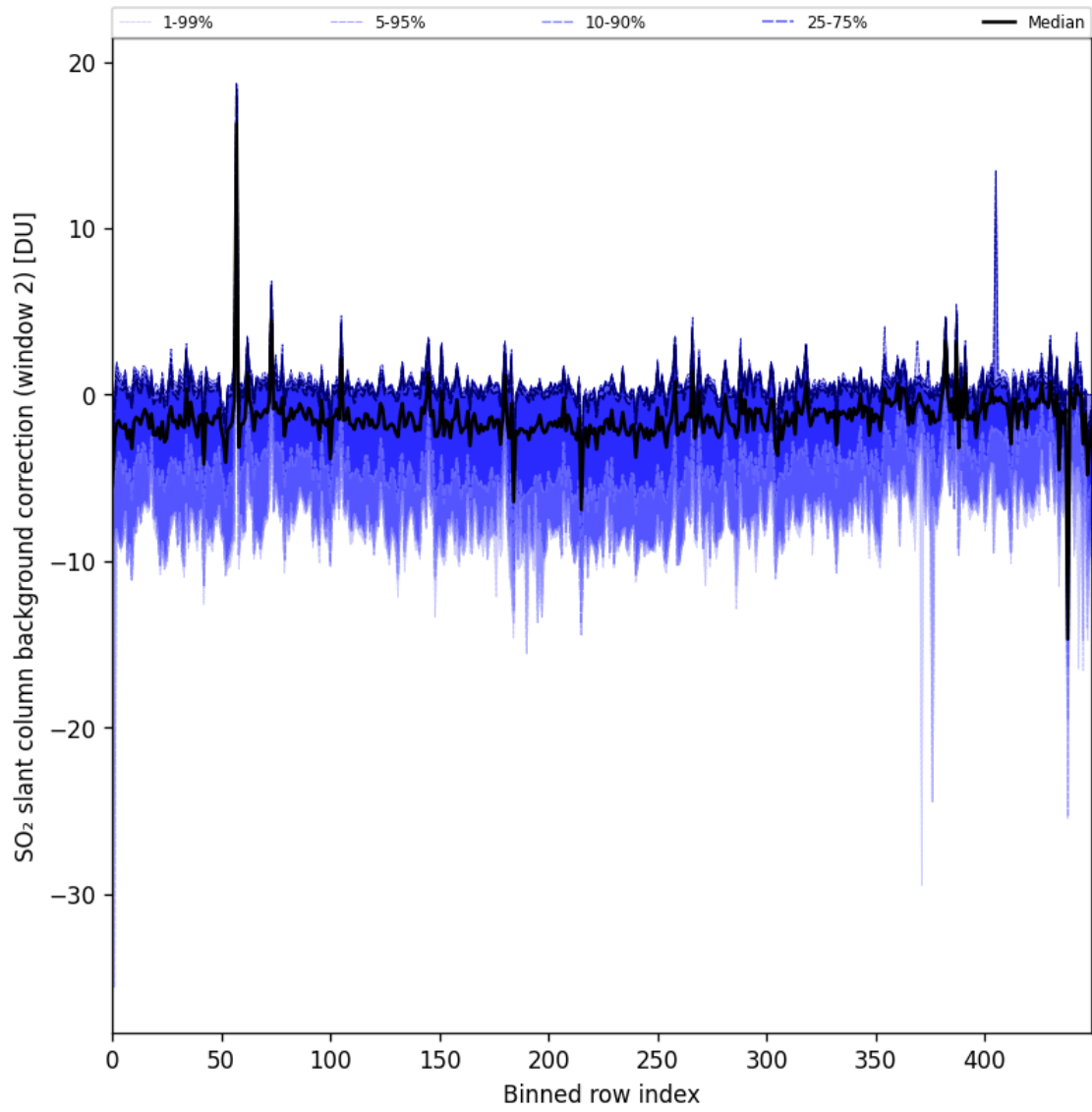
Figure 86: Along track statistics of “SO 2 slant column background correction (window 2)” for 2024-08-29 to 2024-08-31
