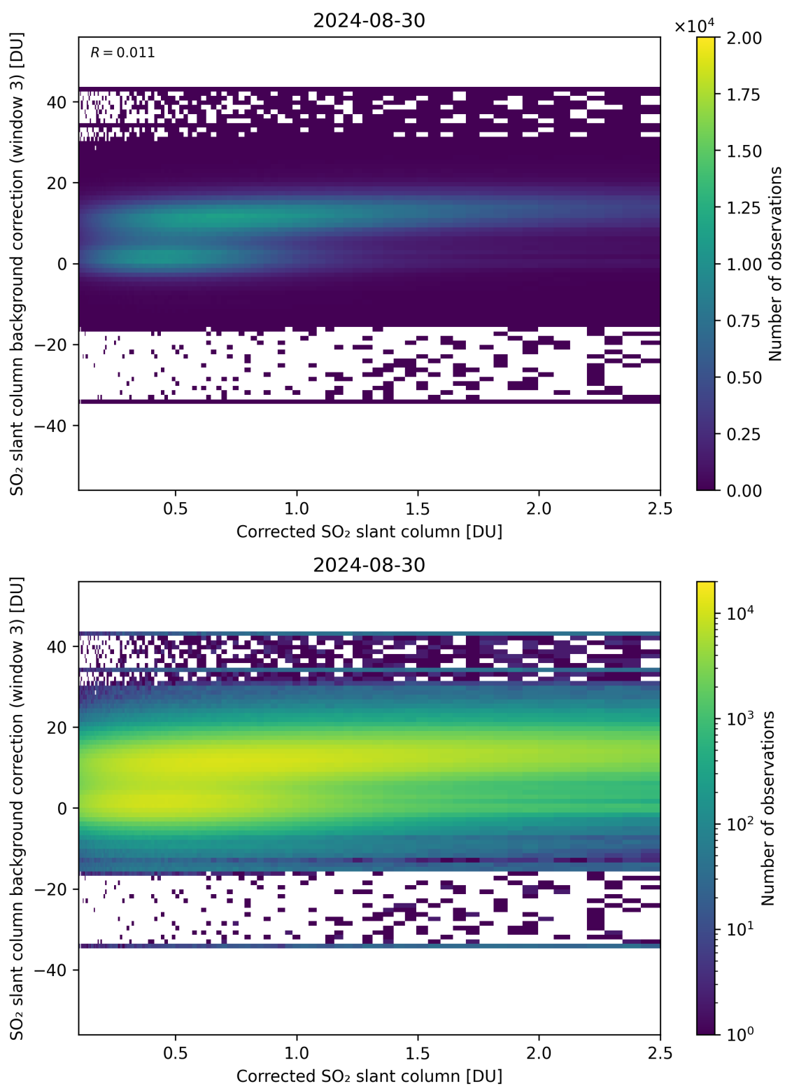
Figure 180: Scatter density plot of “Corrected SO 2 slant column” against “SO 2 slant column background correction (window 3)” for 2024-08-29 to 2024-08-31.
