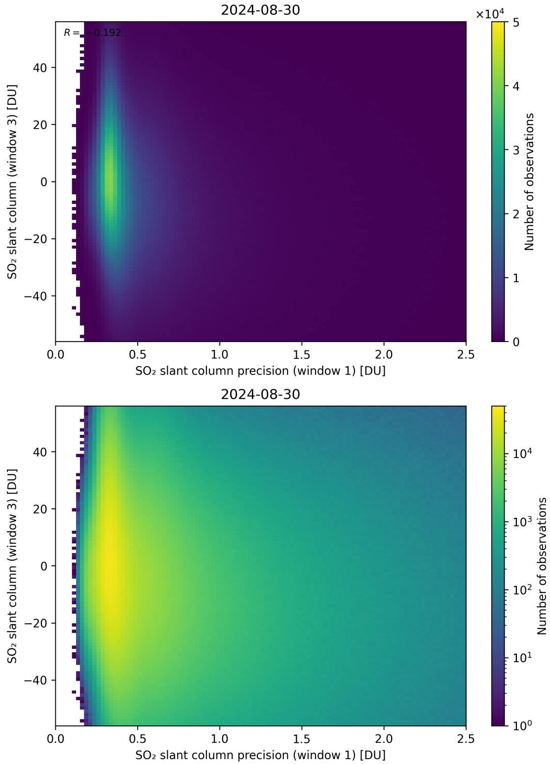
Figure 228: Scatter density plot of “SO 2 slant column precision (window 1)” against “SO 2 slant column (window 3)” for 2024-08-29 to 2024-08-31.
