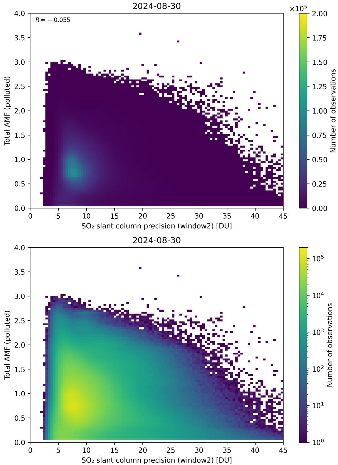
Figure 251: Scatter density plot of “SO 2 slant column precision (window2)” against “Total AMF (polluted)” for 2024-08-29 to 2024-08-31.
