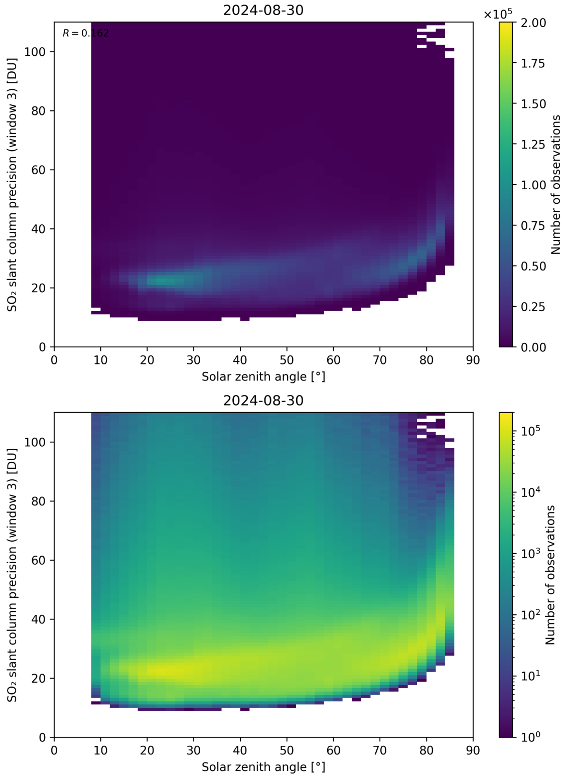
Figure 173: Scatter density plot of “Solar zenith angle” against “SO 2 slant column precision (window 3)” for 2024-08-29 to 2024-08-31.
