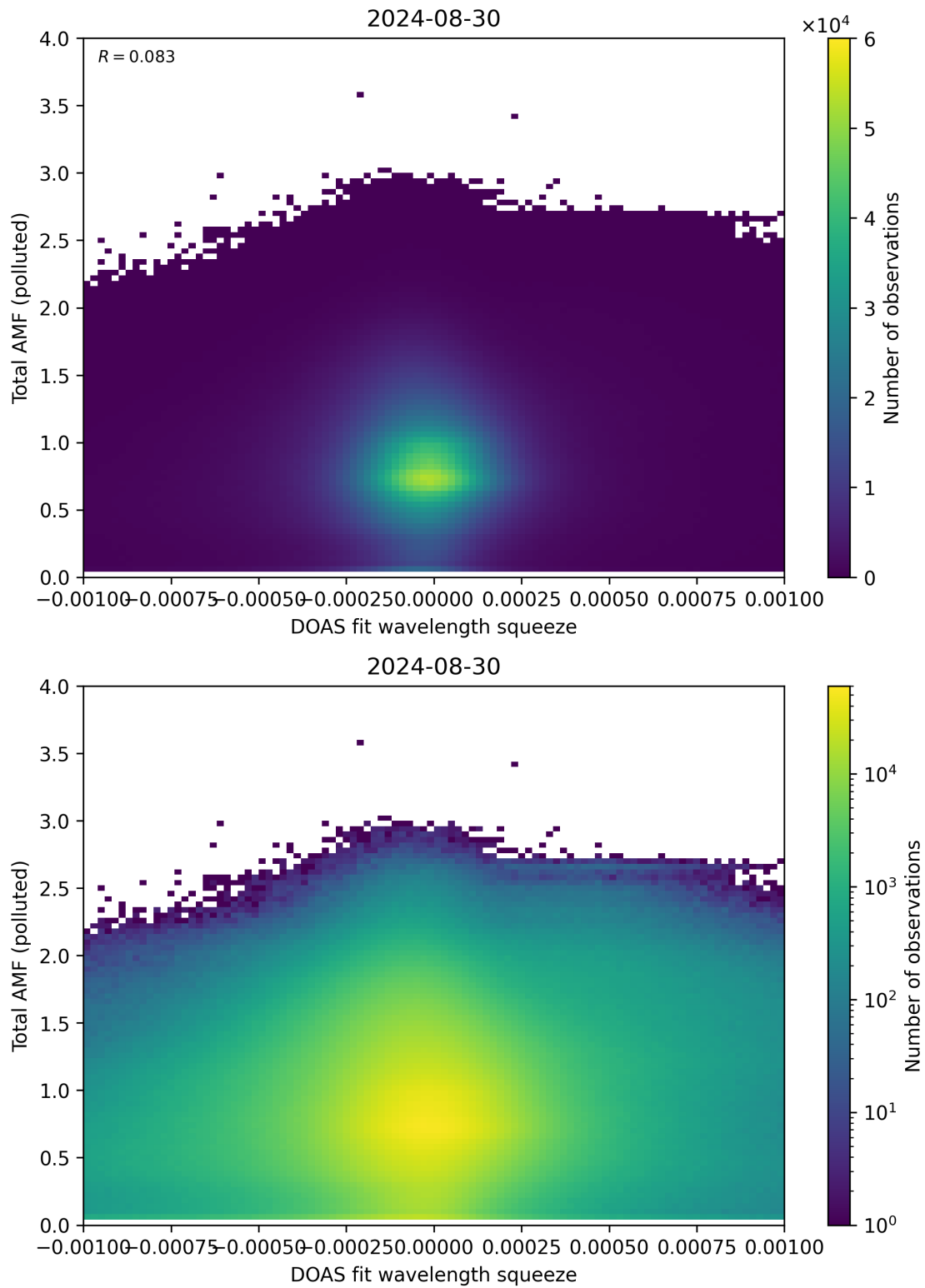
Figure 134: Scatter density plot of “DOAS fit wavelength squeeze” against “Total AMF (polluted)” for 2024-08-29 to 2024-08-31.
