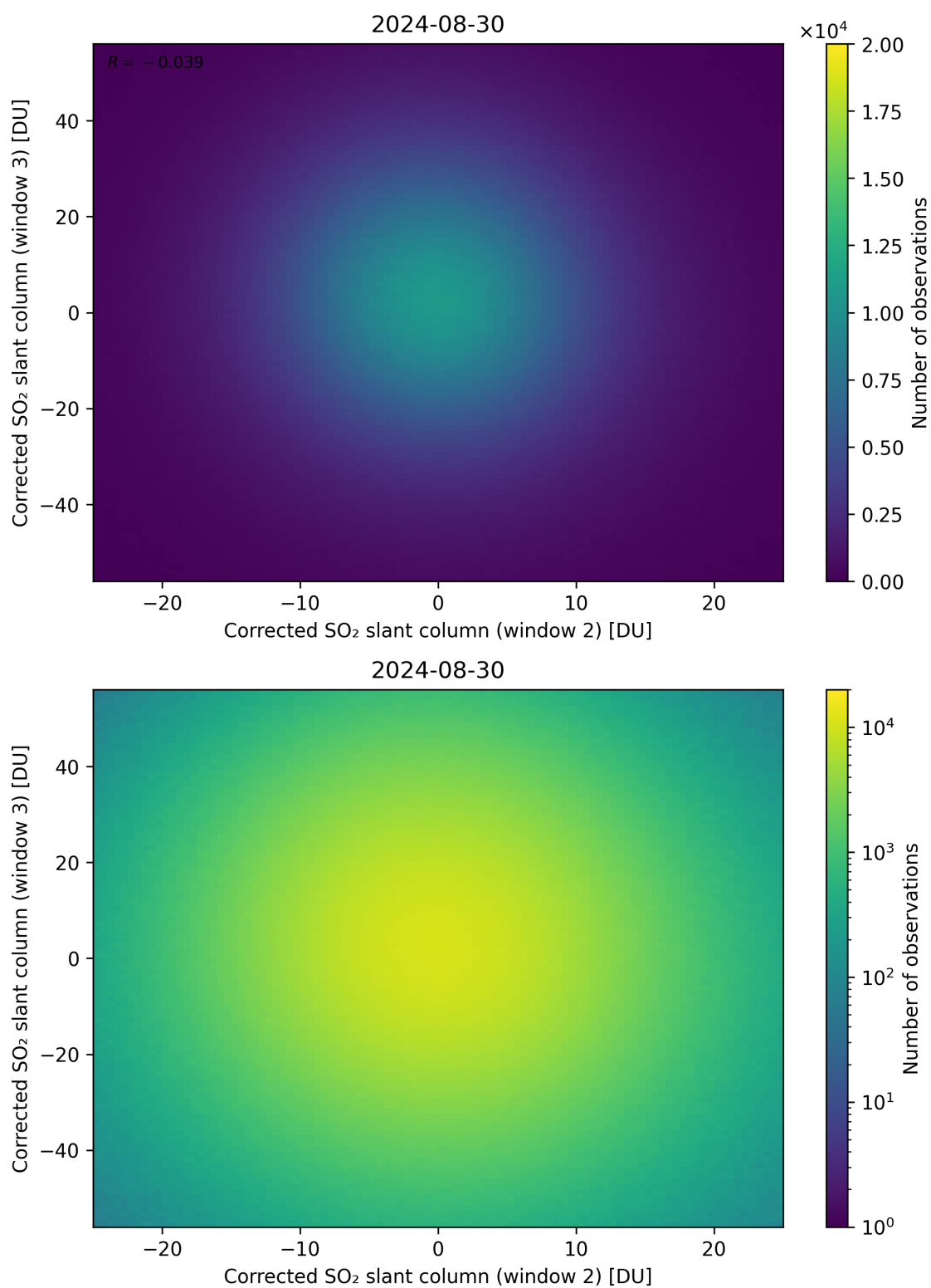
Figure 200: Scatter density plot of “Corrected SO 2 slant column (window 2)” against “Corrected SO 2 slant column (window 3)” for 2024-08-29 to 2024-08-31.
