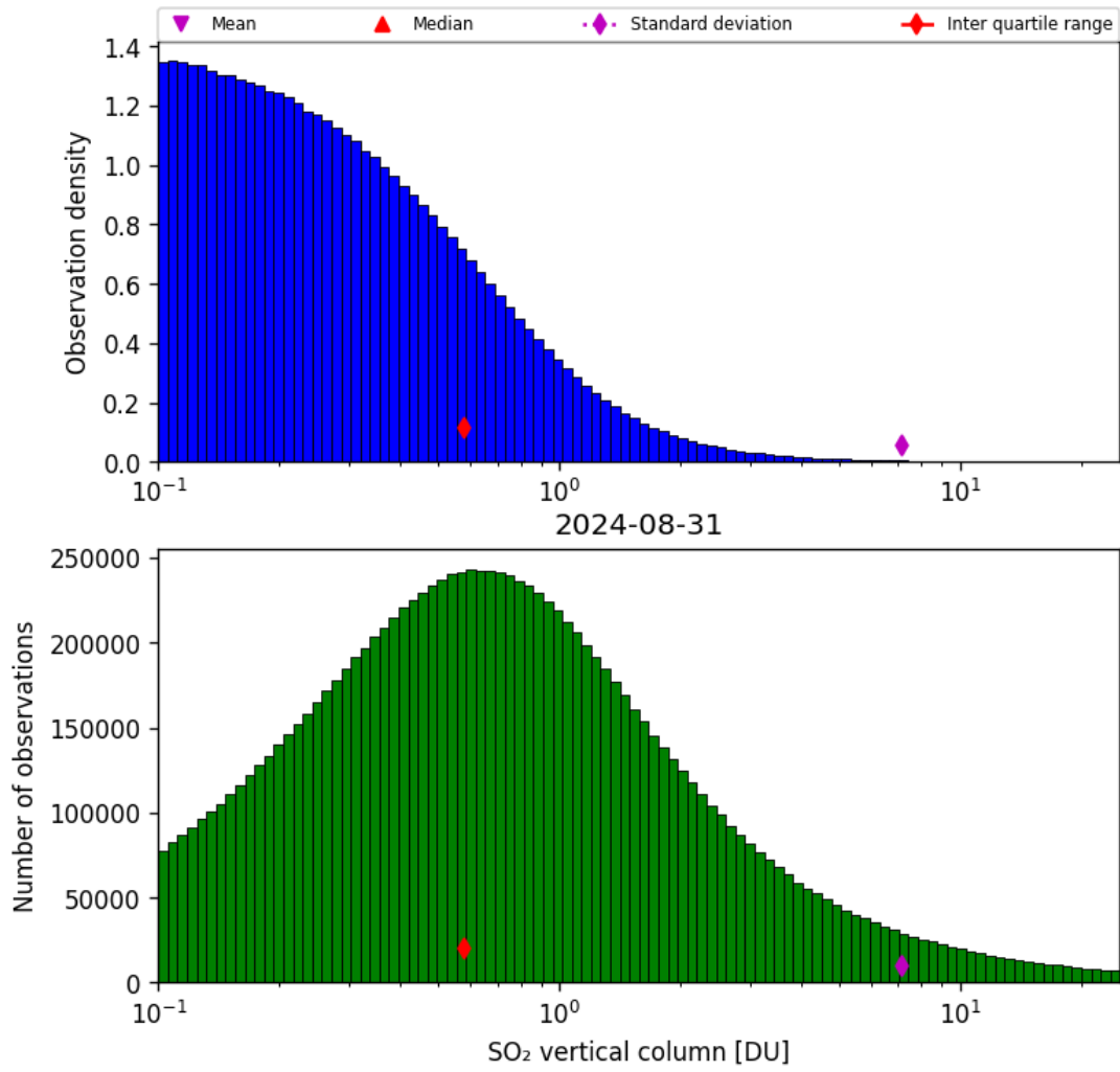
Figure 53: Histogram of “SO 2 vertical column” for 2024-08-30 to 2024-09-01
