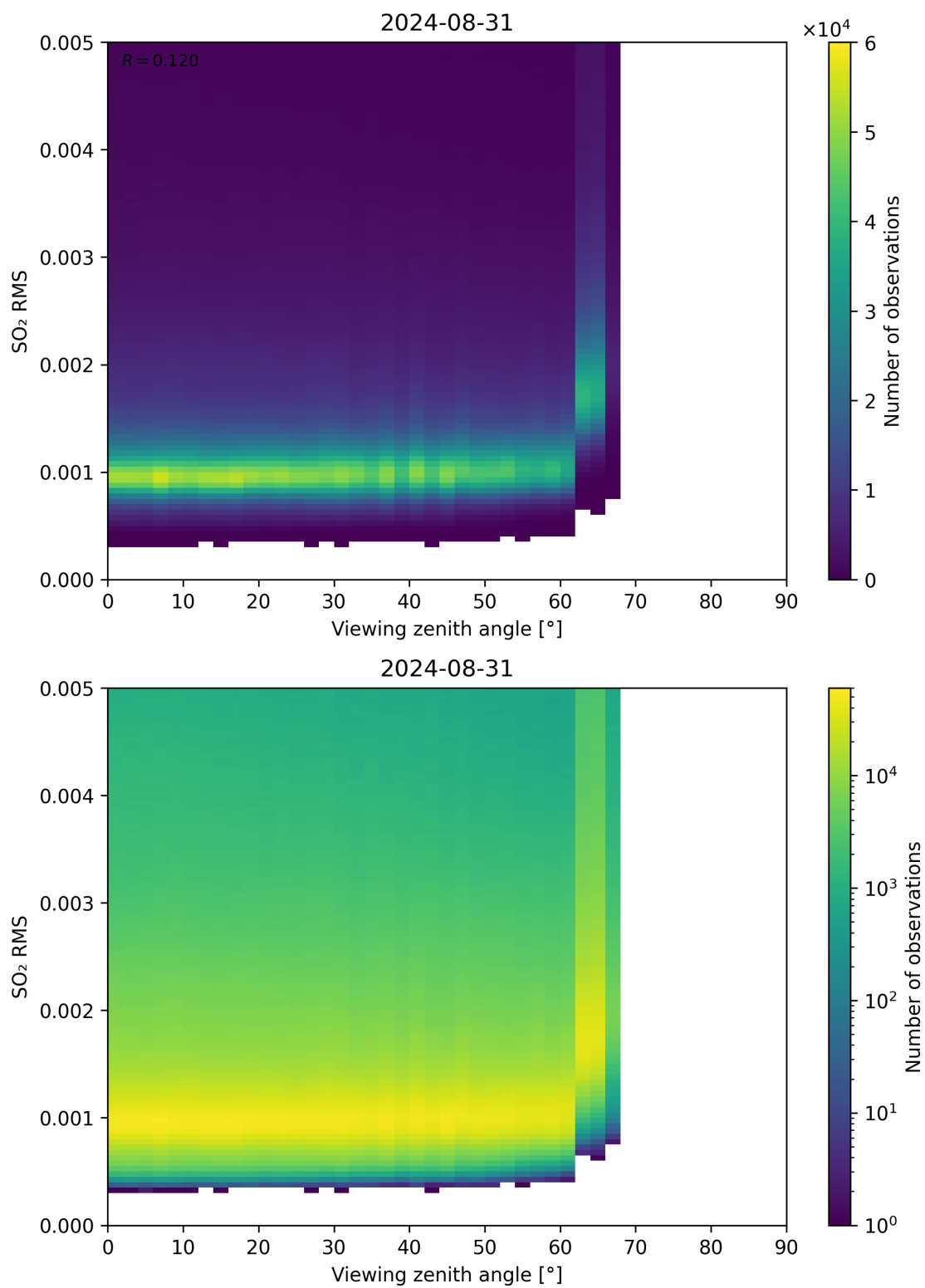
Figure 313: Scatter density plot of “Viewing zenith angle” against “SO 2 RMS” for 2024-08-30 to 2024-09-01.
