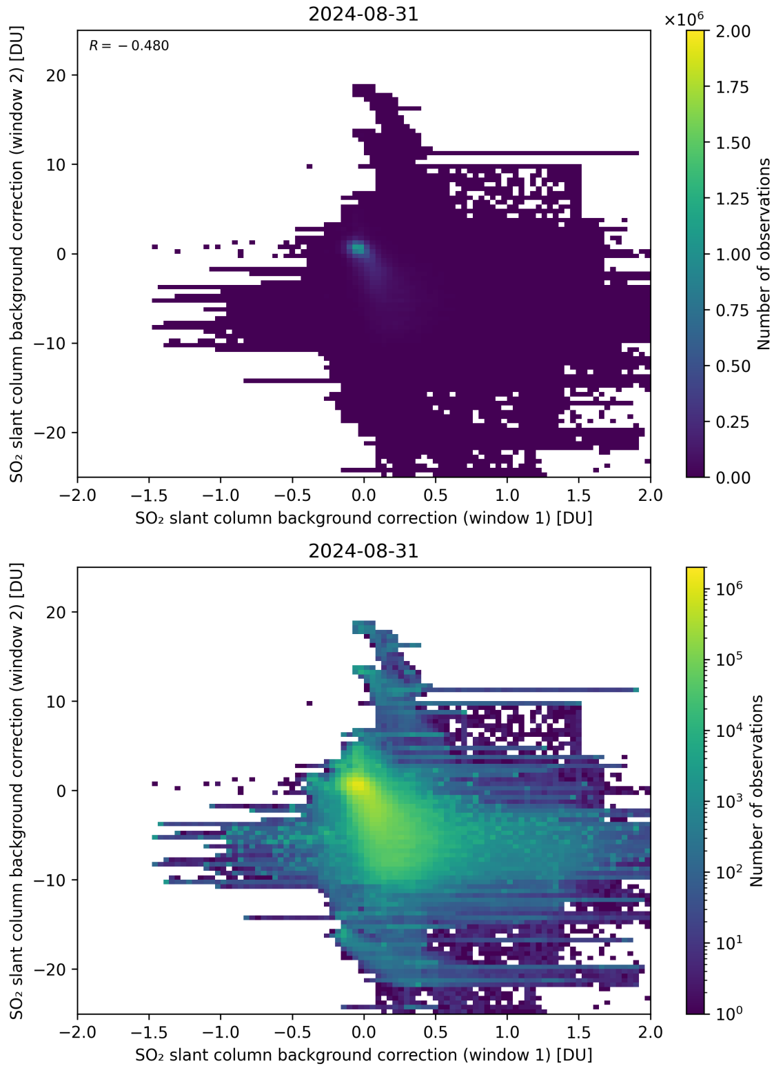
Figure 98: Scatter density plot of “SO 2 slant column background correction (window 1)” against “SO 2 slant column background correction (window 2)” for 2024-08-30 to 2024-09-01.
