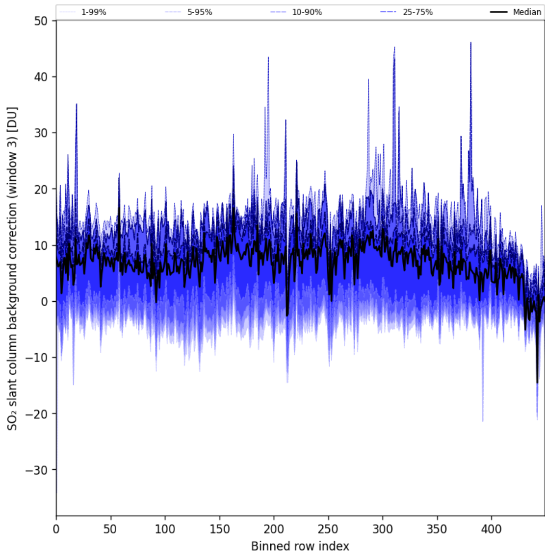
Figure 90: Along track statistics of “SO 2 slant column background correction (window 3)” for 2024-08-30 to 2024-09-01
