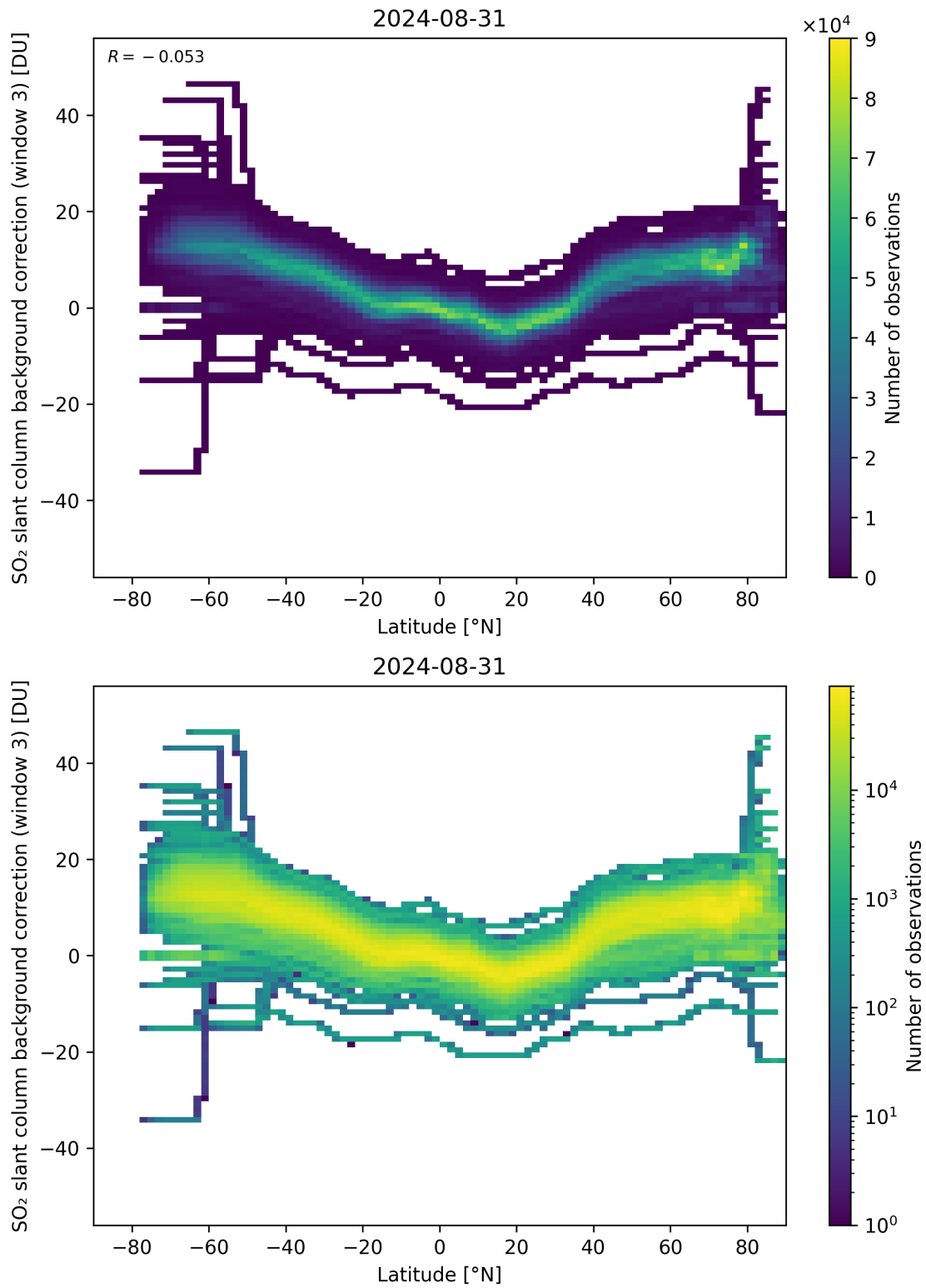
Figure 141: Scatter density plot of “Latitude” against “SO 2 slant column background correction (window 3)” for 2024-08-30 to 2024-09-01.
