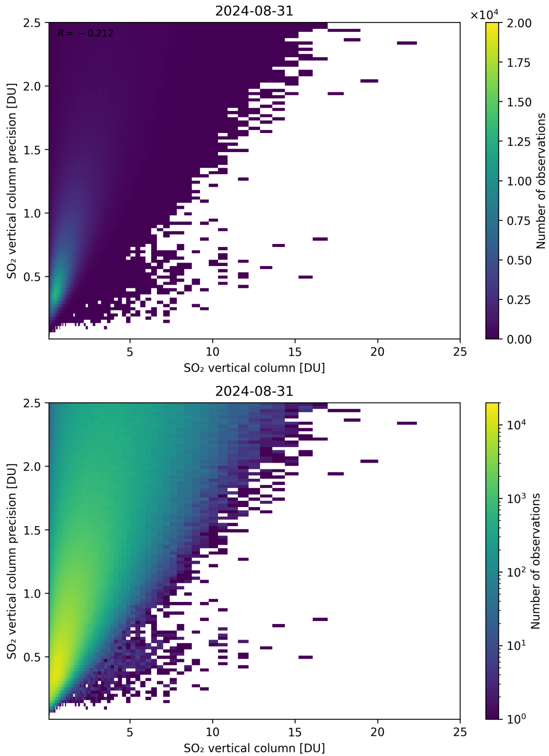
Figure 307: Scatter density plot of “SO 2 vertical column” against “SO 2 vertical column precision” for 2024-08-30 to 2024-09-01.
