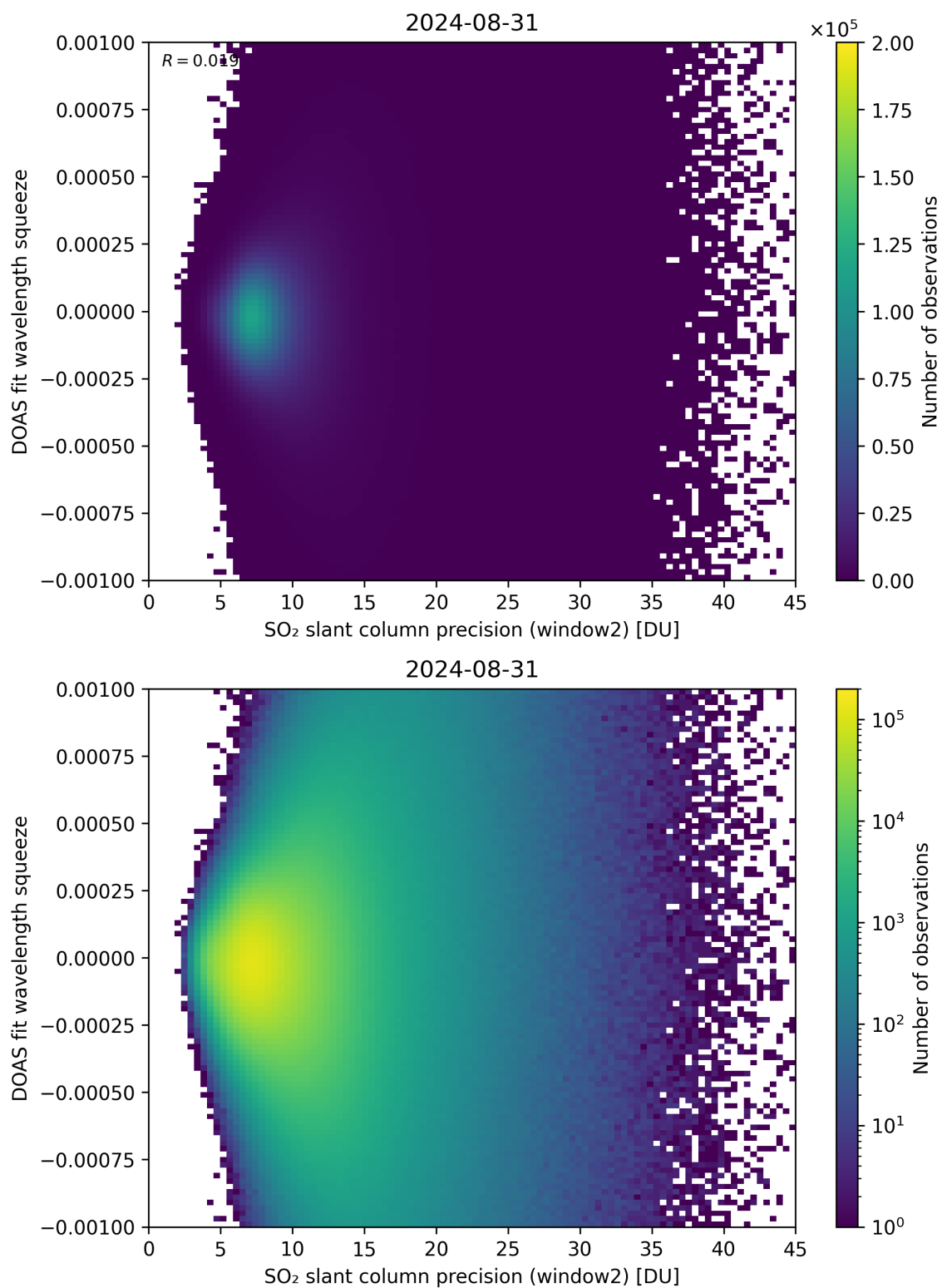
Figure 244: Scatter density plot of “SO 2 slant column precision (window2)” against “DOAS fit wavelength squeeze” for 2024-08-30 to 2024-09-01.
