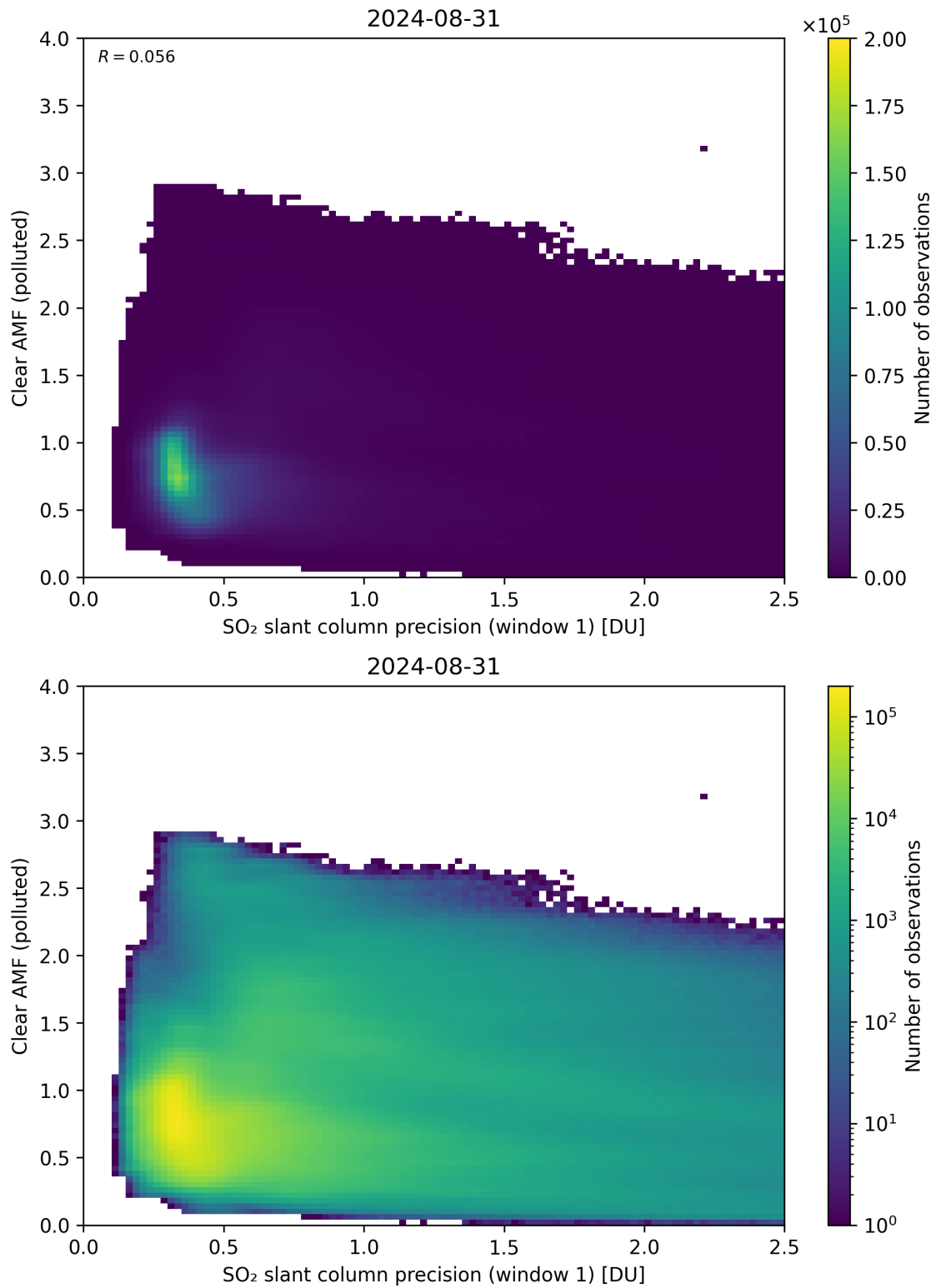
Figure 224: Scatter density plot of “SO 2 slant column precision (window 1)” against “Clear AMF (polluted)” for 2024-08-30 to 2024-09-01.
