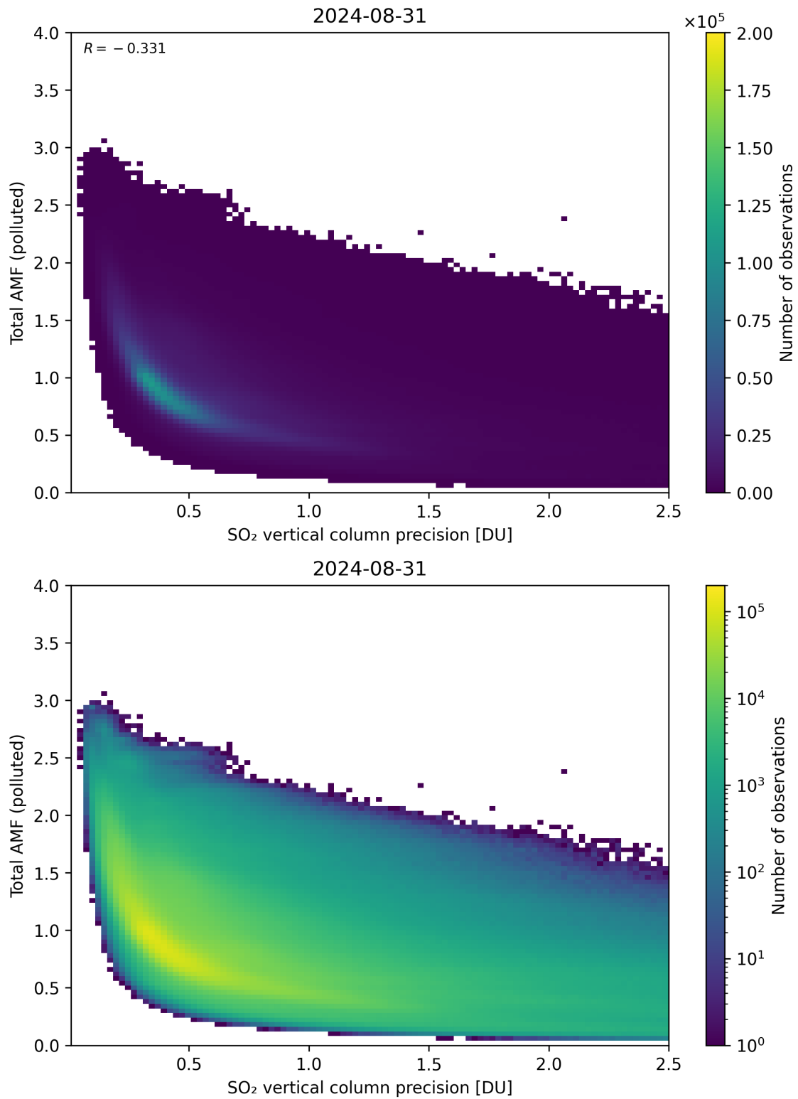
Figure 294: Scatter density plot of “SO 2 vertical column precision” against “Total AMF (polluted)” for 2024-08-30 to 2024-09-01.
