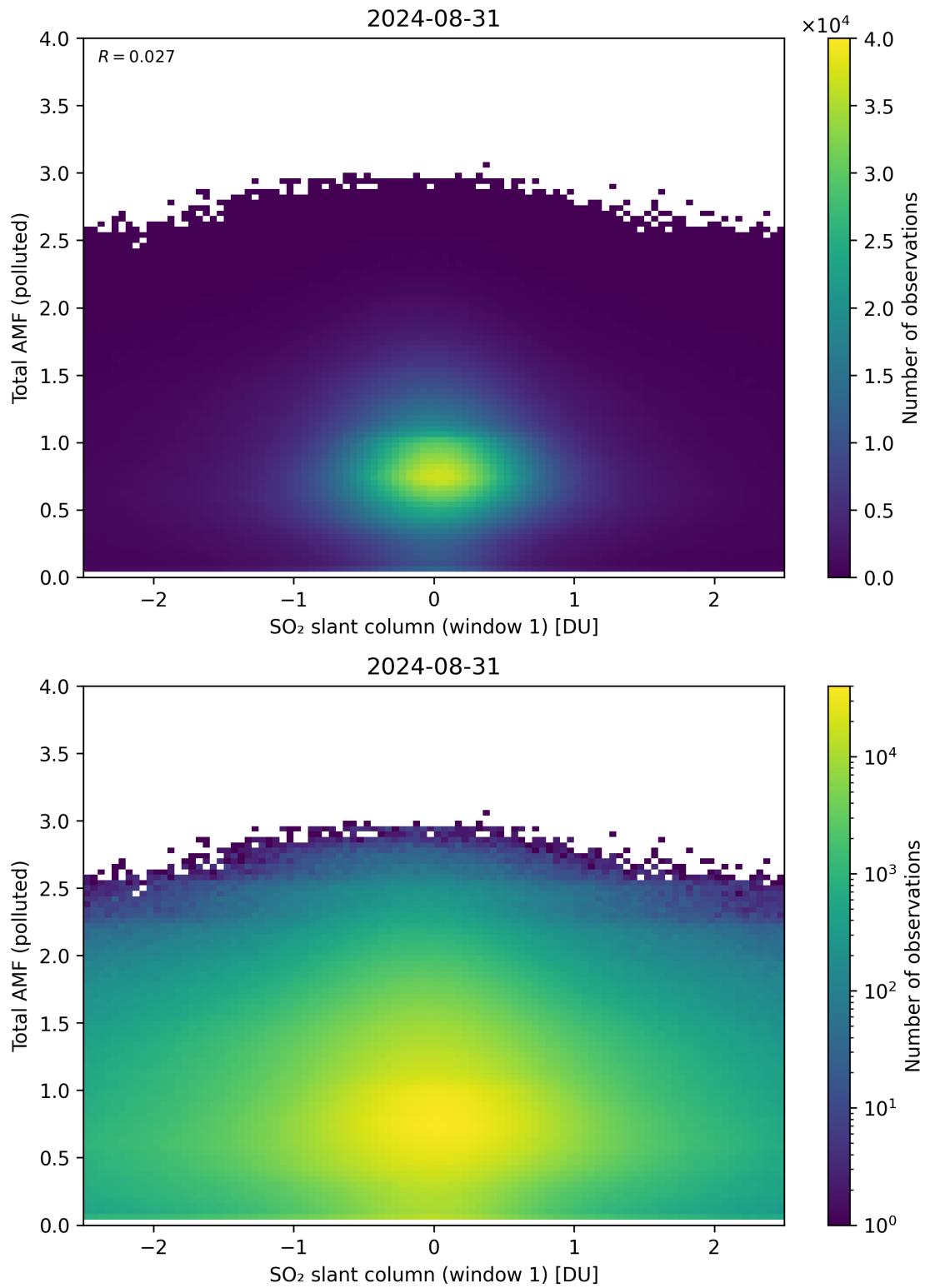
Figure 239: Scatter density plot of “SO 2 slant column (window 1)” against “Total AMF (polluted)” for 2024-08-30 to 2024-09-01.
