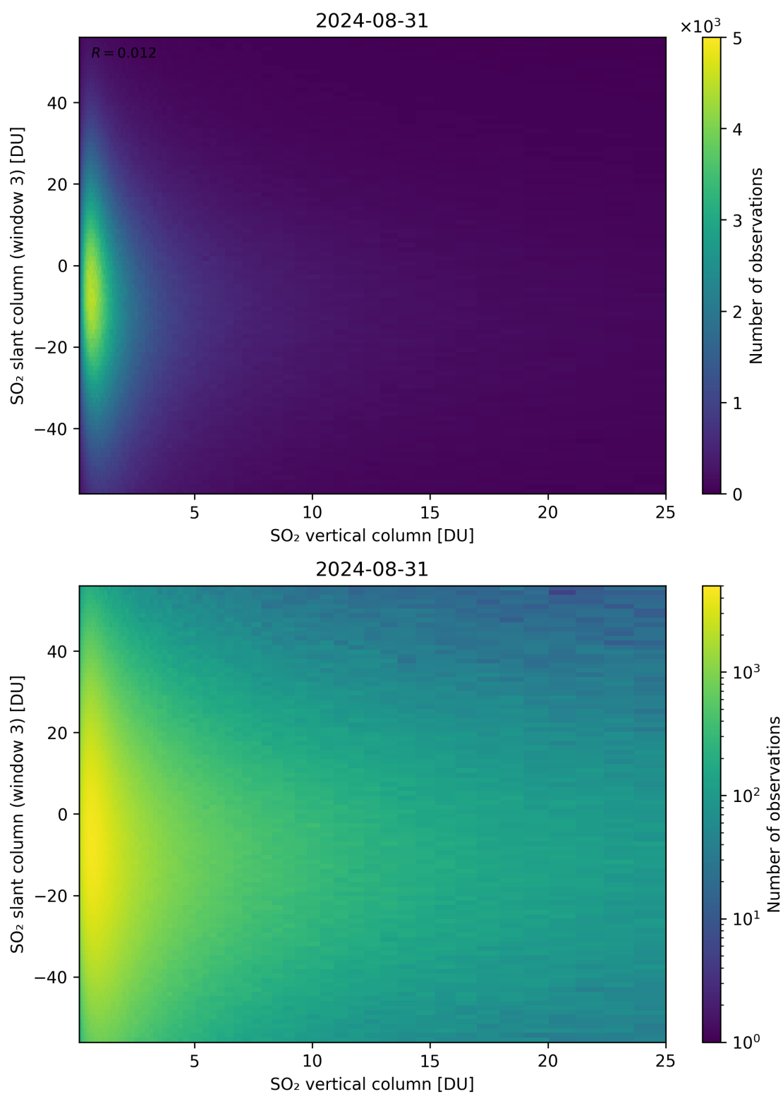
Figure 303: Scatter density plot of “SO 2 vertical column” against “SO 2 slant column (window 3)” for 2024-08-30 to 2024-09-01.
