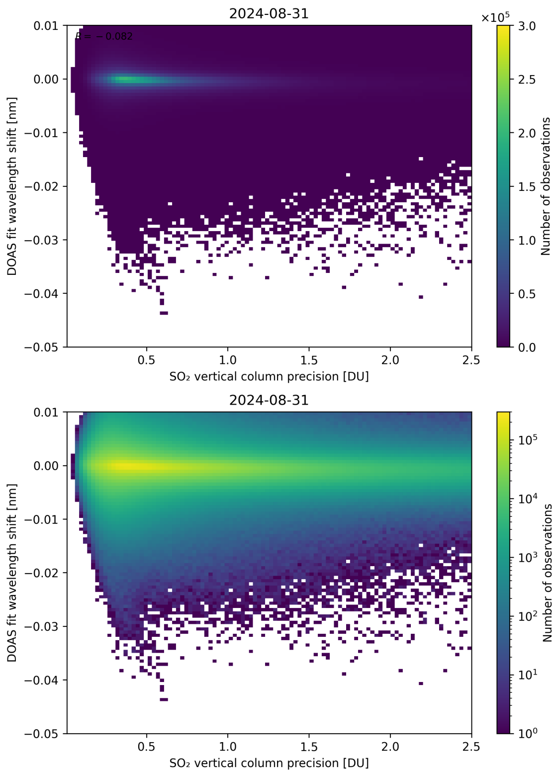
Figure 282: Scatter density plot of “SO 2 vertical column precision” against “DOAS fit wavelength shift” for 2024-08-30 to 2024-09-01.
