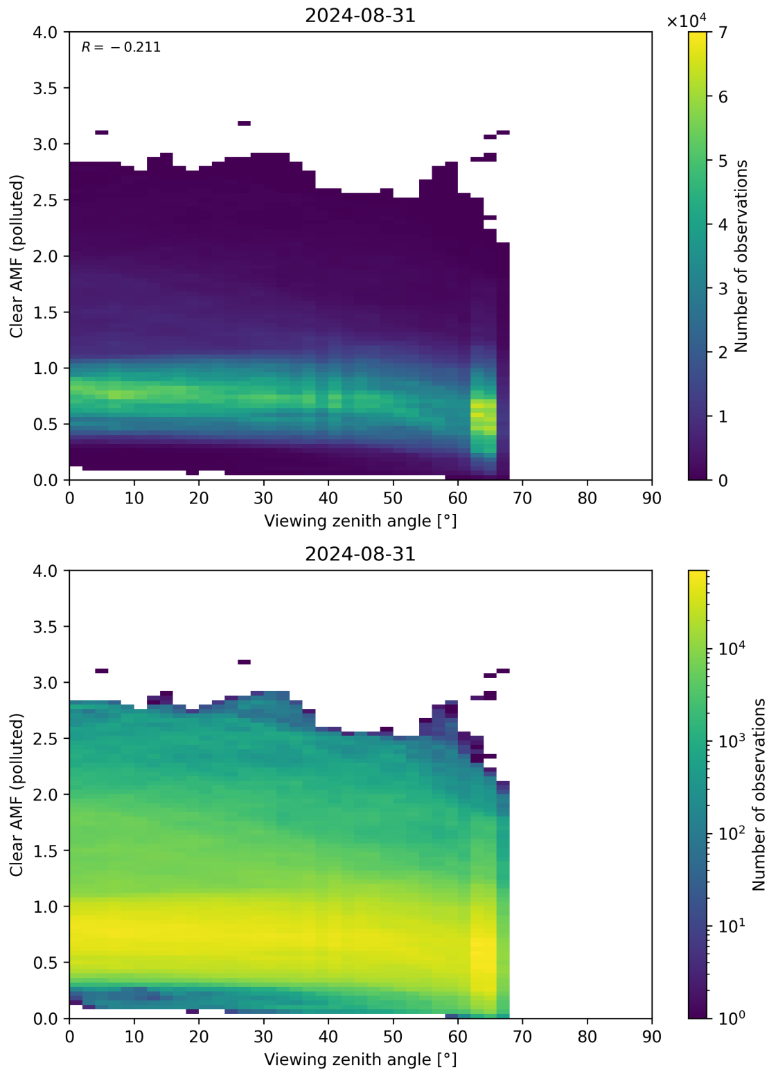
Figure 316: Scatter density plot of “Viewing zenith angle” against “Clear AMF (polluted)” for 2024-08-30 to 2024-09-01.
