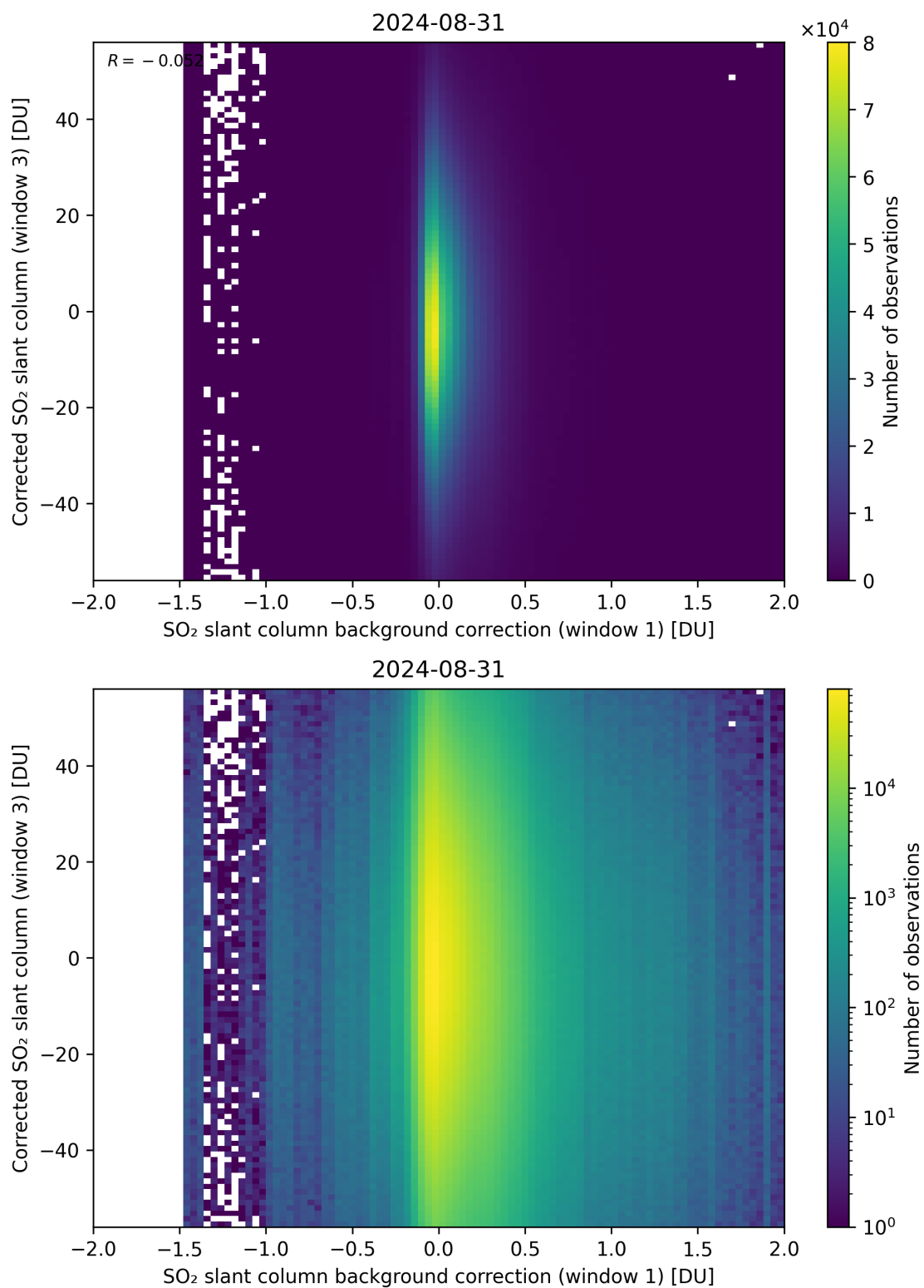
Figure 105: Scatter density plot of “SO 2 slant column background correction (window 1)” against “Corrected SO 2 slant column (window 3)” for 2024-08-30 to 2024-09-01.
