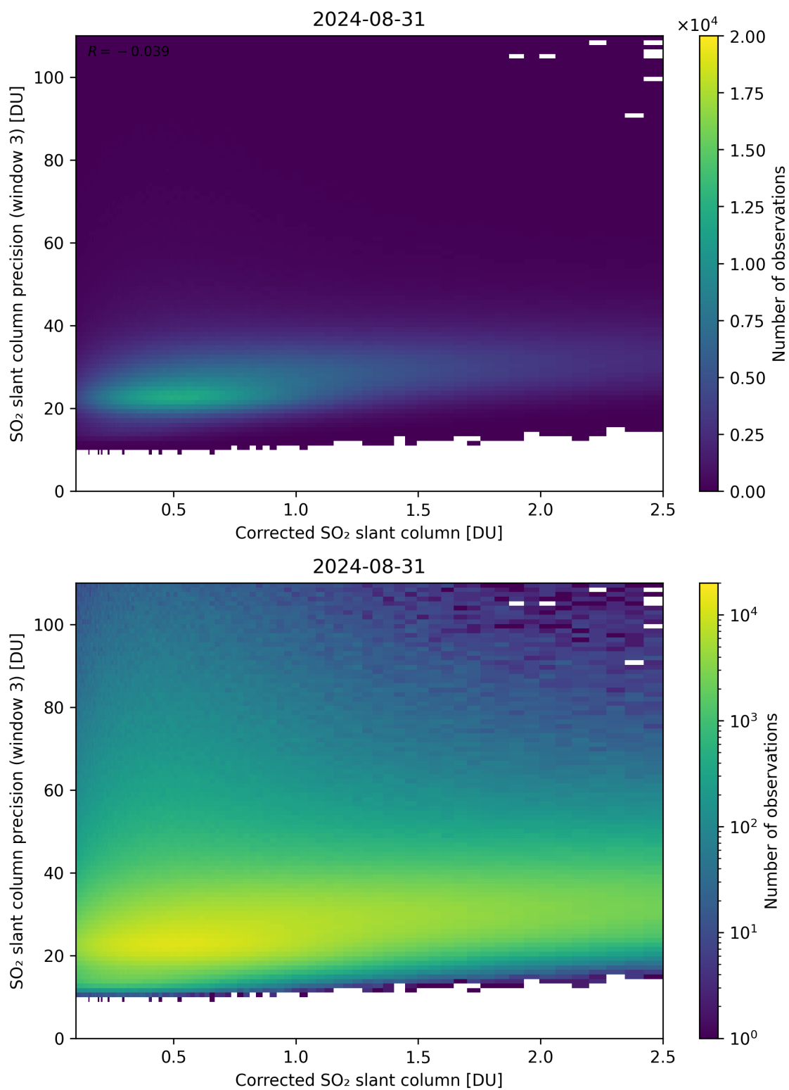
Figure 191: Scatter density plot of “Corrected SO 2 slant column” against “SO 2 slant column precision (window 3)” for 2024-08-30 to 2024-09-01.
