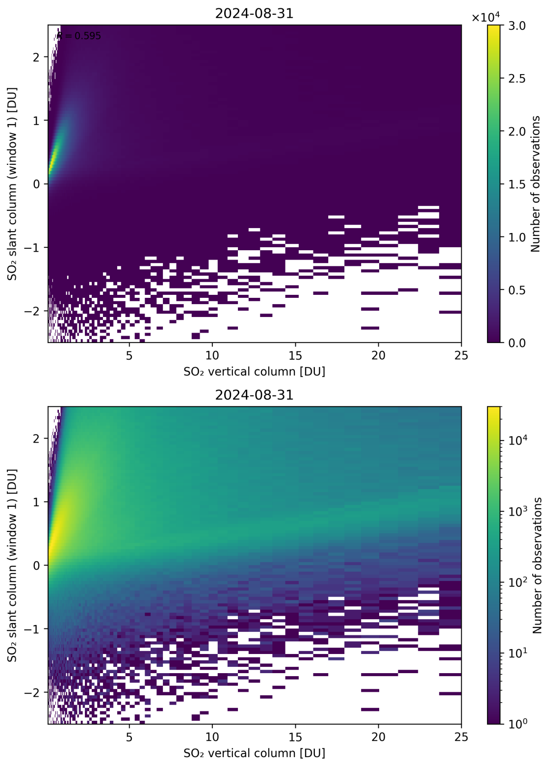
Figure 300: Scatter density plot of “SO 2 vertical column” against “SO 2 slant column (window 1)” for 2024-08-30 to 2024-09-01.
