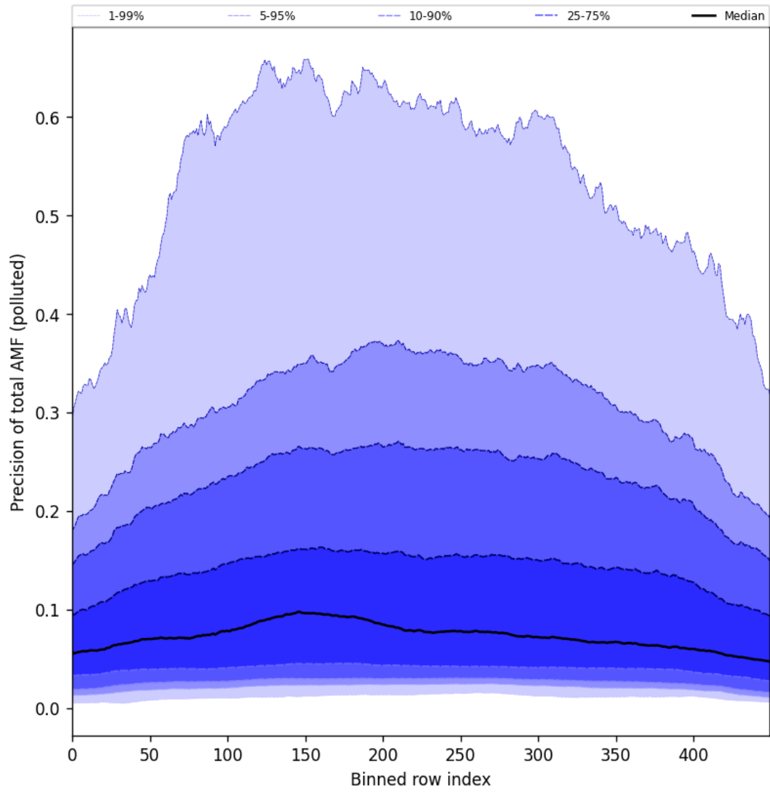
Figure 95: Along track statistics of “Precision of total AMF (polluted)” for 2024-08-30 to 2024-09-01
