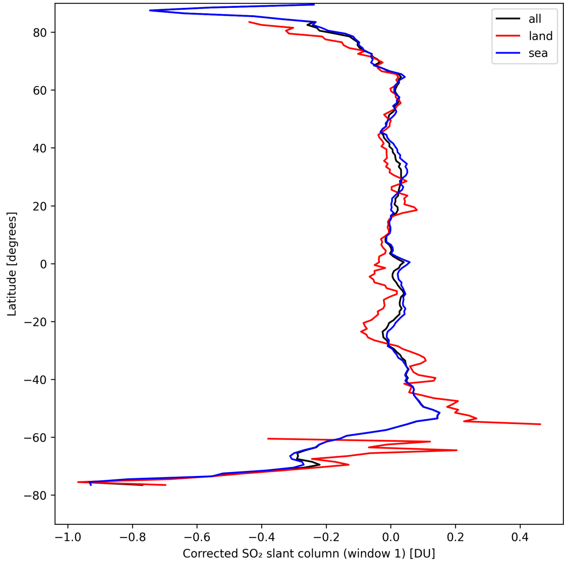
Figure 35: Zonal average of “Corrected SO 2 slant column (window 1)” for 2024-08-30 to 2024-09-01.
