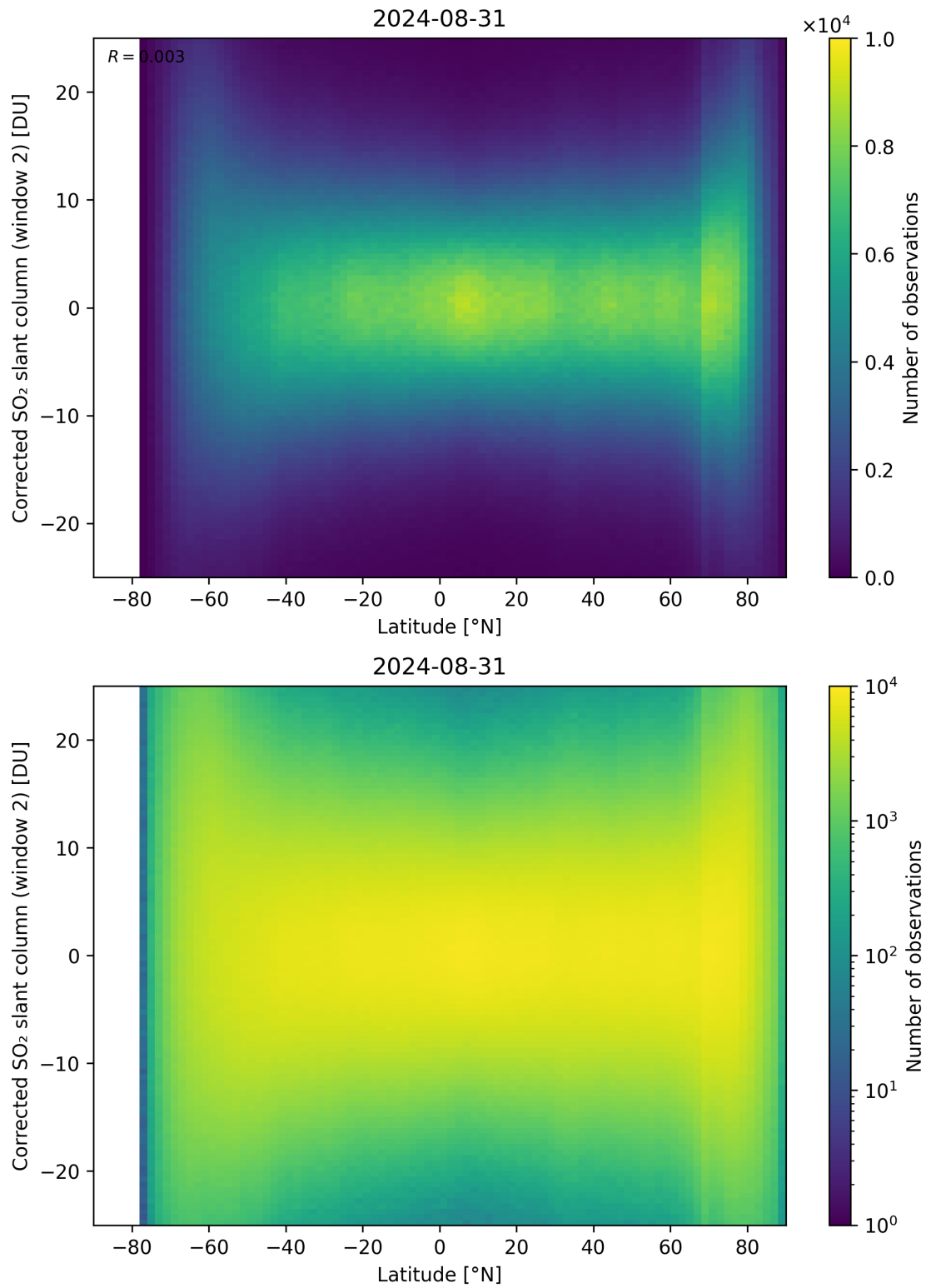
Figure 147: Scatter density plot of “Latitude” against “Corrected SO 2 slant column (window 2)” for 2024-08-30 to 2024-09-01.
