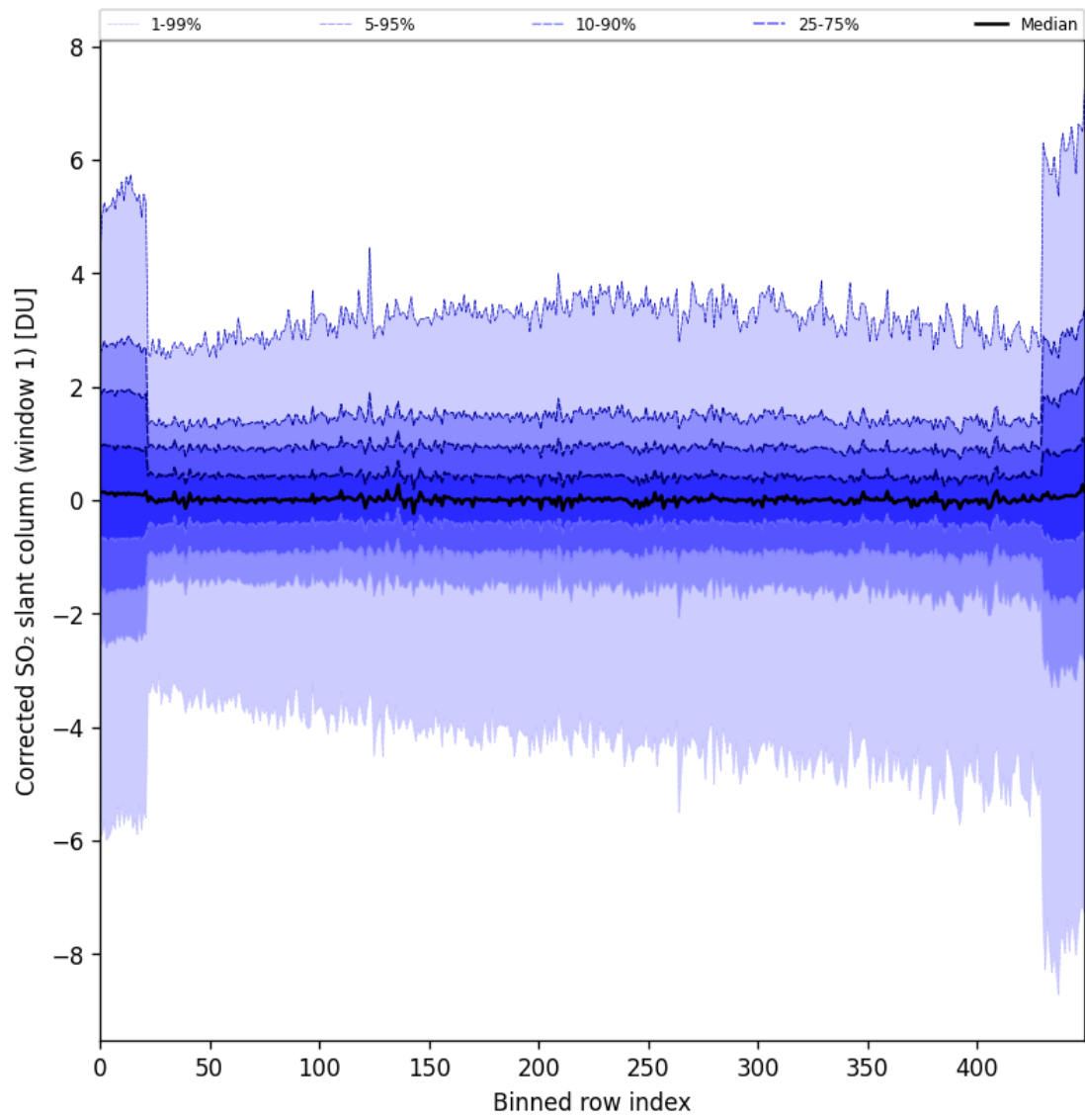
Figure 81: Along track statistics of “Corrected SO 2 slant column (window 1)” for 2024-08-30 to 2024-09-01
