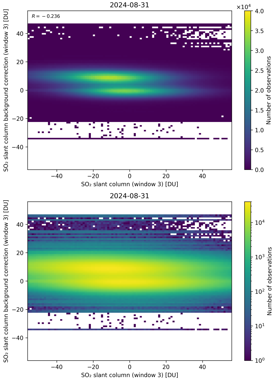
Figure 253: Scatter density plot of “SO 2 slant column (window 3)” against “SO 2 slant column background correction (window 3)” for 2024-08-30 to 2024-09-01.
