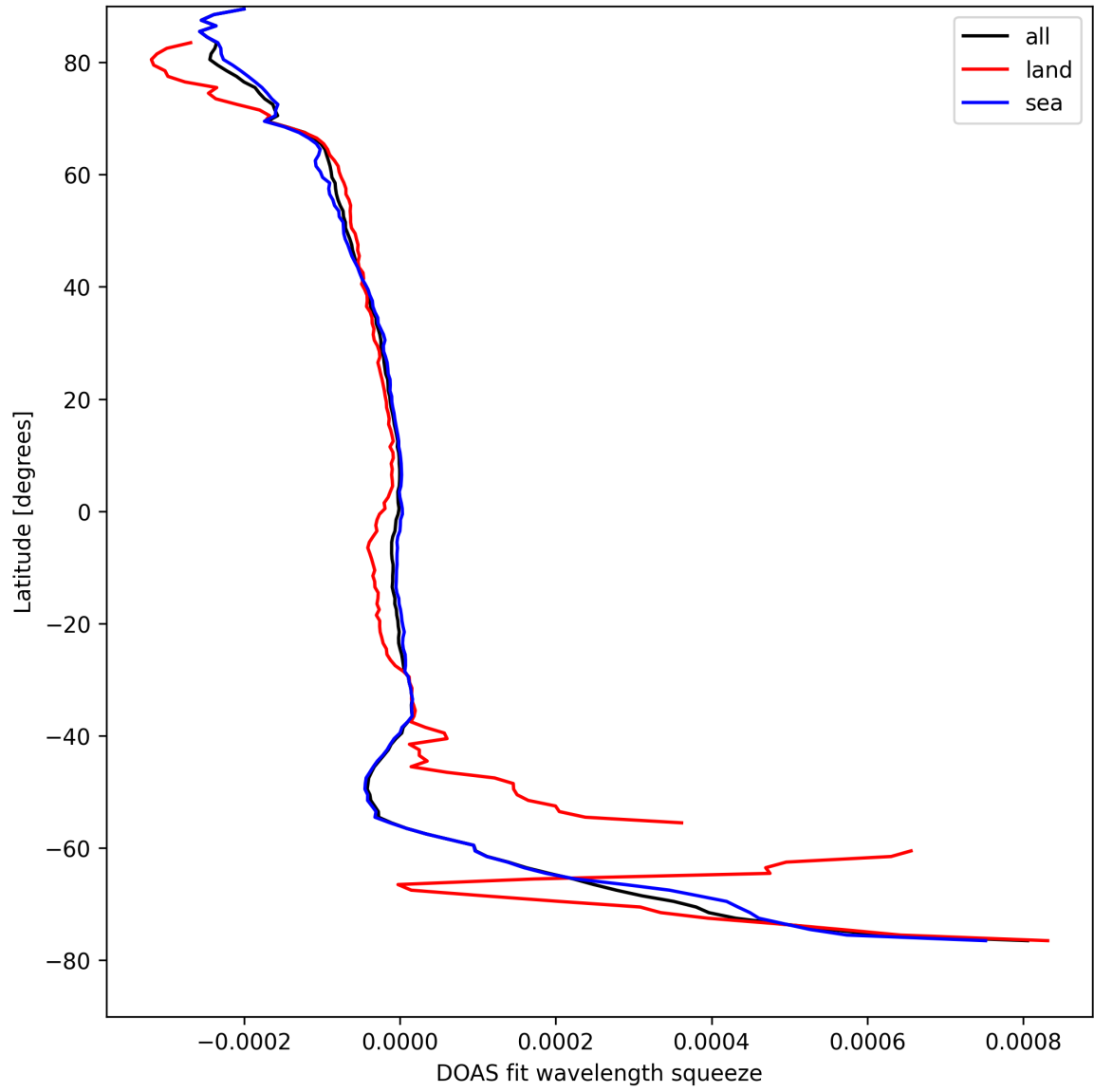
Figure 46: Zonal average of “DOAS fit wavelength squeeze” for 2024-08-30 to 2024-09-01.
