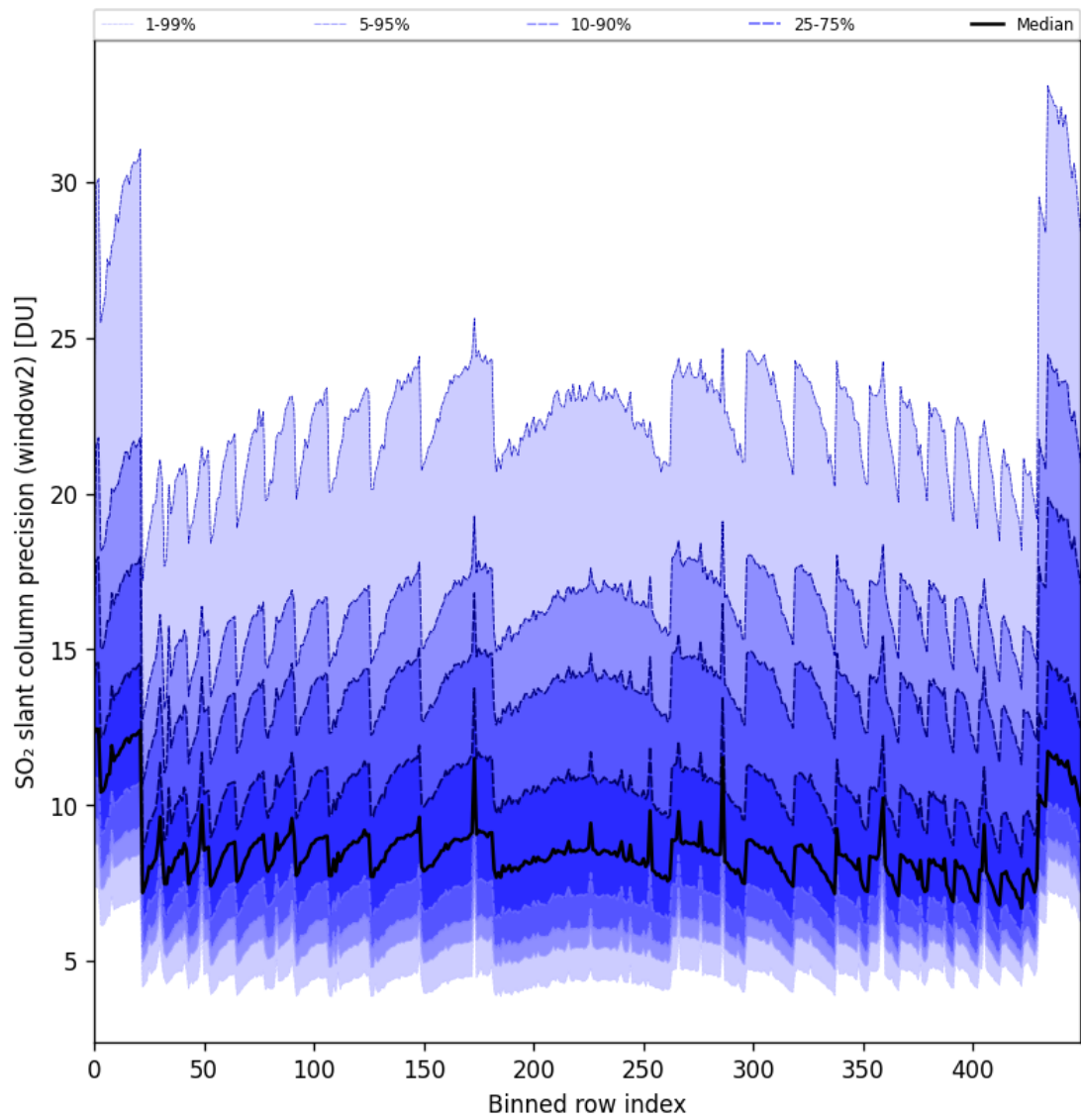
Figure 84: Along track statistics of “SO 2 slant column precision (window2)” for 2024-08-30 to 2024-09-01
