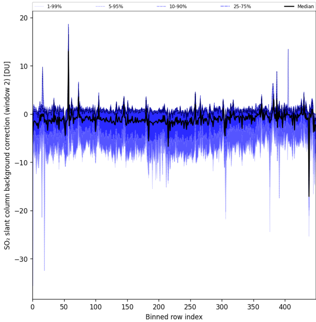
Figure 86: Along track statistics of “SO 2 slant column background correction (window 2)” for 2024-08-30 to 2024-09-01
