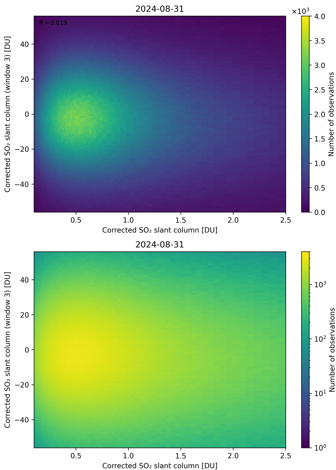
Figure 186: Scatter density plot of “Corrected SO 2 slant column” against “Corrected SO 2 slant column (window 3)” for 2024-08-30 to 2024-09-01.
