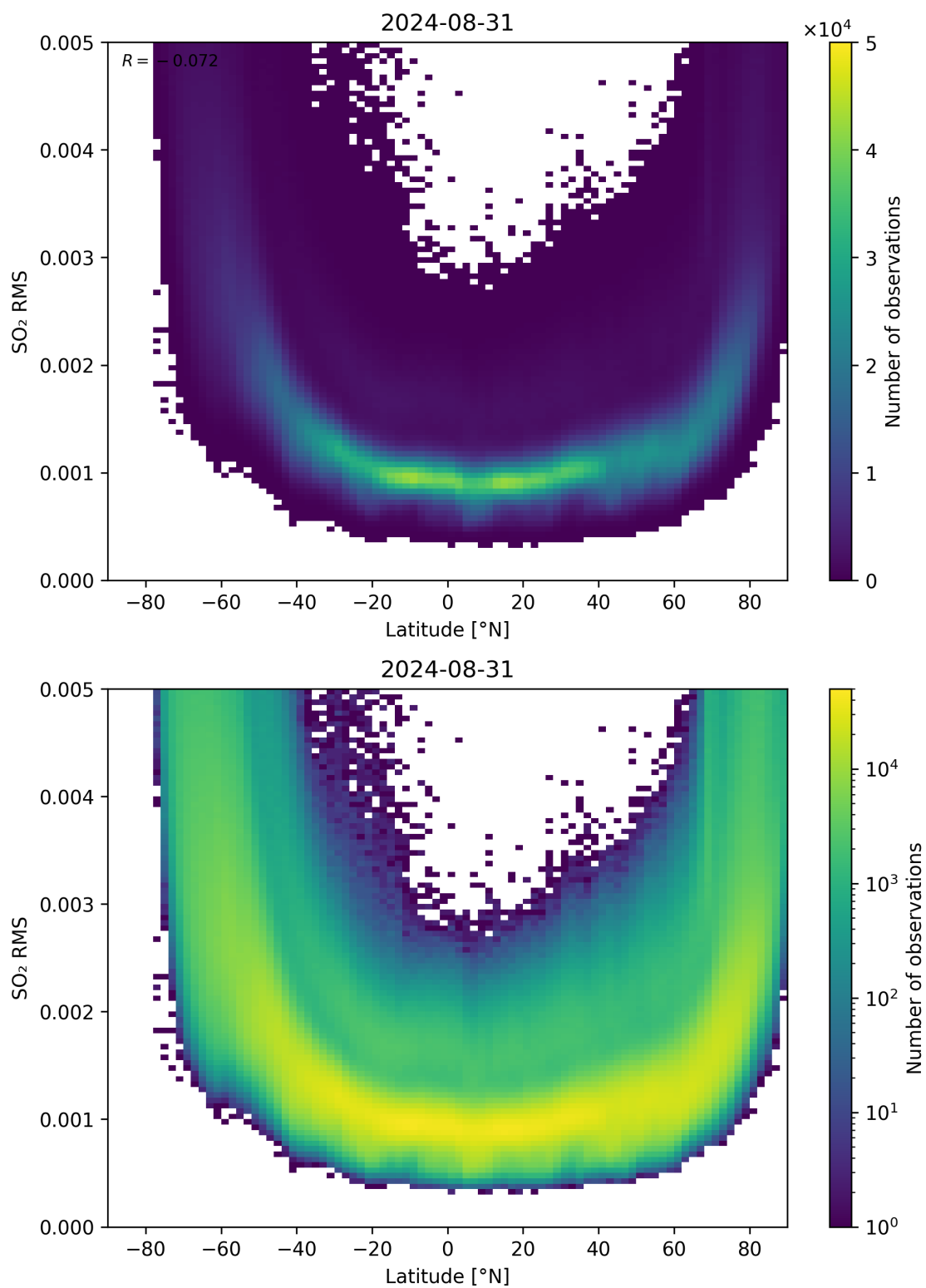
Figure 144: Scatter density plot of “Latitude” against “SO 2 RMS” for 2024-08-30 to 2024-09-01.
