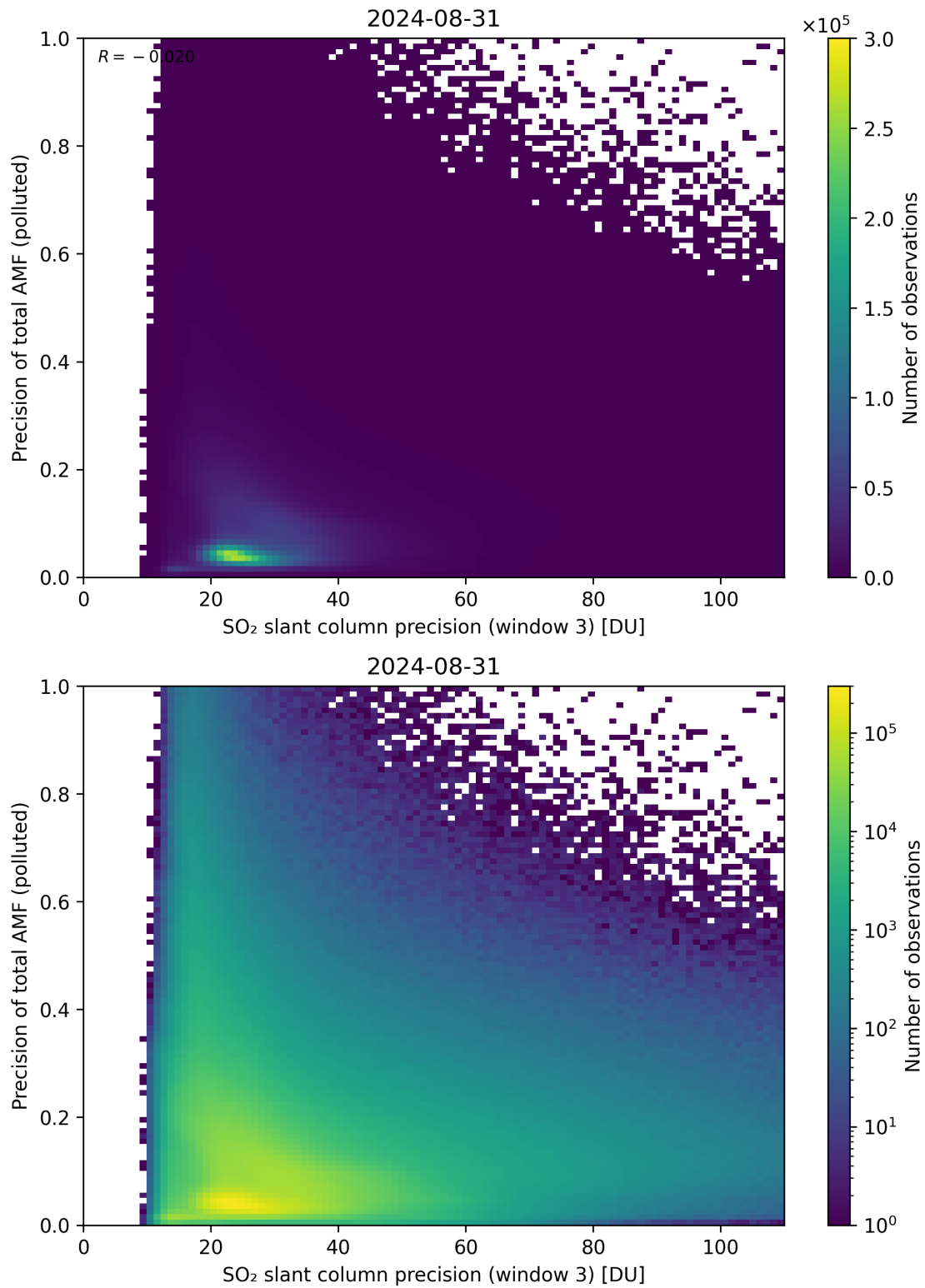
Figure 264: Scatter density plot of “SO 2 slant column precision (window 3)” against “Precision of total AMF (polluted)” for 2024-08-30 to 2024-09-01.
