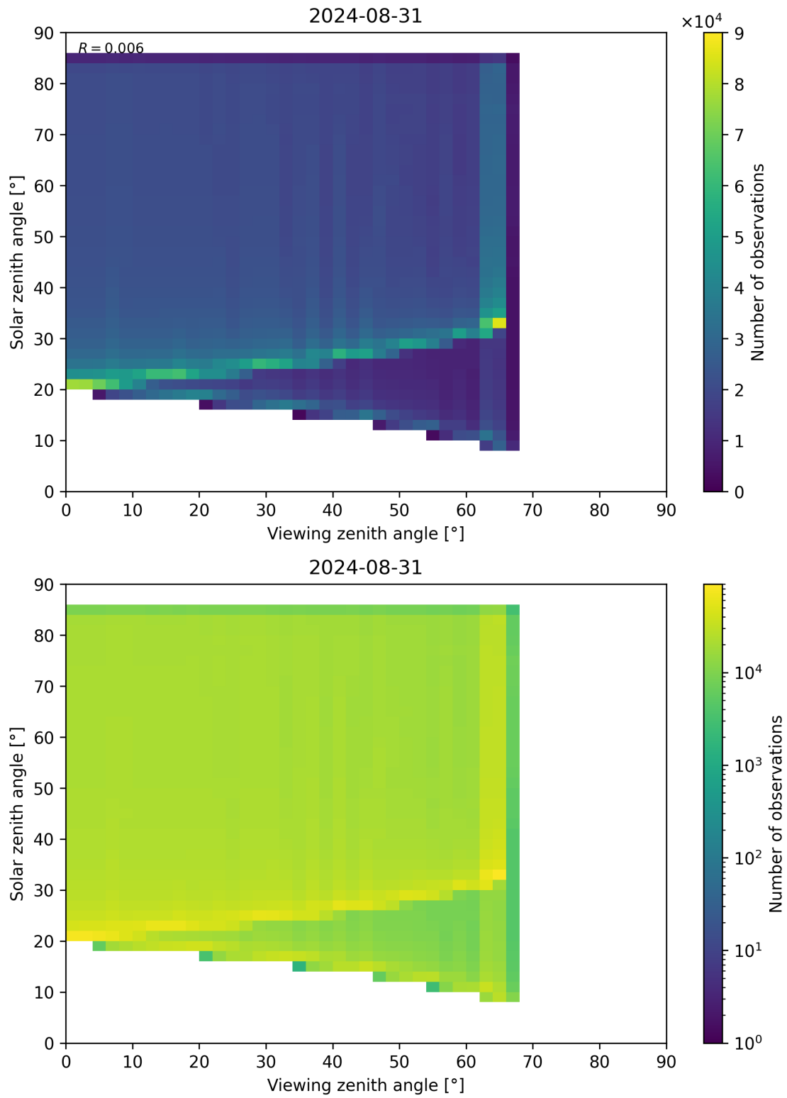
Figure 315: Scatter density plot of “Viewing zenith angle” against “Solar zenith angle” for 2024-08-30 to 2024-09-01.
