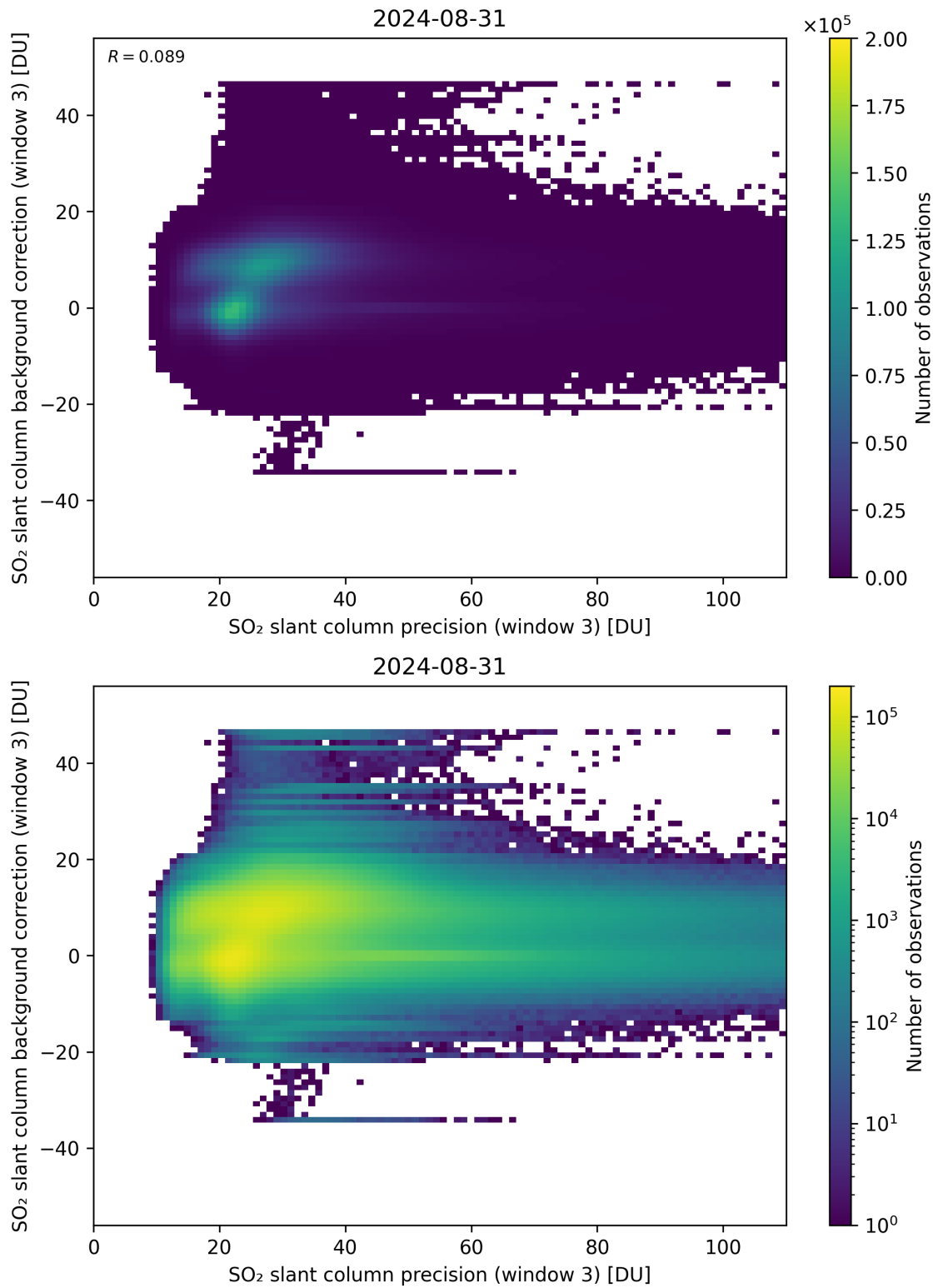
Figure 257: Scatter density plot of “SO 2 slant column precision (window 3)” against “SO 2 slant column background correction (window 3)” for 2024-08-30 to 2024-09-01.
