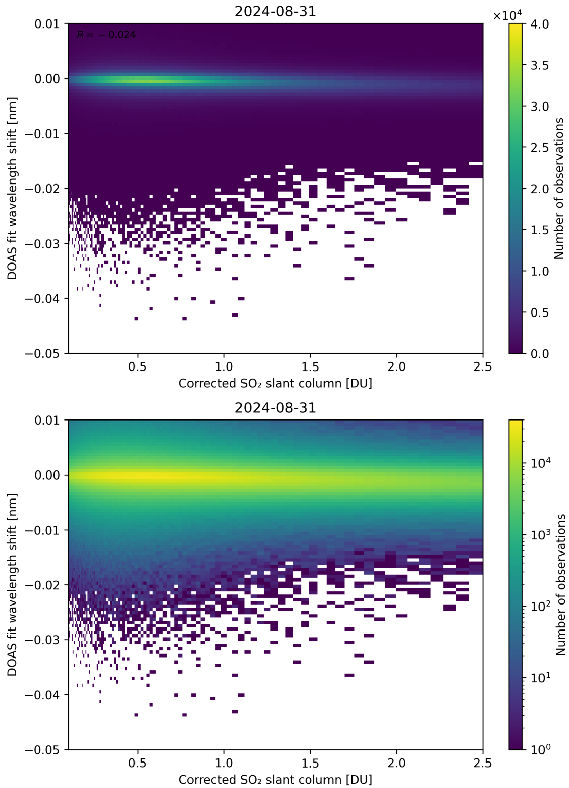
Figure 181: Scatter density plot of “Corrected SO 2 slant column” against “DOAS fit wavelength shift” for 2024-08-30 to 2024-09-01.
