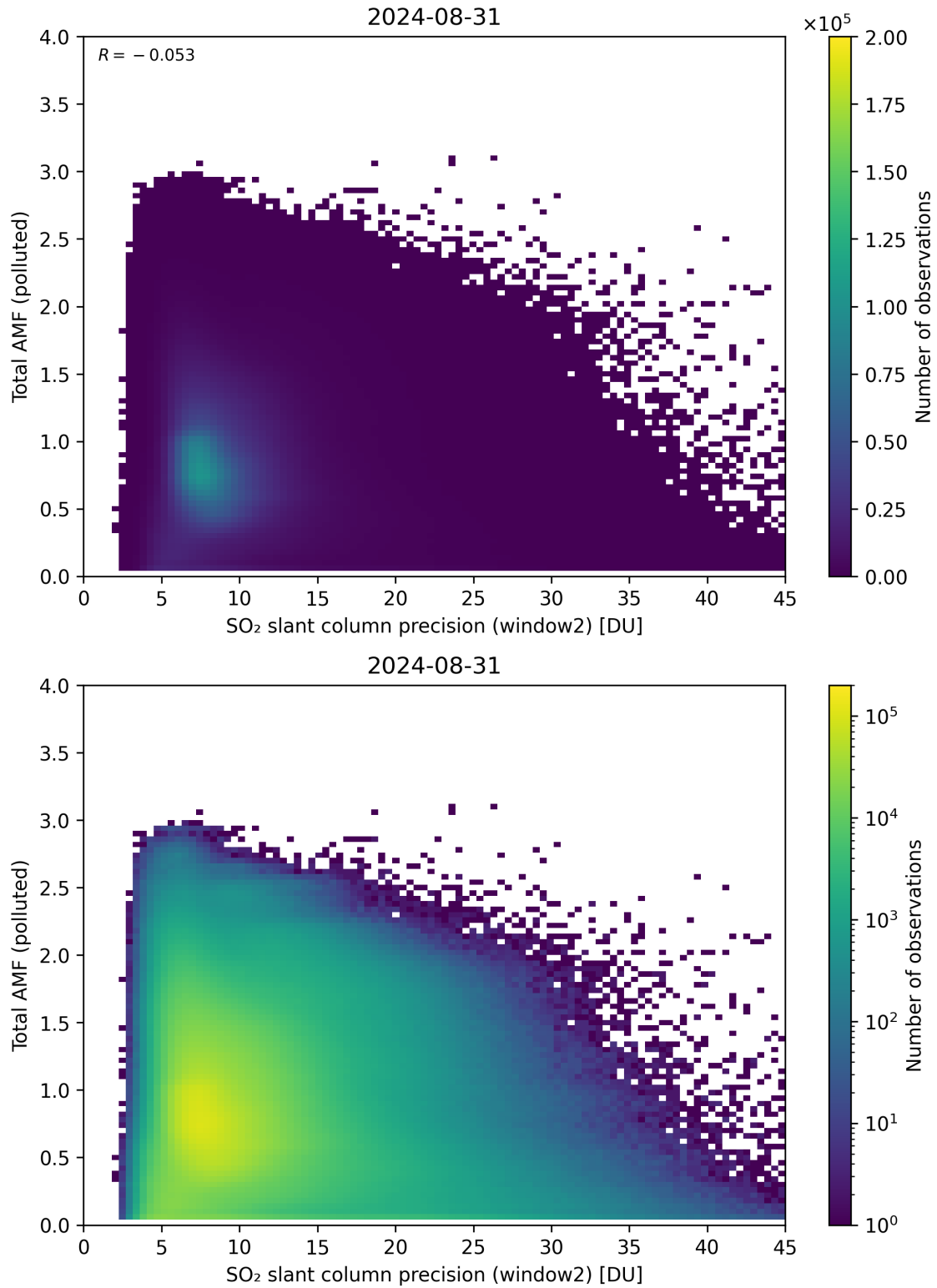
Figure 251: Scatter density plot of “SO 2 slant column precision (window2)” against “Total AMF (polluted)” for 2024-08-30 to 2024-09-01.
