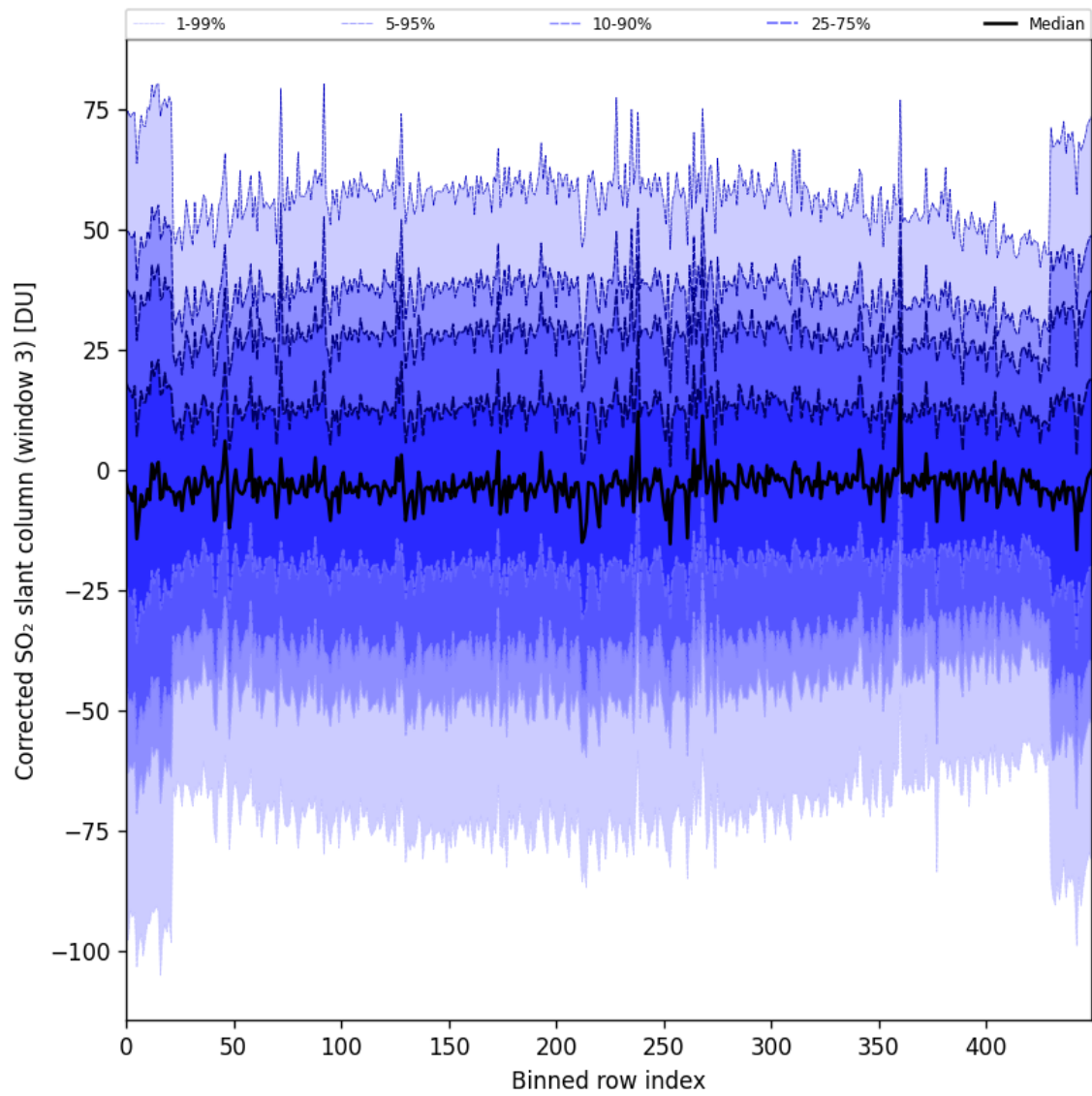
Figure 89: Along track statistics of “Corrected SO 2 slant column (window 3)” for 2024-08-30 to 2024-09-01
