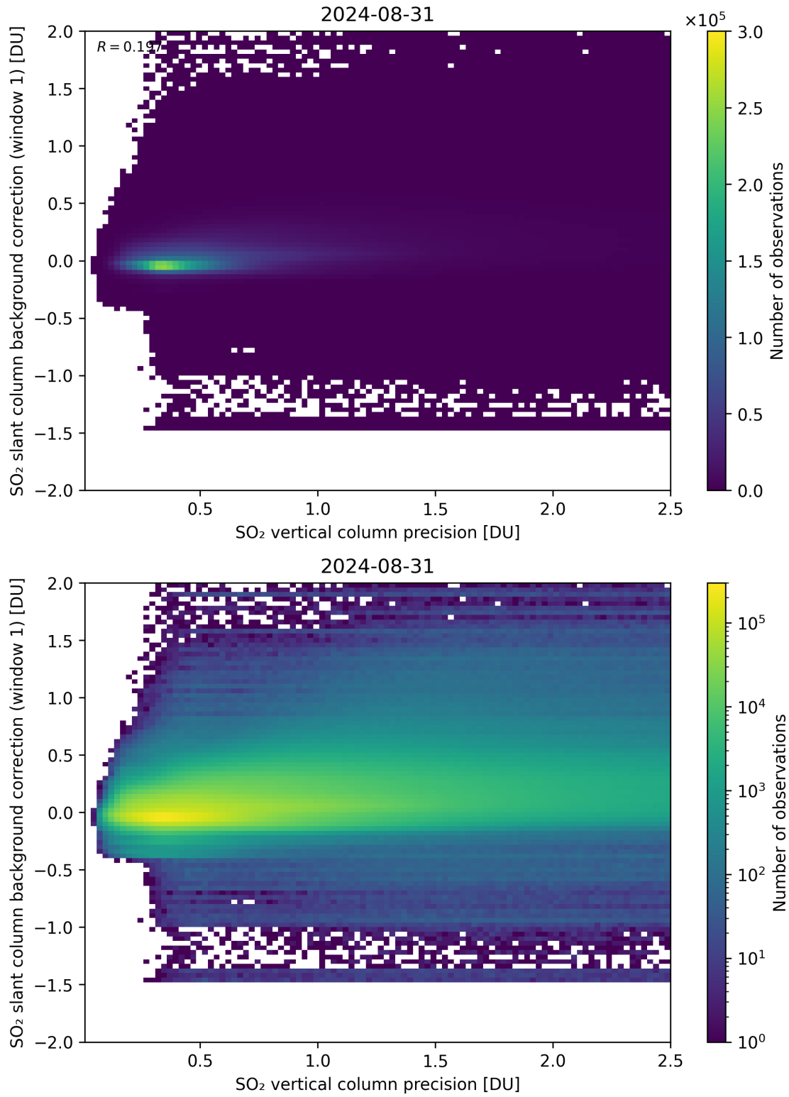
Figure 279: Scatter density plot of “SO 2 vertical column precision” against “SO 2 slant column background correction (window 1)” for 2024-08-30 to 2024-09-01.
