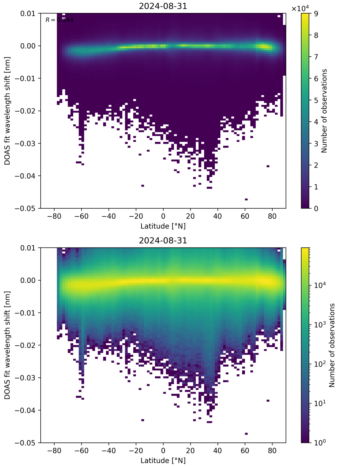
Figure 142: Scatter density plot of “Latitude” against “DOAS fit wavelength shift” for 2024-08-30 to 2024-09-01.
