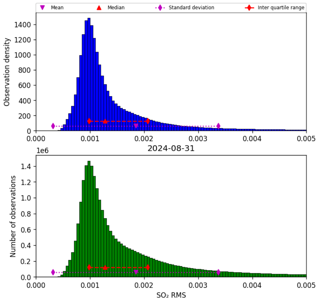
Figure 70: Histogram of “SO 2 RMS” for 2024-08-30 to 2024-09-01
