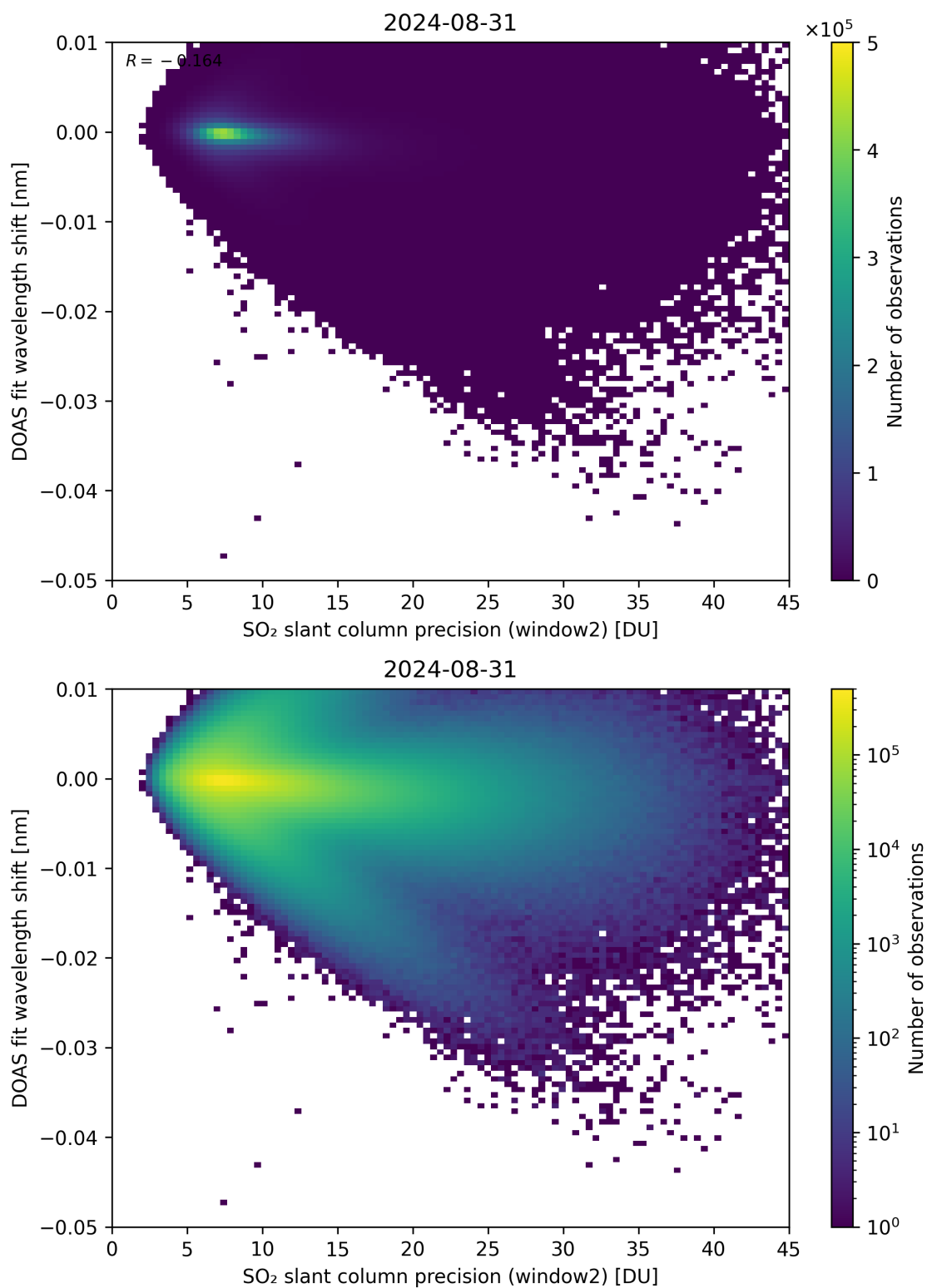
Figure 243: Scatter density plot of “SO 2 slant column precision (window2)” against “DOAS fit wavelength shift” for 2024-08-30 to 2024-09-01.
