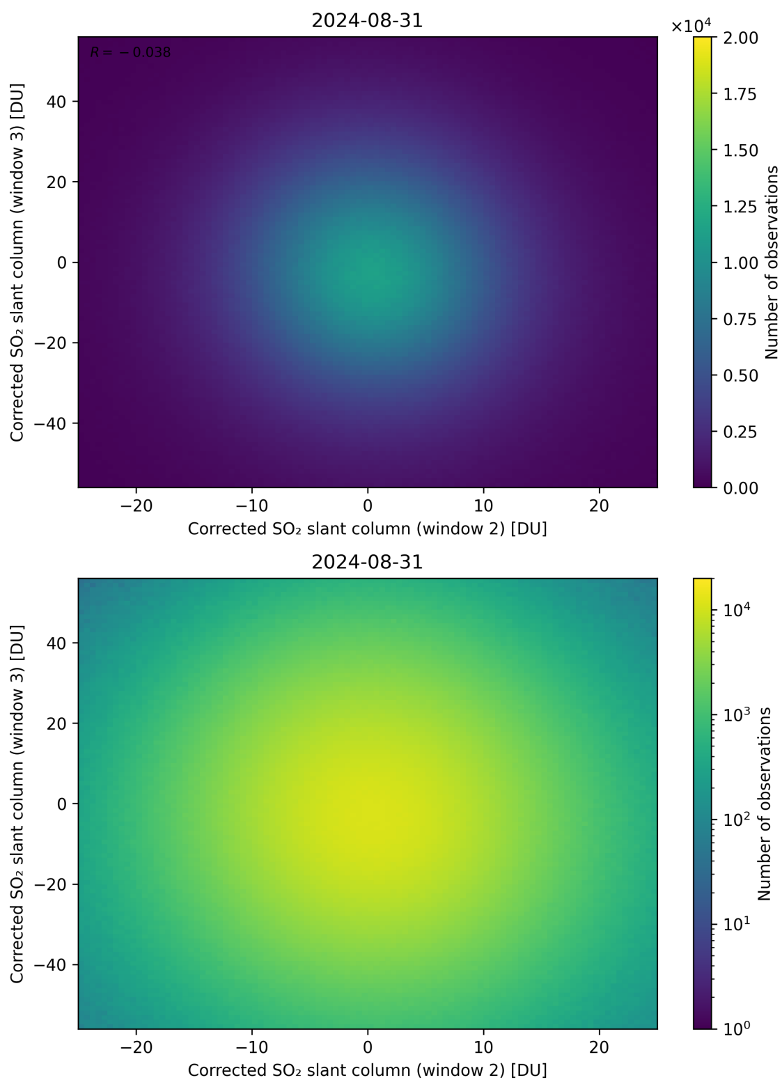
Figure 200: Scatter density plot of “Corrected SO 2 slant column (window 2)” against “Corrected SO 2 slant column (window 3)” for 2024-08-30 to 2024-09-01.
