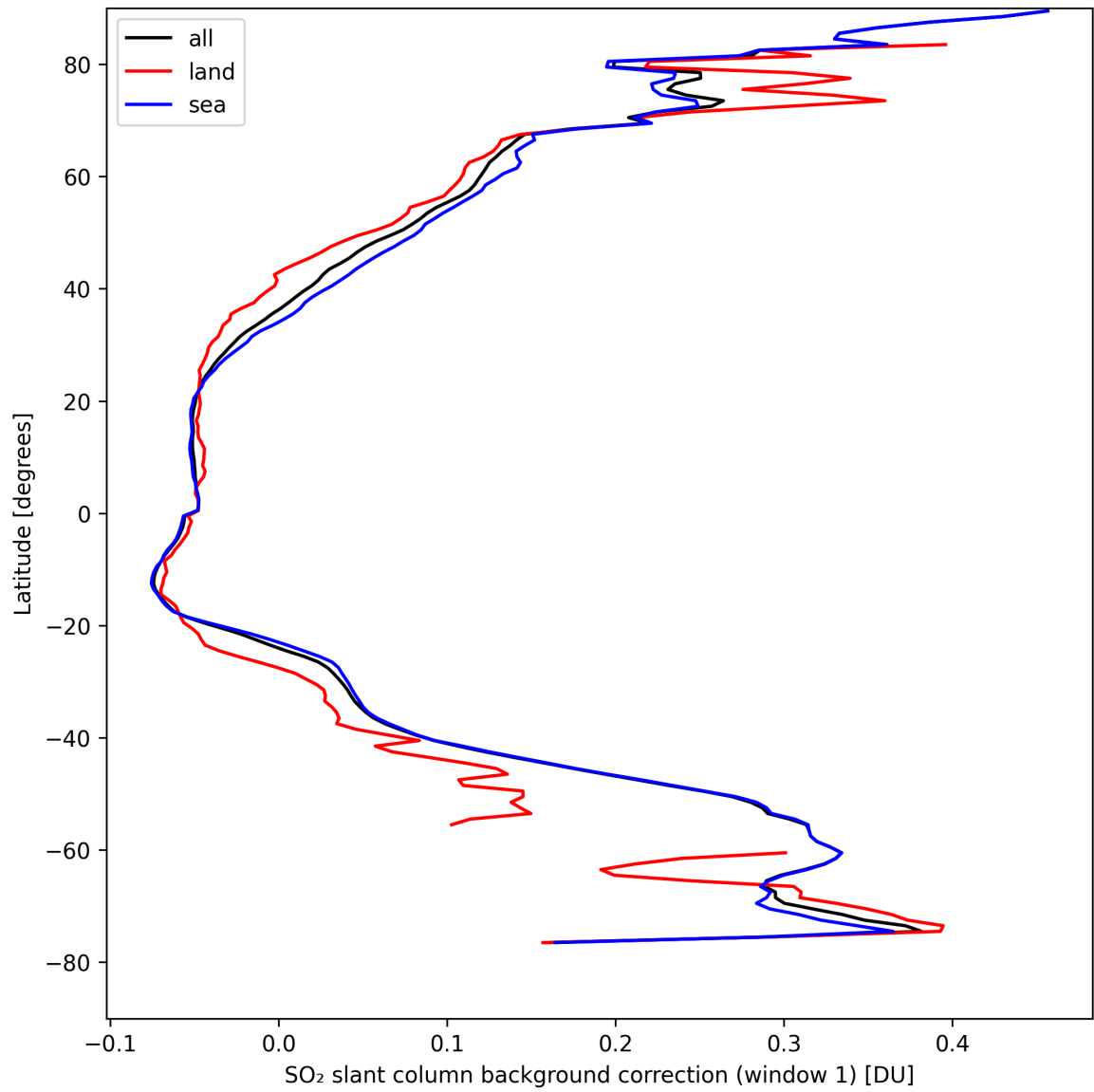
Figure 36: Zonal average of “SO 2 slant column background correction (window 1)” for 2024-08-30 to 2024-09-01.
