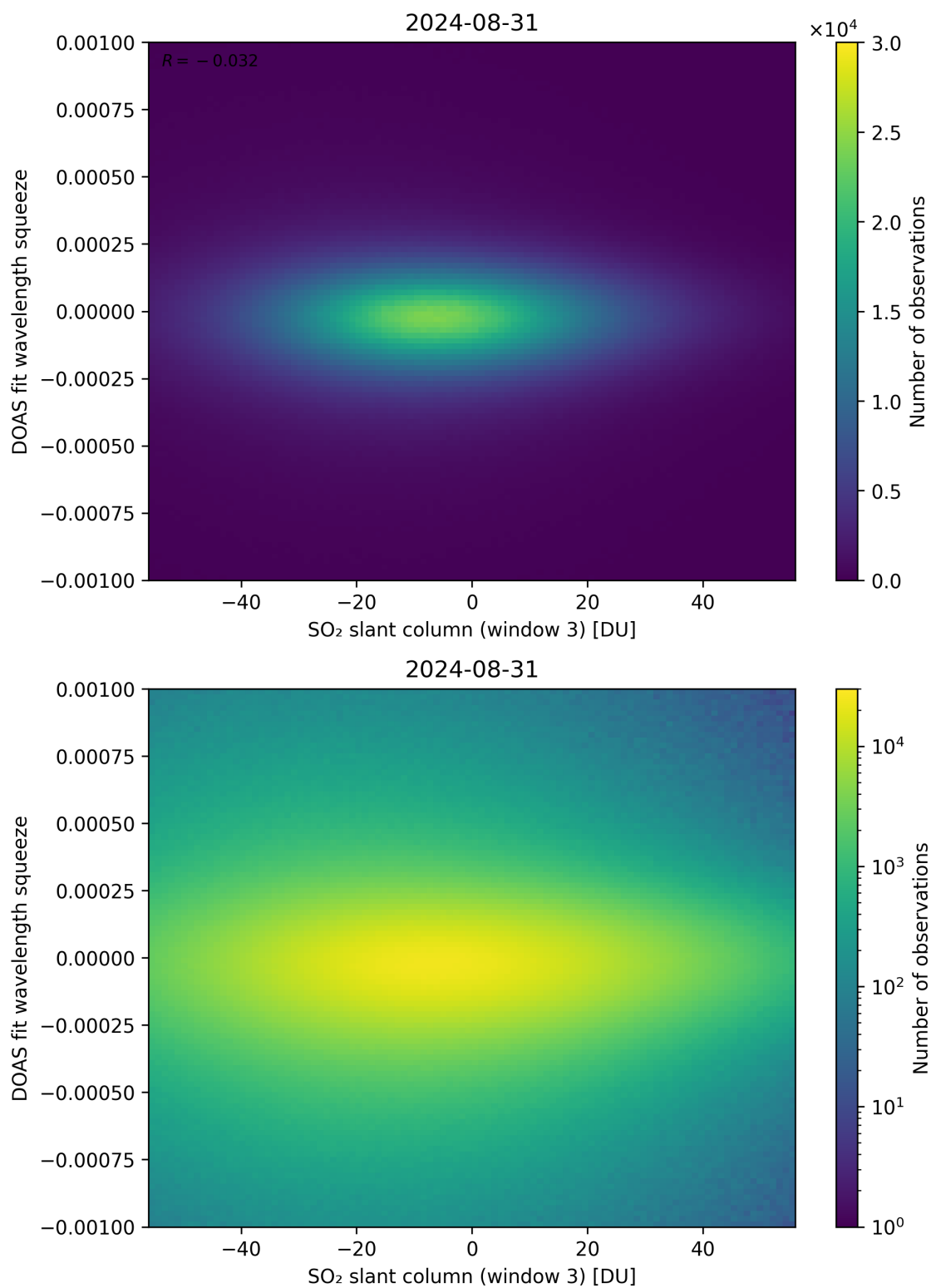
Figure 255: Scatter density plot of “SO 2 slant column (window 3)” against “DOAS fit wavelength squeeze” for 2024-08-30 to 2024-09-01.
