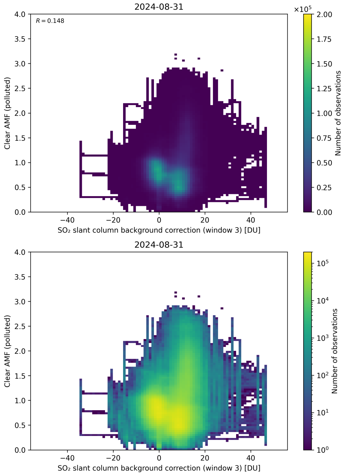
Figure 124: Scatter density plot of “SO 2 slant column background correction (window 3)” against “Clear AMF (polluted)” for 2024-08-30 to 2024-09-01.
