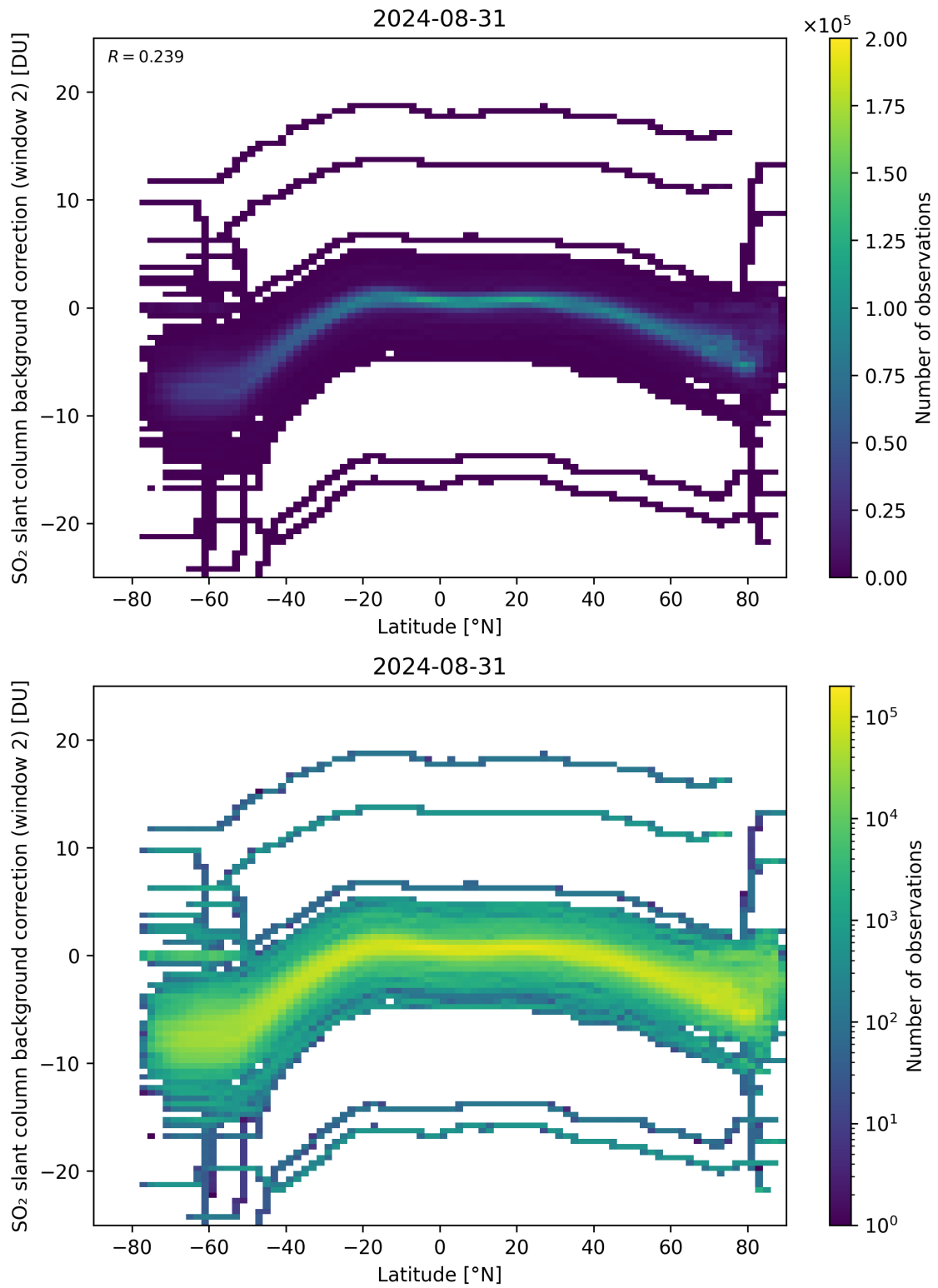
Figure 140: Scatter density plot of “Latitude” against “SO 2 slant column background correction (window 2)” for 2024-08-30 to 2024-09-01.
