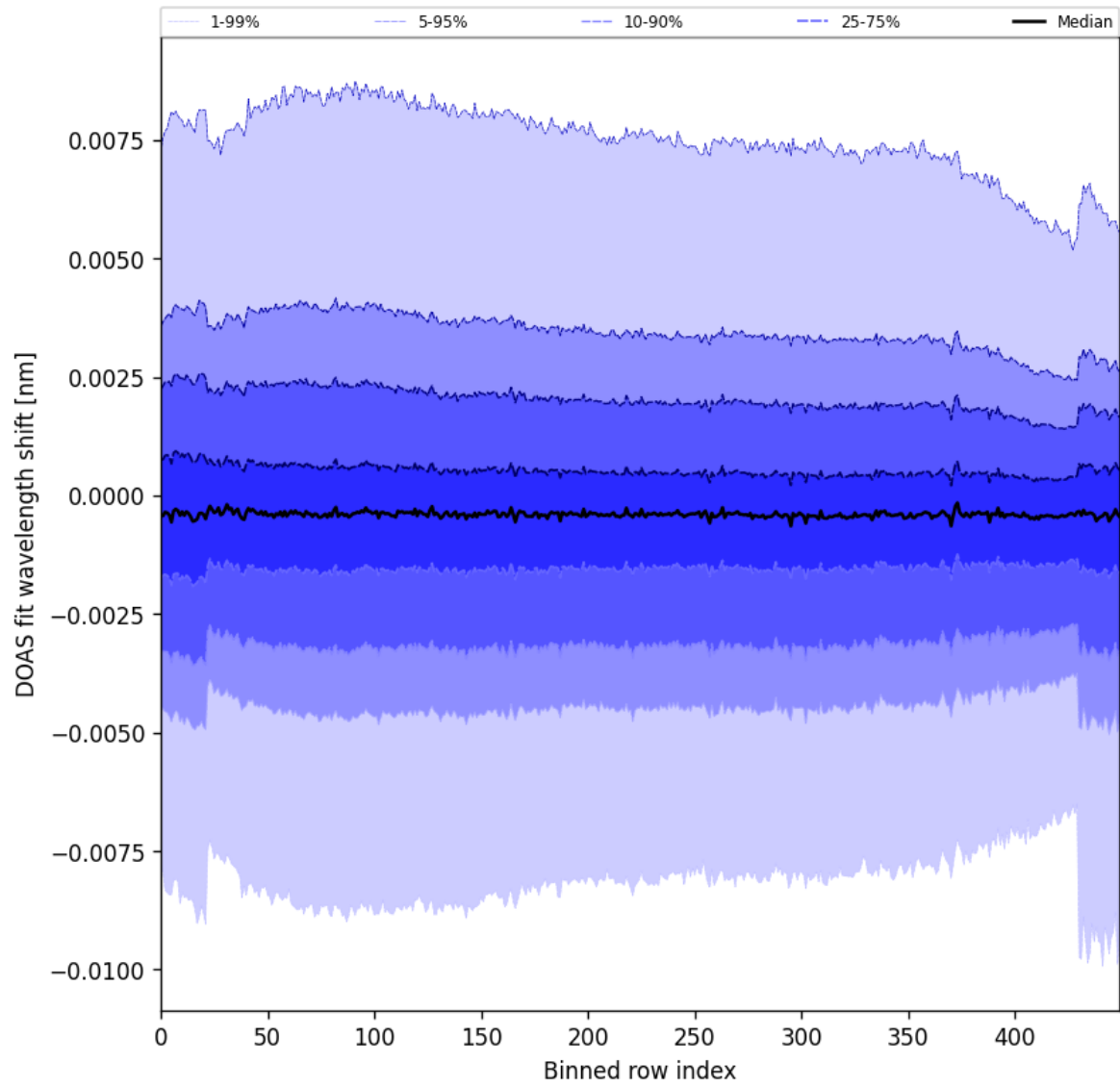
Figure 91: Along track statistics of “DOAS fit wavelength shift” for 2024-08-30 to 2024-09-01
