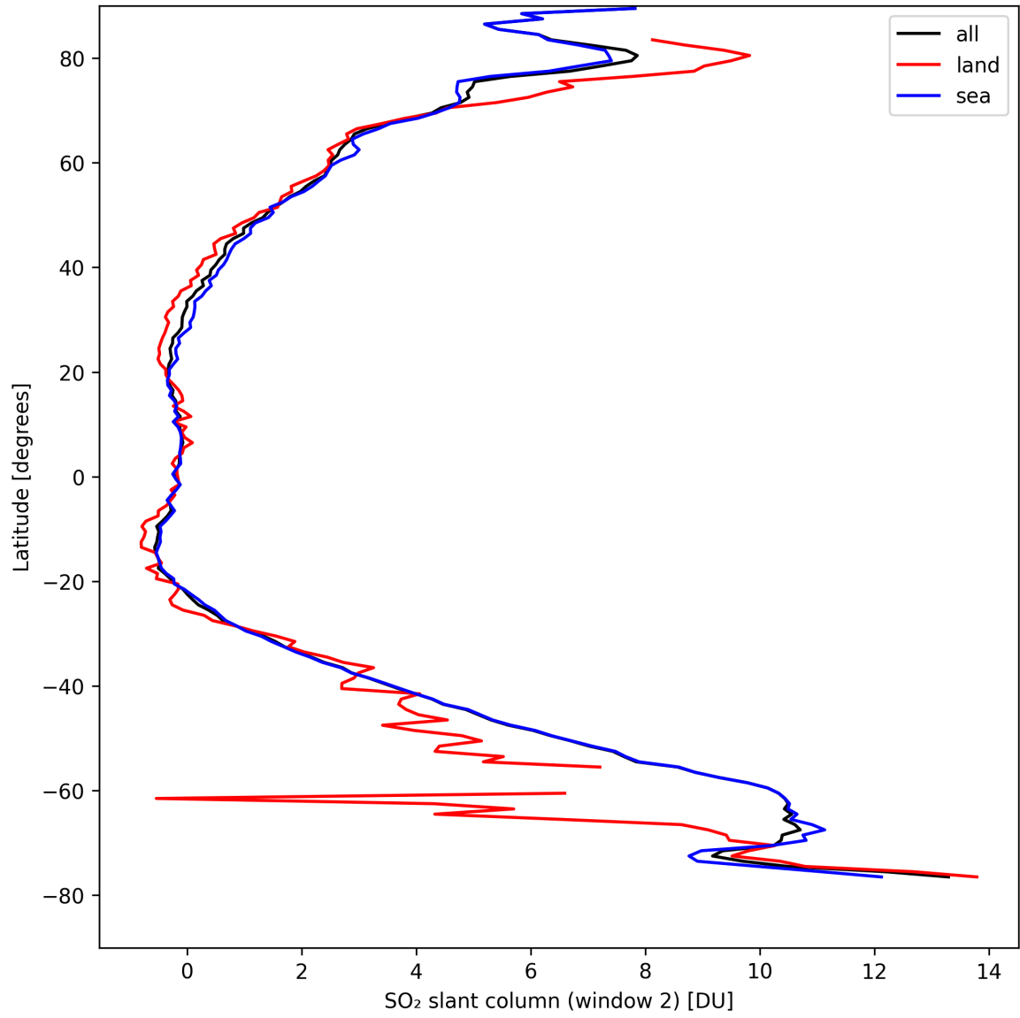
Figure 37: Zonal average of “SO 2 slant column (window 2)” for 2024-08-30 to 2024-09-01.
