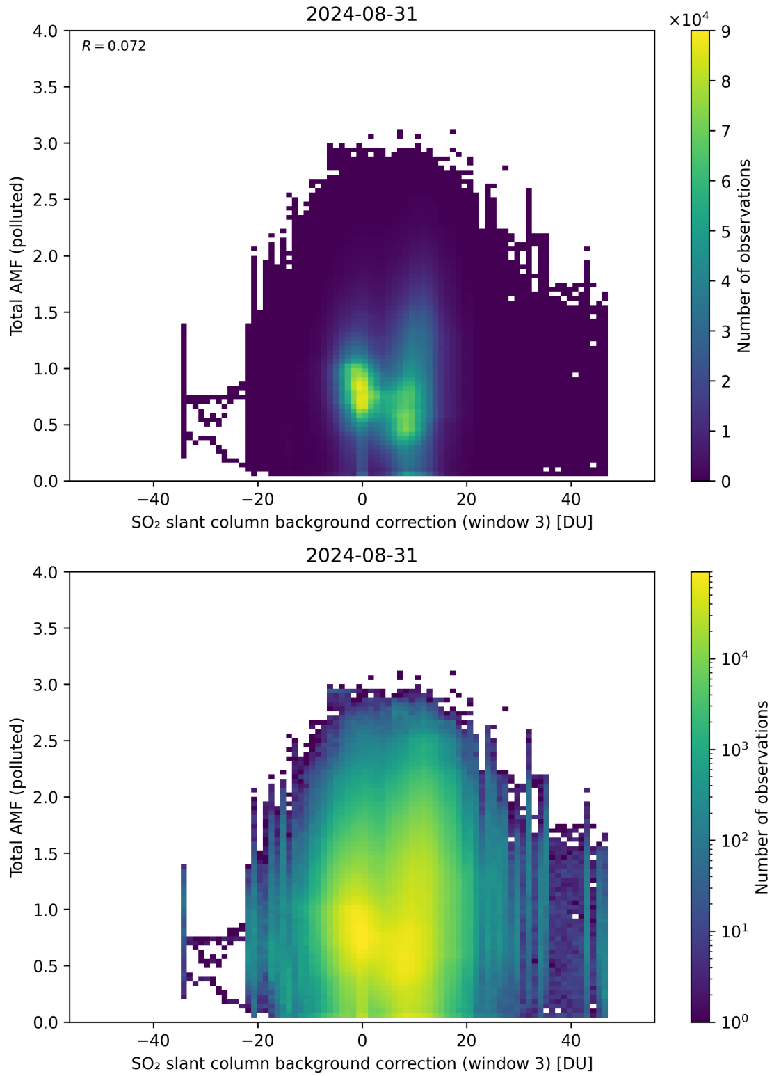
Figure 125: Scatter density plot of “SO 2 slant column background correction (window 3)” against “Total AMF (polluted)” for 2024-08-30 to 2024-09-01.
