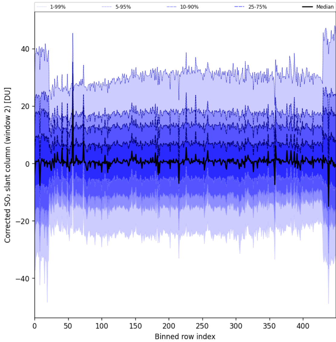
Figure 85: Along track statistics of “Corrected SO 2 slant column (window 2)” for 2024-08-30 to 2024-09-01
