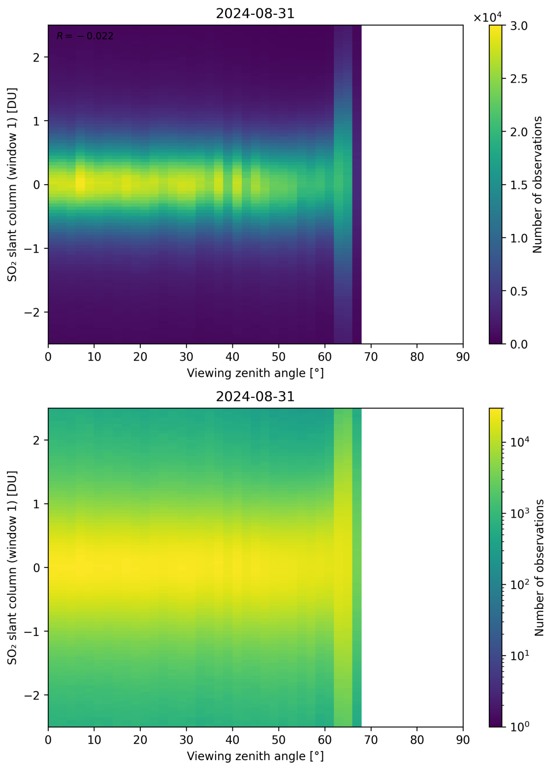
Figure 320: Scatter density plot of “Viewing zenith angle” against “SO 2 slant column (window 1)” for 2024-08-30 to 2024-09-01.
