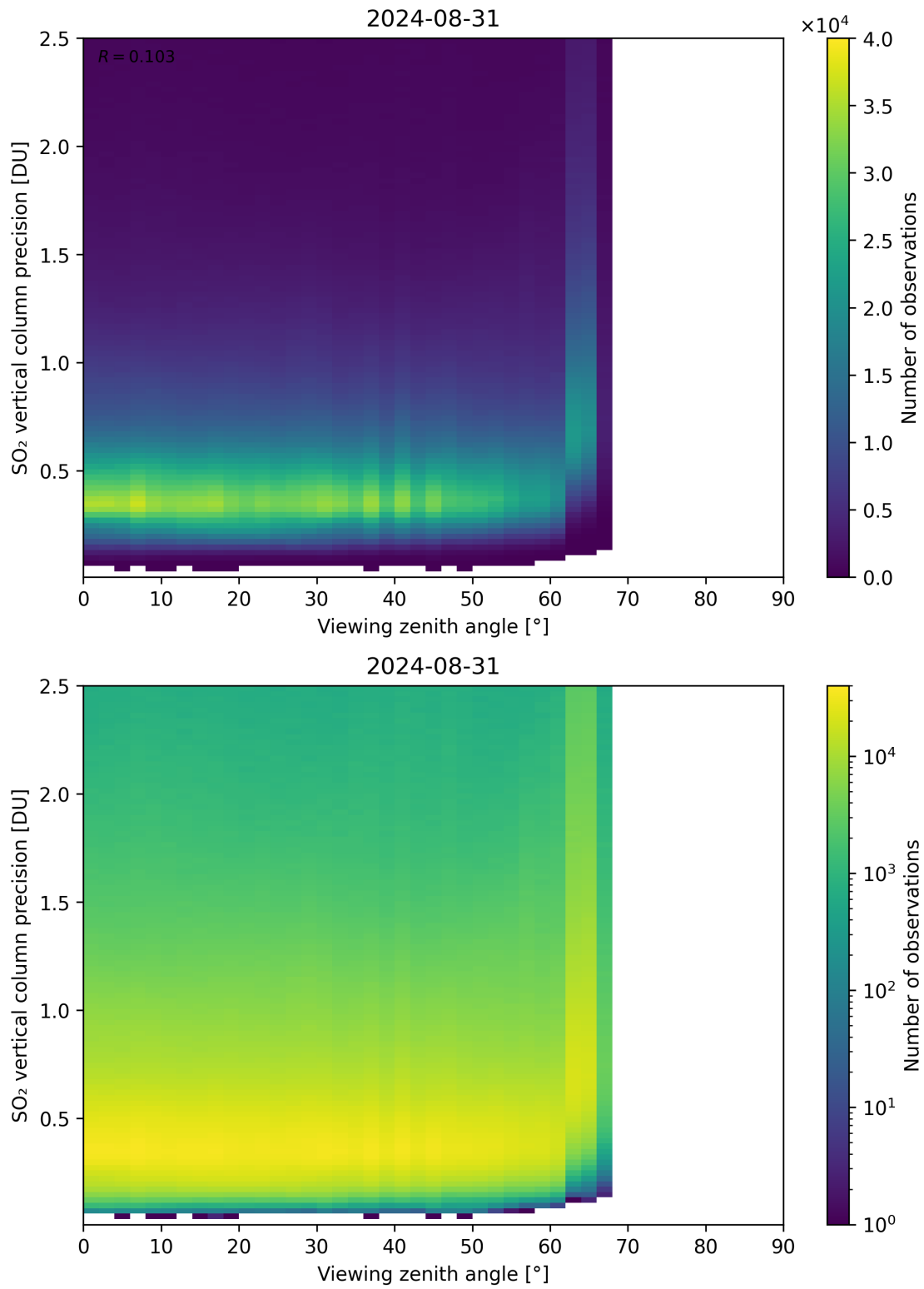
Figure 328: Scatter density plot of “Viewing zenith angle” against “SO 2 vertical column precision” for 2024-08-30 to 2024-09-01.
