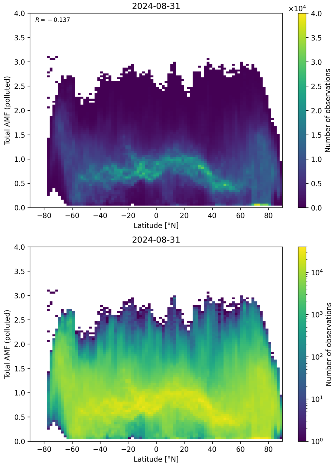
Figure 154: Scatter density plot of “Latitude” against “Total AMF (polluted)” for 2024-08-30 to 2024-09-01.
