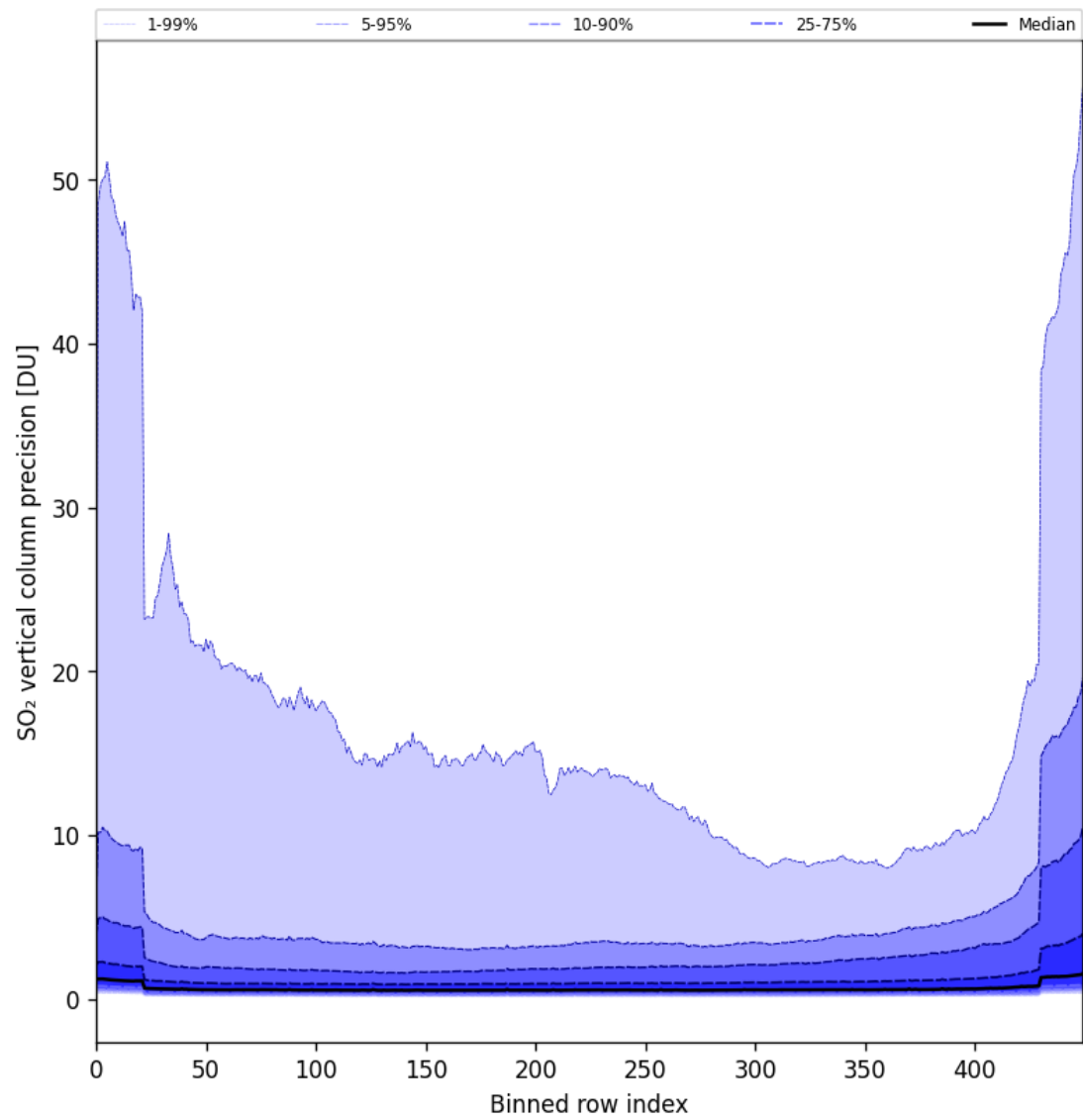
Figure 77: Along track statistics of “SO 2 vertical column precision” for 2024-08-30 to 2024-09-01
