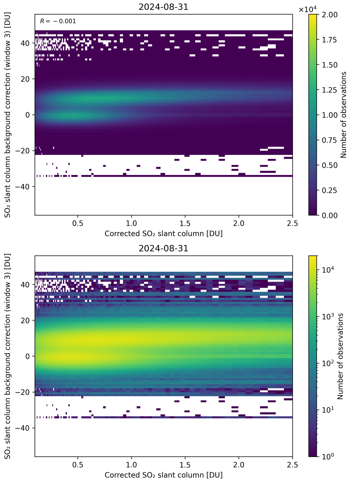
Figure 180: Scatter density plot of “Corrected SO 2 slant column” against “SO 2 slant column background correction (window 3)” for 2024-08-30 to 2024-09-01.
