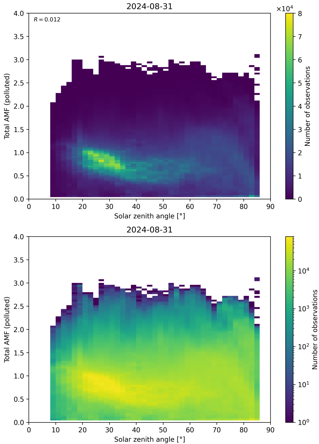
Figure 174: Scatter density plot of “Solar zenith angle” against “Total AMF (polluted)” for 2024-08-30 to 2024-09-01.
