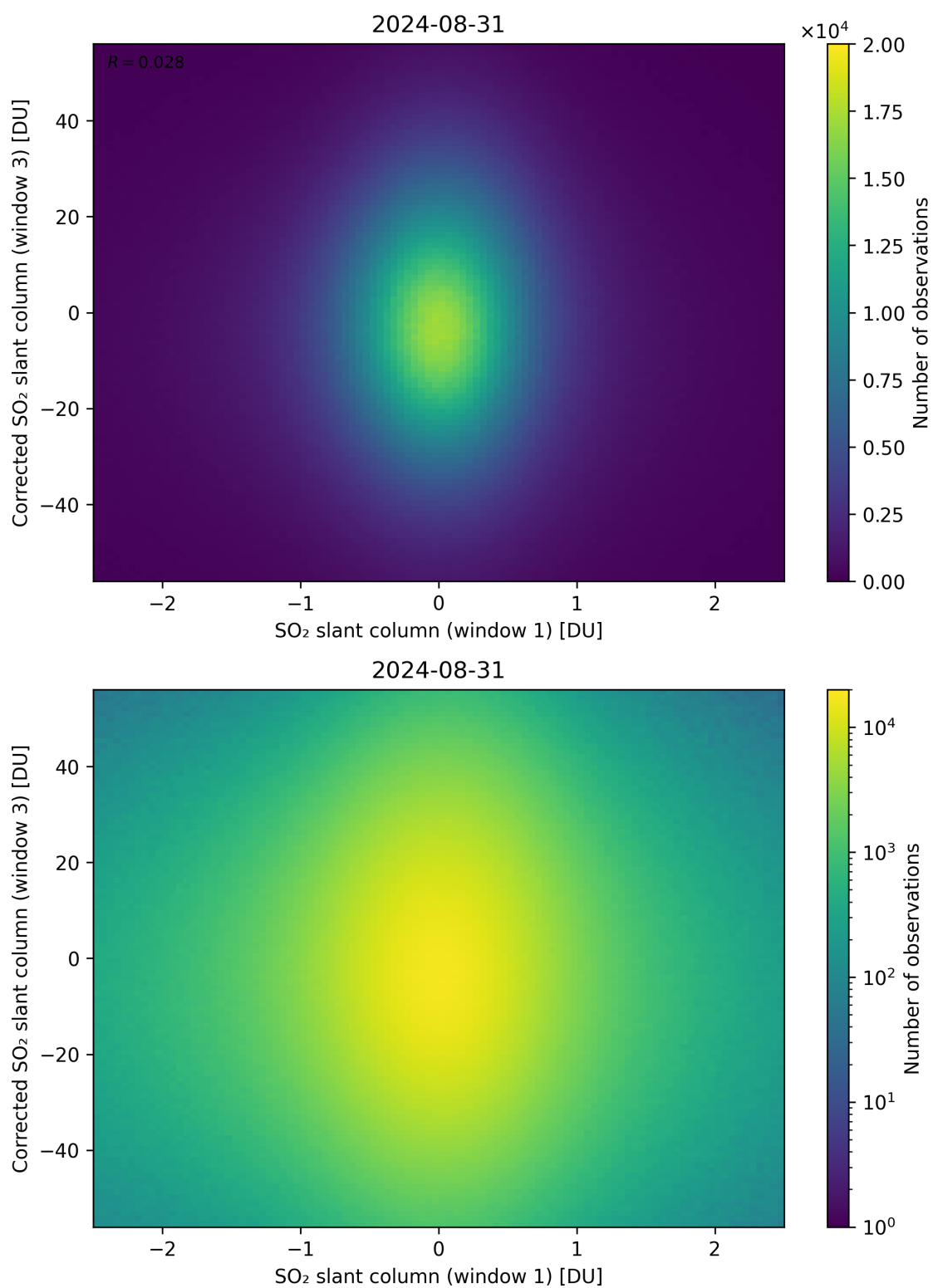
Figure 234: Scatter density plot of “SO 2 slant column (window 1)” against “Corrected SO 2 slant column (window 3)” for 2024-08-30 to 2024-09-01.
