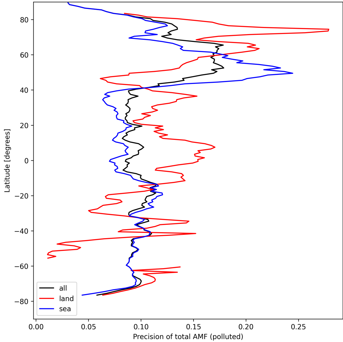
Figure 49: Zonal average of “Precision of total AMF (polluted)” for 2024-08-30 to 2024-09-01.
