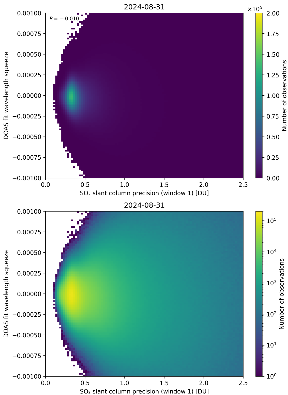
Figure 222: Scatter density plot of “SO 2 slant column precision (window 1)” against “DOAS fit wavelength squeeze” for 2024-08-30 to 2024-09-01.
