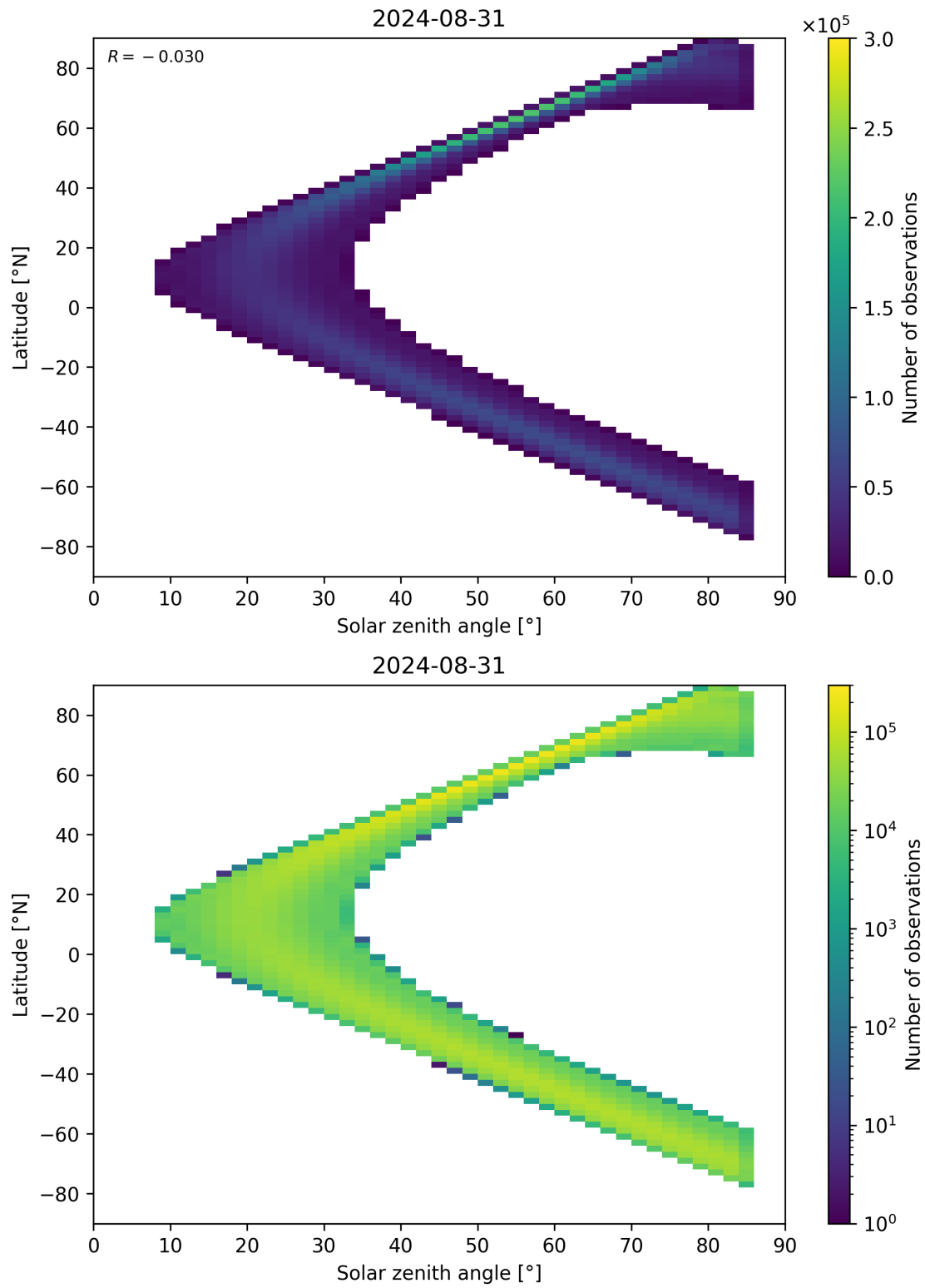
Figure 164: Scatter density plot of “Solar zenith angle” against “Latitude” for 2024-08-30 to 2024-09-01.
