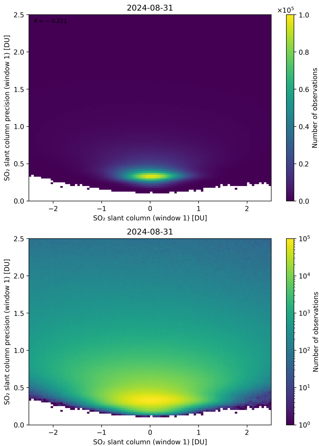
Figure 235: Scatter density plot of “SO 2 slant column (window 1)” against “SO 2 slant column precision (window 1)” for 2024-08-30 to 2024-09-01.
