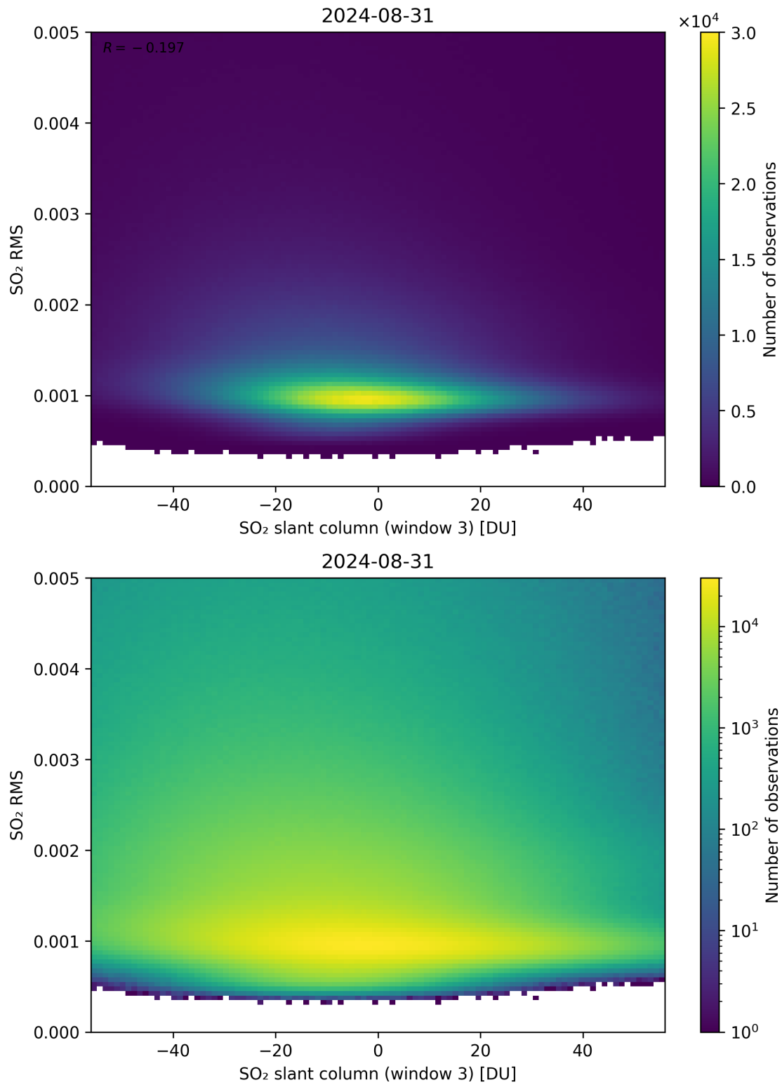
Figure 256: Scatter density plot of “SO 2 slant column (window 3)” against “SO 2 RMS” for 2024-08-30 to 2024-09-01.
