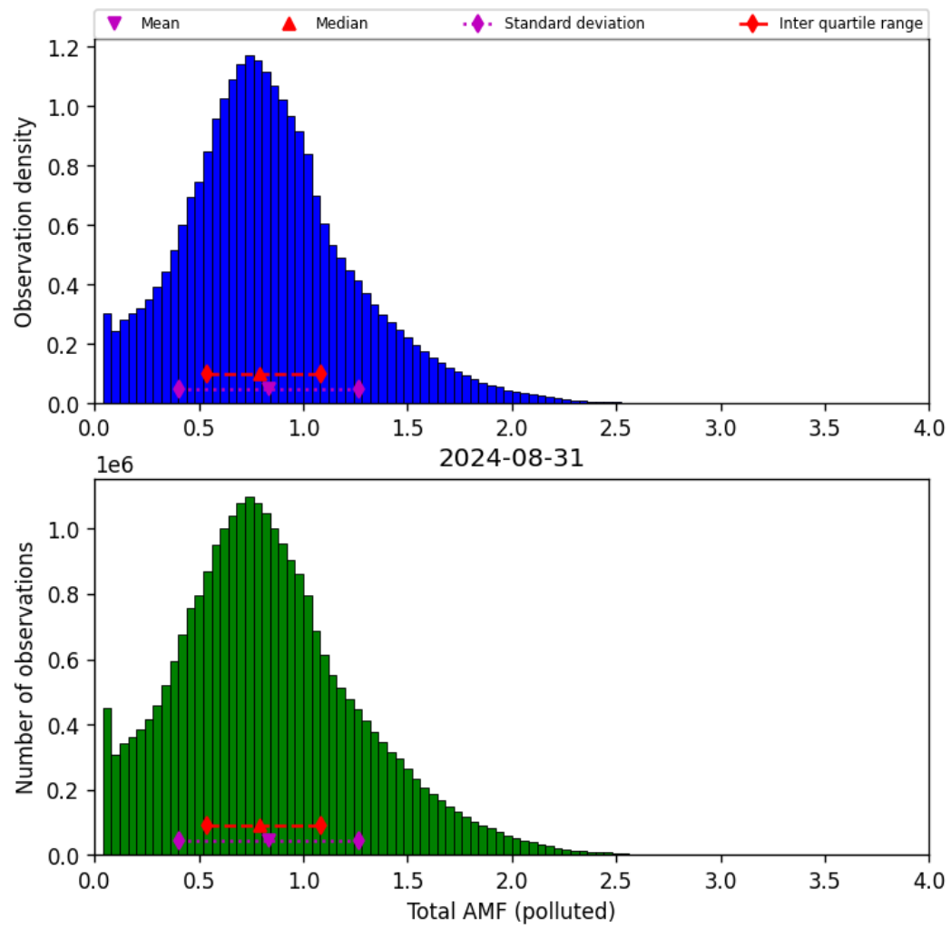
Figure 71: Histogram of “Total AMF (polluted)” for 2024-08-30 to 2024-09-01
