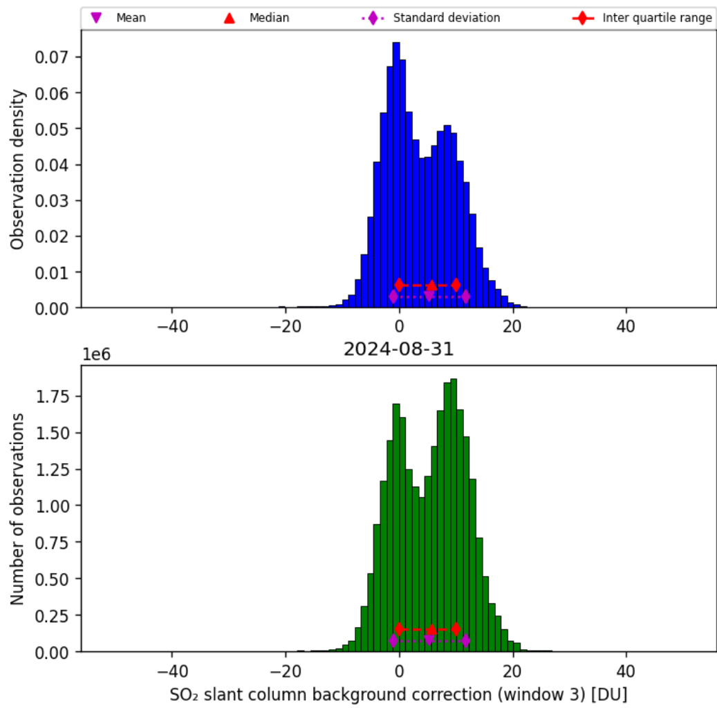
Figure 67: Histogram of “SO 2 slant column background correction (window 3)” for 2024-08-30 to 2024-09-01
