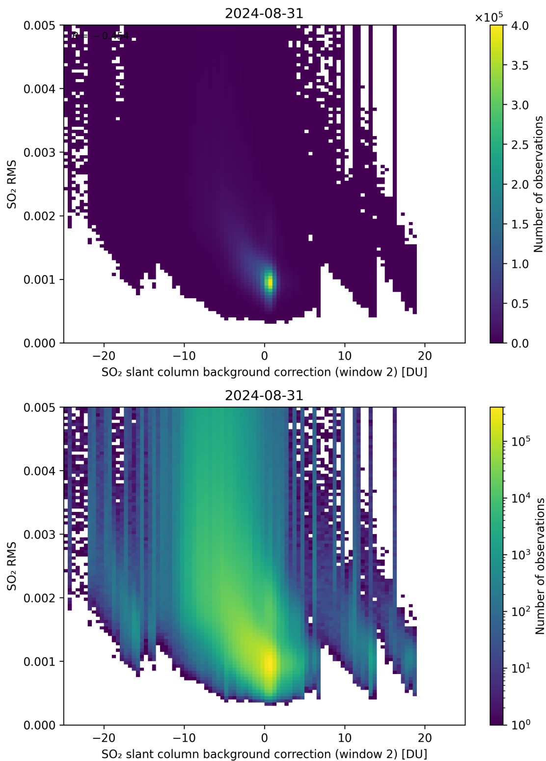
Figure 114: Scatter density plot of “SO 2 slant column background correction (window 2)” against “SO 2 RMS” for 2024-08-30 to 2024-09-01.
