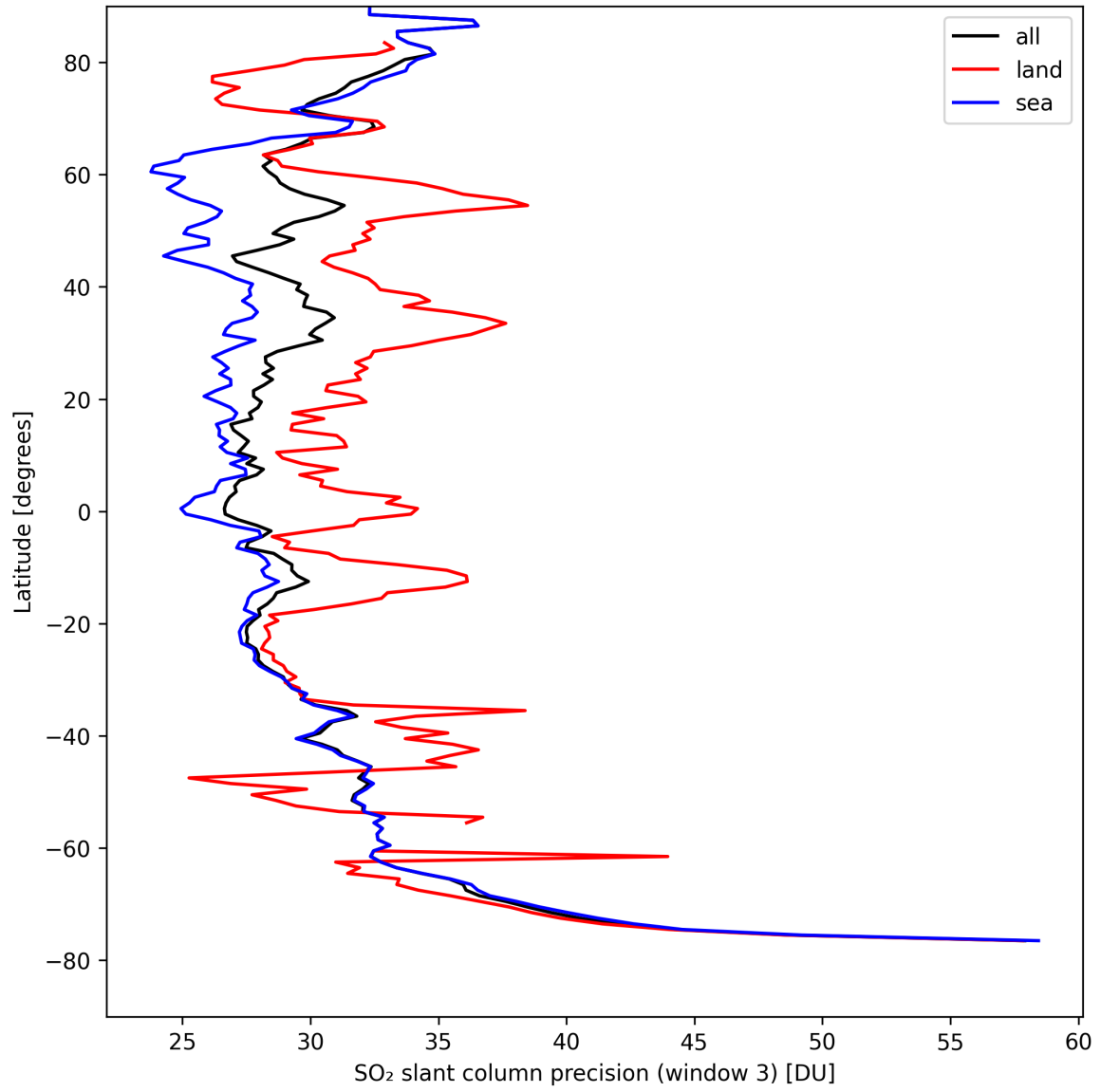
Figure 42: Zonal average of “SO 2 slant column precision (window 3)” for 2024-08-30 to 2024-09-01.
