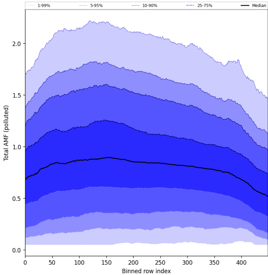
Figure 94: Along track statistics of “Total AMF (polluted)” for 2024-08-30 to 2024-09-01
