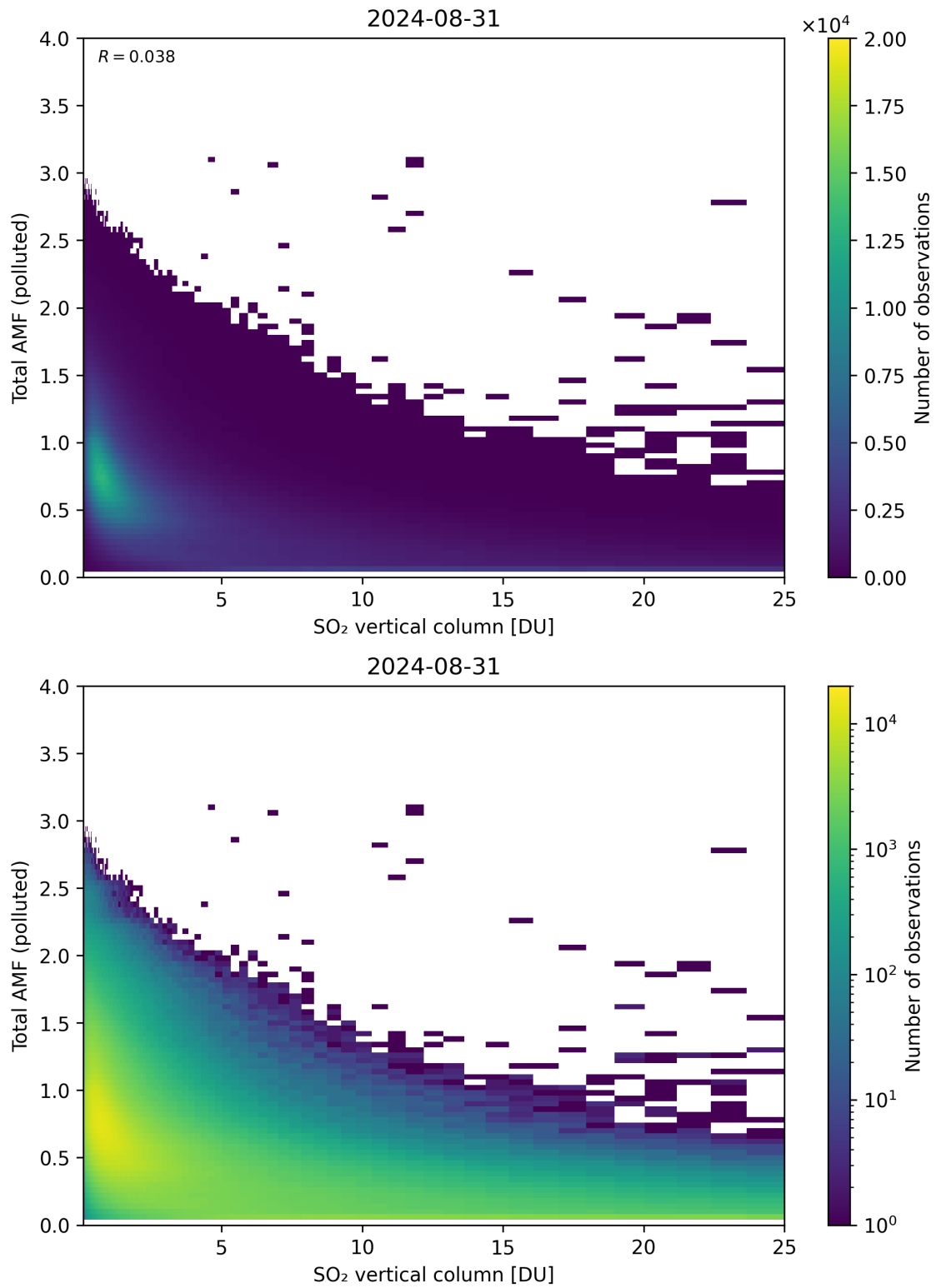
Figure 305: Scatter density plot of “SO 2 vertical column” against “Total AMF (polluted)” for 2024-08-30 to 2024-09-01.
