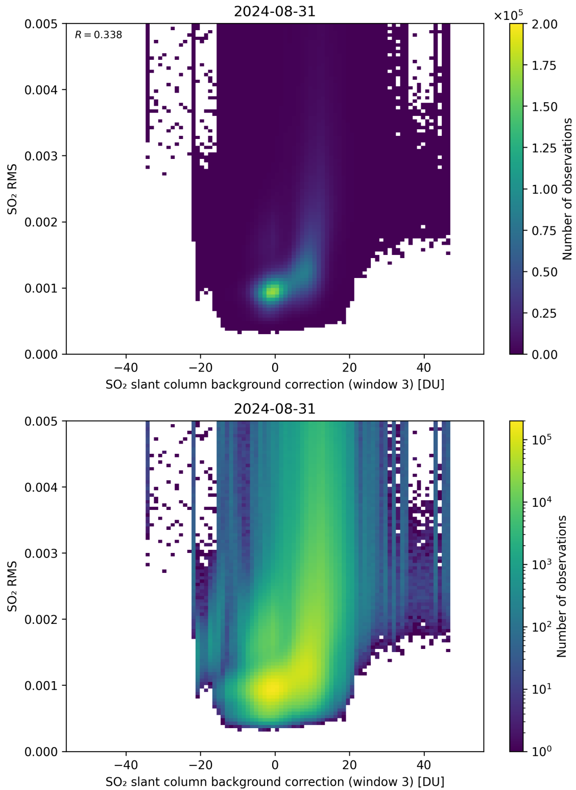
Figure 123: Scatter density plot of “SO 2 slant column background correction (window 3)” against “SO 2 RMS” for 2024-08-30 to 2024-09-01.
