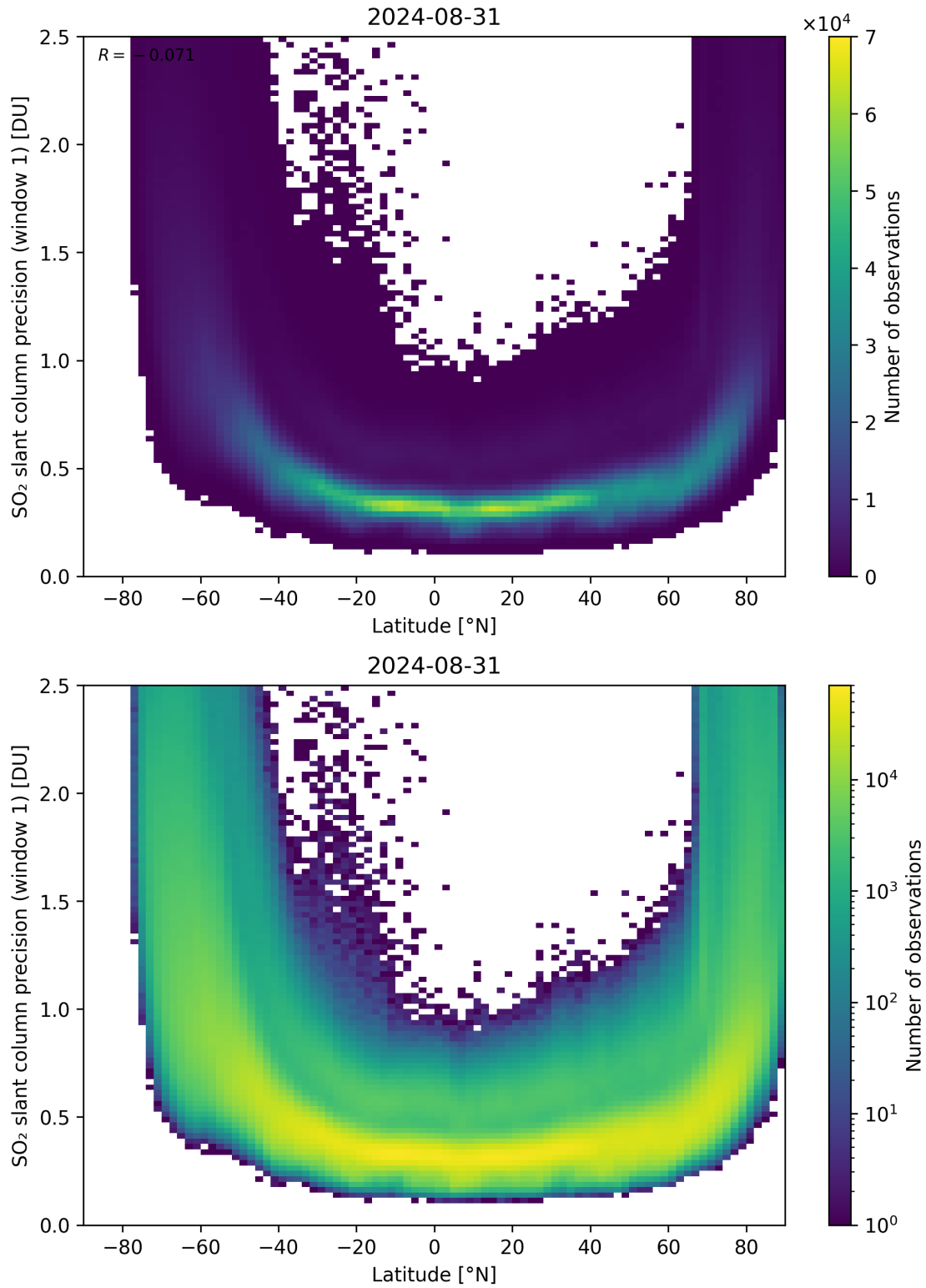
Figure 150: Scatter density plot of “Latitude” against “SO 2 slant column precision (window 1)” for 2024-08-30 to 2024-09-01.
