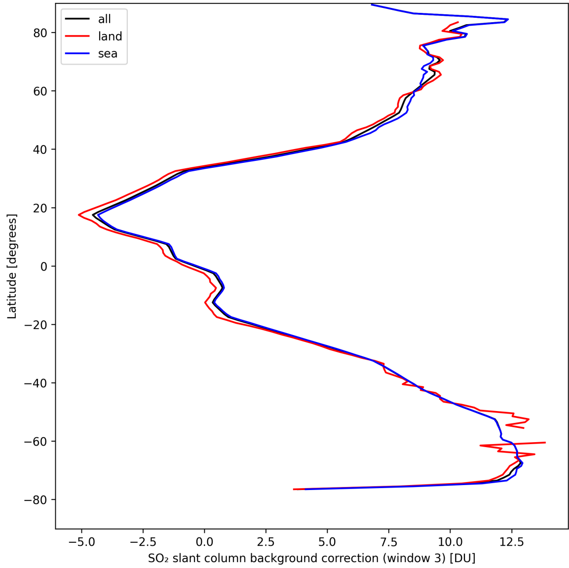
Figure 44: Zonal average of “SO 2 slant column background correction (window 3)” for 2024-08-30 to 2024-09-01.
