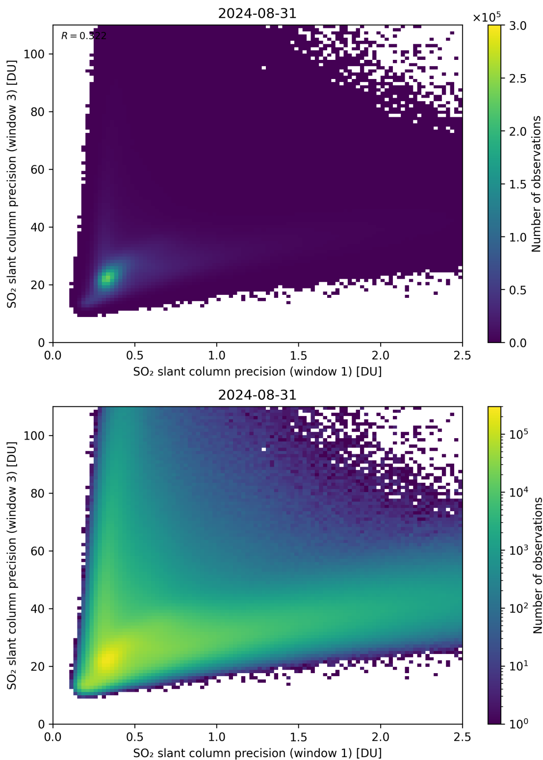
Figure 229: Scatter density plot of “SO 2 slant column precision (window 1)” against “SO 2 slant column precision (window 3)” for 2024-08-30 to 2024-09-01.
