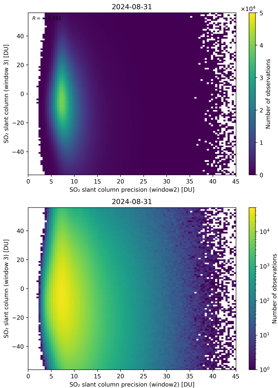
Figure 249: Scatter density plot of “SO 2 slant column precision (window2)” against “SO 2 slant column (window 3)” for 2024-08-30 to 2024-09-01.
