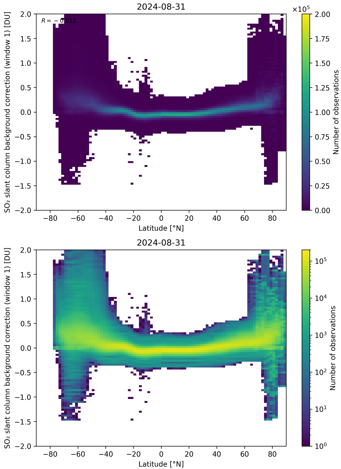
Figure 139: Scatter density plot of “Latitude” against “SO 2 slant column background correction (window 1)” for 2024-08-30 to 2024-09-01.
