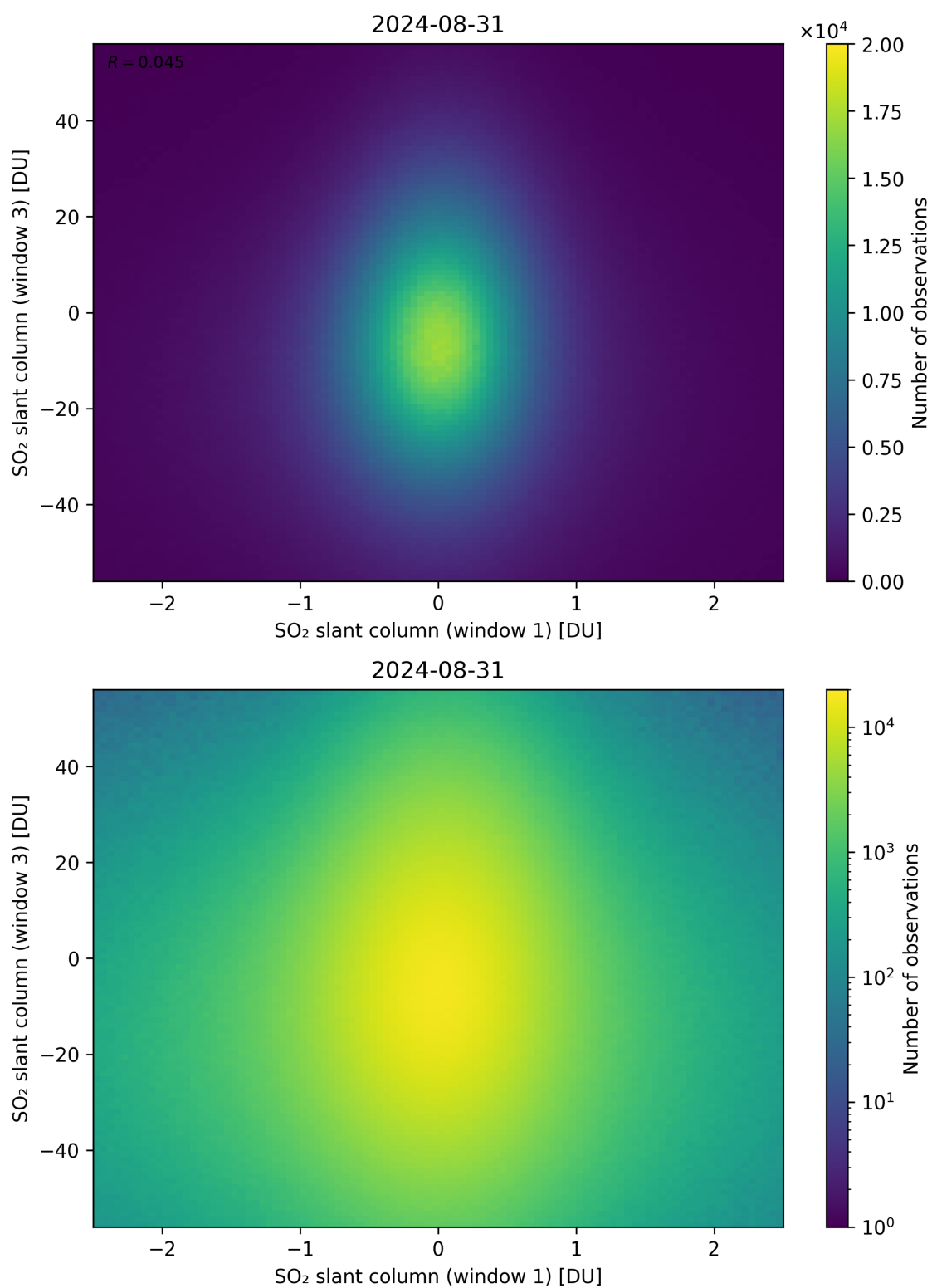
Figure 237: Scatter density plot of “SO 2 slant column (window 1)” against “SO 2 slant column (window 3)” for 2024-08-30 to 2024-09-01.
