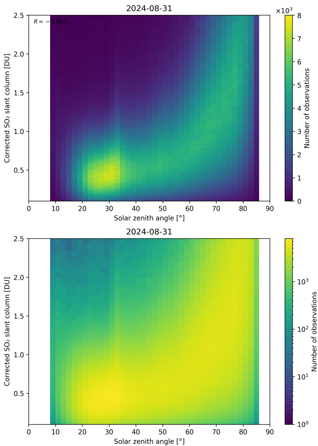
Figure 166: Scatter density plot of “Solar zenith angle” against “Corrected SO 2 slant column” for 2024-08-30 to 2024-09-01.
