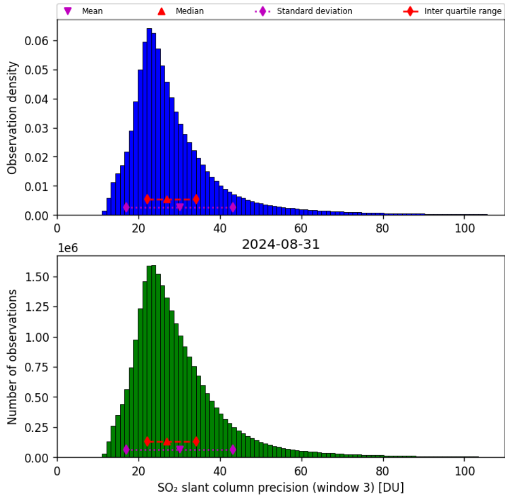
Figure 65: Histogram of “SO 2 slant column precision (window 3)” for 2024-08-30 to 2024-09-01
