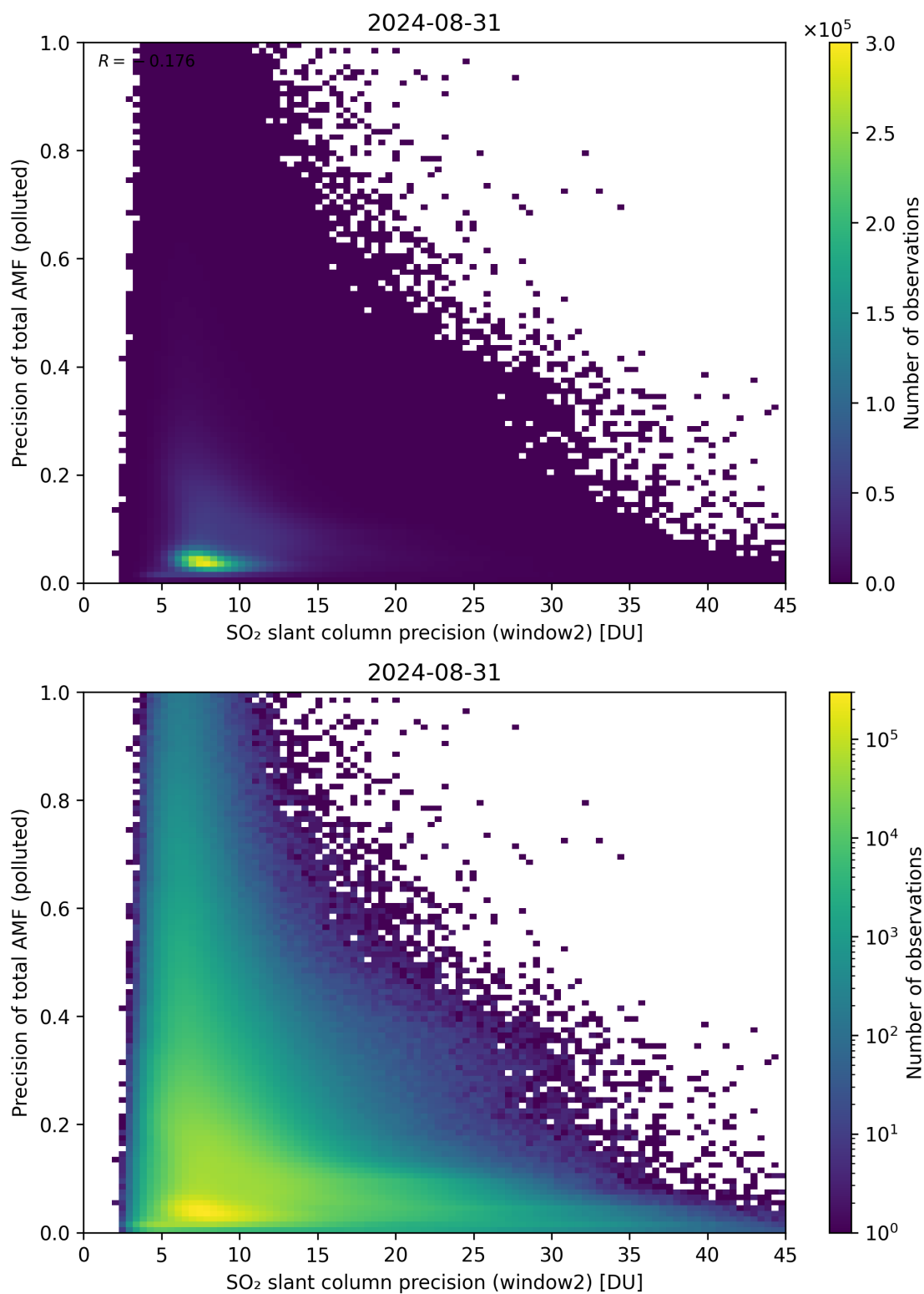
Figure 252: Scatter density plot of “SO 2 slant column precision (window2)” against “Precision of total AMF (polluted)” for 2024-08-30 to 2024-09-01.
