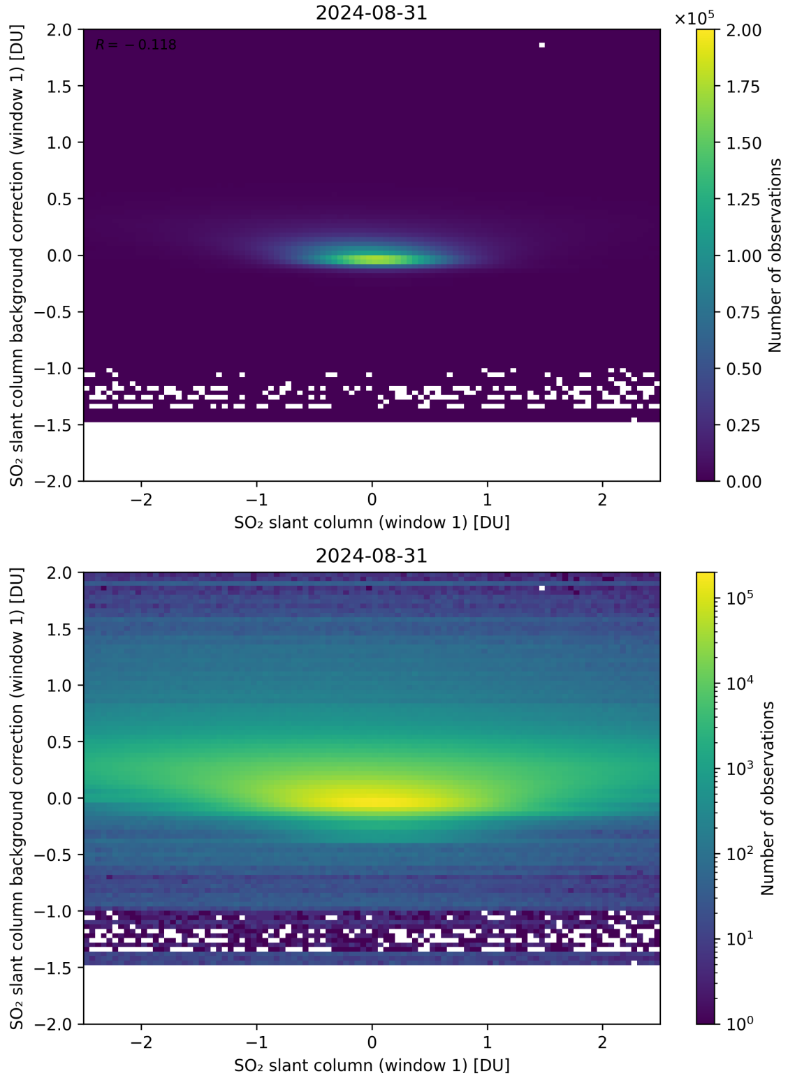
Figure 212: Scatter density plot of “SO 2 slant column (window 1)” against “SO 2 slant column background correction (window 1)” for 2024-08-30 to 2024-09-01.
