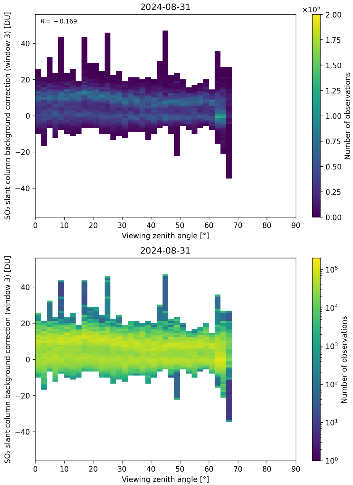
Figure 310: Scatter density plot of “Viewing zenith angle” against “SO 2 slant column background correction (window 3)” for 2024-08-30 to 2024-09-01.
