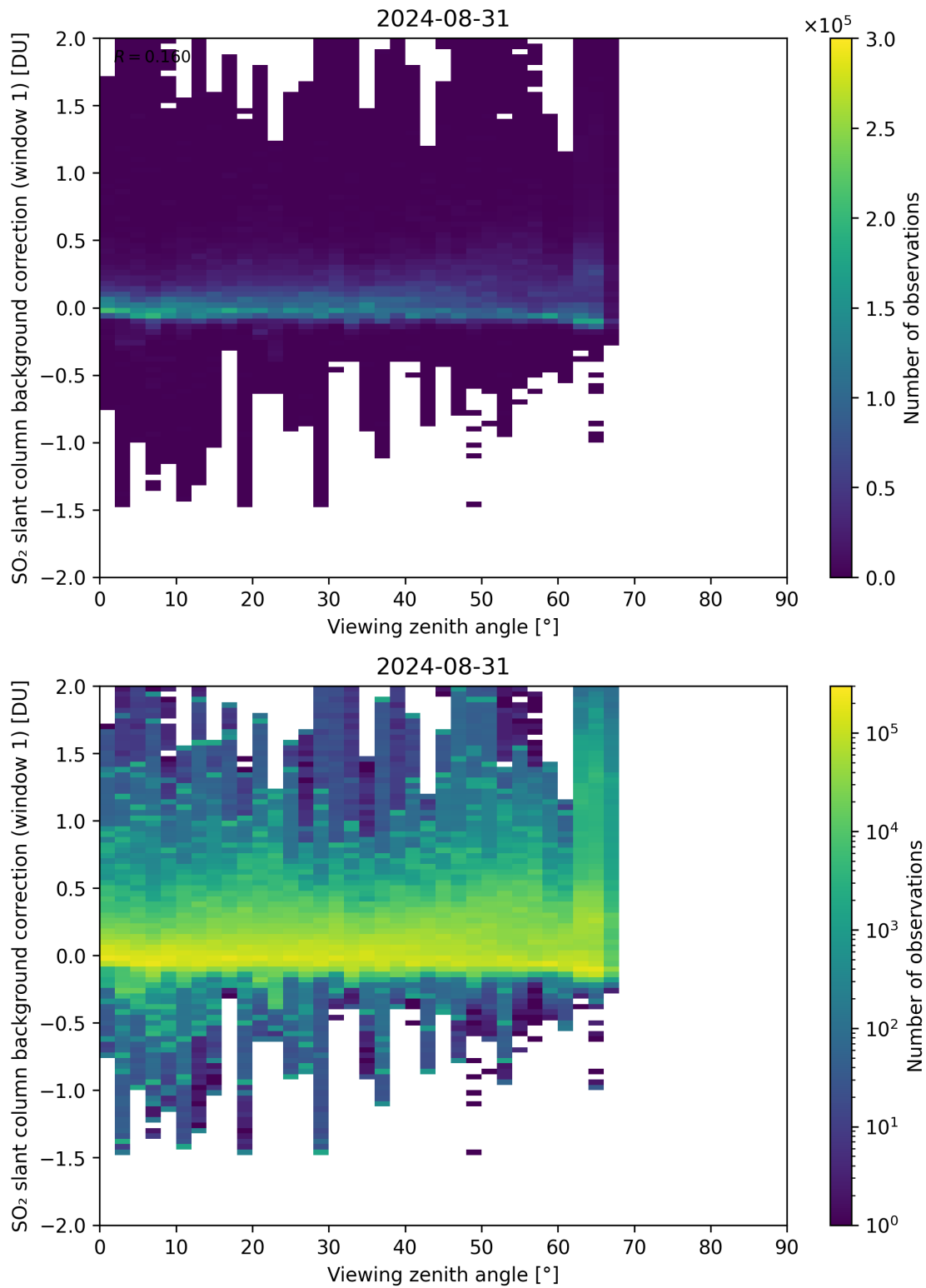
Figure 308: Scatter density plot of “Viewing zenith angle” against “SO 2 slant column background correction (window 1)” for 2024-08-30 to 2024-09-01.
