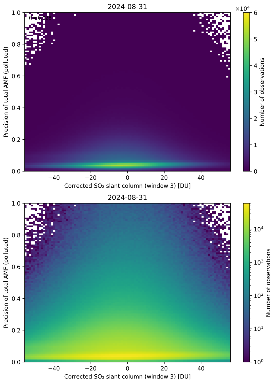
Figure 211: Scatter density plot of “Corrected SO 2 slant column (window 3)” against “Precision of total AMF (polluted)” for 2024-08-30 to 2024-09-01.
