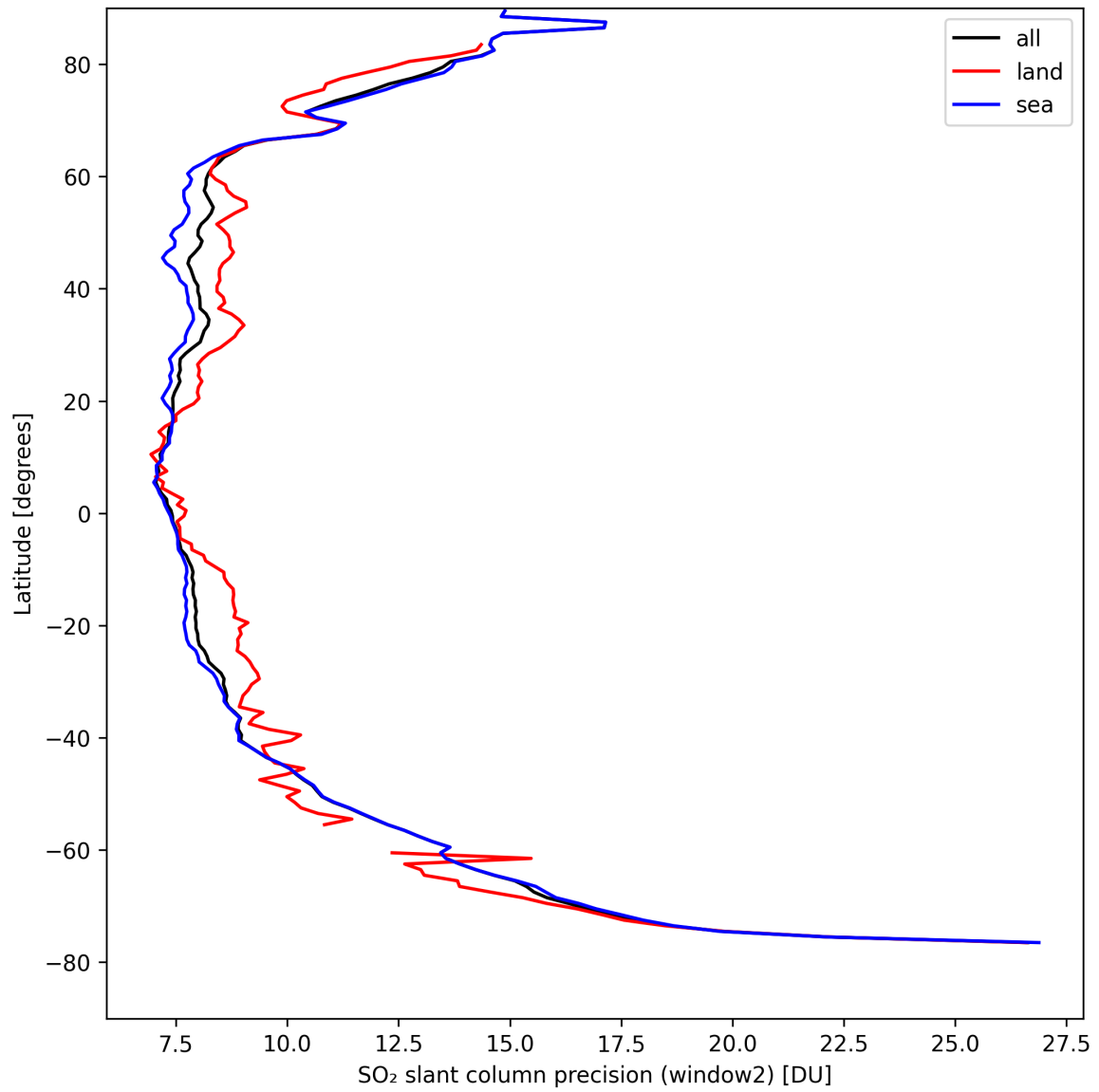
Figure 38: Zonal average of “SO 2 slant column precision (window2)” for 2024-08-30 to 2024-09-01.
