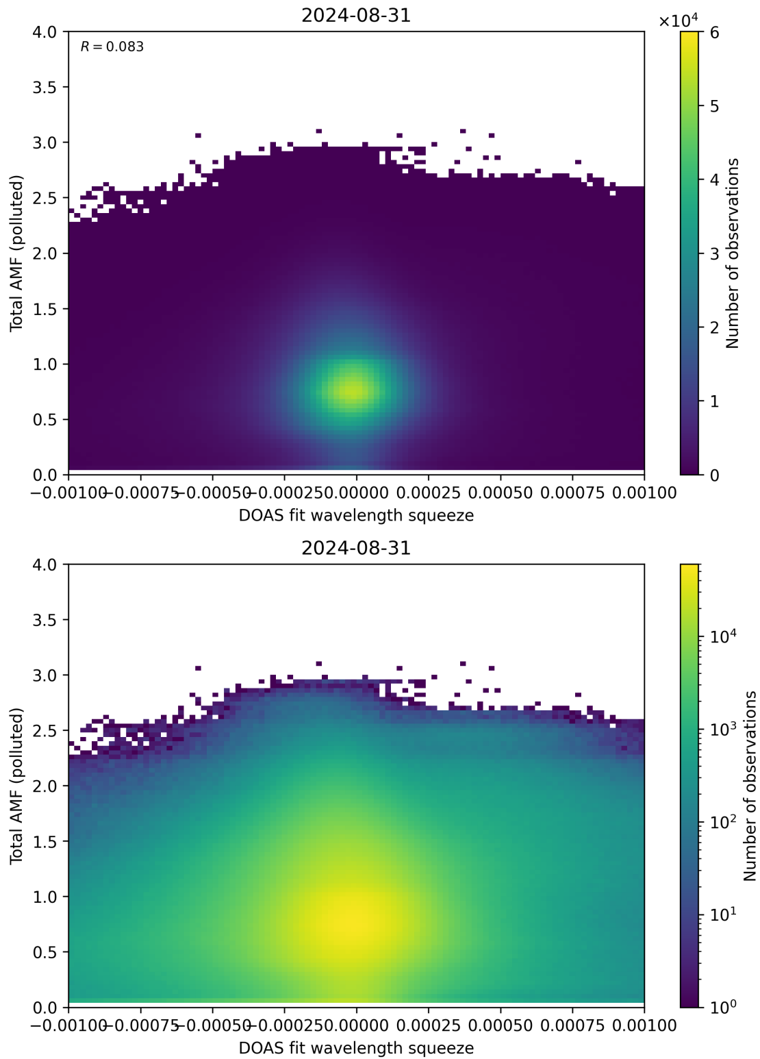
Figure 134: Scatter density plot of “DOAS fit wavelength squeeze” against “Total AMF (polluted)” for 2024-08-30 to 2024-09-01.
