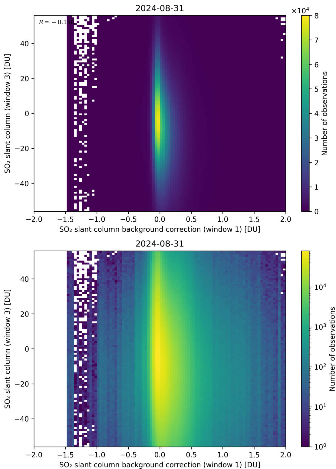
Figure 107: Scatter density plot of “SO 2 slant column background correction (window 1)” against “SO 2 slant column (window 3)” for 2024-08-30 to 2024-09-01.
