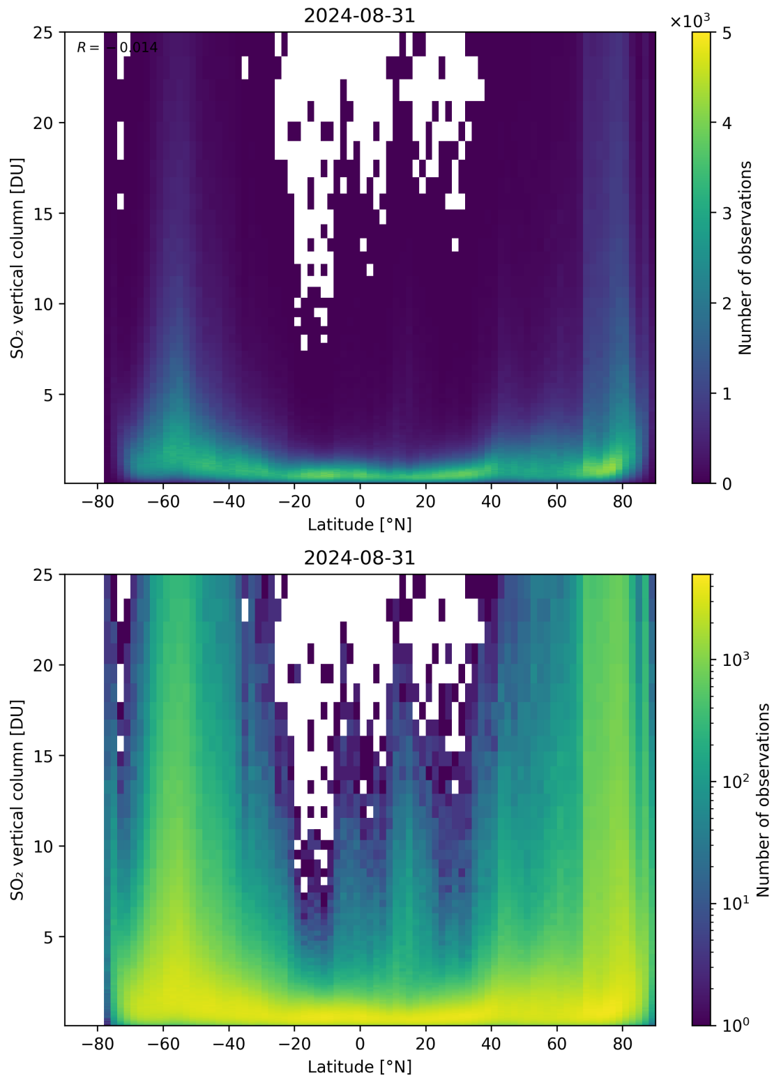
Figure 156: Scatter density plot of “Latitude” against “SO 2 vertical column” for 2024-08-30 to 2024-09-01.
