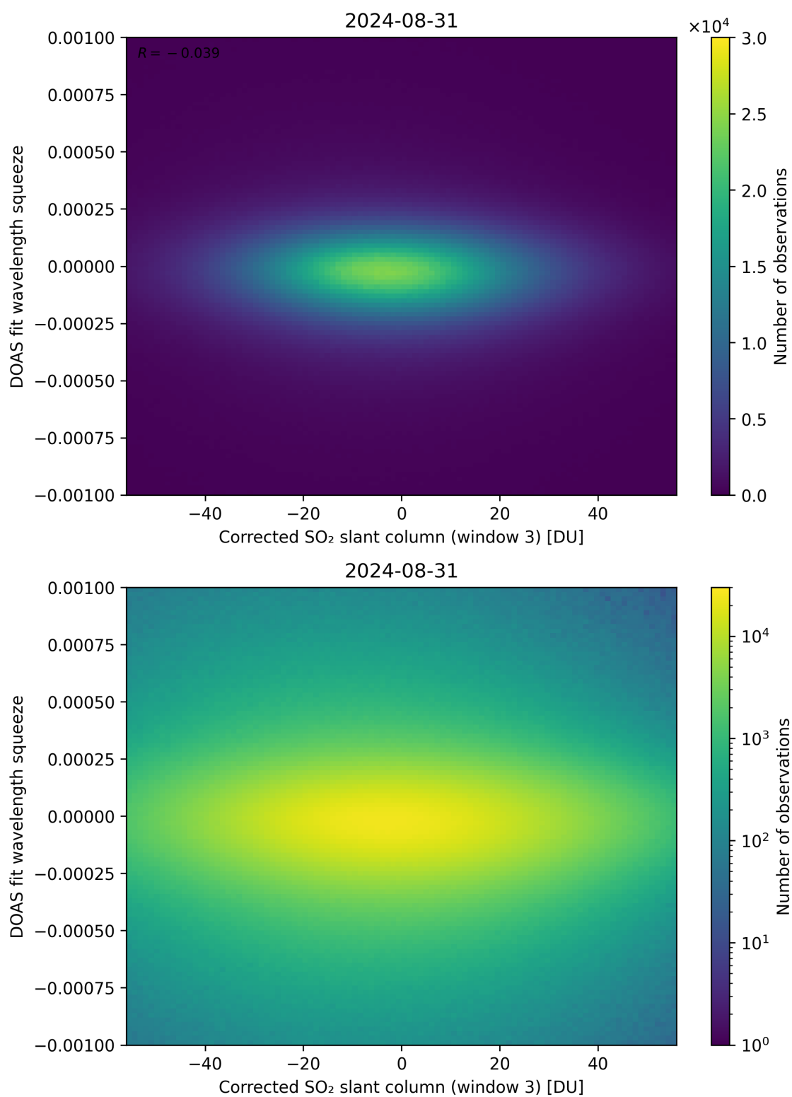
Figure 207: Scatter density plot of “Corrected SO 2 slant column (window 3)” against “DOAS fit wavelength squeeze” for 2024-08-30 to 2024-09-01.
