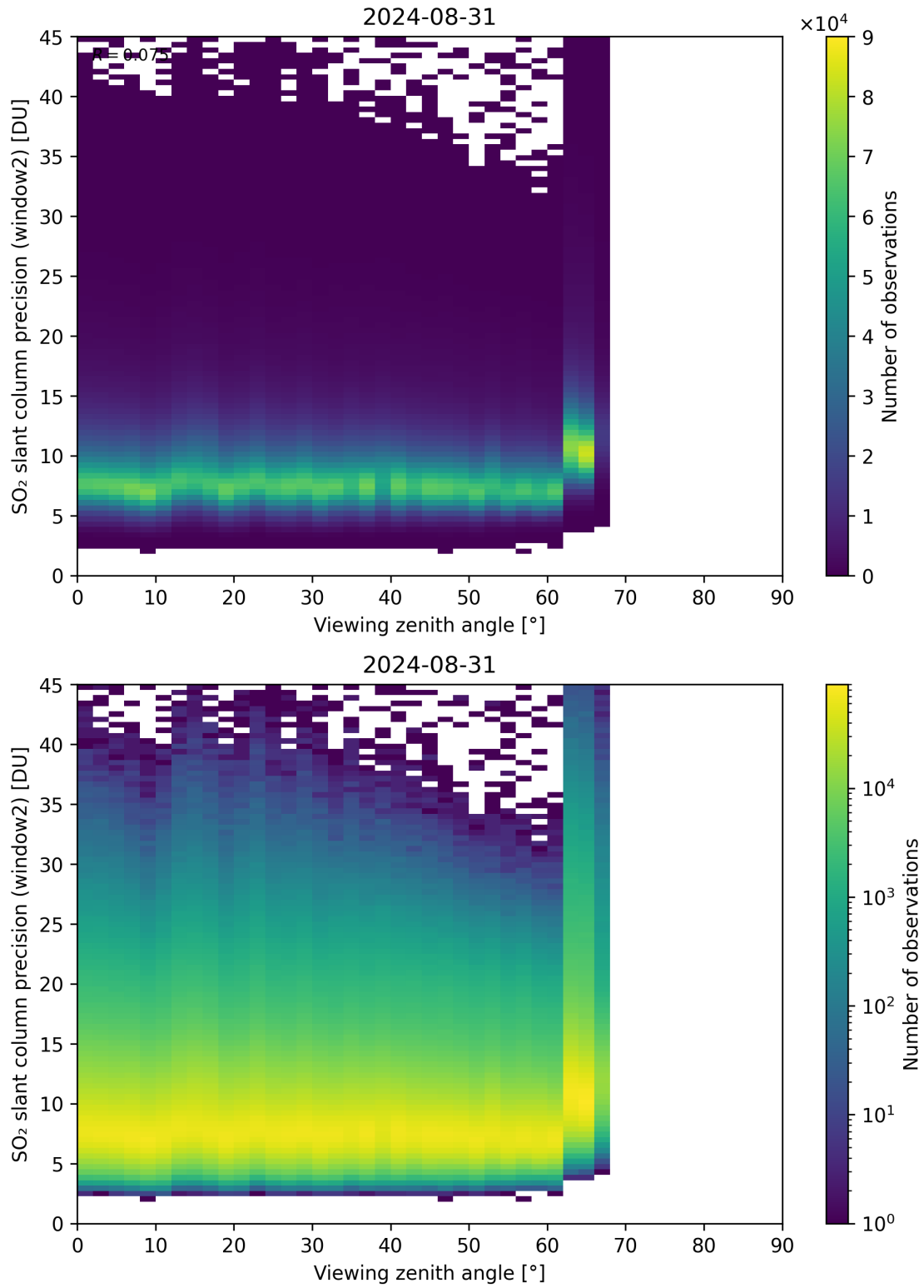
Figure 322: Scatter density plot of “Viewing zenith angle” against “SO 2 slant column precision (window2)” for 2024-08-30 to 2024-09-01.
