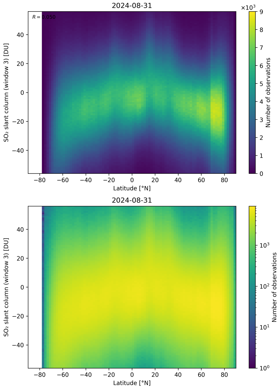
Figure 152: Scatter density plot of “Latitude” against “SO 2 slant column (window 3)” for 2024-08-30 to 2024-09-01.
