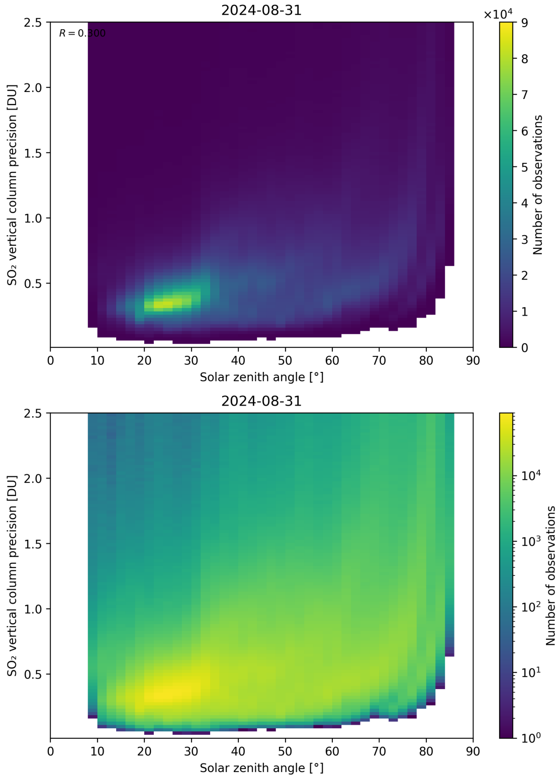
Figure 177: Scatter density plot of “Solar zenith angle” against “SO 2 vertical column precision” for 2024-08-30 to 2024-09-01.
