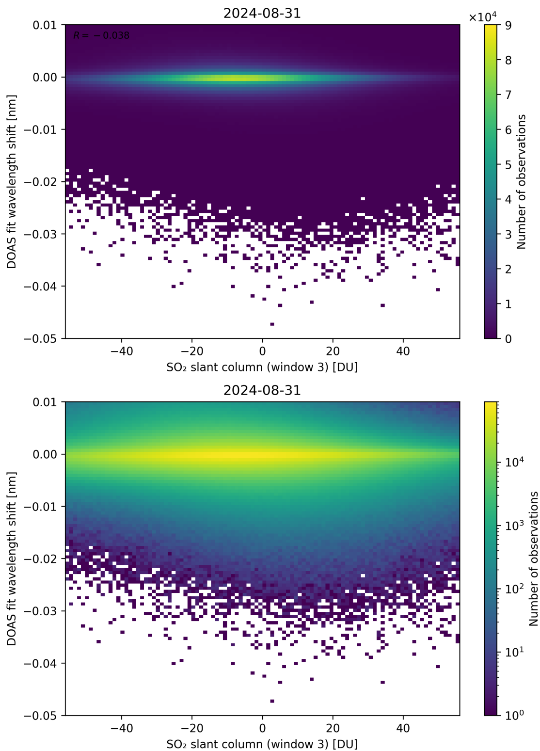
Figure 254: Scatter density plot of “SO 2 slant column (window 3)” against “DOAS fit wavelength shift” for 2024-08-30 to 2024-09-01.
