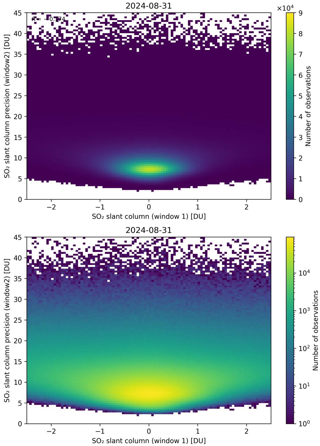
Figure 236: Scatter density plot of “SO 2 slant column (window 1)” against “SO 2 slant column precision (window2)” for 2024-08-30 to 2024-09-01.
