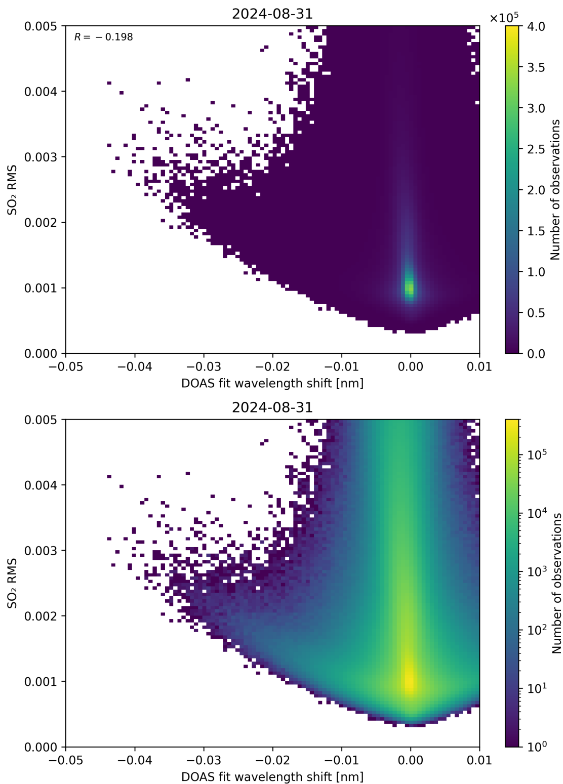
Figure 128: Scatter density plot of “DOAS fit wavelength shift” against “SO 2 RMS” for 2024-08-30 to 2024-09-01.
