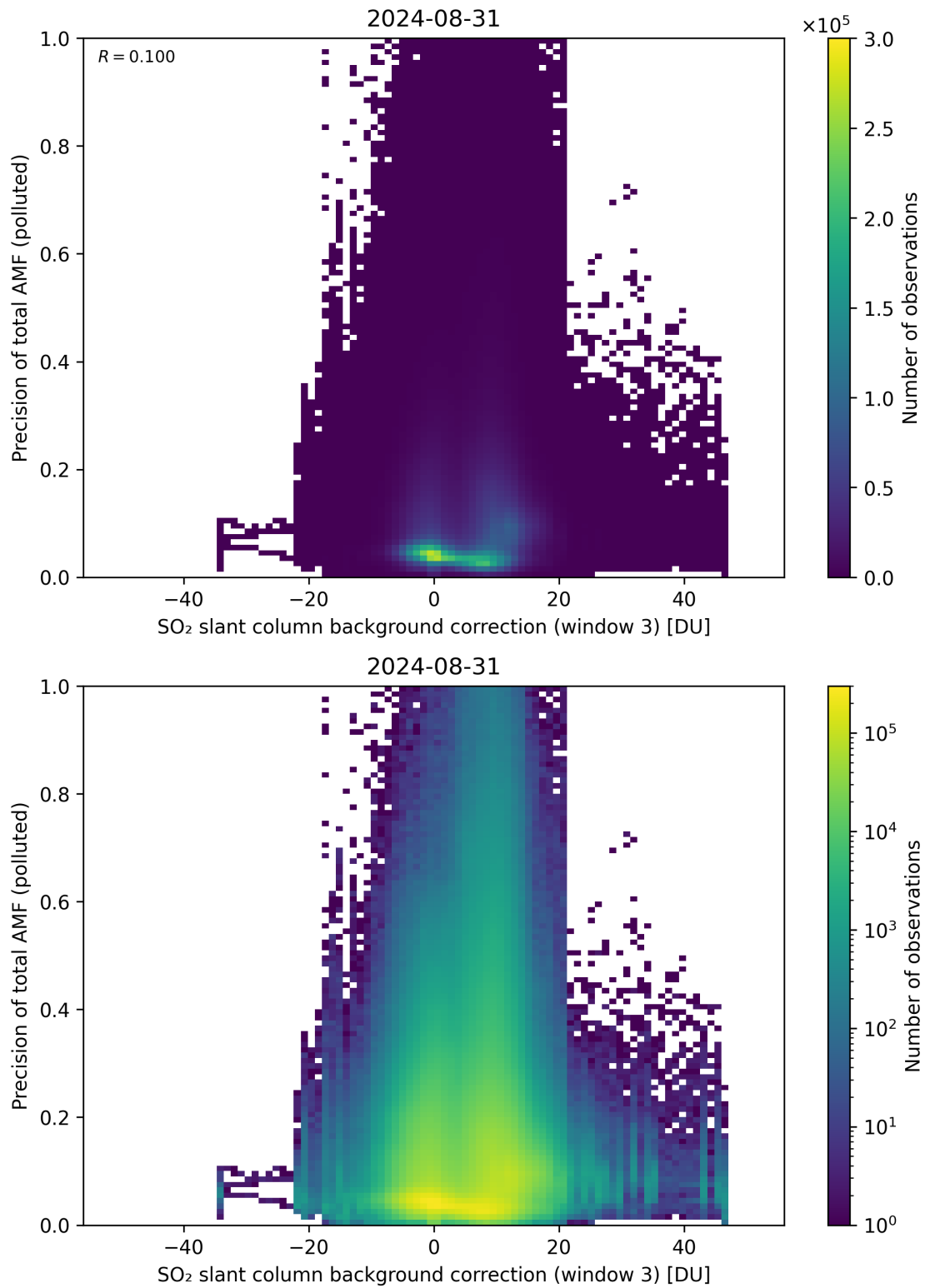
Figure 126: Scatter density plot of “SO 2 slant column background correction (window 3)” against “Precision of total AMF (polluted)” for 2024-08-30 to 2024-09-01.
