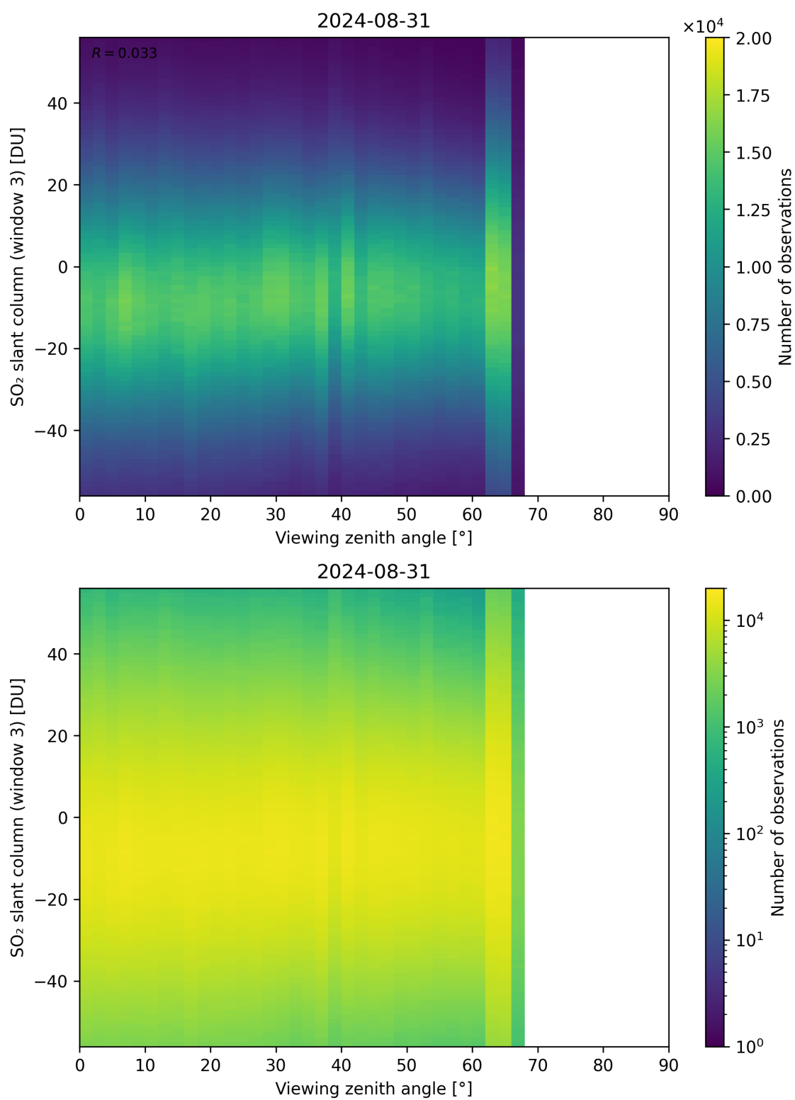
Figure 323: Scatter density plot of “Viewing zenith angle” against “SO 2 slant column (window 3)” for 2024-08-30 to 2024-09-01.
