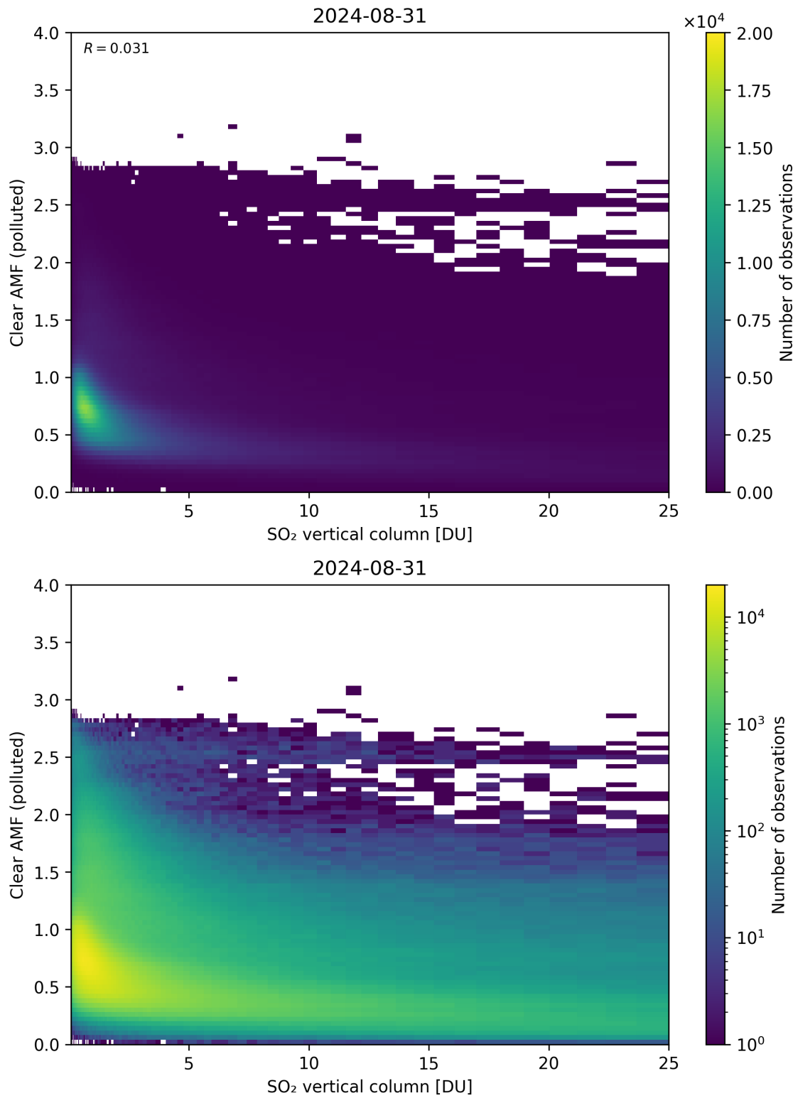
Figure 296: Scatter density plot of “SO 2 vertical column” against “Clear AMF (polluted)” for 2024-08-30 to 2024-09-01.
