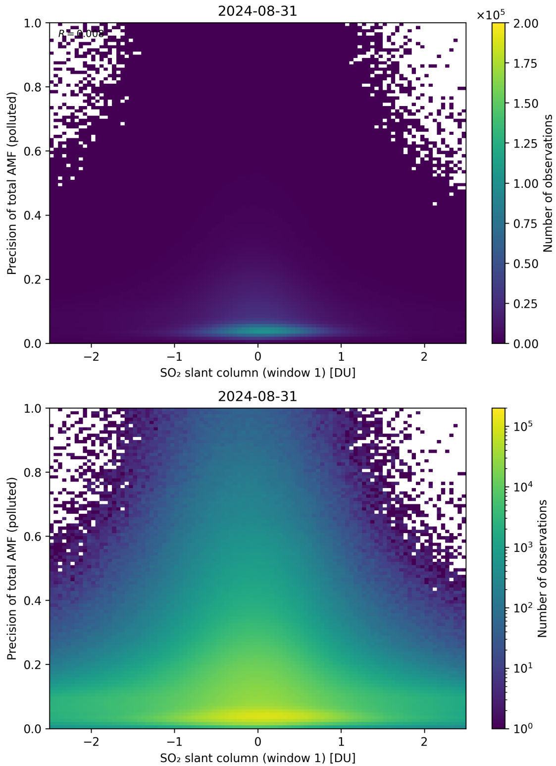
Figure 240: Scatter density plot of “SO 2 slant column (window 1)” against “Precision of total AMF (polluted)” for 2024-08-30 to 2024-09-01.
