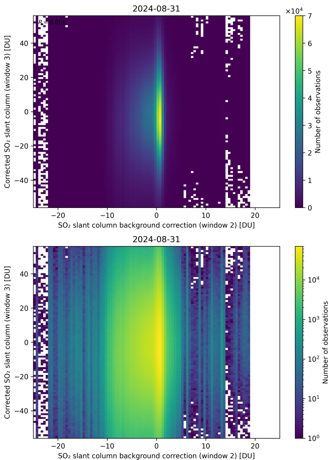
Figure 116: Scatter density plot of “SO 2 slant column background correction (window 2)” against “Corrected SO 2 slant column (window 3)” for 2024-08-30 to 2024-09-01.
