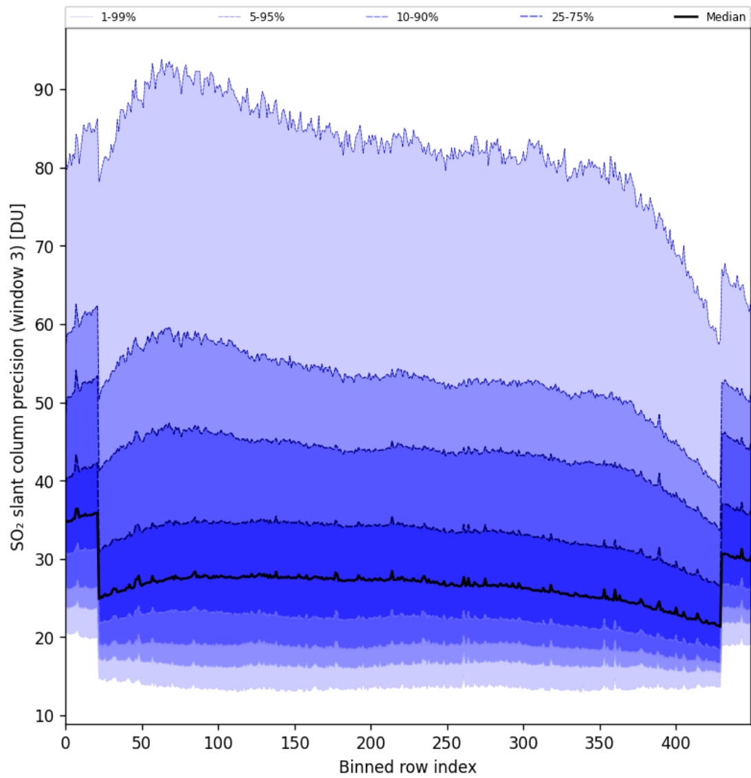
Figure 88: Along track statistics of “SO 2 slant column precision (window 3)” for 2024-08-30 to 2024-09-01
