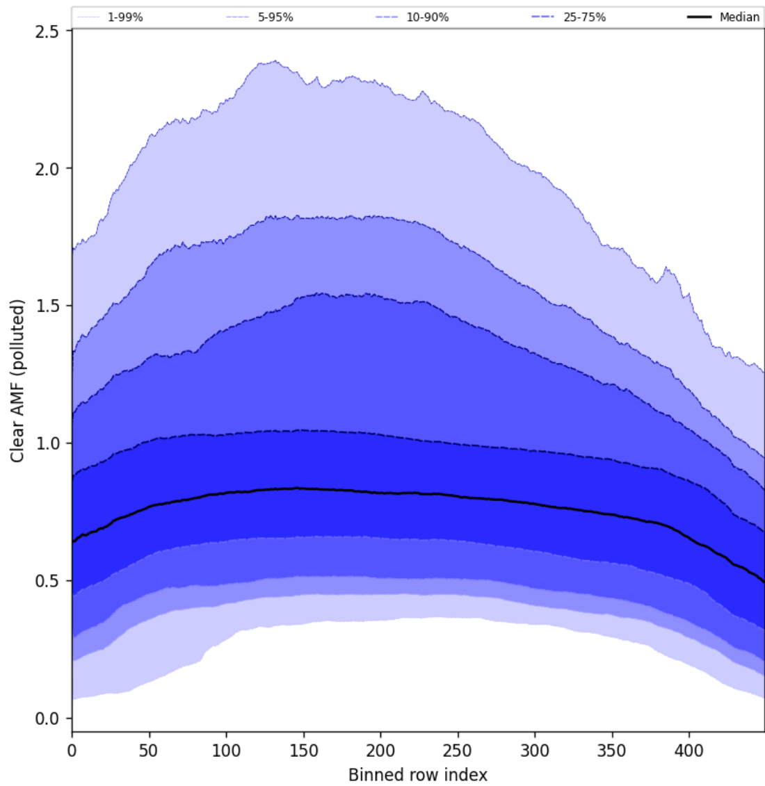
Figure 96: Along track statistics of “Clear AMF (polluted)” for 2024-08-30 to 2024-09-01
