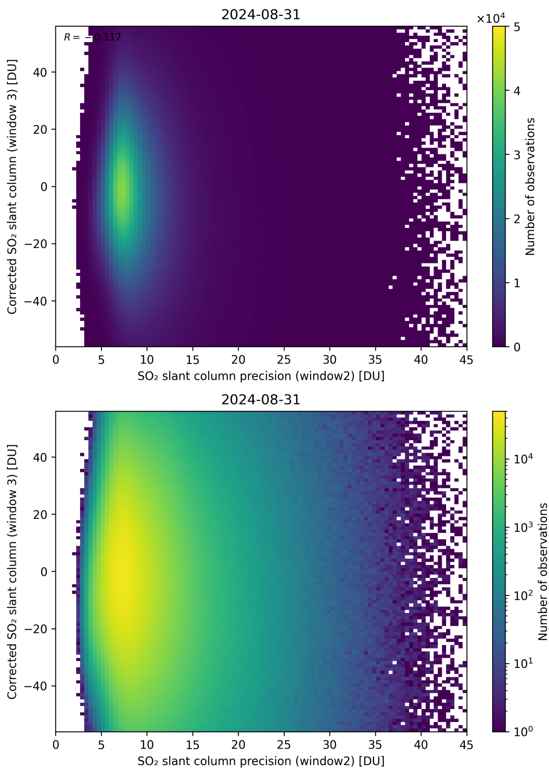
Figure 248: Scatter density plot of “SO 2 slant column precision (window2)” against “Corrected SO 2 slant column (window 3)” for 2024-08-30 to 2024-09-01.
