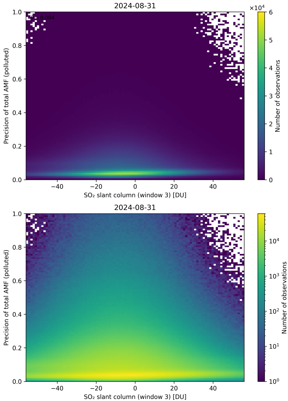
Figure 269: Scatter density plot of “SO 2 slant column (window 3)” against “Precision of total AMF (polluted)” for 2024-08-30 to 2024-09-01.
