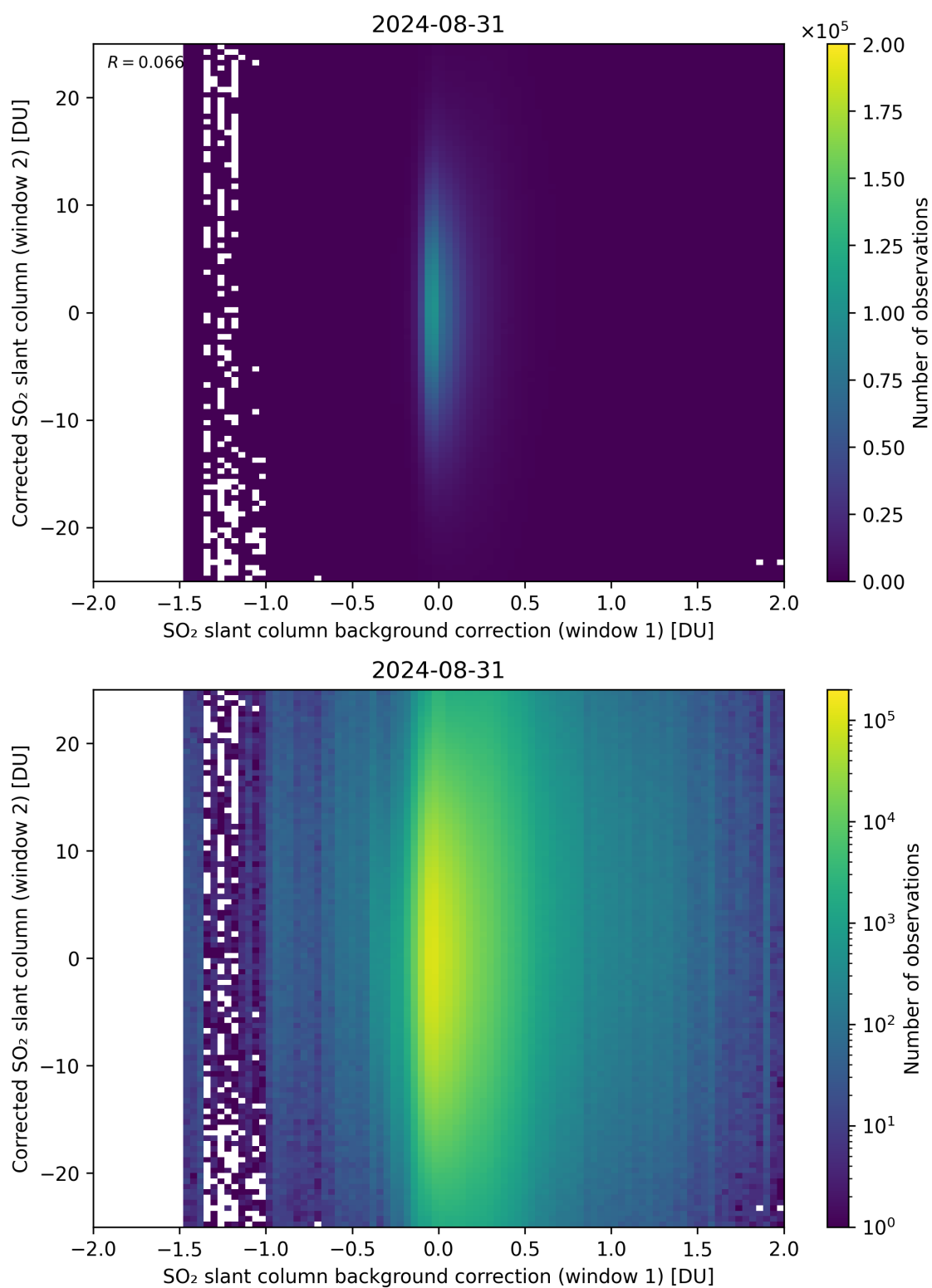
Figure 104: Scatter density plot of “SO 2 slant column background correction (window 1)” against “Corrected SO 2 slant column (window 2)” for 2024-08-30 to 2024-09-01.
