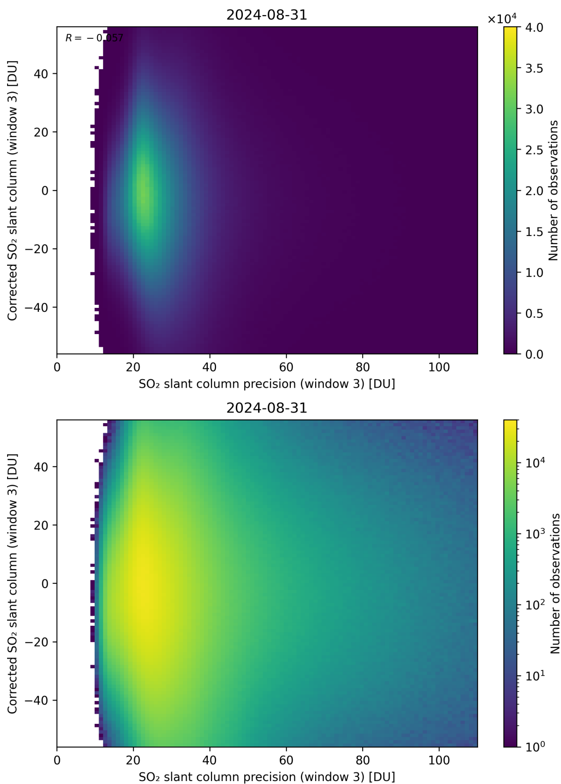
Figure 262: Scatter density plot of “SO 2 slant column precision (window 3)” against “Corrected SO 2 slant column (window 3)” for 2024-08-30 to 2024-09-01.
