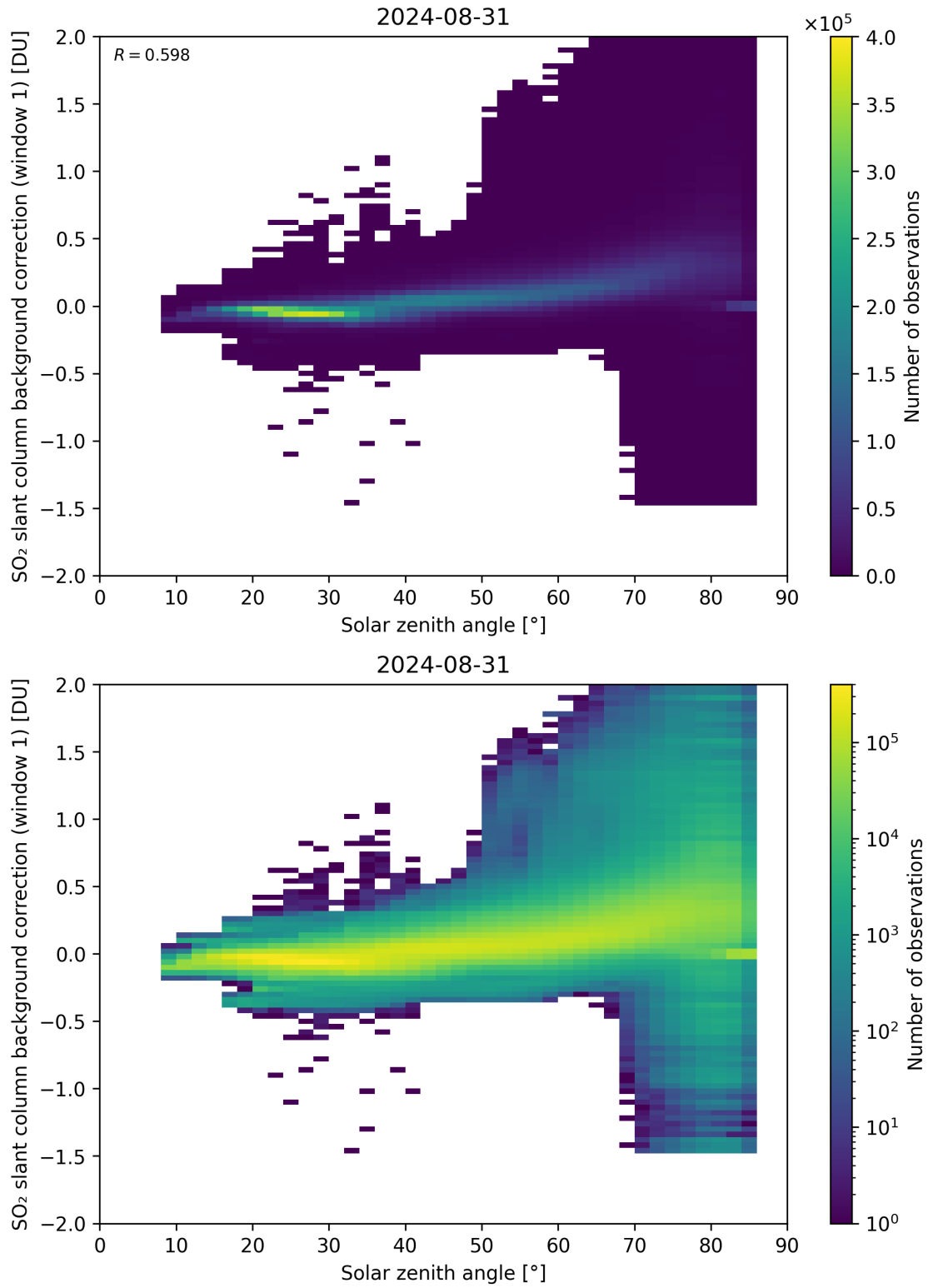
Figure 158: Scatter density plot of “Solar zenith angle” against “SO 2 slant column background correction (window 1)” for 2024-08-30 to 2024-09-01.
