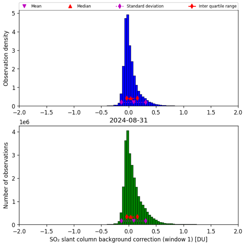
Figure 59: Histogram of “SO 2 slant column background correction (window 1)” for 2024-08-30 to 2024-09-01
