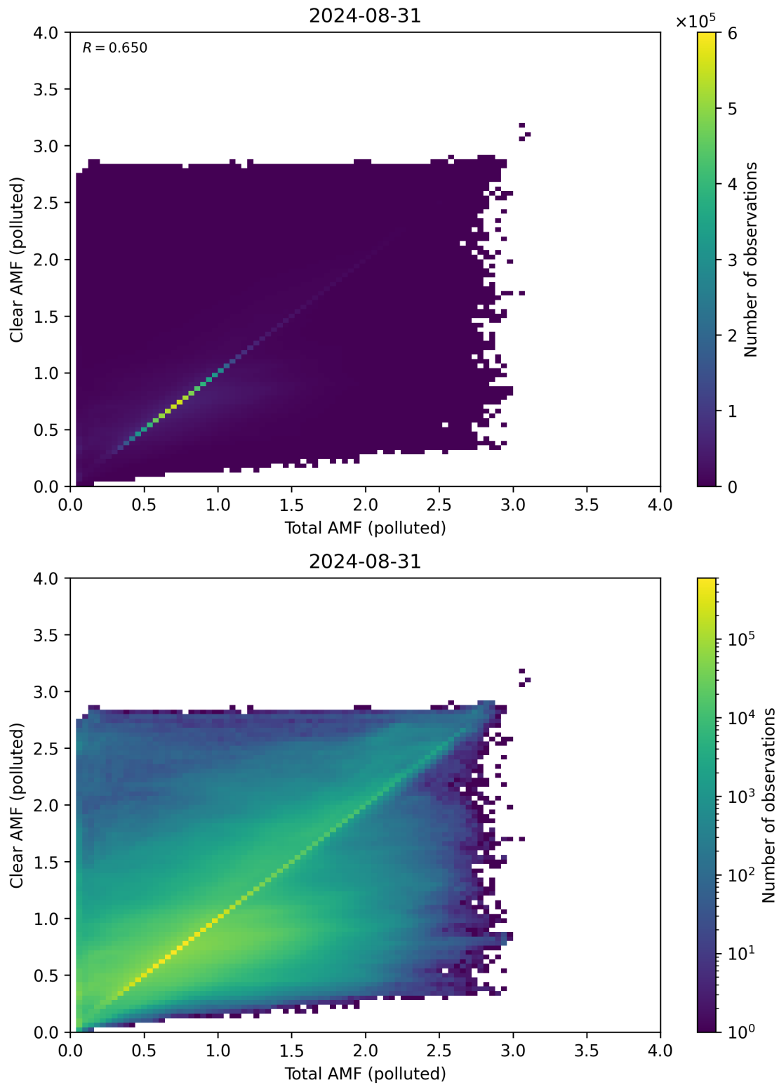
Figure 271: Scatter density plot of “Total AMF (polluted)” against “Clear AMF (polluted)” for 2024-08-30 to 2024-09-01.
