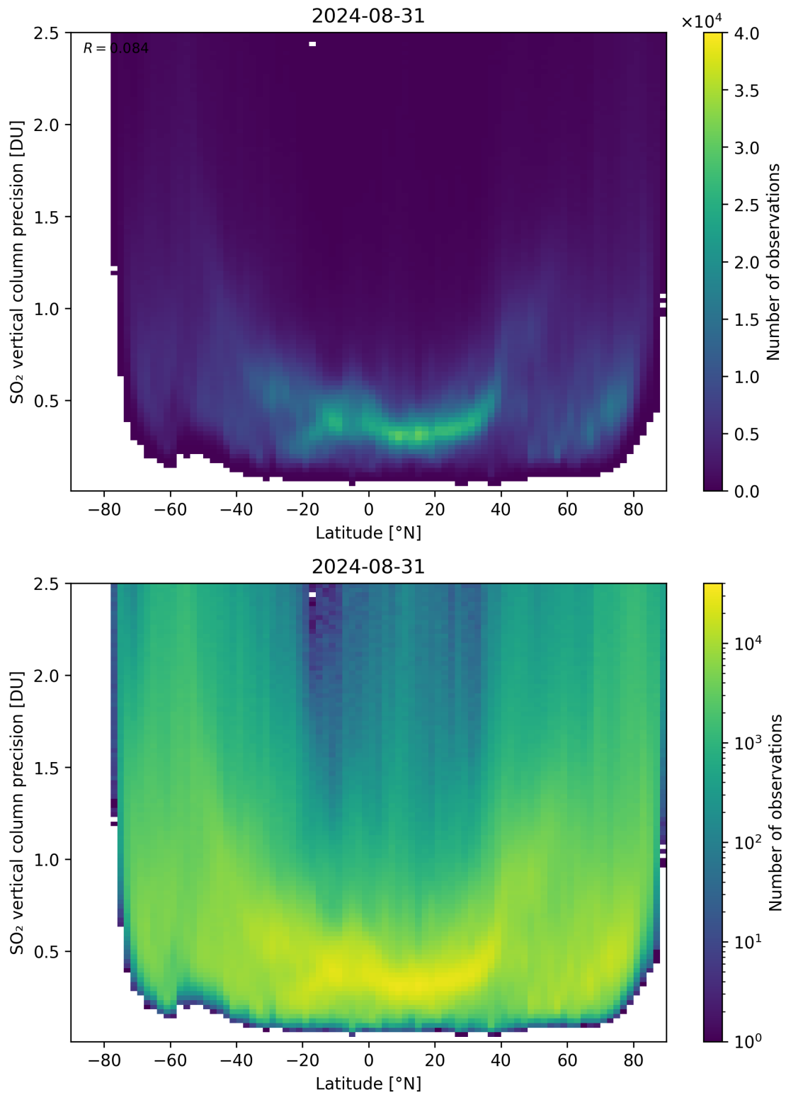
Figure 157: Scatter density plot of “Latitude” against “SO 2 vertical column precision” for 2024-08-30 to 2024-09-01.
