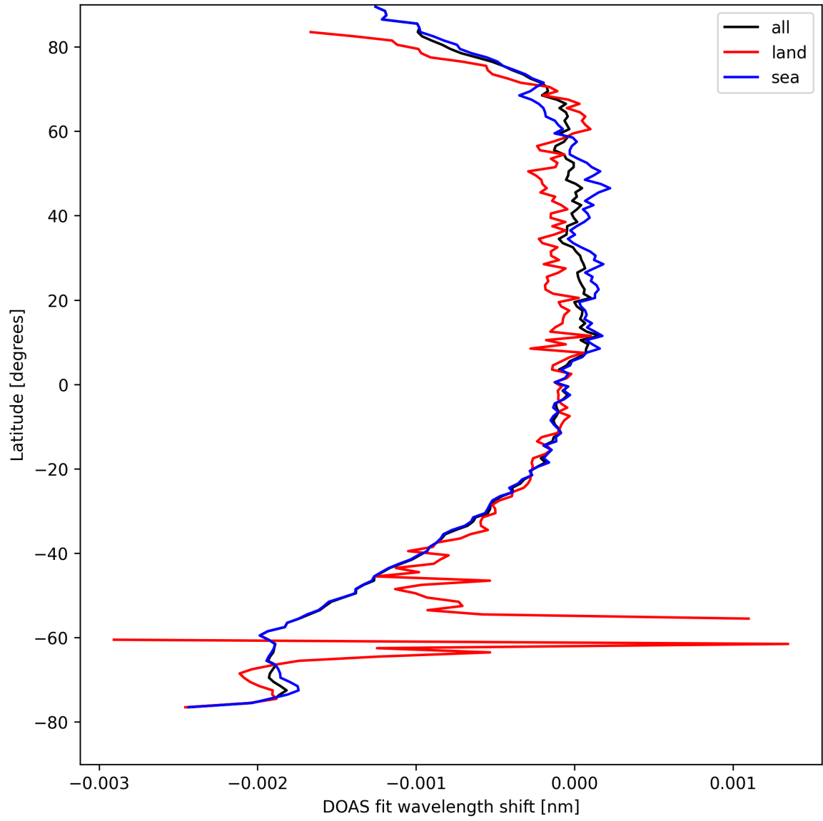
Figure 45: Zonal average of “DOAS fit wavelength shift” for 2024-08-30 to 2024-09-01.
