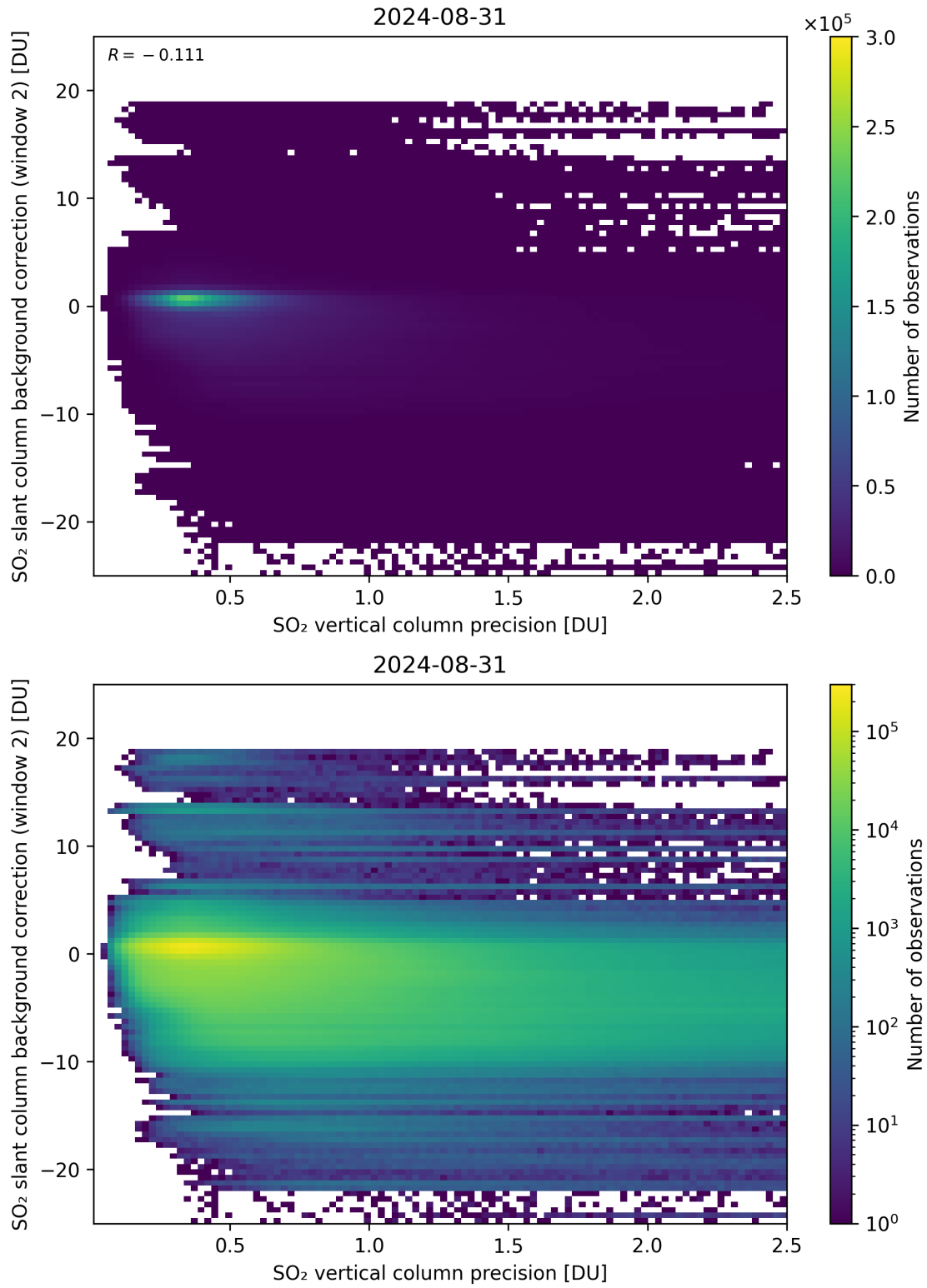
Figure 280: Scatter density plot of “SO 2 vertical column precision” against “SO 2 slant column background correction (window 2)” for 2024-08-30 to 2024-09-01.
