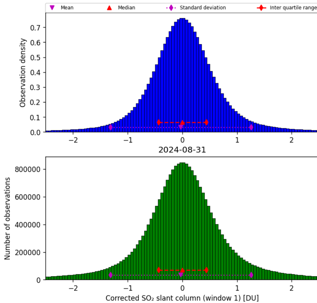
Figure 58: Histogram of “Corrected SO 2 slant column (window 1)” for 2024-08-30 to 2024-09-01
