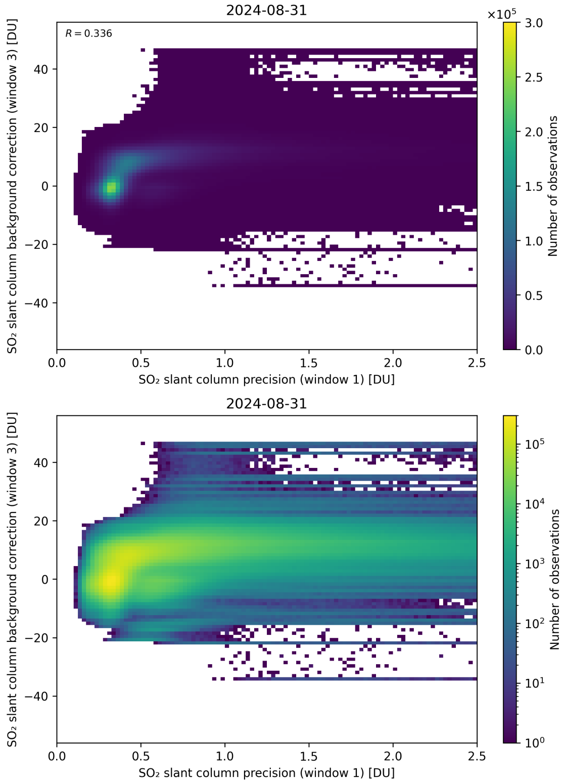
Figure 220: Scatter density plot of “SO 2 slant column precision (window 1)” against “SO 2 slant column background correction (window 3)” for 2024-08-30 to 2024-09-01.
