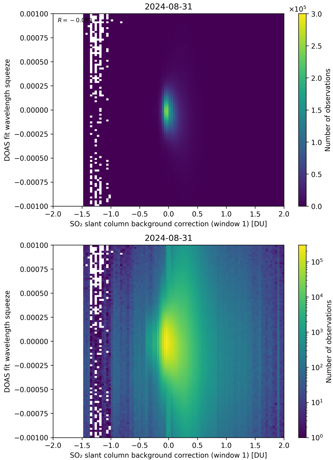
Figure 101: Scatter density plot of “SO 2 slant column background correction (window 1)” against “DOAS fit wavelength squeeze” for 2024-08-30 to 2024-09-01.
