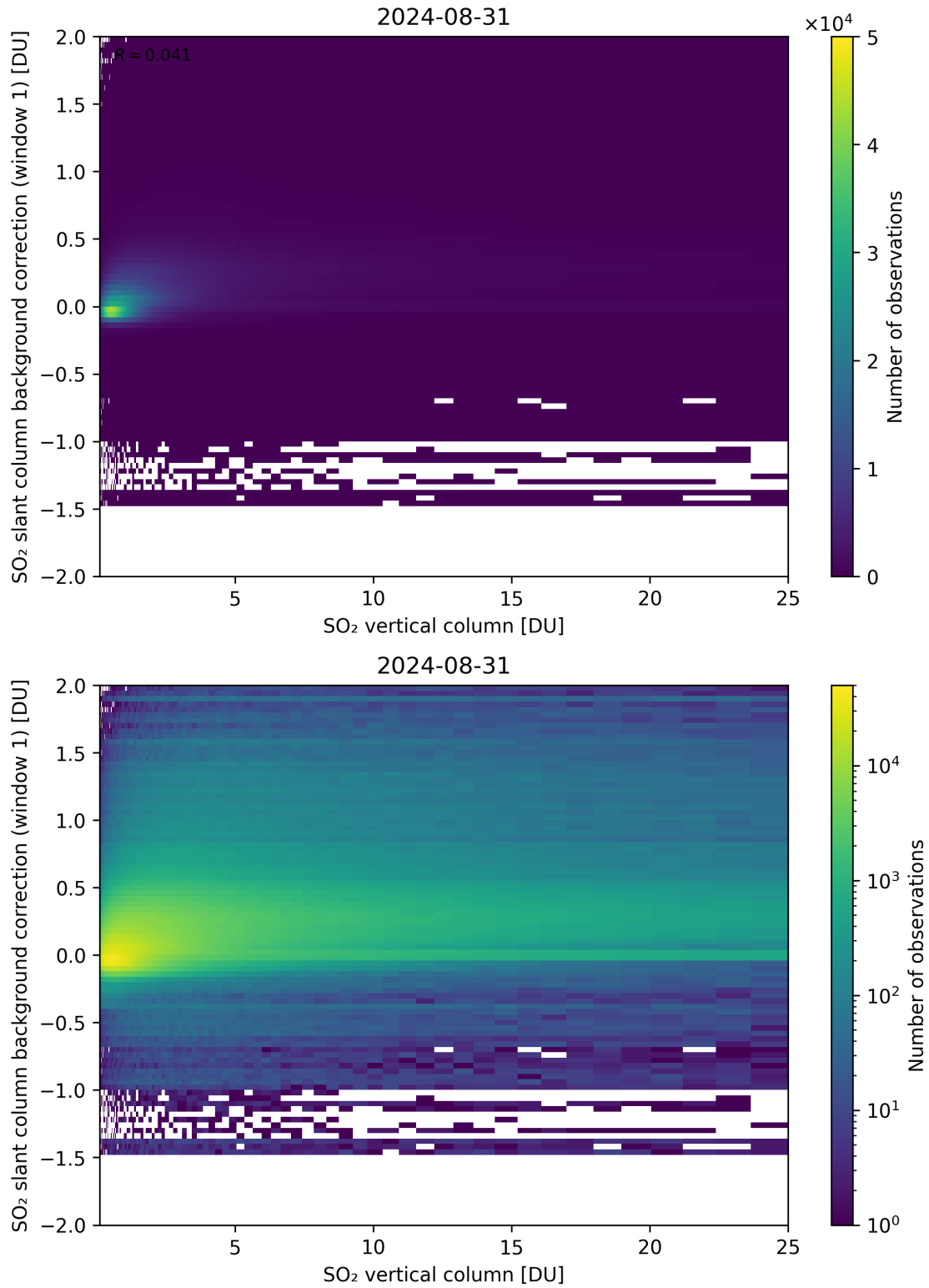
Figure 273: Scatter density plot of “SO 2 vertical column” against “SO 2 slant column background correction (window 1)” for 2024-08-30 to 2024-09-01.
