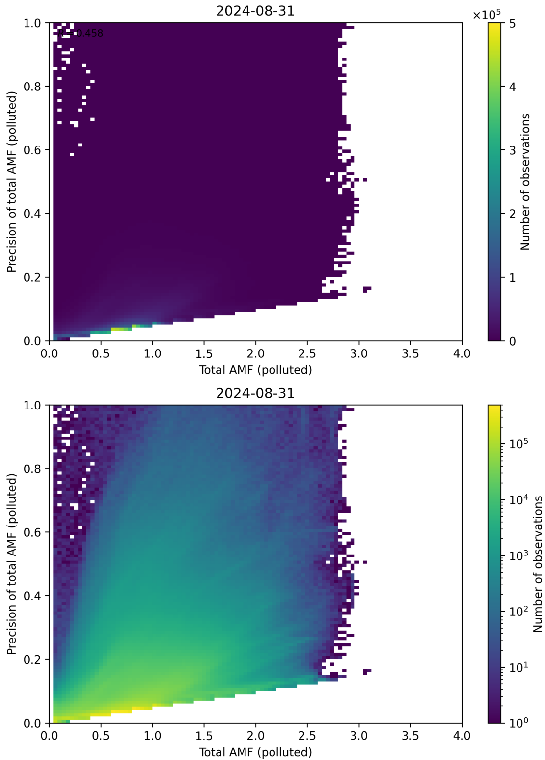
Figure 272: Scatter density plot of “Total AMF (polluted)” against “Precision of total AMF (polluted)” for 2024-08-30 to 2024-09-01.
