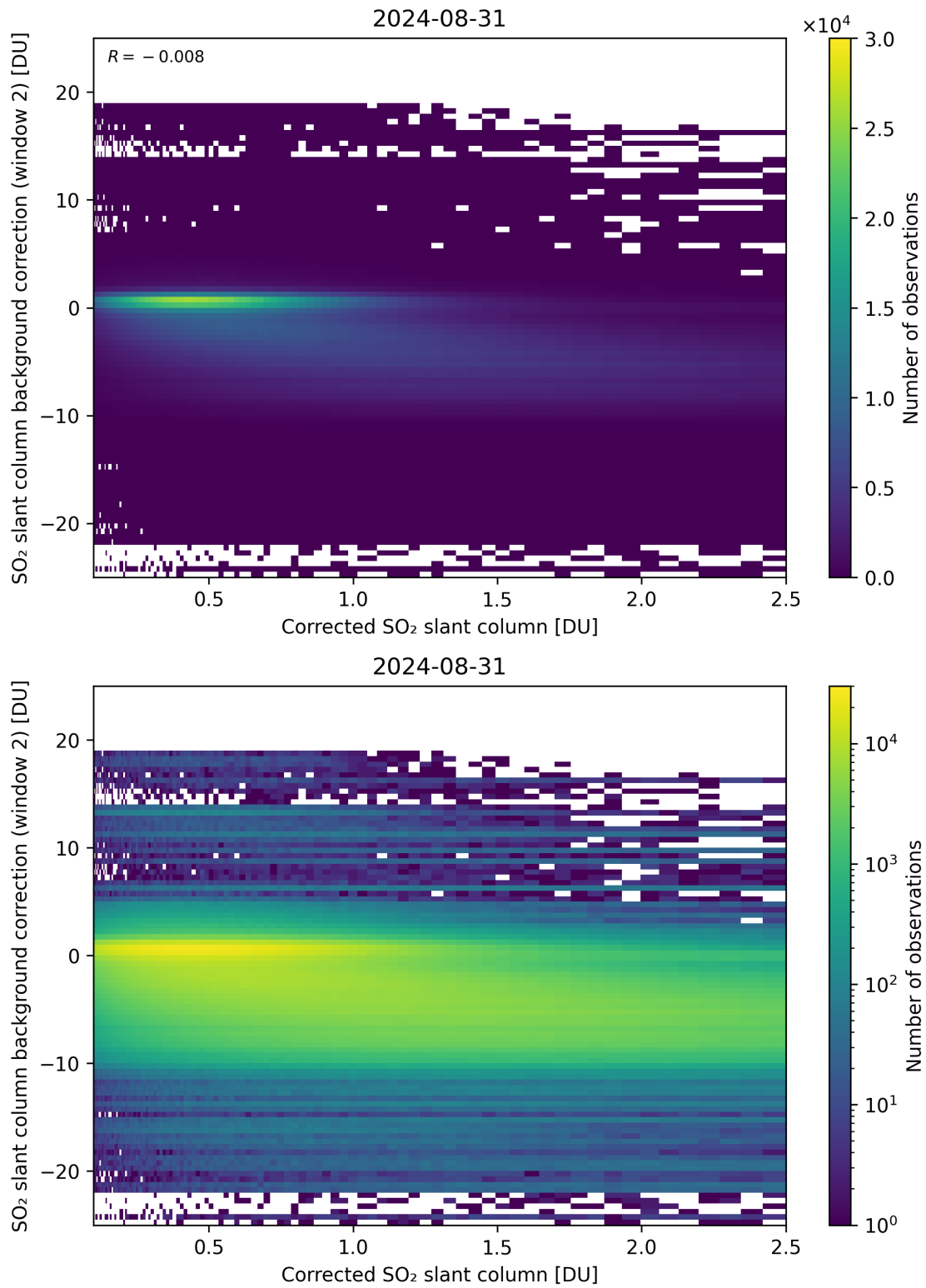
Figure 179: Scatter density plot of “Corrected SO 2 slant column” against “SO 2 slant column background correction (window 2)” for 2024-08-30 to 2024-09-01.
