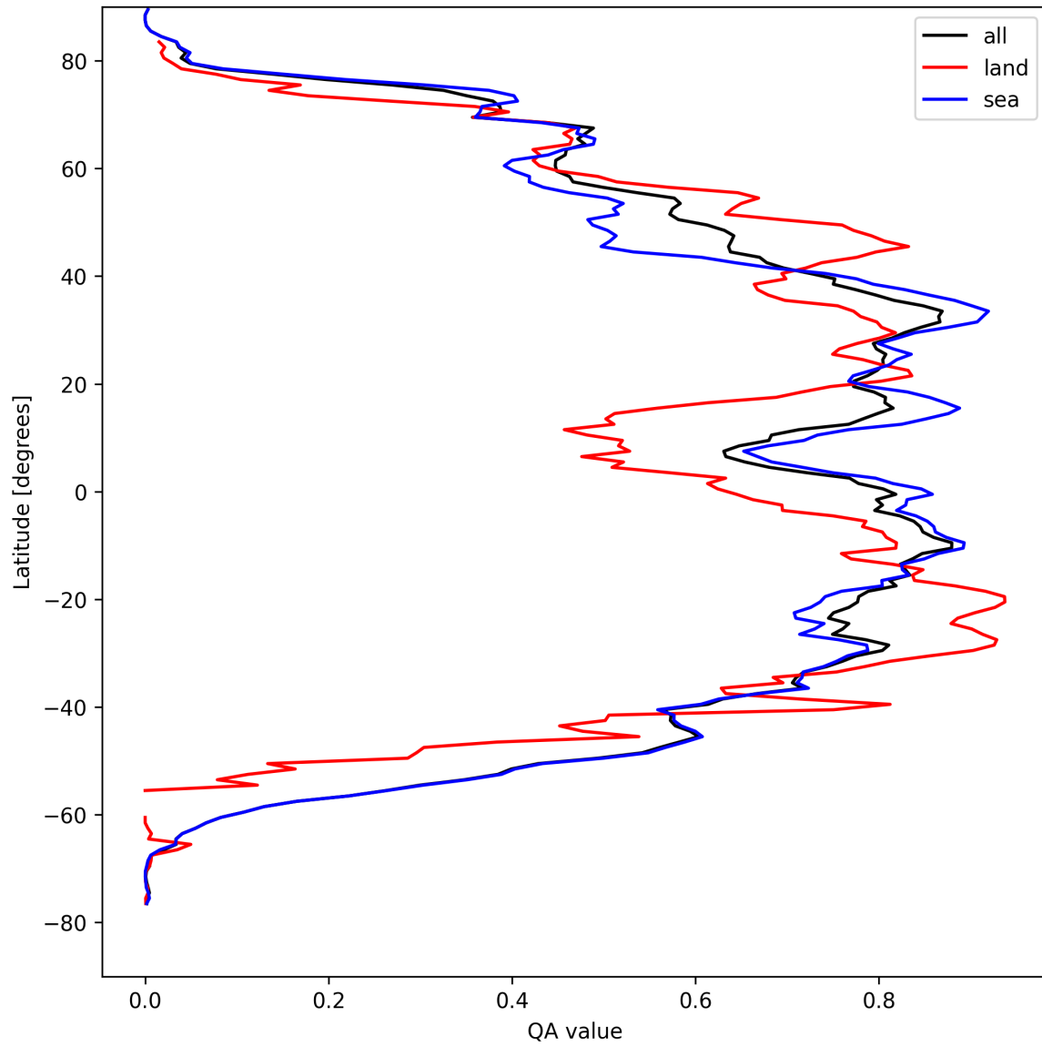
Figure 29: Zonal average of “QA value” for 2024-08-30 to 2024-09-01.
