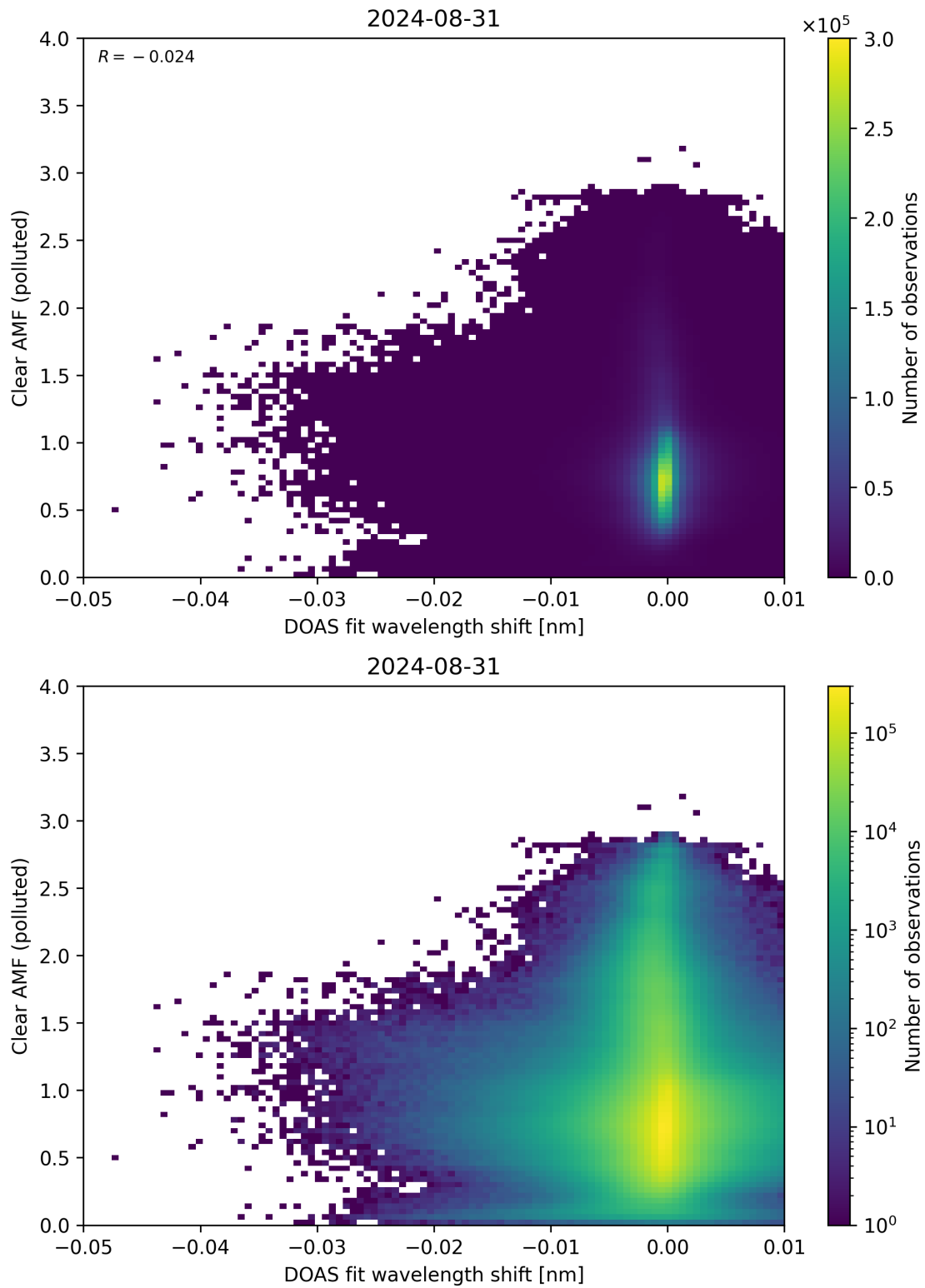
Figure 129: Scatter density plot of “DOAS fit wavelength shift” against “Clear AMF (polluted)” for 2024-08-30 to 2024-09-01.
