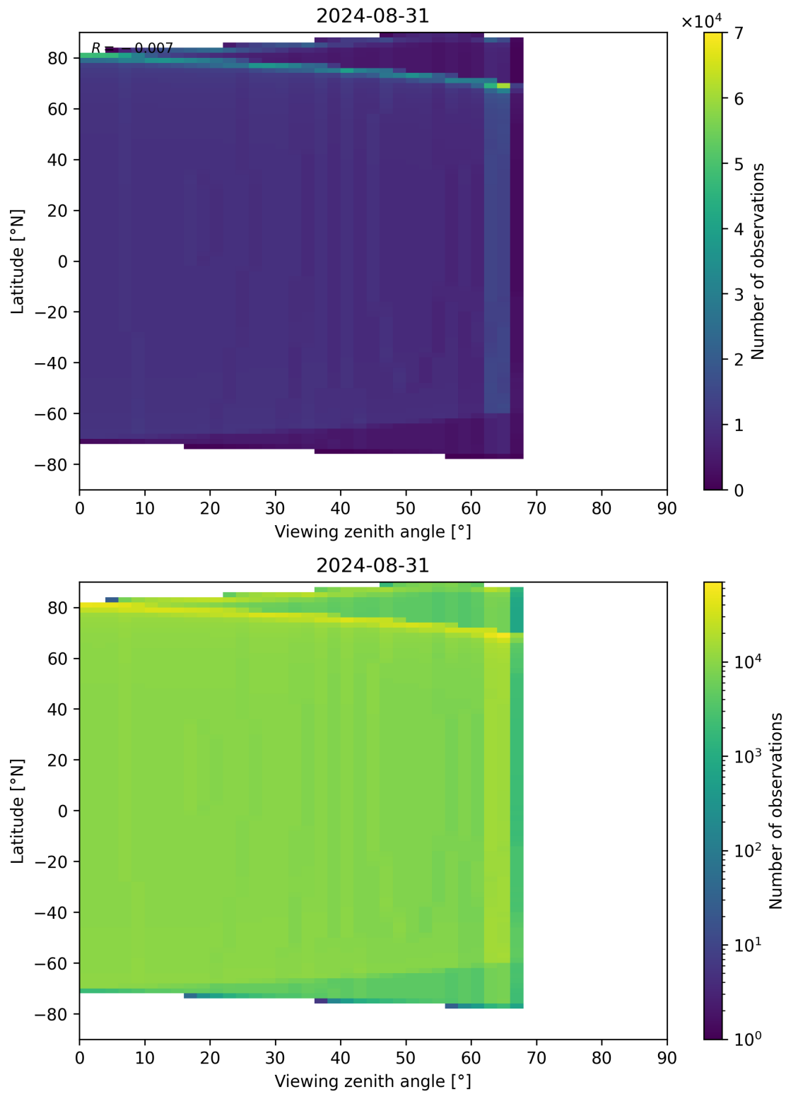
Figure 314: Scatter density plot of “Viewing zenith angle” against “Latitude” for 2024-08-30 to 2024-09-01.
