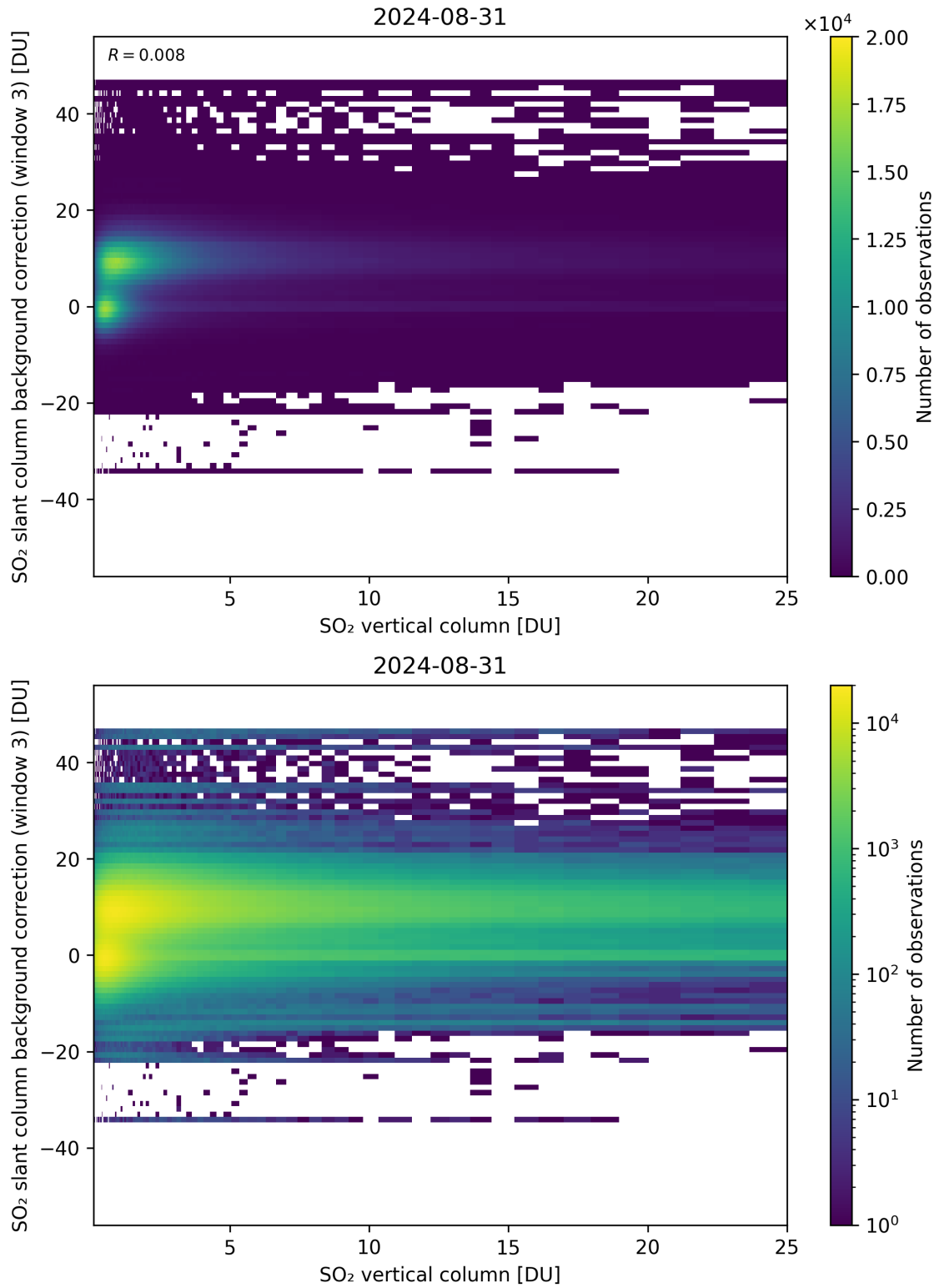
Figure 275: Scatter density plot of “SO 2 vertical column” against “SO 2 slant column background correction (window 3)” for 2024-08-30 to 2024-09-01.
