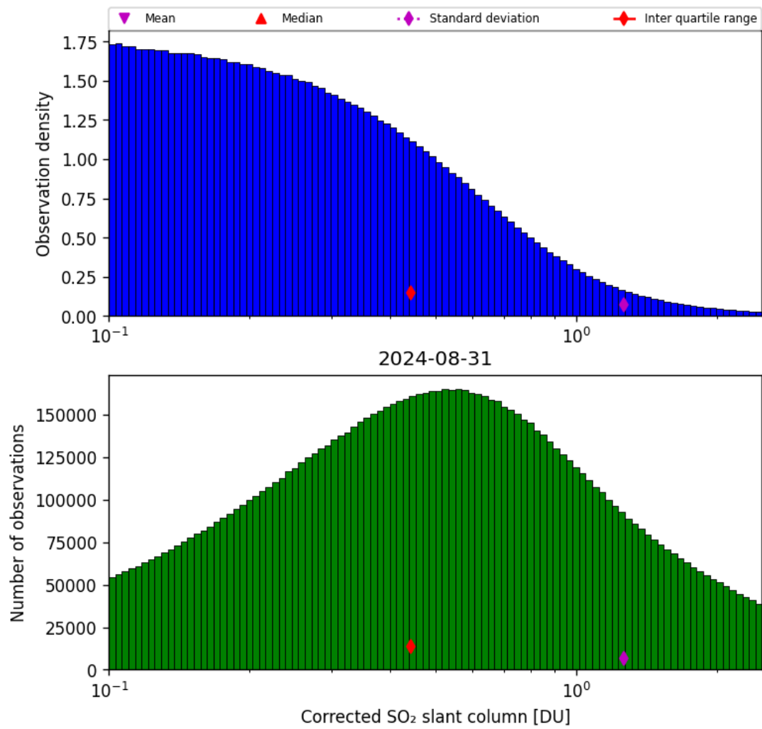
Figure 55: Histogram of “Corrected SO 2 slant column” for 2024-08-30 to 2024-09-01
