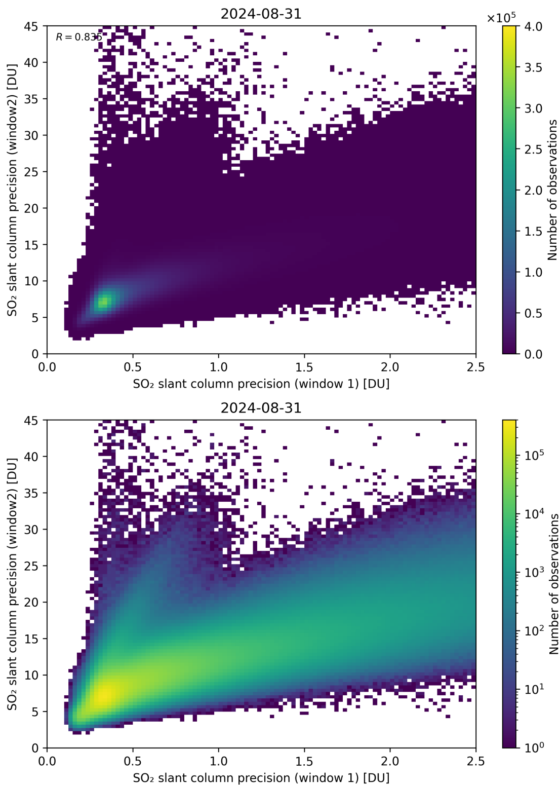
Figure 227: Scatter density plot of “SO 2 slant column precision (window 1)” against “SO 2 slant column precision (window2)” for 2024-08-30 to 2024-09-01.
