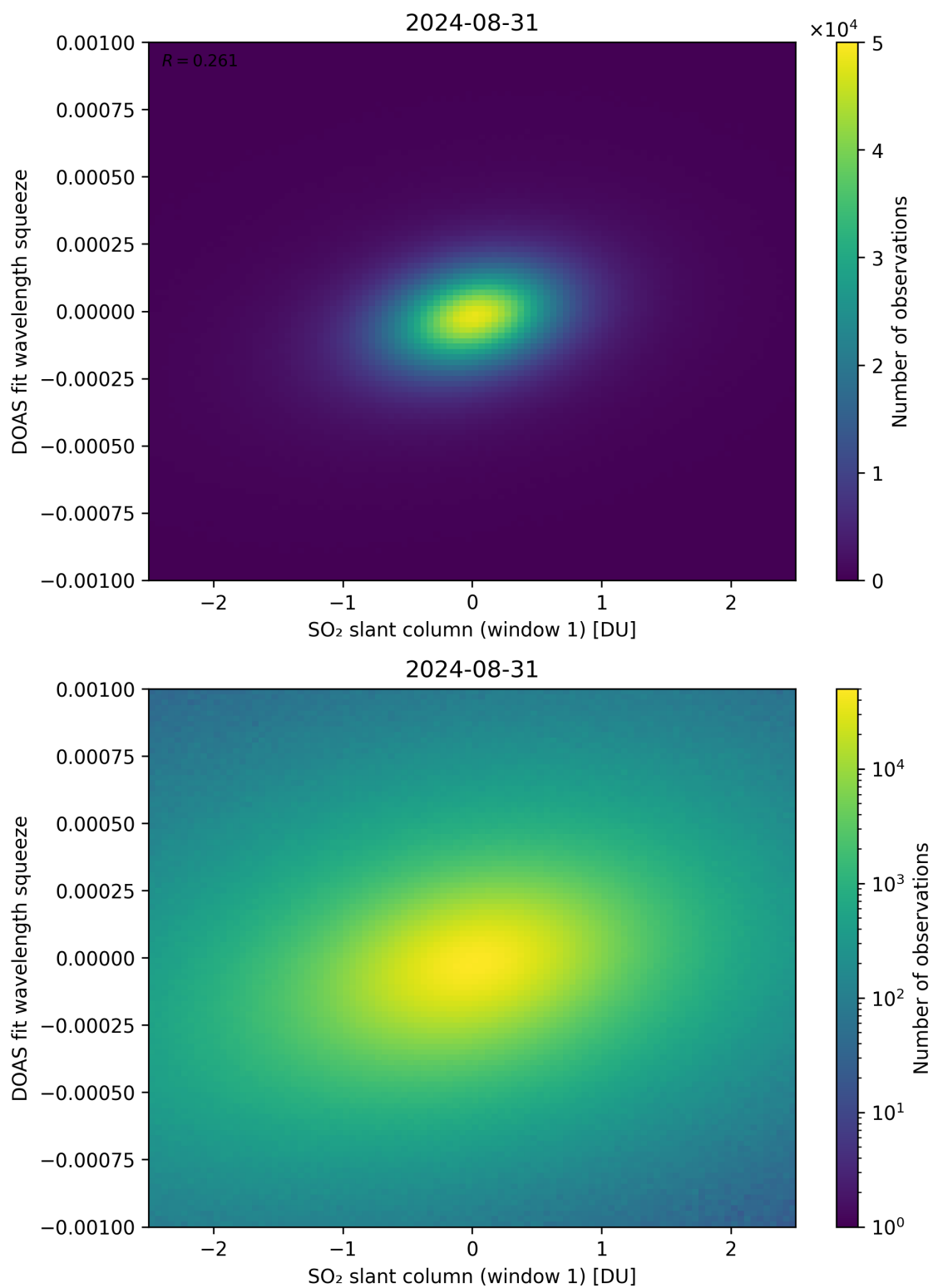
Figure 216: Scatter density plot of “SO 2 slant column (window 1)” against “DOAS fit wavelength squeeze” for 2024-08-30 to 2024-09-01.
