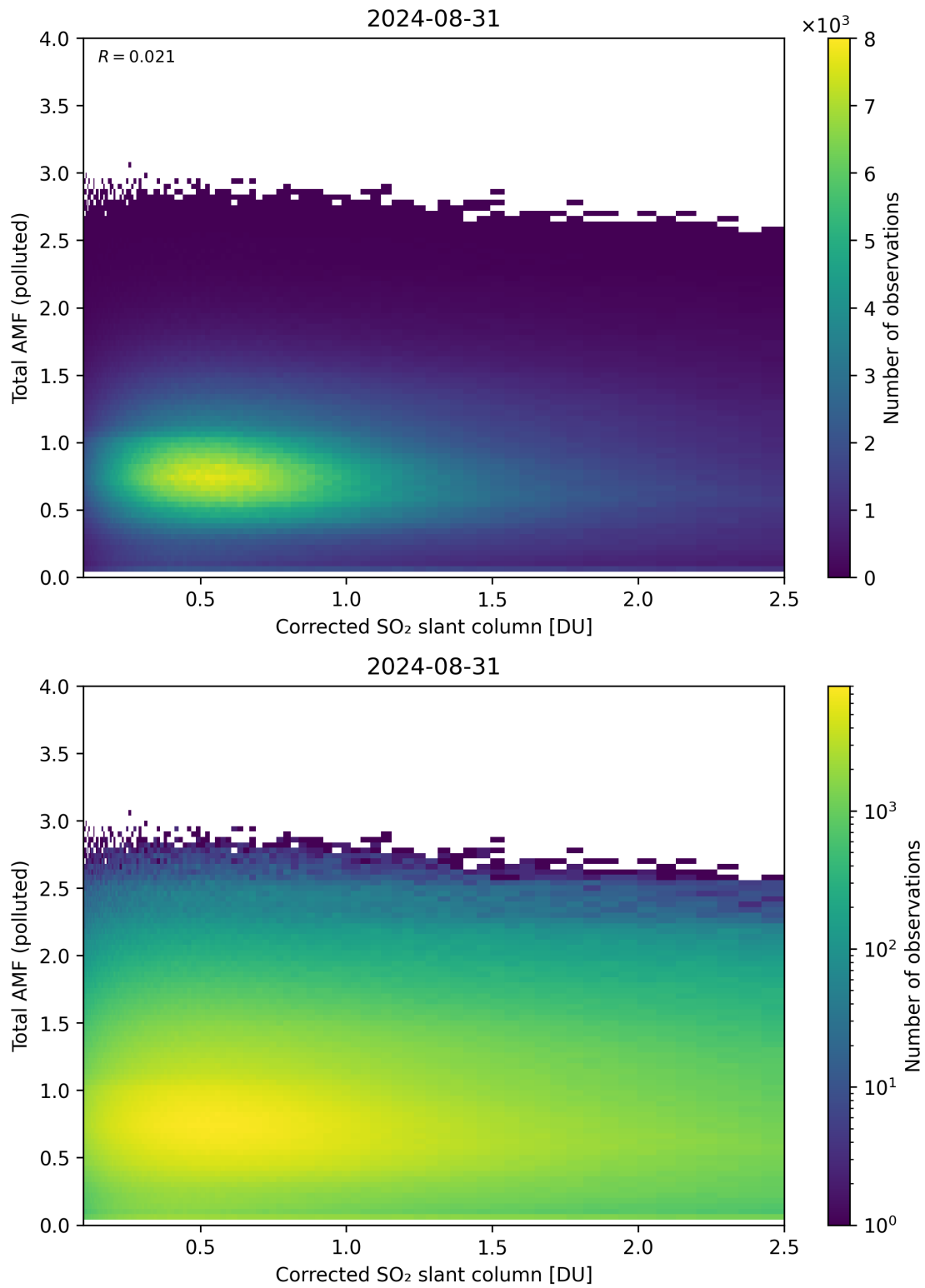
Figure 192: Scatter density plot of “Corrected SO 2 slant column” against “Total AMF (polluted)” for 2024-08-30 to 2024-09-01.
