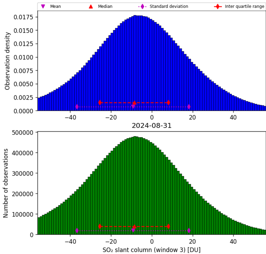
Figure 64: Histogram of “SO 2 slant column (window 3)” for 2024-08-30 to 2024-09-01
