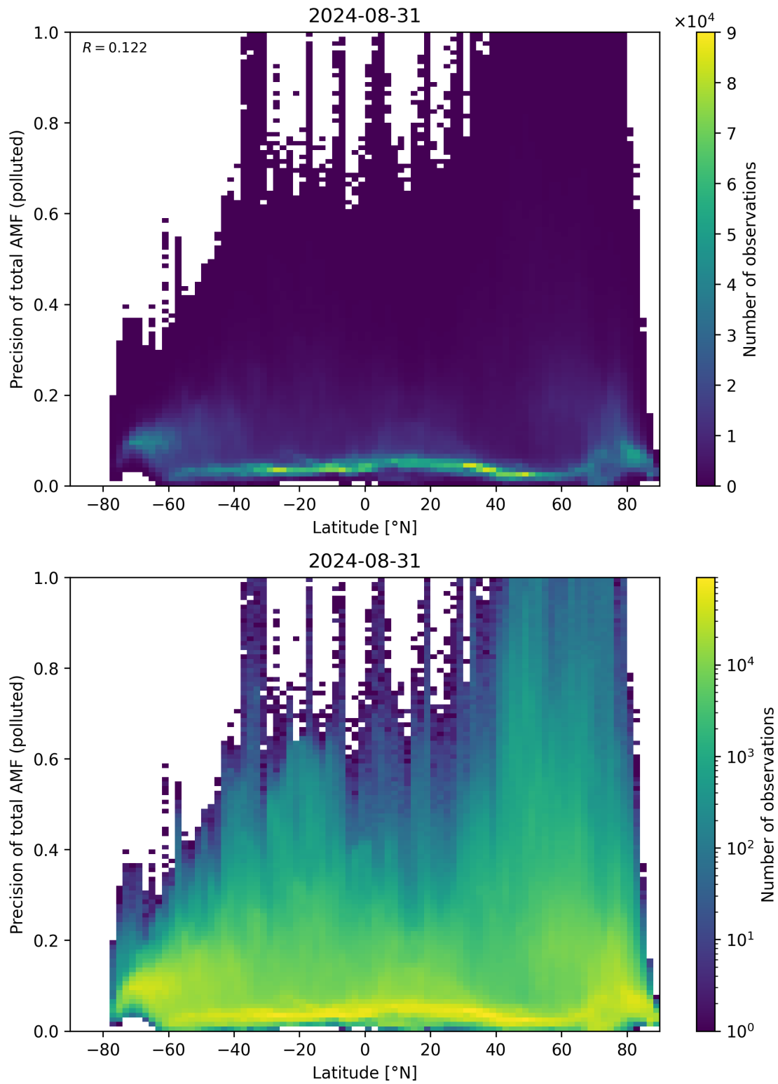
Figure 155: Scatter density plot of “Latitude” against “Precision of total AMF (polluted)” for 2024-08-30 to 2024-09-01.
