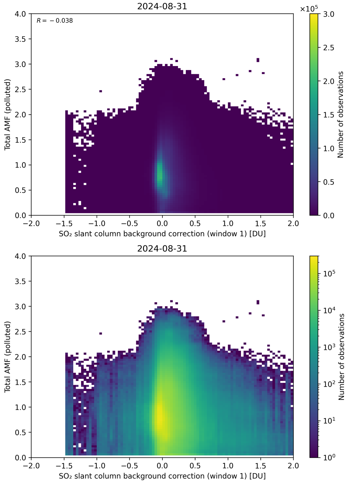
Figure 109: Scatter density plot of “SO 2 slant column background correction (window 1)” against “Total AMF (polluted)” for 2024-08-30 to 2024-09-01.
