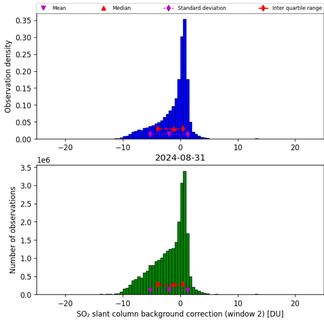
Figure 63: Histogram of “SO 2 slant column background correction (window 2)” for 2024-08-30 to 2024-09-01
