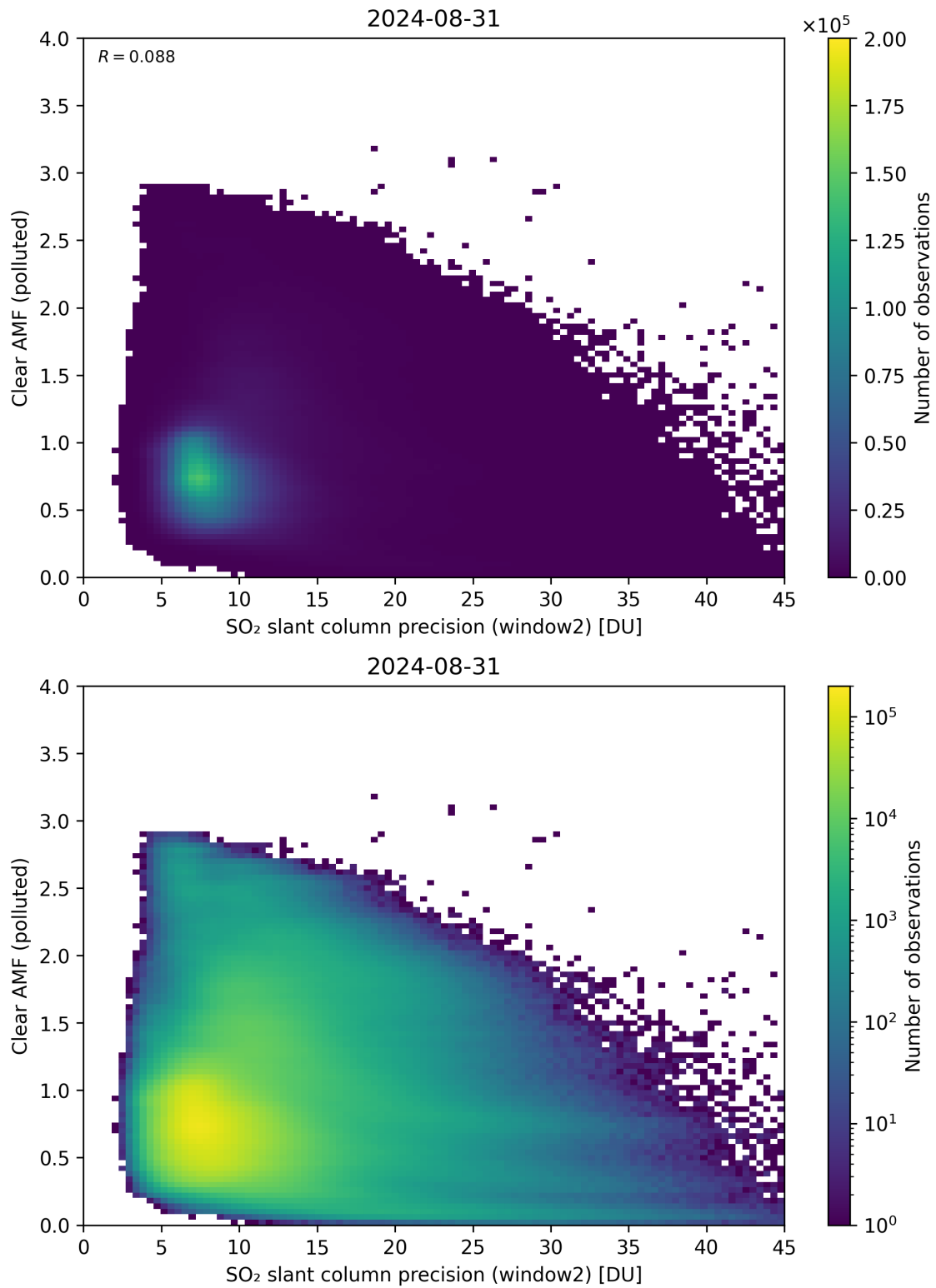
Figure 246: Scatter density plot of “SO 2 slant column precision (window2)” against “Clear AMF (polluted)” for 2024-08-30 to 2024-09-01.
