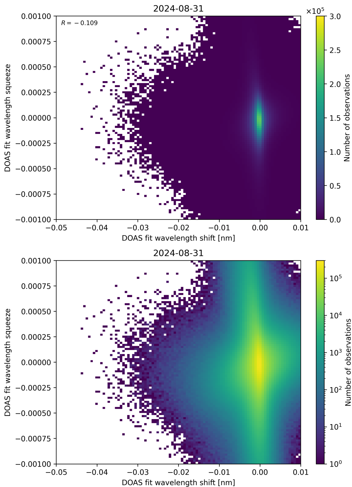
Figure 127: Scatter density plot of “DOAS fit wavelength shift” against “DOAS fit wavelength squeeze” for 2024-08-30 to 2024-09-01.
