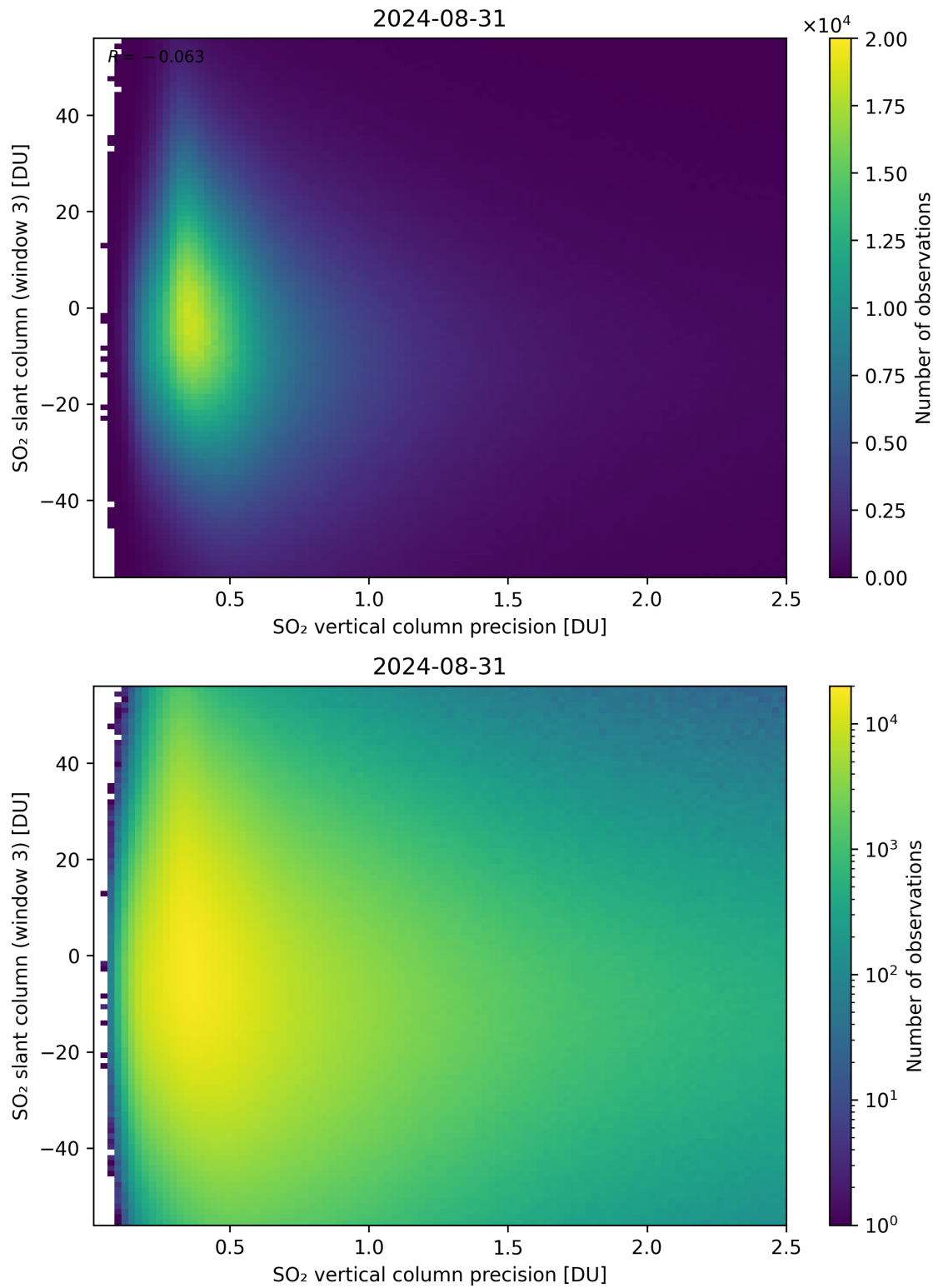
Figure 292: Scatter density plot of “SO 2 vertical column precision” against “SO 2 slant column (window 3)” for 2024-08-30 to 2024-09-01.
