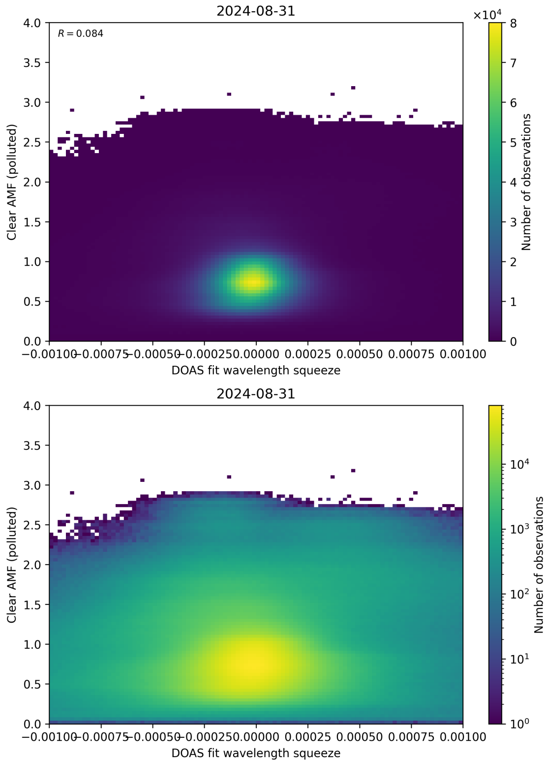
Figure 133: Scatter density plot of “DOAS fit wavelength squeeze” against “Clear AMF (polluted)” for 2024-08-30 to 2024-09-01.
