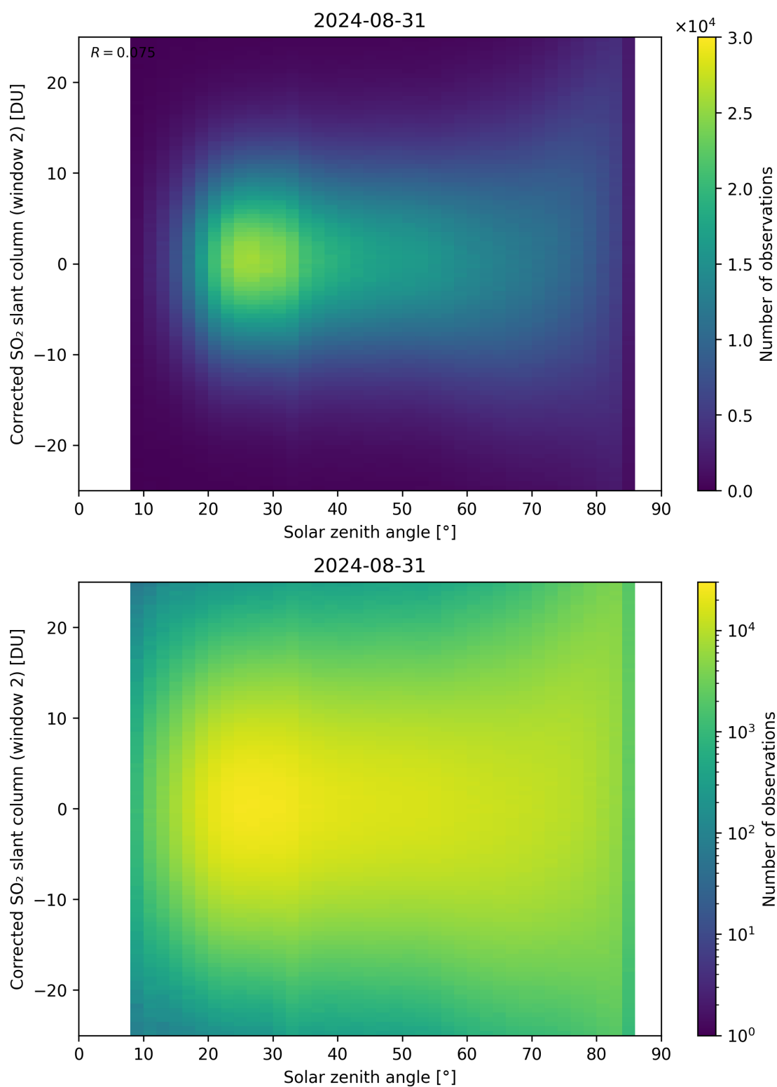
Figure 167: Scatter density plot of “Solar zenith angle” against “Corrected SO 2 slant column (window 2)” for 2024-08-30 to 2024-09-01.
