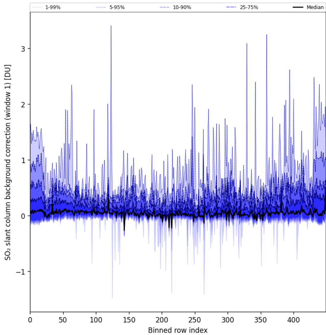
Figure 82: Along track statistics of “SO 2 slant column background correction (window 1)” for 2024-08-30 to 2024-09-01
