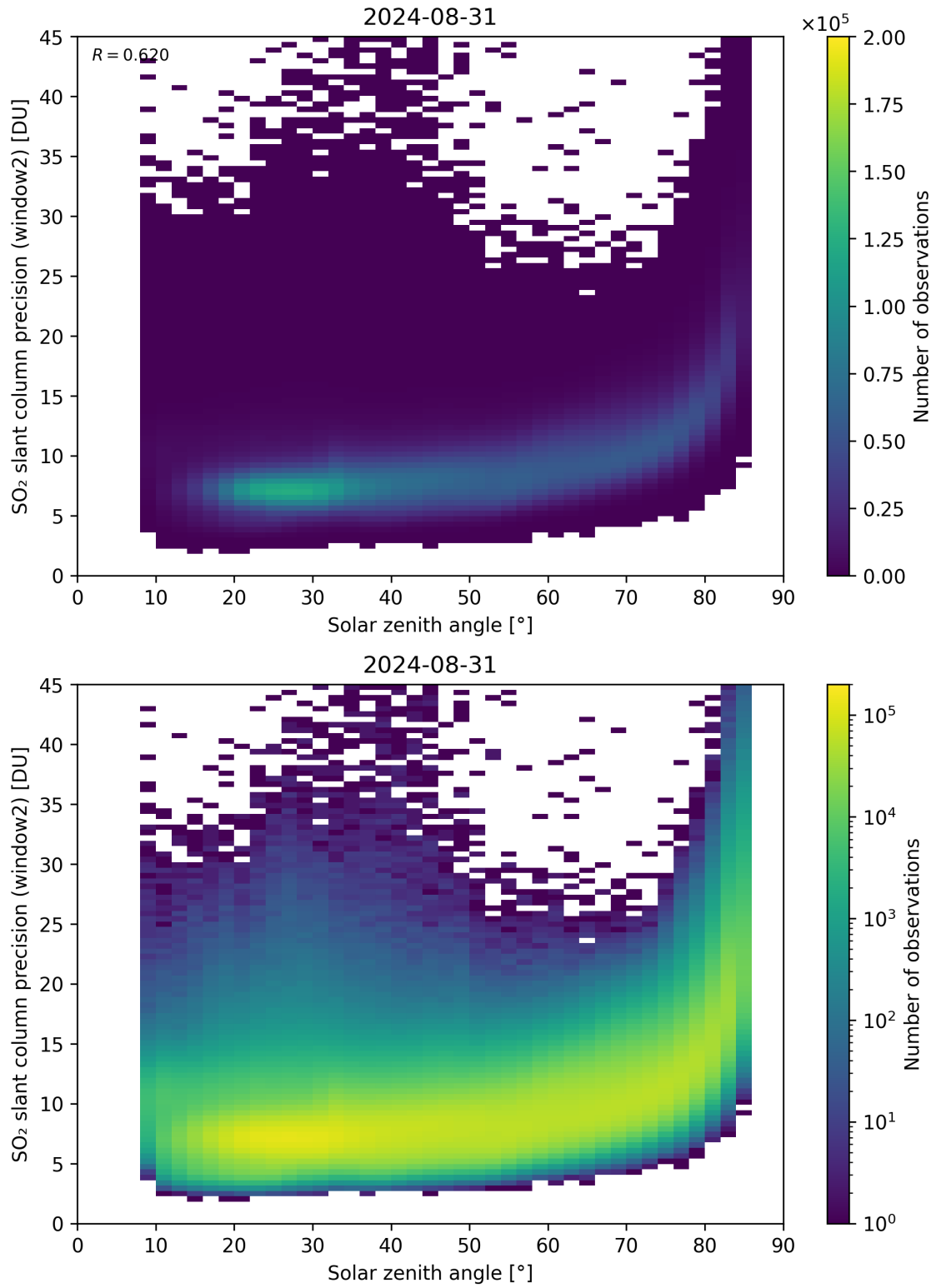
Figure 171: Scatter density plot of “Solar zenith angle” against “SO 2 slant column precision (window2)” for 2024-08-30 to 2024-09-01.
