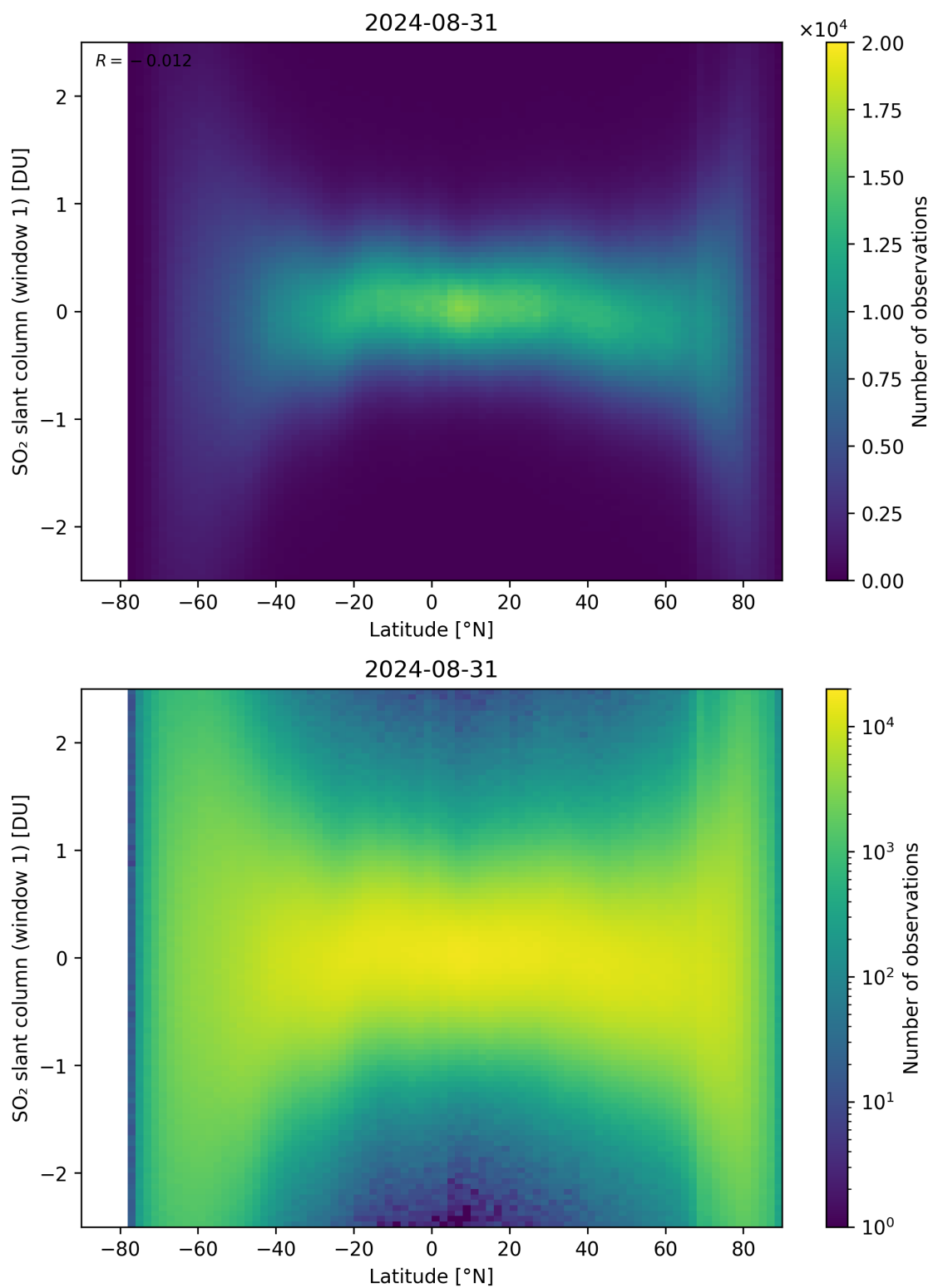
Figure 149: Scatter density plot of “Latitude” against “SO 2 slant column (window 1)” for 2024-08-30 to 2024-09-01.
