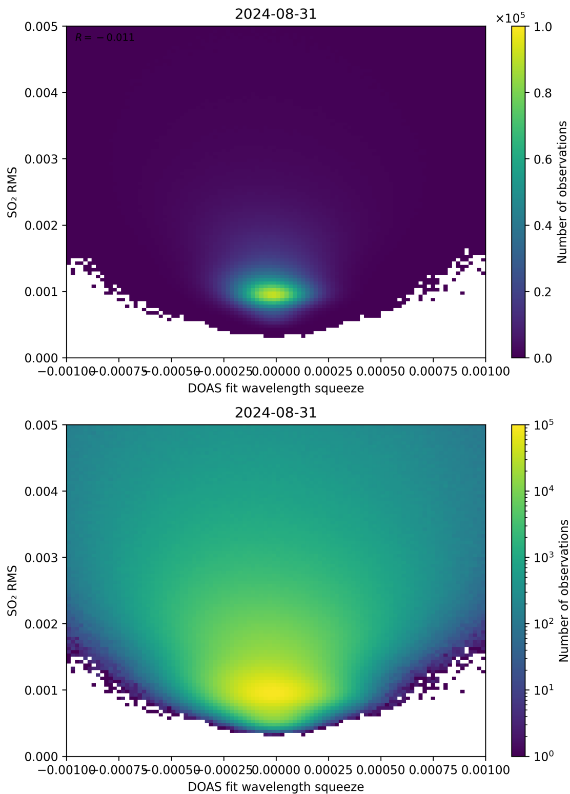
Figure 132: Scatter density plot of “DOAS fit wavelength squeeze” against “SO 2 RMS” for 2024-08-30 to 2024-09-01.
