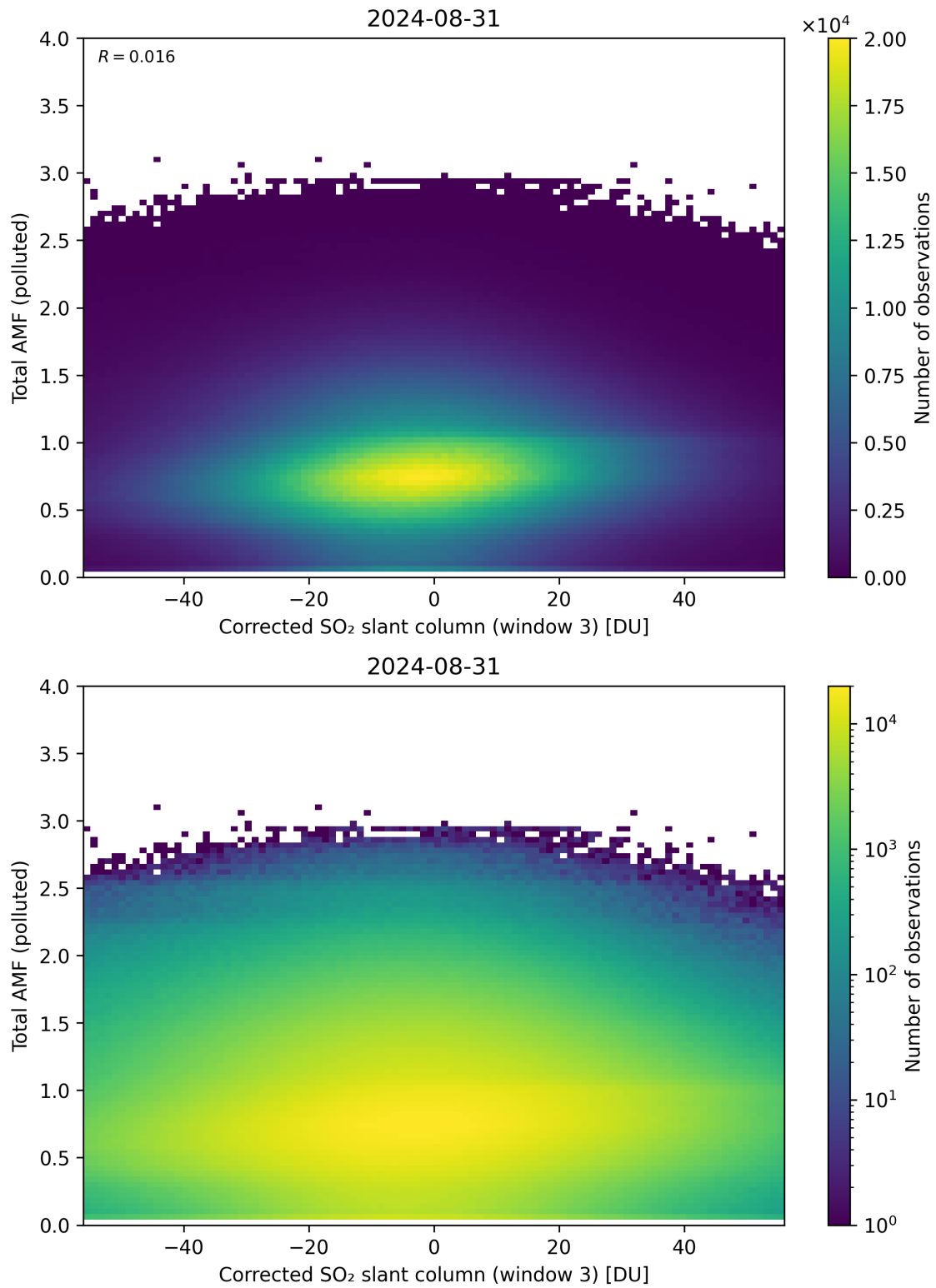
Figure 210: Scatter density plot of “Corrected SO 2 slant column (window 3)” against “Total AMF (polluted)” for 2024-08-30 to 2024-09-01.
