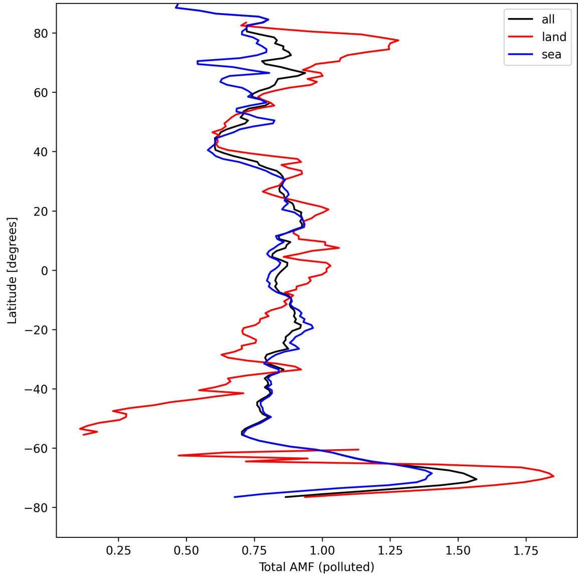
Figure 48: Zonal average of “Total AMF (polluted)” for 2024-08-30 to 2024-09-01.
