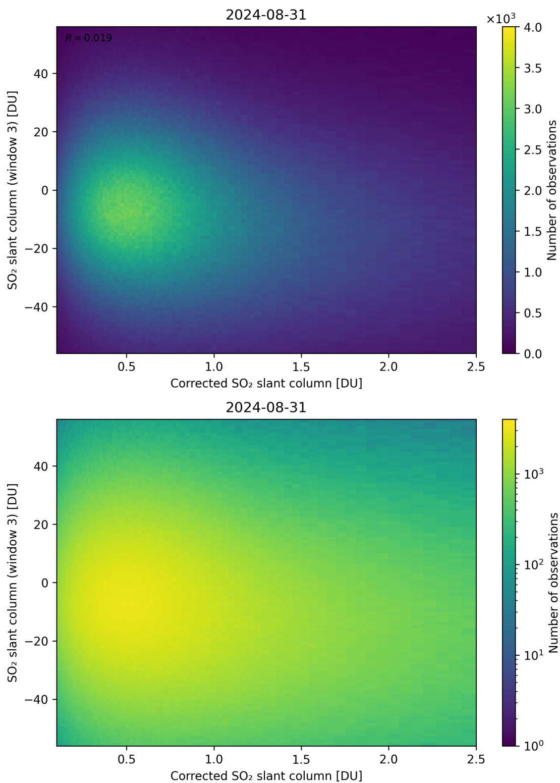
Figure 190: Scatter density plot of “Corrected SO 2 slant column” against “SO 2 slant column (window 3)” for 2024-08-30 to 2024-09-01.
