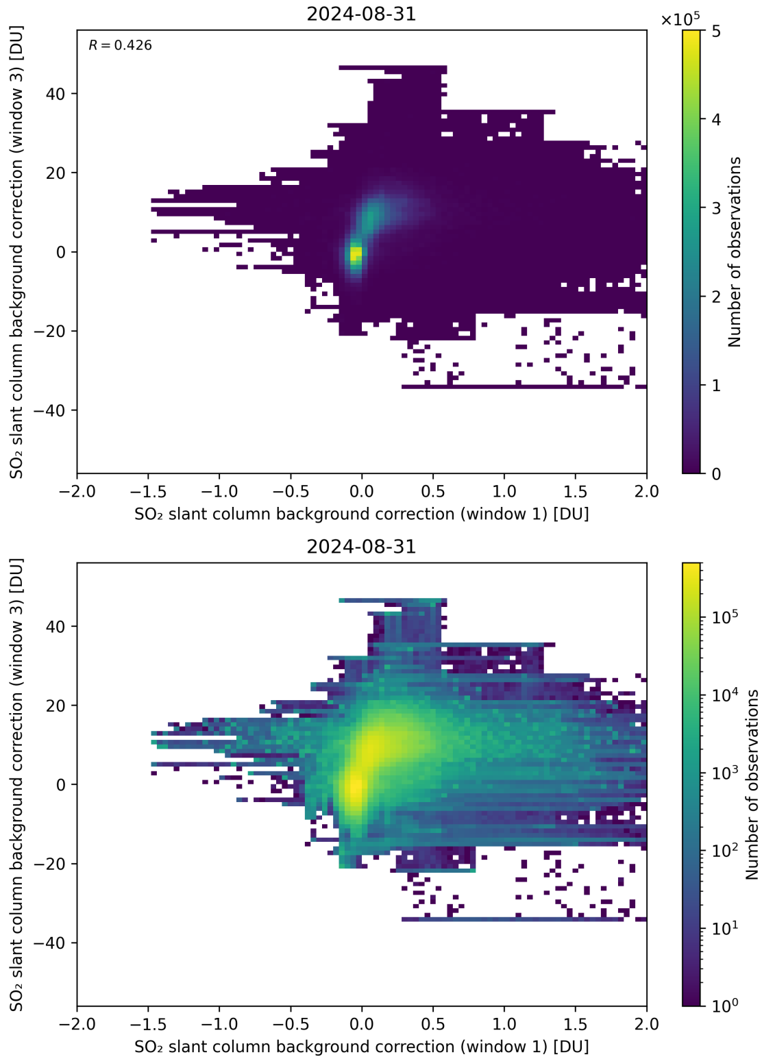
Figure 99: Scatter density plot of “SO 2 slant column background correction (window 1)” against “SO 2 slant column background correction (window 3)” for 2024-08-30 to 2024-09-01.
