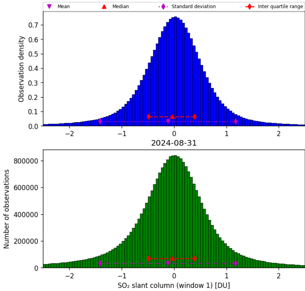
Figure 56: Histogram of “SO 2 slant column (window 1)” for 2024-08-30 to 2024-09-01
