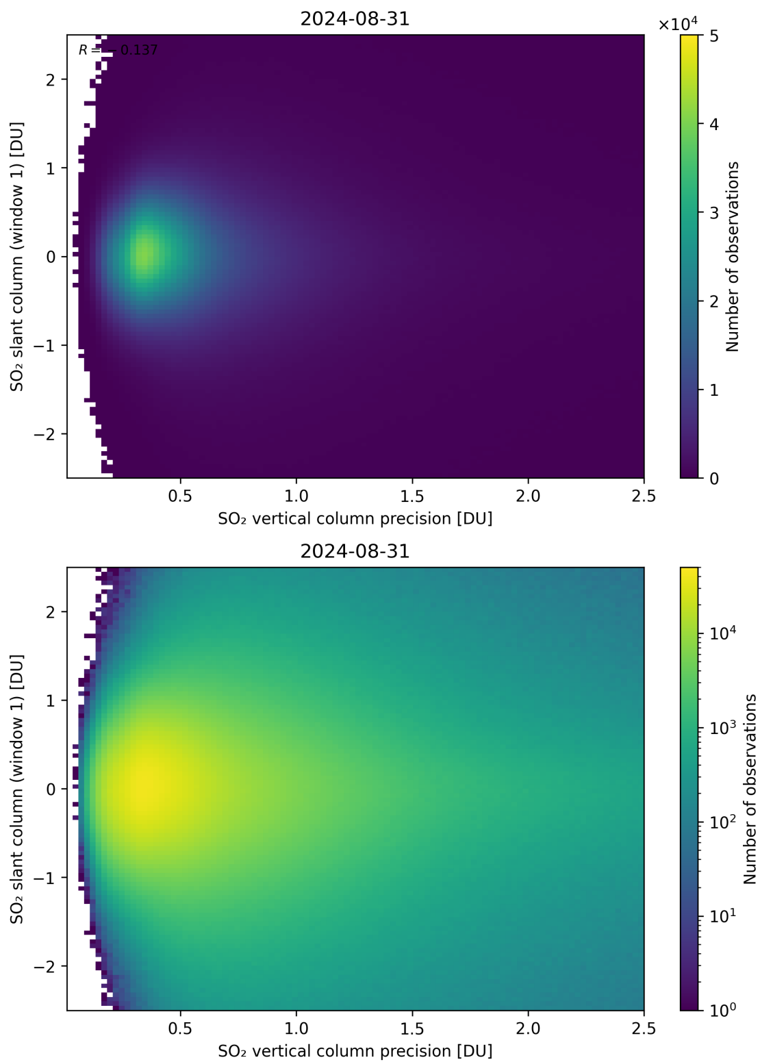
Figure 289: Scatter density plot of “SO 2 vertical column precision” against “SO 2 slant column (window 1)” for 2024-08-30 to 2024-09-01.
