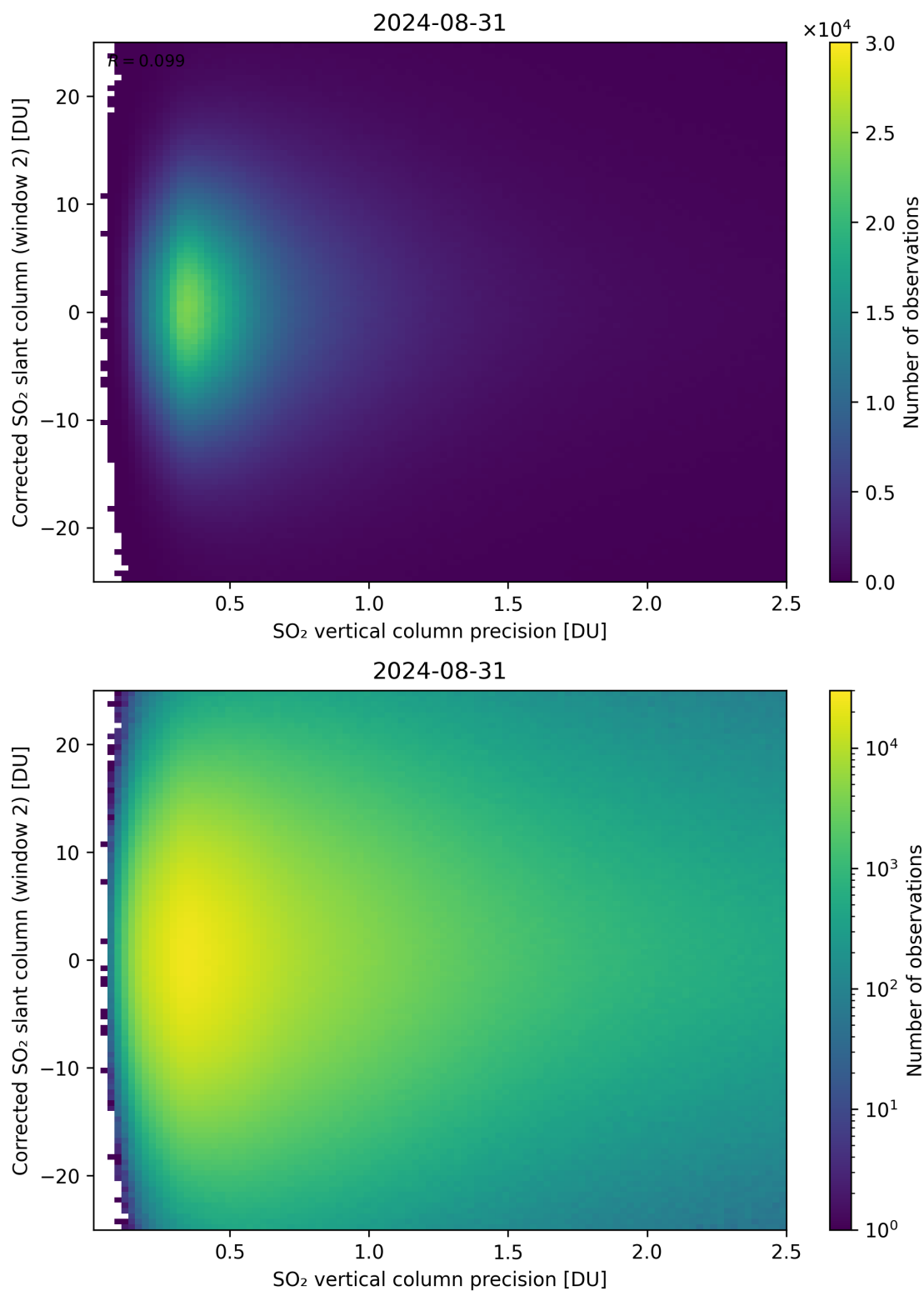
Figure 287: Scatter density plot of “SO 2 vertical column precision” against “Corrected SO 2 slant column (window 2)” for 2024-08-30 to 2024-09-01.
