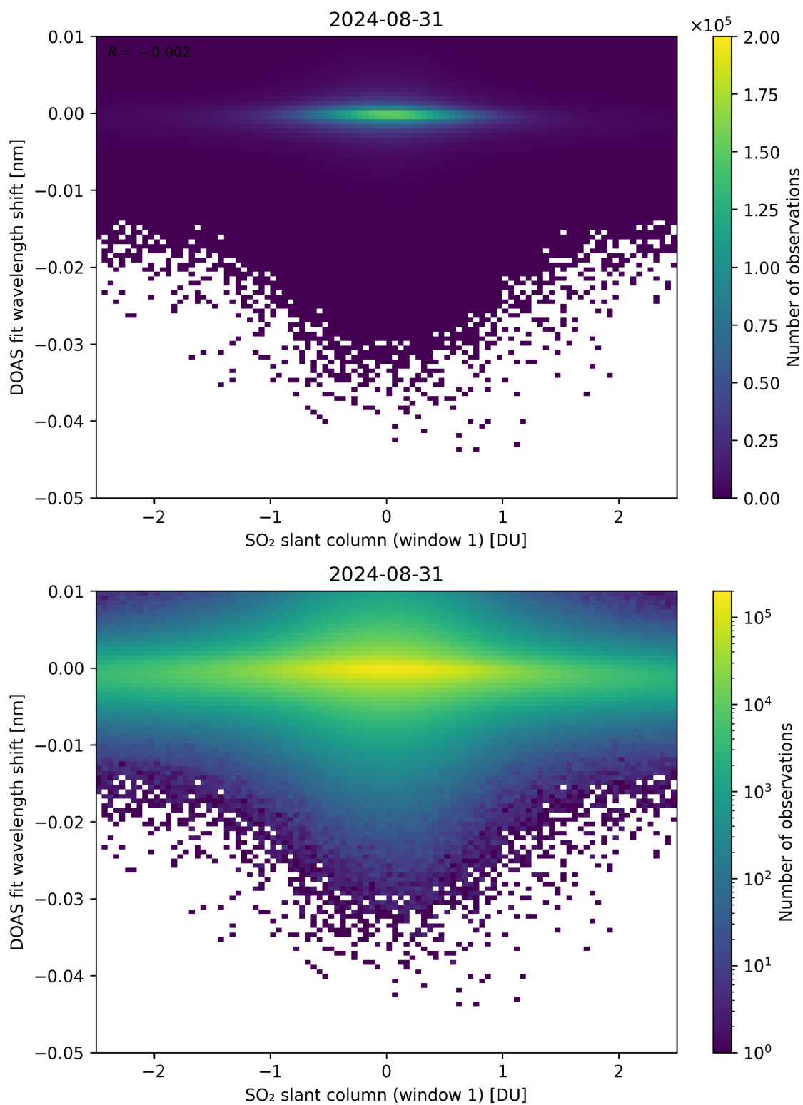
Figure 215: Scatter density plot of “SO 2 slant column (window 1)” against “DOAS fit wavelength shift” for 2024-08-30 to 2024-09-01.
