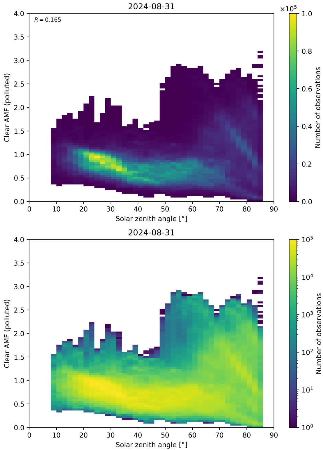
Figure 165: Scatter density plot of “Solar zenith angle” against “Clear AMF (polluted)” for 2024-08-30 to 2024-09-01.
