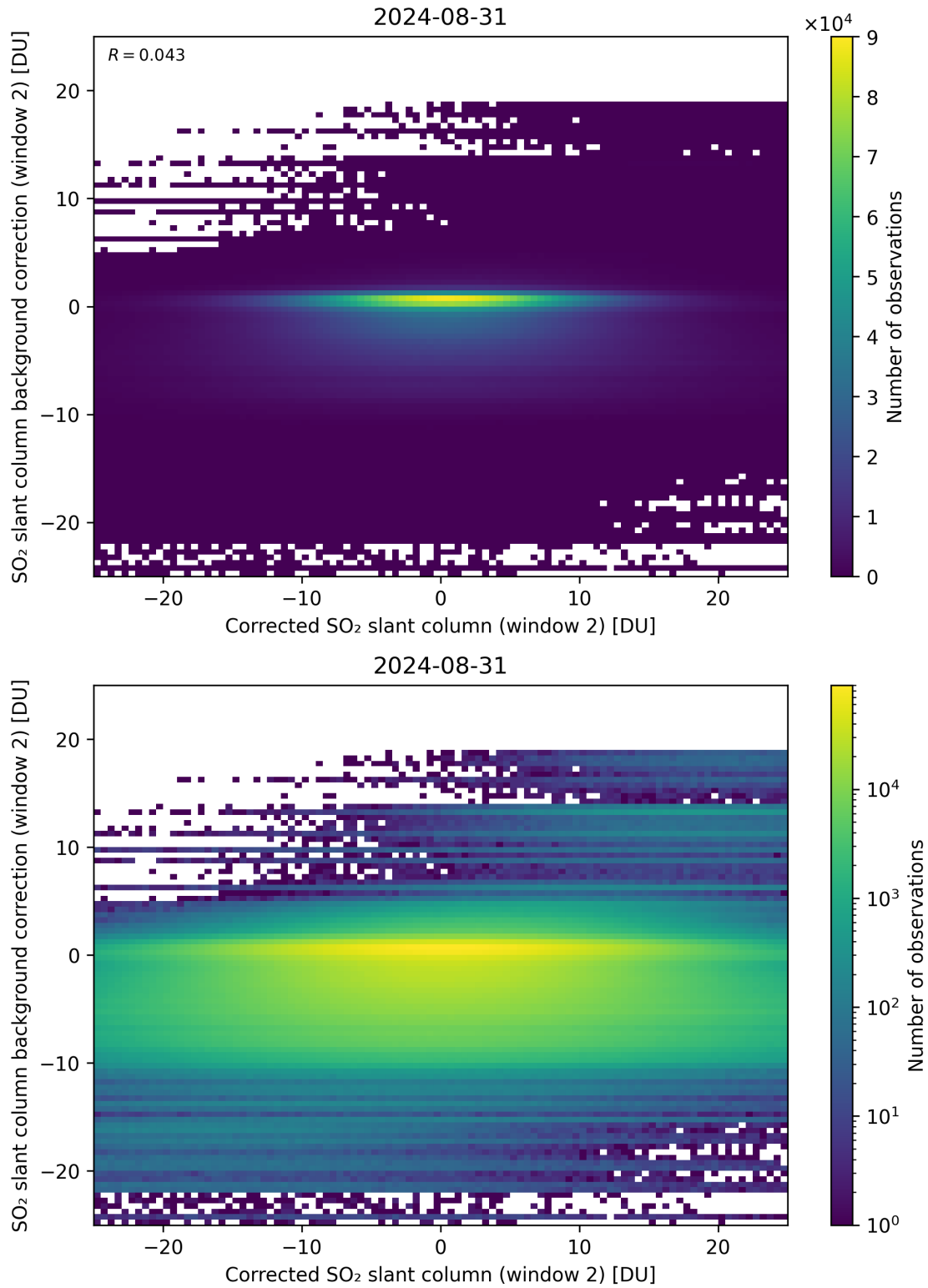
Figure 194: Scatter density plot of “Corrected SO 2 slant column (window 2)” against “SO 2 slant column background correction (window 2)” for 2024-08-30 to 2024-09-01.
