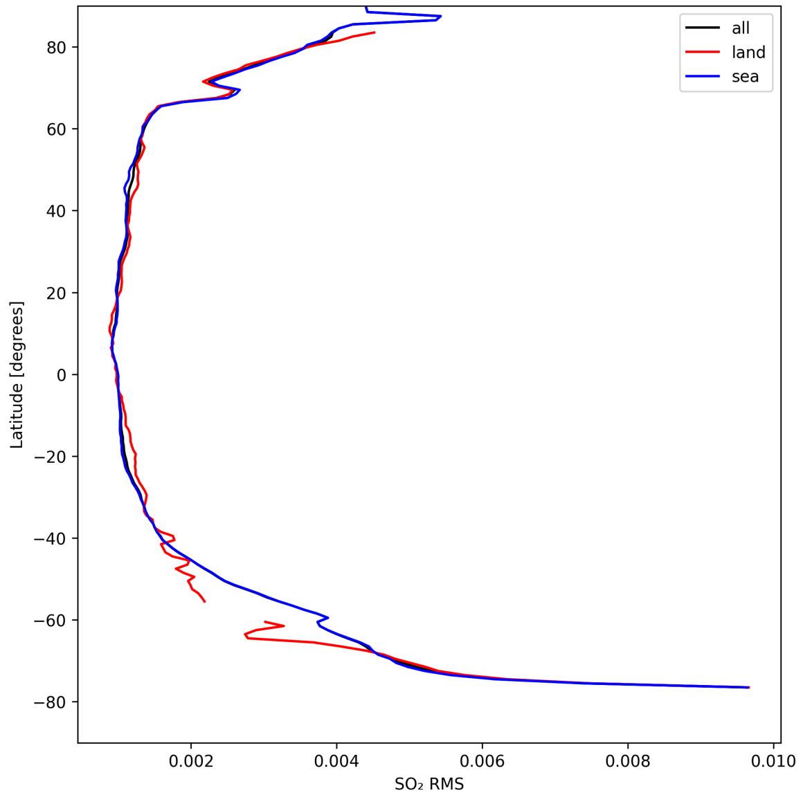
Figure 47: Zonal average of “SO 2 RMS” for 2024-08-30 to 2024-09-01.
