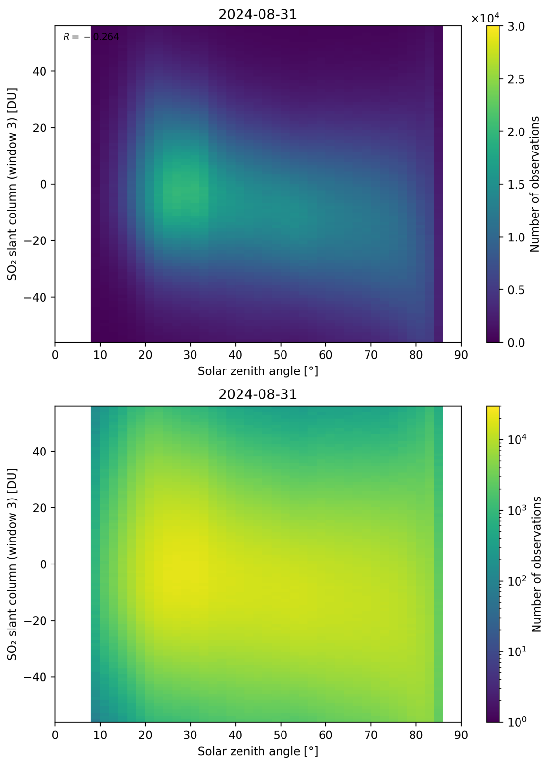
Figure 172: Scatter density plot of “Solar zenith angle” against “SO 2 slant column (window 3)” for 2024-08-30 to 2024-09-01.
