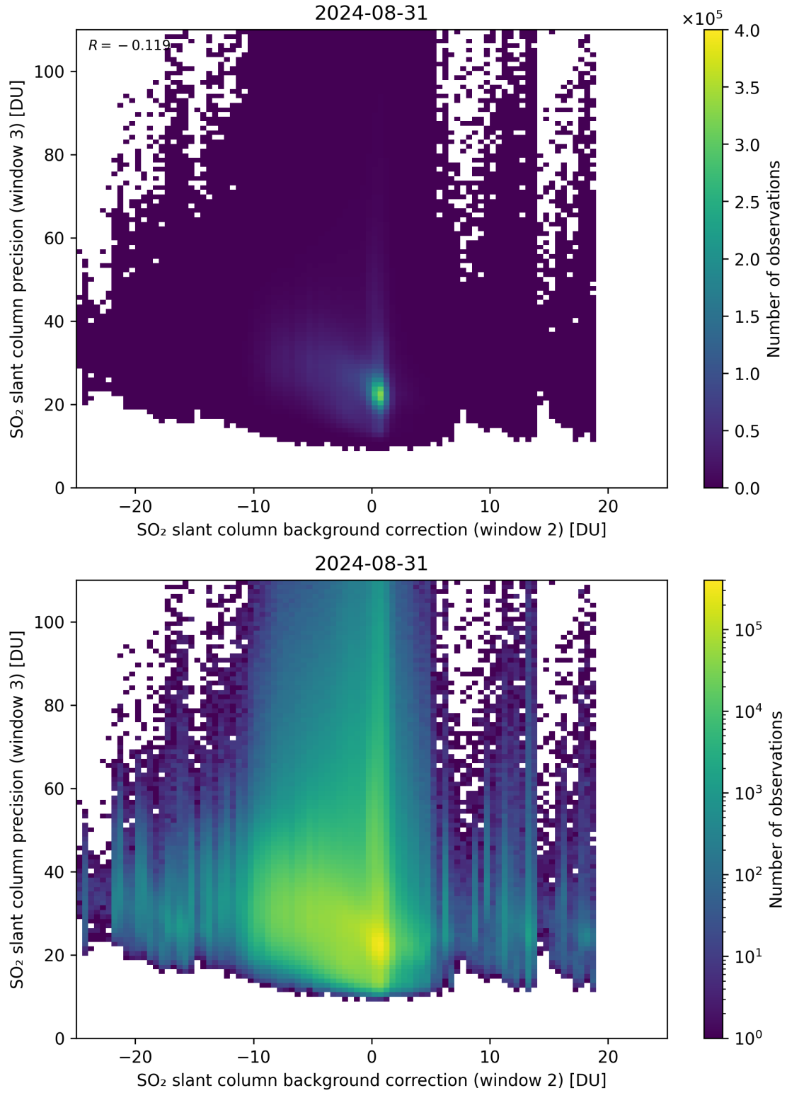
Figure 118: Scatter density plot of “SO 2 slant column background correction (window 2)” against “SO 2 slant column precision (window 3)” for 2024-08-30 to 2024-09-01.
