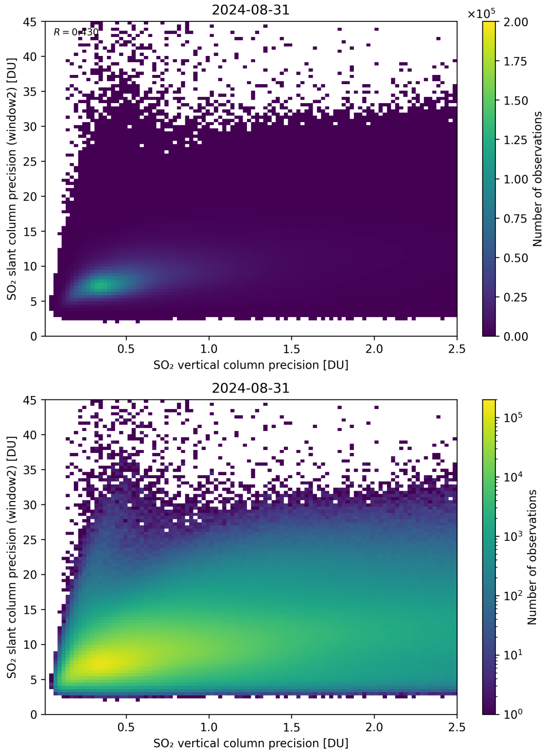
Figure 291: Scatter density plot of “SO 2 vertical column precision” against “SO 2 slant column precision (window2)” for 2024-08-30 to 2024-09-01.
