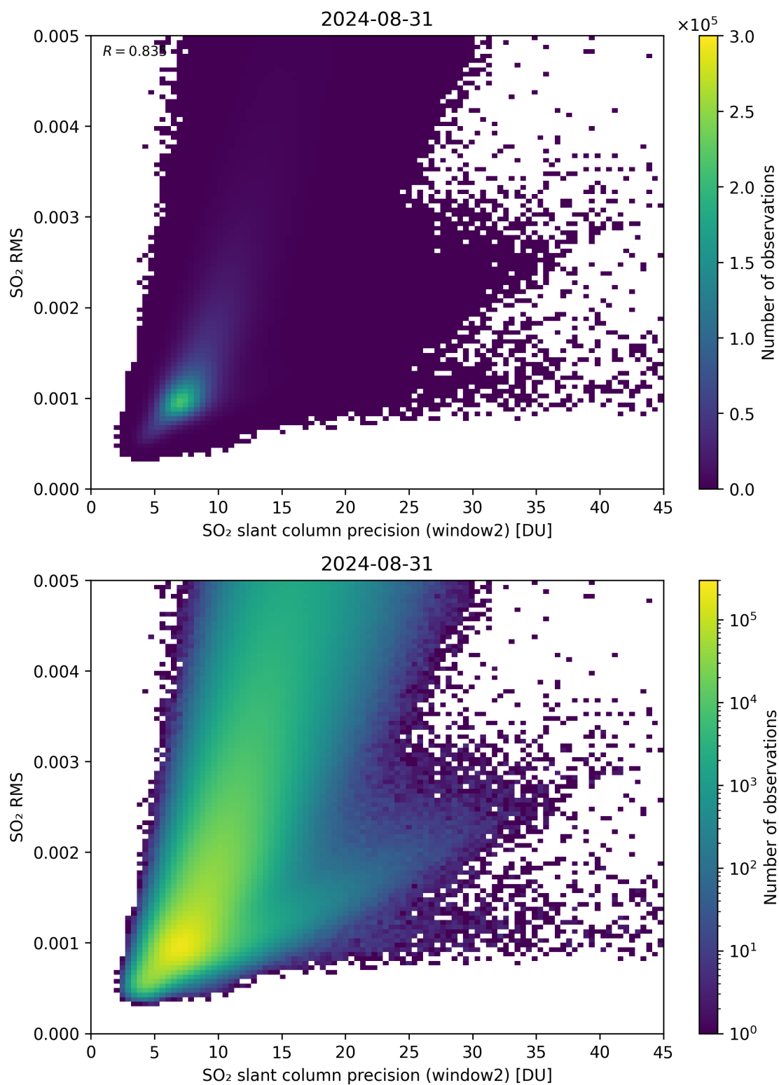
Figure 245: Scatter density plot of “SO 2 slant column precision (window2)” against “SO 2 RMS” for 2024-08-30 to 2024-09-01.
