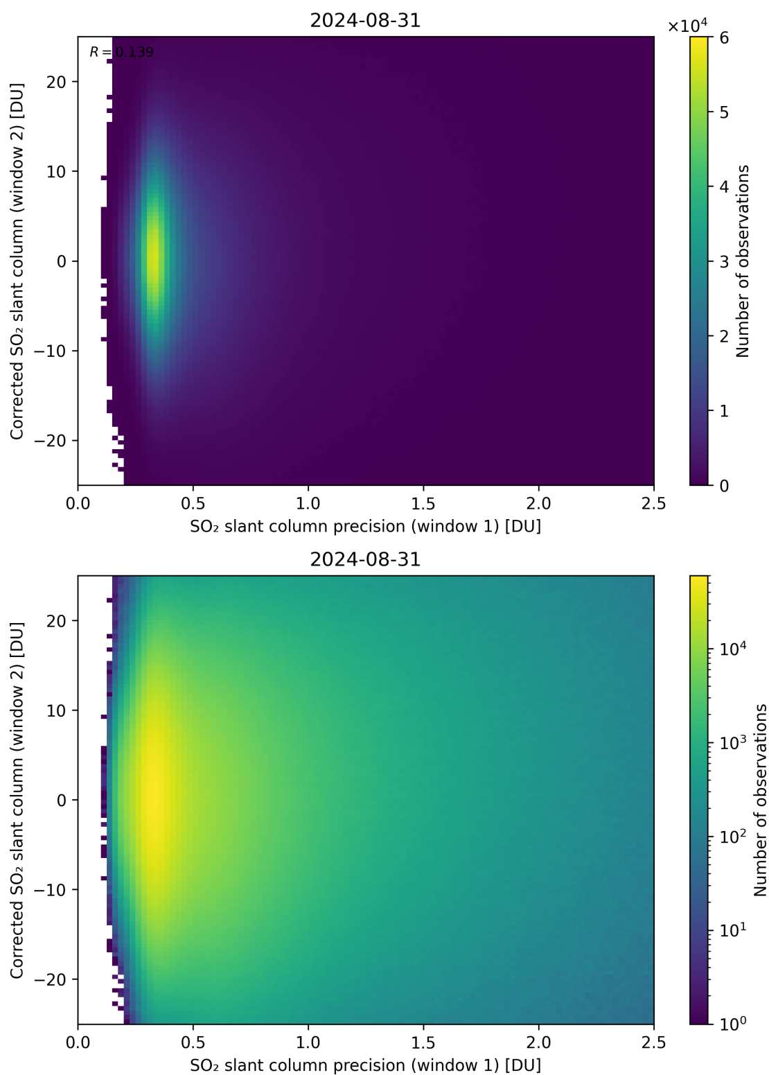
Figure 225: Scatter density plot of “SO 2 slant column precision (window 1)” against “Corrected SO 2 slant column (window 2)” for 2024-08-30 to 2024-09-01.
