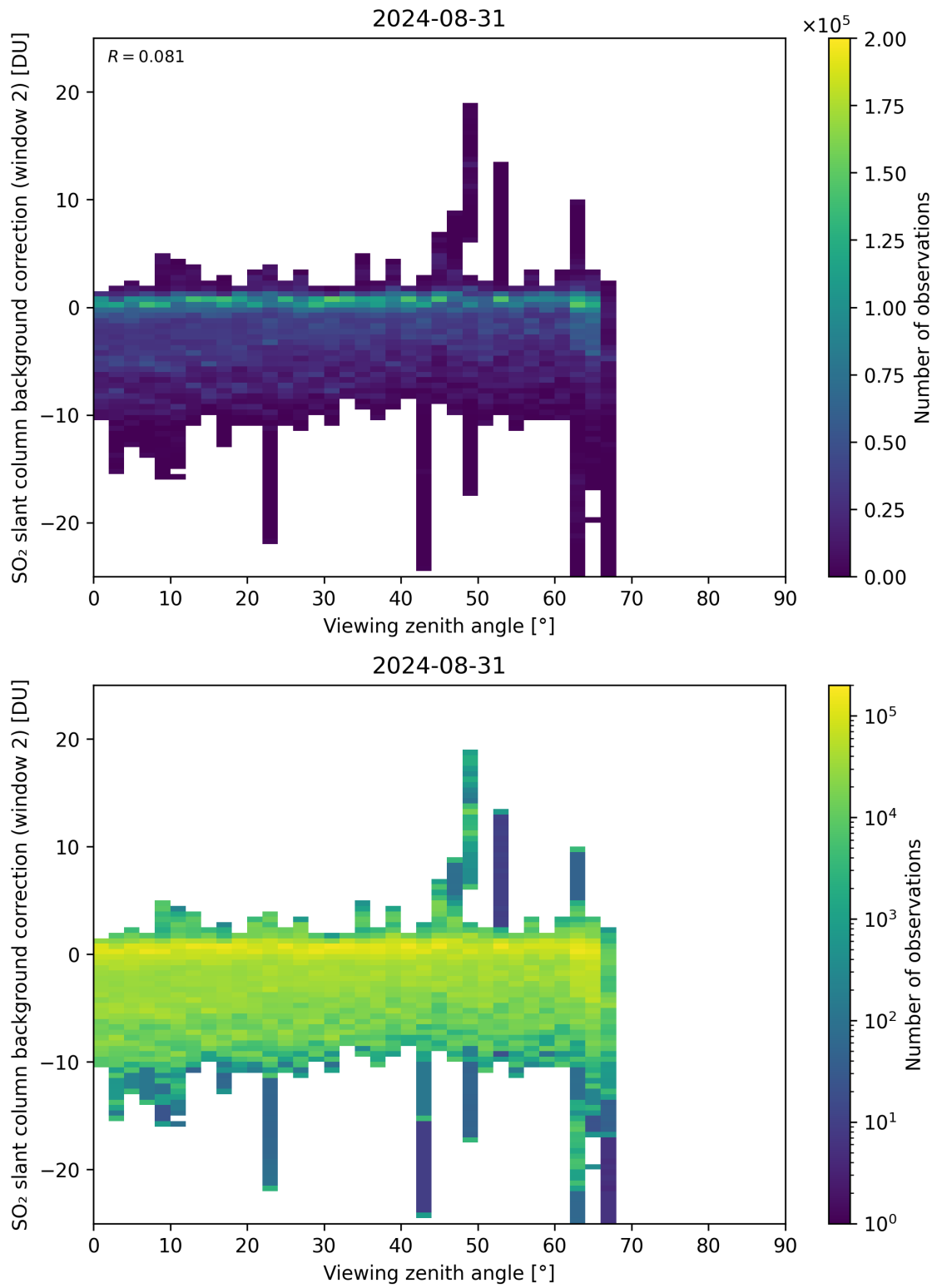
Figure 309: Scatter density plot of “Viewing zenith angle” against “SO 2 slant column background correction (window 2)” for 2024-08-30 to 2024-09-01.
