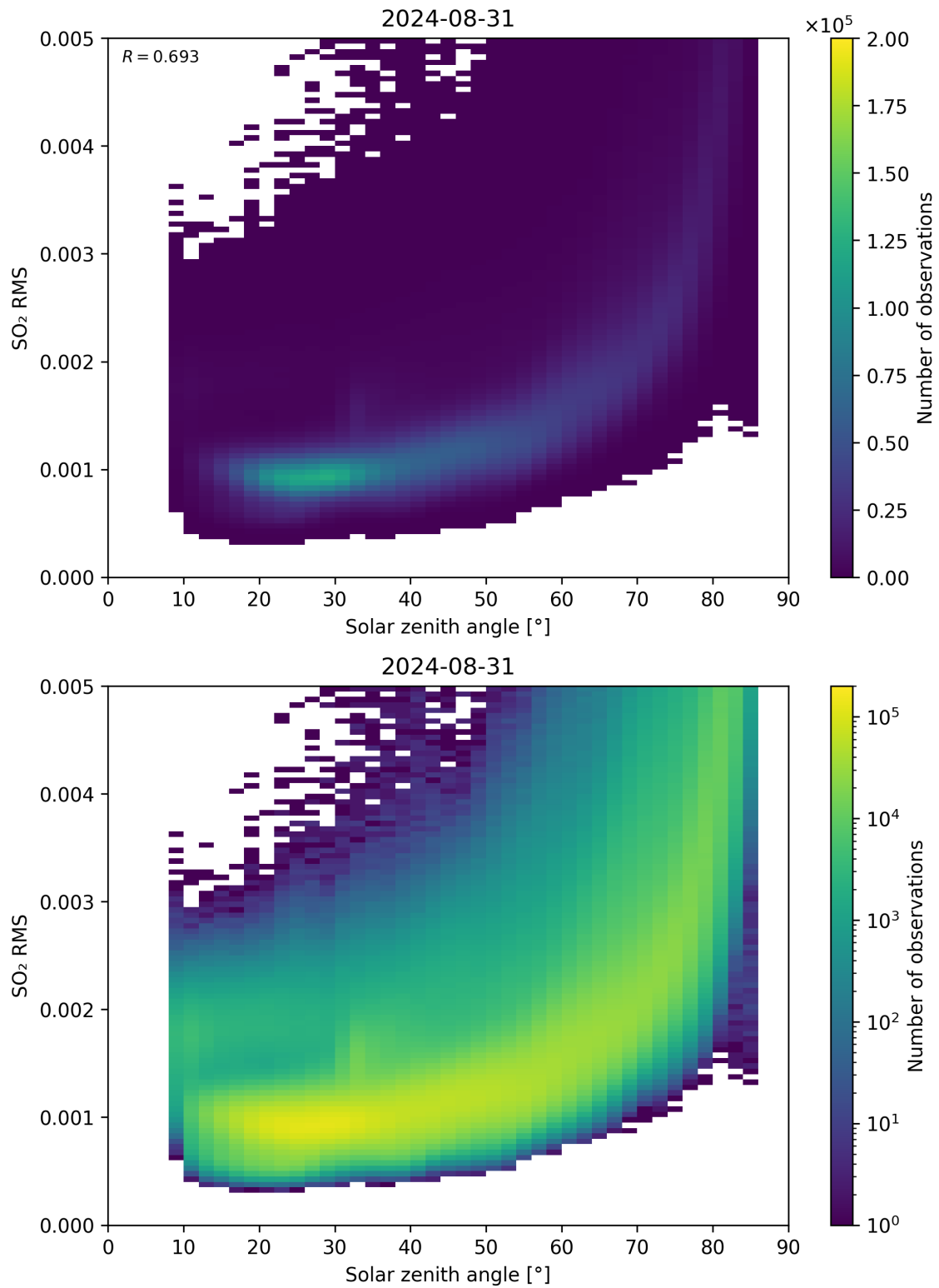
Figure 163: Scatter density plot of “Solar zenith angle” against “SO 2 RMS” for 2024-08-30 to 2024-09-01.
