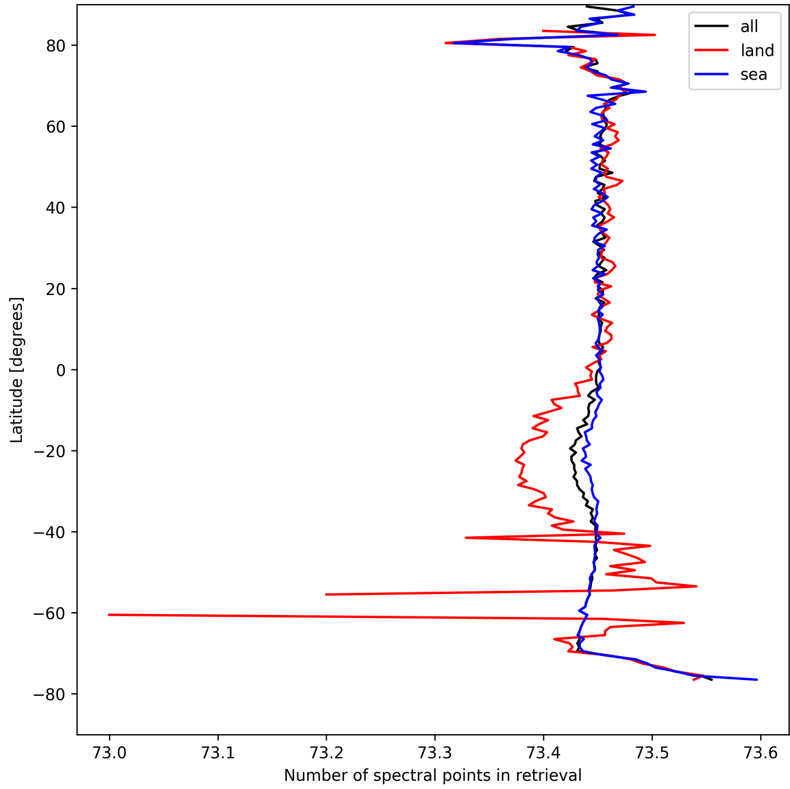
Figure 51: Zonal average of “Number of spectral points in retrieval” for 2024-08-30 to 2024-09-01.
