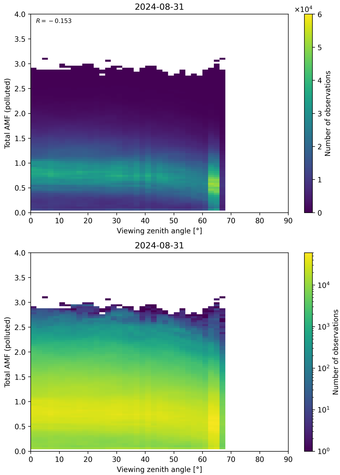
Figure 325: Scatter density plot of “Viewing zenith angle” against “Total AMF (polluted)” for 2024-08-30 to 2024-09-01.
