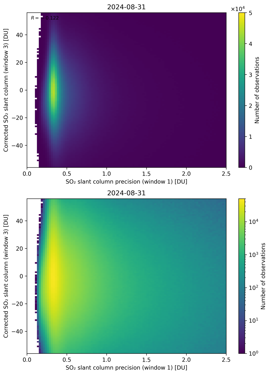
Figure 226: Scatter density plot of “SO 2 slant column precision (window 1)” against “Corrected SO 2 slant column (window 3)” for 2024-08-30 to 2024-09-01.
