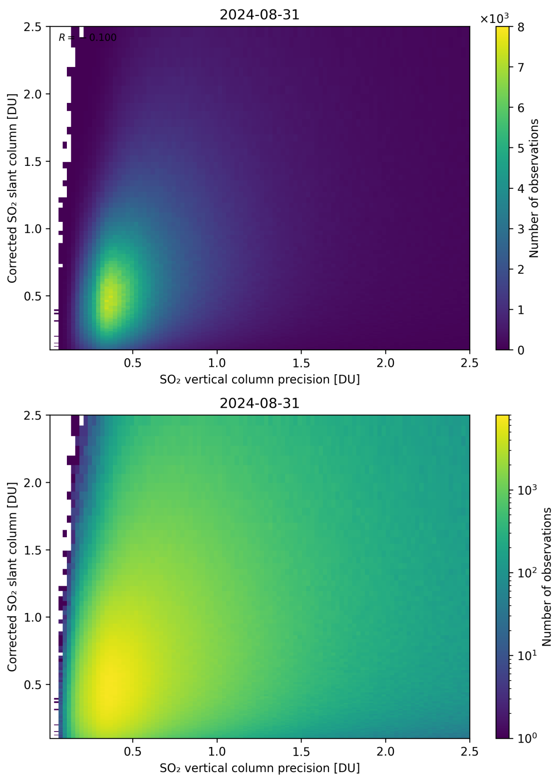
Figure 286: Scatter density plot of “SO 2 vertical column precision” against “Corrected SO 2 slant column” for 2024-08-30 to 2024-09-01.
