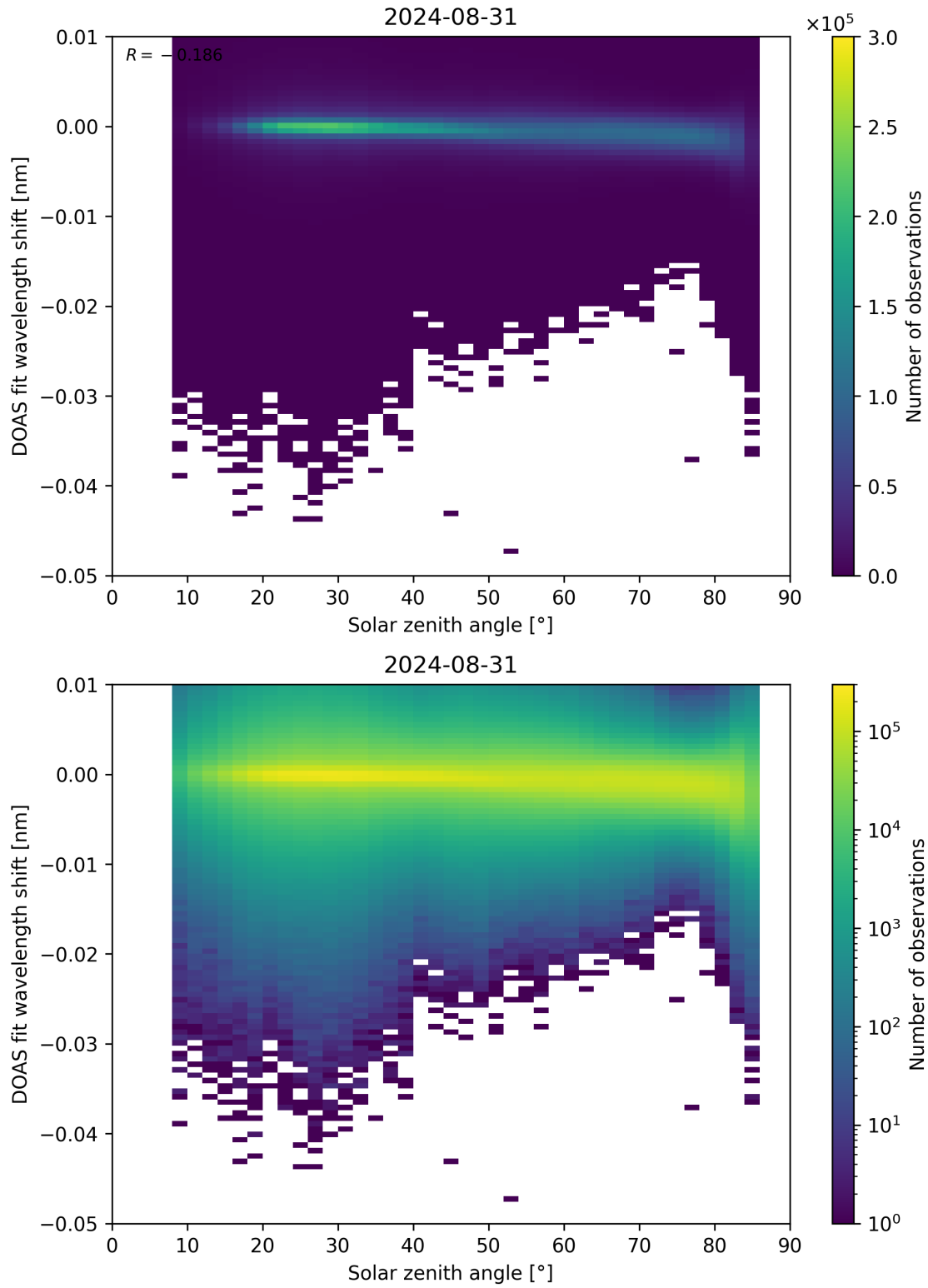
Figure 161: Scatter density plot of “Solar zenith angle” against “DOAS fit wavelength shift” for 2024-08-30 to 2024-09-01.
