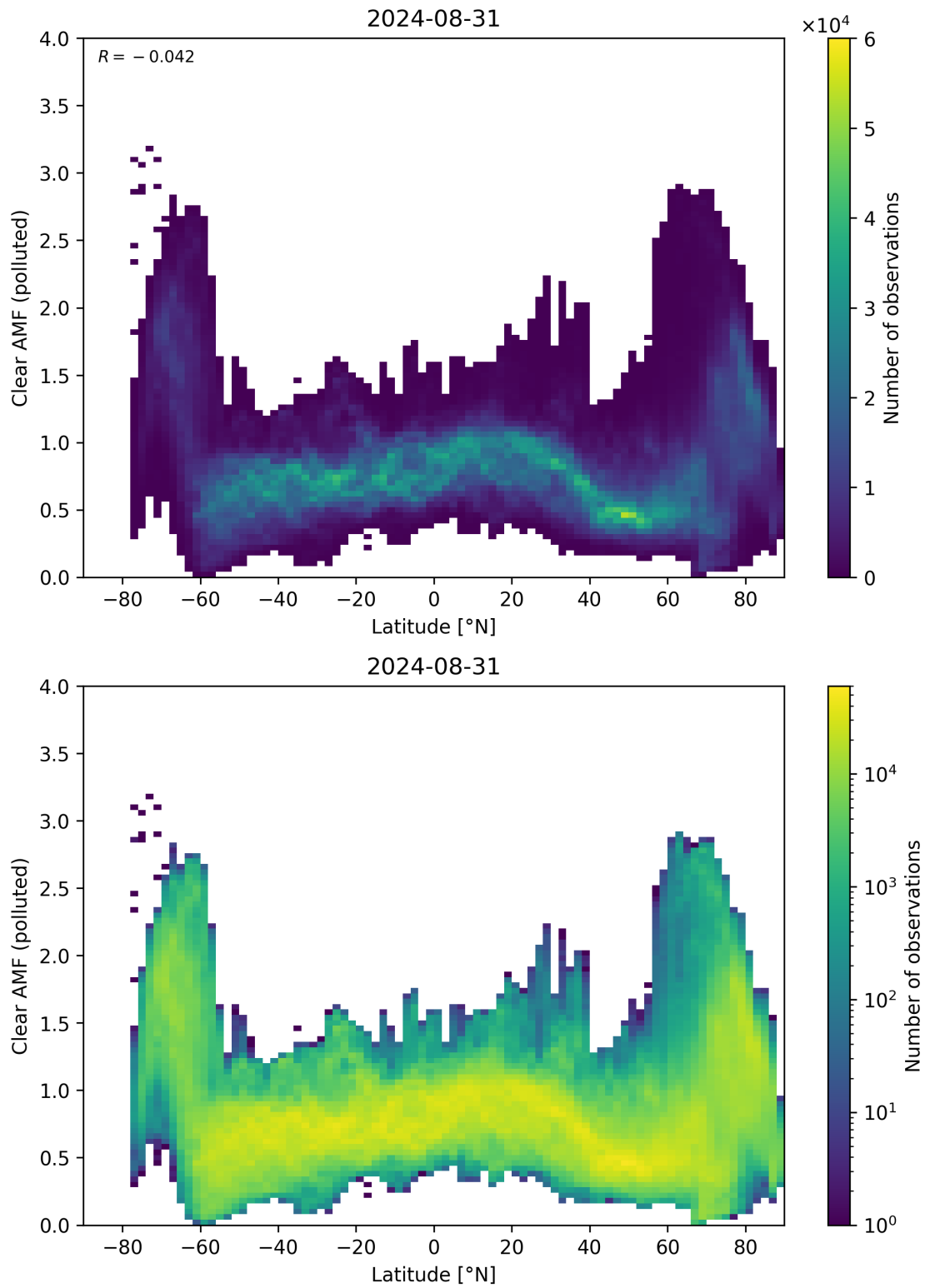
Figure 145: Scatter density plot of “Latitude” against “Clear AMF (polluted)” for 2024-08-30 to 2024-09-01.
