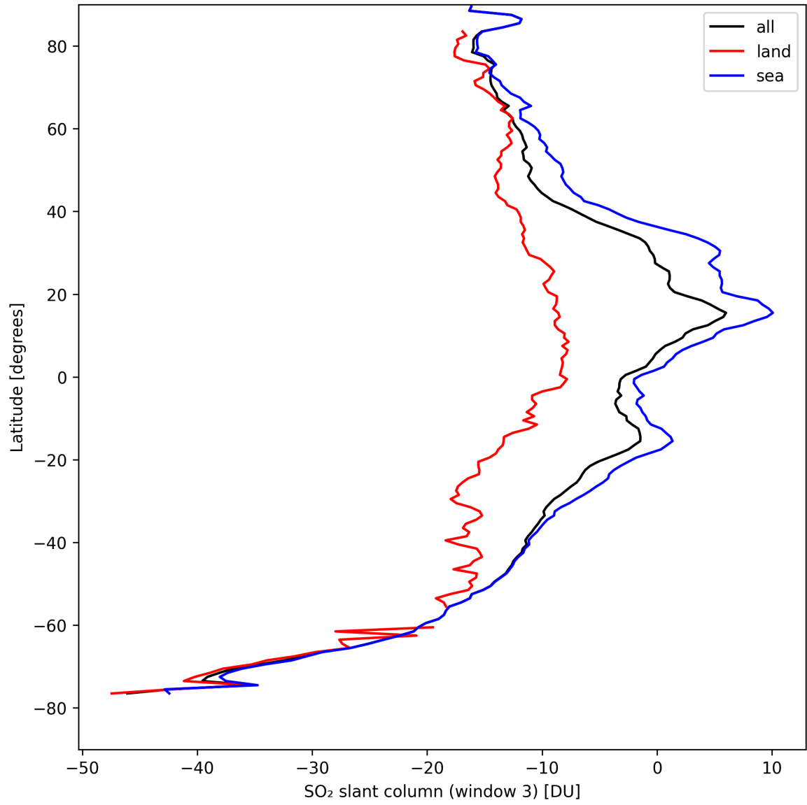
Figure 41: Zonal average of “SO 2 slant column (window 3)” for 2024-08-30 to 2024-09-01.
