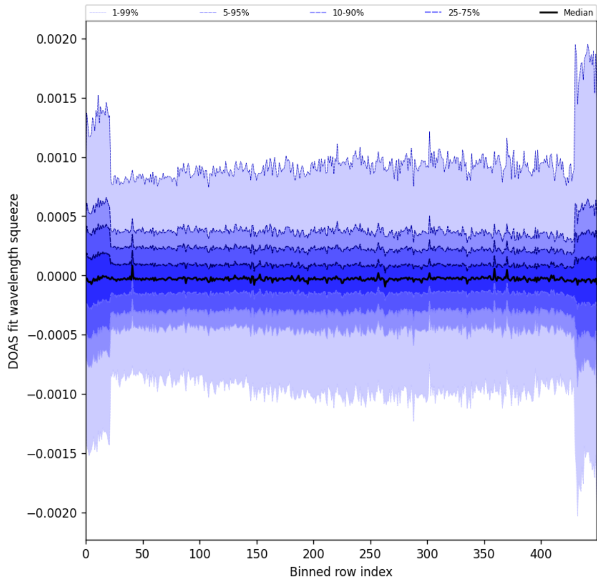
Figure 92: Along track statistics of “DOAS fit wavelength squeeze” for 2024-08-30 to 2024-09-01
