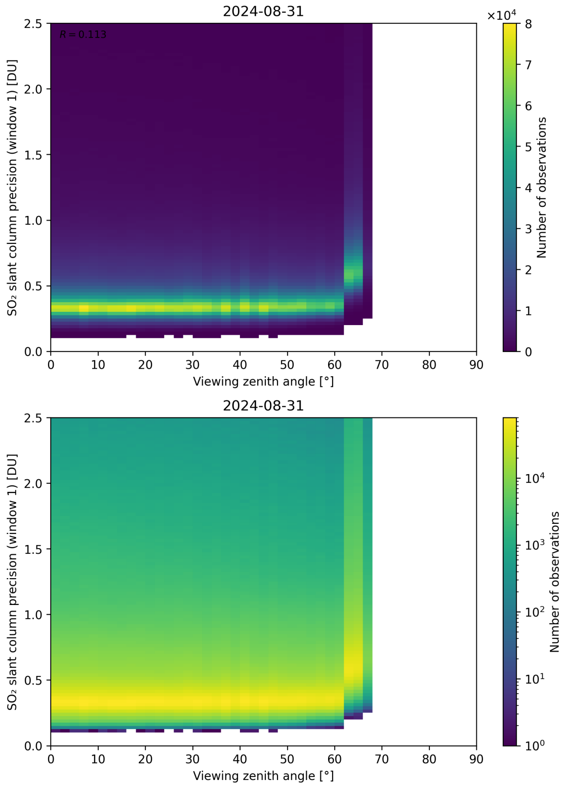
Figure 321: Scatter density plot of “Viewing zenith angle” against “SO 2 slant column precision (window 1)” for 2024-08-30 to 2024-09-01.
