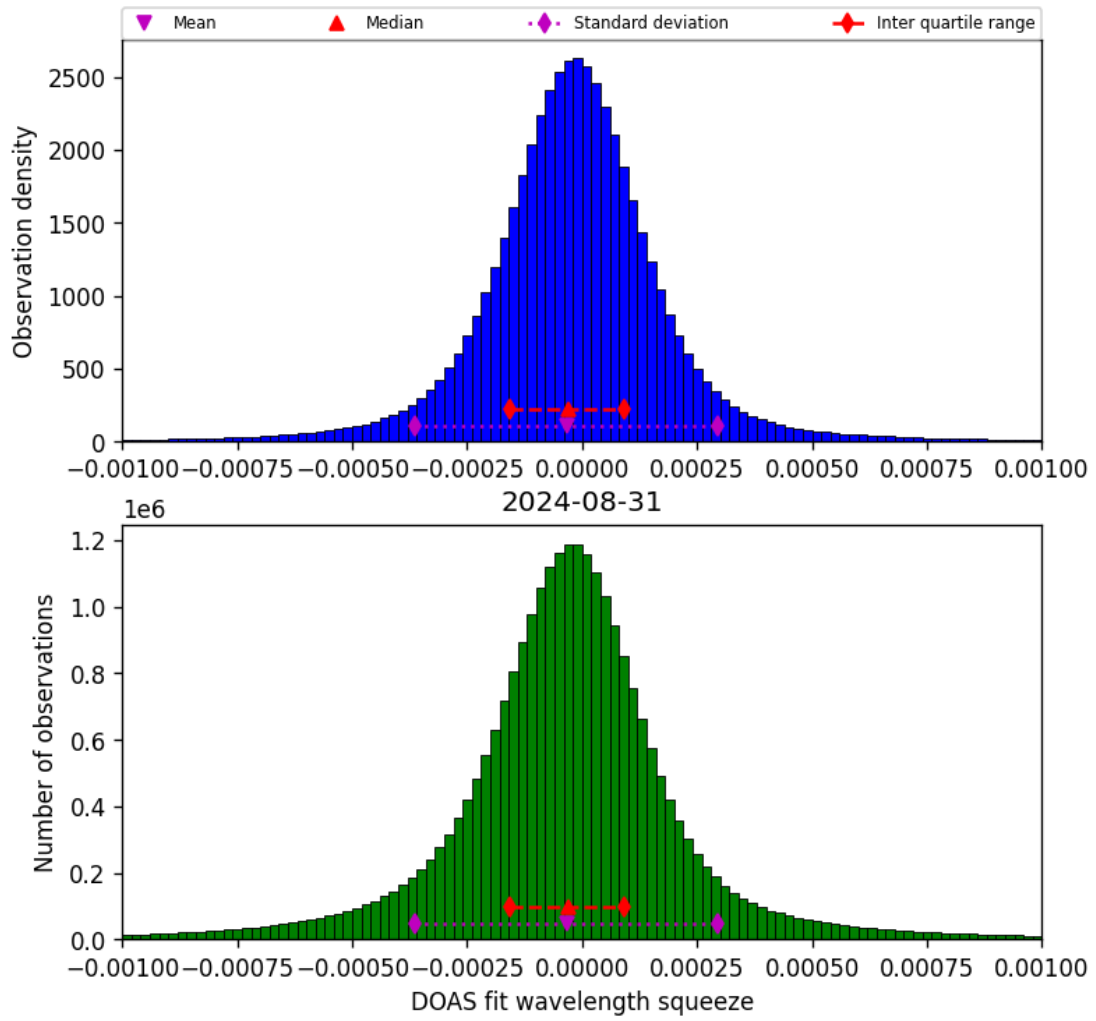
Figure 69: Histogram of “DOAS fit wavelength squeeze” for 2024-08-30 to 2024-09-01
