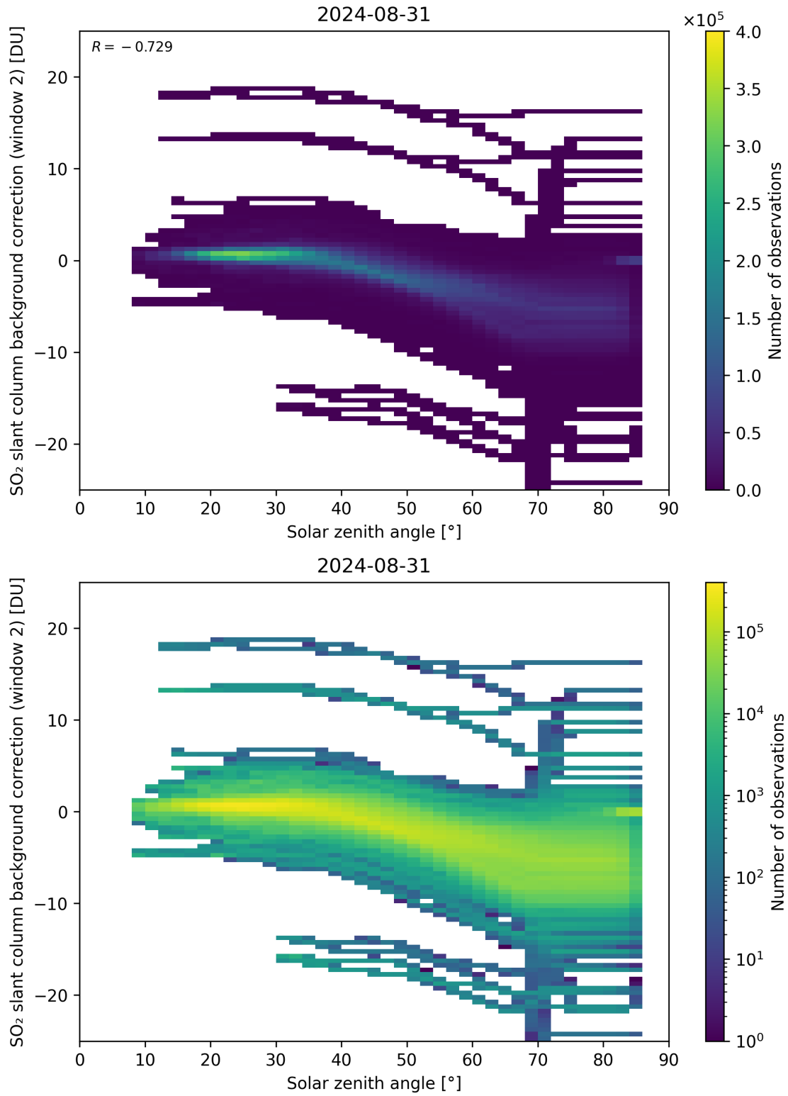
Figure 159: Scatter density plot of “Solar zenith angle” against “SO 2 slant column background correction (window 2)” for 2024-08-30 to 2024-09-01.
