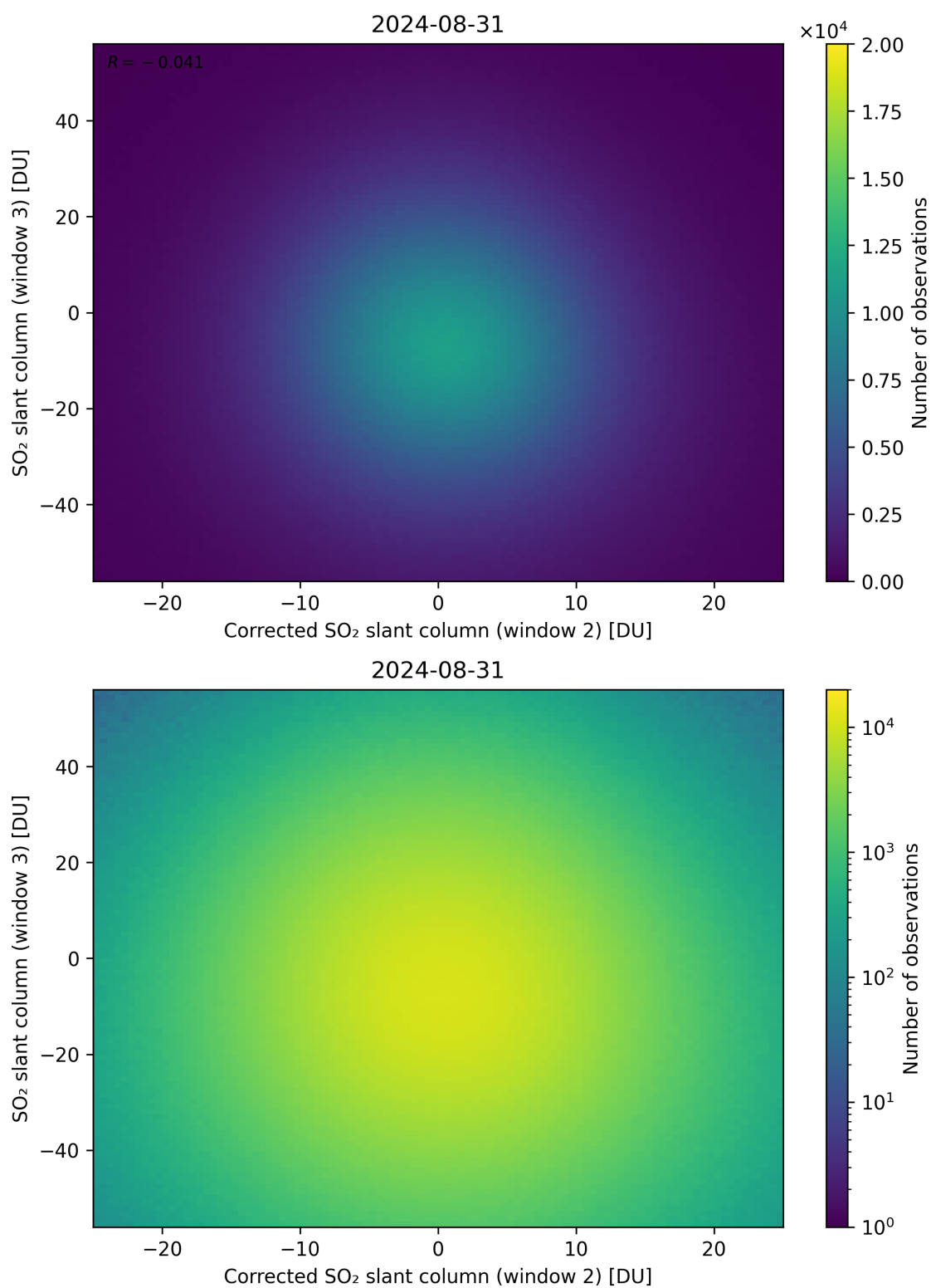
Figure 201: Scatter density plot of “Corrected SO 2 slant column (window 2)” against “SO 2 slant column (window 3)” for 2024-08-30 to 2024-09-01.
