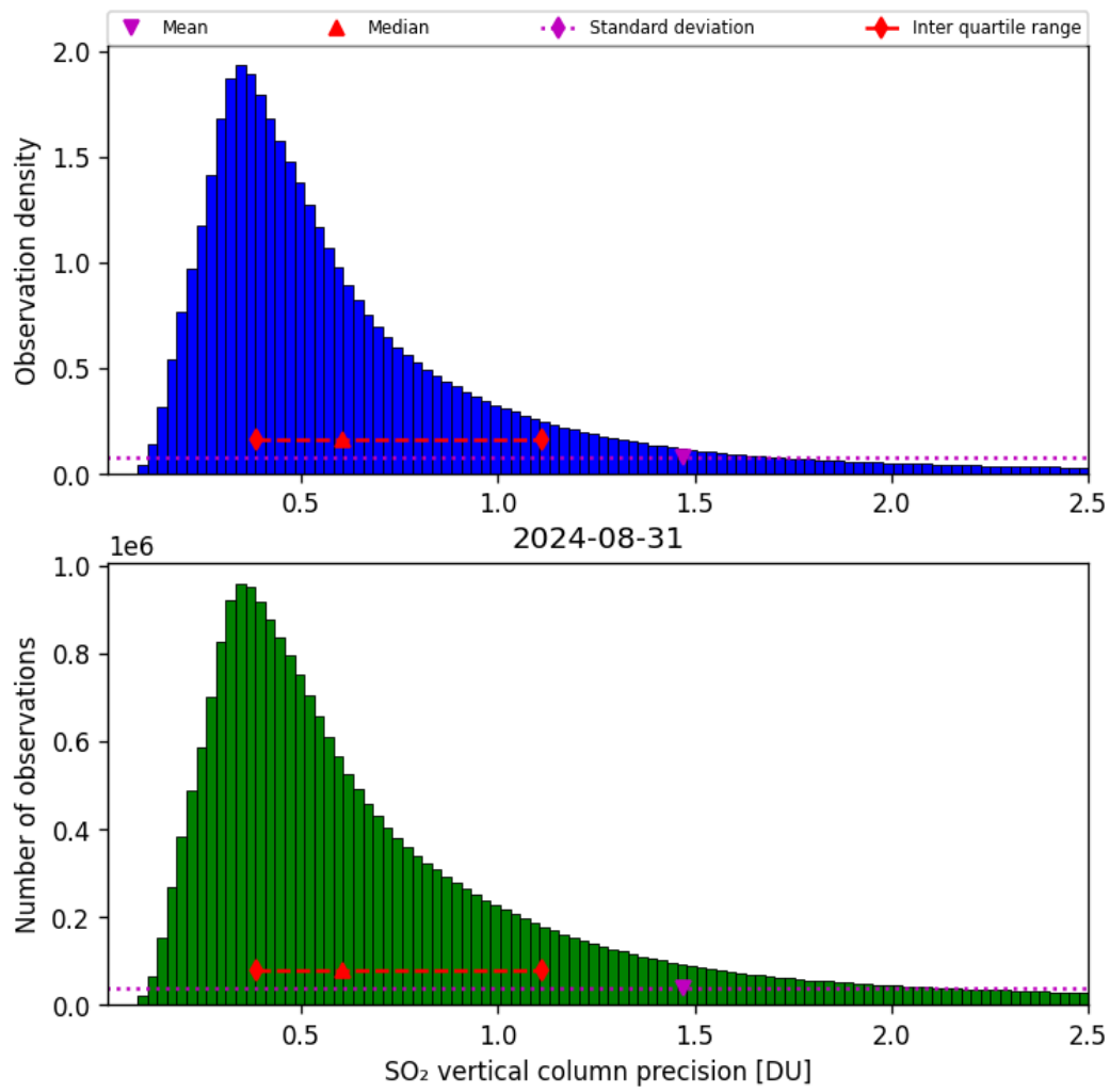
Figure 54: Histogram of “SO 2 vertical column precision” for 2024-08-30 to 2024-09-01
