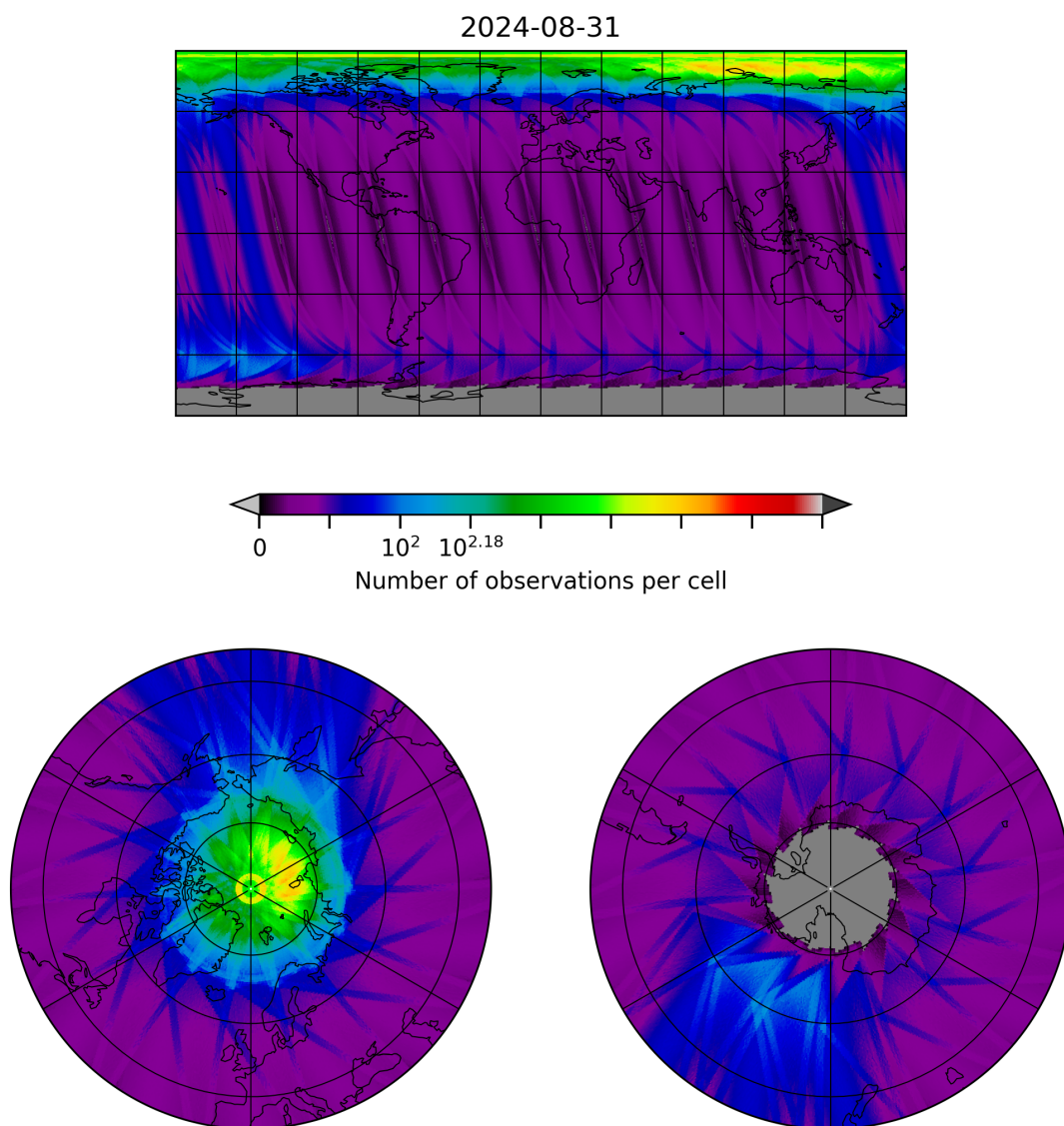
Figure 28: Map of the number of observations for 2024-08-30 to 2024-09-01
