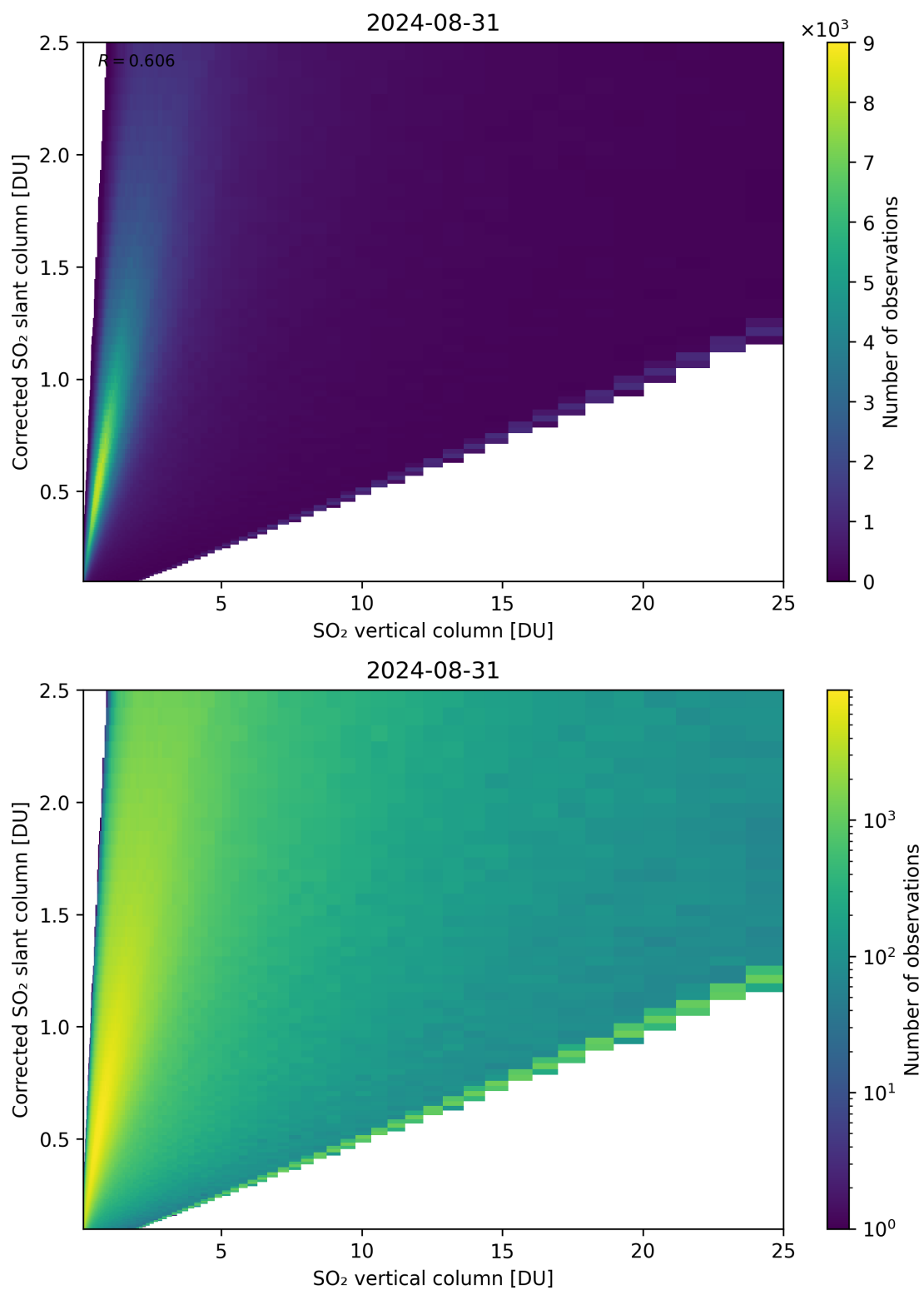
Figure 297: Scatter density plot of “SO 2 vertical column” against “Corrected SO 2 slant column” for 2024-08-30 to 2024-09-01.
