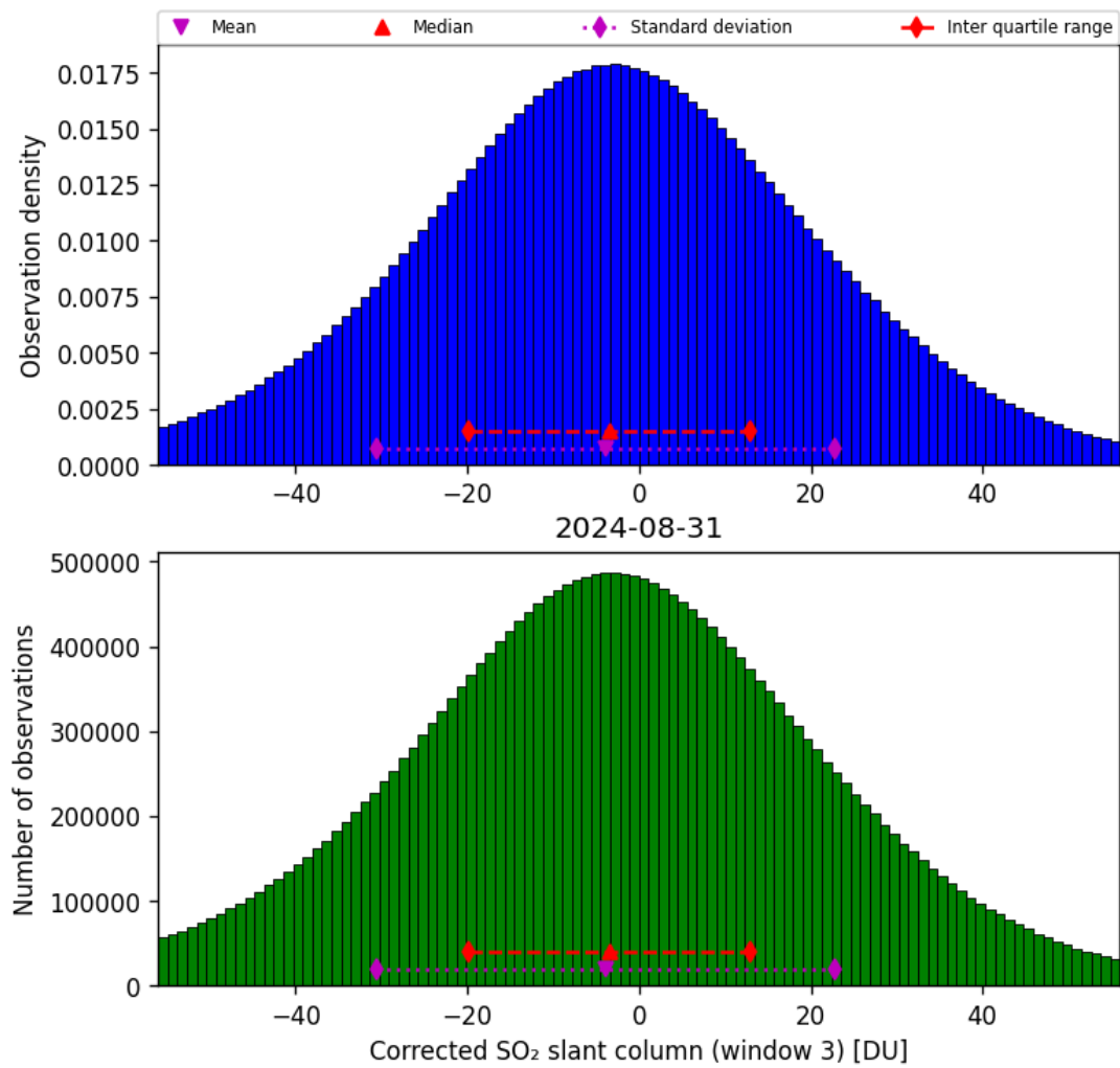
Figure 66: Histogram of “Corrected SO 2 slant column (window 3)” for 2024-08-30 to 2024-09-01
