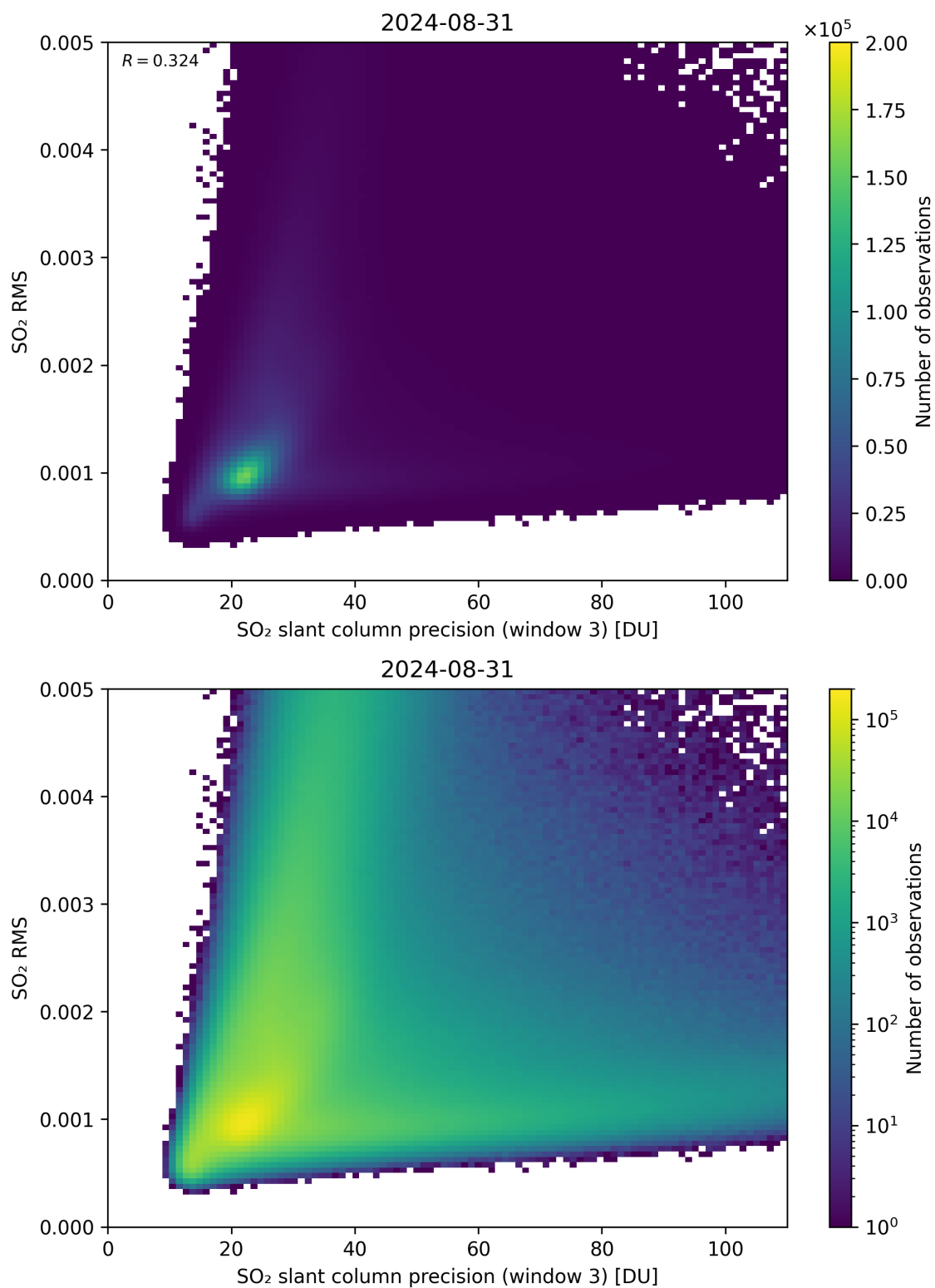
Figure 260: Scatter density plot of “SO 2 slant column precision (window 3)” against “SO 2 RMS” for 2024-08-30 to 2024-09-01.
