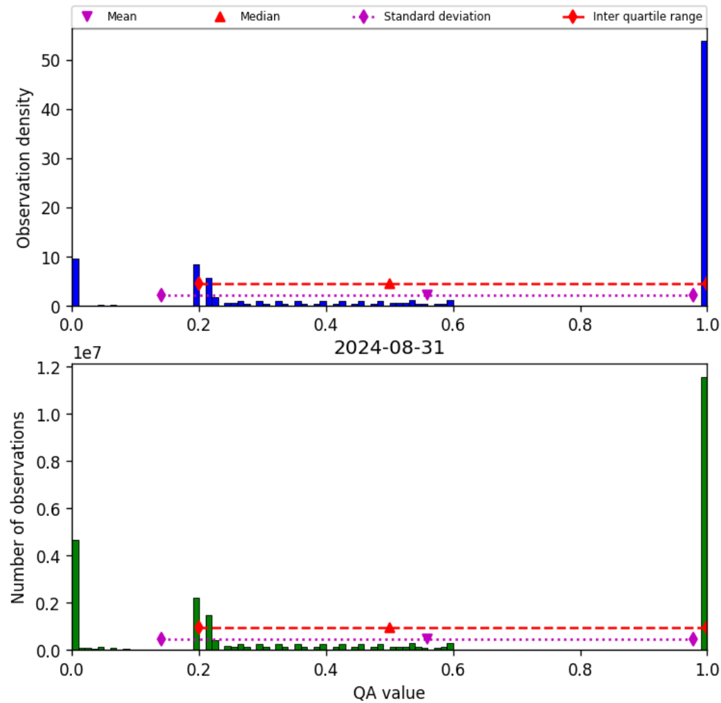
Figure 52: Histogram of “QA value” for 2024-08-30 to 2024-09-01
