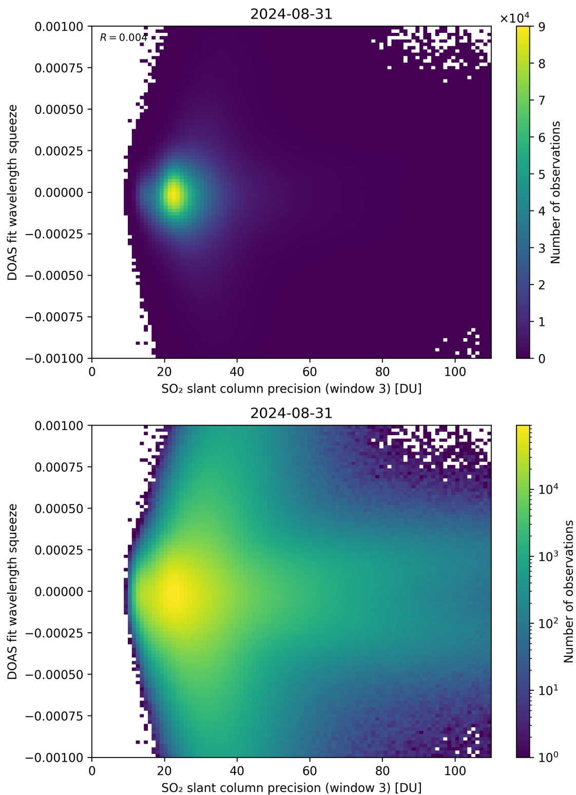
Figure 259: Scatter density plot of “SO 2 slant column precision (window 3)” against “DOAS fit wavelength squeeze” for 2024-08-30 to 2024-09-01.
