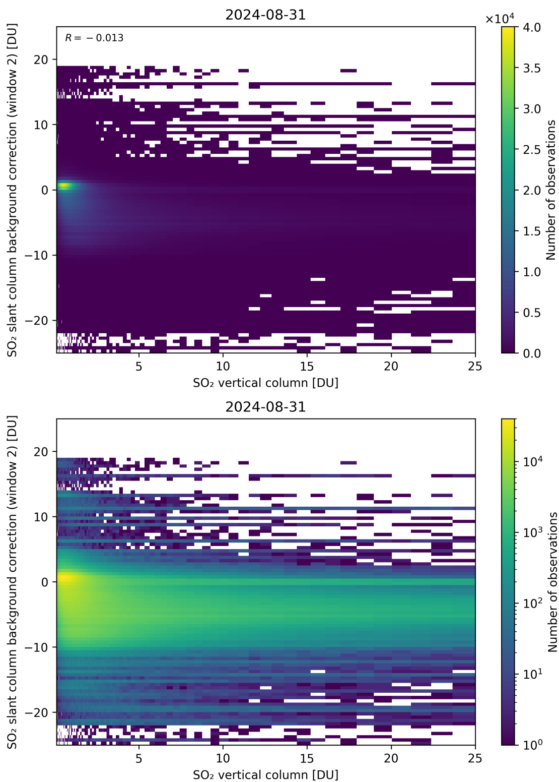
Figure 274: Scatter density plot of “SO 2 vertical column” against “SO 2 slant column background correction (window 2)” for 2024-08-30 to 2024-09-01.
