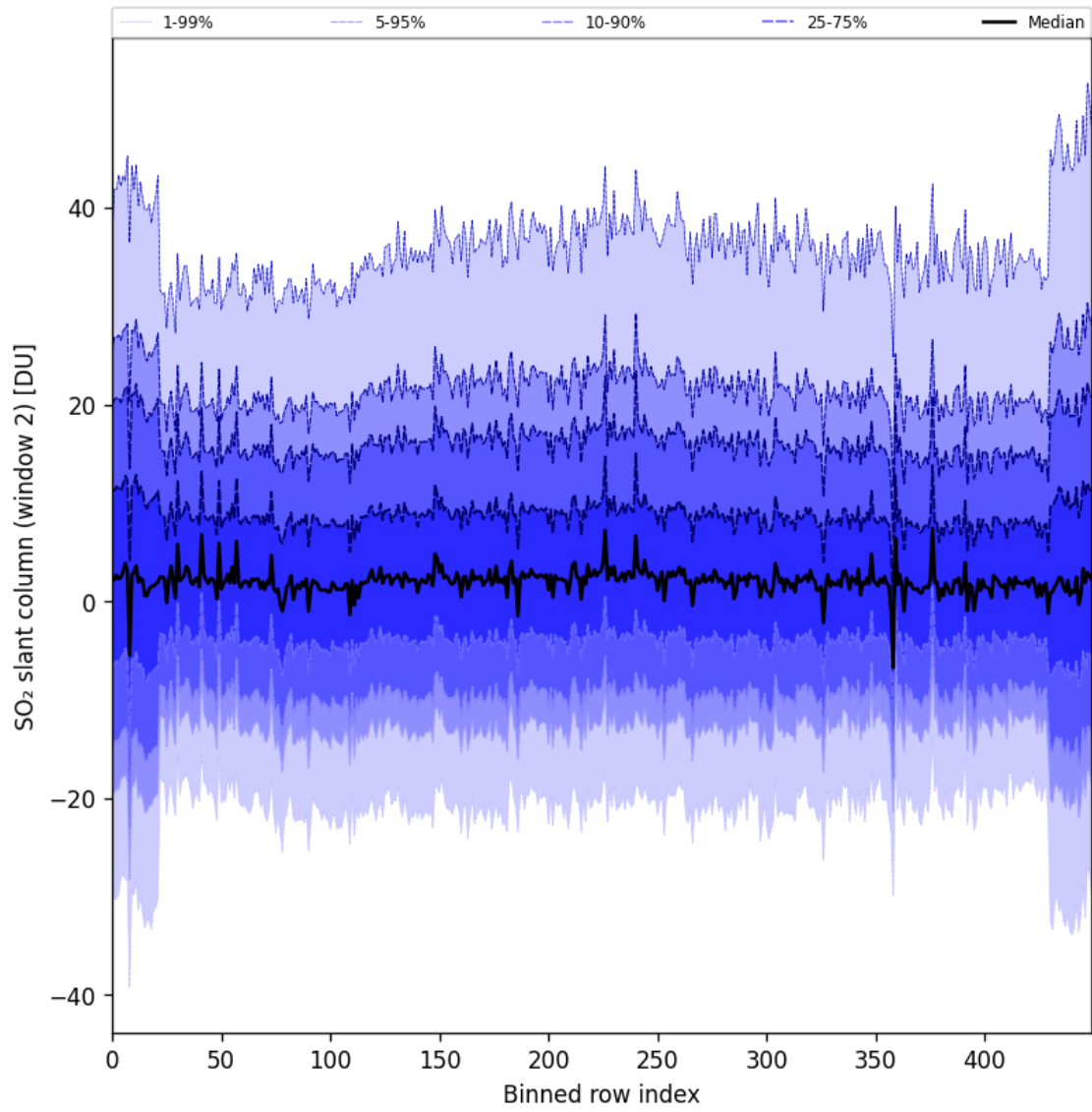
Figure 83: Along track statistics of “SO 2 slant column (window 2)” for 2024-08-30 to 2024-09-01
