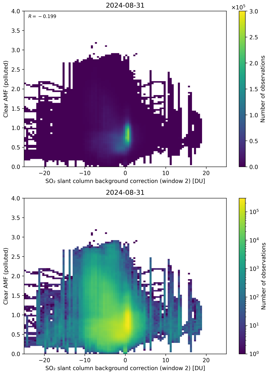
Figure 115: Scatter density plot of “SO 2 slant column background correction (window 2)” against “Clear AMF (polluted)” for 2024-08-30 to 2024-09-01.
