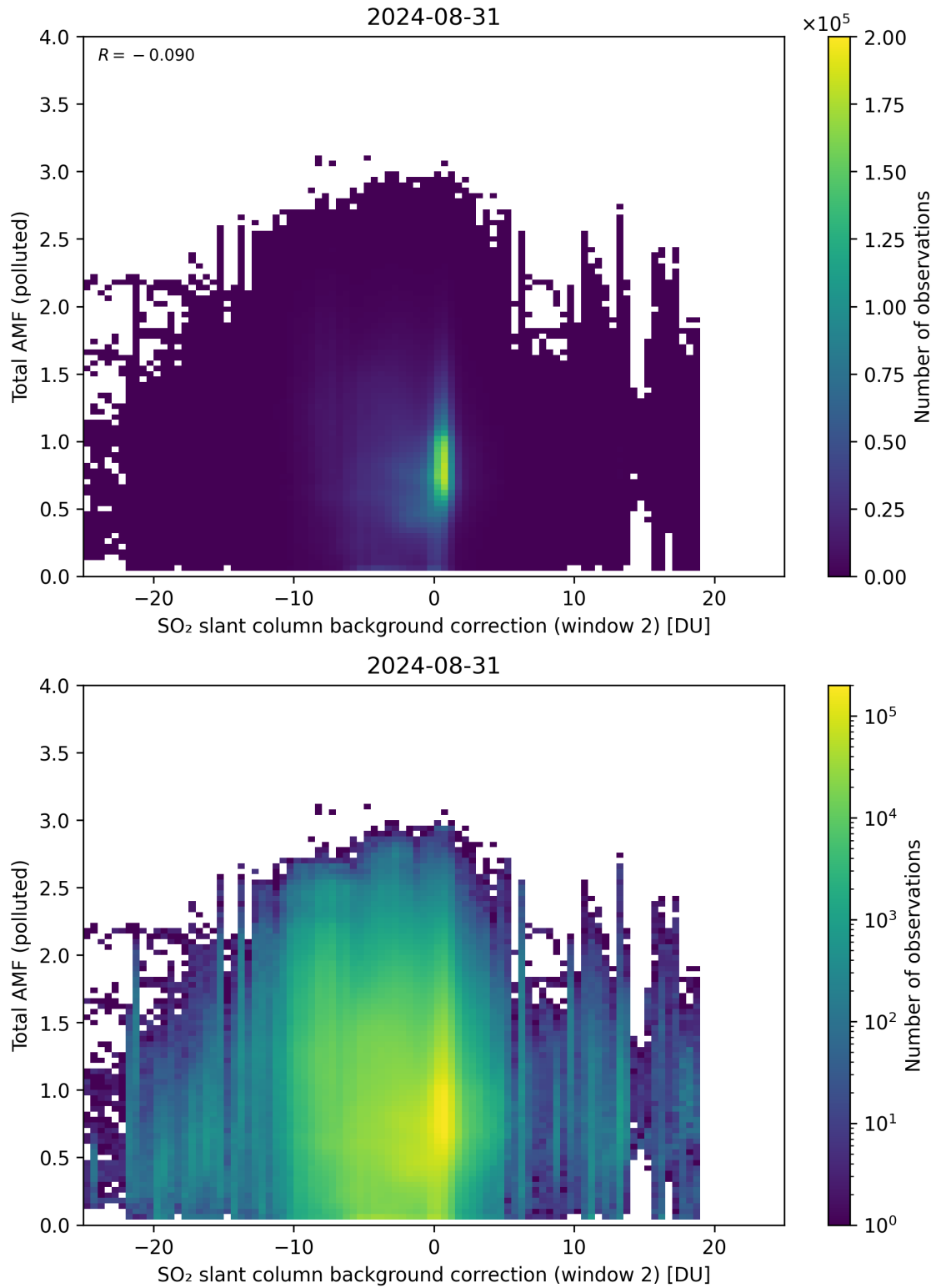
Figure 119: Scatter density plot of “SO 2 slant column background correction (window 2)” against “Total AMF (polluted)” for 2024-08-30 to 2024-09-01.
