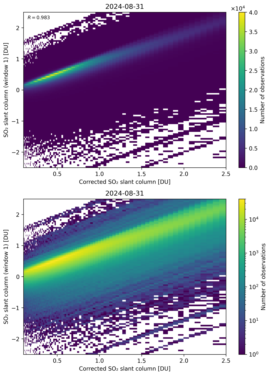
Figure 187: Scatter density plot of “Corrected SO 2 slant column” against “SO 2 slant column (window 1)” for 2024-08-30 to 2024-09-01.
