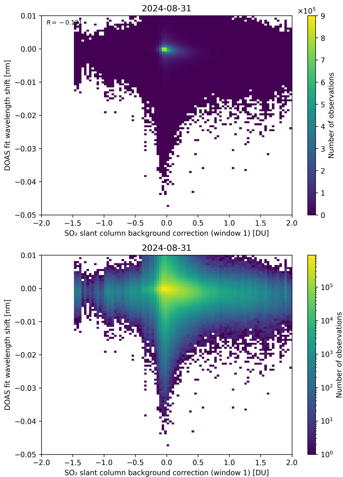
Figure 100: Scatter density plot of “SO 2 slant column background correction (window 1)” against “DOAS fit wavelength shift” for 2024-08-30 to 2024-09-01.
