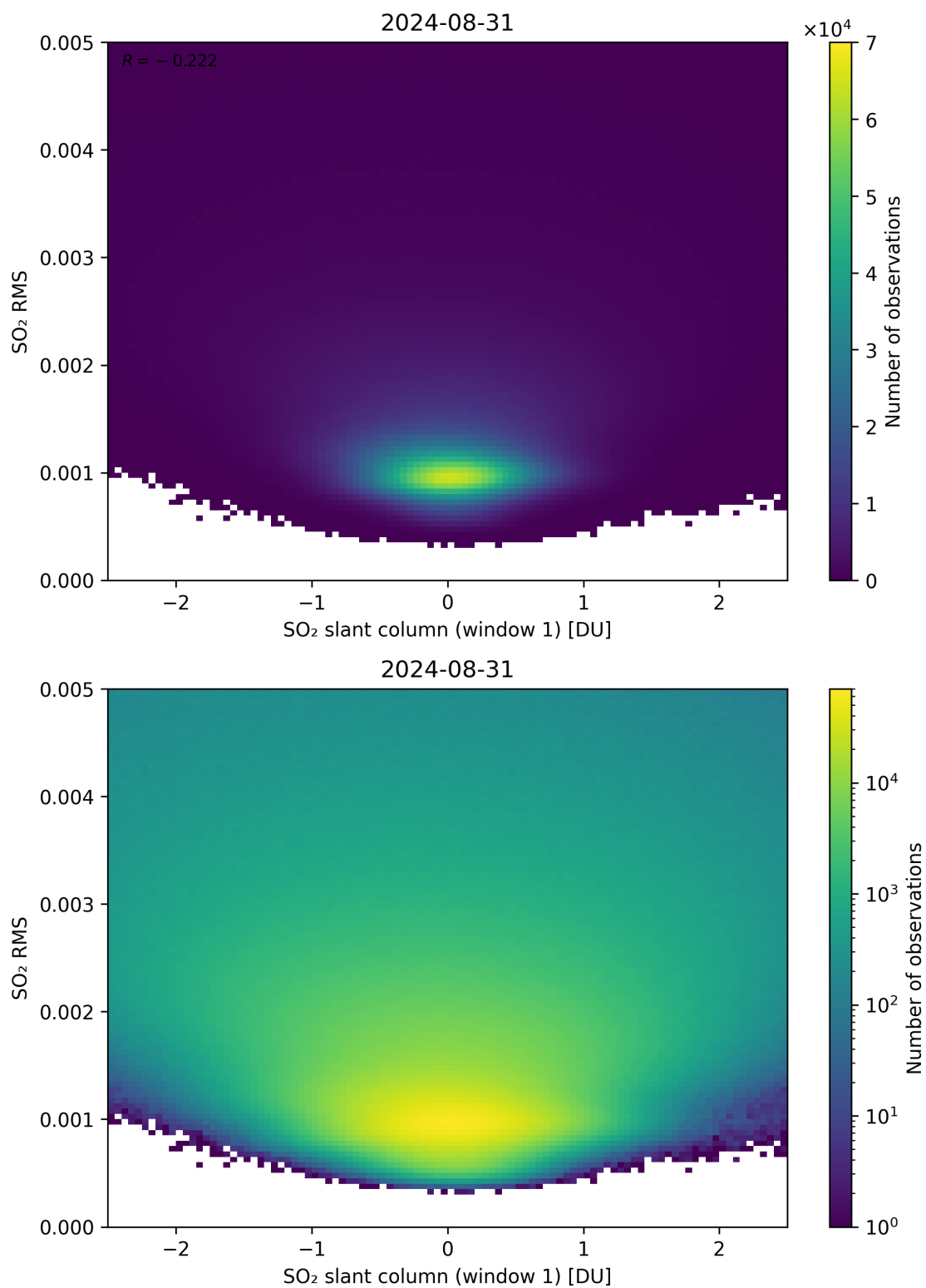
Figure 217: Scatter density plot of “SO 2 slant column (window 1)” against “SO 2 RMS” for 2024-08-30 to 2024-09-01.
