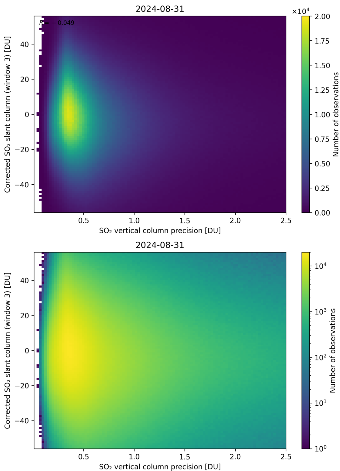
Figure 288: Scatter density plot of “SO 2 vertical column precision” against “Corrected SO 2 slant column (window 3)” for 2024-08-30 to 2024-09-01.
