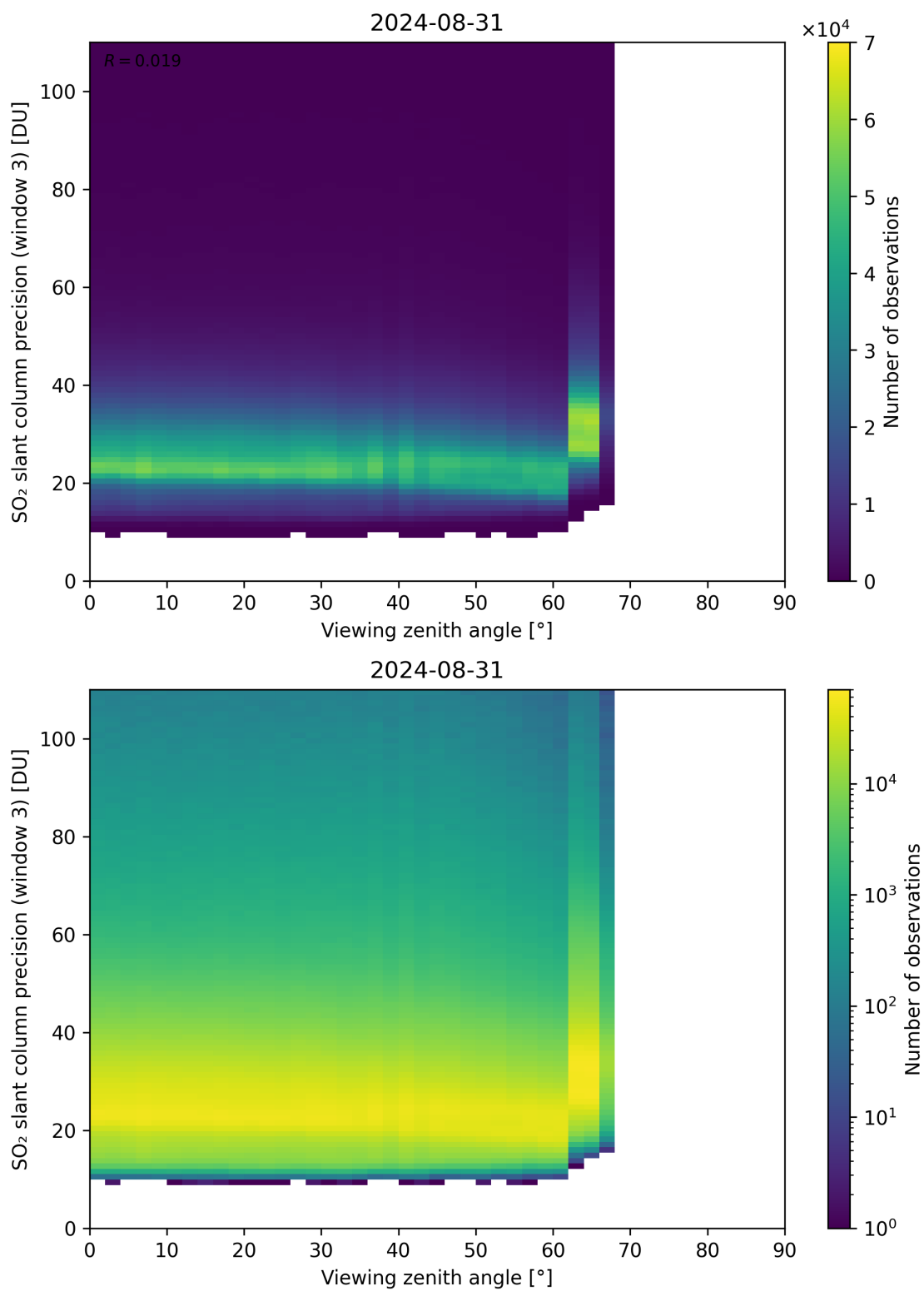
Figure 324: Scatter density plot of “Viewing zenith angle” against “SO 2 slant column precision (window 3)” for 2024-08-30 to 2024-09-01.
