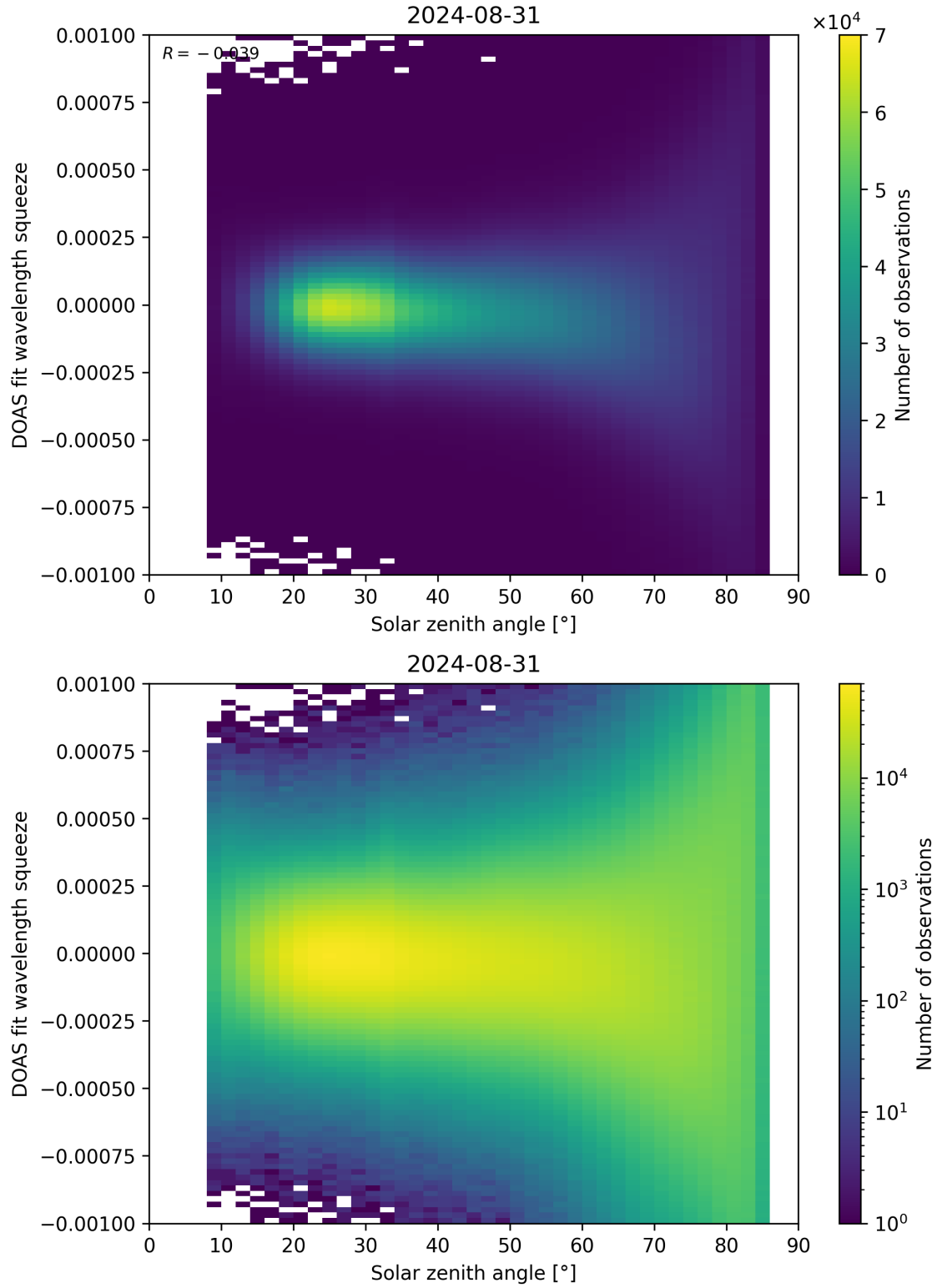
Figure 162: Scatter density plot of “Solar zenith angle” against “DOAS fit wavelength squeeze” for 2024-08-30 to 2024-09-01.
