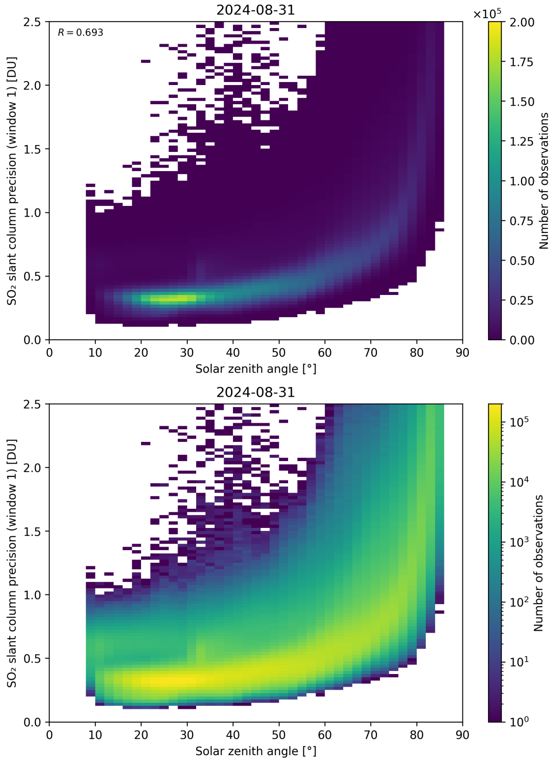
Figure 170: Scatter density plot of “Solar zenith angle” against “SO 2 slant column precision (window 1)” for 2024-08-30 to 2024-09-01.
