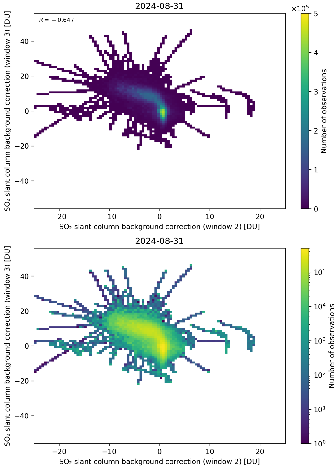
Figure 111: Scatter density plot of “SO 2 slant column background correction (window 2)” against “SO 2 slant column background correction (window 3)” for 2024-08-30 to 2024-09-01.
