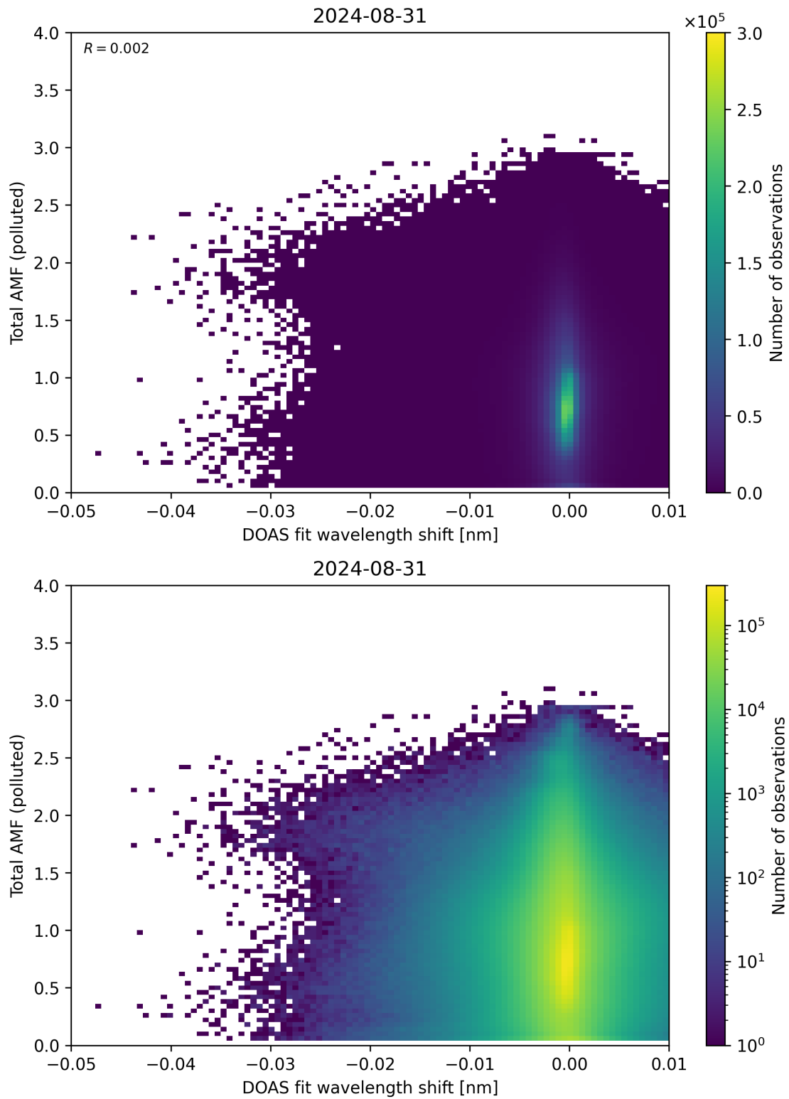
Figure 130: Scatter density plot of “DOAS fit wavelength shift” against “Total AMF (polluted)” for 2024-08-30 to 2024-09-01.
