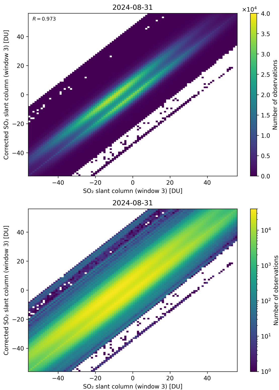
Figure 266: Scatter density plot of “SO 2 slant column (window 3)” against “Corrected SO 2 slant column (window 3)” for 2024-08-30 to 2024-09-01.
