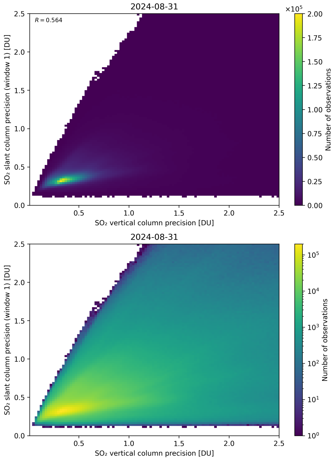
Figure 290: Scatter density plot of “SO 2 vertical column precision” against “SO 2 slant column precision (window 1)” for 2024-08-30 to 2024-09-01.
