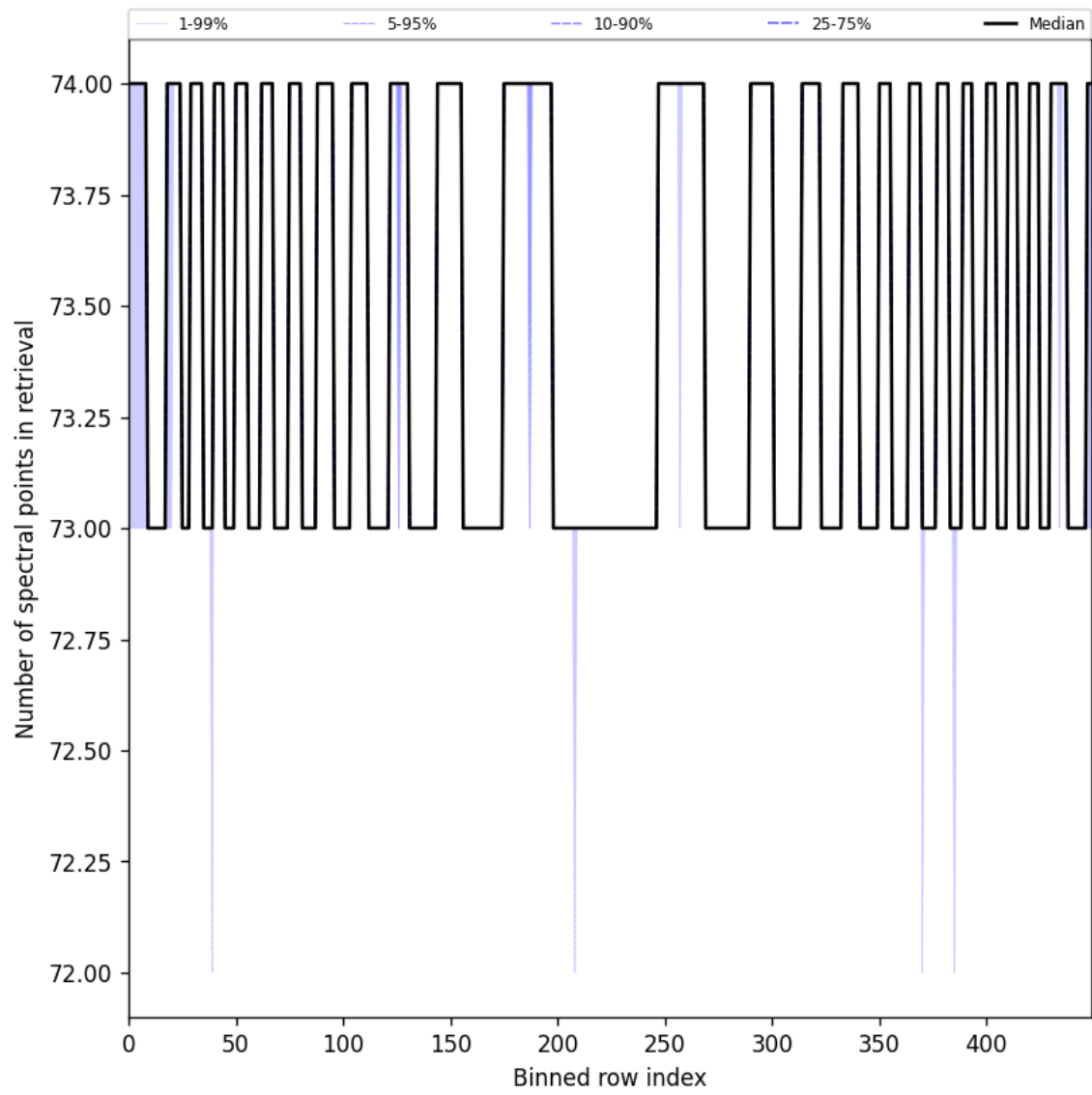
Figure 97: Along track statistics of “Number of spectral points in retrieval” for 2024-08-30 to 2024-09-01
