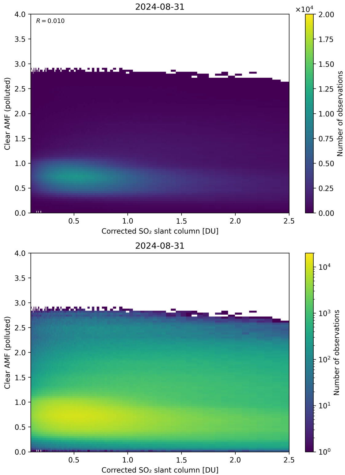
Figure 184: Scatter density plot of “Corrected SO 2 slant column” against “Clear AMF (polluted)” for 2024-08-30 to 2024-09-01.
