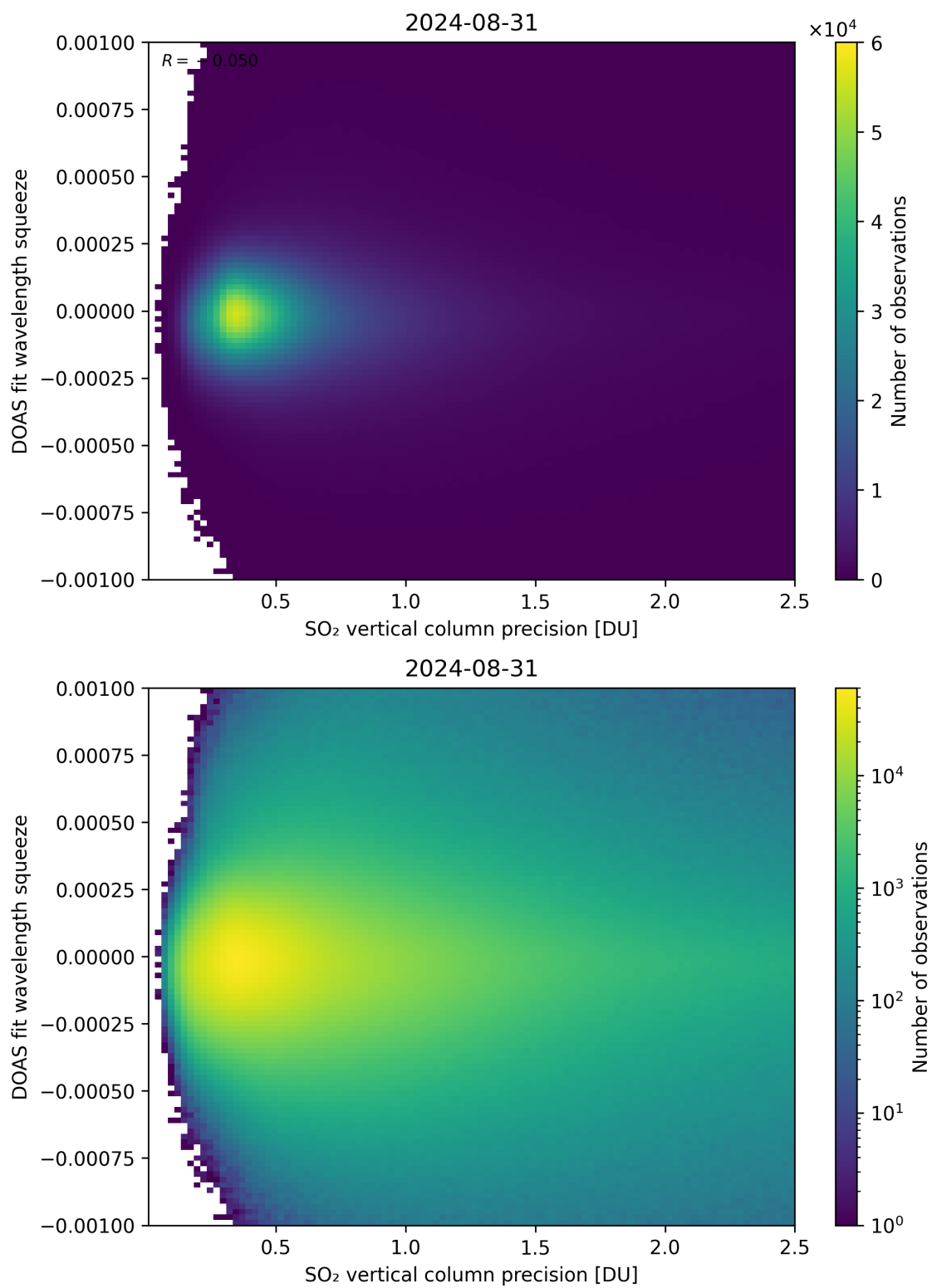
Figure 283: Scatter density plot of “SO 2 vertical column precision” against “DOAS fit wavelength squeeze” for 2024-08-30 to 2024-09-01.
