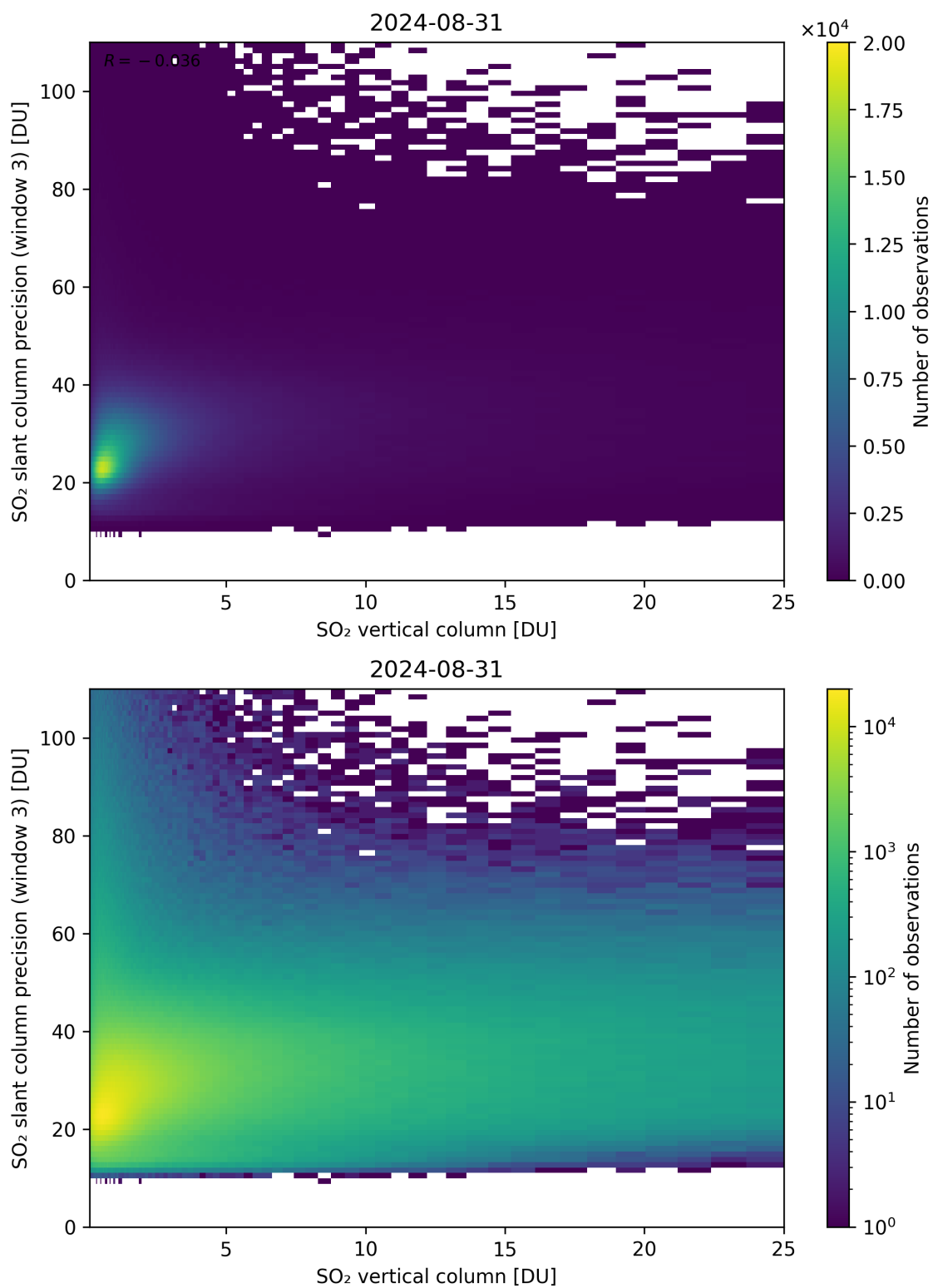
Figure 304: Scatter density plot of “SO 2 vertical column” against “SO 2 slant column precision (window 3)” for 2024-08-30 to 2024-09-01.
