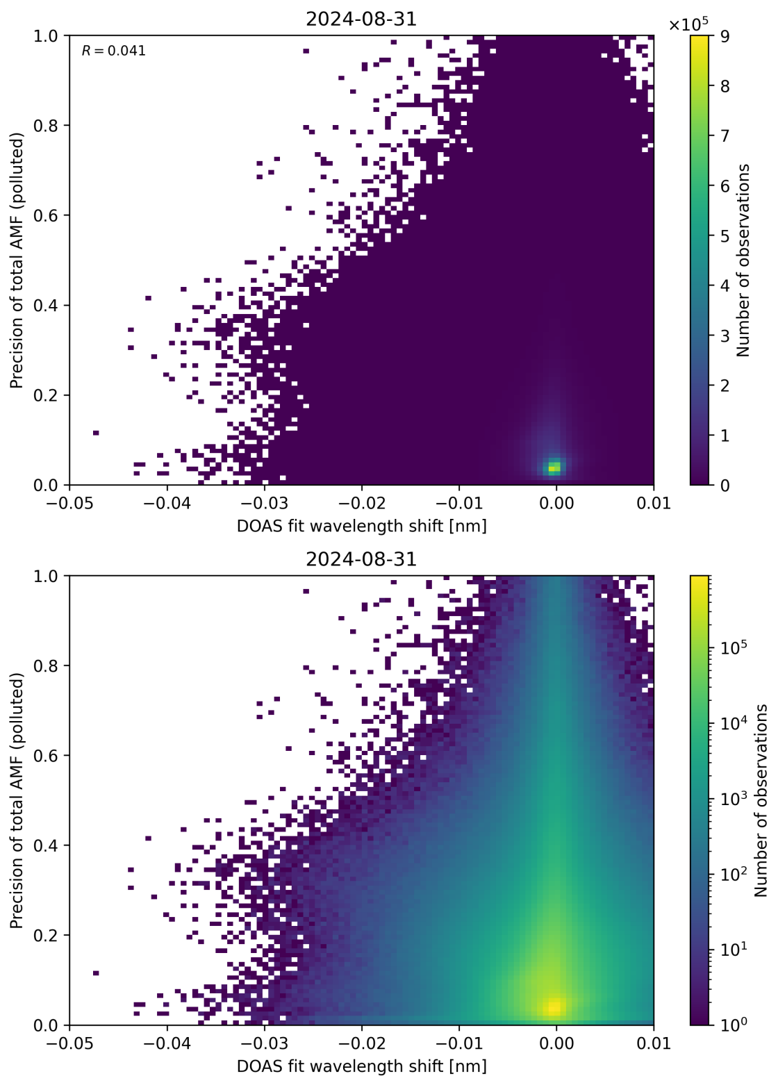
Figure 131: Scatter density plot of “DOAS fit wavelength shift” against “Precision of total AMF (polluted)” for 2024-08-30 to 2024-09-01.
