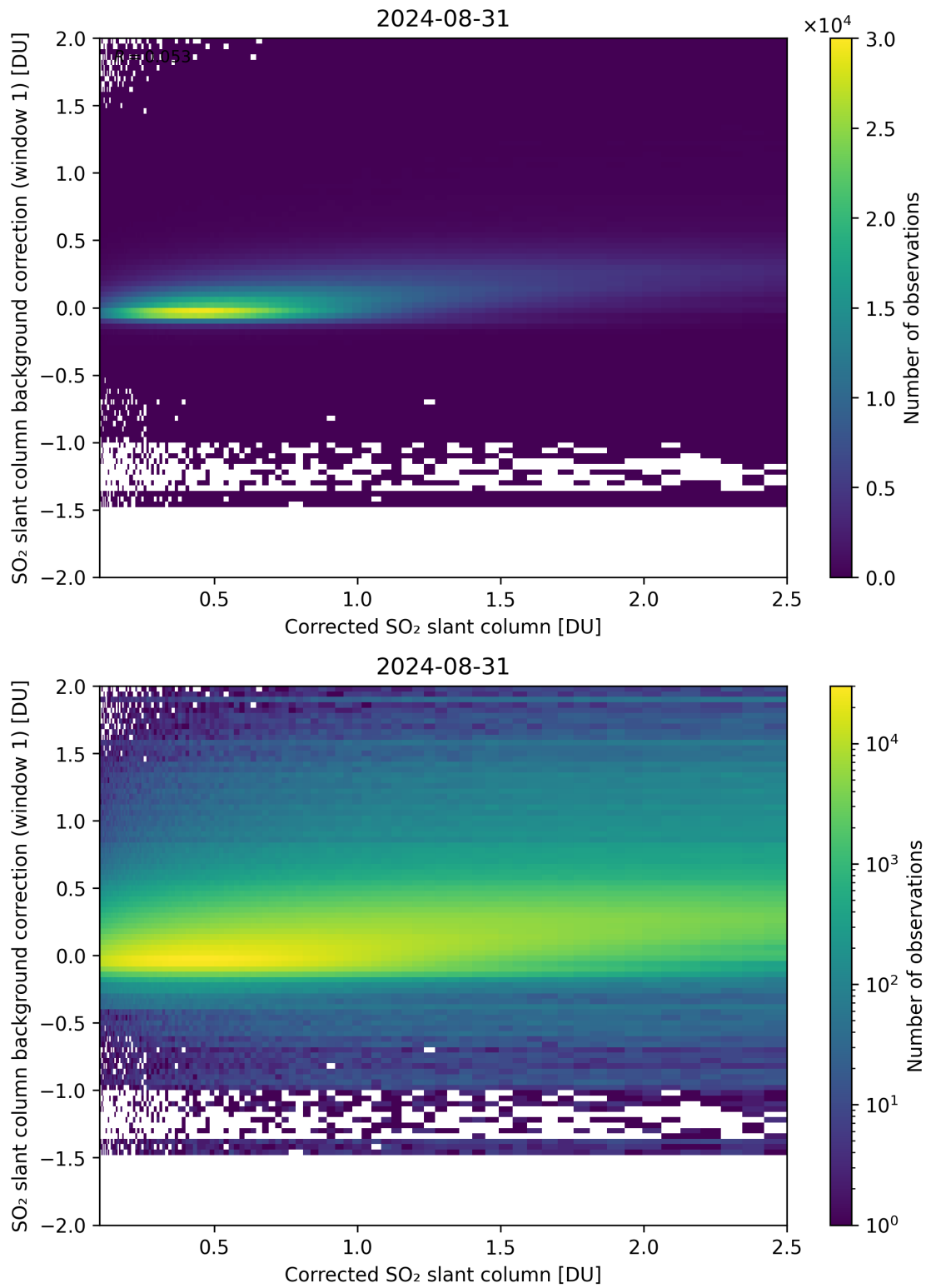
Figure 178: Scatter density plot of “Corrected SO 2 slant column” against “SO 2 slant column background correction (window 1)” for 2024-08-30 to 2024-09-01.
