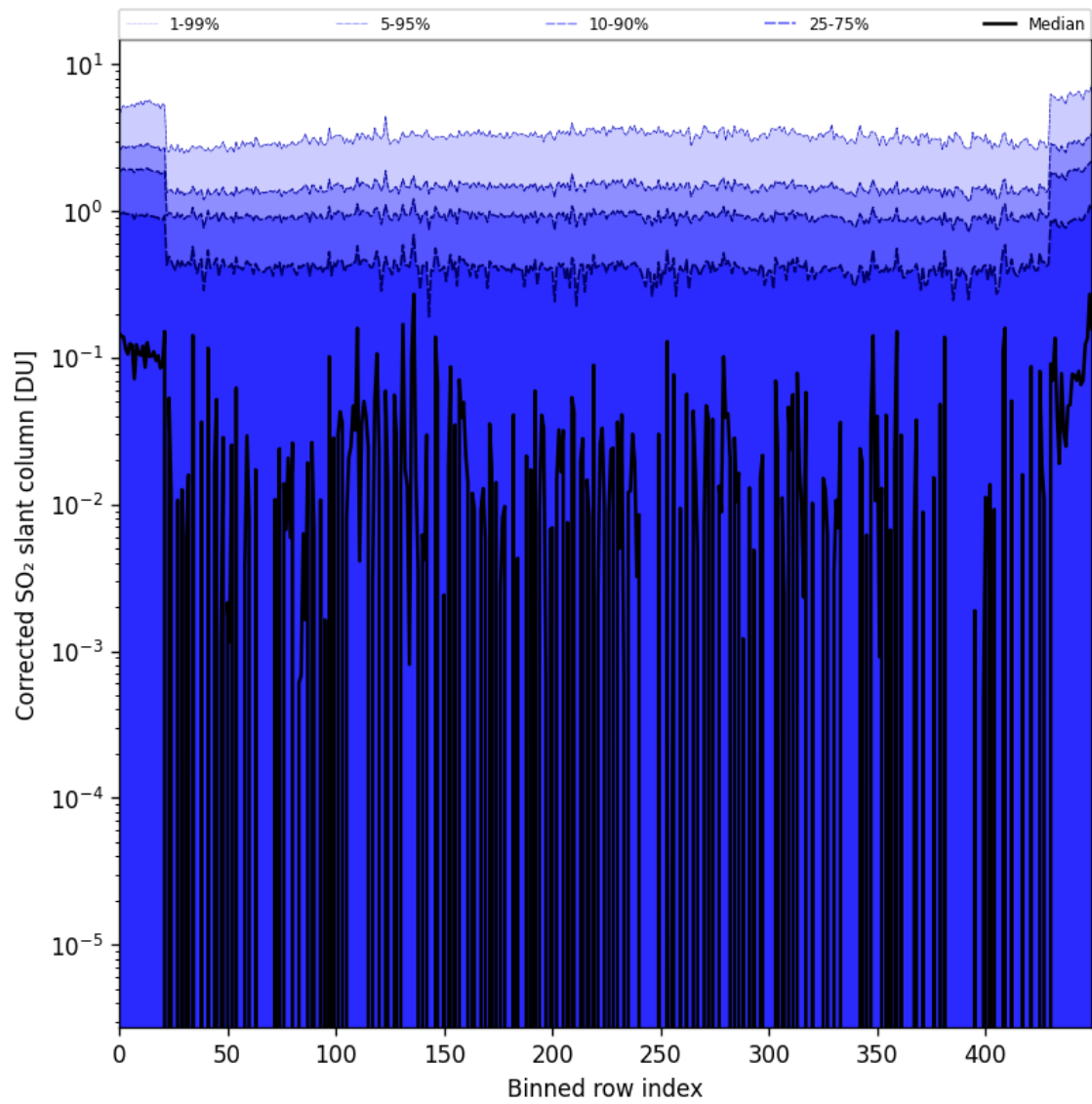
Figure 78: Along track statistics of “Corrected SO 2 slant column” for 2024-08-30 to 2024-09-01
