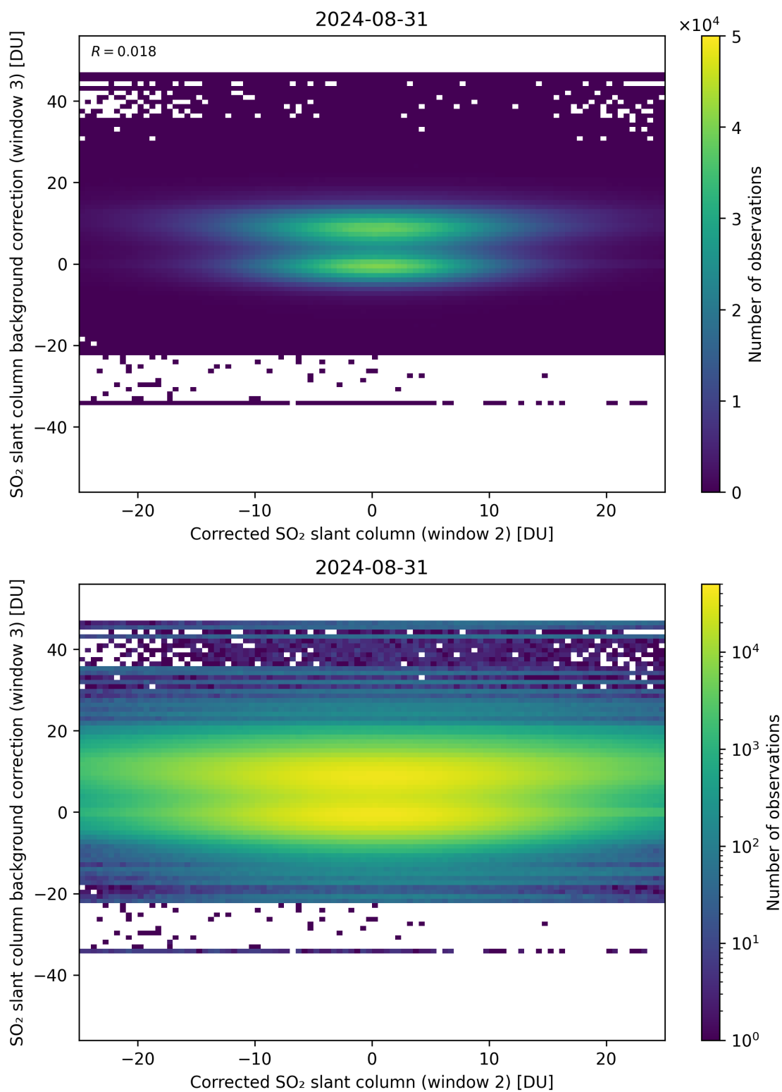
Figure 195: Scatter density plot of “Corrected SO 2 slant column (window 2)” against “SO 2 slant column background correction (window 3)” for 2024-08-30 to 2024-09-01.
