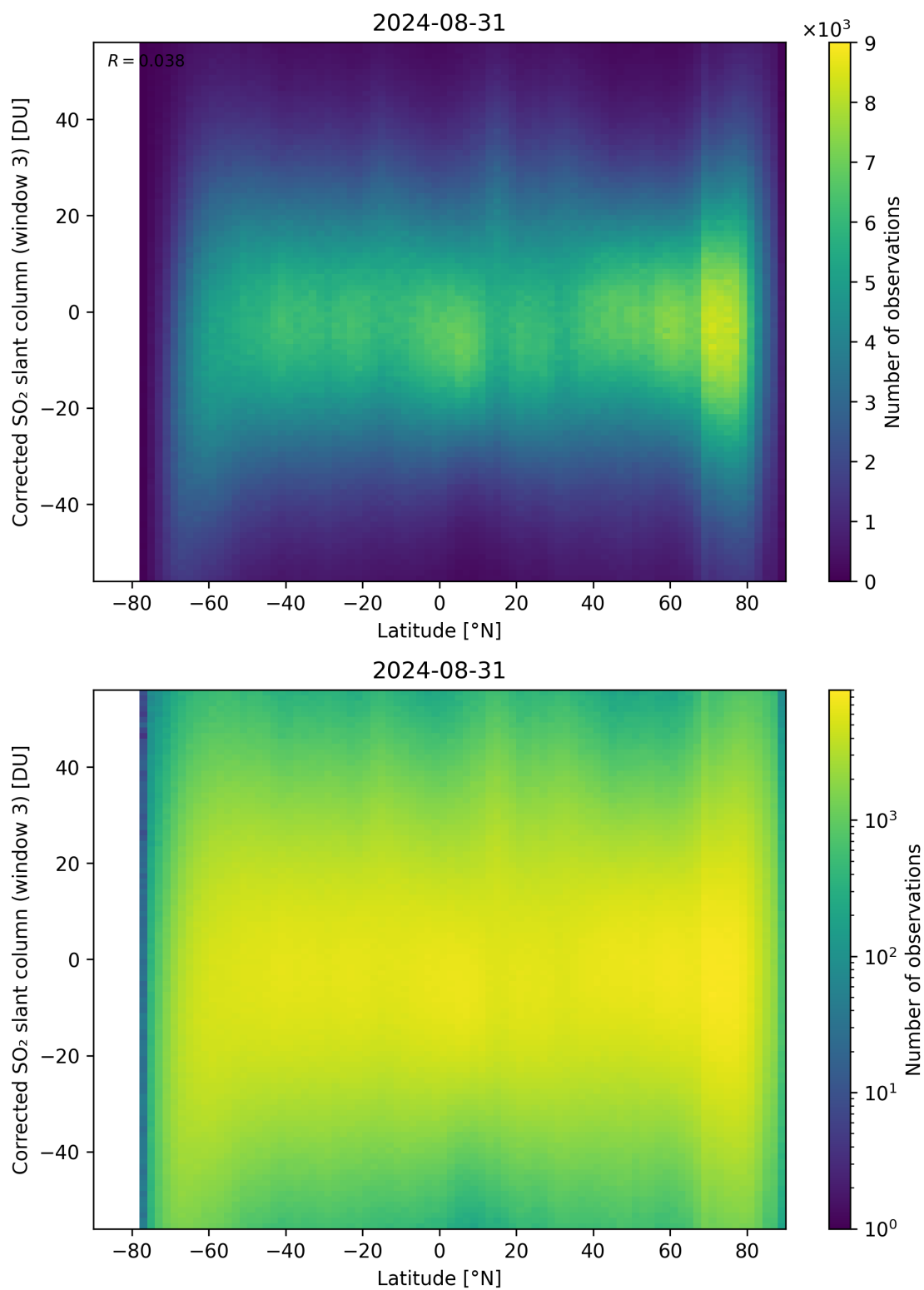
Figure 148: Scatter density plot of “Latitude” against “Corrected SO 2 slant column (window 3)” for 2024-08-30 to 2024-09-01.
