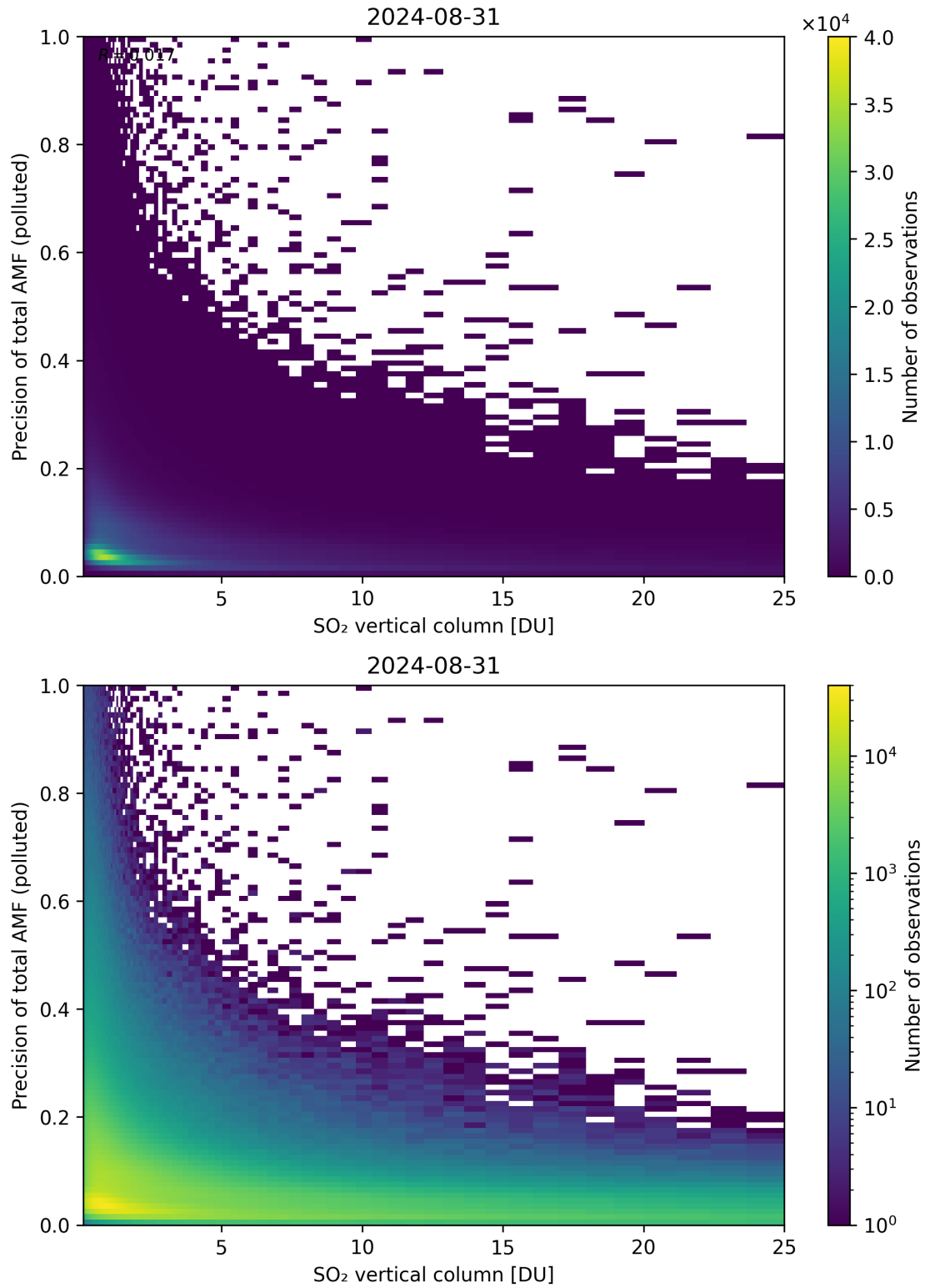
Figure 306: Scatter density plot of “SO 2 vertical column” against “Precision of total AMF (polluted)” for 2024-08-30 to 2024-09-01.
