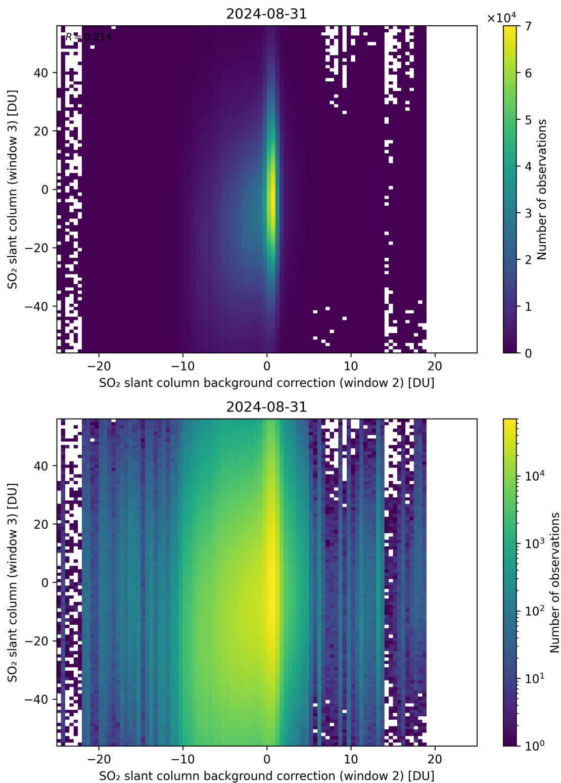
Figure 117: Scatter density plot of “SO 2 slant column background correction (window 2)” against “SO 2 slant column (window 3)” for 2024-08-30 to 2024-09-01.
