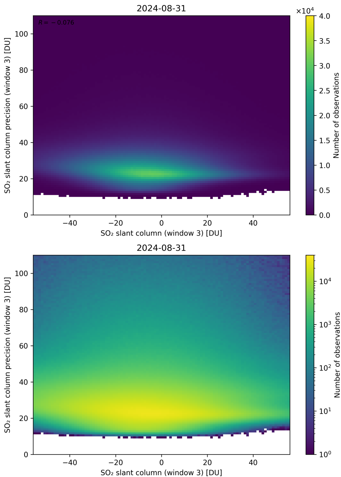
Figure 267: Scatter density plot of “SO 2 slant column (window 3)” against “SO 2 slant column precision (window 3)” for 2024-08-30 to 2024-09-01.
