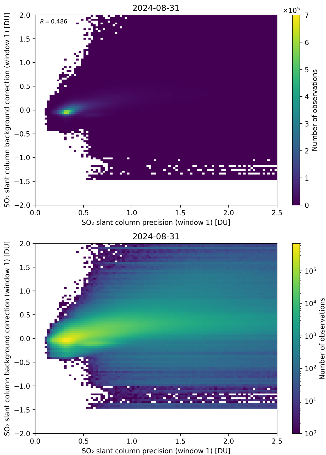
Figure 218: Scatter density plot of “SO 2 slant column precision (window 1)” against “SO 2 slant column background correction (window 1)” for 2024-08-30 to 2024-09-01.
