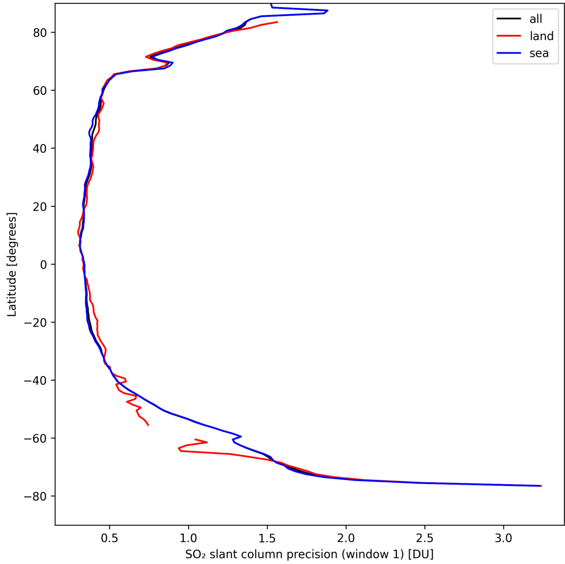
Figure 34: Zonal average of “SO 2 slant column precision (window 1)” for 2024-08-30 to 2024-09-01.
