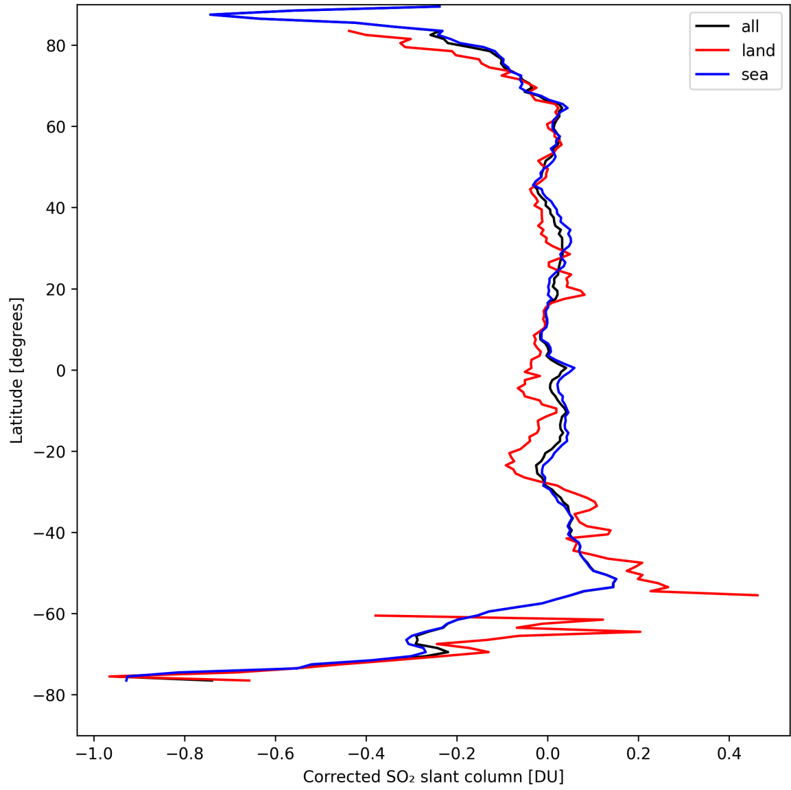
Figure 32: Zonal average of “Corrected SO 2 slant column” for 2024-08-30 to 2024-09-01.
