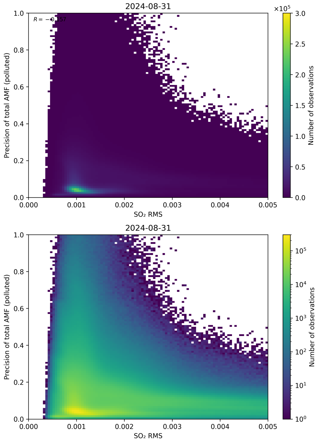
Figure 138: Scatter density plot of “SO 2 RMS” against “Precision of total AMF (polluted)” for 2024-08-30 to 2024-09-01.
