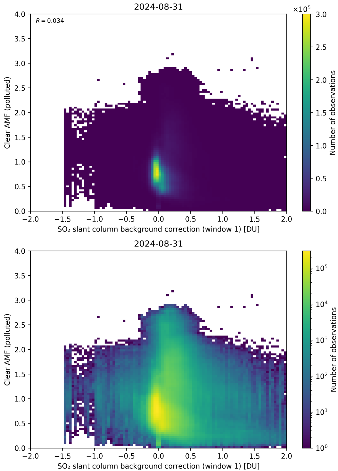
Figure 103: Scatter density plot of “SO 2 slant column background correction (window 1)” against “Clear AMF (polluted)” for 2024-08-30 to 2024-09-01.
