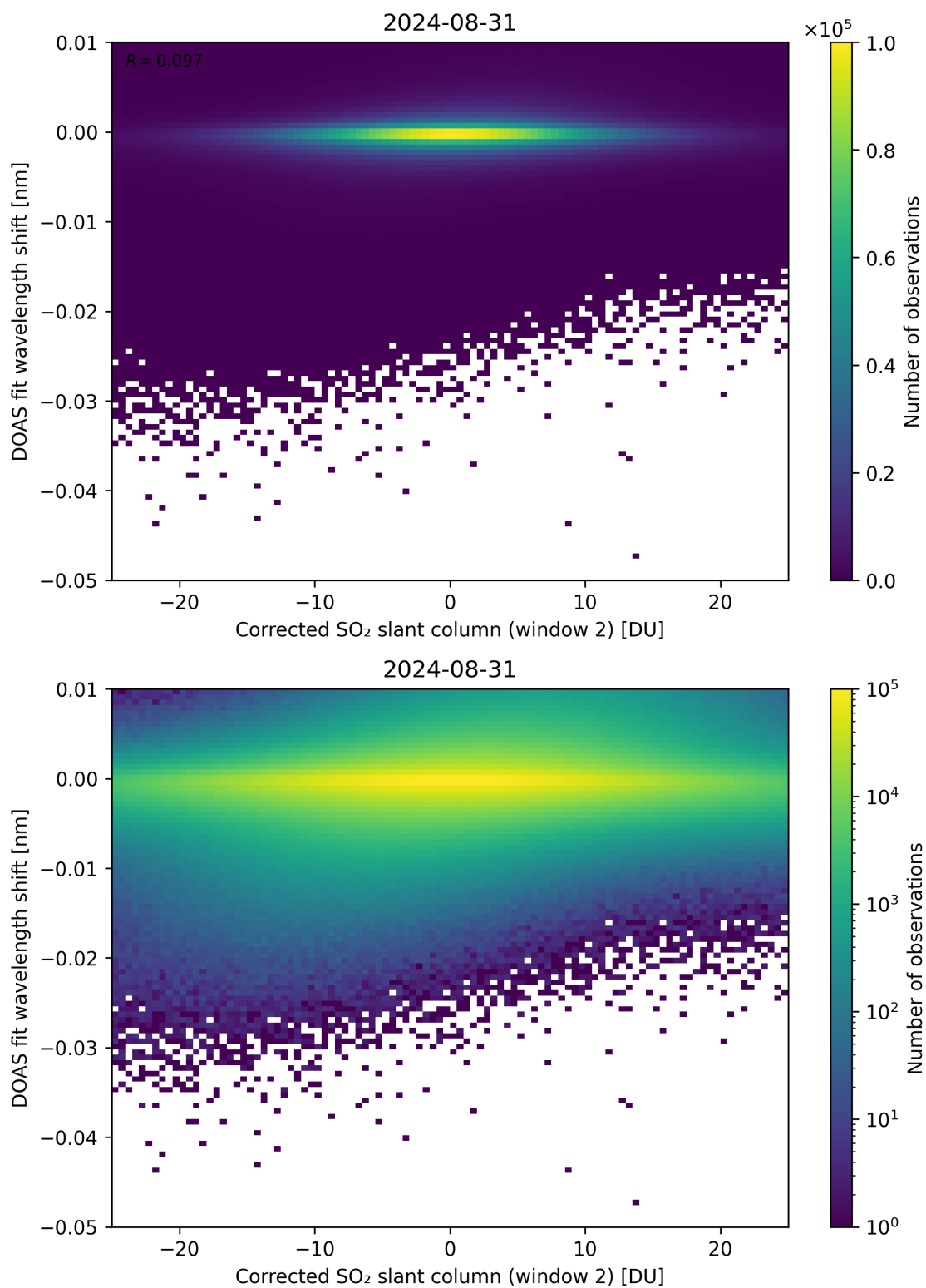
Figure 196: Scatter density plot of “Corrected SO 2 slant column (window 2)” against “DOAS fit wavelength shift” for 2024-08-30 to 2024-09-01.
