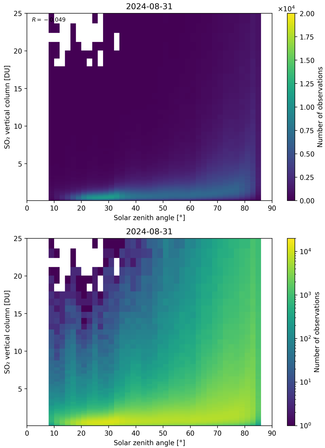
Figure 176: Scatter density plot of “Solar zenith angle” against “SO 2 vertical column” for 2024-08-30 to 2024-09-01.
