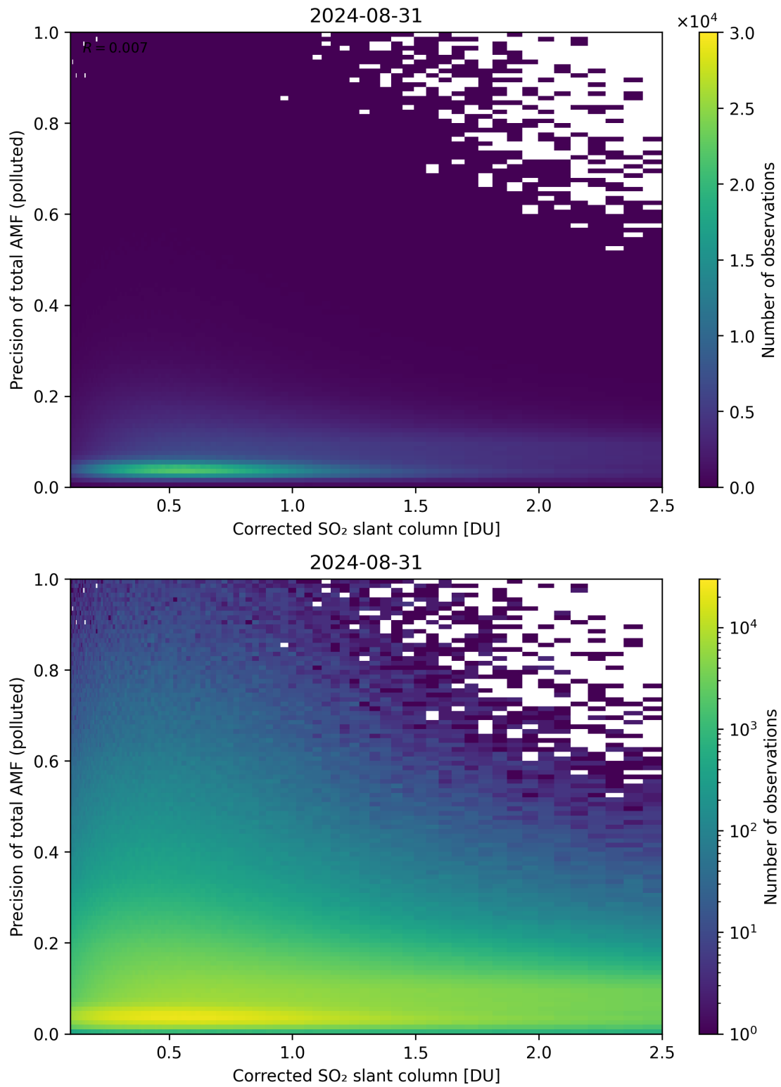
Figure 193: Scatter density plot of “Corrected SO 2 slant column” against “Precision of total AMF (polluted)” for 2024-08-30 to 2024-09-01.
