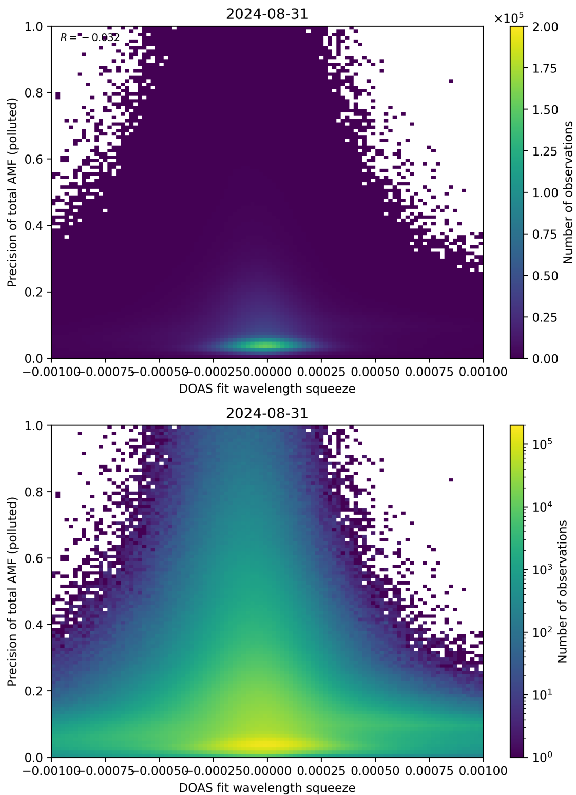
Figure 135: Scatter density plot of “DOAS fit wavelength squeeze” against “Precision of total AMF (polluted)” for 2024-08-30 to 2024-09-01.
