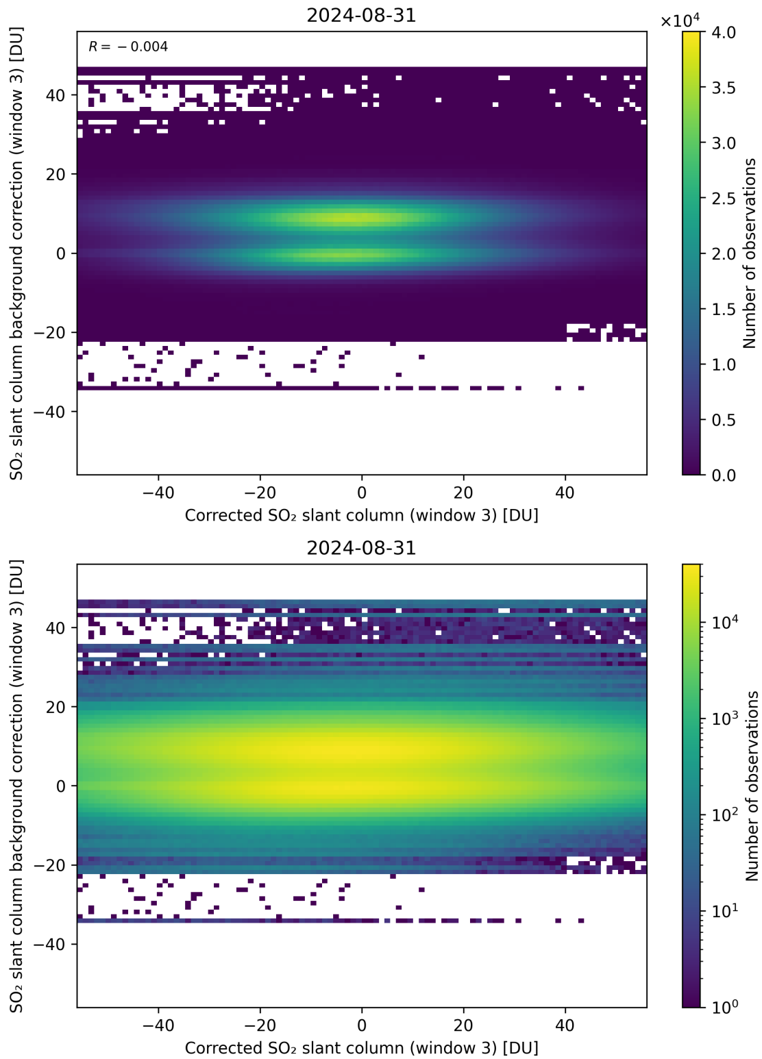
Figure 205: Scatter density plot of “Corrected SO 2 slant column (window 3)” against “SO 2 slant column background correction (window 3)” for 2024-08-30 to 2024-09-01.
