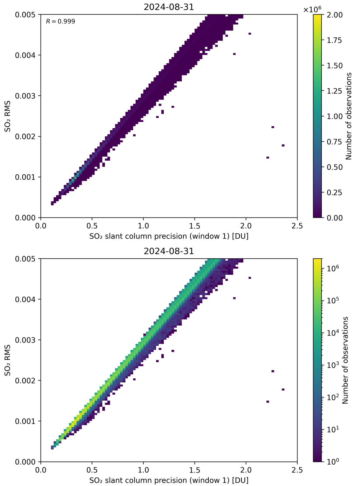
Figure 223: Scatter density plot of “SO 2 slant column precision (window 1)” against “SO 2 RMS” for 2024-08-30 to 2024-09-01.
