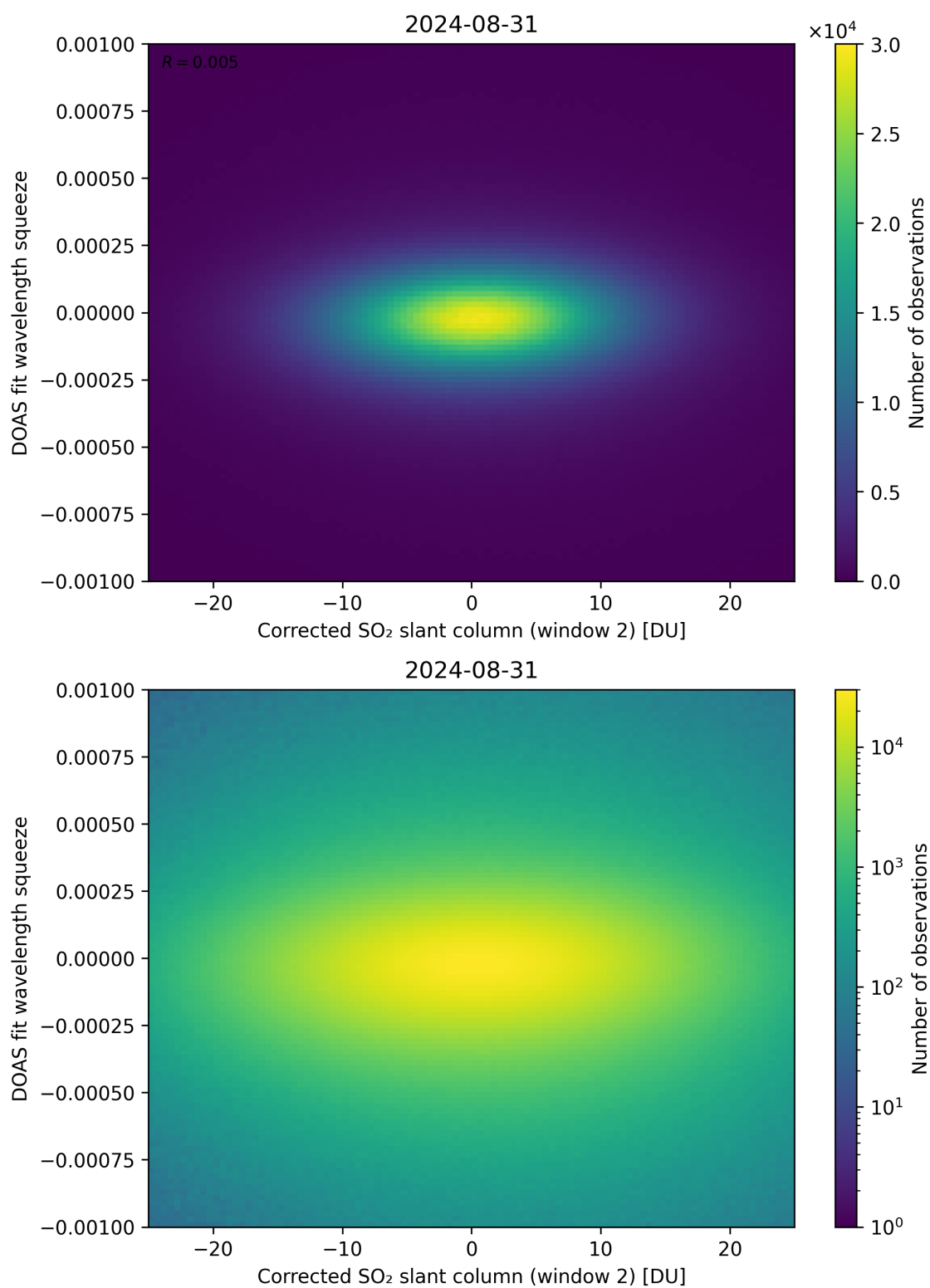
Figure 197: Scatter density plot of “Corrected SO 2 slant column (window 2)” against “DOAS fit wavelength squeeze” for 2024-08-30 to 2024-09-01.
