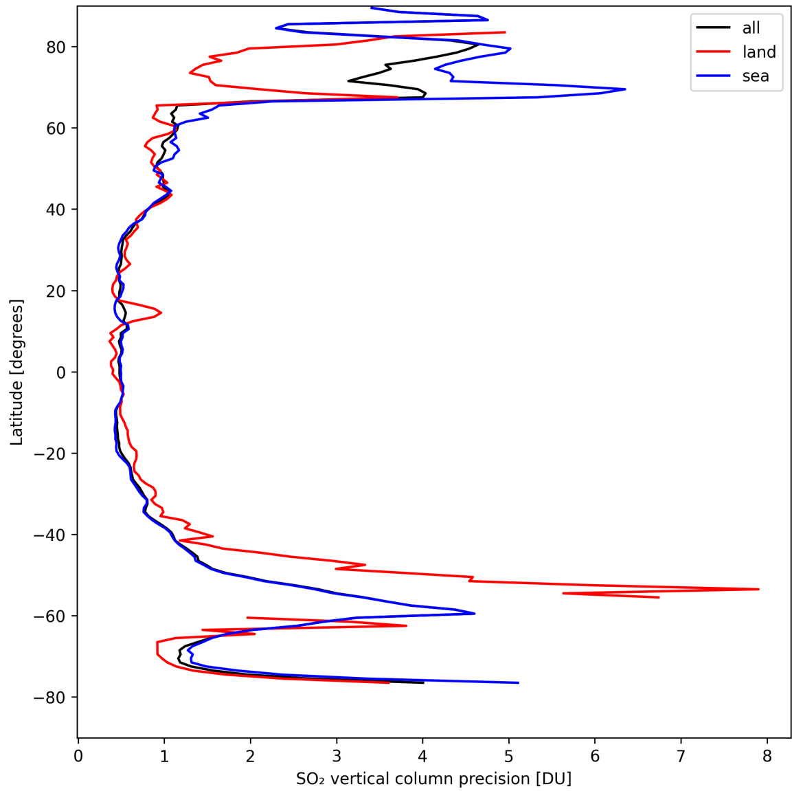
Figure 31: Zonal average of “SO 2 vertical column precision” for 2024-08-30 to 2024-09-01.
