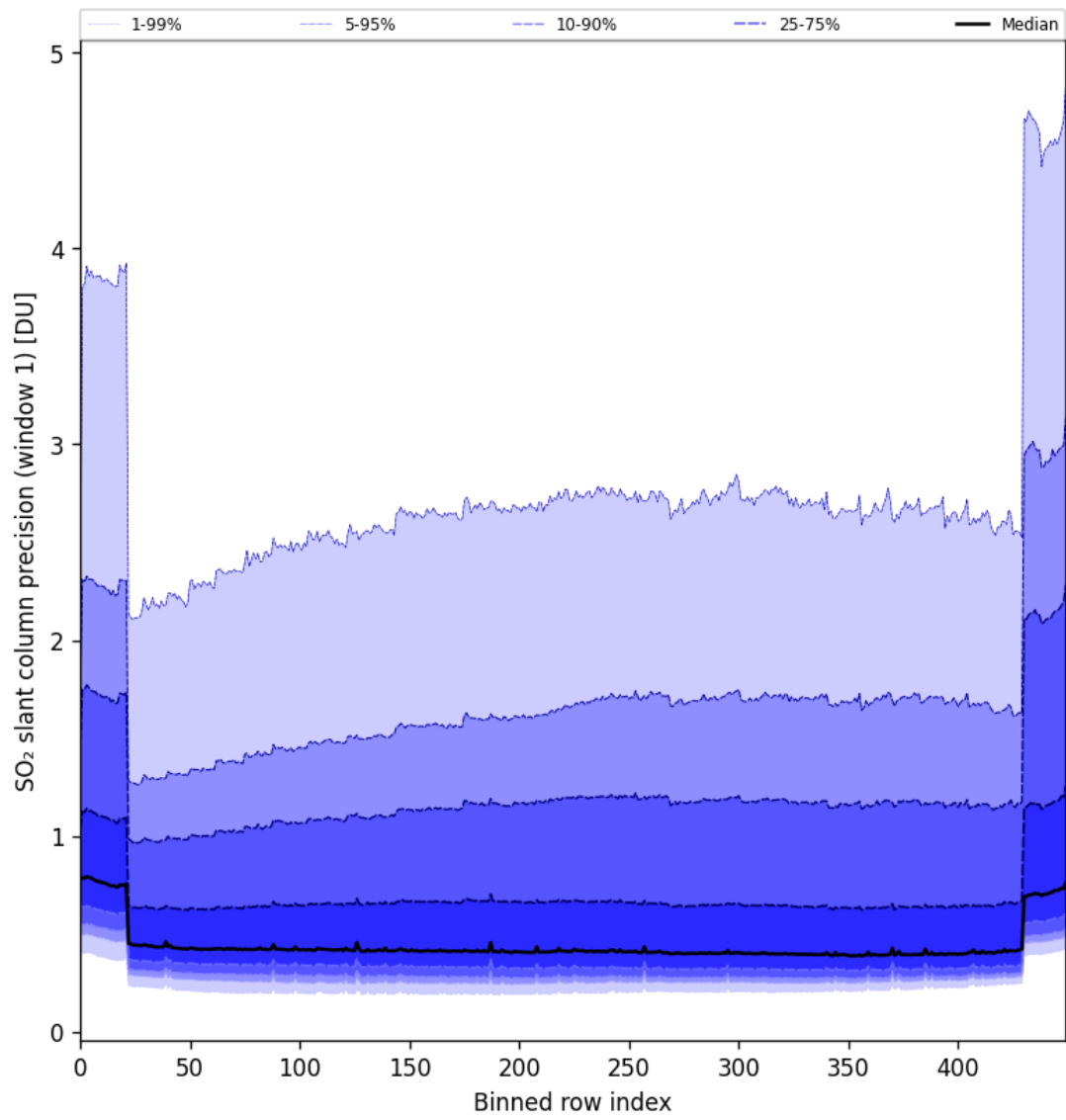
Figure 80: Along track statistics of “SO 2 slant column precision (window 1)” for 2024-08-30 to 2024-09-01
