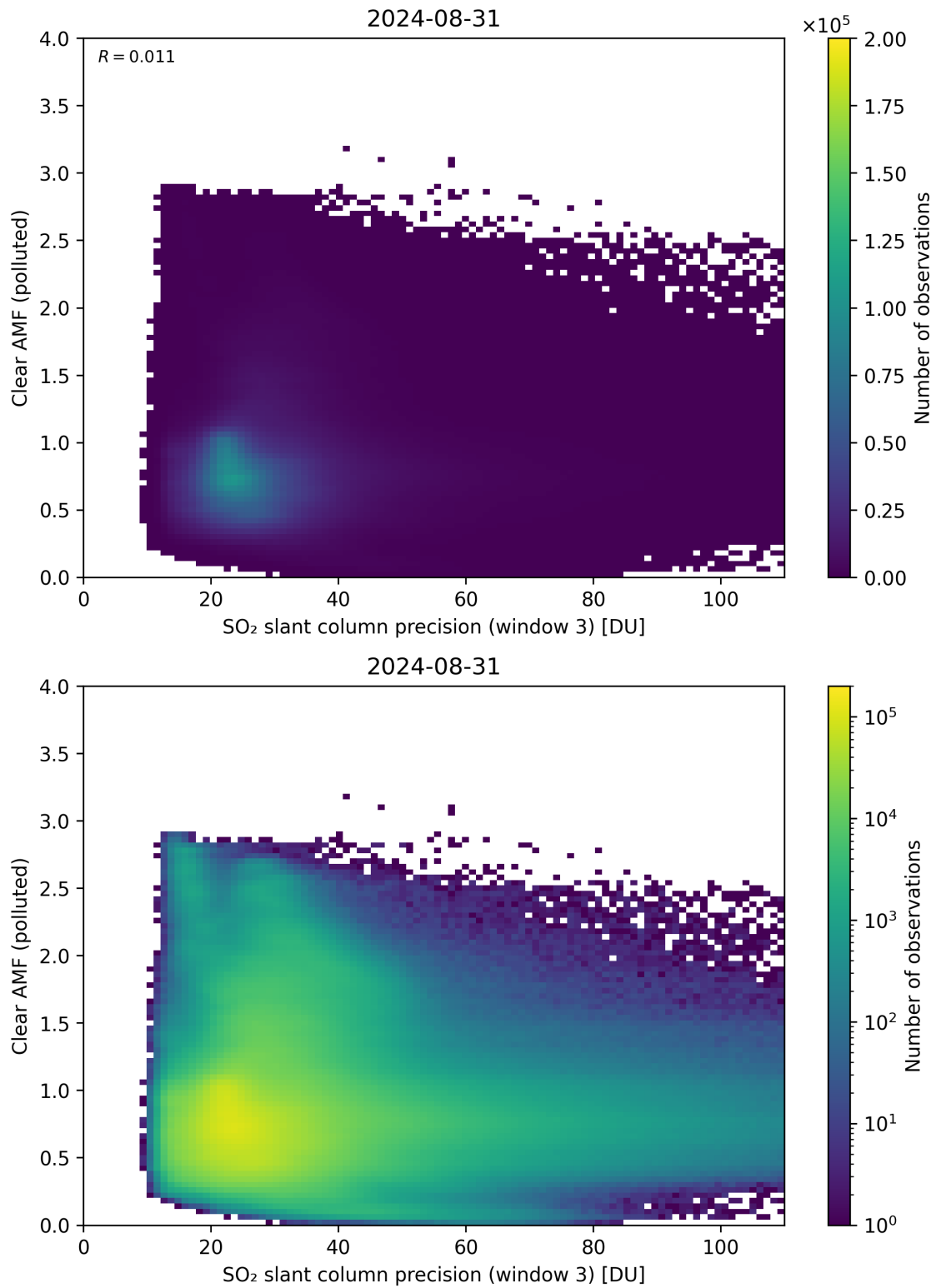
Figure 261: Scatter density plot of “SO 2 slant column precision (window 3)” against “Clear AMF (polluted)” for 2024-08-30 to 2024-09-01.
