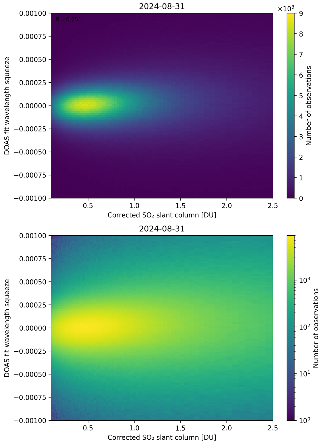
Figure 182: Scatter density plot of “Corrected SO 2 slant column” against “DOAS fit wavelength squeeze” for 2024-08-30 to 2024-09-01.
