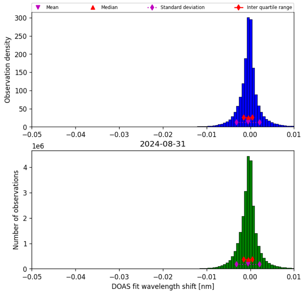
Figure 68: Histogram of “DOAS fit wavelength shift” for 2024-08-30 to 2024-09-01
