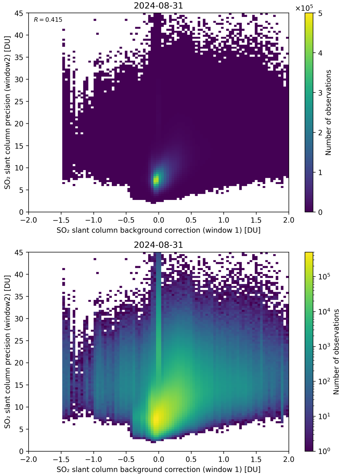
Figure 106: Scatter density plot of “SO 2 slant column background correction (window 1)” against “SO 2 slant column precision (window2)” for 2024-08-30 to 2024-09-01.
