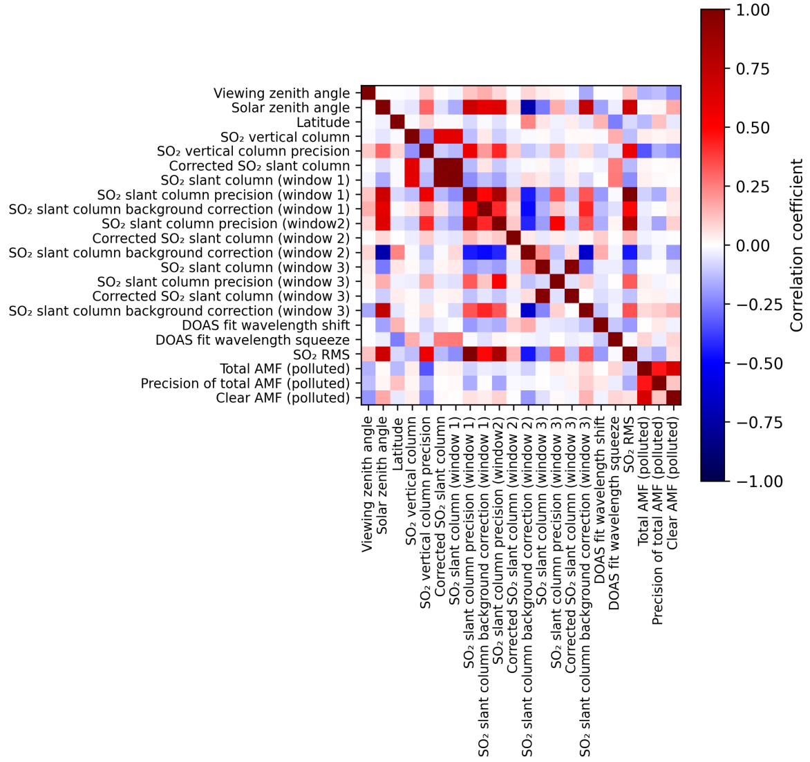
Figure 2: Map of correlation matrix for 2024-08-30 to 2024-09-01.
