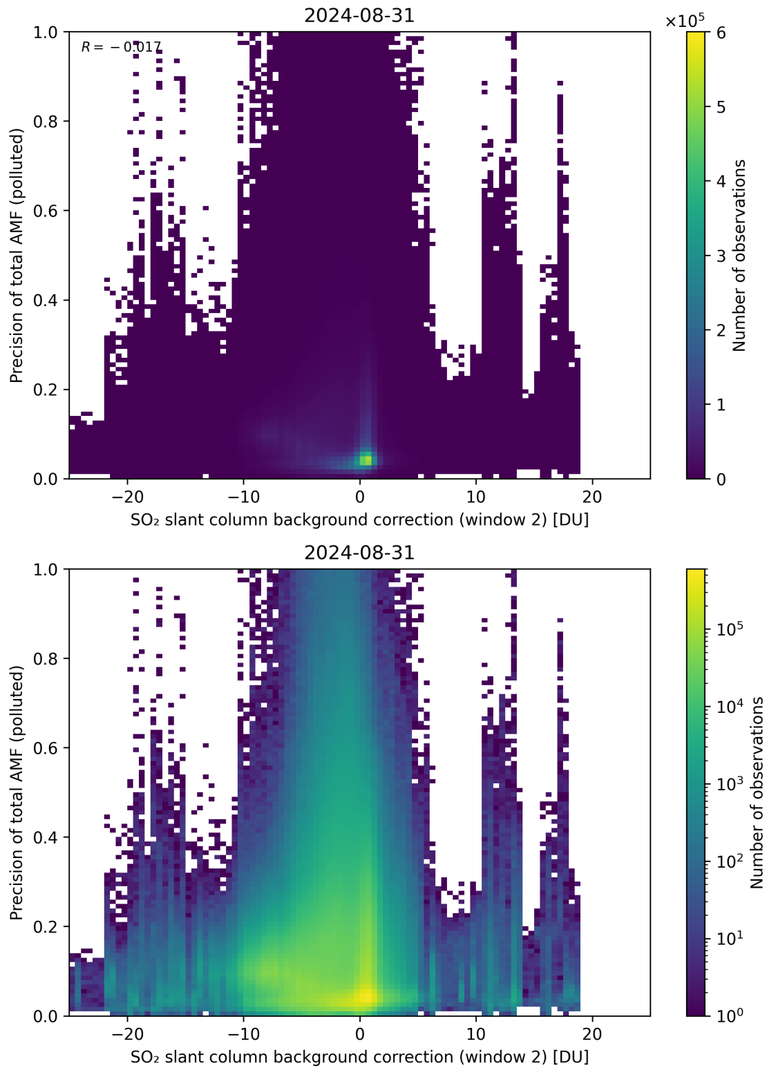
Figure 120: Scatter density plot of “SO 2 slant column background correction (window 2)” against “Precision of total AMF (polluted)” for 2024-08-30 to 2024-09-01.
