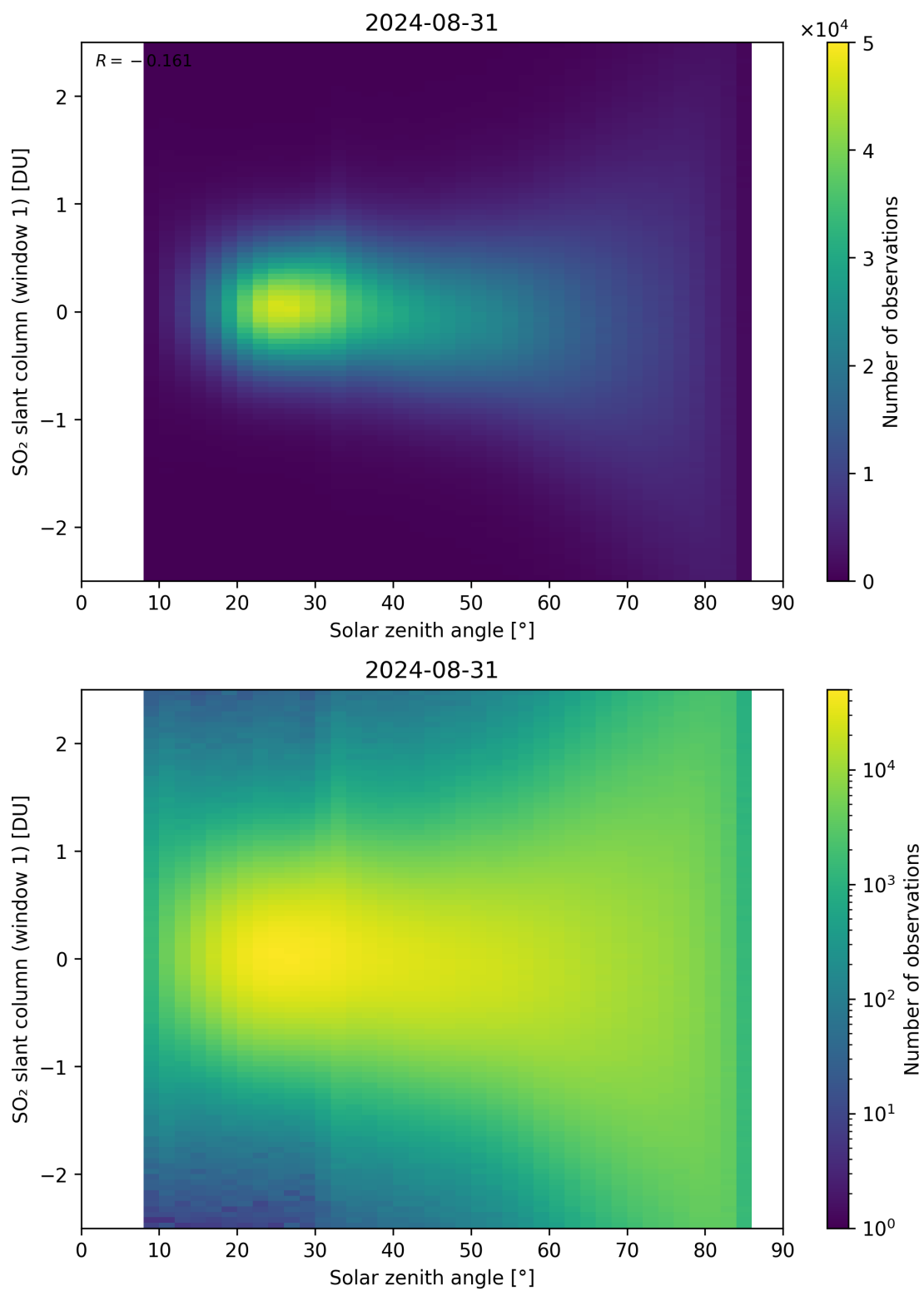
Figure 169: Scatter density plot of “Solar zenith angle” against “SO 2 slant column (window 1)” for 2024-08-30 to 2024-09-01.
