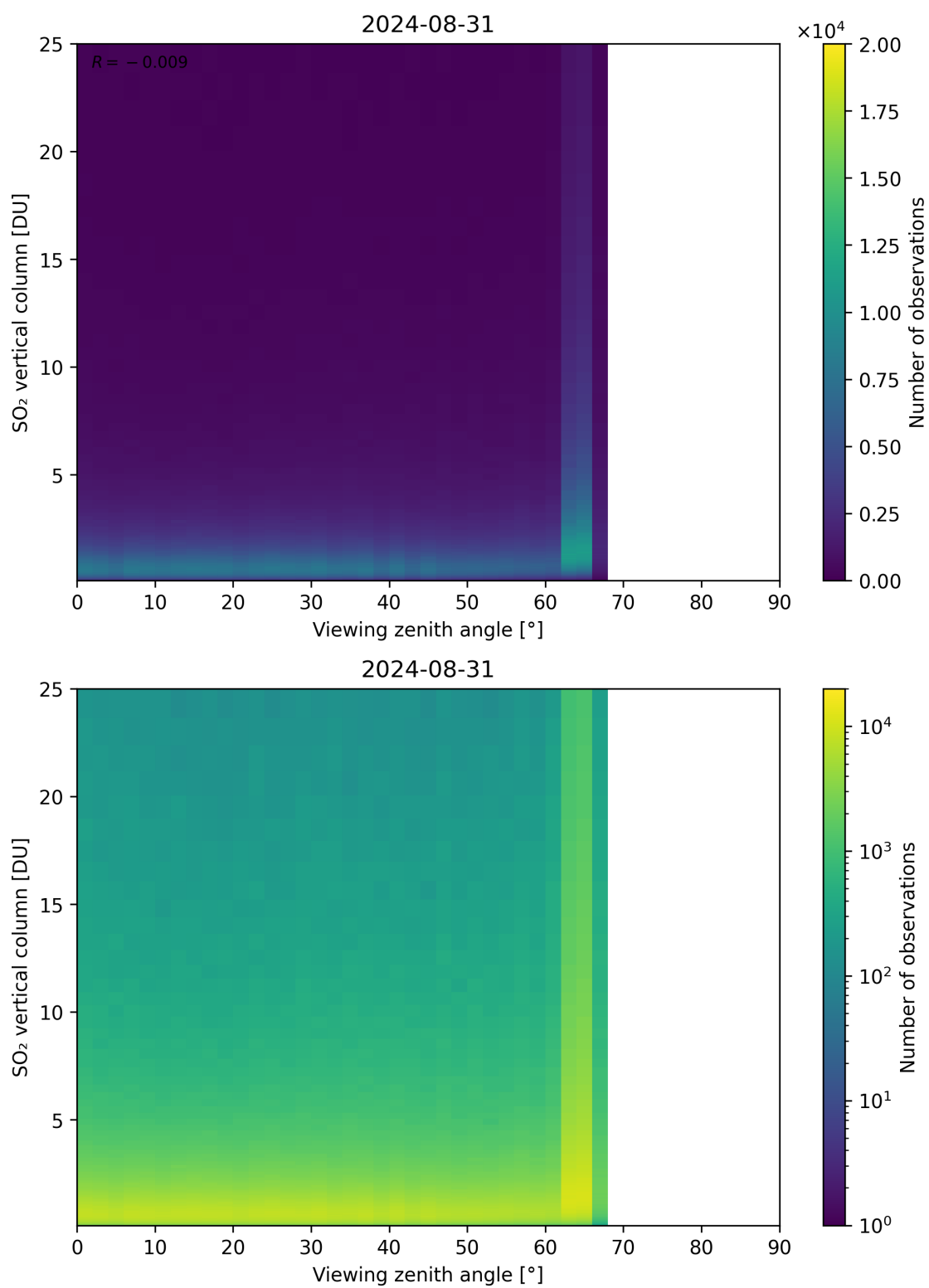
Figure 327: Scatter density plot of “Viewing zenith angle” against “SO 2 vertical column” for 2024-08-30 to 2024-09-01.
