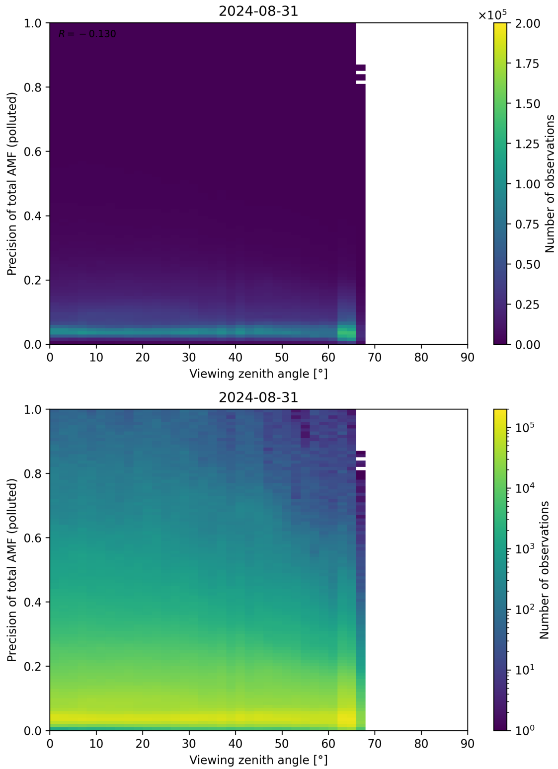
Figure 326: Scatter density plot of “Viewing zenith angle” against “Precision of total AMF (polluted)” for 2024-08-30 to 2024-09-01.
