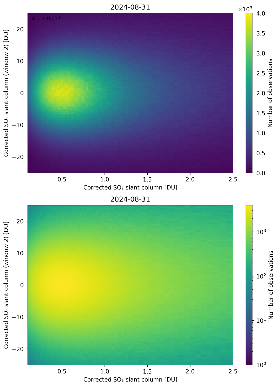
Figure 185: Scatter density plot of “Corrected SO 2 slant column” against “Corrected SO 2 slant column (window 2)” for 2024-08-30 to 2024-09-01.
