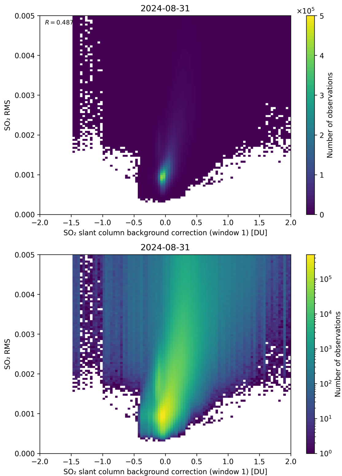
Figure 102: Scatter density plot of “SO 2 slant column background correction (window 1)” against “SO 2 RMS” for 2024-08-30 to 2024-09-01.
