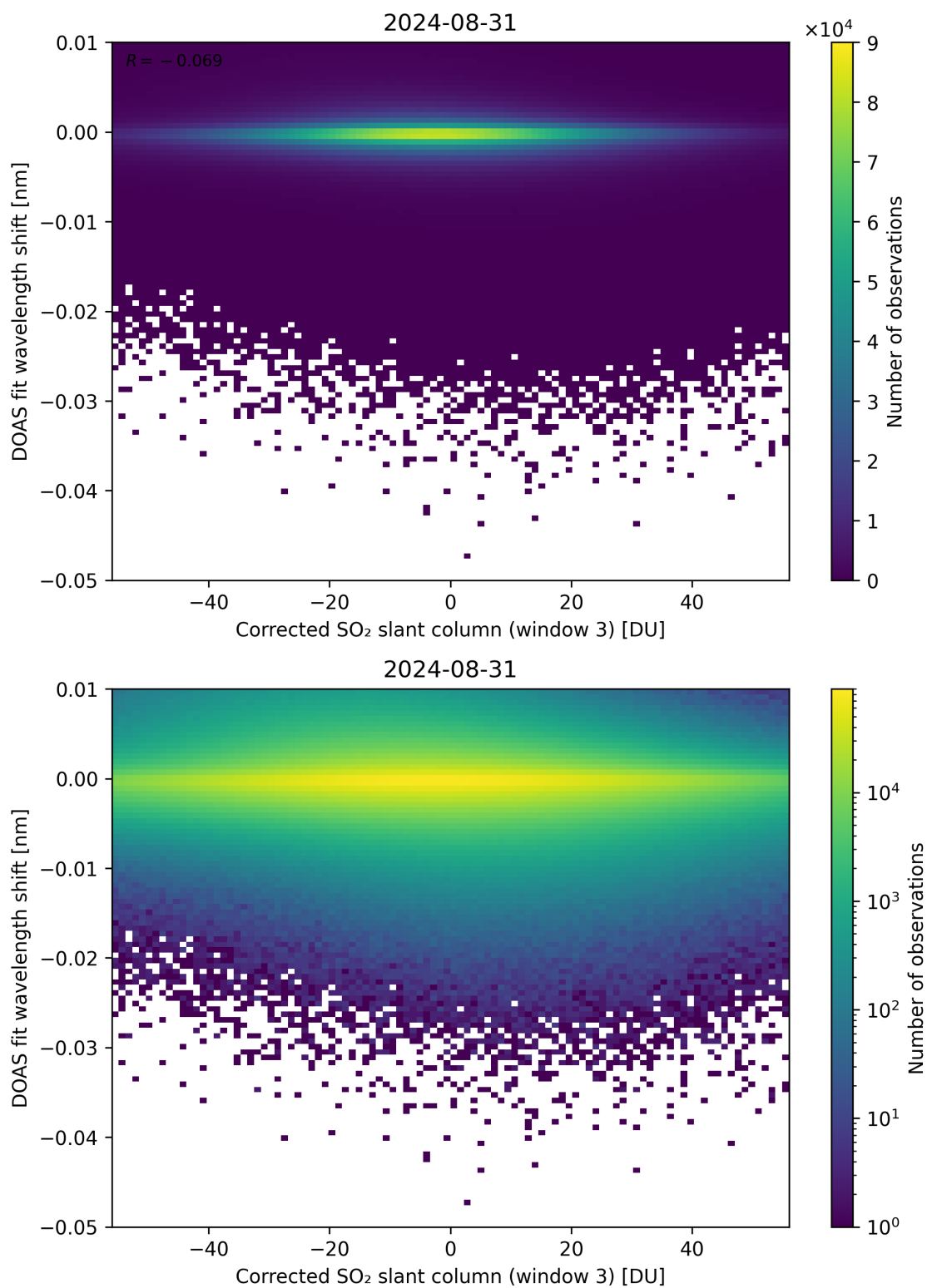
Figure 206: Scatter density plot of “Corrected SO 2 slant column (window 3)” against “DOAS fit wavelength shift” for 2024-08-30 to 2024-09-01.
