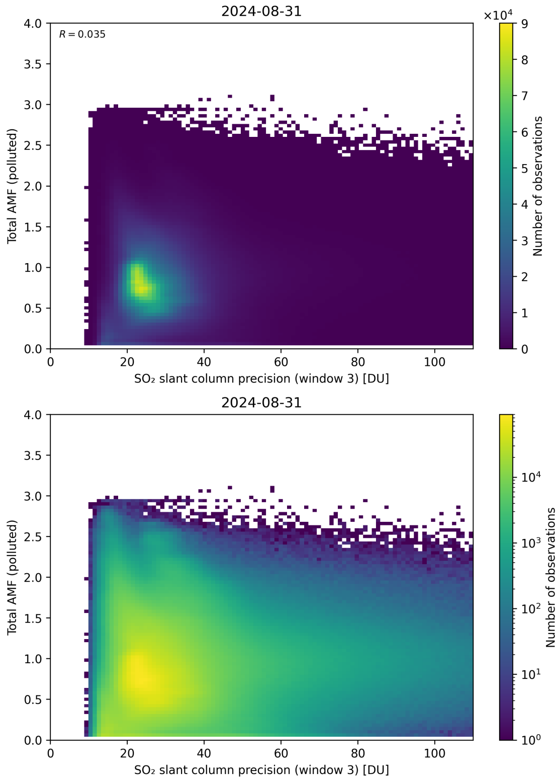
Figure 263: Scatter density plot of “SO 2 slant column precision (window 3)” against “Total AMF (polluted)” for 2024-08-30 to 2024-09-01.
