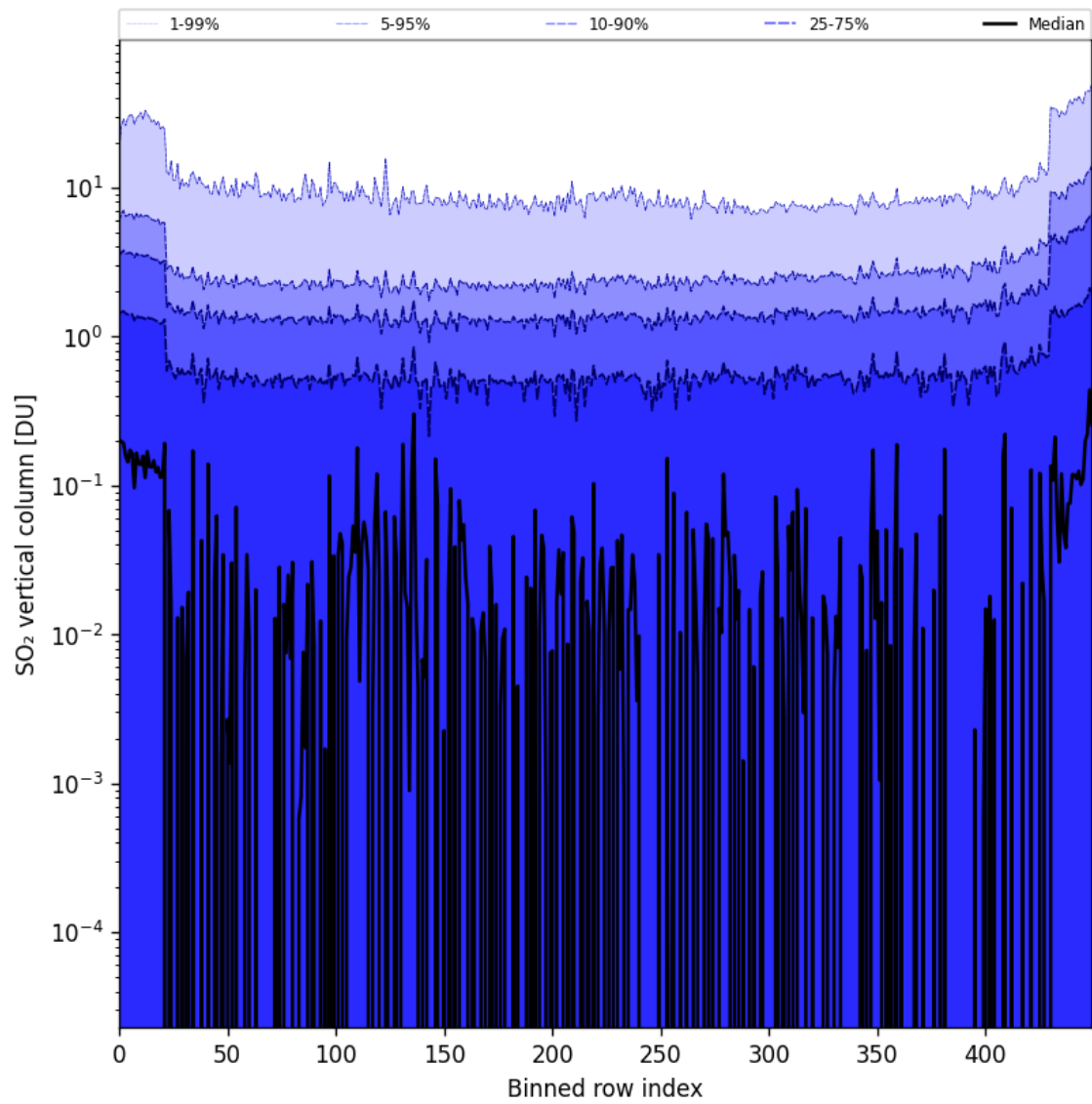
Figure 76: Along track statistics of “SO 2 vertical column” for 2024-08-30 to 2024-09-01
