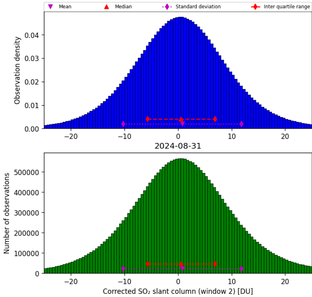
Figure 62: Histogram of “Corrected SO 2 slant column (window 2)” for 2024-08-30 to 2024-09-01
