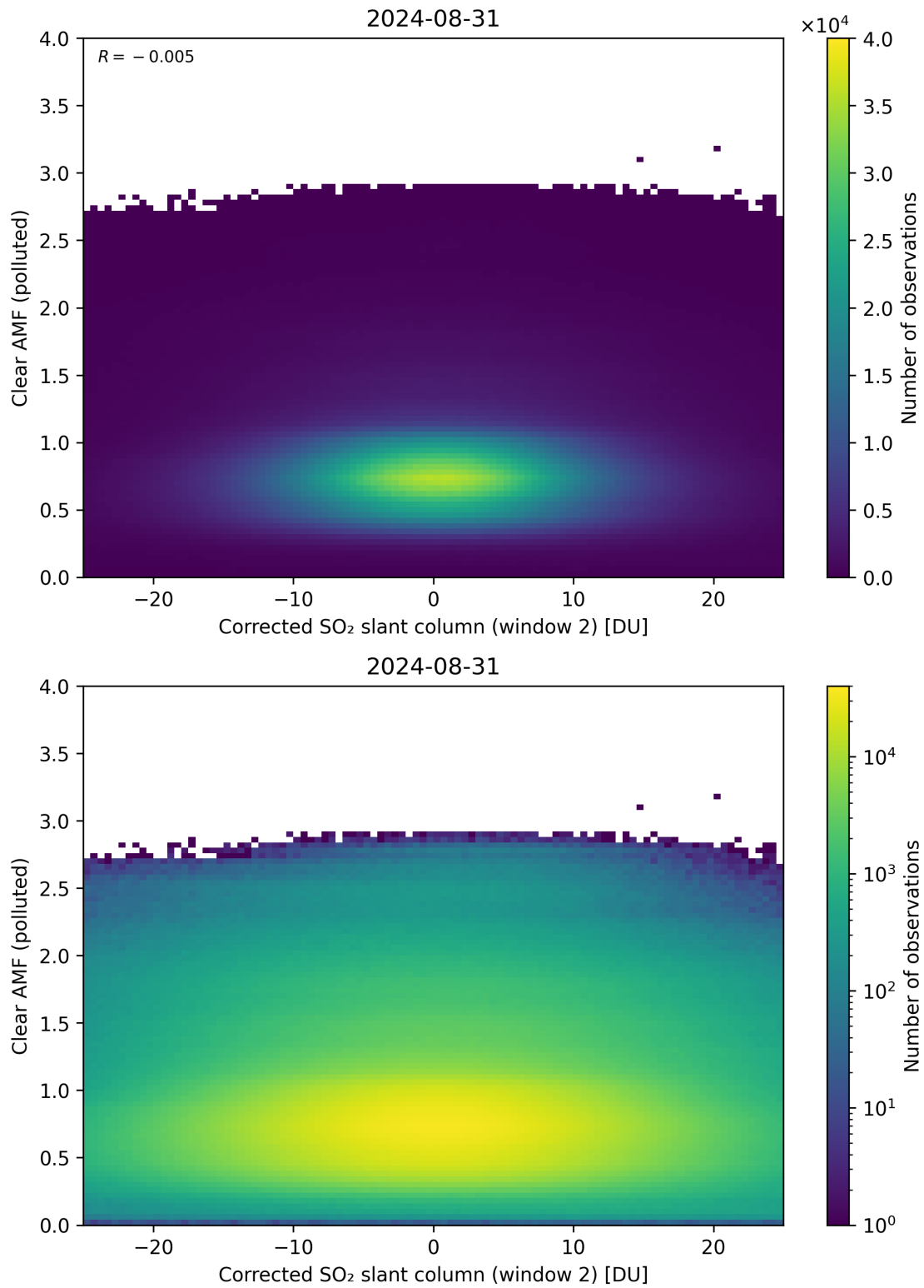
Figure 199: Scatter density plot of “Corrected SO 2 slant column (window 2)” against “Clear AMF (polluted)” for 2024-08-30 to 2024-09-01.
