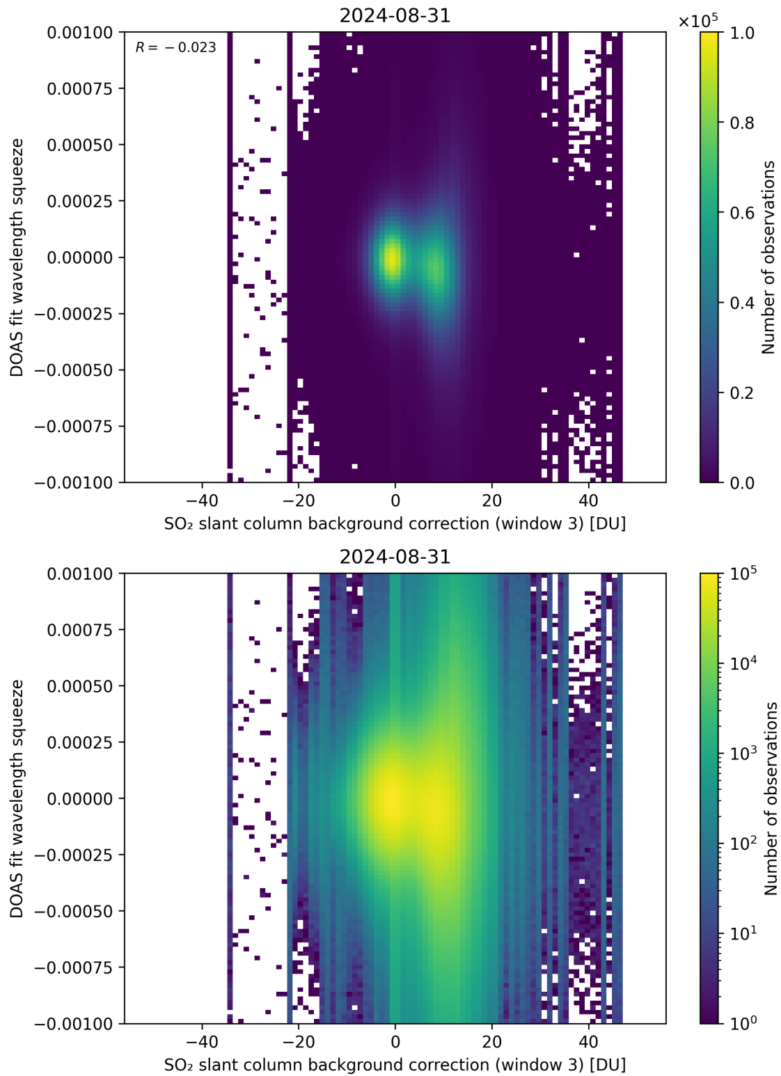
Figure 122: Scatter density plot of “SO 2 slant column background correction (window 3)” against “DOAS fit wavelength squeeze” for 2024-08-30 to 2024-09-01.
