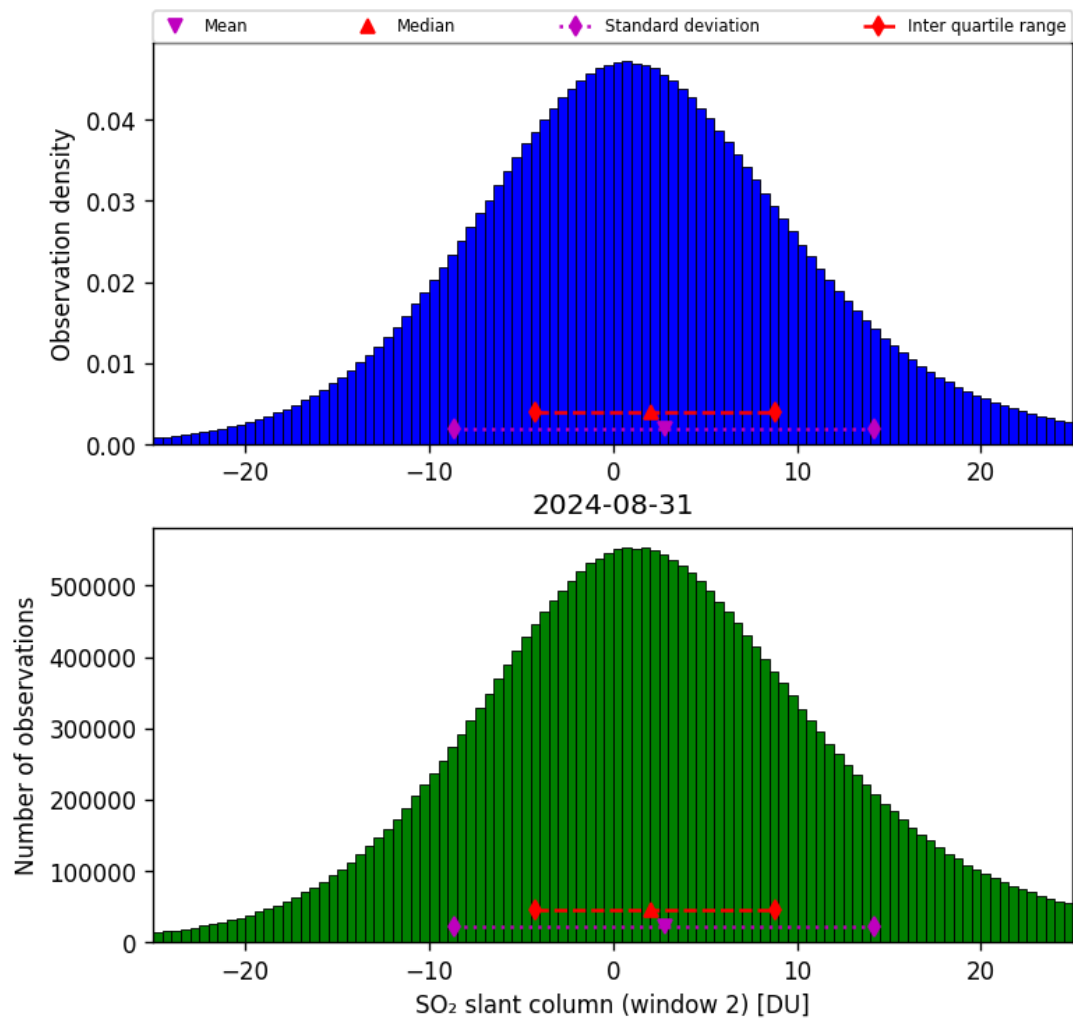
Figure 60: Histogram of “SO 2 slant column (window 2)” for 2024-08-30 to 2024-09-01
