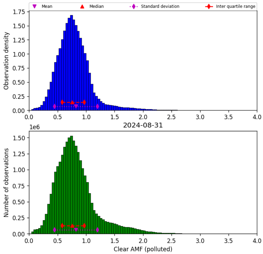
Figure 73: Histogram of “Clear AMF (polluted)” for 2024-08-30 to 2024-09-01
