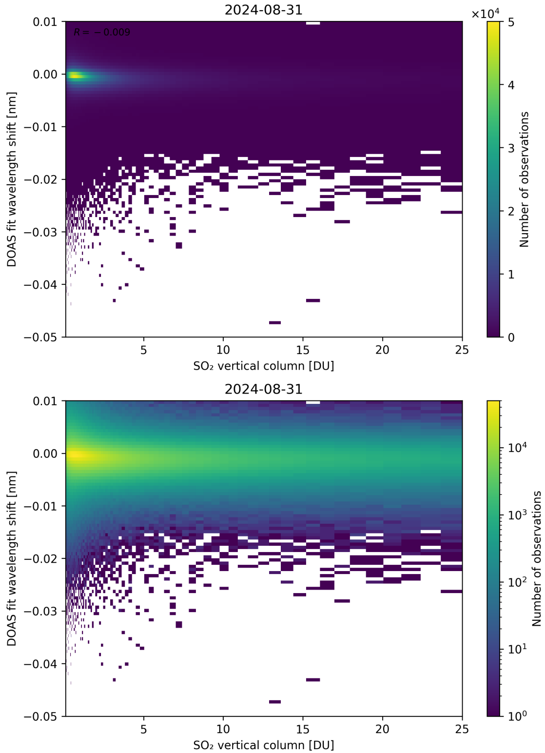
Figure 276: Scatter density plot of “SO 2 vertical column” against “DOAS fit wavelength shift” for 2024-08-30 to 2024-09-01.
