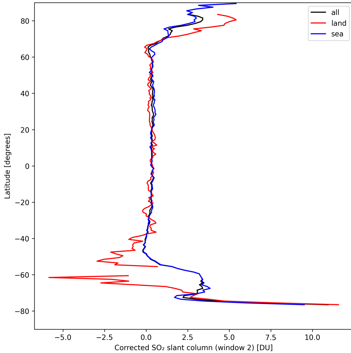
Figure 39: Zonal average of “Corrected SO 2 slant column (window 2)” for 2024-08-30 to 2024-09-01.
