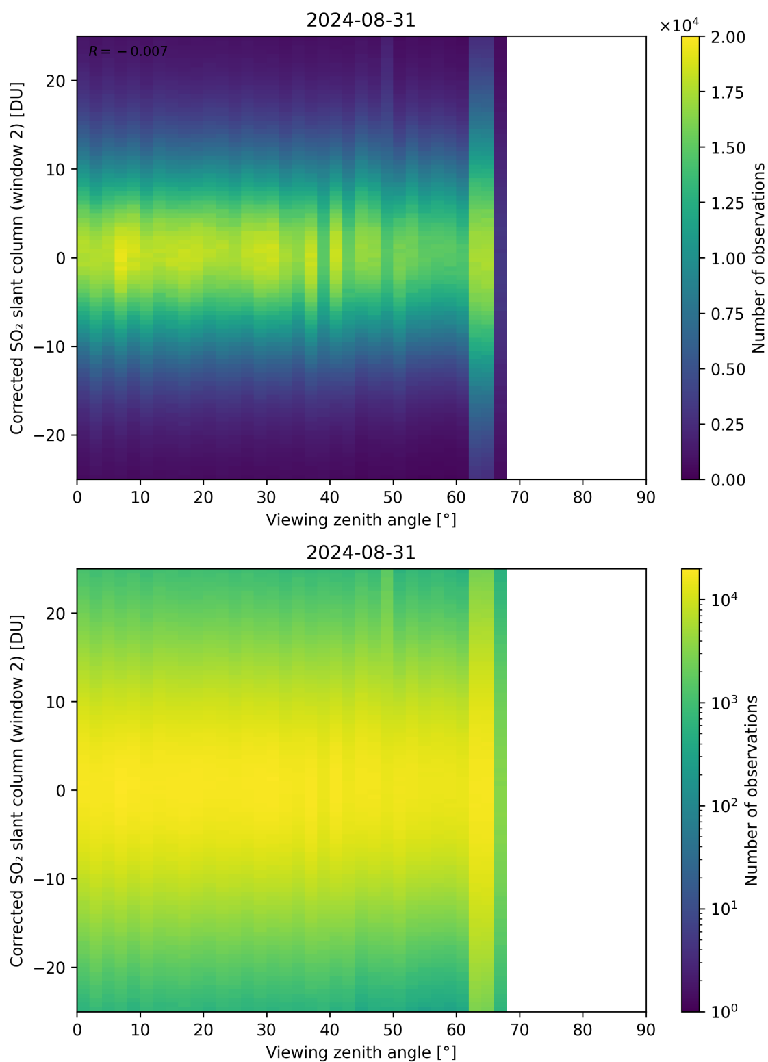
Figure 318: Scatter density plot of “Viewing zenith angle” against “Corrected SO 2 slant column (window 2)” for 2024-08-30 to 2024-09-01.
