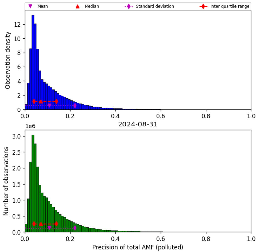
Figure 72: Histogram of “Precision of total AMF (polluted)” for 2024-08-30 to 2024-09-01
