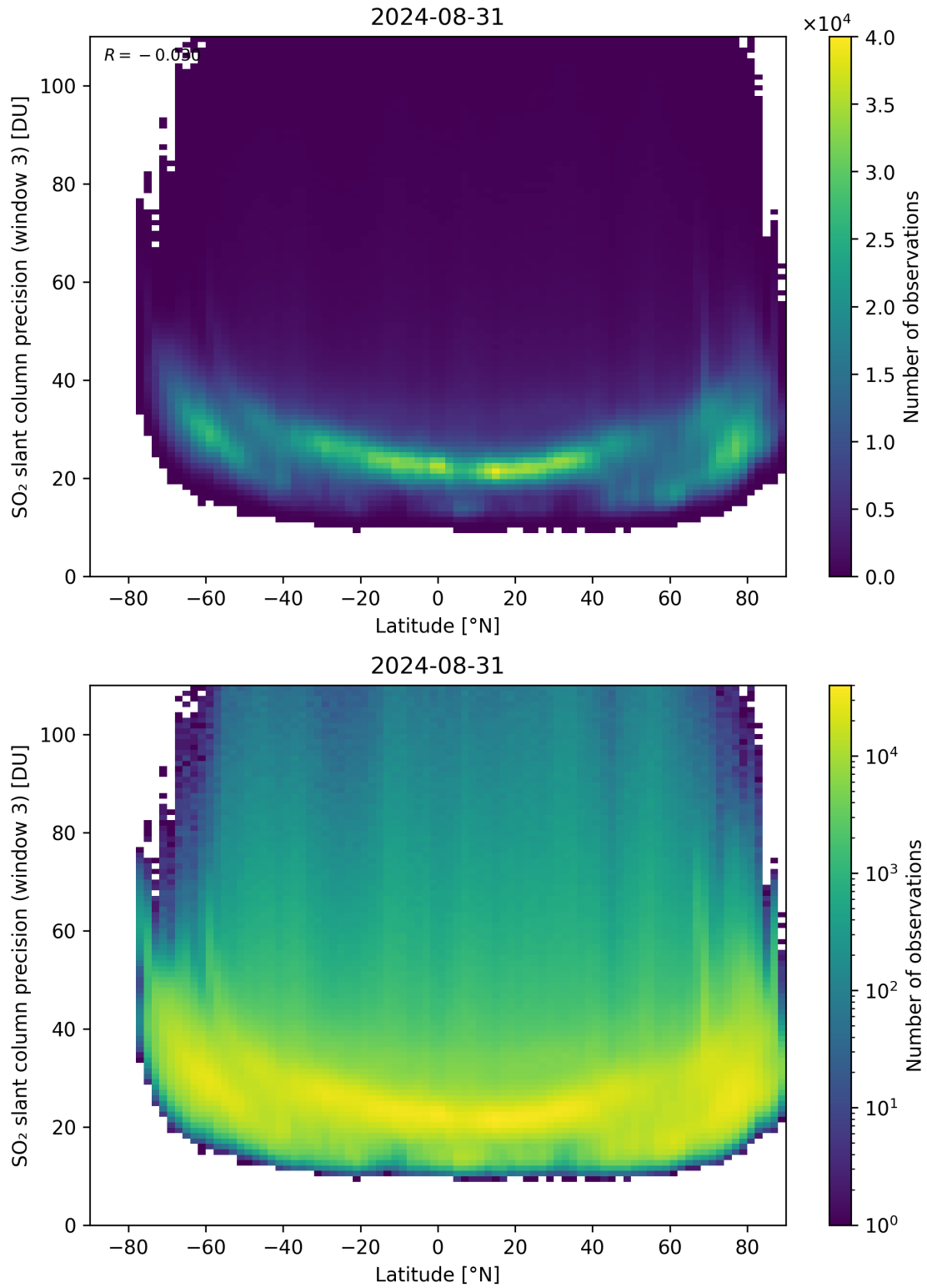
Figure 153: Scatter density plot of “Latitude” against “SO 2 slant column precision (window 3)” for 2024-08-30 to 2024-09-01.
