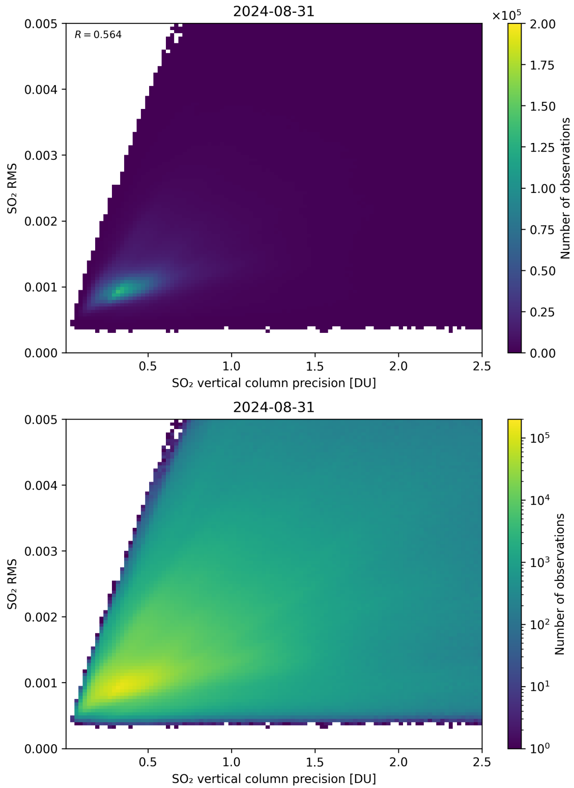
Figure 284: Scatter density plot of “SO 2 vertical column precision” against “SO 2 RMS” for 2024-08-30 to 2024-09-01.
