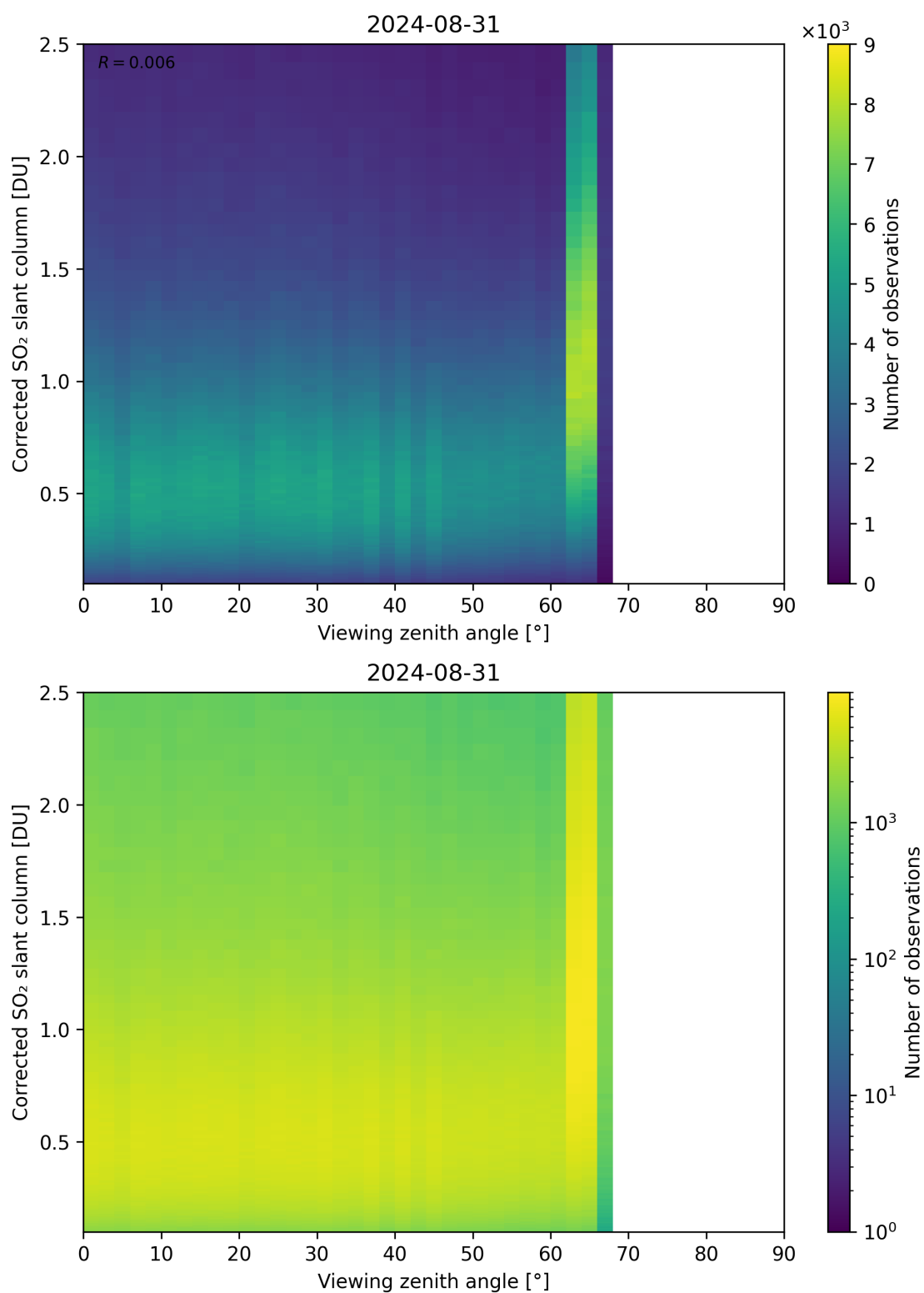
Figure 317: Scatter density plot of “Viewing zenith angle” against “Corrected SO 2 slant column” for 2024-08-30 to 2024-09-01.
