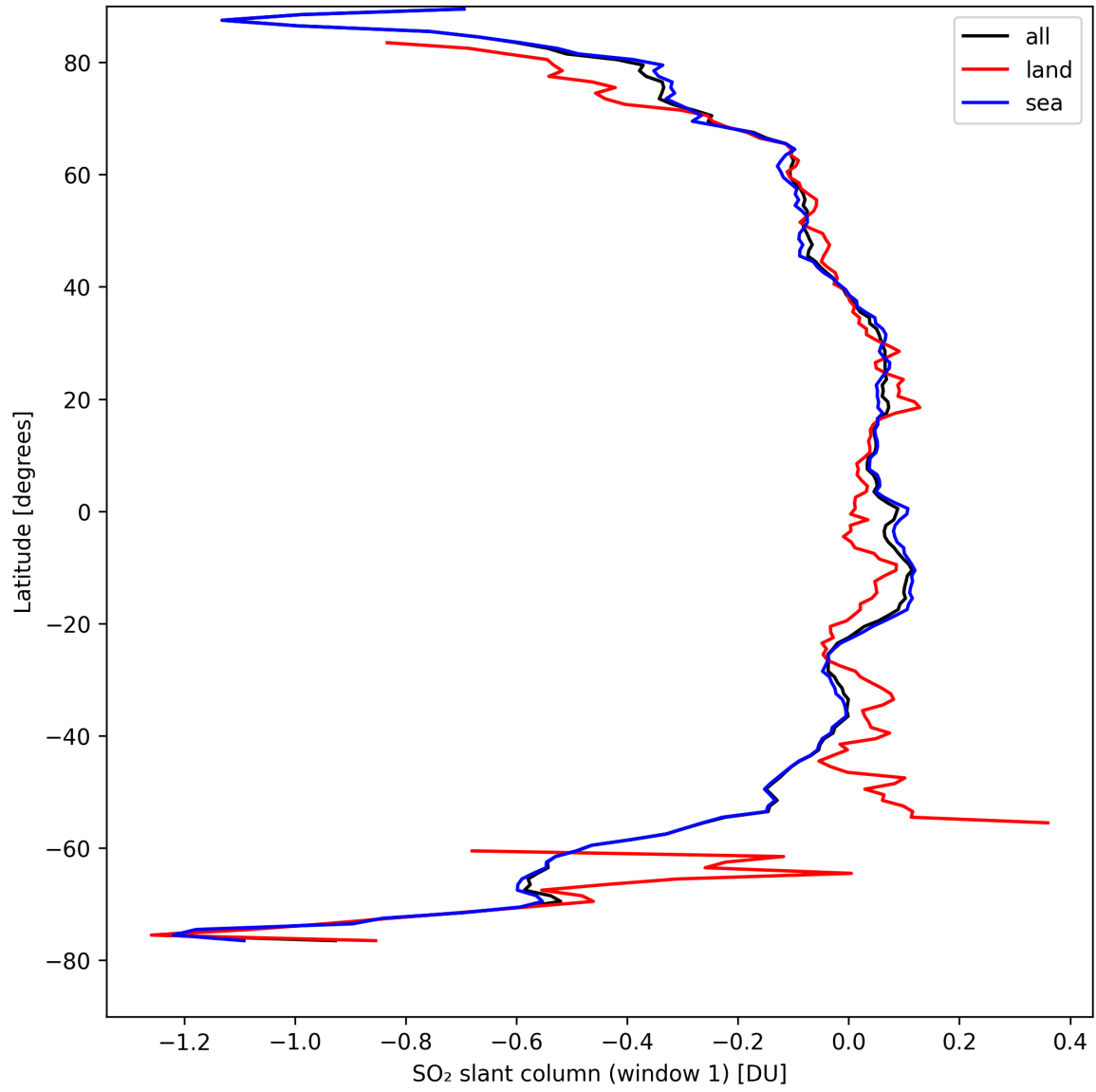
Figure 33: Zonal average of “SO 2 slant column (window 1)” for 2024-08-30 to 2024-09-01.
