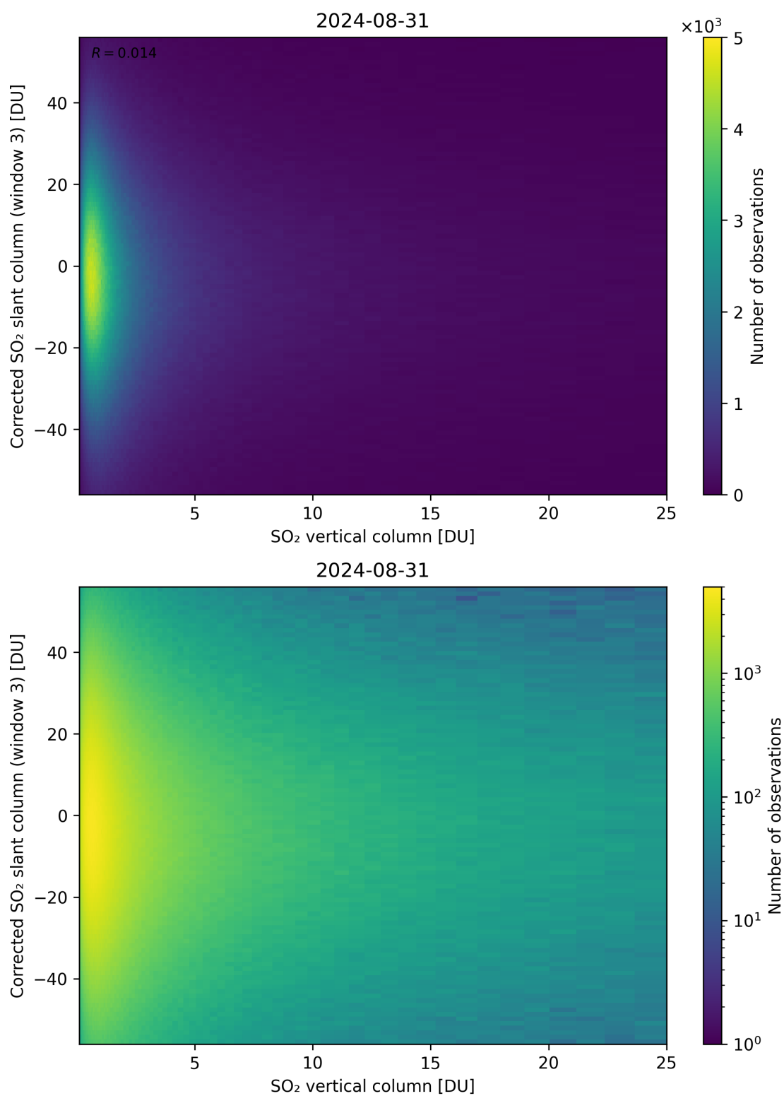
Figure 299: Scatter density plot of “SO 2 vertical column” against “Corrected SO 2 slant column (window 3)” for 2024-08-30 to 2024-09-01.
