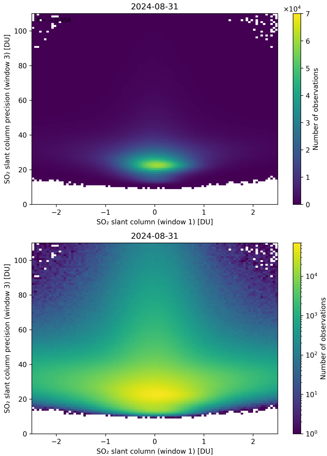
Figure 238: Scatter density plot of “SO 2 slant column (window 1)” against “SO 2 slant column precision (window 3)” for 2024-08-30 to 2024-09-01.
