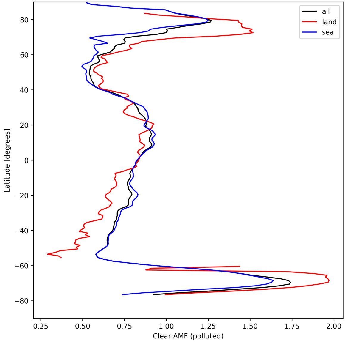
Figure 50: Zonal average of “Clear AMF (polluted)” for 2024-08-30 to 2024-09-01.
