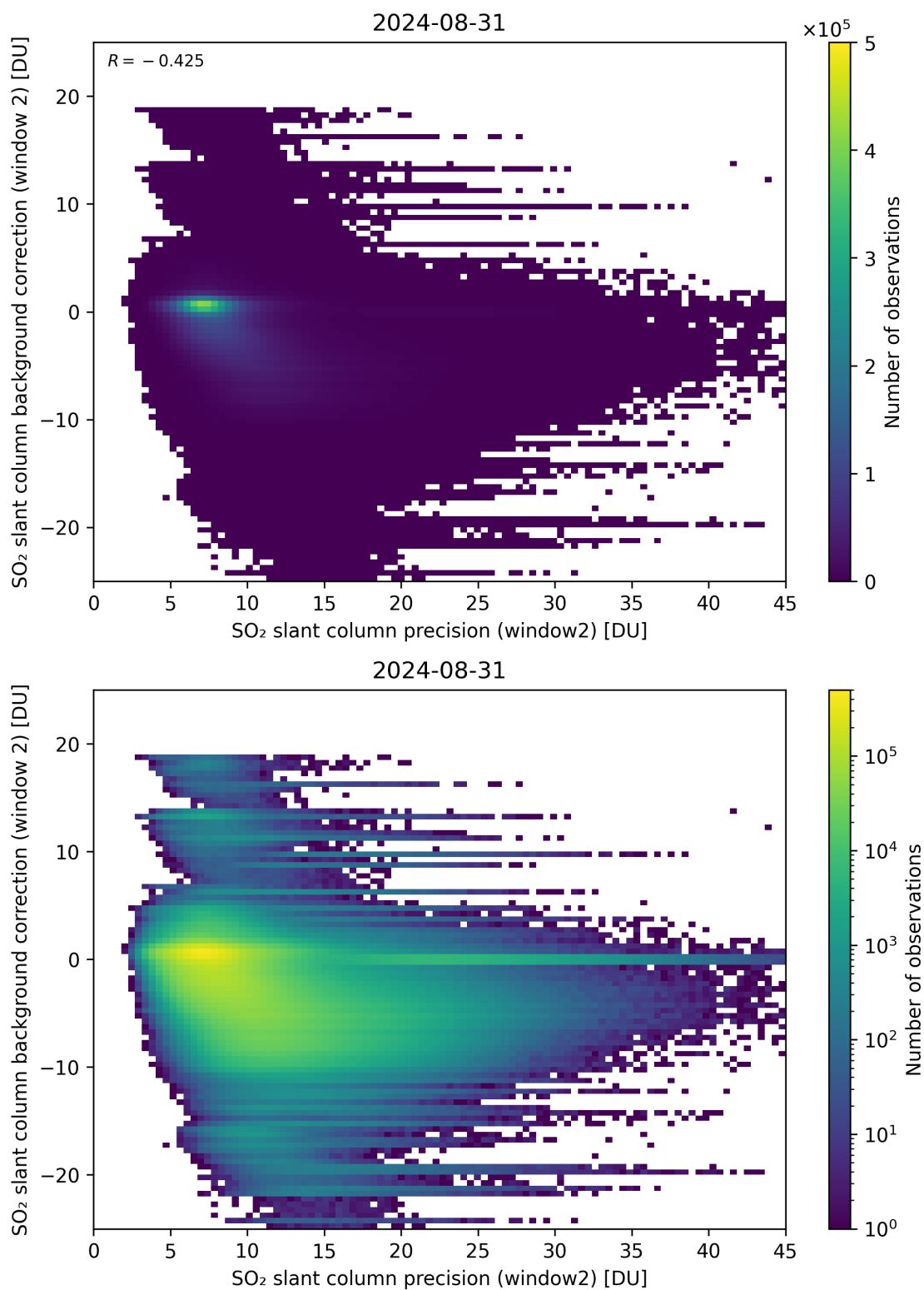
Figure 241: Scatter density plot of “SO 2 slant column precision (window2)” against “SO 2 slant column background correction (window 2)” for 2024-08-30 to 2024-09-01.
