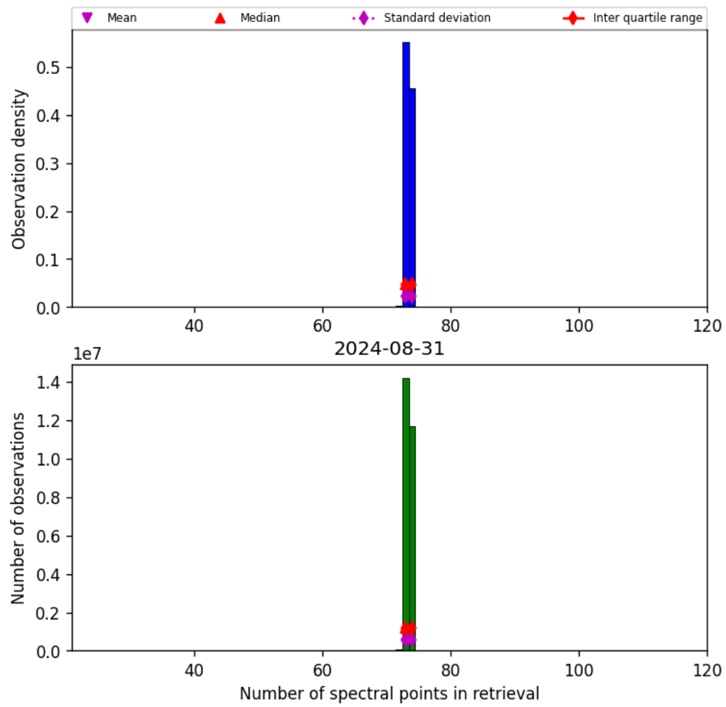
Figure 74: Histogram of “Number of spectral points in retrieval” for 2024-08-30 to 2024-09-01
