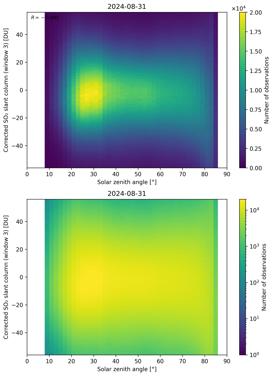
Figure 168: Scatter density plot of “Solar zenith angle” against “Corrected SO 2 slant column (window 3)” for 2024-08-30 to 2024-09-01.
