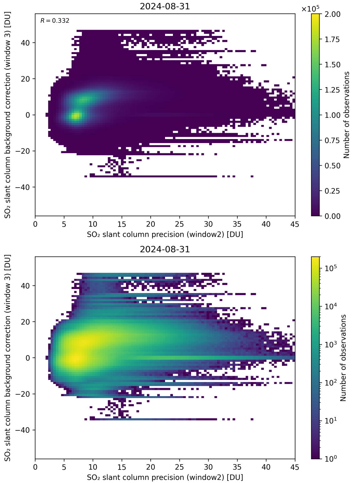
Figure 242: Scatter density plot of “SO 2 slant column precision (window2)” against “SO 2 slant column background correction (window 3)” for 2024-08-30 to 2024-09-01.
