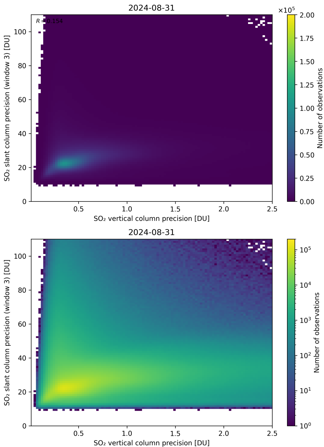
Figure 293: Scatter density plot of “SO 2 vertical column precision” against “SO 2 slant column precision (window 3)” for 2024-08-30 to 2024-09-01.
