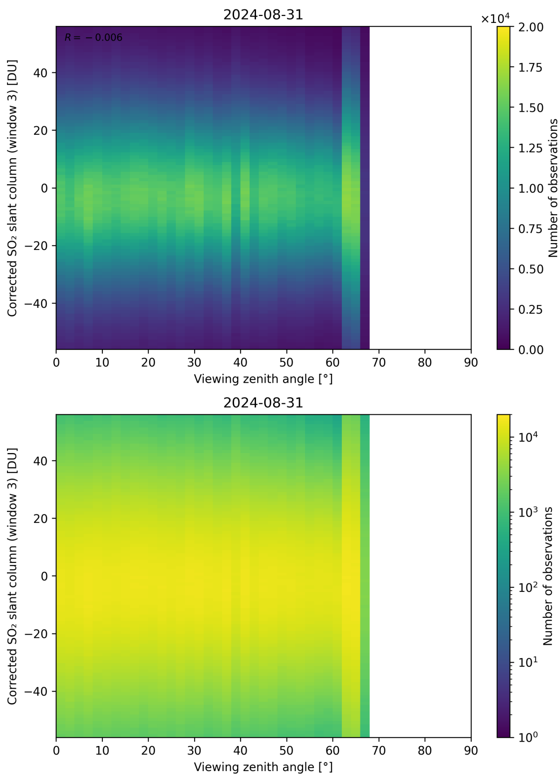
Figure 319: Scatter density plot of “Viewing zenith angle” against “Corrected SO 2 slant column (window 3)” for 2024-08-30 to 2024-09-01.
