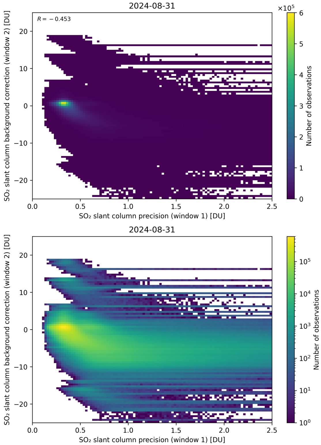
Figure 219: Scatter density plot of “SO 2 slant column precision (window 1)” against “SO 2 slant column background correction (window 2)” for 2024-08-30 to 2024-09-01.
