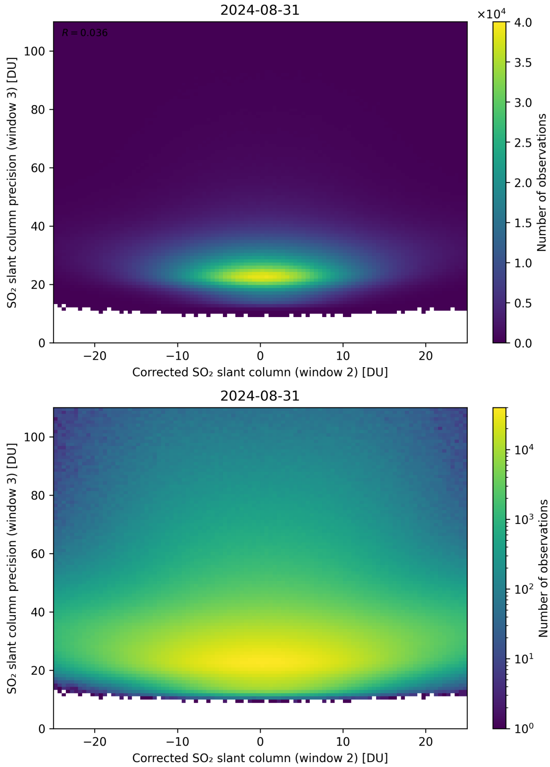
Figure 202: Scatter density plot of “Corrected SO 2 slant column (window 2)” against “SO 2 slant column precision (window 3)” for 2024-08-30 to 2024-09-01.
