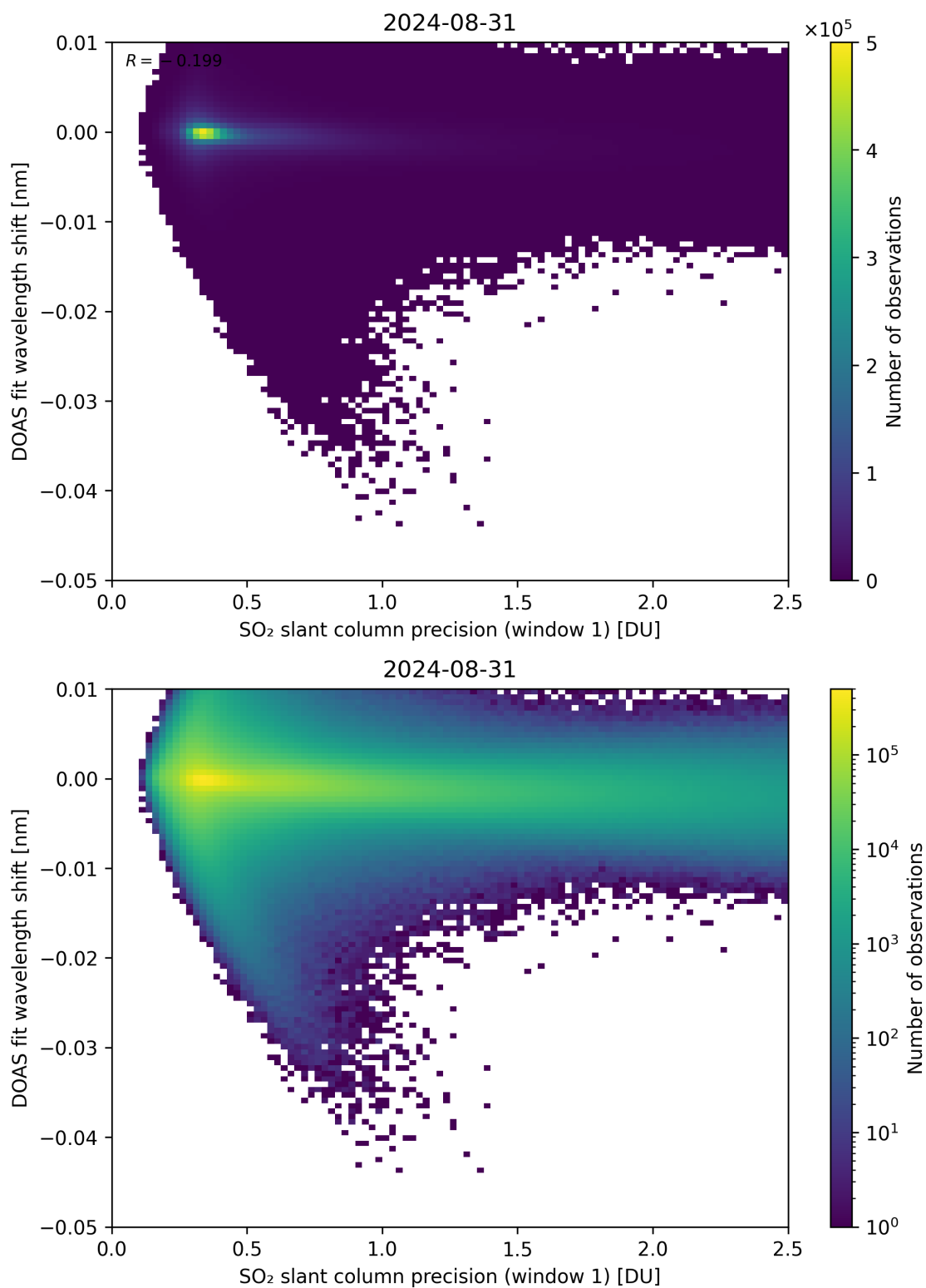
Figure 221: Scatter density plot of “SO 2 slant column precision (window 1)” against “DOAS fit wavelength shift” for 2024-08-30 to 2024-09-01.
