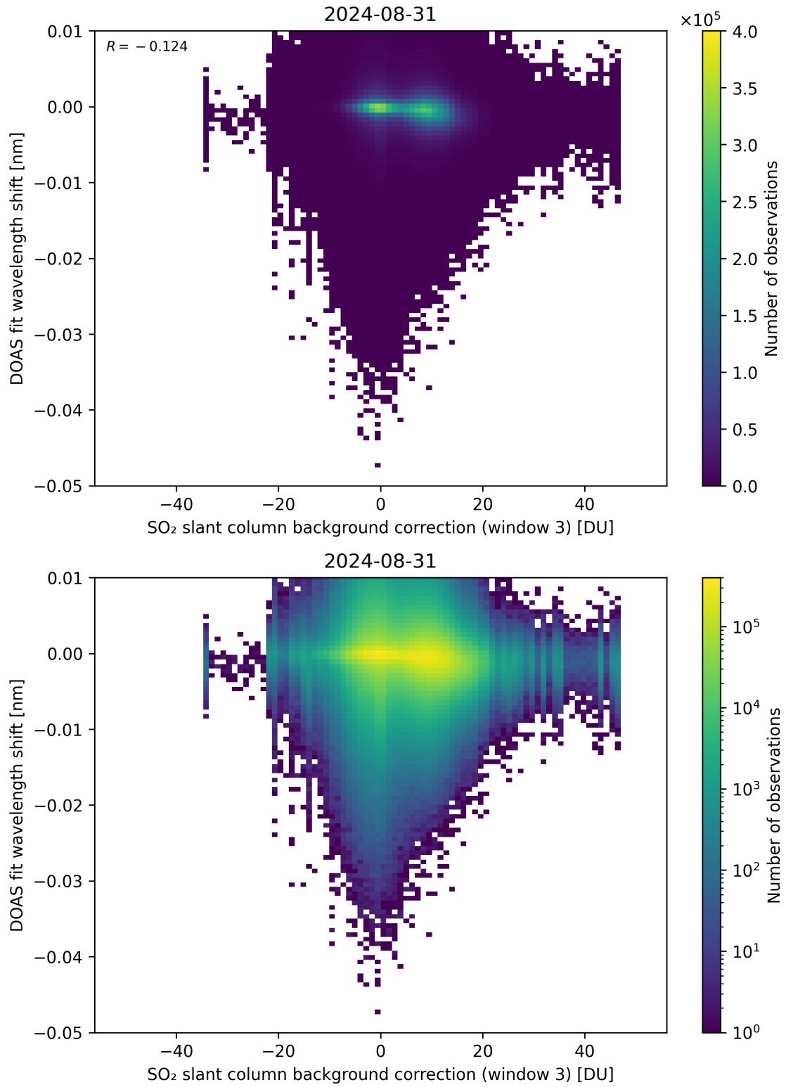
Figure 121: Scatter density plot of “SO 2 slant column background correction (window 3)” against “DOAS fit wavelength shift” for 2024-08-30 to 2024-09-01.
