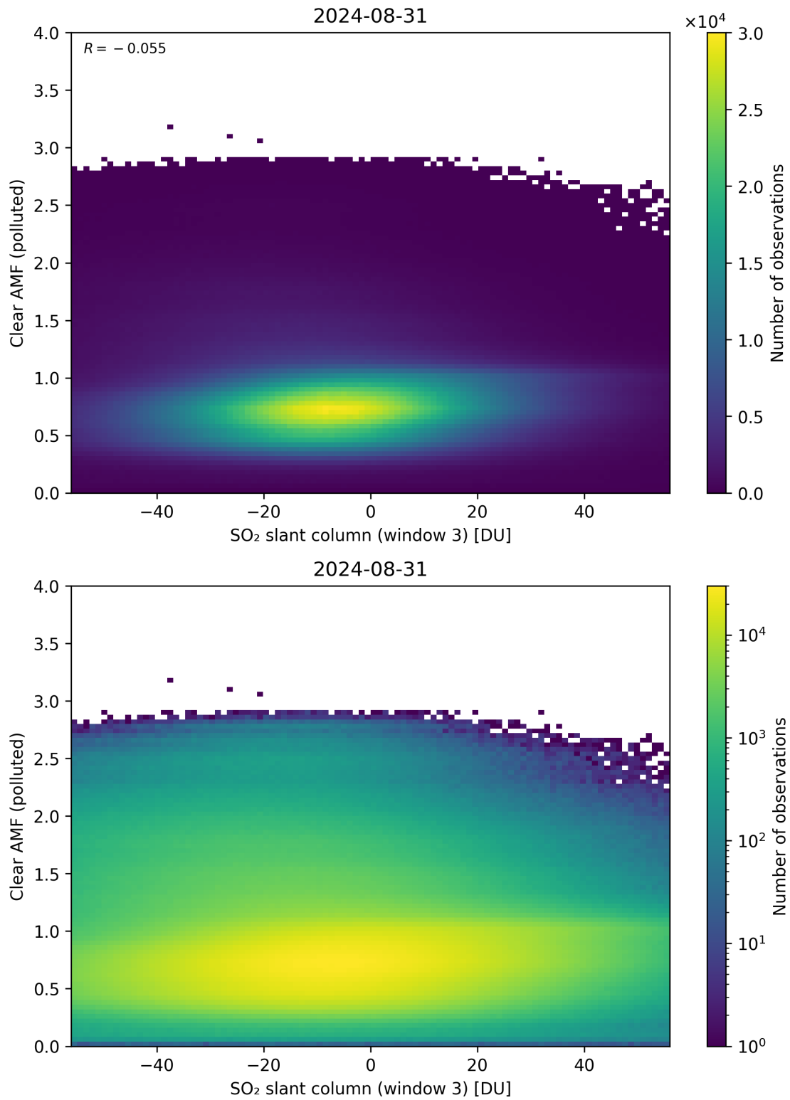
Figure 265: Scatter density plot of “SO 2 slant column (window 3)” against “Clear AMF (polluted)” for 2024-08-30 to 2024-09-01.
