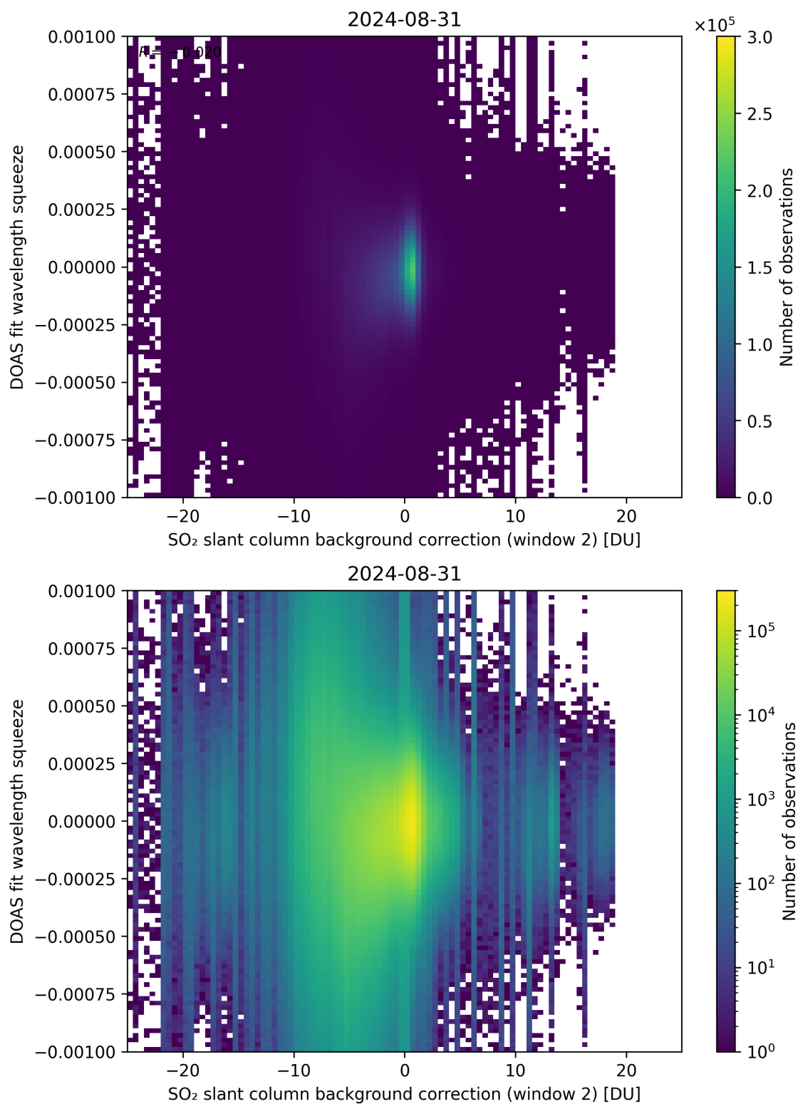
Figure 113: Scatter density plot of “SO 2 slant column background correction (window 2)” against “DOAS fit wavelength squeeze” for 2024-08-30 to 2024-09-01.
