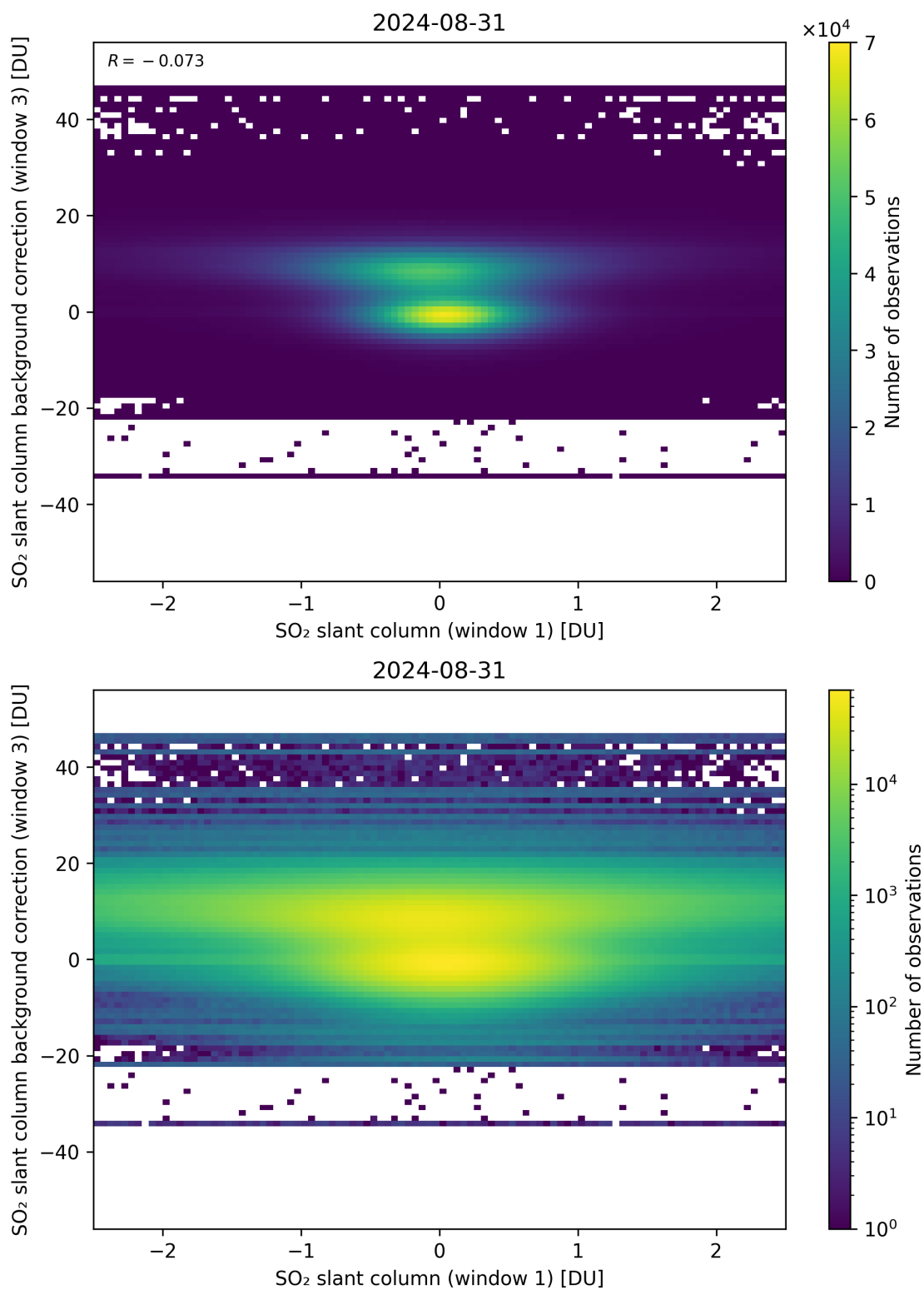
Figure 214: Scatter density plot of “SO 2 slant column (window 1)” against “SO 2 slant column background correction (window 3)” for 2024-08-30 to 2024-09-01.
