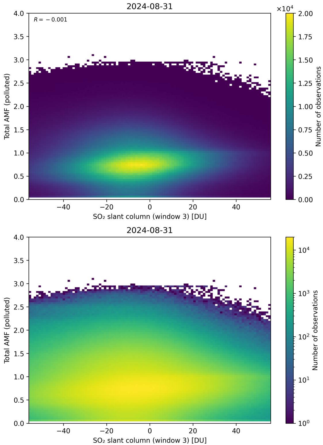
Figure 268: Scatter density plot of “SO 2 slant column (window 3)” against “Total AMF (polluted)” for 2024-08-30 to 2024-09-01.
