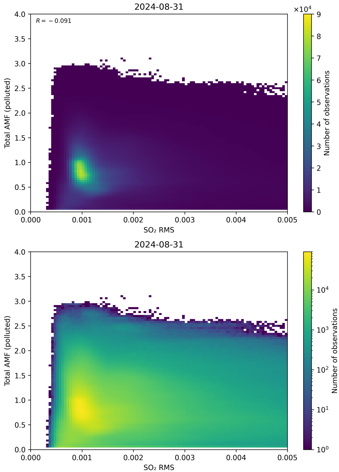
Figure 137: Scatter density plot of “SO 2 RMS” against “Total AMF (polluted)” for 2024-08-30 to 2024-09-01.
