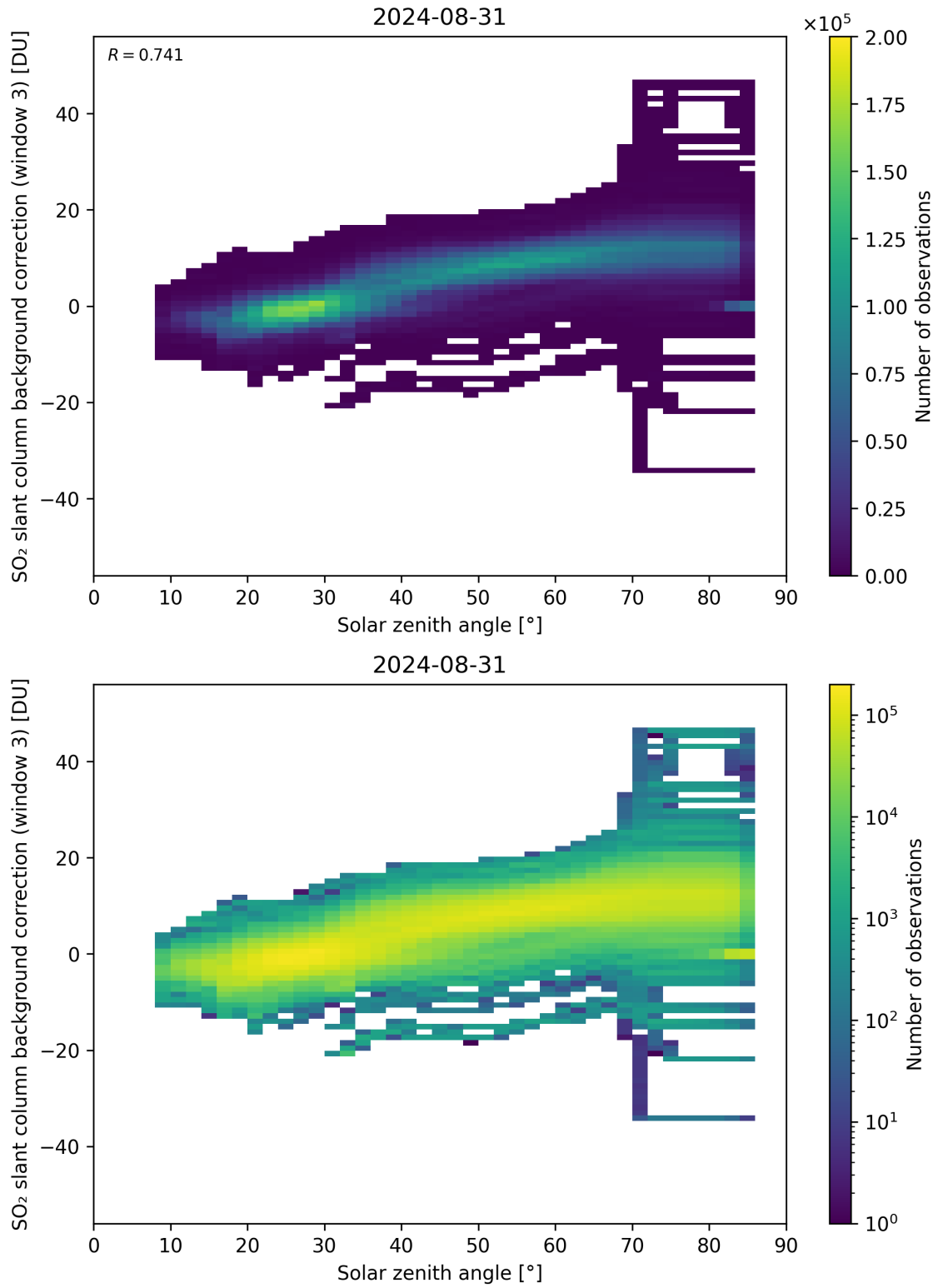
Figure 160: Scatter density plot of “Solar zenith angle” against “SO 2 slant column background correction (window 3)” for 2024-08-30 to 2024-09-01.
