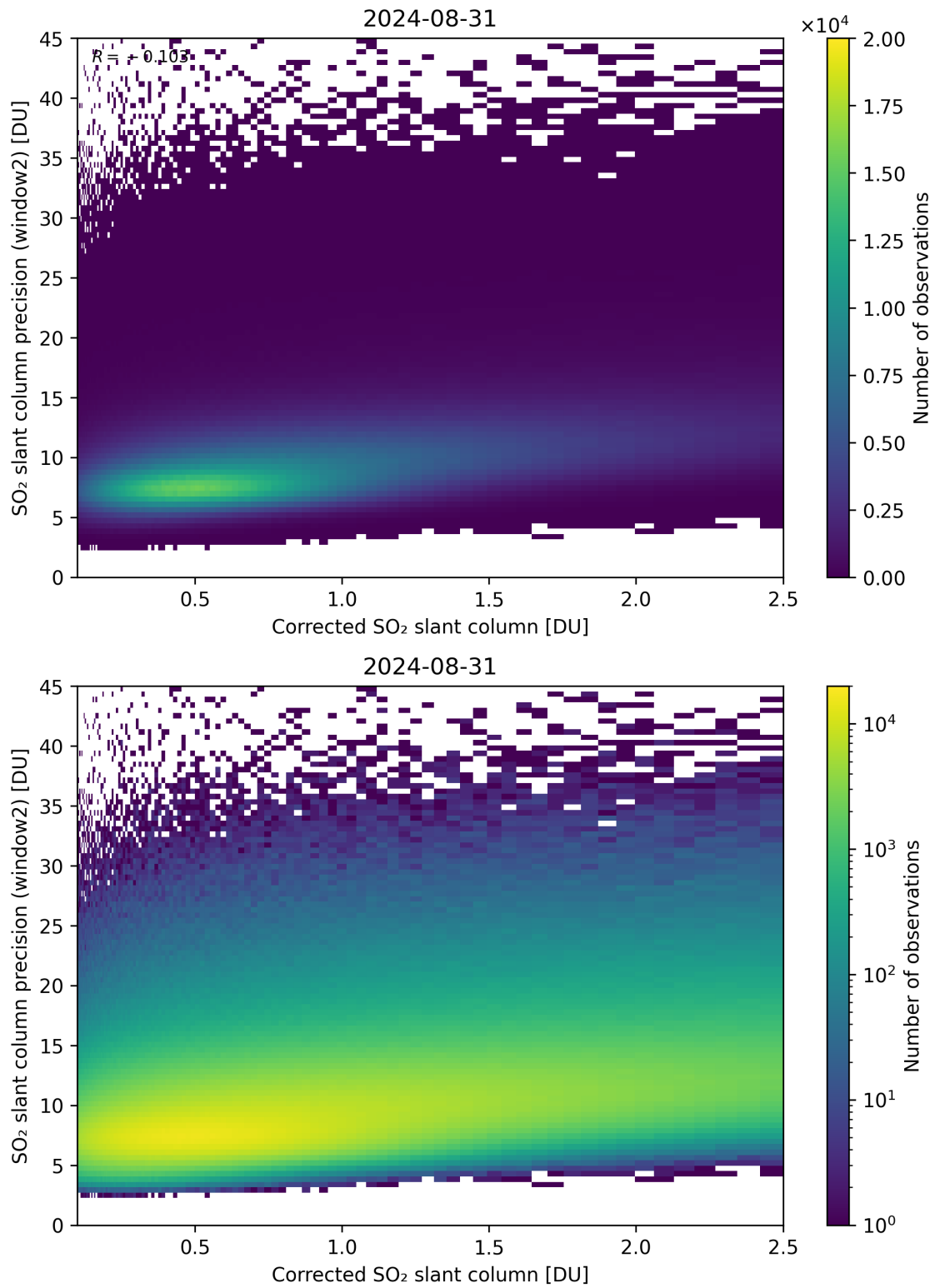
Figure 189: Scatter density plot of “Corrected SO 2 slant column” against “SO 2 slant column precision (window2)” for 2024-08-30 to 2024-09-01.
