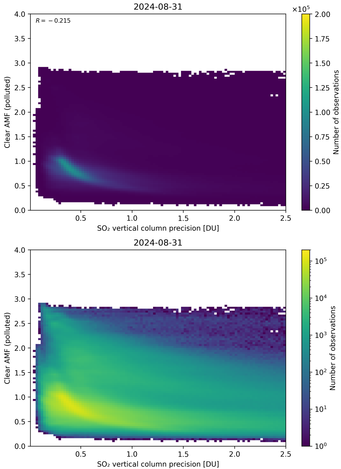
Figure 285: Scatter density plot of “SO 2 vertical column precision” against “Clear AMF (polluted)” for 2024-08-30 to 2024-09-01.
