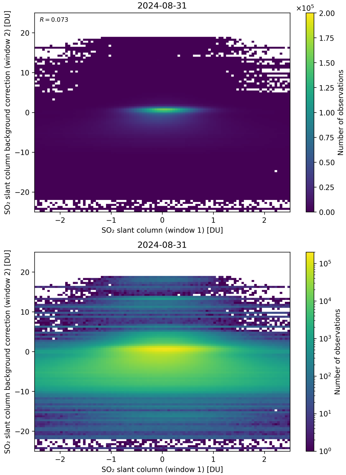
Figure 213: Scatter density plot of “SO 2 slant column (window 1)” against “SO 2 slant column background correction (window 2)” for 2024-08-30 to 2024-09-01.
