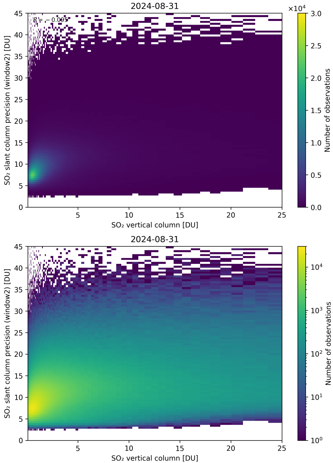
Figure 302: Scatter density plot of “SO 2 vertical column” against “SO 2 slant column precision (window2)” for 2024-08-30 to 2024-09-01.
