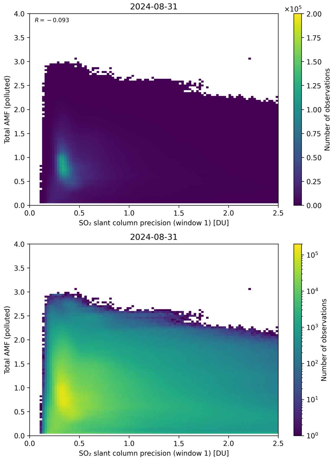
Figure 230: Scatter density plot of “SO 2 slant column precision (window 1)” against “Total AMF (polluted)” for 2024-08-30 to 2024-09-01.
