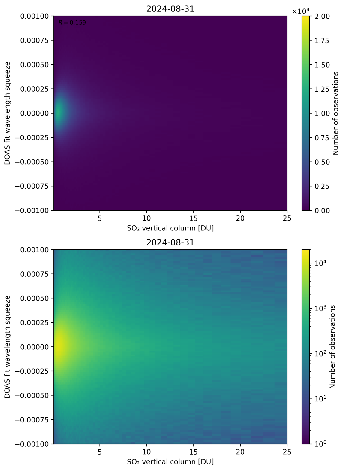
Figure 277: Scatter density plot of “SO 2 vertical column” against “DOAS fit wavelength squeeze” for 2024-08-30 to 2024-09-01.
