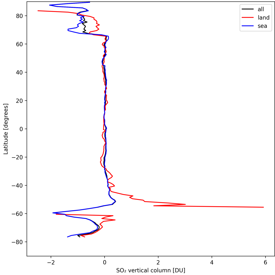
Figure 30: Zonal average of “SO 2 vertical column” for 2024-08-30 to 2024-09-01.
