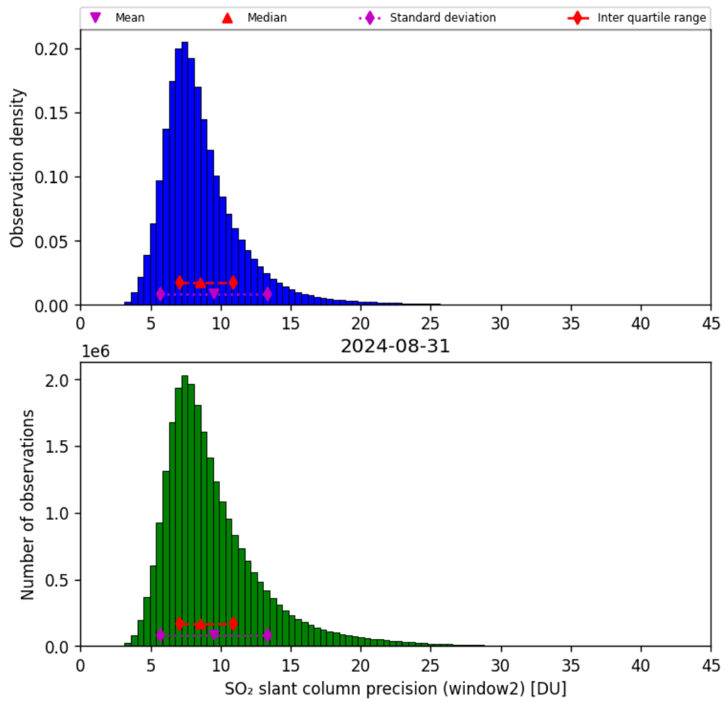
Figure 61: Histogram of “SO 2 slant column precision (window2)” for 2024-08-30 to 2024-09-01
