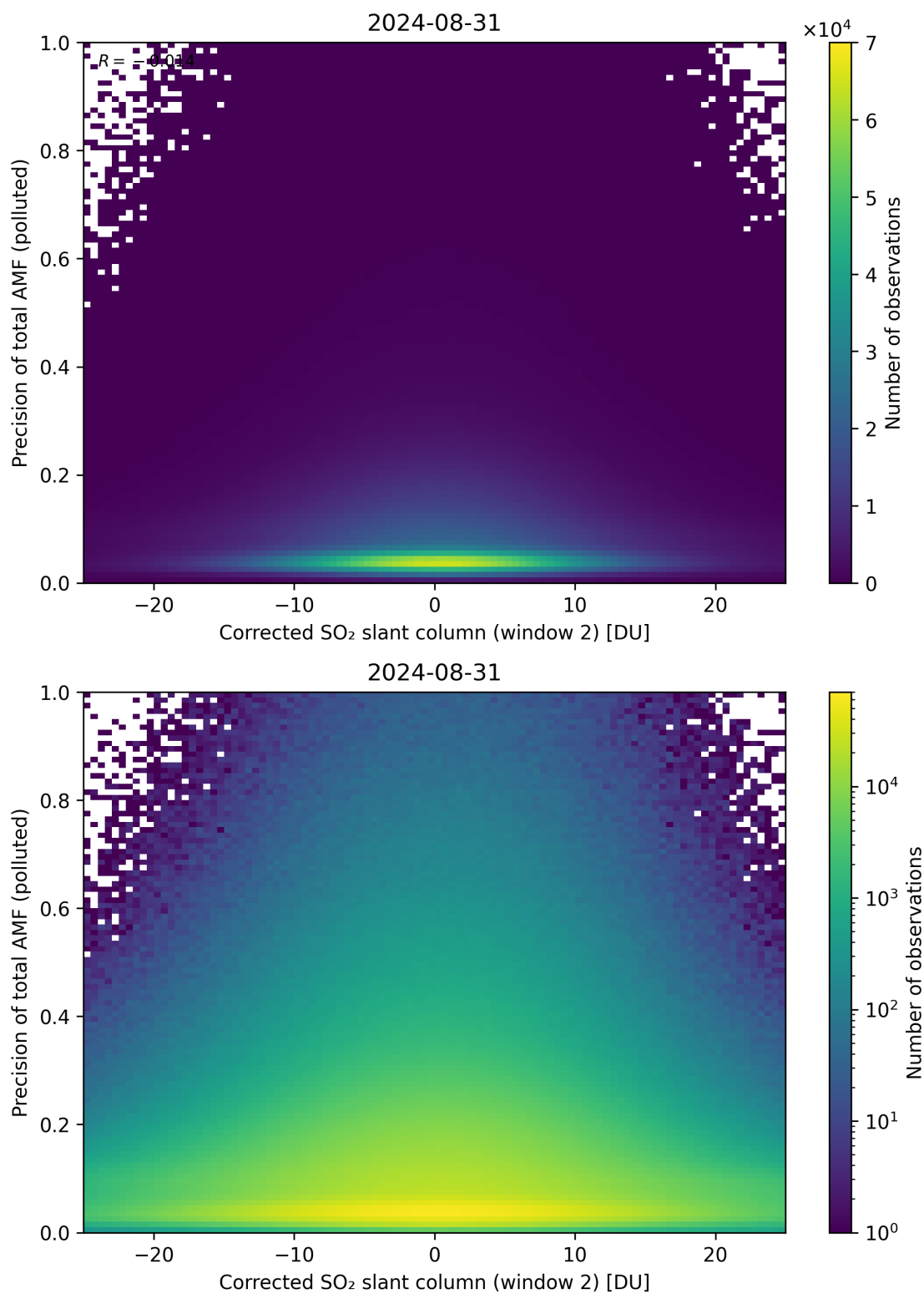
Figure 204: Scatter density plot of “Corrected SO 2 slant column (window 2)” against “Precision of total AMF (polluted)” for 2024-08-30 to 2024-09-01.
