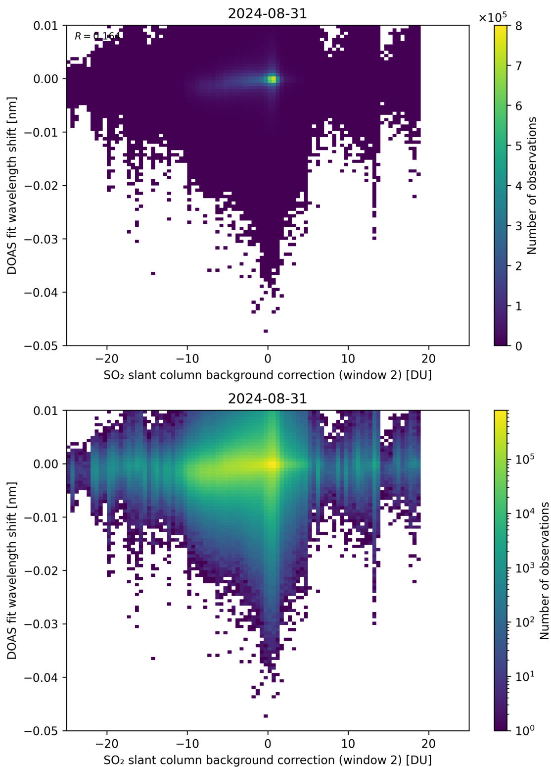
Figure 112: Scatter density plot of “SO 2 slant column background correction (window 2)” against “DOAS fit wavelength shift” for 2024-08-30 to 2024-09-01.
