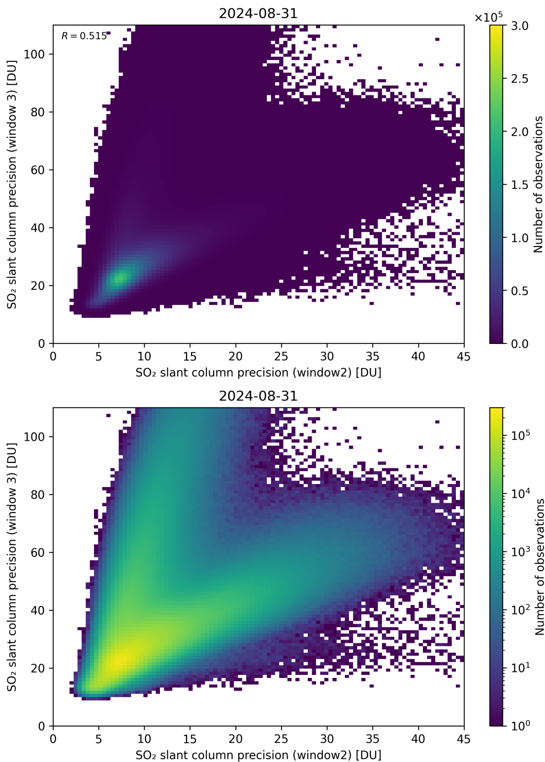
Figure 250: Scatter density plot of “SO 2 slant column precision (window2)” against “SO 2 slant column precision (window 3)” for 2024-08-30 to 2024-09-01.
