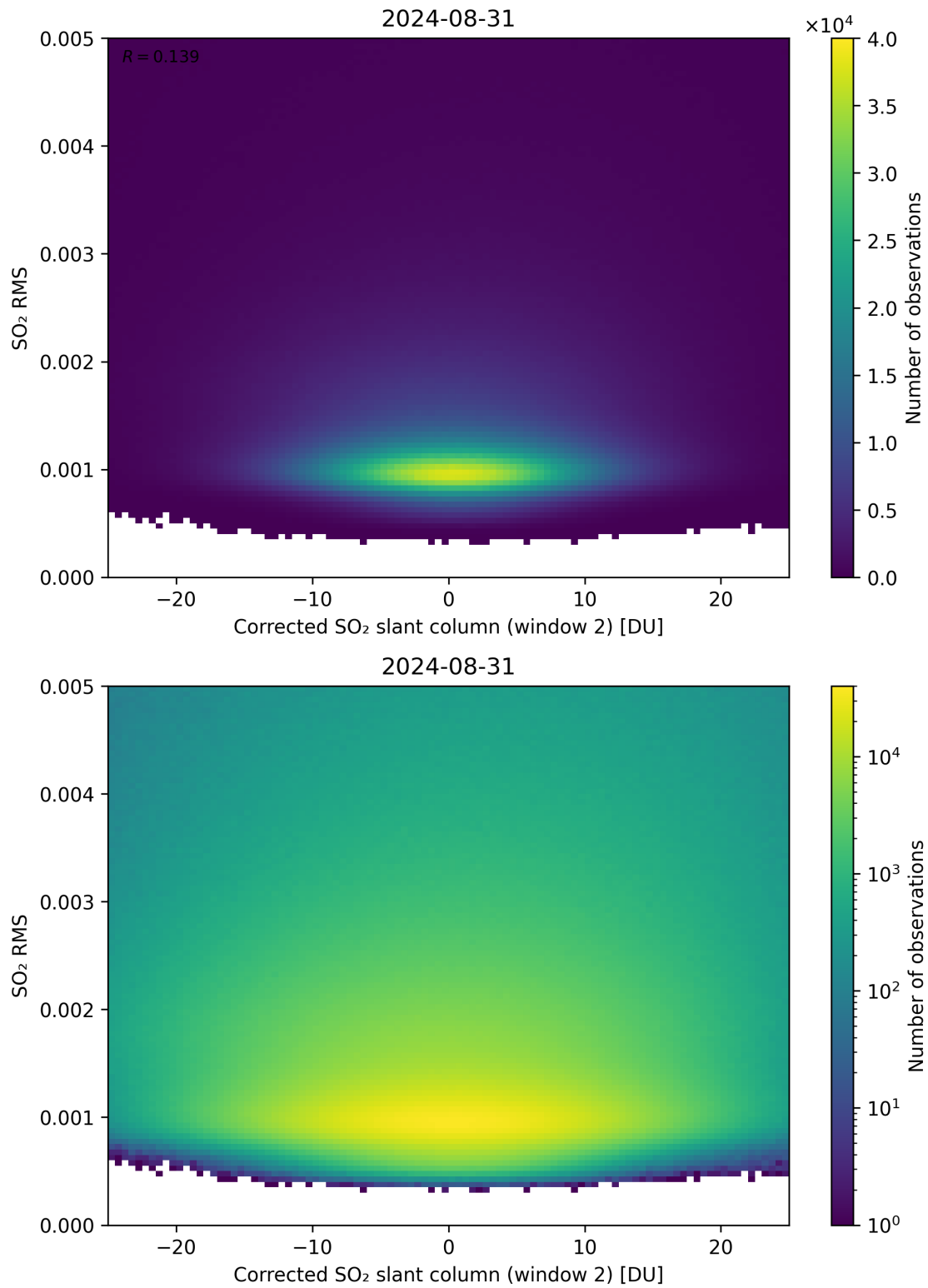
Figure 198: Scatter density plot of “Corrected SO 2 slant column (window 2)” against “SO 2 RMS” for 2024-08-30 to 2024-09-01.
