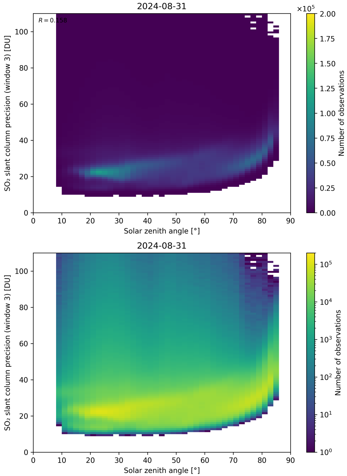
Figure 173: Scatter density plot of “Solar zenith angle” against “SO 2 slant column precision (window 3)” for 2024-08-30 to 2024-09-01.
