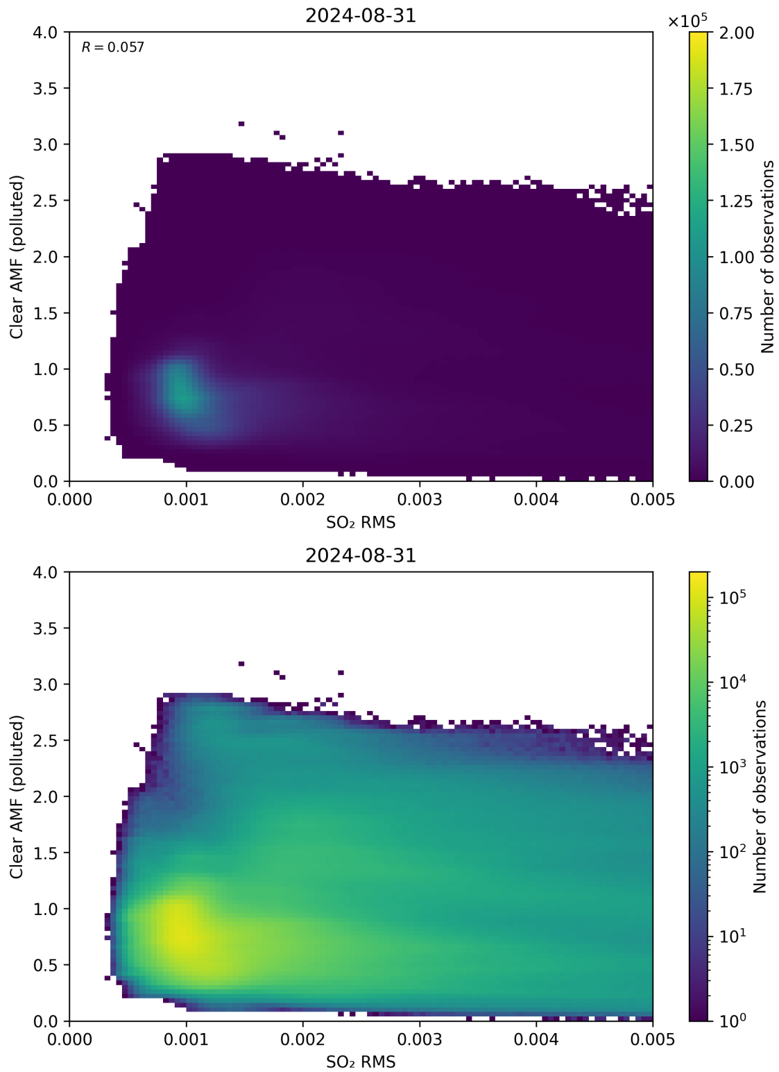
Figure 136: Scatter density plot of “SO 2 RMS” against “Clear AMF (polluted)” for 2024-08-30 to 2024-09-01.
