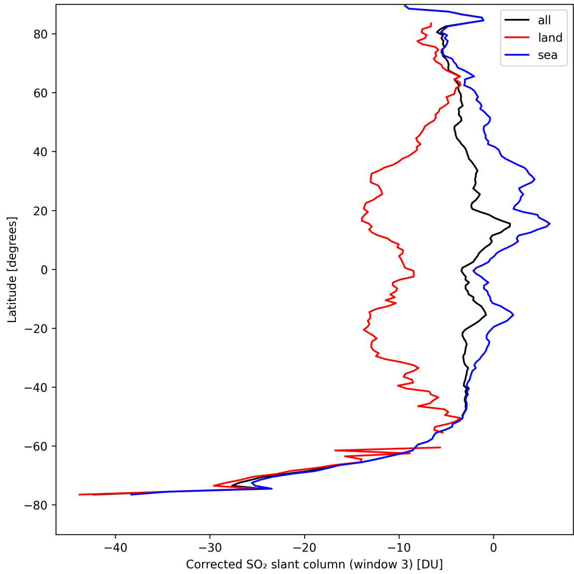
Figure 43: Zonal average of “Corrected SO 2 slant column (window 3)” for 2024-08-30 to 2024-09-01.
