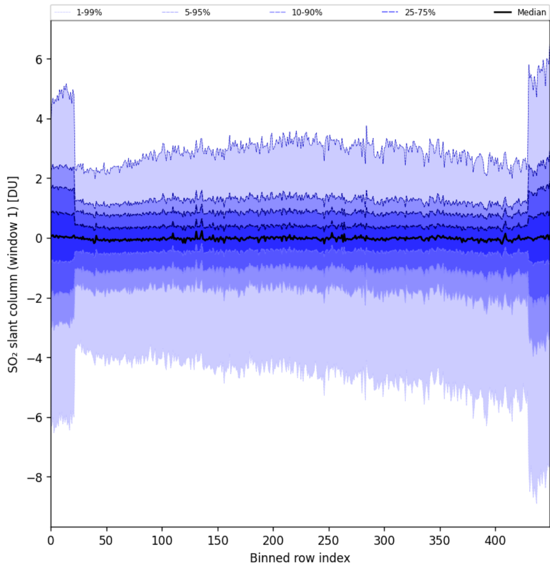
Figure 79: Along track statistics of “SO 2 slant column (window 1)” for 2024-08-30 to 2024-09-01
