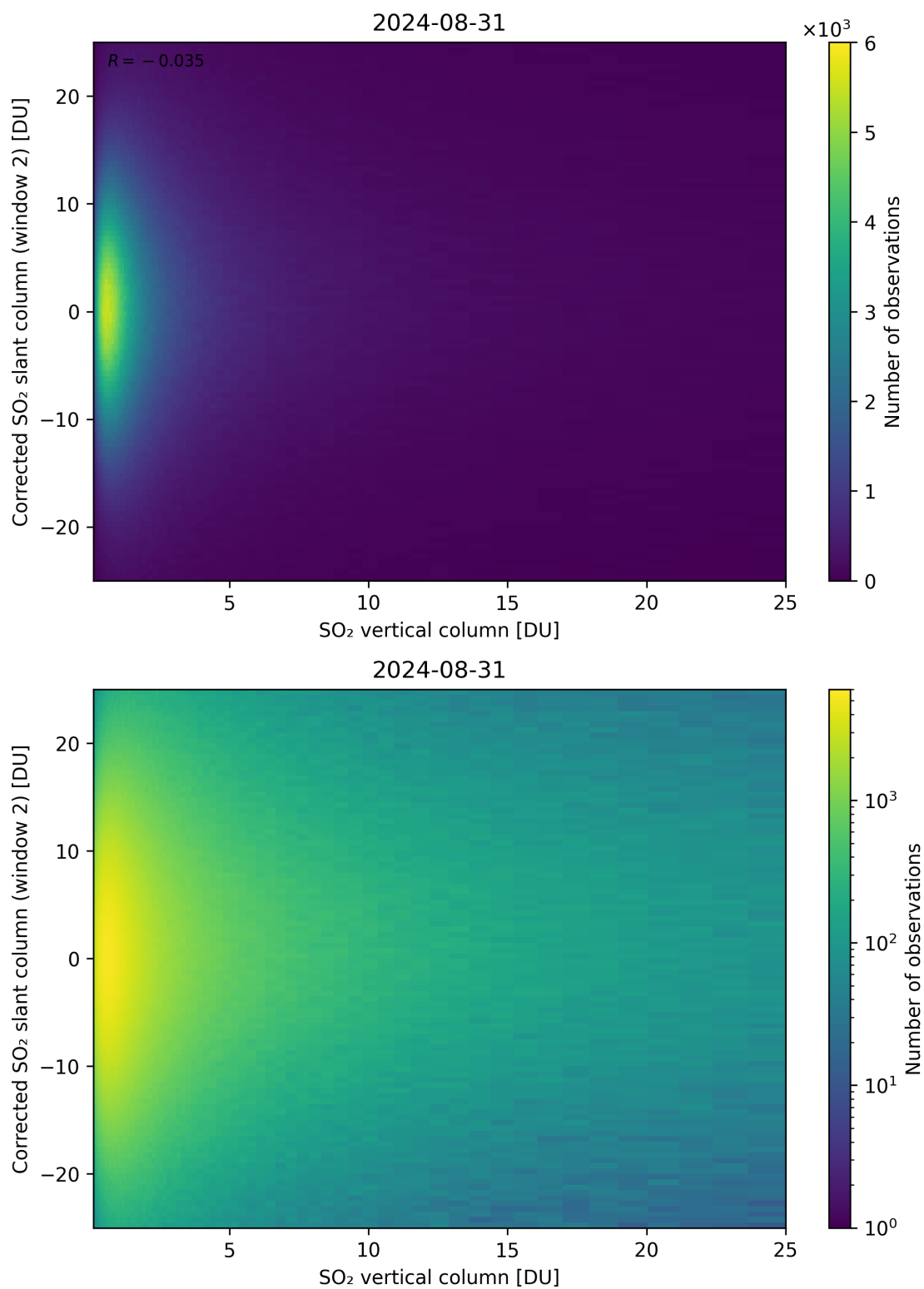
Figure 298: Scatter density plot of “SO 2 vertical column” against “Corrected SO 2 slant column (window 2)” for 2024-08-30 to 2024-09-01.
