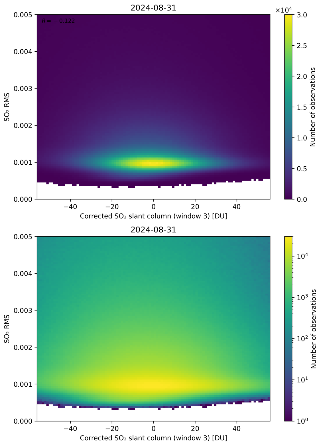
Figure 208: Scatter density plot of “Corrected SO 2 slant column (window 3)” against “SO 2 RMS” for 2024-08-30 to 2024-09-01.
