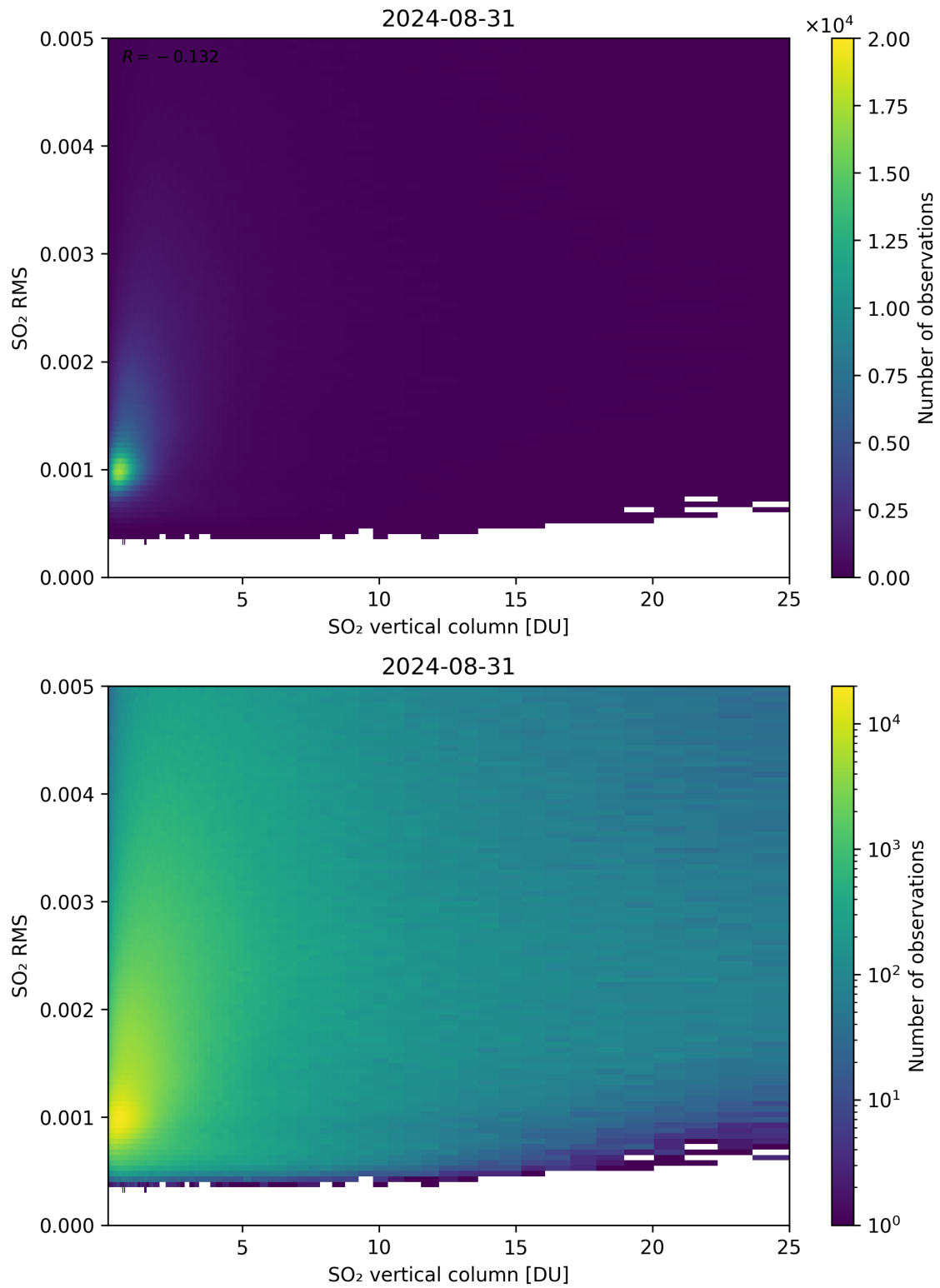
Figure 278: Scatter density plot of “SO 2 vertical column” against “SO 2 RMS” for 2024-08-30 to 2024-09-01.
