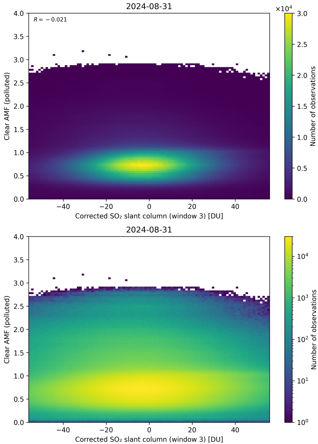
Figure 209: Scatter density plot of “Corrected SO 2 slant column (window 3)” against “Clear AMF (polluted)” for 2024-08-30 to 2024-09-01.
