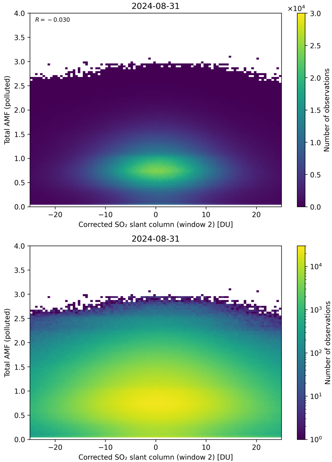
Figure 203: Scatter density plot of “Corrected SO 2 slant column (window 2)” against “Total AMF (polluted)” for 2024-08-30 to 2024-09-01.
