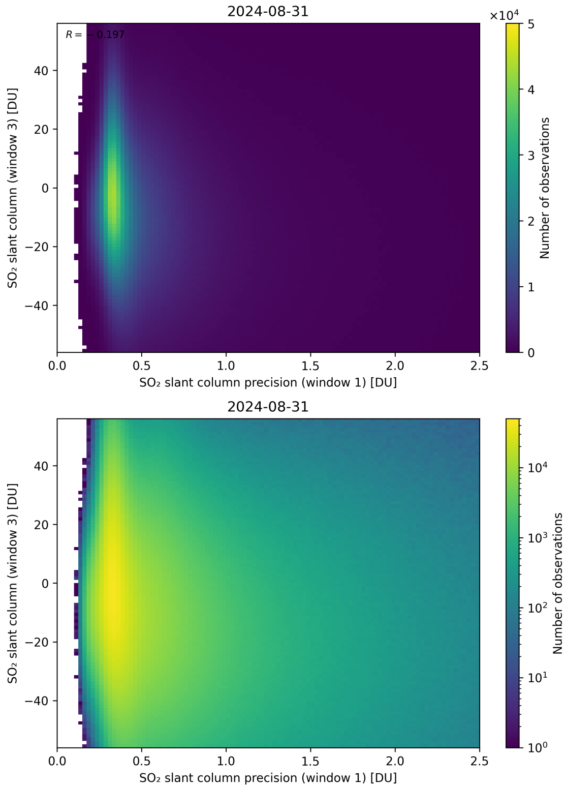
Figure 228: Scatter density plot of “SO 2 slant column precision (window 1)” against “SO 2 slant column (window 3)” for 2024-08-30 to 2024-09-01.
