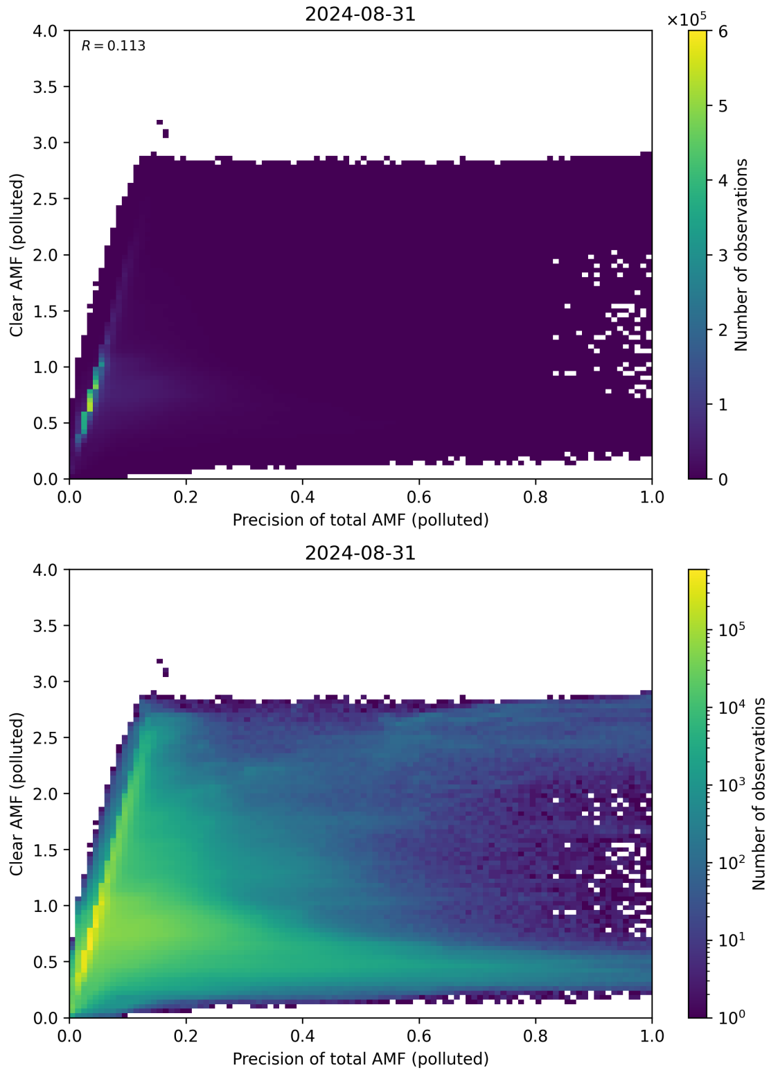
Figure 270: Scatter density plot of “Precision of total AMF (polluted)” against “Clear AMF (polluted)” for 2024-08-30 to 2024-09-01.
