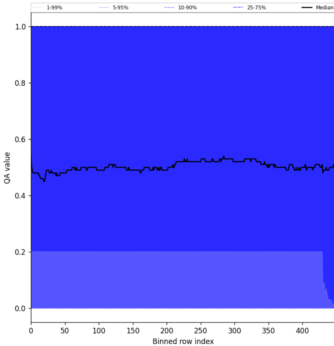
Figure 75: Along track statistics of “QA value” for 2024-08-30 to 2024-09-01
