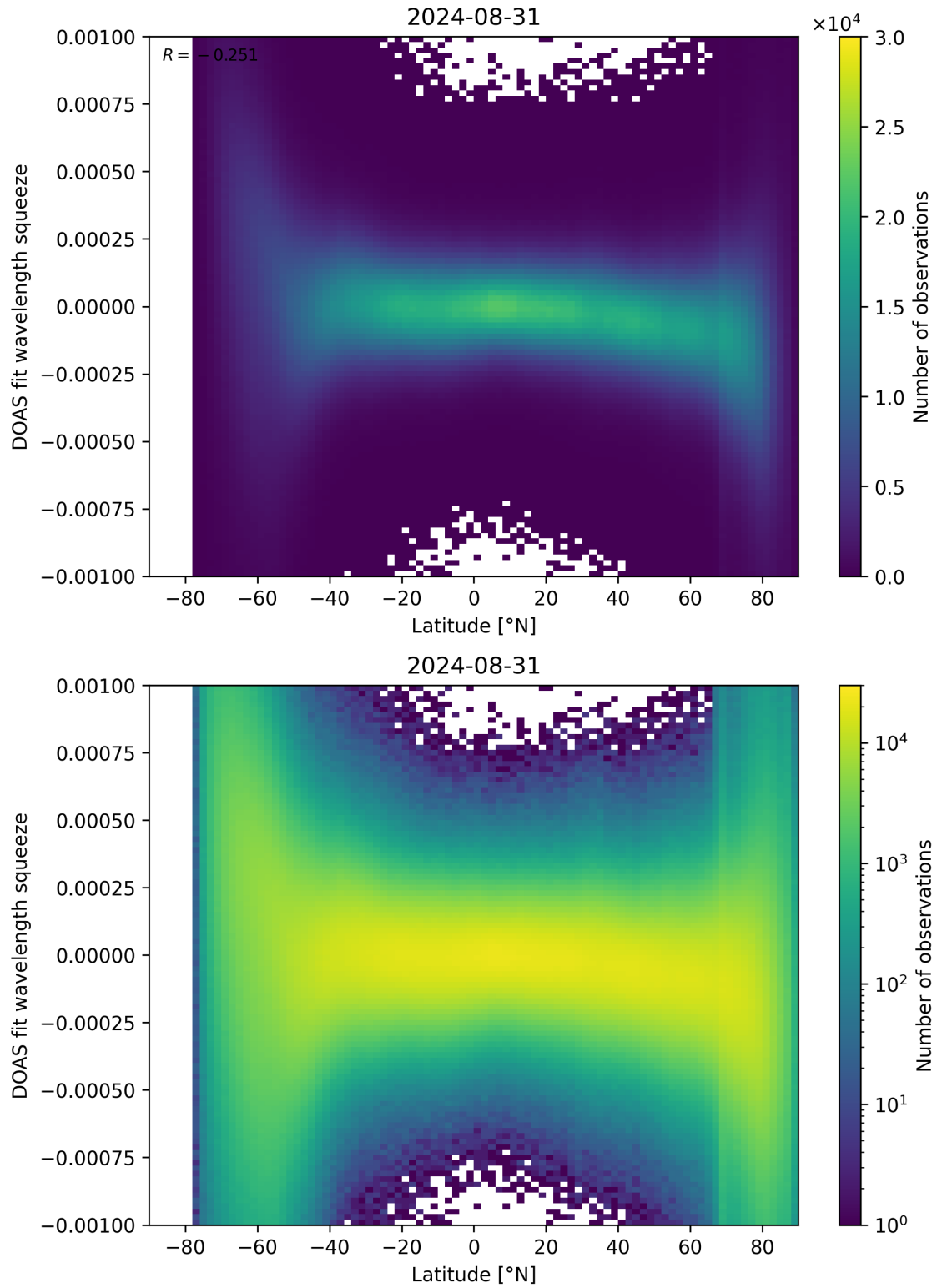
Figure 143: Scatter density plot of “Latitude” against “DOAS fit wavelength squeeze” for 2024-08-30 to 2024-09-01.
