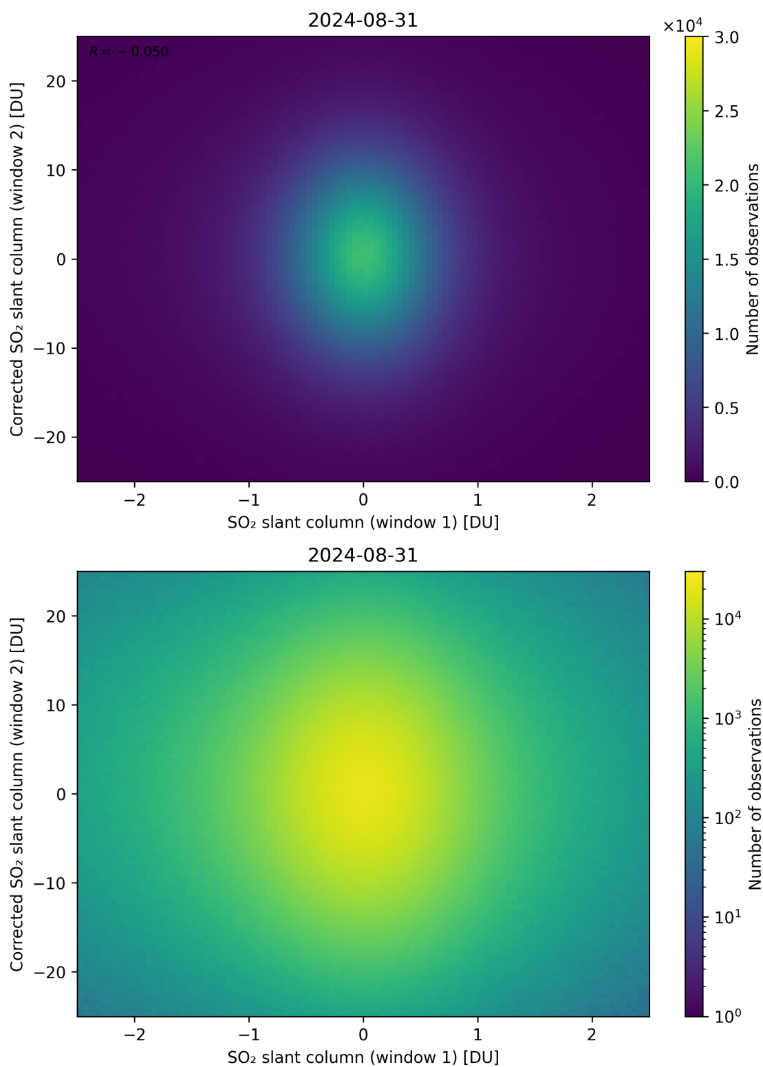
Figure 233: Scatter density plot of “SO 2 slant column (window 1)” against “Corrected SO 2 slant column (window 2)” for 2024-08-30 to 2024-09-01.
