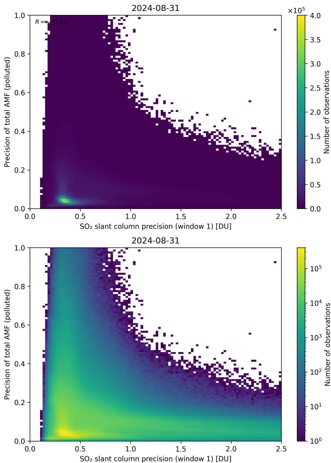
Figure 231: Scatter density plot of “SO 2 slant column precision (window 1)” against “Precision of total AMF (polluted)” for 2024-08-30 to 2024-09-01.
