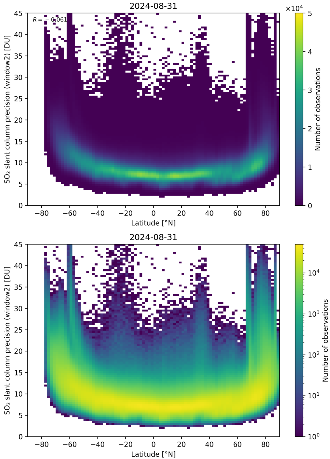
Figure 151: Scatter density plot of “Latitude” against “SO 2 slant column precision (window2)” for 2024-08-30 to 2024-09-01.
