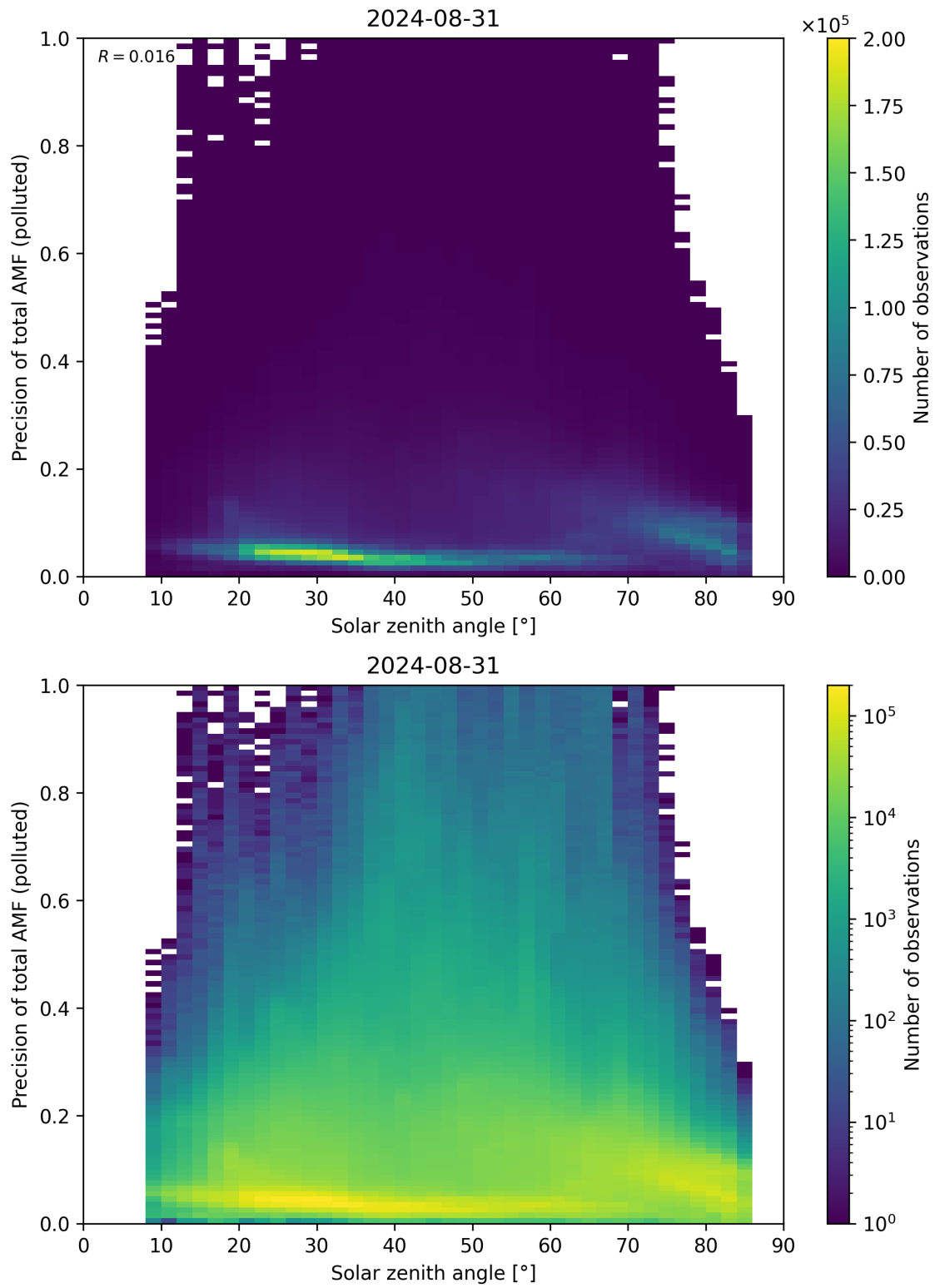
Figure 175: Scatter density plot of “Solar zenith angle” against “Precision of total AMF (polluted)” for 2024-08-30 to 2024-09-01.
