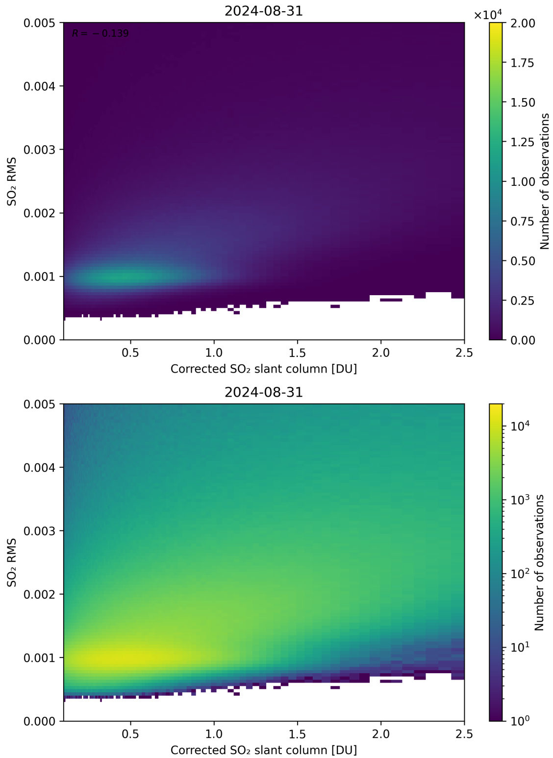
Figure 183: Scatter density plot of “Corrected SO 2 slant column” against “SO 2 RMS” for 2024-08-30 to 2024-09-01.
