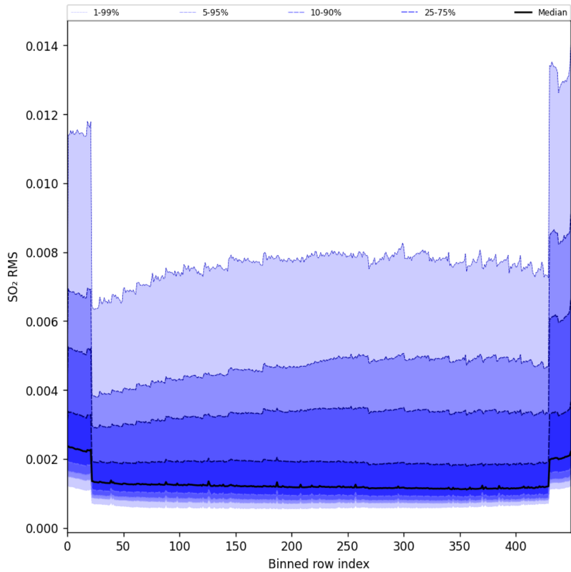
Figure 93: Along track statistics of “SO 2 RMS” for 2024-08-30 to 2024-09-01
