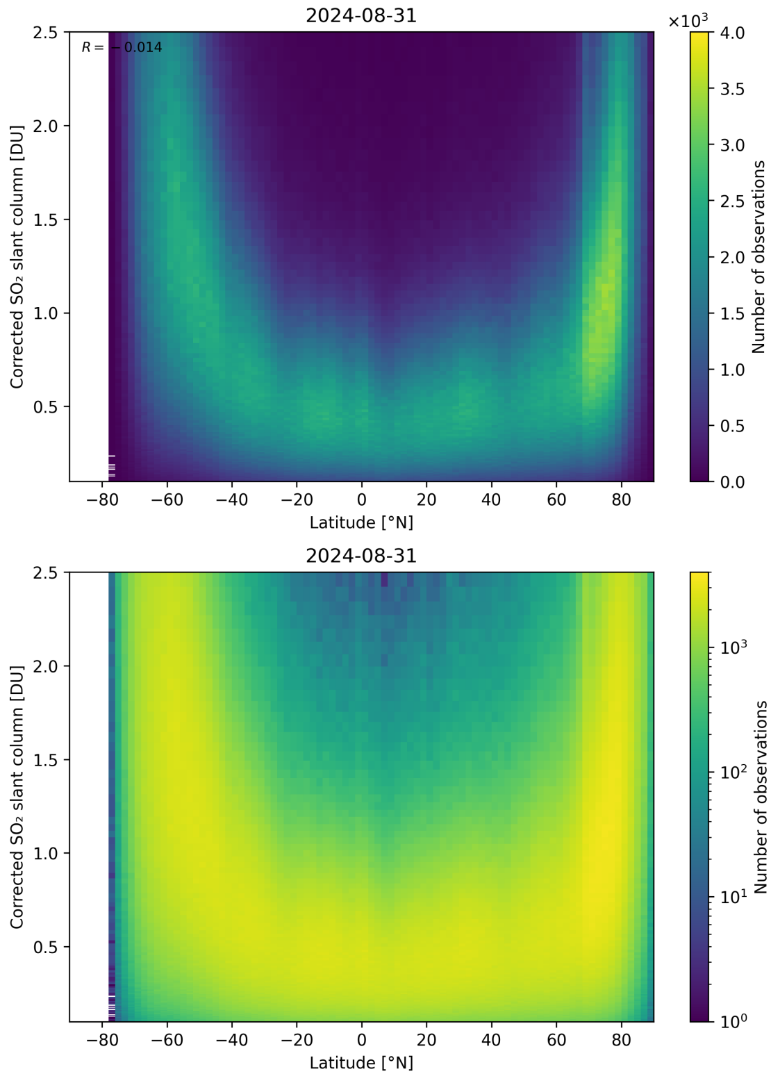
Figure 146: Scatter density plot of “Latitude” against “Corrected SO 2 slant column” for 2024-08-30 to 2024-09-01.
