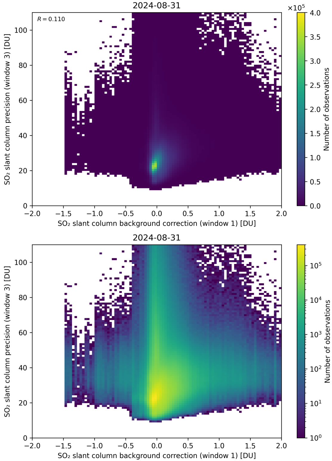
Figure 108: Scatter density plot of “SO 2 slant column background correction (window 1)” against “SO 2 slant column precision (window 3)” for 2024-08-30 to 2024-09-01.
