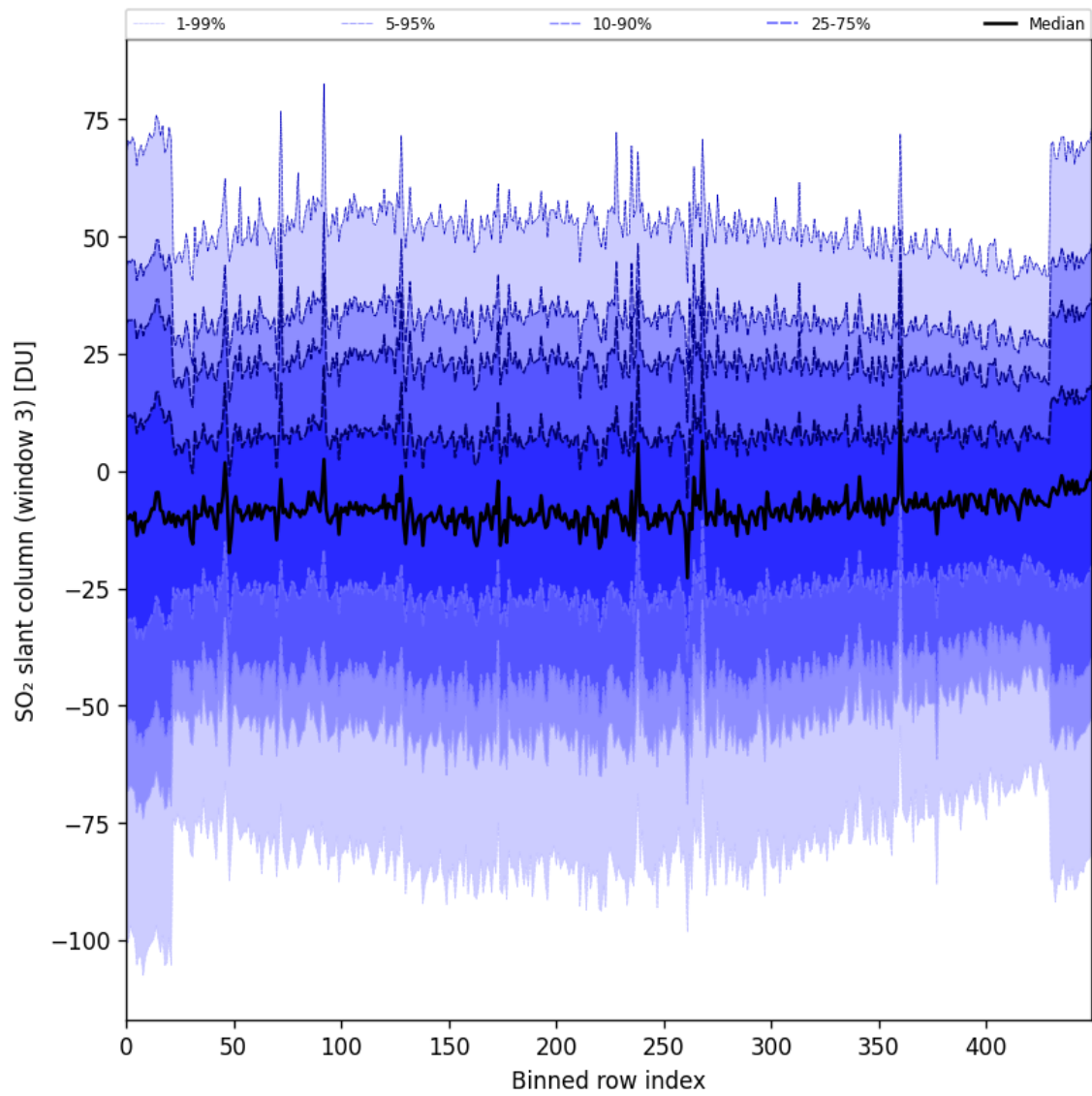
Figure 87: Along track statistics of “SO 2 slant column (window 3)” for 2024-08-30 to 2024-09-01
