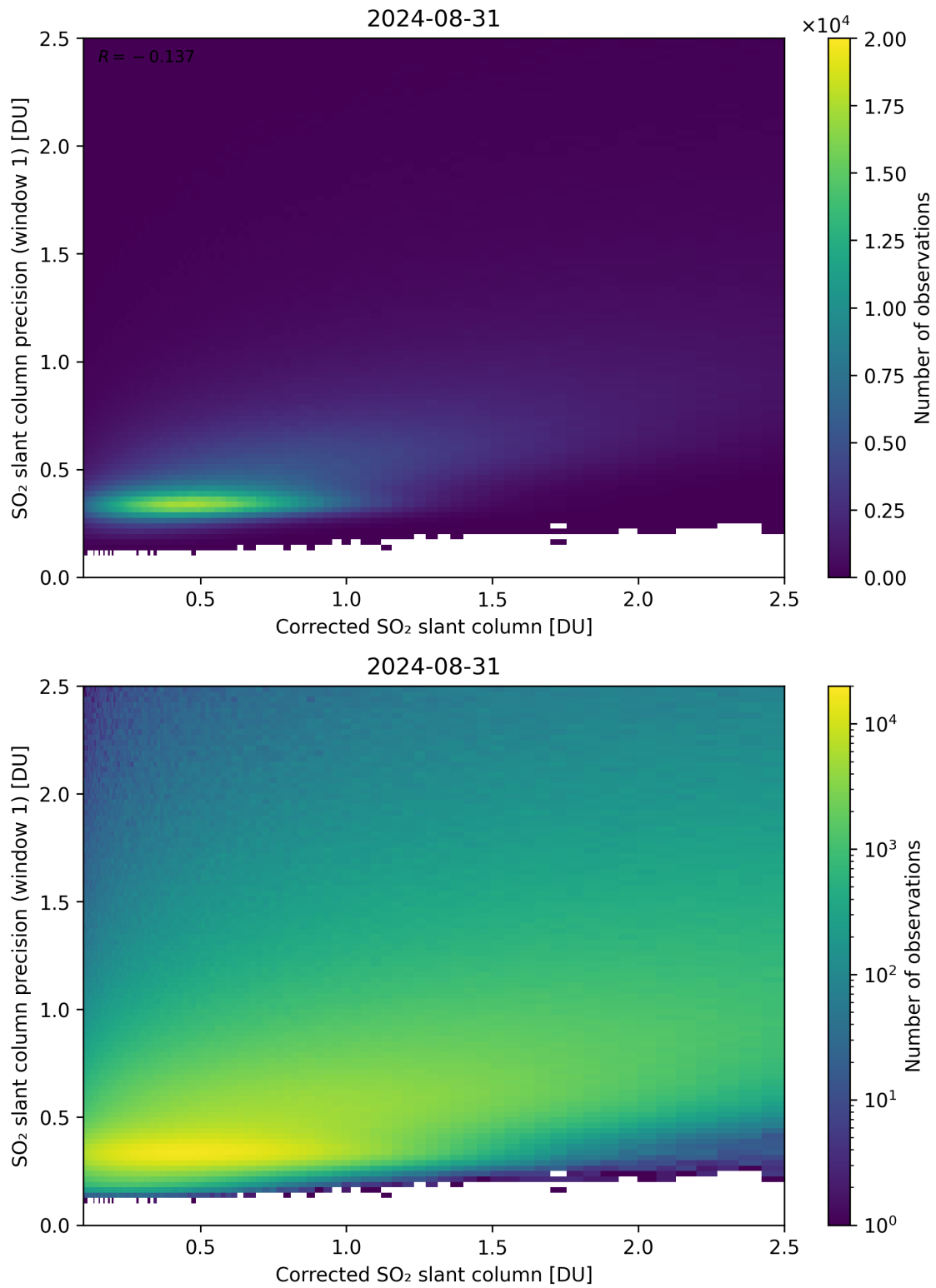
Figure 188: Scatter density plot of “Corrected SO 2 slant column” against “SO 2 slant column precision (window 1)” for 2024-08-30 to 2024-09-01.
