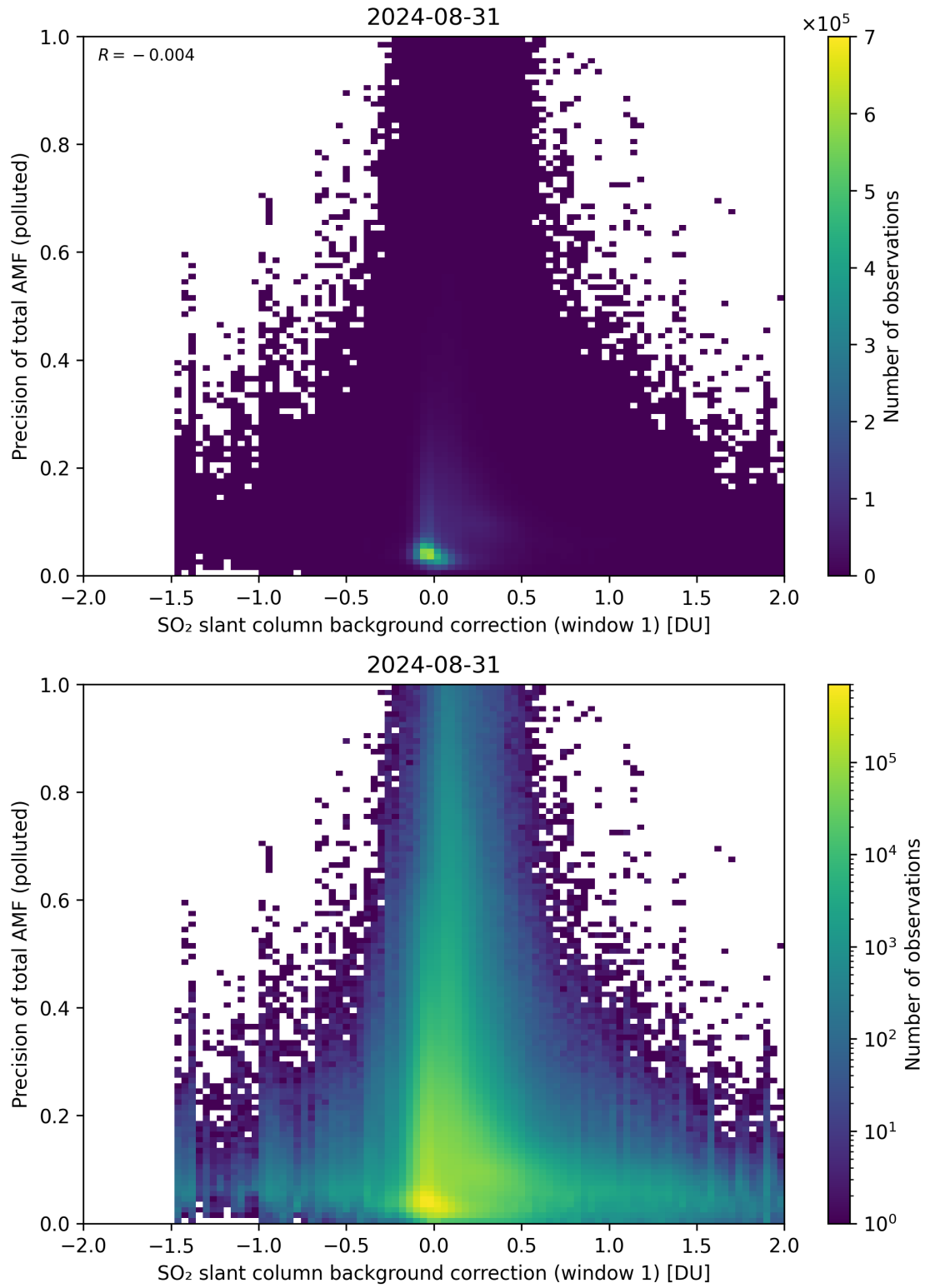
Figure 110: Scatter density plot of “SO 2 slant column background correction (window 1)” against “Precision of total AMF (polluted)” for 2024-08-30 to 2024-09-01.
