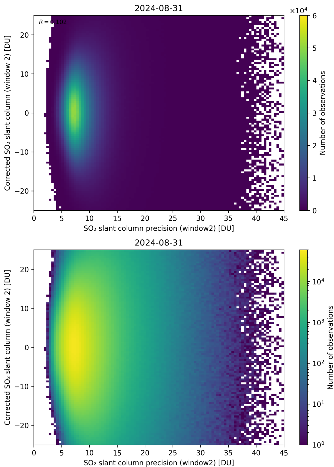
Figure 247: Scatter density plot of “SO 2 slant column precision (window2)” against “Corrected SO 2 slant column (window 2)” for 2024-08-30 to 2024-09-01.
