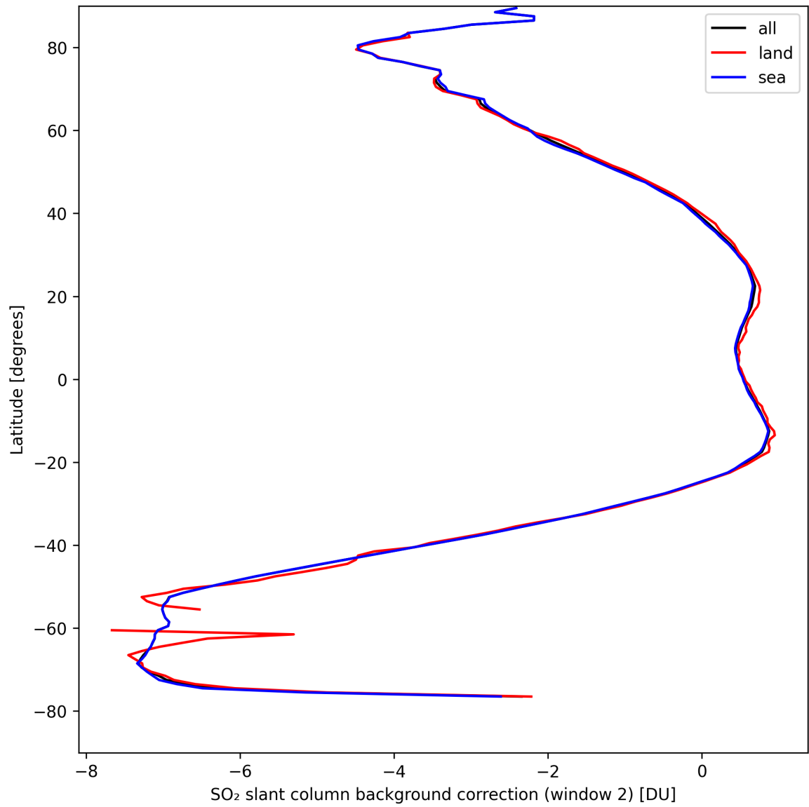
Figure 40: Zonal average of “SO 2 slant column background correction (window 2)” for 2024-08-30 to 2024-09-01.
