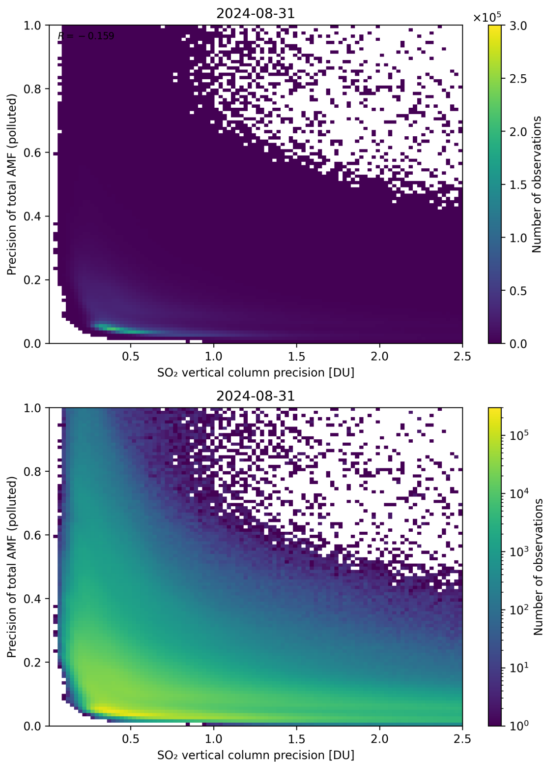
Figure 295: Scatter density plot of “SO 2 vertical column precision” against “Precision of total AMF (polluted)” for 2024-08-30 to 2024-09-01.
