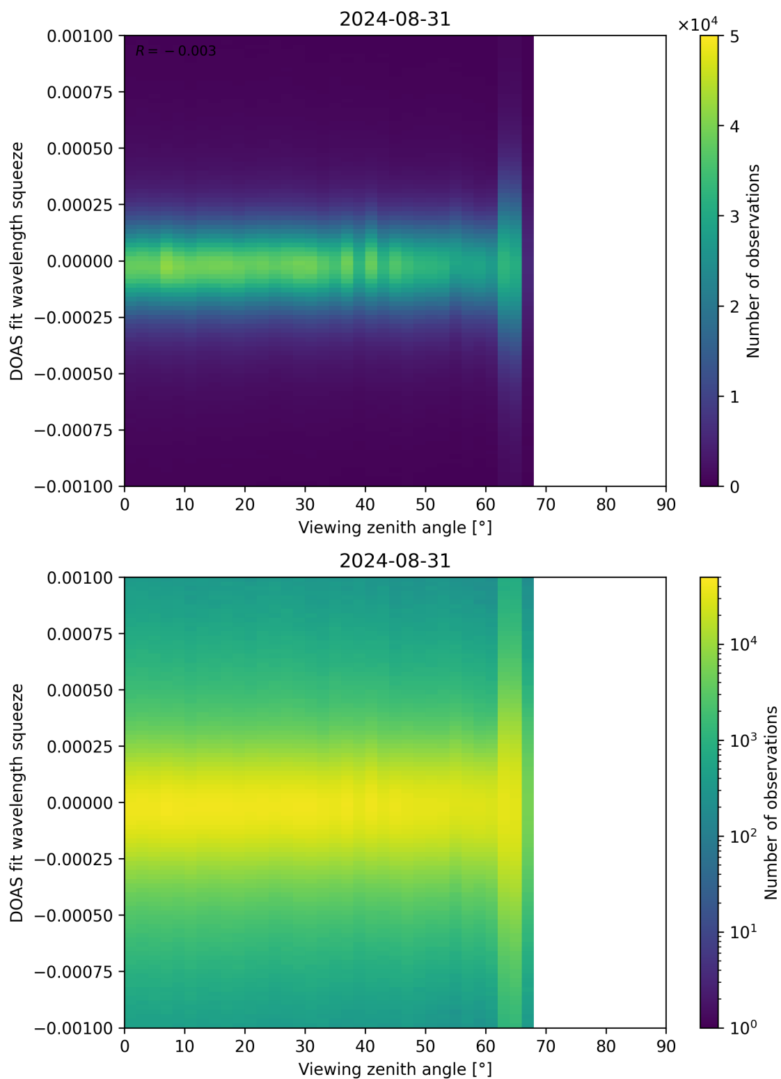
Figure 312: Scatter density plot of “Viewing zenith angle” against “DOAS fit wavelength squeeze” for 2024-08-30 to 2024-09-01.
