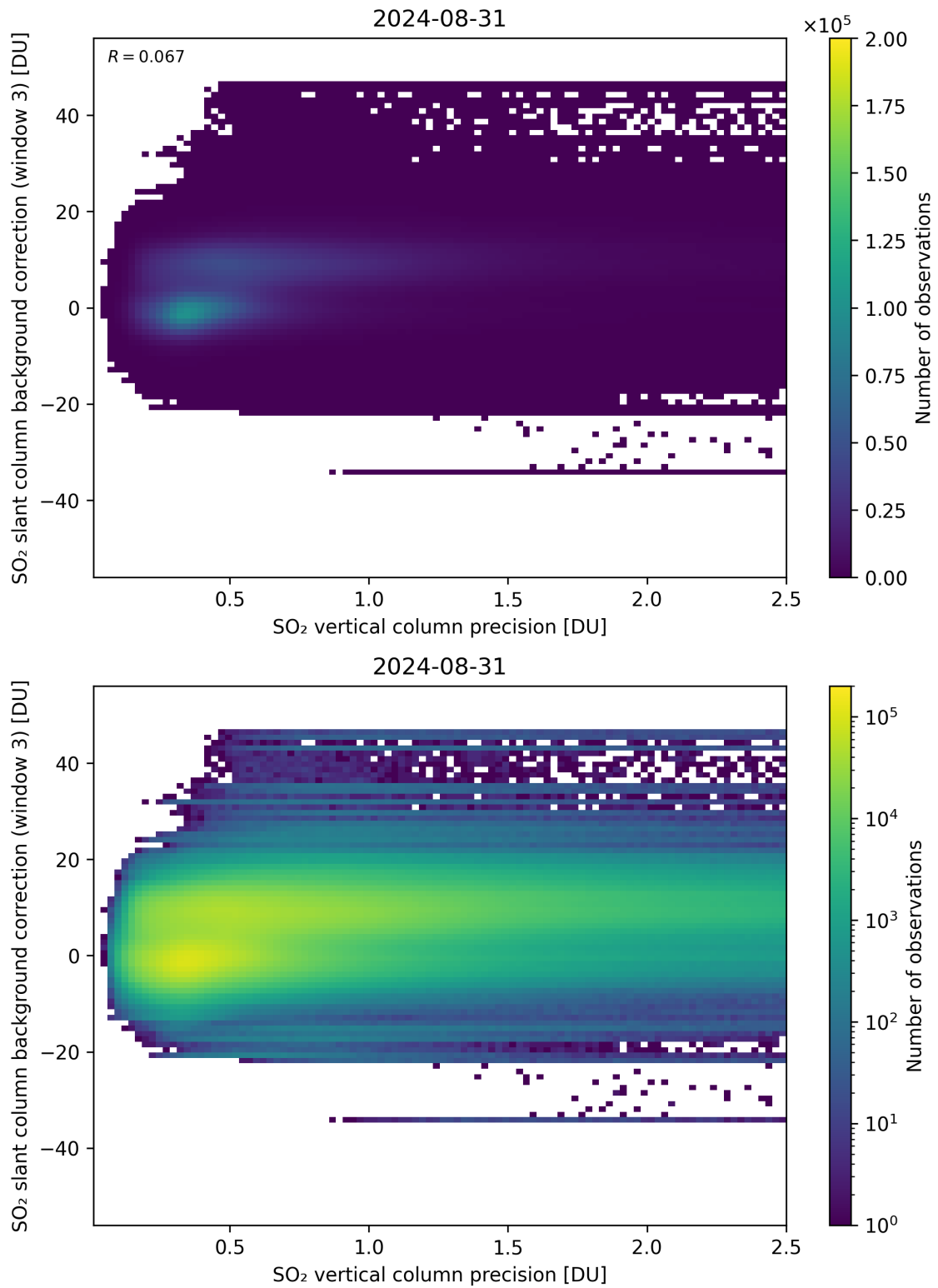
Figure 281: Scatter density plot of “SO 2 vertical column precision” against “SO 2 slant column background correction (window 3)” for 2024-08-30 to 2024-09-01.
