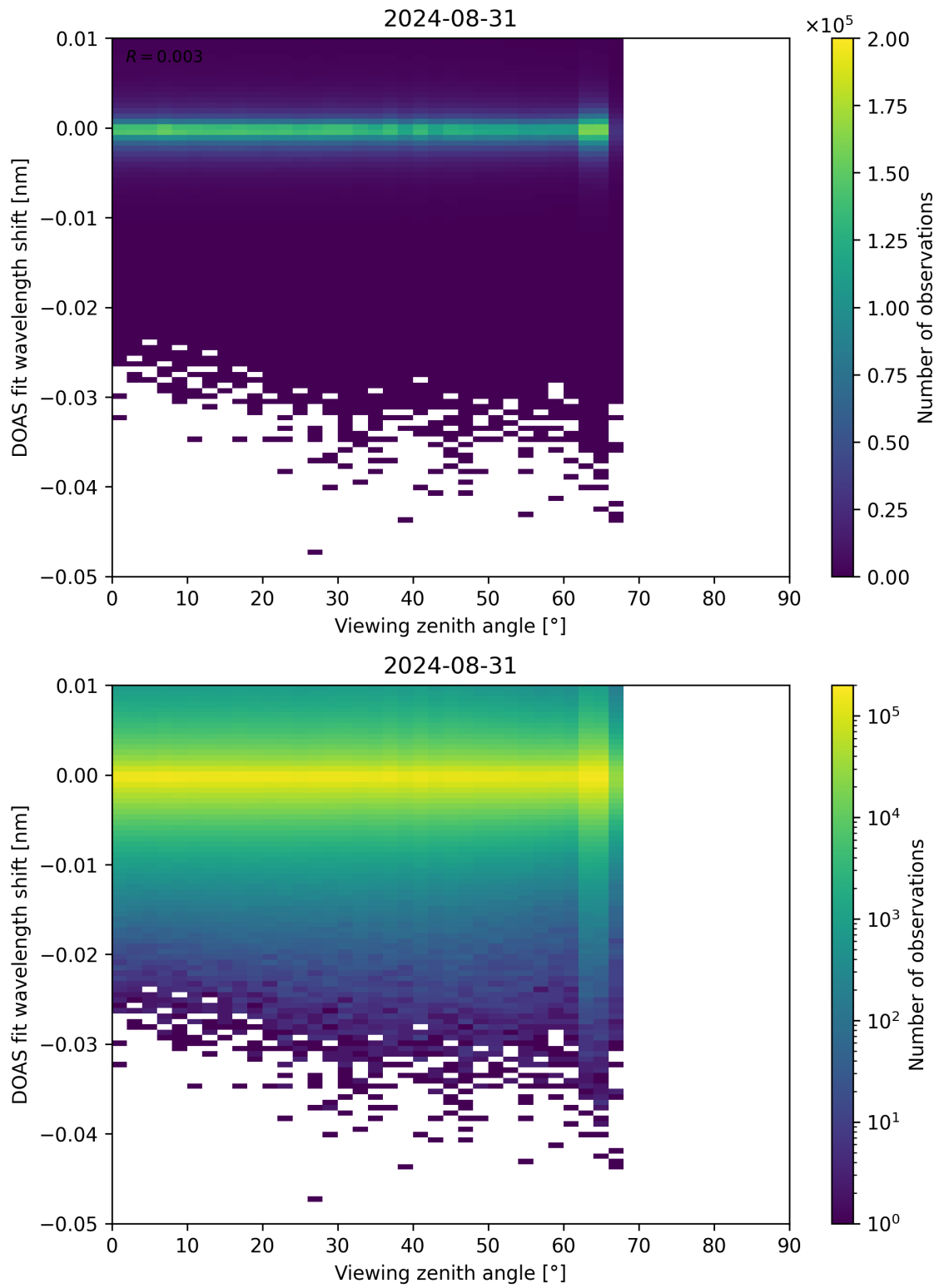
Figure 311: Scatter density plot of “Viewing zenith angle” against “DOAS fit wavelength shift” for 2024-08-30 to 2024-09-01.
