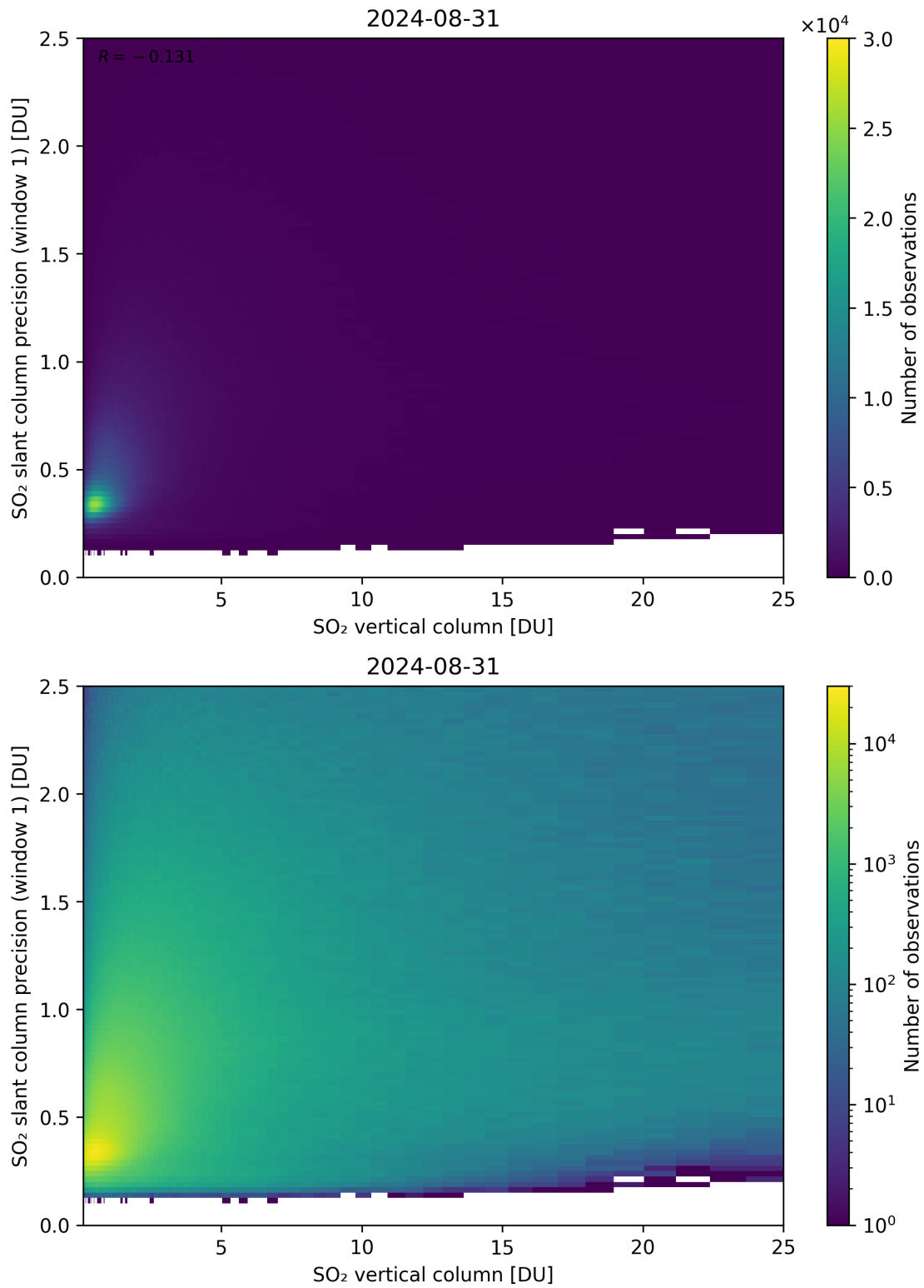
Figure 301: Scatter density plot of “SO 2 vertical column” against “SO 2 slant column precision (window 1)” for 2024-08-30 to 2024-09-01.
