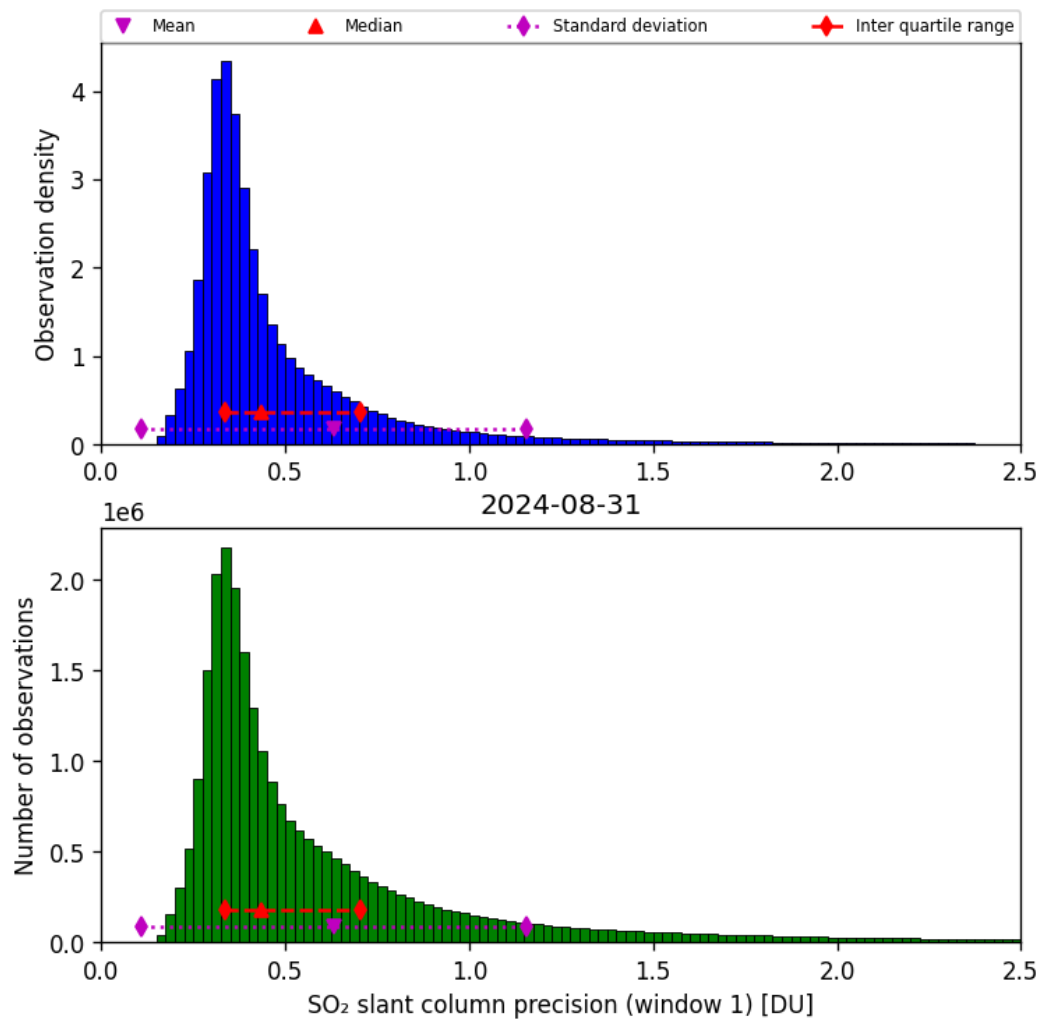
Figure 57: Histogram of "SO 2 slant column precision (window 1)" for 2024-08-30 to 2024-09-01
