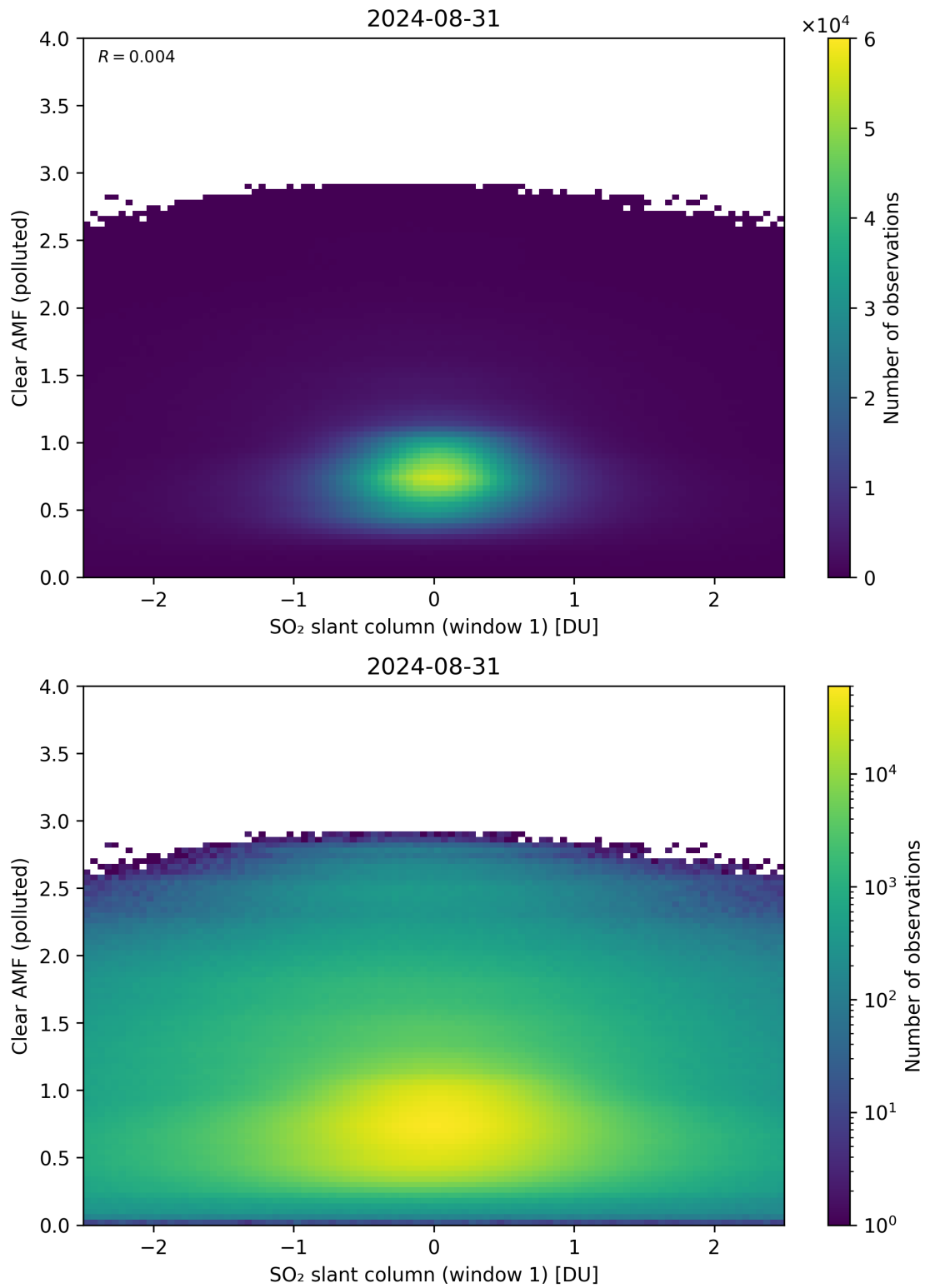
Figure 232: Scatter density plot of “SO 2 slant column (window 1)” against “Clear AMF (polluted)” for 2024-08-30 to 2024-09-01.
