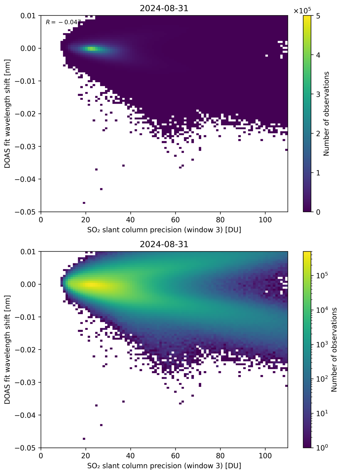
Figure 258: Scatter density plot of “SO 2 slant column precision (window 3)” against “DOAS fit wavelength shift” for 2024-08-30 to 2024-09-01.
