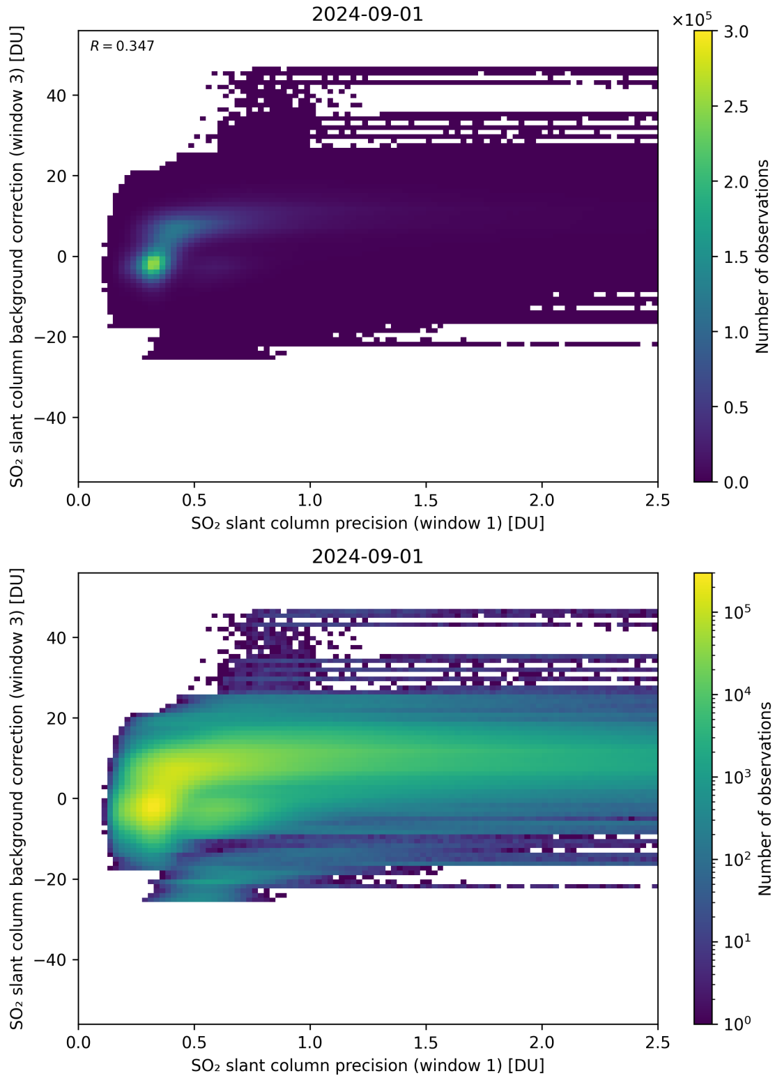
Figure 220: Scatter density plot of “SO 2 slant column precision (window 1)” against “SO 2 slant column background correction (window 3)” for 2024-09-01 to 2024-09-02.
