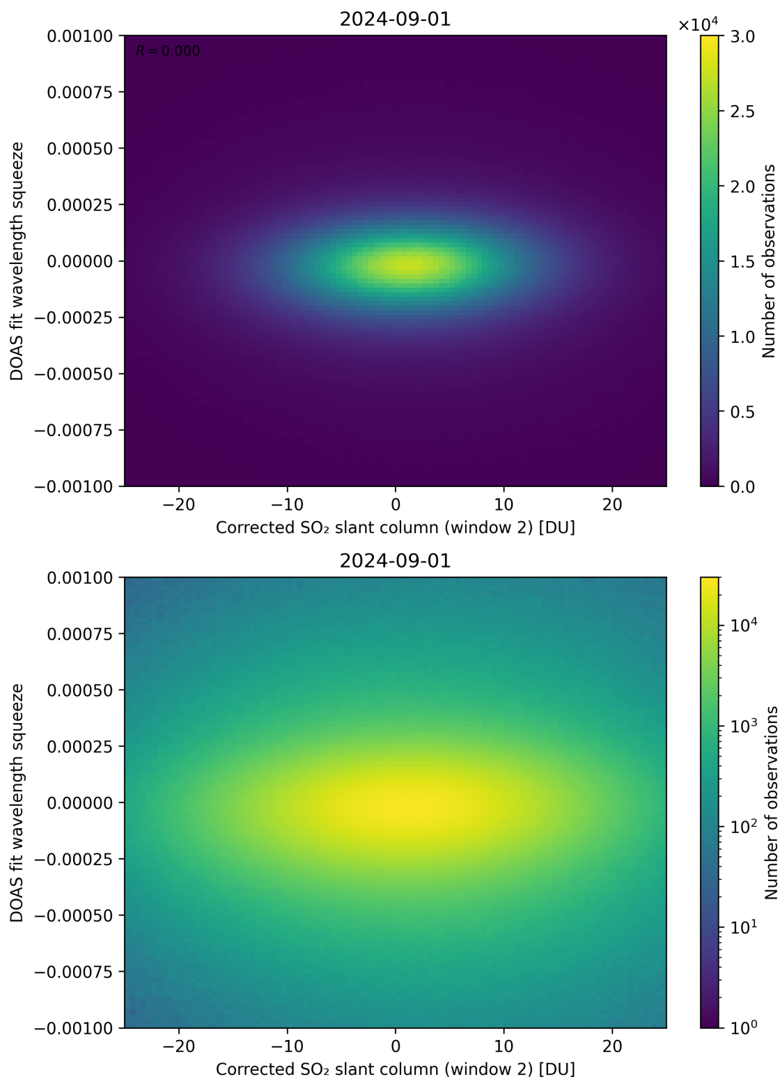
Figure 197: Scatter density plot of “Corrected SO 2 slant column (window 2)” against “DOAS fit wavelength squeeze” for 2024-09-01 to 2024-09-02.
