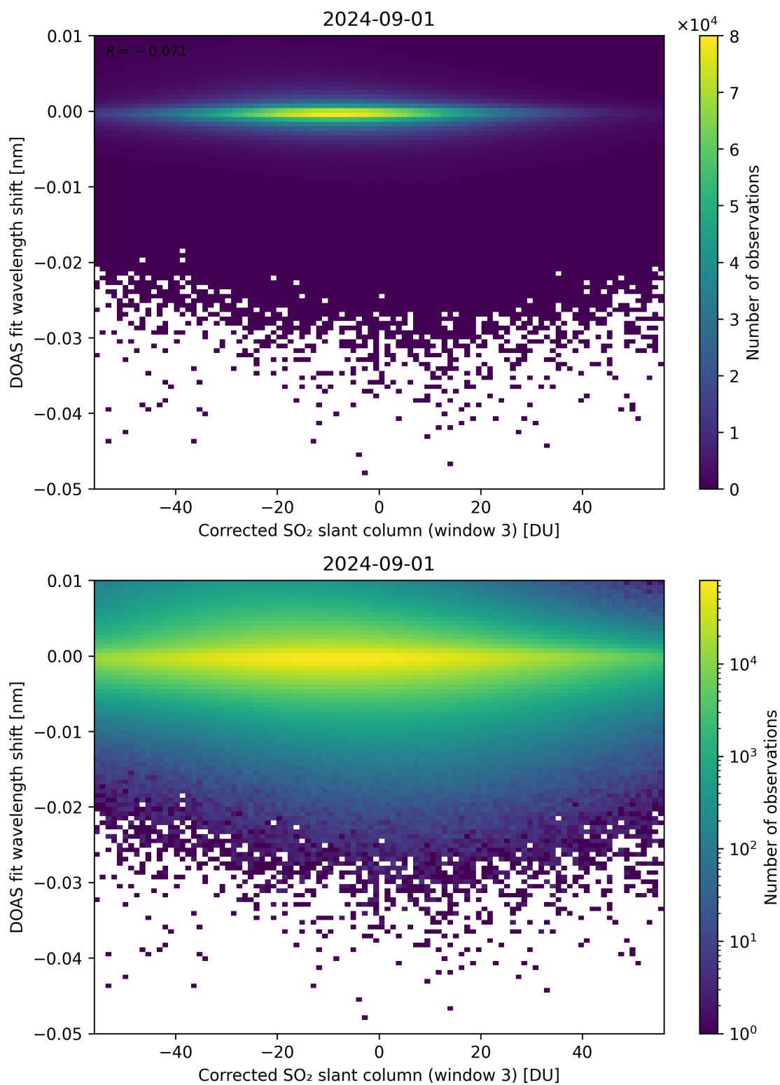
Figure 206: Scatter density plot of “Corrected SO 2 slant column (window 3)” against “DOAS fit wavelength shift” for 2024-09-01 to 2024-09-02.
