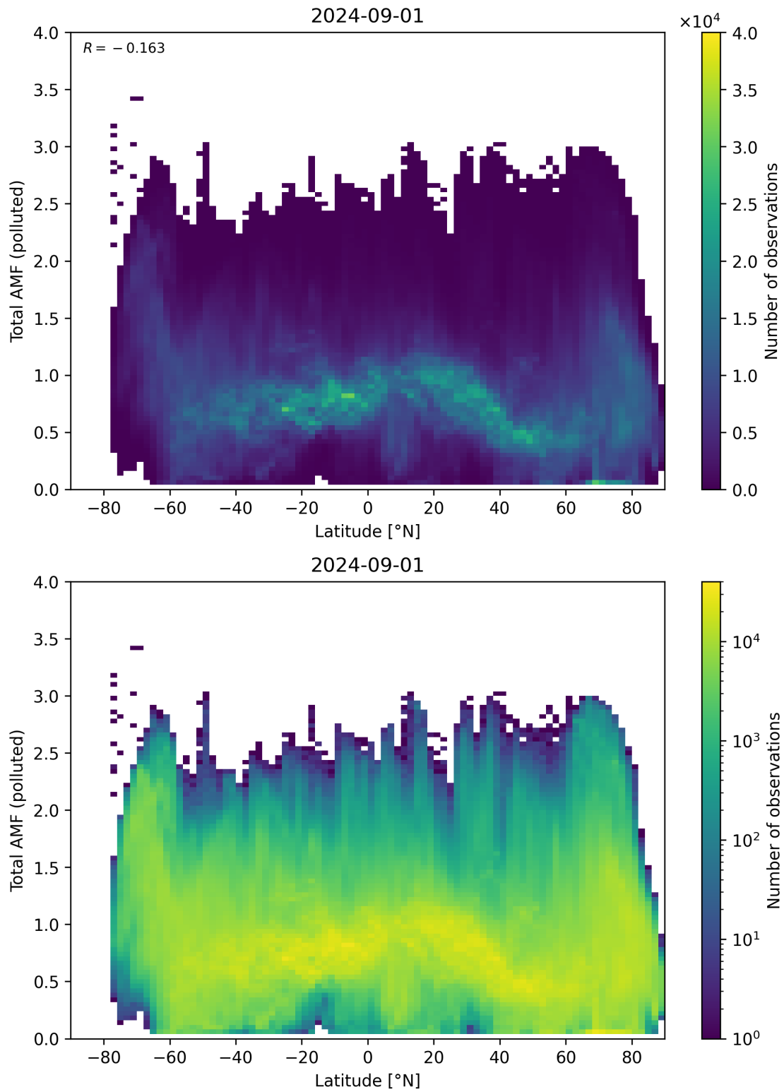
Figure 154: Scatter density plot of “Latitude” against “Total AMF (polluted)” for 2024-09-01 to 2024-09-02.
