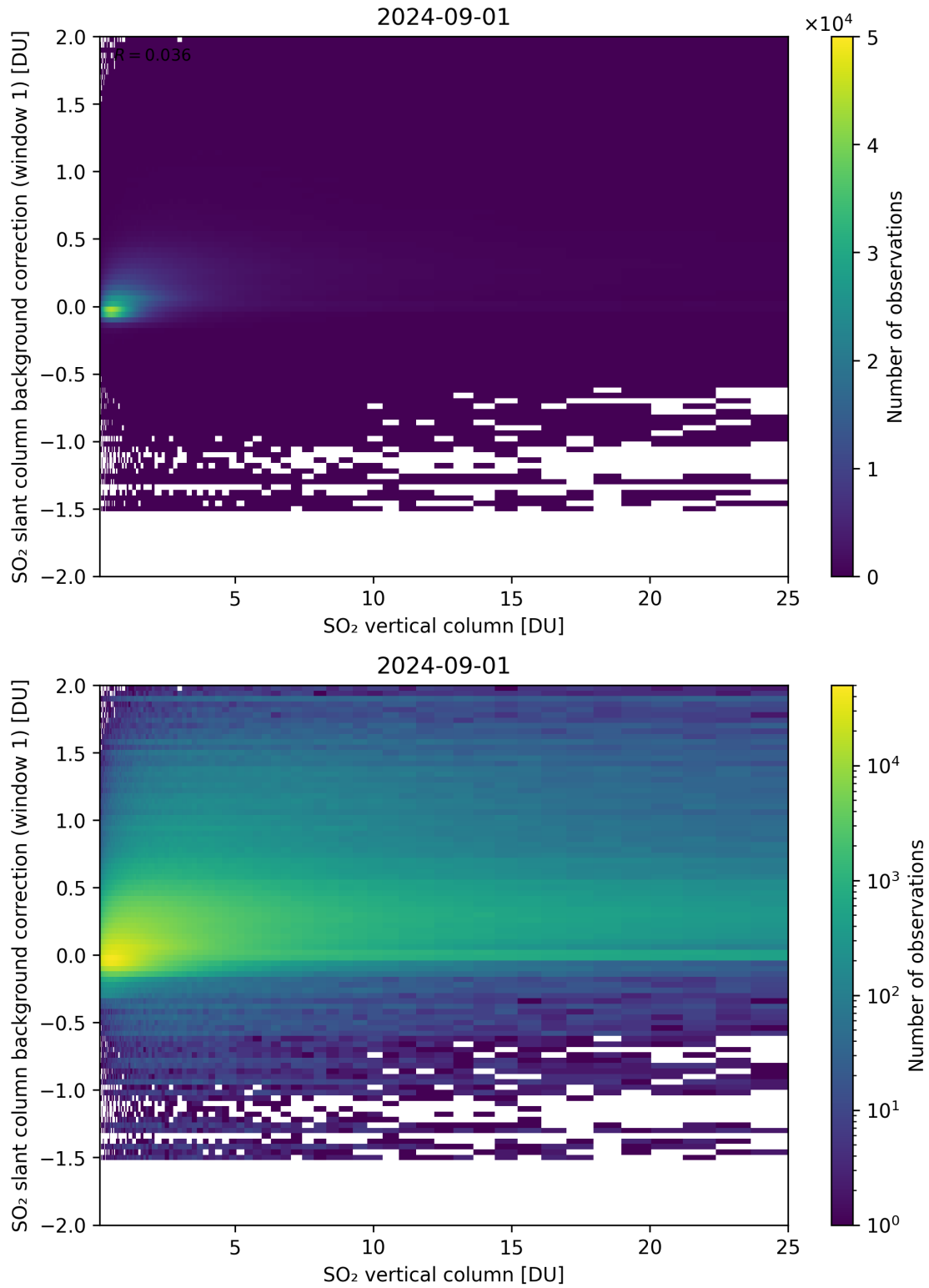
Figure 273: Scatter density plot of “SO 2 vertical column” against “SO 2 slant column background correction (window 1)” for 2024-09-01 to 2024-09-02.
