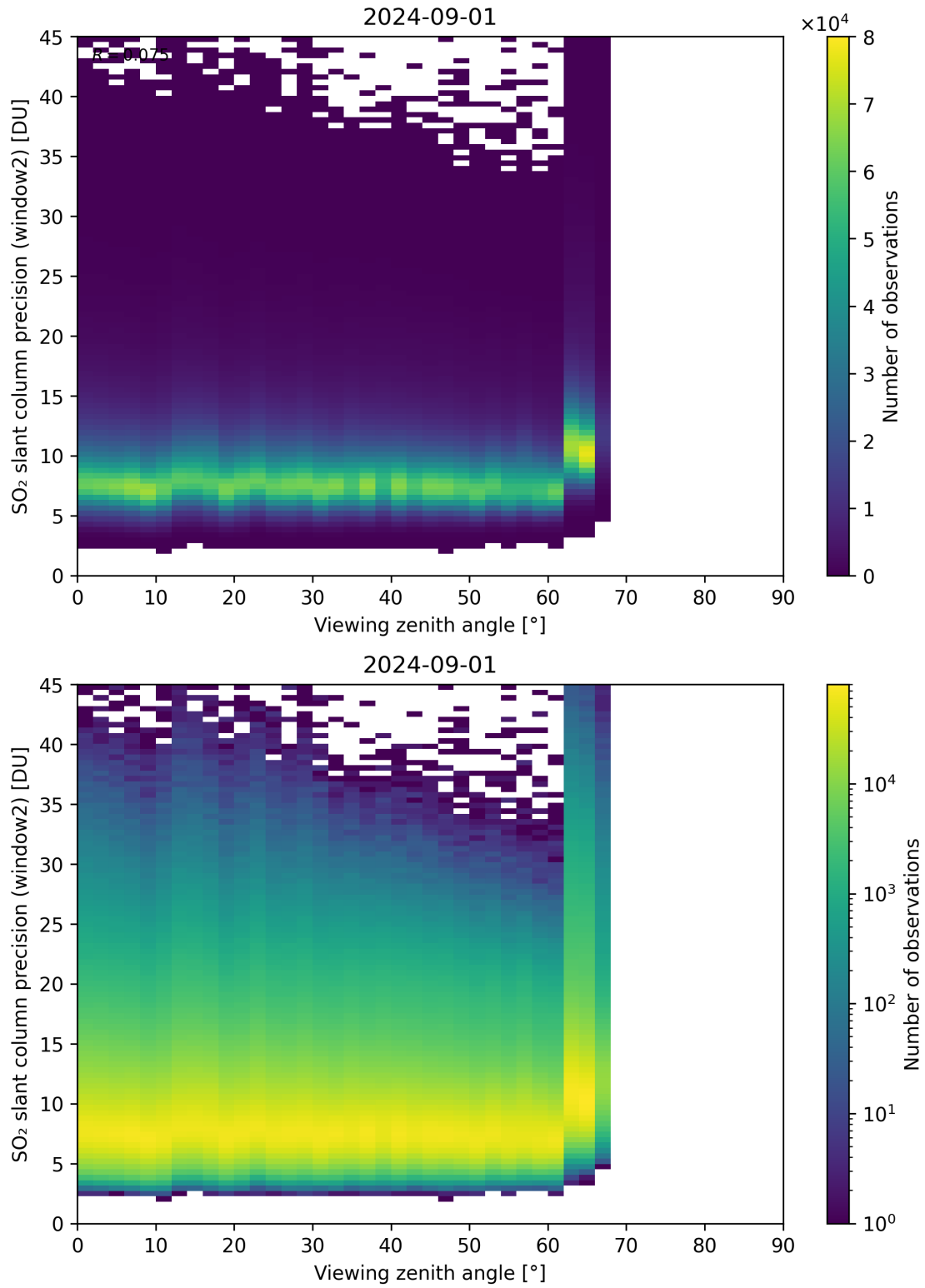
Figure 322: Scatter density plot of “Viewing zenith angle” against “SO 2 slant column precision (window2)” for 2024-09-01 to 2024-09-02.
