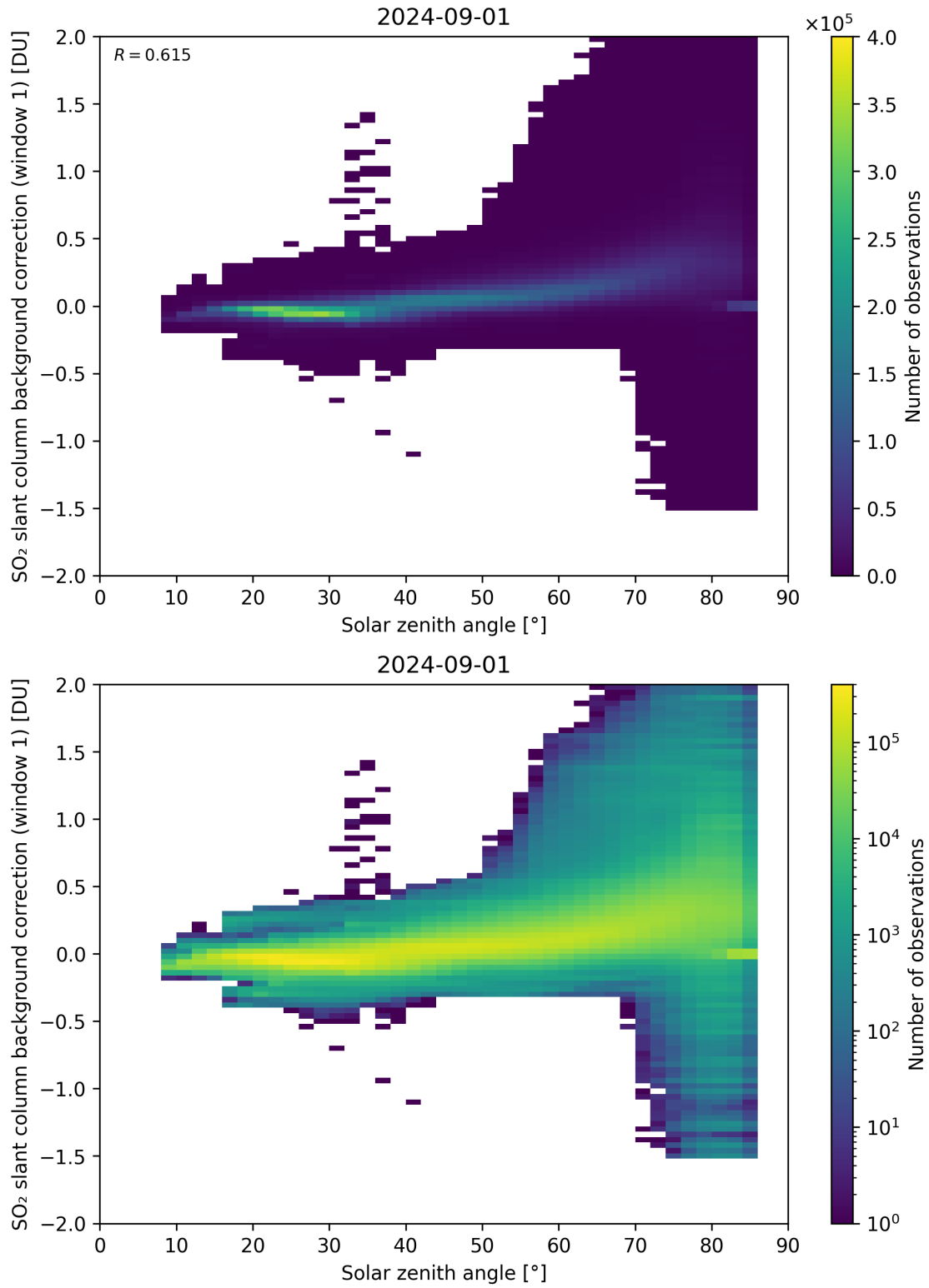
Figure 158: Scatter density plot of “Solar zenith angle” against “SO 2 slant column background correction (window 1)” for 2024-09-01 to 2024-09-02.
