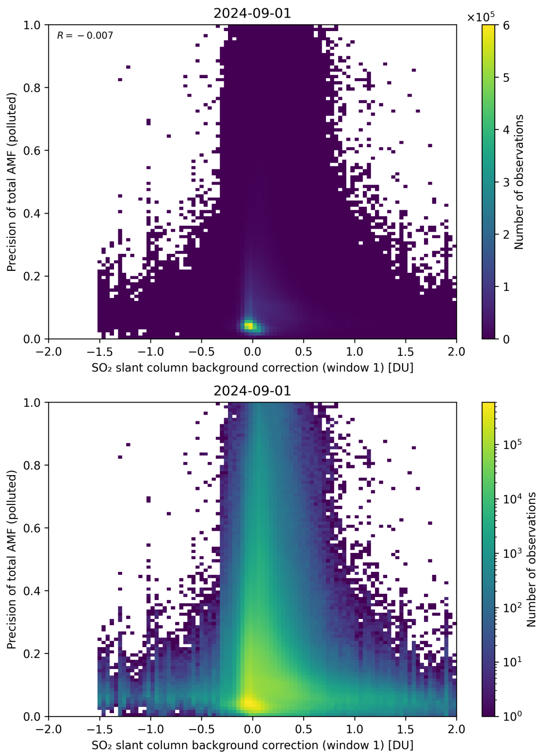
Figure 110: Scatter density plot of “SO 2 slant column background correction (window 1)” against “Precision of total AMF (polluted)” for 2024-09-01 to 2024-09-02.
