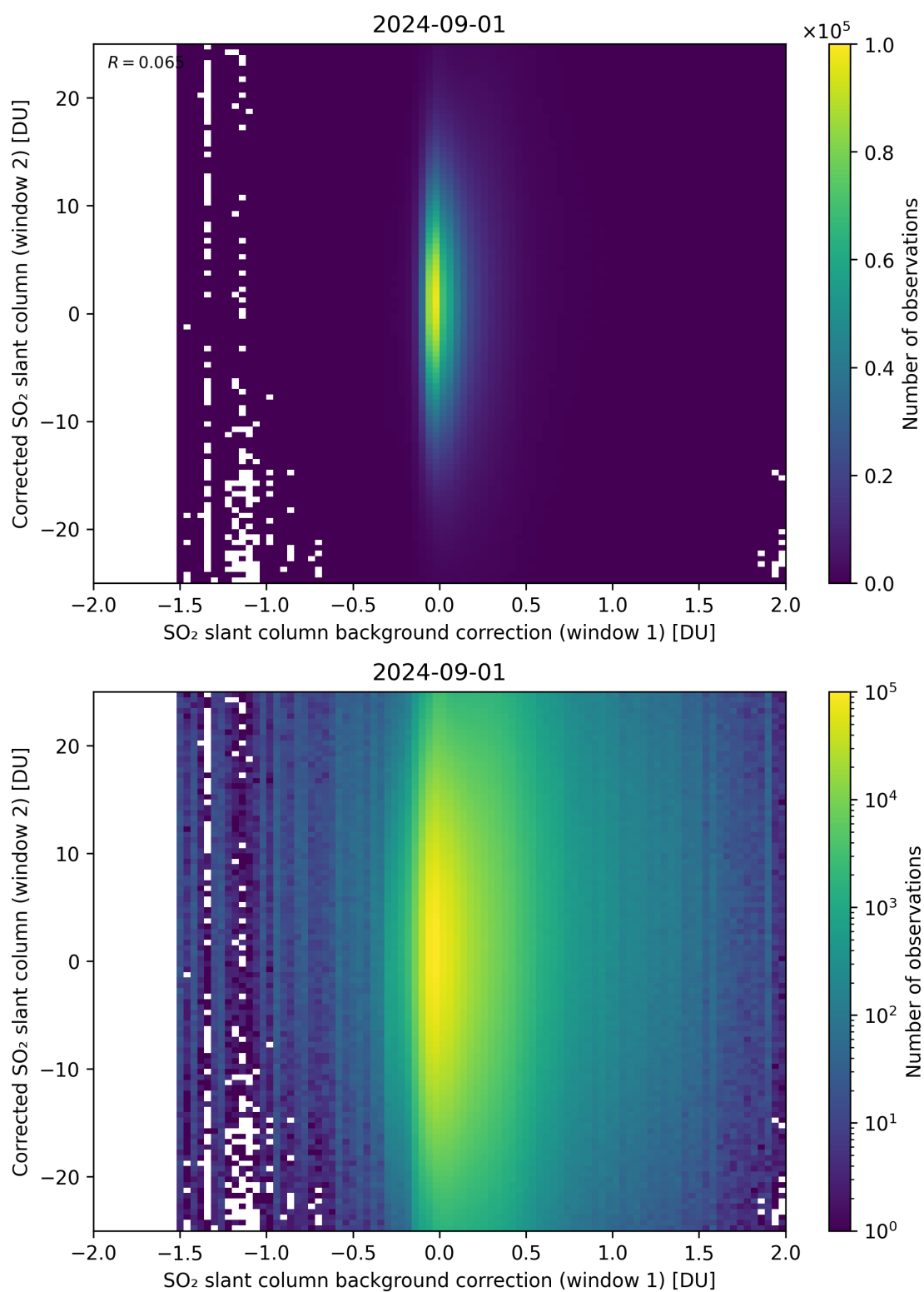
Figure 104: Scatter density plot of “SO 2 slant column background correction (window 1)” against “Corrected SO 2 slant column (window 2)” for 2024-09-01 to 2024-09-02.
