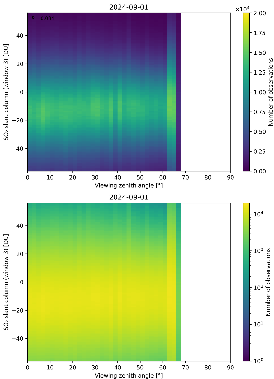
Figure 323: Scatter density plot of “Viewing zenith angle” against “SO 2 slant column (window 3)” for 2024-09-01 to 2024-09-02.
