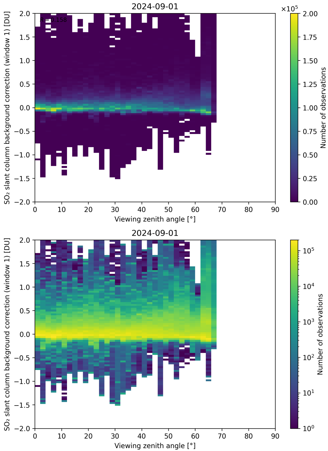
Figure 308: Scatter density plot of “Viewing zenith angle” against “SO 2 slant column background correction (window 1)” for 2024-09-01 to 2024-09-02.
