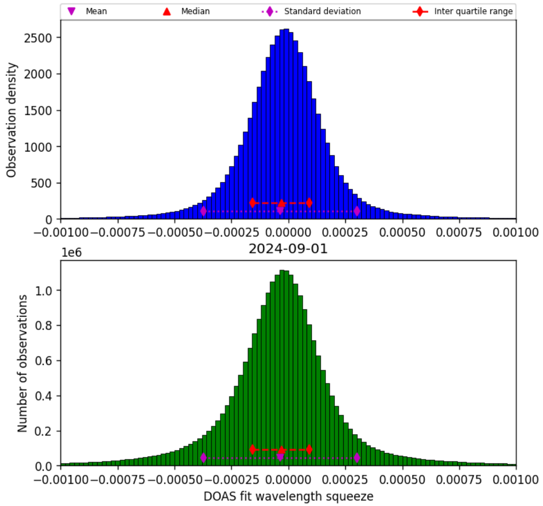
Figure 69: Histogram of “DOAS fit wavelength squeeze” for 2024-09-01 to 2024-09-02
