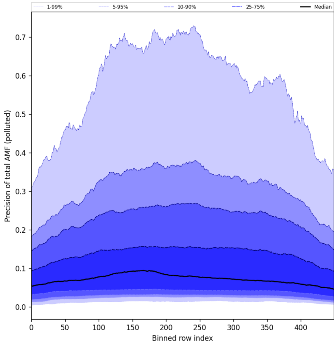
Figure 95: Along track statistics of “Precision of total AMF (polluted)” for 2024-09-01 to 2024-09-02
