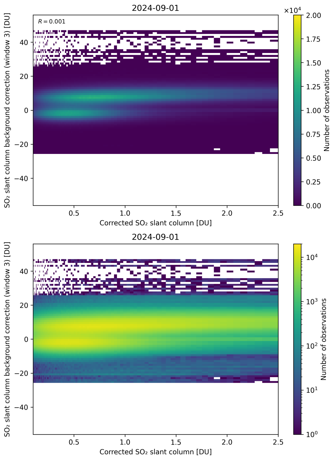
Figure 180: Scatter density plot of “Corrected SO 2 slant column” against “SO 2 slant column background correction (window 3)” for 2024-09-01 to 2024-09-02.
