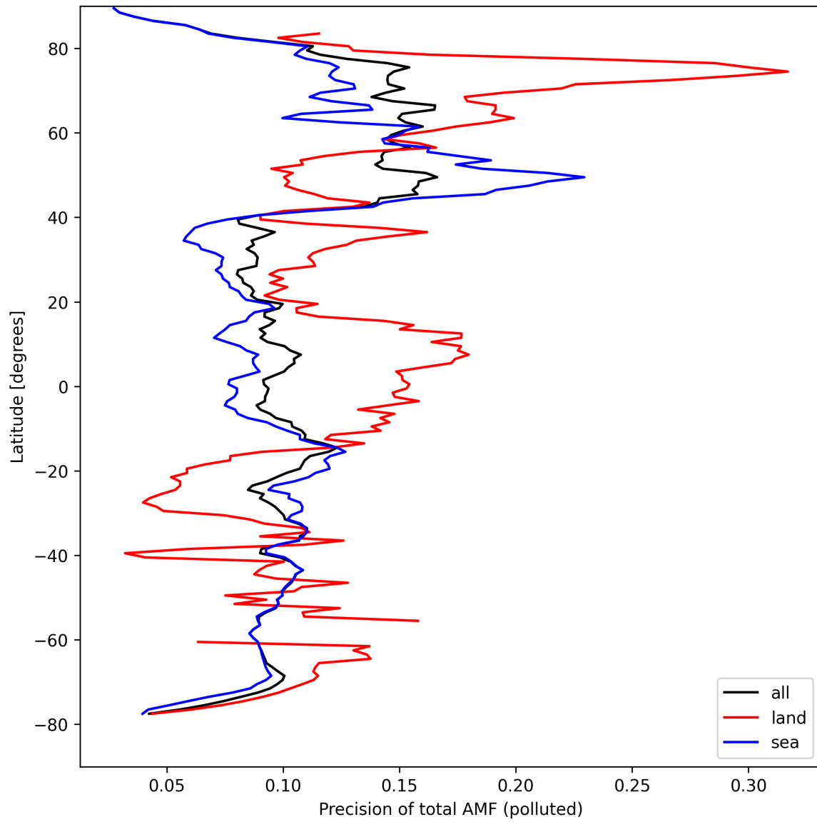
Figure 49: Zonal average of “Precision of total AMF (polluted)” for 2024-09-01 to 2024-09-02.
