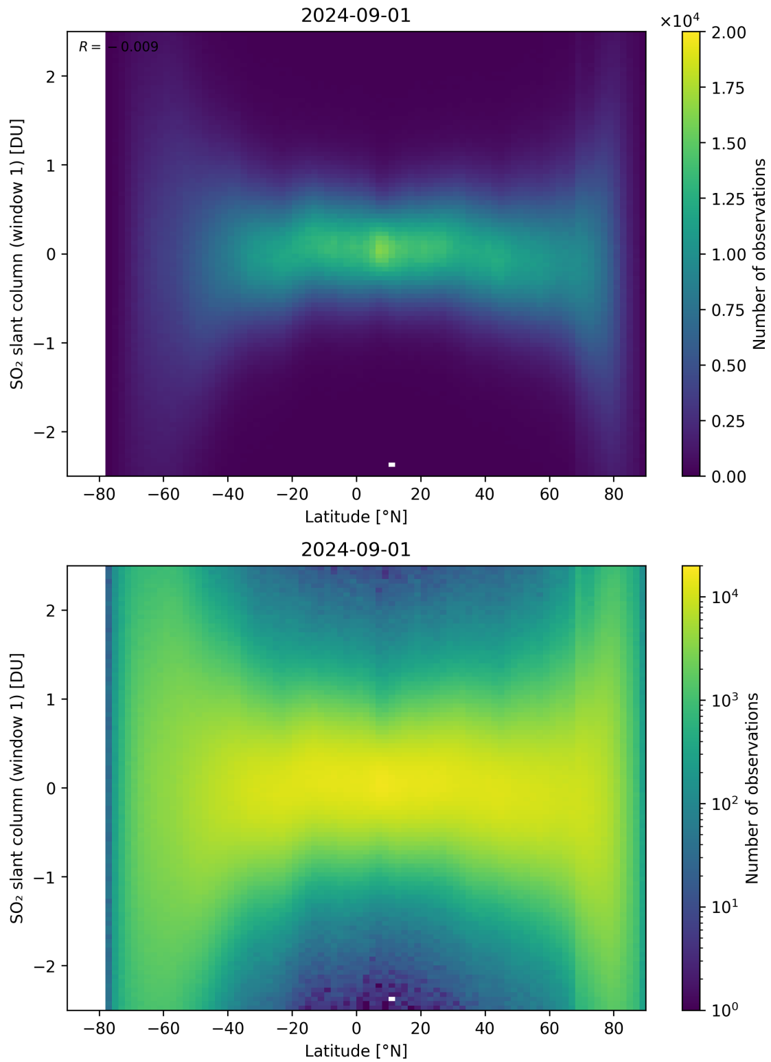
Figure 149: Scatter density plot of “Latitude” against “SO 2 slant column (window 1)” for 2024-09-01 to 2024-09-02.
