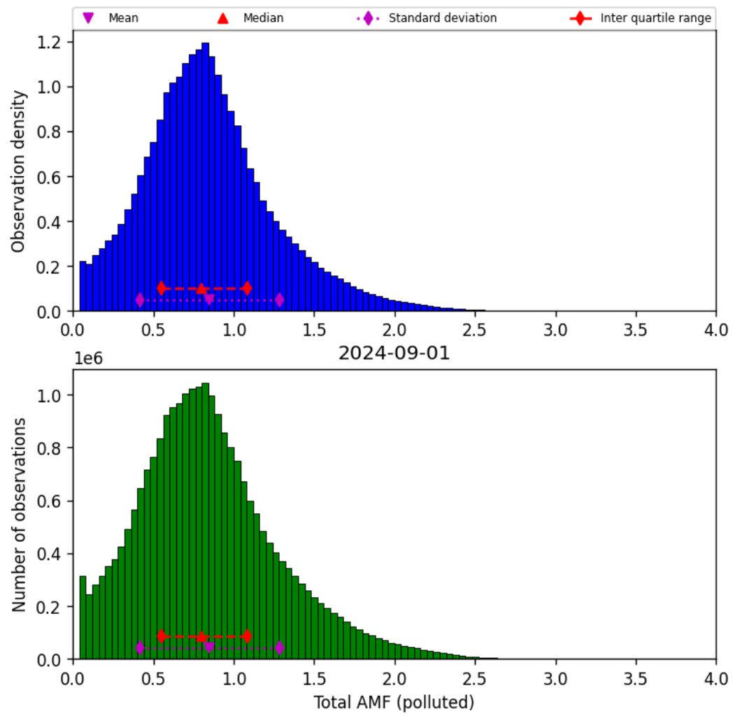
Figure 71: Histogram of “Total AMF (polluted)” for 2024-09-01 to 2024-09-02
