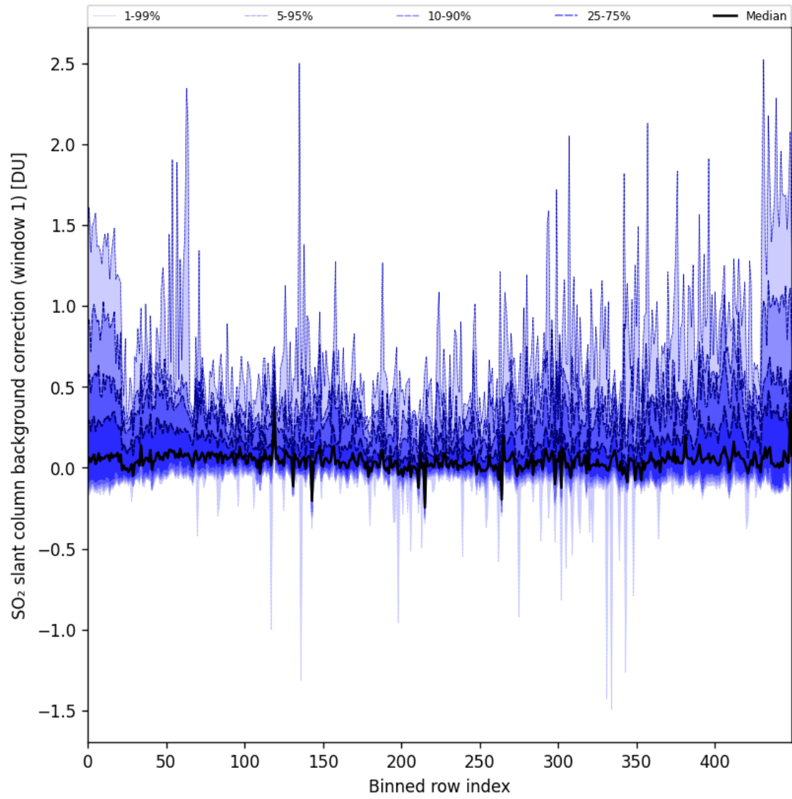
Figure 82: Along track statistics of “SO 2 slant column background correction (window 1)” for 2024-09-01 to 2024-09-02
