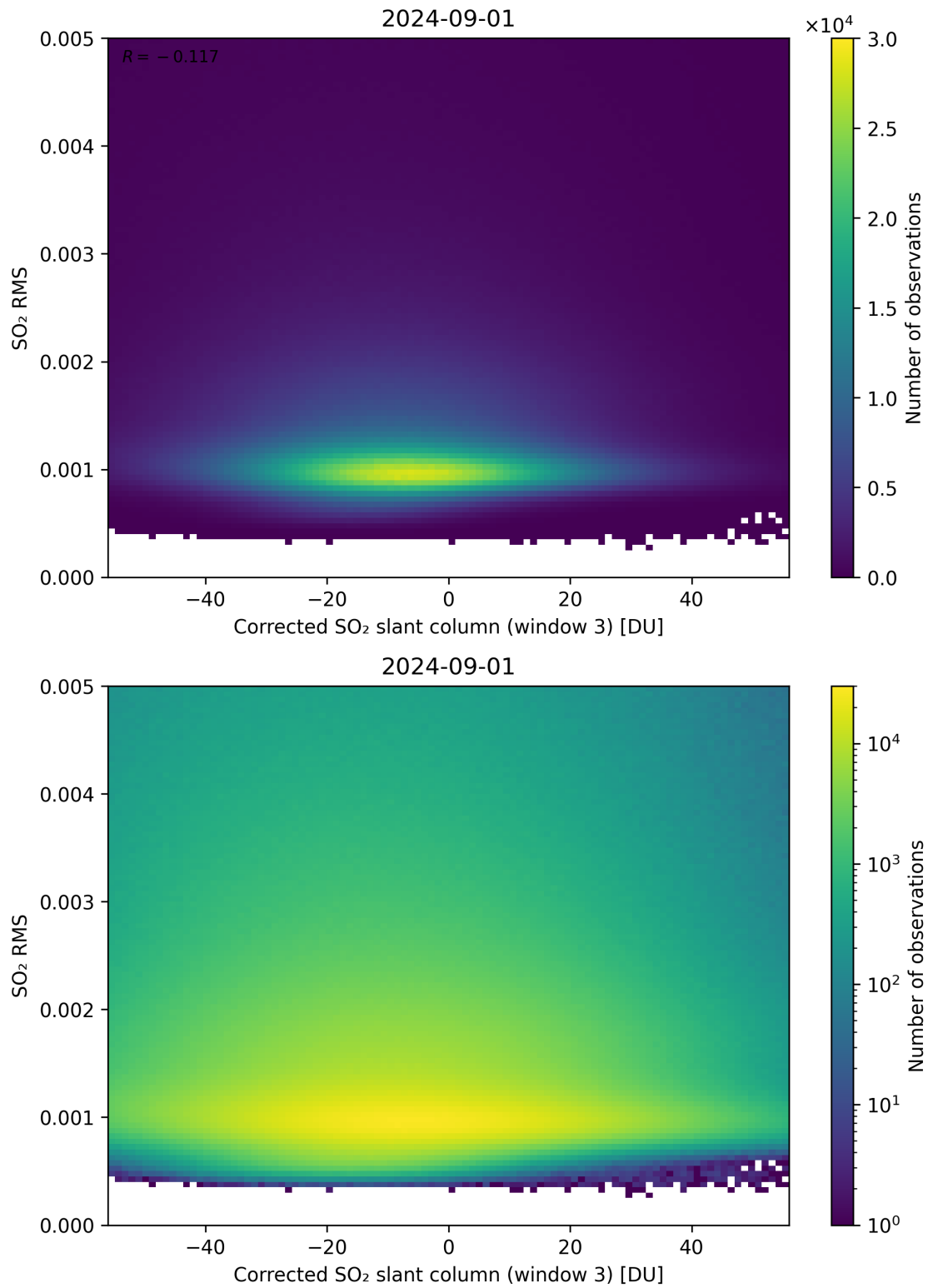
Figure 208: Scatter density plot of “Corrected SO 2 slant column (window 3)” against “SO 2 RMS” for 2024-09-01 to 2024-09-02.
