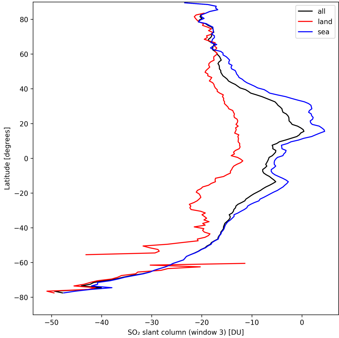
Figure 41: Zonal average of “SO 2 slant column (window 3)” for 2024-09-01 to 2024-09-02.
