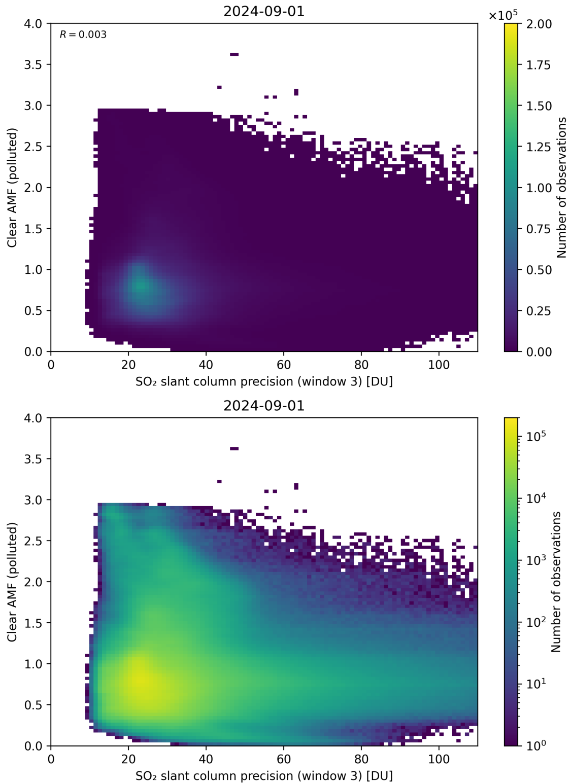
Figure 261: Scatter density plot of “SO 2 slant column precision (window 3)” against “Clear AMF (polluted)” for 2024-09-01 to 2024-09-02.
