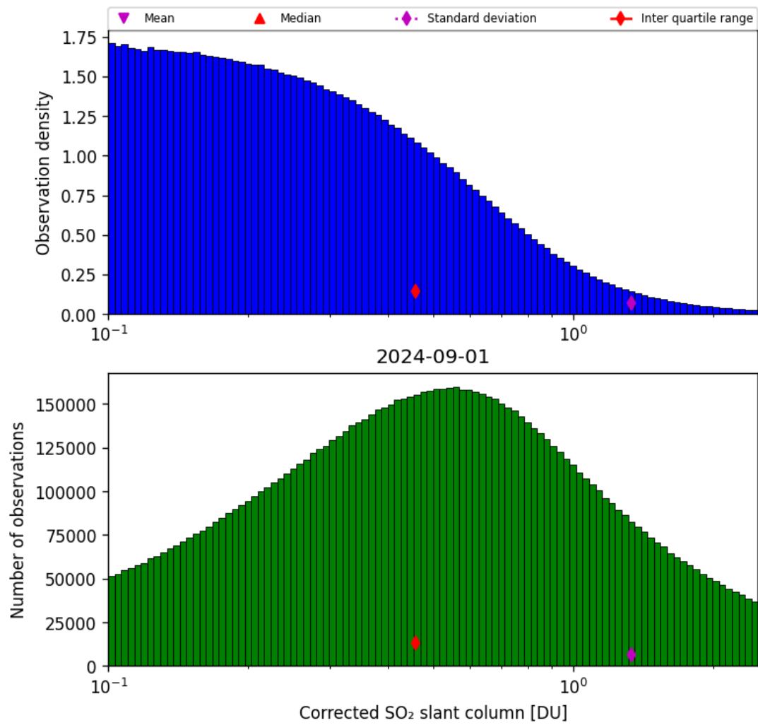
Figure 55: Histogram of “Corrected SO 2 slant column” for 2024-09-01 to 2024-09-02
