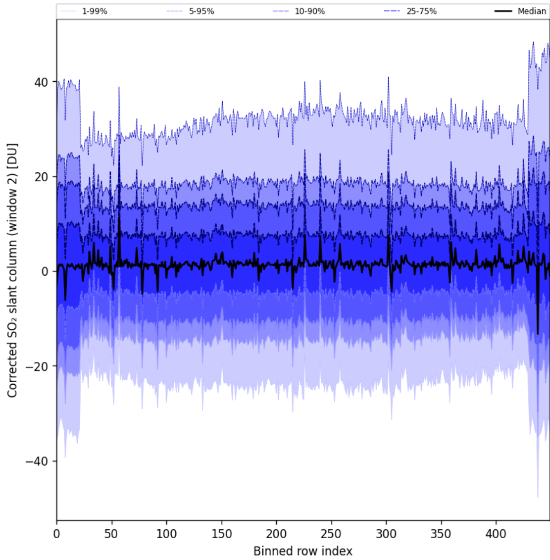
Figure 85: Along track statistics of “Corrected SO 2 slant column (window 2)” for 2024-09-01 to 2024-09-02
