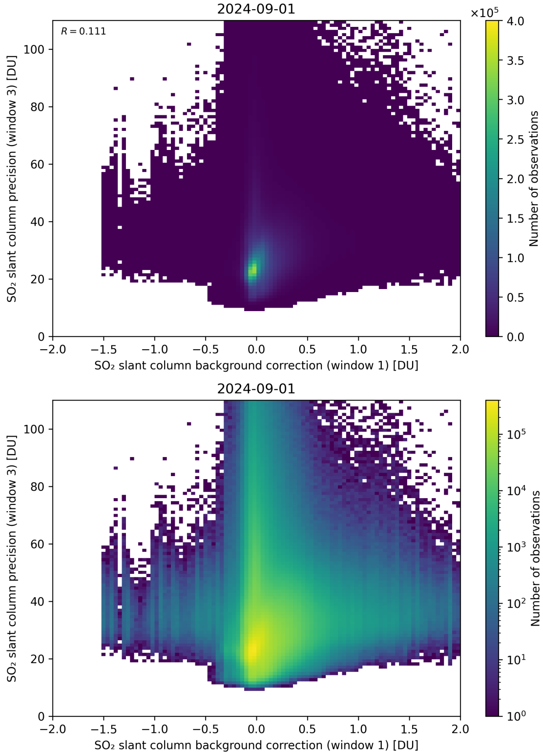
Figure 108: Scatter density plot of “SO 2 slant column background correction (window 1)” against “SO 2 slant column precision (window 3)” for 2024-09-01 to 2024-09-02.
