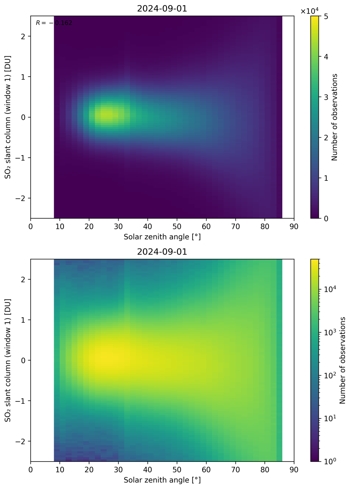
Figure 169: Scatter density plot of “Solar zenith angle” against “SO 2 slant column (window 1)” for 2024-09-01 to 2024-09-02.
