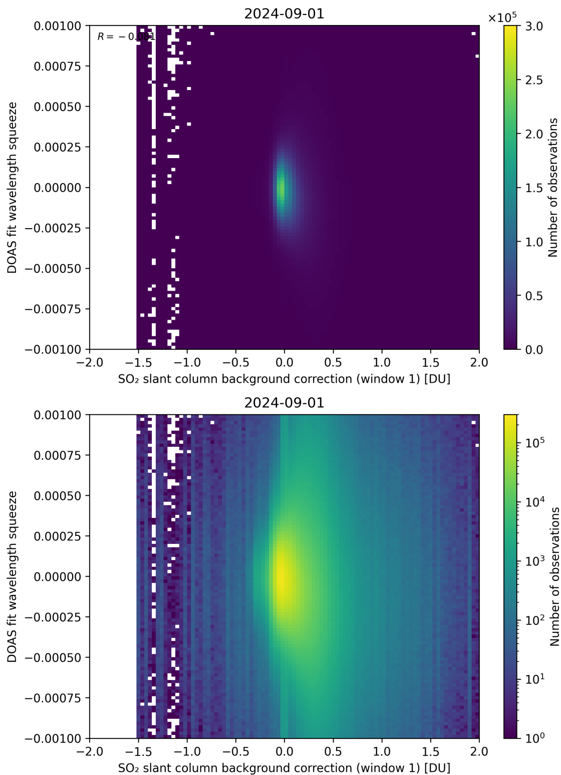
Figure 101: Scatter density plot of “SO 2 slant column background correction (window 1)” against “DOAS fit wavelength squeeze” for 2024-09-01 to 2024-09-02.
