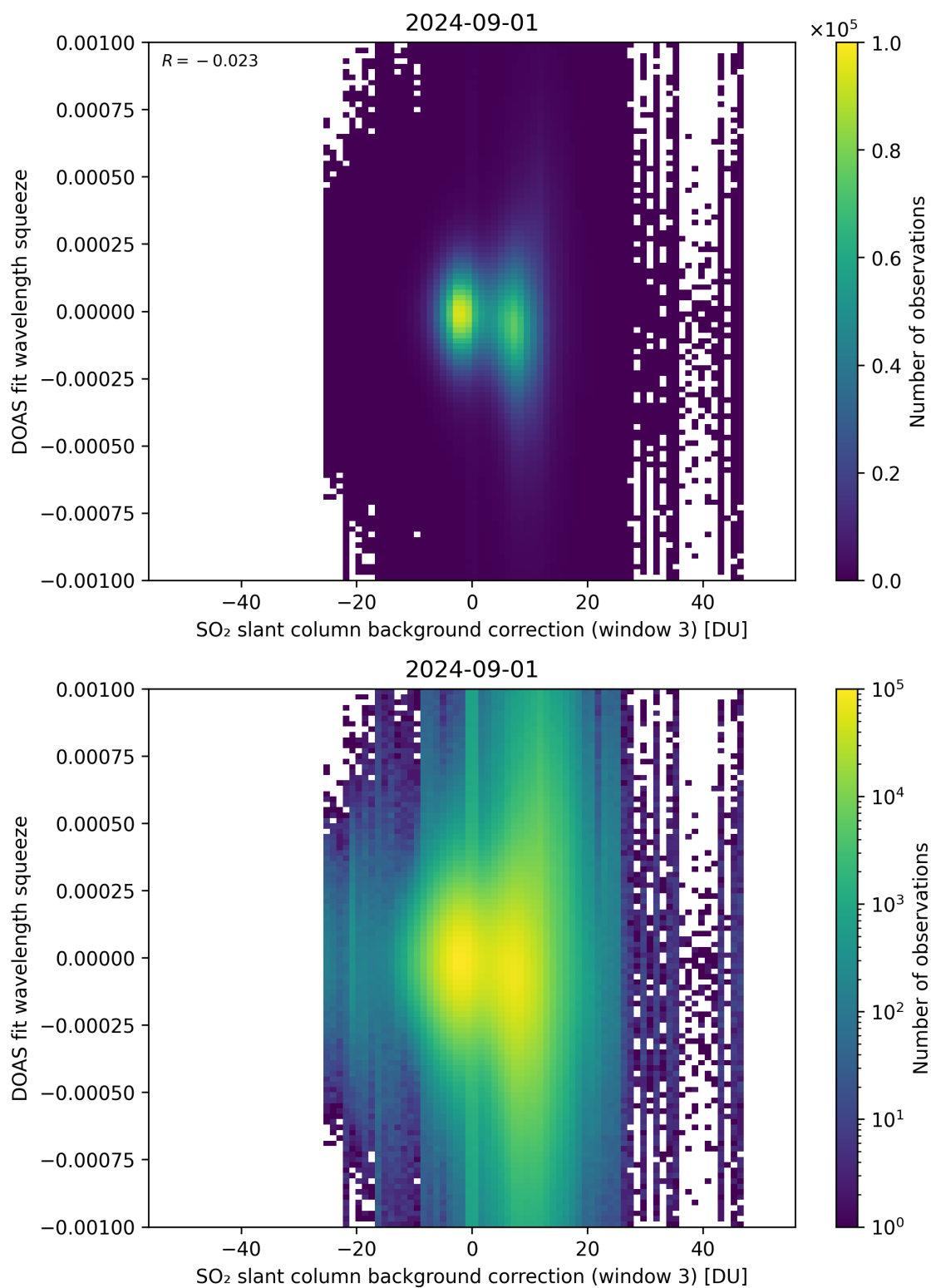
Figure 122: Scatter density plot of “SO 2 slant column background correction (window 3)” against “DOAS fit wavelength squeeze” for 2024-09-01 to 2024-09-02.
