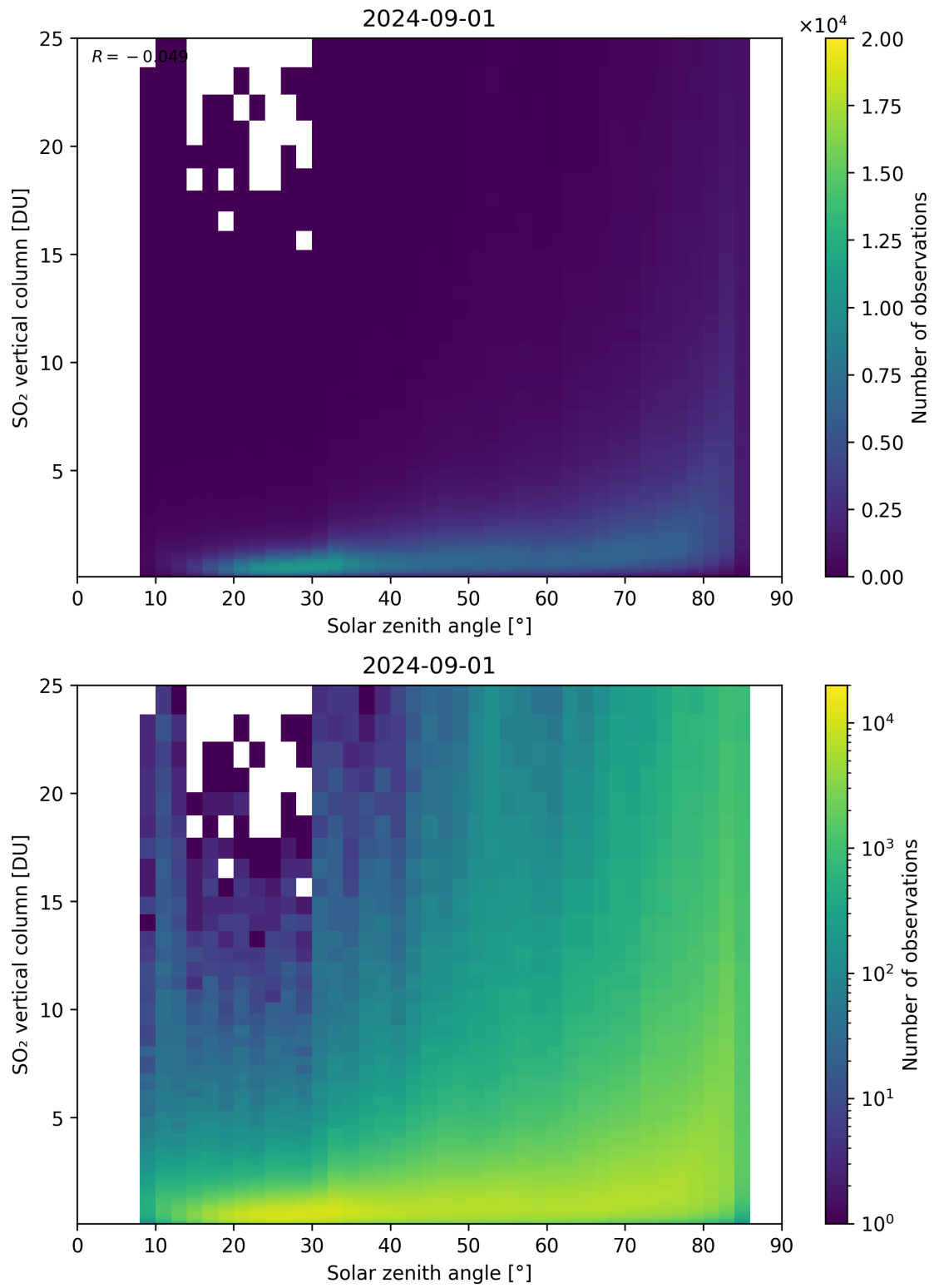
Figure 176: Scatter density plot of “Solar zenith angle” against “SO 2 vertical column” for 2024-09-01 to 2024-09-02.
