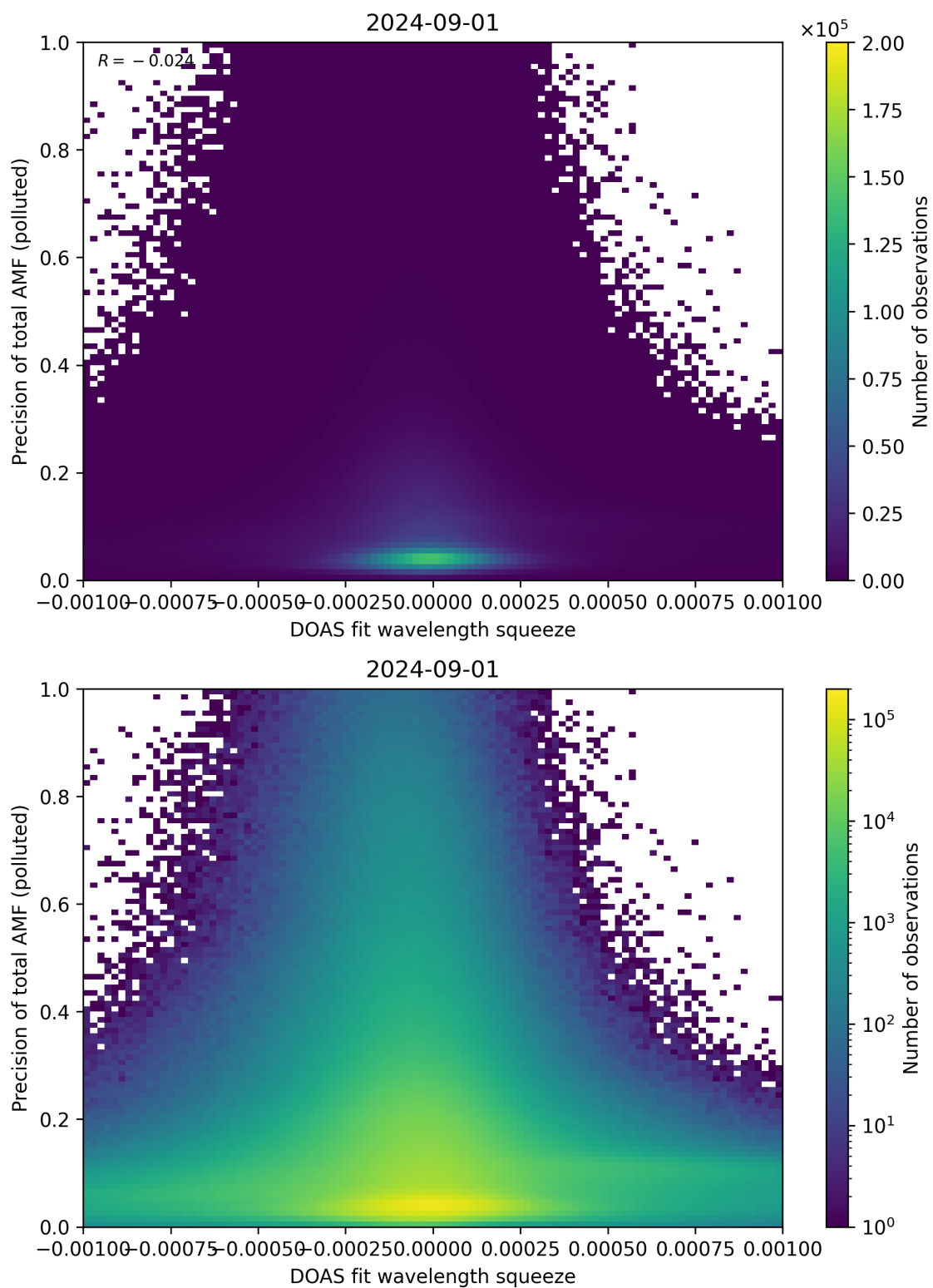
Figure 135: Scatter density plot of “DOAS fit wavelength squeeze” against “Precision of total AMF (polluted)” for 2024-09-01 to 2024-09-02.
