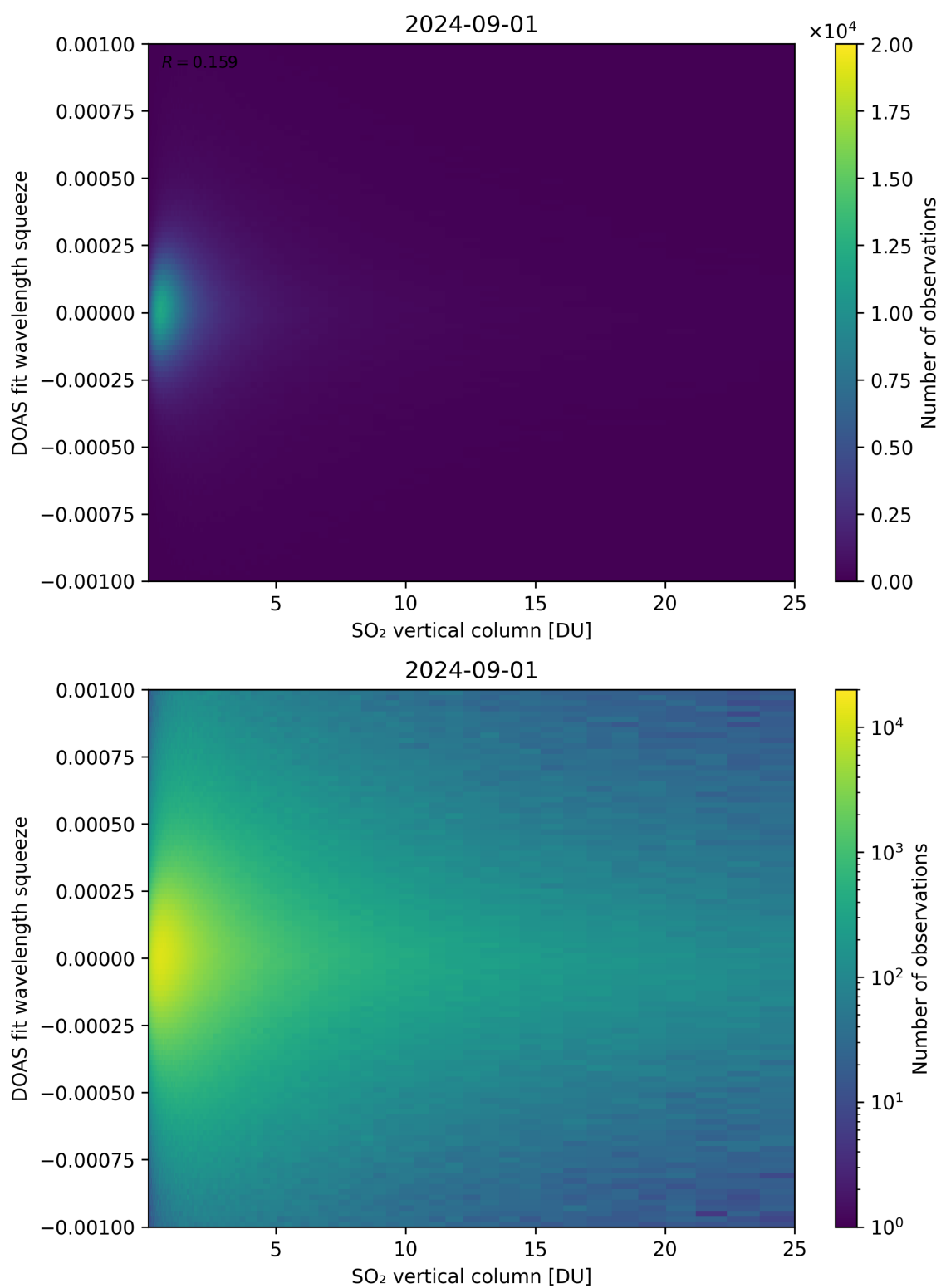
Figure 277: Scatter density plot of “SO 2 vertical column” against “DOAS fit wavelength squeeze” for 2024-09-01 to 2024-09-02.
