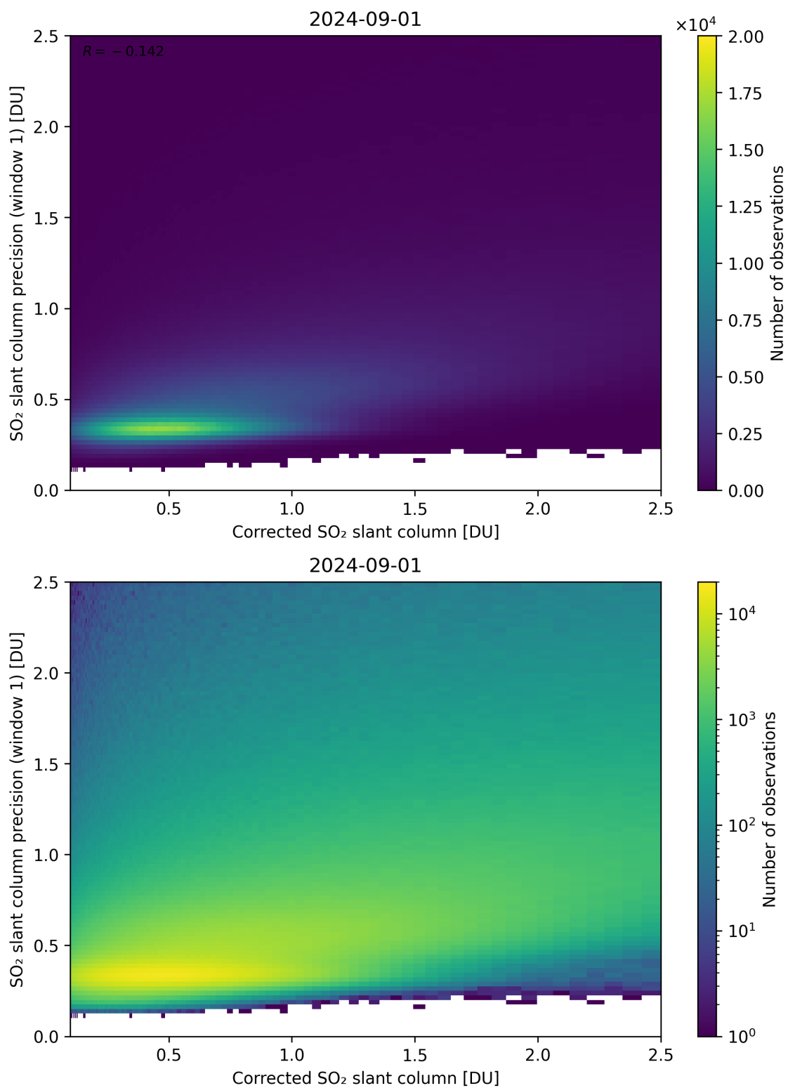
Figure 188: Scatter density plot of “Corrected SO 2 slant column” against “SO 2 slant column precision (window 1)” for 2024-09-01 to 2024-09-02.
