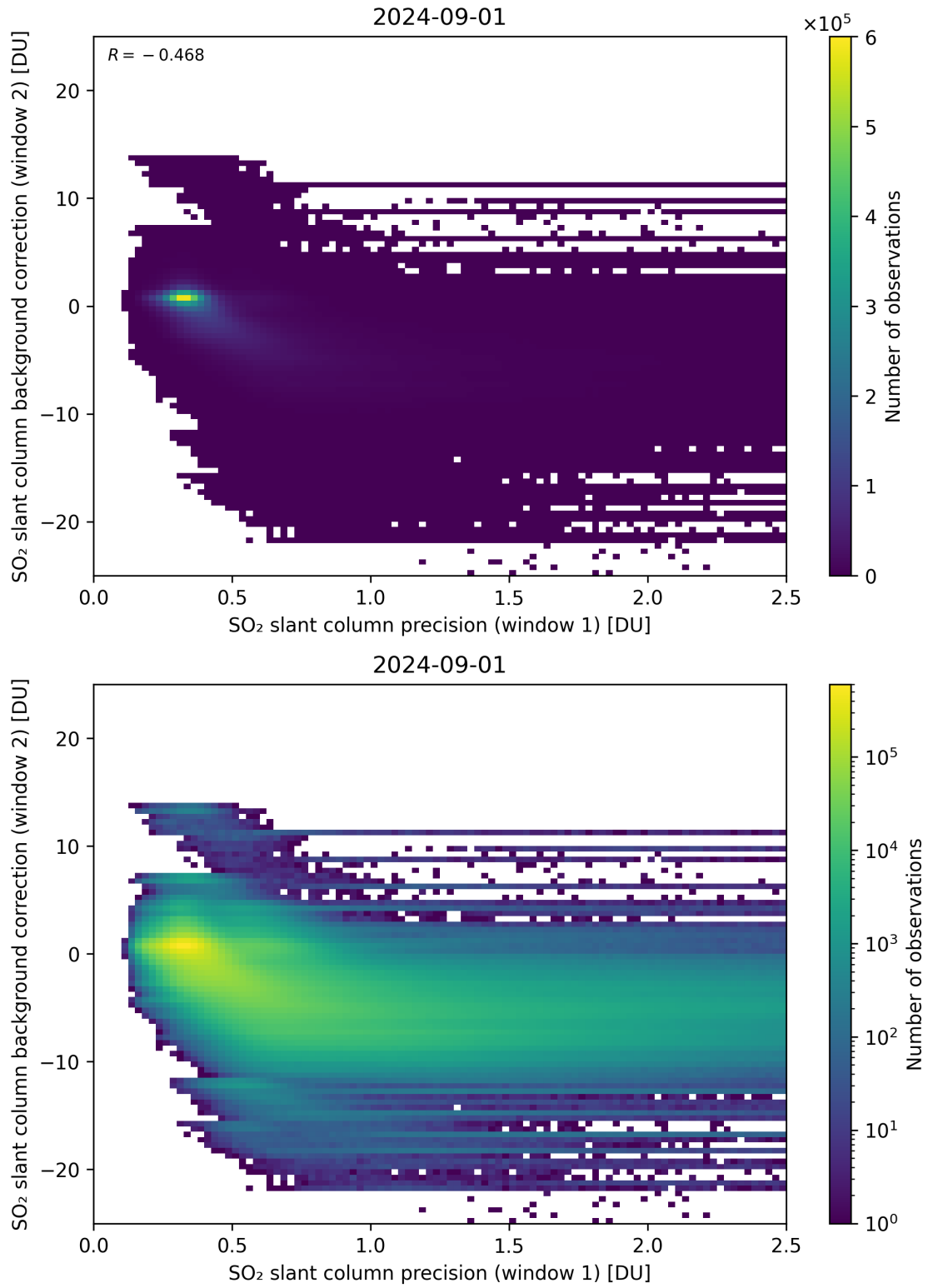
Figure 219: Scatter density plot of “SO 2 slant column precision (window 1)” against “SO 2 slant column background correction (window 2)” for 2024-09-01 to 2024-09-02.
