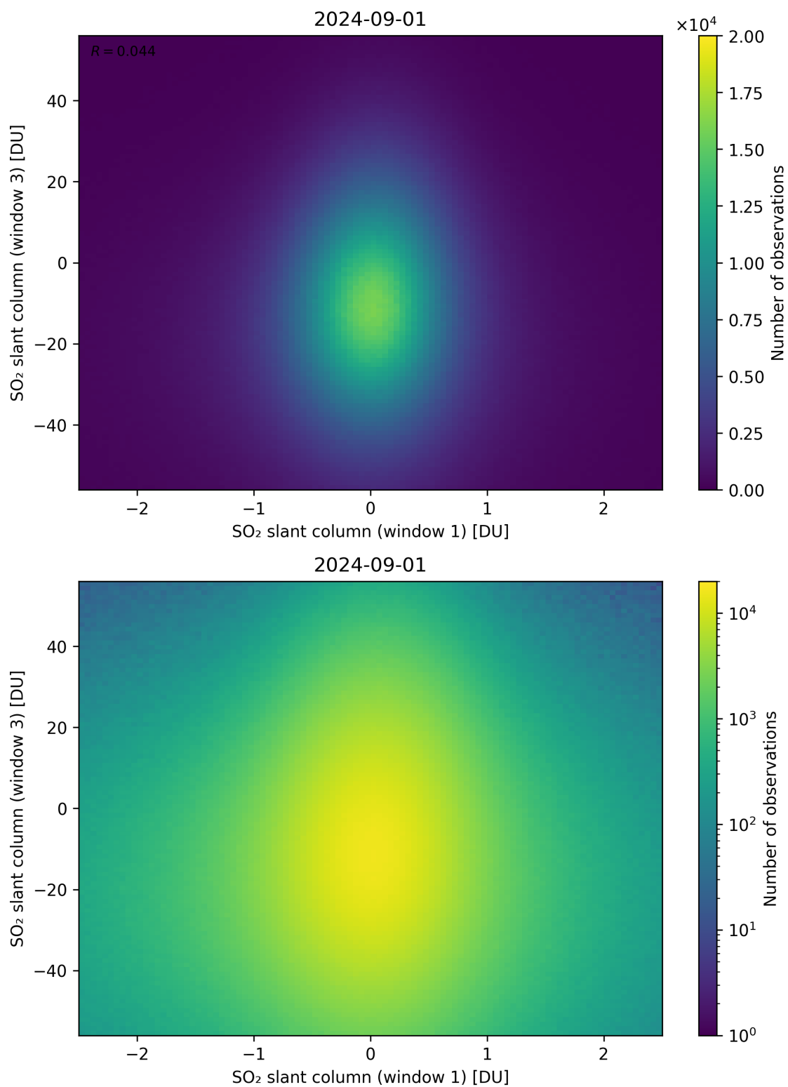
Figure 237: Scatter density plot of “SO 2 slant column (window 1)” against “SO 2 slant column (window 3)” for 2024-09-01 to 2024-09-02.
