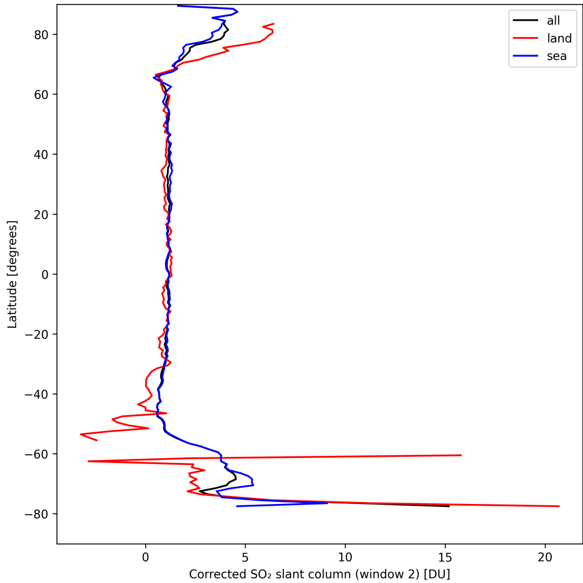
Figure 39: Zonal average of “Corrected SO 2 slant column (window 2)” for 2024-09-01 to 2024-09-02.
