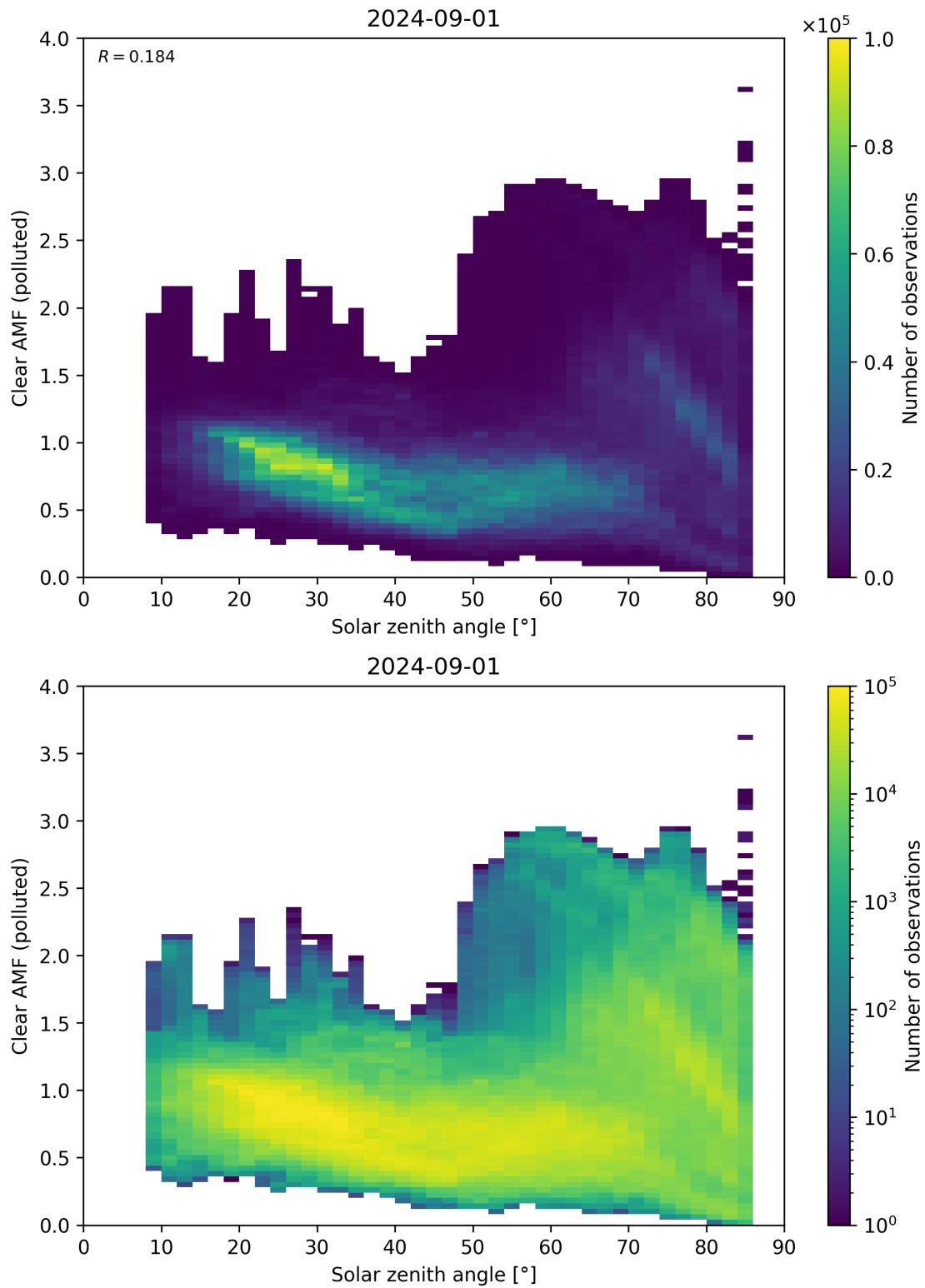
Figure 165: Scatter density plot of “Solar zenith angle” against “Clear AMF (polluted)” for 2024-09-01 to 2024-09-02.
