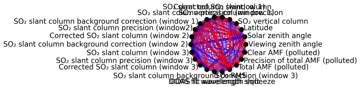
Figure 1: Map of correlation graph for 2024-09-01 to 2024-09-02.
