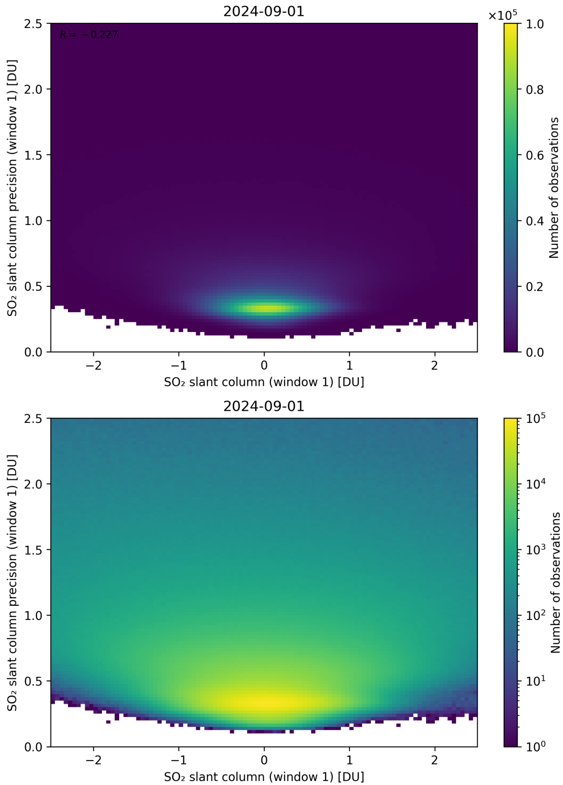
Figure 235: Scatter density plot of “SO 2 slant column (window 1)” against “SO 2 slant column precision (window 1)” for 2024-09-01 to 2024-09-02.
