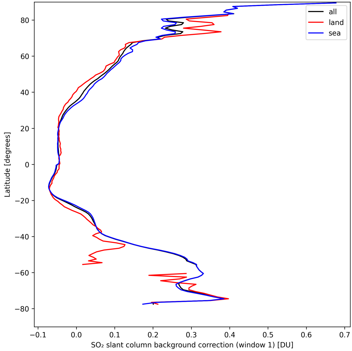
Figure 36: Zonal average of “SO 2 slant column background correction (window 1)” for 2024-09-01 to 2024-09-02.
