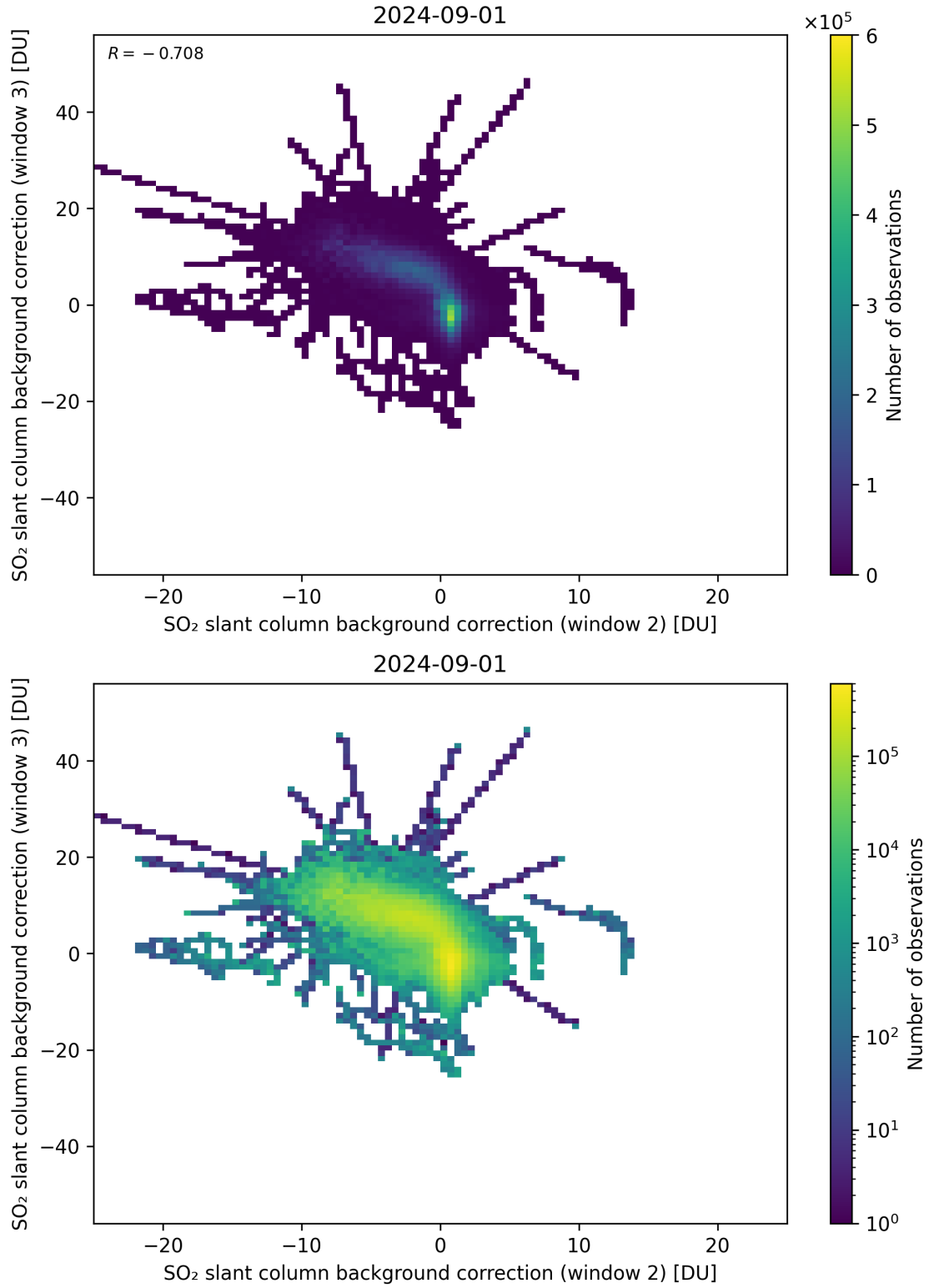
Figure 111: Scatter density plot of “SO 2 slant column background correction (window 2)” against “SO 2 slant column background correction (window 3)” for 2024-09-01 to 2024-09-02.
