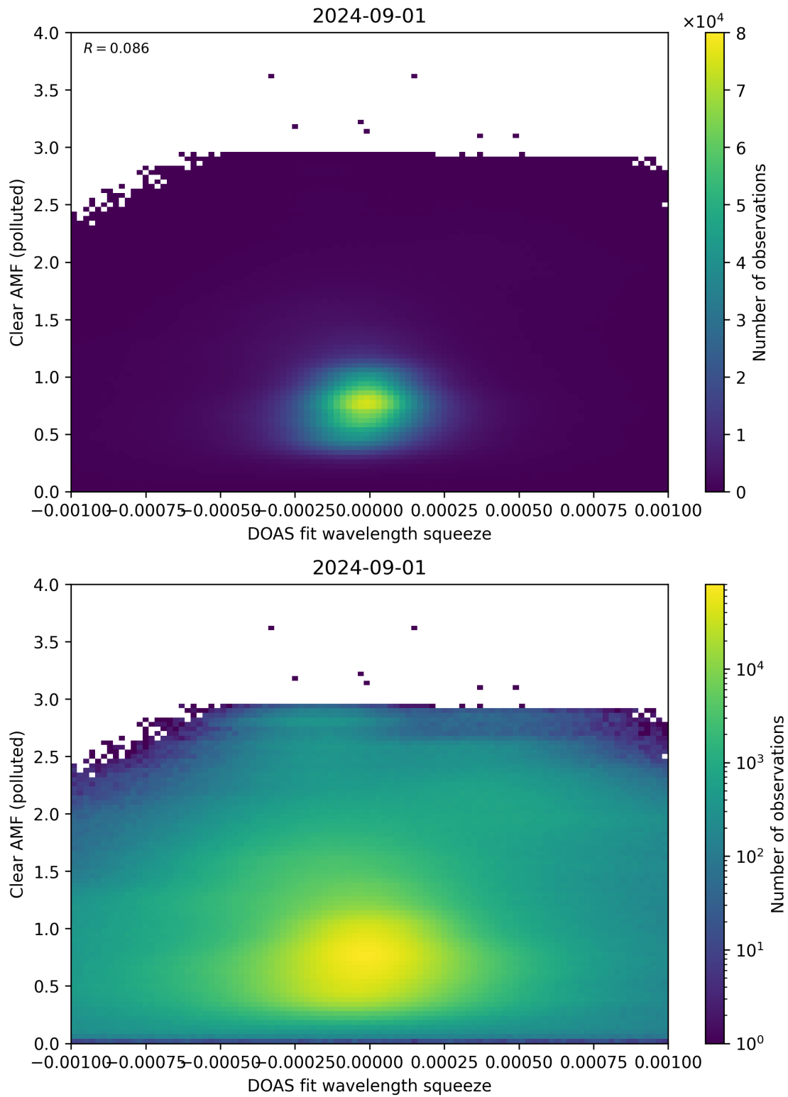
Figure 133: Scatter density plot of “DOAS fit wavelength squeeze” against “Clear AMF (polluted)” for 2024-09-01 to 2024-09-02.
