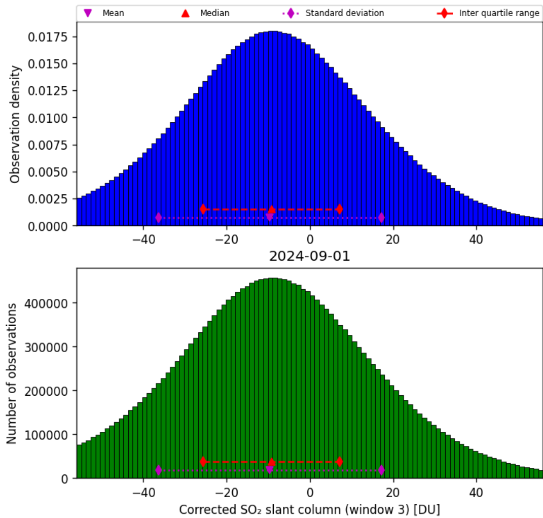
Figure 66: Histogram of “Corrected SO 2 slant column (window 3)” for 2024-09-01 to 2024-09-02
