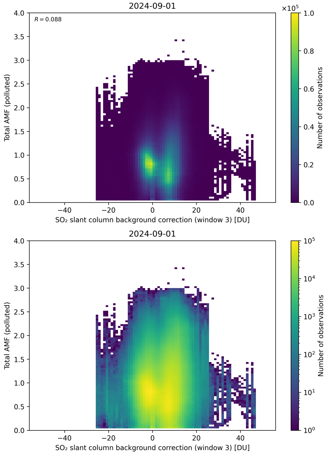
Figure 125: Scatter density plot of “SO 2 slant column background correction (window 3)” against “Total AMF (polluted)” for 2024-09-01 to 2024-09-02.
