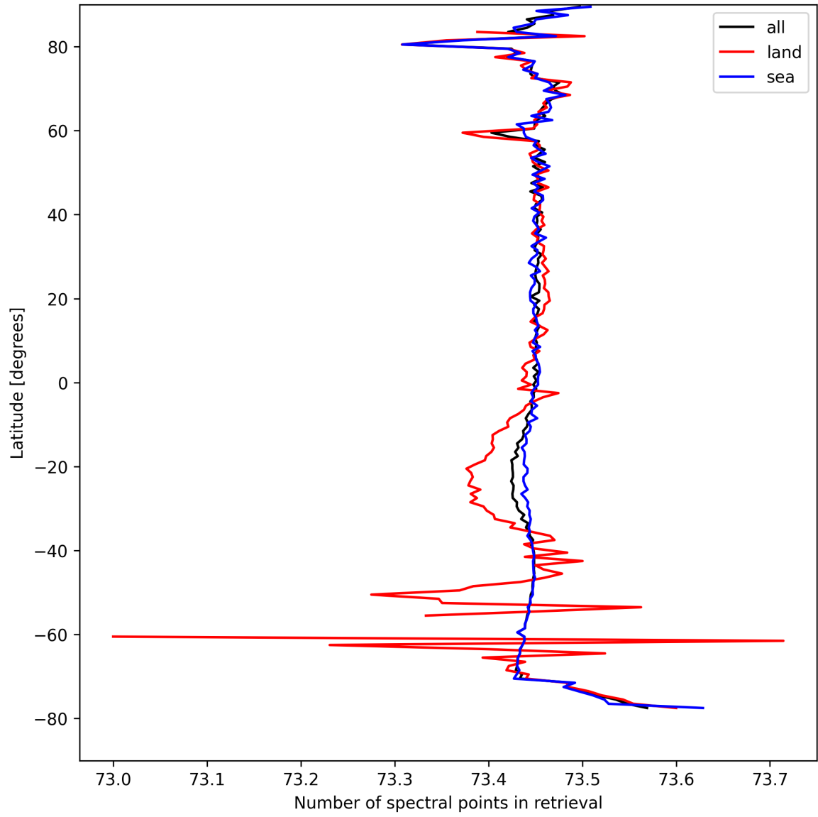
Figure 51: Zonal average of “Number of spectral points in retrieval” for 2024-09-01 to 2024-09-02.
