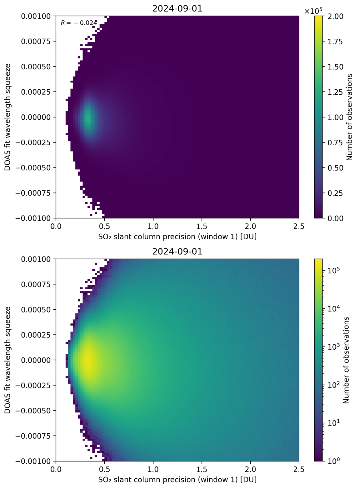
Figure 222: Scatter density plot of “SO 2 slant column precision (window 1)” against “DOAS fit wavelength squeeze” for 2024-09-01 to 2024-09-02.
