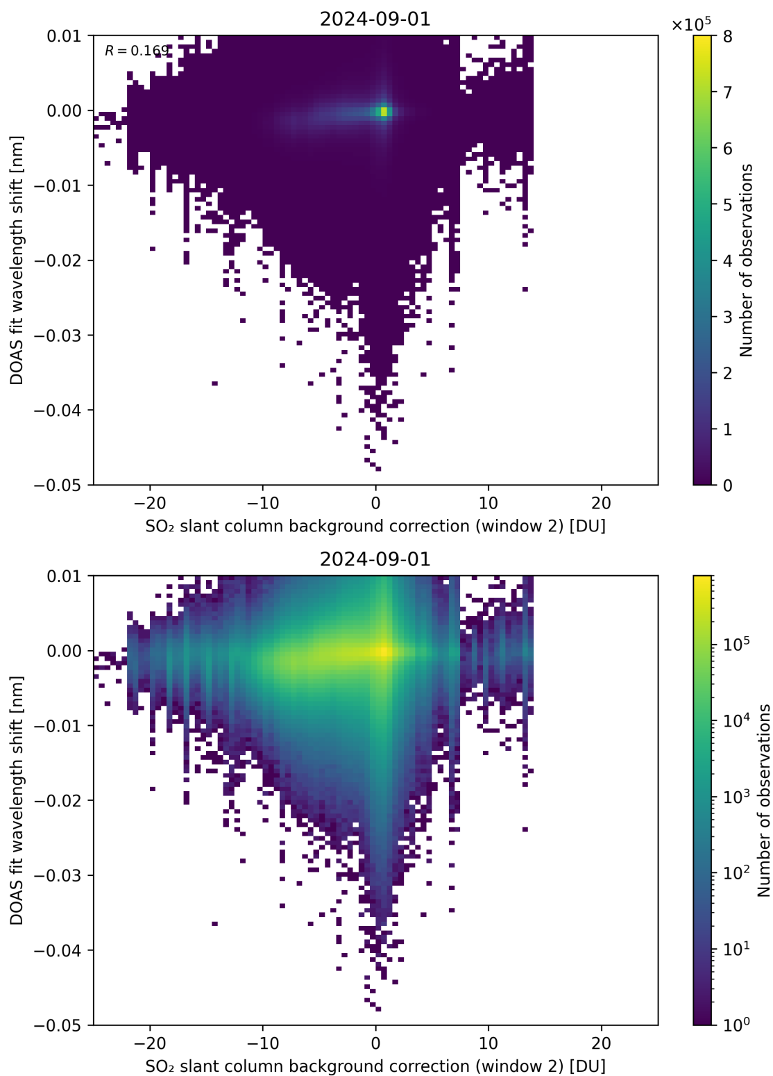
Figure 112: Scatter density plot of “SO 2 slant column background correction (window 2)” against “DOAS fit wavelength shift” for 2024-09-01 to 2024-09-02.
