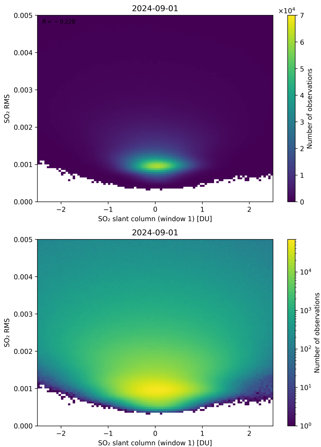
Figure 217: Scatter density plot of “SO 2 slant column (window 1)” against “SO 2 RMS” for 2024-09-01 to 2024-09-02.
