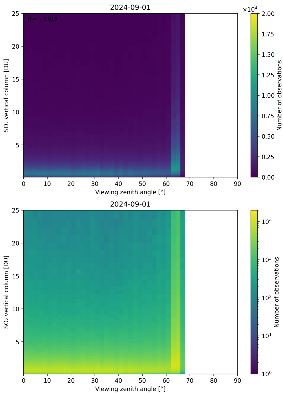
Figure 327: Scatter density plot of “Viewing zenith angle” against “SO 2 vertical column” for 2024-09-01 to 2024-09-02.
