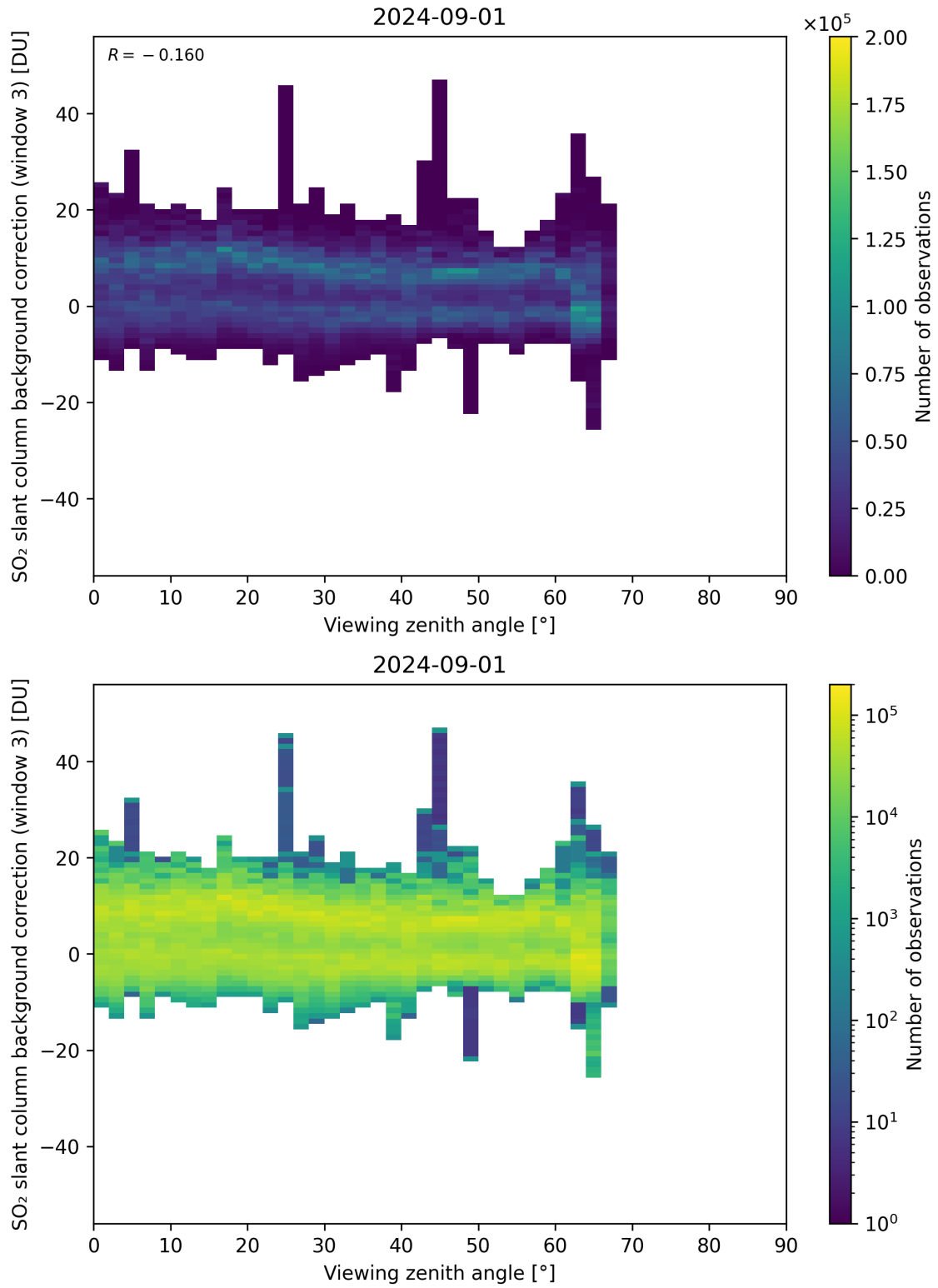
Figure 310: Scatter density plot of “Viewing zenith angle” against “SO 2 slant column background correction (window 3)” for 2024-09-01 to 2024-09-02.
