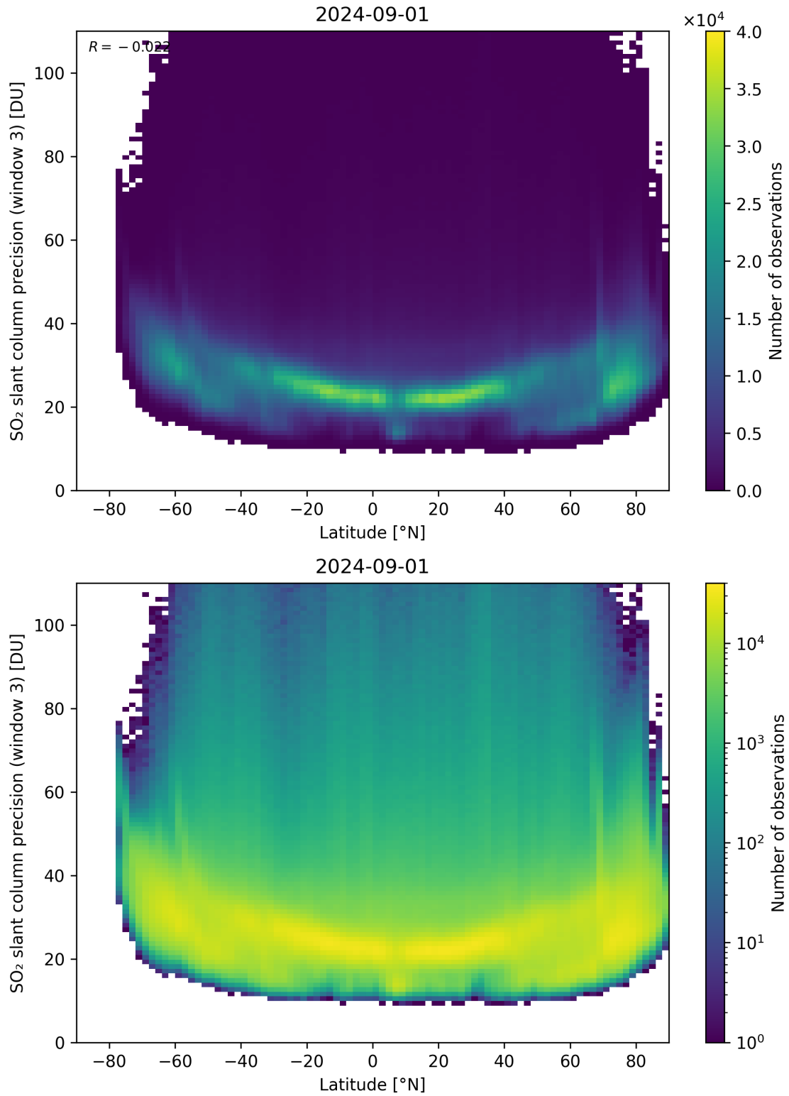
Figure 153: Scatter density plot of “Latitude” against “SO 2 slant column precision (window 3)” for 2024-09-01 to 2024-09-02.
