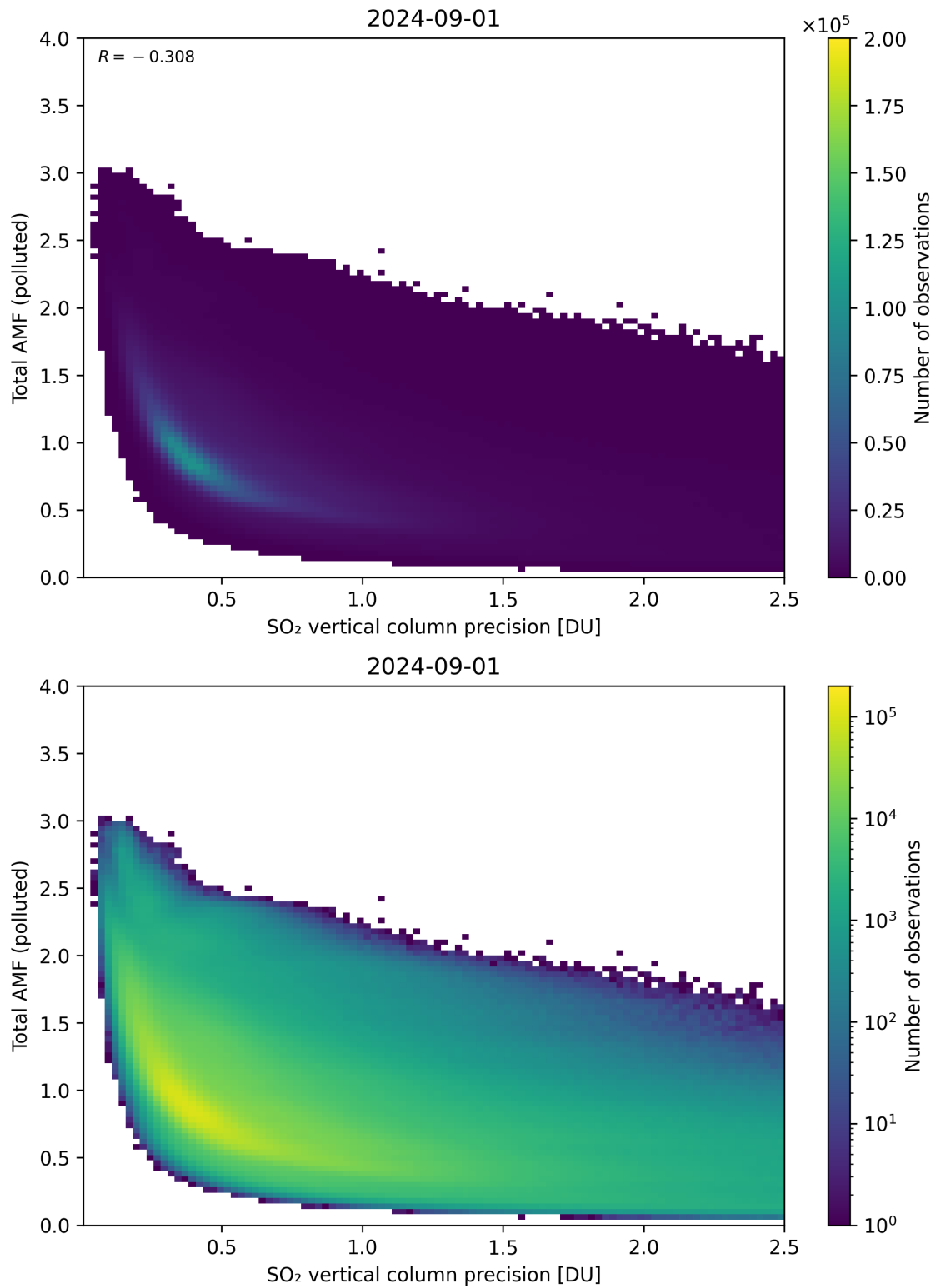
Figure 294: Scatter density plot of “SO 2 vertical column precision” against “Total AMF (polluted)” for 2024-09-01 to 2024-09-02.
