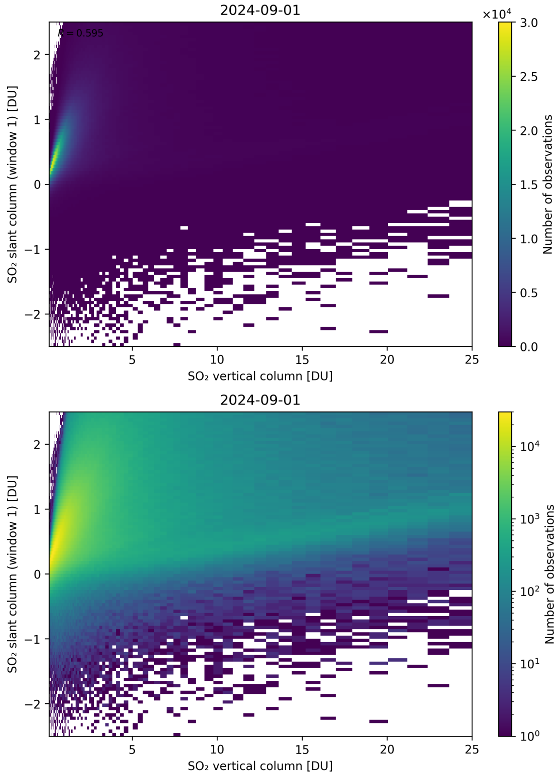
Figure 300: Scatter density plot of “SO 2 vertical column” against “SO 2 slant column (window 1)” for 2024-09-01 to 2024-09-02.
