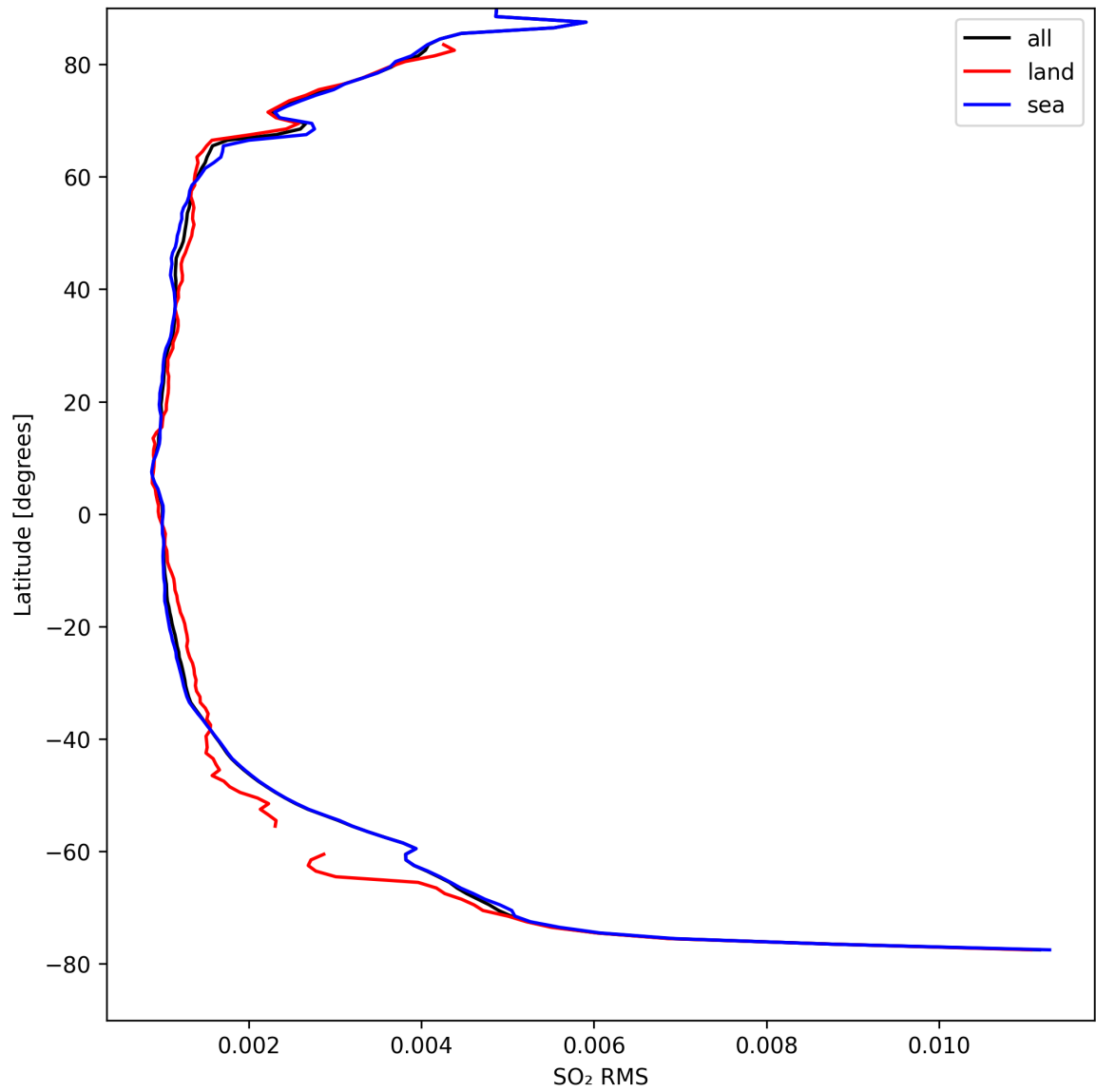
Figure 47: Zonal average of “SO 2 RMS” for 2024-09-01 to 2024-09-02.
