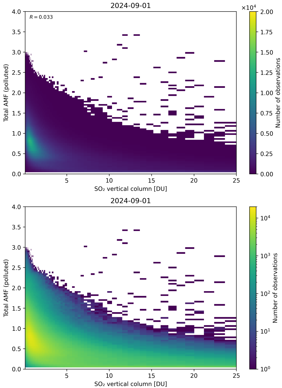
Figure 305: Scatter density plot of “SO 2 vertical column” against “Total AMF (polluted)” for 2024-09-01 to 2024-09-02.
