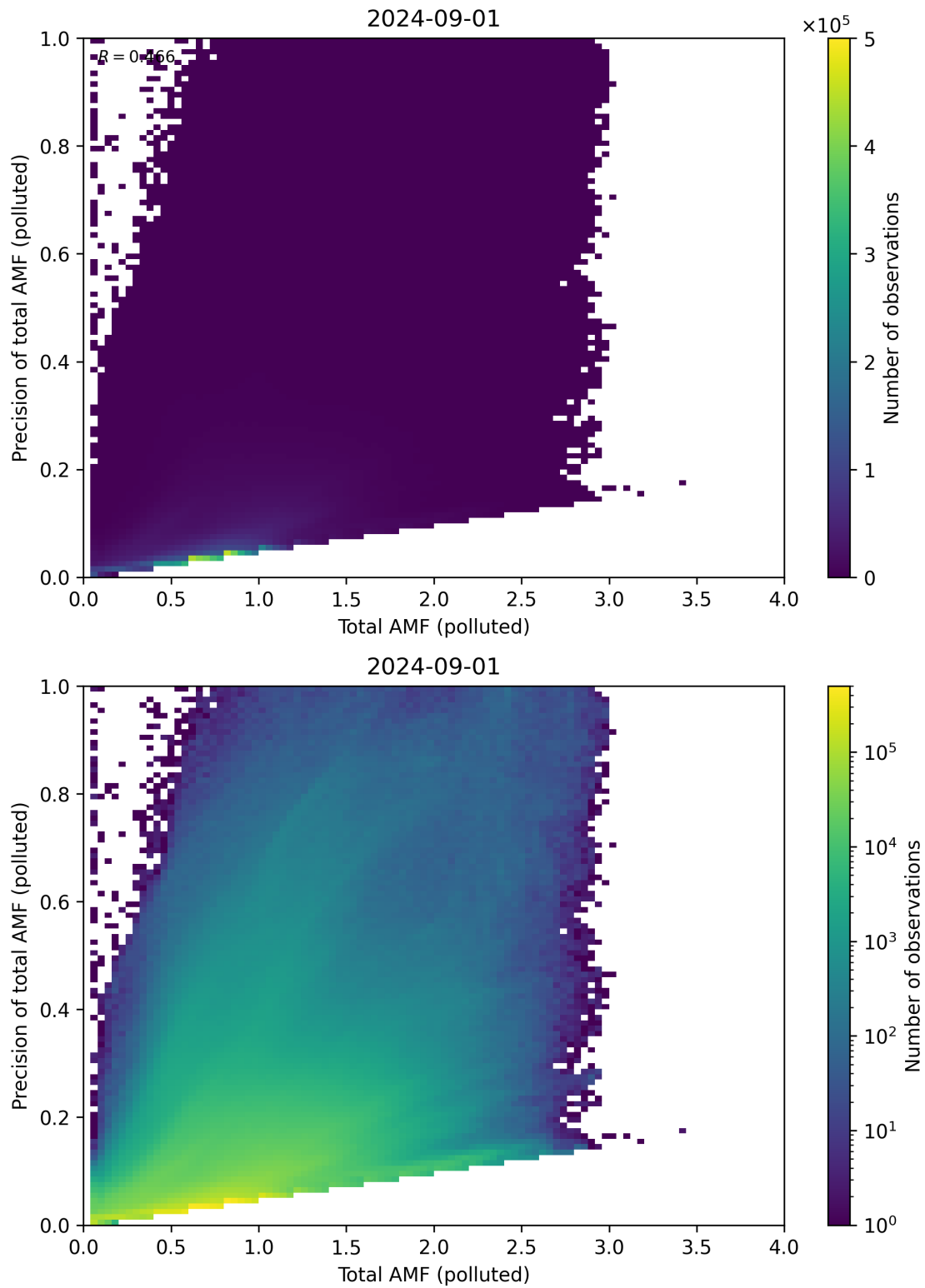
Figure 272: Scatter density plot of “Total AMF (polluted)” against “Precision of total AMF (polluted)” for 2024-09-01 to 2024-09-02.
