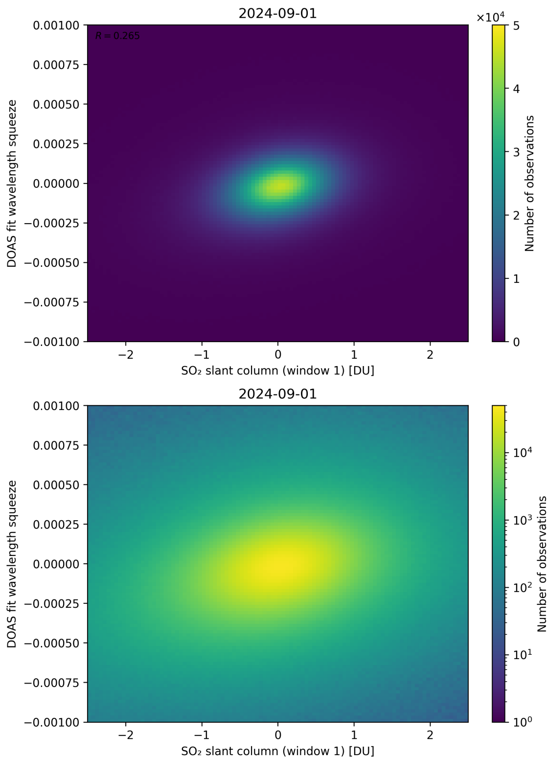
Figure 216: Scatter density plot of “SO 2 slant column (window 1)” against “DOAS fit wavelength squeeze” for 2024-09-01 to 2024-09-02.
