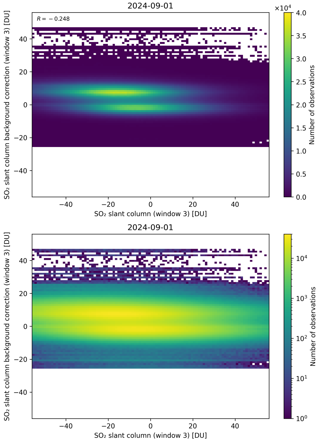
Figure 253: Scatter density plot of “SO 2 slant column (window 3)” against “SO 2 slant column background correction (window 3)” for 2024-09-01 to 2024-09-02.
