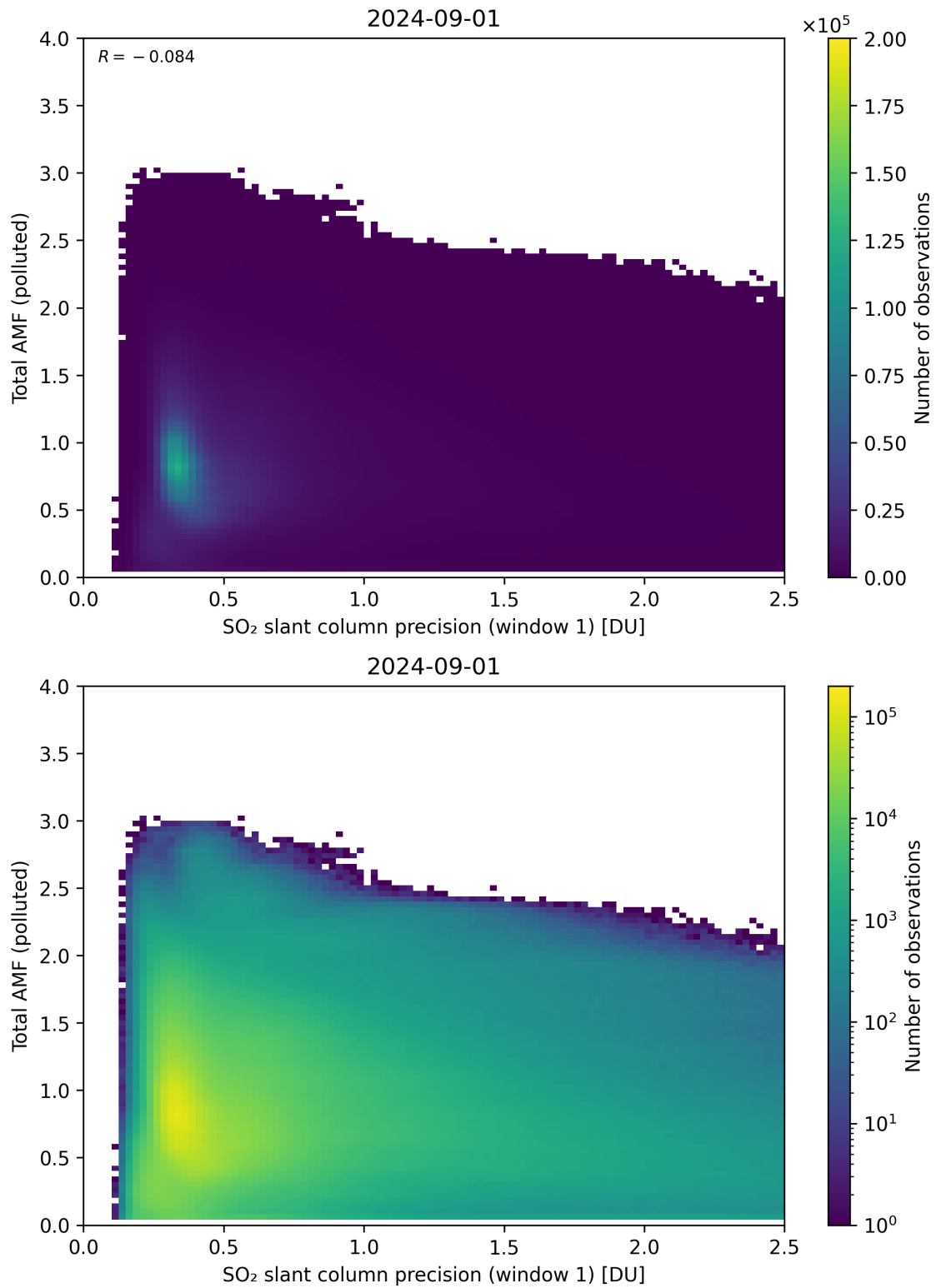
Figure 230: Scatter density plot of “SO 2 slant column precision (window 1)” against “Total AMF (polluted)” for 2024-09-01 to 2024-09-02.
