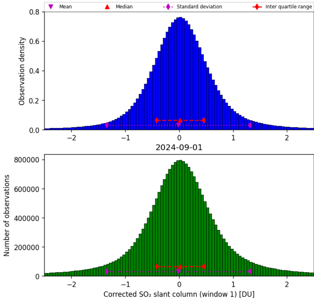
Figure 58: Histogram of “Corrected SO 2 slant column (window 1)” for 2024-09-01 to 2024-09-02
