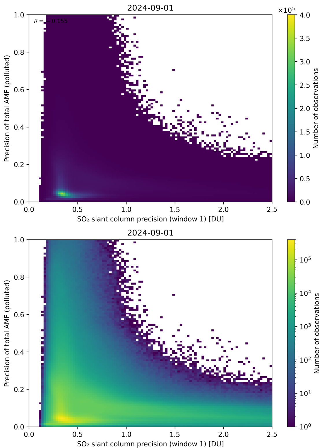
Figure 231: Scatter density plot of “SO 2 slant column precision (window 1)” against “Precision of total AMF (polluted)” for 2024-09-01 to 2024-09-02.
