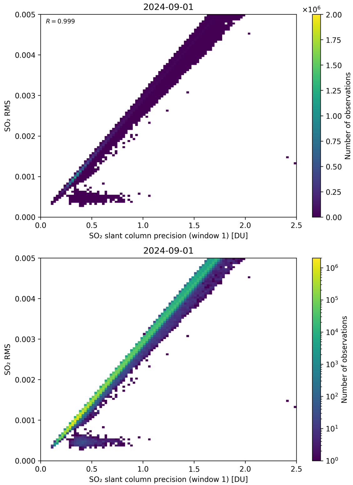
Figure 223: Scatter density plot of “SO 2 slant column precision (window 1)” against “SO 2 RMS” for 2024-09-01 to 2024-09-02.
