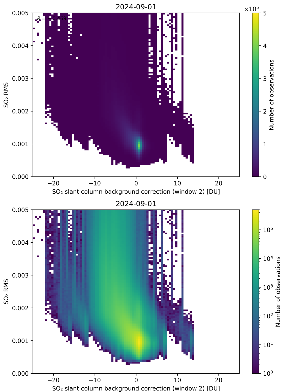
Figure 114: Scatter density plot of “SO 2 slant column background correction (window 2)” against “SO 2 RMS” for 2024-09-01 to 2024-09-02.
