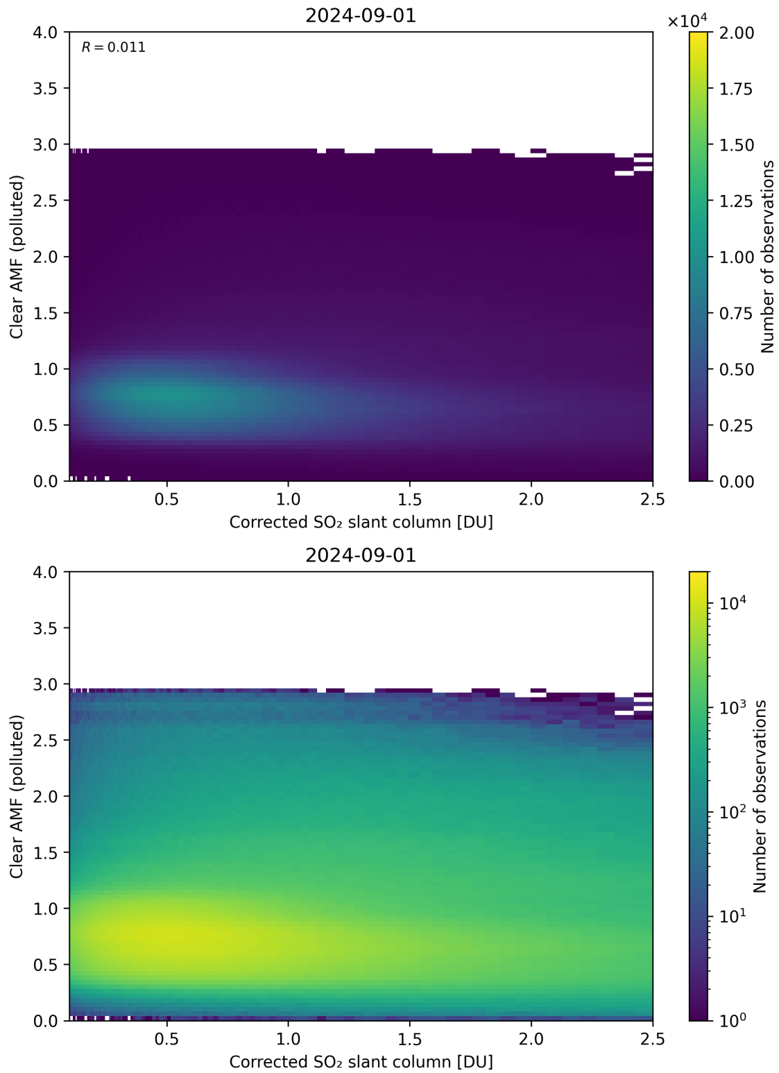
Figure 184: Scatter density plot of “Corrected SO 2 slant column” against “Clear AMF (polluted)” for 2024-09-01 to 2024-09-02.
