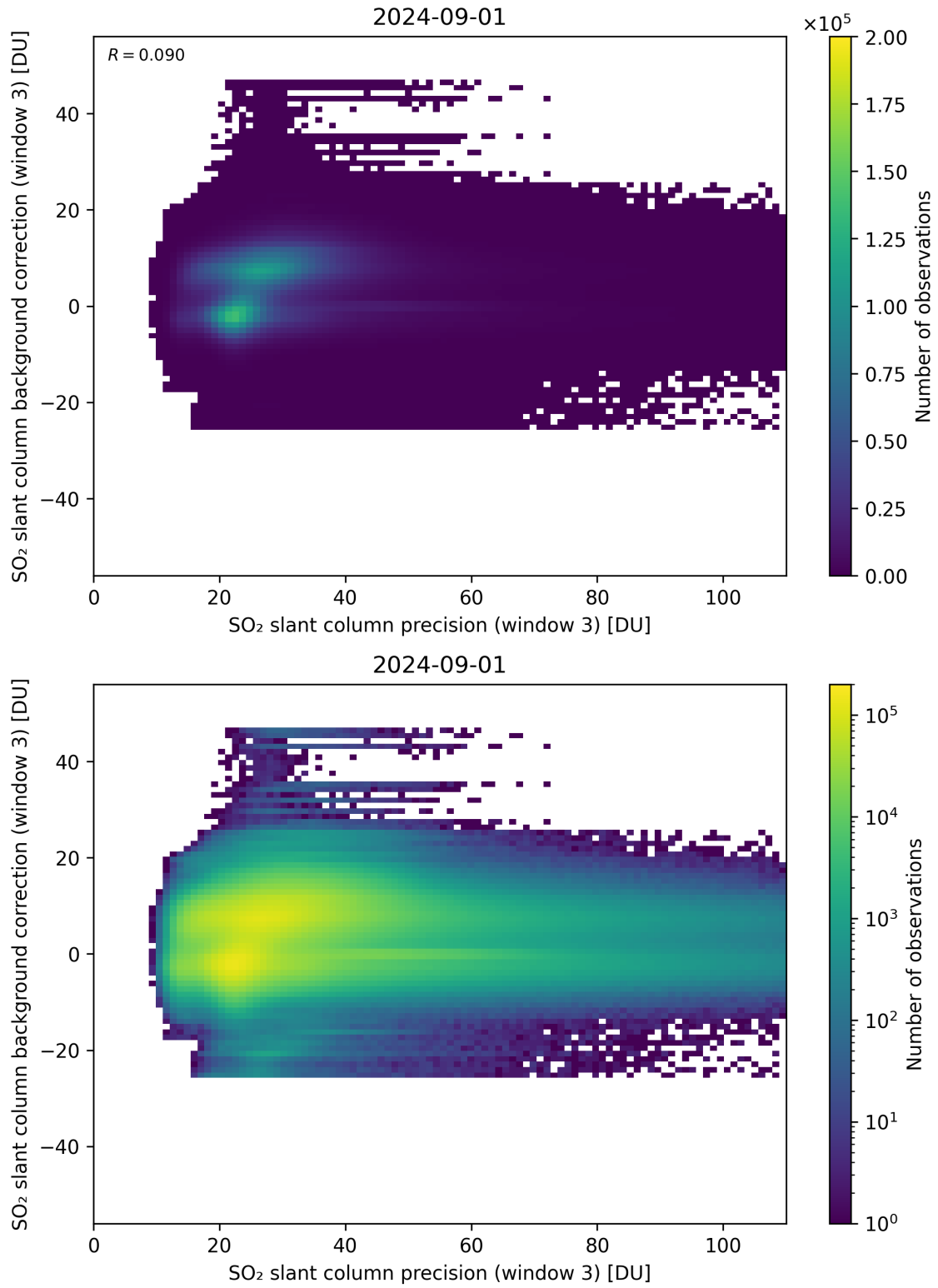
Figure 257: Scatter density plot of “SO 2 slant column precision (window 3)” against “SO 2 slant column background correction (window 3)” for 2024-09-01 to 2024-09-02.
