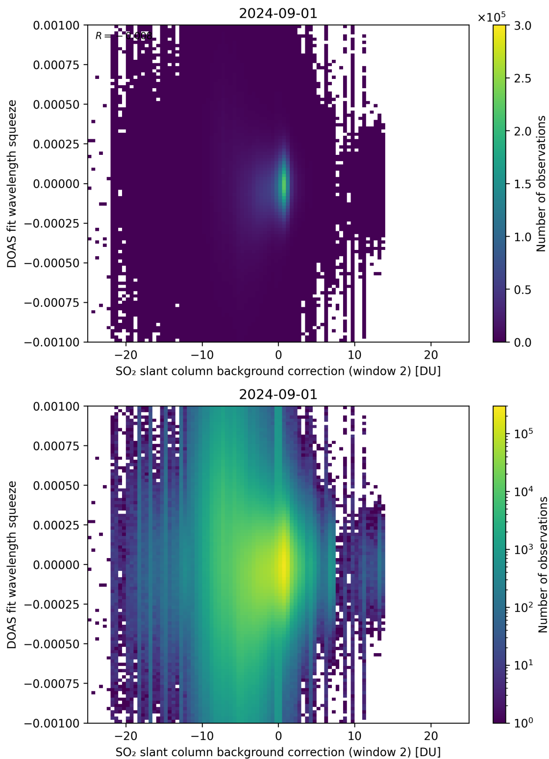
Figure 113: Scatter density plot of “SO 2 slant column background correction (window 2)” against “DOAS fit wavelength squeeze” for 2024-09-01 to 2024-09-02.
