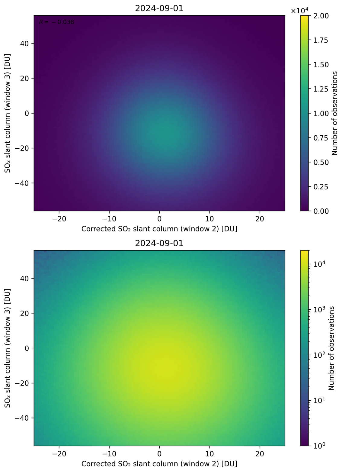
Figure 201: Scatter density plot of “Corrected SO 2 slant column (window 2)” against “SO 2 slant column (window 3)” for 2024-09-01 to 2024-09-02.
