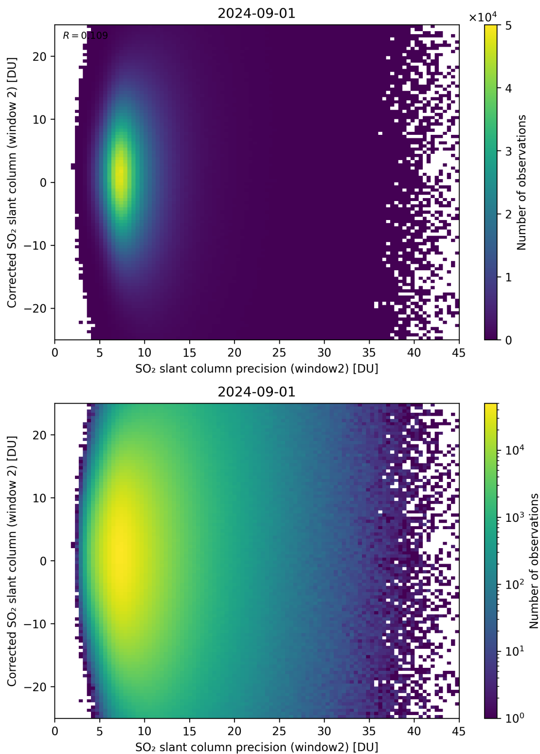
Figure 247: Scatter density plot of “SO 2 slant column precision (window2)” against “Corrected SO 2 slant column (window 2)” for 2024-09-01 to 2024-09-02.
