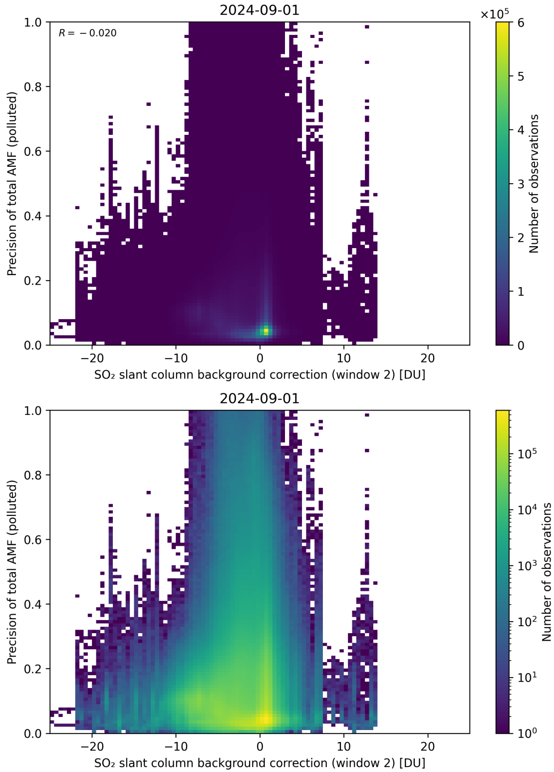
Figure 120: Scatter density plot of “SO 2 slant column background correction (window 2)” against “Precision of total AMF (polluted)” for 2024-09-01 to 2024-09-02.
