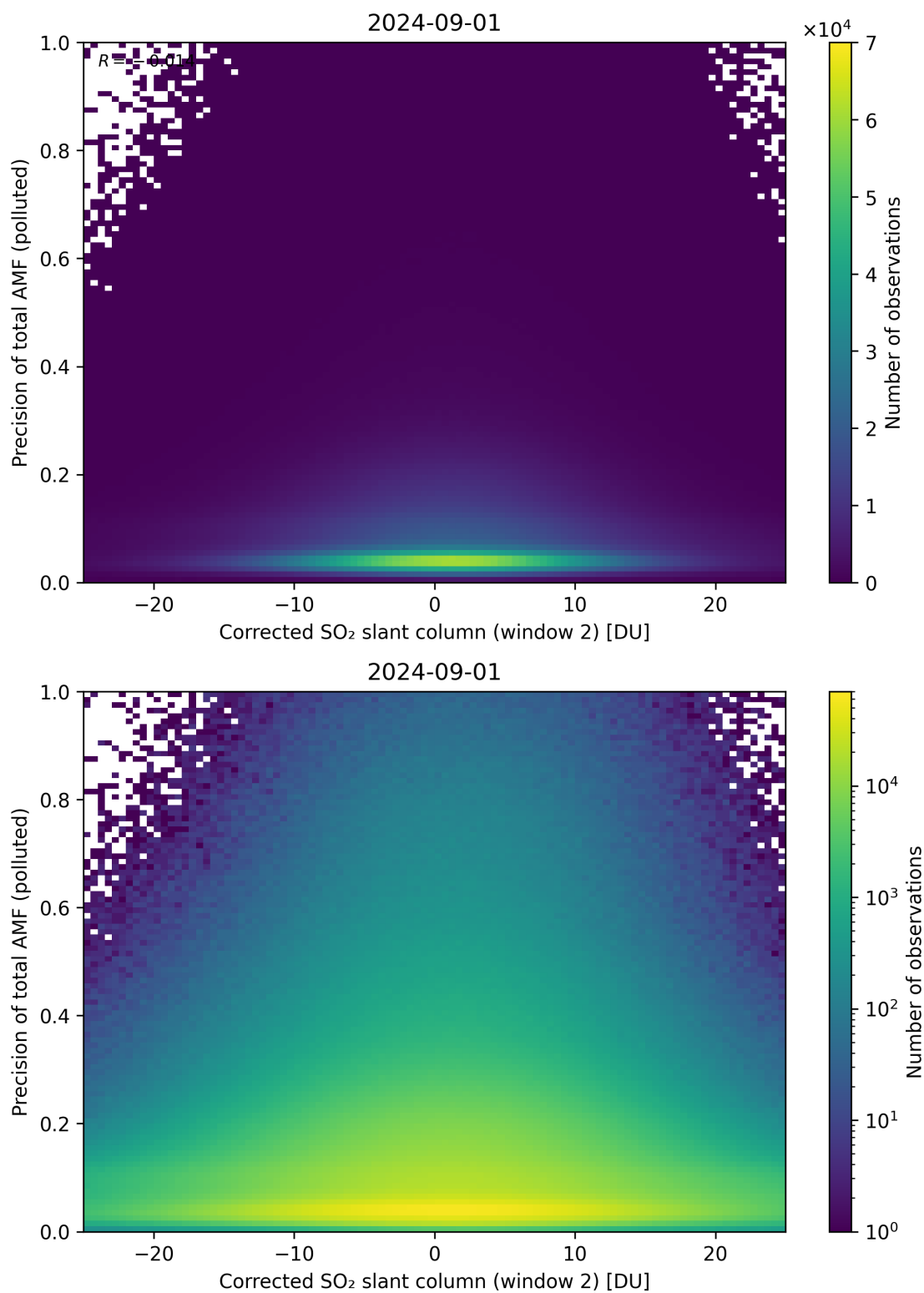
Figure 204: Scatter density plot of “Corrected SO 2 slant column (window 2)” against “Precision of total AMF (polluted)” for 2024-09-01 to 2024-09-02.
