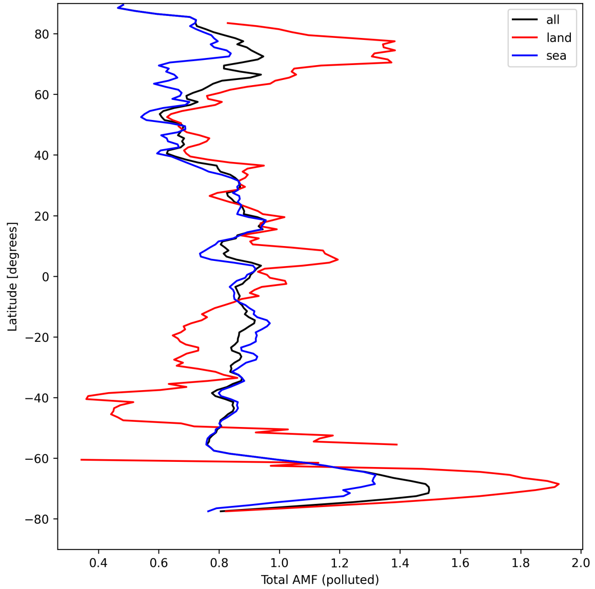
Figure 48: Zonal average of “Total AMF (polluted)” for 2024-09-01 to 2024-09-02.
