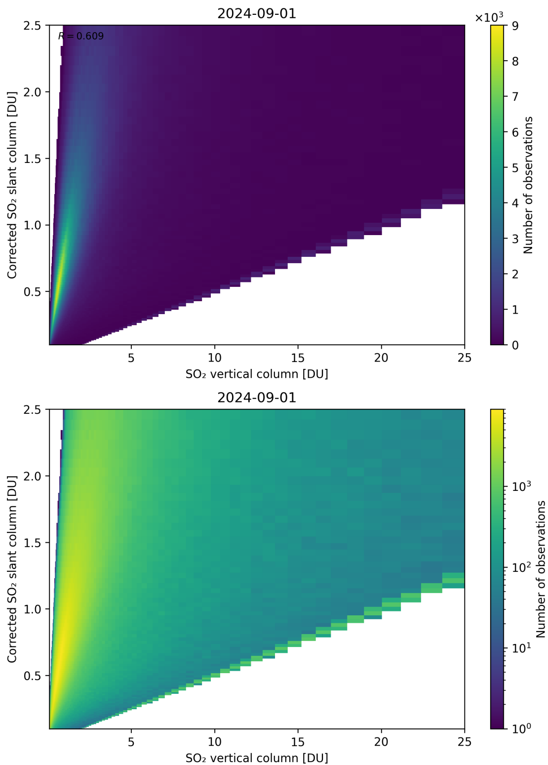
Figure 297: Scatter density plot of “SO 2 vertical column” against “Corrected SO 2 slant column” for 2024-09-01 to 2024-09-02.
