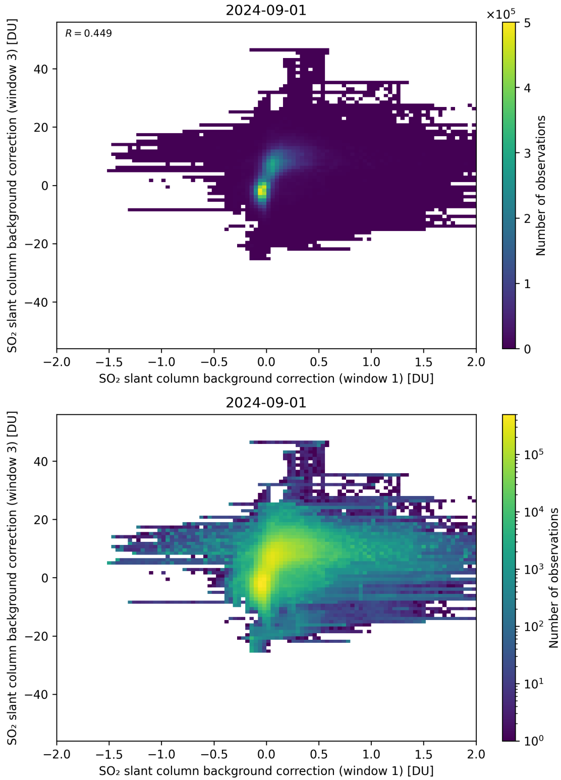
Figure 99: Scatter density plot of “SO 2 slant column background correction (window 1)” against “SO 2 slant column background correction (window 3)” for 2024-09-01 to 2024-09-02.
