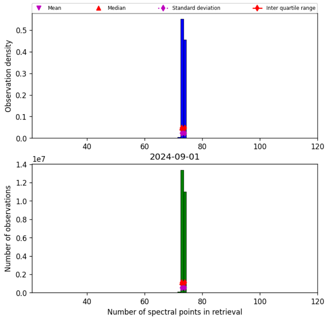
Figure 74: Histogram of “Number of spectral points in retrieval” for 2024-09-01 to 2024-09-02
