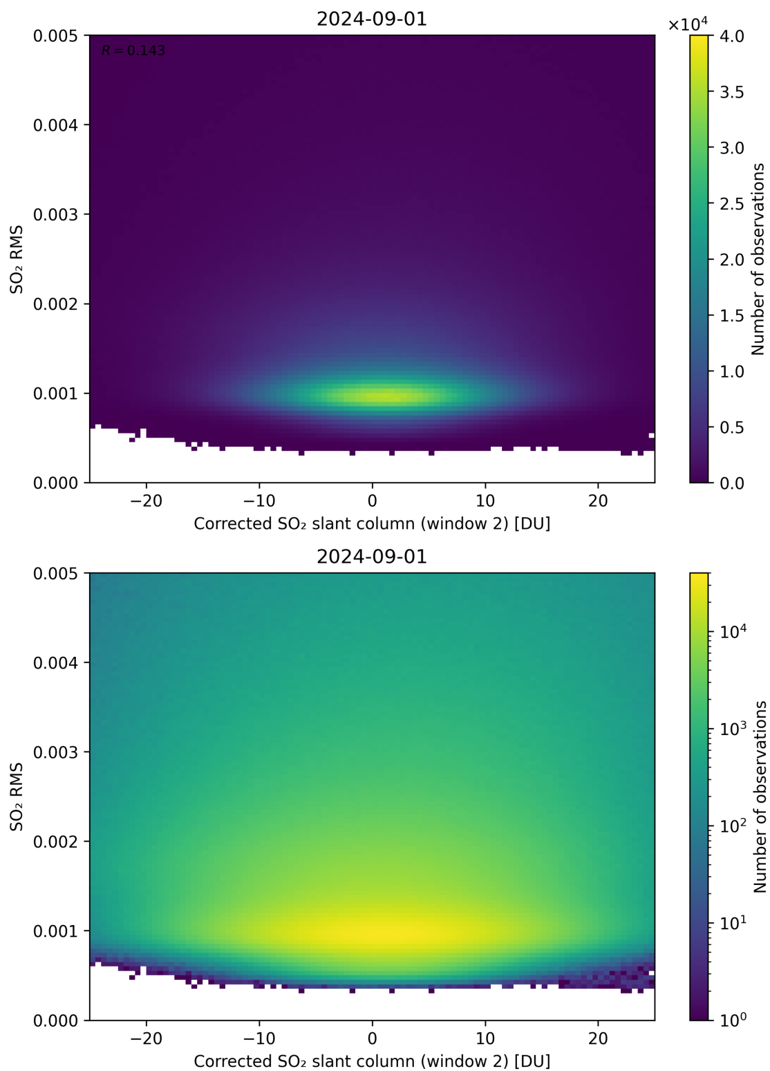
Figure 198: Scatter density plot of “Corrected SO 2 slant column (window 2)” against “SO 2 RMS” for 2024-09-01 to 2024-09-02.
