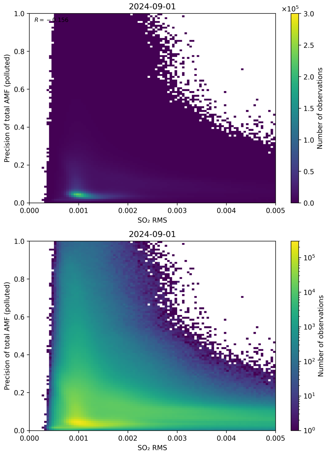
Figure 138: Scatter density plot of “SO 2 RMS” against “Precision of total AMF (polluted)” for 2024-09-01 to 2024-09-02.
