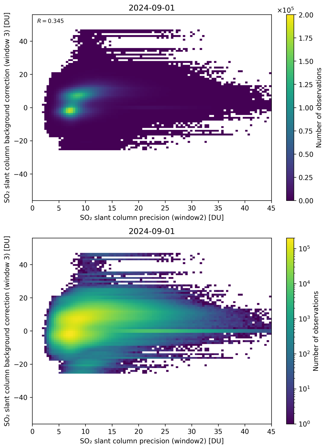
Figure 242: Scatter density plot of “SO 2 slant column precision (window2)” against “SO 2 slant column background correction (window 3)” for 2024-09-01 to 2024-09-02.
