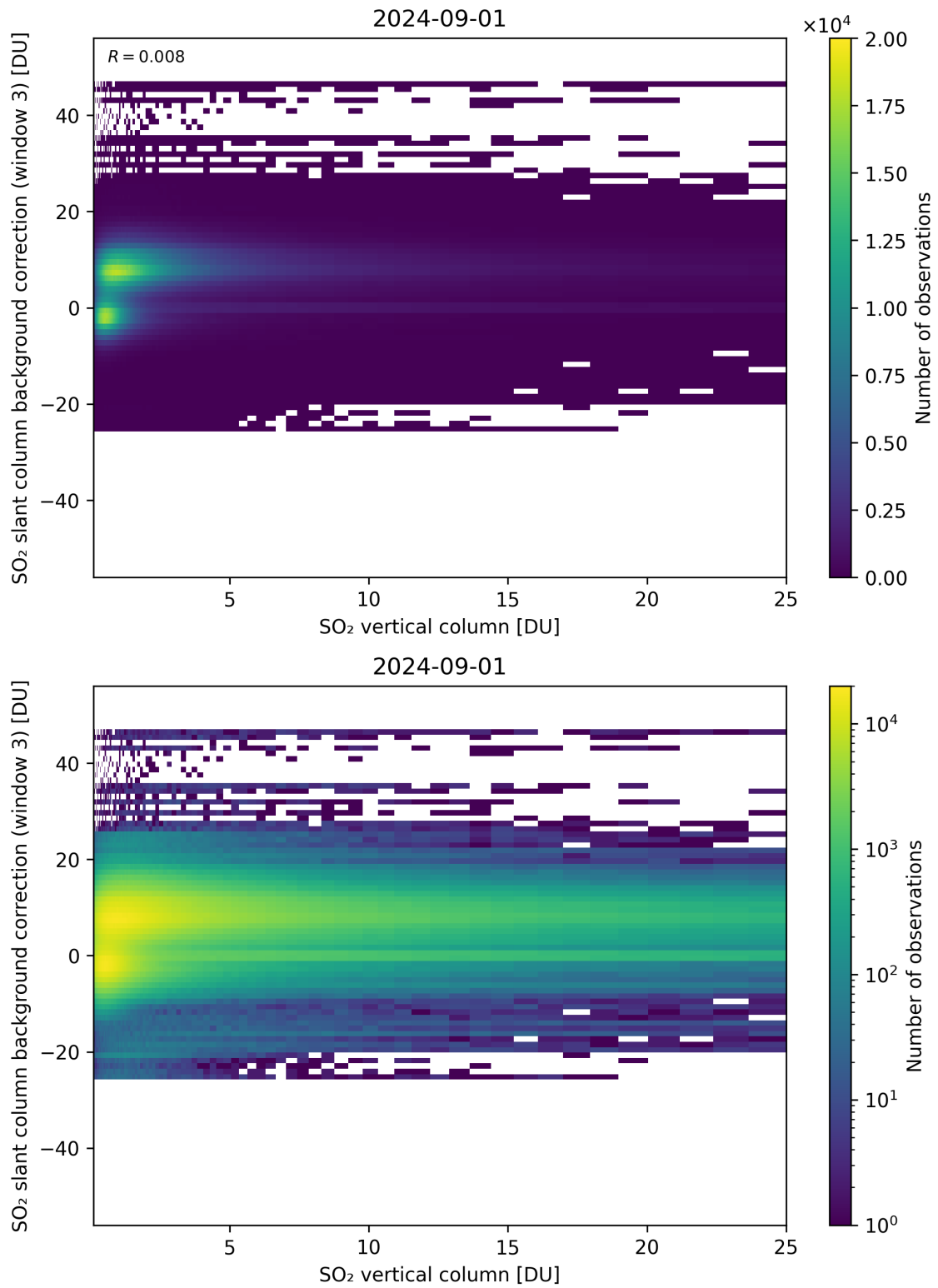
Figure 275: Scatter density plot of “SO 2 vertical column” against “SO 2 slant column background correction (window 3)” for 2024-09-01 to 2024-09-02.
