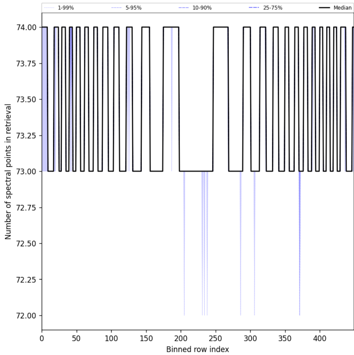
Figure 97: Along track statistics of “Number of spectral points in retrieval” for 2024-09-01 to 2024-09-02
