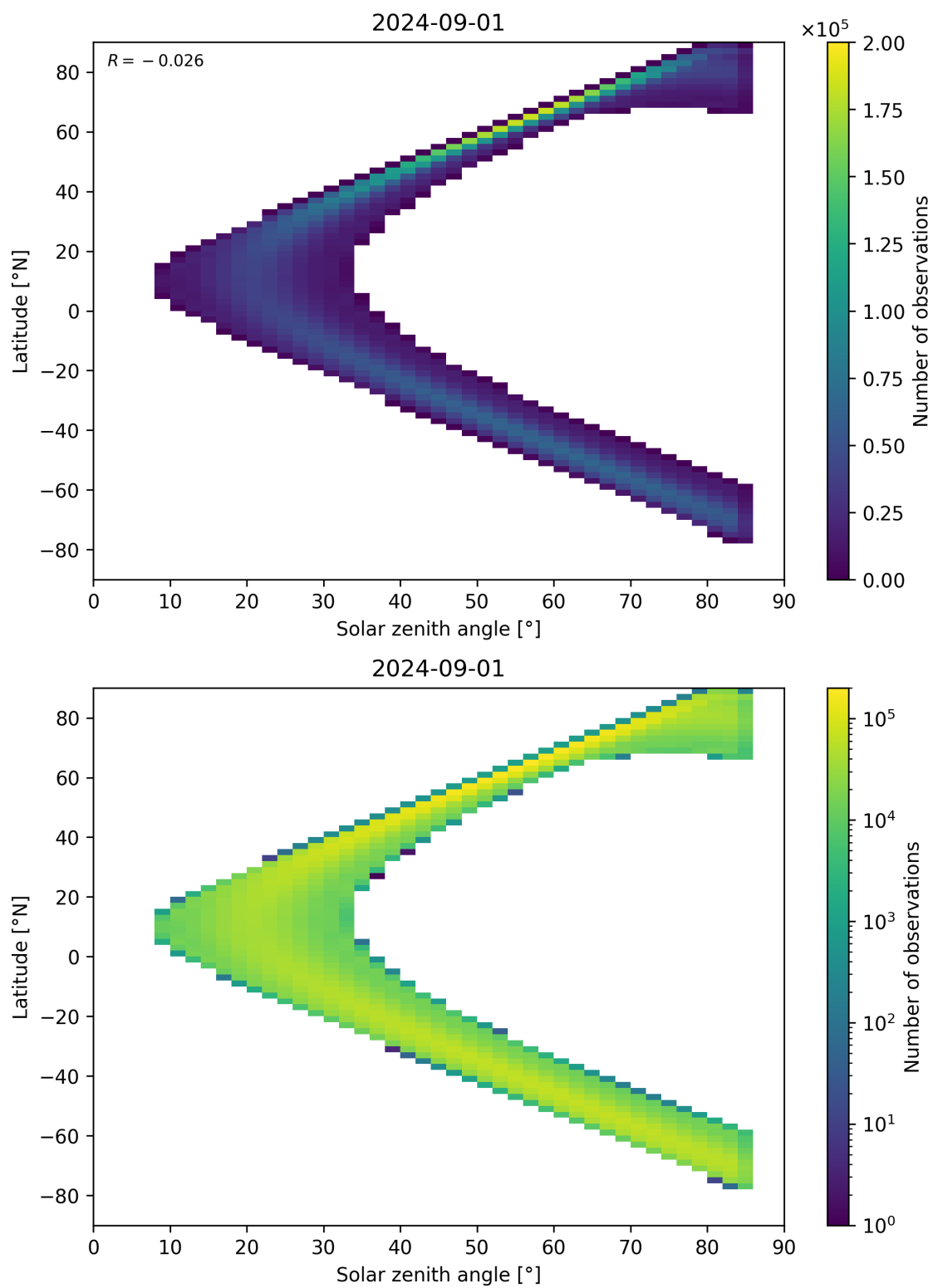
Figure 164: Scatter density plot of “Solar zenith angle” against “Latitude” for 2024-09-01 to 2024-09-02.
