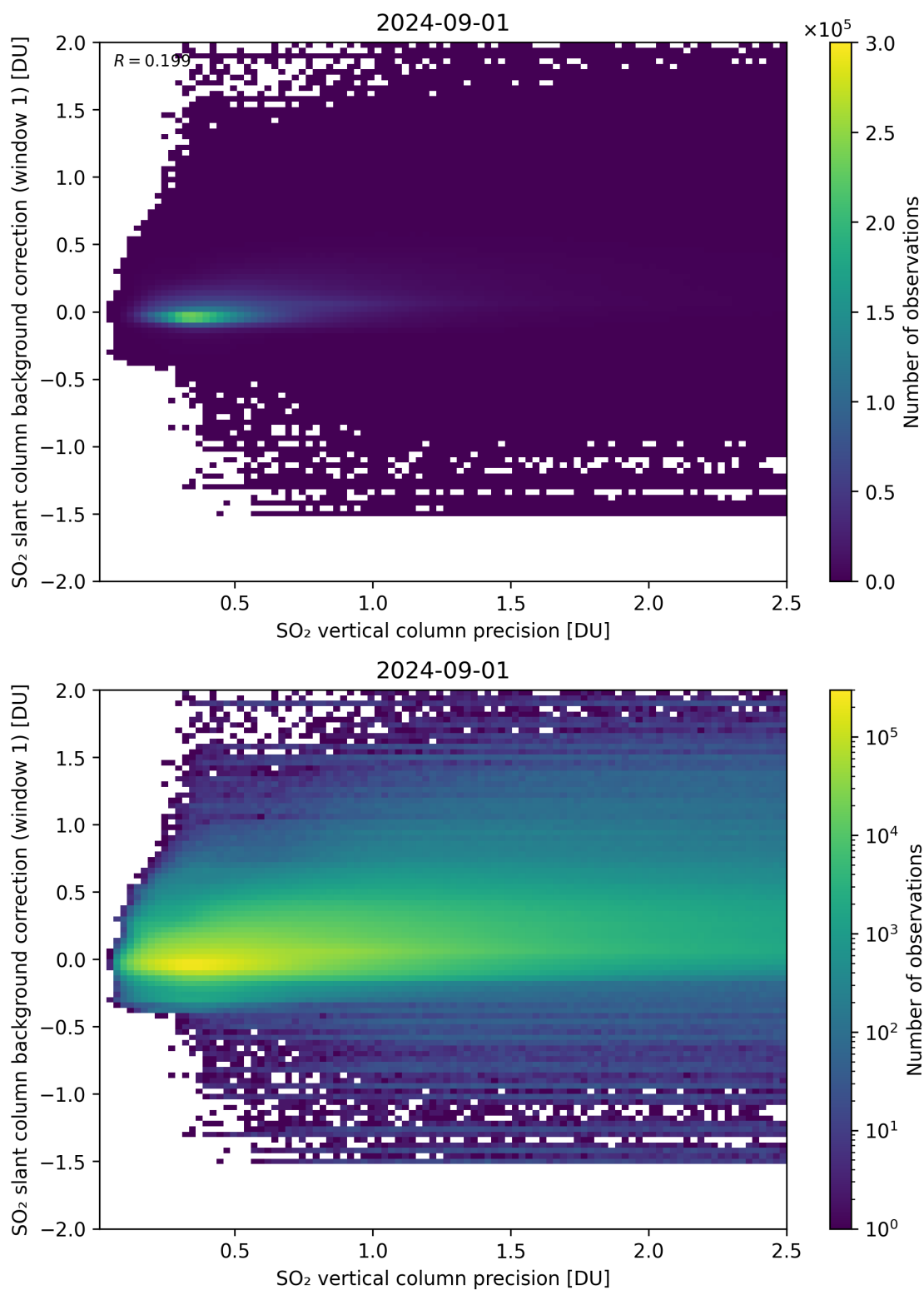
Figure 279: Scatter density plot of “SO 2 vertical column precision” against “SO 2 slant column background correction (window 1)” for 2024-09-01 to 2024-09-02.
