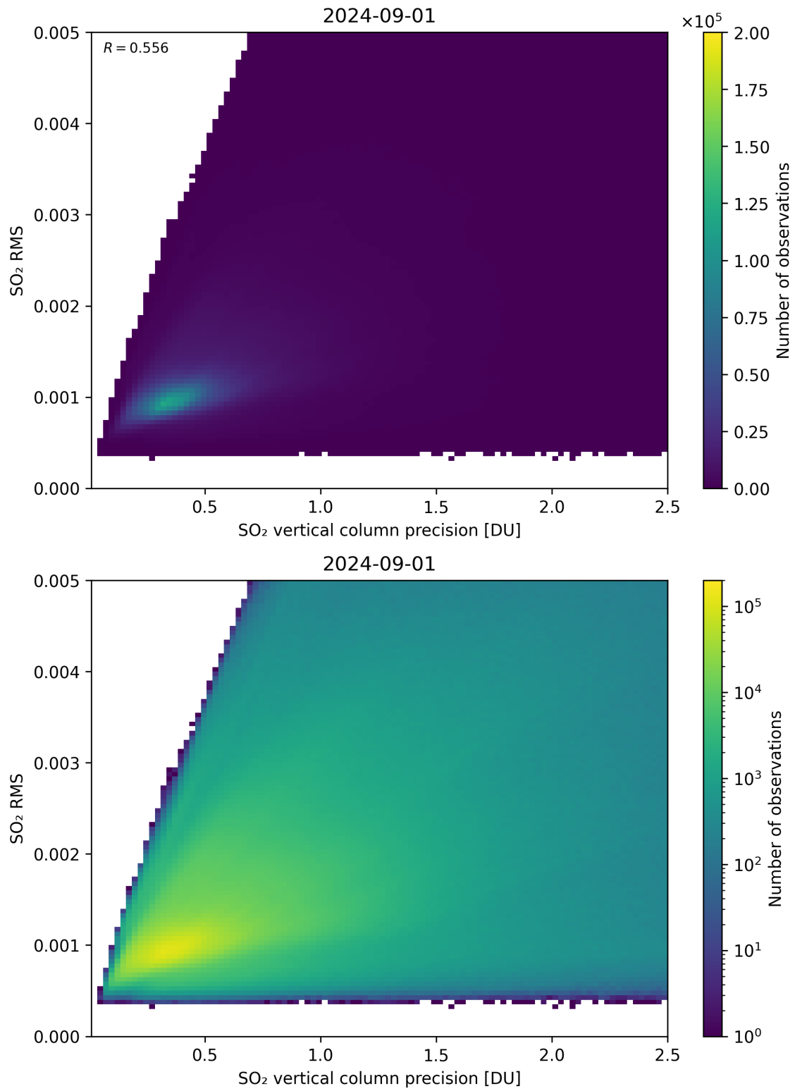
Figure 284: Scatter density plot of “SO 2 vertical column precision” against “SO 2 RMS” for 2024-09-01 to 2024-09-02.
