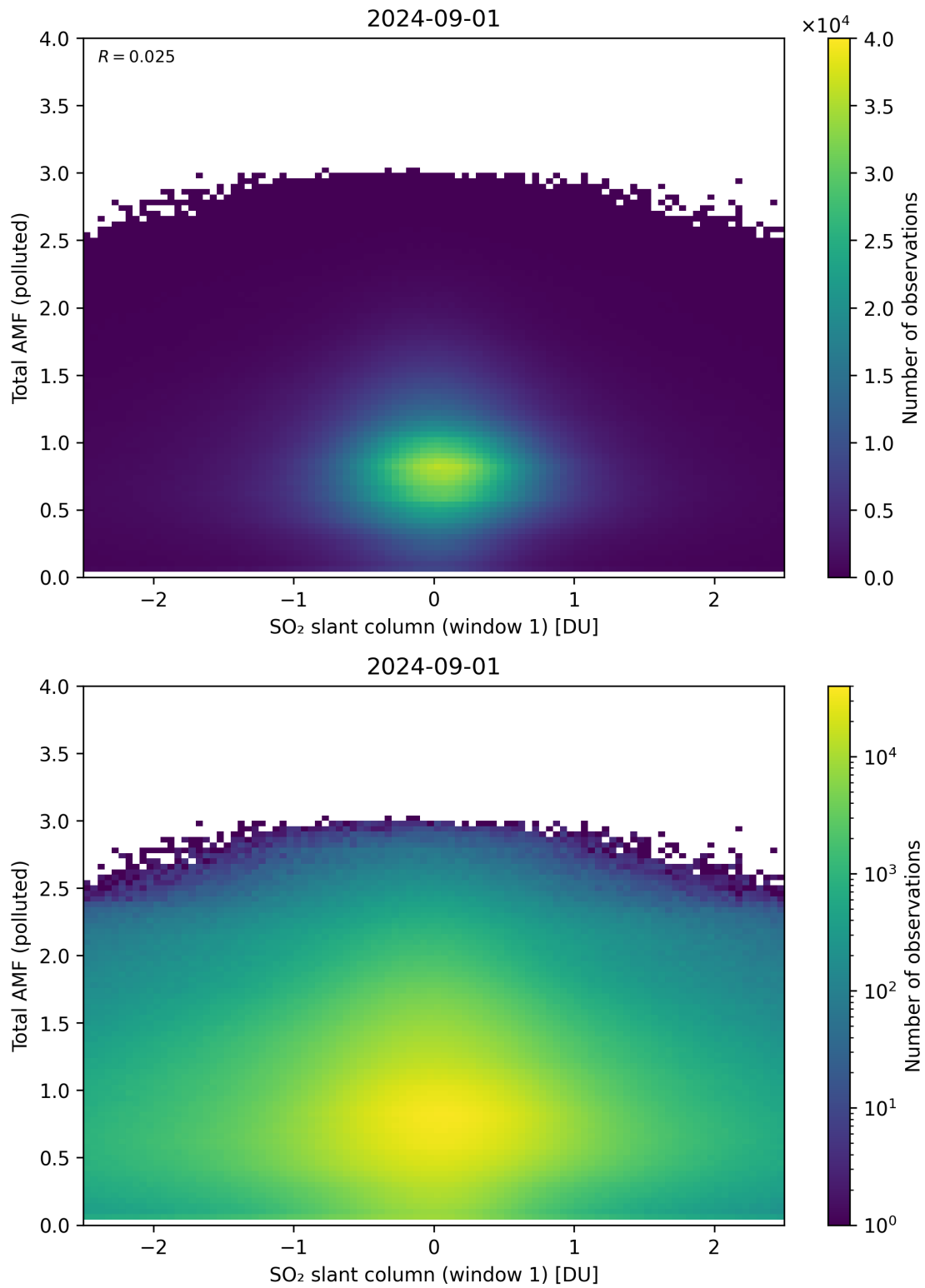
Figure 239: Scatter density plot of “SO 2 slant column (window 1)” against “Total AMF (polluted)” for 2024-09-01 to 2024-09-02.
