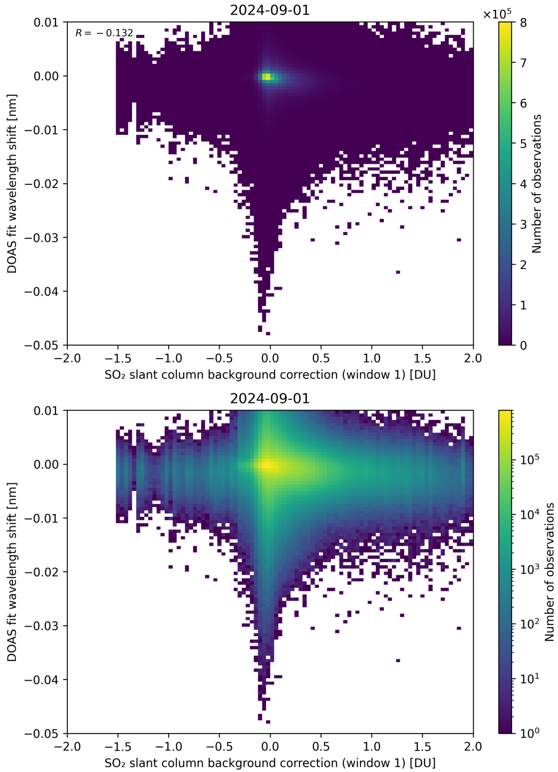
Figure 100: Scatter density plot of “SO 2 slant column background correction (window 1)” against “DOAS fit wavelength shift” for 2024-09-01 to 2024-09-02.
