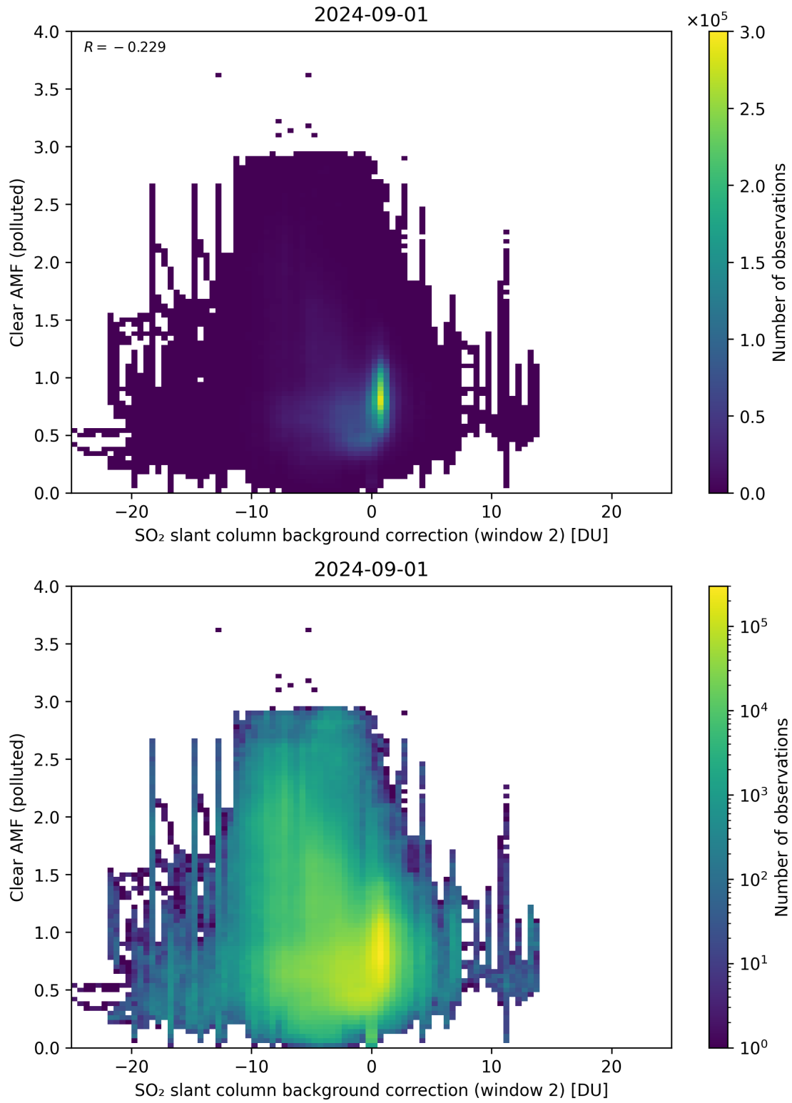
Figure 115: Scatter density plot of “SO 2 slant column background correction (window 2)” against “Clear AMF (polluted)” for 2024-09-01 to 2024-09-02.
