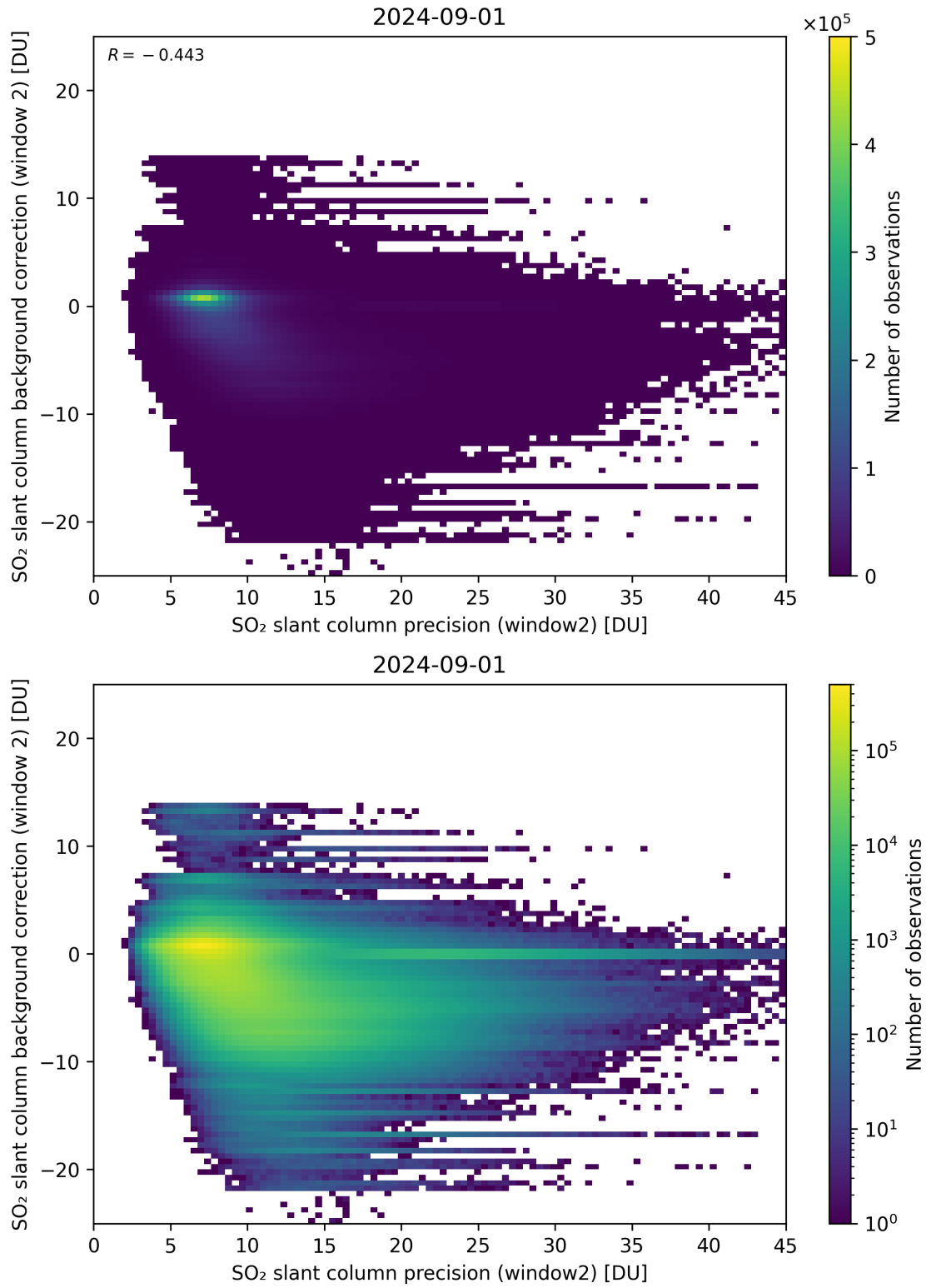
Figure 241: Scatter density plot of “SO 2 slant column precision (window2)” against “SO 2 slant column background correction (window 2)” for 2024-09-01 to 2024-09-02.
