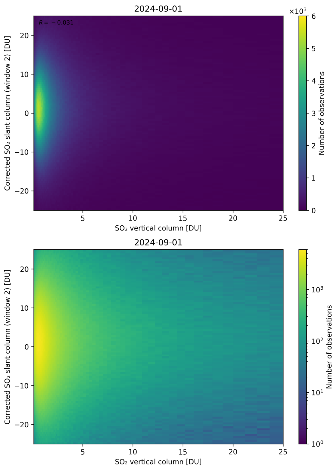
Figure 298: Scatter density plot of “SO 2 vertical column” against “Corrected SO 2 slant column (window 2)” for 2024-09-01 to 2024-09-02.
