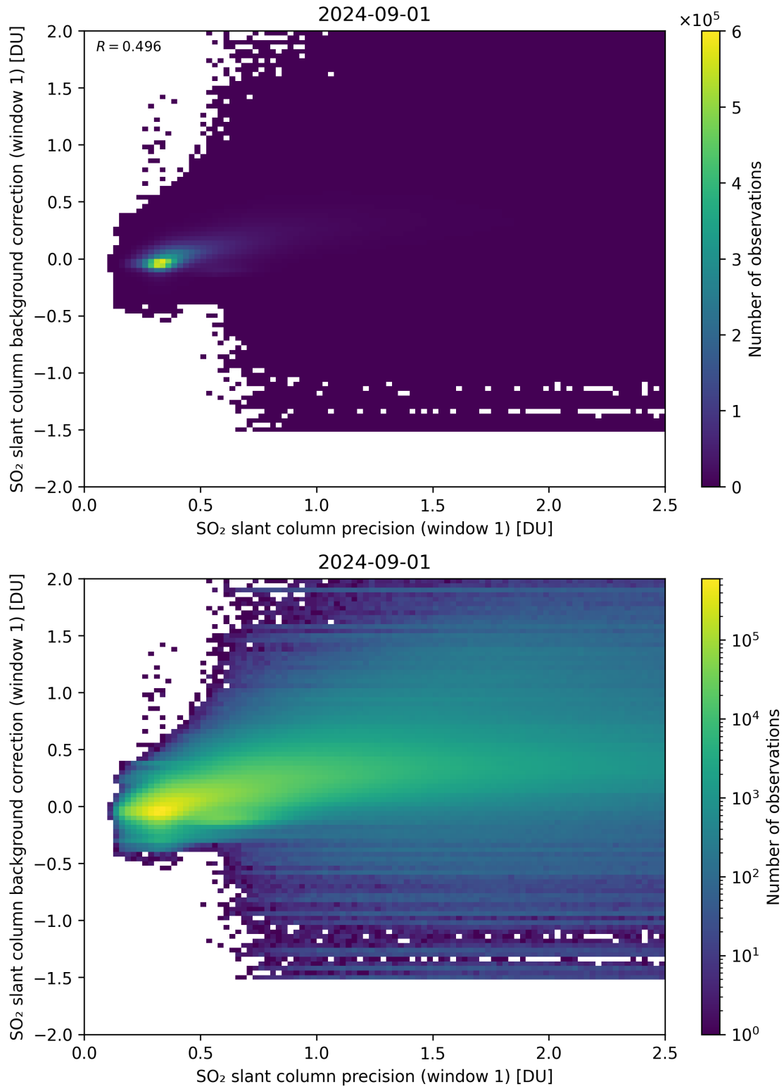
Figure 218: Scatter density plot of “SO 2 slant column precision (window 1)” against “SO 2 slant column background correction (window 1)” for 2024-09-01 to 2024-09-02.
