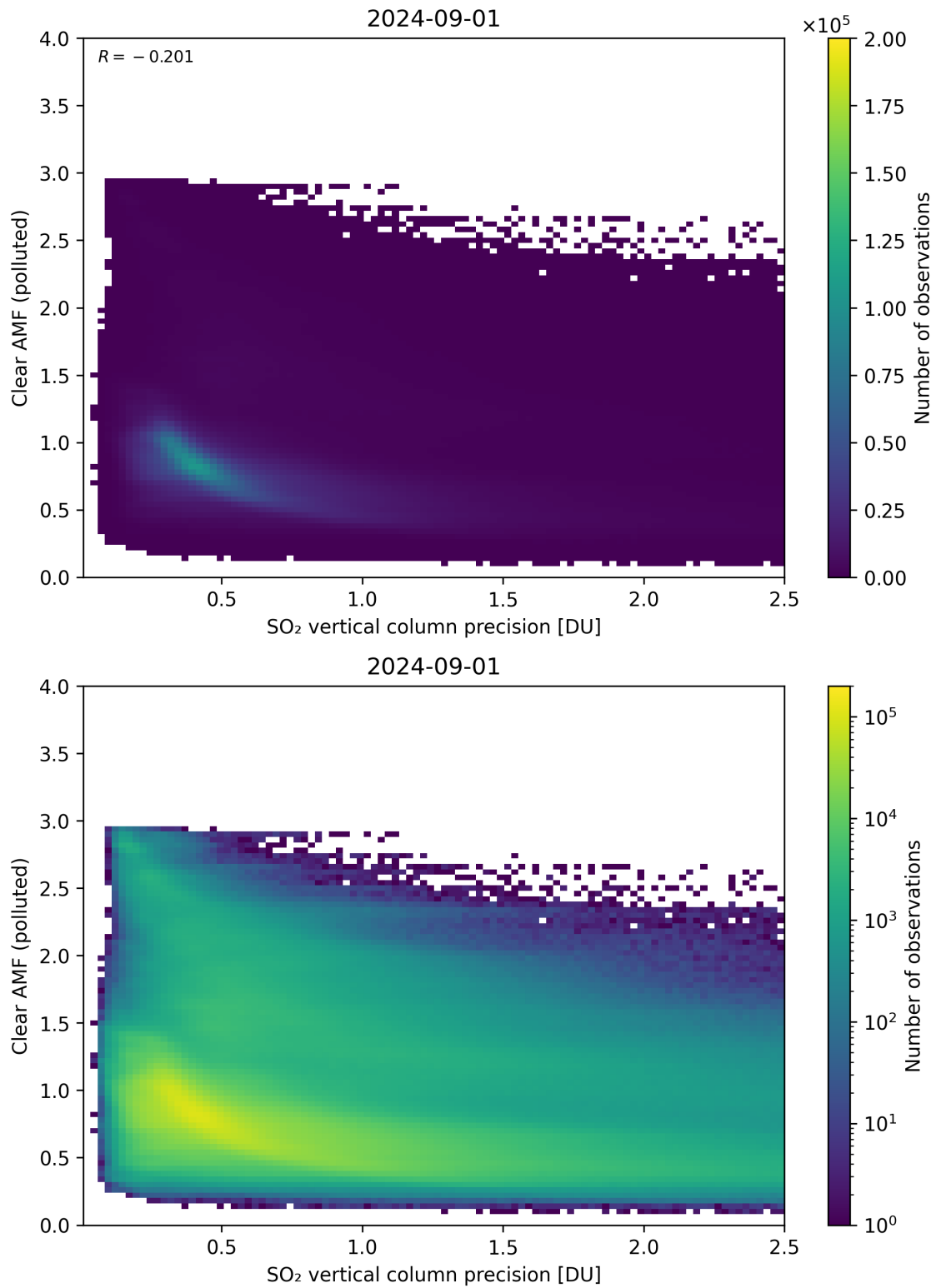
Figure 285: Scatter density plot of “SO 2 vertical column precision” against “Clear AMF (polluted)” for 2024-09-01 to 2024-09-02.
