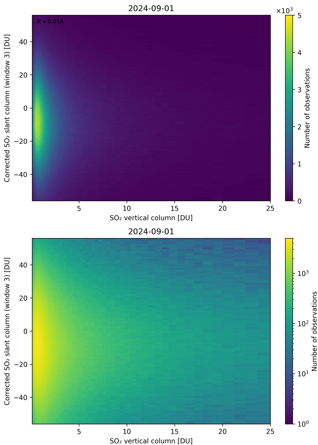
Figure 299: Scatter density plot of “SO 2 vertical column” against “Corrected SO 2 slant column (window 3)” for 2024-09-01 to 2024-09-02.
