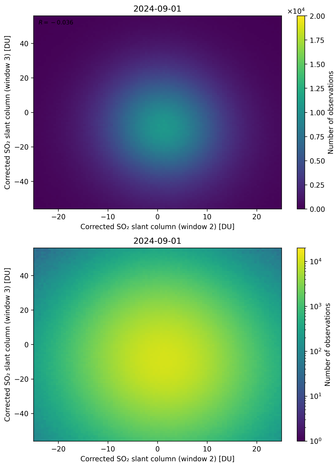
Figure 200: Scatter density plot of “Corrected SO 2 slant column (window 2)” against “Corrected SO 2 slant column (window 3)” for 2024-09-01 to 2024-09-02.
