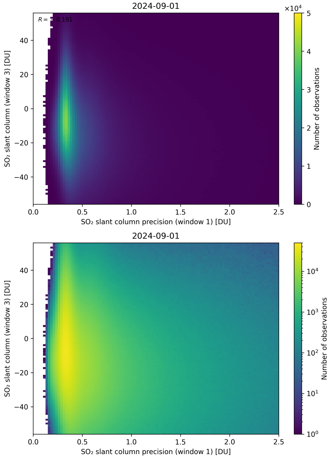
Figure 228: Scatter density plot of “SO 2 slant column precision (window 1)” against “SO 2 slant column (window 3)” for 2024-09-01 to 2024-09-02.
