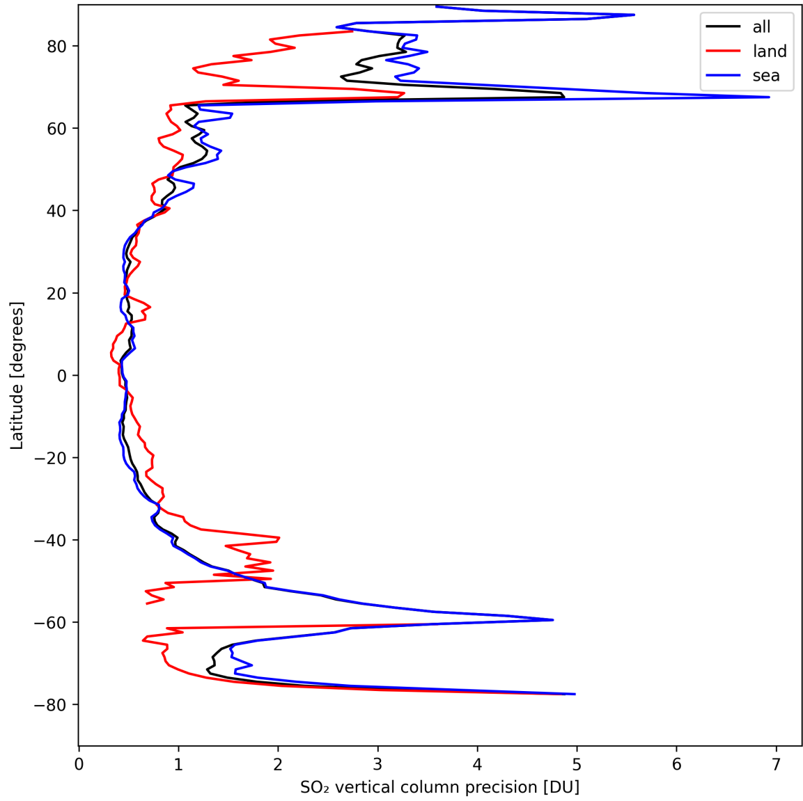
Figure 31: Zonal average of “SO 2 vertical column precision” for 2024-09-01 to 2024-09-02.
