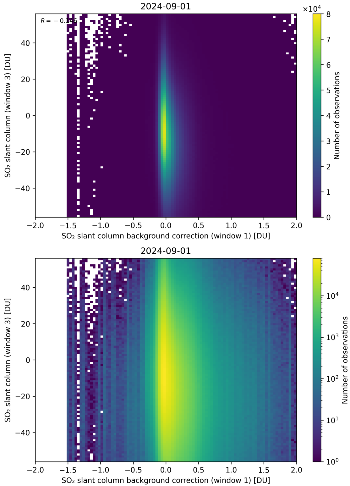
Figure 107: Scatter density plot of “SO 2 slant column background correction (window 1)” against “SO 2 slant column (window 3)” for 2024-09-01 to 2024-09-02.
