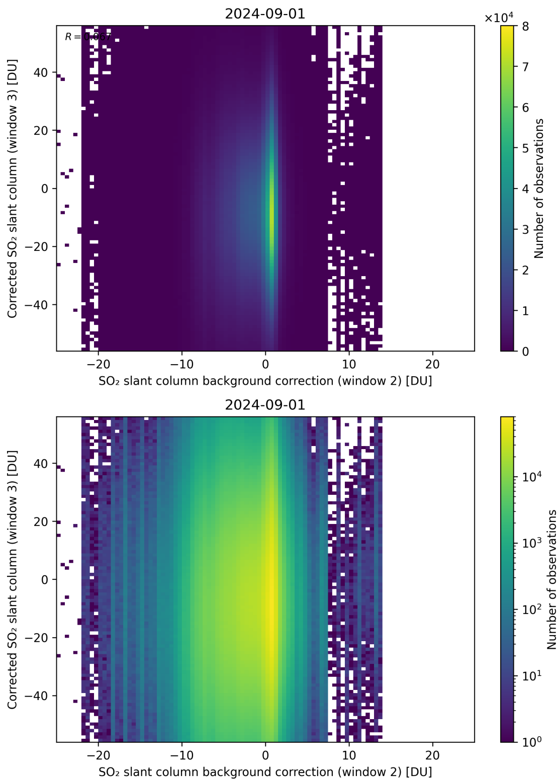
Figure 116: Scatter density plot of “SO 2 slant column background correction (window 2)” against “Corrected SO 2 slant column (window 3)” for 2024-09-01 to 2024-09-02.
