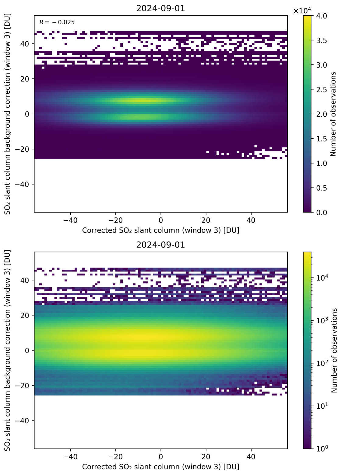
Figure 205: Scatter density plot of “Corrected SO 2 slant column (window 3)” against “SO 2 slant column background correction (window 3)” for 2024-09-01 to 2024-09-02.
