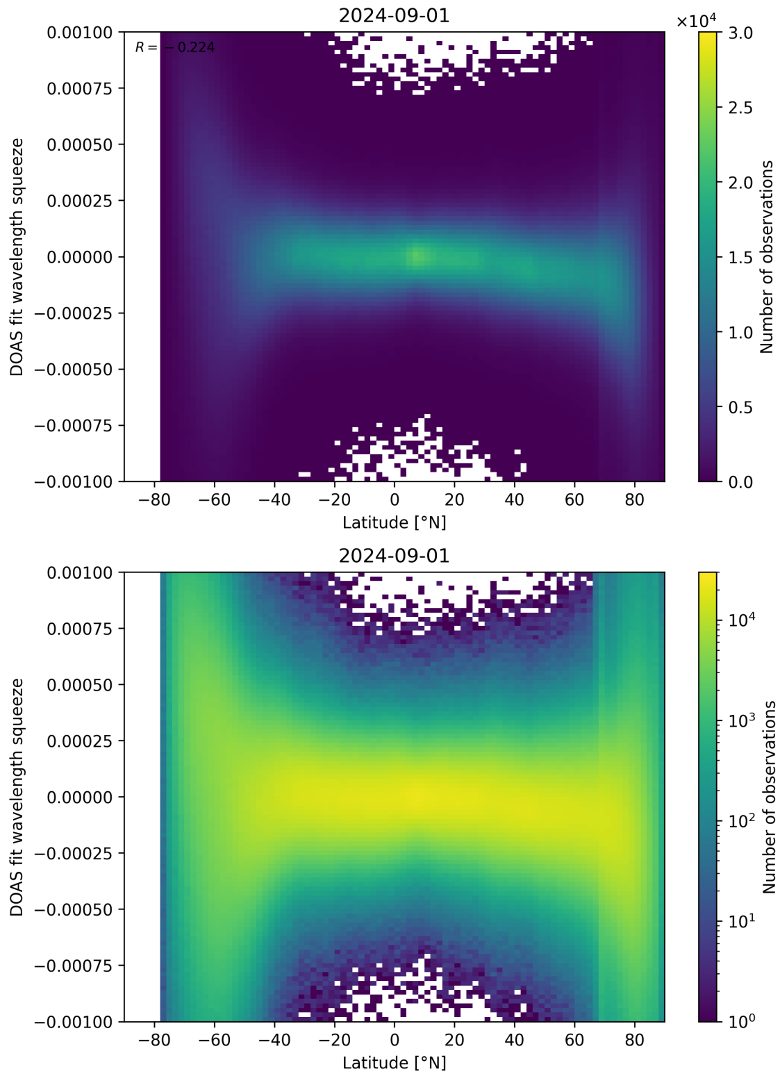
Figure 143: Scatter density plot of “Latitude” against “DOAS fit wavelength squeeze” for 2024-09-01 to 2024-09-02.
