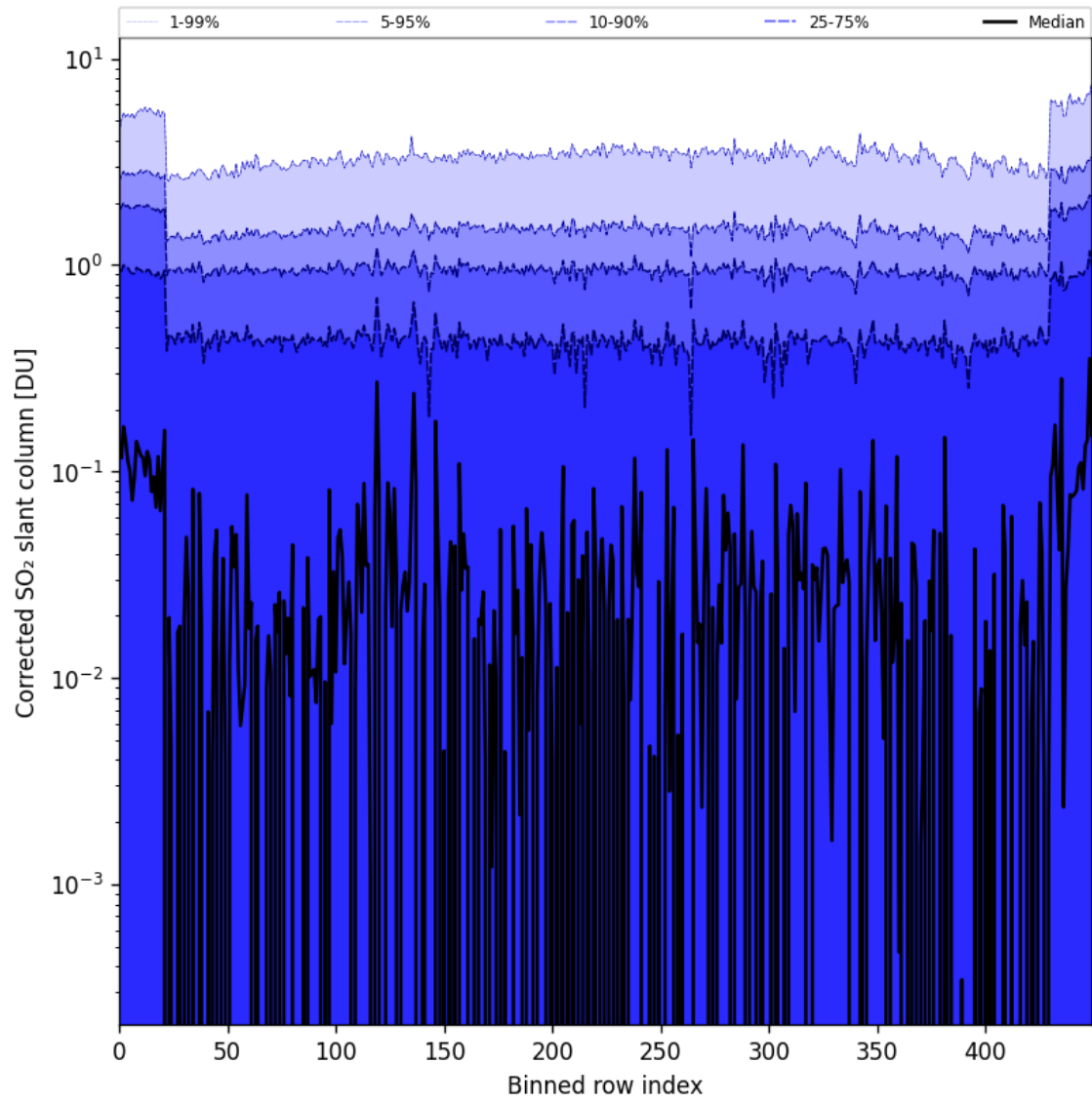
Figure 78: Along track statistics of “Corrected SO 2 slant column” for 2024-09-01 to 2024-09-02
