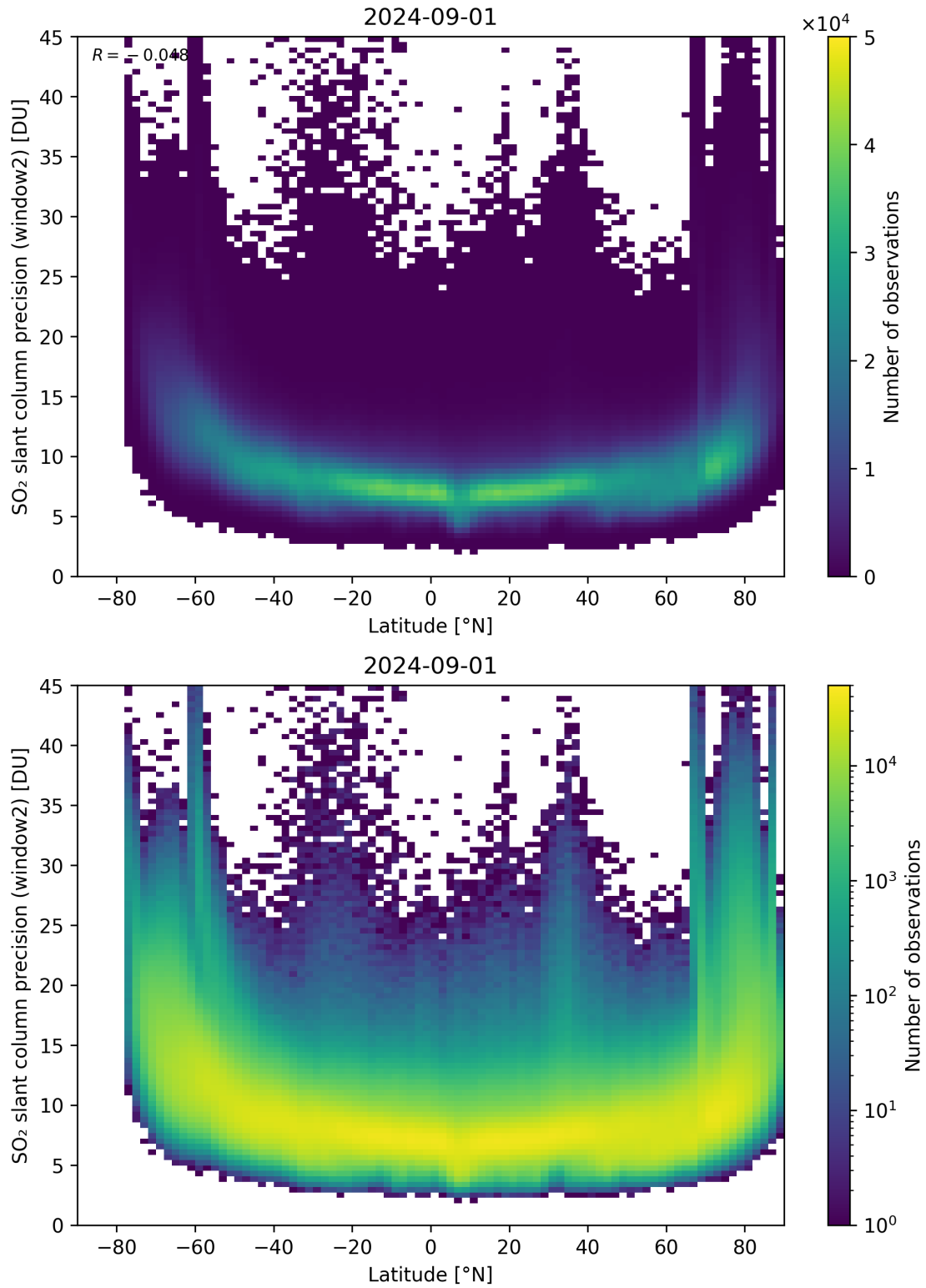
Figure 151: Scatter density plot of “Latitude” against “SO 2 slant column precision (window2)” for 2024-09-01 to 2024-09-02.
