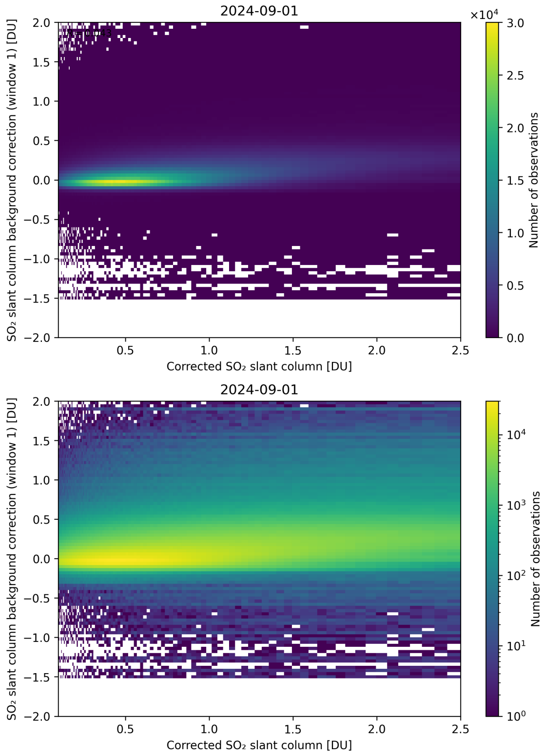
Figure 178: Scatter density plot of “Corrected SO 2 slant column” against “SO 2 slant column background correction (window 1)” for 2024-09-01 to 2024-09-02.
