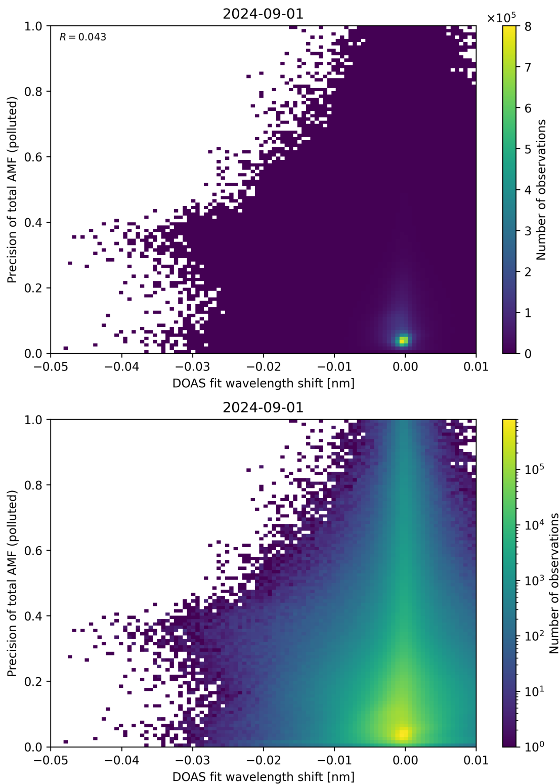
Figure 131: Scatter density plot of “DOAS fit wavelength shift” against “Precision of total AMF (polluted)” for 2024-09-01 to 2024-09-02.
