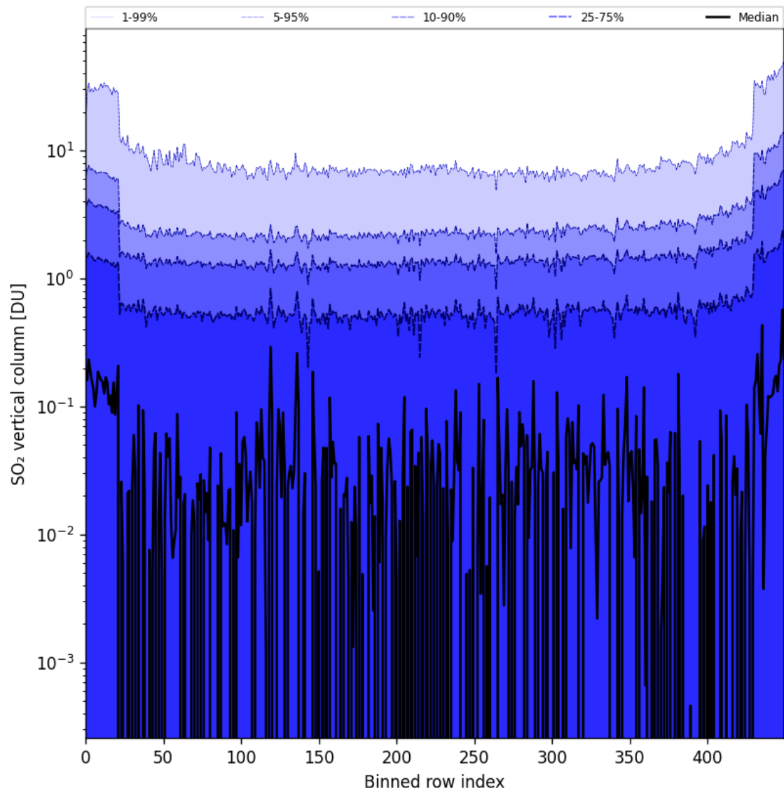
Figure 76: Along track statistics of “SO 2 vertical column” for 2024-09-01 to 2024-09-02
