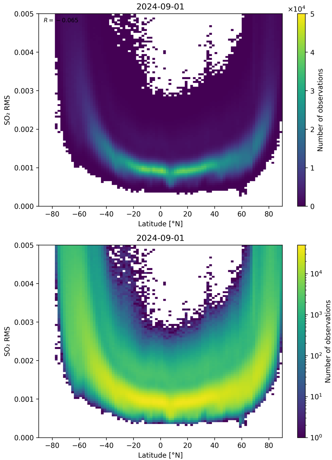
Figure 144: Scatter density plot of “Latitude” against “SO 2 RMS” for 2024-09-01 to 2024-09-02.
