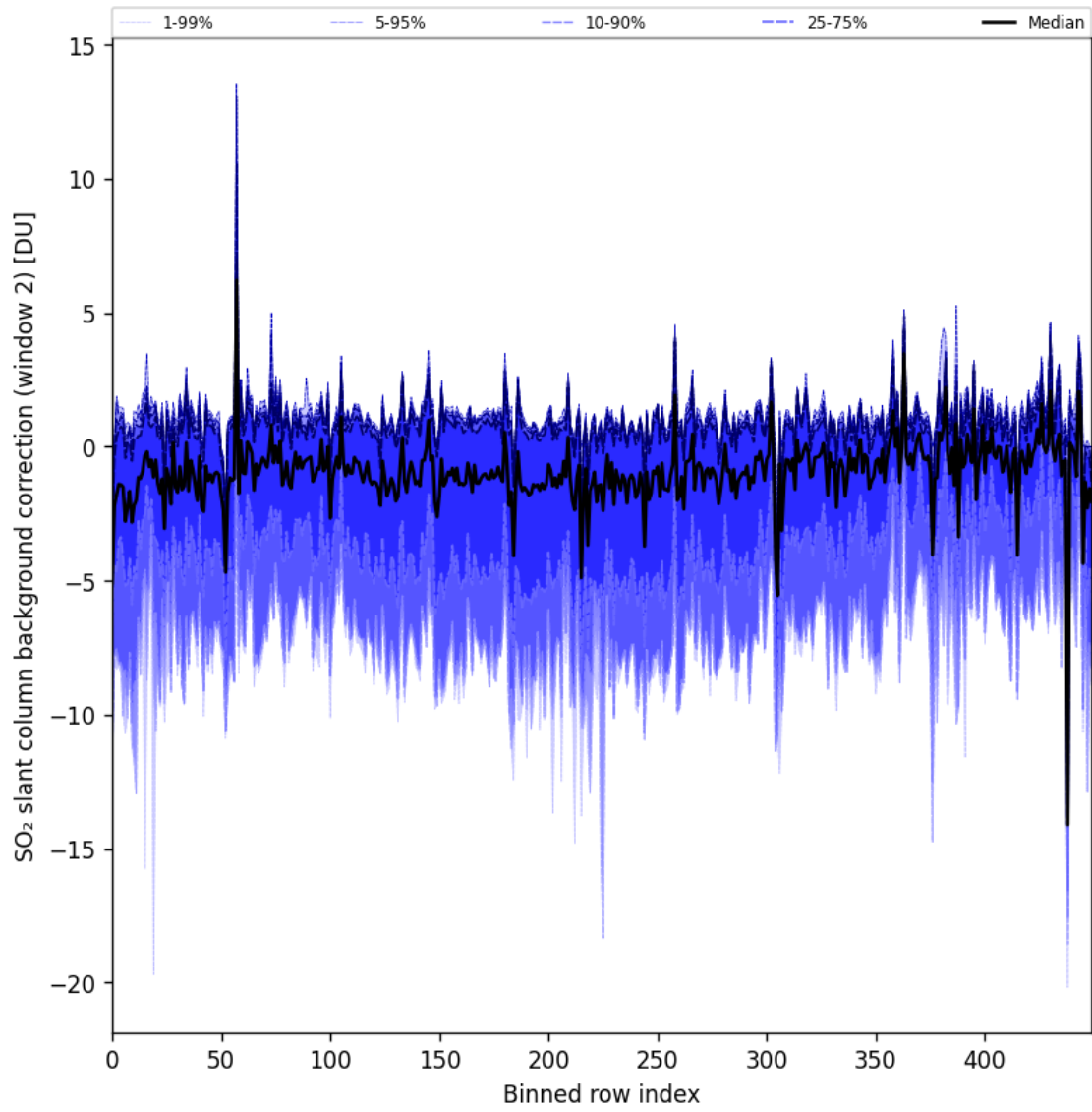
Figure 86: Along track statistics of “SO 2 slant column background correction (window 2)” for 2024-09-01 to 2024-09-02
