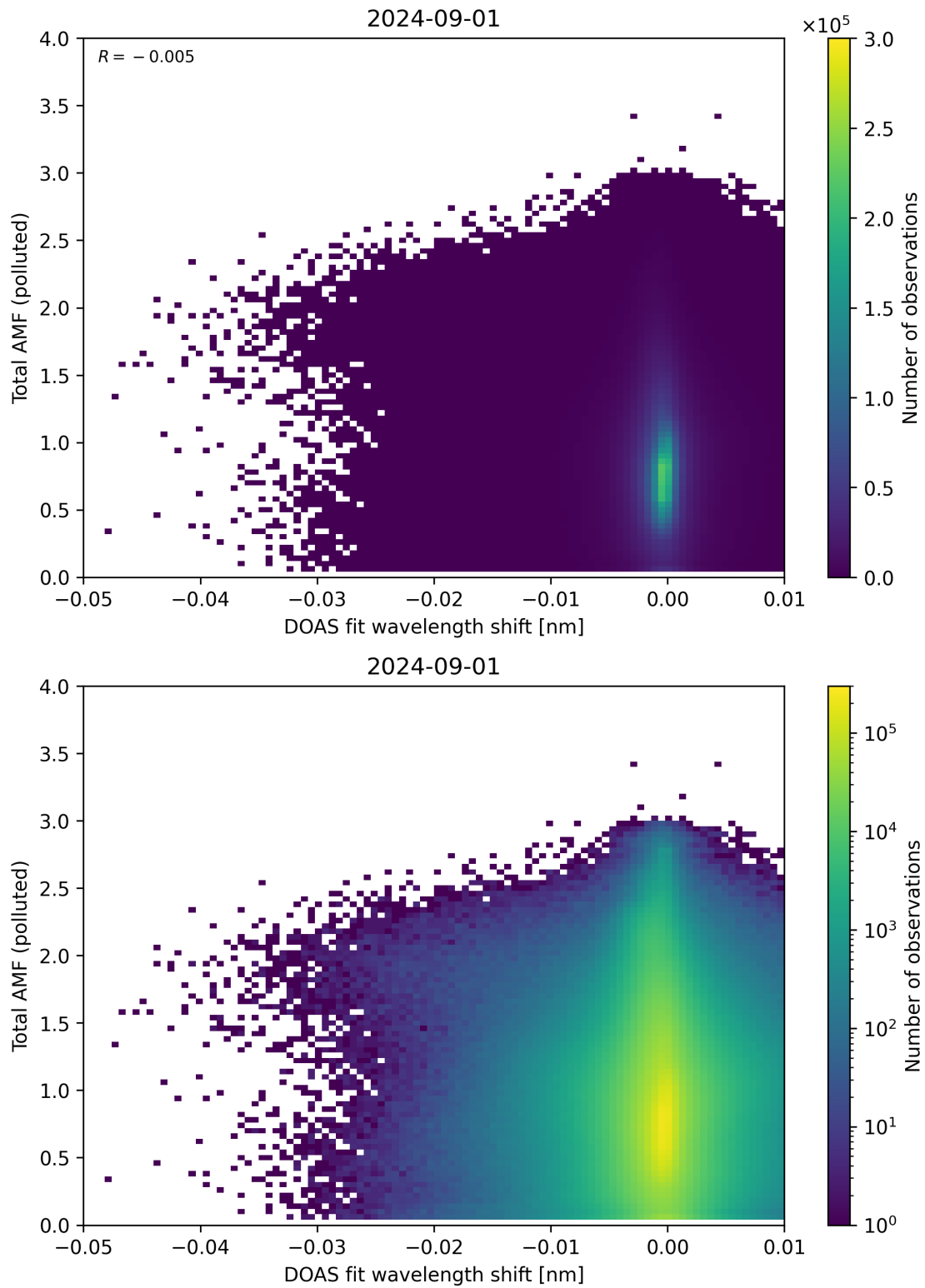
Figure 130: Scatter density plot of “DOAS fit wavelength shift” against “Total AMF (polluted)” for 2024-09-01 to 2024-09-02.
