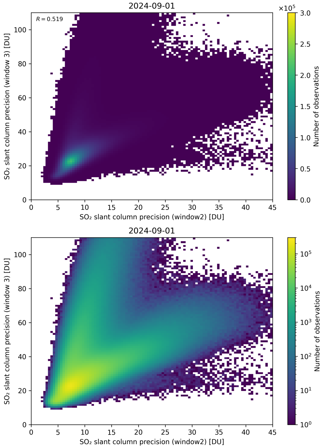
Figure 250: Scatter density plot of “SO 2 slant column precision (window2)” against “SO 2 slant column precision (window 3)” for 2024-09-01 to 2024-09-02.
