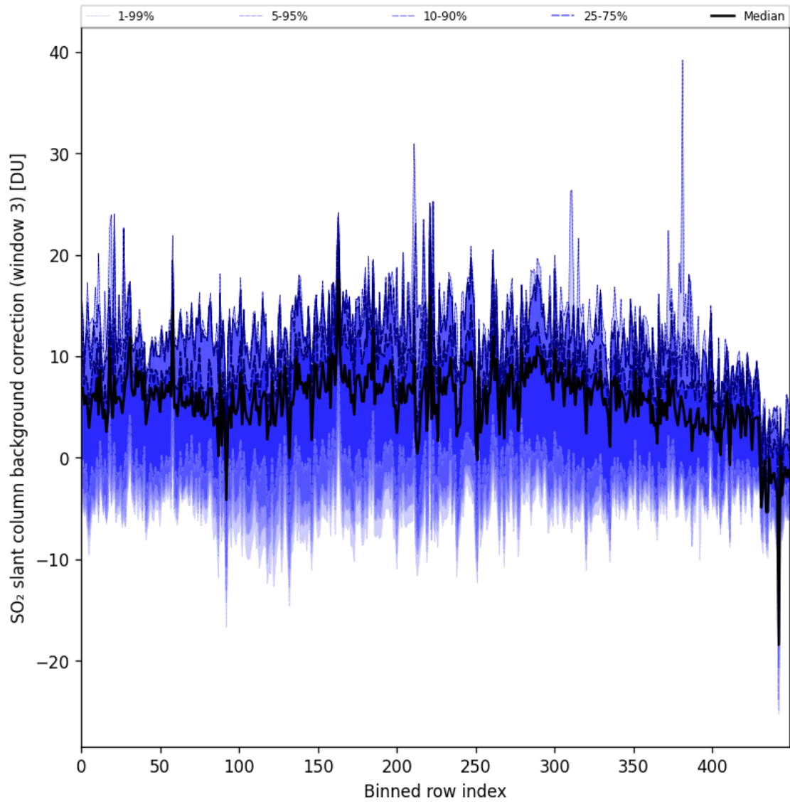
Figure 90: Along track statistics of “SO 2 slant column background correction (window 3)” for 2024-09-01 to 2024-09-02
