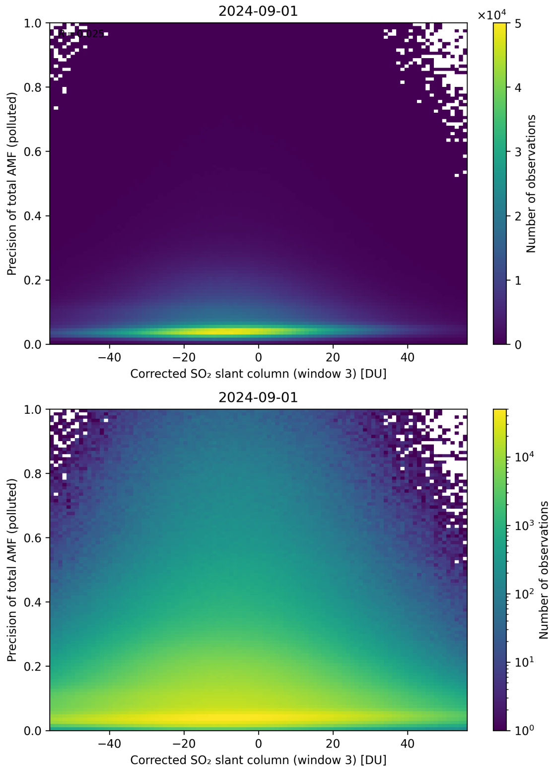
Figure 211: Scatter density plot of “Corrected SO 2 slant column (window 3)” against “Precision of total AMF (polluted)” for 2024-09-01 to 2024-09-02.
