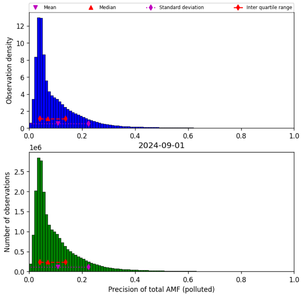
Figure 72: Histogram of “Precision of total AMF (polluted)” for 2024-09-01 to 2024-09-02
