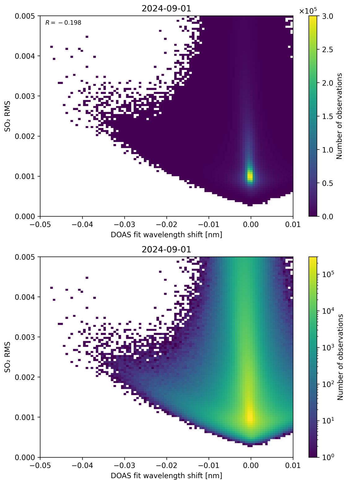
Figure 128: Scatter density plot of “DOAS fit wavelength shift” against “SO 2 RMS” for 2024-09-01 to 2024-09-02.
