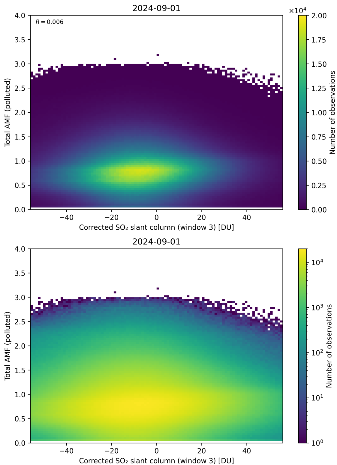
Figure 210: Scatter density plot of “Corrected SO 2 slant column (window 3)” against “Total AMF (polluted)” for 2024-09-01 to 2024-09-02.
