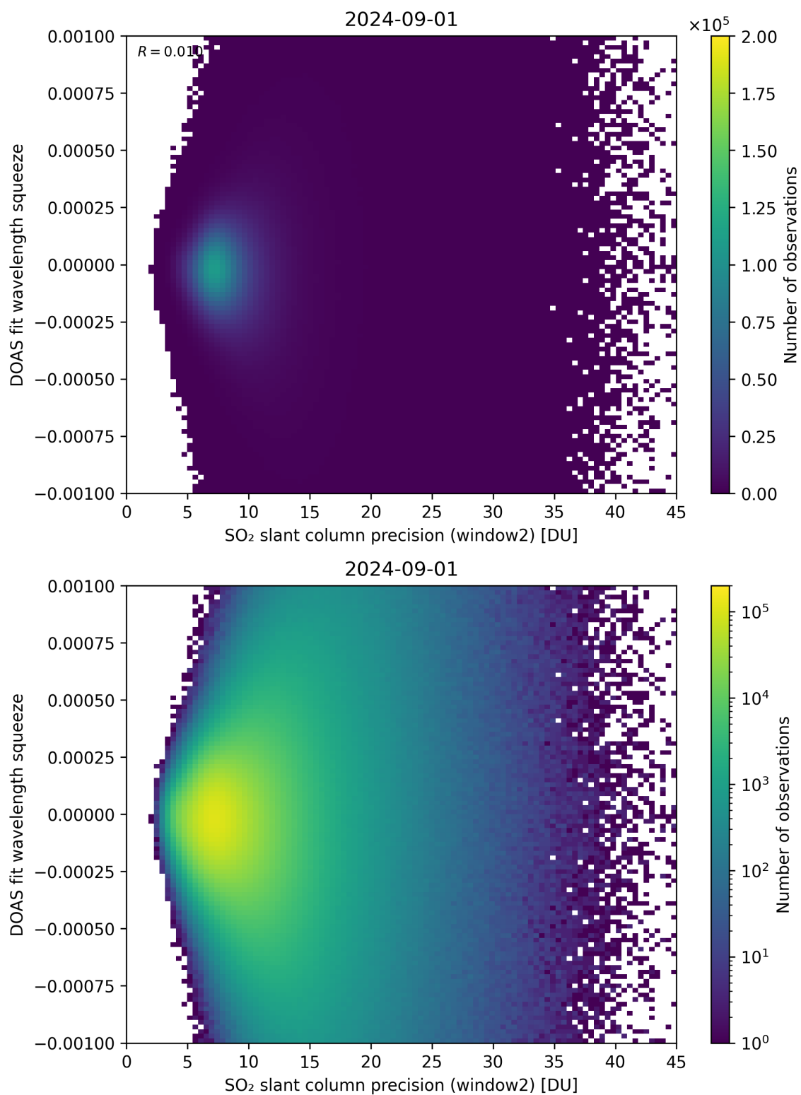
Figure 244: Scatter density plot of “SO 2 slant column precision (window2)” against “DOAS fit wavelength squeeze” for 2024-09-01 to 2024-09-02.
