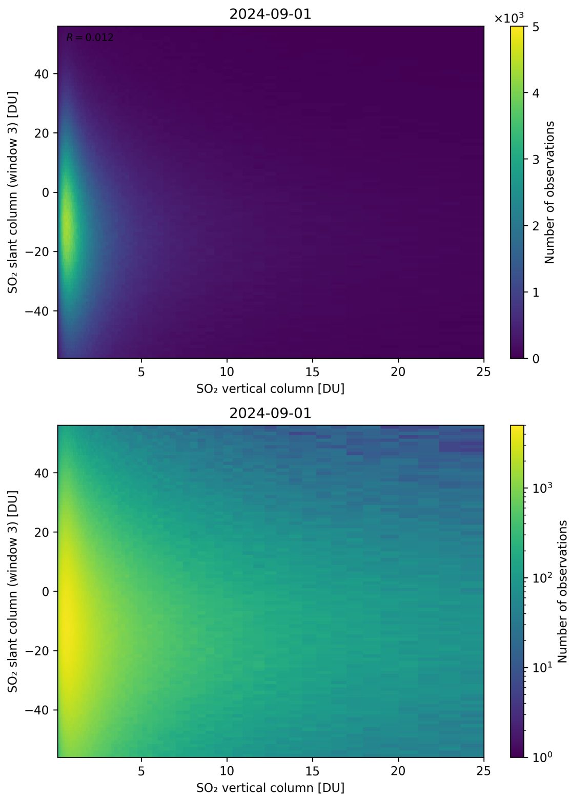
Figure 303: Scatter density plot of “SO 2 vertical column” against “SO 2 slant column (window 3)” for 2024-09-01 to 2024-09-02.
