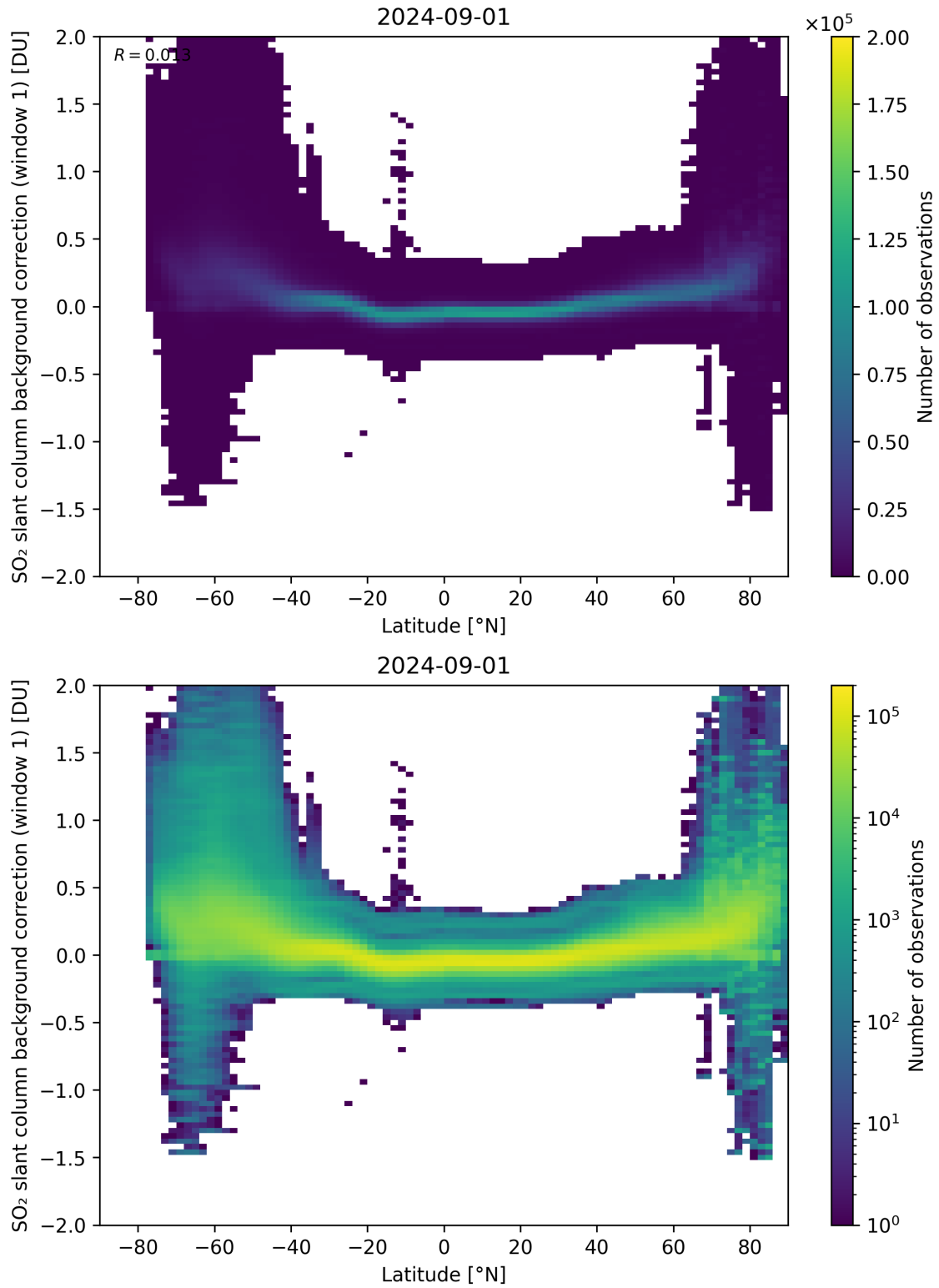
Figure 139: Scatter density plot of “Latitude” against “SO 2 slant column background correction (window 1)” for 2024-09-01 to 2024-09-02.
