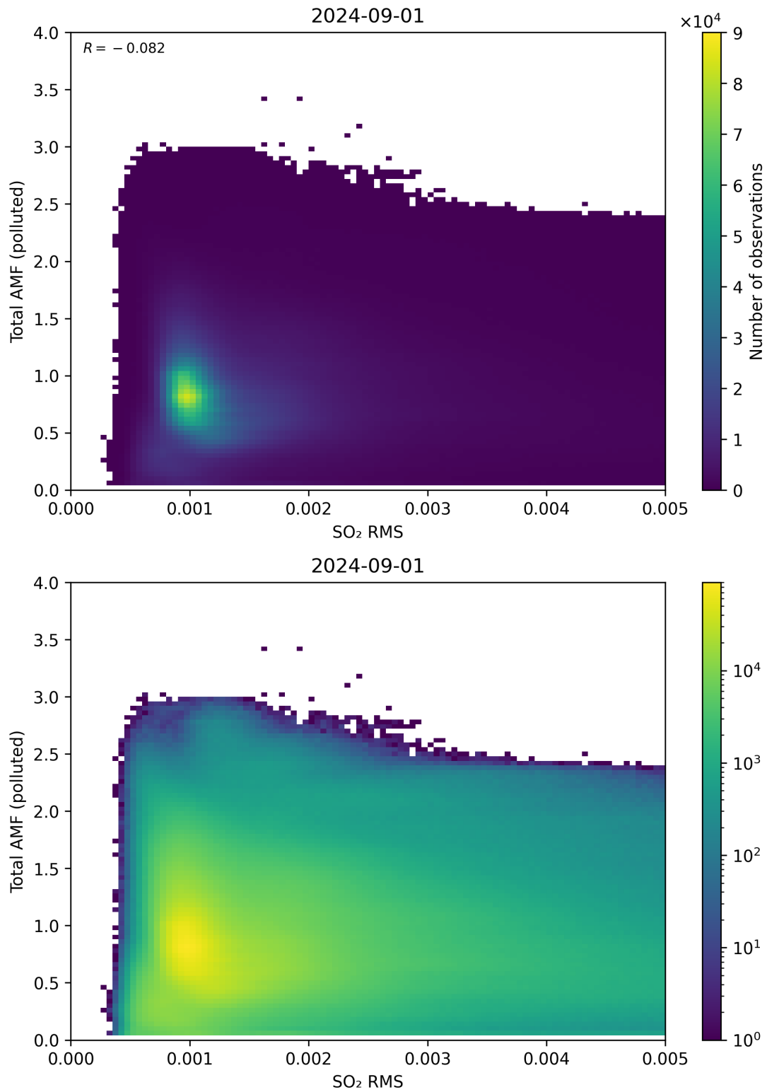
Figure 137: Scatter density plot of “SO 2 RMS” against “Total AMF (polluted)” for 2024-09-01 to 2024-09-02.
