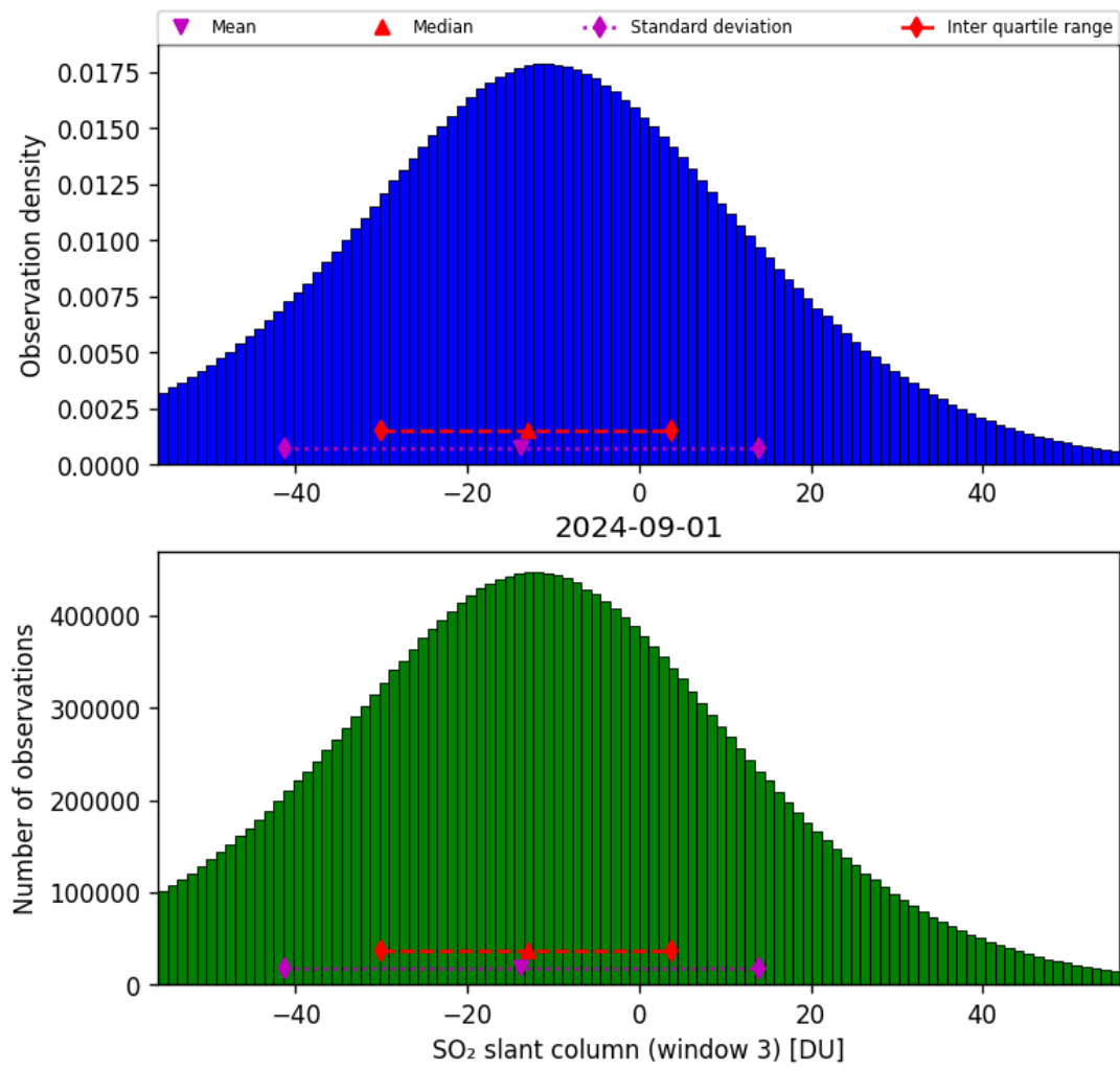
Figure 64: Histogram of “SO 2 slant column (window 3)” for 2024-09-01 to 2024-09-02
