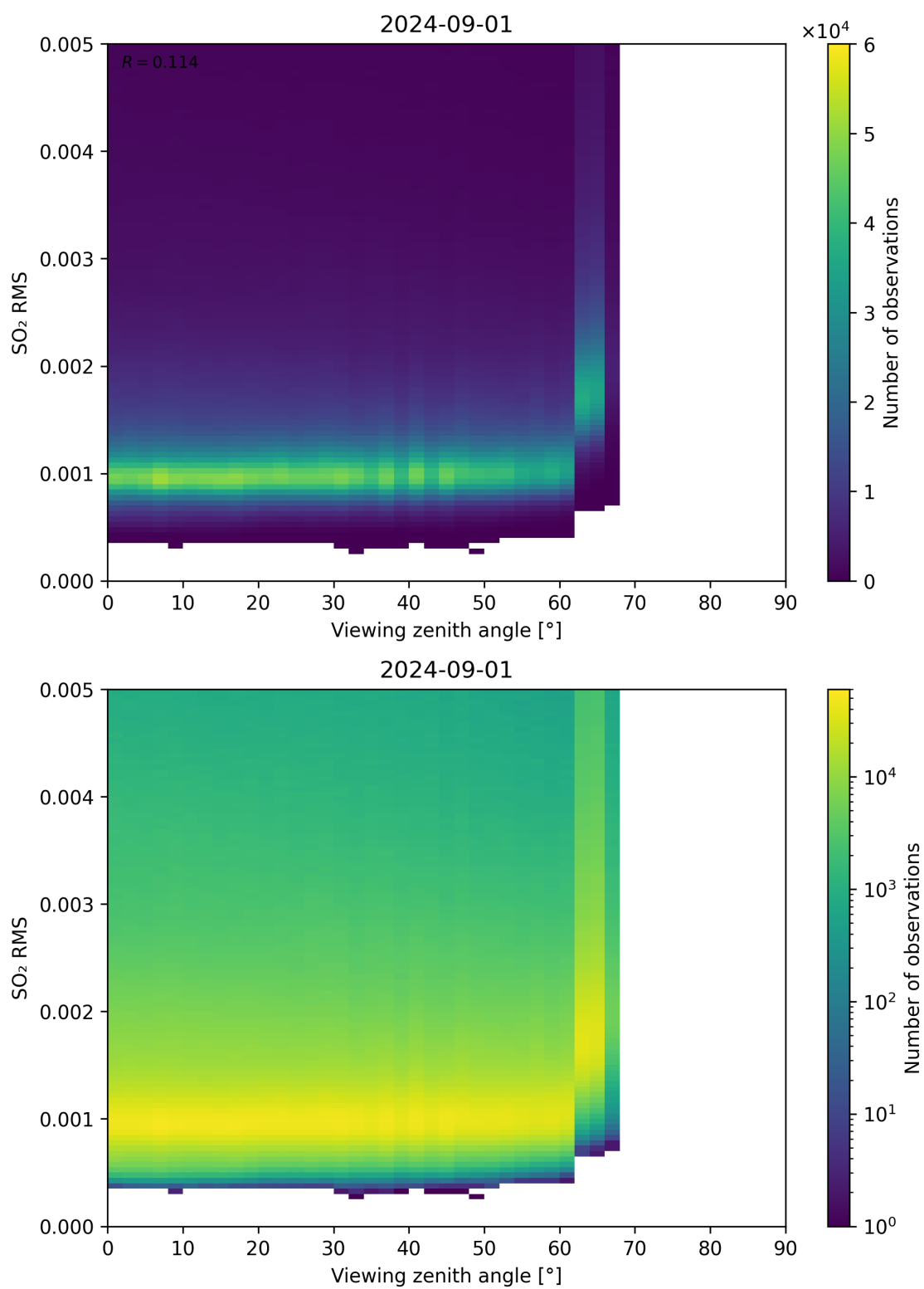
Figure 313: Scatter density plot of “Viewing zenith angle” against “SO 2 RMS” for 2024-09-01 to 2024-09-02.
