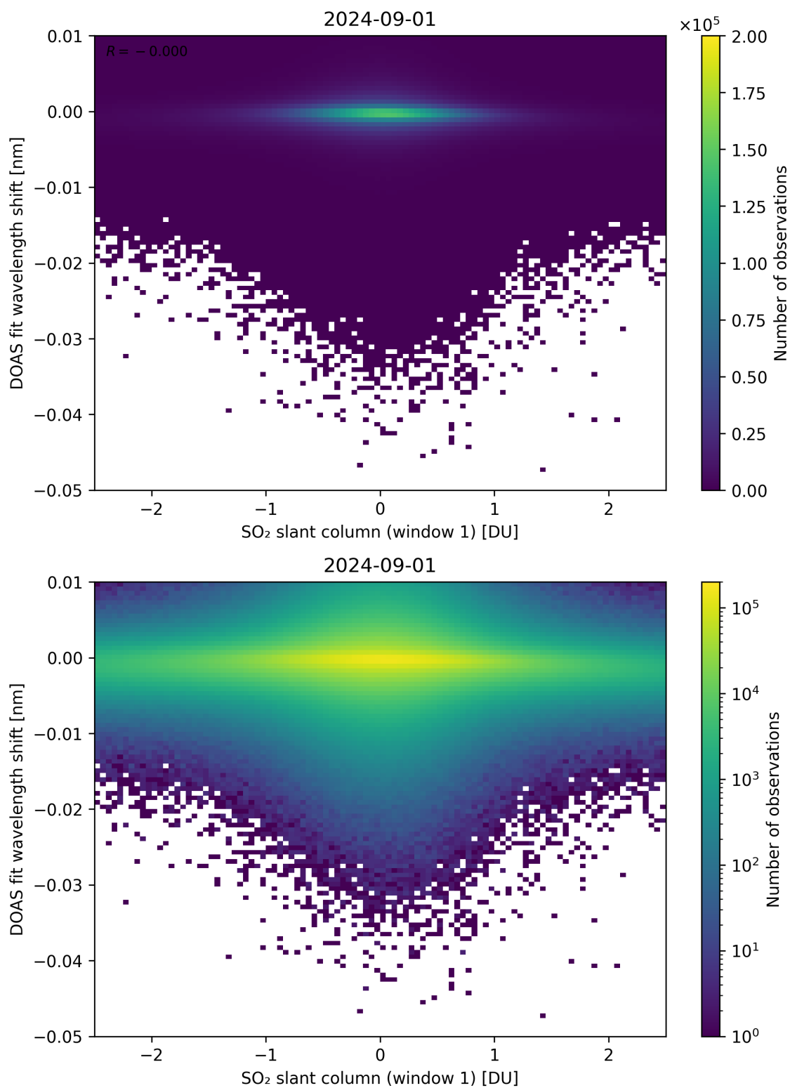
Figure 215: Scatter density plot of “SO 2 slant column (window 1)” against “DOAS fit wavelength shift” for 2024-09-01 to 2024-09-02.
