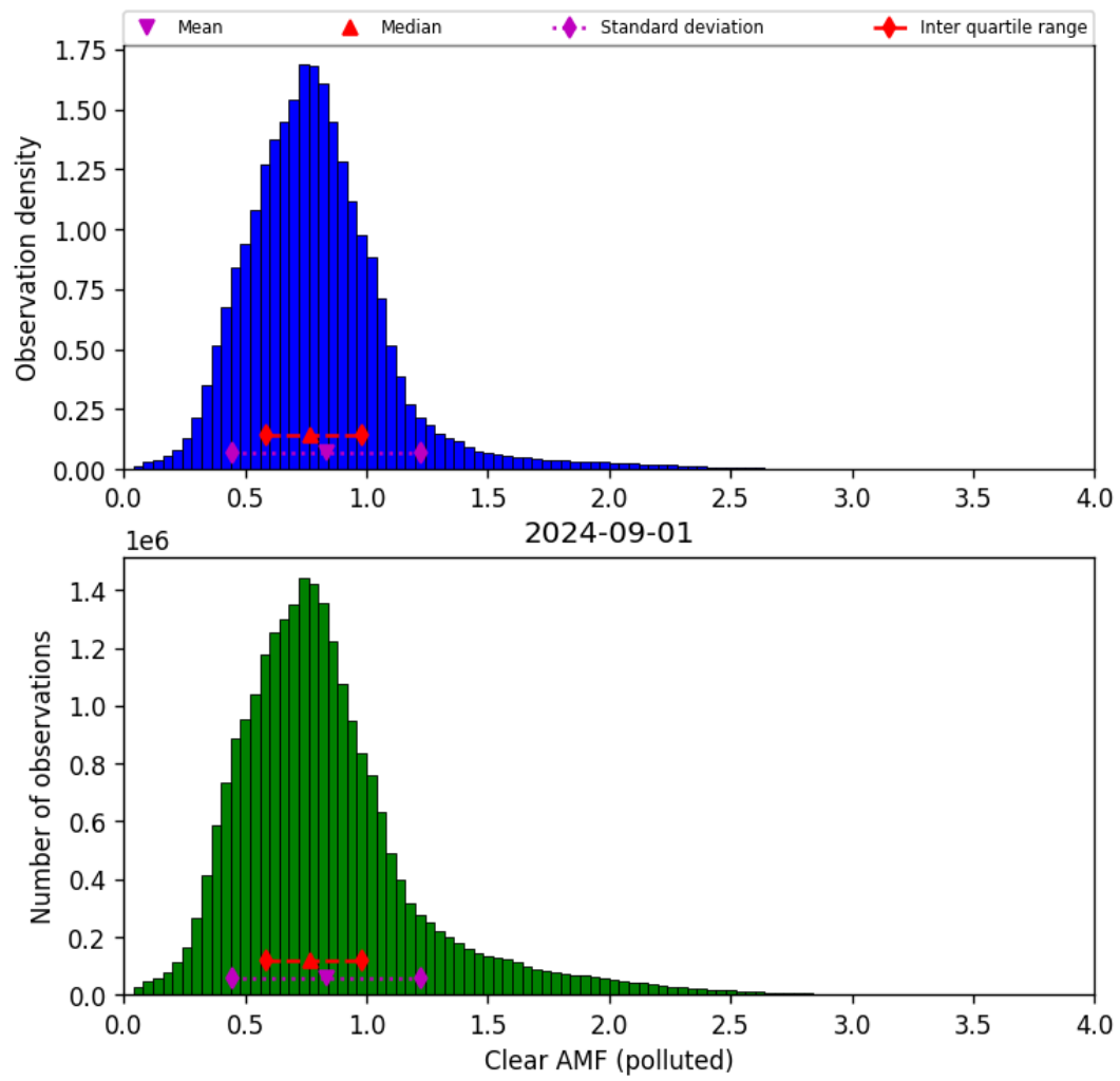
Figure 73: Histogram of “Clear AMF (polluted)” for 2024-09-01 to 2024-09-02
