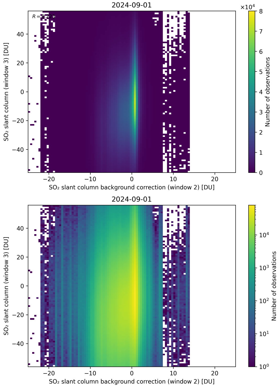
Figure 117: Scatter density plot of “SO 2 slant column background correction (window 2)” against “SO 2 slant column (window 3)” for 2024-09-01 to 2024-09-02.
