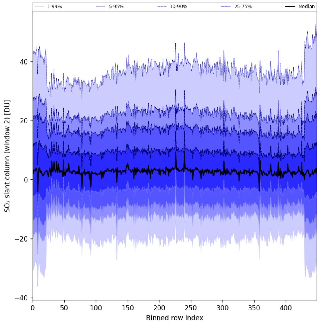
Figure 83: Along track statistics of “SO 2 slant column (window 2)” for 2024-09-01 to 2024-09-02
