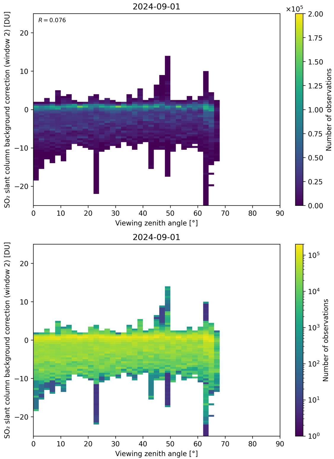
Figure 309: Scatter density plot of “Viewing zenith angle” against “SO 2 slant column background correction (window 2)” for 2024-09-01 to 2024-09-02.
