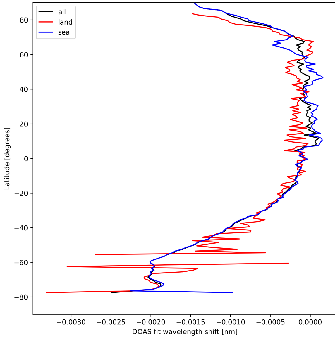
Figure 45: Zonal average of “DOAS fit wavelength shift” for 2024-09-01 to 2024-09-02.
