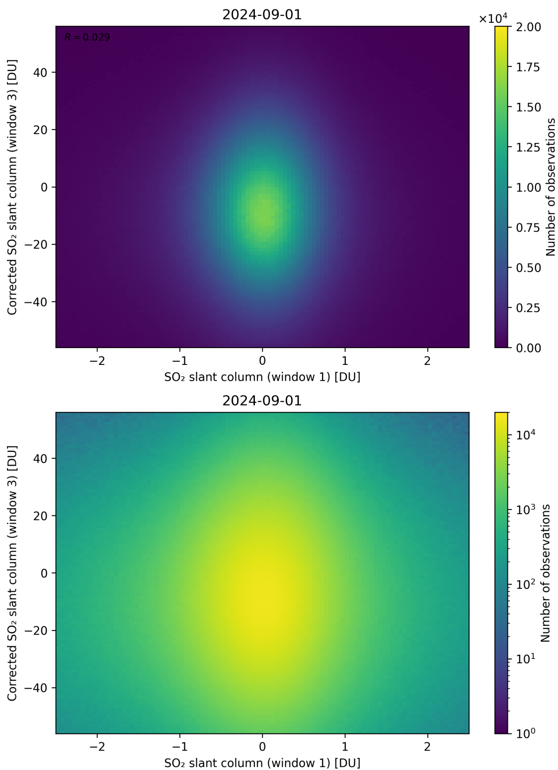
Figure 234: Scatter density plot of “SO 2 slant column (window 1)” against “Corrected SO 2 slant column (window 3)” for 2024-09-01 to 2024-09-02.
