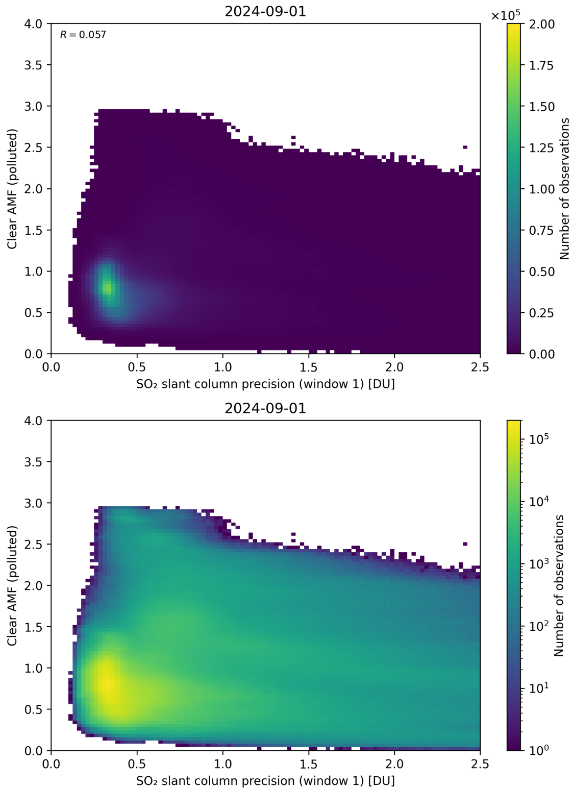
Figure 224: Scatter density plot of “SO 2 slant column precision (window 1)” against “Clear AMF (polluted)” for 2024-09-01 to 2024-09-02.
