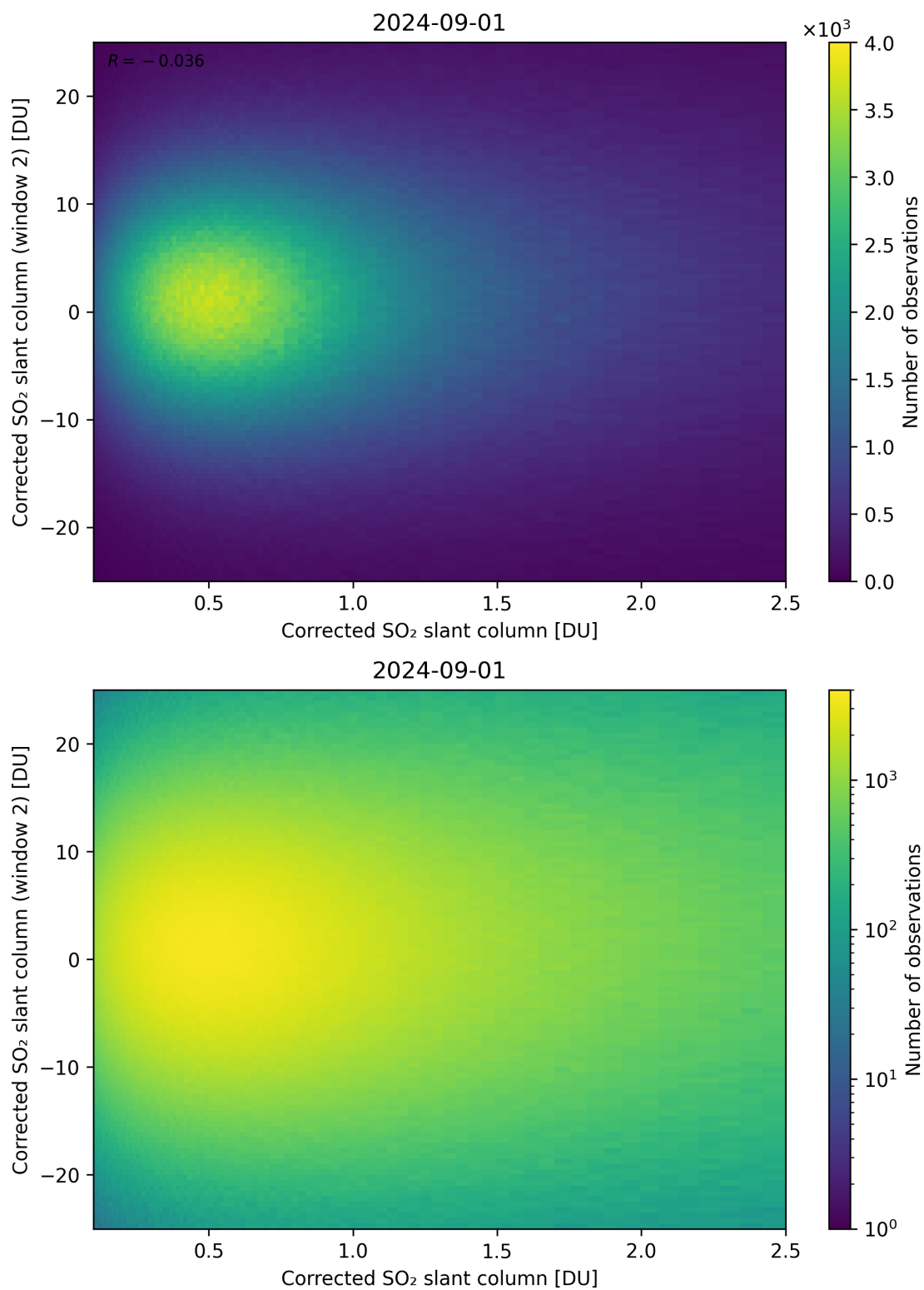
Figure 185: Scatter density plot of “Corrected SO 2 slant column” against “Corrected SO 2 slant column (window 2)” for 2024-09-01 to 2024-09-02.
