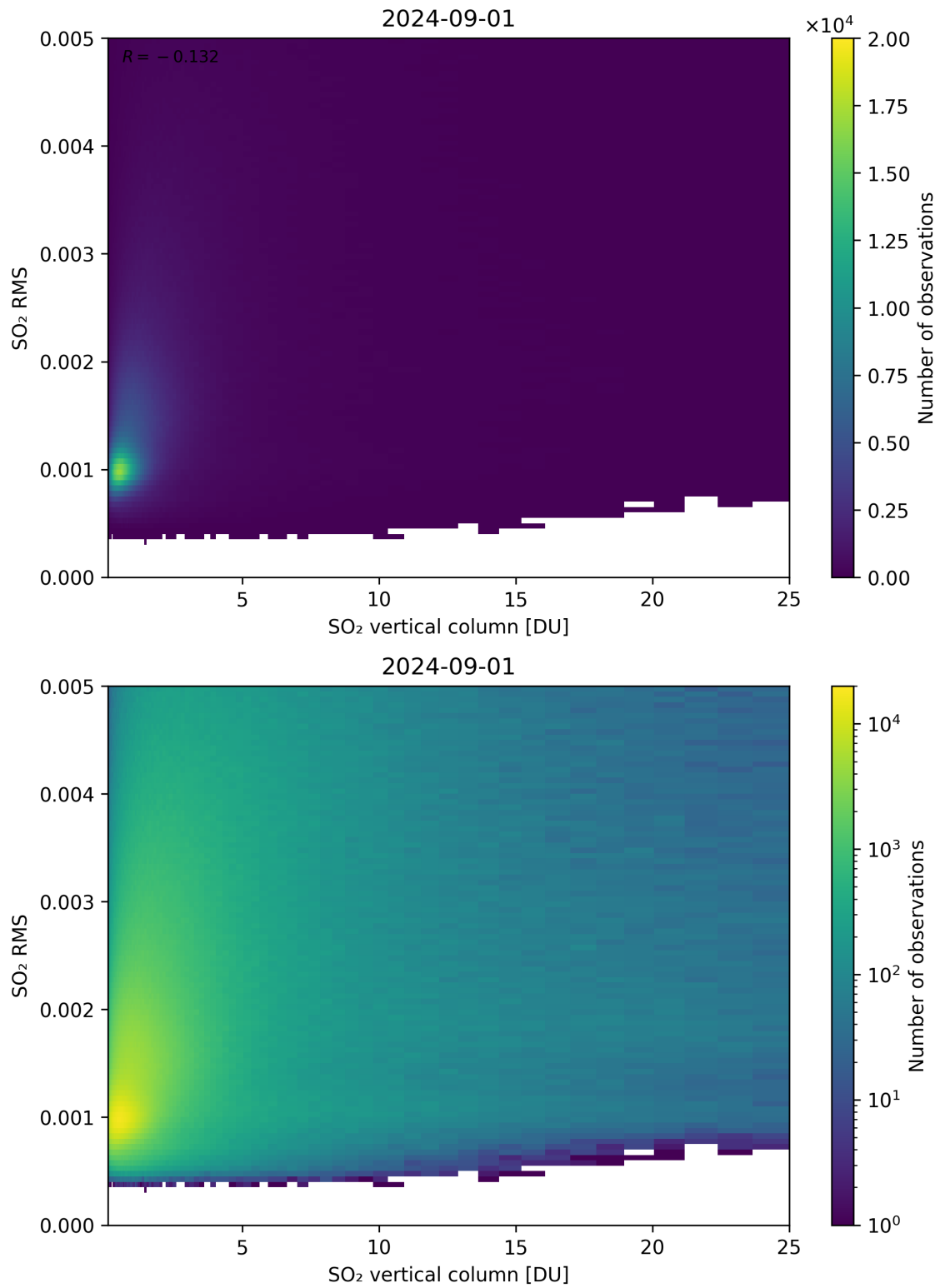
Figure 278: Scatter density plot of “SO 2 vertical column” against “SO 2 RMS” for 2024-09-01 to 2024-09-02.
