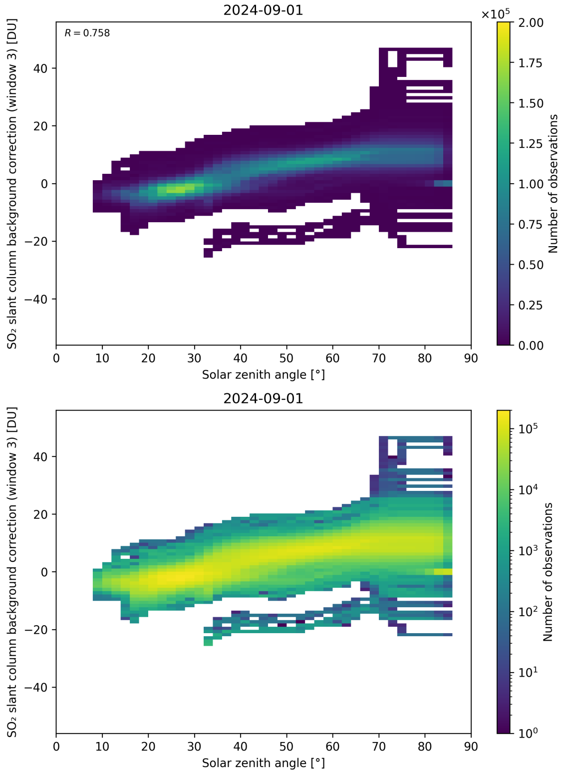
Figure 160: Scatter density plot of “Solar zenith angle” against “SO 2 slant column background correction (window 3)” for 2024-09-01 to 2024-09-02.
