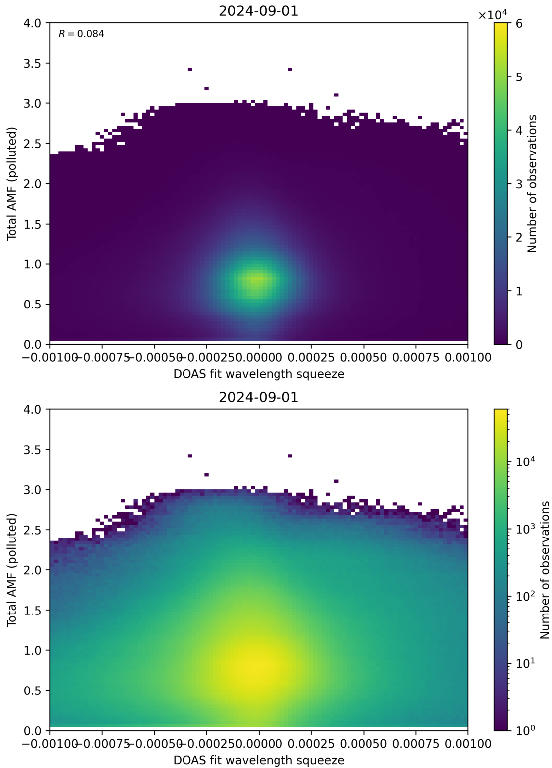
Figure 134: Scatter density plot of “DOAS fit wavelength squeeze” against “Total AMF (polluted)” for 2024-09-01 to 2024-09-02.
