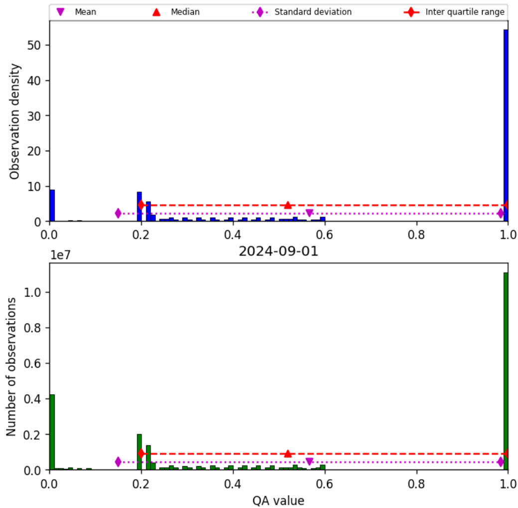
Figure 52: Histogram of “QA value” for 2024-09-01 to 2024-09-02
