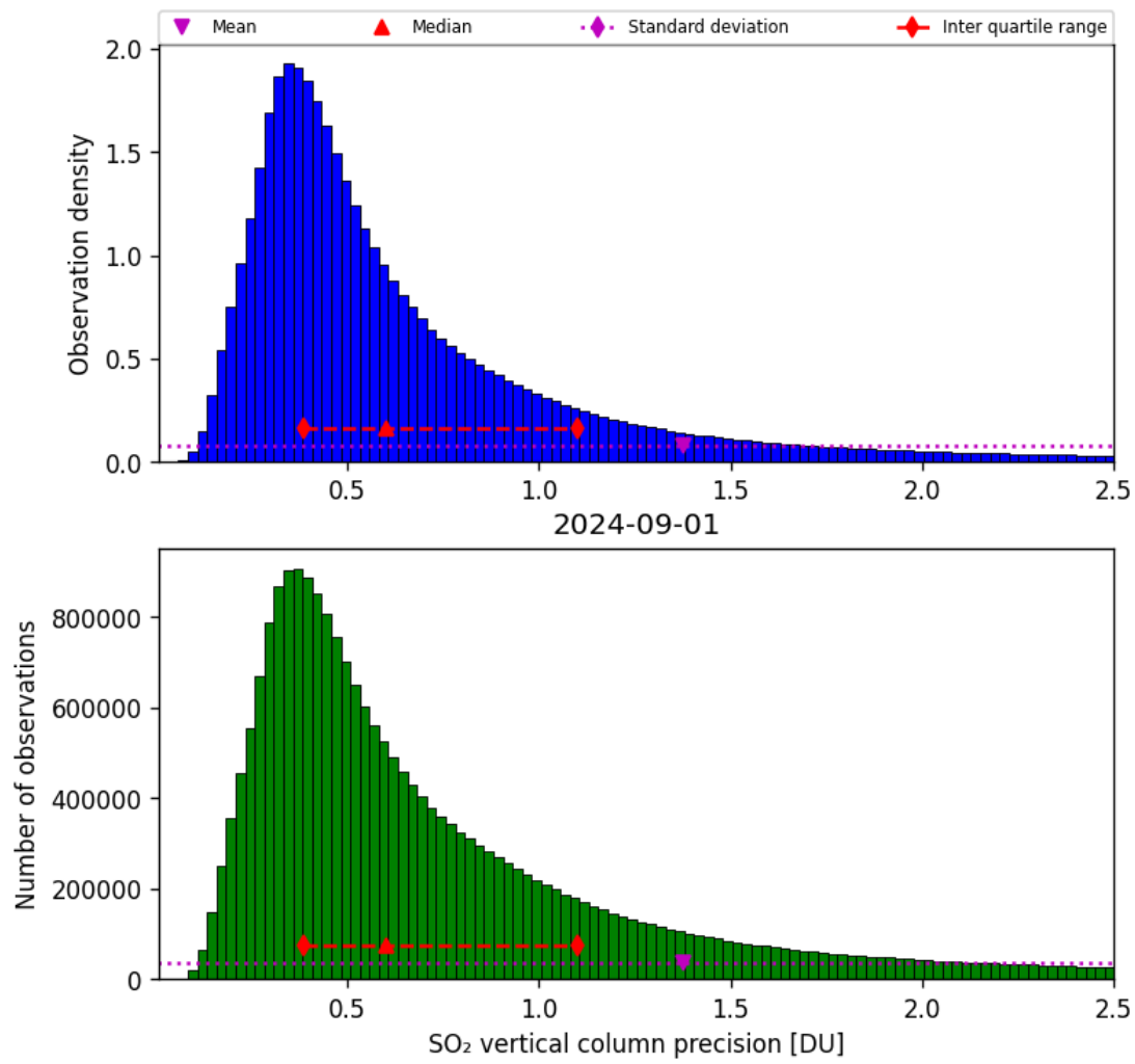
Figure 54: Histogram of “SO 2 vertical column precision” for 2024-09-01 to 2024-09-02
