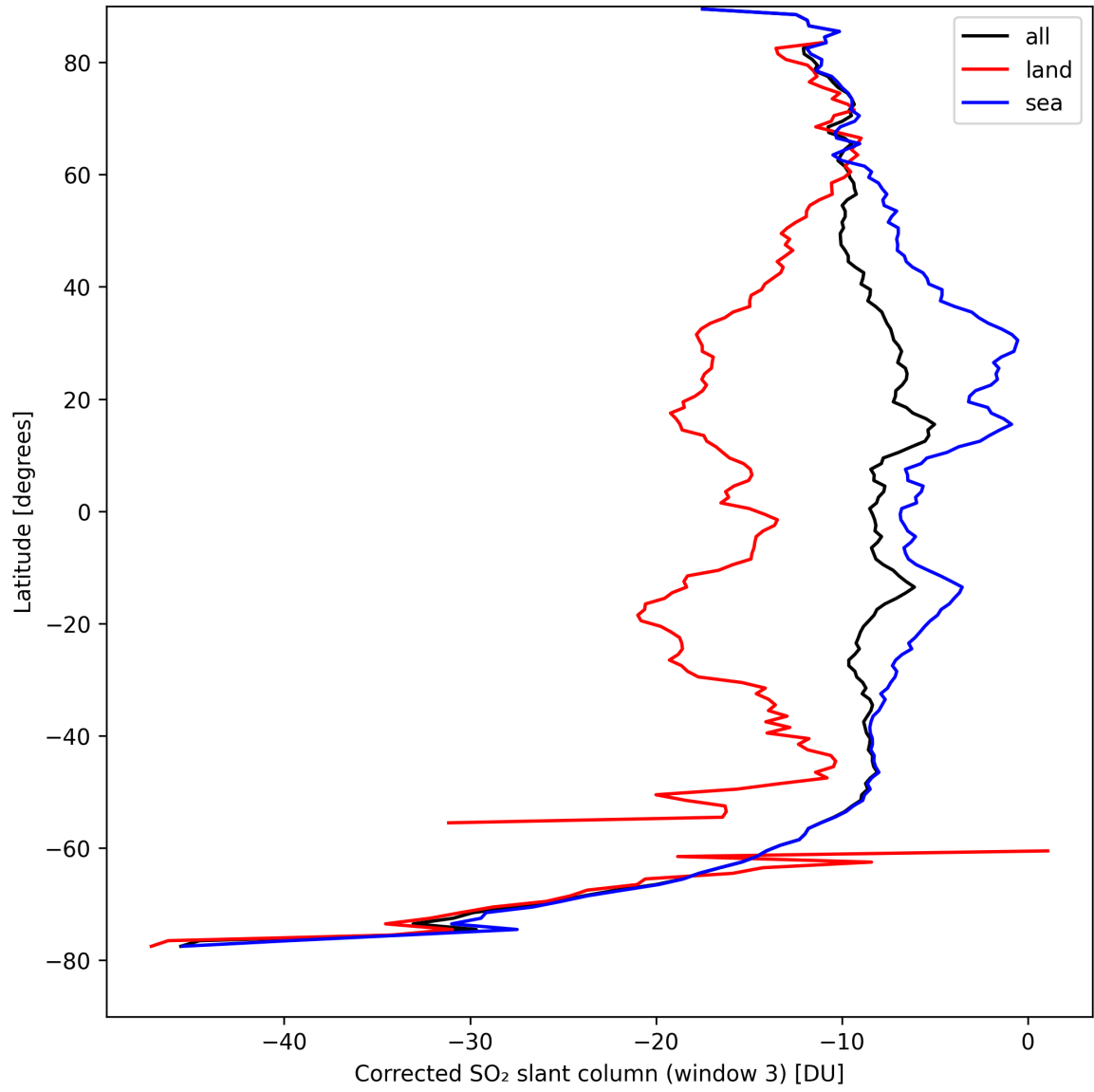
Figure 43: Zonal average of “Corrected SO 2 slant column (window 3)” for 2024-09-01 to 2024-09-02.
