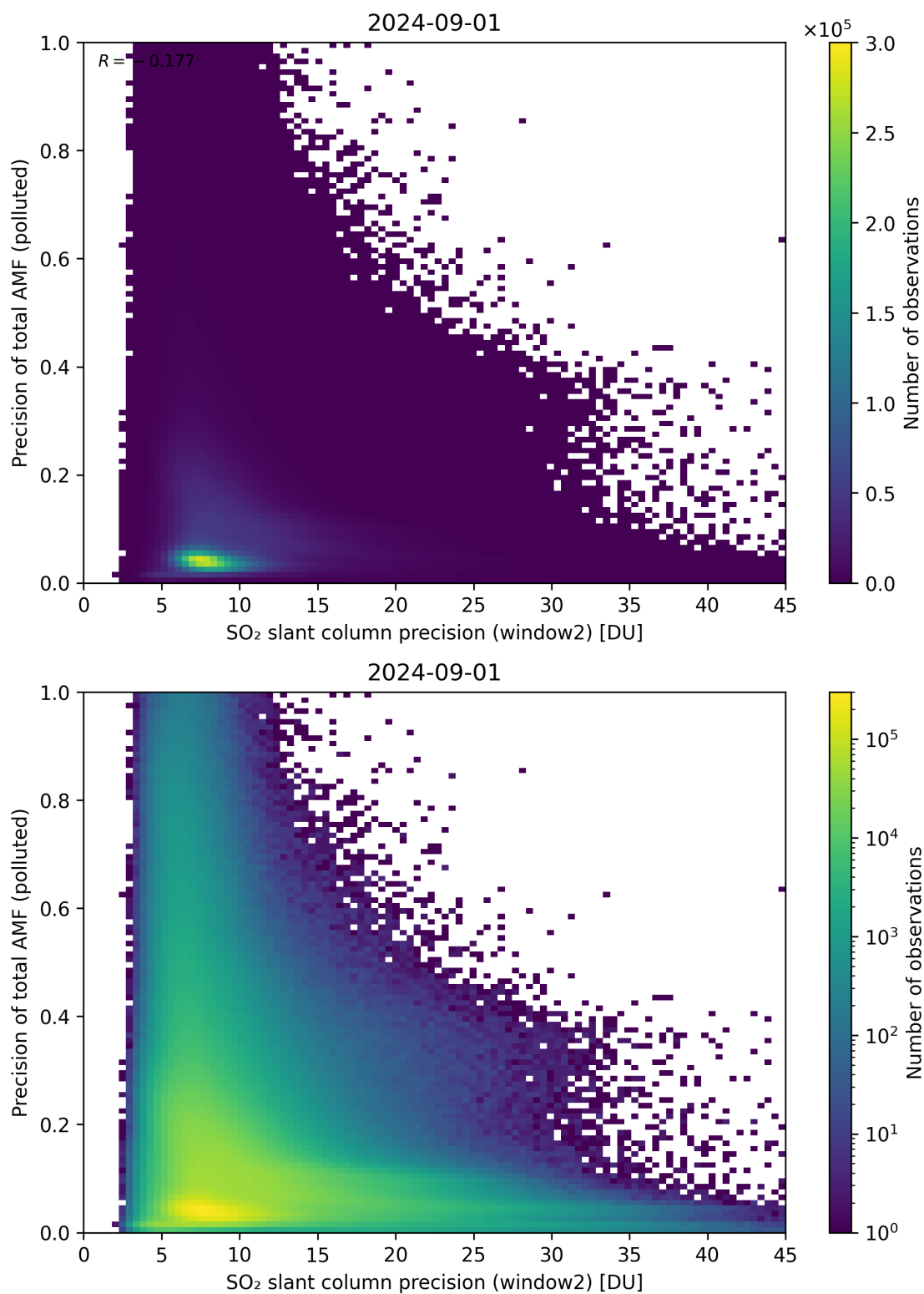
Figure 252: Scatter density plot of “SO 2 slant column precision (window2)” against “Precision of total AMF (polluted)” for 2024-09-01 to 2024-09-02.
