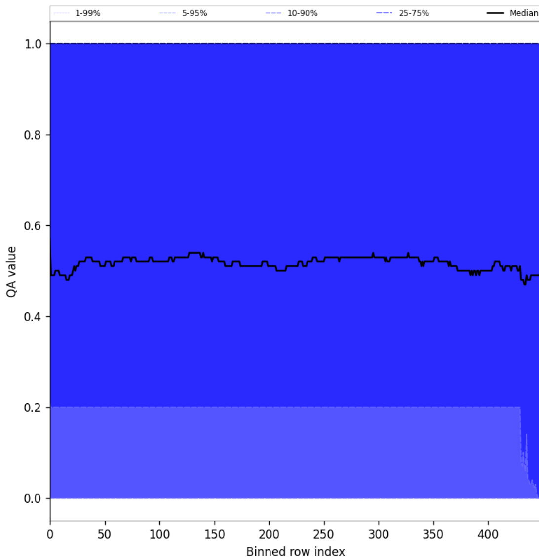
Figure 75: Along track statistics of “QA value” for 2024-09-01 to 2024-09-02
