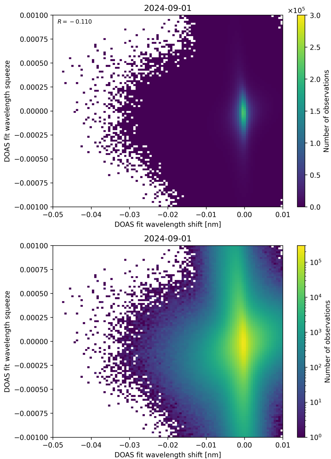
Figure 127: Scatter density plot of “DOAS fit wavelength shift” against “DOAS fit wavelength squeeze” for 2024-09-01 to 2024-09-02.
