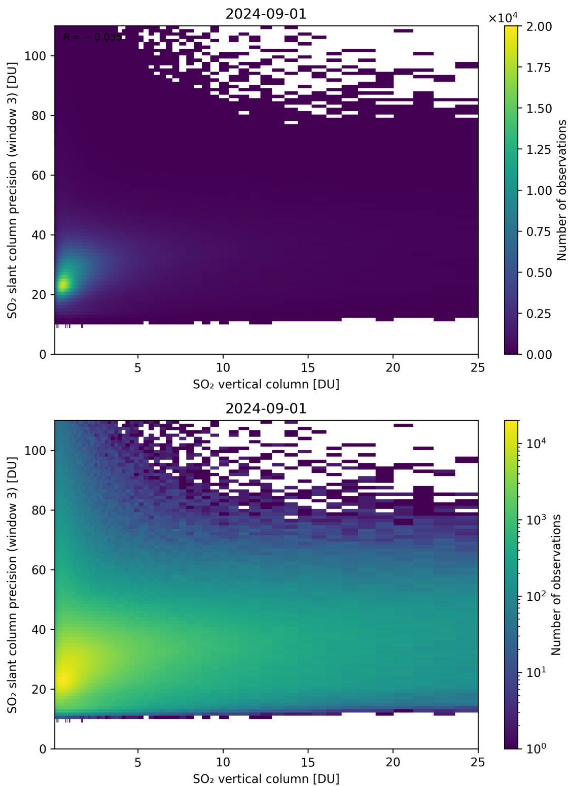
Figure 304: Scatter density plot of “SO 2 vertical column” against “SO 2 slant column precision (window 3)” for 2024-09-01 to 2024-09-02.
