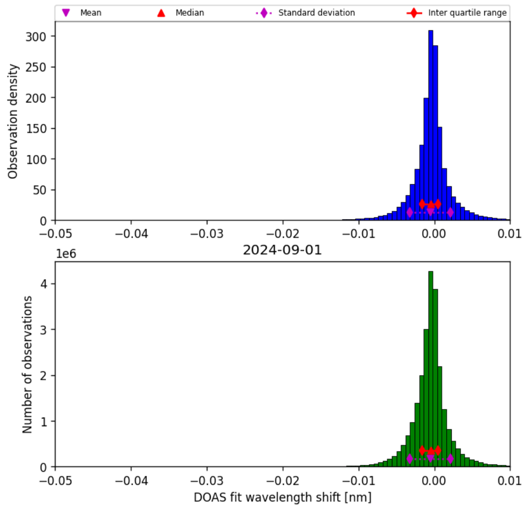
Figure 68: Histogram of “DOAS fit wavelength shift” for 2024-09-01 to 2024-09-02
