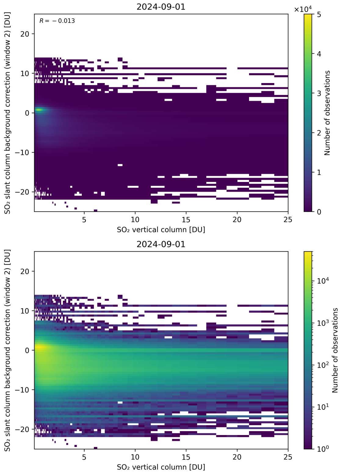
Figure 274: Scatter density plot of “SO 2 vertical column” against “SO 2 slant column background correction (window 2)” for 2024-09-01 to 2024-09-02.
