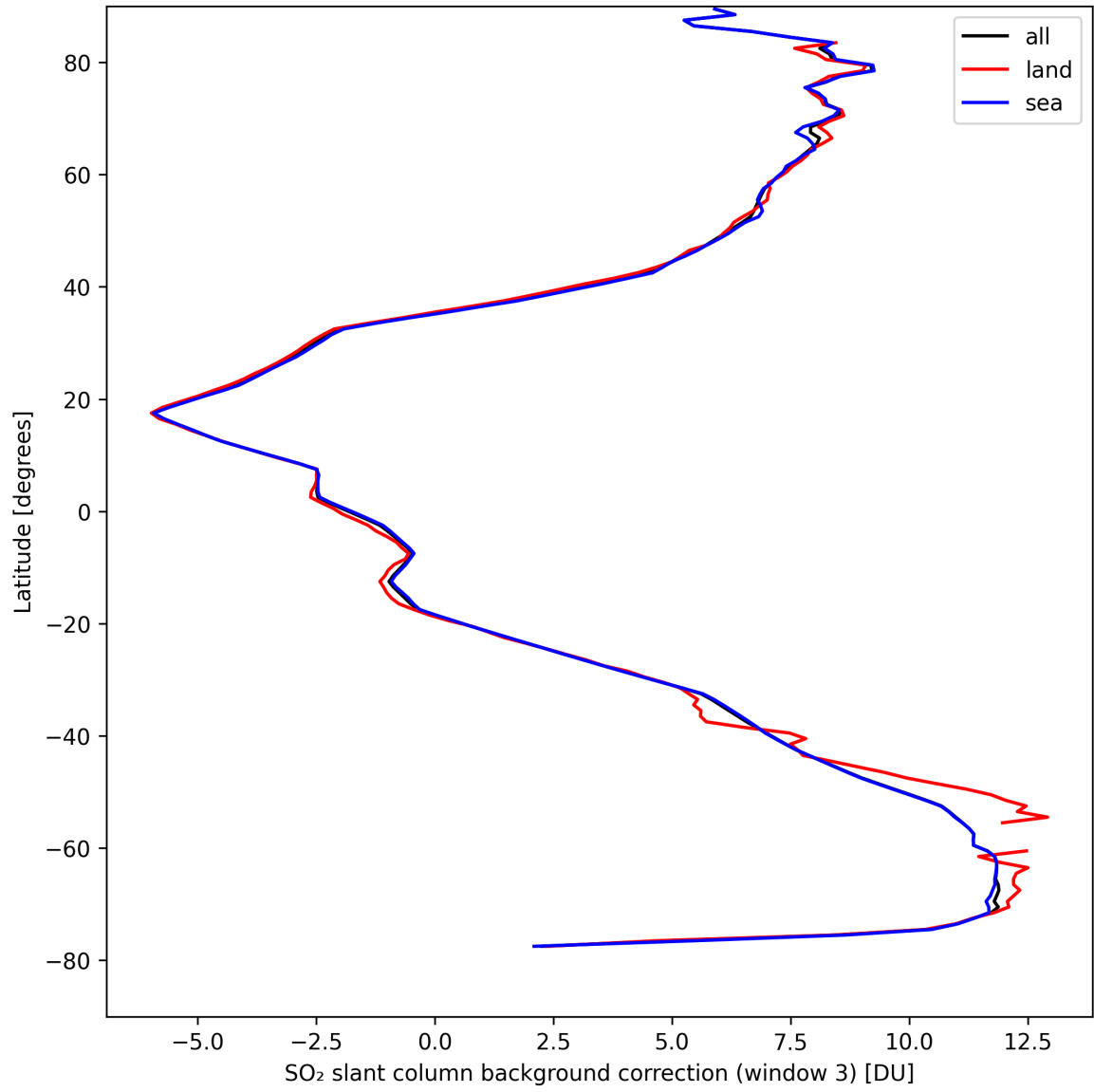
Figure 44: Zonal average of “SO 2 slant column background correction (window 3)” for 2024-09-01 to 2024-09-02.
