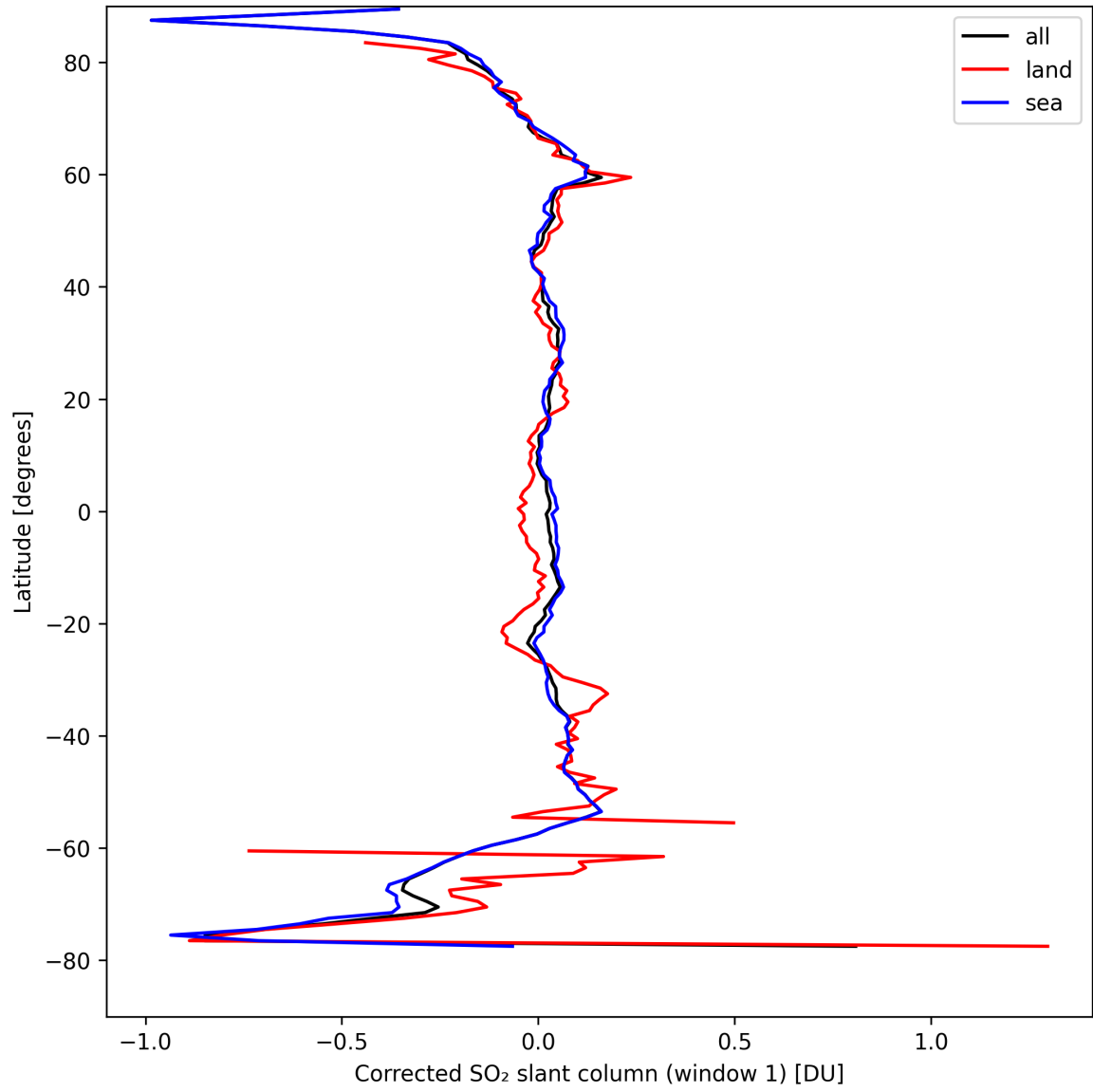
Figure 35: Zonal average of “Corrected SO 2 slant column (window 1)” for 2024-09-01 to 2024-09-02.
