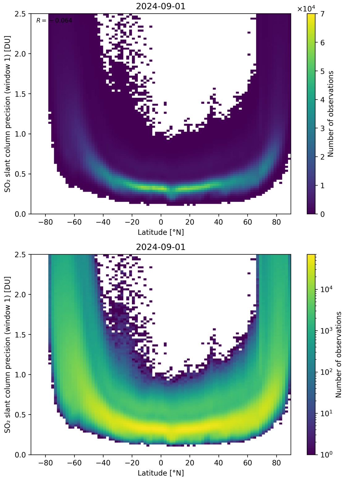
Figure 150: Scatter density plot of “Latitude” against “SO 2 slant column precision (window 1)” for 2024-09-01 to 2024-09-02.
