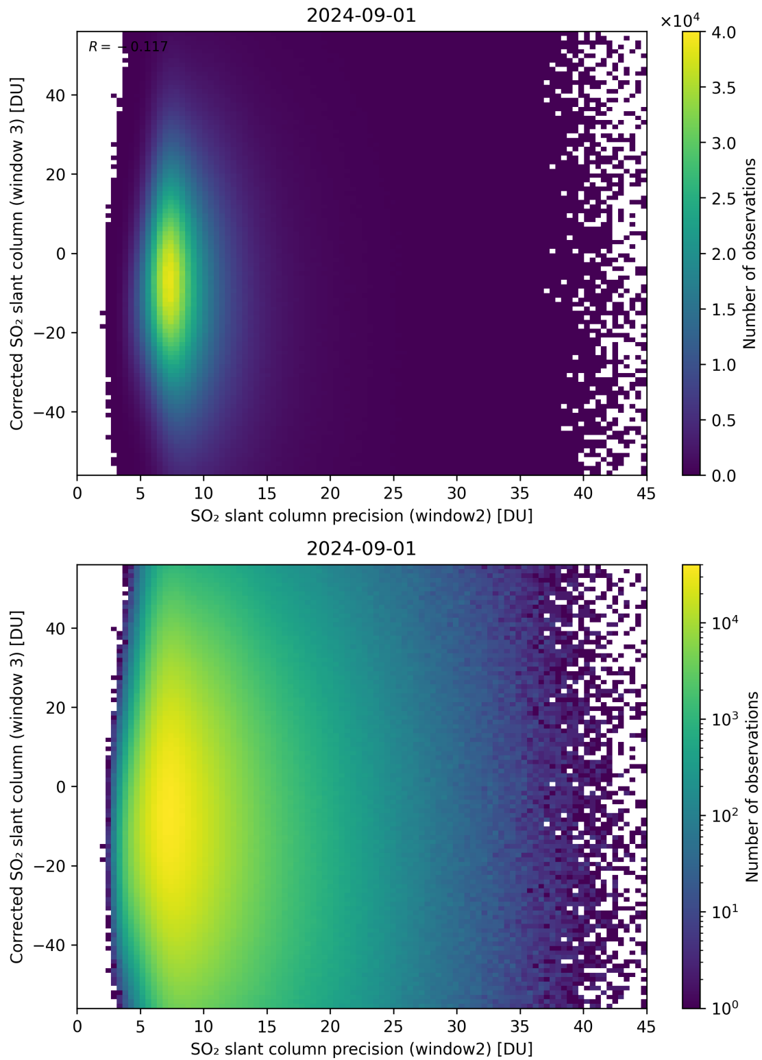
Figure 248: Scatter density plot of “SO 2 slant column precision (window2)” against “Corrected SO 2 slant column (window 3)” for 2024-09-01 to 2024-09-02.
