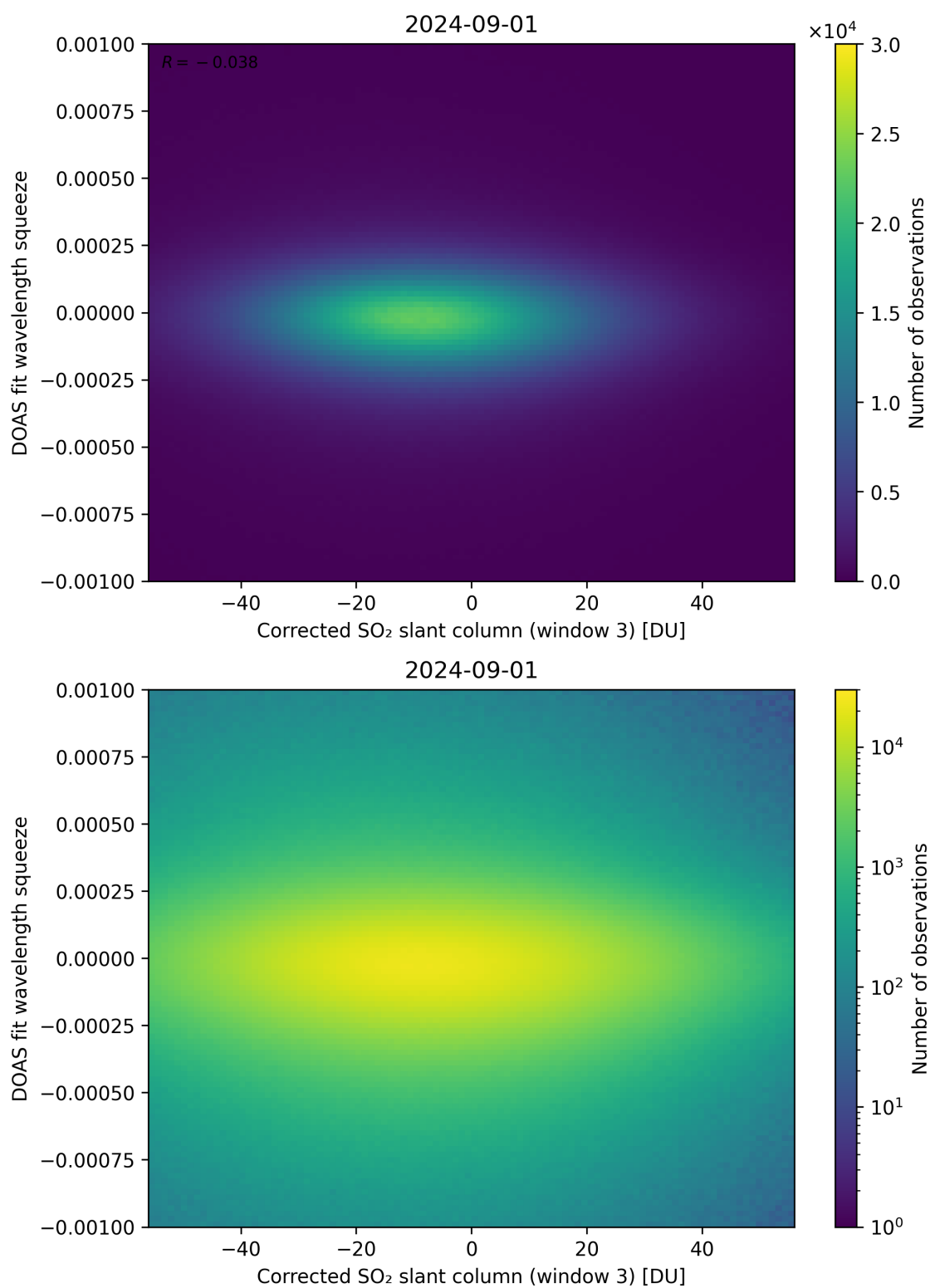
Figure 207: Scatter density plot of “Corrected SO 2 slant column (window 3)” against “DOAS fit wavelength squeeze” for 2024-09-01 to 2024-09-02.
