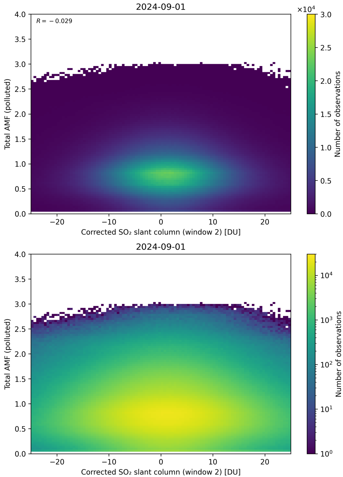
Figure 203: Scatter density plot of “Corrected SO 2 slant column (window 2)” against “Total AMF (polluted)” for 2024-09-01 to 2024-09-02.
