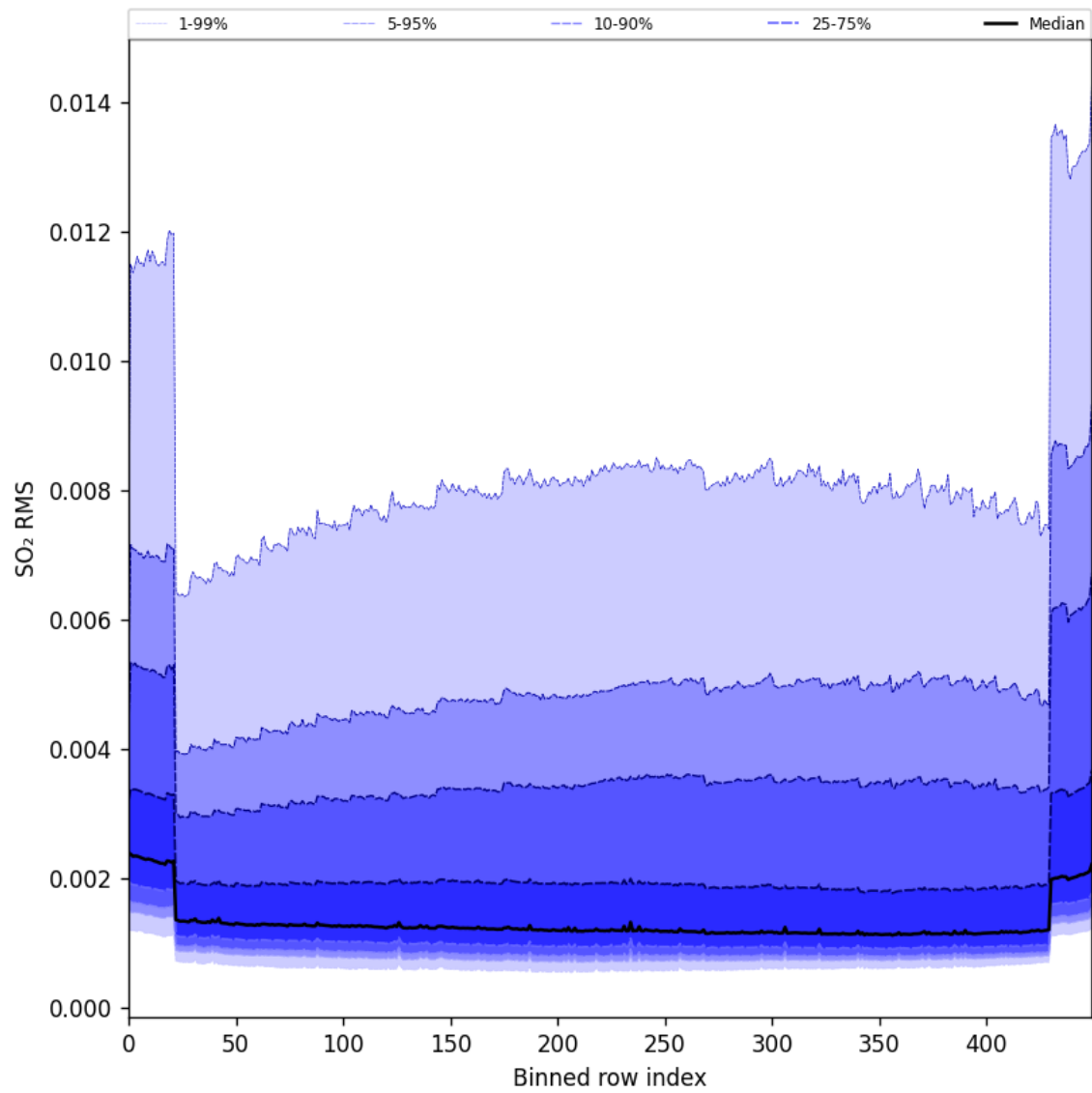
Figure 93: Along track statistics of “SO 2 RMS” for 2024-09-01 to 2024-09-02
