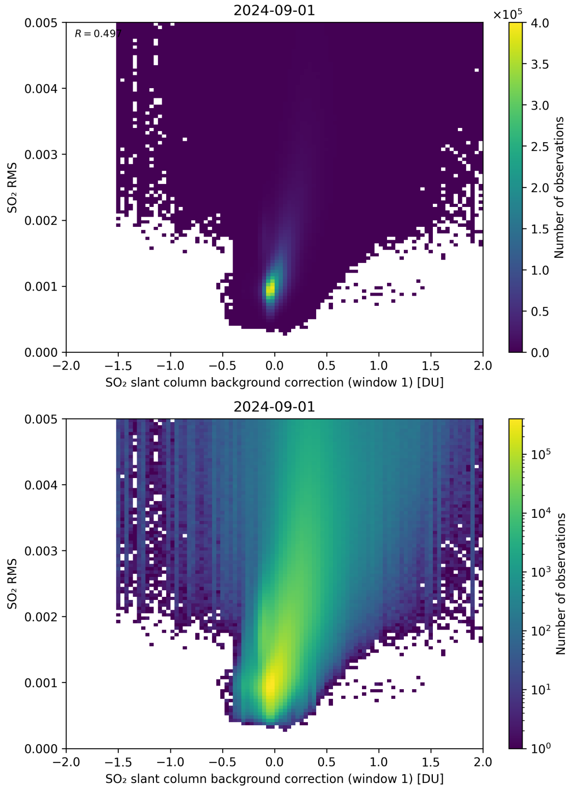
Figure 102: Scatter density plot of “SO 2 slant column background correction (window 1)” against “SO 2 RMS” for 2024-09-01 to 2024-09-02.
