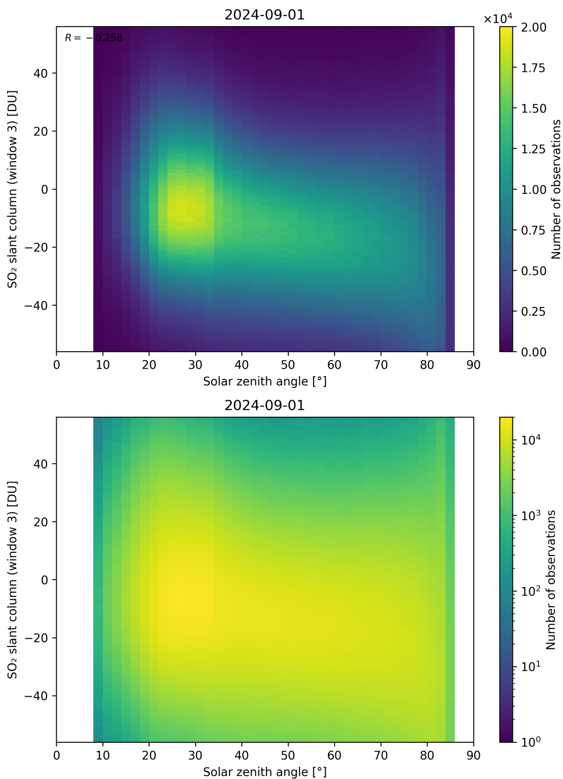
Figure 172: Scatter density plot of “Solar zenith angle” against “SO 2 slant column (window 3)” for 2024-09-01 to 2024-09-02.
