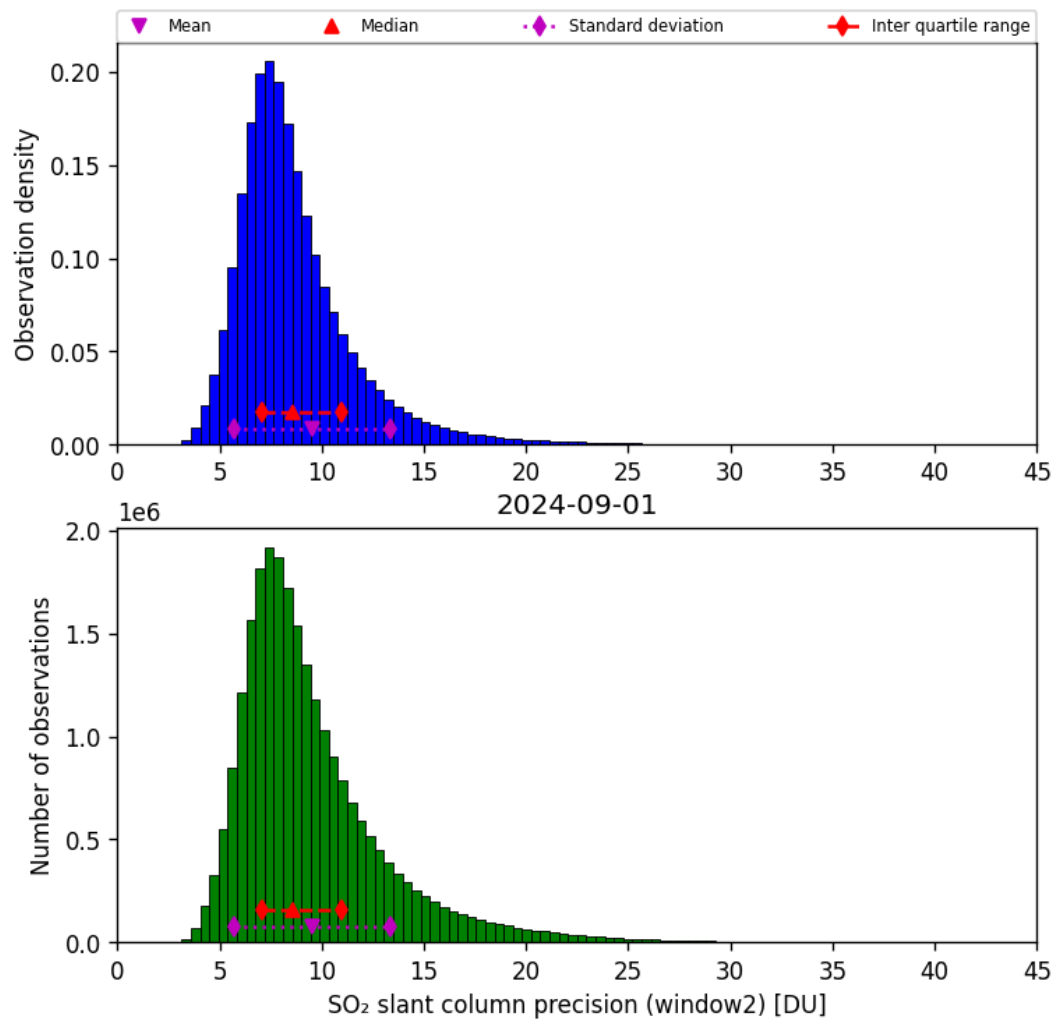
Figure 61: Histogram of “SO 2 slant column precision (window2)” for 2024-09-01 to 2024-09-02
