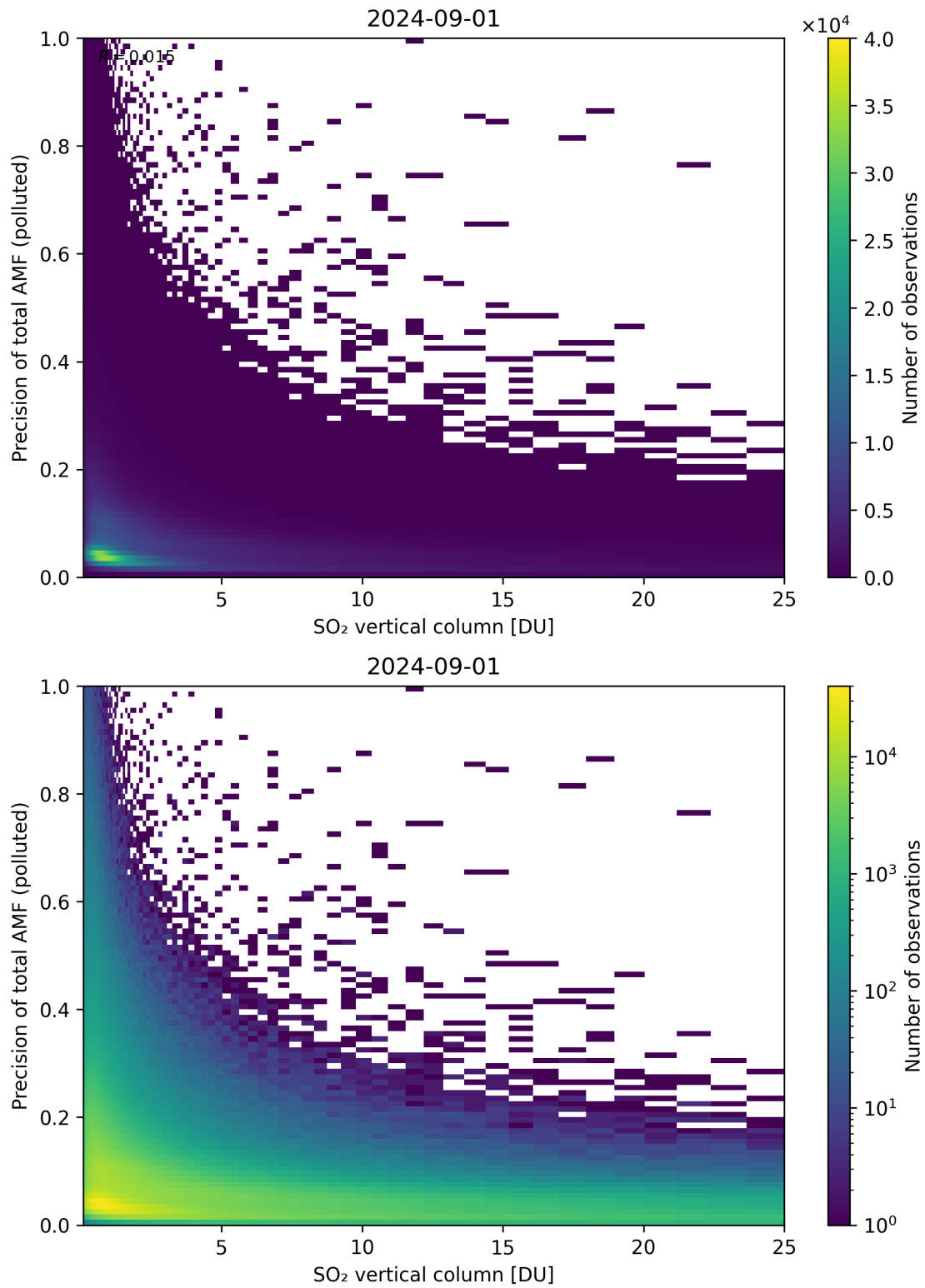
Figure 306: Scatter density plot of “SO 2 vertical column” against “Precision of total AMF (polluted)” for 2024-09-01 to 2024-09-02.
