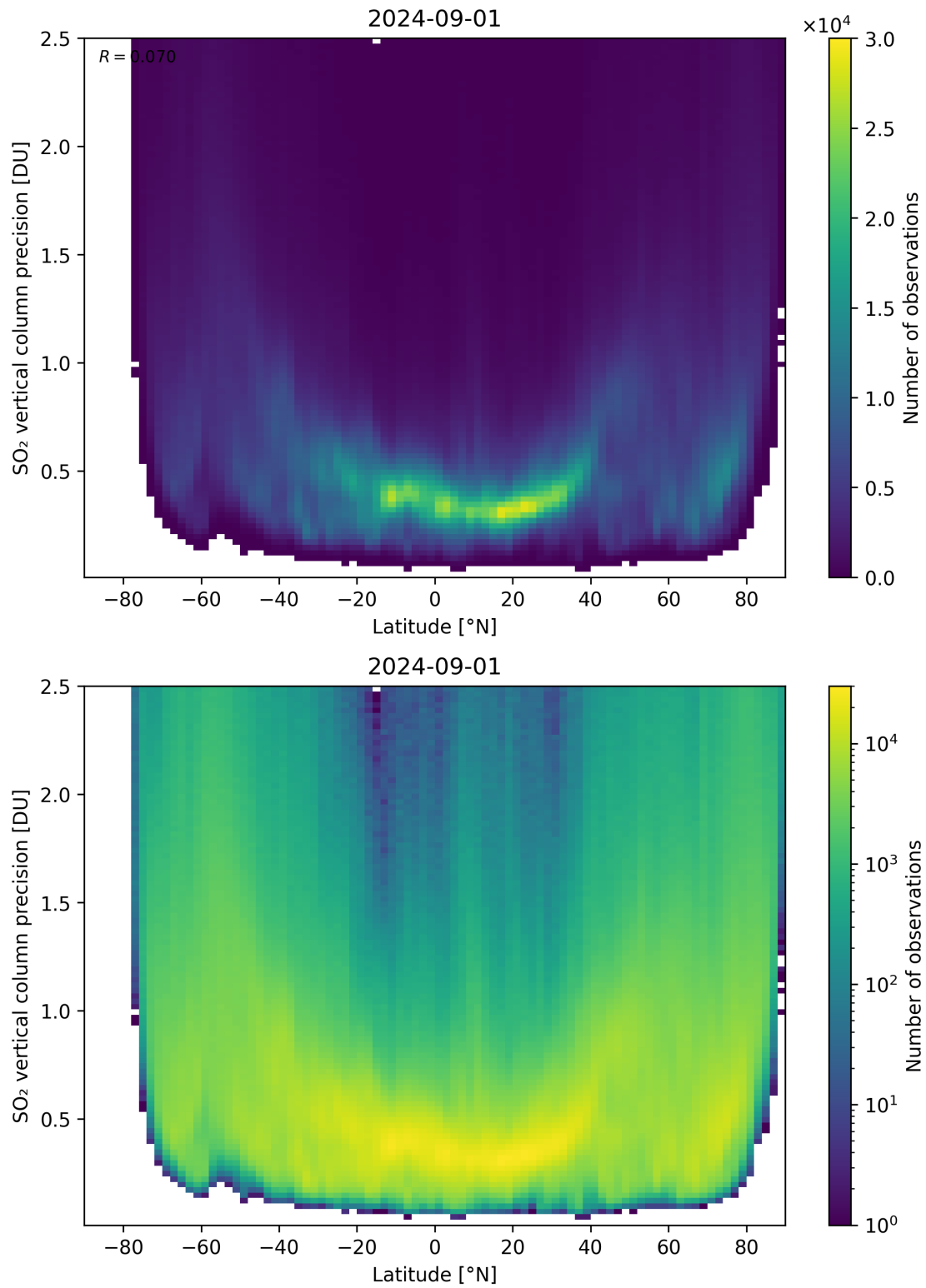
Figure 157: Scatter density plot of “Latitude” against “SO 2 vertical column precision” for 2024-09-01 to 2024-09-02.
