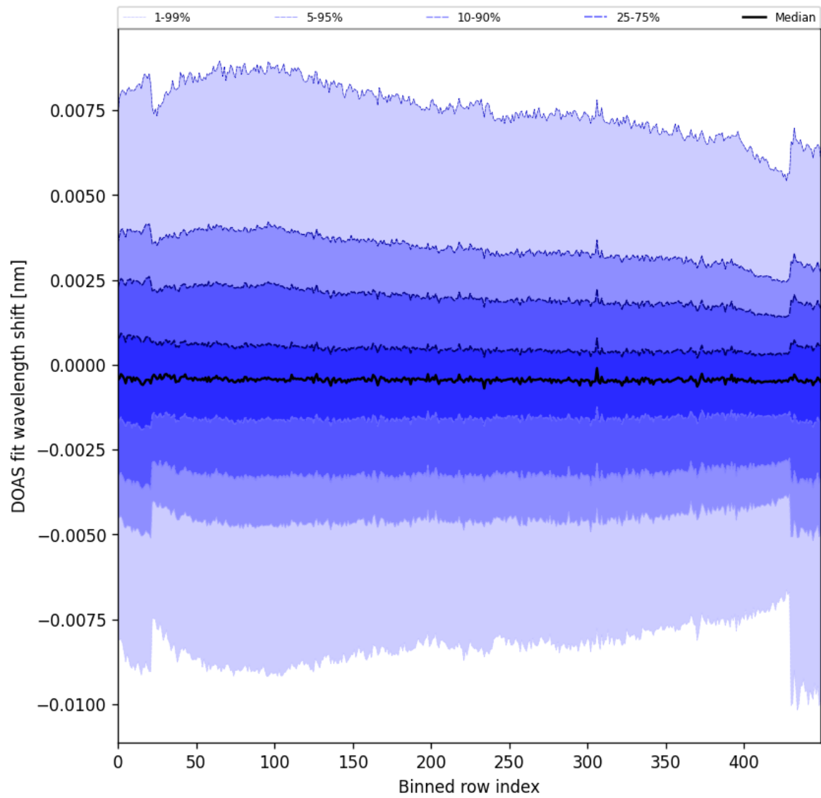
Figure 91: Along track statistics of “DOAS fit wavelength shift” for 2024-09-01 to 2024-09-02
