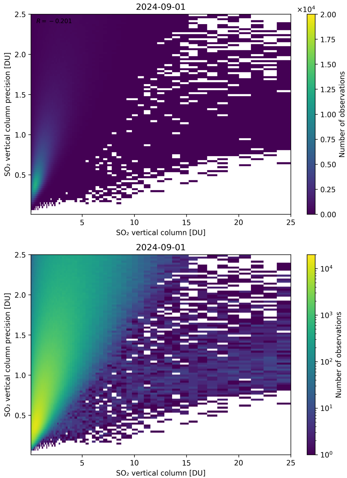
Figure 307: Scatter density plot of “SO 2 vertical column” against “SO 2 vertical column precision” for 2024-09-01 to 2024-09-02.
