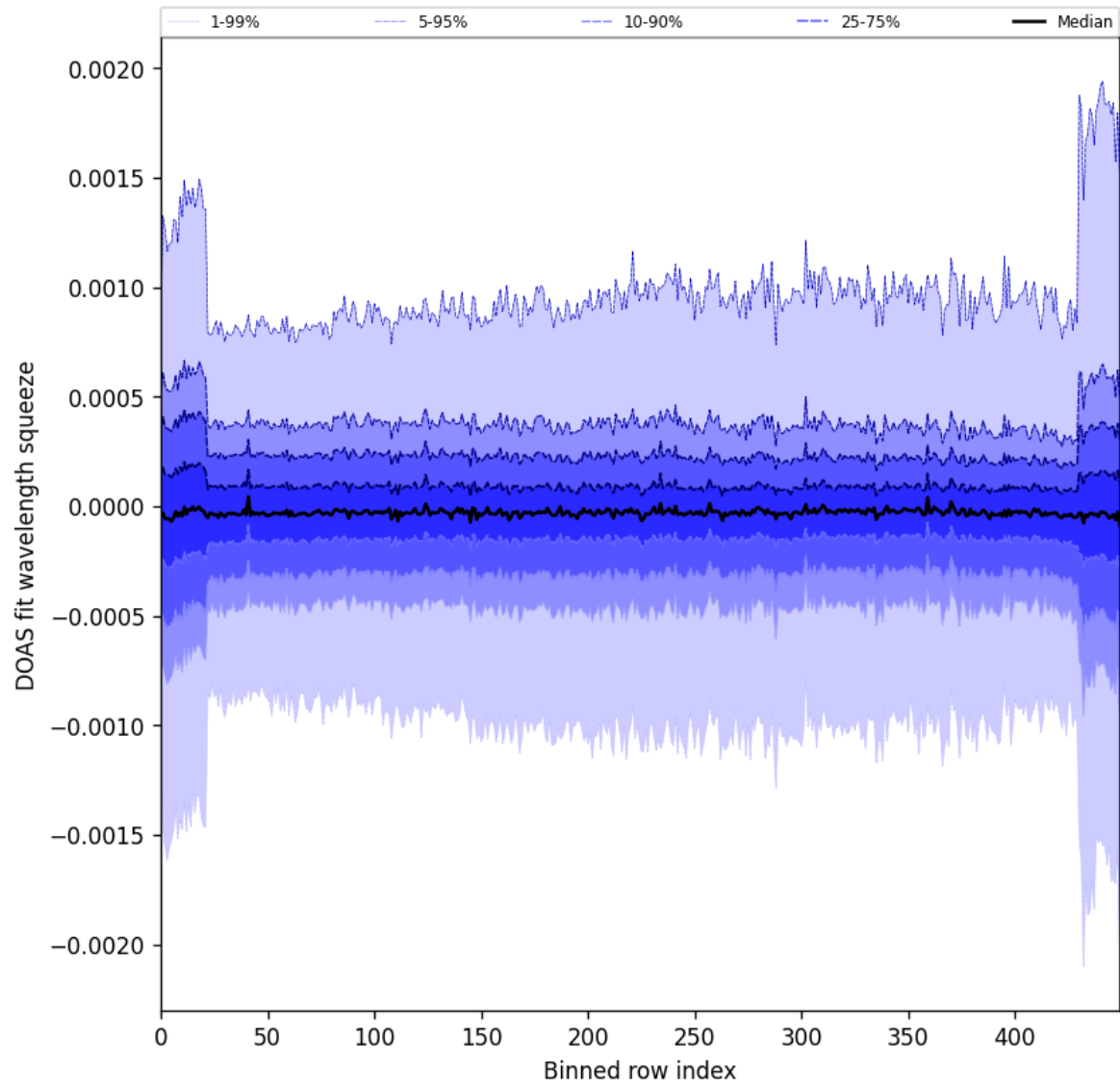
Figure 92: Along track statistics of “DOAS fit wavelength squeeze” for 2024-09-01 to 2024-09-02
