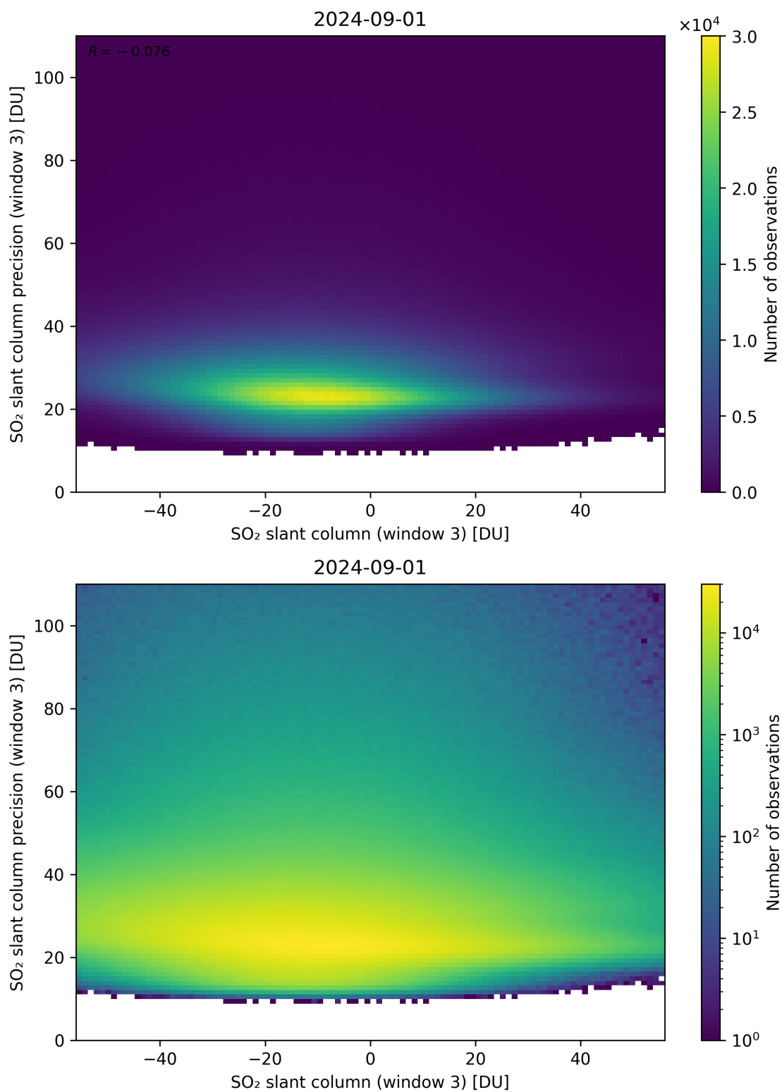
Figure 267: Scatter density plot of “SO 2 slant column (window 3)” against “SO 2 slant column precision (window 3)” for 2024-09-01 to 2024-09-02.
