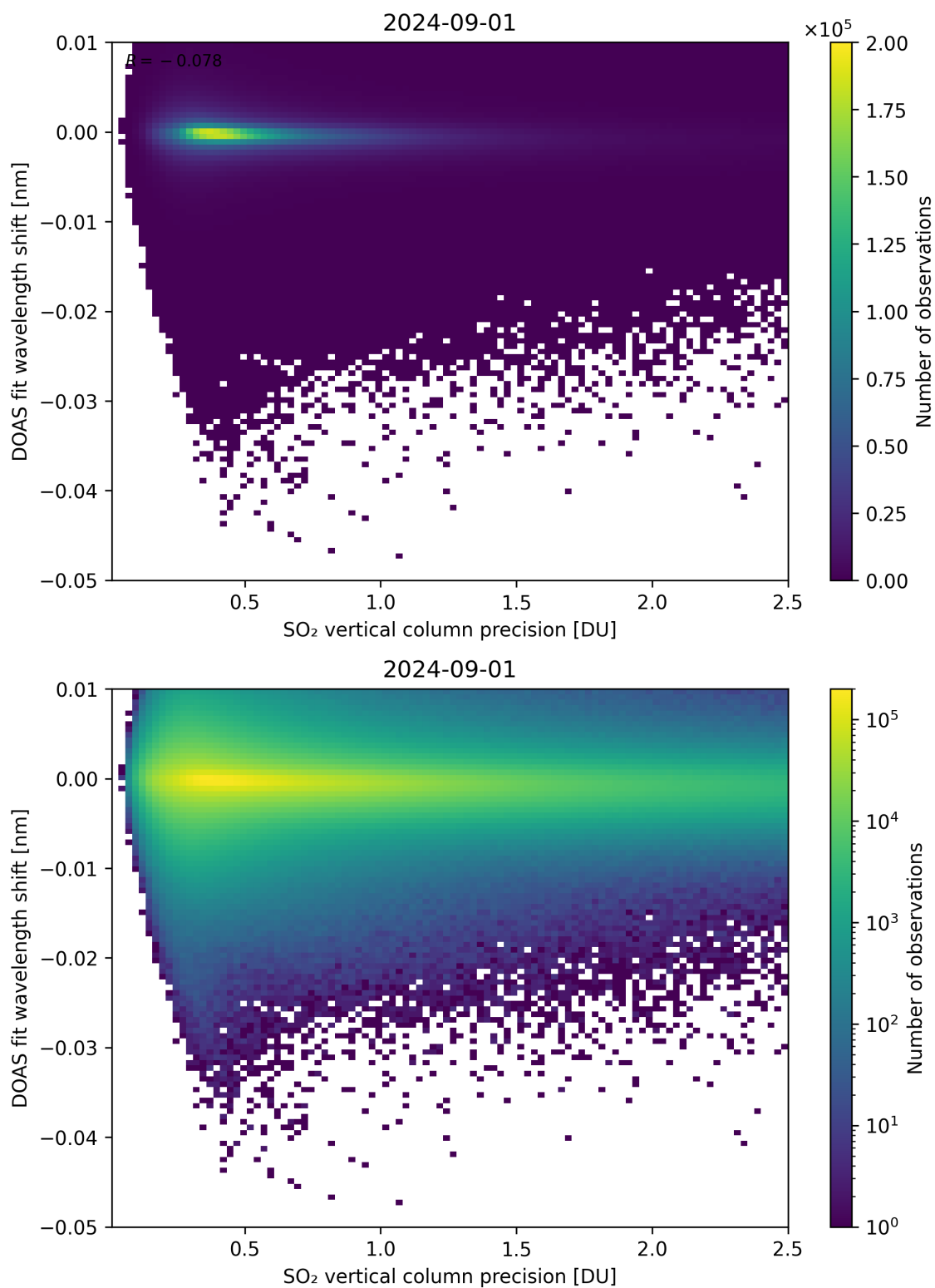
Figure 282: Scatter density plot of “SO 2 vertical column precision” against “DOAS fit wavelength shift” for 2024-09-01 to 2024-09-02.
