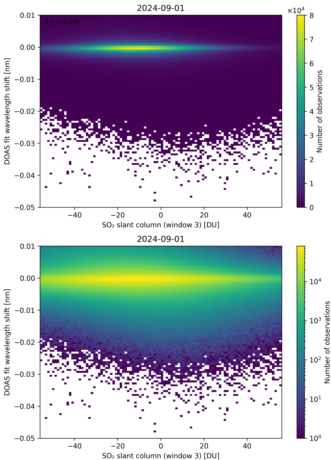
Figure 254: Scatter density plot of “SO 2 slant column (window 3)” against “DOAS fit wavelength shift” for 2024-09-01 to 2024-09-02.
