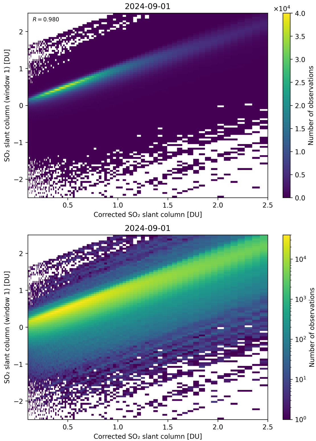
Figure 187: Scatter density plot of “Corrected SO 2 slant column” against “SO 2 slant column (window 1)” for 2024-09-01 to 2024-09-02.
