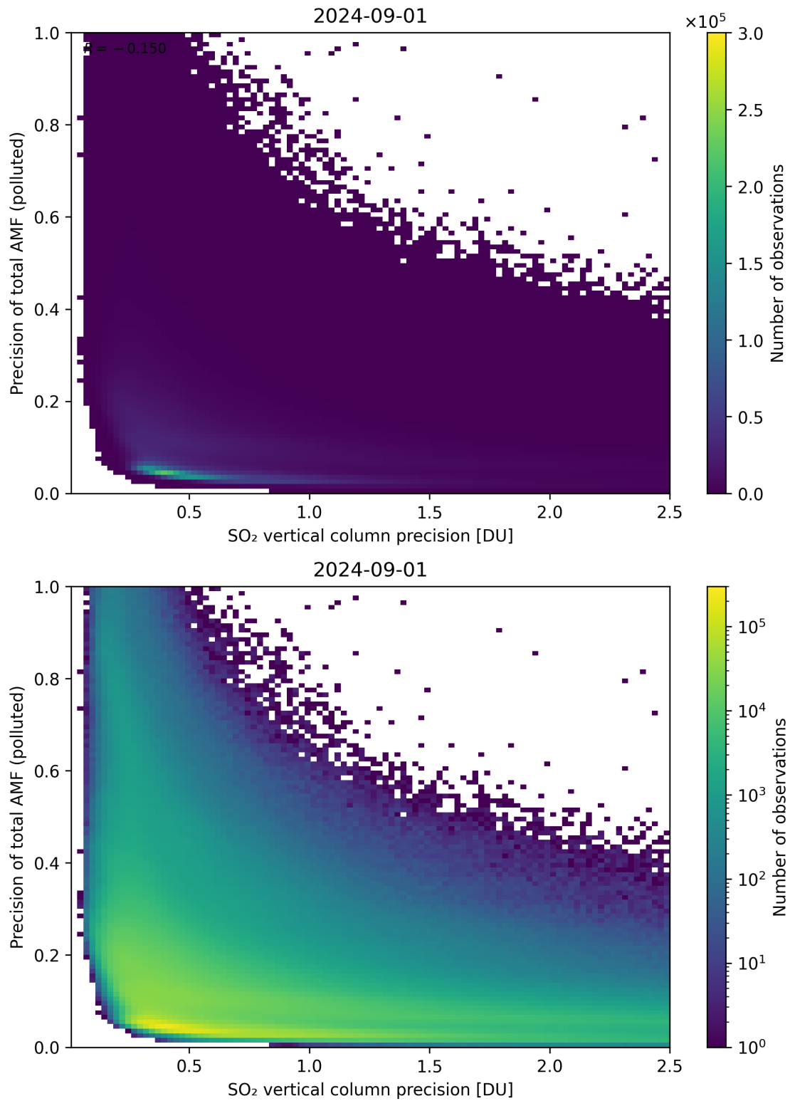
Figure 295: Scatter density plot of “SO 2 vertical column precision” against “Precision of total AMF (polluted)” for 2024-09-01 to 2024-09-02.
