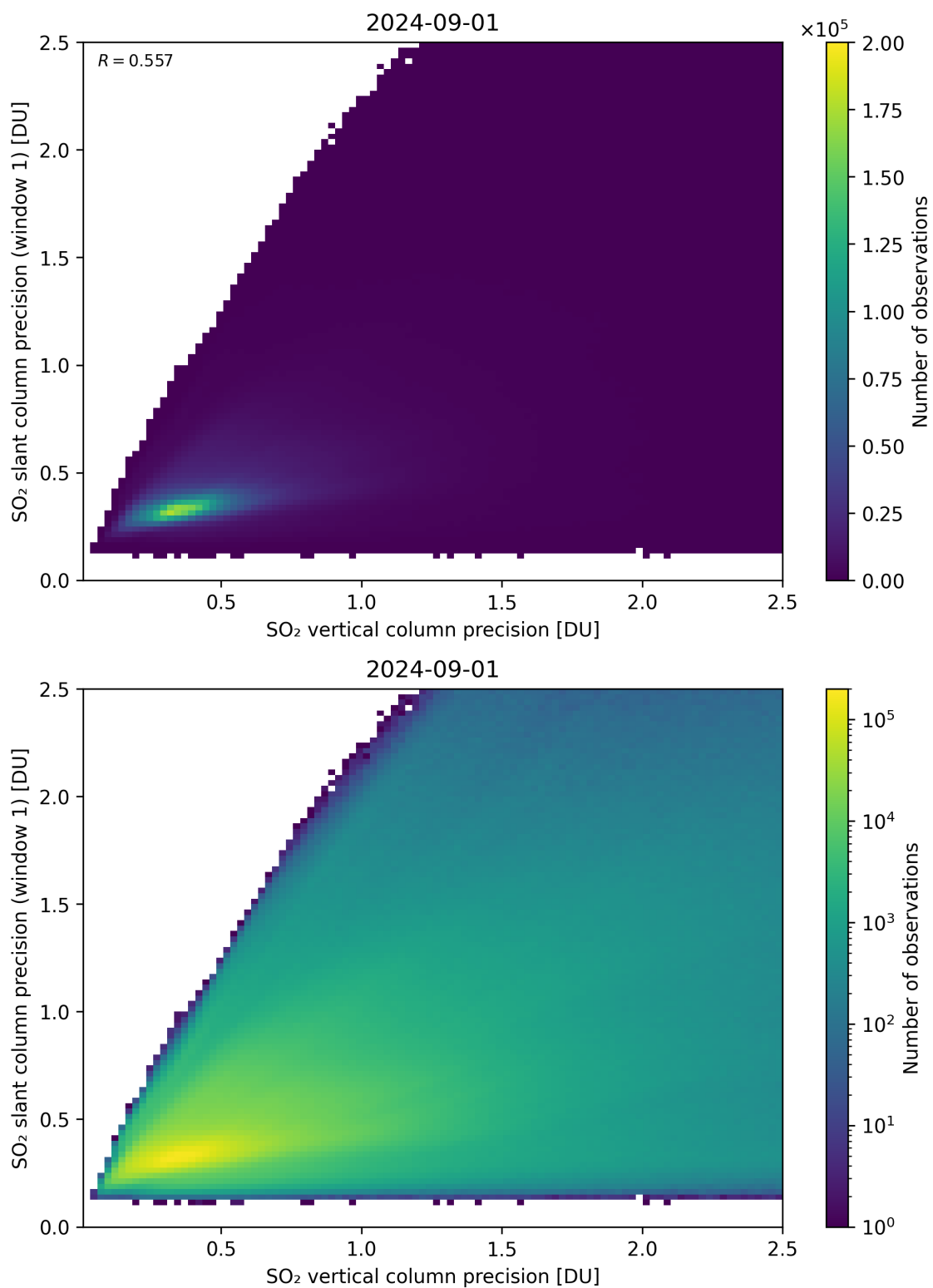
Figure 290: Scatter density plot of “SO 2 vertical column precision” against “SO 2 slant column precision (window 1)” for 2024-09-01 to 2024-09-02.
