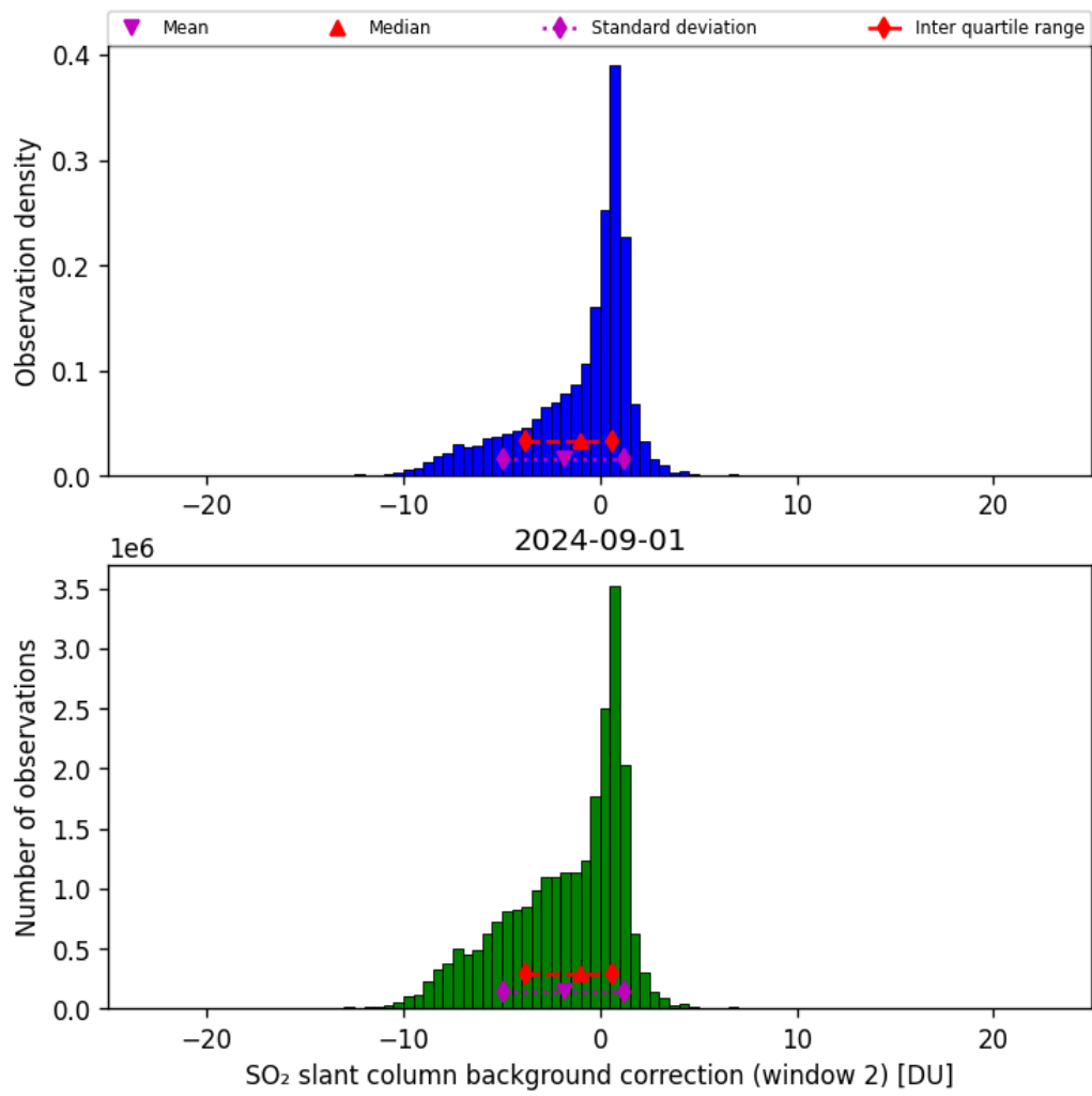
Figure 63: Histogram of “SO 2 slant column background correction (window 2)” for 2024-09-01 to 2024-09-02
