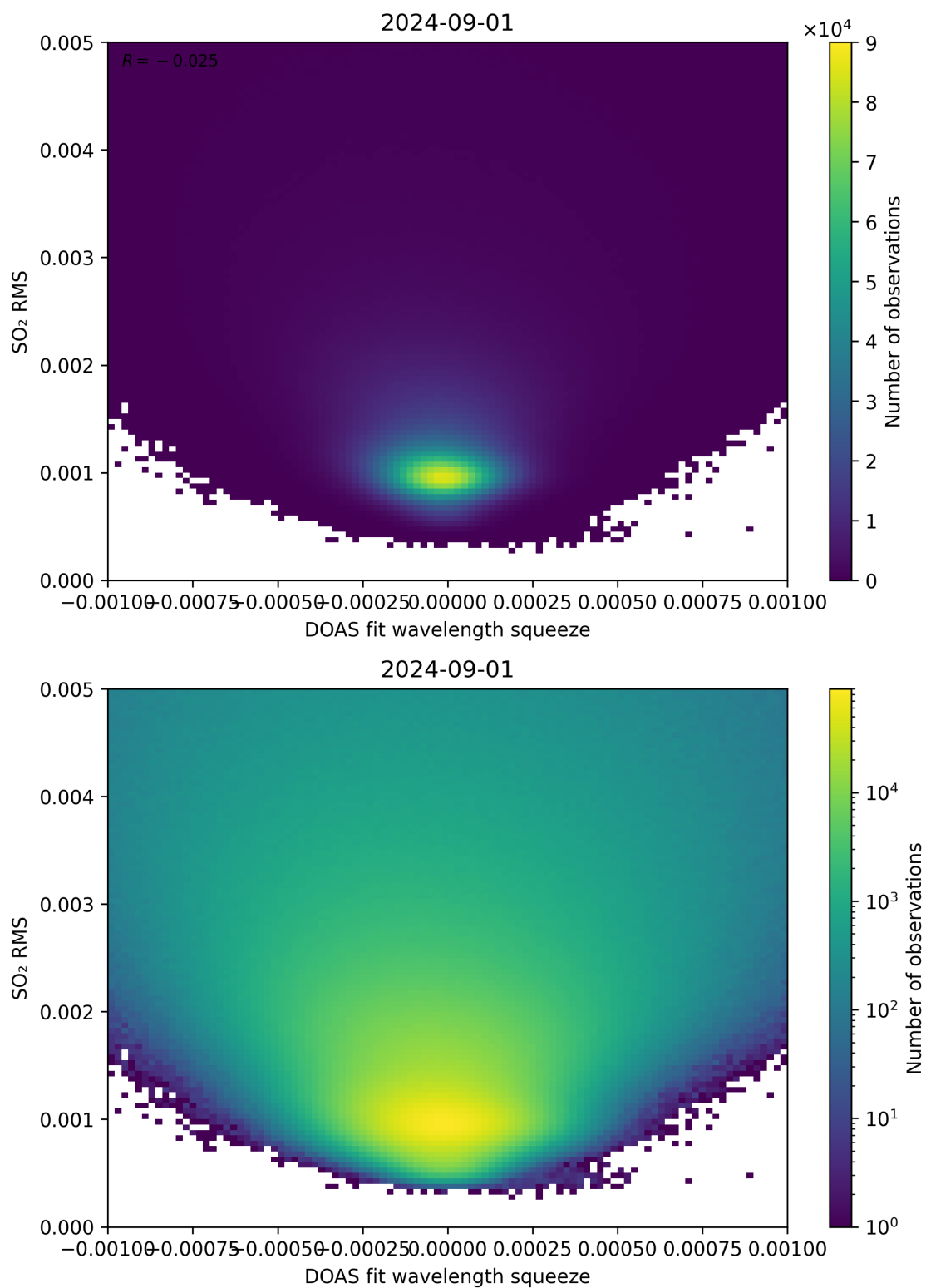
Figure 132: Scatter density plot of “DOAS fit wavelength squeeze” against “SO 2 RMS” for 2024-09-01 to 2024-09-02.
