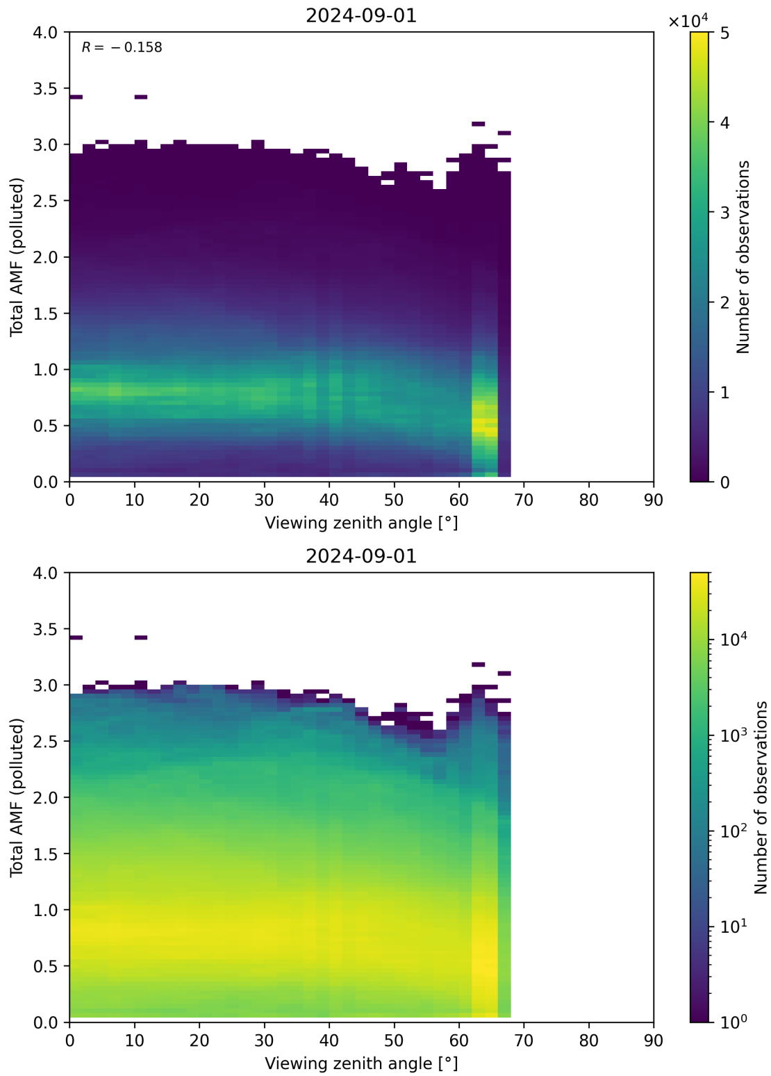
Figure 325: Scatter density plot of “Viewing zenith angle” against “Total AMF (polluted)” for 2024-09-01 to 2024-09-02.
