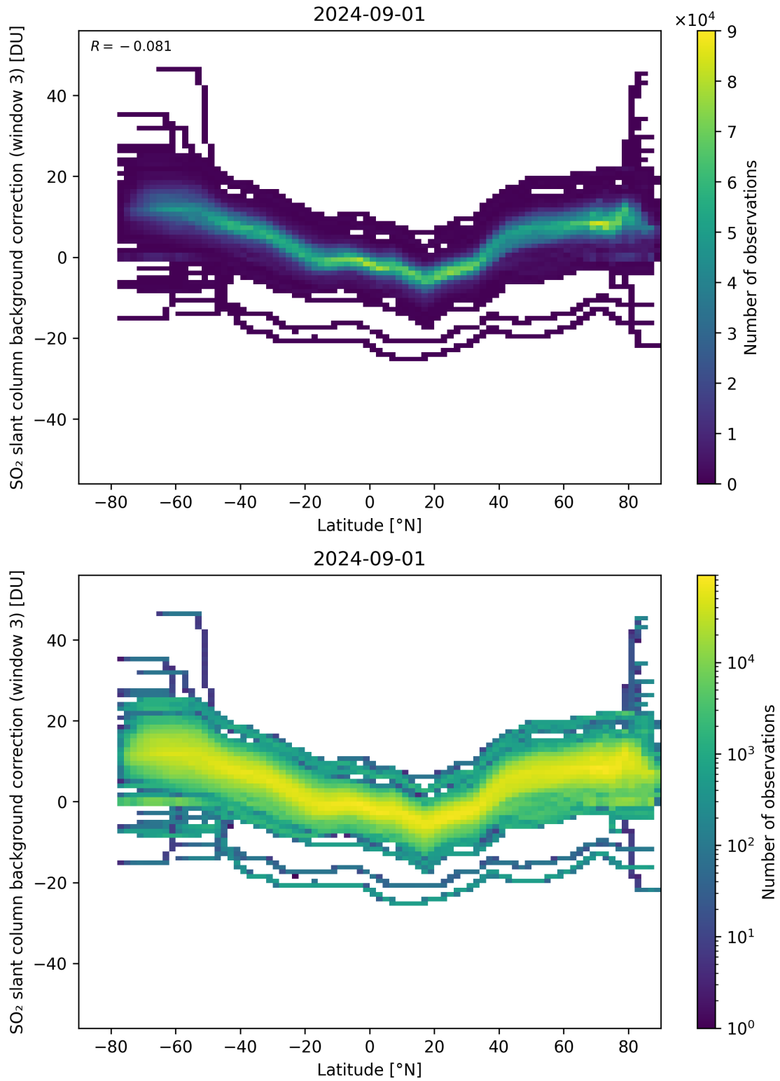
Figure 141: Scatter density plot of “Latitude” against “SO 2 slant column background correction (window 3)” for 2024-09-01 to 2024-09-02.
