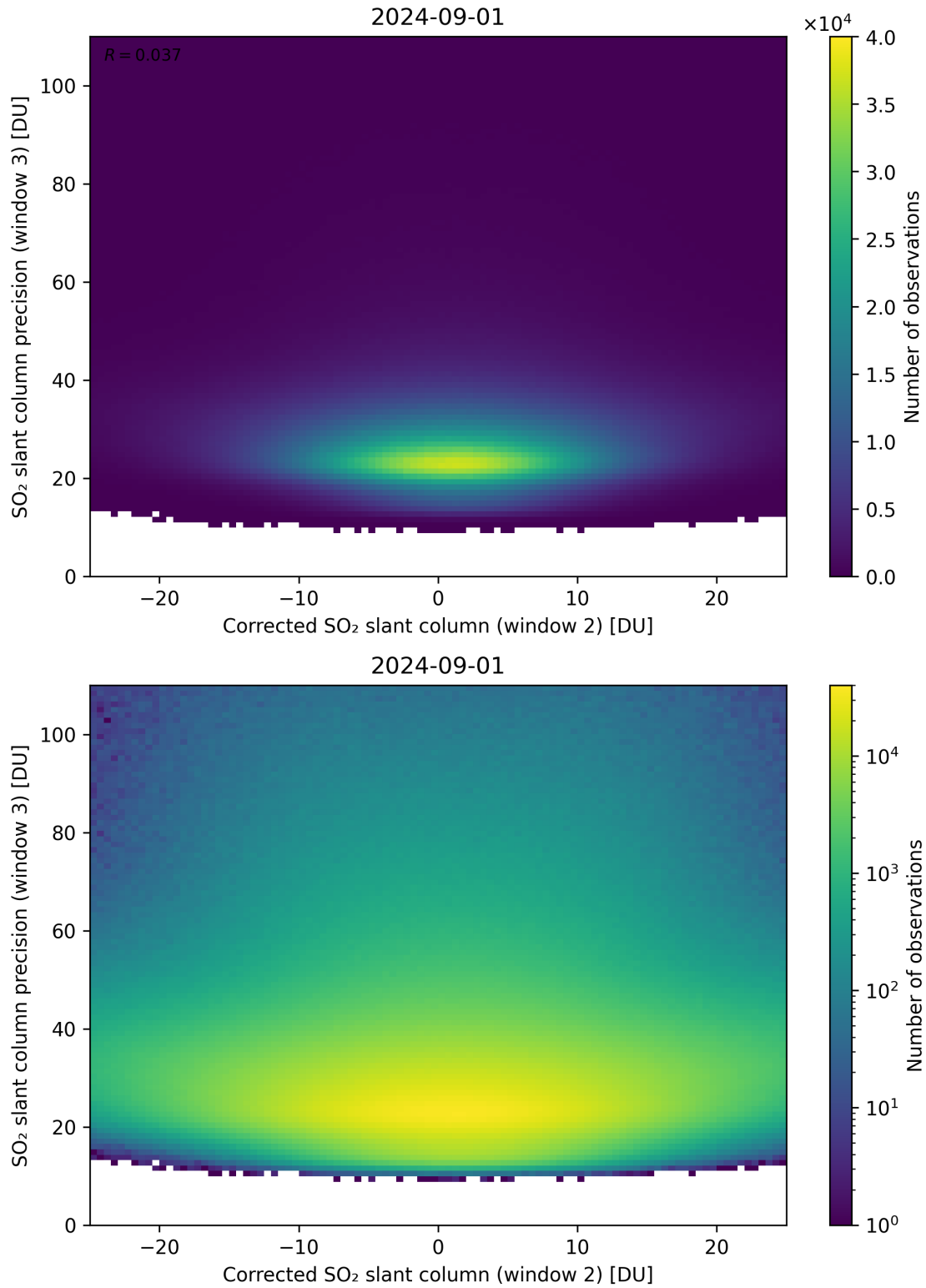
Figure 202: Scatter density plot of “Corrected SO 2 slant column (window 2)” against “SO 2 slant column precision (window 3)” for 2024-09-01 to 2024-09-02.
