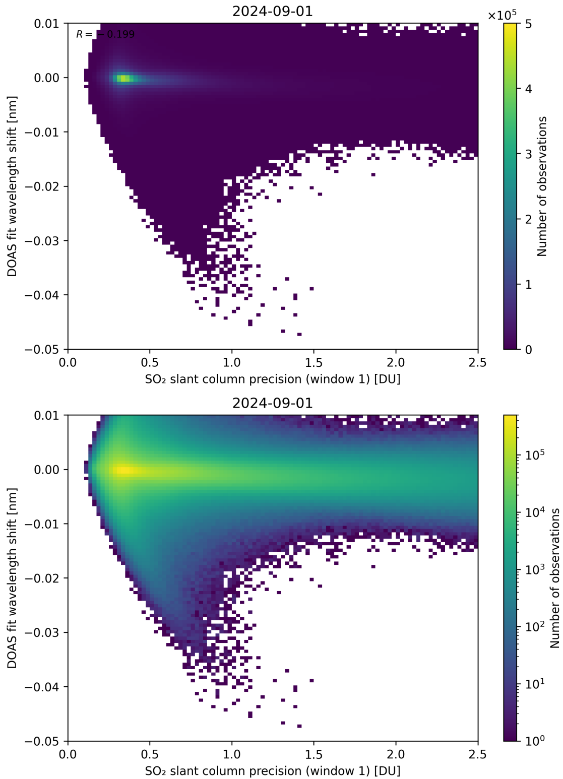
Figure 221: Scatter density plot of “SO 2 slant column precision (window 1)” against “DOAS fit wavelength shift” for 2024-09-01 to 2024-09-02.
