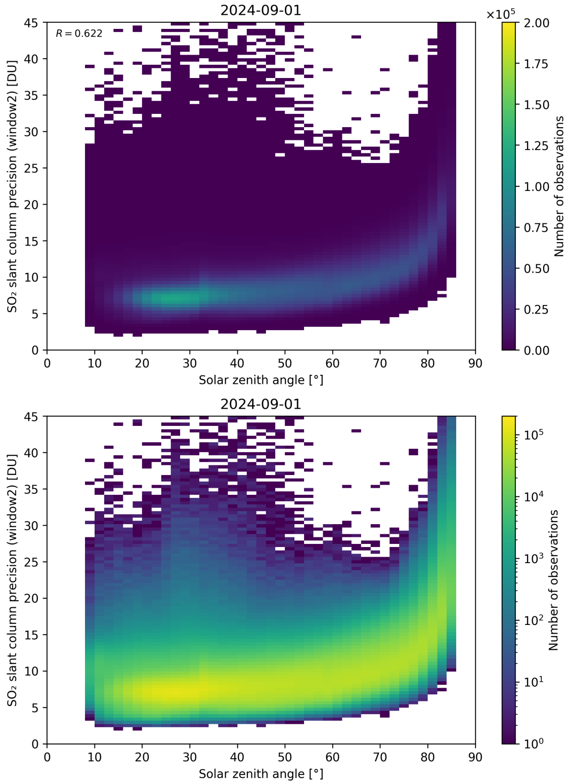
Figure 171: Scatter density plot of “Solar zenith angle” against “SO 2 slant column precision (window2)” for 2024-09-01 to 2024-09-02.
