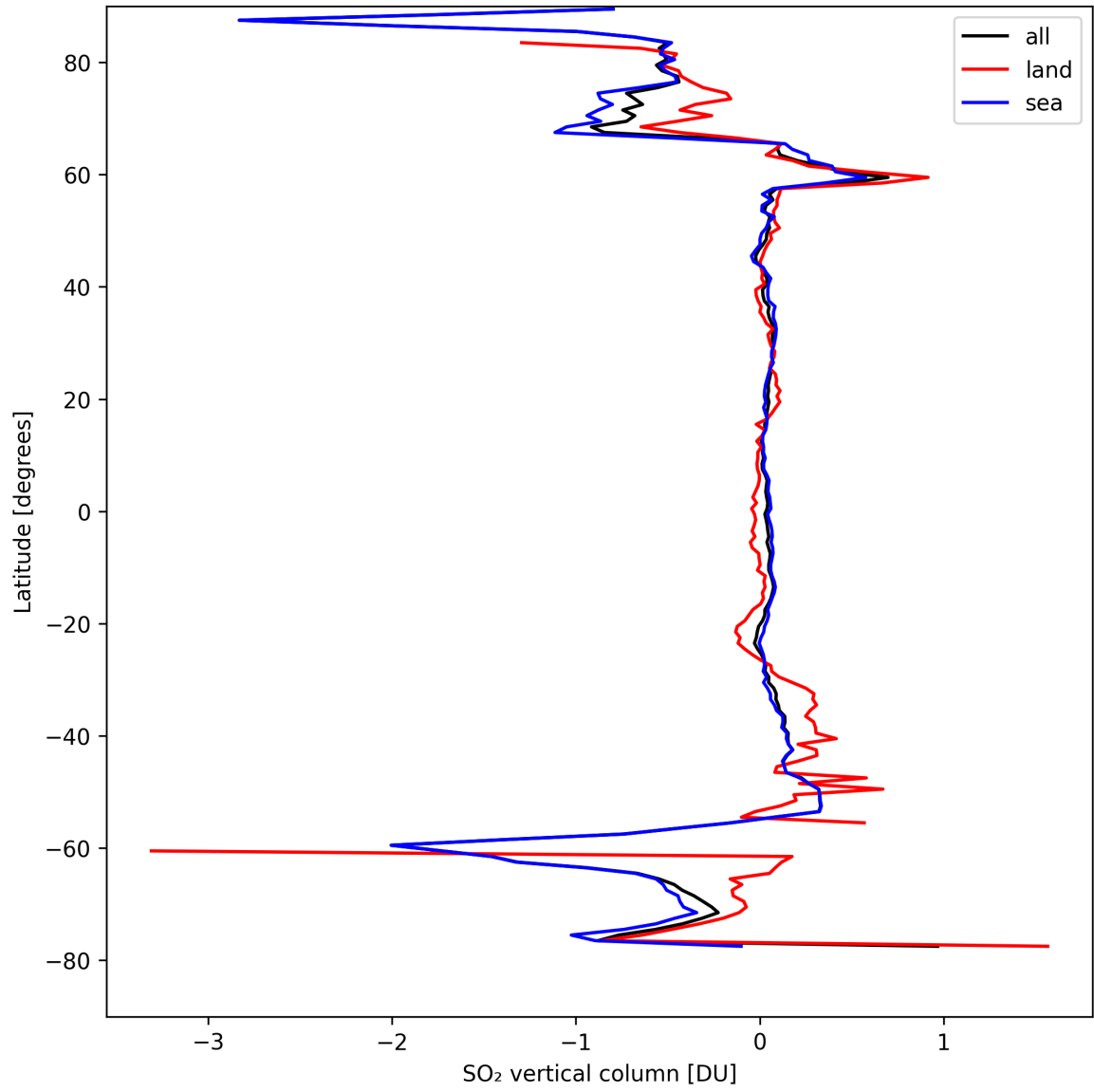
Figure 30: Zonal average of “SO 2 vertical column” for 2024-09-01 to 2024-09-02.
