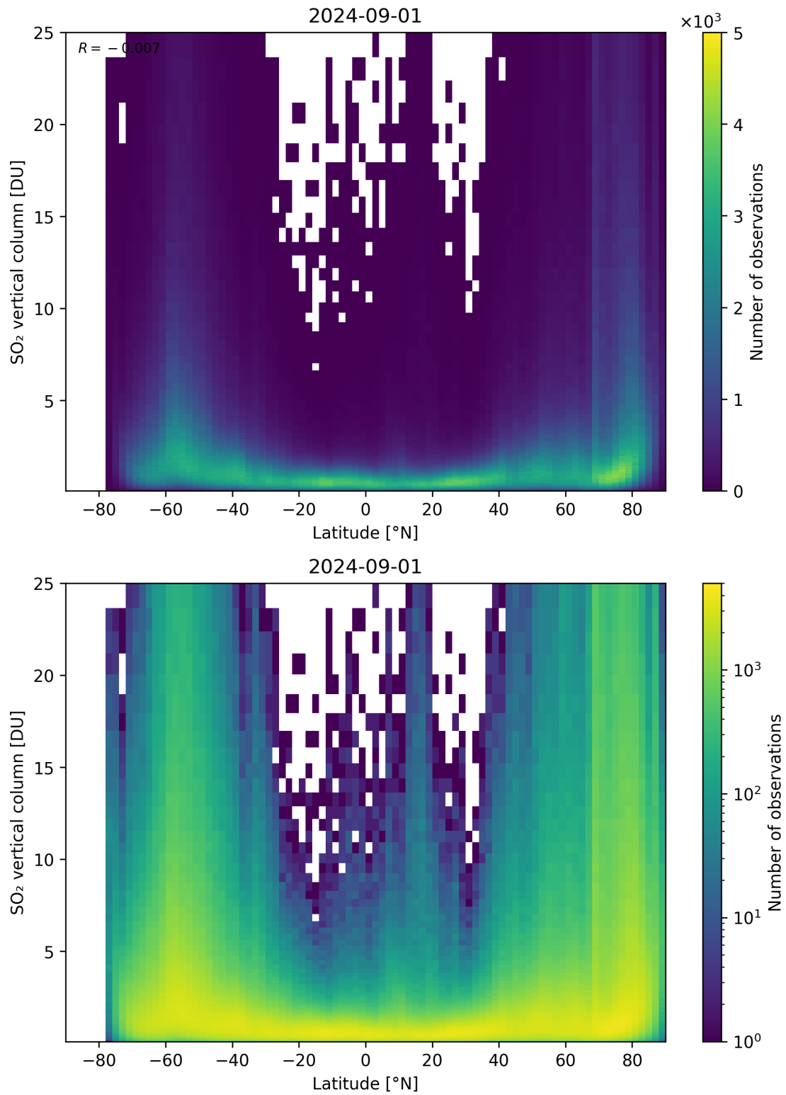
Figure 156: Scatter density plot of “Latitude” against “SO 2 vertical column” for 2024-09-01 to 2024-09-02.
