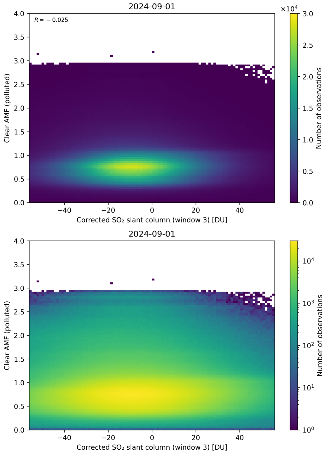
Figure 209: Scatter density plot of “Corrected SO 2 slant column (window 3)” against “Clear AMF (polluted)” for 2024-09-01 to 2024-09-02.
