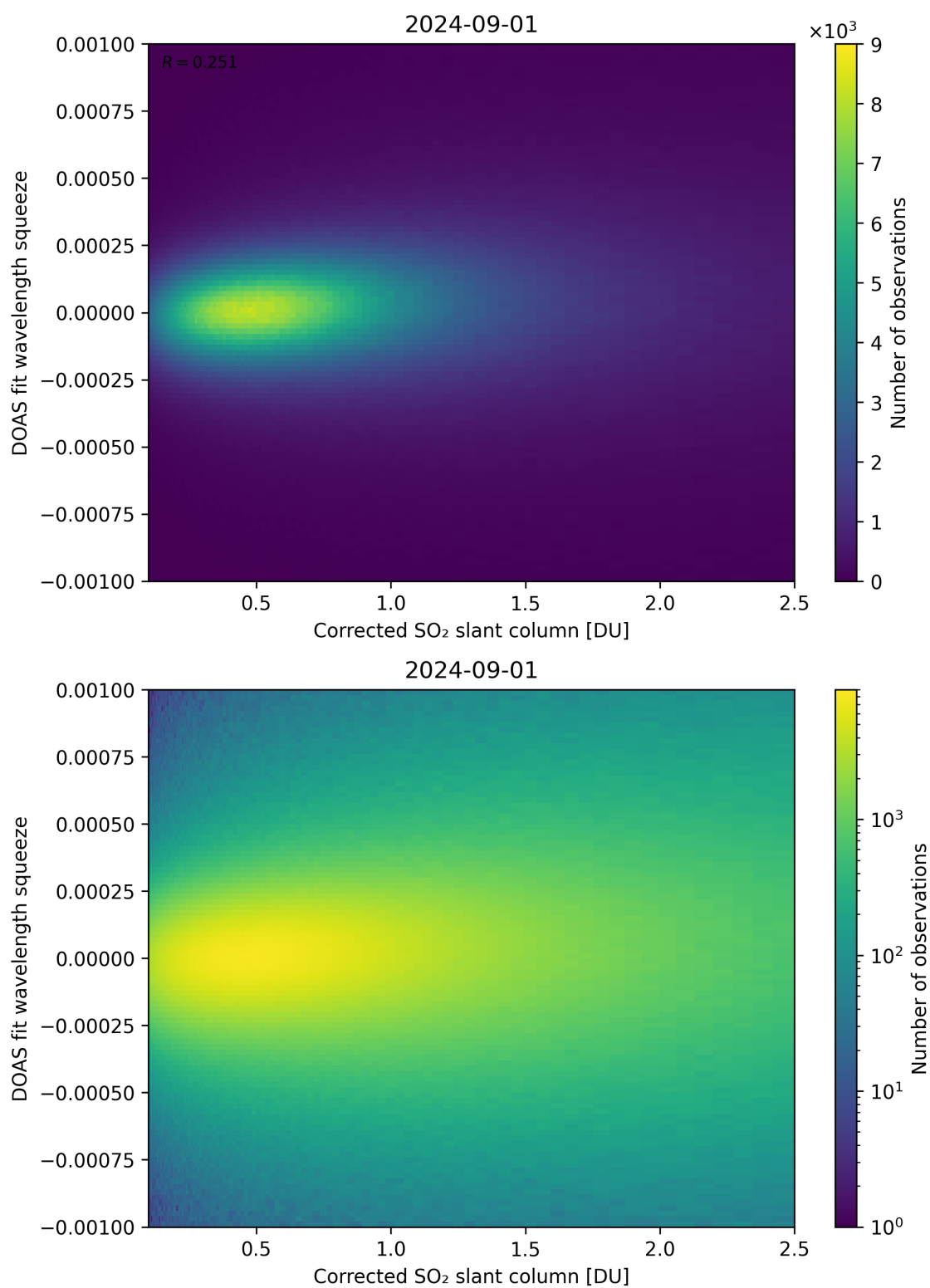
Figure 182: Scatter density plot of “Corrected SO 2 slant column” against “DOAS fit wavelength squeeze” for 2024-09-01 to 2024-09-02.
