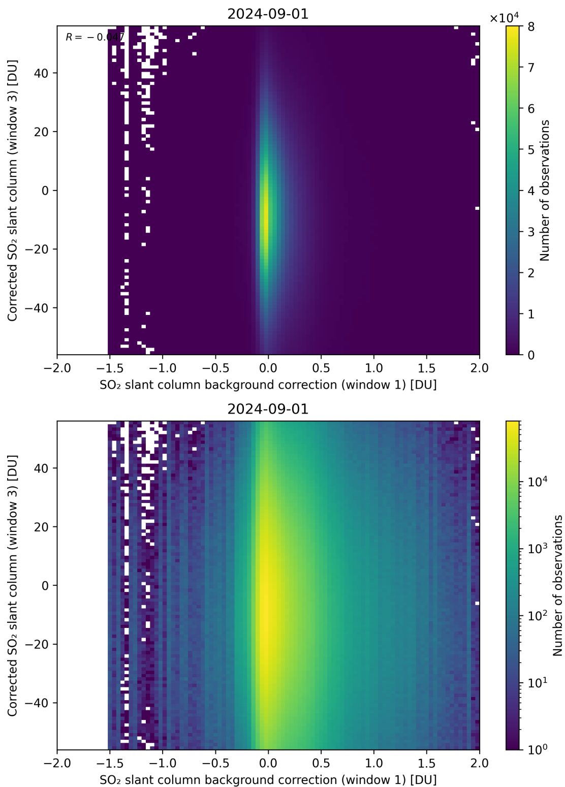
Figure 105: Scatter density plot of “SO 2 slant column background correction (window 1)” against “Corrected SO 2 slant column (window 3)” for 2024-09-01 to 2024-09-02.
