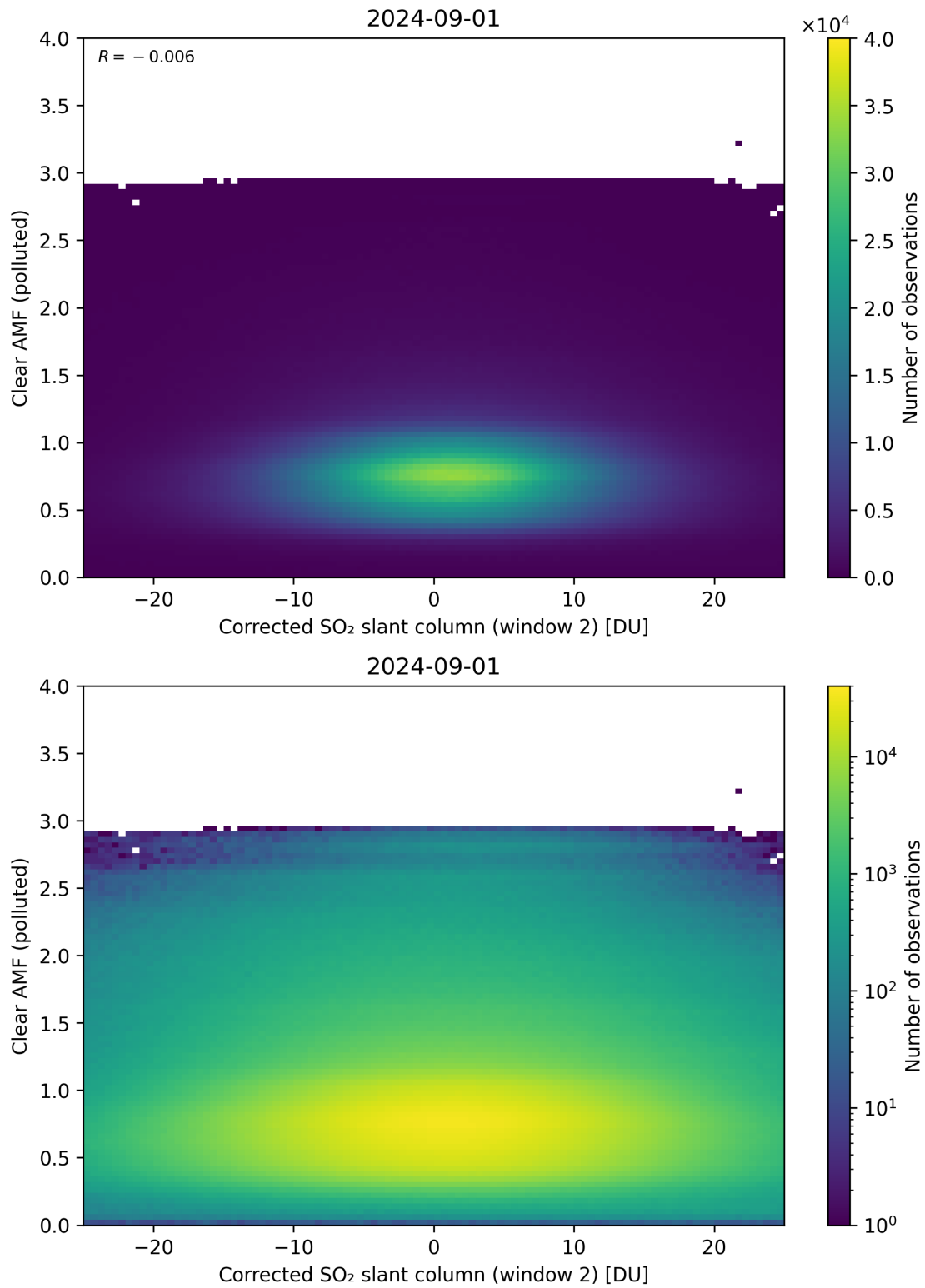
Figure 199: Scatter density plot of “Corrected SO 2 slant column (window 2)” against “Clear AMF (polluted)” for 2024-09-01 to 2024-09-02.
