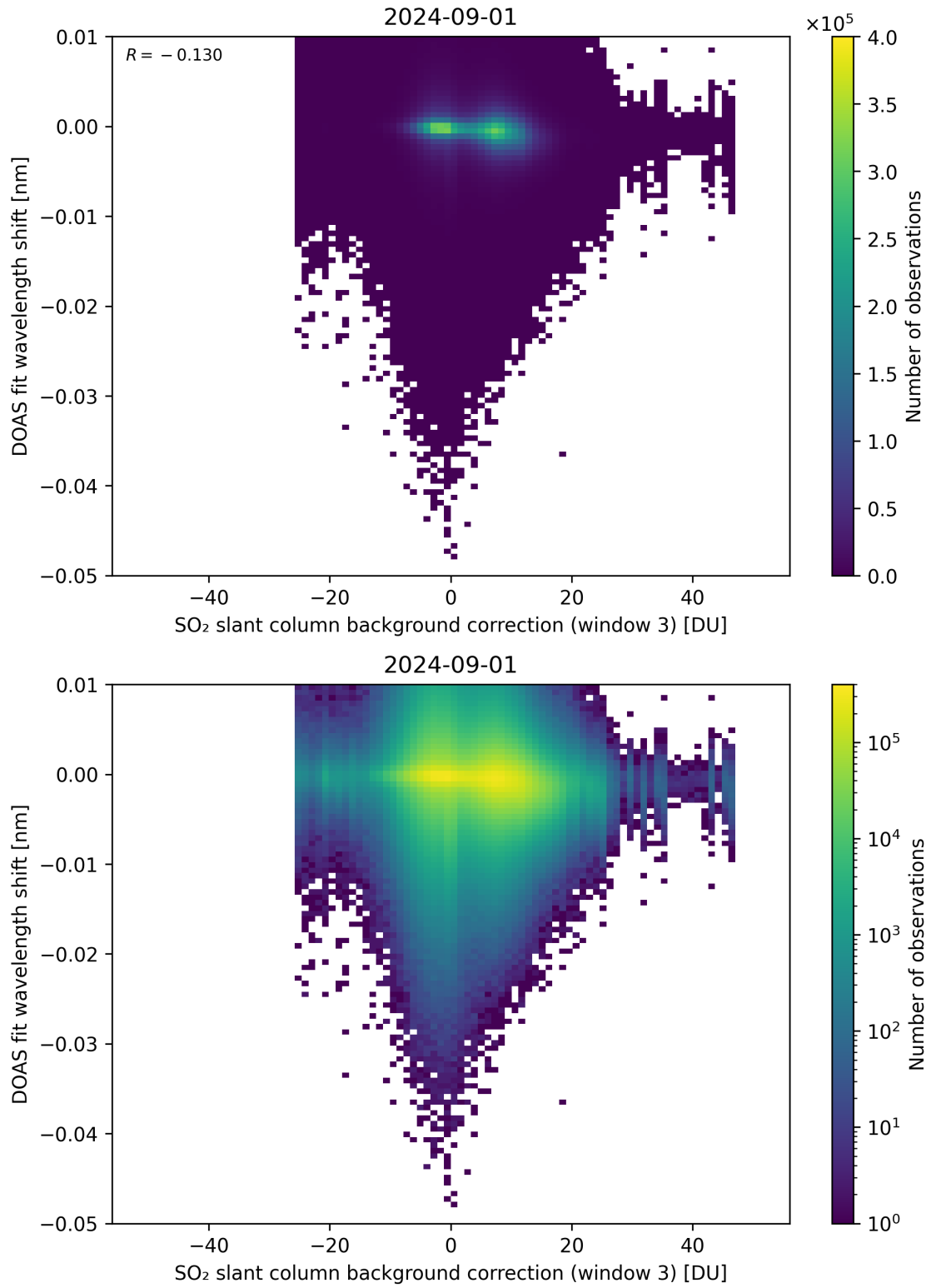
Figure 121: Scatter density plot of “SO 2 slant column background correction (window 3)” against “DOAS fit wavelength shift” for 2024-09-01 to 2024-09-02.
