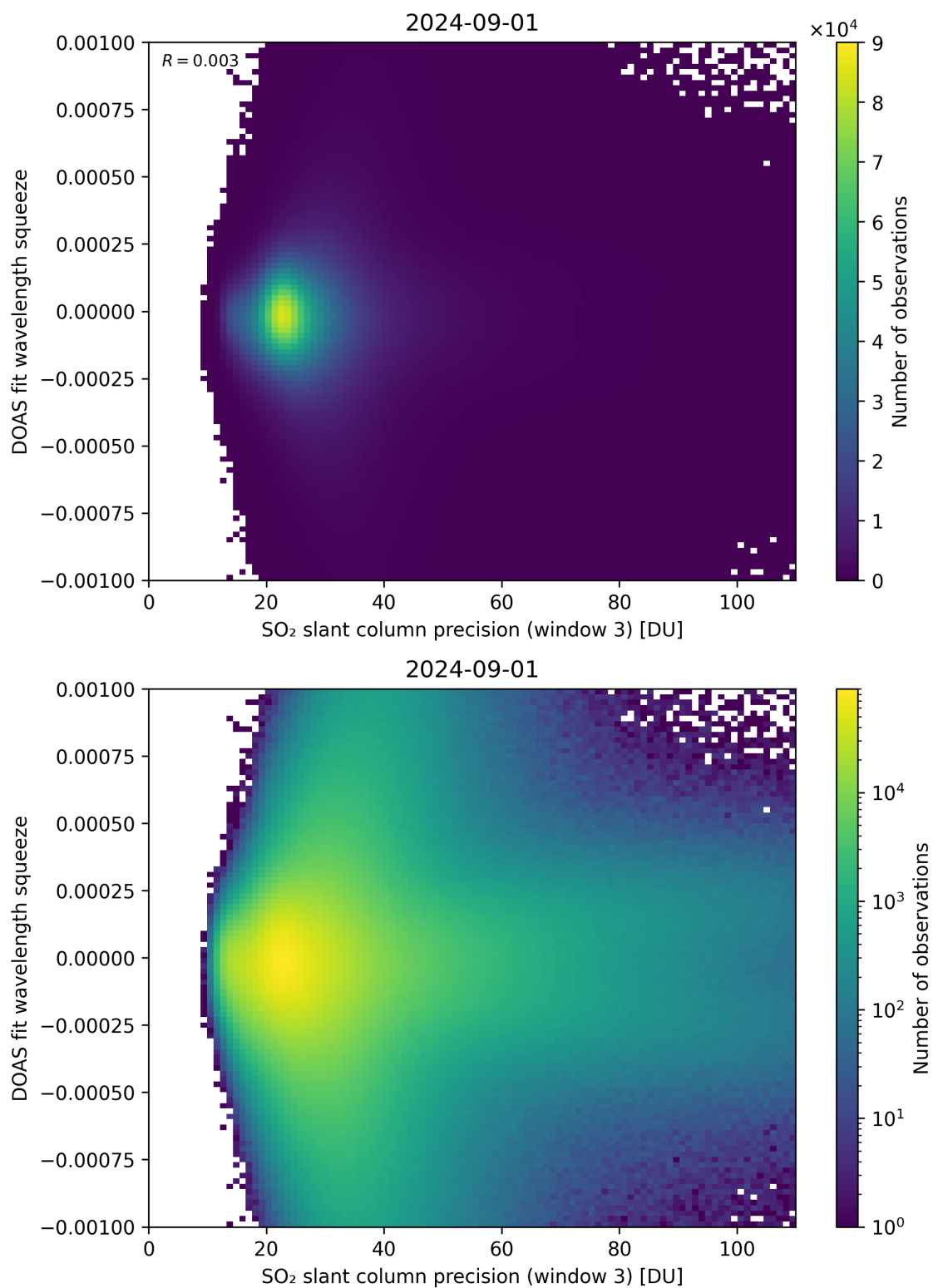
Figure 259: Scatter density plot of “SO 2 slant column precision (window 3)” against “DOAS fit wavelength squeeze” for 2024-09-01 to 2024-09-02.
