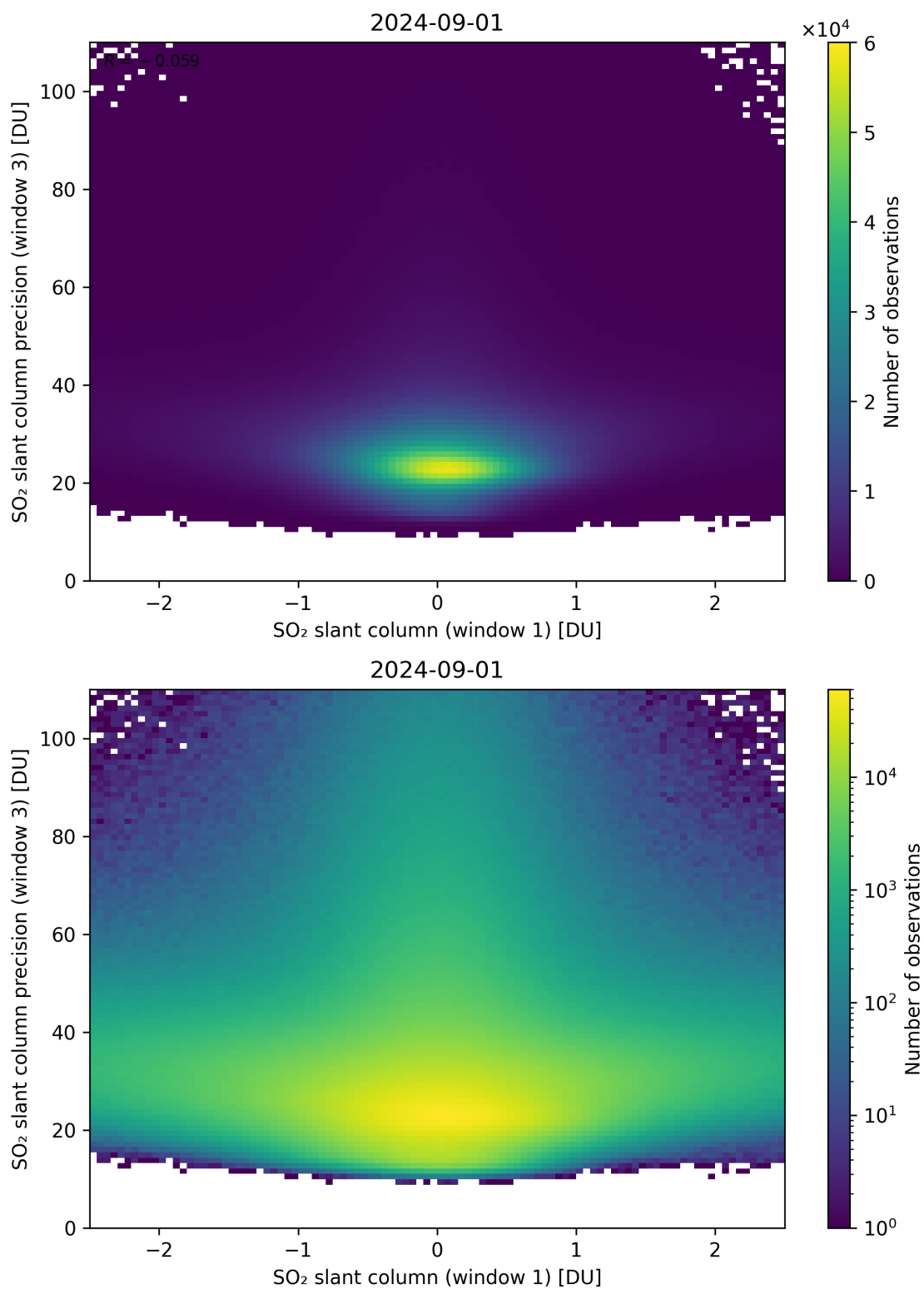
Figure 238: Scatter density plot of “SO 2 slant column (window 1)” against “SO 2 slant column precision (window 3)” for 2024-09-01 to 2024-09-02.
