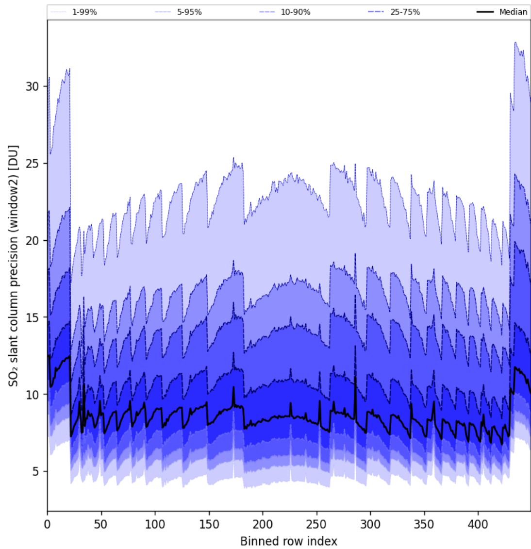
Figure 84: Along track statistics of “SO 2 slant column precision (window2)” for 2024-09-01 to 2024-09-02
