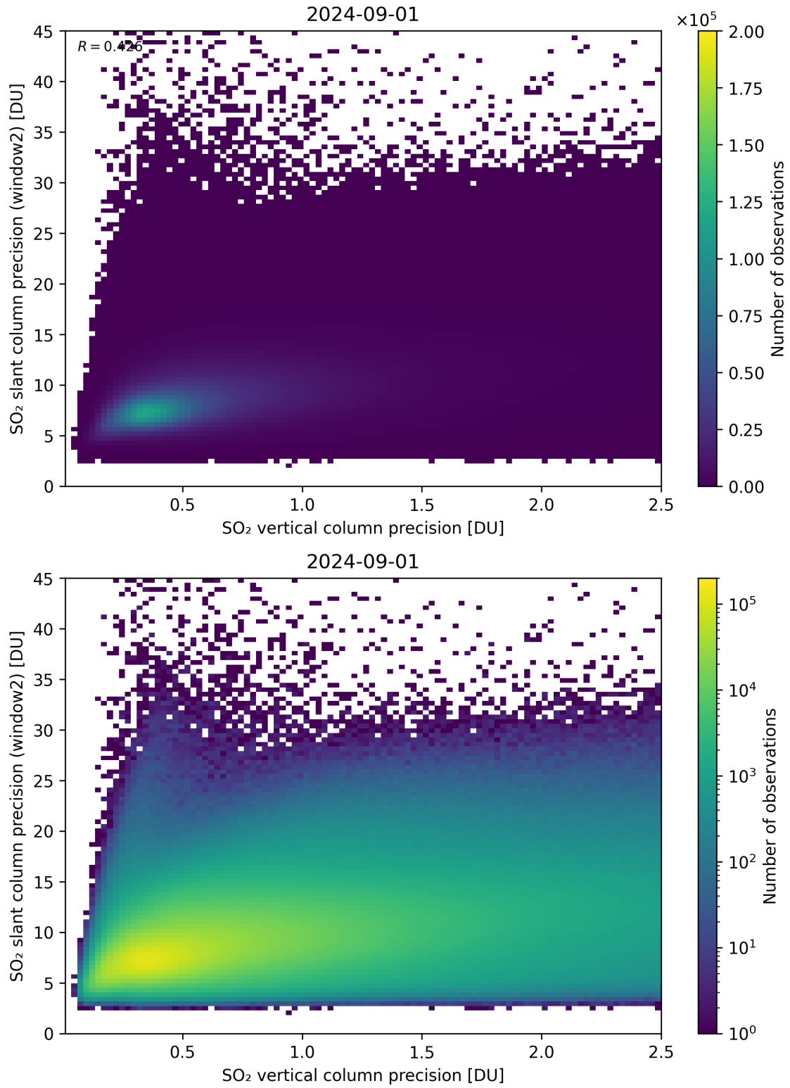
Figure 291: Scatter density plot of “SO 2 vertical column precision” against “SO 2 slant column precision (window2)” for 2024-09-01 to 2024-09-02.
