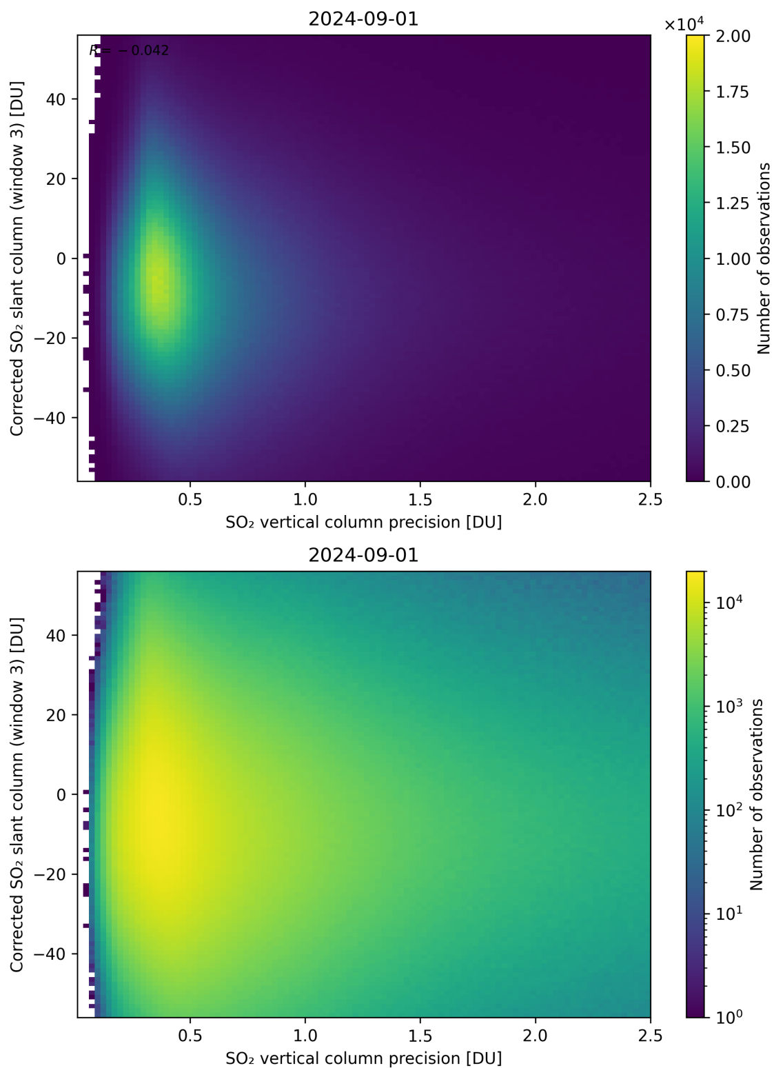
Figure 288: Scatter density plot of “SO 2 vertical column precision” against “Corrected SO 2 slant column (window 3)” for 2024-09-01 to 2024-09-02.
