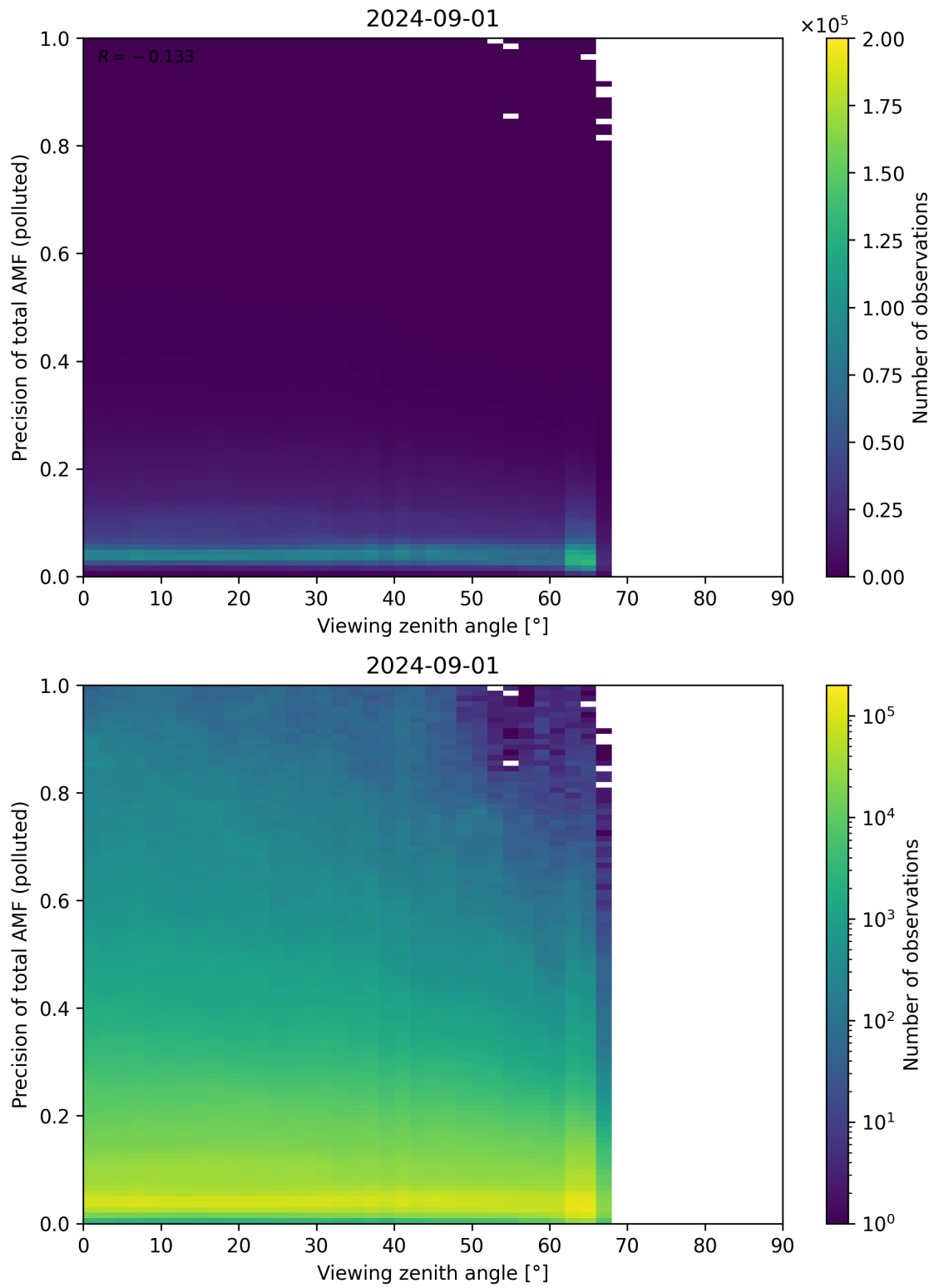
Figure 326: Scatter density plot of “Viewing zenith angle” against “Precision of total AMF (polluted)” for 2024-09-01 to 2024-09-02.
