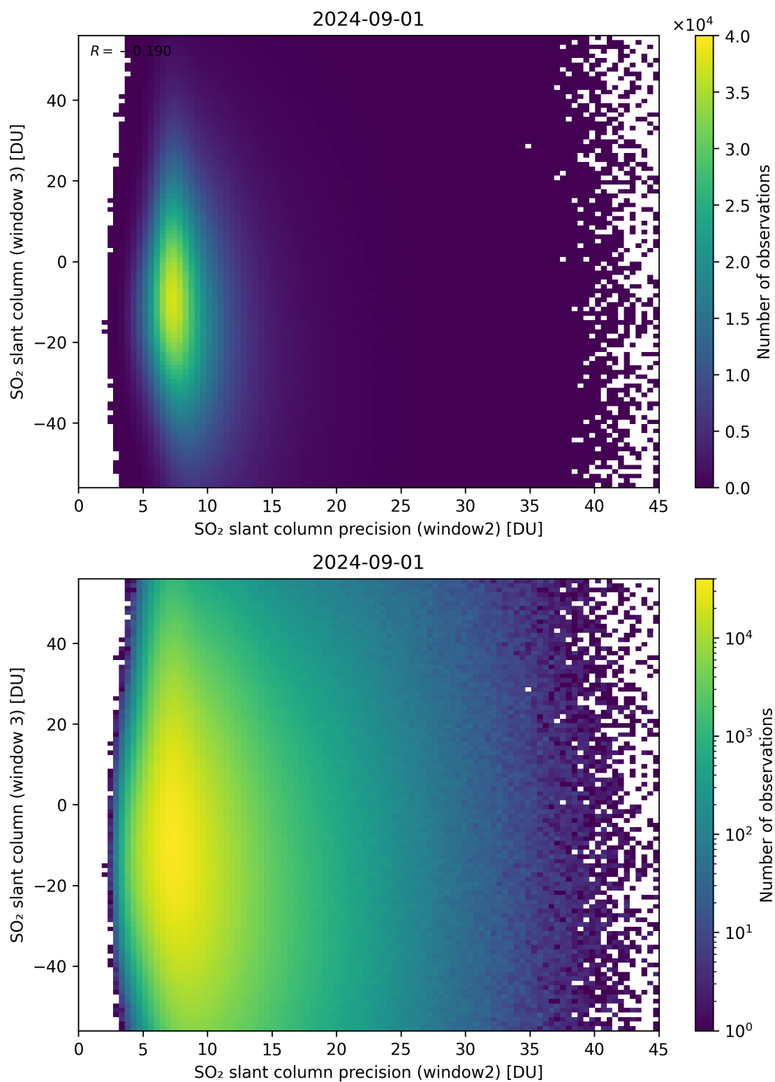
Figure 249: Scatter density plot of “SO 2 slant column precision (window2)” against “SO 2 slant column (window 3)” for 2024-09-01 to 2024-09-02.
