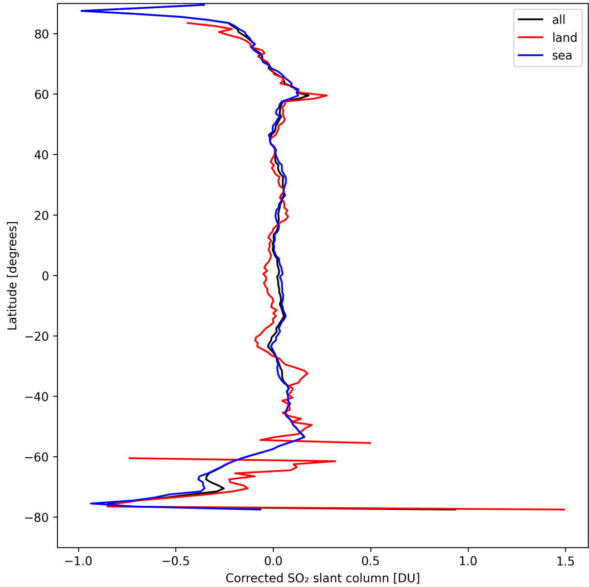
Figure 32: Zonal average of “Corrected SO 2 slant column” for 2024-09-01 to 2024-09-02.
