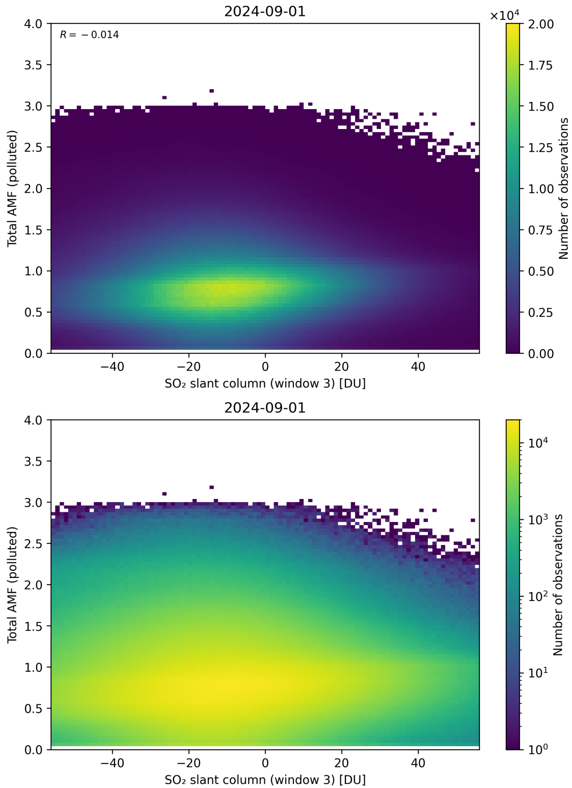
Figure 268: Scatter density plot of “SO 2 slant column (window 3)” against “Total AMF (polluted)” for 2024-09-01 to 2024-09-02.
