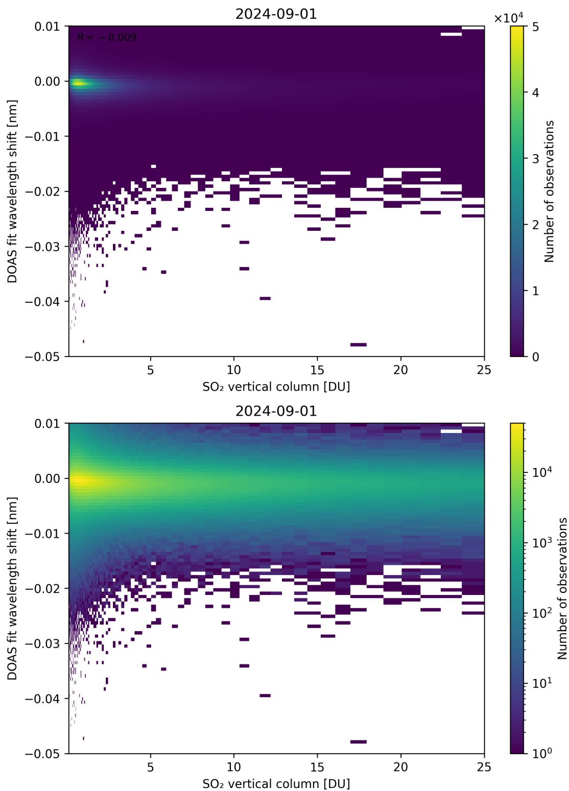
Figure 276: Scatter density plot of “SO 2 vertical column” against “DOAS fit wavelength shift” for 2024-09-01 to 2024-09-02.
