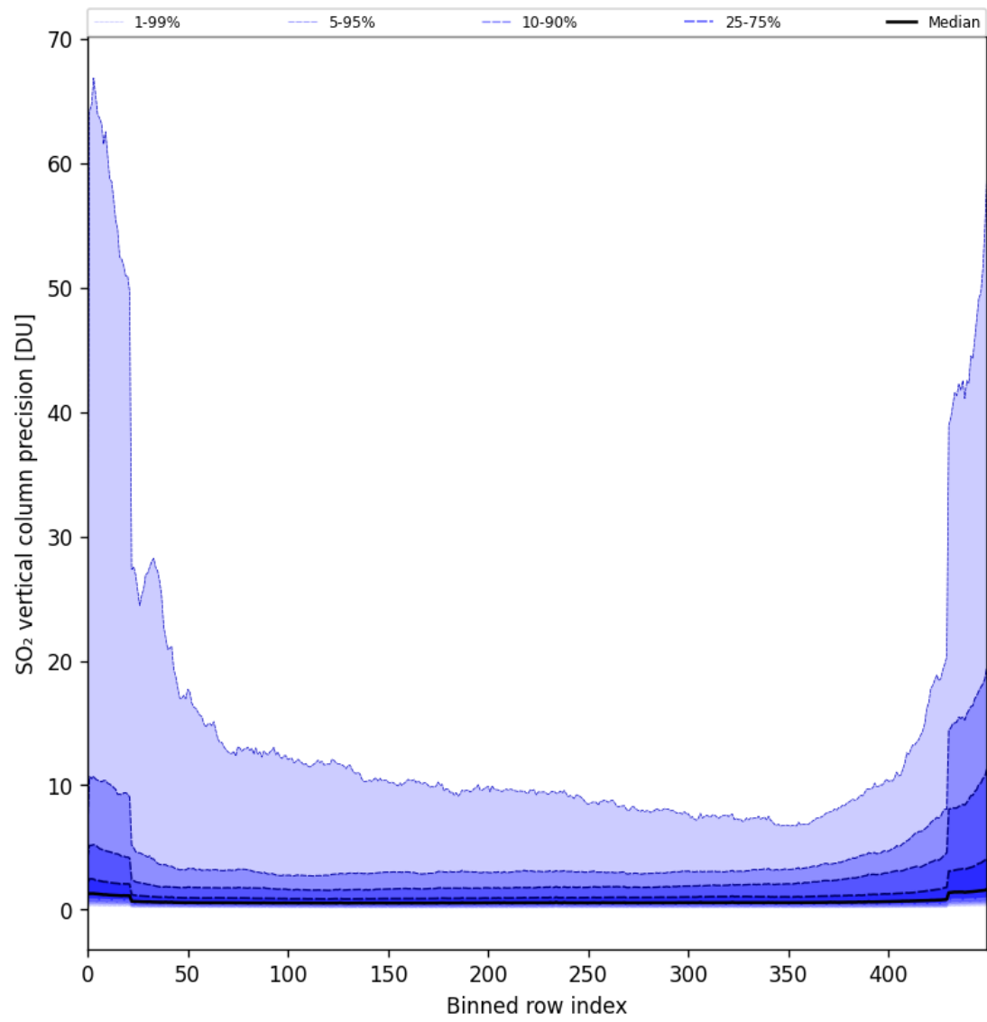
Figure 77: Along track statistics of “SO 2 vertical column precision” for 2024-09-01 to 2024-09-02
