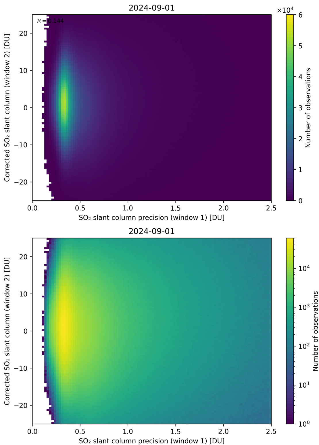
Figure 225: Scatter density plot of “SO 2 slant column precision (window 1)” against “Corrected SO 2 slant column (window 2)” for 2024-09-01 to 2024-09-02.
