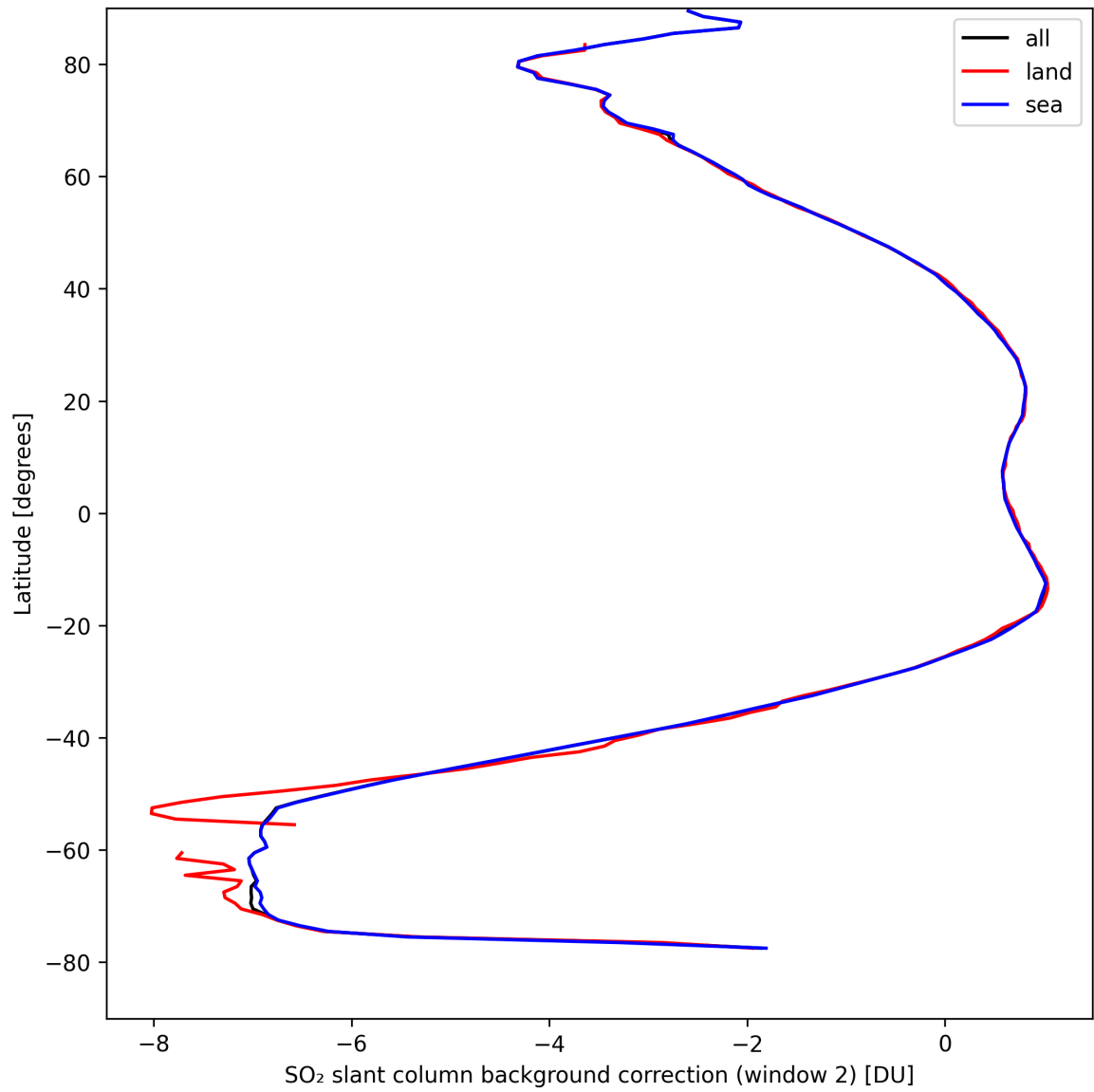
Figure 40: Zonal average of “SO 2 slant column background correction (window 2)” for 2024-09-01 to 2024-09-02.
