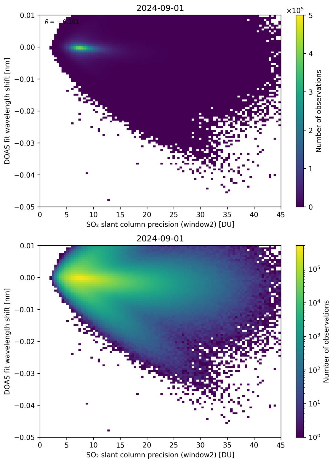
Figure 243: Scatter density plot of “SO 2 slant column precision (window2)” against “DOAS fit wavelength shift” for 2024-09-01 to 2024-09-02.
