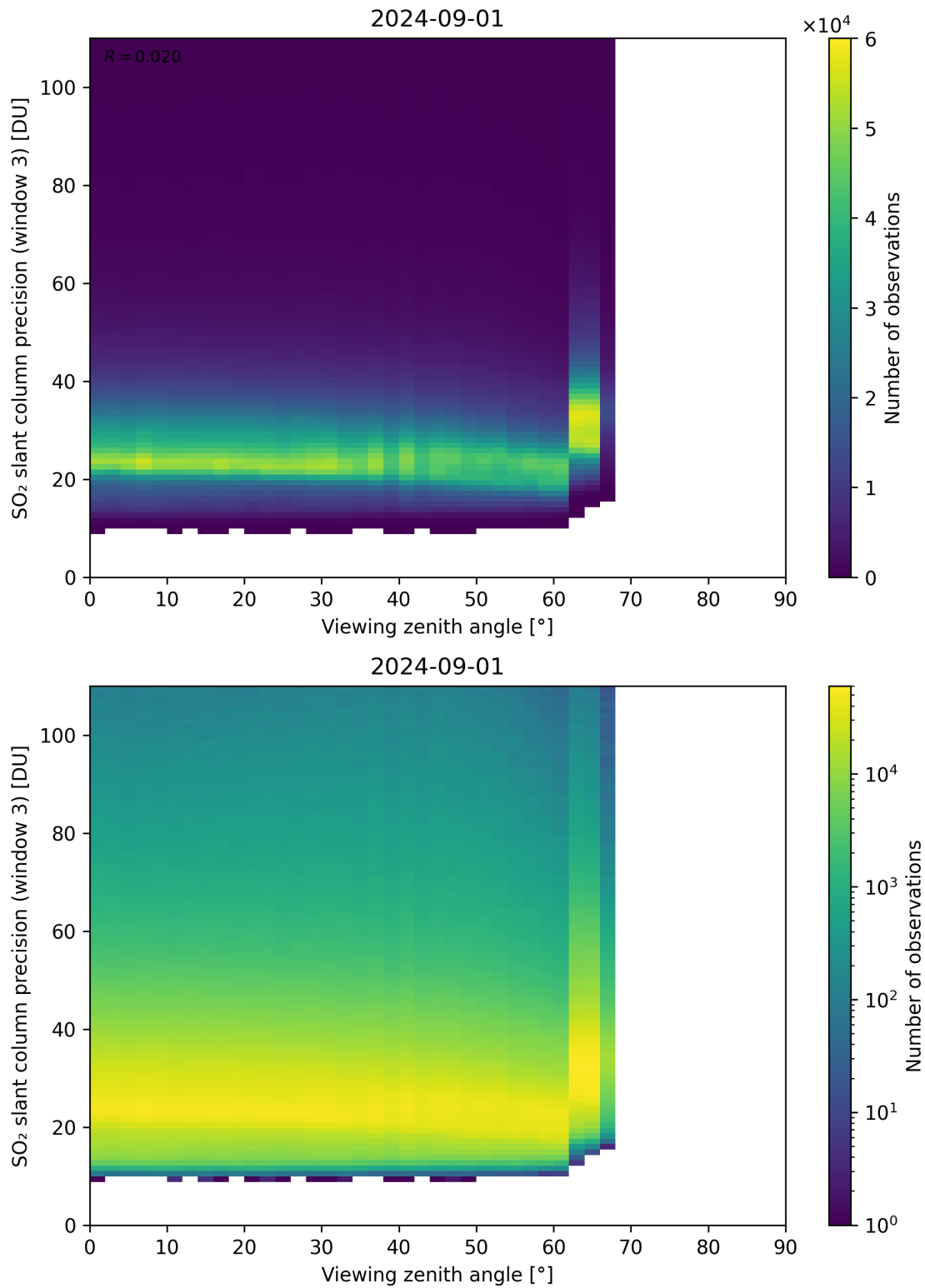
Figure 324: Scatter density plot of “Viewing zenith angle” against “SO 2 slant column precision (window 3)” for 2024-09-01 to 2024-09-02.
