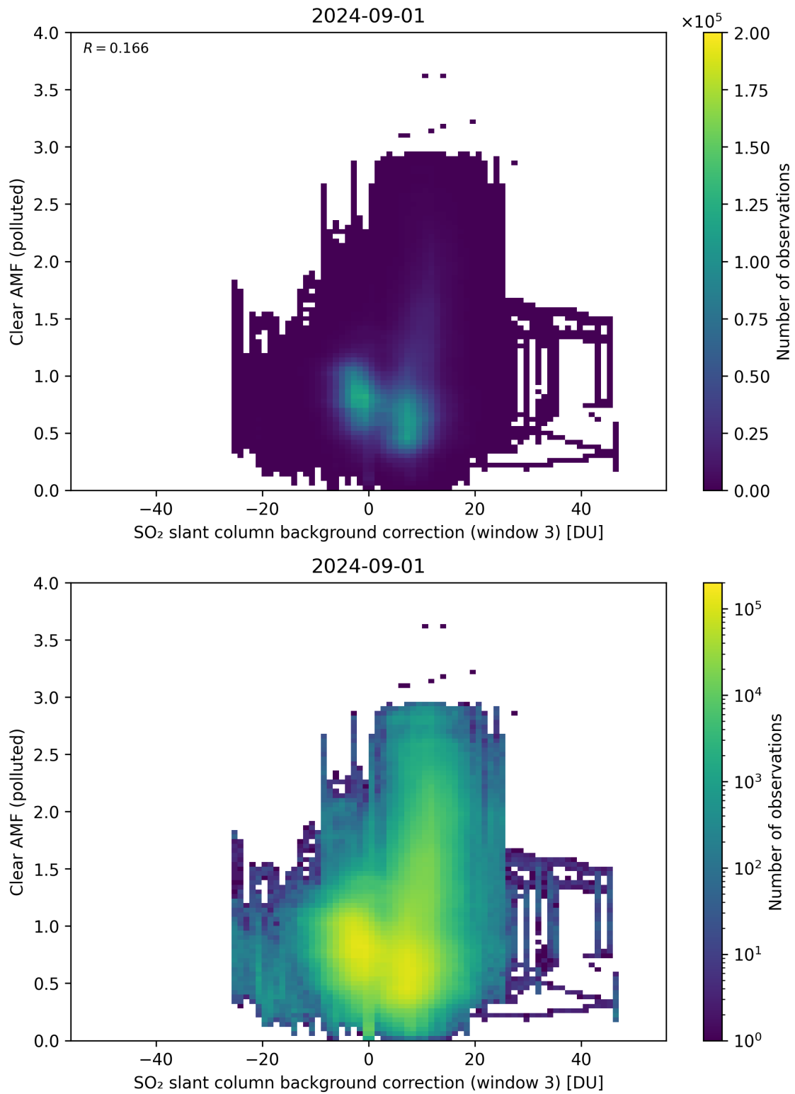
Figure 124: Scatter density plot of “SO 2 slant column background correction (window 3)” against “Clear AMF (polluted)” for 2024-09-01 to 2024-09-02.
