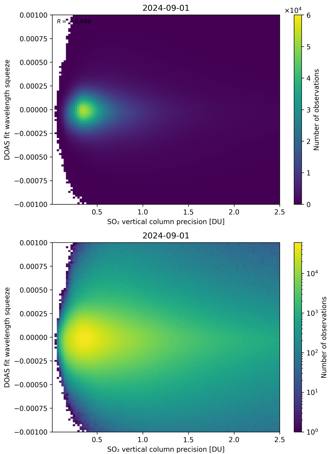
Figure 283: Scatter density plot of “SO 2 vertical column precision” against “DOAS fit wavelength squeeze” for 2024-09-01 to 2024-09-02.
