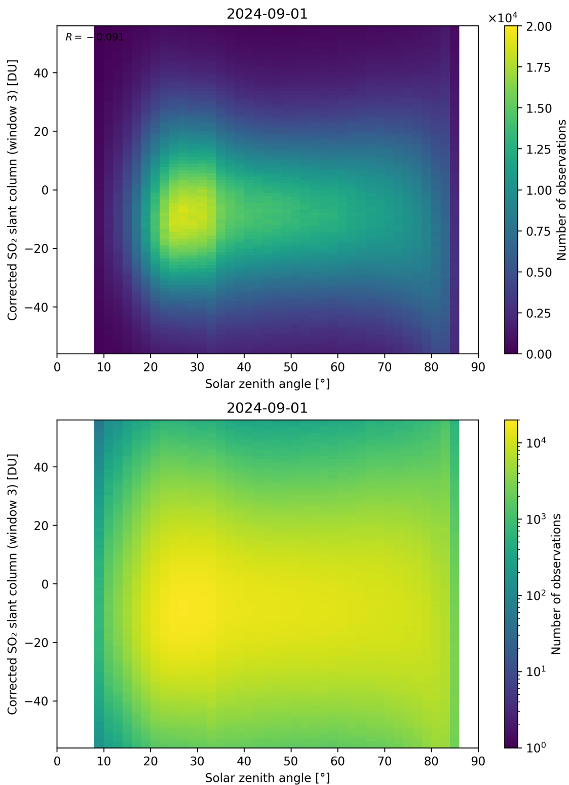
Figure 168: Scatter density plot of “Solar zenith angle” against “Corrected SO 2 slant column (window 3)” for 2024-09-01 to 2024-09-02.
