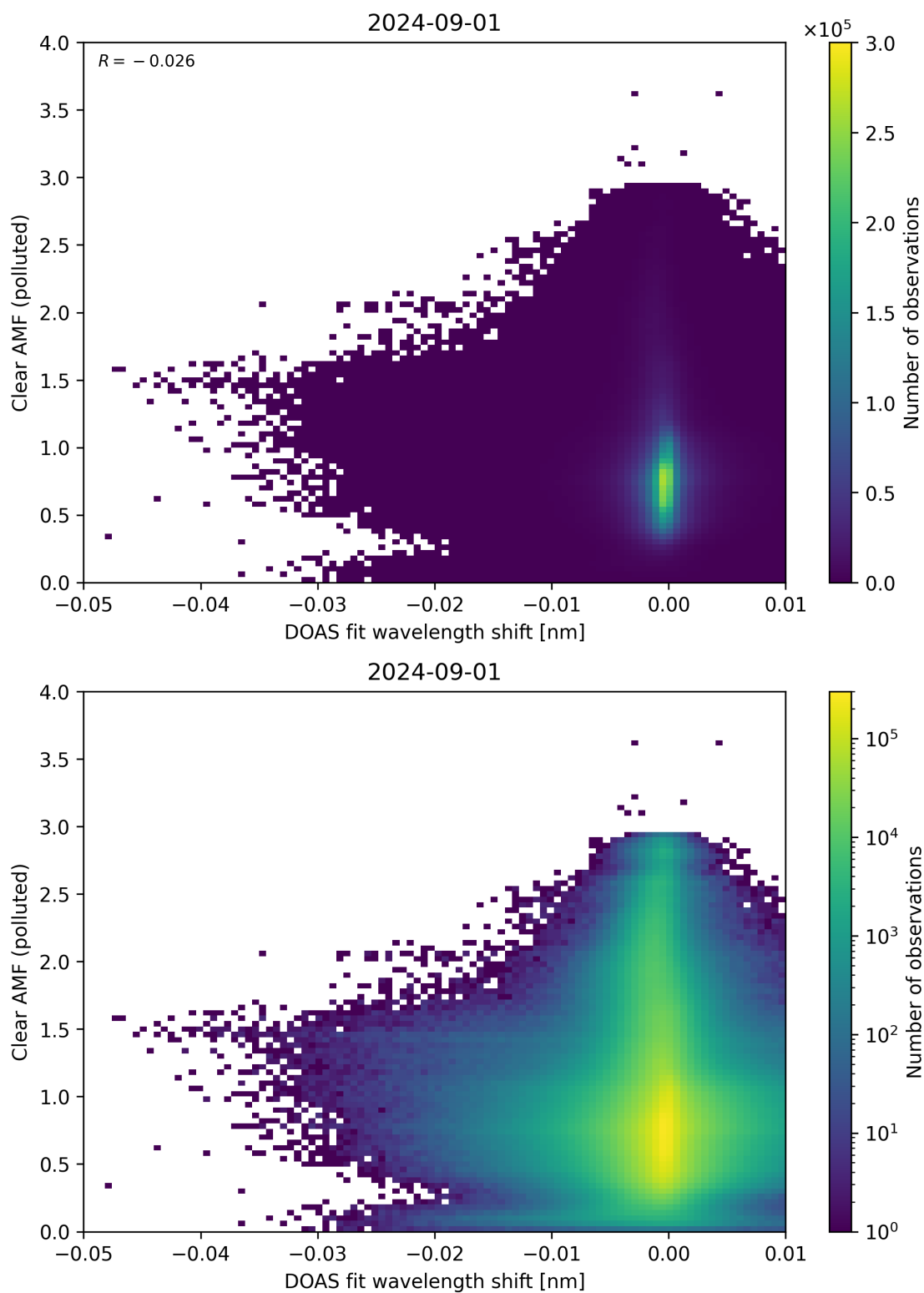
Figure 129: Scatter density plot of “DOAS fit wavelength shift” against “Clear AMF (polluted)” for 2024-09-01 to 2024-09-02.
