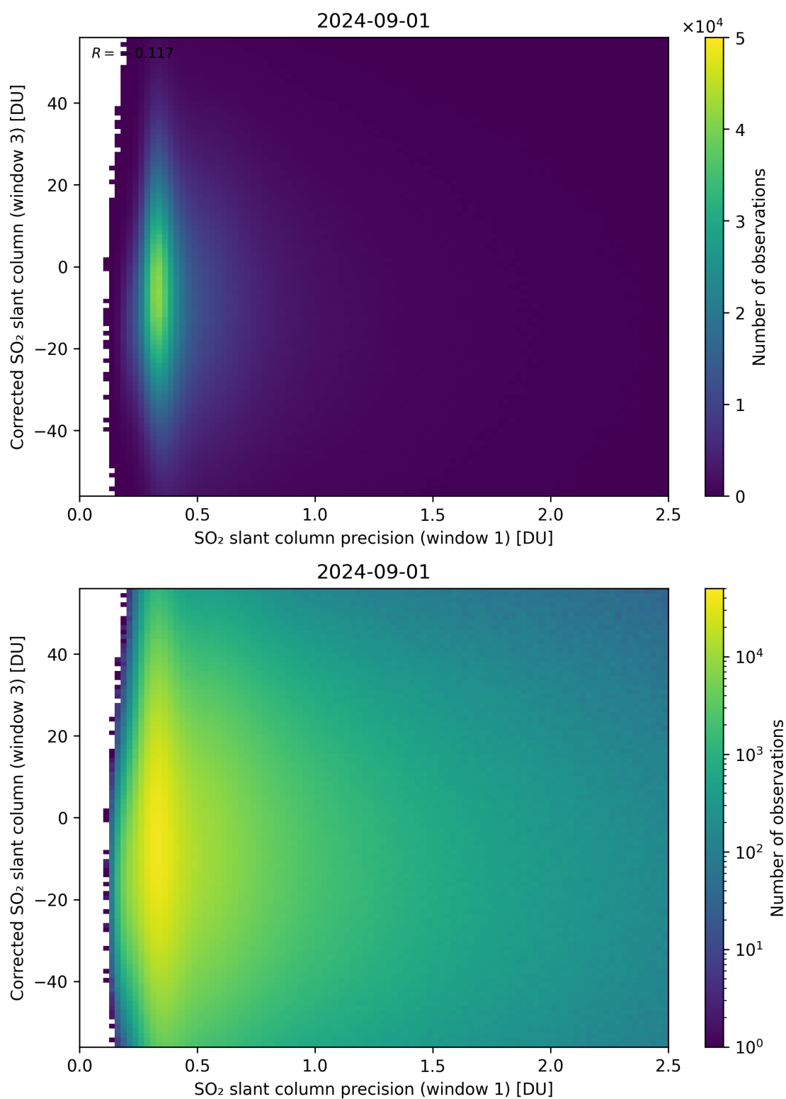
Figure 226: Scatter density plot of “SO 2 slant column precision (window 1)” against “Corrected SO 2 slant column (window 3)” for 2024-09-01 to 2024-09-02.
