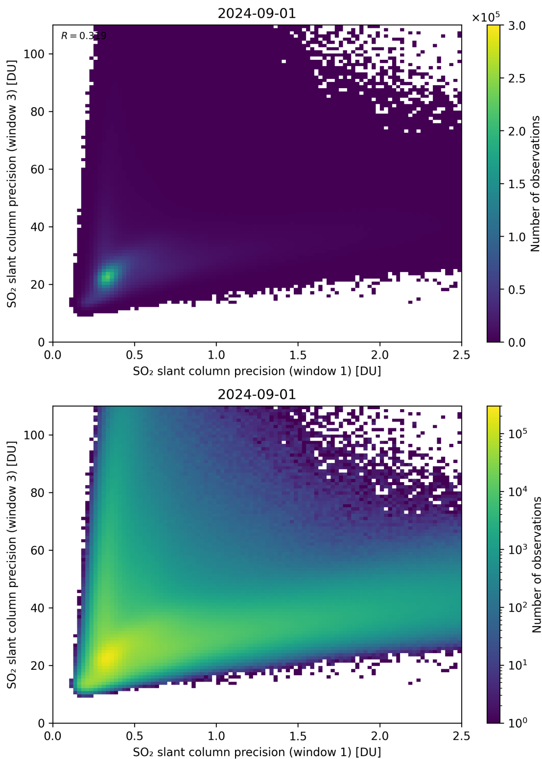
Figure 229: Scatter density plot of “SO 2 slant column precision (window 1)” against “SO 2 slant column precision (window 3)” for 2024-09-01 to 2024-09-02.
