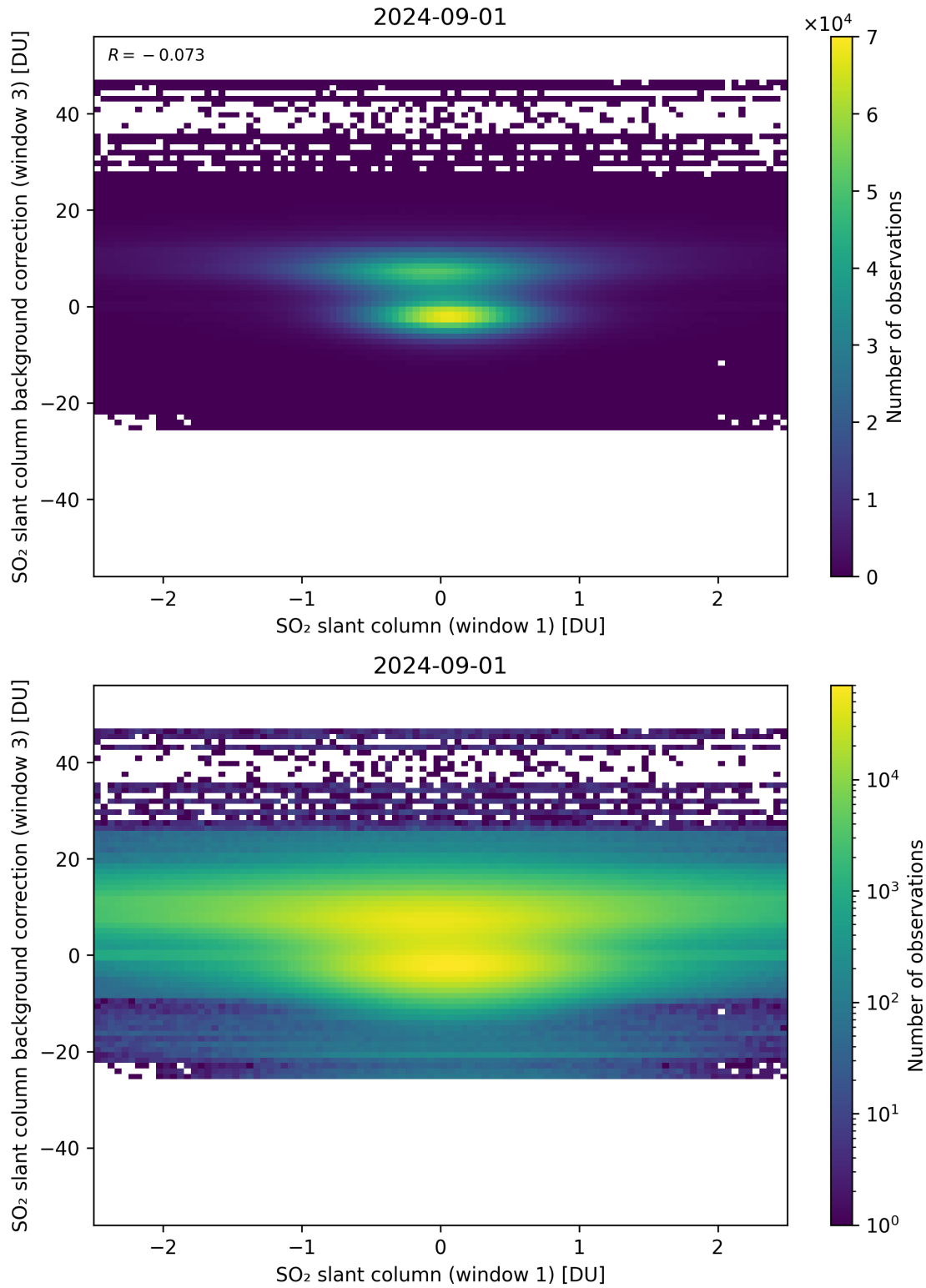
Figure 214: Scatter density plot of “SO 2 slant column (window 1)” against “SO 2 slant column background correction (window 3)” for 2024-09-01 to 2024-09-02.
