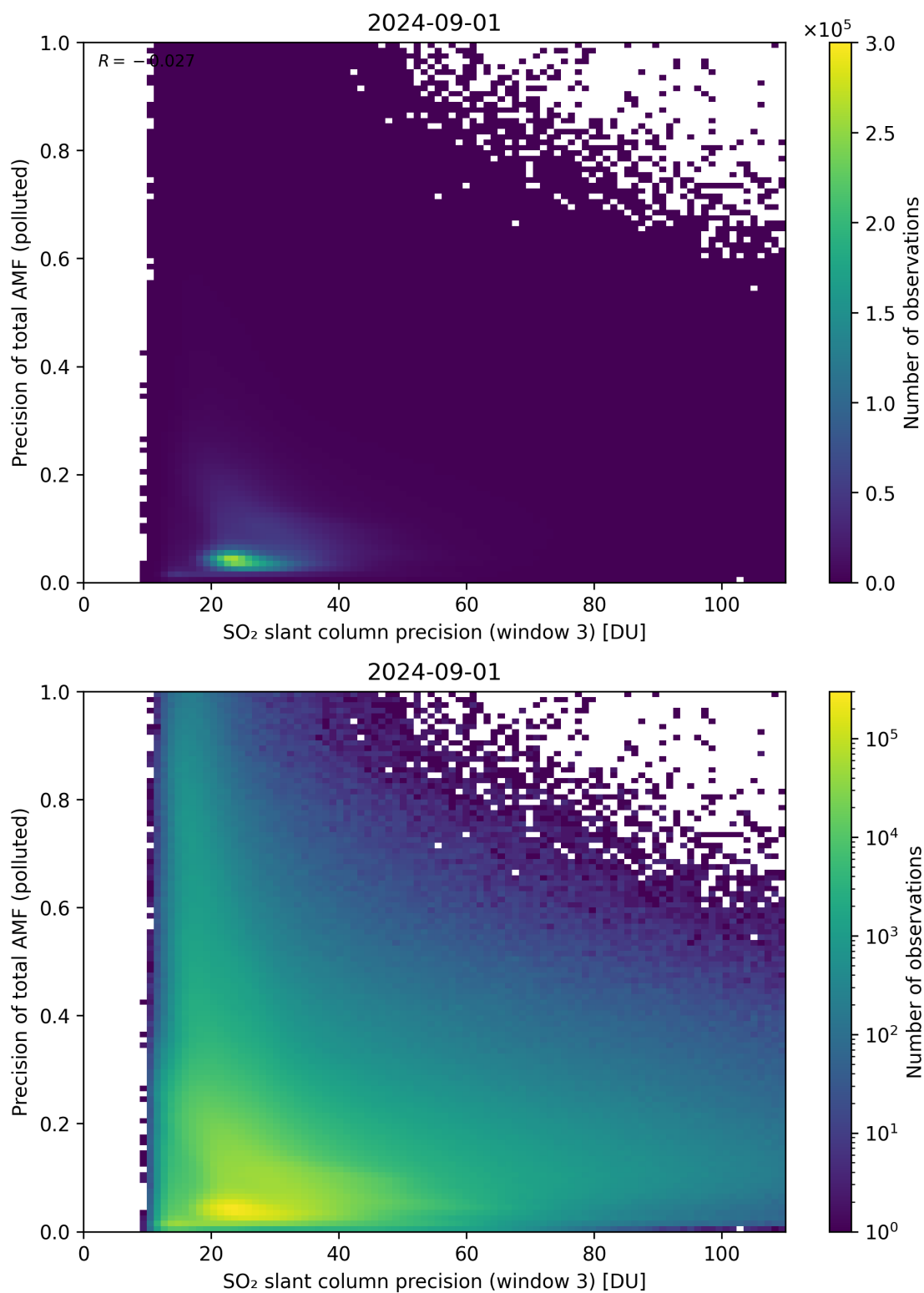
Figure 264: Scatter density plot of “SO 2 slant column precision (window 3)” against “Precision of total AMF (polluted)” for 2024-09-01 to 2024-09-02.
