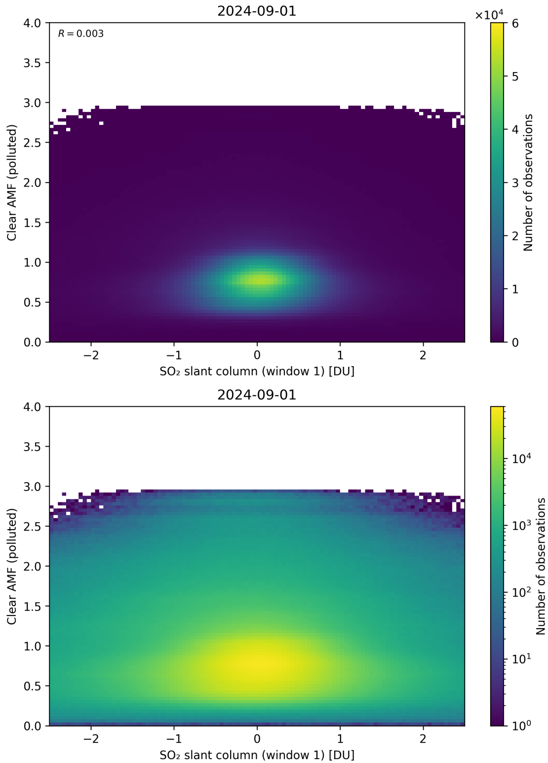
Figure 232: Scatter density plot of “SO 2 slant column (window 1)” against “Clear AMF (polluted)” for 2024-09-01 to 2024-09-02.
