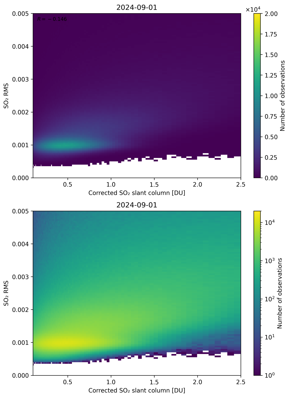
Figure 183: Scatter density plot of “Corrected SO 2 slant column” against “SO 2 RMS” for 2024-09-01 to 2024-09-02.
