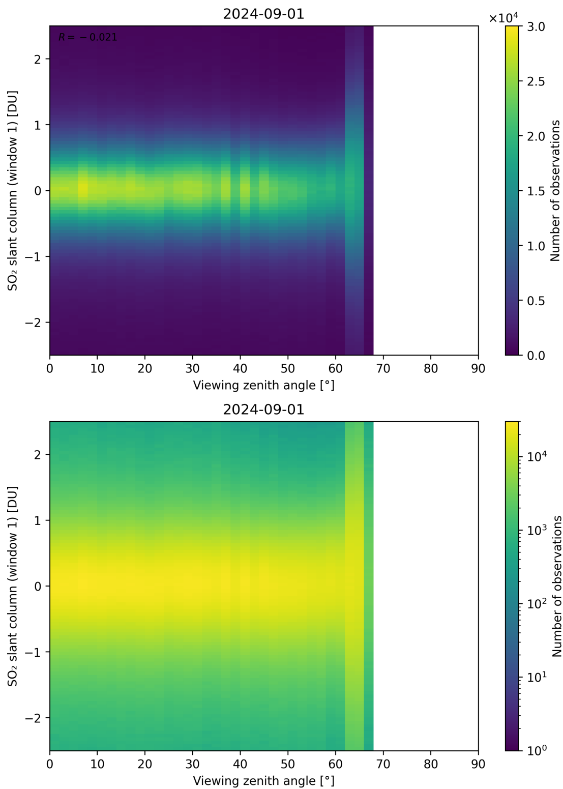
Figure 320: Scatter density plot of “Viewing zenith angle” against “SO 2 slant column (window 1)” for 2024-09-01 to 2024-09-02.
