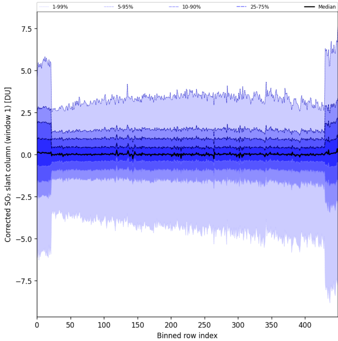
Figure 81: Along track statistics of “Corrected SO 2 slant column (window 1)” for 2024-09-01 to 2024-09-02
