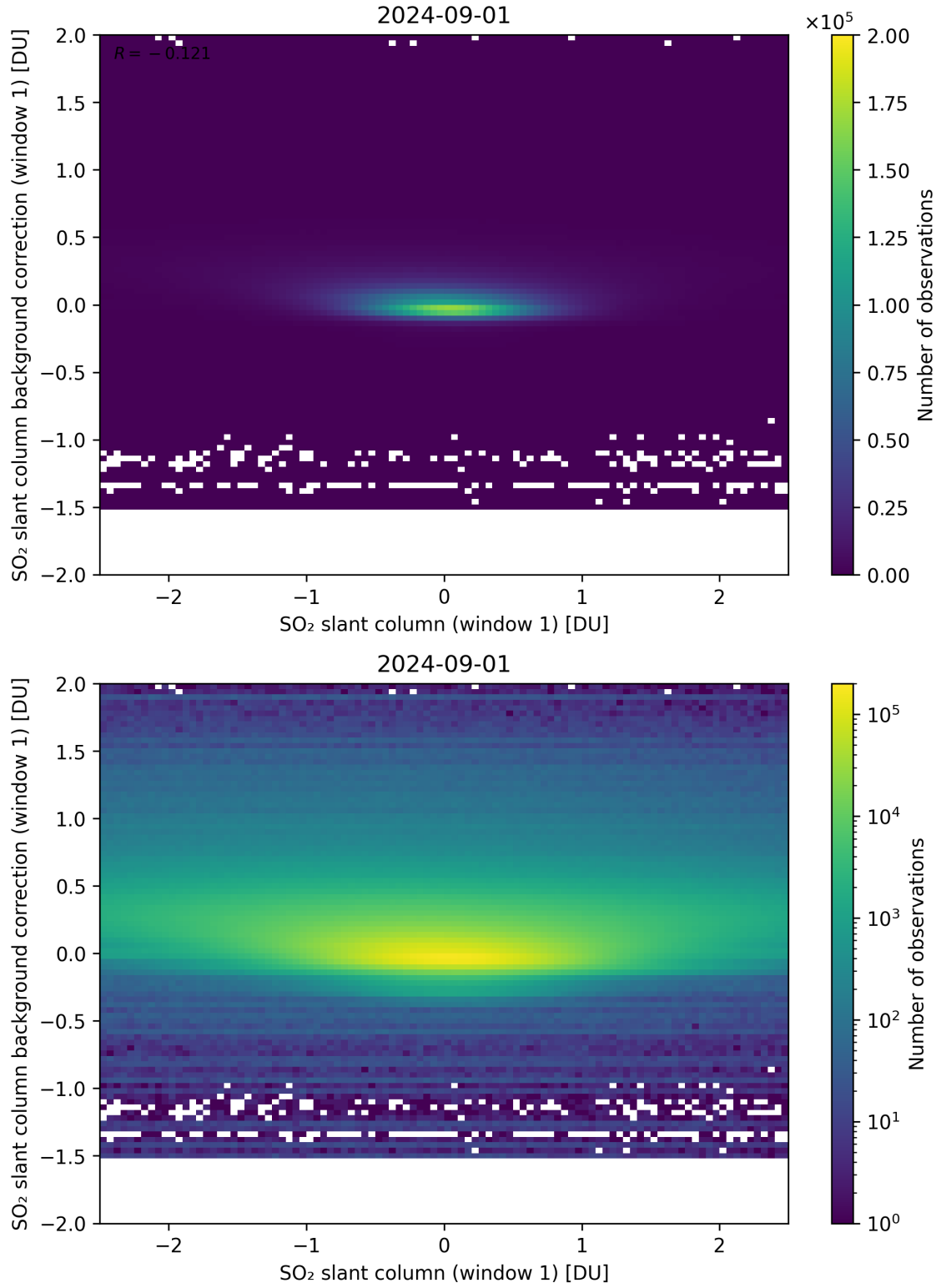
Figure 212: Scatter density plot of “SO 2 slant column (window 1)” against “SO 2 slant column background correction (window 1)” for 2024-09-01 to 2024-09-02.
