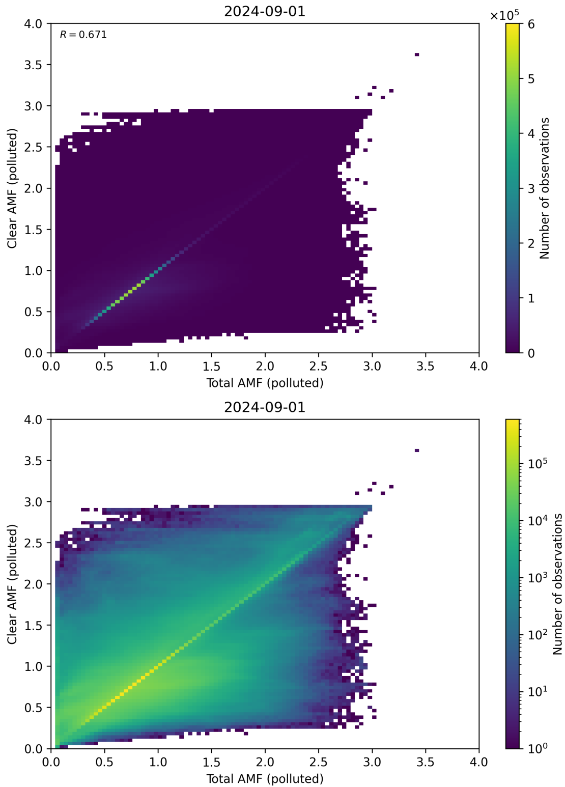
Figure 271: Scatter density plot of “Total AMF (polluted)” against “Clear AMF (polluted)” for 2024-09-01 to 2024-09-02.
