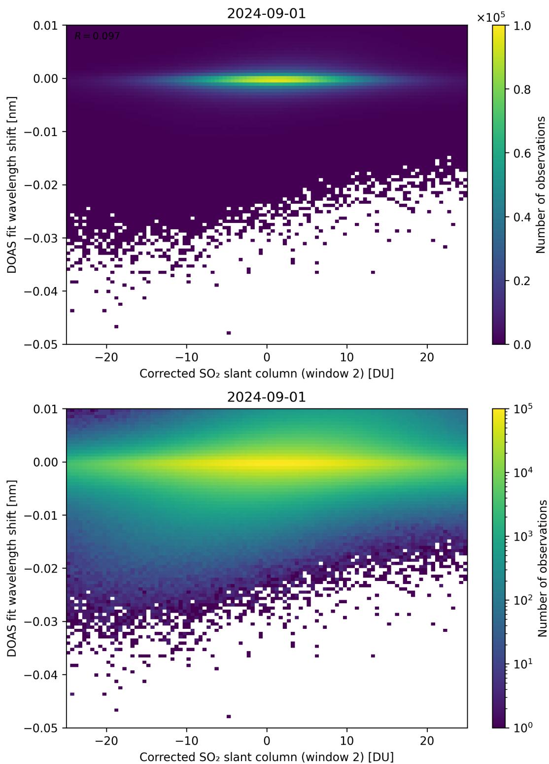
Figure 196: Scatter density plot of “Corrected SO 2 slant column (window 2)” against “DOAS fit wavelength shift” for 2024-09-01 to 2024-09-02.
