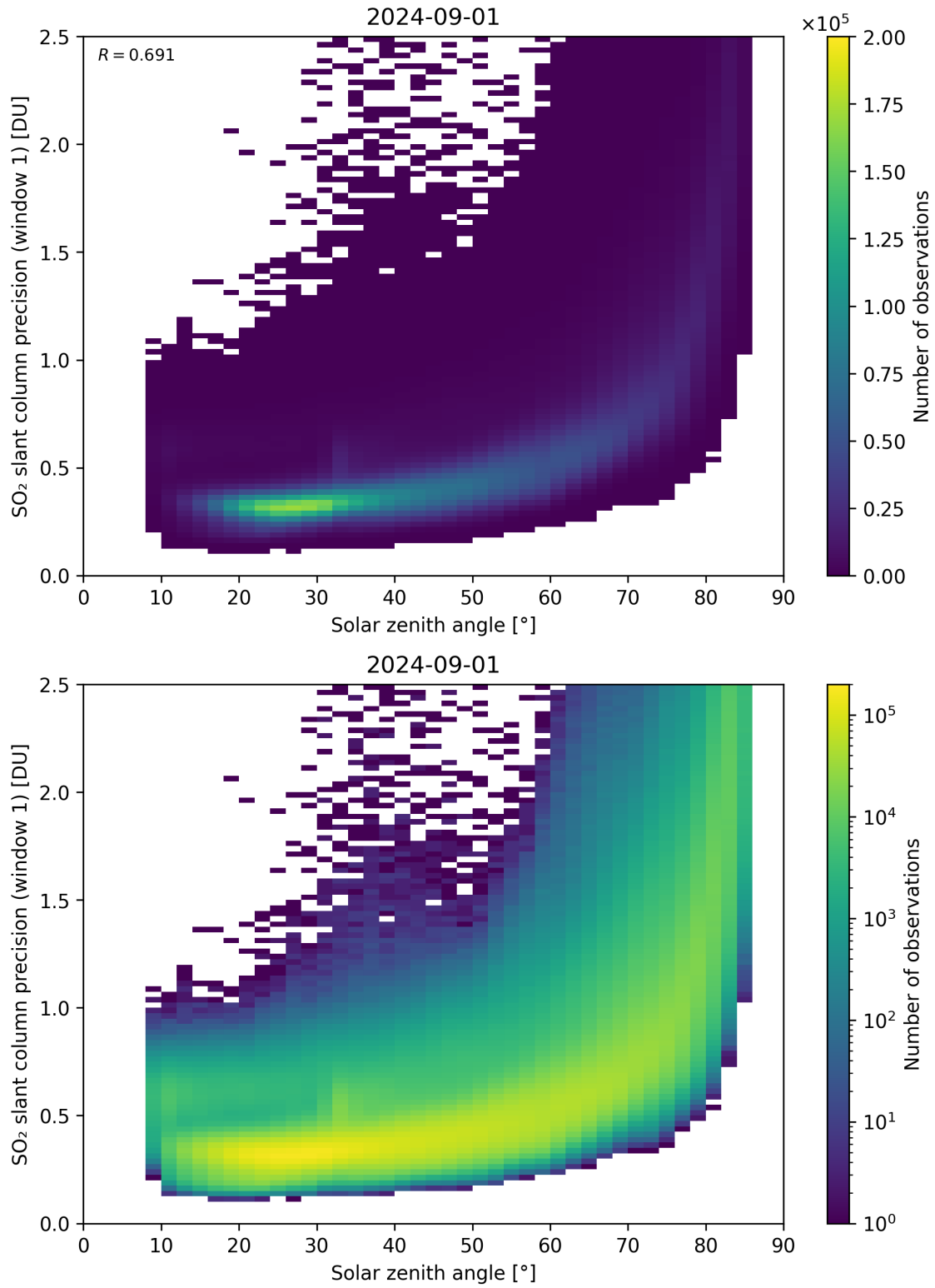
Figure 170: Scatter density plot of “Solar zenith angle” against “SO 2 slant column precision (window 1)” for 2024-09-01 to 2024-09-02.
