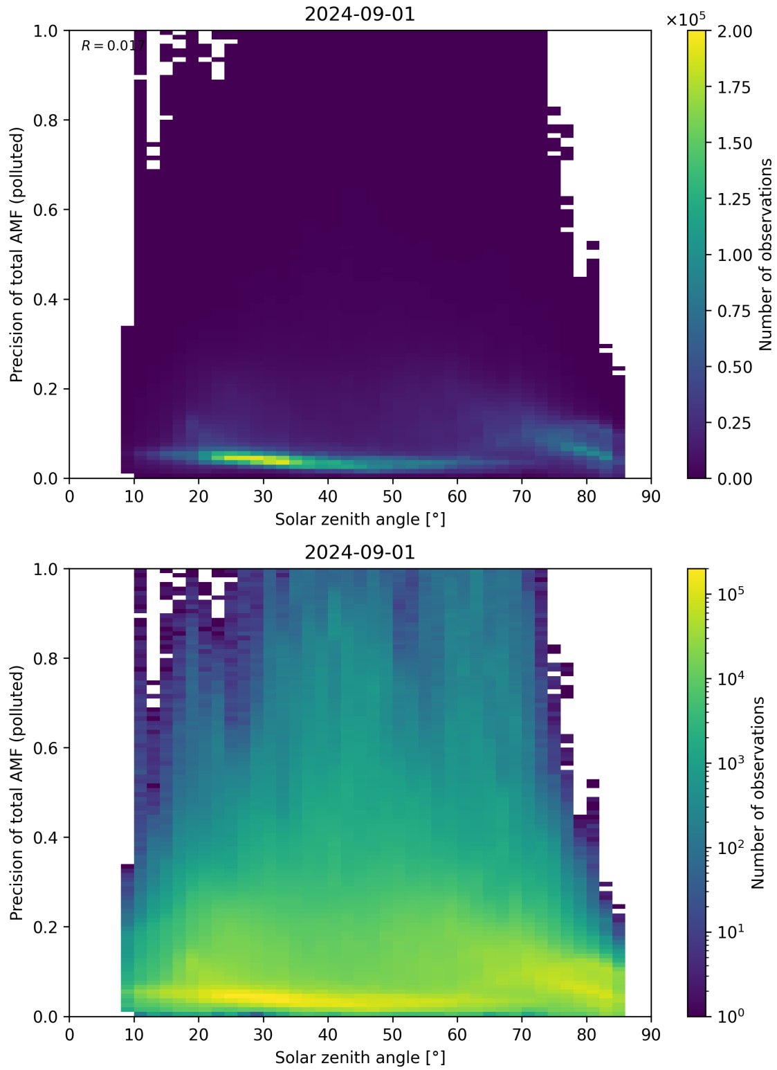
Figure 175: Scatter density plot of “Solar zenith angle” against “Precision of total AMF (polluted)” for 2024-09-01 to 2024-09-02.
