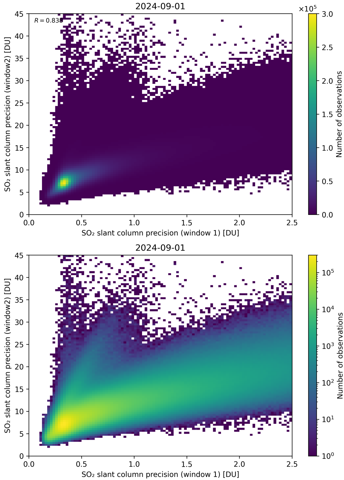
Figure 227: Scatter density plot of “SO 2 slant column precision (window 1)” against “SO 2 slant column precision (window2)” for 2024-09-01 to 2024-09-02.
