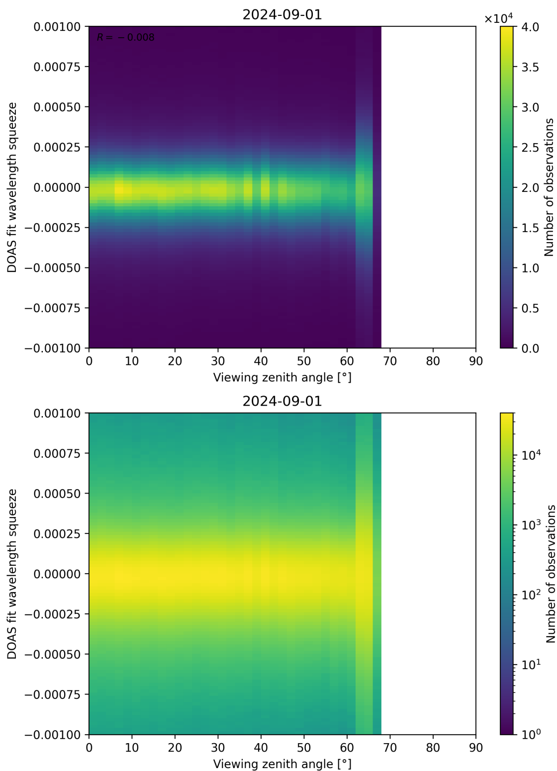
Figure 312: Scatter density plot of “Viewing zenith angle” against “DOAS fit wavelength squeeze” for 2024-09-01 to 2024-09-02.
