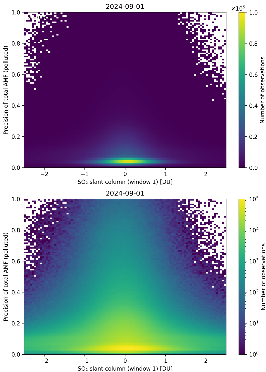
Figure 240: Scatter density plot of “SO 2 slant column (window 1)” against “Precision of total AMF (polluted)” for 2024-09-01 to 2024-09-02.
