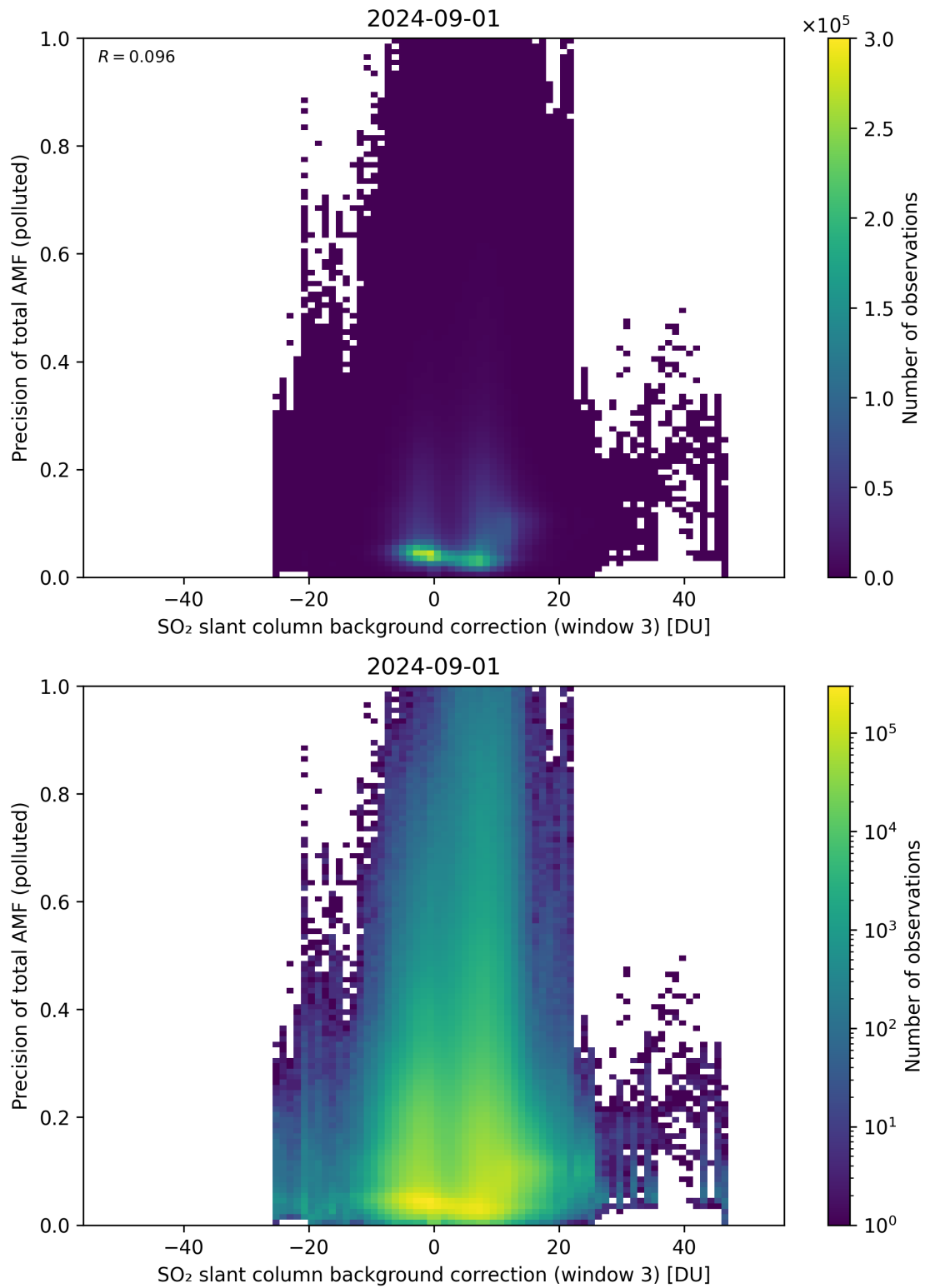
Figure 126: Scatter density plot of “SO 2 slant column background correction (window 3)” against “Precision of total AMF (polluted)” for 2024-09-01 to 2024-09-02.
