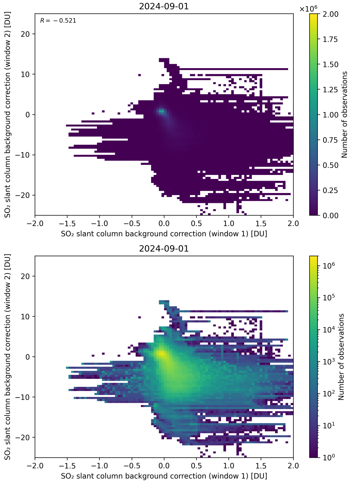
Figure 98: Scatter density plot of “SO 2 slant column background correction (window 1)” against “SO 2 slant column background correction (window 2)” for 2024-09-01 to 2024-09-02.
