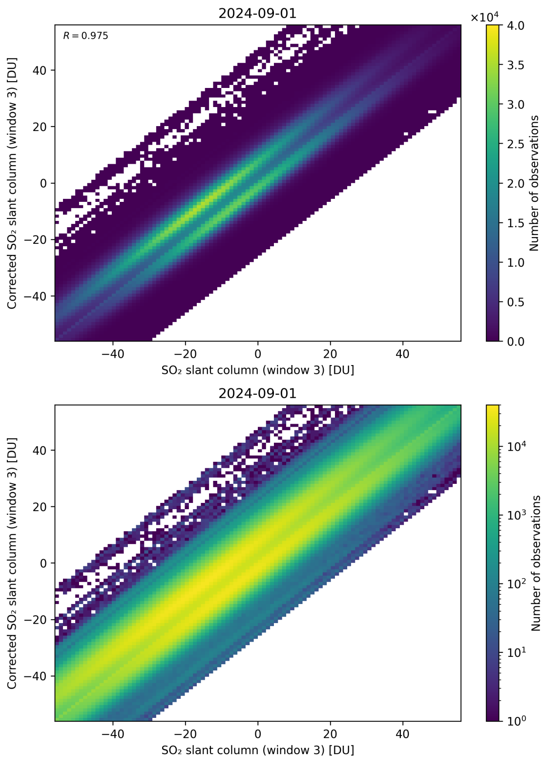
Figure 266: Scatter density plot of “SO 2 slant column (window 3)” against “Corrected SO 2 slant column (window 3)” for 2024-09-01 to 2024-09-02.
