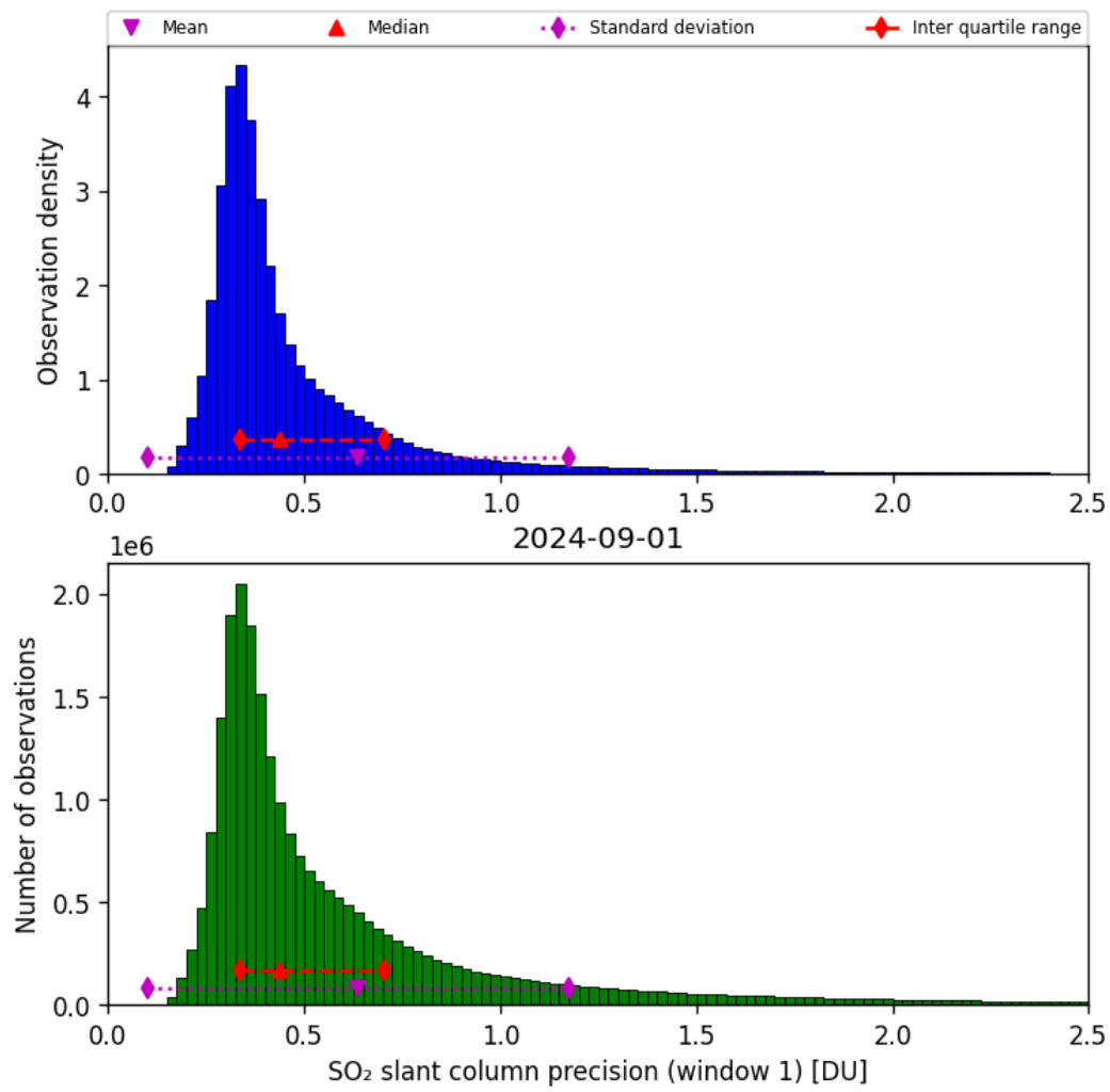
Figure 57: Histogram of “SO 2 slant column precision (window 1)” for 2024-09-01 to 2024-09-02
