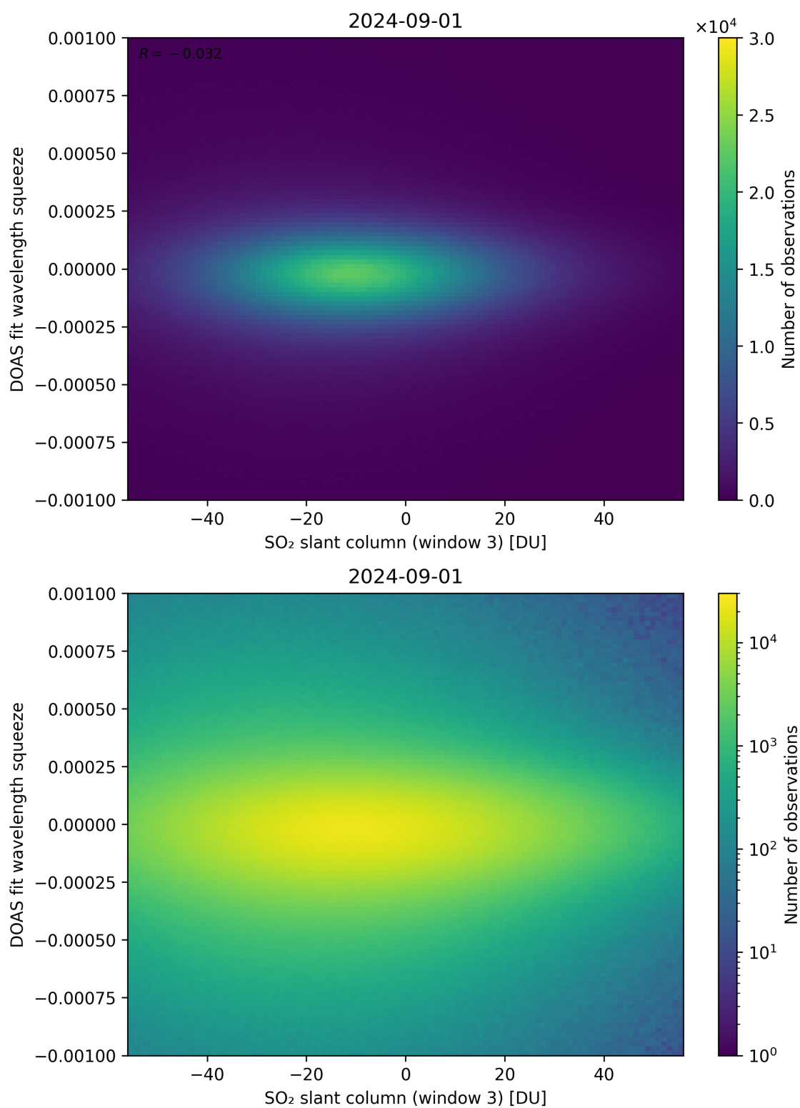
Figure 255: Scatter density plot of “SO 2 slant column (window 3)” against “DOAS fit wavelength squeeze” for 2024-09-01 to 2024-09-02.
