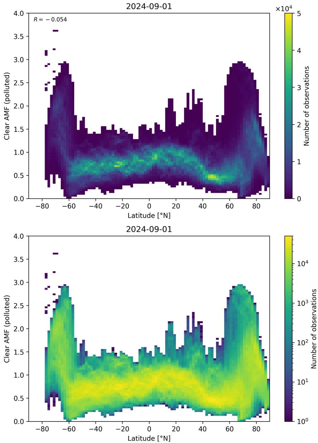
Figure 145: Scatter density plot of “Latitude” against “Clear AMF (polluted)” for 2024-09-01 to 2024-09-02.
