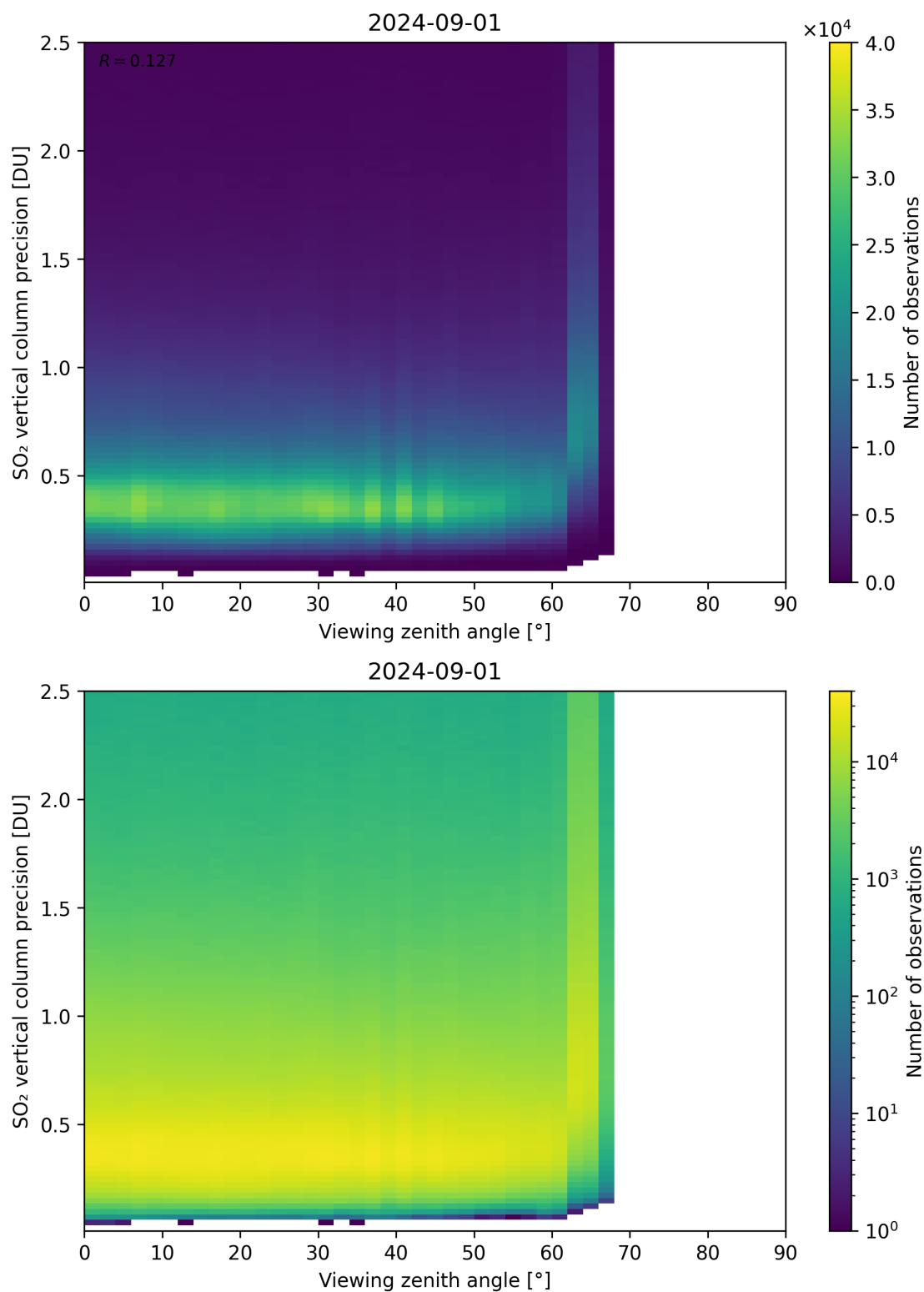
Figure 328: Scatter density plot of “Viewing zenith angle” against “SO 2 vertical column precision” for 2024-09-01 to 2024-09-02.
