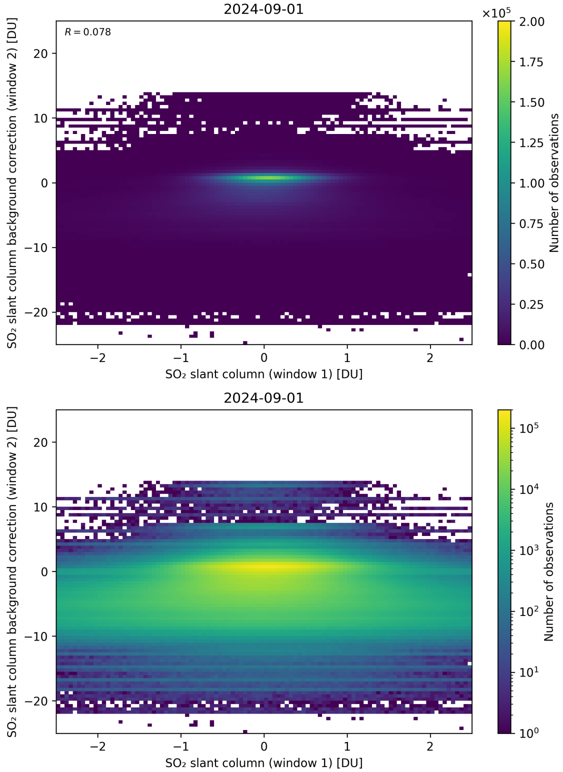
Figure 213: Scatter density plot of “SO 2 slant column (window 1)” against “SO 2 slant column background correction (window 2)” for 2024-09-01 to 2024-09-02.
