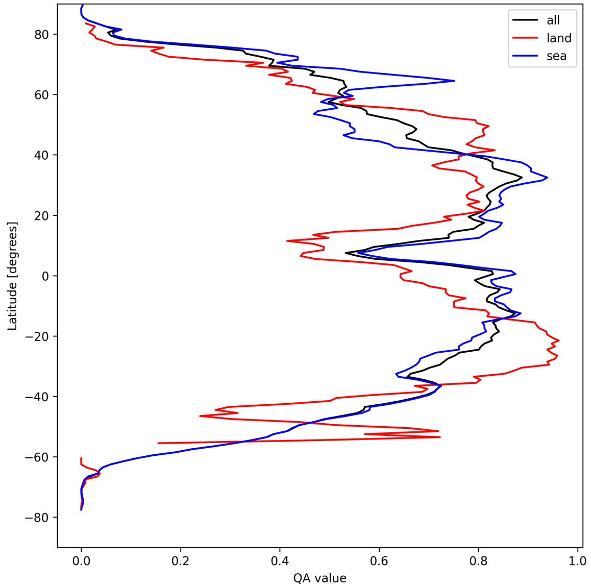
Figure 29: Zonal average of “QA value” for 2024-09-01 to 2024-09-02.
