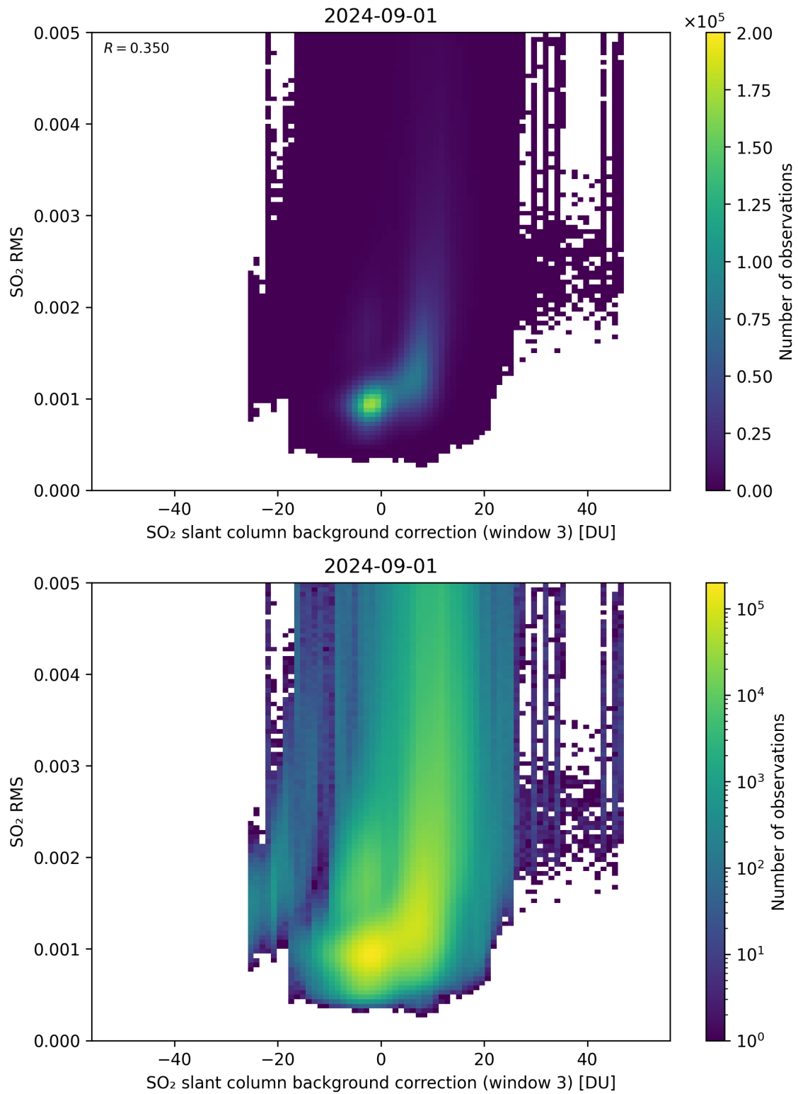
Figure 123: Scatter density plot of “SO 2 slant column background correction (window 3)” against “SO 2 RMS” for 2024-09-01 to 2024-09-02.
