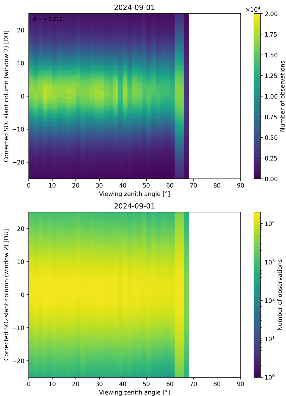
Figure 318: Scatter density plot of “Viewing zenith angle” against “Corrected SO 2 slant column (window 2)” for 2024-09-01 to 2024-09-02.
