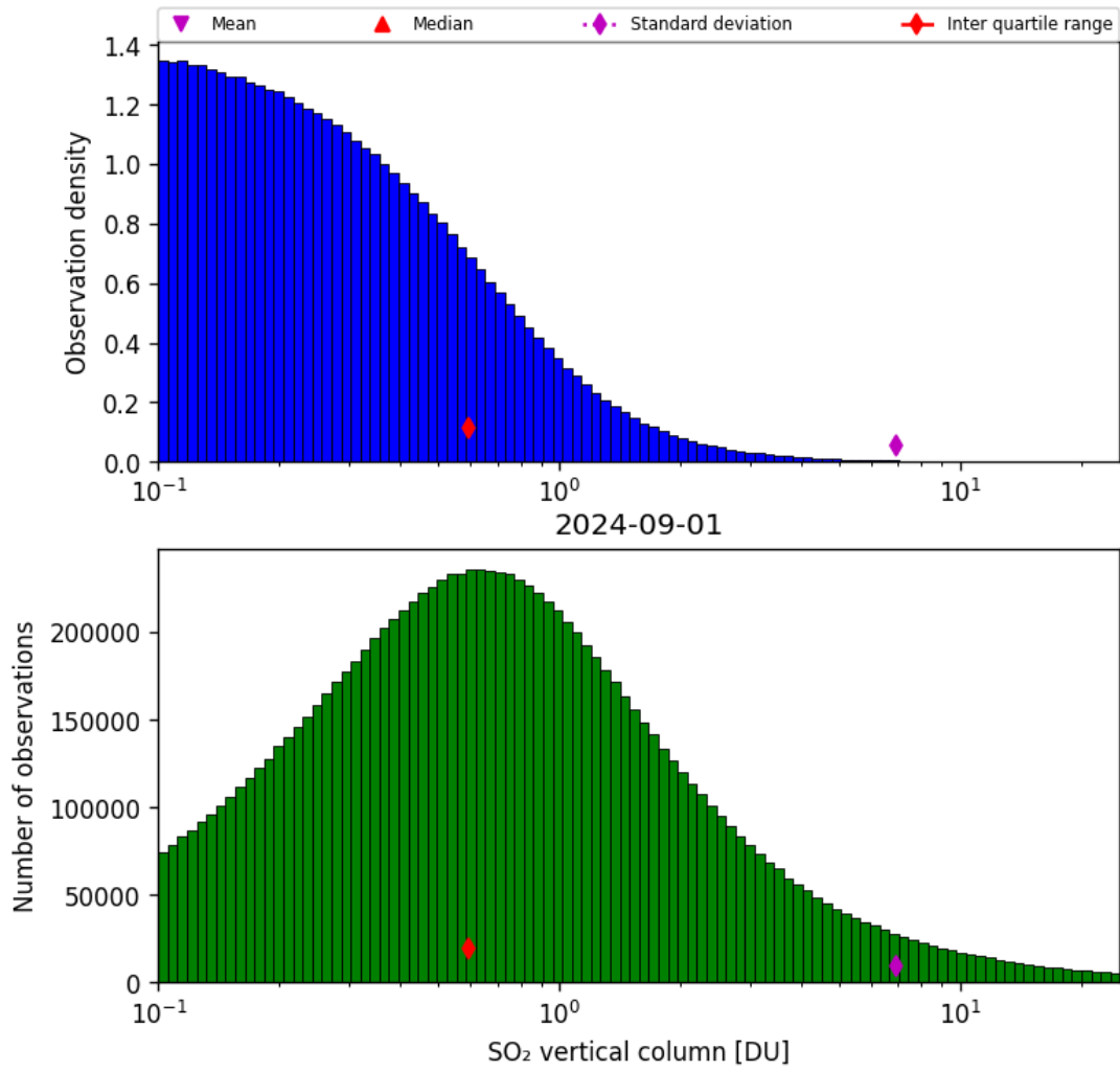
Figure 53: Histogram of “SO 2 vertical column” for 2024-09-01 to 2024-09-02
