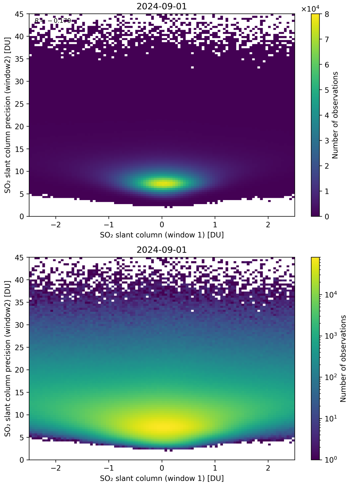
Figure 236: Scatter density plot of “SO 2 slant column (window 1)” against “SO 2 slant column precision (window2)” for 2024-09-01 to 2024-09-02.
