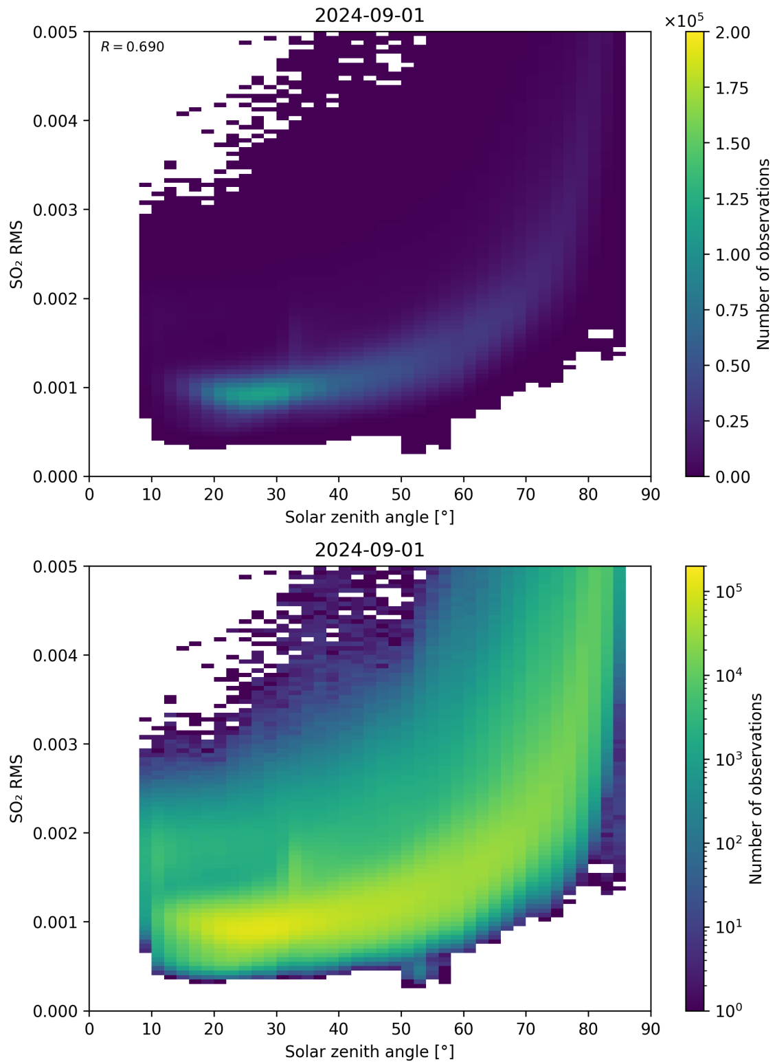
Figure 163: Scatter density plot of “Solar zenith angle” against “SO 2 RMS” for 2024-09-01 to 2024-09-02.
