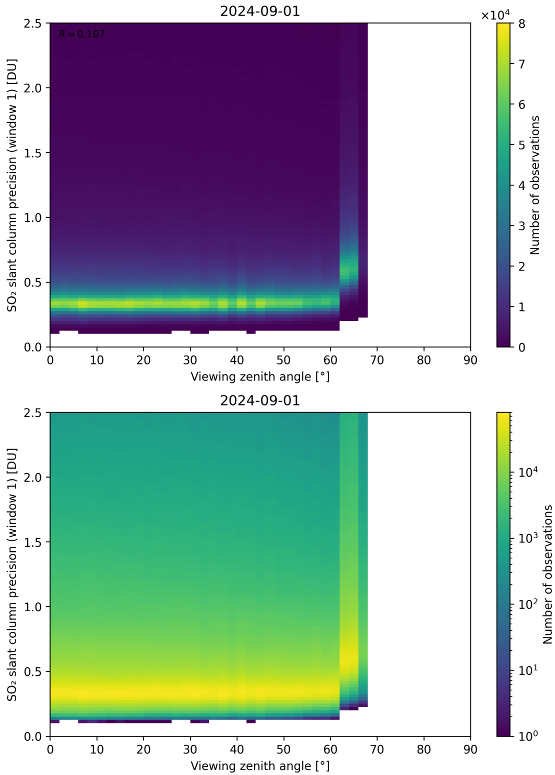
Figure 321: Scatter density plot of “Viewing zenith angle” against “SO 2 slant column precision (window 1)” for 2024-09-01 to 2024-09-02.
