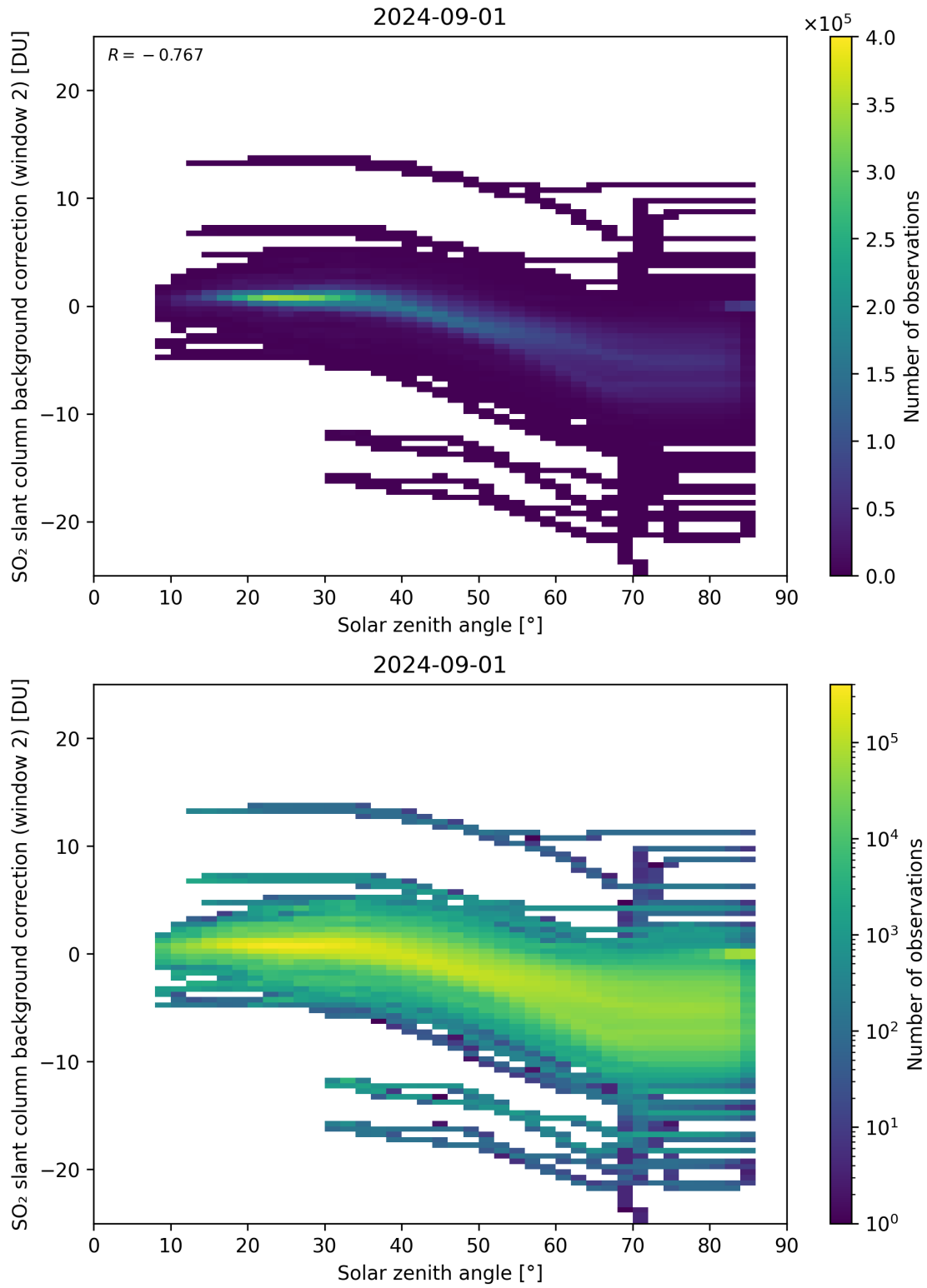
Figure 159: Scatter density plot of “Solar zenith angle” against “SO 2 slant column background correction (window 2)” for 2024-09-01 to 2024-09-02.
