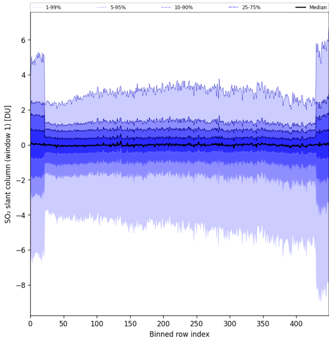
Figure 79: Along track statistics of “SO 2 slant column (window 1)” for 2024-09-01 to 2024-09-02
