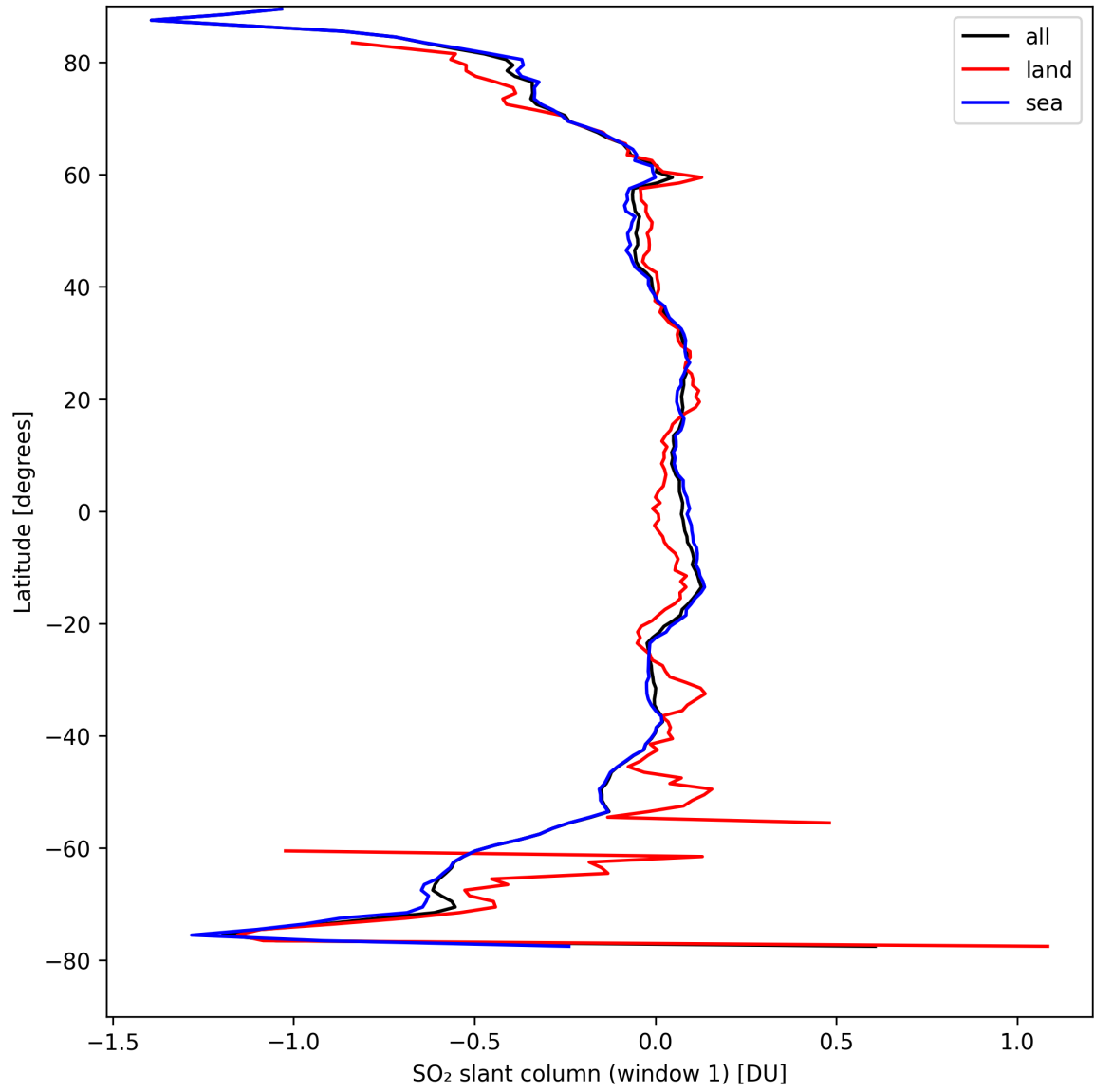
Figure 33: Zonal average of “SO 2 slant column (window 1)” for 2024-09-01 to 2024-09-02.
