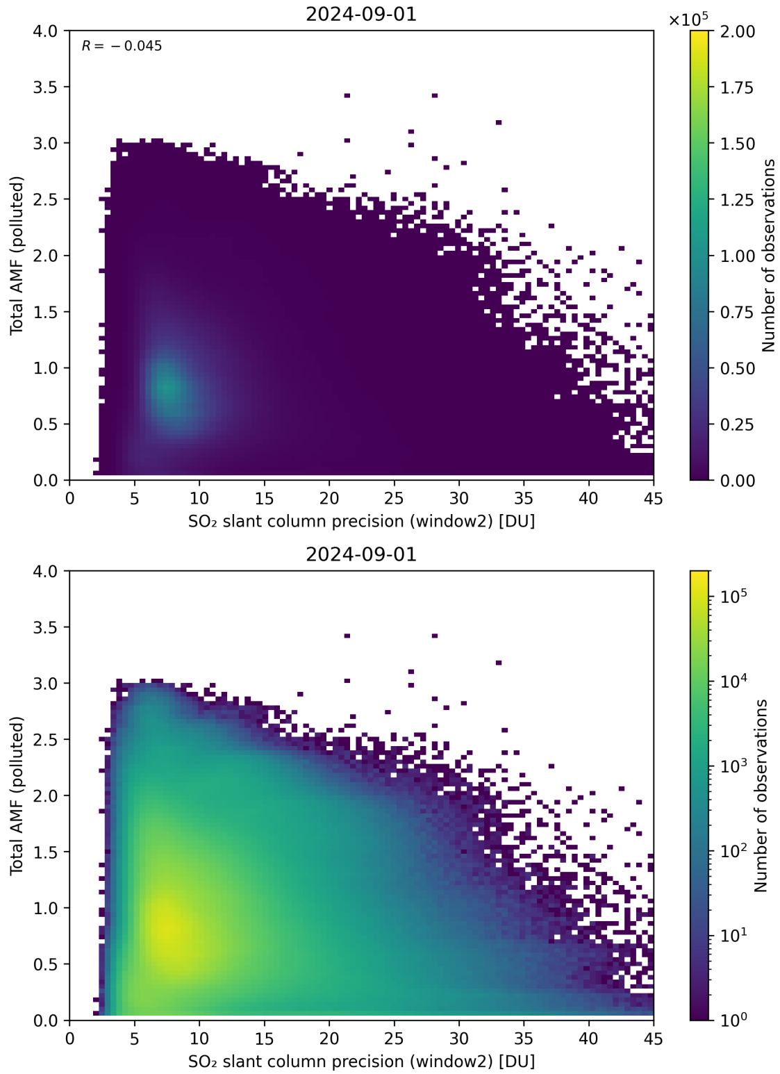
Figure 251: Scatter density plot of “SO 2 slant column precision (window2)” against “Total AMF (polluted)” for 2024-09-01 to 2024-09-02.
