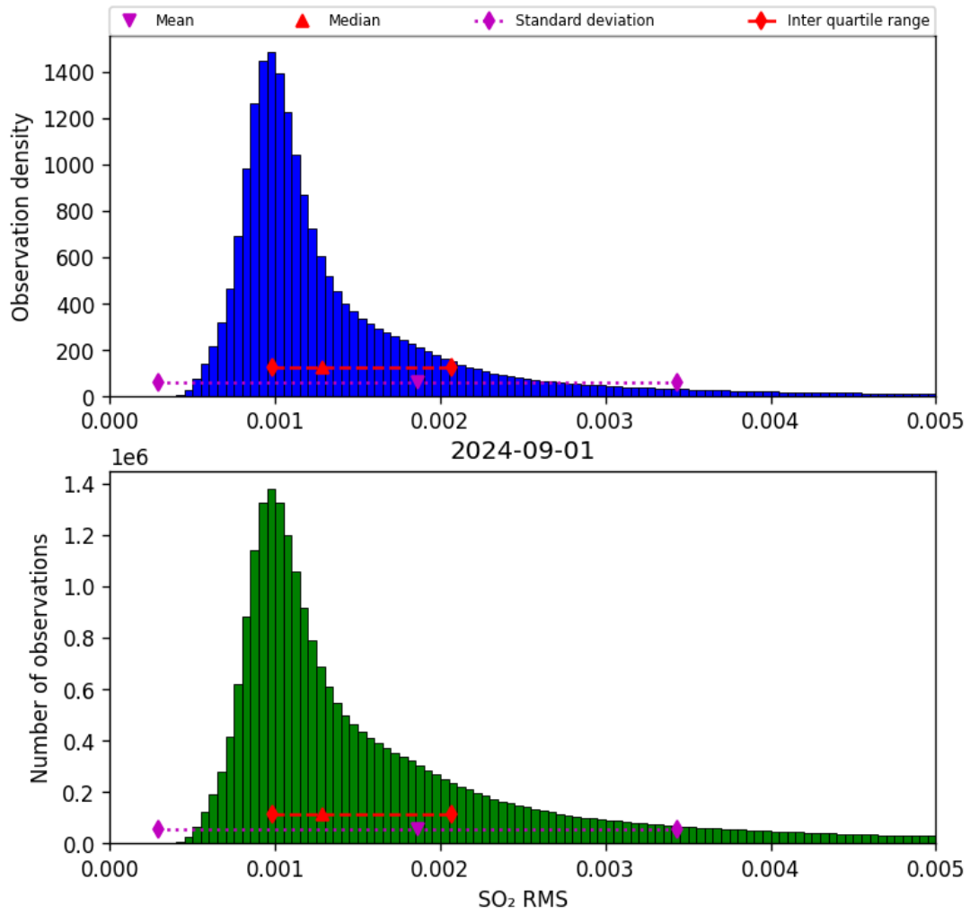
Figure 70: Histogram of “SO 2 RMS” for 2024-09-01 to 2024-09-02
