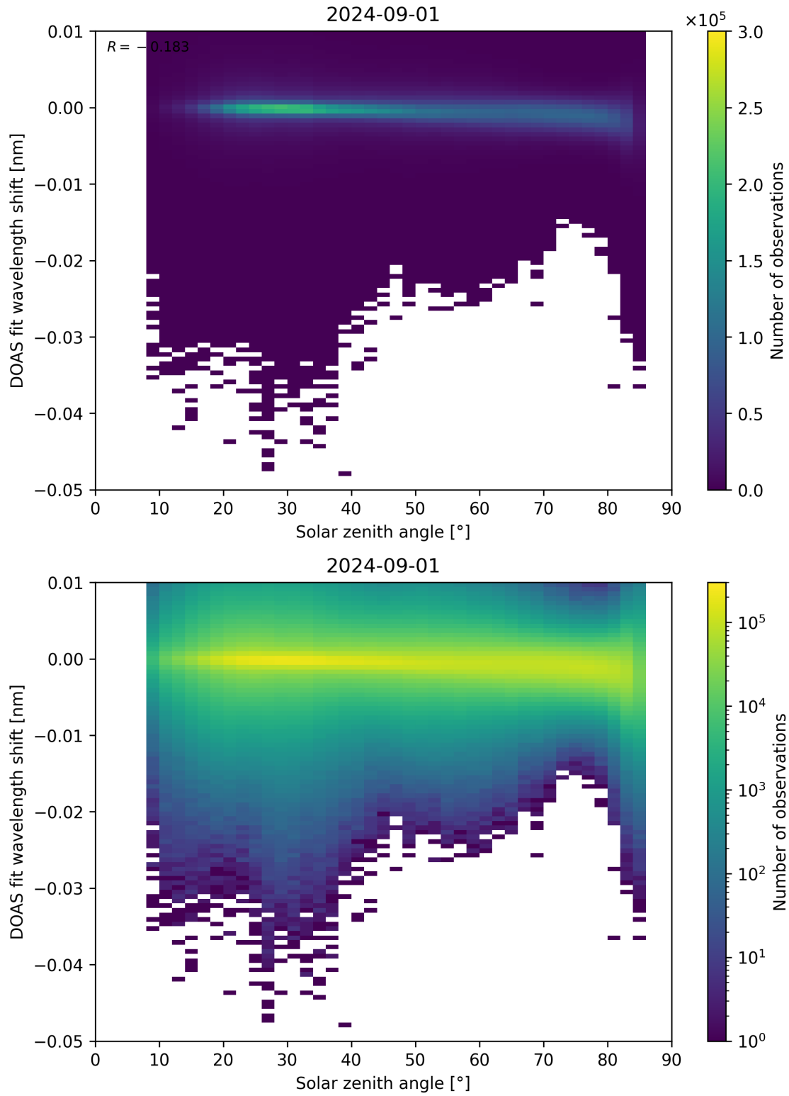
Figure 161: Scatter density plot of “Solar zenith angle” against “DOAS fit wavelength shift” for 2024-09-01 to 2024-09-02.
