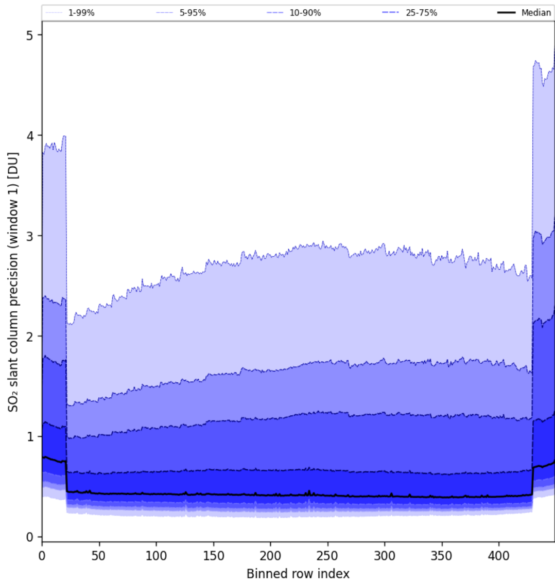
Figure 80: Along track statistics of “SO 2 slant column precision (window 1)” for 2024-09-01 to 2024-09-02
