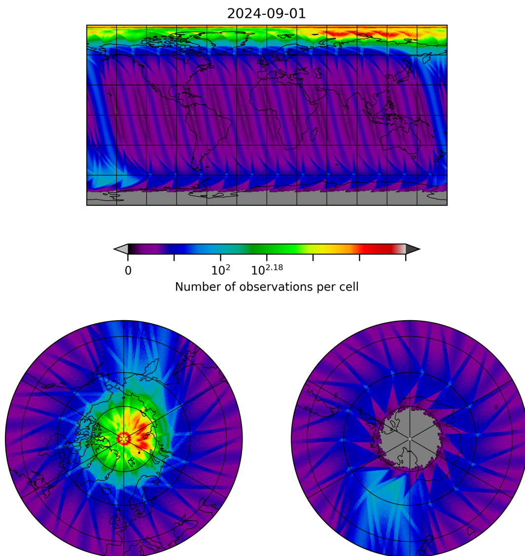
Figure 28: Map of the number of observations for 2024-09-01 to 2024-09-02
