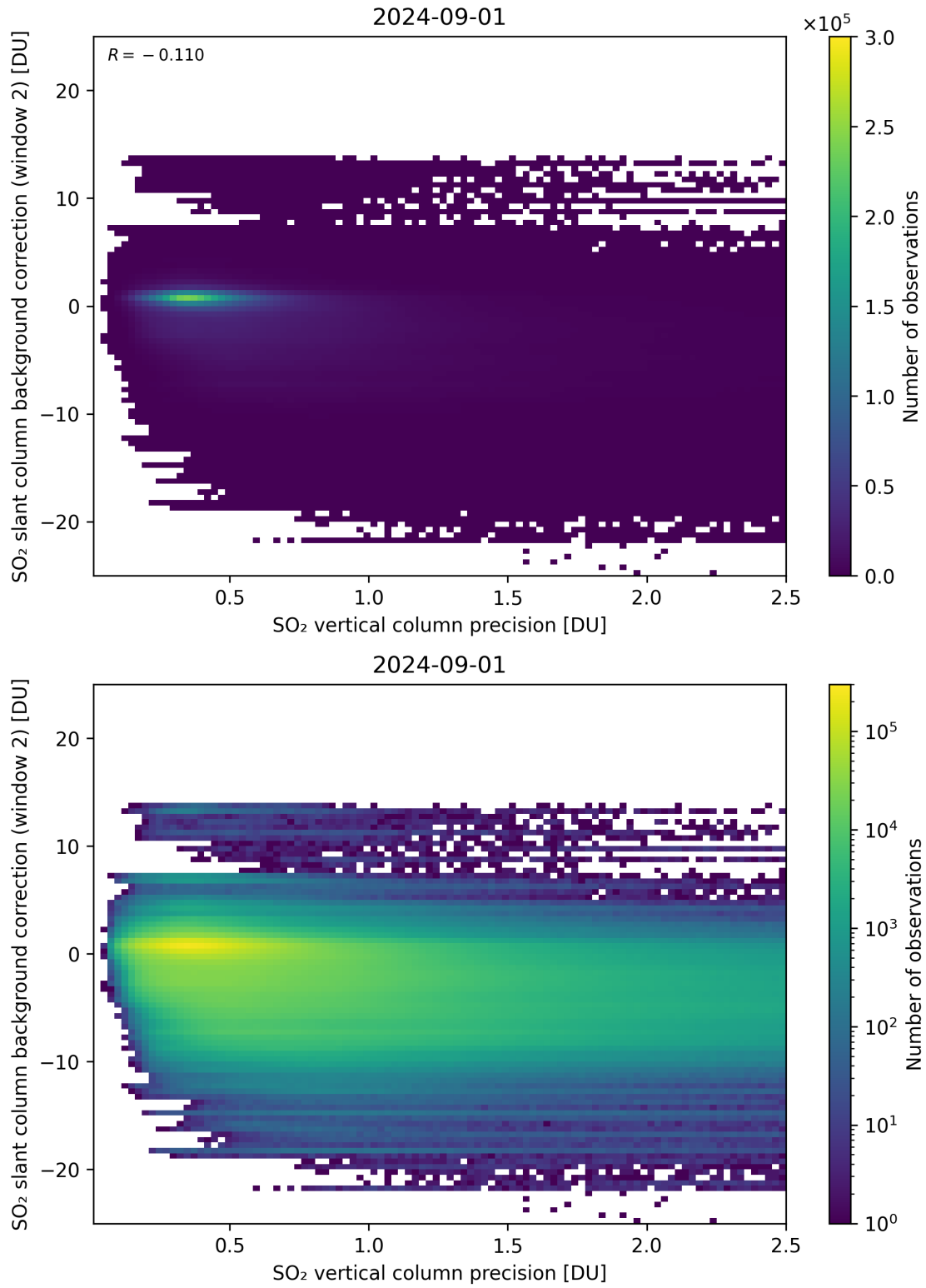
Figure 280: Scatter density plot of “SO 2 vertical column precision” against “SO 2 slant column background correction (window 2)” for 2024-09-01 to 2024-09-02.
