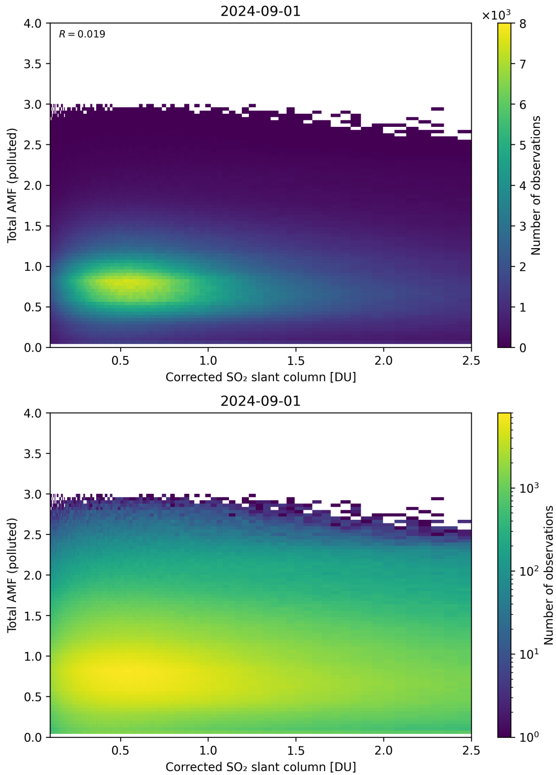
Figure 192: Scatter density plot of “Corrected SO 2 slant column” against “Total AMF (polluted)” for 2024-09-01 to 2024-09-02.
