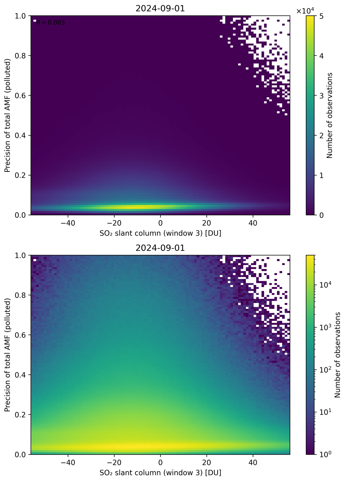
Figure 269: Scatter density plot of “SO 2 slant column (window 3)” against “Precision of total AMF (polluted)” for 2024-09-01 to 2024-09-02.
