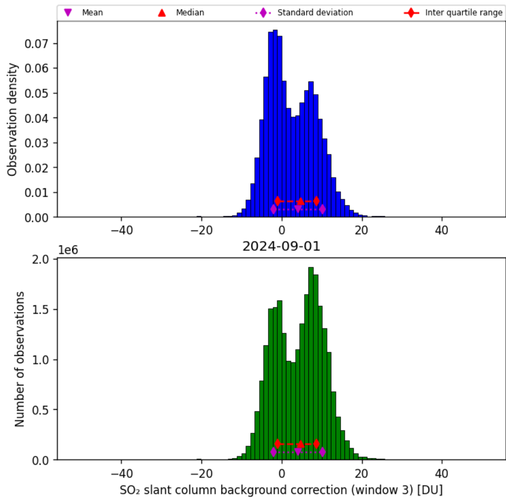
Figure 67: Histogram of “SO 2 slant column background correction (window 3)” for 2024-09-01 to 2024-09-02
