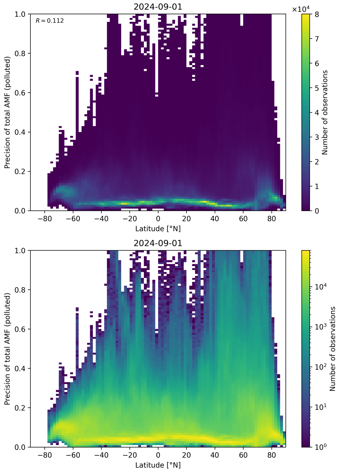
Figure 155: Scatter density plot of “Latitude” against “Precision of total AMF (polluted)” for 2024-09-01 to 2024-09-02.
