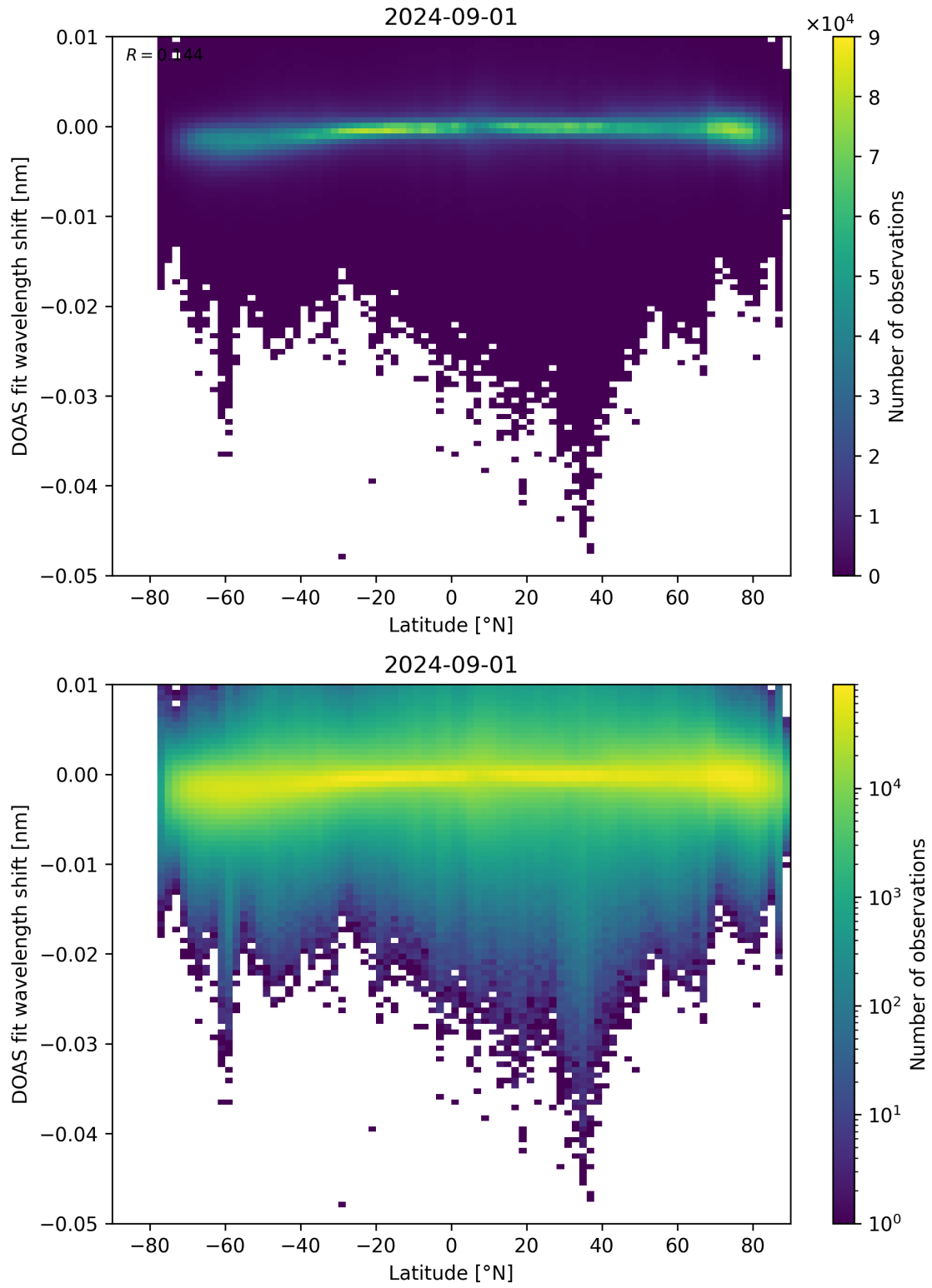
Figure 142: Scatter density plot of “Latitude” against “DOAS fit wavelength shift” for 2024-09-01 to 2024-09-02.
