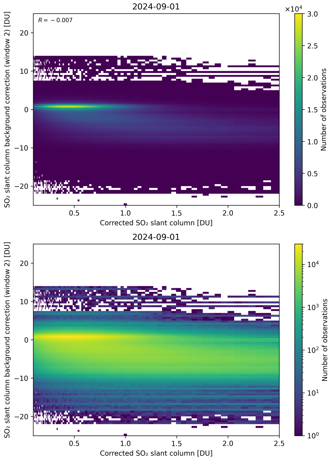
Figure 179: Scatter density plot of “Corrected SO 2 slant column” against “SO 2 slant column background correction (window 2)” for 2024-09-01 to 2024-09-02.
