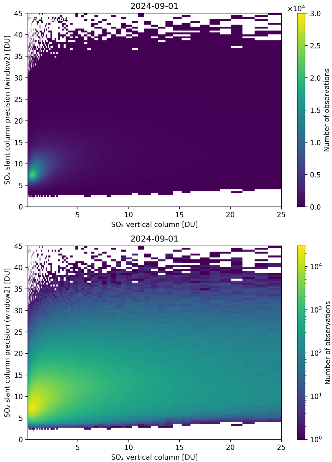
Figure 302: Scatter density plot of “SO 2 vertical column” against “SO 2 slant column precision (window2)” for 2024-09-01 to 2024-09-02.
