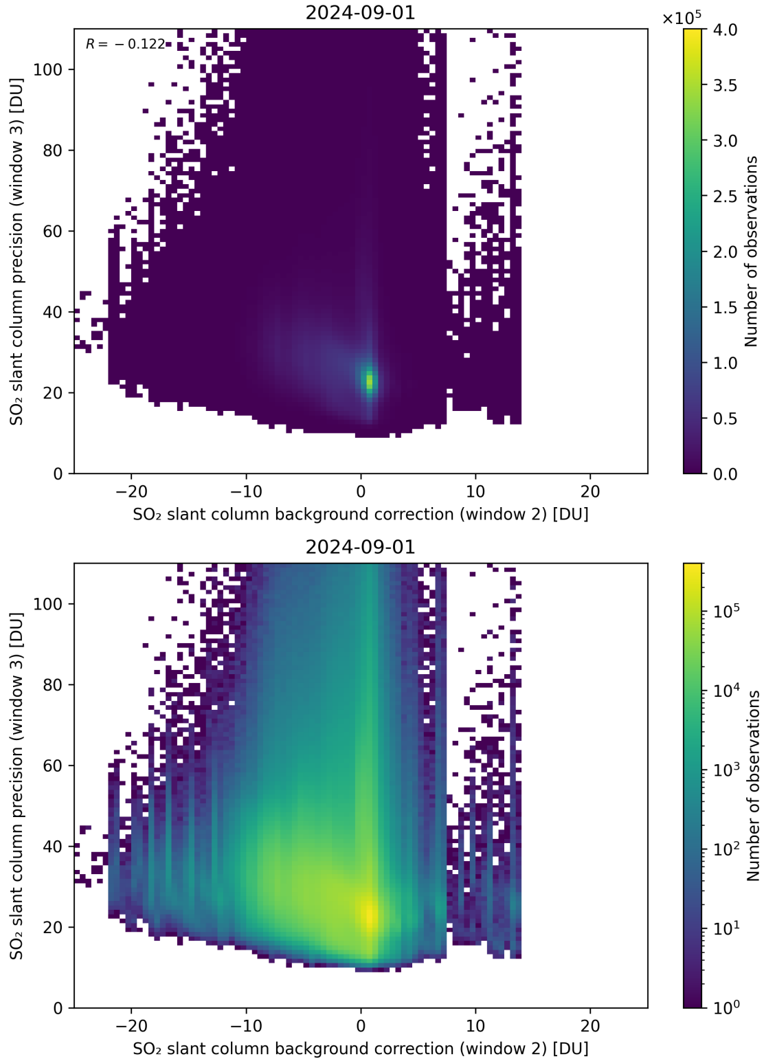
Figure 118: Scatter density plot of “SO 2 slant column background correction (window 2)” against “SO 2 slant column precision (window 3)” for 2024-09-01 to 2024-09-02.
