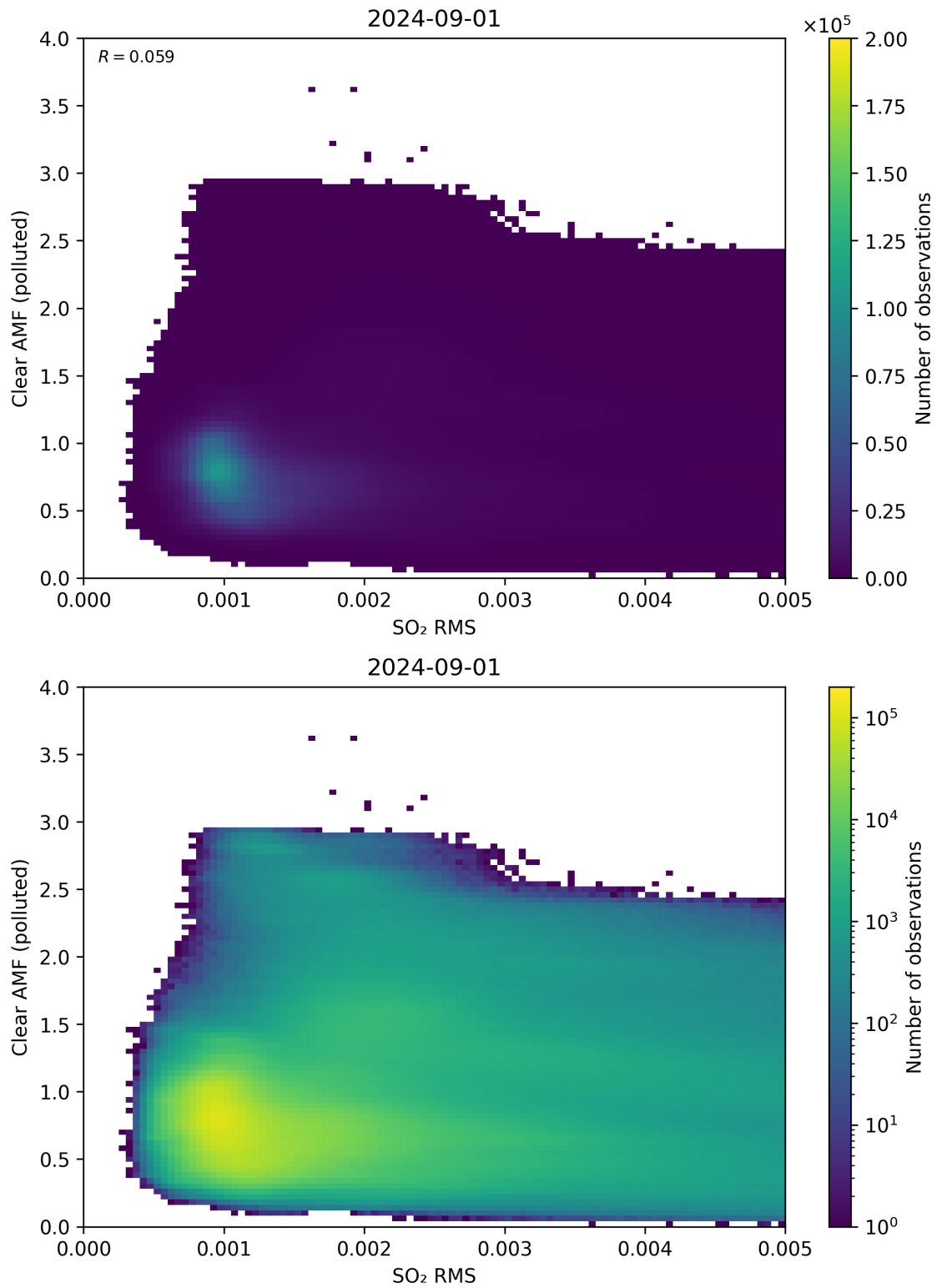
Figure 136: Scatter density plot of “SO 2 RMS” against “Clear AMF (polluted)” for 2024-09-01 to 2024-09-02.
