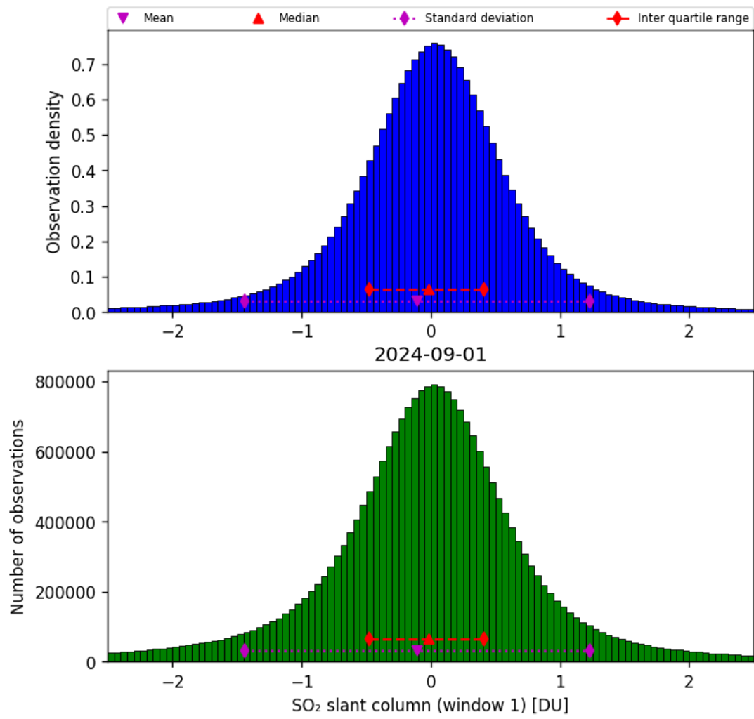
Figure 56: Histogram of “SO 2 slant column (window 1)” for 2024-09-01 to 2024-09-02
