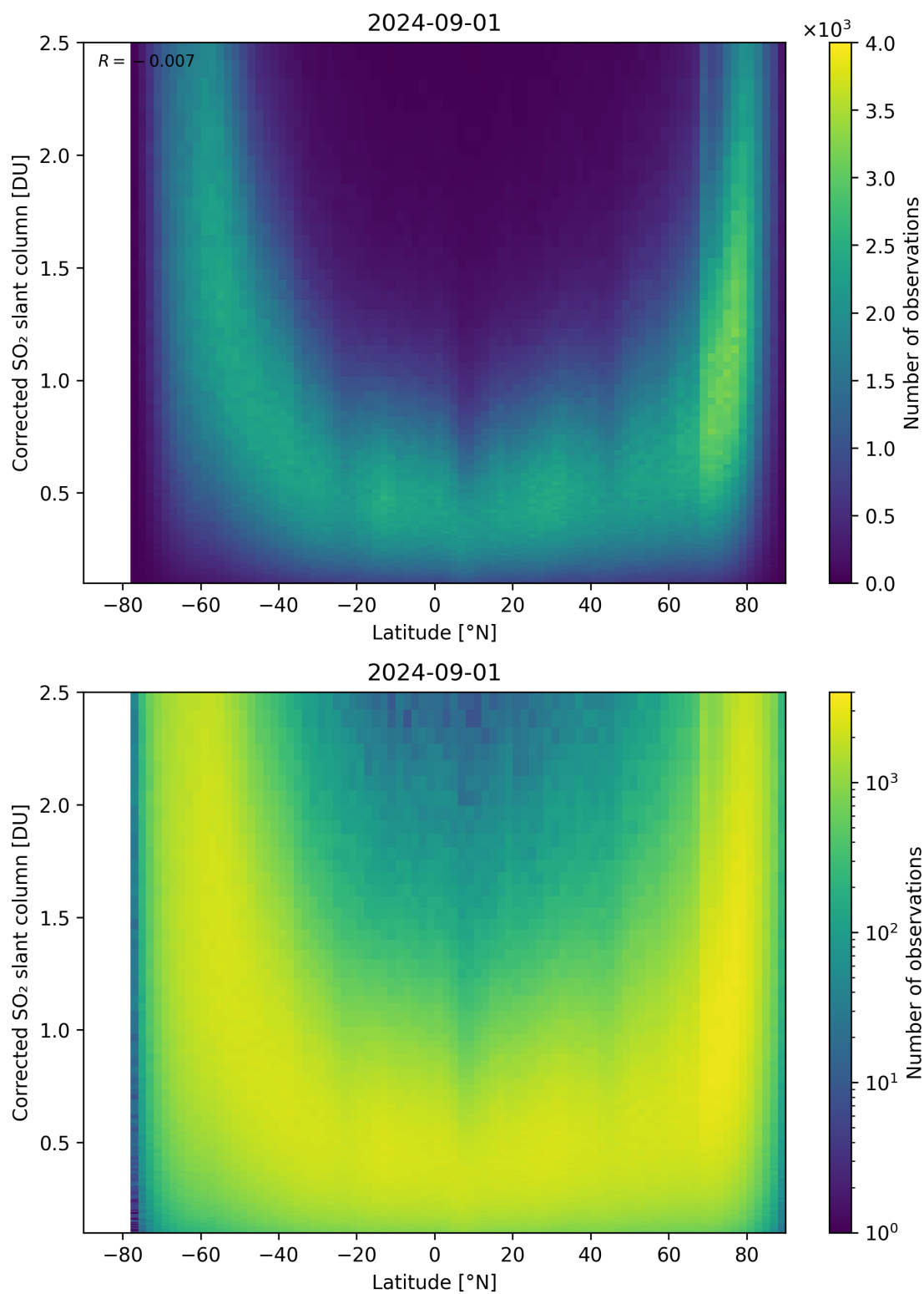
Figure 146: Scatter density plot of “Latitude” against “Corrected SO 2 slant column” for 2024-09-01 to 2024-09-02.
