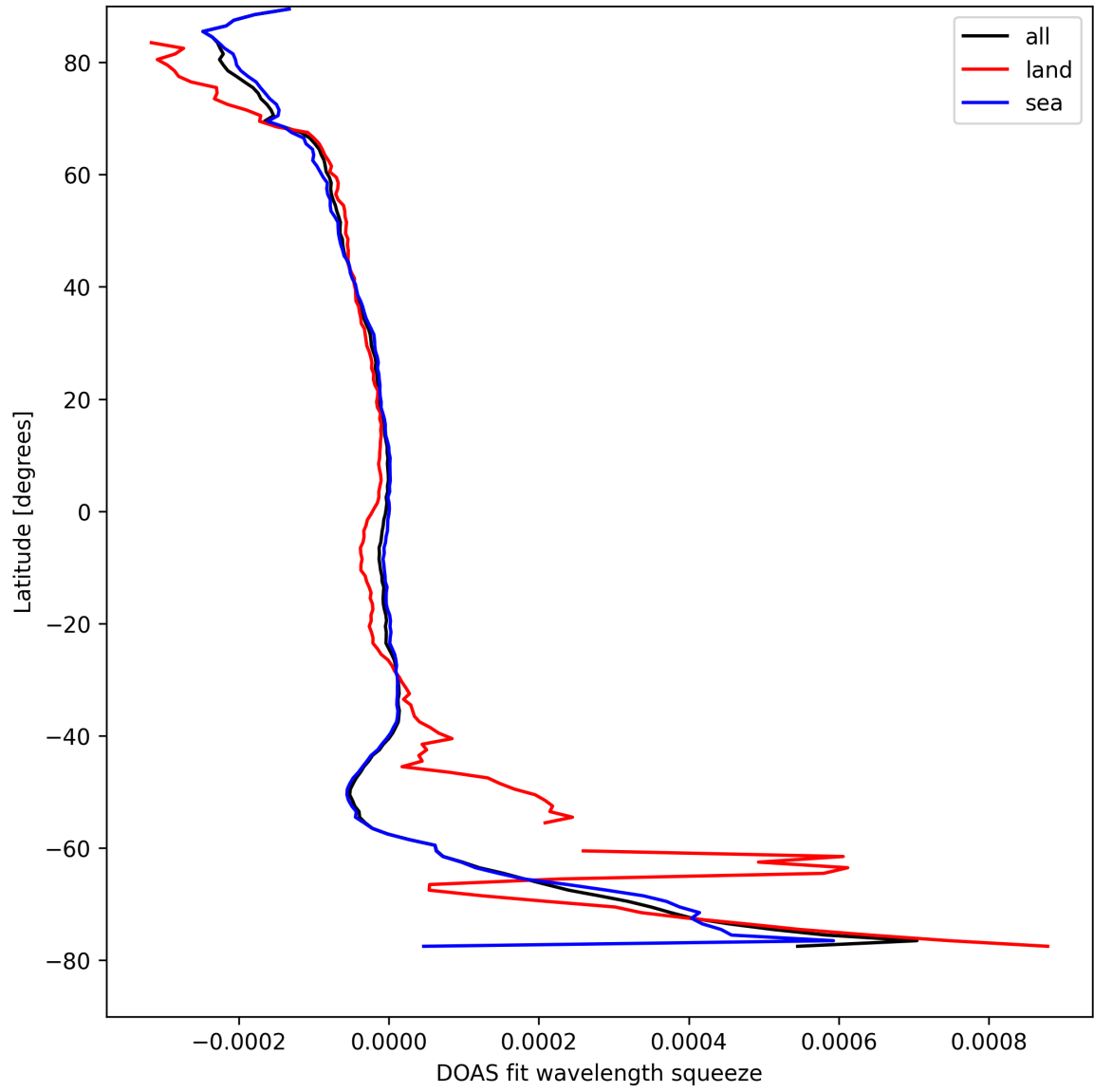
Figure 46: Zonal average of “DOAS fit wavelength squeeze” for 2024-09-01 to 2024-09-02.
