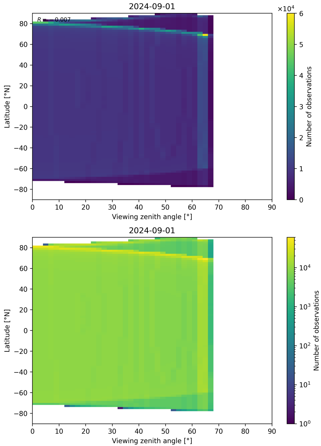
Figure 314: Scatter density plot of “Viewing zenith angle” against “Latitude” for 2024-09-01 to 2024-09-02.
