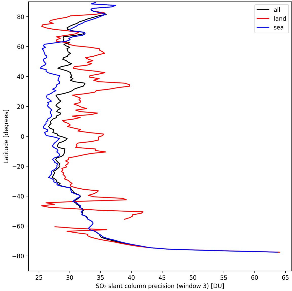
Figure 42: Zonal average of “SO 2 slant column precision (window 3)” for 2024-09-01 to 2024-09-02.
