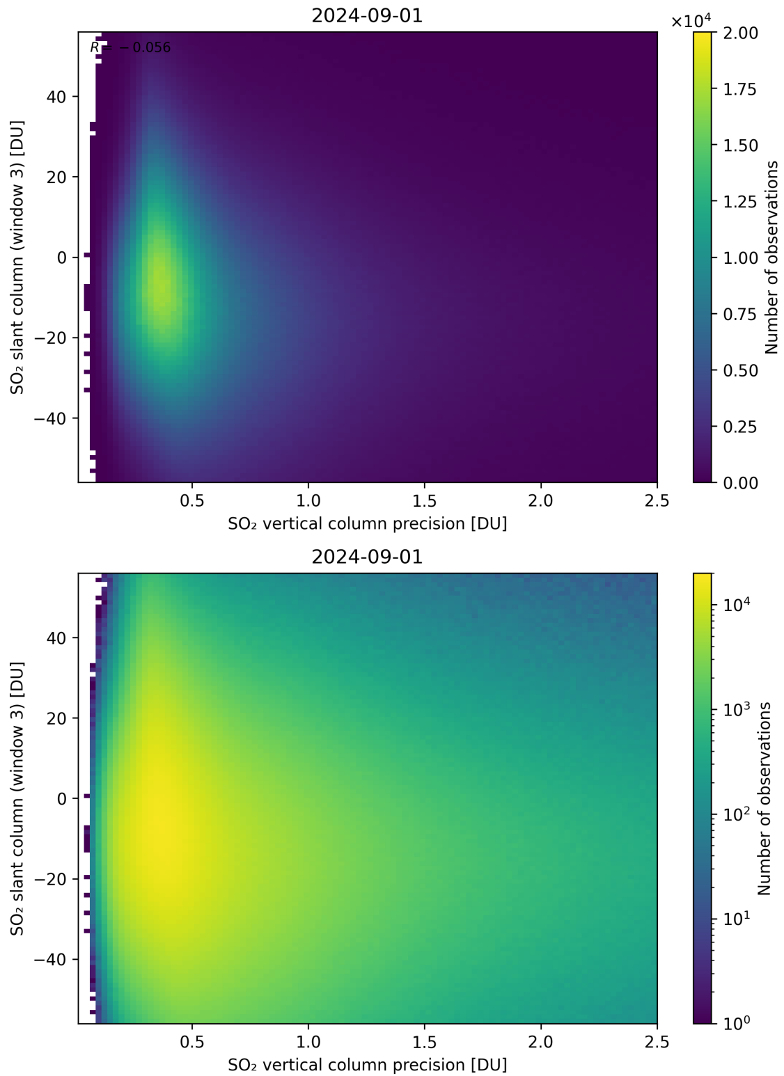
Figure 292: Scatter density plot of “SO 2 vertical column precision” against “SO 2 slant column (window 3)” for 2024-09-01 to 2024-09-02.
