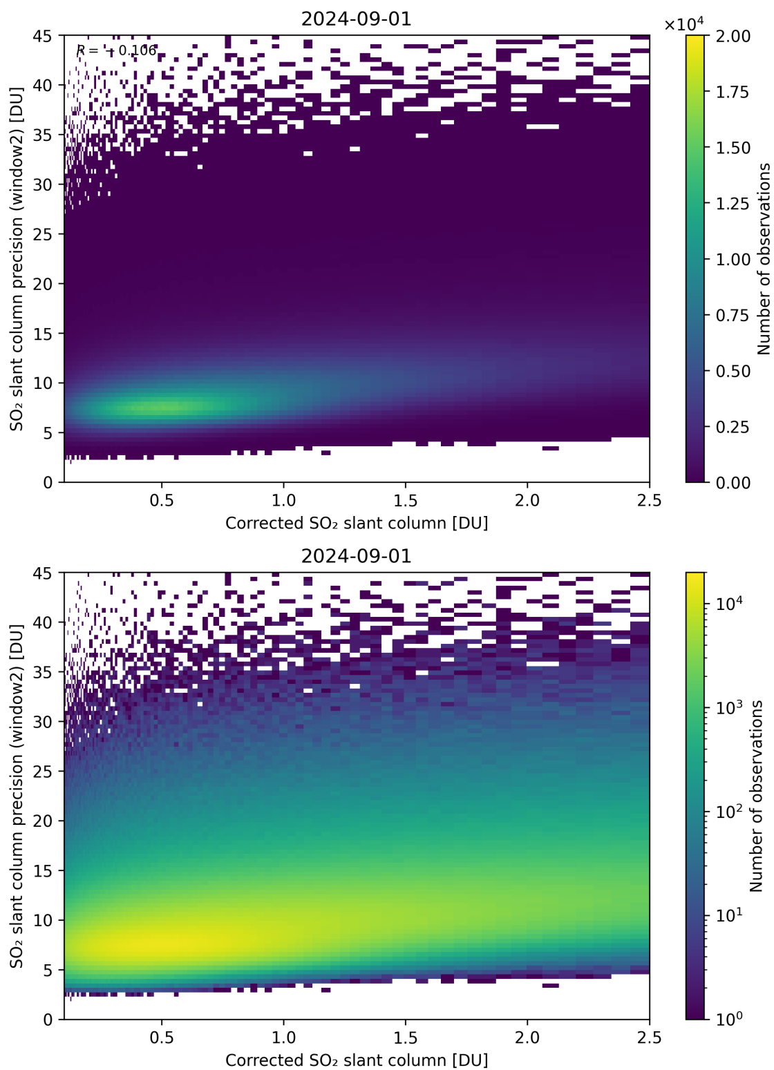
Figure 189: Scatter density plot of “Corrected SO 2 slant column” against “SO 2 slant column precision (window2)” for 2024-09-01 to 2024-09-02.
