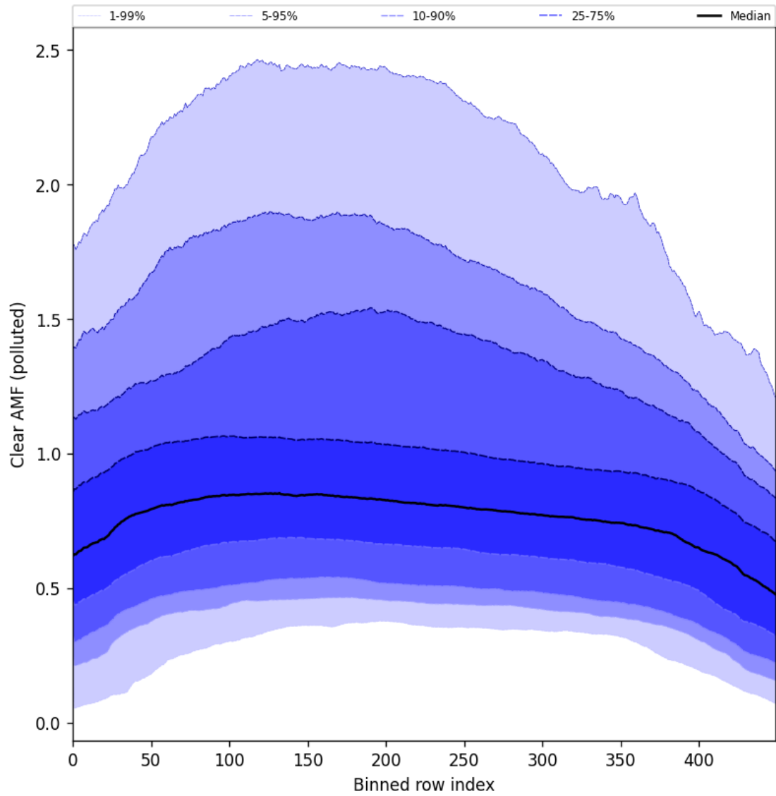
Figure 96: Along track statistics of “Clear AMF (polluted)” for 2024-09-01 to 2024-09-02
