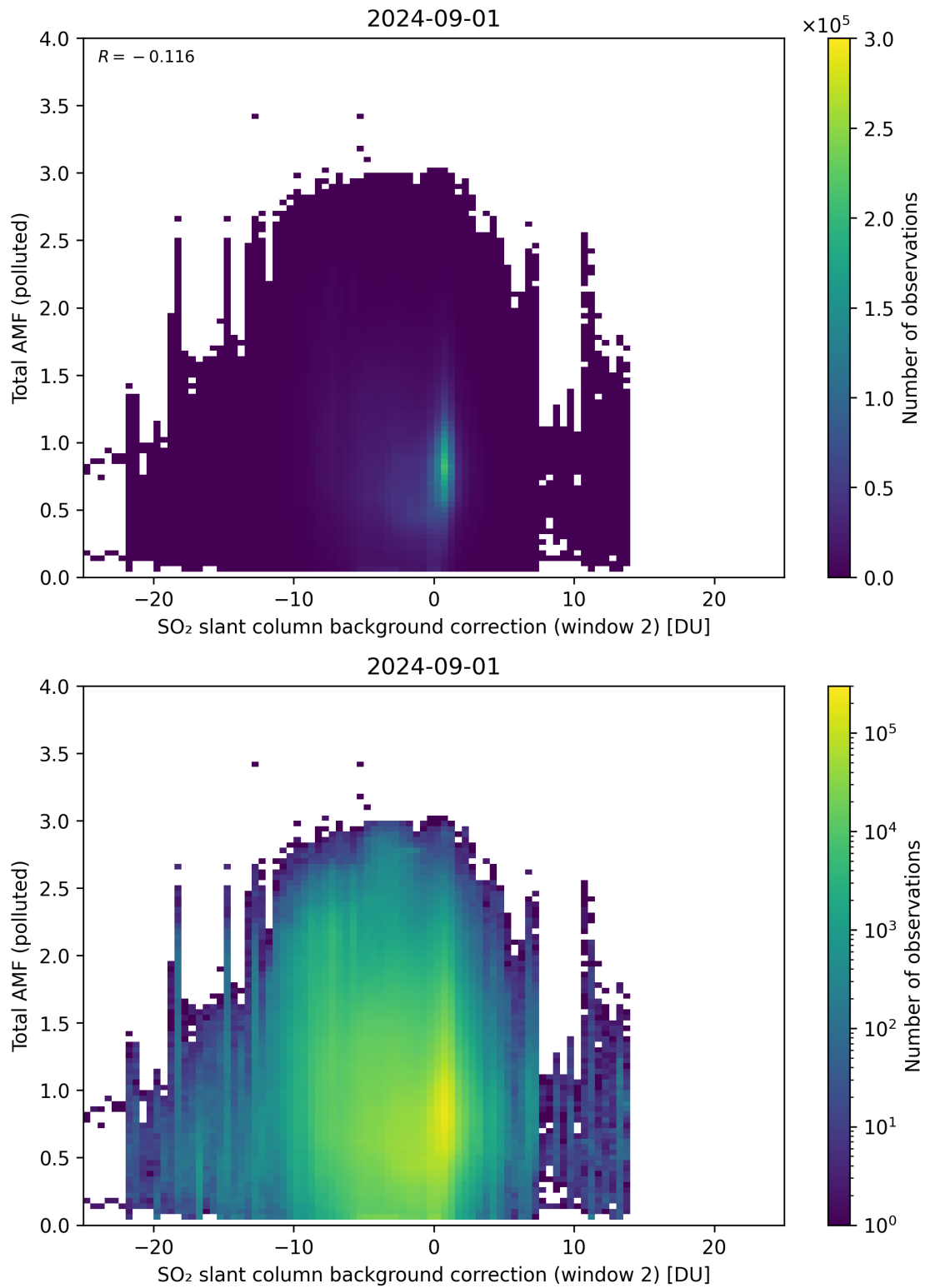
Figure 119: Scatter density plot of “SO 2 slant column background correction (window 2)” against “Total AMF (polluted)” for 2024-09-01 to 2024-09-02.
