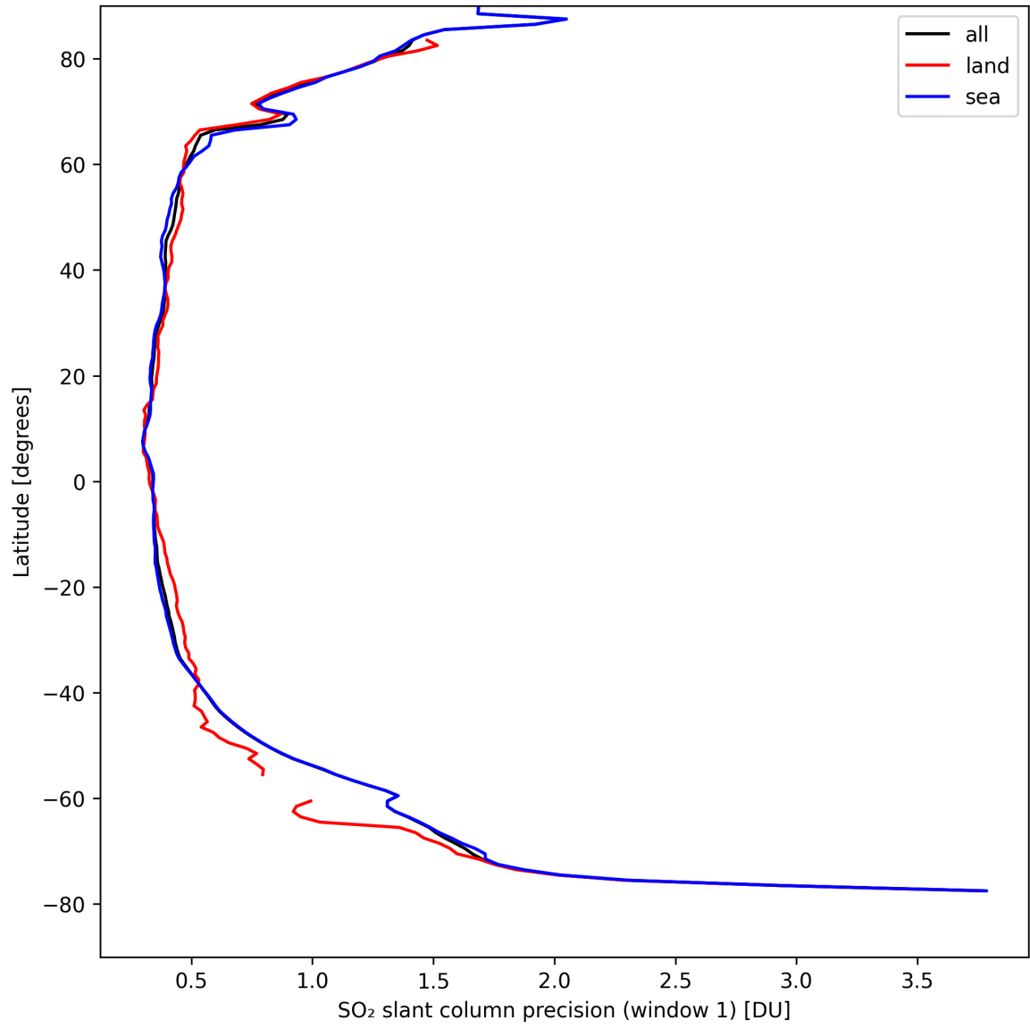
Figure 34: Zonal average of “SO 2 slant column precision (window 1)” for 2024-09-01 to 2024-09-02.
