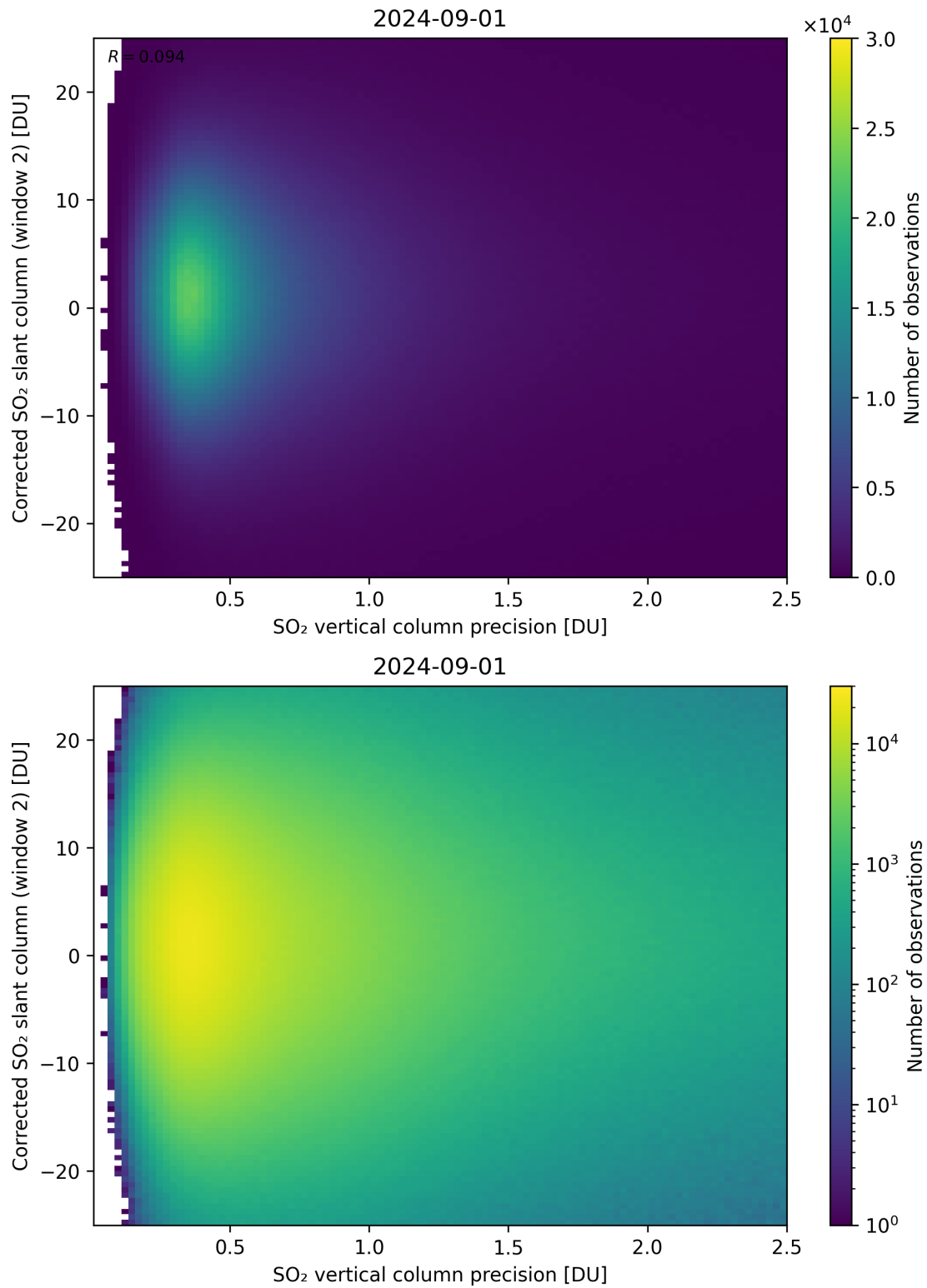
Figure 287: Scatter density plot of “SO 2 vertical column precision” against “Corrected SO 2 slant column (window 2)” for 2024-09-01 to 2024-09-02.
