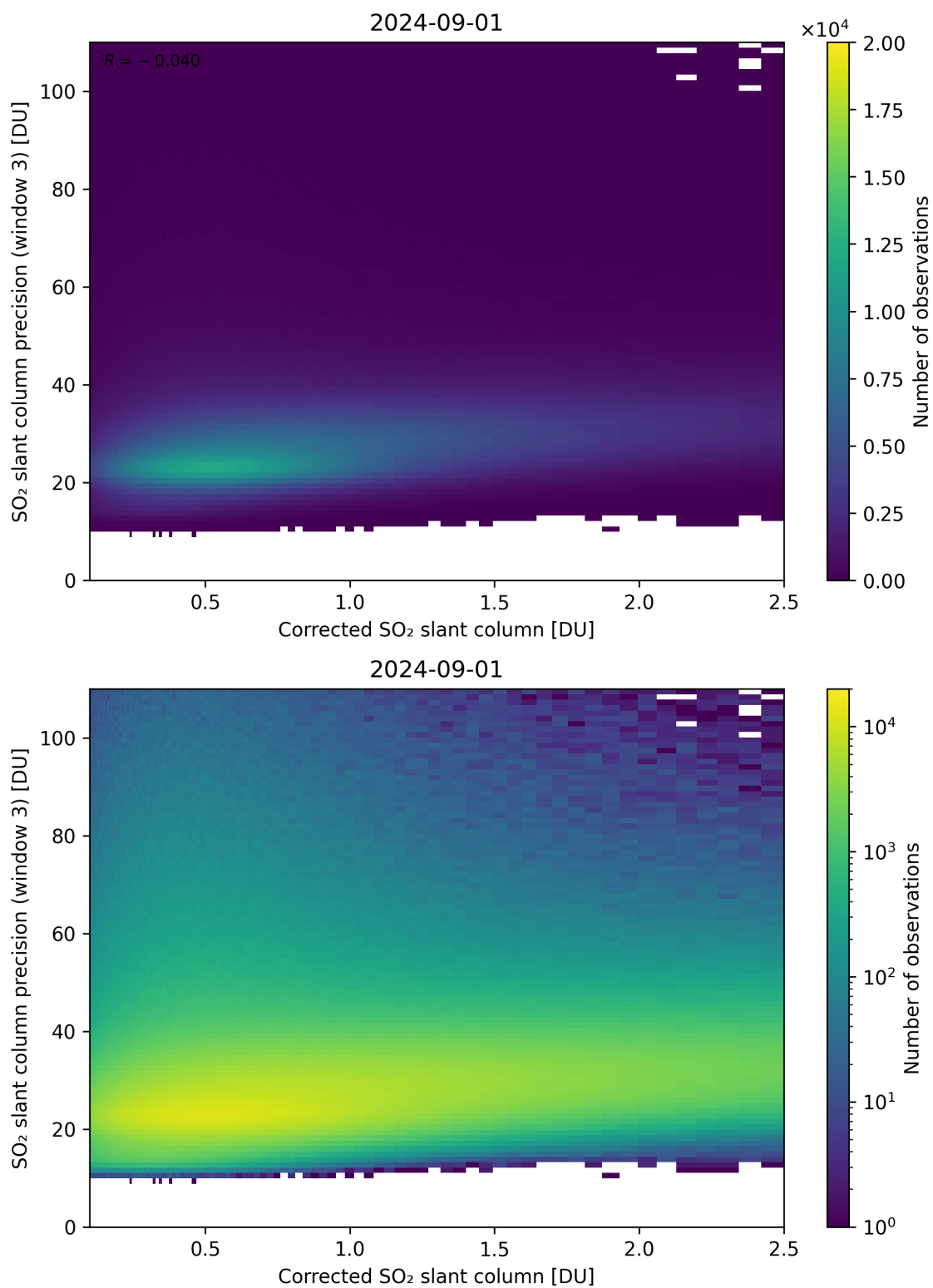
Figure 191: Scatter density plot of “Corrected SO 2 slant column” against “SO 2 slant column precision (window 3)” for 2024-09-01 to 2024-09-02.
