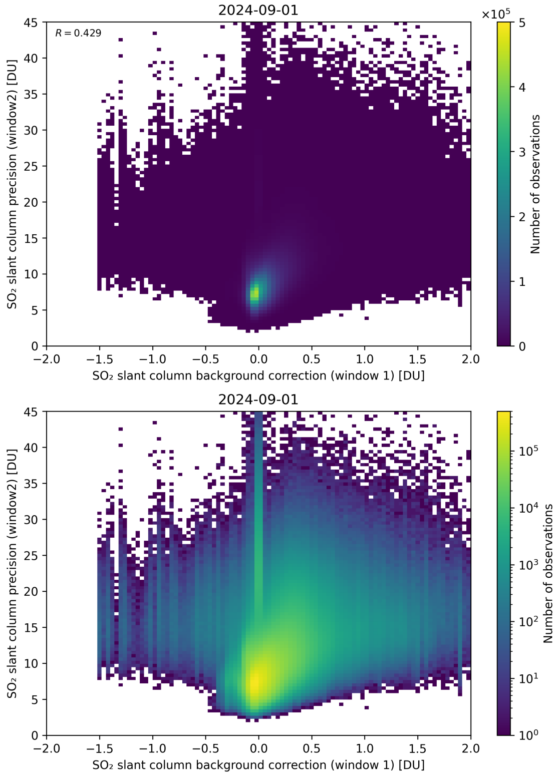
Figure 106: Scatter density plot of “SO 2 slant column background correction (window 1)” against “SO 2 slant column precision (window2)” for 2024-09-01 to 2024-09-02.
