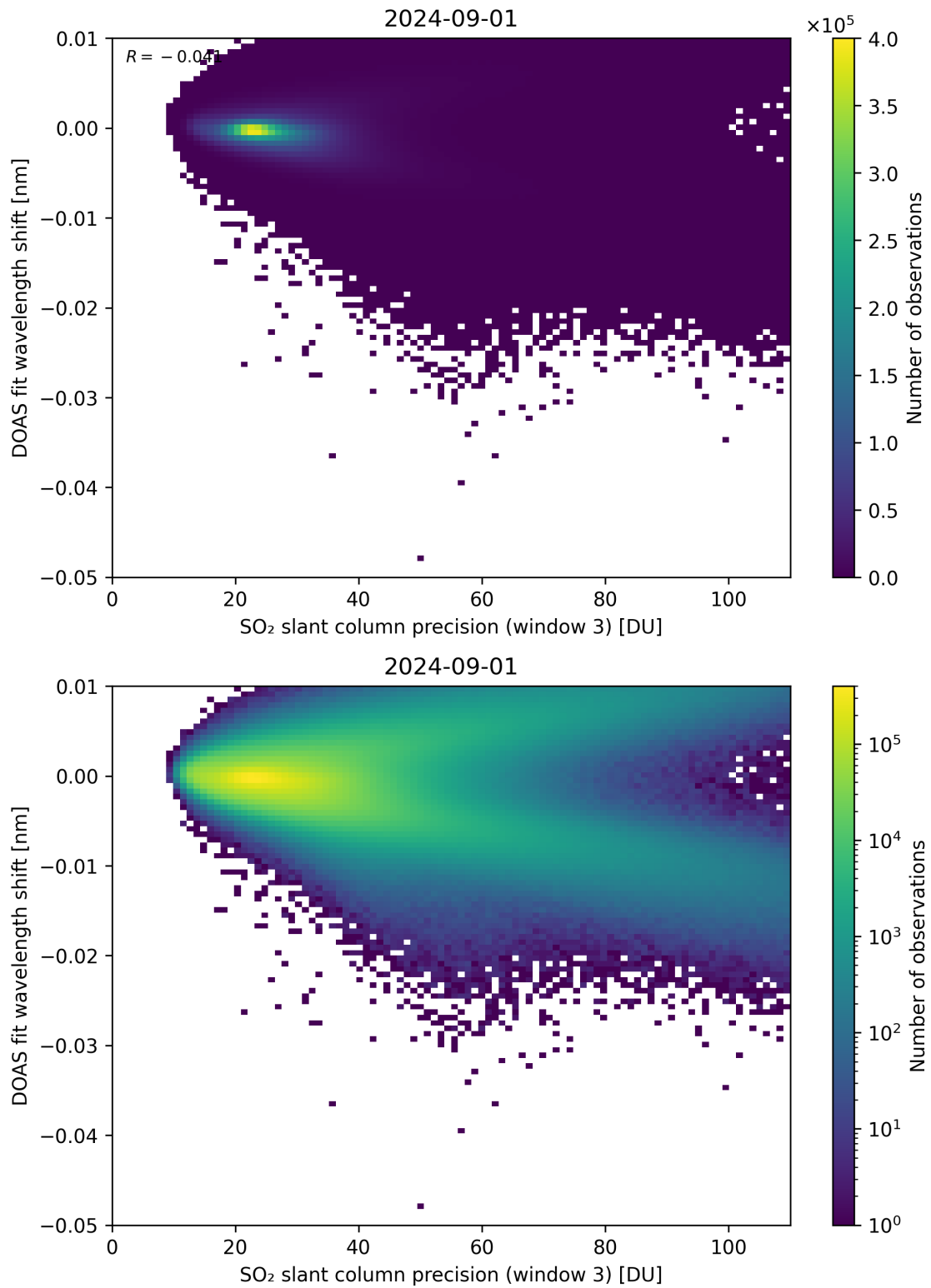
Figure 258: Scatter density plot of “SO 2 slant column precision (window 3)” against “DOAS fit wavelength shift” for 2024-09-01 to 2024-09-02.
