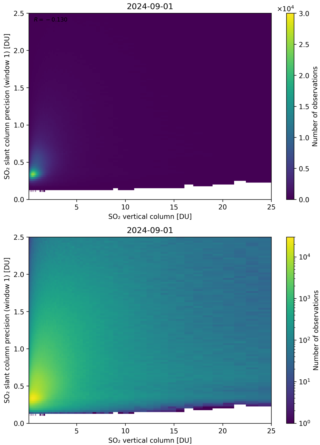
Figure 301: Scatter density plot of “SO 2 vertical column” against “SO 2 slant column precision (window 1)” for 2024-09-01 to 2024-09-02.
