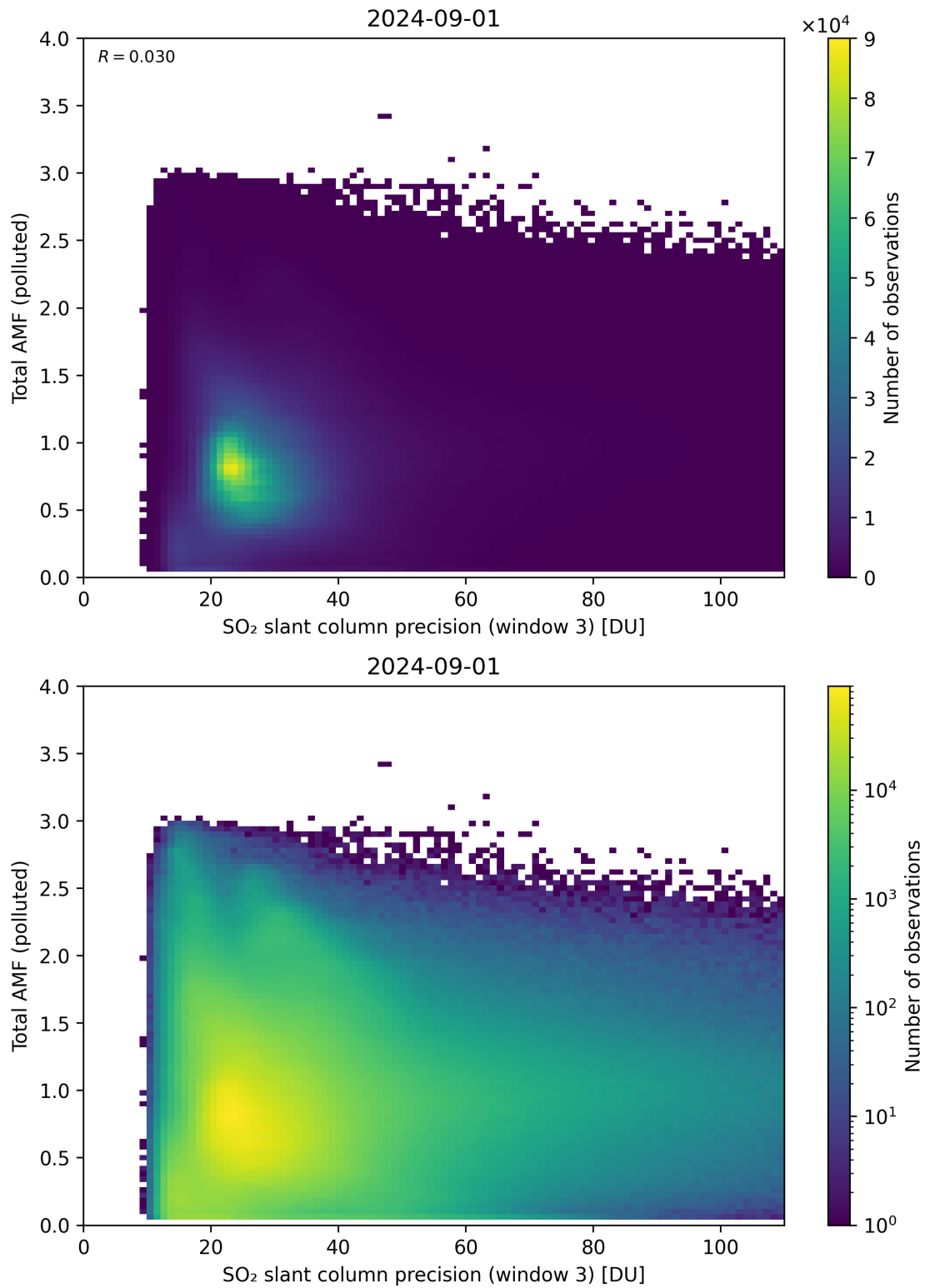
Figure 263: Scatter density plot of “SO 2 slant column precision (window 3)” against “Total AMF (polluted)” for 2024-09-01 to 2024-09-02.
