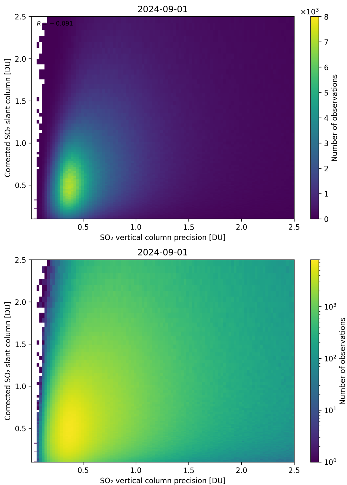
Figure 286: Scatter density plot of “SO 2 vertical column precision” against “Corrected SO 2 slant column” for 2024-09-01 to 2024-09-02.
