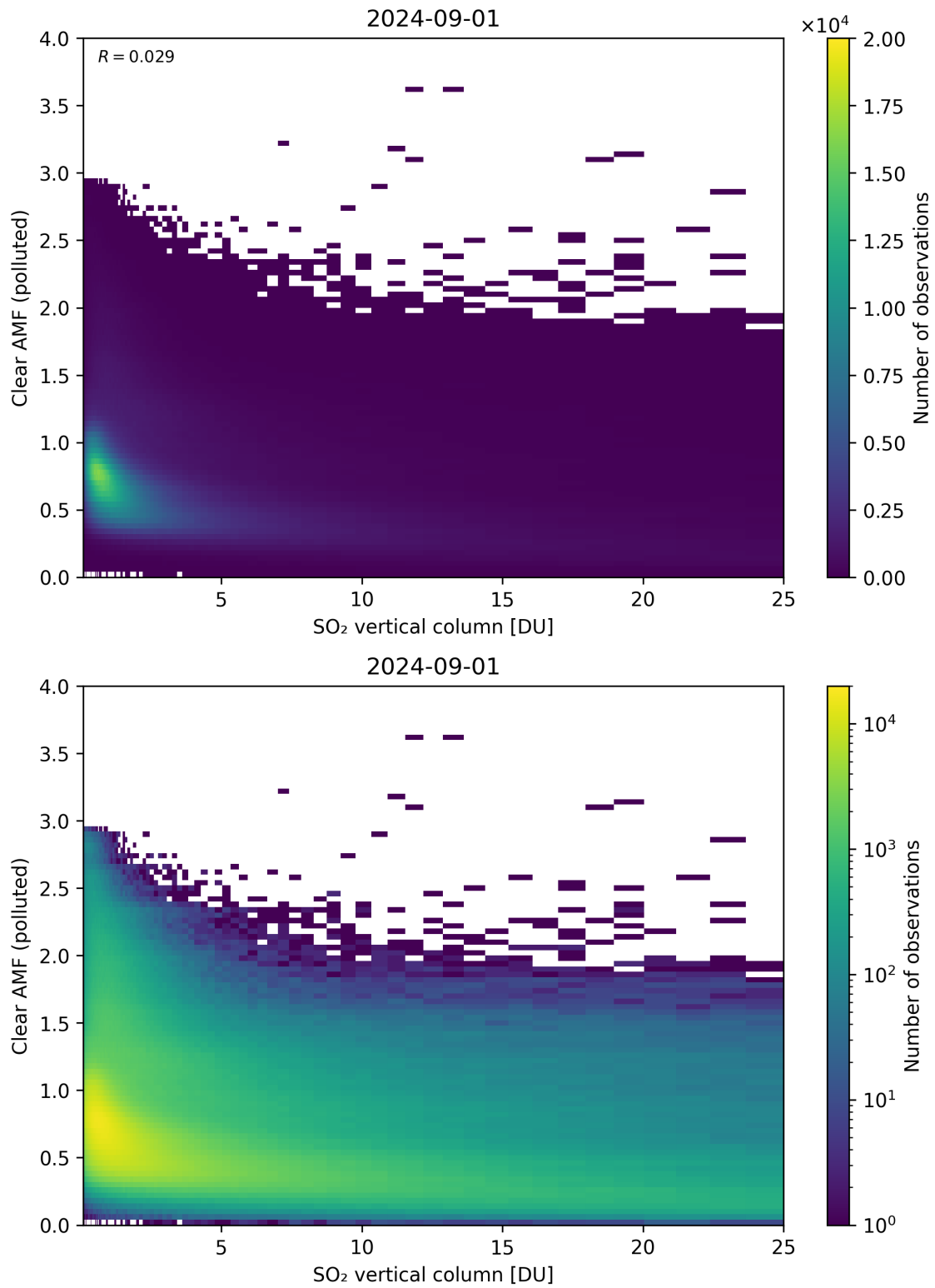
Figure 296: Scatter density plot of “SO 2 vertical column” against “Clear AMF (polluted)” for 2024-09-01 to 2024-09-02.
