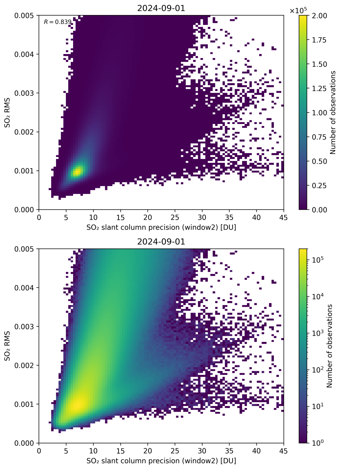
Figure 245: Scatter density plot of “SO 2 slant column precision (window2)” against “SO 2 RMS” for 2024-09-01 to 2024-09-02.
