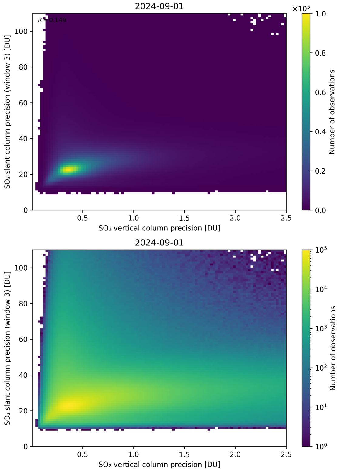
Figure 293: Scatter density plot of “SO 2 vertical column precision” against “SO 2 slant column precision (window 3)” for 2024-09-01 to 2024-09-02.
