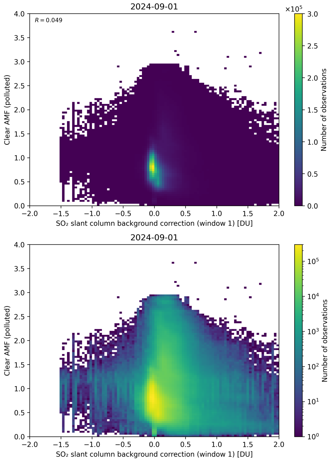
Figure 103: Scatter density plot of “SO 2 slant column background correction (window 1)” against “Clear AMF (polluted)” for 2024-09-01 to 2024-09-02.
