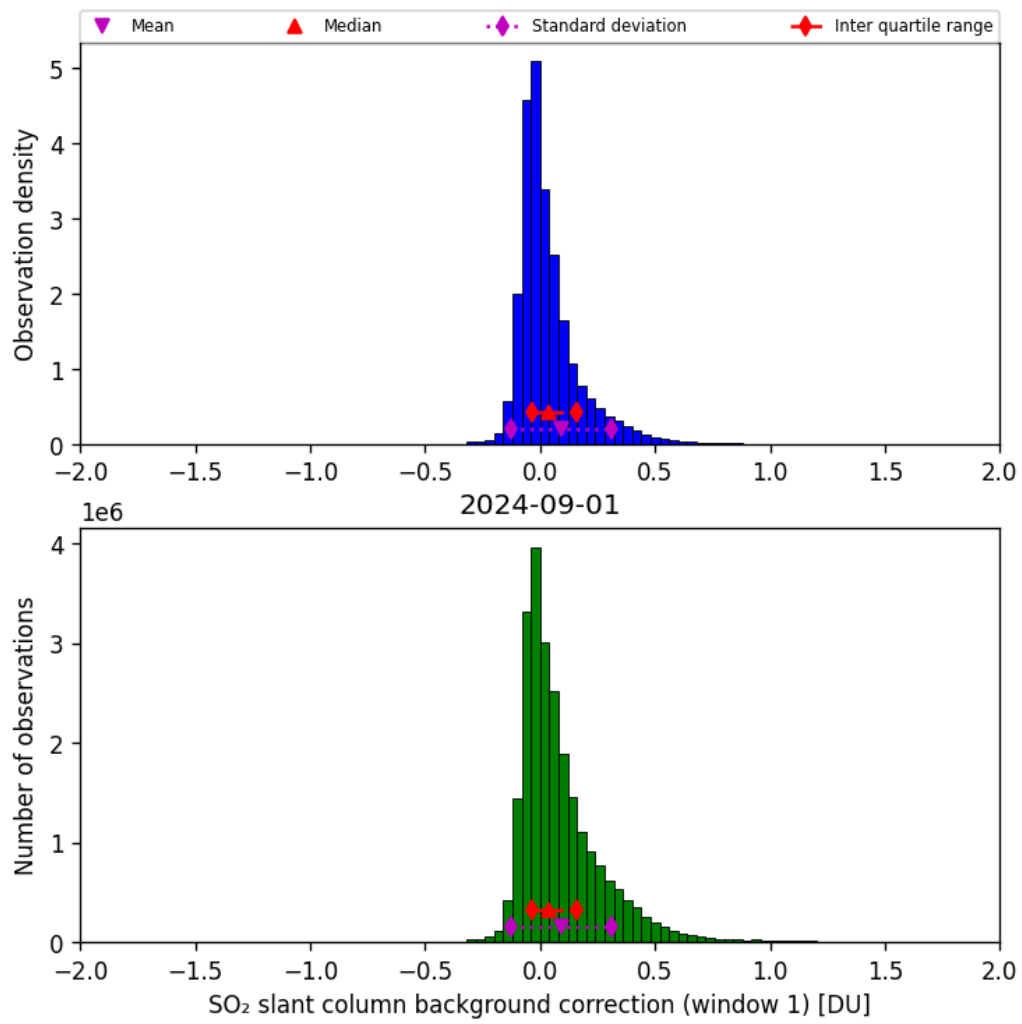
Figure 59: Histogram of “SO 2 slant column background correction (window 1)” for 2024-09-01 to 2024-09-02
