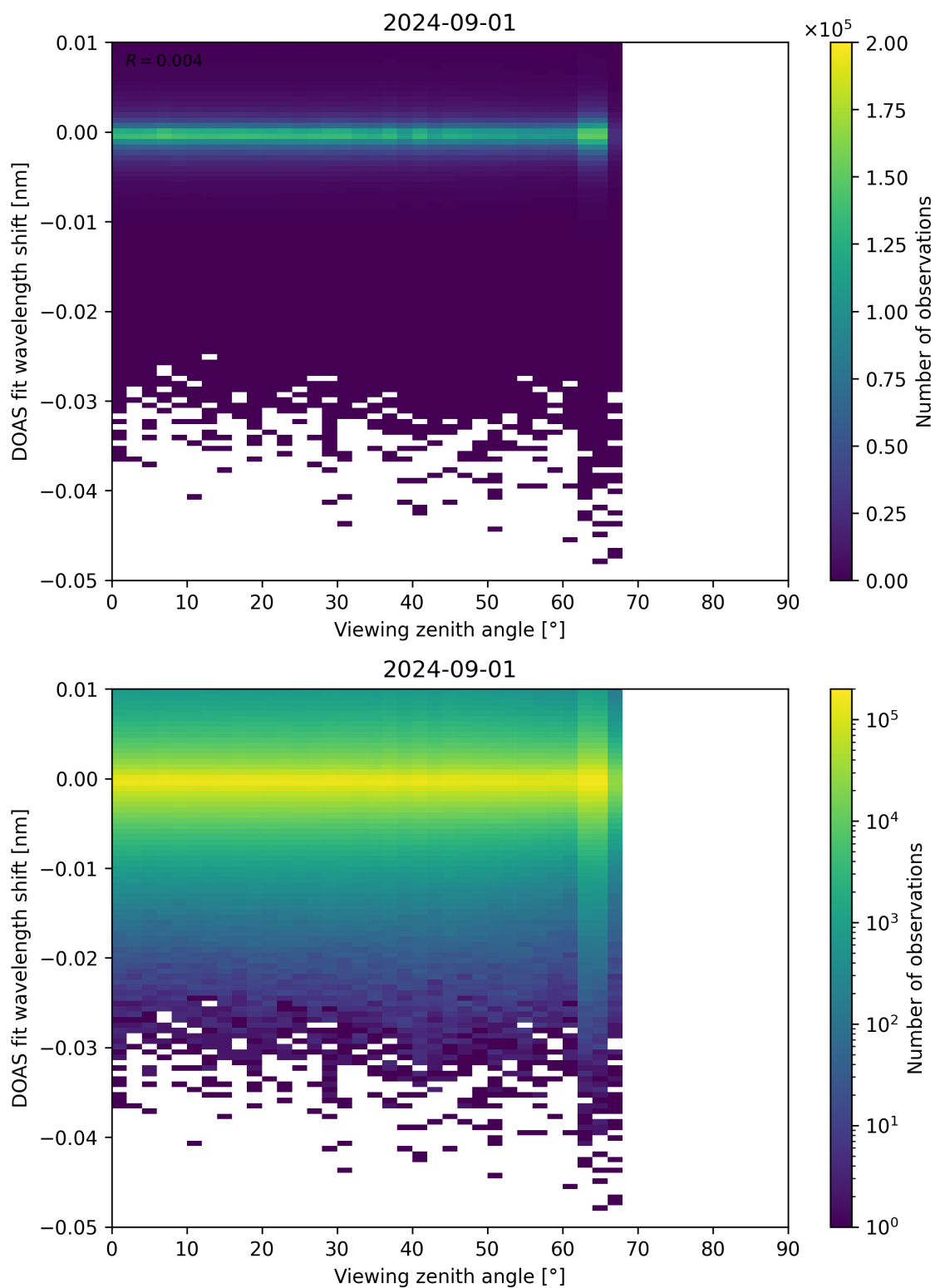
Figure 311: Scatter density plot of “Viewing zenith angle” against “DOAS fit wavelength shift” for 2024-09-01 to 2024-09-02.
