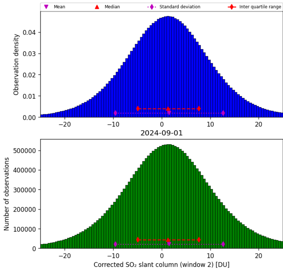
Figure 62: Histogram of “Corrected SO 2 slant column (window 2)” for 2024-09-01 to 2024-09-02
