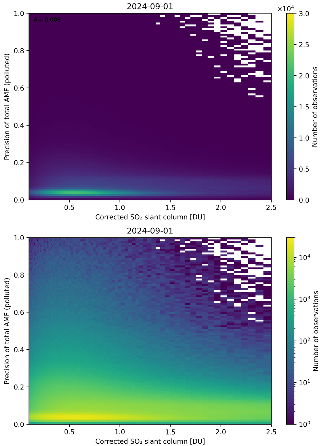
Figure 193: Scatter density plot of “Corrected SO 2 slant column” against “Precision of total AMF (polluted)” for 2024-09-01 to 2024-09-02.
