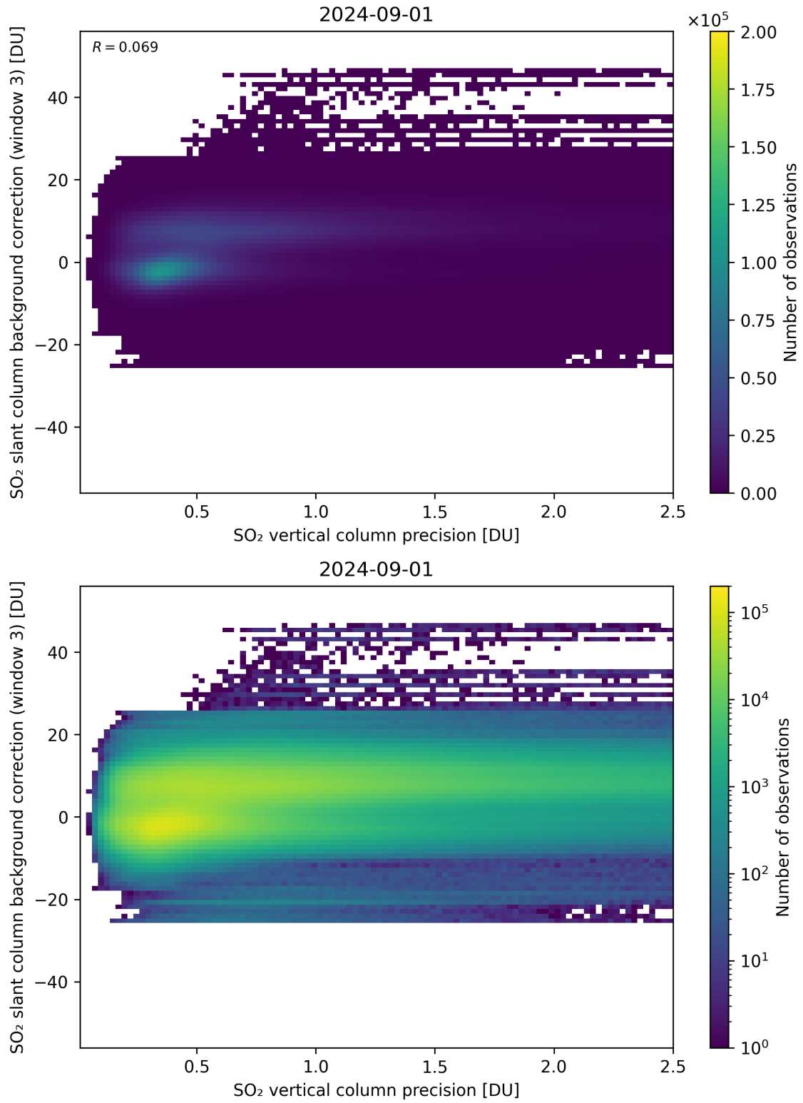
Figure 281: Scatter density plot of “SO 2 vertical column precision” against “SO 2 slant column background correction (window 3)” for 2024-09-01 to 2024-09-02.
