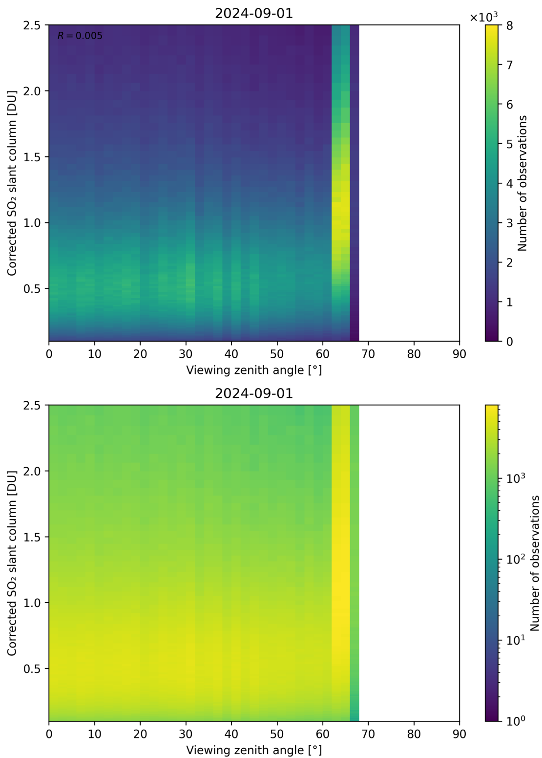
Figure 317: Scatter density plot of “Viewing zenith angle” against “Corrected SO 2 slant column” for 2024-09-01 to 2024-09-02.
