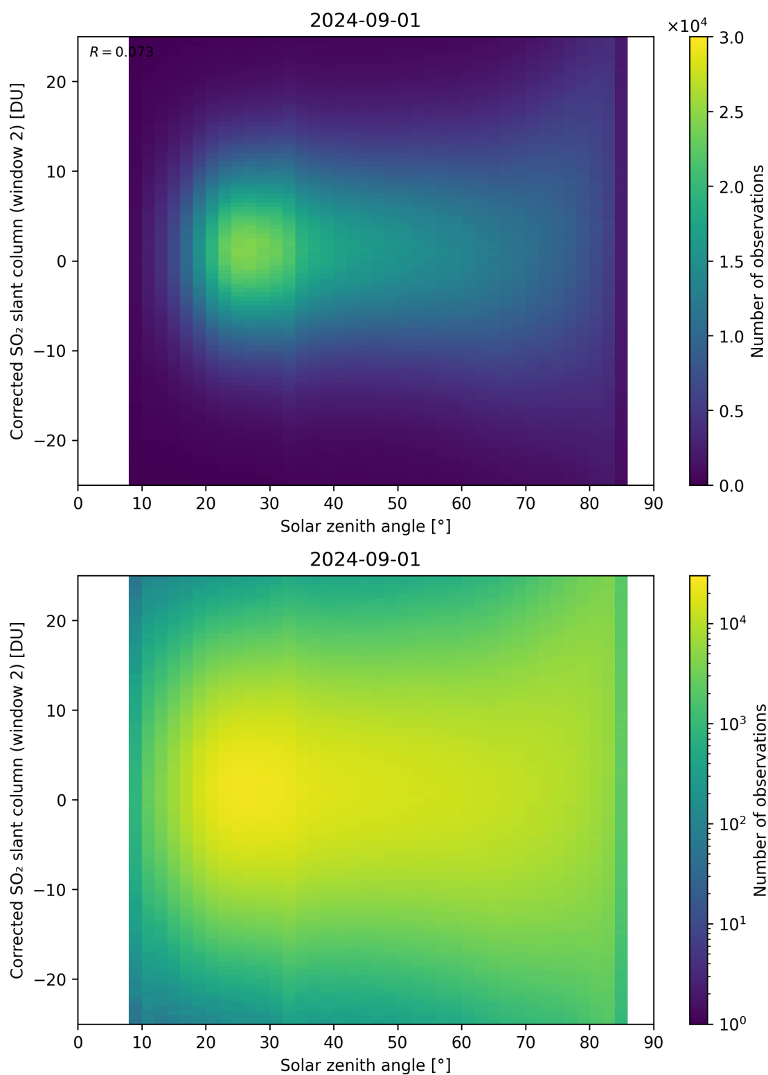
Figure 167: Scatter density plot of “Solar zenith angle” against “Corrected SO 2 slant column (window 2)” for 2024-09-01 to 2024-09-02.
