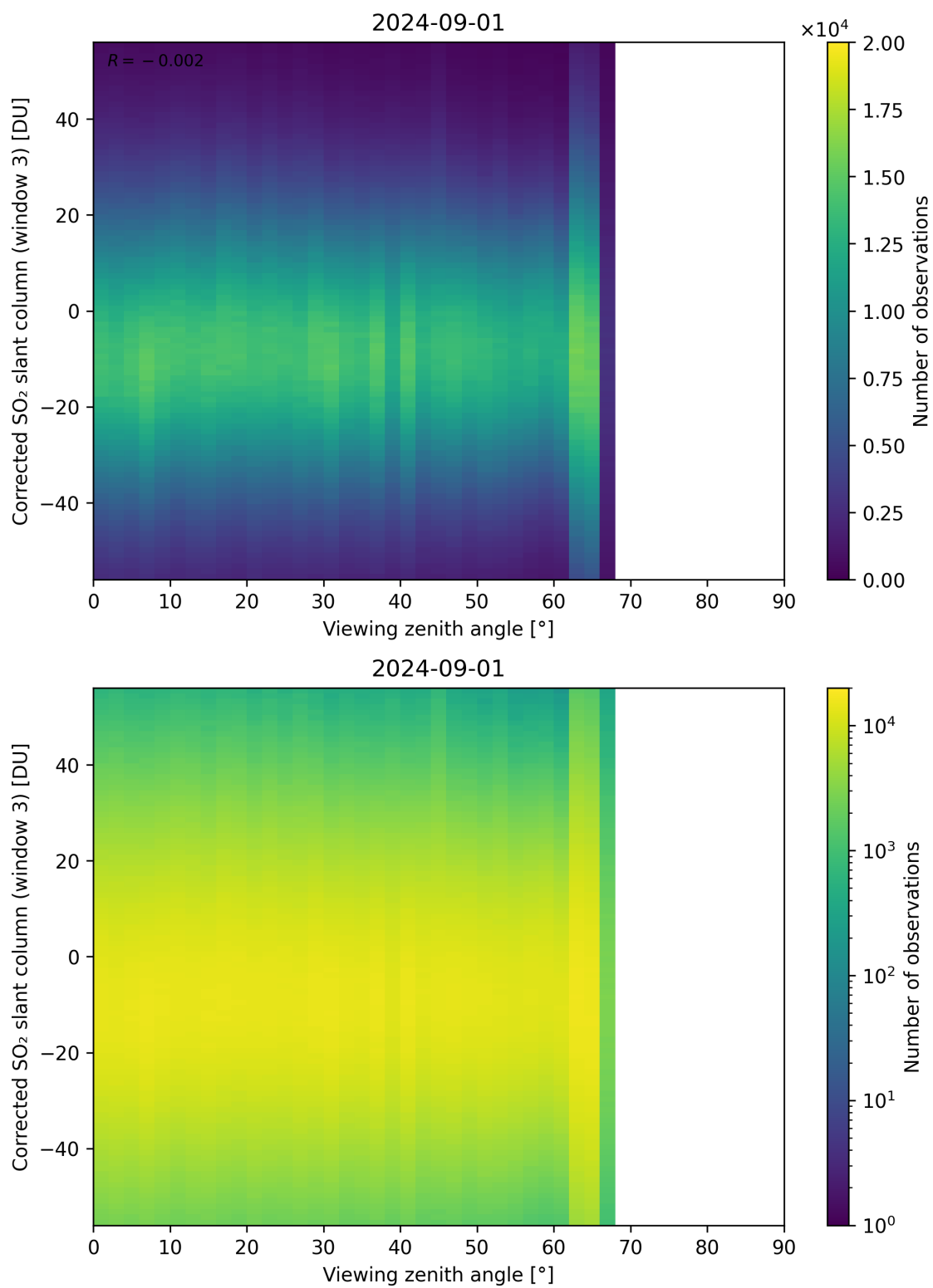
Figure 319: Scatter density plot of “Viewing zenith angle” against “Corrected SO 2 slant column (window 3)” for 2024-09-01 to 2024-09-02.
