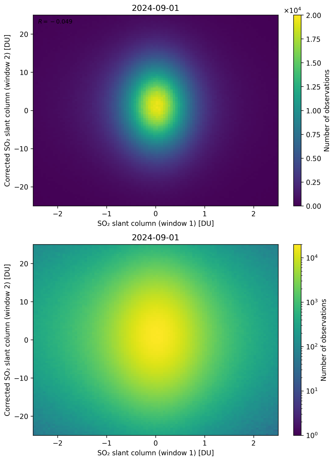
Figure 233: Scatter density plot of “SO 2 slant column (window 1)” against “Corrected SO 2 slant column (window 2)” for 2024-09-01 to 2024-09-02.
