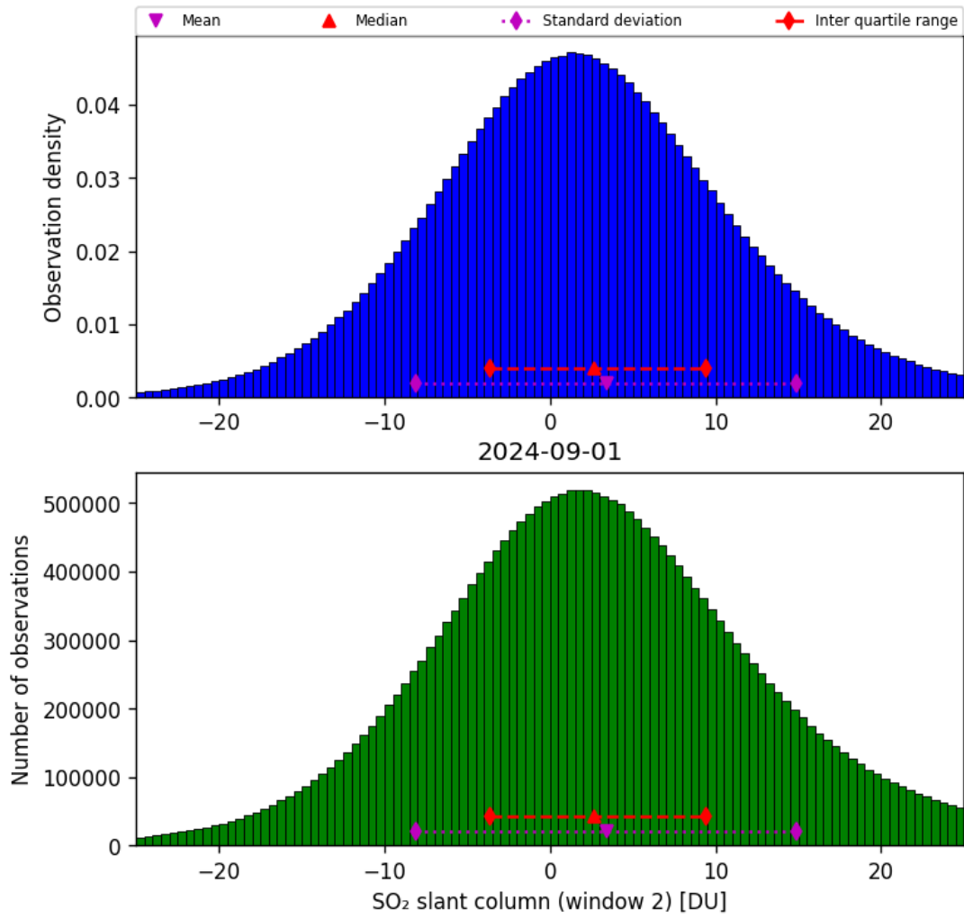
Figure 60: Histogram of “SO 2 slant column (window 2)” for 2024-09-01 to 2024-09-02
