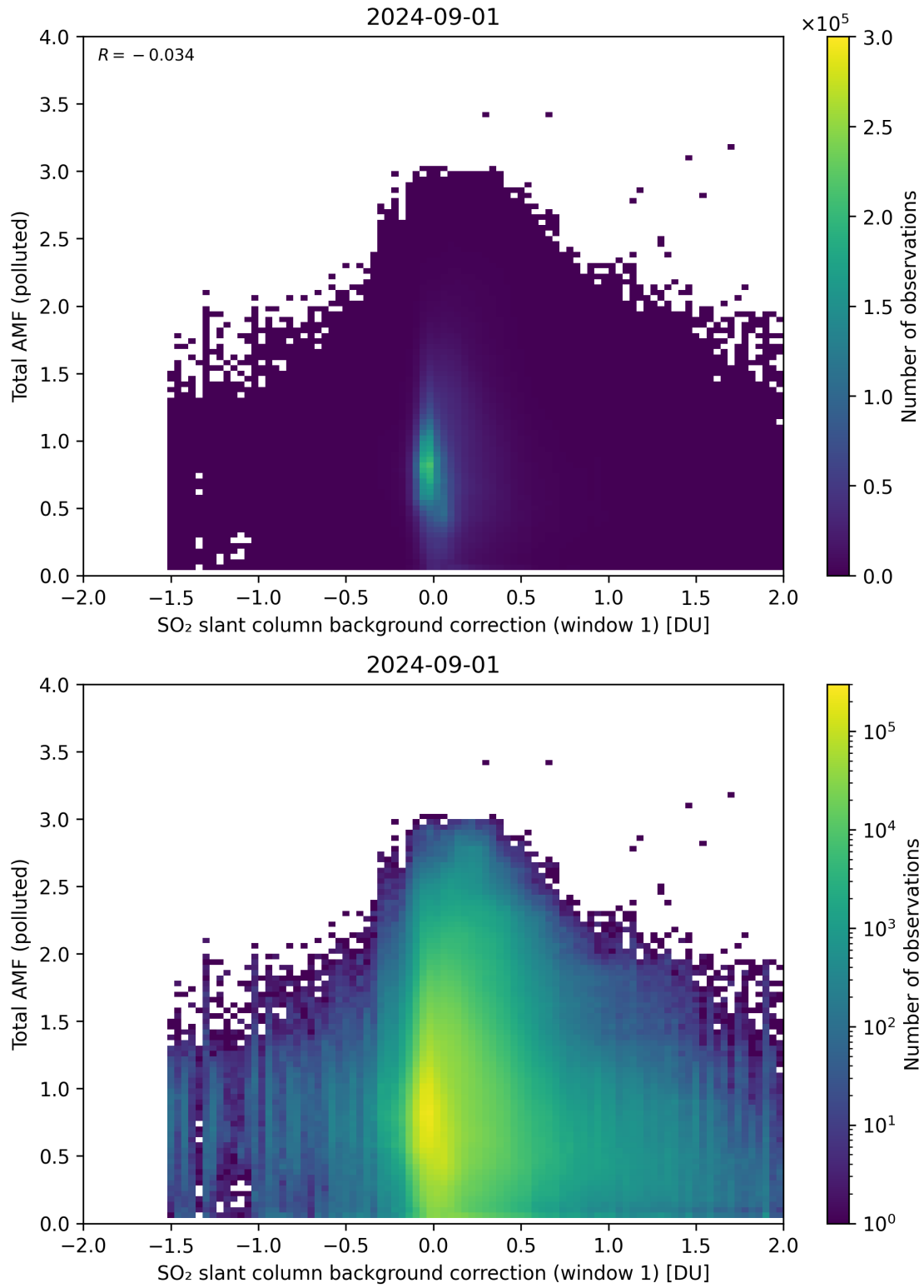
Figure 109: Scatter density plot of “SO 2 slant column background correction (window 1)” against “Total AMF (polluted)” for 2024-09-01 to 2024-09-02.
