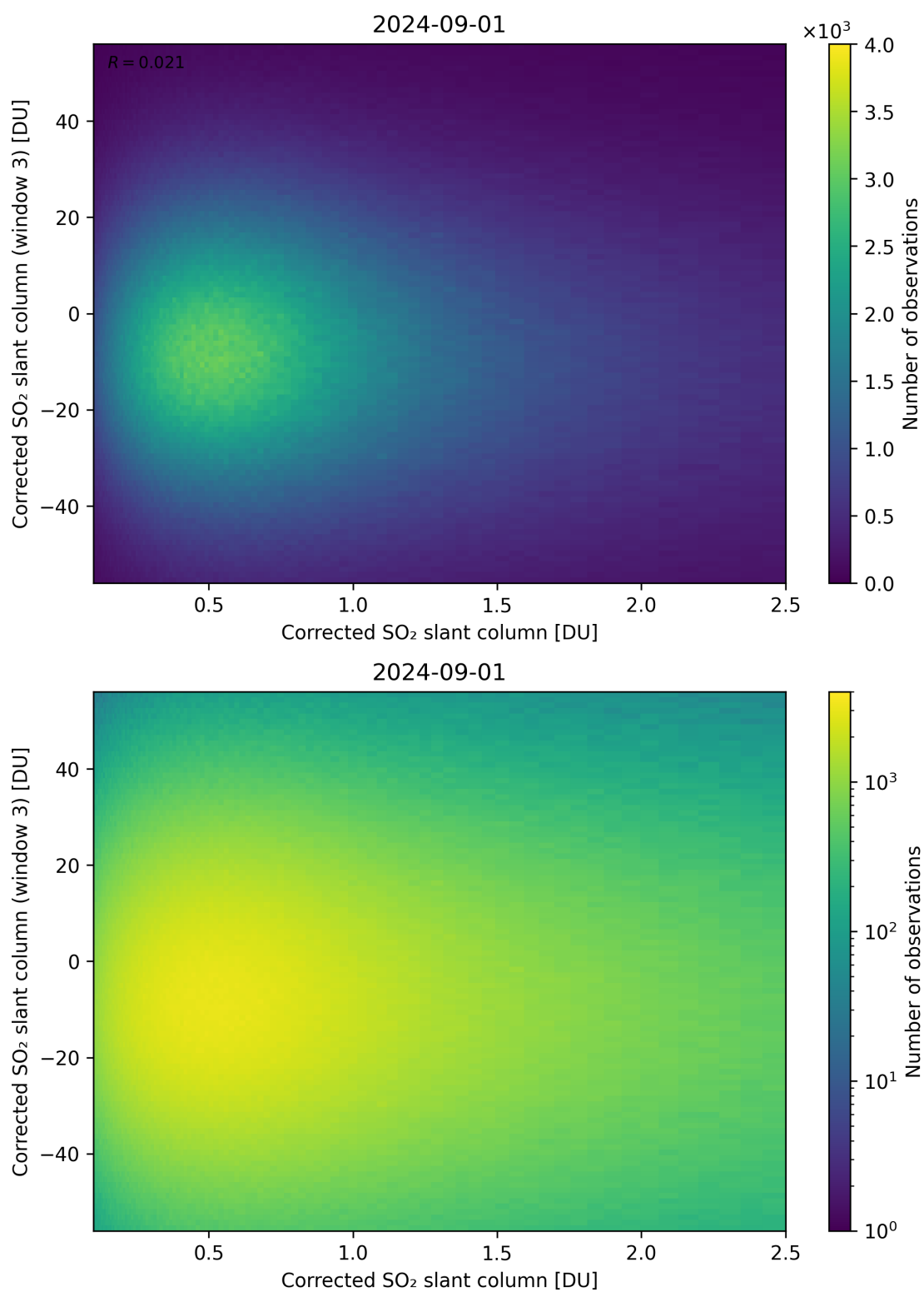
Figure 186: Scatter density plot of “Corrected SO 2 slant column” against “Corrected SO 2 slant column (window 3)” for 2024-09-01 to 2024-09-02.
