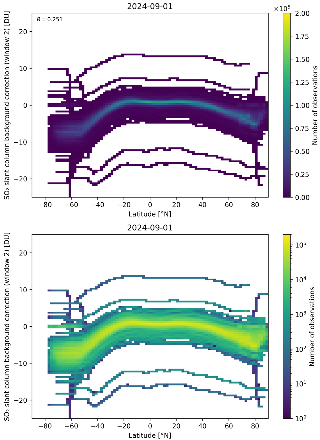
Figure 140: Scatter density plot of “Latitude” against “SO 2 slant column background correction (window 2)” for 2024-09-01 to 2024-09-02.
