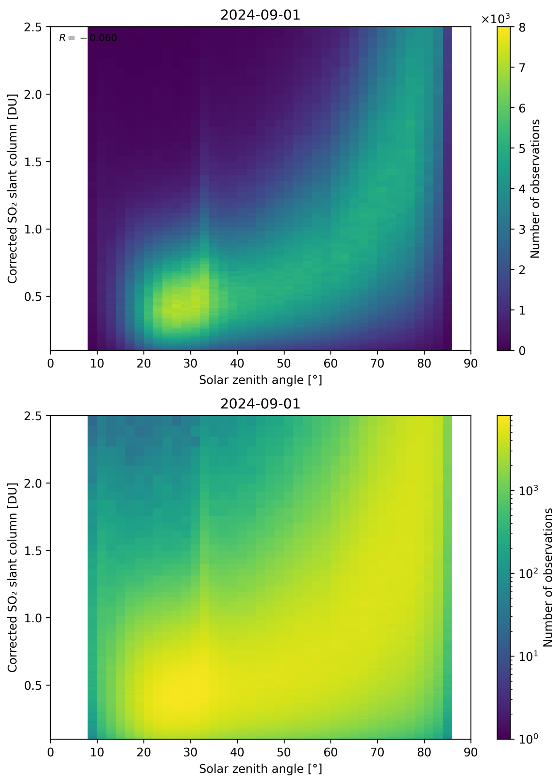
Figure 166: Scatter density plot of “Solar zenith angle” against “Corrected SO 2 slant column” for 2024-09-01 to 2024-09-02.
