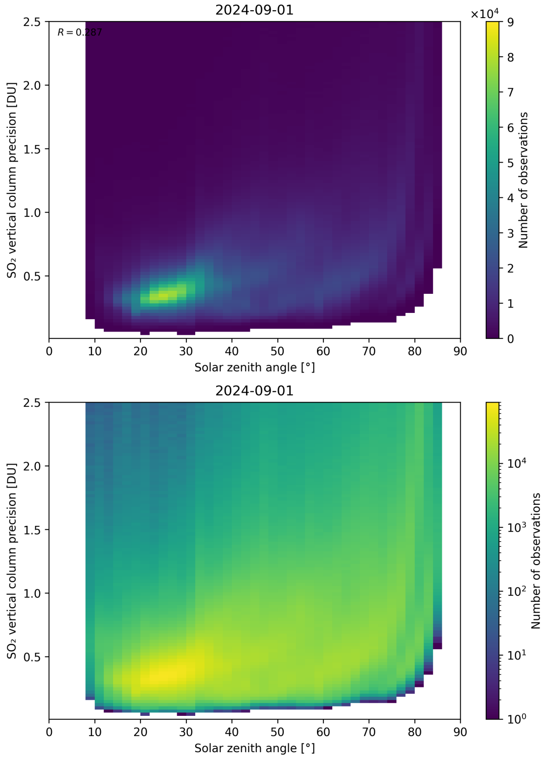
Figure 177: Scatter density plot of “Solar zenith angle” against “SO 2 vertical column precision” for 2024-09-01 to 2024-09-02.
