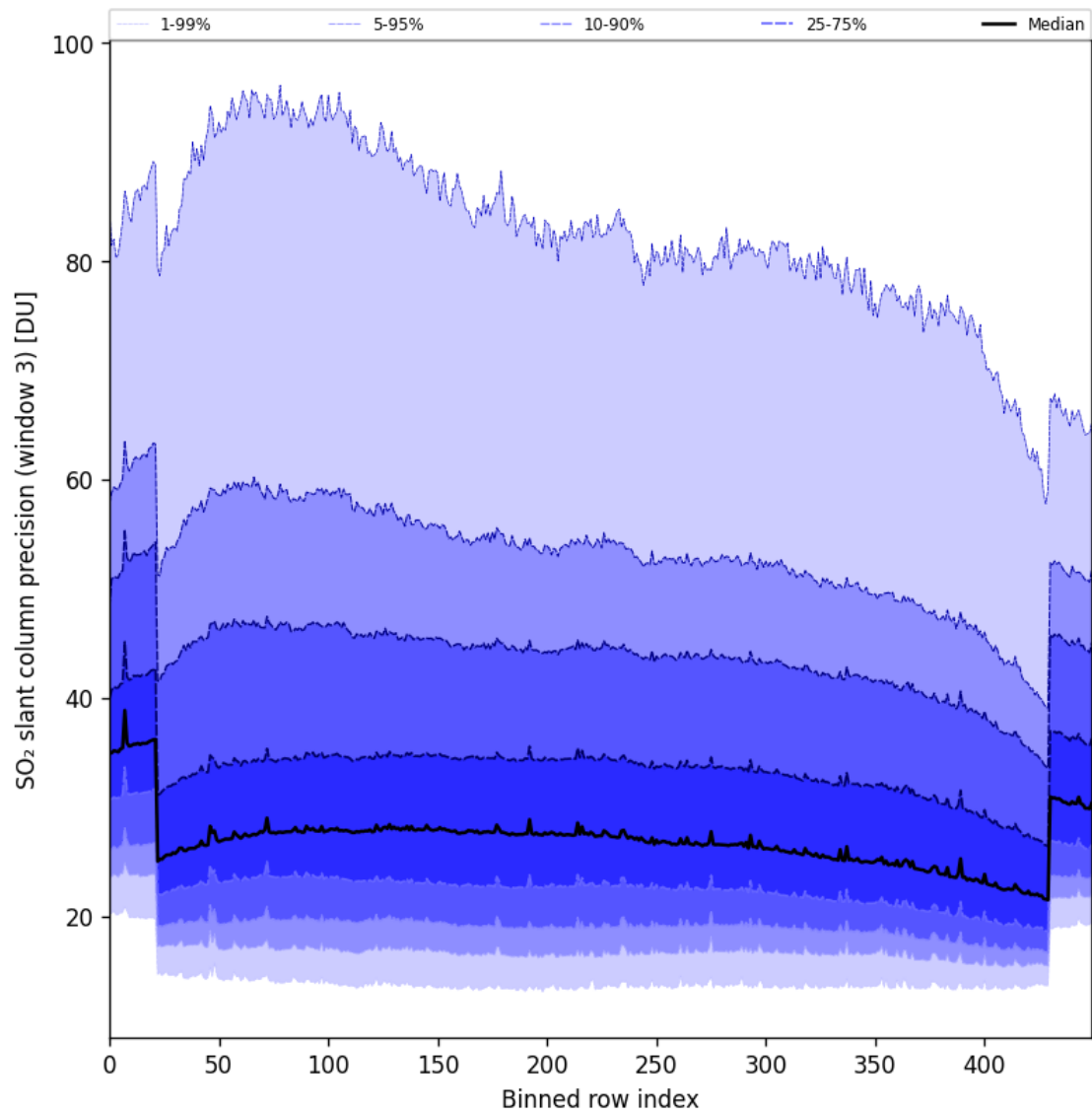
Figure 88: Along track statistics of “SO 2 slant column precision (window 3)” for 2024-09-01 to 2024-09-02
