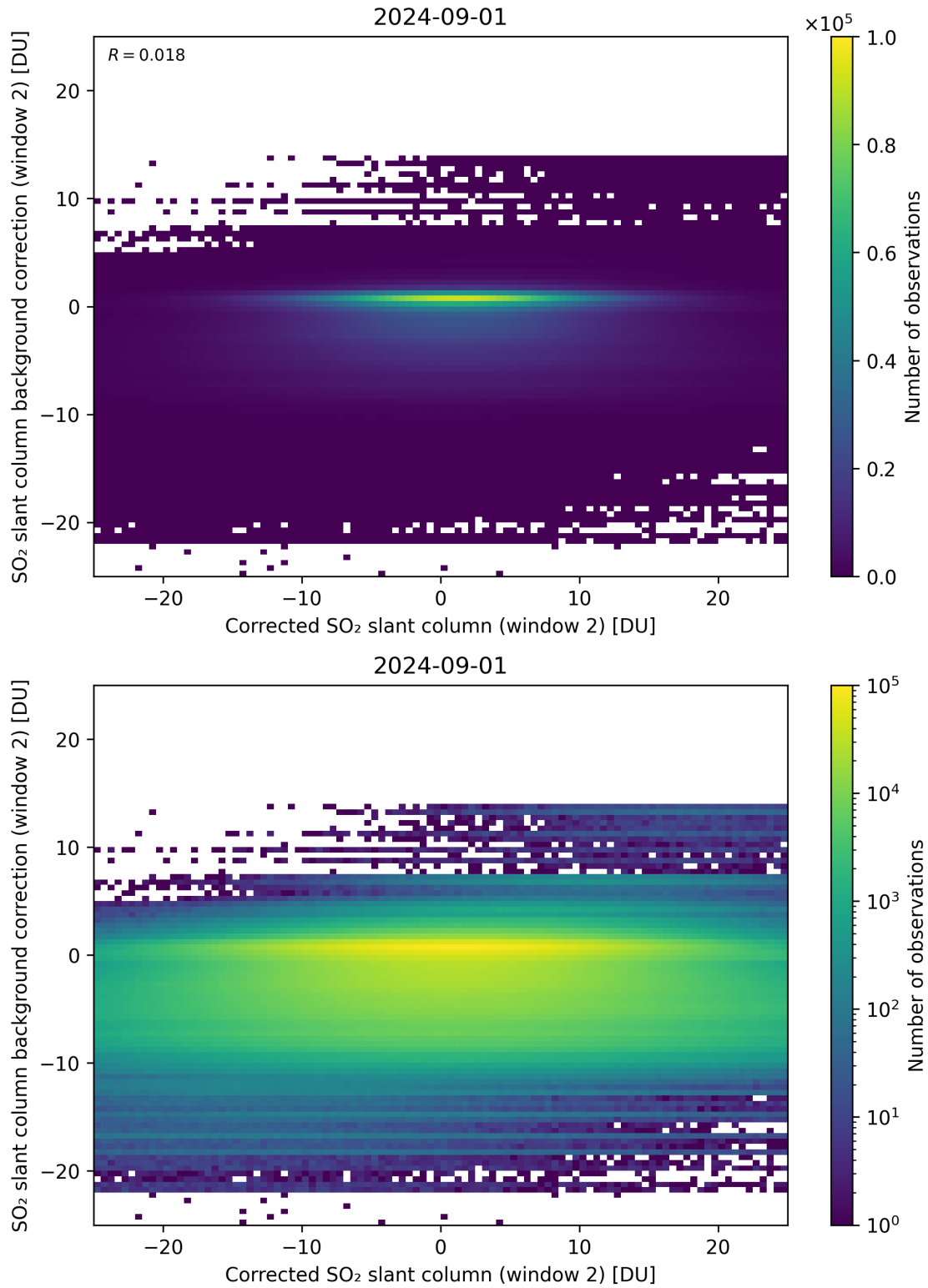
Figure 194: Scatter density plot of “Corrected SO 2 slant column (window 2)” against “SO 2 slant column background correction (window 2)” for 2024-09-01 to 2024-09-02.
