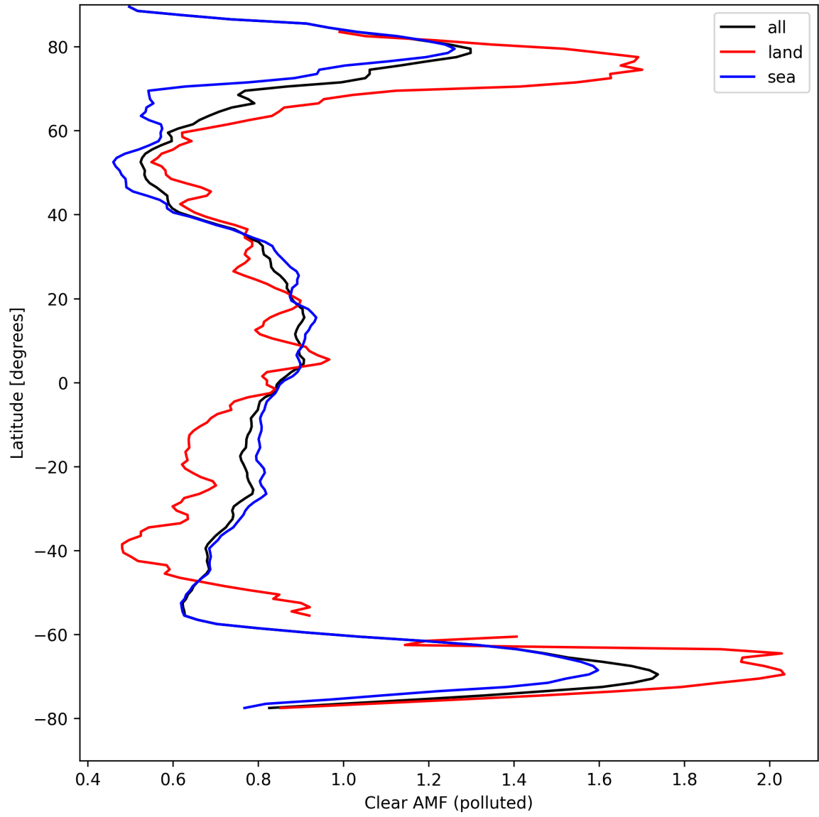
Figure 50: Zonal average of “Clear AMF (polluted)” for 2024-09-01 to 2024-09-02.
