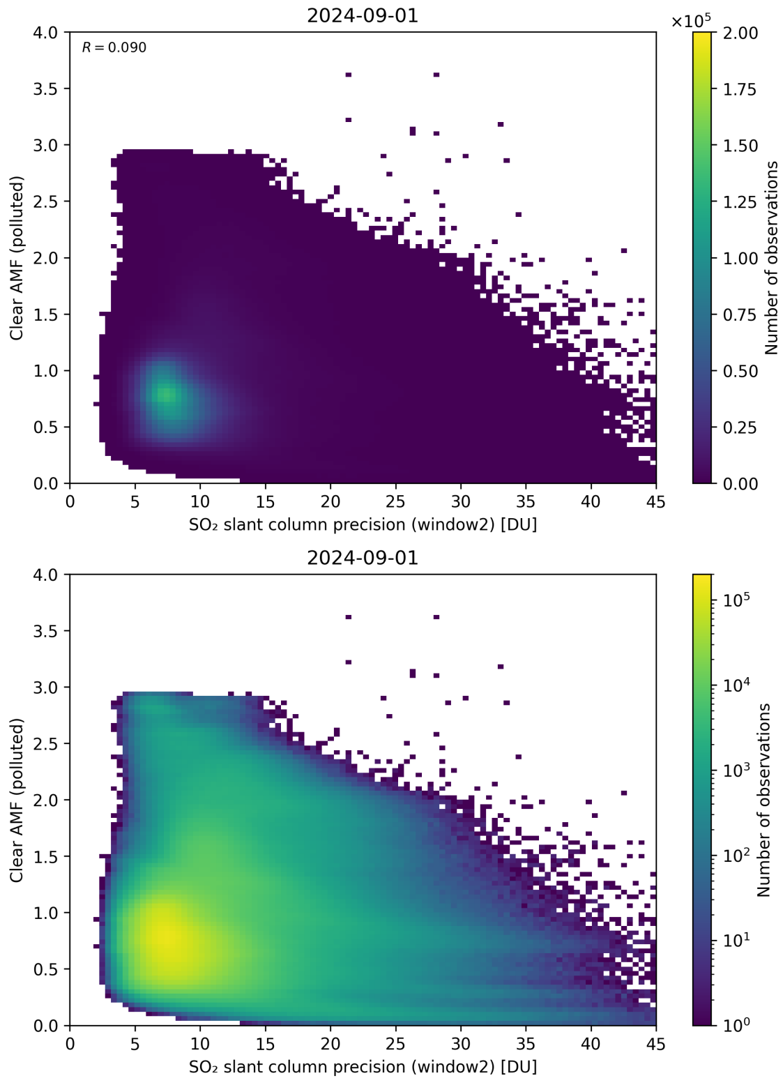
Figure 246: Scatter density plot of “SO 2 slant column precision (window2)” against “Clear AMF (polluted)” for 2024-09-01 to 2024-09-02.
