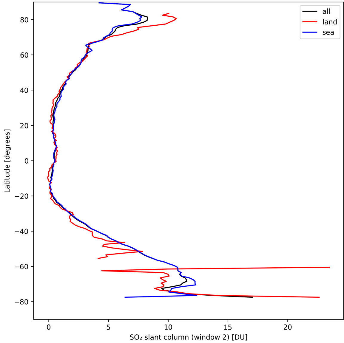
Figure 37: Zonal average of “SO 2 slant column (window 2)” for 2024-09-01 to 2024-09-02.
