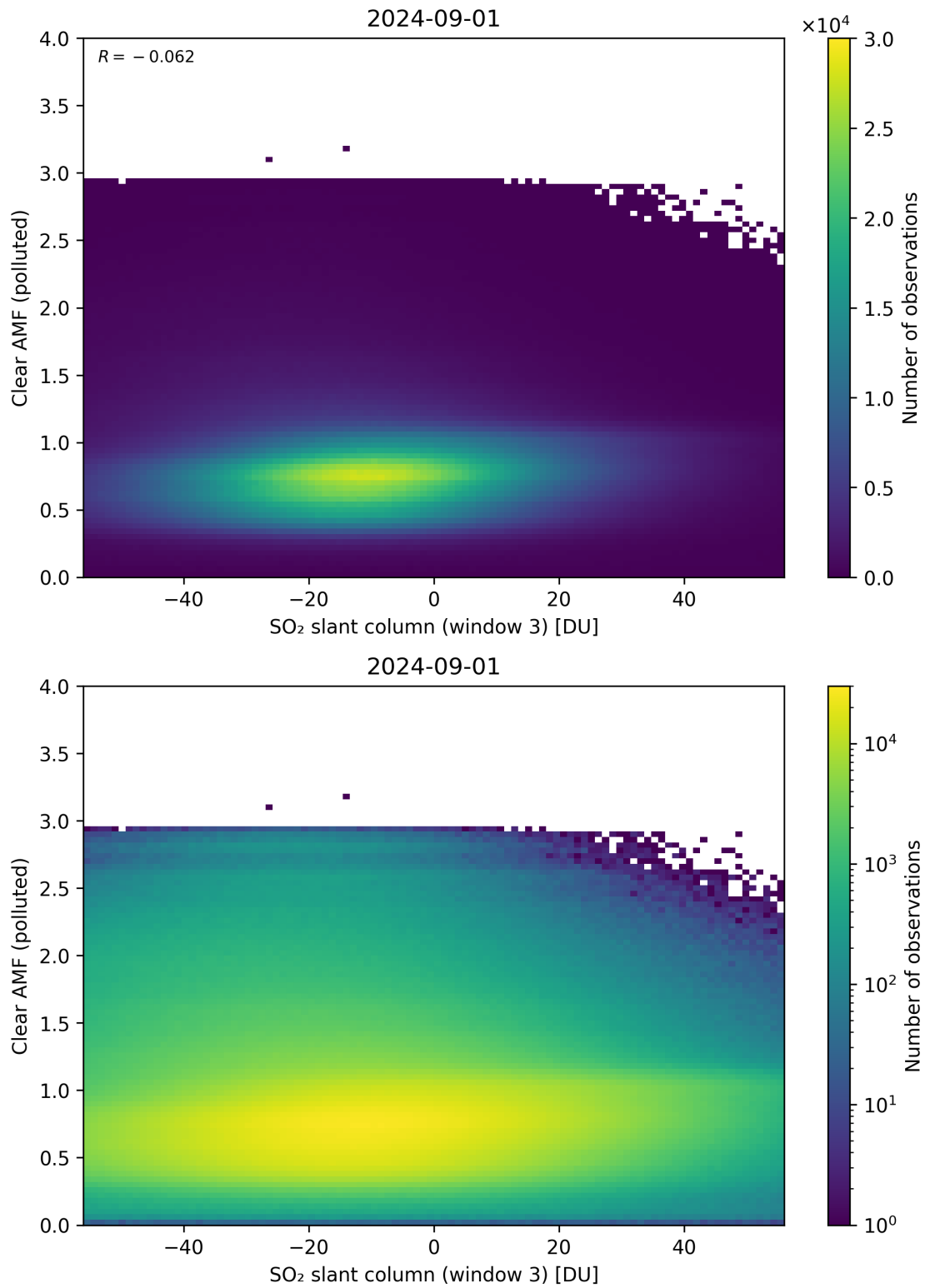
Figure 265: Scatter density plot of “SO 2 slant column (window 3)” against “Clear AMF (polluted)” for 2024-09-01 to 2024-09-02.
