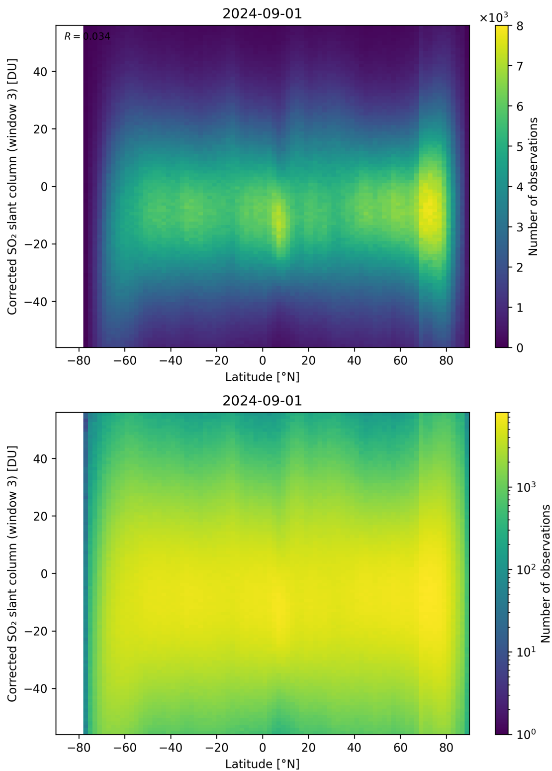
Figure 148: Scatter density plot of “Latitude” against “Corrected SO 2 slant column (window 3)” for 2024-09-01 to 2024-09-02.
