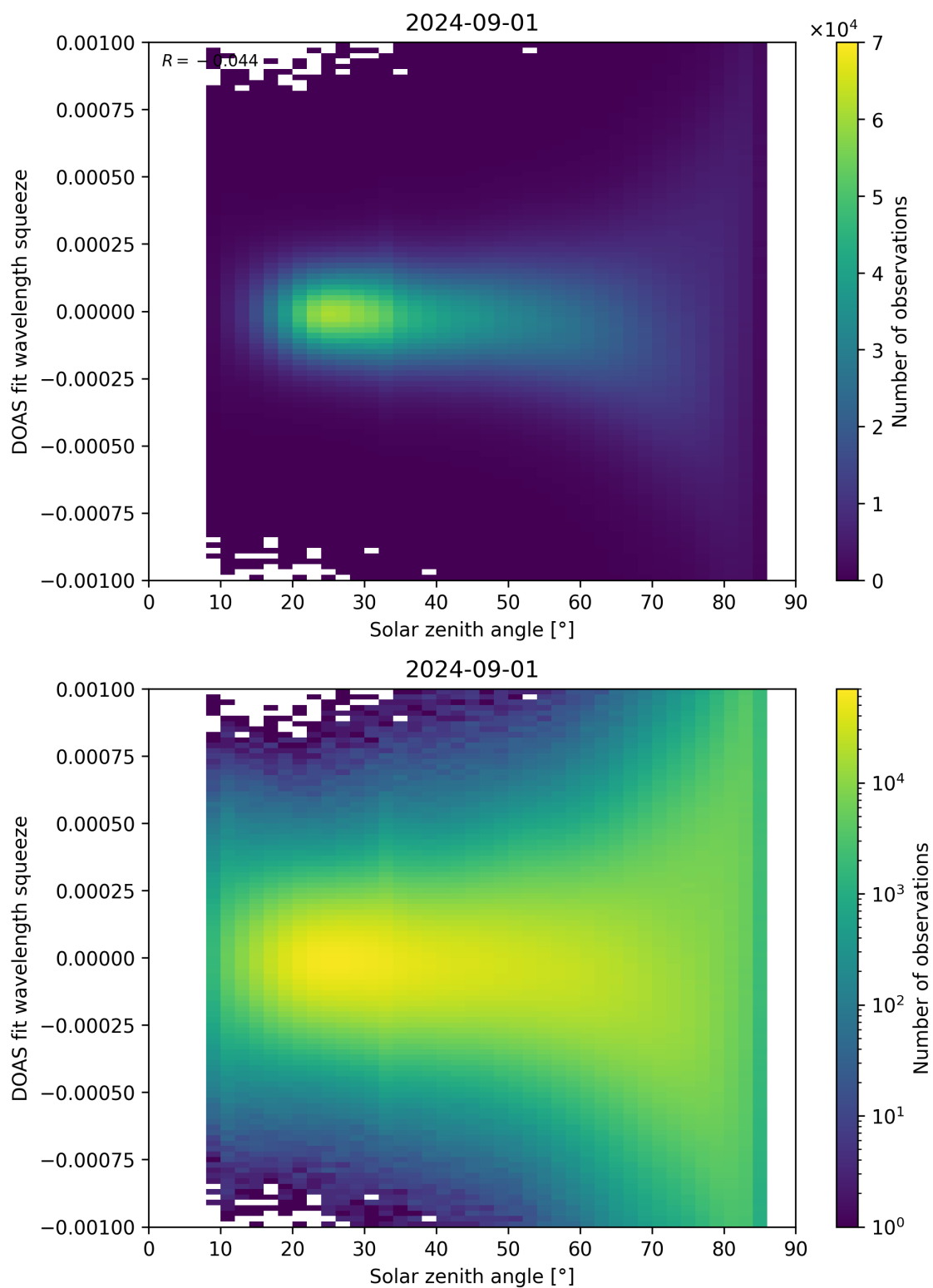
Figure 162: Scatter density plot of “Solar zenith angle” against “DOAS fit wavelength squeeze” for 2024-09-01 to 2024-09-02.
