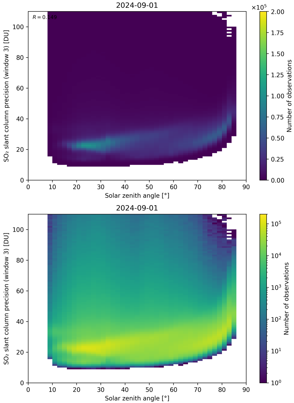
Figure 173: Scatter density plot of “Solar zenith angle” against “SO 2 slant column precision (window 3)” for 2024-09-01 to 2024-09-02.
