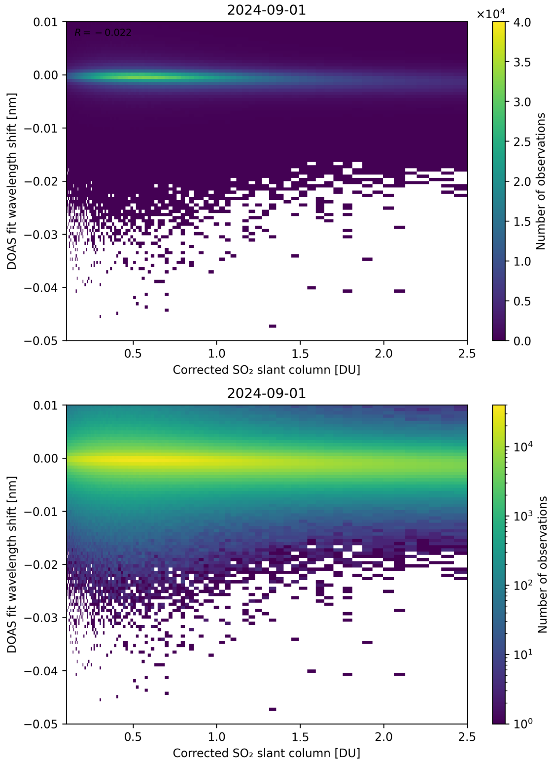
Figure 181: Scatter density plot of “Corrected SO 2 slant column” against “DOAS fit wavelength shift” for 2024-09-01 to 2024-09-02.
