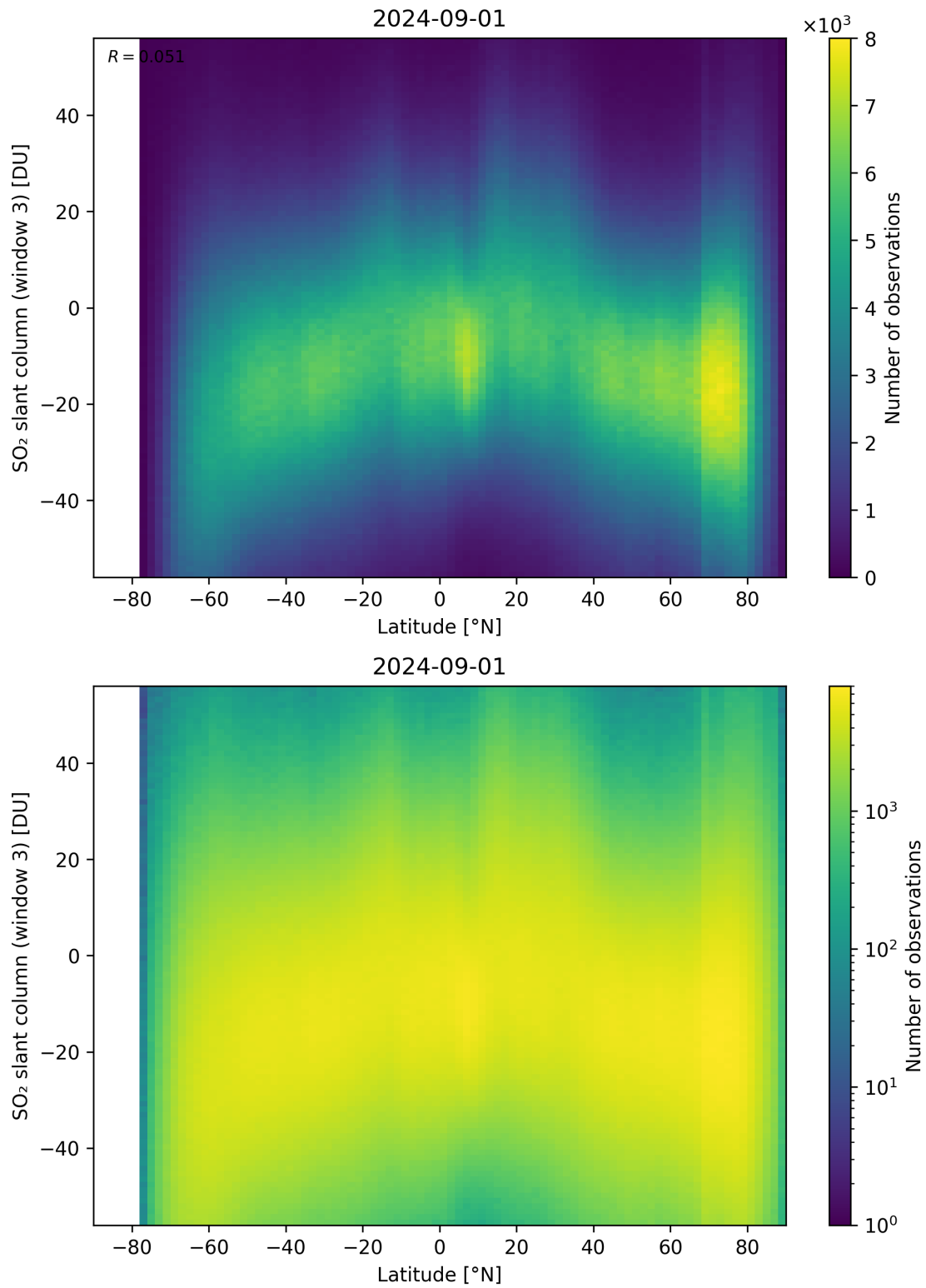
Figure 152: Scatter density plot of “Latitude” against “SO 2 slant column (window 3)” for 2024-09-01 to 2024-09-02.
