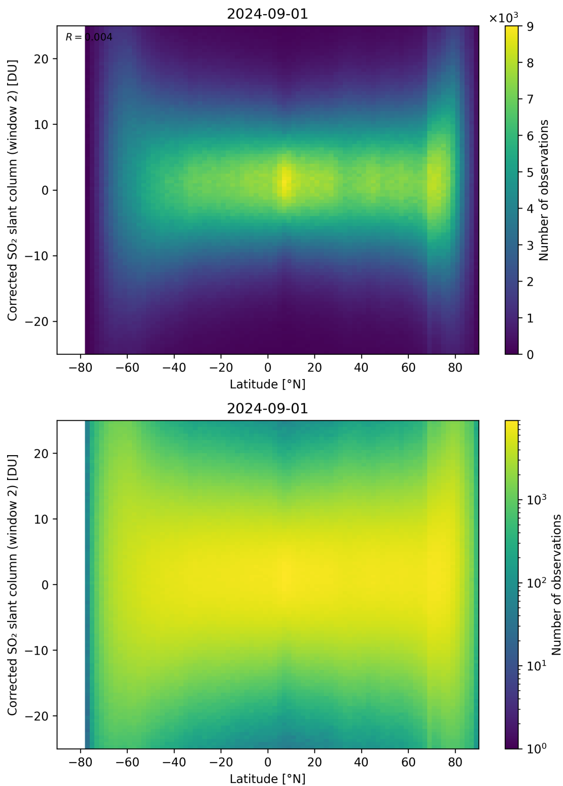
Figure 147: Scatter density plot of “Latitude” against “Corrected SO 2 slant column (window 2)” for 2024-09-01 to 2024-09-02.
