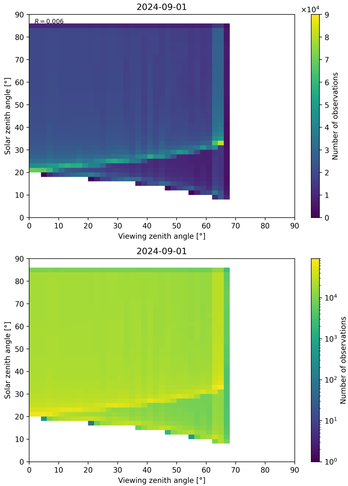
Figure 315: Scatter density plot of “Viewing zenith angle” against “Solar zenith angle” for 2024-09-01 to 2024-09-02.
