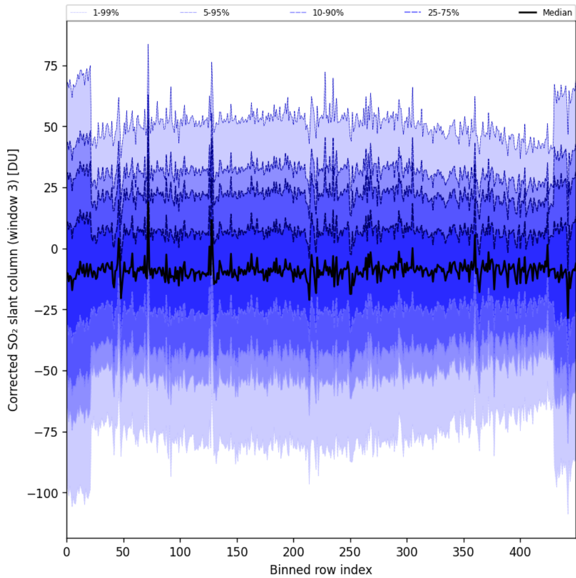
Figure 89: Along track statistics of “Corrected SO 2 slant column (window 3)” for 2024-09-01 to 2024-09-02
