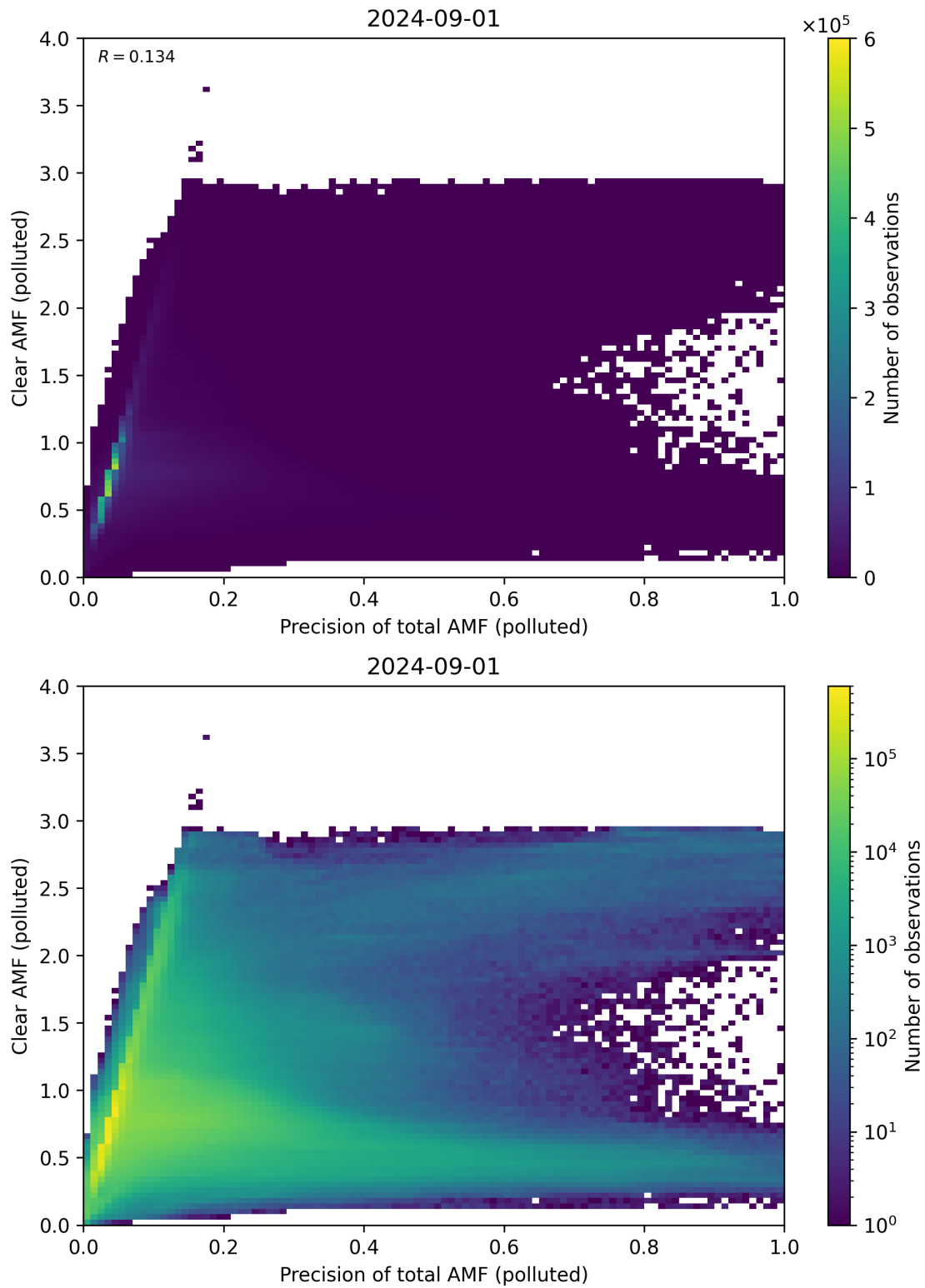
Figure 270: Scatter density plot of “Precision of total AMF (polluted)” against “Clear AMF (polluted)” for 2024-09-01 to 2024-09-02.
