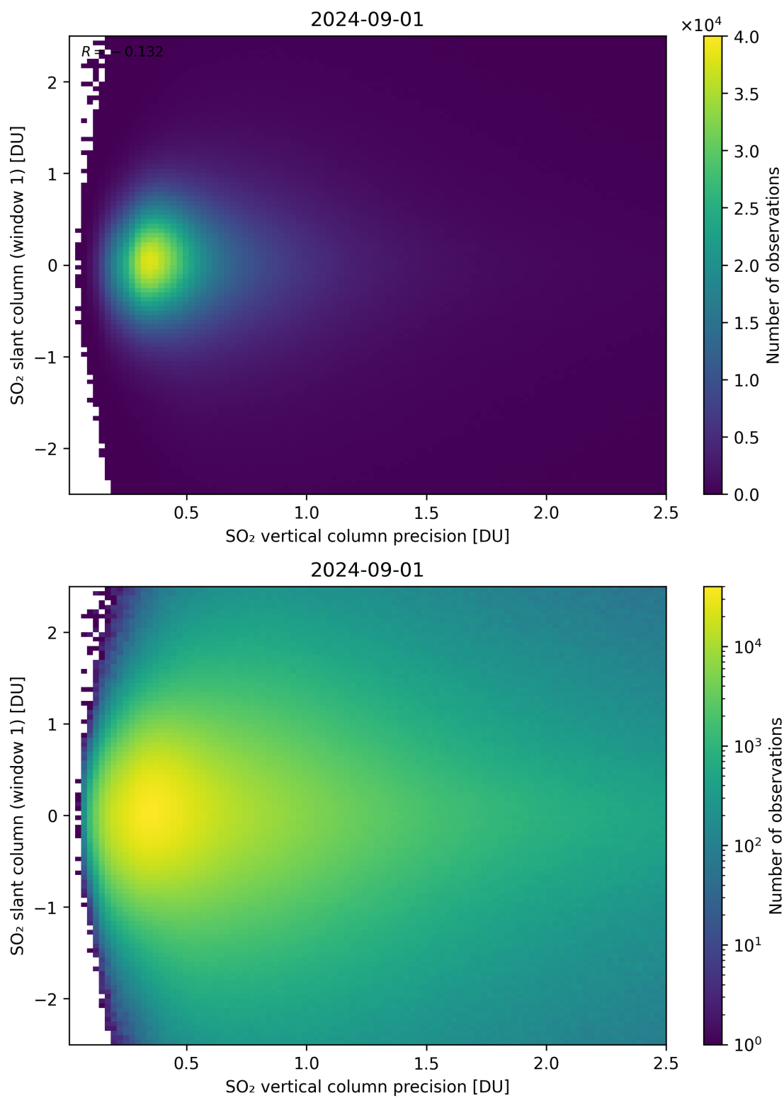
Figure 289: Scatter density plot of “SO 2 vertical column precision” against “SO 2 slant column (window 1)” for 2024-09-01 to 2024-09-02.
