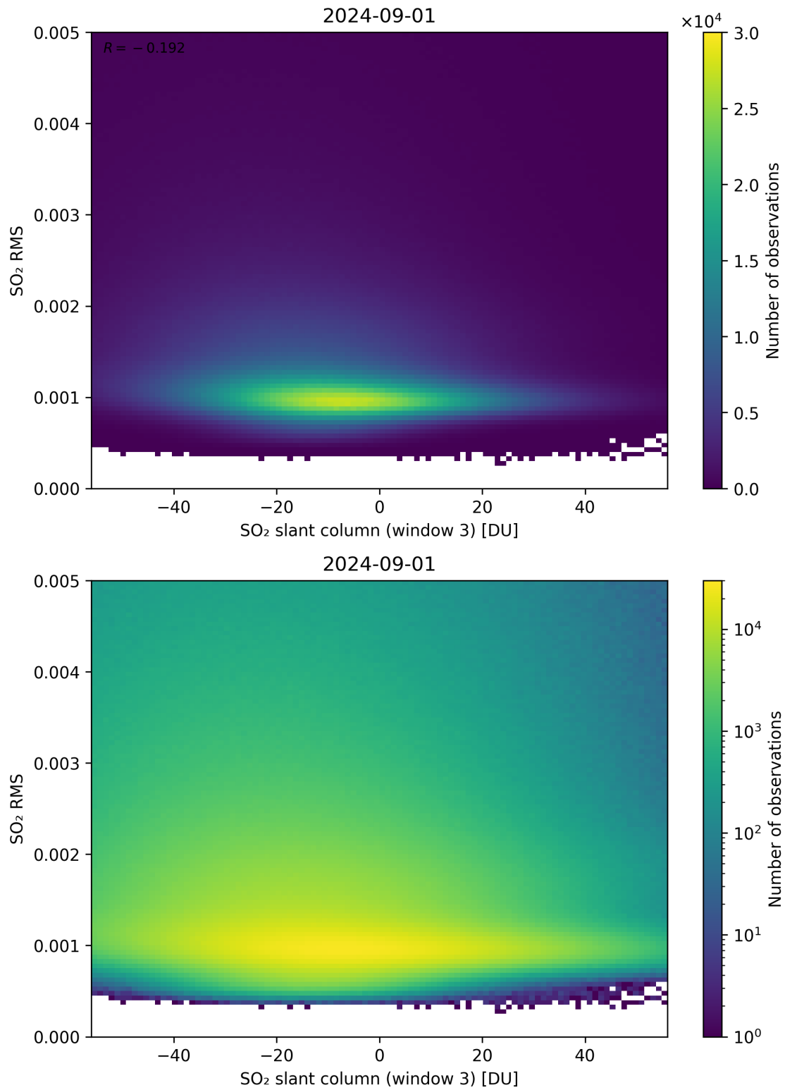
Figure 256: Scatter density plot of “SO 2 slant column (window 3)” against “SO 2 RMS” for 2024-09-01 to 2024-09-02.
