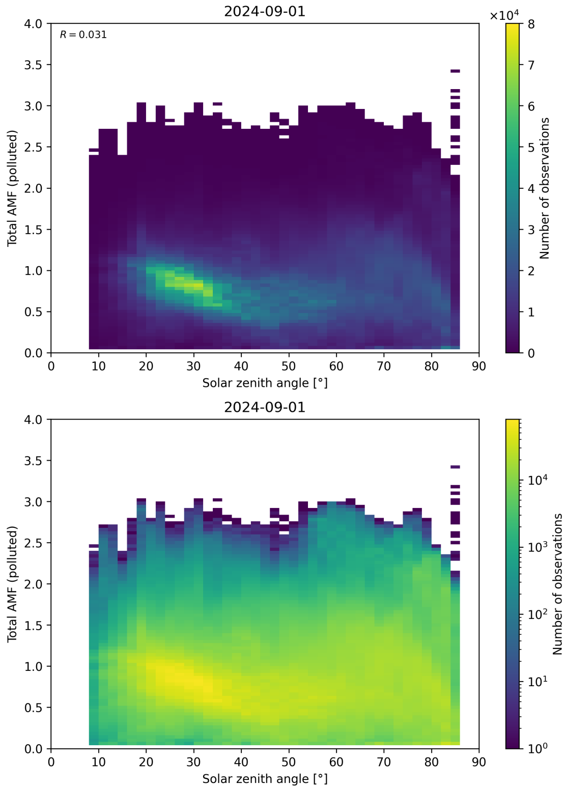
Figure 174: Scatter density plot of “Solar zenith angle” against “Total AMF (polluted)” for 2024-09-01 to 2024-09-02.
