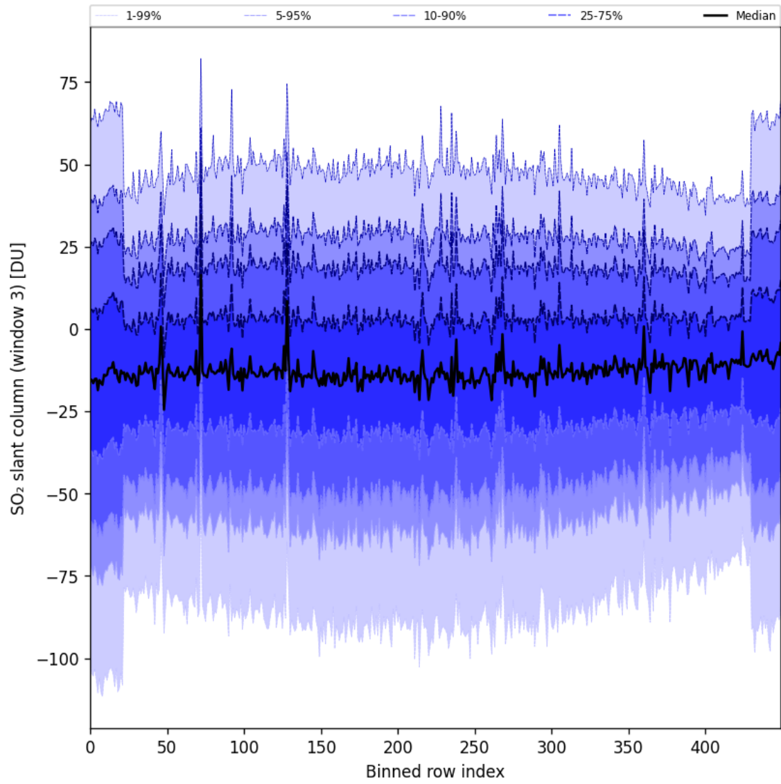
Figure 87: Along track statistics of “SO 2 slant column (window 3)” for 2024-09-01 to 2024-09-02
