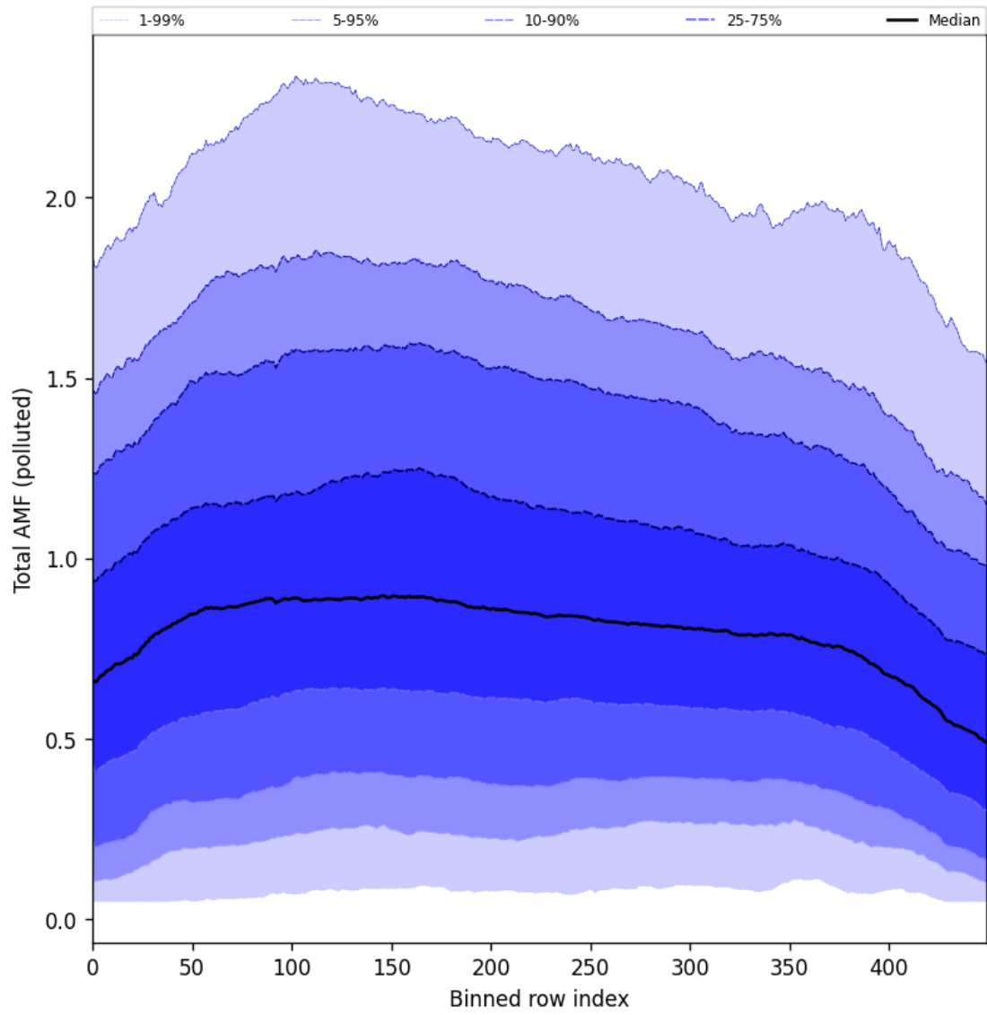
Figure 94: Along track statistics of “Total AMF (polluted)” for 2024-09-01 to 2024-09-02
