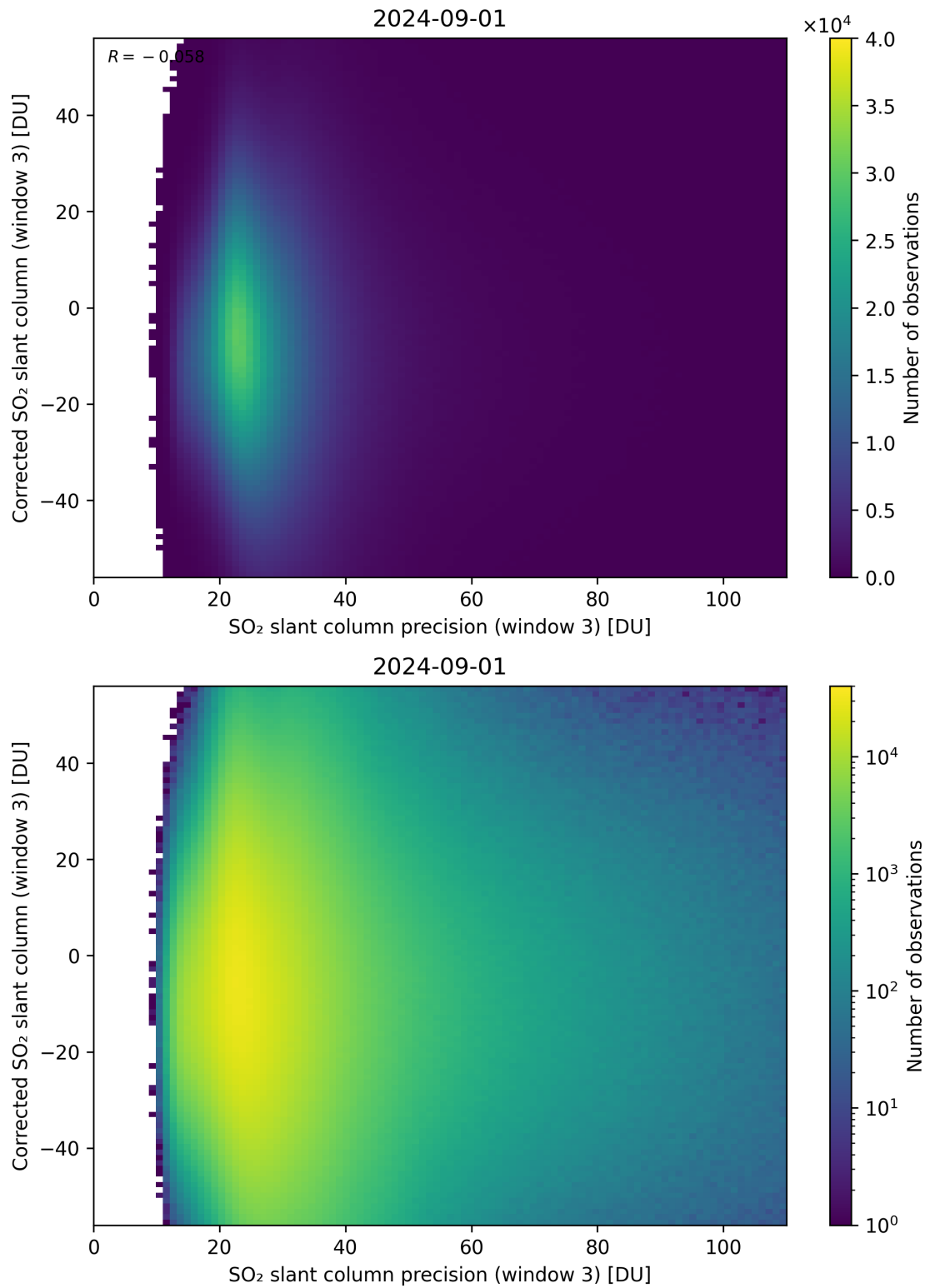
Figure 262: Scatter density plot of “SO 2 slant column precision (window 3)” against “Corrected SO 2 slant column (window 3)” for 2024-09-01 to 2024-09-02.
