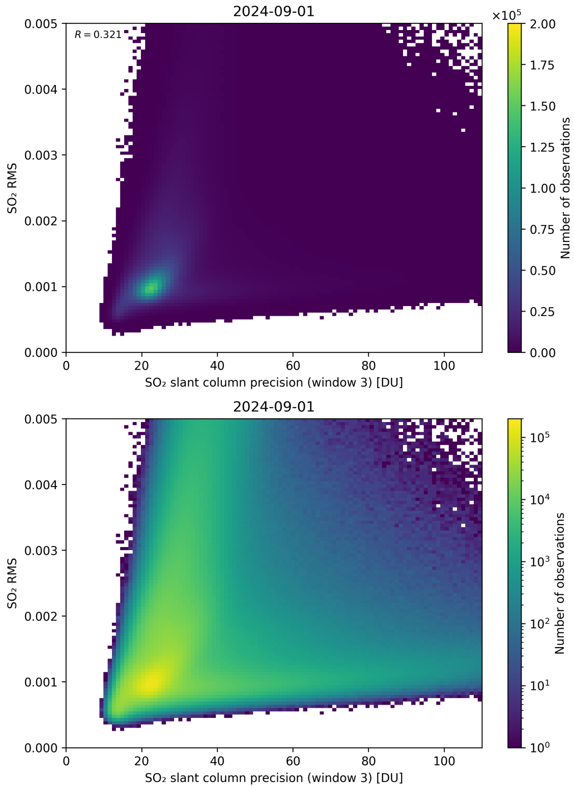
Figure 260: Scatter density plot of “SO 2 slant column precision (window 3)” against “SO 2 RMS” for 2024-09-01 to 2024-09-02.
