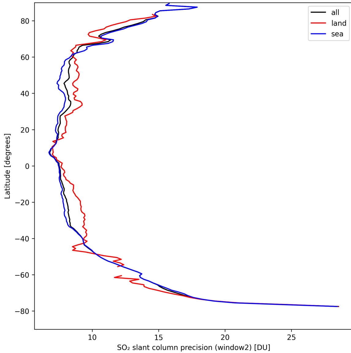
Figure 38: Zonal average of “SO 2 slant column precision (window2)” for 2024-09-01 to 2024-09-02.
