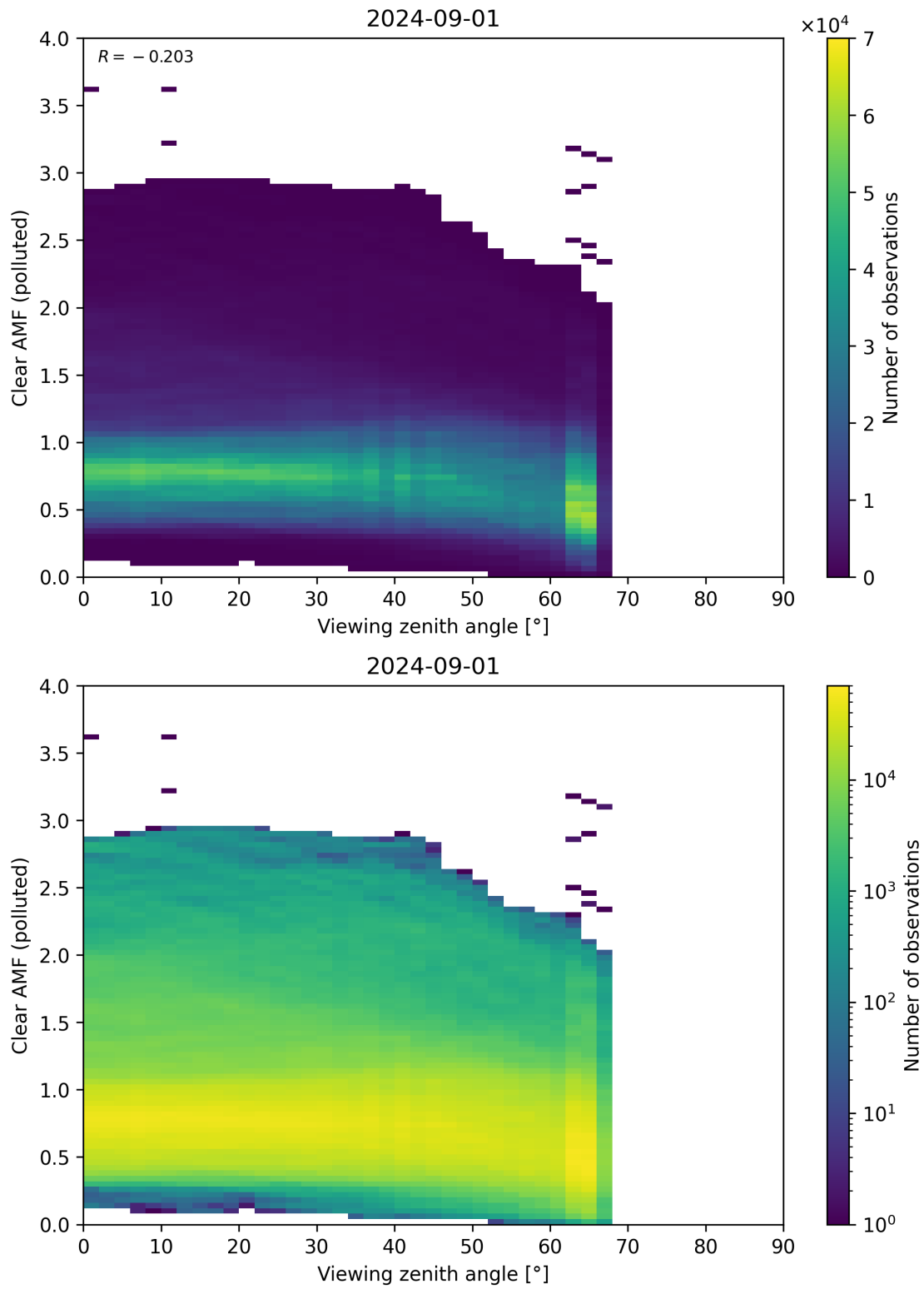
Figure 316: Scatter density plot of “Viewing zenith angle” against “Clear AMF (polluted)” for 2024-09-01 to 2024-09-02.
