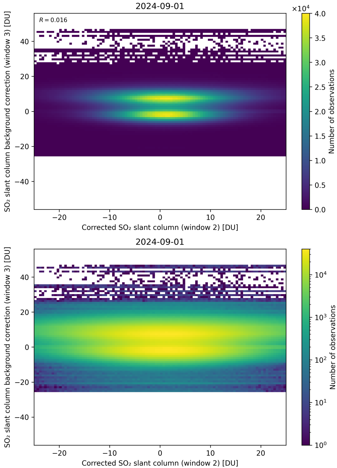
Figure 195: Scatter density plot of “Corrected SO 2 slant column (window 2)” against “SO 2 slant column background correction (window 3)” for 2024-09-01 to 2024-09-02.
