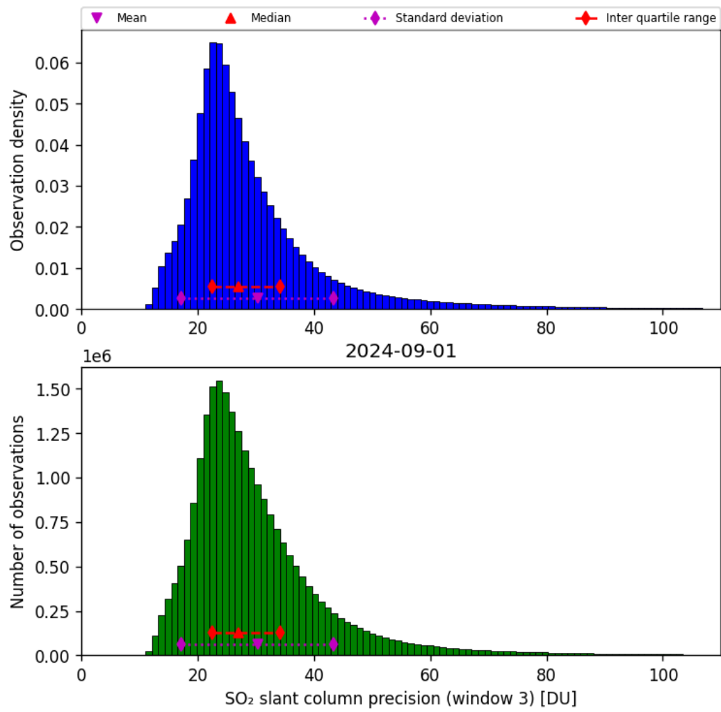
Figure 65: Histogram of “SO 2 slant column precision (window 3)” for 2024-09-01 to 2024-09-02
