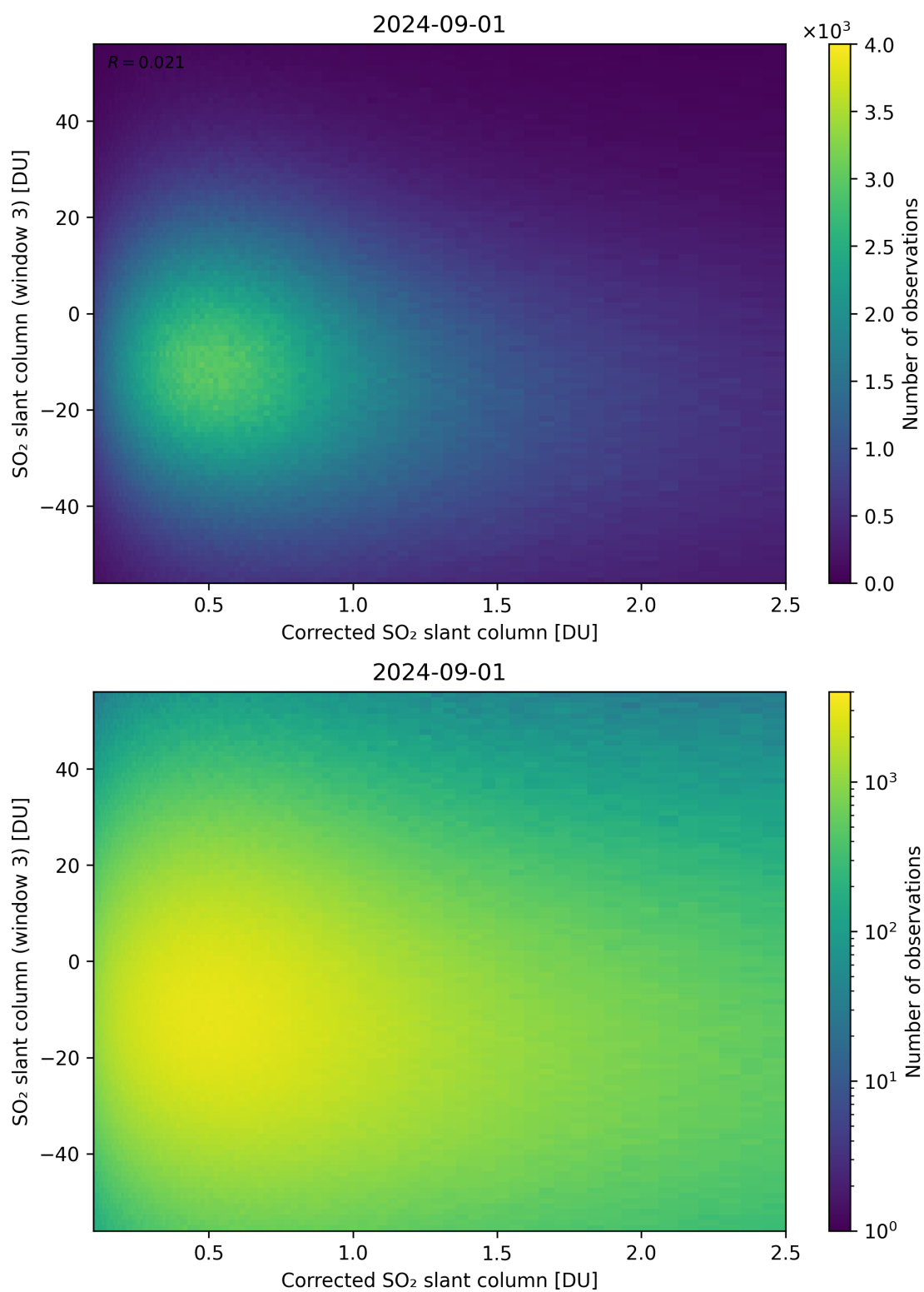
Figure 190: Scatter density plot of “Corrected SO 2 slant column” against “SO 2 slant column (window 3)” for 2024-09-01 to 2024-09-02.
