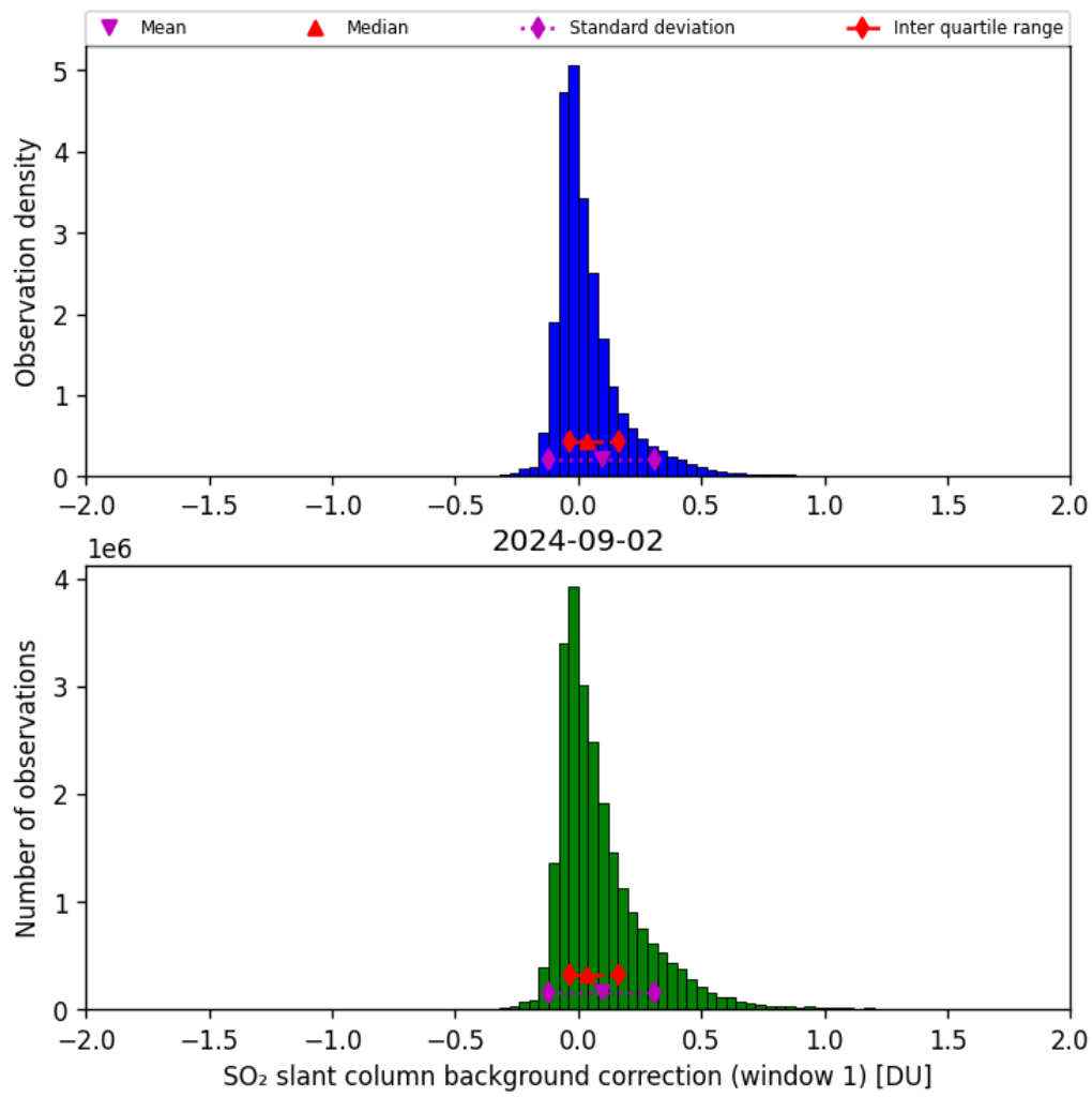
Figure 59: Histogram of “SO 2 slant column background correction (window 1)” for 2024-09-01 to 2024-09-03
