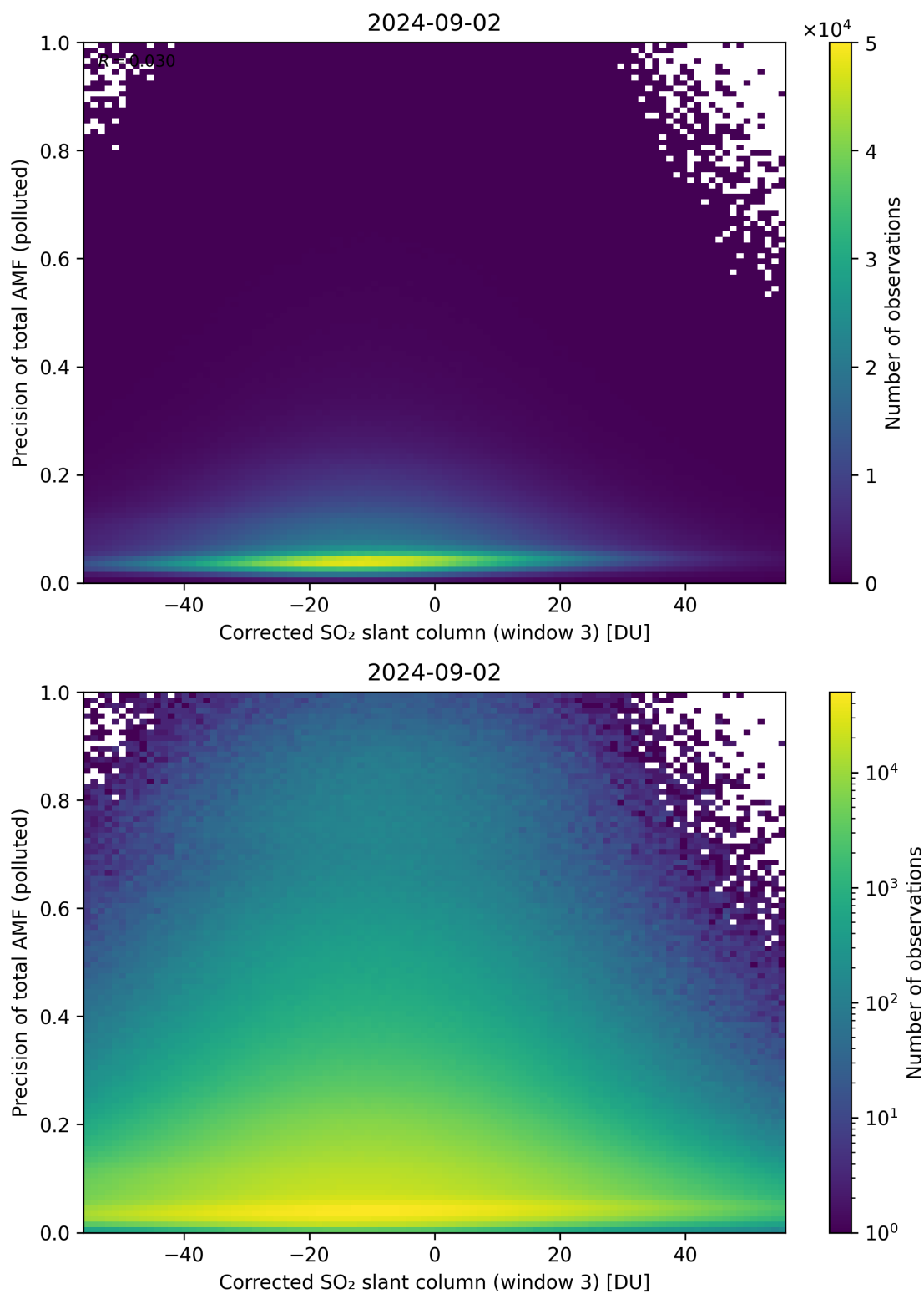
Figure 211: Scatter density plot of “Corrected SO 2 slant column (window 3)” against “Precision of total AMF (polluted)” for 2024-09-01 to 2024-09-03.
