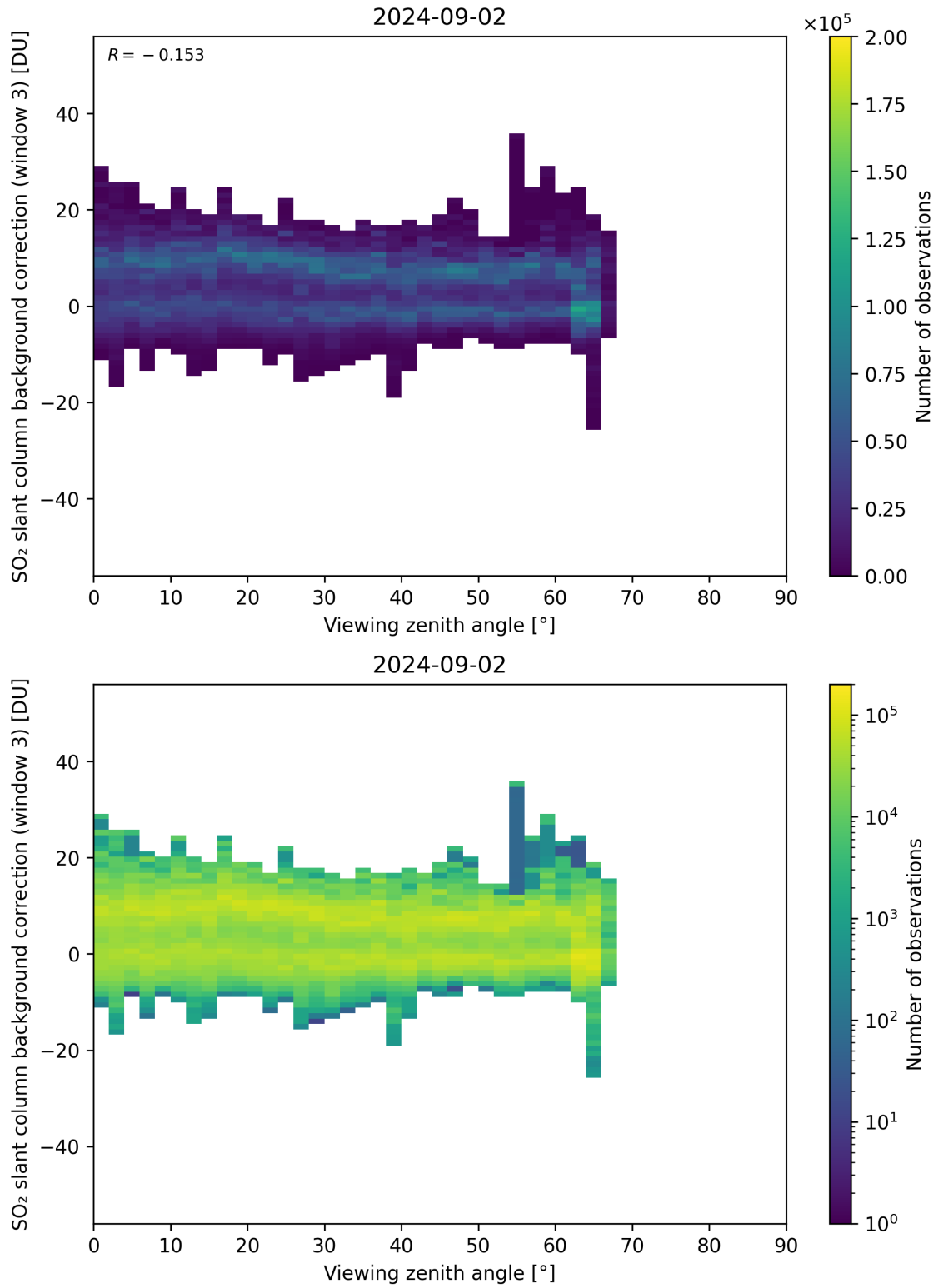
Figure 310: Scatter density plot of “Viewing zenith angle” against “SO 2 slant column background correction (window 3)” for 2024-09-01 to 2024-09-03.
