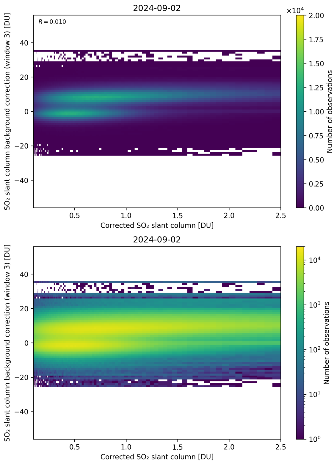
Figure 180: Scatter density plot of “Corrected SO 2 slant column” against “SO 2 slant column background correction (window 3)” for 2024-09-01 to 2024-09-03.
