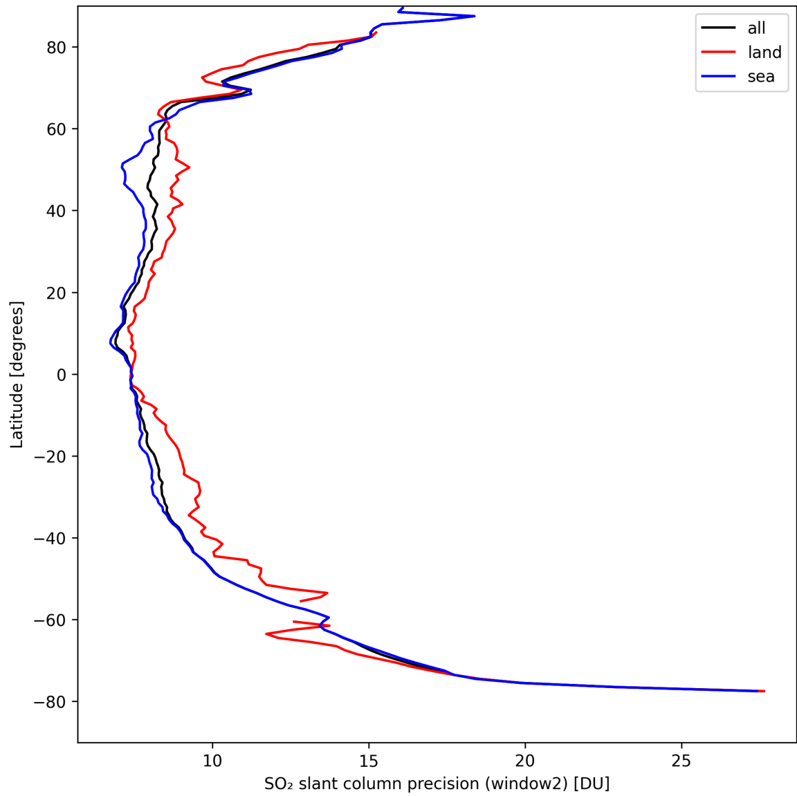
Figure 38: Zonal average of “SO 2 slant column precision (window2)” for 2024-09-01 to 2024-09-03.
