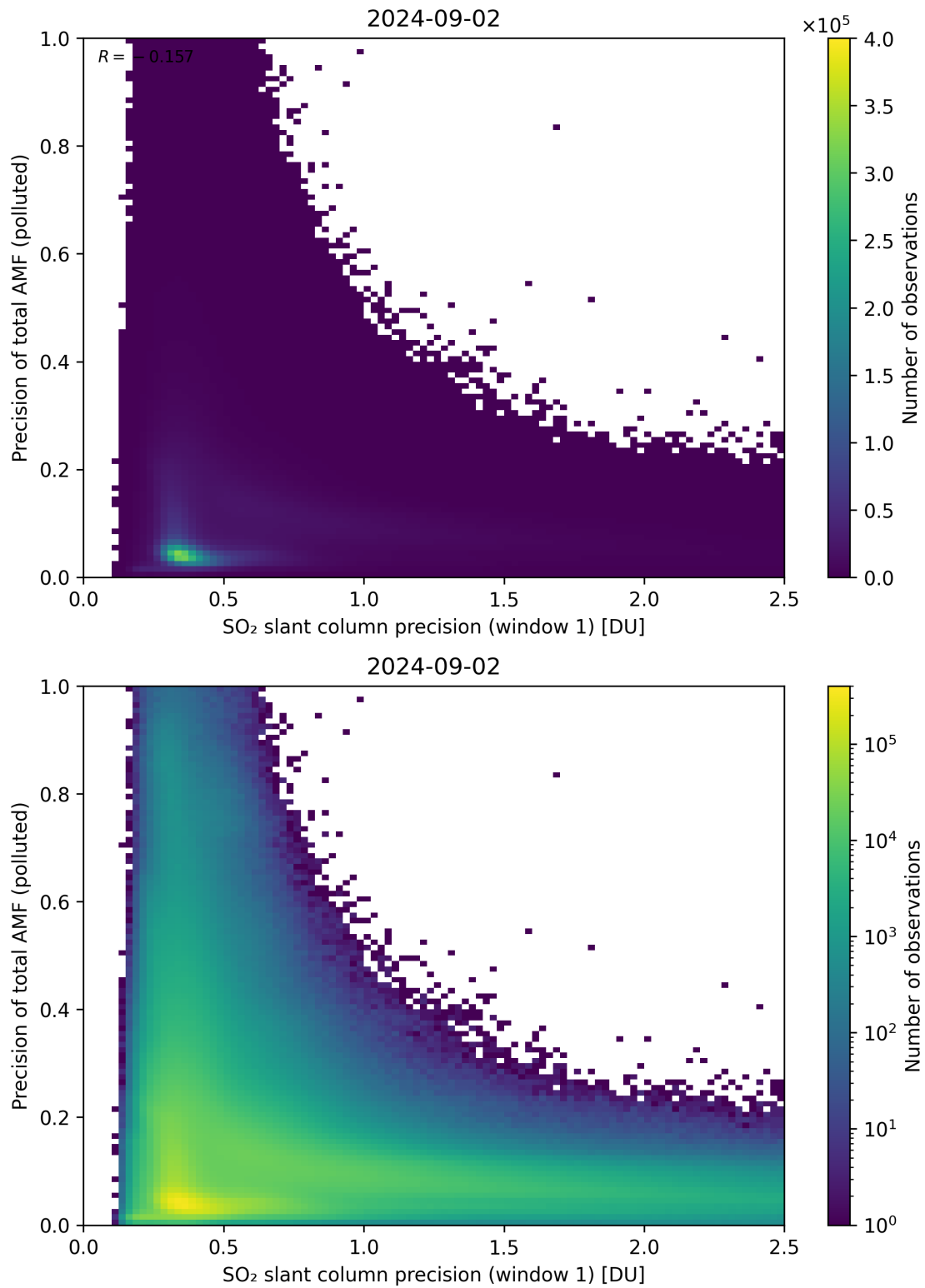
Figure 231: Scatter density plot of “SO 2 slant column precision (window 1)” against “Precision of total AMF (polluted)” for 2024-09-01 to 2024-09-03.
