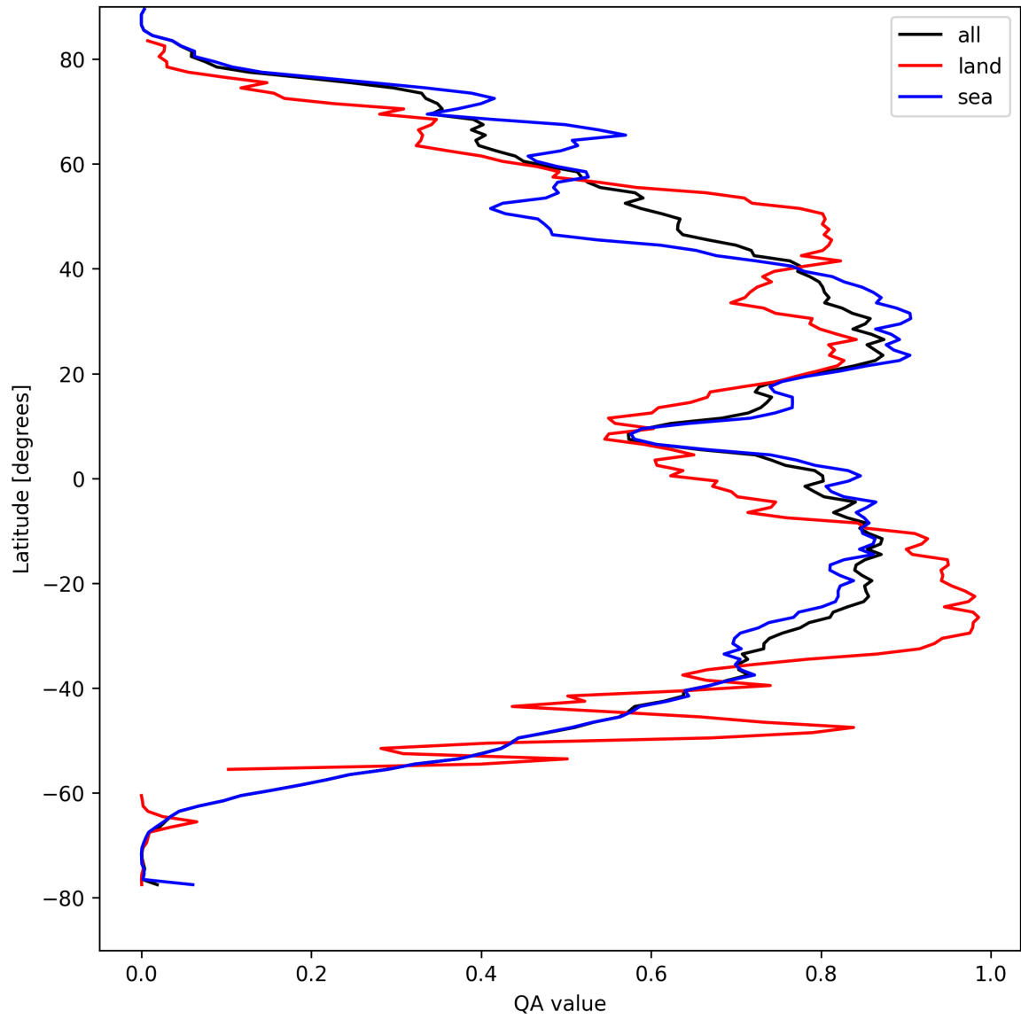
Figure 29: Zonal average of “QA value” for 2024-09-01 to 2024-09-03.
