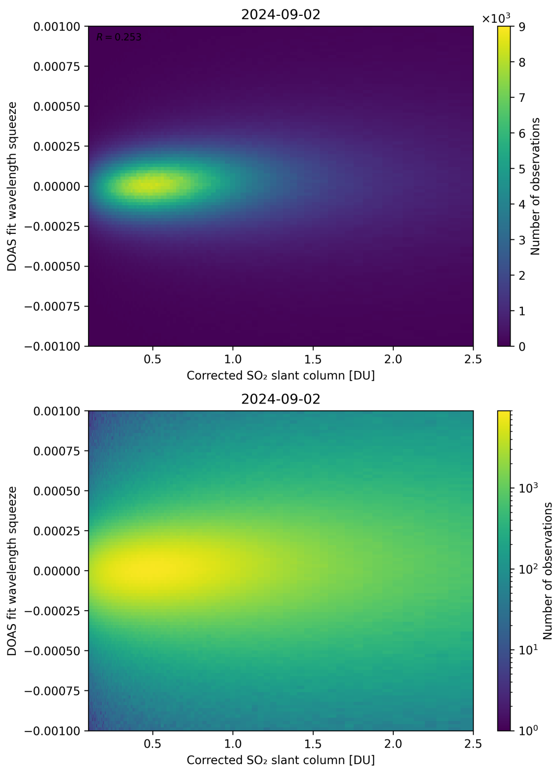
Figure 182: Scatter density plot of “Corrected SO 2 slant column” against “DOAS fit wavelength squeeze” for 2024-09-01 to 2024-09-03.
