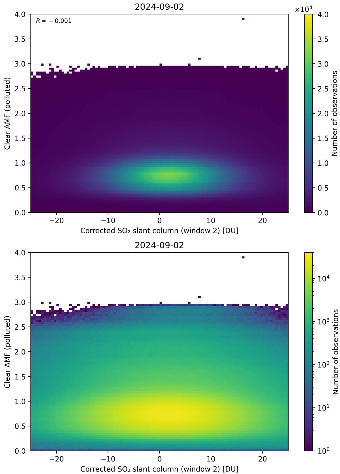
Figure 199: Scatter density plot of “Corrected SO 2 slant column (window 2)” against “Clear AMF (polluted)” for 2024-09-01 to 2024-09-03.
