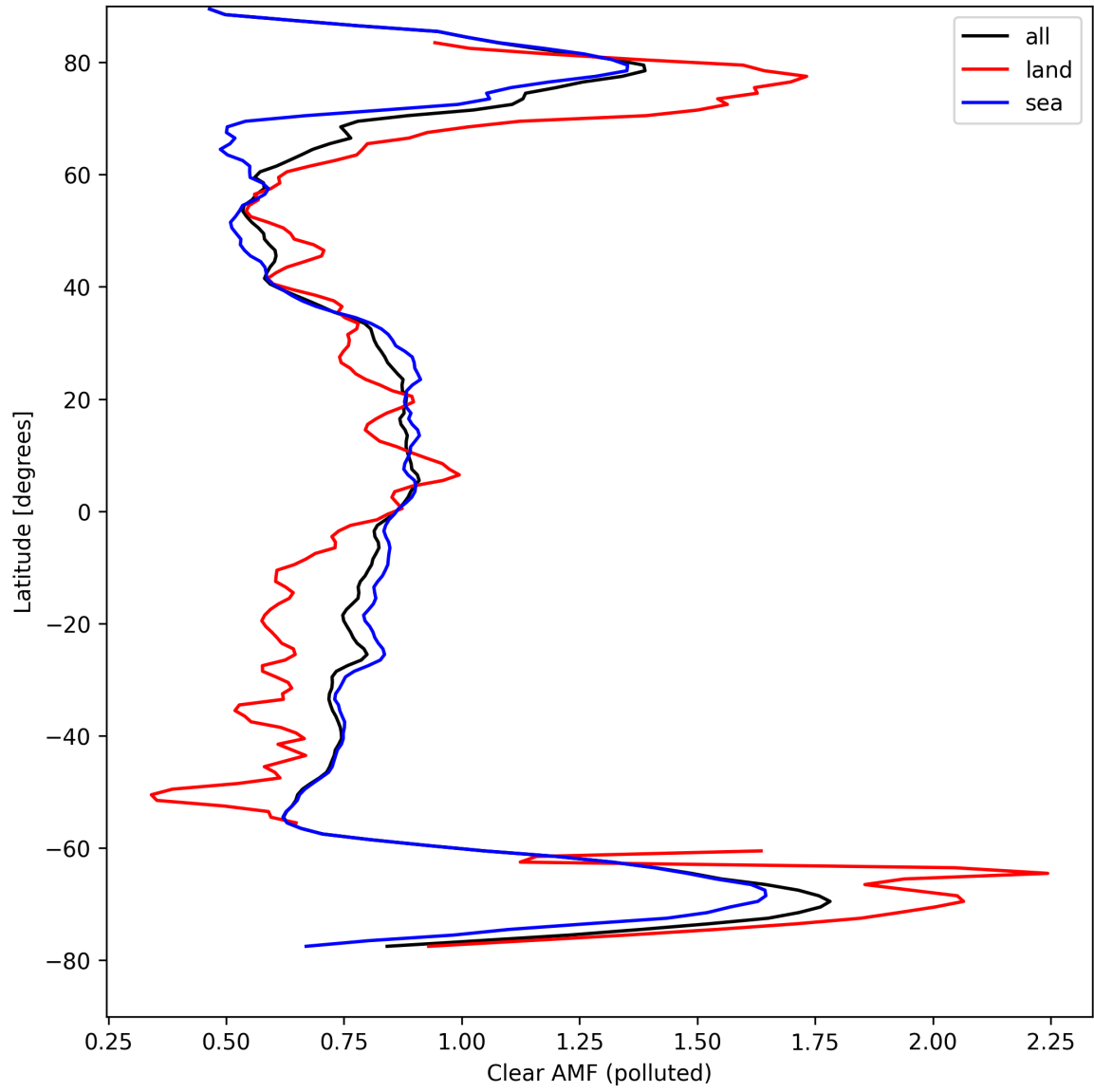
Figure 50: Zonal average of “Clear AMF (polluted)” for 2024-09-01 to 2024-09-03.
