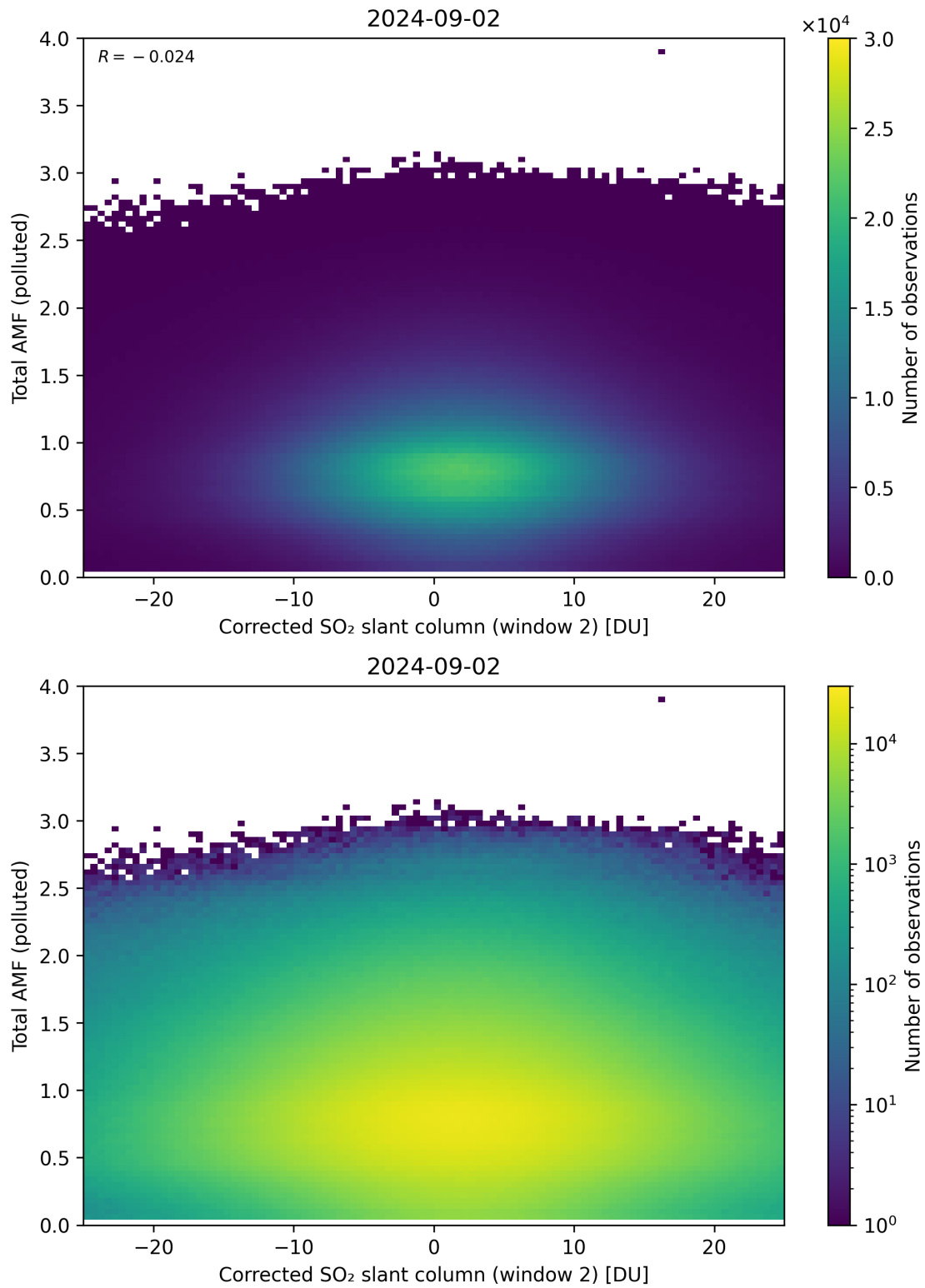
Figure 203: Scatter density plot of “Corrected SO 2 slant column (window 2)” against “Total AMF (polluted)” for 2024-09-01 to 2024-09-03.
