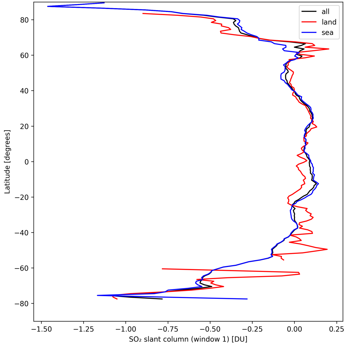
Figure 33: Zonal average of “SO 2 slant column (window 1)” for 2024-09-01 to 2024-09-03.
