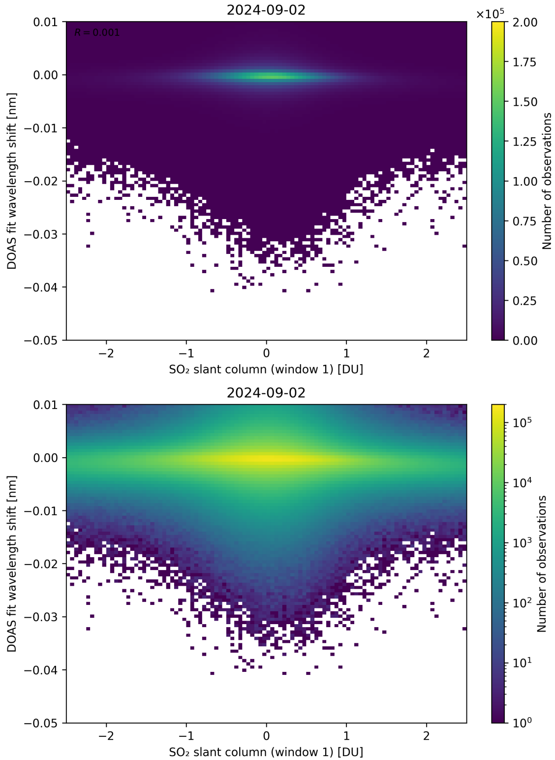
Figure 215: Scatter density plot of “SO 2 slant column (window 1)” against “DOAS fit wavelength shift” for 2024-09-01 to 2024-09-03.
