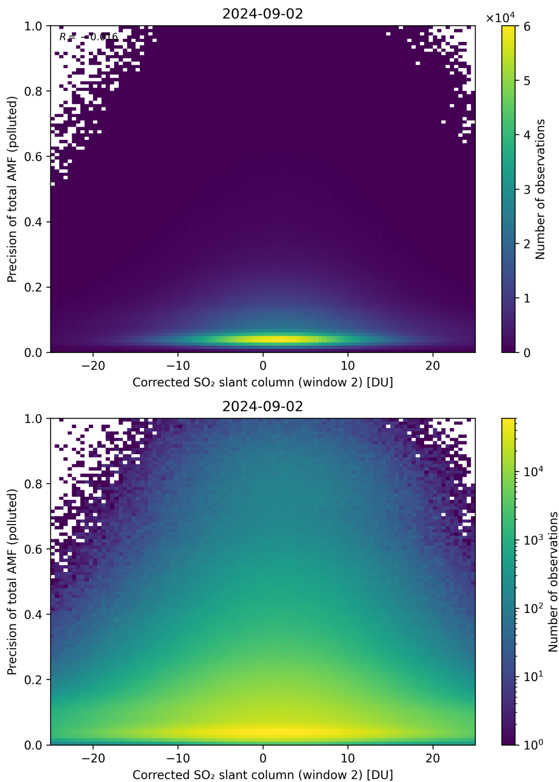
Figure 204: Scatter density plot of “Corrected SO 2 slant column (window 2)” against “Precision of total AMF (polluted)” for 2024-09-01 to 2024-09-03.
