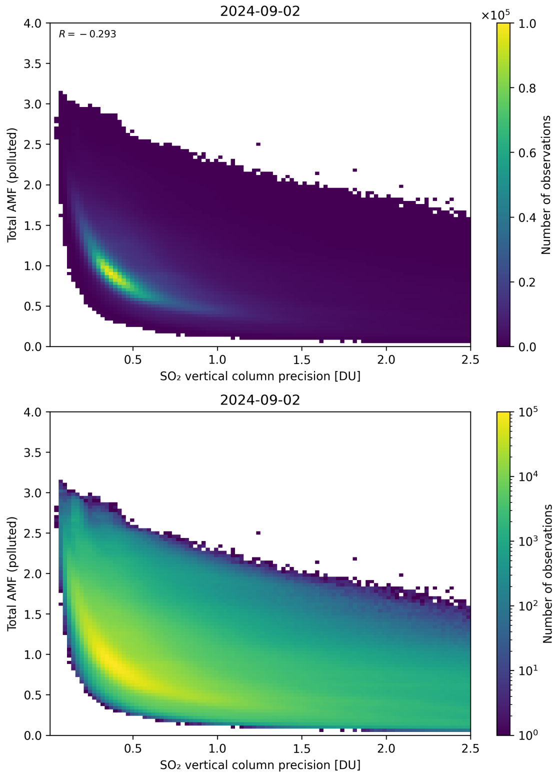
Figure 294: Scatter density plot of “SO 2 vertical column precision” against “Total AMF (polluted)” for 2024-09-01 to 2024-09-03.
