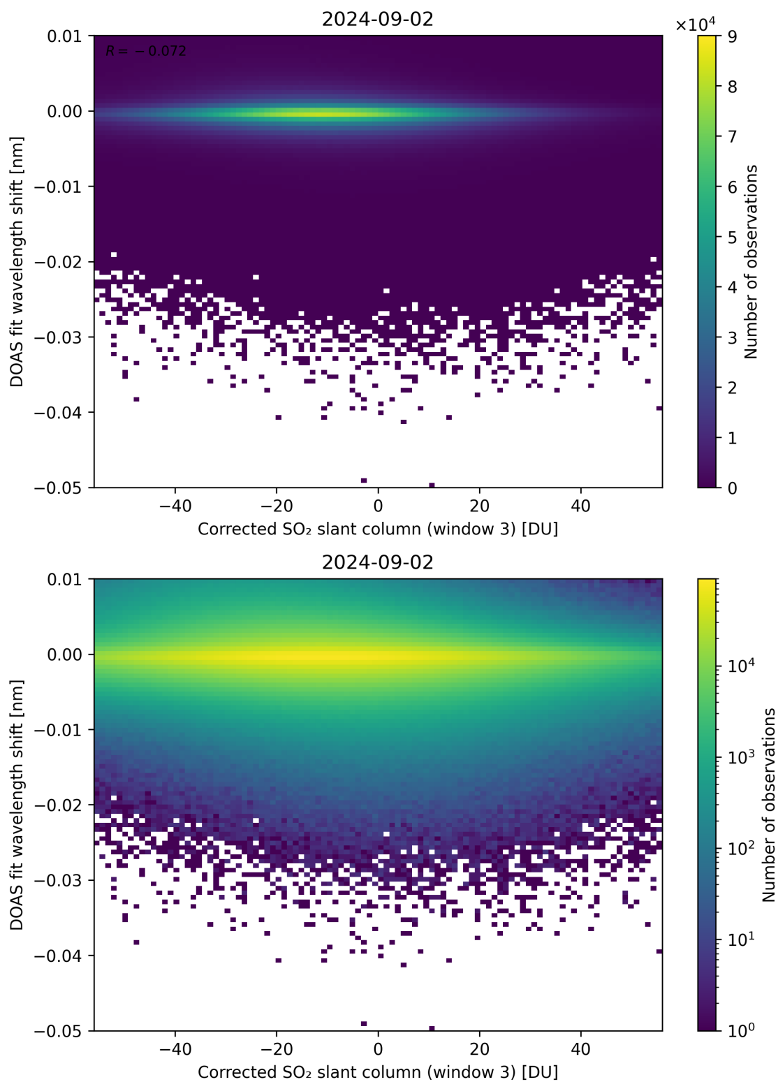
Figure 206: Scatter density plot of “Corrected SO 2 slant column (window 3)” against “DOAS fit wavelength shift” for 2024-09-01 to 2024-09-03.
