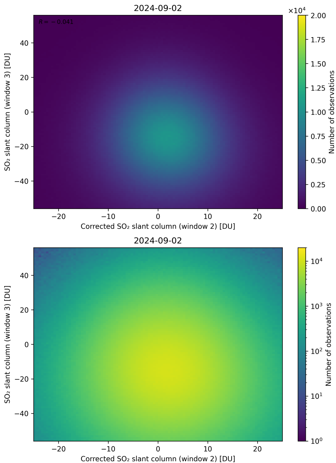
Figure 201: Scatter density plot of “Corrected SO 2 slant column (window 2)” against “SO 2 slant column (window 3)” for 2024-09-01 to 2024-09-03.
