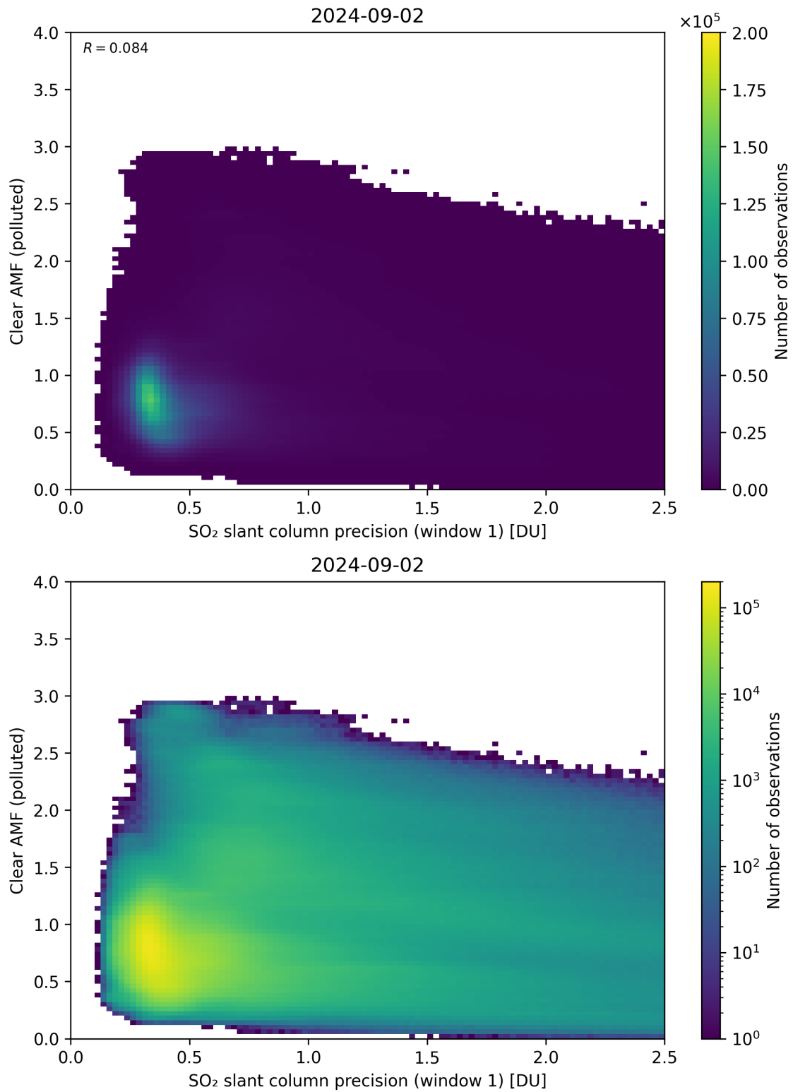
Figure 224: Scatter density plot of “SO 2 slant column precision (window 1)” against “Clear AMF (polluted)” for 2024-09-01 to 2024-09-03.
