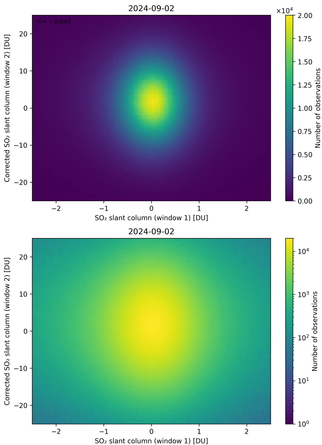
Figure 233: Scatter density plot of “SO 2 slant column (window 1)” against “Corrected SO 2 slant column (window 2)” for 2024-09-01 to 2024-09-03.
