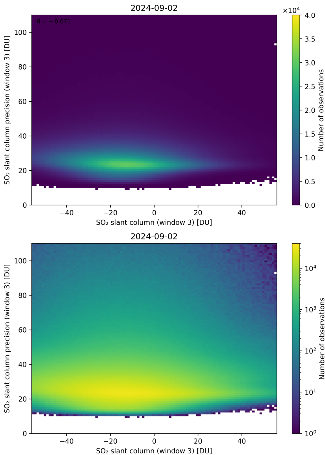
Figure 267: Scatter density plot of “SO 2 slant column (window 3)” against “SO 2 slant column precision (window 3)” for 2024-09-01 to 2024-09-03.
