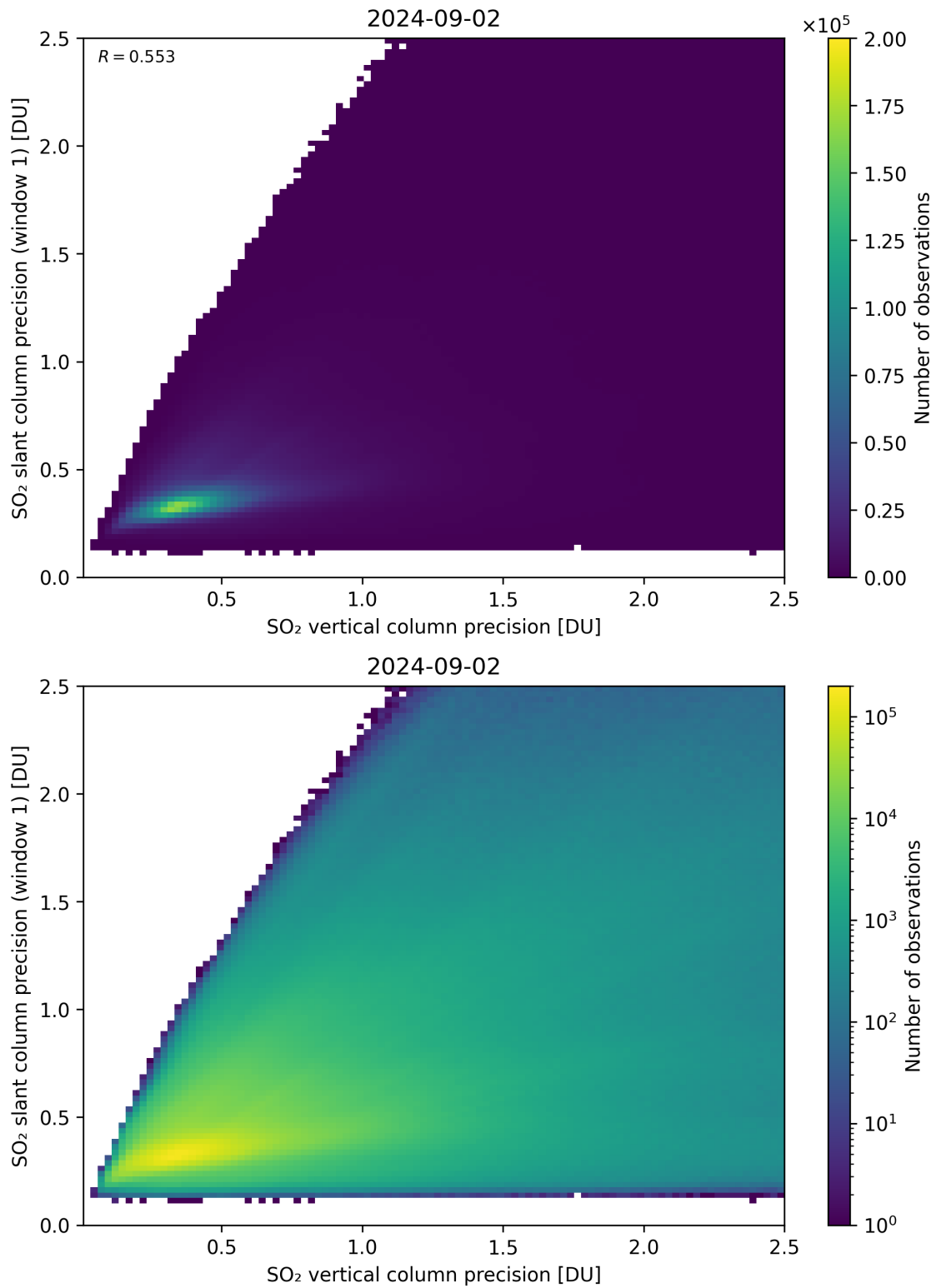
Figure 290: Scatter density plot of “SO 2 vertical column precision” against “SO 2 slant column precision (window 1)” for 2024-09-01 to 2024-09-03.
