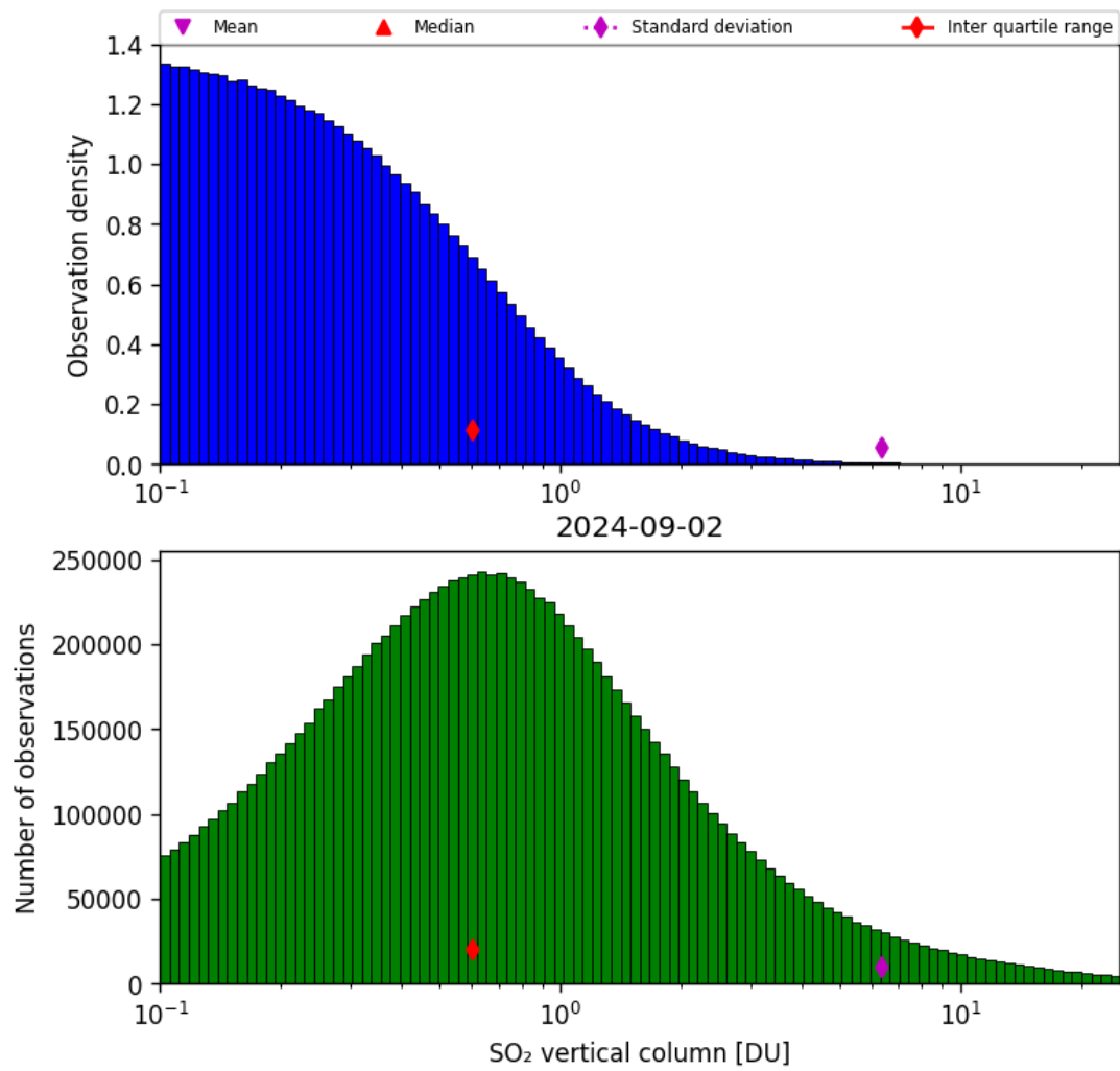
Figure 53: Histogram of “SO 2 vertical column” for 2024-09-01 to 2024-09-03
