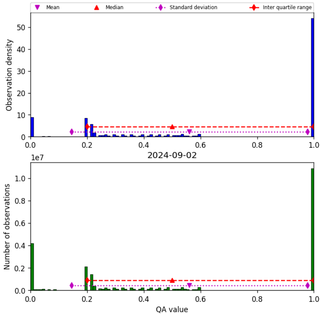
Figure 52: Histogram of “QA value” for 2024-09-01 to 2024-09-03
