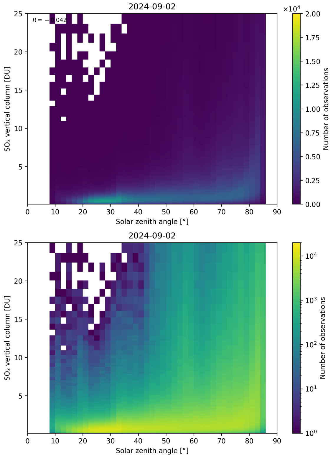
Figure 176: Scatter density plot of “Solar zenith angle” against “SO 2 vertical column” for 2024-09-01 to 2024-09-03.
