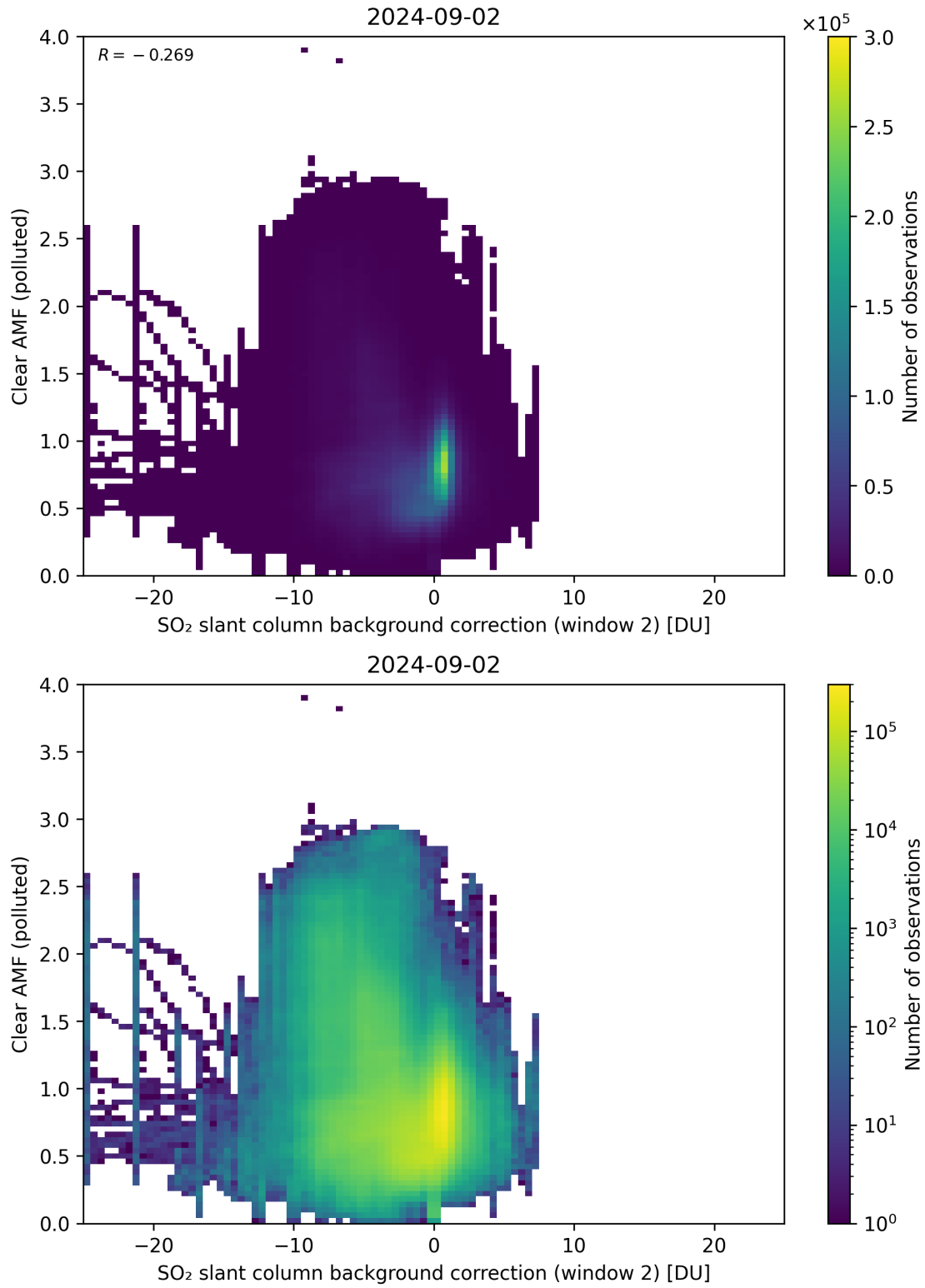
Figure 115: Scatter density plot of “SO 2 slant column background correction (window 2)” against “Clear AMF (polluted)” for 2024-09-01 to 2024-09-03.
