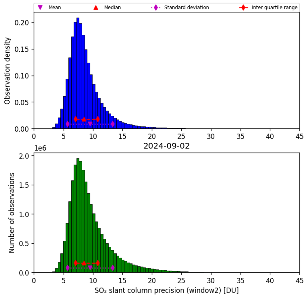
Figure 61: Histogram of “SO 2 slant column precision (window2)” for 2024-09-01 to 2024-09-03
