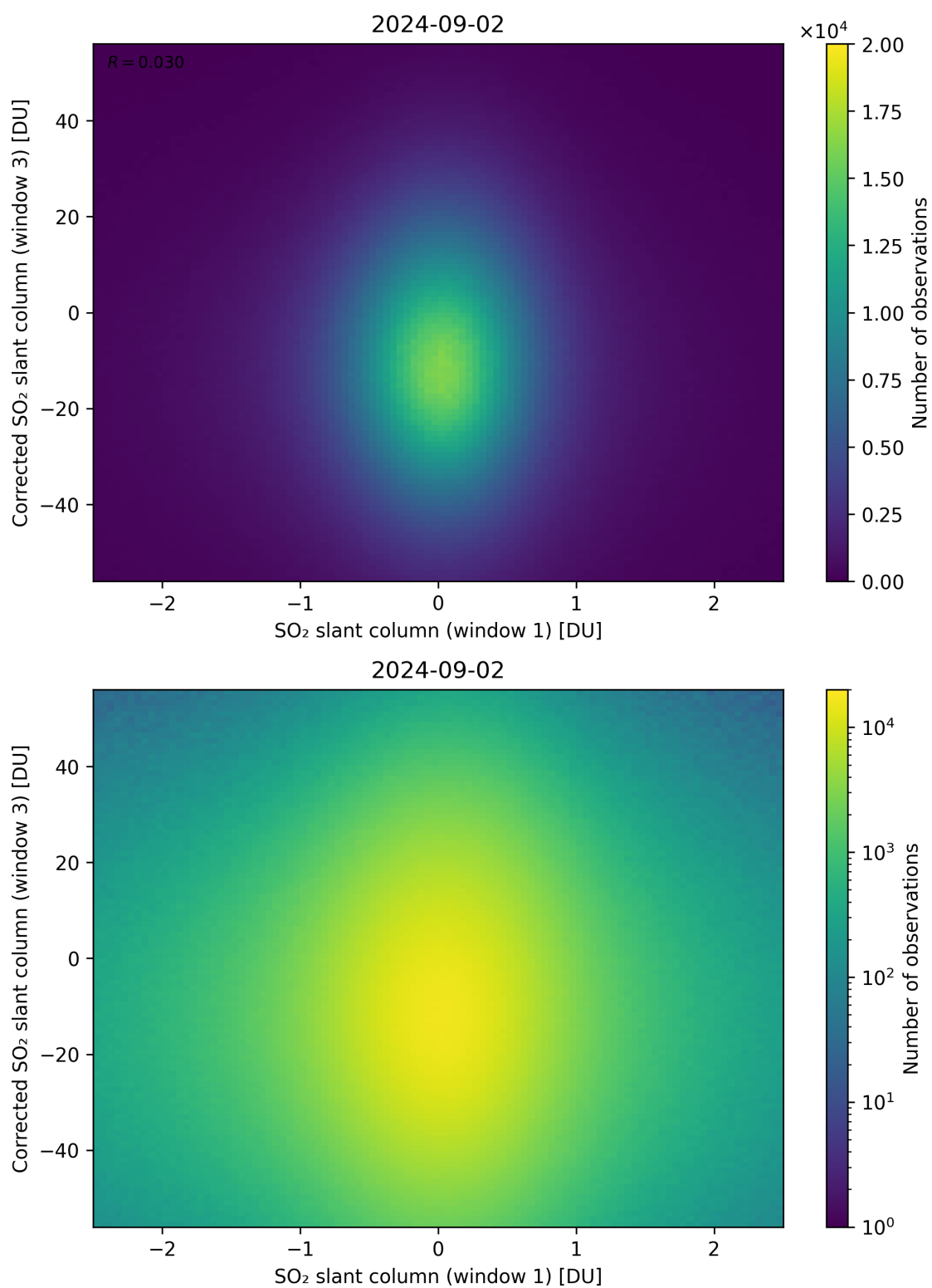
Figure 234: Scatter density plot of “SO 2 slant column (window 1)” against “Corrected SO 2 slant column (window 3)” for 2024-09-01 to 2024-09-03.
