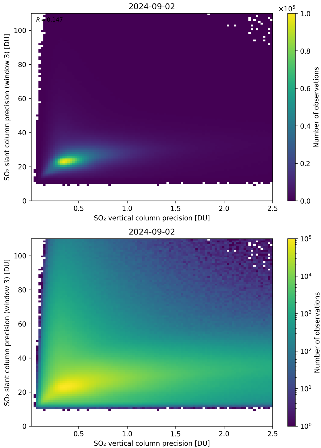
Figure 293: Scatter density plot of “SO 2 vertical column precision” against “SO 2 slant column precision (window 3)” for 2024-09-01 to 2024-09-03.
