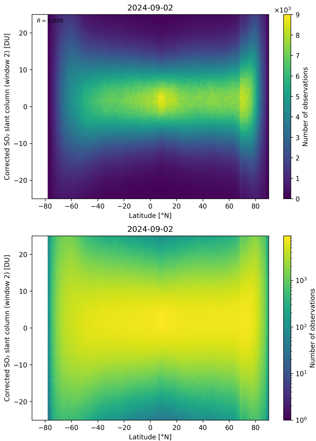
Figure 147: Scatter density plot of “Latitude” against “Corrected SO 2 slant column (window 2)” for 2024-09-01 to 2024-09-03.
