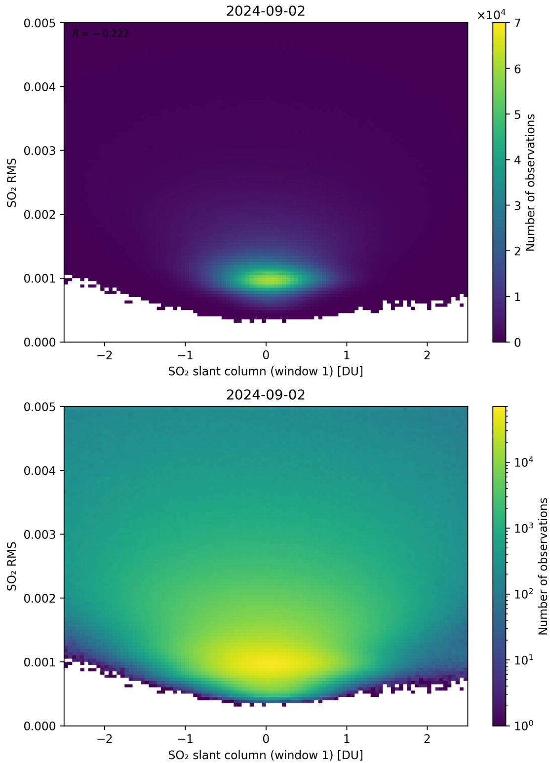
Figure 217: Scatter density plot of “SO 2 slant column (window 1)” against “SO 2 RMS” for 2024-09-01 to 2024-09-03.
