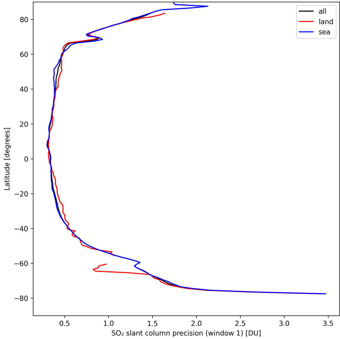
Figure 34: Zonal average of “SO 2 slant column precision (window 1)” for 2024-09-01 to 2024-09-03.
