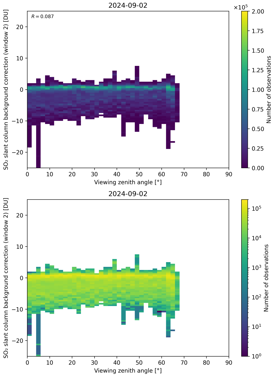
Figure 309: Scatter density plot of “Viewing zenith angle” against “SO 2 slant column background correction (window 2)” for 2024-09-01 to 2024-09-03.
