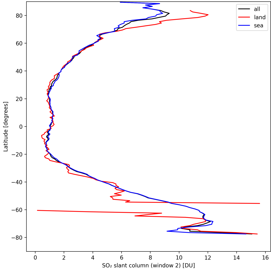
Figure 37: Zonal average of “SO 2 slant column (window 2)” for 2024-09-01 to 2024-09-03.
