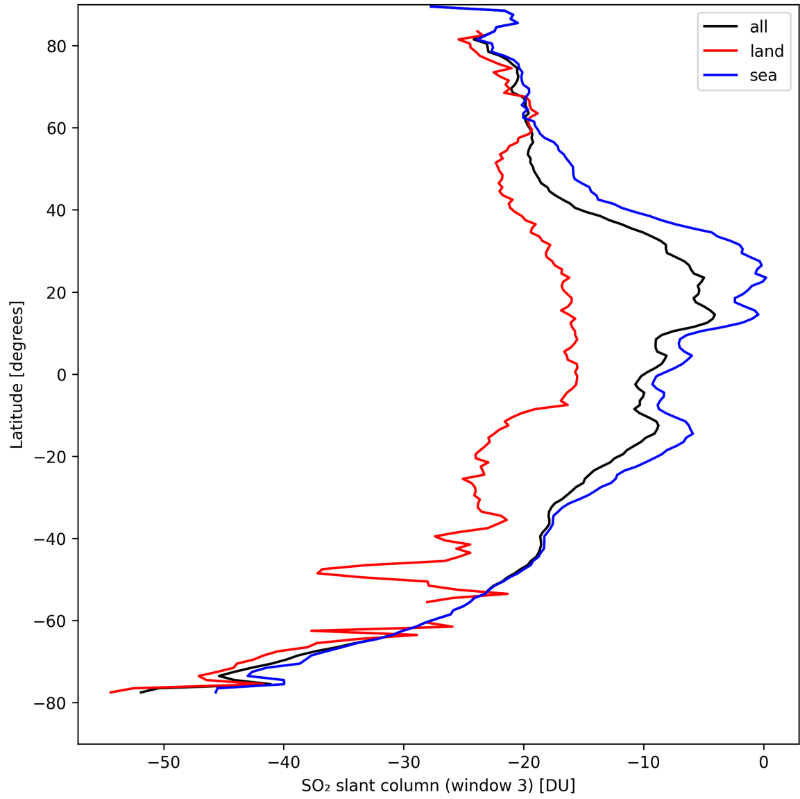
Figure 41: Zonal average of “SO 2 slant column (window 3)” for 2024-09-01 to 2024-09-03.
