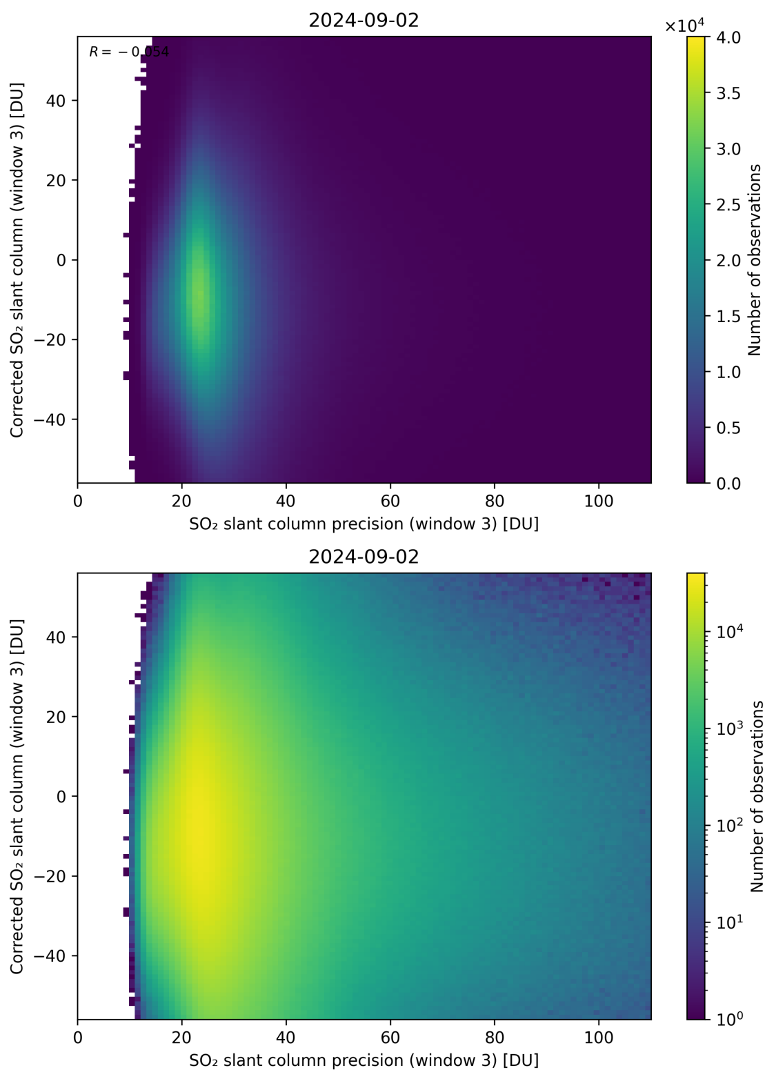
Figure 262: Scatter density plot of “SO 2 slant column precision (window 3)” against “Corrected SO 2 slant column (window 3)” for 2024-09-01 to 2024-09-03.
