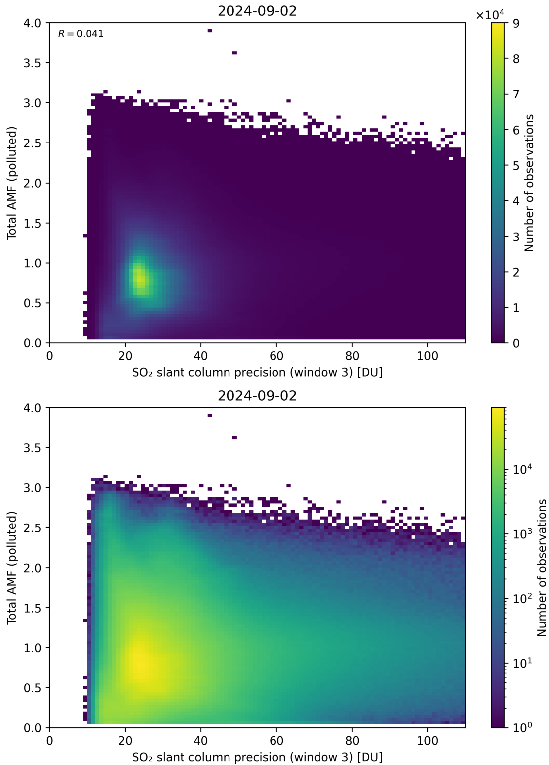
Figure 263: Scatter density plot of “SO 2 slant column precision (window 3)” against “Total AMF (polluted)” for 2024-09-01 to 2024-09-03.
