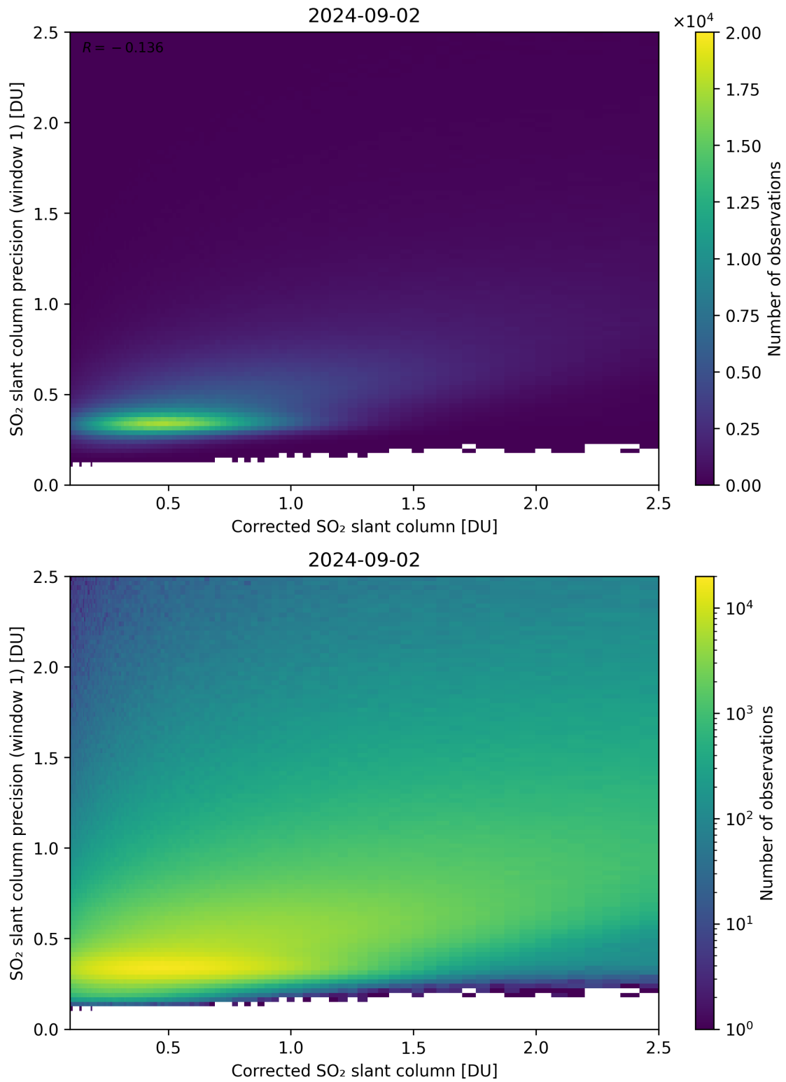
Figure 188: Scatter density plot of “Corrected SO 2 slant column” against “SO 2 slant column precision (window 1)” for 2024-09-01 to 2024-09-03.
