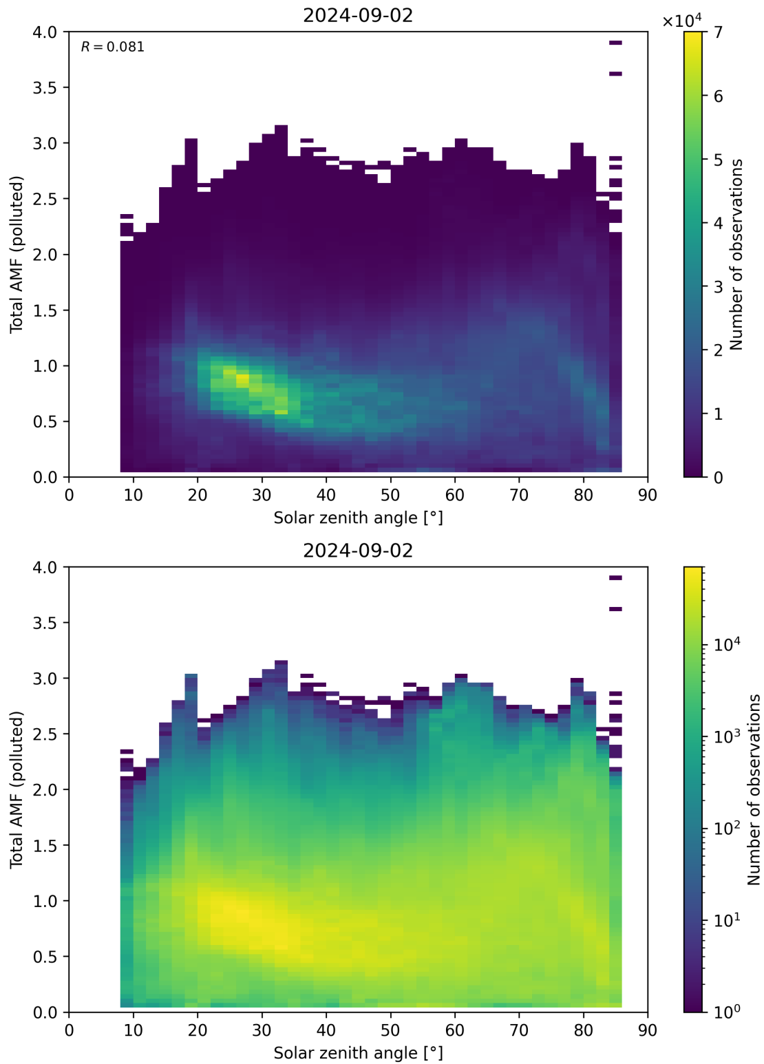
Figure 174: Scatter density plot of “Solar zenith angle” against “Total AMF (polluted)” for 2024-09-01 to 2024-09-03.
