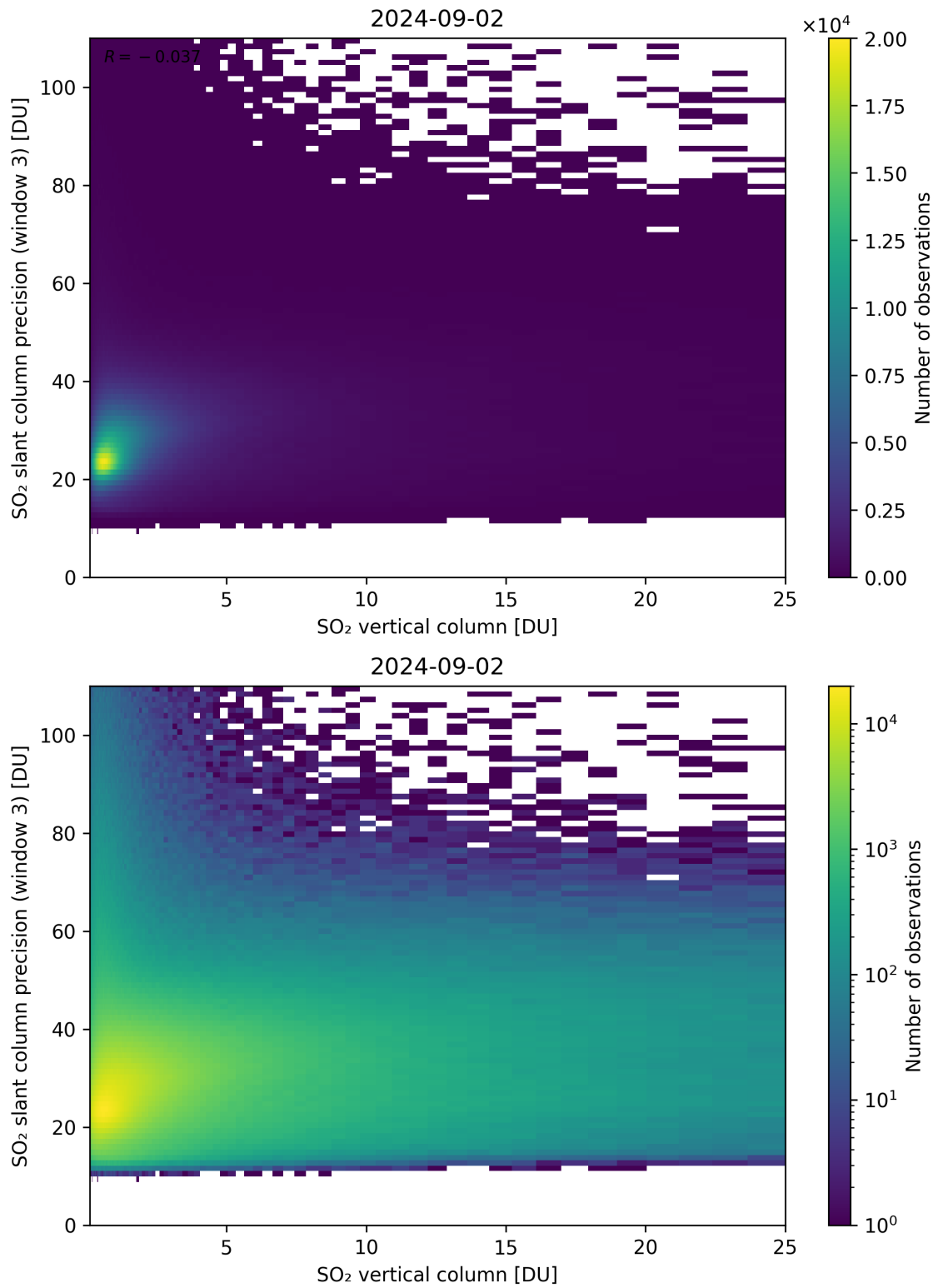
Figure 304: Scatter density plot of “SO 2 vertical column” against “SO 2 slant column precision (window 3)” for 2024-09-01 to 2024-09-03.
