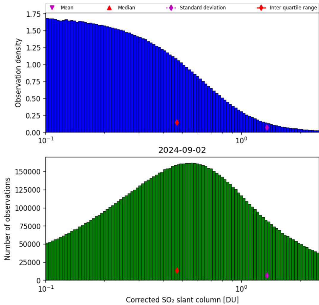
Figure 55: Histogram of “Corrected SO 2 slant column” for 2024-09-01 to 2024-09-03
