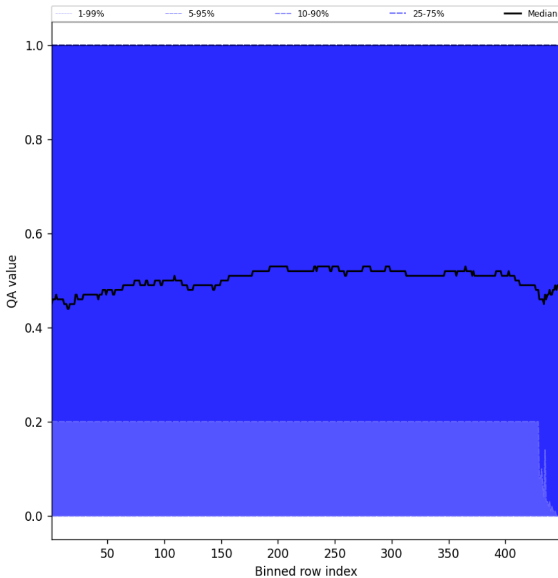
Figure 75: Along track statistics of “QA value” for 2024-09-01 to 2024-09-03
