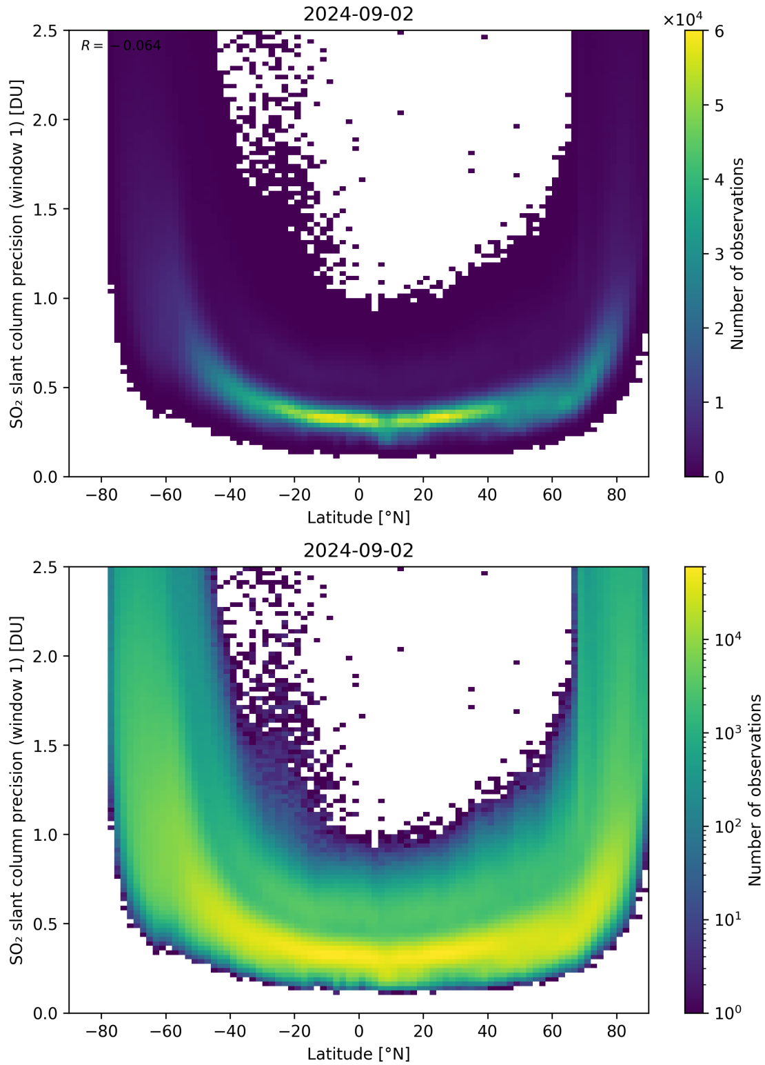
Figure 150: Scatter density plot of “Latitude” against “SO 2 slant column precision (window 1)” for 2024-09-01 to 2024-09-03.
