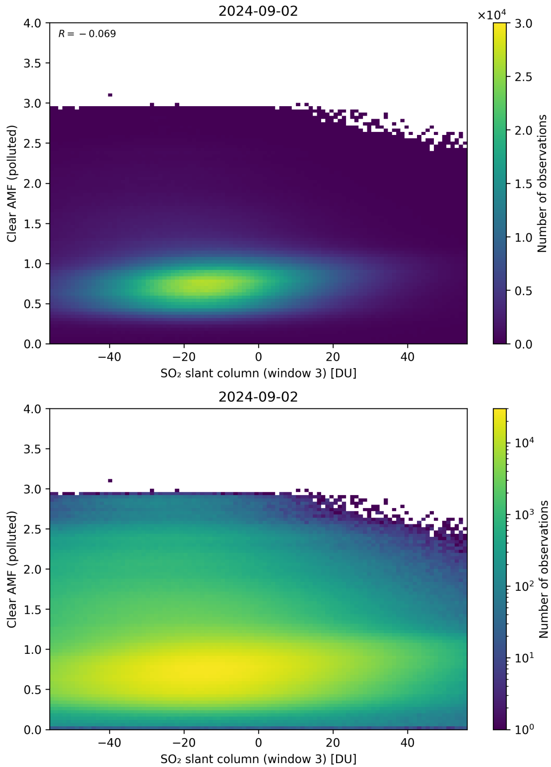
Figure 265: Scatter density plot of “SO 2 slant column (window 3)” against “Clear AMF (polluted)” for 2024-09-01 to 2024-09-03.
