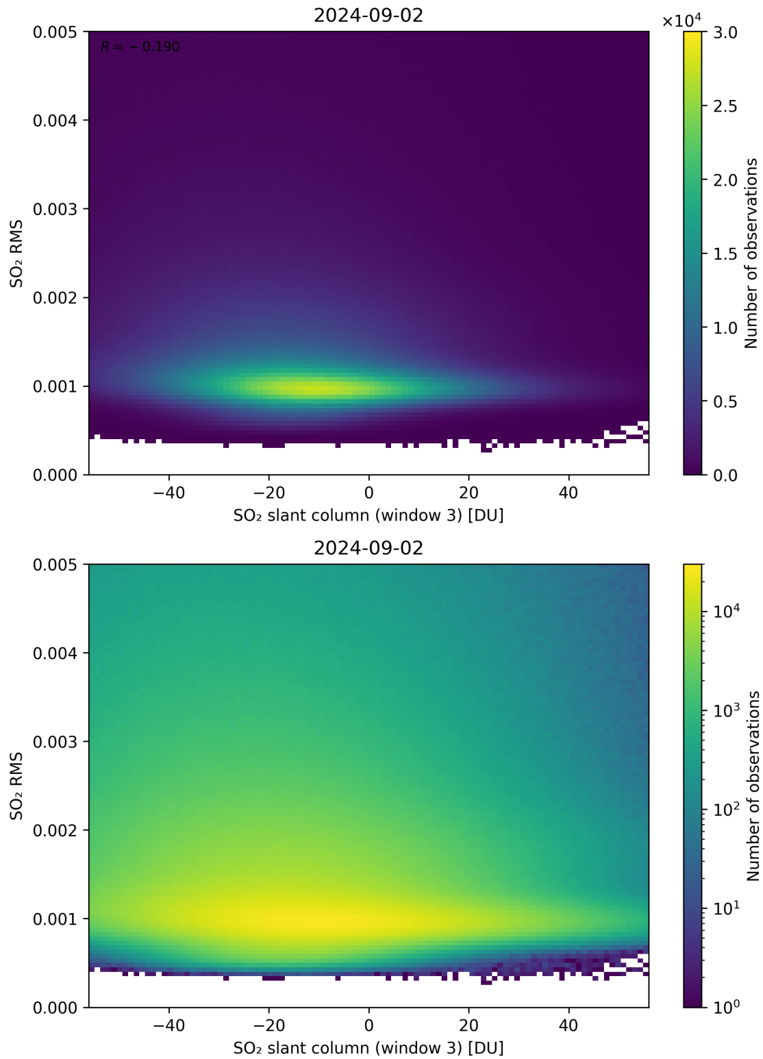
Figure 256: Scatter density plot of “SO 2 slant column (window 3)” against “SO 2 RMS” for 2024-09-01 to 2024-09-03.
