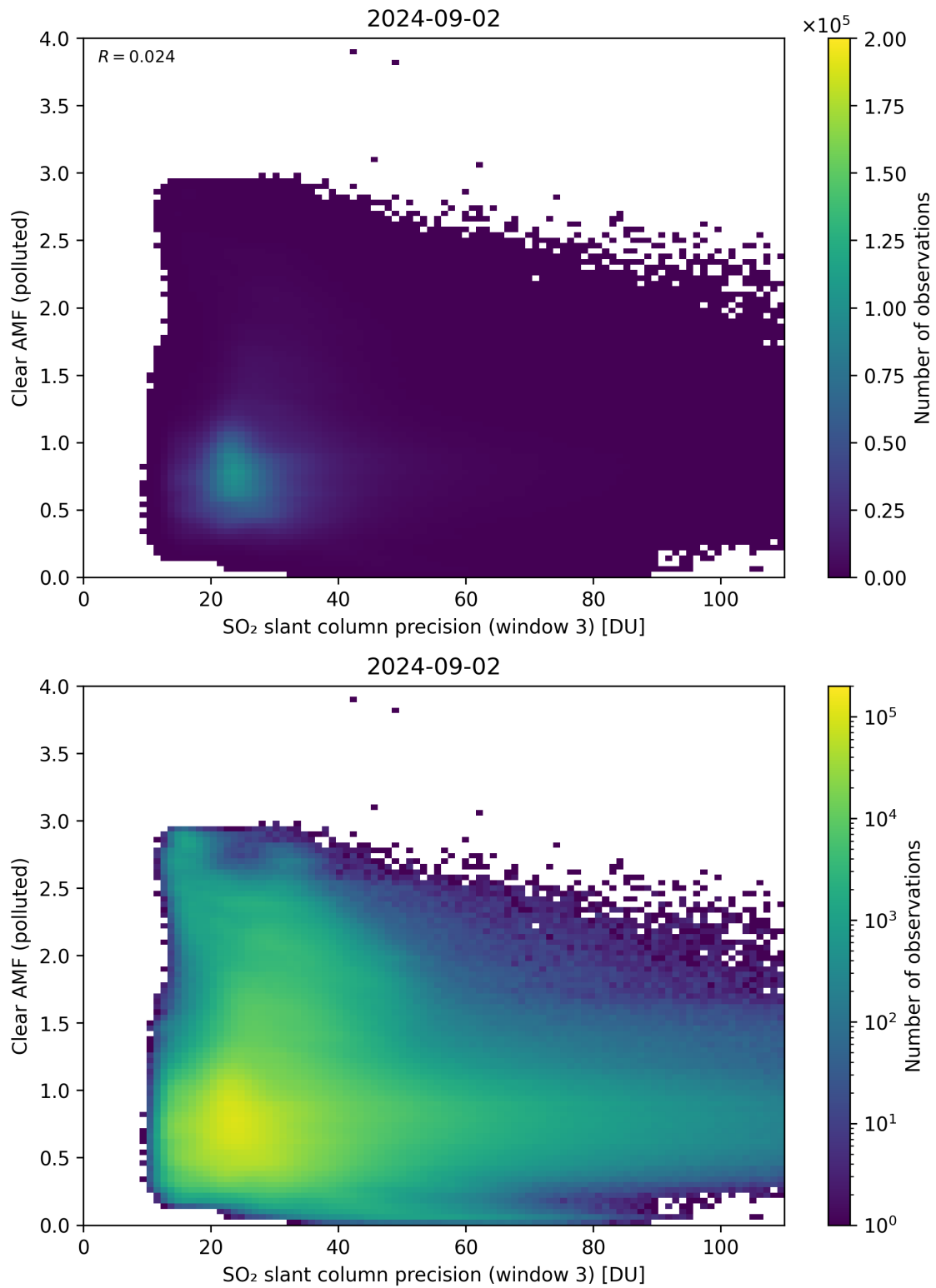
Figure 261: Scatter density plot of “SO 2 slant column precision (window 3)” against “Clear AMF (polluted)” for 2024-09-01 to 2024-09-03.
