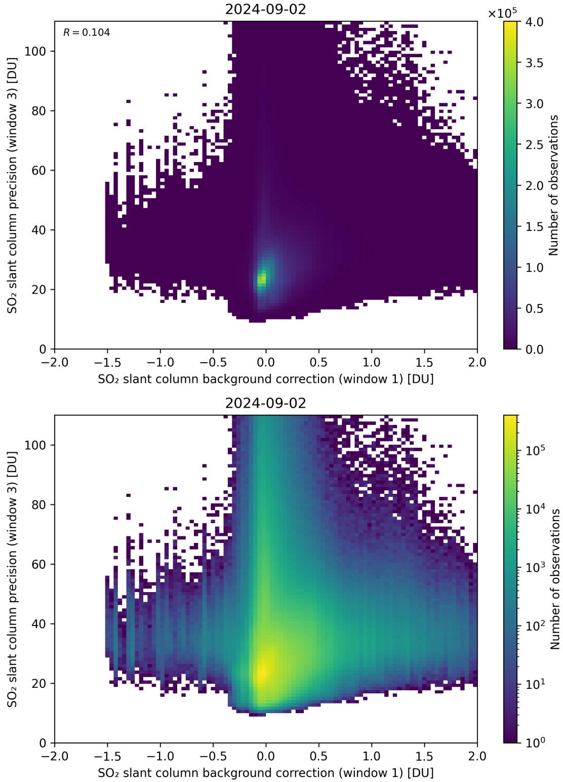
Figure 108: Scatter density plot of “SO 2 slant column background correction (window 1)” against “SO 2 slant column precision (window 3)” for 2024-09-01 to 2024-09-03.
