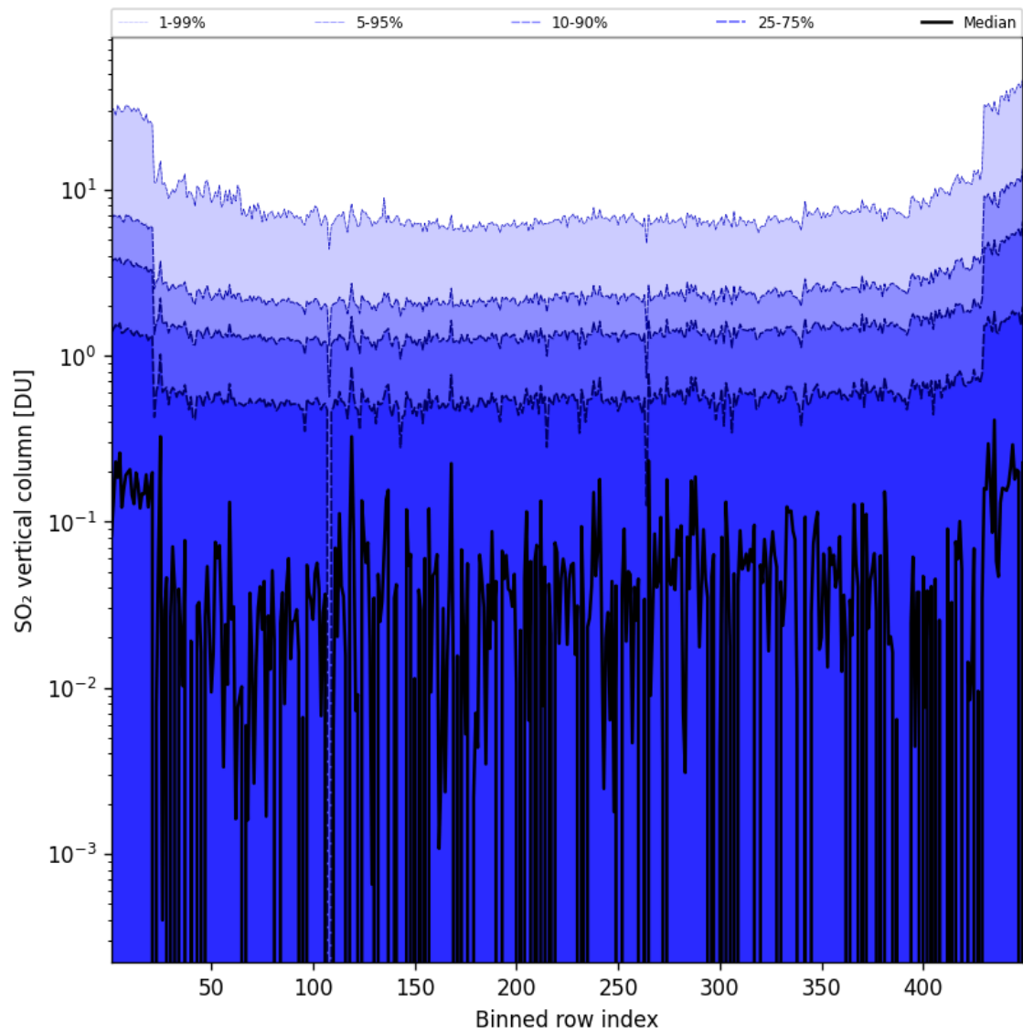
Figure 76: Along track statistics of “SO 2 vertical column” for 2024-09-01 to 2024-09-03
