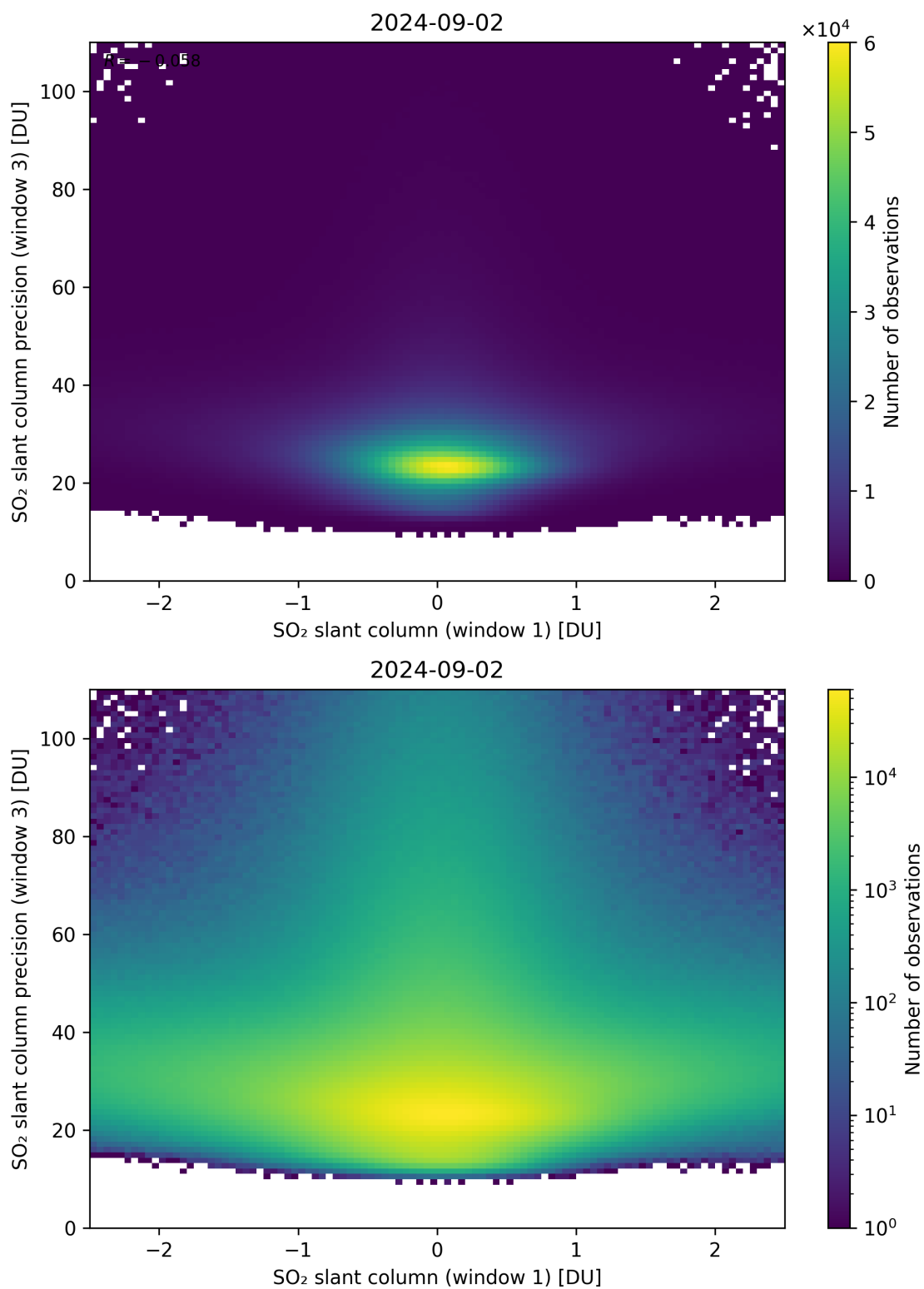
Figure 238: Scatter density plot of “SO 2 slant column (window 1)” against “SO 2 slant column precision (window 3)” for 2024-09-01 to 2024-09-03.
