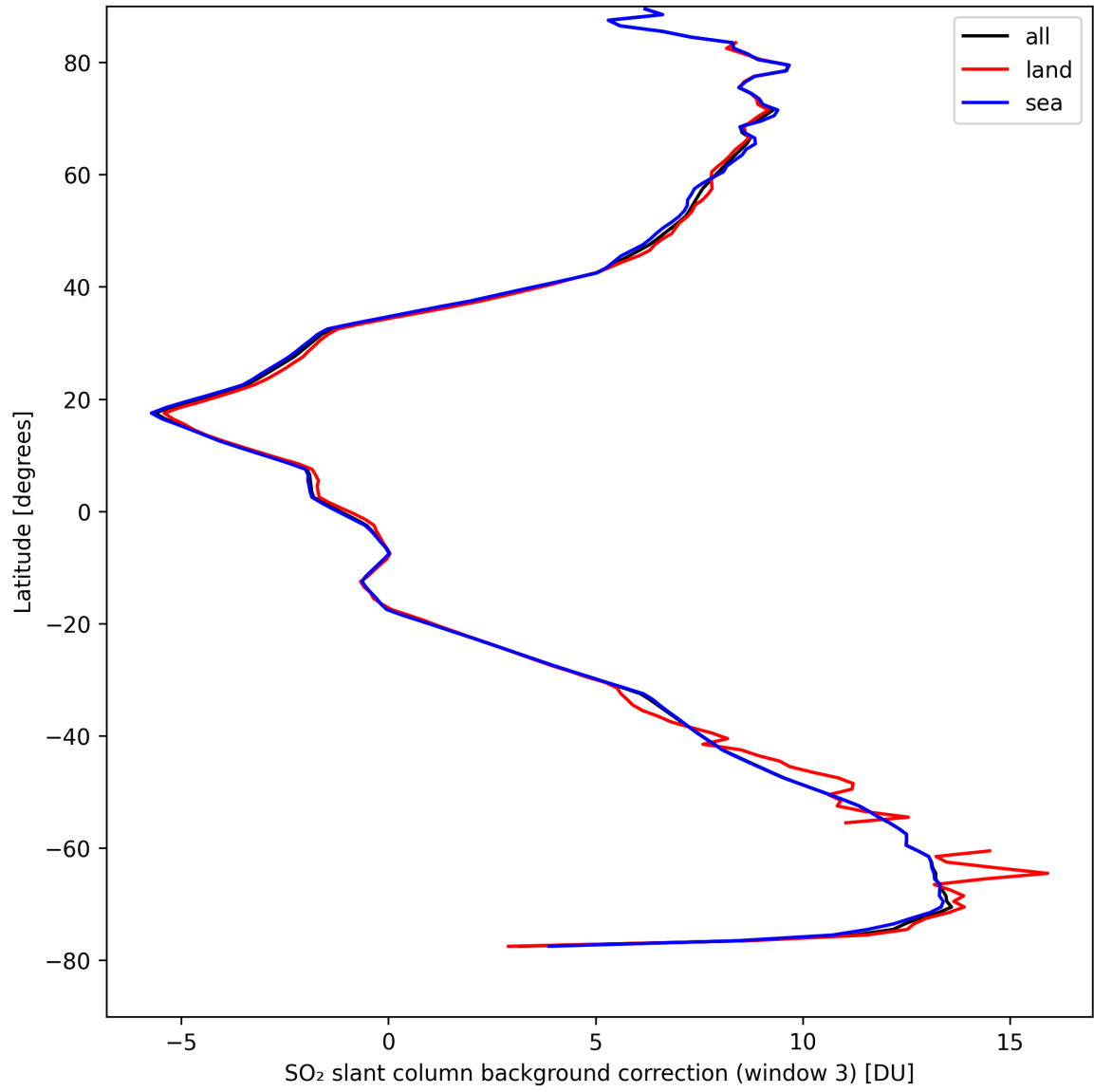
Figure 44: Zonal average of “SO 2 slant column background correction (window 3)” for 2024-09-01 to 2024-09-03.
