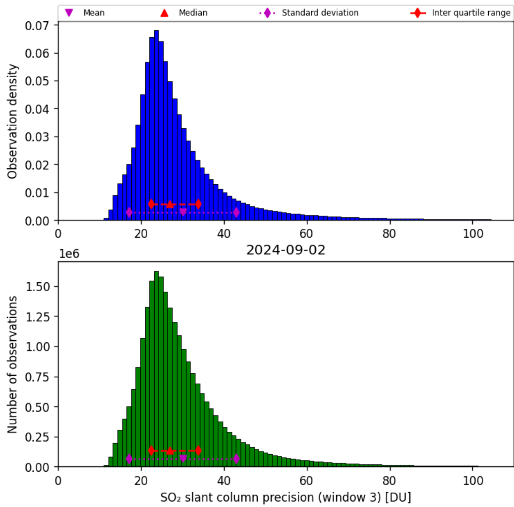
Figure 65: Histogram of “SO 2 slant column precision (window 3)” for 2024-09-01 to 2024-09-03
