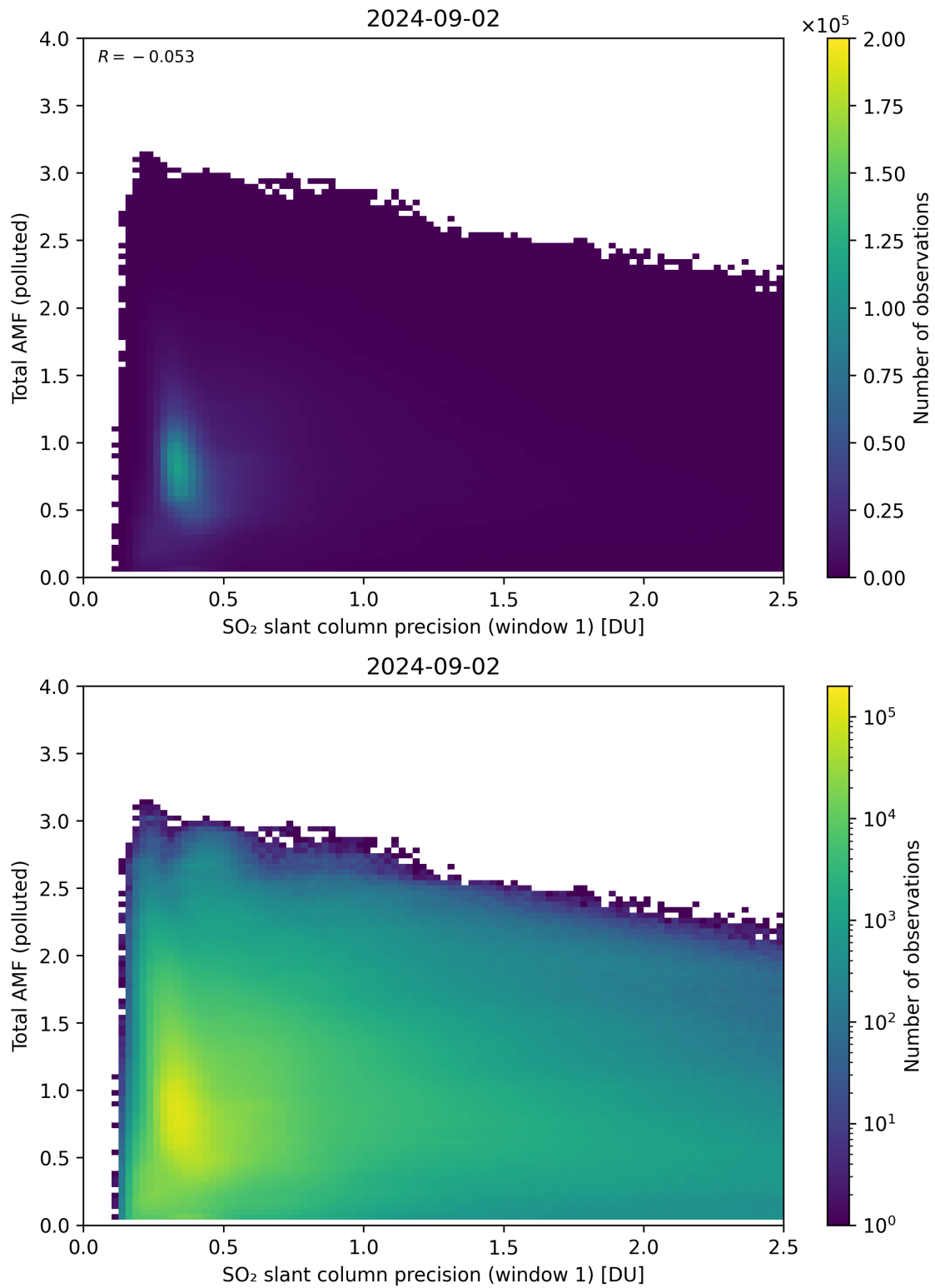
Figure 230: Scatter density plot of “SO 2 slant column precision (window 1)” against “Total AMF (polluted)” for 2024-09-01 to 2024-09-03.
