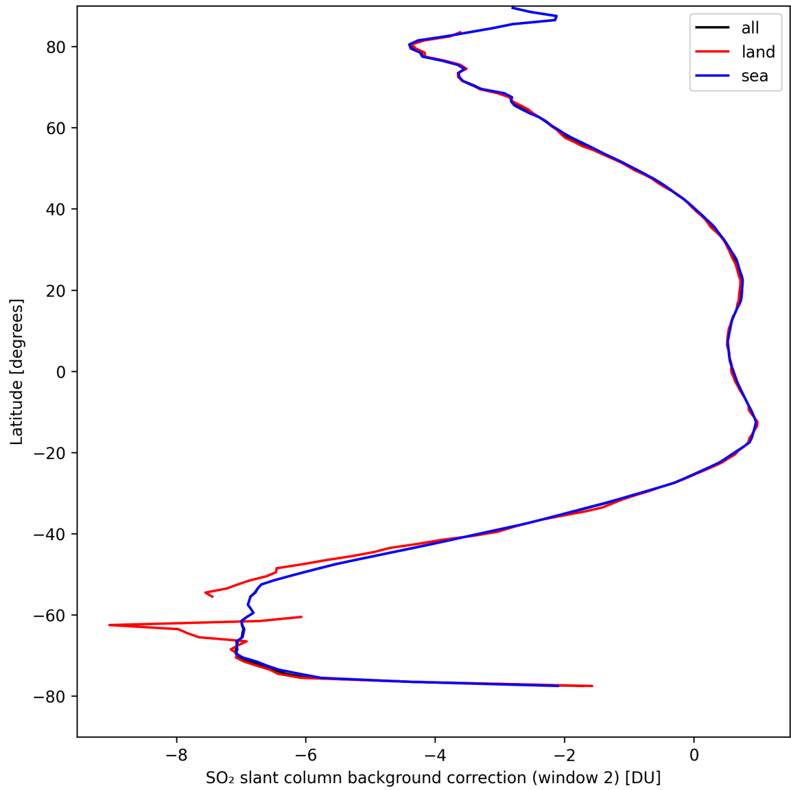
Figure 40: Zonal average of “SO 2 slant column background correction (window 2)” for 2024-09-01 to 2024-09-03.
