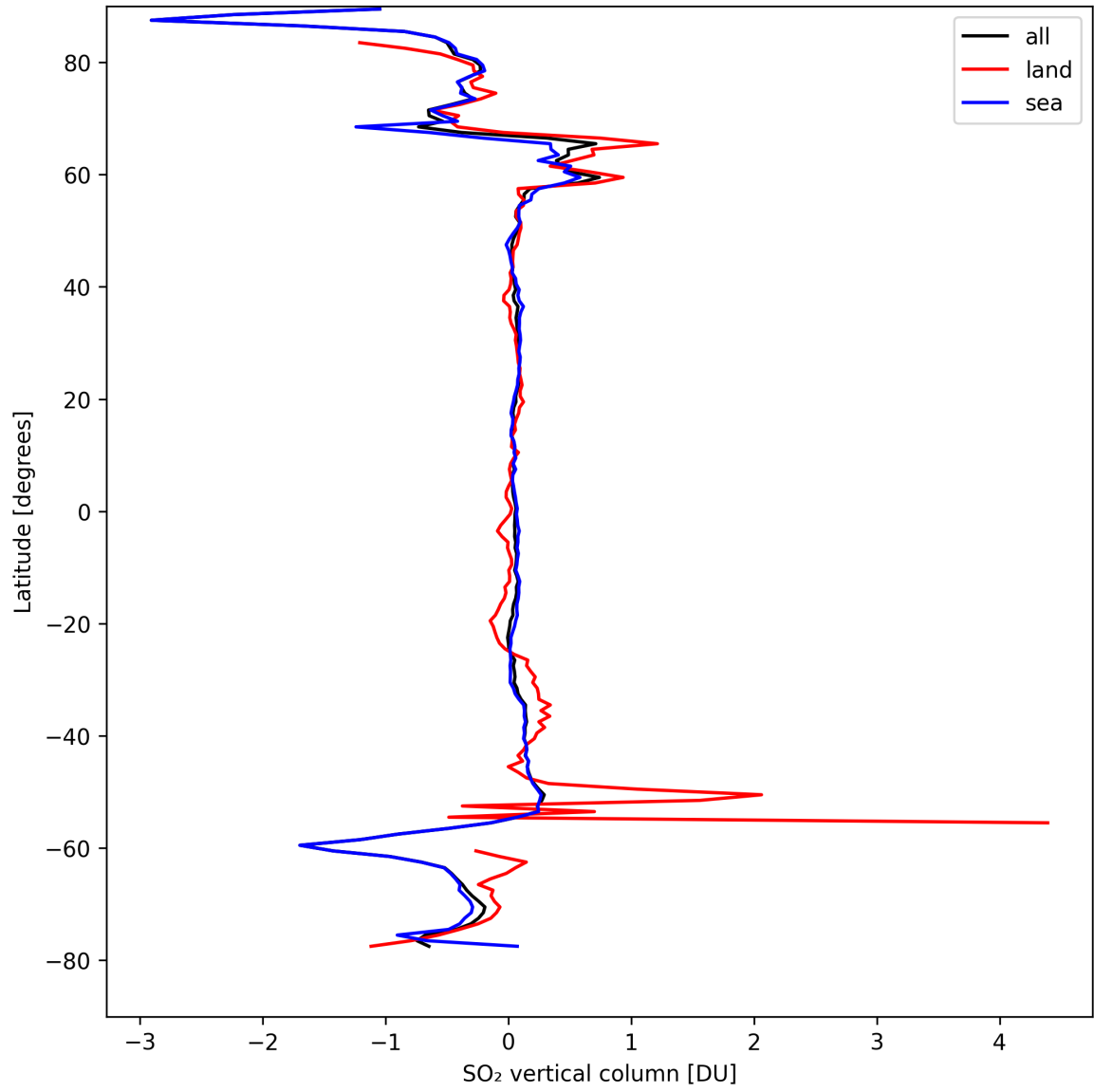
Figure 30: Zonal average of “SO 2 vertical column” for 2024-09-01 to 2024-09-03.
