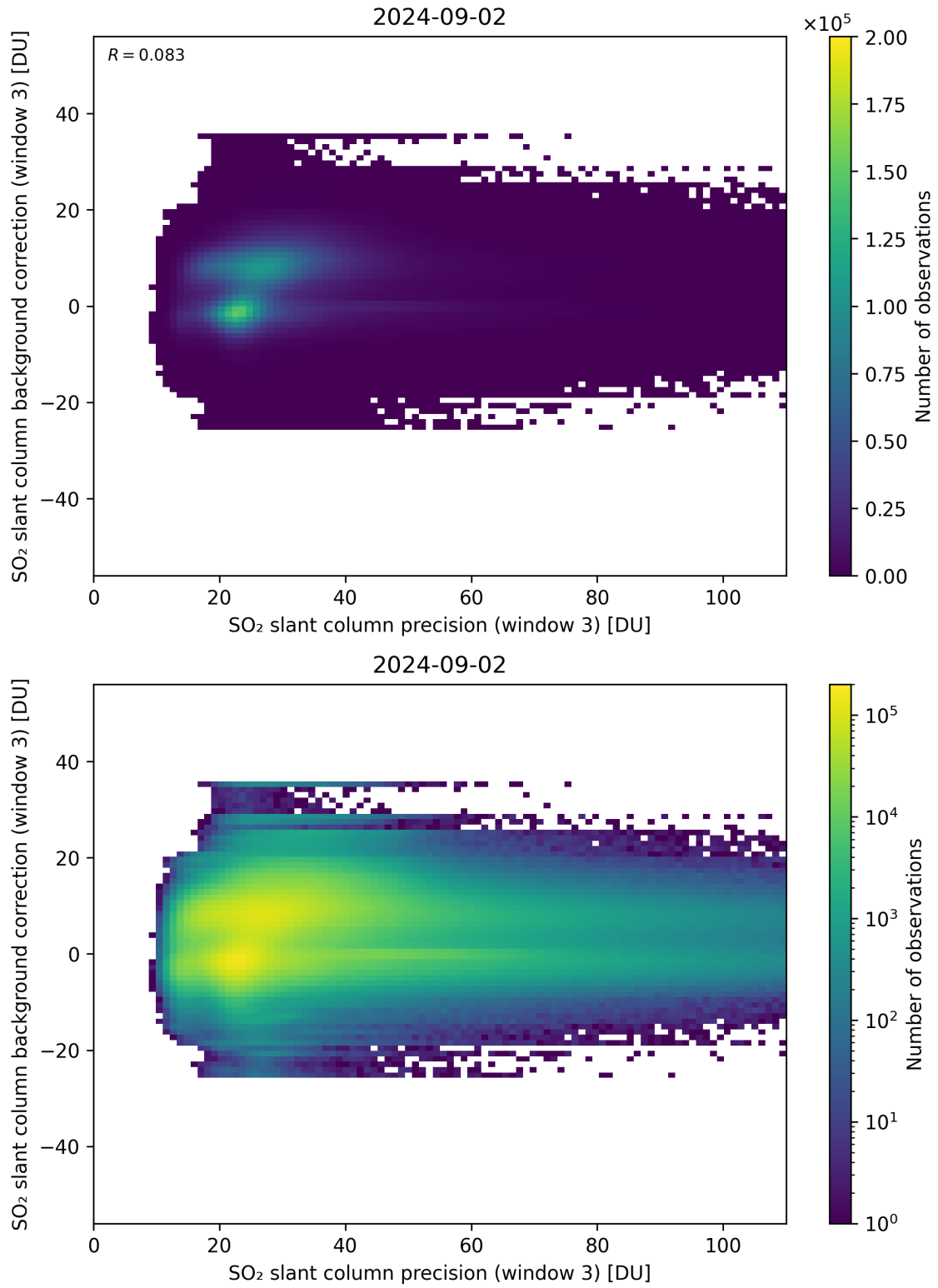
Figure 257: Scatter density plot of “SO 2 slant column precision (window 3)” against “SO 2 slant column background correction (window 3)” for 2024-09-01 to 2024-09-03.
