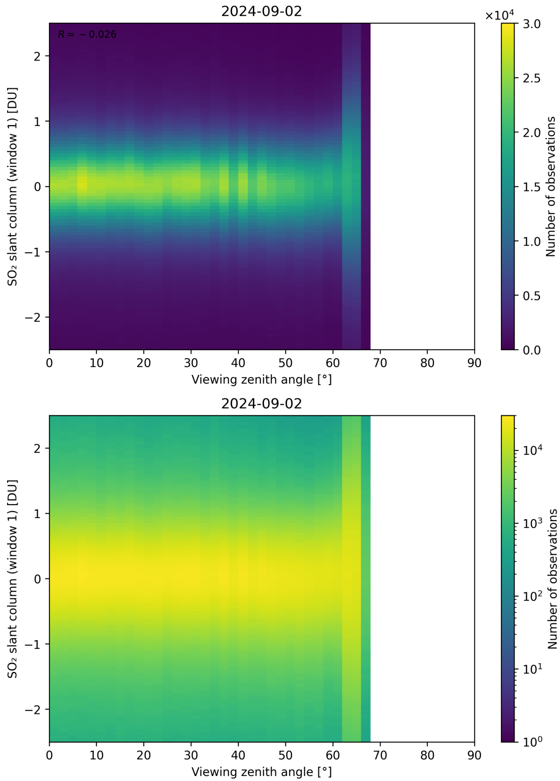
Figure 320: Scatter density plot of “Viewing zenith angle” against “SO 2 slant column (window 1)” for 2024-09-01 to 2024-09-03.
