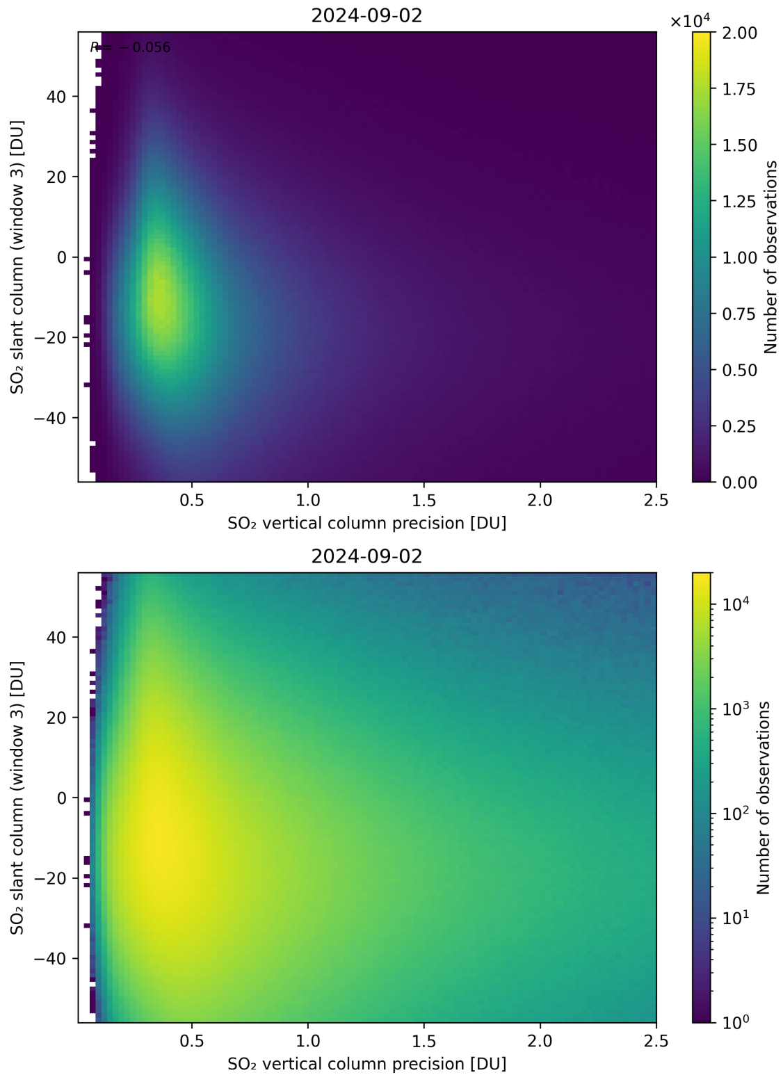
Figure 292: Scatter density plot of “SO 2 vertical column precision” against “SO 2 slant column (window 3)” for 2024-09-01 to 2024-09-03.
