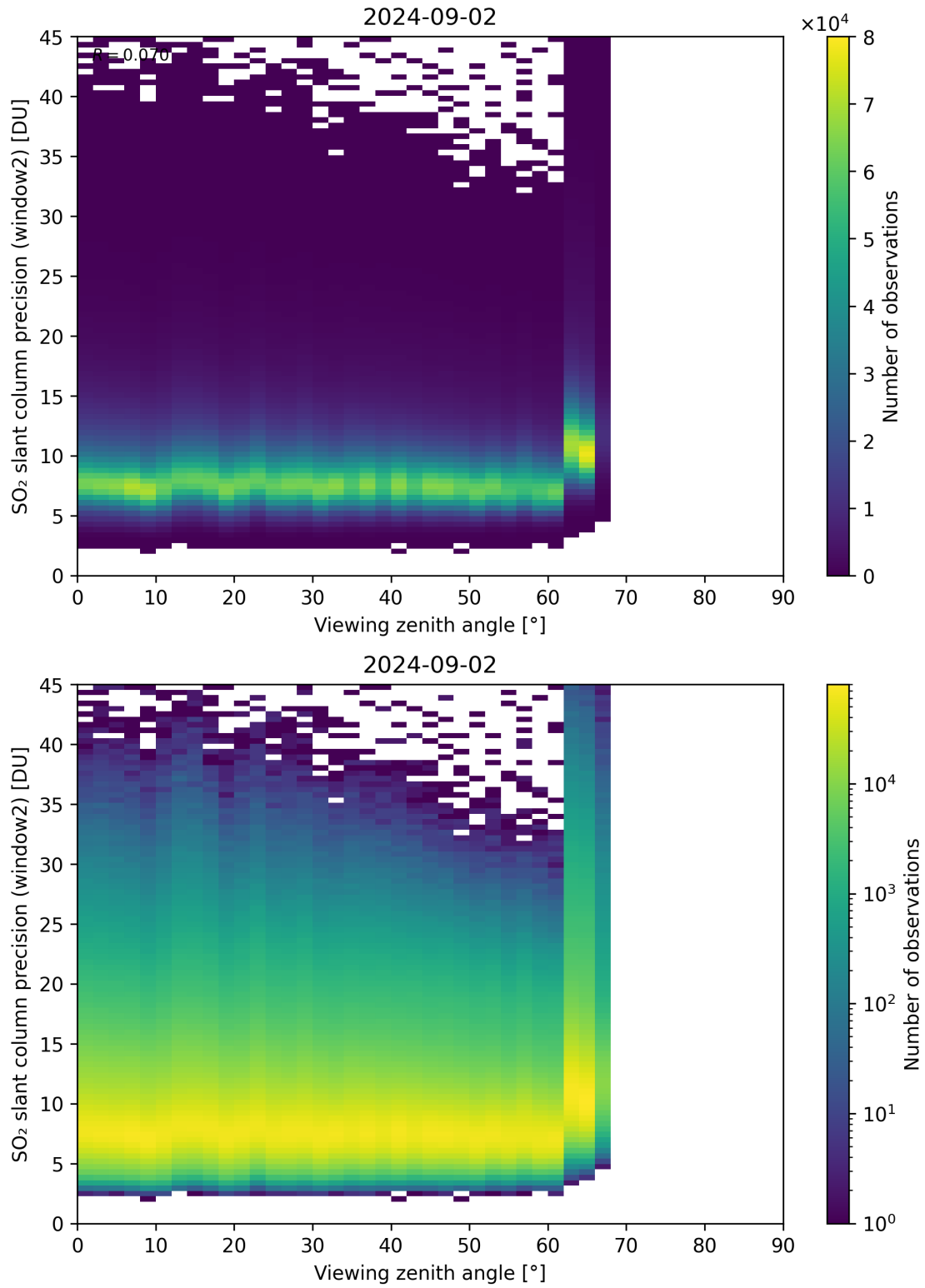
Figure 322: Scatter density plot of “Viewing zenith angle” against “SO 2 slant column precision (window2)” for 2024-09-01 to 2024-09-03.
