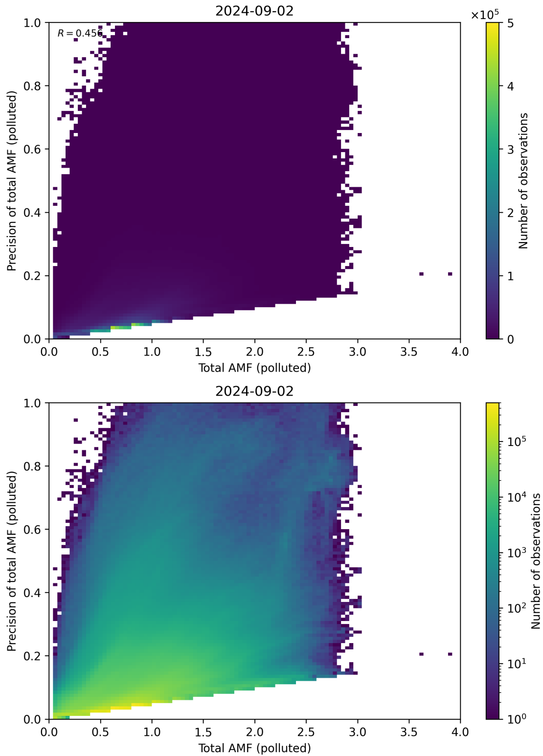
Figure 272: Scatter density plot of “Total AMF (polluted)” against “Precision of total AMF (polluted)” for 2024-09-01 to 2024-09-03.
