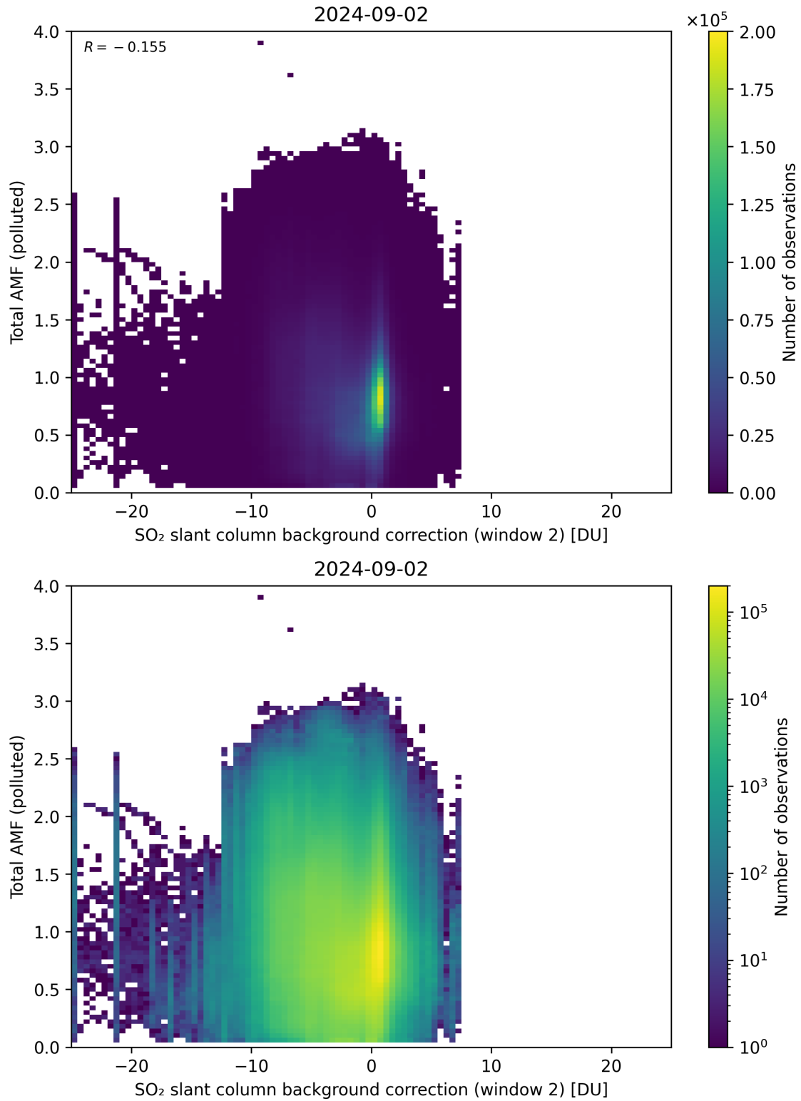
Figure 119: Scatter density plot of “SO 2 slant column background correction (window 2)” against “Total AMF (polluted)” for 2024-09-01 to 2024-09-03.
