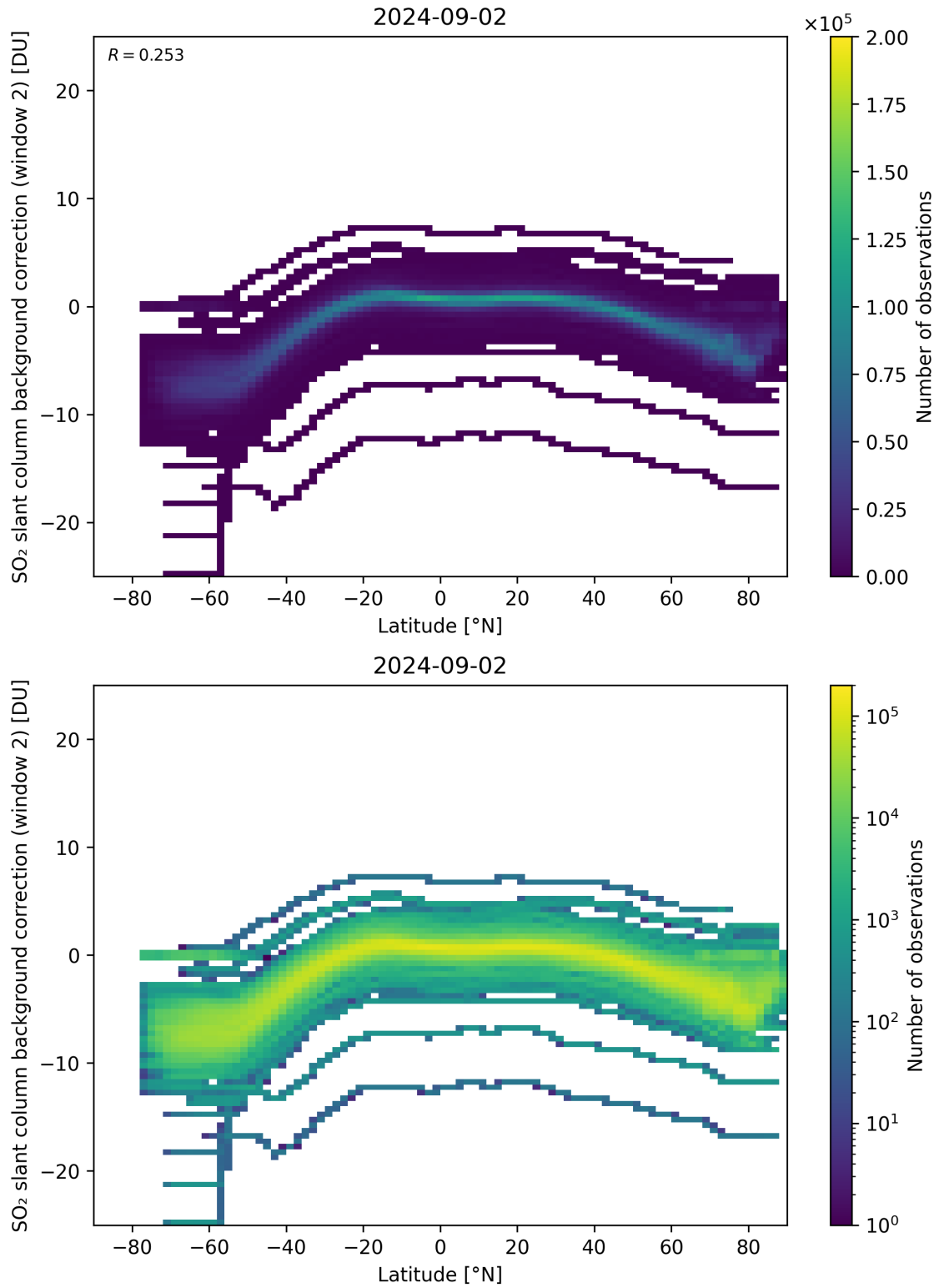
Figure 140: Scatter density plot of “Latitude” against “SO 2 slant column background correction (window 2)” for 2024-09-01 to 2024-09-03.
