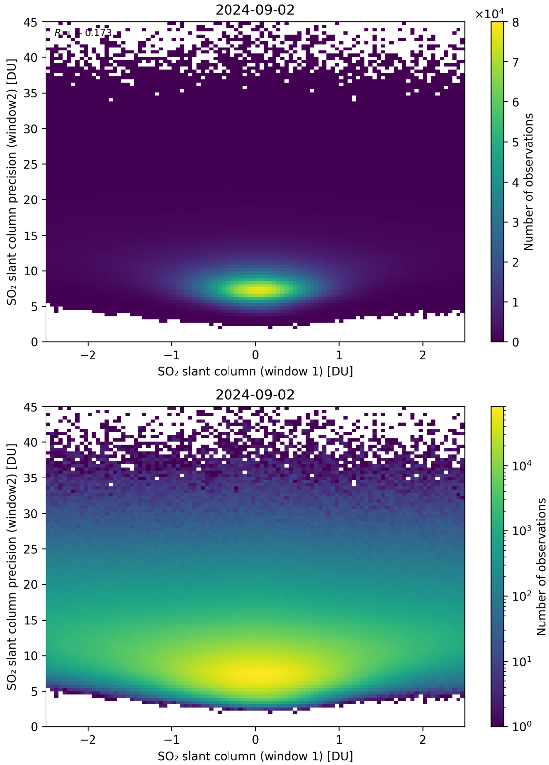
Figure 236: Scatter density plot of “SO 2 slant column (window 1)” against “SO 2 slant column precision (window2)” for 2024-09-01 to 2024-09-03.
