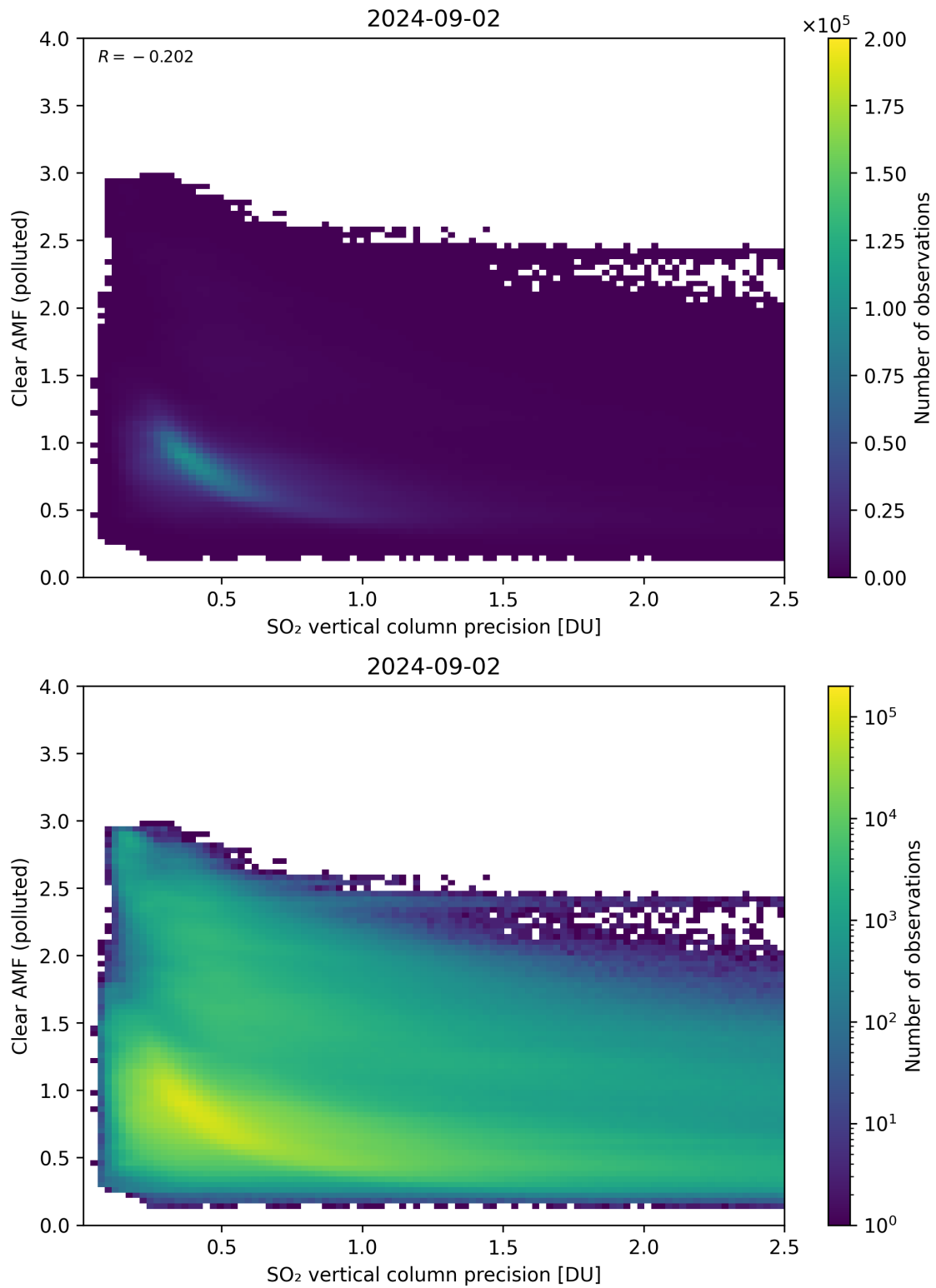
Figure 285: Scatter density plot of “SO 2 vertical column precision” against “Clear AMF (polluted)” for 2024-09-01 to 2024-09-03.
