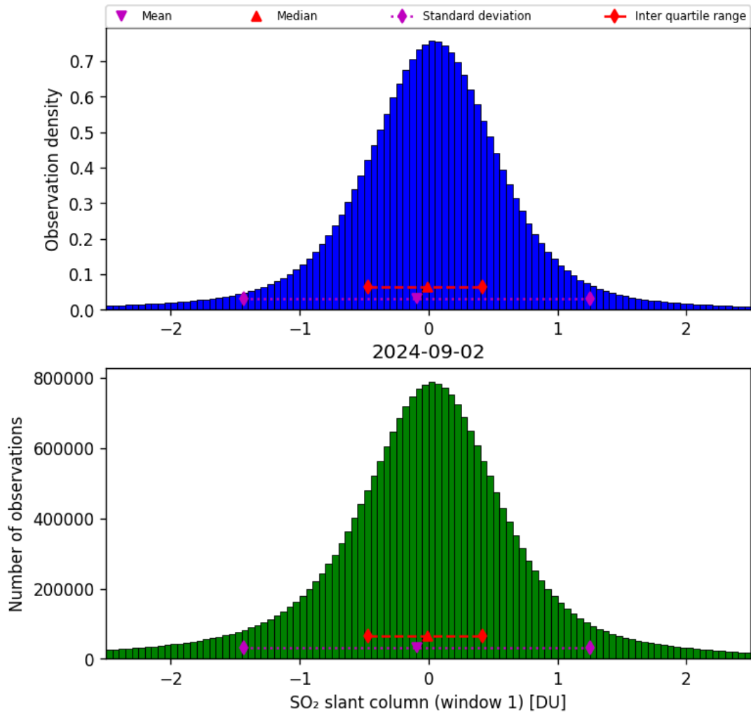
Figure 56: Histogram of “SO 2 slant column (window 1)” for 2024-09-01 to 2024-09-03
