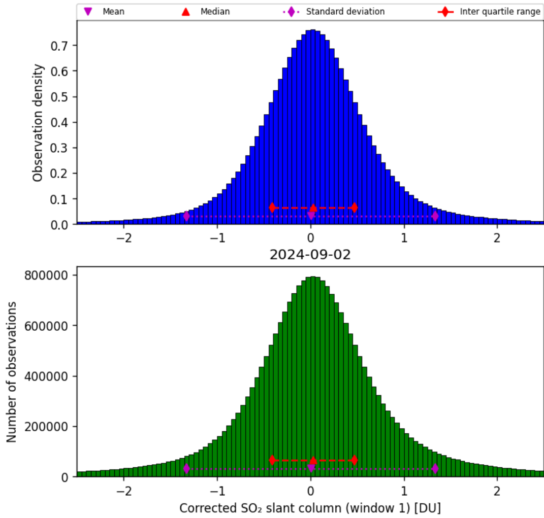
Figure 58: Histogram of “Corrected SO 2 slant column (window 1)” for 2024-09-01 to 2024-09-03
