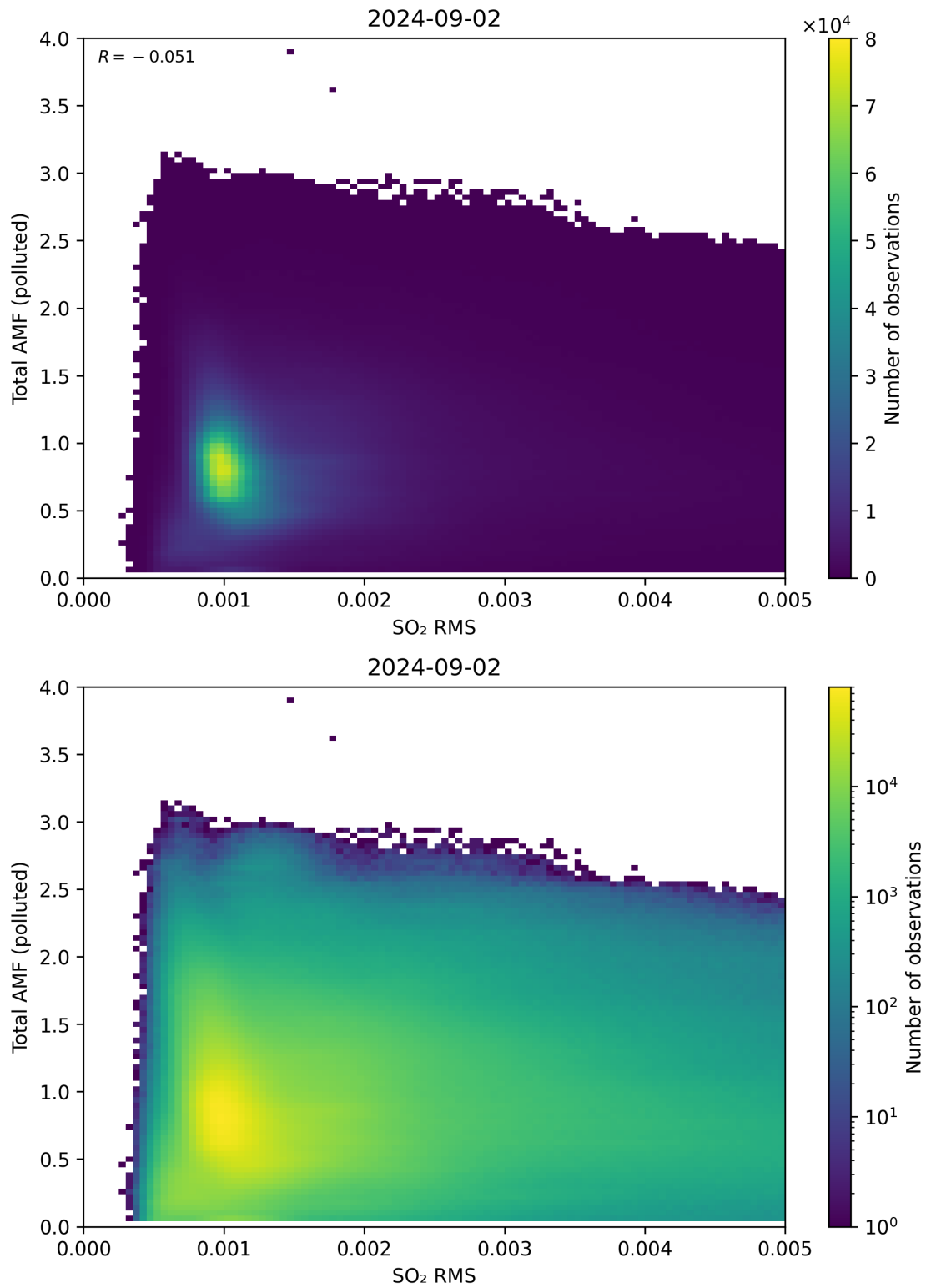
Figure 137: Scatter density plot of “SO 2 RMS” against “Total AMF (polluted)” for 2024-09-01 to 2024-09-03.
