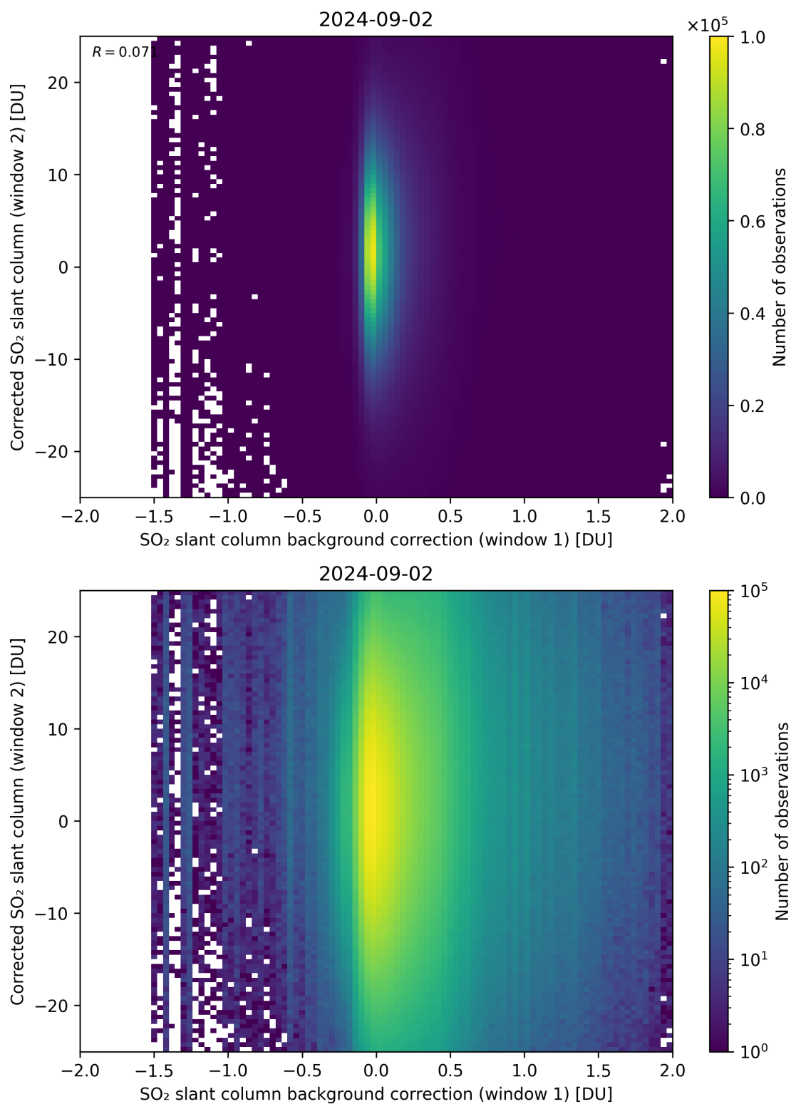
Figure 104: Scatter density plot of “SO 2 slant column background correction (window 1)” against “Corrected SO 2 slant column (window 2)” for 2024-09-01 to 2024-09-03.
