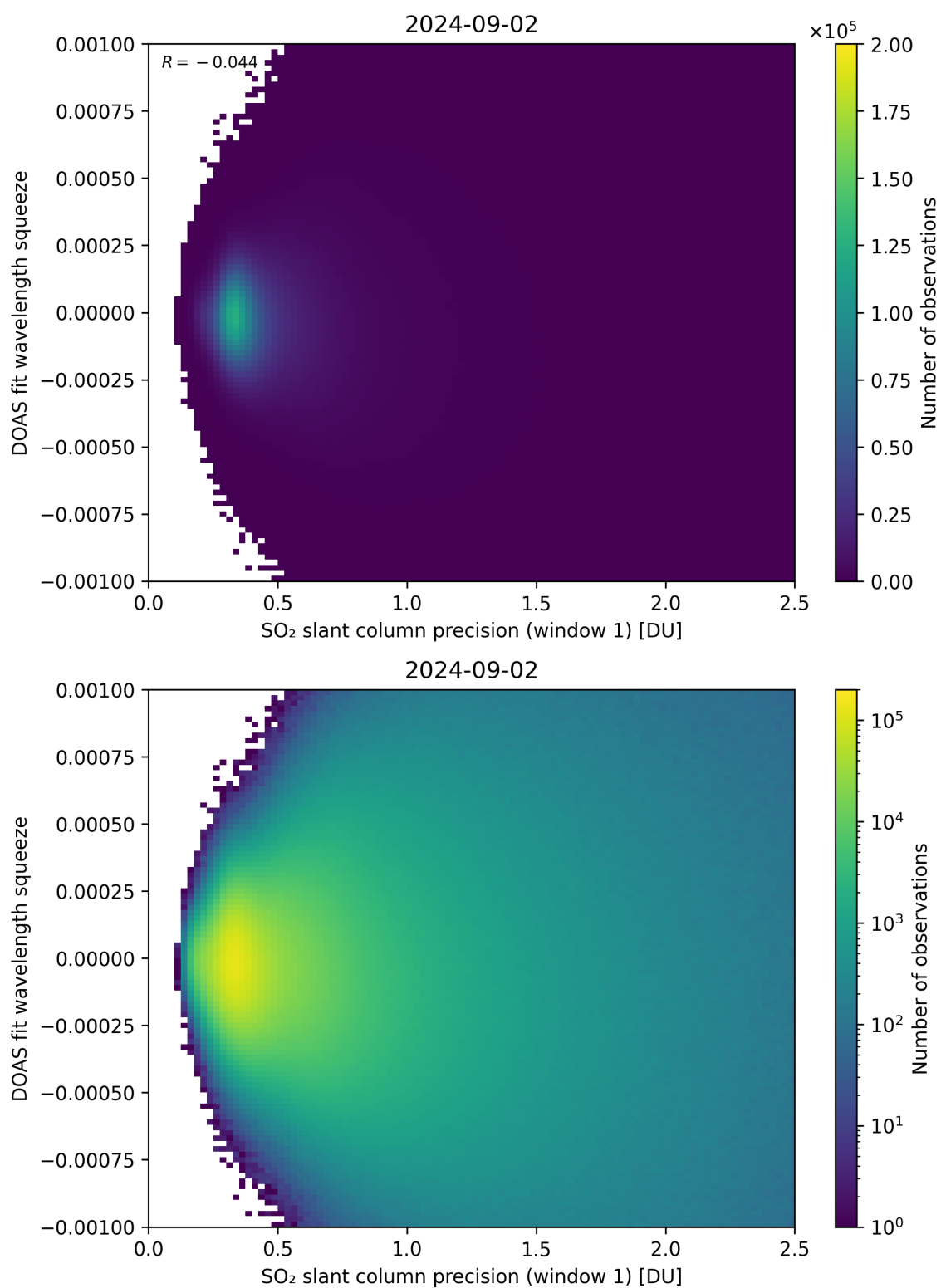
Figure 222: Scatter density plot of “SO 2 slant column precision (window 1)” against “DOAS fit wavelength squeeze” for 2024-09-01 to 2024-09-03.
