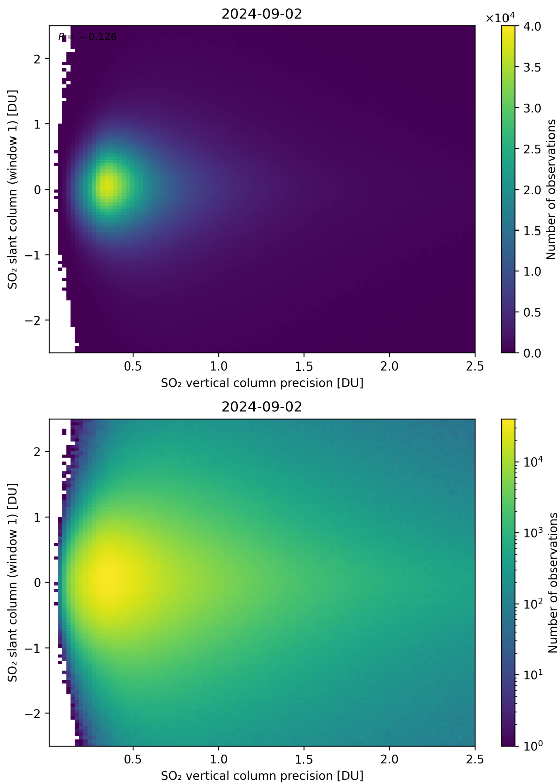
Figure 289: Scatter density plot of “SO 2 vertical column precision” against “SO 2 slant column (window 1)” for 2024-09-01 to 2024-09-03.
