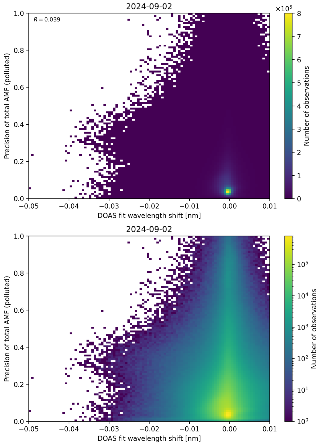
Figure 131: Scatter density plot of “DOAS fit wavelength shift” against “Precision of total AMF (polluted)” for 2024-09-01 to 2024-09-03.
