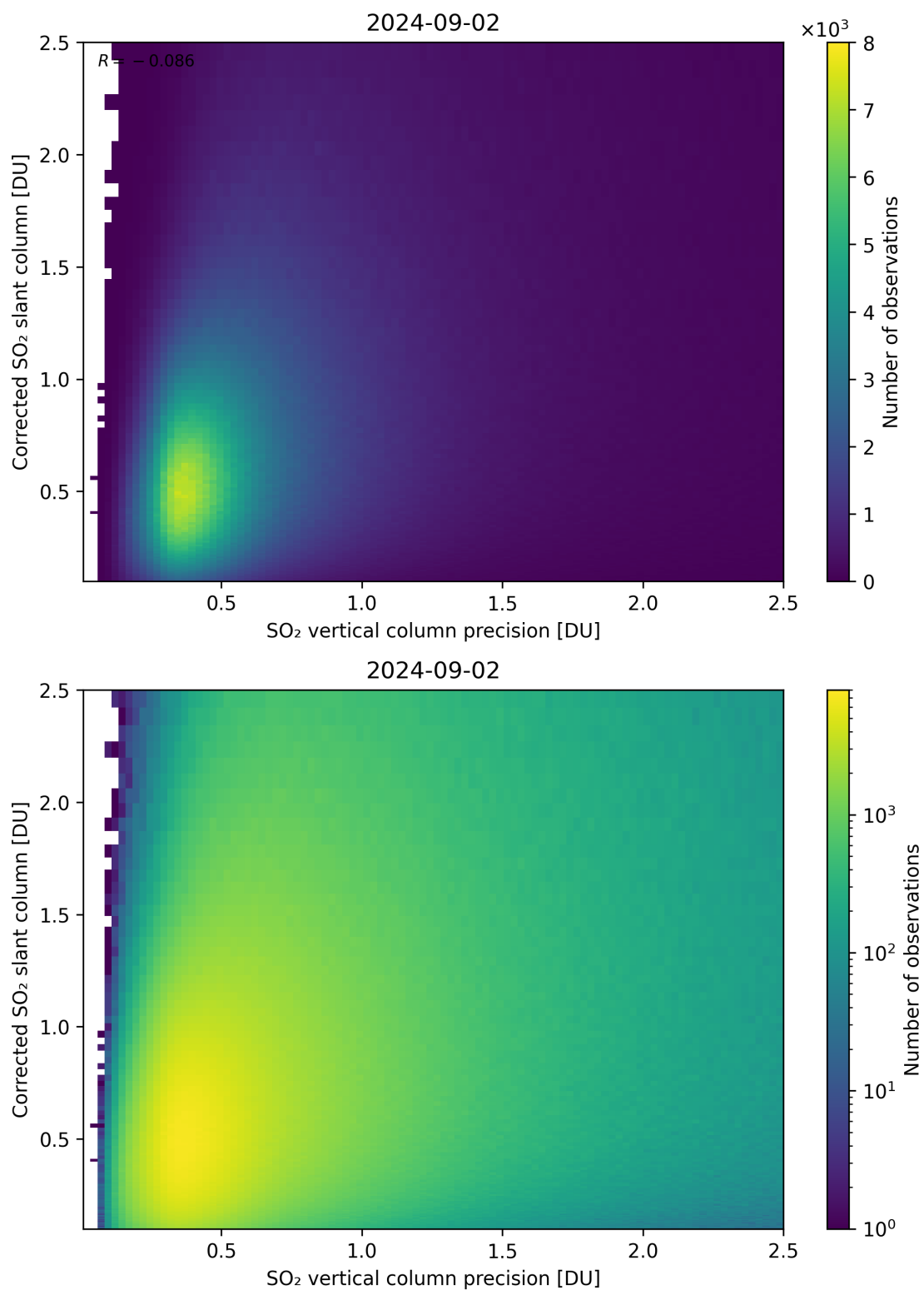
Figure 286: Scatter density plot of “SO 2 vertical column precision” against “Corrected SO 2 slant column” for 2024-09-01 to 2024-09-03.
