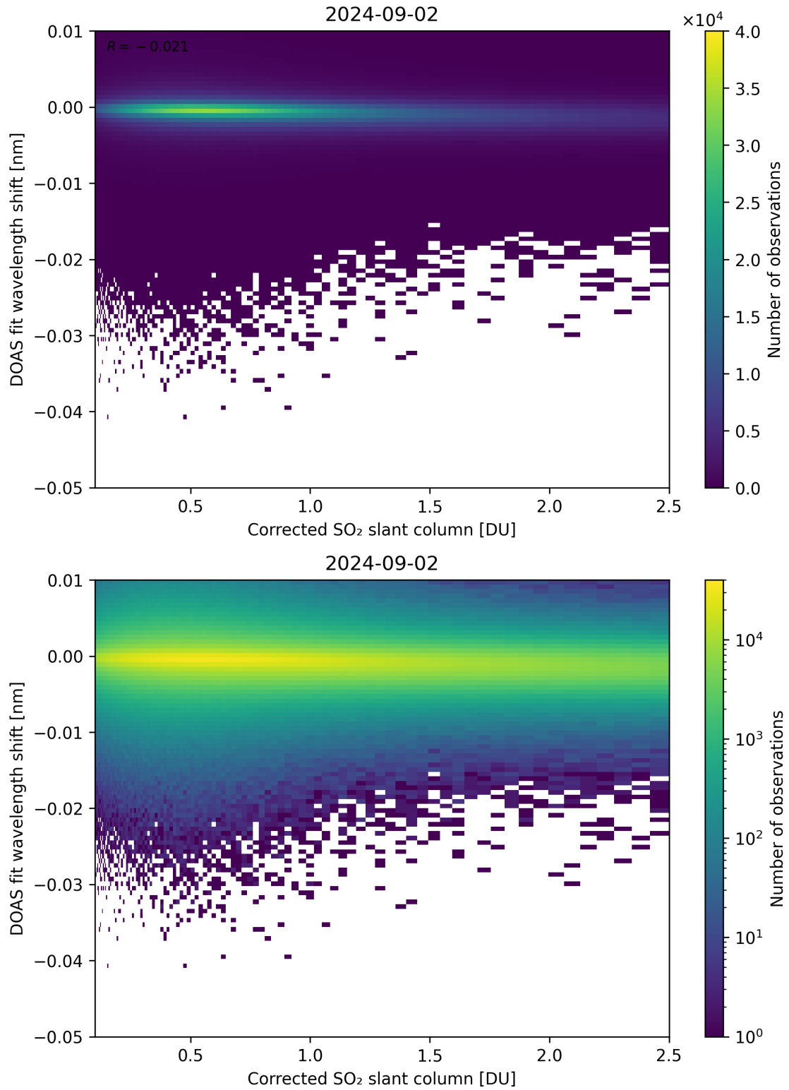
Figure 181: Scatter density plot of “Corrected SO 2 slant column” against “DOAS fit wavelength shift” for 2024-09-01 to 2024-09-03.
