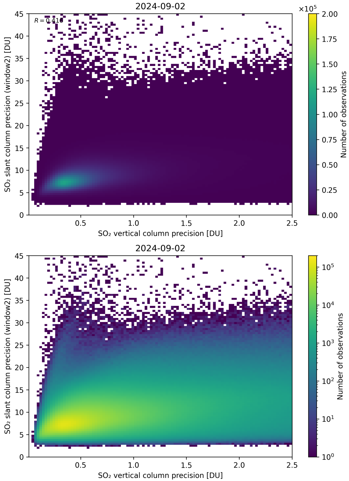
Figure 291: Scatter density plot of “SO 2 vertical column precision” against “SO 2 slant column precision (window2)” for 2024-09-01 to 2024-09-03.
