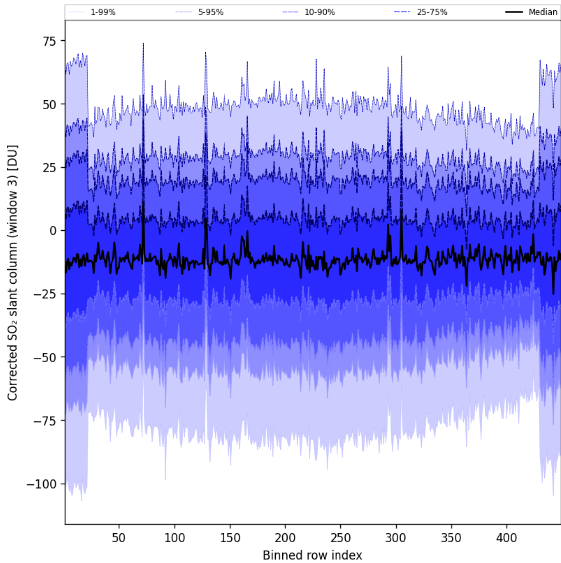
Figure 89: Along track statistics of “Corrected SO 2 slant column (window 3)” for 2024-09-01 to 2024-09-03
