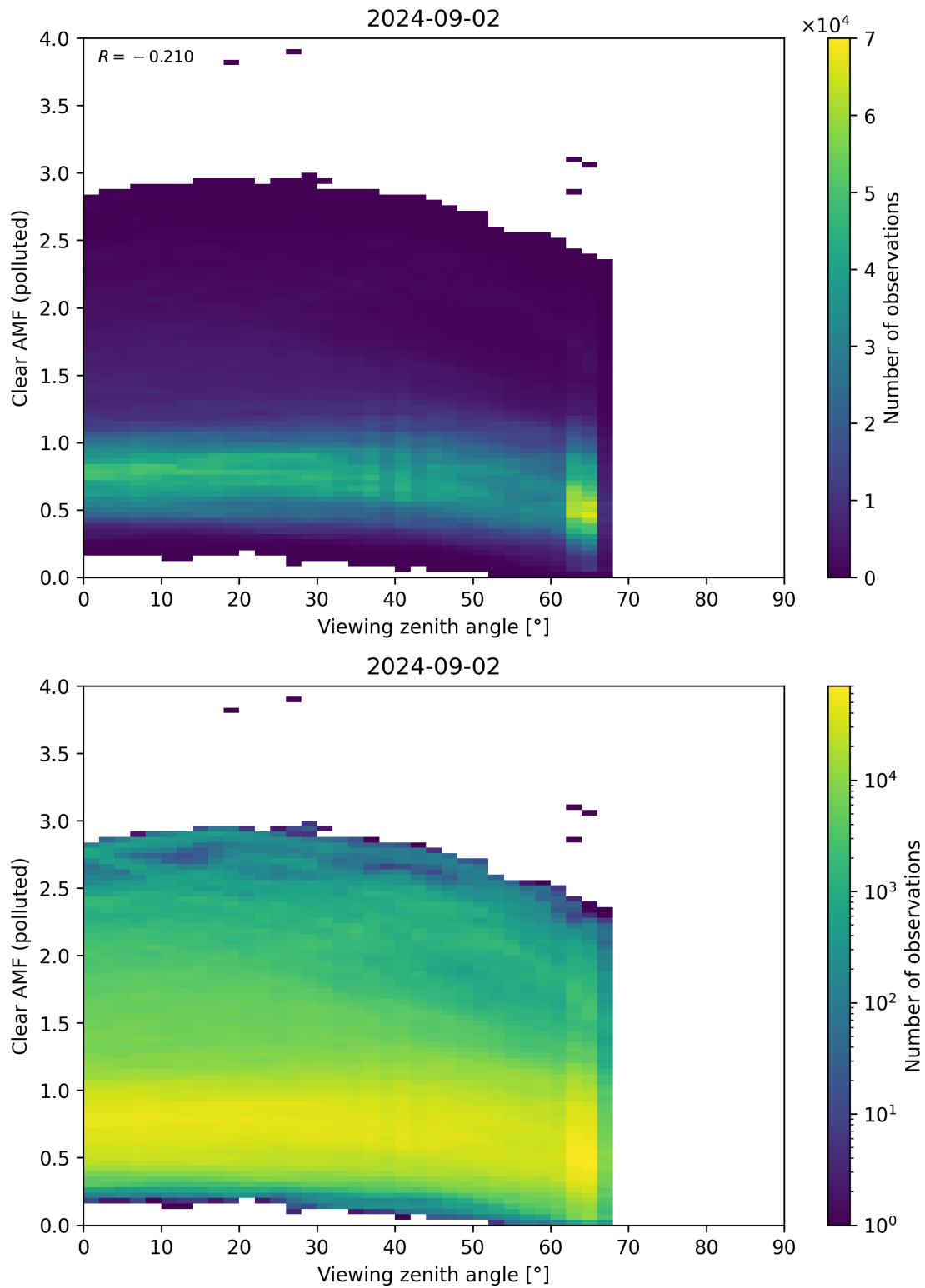
Figure 316: Scatter density plot of “Viewing zenith angle” against “Clear AMF (polluted)” for 2024-09-01 to 2024-09-03.
