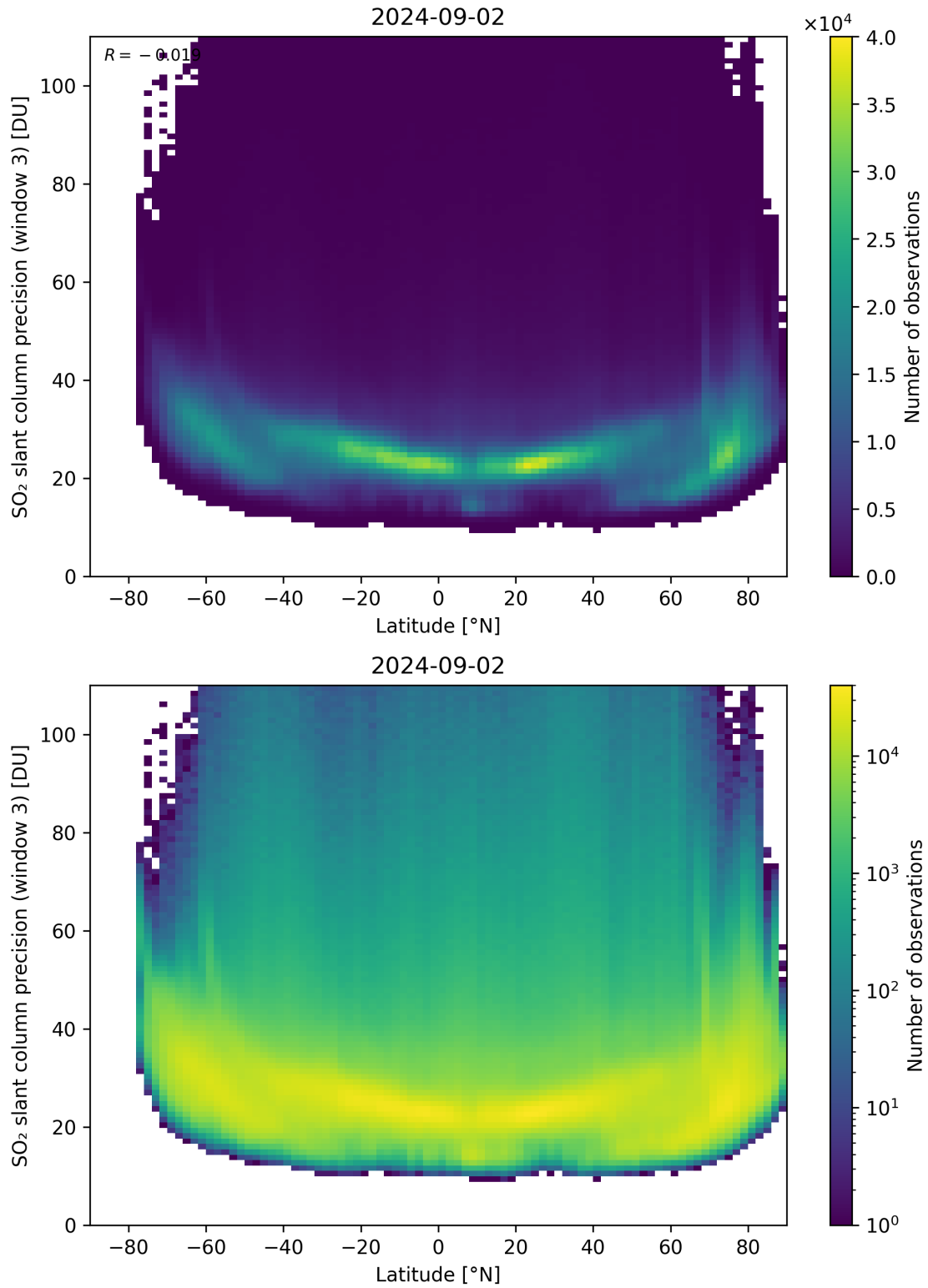
Figure 153: Scatter density plot of “Latitude” against “SO 2 slant column precision (window 3)” for 2024-09-01 to 2024-09-03.
