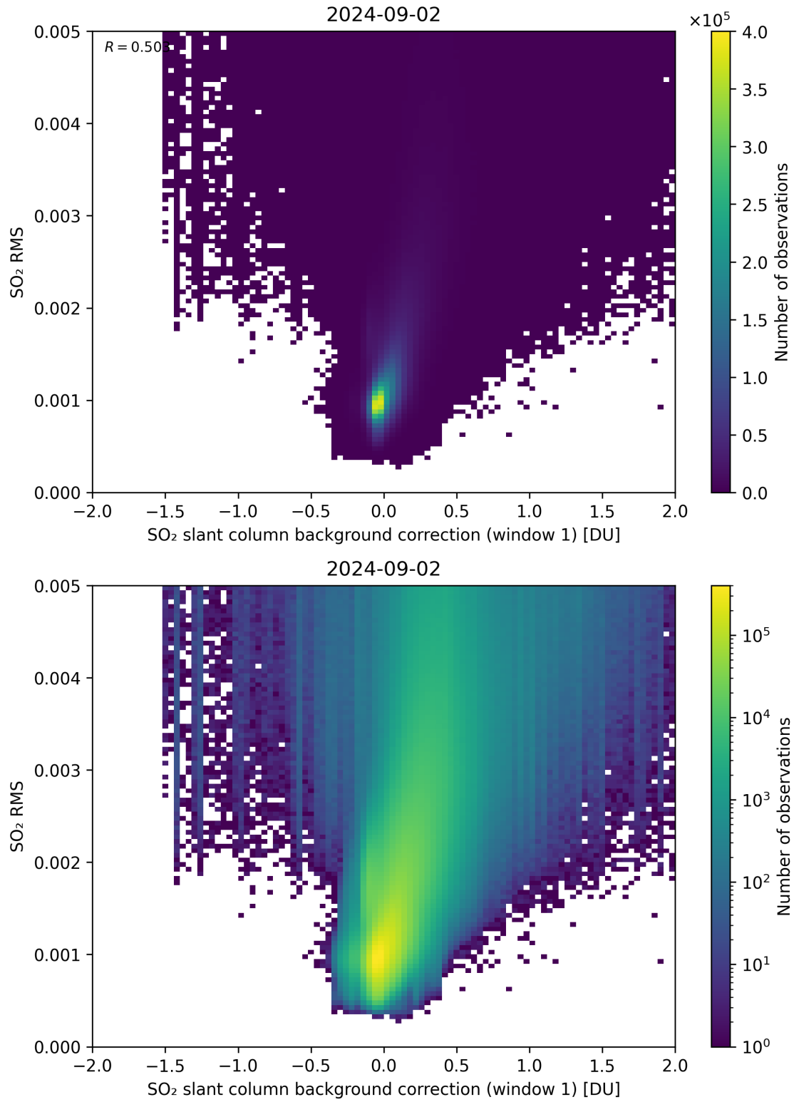
Figure 102: Scatter density plot of “SO 2 slant column background correction (window 1)” against “SO 2 RMS” for 2024-09-01 to 2024-09-03.
