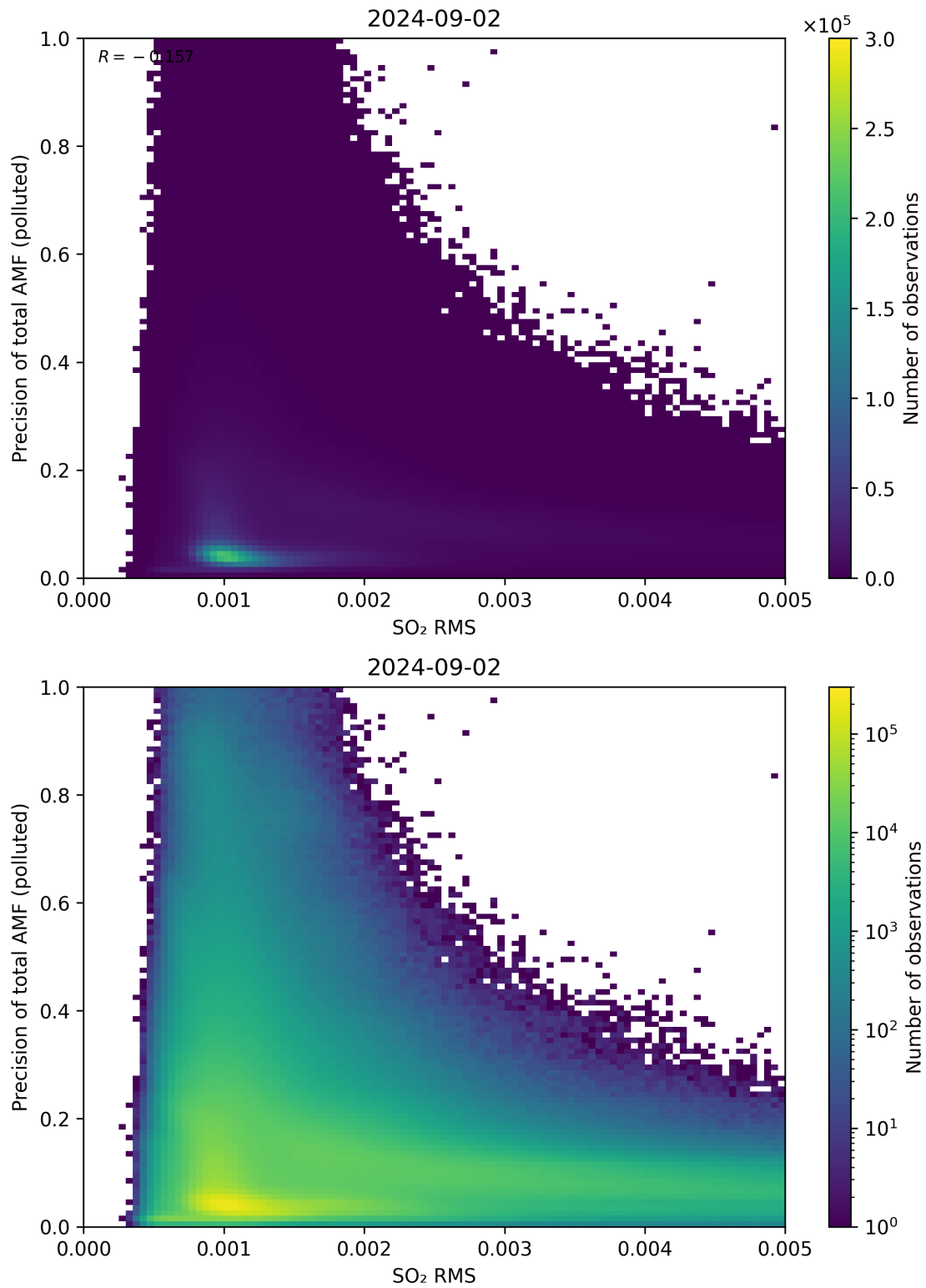
Figure 138: Scatter density plot of “SO 2 RMS” against “Precision of total AMF (polluted)” for 2024-09-01 to 2024-09-03.
