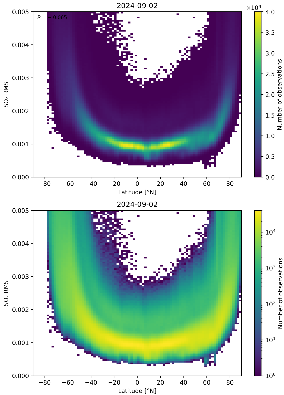
Figure 144: Scatter density plot of “Latitude” against “SO 2 RMS” for 2024-09-01 to 2024-09-03.
