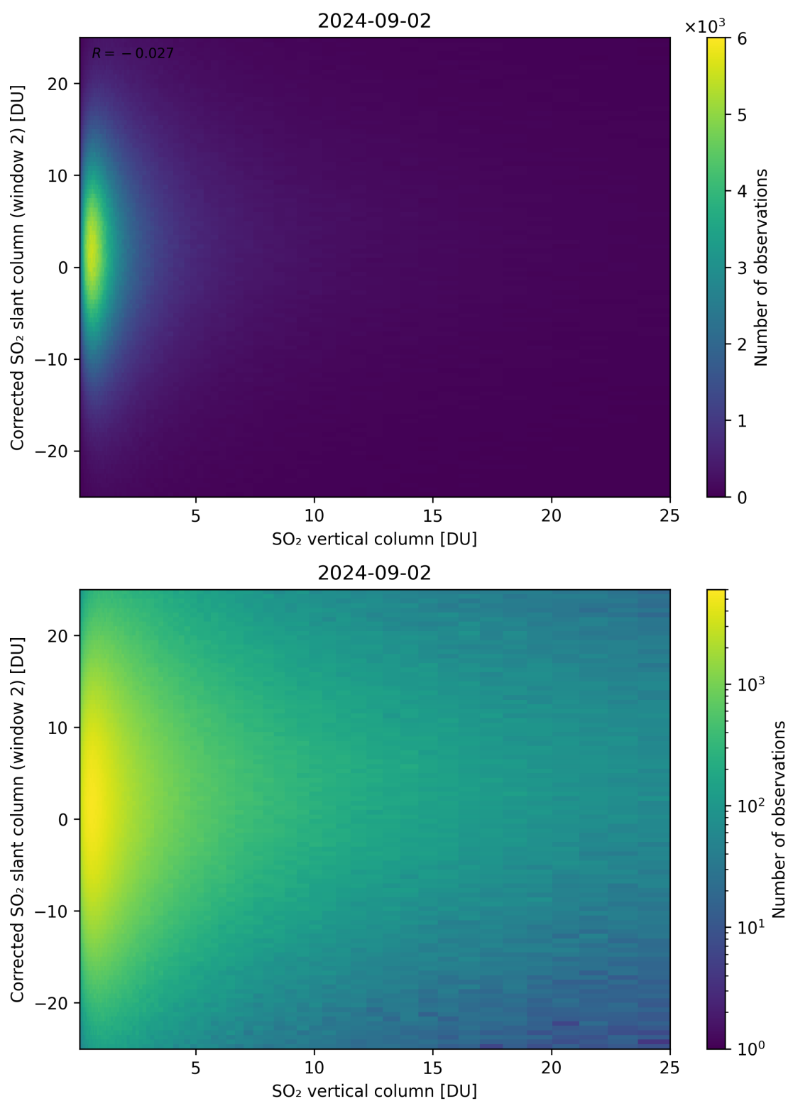
Figure 298: Scatter density plot of “SO 2 vertical column” against “Corrected SO 2 slant column (window 2)” for 2024-09-01 to 2024-09-03.
