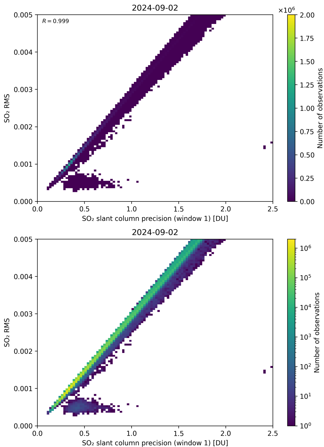
Figure 223: Scatter density plot of “SO 2 slant column precision (window 1)” against “SO 2 RMS” for 2024-09-01 to 2024-09-03.
