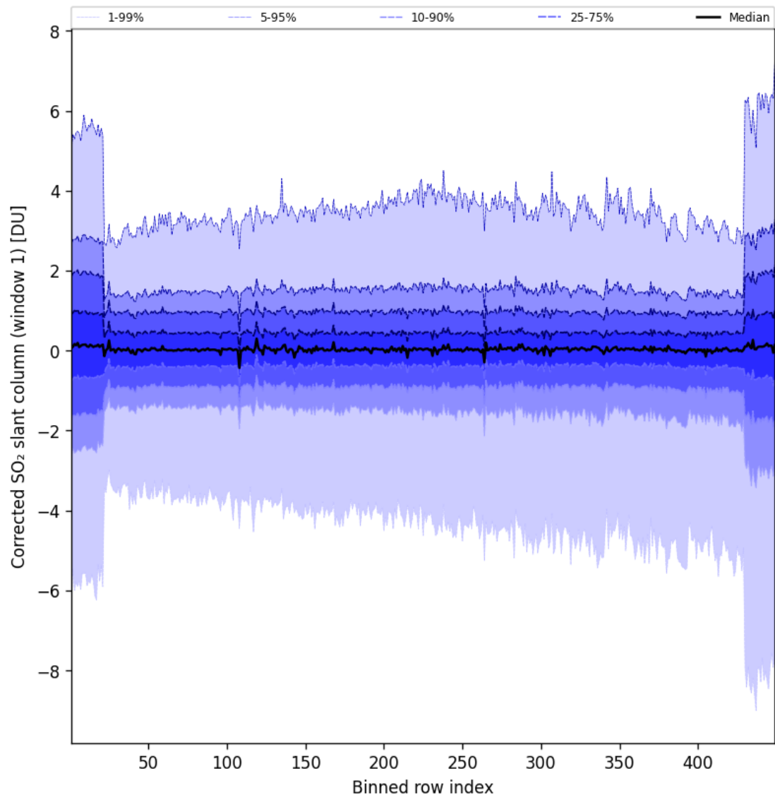
Figure 81: Along track statistics of “Corrected SO 2 slant column (window 1)” for 2024-09-01 to 2024-09-03
