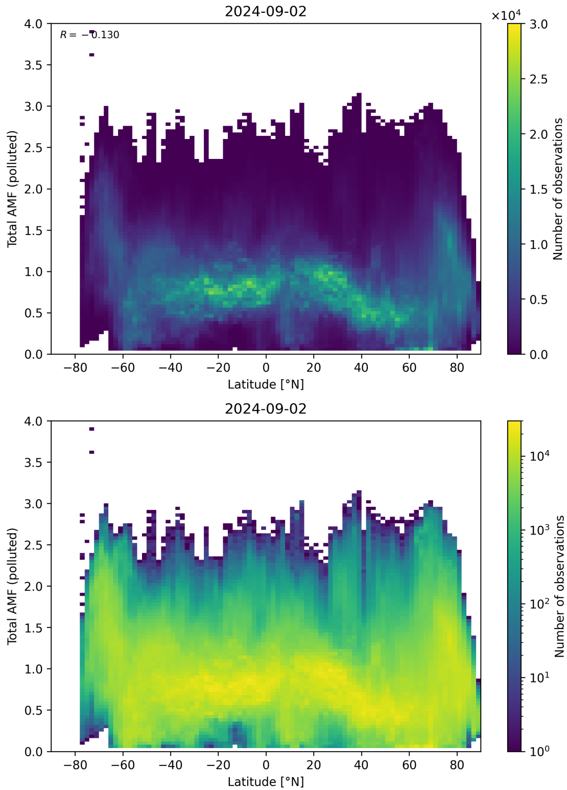
Figure 154: Scatter density plot of “Latitude” against “Total AMF (polluted)” for 2024-09-01 to 2024-09-03.
