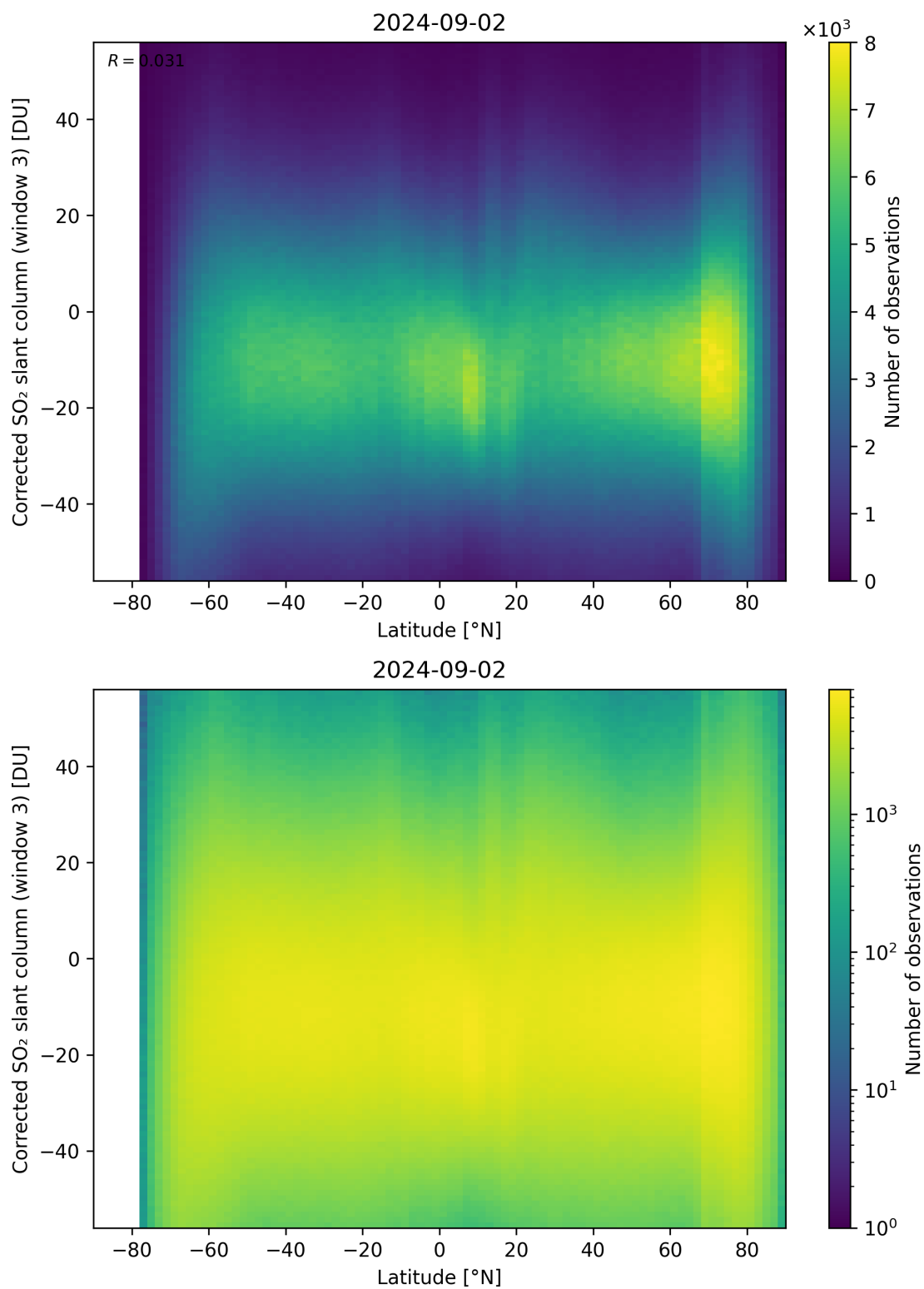
Figure 148: Scatter density plot of “Latitude” against “Corrected SO 2 slant column (window 3)” for 2024-09-01 to 2024-09-03.
