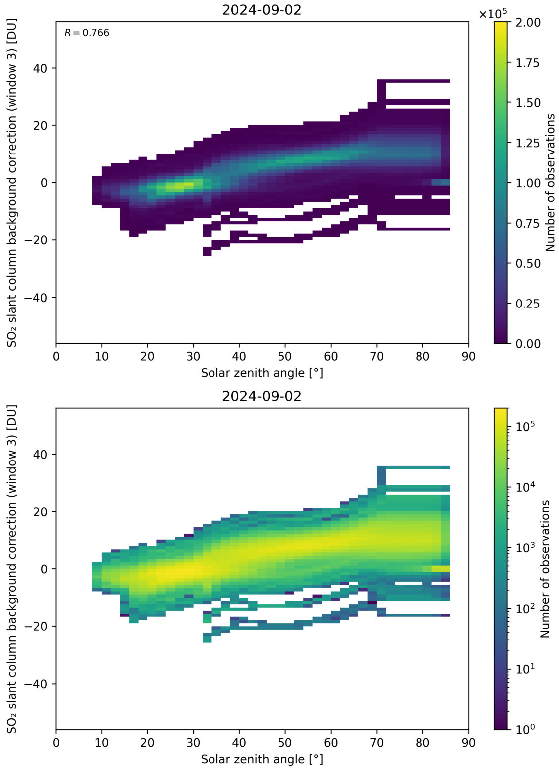
Figure 160: Scatter density plot of “Solar zenith angle” against “SO 2 slant column background correction (window 3)” for 2024-09-01 to 2024-09-03.
