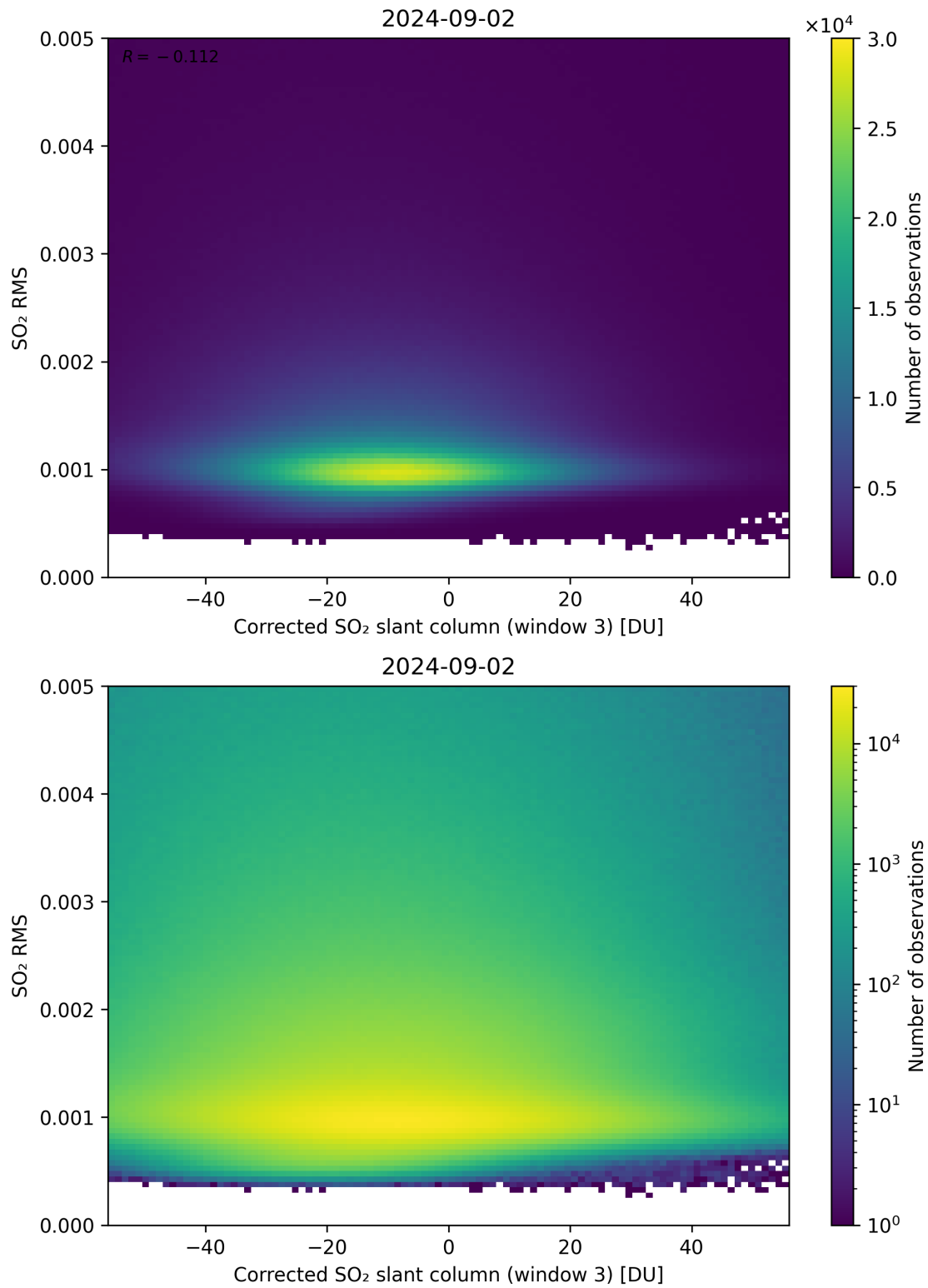
Figure 208: Scatter density plot of “Corrected SO 2 slant column (window 3)” against “SO 2 RMS” for 2024-09-01 to 2024-09-03.
