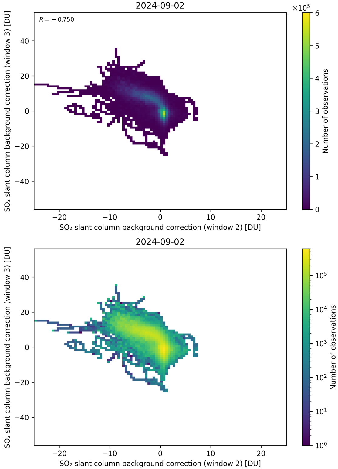
Figure 111: Scatter density plot of “SO 2 slant column background correction (window 2)” against “SO 2 slant column background correction (window 3)” for 2024-09-01 to 2024-09-03.
