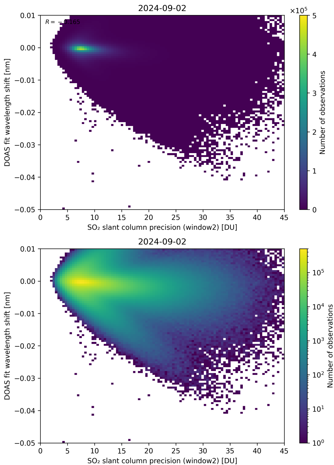
Figure 243: Scatter density plot of “SO 2 slant column precision (window2)” against “DOAS fit wavelength shift” for 2024-09-01 to 2024-09-03.
