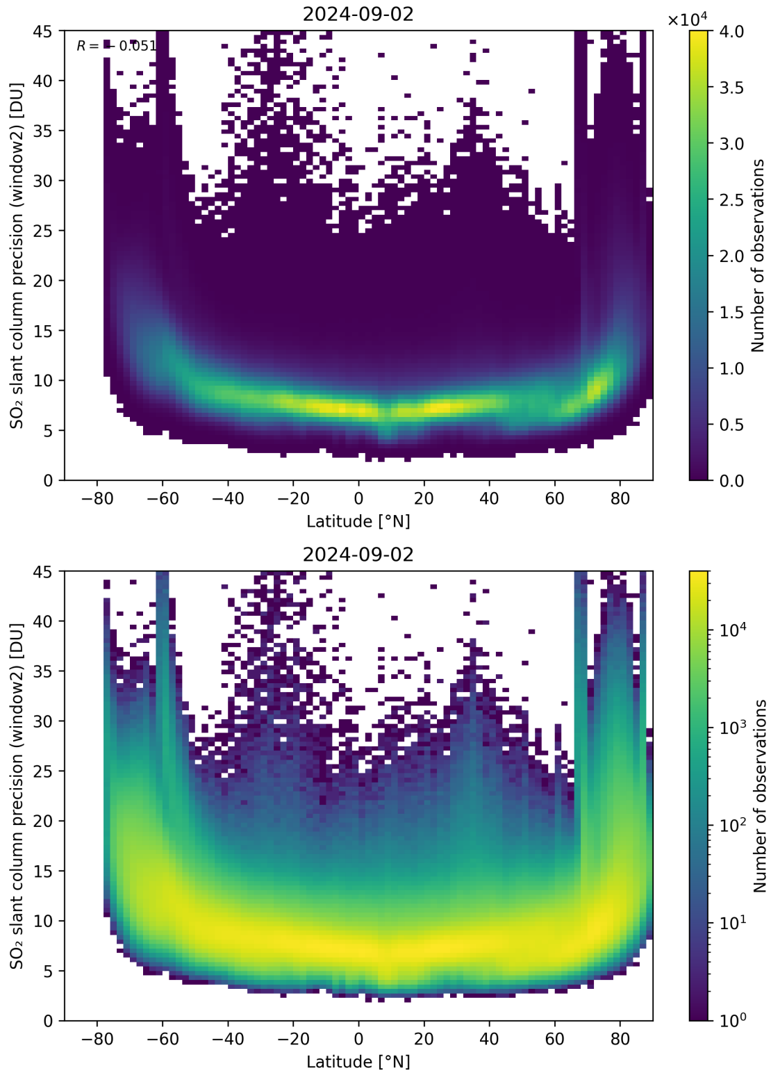
Figure 151: Scatter density plot of “Latitude” against “SO 2 slant column precision (window2)” for 2024-09-01 to 2024-09-03.
