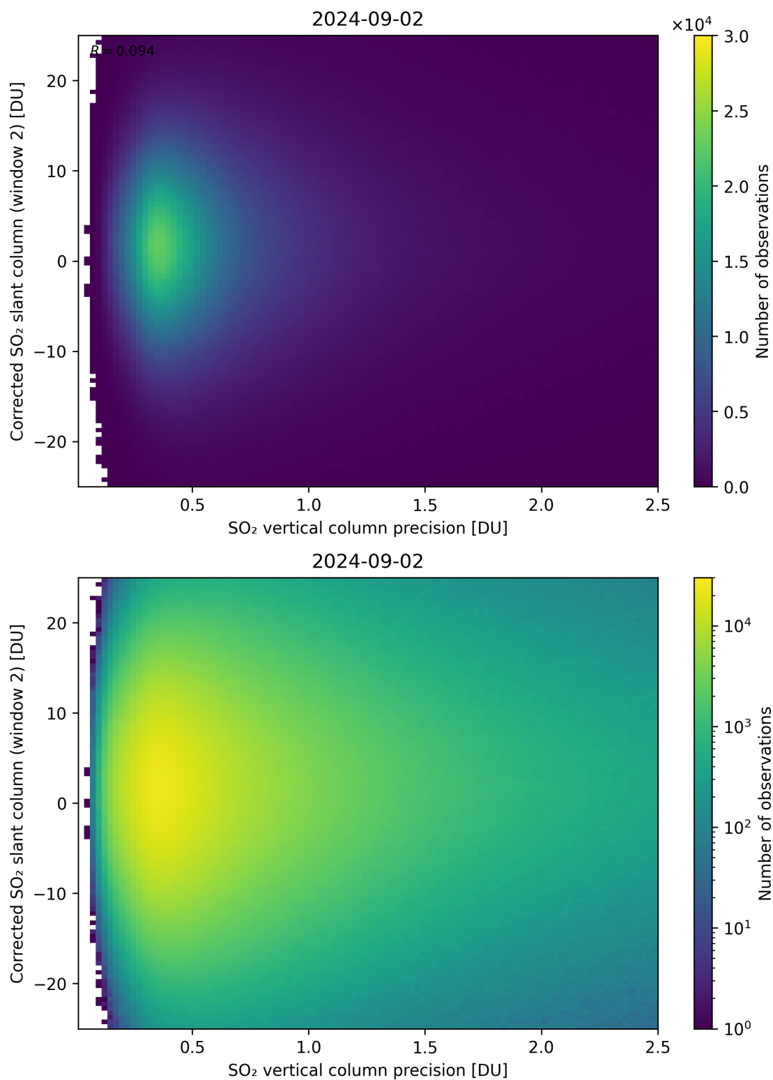
Figure 287: Scatter density plot of “SO 2 vertical column precision” against “Corrected SO 2 slant column (window 2)” for 2024-09-01 to 2024-09-03.
