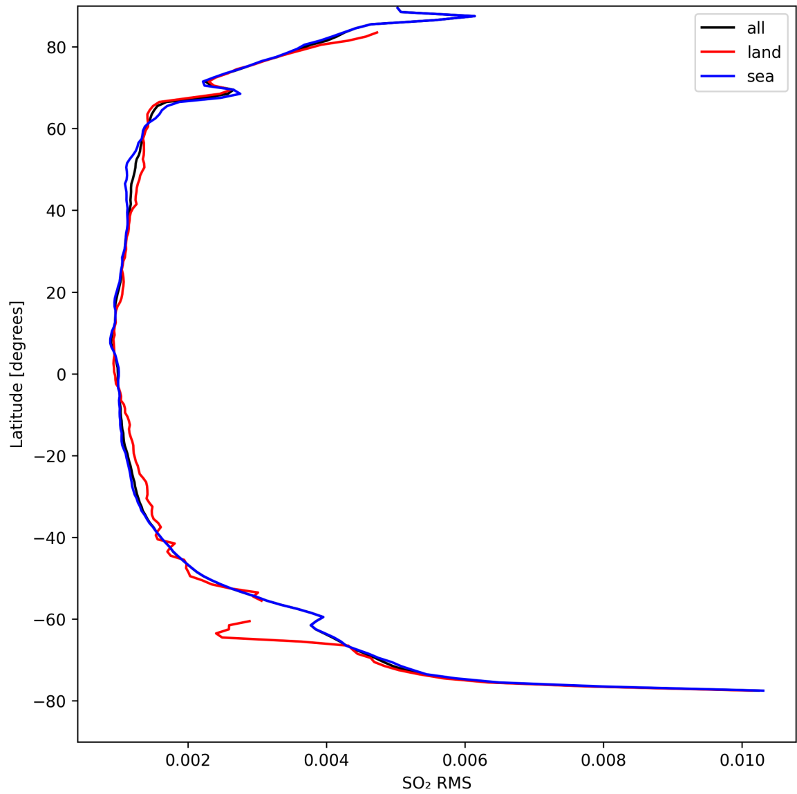
Figure 47: Zonal average of “SO 2 RMS” for 2024-09-01 to 2024-09-03.
