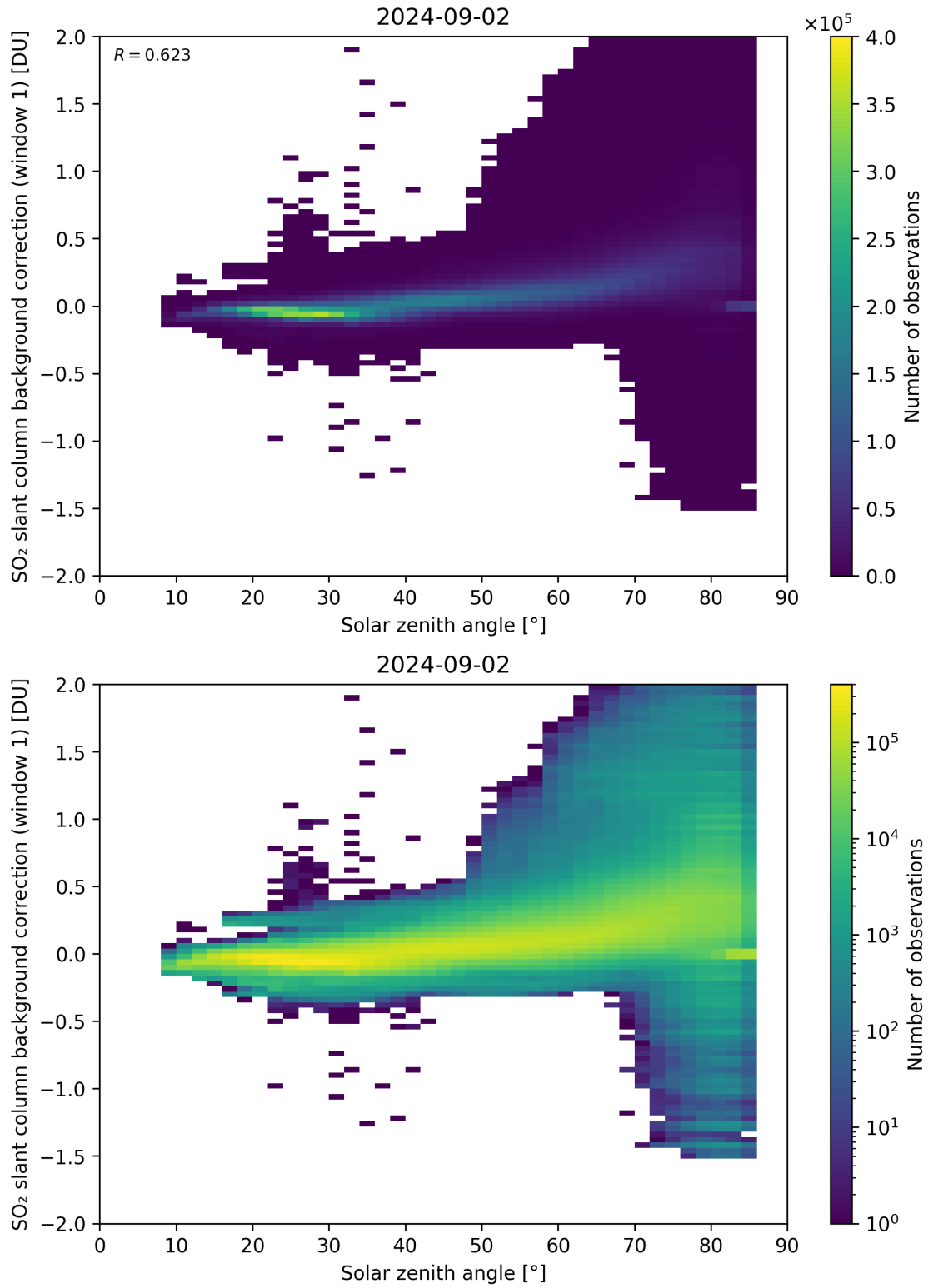
Figure 158: Scatter density plot of “Solar zenith angle” against “SO 2 slant column background correction (window 1)” for 2024-09-01 to 2024-09-03.
