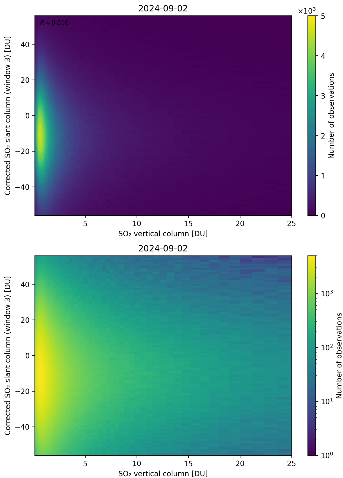
Figure 299: Scatter density plot of “SO 2 vertical column” against “Corrected SO 2 slant column (window 3)” for 2024-09-01 to 2024-09-03.
