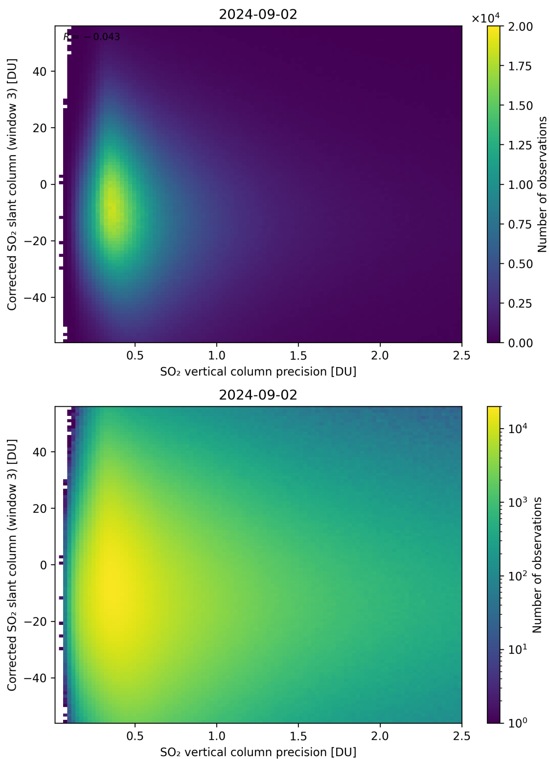
Figure 288: Scatter density plot of “SO 2 vertical column precision” against “Corrected SO 2 slant column (window 3)” for 2024-09-01 to 2024-09-03.
