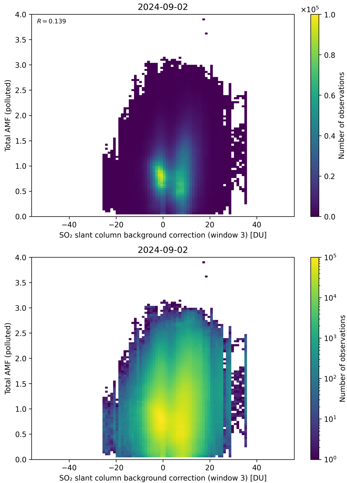
Figure 125: Scatter density plot of “SO 2 slant column background correction (window 3)” against “Total AMF (polluted)” for 2024-09-01 to 2024-09-03.
