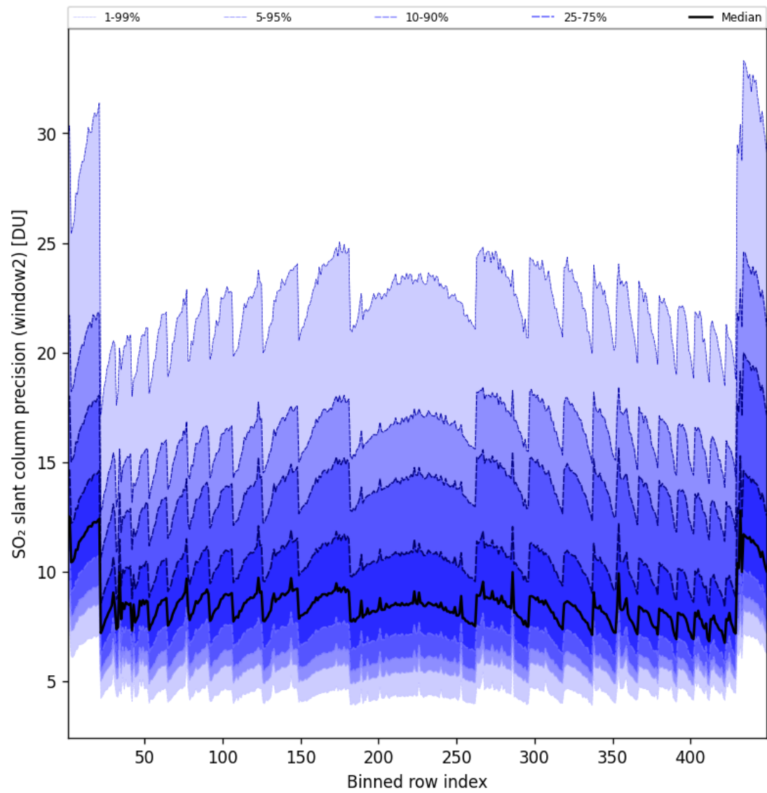
Figure 84: Along track statistics of “SO 2 slant column precision (window2)” for 2024-09-01 to 2024-09-03
