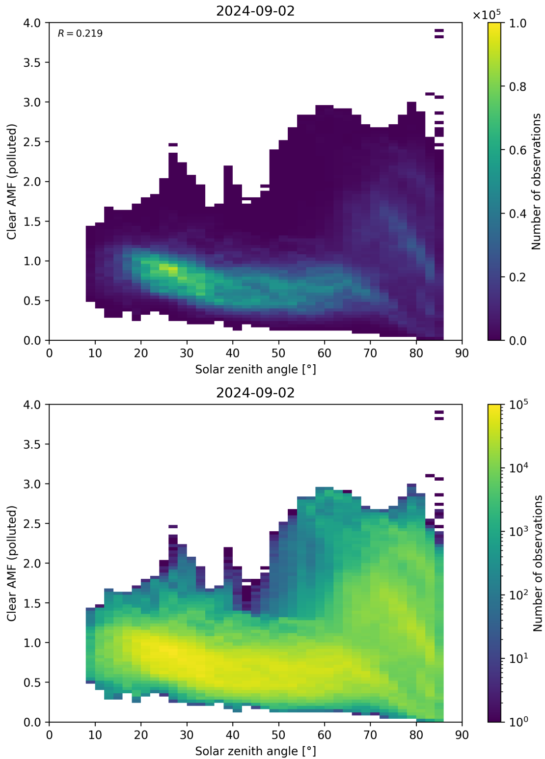
Figure 165: Scatter density plot of “Solar zenith angle” against “Clear AMF (polluted)” for 2024-09-01 to 2024-09-03.
