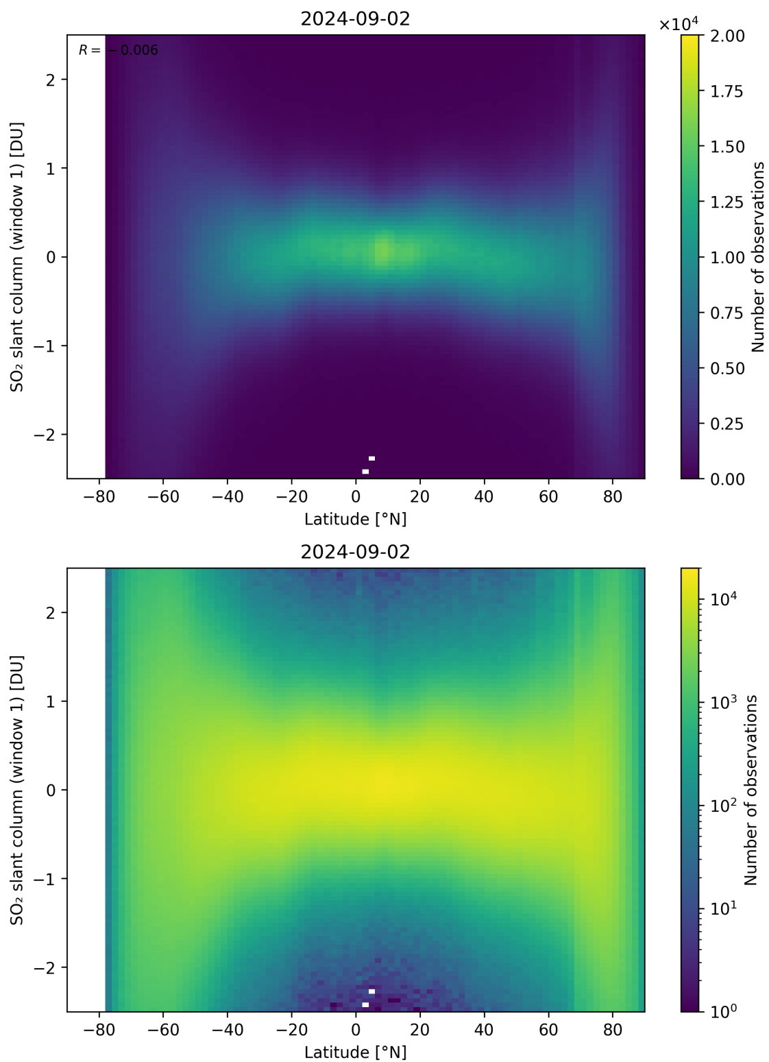
Figure 149: Scatter density plot of “Latitude” against “SO 2 slant column (window 1)” for 2024-09-01 to 2024-09-03.
