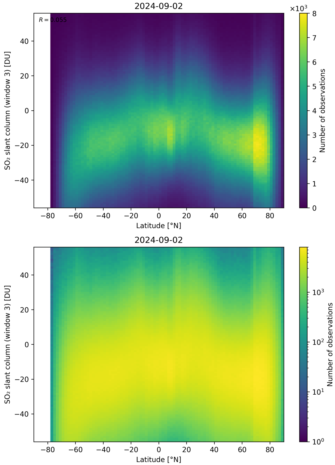
Figure 152: Scatter density plot of “Latitude” against “SO 2 slant column (window 3)” for 2024-09-01 to 2024-09-03.
