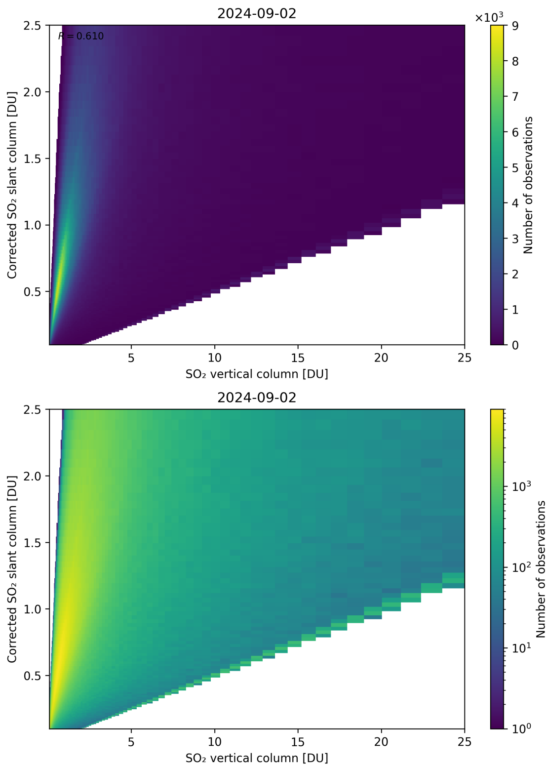
Figure 297: Scatter density plot of “SO 2 vertical column” against “Corrected SO 2 slant column” for 2024-09-01 to 2024-09-03.
