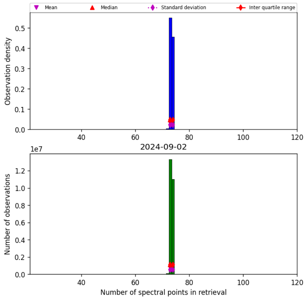
Figure 74: Histogram of “Number of spectral points in retrieval” for 2024-09-01 to 2024-09-03
