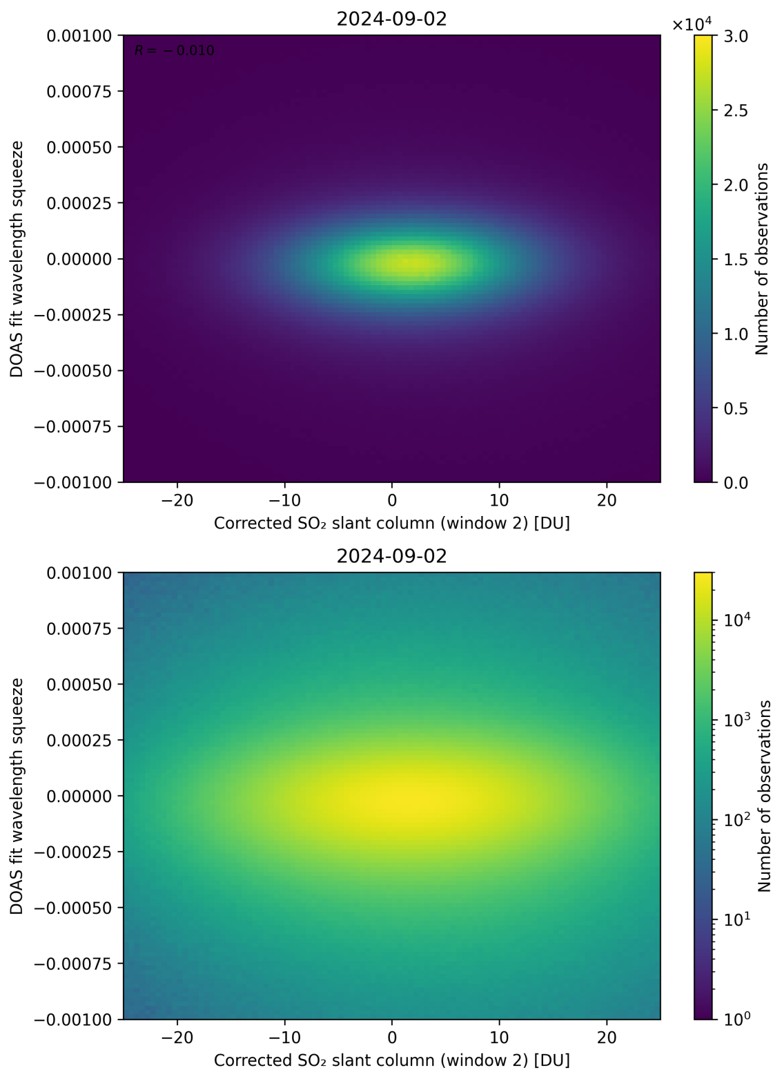
Figure 197: Scatter density plot of “Corrected SO 2 slant column (window 2)” against “DOAS fit wavelength squeeze” for 2024-09-01 to 2024-09-03.
