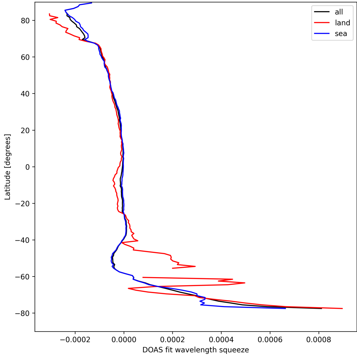
Figure 46: Zonal average of “DOAS fit wavelength squeeze” for 2024-09-01 to 2024-09-03.
