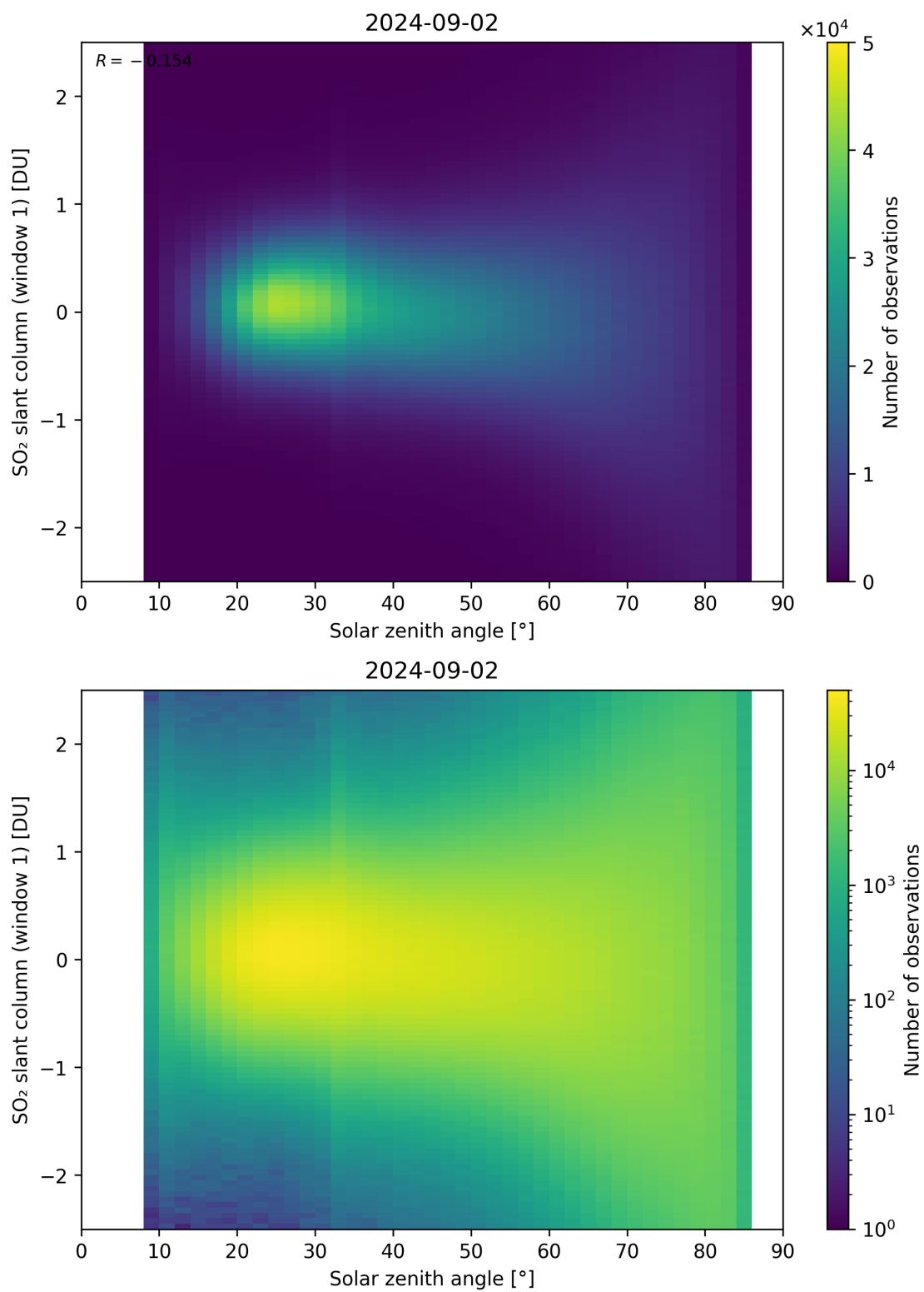
Figure 169: Scatter density plot of “Solar zenith angle” against “SO 2 slant column (window 1)” for 2024-09-01 to 2024-09-03.
