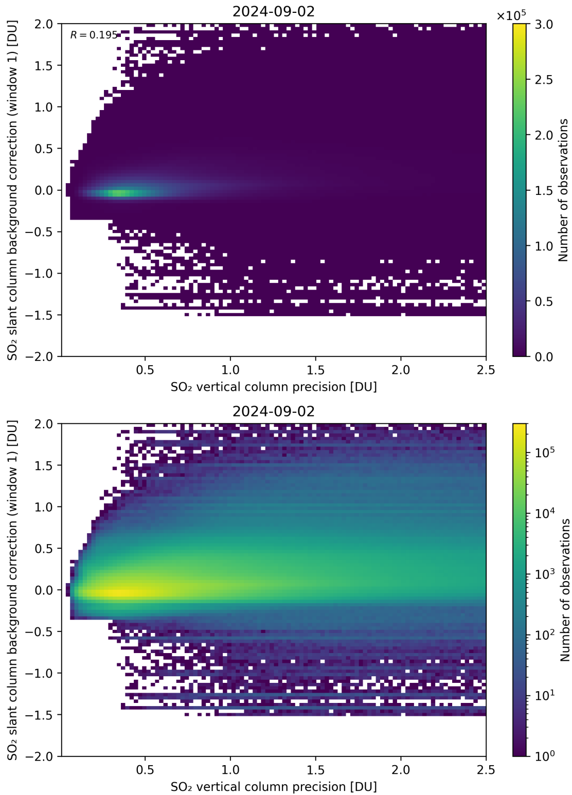
Figure 279: Scatter density plot of “SO 2 vertical column precision” against “SO 2 slant column background correction (window 1)” for 2024-09-01 to 2024-09-03.
