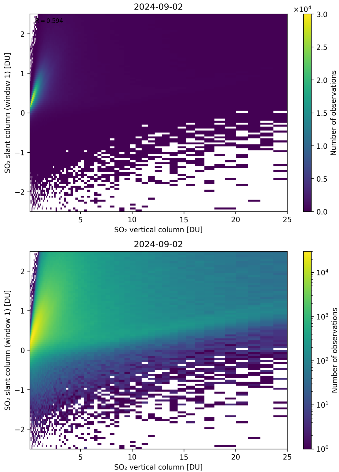
Figure 300: Scatter density plot of “SO 2 vertical column” against “SO 2 slant column (window 1)” for 2024-09-01 to 2024-09-03.
