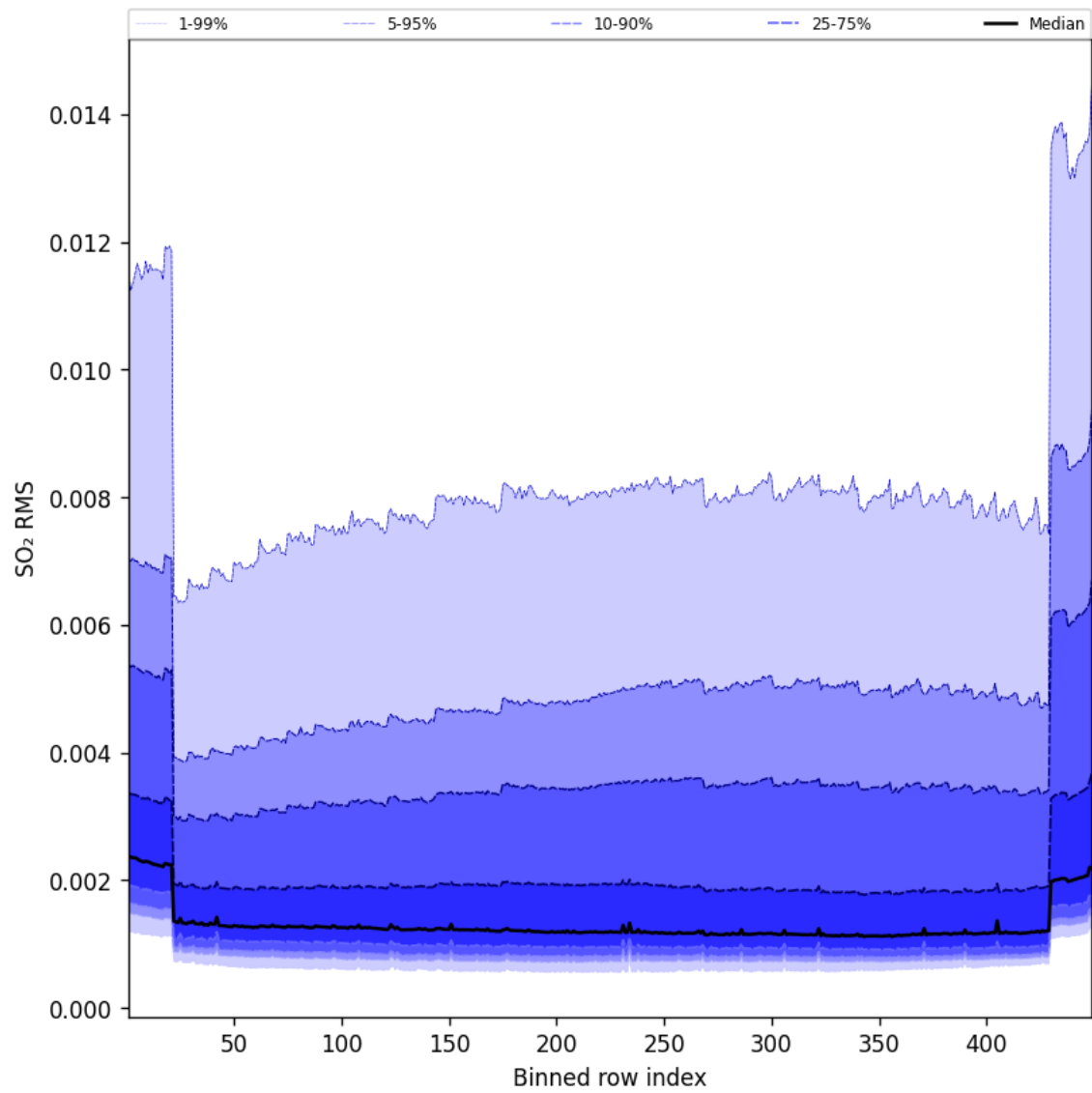
Figure 93: Along track statistics of “SO 2 RMS” for 2024-09-01 to 2024-09-03
