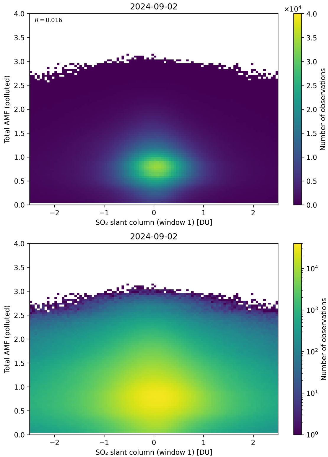
Figure 239: Scatter density plot of “SO 2 slant column (window 1)” against “Total AMF (polluted)” for 2024-09-01 to 2024-09-03.
