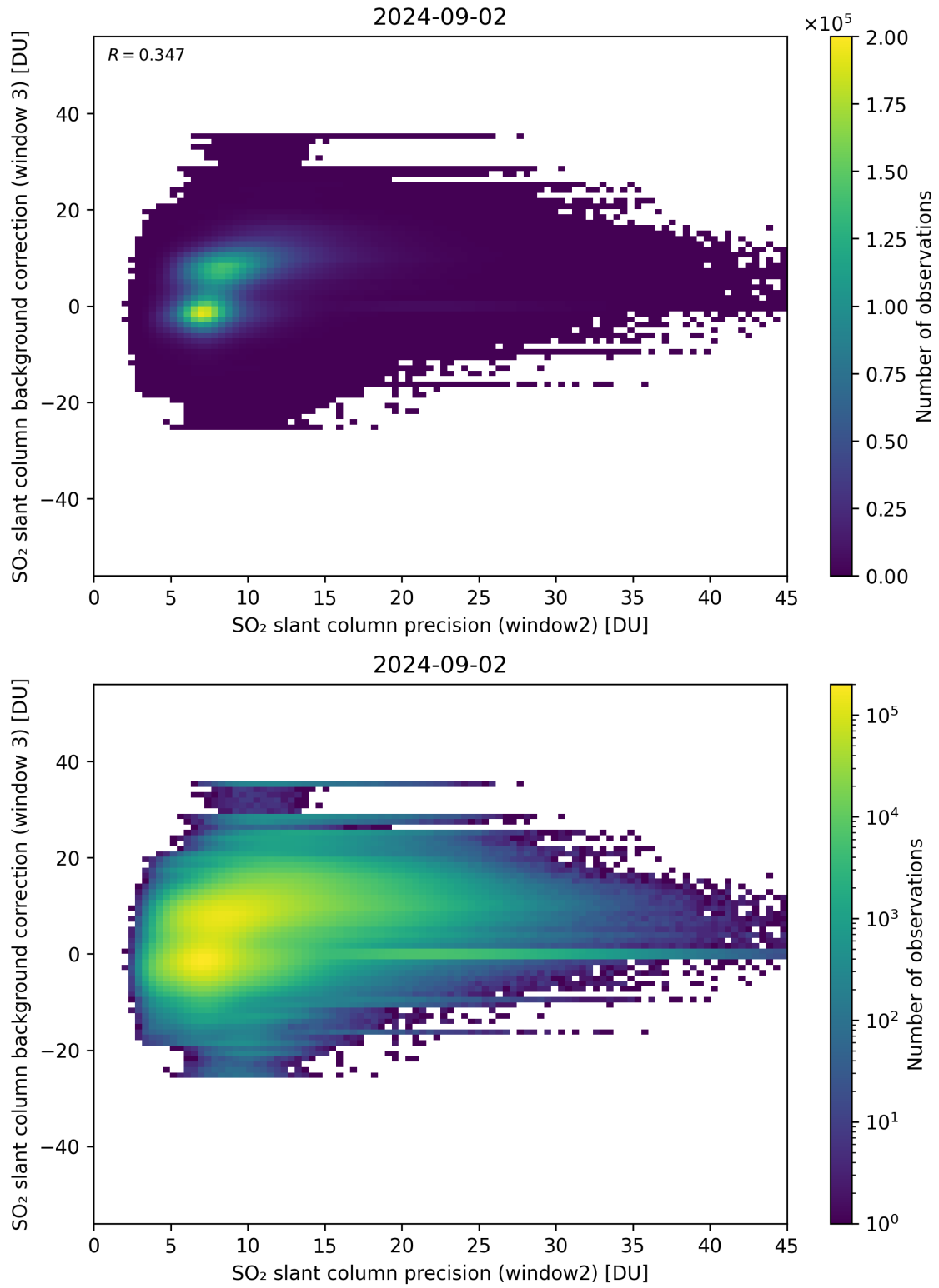
Figure 242: Scatter density plot of “SO 2 slant column precision (window2)” against “SO 2 slant column background correction (window 3)” for 2024-09-01 to 2024-09-03.
