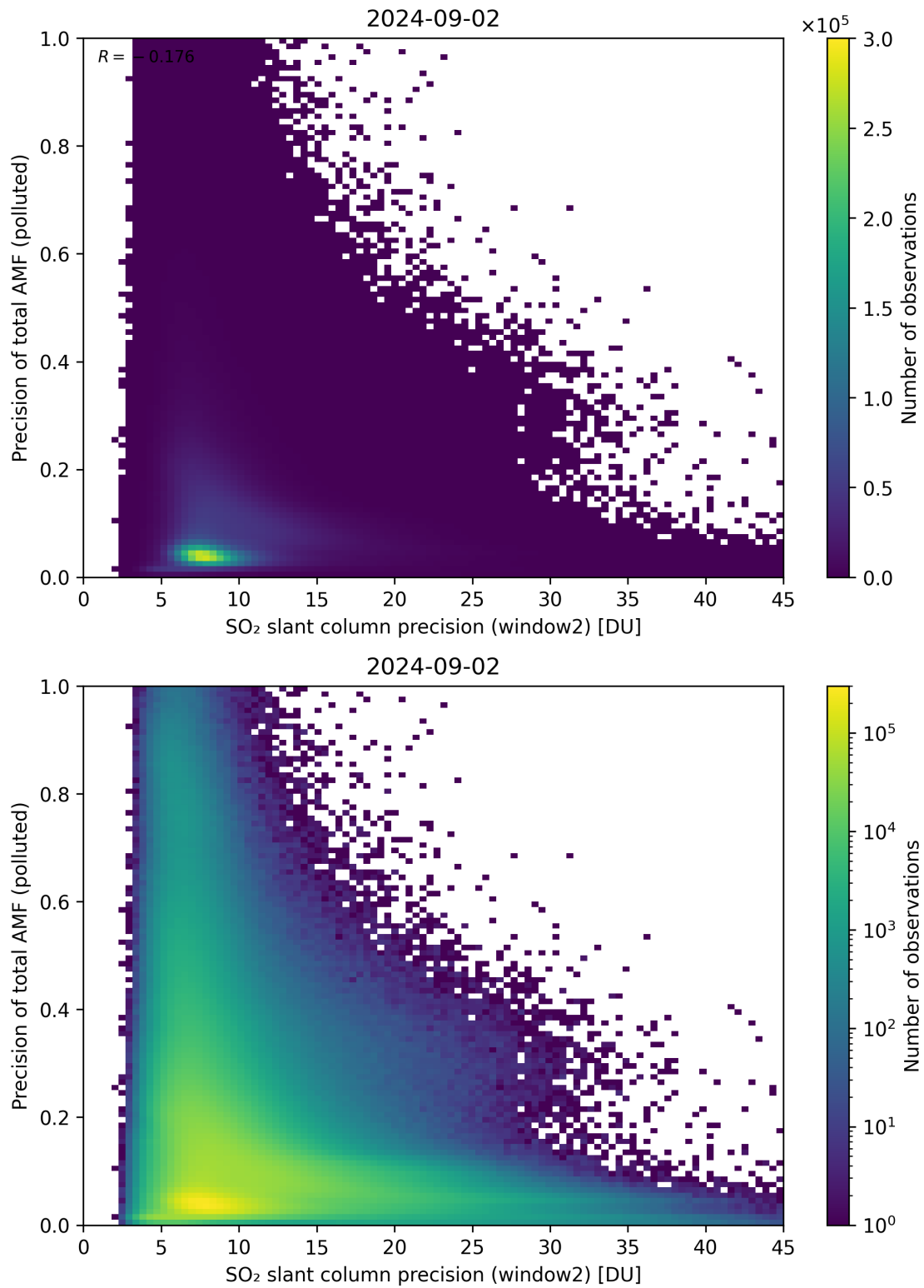
Figure 252: Scatter density plot of “SO 2 slant column precision (window2)” against “Precision of total AMF (polluted)” for 2024-09-01 to 2024-09-03.
