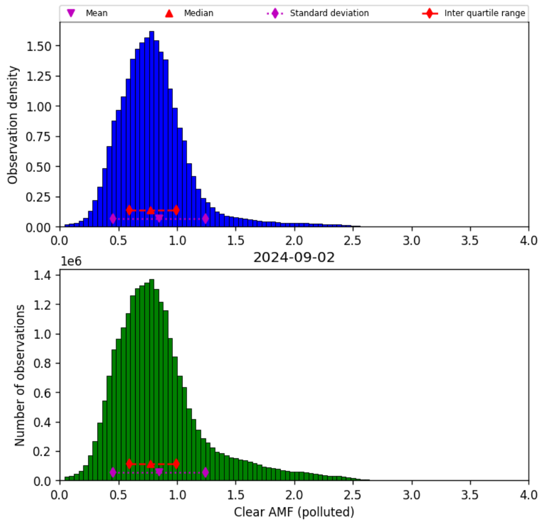
Figure 73: Histogram of “Clear AMF (polluted)” for 2024-09-01 to 2024-09-03
