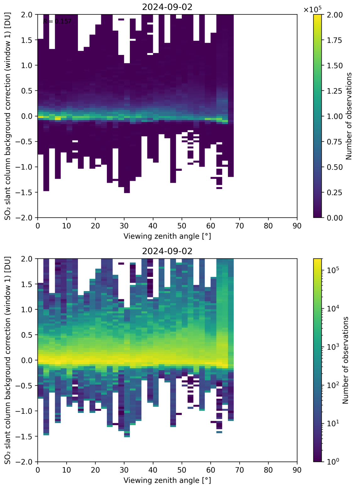
Figure 308: Scatter density plot of “Viewing zenith angle” against “SO 2 slant column background correction (window 1)” for 2024-09-01 to 2024-09-03.
