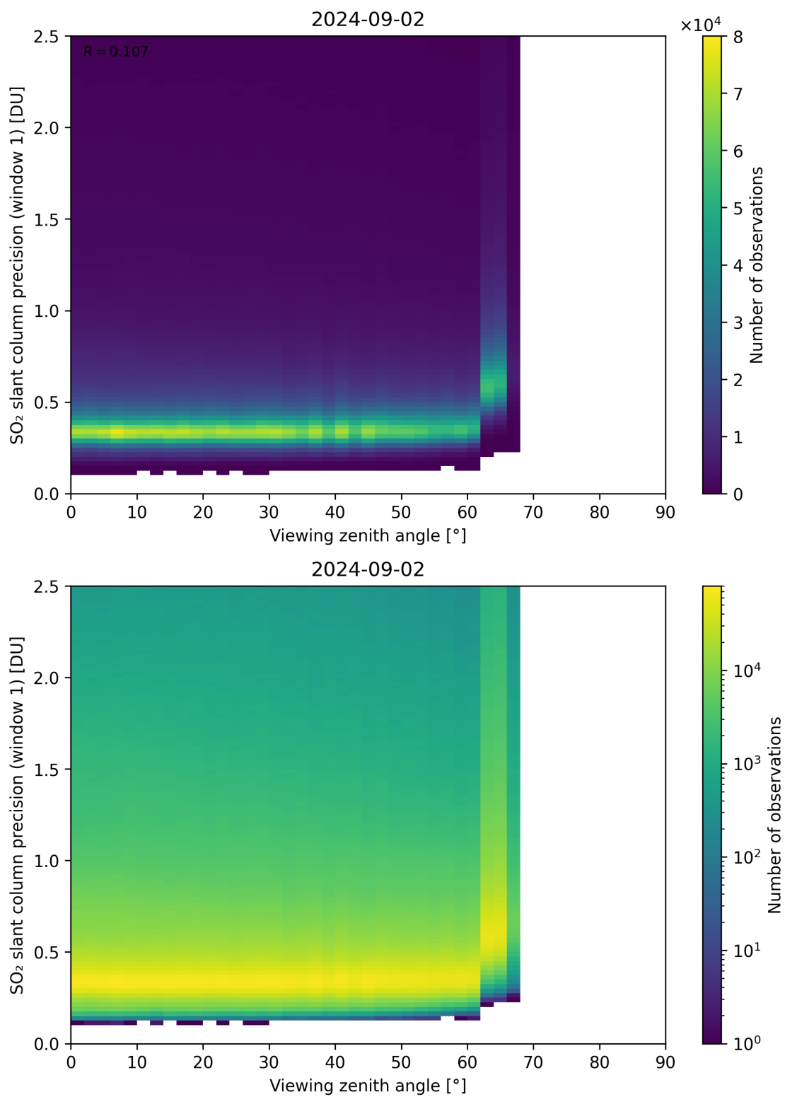
Figure 321: Scatter density plot of “Viewing zenith angle” against “SO 2 slant column precision (window 1)” for 2024-09-01 to 2024-09-03.
