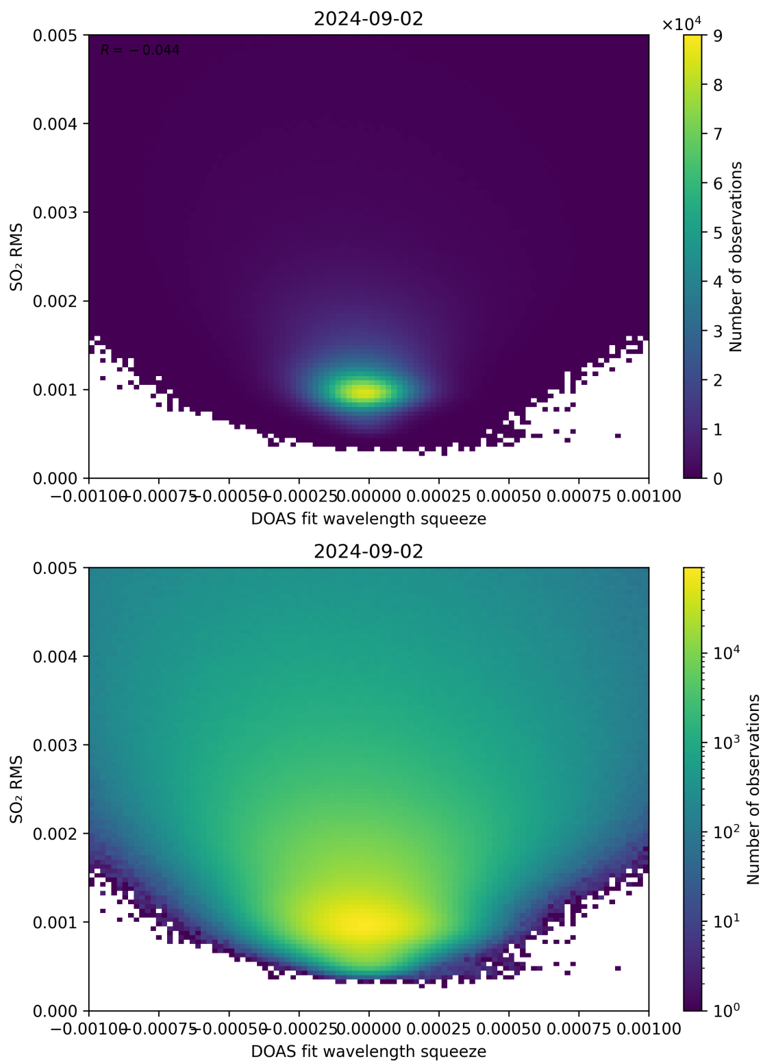
Figure 132: Scatter density plot of “DOAS fit wavelength squeeze” against “SO 2 RMS” for 2024-09-01 to 2024-09-03.
