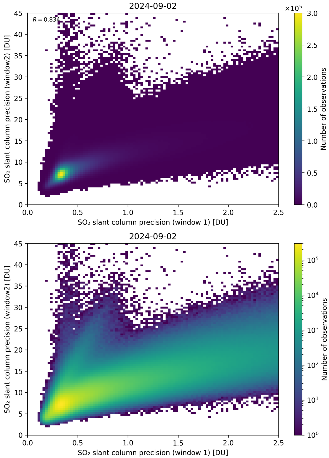
Figure 227: Scatter density plot of “SO 2 slant column precision (window 1)” against “SO 2 slant column precision (window 2)” for 2024-09-01 to 2024-09-03.
