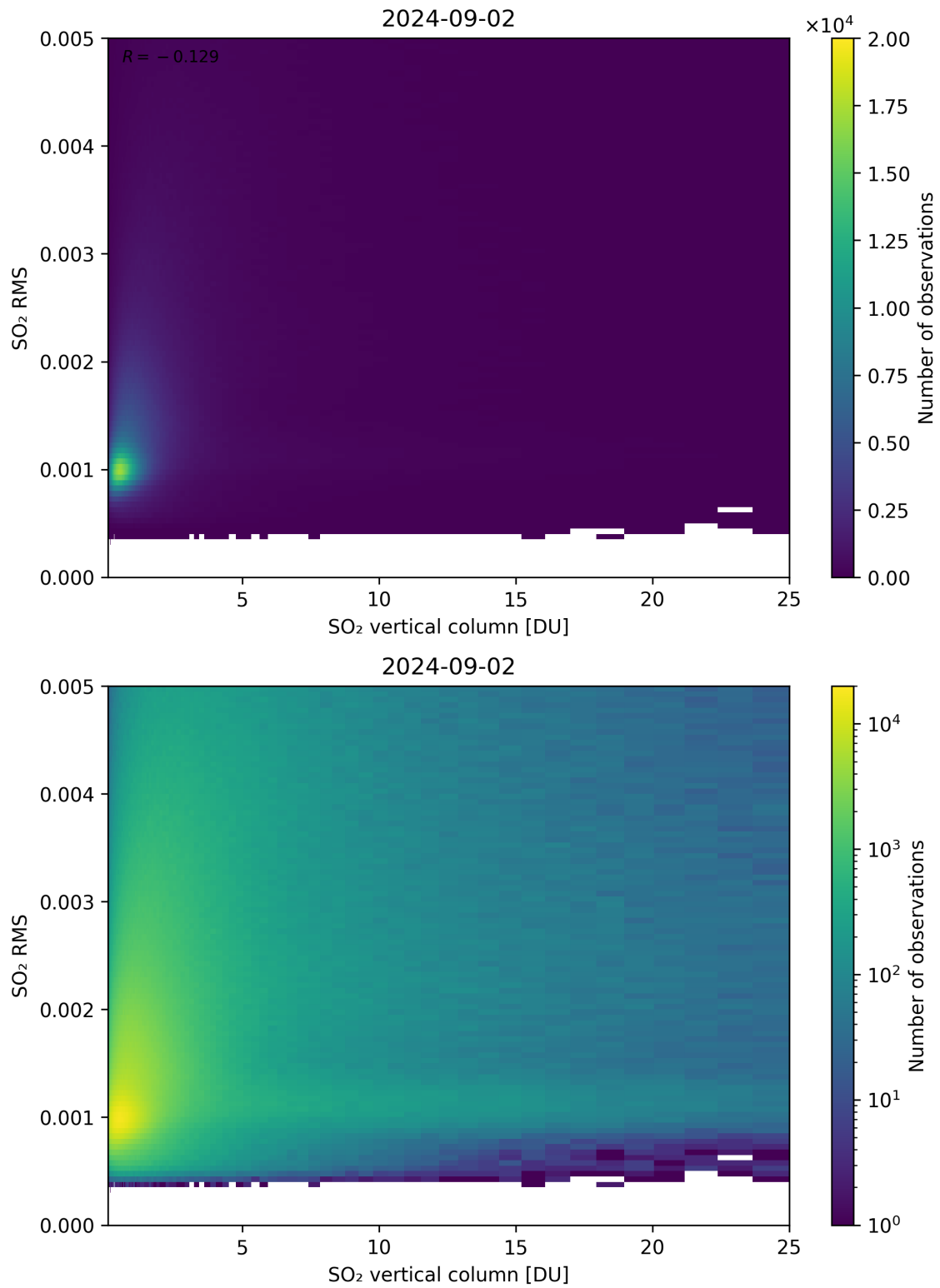
Figure 278: Scatter density plot of “SO 2 vertical column” against “SO 2 RMS” for 2024-09-01 to 2024-09-03.
