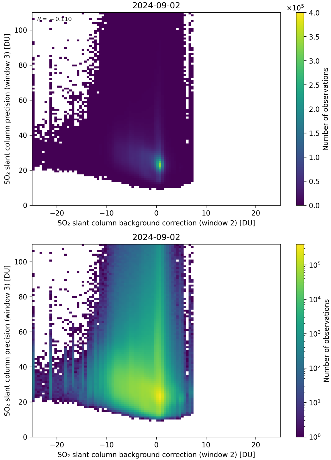
Figure 118: Scatter density plot of “SO 2 slant column background correction (window 2)” against “SO 2 slant column precision (window 3)” for 2024-09-01 to 2024-09-03.
