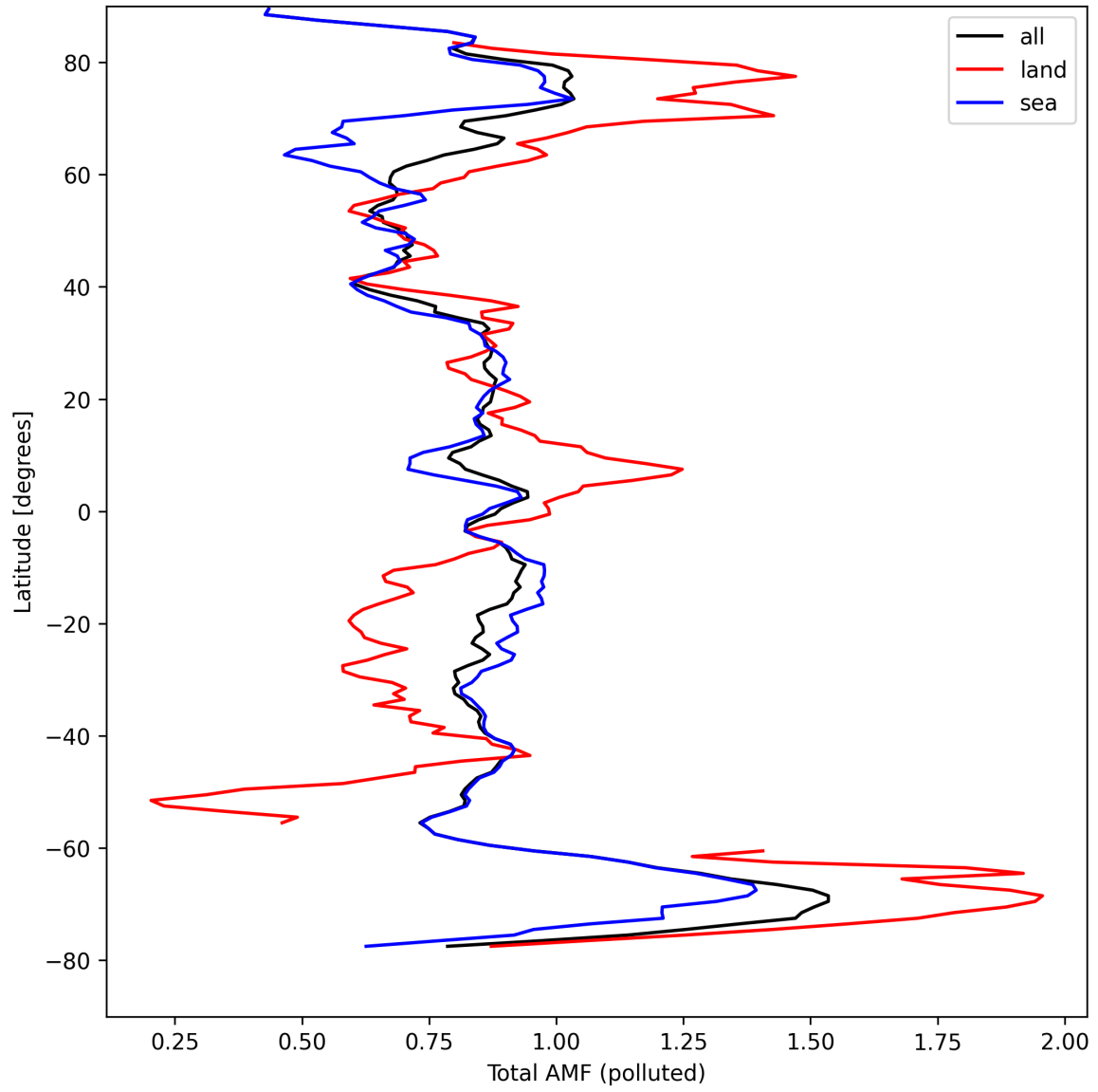
Figure 48: Zonal average of “Total AMF (polluted)” for 2024-09-01 to 2024-09-03.
