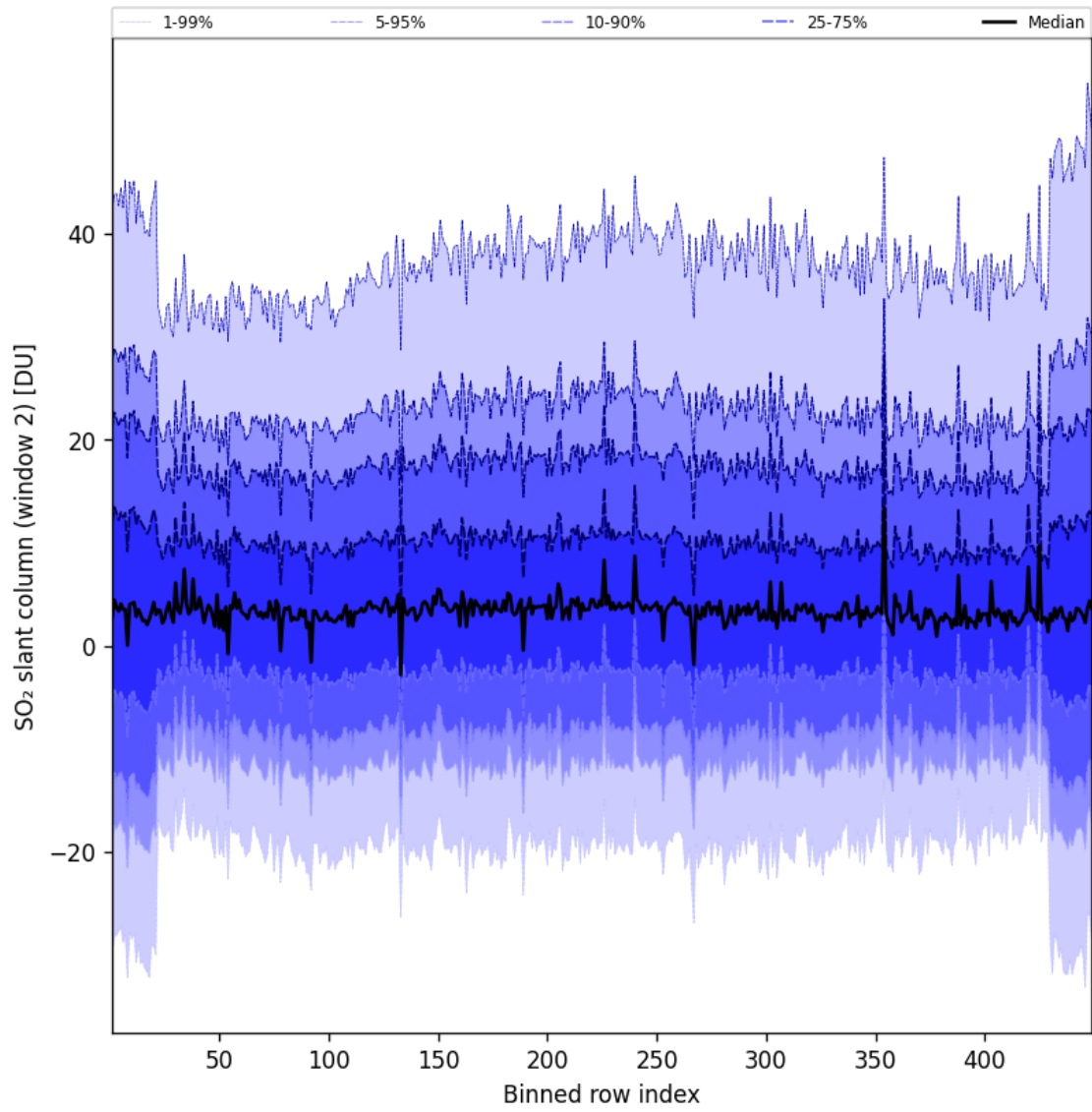
Figure 83: Along track statistics of “SO 2 slant column (window 2)” for 2024-09-01 to 2024-09-03
