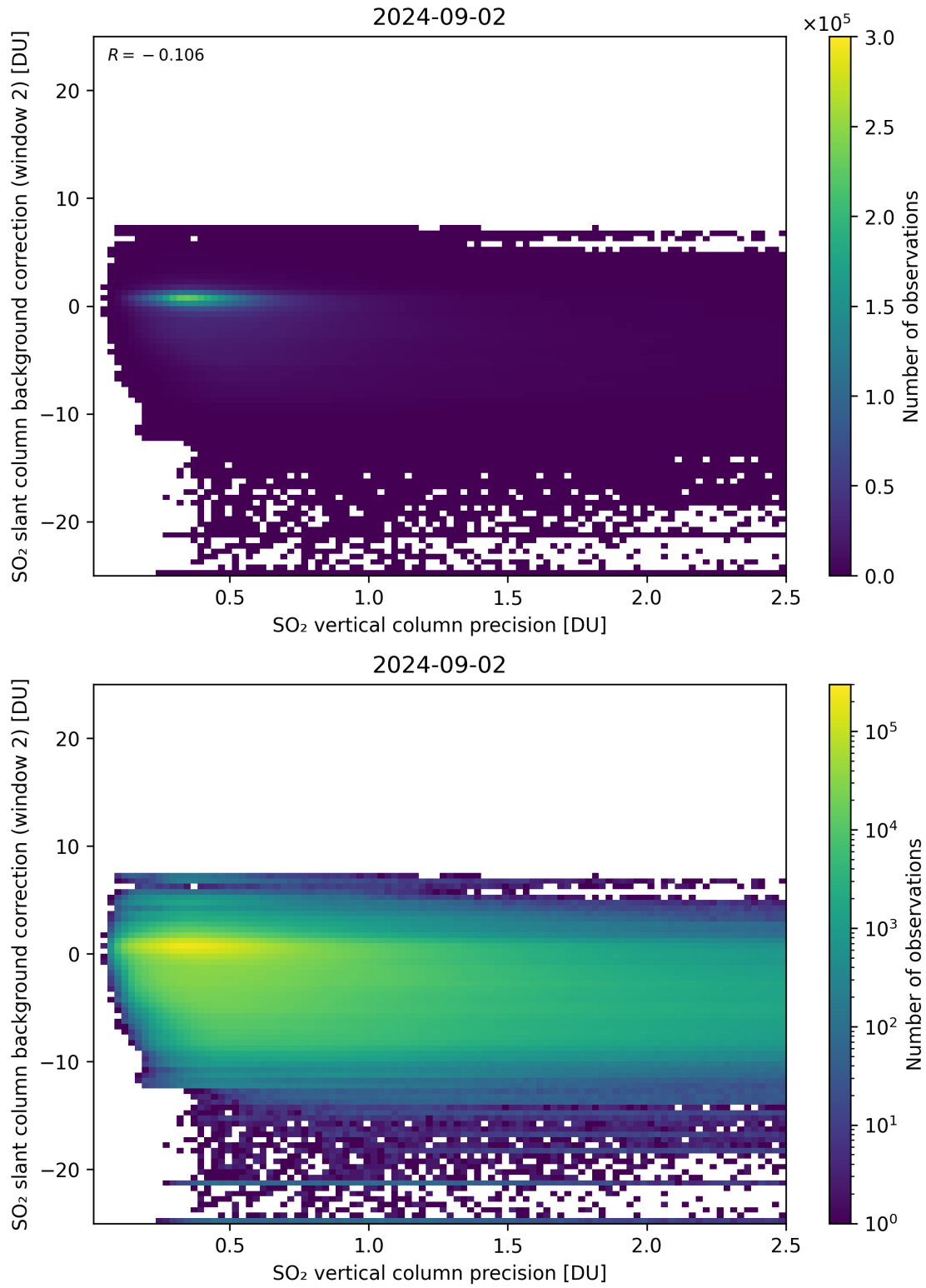
Figure 280: Scatter density plot of “SO 2 vertical column precision” against “SO 2 slant column background correction (window 2)” for 2024-09-01 to 2024-09-03.
