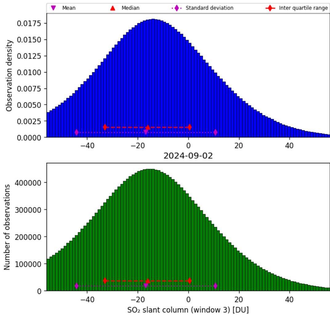
Figure 64: Histogram of “SO 2 slant column (window 3)” for 2024-09-01 to 2024-09-03
