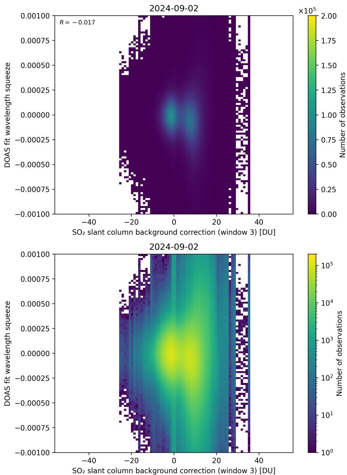
Figure 122: Scatter density plot of “SO 2 slant column background correction (window 3)” against “DOAS fit wavelength squeeze” for 2024-09-01 to 2024-09-03.
