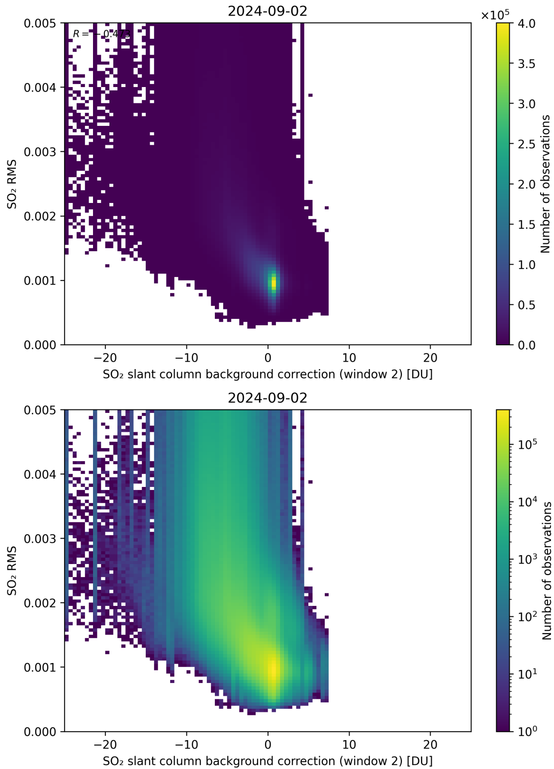
Figure 114: Scatter density plot of “SO 2 slant column background correction (window 2)” against “SO 2 RMS” for 2024-09-01 to 2024-09-03.
