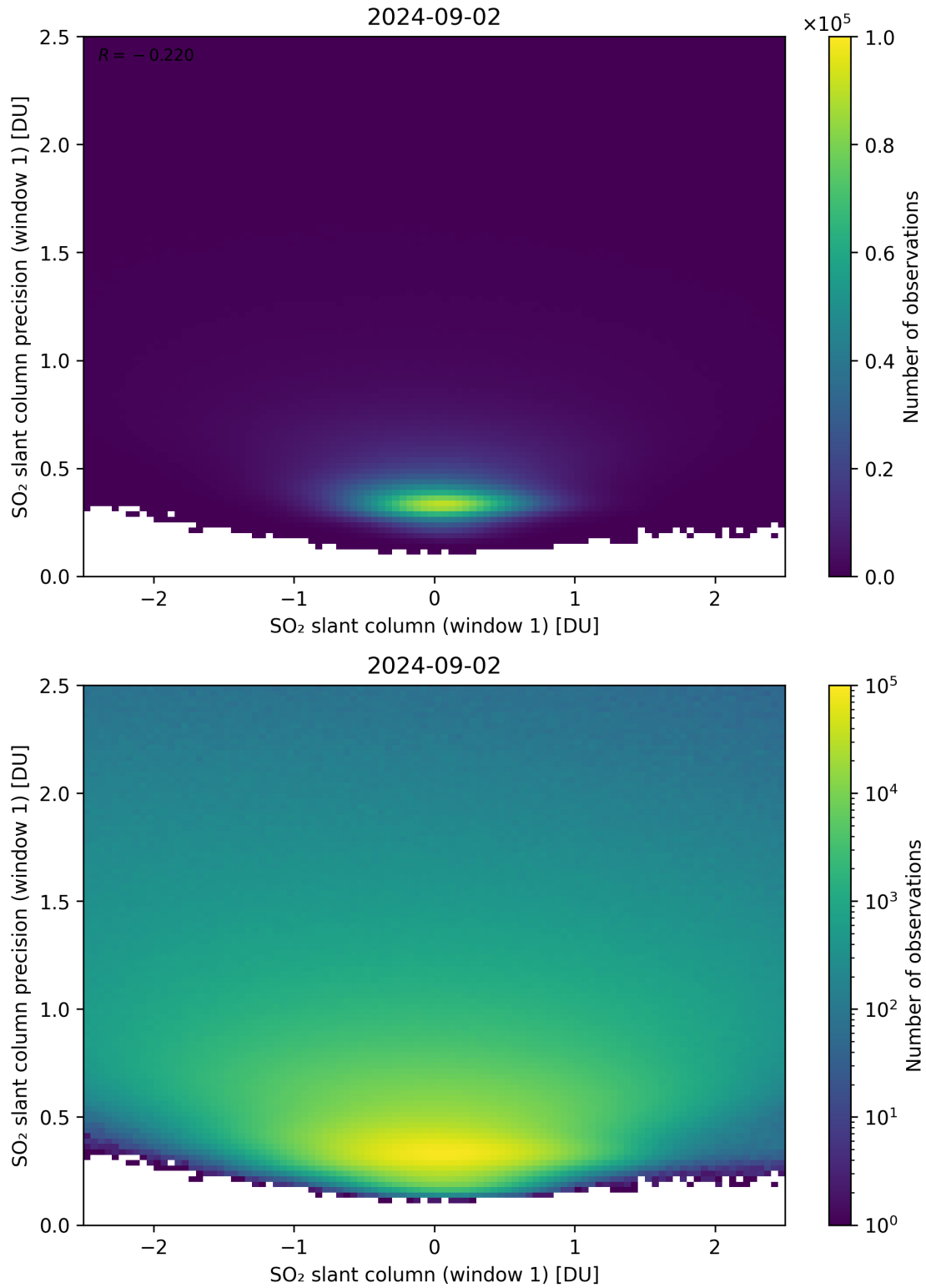
Figure 235: Scatter density plot of “SO 2 slant column (window 1)” against “SO 2 slant column precision (window 1)” for 2024-09-01 to 2024-09-03.
