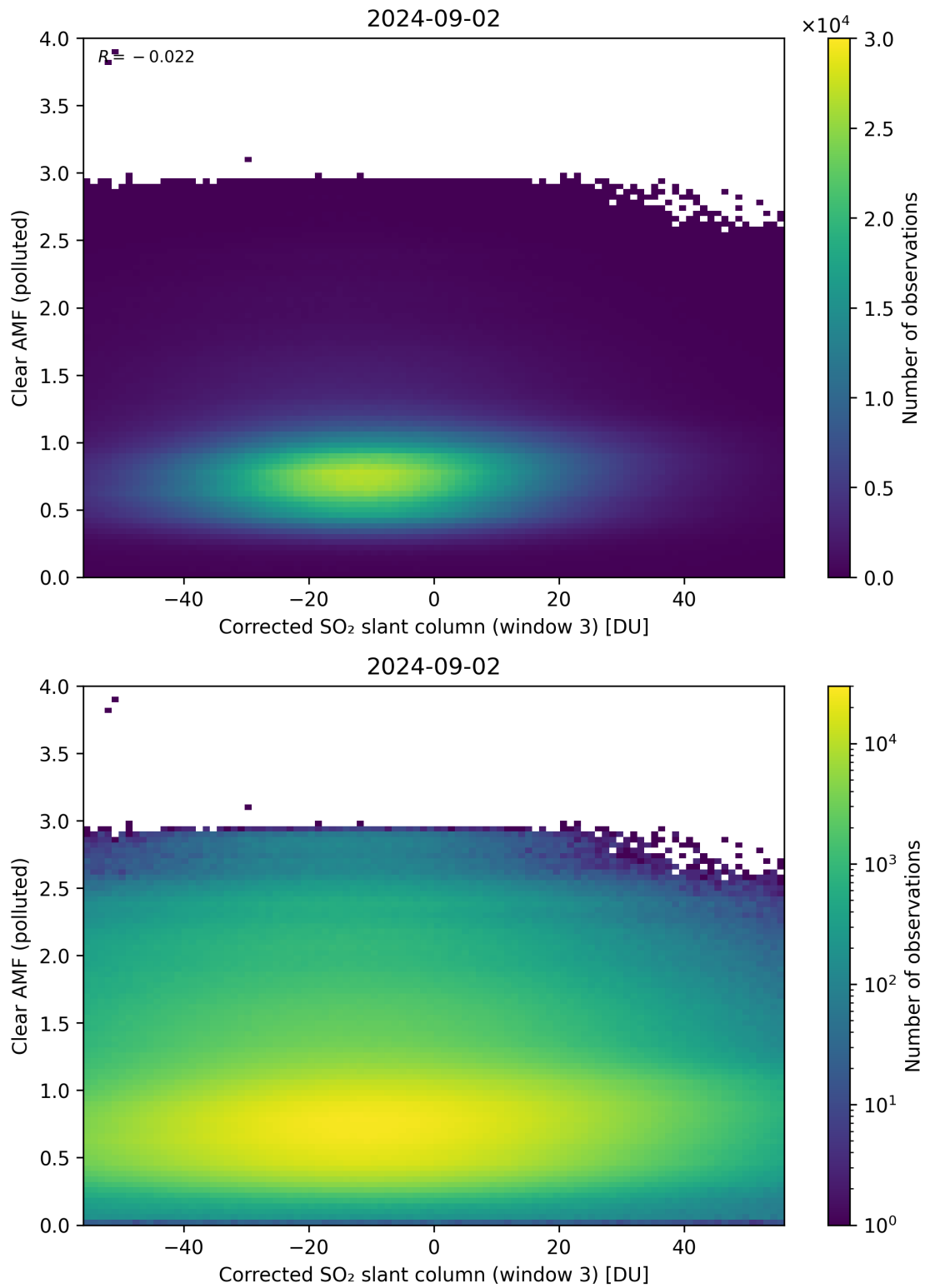
Figure 209: Scatter density plot of “Corrected SO 2 slant column (window 3)” against “Clear AMF (polluted)” for 2024-09-01 to 2024-09-03.
