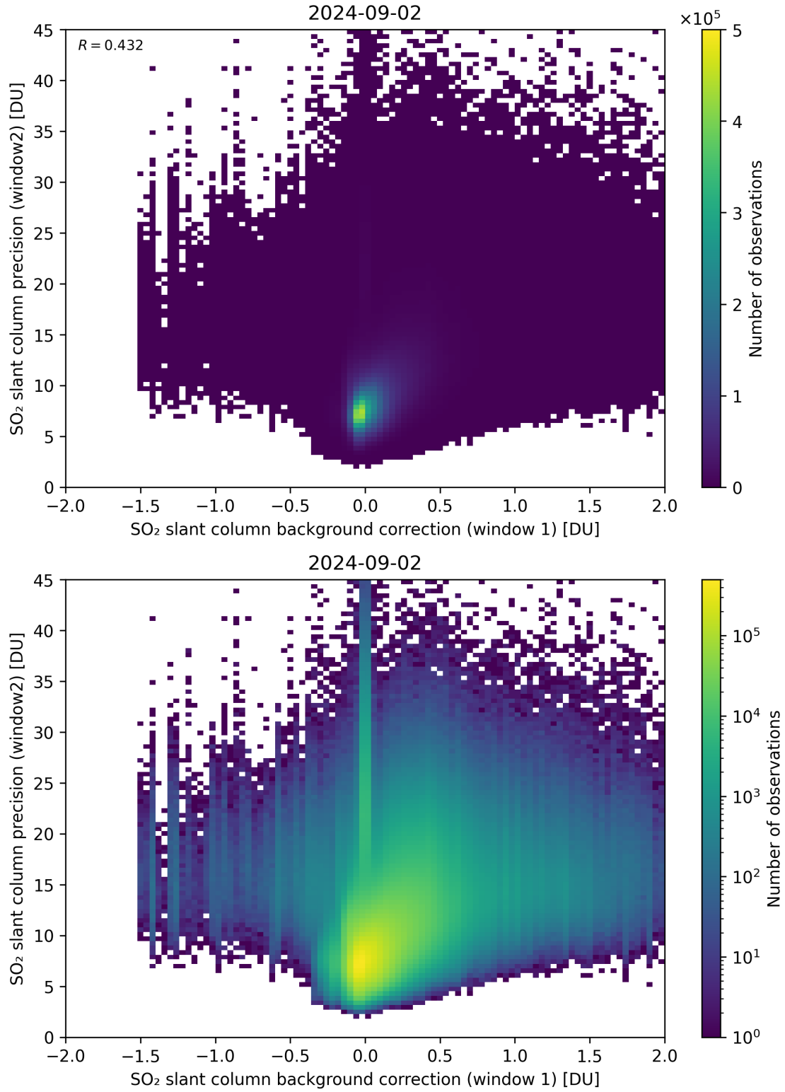
Figure 106: Scatter density plot of “SO 2 slant column background correction (window 1)” against “SO 2 slant column precision (window2)” for 2024-09-01 to 2024-09-03.
