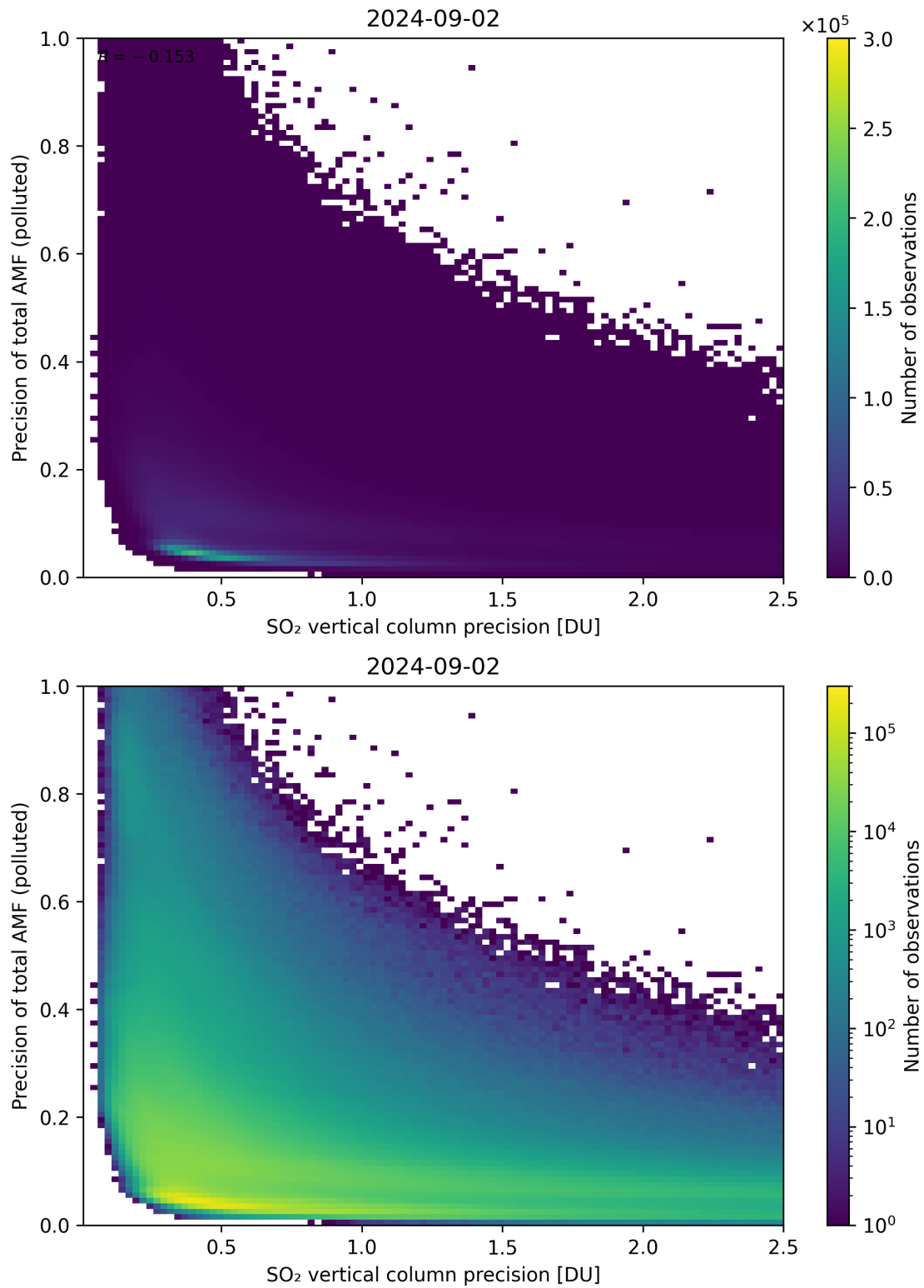
Figure 295: Scatter density plot of “SO 2 vertical column precision” against “Precision of total AMF (polluted)” for 2024-09-01 to 2024-09-03.
