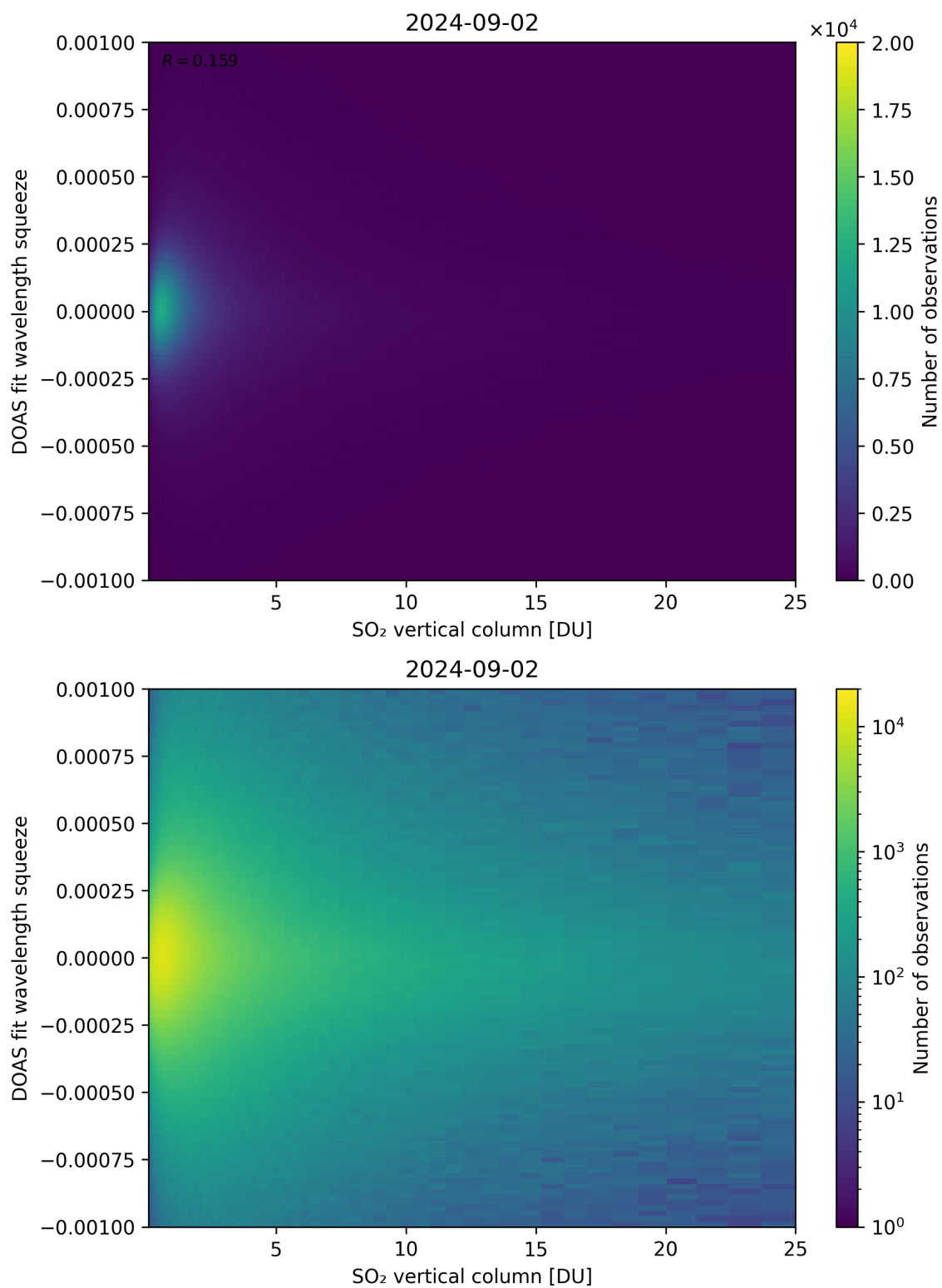
Figure 277: Scatter density plot of “SO 2 vertical column” against “DOAS fit wavelength squeeze” for 2024-09-01 to 2024-09-03.
