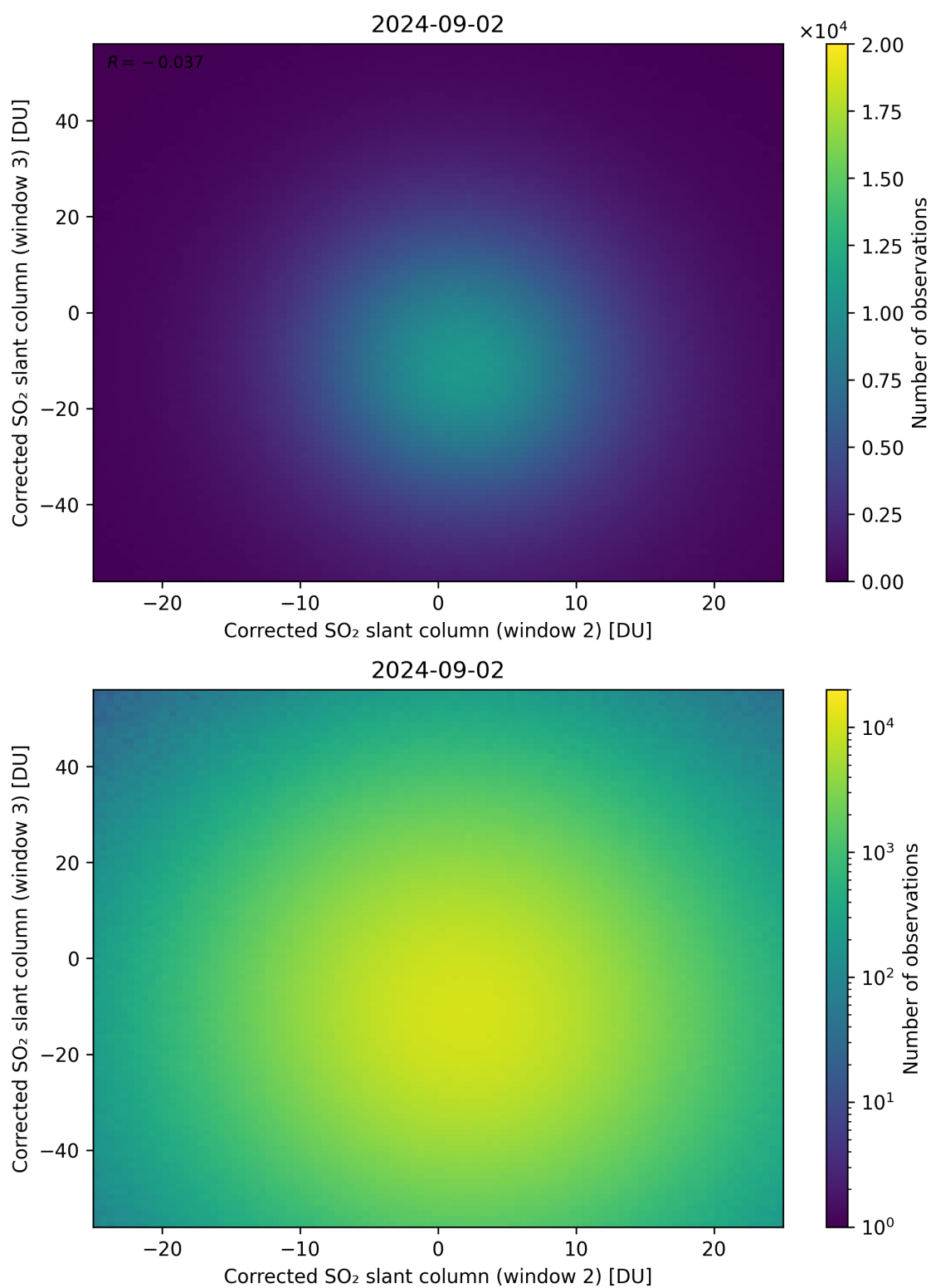
Figure 200: Scatter density plot of “Corrected SO 2 slant column (window 2)” against “Corrected SO 2 slant column (window 3)” for 2024-09-01 to 2024-09-03.
