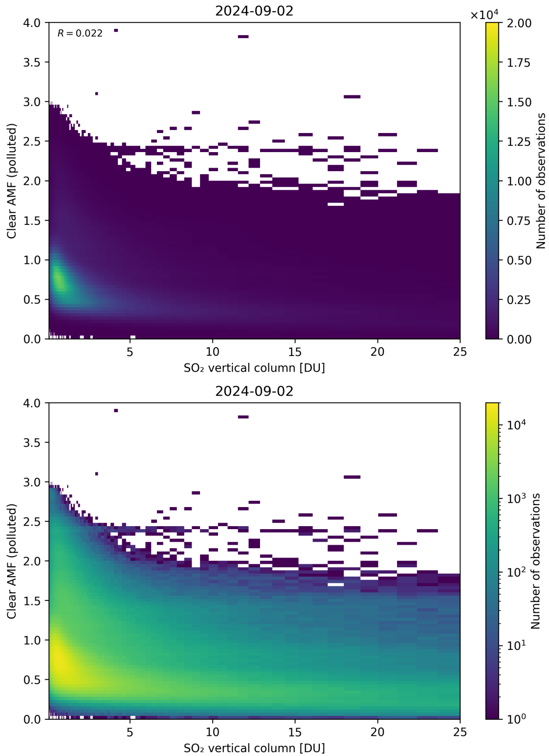
Figure 296: Scatter density plot of “SO 2 vertical column” against “Clear AMF (polluted)” for 2024-09-01 to 2024-09-03.
