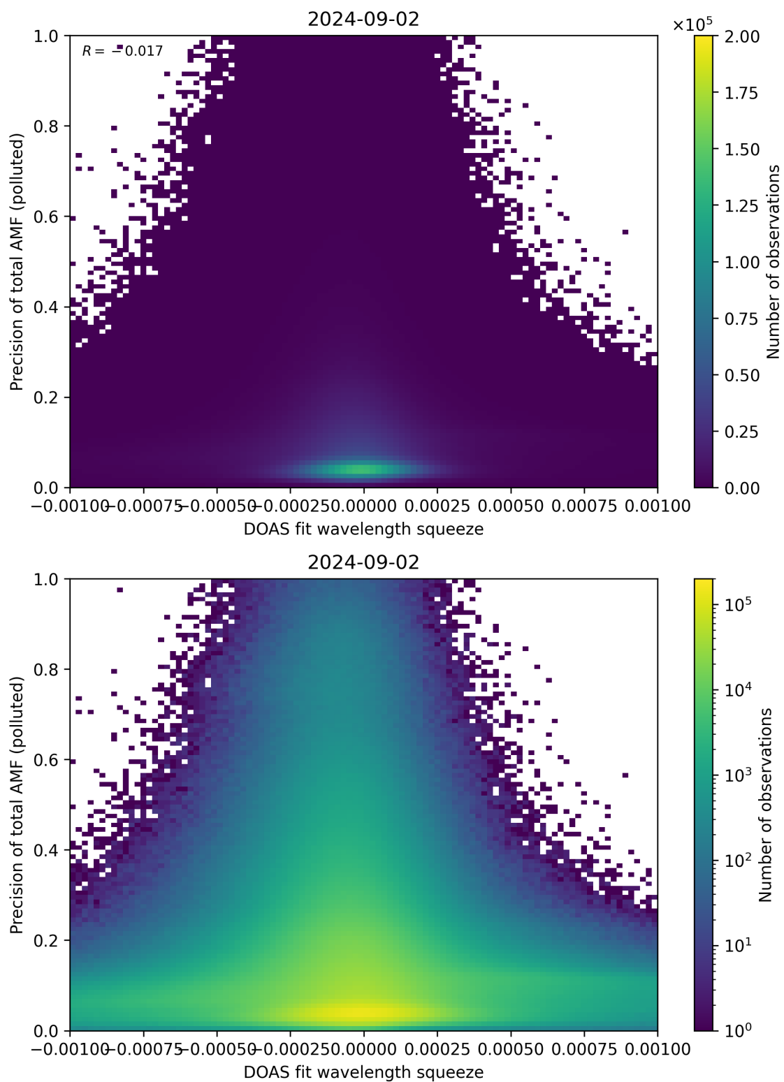
Figure 135: Scatter density plot of “DOAS fit wavelength squeeze” against “Precision of total AMF (polluted)” for 2024-09-01 to 2024-09-03.
