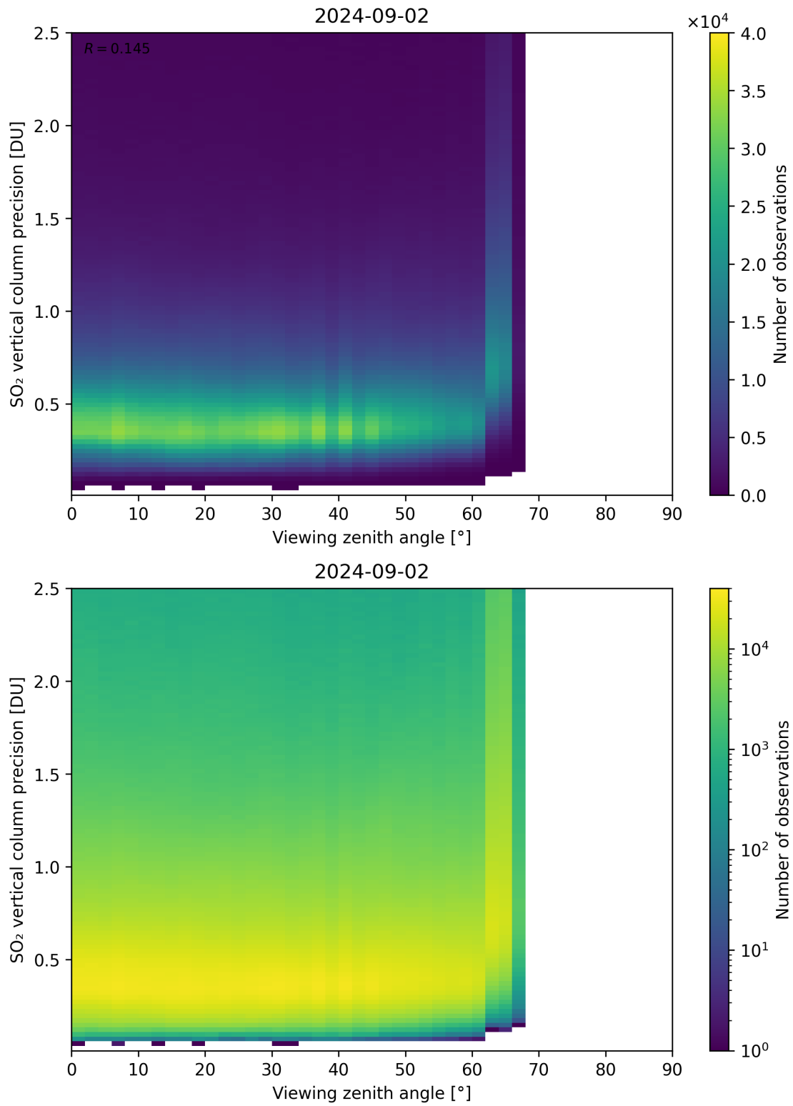
Figure 328: Scatter density plot of “Viewing zenith angle” against “SO 2 vertical column precision” for 2024-09-01 to 2024-09-03.
