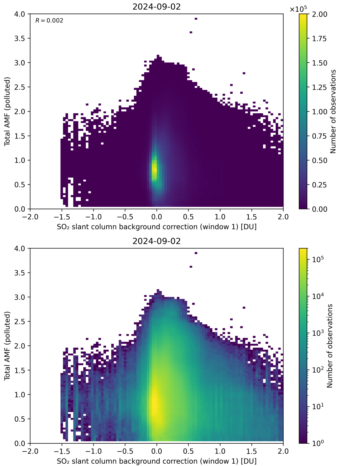
Figure 109: Scatter density plot of “SO 2 slant column background correction (window 1)” against “Total AMF (polluted)” for 2024-09-01 to 2024-09-03.
