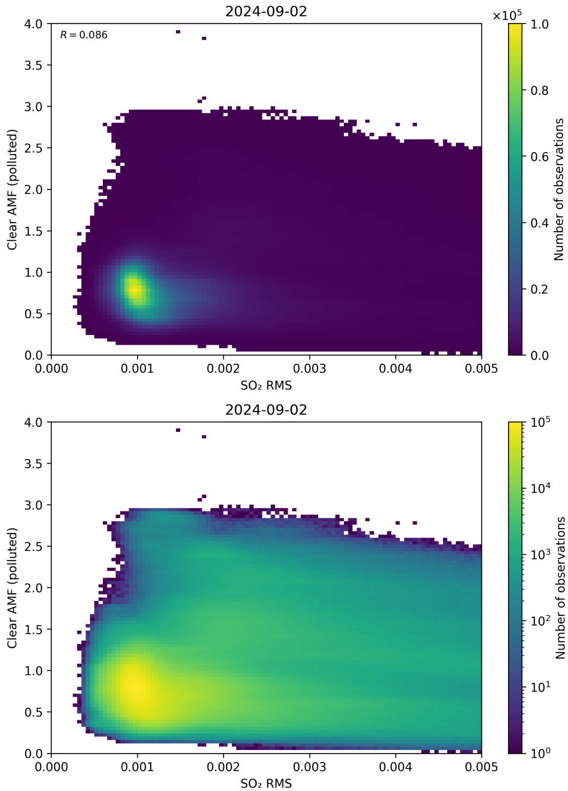
Figure 136: Scatter density plot of “SO 2 RMS” against “Clear AMF (polluted)” for 2024-09-01 to 2024-09-03.
