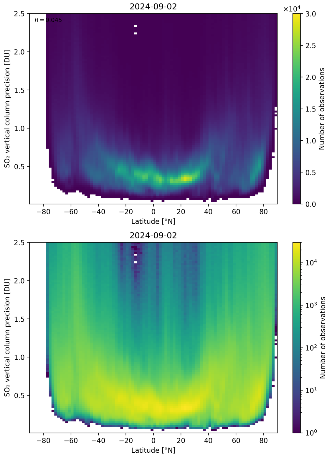
Figure 157: Scatter density plot of “Latitude” against “SO 2 vertical column precision” for 2024-09-01 to 2024-09-03.
