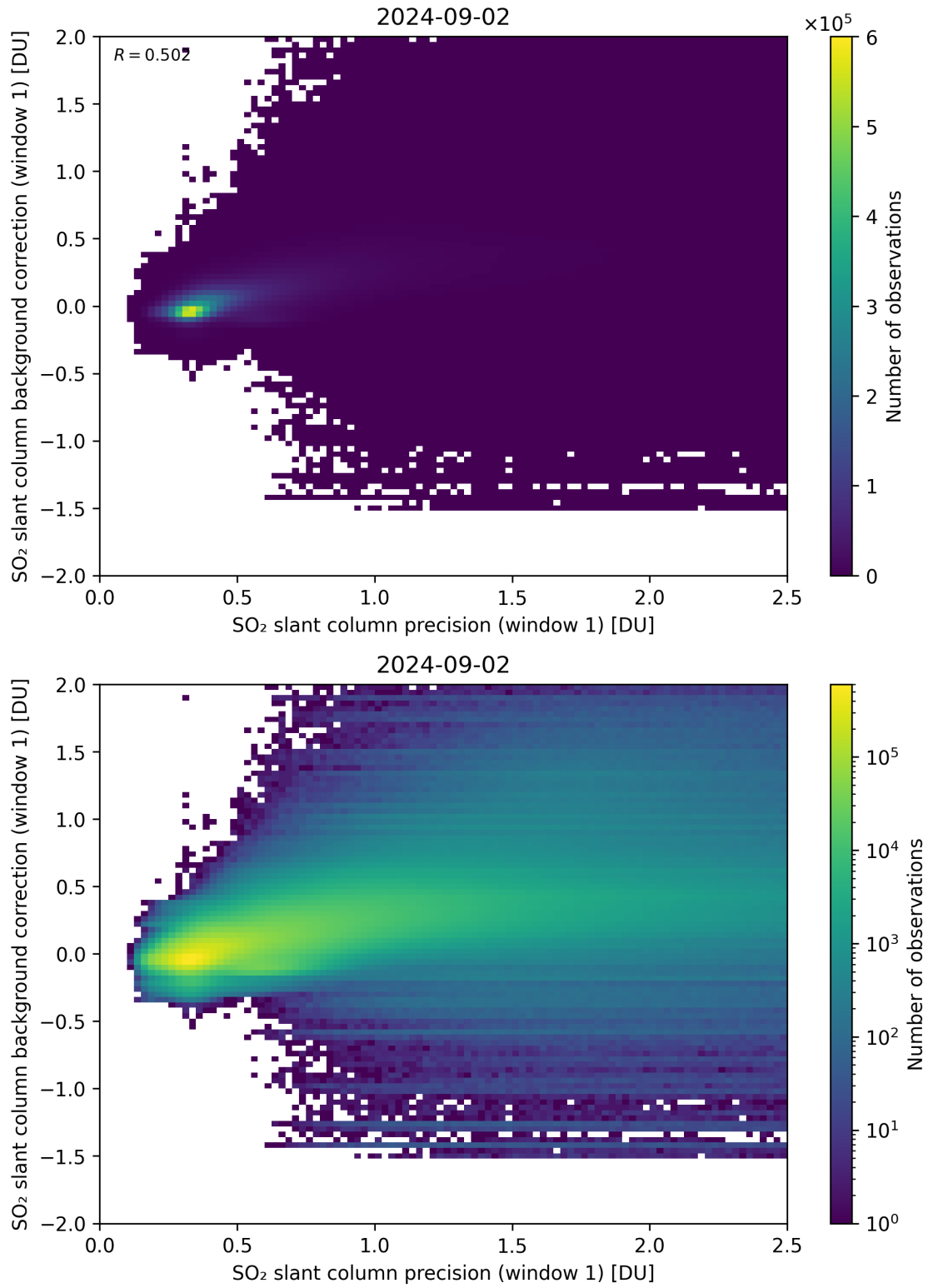
Figure 218: Scatter density plot of “SO 2 slant column precision (window 1)” against “SO 2 slant column background correction (window 1)” for 2024-09-01 to 2024-09-03.
