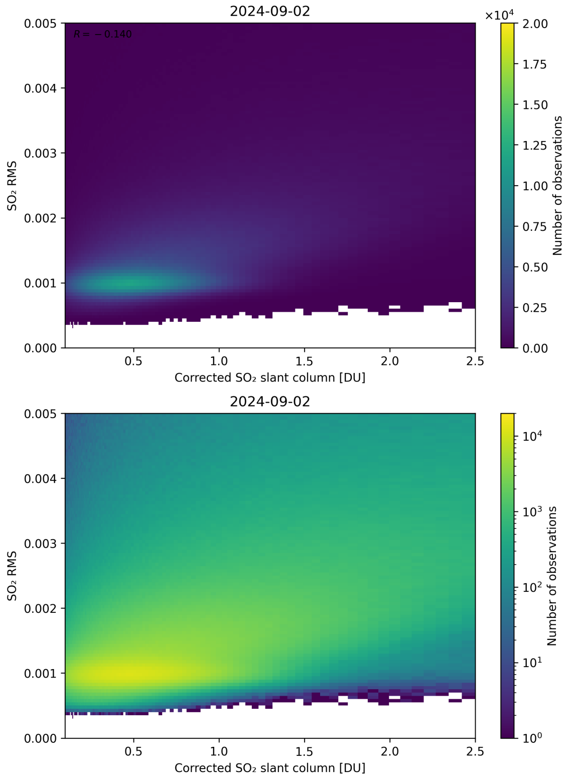
Figure 183: Scatter density plot of “Corrected SO 2 slant column” against “SO 2 RMS” for 2024-09-01 to 2024-09-03.
