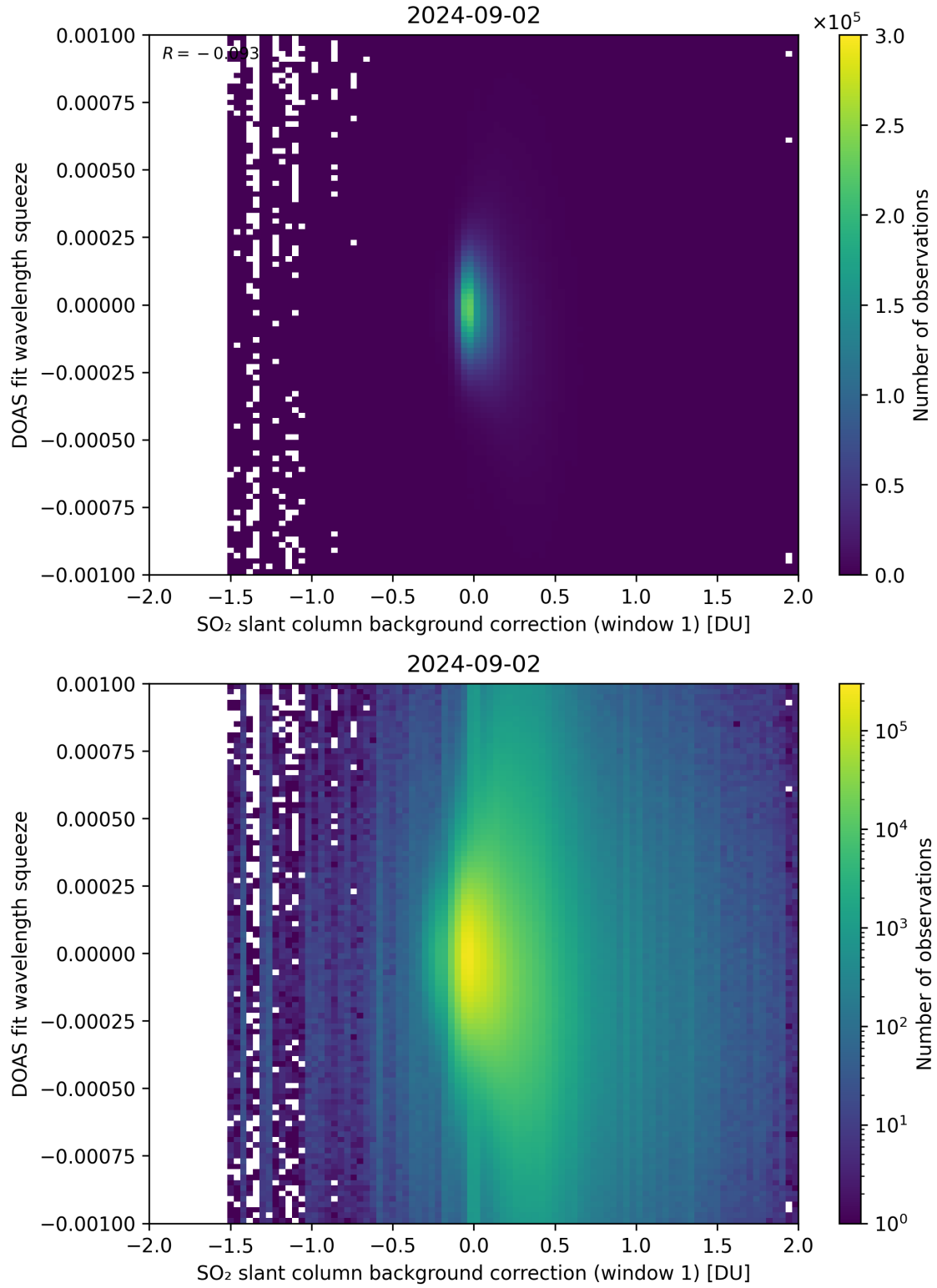
Figure 101: Scatter density plot of “SO 2 slant column background correction (window 1)” against “DOAS fit wavelength squeeze” for 2024-09-01 to 2024-09-03.
