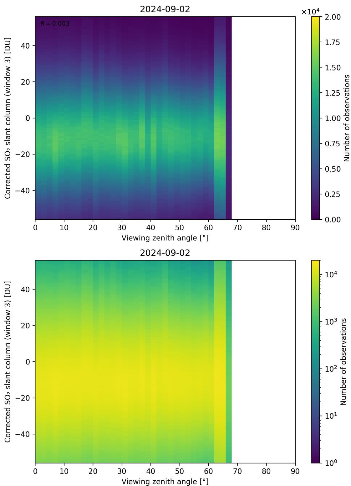
Figure 319: Scatter density plot of “Viewing zenith angle” against “Corrected SO 2 slant column (window 3)” for 2024-09-01 to 2024-09-03.
