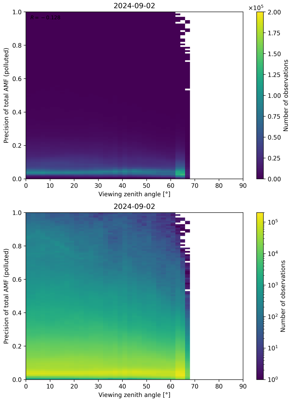
Figure 326: Scatter density plot of “Viewing zenith angle” against “Precision of total AMF (polluted)” for 2024-09-01 to 2024-09-03.
