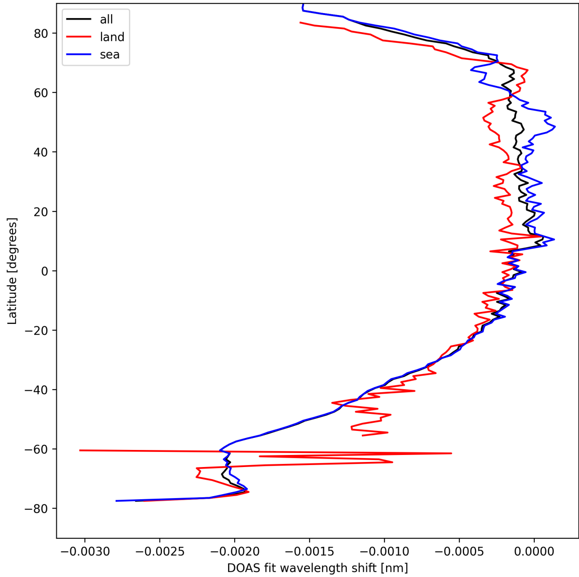
Figure 45: Zonal average of "DOAS fit wavelength shift" for 2024-09-01 to 2024-09-03.
