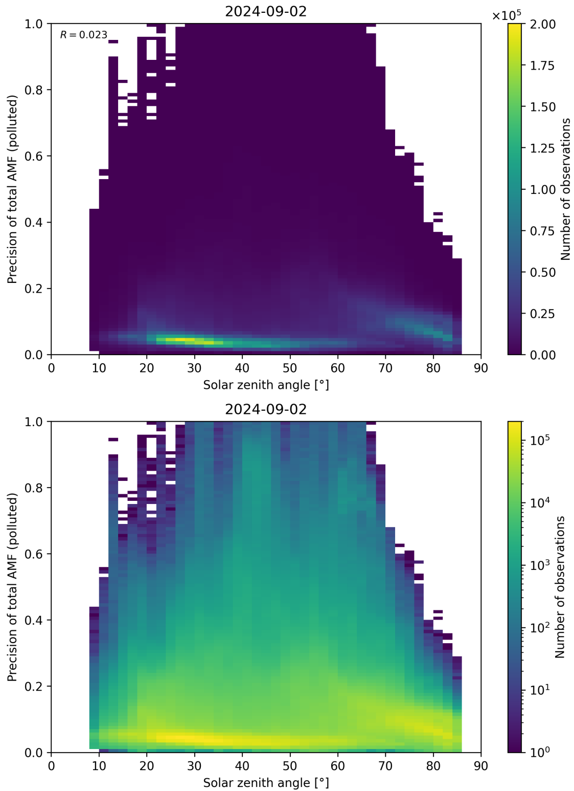
Figure 175: Scatter density plot of “Solar zenith angle” against “Precision of total AMF (polluted)” for 2024-09-01 to 2024-09-03.
