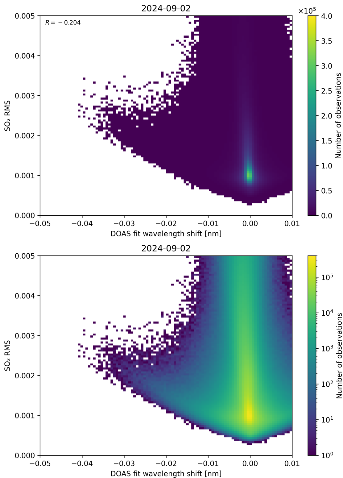
Figure 128: Scatter density plot of “DOAS fit wavelength shift” against “SO 2 RMS” for 2024-09-01 to 2024-09-03.
