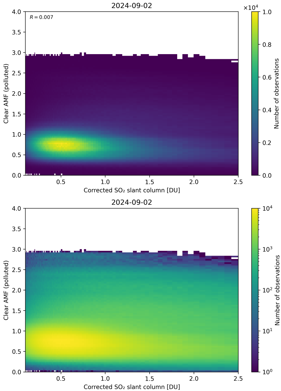
Figure 184: Scatter density plot of “Corrected SO 2 slant column” against “Clear AMF (polluted)” for 2024-09-01 to 2024-09-03.
