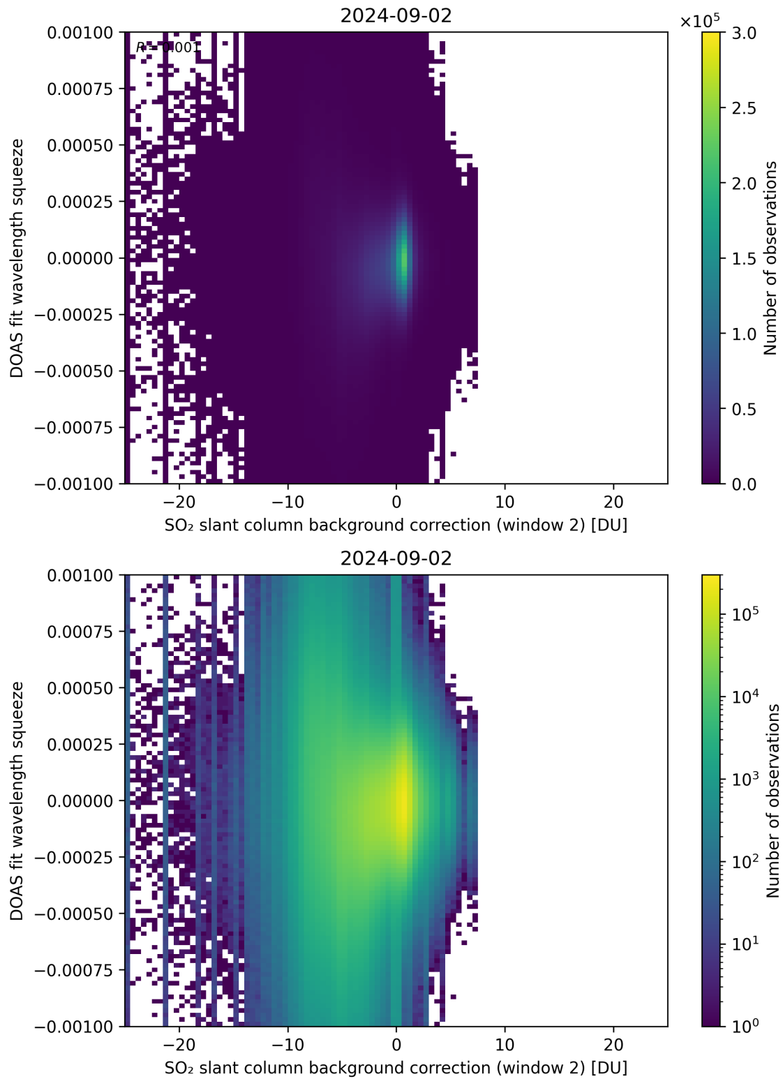
Figure 113: Scatter density plot of “SO 2 slant column background correction (window 2)” against “DOAS fit wavelength squeeze” for 2024-09-01 to 2024-09-03.
