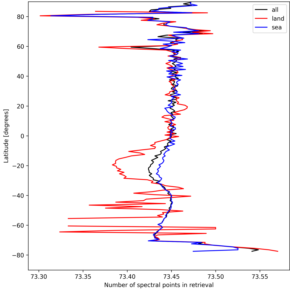
Figure 51: Zonal average of “Number of spectral points in retrieval” for 2024-09-01 to 2024-09-03.
