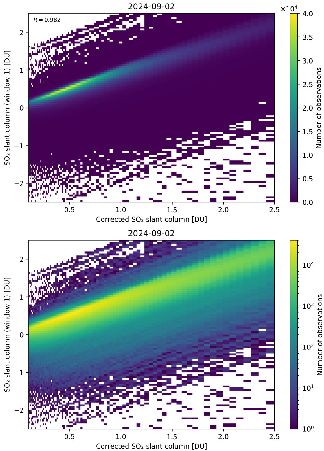
Figure 187: Scatter density plot of “Corrected SO 2 slant column” against “SO 2 slant column (window 1)” for 2024-09-01 to 2024-09-03.
