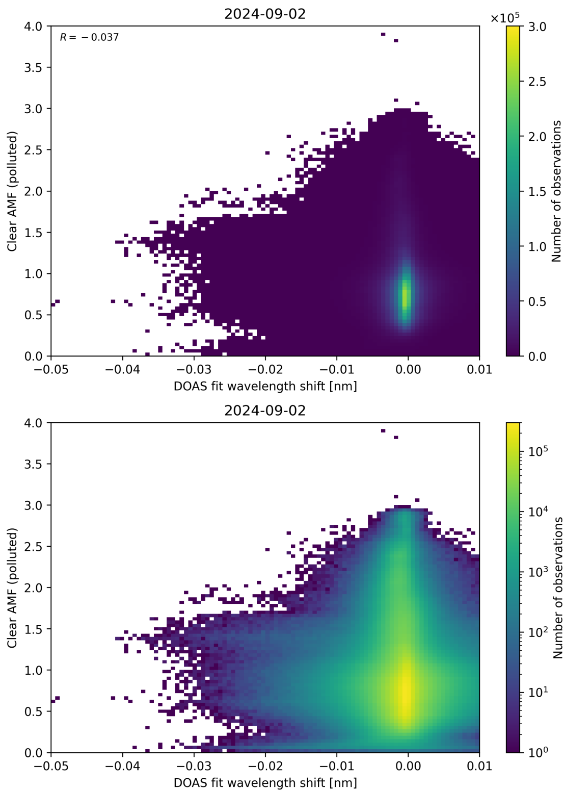
Figure 129: Scatter density plot of “DOAS fit wavelength shift” against “Clear AMF (polluted)” for 2024-09-01 to 2024-09-03.
