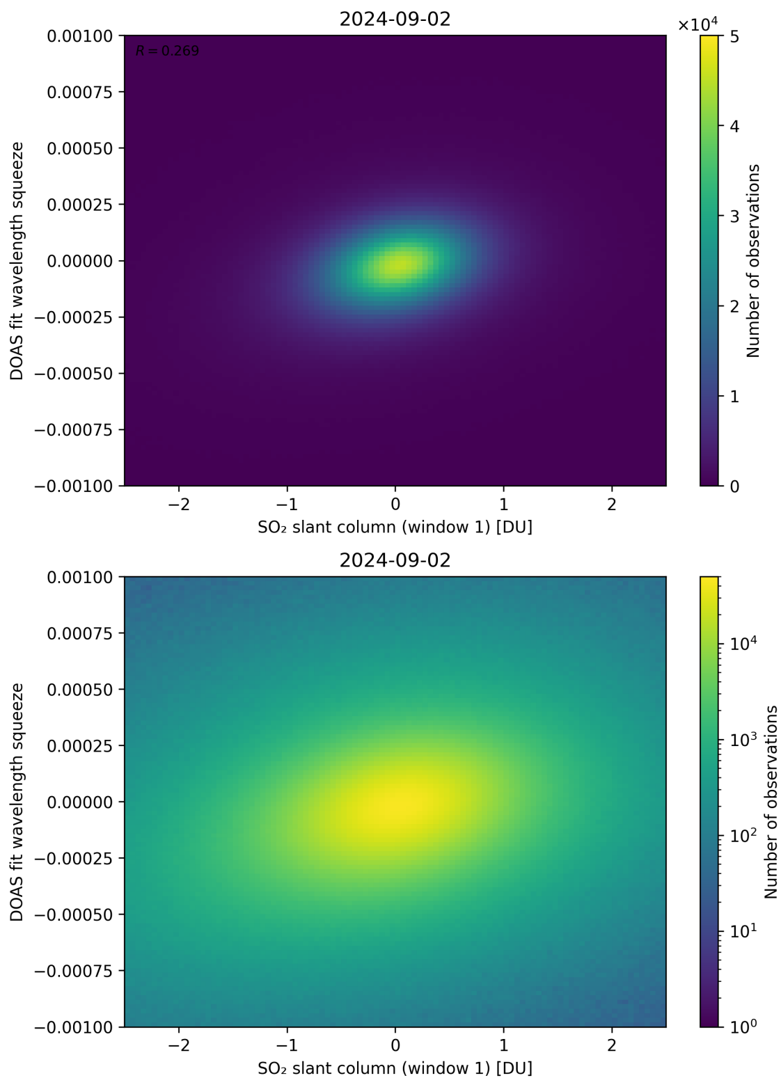
Figure 216: Scatter density plot of “SO 2 slant column (window 1)” against “DOAS fit wavelength squeeze” for 2024-09-01 to 2024-09-03.
