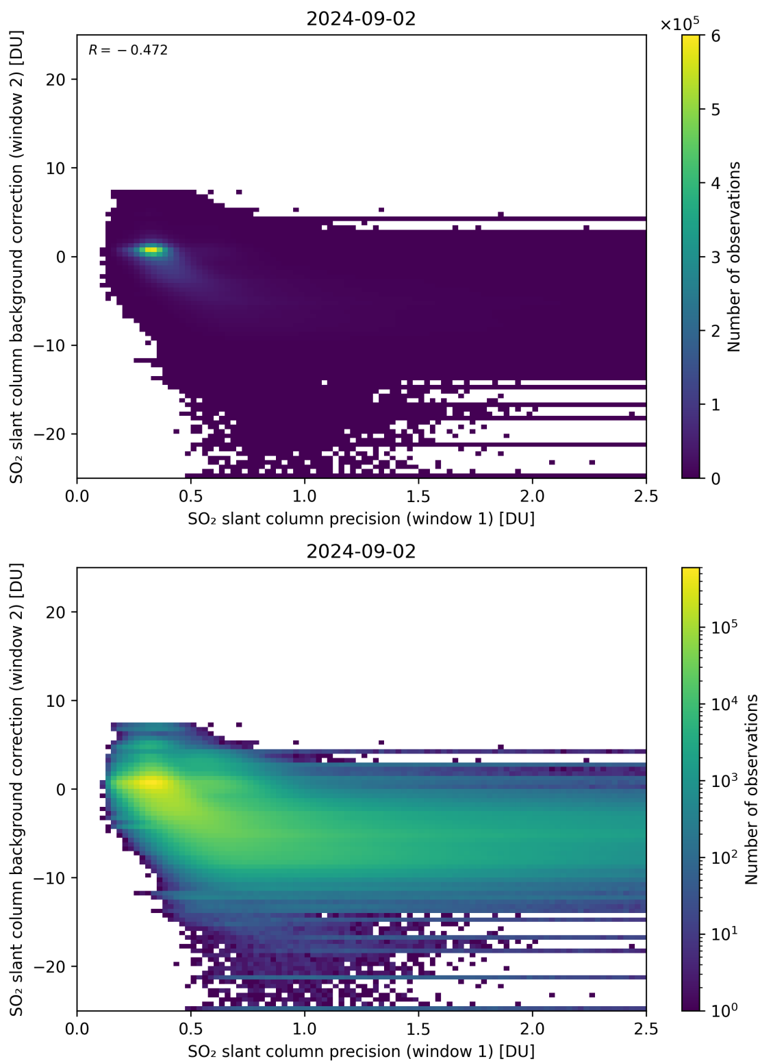
Figure 219: Scatter density plot of “SO 2 slant column precision (window 1)” against “SO 2 slant column background correction (window 2)” for 2024-09-01 to 2024-09-03.
