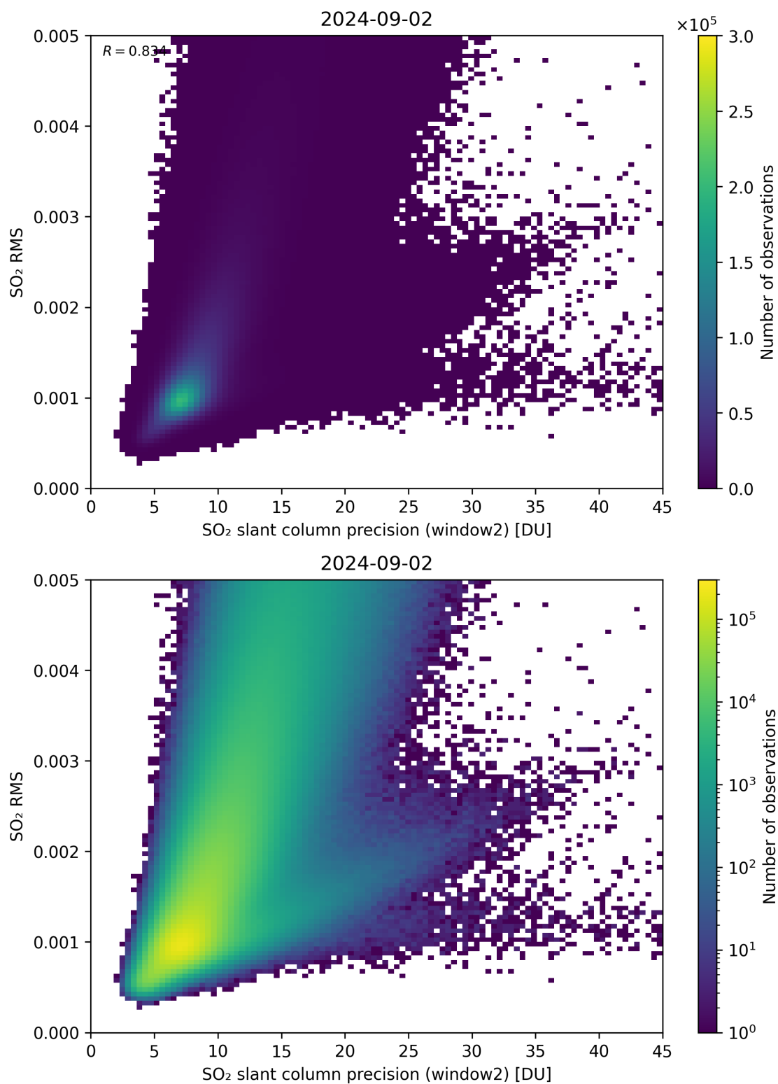
Figure 245: Scatter density plot of “SO 2 slant column precision (window2)” against “SO 2 RMS” for 2024-09-01 to 2024-09-03.
