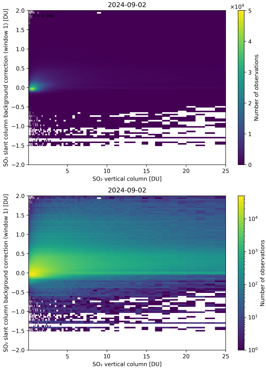
Figure 273: Scatter density plot of “SO 2 vertical column” against “SO 2 slant column background correction (window 1)” for 2024-09-01 to 2024-09-03.
