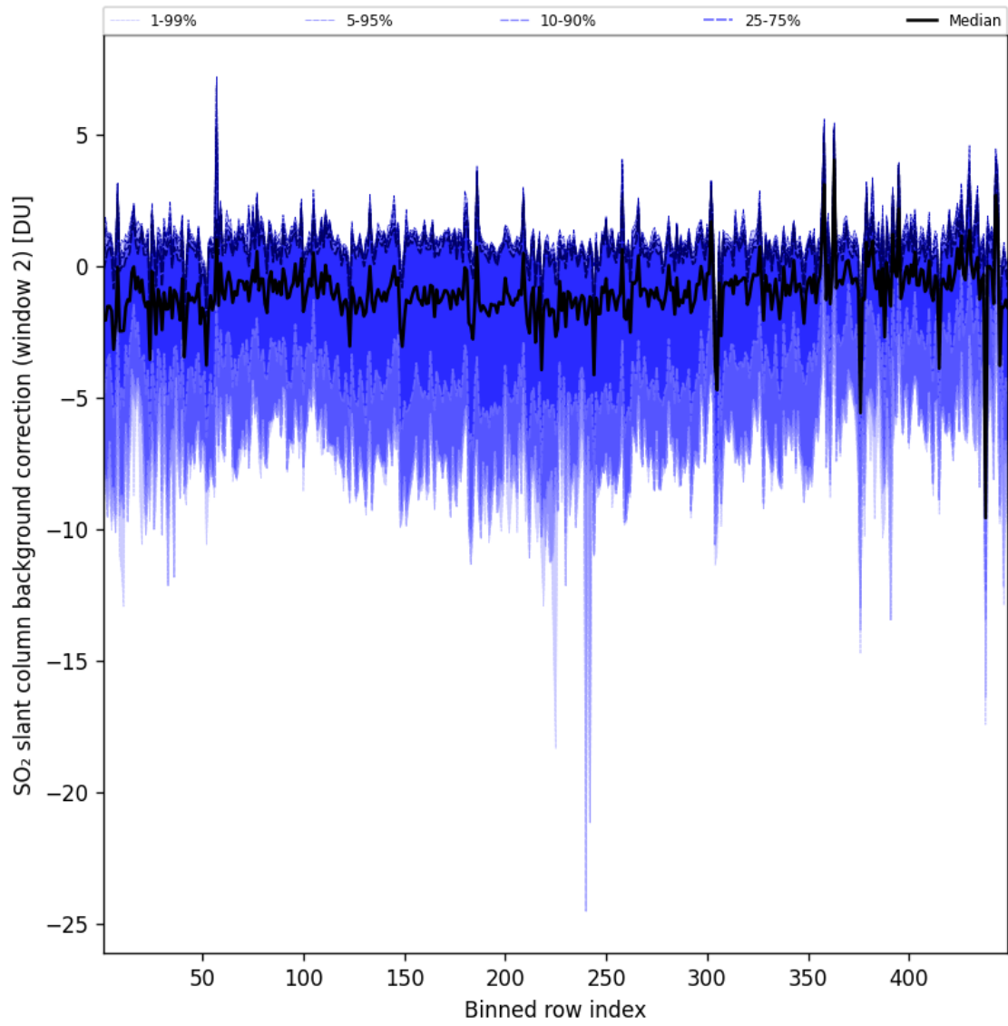
Figure 86: Along track statistics of “SO 2 slant column background correction (window 2)” for 2024-09-01 to 2024-09-03
