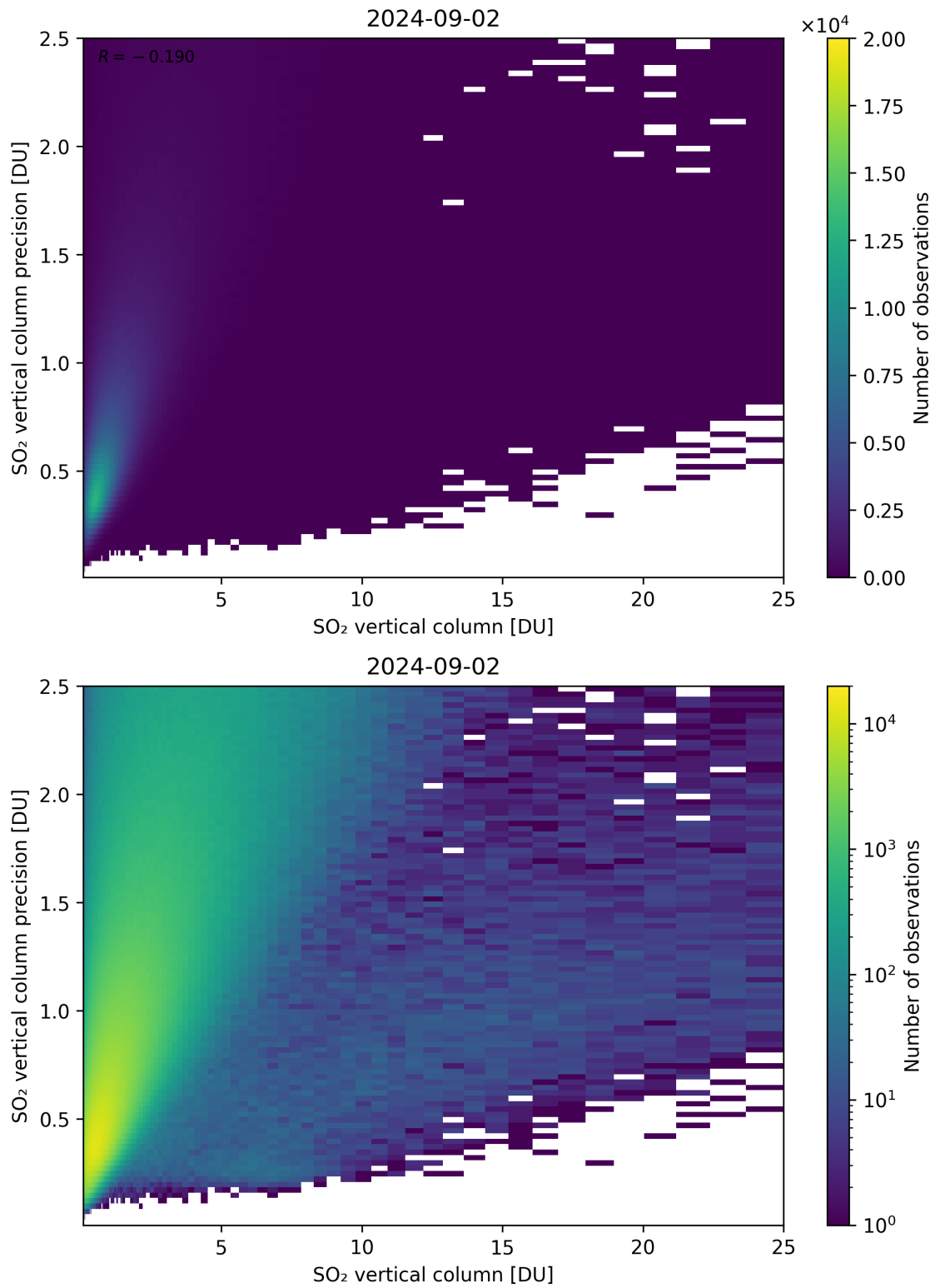
Figure 307: Scatter density plot of “SO 2 vertical column” against “SO 2 vertical column precision” for 2024-09-01 to 2024-09-03.
