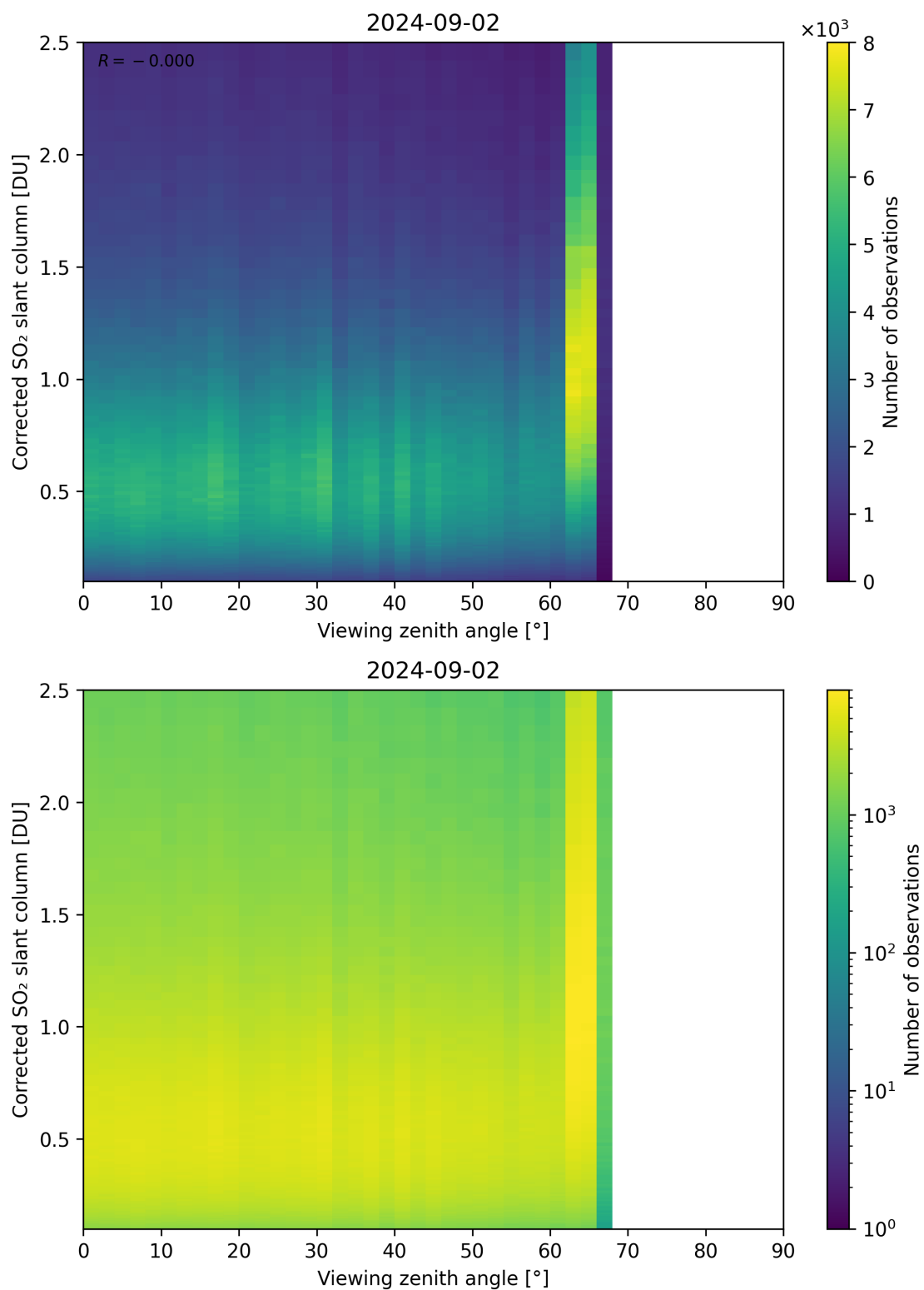
Figure 317: Scatter density plot of “Viewing zenith angle” against “Corrected SO 2 slant column” for 2024-09-01 to 2024-09-03.
