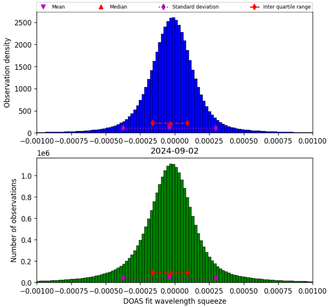
Figure 69: Histogram of “DOAS fit wavelength squeeze” for 2024-09-01 to 2024-09-03
