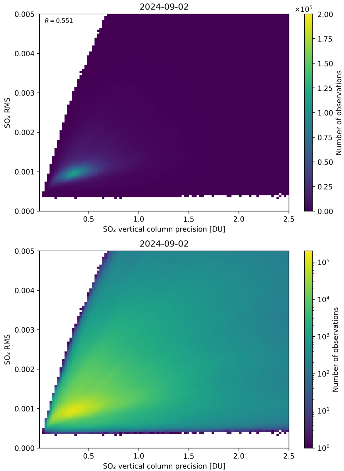
Figure 284: Scatter density plot of “SO 2 vertical column precision” against “SO 2 RMS” for 2024-09-01 to 2024-09-03.
