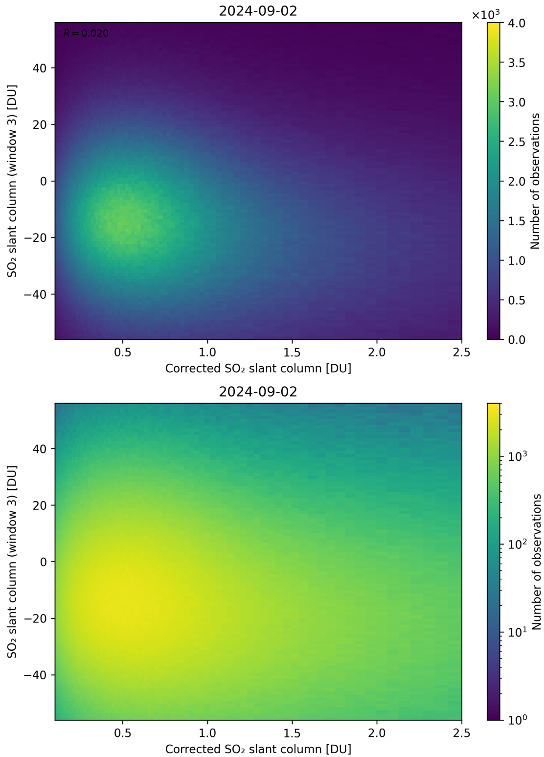
Figure 190: Scatter density plot of “Corrected SO 2 slant column” against “SO 2 slant column (window 3)” for 2024-09-01 to 2024-09-03.
