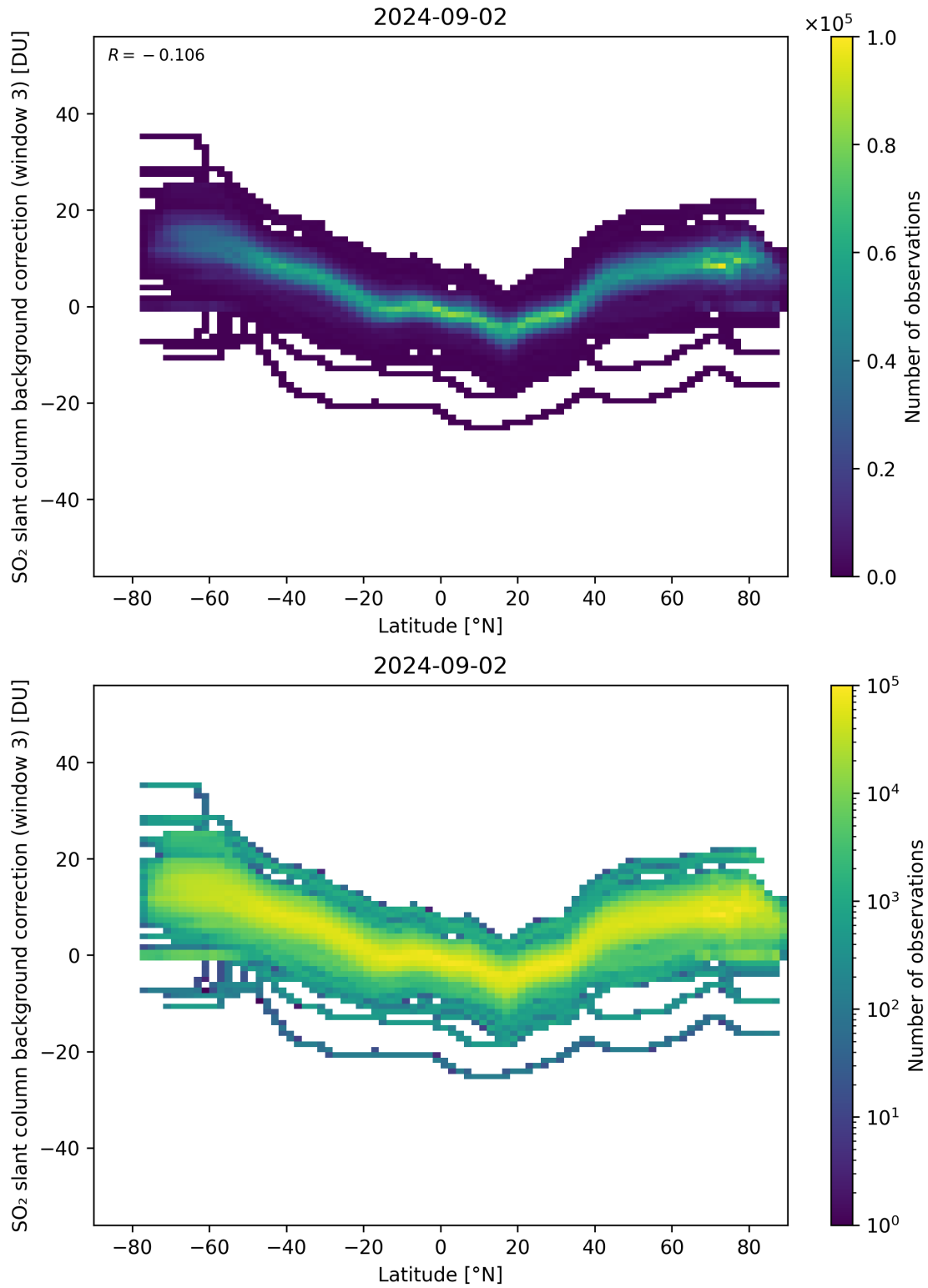
Figure 141: Scatter density plot of “Latitude” against “SO 2 slant column background correction (window 3)” for 2024-09-01 to 2024-09-03.
