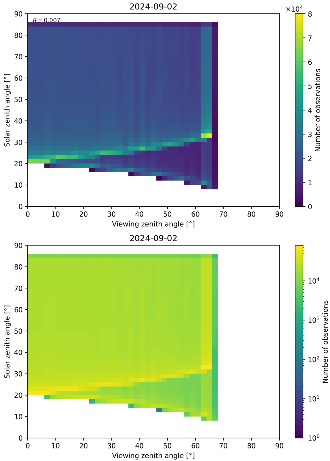
Figure 315: Scatter density plot of “Viewing zenith angle” against “Solar zenith angle” for 2024-09-01 to 2024-09-03.
