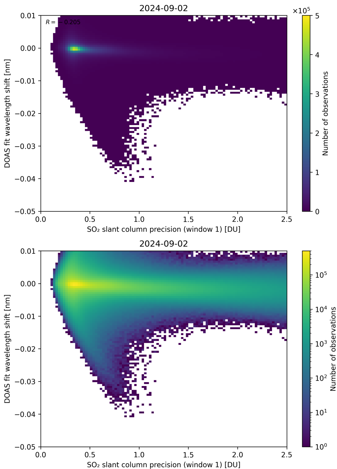
Figure 221: Scatter density plot of “SO 2 slant column precision (window 1)” against “DOAS fit wavelength shift” for 2024-09-01 to 2024-09-03.
