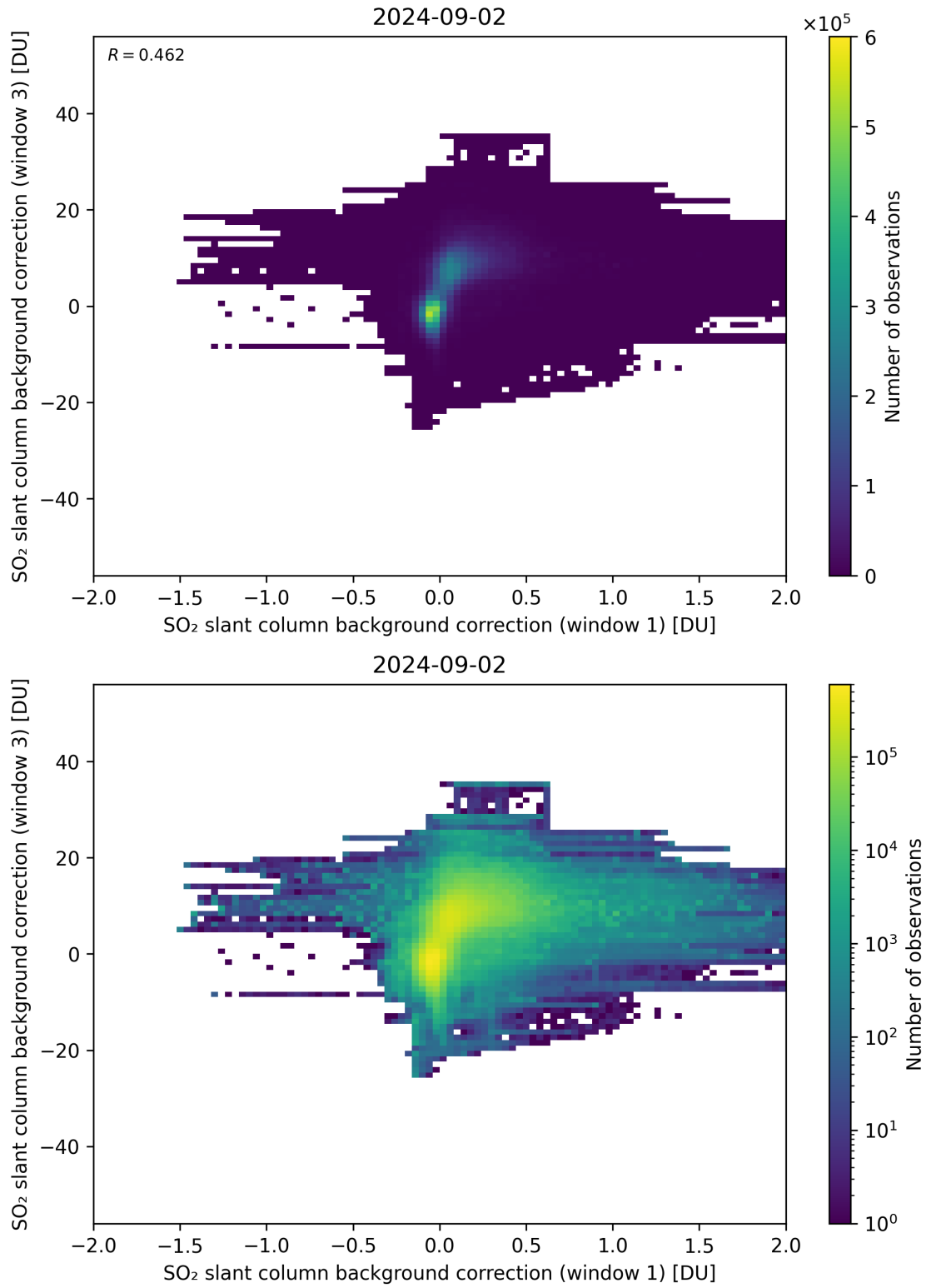
Figure 99: Scatter density plot of “SO 2 slant column background correction (window 1)” against “SO 2 slant column background correction (window 3)” for 2024-09-01 to 2024-09-03.
