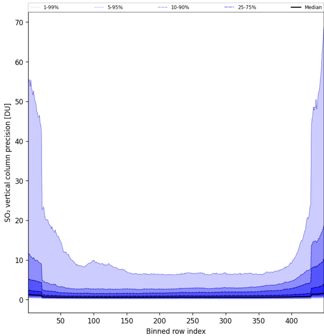
Figure 77: Along track statistics of “SO 2 vertical column precision” for 2024-09-01 to 2024-09-03
