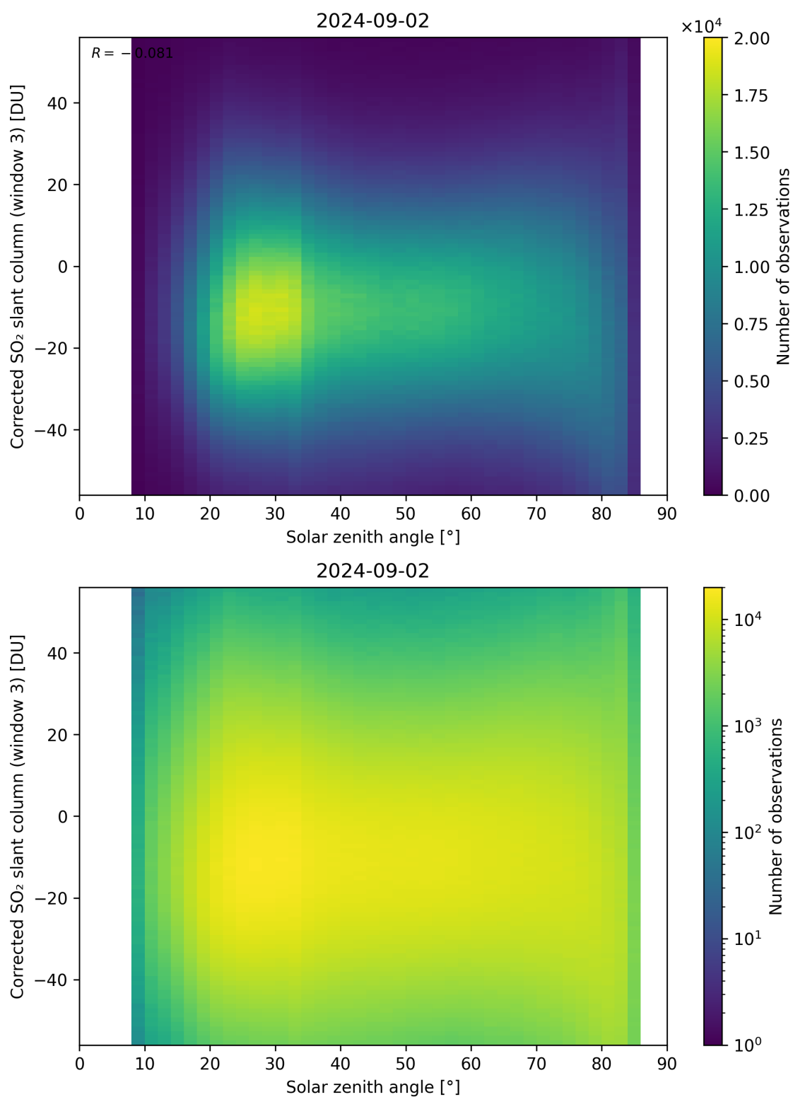
Figure 168: Scatter density plot of “Solar zenith angle” against “Corrected SO 2 slant column (window 3)” for 2024-09-01 to 2024-09-03.
