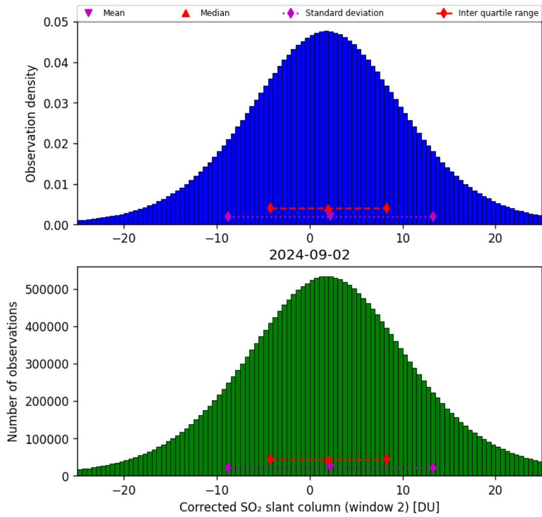
Figure 62: Histogram of “Corrected SO 2 slant column (window 2)” for 2024-09-01 to 2024-09-03
