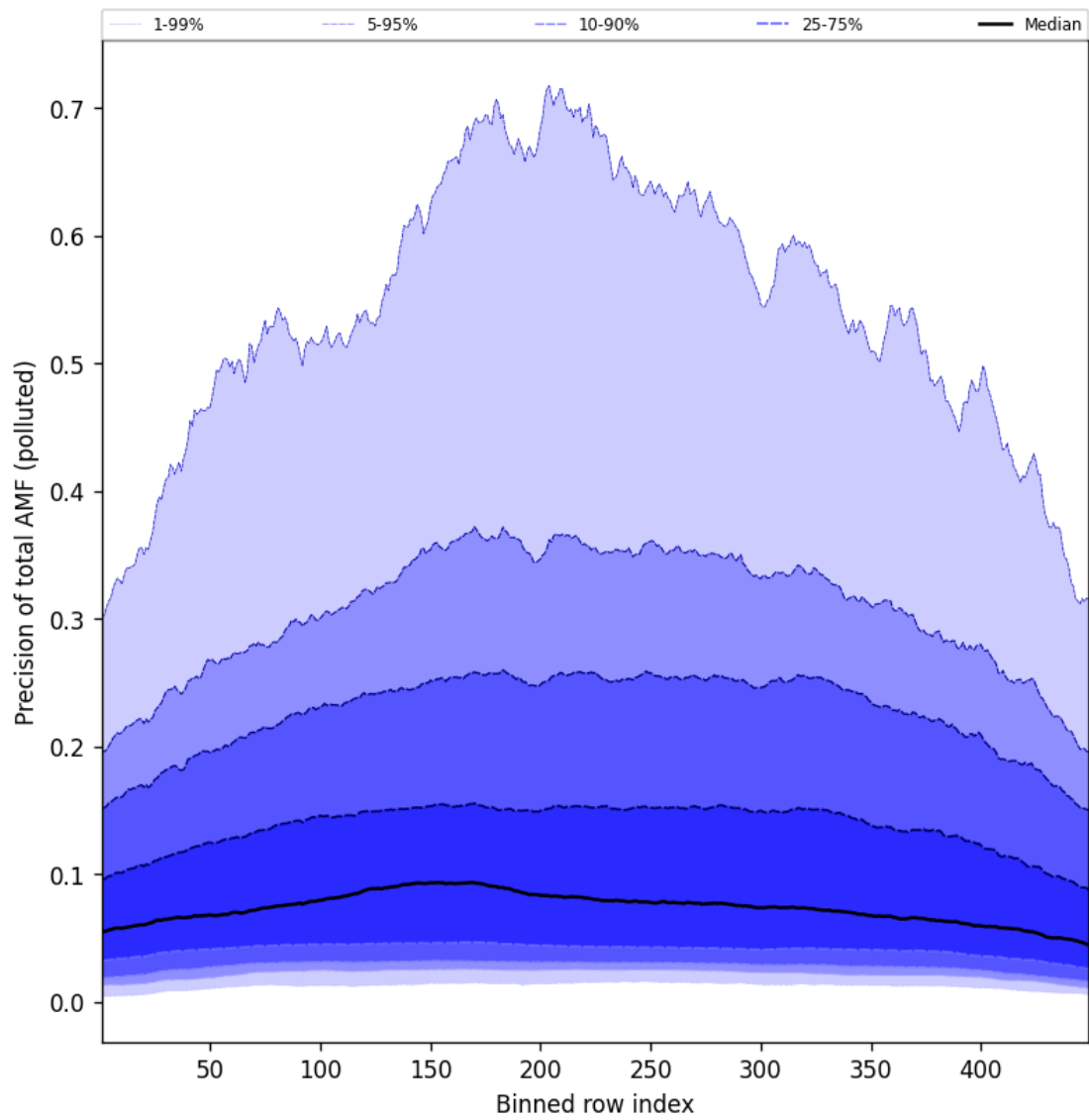
Figure 95: Along track statistics of “Precision of total AMF (polluted)” for 2024-09-01 to 2024-09-03
