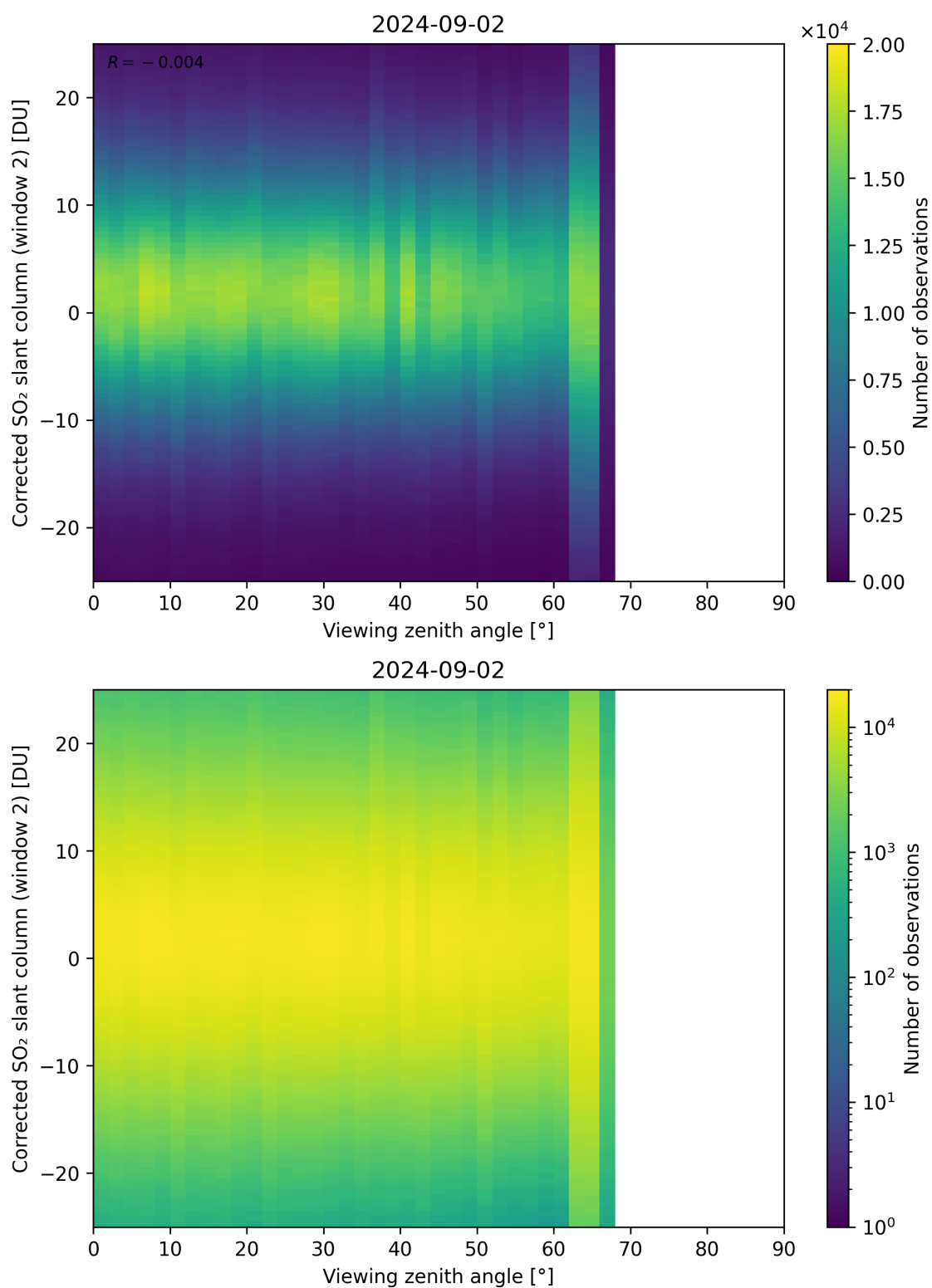
Figure 318: Scatter density plot of “Viewing zenith angle” against “Corrected SO 2 slant column (window 2)” for 2024-09-01 to 2024-09-03.
