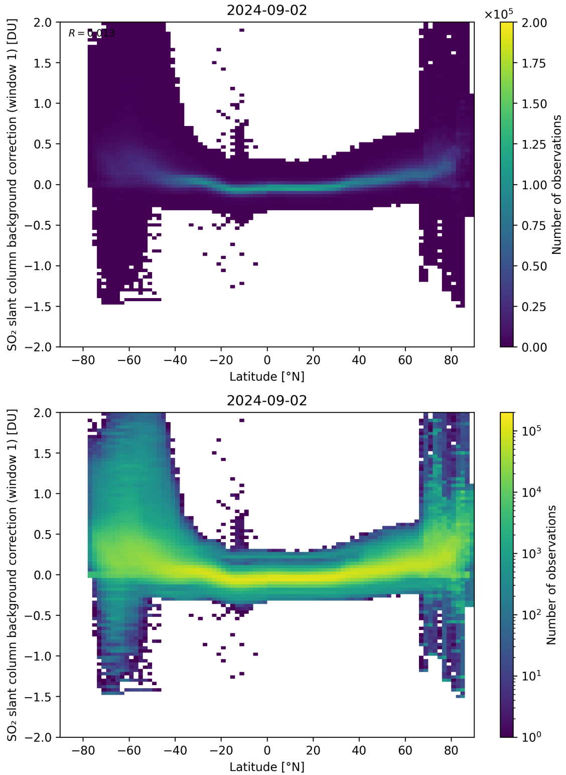
Figure 139: Scatter density plot of “Latitude” against “SO 2 slant column background correction (window 1)” for 2024-09-01 to 2024-09-03.
