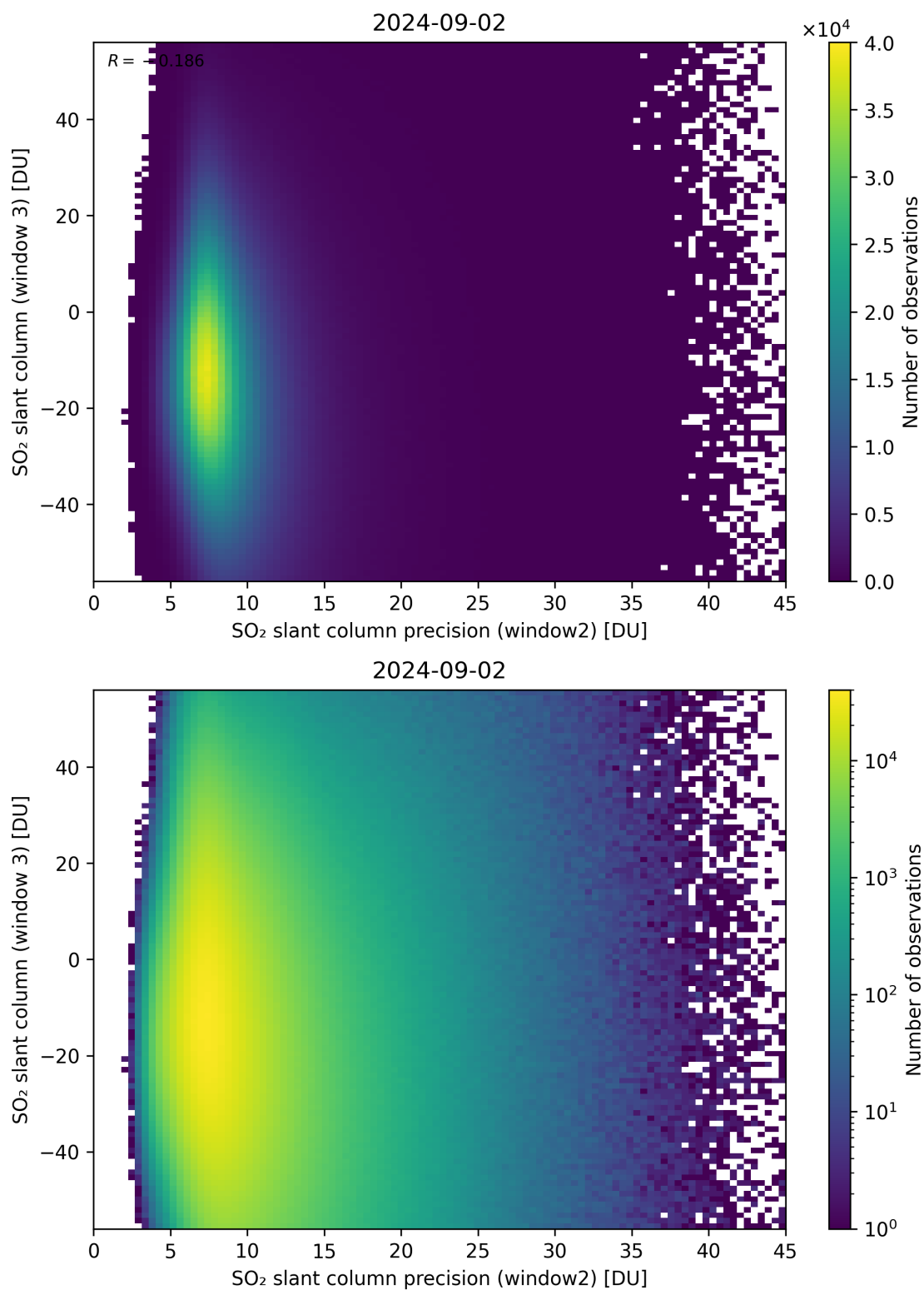
Figure 249: Scatter density plot of “SO 2 slant column precision (window2)” against “SO 2 slant column (window 3)” for 2024-09-01 to 2024-09-03.
