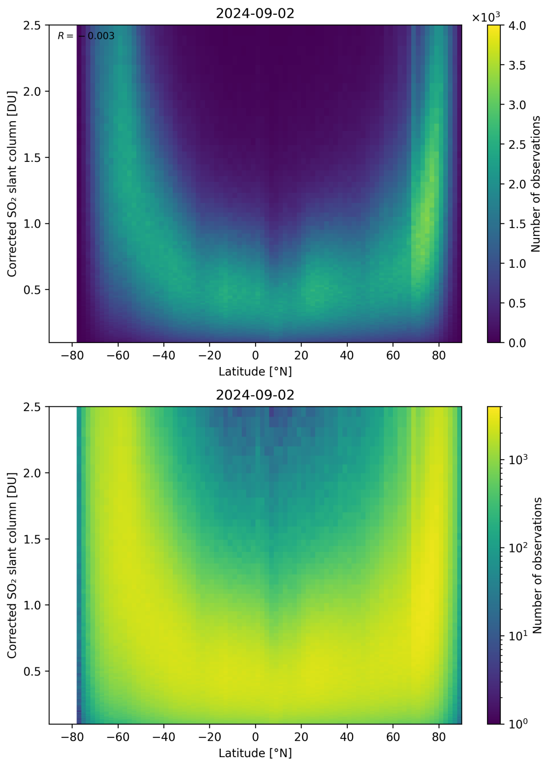
Figure 146: Scatter density plot of “Latitude” against “Corrected SO 2 slant column” for 2024-09-01 to 2024-09-03.
