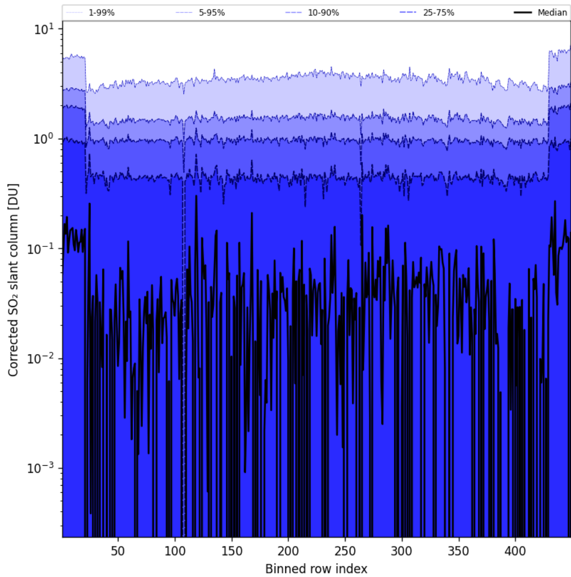
Figure 78: Along track statistics of "Corrected SO 2 slant column" for 2024-09-01 to 2024-09-03
