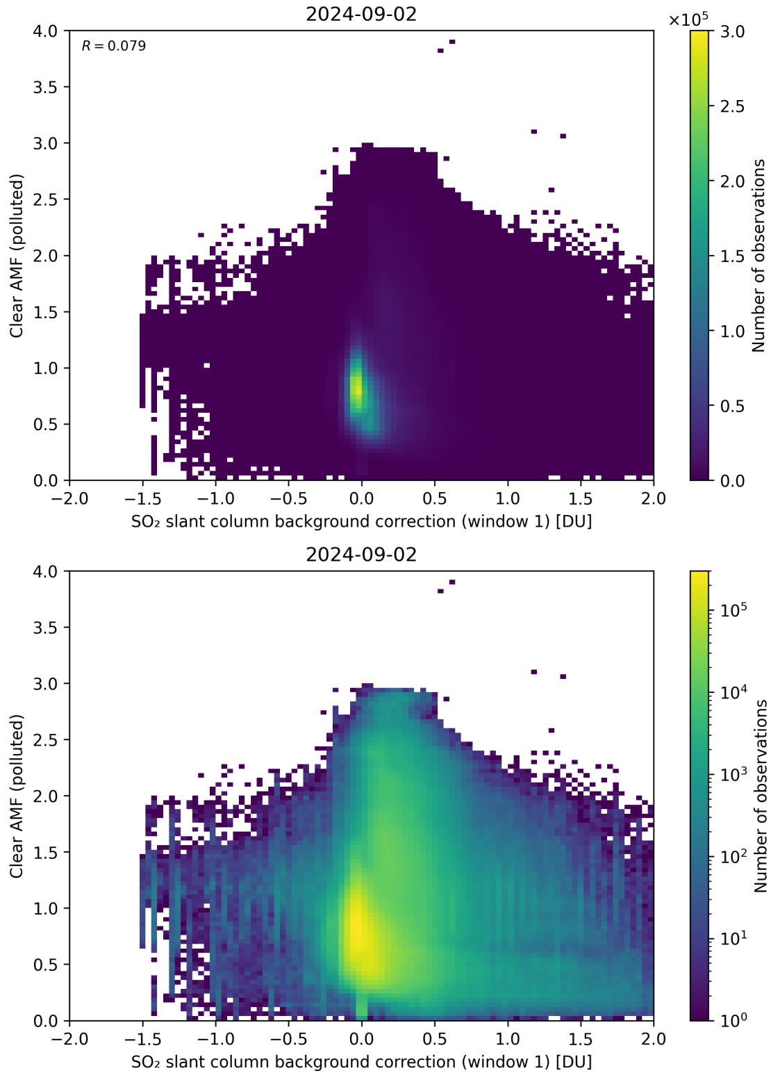
Figure 103: Scatter density plot of “SO 2 slant column background correction (window 1)” against “Clear AMF (polluted)” for 2024-09-01 to 2024-09-03.
