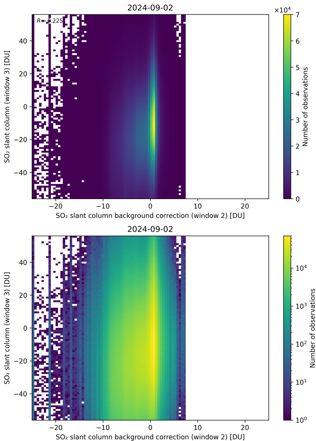
Figure 117: Scatter density plot of “SO 2 slant column background correction (window 2)” against “SO 2 slant column (window 3)” for 2024-09-01 to 2024-09-03.
