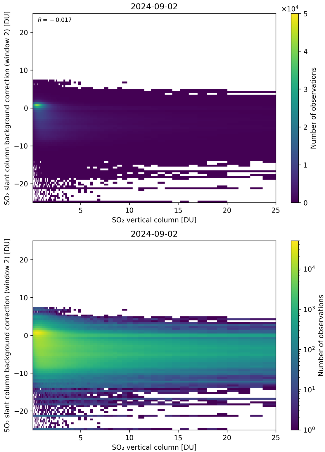
Figure 274: Scatter density plot of “SO 2 vertical column” against “SO 2 slant column background correction (window 2)” for 2024-09-01 to 2024-09-03.
