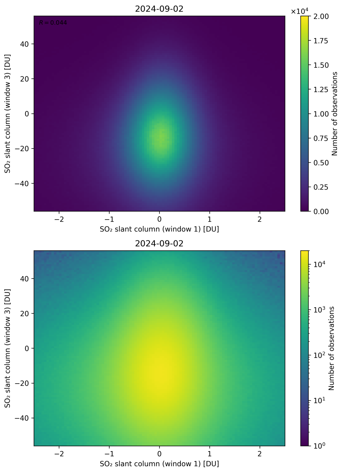
Figure 237: Scatter density plot of “SO 2 slant column (window 1)” against “SO 2 slant column (window 3)” for 2024-09-01 to 2024-09-03.
