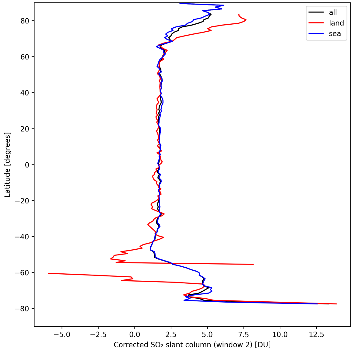
Figure 39: Zonal average of “Corrected SO 2 slant column (window 2)” for 2024-09-01 to 2024-09-03.
