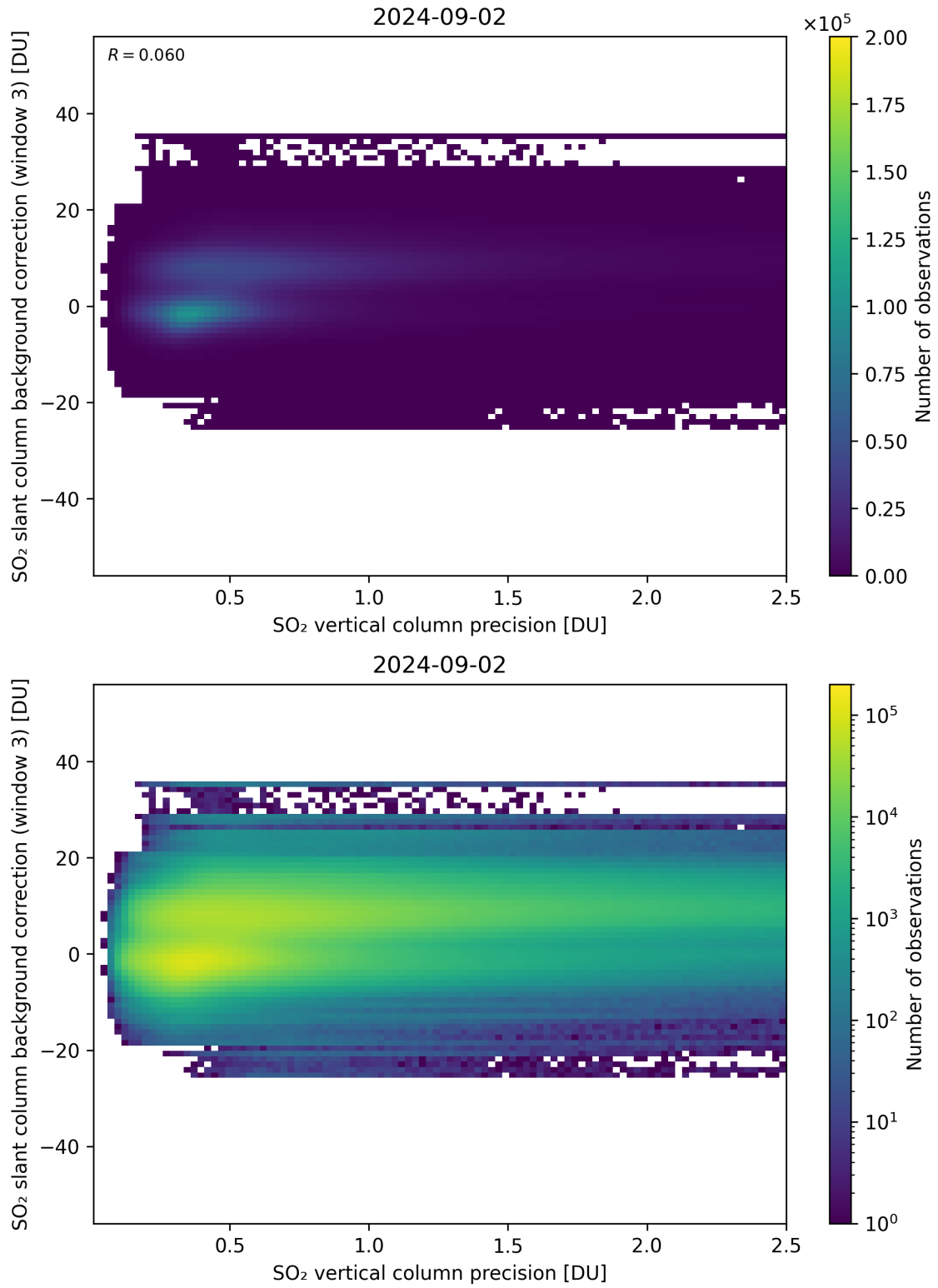
Figure 281: Scatter density plot of “SO 2 vertical column precision” against “SO 2 slant column background correction (window 3)” for 2024-09-01 to 2024-09-03.
