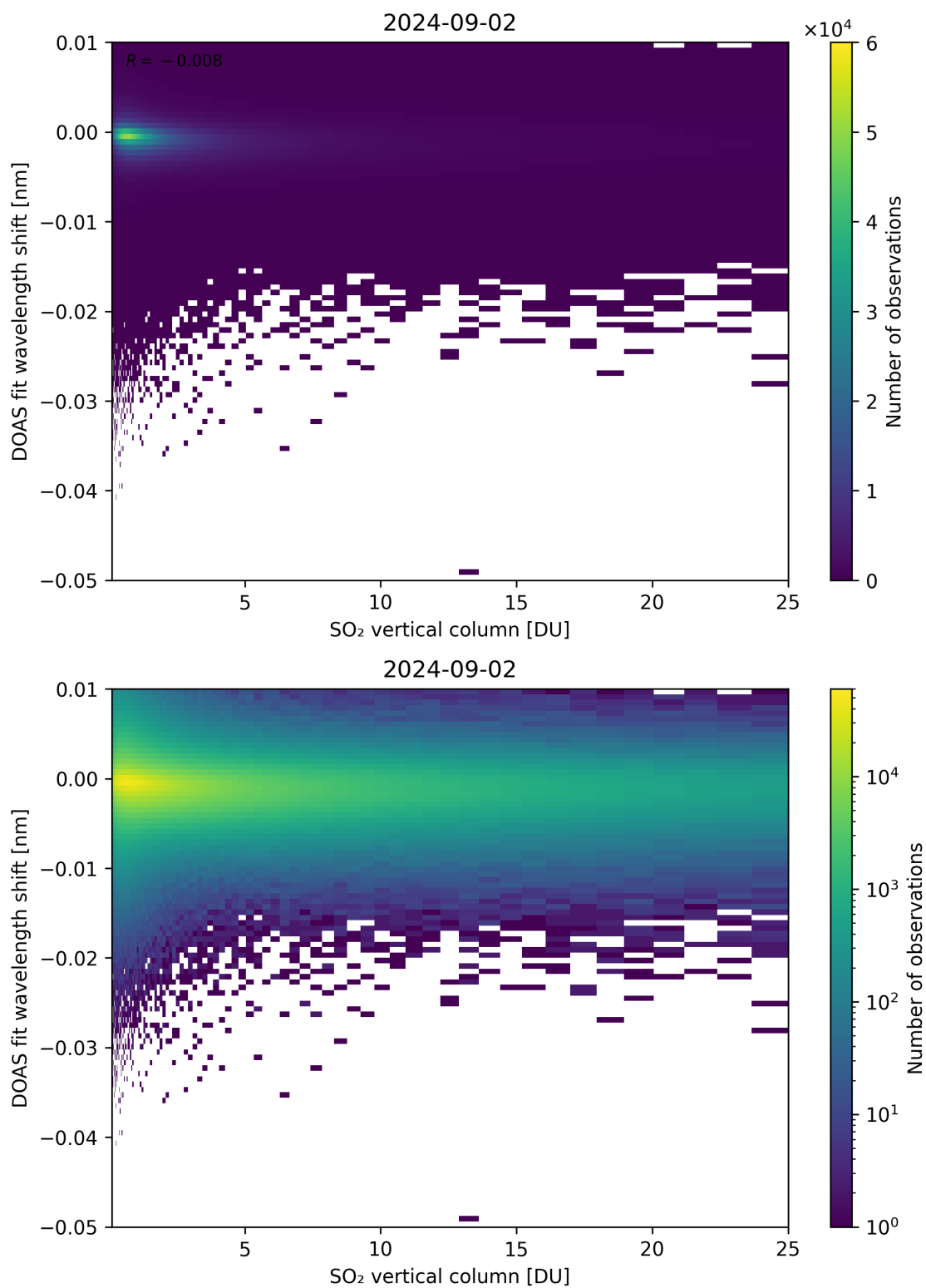
Figure 276: Scatter density plot of “SO 2 vertical column” against “DOAS fit wavelength shift” for 2024-09-01 to 2024-09-03.
