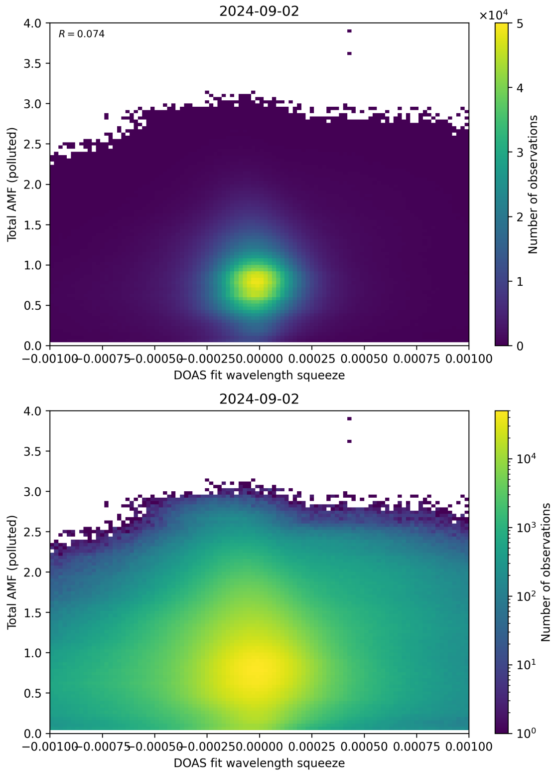
Figure 134: Scatter density plot of “DOAS fit wavelength squeeze” against “Total AMF (polluted)” for 2024-09-01 to 2024-09-03.
