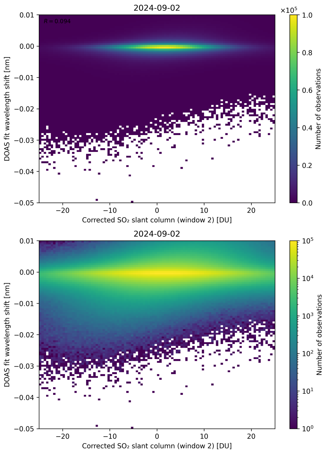
Figure 196: Scatter density plot of “Corrected SO 2 slant column (window 2)” against “DOAS fit wavelength shift” for 2024-09-01 to 2024-09-03.
