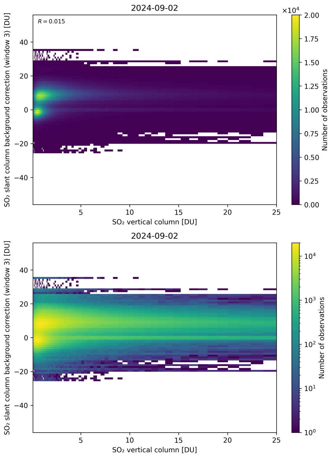
Figure 275: Scatter density plot of “SO 2 vertical column” against “SO 2 slant column background correction (window 3)” for 2024-09-01 to 2024-09-03.
