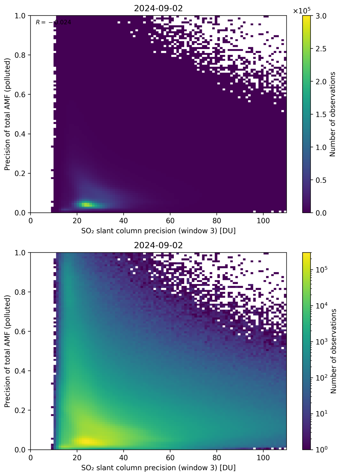
Figure 264: Scatter density plot of “SO 2 slant column precision (window 3)” against “Precision of total AMF (polluted)” for 2024-09-01 to 2024-09-03.
