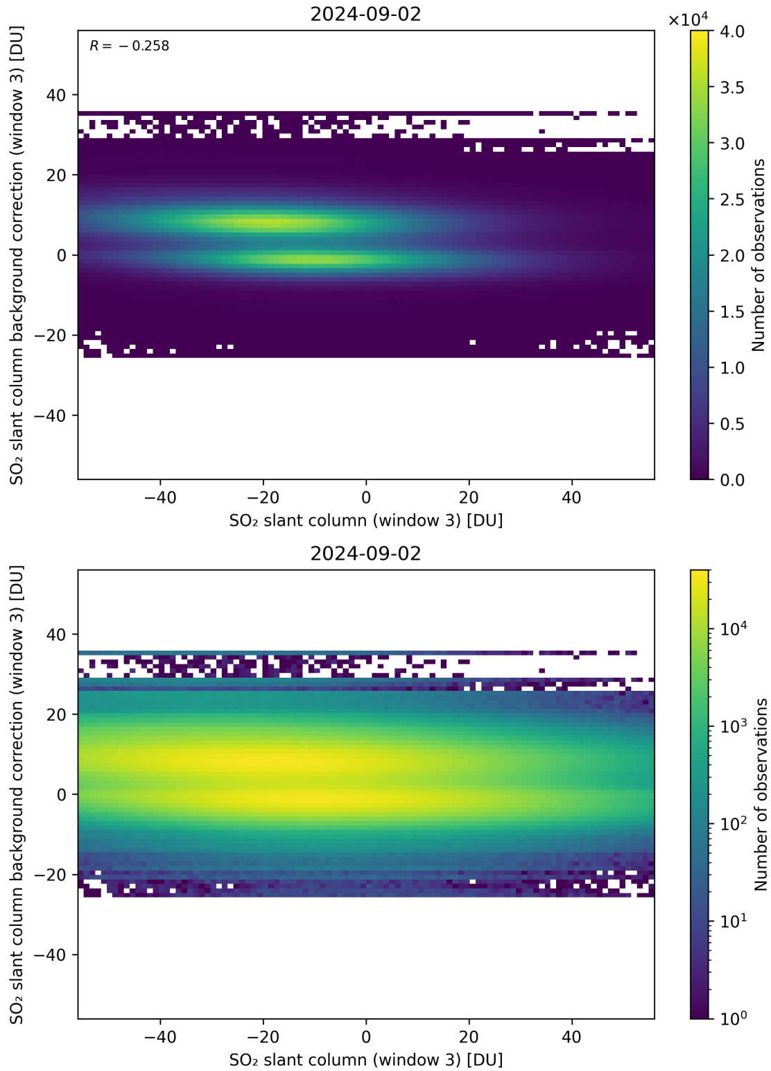
Figure 253: Scatter density plot of “SO 2 slant column (window 3)” against “SO 2 slant column background correction (window 3)” for 2024-09-01 to 2024-09-03.
