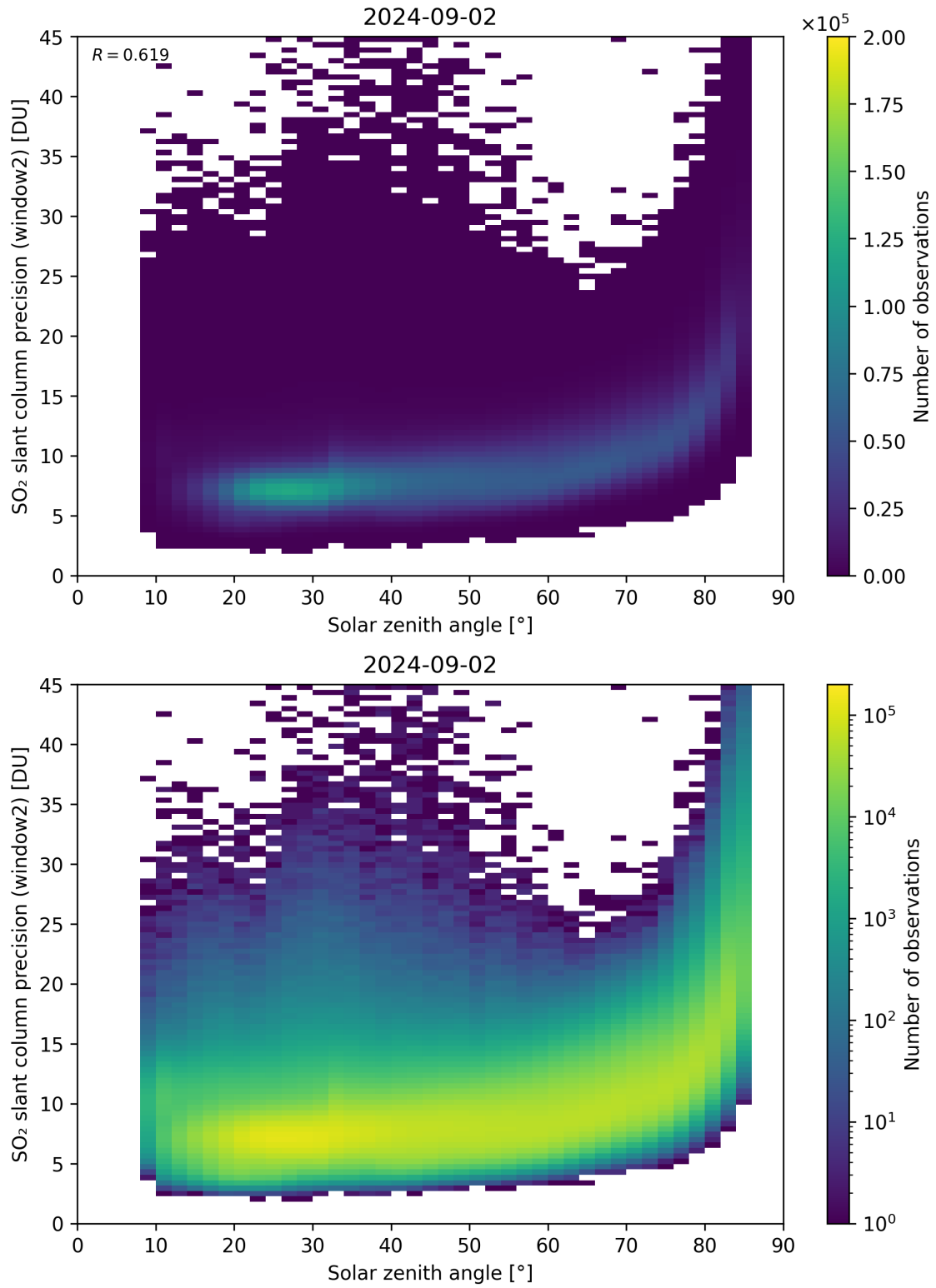
Figure 171: Scatter density plot of “Solar zenith angle” against “SO 2 slant column precision (window2)” for 2024-09-01 to 2024-09-03.
