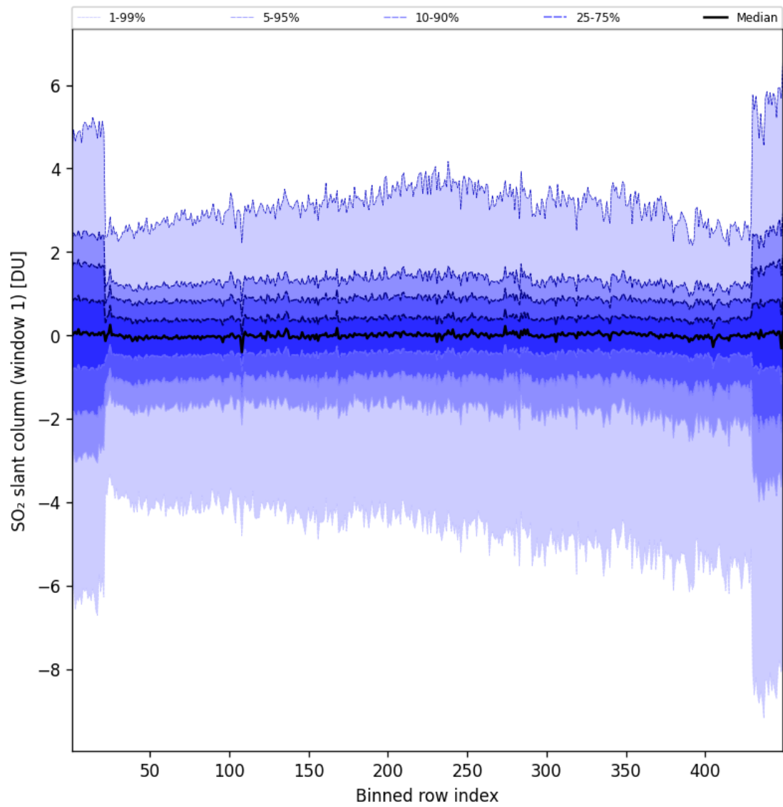
Figure 79: Along track statistics of “SO 2 slant column (window 1)” for 2024-09-01 to 2024-09-03
