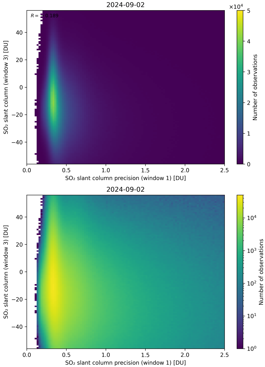
Figure 228: Scatter density plot of “SO 2 slant column precision (window 1)” against “SO 2 slant column (window 3)” for 2024-09-01 to 2024-09-03.
