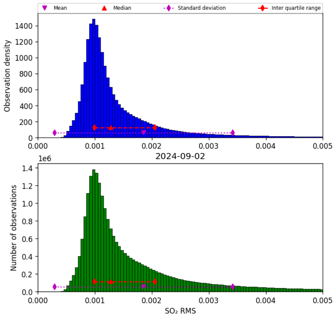
Figure 70: Histogram of “SO 2 RMS” for 2024-09-01 to 2024-09-03
