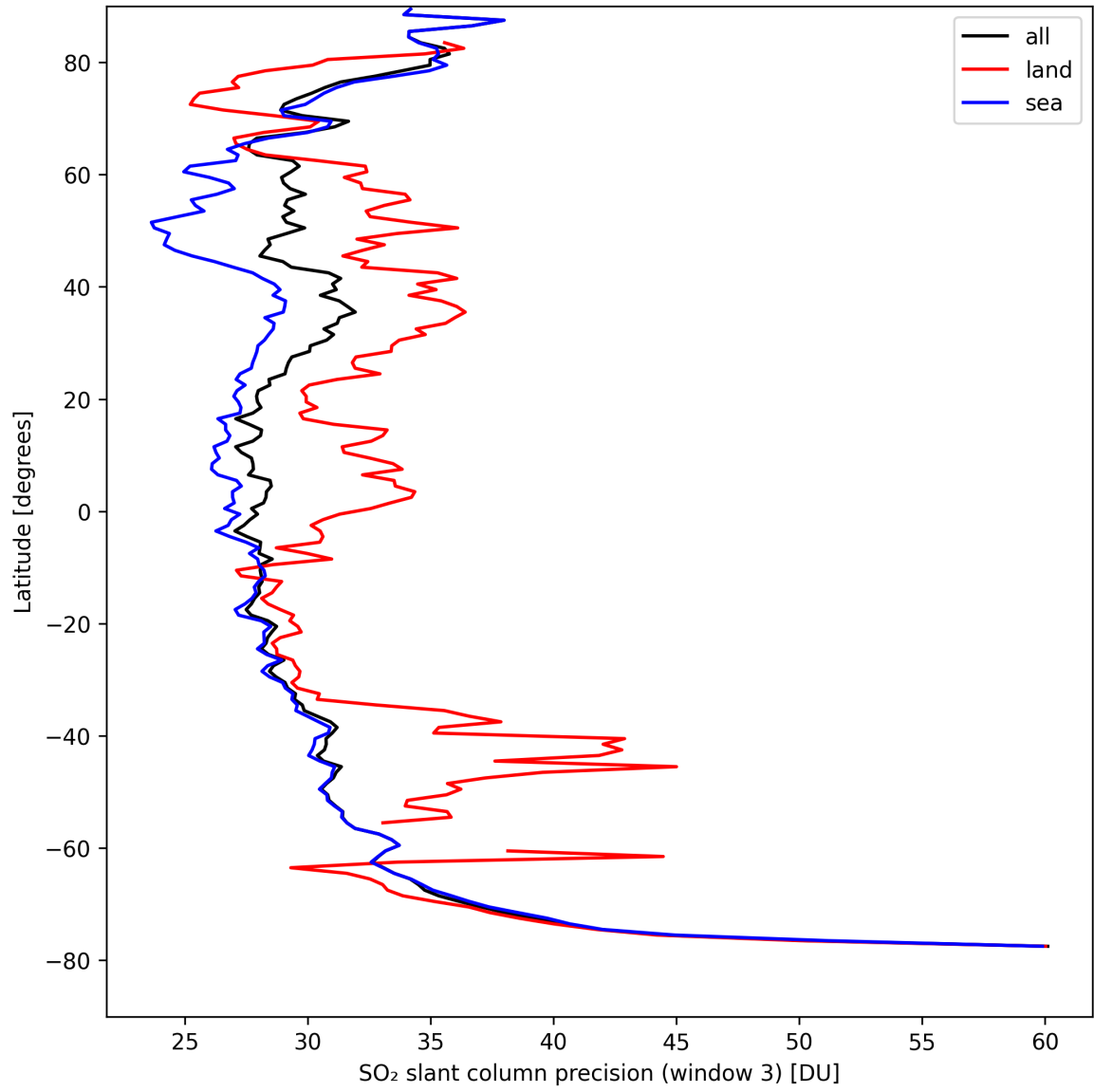
Figure 42: Zonal average of “SO 2 slant column precision (window 3)” for 2024-09-01 to 2024-09-03.
