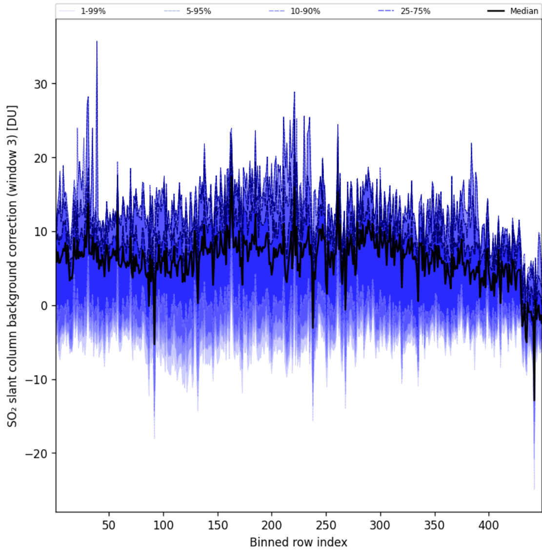
Figure 90: Along track statistics of “SO 2 slant column background correction (window 3)” for 2024-09-01 to 2024-09-03
