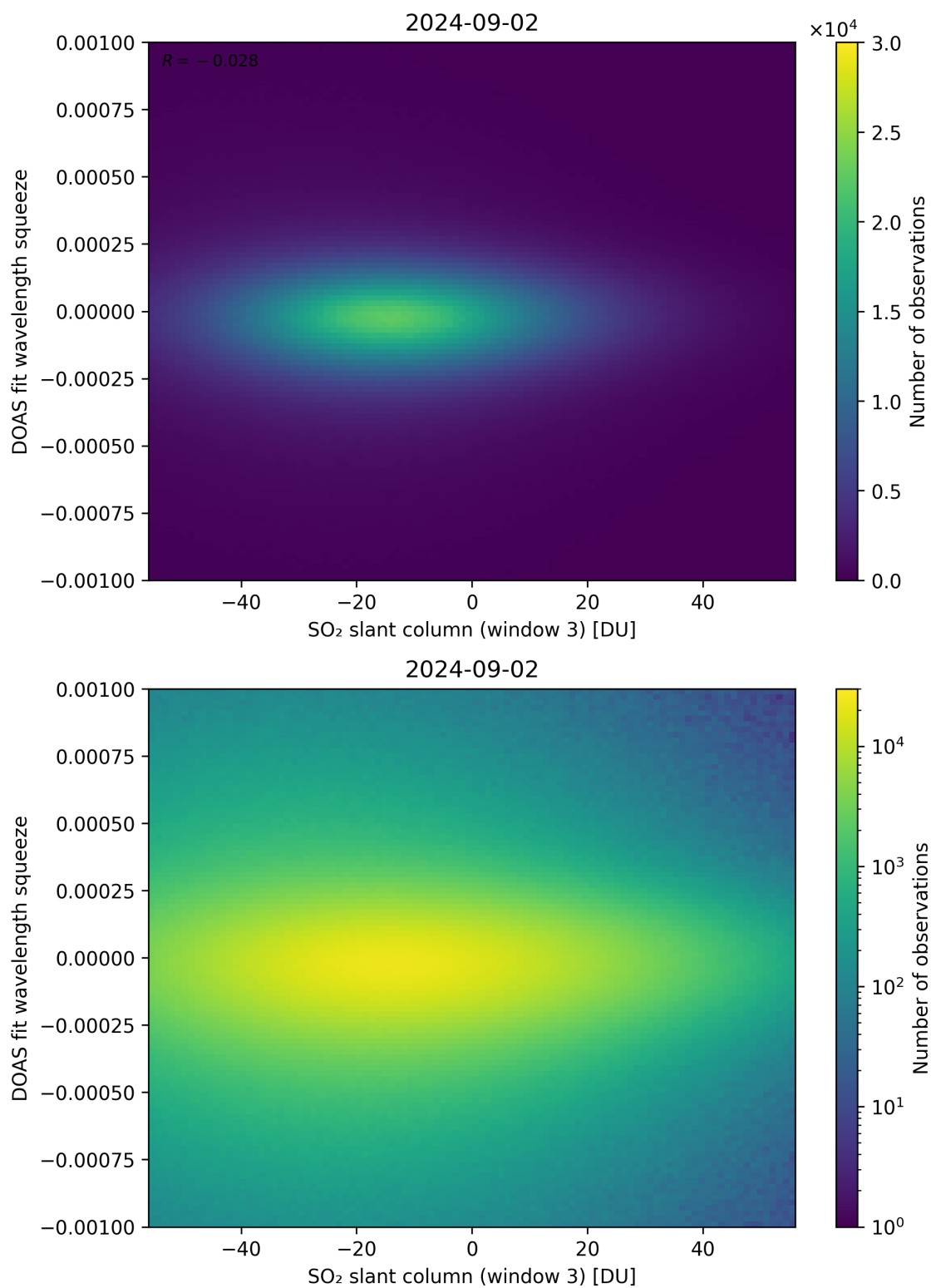
Figure 255: Scatter density plot of “SO 2 slant column (window 3)” against “DOAS fit wavelength squeeze” for 2024-09-01 to 2024-09-03.
