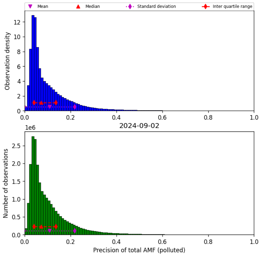
Figure 72: Histogram of “Precision of total AMF (polluted)” for 2024-09-01 to 2024-09-03
