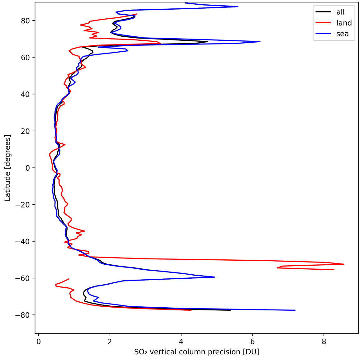
Figure 31: Zonal average of “SO 2 vertical column precision” for 2024-09-01 to 2024-09-03.
