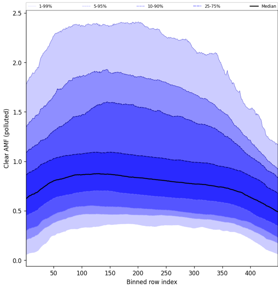
Figure 96: Along track statistics of “Clear AMF (polluted)” for 2024-09-01 to 2024-09-03
