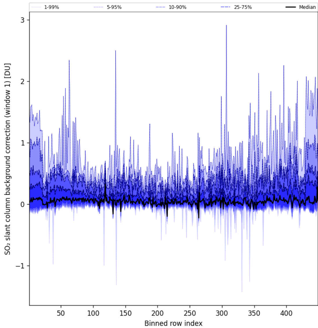
Figure 82: Along track statistics of “SO 2 slant column background correction (window 1)” for 2024-09-01 to 2024-09-03
