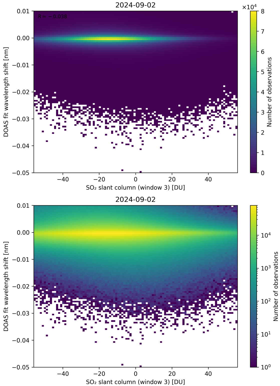
Figure 254: Scatter density plot of “SO 2 slant column (window 3)” against “DOAS fit wavelength shift” for 2024-09-01 to 2024-09-03.
