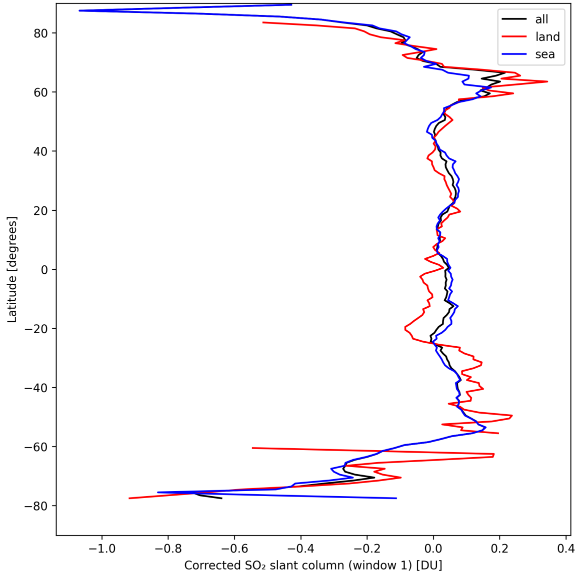
Figure 35: Zonal average of “Corrected SO 2 slant column (window 1)” for 2024-09-01 to 2024-09-03.
