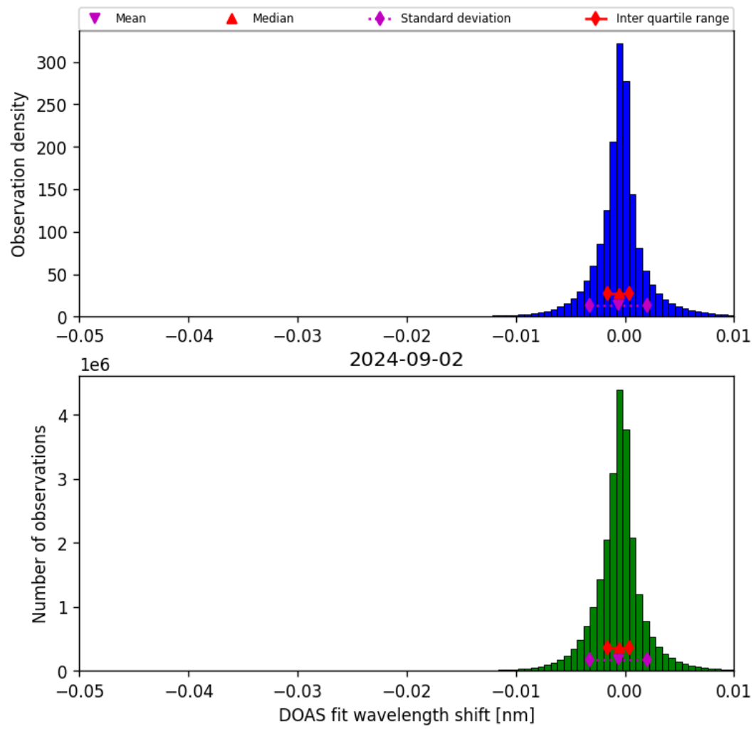
Figure 68: Histogram of “DOAS fit wavelength shift” for 2024-09-01 to 2024-09-03
