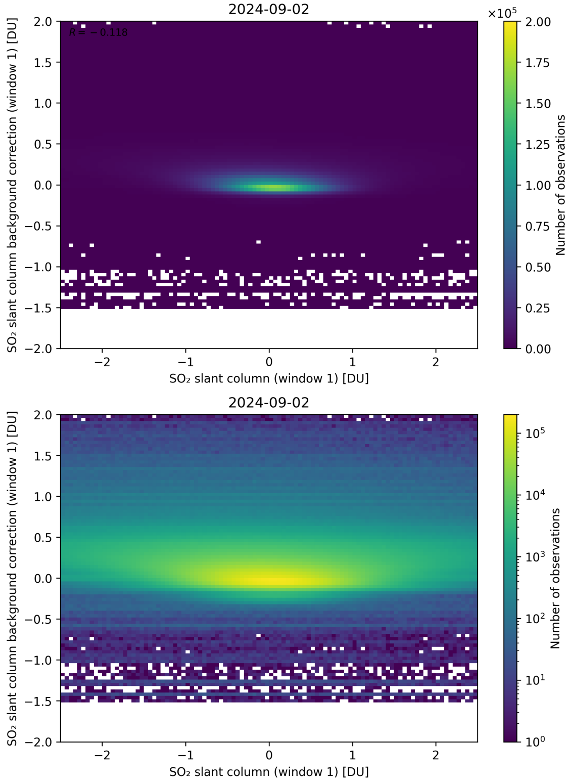
Figure 212: Scatter density plot of “SO 2 slant column (window 1)” against “SO 2 slant column background correction (window 1)” for 2024-09-01 to 2024-09-03.
