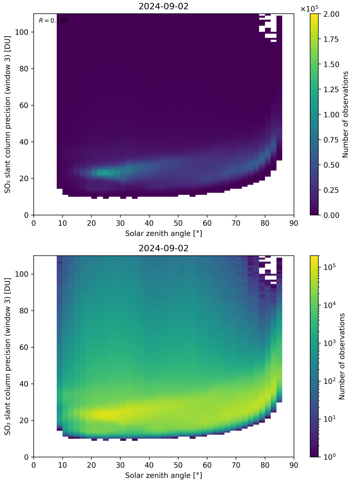
Figure 173: Scatter density plot of “Solar zenith angle” against “SO 2 slant column precision (window 3)” for 2024-09-01 to 2024-09-03.
