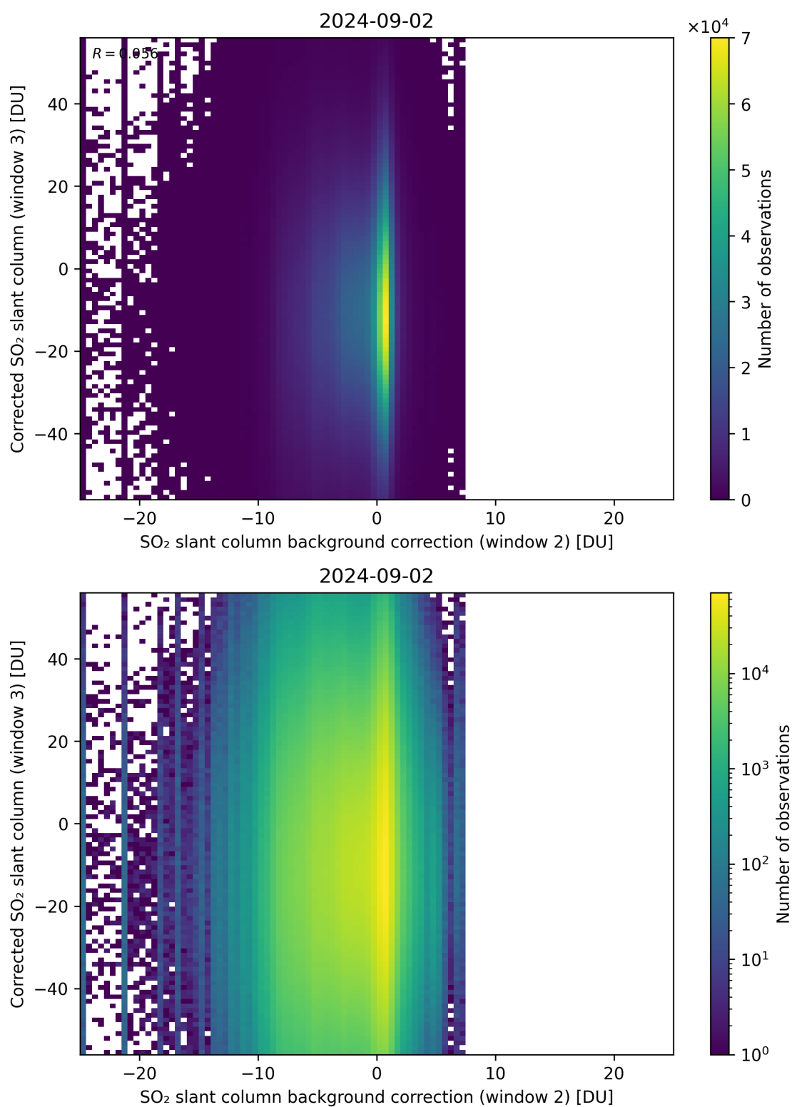
Figure 116: Scatter density plot of “SO 2 slant column background correction (window 2)” against “Corrected SO 2 slant column (window 3)” for 2024-09-01 to 2024-09-03.
