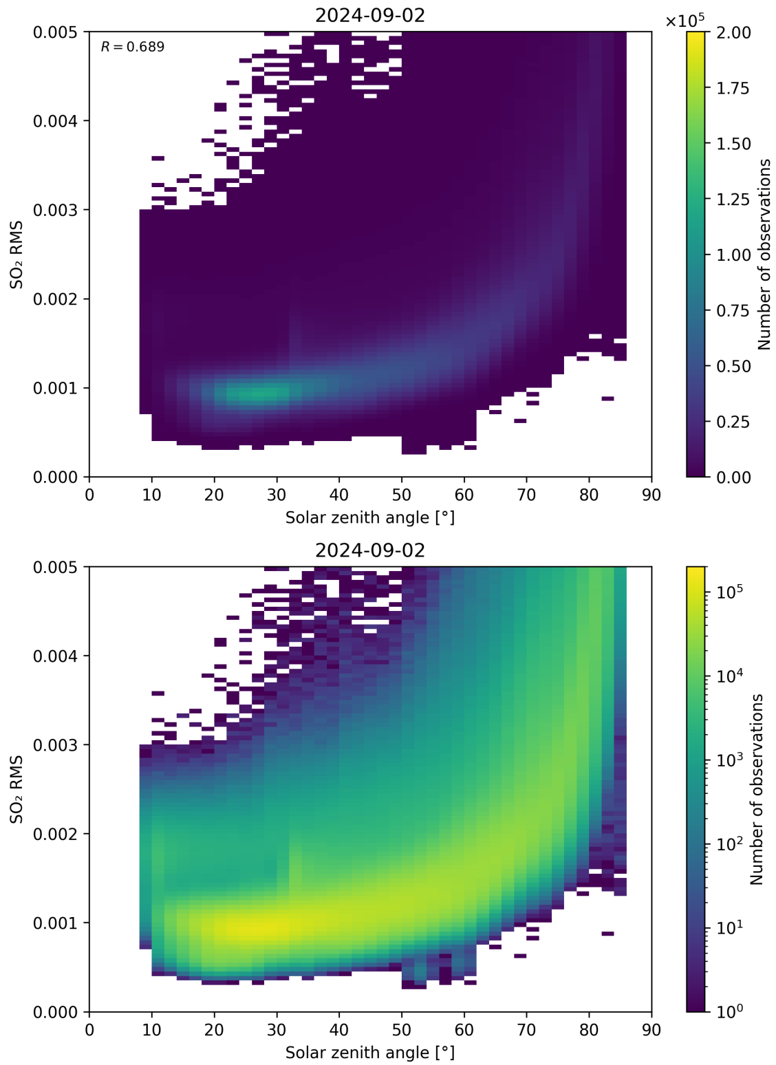
Figure 163: Scatter density plot of “Solar zenith angle” against “SO 2 RMS” for 2024-09-01 to 2024-09-03.
