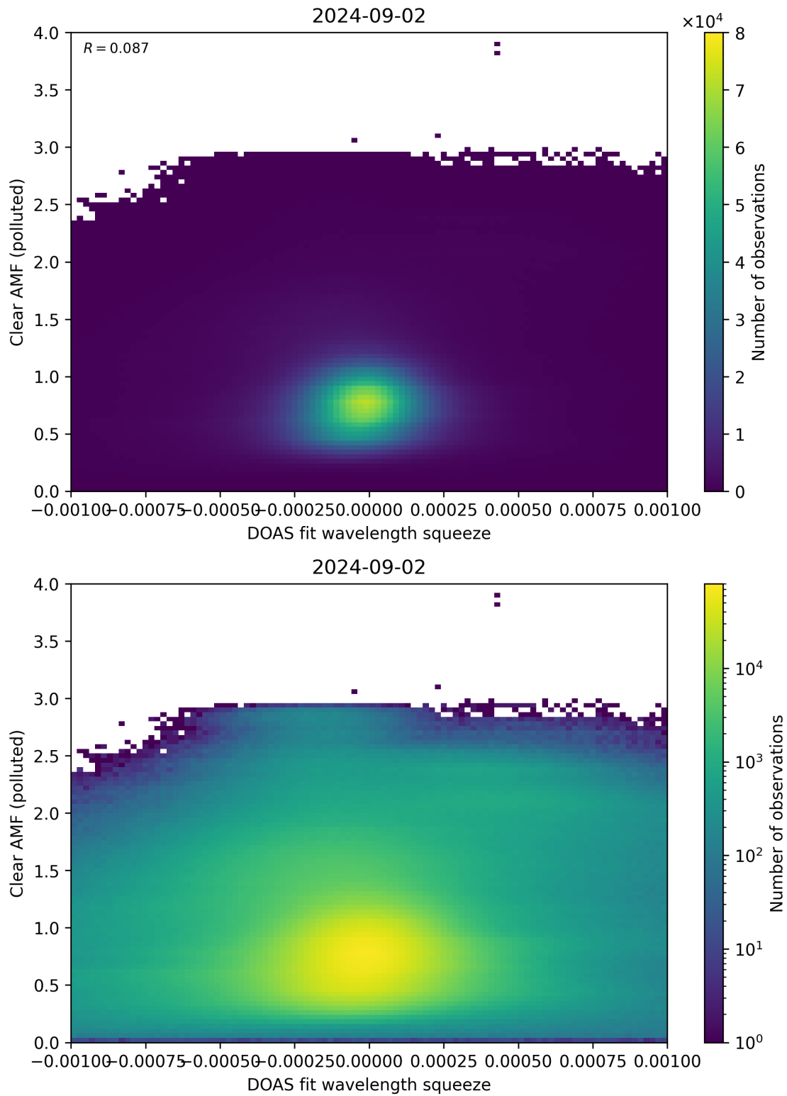
Figure 133: Scatter density plot of “DOAS fit wavelength squeeze” against “Clear AMF (polluted)” for 2024-09-01 to 2024-09-03.
