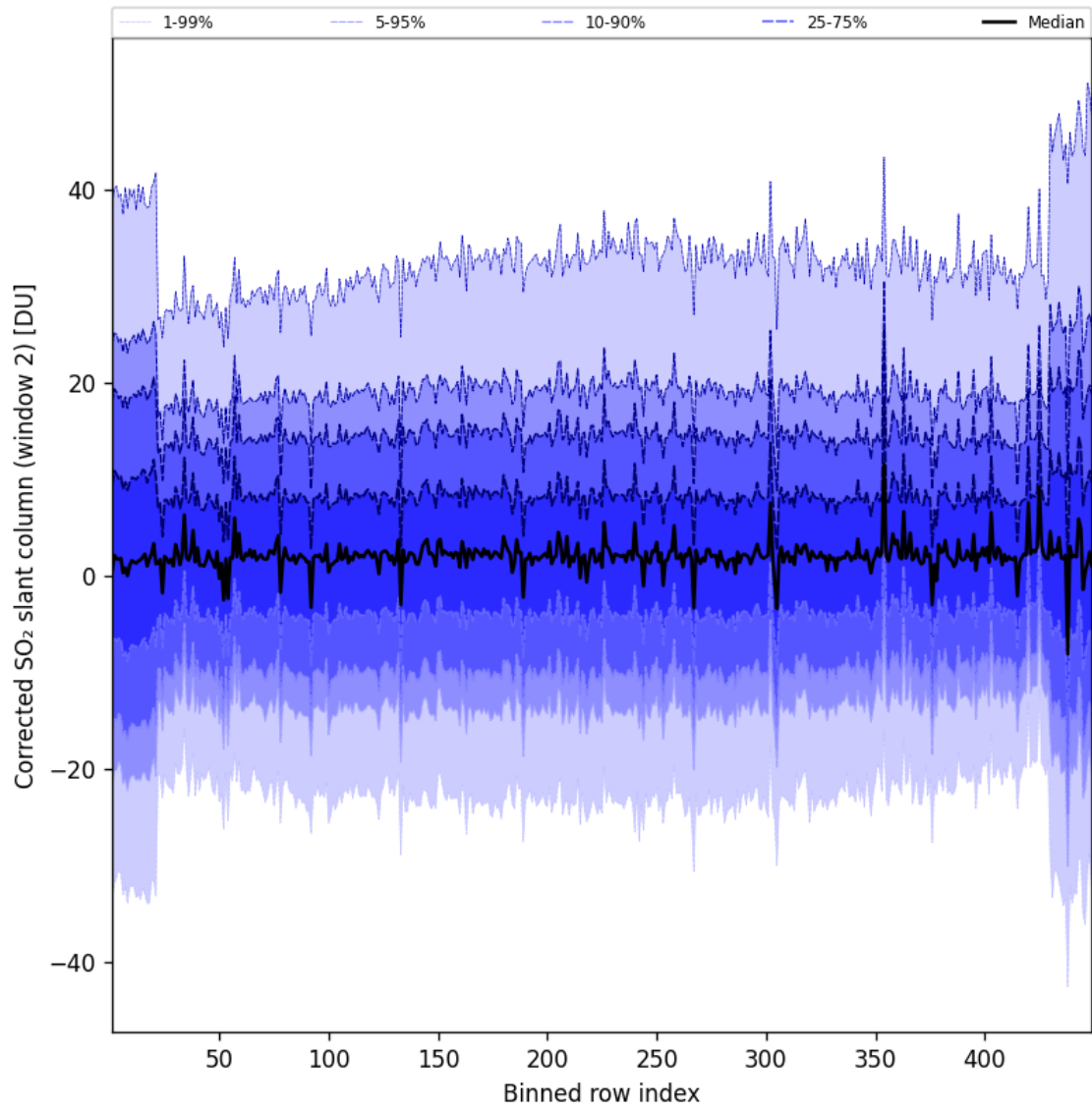
Figure 85: Along track statistics of “Corrected SO 2 slant column (window 2)” for 2024-09-01 to 2024-09-03
