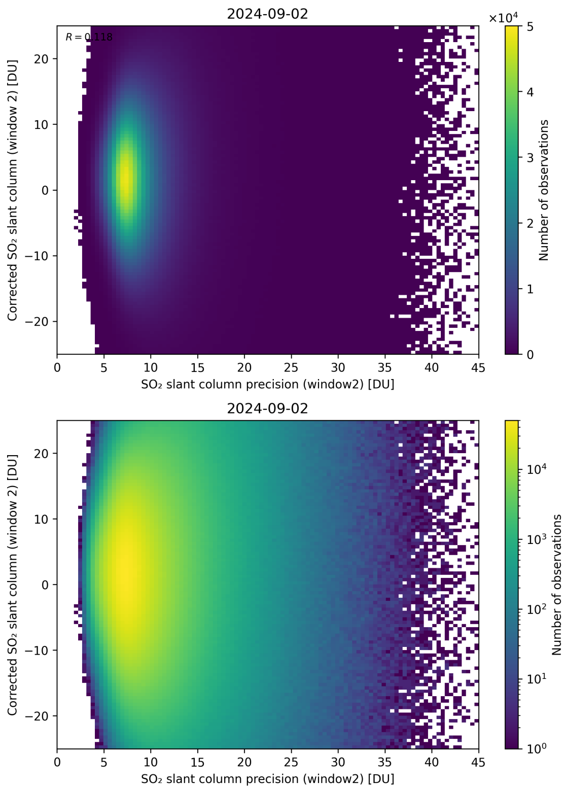
Figure 247: Scatter density plot of “SO 2 slant column precision (window2)” against “Corrected SO 2 slant column (window 2)” for 2024-09-01 to 2024-09-03.
