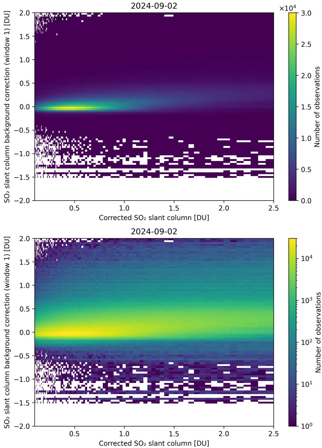
Figure 178: Scatter density plot of “Corrected SO 2 slant column” against “SO 2 slant column background correction (window 1)” for 2024-09-01 to 2024-09-03.
