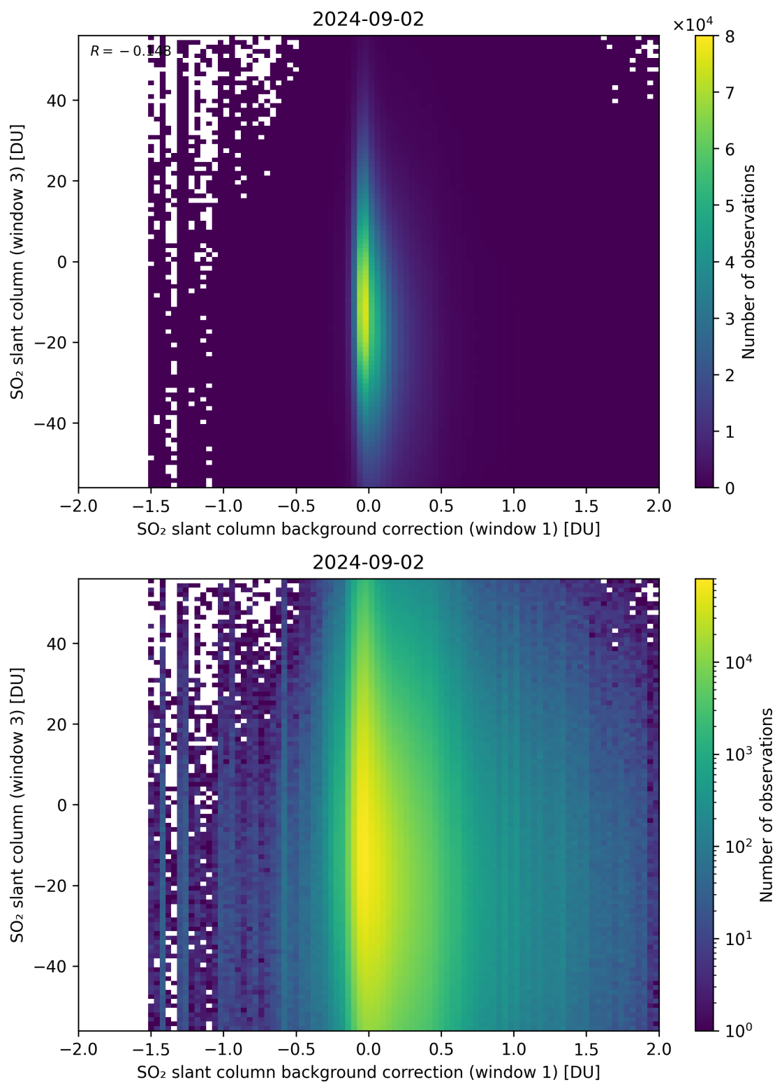
Figure 107: Scatter density plot of “SO 2 slant column background correction (window 1)” against “SO 2 slant column (window 3)” for 2024-09-01 to 2024-09-03.
