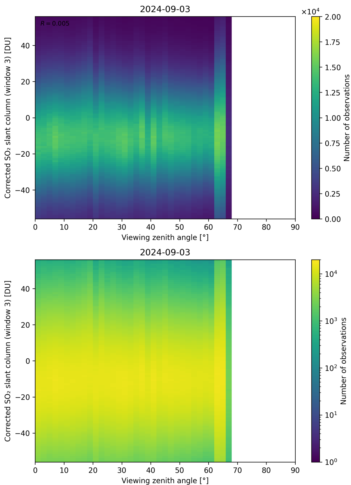
Figure 319: Scatter density plot of “Viewing zenith angle” against “Corrected SO 2 slant column (window 3)” for 2024-09-02 to 2024-09-04.
