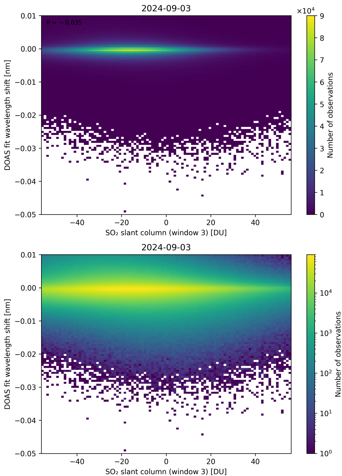
Figure 254: Scatter density plot of “SO 2 slant column (window 3)” against “DOAS fit wavelength shift” for 2024-09-02 to 2024-09-04.
