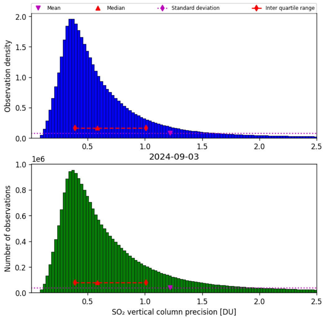
Figure 54: Histogram of “SO 2 vertical column precision” for 2024-09-02 to 2024-09-04
