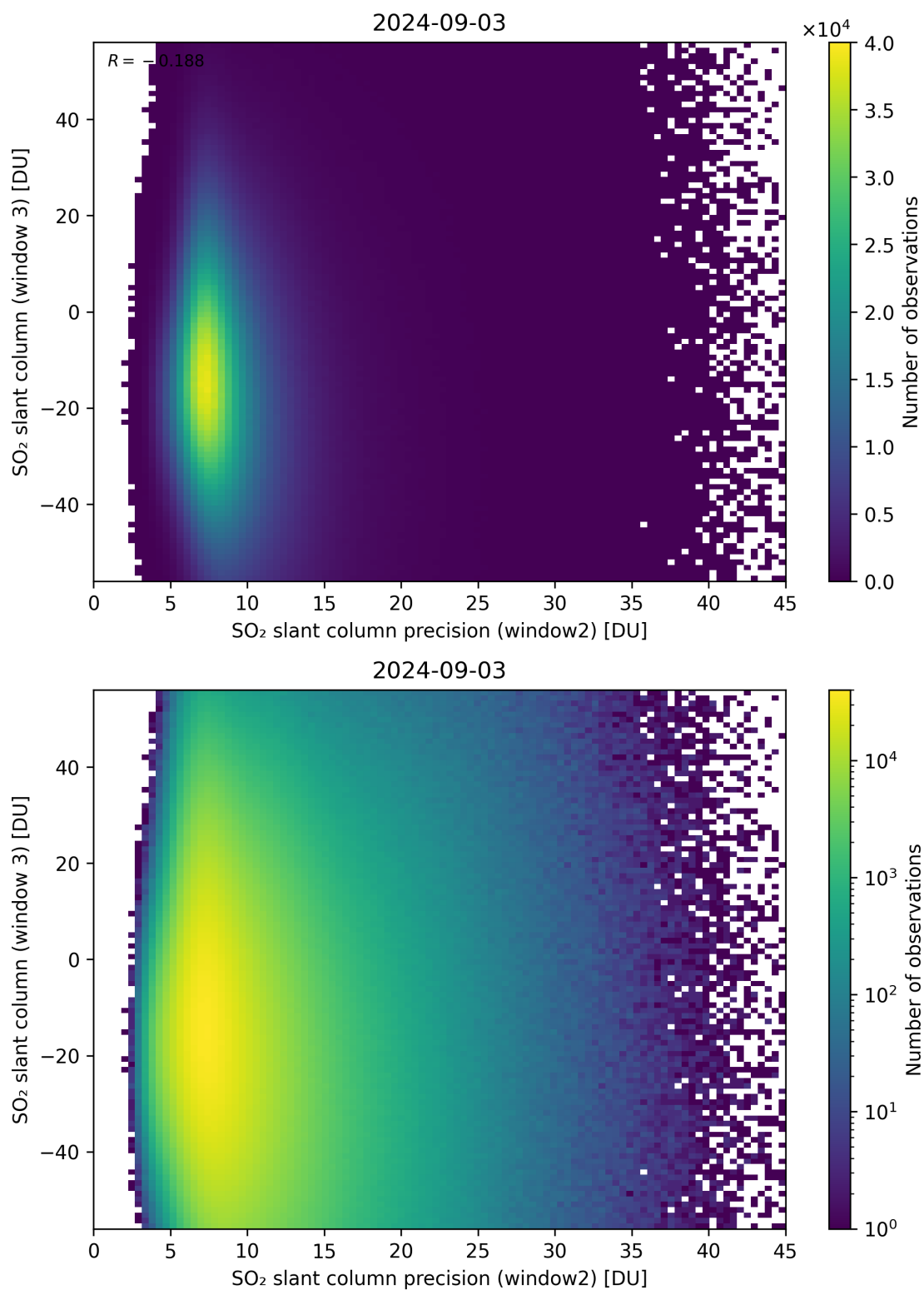
Figure 249: Scatter density plot of “SO 2 slant column precision (window2)” against “SO 2 slant column (window 3)” for 2024-09-02 to 2024-09-04.
