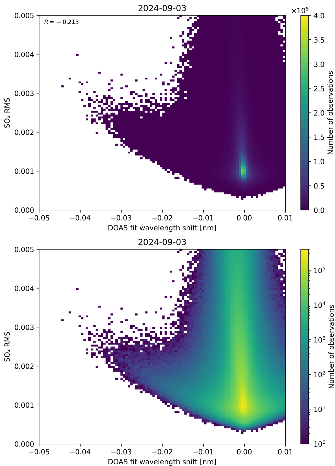
Figure 128: Scatter density plot of “DOAS fit wavelength shift” against “SO 2 RMS” for 2024-09-02 to 2024-09-04.
