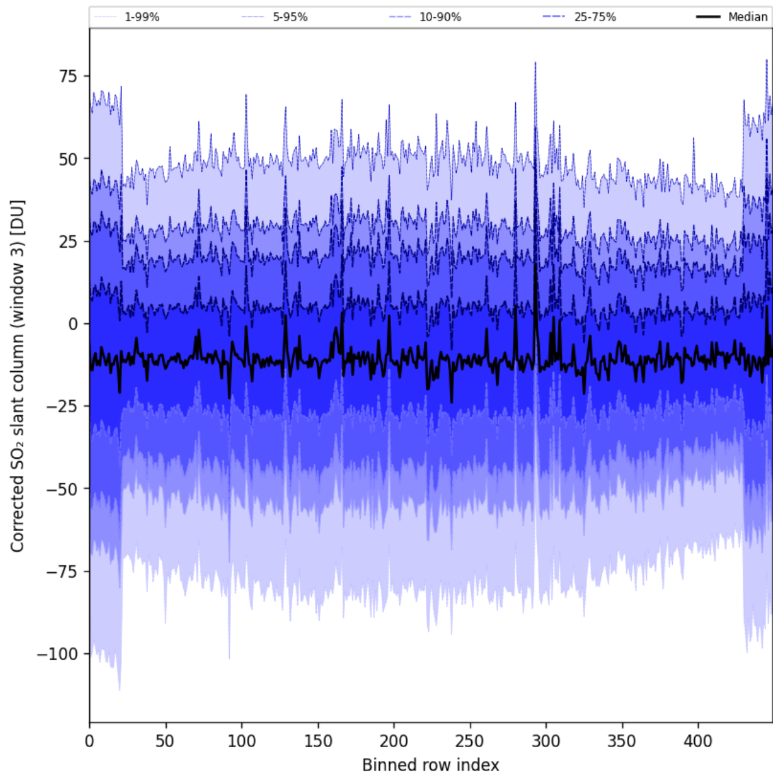
Figure 89: Along track statistics of “Corrected SO 2 slant column (window 3)” for 2024-09-02 to 2024-09-04
