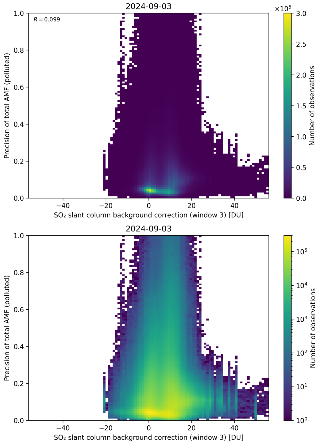
Figure 126: Scatter density plot of “SO 2 slant column background correction (window 3)” against “Precision of total AMF (polluted)” for 2024-09-02 to 2024-09-04.
