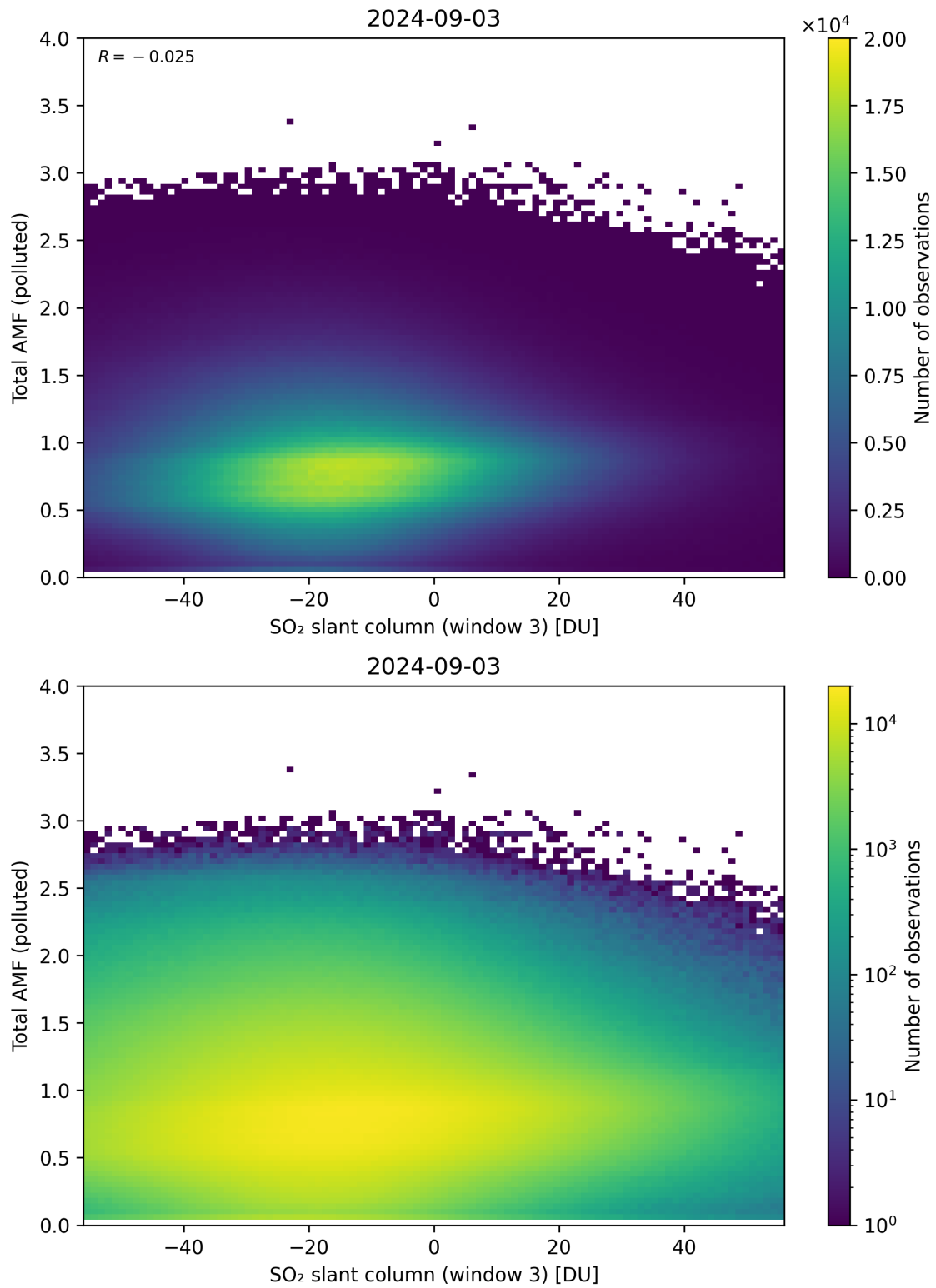
Figure 268: Scatter density plot of “SO 2 slant column (window 3)” against “Total AMF (polluted)” for 2024-09-02 to 2024-09-04.
