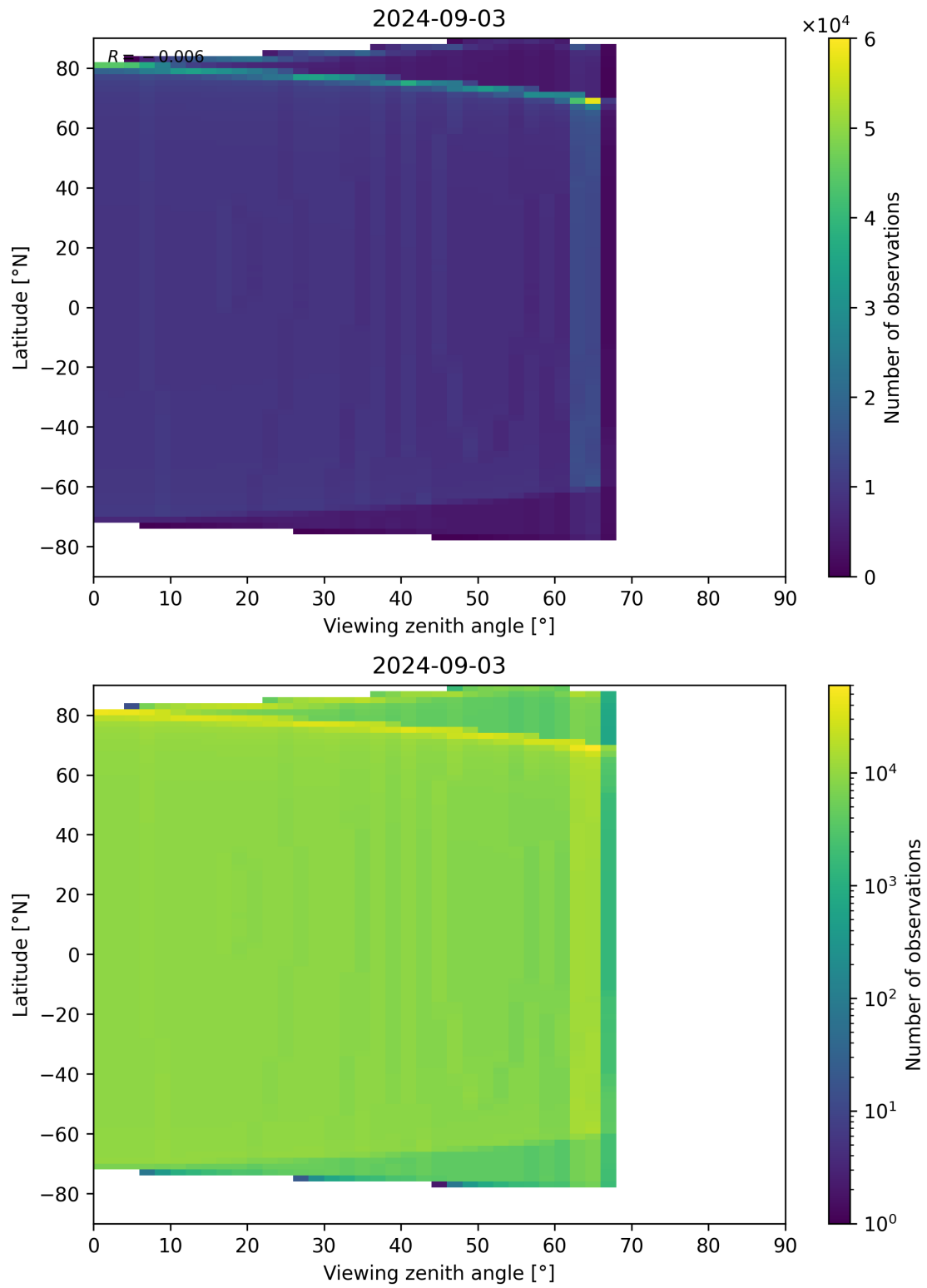
Figure 314: Scatter density plot of “Viewing zenith angle” against “Latitude” for 2024-09-02 to 2024-09-04.
