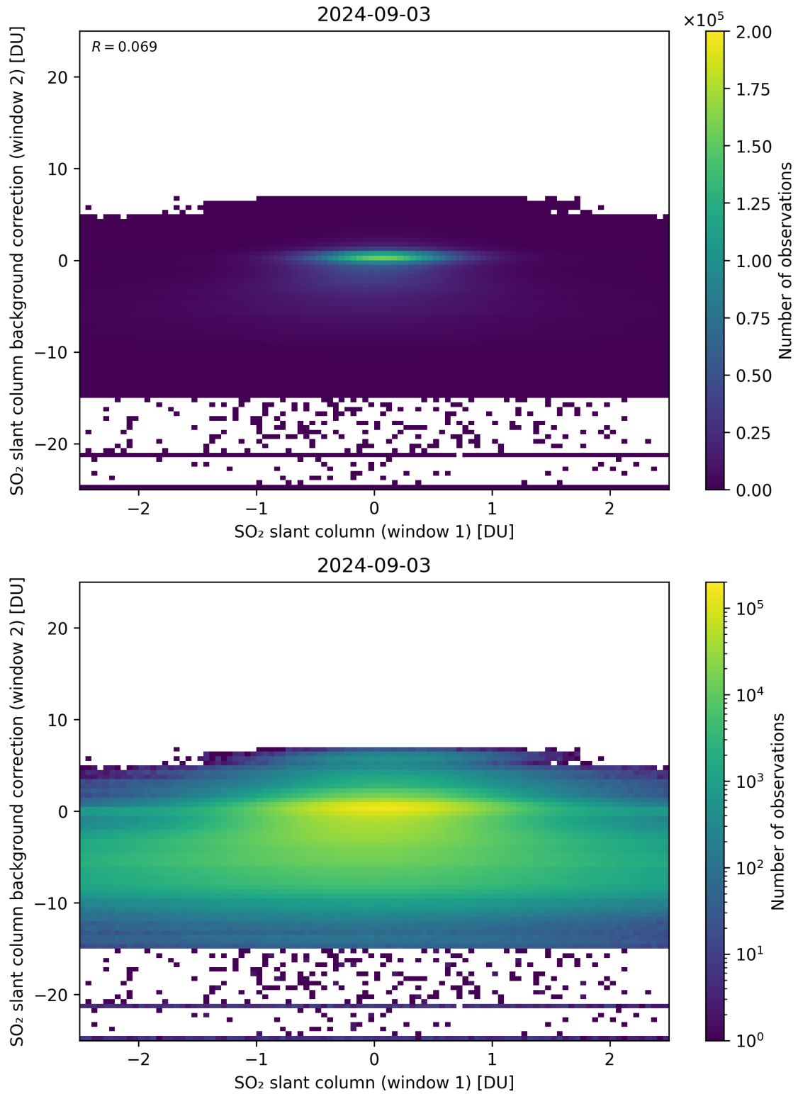
Figure 213: Scatter density plot of “SO 2 slant column (window 1)” against “SO 2 slant column background correction (window 2)” for 2024-09-02 to 2024-09-04.
