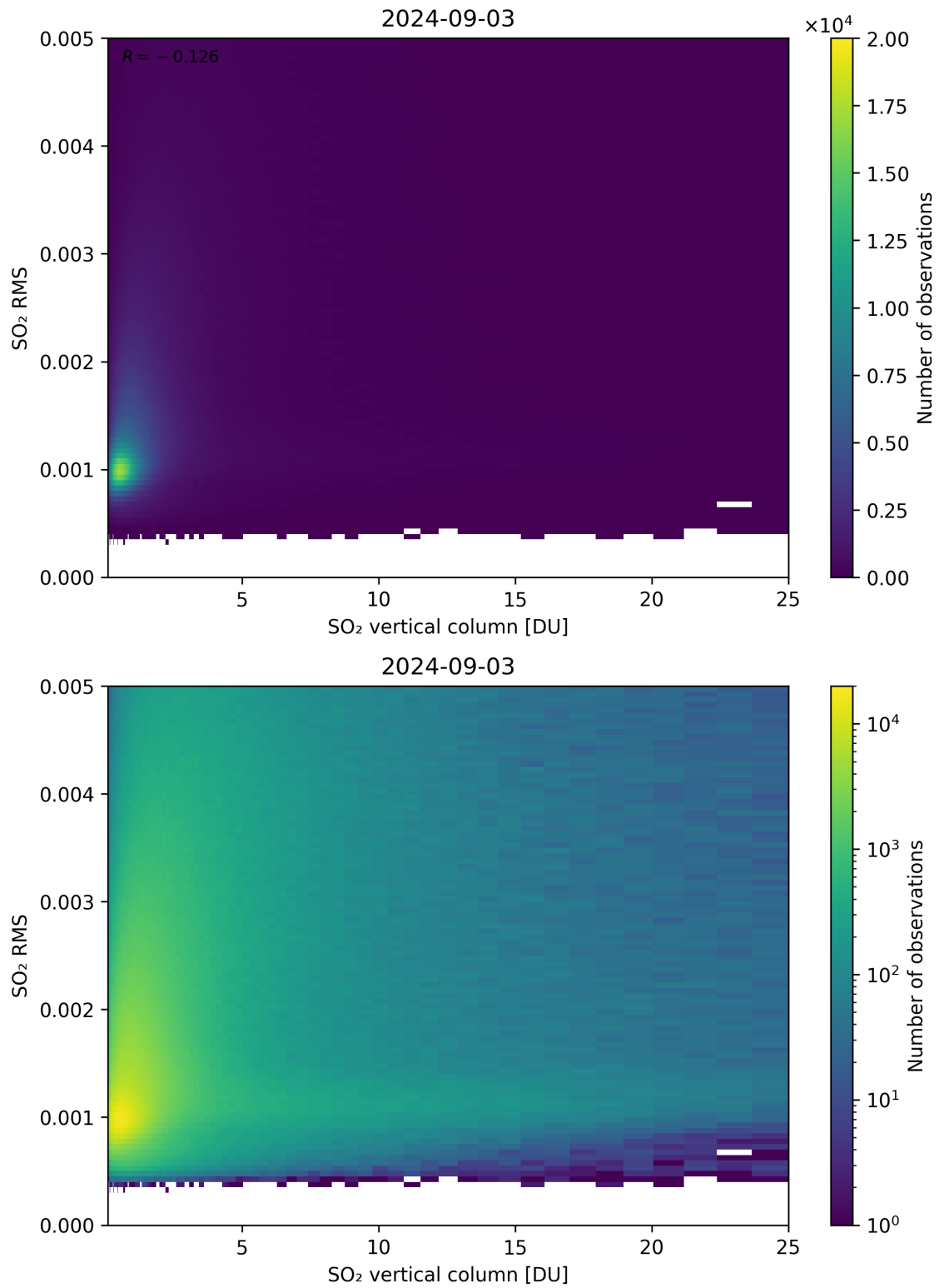
Figure 278: Scatter density plot of “SO 2 vertical column” against “SO 2 RMS” for 2024-09-02 to 2024-09-04.
