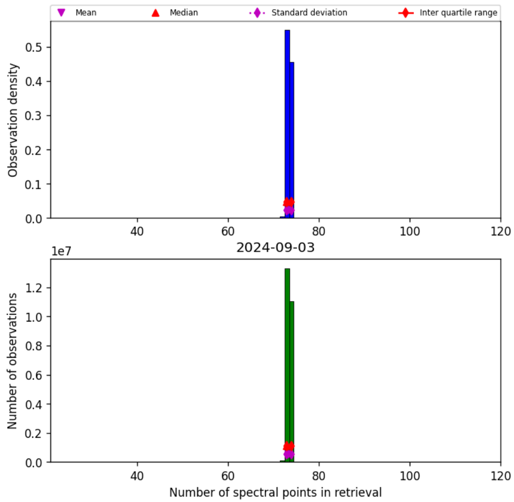
Figure 74: Histogram of “Number of spectral points in retrieval” for 2024-09-02 to 2024-09-04
