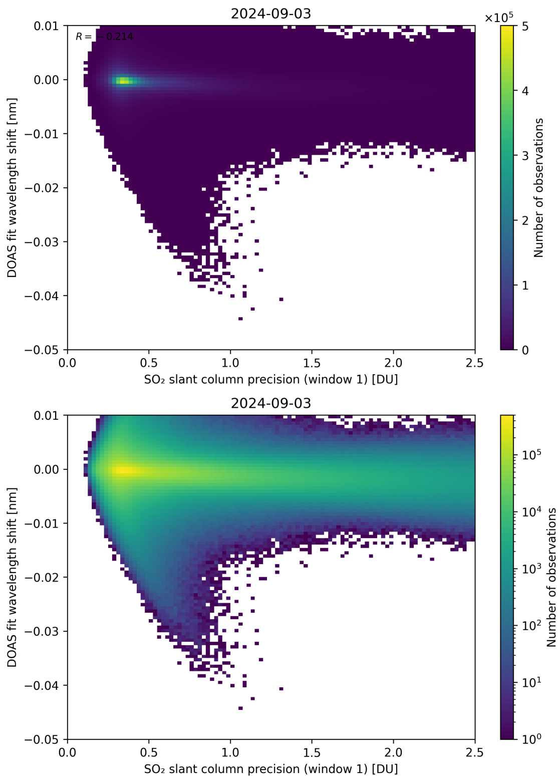
Figure 221: Scatter density plot of “SO 2 slant column precision (window 1)” against “DOAS fit wavelength shift” for 2024-09-02 to 2024-09-04.
