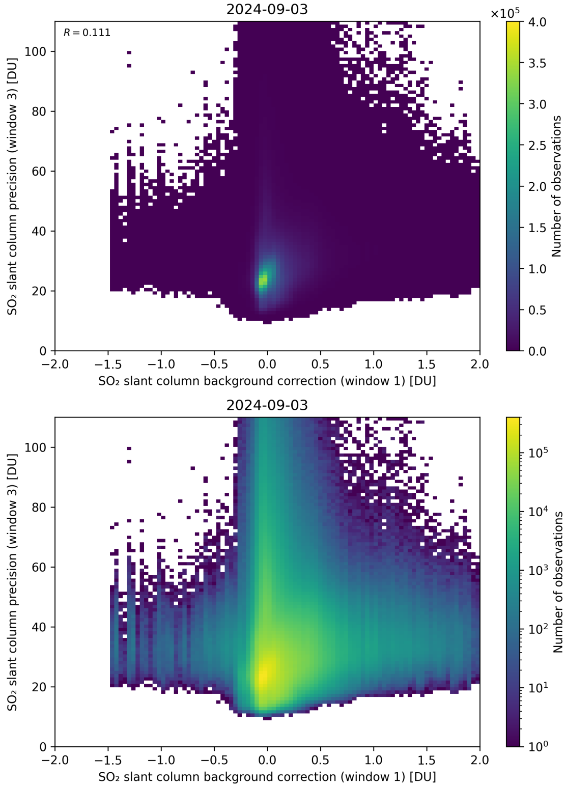
Figure 108: Scatter density plot of “SO 2 slant column background correction (window 1)” against “SO 2 slant column precision (window 3)” for 2024-09-02 to 2024-09-04.
