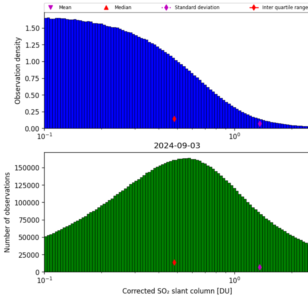
Figure 55: Histogram of “Corrected SO 2 slant column” for 2024-09-02 to 2024-09-04
