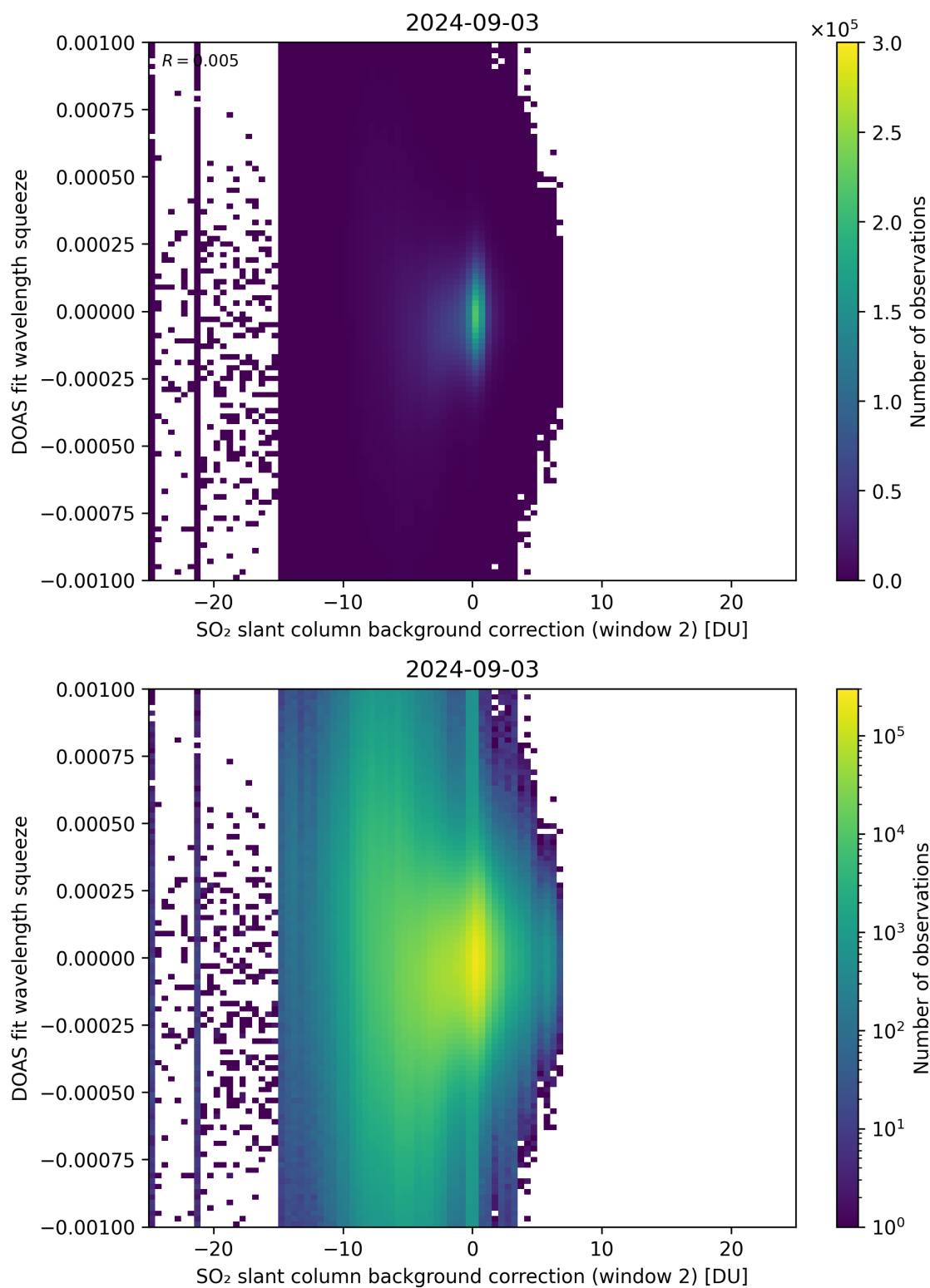
Figure 113: Scatter density plot of “SO 2 slant column background correction (window 2)” against “DOAS fit wavelength squeeze” for 2024-09-02 to 2024-09-04.
