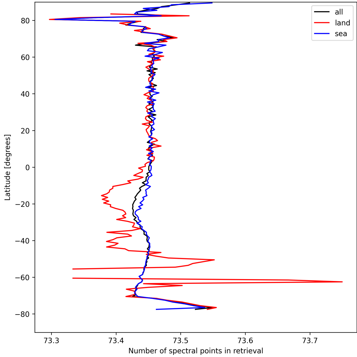
Figure 51: Zonal average of “Number of spectral points in retrieval” for 2024-09-02 to 2024-09-04.
