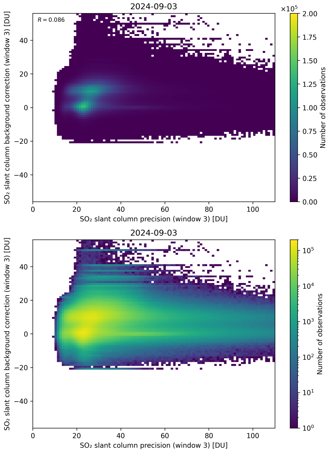
Figure 257: Scatter density plot of “SO 2 slant column precision (window 3)” against “SO 2 slant column background correction (window 3)” for 2024-09-02 to 2024-09-04.
