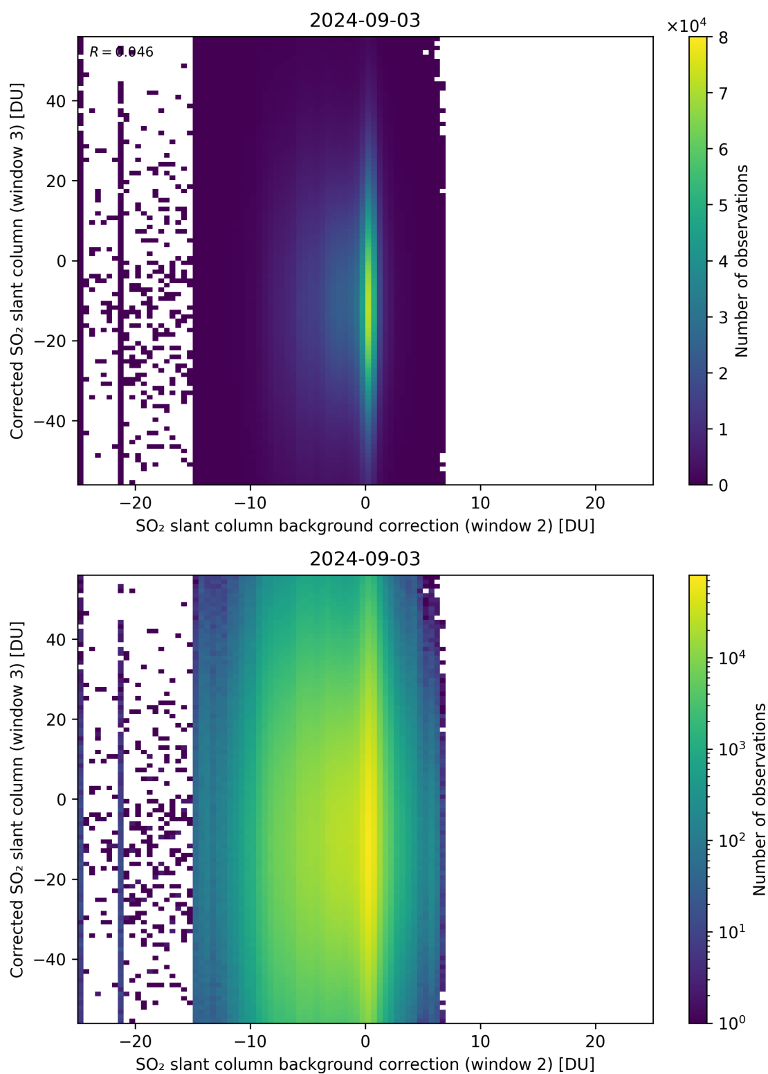
Figure 116: Scatter density plot of “SO 2 slant column background correction (window 2)” against “Corrected SO 2 slant column (window 3)” for 2024-09-02 to 2024-09-04.
