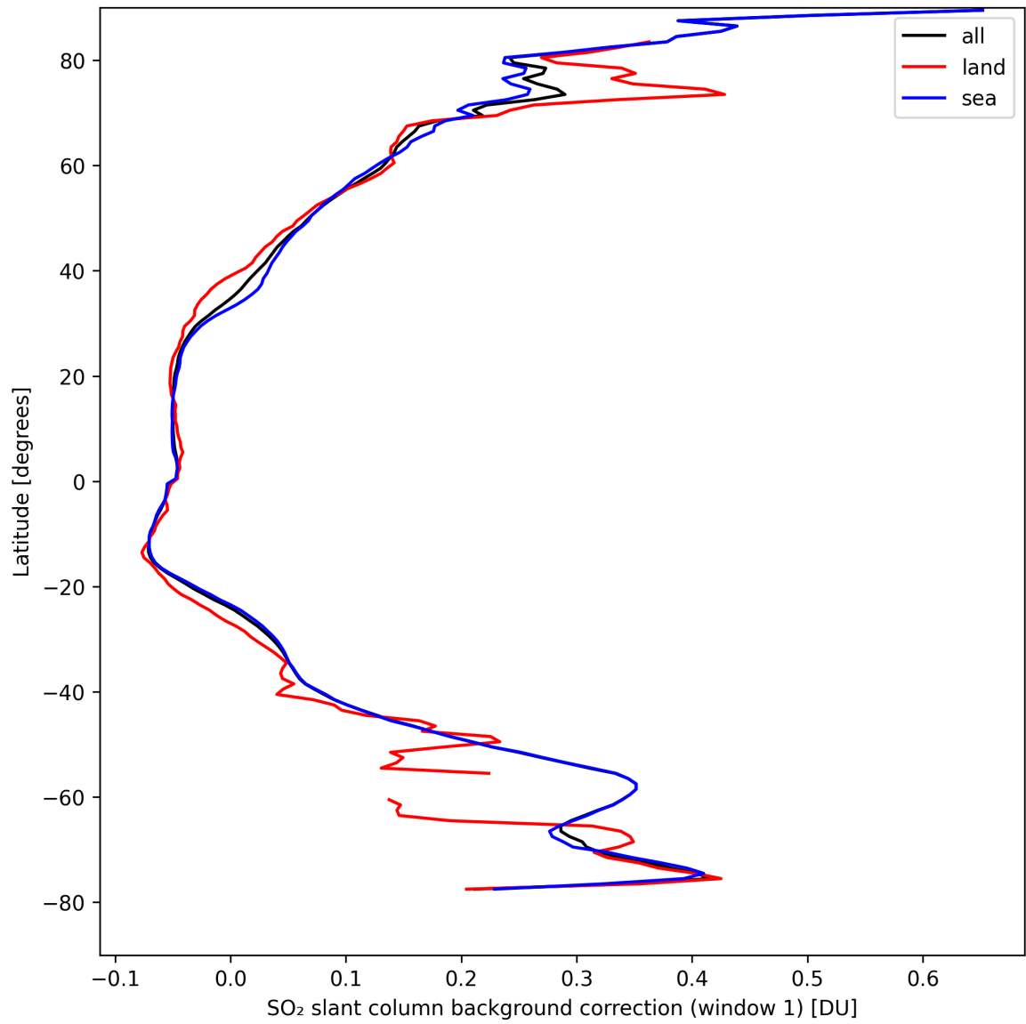
Figure 36: Zonal average of “SO 2 slant column background correction (window 1)” for 2024-09-02 to 2024-09-04.
