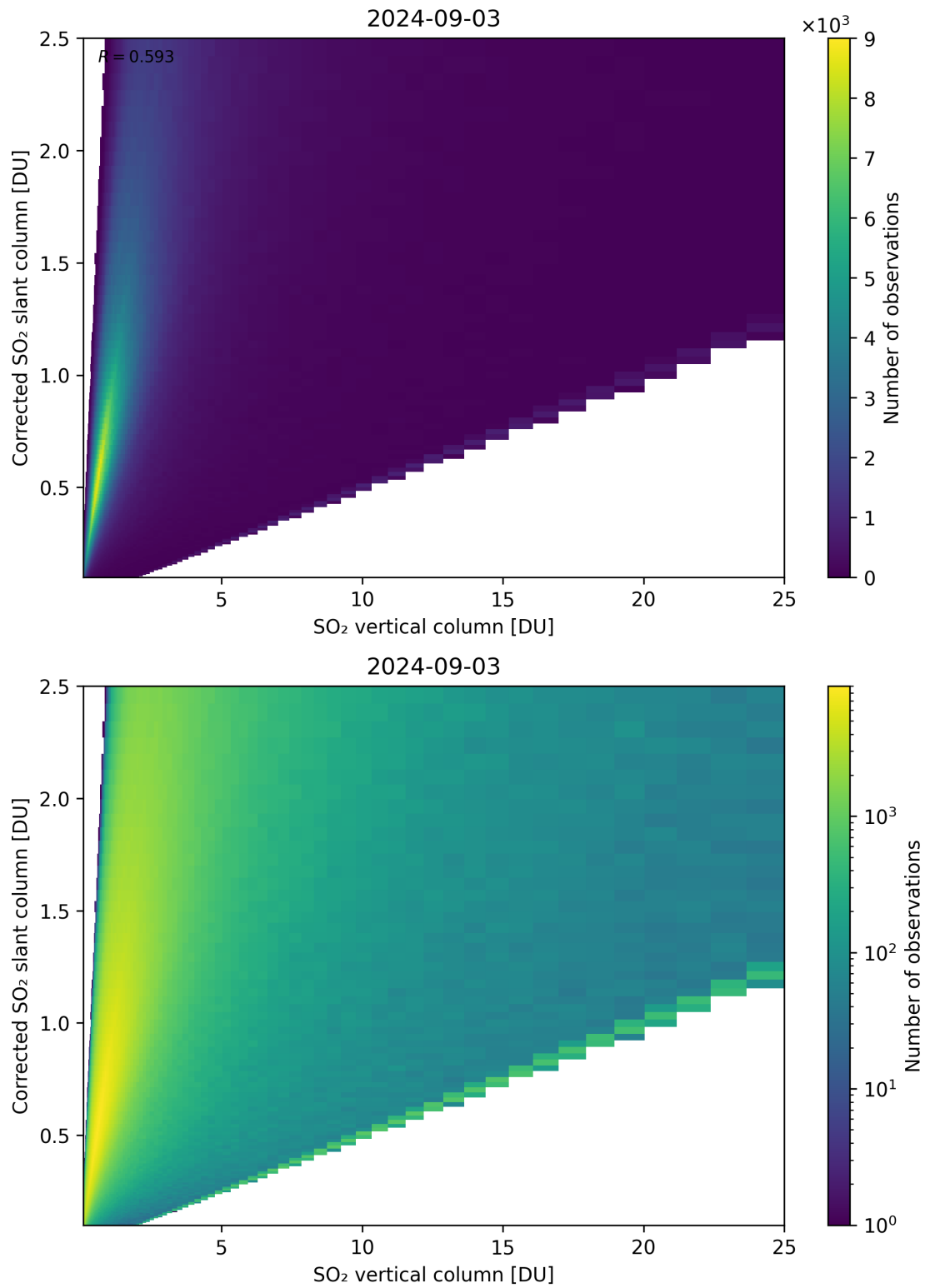
Figure 297: Scatter density plot of “SO 2 vertical column” against “Corrected SO 2 slant column” for 2024-09-02 to 2024-09-04.
