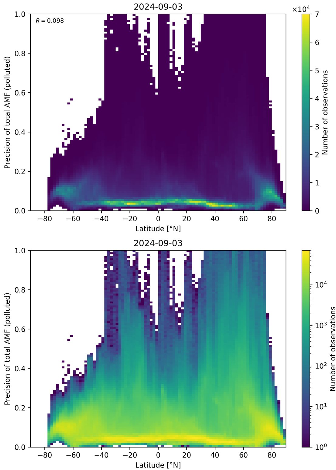
Figure 155: Scatter density plot of “Latitude” against “Precision of total AMF (polluted)” for 2024-09-02 to 2024-09-04.
