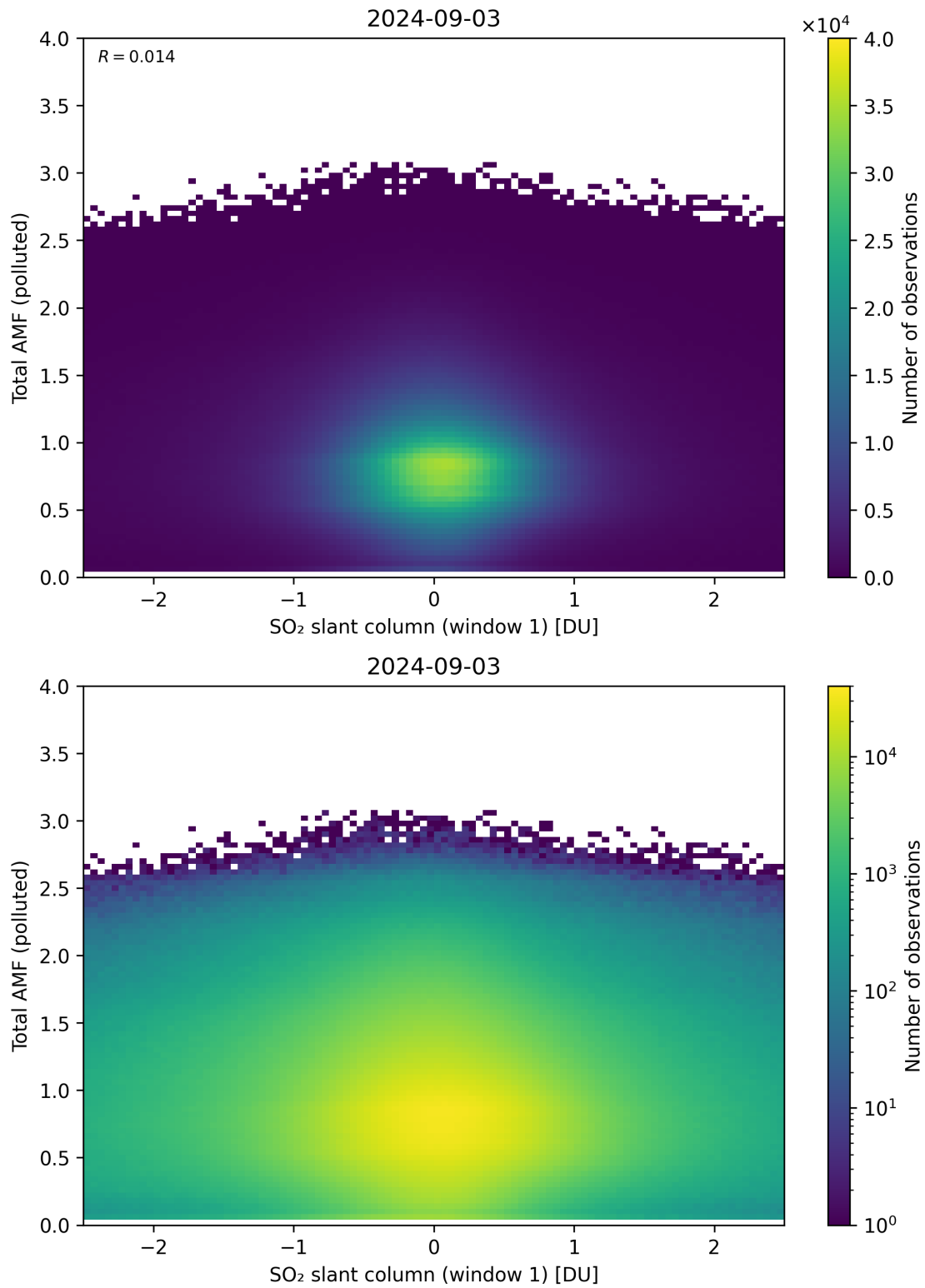
Figure 239: Scatter density plot of “SO 2 slant column (window 1)” against “Total AMF (polluted)” for 2024-09-02 to 2024-09-04.
