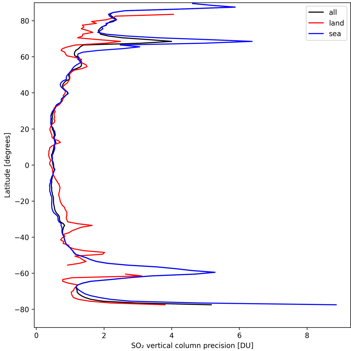
Figure 31: Zonal average of “SO 2 vertical column precision” for 2024-09-02 to 2024-09-04.
