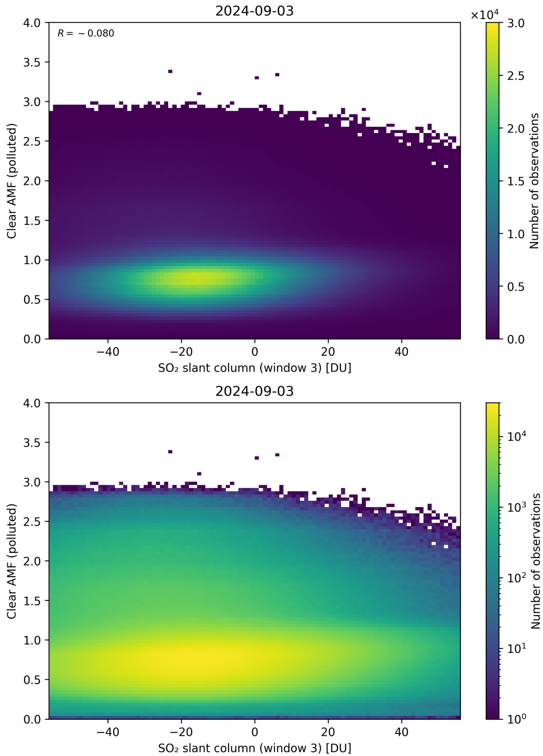
Figure 265: Scatter density plot of “SO 2 slant column (window 3)” against “Clear AMF (polluted)” for 2024-09-02 to 2024-09-04.
