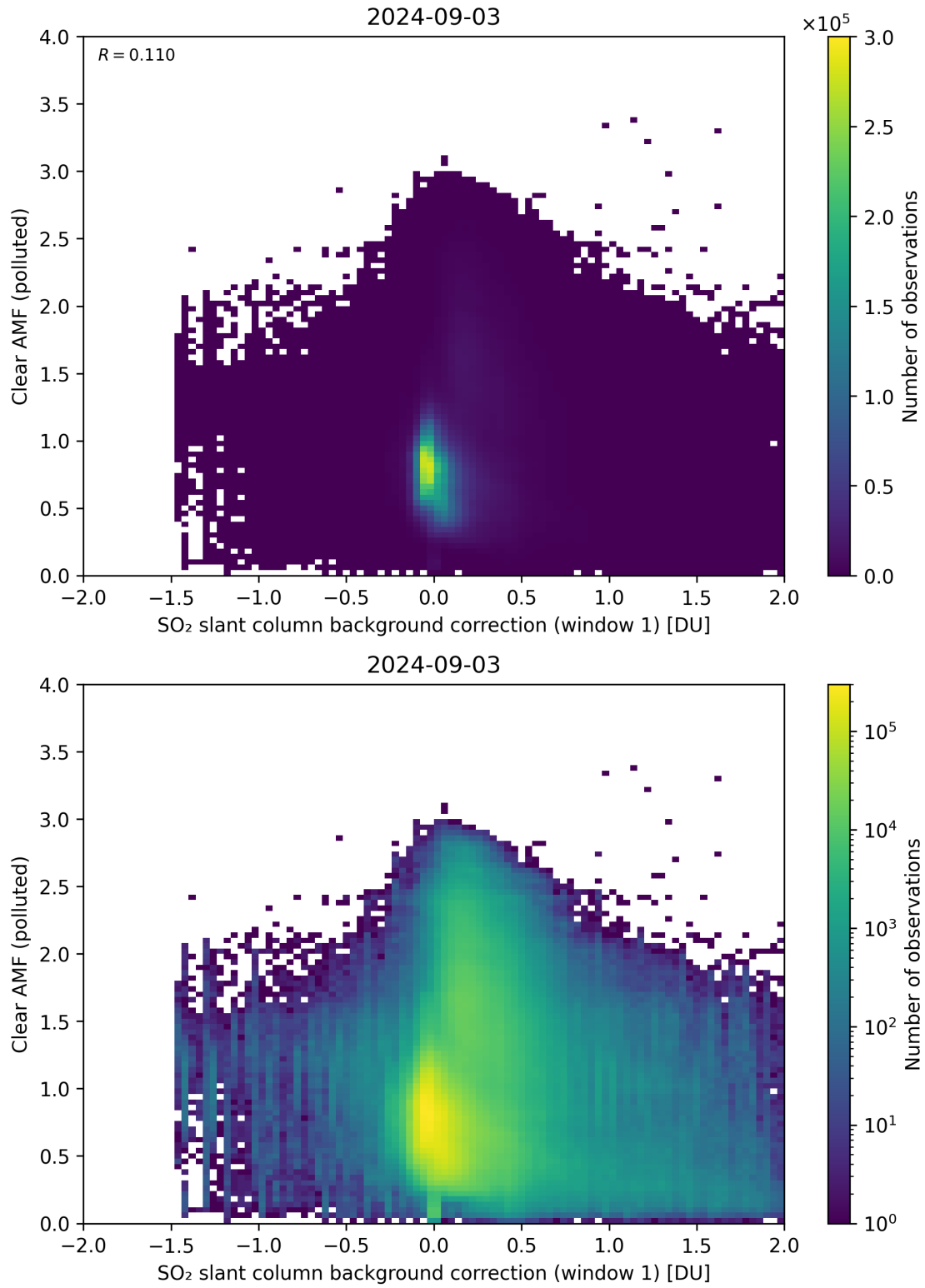
Figure 103: Scatter density plot of “SO 2 slant column background correction (window 1)” against “Clear AMF (polluted)” for 2024-09-02 to 2024-09-04.
