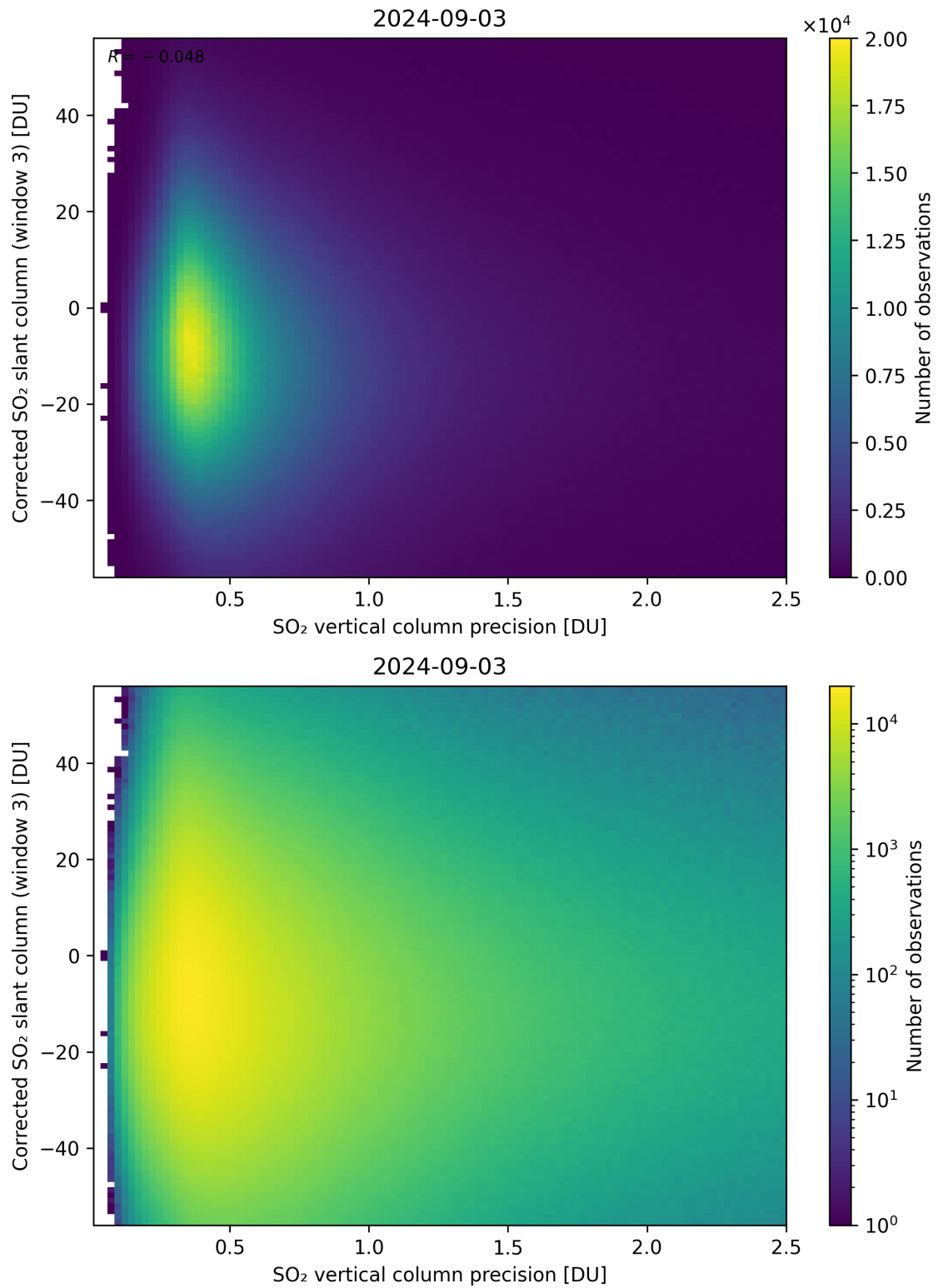
Figure 288: Scatter density plot of “SO 2 vertical column precision” against “Corrected SO 2 slant column (window 3)” for 2024-09-02 to 2024-09-04.
