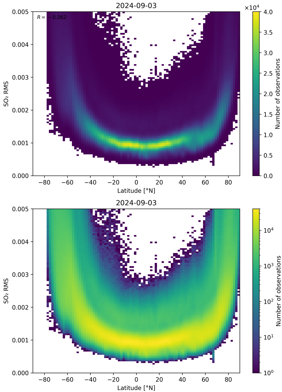
Figure 144: Scatter density plot of “Latitude” against “SO 2 RMS” for 2024-09-02 to 2024-09-04.
