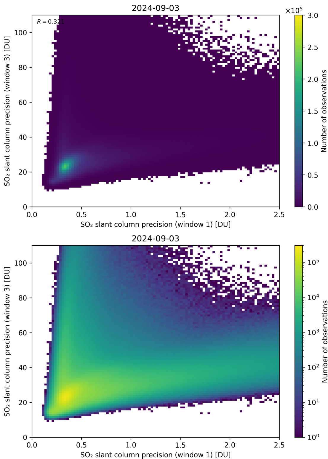
Figure 229: Scatter density plot of “SO 2 slant column precision (window 1)” against “SO 2 slant column precision (window 3)” for 2024-09-02 to 2024-09-04.
