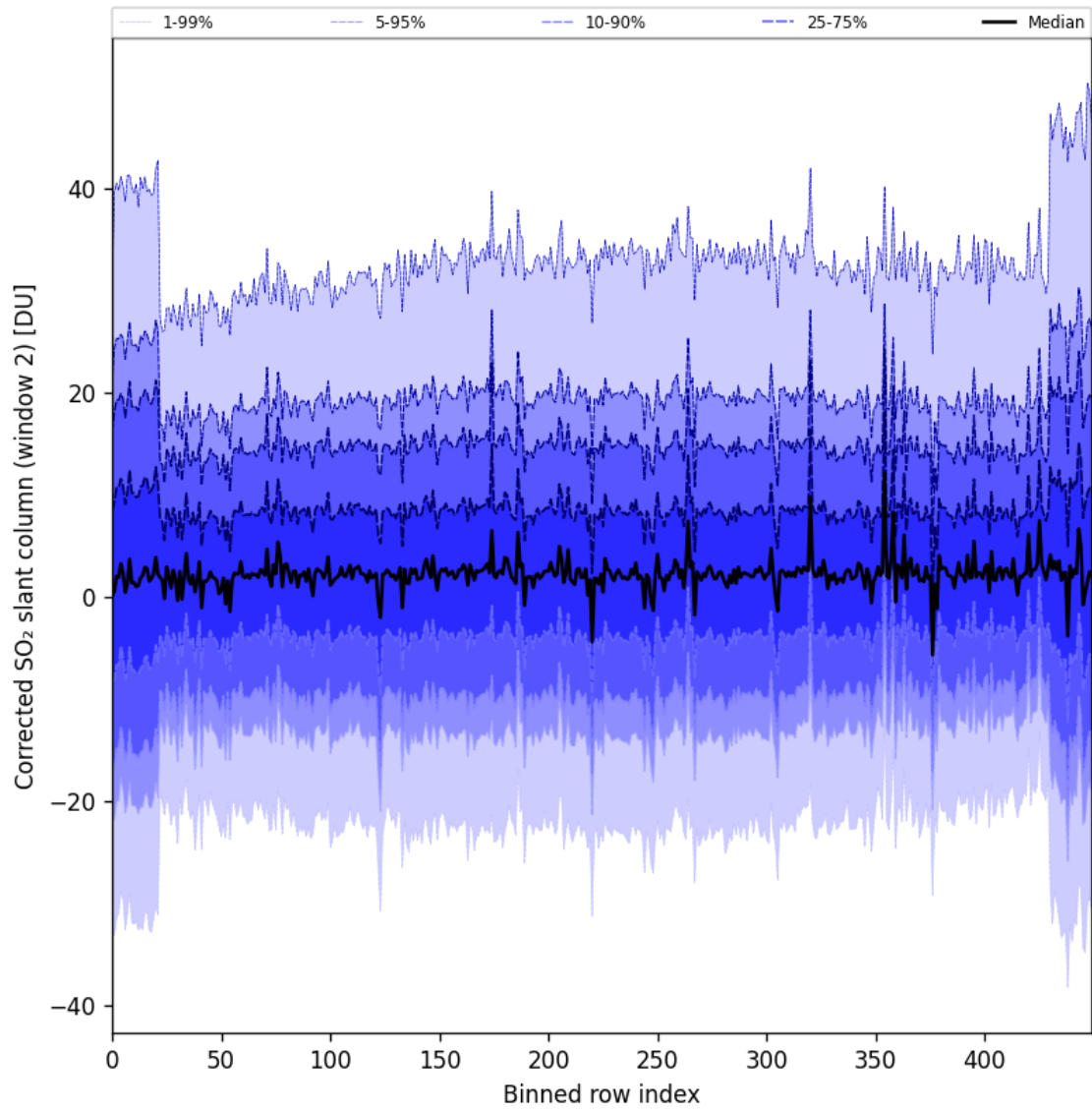
Figure 85: Along track statistics of “Corrected SO 2 slant column (window 2)” for 2024-09-02 to 2024-09-04
