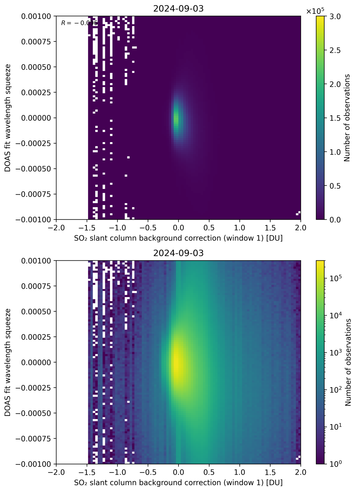
Figure 101: Scatter density plot of “SO 2 slant column background correction (window 1)” against “DOAS fit wavelength squeeze” for 2024-09-02 to 2024-09-04.
