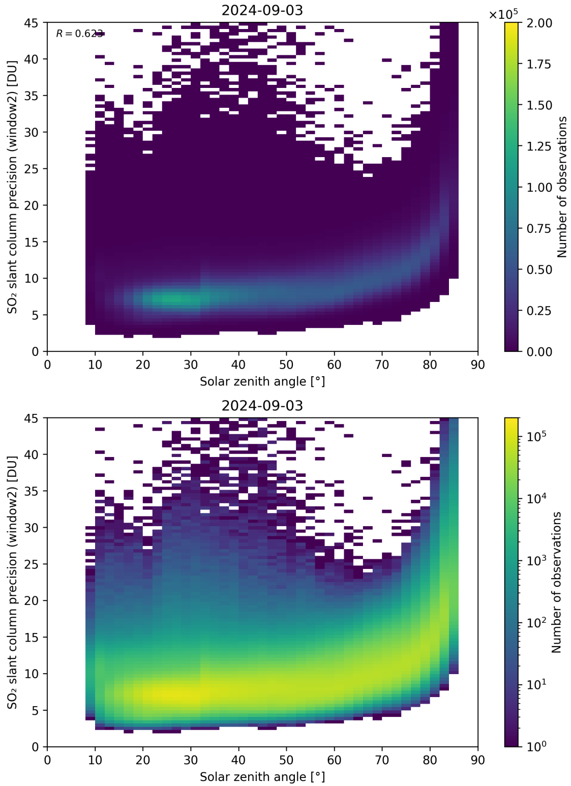
Figure 171: Scatter density plot of “Solar zenith angle” against “SO 2 slant column precision (window2)” for 2024-09-02 to 2024-09-04.
