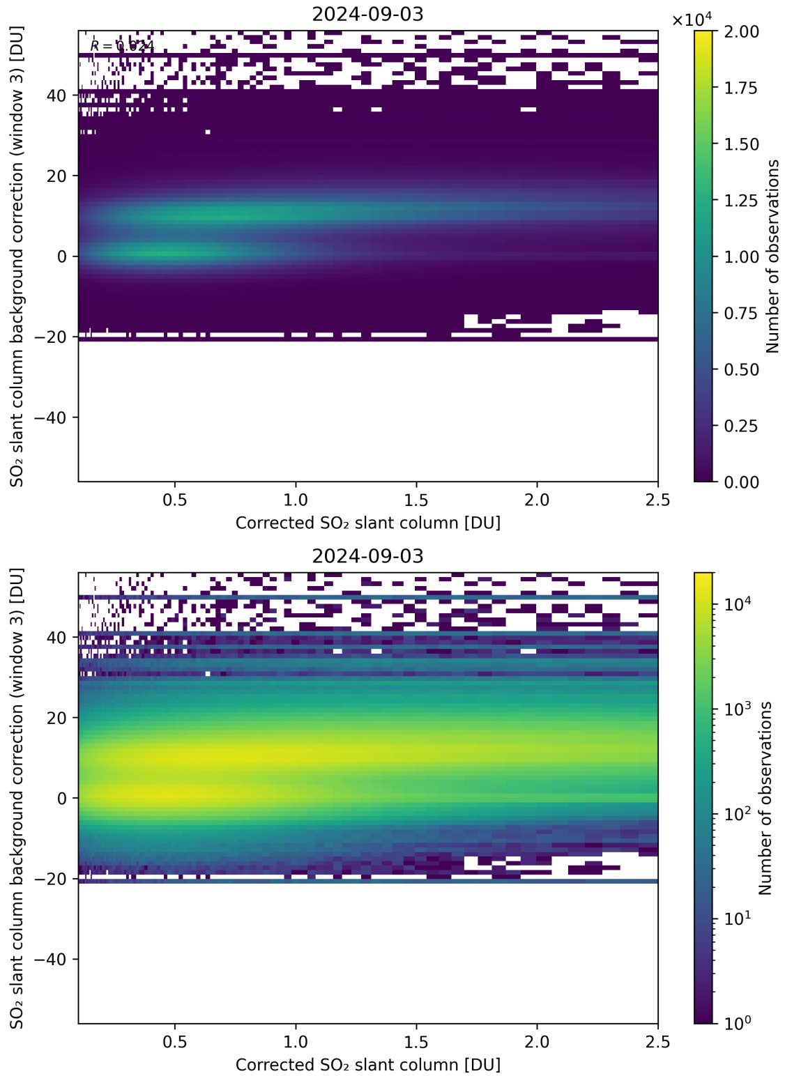
Figure 180: Scatter density plot of “Corrected SO 2 slant column” against “SO 2 slant column background correction (window 3)” for 2024-09-02 to 2024-09-04.
