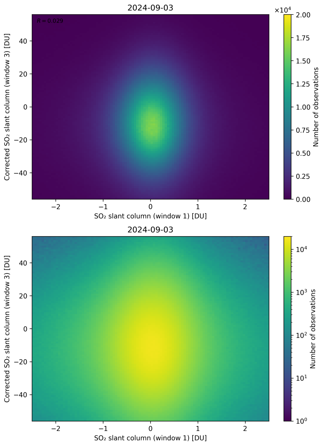
Figure 234: Scatter density plot of “SO 2 slant column (window 1)” against “Corrected SO 2 slant column (window 3)” for 2024-09-02 to 2024-09-04.
