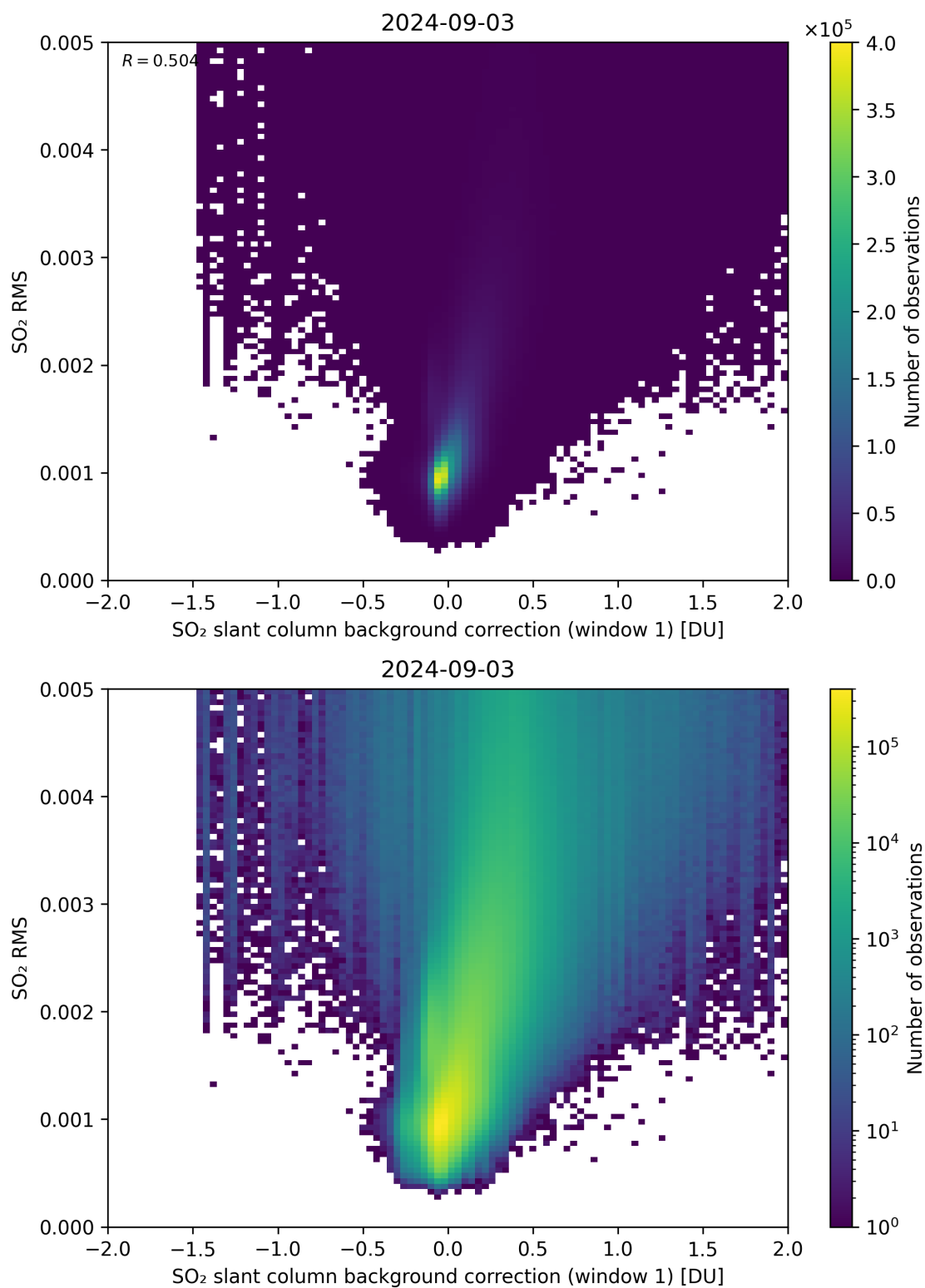
Figure 102: Scatter density plot of “SO 2 slant column background correction (window 1)” against “SO 2 RMS” for 2024-09-02 to 2024-09-04.
