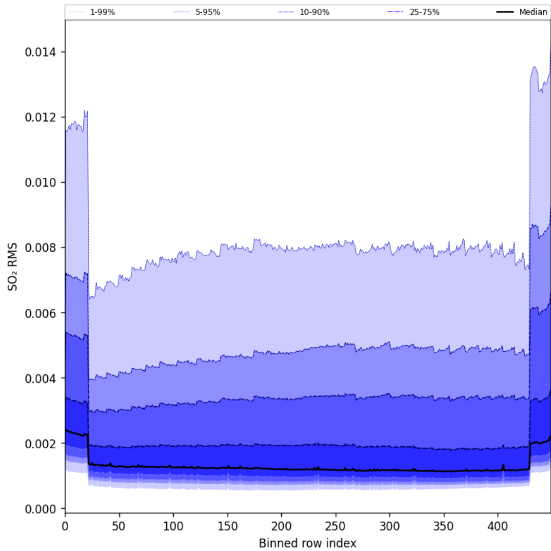
Figure 93: Along track statistics of “SO 2 RMS” for 2024-09-02 to 2024-09-04
