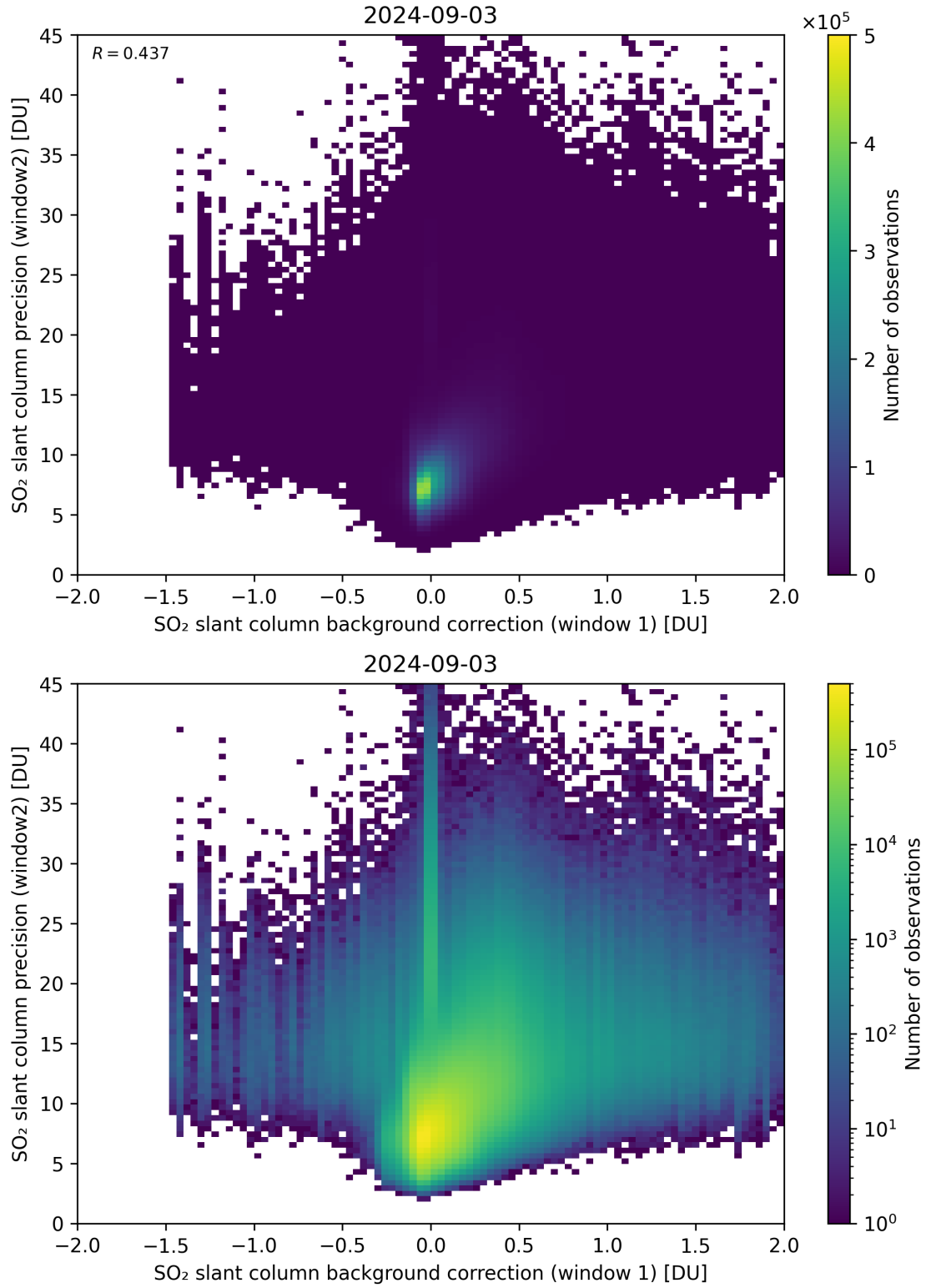
Figure 106: Scatter density plot of “SO 2 slant column background correction (window 1)” against “SO 2 slant column precision (window2)” for 2024-09-02 to 2024-09-04.
