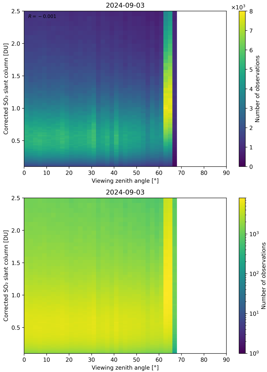
Figure 317: Scatter density plot of “Viewing zenith angle” against “Corrected SO 2 slant column” for 2024-09-02 to 2024-09-04.
