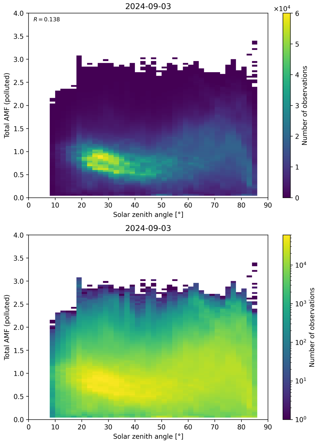
Figure 174: Scatter density plot of “Solar zenith angle” against “Total AMF (polluted)” for 2024-09-02 to 2024-09-04.
