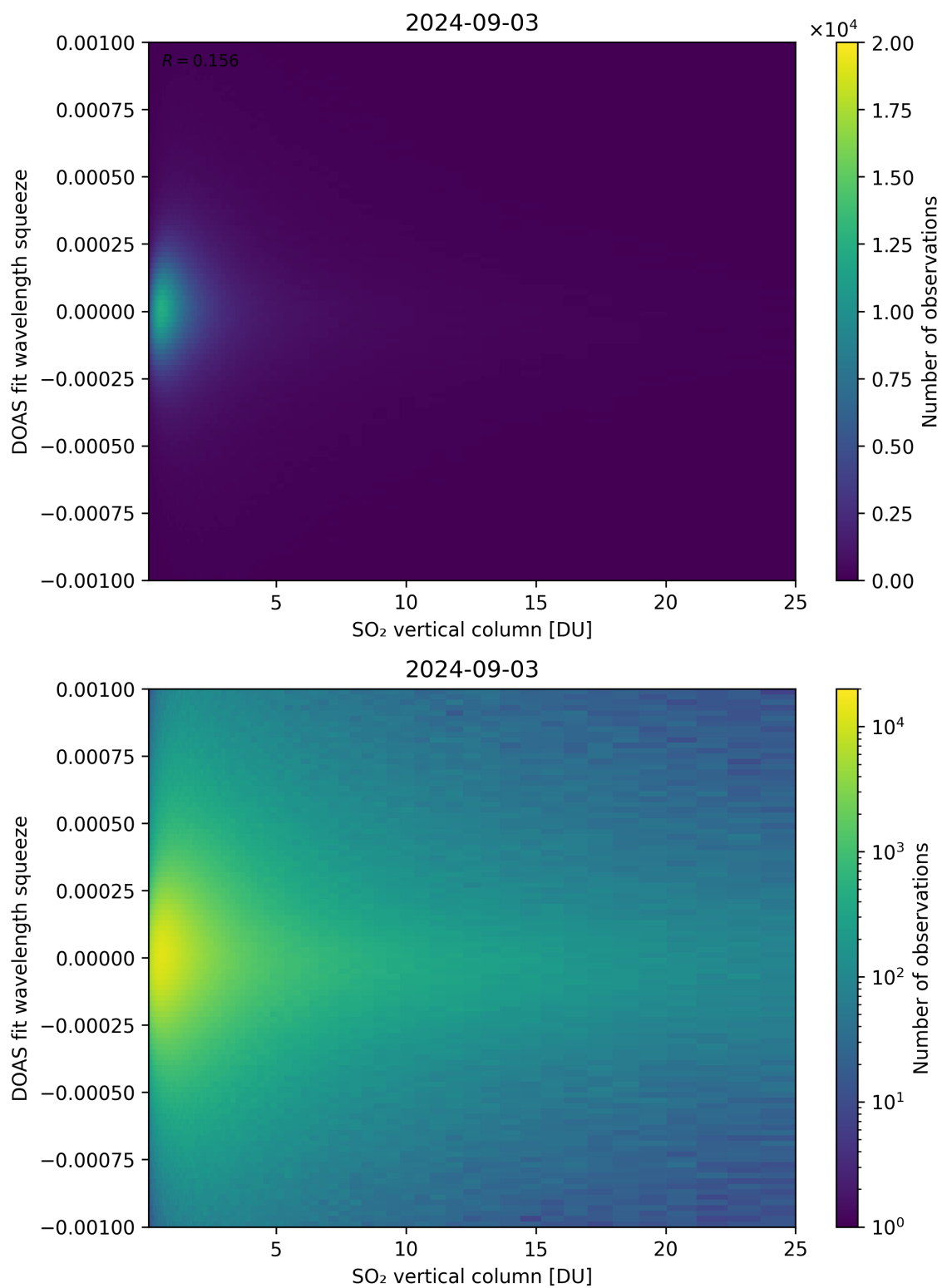
Figure 277: Scatter density plot of “SO 2 vertical column” against “DOAS fit wavelength squeeze” for 2024-09-02 to 2024-09-04.
