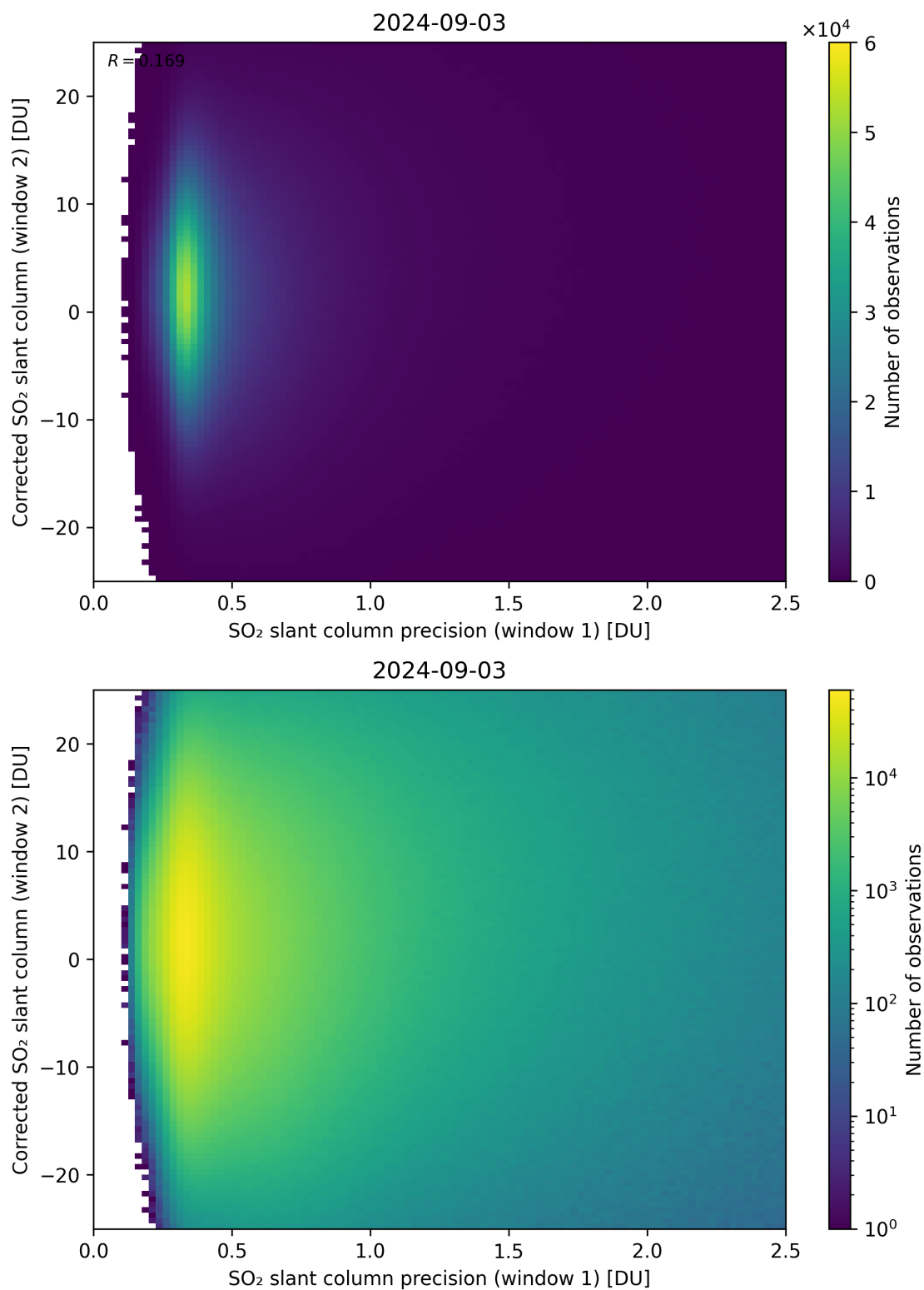
Figure 225: Scatter density plot of “SO 2 slant column precision (window 1)” against “Corrected SO 2 slant column (window 2)” for 2024-09-02 to 2024-09-04.
