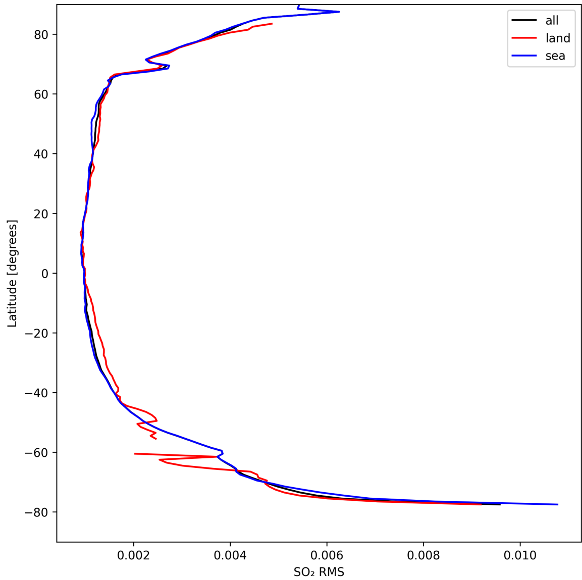
Figure 47: Zonal average of “SO 2 RMS” for 2024-09-02 to 2024-09-04.
