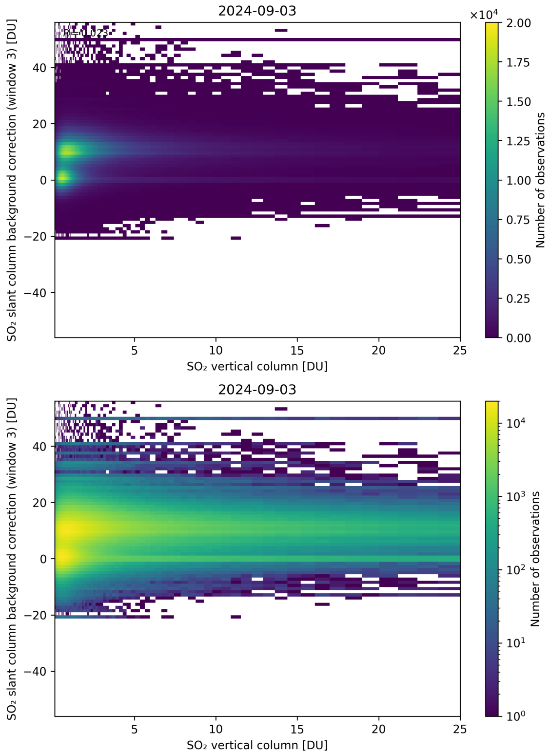
Figure 275: Scatter density plot of “SO 2 vertical column” against “SO 2 slant column background correction (window 3)” for 2024-09-02 to 2024-09-04.
