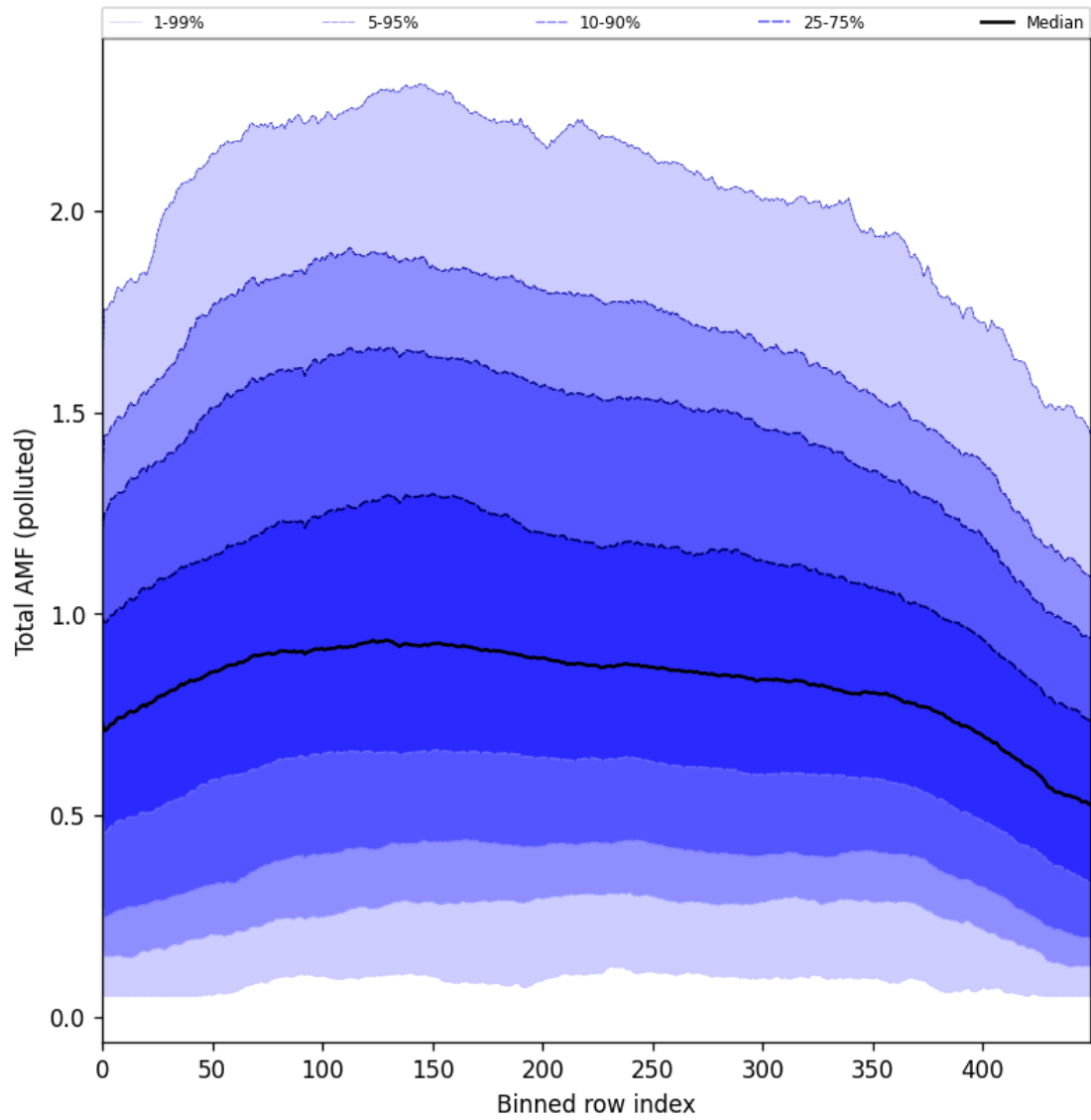
Figure 94: Along track statistics of “Total AMF (polluted)” for 2024-09-02 to 2024-09-04
