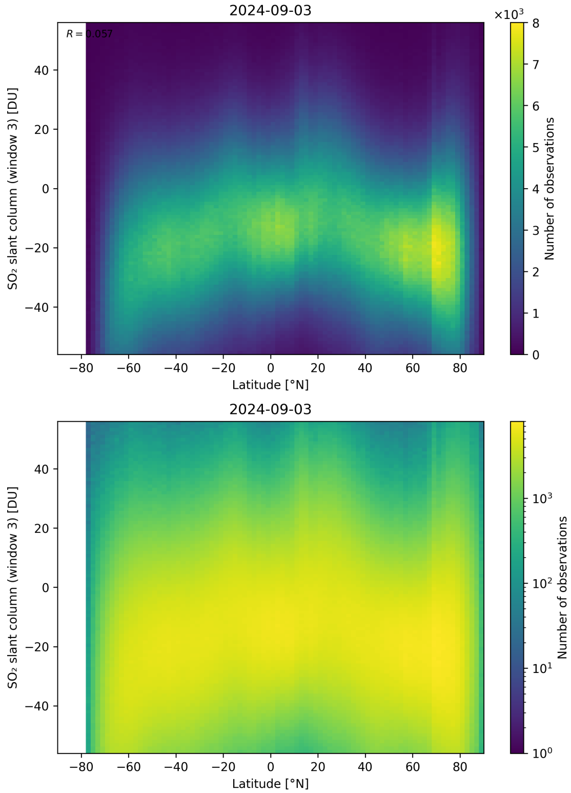
Figure 152: Scatter density plot of “Latitude” against “SO 2 slant column (window 3)” for 2024-09-02 to 2024-09-04.
