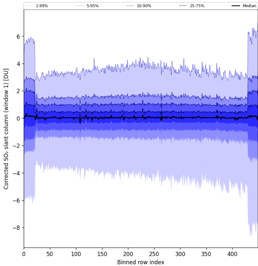
Figure 81: Along track statistics of “Corrected SO 2 slant column (window 1)” for 2024-09-02 to 2024-09-04
