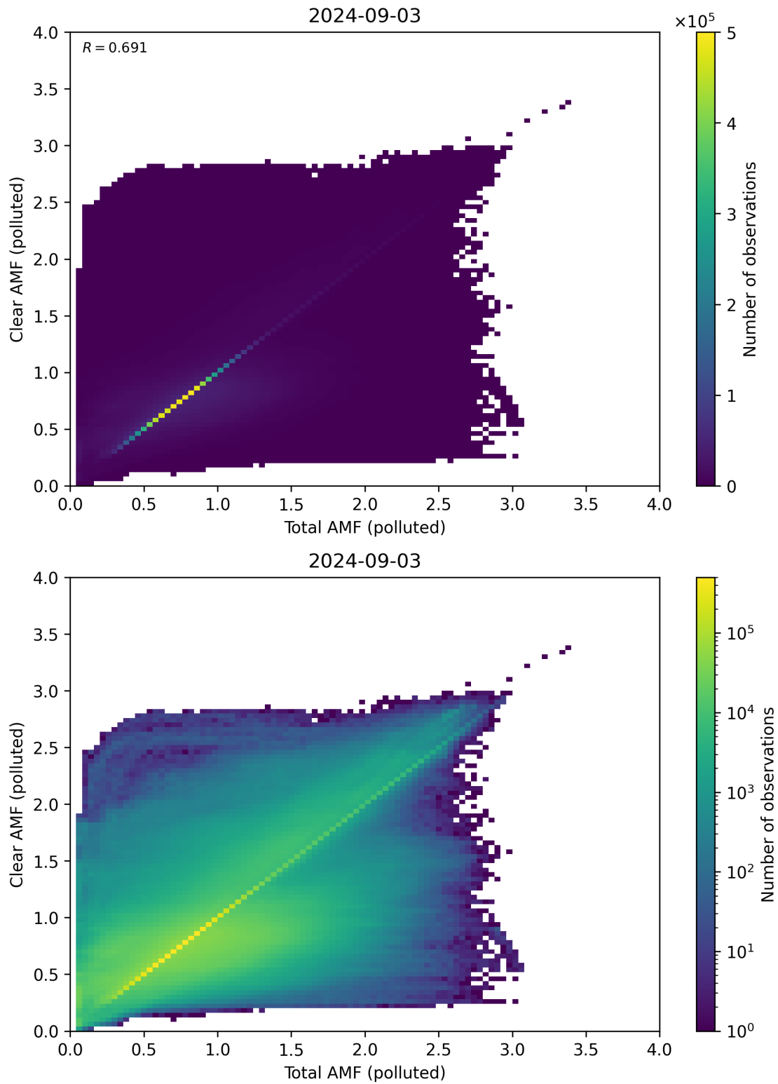
Figure 271: Scatter density plot of “Total AMF (polluted)” against “Clear AMF (polluted)” for 2024-09-02 to 2024-09-04.
