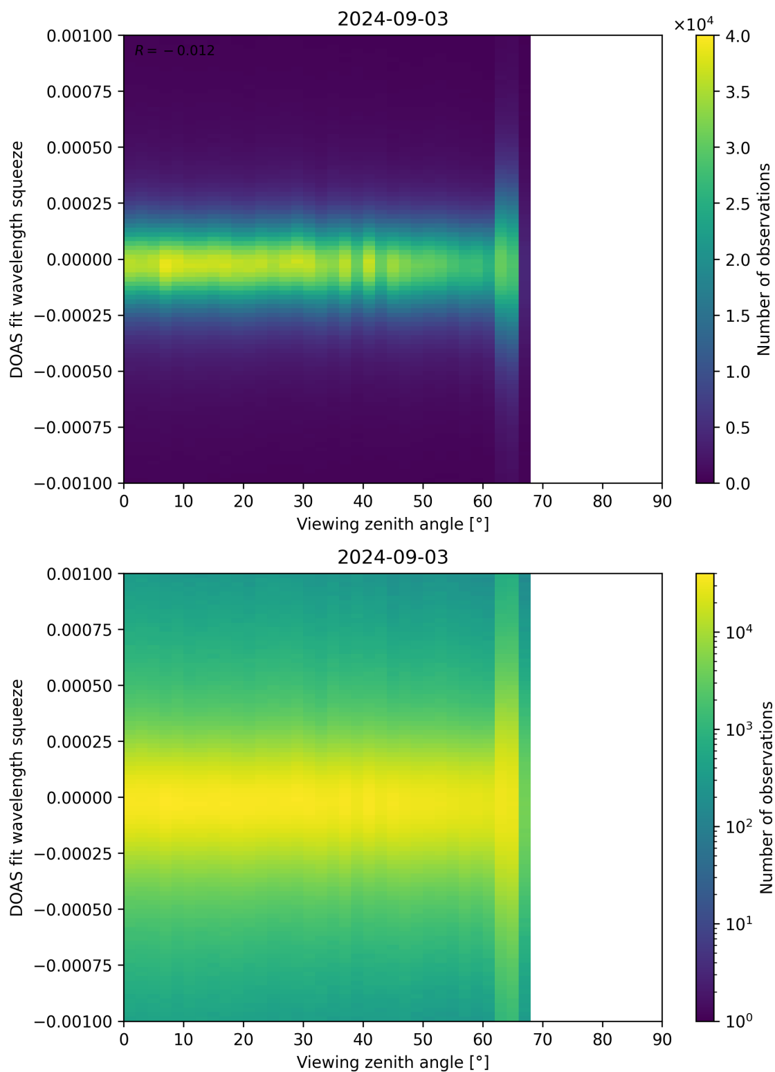
Figure 312: Scatter density plot of “Viewing zenith angle” against “DOAS fit wavelength squeeze” for 2024-09-02 to 2024-09-04.
