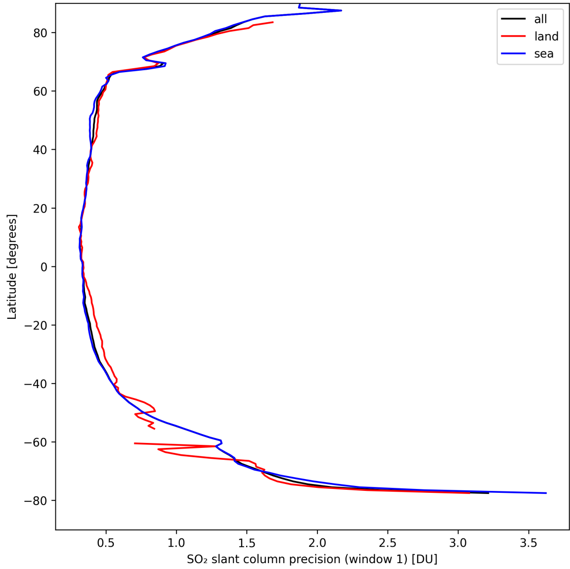
Figure 34: Zonal average of “SO 2 slant column precision (window 1)” for 2024-09-02 to 2024-09-04.
