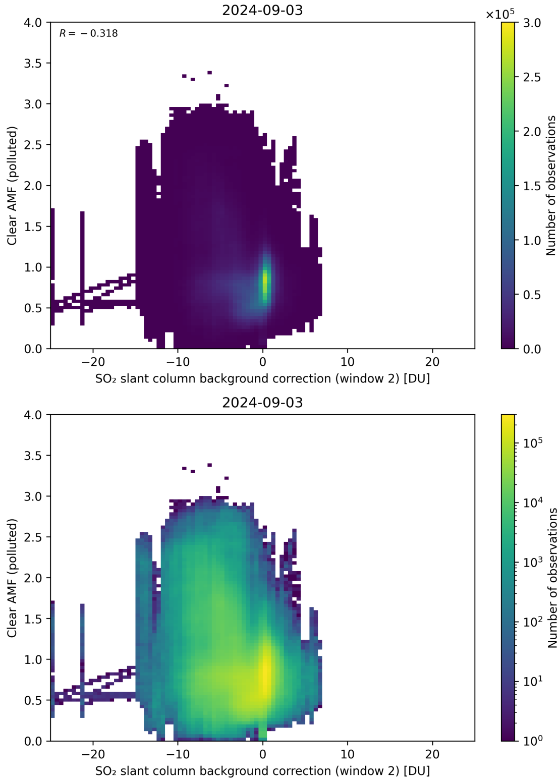
Figure 115: Scatter density plot of “SO 2 slant column background correction (window 2)” against “Clear AMF (polluted)” for 2024-09-02 to 2024-09-04.
