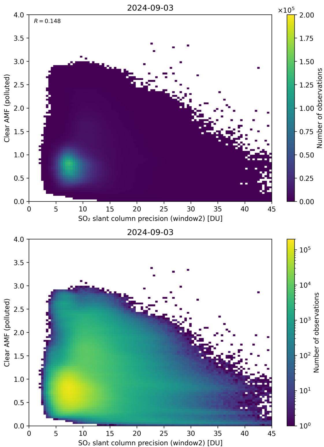
Figure 246: Scatter density plot of “SO 2 slant column precision (window2)” against “Clear AMF (polluted)” for 2024-09-02 to 2024-09-04.
