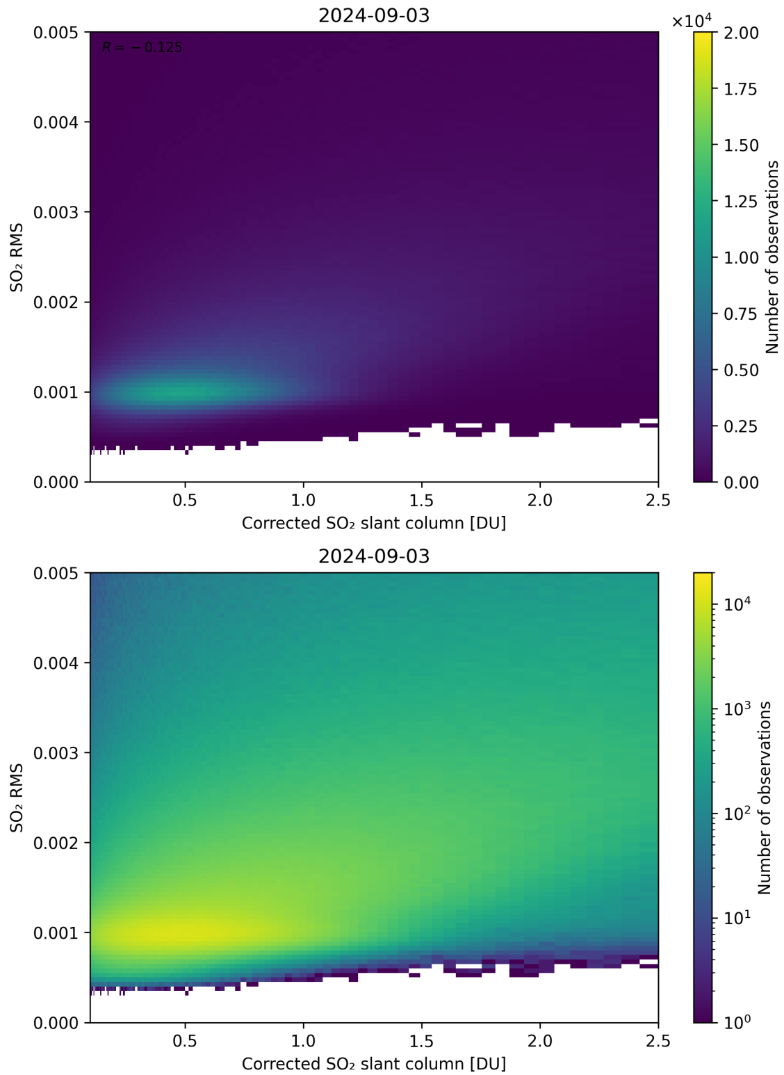
Figure 183: Scatter density plot of “Corrected SO 2 slant column” against “SO 2 RMS” for 2024-09-02 to 2024-09-04.
