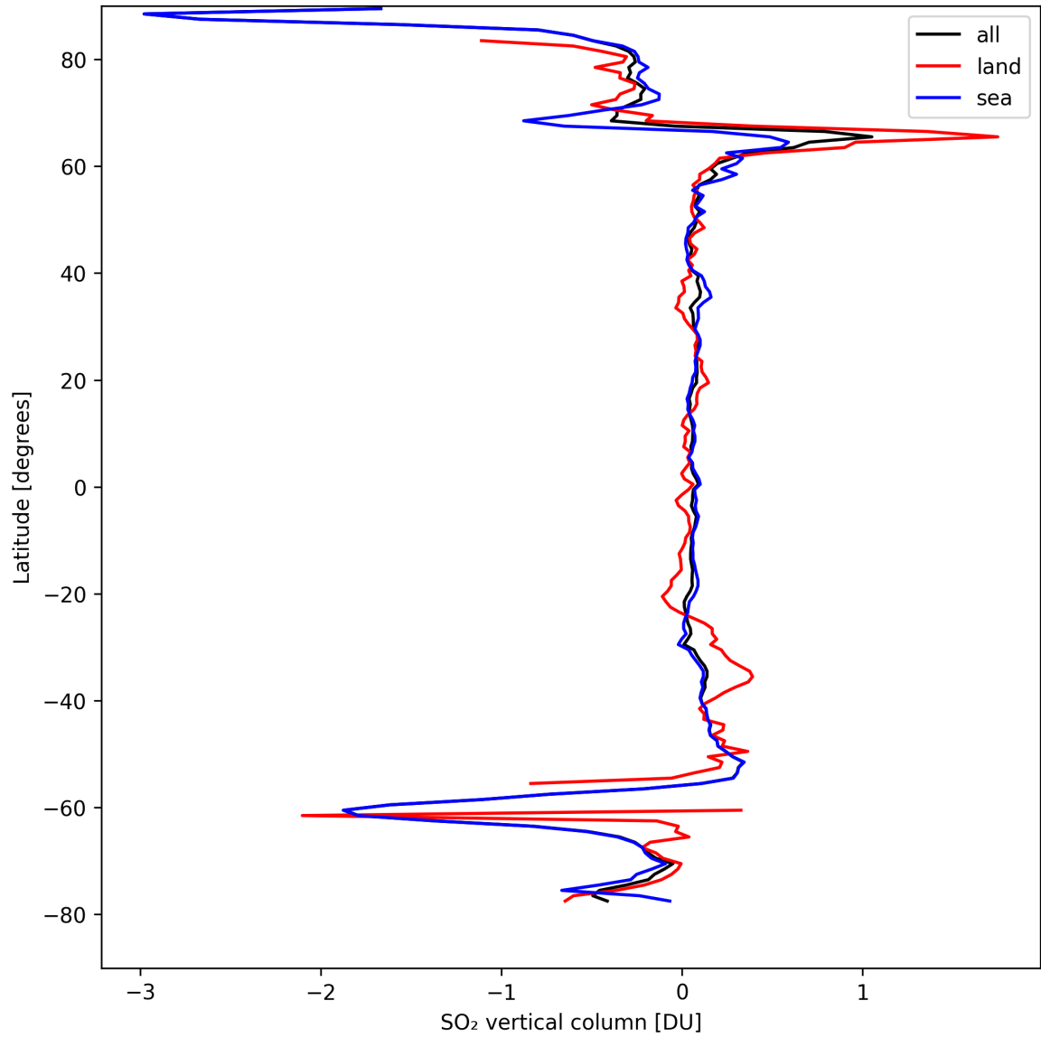
Figure 30: Zonal average of “SO 2 vertical column” for 2024-09-02 to 2024-09-04.
