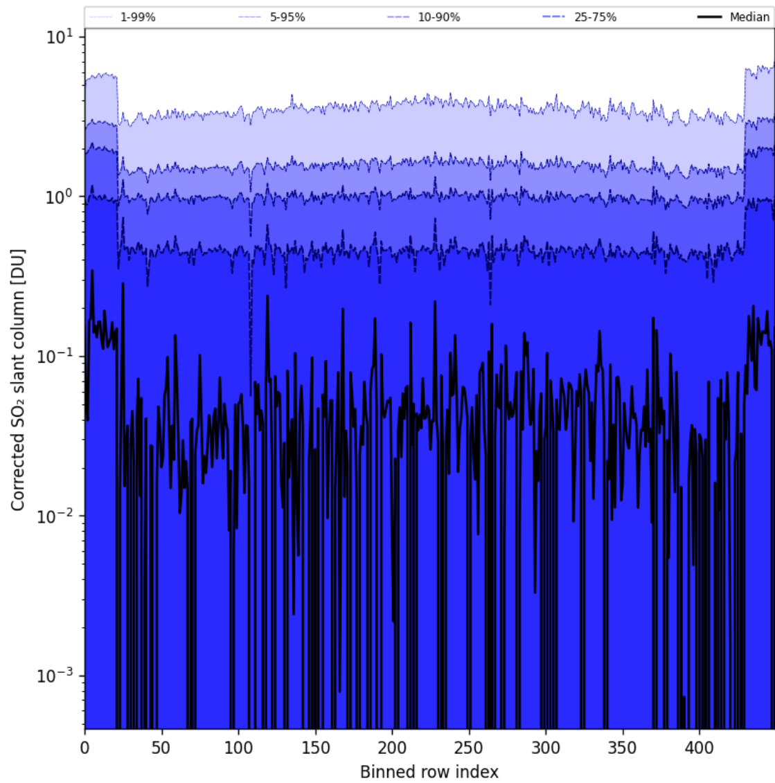
Figure 78: Along track statistics of “Corrected SO 2 slant column” for 2024-09-02 to 2024-09-04
