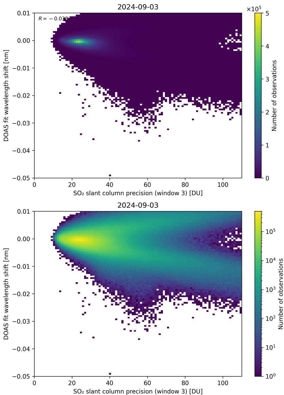
Figure 258: Scatter density plot of “SO 2 slant column precision (window 3)” against “DOAS fit wavelength shift” for 2024-09-02 to 2024-09-04.
