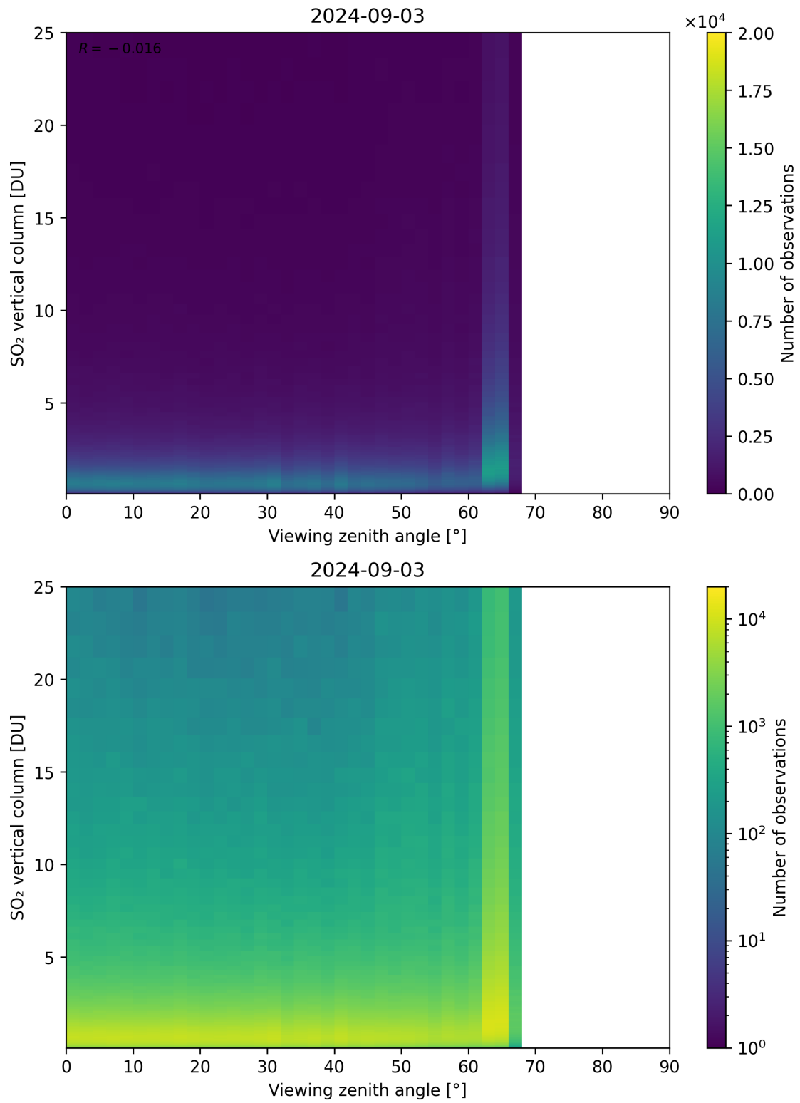
Figure 327: Scatter density plot of “Viewing zenith angle” against “SO 2 vertical column” for 2024-09-02 to 2024-09-04.
