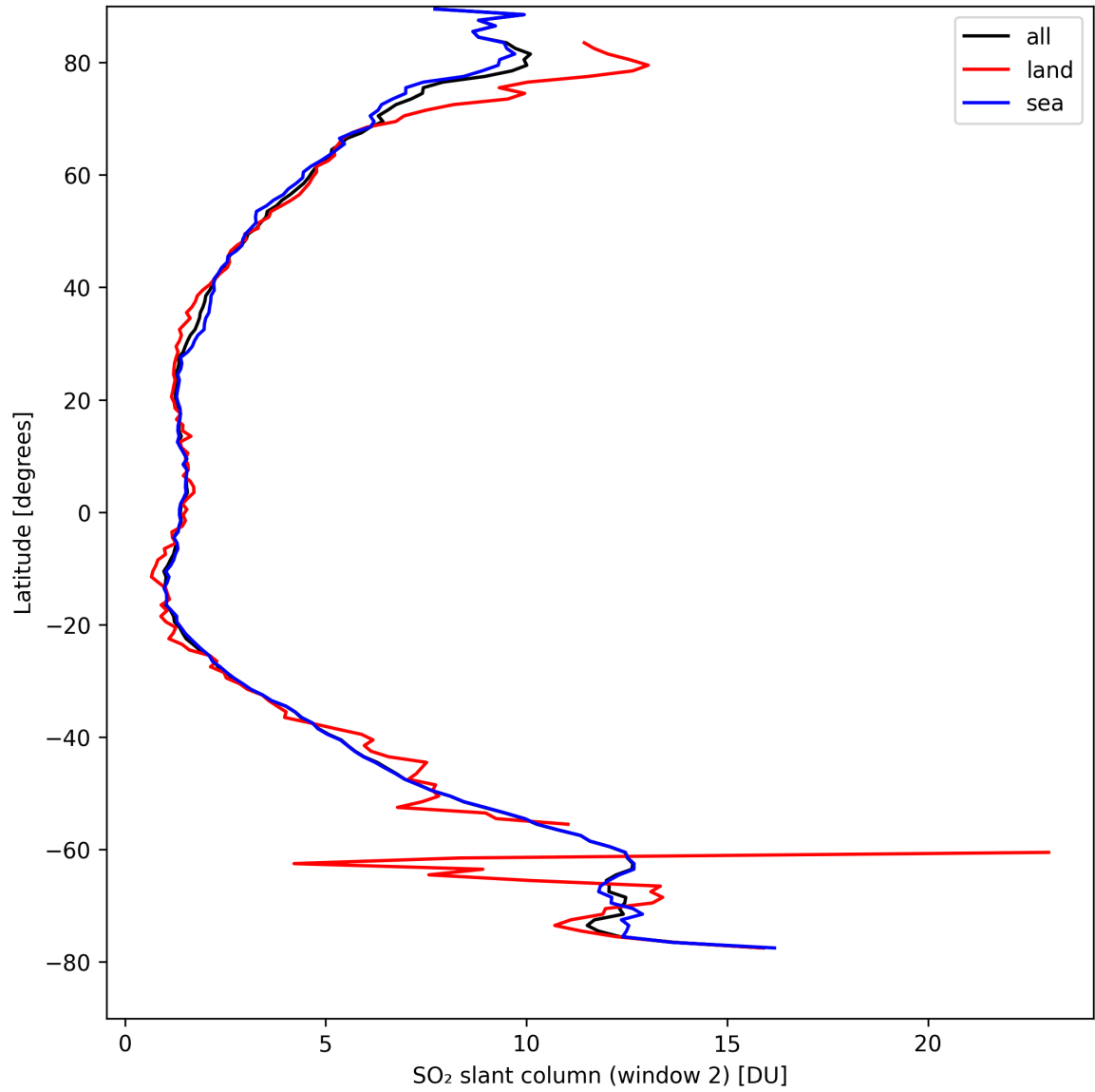
Figure 37: Zonal average of “SO 2 slant column (window 2)” for 2024-09-02 to 2024-09-04.
