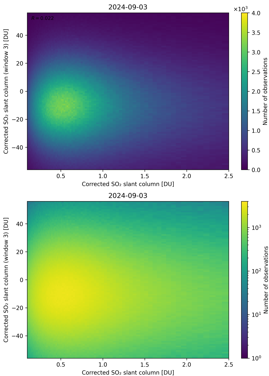
Figure 186: Scatter density plot of “Corrected SO 2 slant column” against “Corrected SO 2 slant column (window 3)” for 2024-09-02 to 2024-09-04.
