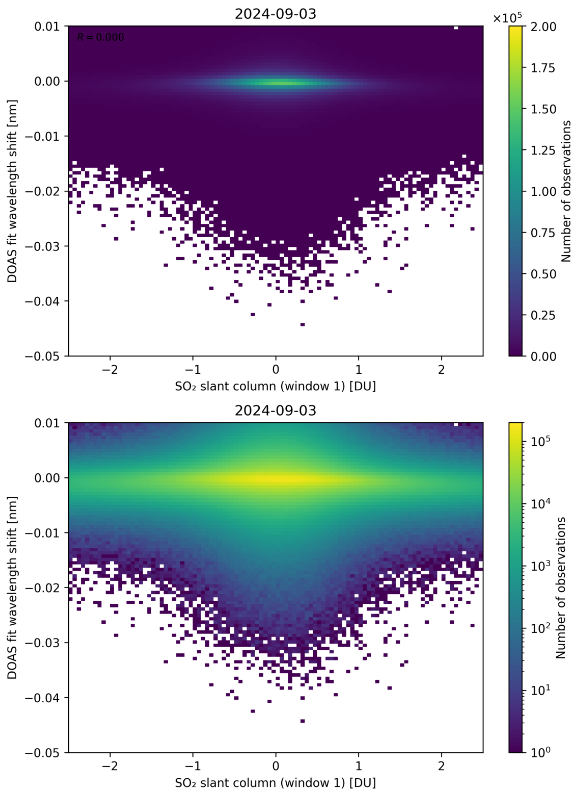
Figure 215: Scatter density plot of “SO 2 slant column (window 1)” against “DOAS fit wavelength shift” for 2024-09-02 to 2024-09-04.
