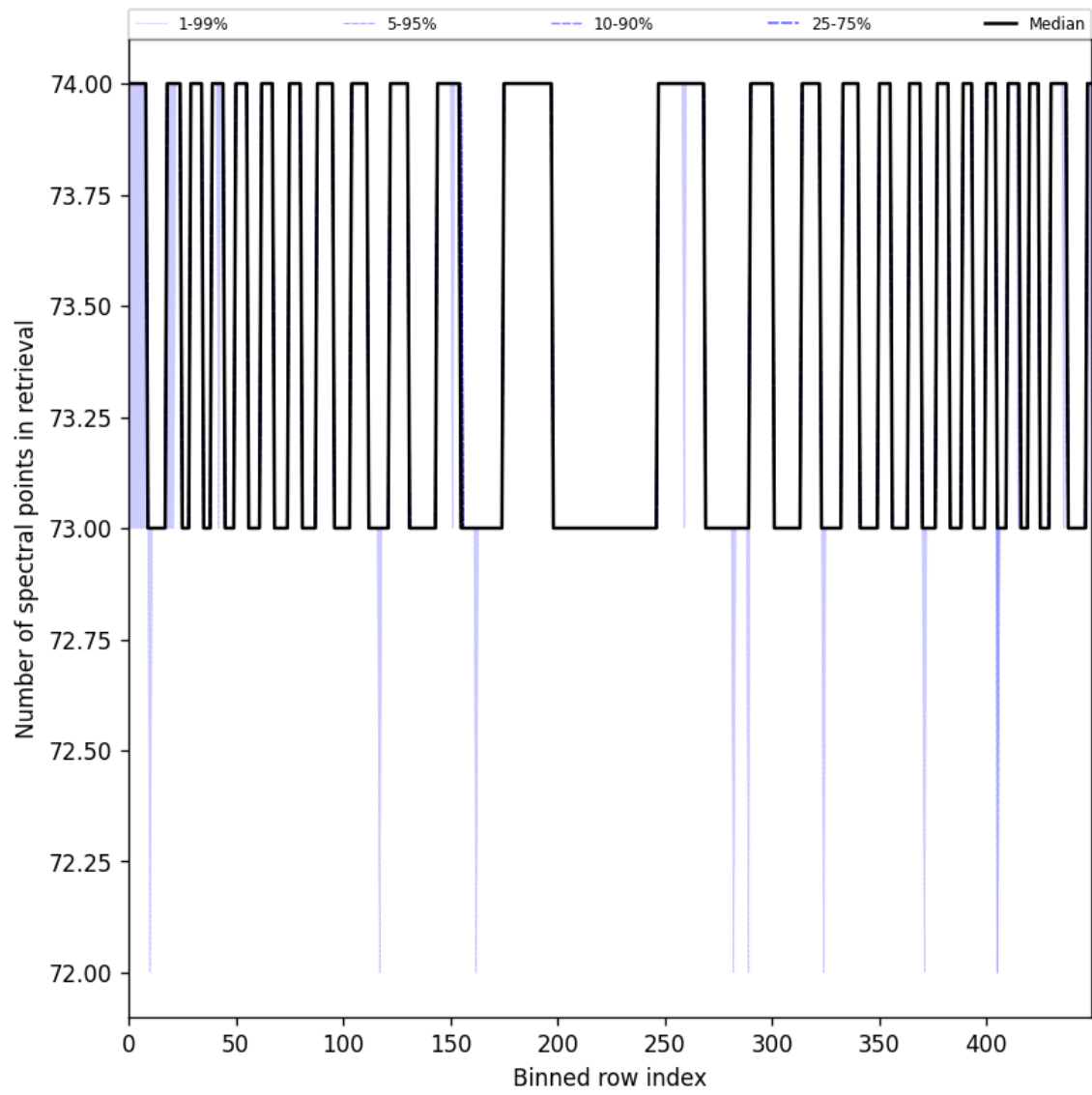
Figure 97: Along track statistics of “Number of spectral points in retrieval” for 2024-09-02 to 2024-09-04
