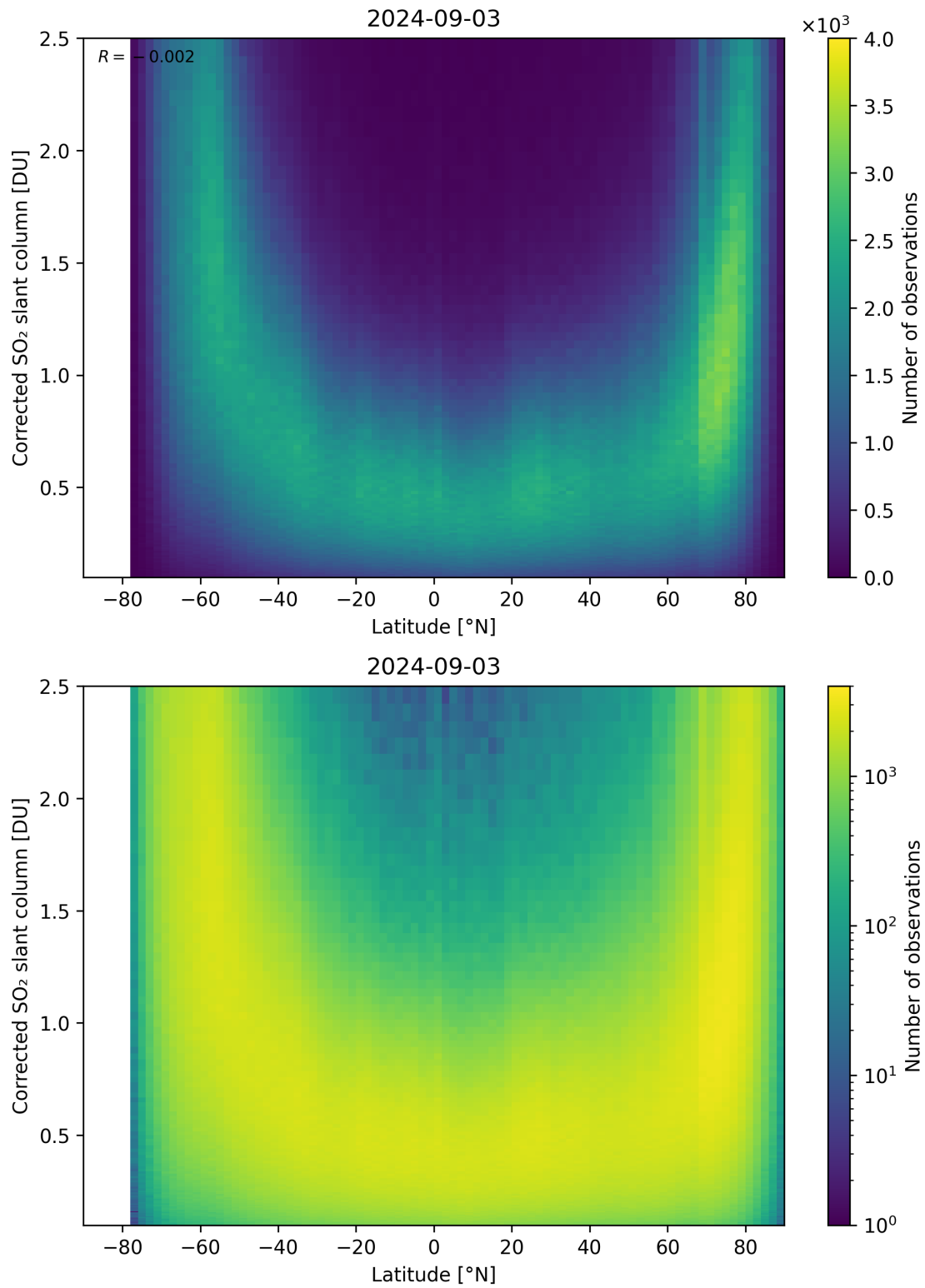
Figure 146: Scatter density plot of “Latitude” against “Corrected SO 2 slant column” for 2024-09-02 to 2024-09-04.
