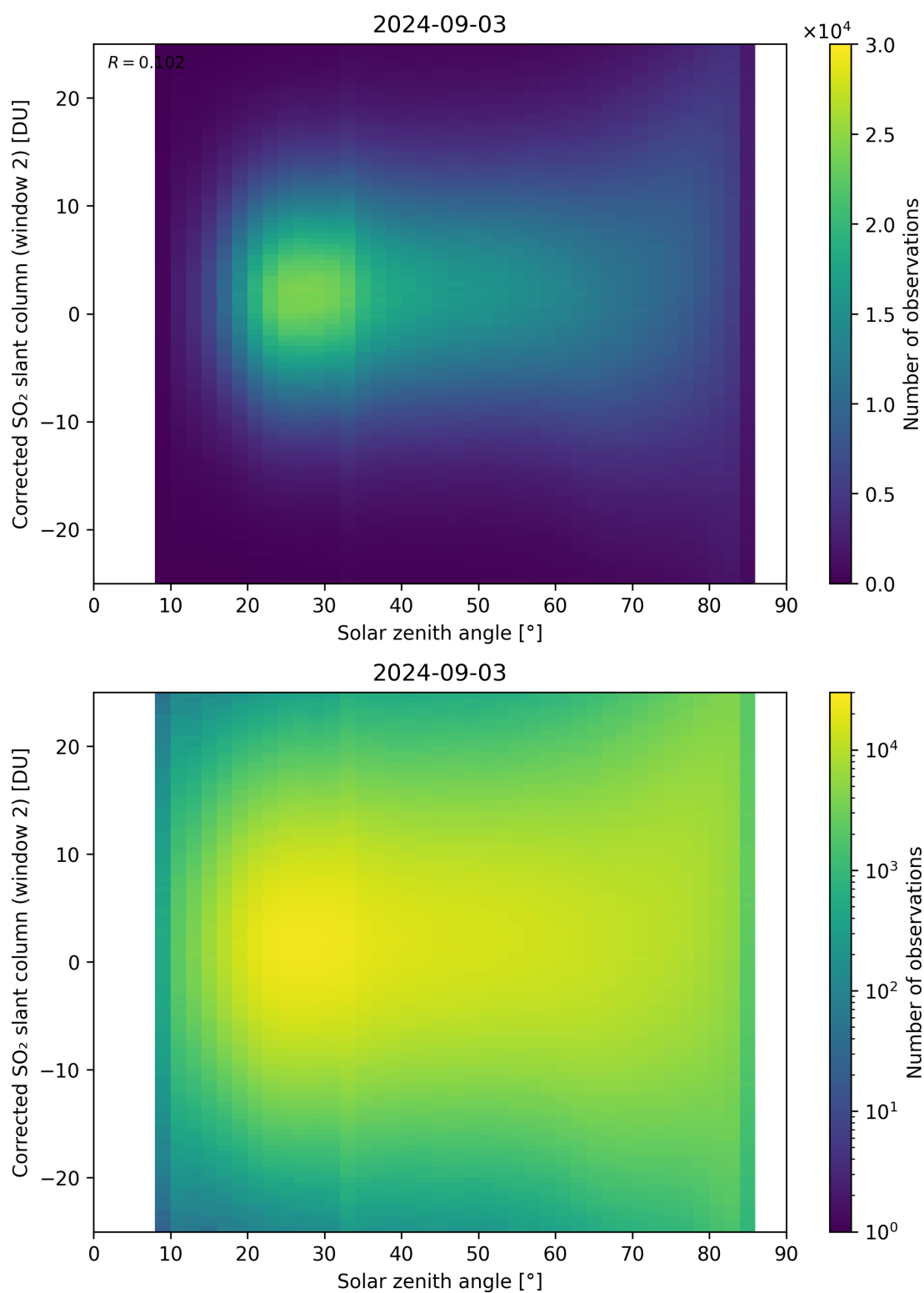
Figure 167: Scatter density plot of “Solar zenith angle” against “Corrected SO 2 slant column (window 2)” for 2024-09-02 to 2024-09-04.
