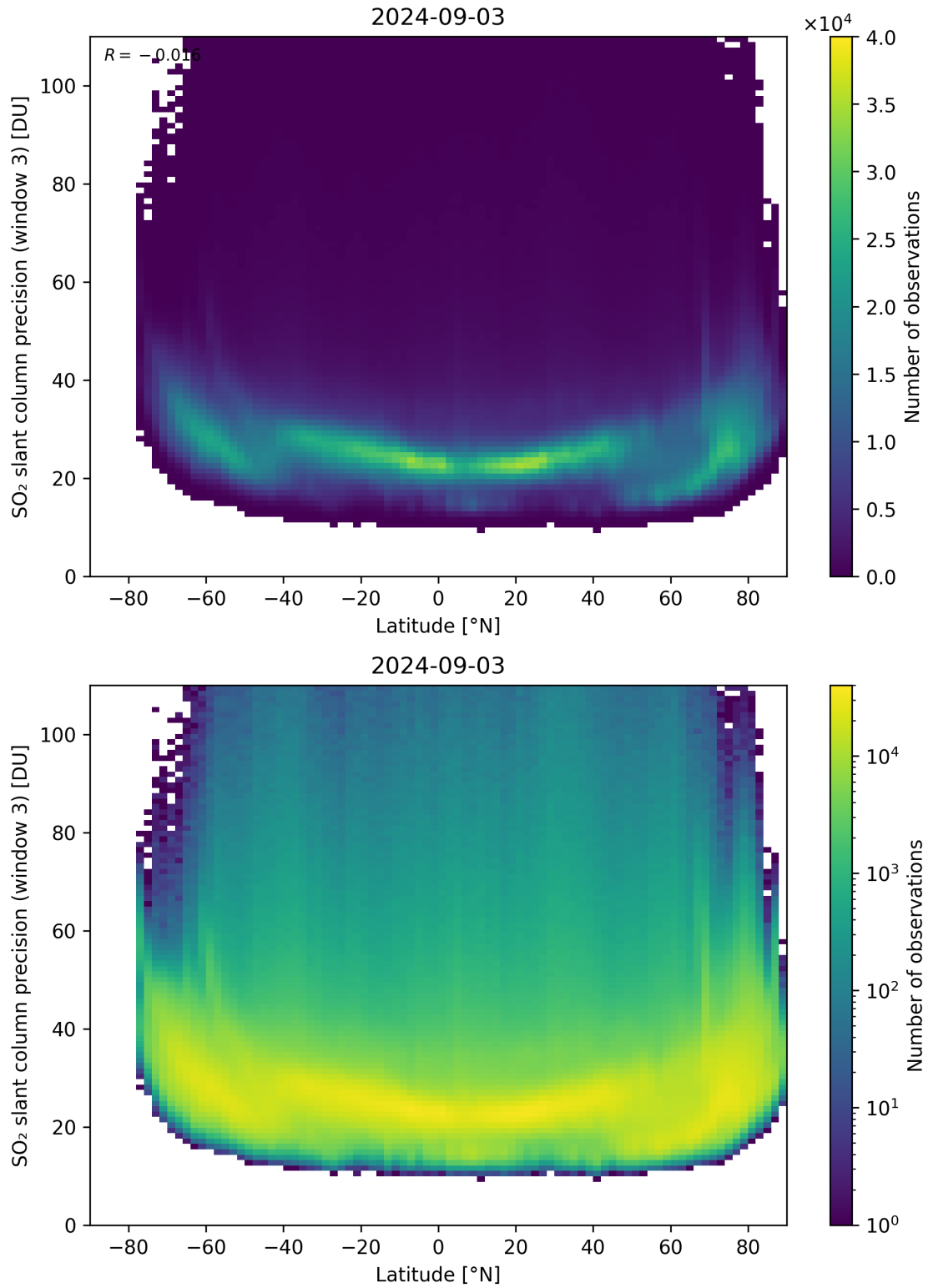
Figure 153: Scatter density plot of “Latitude” against “SO 2 slant column precision (window 3)” for 2024-09-02 to 2024-09-04.
