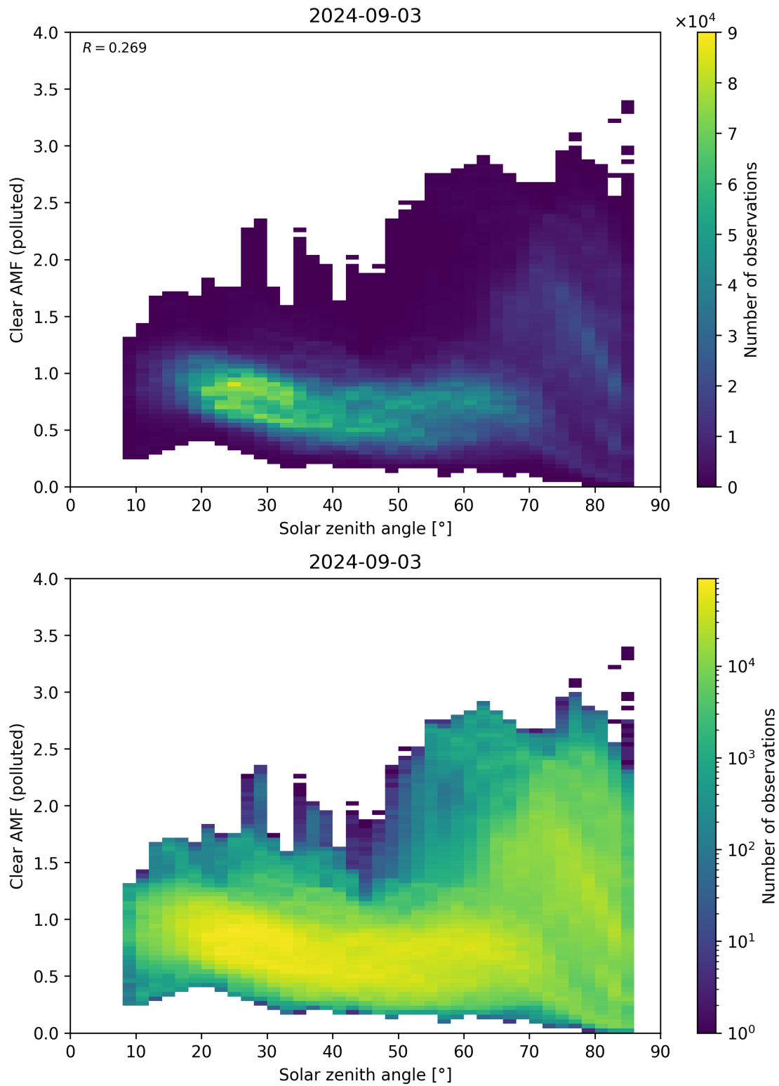
Figure 165: Scatter density plot of “Solar zenith angle” against “Clear AMF (polluted)” for 2024-09-02 to 2024-09-04.
