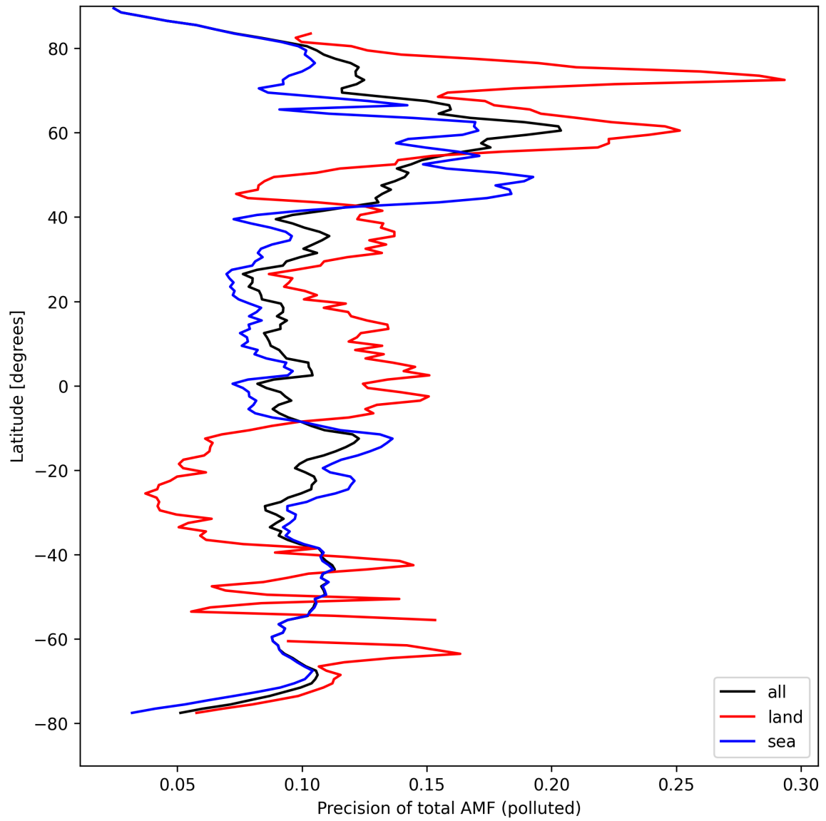
Figure 49: Zonal average of “Precision of total AMF (polluted)” for 2024-09-02 to 2024-09-04.
