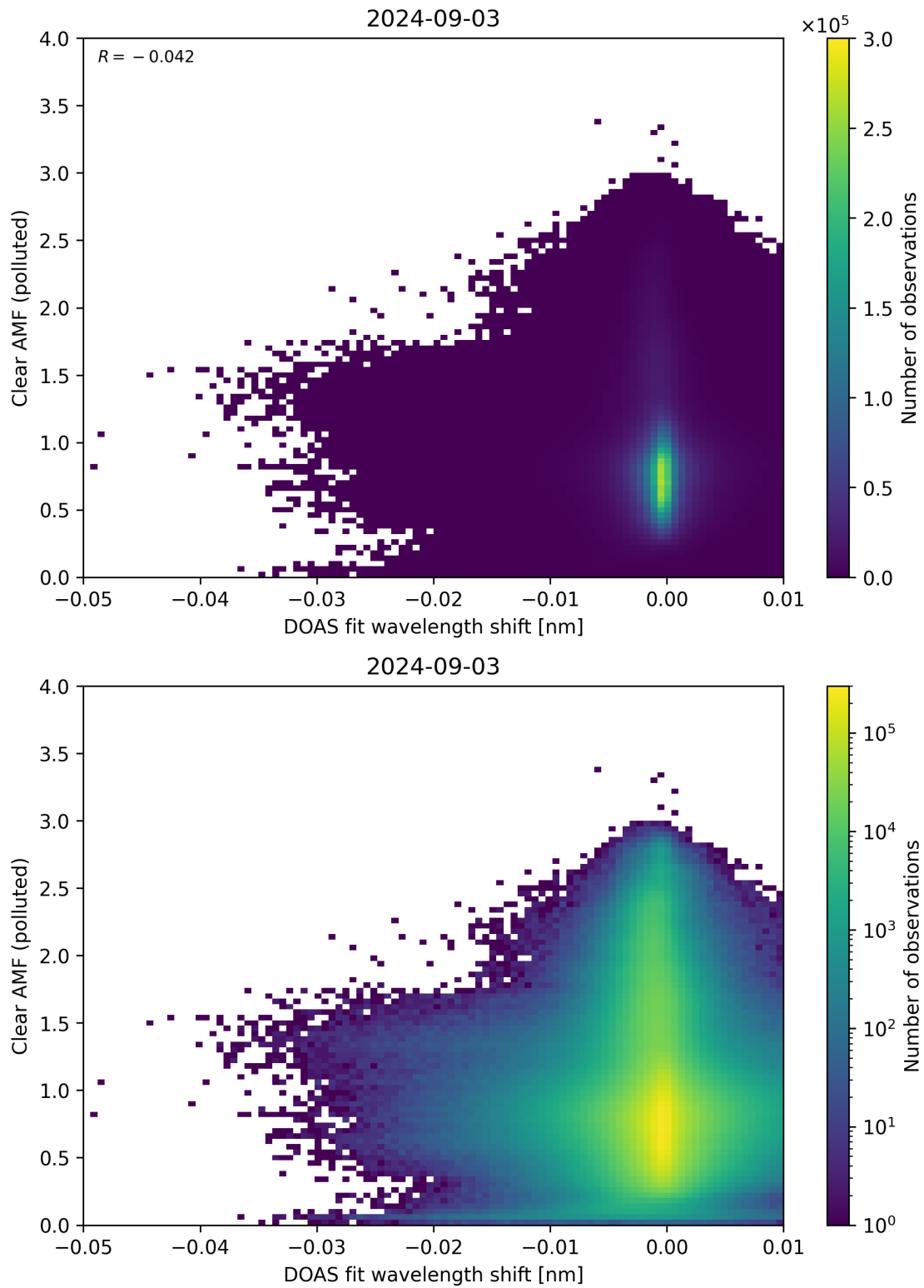
Figure 129: Scatter density plot of “DOAS fit wavelength shift” against “Clear AMF (polluted)” for 2024-09-02 to 2024-09-04.
