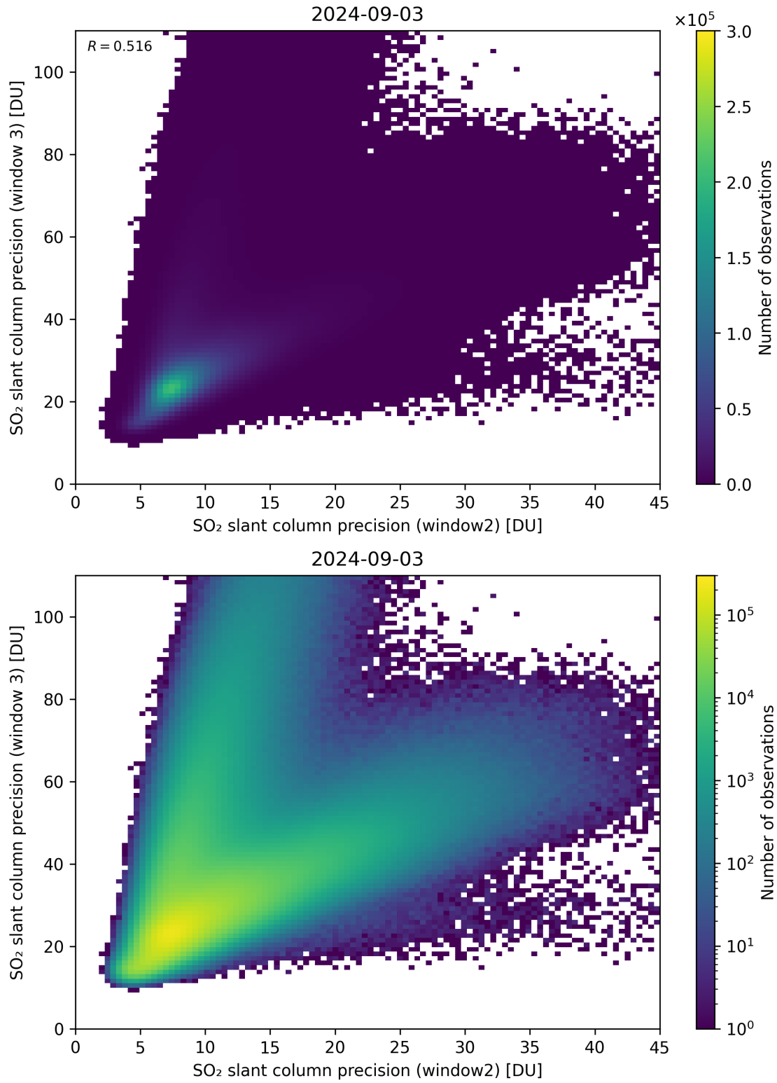
Figure 250: Scatter density plot of “SO 2 slant column precision (window2)” against “SO 2 slant column precision (window 3)” for 2024-09-02 to 2024-09-04.
