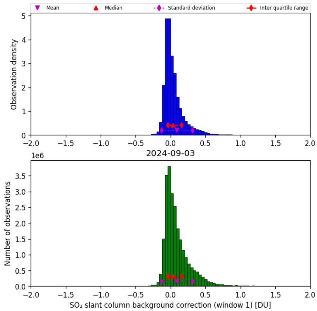
Figure 59: Histogram of “SO 2 slant column background correction (window 1)” for 2024-09-02 to 2024-09-04
