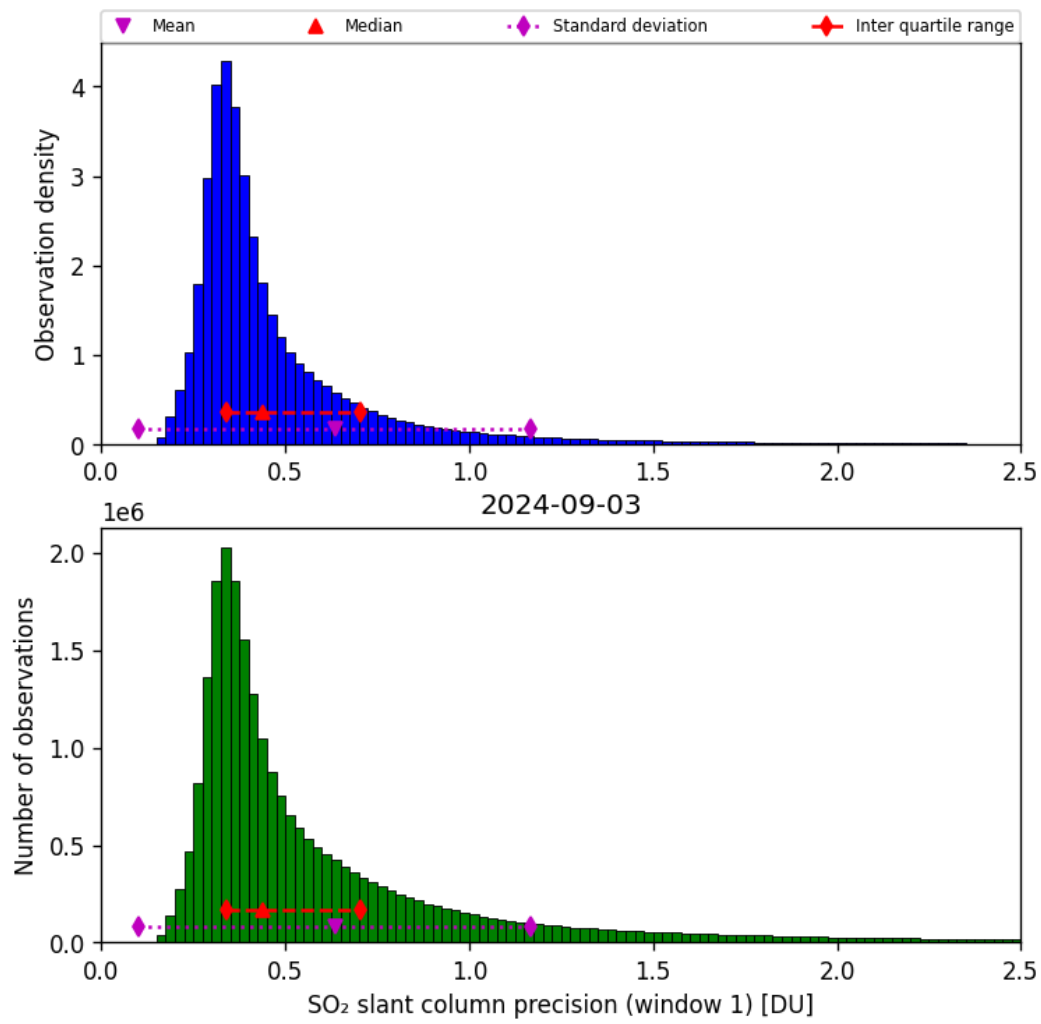
Figure 57: Histogram of “SO 2 slant column precision (window 1)” for 2024-09-02 to 2024-09-04
