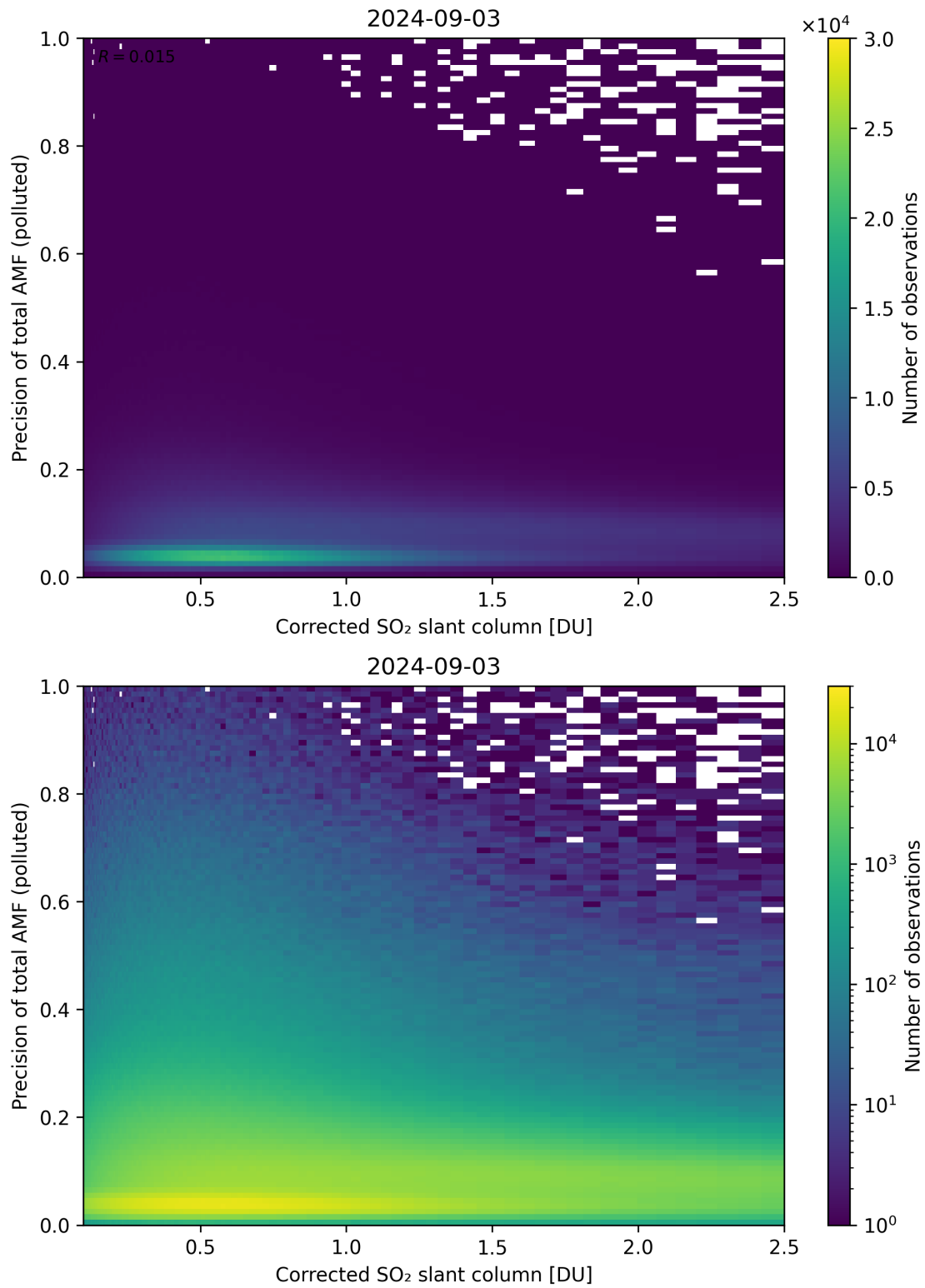
Figure 193: Scatter density plot of “Corrected SO 2 slant column” against “Precision of total AMF (polluted)” for 2024-09-02 to 2024-09-04.
