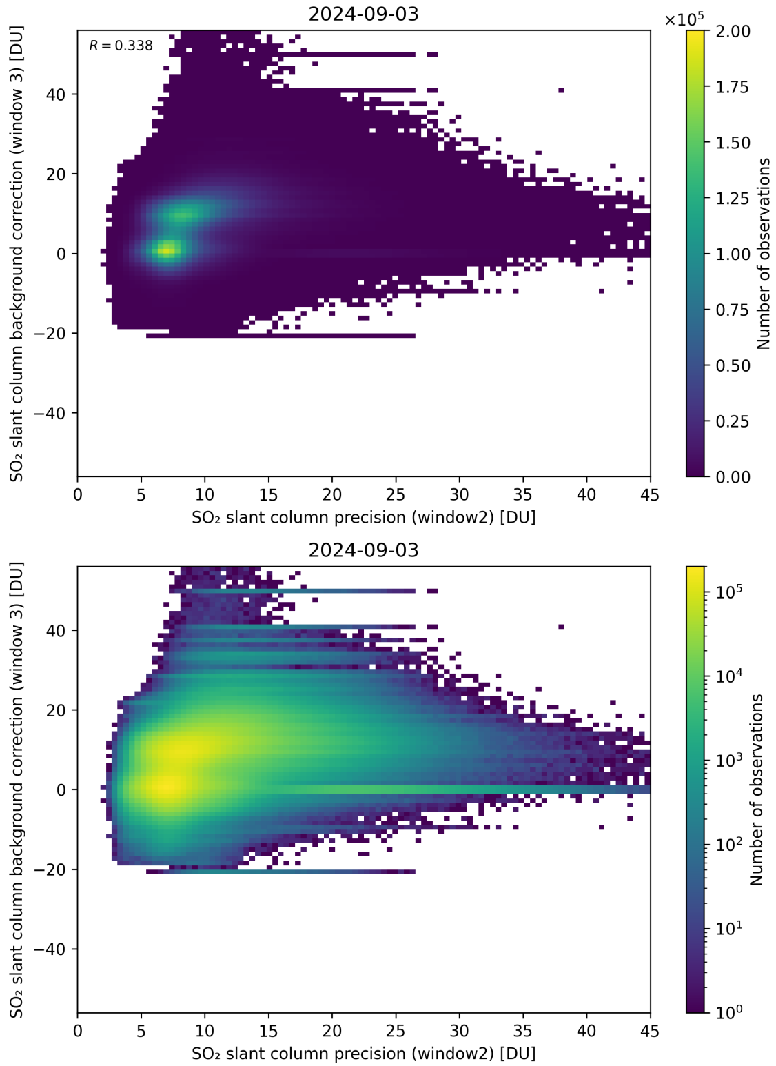
Figure 242: Scatter density plot of “SO 2 slant column precision (window2)” against “SO 2 slant column background correction (window 3)” for 2024-09-02 to 2024-09-04.
