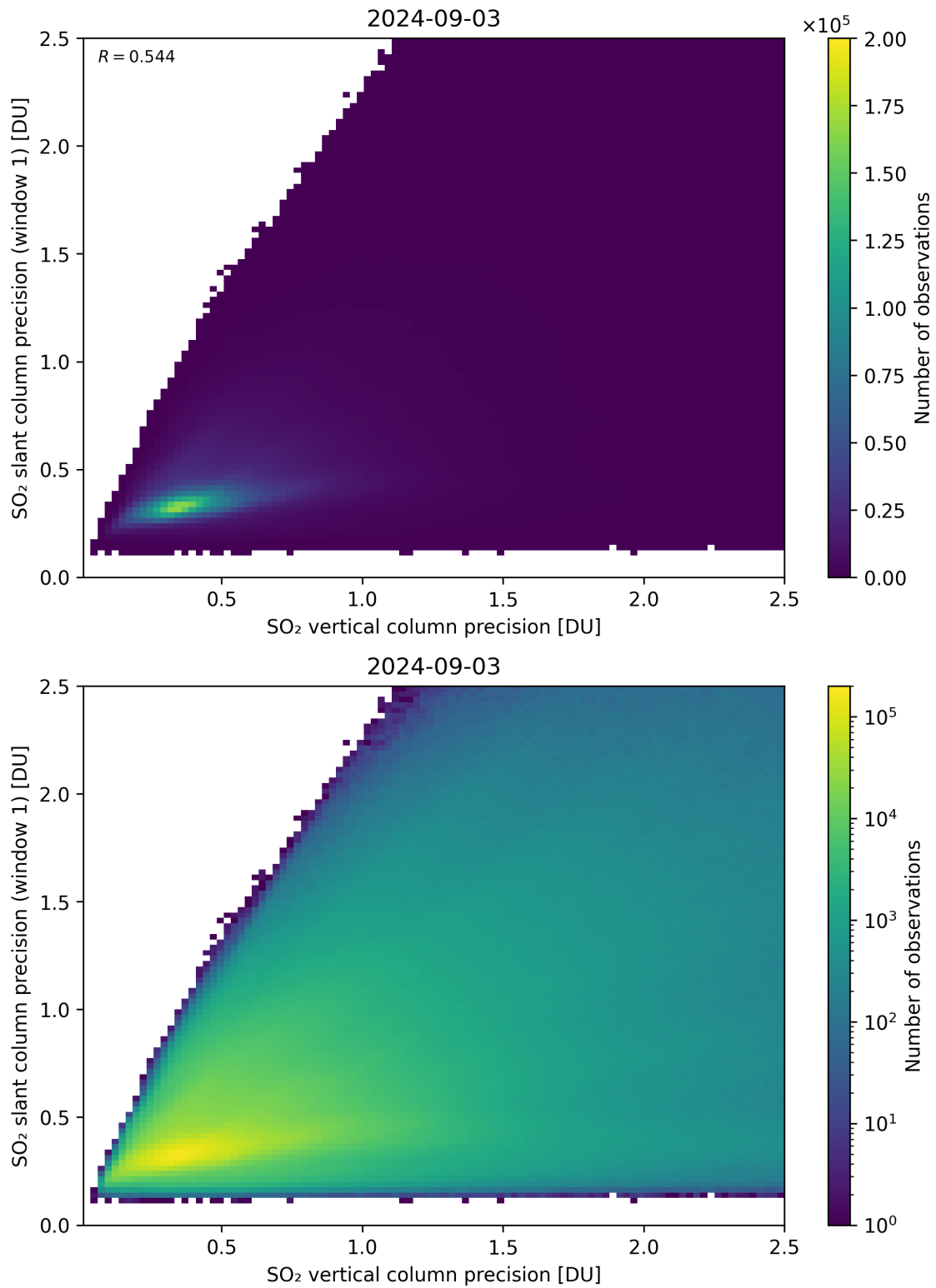
Figure 290: Scatter density plot of “SO 2 vertical column precision” against “SO 2 slant column precision (window 1)” for 2024-09-02 to 2024-09-04.
