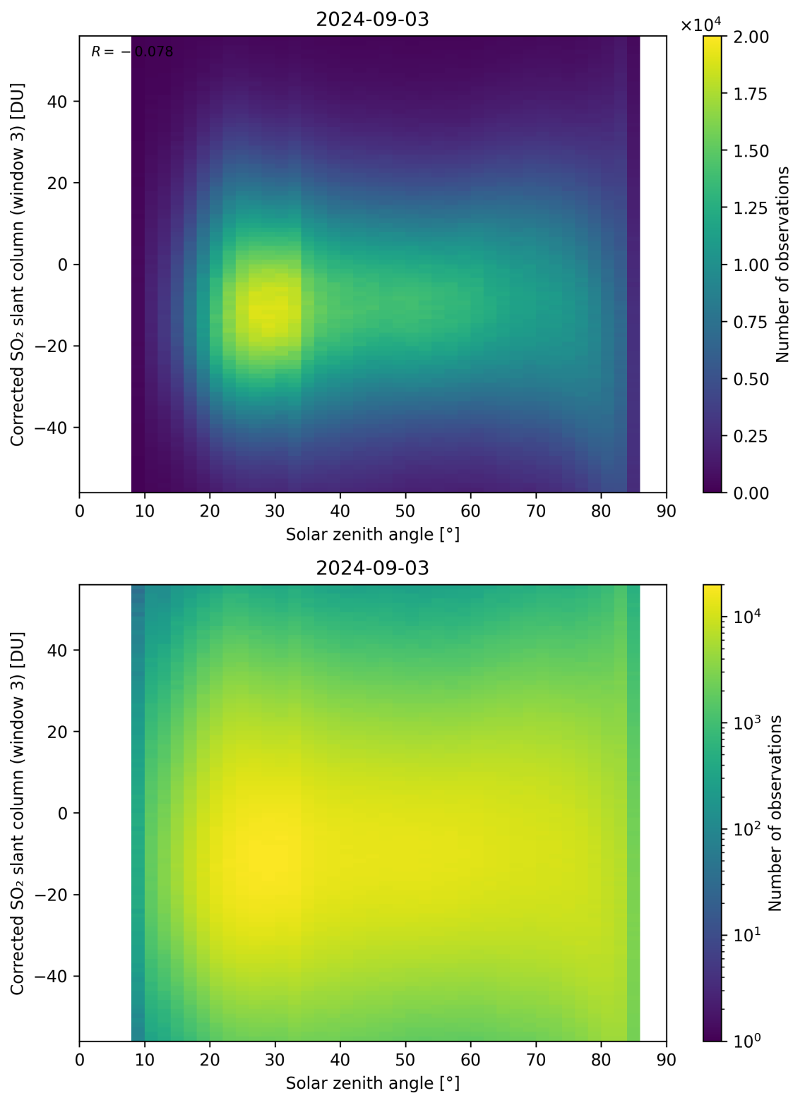
Figure 168: Scatter density plot of “Solar zenith angle” against “Corrected SO 2 slant column (window 3)” for 2024-09-02 to 2024-09-04.
