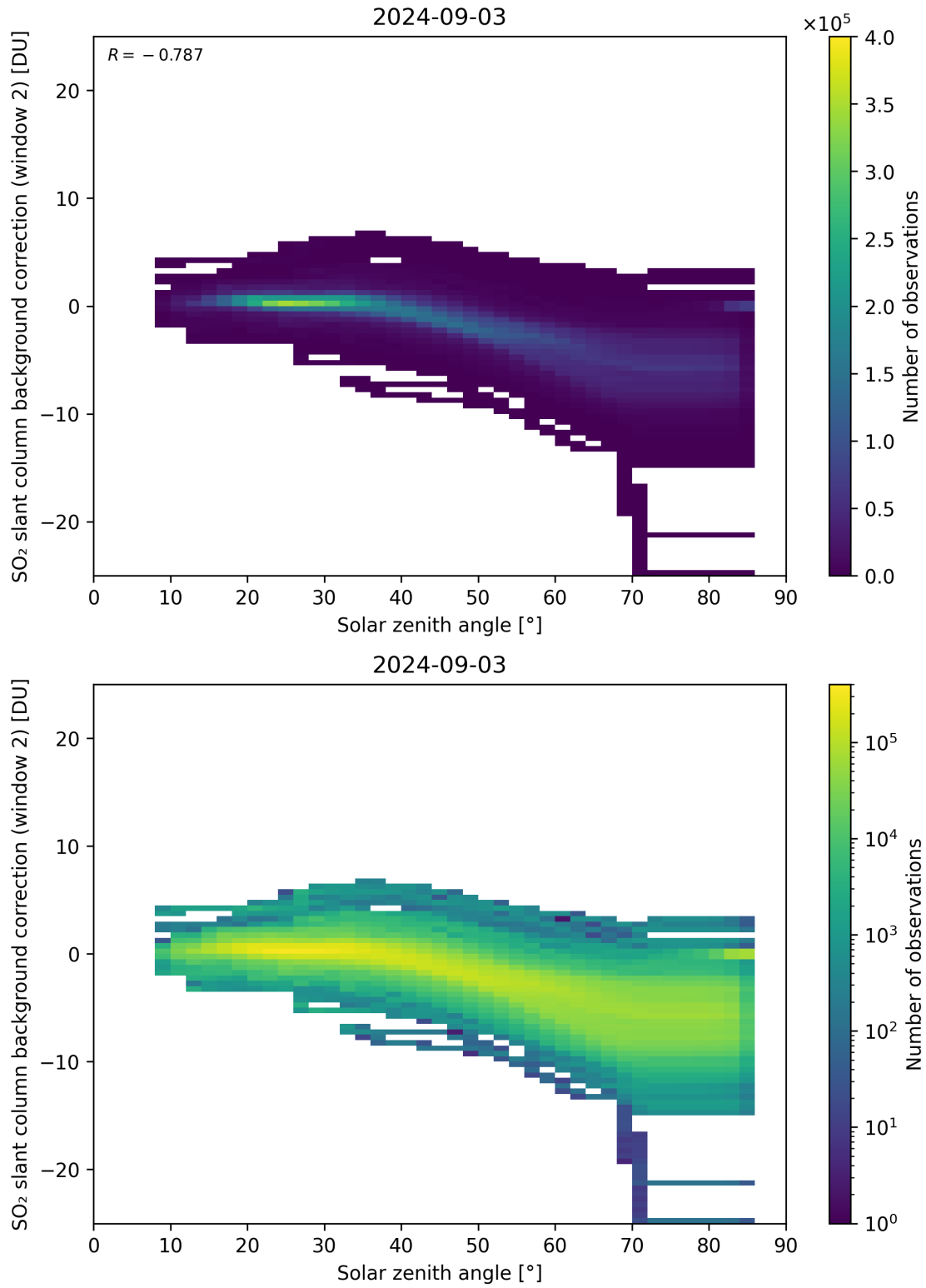
Figure 159: Scatter density plot of “Solar zenith angle” against “SO 2 slant column background correction (window 2)” for 2024-09-02 to 2024-09-04.
