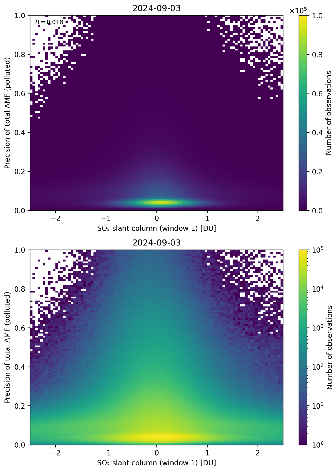
Figure 240: Scatter density plot of “SO 2 slant column (window 1)” against “Precision of total AMF (polluted)” for 2024-09-02 to 2024-09-04.
