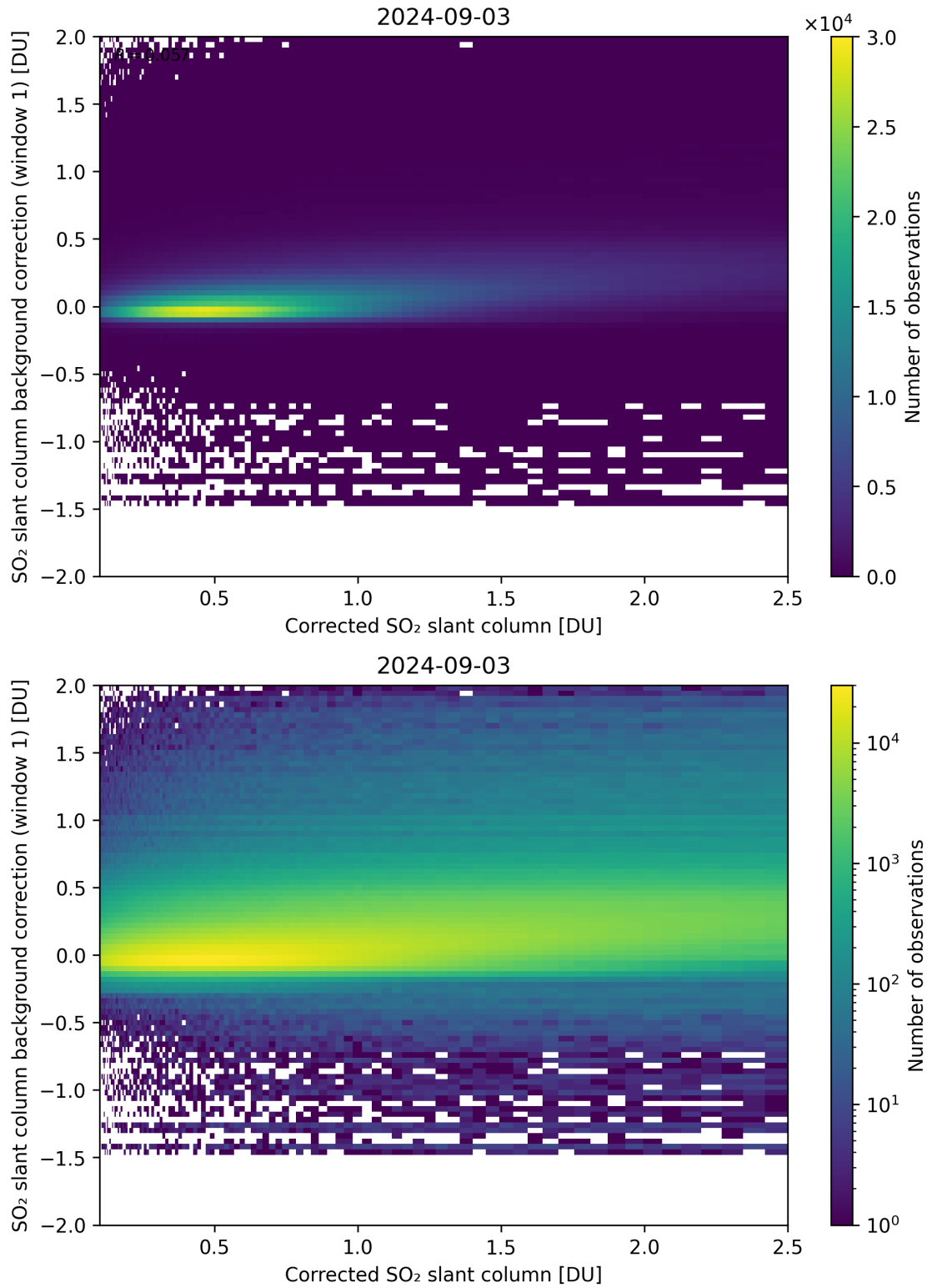
Figure 178: Scatter density plot of “Corrected SO 2 slant column” against “SO 2 slant column background correction (window 1)” for 2024-09-02 to 2024-09-04.
