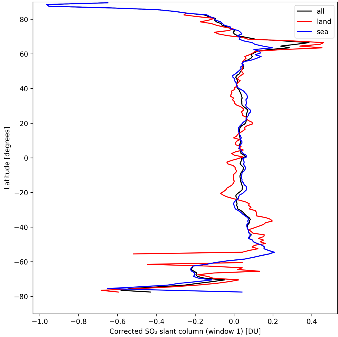
Figure 35: Zonal average of “Corrected SO 2 slant column (window 1)” for 2024-09-02 to 2024-09-04.
