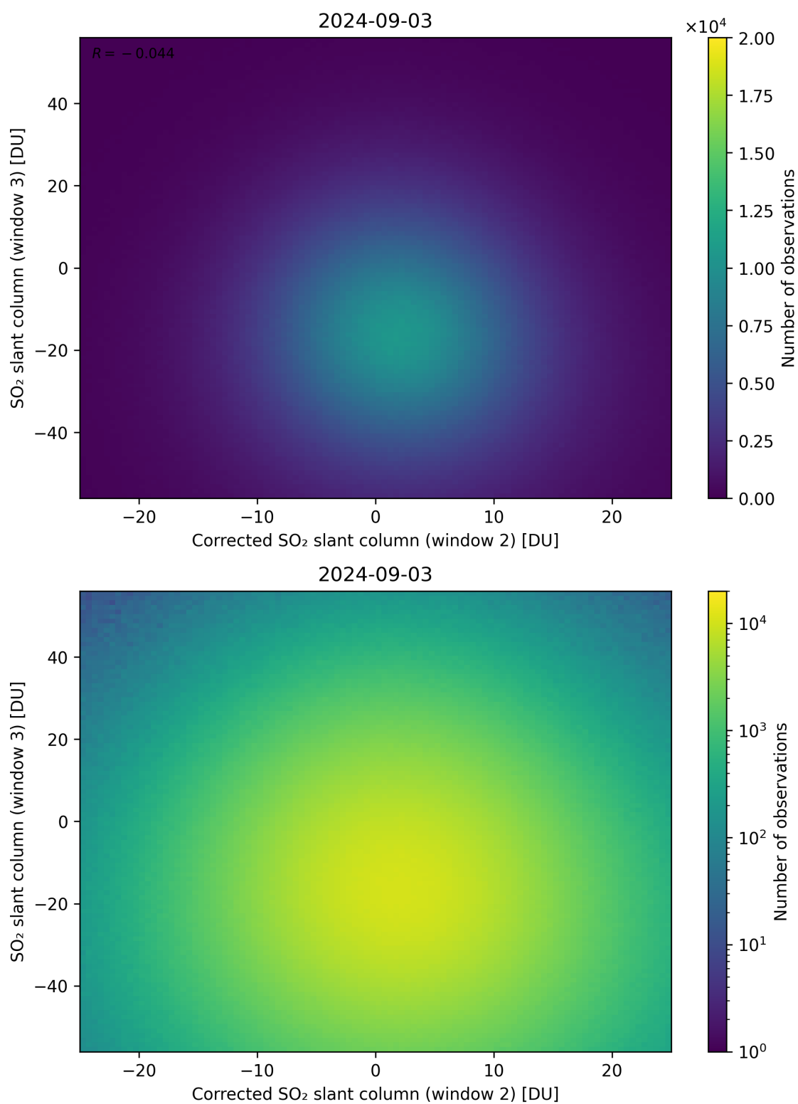
Figure 201: Scatter density plot of “Corrected SO 2 slant column (window 2)” against “SO 2 slant column (window 3)” for 2024-09-02 to 2024-09-04.
