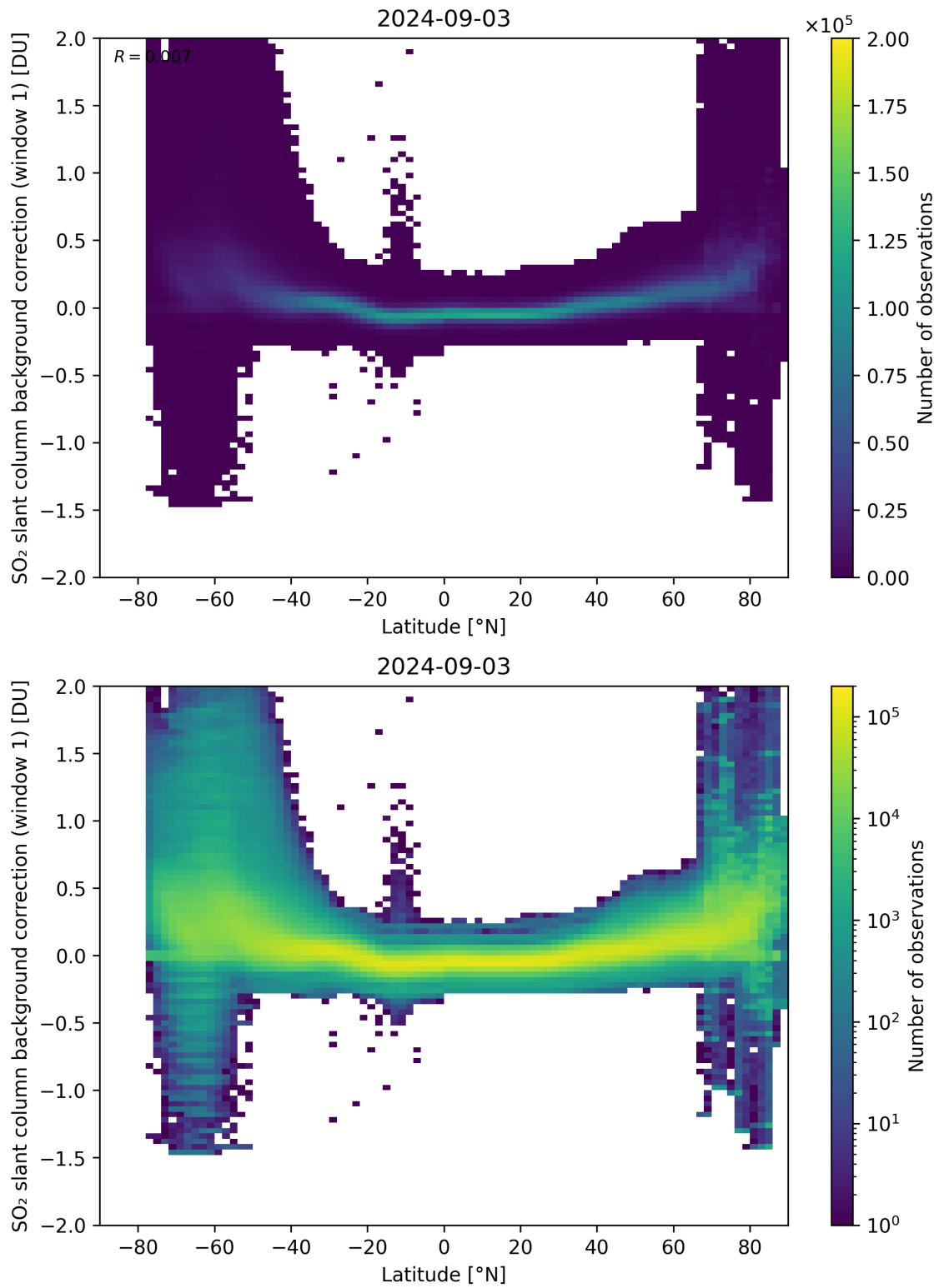
Figure 139: Scatter density plot of “Latitude” against “SO 2 slant column background correction (window 1)” for 2024-09-02 to 2024-09-04.
