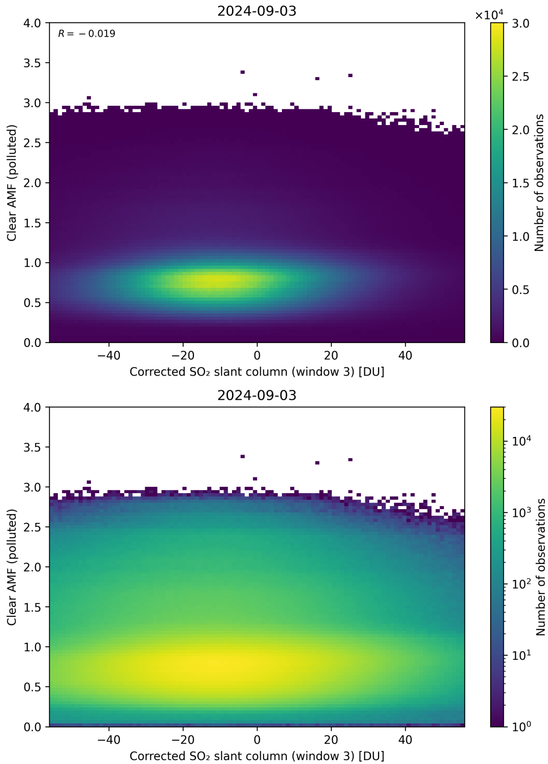
Figure 209: Scatter density plot of “Corrected SO 2 slant column (window 3)” against “Clear AMF (polluted)” for 2024-09-02 to 2024-09-04.
