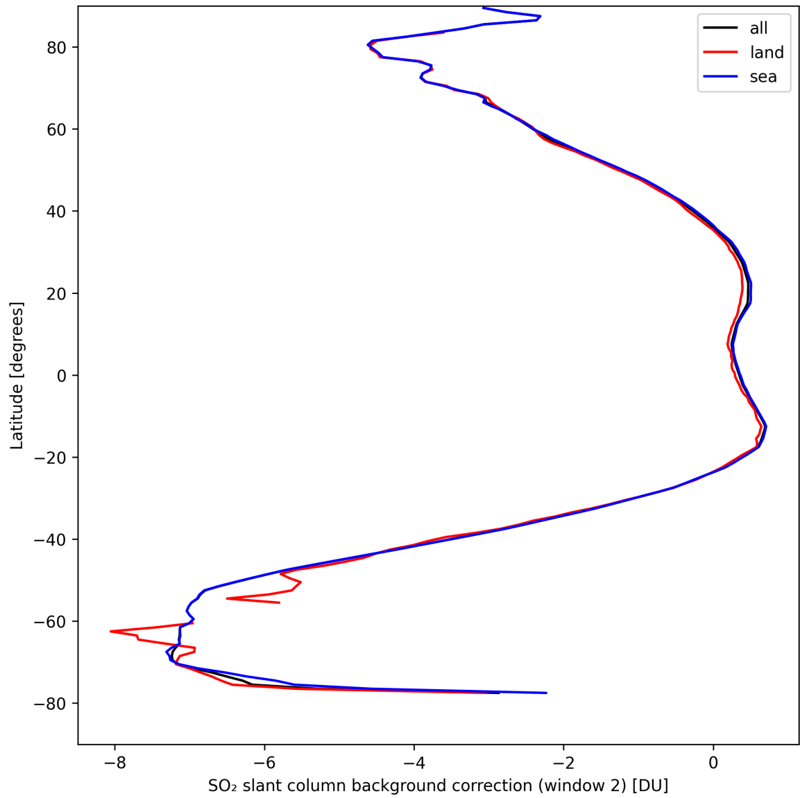
Figure 40: Zonal average of “SO 2 slant column background correction (window 2)” for 2024-09-02 to 2024-09-04.
