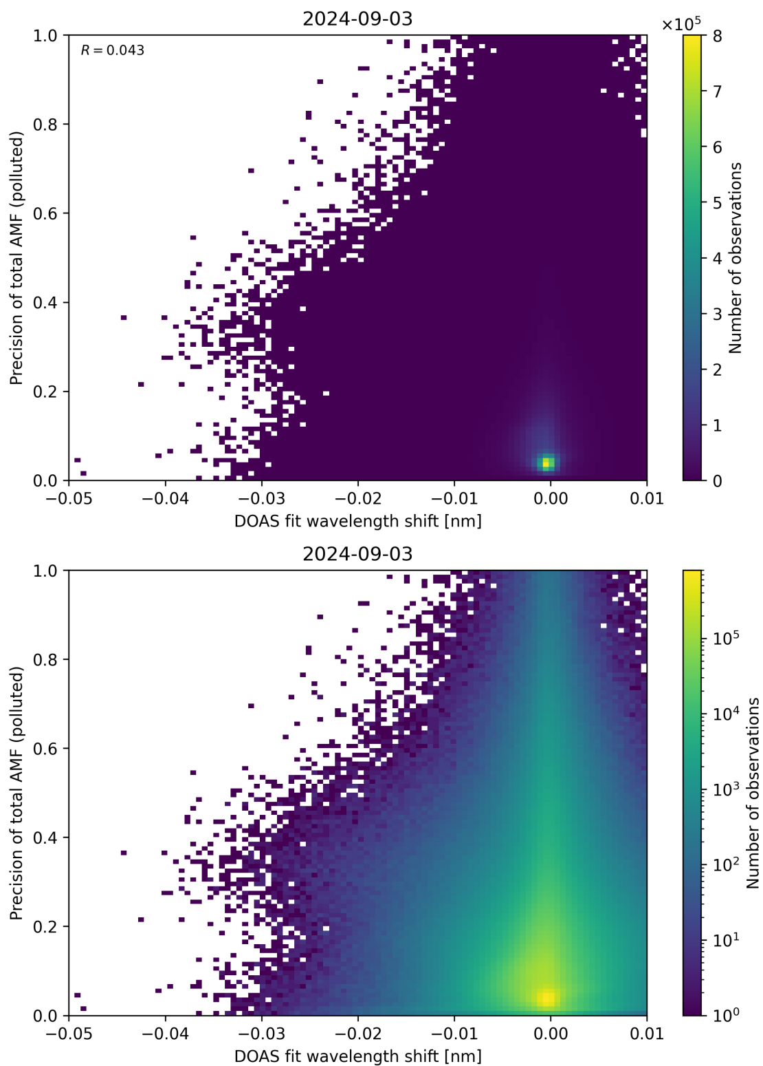
Figure 131: Scatter density plot of “DOAS fit wavelength shift” against “Precision of total AMF (polluted)” for 2024-09-02 to 2024-09-04.
