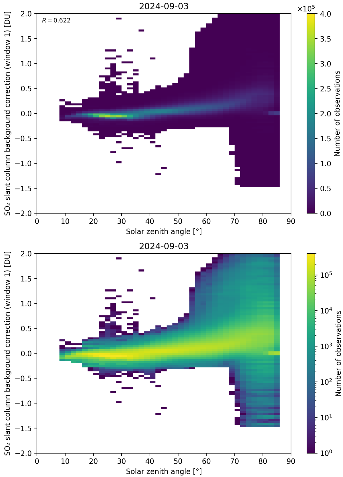
Figure 158: Scatter density plot of “Solar zenith angle” against “SO 2 slant column background correction (window 1)” for 2024-09-02 to 2024-09-04.
