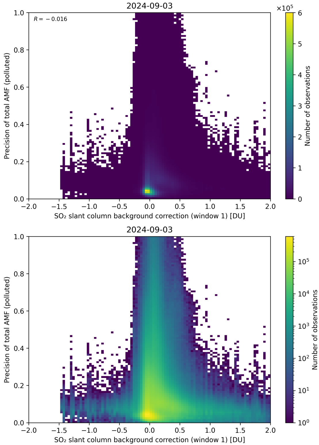
Figure 110: Scatter density plot of “SO 2 slant column background correction (window 1)” against “Precision of total AMF (polluted)” for 2024-09-02 to 2024-09-04.
