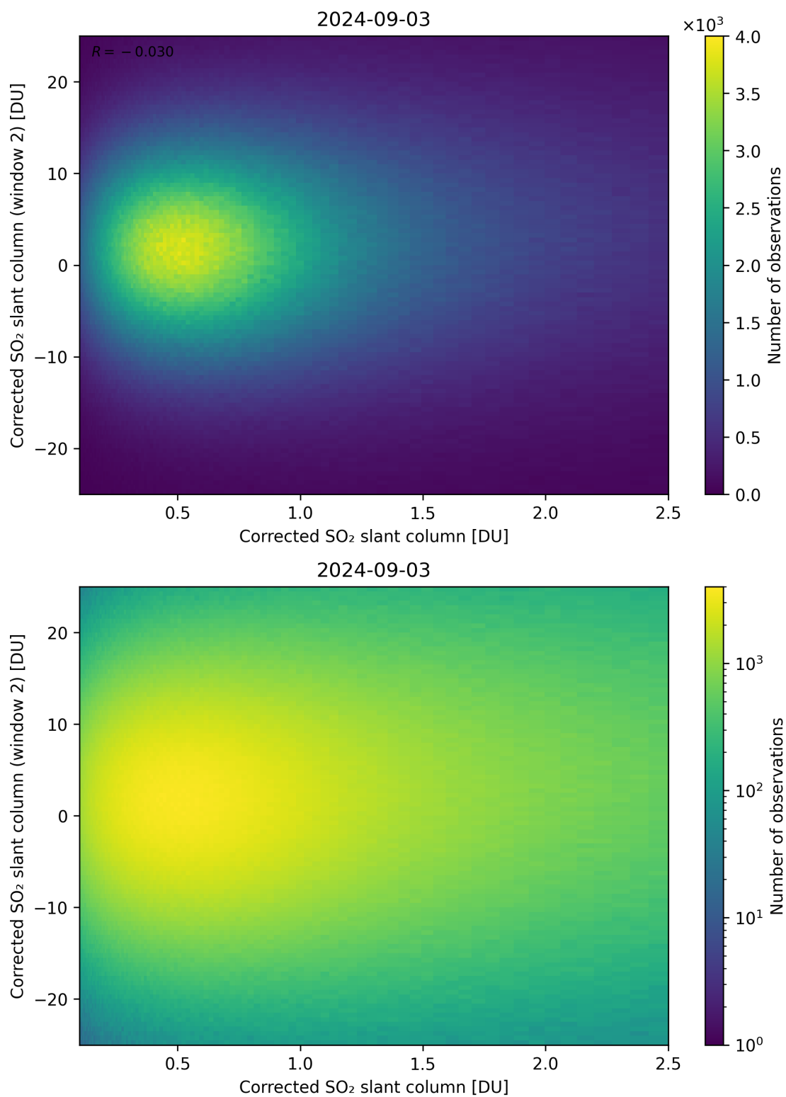
Figure 185: Scatter density plot of “Corrected SO 2 slant column” against “Corrected SO 2 slant column (window 2)” for 2024-09-02 to 2024-09-04.
