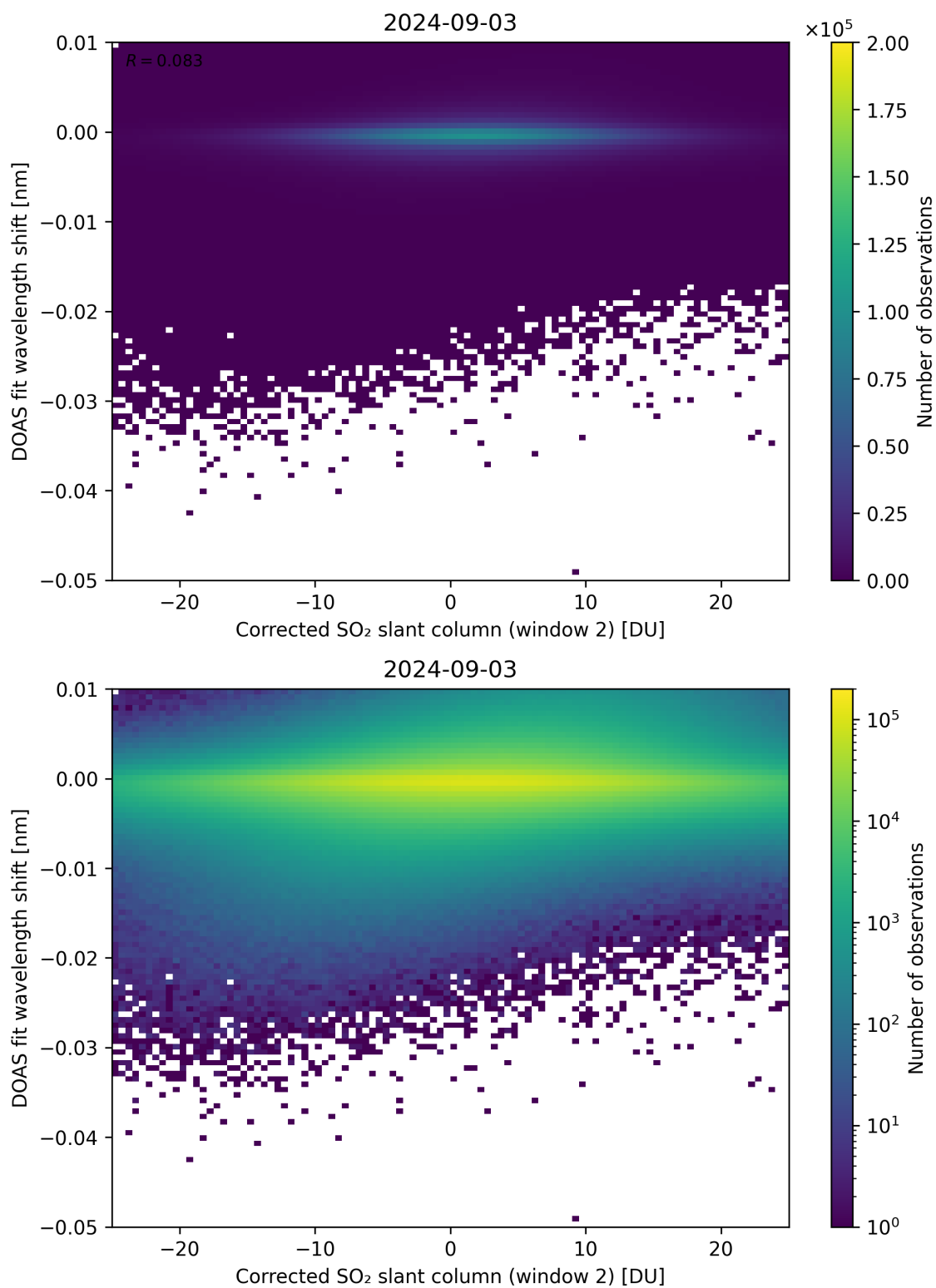
Figure 196: Scatter density plot of “Corrected SO 2 slant column (window 2)” against “DOAS fit wavelength shift” for 2024-09-02 to 2024-09-04.
