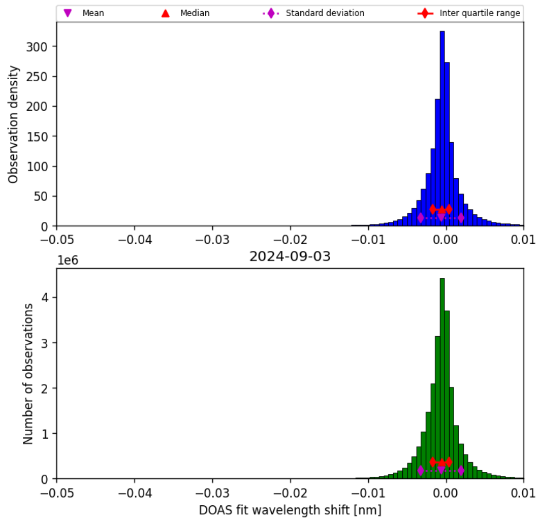
Figure 68: Histogram of “DOAS fit wavelength shift” for 2024-09-02 to 2024-09-04
