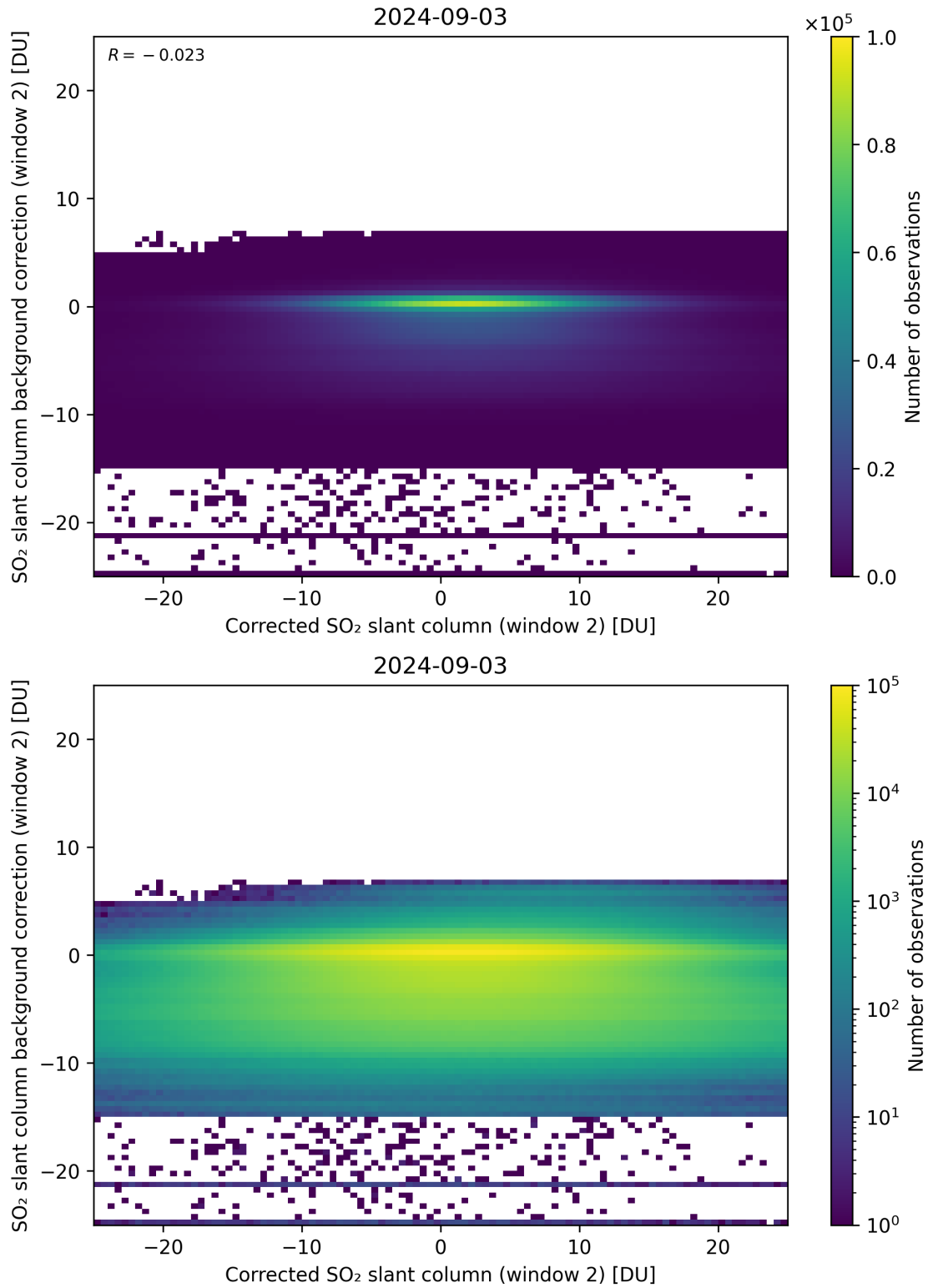
Figure 194: Scatter density plot of “Corrected SO 2 slant column (window 2)” against “SO 2 slant column background correction (window 2)” for 2024-09-02 to 2024-09-04.
