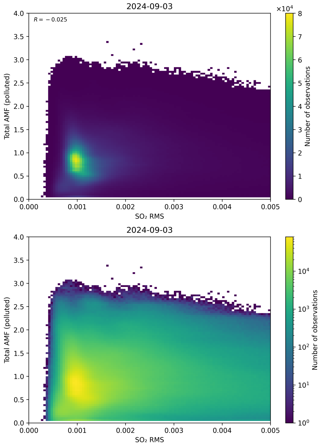
Figure 137: Scatter density plot of “SO 2 RMS” against “Total AMF (polluted)” for 2024-09-02 to 2024-09-04.
