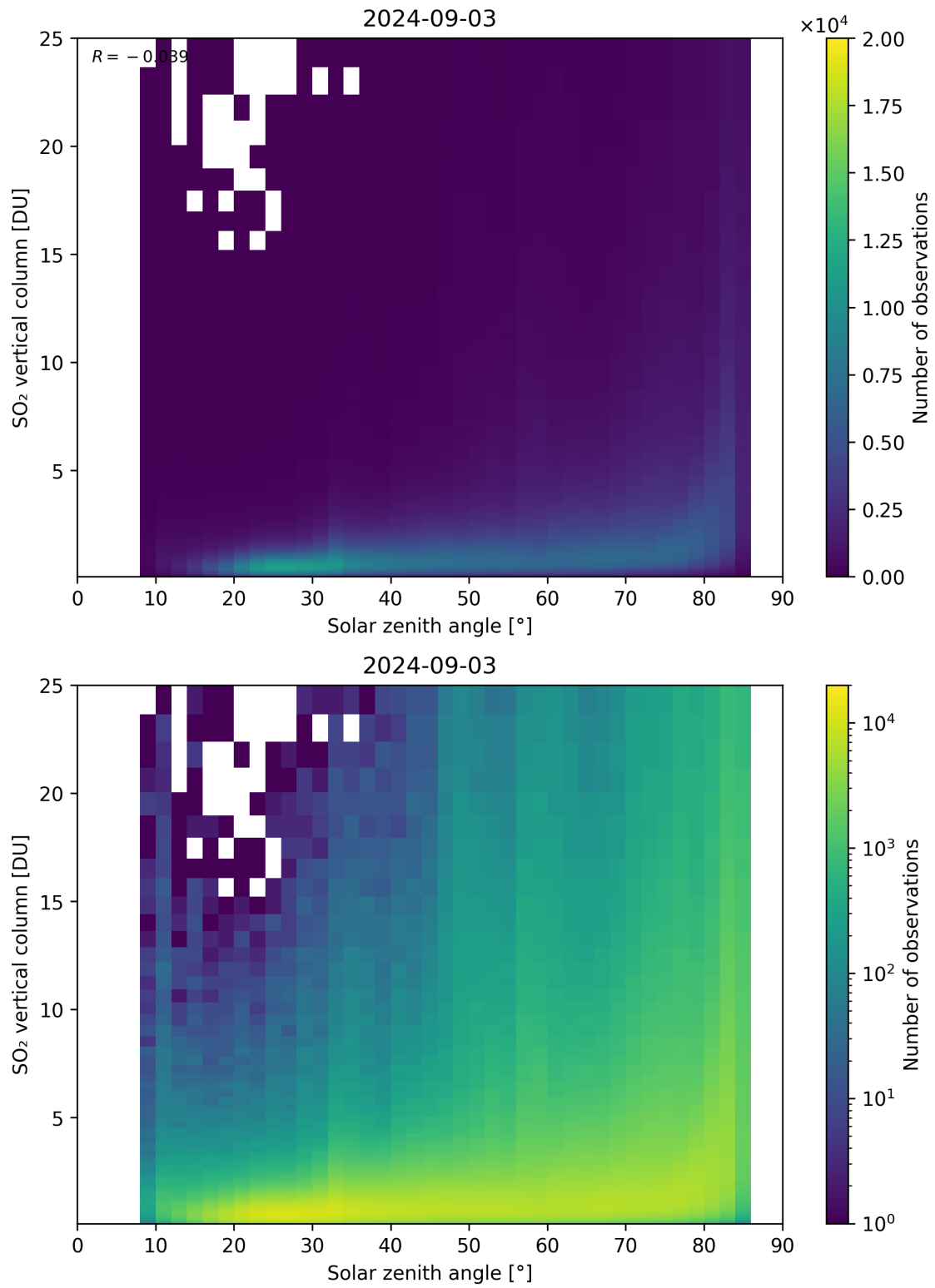
Figure 176: Scatter density plot of “Solar zenith angle” against “SO 2 vertical column” for 2024-09-02 to 2024-09-04.
