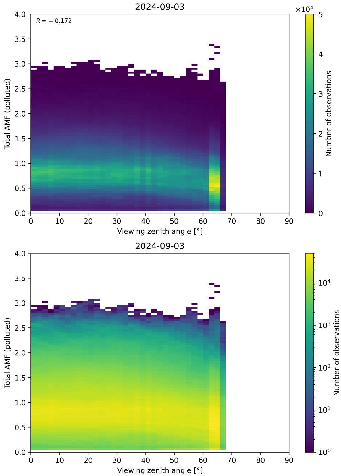
Figure 325: Scatter density plot of “Viewing zenith angle” against “Total AMF (polluted)” for 2024-09-02 to 2024-09-04.
