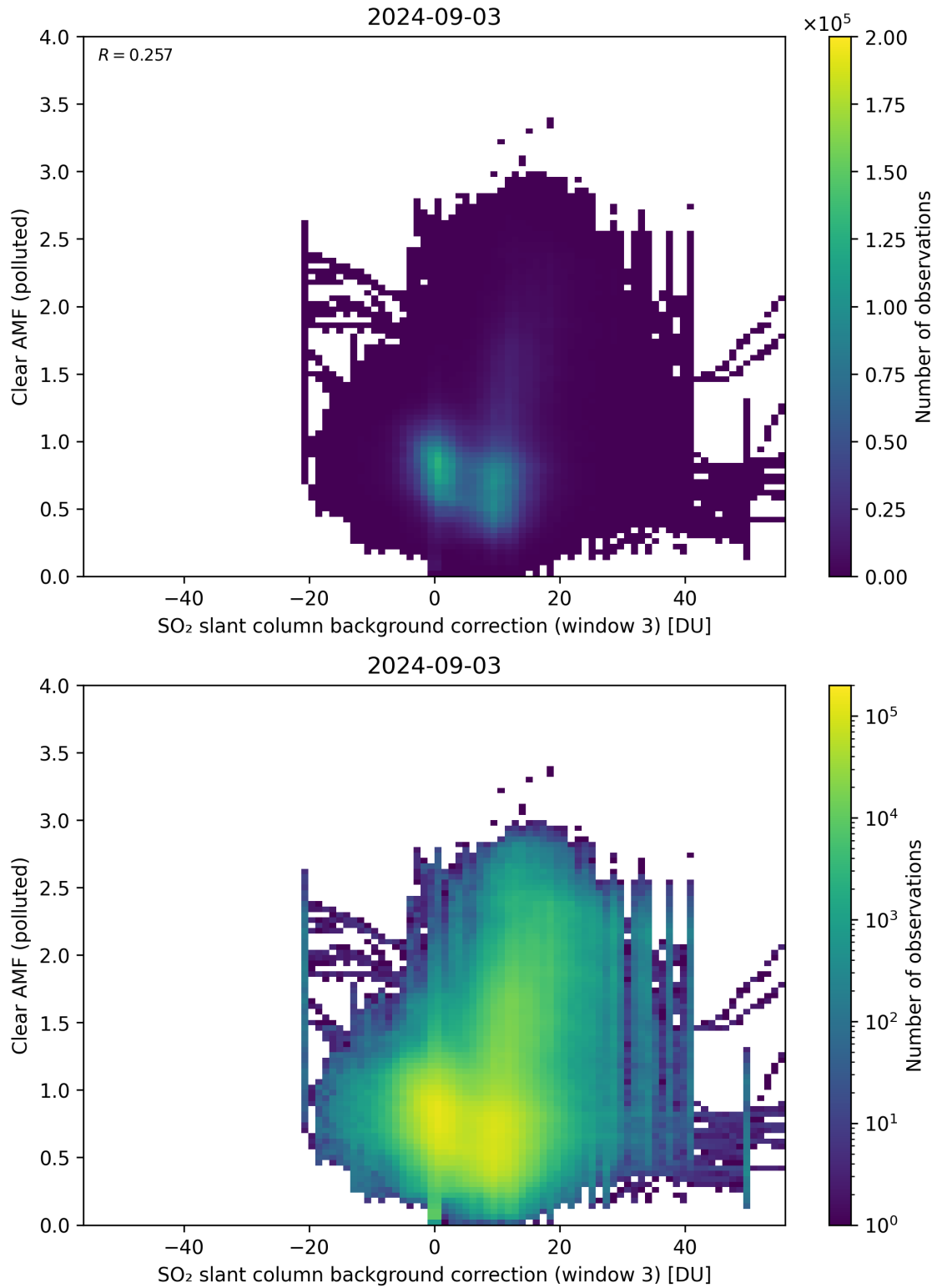
Figure 124: Scatter density plot of “SO 2 slant column background correction (window 3)” against “Clear AMF (polluted)” for 2024-09-02 to 2024-09-04.
