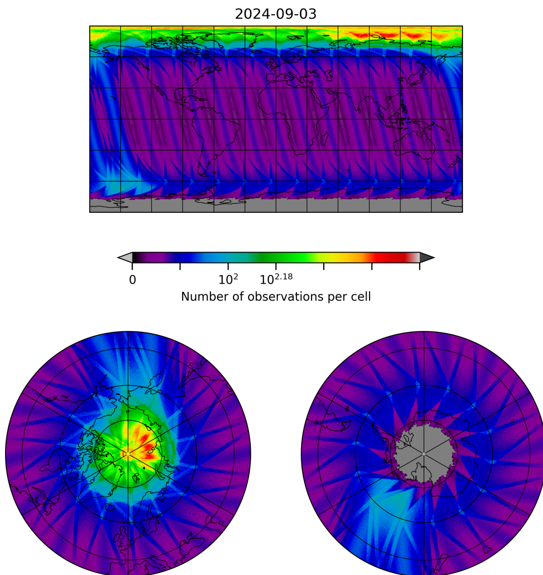
Figure 28: Map of the number of observations for 2024-09-02 to 2024-09-04
