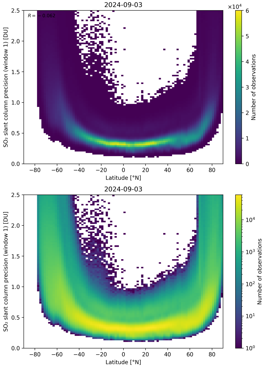
Figure 150: Scatter density plot of “Latitude” against “SO 2 slant column precision (window 1)” for 2024-09-02 to 2024-09-04.
