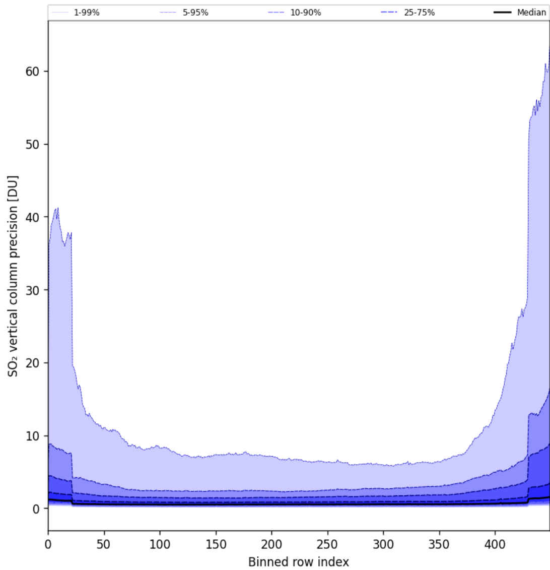
Figure 77: Along track statistics of “SO 2 vertical column precision” for 2024-09-02 to 2024-09-04
