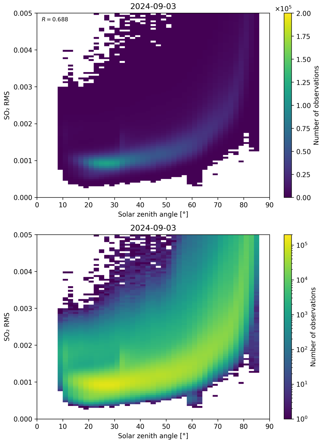
Figure 163: Scatter density plot of “Solar zenith angle” against “SO 2 RMS” for 2024-09-02 to 2024-09-04.
