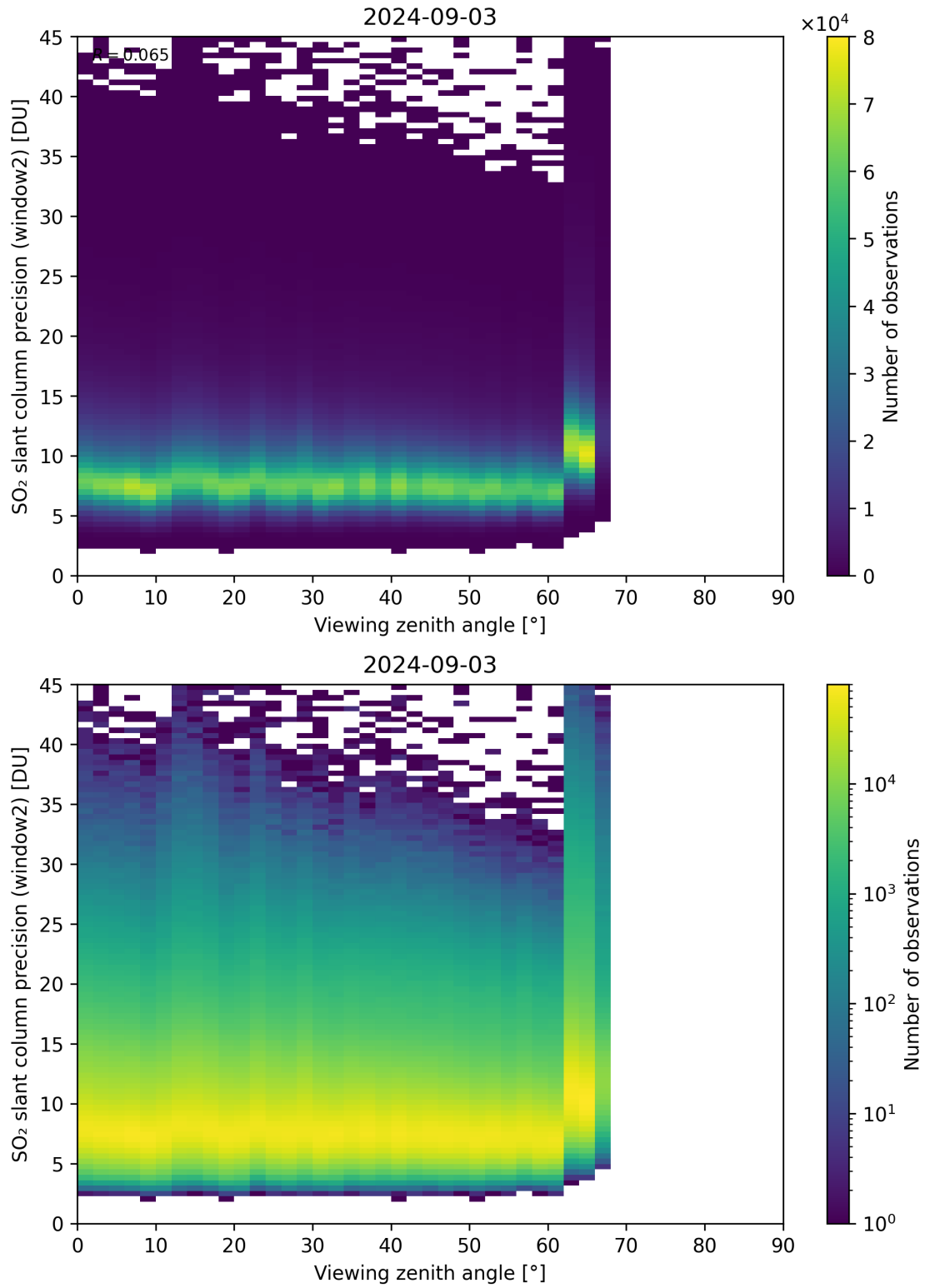
Figure 322: Scatter density plot of “Viewing zenith angle” against “SO 2 slant column precision (window2)” for 2024-09-02 to 2024-09-04.
