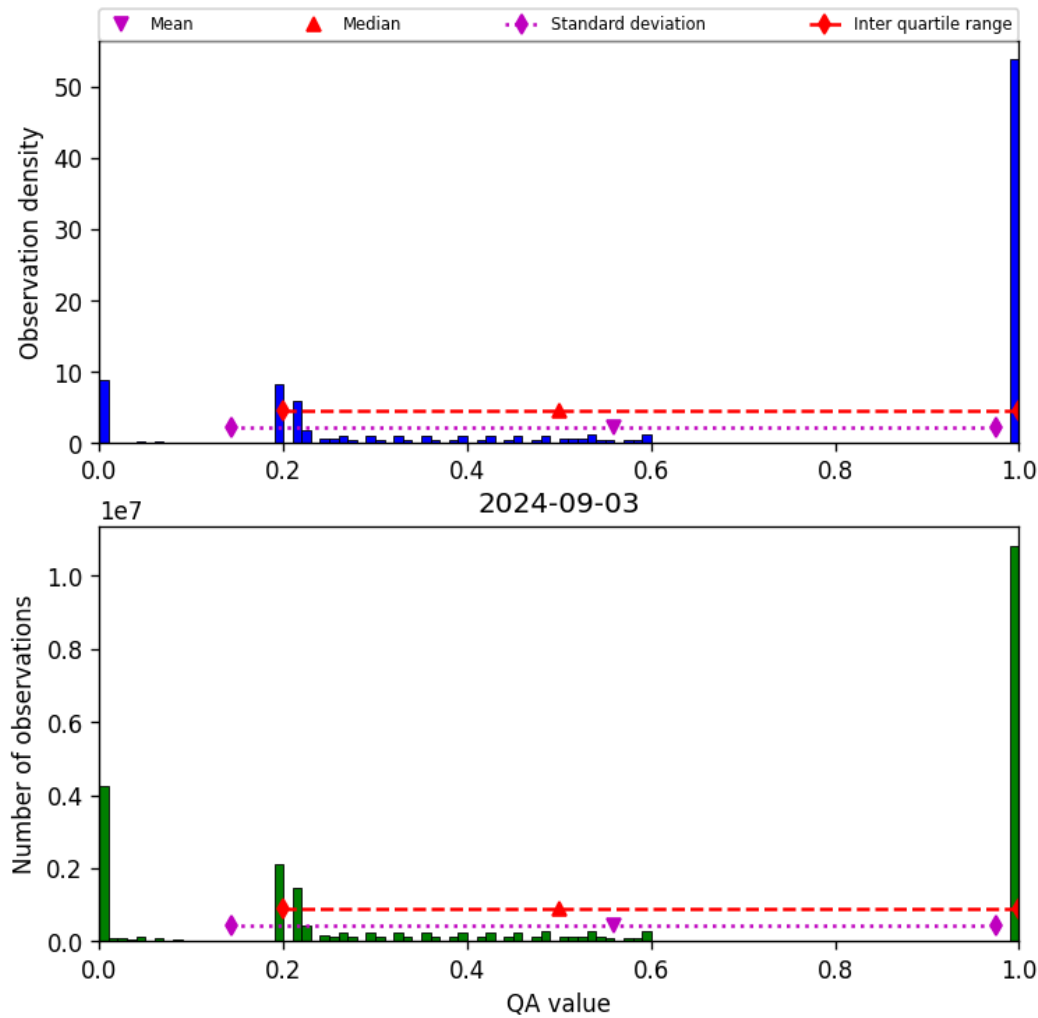
Figure 52: Histogram of “QA value” for 2024-09-02 to 2024-09-04
