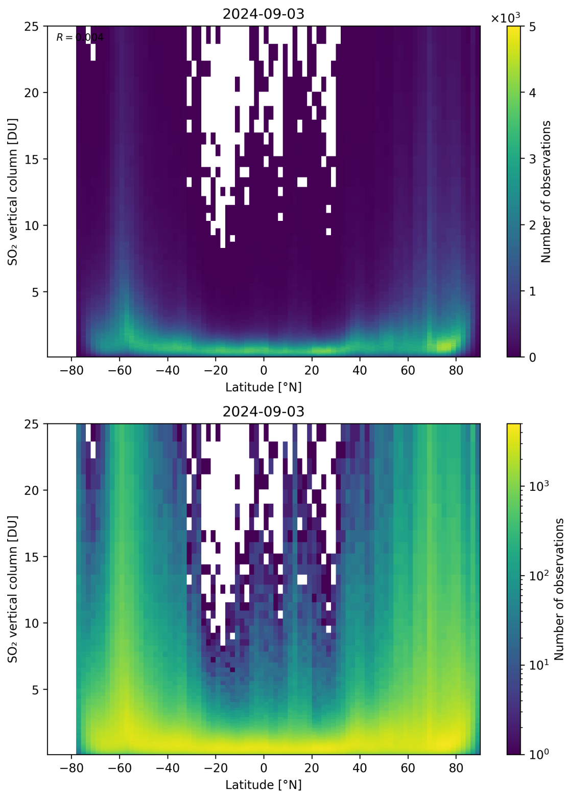
Figure 156: Scatter density plot of “Latitude” against “SO 2 vertical column” for 2024-09-02 to 2024-09-04.
