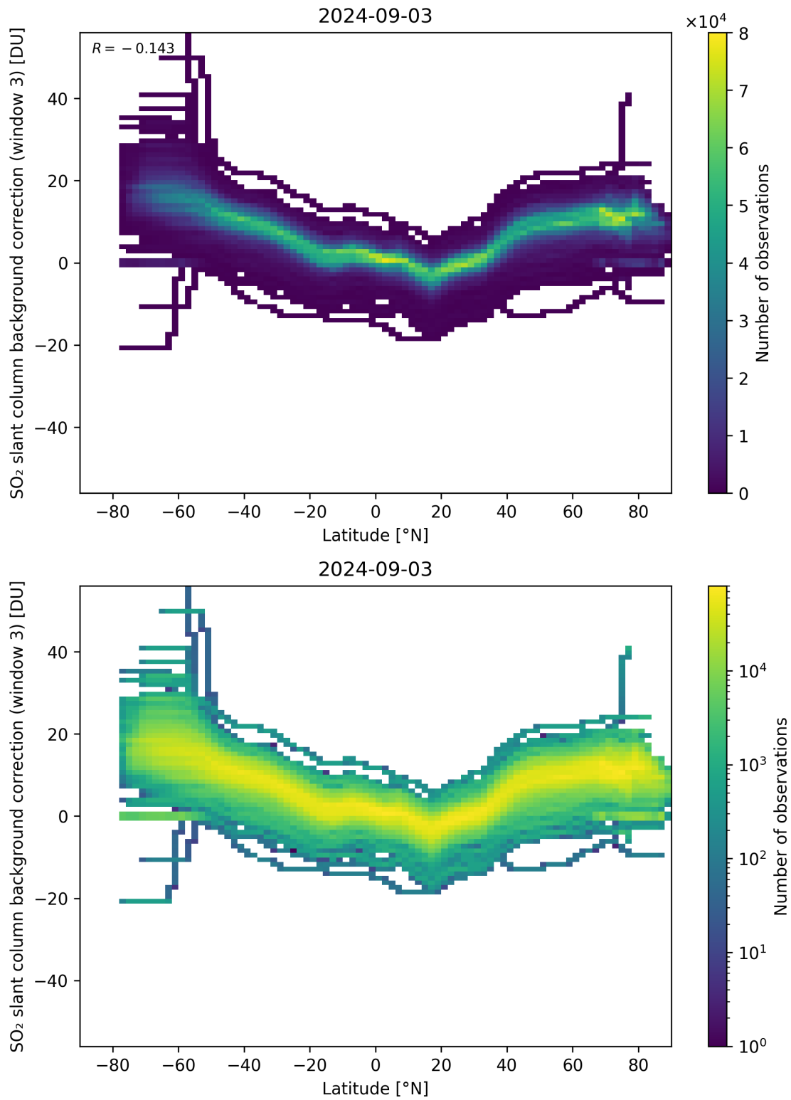
Figure 141: Scatter density plot of “Latitude” against “SO 2 slant column background correction (window 3)” for 2024-09-02 to 2024-09-04.
