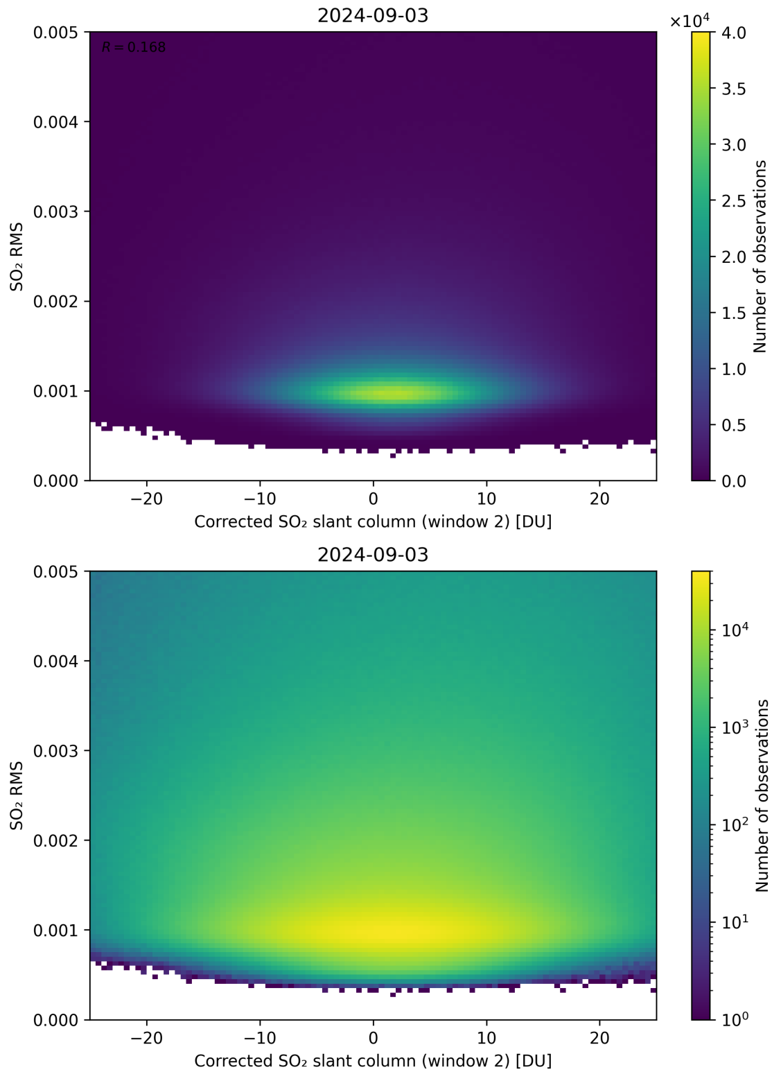
Figure 198: Scatter density plot of “Corrected SO 2 slant column (window 2)” against “SO 2 RMS” for 2024-09-02 to 2024-09-04.
