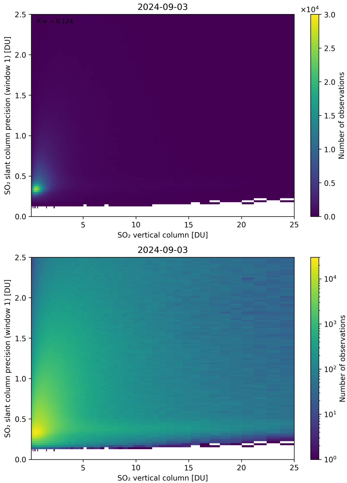
Figure 301: Scatter density plot of “SO 2 vertical column” against “SO 2 slant column precision (window 1)” for 2024-09-02 to 2024-09-04.
