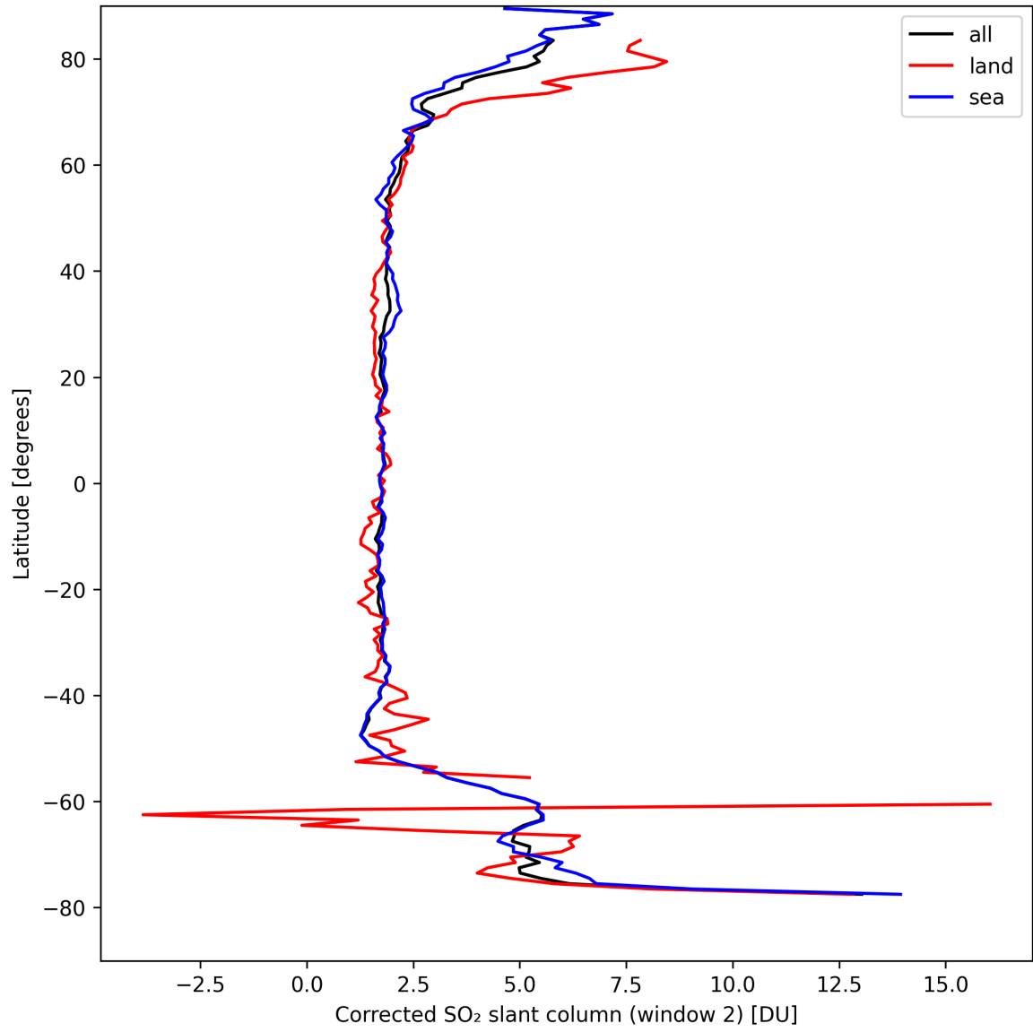
Figure 39: Zonal average of “Corrected SO 2 slant column (window 2)” for 2024-09-02 to 2024-09-04.
