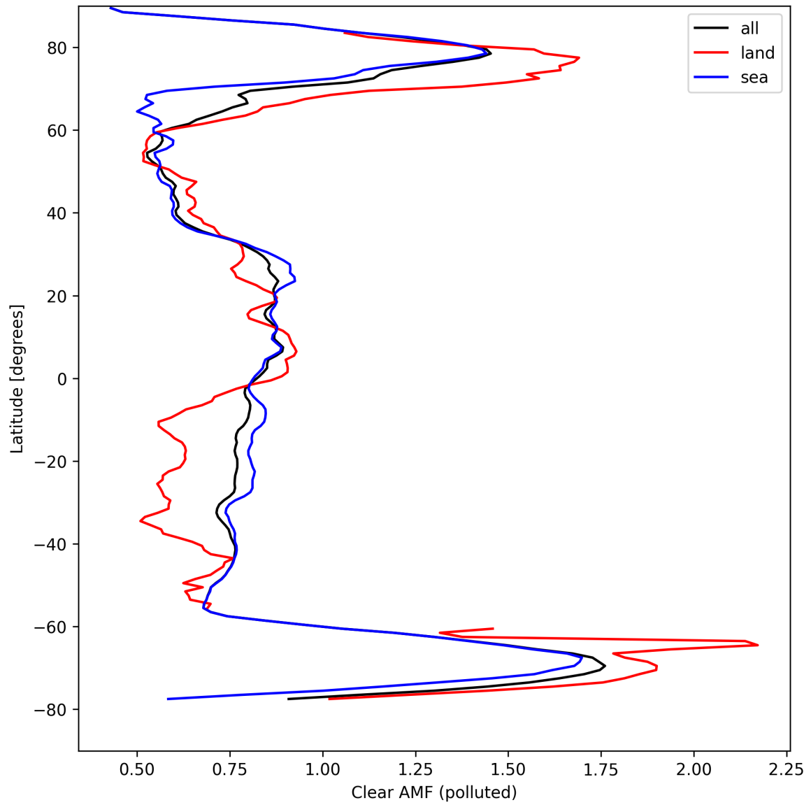
Figure 50: Zonal average of “Clear AMF (polluted)” for 2024-09-02 to 2024-09-04.
