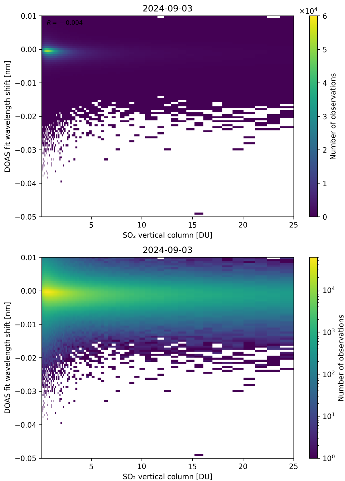
Figure 276: Scatter density plot of “SO 2 vertical column” against “DOAS fit wavelength shift” for 2024-09-02 to 2024-09-04.
