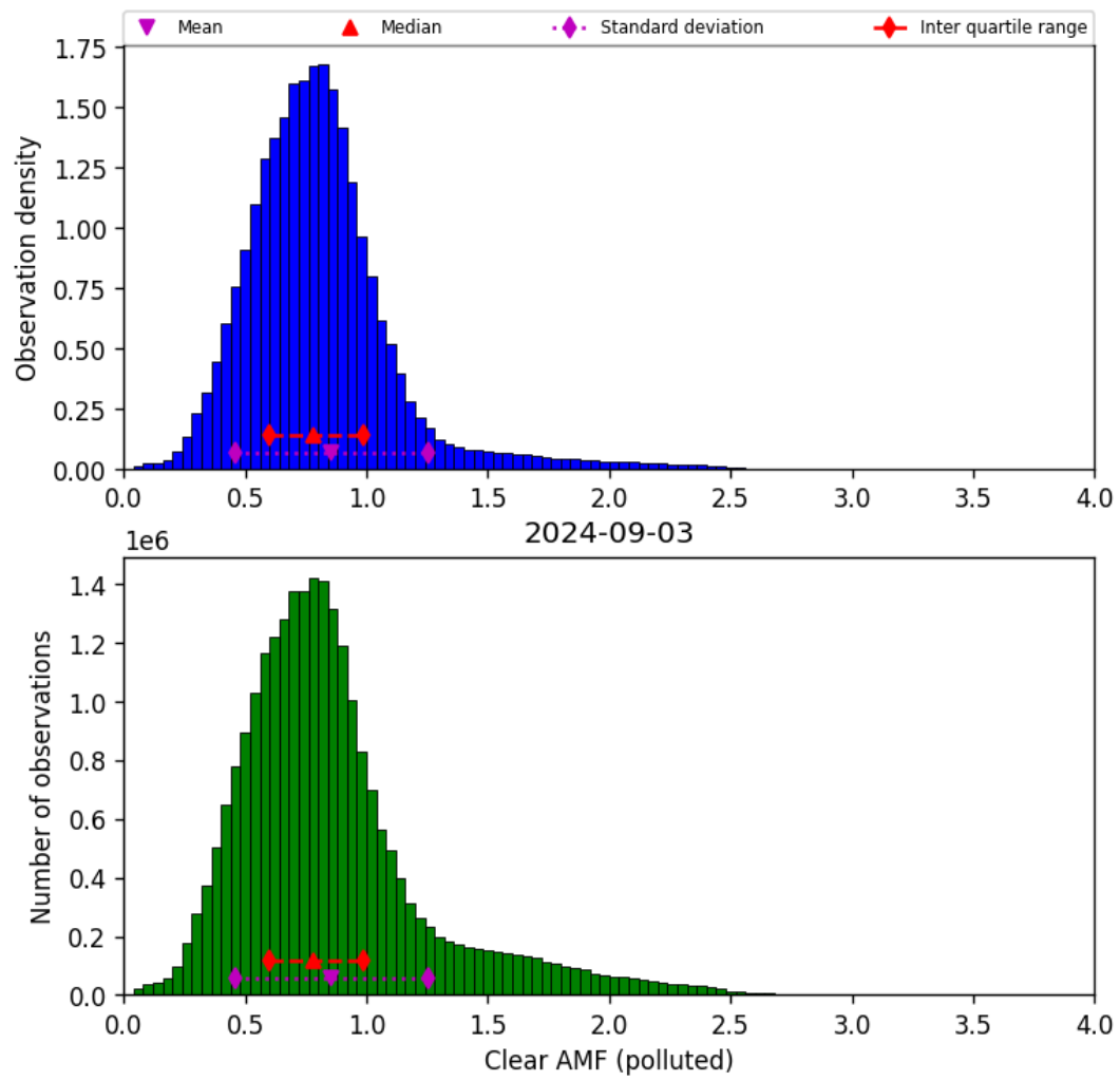
Figure 73: Histogram of “Clear AMF (polluted)” for 2024-09-02 to 2024-09-04
