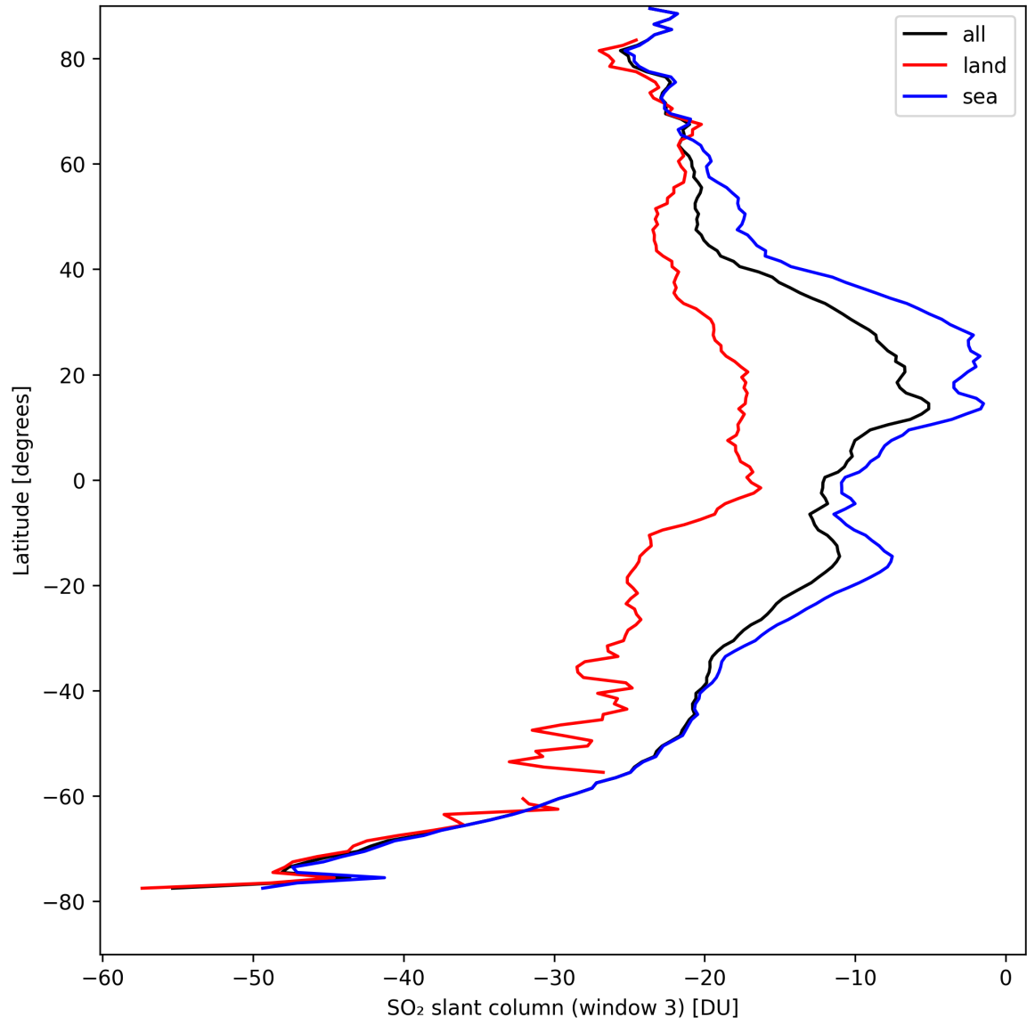
Figure 41: Zonal average of “SO 2 slant column (window 3)” for 2024-09-02 to 2024-09-04.
