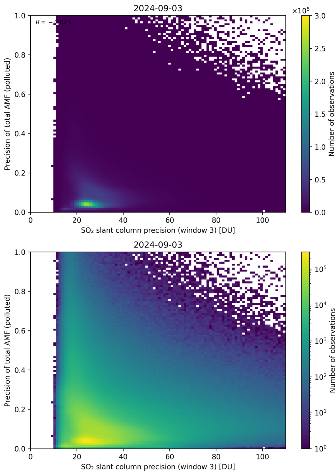
Figure 264: Scatter density plot of “SO 2 slant column precision (window 3)” against “Precision of total AMF (polluted)” for 2024-09-02 to 2024-09-04.
