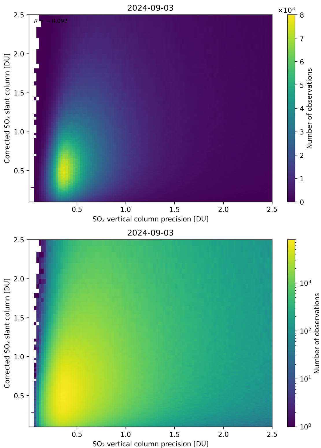
Figure 286: Scatter density plot of “SO 2 vertical column precision” against “Corrected SO 2 slant column” for 2024-09-02 to 2024-09-04.
