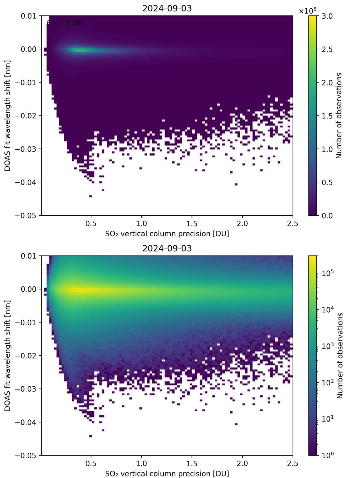
Figure 282: Scatter density plot of “SO 2 vertical column precision” against “DOAS fit wavelength shift” for 2024-09-02 to 2024-09-04.
