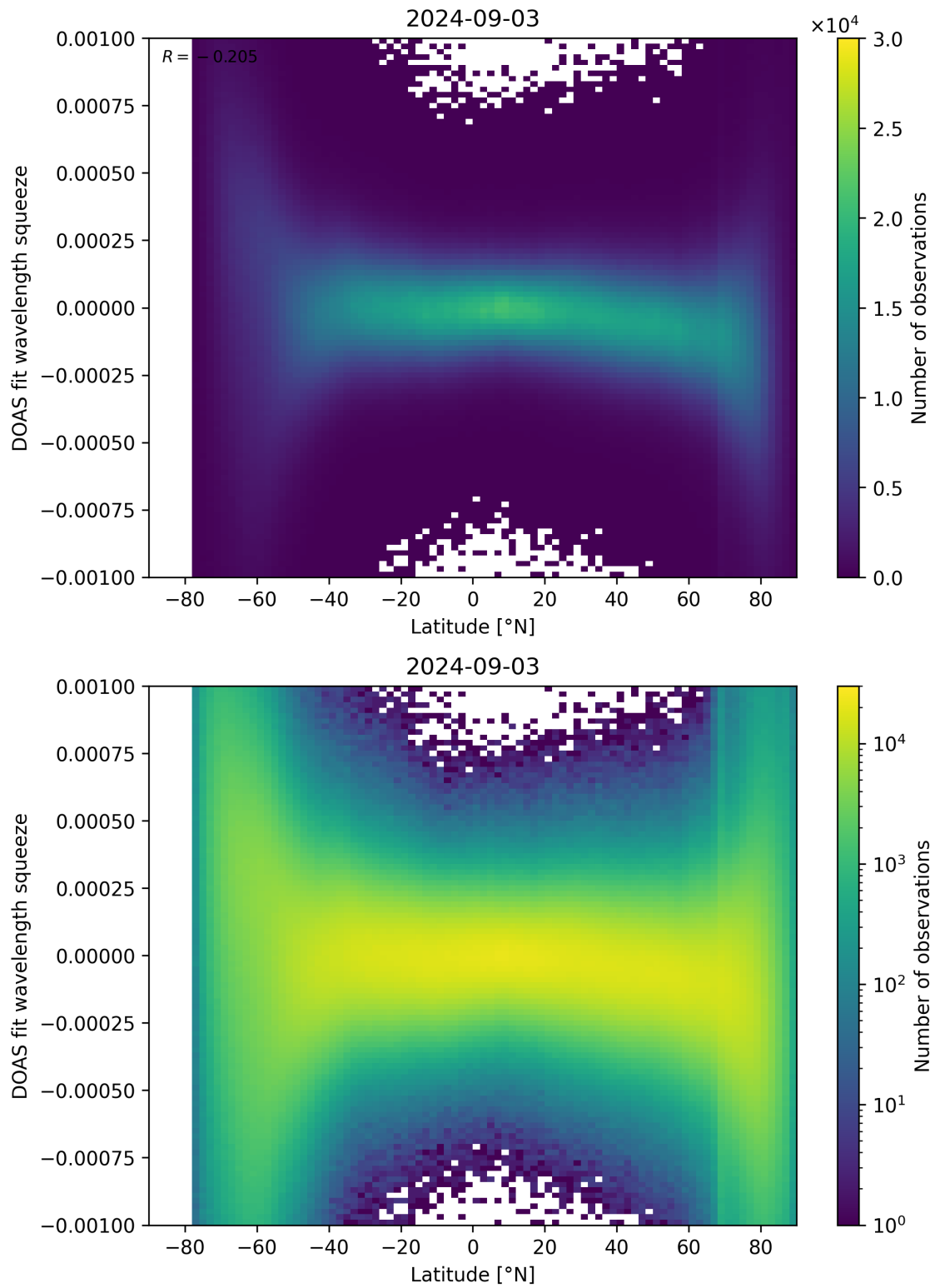
Figure 143: Scatter density plot of “Latitude” against “DOAS fit wavelength squeeze” for 2024-09-02 to 2024-09-04.
