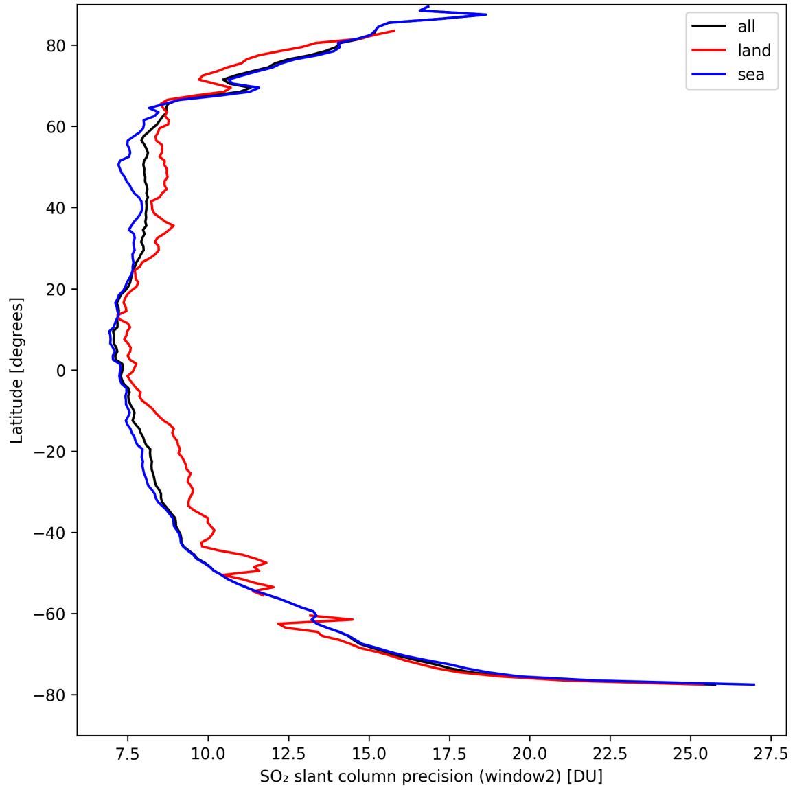
Figure 38: Zonal average of “SO 2 slant column precision (window2)” for 2024-09-02 to 2024-09-04.
