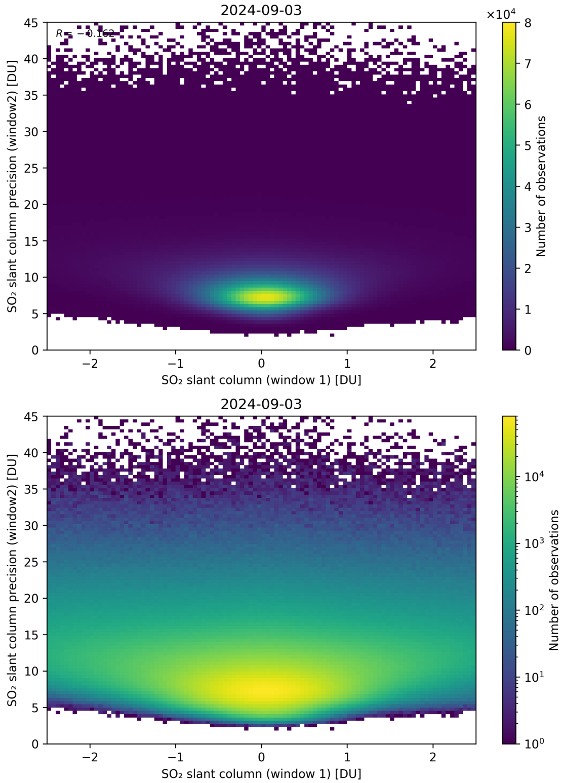
Figure 236: Scatter density plot of “SO 2 slant column (window 1)” against “SO 2 slant column precision (window2)” for 2024-09-02 to 2024-09-04.
