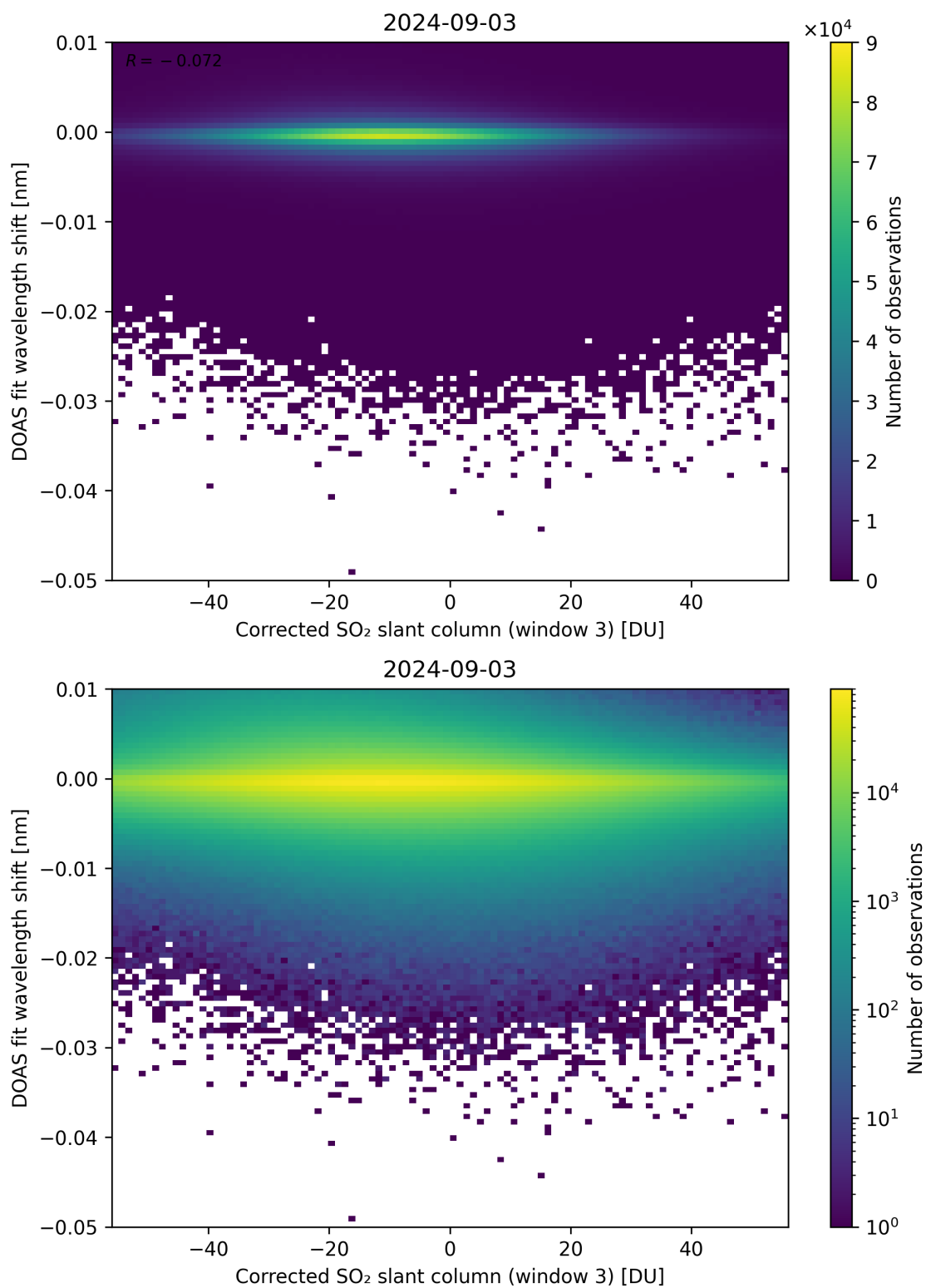
Figure 206: Scatter density plot of “Corrected SO 2 slant column (window 3)” against “DOAS fit wavelength shift” for 2024-09-02 to 2024-09-04.
