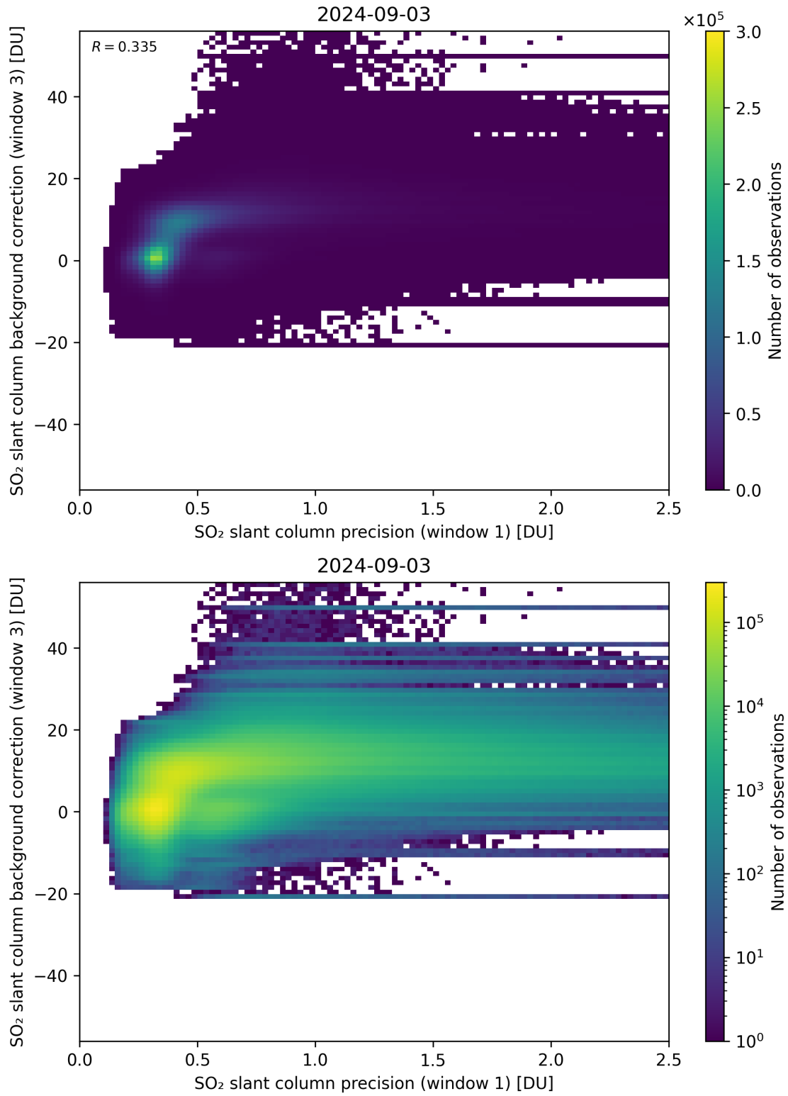
Figure 220: Scatter density plot of “SO 2 slant column precision (window 1)” against “SO 2 slant column background correction (window 3)” for 2024-09-02 to 2024-09-04.
