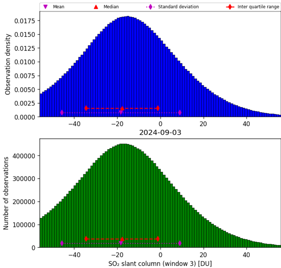
Figure 64: Histogram of “SO 2 slant column (window 3)” for 2024-09-02 to 2024-09-04
