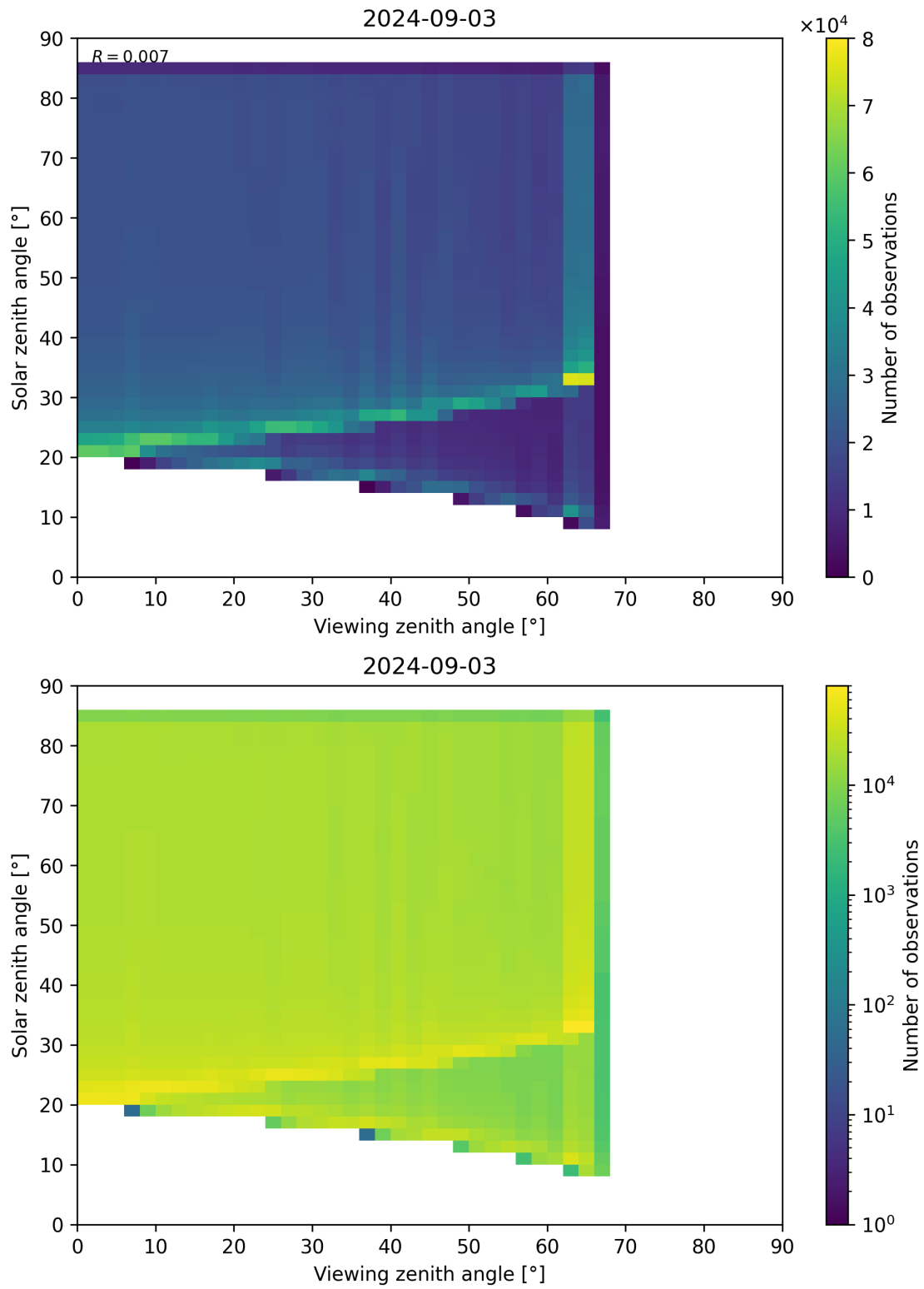
Figure 315: Scatter density plot of “Viewing zenith angle” against “Solar zenith angle” for 2024-09-02 to 2024-09-04.
