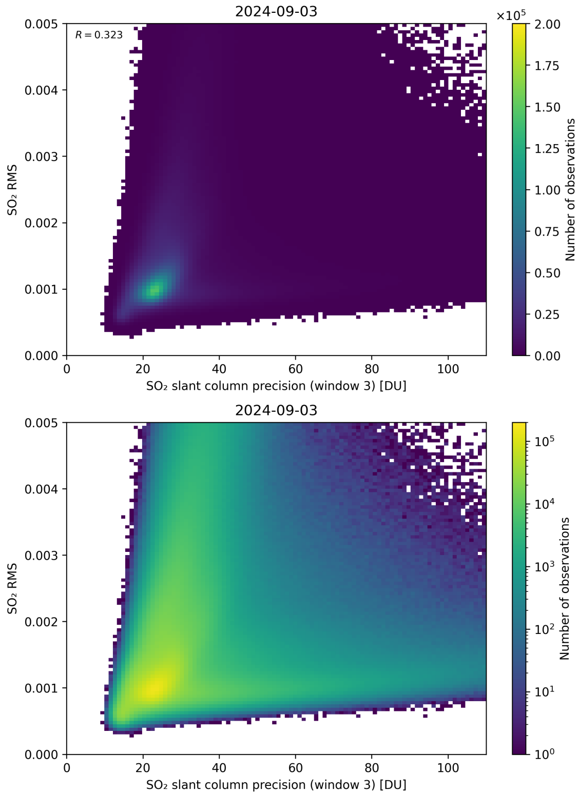
Figure 260: Scatter density plot of “SO 2 slant column precision (window 3)” against “SO 2 RMS” for 2024-09-02 to 2024-09-04.
