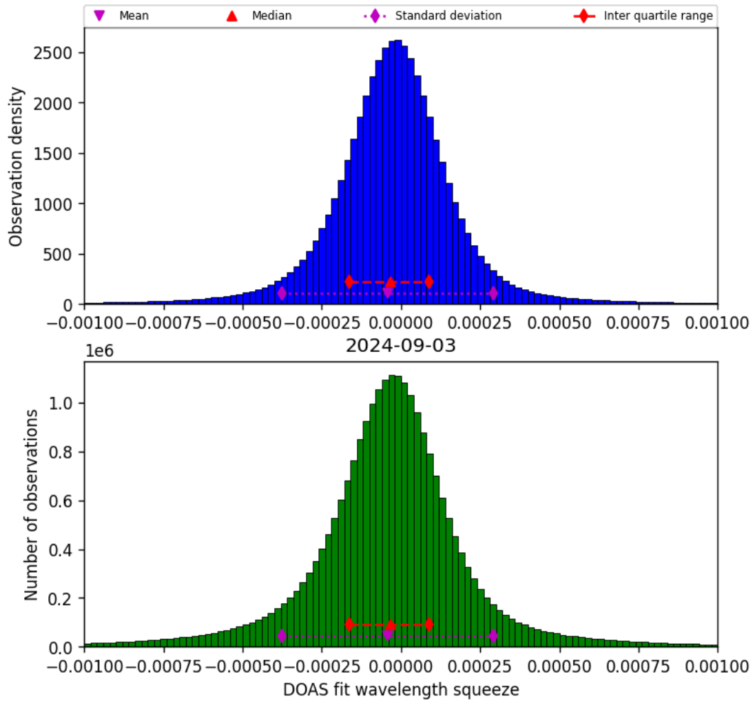
Figure 69: Histogram of “DOAS fit wavelength squeeze” for 2024-09-02 to 2024-09-04
