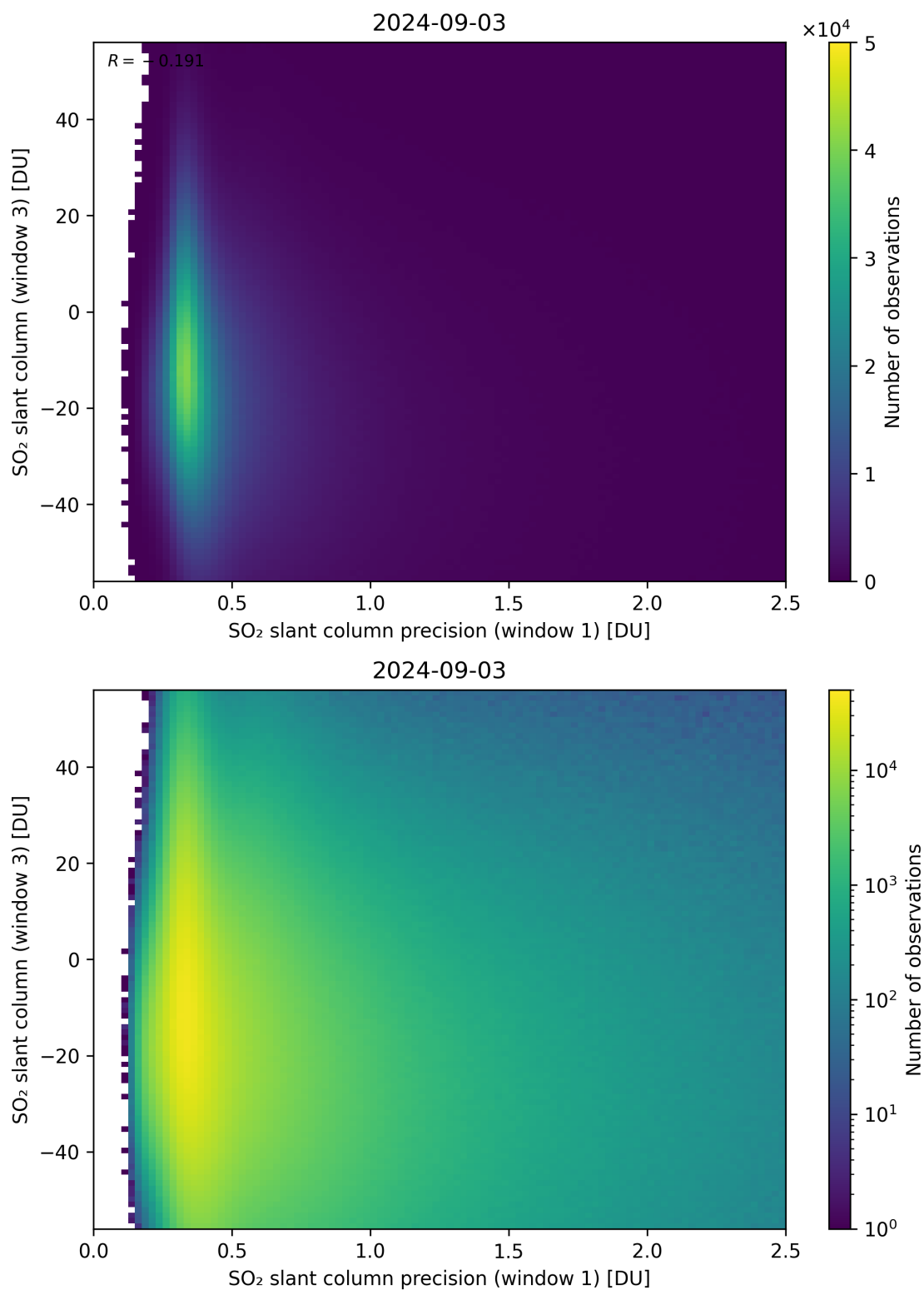
Figure 228: Scatter density plot of “SO 2 slant column precision (window 1)” against “SO 2 slant column (window 3)” for 2024-09-02 to 2024-09-04.
