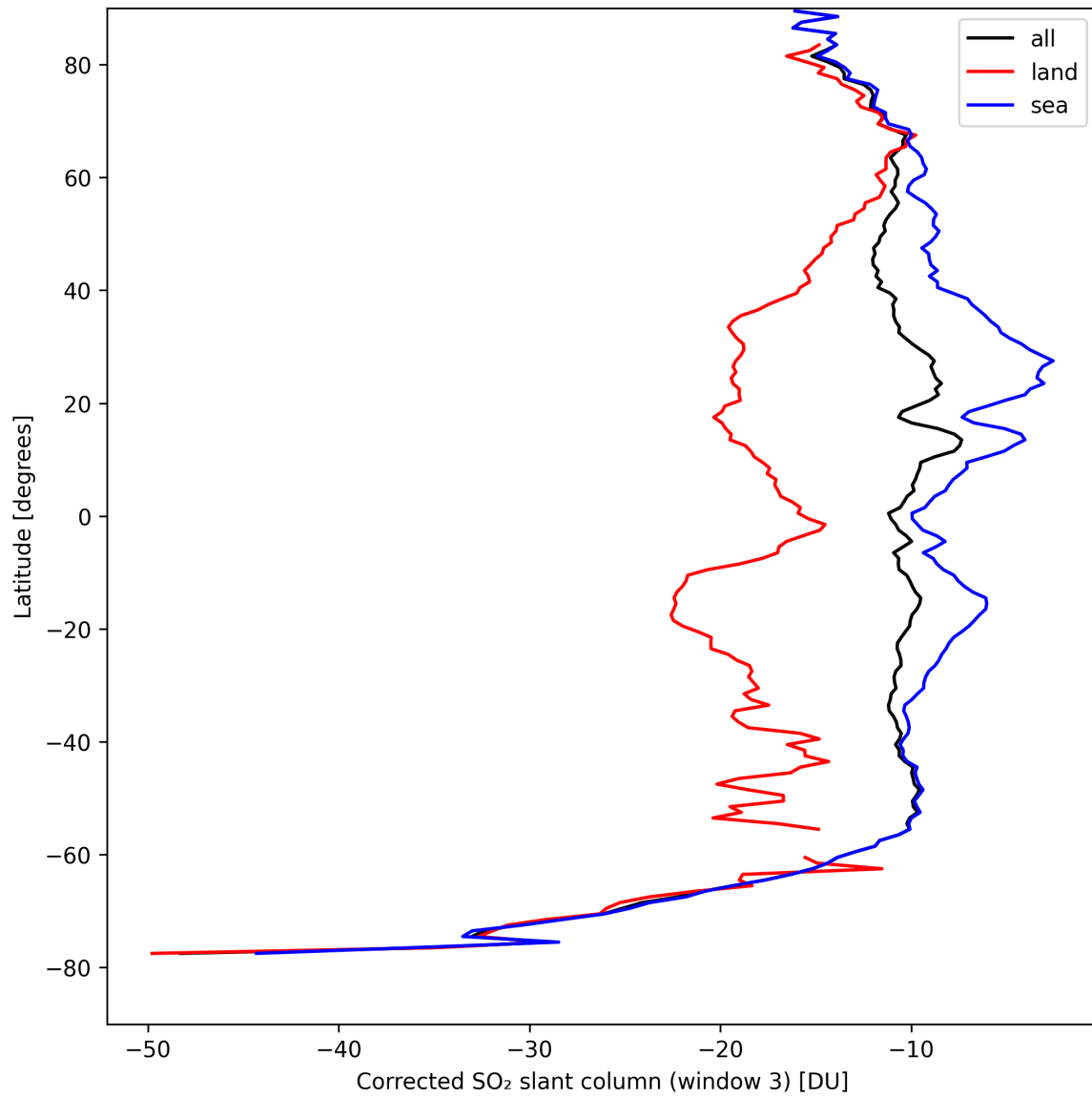
Figure 43: Zonal average of “Corrected SO 2 slant column (window 3)” for 2024-09-02 to 2024-09-04.
