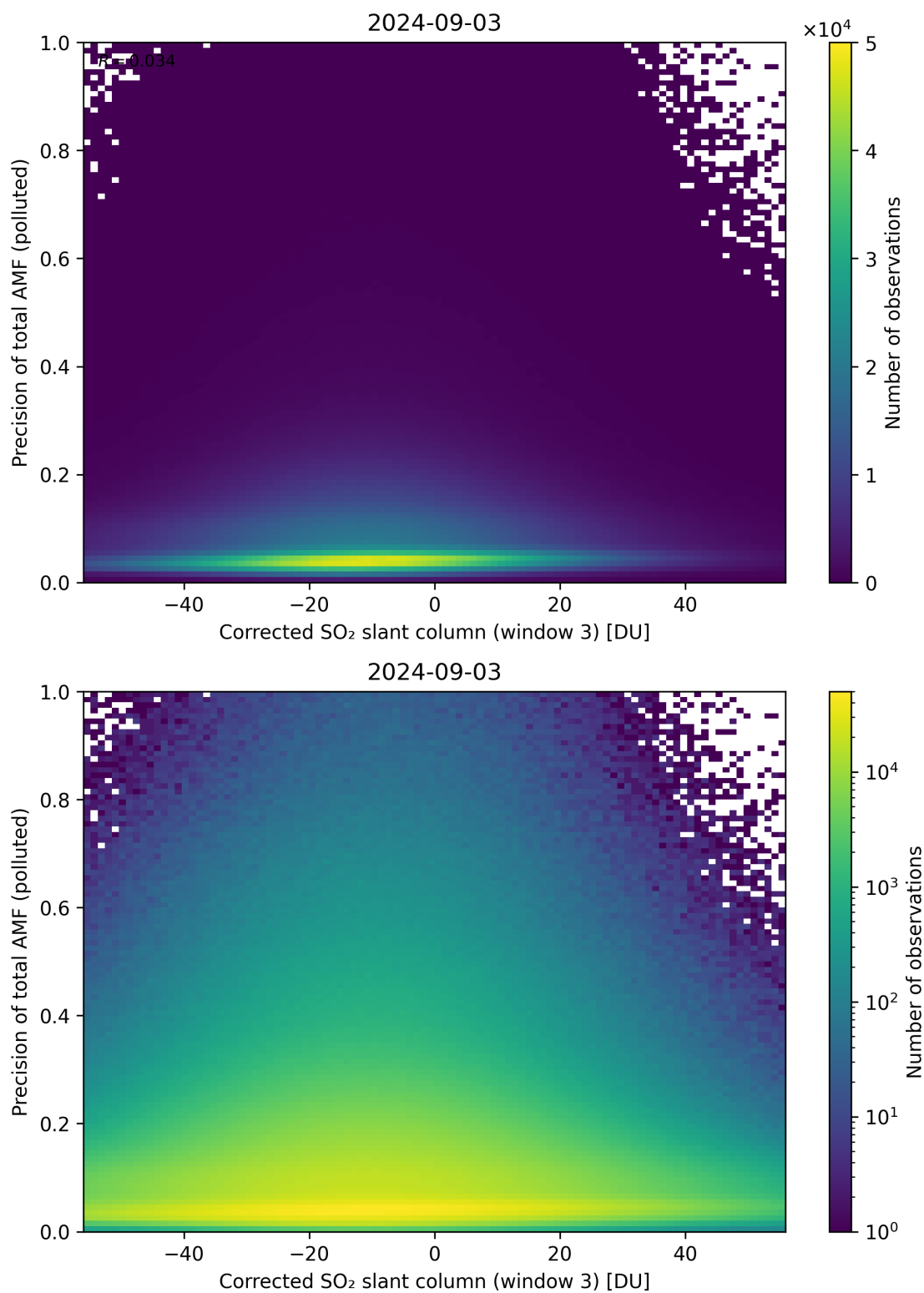
Figure 211: Scatter density plot of “Corrected SO 2 slant column (window 3)” against “Precision of total AMF (polluted)” for 2024-09-02 to 2024-09-04.
