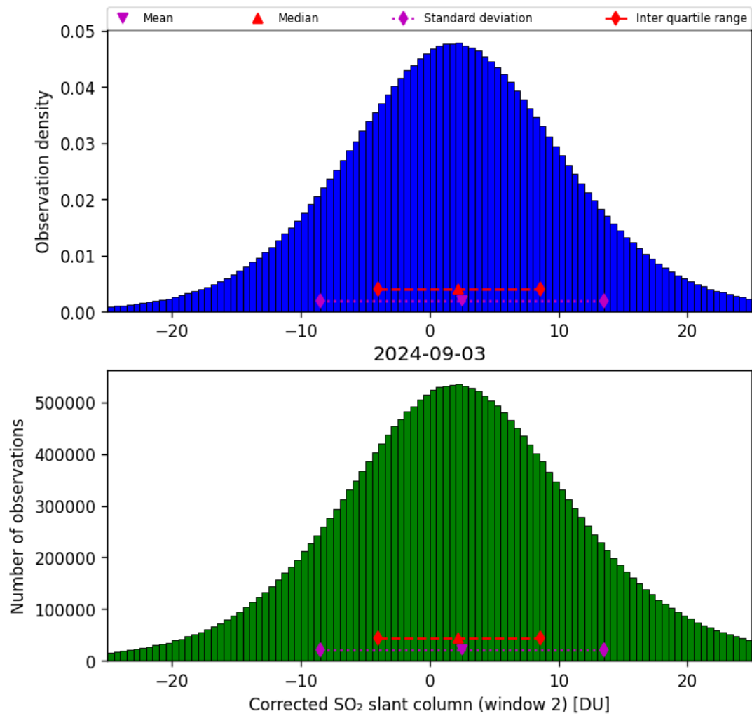
Figure 62: Histogram of “Corrected SO 2 slant column (window 2)” for 2024-09-02 to 2024-09-04
