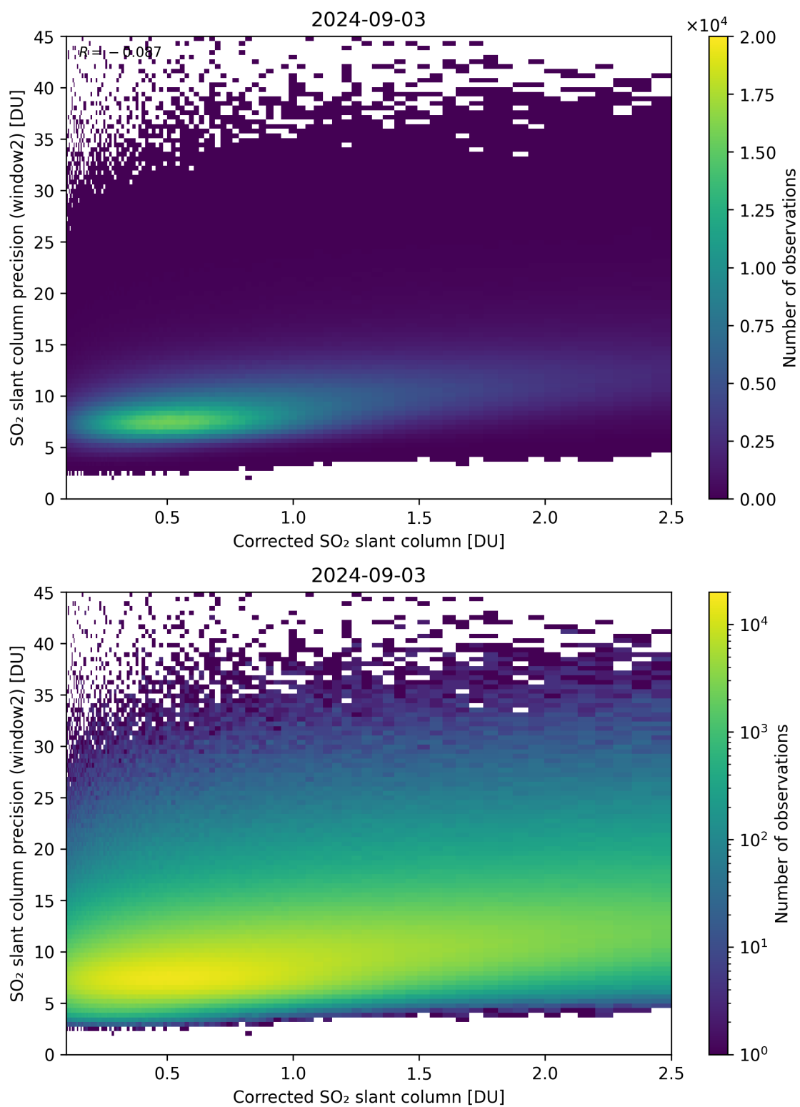
Figure 189: Scatter density plot of “Corrected SO 2 slant column” against “SO 2 slant column precision (window2)” for 2024-09-02 to 2024-09-04.
