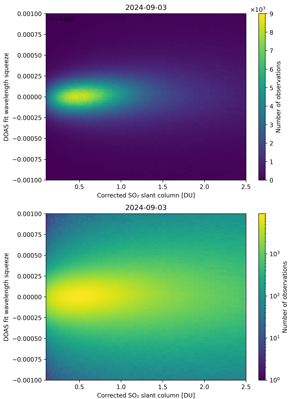
Figure 182: Scatter density plot of “Corrected SO 2 slant column” against “DOAS fit wavelength squeeze” for 2024-09-02 to 2024-09-04.
