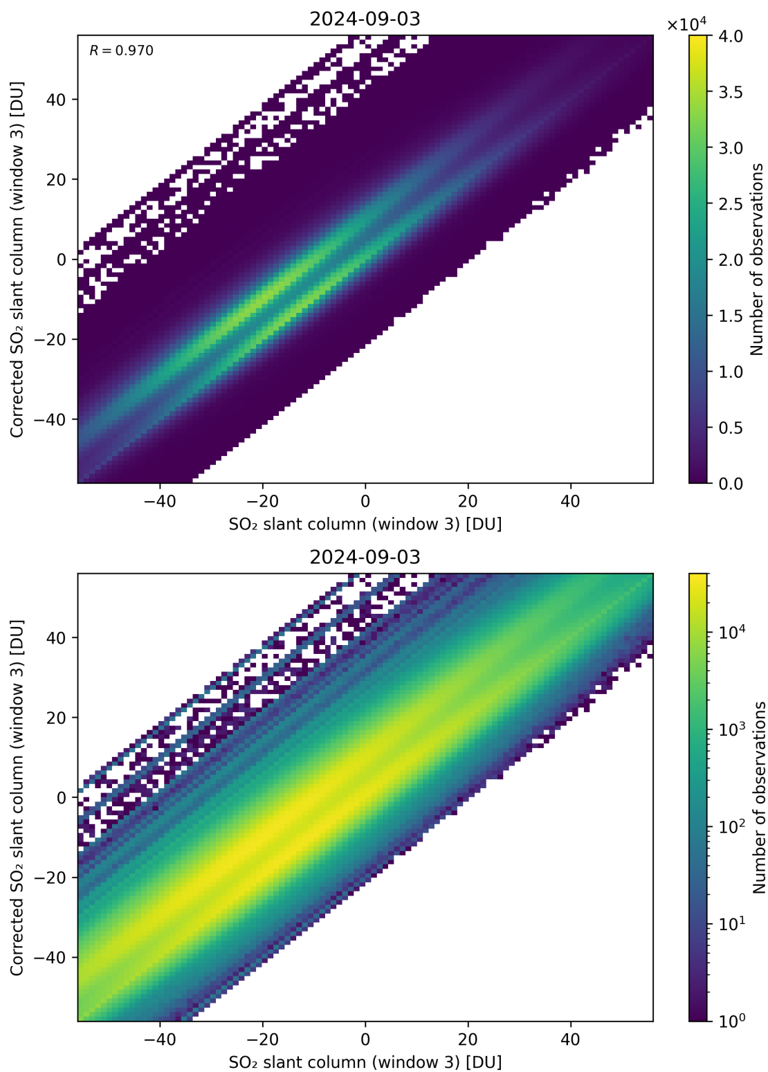
Figure 266: Scatter density plot of “SO 2 slant column (window 3)” against “Corrected SO 2 slant column (window 3)” for 2024-09-02 to 2024-09-04.
