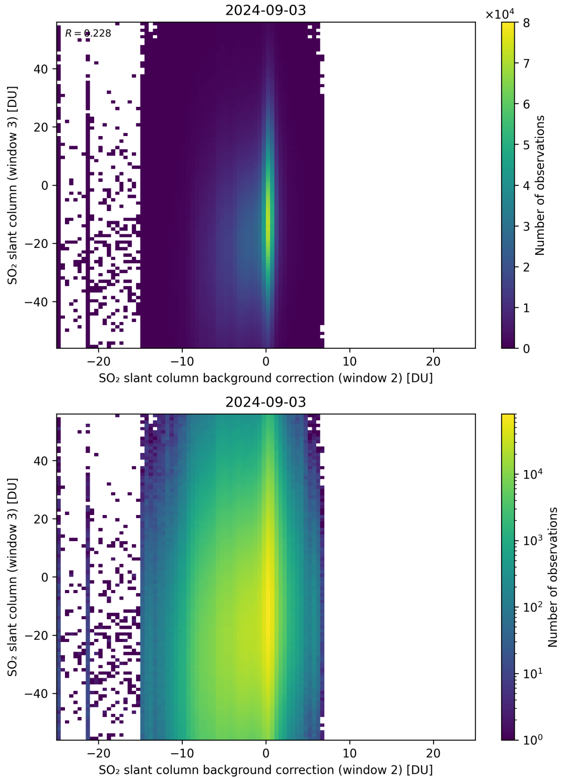
Figure 117: Scatter density plot of “SO 2 slant column background correction (window 2)” against “SO 2 slant column (window 3)” for 2024-09-02 to 2024-09-04.
