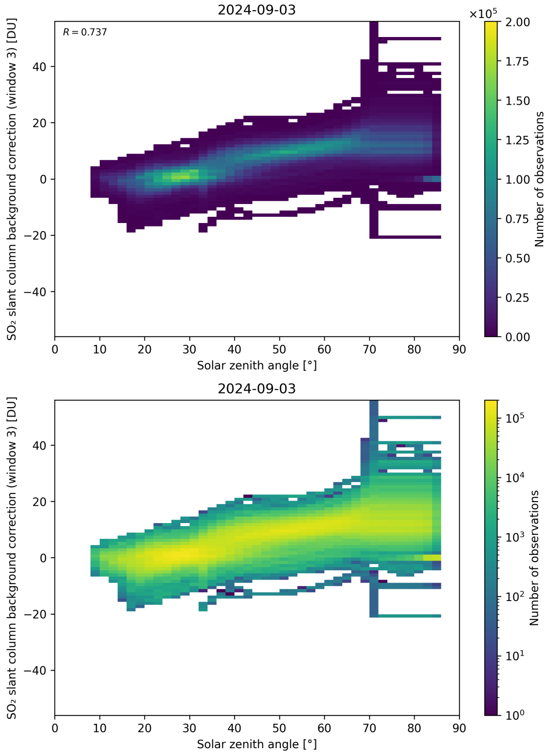
Figure 160: Scatter density plot of “Solar zenith angle” against “SO 2 slant column background correction (window 3)” for 2024-09-02 to 2024-09-04.
