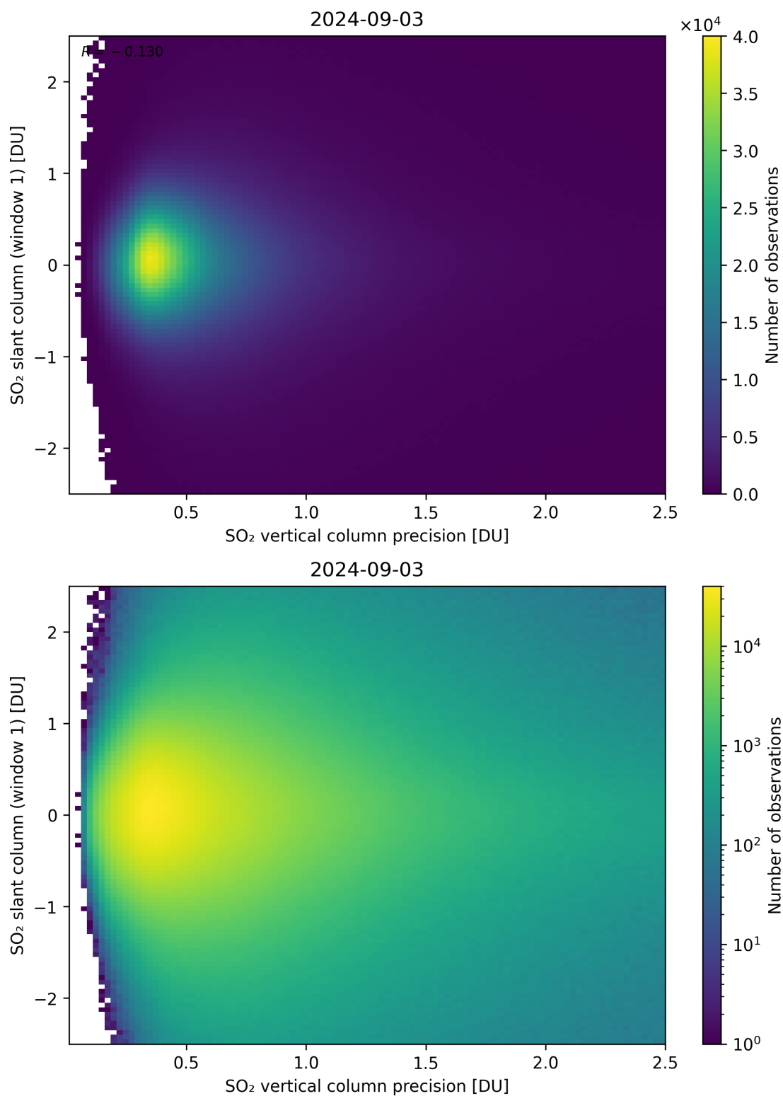
Figure 289: Scatter density plot of “SO 2 vertical column precision” against “SO 2 slant column (window 1)” for 2024-09-02 to 2024-09-04.
