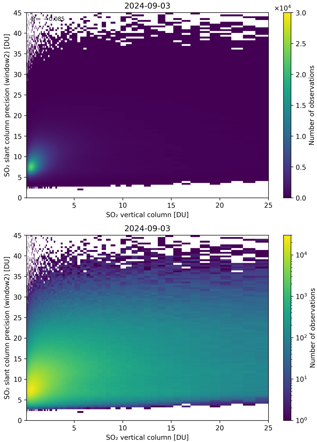
Figure 302: Scatter density plot of “SO 2 vertical column” against “SO 2 slant column precision (window2)” for 2024-09-02 to 2024-09-04.
