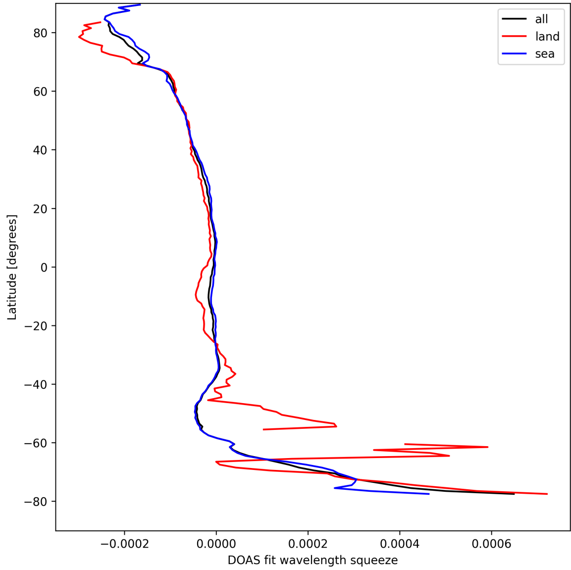
Figure 46: Zonal average of “DOAS fit wavelength squeeze” for 2024-09-02 to 2024-09-04.
