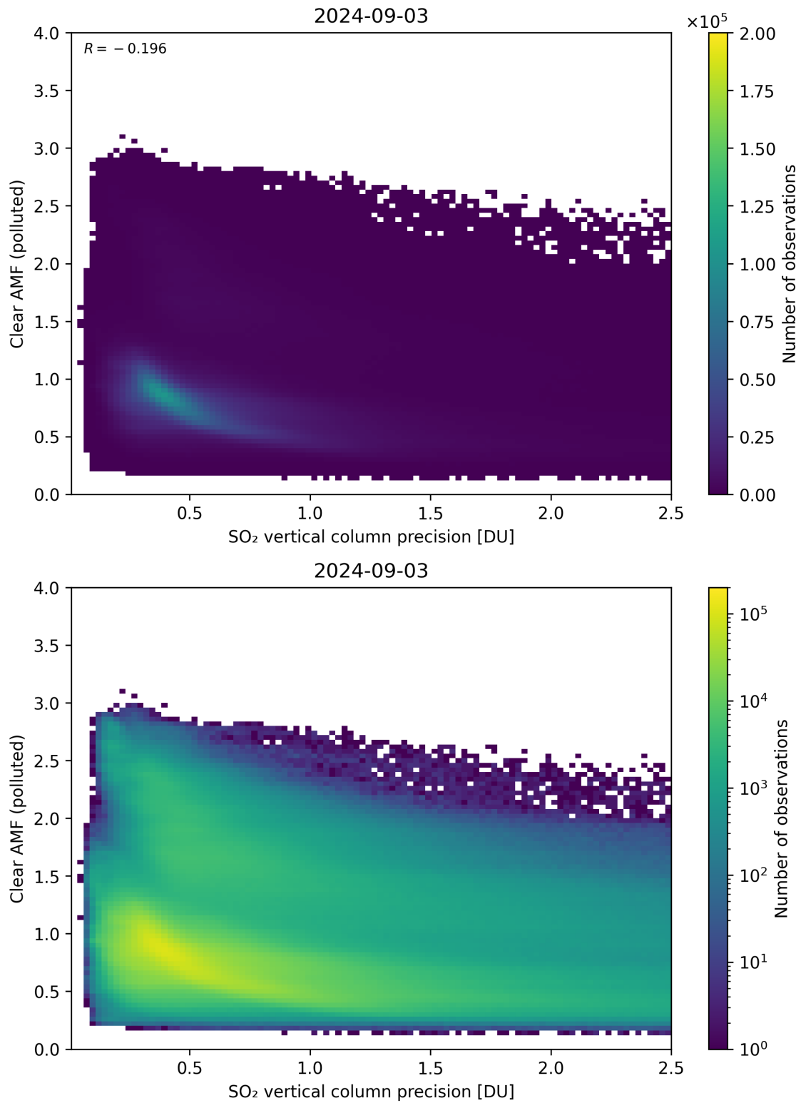
Figure 285: Scatter density plot of “SO 2 vertical column precision” against “Clear AMF (polluted)” for 2024-09-02 to 2024-09-04.
