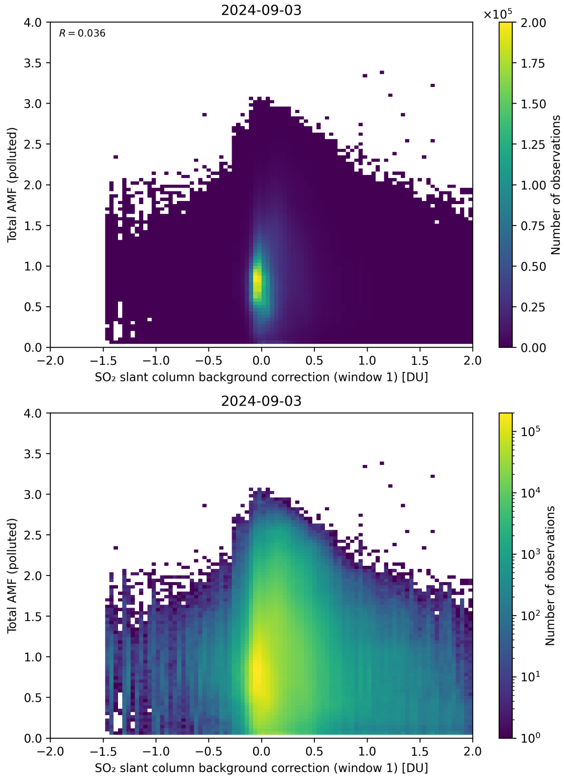
Figure 109: Scatter density plot of “SO 2 slant column background correction (window 1)” against “Total AMF (polluted)” for 2024-09-02 to 2024-09-04.
