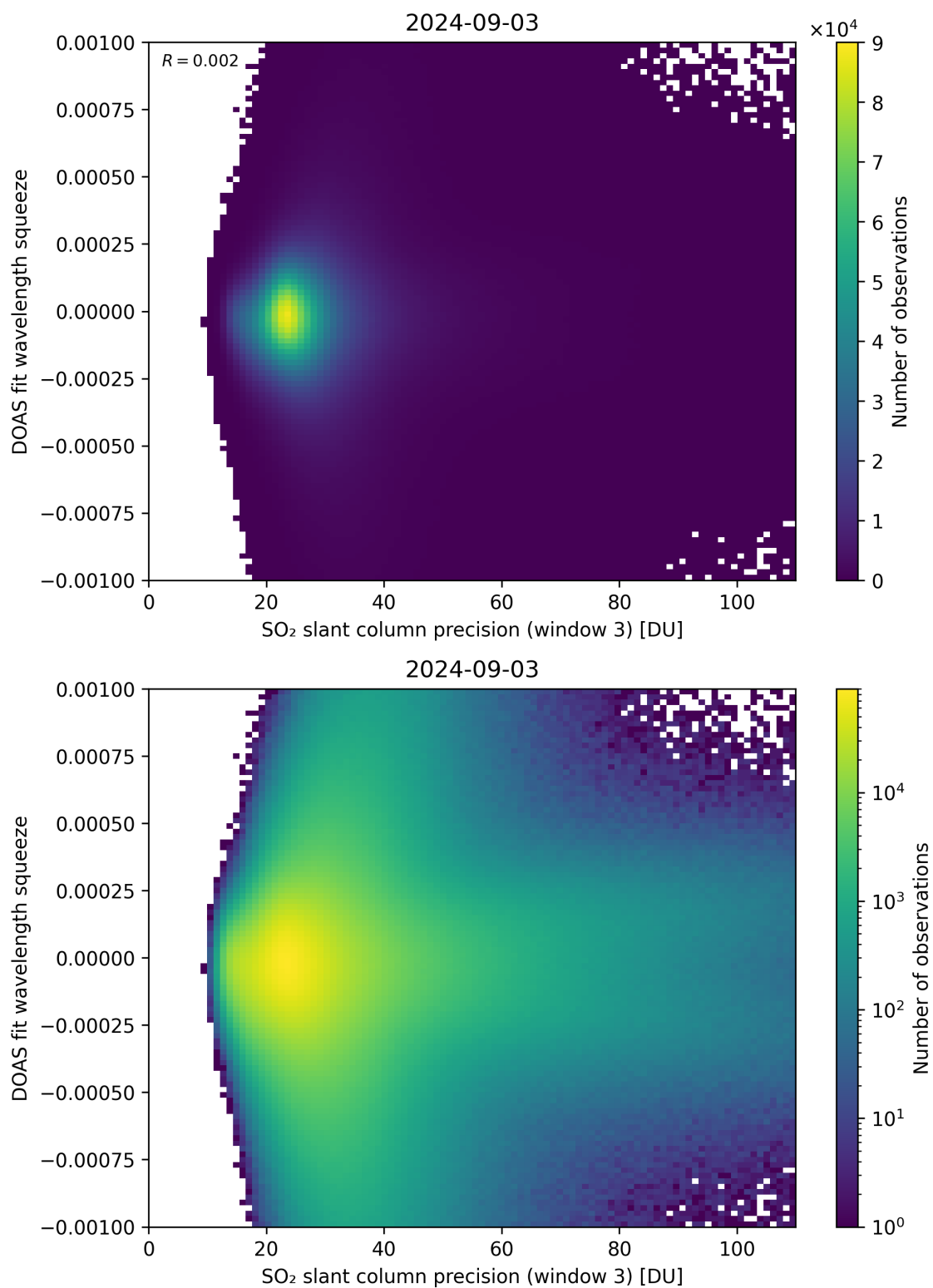
Figure 259: Scatter density plot of “SO 2 slant column precision (window 3)” against “DOAS fit wavelength squeeze” for 2024-09-02 to 2024-09-04.
