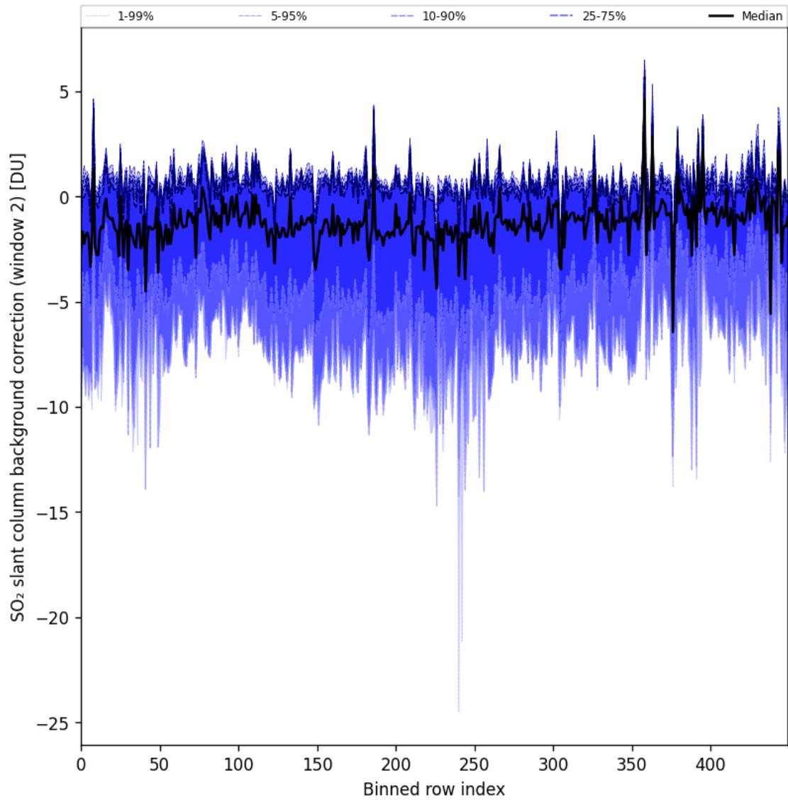
Figure 86: Along track statistics of “SO 2 slant column background correction (window 2)” for 2024-09-02 to 2024-09-04
