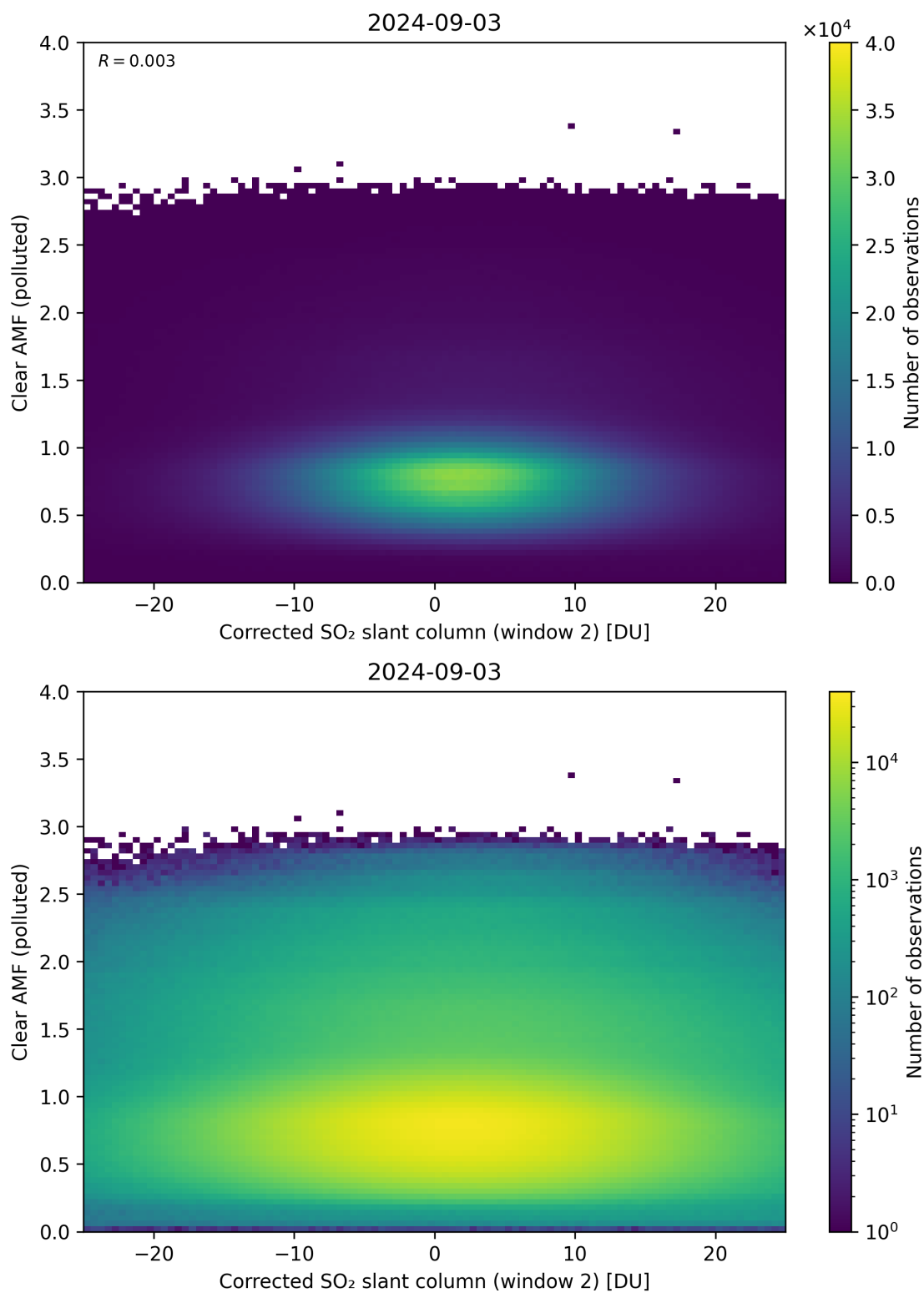
Figure 199: Scatter density plot of “Corrected SO 2 slant column (window 2)” against “Clear AMF (polluted)” for 2024-09-02 to 2024-09-04.
