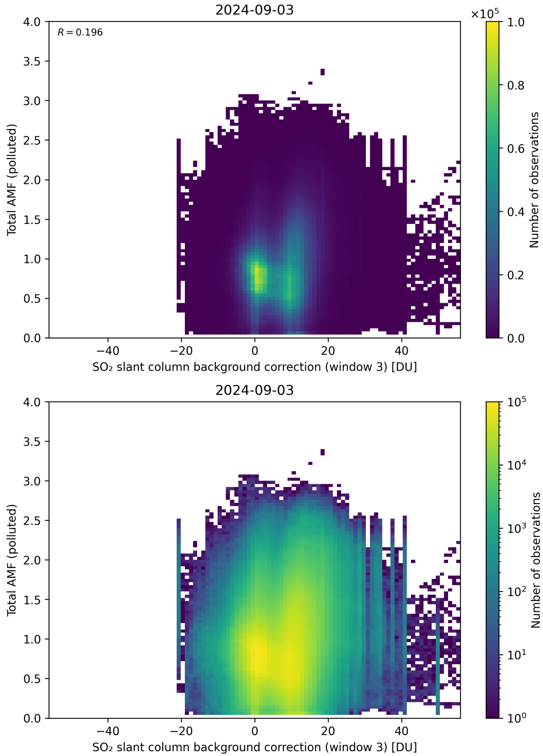
Figure 125: Scatter density plot of “SO 2 slant column background correction (window 3)” against “Total AMF (polluted)” for 2024-09-02 to 2024-09-04.
