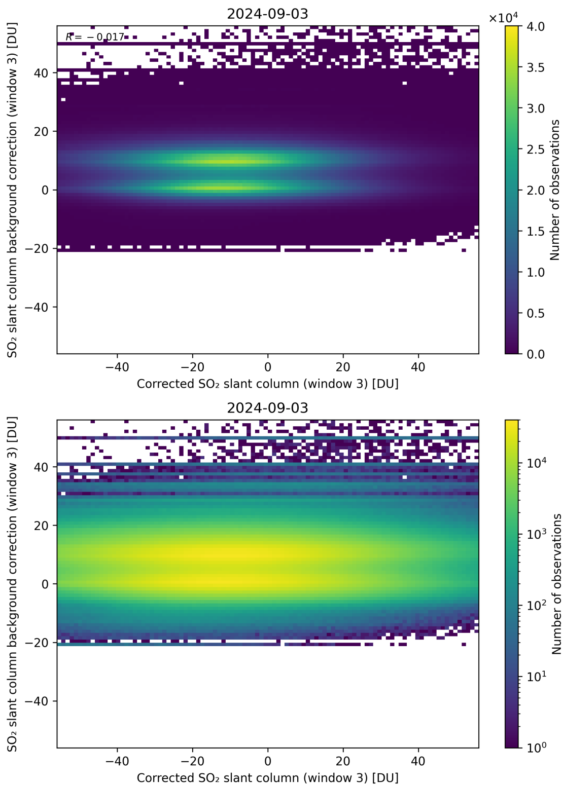
Figure 205: Scatter density plot of “Corrected SO 2 slant column (window 3)” against “SO 2 slant column background correction (window 3)” for 2024-09-02 to 2024-09-04.
