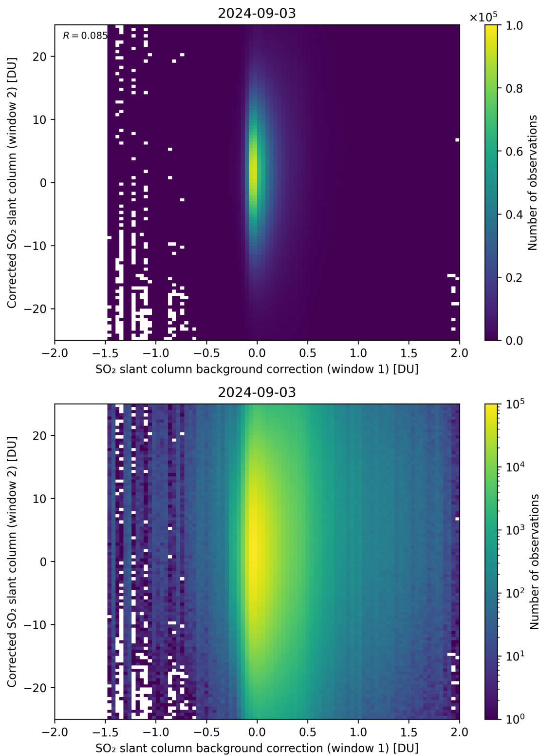
Figure 104: Scatter density plot of “SO 2 slant column background correction (window 1)” against “Corrected SO 2 slant column (window 2)” for 2024-09-02 to 2024-09-04.
