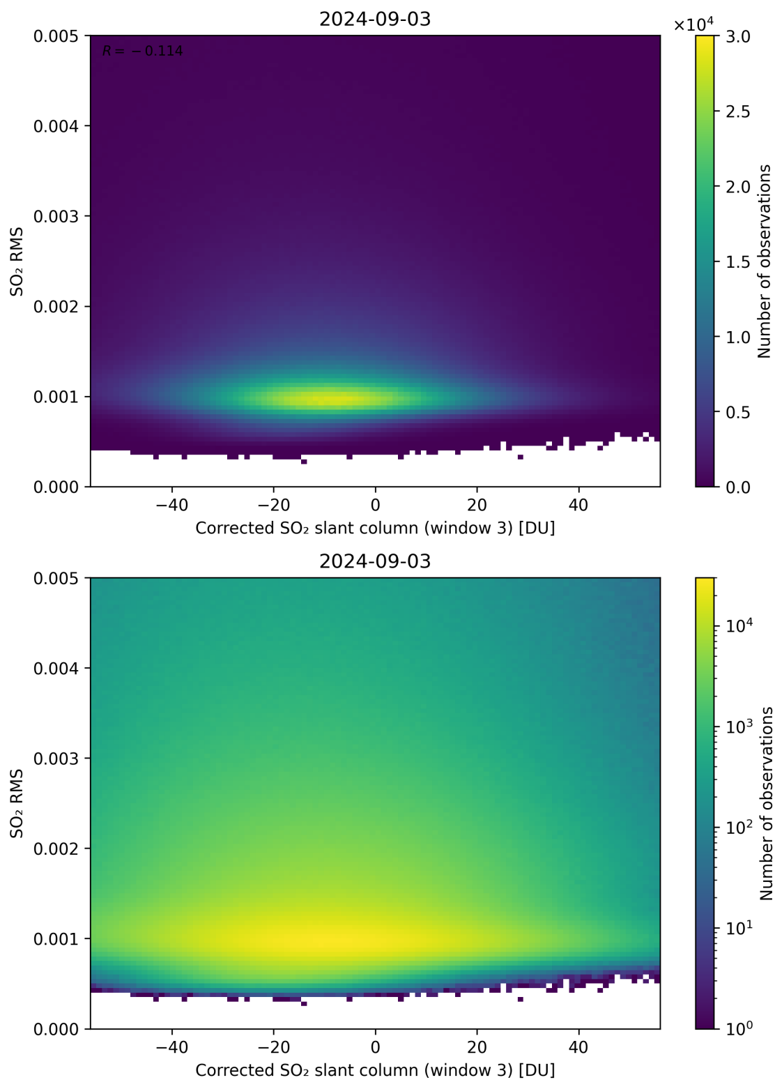
Figure 208: Scatter density plot of “Corrected SO 2 slant column (window 3)” against “SO 2 RMS” for 2024-09-02 to 2024-09-04.
