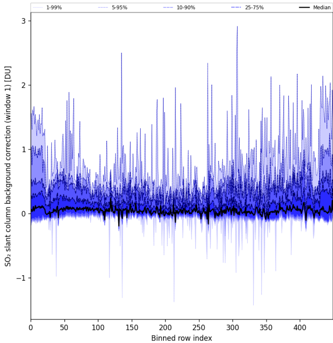
Figure 82: Along track statistics of “SO 2 slant column background correction (window 1)” for 2024-09-02 to 2024-09-04
