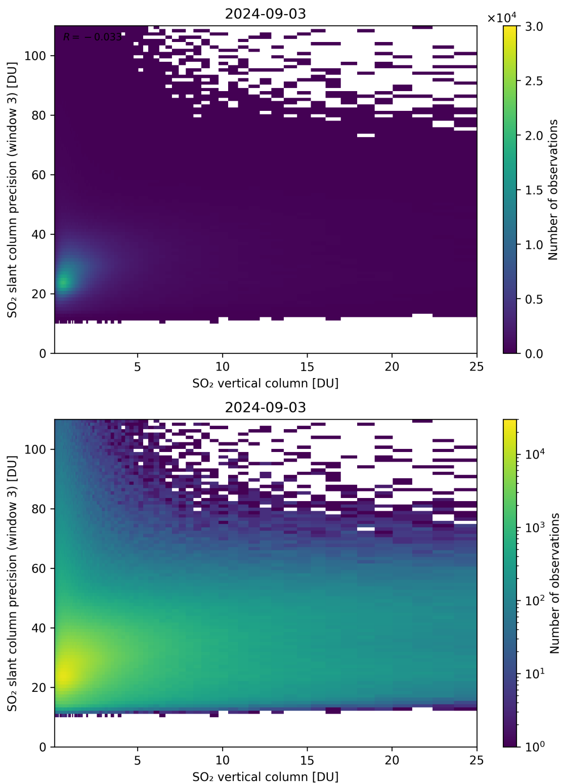
Figure 304: Scatter density plot of “SO 2 vertical column” against “SO 2 slant column precision (window 3)” for 2024-09-02 to 2024-09-04.
