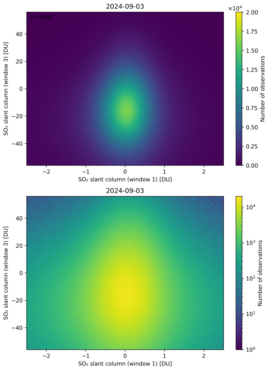
Figure 237: Scatter density plot of “SO 2 slant column (window 1)” against “SO 2 slant column (window 3)” for 2024-09-02 to 2024-09-04.
