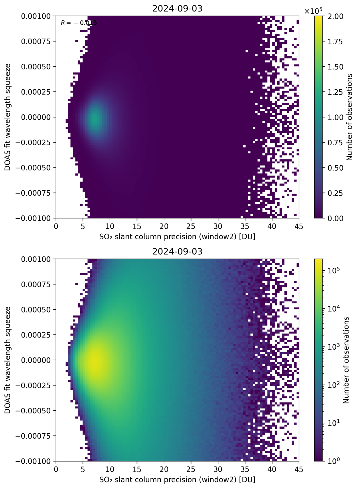
Figure 244: Scatter density plot of “SO 2 slant column precision (window2)” against “DOAS fit wavelength squeeze” for 2024-09-02 to 2024-09-04.
