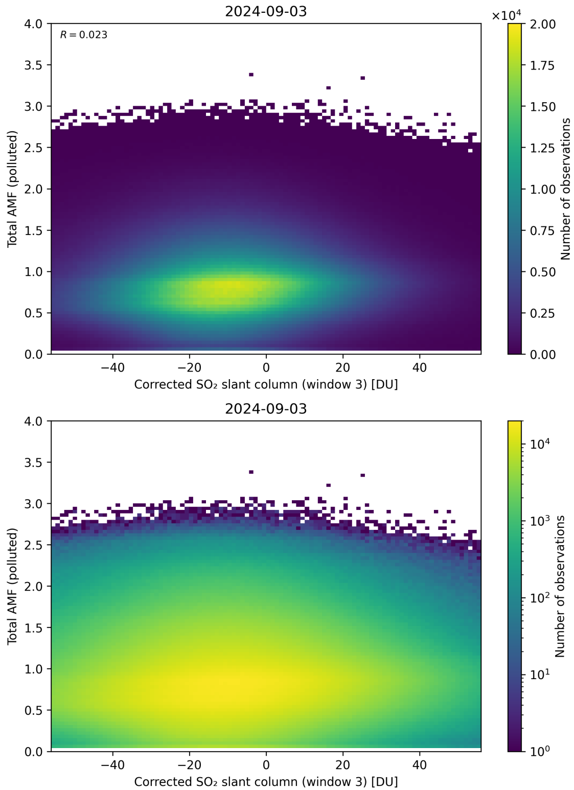
Figure 210: Scatter density plot of “Corrected SO 2 slant column (window 3)” against “Total AMF (polluted)” for 2024-09-02 to 2024-09-04.
