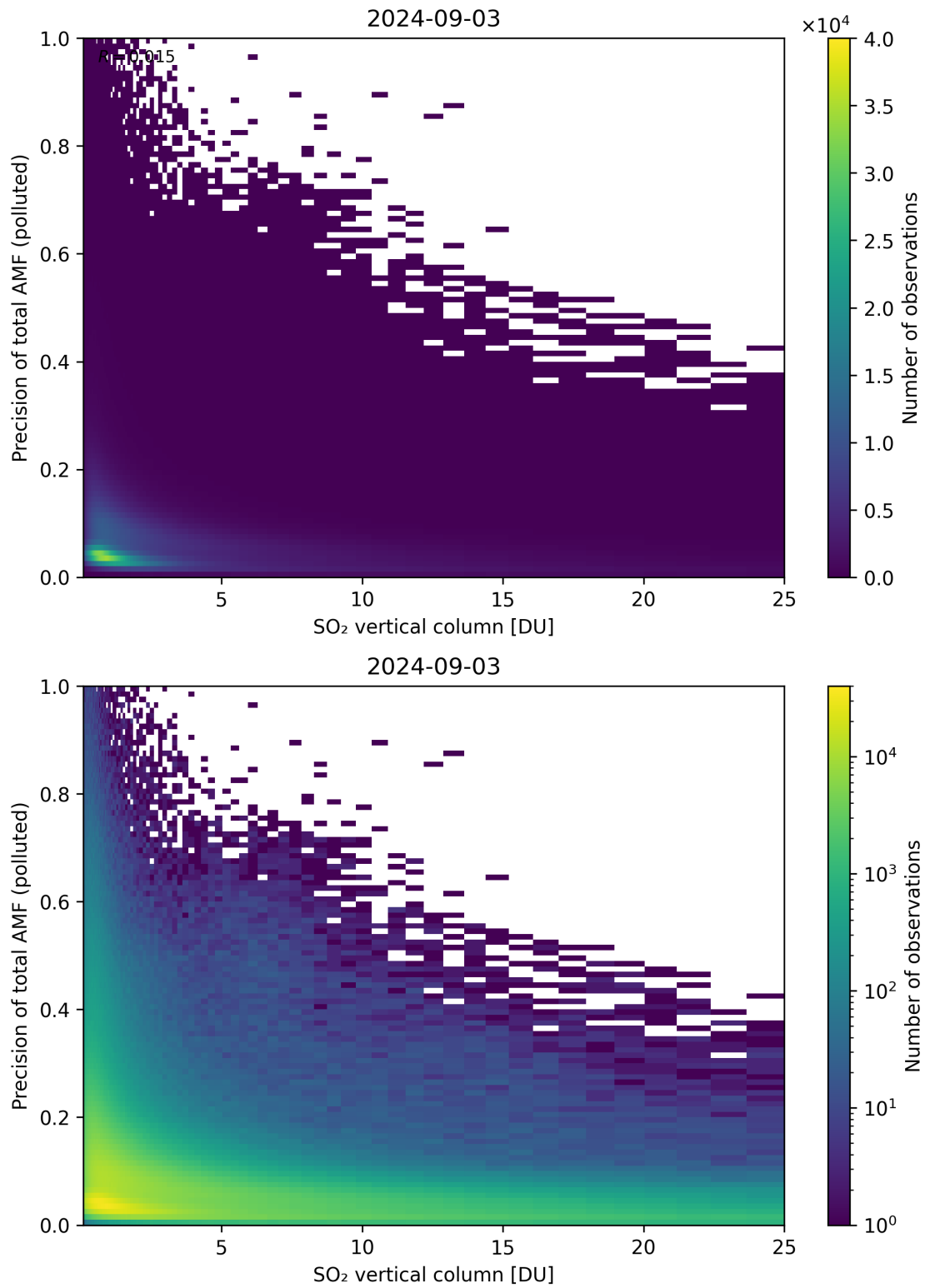
Figure 306: Scatter density plot of “SO 2 vertical column” against “Precision of total AMF (polluted)” for 2024-09-02 to 2024-09-04.
