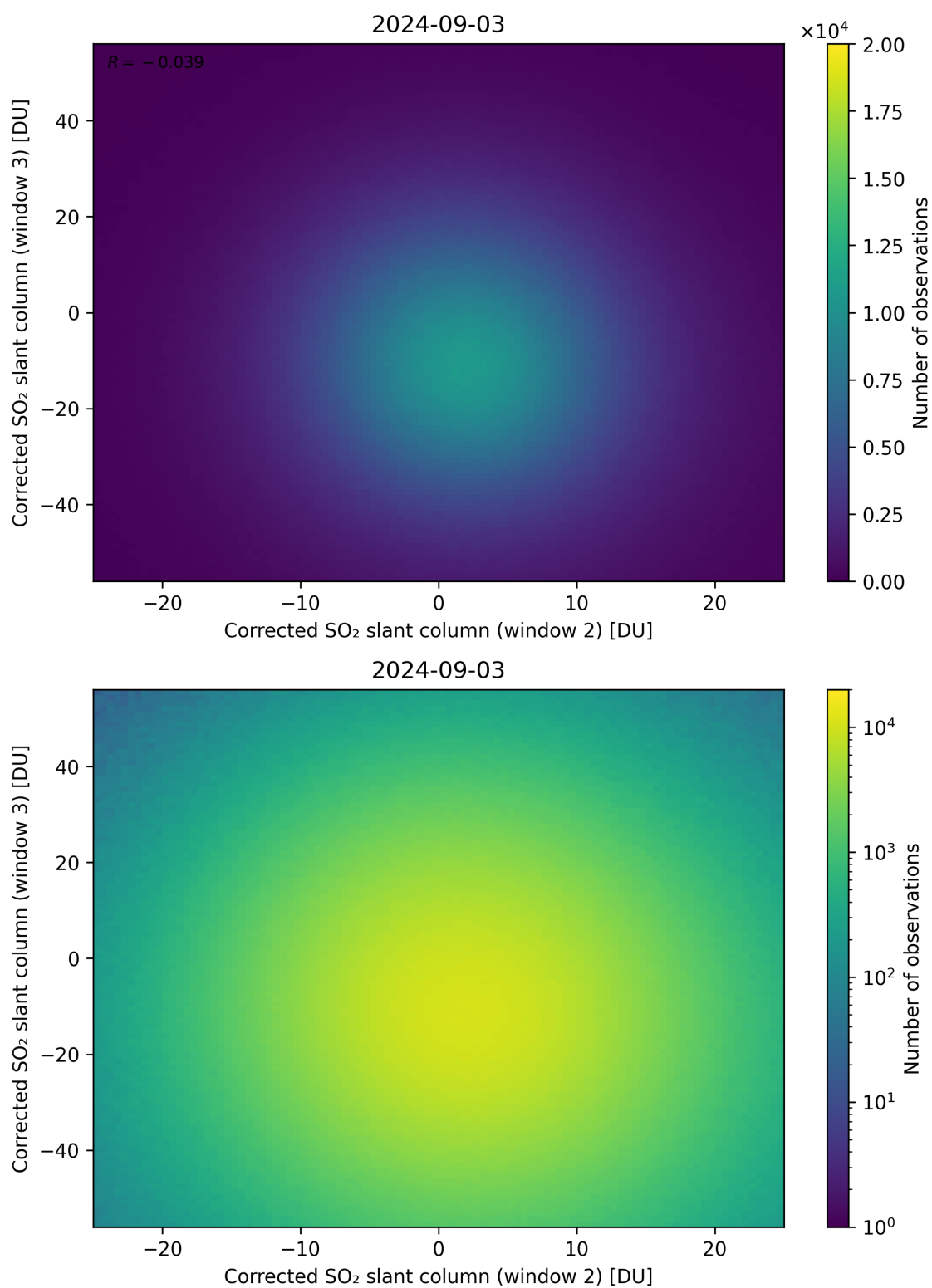
Figure 200: Scatter density plot of “Corrected SO 2 slant column (window 2)” against “Corrected SO 2 slant column (window 3)” for 2024-09-02 to 2024-09-04.
