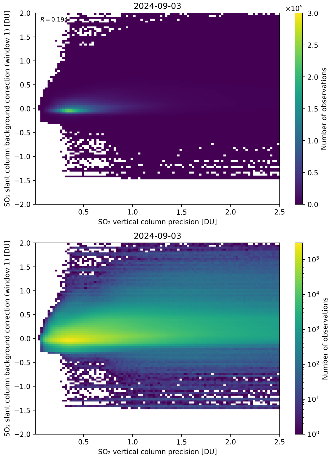
Figure 279: Scatter density plot of “SO 2 vertical column precision” against “SO 2 slant column background correction (window 1)” for 2024-09-02 to 2024-09-04.
