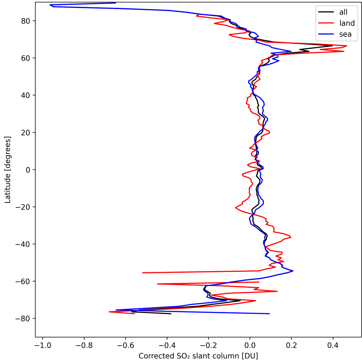
Figure 32: Zonal average of “Corrected SO 2 slant column” for 2024-09-02 to 2024-09-04.
