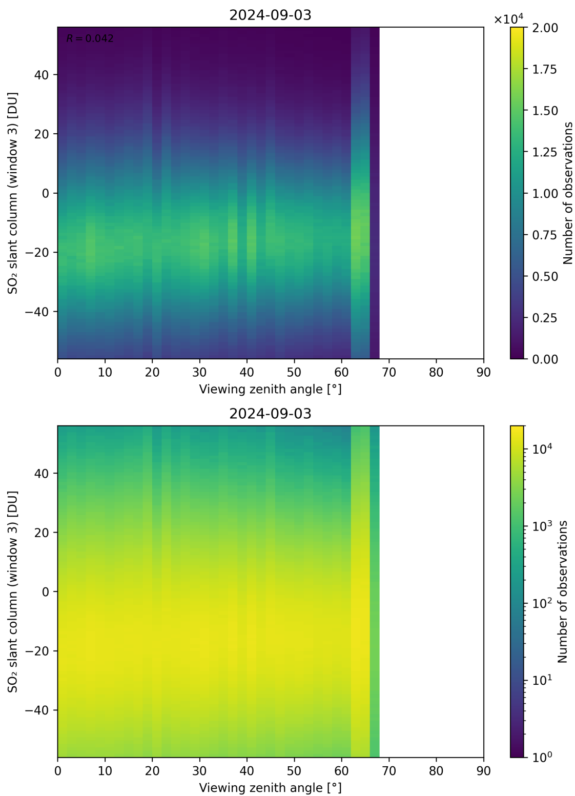
Figure 323: Scatter density plot of “Viewing zenith angle” against “SO 2 slant column (window 3)” for 2024-09-02 to 2024-09-04.
