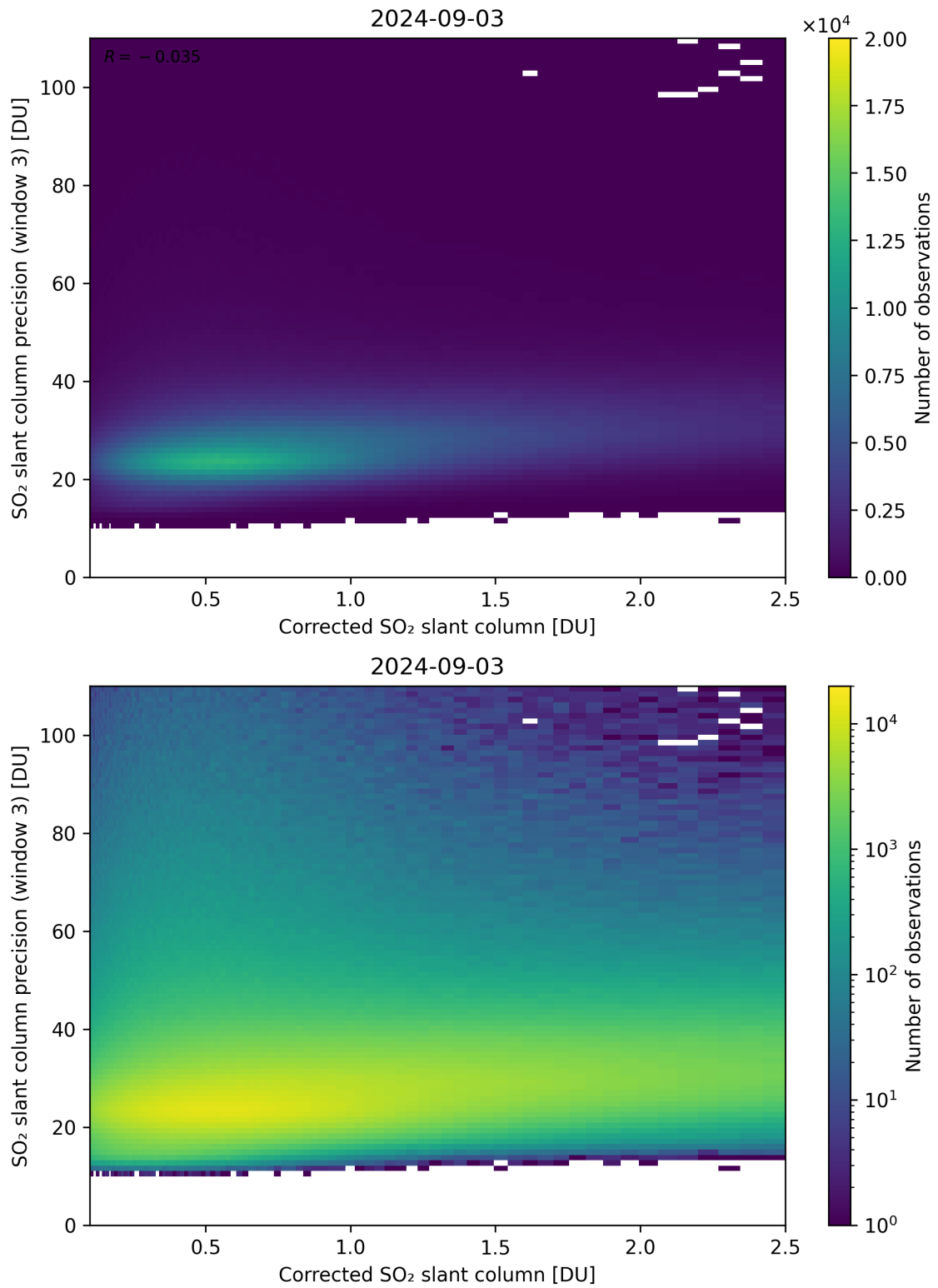
Figure 191: Scatter density plot of “Corrected SO 2 slant column” against “SO 2 slant column precision (window 3)” for 2024-09-02 to 2024-09-04.
