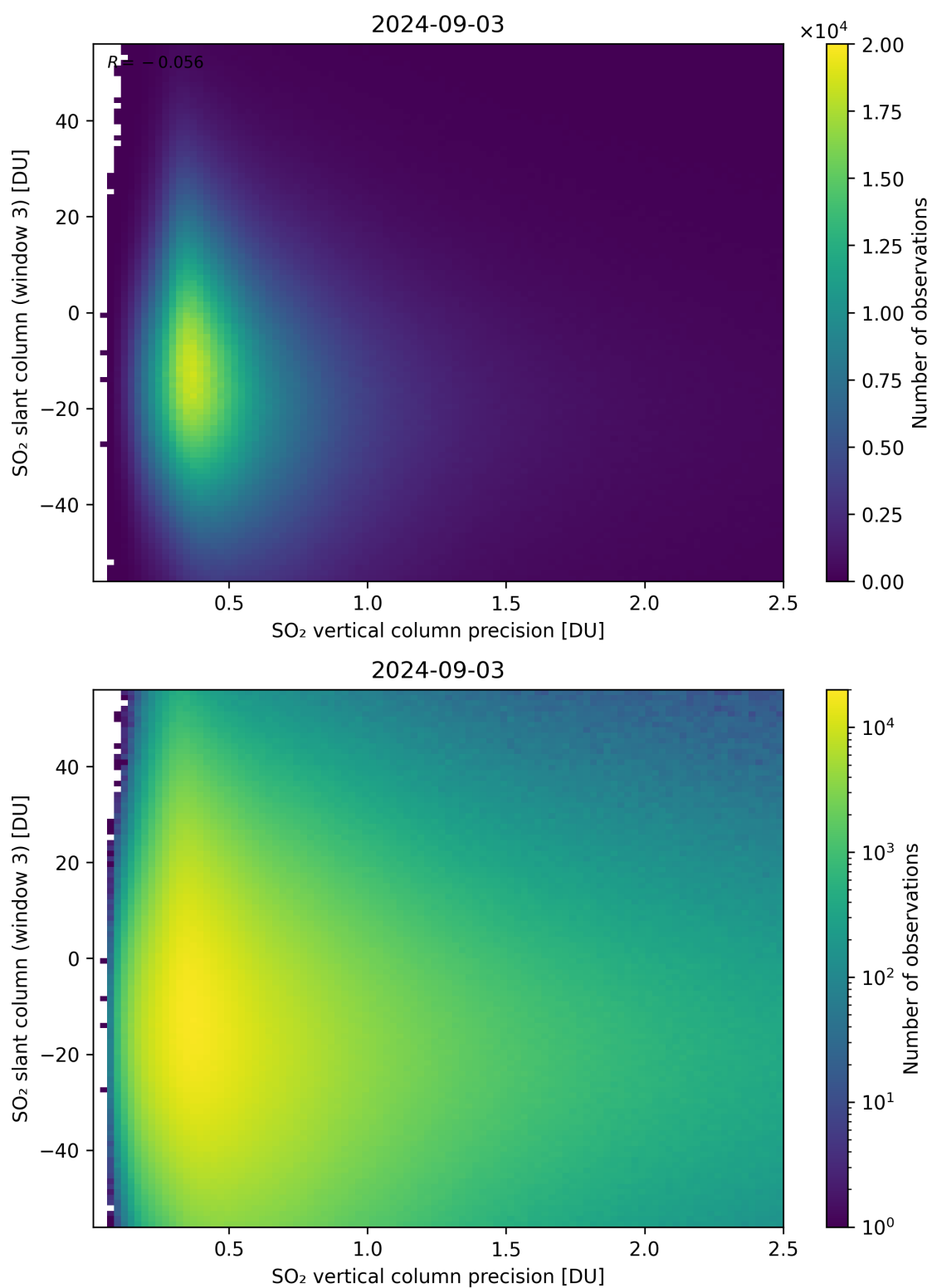
Figure 292: Scatter density plot of “SO 2 vertical column precision” against “SO 2 slant column (window 3)” for 2024-09-02 to 2024-09-04.
