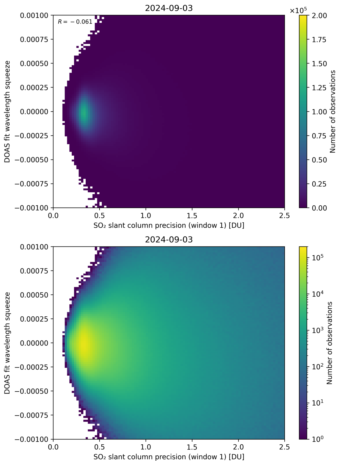
Figure 222: Scatter density plot of “SO 2 slant column precision (window 1)” against “DOAS fit wavelength squeeze” for 2024-09-02 to 2024-09-04.
