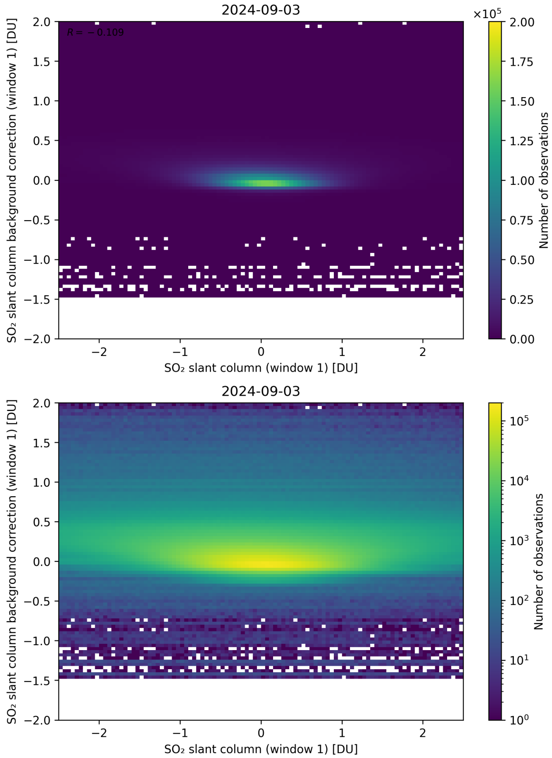
Figure 212: Scatter density plot of “SO 2 slant column (window 1)” against “SO 2 slant column background correction (window 1)” for 2024-09-02 to 2024-09-04.
