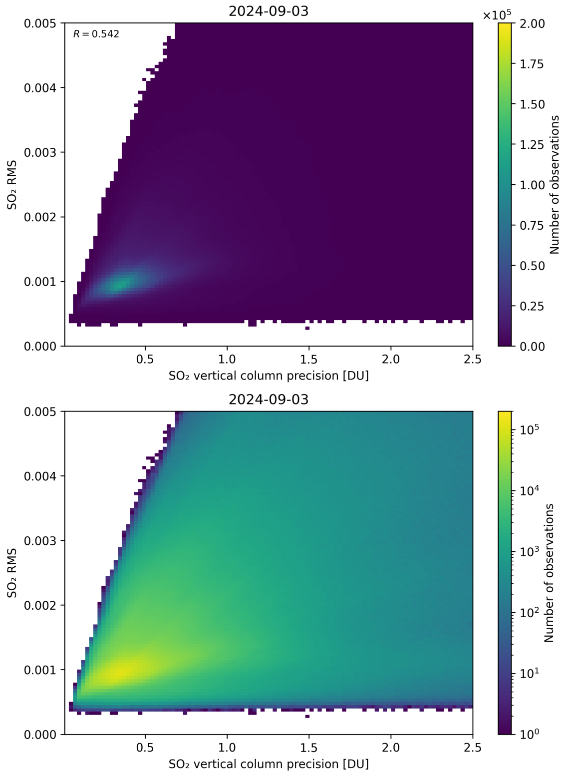
Figure 284: Scatter density plot of “SO 2 vertical column precision” against “SO 2 RMS” for 2024-09-02 to 2024-09-04.
