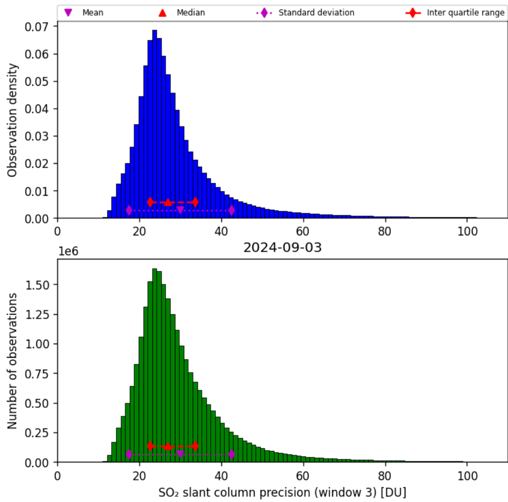
Figure 65: Histogram of “SO 2 slant column precision (window 3)” for 2024-09-02 to 2024-09-04
