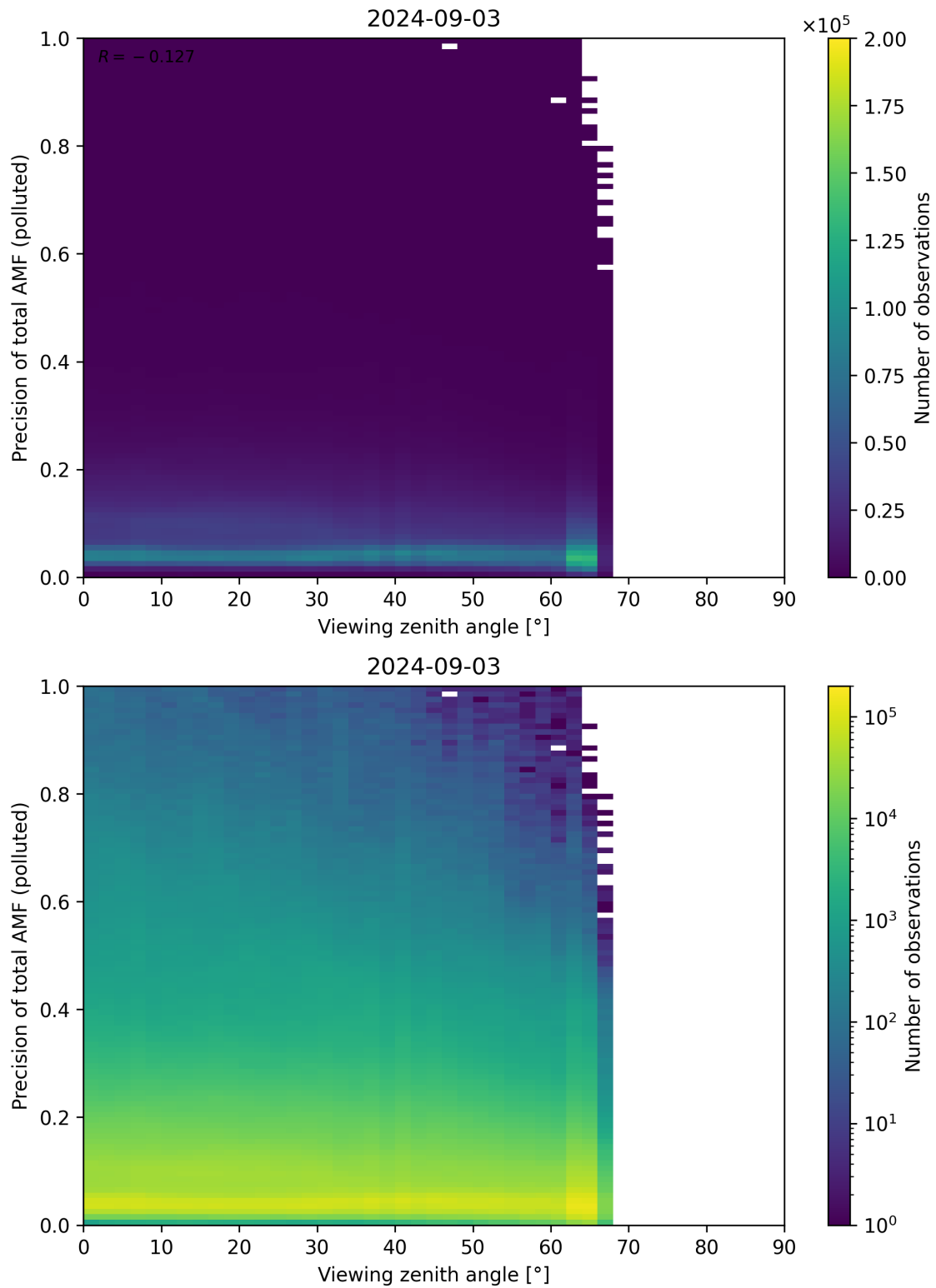
Figure 326: Scatter density plot of “Viewing zenith angle” against “Precision of total AMF (polluted)” for 2024-09-02 to 2024-09-04.
