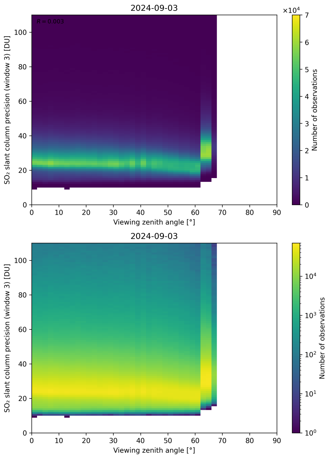
Figure 324: Scatter density plot of “Viewing zenith angle” against “SO 2 slant column precision (window 3)” for 2024-09-02 to 2024-09-04.
