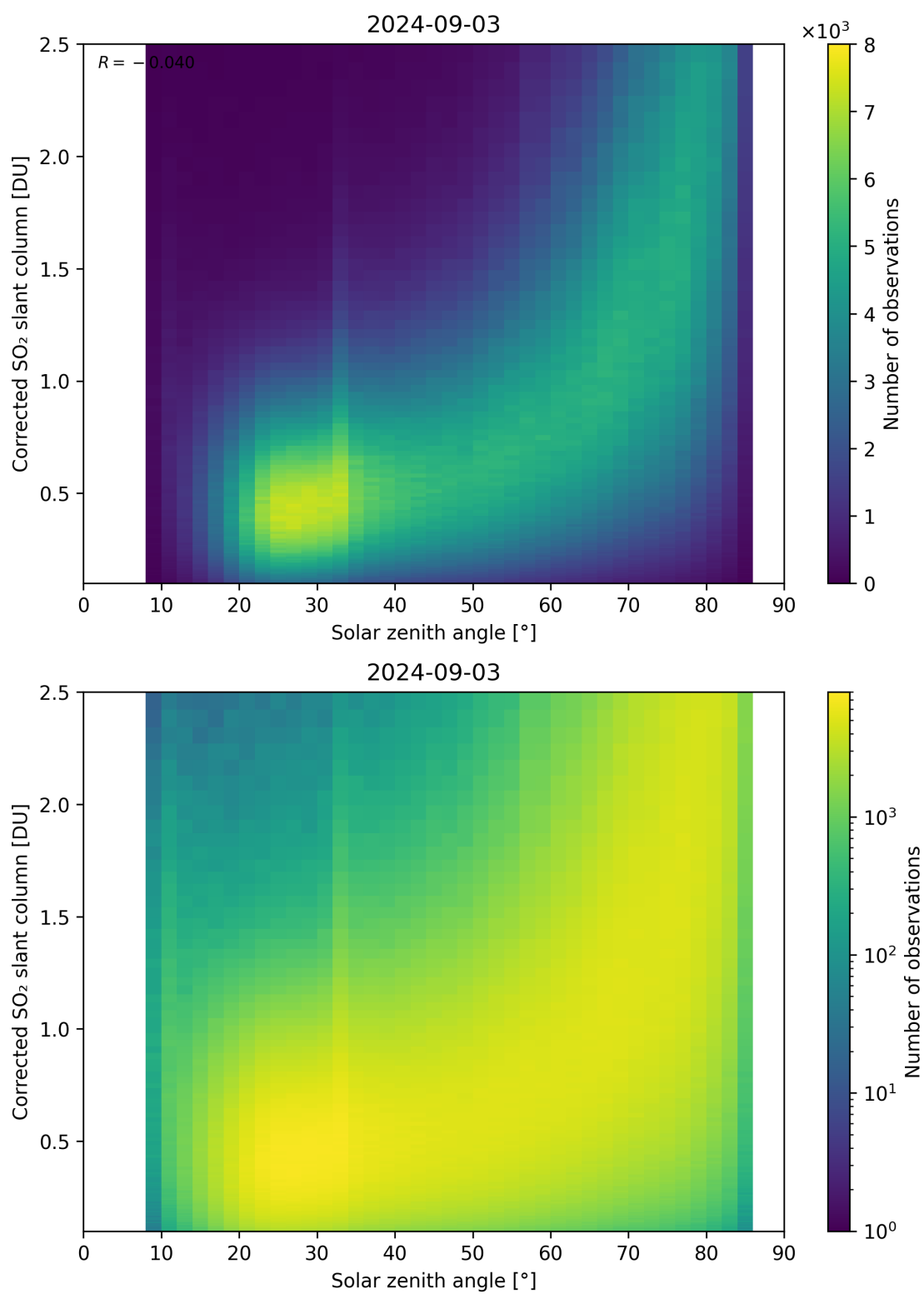
Figure 166: Scatter density plot of “Solar zenith angle” against “Corrected SO 2 slant column” for 2024-09-02 to 2024-09-04.
