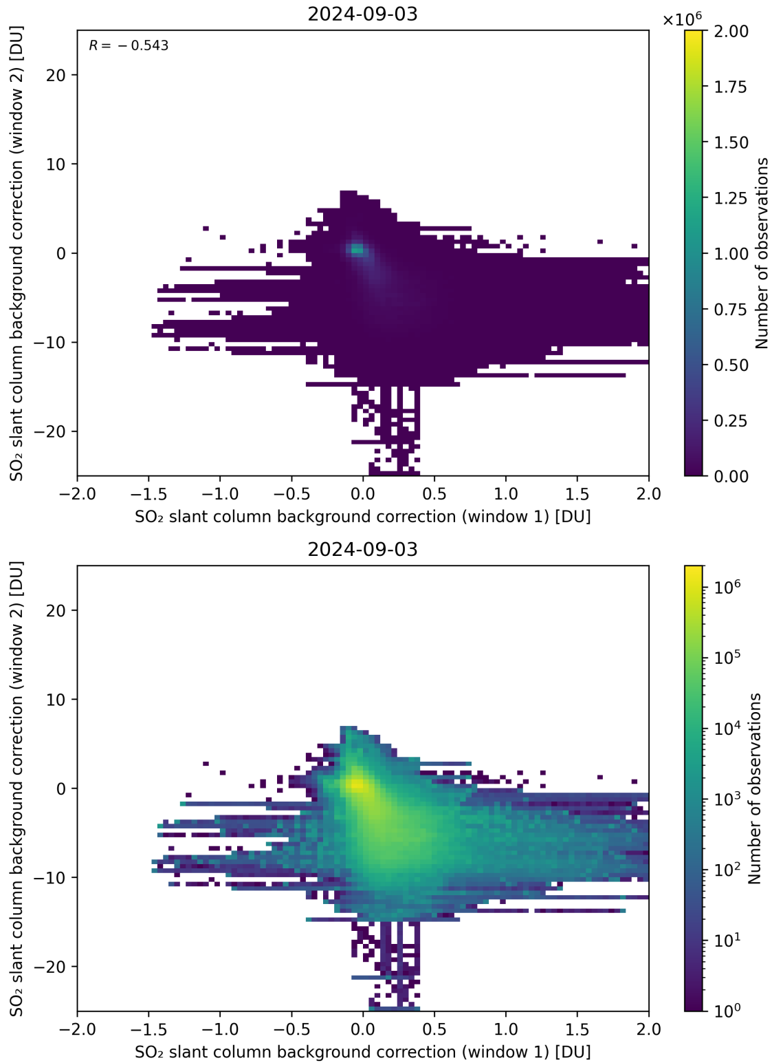
Figure 98: Scatter density plot of “SO 2 slant column background correction (window 1)” against “SO 2 slant column background correction (window 2)” for 2024-09-02 to 2024-09-04.
