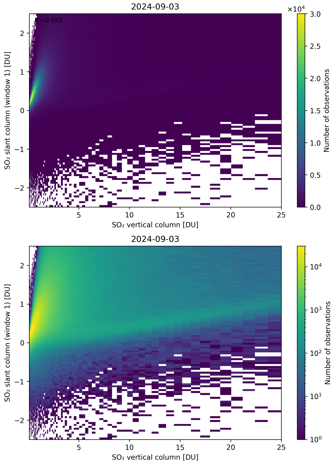
Figure 300: Scatter density plot of “SO 2 vertical column” against “SO 2 slant column (window 1)” for 2024-09-02 to 2024-09-04.
