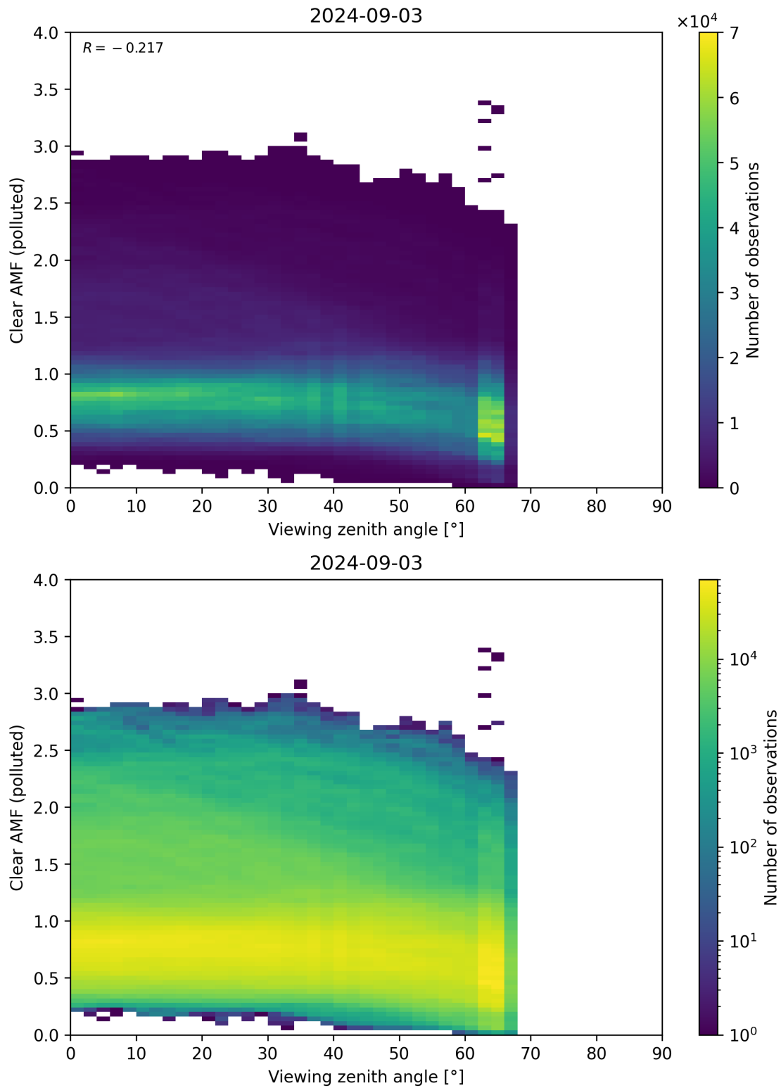
Figure 316: Scatter density plot of “Viewing zenith angle” against “Clear AMF (polluted)” for 2024-09-02 to 2024-09-04.
