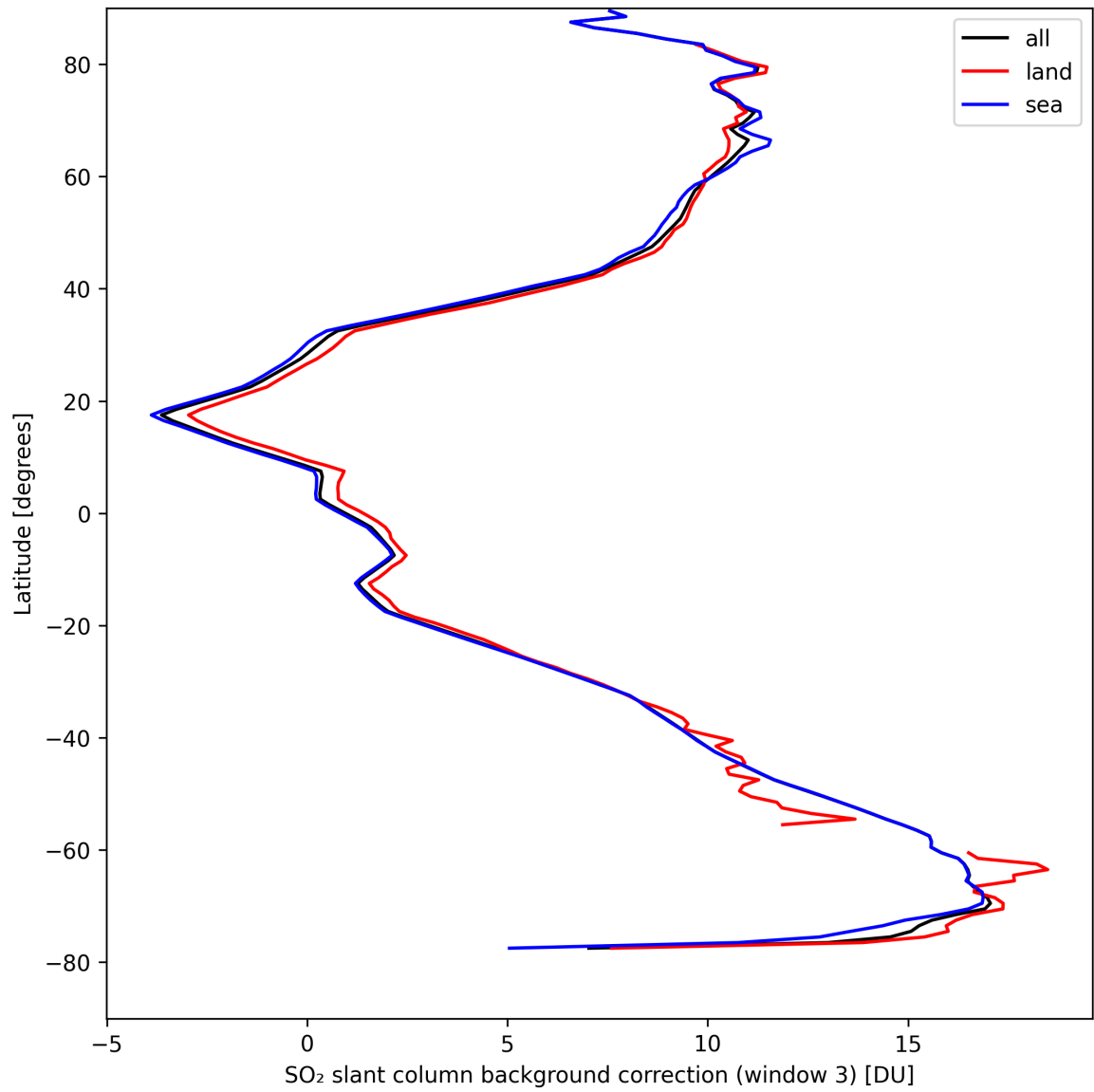
Figure 44: Zonal average of “SO 2 slant column background correction (window 3)” for 2024-09-02 to 2024-09-04.
