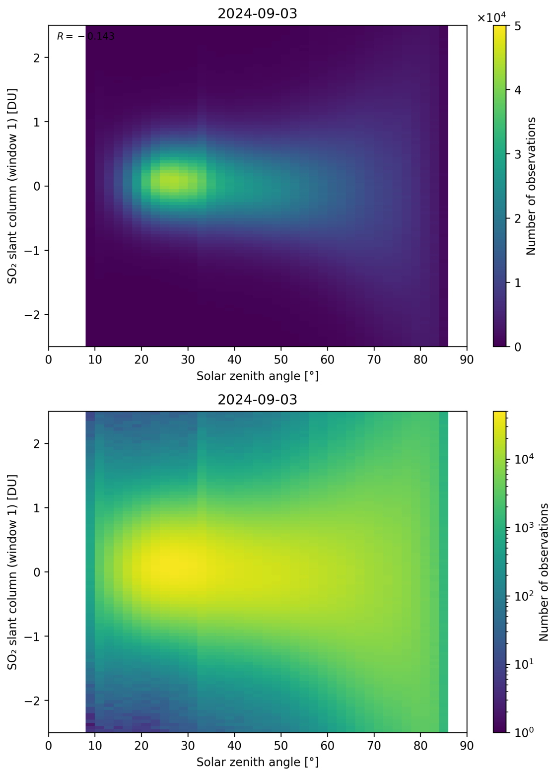
Figure 169: Scatter density plot of “Solar zenith angle” against “SO 2 slant column (window 1)” for 2024-09-02 to 2024-09-04.
