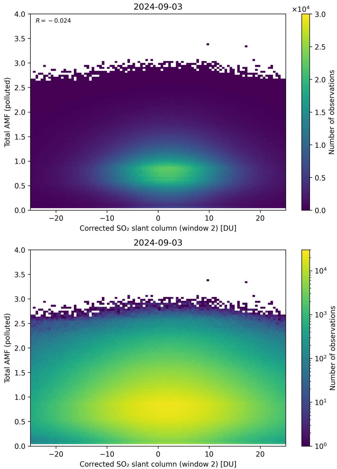
Figure 203: Scatter density plot of “Corrected SO 2 slant column (window 2)” against “Total AMF (polluted)” for 2024-09-02 to 2024-09-04.
