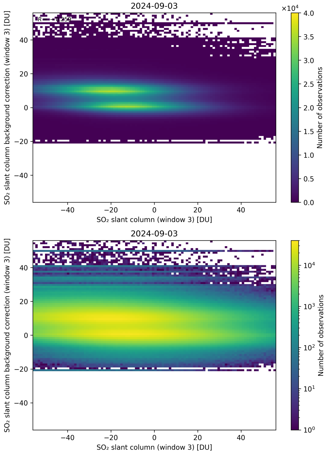
Figure 253: Scatter density plot of “SO 2 slant column (window 3)” against “SO 2 slant column background correction (window 3)” for 2024-09-02 to 2024-09-04.
