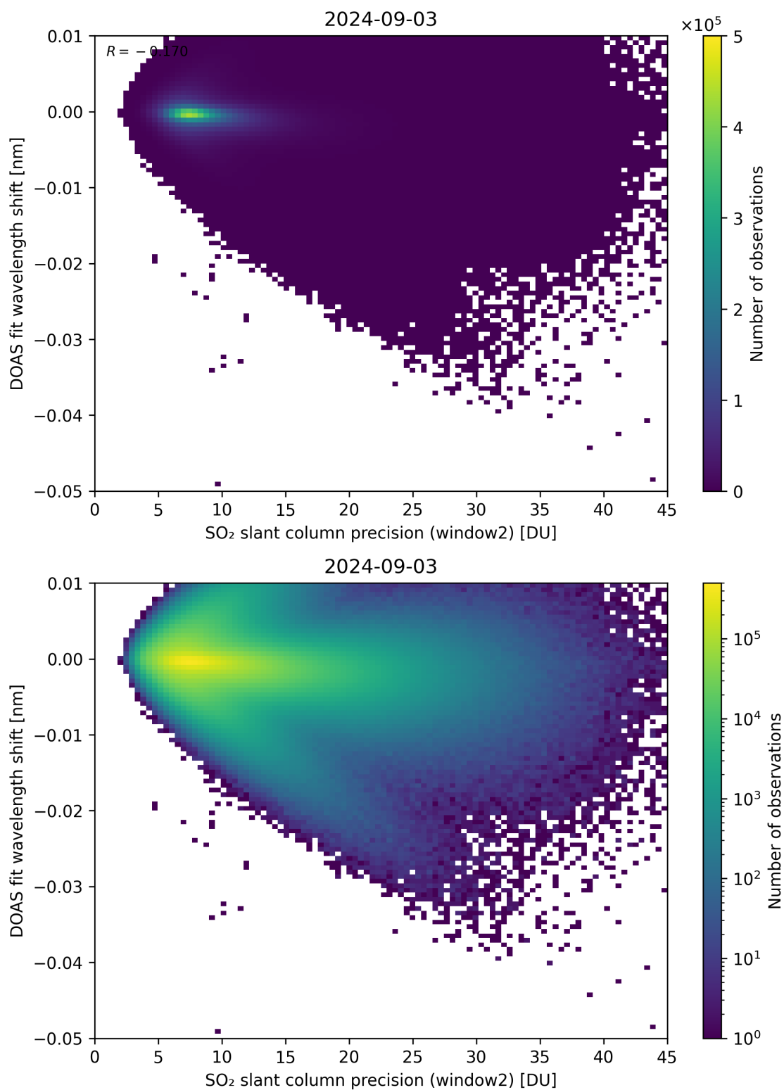
Figure 243: Scatter density plot of “SO 2 slant column precision (window2)” against “DOAS fit wavelength shift” for 2024-09-02 to 2024-09-04.
