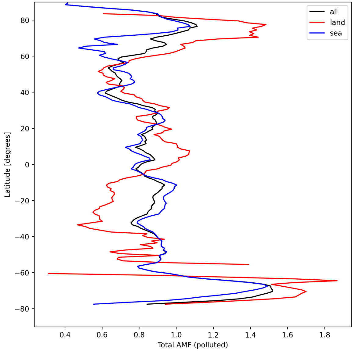
Figure 48: Zonal average of “Total AMF (polluted)” for 2024-09-02 to 2024-09-04.
