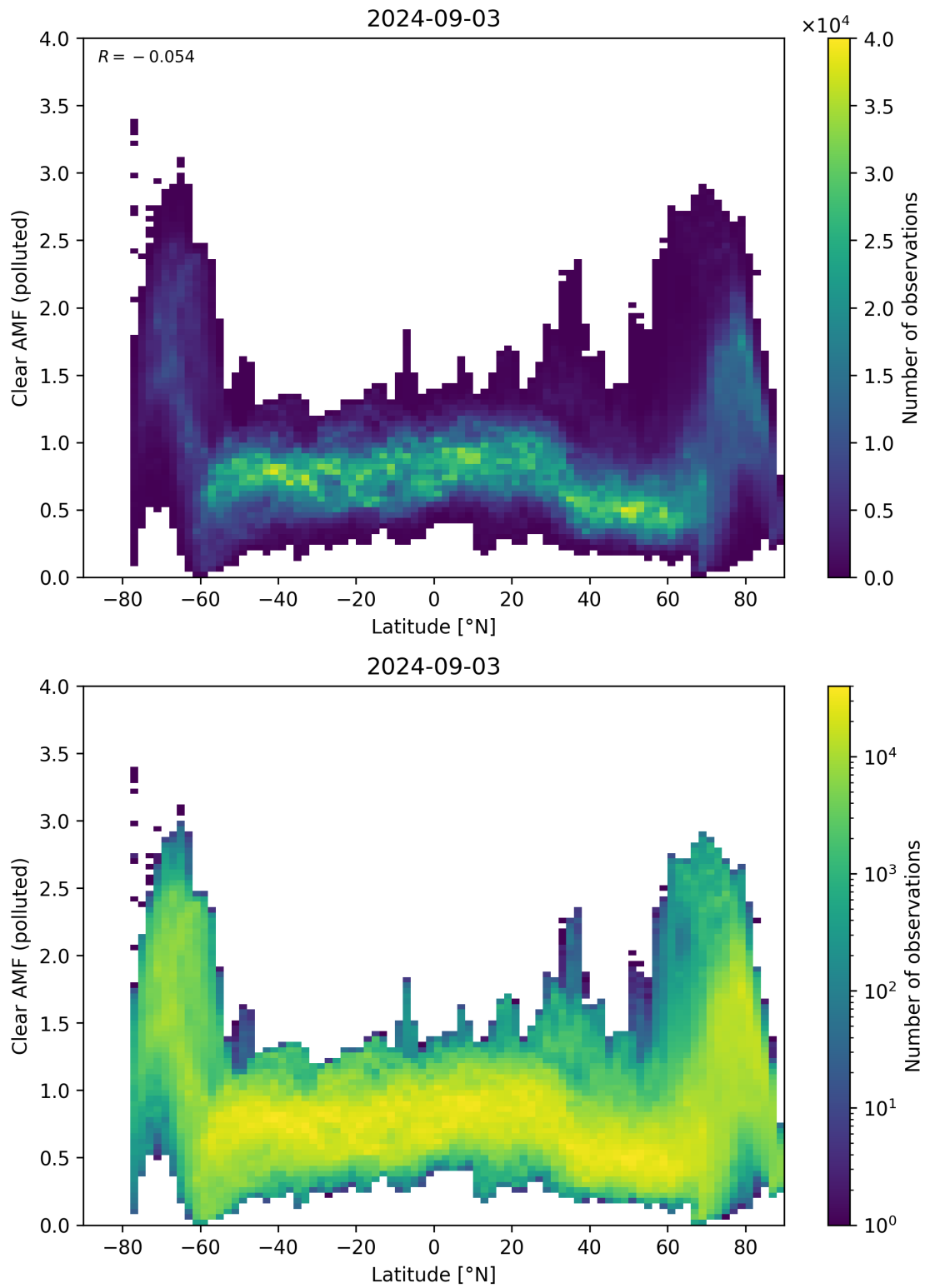
Figure 145: Scatter density plot of “Latitude” against “Clear AMF (polluted)” for 2024-09-02 to 2024-09-04.
