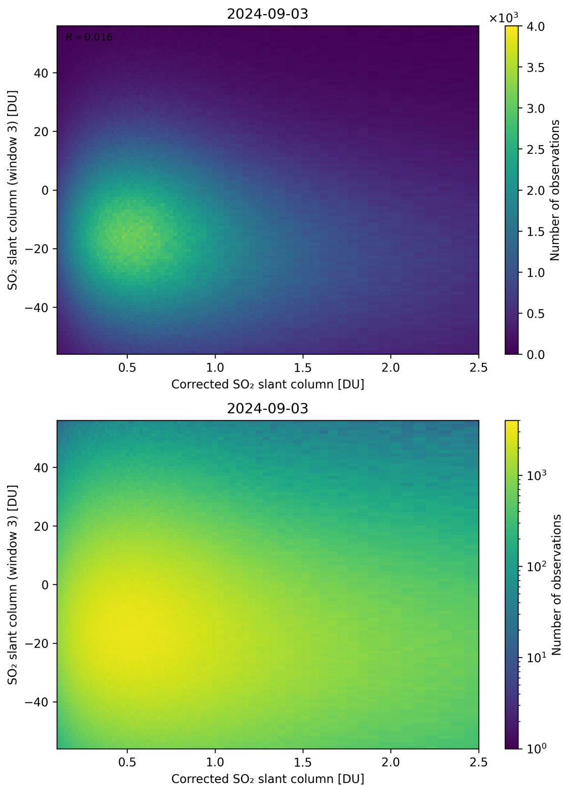
Figure 190: Scatter density plot of “Corrected SO 2 slant column” against “SO 2 slant column (window 3)” for 2024-09-02 to 2024-09-04.
