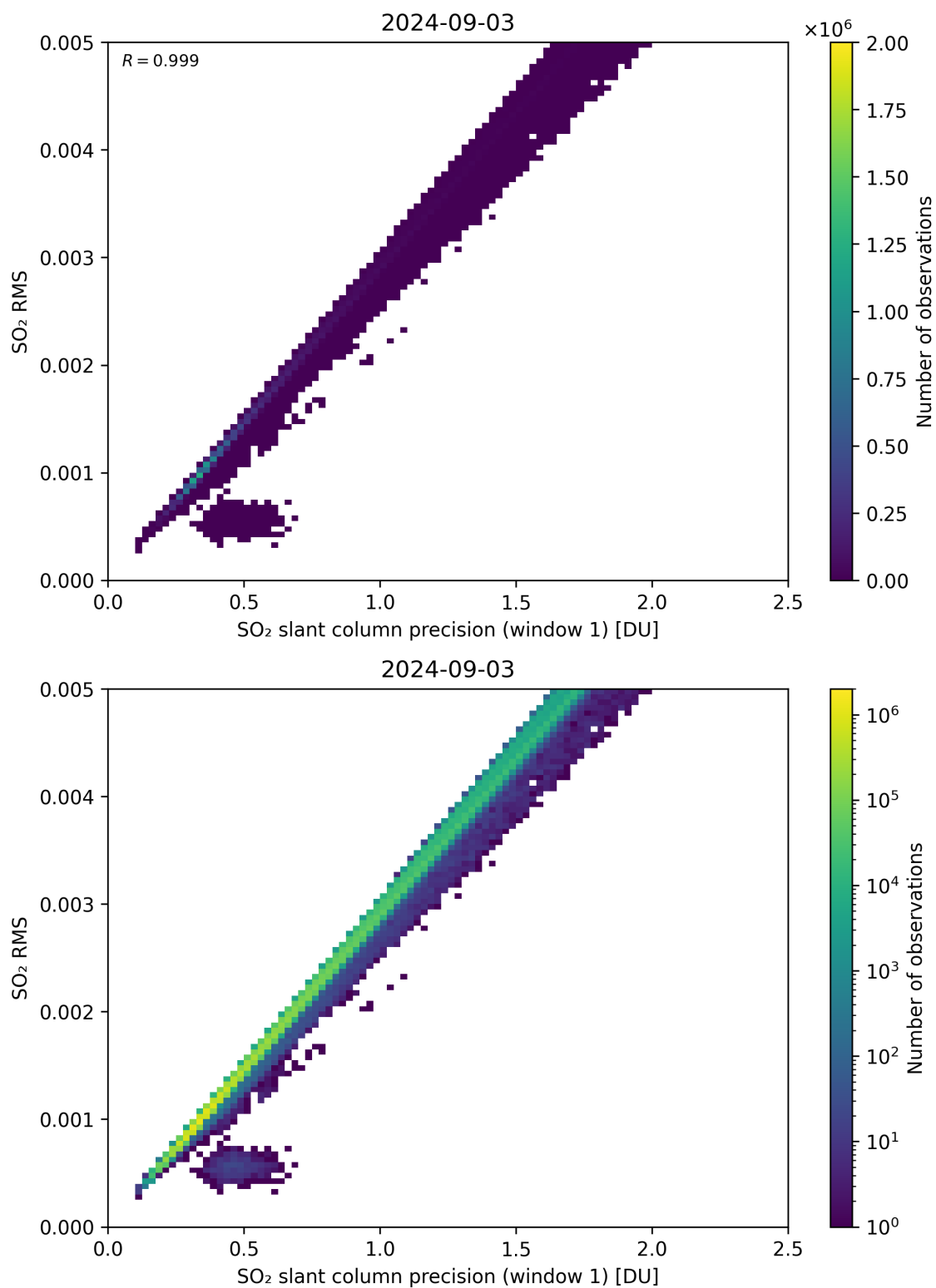
Figure 223: Scatter density plot of “SO 2 slant column precision (window 1)” against “SO 2 RMS” for 2024-09-02 to 2024-09-04.
