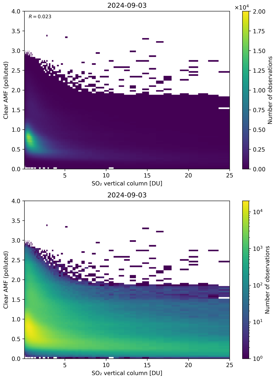
Figure 296: Scatter density plot of “SO 2 vertical column” against “Clear AMF (polluted)” for 2024-09-02 to 2024-09-04.
