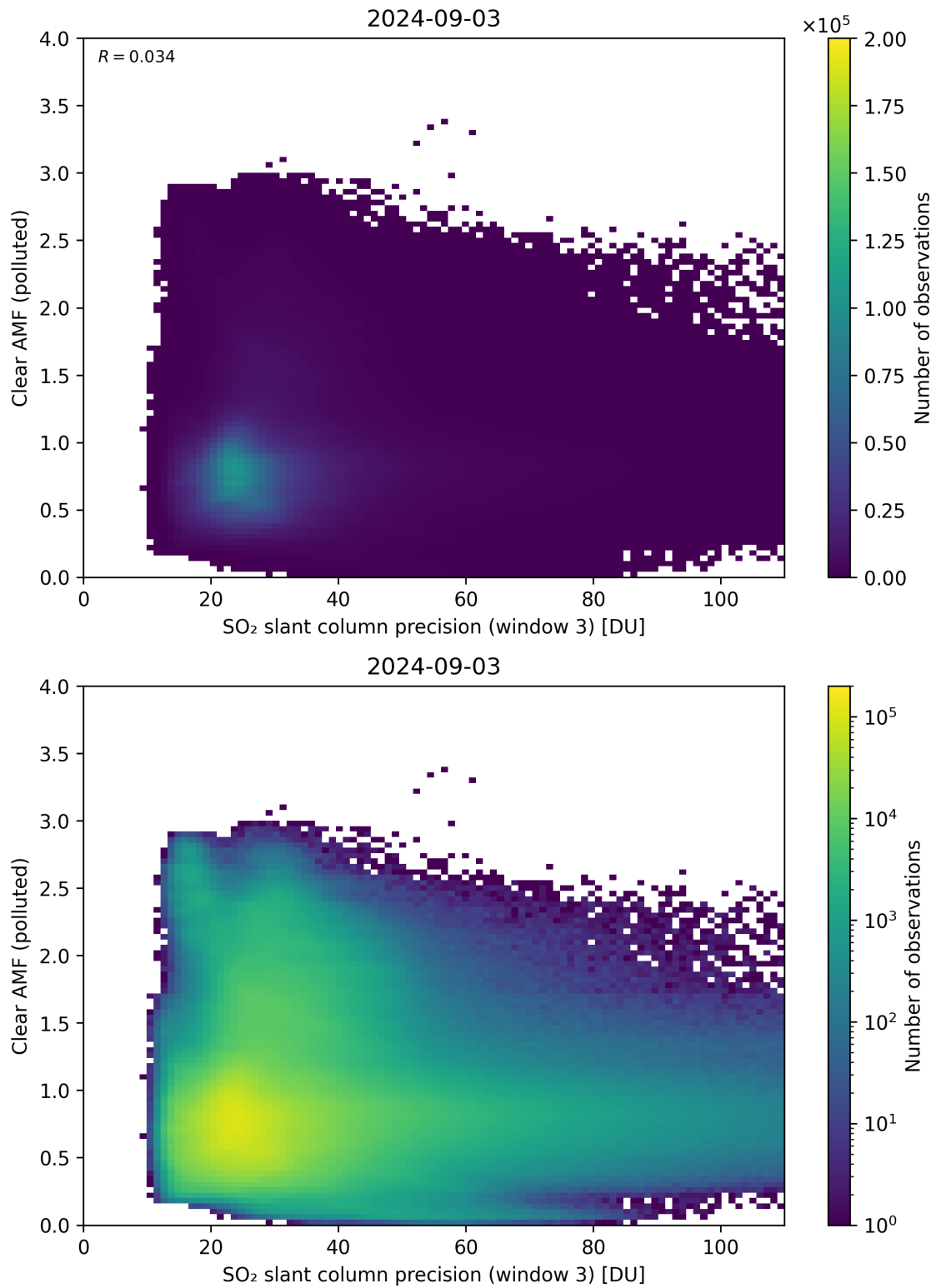
Figure 261: Scatter density plot of “SO 2 slant column precision (window 3)” against “Clear AMF (polluted)” for 2024-09-02 to 2024-09-04.
