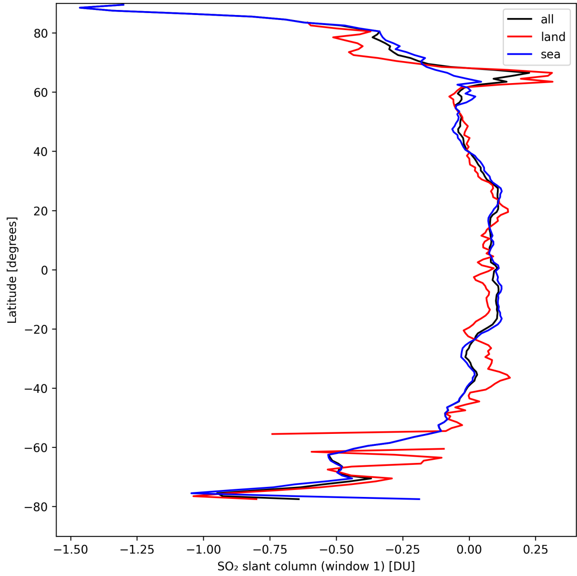
Figure 33: Zonal average of “SO 2 slant column (window 1)” for 2024-09-02 to 2024-09-04.
