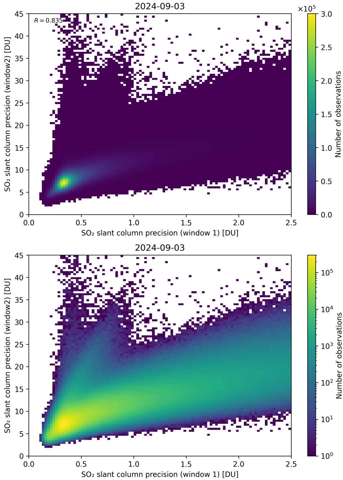
Figure 227: Scatter density plot of “SO 2 slant column precision (window 1)” against “SO 2 slant column precision (window2)” for 2024-09-02 to 2024-09-04.
