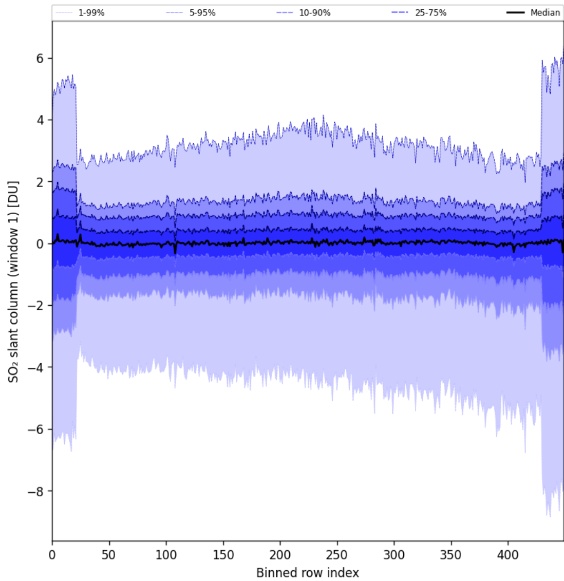
Figure 79: Along track statistics of “SO 2 slant column (window 1)” for 2024-09-02 to 2024-09-04
