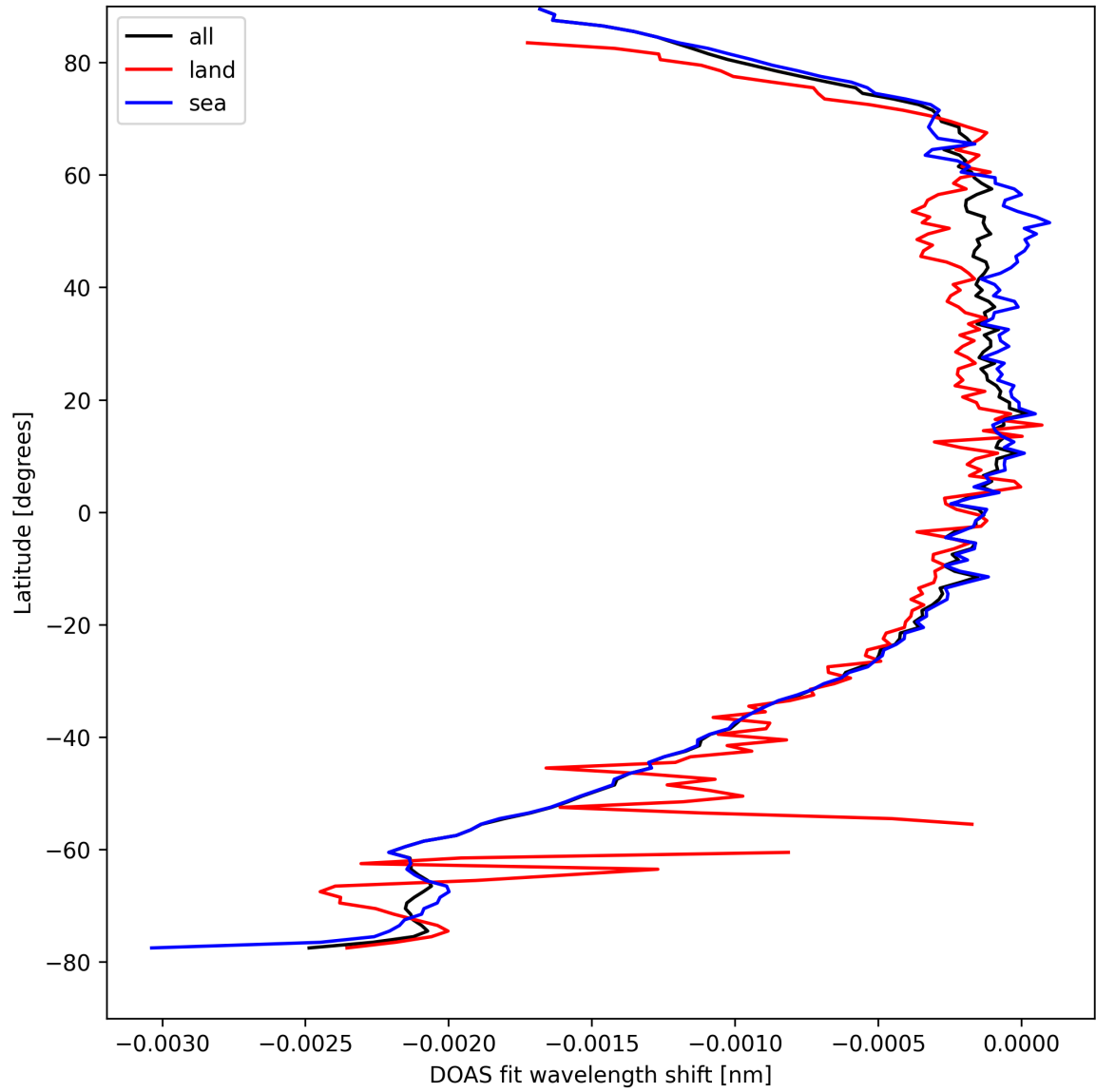
Figure 45: Zonal average of “DOAS fit wavelength shift” for 2024-09-02 to 2024-09-04.
