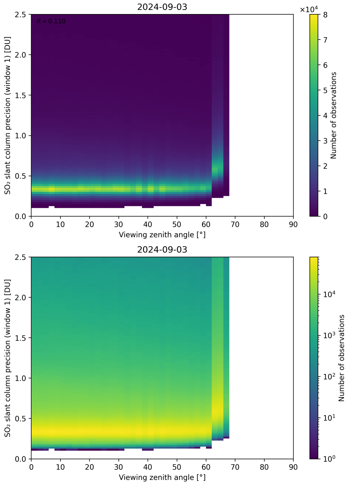
Figure 321: Scatter density plot of “Viewing zenith angle” against “SO 2 slant column precision (window 1)” for 2024-09-02 to 2024-09-04.
