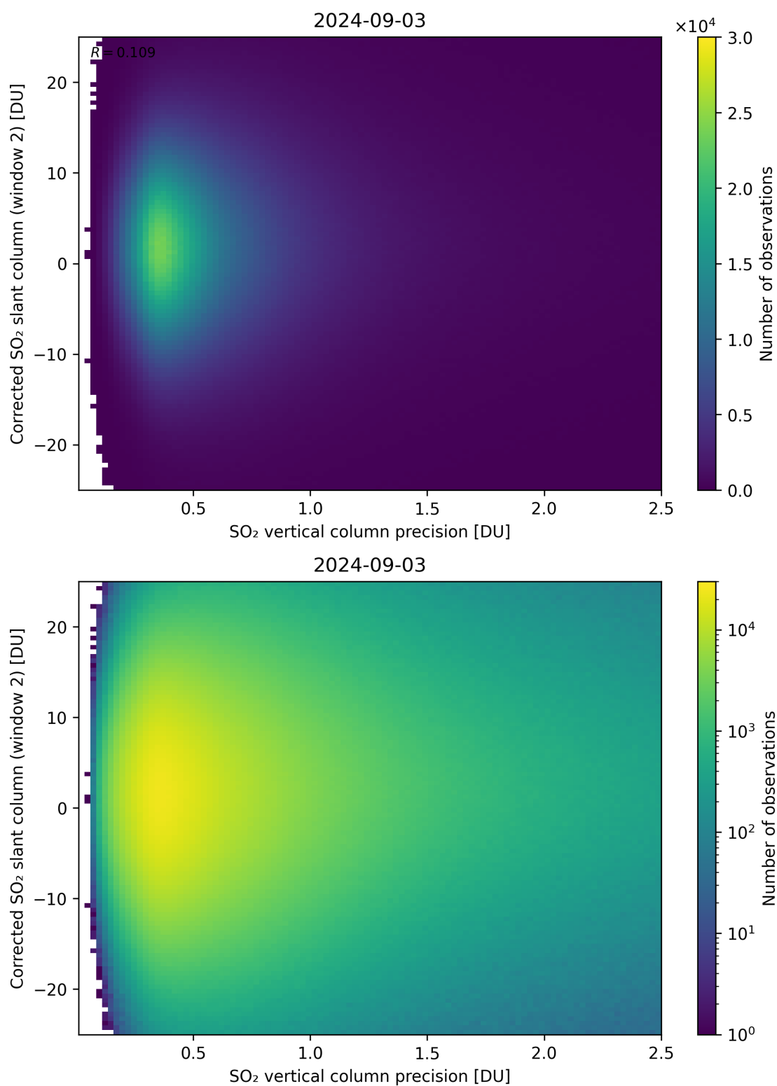
Figure 287: Scatter density plot of “SO 2 vertical column precision” against “Corrected SO 2 slant column (window 2)” for 2024-09-02 to 2024-09-04.
