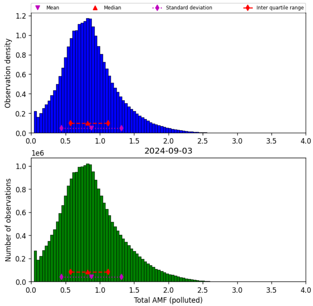
Figure 71: Histogram of “Total AMF (polluted)” for 2024-09-02 to 2024-09-04
