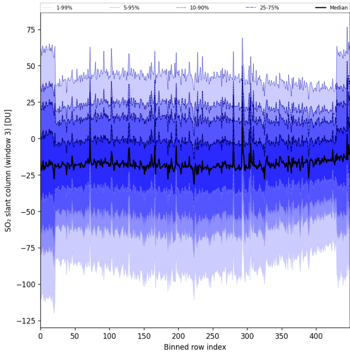
Figure 87: Along track statistics of “SO 2 slant column (window 3)” for 2024-09-02 to 2024-09-04
