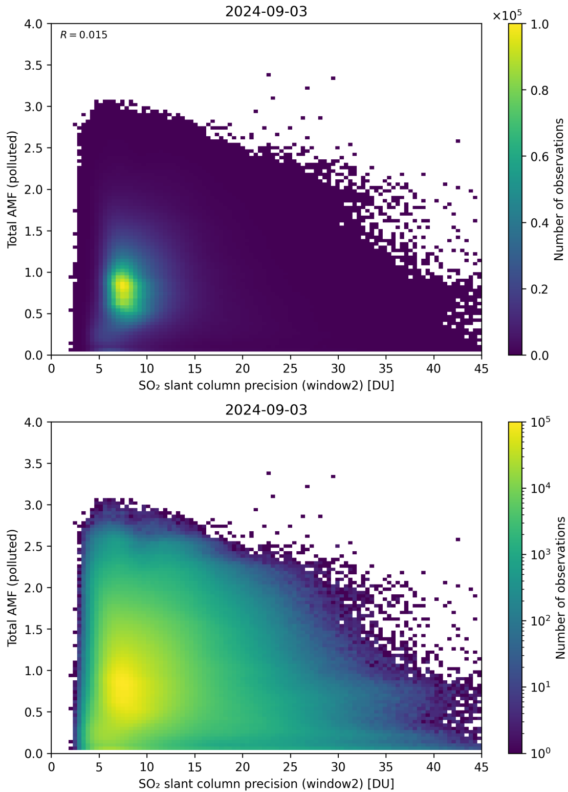
Figure 251: Scatter density plot of “SO 2 slant column precision (window2)” against “Total AMF (polluted)” for 2024-09-02 to 2024-09-04.
