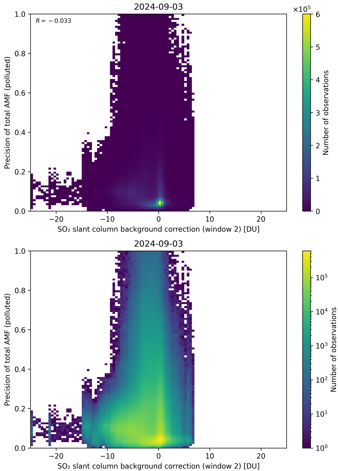
Figure 120: Scatter density plot of “SO 2 slant column background correction (window 2)” against “Precision of total AMF (polluted)” for 2024-09-02 to 2024-09-04.
