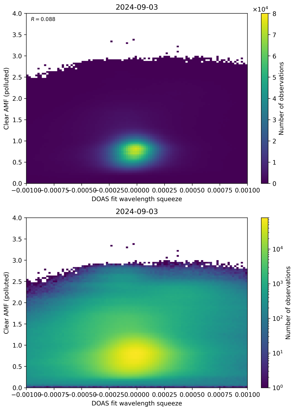
Figure 133: Scatter density plot of “DOAS fit wavelength squeeze” against “Clear AMF (polluted)” for 2024-09-02 to 2024-09-04.
