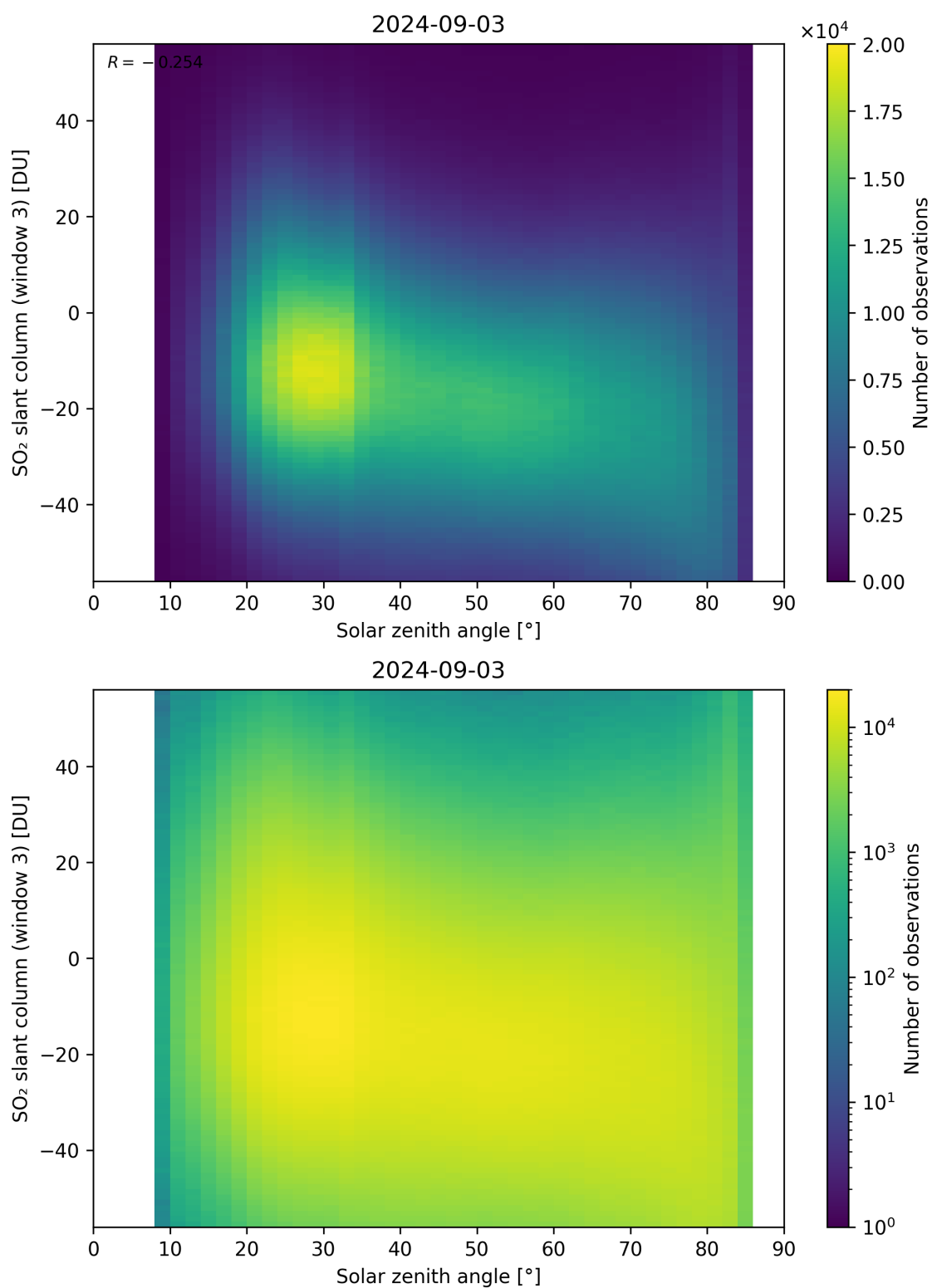
Figure 172: Scatter density plot of “Solar zenith angle” against “SO 2 slant column (window 3)” for 2024-09-02 to 2024-09-04.
