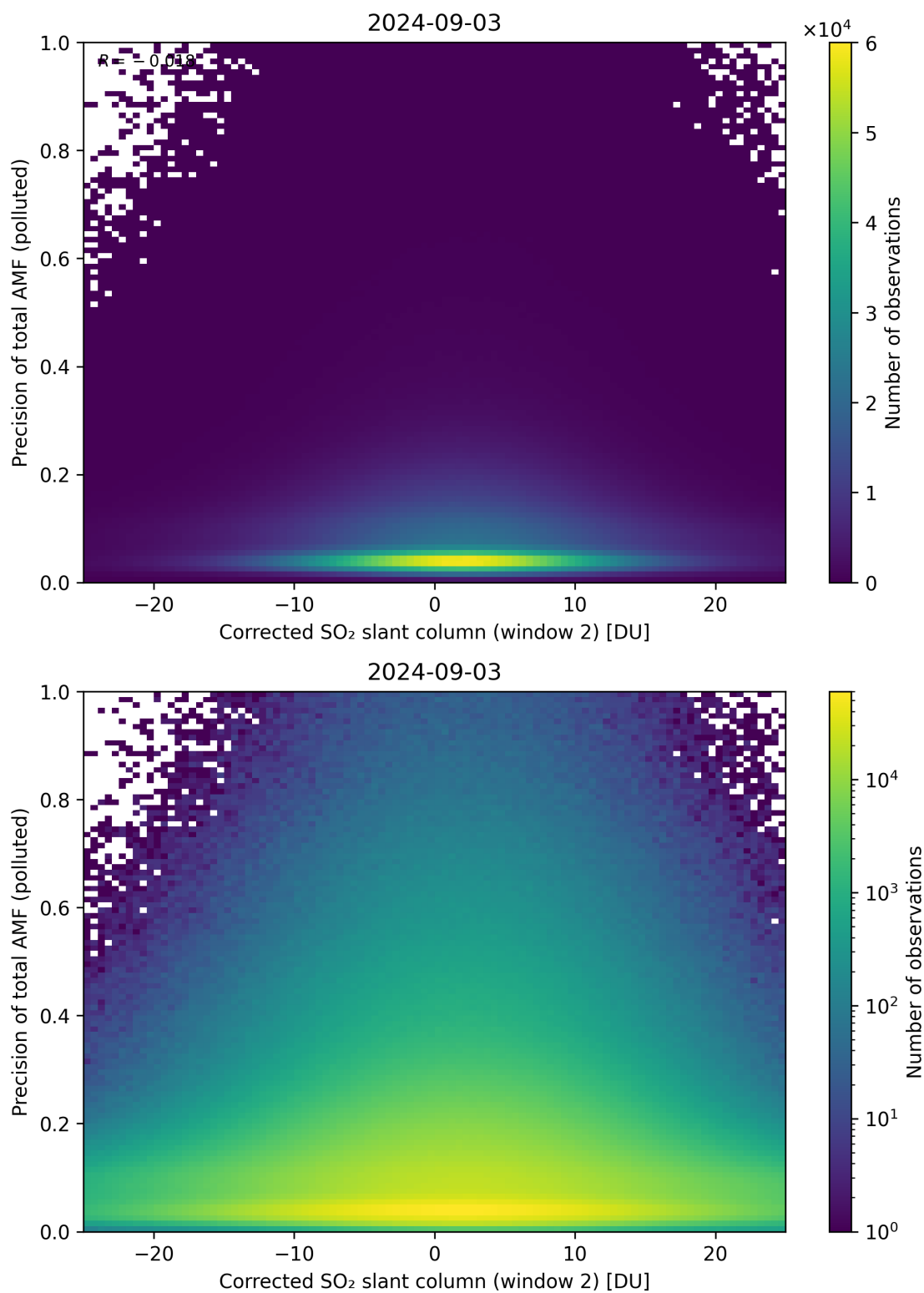
Figure 204: Scatter density plot of “Corrected SO 2 slant column (window 2)” against “Precision of total AMF (polluted)” for 2024-09-02 to 2024-09-04.
