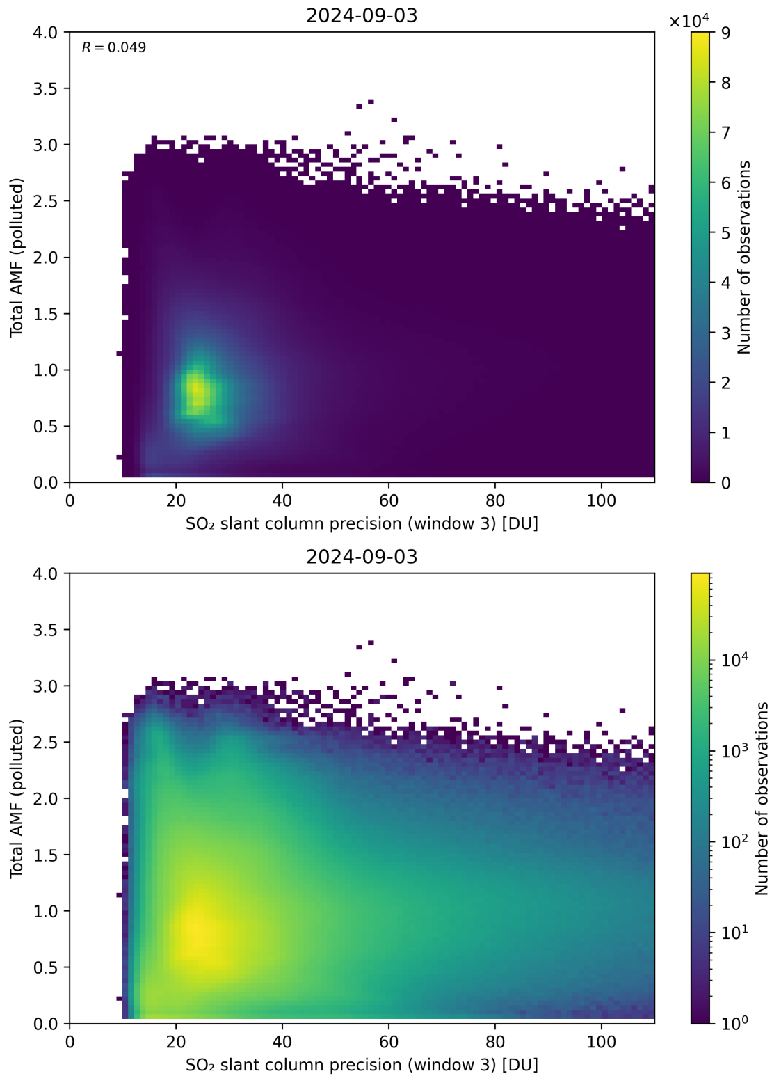
Figure 263: Scatter density plot of “SO 2 slant column precision (window 3)” against “Total AMF (polluted)” for 2024-09-02 to 2024-09-04.
