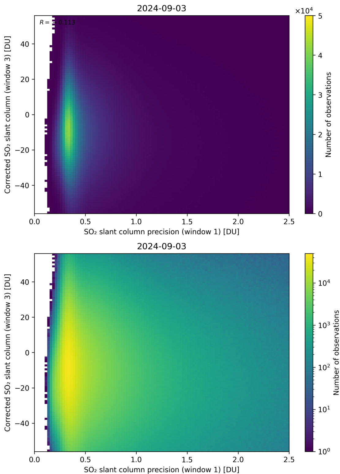
Figure 226: Scatter density plot of “SO 2 slant column precision (window 1)” against “Corrected SO 2 slant column (window 3)” for 2024-09-02 to 2024-09-04.
