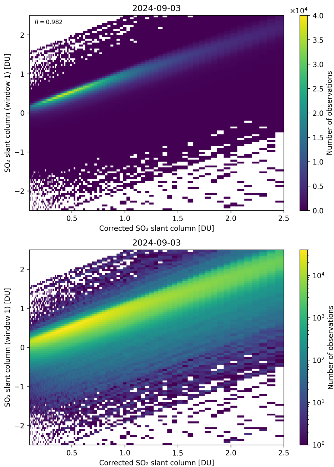
Figure 187: Scatter density plot of “Corrected SO 2 slant column” against “SO 2 slant column (window 1)” for 2024-09-02 to 2024-09-04.
