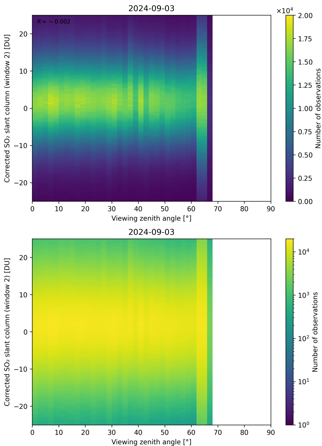
Figure 318: Scatter density plot of “Viewing zenith angle” against “Corrected SO 2 slant column (window 2)” for 2024-09-02 to 2024-09-04.
