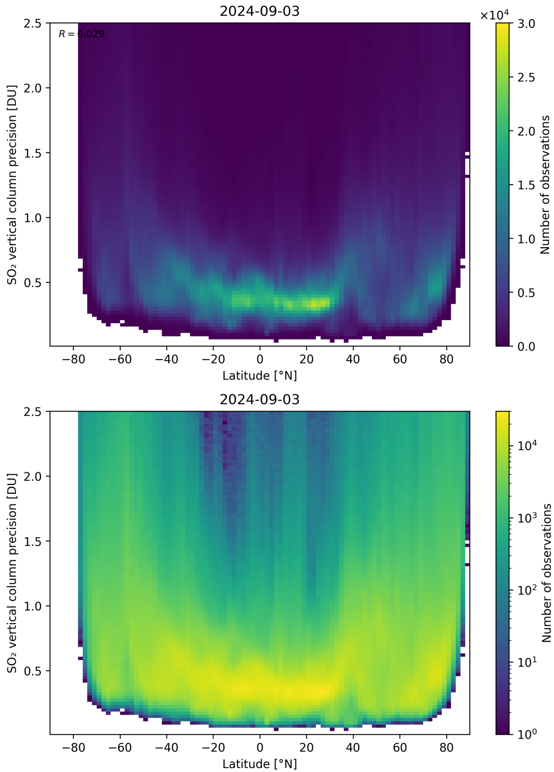
Figure 157: Scatter density plot of “Latitude” against “SO 2 vertical column precision” for 2024-09-02 to 2024-09-04.
