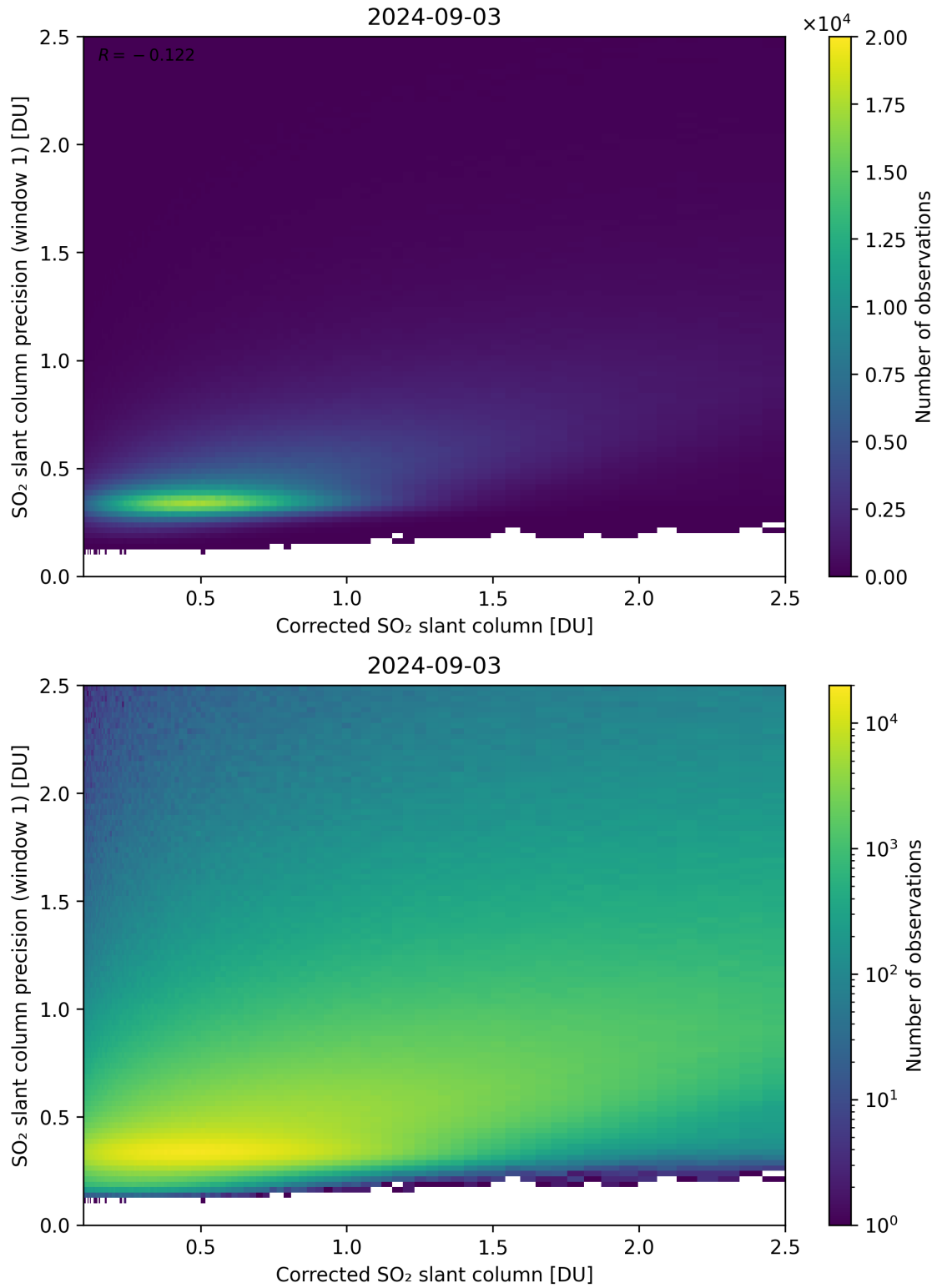
Figure 188: Scatter density plot of “Corrected SO 2 slant column” against “SO 2 slant column precision (window 1)” for 2024-09-02 to 2024-09-04.
