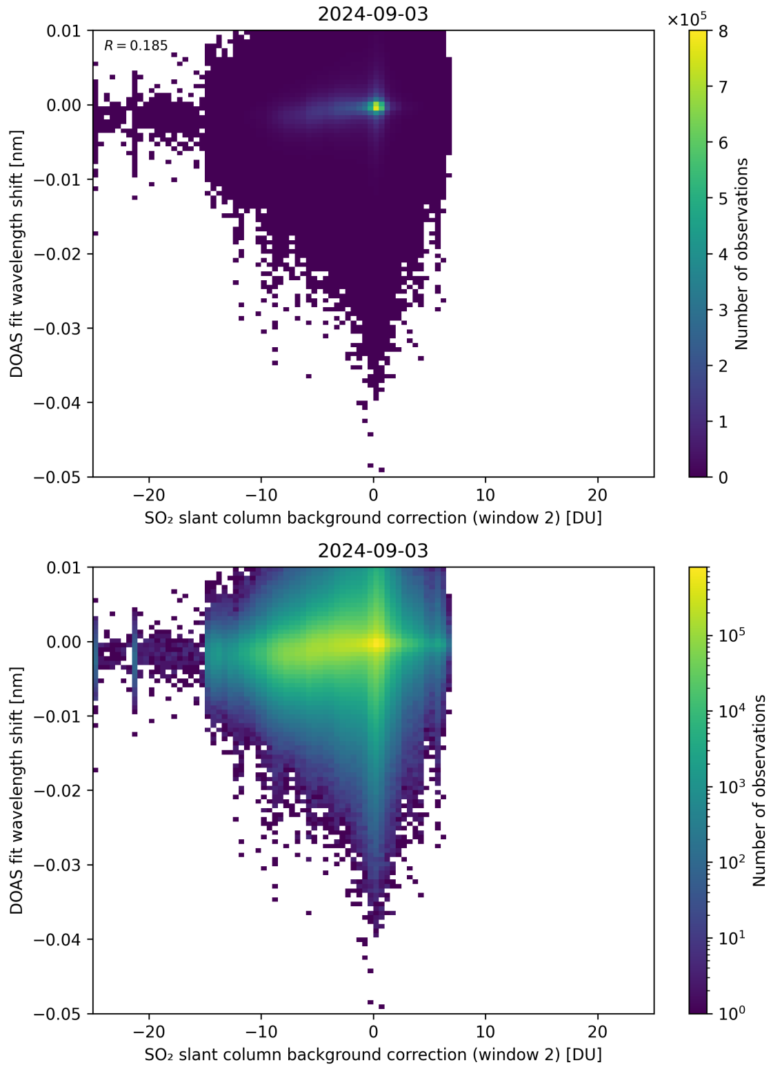
Figure 112: Scatter density plot of “SO 2 slant column background correction (window 2)” against “DOAS fit wavelength shift” for 2024-09-02 to 2024-09-04.
