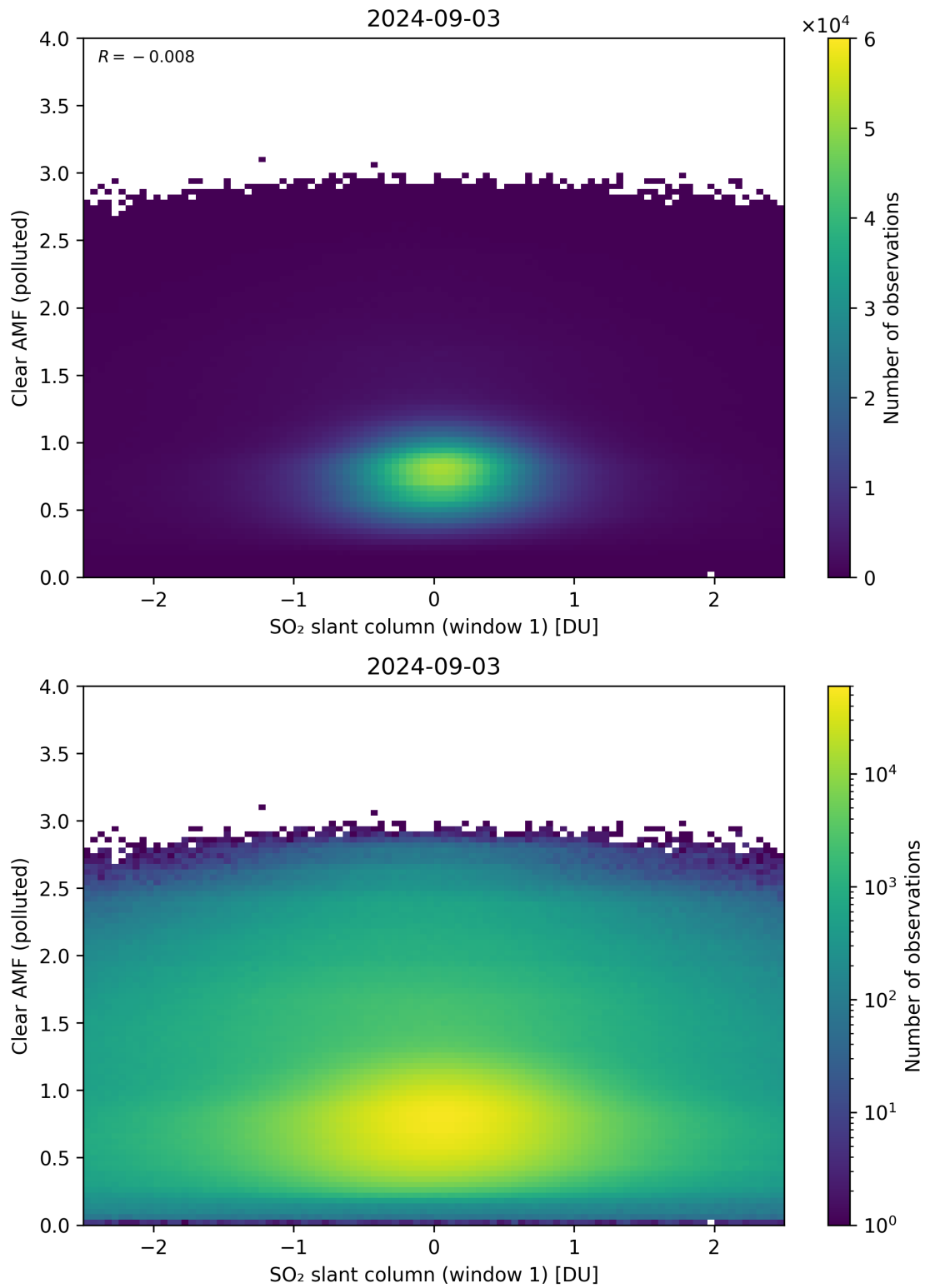
Figure 232: Scatter density plot of “SO 2 slant column (window 1)” against “Clear AMF (polluted)” for 2024-09-02 to 2024-09-04.
