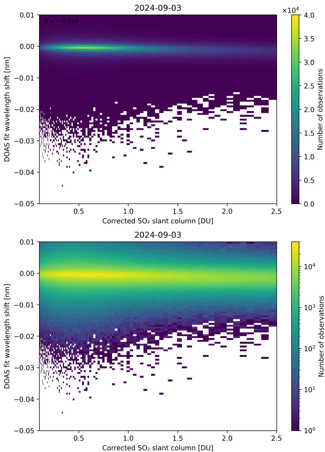
Figure 181: Scatter density plot of “Corrected SO 2 slant column” against “DOAS fit wavelength shift” for 2024-09-02 to 2024-09-04.
