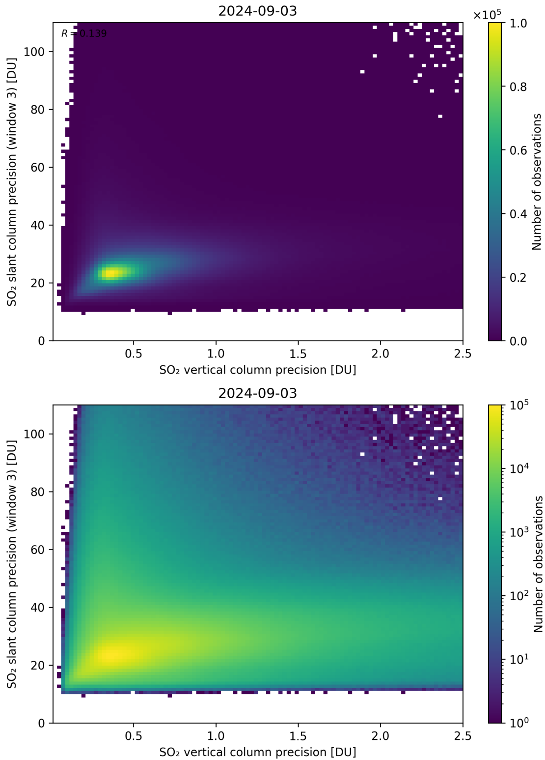
Figure 293: Scatter density plot of “SO 2 vertical column precision” against “SO 2 slant column precision (window 3)” for 2024-09-02 to 2024-09-04.
