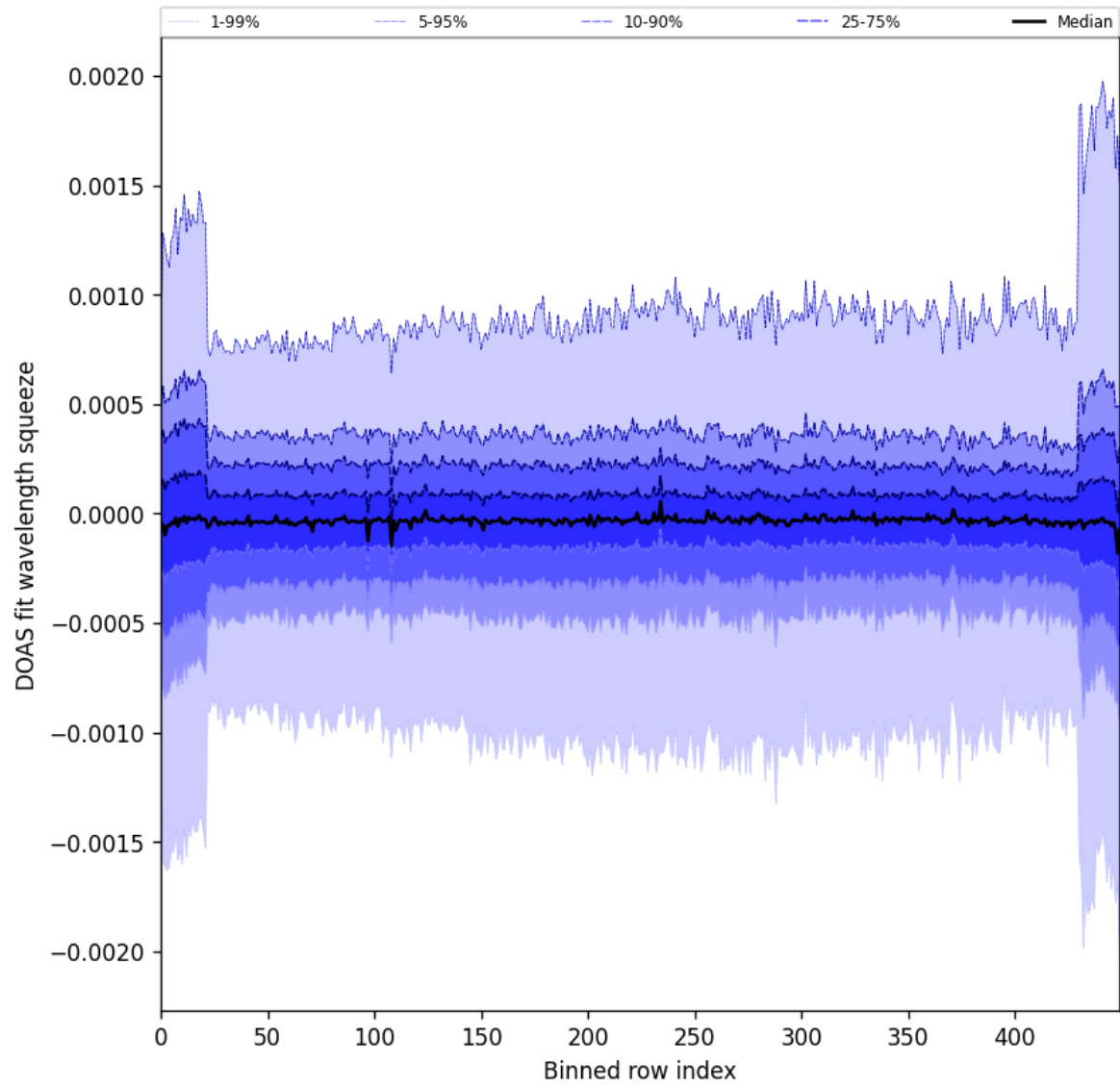
Figure 92: Along track statistics of “DOAS fit wavelength squeeze” for 2024-09-02 to 2024-09-04
