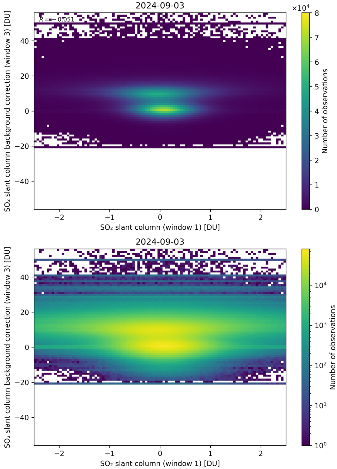
Figure 214: Scatter density plot of “SO 2 slant column (window 1)” against “SO 2 slant column background correction (window 3)” for 2024-09-02 to 2024-09-04.
