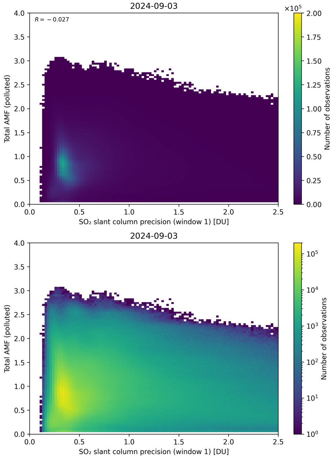
Figure 230: Scatter density plot of “SO 2 slant column precision (window 1)” against “Total AMF (polluted)” for 2024-09-02 to 2024-09-04.
