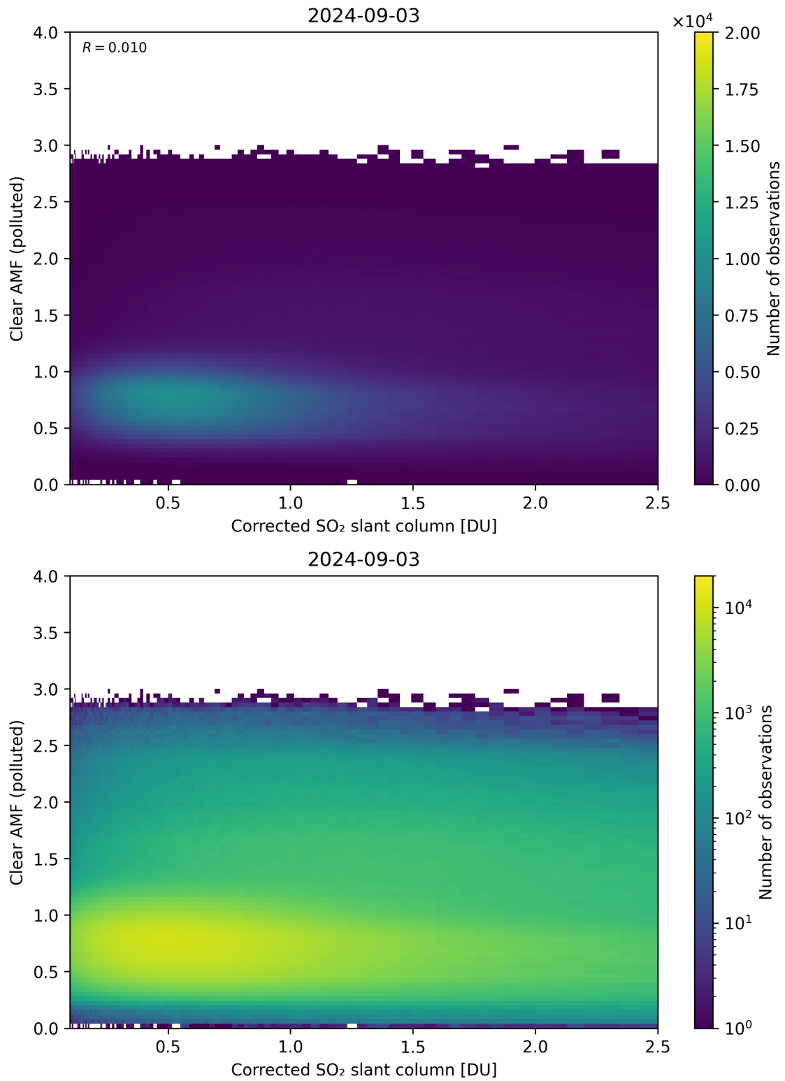
Figure 184: Scatter density plot of “Corrected SO 2 slant column” against “Clear AMF (polluted)” for 2024-09-02 to 2024-09-04.
