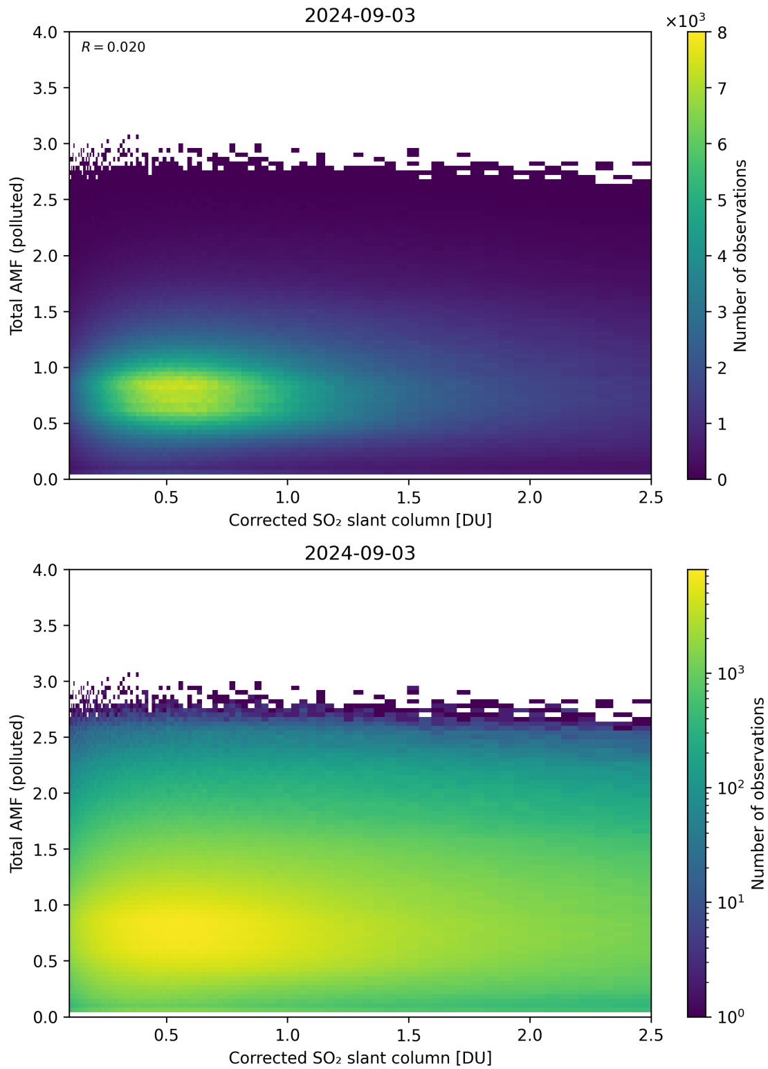
Figure 192: Scatter density plot of “Corrected SO 2 slant column” against “Total AMF (polluted)” for 2024-09-02 to 2024-09-04.
