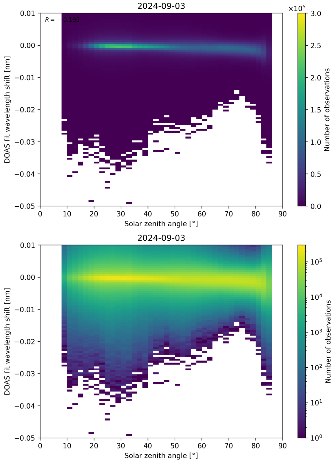
Figure 161: Scatter density plot of “Solar zenith angle” against “DOAS fit wavelength shift” for 2024-09-02 to 2024-09-04.
