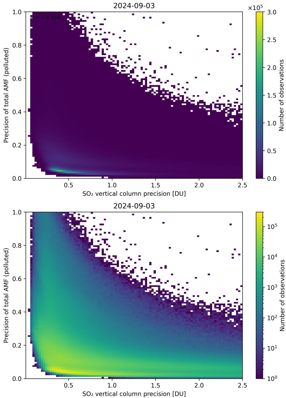
Figure 295: Scatter density plot of “SO 2 vertical column precision” against “Precision of total AMF (polluted)” for 2024-09-02 to 2024-09-04.
