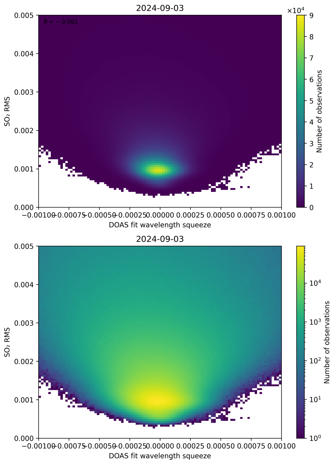
Figure 132: Scatter density plot of “DOAS fit wavelength squeeze” against “SO 2 RMS” for 2024-09-02 to 2024-09-04.
