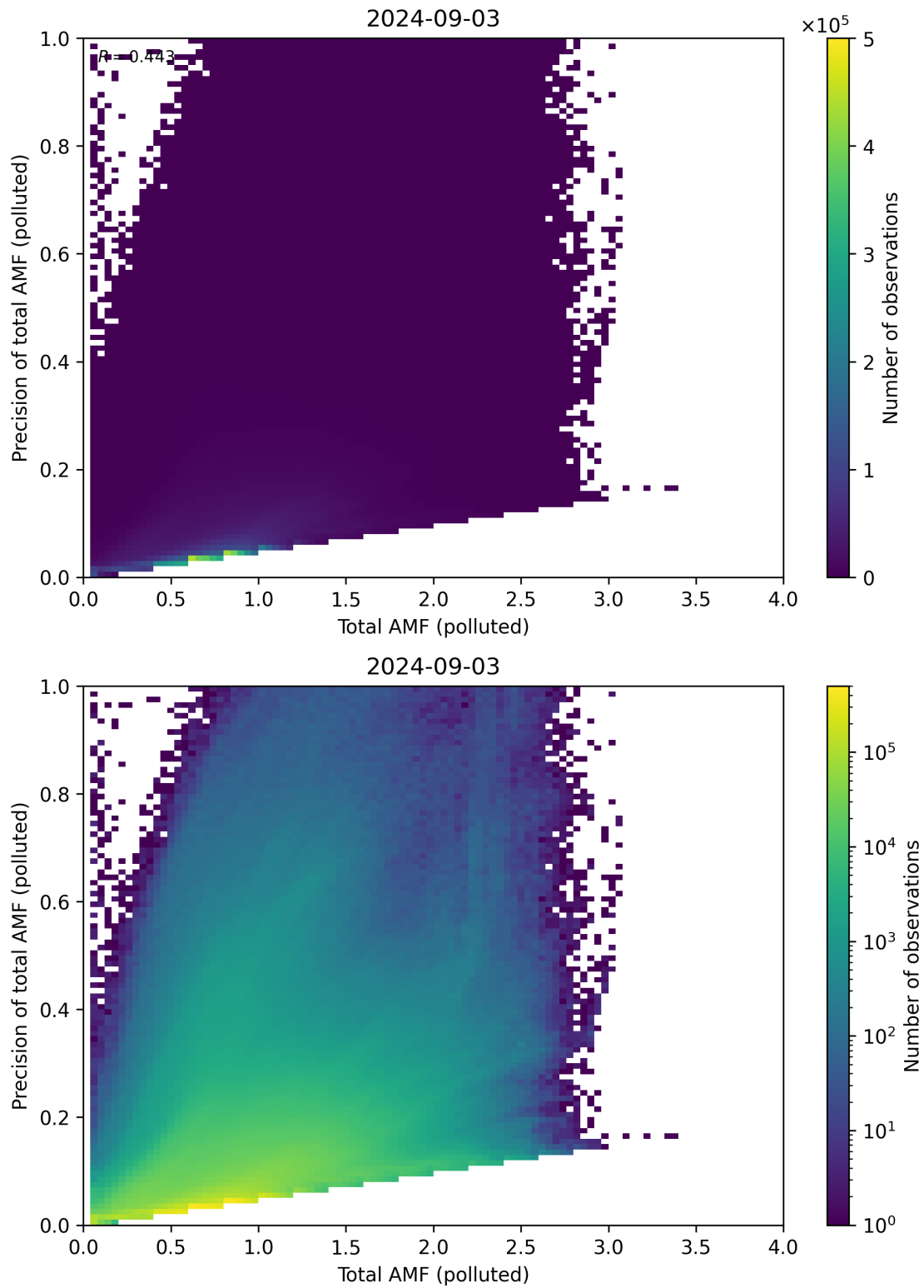
Figure 272: Scatter density plot of “Total AMF (polluted)” against “Precision of total AMF (polluted)” for 2024-09-02 to 2024-09-04.
