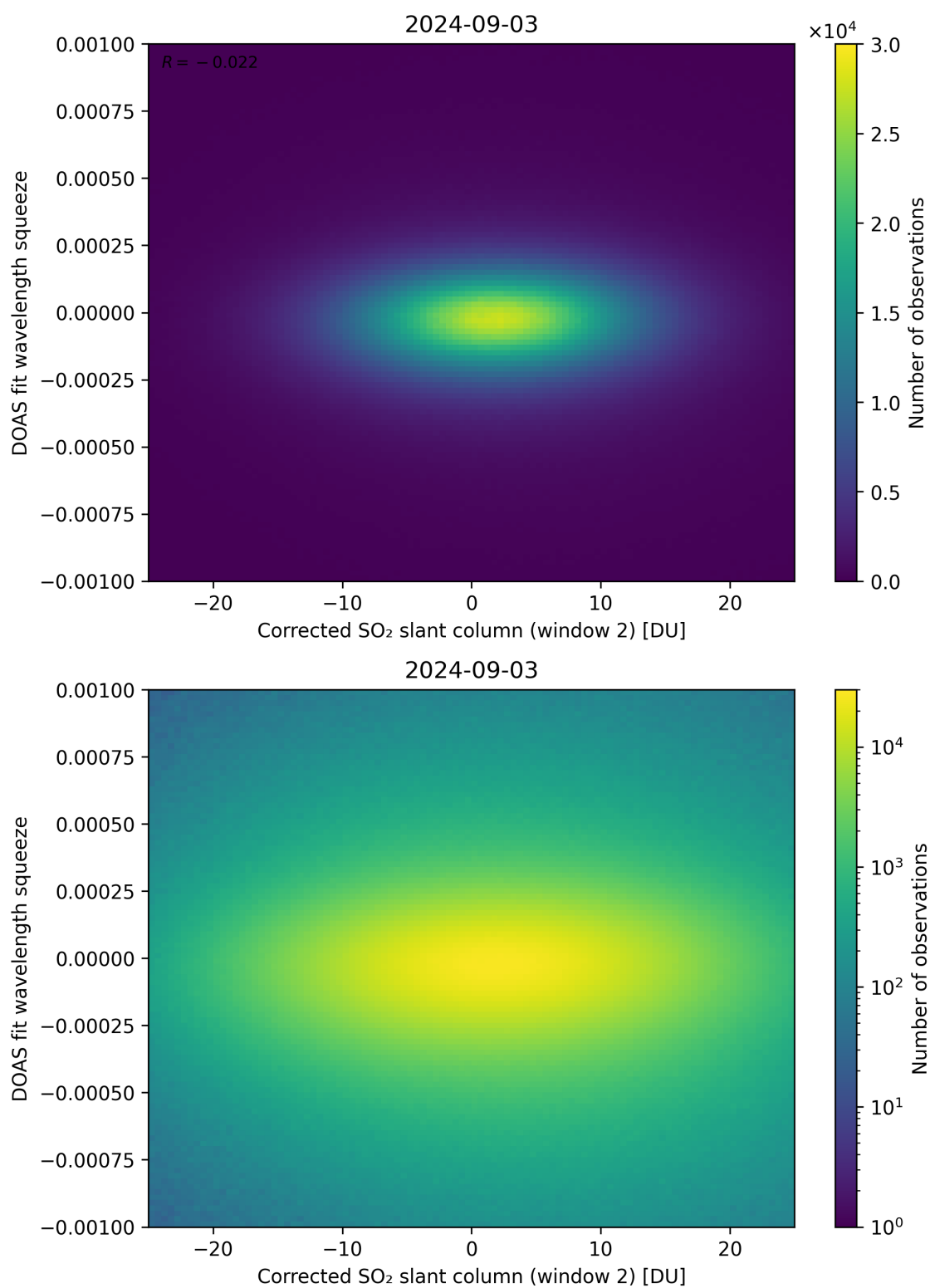
Figure 197: Scatter density plot of “Corrected SO 2 slant column (window 2)” against “DOAS fit wavelength squeeze” for 2024-09-02 to 2024-09-04.
