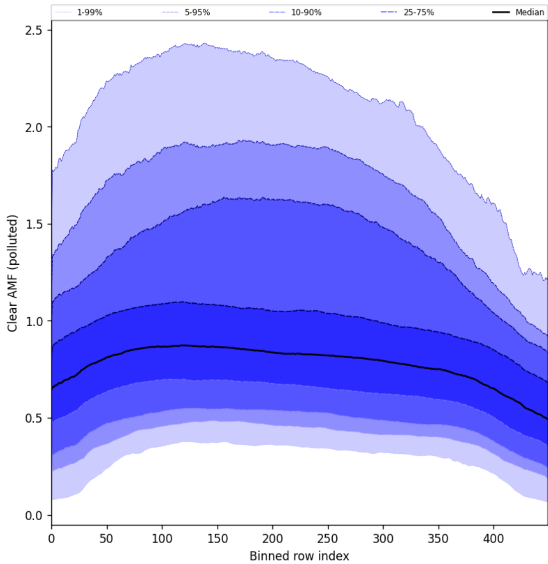
Figure 96: Along track statistics of “Clear AMF (polluted)” for 2024-09-02 to 2024-09-04
