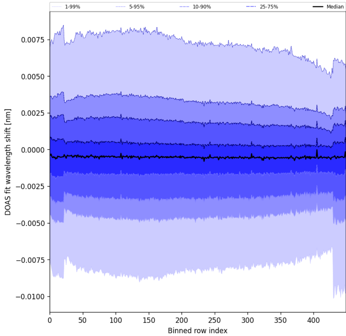
Figure 91: Along track statistics of “DOAS fit wavelength shift” for 2024-09-02 to 2024-09-04
