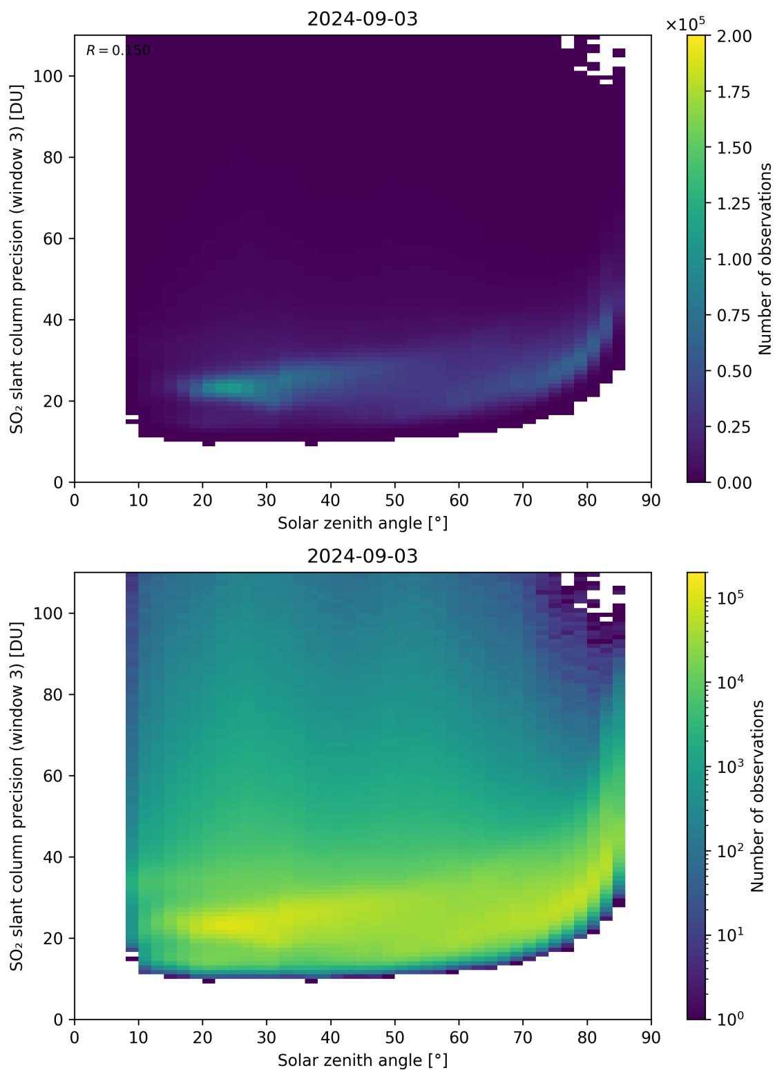
Figure 173: Scatter density plot of “Solar zenith angle” against “SO 2 slant column precision (window 3)” for 2024-09-02 to 2024-09-04.
