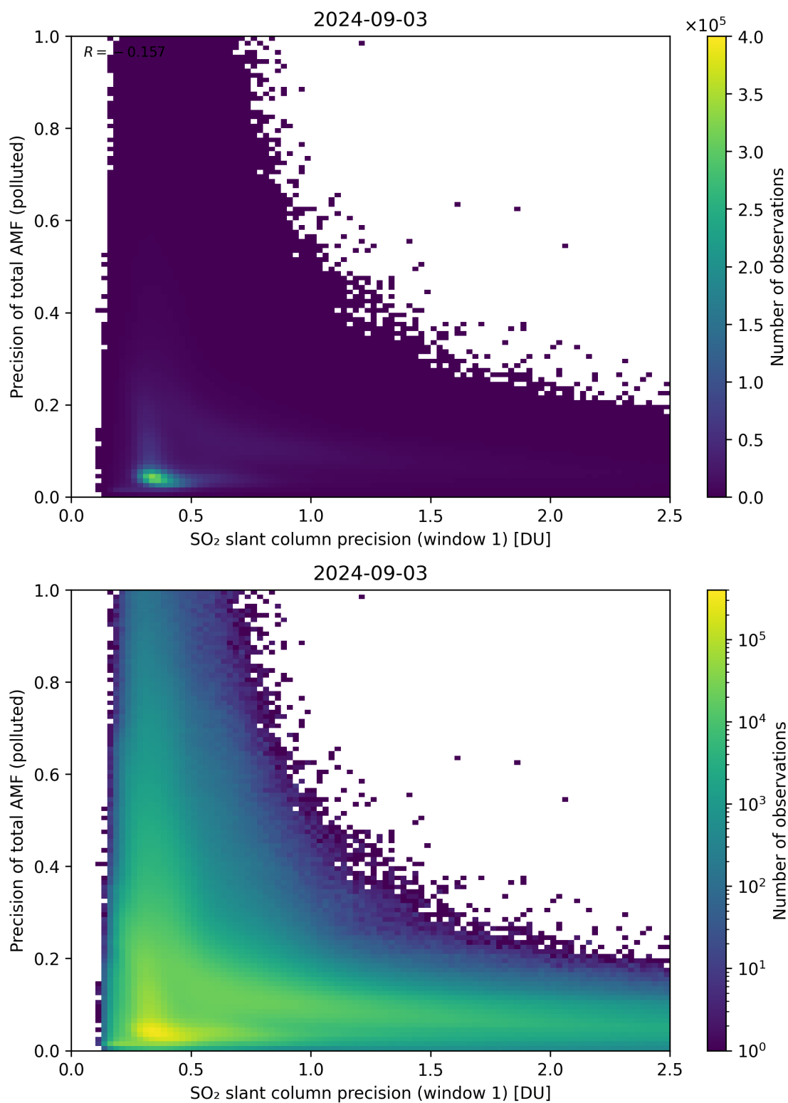
Figure 231: Scatter density plot of “SO 2 slant column precision (window 1)” against “Precision of total AMF (polluted)” for 2024-09-02 to 2024-09-04.
