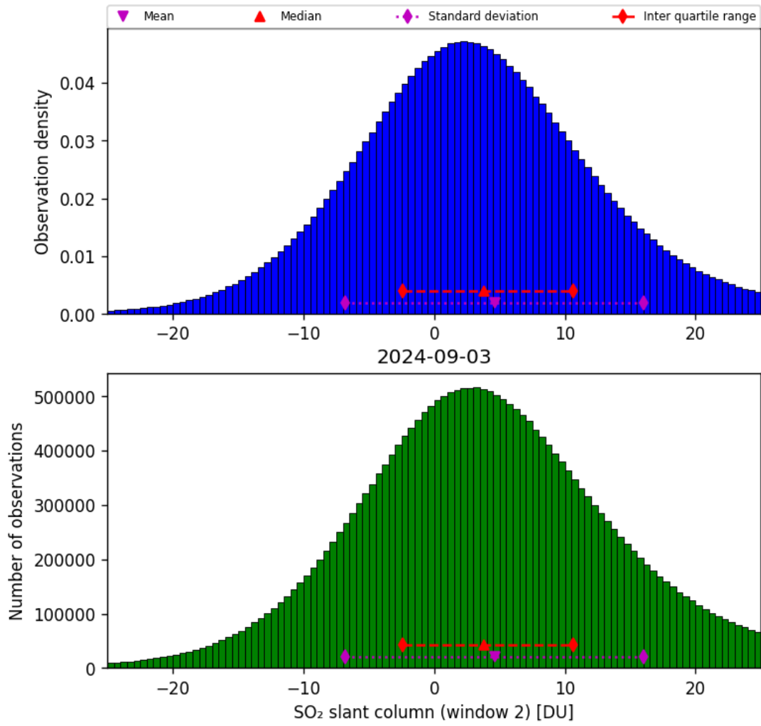
Figure 60: Histogram of “SO 2 slant column (window 2)” for 2024-09-02 to 2024-09-04
