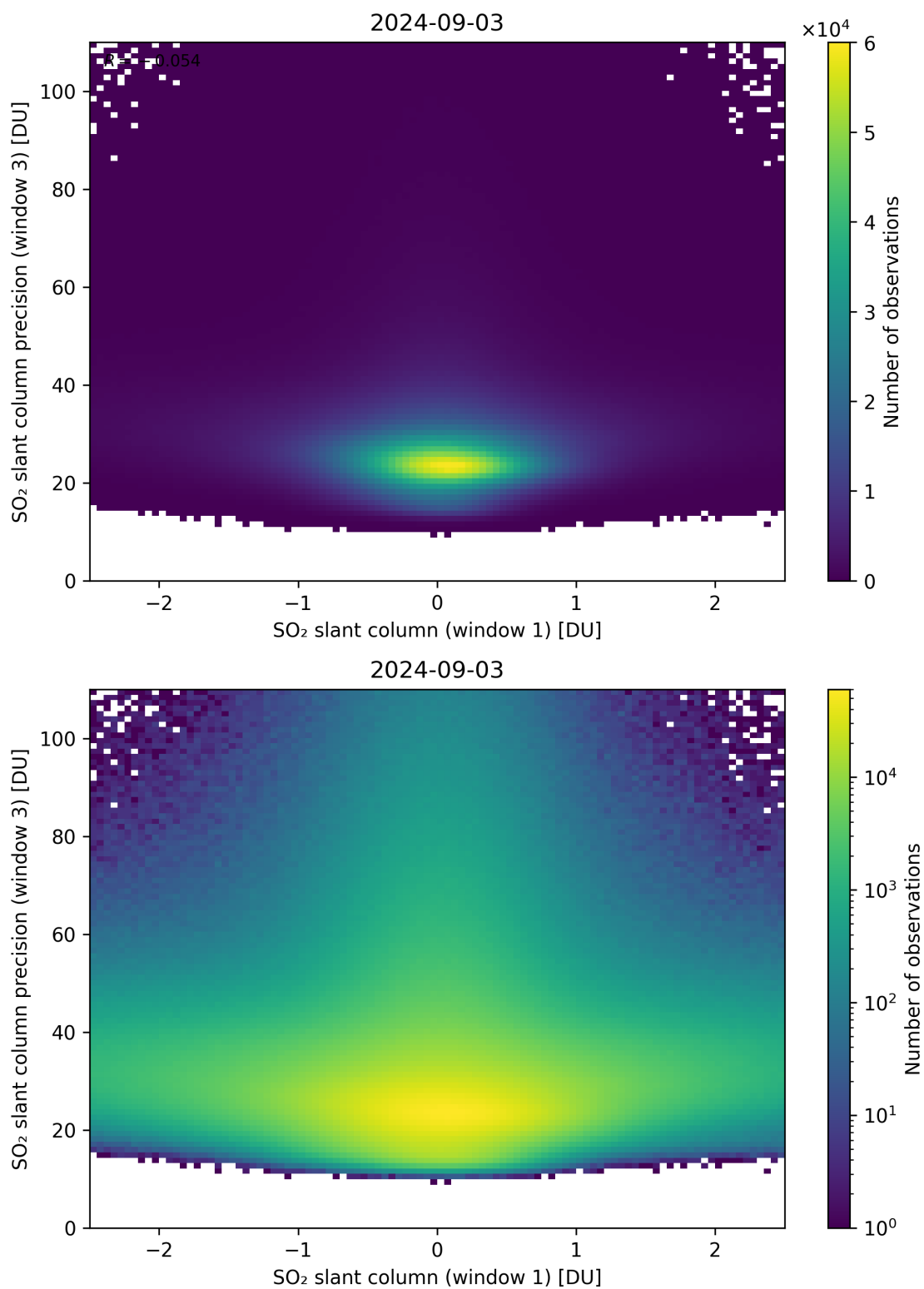
Figure 238: Scatter density plot of “SO 2 slant column (window 1)” against “SO 2 slant column precision (window 3)” for 2024-09-02 to 2024-09-04.
