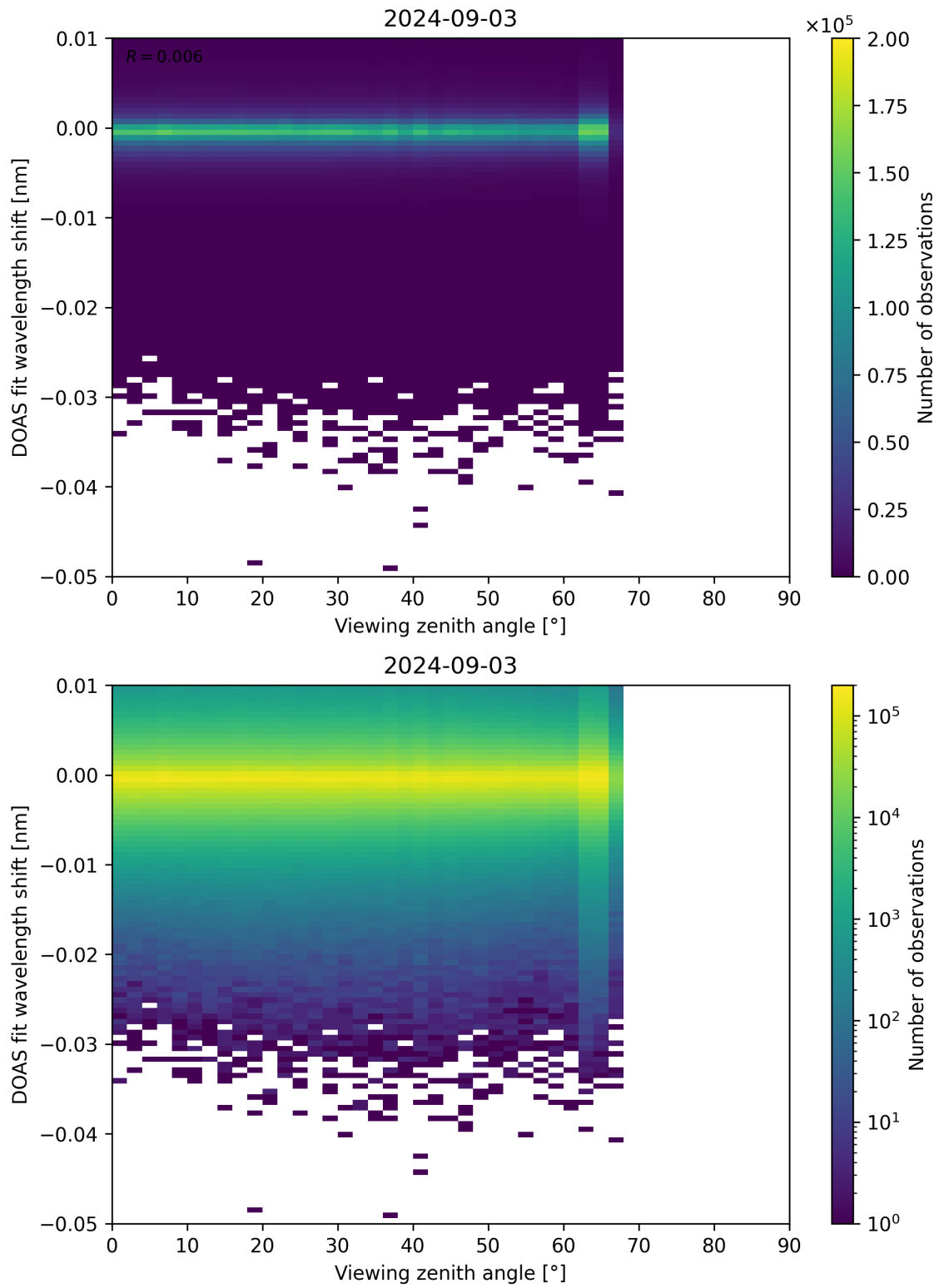
Figure 311: Scatter density plot of “Viewing zenith angle” against “DOAS fit wavelength shift” for 2024-09-02 to 2024-09-04.
