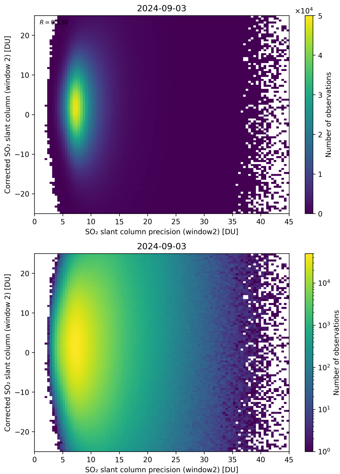
Figure 247: Scatter density plot of “SO 2 slant column precision (window2)” against “Corrected SO 2 slant column (window 2)” for 2024-09-02 to 2024-09-04.
