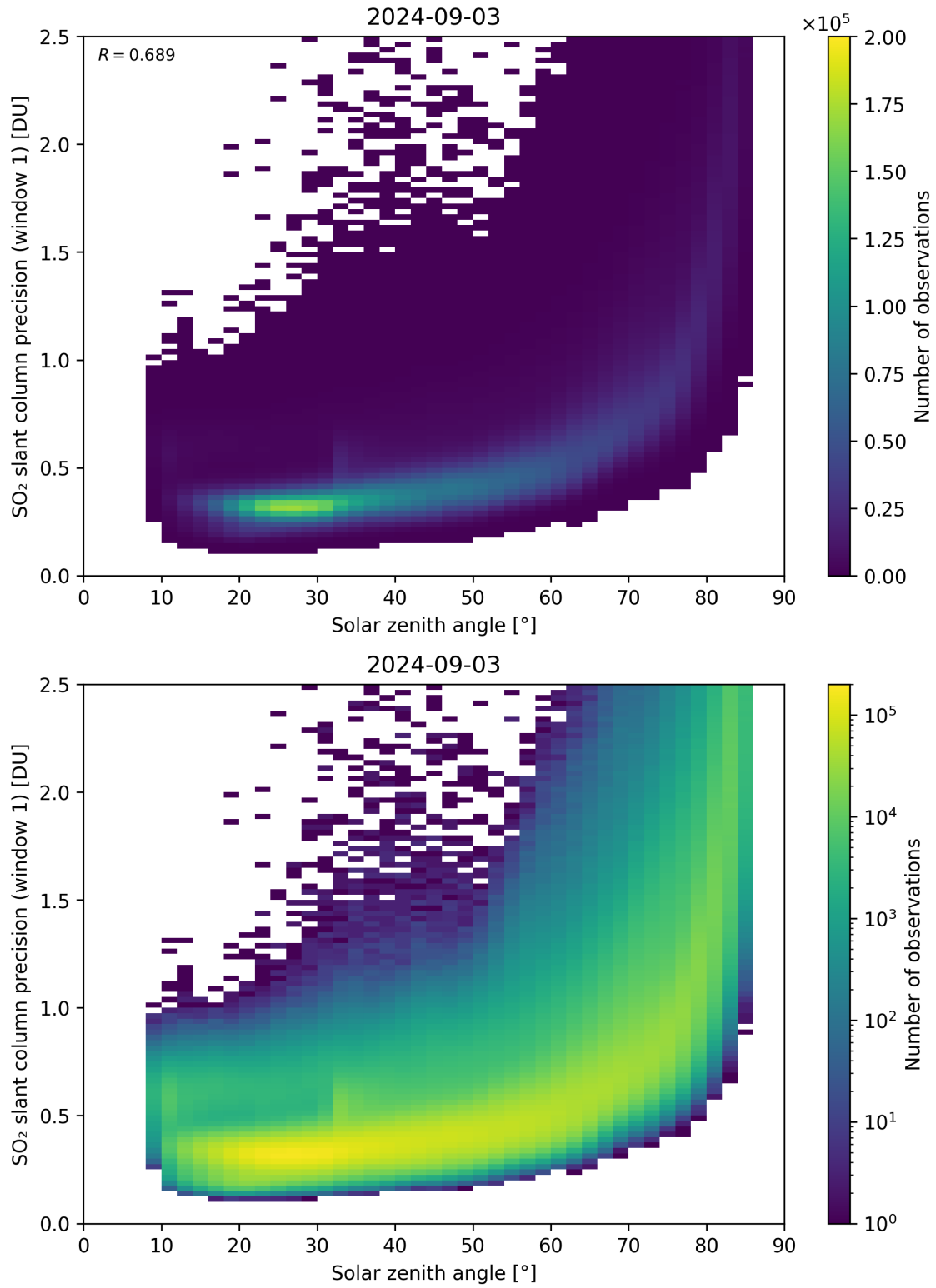
Figure 170: Scatter density plot of “Solar zenith angle” against “SO 2 slant column precision (window 1)” for 2024-09-02 to 2024-09-04.
