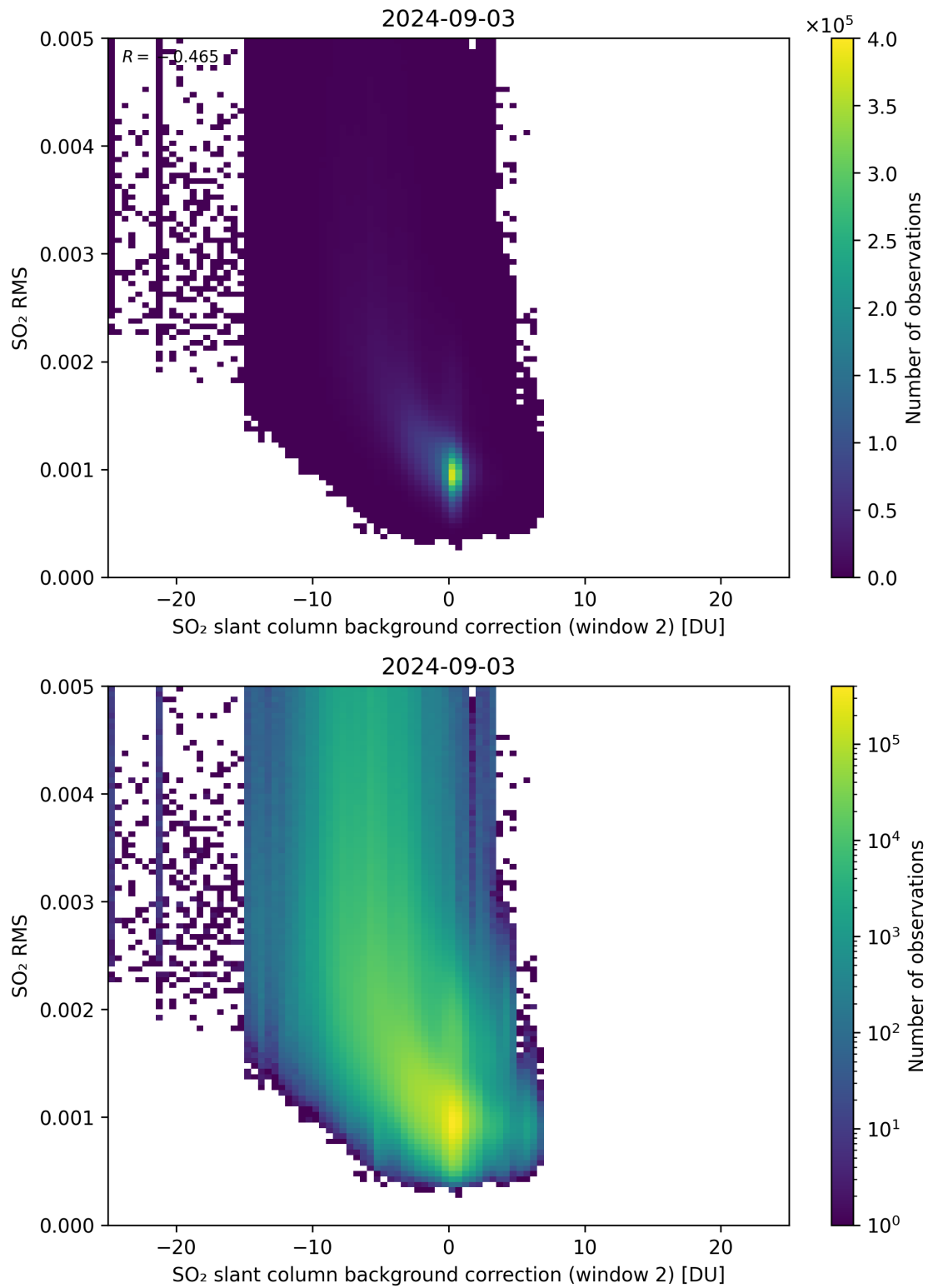
Figure 114: Scatter density plot of “SO 2 slant column background correction (window 2)” against “SO 2 RMS” for 2024-09-02 to 2024-09-04.
