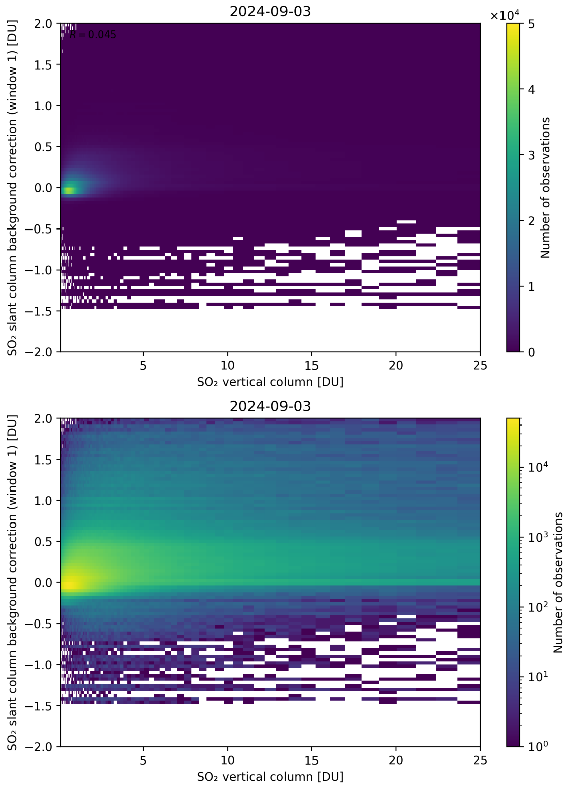
Figure 273: Scatter density plot of “SO 2 vertical column” against “SO 2 slant column background correction (window 1)” for 2024-09-02 to 2024-09-04.
