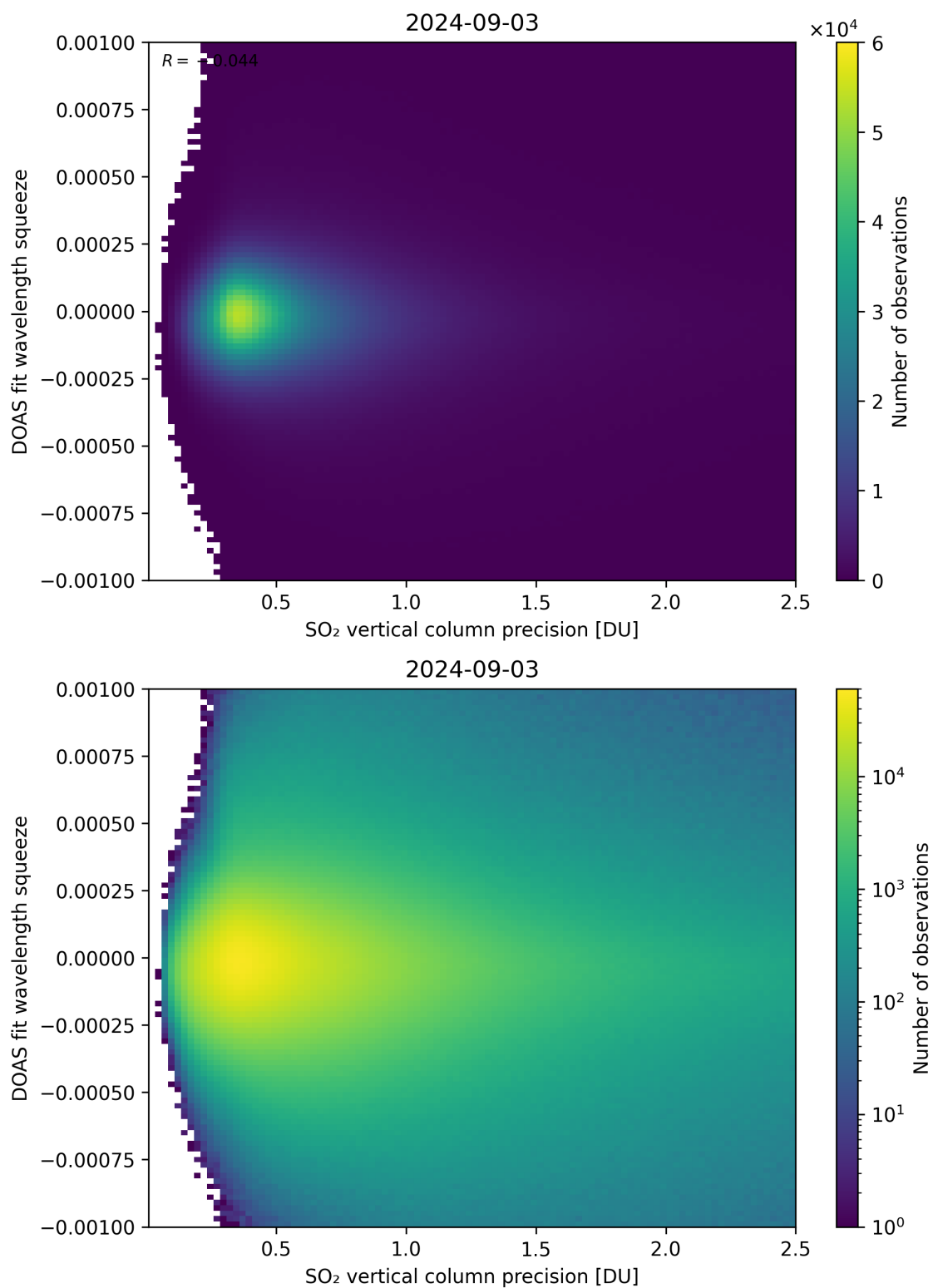
Figure 283: Scatter density plot of “SO 2 vertical column precision” against “DOAS fit wavelength squeeze” for 2024-09-02 to 2024-09-04.
