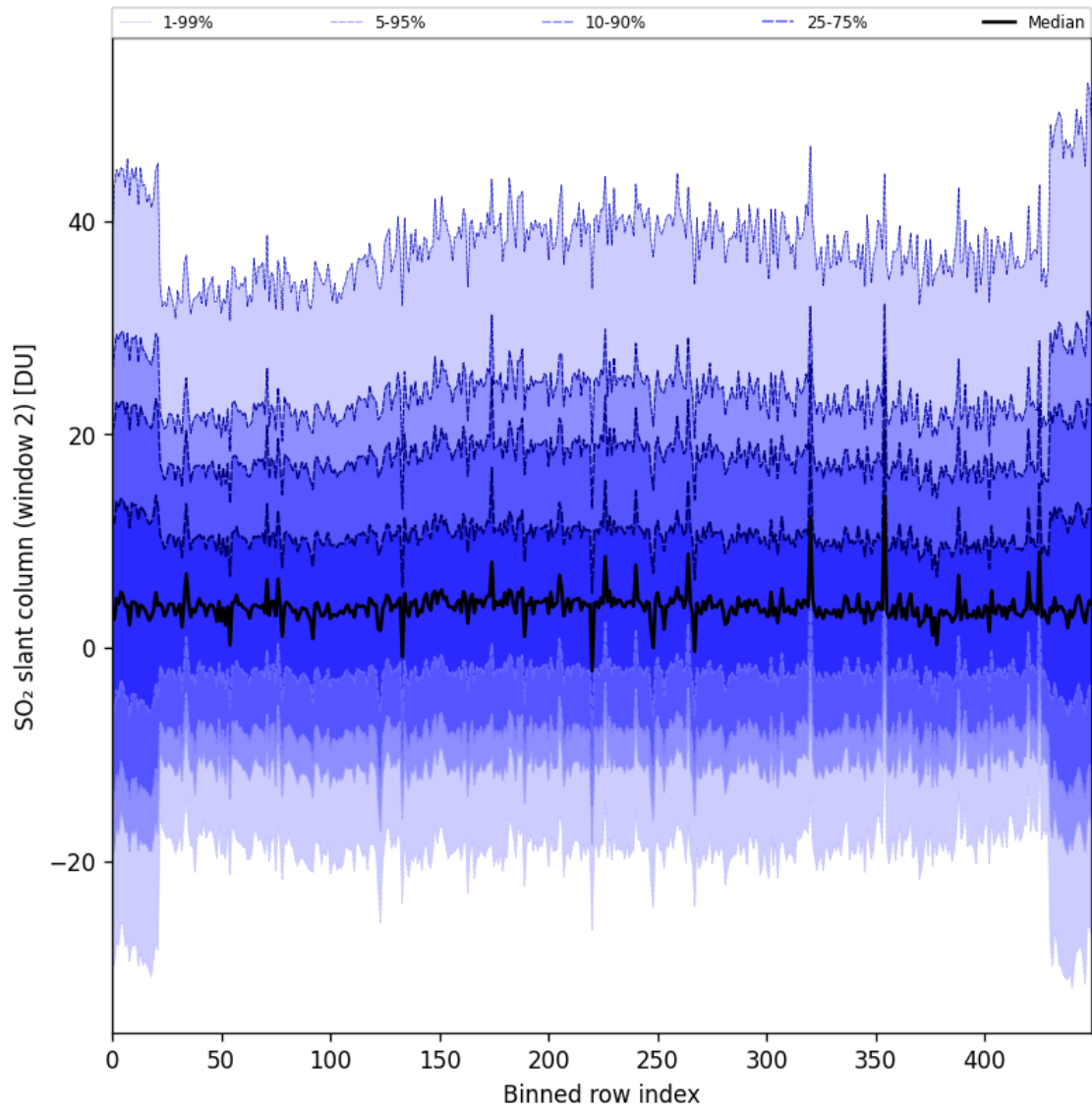
Figure 83: Along track statistics of “SO 2 slant column (window 2)” for 2024-09-02 to 2024-09-04
