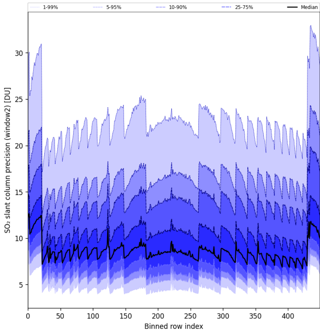
Figure 84: Along track statistics of “SO 2 slant column precision (window2)” for 2024-09-02 to 2024-09-04
