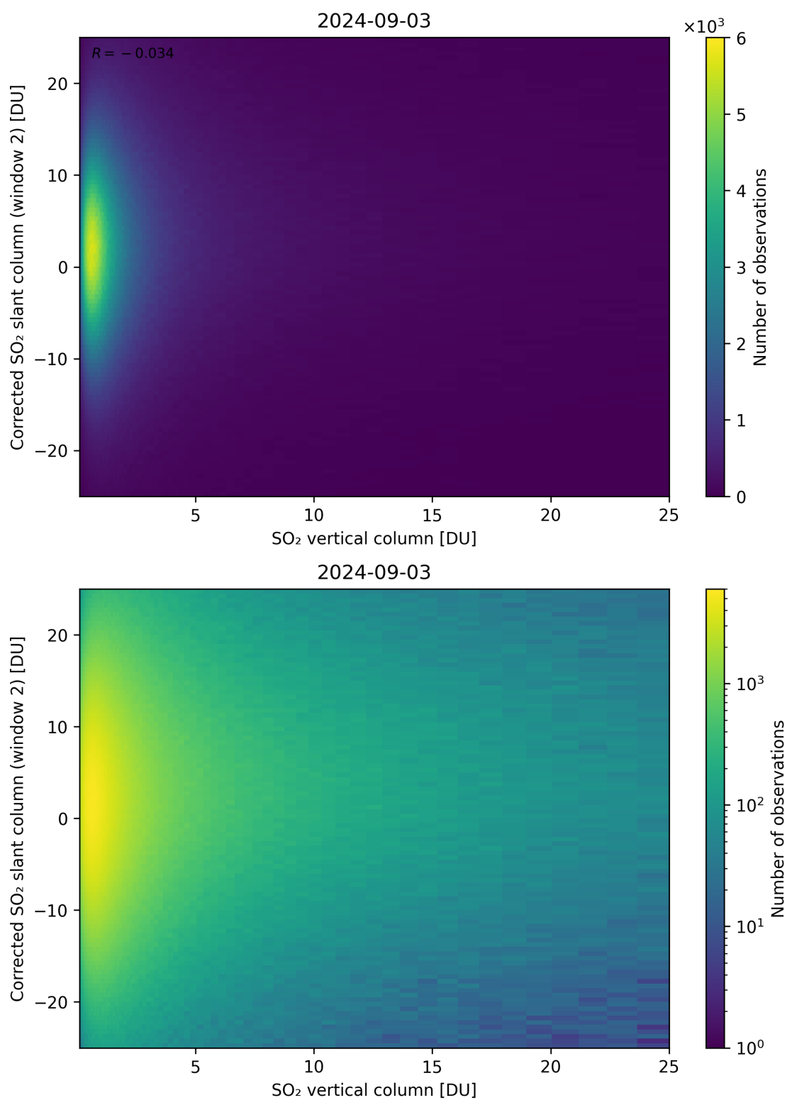
Figure 298: Scatter density plot of “SO 2 vertical column” against “Corrected SO 2 slant column (window 2)” for 2024-09-02 to 2024-09-04.
