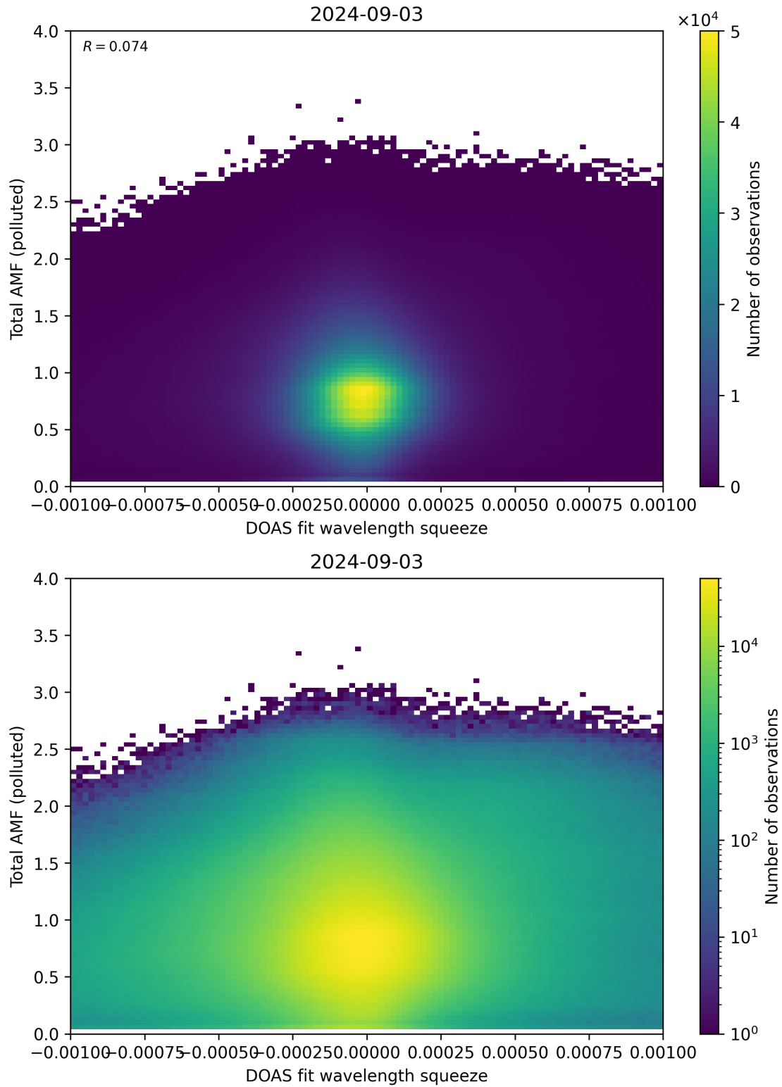
Figure 134: Scatter density plot of “DOAS fit wavelength squeeze” against “Total AMF (polluted)” for 2024-09-02 to 2024-09-04.
