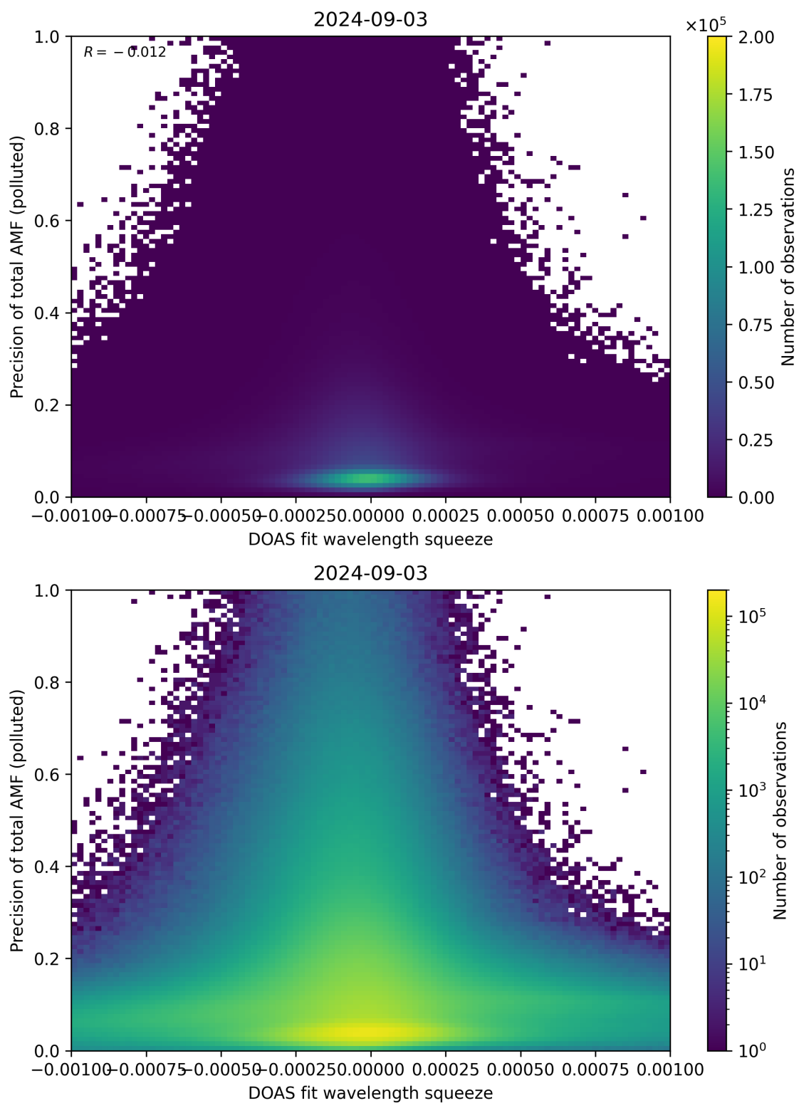
Figure 135: Scatter density plot of “DOAS fit wavelength squeeze” against “Precision of total AMF (polluted)” for 2024-09-02 to 2024-09-04.
