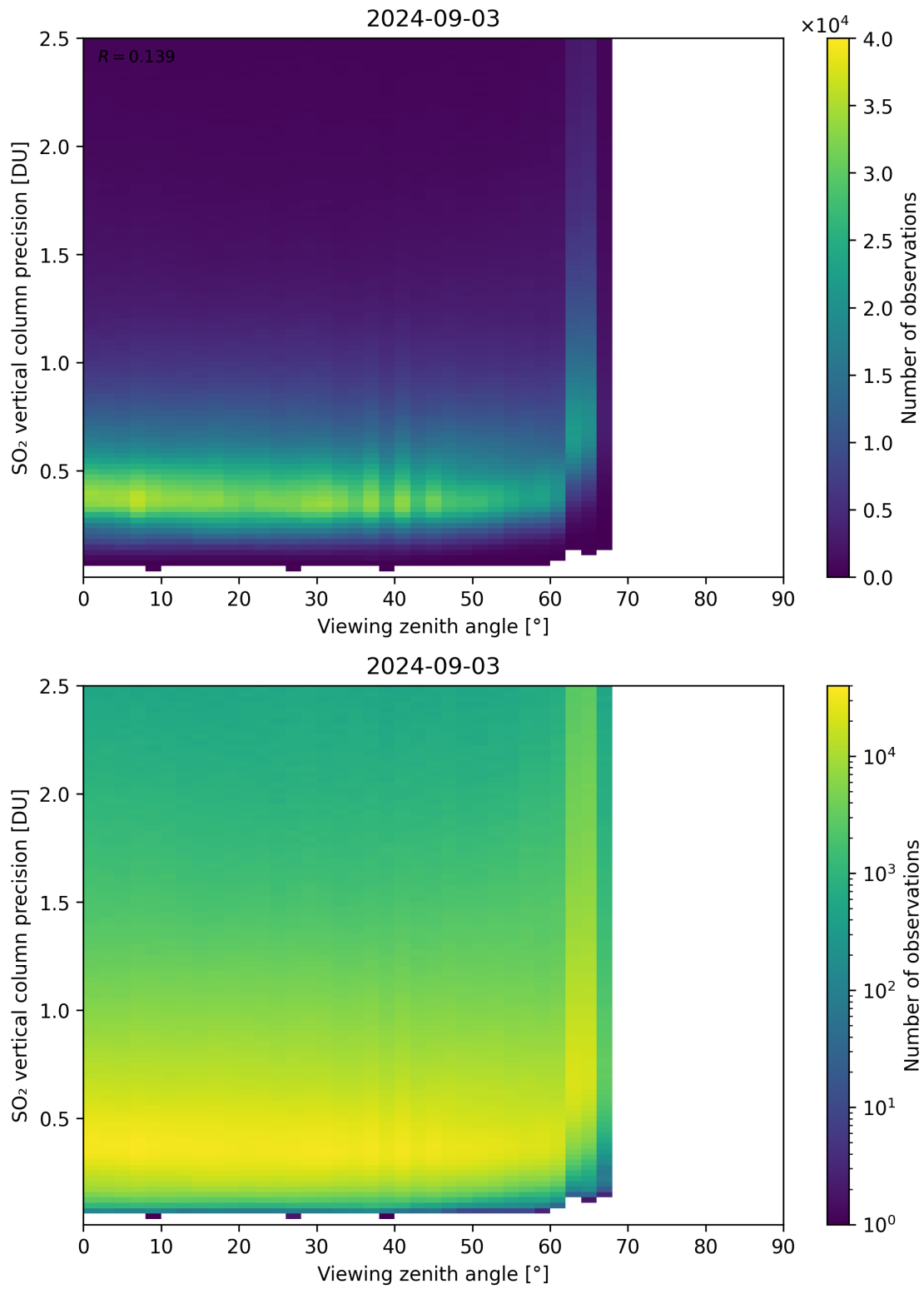
Figure 328: Scatter density plot of “Viewing zenith angle” against “SO 2 vertical column precision” for 2024-09-02 to 2024-09-04.
