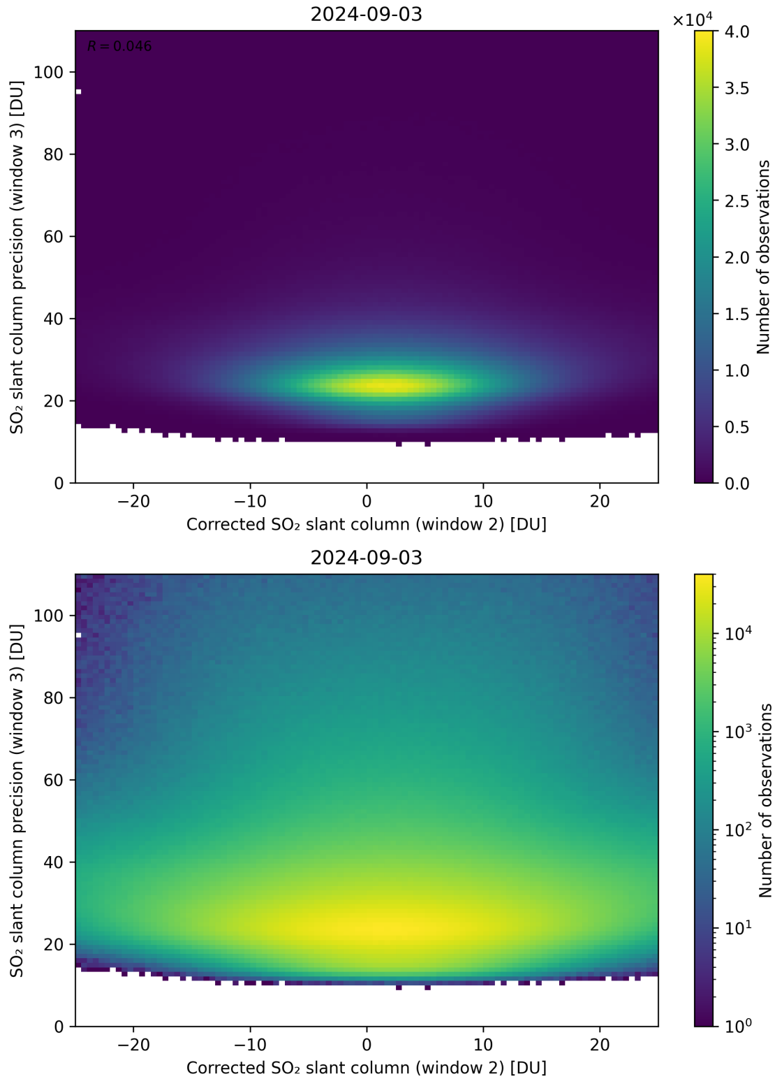
Figure 202: Scatter density plot of “Corrected SO 2 slant column (window 2)” against “SO 2 slant column precision (window 3)” for 2024-09-02 to 2024-09-04.
