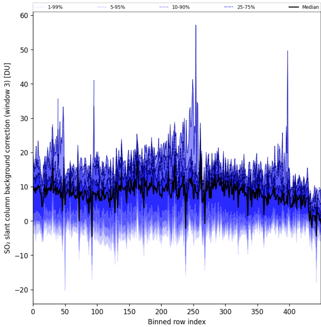
Figure 90: Along track statistics of “SO 2 slant column background correction (window 3)” for 2024-09-02 to 2024-09-04
