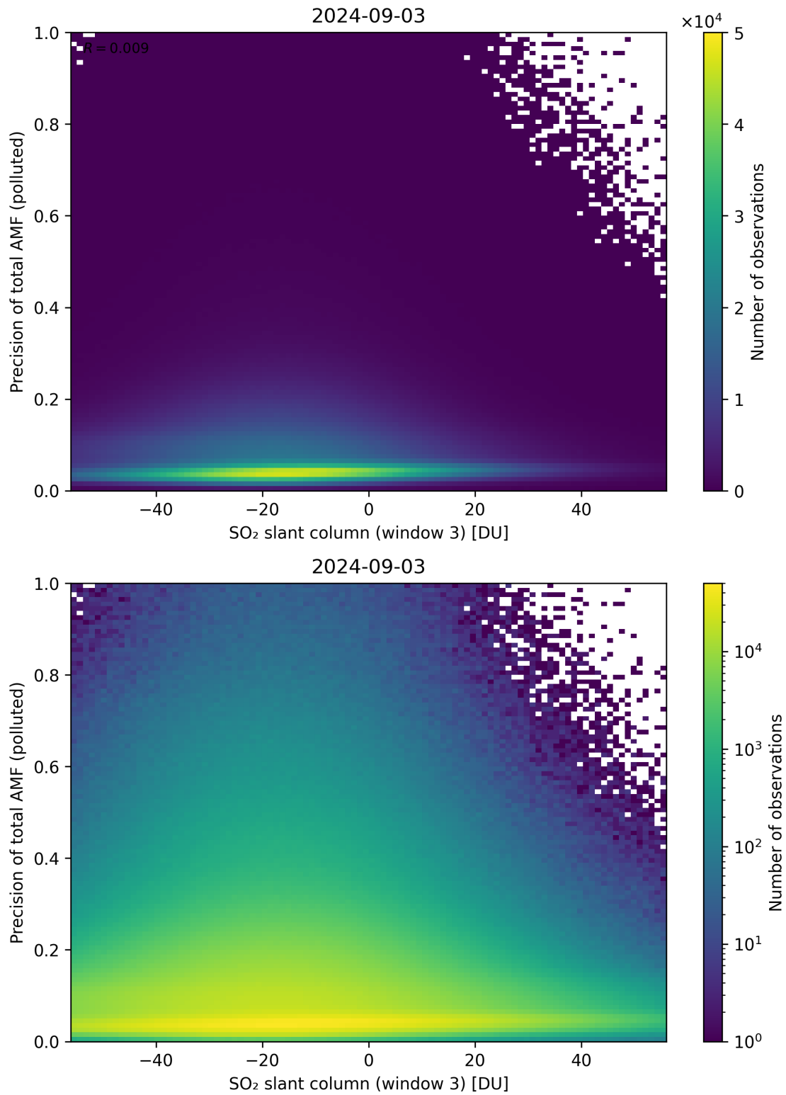
Figure 269: Scatter density plot of “SO 2 slant column (window 3)” against “Precision of total AMF (polluted)” for 2024-09-02 to 2024-09-04.
