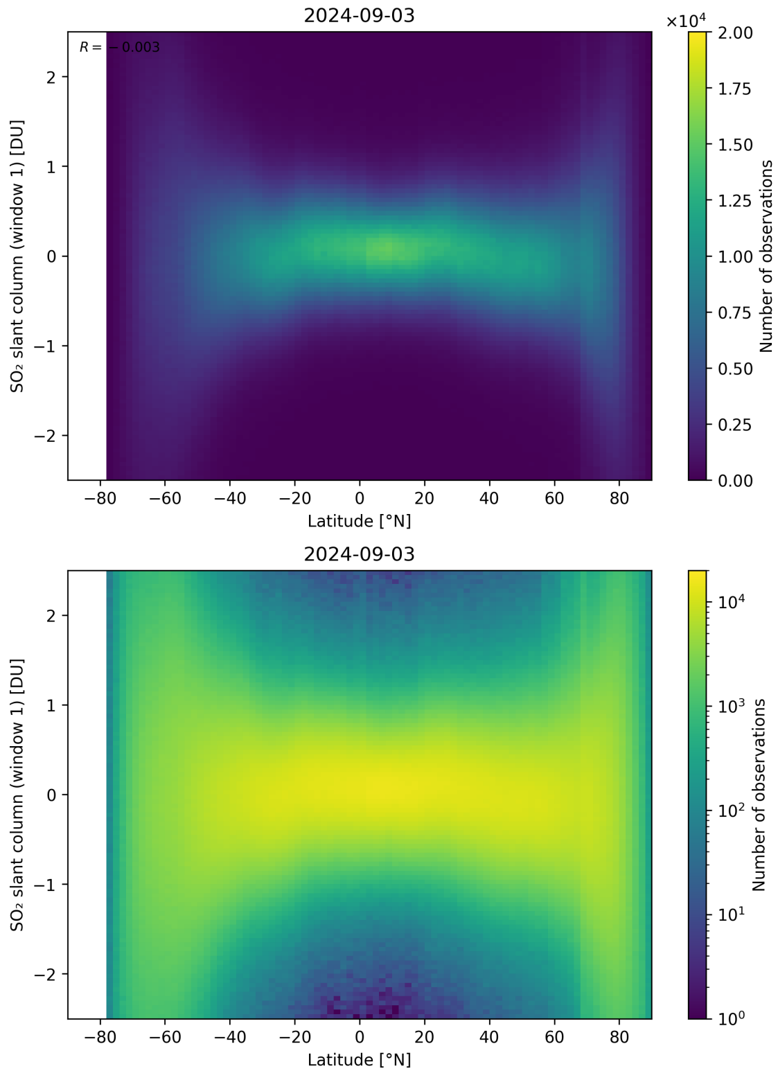
Figure 149: Scatter density plot of “Latitude” against “SO 2 slant column (window 1)” for 2024-09-02 to 2024-09-04.
