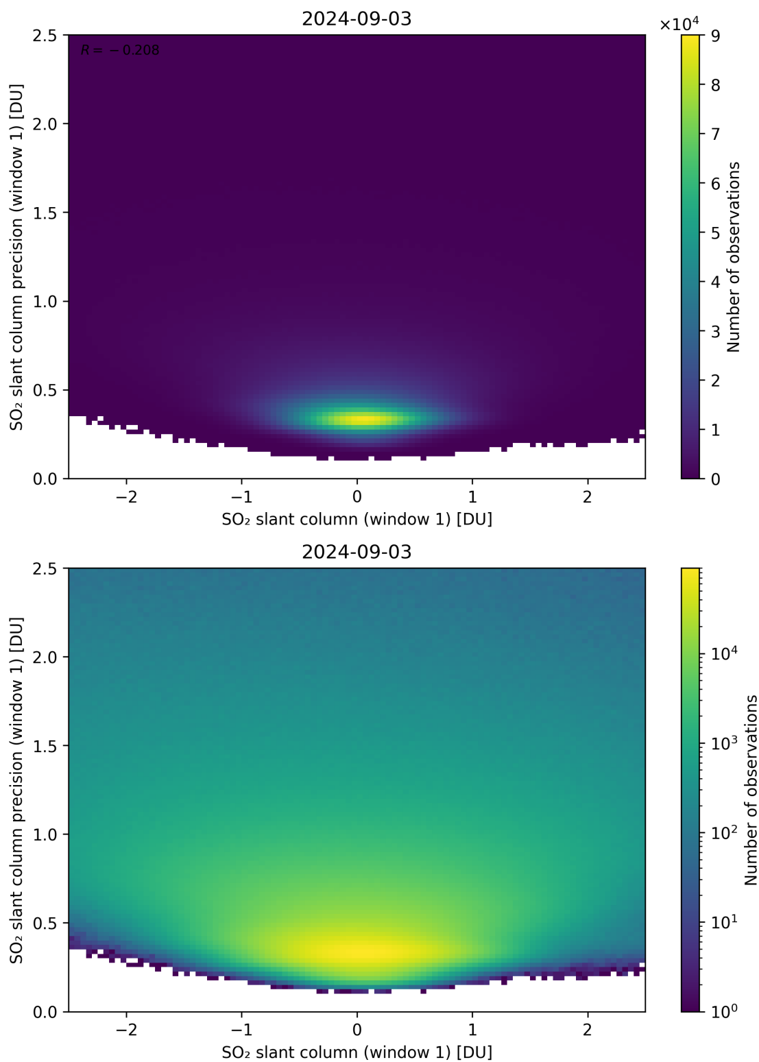
Figure 235: Scatter density plot of “SO 2 slant column (window 1)” against “SO 2 slant column precision (window 1)” for 2024-09-02 to 2024-09-04.
