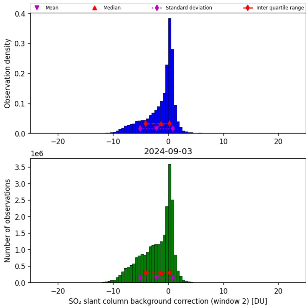
Figure 63: Histogram of “SO 2 slant column background correction (window 2)” for 2024-09-02 to 2024-09-04
