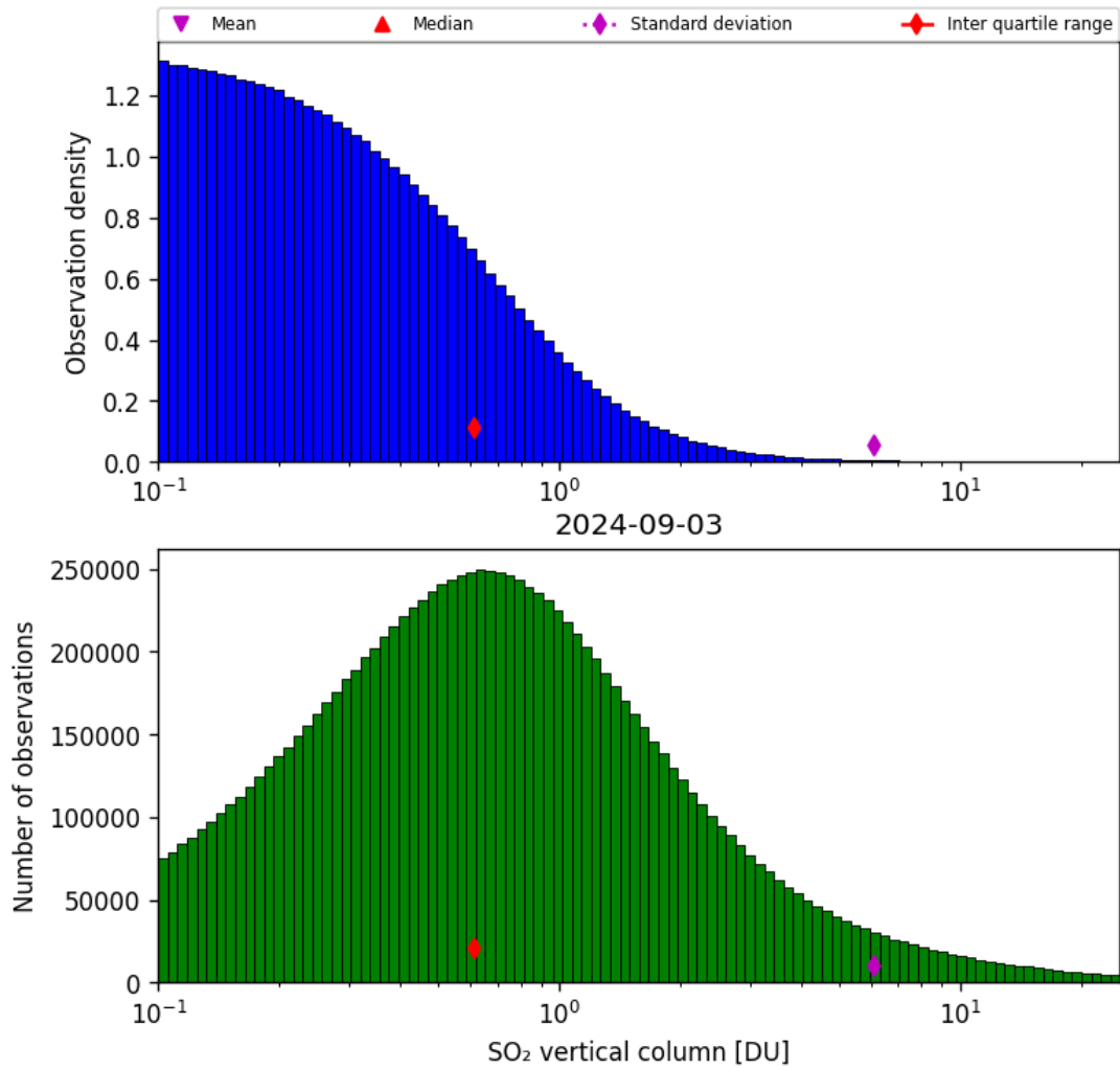
Figure 53: Histogram of “SO 2 vertical column” for 2024-09-02 to 2024-09-04
