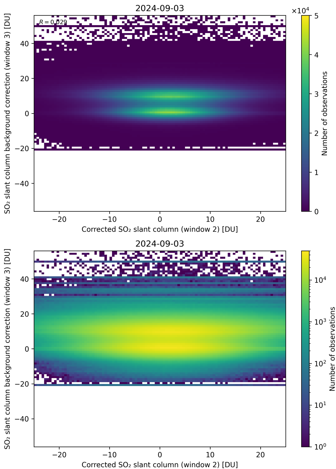
Figure 195: Scatter density plot of “Corrected SO 2 slant column (window 2)” against “SO 2 slant column background correction (window 3)” for 2024-09-02 to 2024-09-04.
