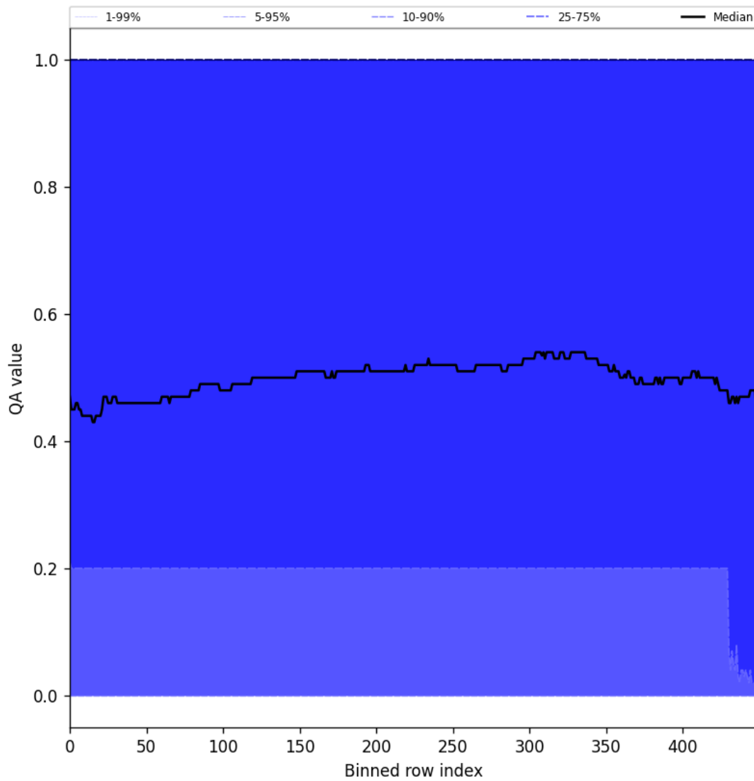
Figure 75: Along track statistics of “QA value” for 2024-09-02 to 2024-09-04
