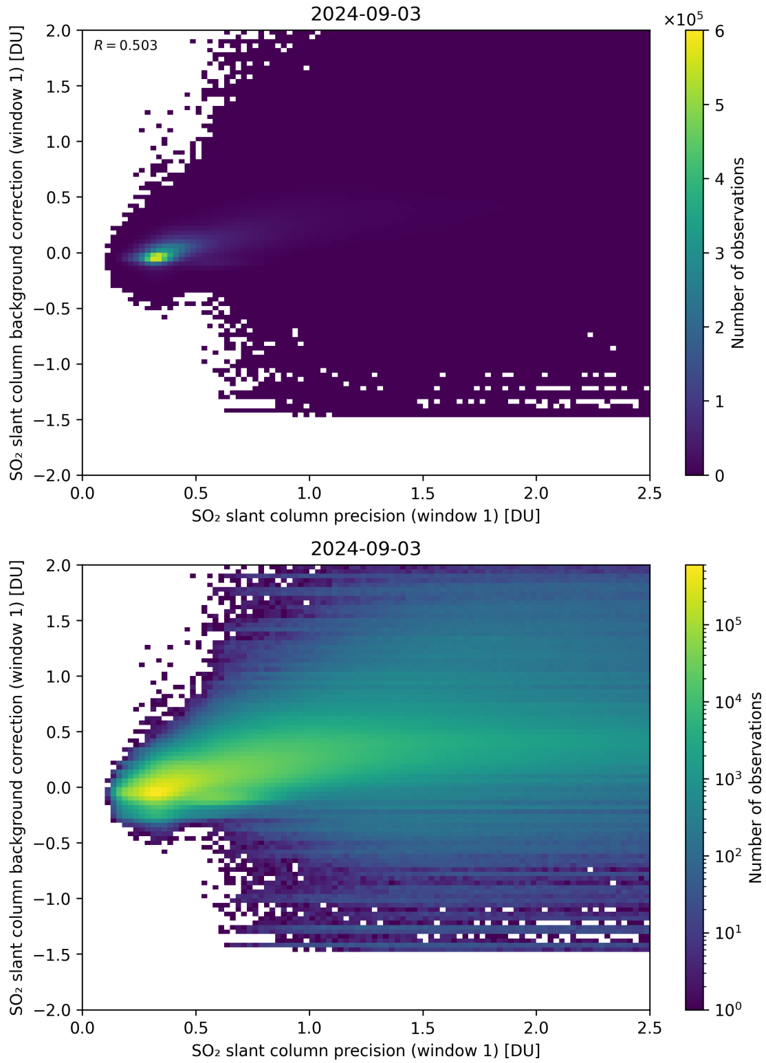
Figure 218: Scatter density plot of “SO 2 slant column precision (window 1)” against “SO 2 slant column background correction (window 1)” for 2024-09-02 to 2024-09-04.
