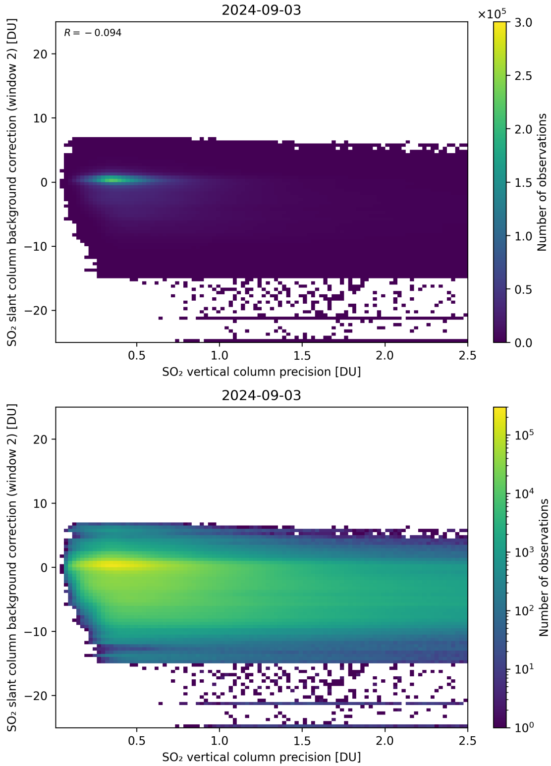
Figure 280: Scatter density plot of “SO 2 vertical column precision” against “SO 2 slant column background correction (window 2)” for 2024-09-02 to 2024-09-04.
