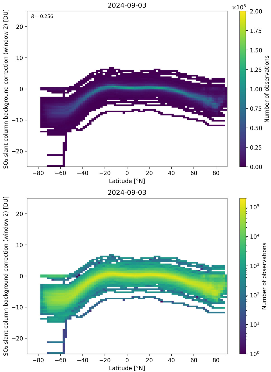
Figure 140: Scatter density plot of “Latitude” against “SO 2 slant column background correction (window 2)” for 2024-09-02 to 2024-09-04.
