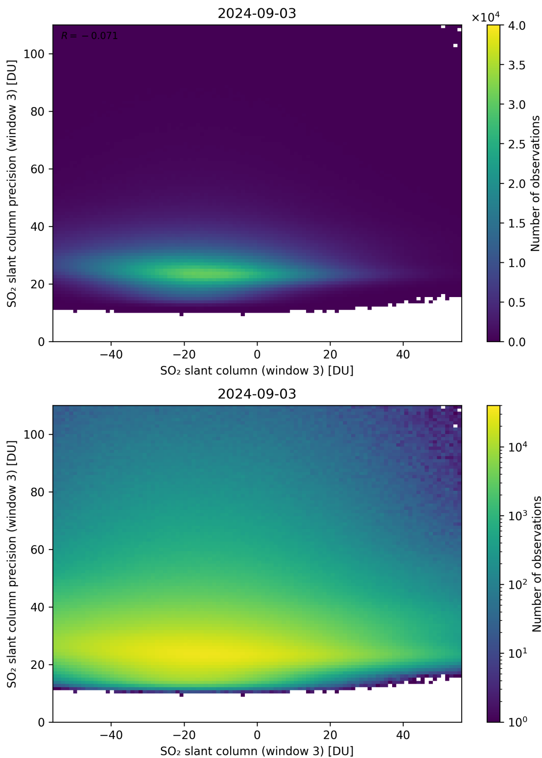
Figure 267: Scatter density plot of “SO 2 slant column (window 3)” against “SO 2 slant column precision (window 3)” for 2024-09-02 to 2024-09-04.
