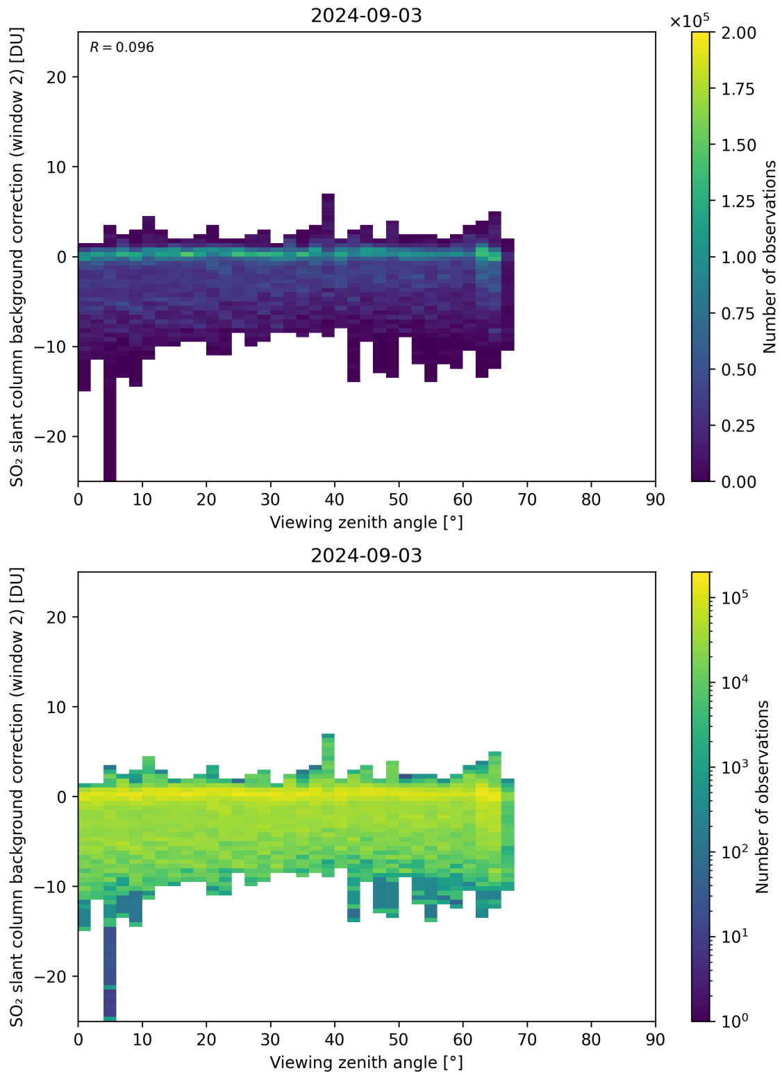
Figure 309: Scatter density plot of “Viewing zenith angle” against “SO 2 slant column background correction (window 2)” for 2024-09-02 to 2024-09-04.
