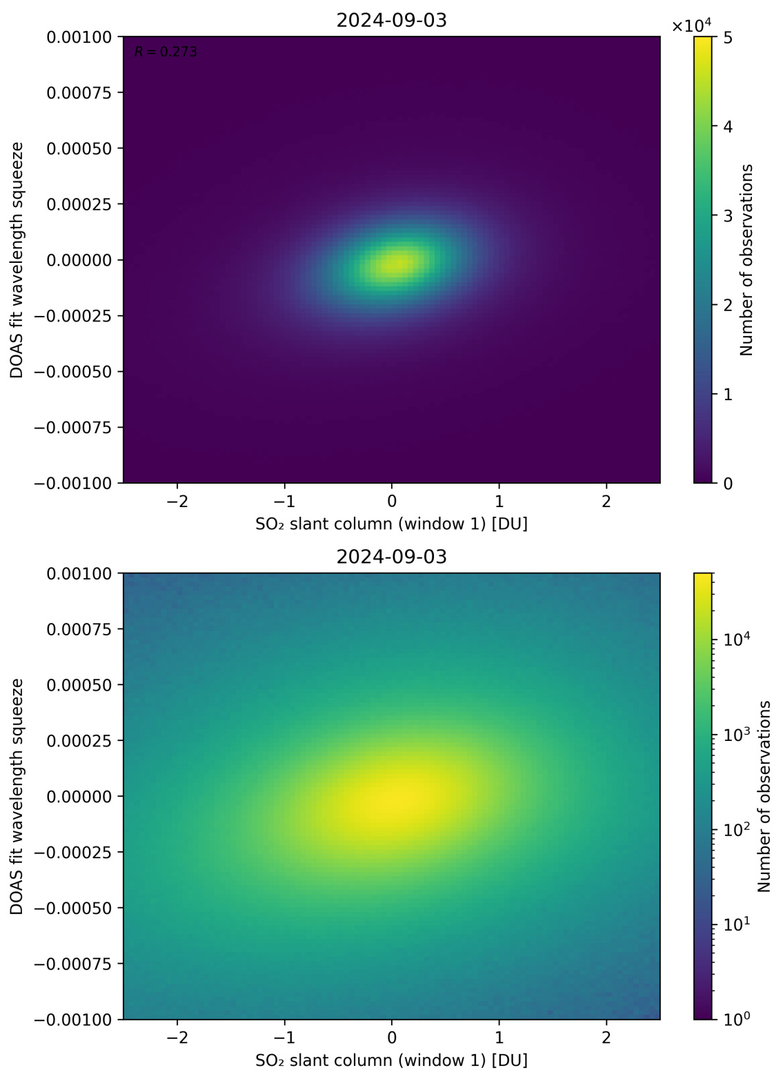
Figure 216: Scatter density plot of “SO 2 slant column (window 1)” against “DOAS fit wavelength squeeze” for 2024-09-02 to 2024-09-04.
