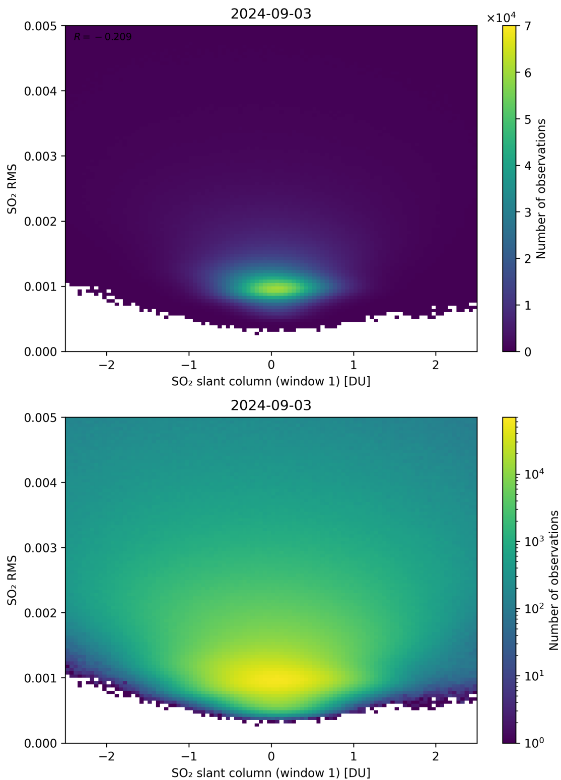
Figure 217: Scatter density plot of “SO 2 slant column (window 1)” against “SO 2 RMS” for 2024-09-02 to 2024-09-04.
