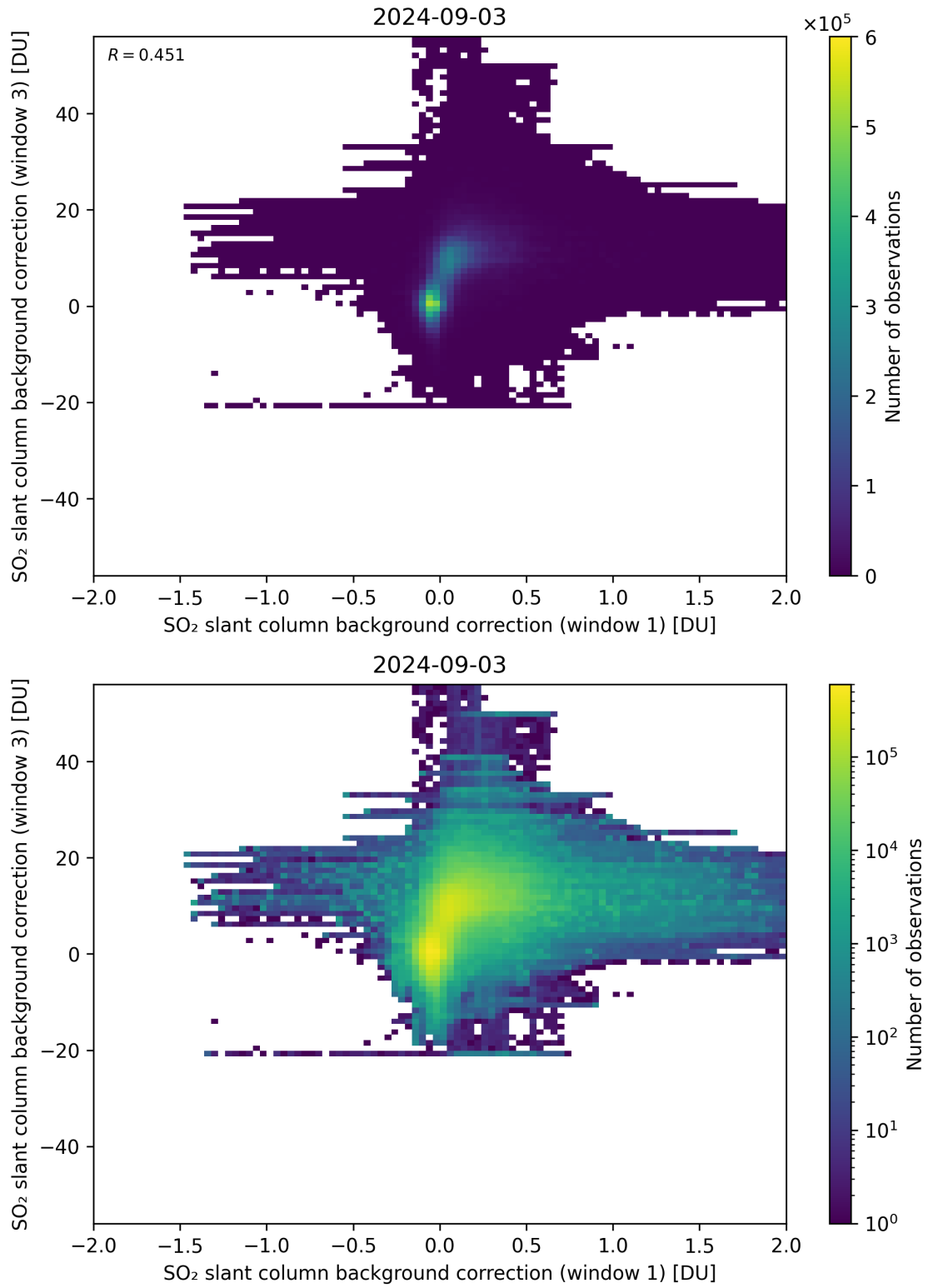
Figure 99: Scatter density plot of “SO 2 slant column background correction (window 1)” against “SO 2 slant column background correction (window 3)” for 2024-09-02 to 2024-09-04.
