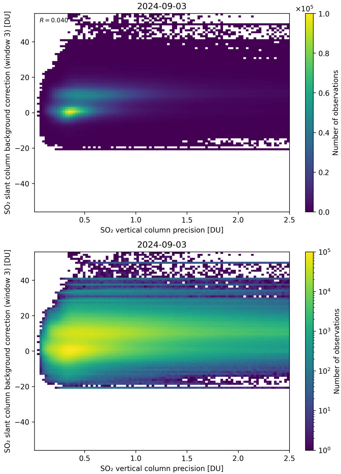
Figure 281: Scatter density plot of “SO 2 vertical column precision” against “SO 2 slant column background correction (window 3)” for 2024-09-02 to 2024-09-04.
