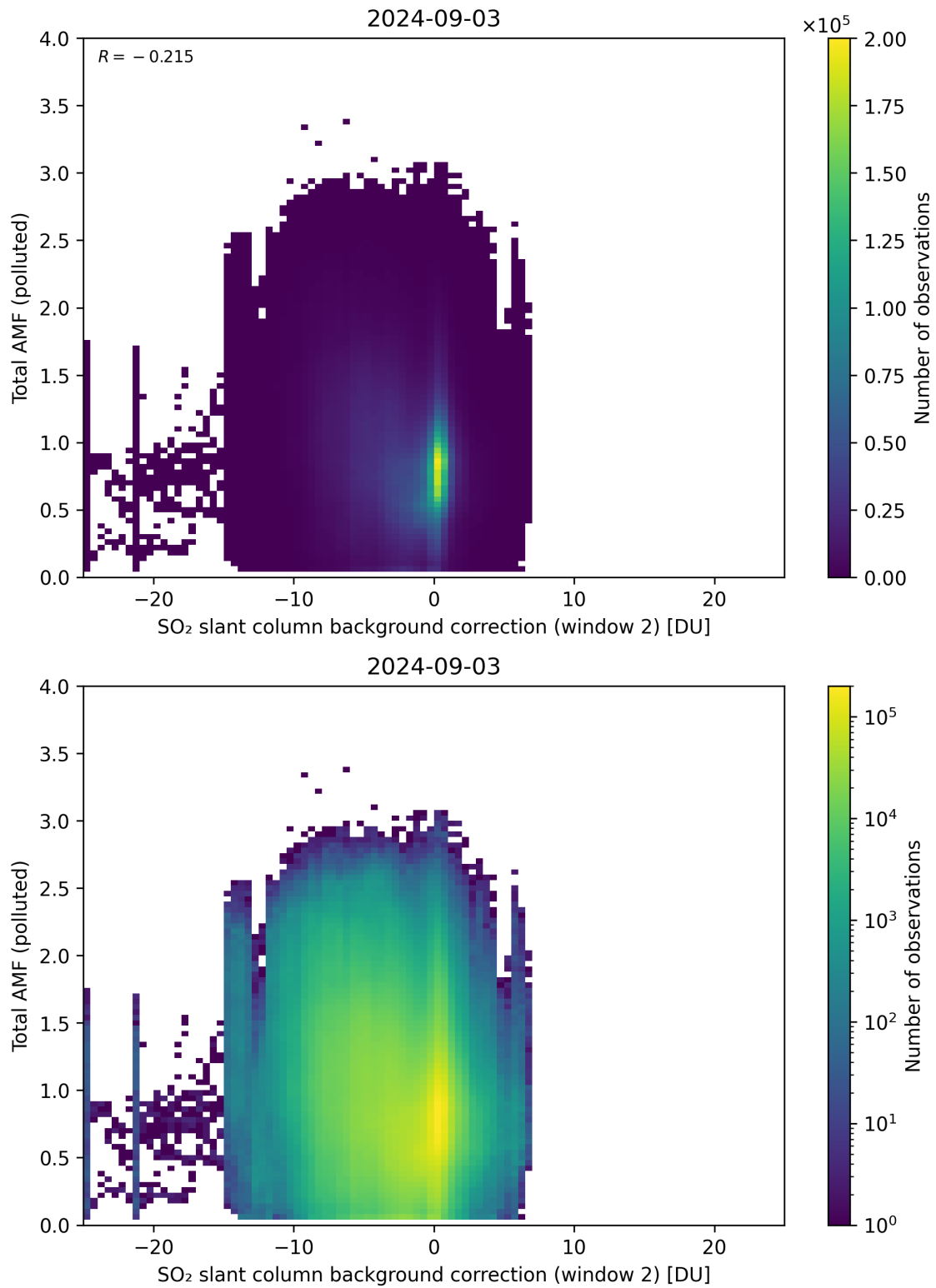
Figure 119: Scatter density plot of “SO 2 slant column background correction (window 2)” against “Total AMF (polluted)” for 2024-09-02 to 2024-09-04.
