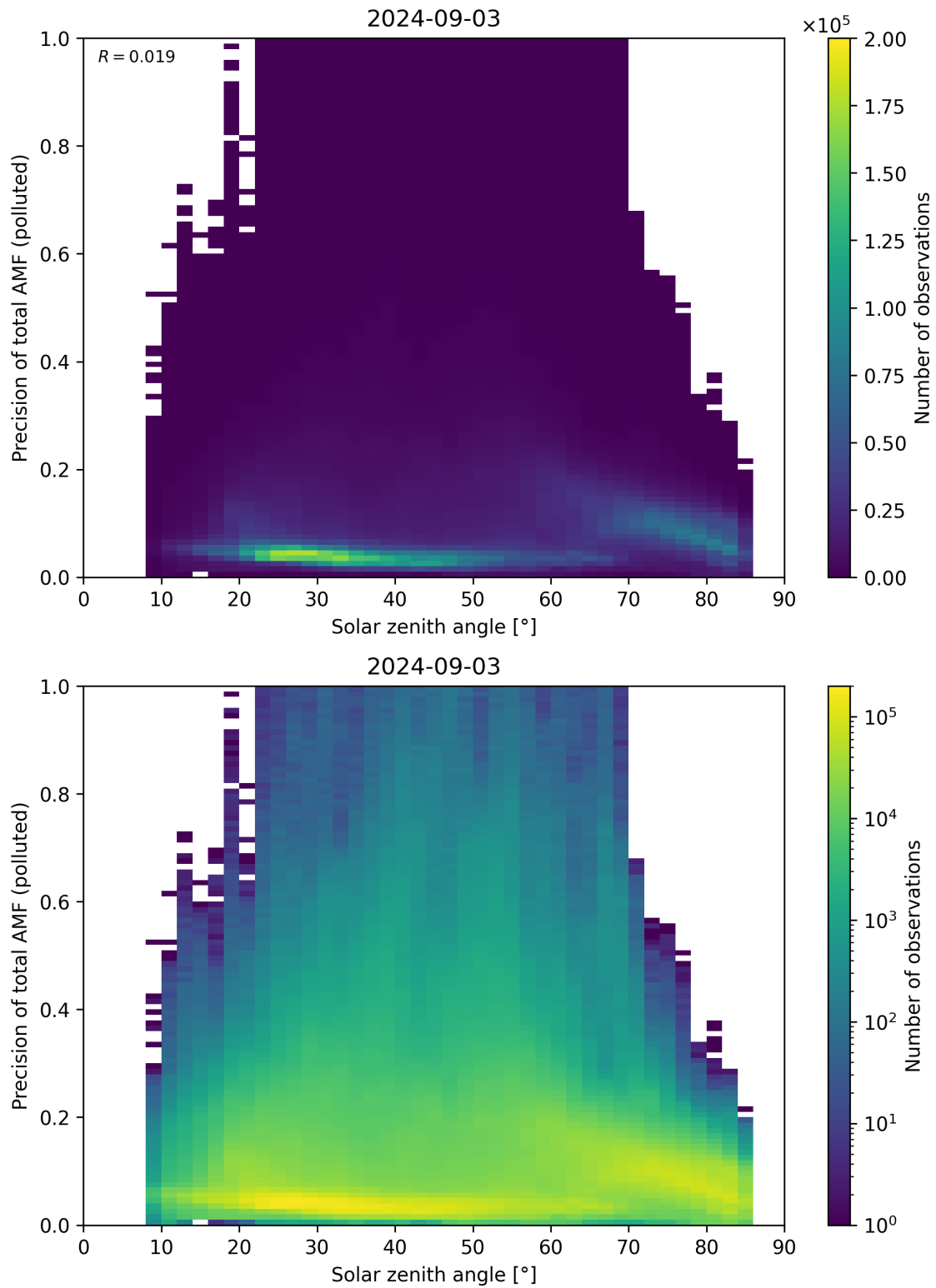
Figure 175: Scatter density plot of “Solar zenith angle” against “Precision of total AMF (polluted)” for 2024-09-02 to 2024-09-04.
