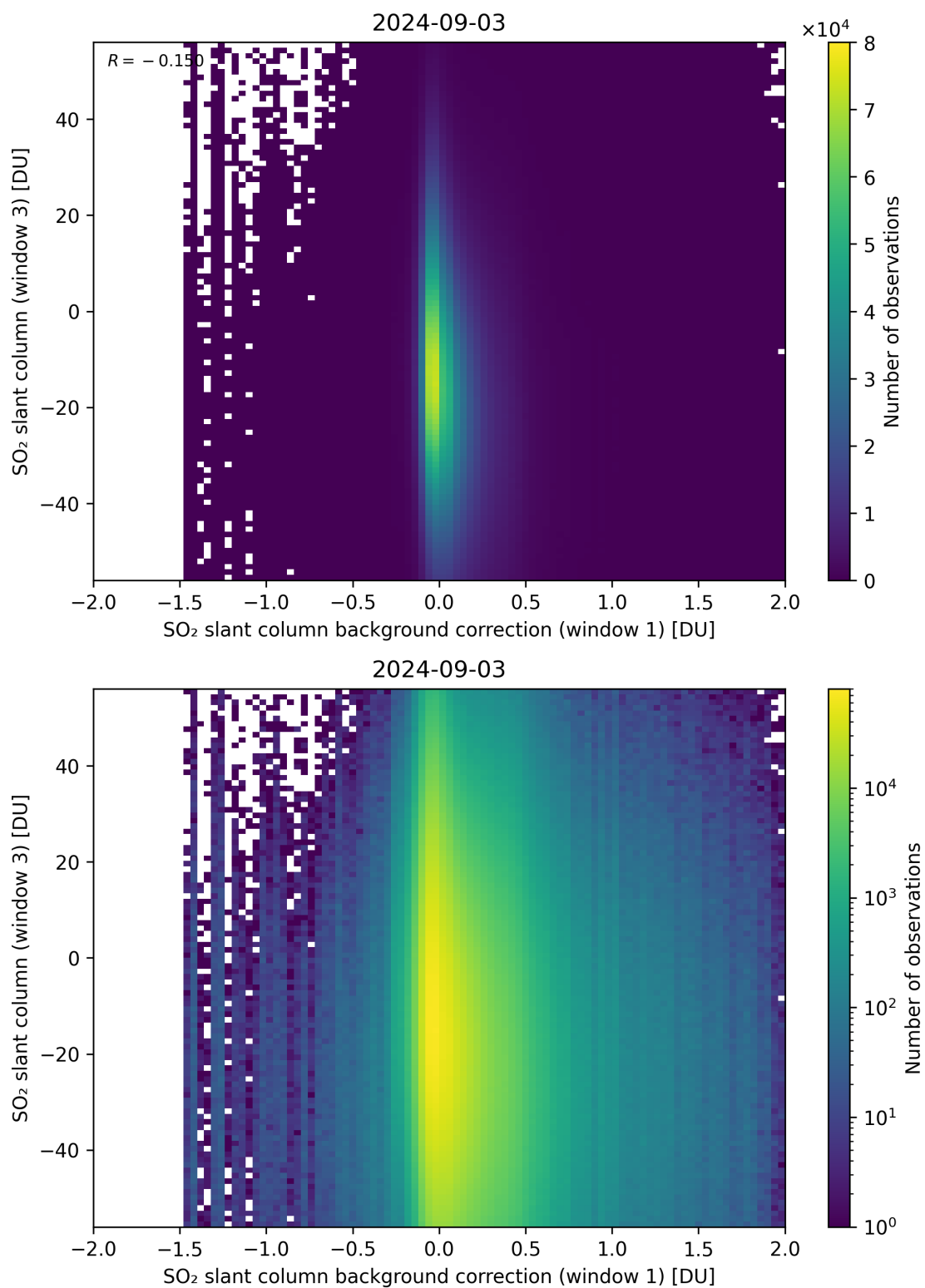
Figure 107: Scatter density plot of “SO 2 slant column background correction (window 1)” against “SO 2 slant column (window 3)” for 2024-09-02 to 2024-09-04.
