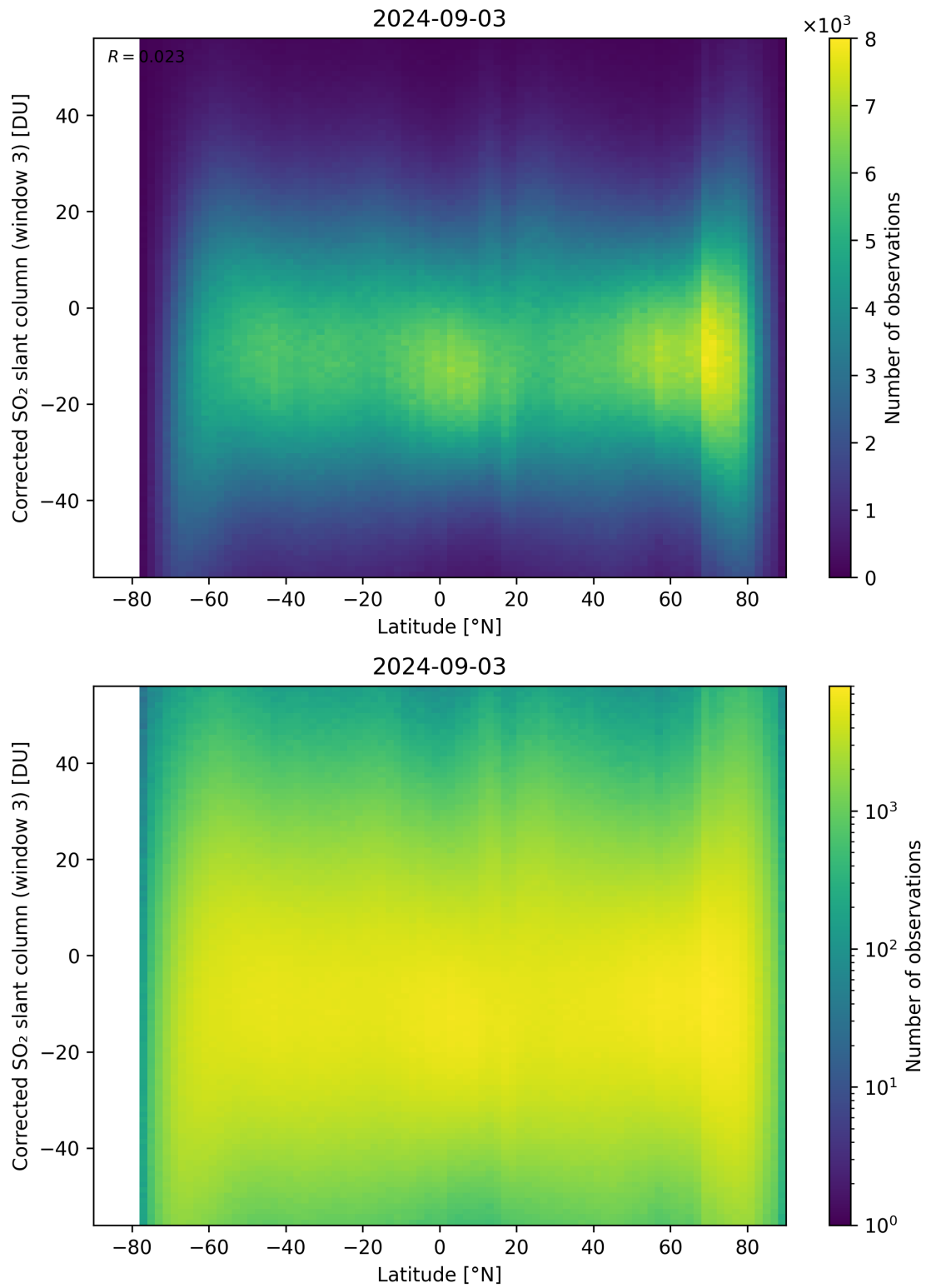
Figure 148: Scatter density plot of “Latitude” against “Corrected SO 2 slant column (window 3)” for 2024-09-02 to 2024-09-04.
