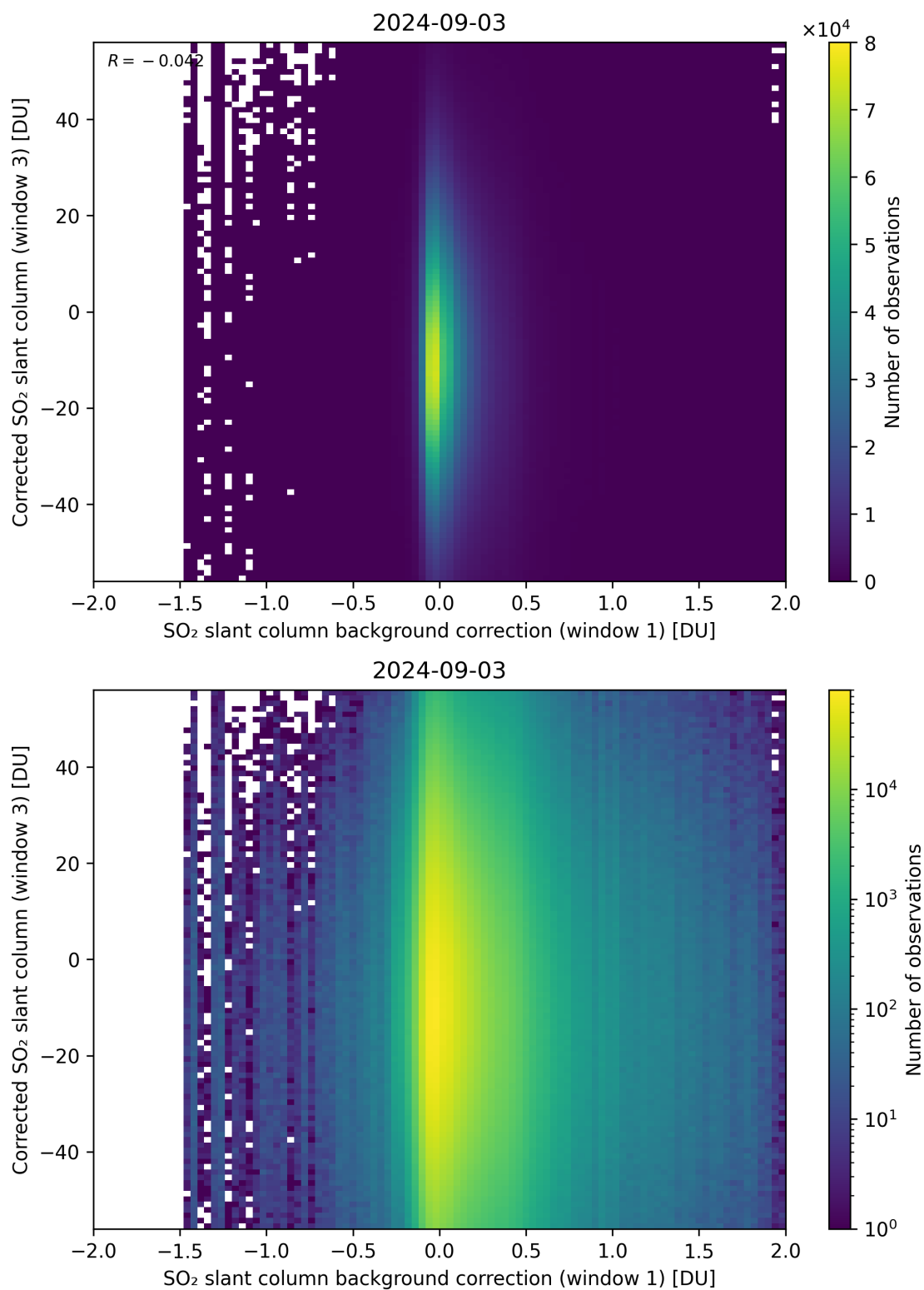
Figure 105: Scatter density plot of “SO 2 slant column background correction (window 1)” against “Corrected SO 2 slant column (window 3)” for 2024-09-02 to 2024-09-04.
