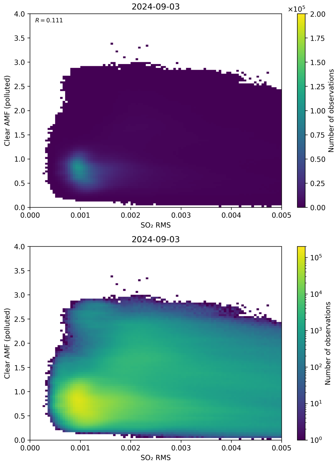
Figure 136: Scatter density plot of “SO 2 RMS” against “Clear AMF (polluted)” for 2024-09-02 to 2024-09-04.
