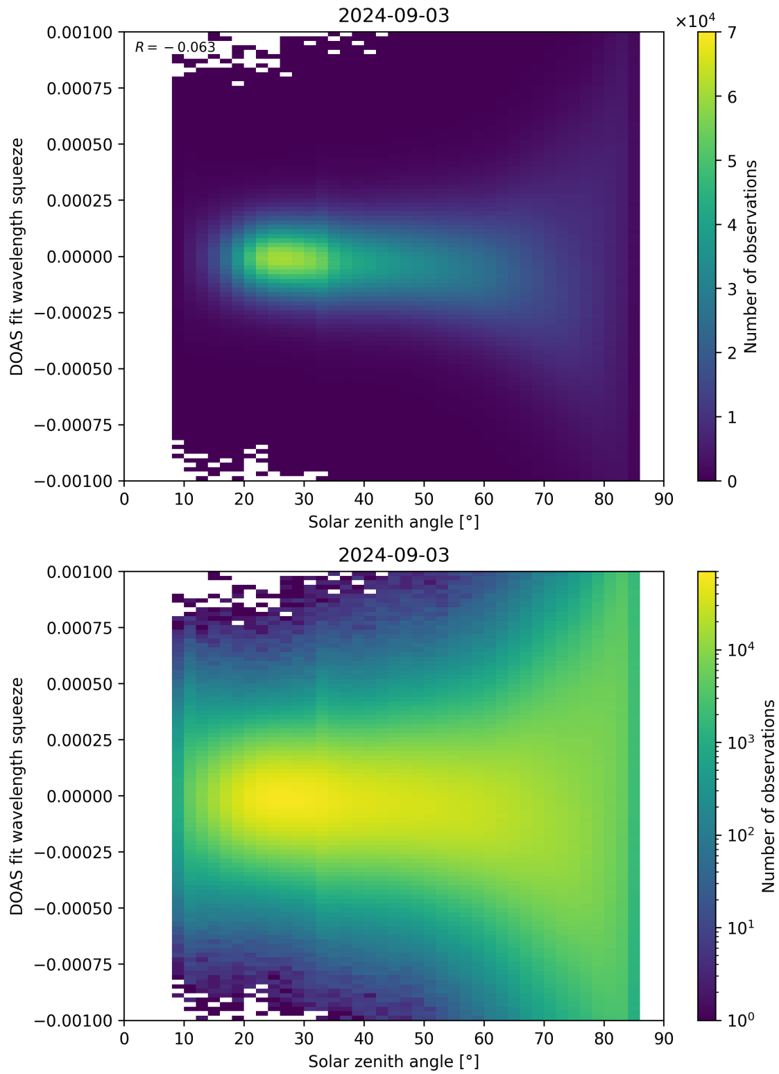
Figure 162: Scatter density plot of “Solar zenith angle” against “DOAS fit wavelength squeeze” for 2024-09-02 to 2024-09-04.
