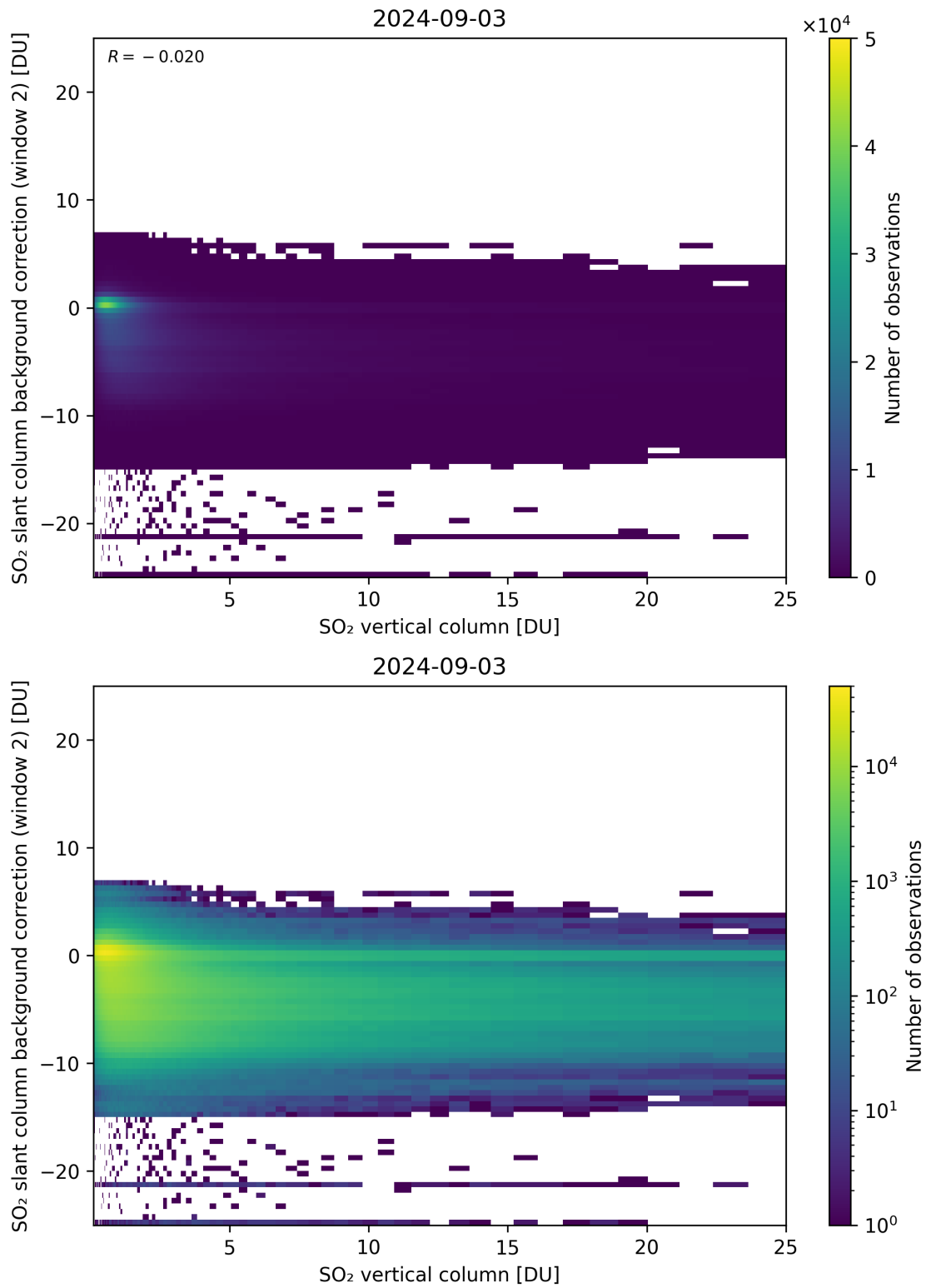
Figure 274: Scatter density plot of “SO 2 vertical column” against “SO 2 slant column background correction (window 2)” for 2024-09-02 to 2024-09-04.
