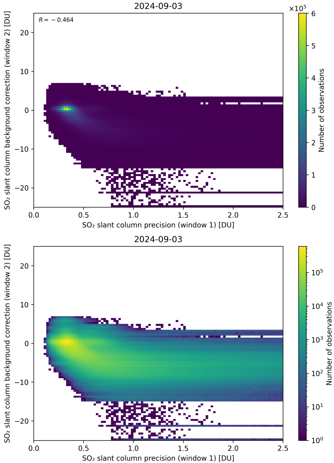
Figure 219: Scatter density plot of “SO 2 slant column precision (window 1)” against “SO 2 slant column background correction (window 2)” for 2024-09-02 to 2024-09-04.
