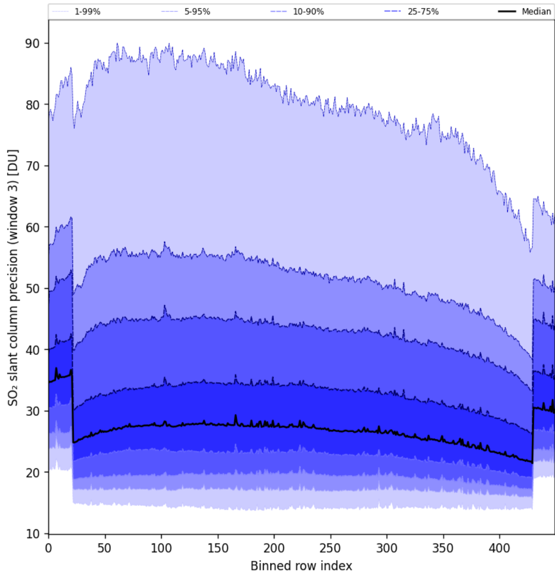
Figure 88: Along track statistics of “SO 2 slant column precision (window 3)” for 2024-09-02 to 2024-09-04
