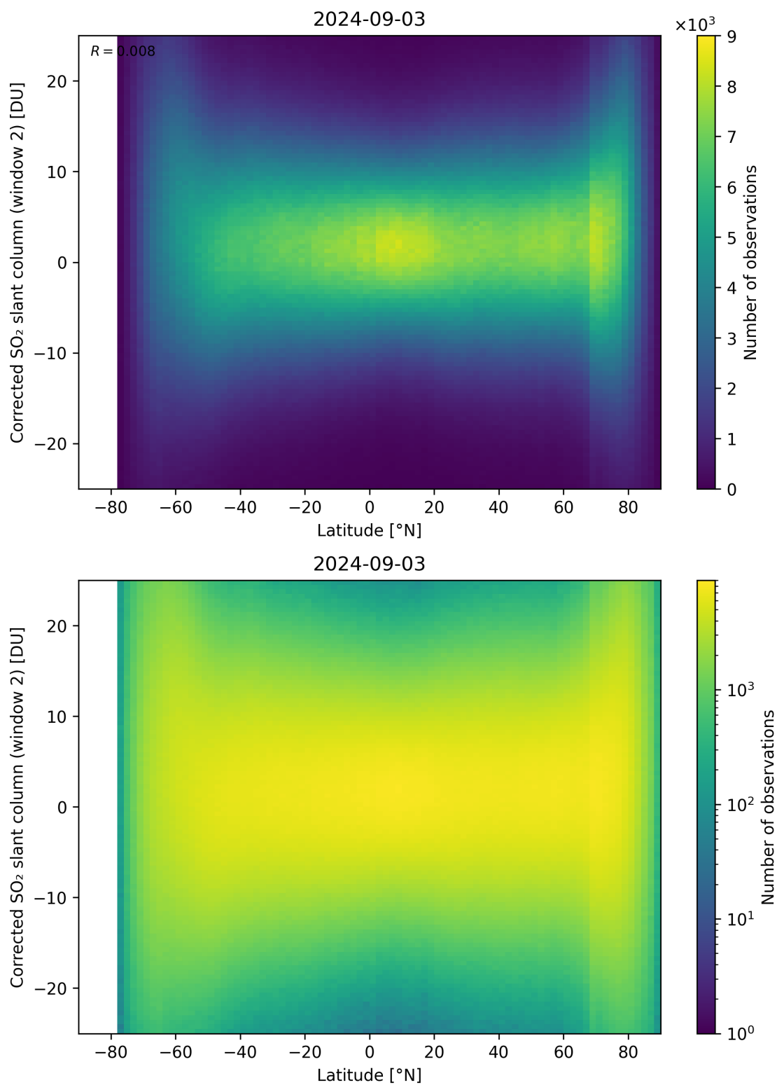
Figure 147: Scatter density plot of “Latitude” against “Corrected SO 2 slant column (window 2)” for 2024-09-02 to 2024-09-04.
