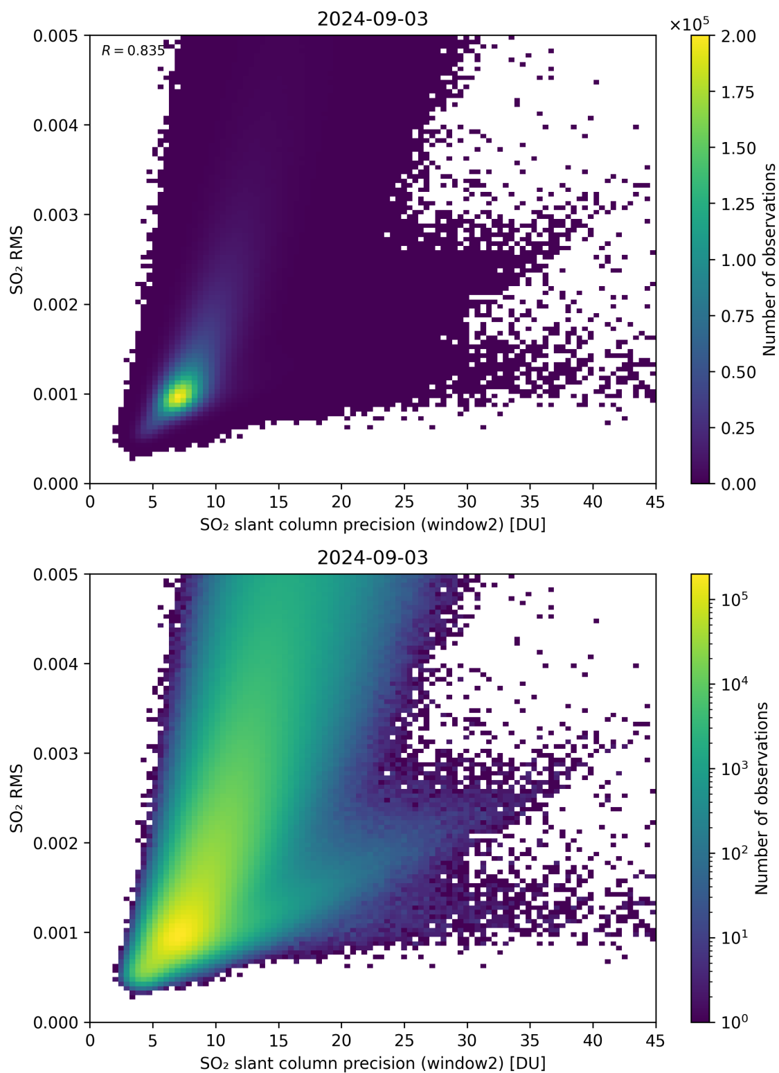
Figure 245: Scatter density plot of “SO 2 slant column precision (window2)” against “SO 2 RMS” for 2024-09-02 to 2024-09-04.
