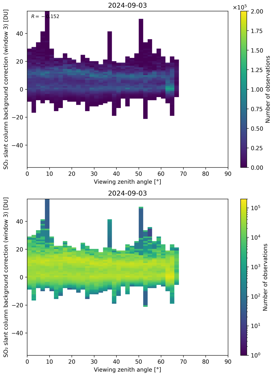
Figure 310: Scatter density plot of “Viewing zenith angle” against “SO 2 slant column background correction (window 3)” for 2024-09-02 to 2024-09-04.
