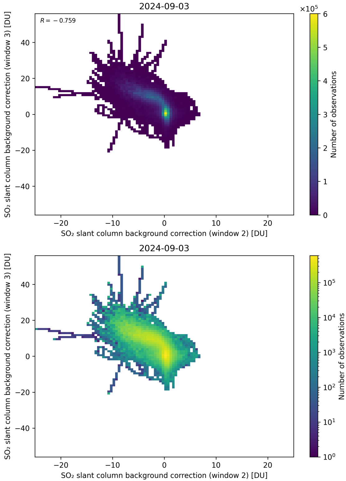
Figure 111: Scatter density plot of “SO 2 slant column background correction (window 2)” against “SO 2 slant column background correction (window 3)” for 2024-09-02 to 2024-09-04.
