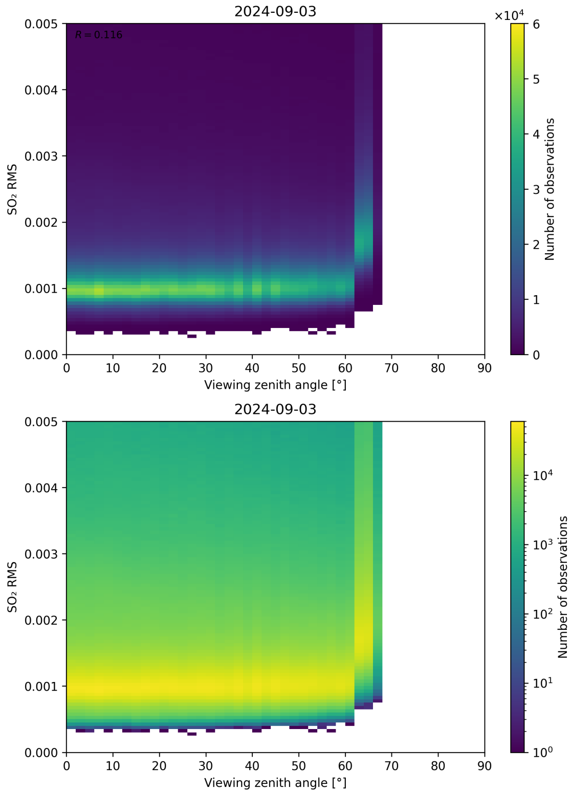
Figure 313: Scatter density plot of “Viewing zenith angle” against “SO 2 RMS” for 2024-09-02 to 2024-09-04.
