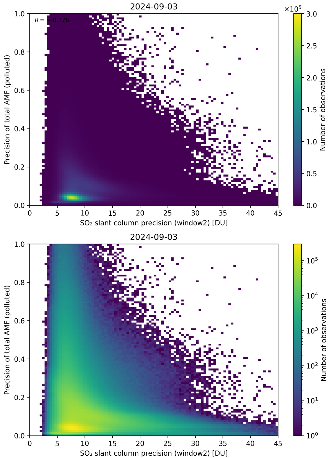
Figure 252: Scatter density plot of “SO 2 slant column precision (window2)” against “Precision of total AMF (polluted)” for 2024-09-02 to 2024-09-04.
