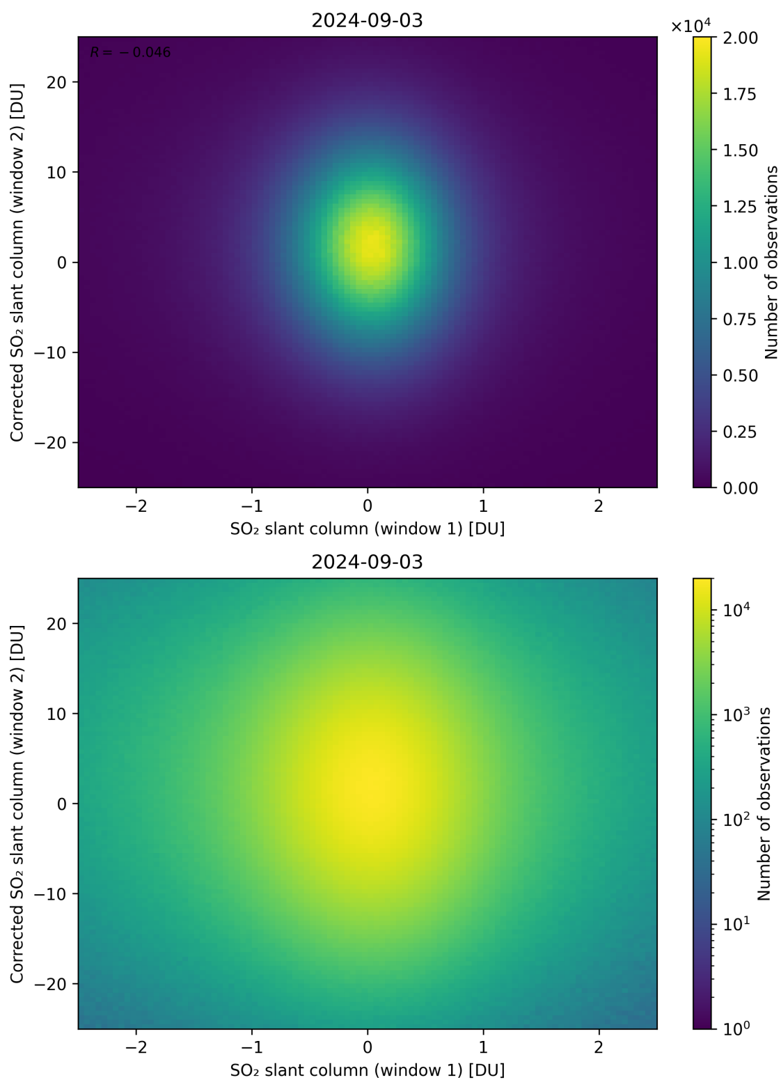
Figure 233: Scatter density plot of “SO 2 slant column (window 1)” against “Corrected SO 2 slant column (window 2)” for 2024-09-02 to 2024-09-04.
