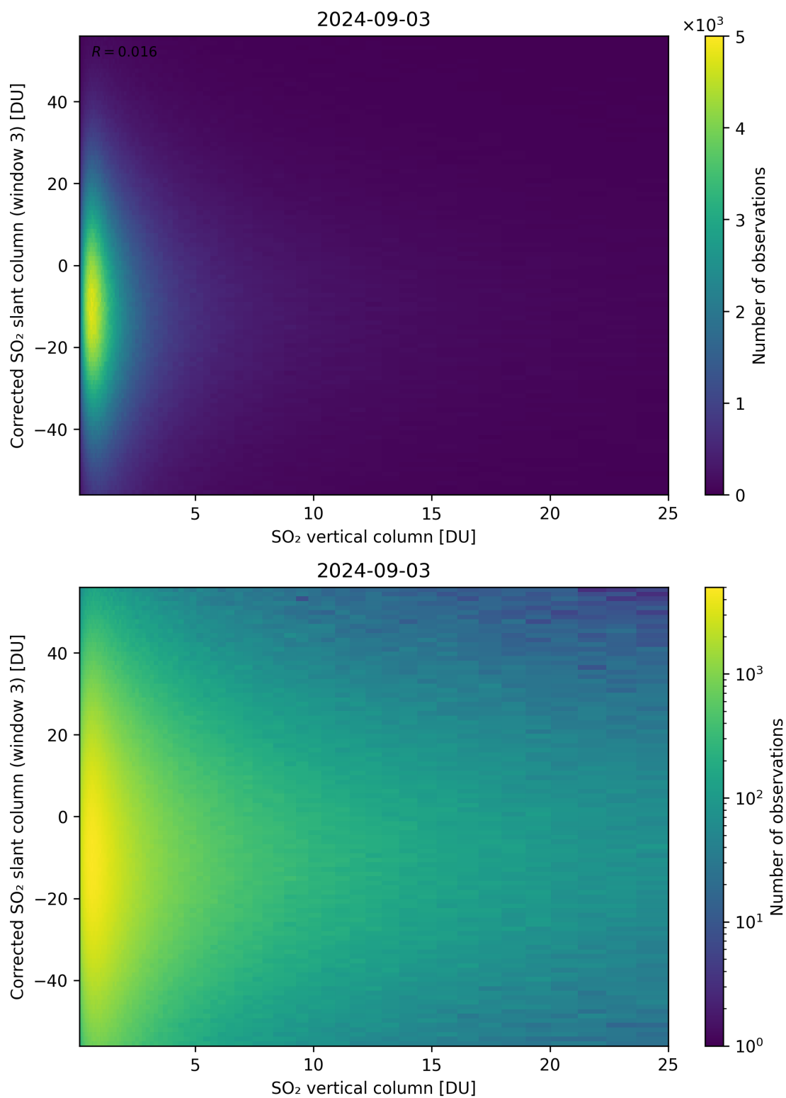
Figure 299: Scatter density plot of “SO 2 vertical column” against “Corrected SO 2 slant column (window 3)” for 2024-09-02 to 2024-09-04.
