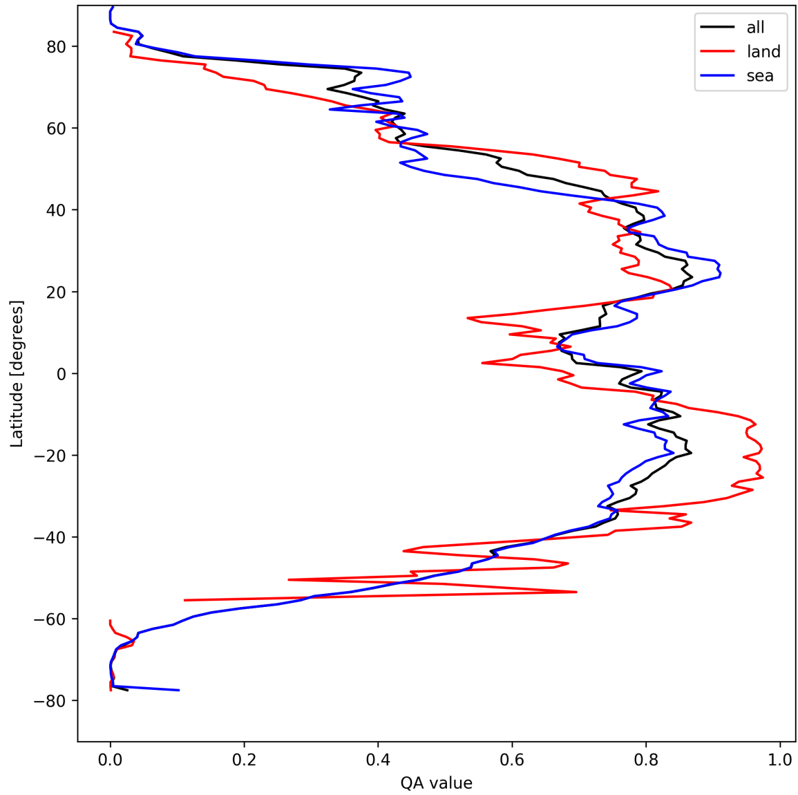
Figure 29: Zonal average of “QA value” for 2024-09-02 to 2024-09-04.
