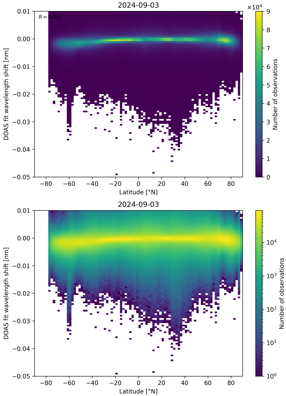
Figure 142: Scatter density plot of “Latitude” against “DOAS fit wavelength shift” for 2024-09-02 to 2024-09-04.
