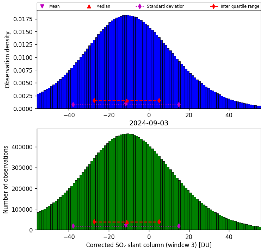
Figure 66: Histogram of "Corrected SO 2 slant column (window 3)" for 2024-09-02 to 2024-09-04
