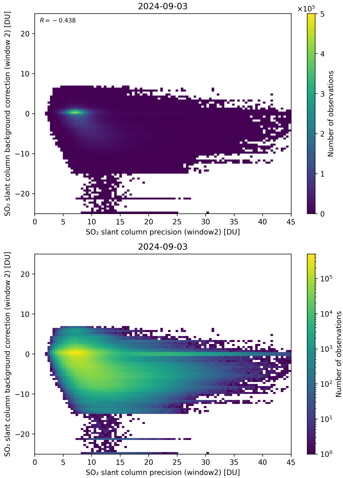
Figure 241: Scatter density plot of “SO 2 slant column precision (window2)” against “SO 2 slant column background correction (window 2)” for 2024-09-02 to 2024-09-04.
