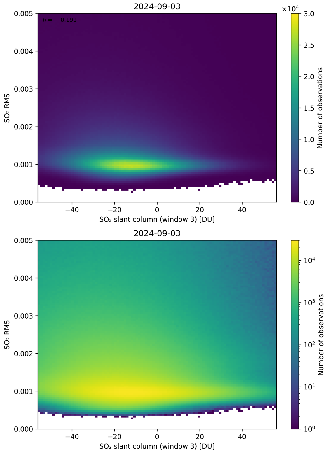
Figure 256: Scatter density plot of “SO 2 slant column (window 3)” against “SO 2 RMS” for 2024-09-02 to 2024-09-04.
