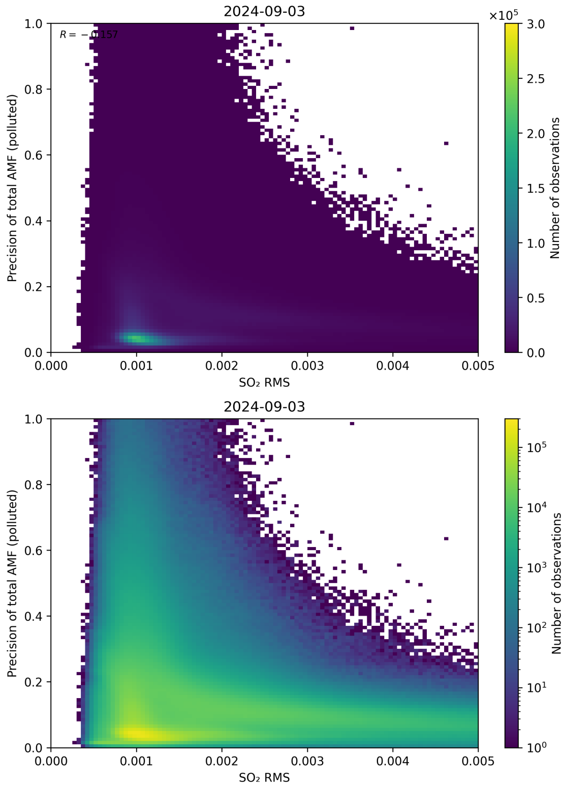
Figure 138: Scatter density plot of “SO 2 RMS” against “Precision of total AMF (polluted)” for 2024-09-02 to 2024-09-04.
