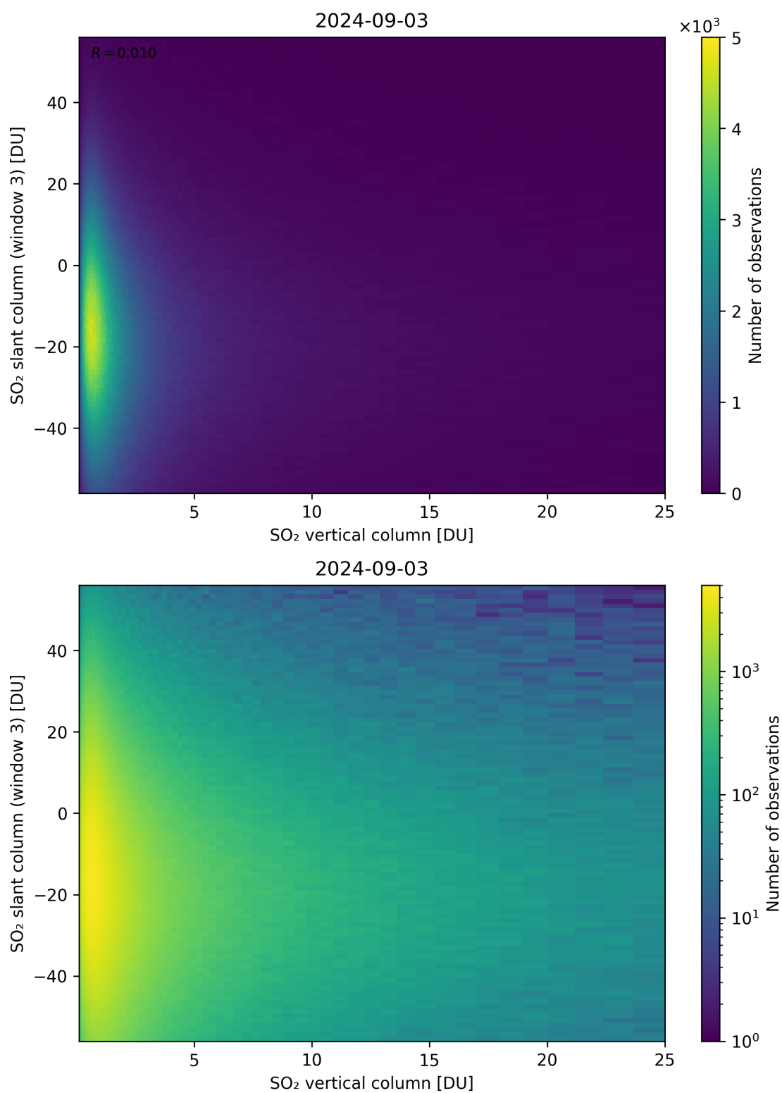
Figure 303: Scatter density plot of “SO 2 vertical column” against “SO 2 slant column (window 3)” for 2024-09-02 to 2024-09-04.
