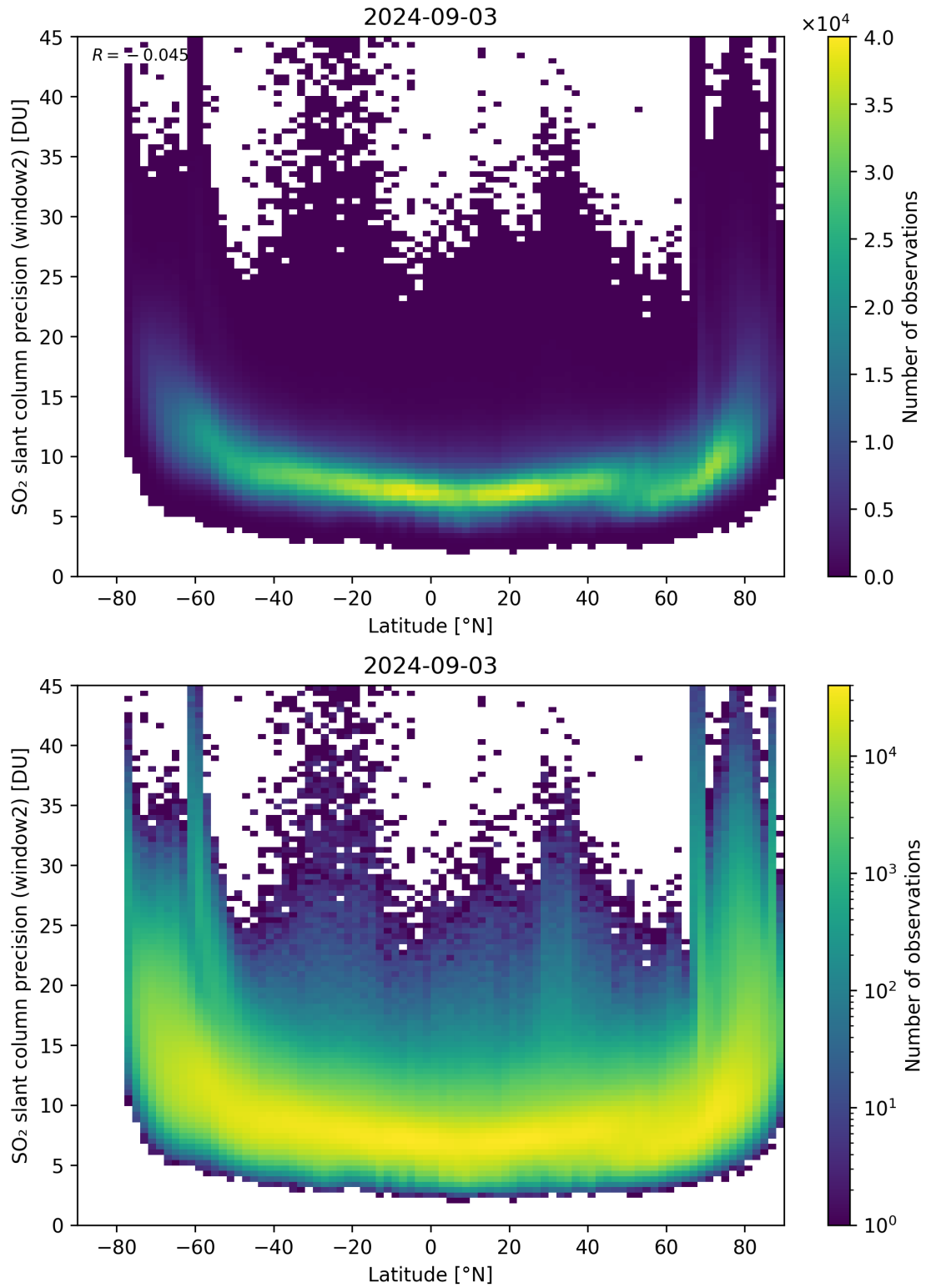
Figure 151: Scatter density plot of “Latitude” against “SO 2 slant column precision (window2)” for 2024-09-02 to 2024-09-04.
