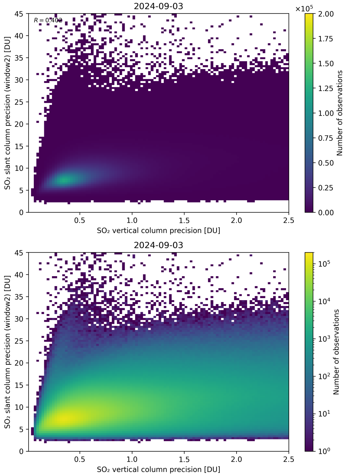
Figure 291: Scatter density plot of “SO 2 vertical column precision” against “SO 2 slant column precision (window2)” for 2024-09-02 to 2024-09-04.
