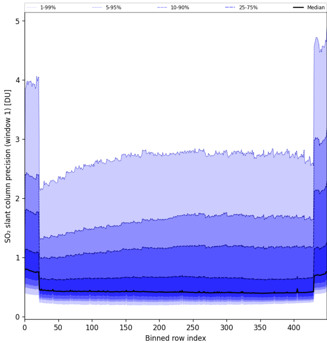
Figure 80: Along track statistics of “SO 2 slant column precision (window 1)” for 2024-09-02 to 2024-09-04
