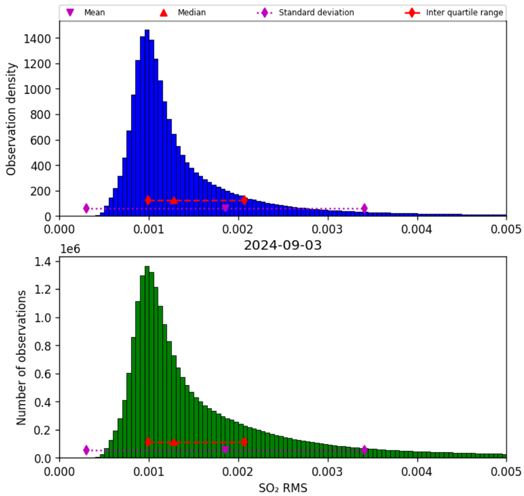
Figure 70: Histogram of “SO 2 RMS” for 2024-09-02 to 2024-09-04
