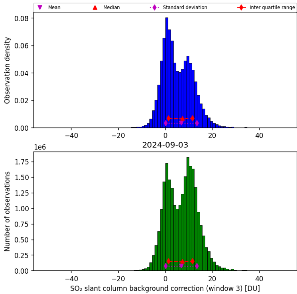
Figure 67: Histogram of “SO 2 slant column background correction (window 3)” for 2024-09-02 to 2024-09-04
