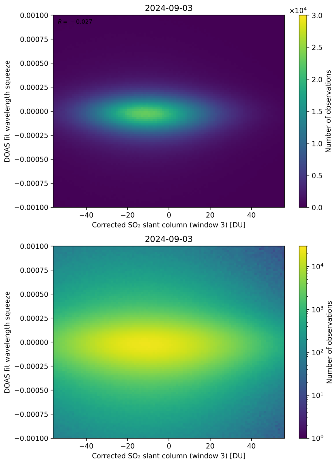
Figure 207: Scatter density plot of “Corrected SO 2 slant column (window 3)” against “DOAS fit wavelength squeeze” for 2024-09-02 to 2024-09-04.
