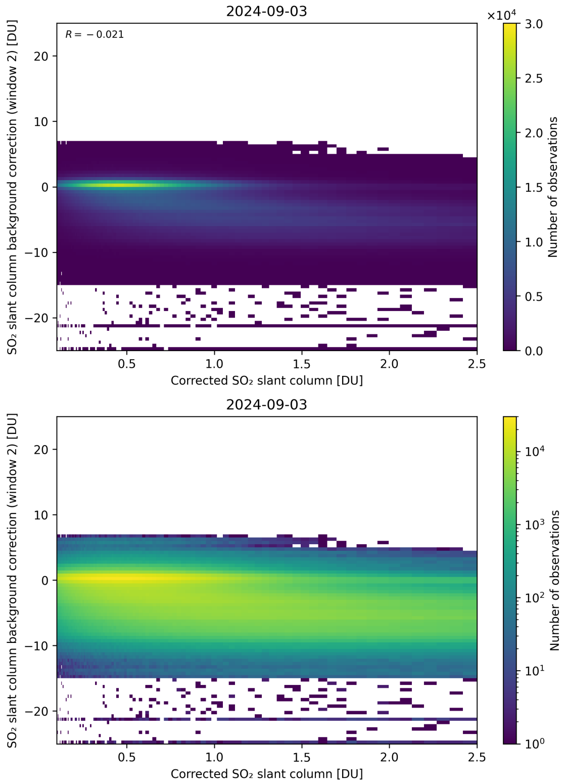
Figure 179: Scatter density plot of “Corrected SO 2 slant column” against “SO 2 slant column background correction (window 2)” for 2024-09-02 to 2024-09-04.
