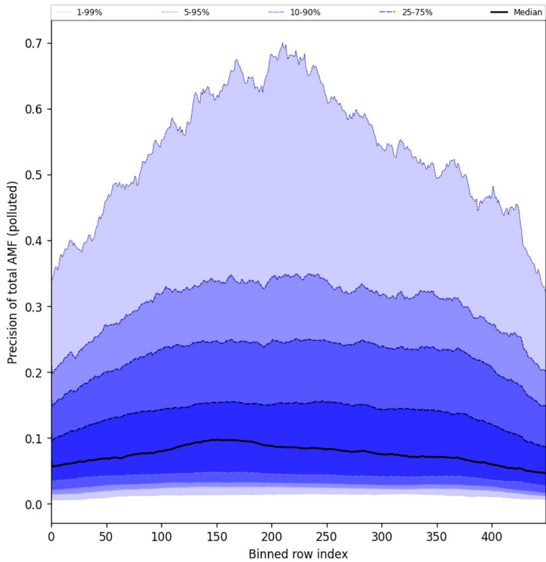
Figure 95: Along track statistics of “Precision of total AMF (polluted)” for 2024-09-02 to 2024-09-04
