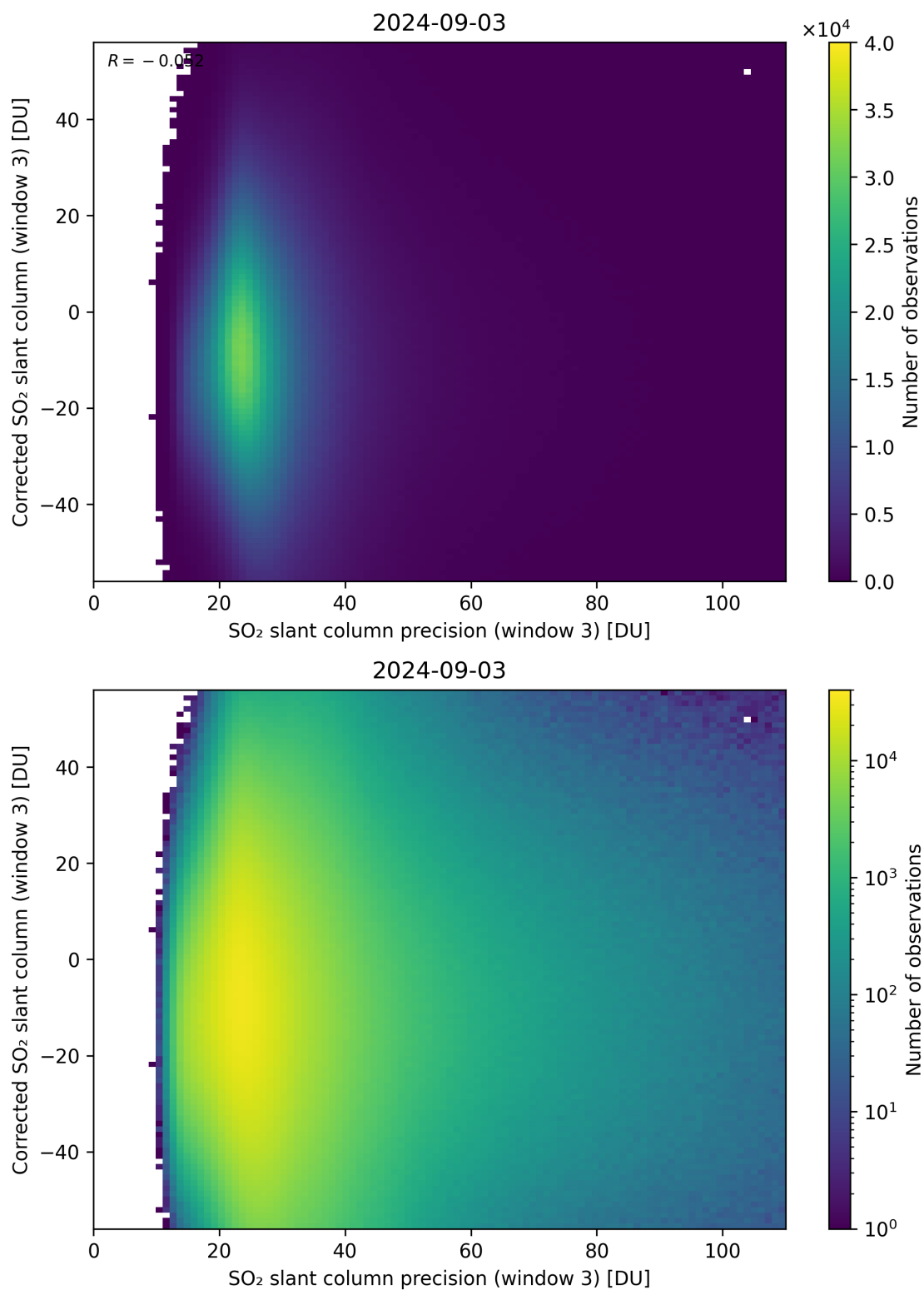
Figure 262: Scatter density plot of “SO 2 slant column precision (window 3)” against “Corrected SO 2 slant column (window 3)” for 2024-09-02 to 2024-09-04.
