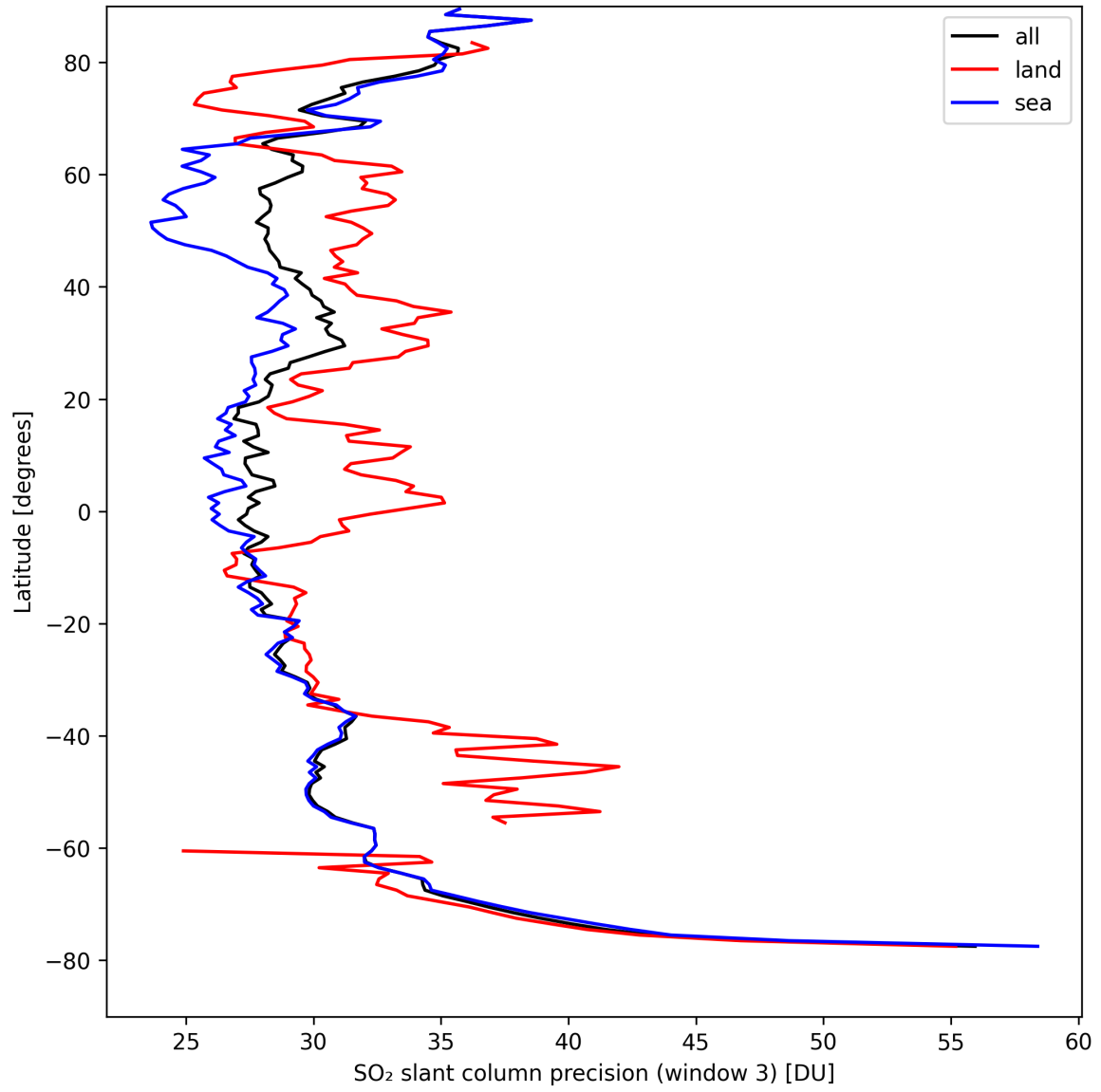
Figure 42: Zonal average of “SO 2 slant column precision (window 3)” for 2024-09-02 to 2024-09-04.
