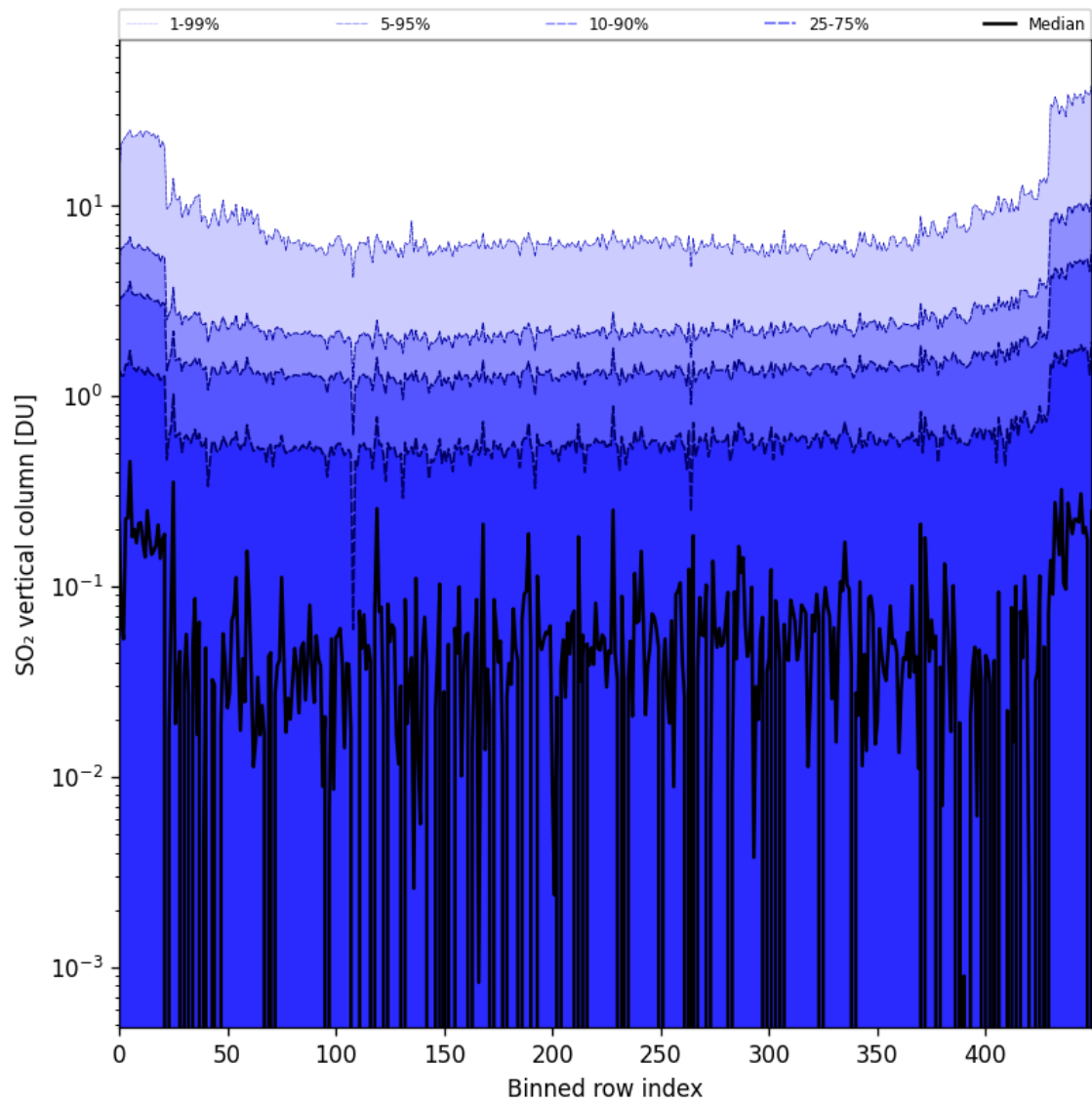
Figure 76: Along track statistics of “SO 2 vertical column” for 2024-09-02 to 2024-09-04
