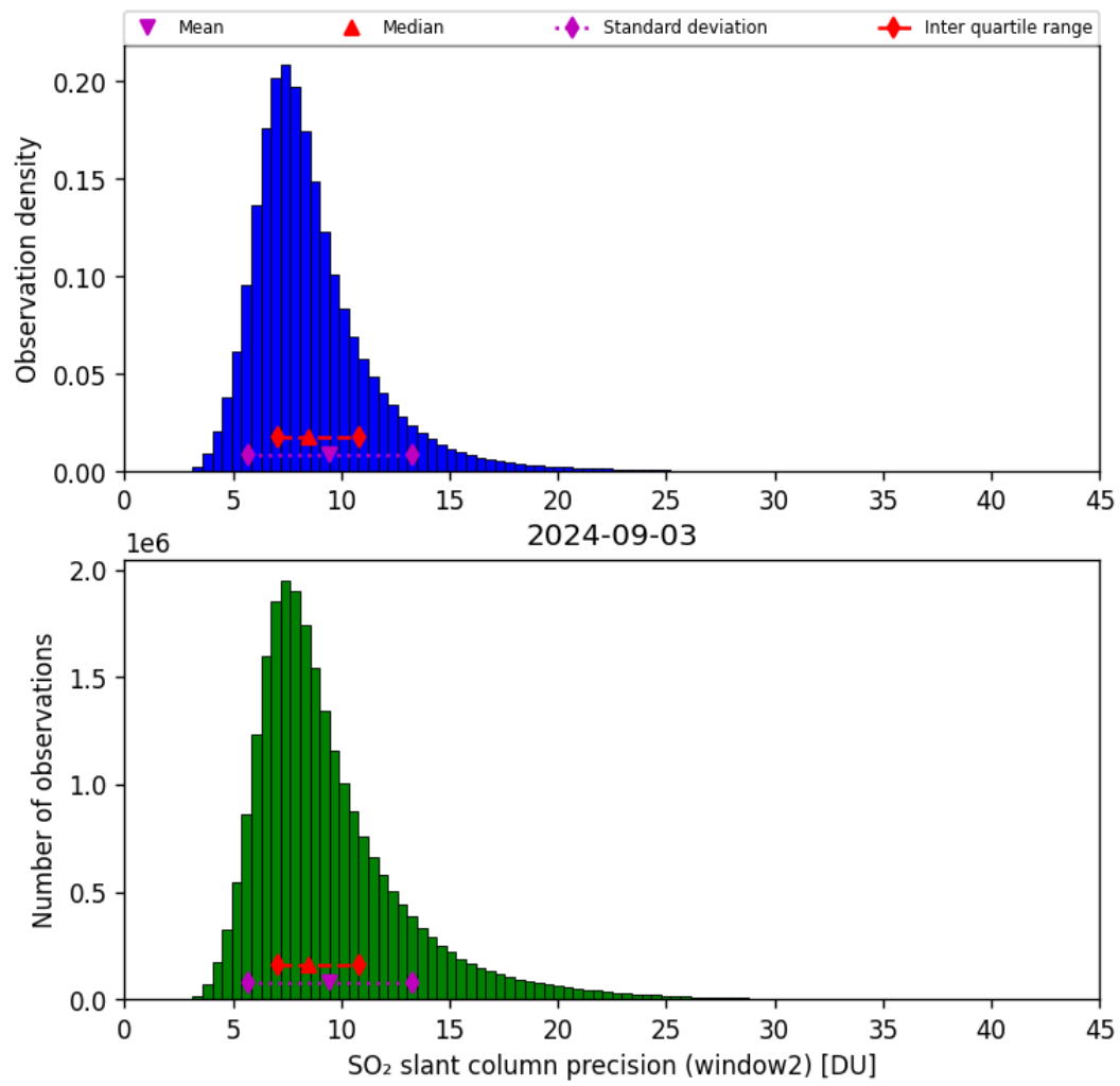
Figure 61: Histogram of “SO 2 slant column precision (window2)” for 2024-09-02 to 2024-09-04
