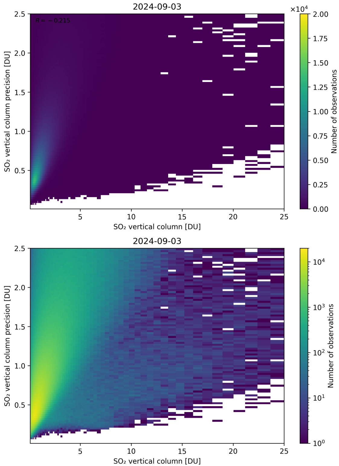
Figure 307: Scatter density plot of “SO 2 vertical column” against “SO 2 vertical column precision” for 2024-09-02 to 2024-09-04.
