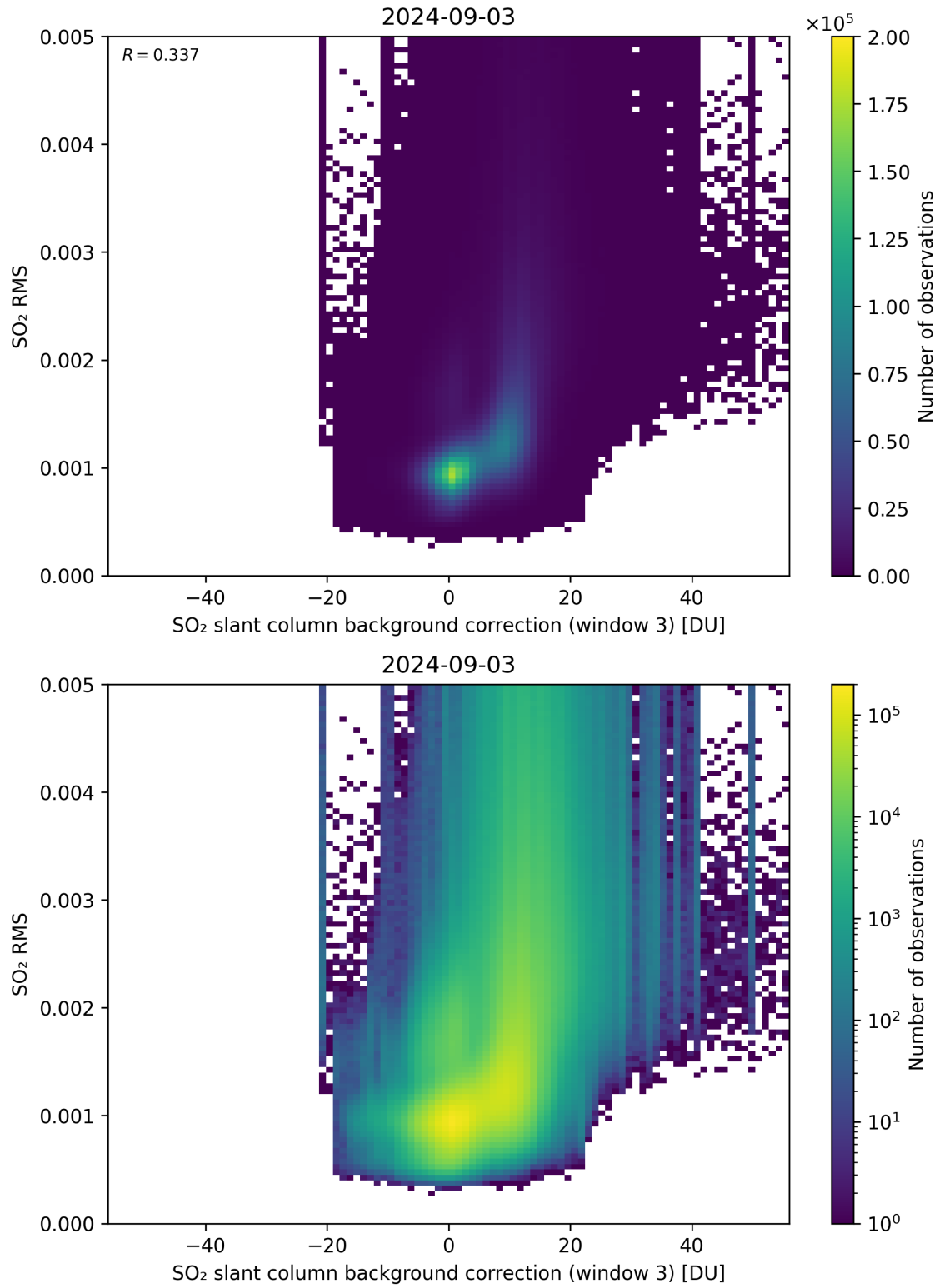
Figure 123: Scatter density plot of “SO 2 slant column background correction (window 3)” against “SO 2 RMS” for 2024-09-02 to 2024-09-04.
