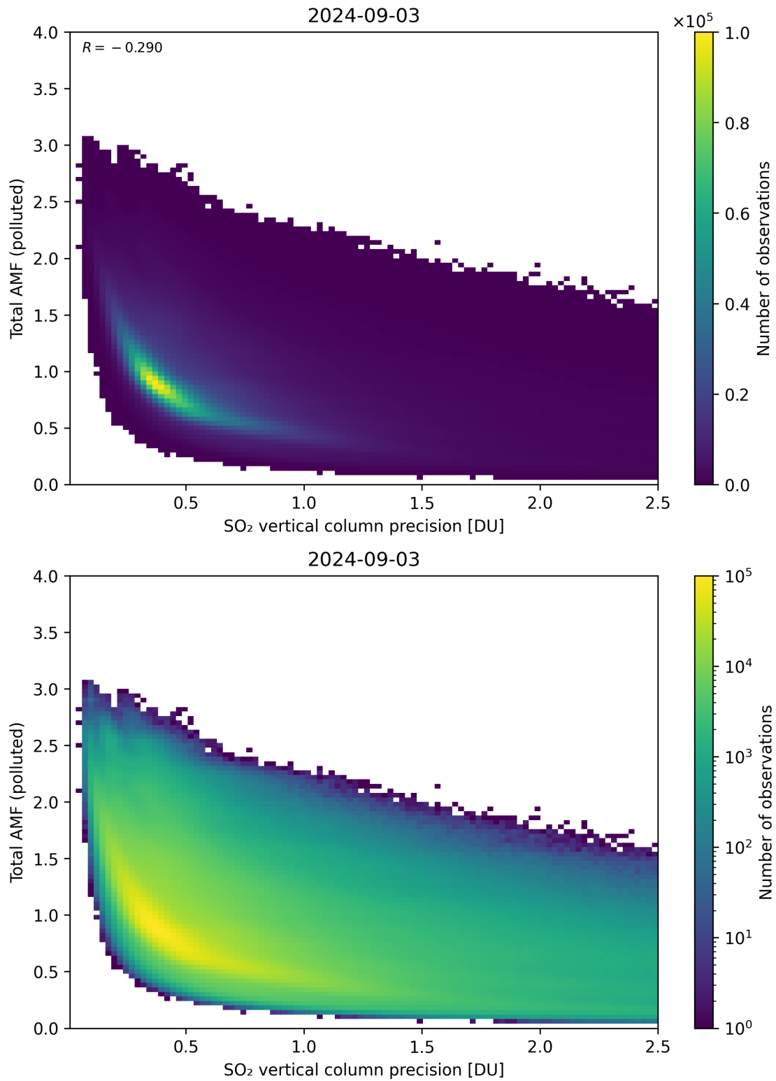
Figure 294: Scatter density plot of “SO 2 vertical column precision” against “Total AMF (polluted)” for 2024-09-02 to 2024-09-04.
