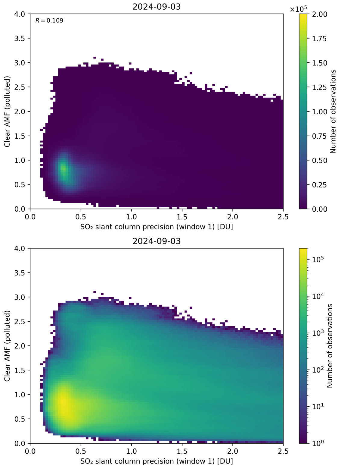
Figure 224: Scatter density plot of “SO 2 slant column precision (window 1)” against “Clear AMF (polluted)” for 2024-09-02 to 2024-09-04.
