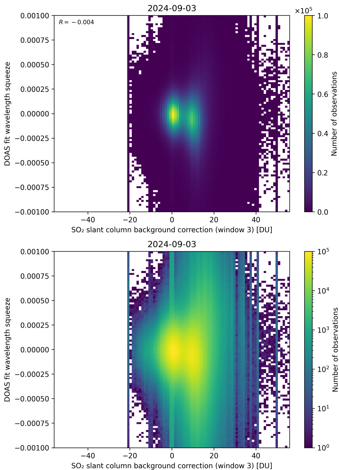
Figure 122: Scatter density plot of “SO 2 slant column background correction (window 3)” against “DOAS fit wavelength squeeze” for 2024-09-02 to 2024-09-04.
