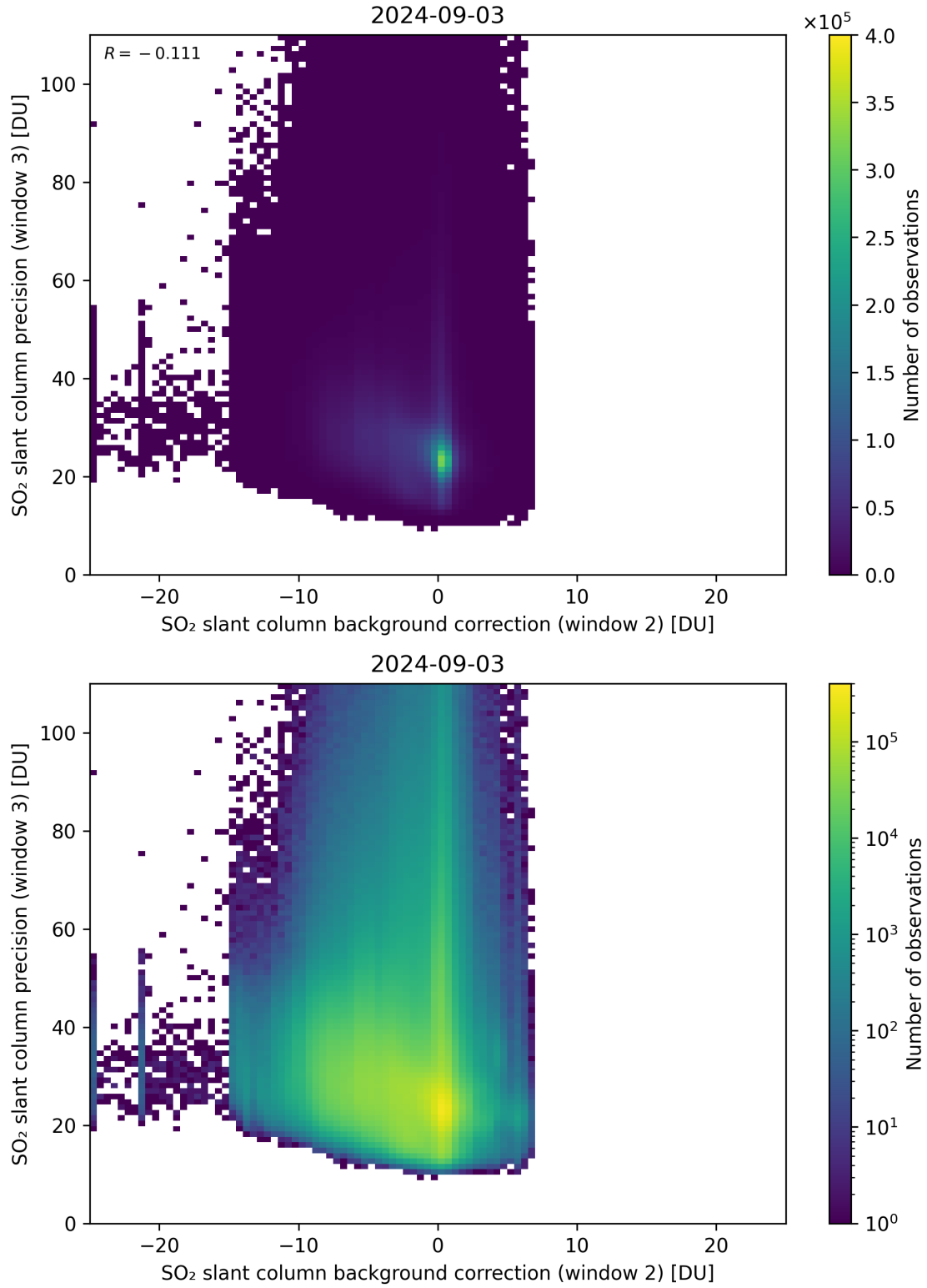
Figure 118: Scatter density plot of “SO 2 slant column background correction (window 2)” against “SO 2 slant column precision (window 3)” for 2024-09-02 to 2024-09-04.
