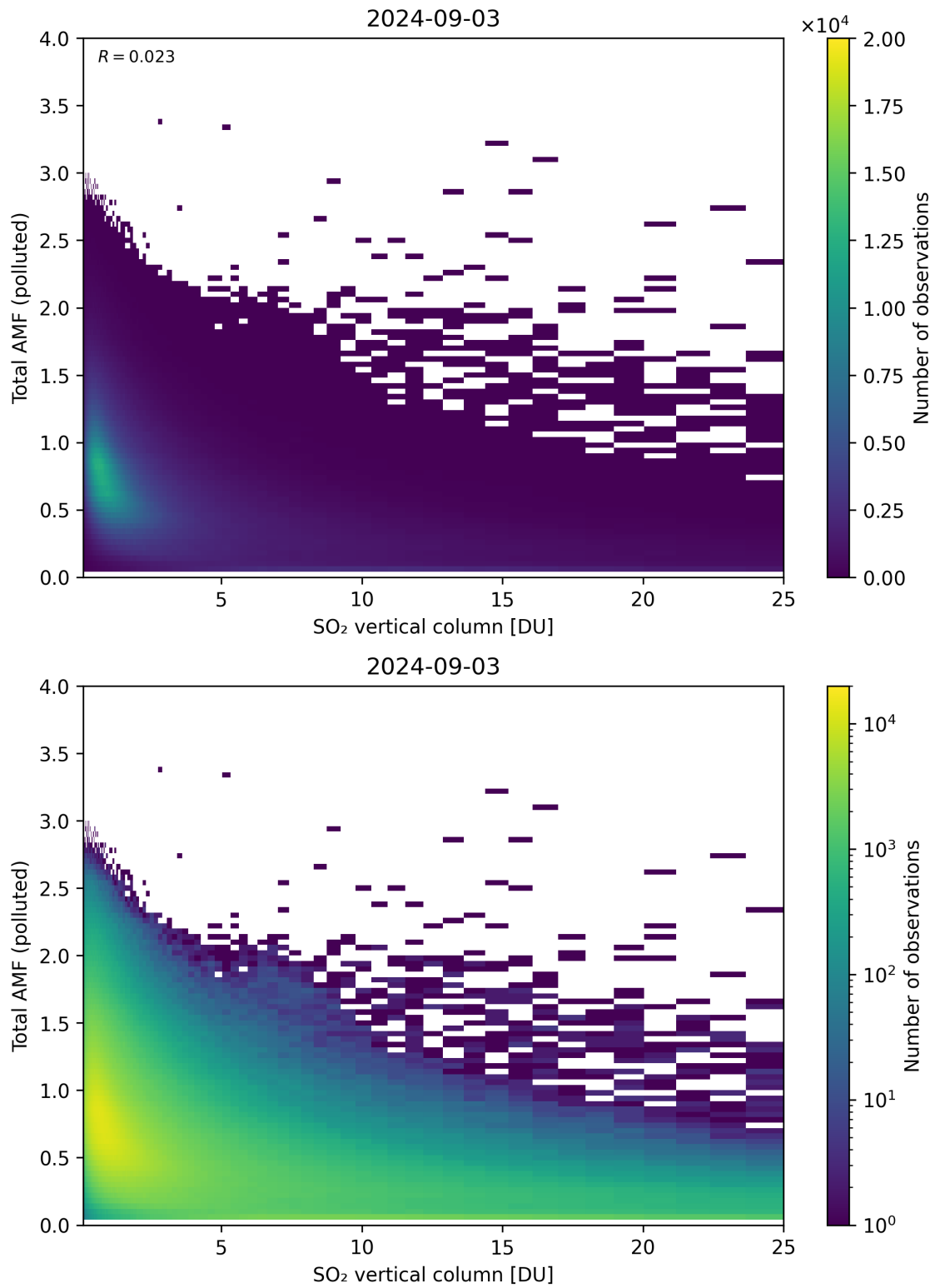
Figure 305: Scatter density plot of “SO 2 vertical column” against “Total AMF (polluted)” for 2024-09-02 to 2024-09-04.
