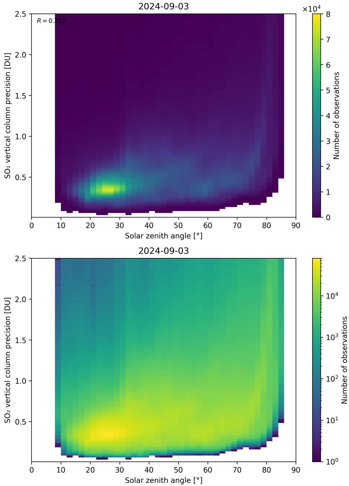
Figure 177: Scatter density plot of “Solar zenith angle” against “SO 2 vertical column precision” for 2024-09-02 to 2024-09-04.
