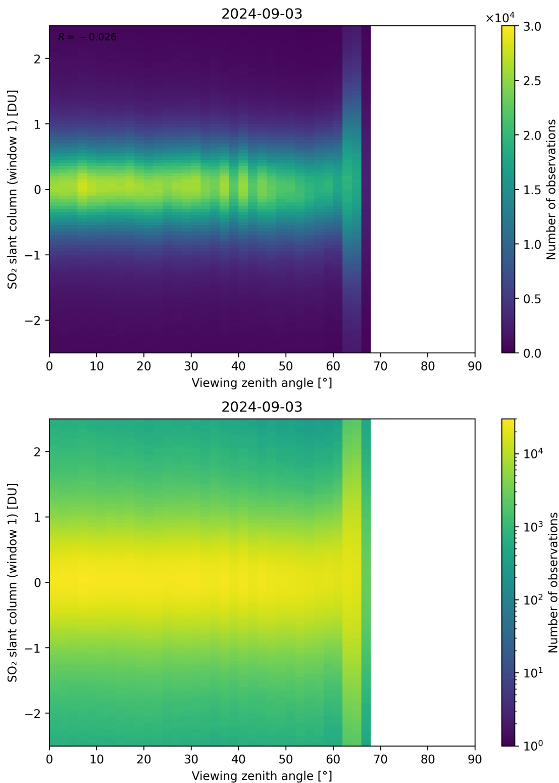
Figure 320: Scatter density plot of “Viewing zenith angle” against “SO 2 slant column (window 1)” for 2024-09-02 to 2024-09-04.
