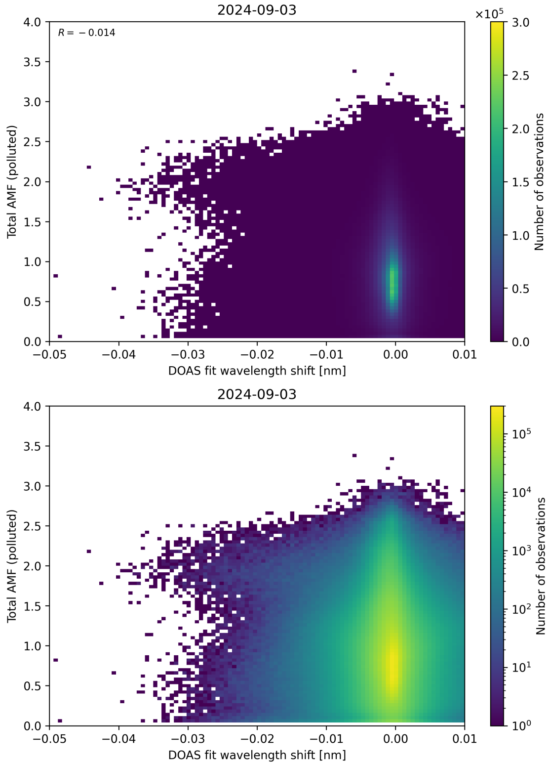
Figure 130: Scatter density plot of “DOAS fit wavelength shift” against “Total AMF (polluted)” for 2024-09-02 to 2024-09-04.
