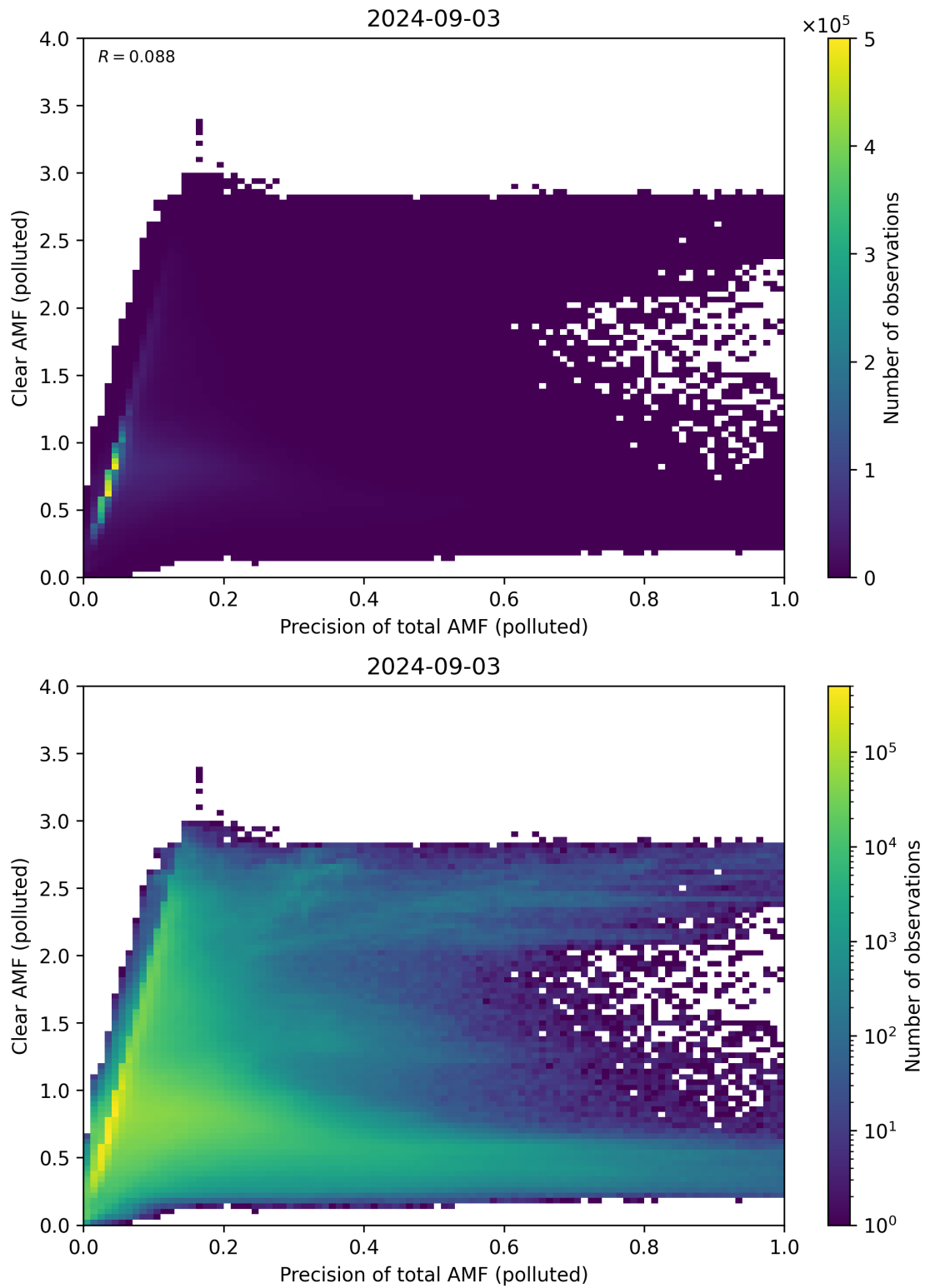
Figure 270: Scatter density plot of “Precision of total AMF (polluted)” against “Clear AMF (polluted)” for 2024-09-02 to 2024-09-04.
