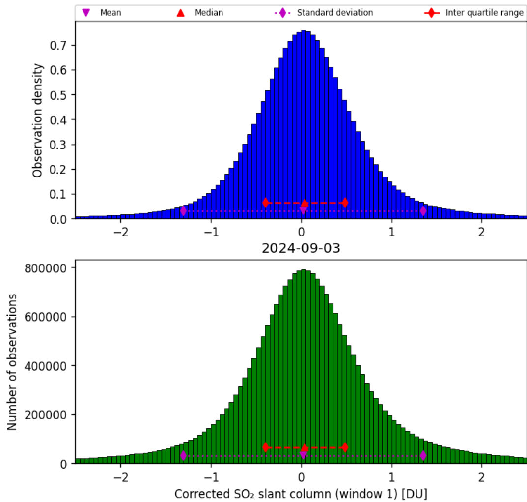
Figure 58: Histogram of “Corrected SO 2 slant column (window 1)” for 2024-09-02 to 2024-09-04
