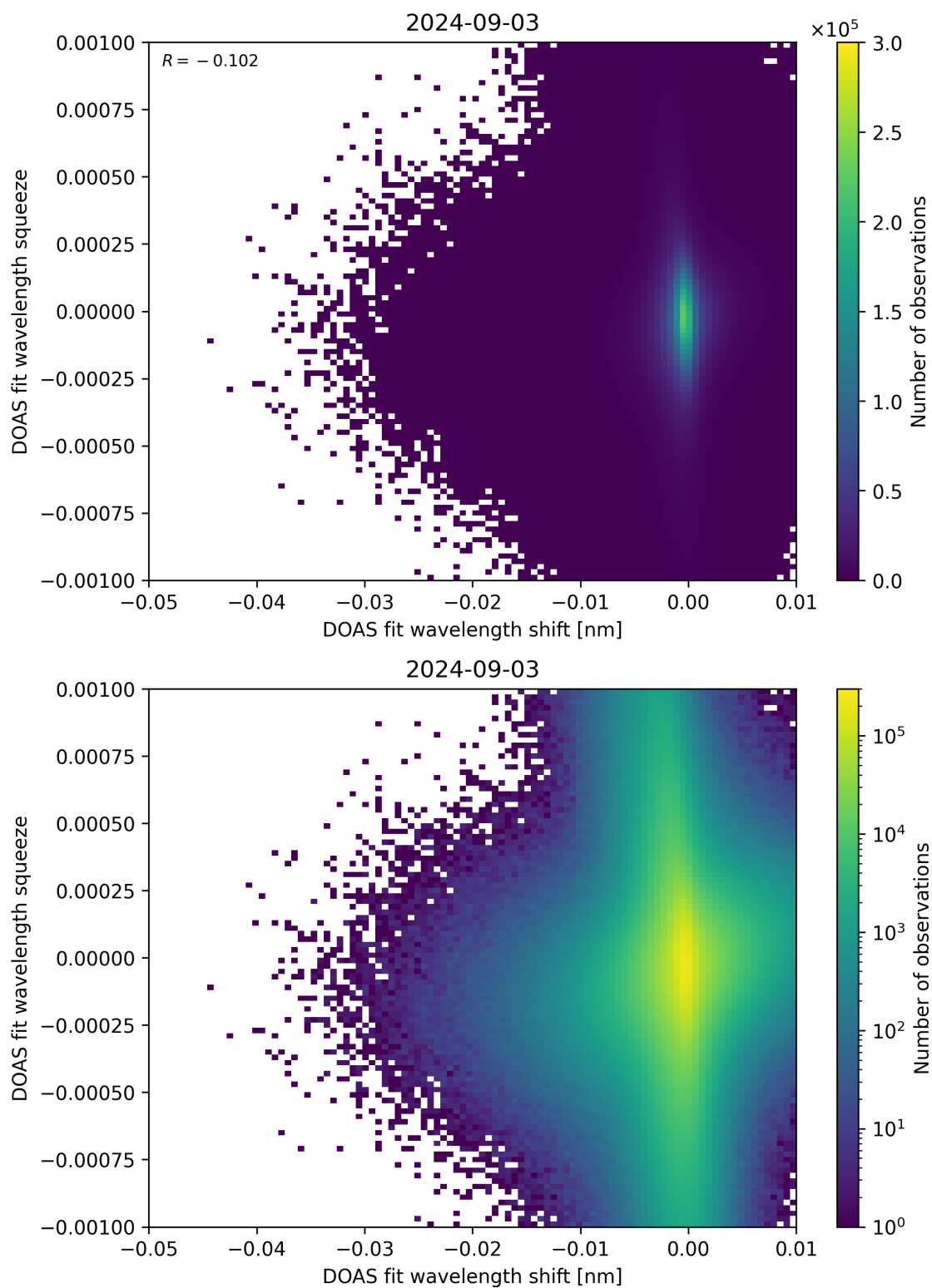
Figure 127: Scatter density plot of “DOAS fit wavelength shift” against “DOAS fit wavelength squeeze” for 2024-09-02 to 2024-09-04.
