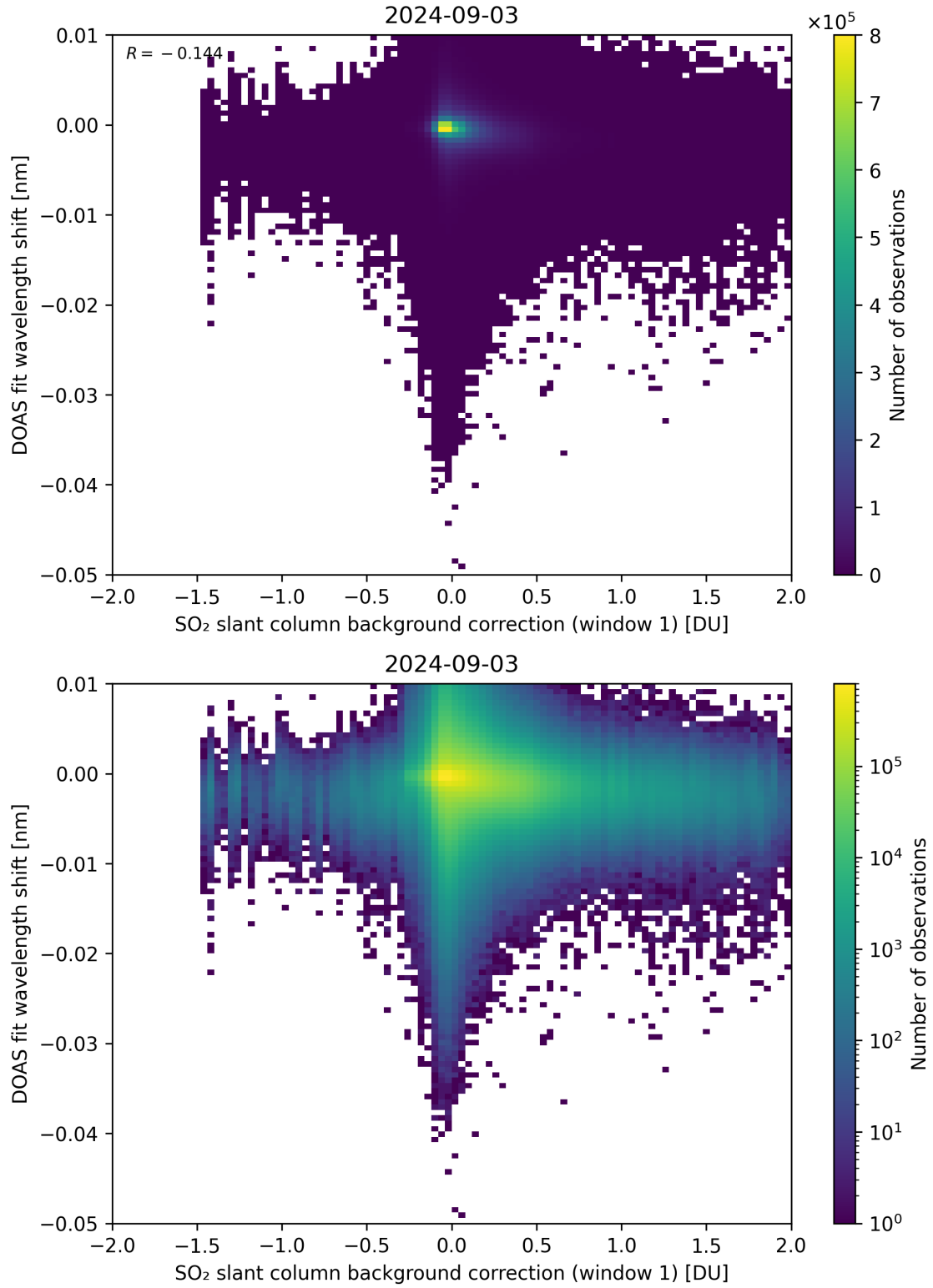
Figure 100: Scatter density plot of “SO 2 slant column background correction (window 1)” against “DOAS fit wavelength shift” for 2024-09-02 to 2024-09-04.
