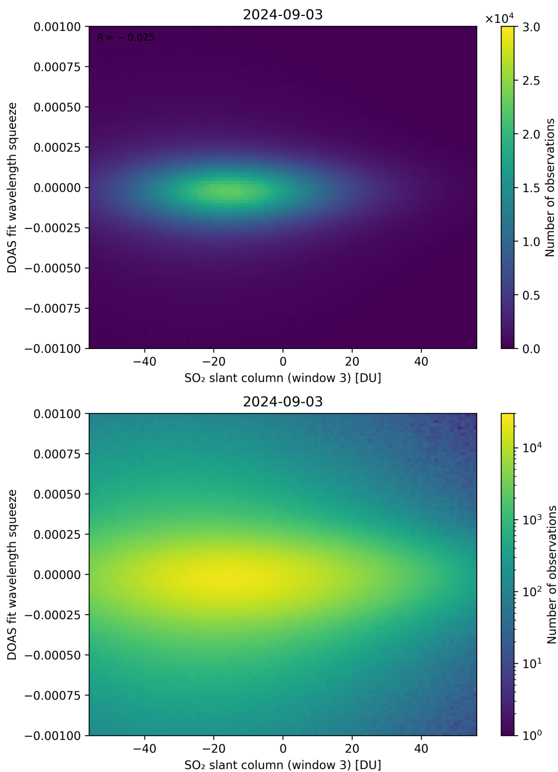
Figure 255: Scatter density plot of “SO 2 slant column (window 3)” against “DOAS fit wavelength squeeze” for 2024-09-02 to 2024-09-04.
