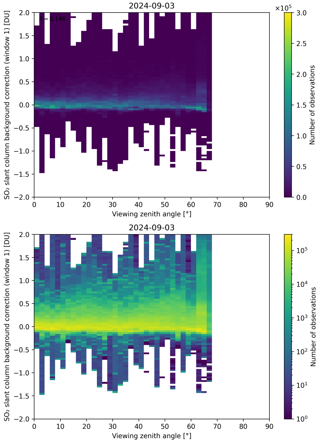
Figure 308: Scatter density plot of “Viewing zenith angle” against “SO 2 slant column background correction (window 1)” for 2024-09-02 to 2024-09-04.
