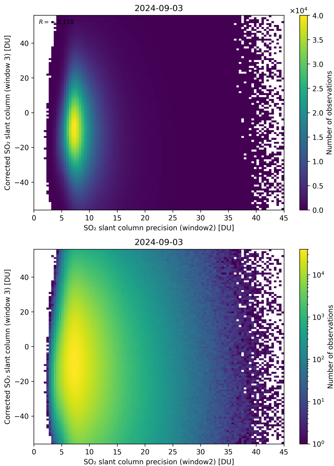
Figure 248: Scatter density plot of “SO 2 slant column precision (window2)” against “Corrected SO 2 slant column (window 3)” for 2024-09-02 to 2024-09-04.
