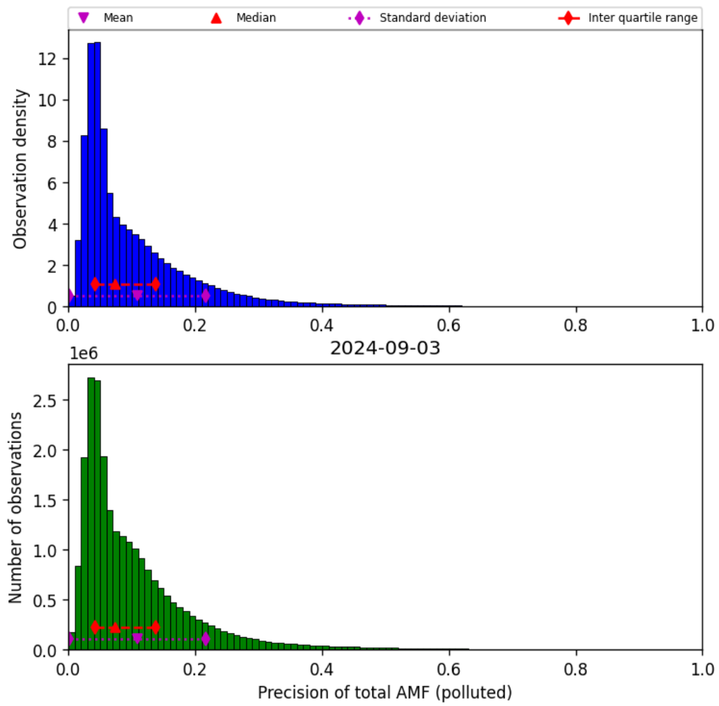
Figure 72: Histogram of “Precision of total AMF (polluted)” for 2024-09-02 to 2024-09-04
