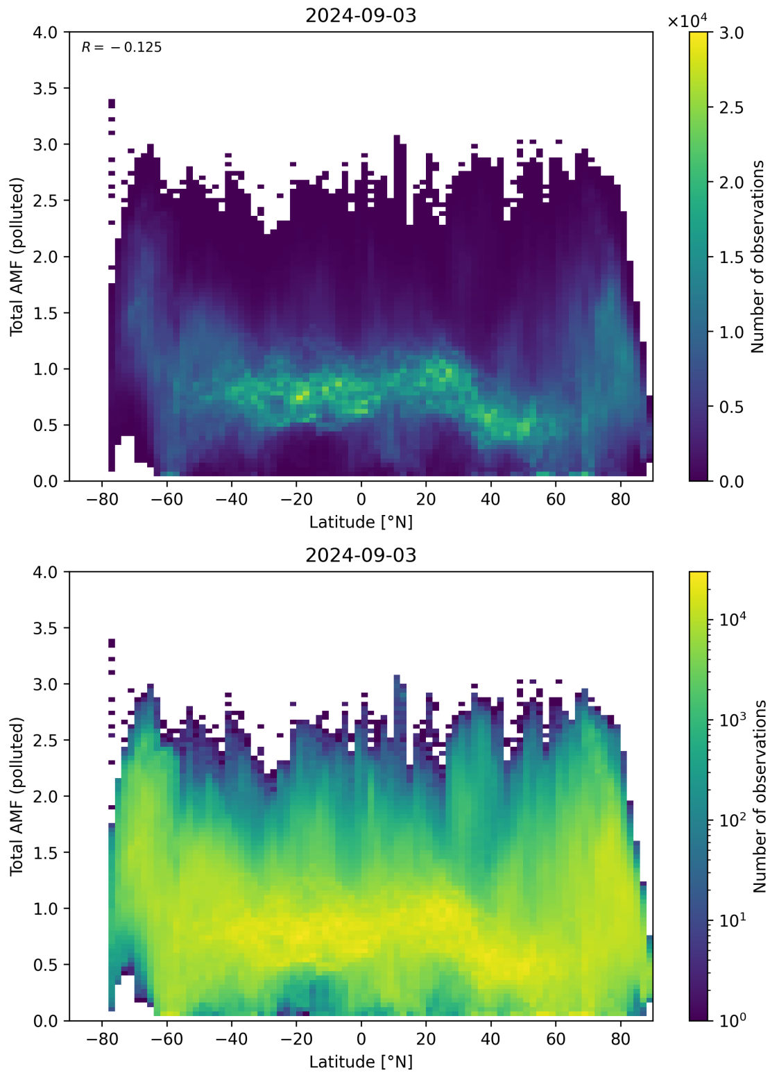
Figure 154: Scatter density plot of “Latitude” against “Total AMF (polluted)” for 2024-09-02 to 2024-09-04.
