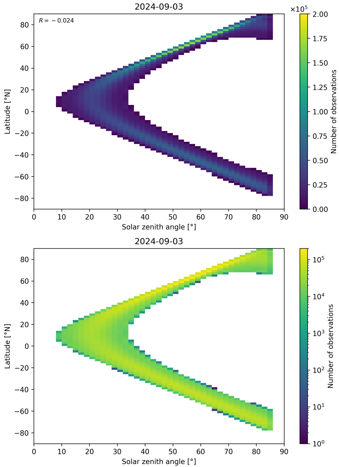
Figure 164: Scatter density plot of “Solar zenith angle” against “Latitude” for 2024-09-02 to 2024-09-04.
