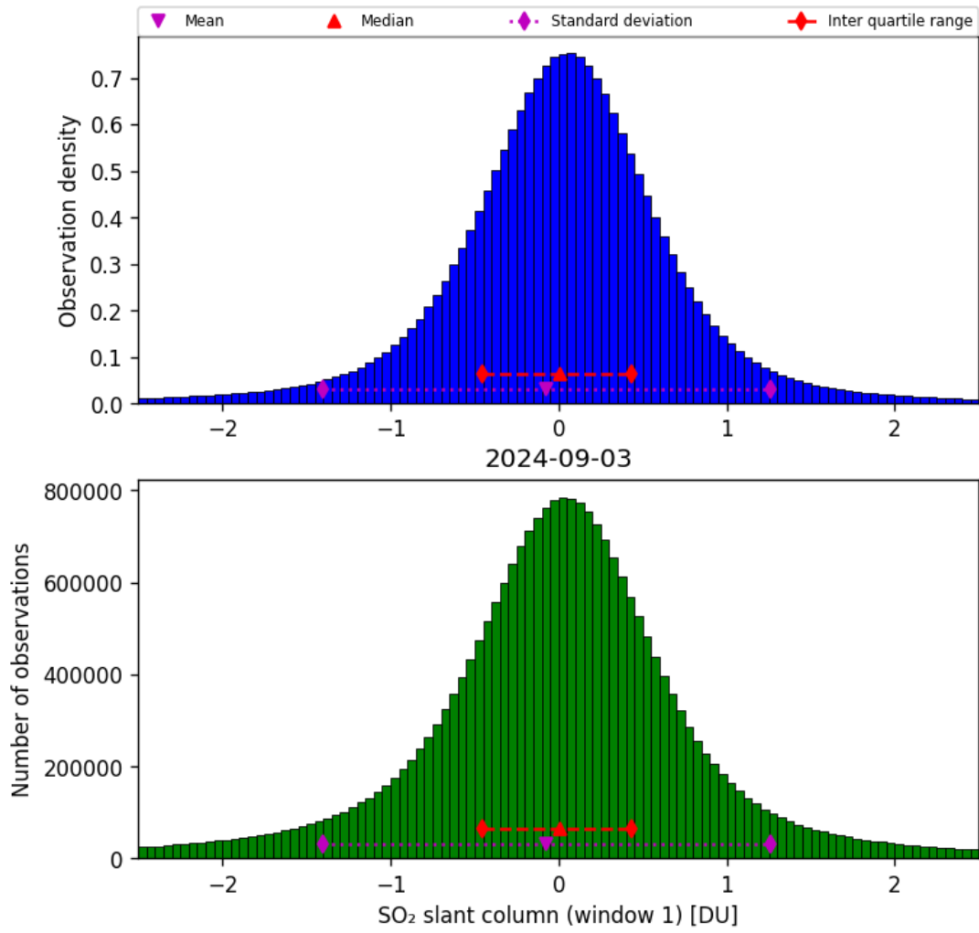
Figure 56: Histogram of “SO 2 slant column (window 1)” for 2024-09-02 to 2024-09-04
