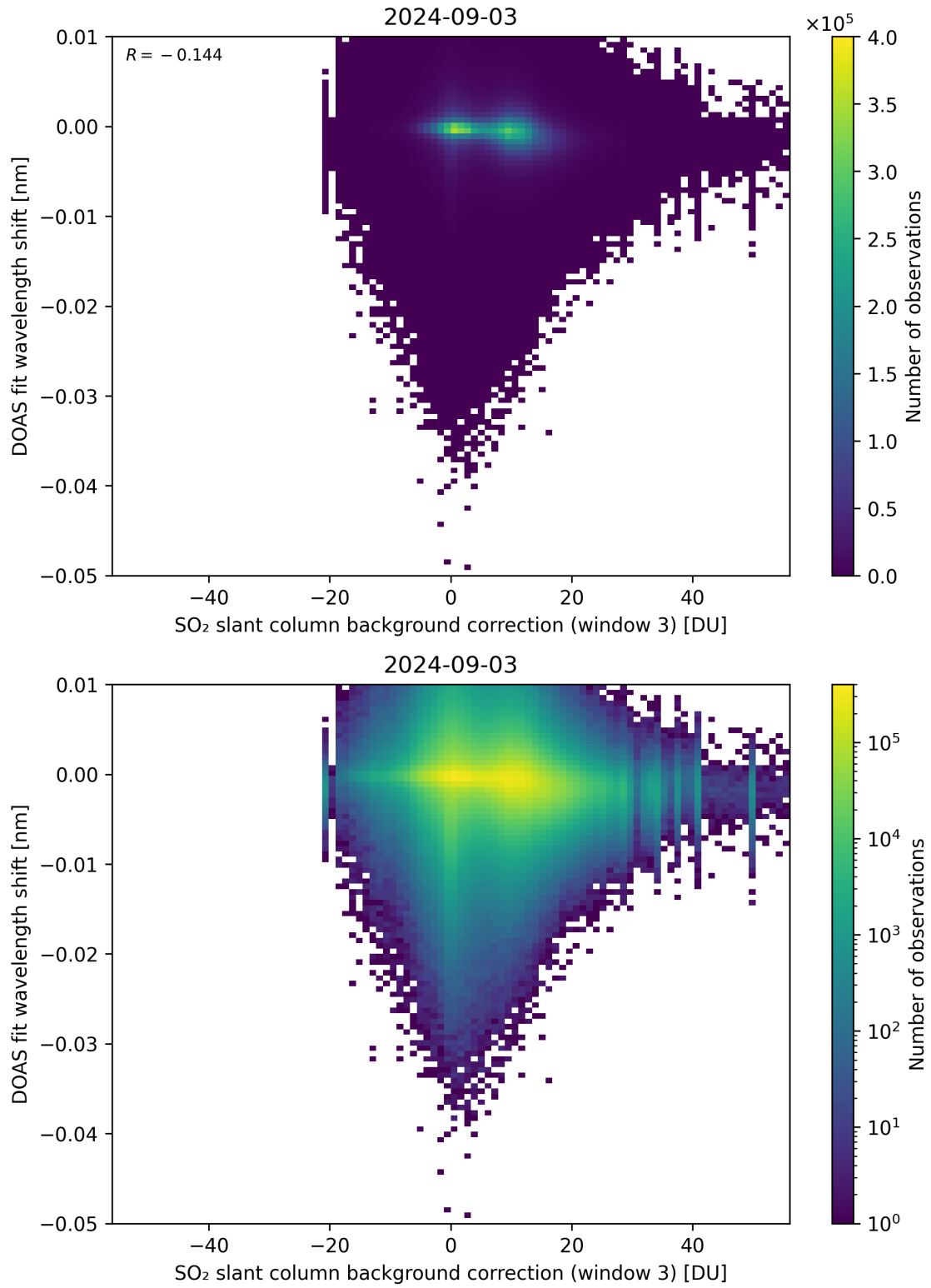
Figure 121: Scatter density plot of “SO 2 slant column background correction (window 3)” against “DOAS fit wavelength shift” for 2024-09-02 to 2024-09-04.
