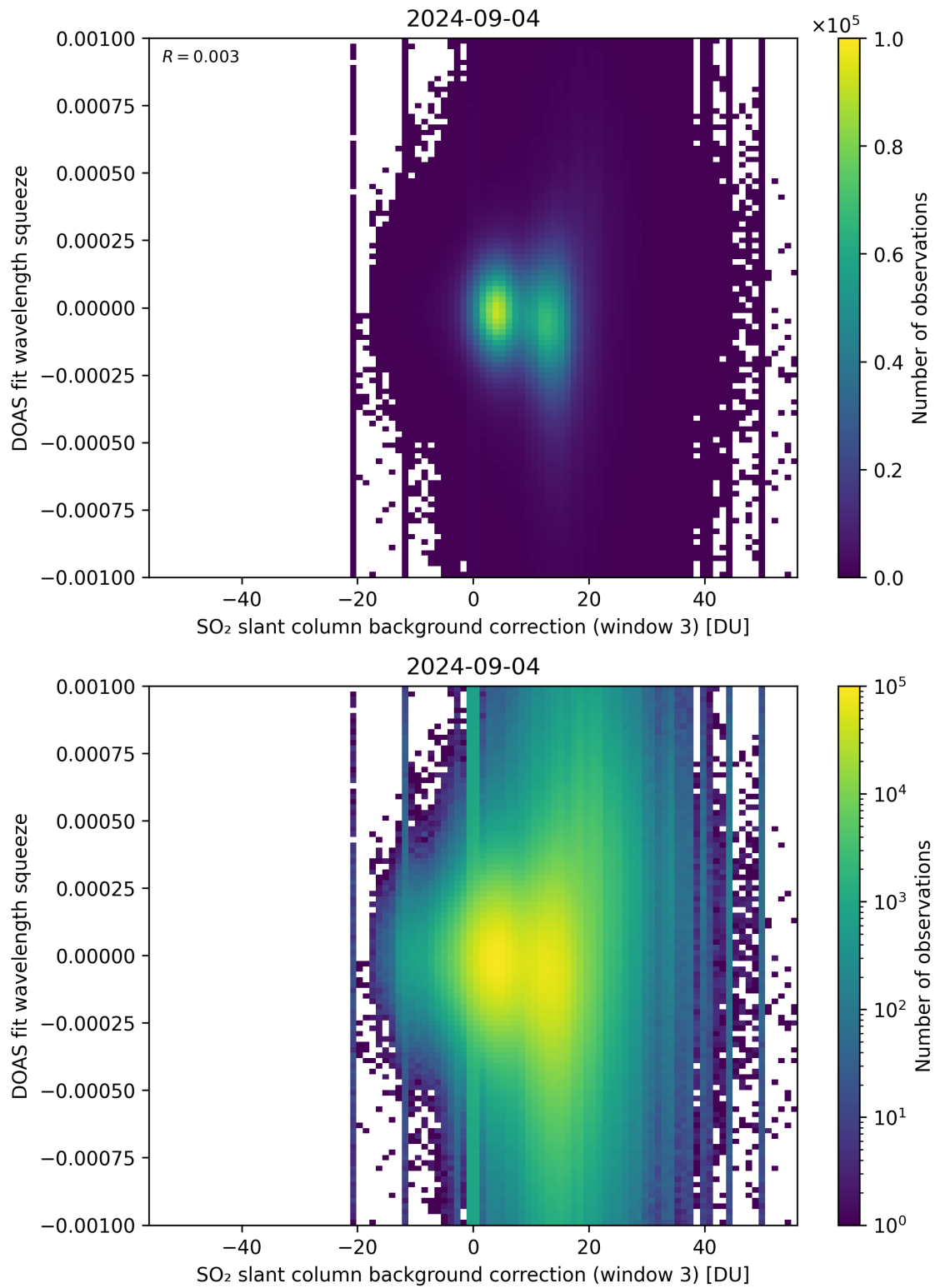
Figure 122: Scatter density plot of “SO 2 slant column background correction (window 3)” against “DOAS fit wavelength squeeze” for 2024-09-03 to 2024-09-05.
