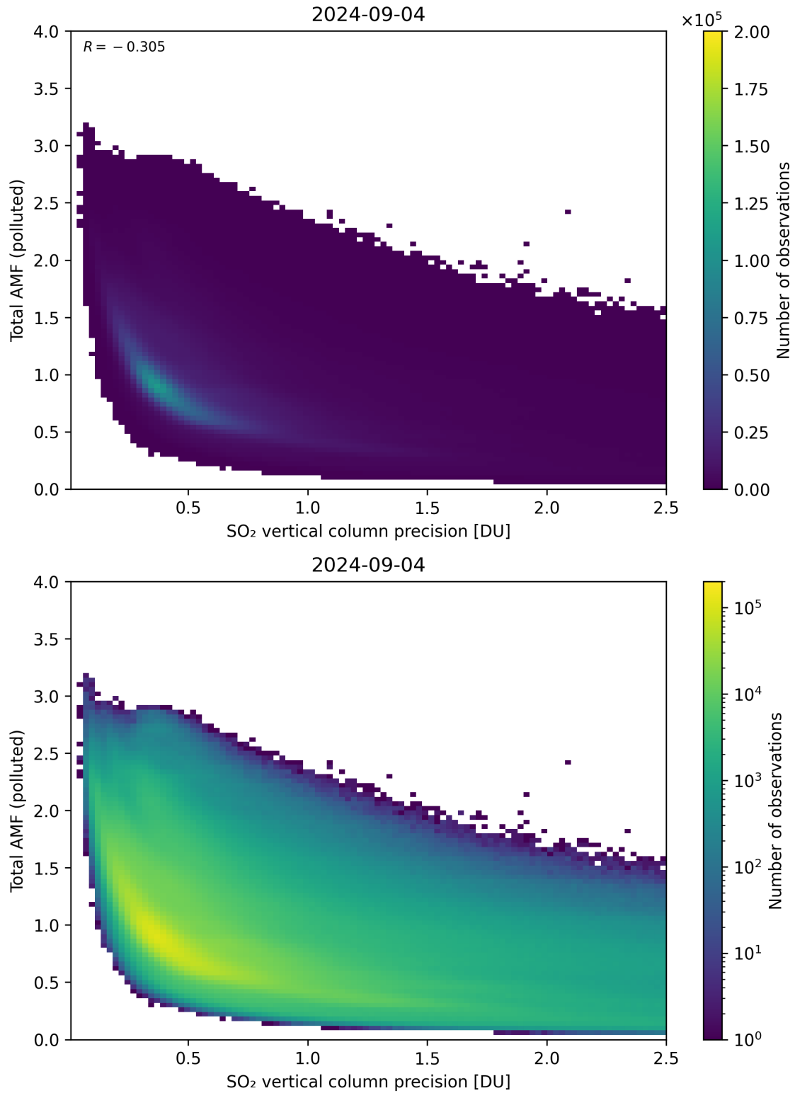
Figure 294: Scatter density plot of “SO 2 vertical column precision” against “Total AMF (polluted)” for 2024-09-03 to 2024-09-05.
