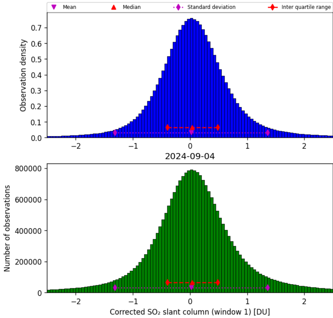
Figure 58: Histogram of “Corrected SO 2 slant column (window 1)” for 2024-09-03 to 2024-09-05
