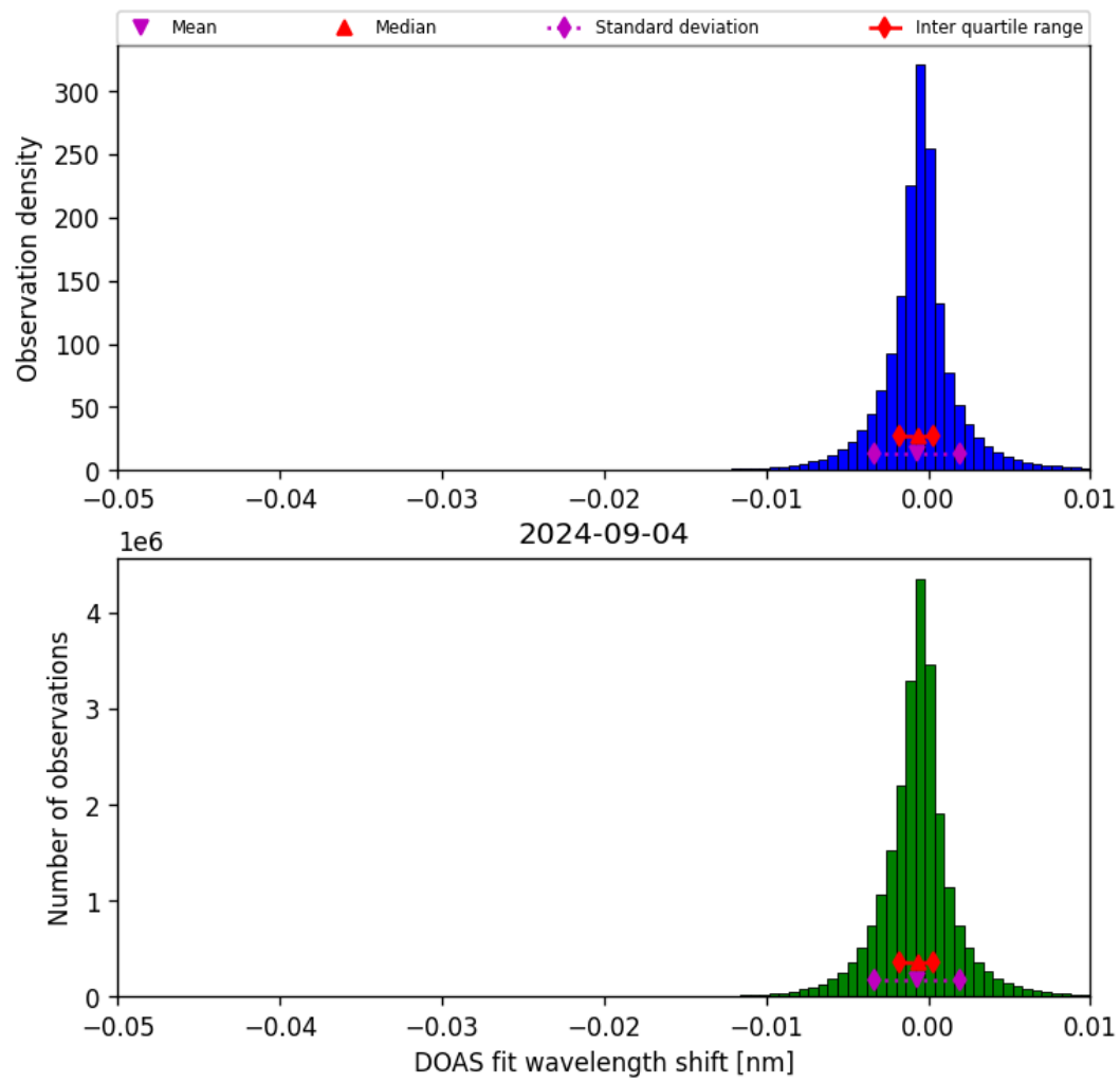
Figure 68: Histogram of “DOAS fit wavelength shift” for 2024-09-03 to 2024-09-05
