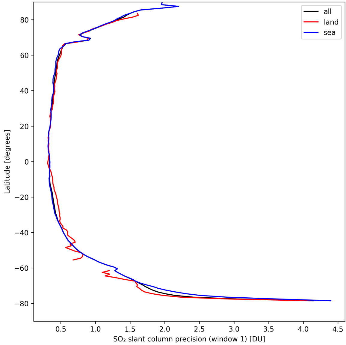
Figure 34: Zonal average of “SO 2 slant column precision (window 1)” for 2024-09-03 to 2024-09-05.
