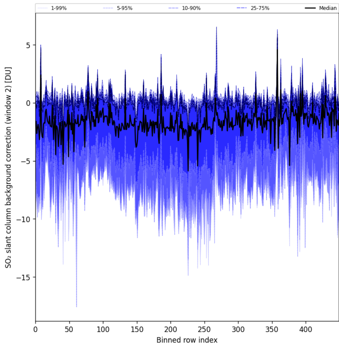
Figure 86: Along track statistics of “SO 2 slant column background correction (window 2)” for 2024-09-03 to 2024-09-05
