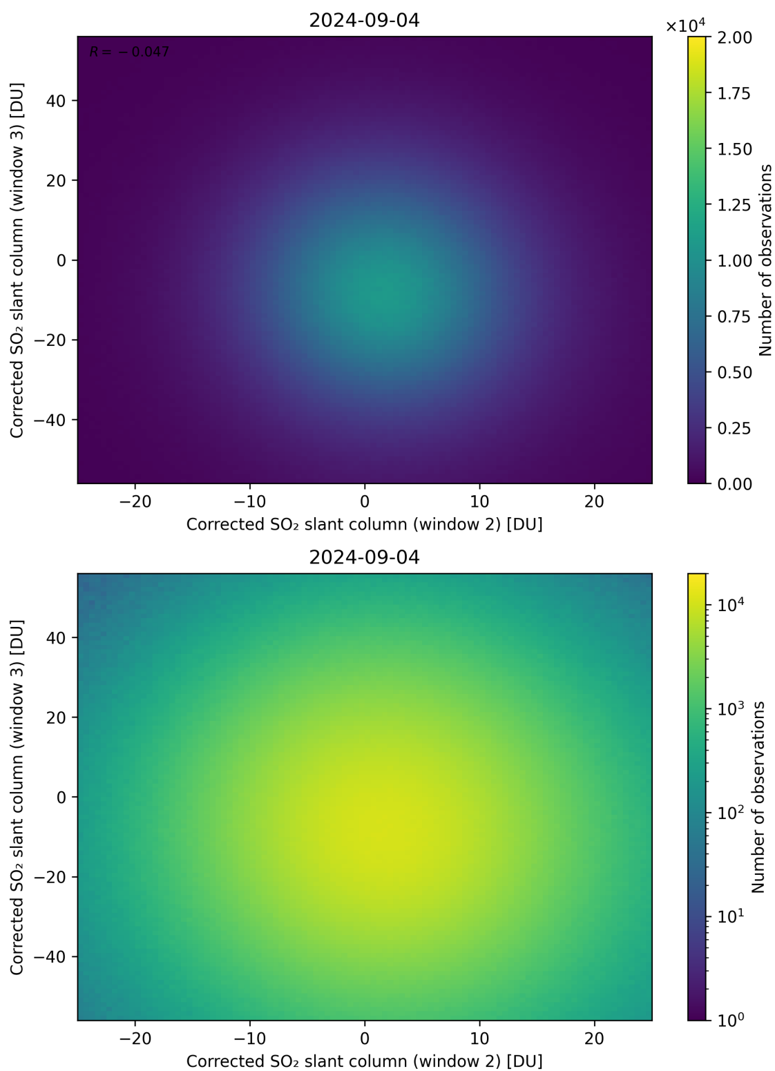
Figure 200: Scatter density plot of “Corrected SO 2 slant column (window 2)” against “Corrected SO 2 slant column (window 3)” for 2024-09-03 to 2024-09-05.
