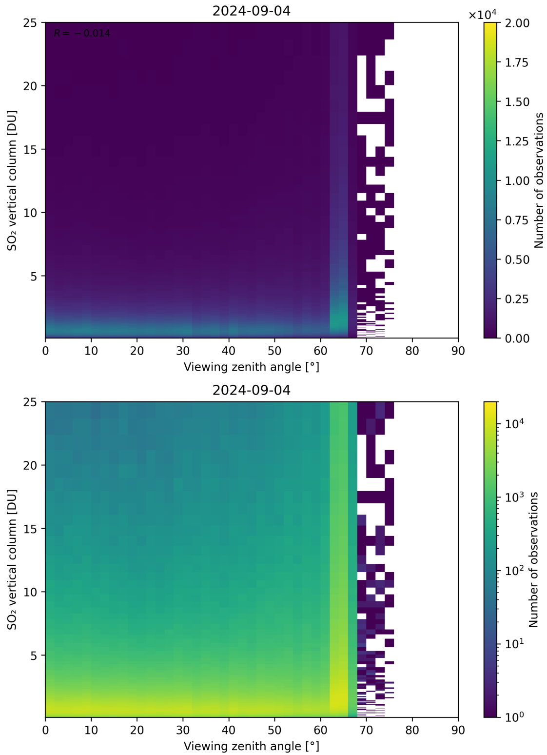
Figure 327: Scatter density plot of “Viewing zenith angle” against “SO 2 vertical column” for 2024-09-03 to 2024-09-05.
