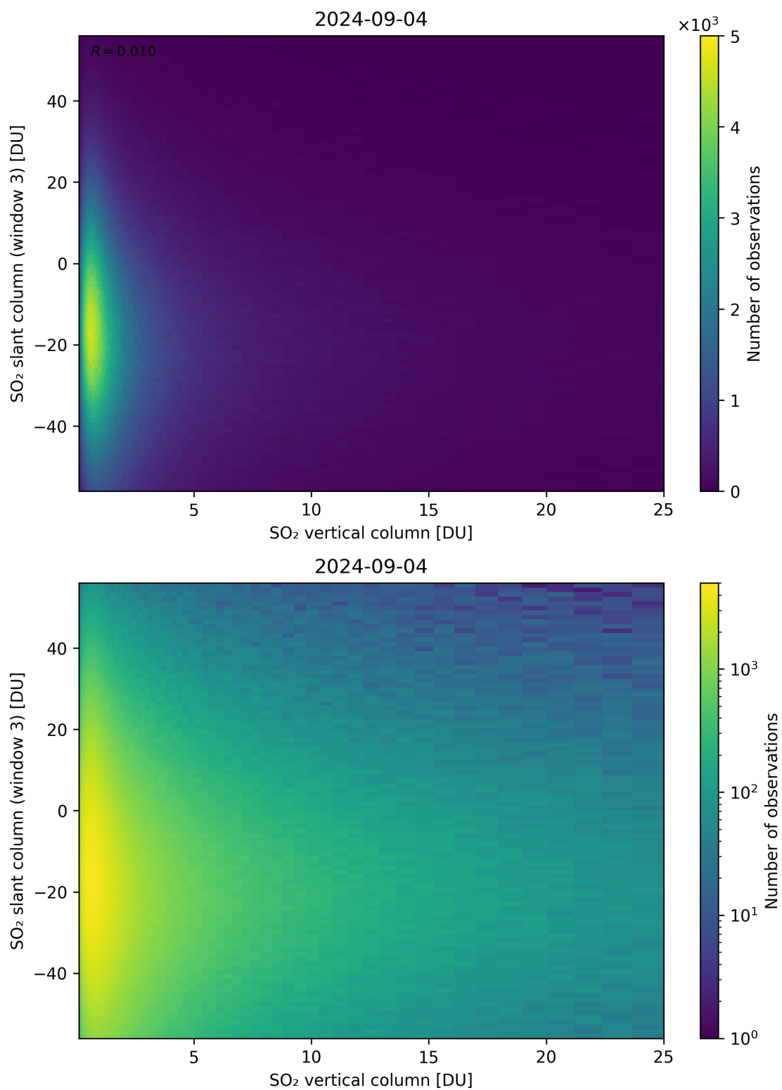
Figure 303: Scatter density plot of “SO 2 vertical column” against “SO 2 slant column (window 3)” for 2024-09-03 to 2024-09-05.
