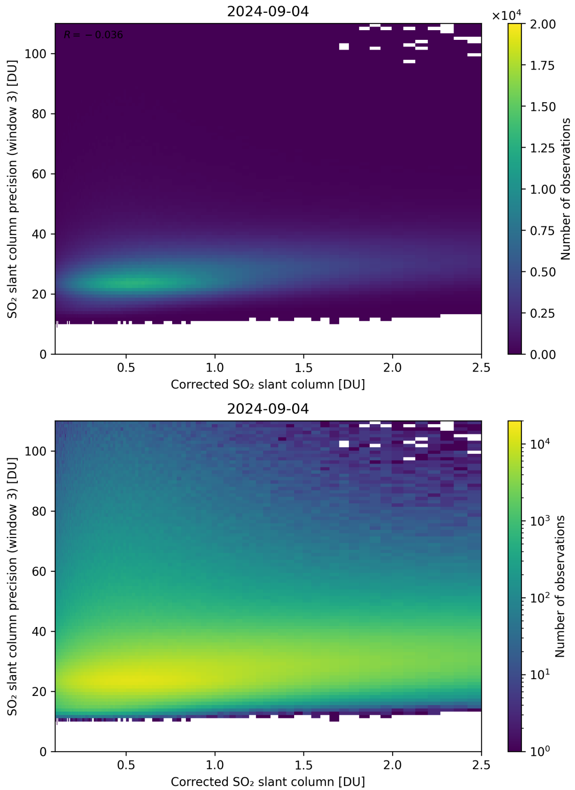
Figure 191: Scatter density plot of “Corrected SO 2 slant column” against “SO 2 slant column precision (window 3)” for 2024-09-03 to 2024-09-05.
