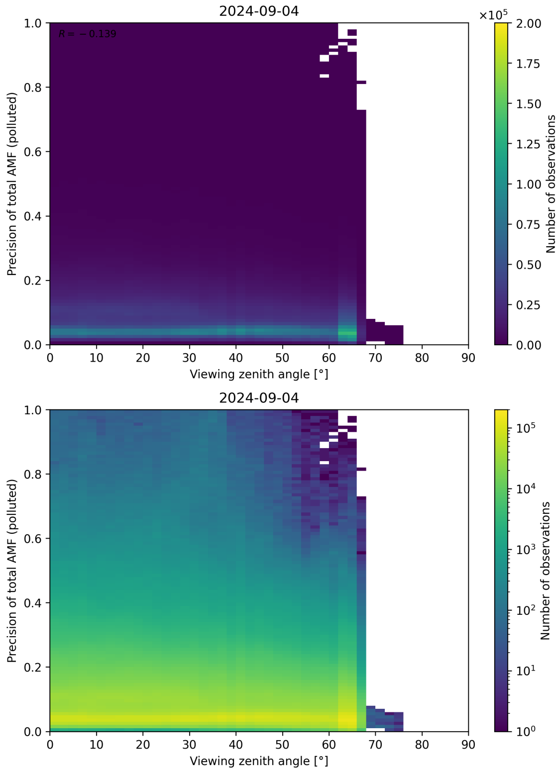
Figure 326: Scatter density plot of “Viewing zenith angle” against “Precision of total AMF (polluted)” for 2024-09-03 to 2024-09-05.
