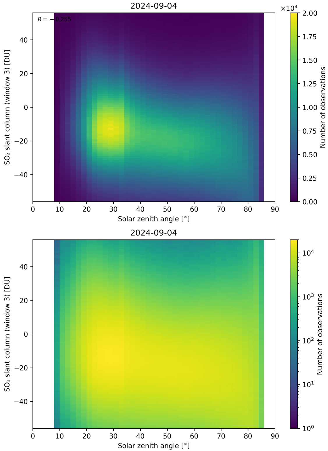
Figure 172: Scatter density plot of “Solar zenith angle” against “SO 2 slant column (window 3)” for 2024-09-03 to 2024-09-05.
