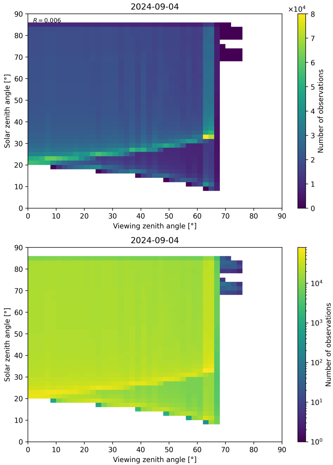
Figure 315: Scatter density plot of “Viewing zenith angle” against “Solar zenith angle” for 2024-09-03 to 2024-09-05.
