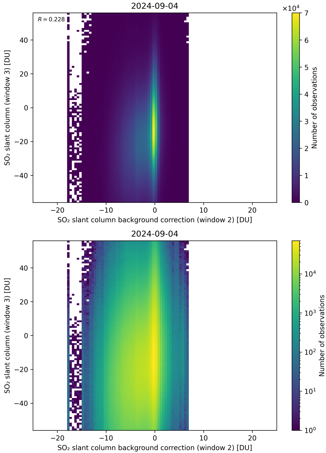
Figure 117: Scatter density plot of “SO 2 slant column background correction (window 2)” against “SO 2 slant column (window 3)” for 2024-09-03 to 2024-09-05.
