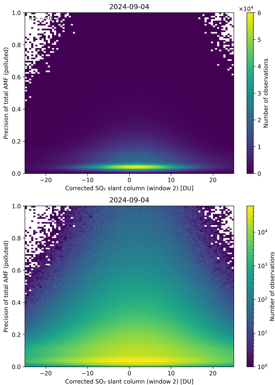
Figure 204: Scatter density plot of “Corrected SO 2 slant column (window 2)” against “Precision of total AMF (polluted)” for 2024-09-03 to 2024-09-05.
