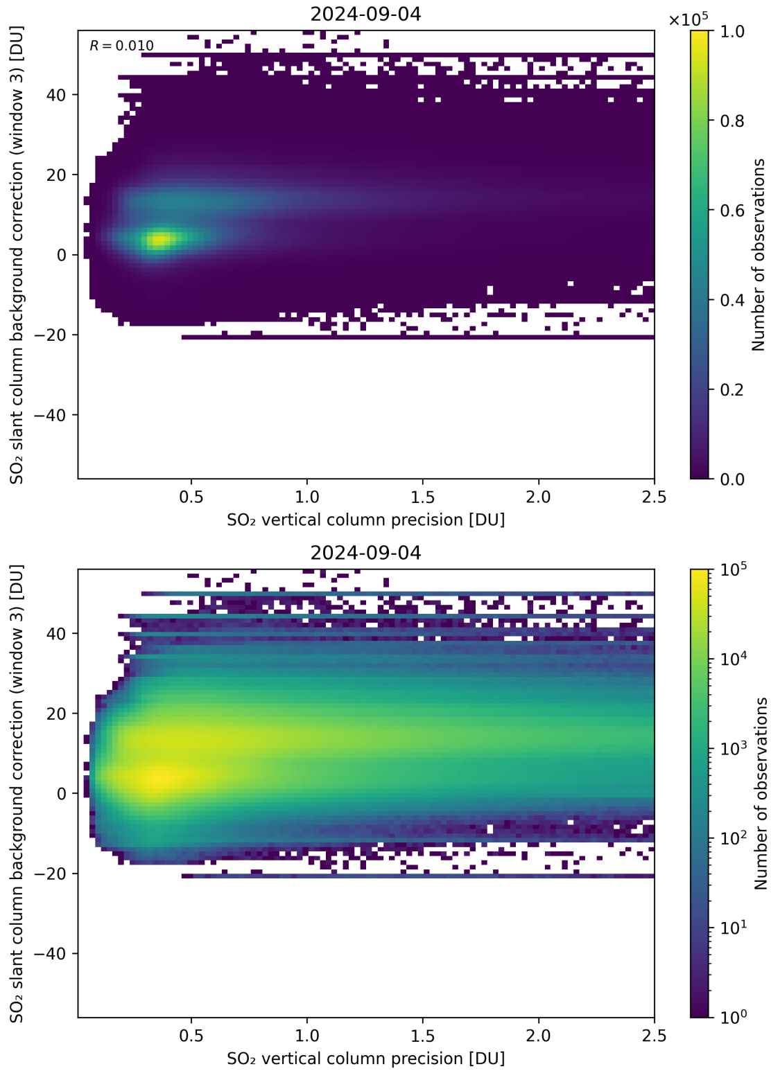
Figure 281: Scatter density plot of “SO 2 vertical column precision” against “SO 2 slant column background correction (window 3)” for 2024-09-03 to 2024-09-05.
