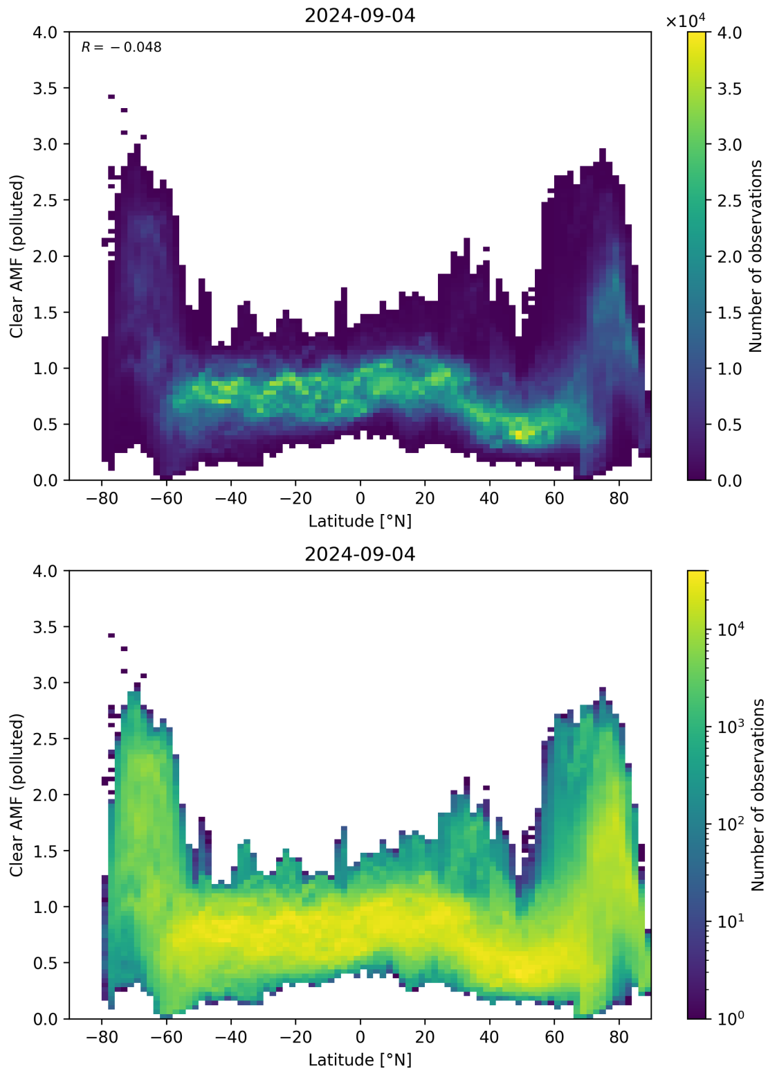
Figure 145: Scatter density plot of “Latitude” against “Clear AMF (polluted)” for 2024-09-03 to 2024-09-05.
