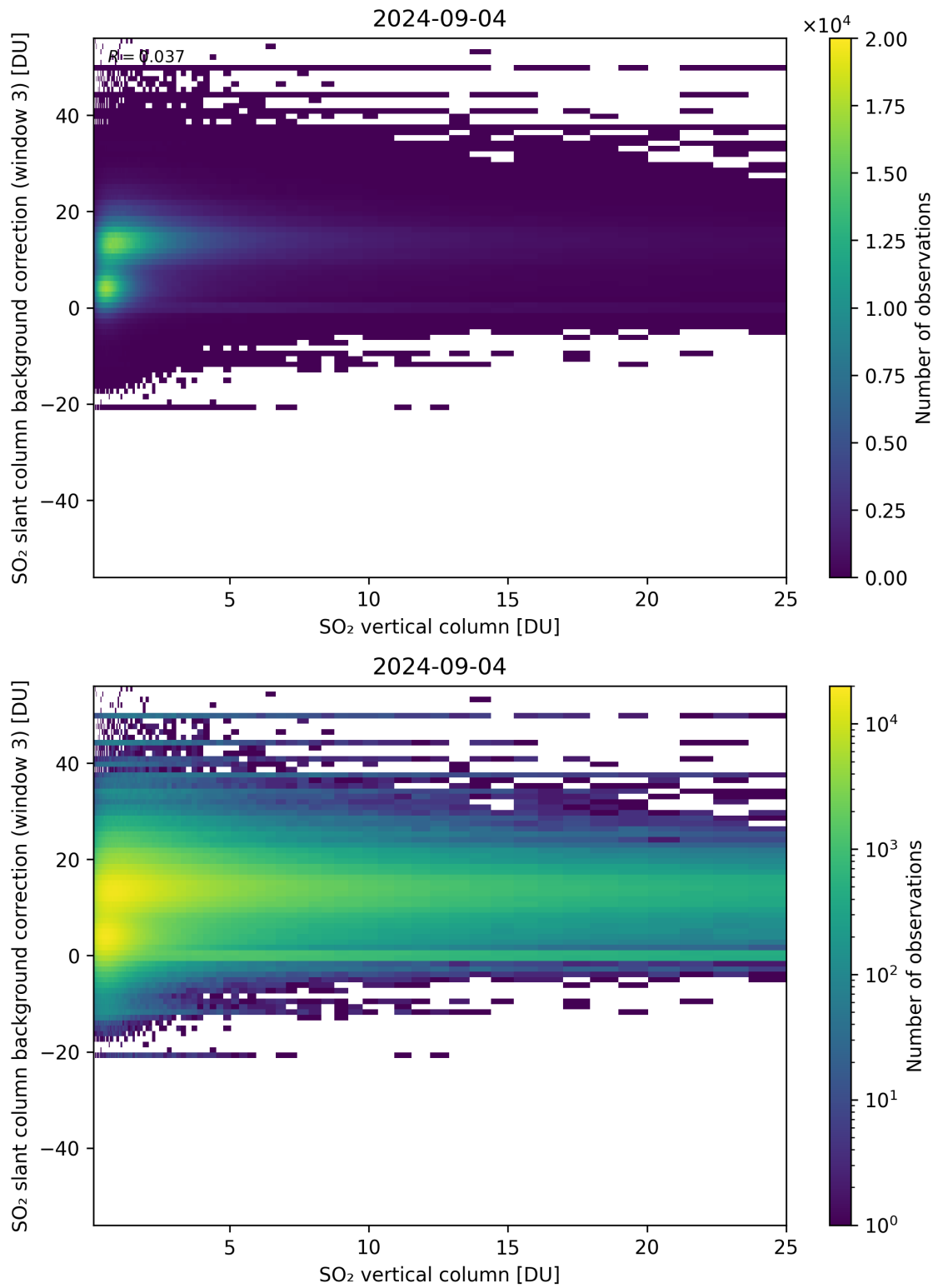
Figure 275: Scatter density plot of “SO 2 vertical column” against “SO 2 slant column background correction (window 3)” for 2024-09-03 to 2024-09-05.
