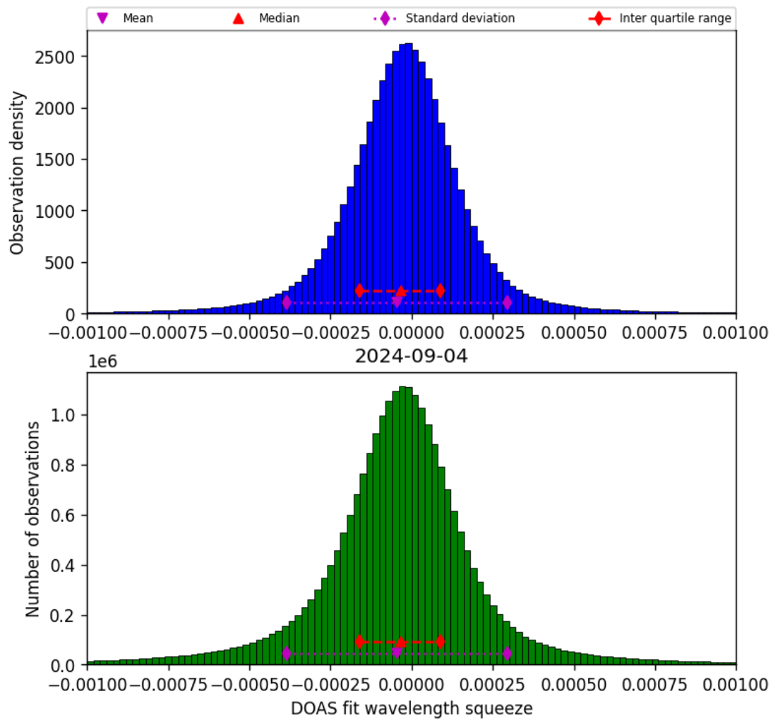
Figure 69: Histogram of “DOAS fit wavelength squeeze” for 2024-09-03 to 2024-09-05
