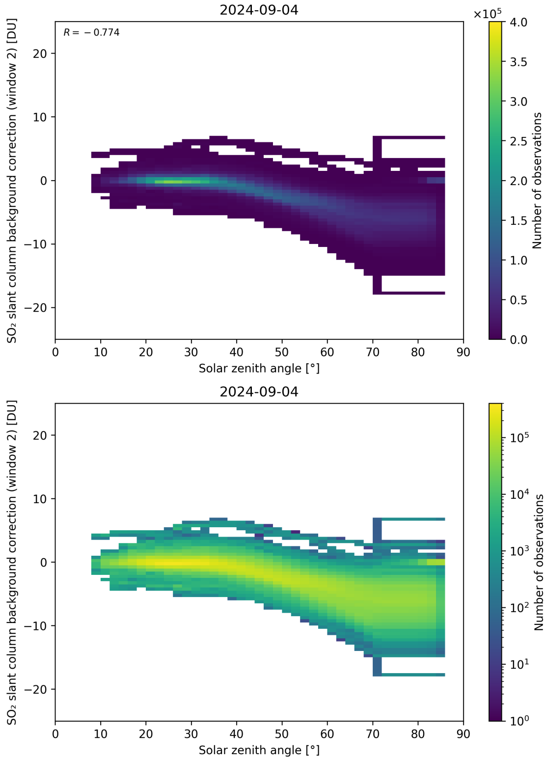
Figure 159: Scatter density plot of “Solar zenith angle” against “SO 2 slant column background correction (window 2)” for 2024-09-03 to 2024-09-05.
