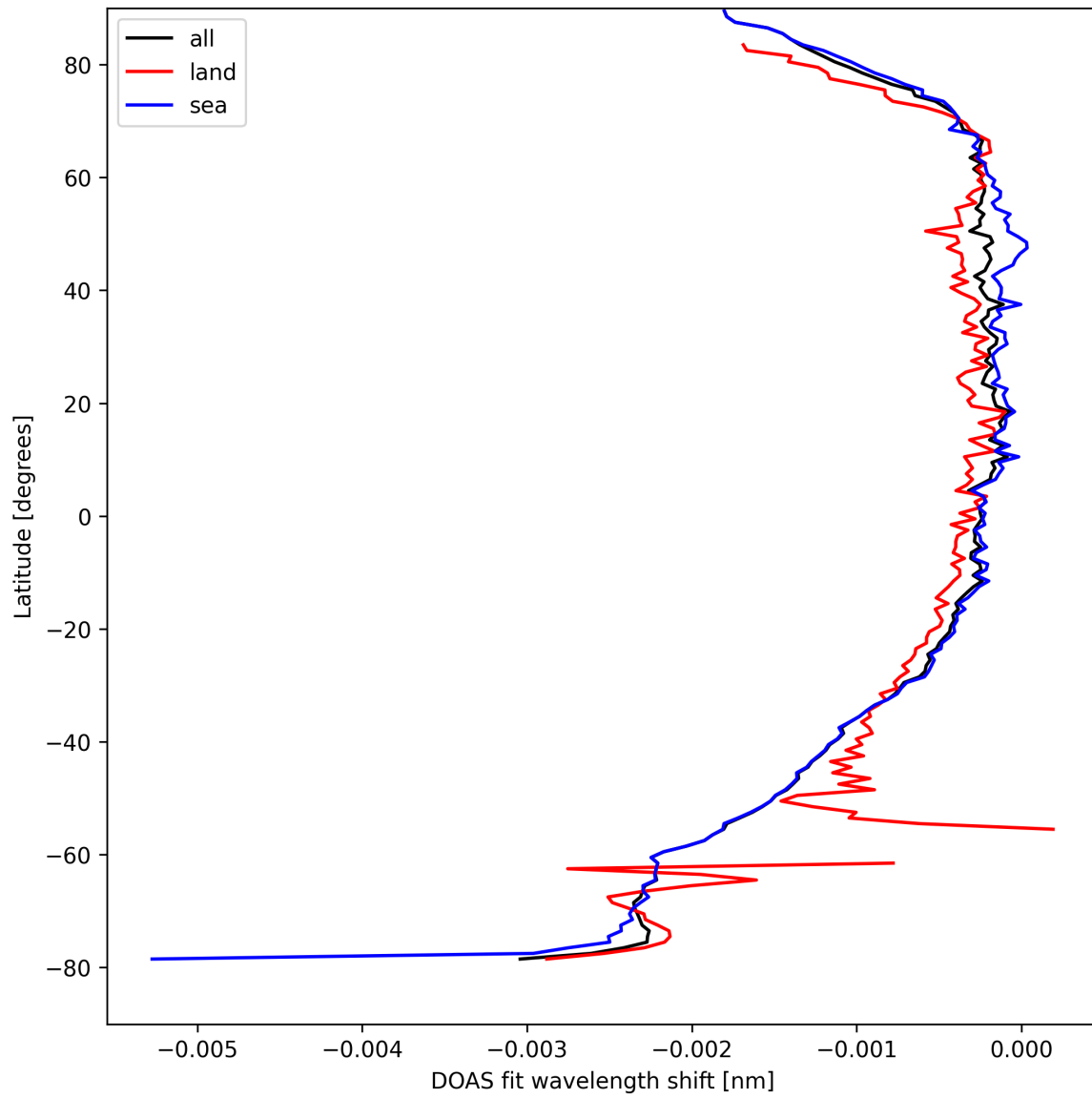
Figure 45: Zonal average of “DOAS fit wavelength shift” for 2024-09-03 to 2024-09-05.
