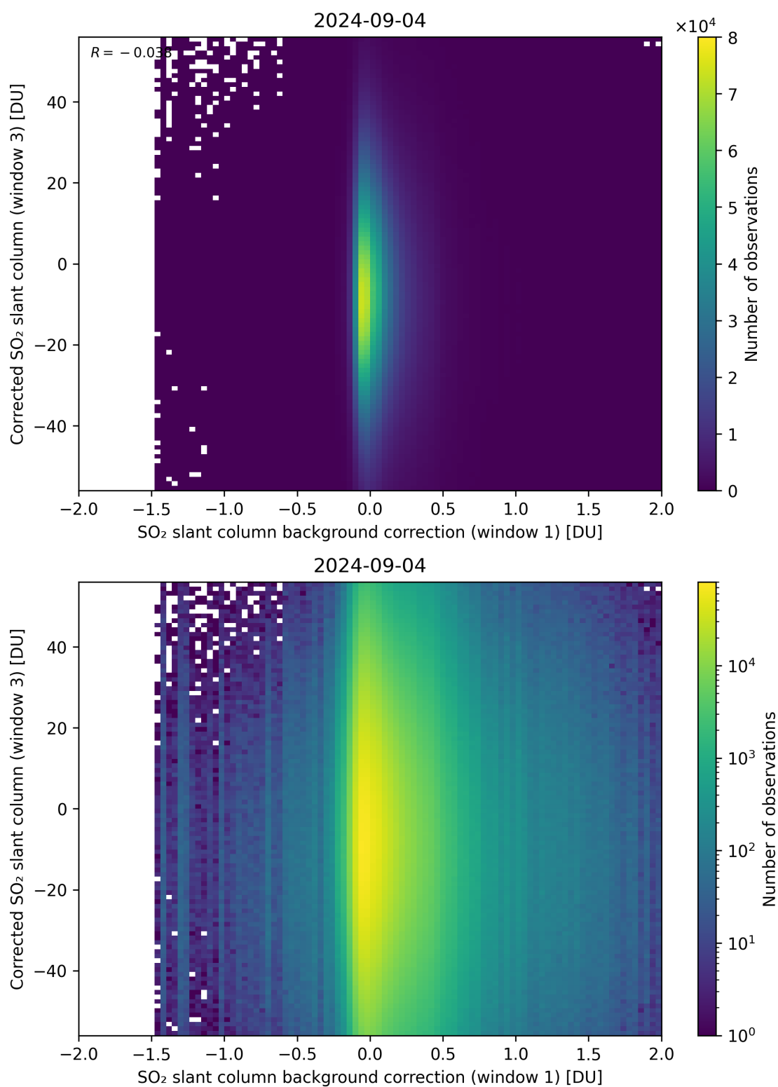
Figure 105: Scatter density plot of “SO 2 slant column background correction (window 1)” against “Corrected SO 2 slant column (window 3)” for 2024-09-03 to 2024-09-05.
