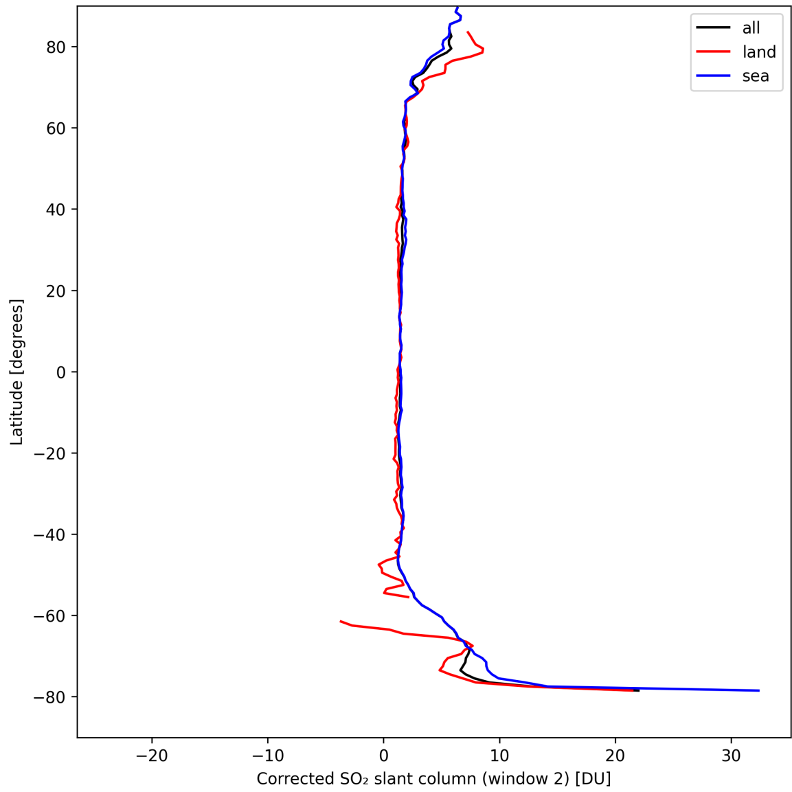
Figure 39: Zonal average of “Corrected SO 2 slant column (window 2)” for 2024-09-03 to 2024-09-05.
