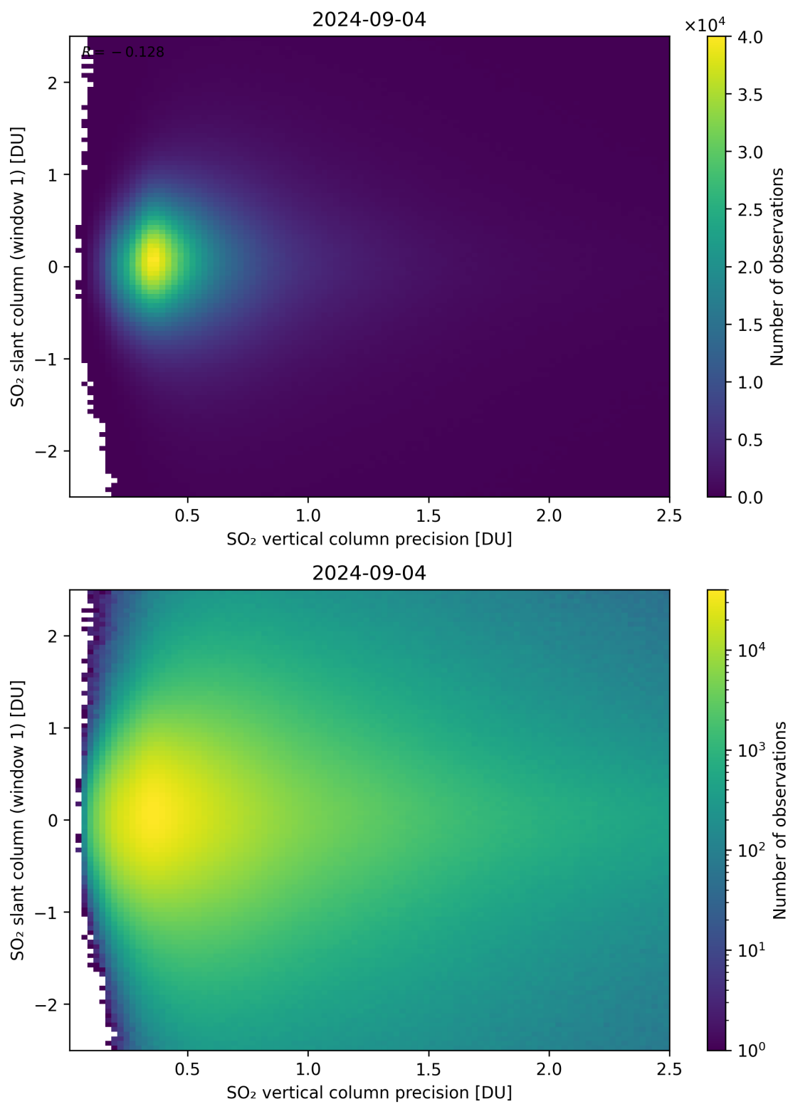
Figure 289: Scatter density plot of “SO 2 vertical column precision” against “SO 2 slant column (window 1)” for 2024-09-03 to 2024-09-05.
