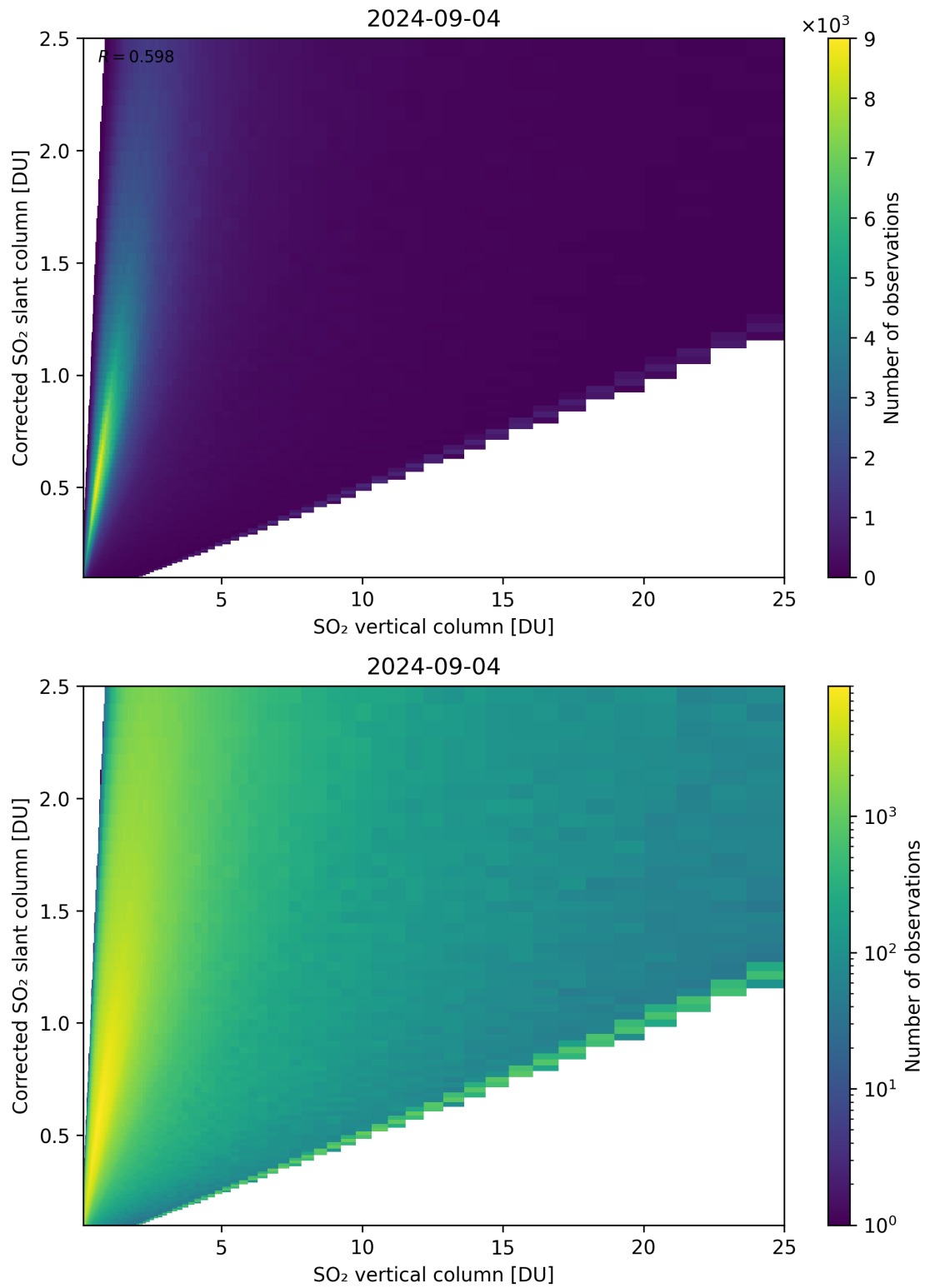
Figure 297: Scatter density plot of “SO 2 vertical column” against “Corrected SO 2 slant column” for 2024-09-03 to 2024-09-05.
