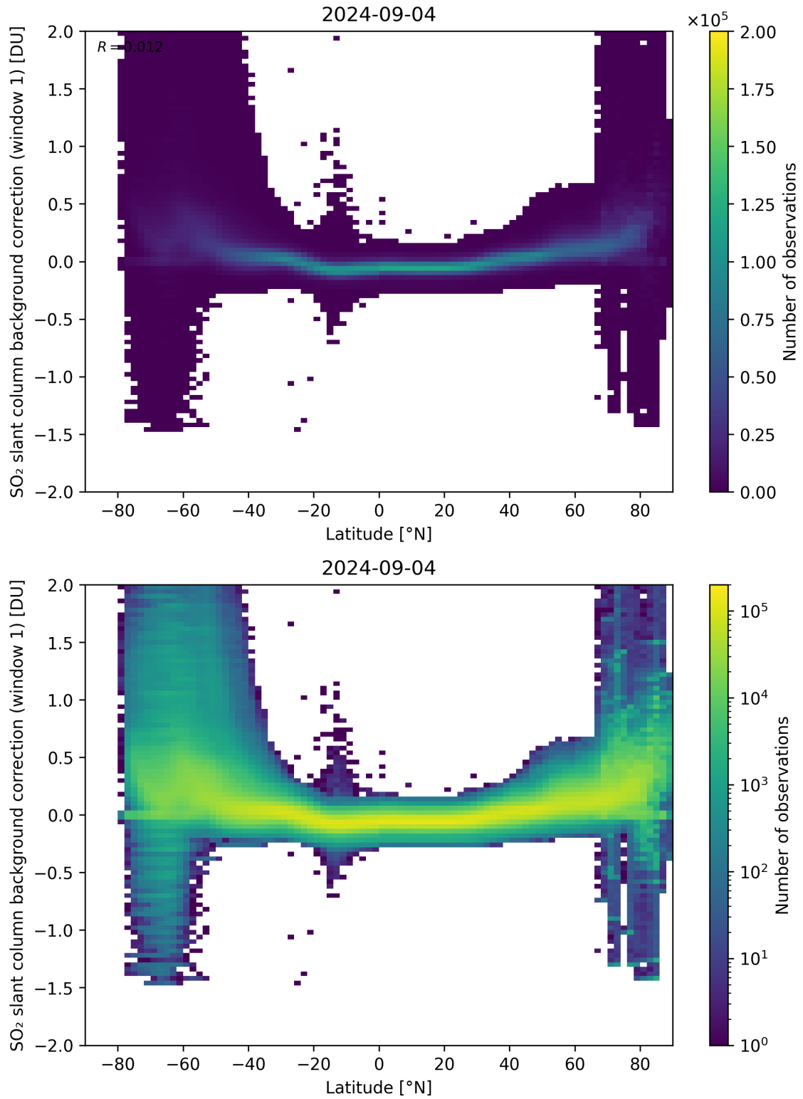
Figure 139: Scatter density plot of “Latitude” against “SO 2 slant column background correction (window 1)” for 2024-09-03 to 2024-09-05.
