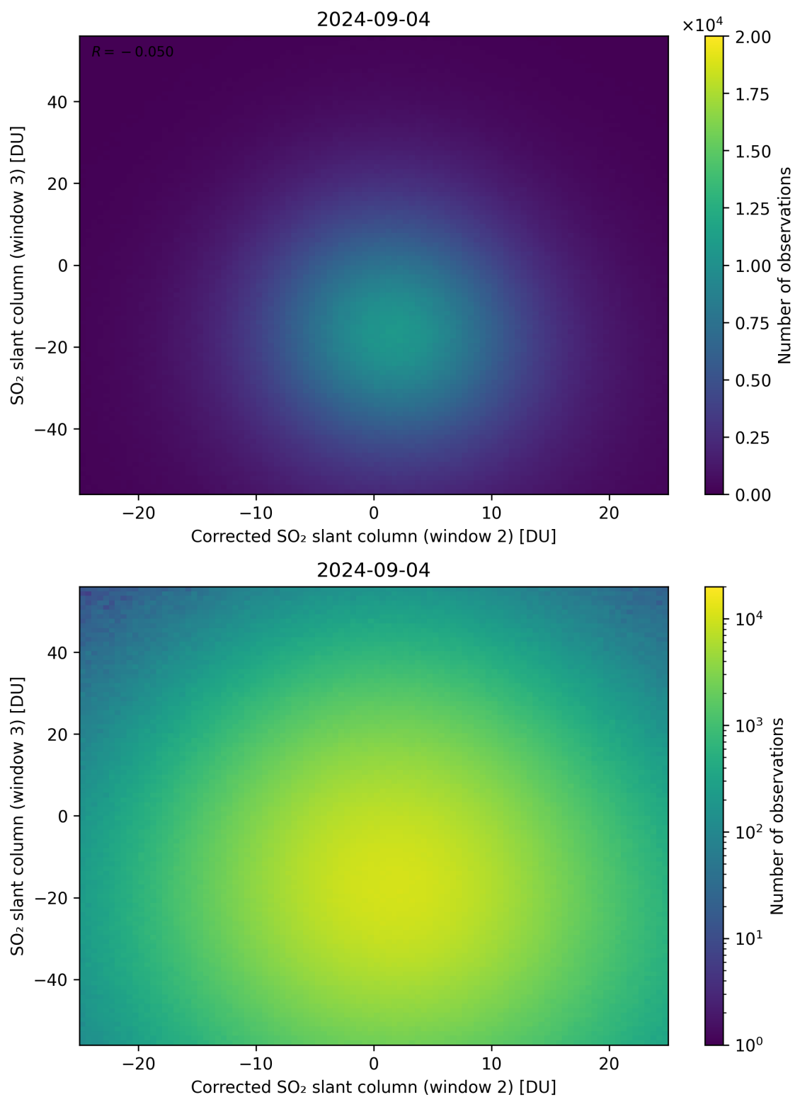
Figure 201: Scatter density plot of “Corrected SO 2 slant column (window 2)” against “SO 2 slant column (window 3)” for 2024-09-03 to 2024-09-05.
