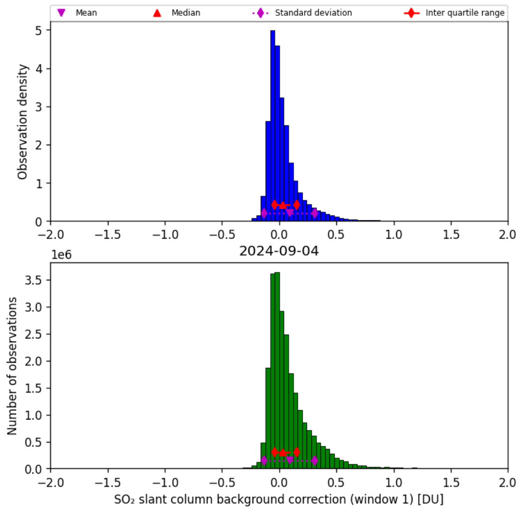
Figure 59: Histogram of “SO 2 slant column background correction (window 1)” for 2024-09-03 to 2024-09-05
