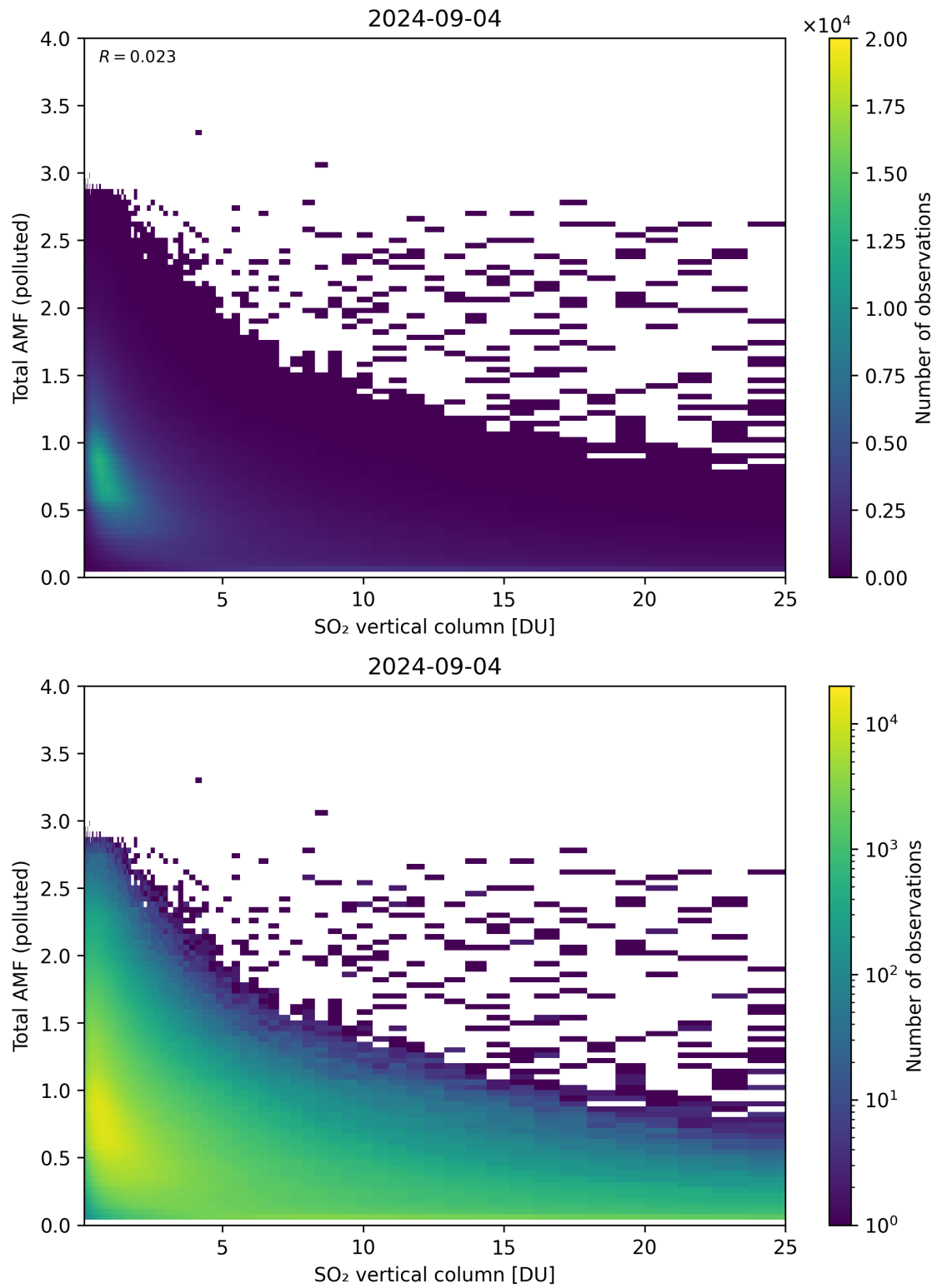
Figure 305: Scatter density plot of “SO 2 vertical column” against “Total AMF (polluted)” for 2024-09-03 to 2024-09-05.
