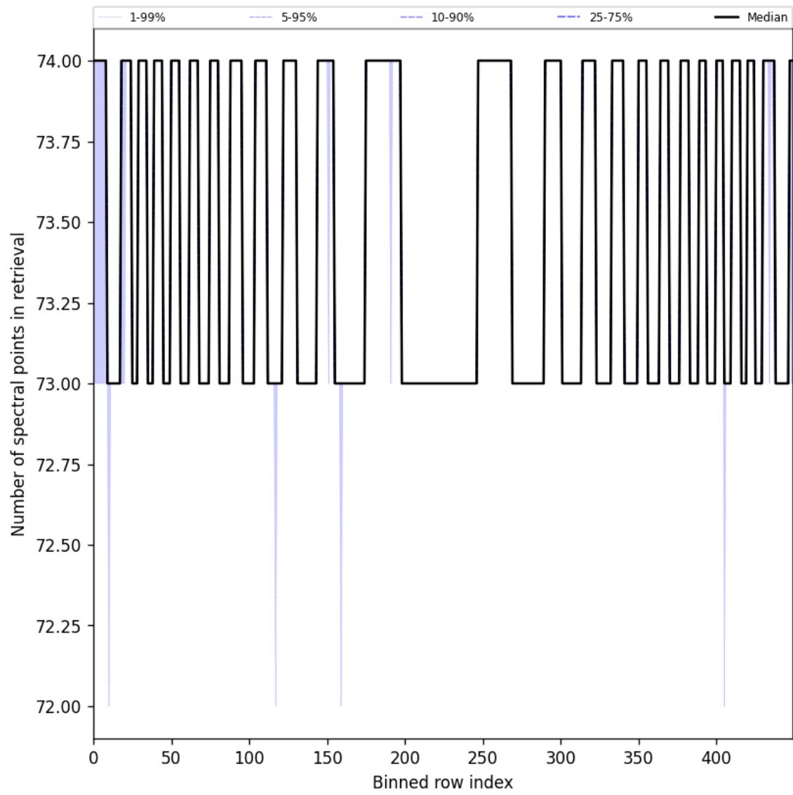
Figure 97: Along track statistics of “Number of spectral points in retrieval” for 2024-09-03 to 2024-09-05
