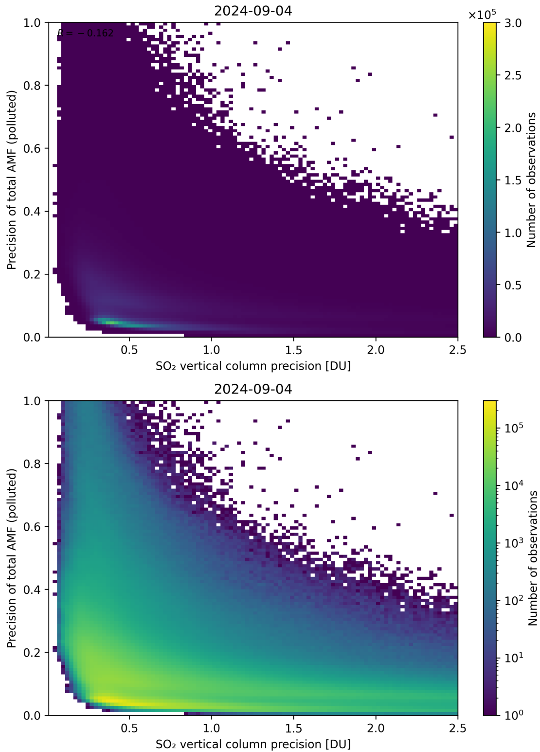
Figure 295: Scatter density plot of “SO 2 vertical column precision” against “Precision of total AMF (polluted)” for 2024-09-03 to 2024-09-05.
