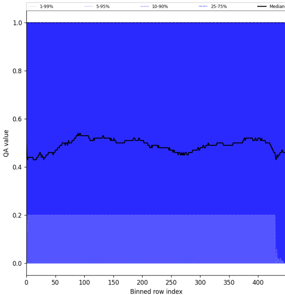
Figure 75: Along track statistics of “QA value” for 2024-09-03 to 2024-09-05
