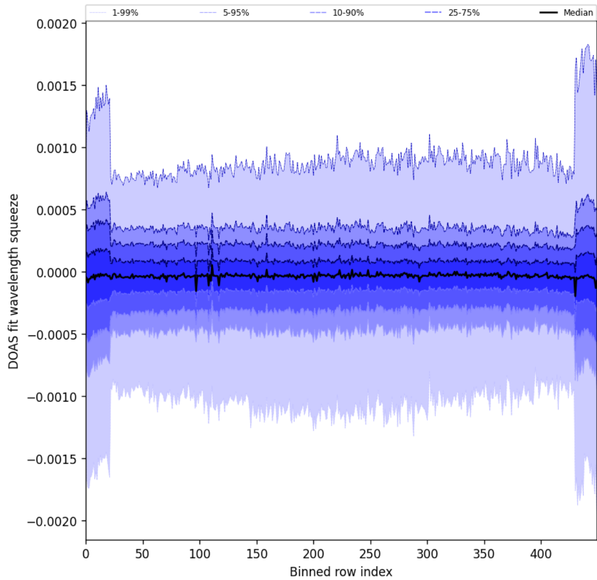
Figure 92: Along track statistics of “DOAS fit wavelength squeeze” for 2024-09-03 to 2024-09-05
