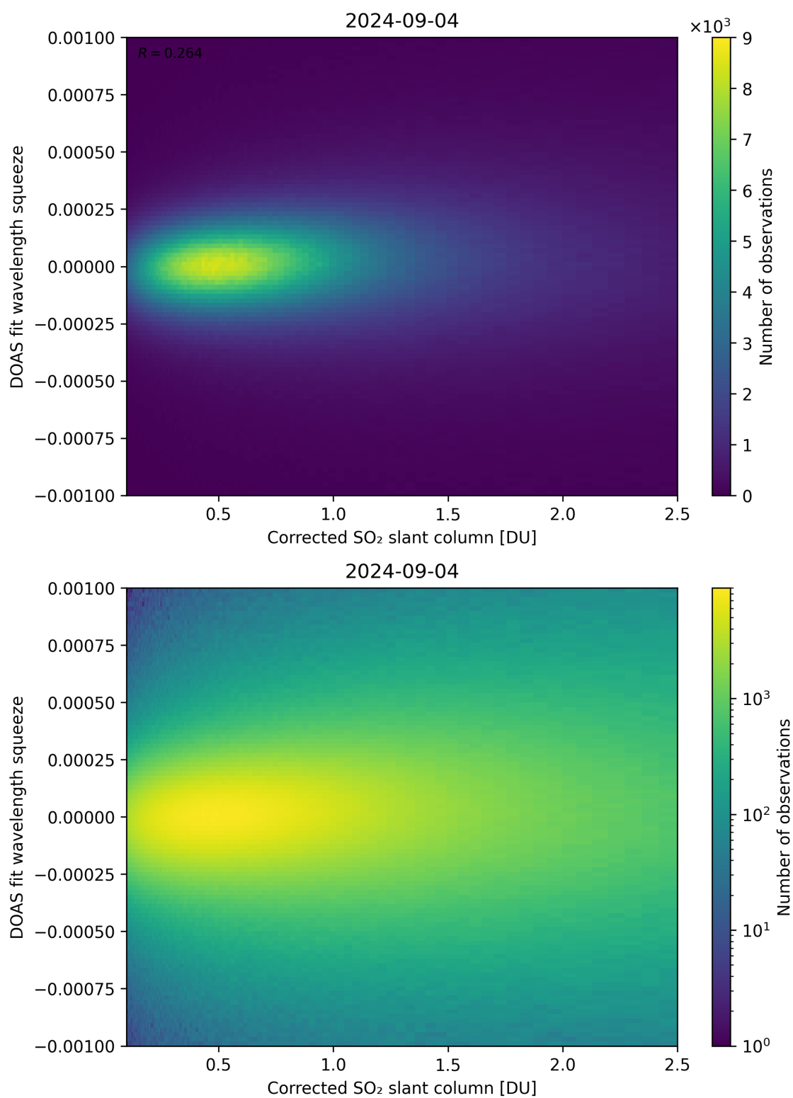
Figure 182: Scatter density plot of “Corrected SO 2 slant column” against “DOAS fit wavelength squeeze” for 2024-09-03 to 2024-09-05.
