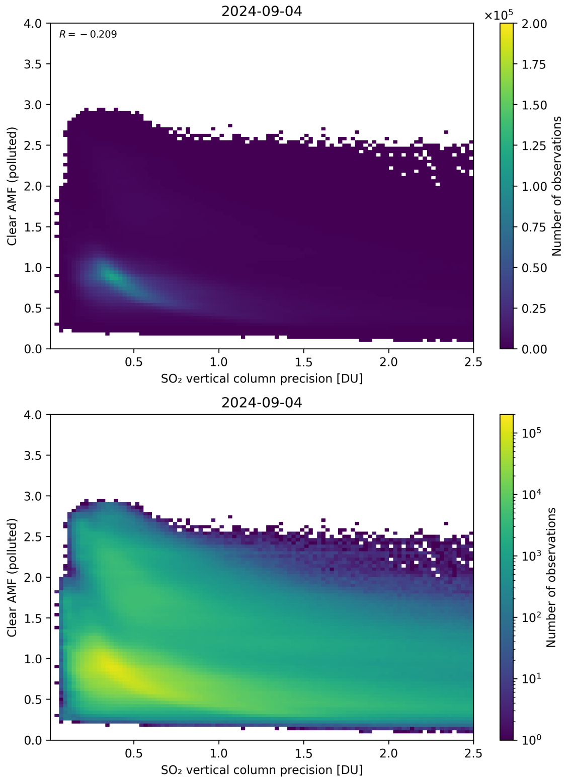
Figure 285: Scatter density plot of “SO 2 vertical column precision” against “Clear AMF (polluted)” for 2024-09-03 to 2024-09-05.
