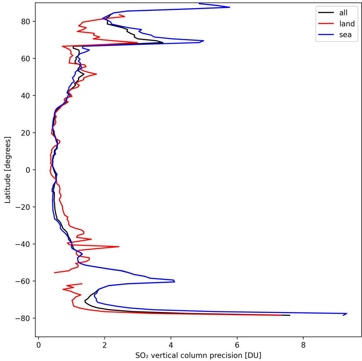
Figure 31: Zonal average of “SO 2 vertical column precision” for 2024-09-03 to 2024-09-05.
