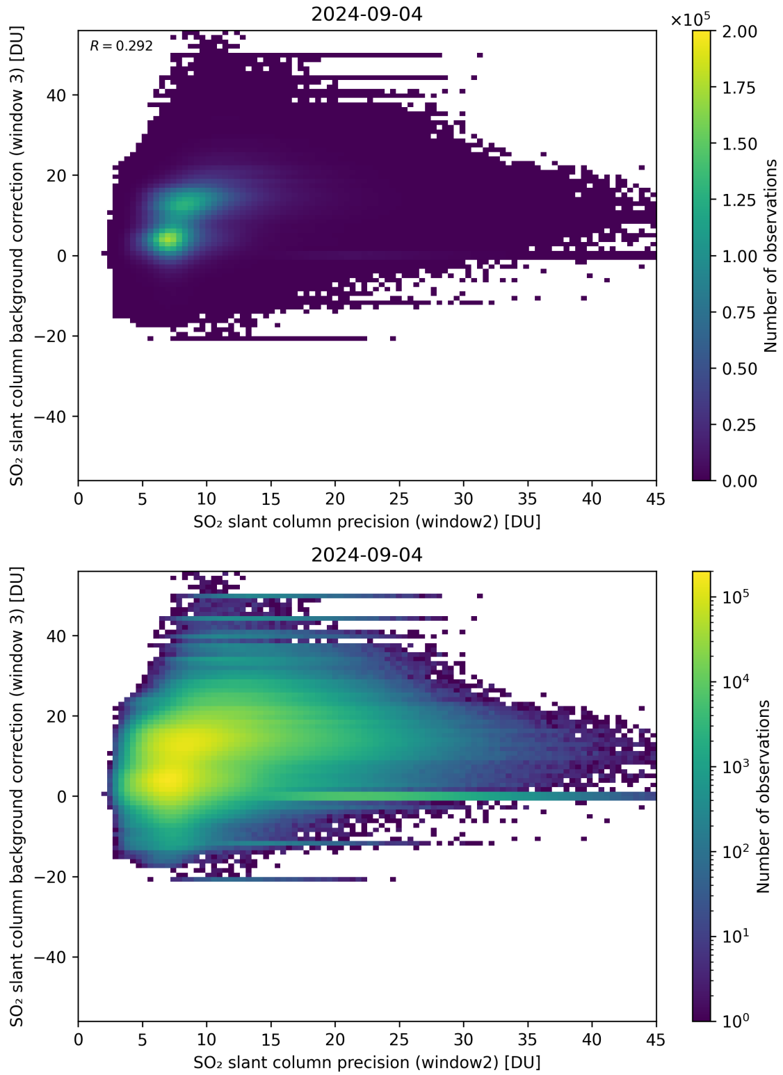
Figure 242: Scatter density plot of “SO 2 slant column precision (window2)” against “SO 2 slant column background correction (window 3)” for 2024-09-03 to 2024-09-05.
