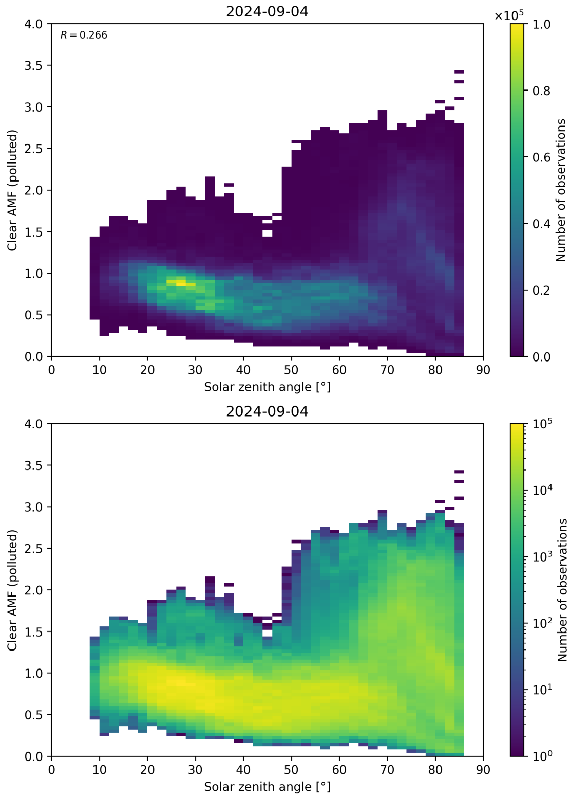
Figure 165: Scatter density plot of “Solar zenith angle” against “Clear AMF (polluted)” for 2024-09-03 to 2024-09-05.
