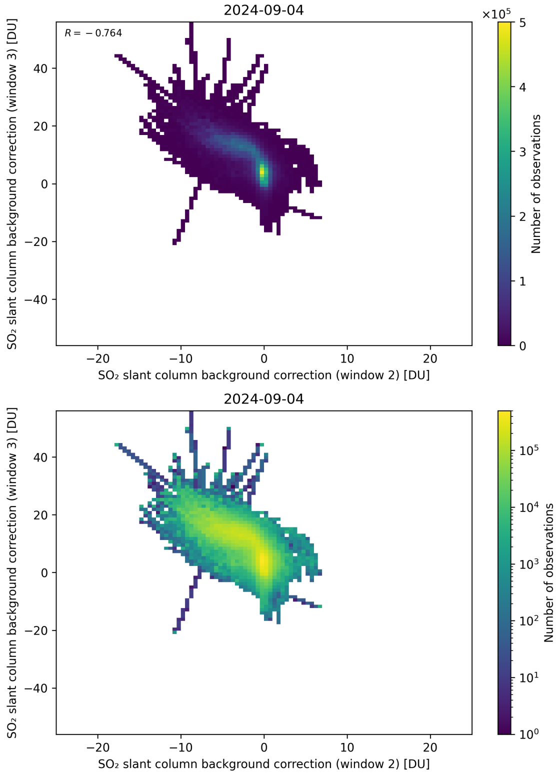
Figure 111: Scatter density plot of “SO 2 slant column background correction (window 2)” against “SO 2 slant column background correction (window 3)” for 2024-09-03 to 2024-09-05.
