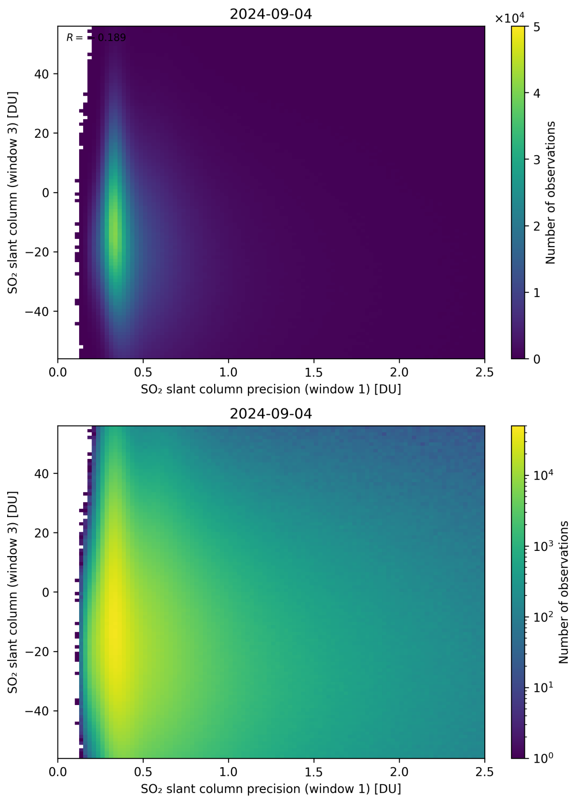
Figure 228: Scatter density plot of “SO 2 slant column precision (window 1)” against “SO 2 slant column (window 3)” for 2024-09-03 to 2024-09-05.
