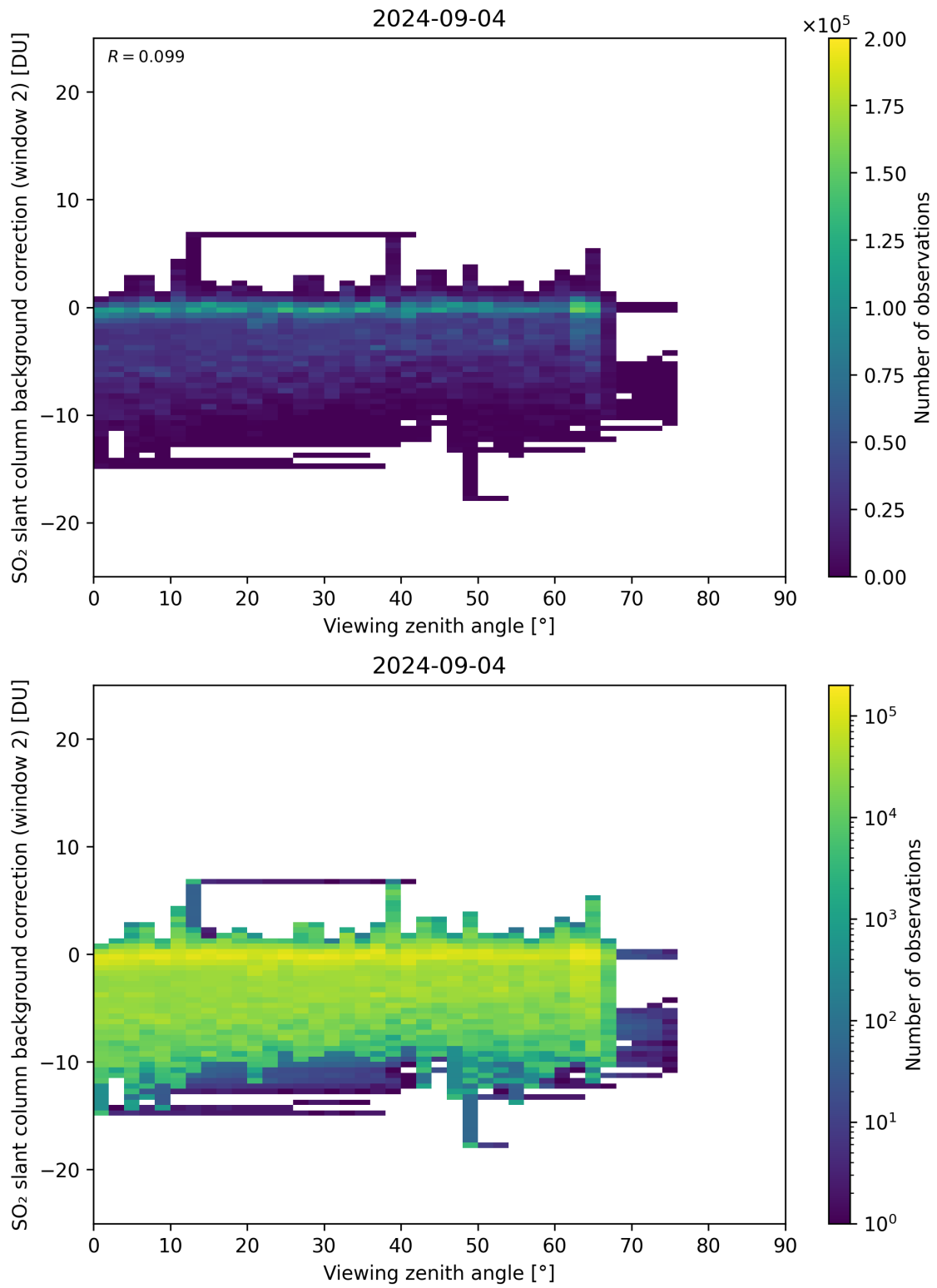
Figure 309: Scatter density plot of “Viewing zenith angle” against “SO 2 slant column background correction (window 2)” for 2024-09-03 to 2024-09-05.
