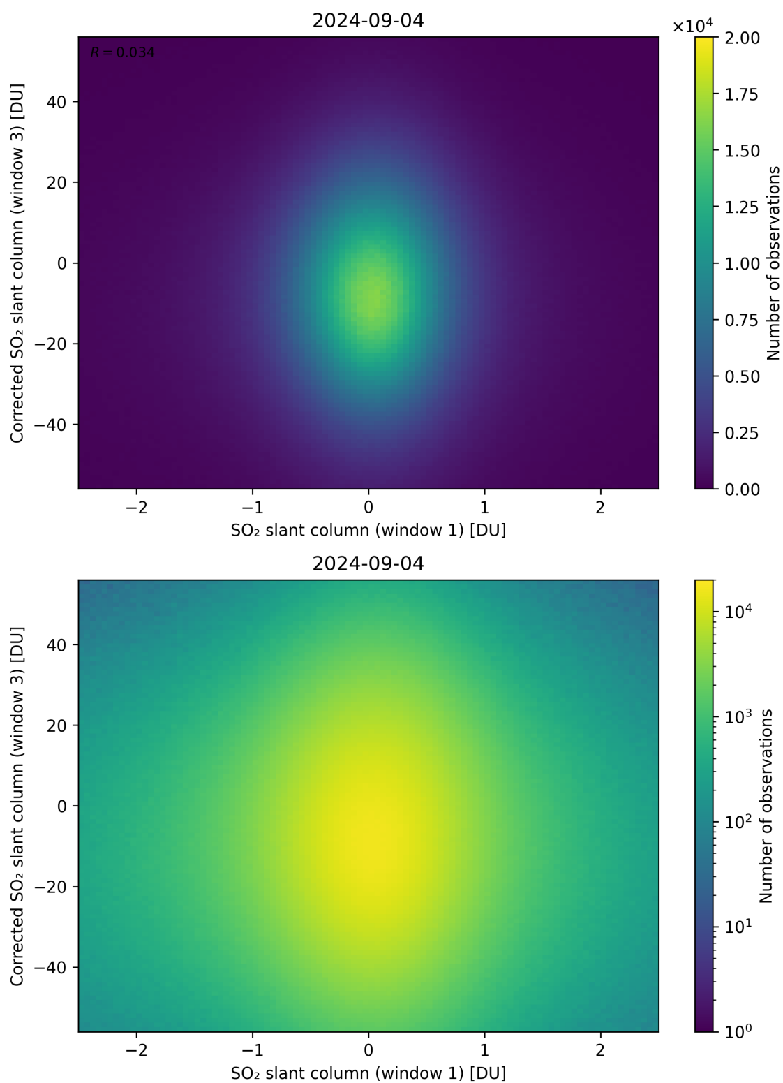
Figure 234: Scatter density plot of “SO 2 slant column (window 1)” against “Corrected SO 2 slant column (window 3)” for 2024-09-03 to 2024-09-05.
