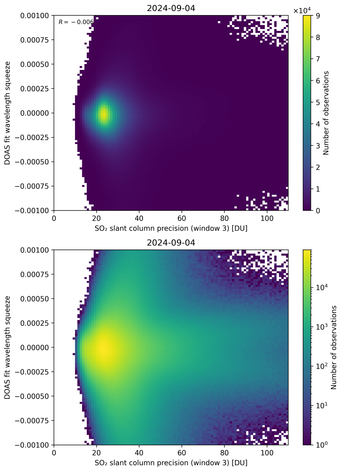
Figure 259: Scatter density plot of “SO 2 slant column precision (window 3)” against “DOAS fit wavelength squeeze” for 2024-09-03 to 2024-09-05.
