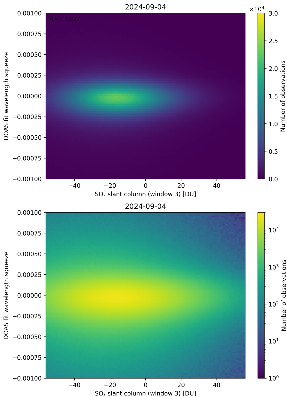
Figure 255: Scatter density plot of “SO 2 slant column (window 3)” against “DOAS fit wavelength squeeze” for 2024-09-03 to 2024-09-05.
