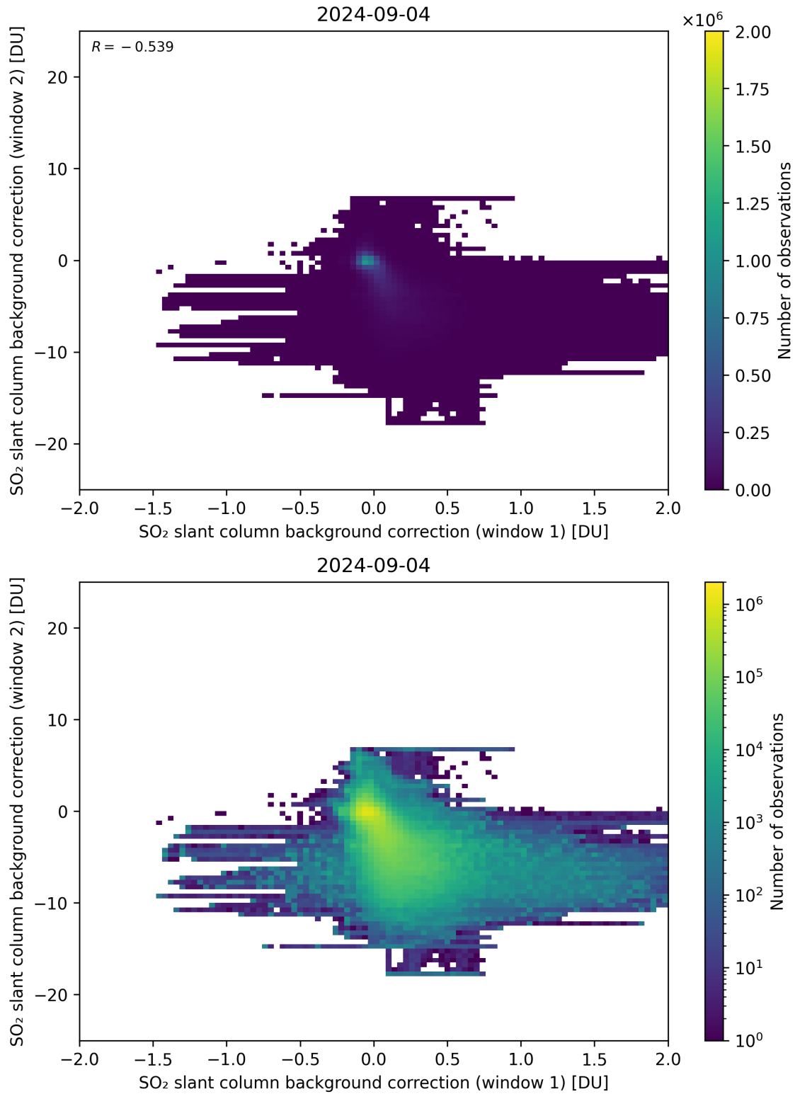
Figure 98: Scatter density plot of “SO 2 slant column background correction (window 1)” against “SO 2 slant column background correction (window 2)” for 2024-09-03 to 2024-09-05.
