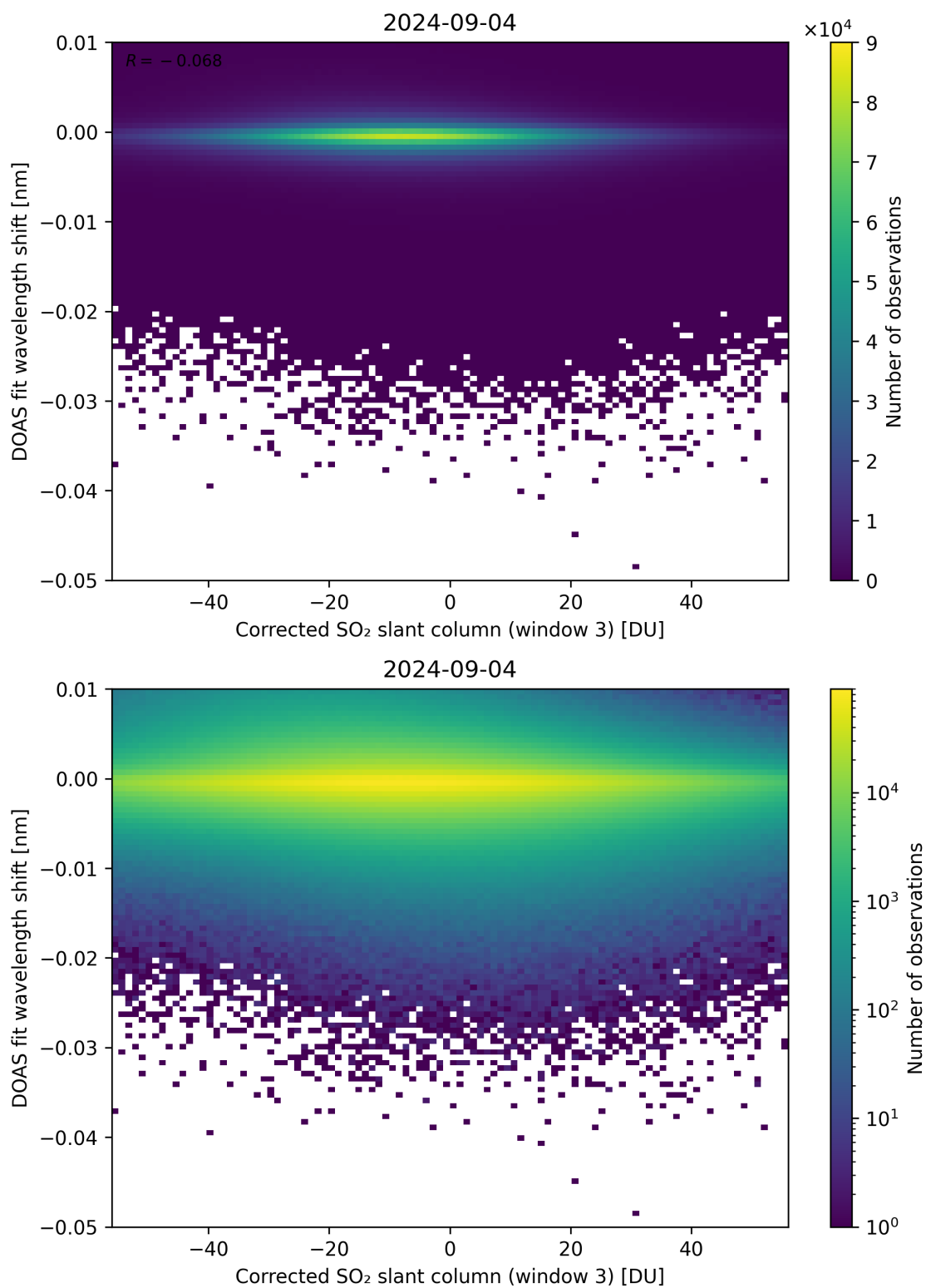
Figure 206: Scatter density plot of “Corrected SO 2 slant column (window 3)” against “DOAS fit wavelength shift” for 2024-09-03 to 2024-09-05.
