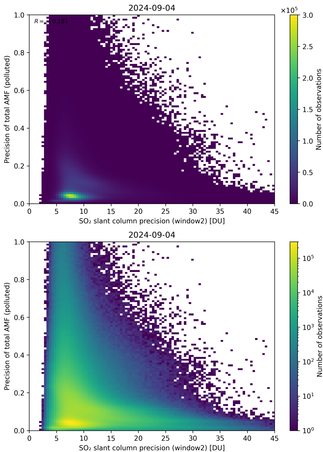
Figure 252: Scatter density plot of “SO 2 slant column precision (window2)” against “Precision of total AMF (polluted)” for 2024-09-03 to 2024-09-05.
