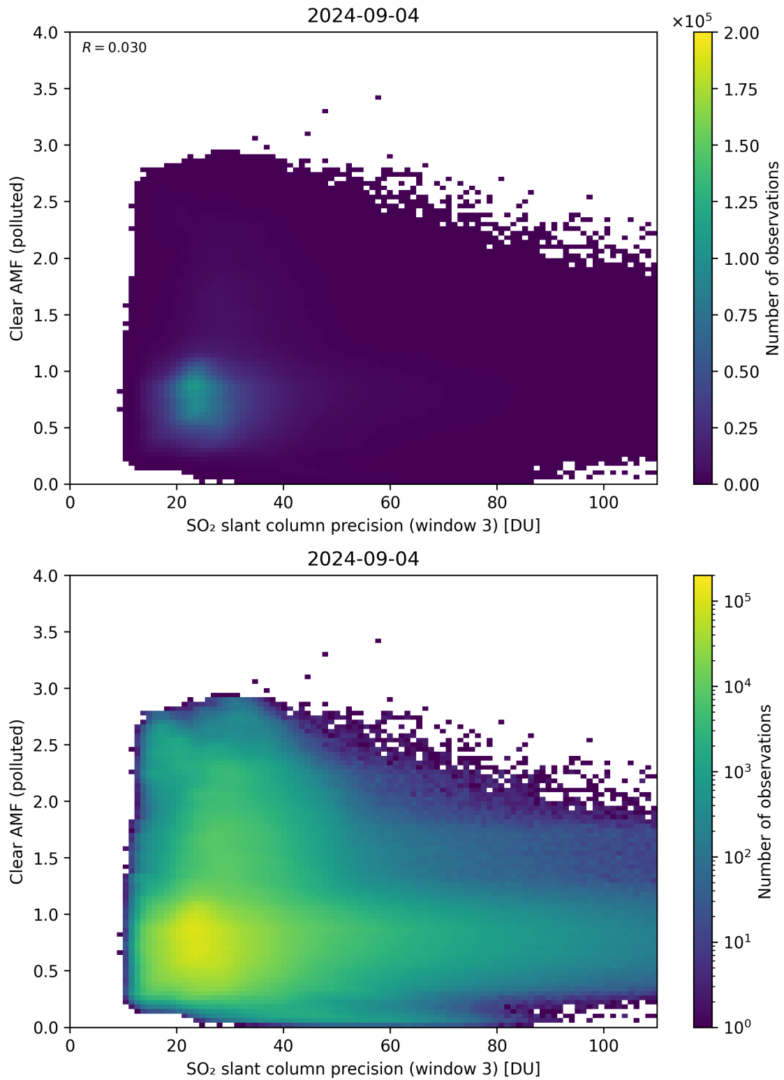
Figure 261: Scatter density plot of “SO 2 slant column precision (window 3)” against “Clear AMF (polluted)” for 2024-09-03 to 2024-09-05.
