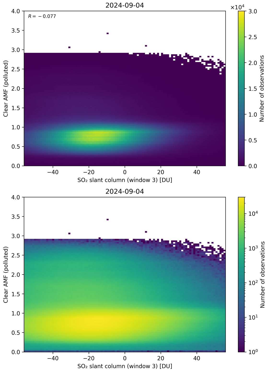
Figure 265: Scatter density plot of “SO 2 slant column (window 3)” against “Clear AMF (polluted)” for 2024-09-03 to 2024-09-05.
