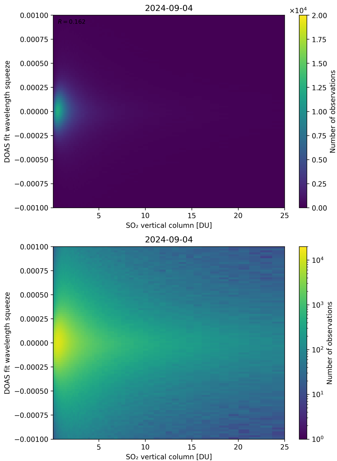
Figure 277: Scatter density plot of “SO 2 vertical column” against “DOAS fit wavelength squeeze” for 2024-09-03 to 2024-09-05.
