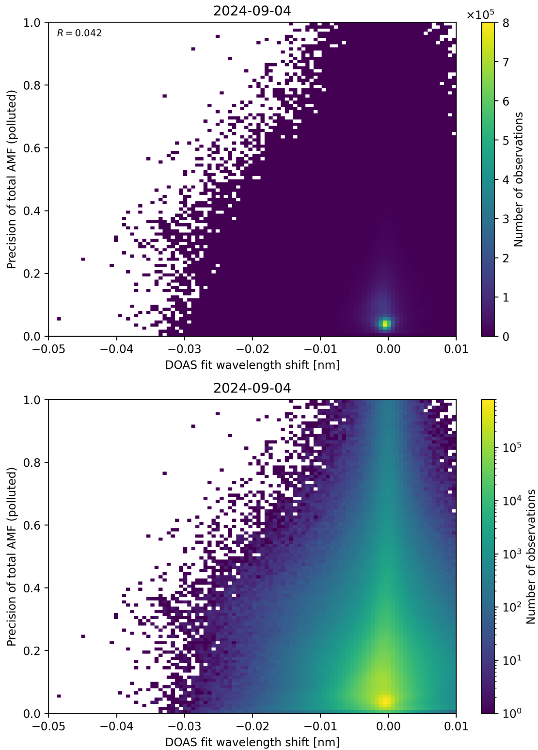
Figure 131: Scatter density plot of “DOAS fit wavelength shift” against “Precision of total AMF (polluted)” for 2024-09-03 to 2024-09-05.
