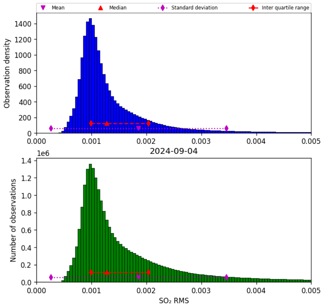
Figure 70: Histogram of “SO 2 RMS” for 2024-09-03 to 2024-09-05
