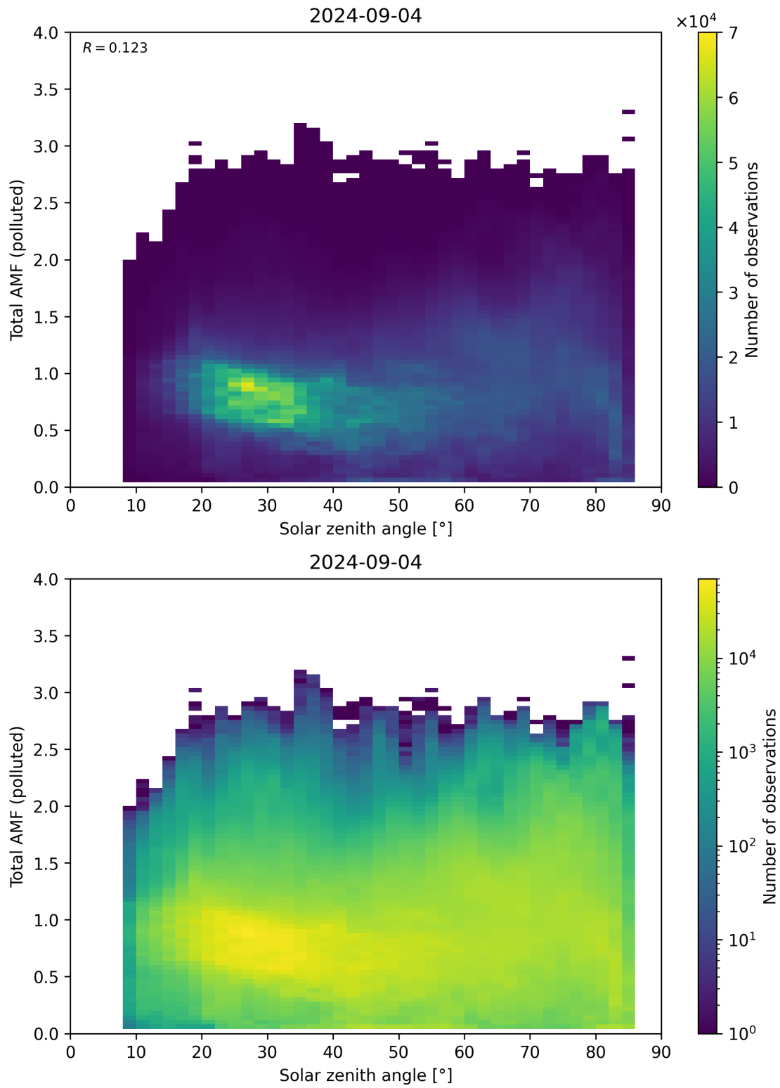
Figure 174: Scatter density plot of “Solar zenith angle” against “Total AMF (polluted)” for 2024-09-03 to 2024-09-05.
