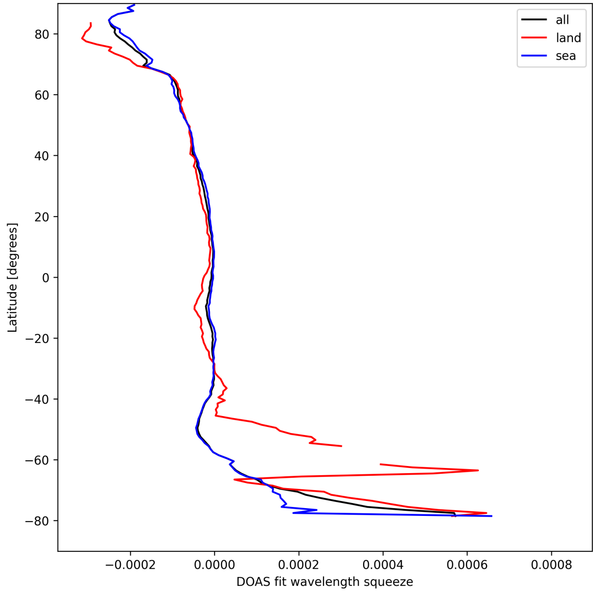
Figure 46: Zonal average of “DOAS fit wavelength squeeze” for 2024-09-03 to 2024-09-05.
