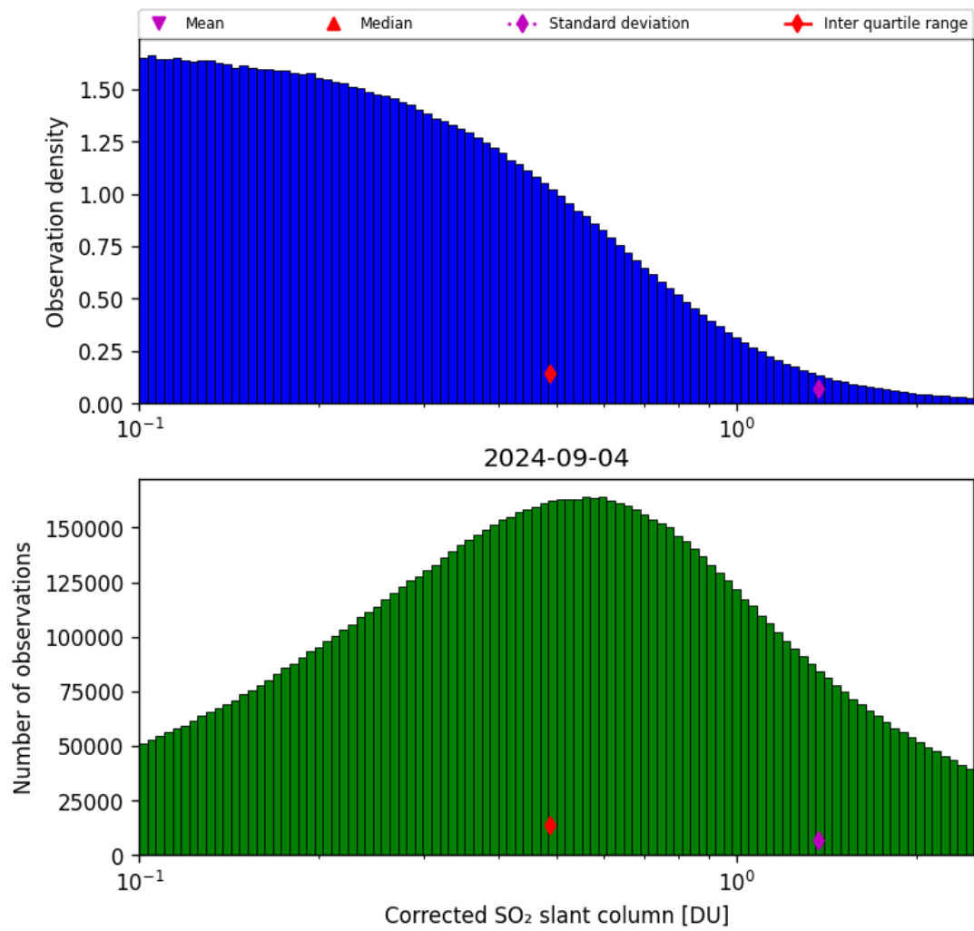
Figure 55: Histogram of "Corrected SO 2 slant column" for 2024-09-03 to 2024-09-05
