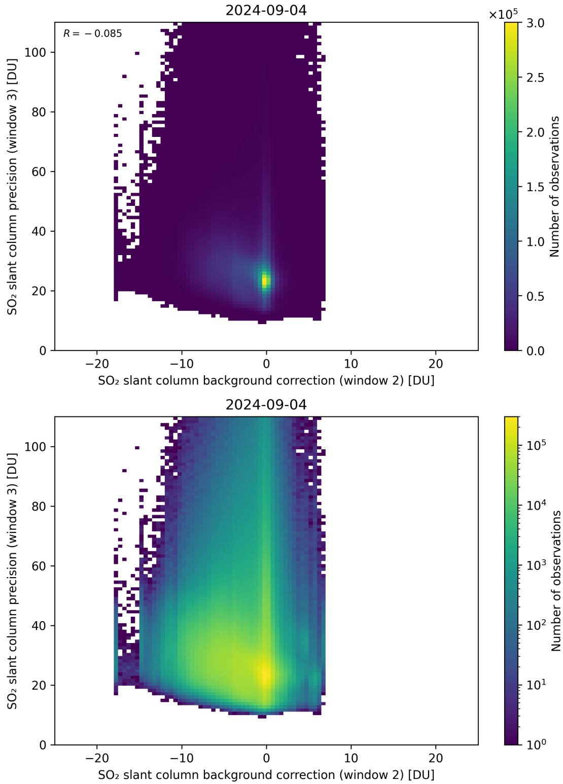
Figure 118: Scatter density plot of “SO 2 slant column background correction (window 2)” against “SO 2 slant column precision (window 3)” for 2024-09-03 to 2024-09-05.
