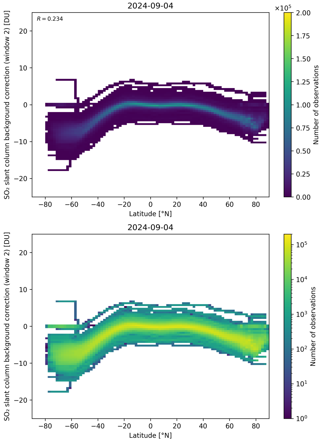
Figure 140: Scatter density plot of “Latitude” against “SO 2 slant column background correction (window 2)” for 2024-09-03 to 2024-09-05.
