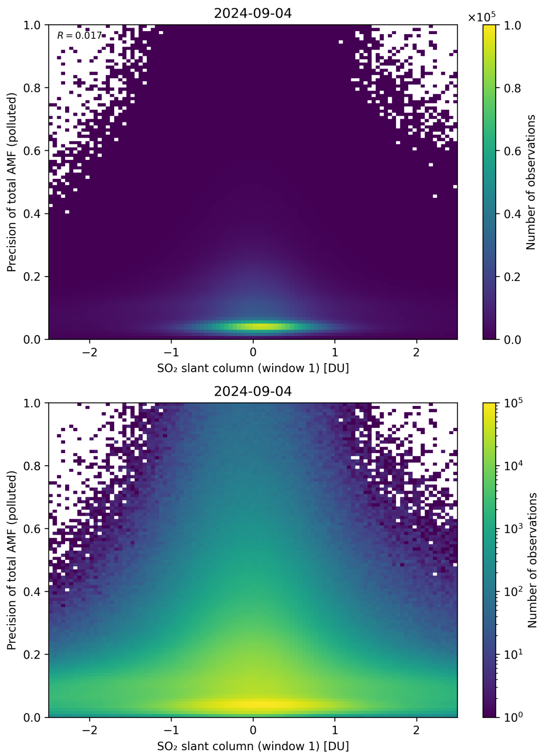
Figure 240: Scatter density plot of “SO 2 slant column (window 1)” against “Precision of total AMF (polluted)” for 2024-09-03 to 2024-09-05.
