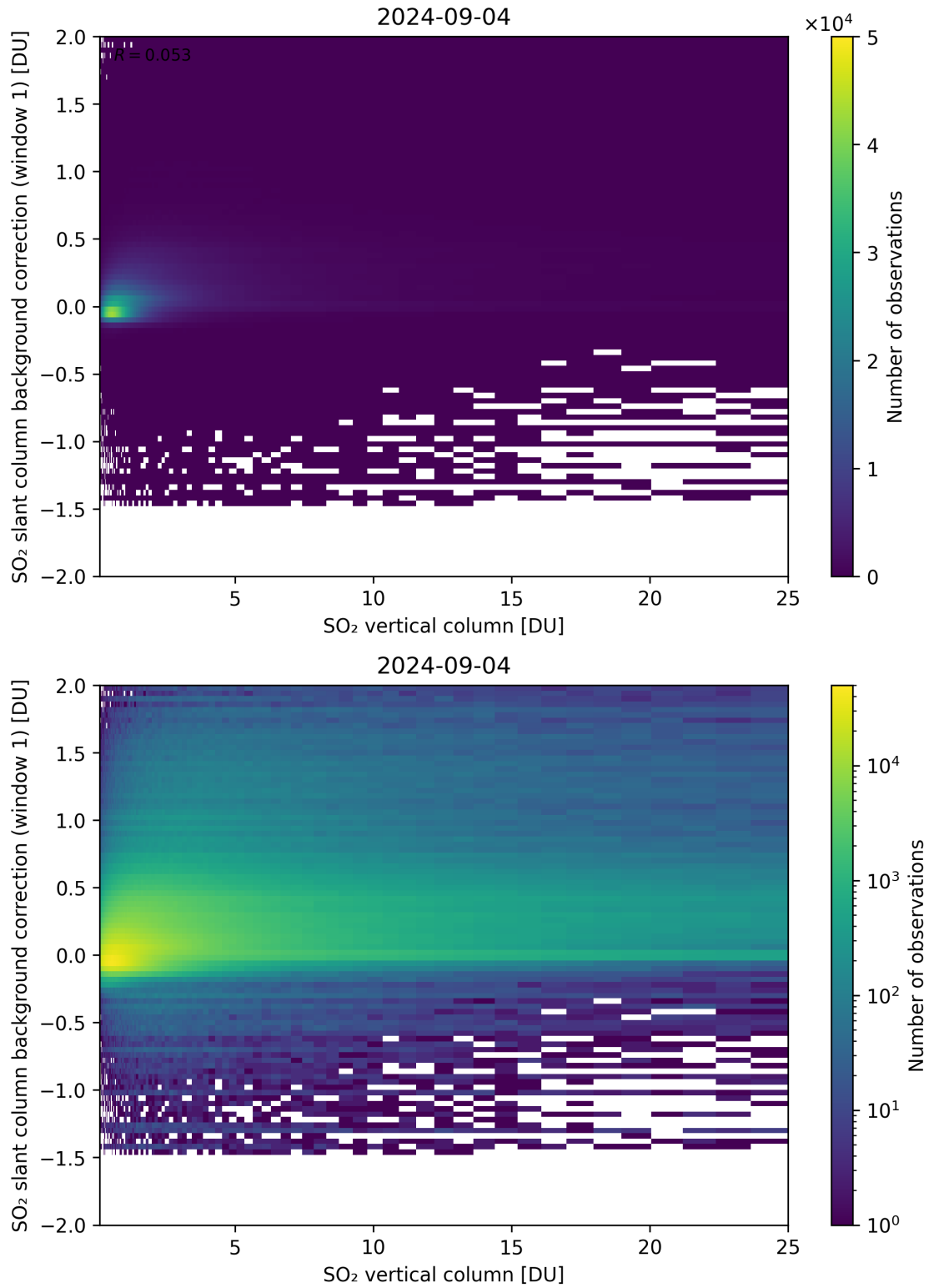
Figure 273: Scatter density plot of “SO 2 vertical column” against “SO 2 slant column background correction (window 1)” for 2024-09-03 to 2024-09-05.
