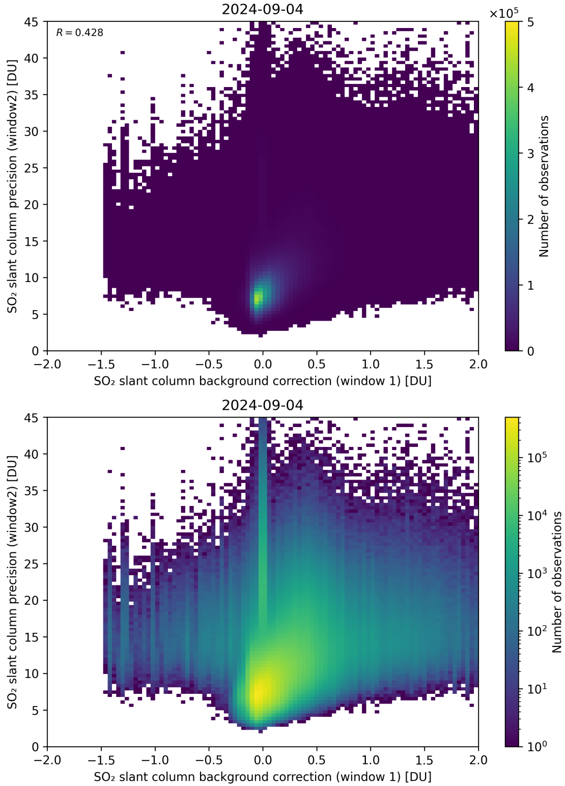
Figure 106: Scatter density plot of “SO 2 slant column background correction (window 1)” against “SO 2 slant column precision (window2)” for 2024-09-03 to 2024-09-05.
