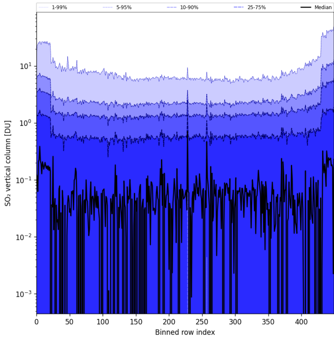
Figure 76: Along track statistics of “SO 2 vertical column” for 2024-09-03 to 2024-09-05
