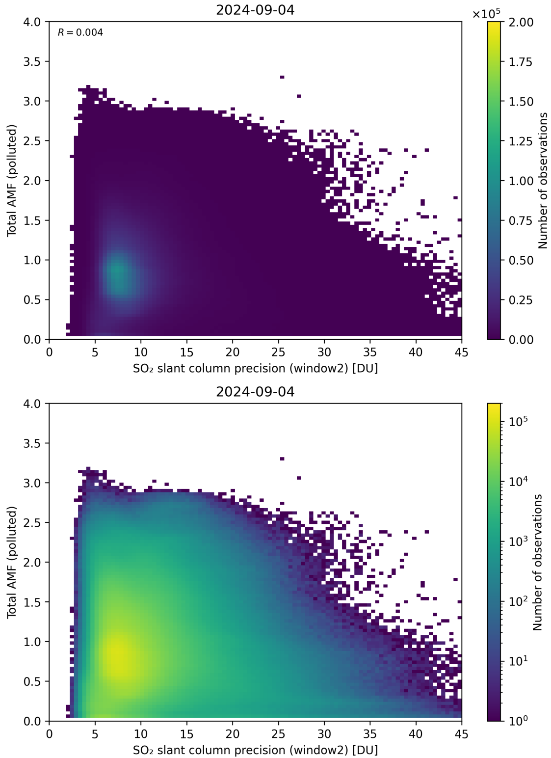
Figure 251: Scatter density plot of “SO 2 slant column precision (window2)” against “Total AMF (polluted)” for 2024-09-03 to 2024-09-05.
