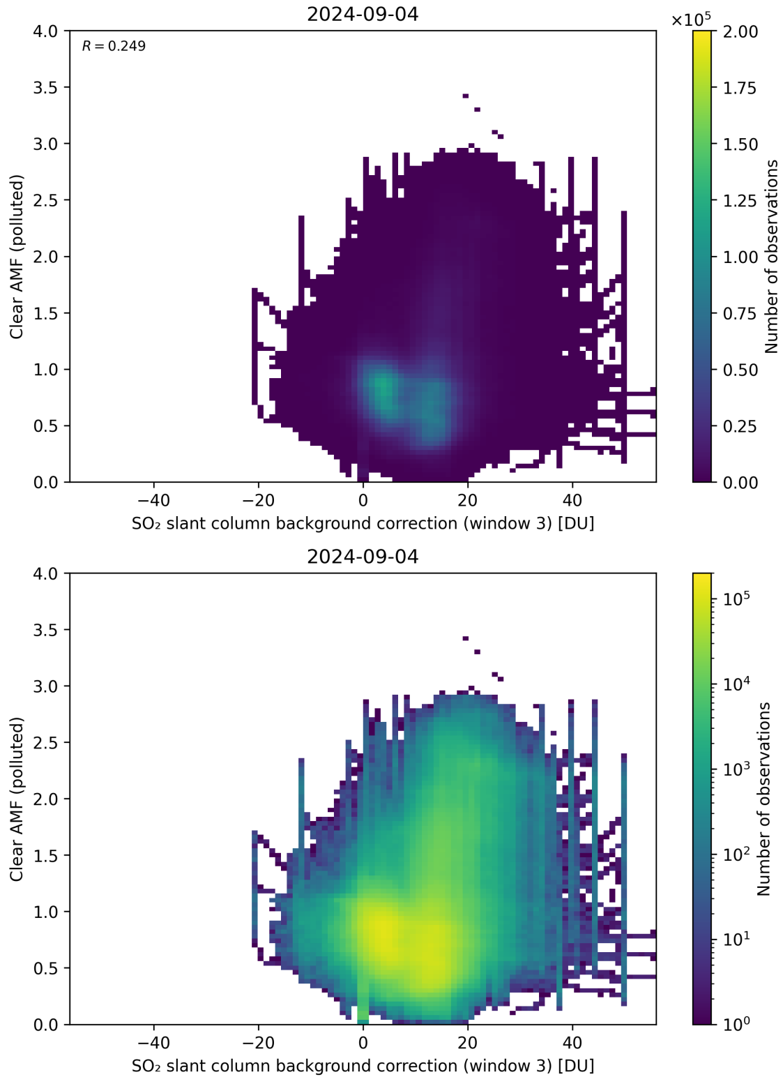
Figure 124: Scatter density plot of “SO 2 slant column background correction (window 3)” against “Clear AMF (polluted)” for 2024-09-03 to 2024-09-05.
