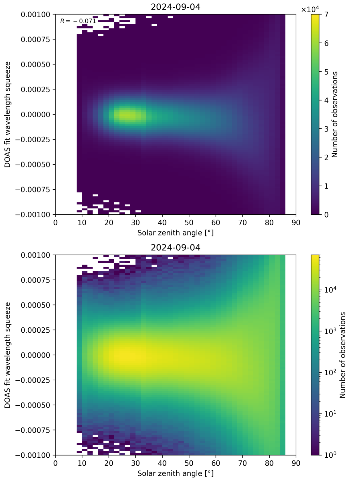
Figure 162: Scatter density plot of “Solar zenith angle” against “DOAS fit wavelength squeeze” for 2024-09-03 to 2024-09-05.
