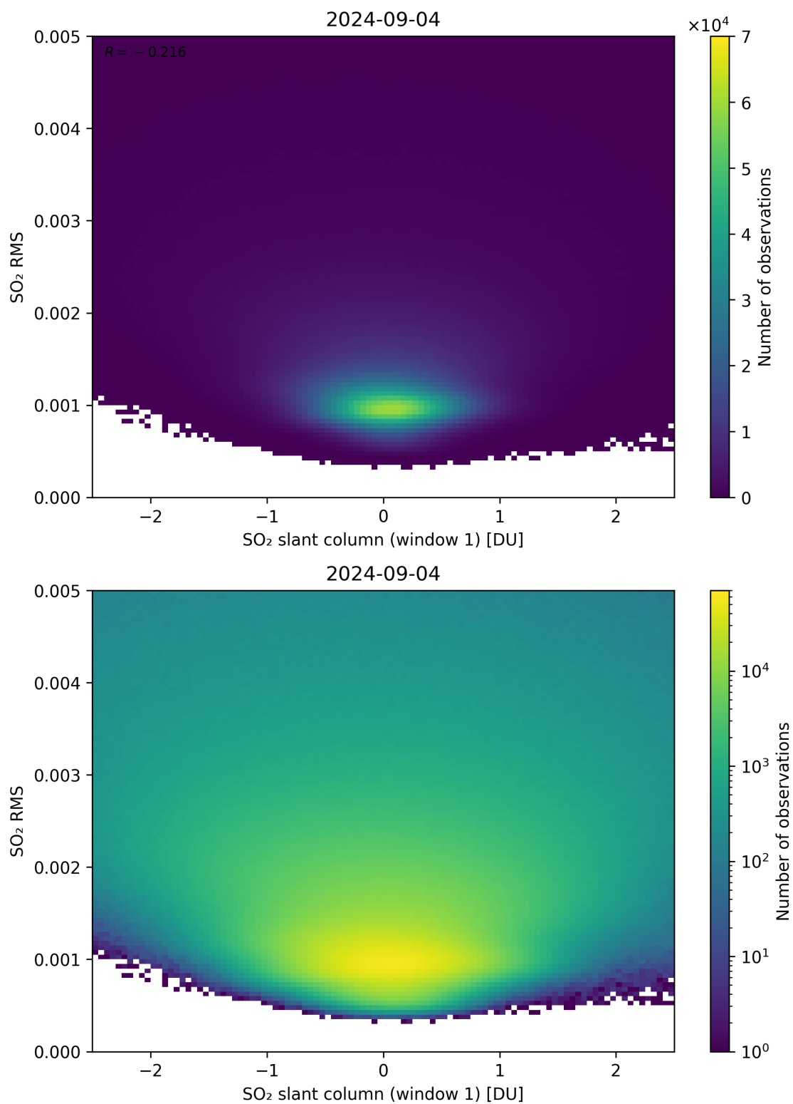
Figure 217: Scatter density plot of “SO 2 slant column (window 1)” against “SO 2 RMS” for 2024-09-03 to 2024-09-05.
