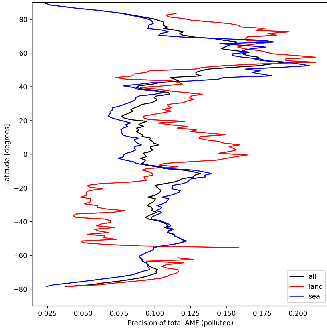
Figure 49: Zonal average of “Precision of total AMF (polluted)” for 2024-09-03 to 2024-09-05.
