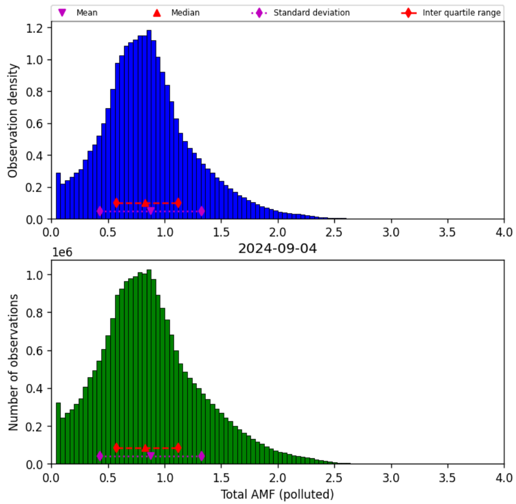
Figure 71: Histogram of “Total AMF (polluted)” for 2024-09-03 to 2024-09-05
