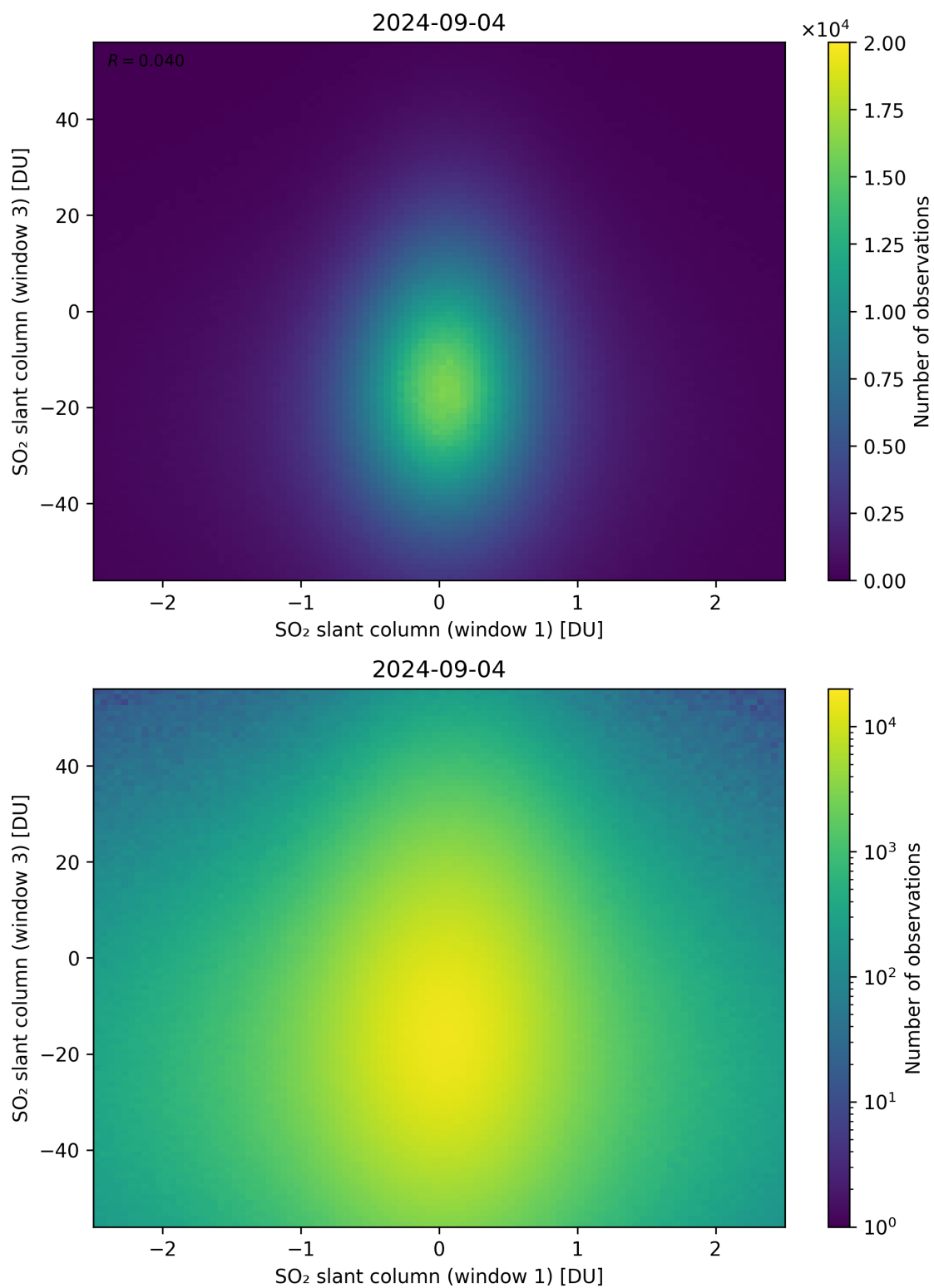
Figure 237: Scatter density plot of “SO 2 slant column (window 1)” against “SO 2 slant column (window 3)” for 2024-09-03 to 2024-09-05.
