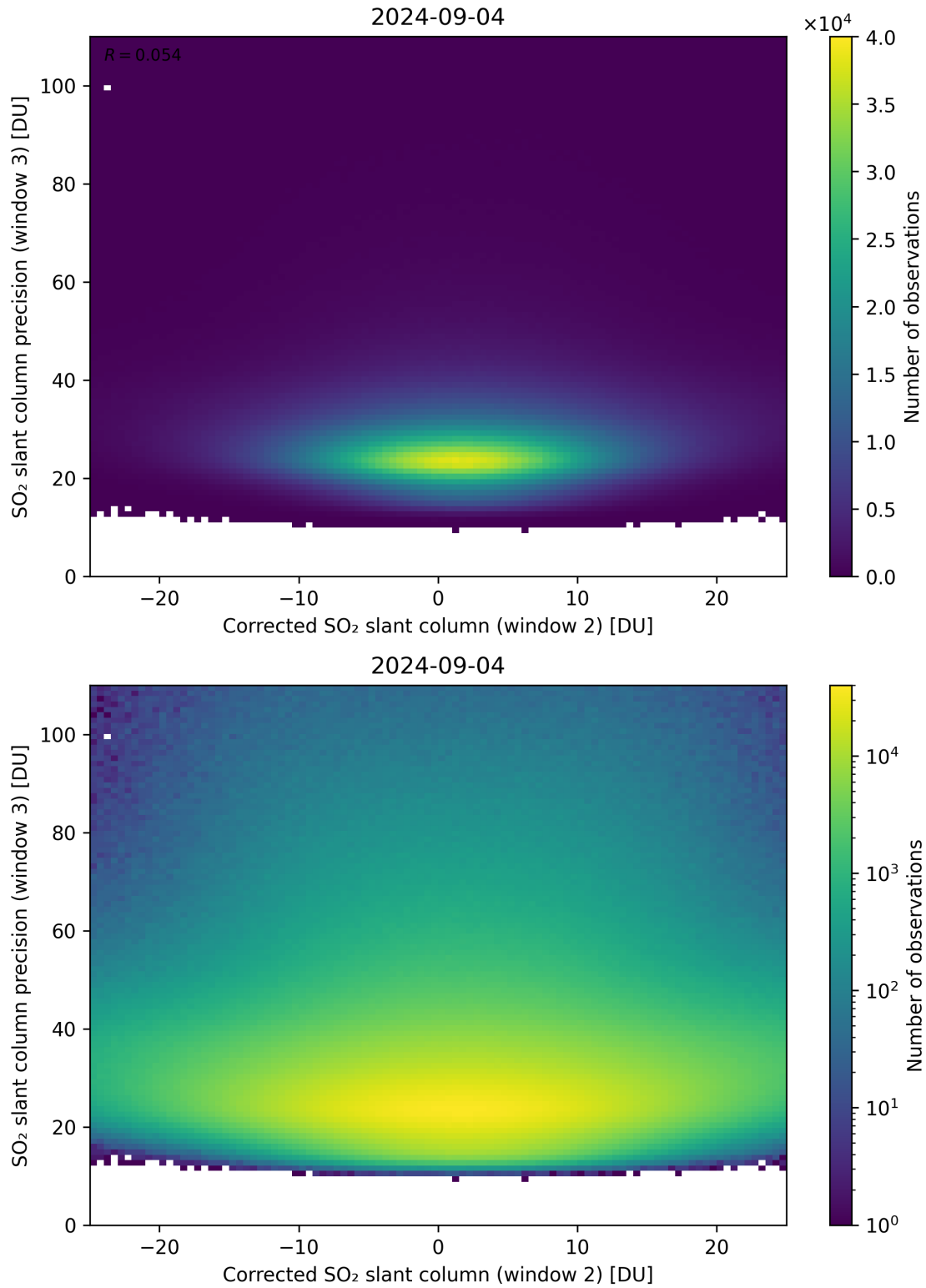
Figure 202: Scatter density plot of “Corrected SO 2 slant column (window 2)” against “SO 2 slant column precision (window 3)” for 2024-09-03 to 2024-09-05.
