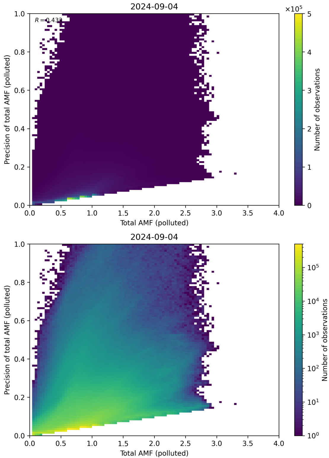
Figure 272: Scatter density plot of “Total AMF (polluted)” against “Precision of total AMF (polluted)” for 2024-09-03 to 2024-09-05.
