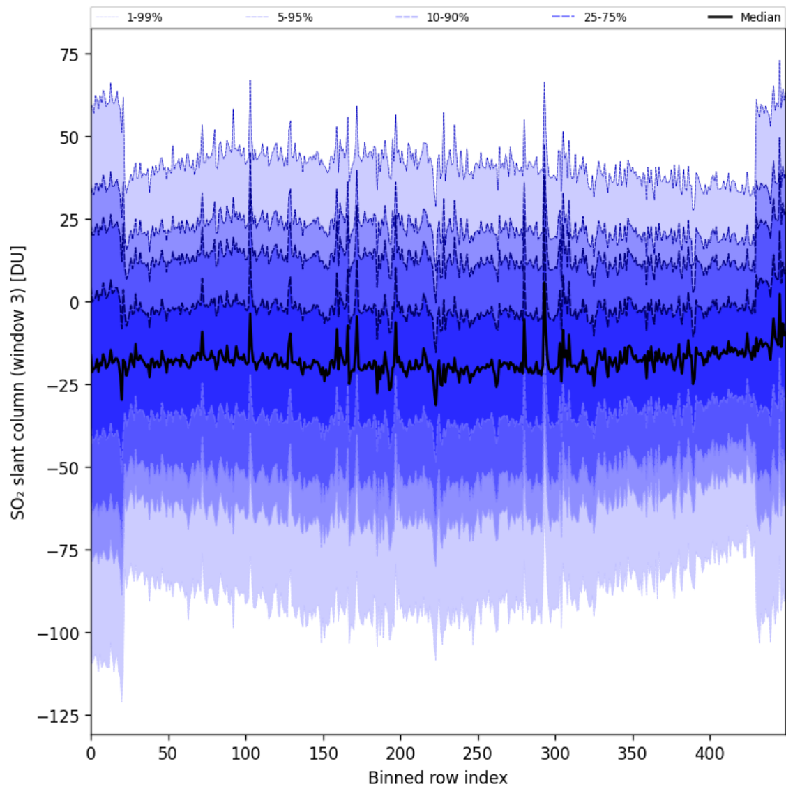
Figure 87: Along track statistics of “SO 2 slant column (window 3)” for 2024-09-03 to 2024-09-05
