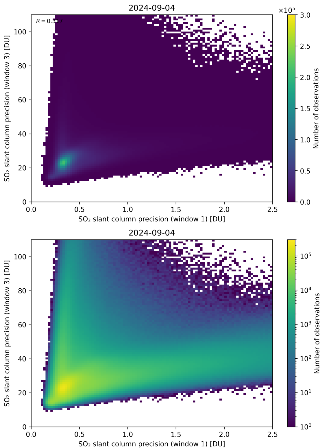
Figure 229: Scatter density plot of “SO 2 slant column precision (window 1)” against “SO 2 slant column precision (window 3)” for 2024-09-03 to 2024-09-05.
