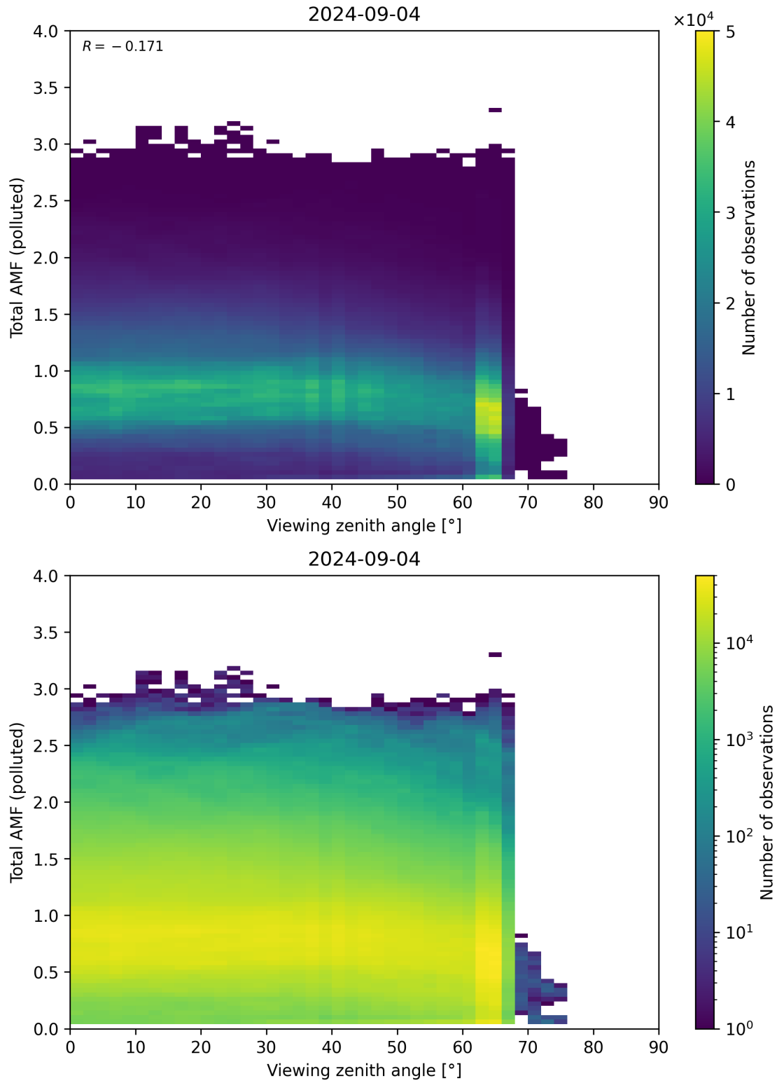
Figure 325: Scatter density plot of “Viewing zenith angle” against “Total AMF (polluted)” for 2024-09-03 to 2024-09-05.
