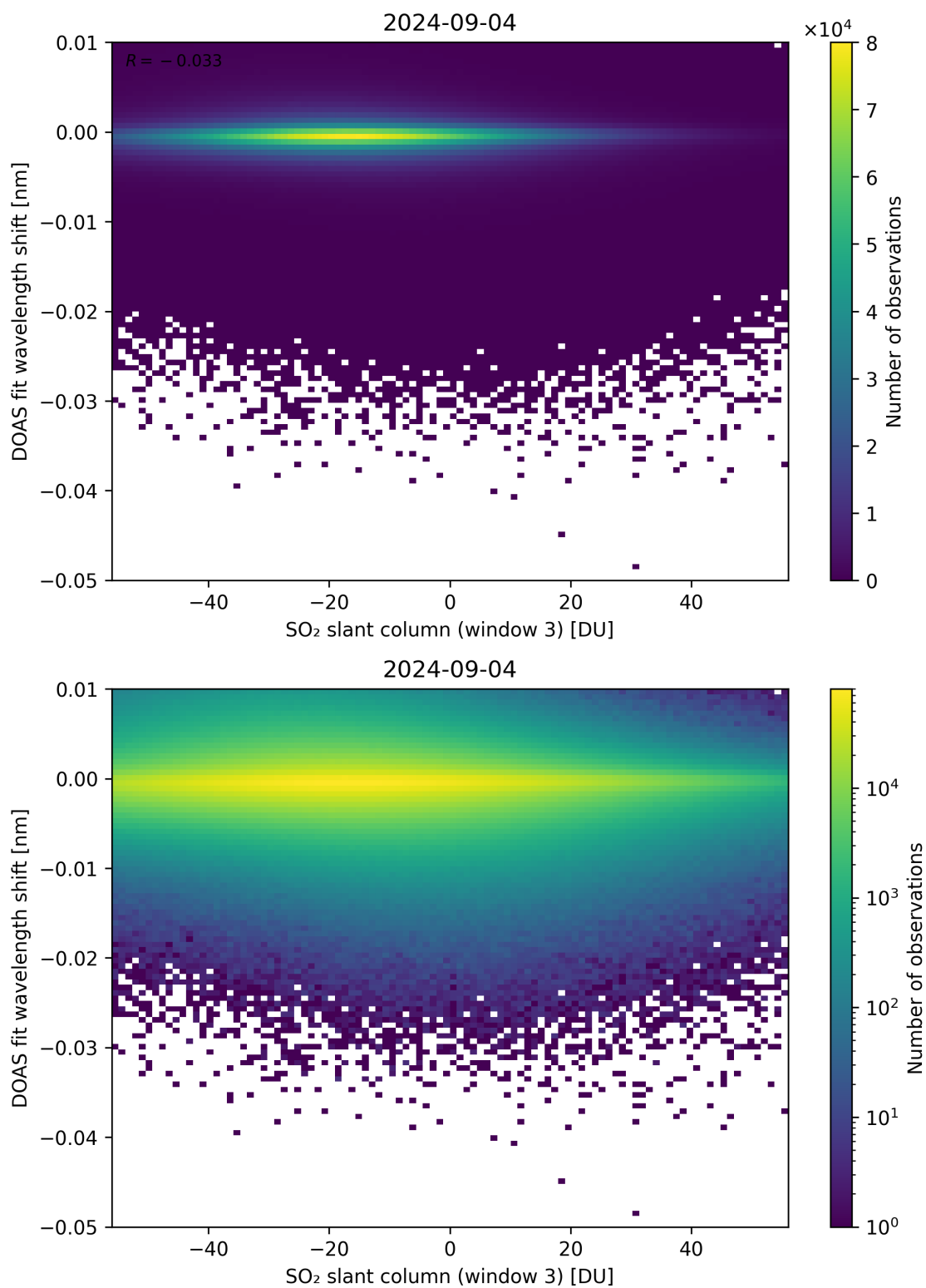
Figure 254: Scatter density plot of “SO 2 slant column (window 3)” against “DOAS fit wavelength shift” for 2024-09-03 to 2024-09-05.
