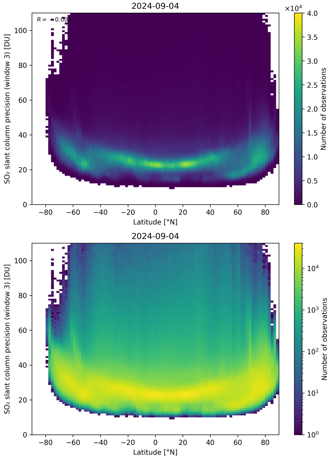
Figure 153: Scatter density plot of “Latitude” against “SO 2 slant column precision (window 3)” for 2024-09-03 to 2024-09-05.
