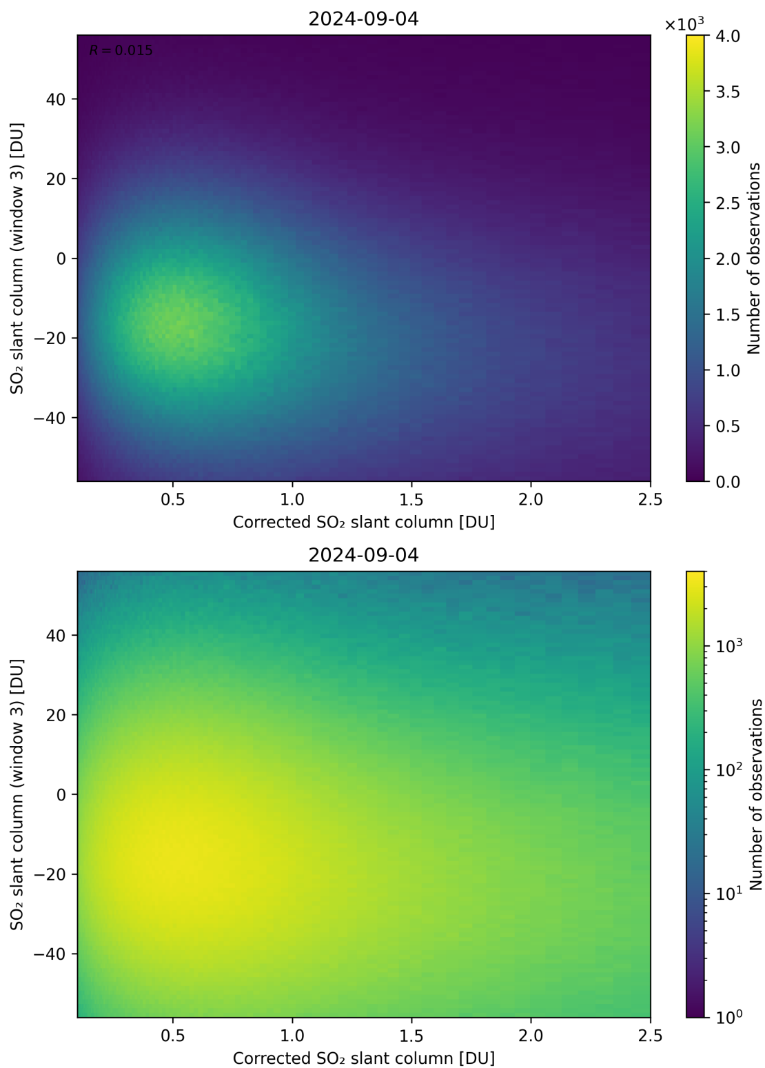
Figure 190: Scatter density plot of “Corrected SO 2 slant column” against “SO 2 slant column (window 3)” for 2024-09-03 to 2024-09-05.
