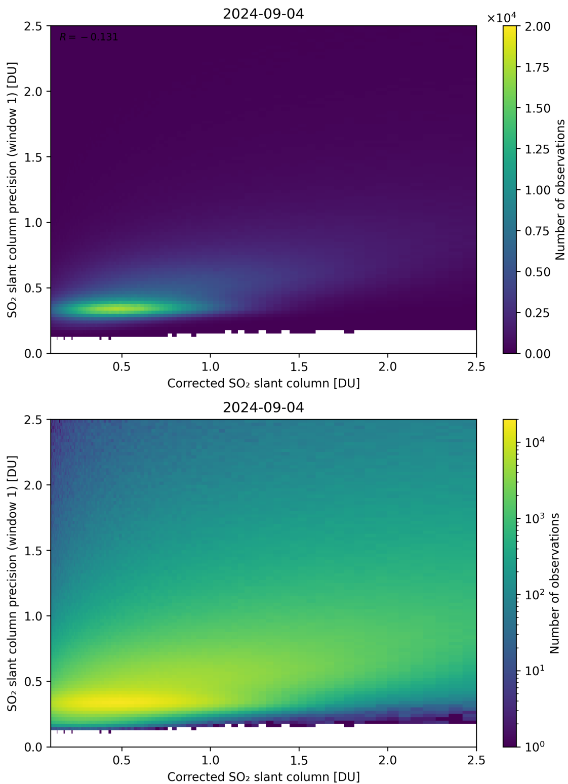
Figure 188: Scatter density plot of “Corrected SO 2 slant column” against “SO 2 slant column precision (window 1)” for 2024-09-03 to 2024-09-05.
