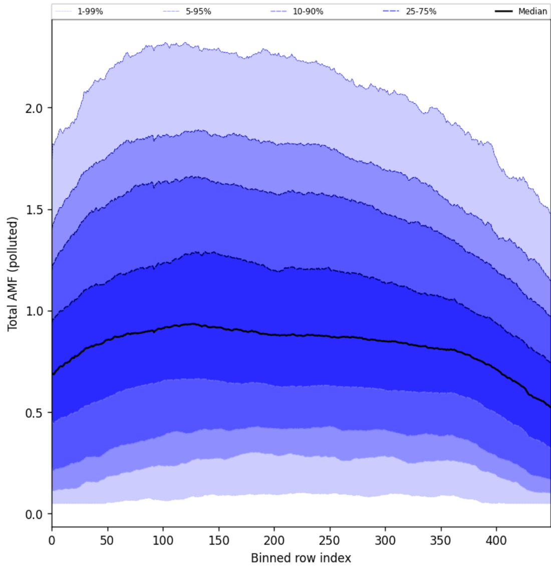
Figure 94: Along track statistics of “Total AMF (polluted)” for 2024-09-03 to 2024-09-05
