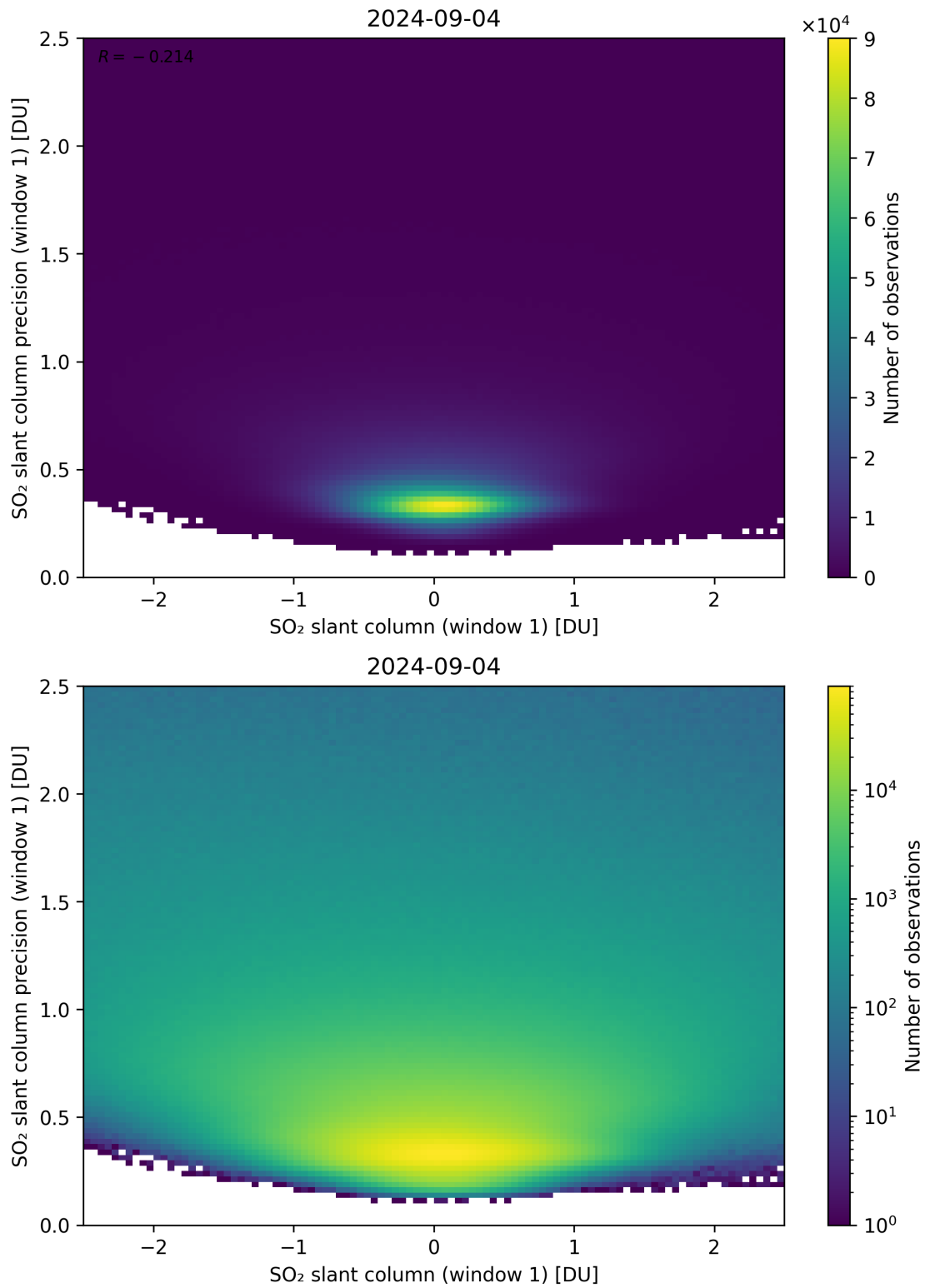
Figure 235: Scatter density plot of “SO 2 slant column (window 1)” against “SO 2 slant column precision (window 1)” for 2024-09-03 to 2024-09-05.
