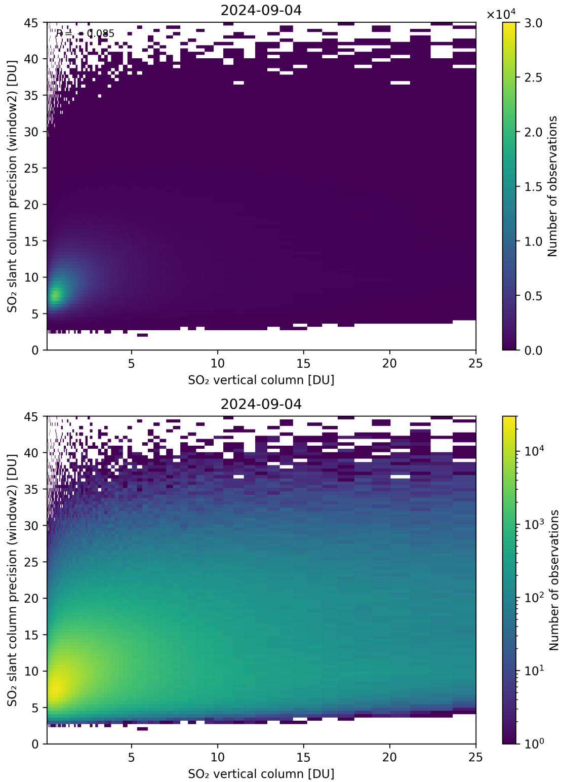
Figure 302: Scatter density plot of “SO 2 vertical column” against “SO 2 slant column precision (window2)” for 2024-09-03 to 2024-09-05.
