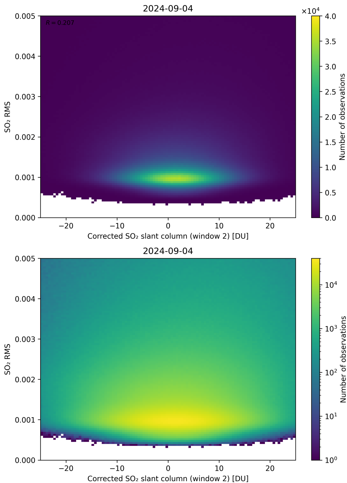
Figure 198: Scatter density plot of “Corrected SO 2 slant column (window 2)” against “SO 2 RMS” for 2024-09-03 to 2024-09-05.
