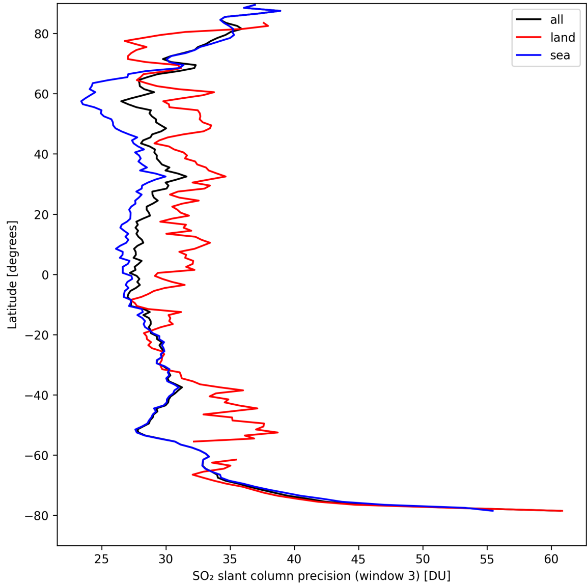
Figure 42: Zonal average of “SO 2 slant column precision (window 3)” for 2024-09-03 to 2024-09-05.
