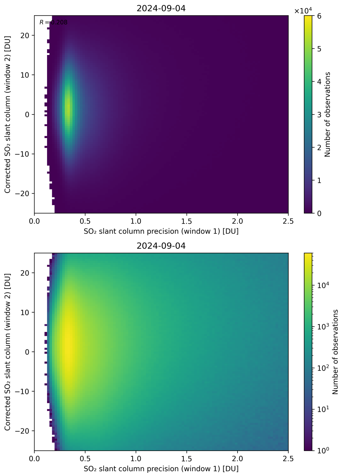
Figure 225: Scatter density plot of “SO 2 slant column precision (window 1)” against “Corrected SO 2 slant column (window 2)” for 2024-09-03 to 2024-09-05.
