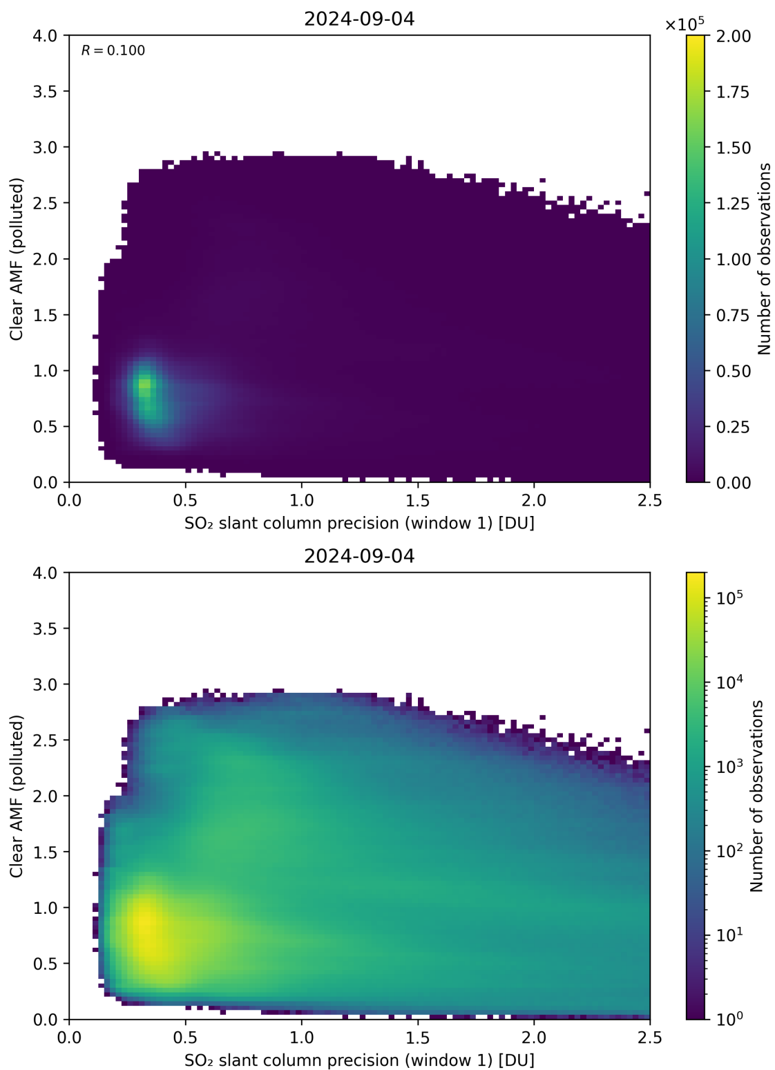
Figure 224: Scatter density plot of “SO 2 slant column precision (window 1)” against “Clear AMF (polluted)” for 2024-09-03 to 2024-09-05.
