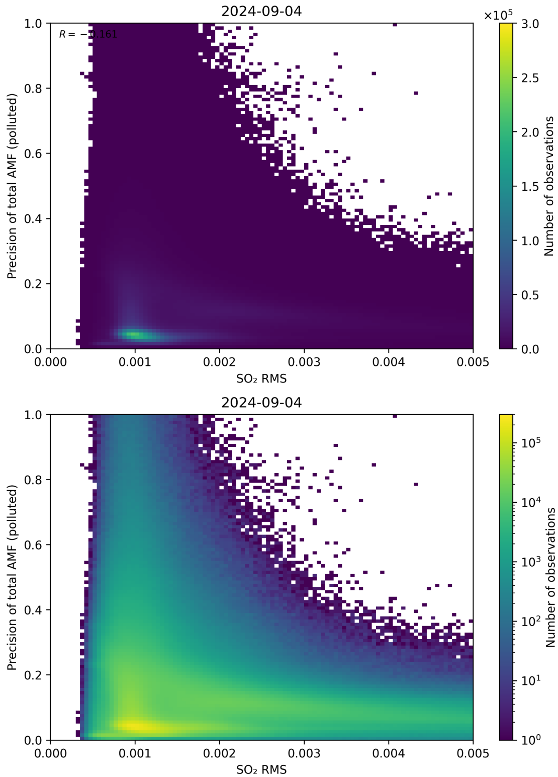
Figure 138: Scatter density plot of “SO 2 RMS” against “Precision of total AMF (polluted)” for 2024-09-03 to 2024-09-05.
