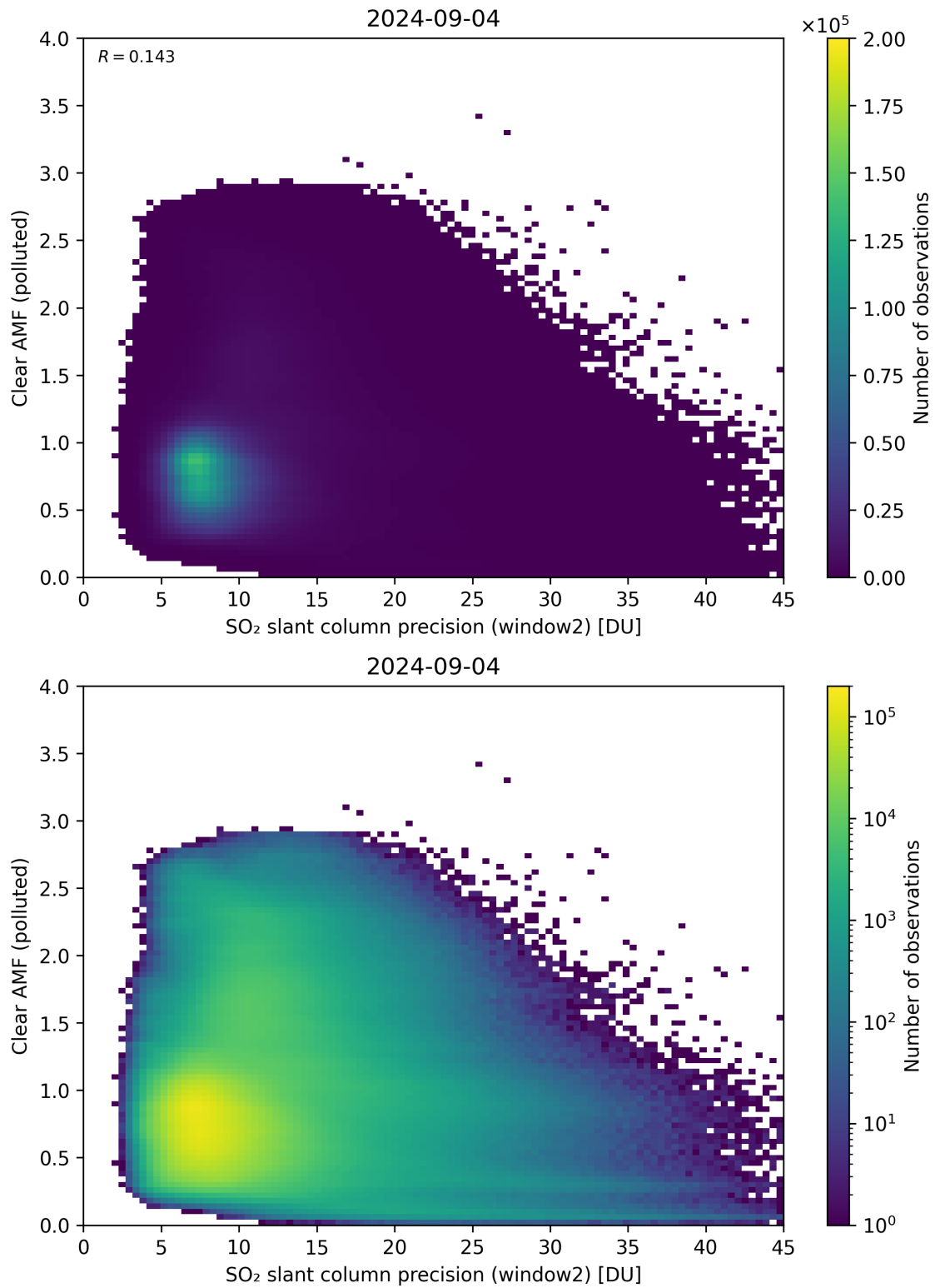
Figure 246: Scatter density plot of “SO 2 slant column precision (window2)” against “Clear AMF (polluted)” for 2024-09-03 to 2024-09-05.
