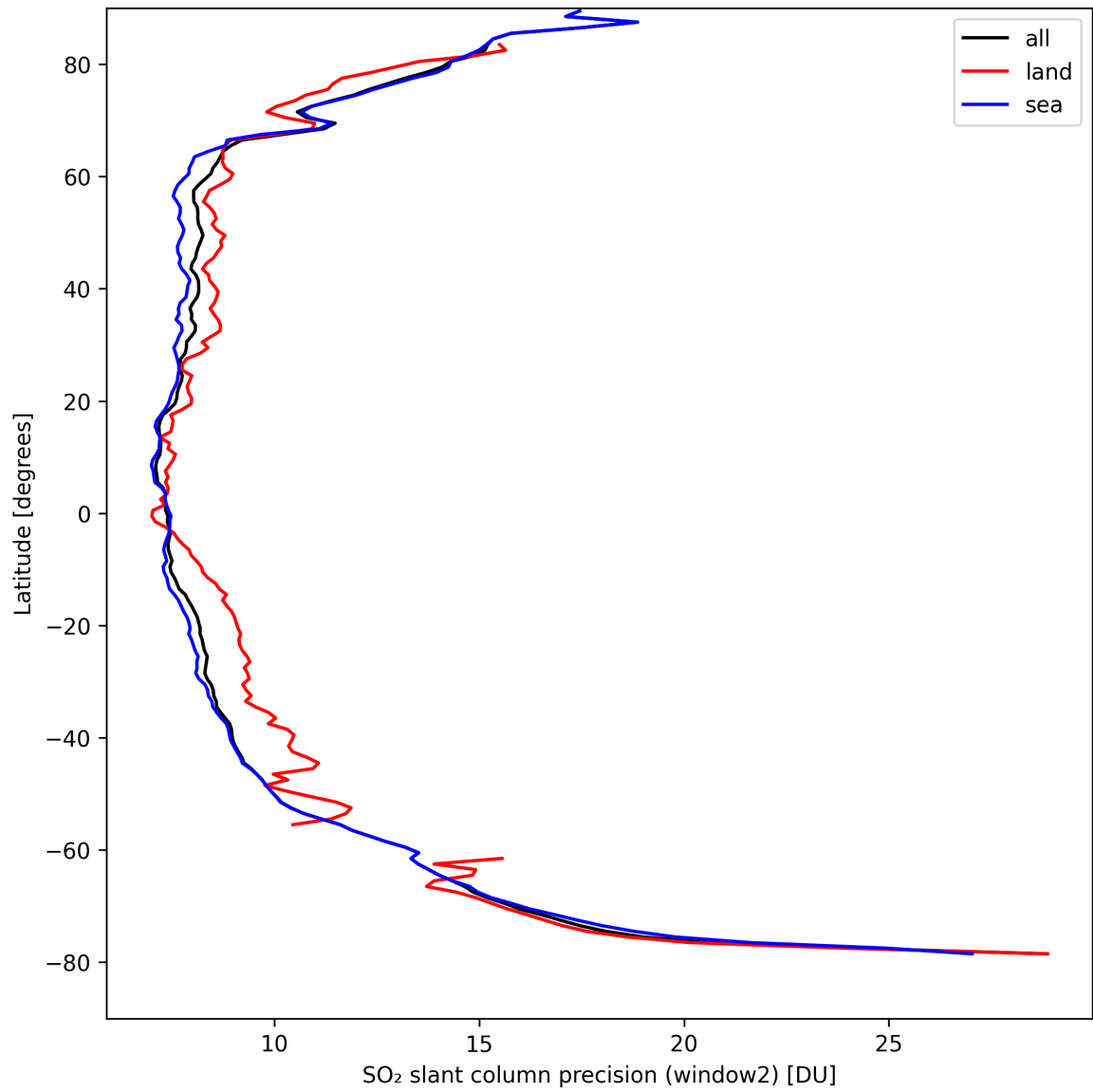
Figure 38: Zonal average of “SO 2 slant column precision (window2)” for 2024-09-03 to 2024-09-05.
