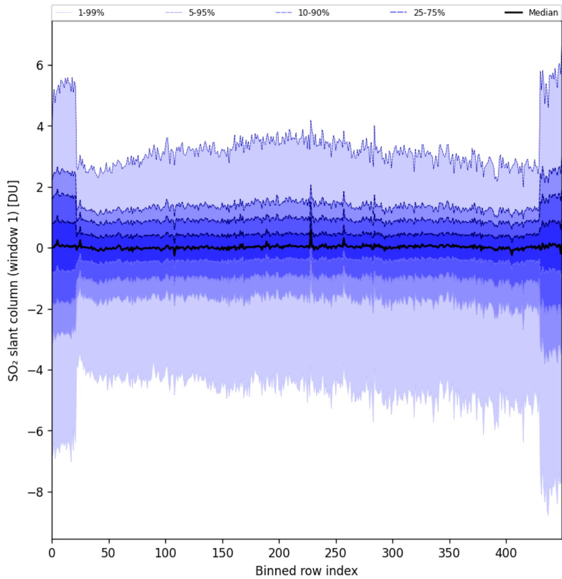
Figure 79: Along track statistics of “SO 2 slant column (window 1)” for 2024-09-03 to 2024-09-05
