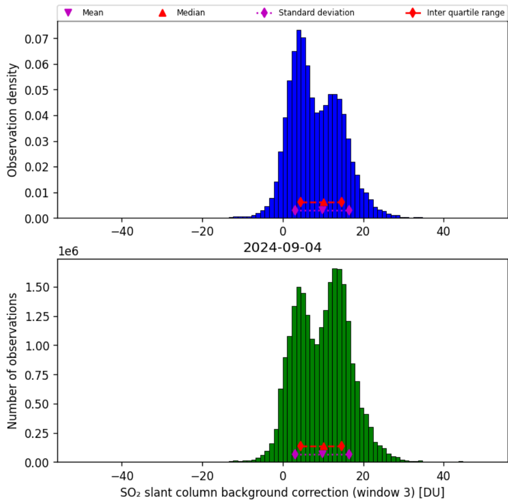
Figure 67: Histogram of “SO 2 slant column background correction (window 3)” for 2024-09-03 to 2024-09-05
