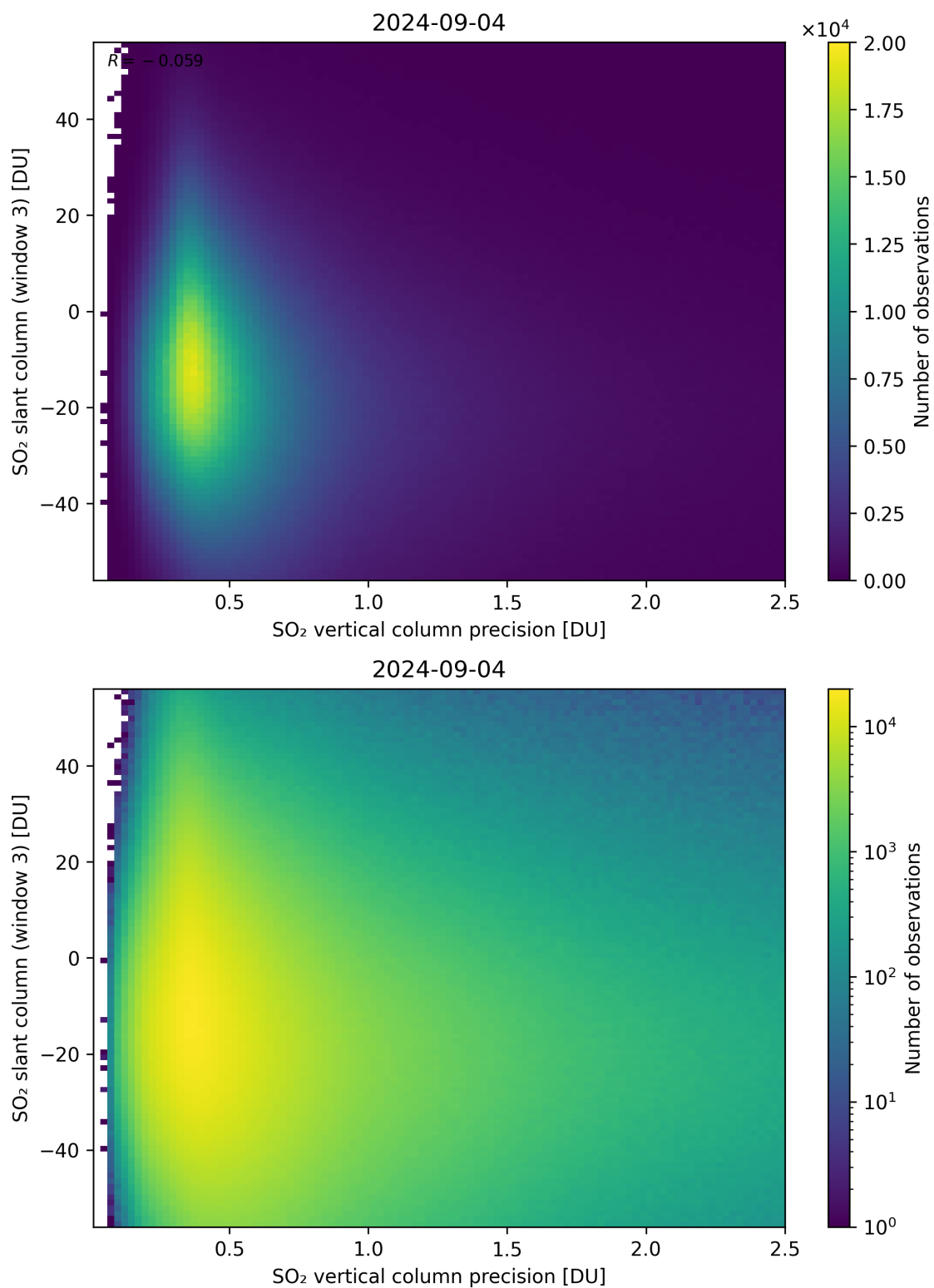
Figure 292: Scatter density plot of “SO 2 vertical column precision” against “SO 2 slant column (window 3)” for 2024-09-03 to 2024-09-05.
