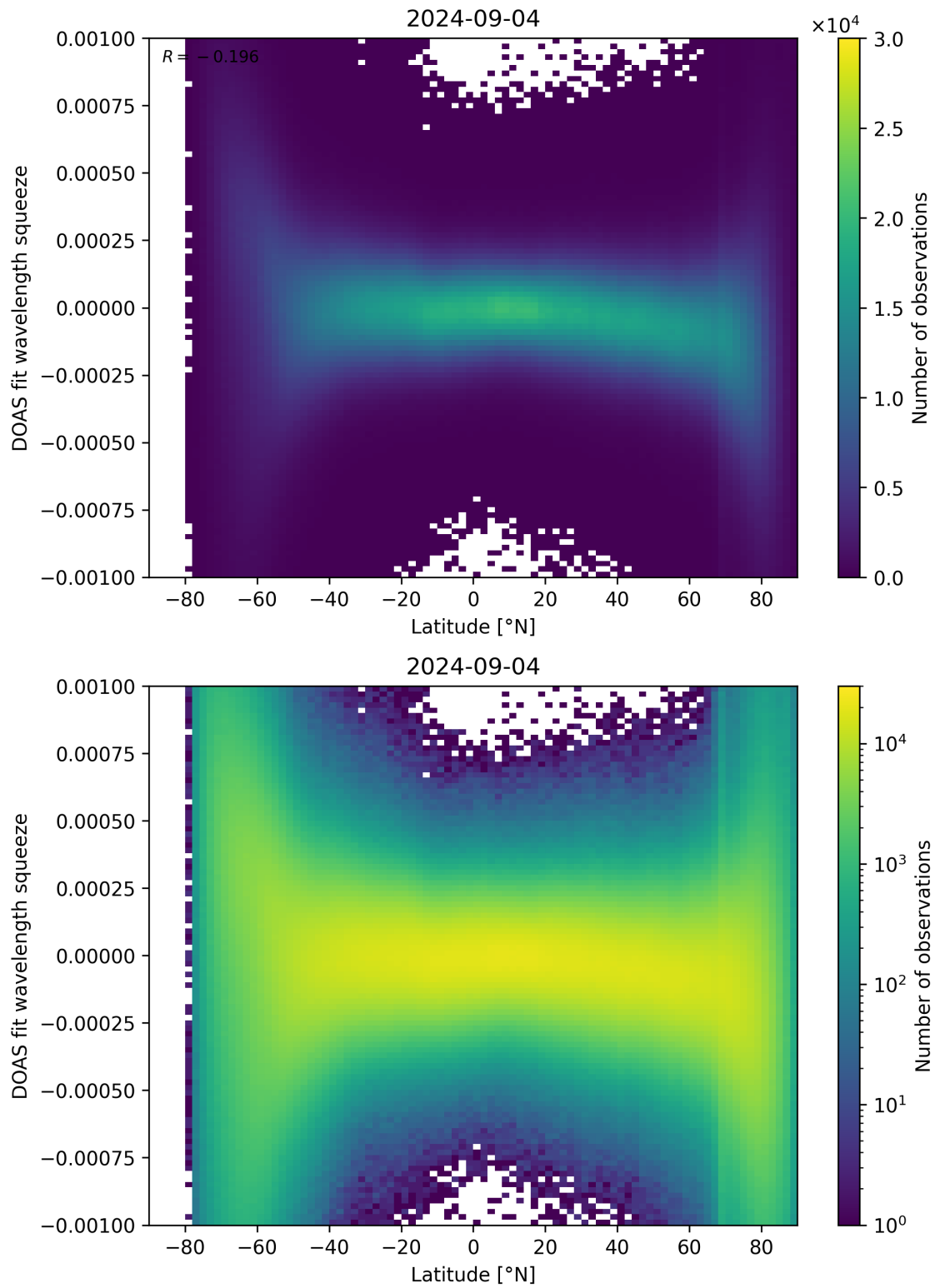
Figure 143: Scatter density plot of “Latitude” against “DOAS fit wavelength squeeze” for 2024-09-03 to 2024-09-05.
