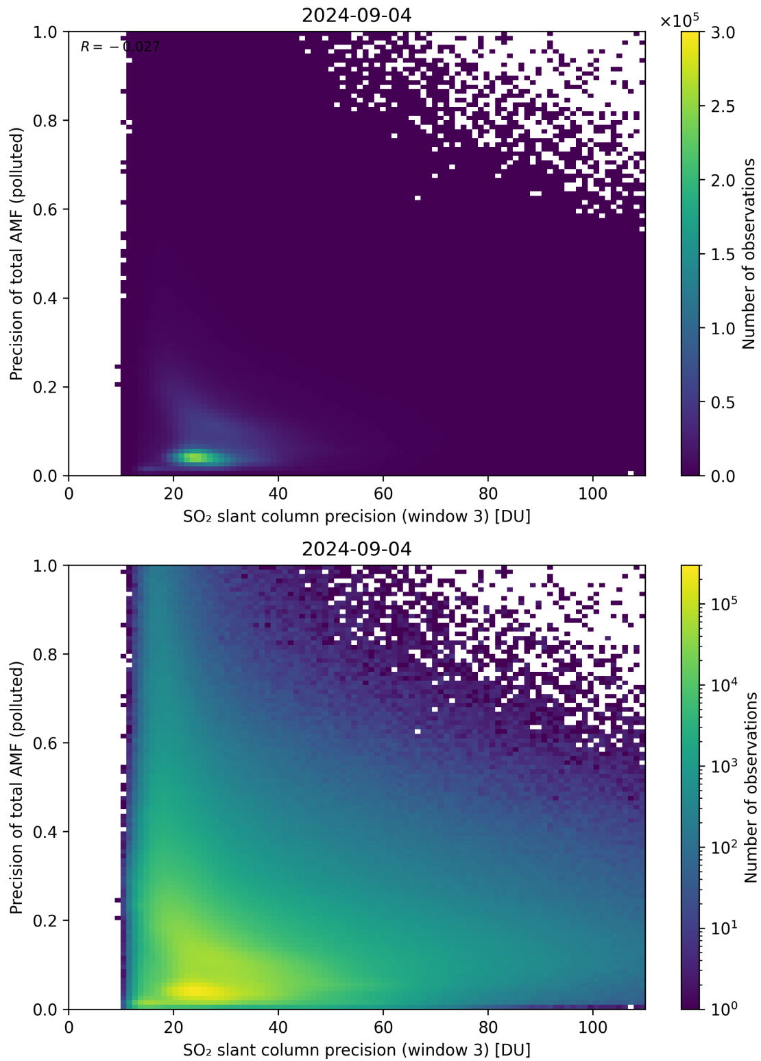
Figure 264: Scatter density plot of “SO 2 slant column precision (window 3)” against “Precision of total AMF (polluted)” for 2024-09-03 to 2024-09-05.
