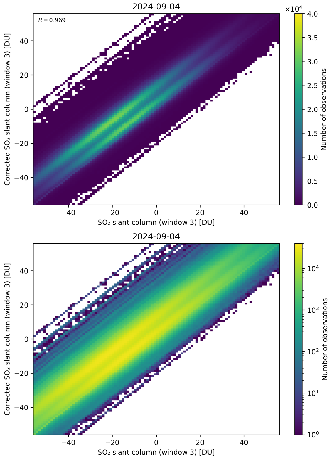
Figure 266: Scatter density plot of “SO 2 slant column (window 3)” against “Corrected SO 2 slant column (window 3)” for 2024-09-03 to 2024-09-05.
