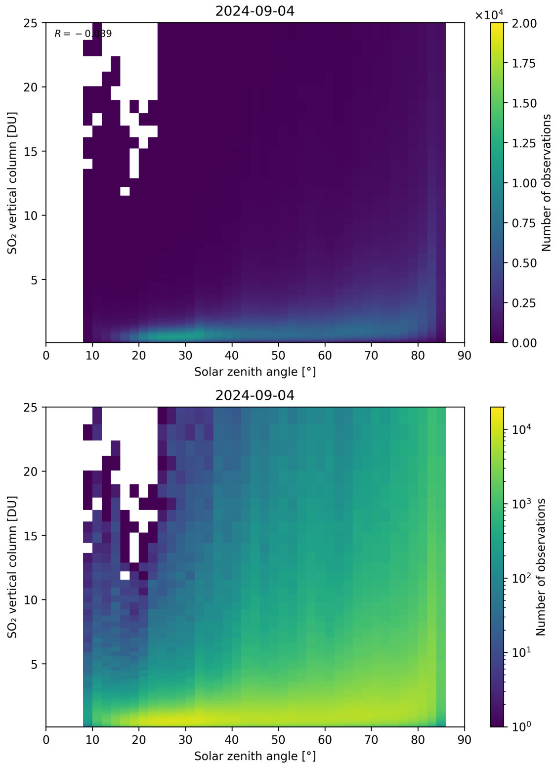
Figure 176: Scatter density plot of “Solar zenith angle” against “SO 2 vertical column” for 2024-09-03 to 2024-09-05.
