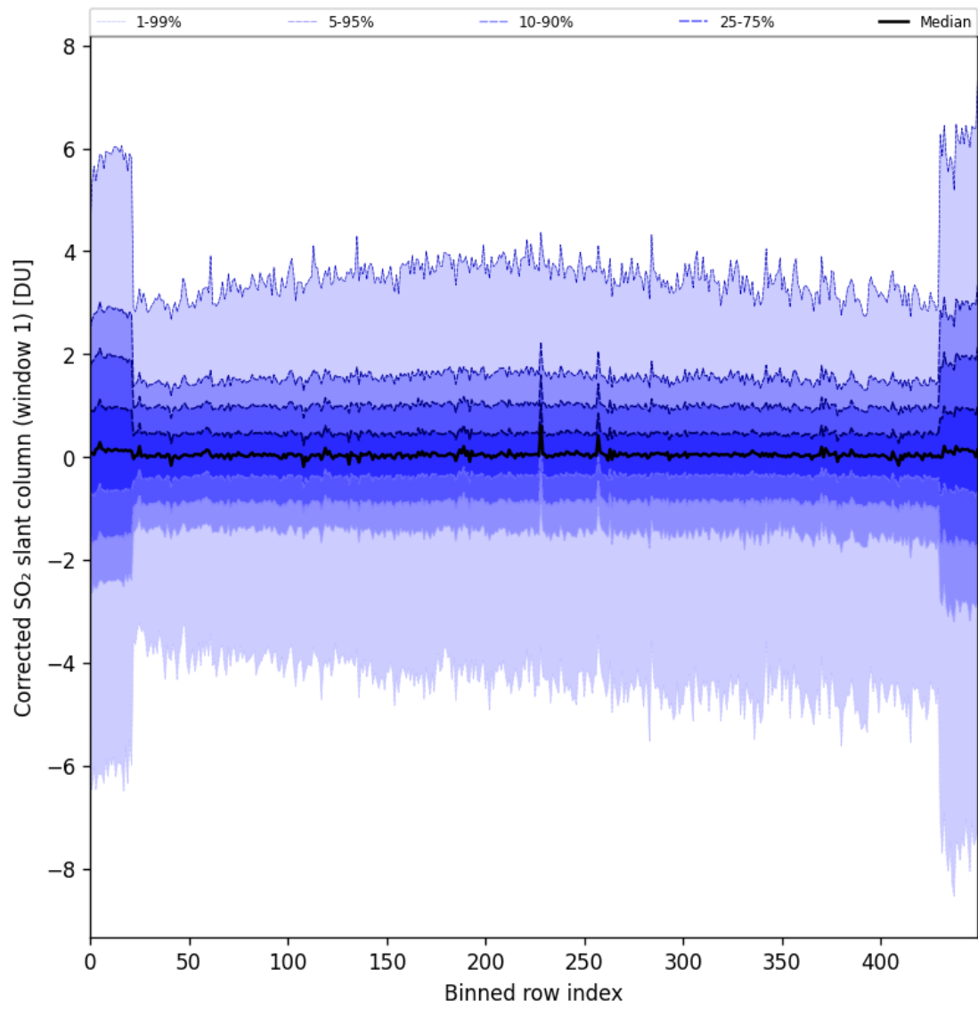
Figure 81: Along track statistics of “Corrected SO 2 slant column (window 1)” for 2024-09-03 to 2024-09-05
