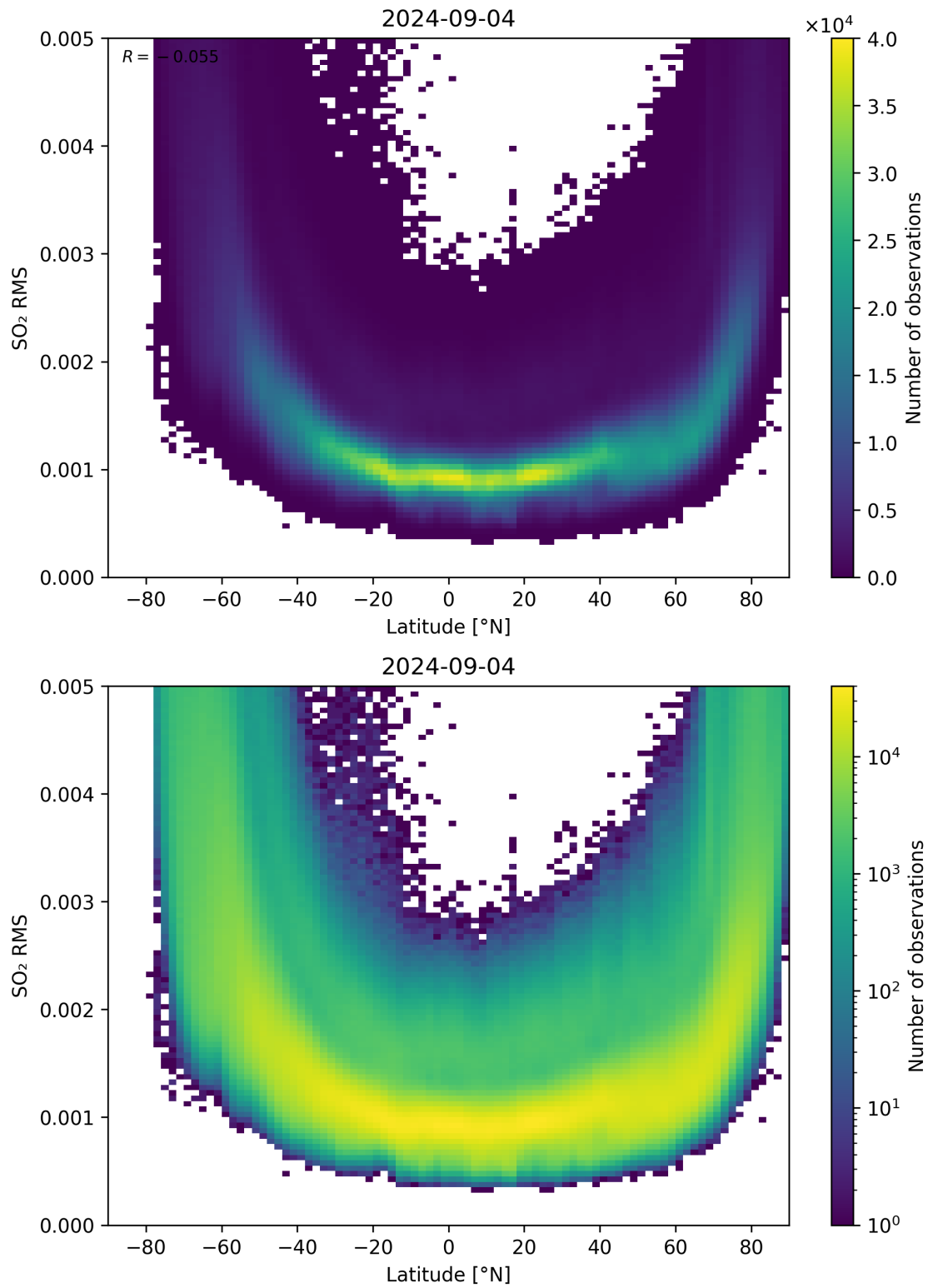
Figure 144: Scatter density plot of “Latitude” against “SO 2 RMS” for 2024-09-03 to 2024-09-05.
