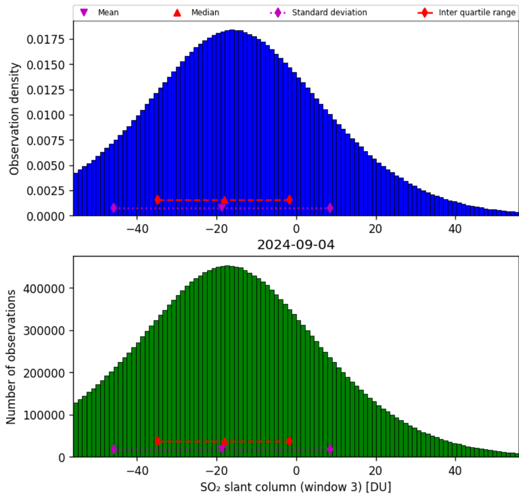
Figure 64: Histogram of “SO 2 slant column (window 3)” for 2024-09-03 to 2024-09-05
