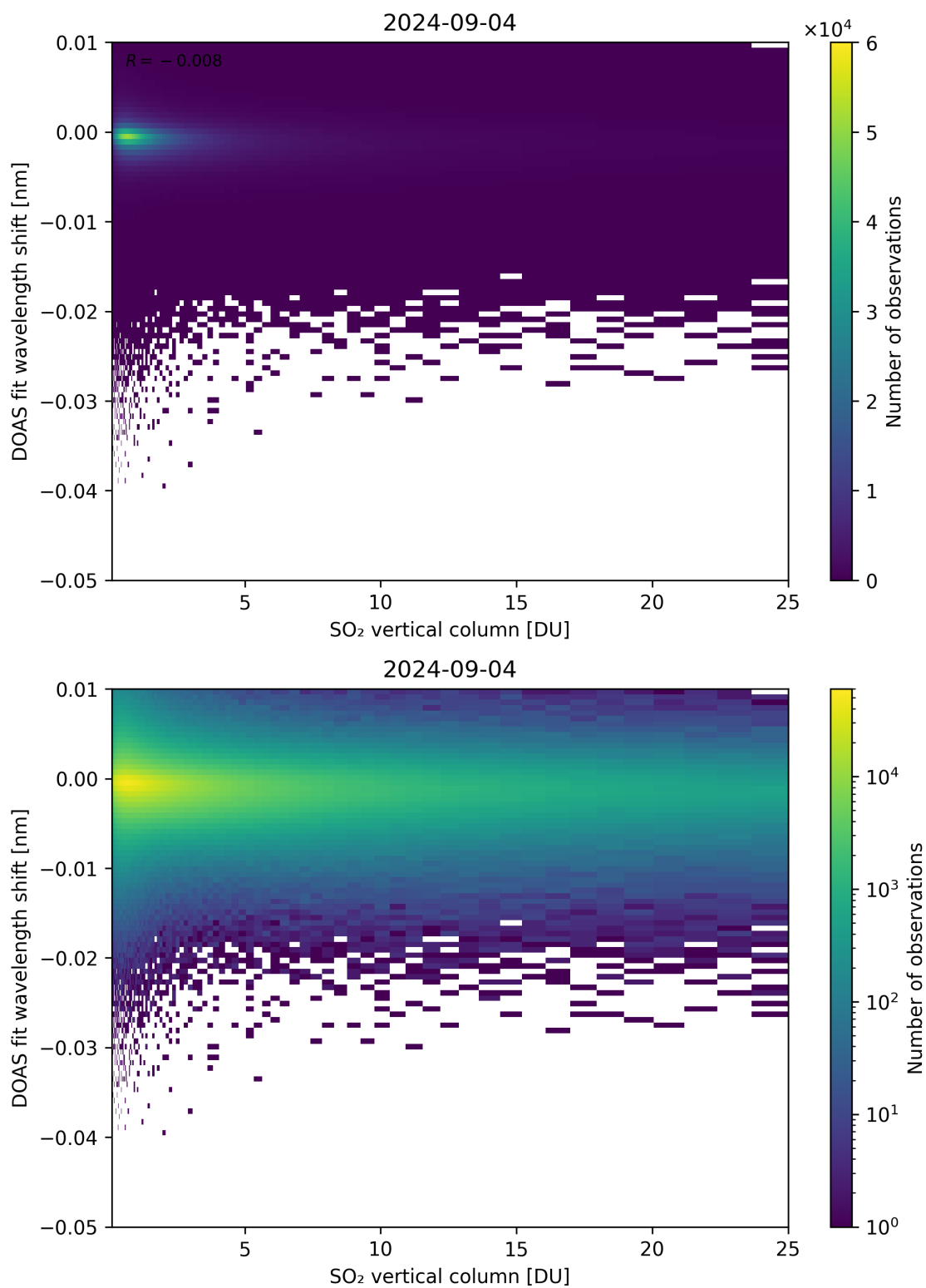
Figure 276: Scatter density plot of “SO 2 vertical column” against “DOAS fit wavelength shift” for 2024-09-03 to 2024-09-05.
