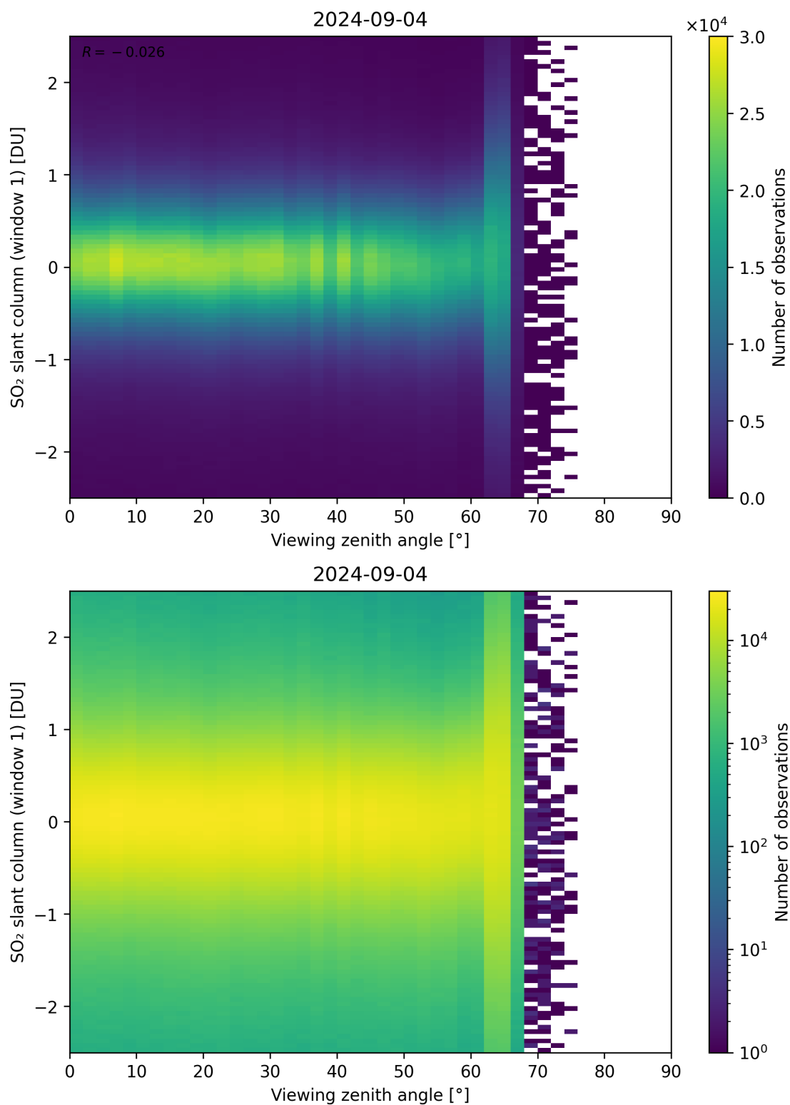
Figure 320: Scatter density plot of “Viewing zenith angle” against “SO 2 slant column (window 1)” for 2024-09-03 to 2024-09-05.
