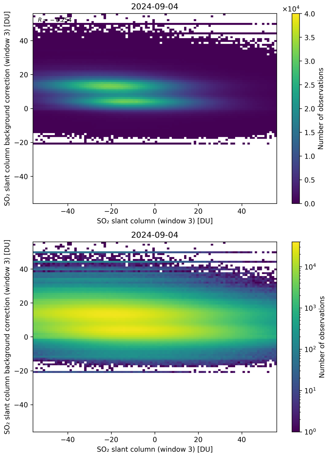
Figure 253: Scatter density plot of “SO 2 slant column (window 3)” against “SO 2 slant column background correction (window 3)” for 2024-09-03 to 2024-09-05.
