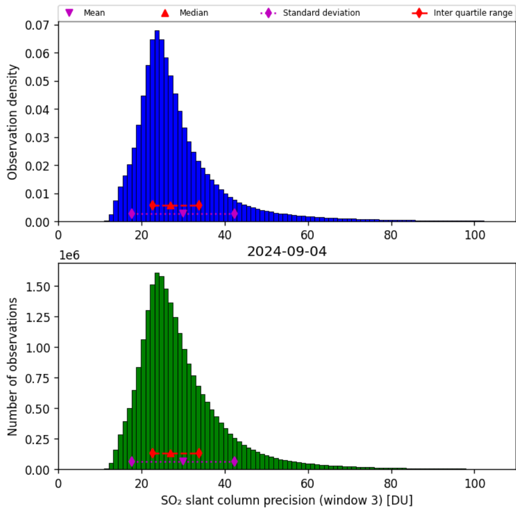
Figure 65: Histogram of “SO 2 slant column precision (window 3)” for 2024-09-03 to 2024-09-05
