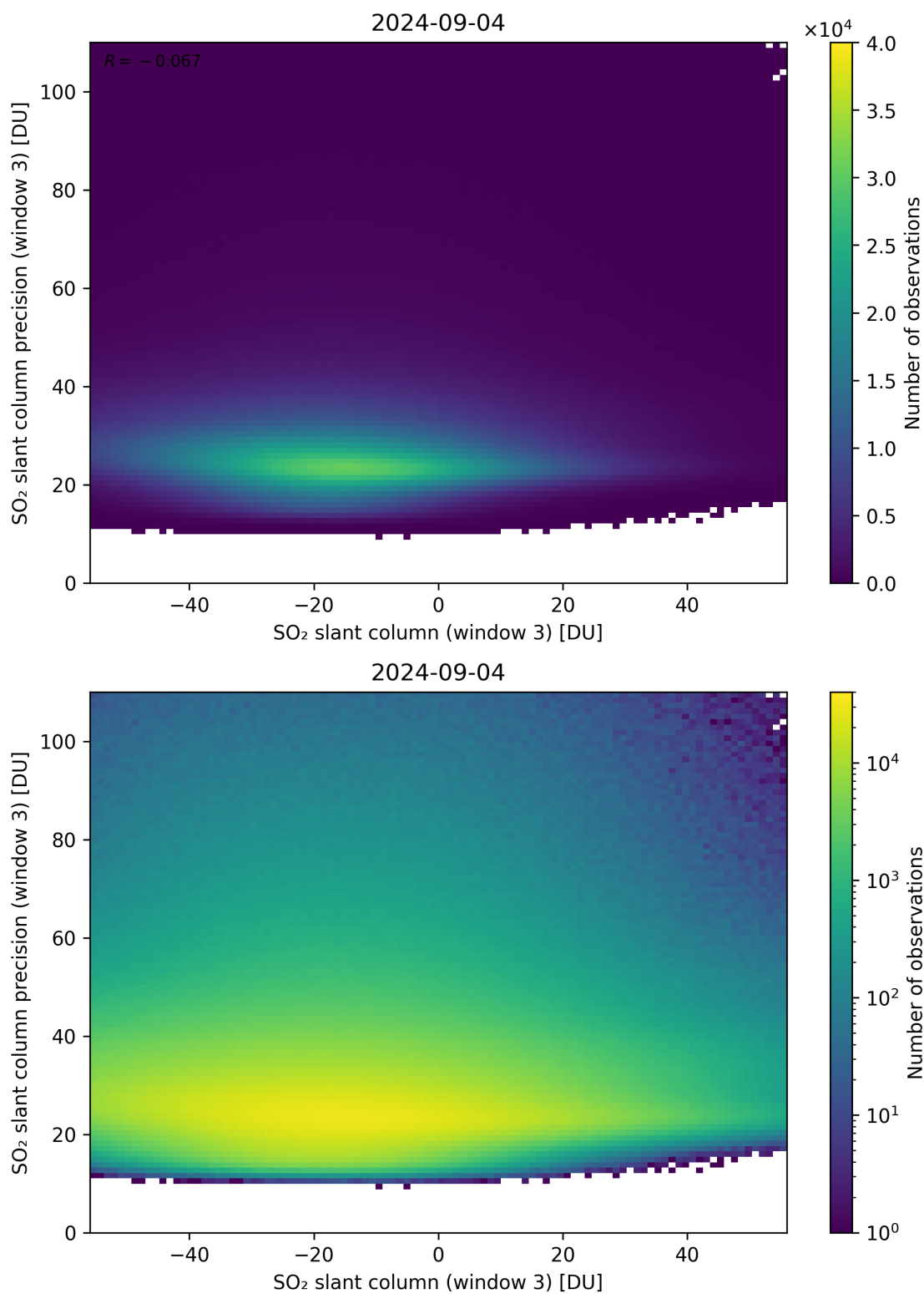
Figure 267: Scatter density plot of “SO 2 slant column (window 3)” against “SO 2 slant column precision (window 3)” for 2024-09-03 to 2024-09-05.
