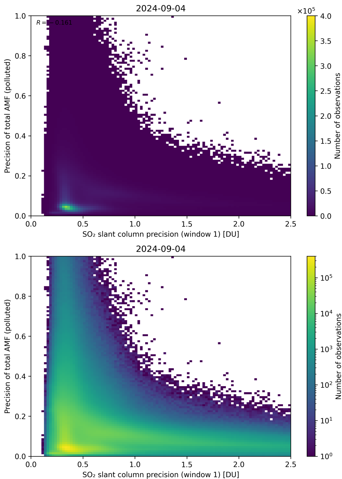
Figure 231: Scatter density plot of “SO 2 slant column precision (window 1)” against “Precision of total AMF (polluted)” for 2024-09-03 to 2024-09-05.
