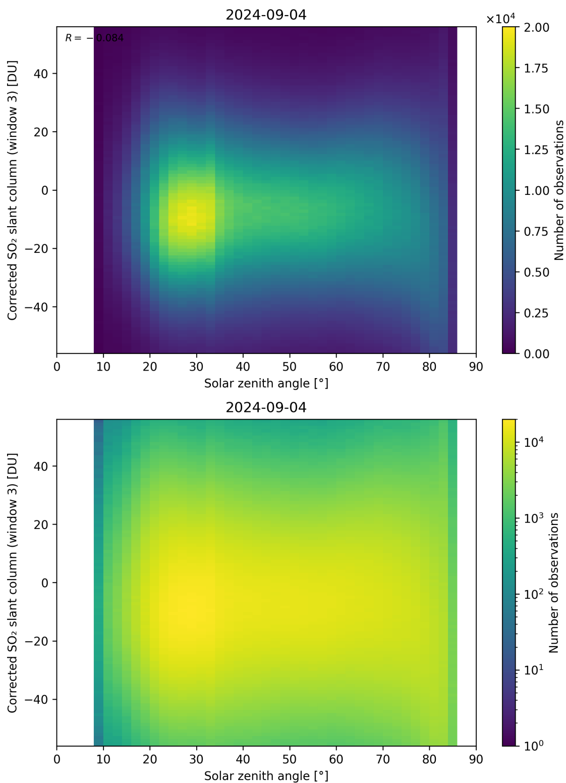
Figure 168: Scatter density plot of “Solar zenith angle” against “Corrected SO 2 slant column (window 3)” for 2024-09-03 to 2024-09-05.
