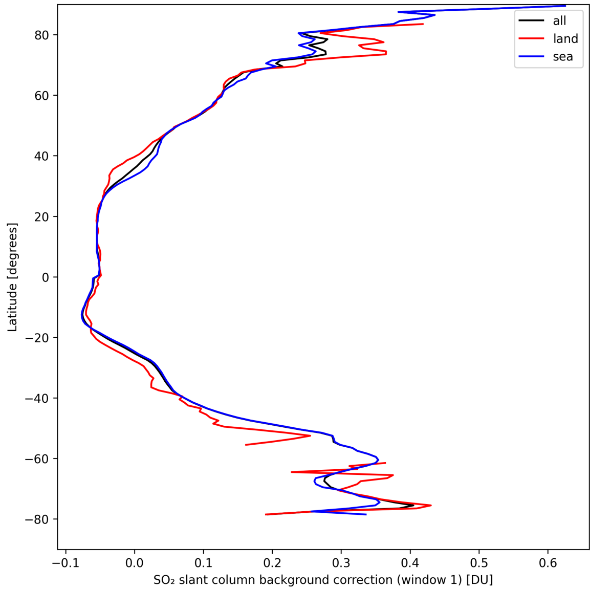
Figure 36: Zonal average of “SO 2 slant column background correction (window 1)” for 2024-09-03 to 2024-09-05.
