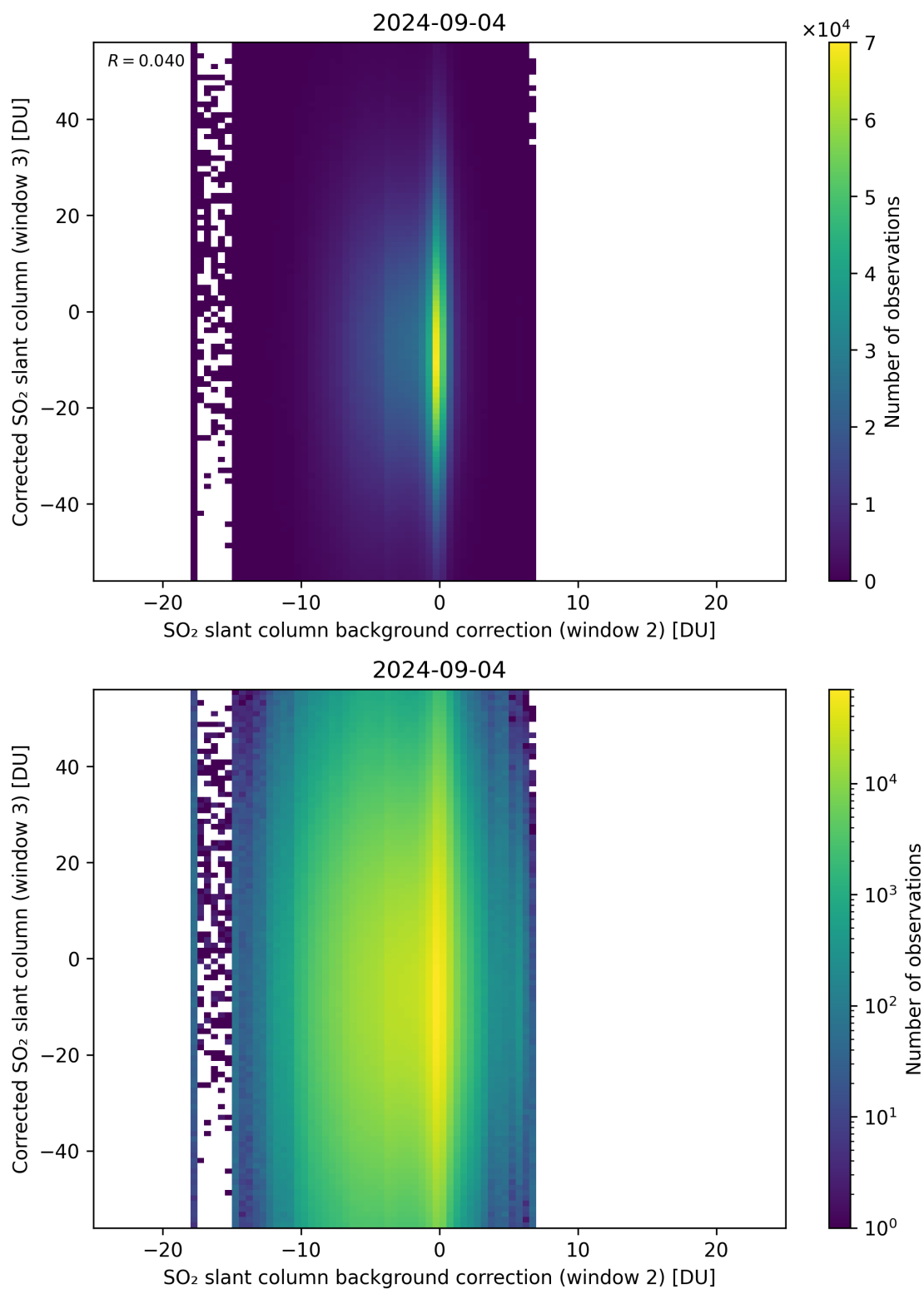
Figure 116: Scatter density plot of “SO 2 slant column background correction (window 2)” against “Corrected SO 2 slant column (window 3)” for 2024-09-03 to 2024-09-05.
