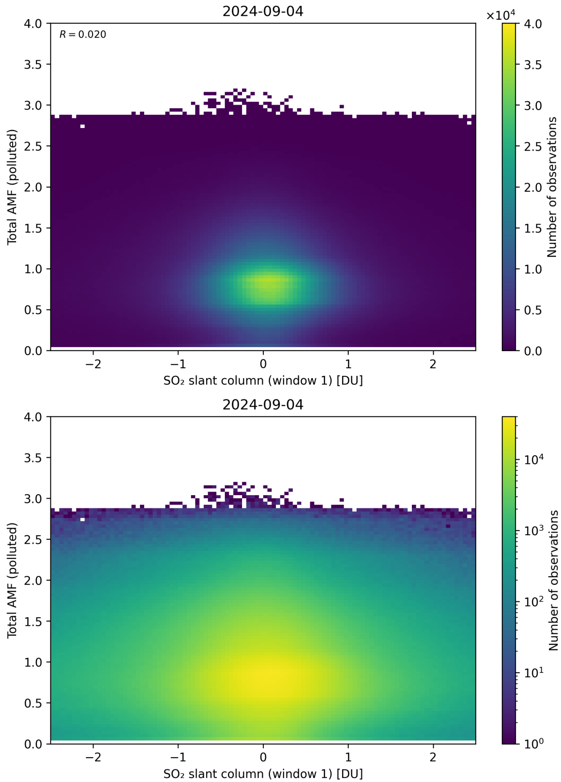
Figure 239: Scatter density plot of “SO 2 slant column (window 1)” against “Total AMF (polluted)” for 2024-09-03 to 2024-09-05.
