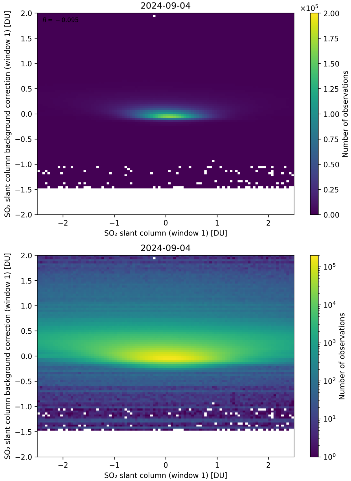
Figure 212: Scatter density plot of “SO 2 slant column (window 1)” against “SO 2 slant column background correction (window 1)” for 2024-09-03 to 2024-09-05.
