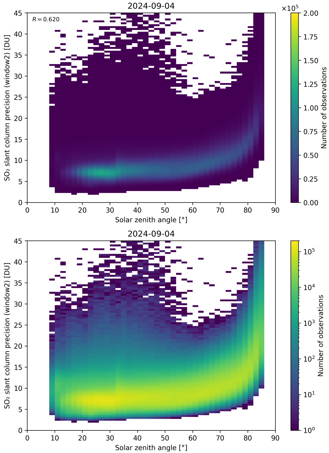
Figure 171: Scatter density plot of “Solar zenith angle” against “SO 2 slant column precision (window2)” for 2024-09-03 to 2024-09-05.
