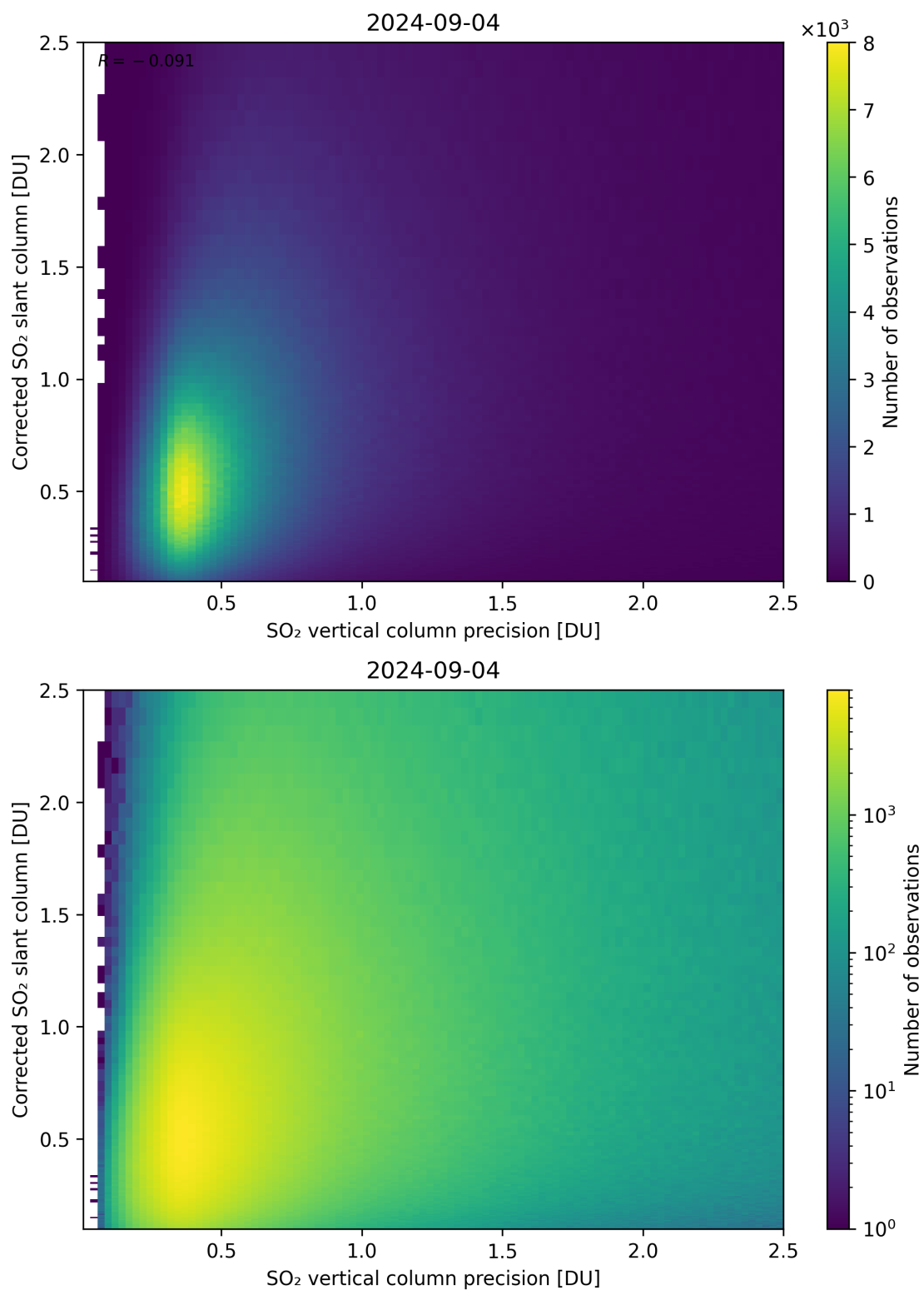
Figure 286: Scatter density plot of “SO 2 vertical column precision” against “Corrected SO 2 slant column” for 2024-09-03 to 2024-09-05.
