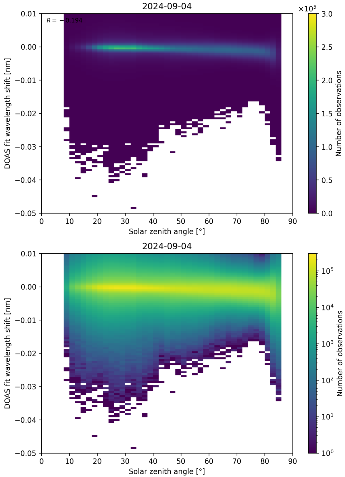
Figure 161: Scatter density plot of “Solar zenith angle” against “DOAS fit wavelength shift” for 2024-09-03 to 2024-09-05.
