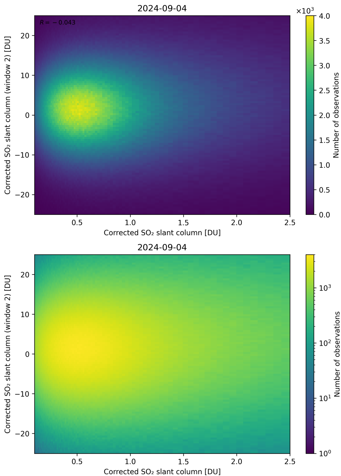
Figure 185: Scatter density plot of “Corrected SO 2 slant column” against “Corrected SO 2 slant column (window 2)” for 2024-09-03 to 2024-09-05.
