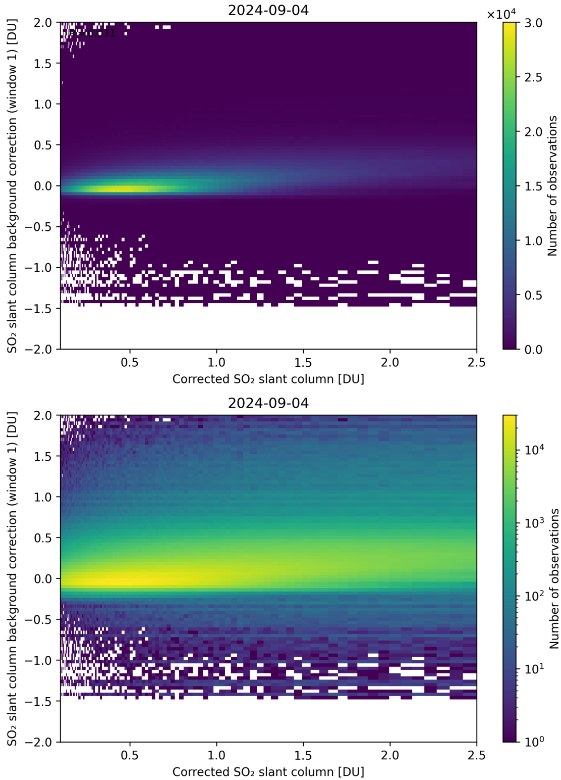
Figure 178: Scatter density plot of “Corrected SO 2 slant column” against “SO 2 slant column background correction (window 1)” for 2024-09-03 to 2024-09-05.
