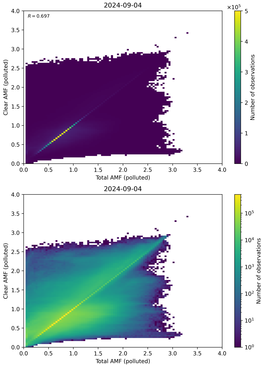
Figure 271: Scatter density plot of “Total AMF (polluted)” against “Clear AMF (polluted)” for 2024-09-03 to 2024-09-05.
