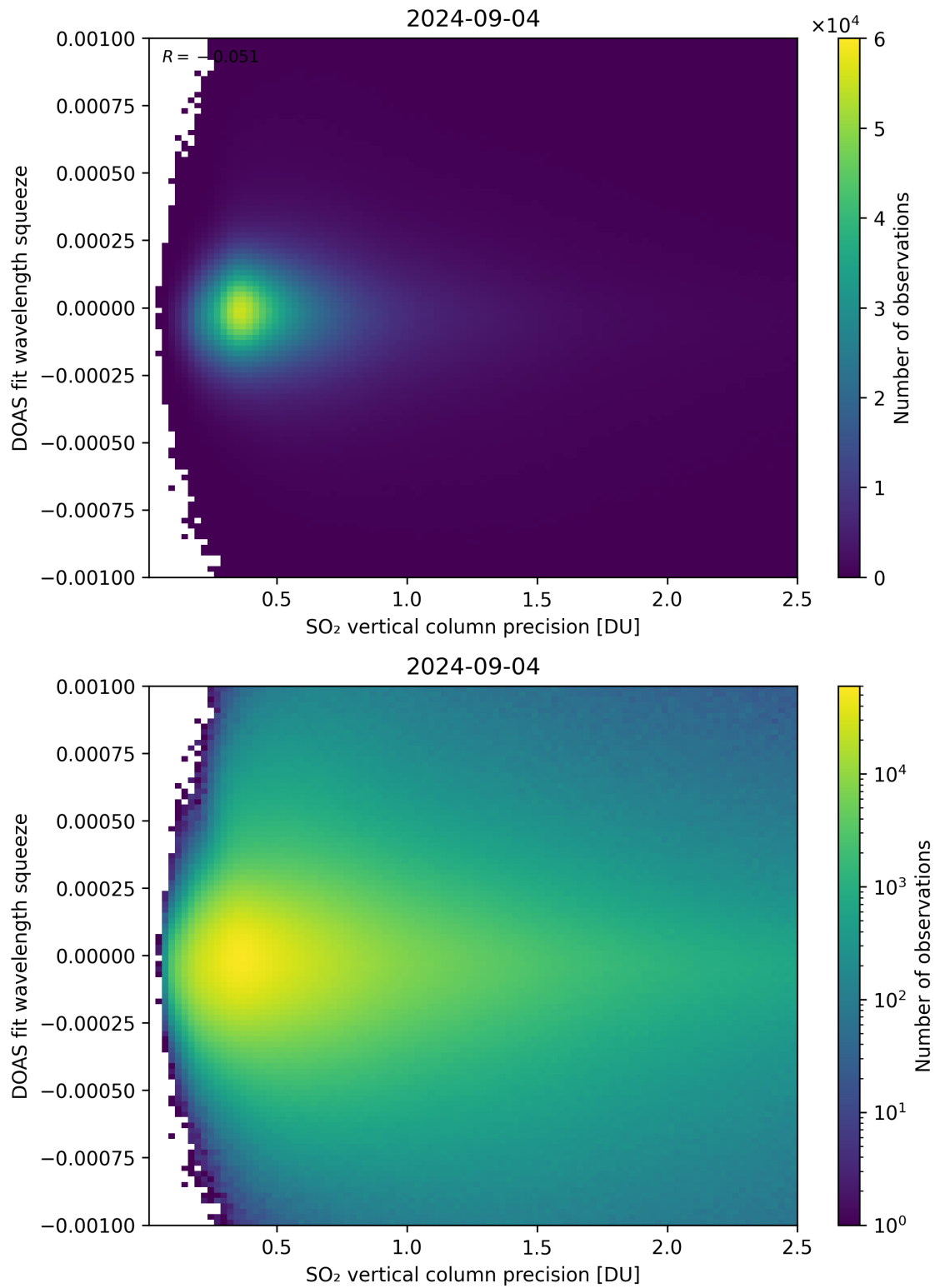
Figure 283: Scatter density plot of “SO 2 vertical column precision” against “DOAS fit wavelength squeeze” for 2024-09-03 to 2024-09-05.
