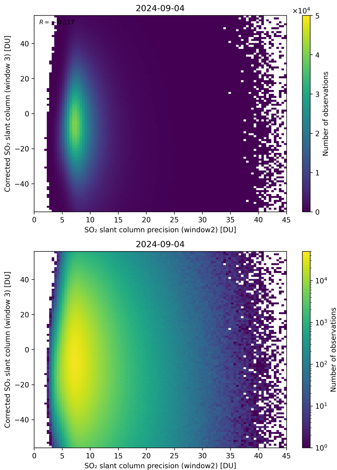
Figure 248: Scatter density plot of “SO 2 slant column precision (window2)” against “Corrected SO 2 slant column (window 3)” for 2024-09-03 to 2024-09-05.
