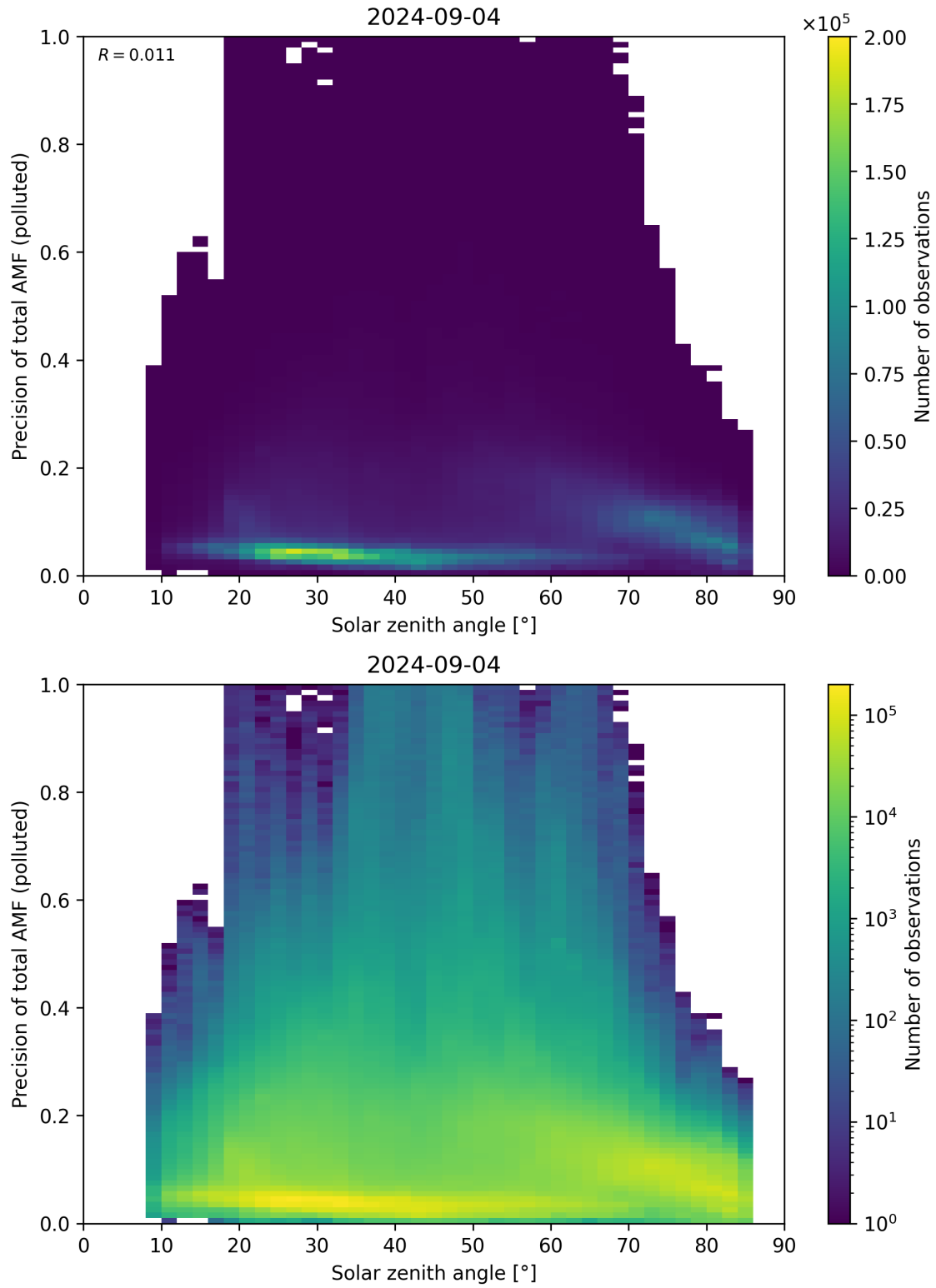
Figure 175: Scatter density plot of “Solar zenith angle” against “Precision of total AMF (polluted)” for 2024-09-03 to 2024-09-05.
