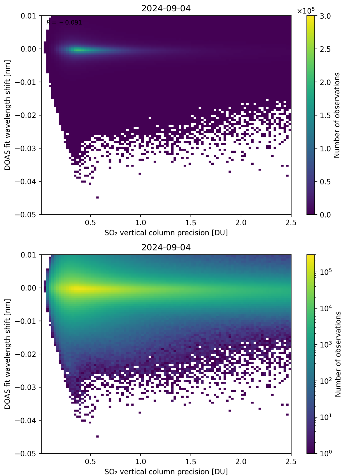
Figure 282: Scatter density plot of “SO 2 vertical column precision” against “DOAS fit wavelength shift” for 2024-09-03 to 2024-09-05.
