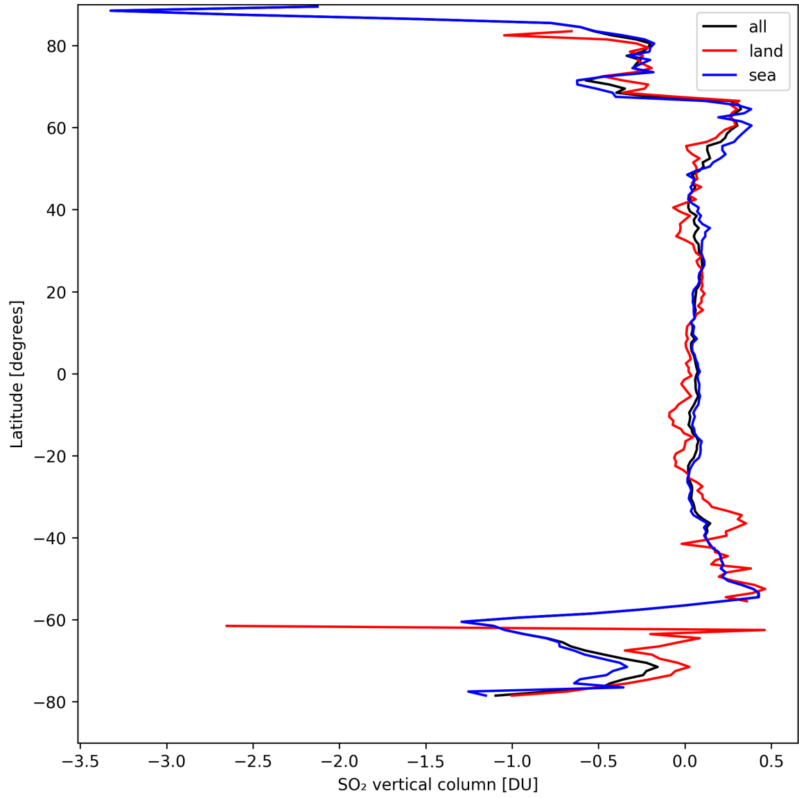
Figure 30: Zonal average of “SO 2 vertical column” for 2024-09-03 to 2024-09-05.
