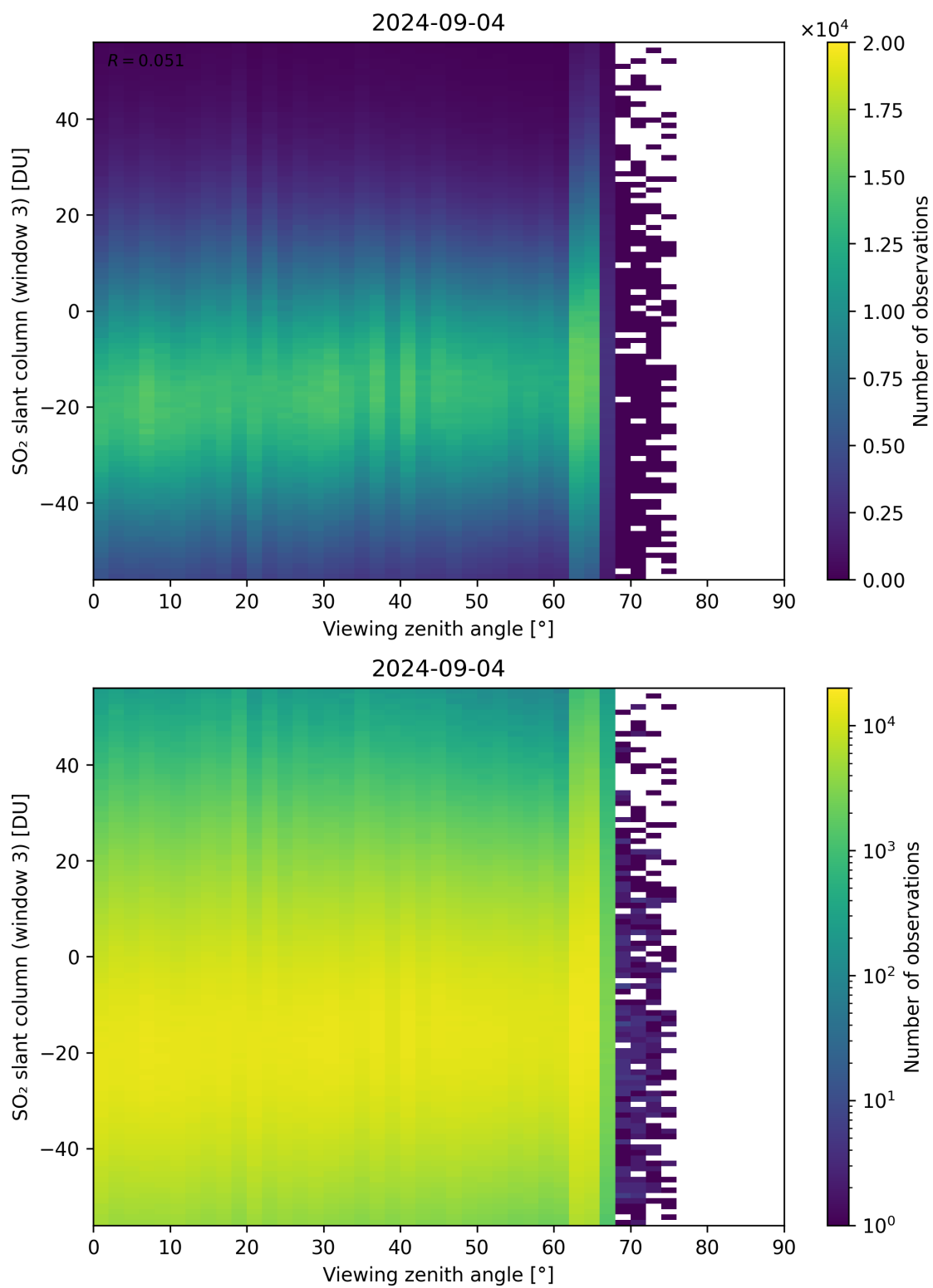
Figure 323: Scatter density plot of “Viewing zenith angle” against “SO 2 slant column (window 3)” for 2024-09-03 to 2024-09-05.
