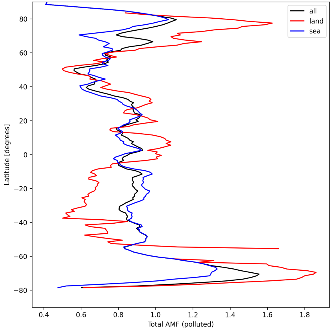
Figure 48: Zonal average of “Total AMF (polluted)” for 2024-09-03 to 2024-09-05.
