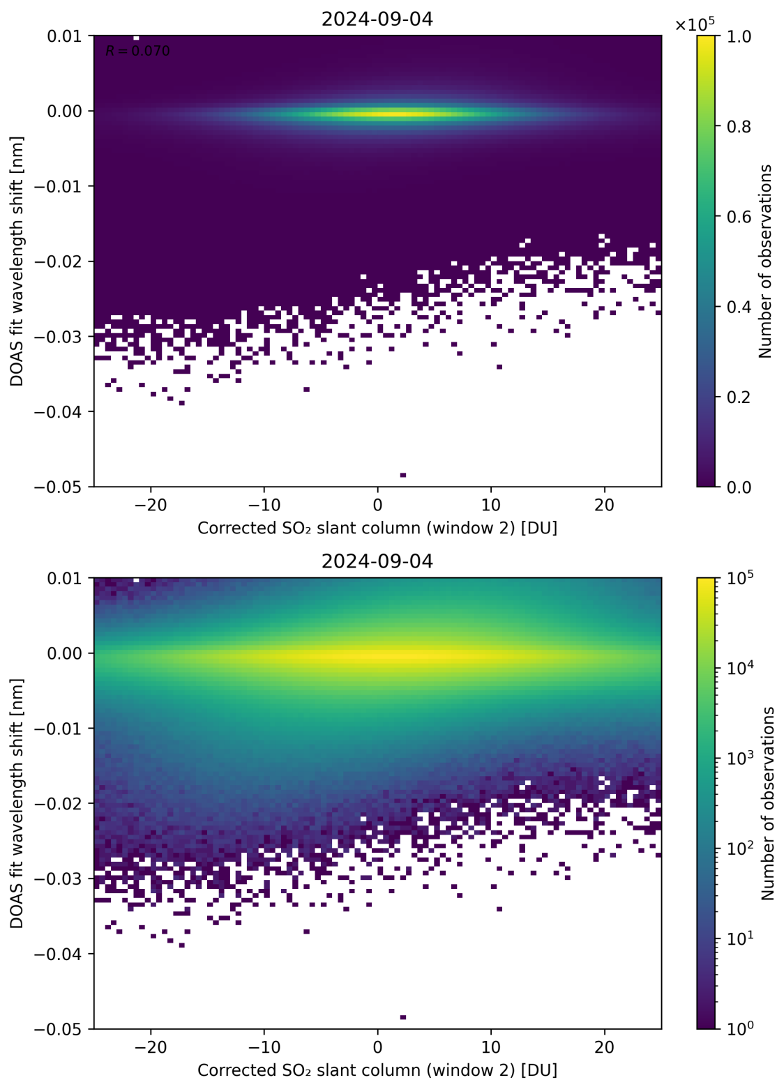
Figure 196: Scatter density plot of “Corrected SO 2 slant column (window 2)” against “DOAS fit wavelength shift” for 2024-09-03 to 2024-09-05.
