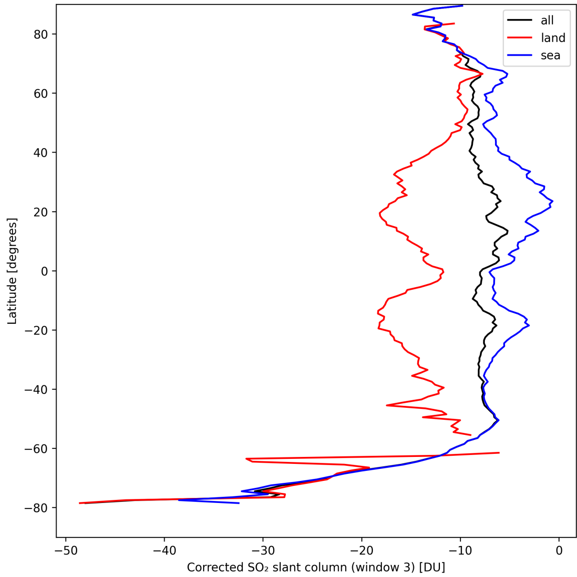
Figure 43: Zonal average of “Corrected SO 2 slant column (window 3)” for 2024-09-03 to 2024-09-05.
