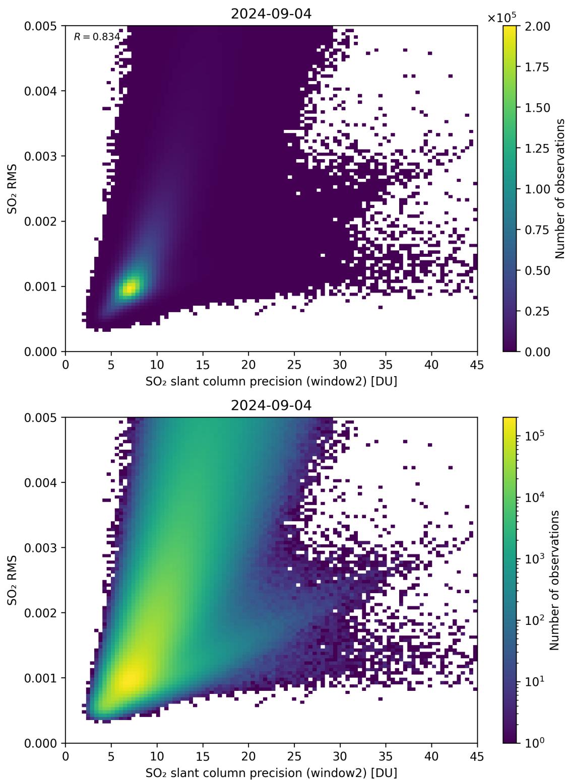
Figure 245: Scatter density plot of “SO 2 slant column precision (window2)” against “SO 2 RMS” for 2024-09-03 to 2024-09-05.
