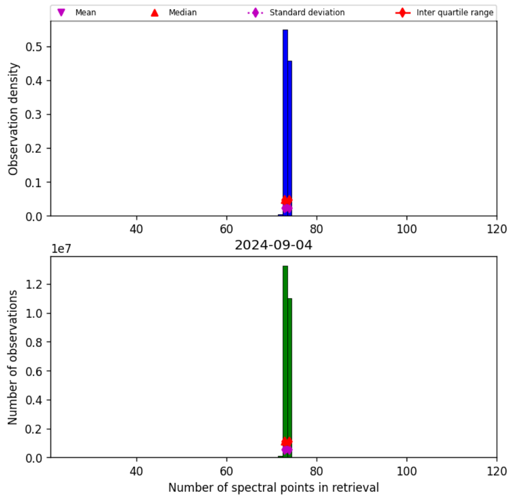
Figure 74: Histogram of “Number of spectral points in retrieval” for 2024-09-03 to 2024-09-05
