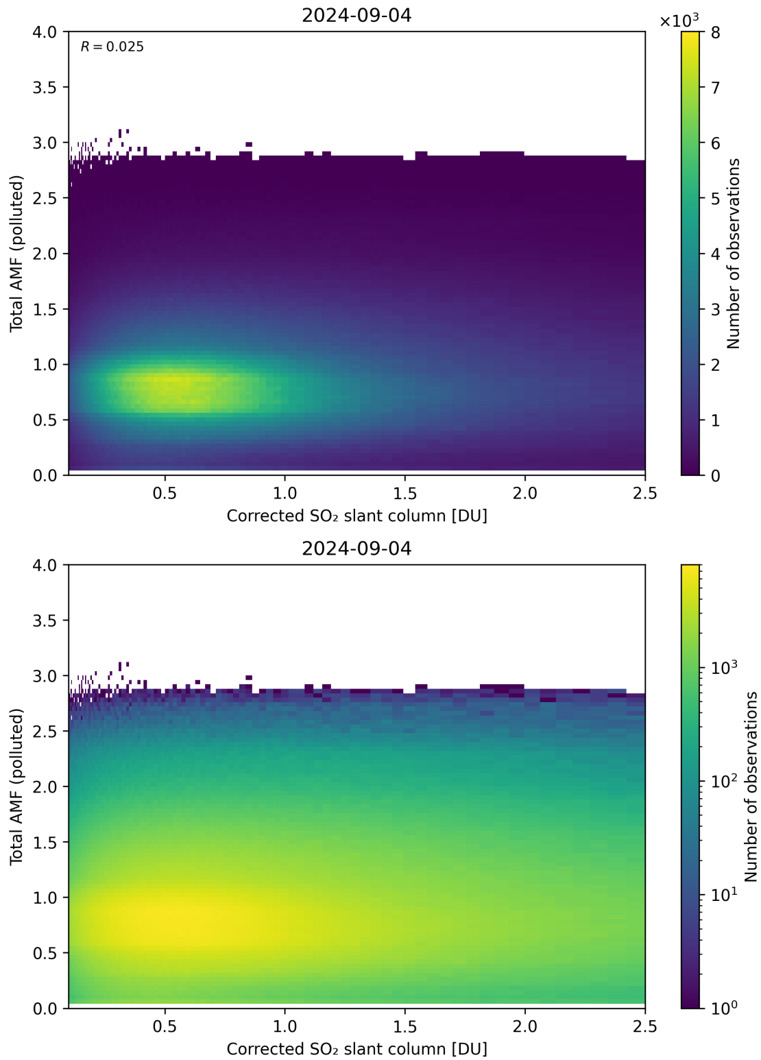
Figure 192: Scatter density plot of “Corrected SO 2 slant column” against “Total AMF (polluted)” for 2024-09-03 to 2024-09-05.
