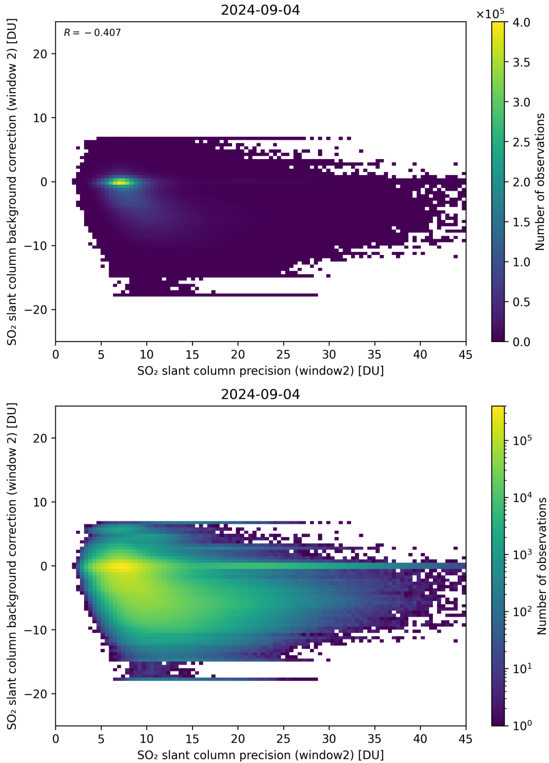
Figure 241: Scatter density plot of “SO 2 slant column precision (window2)” against “SO 2 slant column background correction (window 2)” for 2024-09-03 to 2024-09-05.
