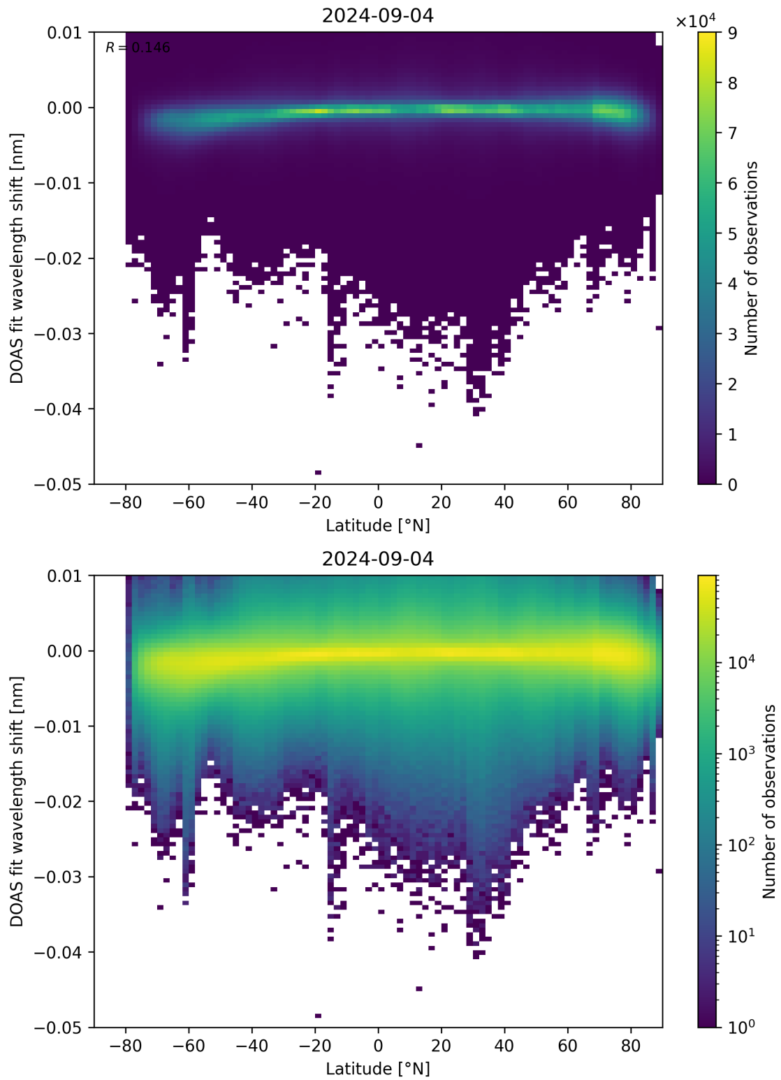
Figure 142: Scatter density plot of “Latitude” against “DOAS fit wavelength shift” for 2024-09-03 to 2024-09-05.
