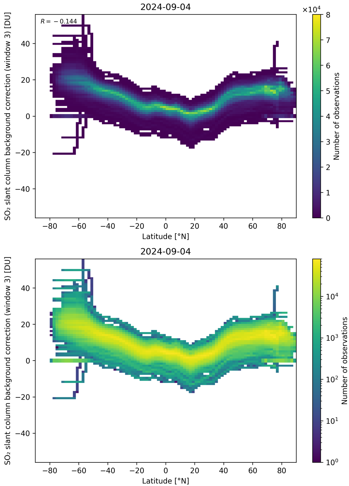
Figure 141: Scatter density plot of “Latitude” against “SO 2 slant column background correction (window 3)” for 2024-09-03 to 2024-09-05.
