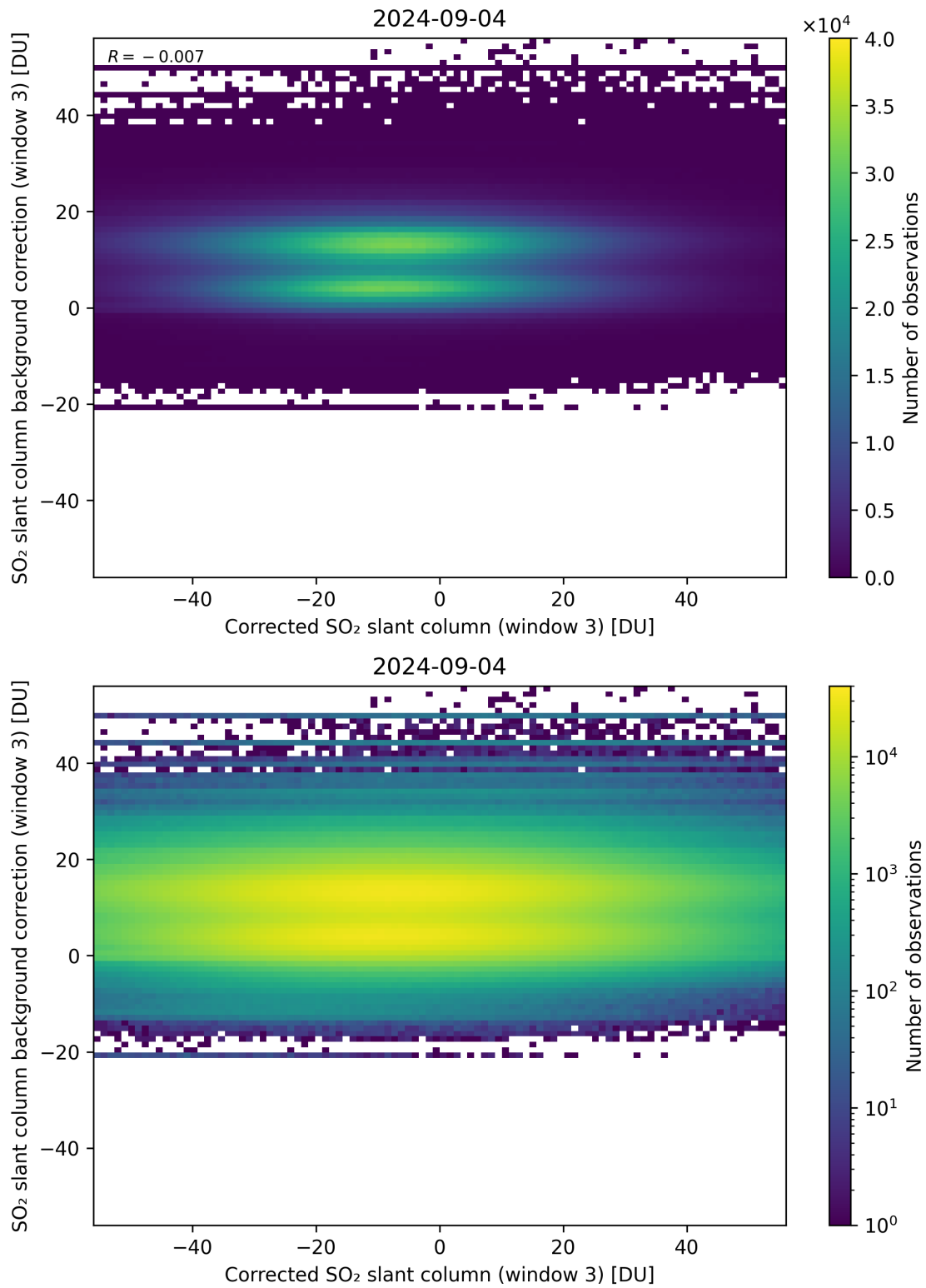
Figure 205: Scatter density plot of “Corrected SO 2 slant column (window 3)” against “SO 2 slant column background correction (window 3)” for 2024-09-03 to 2024-09-05.
