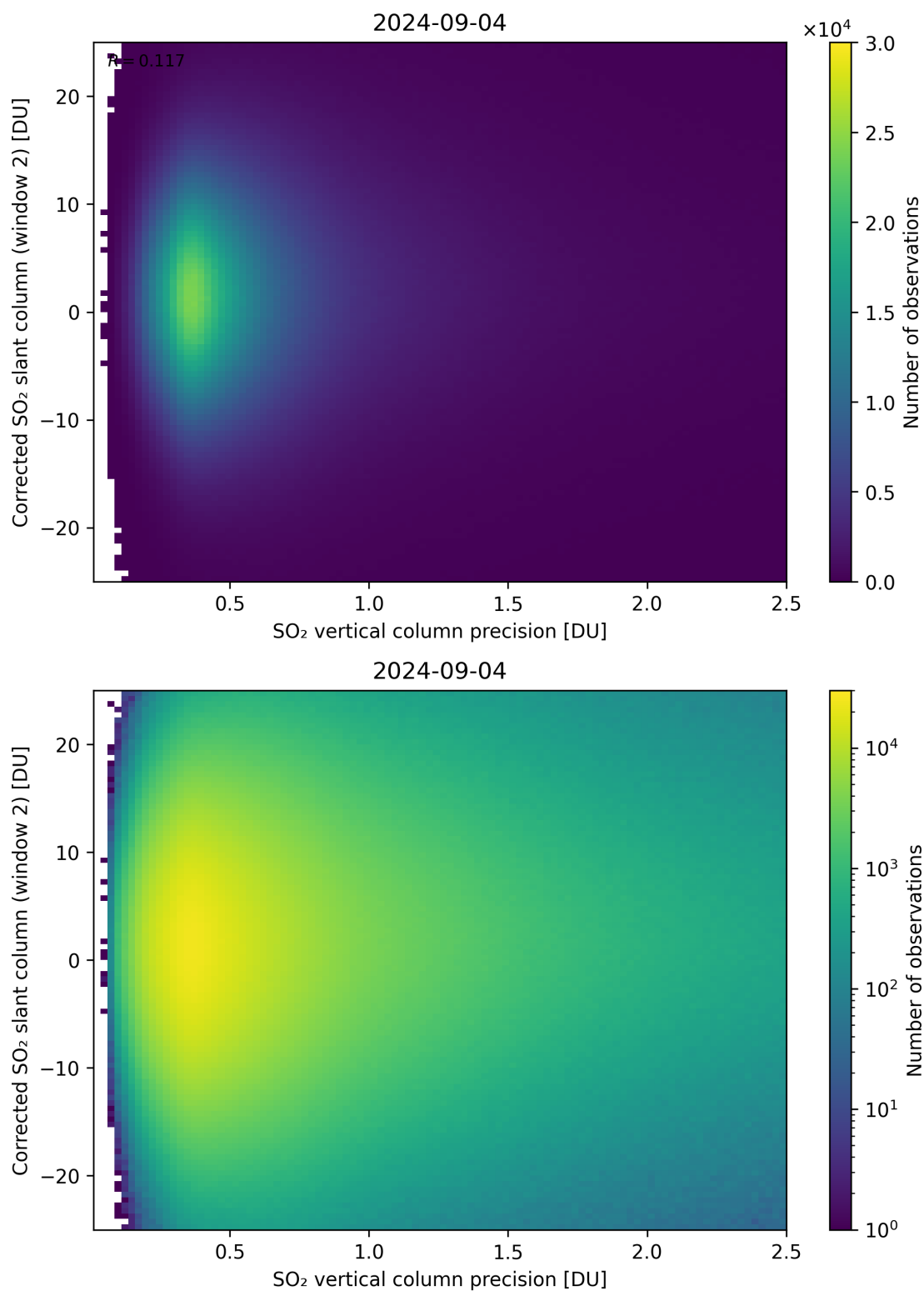
Figure 287: Scatter density plot of “SO 2 vertical column precision” against “Corrected SO 2 slant column (window 2)” for 2024-09-03 to 2024-09-05.
