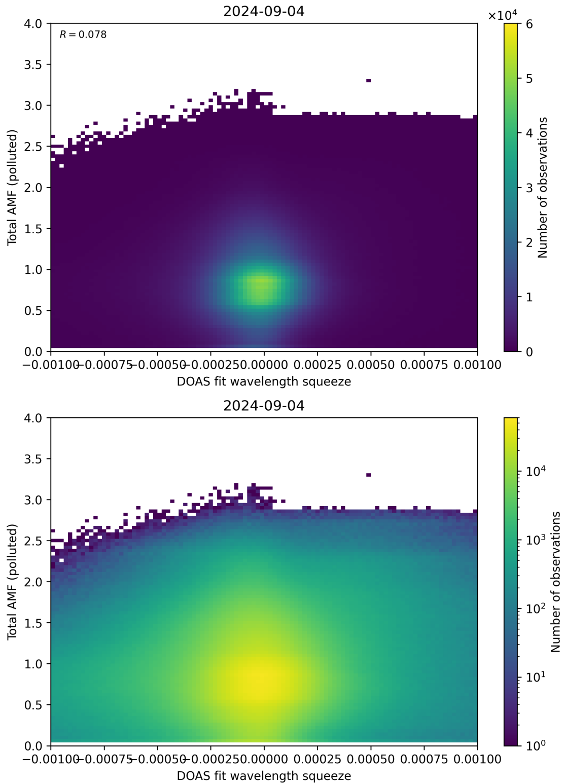
Figure 134: Scatter density plot of “DOAS fit wavelength squeeze” against “Total AMF (polluted)” for 2024-09-03 to 2024-09-05.
