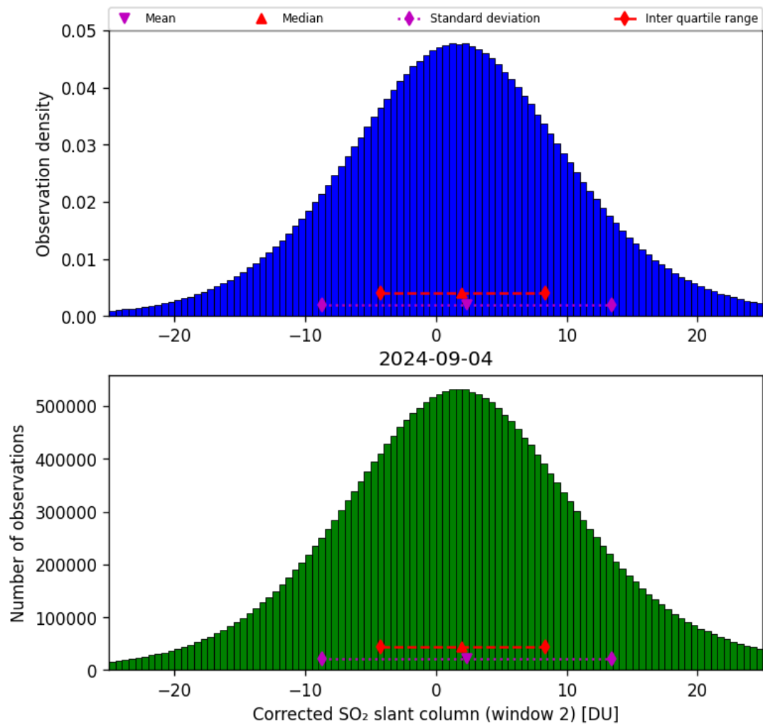
Figure 62: Histogram of “Corrected SO 2 slant column (window 2)” for 2024-09-03 to 2024-09-05
