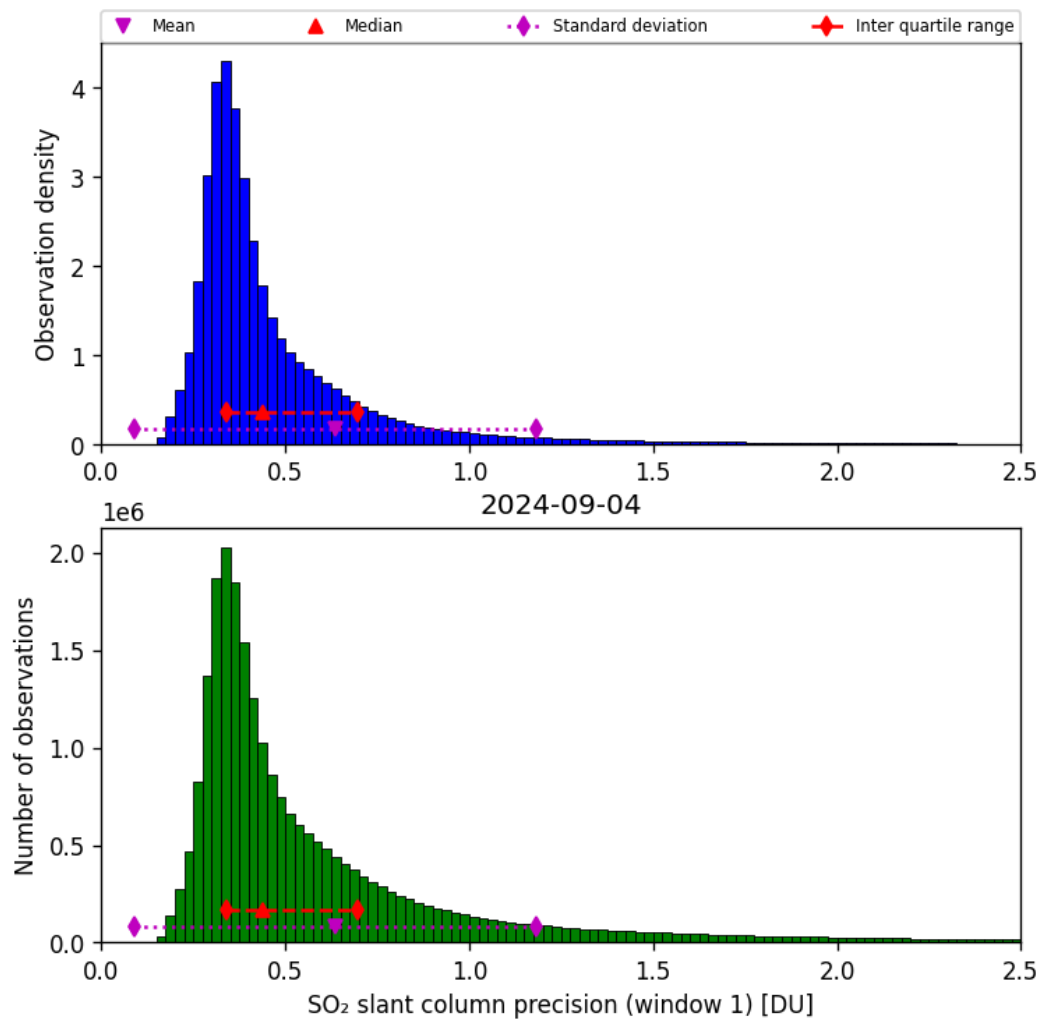
Figure 57: Histogram of “SO 2 slant column precision (window 1)” for 2024-09-03 to 2024-09-05
