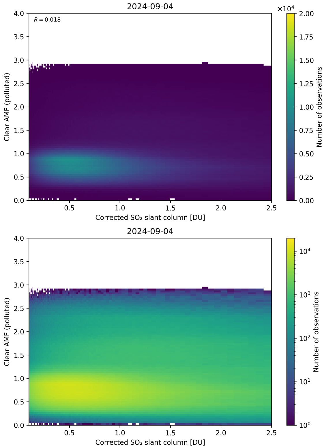
Figure 184: Scatter density plot of “Corrected SO 2 slant column” against “Clear AMF (polluted)” for 2024-09-03 to 2024-09-05.
