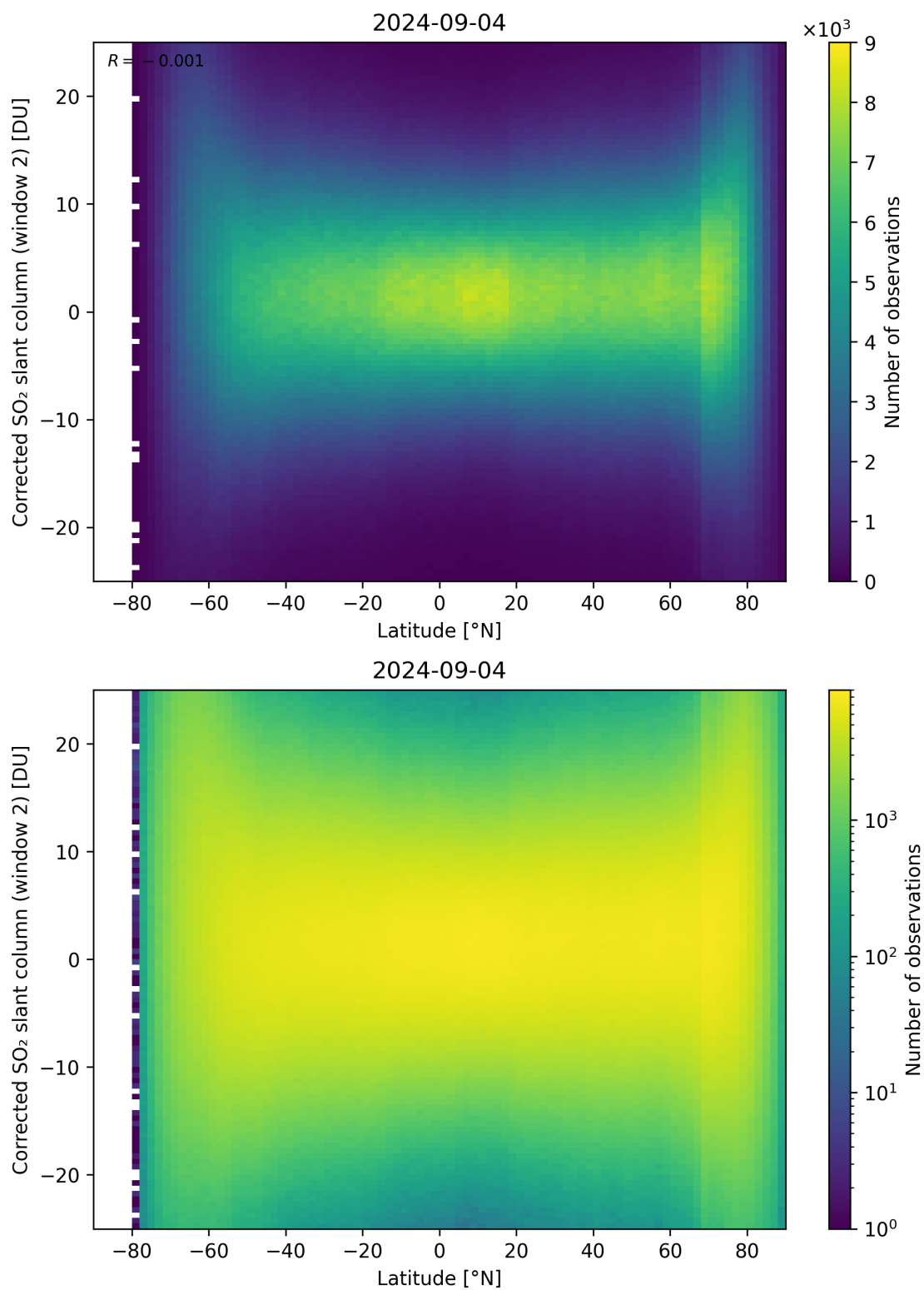
Figure 147: Scatter density plot of “Latitude” against “Corrected SO 2 slant column (window 2)” for 2024-09-03 to 2024-09-05.
