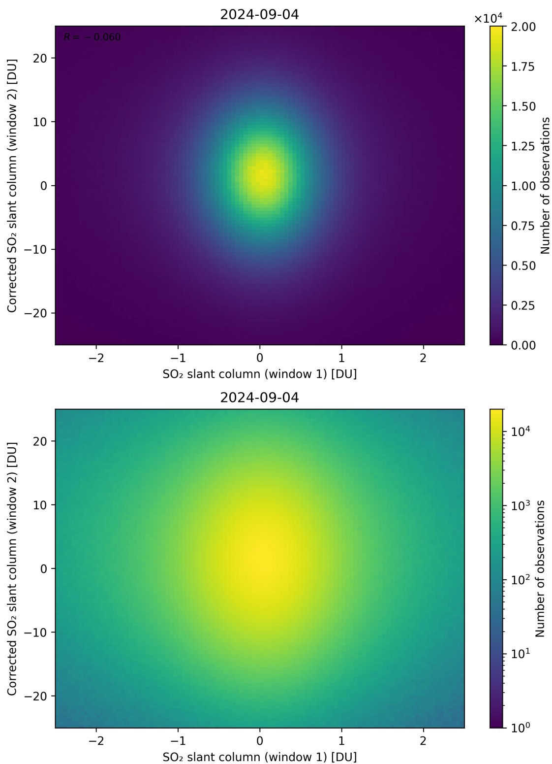
Figure 233: Scatter density plot of “SO 2 slant column (window 1)” against “Corrected SO 2 slant column (window 2)” for 2024-09-03 to 2024-09-05.
