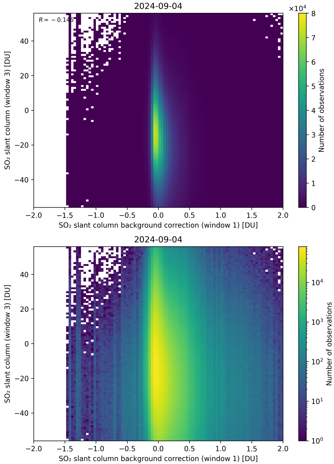
Figure 107: Scatter density plot of “SO 2 slant column background correction (window 1)” against “SO 2 slant column (window 3)” for 2024-09-03 to 2024-09-05.
