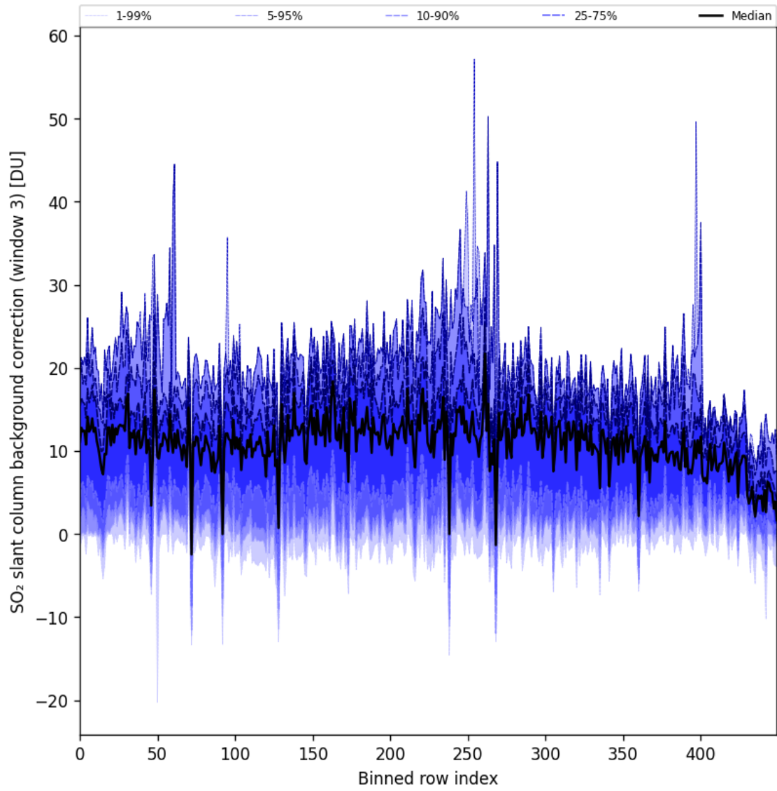
Figure 90: Along track statistics of “SO 2 slant column background correction (window 3)” for 2024-09-03 to 2024-09-05
