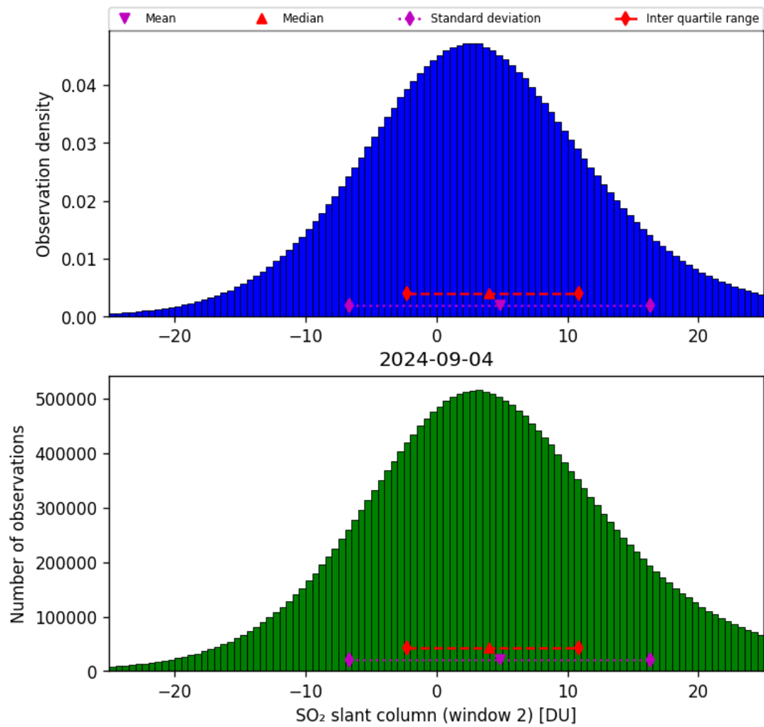
Figure 60: Histogram of “SO 2 slant column (window 2)” for 2024-09-03 to 2024-09-05
