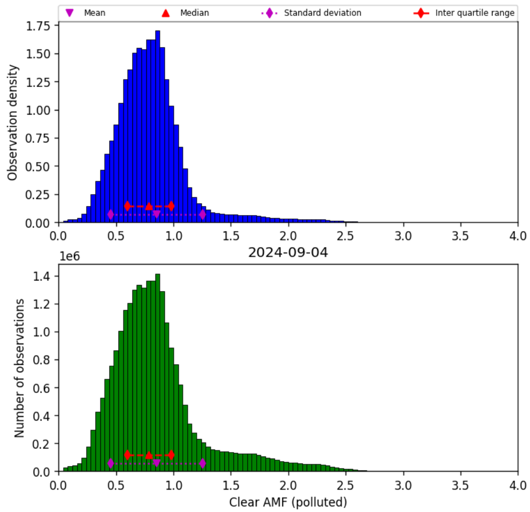
Figure 73: Histogram of “Clear AMF (polluted)” for 2024-09-03 to 2024-09-05
