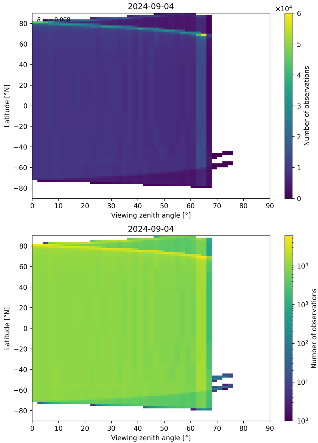
Figure 314: Scatter density plot of “Viewing zenith angle” against “Latitude” for 2024-09-03 to 2024-09-05.
