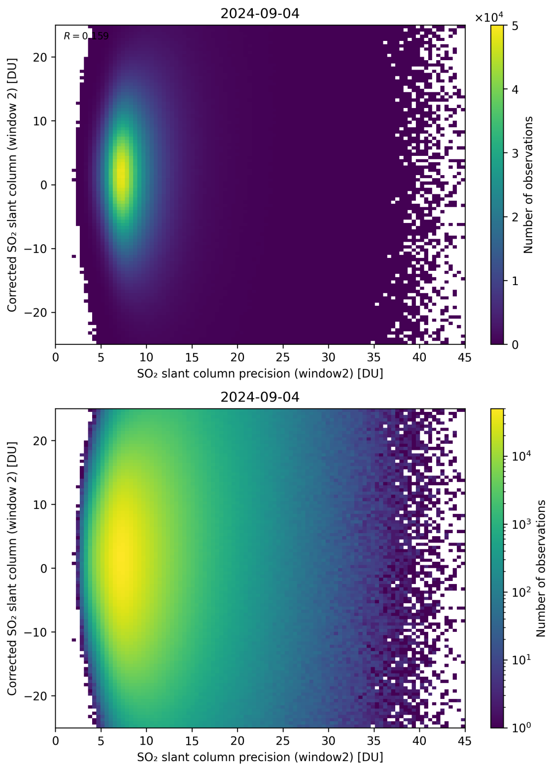
Figure 247: Scatter density plot of “SO 2 slant column precision (window2)” against “Corrected SO 2 slant column (window 2)” for 2024-09-03 to 2024-09-05.
