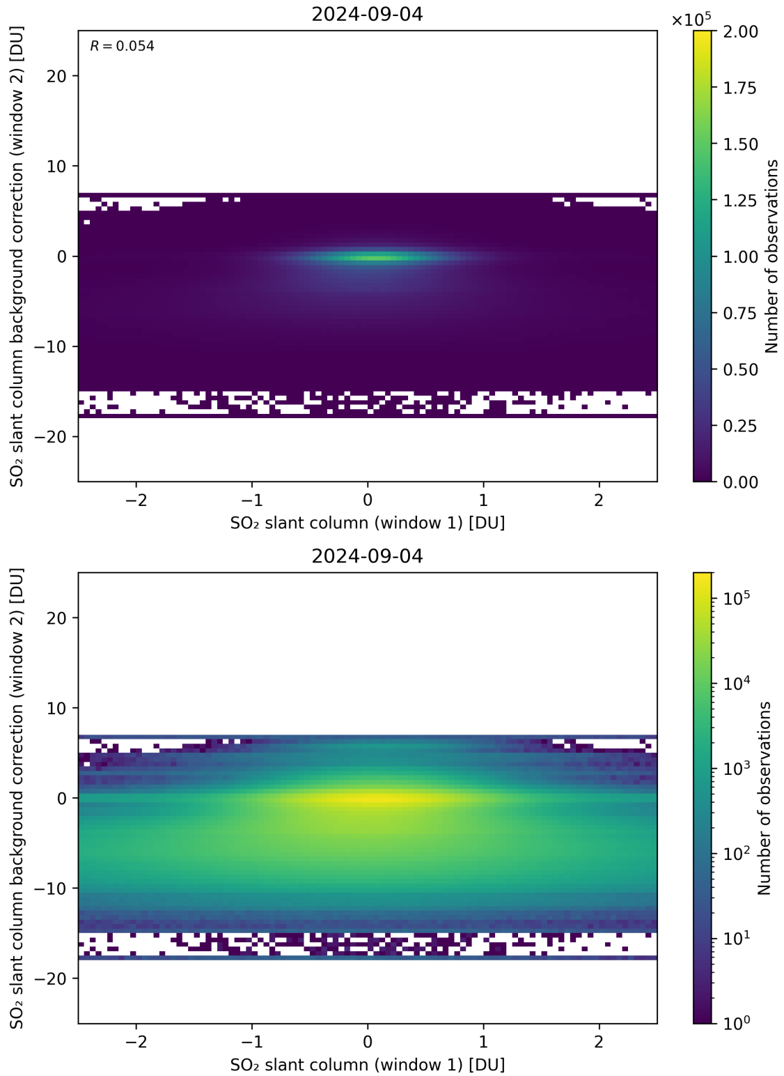
Figure 213: Scatter density plot of “SO 2 slant column (window 1)” against “SO 2 slant column background correction (window 2)” for 2024-09-03 to 2024-09-05.
