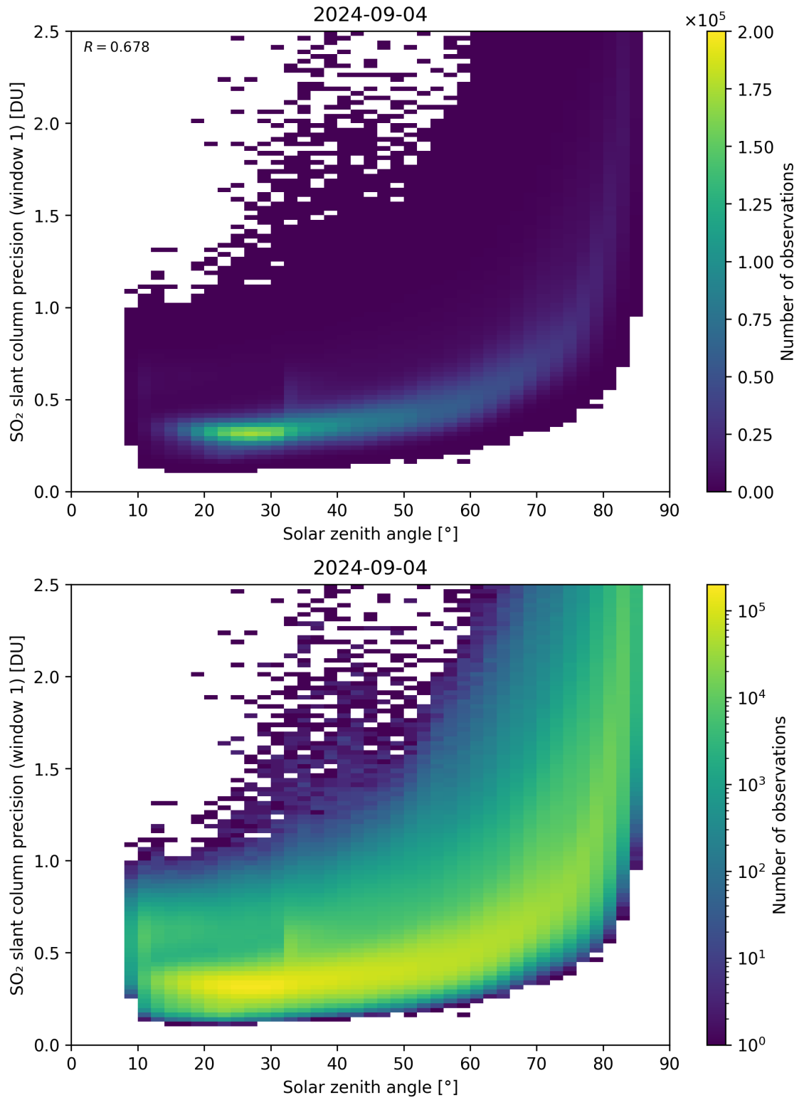
Figure 170: Scatter density plot of “Solar zenith angle” against “SO 2 slant column precision (window 1)” for 2024-09-03 to 2024-09-05.
