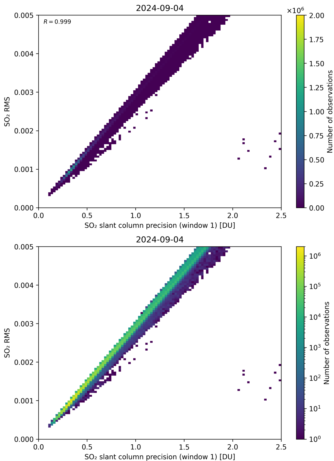
Figure 223: Scatter density plot of “SO 2 slant column precision (window 1)” against “SO 2 RMS” for 2024-09-03 to 2024-09-05.
