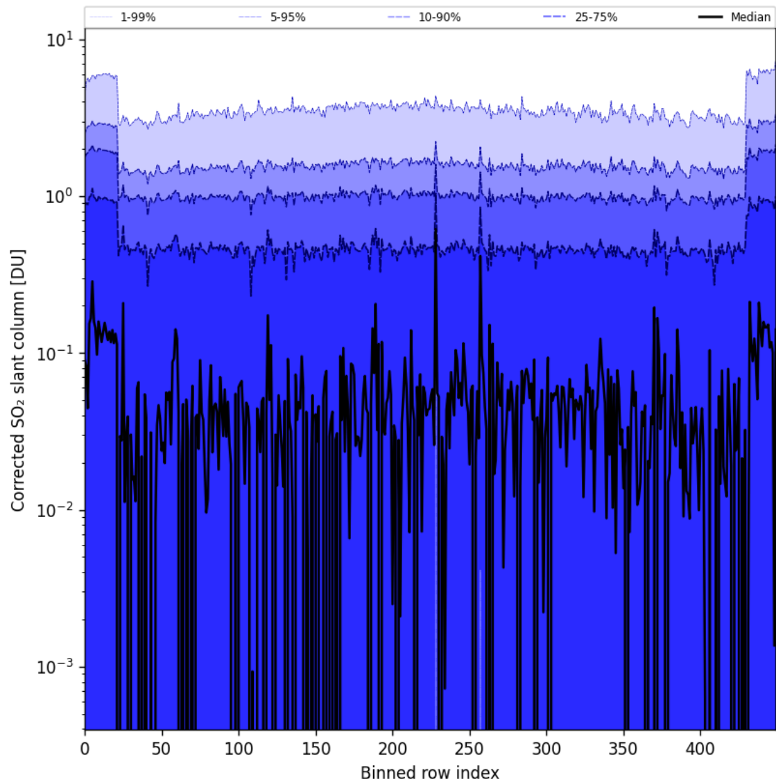
Figure 78: Along track statistics of “Corrected SO 2 slant column” for 2024-09-03 to 2024-09-05
