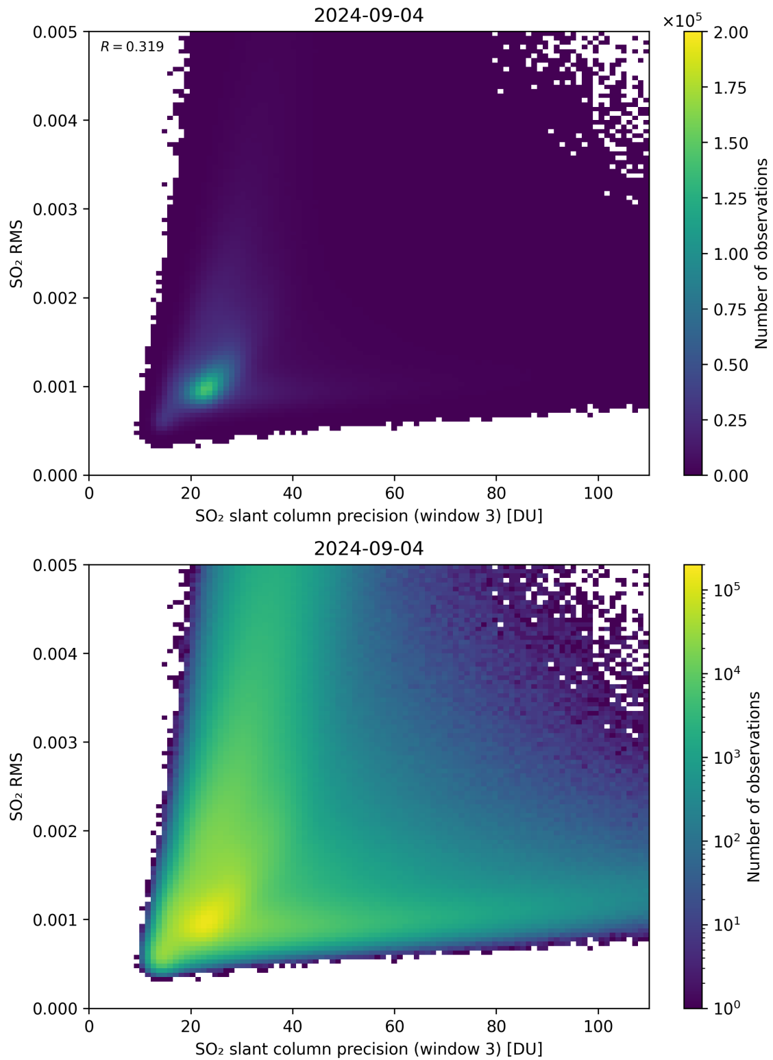
Figure 260: Scatter density plot of “SO 2 slant column precision (window 3)” against “SO 2 RMS” for 2024-09-03 to 2024-09-05.
