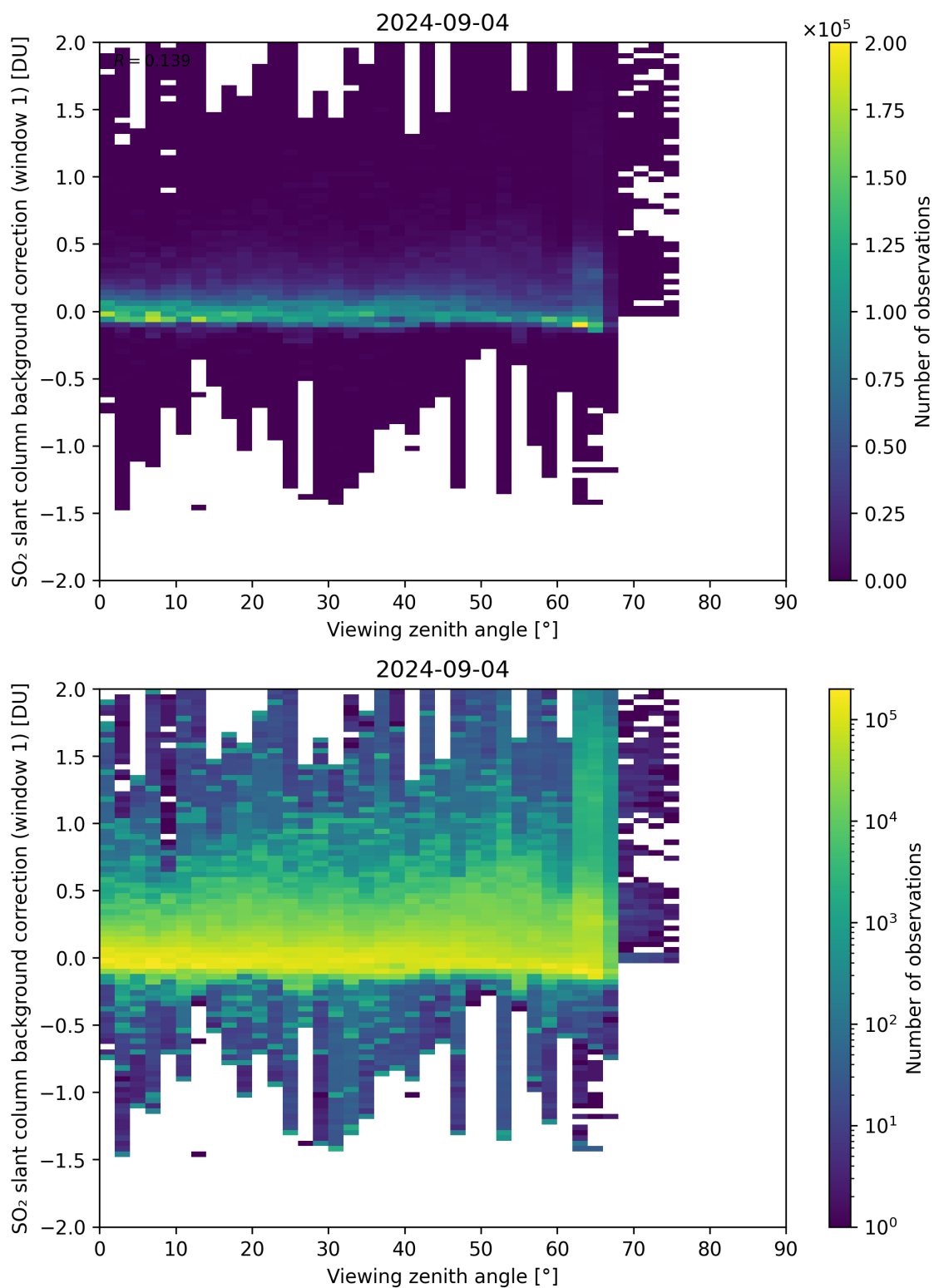
Figure 308: Scatter density plot of “Viewing zenith angle” against “SO 2 slant column background correction (window 1)” for 2024-09-03 to 2024-09-05.
