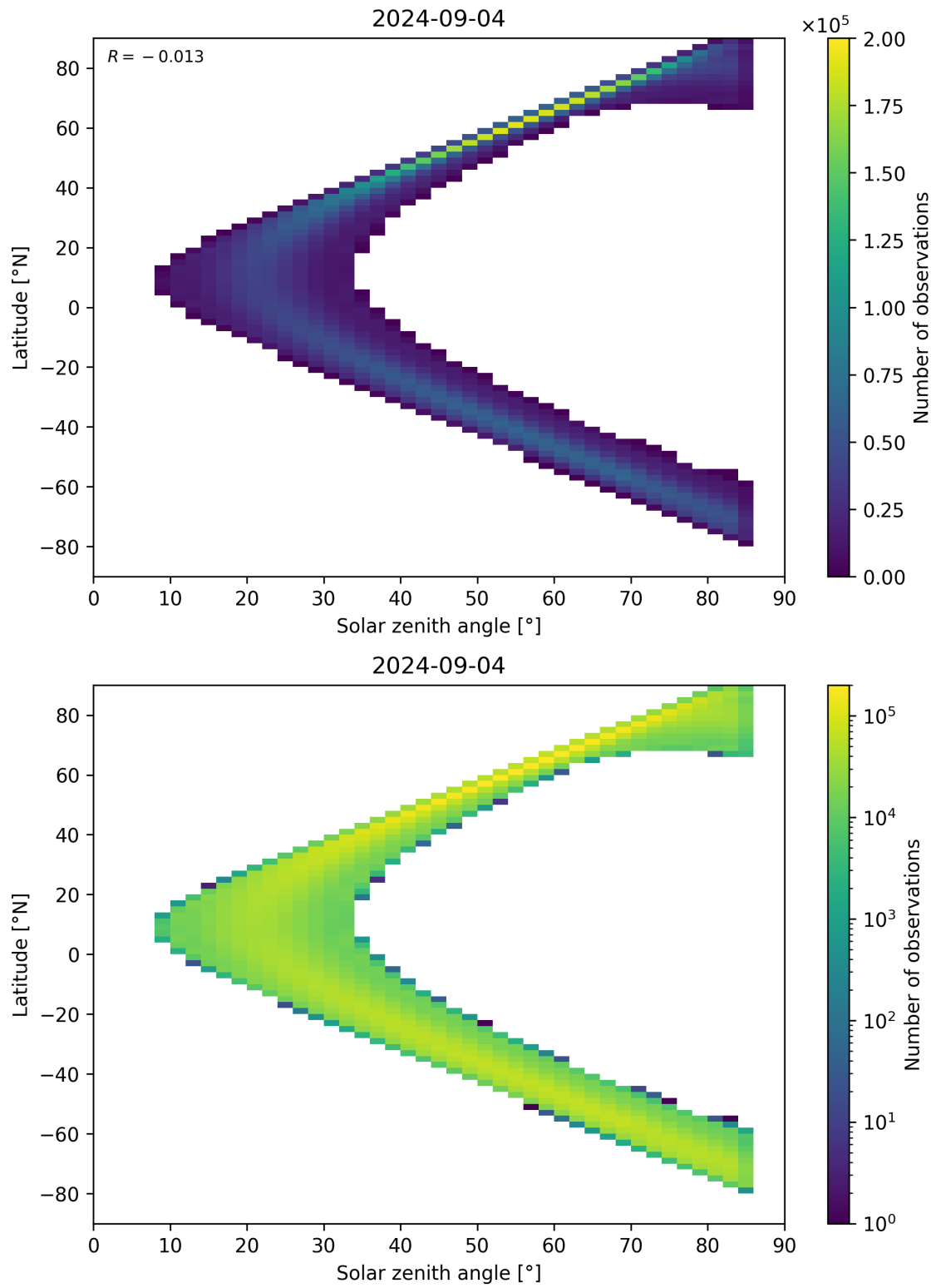
Figure 164: Scatter density plot of “Solar zenith angle” against “Latitude” for 2024-09-03 to 2024-09-05.
