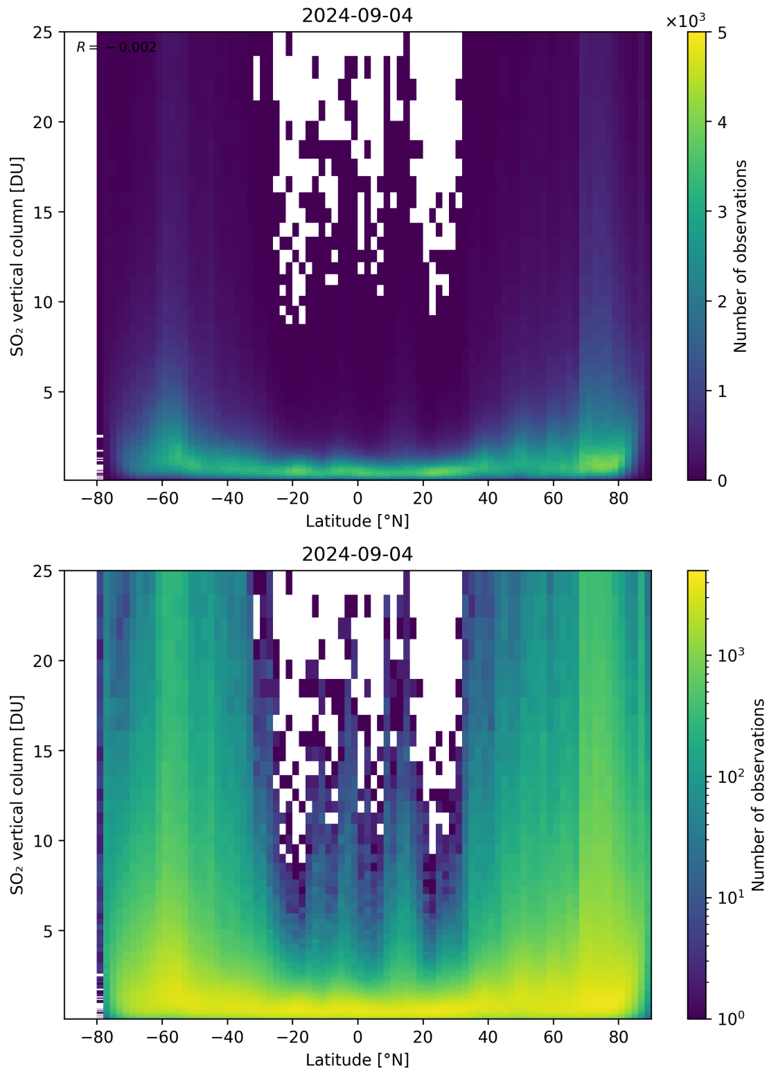
Figure 156: Scatter density plot of “Latitude” against “SO 2 vertical column” for 2024-09-03 to 2024-09-05.
