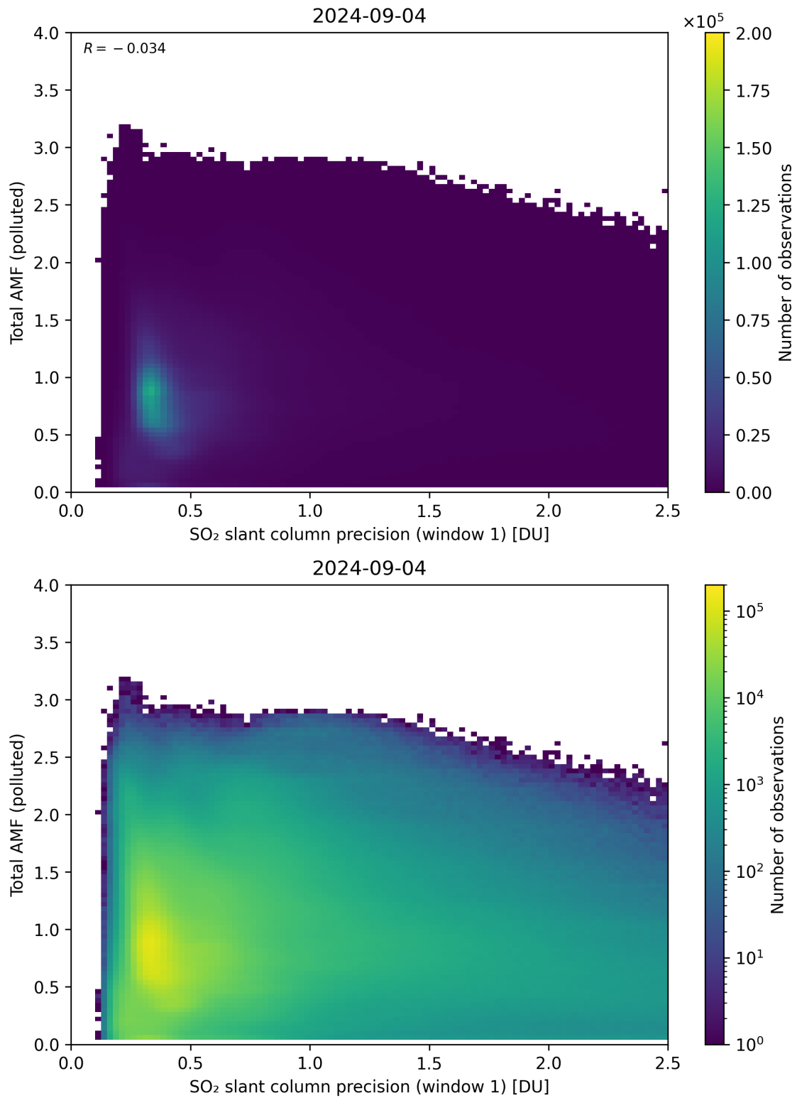
Figure 230: Scatter density plot of “SO 2 slant column precision (window 1)” against “Total AMF (polluted)” for 2024-09-03 to 2024-09-05.
