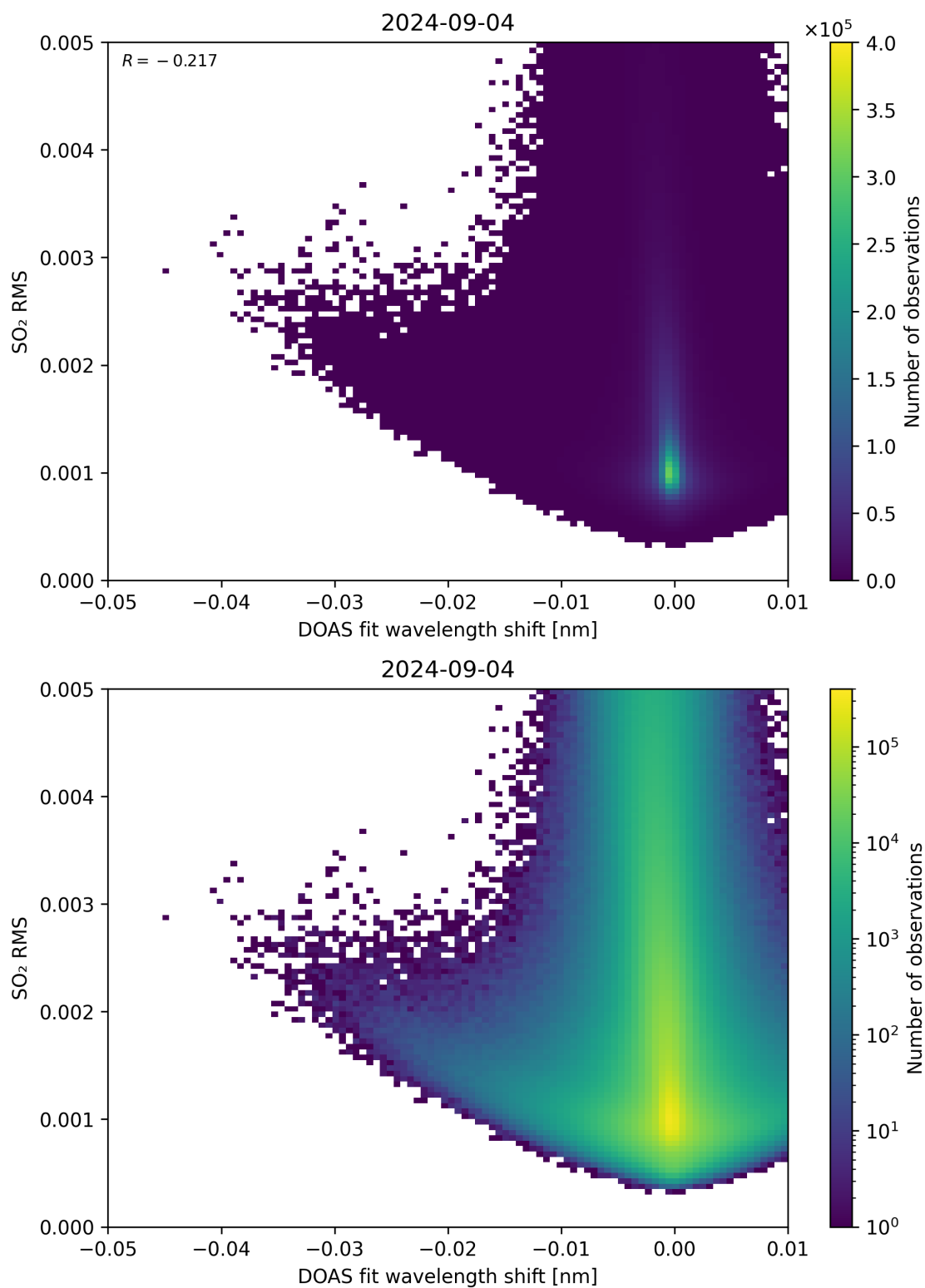
Figure 128: Scatter density plot of “DOAS fit wavelength shift” against “SO 2 RMS” for 2024-09-03 to 2024-09-05.
