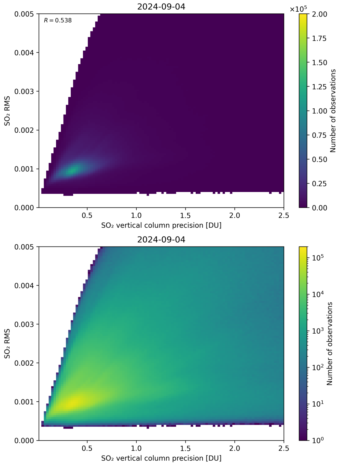
Figure 284: Scatter density plot of “SO 2 vertical column precision” against “SO 2 RMS” for 2024-09-03 to 2024-09-05.
