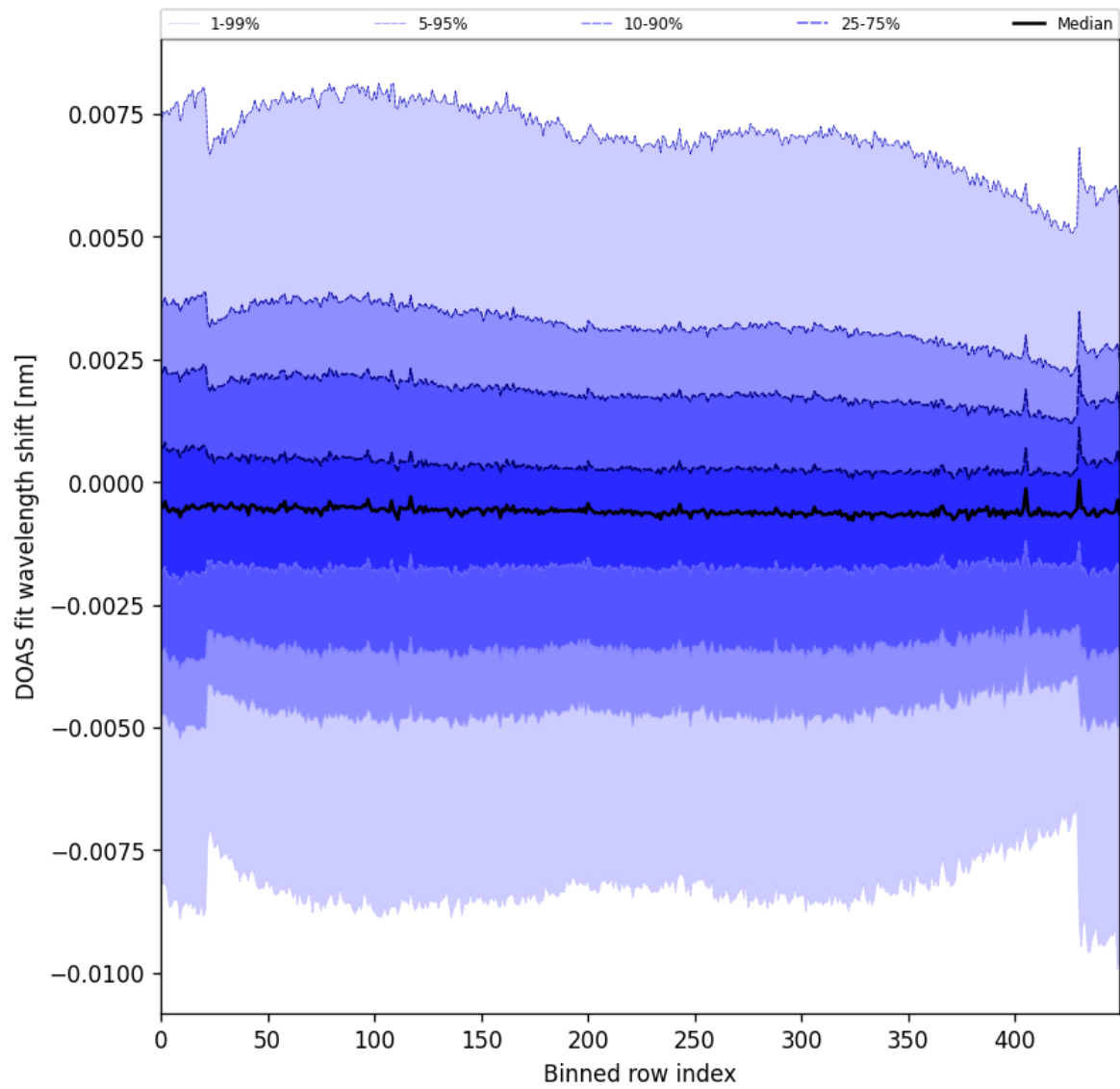
Figure 91: Along track statistics of “DOAS fit wavelength shift” for 2024-09-03 to 2024-09-05
