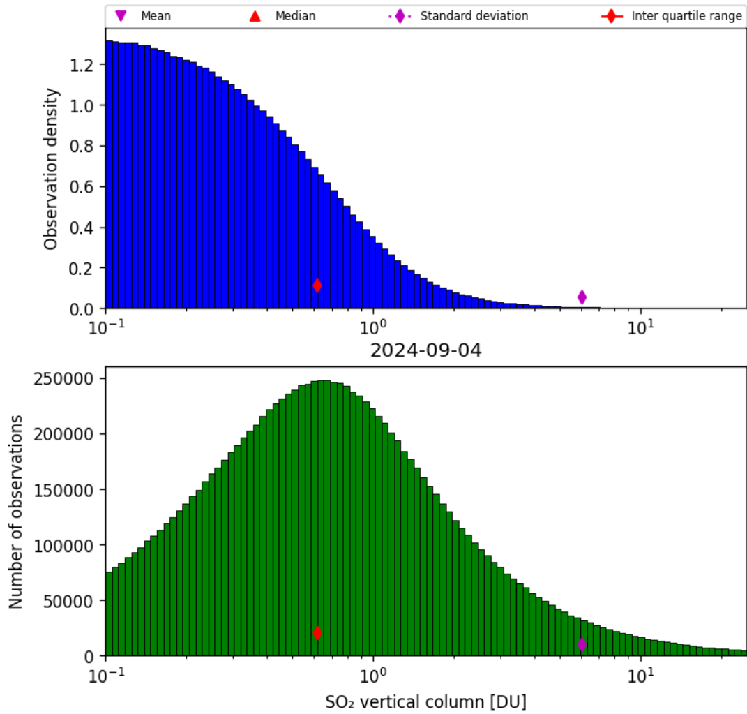
Figure 53: Histogram of “SO 2 vertical column” for 2024-09-03 to 2024-09-05
