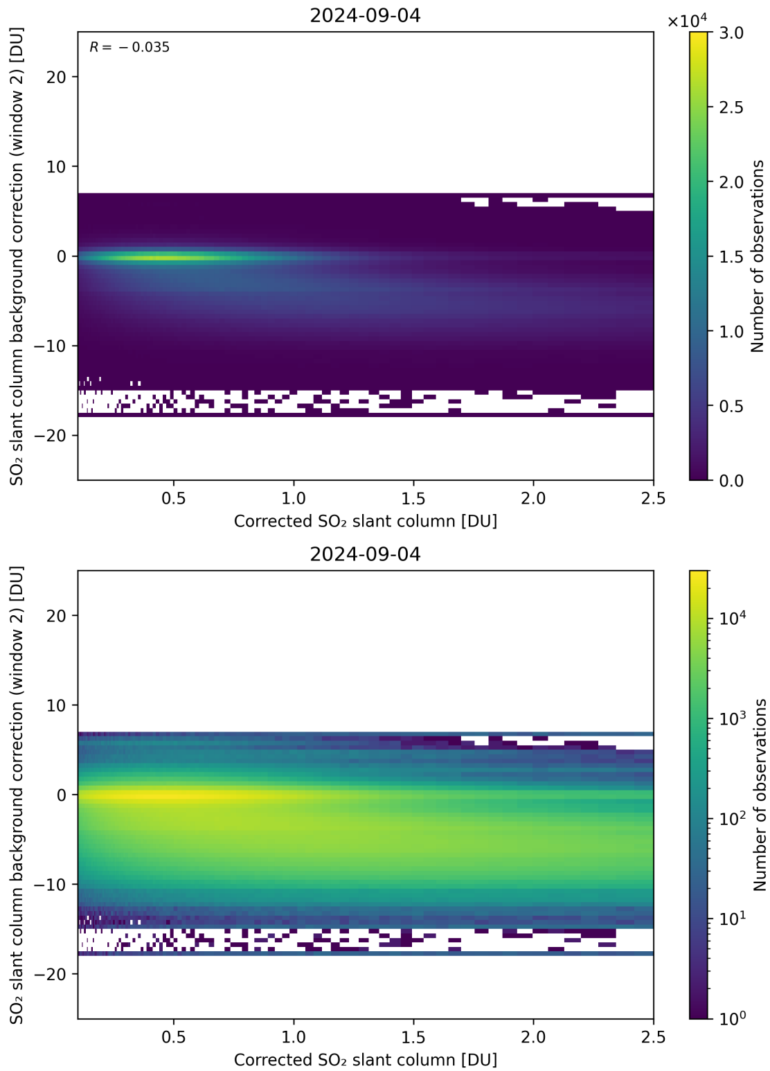
Figure 179: Scatter density plot of “Corrected SO 2 slant column” against “SO 2 slant column background correction (window 2)” for 2024-09-03 to 2024-09-05.
