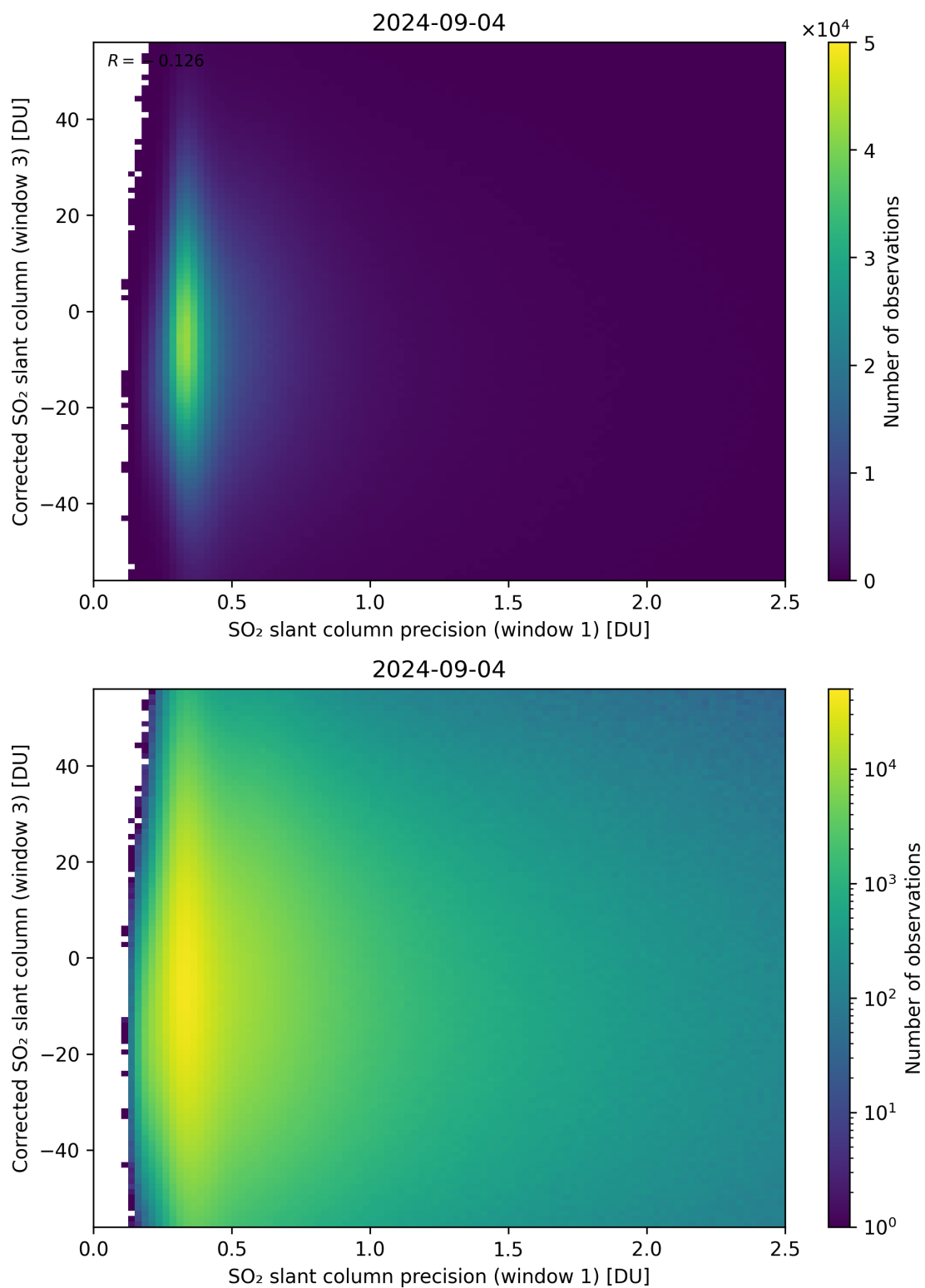
Figure 226: Scatter density plot of “SO 2 slant column precision (window 1)” against “Corrected SO 2 slant column (window 3)” for 2024-09-03 to 2024-09-05.
