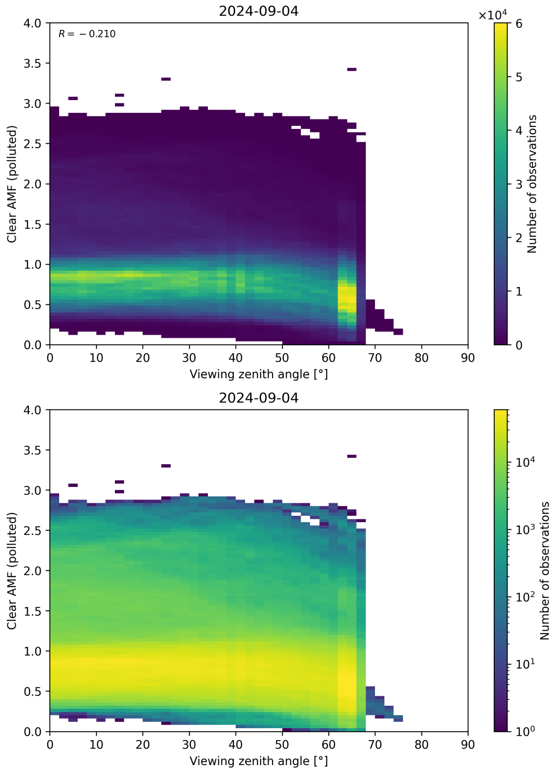
Figure 316: Scatter density plot of “Viewing zenith angle” against “Clear AMF (polluted)” for 2024-09-03 to 2024-09-05.
