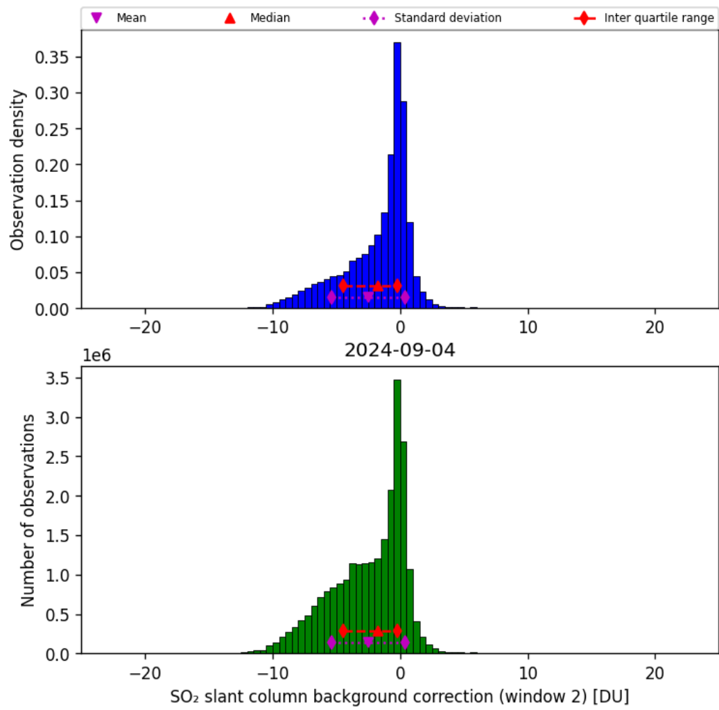
Figure 63: Histogram of “SO 2 slant column background correction (window 2)” for 2024-09-03 to 2024-09-05
