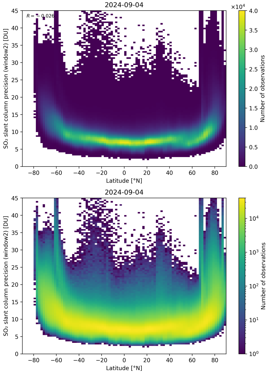
Figure 151: Scatter density plot of “Latitude” against “SO 2 slant column precision (window2)” for 2024-09-03 to 2024-09-05.
