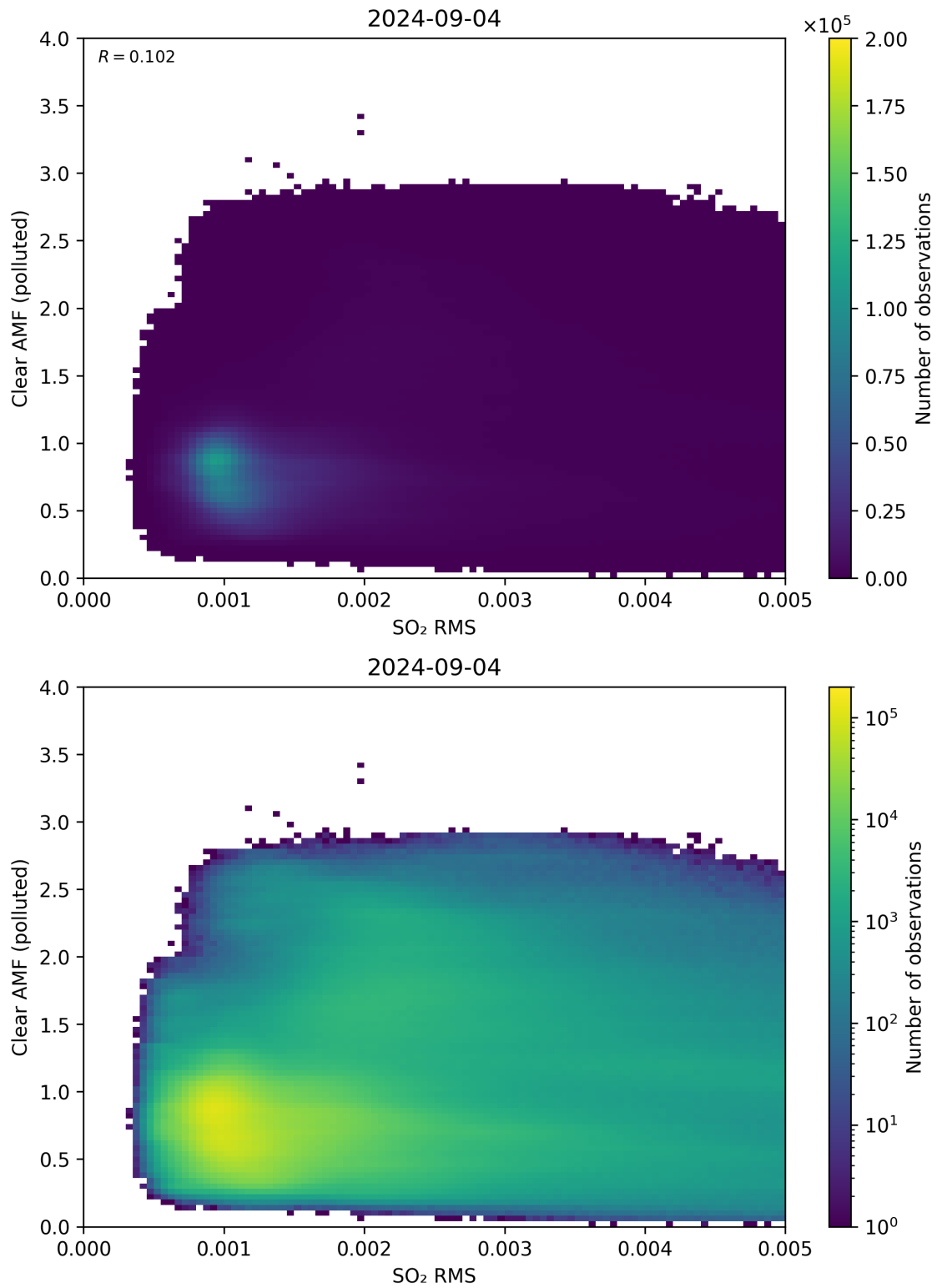
Figure 136: Scatter density plot of “SO 2 RMS” against “Clear AMF (polluted)” for 2024-09-03 to 2024-09-05.
