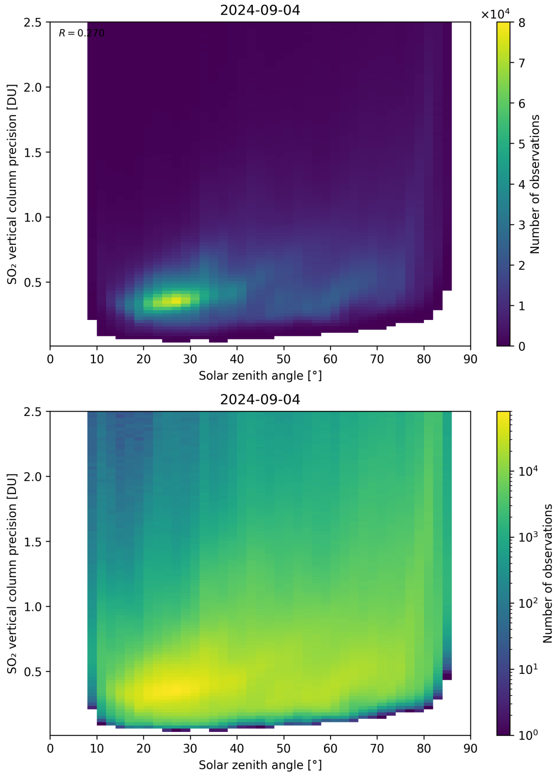
Figure 177: Scatter density plot of “Solar zenith angle” against “SO 2 vertical column precision” for 2024-09-03 to 2024-09-05.
