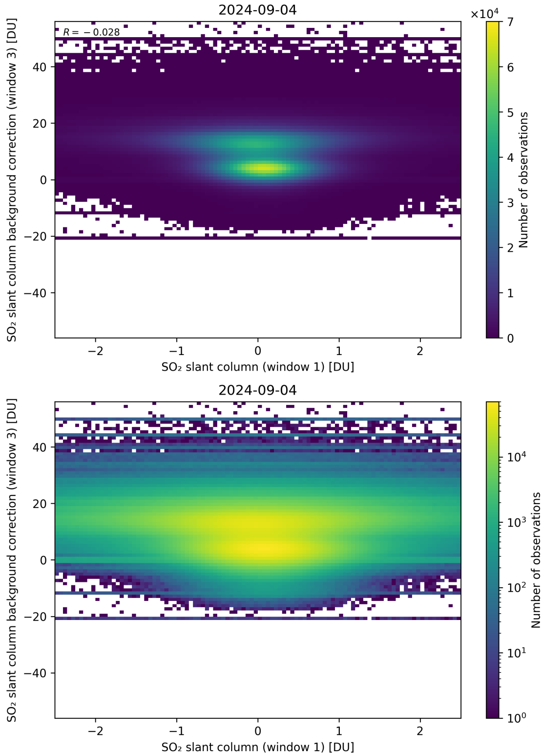
Figure 214: Scatter density plot of “SO 2 slant column (window 1)” against “SO 2 slant column background correction (window 3)” for 2024-09-03 to 2024-09-05.
