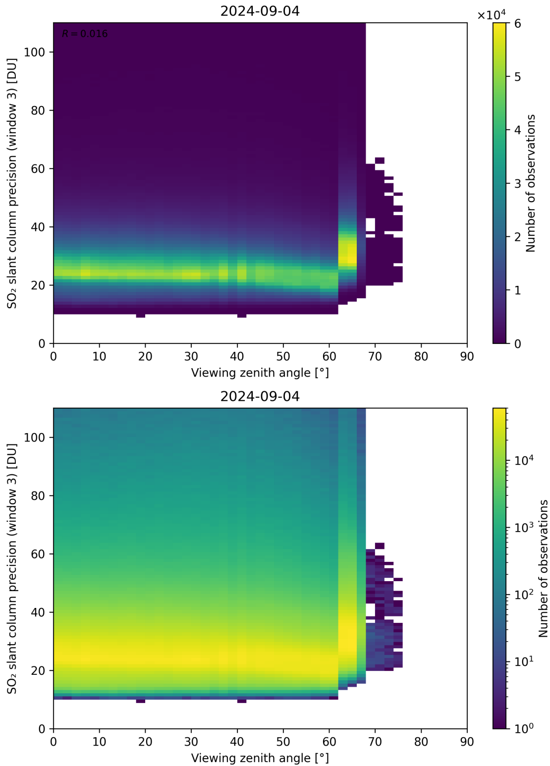
Figure 324: Scatter density plot of “Viewing zenith angle” against “SO 2 slant column precision (window 3)” for 2024-09-03 to 2024-09-05.
