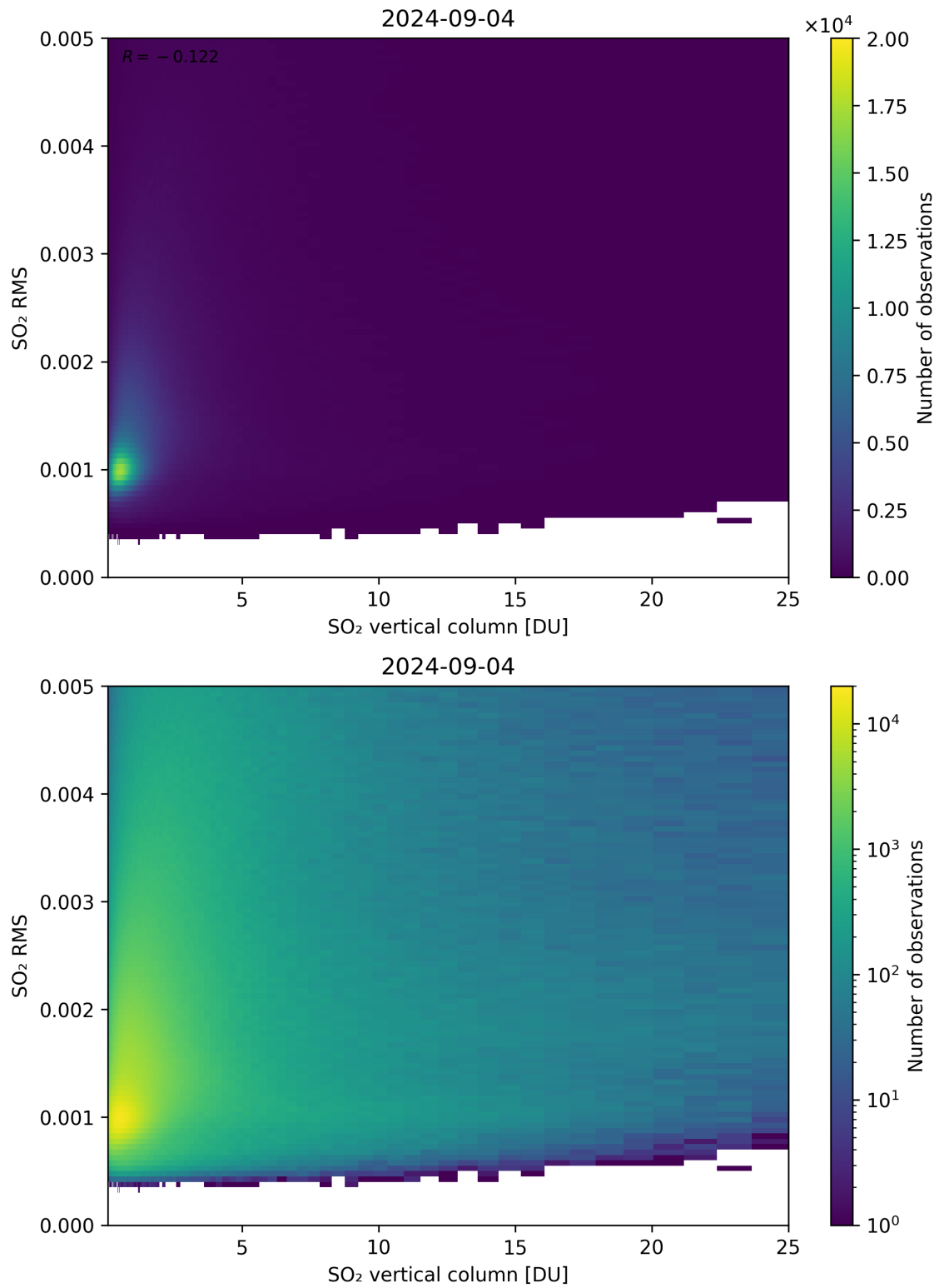
Figure 278: Scatter density plot of “SO 2 vertical column” against “SO 2 RMS” for 2024-09-03 to 2024-09-05.
