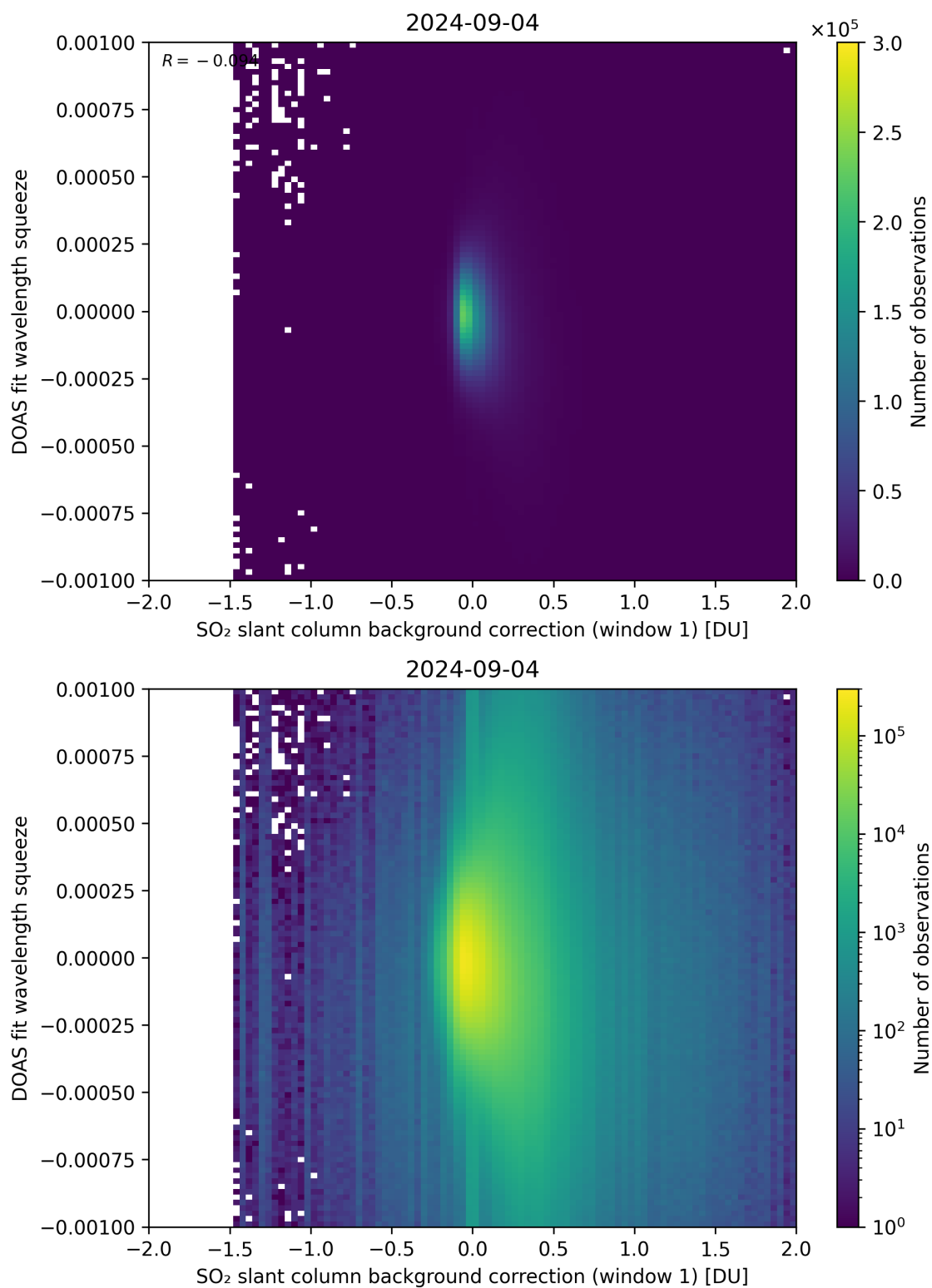
Figure 101: Scatter density plot of “SO 2 slant column background correction (window 1)” against “DOAS fit wavelength squeeze” for 2024-09-03 to 2024-09-05.
