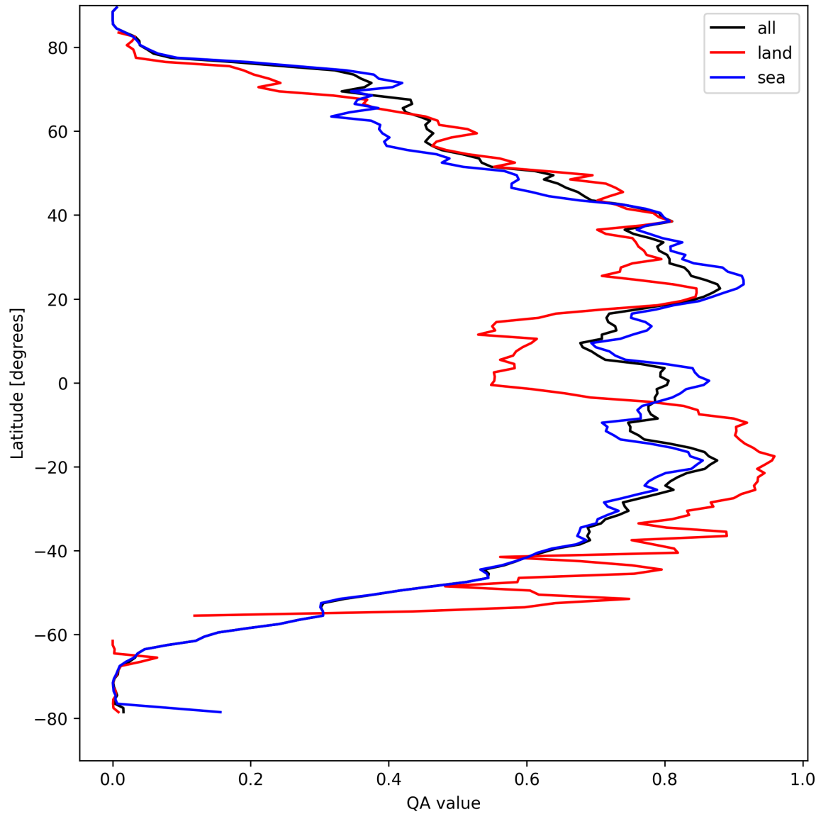
Figure 29: Zonal average of “QA value” for 2024-09-03 to 2024-09-05.
