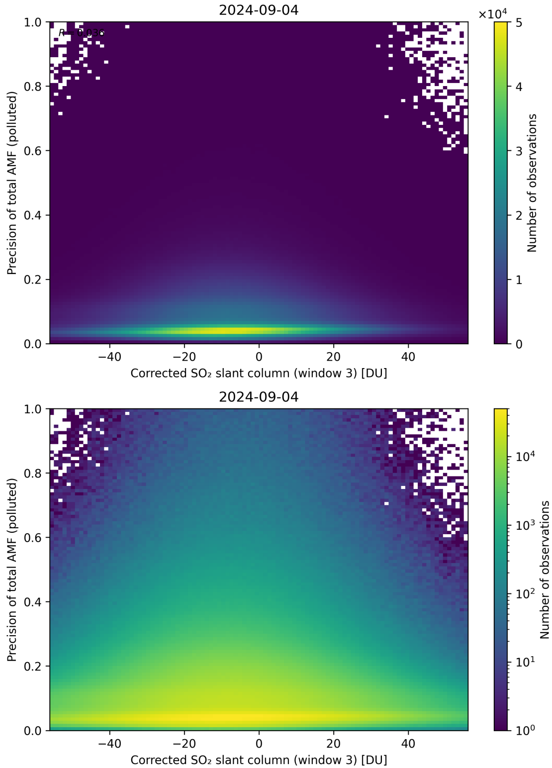
Figure 211: Scatter density plot of “Corrected SO 2 slant column (window 3)” against “Precision of total AMF (polluted)” for 2024-09-03 to 2024-09-05.
