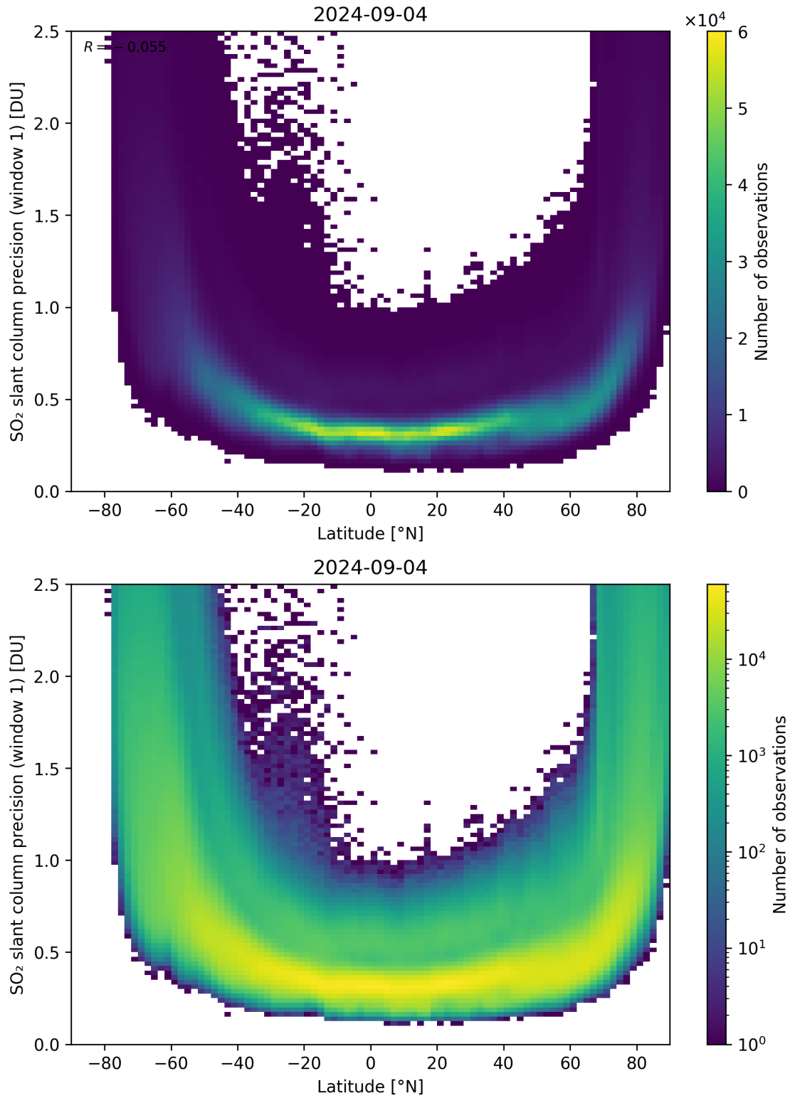
Figure 150: Scatter density plot of “Latitude” against “SO 2 slant column precision (window 1)” for 2024-09-03 to 2024-09-05.
