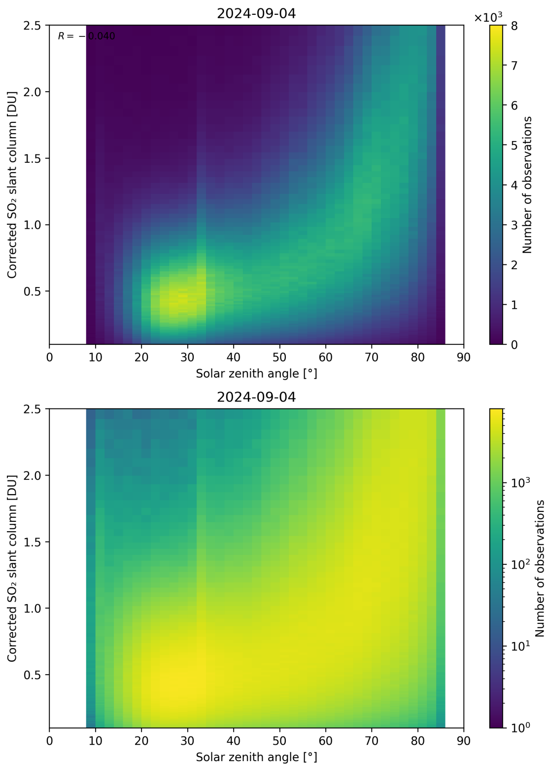
Figure 166: Scatter density plot of “Solar zenith angle” against “Corrected SO 2 slant column” for 2024-09-03 to 2024-09-05.
