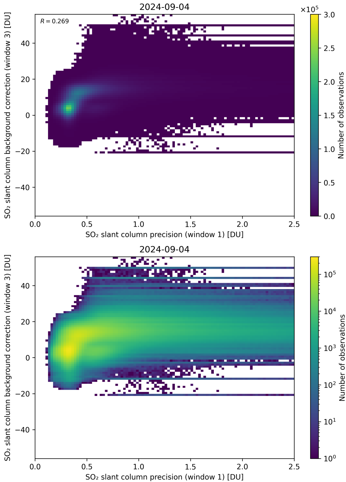
Figure 220: Scatter density plot of “SO 2 slant column precision (window 1)” against “SO 2 slant column background correction (window 3)” for 2024-09-03 to 2024-09-05.
