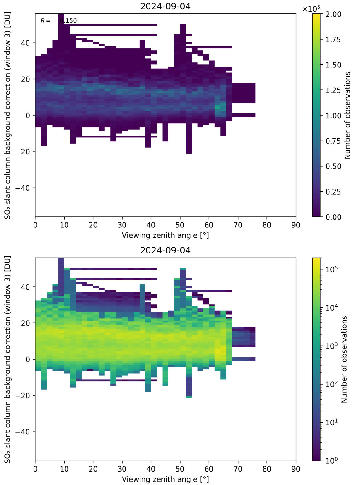
Figure 310: Scatter density plot of “Viewing zenith angle” against “SO 2 slant column background correction (window 3)” for 2024-09-03 to 2024-09-05.
