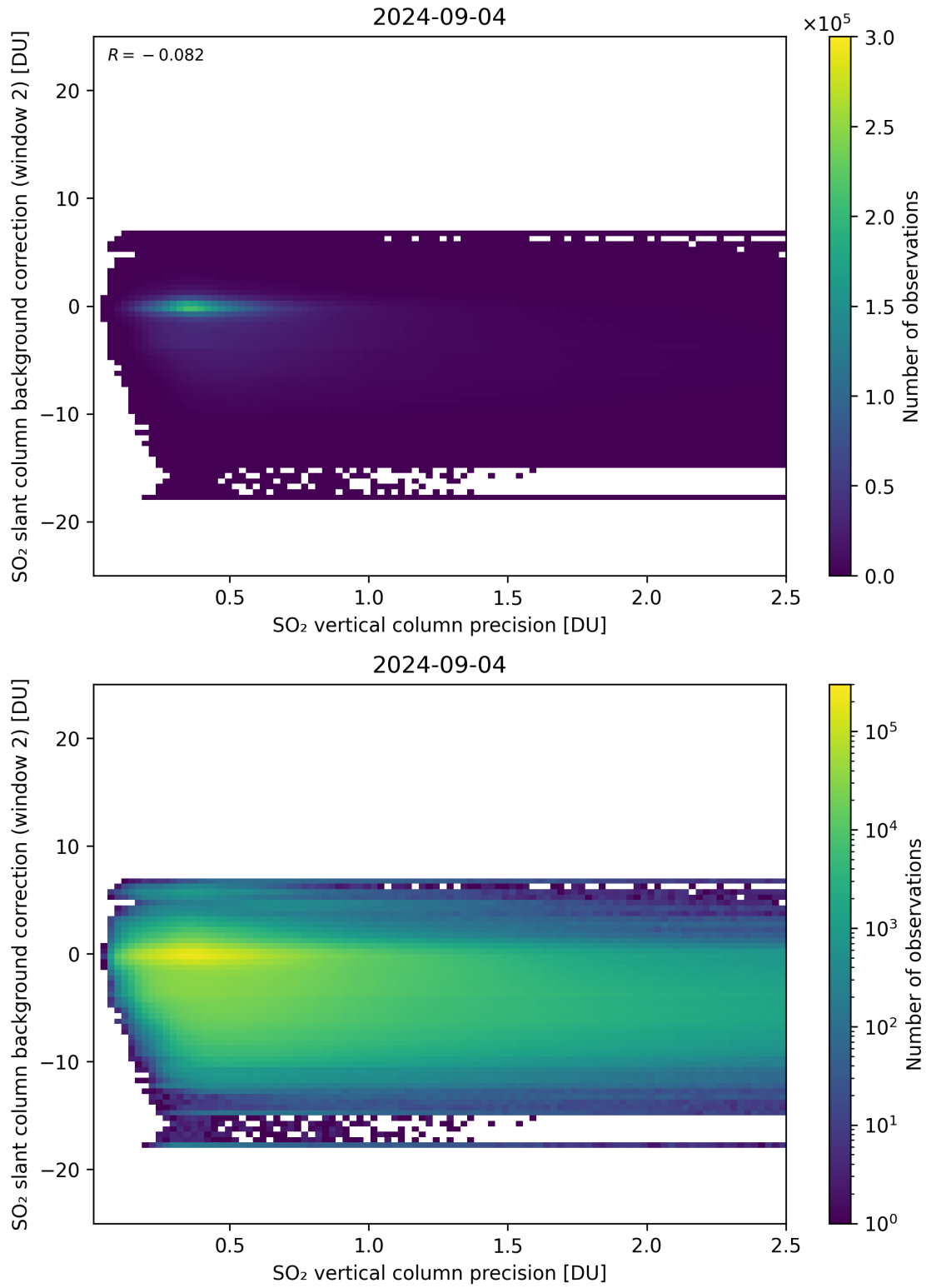
Figure 280: Scatter density plot of “SO 2 vertical column precision” against “SO 2 slant column background correction (window 2)” for 2024-09-03 to 2024-09-05.
