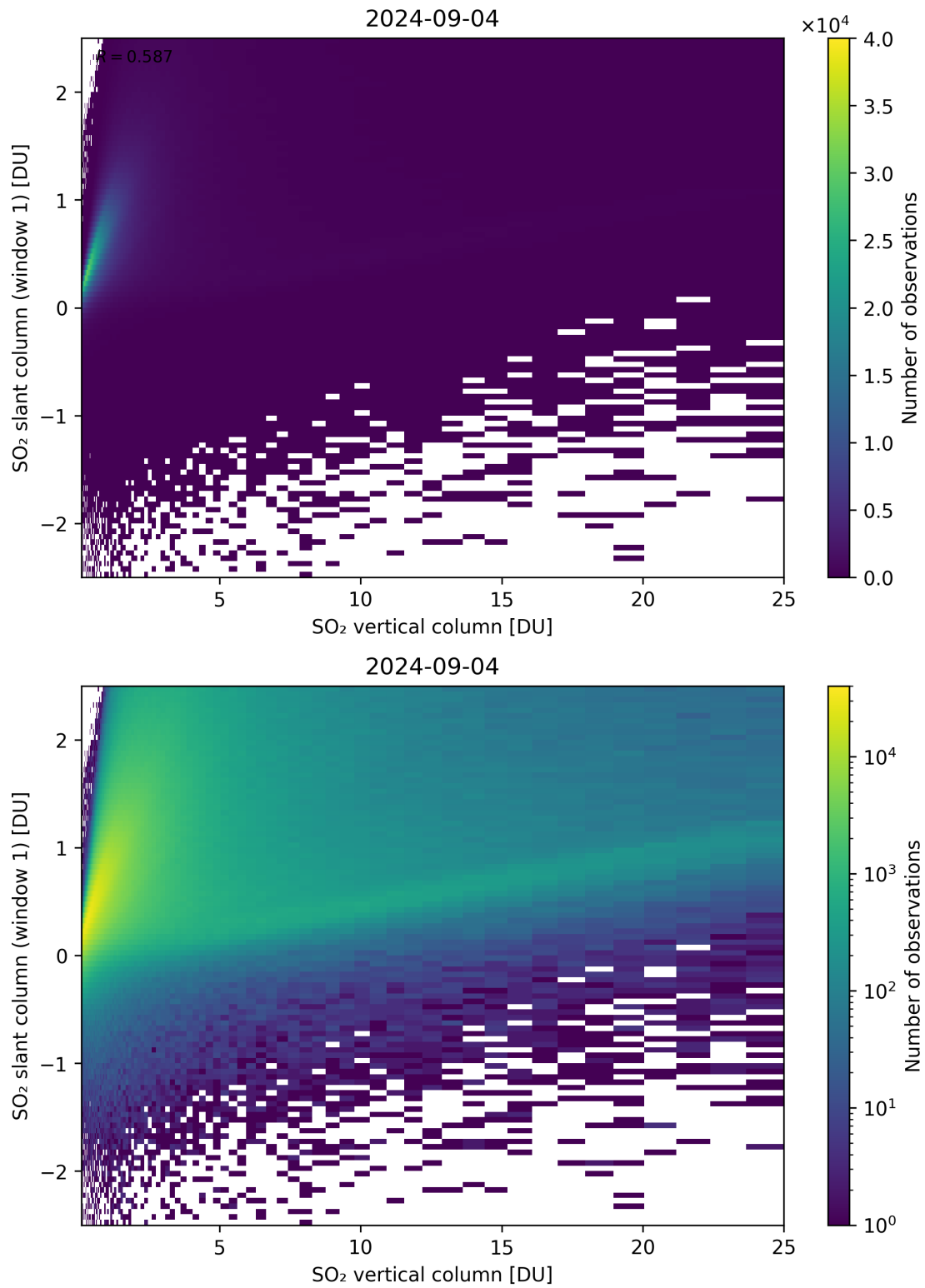
Figure 300: Scatter density plot of “SO 2 vertical column” against “SO 2 slant column (window 1)” for 2024-09-03 to 2024-09-05.
