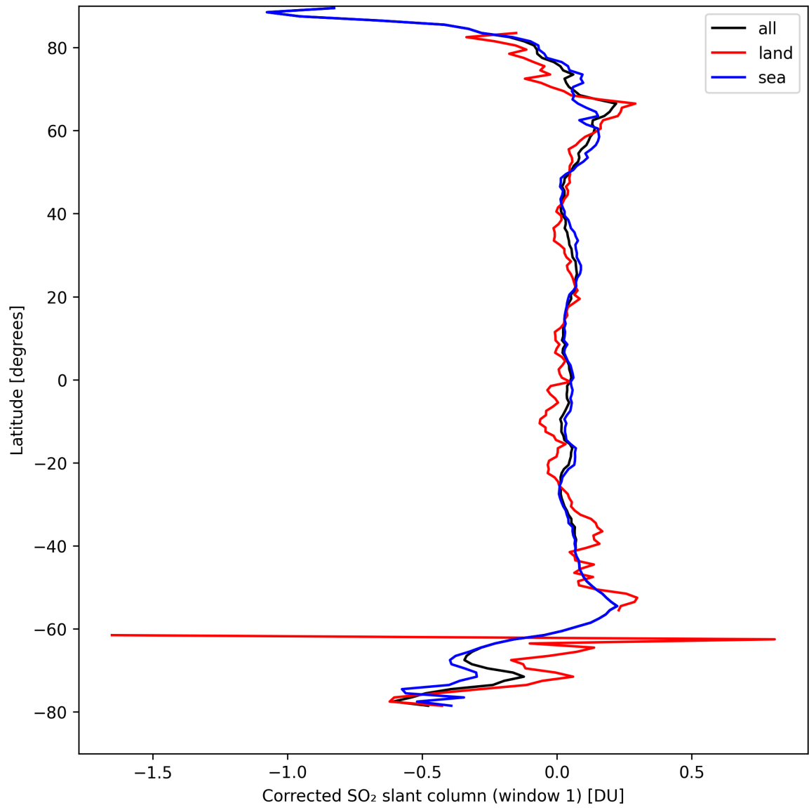
Figure 35: Zonal average of “Corrected SO 2 slant column (window 1)” for 2024-09-03 to 2024-09-05.
