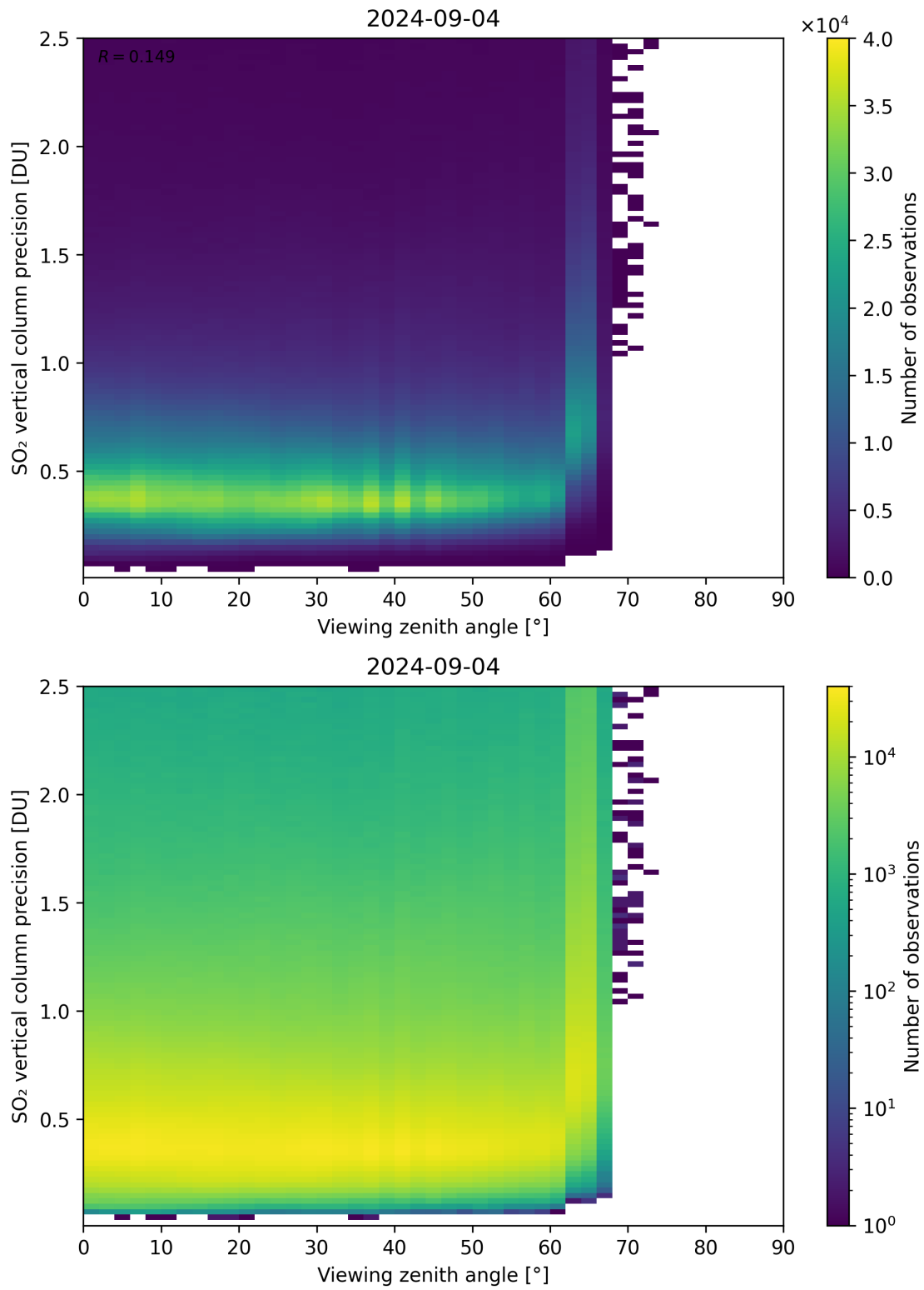
Figure 328: Scatter density plot of “Viewing zenith angle” against “SO 2 vertical column precision” for 2024-09-03 to 2024-09-05.
