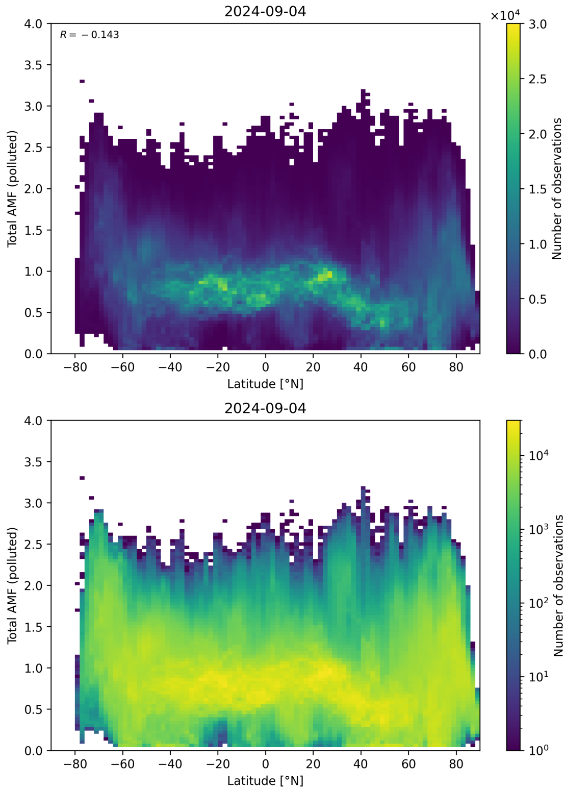
Figure 154: Scatter density plot of “Latitude” against “Total AMF (polluted)” for 2024-09-03 to 2024-09-05.
