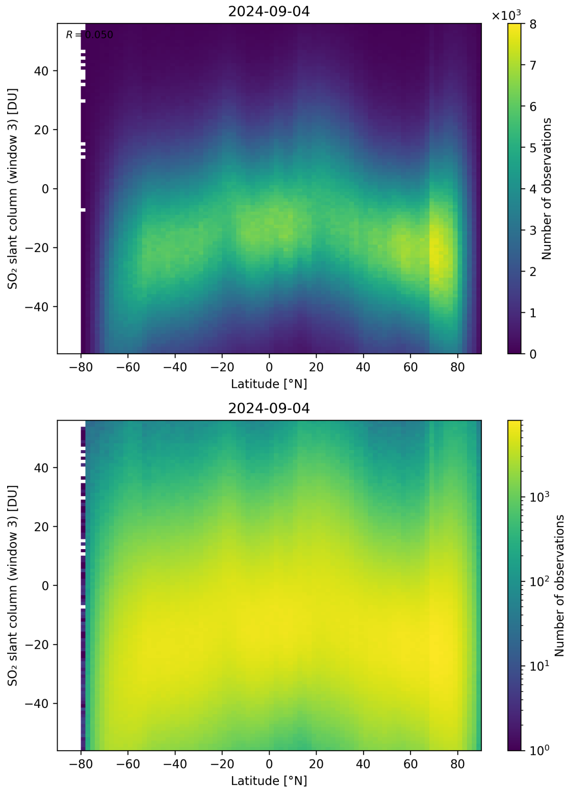
Figure 152: Scatter density plot of “Latitude” against “SO 2 slant column (window 3)” for 2024-09-03 to 2024-09-05.
