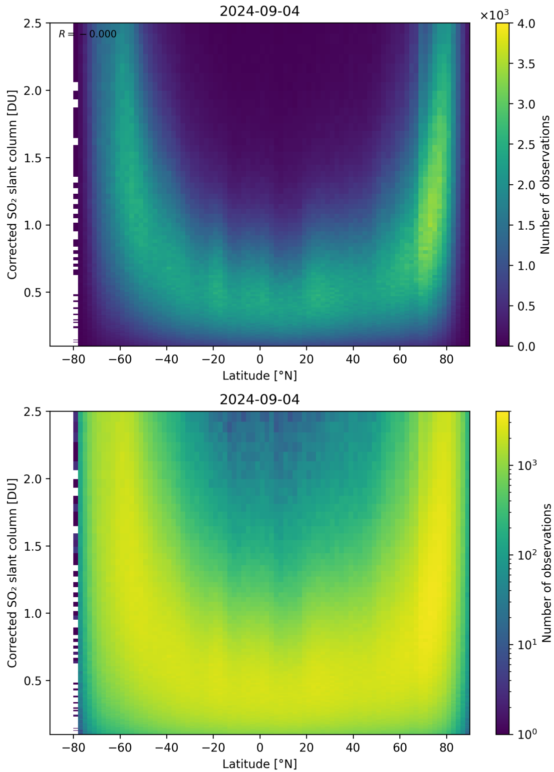
Figure 146: Scatter density plot of “Latitude” against “Corrected SO 2 slant column” for 2024-09-03 to 2024-09-05.
