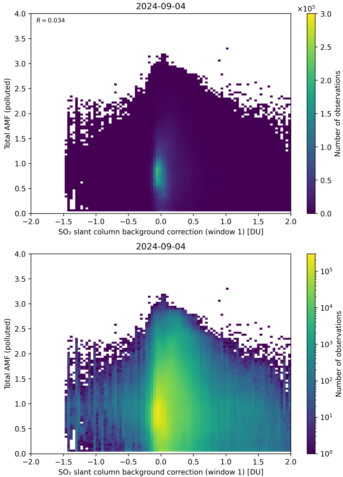
Figure 109: Scatter density plot of “SO 2 slant column background correction (window 1)” against “Total AMF (polluted)” for 2024-09-03 to 2024-09-05.
