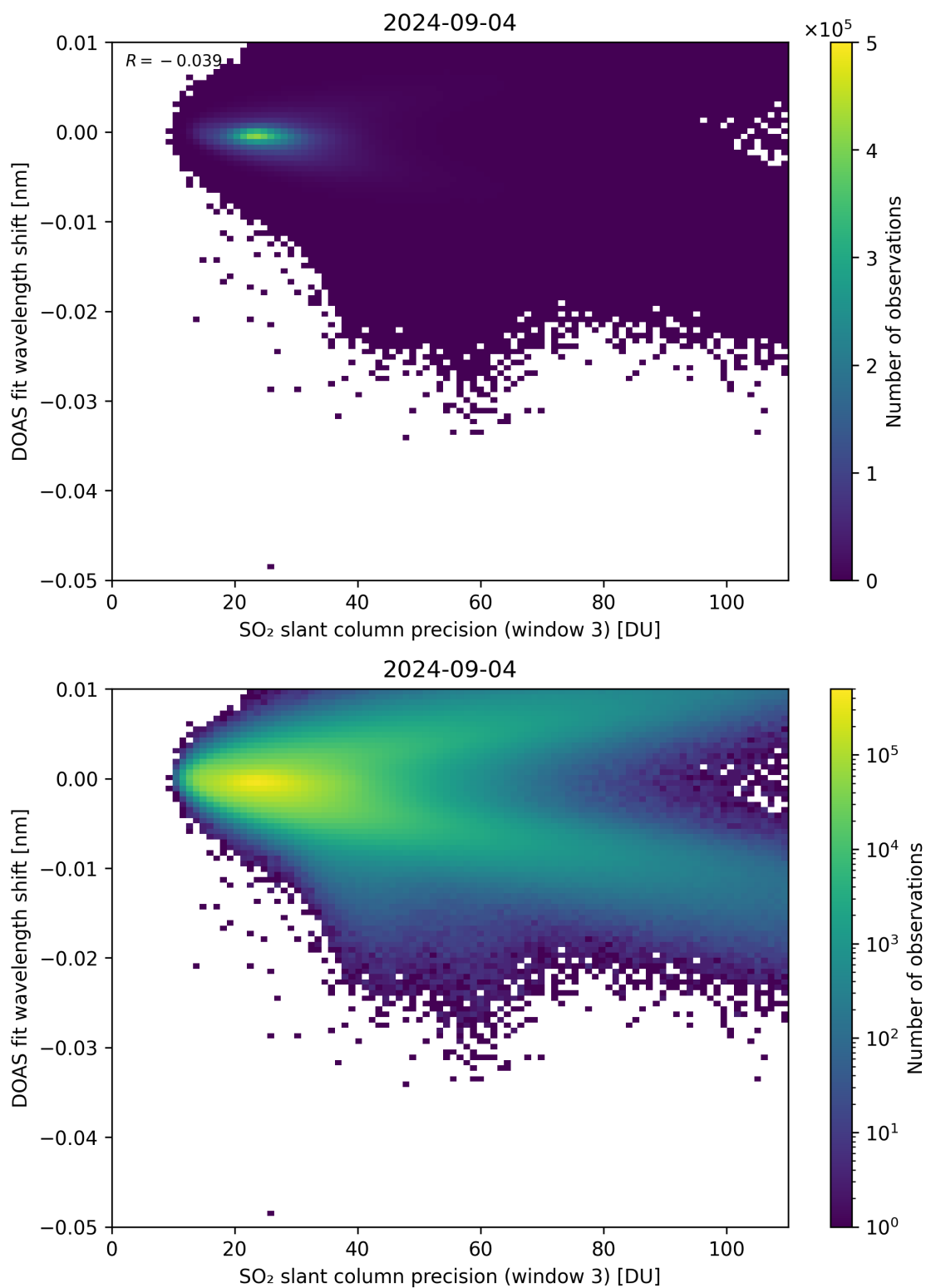
Figure 258: Scatter density plot of “SO 2 slant column precision (window 3)” against “DOAS fit wavelength shift” for 2024-09-03 to 2024-09-05.
