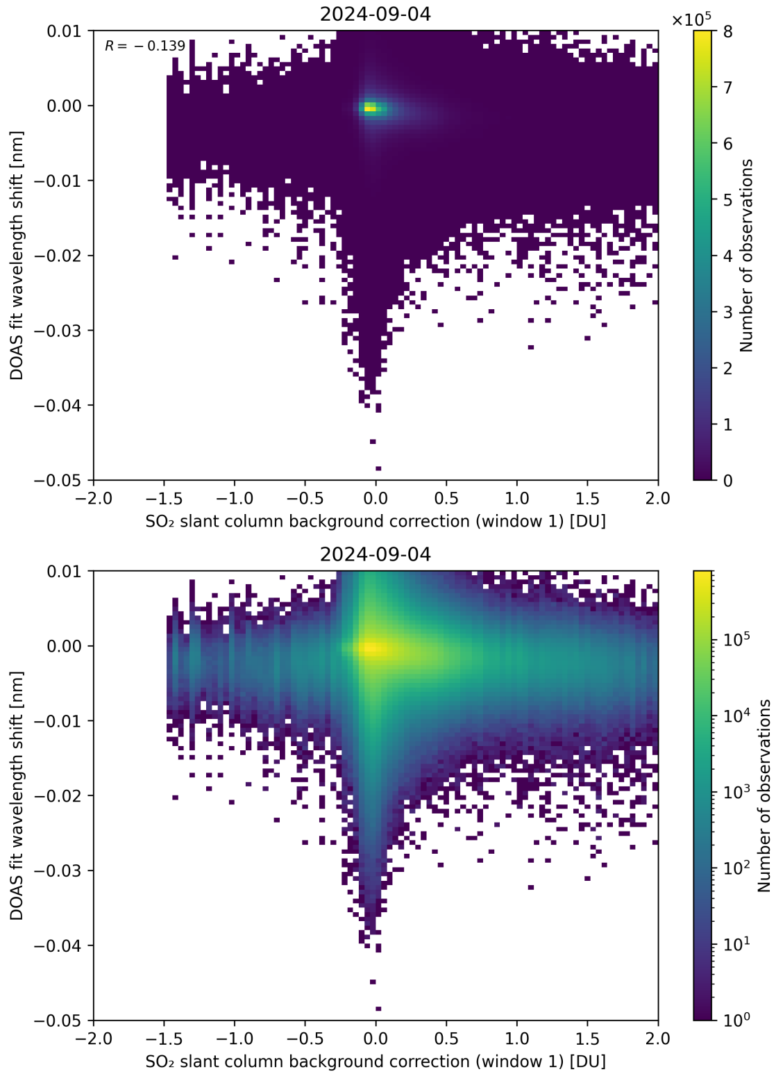
Figure 100: Scatter density plot of “SO 2 slant column background correction (window 1)” against “DOAS fit wavelength shift” for 2024-09-03 to 2024-09-05.
