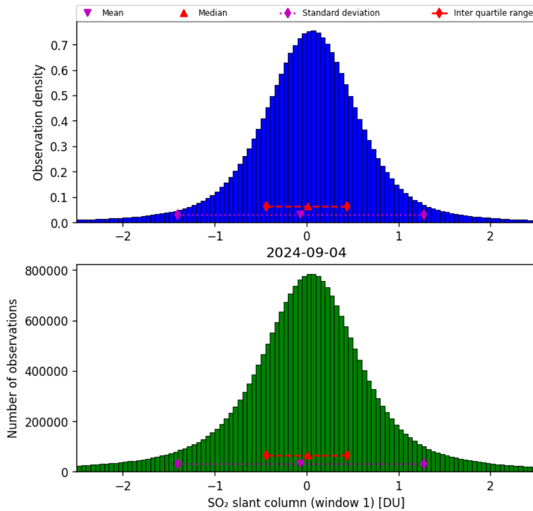
Figure 56: Histogram of “SO 2 slant column (window 1)” for 2024-09-03 to 2024-09-05
