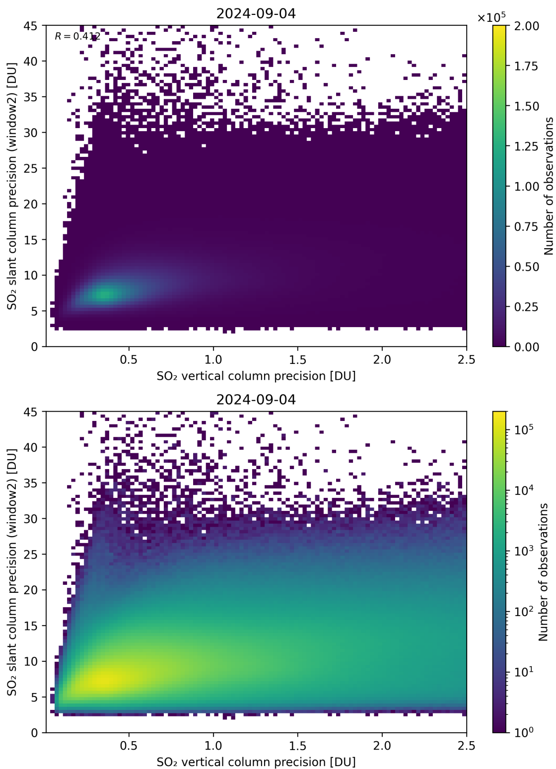
Figure 291: Scatter density plot of “SO 2 vertical column precision” against “SO 2 slant column precision (window2)” for 2024-09-03 to 2024-09-05.
