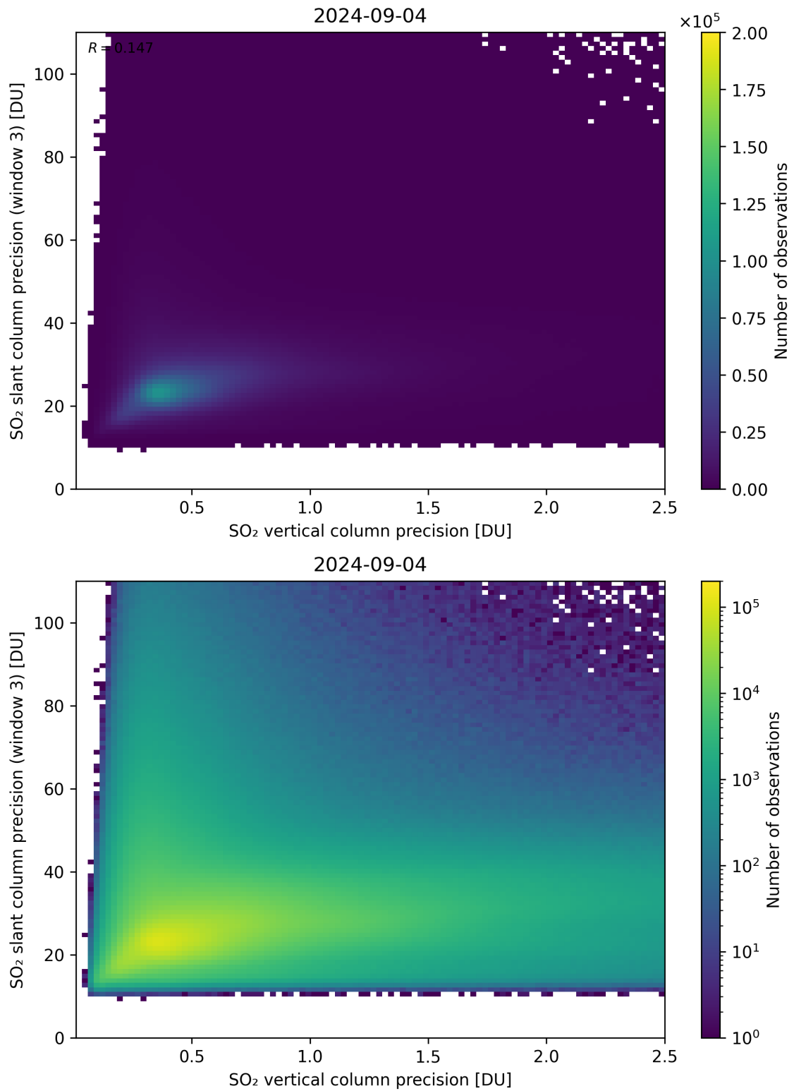
Figure 293: Scatter density plot of “SO 2 vertical column precision” against “SO 2 slant column precision (window 3)” for 2024-09-03 to 2024-09-05.
