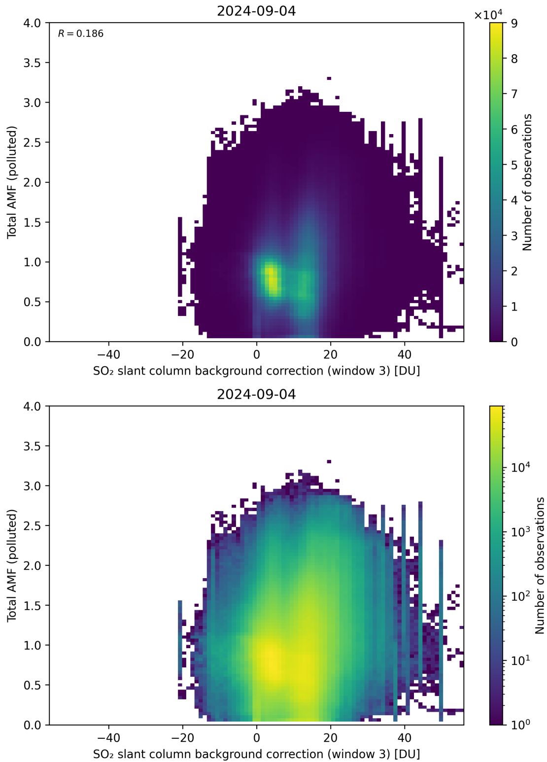
Figure 125: Scatter density plot of “SO 2 slant column background correction (window 3)” against “Total AMF (polluted)” for 2024-09-03 to 2024-09-05.
