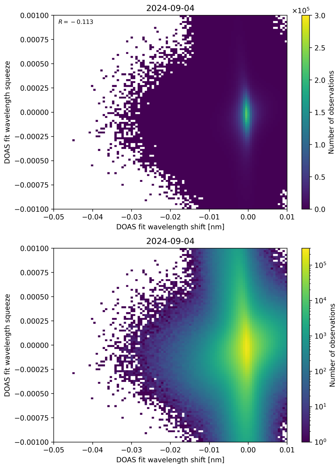
Figure 127: Scatter density plot of “DOAS fit wavelength shift” against “DOAS fit wavelength squeeze” for 2024-09-03 to 2024-09-05.
