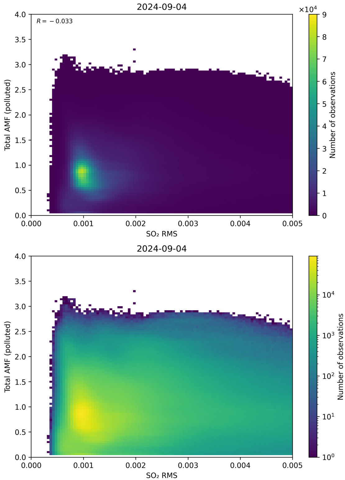
Figure 137: Scatter density plot of “SO 2 RMS” against “Total AMF (polluted)” for 2024-09-03 to 2024-09-05.
