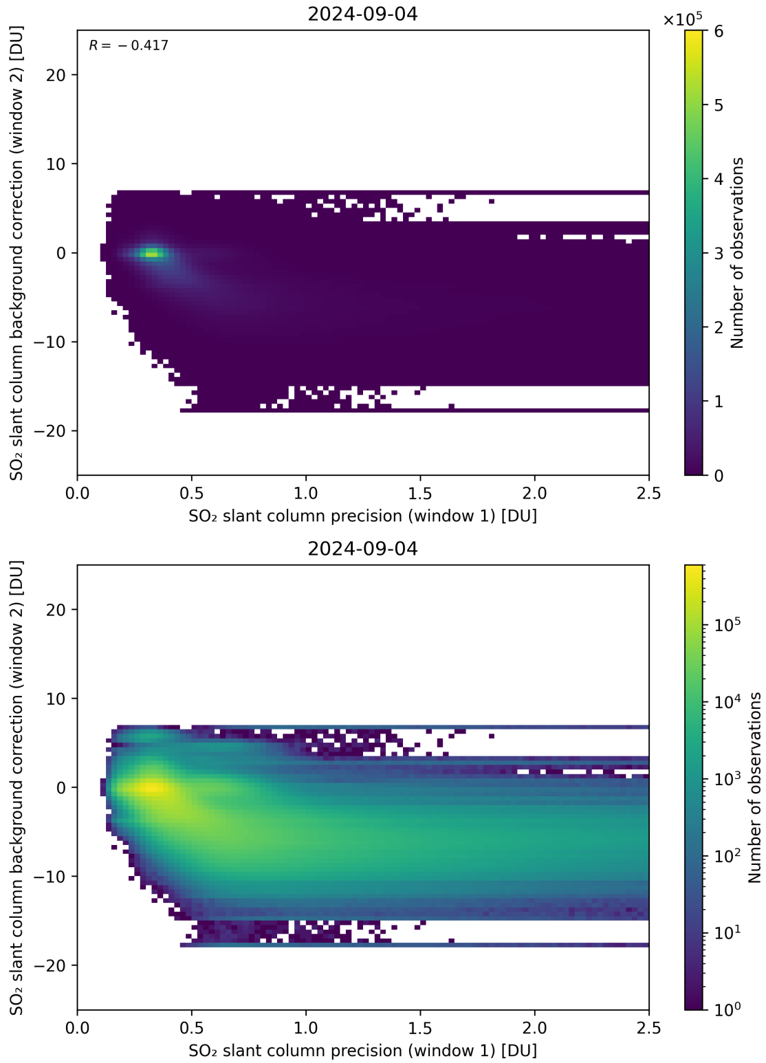
Figure 219: Scatter density plot of “SO 2 slant column precision (window 1)” against “SO 2 slant column background correction (window 2)” for 2024-09-03 to 2024-09-05.
