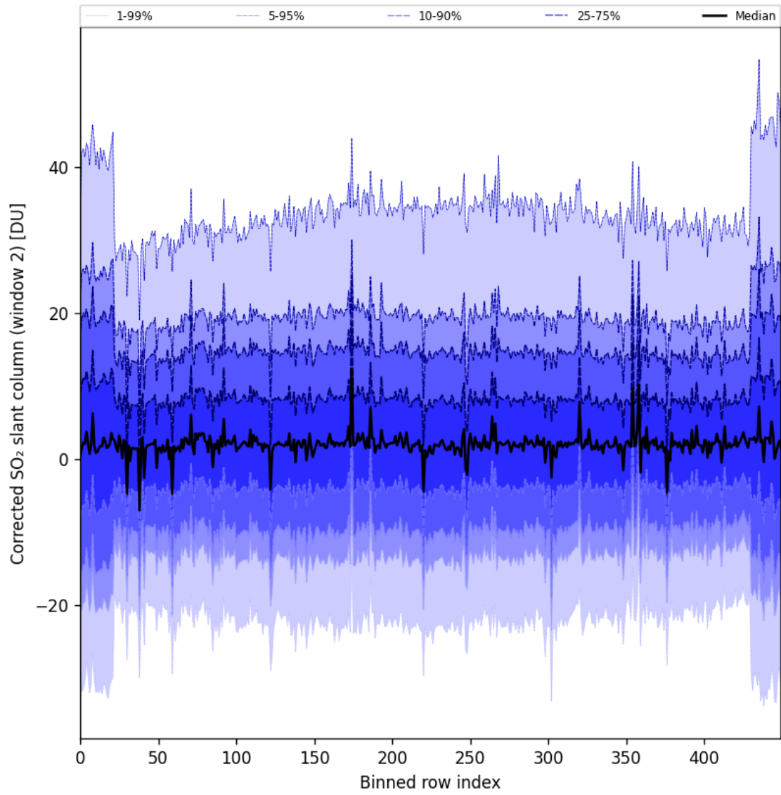
Figure 85: Along track statistics of “Corrected SO 2 slant column (window 2)” for 2024-09-03 to 2024-09-05
