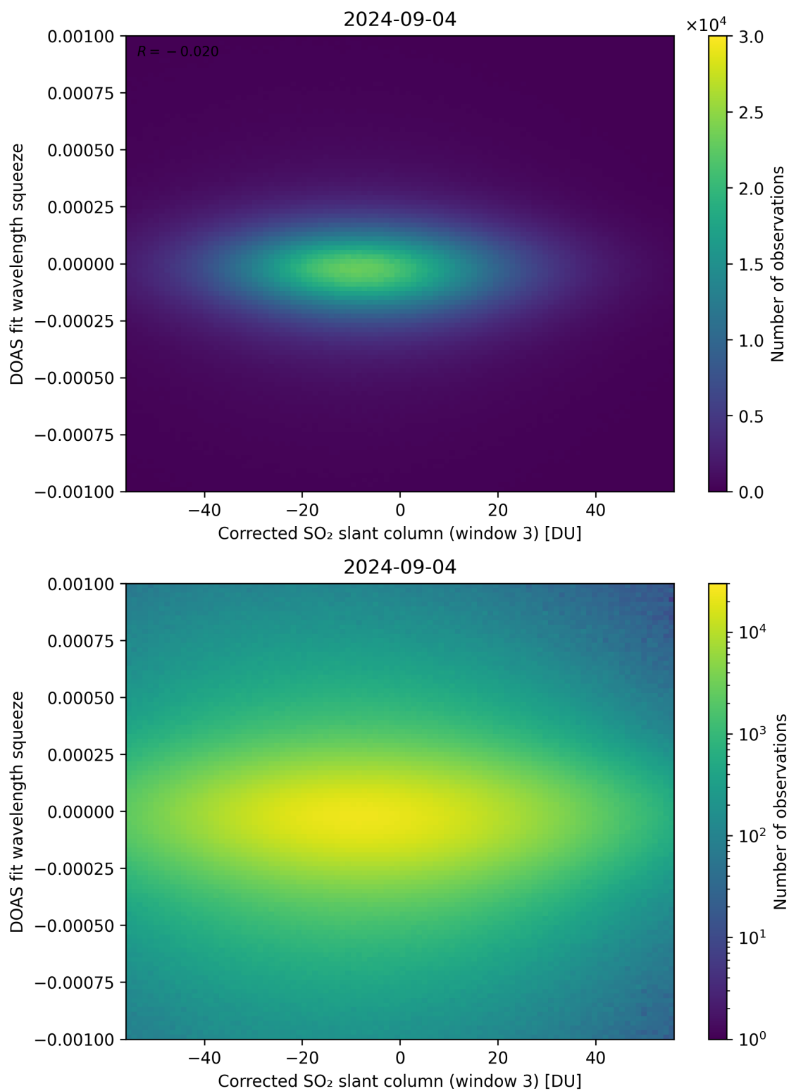
Figure 207: Scatter density plot of “Corrected SO 2 slant column (window 3)” against “DOAS fit wavelength squeeze” for 2024-09-03 to 2024-09-05.
