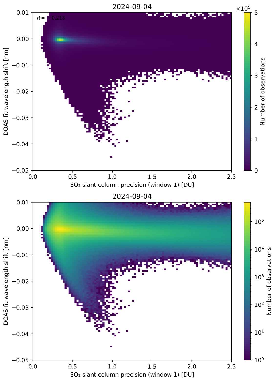
Figure 221: Scatter density plot of “SO 2 slant column precision (window 1)” against “DOAS fit wavelength shift” for 2024-09-03 to 2024-09-05.
