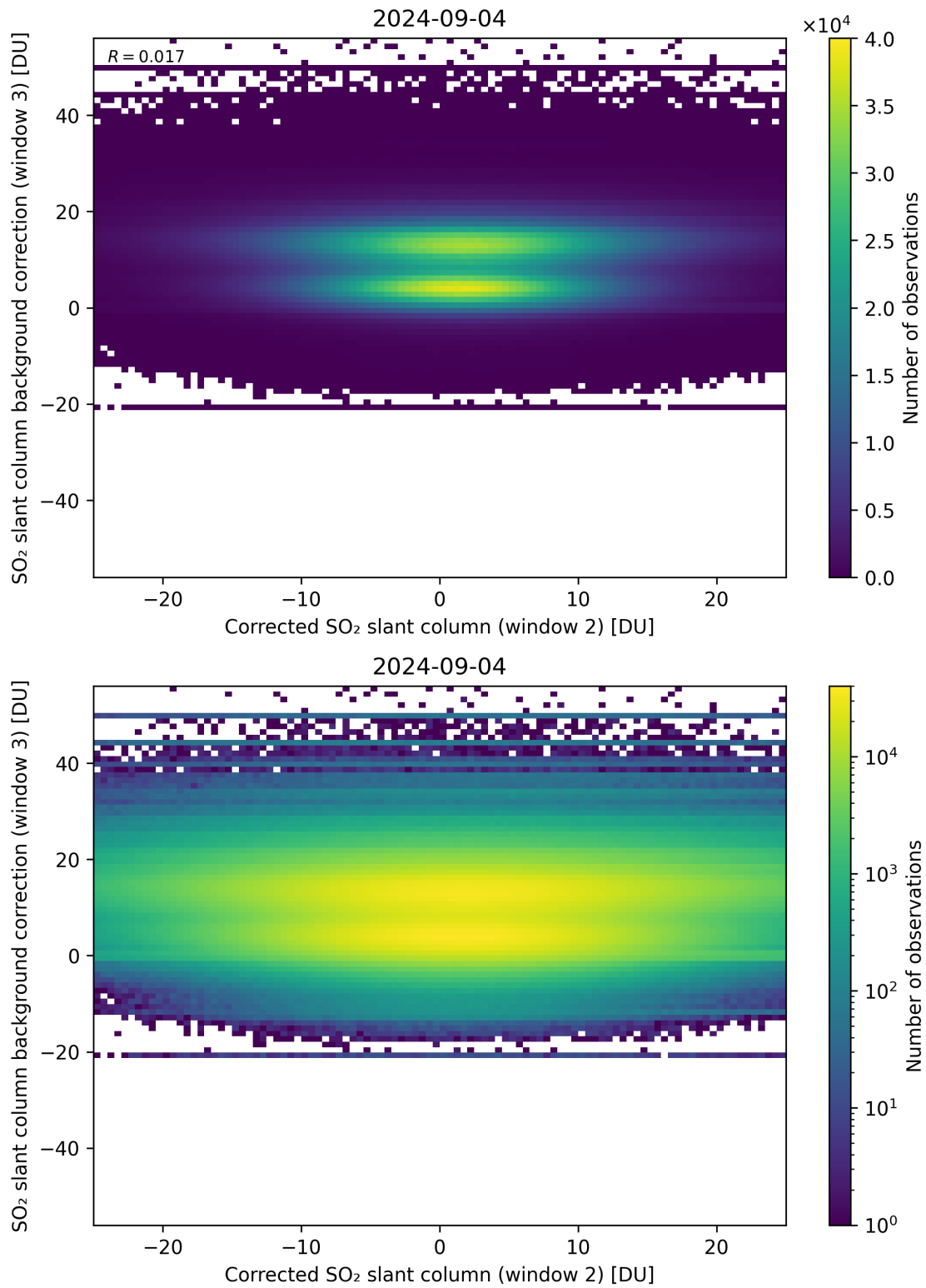
Figure 195: Scatter density plot of “Corrected SO 2 slant column (window 2)” against “SO 2 slant column background correction (window 3)” for 2024-09-03 to 2024-09-05.
