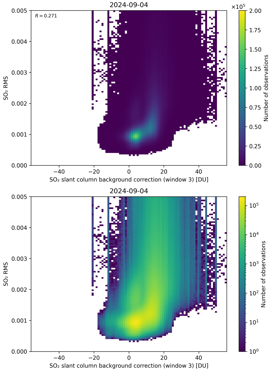
Figure 123: Scatter density plot of “SO 2 slant column background correction (window 3)” against “SO 2 RMS” for 2024-09-03 to 2024-09-05.
