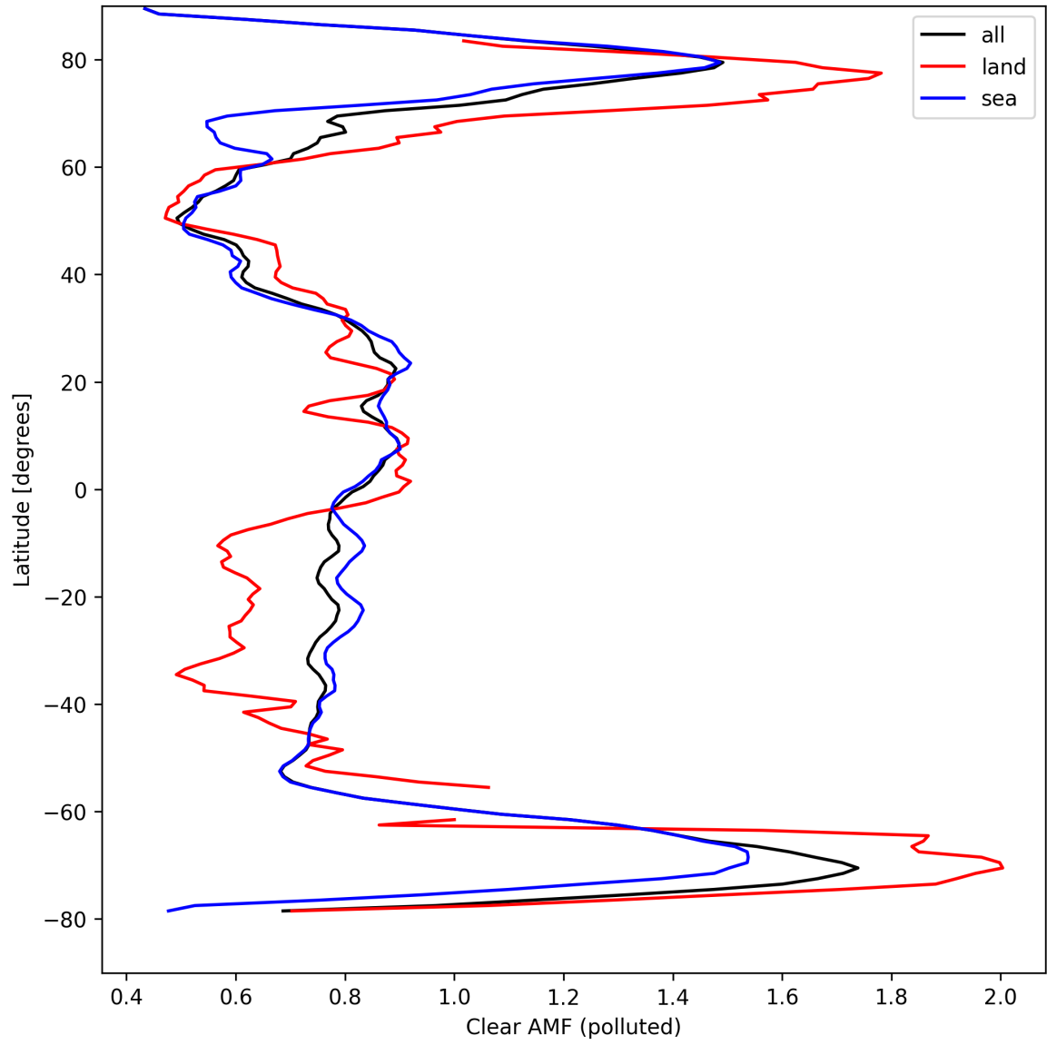
Figure 50: Zonal average of “Clear AMF (polluted)” for 2024-09-03 to 2024-09-05.
