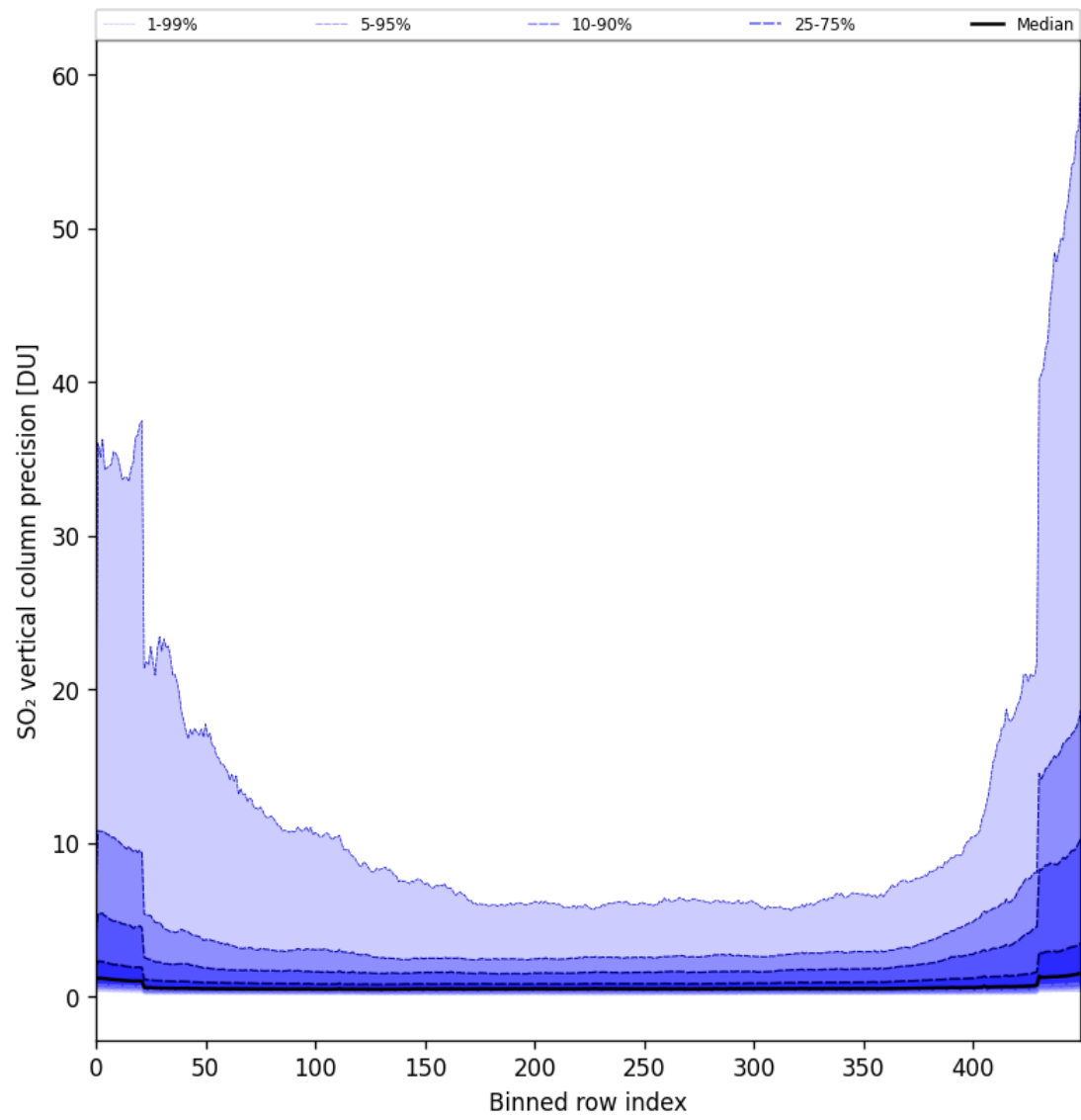
Figure 77: Along track statistics of “SO 2 vertical column precision” for 2024-09-03 to 2024-09-05
