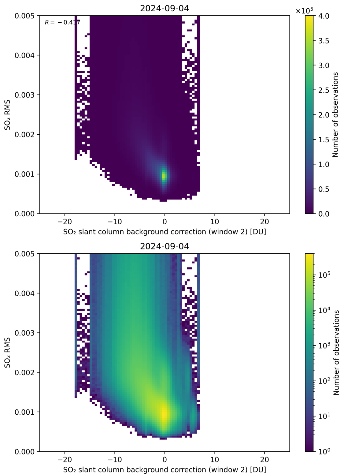
Figure 114: Scatter density plot of “SO 2 slant column background correction (window 2)” against “SO 2 RMS” for 2024-09-03 to 2024-09-05.
