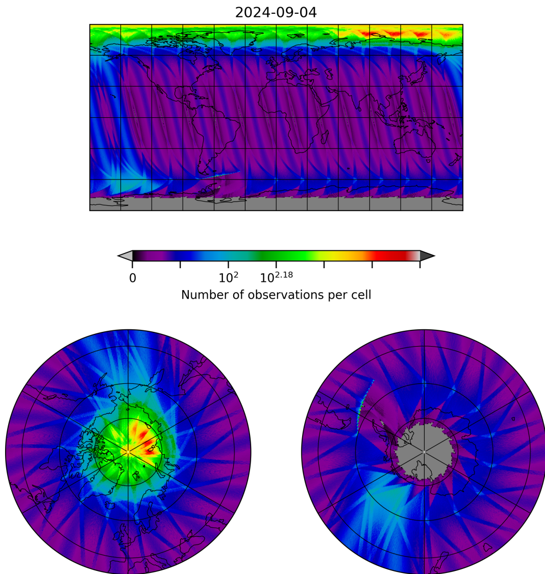
Figure 28: Map of the number of observations for 2024-09-03 to 2024-09-05
