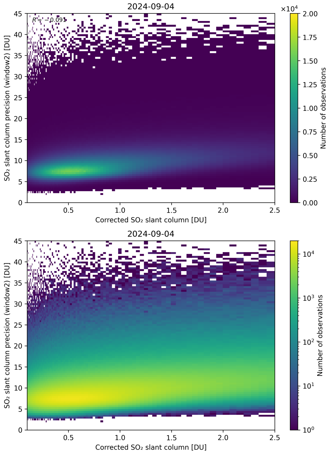
Figure 189: Scatter density plot of “Corrected SO 2 slant column” against “SO 2 slant column precision (window2)” for 2024-09-03 to 2024-09-05.
