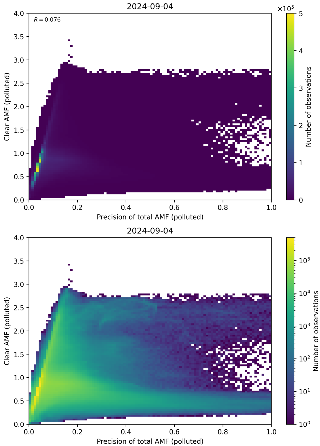
Figure 270: Scatter density plot of “Precision of total AMF (polluted)” against “Clear AMF (polluted)” for 2024-09-03 to 2024-09-05.
