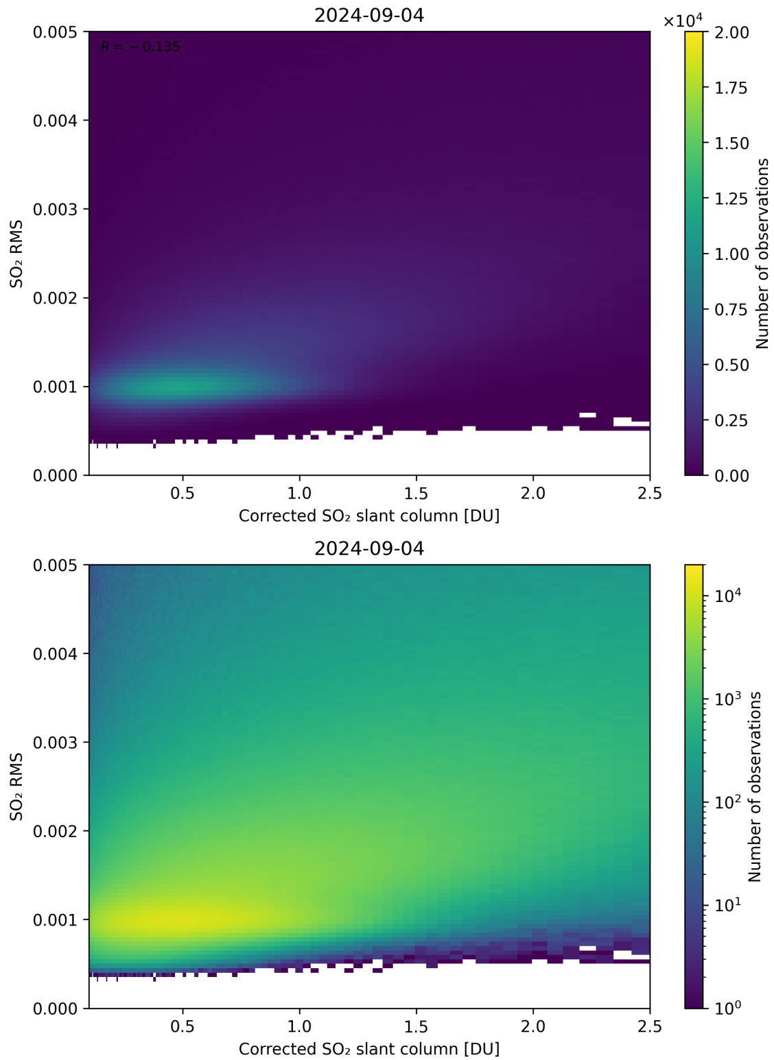
Figure 183: Scatter density plot of “Corrected SO 2 slant column” against “SO 2 RMS” for 2024-09-03 to 2024-09-05.
