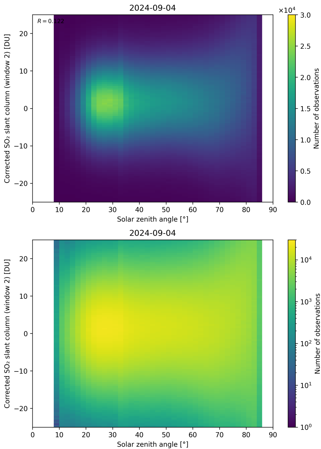
Figure 167: Scatter density plot of “Solar zenith angle” against “Corrected SO 2 slant column (window 2)” for 2024-09-03 to 2024-09-05.
