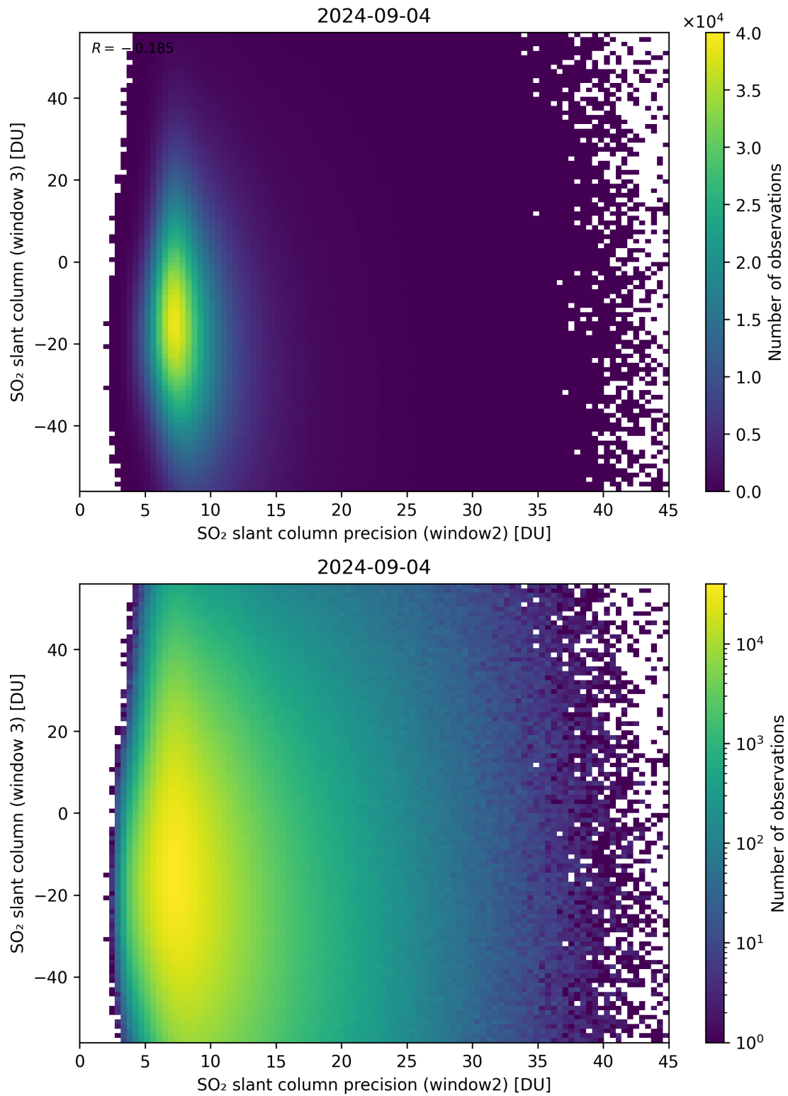
Figure 249: Scatter density plot of “SO 2 slant column precision (window2)” against “SO 2 slant column (window 3)” for 2024-09-03 to 2024-09-05.
