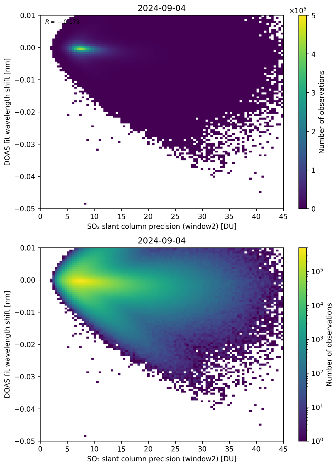
Figure 243: Scatter density plot of “SO 2 slant column precision (window2)” against “DOAS fit wavelength shift” for 2024-09-03 to 2024-09-05.
