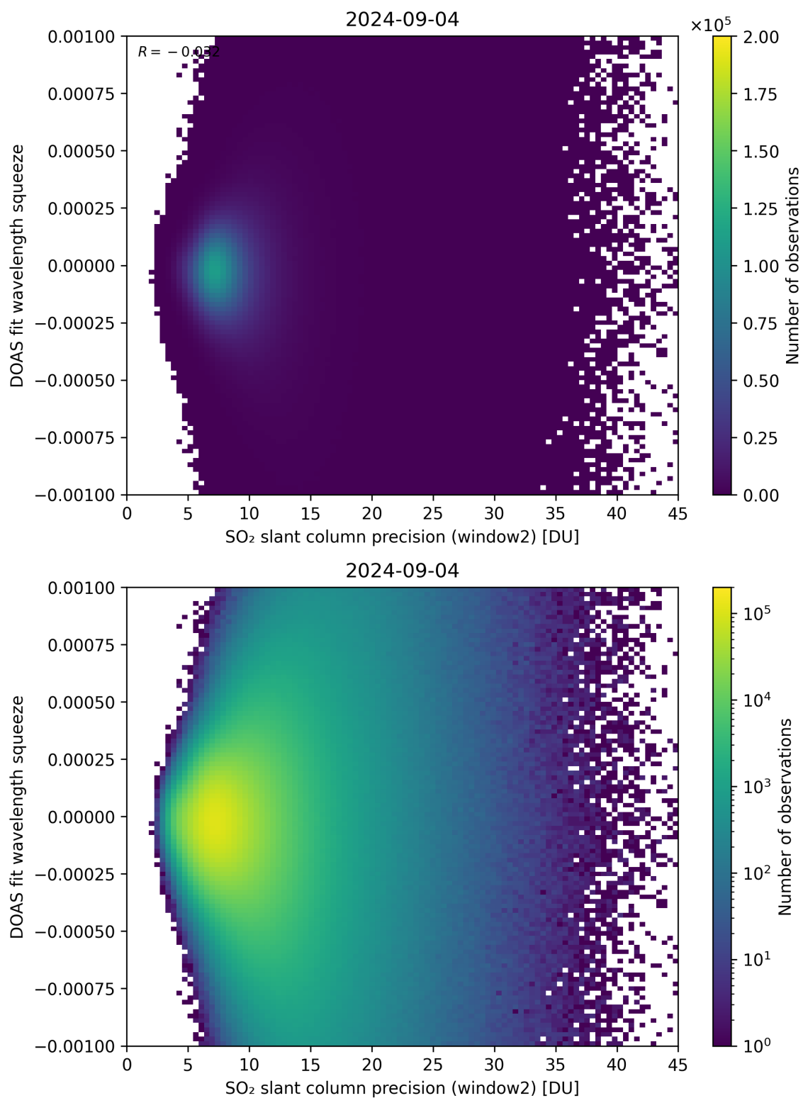
Figure 244: Scatter density plot of “SO 2 slant column precision (window2)” against “DOAS fit wavelength squeeze” for 2024-09-03 to 2024-09-05.
