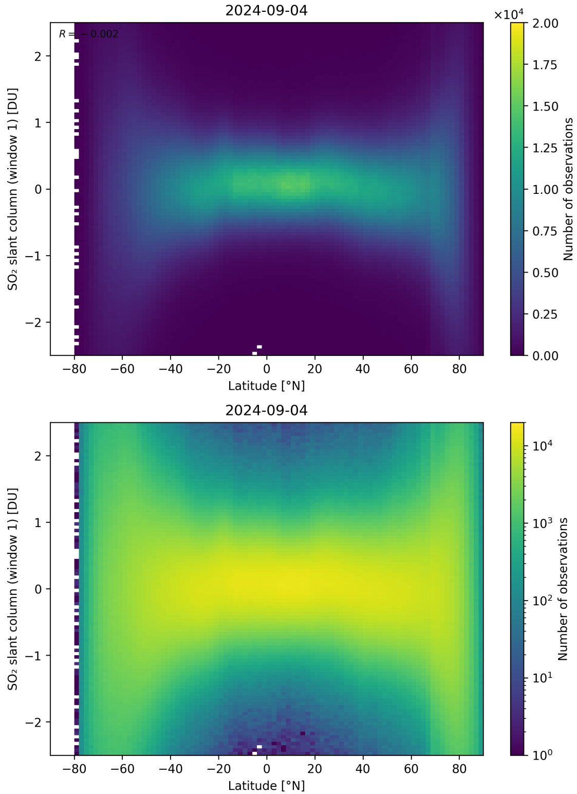
Figure 149: Scatter density plot of “Latitude” against “SO 2 slant column (window 1)” for 2024-09-03 to 2024-09-05.
