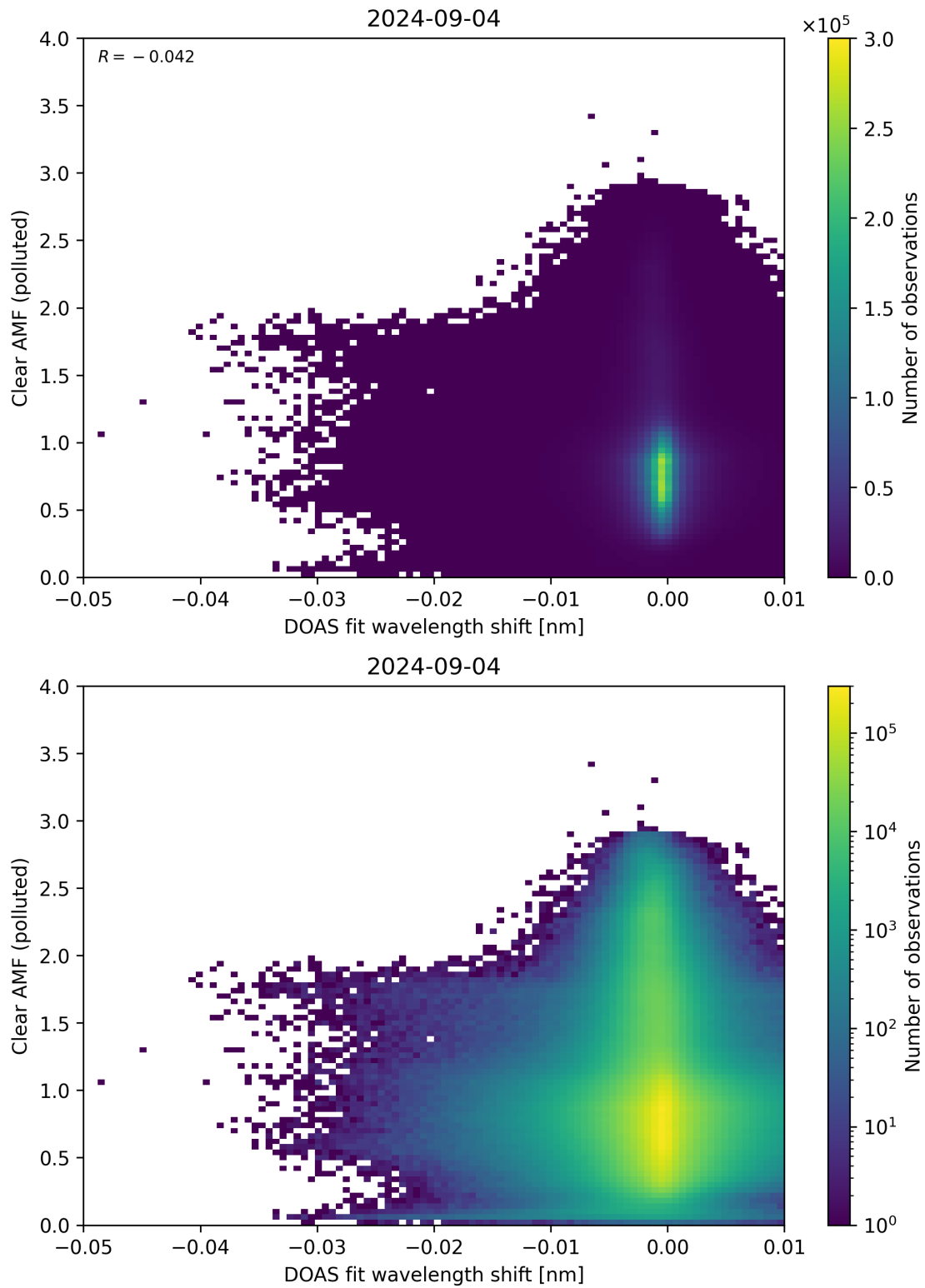
Figure 129: Scatter density plot of “DOAS fit wavelength shift” against “Clear AMF (polluted)” for 2024-09-03 to 2024-09-05.
