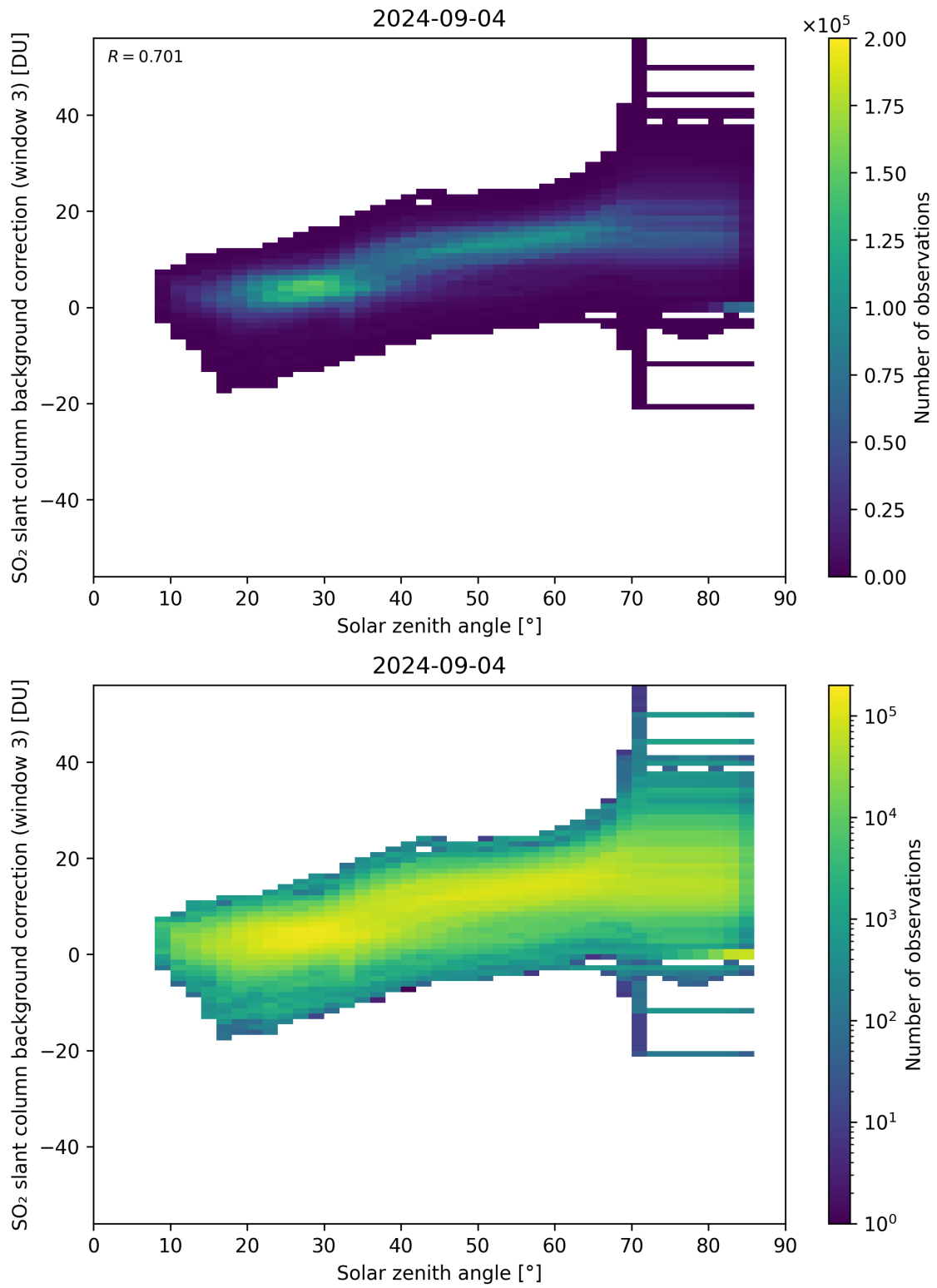
Figure 160: Scatter density plot of “Solar zenith angle” against “SO 2 slant column background correction (window 3)” for 2024-09-03 to 2024-09-05.
