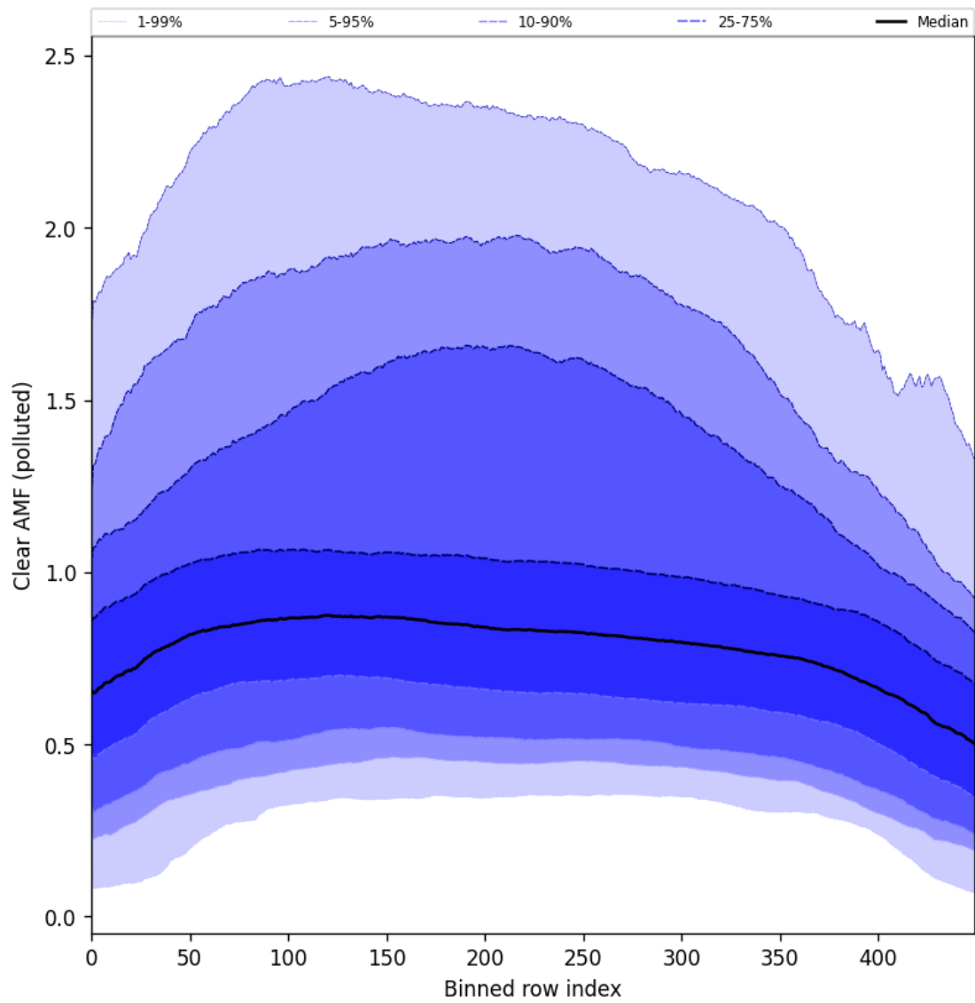
Figure 96: Along track statistics of “Clear AMF (polluted)” for 2024-09-03 to 2024-09-05
