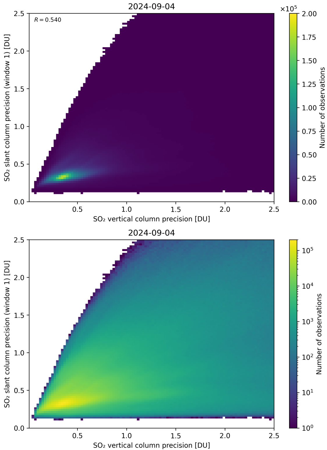
Figure 290: Scatter density plot of “SO 2 vertical column precision” against “SO 2 slant column precision (window 1)” for 2024-09-03 to 2024-09-05.
