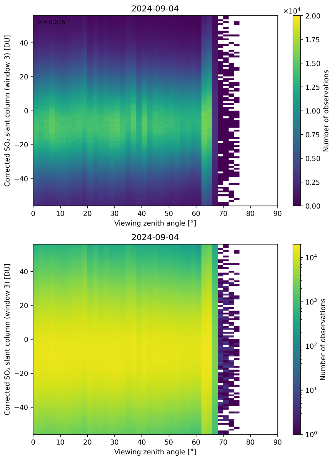
Figure 319: Scatter density plot of “Viewing zenith angle” against “Corrected SO 2 slant column (window 3)” for 2024-09-03 to 2024-09-05.
