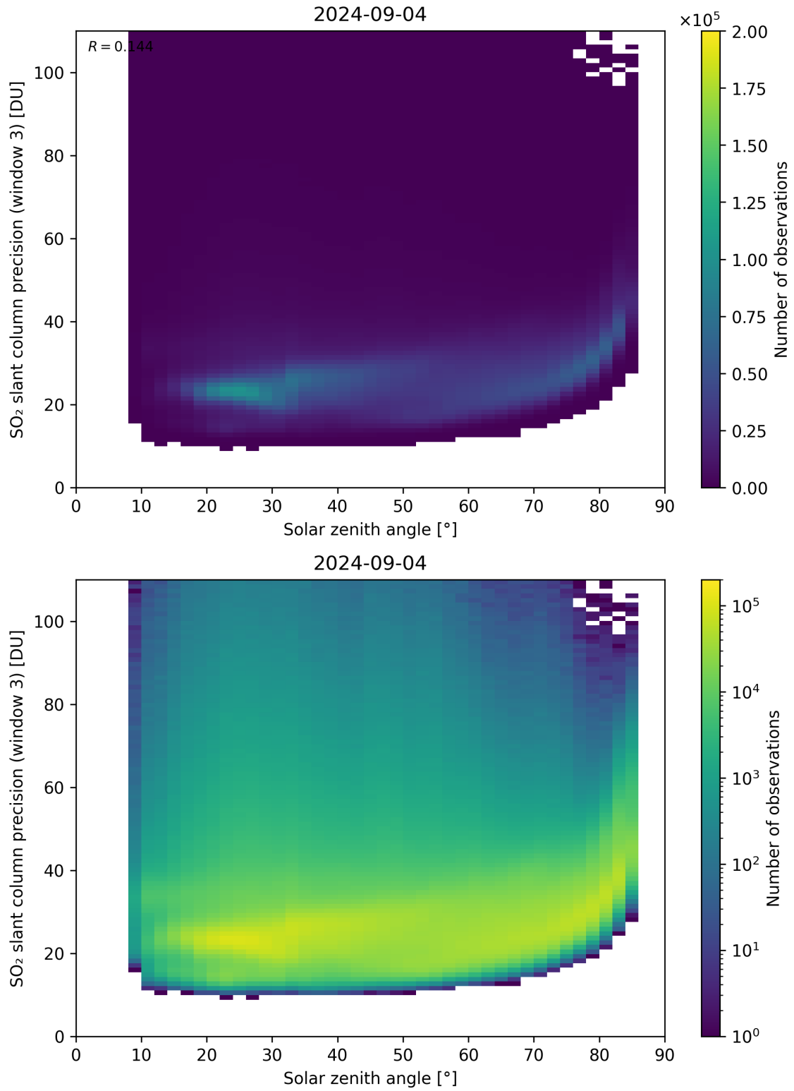
Figure 173: Scatter density plot of “Solar zenith angle” against “SO 2 slant column precision (window 3)” for 2024-09-03 to 2024-09-05.
