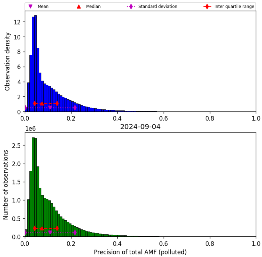
Figure 72: Histogram of “Precision of total AMF (polluted)” for 2024-09-03 to 2024-09-05
