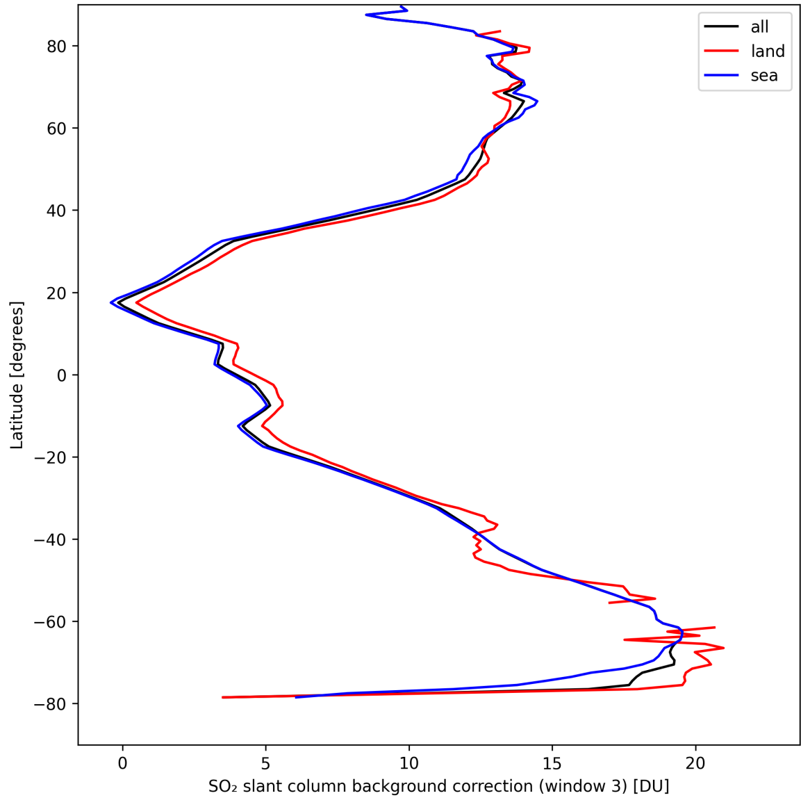
Figure 44: Zonal average of "SO 2 slant column background correction (window 3)" for 2024-09-03 to 2024-09-05.
