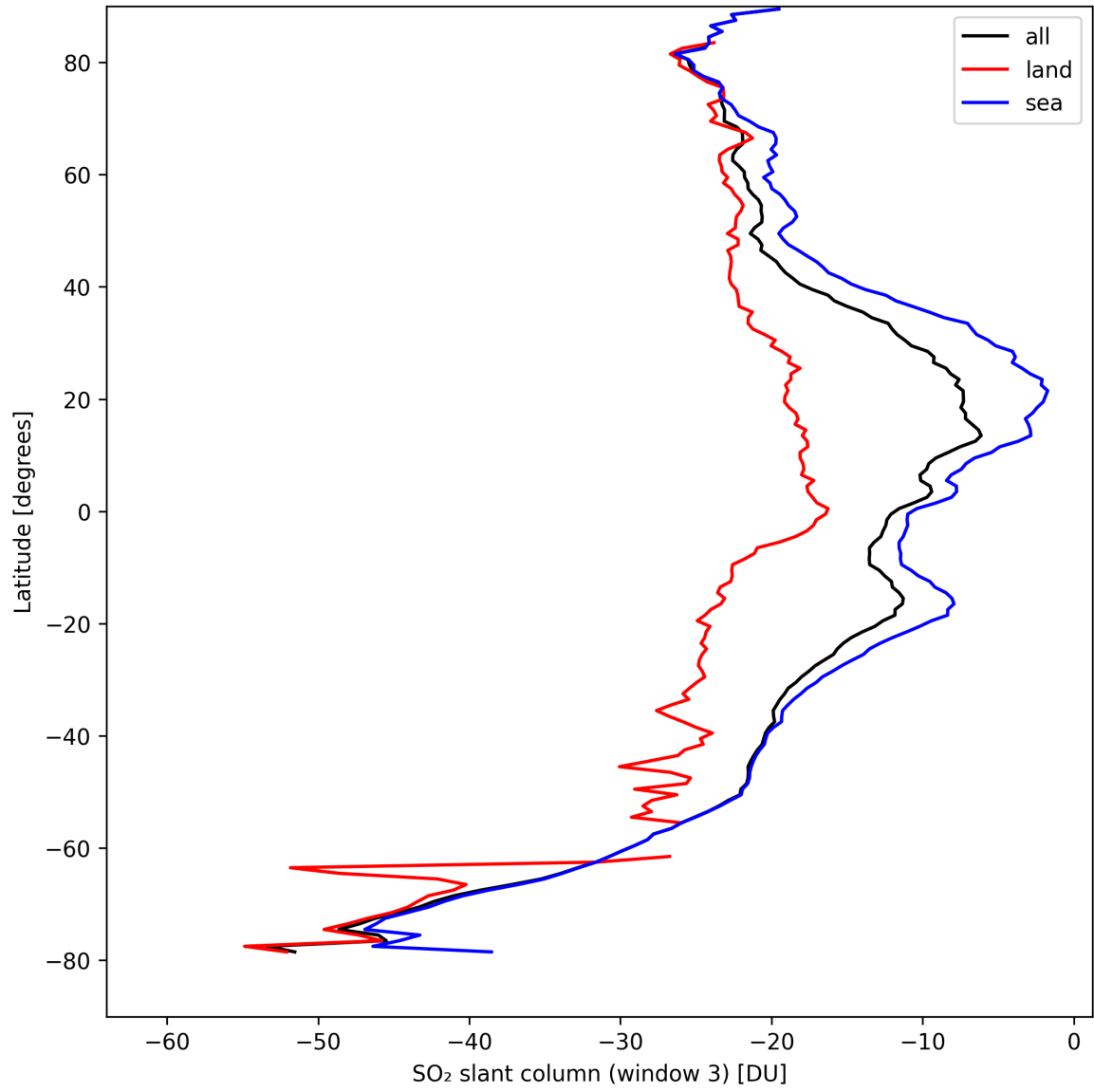
Figure 41: Zonal average of “SO 2 slant column (window 3)” for 2024-09-03 to 2024-09-05.
