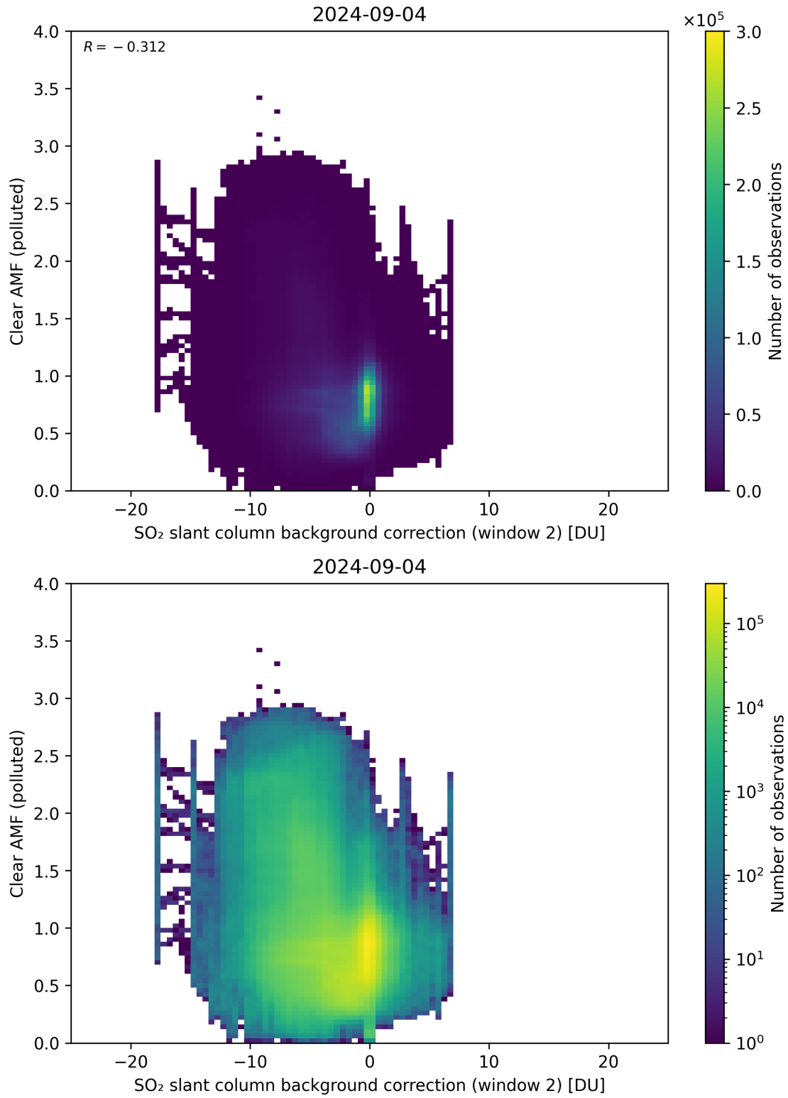
Figure 115: Scatter density plot of “SO 2 slant column background correction (window 2)” against “Clear AMF (polluted)” for 2024-09-03 to 2024-09-05.
