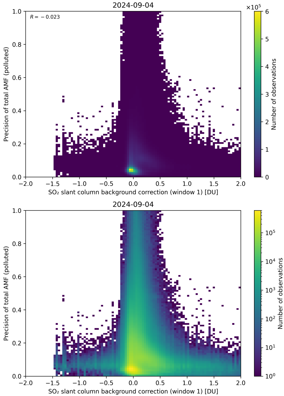
Figure 110: Scatter density plot of “SO 2 slant column background correction (window 1)” against “Precision of total AMF (polluted)” for 2024-09-03 to 2024-09-05.
