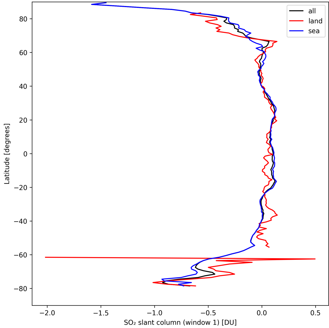
Figure 33: Zonal average of “SO 2 slant column (window 1)” for 2024-09-03 to 2024-09-05.
