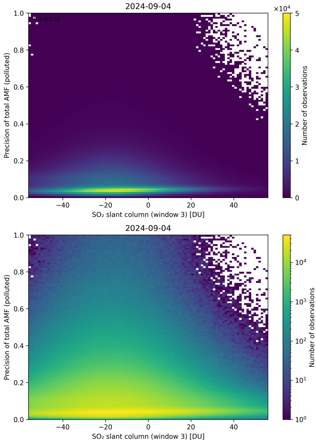
Figure 269: Scatter density plot of “SO 2 slant column (window 3)” against “Precision of total AMF (polluted)” for 2024-09-03 to 2024-09-05.
