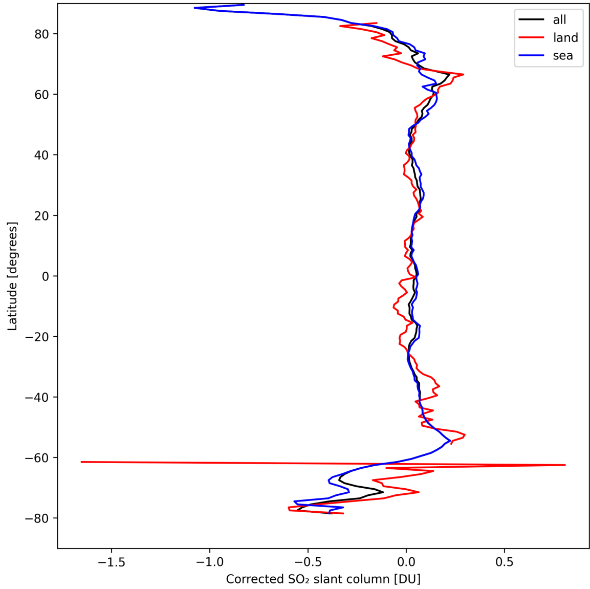
Figure 32: Zonal average of “Corrected SO 2 slant column” for 2024-09-03 to 2024-09-05.
