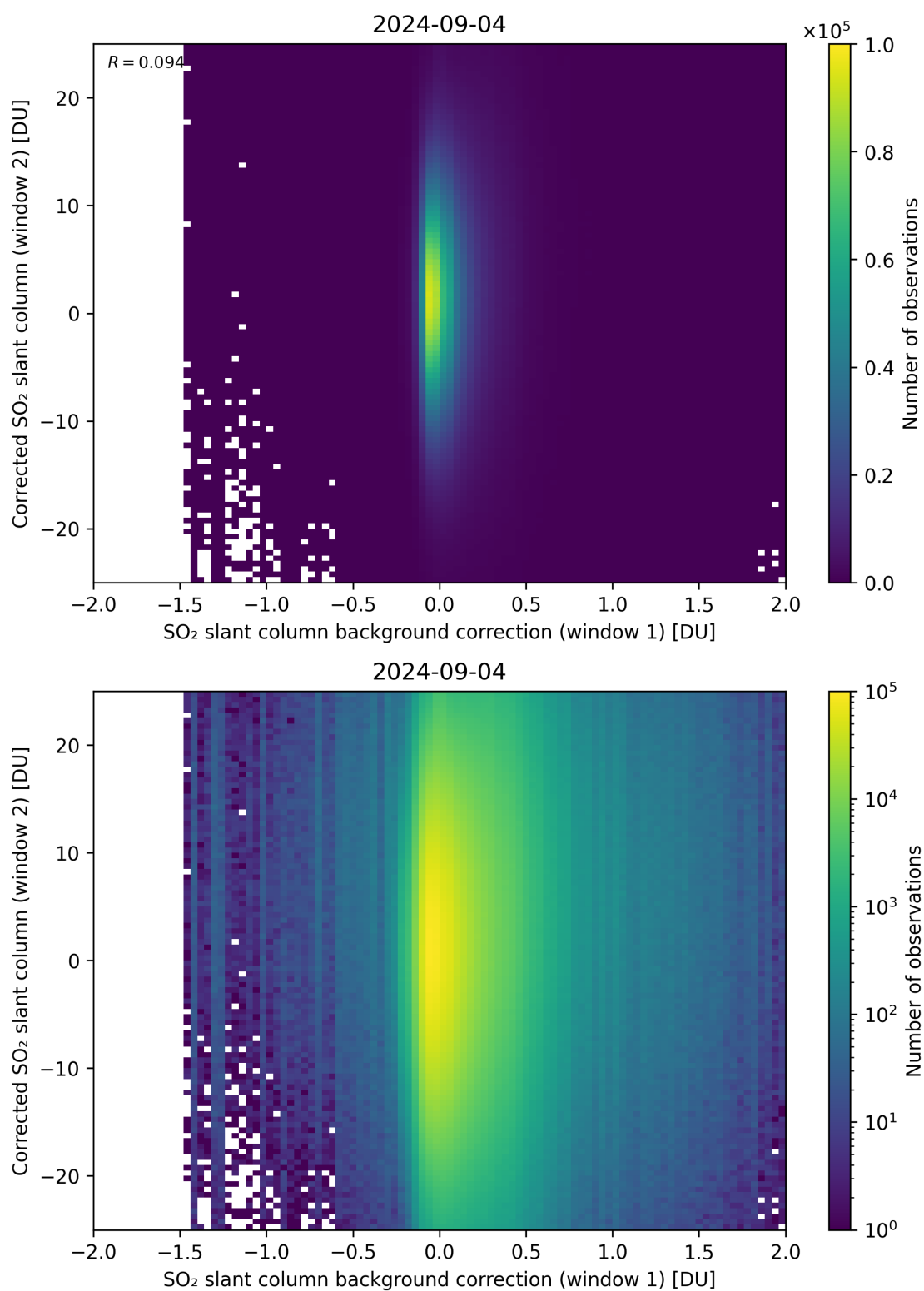
Figure 104: Scatter density plot of “SO 2 slant column background correction (window 1)” against “Corrected SO 2 slant column (window 2)” for 2024-09-03 to 2024-09-05.
