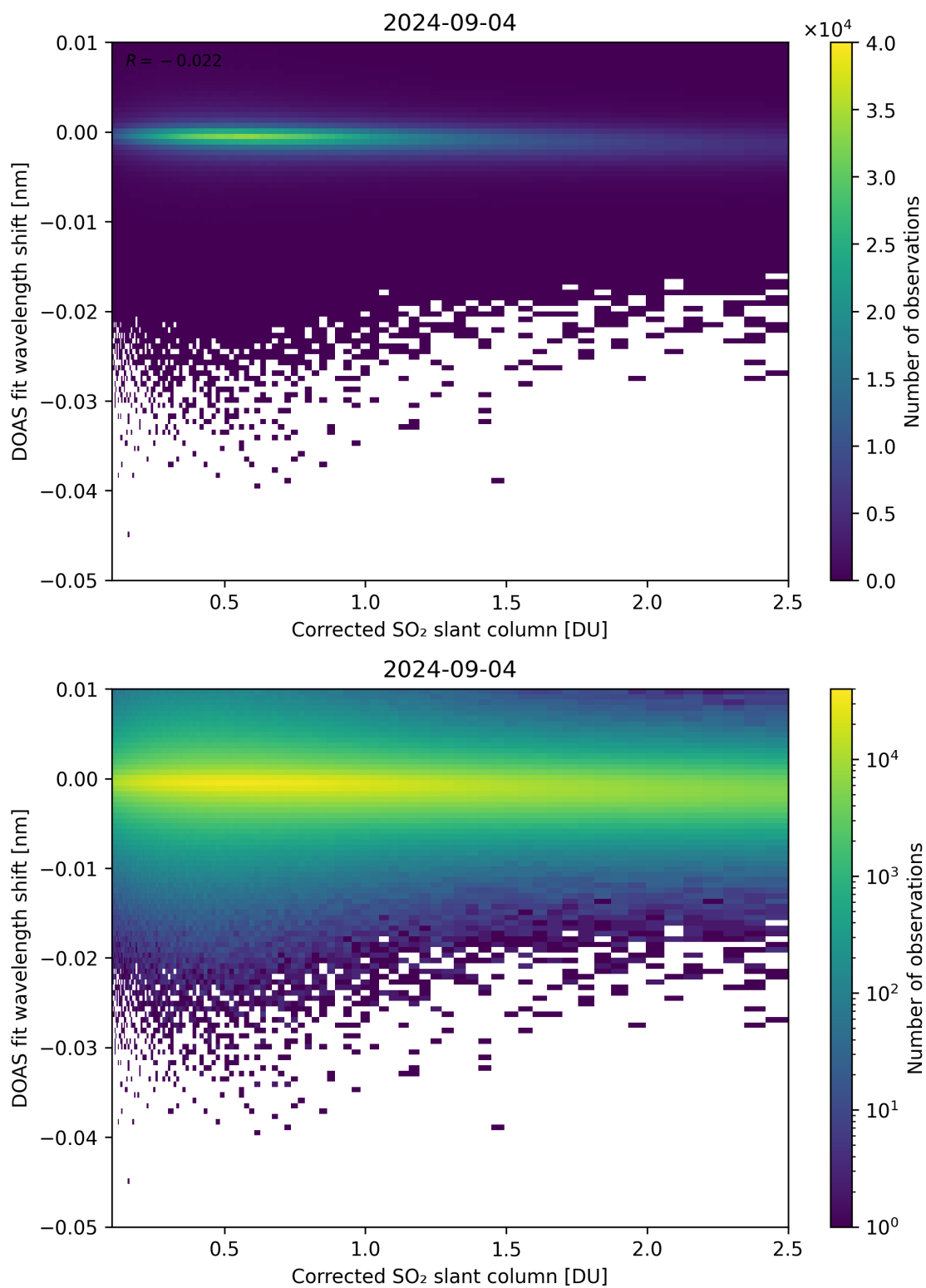
Figure 181: Scatter density plot of “Corrected SO 2 slant column” against “DOAS fit wavelength shift” for 2024-09-03 to 2024-09-05.
