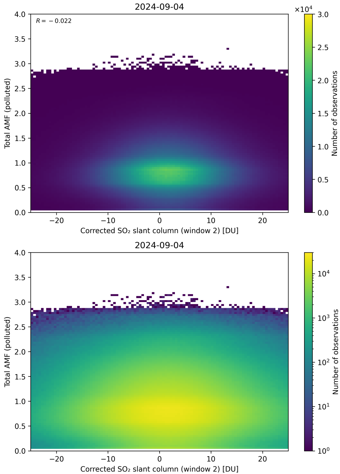
Figure 203: Scatter density plot of “Corrected SO 2 slant column (window 2)” against “Total AMF (polluted)” for 2024-09-03 to 2024-09-05.
