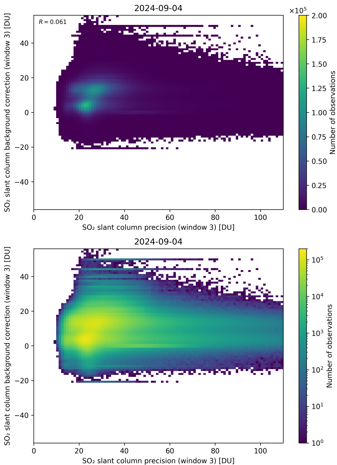
Figure 257: Scatter density plot of “SO 2 slant column precision (window 3)” against “SO 2 slant column background correction (window 3)” for 2024-09-03 to 2024-09-05.
