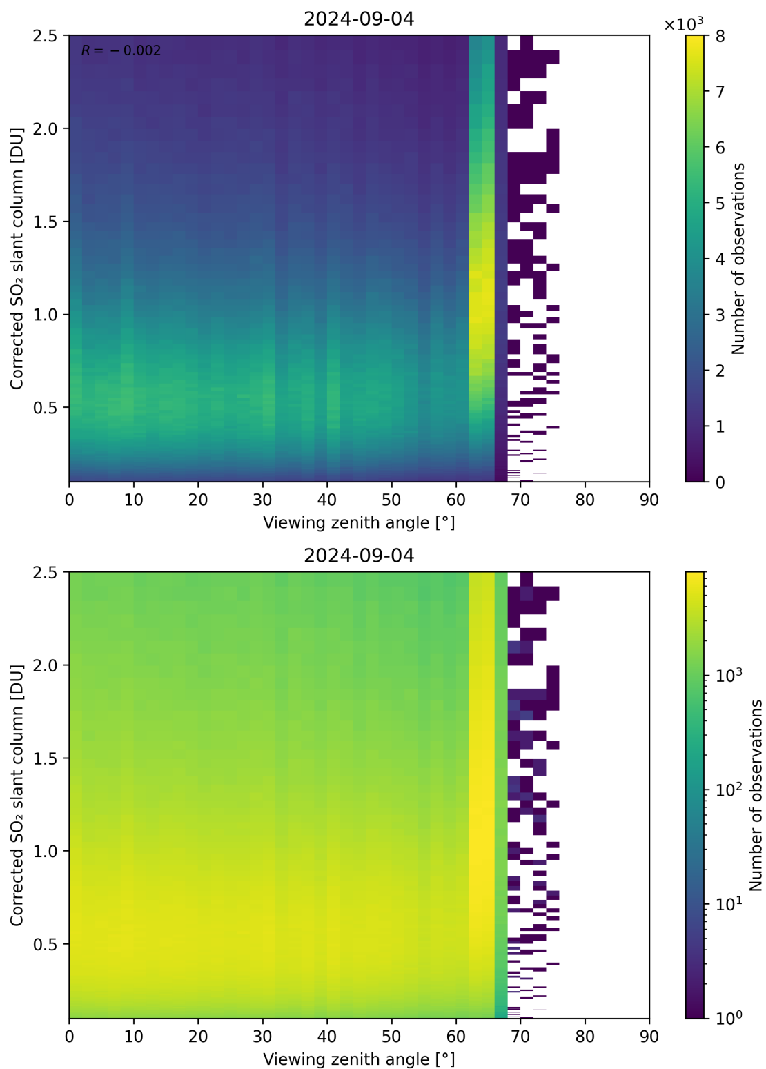
Figure 317: Scatter density plot of “Viewing zenith angle” against “Corrected SO 2 slant column” for 2024-09-03 to 2024-09-05.
