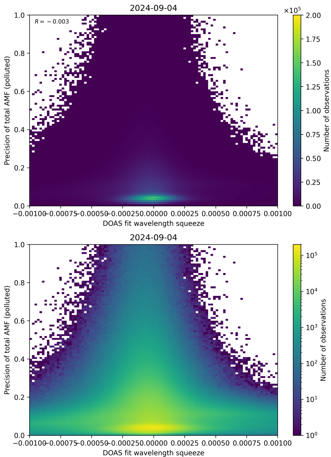
Figure 135: Scatter density plot of “DOAS fit wavelength squeeze” against “Precision of total AMF (polluted)” for 2024-09-03 to 2024-09-05.
