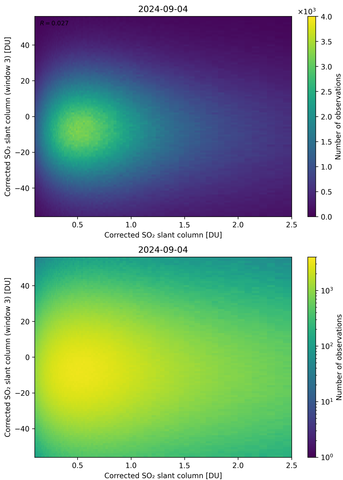
Figure 186: Scatter density plot of “Corrected SO 2 slant column” against “Corrected SO 2 slant column (window 3)” for 2024-09-03 to 2024-09-05.
