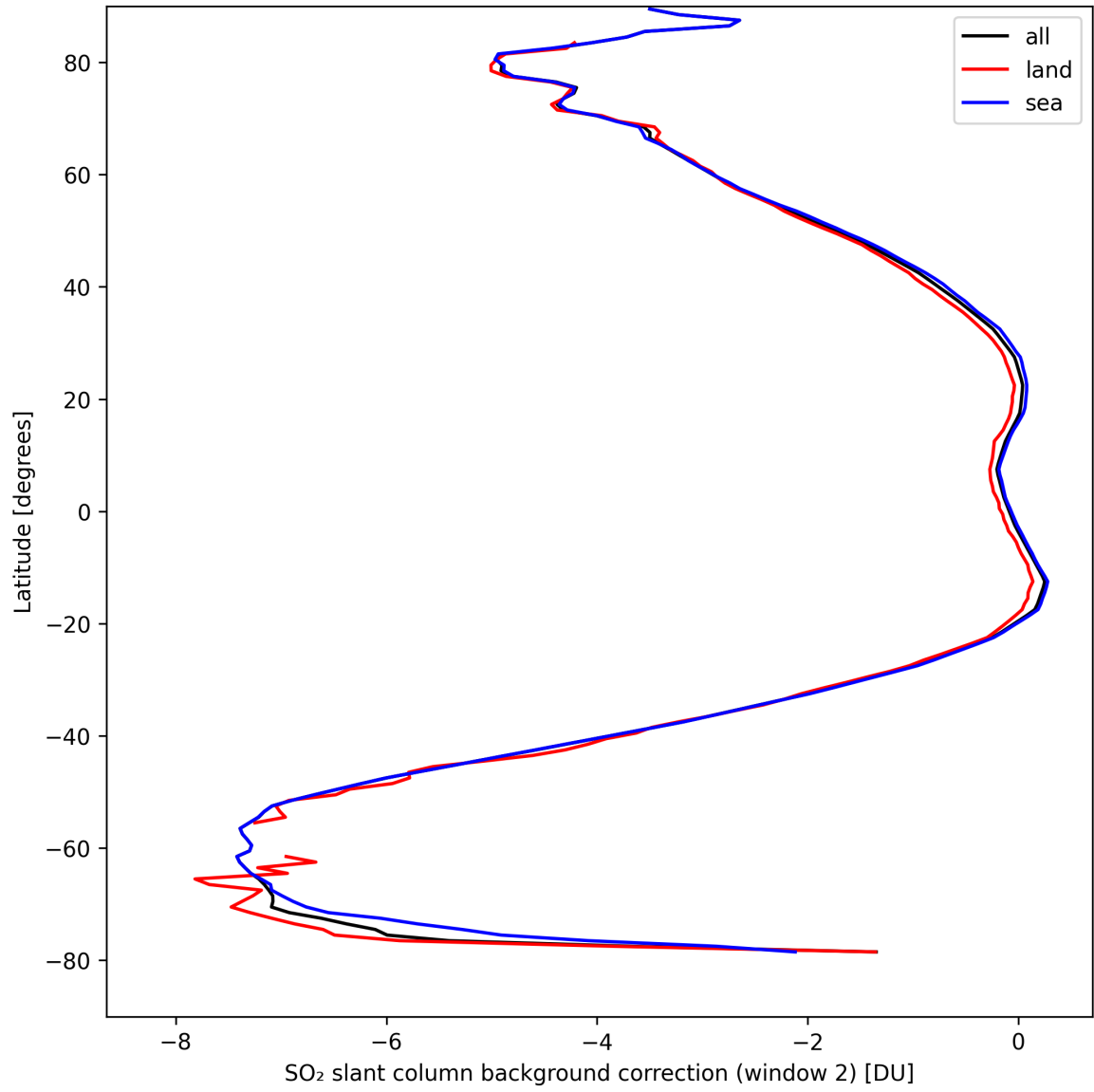
Figure 40: Zonal average of “SO 2 slant column background correction (window 2)” for 2024-09-03 to 2024-09-05.
