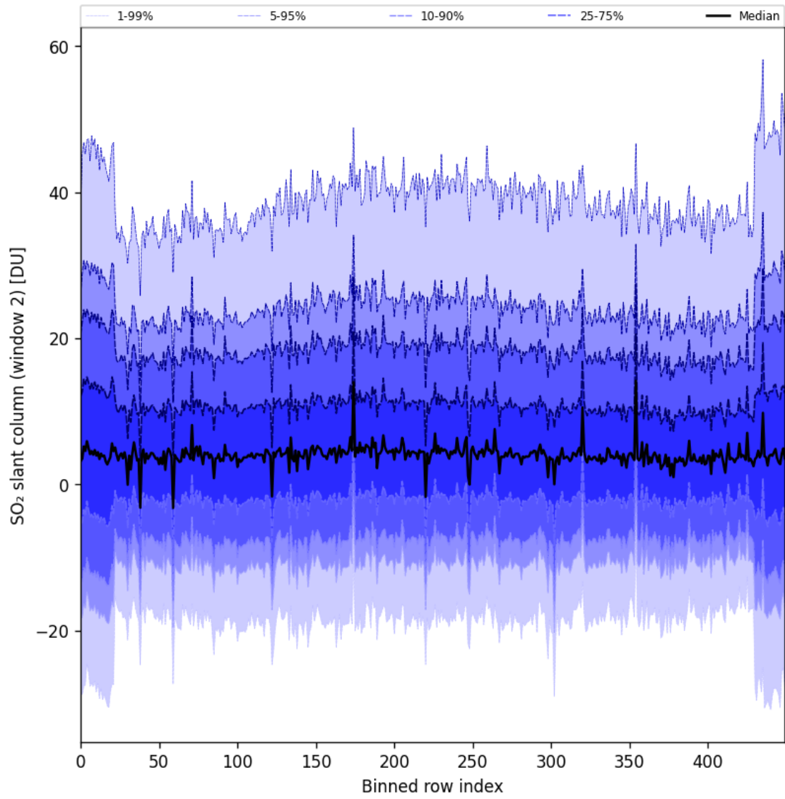
Figure 83: Along track statistics of “SO 2 slant column (window 2)” for 2024-09-03 to 2024-09-05
