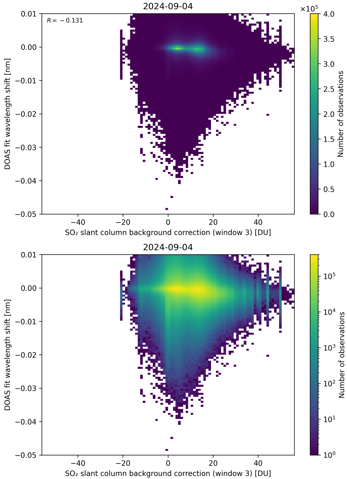
Figure 121: Scatter density plot of “SO 2 slant column background correction (window 3)” against “DOAS fit wavelength shift” for 2024-09-03 to 2024-09-05.
