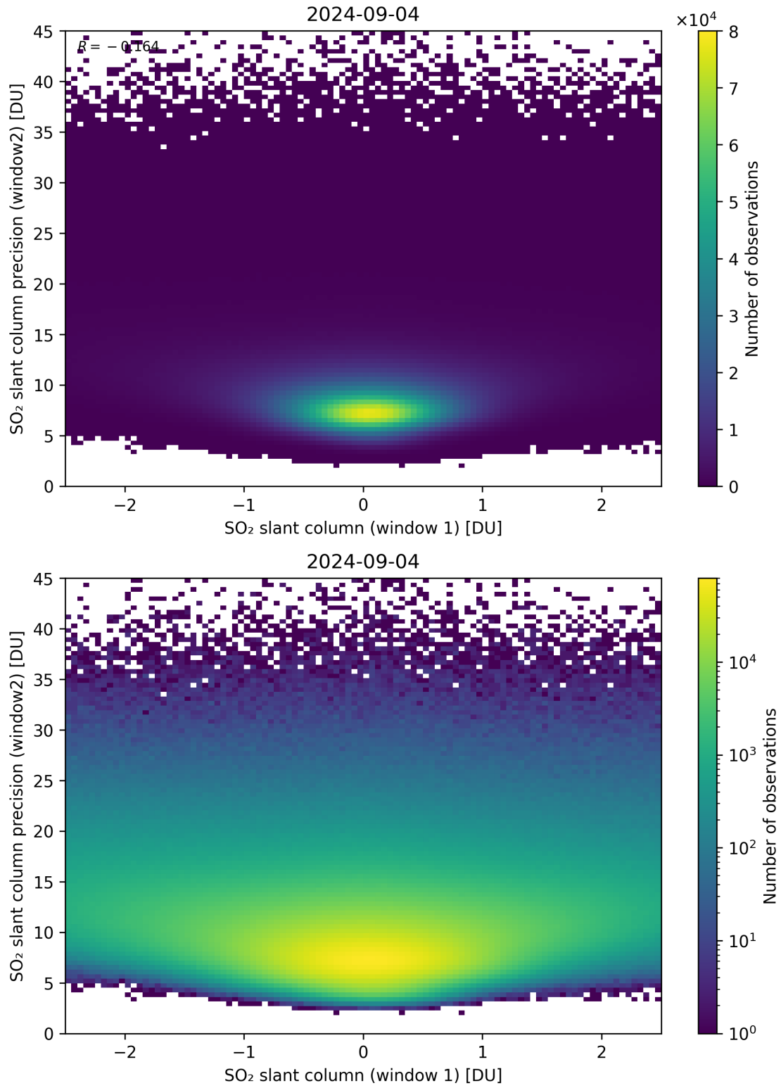
Figure 236: Scatter density plot of “SO 2 slant column (window 1)” against “SO 2 slant column precision (window2)” for 2024-09-03 to 2024-09-05.
