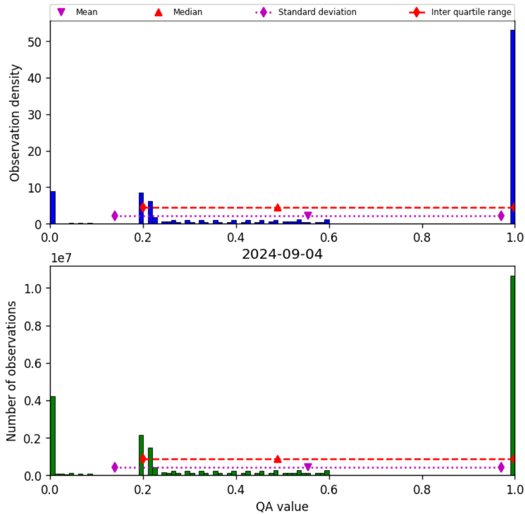
Figure 52: Histogram of “QA value” for 2024-09-03 to 2024-09-05
