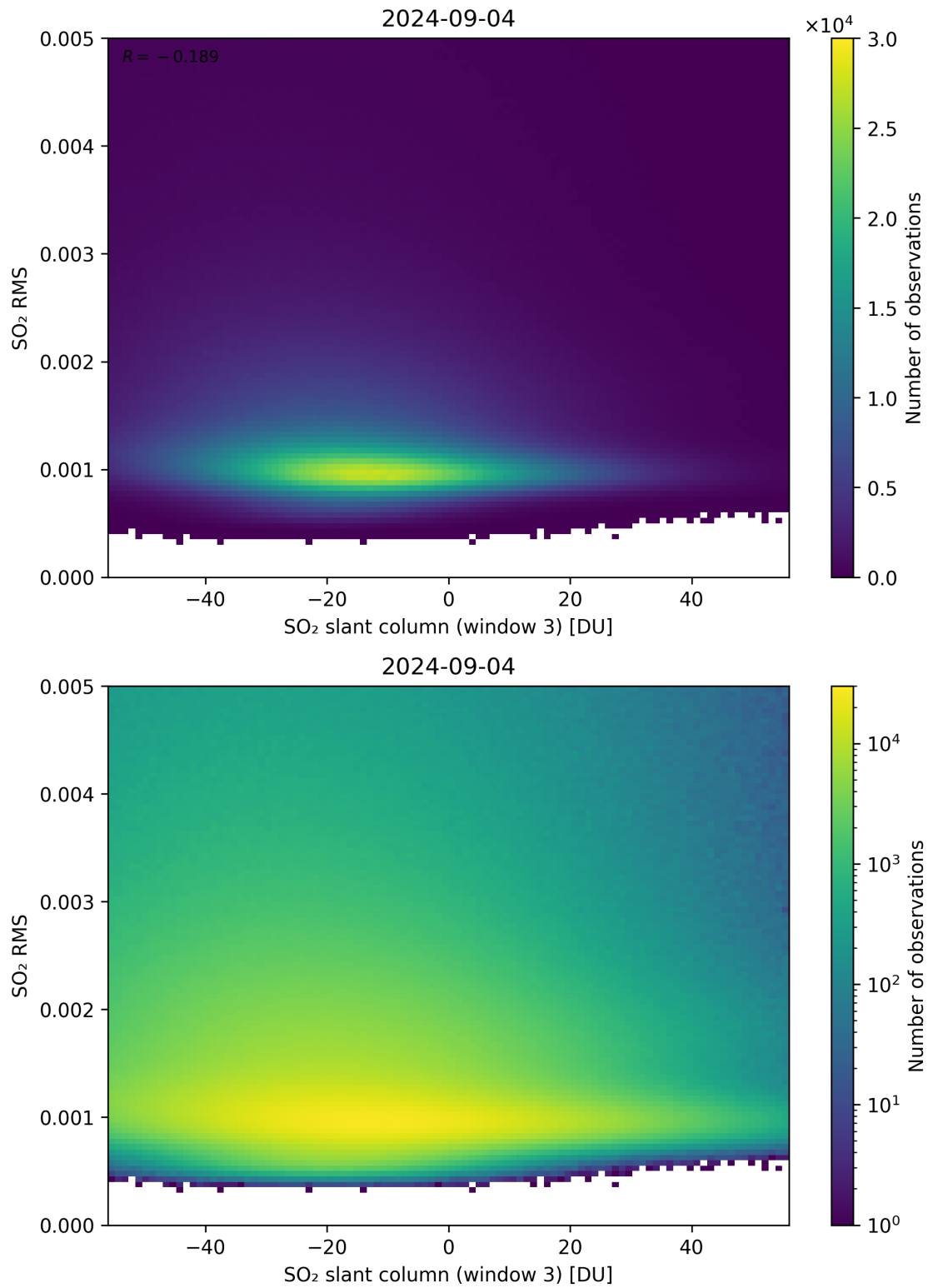
Figure 256: Scatter density plot of “SO 2 slant column (window 3)” against “SO 2 RMS” for 2024-09-03 to 2024-09-05.
