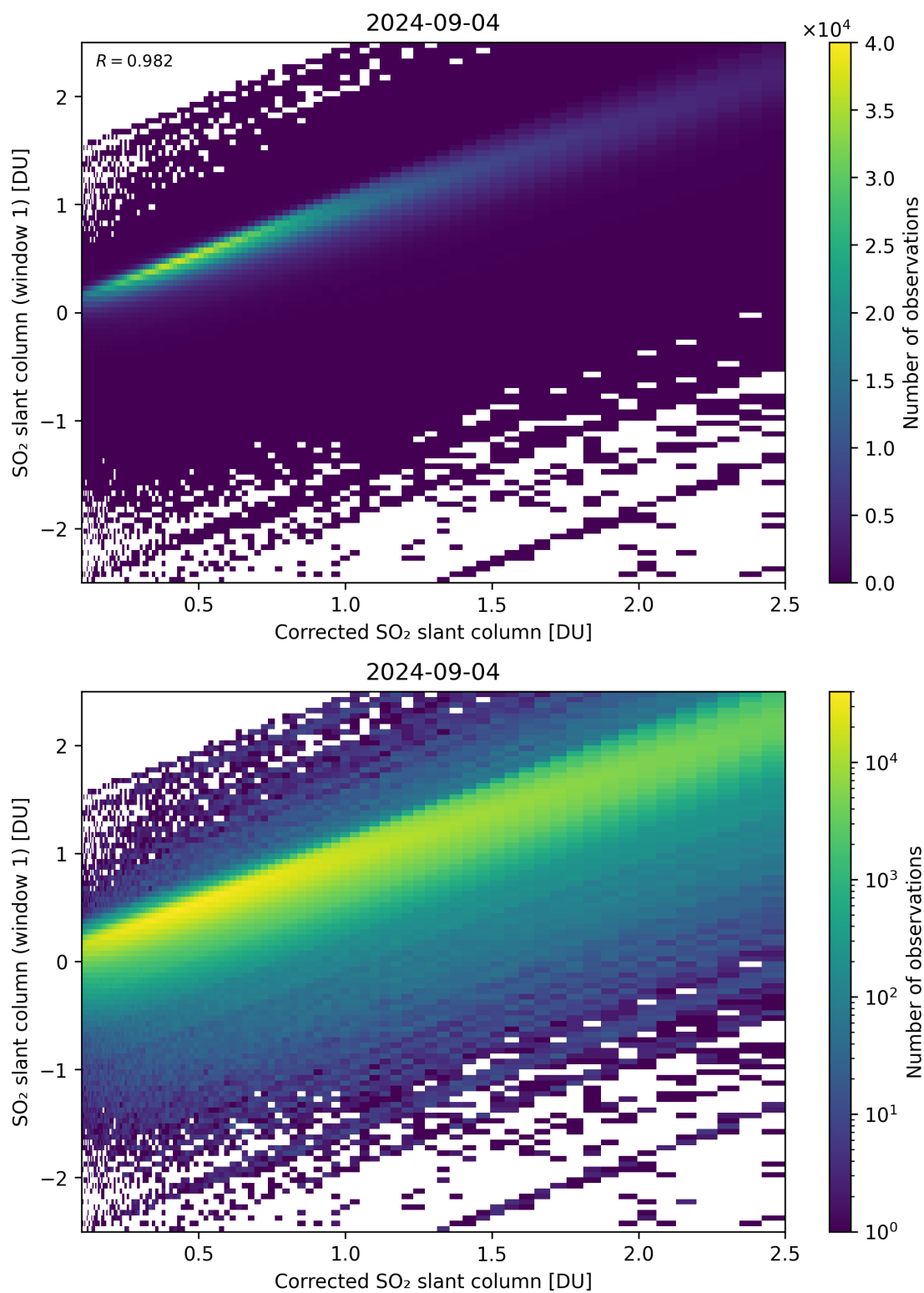
Figure 187: Scatter density plot of “Corrected SO 2 slant column” against “SO 2 slant column (window 1)” for 2024-09-03 to 2024-09-05.
