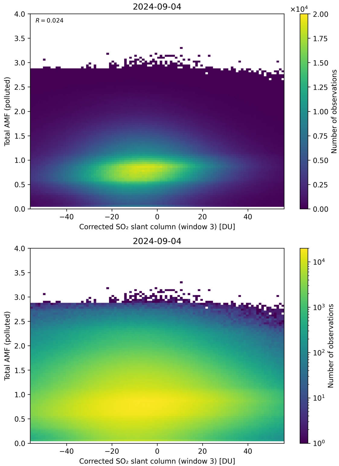
Figure 210: Scatter density plot of “Corrected SO 2 slant column (window 3)” against “Total AMF (polluted)” for 2024-09-03 to 2024-09-05.
