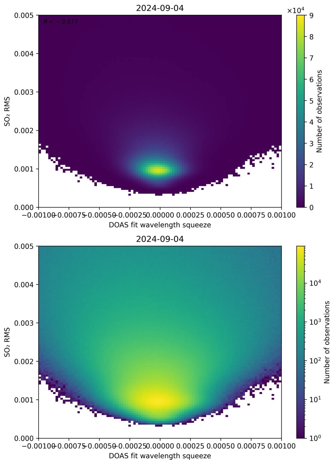
Figure 132: Scatter density plot of “DOAS fit wavelength squeeze” against “SO 2 RMS” for 2024-09-03 to 2024-09-05.
