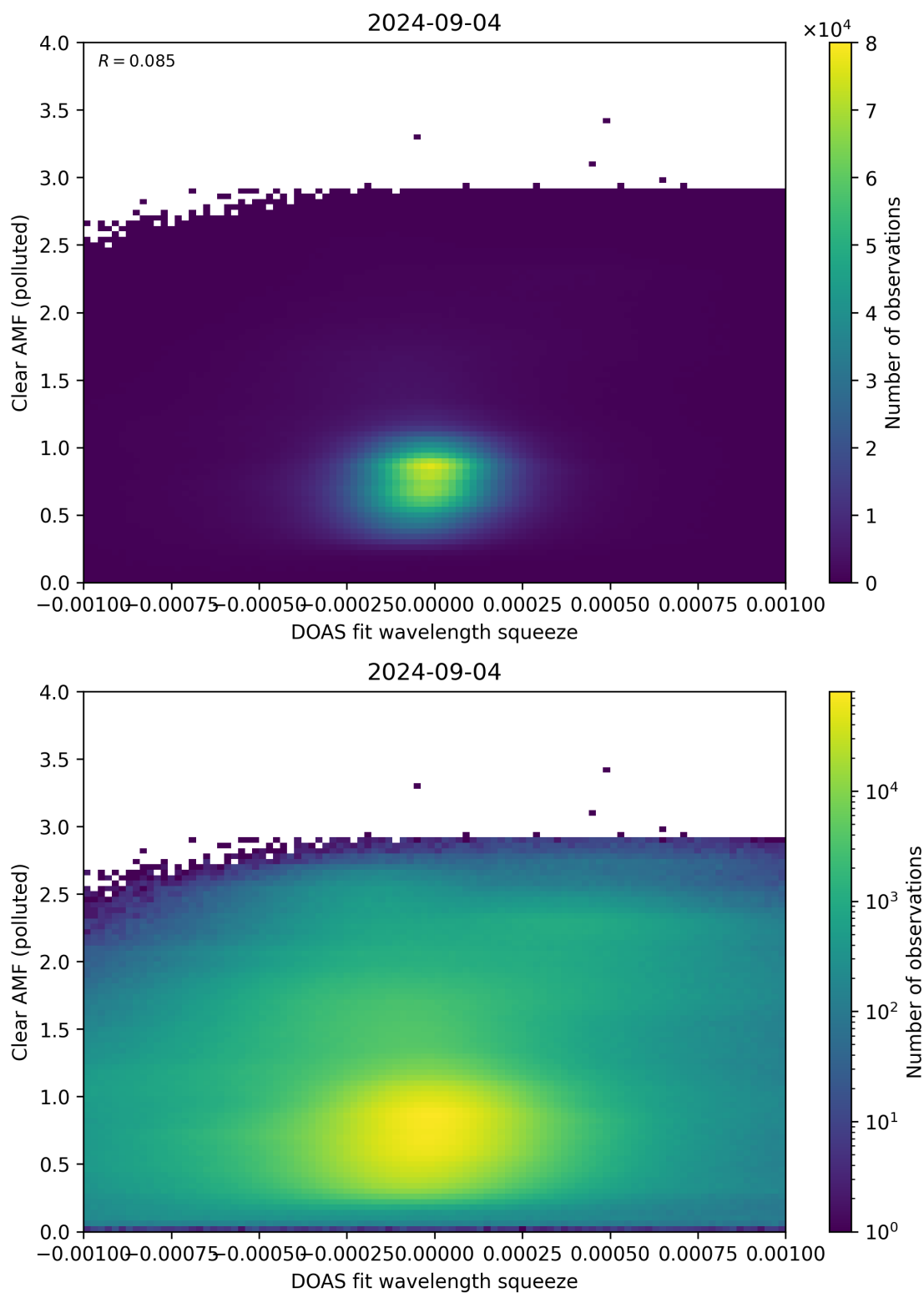
Figure 133: Scatter density plot of “DOAS fit wavelength squeeze” against “Clear AMF (polluted)” for 2024-09-03 to 2024-09-05.
