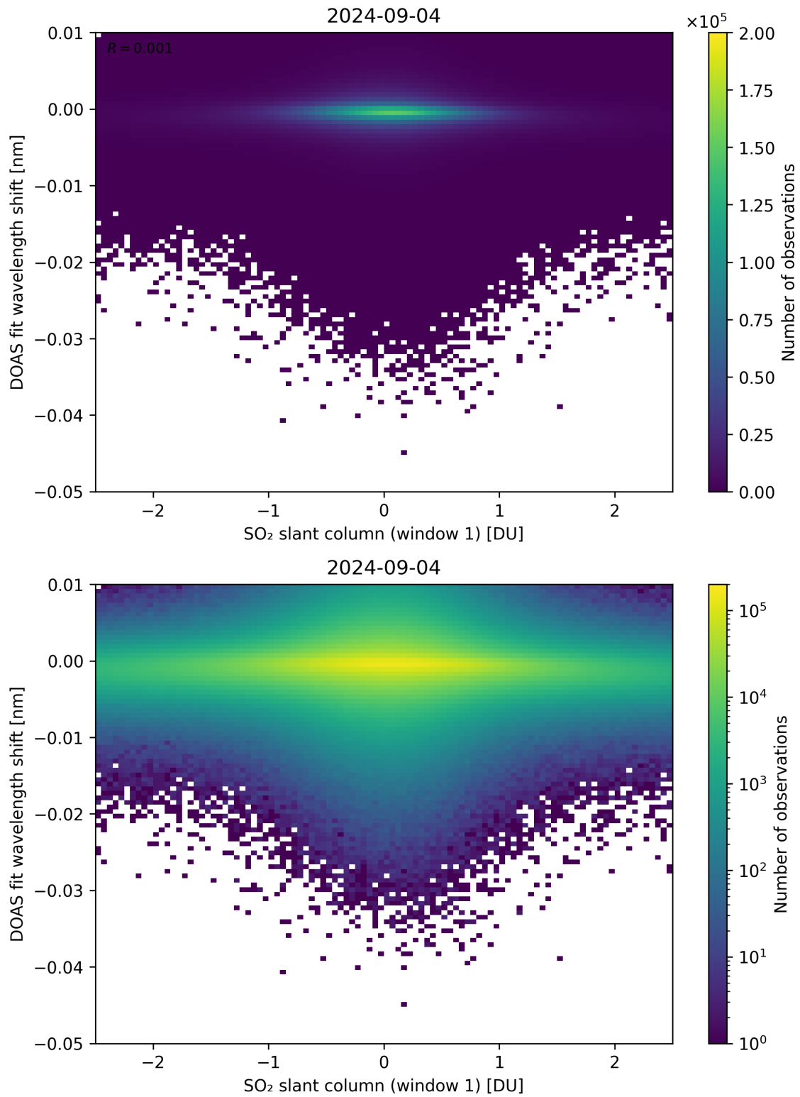
Figure 215: Scatter density plot of “SO 2 slant column (window 1)” against “DOAS fit wavelength shift” for 2024-09-03 to 2024-09-05.
