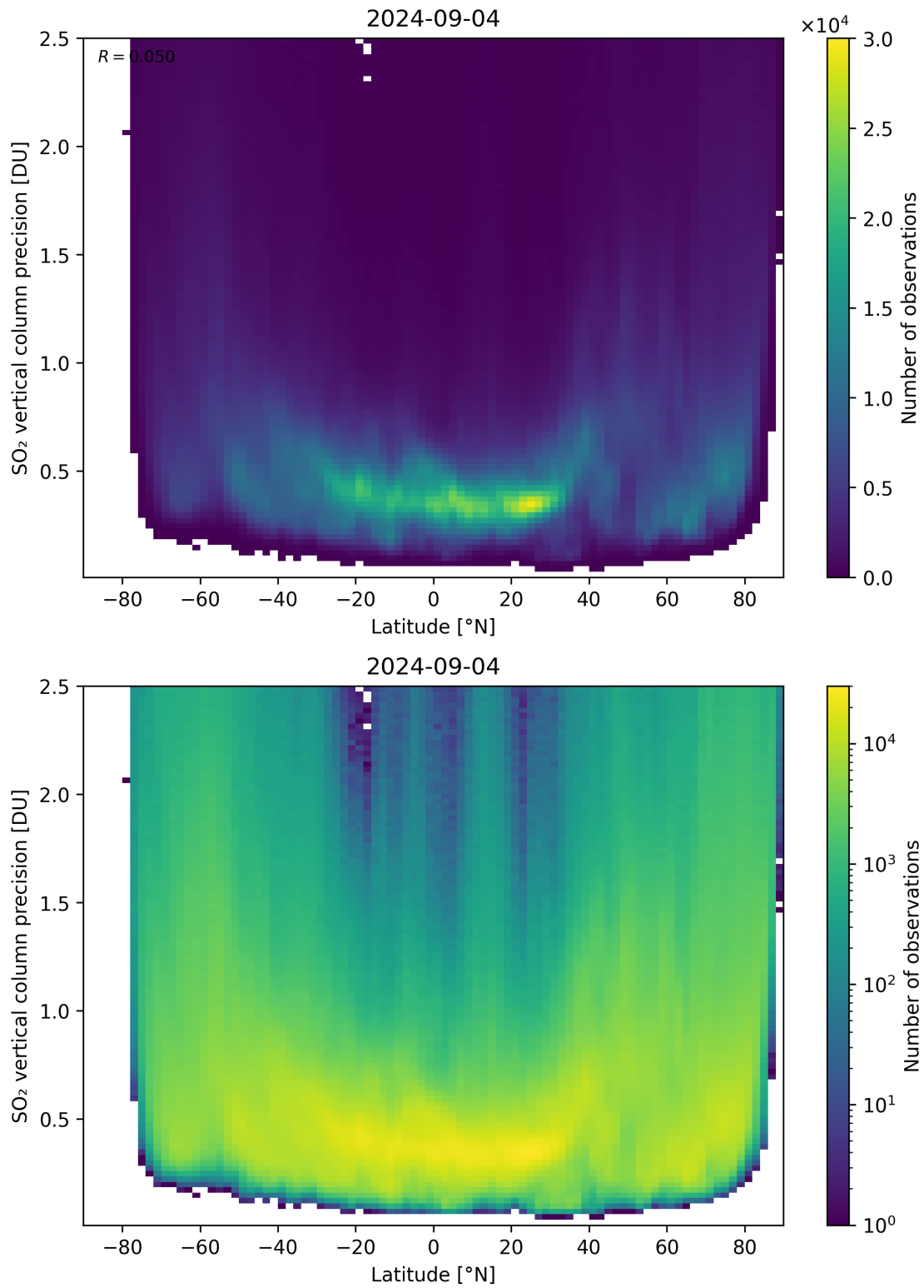
Figure 157: Scatter density plot of “Latitude” against “SO 2 vertical column precision” for 2024-09-03 to 2024-09-05.
