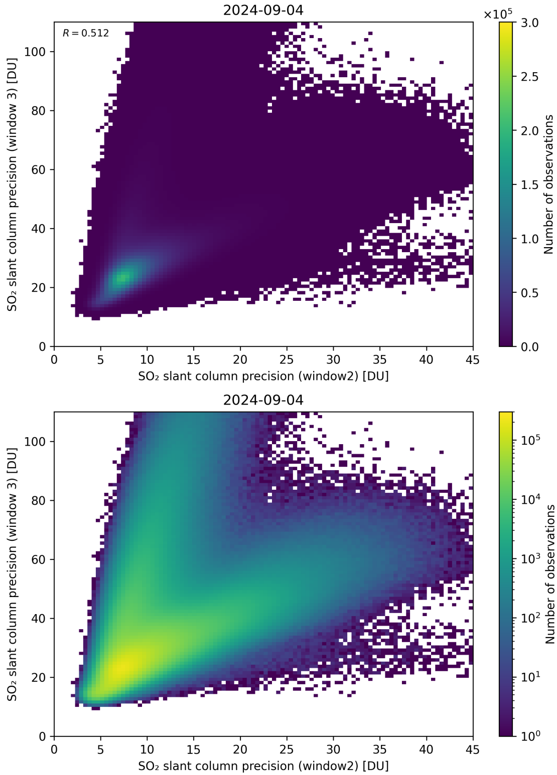
Figure 250: Scatter density plot of “SO 2 slant column precision (window2)” against “SO 2 slant column precision (window 3)” for 2024-09-03 to 2024-09-05.
