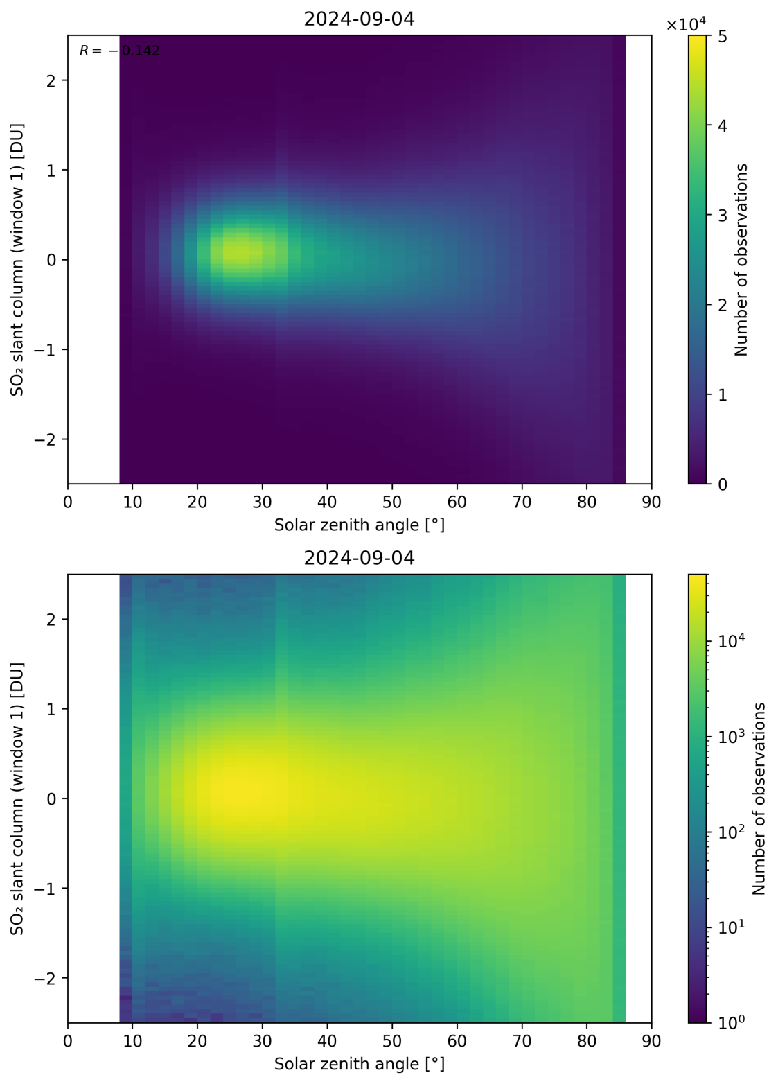
Figure 169: Scatter density plot of “Solar zenith angle” against “SO 2 slant column (window 1)” for 2024-09-03 to 2024-09-05.
