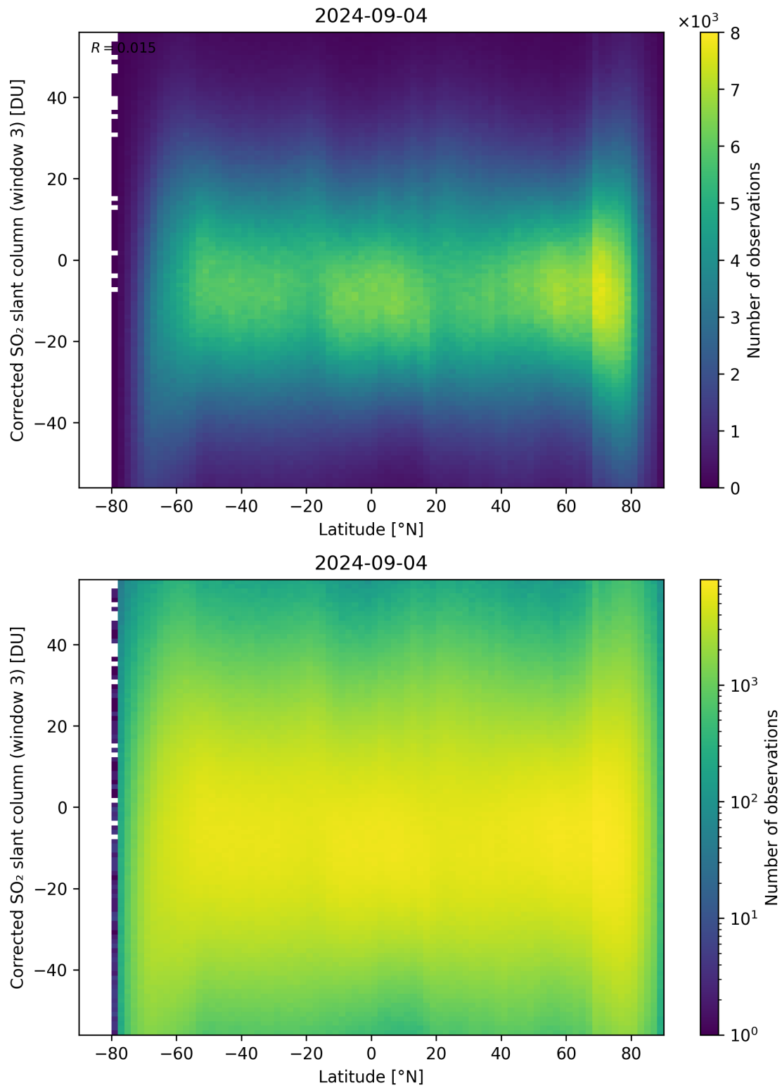
Figure 148: Scatter density plot of “Latitude” against “Corrected SO 2 slant column (window 3)” for 2024-09-03 to 2024-09-05.
