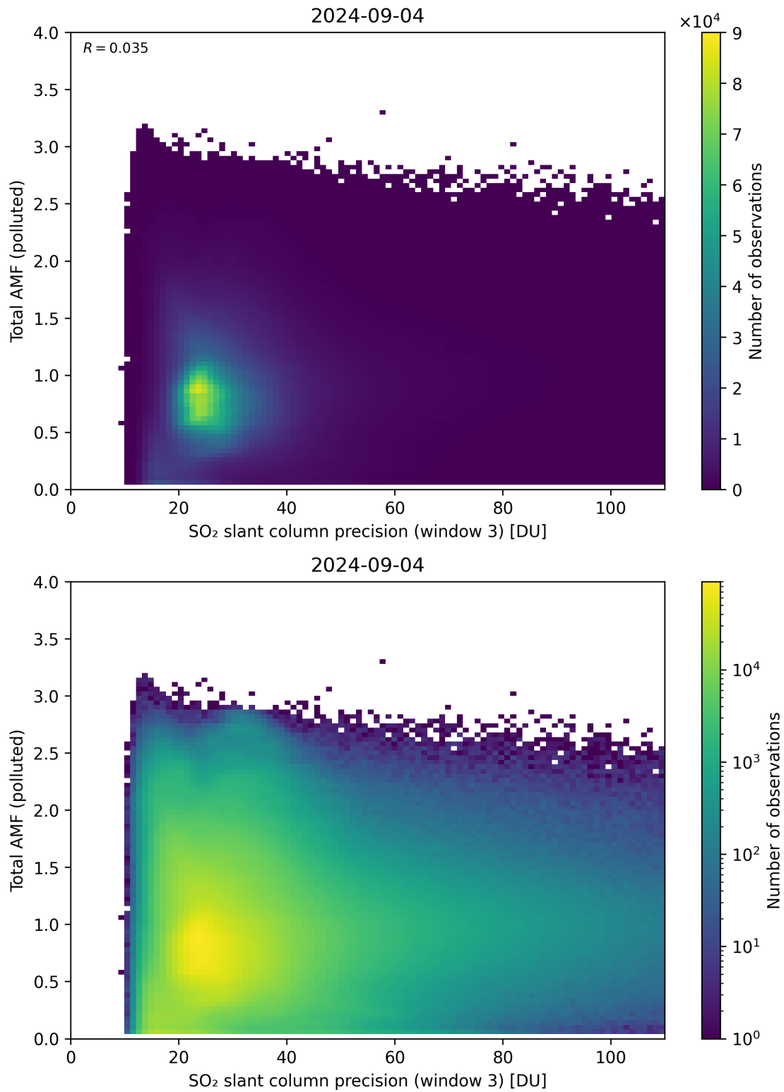
Figure 263: Scatter density plot of “SO 2 slant column precision (window 3)” against “Total AMF (polluted)” for 2024-09-03 to 2024-09-05.
