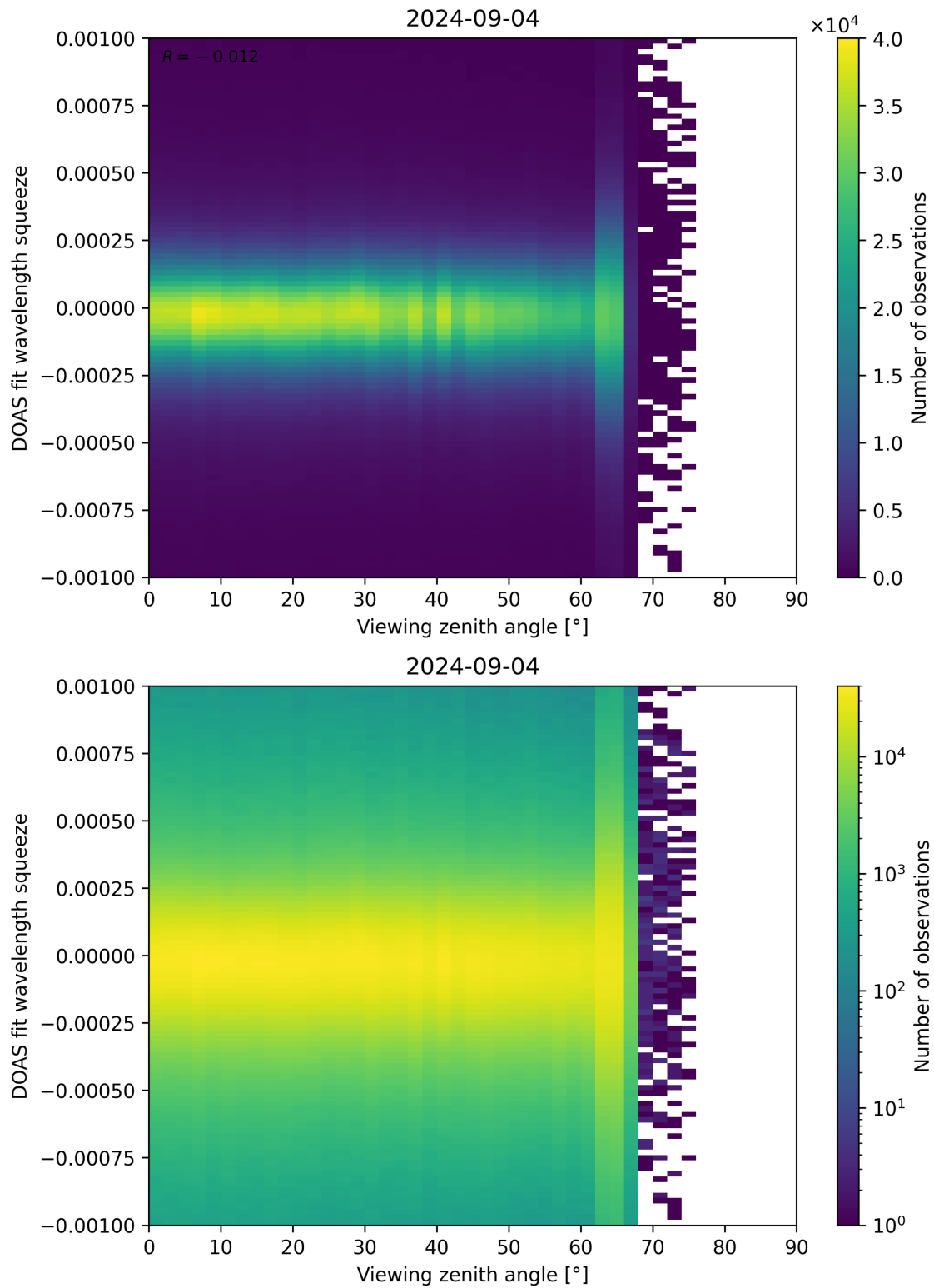
Figure 312: Scatter density plot of “Viewing zenith angle” against “DOAS fit wavelength squeeze” for 2024-09-03 to 2024-09-05.
