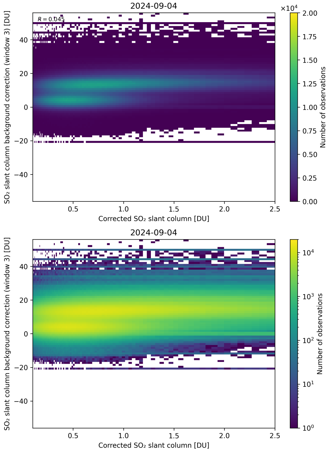
Figure 180: Scatter density plot of “Corrected SO 2 slant column” against “SO 2 slant column background correction (window 3)” for 2024-09-03 to 2024-09-05.
