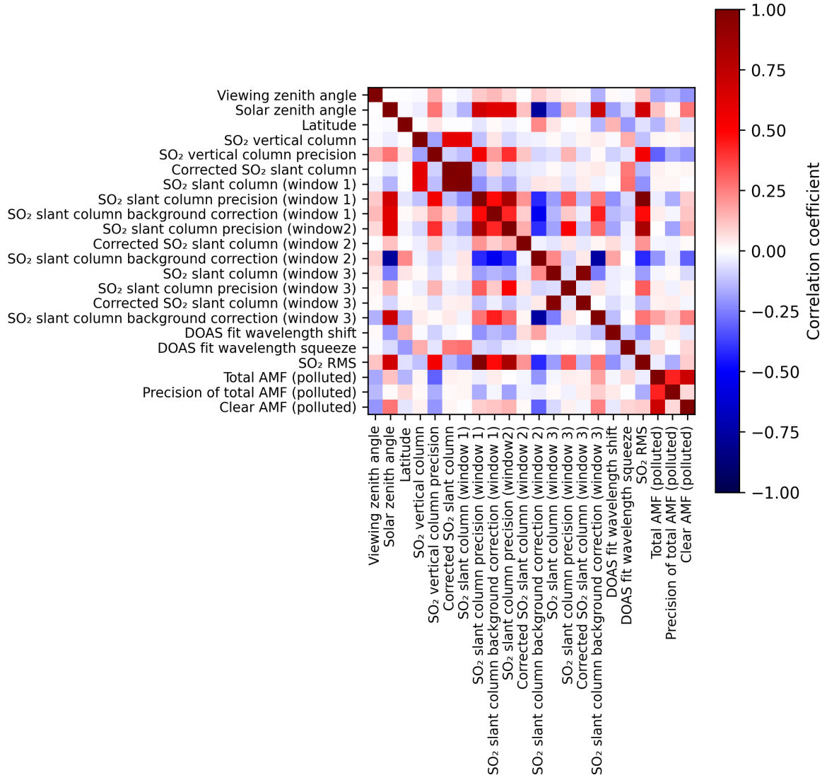
Figure 2: Map of correlation matrix for 2024-09-03 to 2024-09-05.
