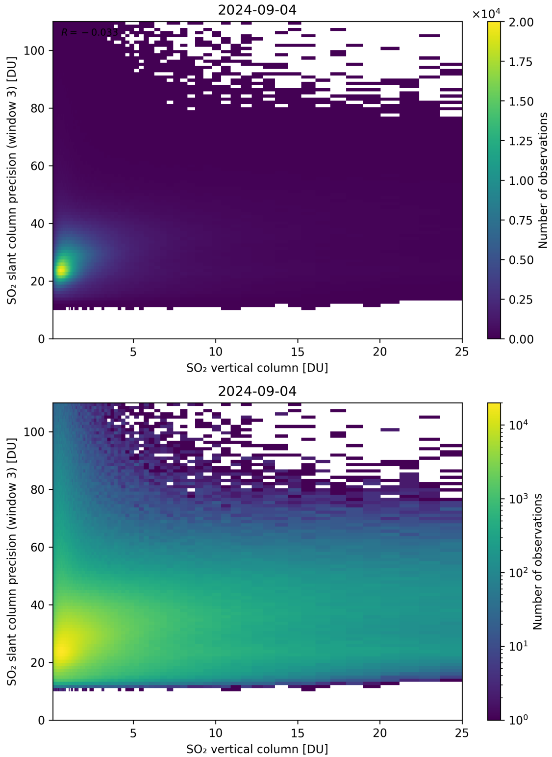
Figure 304: Scatter density plot of “SO 2 vertical column” against “SO 2 slant column precision (window 3)” for 2024-09-03 to 2024-09-05.
