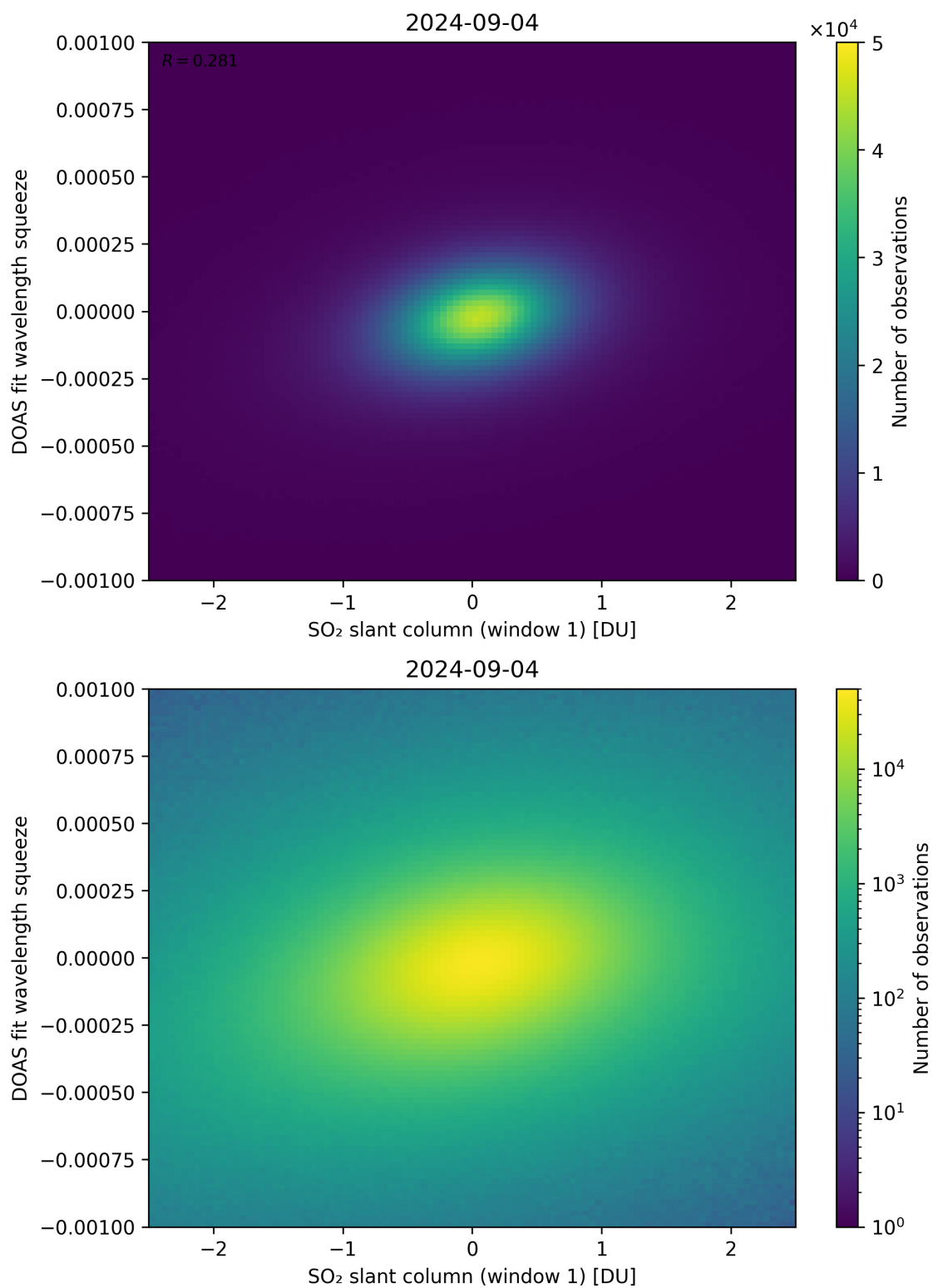
Figure 216: Scatter density plot of “SO 2 slant column (window 1)” against “DOAS fit wavelength squeeze” for 2024-09-03 to 2024-09-05.
