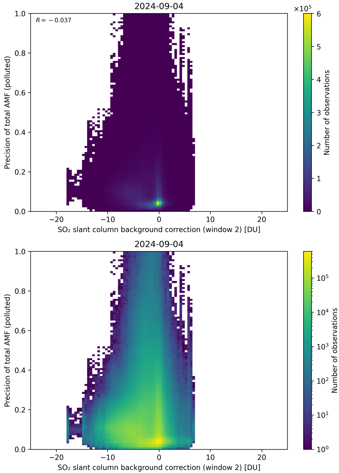
Figure 120: Scatter density plot of “SO 2 slant column background correction (window 2)” against “Precision of total AMF (polluted)” for 2024-09-03 to 2024-09-05.
