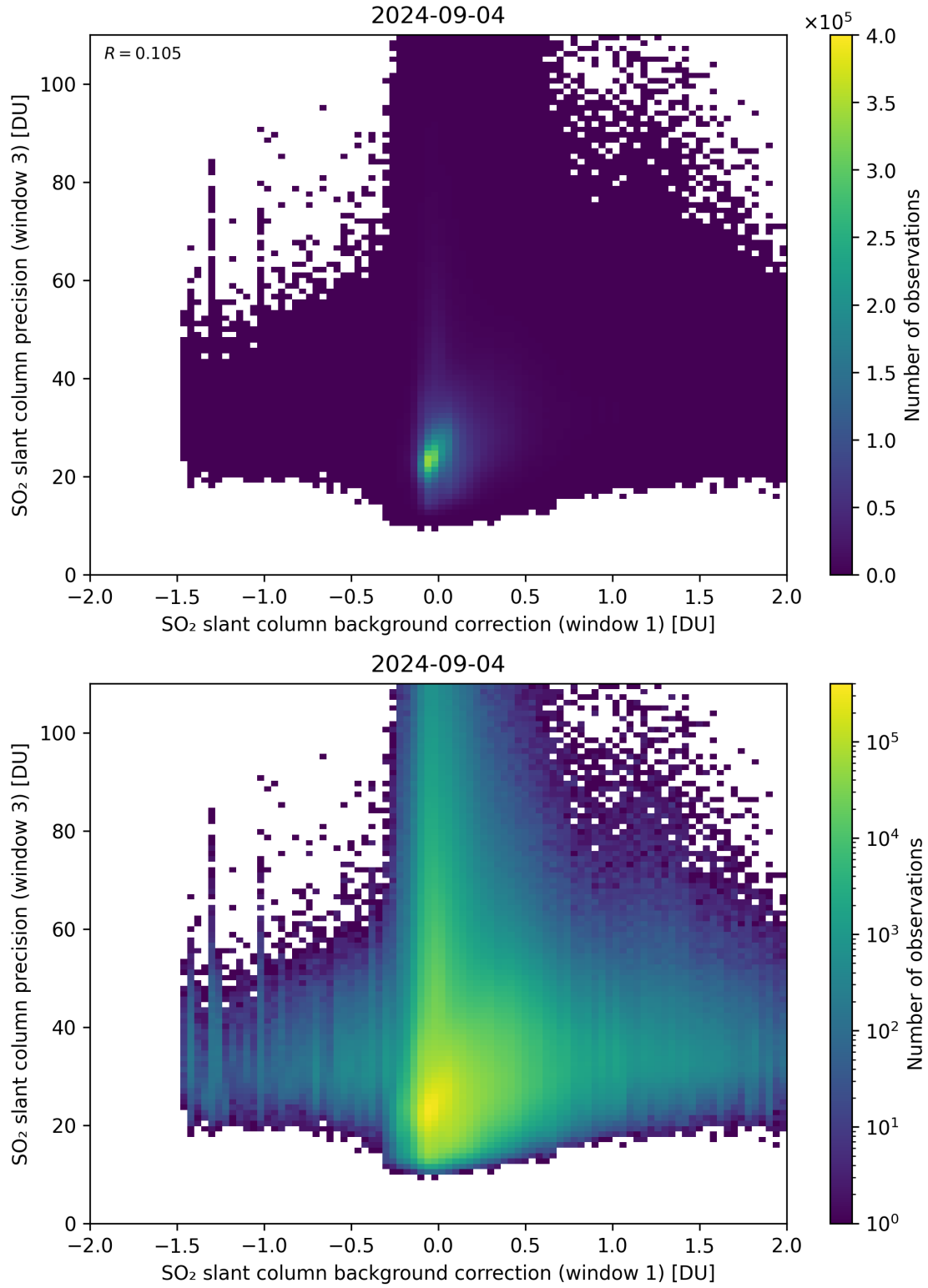
Figure 108: Scatter density plot of “SO 2 slant column background correction (window 1)” against “SO 2 slant column precision (window 3)” for 2024-09-03 to 2024-09-05.
