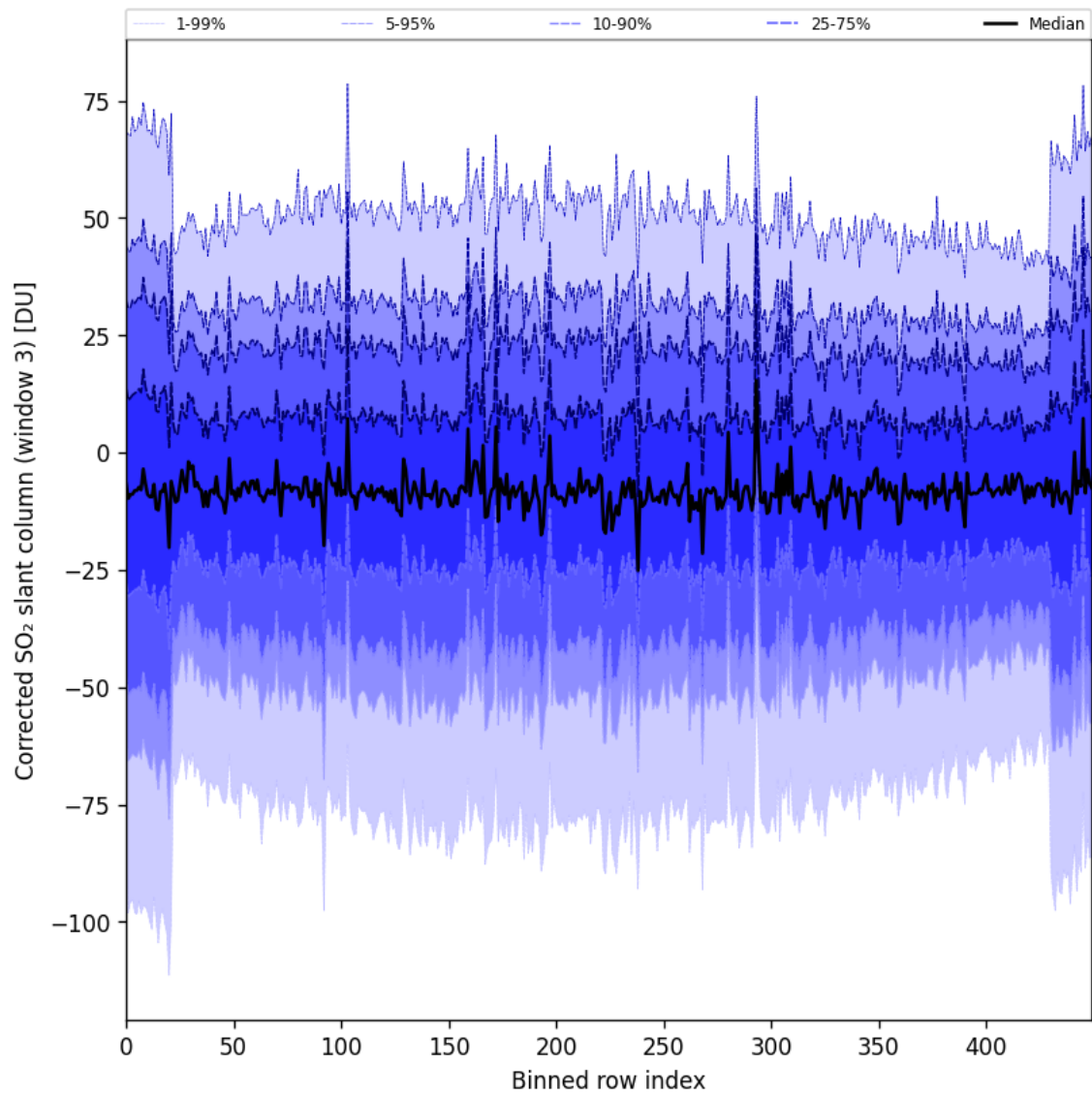
Figure 89: Along track statistics of “Corrected SO 2 slant column (window 3)” for 2024-09-03 to 2024-09-05
