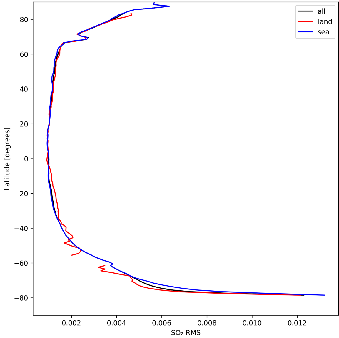
Figure 47: Zonal average of “SO 2 RMS” for 2024-09-03 to 2024-09-05.
