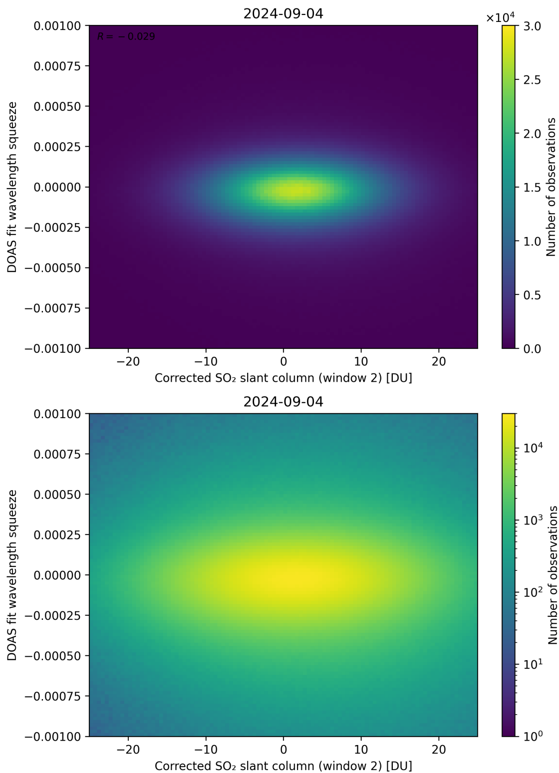
Figure 197: Scatter density plot of “Corrected SO 2 slant column (window 2)” against “DOAS fit wavelength squeeze” for 2024-09-03 to 2024-09-05.
