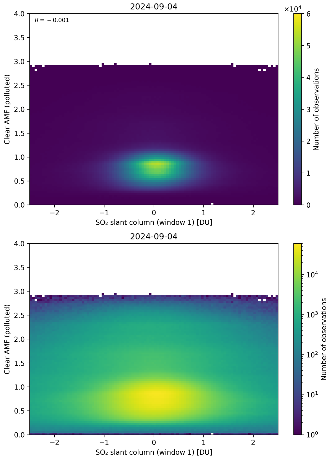
Figure 232: Scatter density plot of “SO 2 slant column (window 1)” against “Clear AMF (polluted)” for 2024-09-03 to 2024-09-05.
