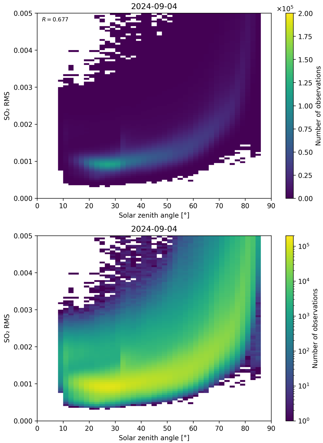
Figure 163: Scatter density plot of “Solar zenith angle” against “SO 2 RMS” for 2024-09-03 to 2024-09-05.
