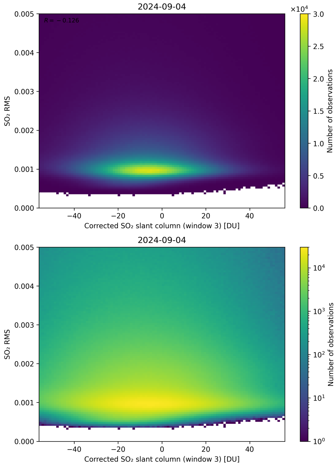
Figure 208: Scatter density plot of “Corrected SO 2 slant column (window 3)” against “SO 2 RMS” for 2024-09-03 to 2024-09-05.
