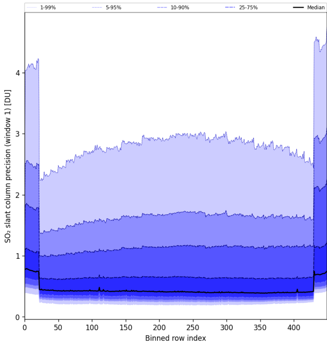
Figure 80: Along track statistics of “SO 2 slant column precision (window 1)” for 2024-09-03 to 2024-09-05
