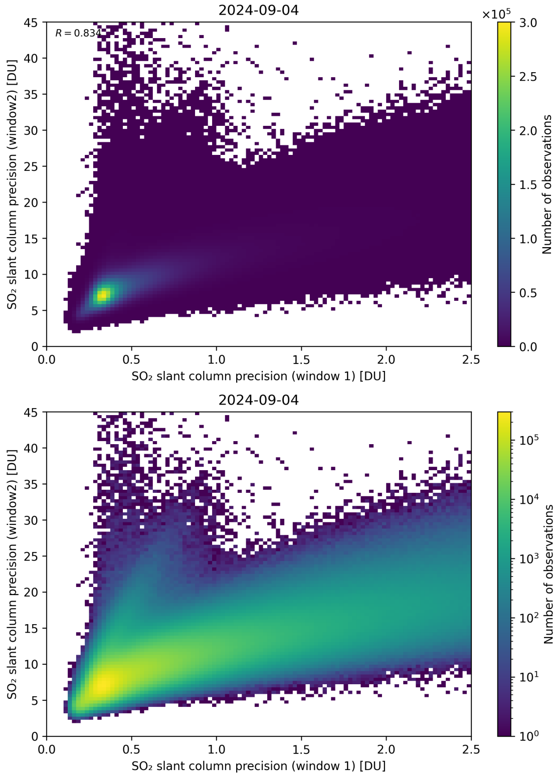
Figure 227: Scatter density plot of “SO 2 slant column precision (window 1)” against “SO 2 slant column precision (window2)” for 2024-09-03 to 2024-09-05.
