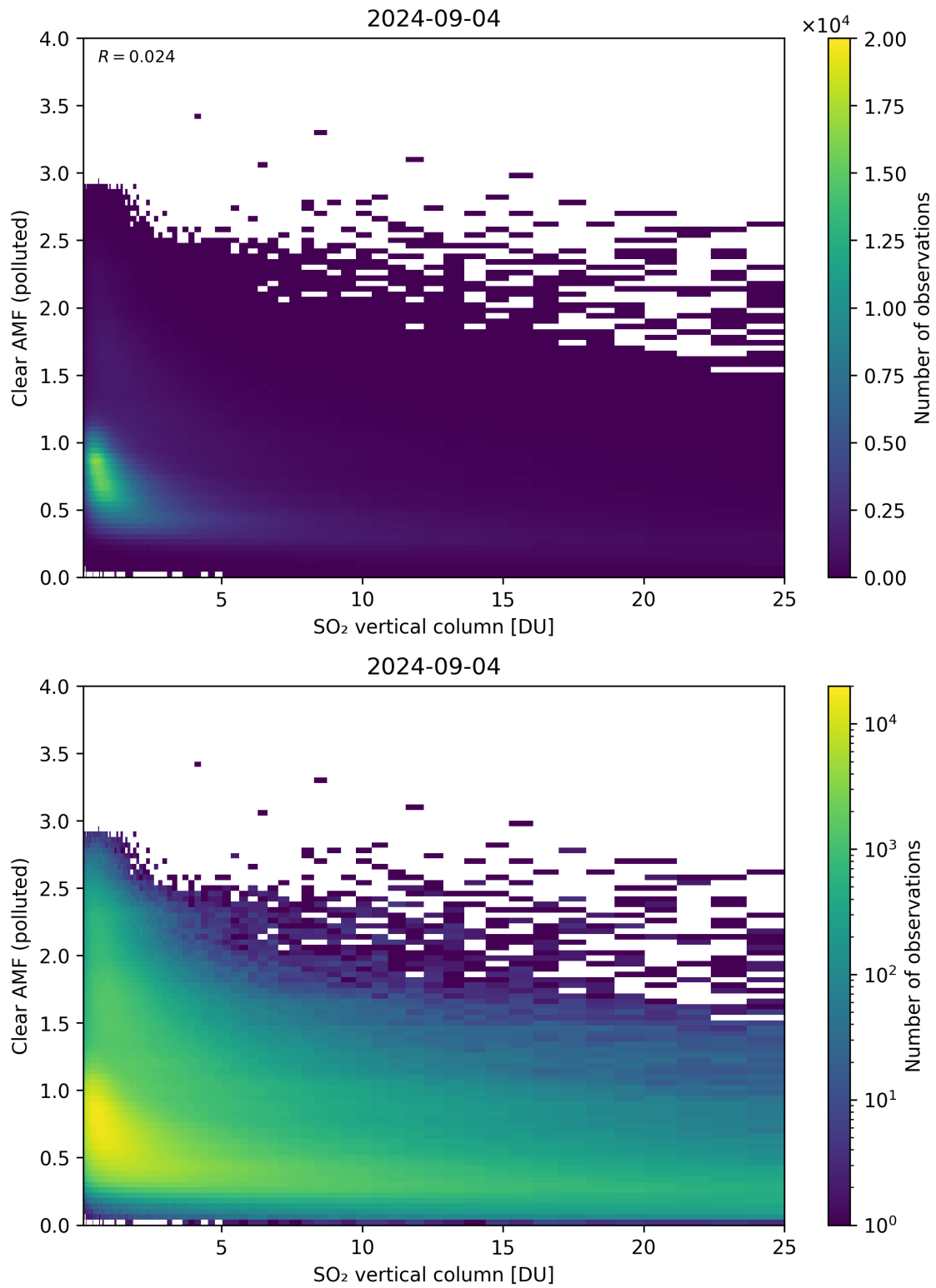
Figure 296: Scatter density plot of “SO 2 vertical column” against “Clear AMF (polluted)” for 2024-09-03 to 2024-09-05.
