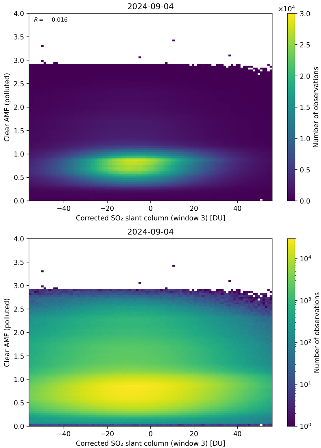
Figure 209: Scatter density plot of “Corrected SO 2 slant column (window 3)” against “Clear AMF (polluted)” for 2024-09-03 to 2024-09-05.
