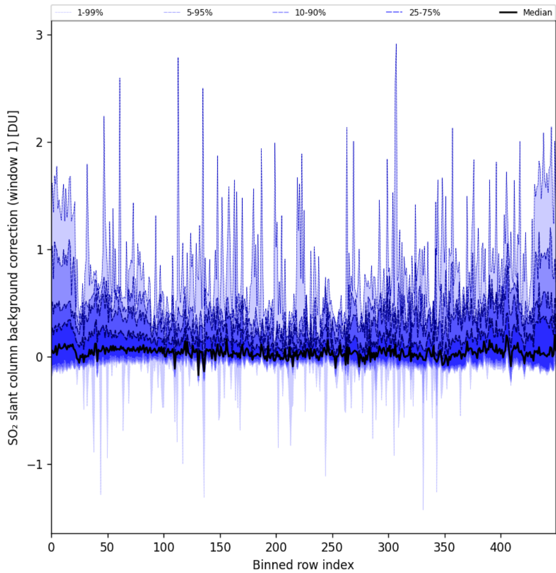
Figure 82: Along track statistics of “SO 2 slant column background correction (window 1)” for 2024-09-03 to 2024-09-05
