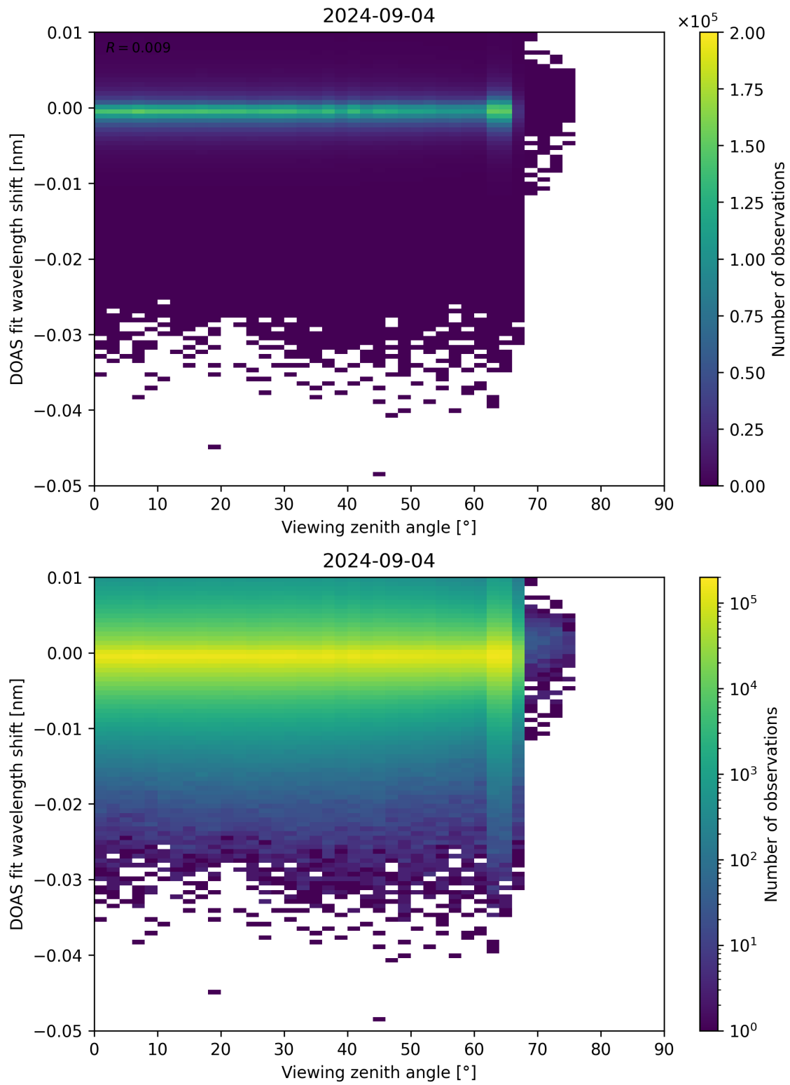
Figure 311: Scatter density plot of “Viewing zenith angle” against “DOAS fit wavelength shift” for 2024-09-03 to 2024-09-05.
