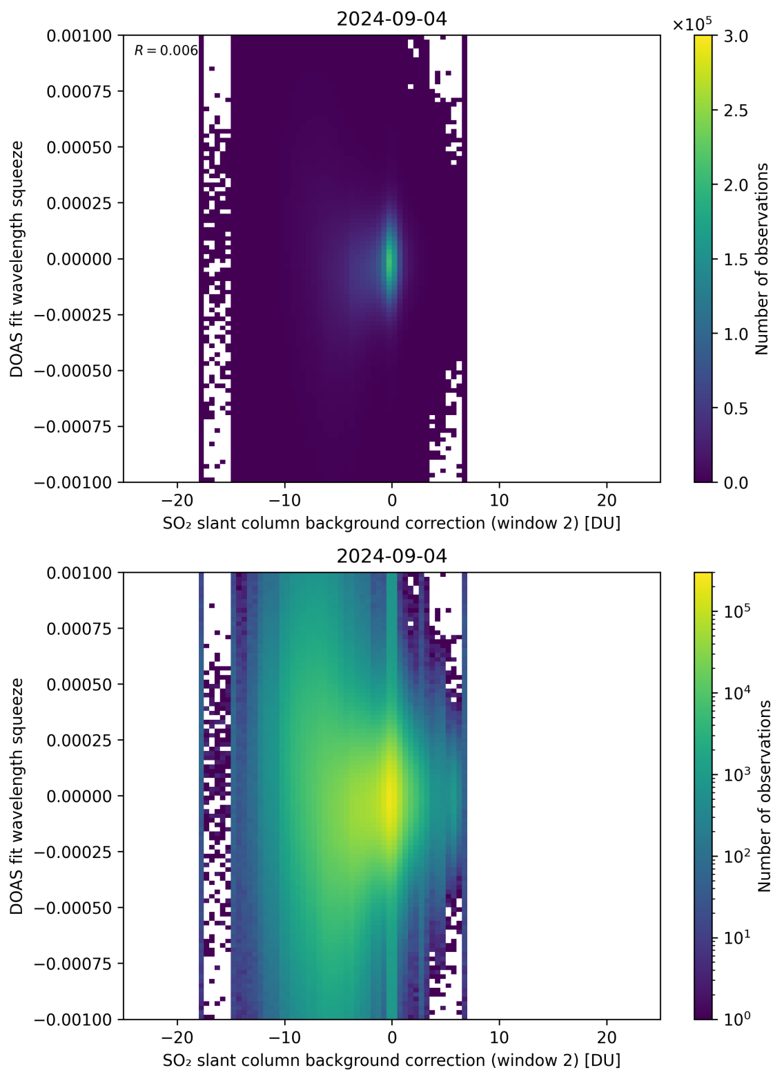
Figure 113: Scatter density plot of “SO 2 slant column background correction (window 2)” against “DOAS fit wavelength squeeze” for 2024-09-03 to 2024-09-05.
