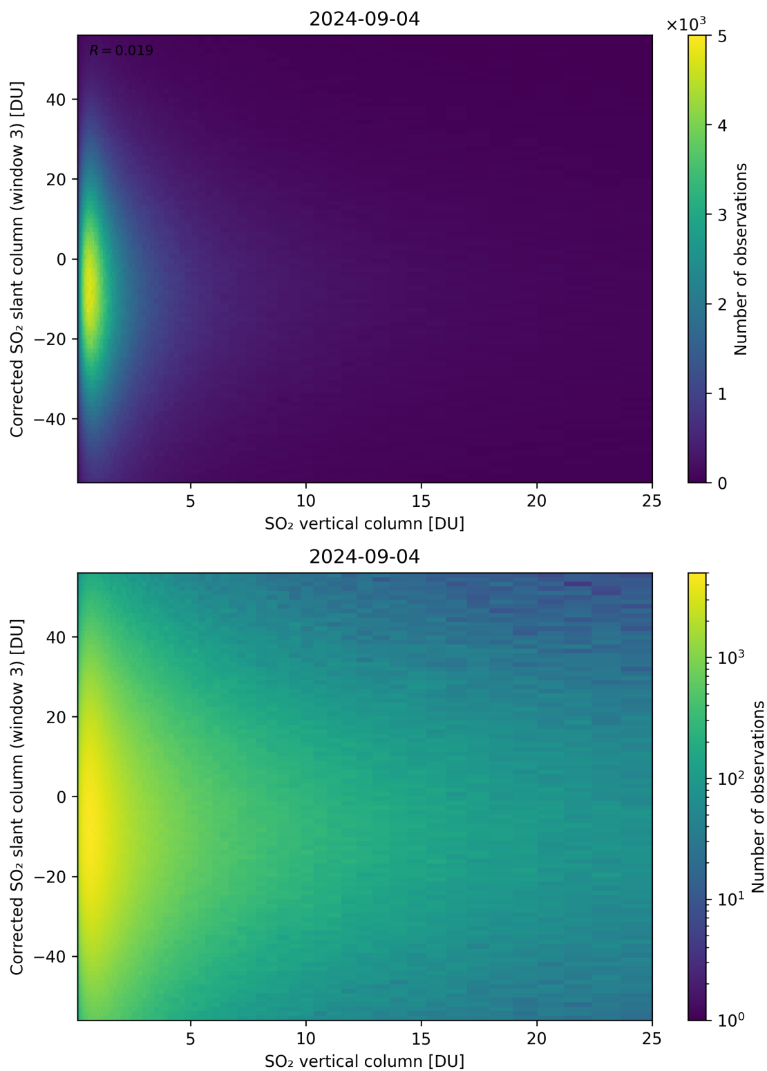
Figure 299: Scatter density plot of “SO 2 vertical column” against “Corrected SO 2 slant column (window 3)” for 2024-09-03 to 2024-09-05.
