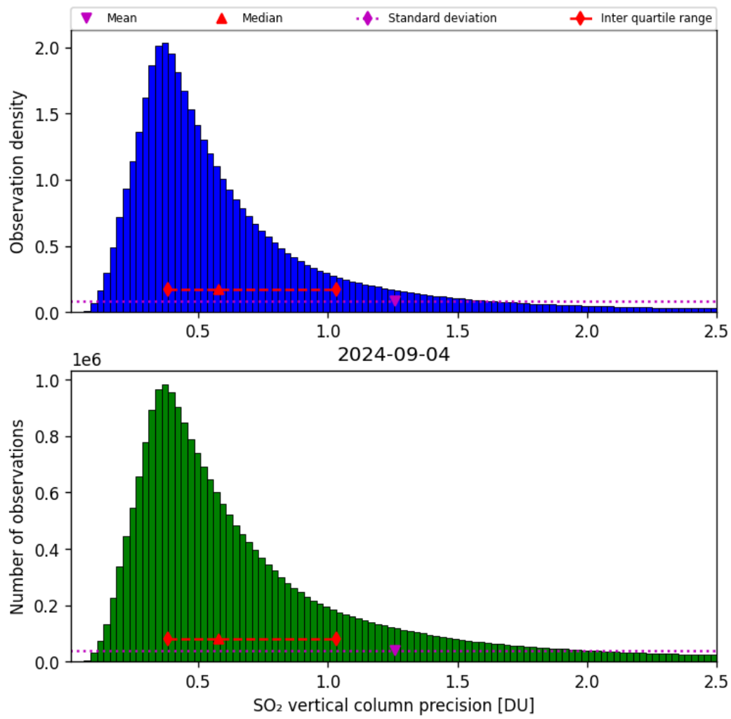
Figure 54: Histogram of "SO 2 vertical column precision" for 2024-09-03 to 2024-09-05
