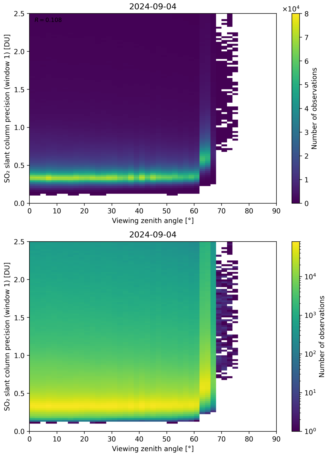
Figure 321: Scatter density plot of “Viewing zenith angle” against “SO 2 slant column precision (window 1)” for 2024-09-03 to 2024-09-05.
