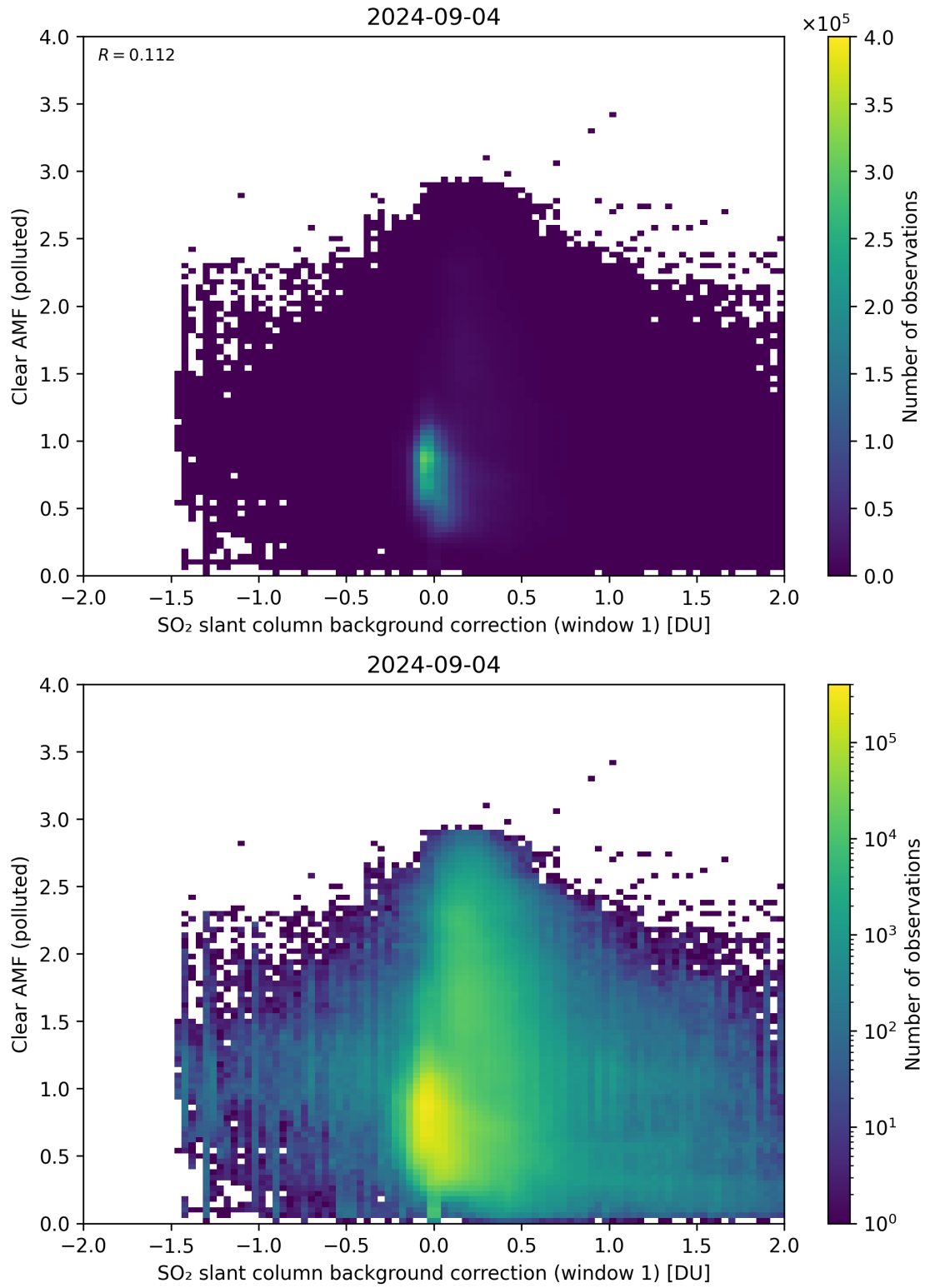
Figure 103: Scatter density plot of “SO 2 slant column background correction (window 1)” against “Clear AMF (polluted)” for 2024-09-03 to 2024-09-05.
