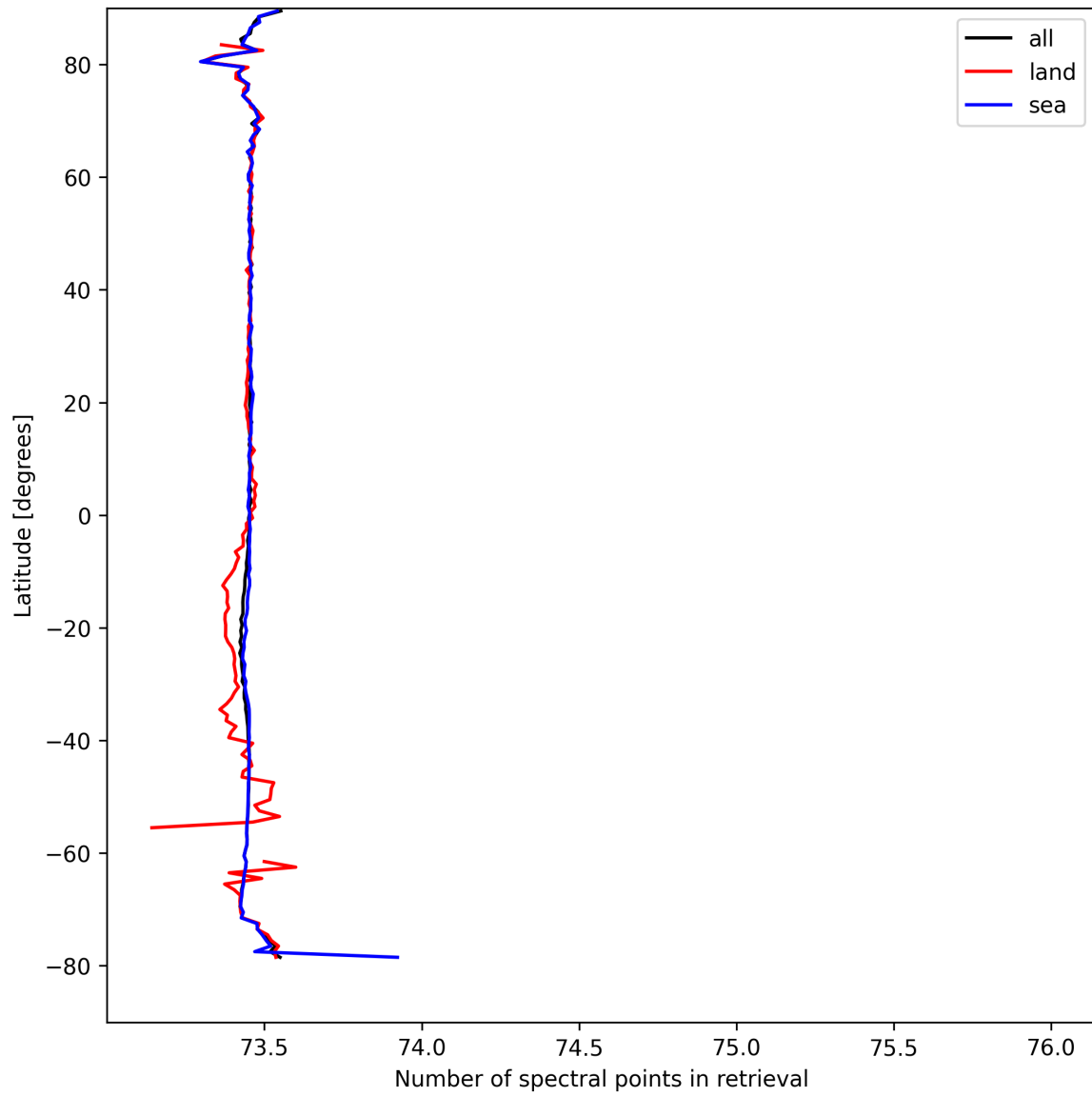
Figure 51: Zonal average of “Number of spectral points in retrieval” for 2024-09-03 to 2024-09-05.
