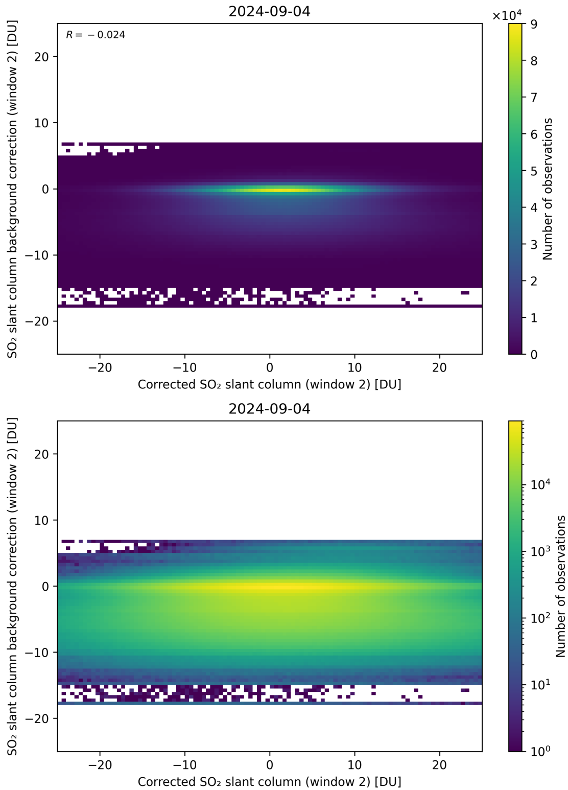
Figure 194: Scatter density plot of “Corrected SO 2 slant column (window 2)” against “SO 2 slant column background correction (window 2)” for 2024-09-03 to 2024-09-05.
