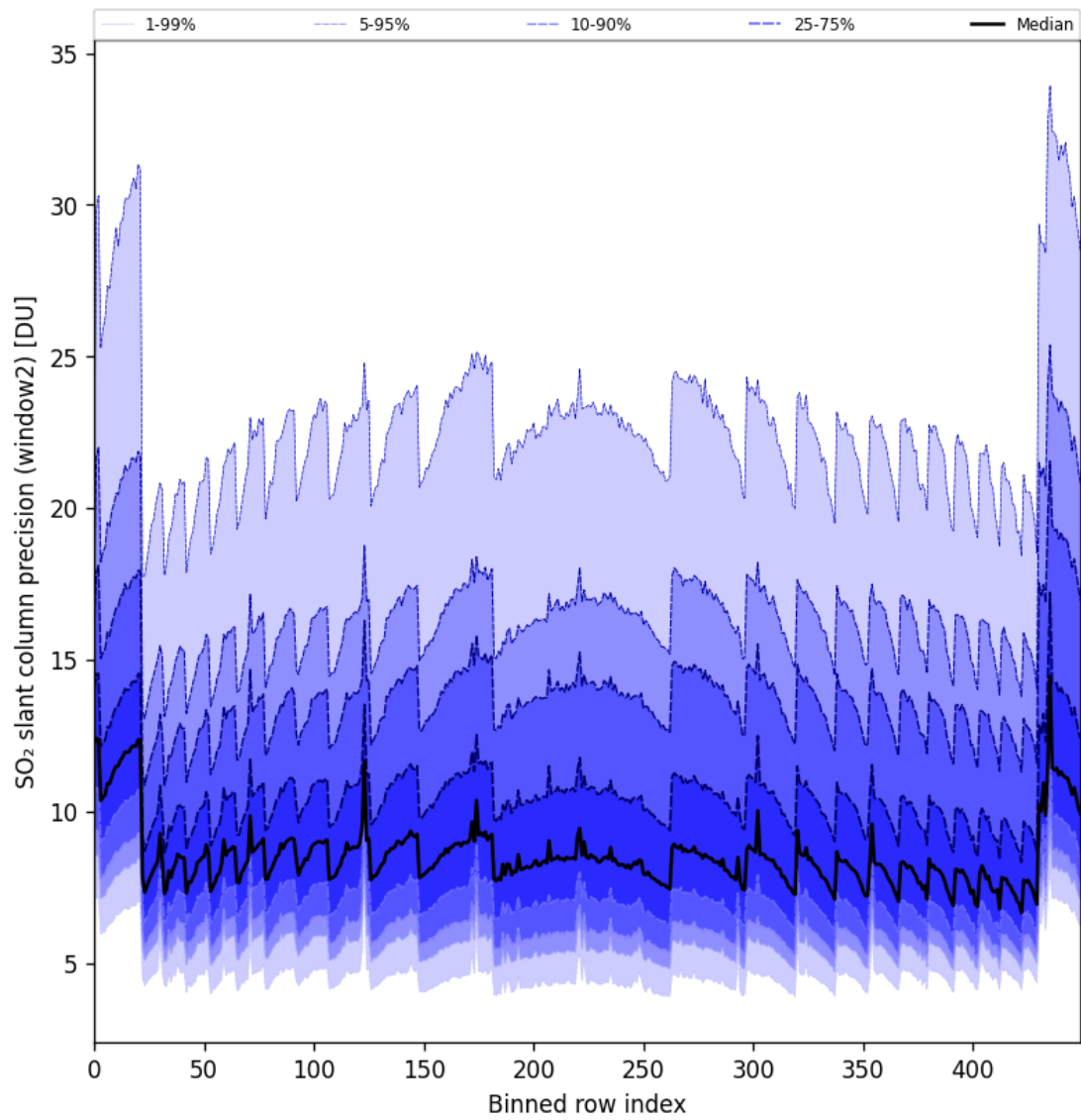
Figure 84: Along track statistics of “SO 2 slant column precision (window2)” for 2024-09-03 to 2024-09-05
