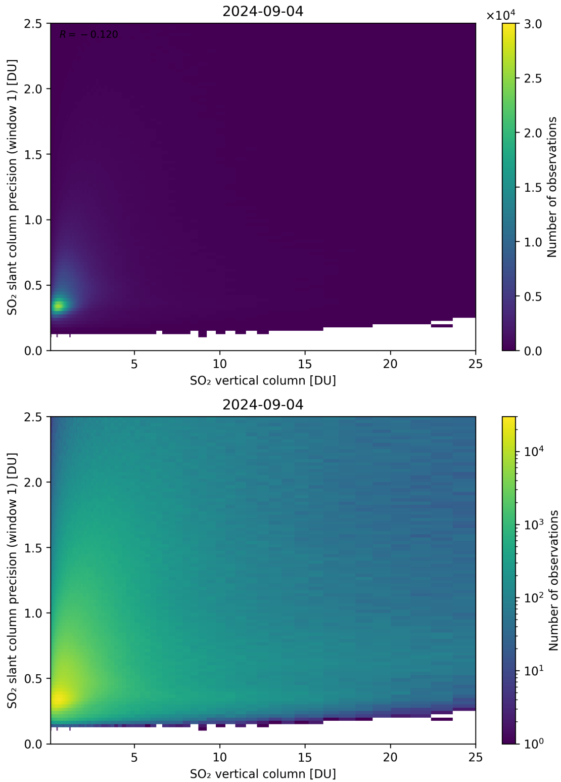
Figure 301: Scatter density plot of “SO 2 vertical column” against “SO 2 slant column precision (window 1)” for 2024-09-03 to 2024-09-05.
