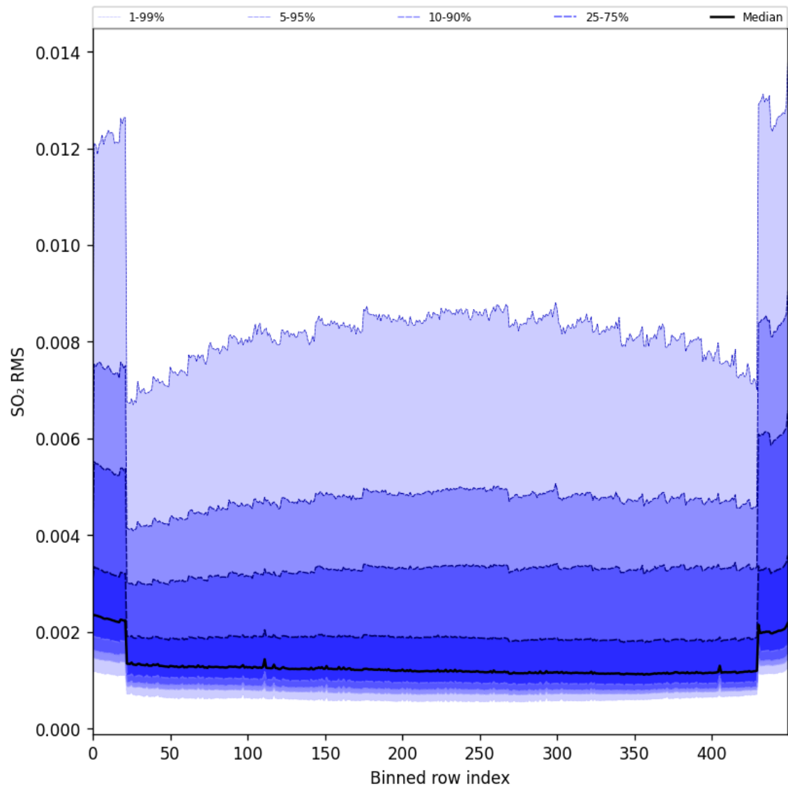
Figure 93: Along track statistics of “SO 2 RMS” for 2024-09-03 to 2024-09-05
