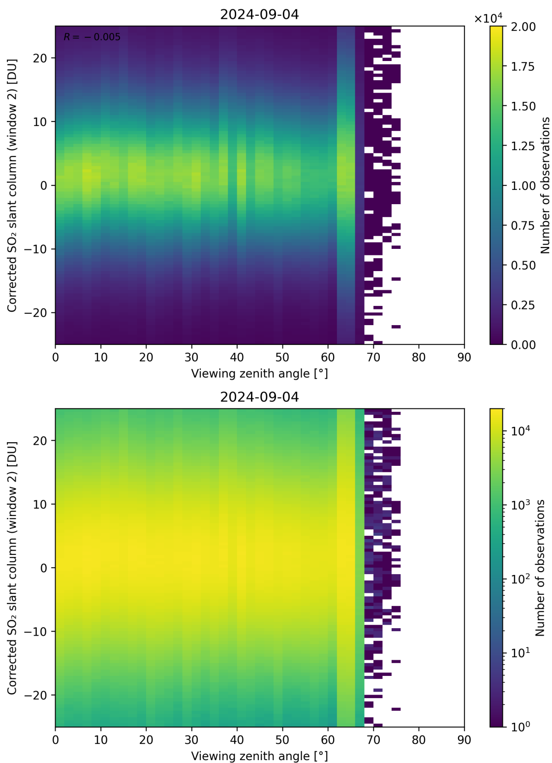
Figure 318: Scatter density plot of “Viewing zenith angle” against “Corrected SO 2 slant column (window 2)” for 2024-09-03 to 2024-09-05.
