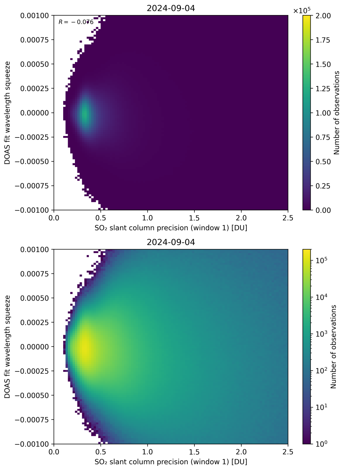
Figure 222: Scatter density plot of “SO 2 slant column precision (window 1)” against “DOAS fit wavelength squeeze” for 2024-09-03 to 2024-09-05.
