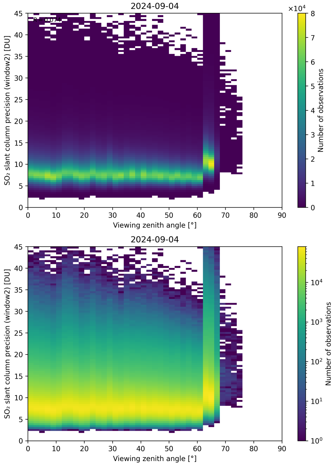
Figure 322: Scatter density plot of “Viewing zenith angle” against “SO 2 slant column precision (window2)” for 2024-09-03 to 2024-09-05.
