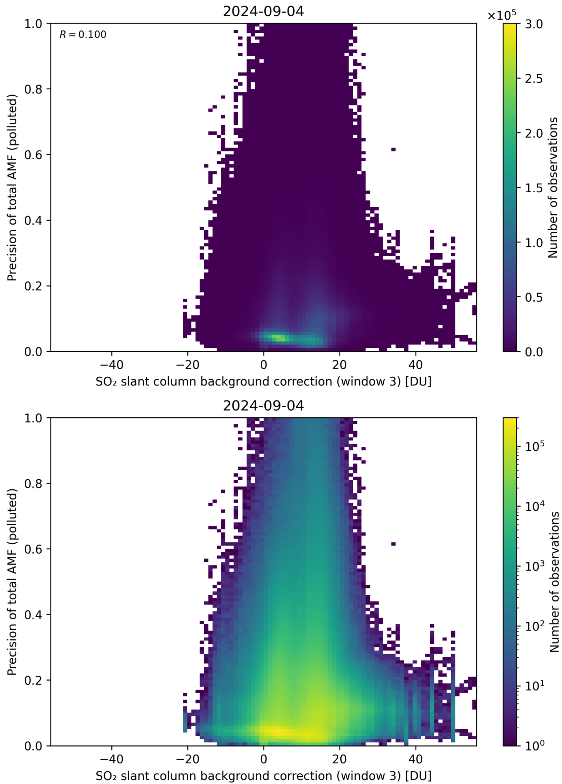
Figure 126: Scatter density plot of “SO 2 slant column background correction (window 3)” against “Precision of total AMF (polluted)” for 2024-09-03 to 2024-09-05.
