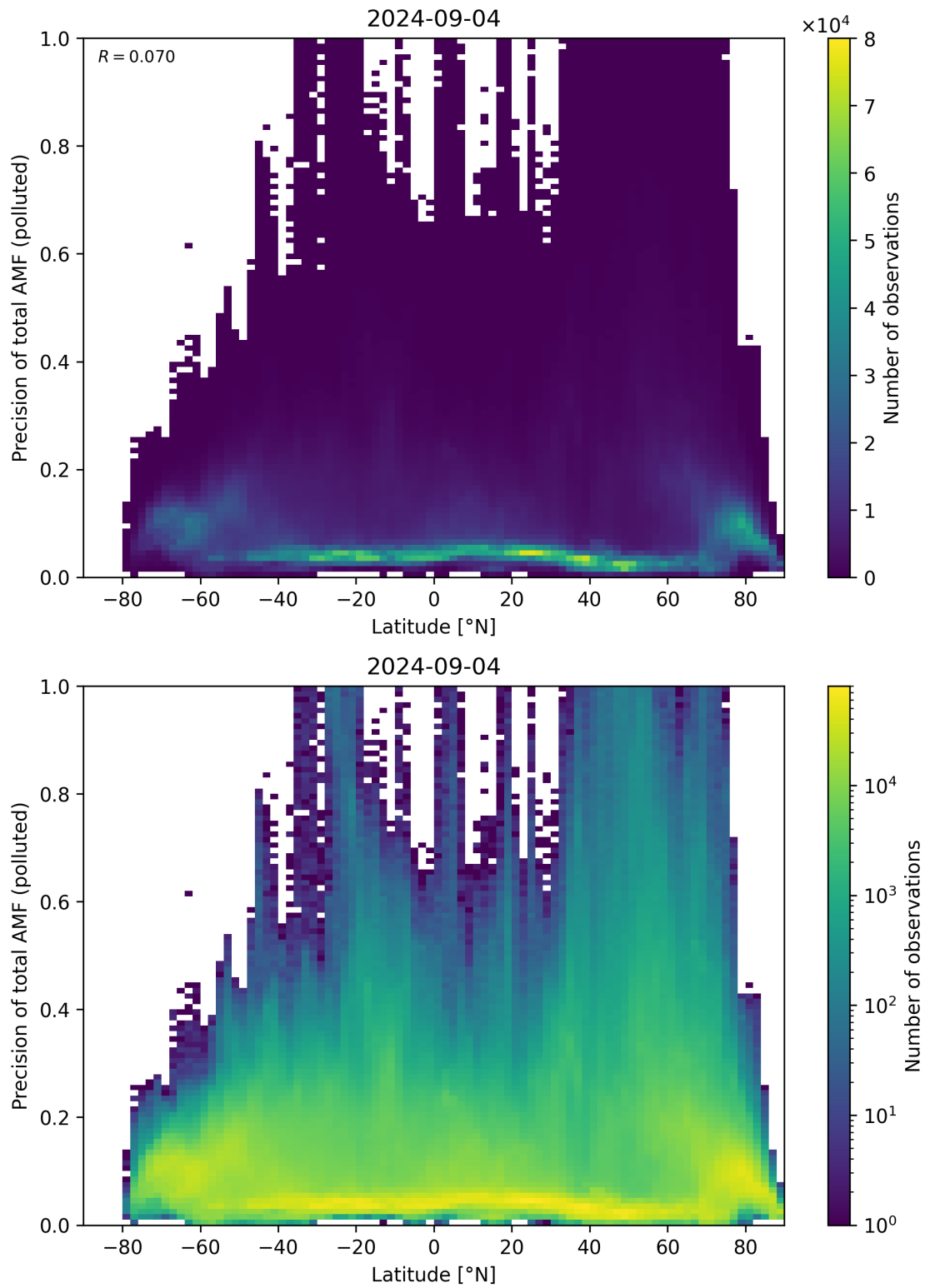
Figure 155: Scatter density plot of “Latitude” against “Precision of total AMF (polluted)” for 2024-09-03 to 2024-09-05.
