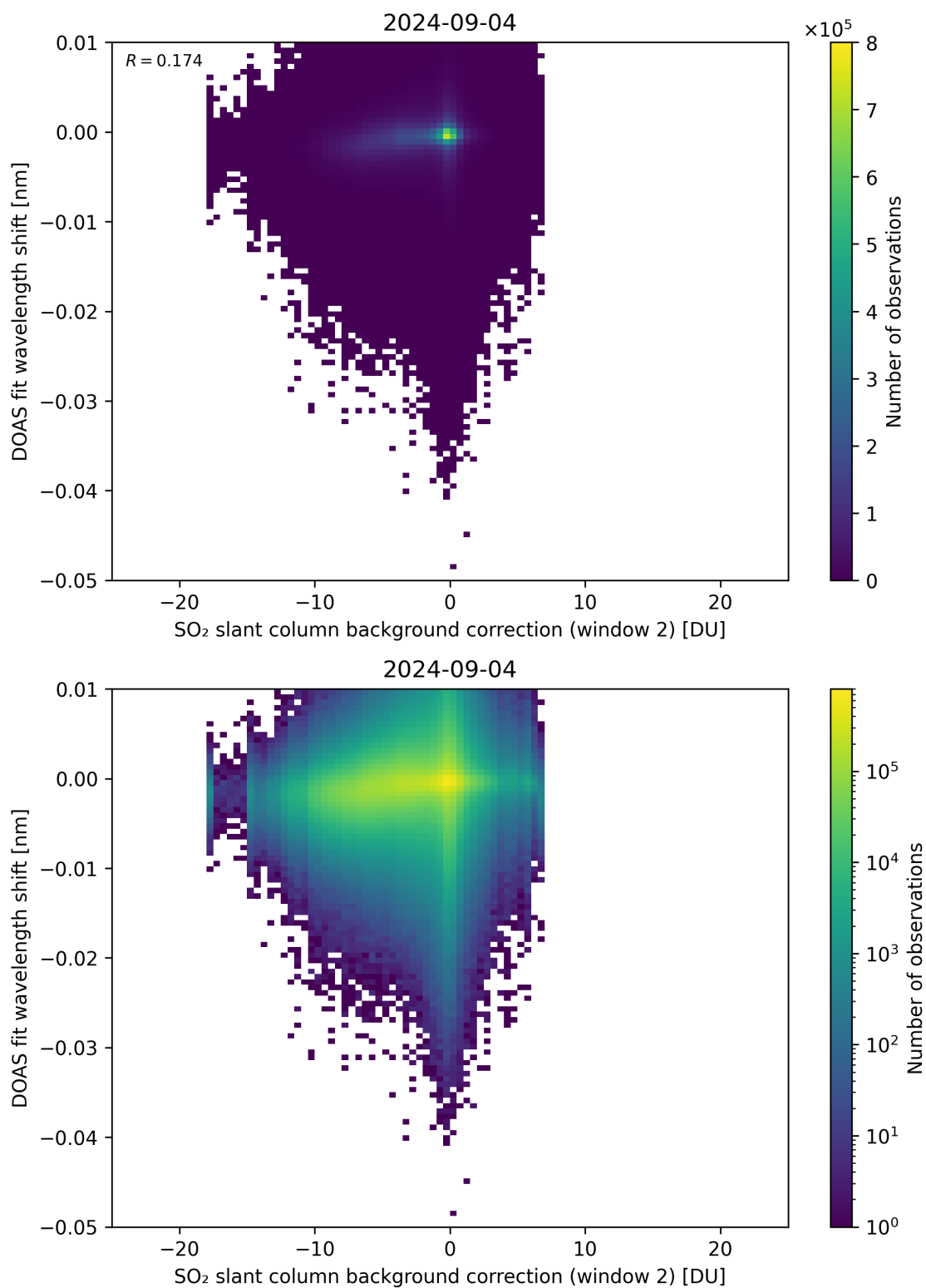
Figure 112: Scatter density plot of “SO 2 slant column background correction (window 2)” against “DOAS fit wavelength shift” for 2024-09-03 to 2024-09-05.
