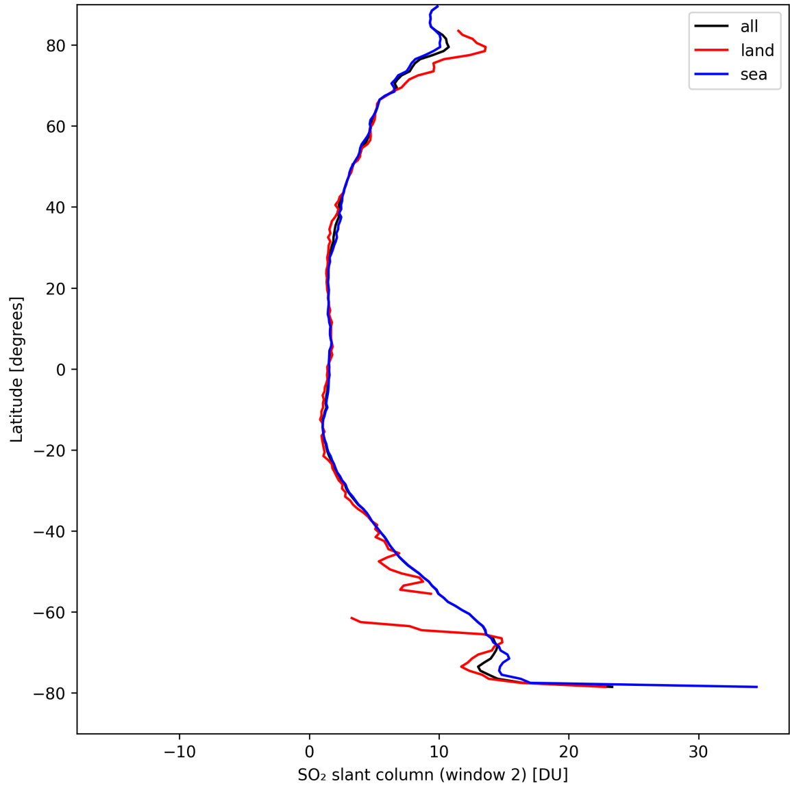
Figure 37: Zonal average of “SO 2 slant column (window 2)” for 2024-09-03 to 2024-09-05.
