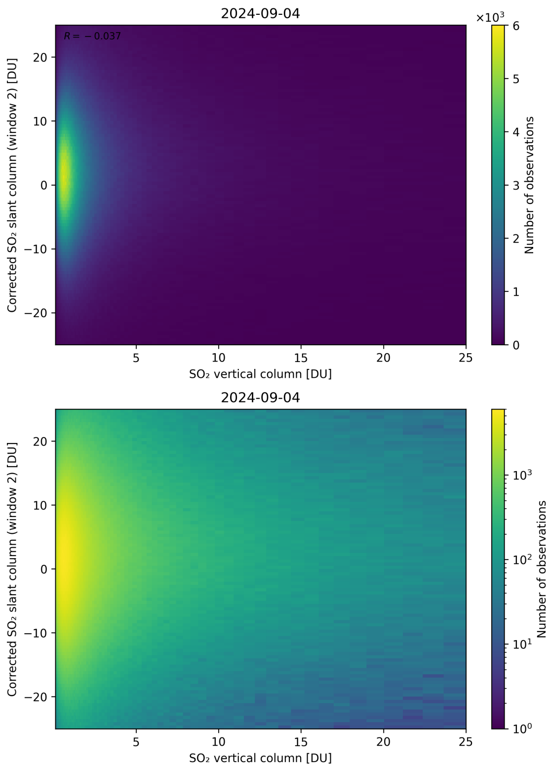
Figure 298: Scatter density plot of “SO 2 vertical column” against “Corrected SO 2 slant column (window 2)” for 2024-09-03 to 2024-09-05.
