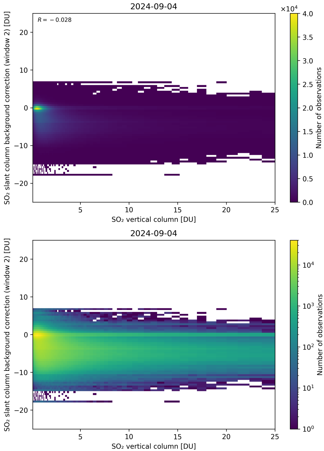
Figure 274: Scatter density plot of “SO 2 vertical column” against “SO 2 slant column background correction (window 2)” for 2024-09-03 to 2024-09-05.
