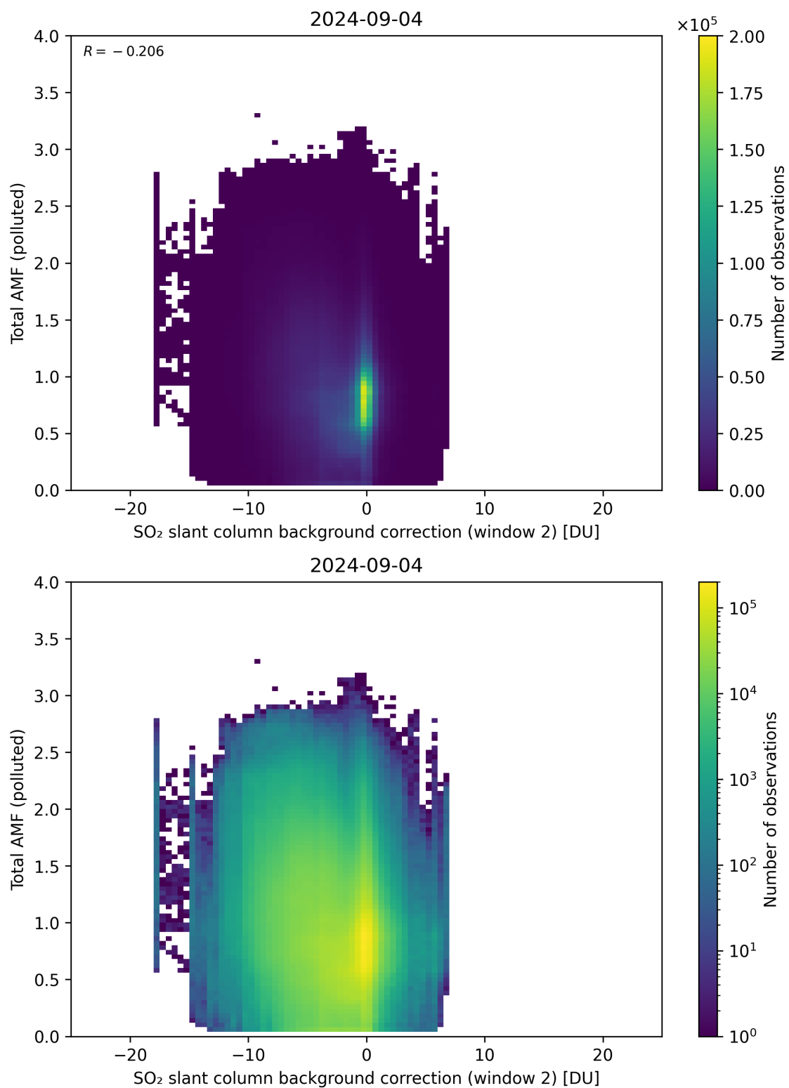
Figure 119: Scatter density plot of “SO 2 slant column background correction (window 2)” against “Total AMF (polluted)” for 2024-09-03 to 2024-09-05.
