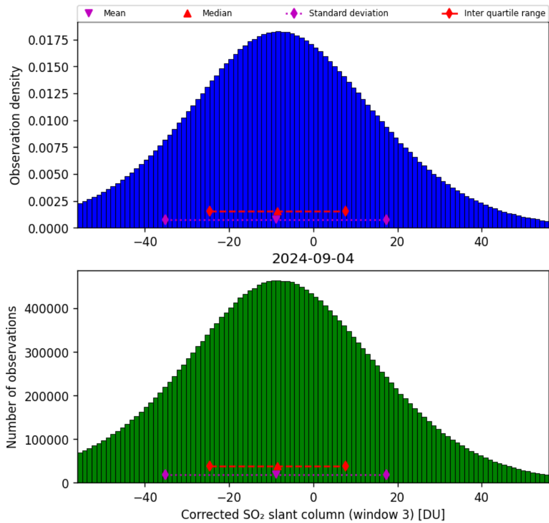
Figure 66: Histogram of “Corrected SO 2 slant column (window 3)” for 2024-09-03 to 2024-09-05
