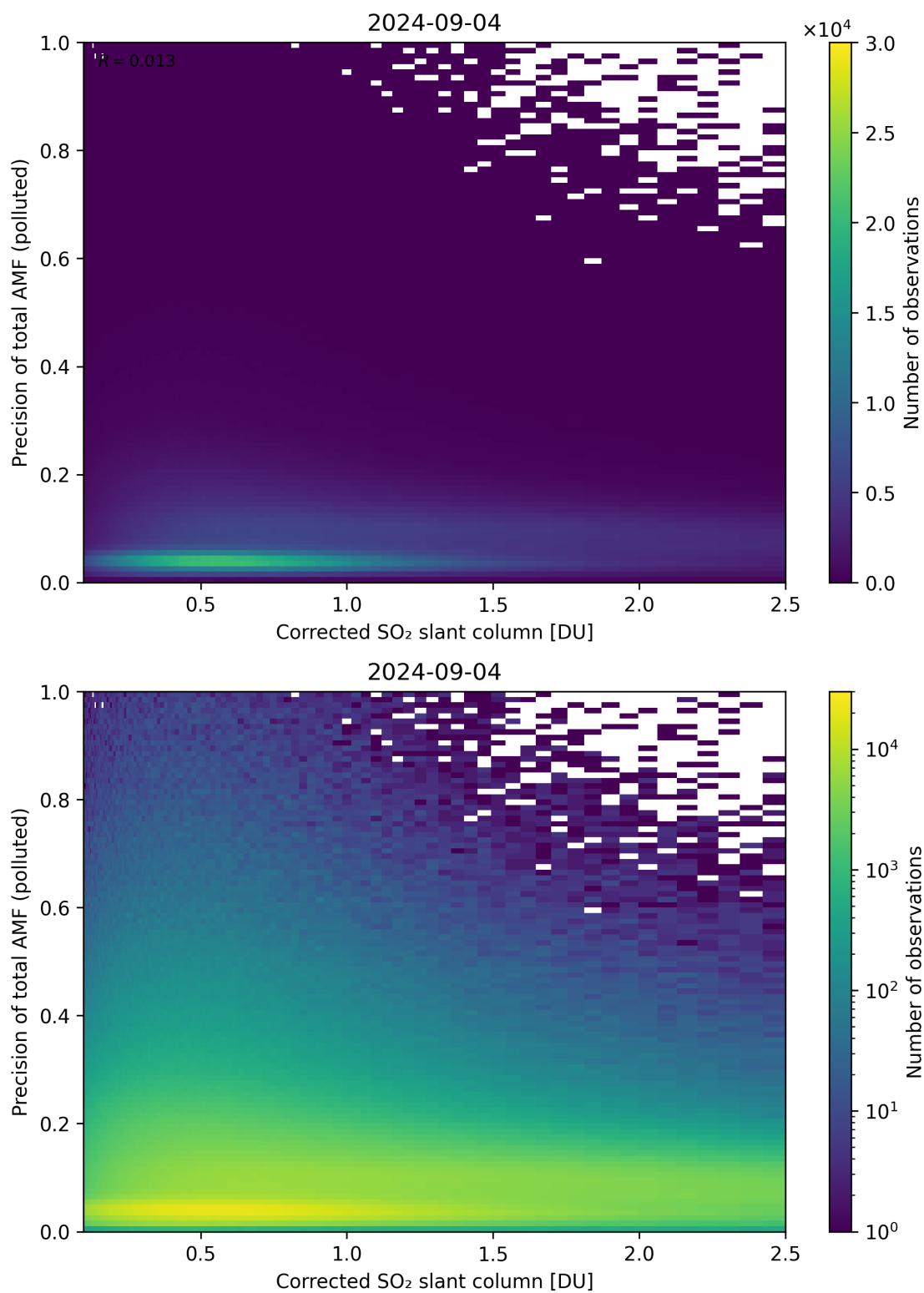
Figure 193: Scatter density plot of “Corrected SO 2 slant column” against “Precision of total AMF (polluted)” for 2024-09-03 to 2024-09-05.
