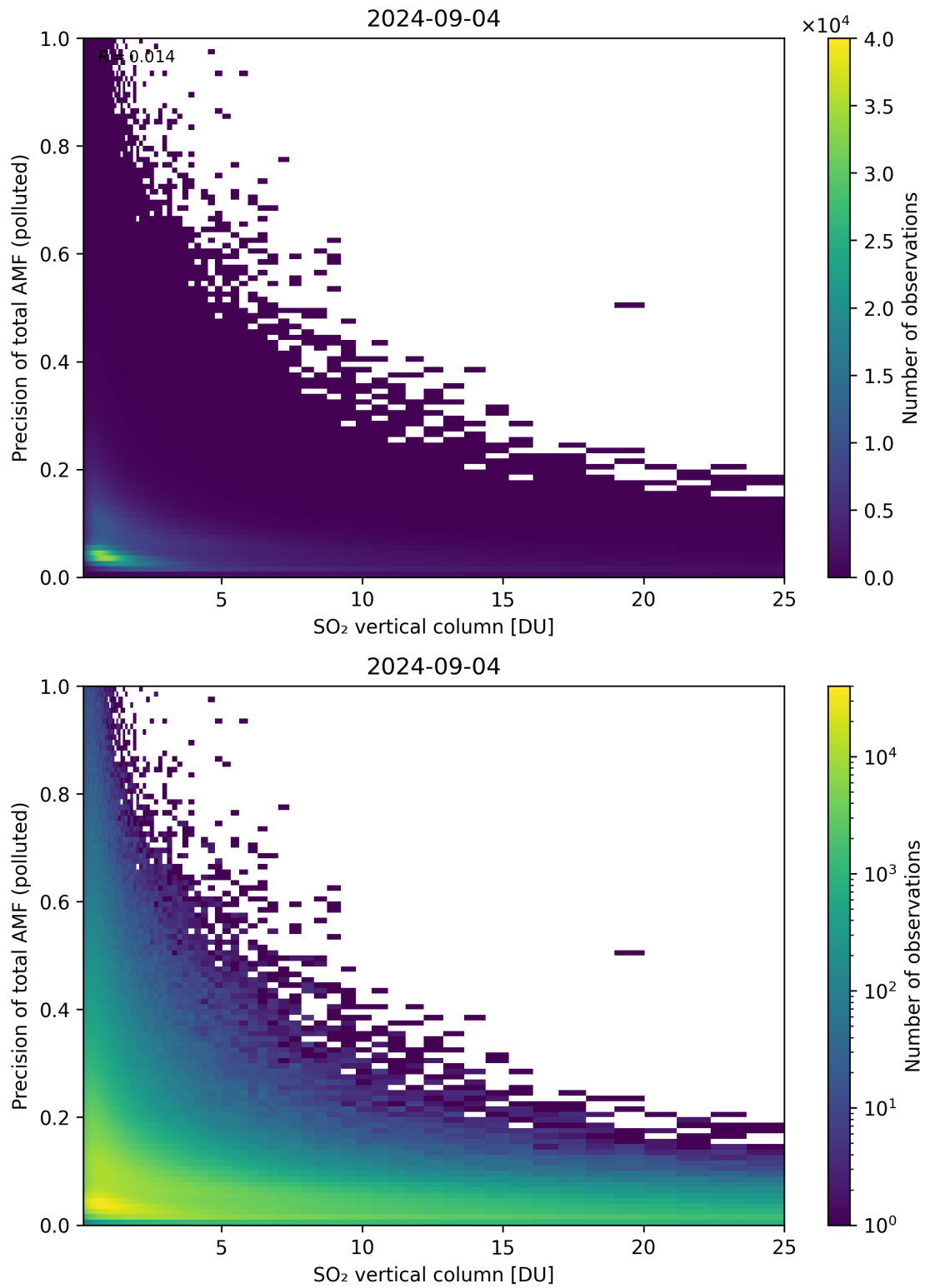
Figure 306: Scatter density plot of “SO 2 vertical column” against “Precision of total AMF (polluted)” for 2024-09-03 to 2024-09-05.
