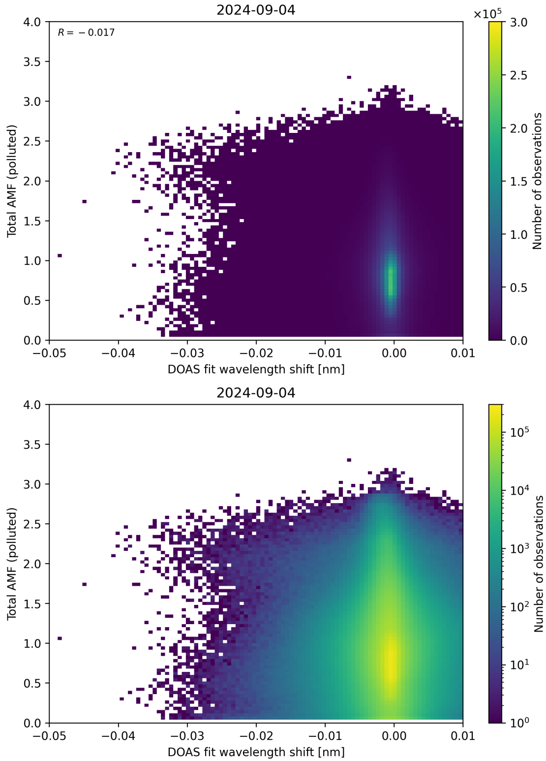
Figure 130: Scatter density plot of “DOAS fit wavelength shift” against “Total AMF (polluted)” for 2024-09-03 to 2024-09-05.
