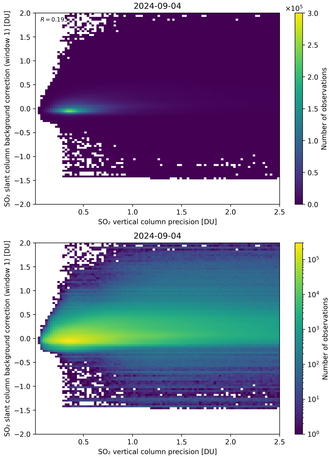
Figure 279: Scatter density plot of “SO 2 vertical column precision” against “SO 2 slant column background correction (window 1)” for 2024-09-03 to 2024-09-05.
