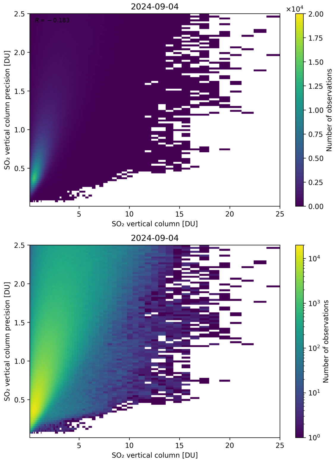
Figure 307: Scatter density plot of “SO 2 vertical column” against “SO 2 vertical column precision” for 2024-09-03 to 2024-09-05.
