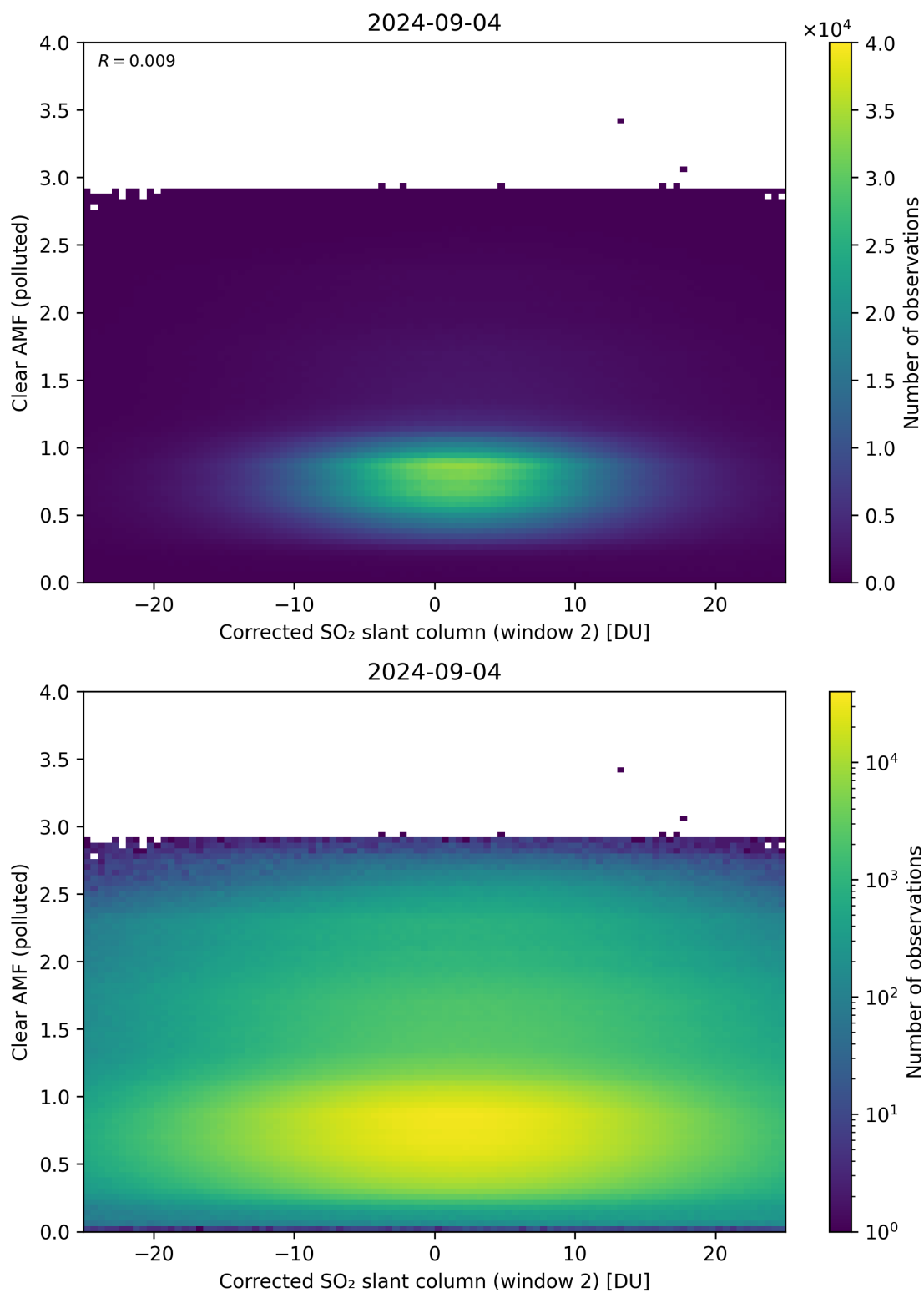
Figure 199: Scatter density plot of “Corrected SO 2 slant column (window 2)” against “Clear AMF (polluted)” for 2024-09-03 to 2024-09-05.
