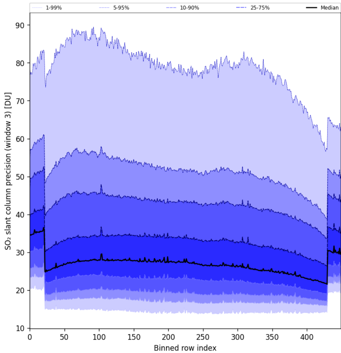
Figure 88: Along track statistics of “SO 2 slant column precision (window 3)” for 2024-09-03 to 2024-09-05
