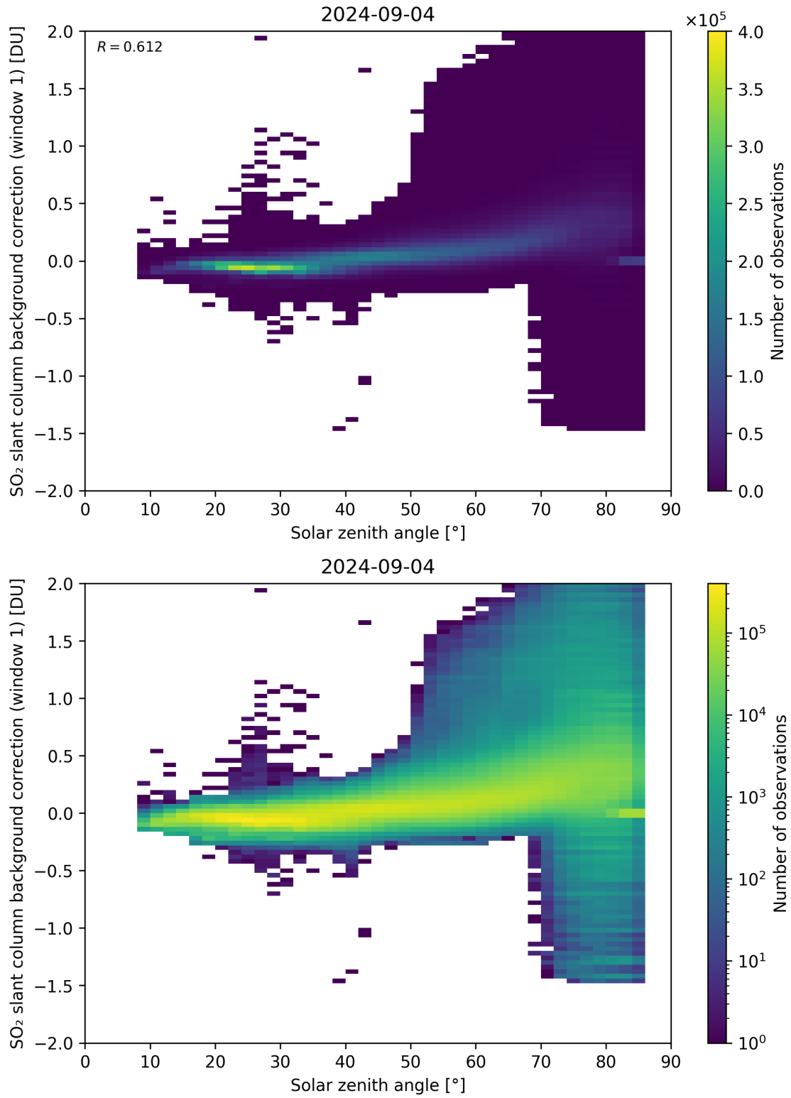
Figure 158: Scatter density plot of “Solar zenith angle” against “SO 2 slant column background correction (window 1)” for 2024-09-03 to 2024-09-05.
