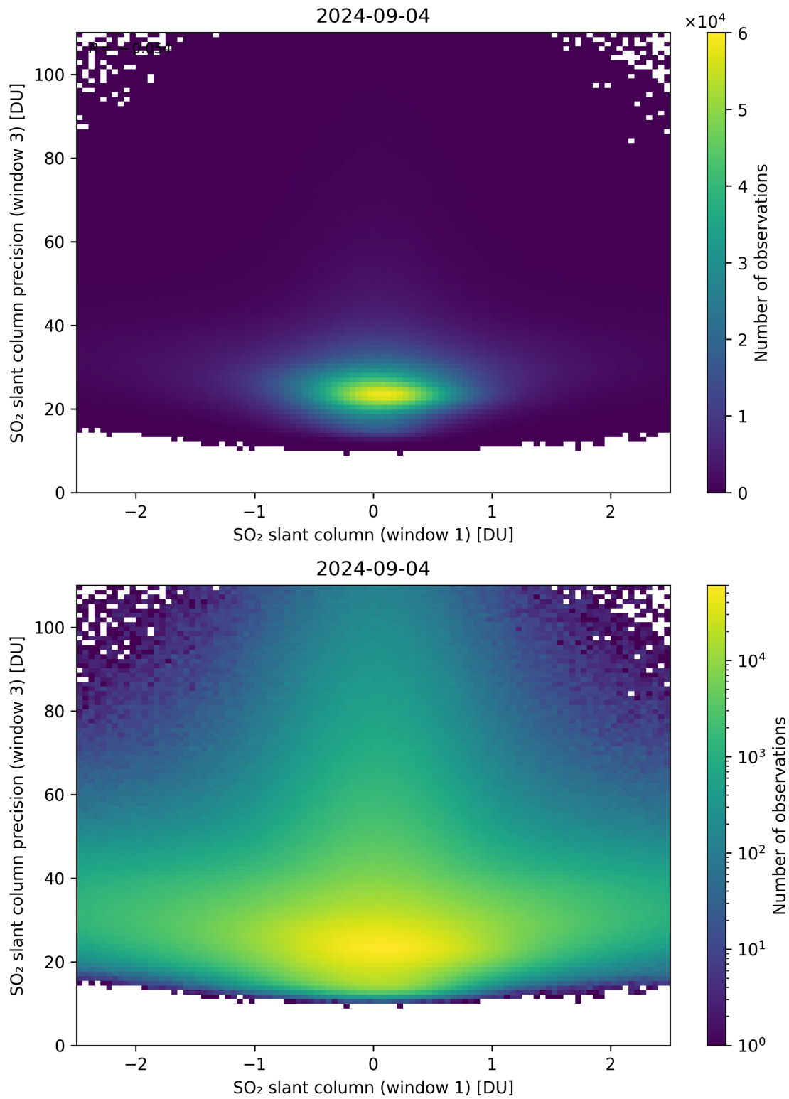
Figure 238: Scatter density plot of “SO 2 slant column (window 1)” against “SO 2 slant column precision (window 3)” for 2024-09-03 to 2024-09-05.
