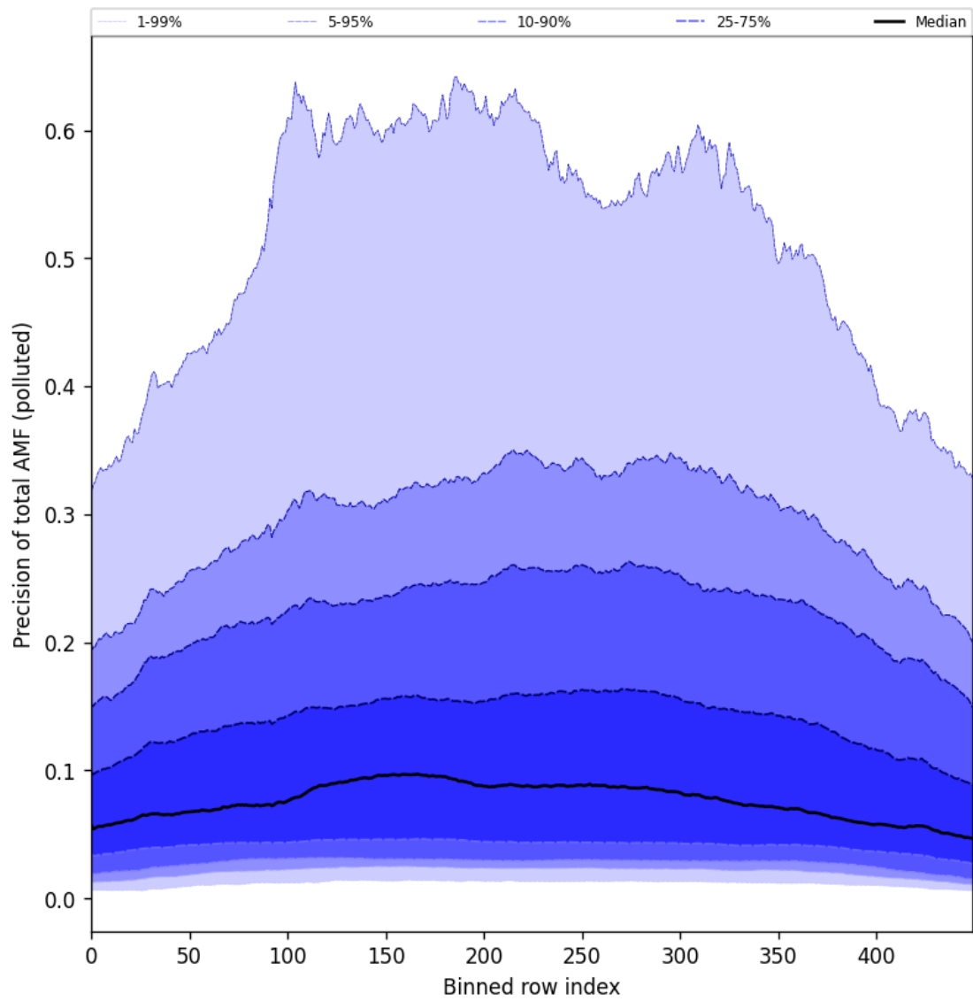
Figure 95: Along track statistics of “Precision of total AMF (polluted)” for 2024-09-03 to 2024-09-05
