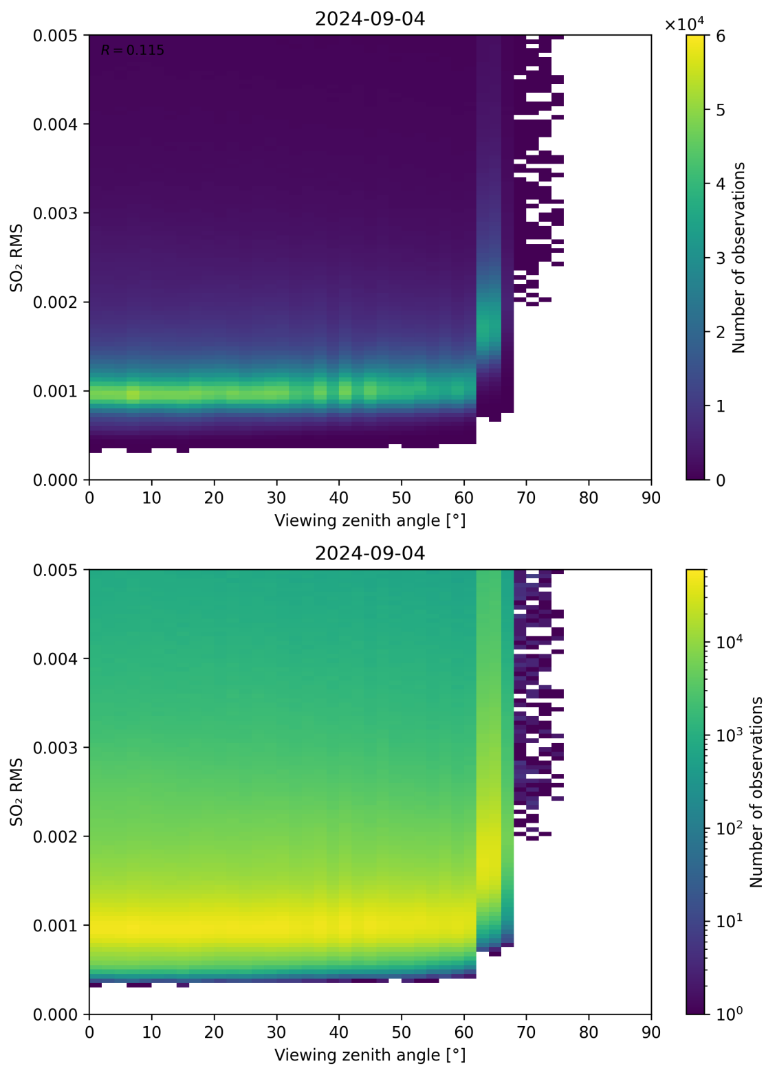
Figure 313: Scatter density plot of “Viewing zenith angle” against “SO 2 RMS” for 2024-09-03 to 2024-09-05.
