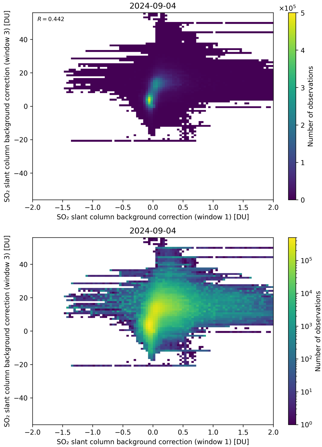
Figure 99: Scatter density plot of “SO 2 slant column background correction (window 1)” against “SO 2 slant column background correction (window 3)” for 2024-09-03 to 2024-09-05.
