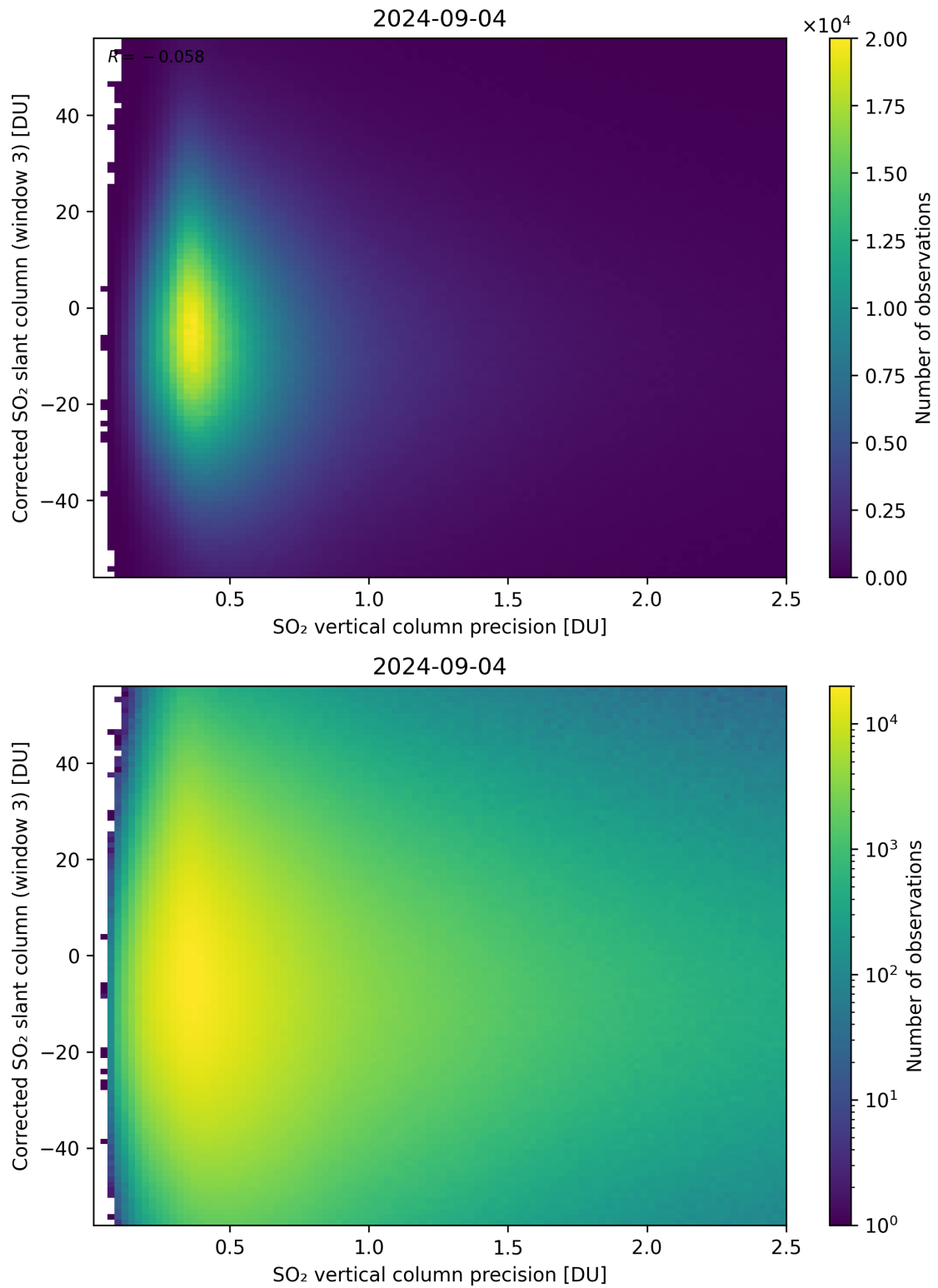
Figure 288: Scatter density plot of “SO 2 vertical column precision” against “Corrected SO 2 slant column (window 3)” for 2024-09-03 to 2024-09-05.
