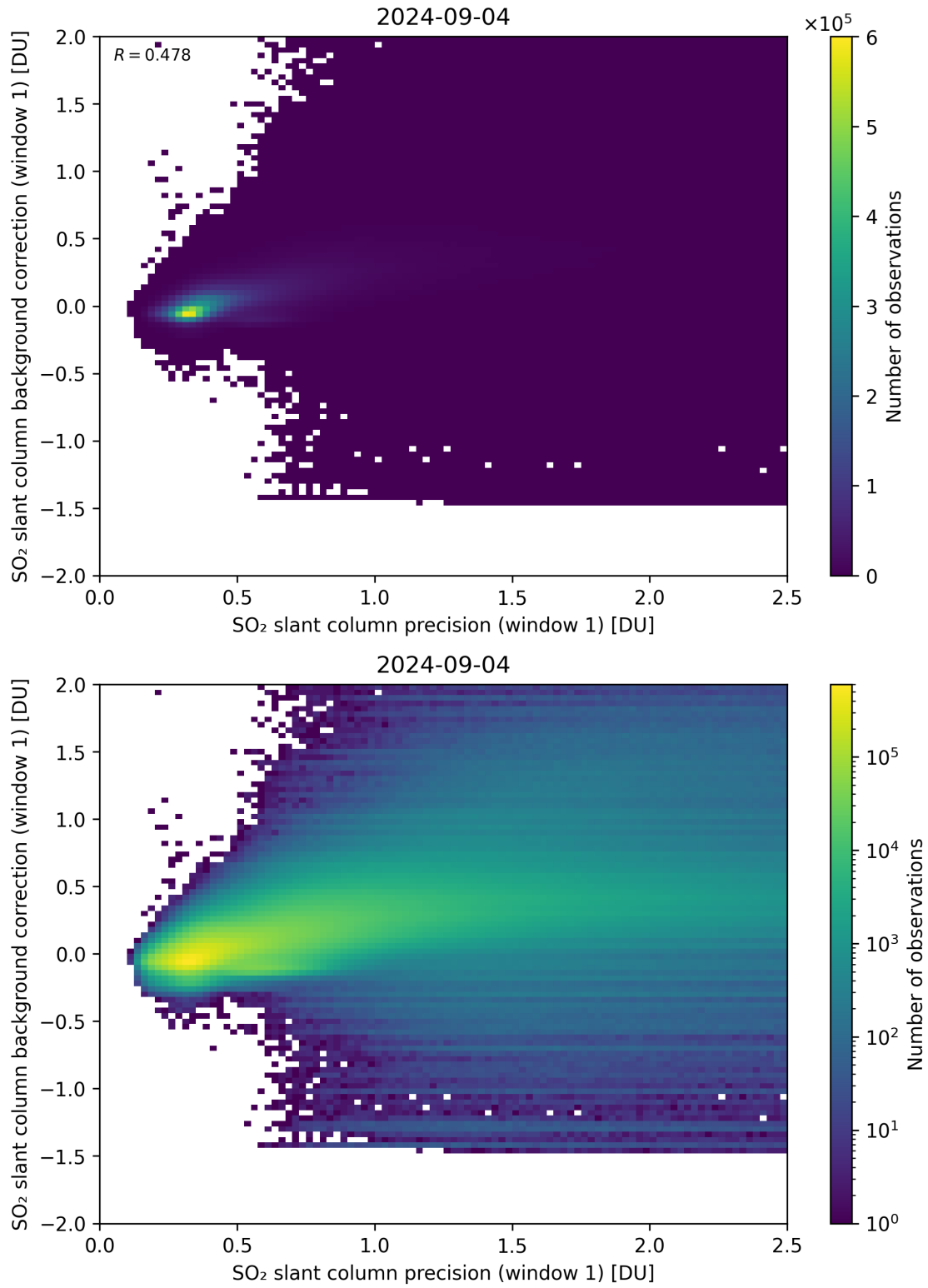
Figure 218: Scatter density plot of “SO 2 slant column precision (window 1)” against “SO 2 slant column background correction (window 1)” for 2024-09-03 to 2024-09-05.
