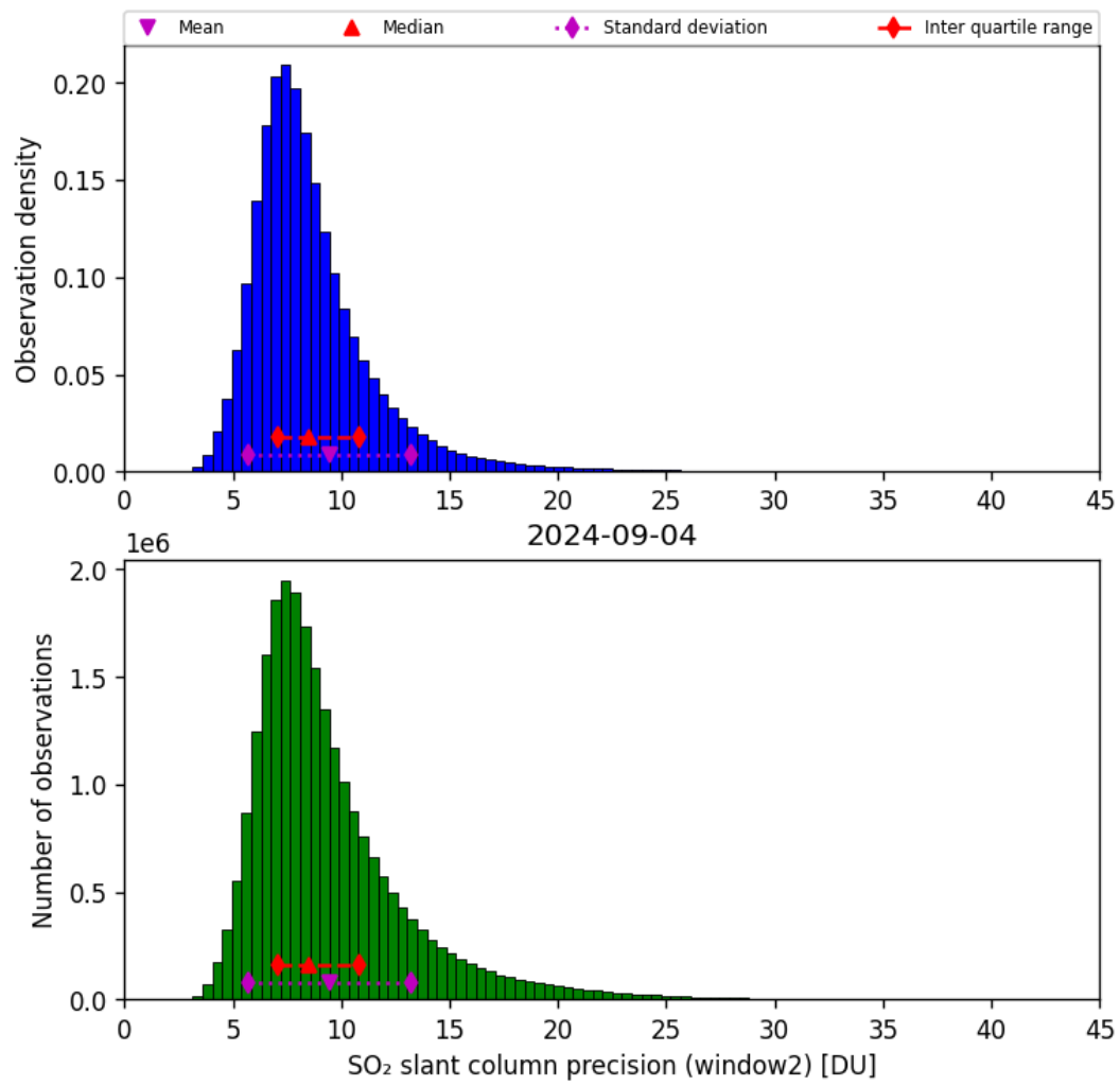
Figure 61: Histogram of “SO 2 slant column precision (window2)” for 2024-09-03 to 2024-09-05
