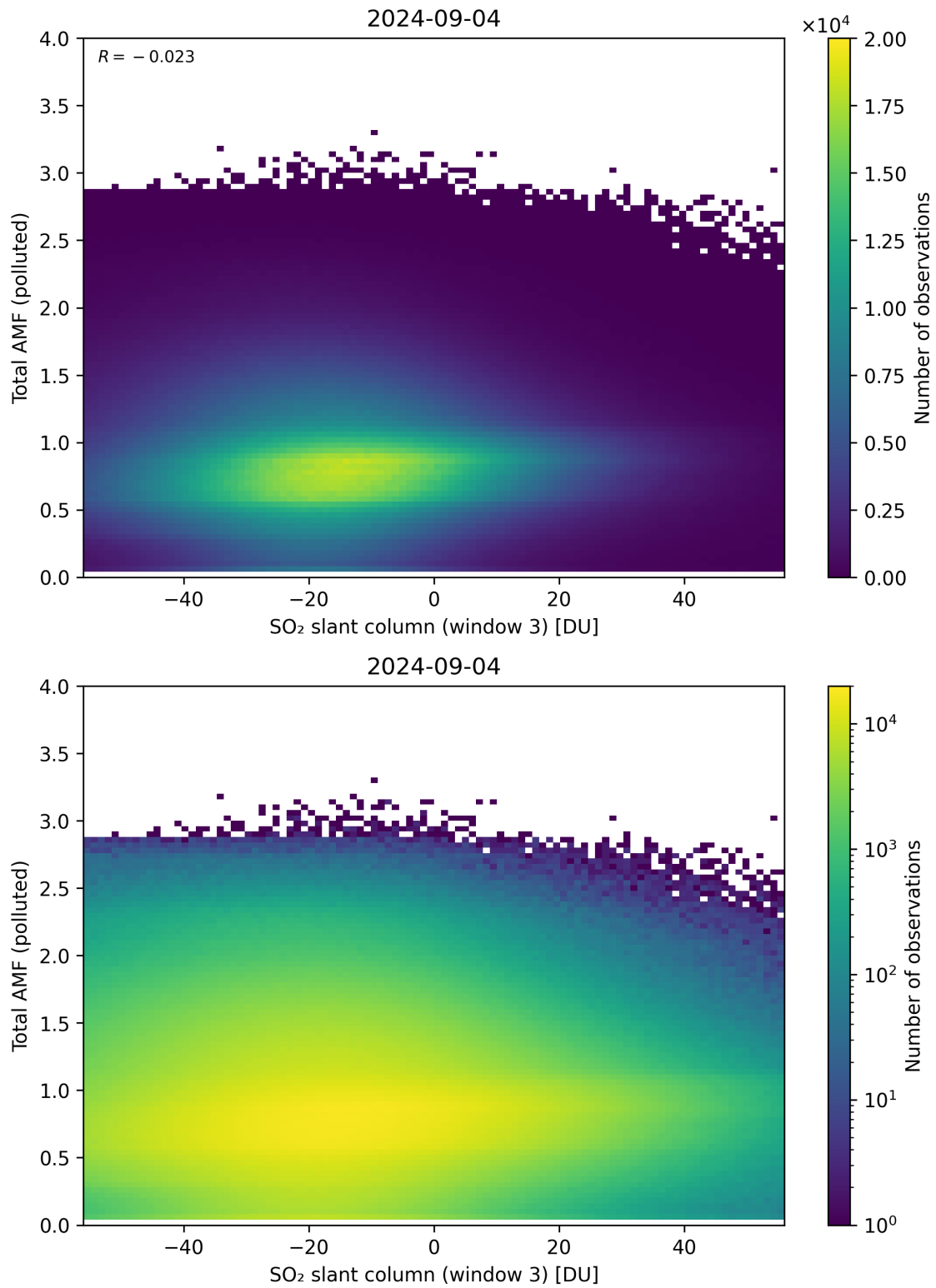
Figure 268: Scatter density plot of “SO 2 slant column (window 3)” against “Total AMF (polluted)” for 2024-09-03 to 2024-09-05.
