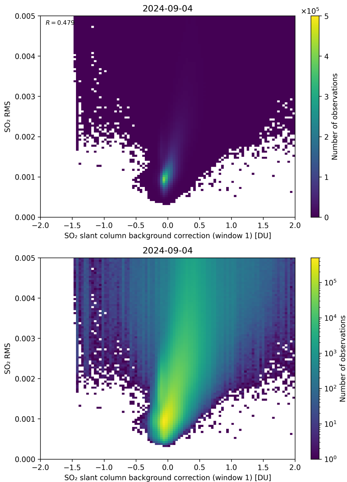
Figure 102: Scatter density plot of “SO 2 slant column background correction (window 1)” against “SO 2 RMS” for 2024-09-03 to 2024-09-05.
