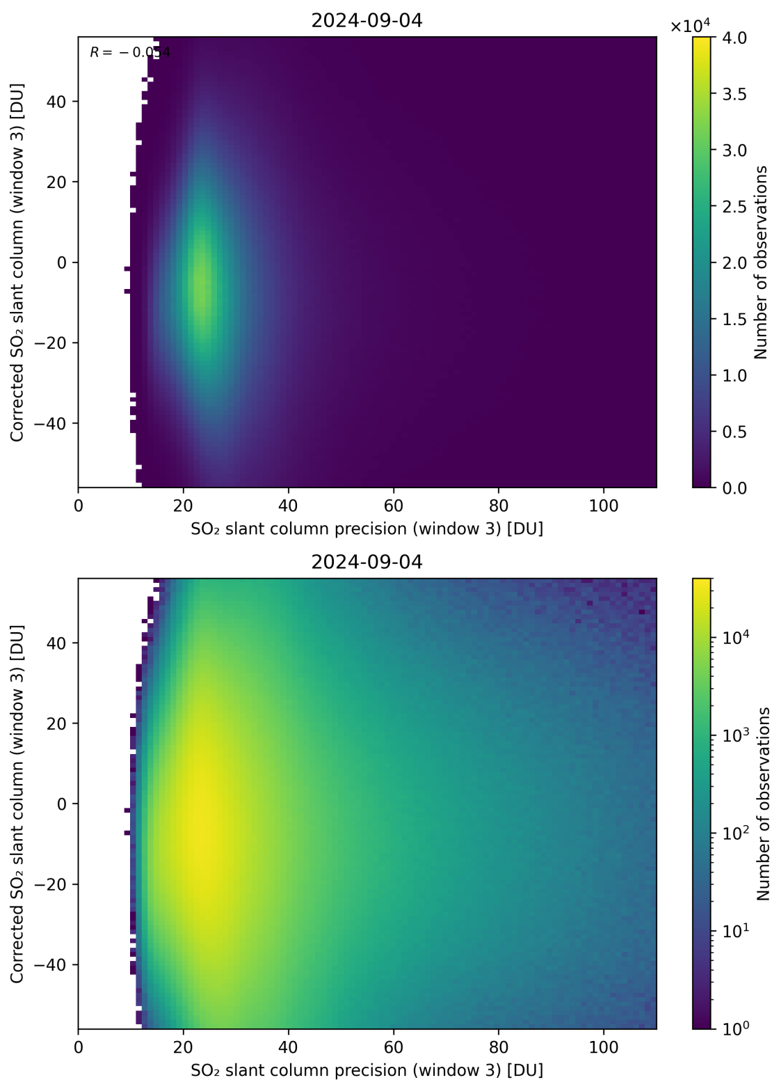
Figure 262: Scatter density plot of “SO 2 slant column precision (window 3)” against “Corrected SO 2 slant column (window 3)” for 2024-09-03 to 2024-09-05.
