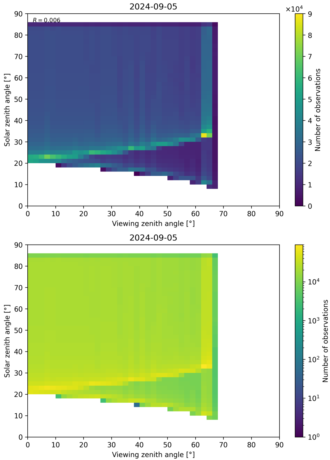
Figure 315: Scatter density plot of “Viewing zenith angle” against “Solar zenith angle” for 2024-09-04 to 2024-09-06.
