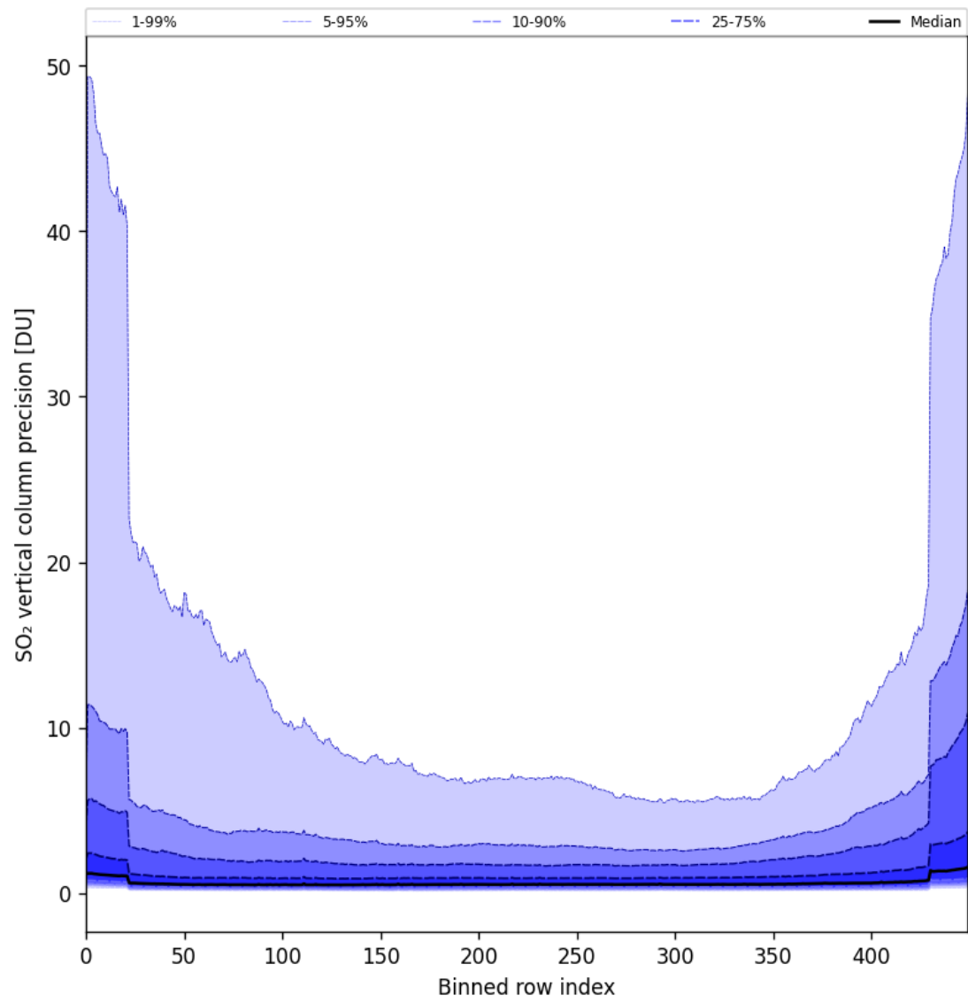
Figure 77: Along track statistics of “SO 2 vertical column precision” for 2024-09-04 to 2024-09-06
