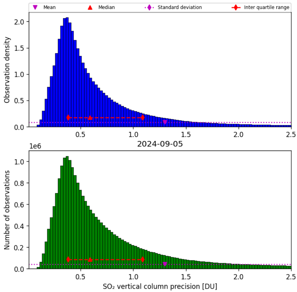
Figure 54: Histogram of “SO 2 vertical column precision” for 2024-09-04 to 2024-09-06
