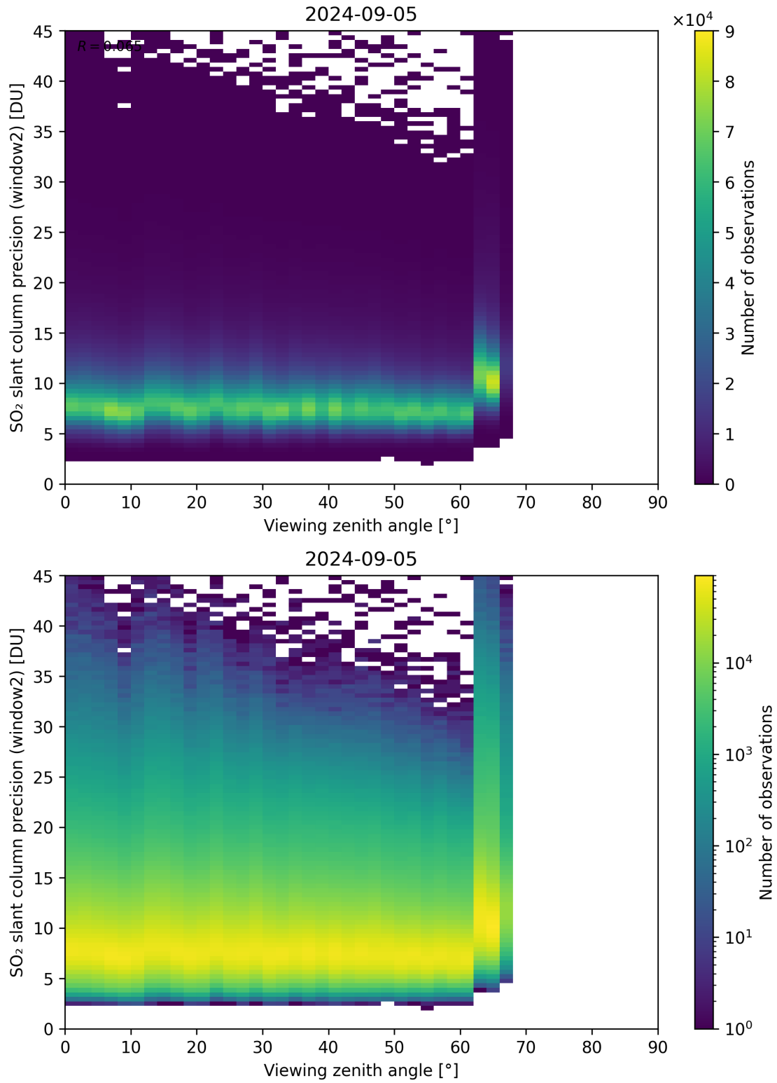
Figure 322: Scatter density plot of “Viewing zenith angle” against “SO 2 slant column precision (window2)” for 2024-09-04 to 2024-09-06.
