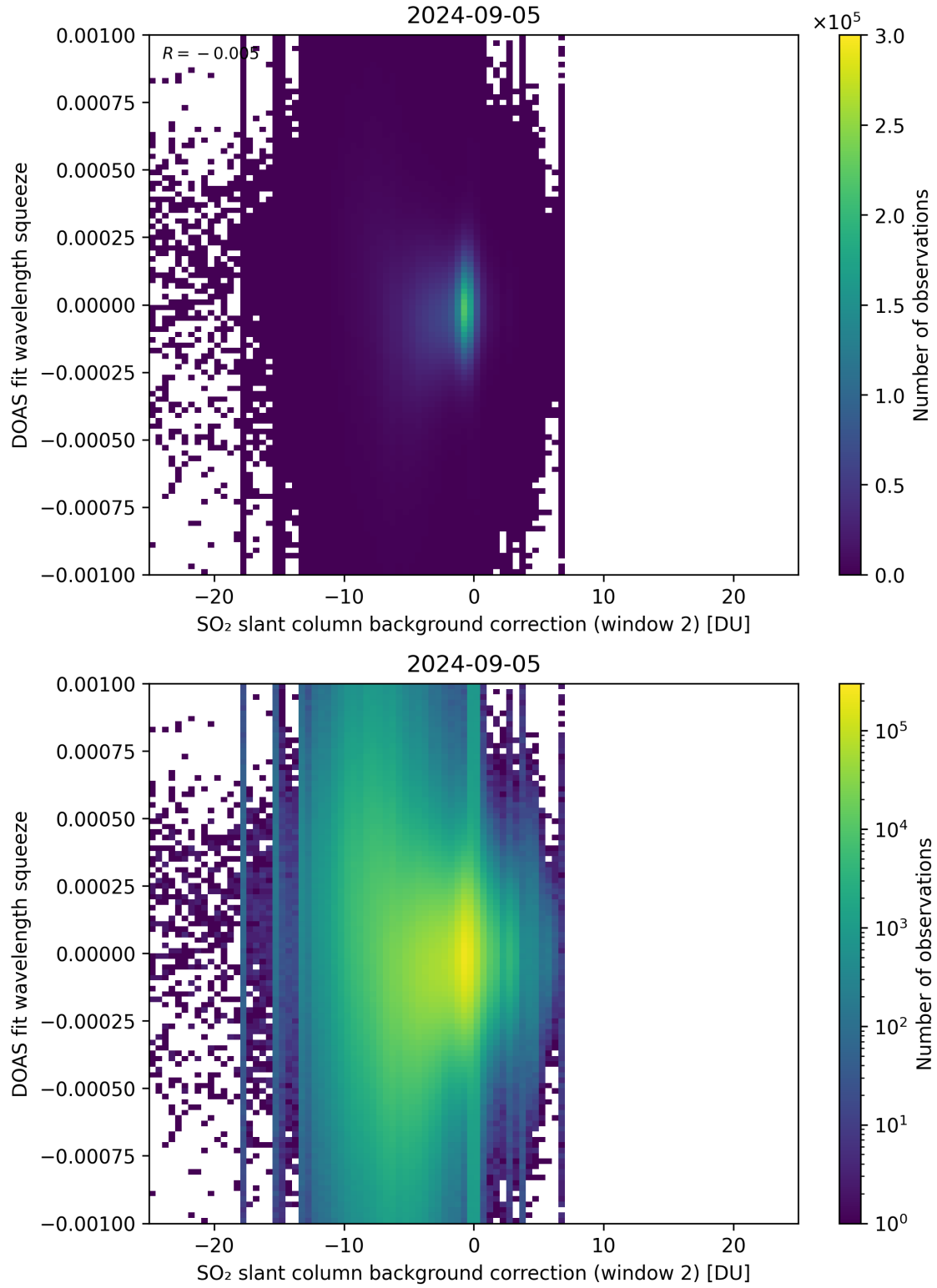
Figure 113: Scatter density plot of “SO 2 slant column background correction (window 2)” against “DOAS fit wavelength squeeze” for 2024-09-04 to 2024-09-06.
