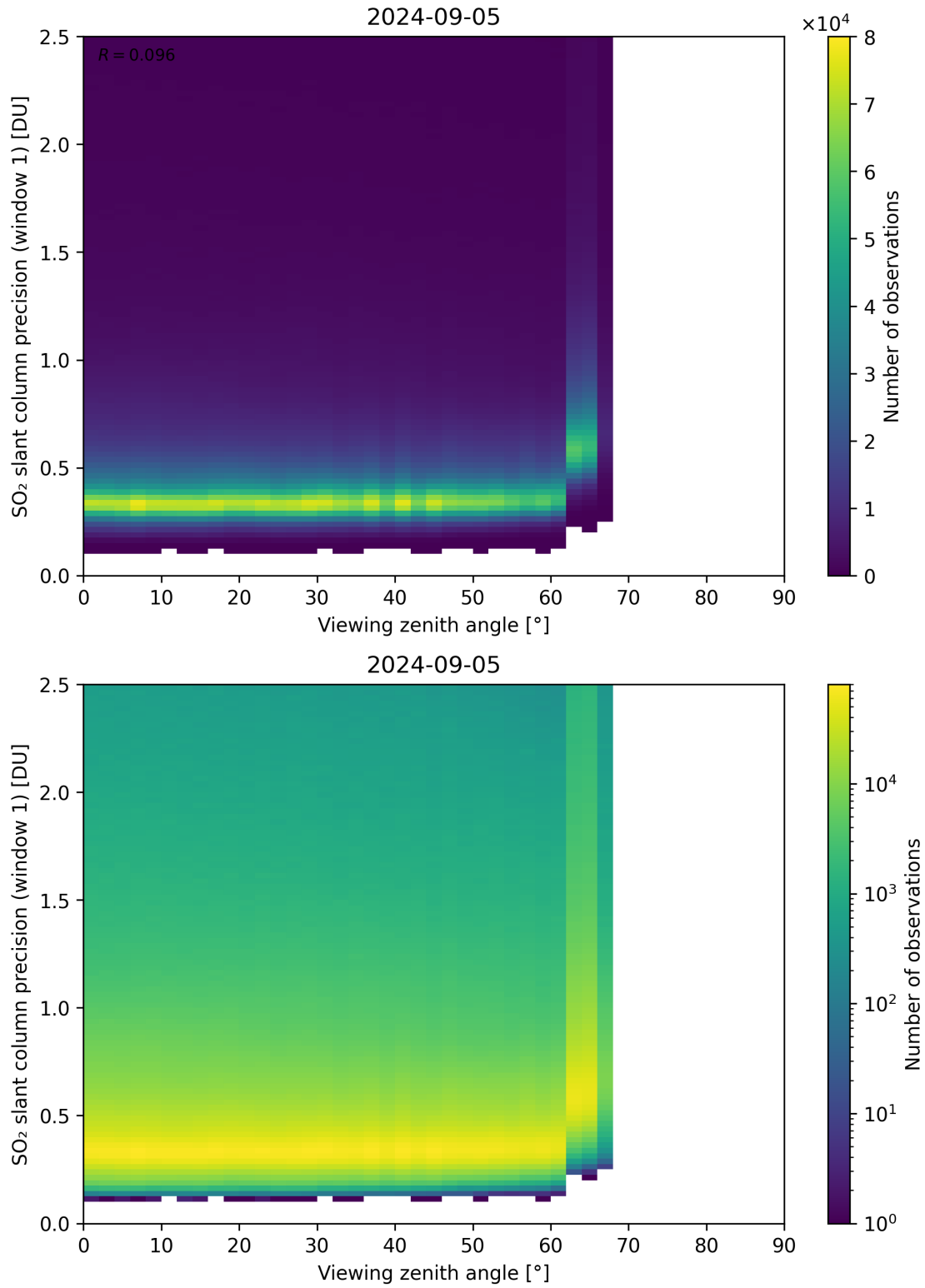
Figure 321: Scatter density plot of “Viewing zenith angle” against “SO 2 slant column precision (window 1)” for 2024-09-04 to 2024-09-06.
