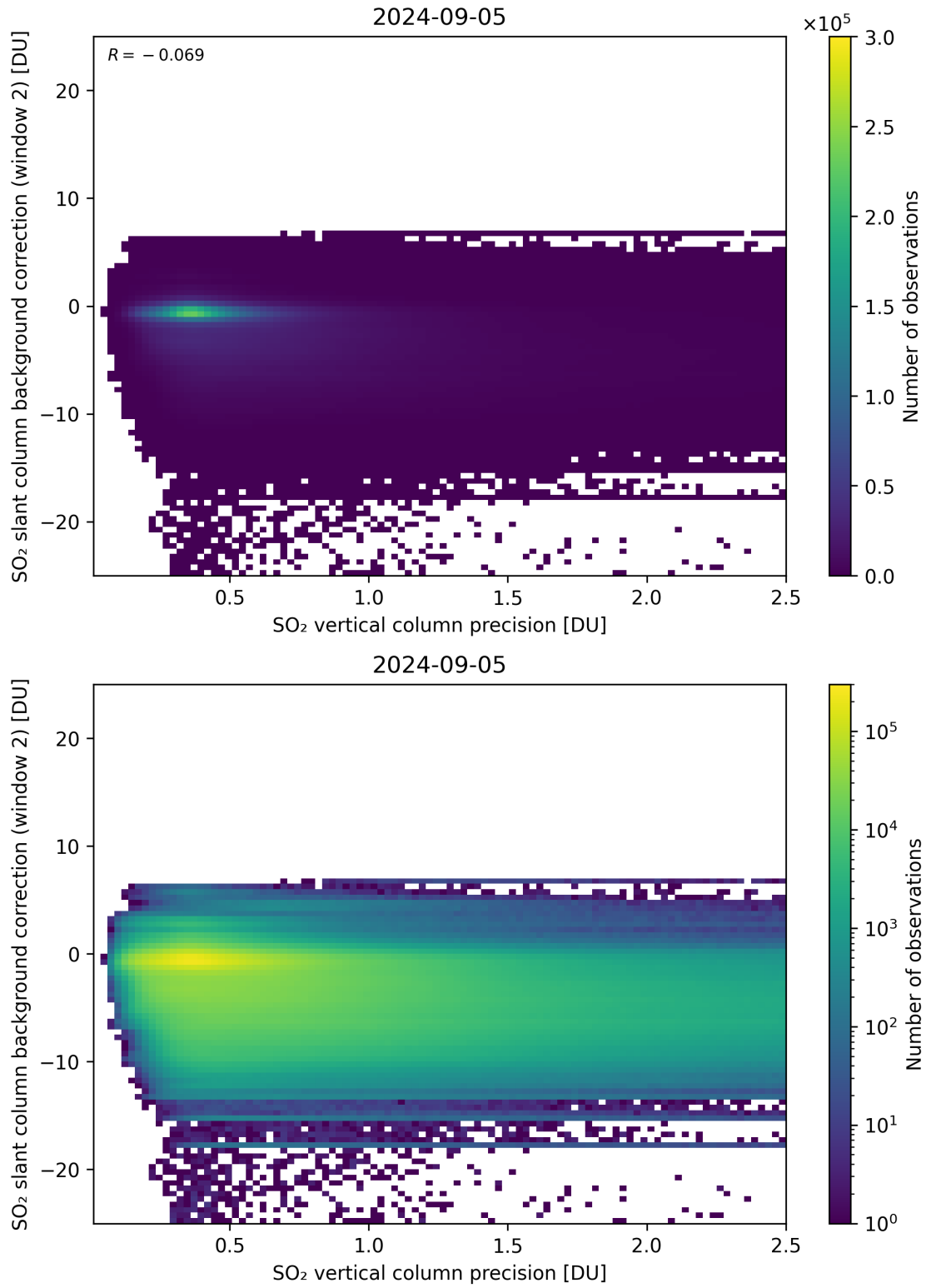
Figure 280: Scatter density plot of “SO 2 vertical column precision” against “SO 2 slant column background correction (window 2)” for 2024-09-04 to 2024-09-06.
