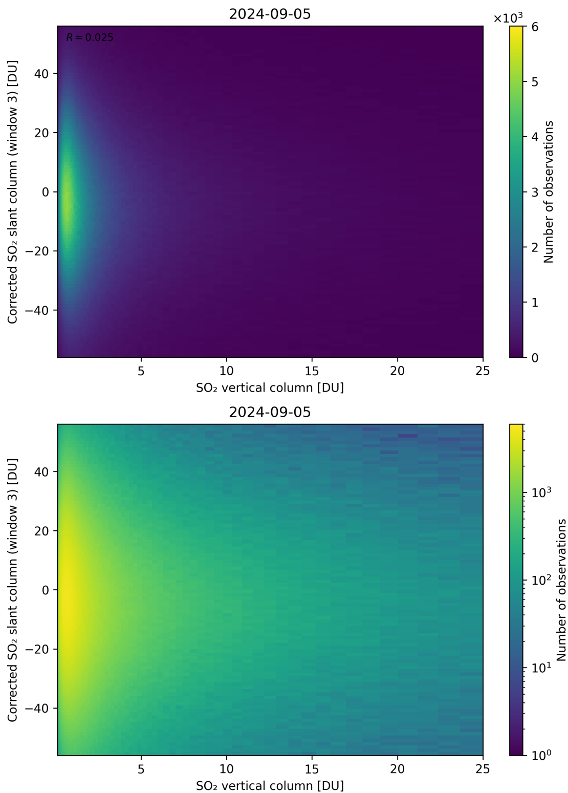
Figure 299: Scatter density plot of “SO 2 vertical column” against “Corrected SO 2 slant column (window 3)” for 2024-09-04 to 2024-09-06.
