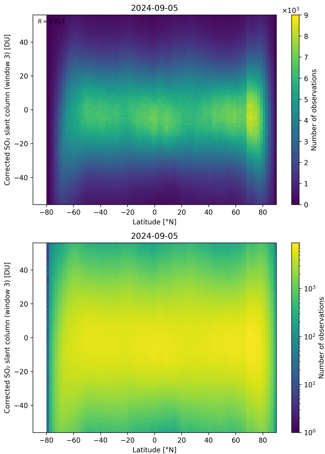
Figure 148: Scatter density plot of “Latitude” against “Corrected SO 2 slant column (window 3)” for 2024-09-04 to 2024-09-06.
