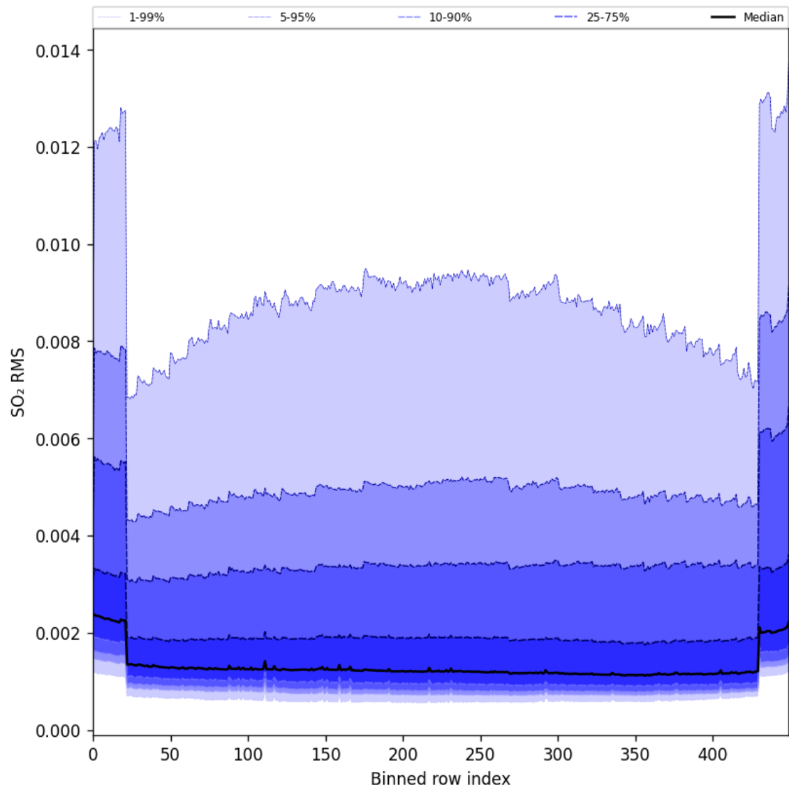
Figure 93: Along track statistics of “SO 2 RMS” for 2024-09-04 to 2024-09-06
