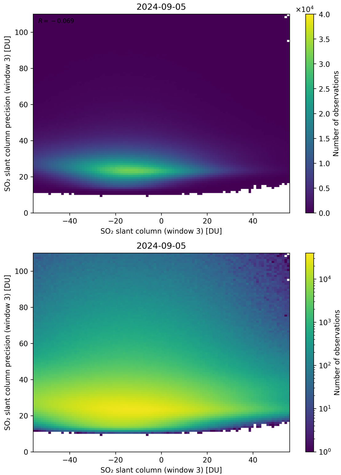
Figure 267: Scatter density plot of “SO 2 slant column (window 3)” against “SO 2 slant column precision (window 3)” for 2024-09-04 to 2024-09-06.
