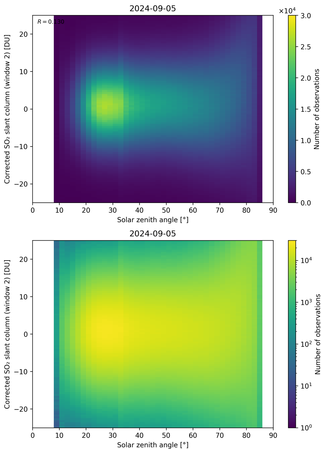
Figure 167: Scatter density plot of “Solar zenith angle” against “Corrected SO 2 slant column (window 2)” for 2024-09-04 to 2024-09-06.
