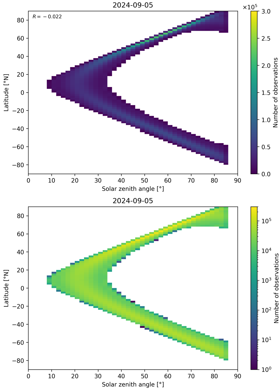
Figure 164: Scatter density plot of “Solar zenith angle” against “Latitude” for 2024-09-04 to 2024-09-06.
