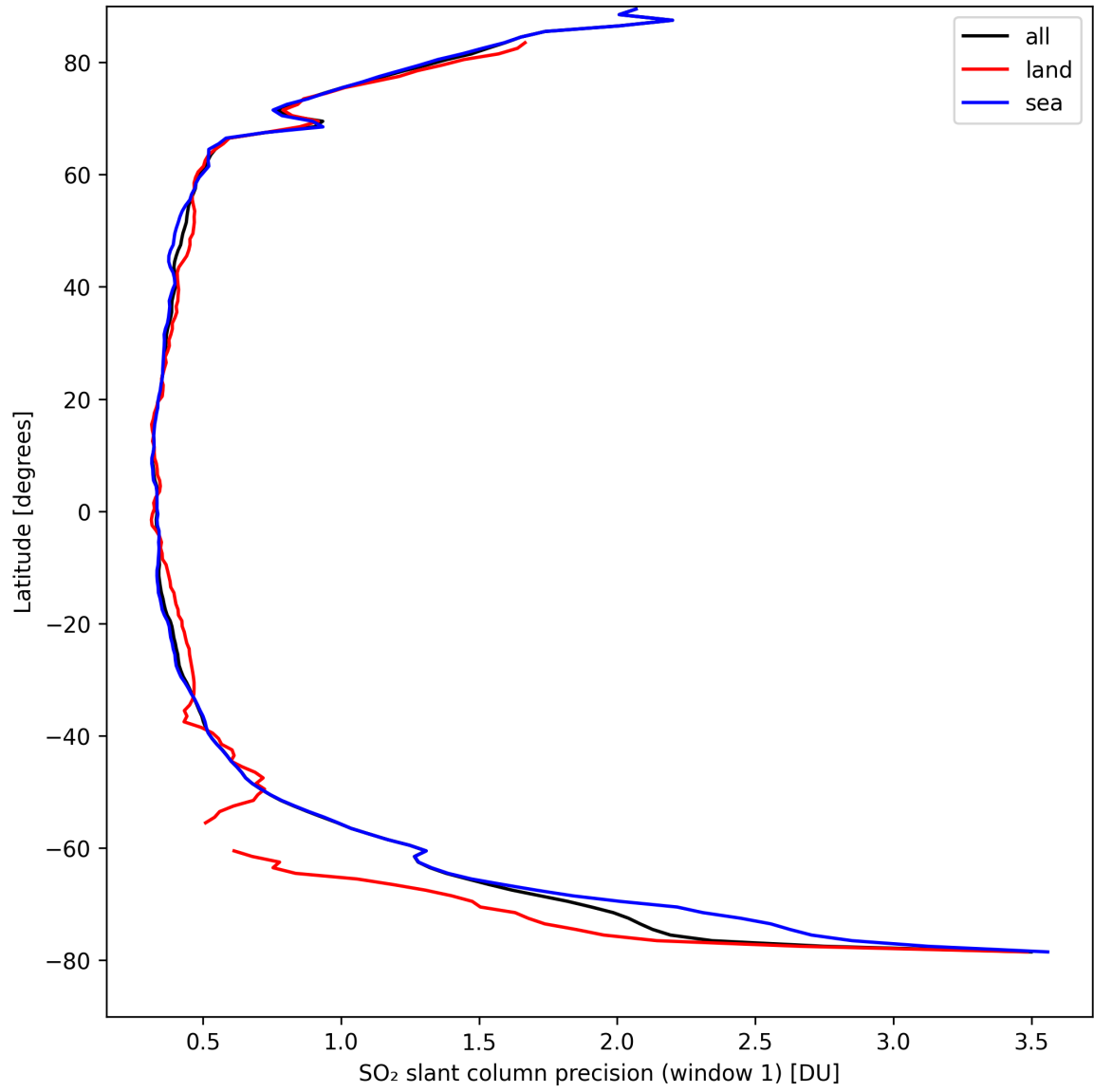
Figure 34: Zonal average of “SO 2 slant column precision (window 1)” for 2024-09-04 to 2024-09-06.
