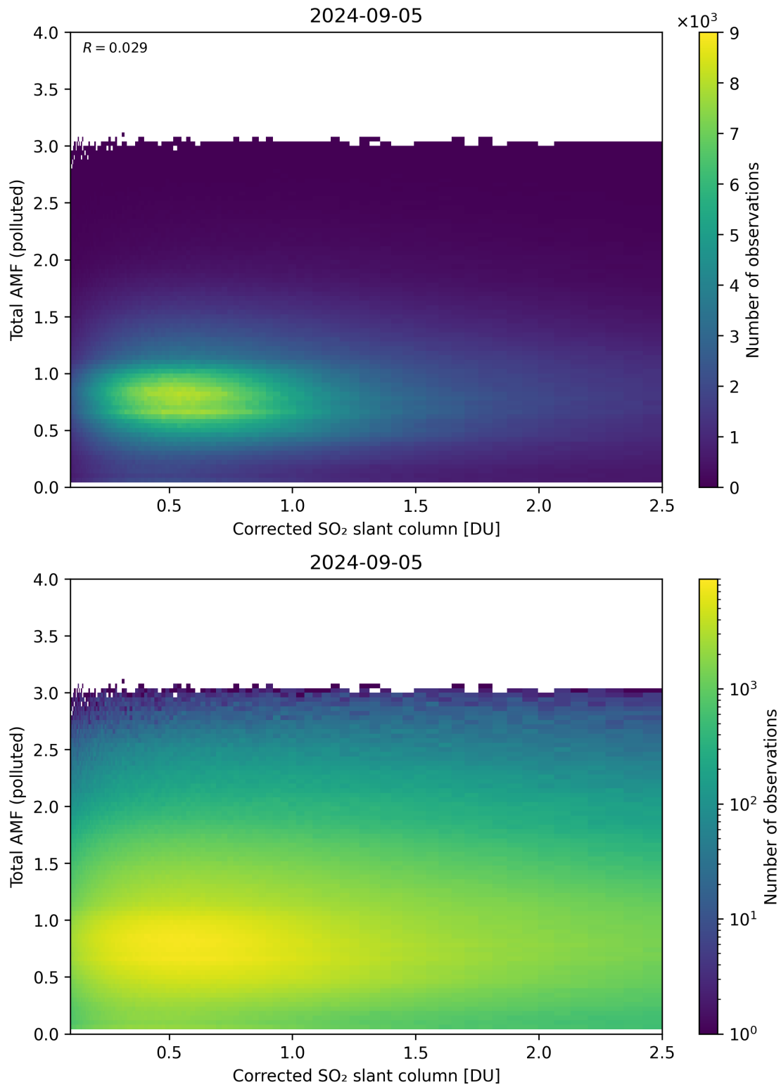
Figure 192: Scatter density plot of “Corrected SO 2 slant column” against “Total AMF (polluted)” for 2024-09-04 to 2024-09-06.
