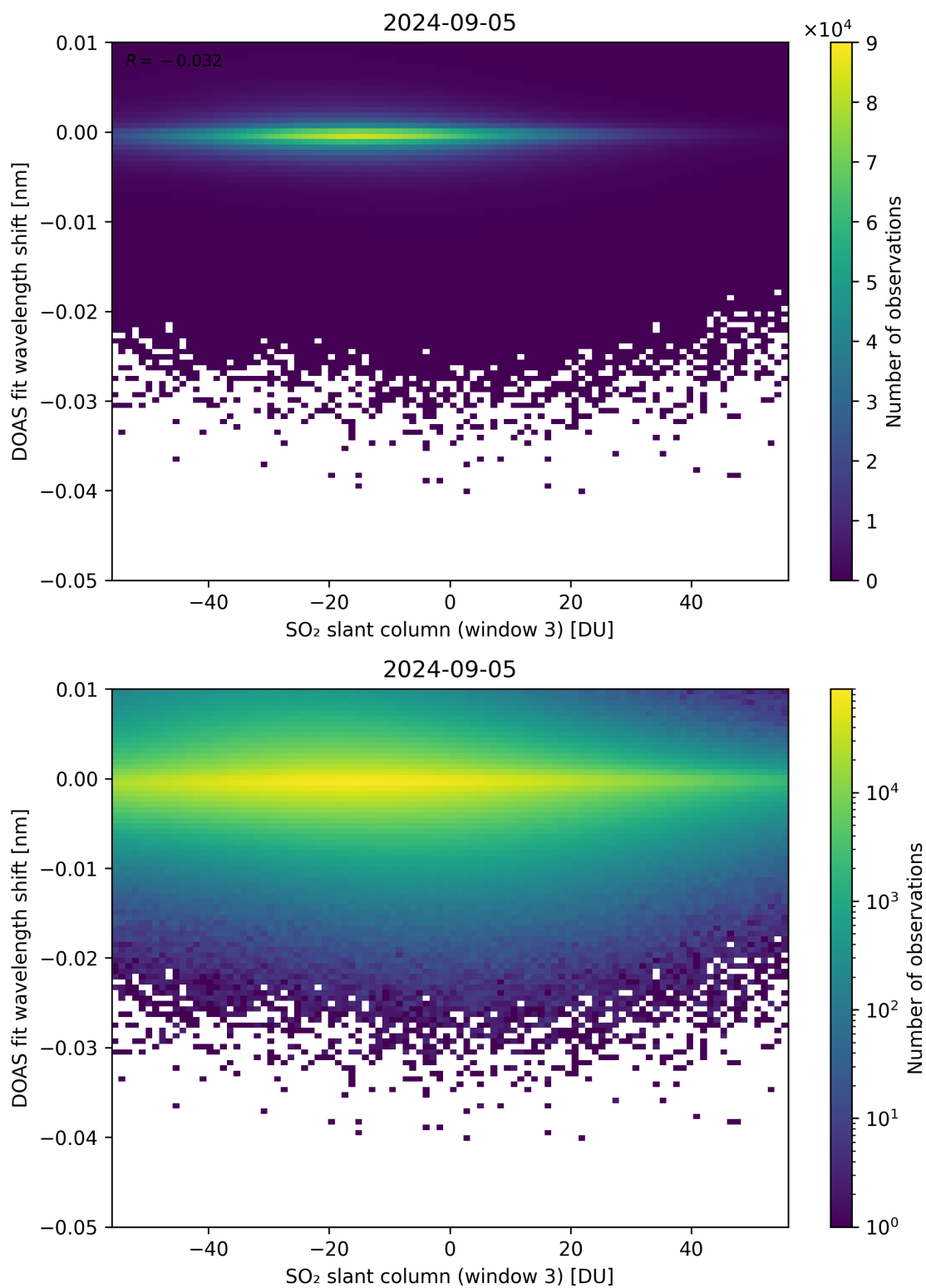
Figure 254: Scatter density plot of “SO 2 slant column (window 3)” against “DOAS fit wavelength shift” for 2024-09-04 to 2024-09-06.
