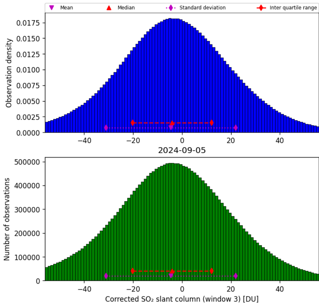
Figure 66: Histogram of “Corrected SO 2 slant column (window 3)” for 2024-09-04 to 2024-09-06
