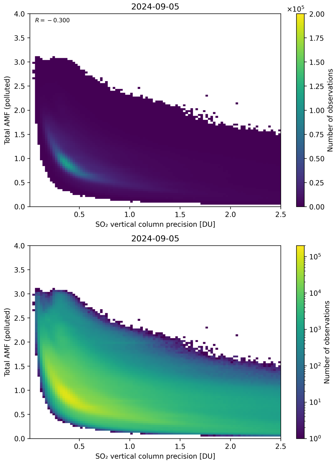
Figure 294: Scatter density plot of “SO 2 vertical column precision” against “Total AMF (polluted)” for 2024-09-04 to 2024-09-06.
