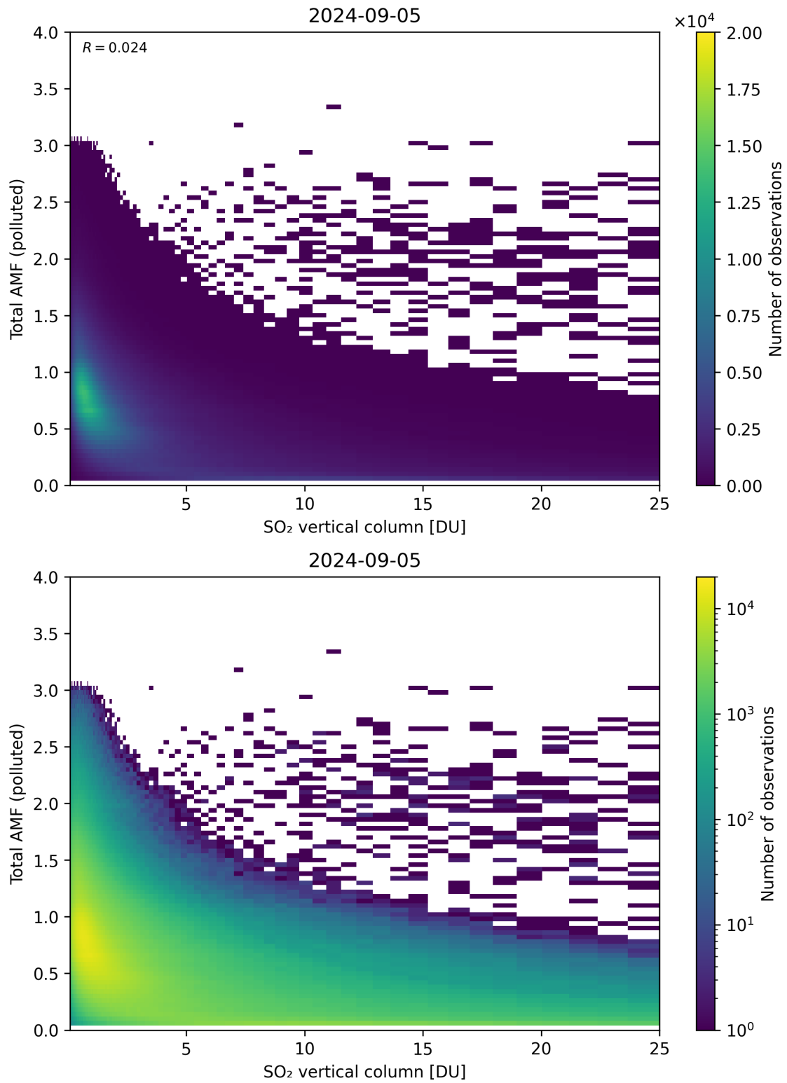
Figure 305: Scatter density plot of “SO 2 vertical column” against “Total AMF (polluted)” for 2024-09-04 to 2024-09-06.
