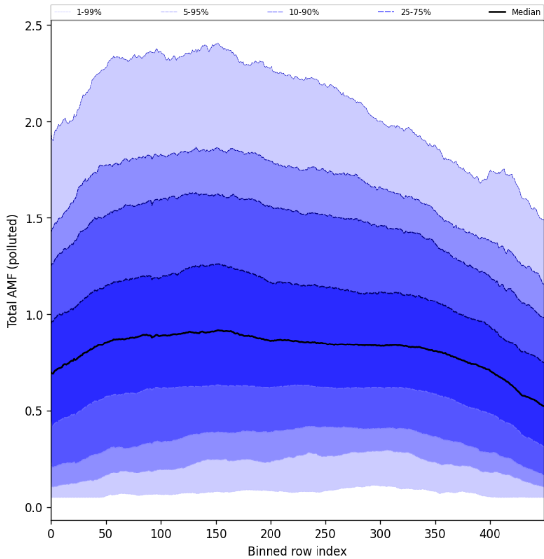
Figure 94: Along track statistics of “Total AMF (polluted)” for 2024-09-04 to 2024-09-06
