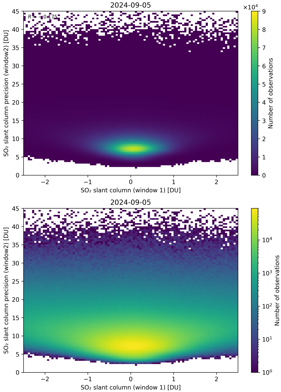
Figure 236: Scatter density plot of “SO 2 slant column (window 1)” against “SO 2 slant column precision (window2)” for 2024-09-04 to 2024-09-06.
