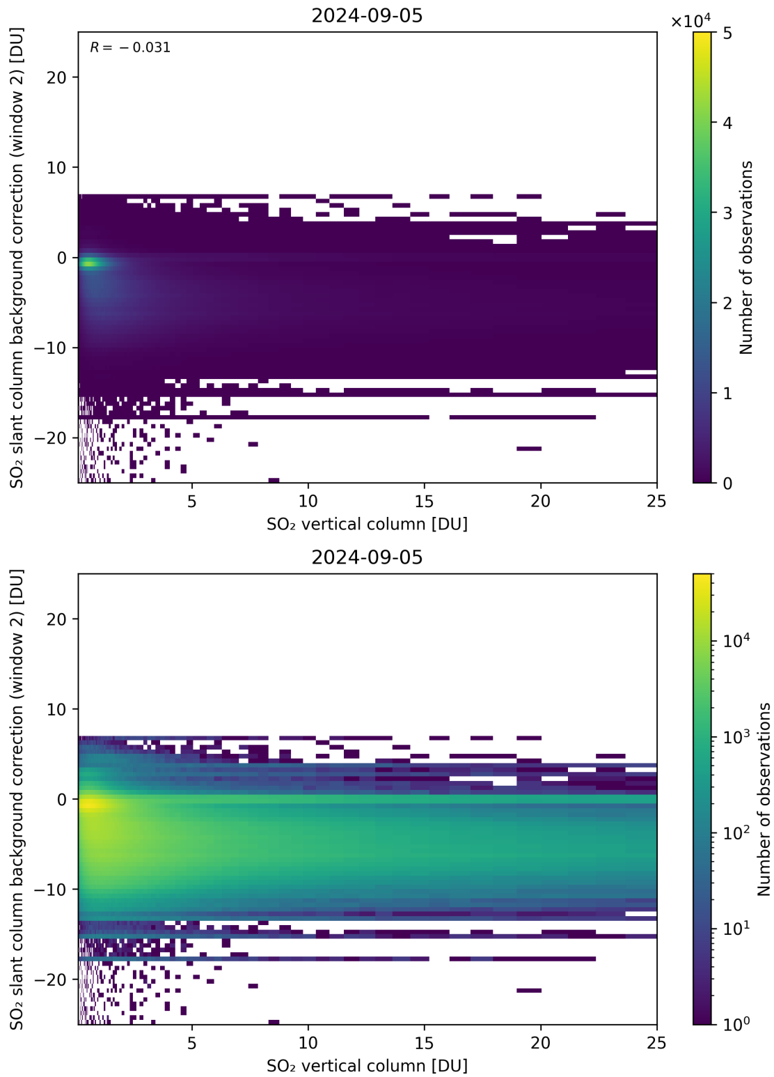
Figure 274: Scatter density plot of “SO 2 vertical column” against “SO 2 slant column background correction (window 2)” for 2024-09-04 to 2024-09-06.
