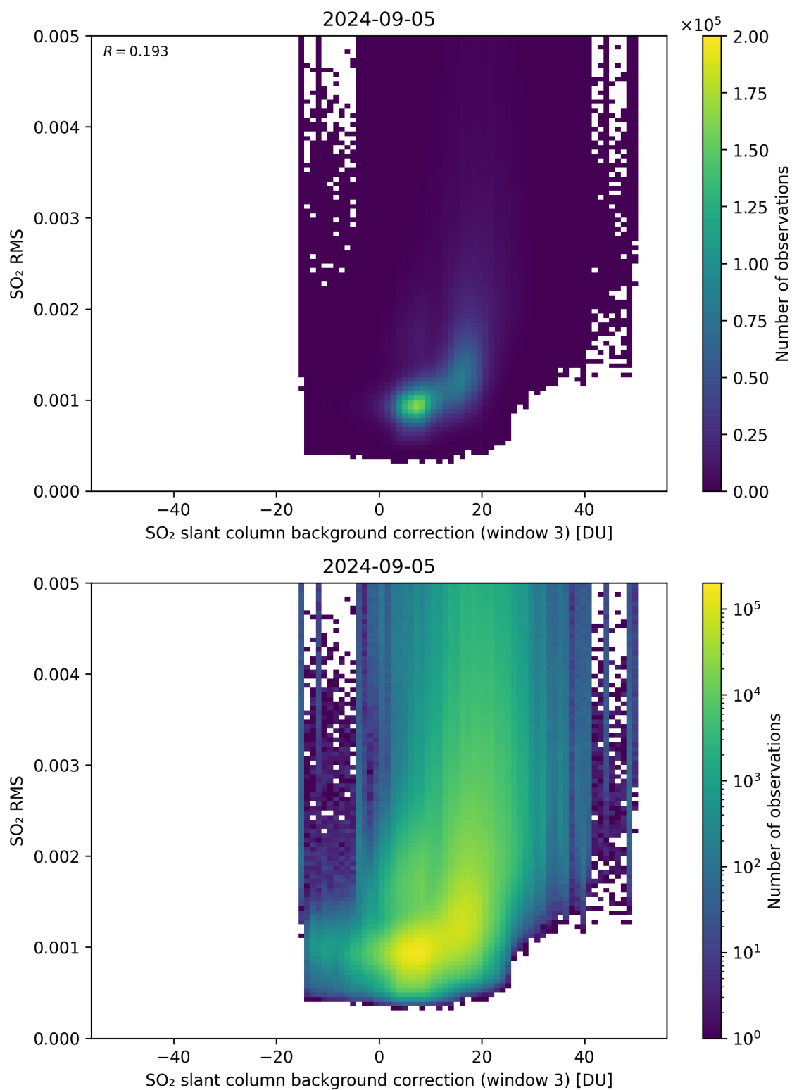
Figure 123: Scatter density plot of “SO 2 slant column background correction (window 3)” against “SO 2 RMS” for 2024-09-04 to 2024-09-06.
