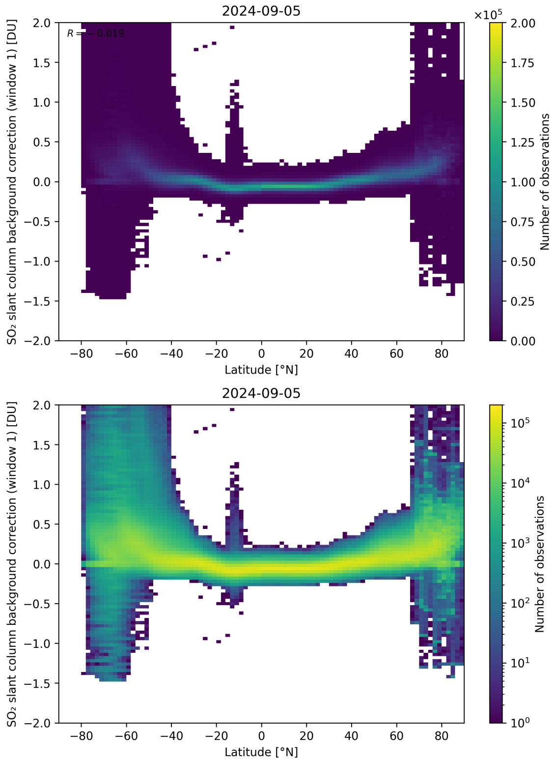
Figure 139: Scatter density plot of “Latitude” against “SO 2 slant column background correction (window 1)” for 2024-09-04 to 2024-09-06.
