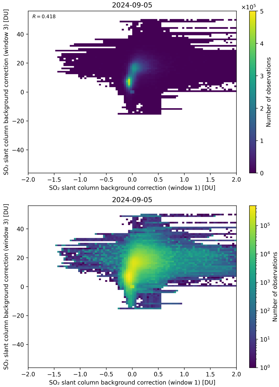
Figure 99: Scatter density plot of “SO 2 slant column background correction (window 1)” against “SO 2 slant column background correction (window 3)” for 2024-09-04 to 2024-09-06.
