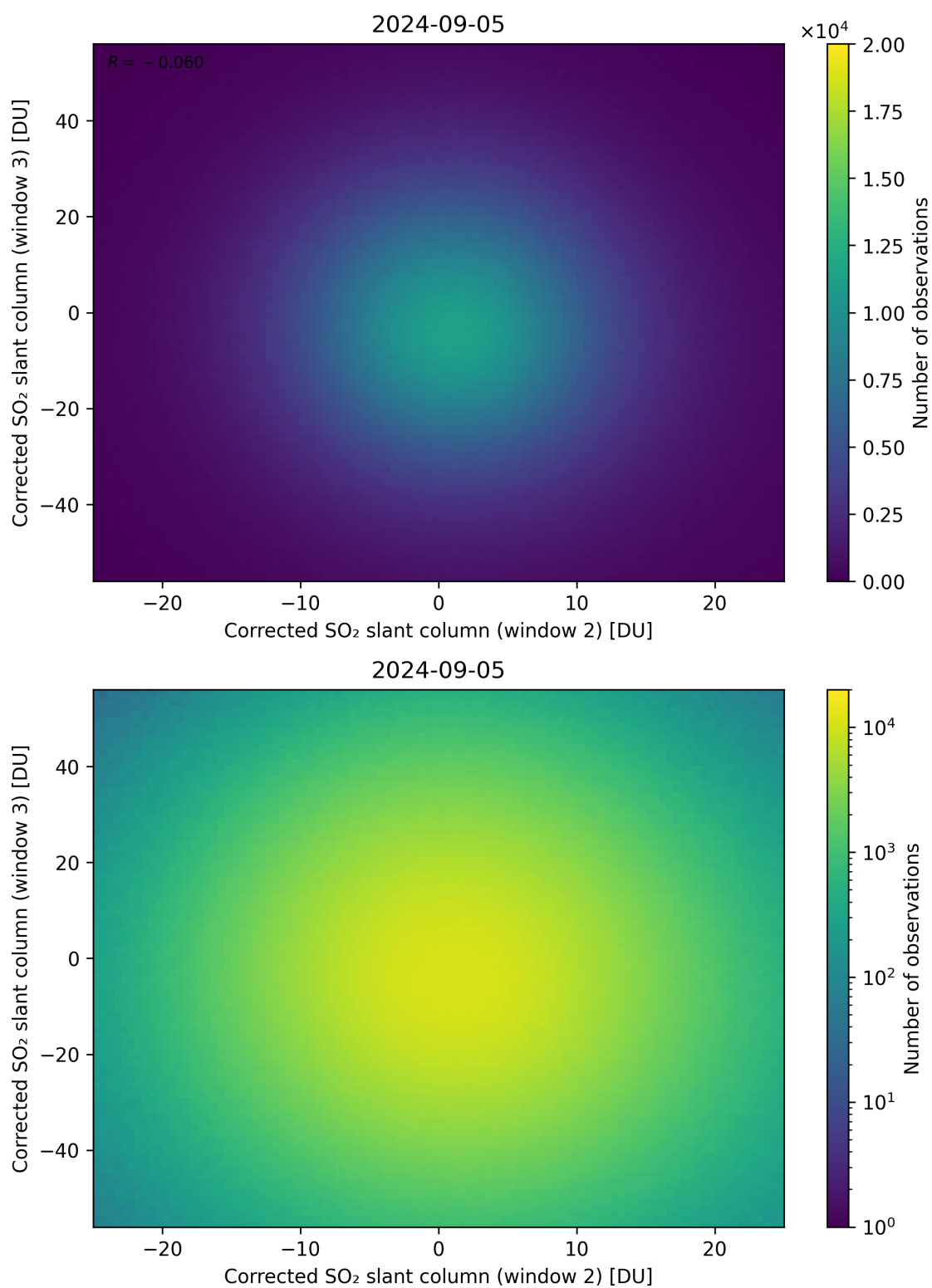
Figure 200: Scatter density plot of “Corrected SO 2 slant column (window 2)” against “Corrected SO 2 slant column (window 3)” for 2024-09-04 to 2024-09-06.
