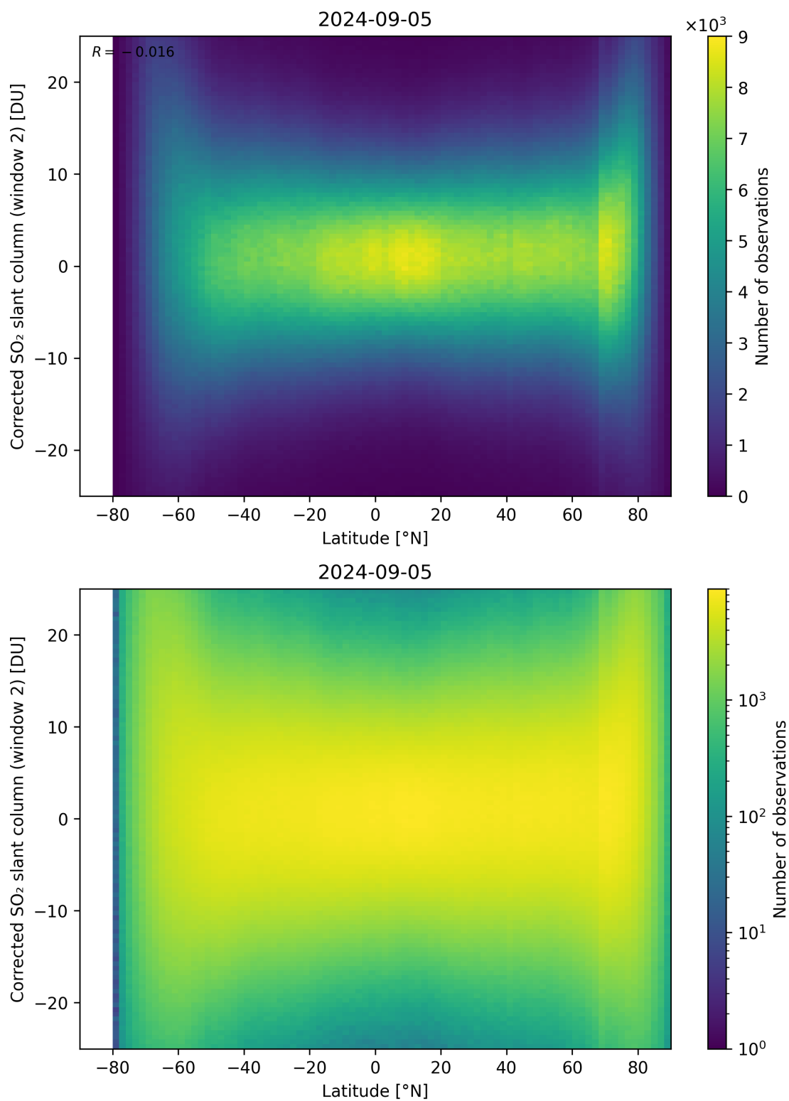
Figure 147: Scatter density plot of “Latitude” against “Corrected SO 2 slant column (window 2)” for 2024-09-04 to 2024-09-06.
