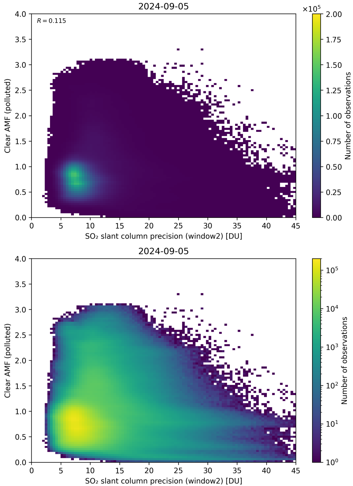
Figure 246: Scatter density plot of “SO 2 slant column precision (window2)” against “Clear AMF (polluted)” for 2024-09-04 to 2024-09-06.
