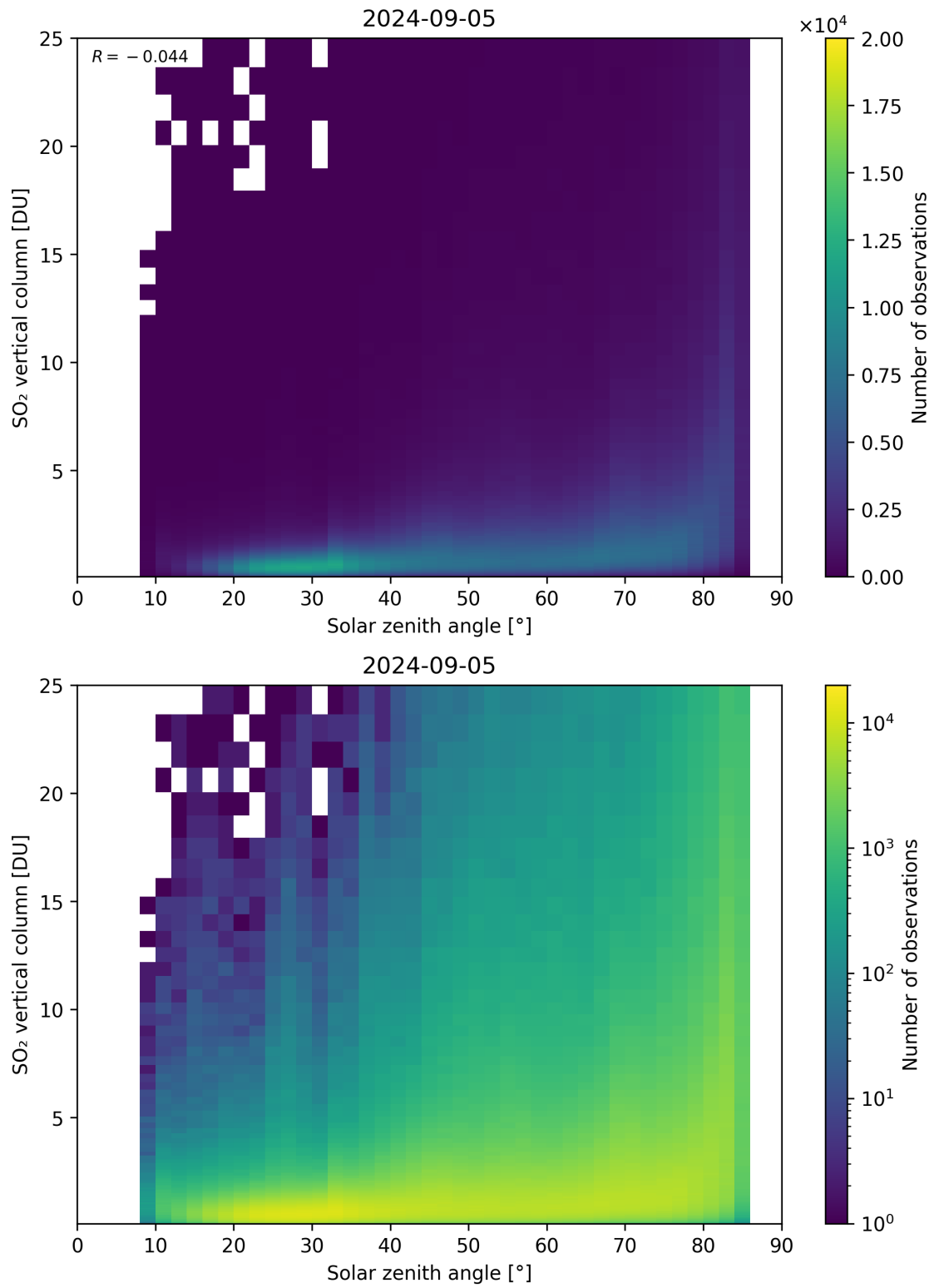
Figure 176: Scatter density plot of “Solar zenith angle” against “SO 2 vertical column” for 2024-09-04 to 2024-09-06.
