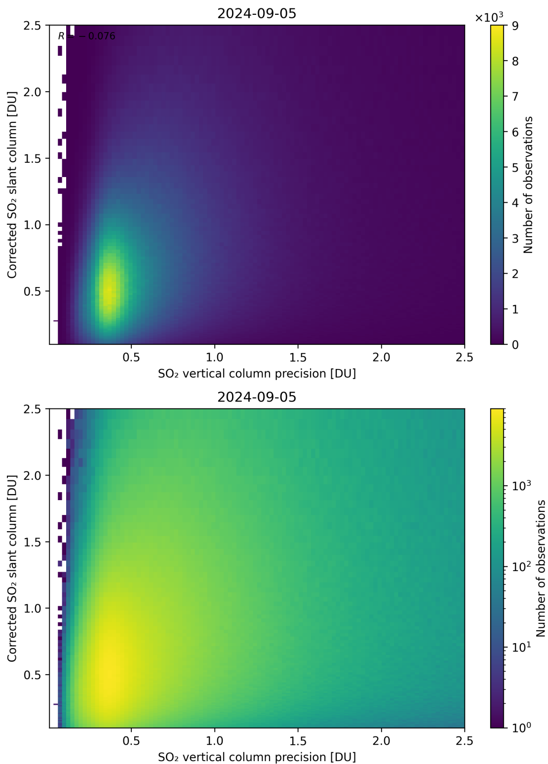
Figure 286: Scatter density plot of “SO 2 vertical column precision” against “Corrected SO 2 slant column” for 2024-09-04 to 2024-09-06.
