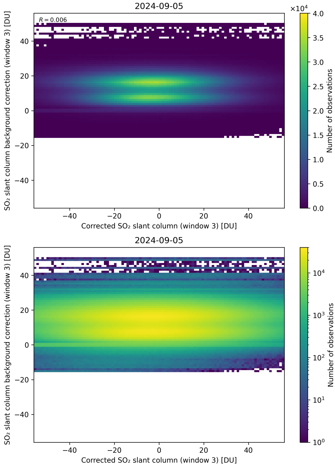
Figure 205: Scatter density plot of “Corrected SO 2 slant column (window 3)” against “SO 2 slant column background correction (window 3)” for 2024-09-04 to 2024-09-06.
