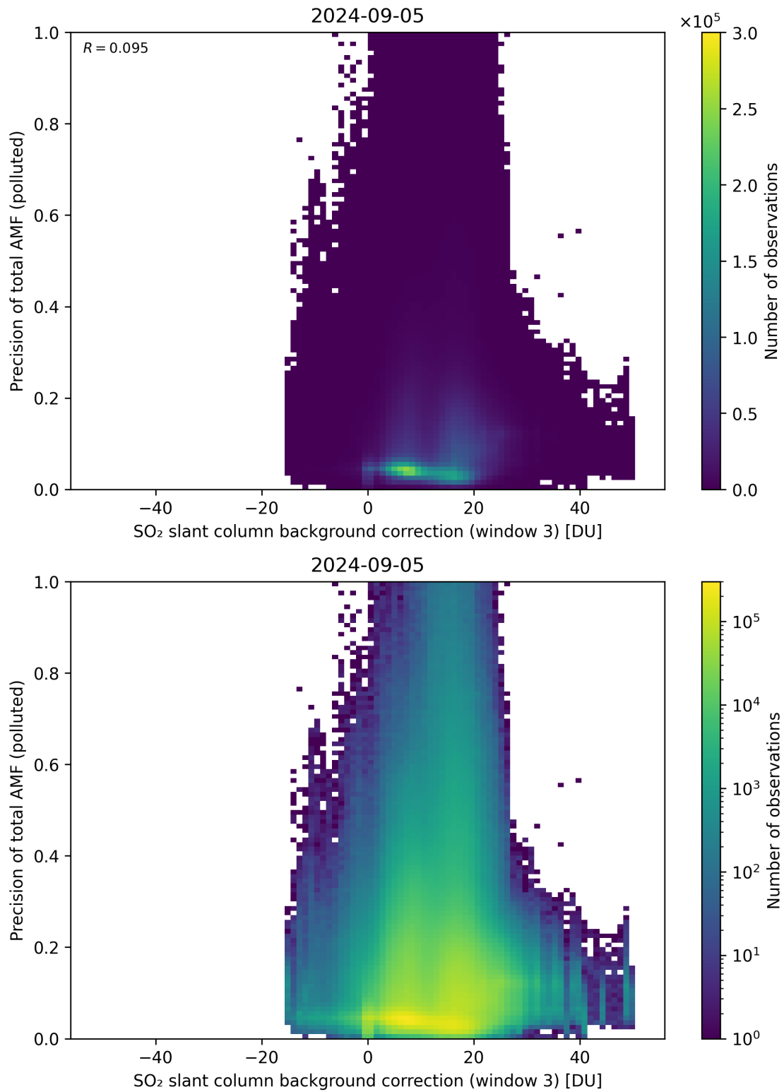
Figure 126: Scatter density plot of “SO 2 slant column background correction (window 3)” against “Precision of total AMF (polluted)” for 2024-09-04 to 2024-09-06.
