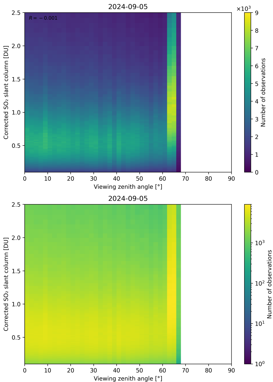
Figure 317: Scatter density plot of “Viewing zenith angle” against “Corrected SO 2 slant column” for 2024-09-04 to 2024-09-06.
