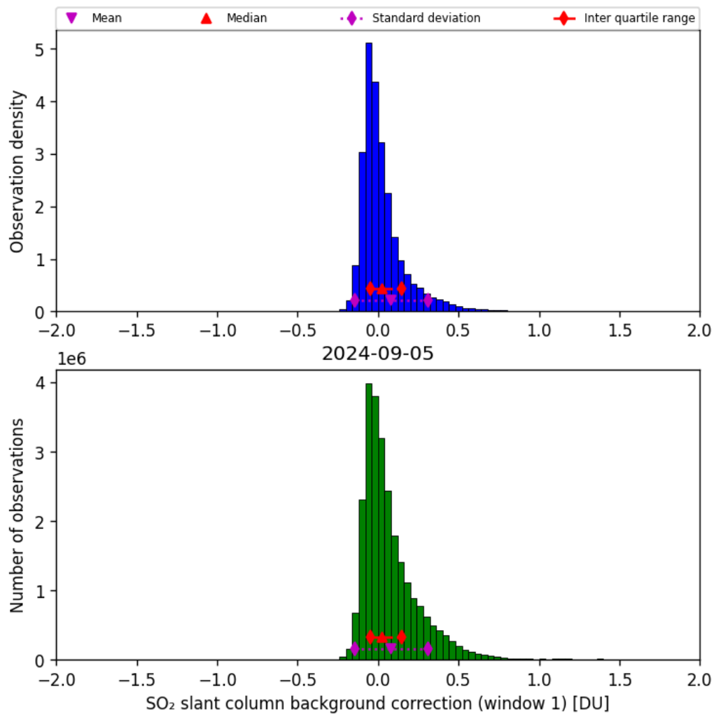
Figure 59: Histogram of “SO 2 slant column background correction (window 1)” for 2024-09-04 to 2024-09-06
