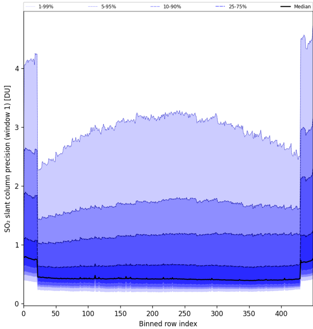
Figure 80: Along track statistics of “SO 2 slant column precision (window 1)” for 2024-09-04 to 2024-09-06
