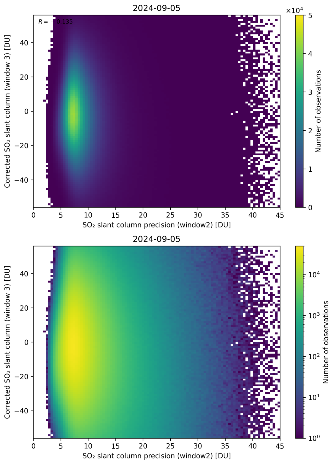
Figure 248: Scatter density plot of “SO 2 slant column precision (window2)” against “Corrected SO 2 slant column (window 3)” for 2024-09-04 to 2024-09-06.
