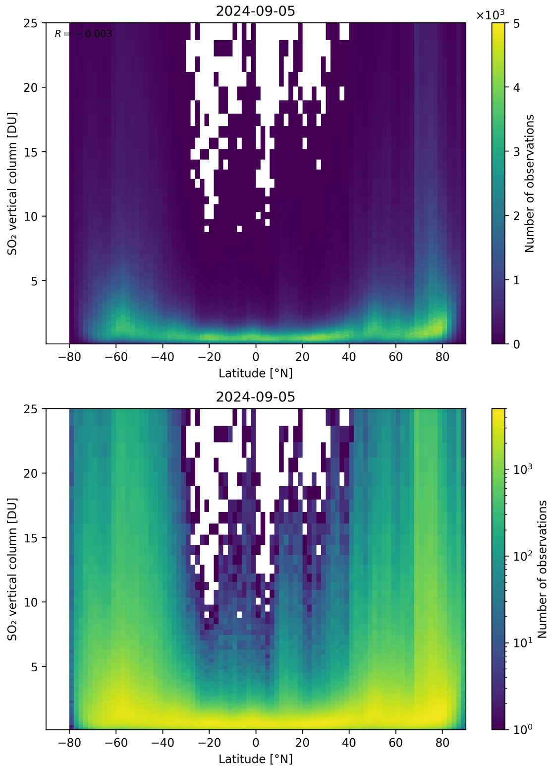
Figure 156: Scatter density plot of “Latitude” against “SO 2 vertical column” for 2024-09-04 to 2024-09-06.
