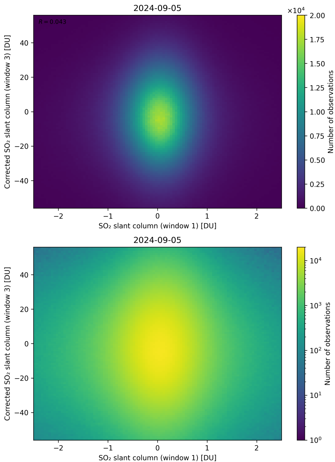
Figure 234: Scatter density plot of “SO 2 slant column (window 1)” against “Corrected SO 2 slant column (window 3)” for 2024-09-04 to 2024-09-06.
