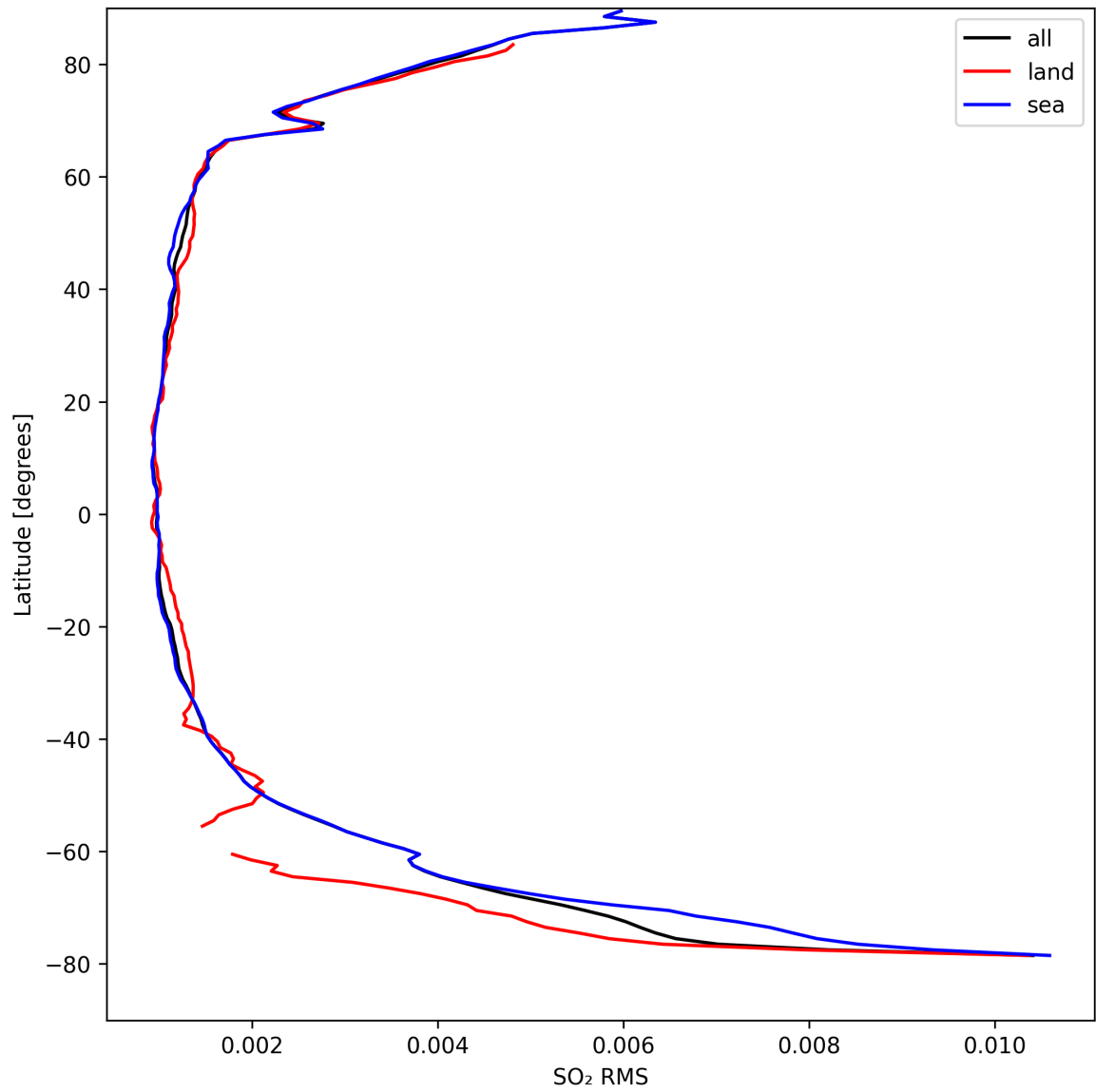
Figure 47: Zonal average of “SO 2 RMS” for 2024-09-04 to 2024-09-06.
