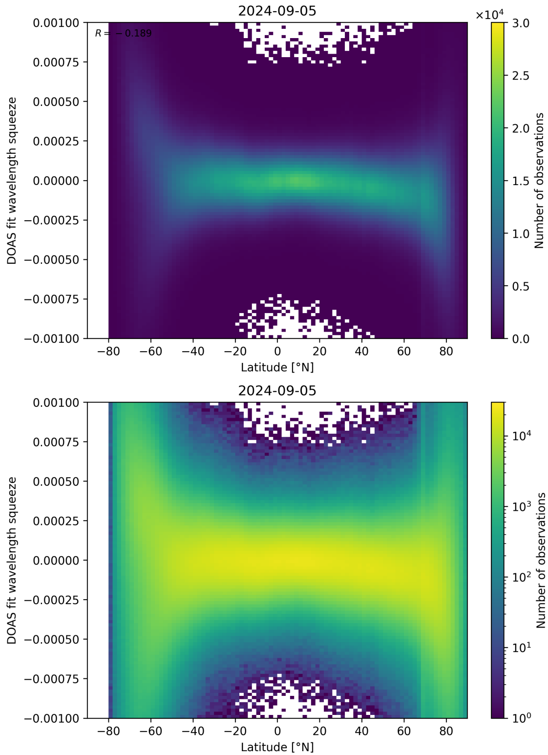
Figure 143: Scatter density plot of “Latitude” against “DOAS fit wavelength squeeze” for 2024-09-04 to 2024-09-06.
