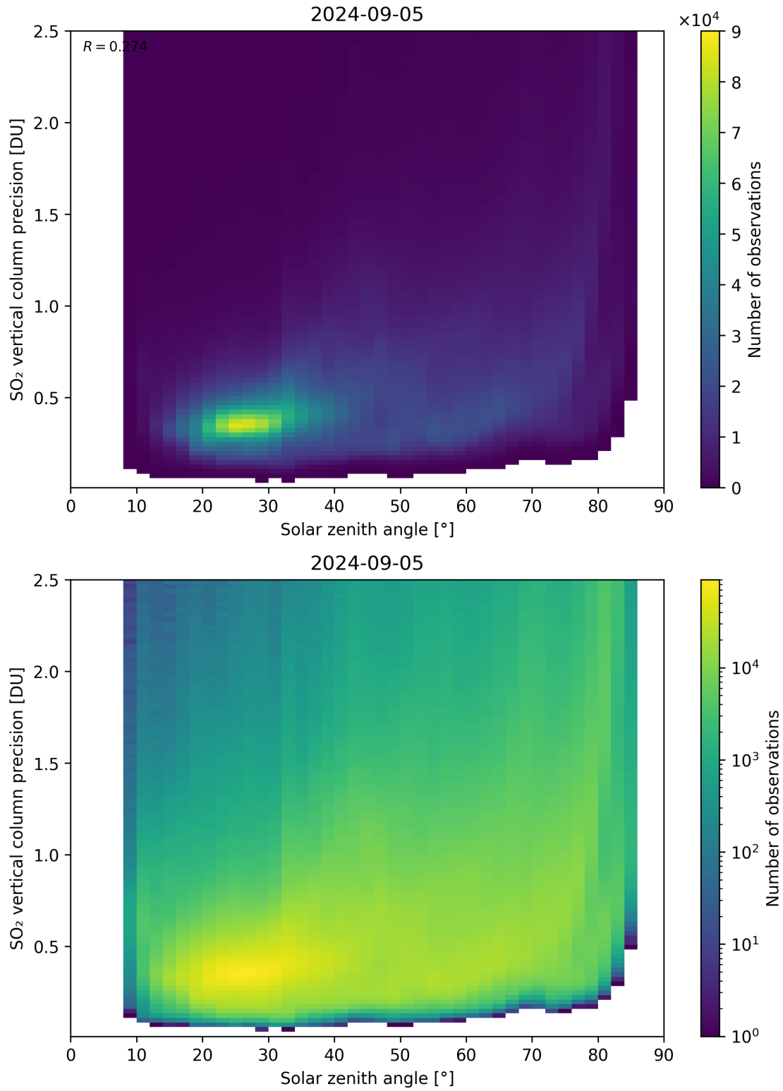
Figure 177: Scatter density plot of “Solar zenith angle” against “SO 2 vertical column precision” for 2024-09-04 to 2024-09-06.
