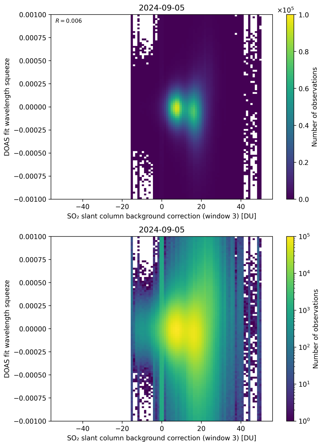
Figure 122: Scatter density plot of “SO 2 slant column background correction (window 3)” against “DOAS fit wavelength squeeze” for 2024-09-04 to 2024-09-06.
