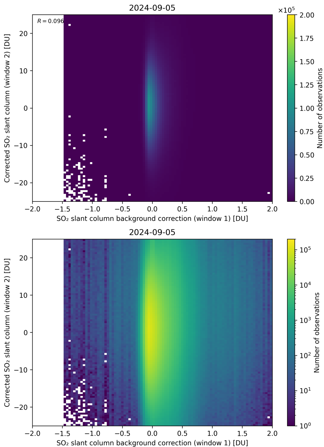
Figure 104: Scatter density plot of “SO 2 slant column background correction (window 1)” against “Corrected SO 2 slant column (window 2)” for 2024-09-04 to 2024-09-06.
