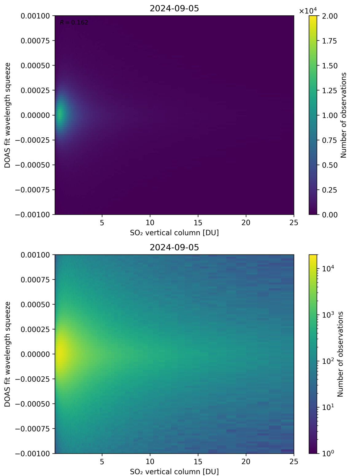
Figure 277: Scatter density plot of “SO 2 vertical column” against “DOAS fit wavelength squeeze” for 2024-09-04 to 2024-09-06.
