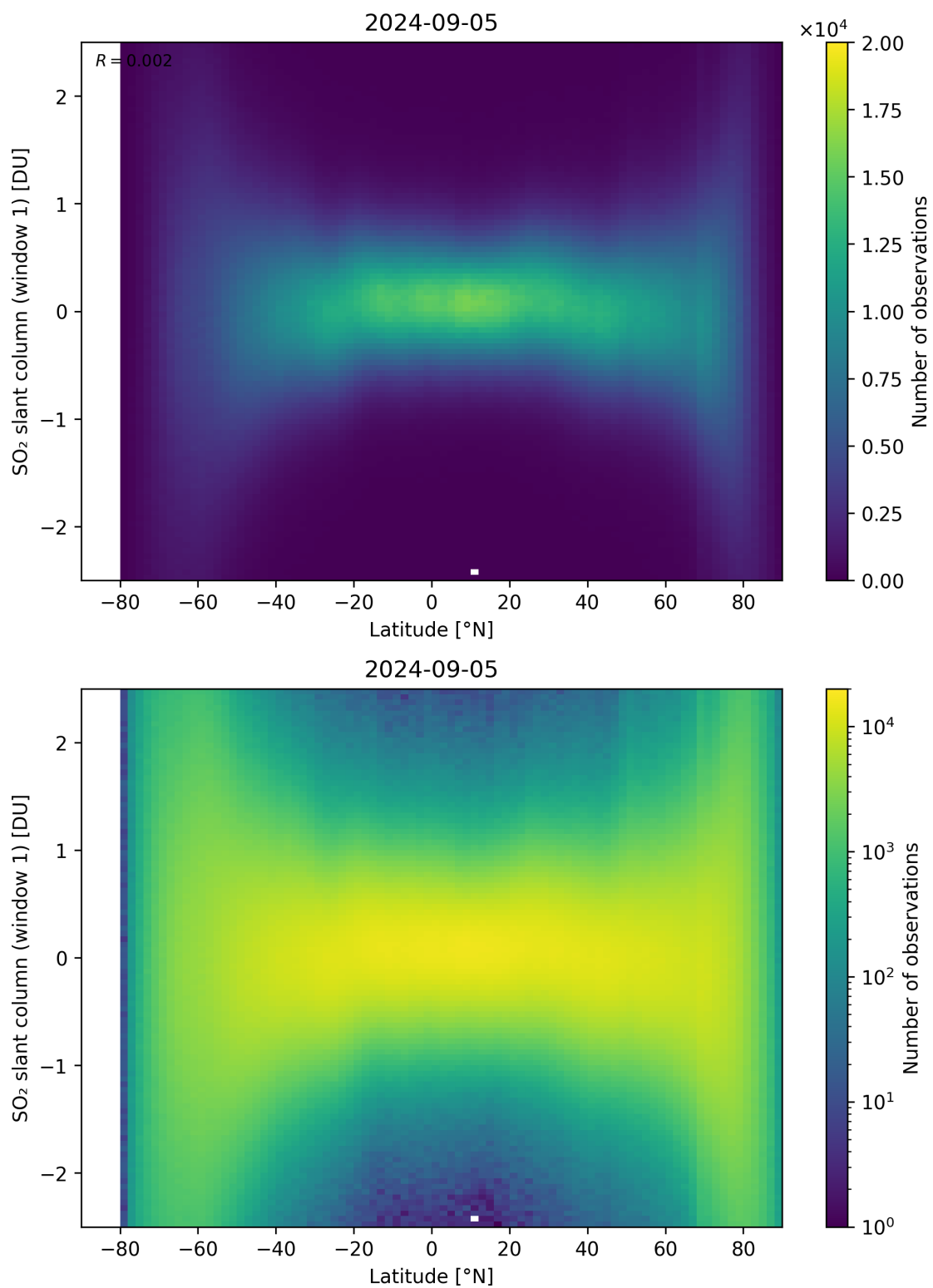
Figure 149: Scatter density plot of “Latitude” against “SO 2 slant column (window 1)” for 2024-09-04 to 2024-09-06.
