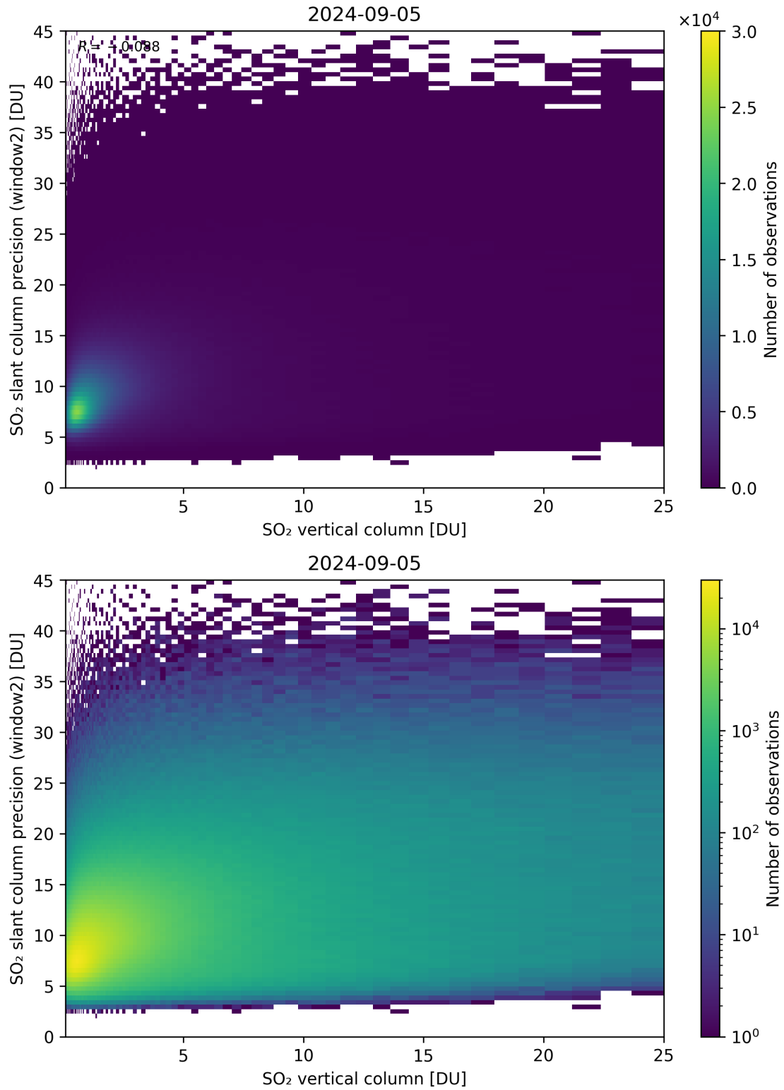
Figure 302: Scatter density plot of “SO 2 vertical column” against “SO 2 slant column precision (window2)” for 2024-09-04 to 2024-09-06.
