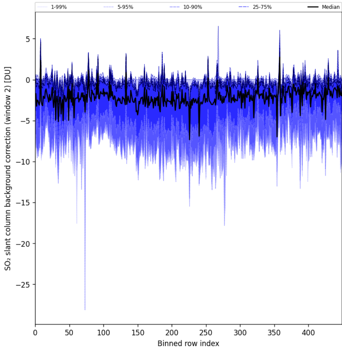
Figure 86: Along track statistics of “SO 2 slant column background correction (window 2)” for 2024-09-04 to 2024-09-06
