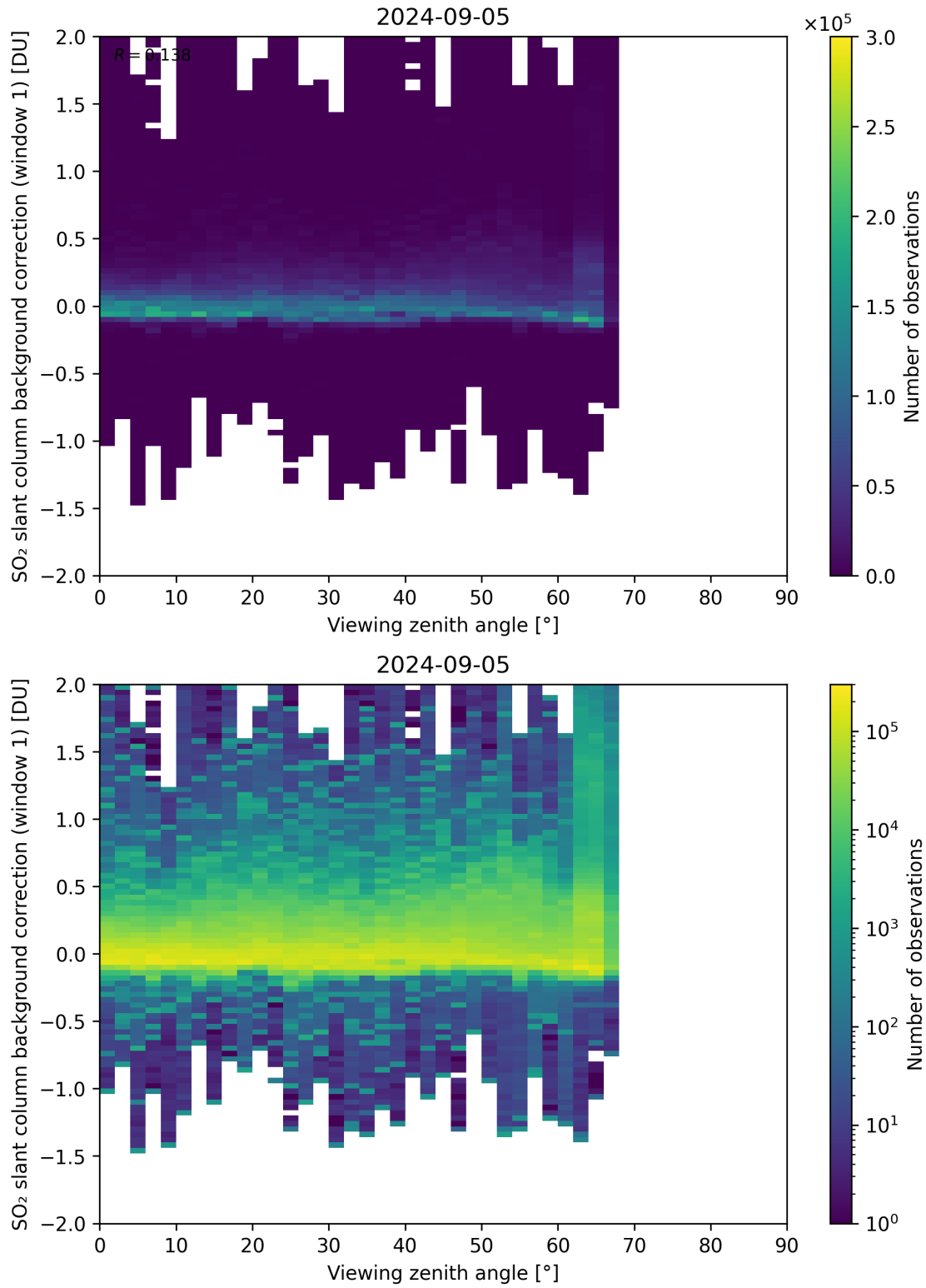
Figure 308: Scatter density plot of “Viewing zenith angle” against “SO 2 slant column background correction (window 1)” for 2024-09-04 to 2024-09-06.
