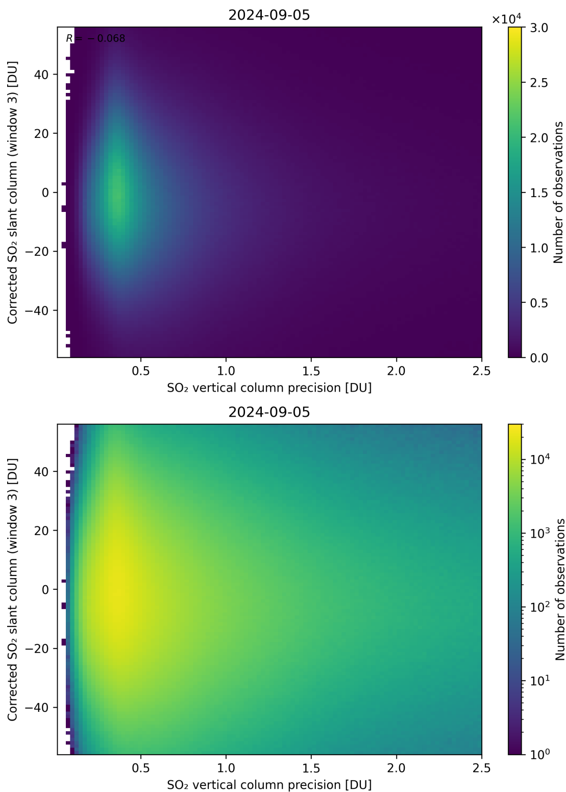
Figure 288: Scatter density plot of “SO 2 vertical column precision” against “Corrected SO 2 slant column (window 3)” for 2024-09-04 to 2024-09-06.
