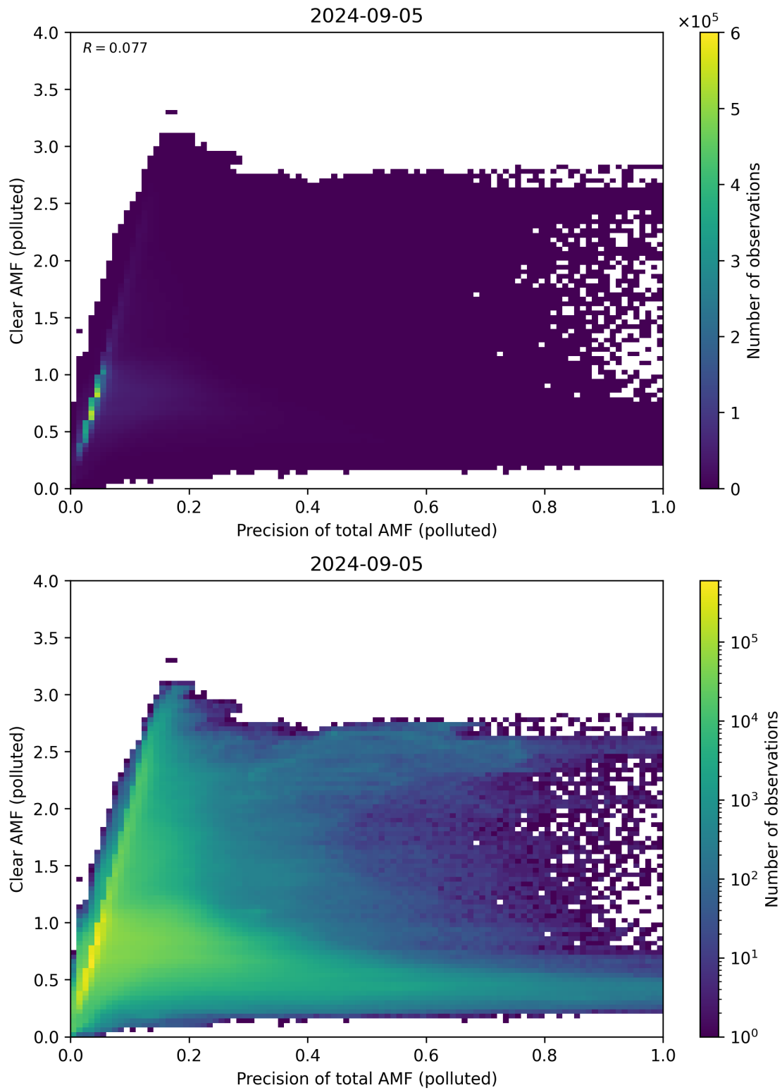
Figure 270: Scatter density plot of “Precision of total AMF (polluted)” against “Clear AMF (polluted)” for 2024-09-04 to 2024-09-06.
