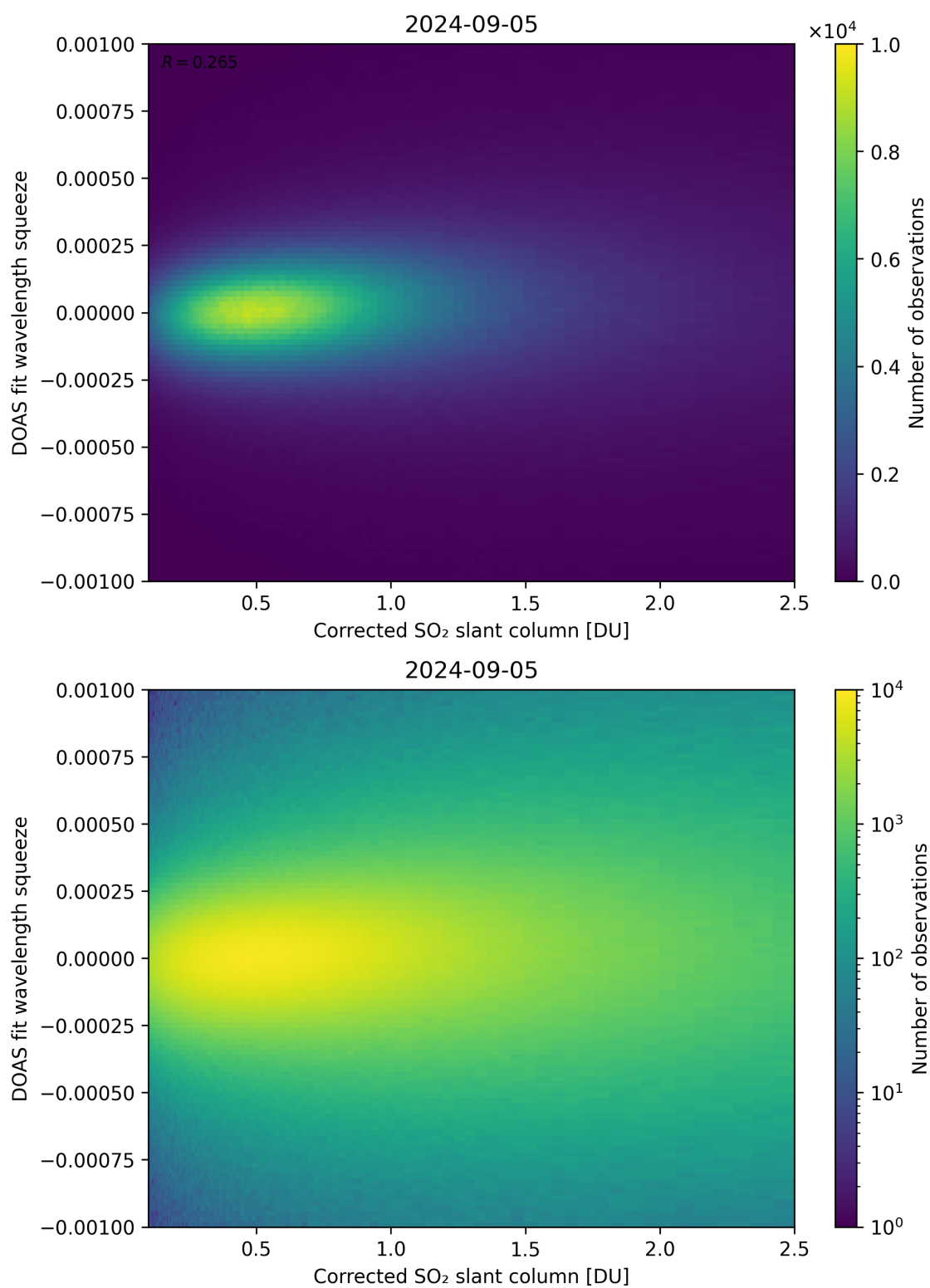
Figure 182: Scatter density plot of “Corrected SO 2 slant column” against “DOAS fit wavelength squeeze” for 2024-09-04 to 2024-09-06.
