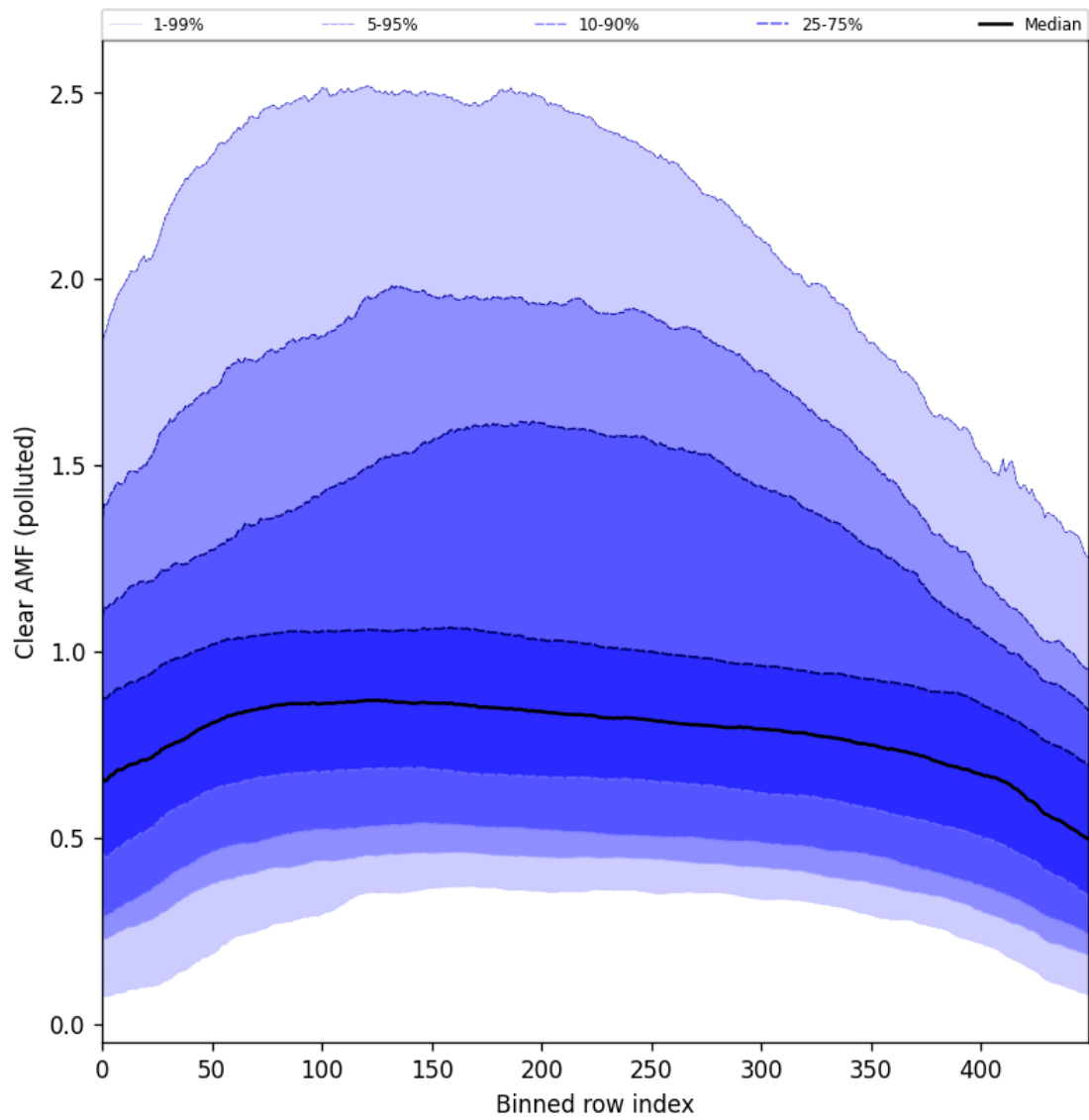
Figure 96: Along track statistics of “Clear AMF (polluted)” for 2024-09-04 to 2024-09-06
