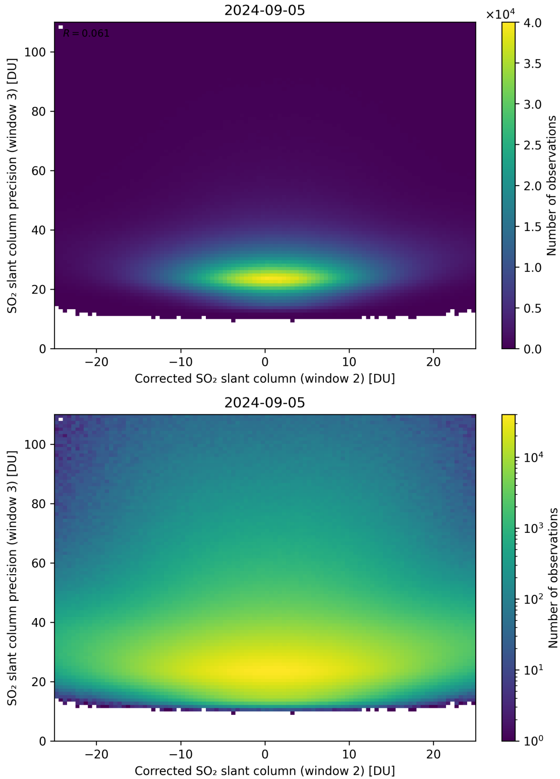
Figure 202: Scatter density plot of “Corrected SO 2 slant column (window 2)” against “SO 2 slant column precision (window 3)” for 2024-09-04 to 2024-09-06.
