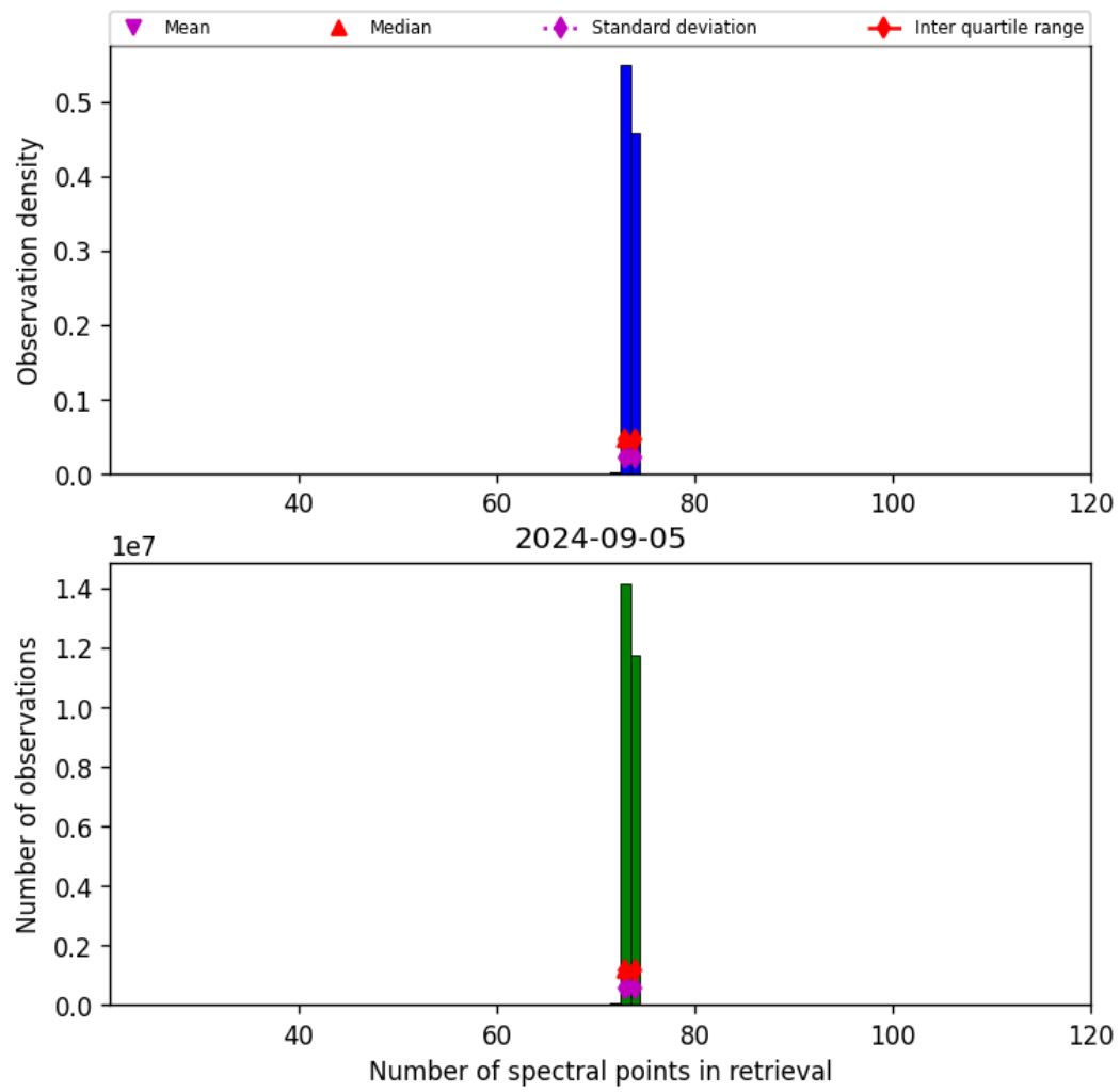
Figure 74: Histogram of “Number of spectral points in retrieval” for 2024-09-04 to 2024-09-06
