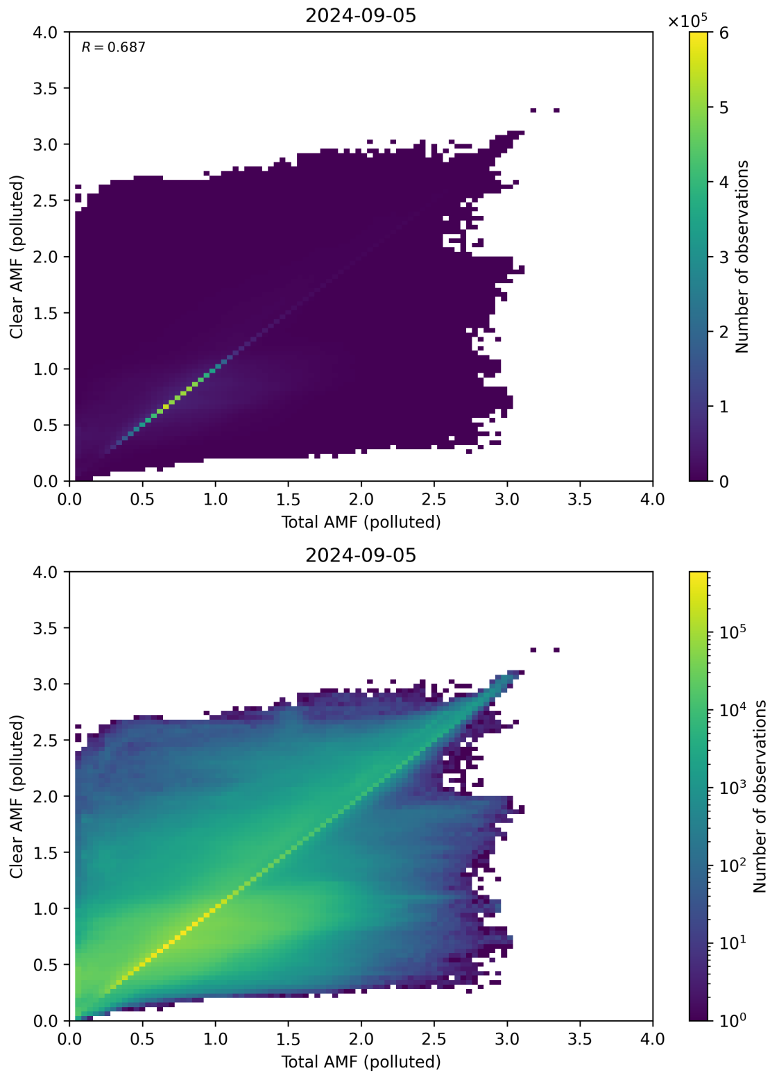
Figure 271: Scatter density plot of “Total AMF (polluted)” against “Clear AMF (polluted)” for 2024-09-04 to 2024-09-06.
