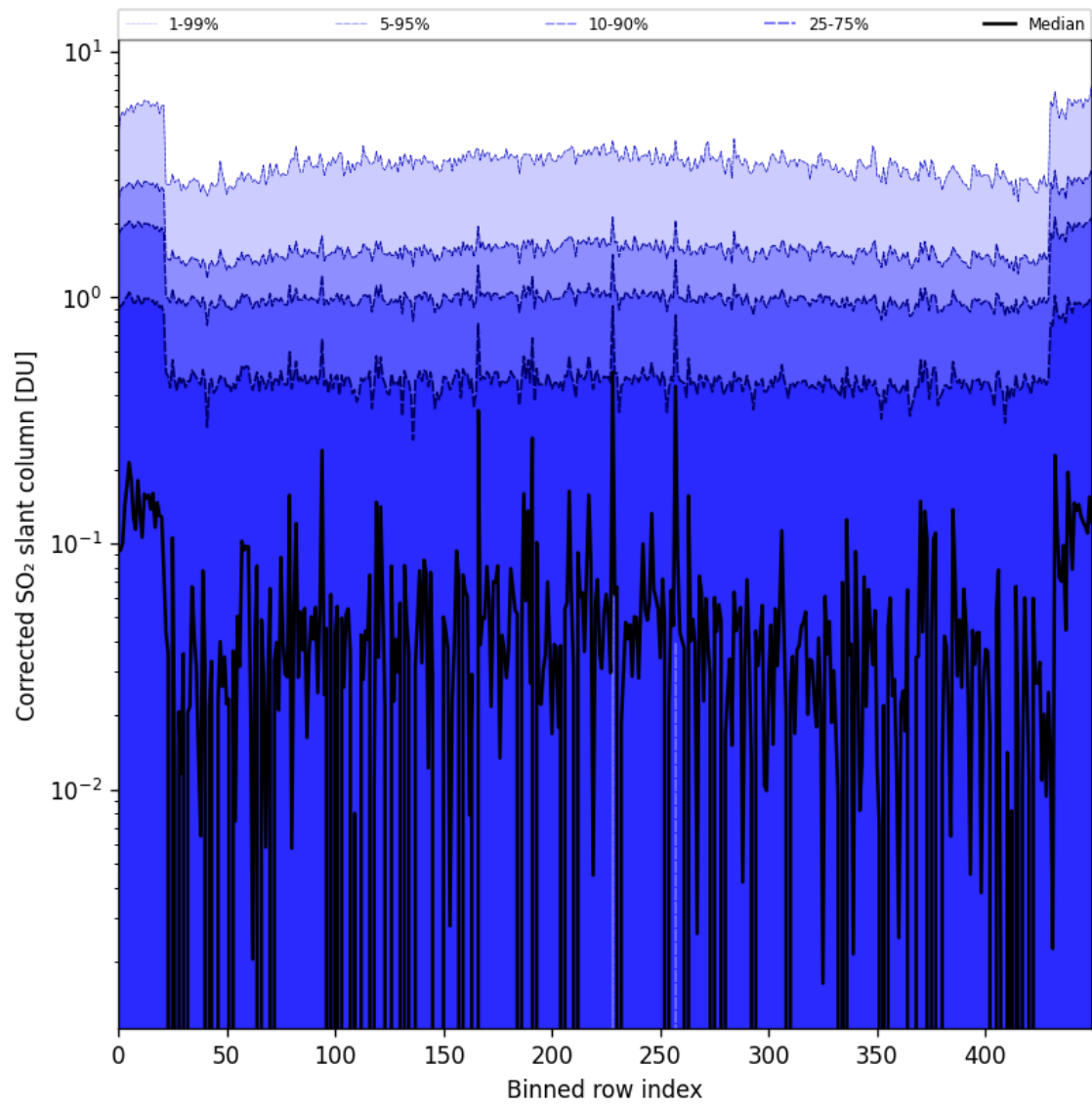
Figure 78: Along track statistics of "Corrected SO 2 slant column" for 2024-09-04 to 2024-09-06
