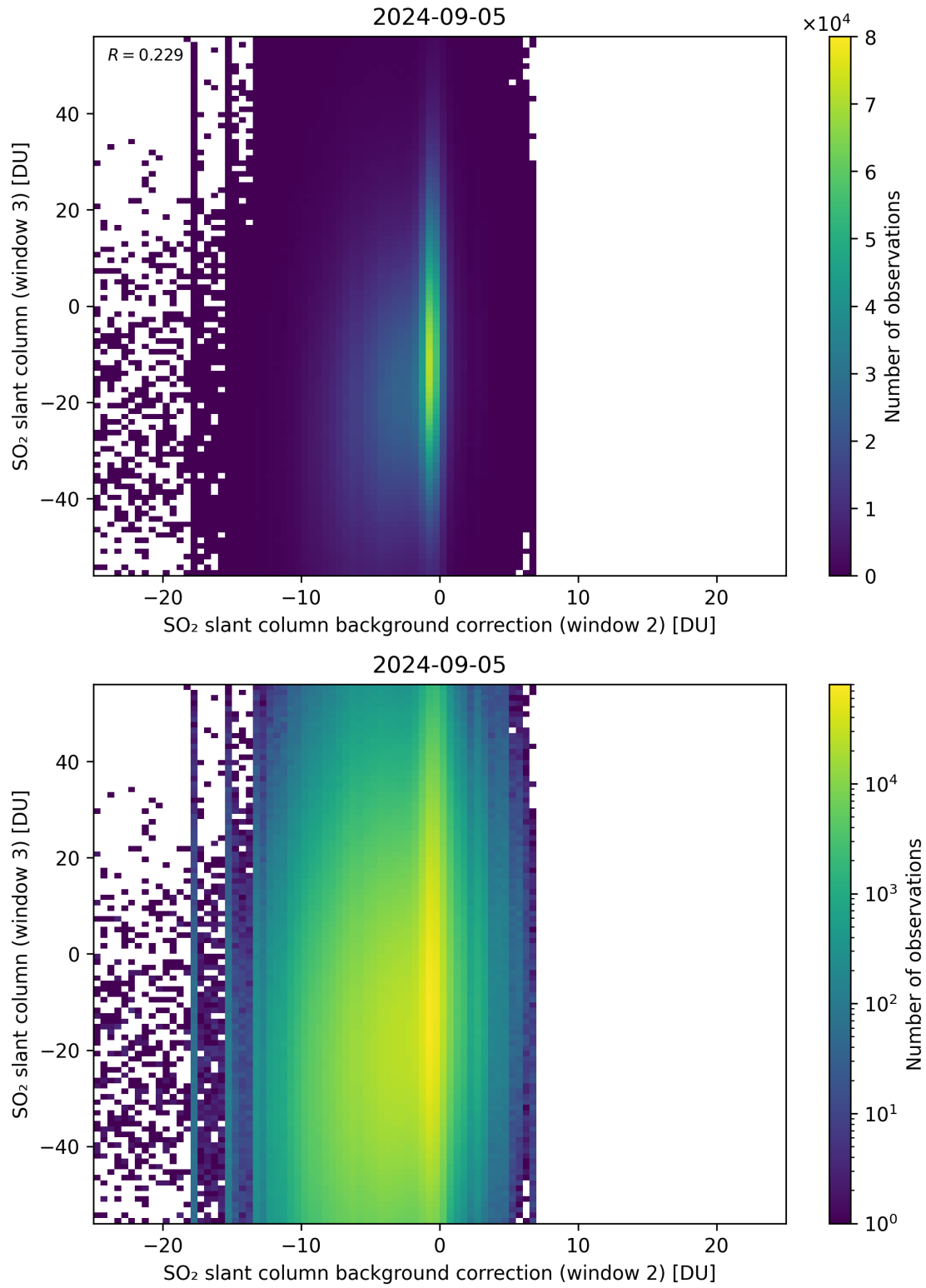
Figure 117: Scatter density plot of “SO 2 slant column background correction (window 2)” against “SO 2 slant column (window 3)” for 2024-09-04 to 2024-09-06.
