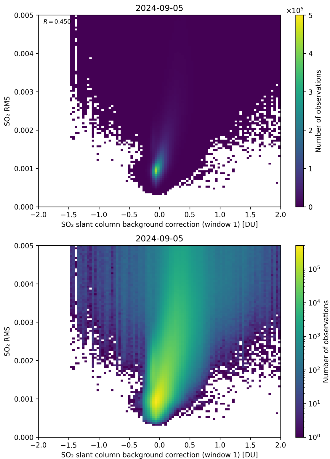
Figure 102: Scatter density plot of “SO 2 slant column background correction (window 1)” against “SO 2 RMS” for 2024-09-04 to 2024-09-06.
