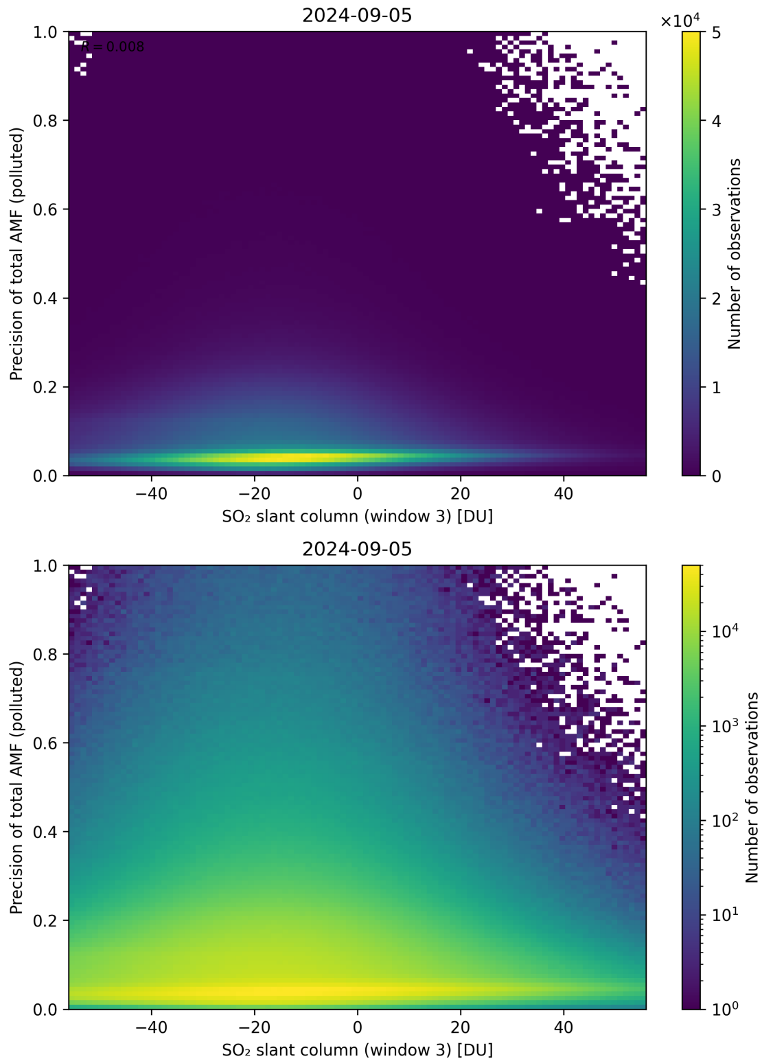
Figure 269: Scatter density plot of “SO 2 slant column (window 3)” against “Precision of total AMF (polluted)” for 2024-09-04 to 2024-09-06.
