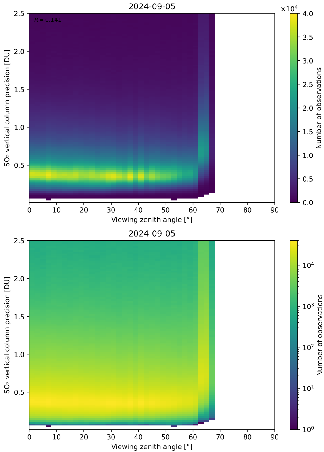
Figure 328: Scatter density plot of “Viewing zenith angle” against “SO 2 vertical column precision” for 2024-09-04 to 2024-09-06.
