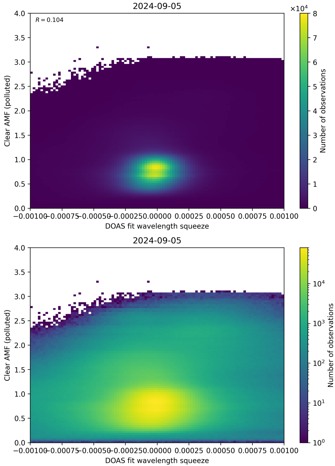
Figure 133: Scatter density plot of “DOAS fit wavelength squeeze” against “Clear AMF (polluted)” for 2024-09-04 to 2024-09-06.
