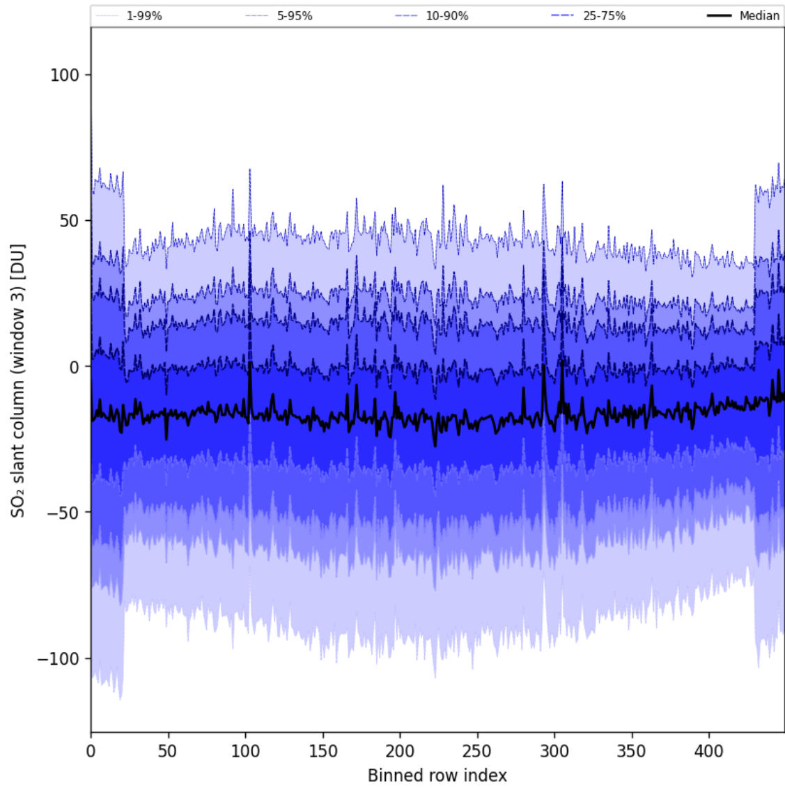
Figure 87: Along track statistics of “SO 2 slant column (window 3)” for 2024-09-04 to 2024-09-06
