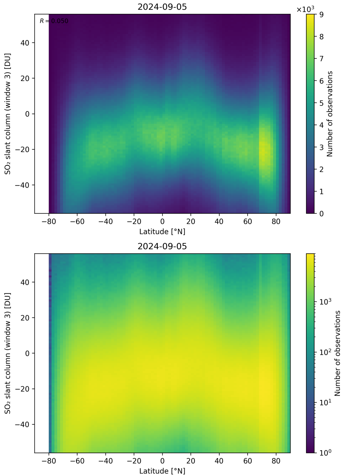
Figure 152: Scatter density plot of “Latitude” against “SO 2 slant column (window 3)” for 2024-09-04 to 2024-09-06.
