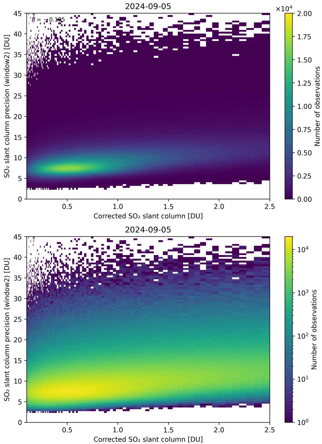
Figure 189: Scatter density plot of “Corrected SO 2 slant column” against “SO 2 slant column precision (window2)” for 2024-09-04 to 2024-09-06.
