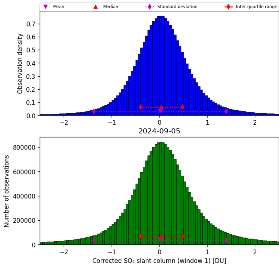
Figure 58: Histogram of “Corrected SO 2 slant column (window 1)” for 2024-09-04 to 2024-09-06
