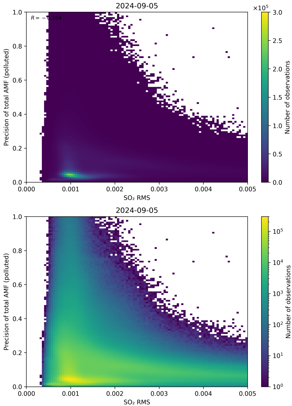
Figure 138: Scatter density plot of “SO 2 RMS” against “Precision of total AMF (polluted)” for 2024-09-04 to 2024-09-06.
