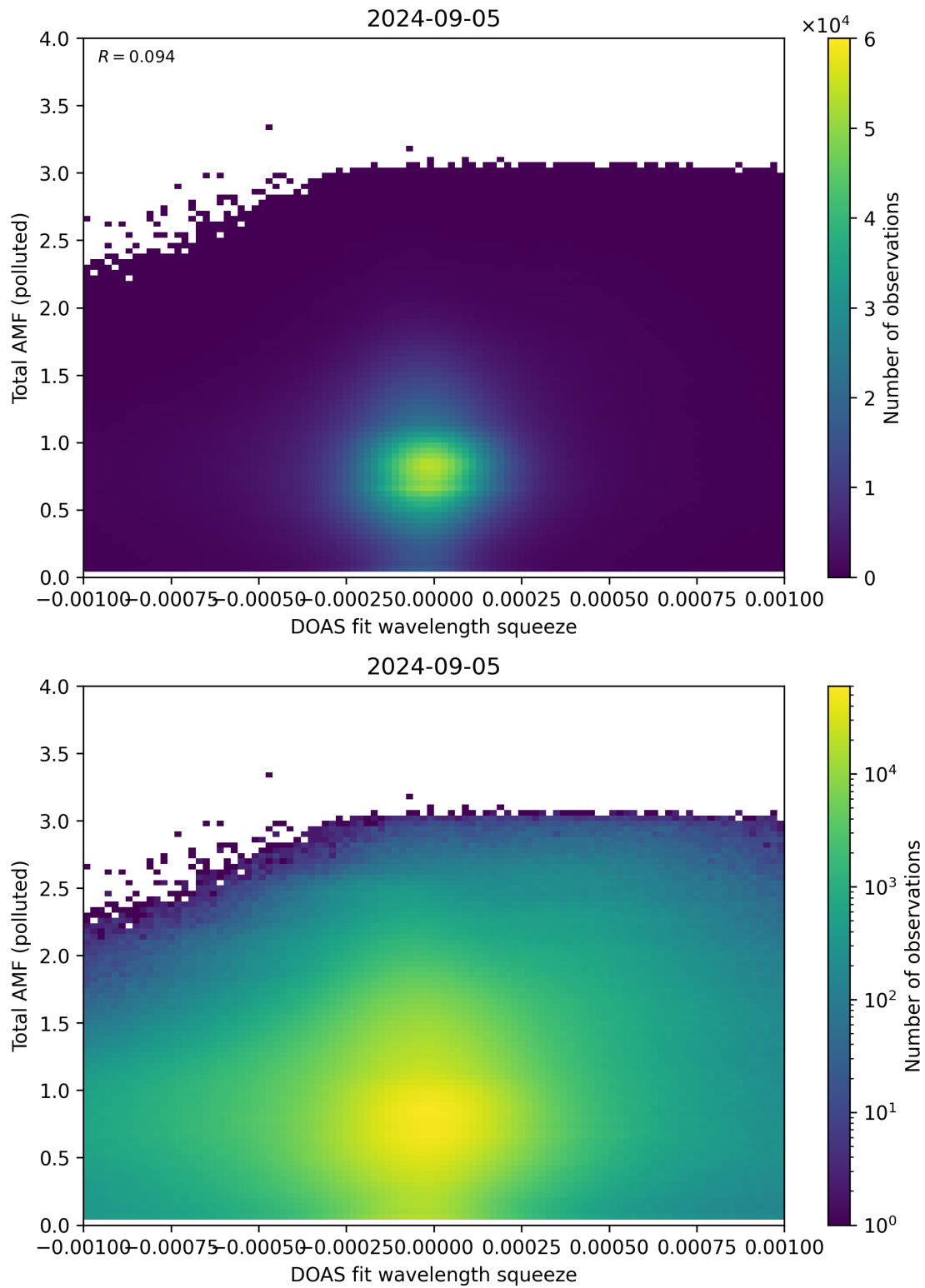
Figure 134: Scatter density plot of “DOAS fit wavelength squeeze” against “Total AMF (polluted)” for 2024-09-04 to 2024-09-06.
