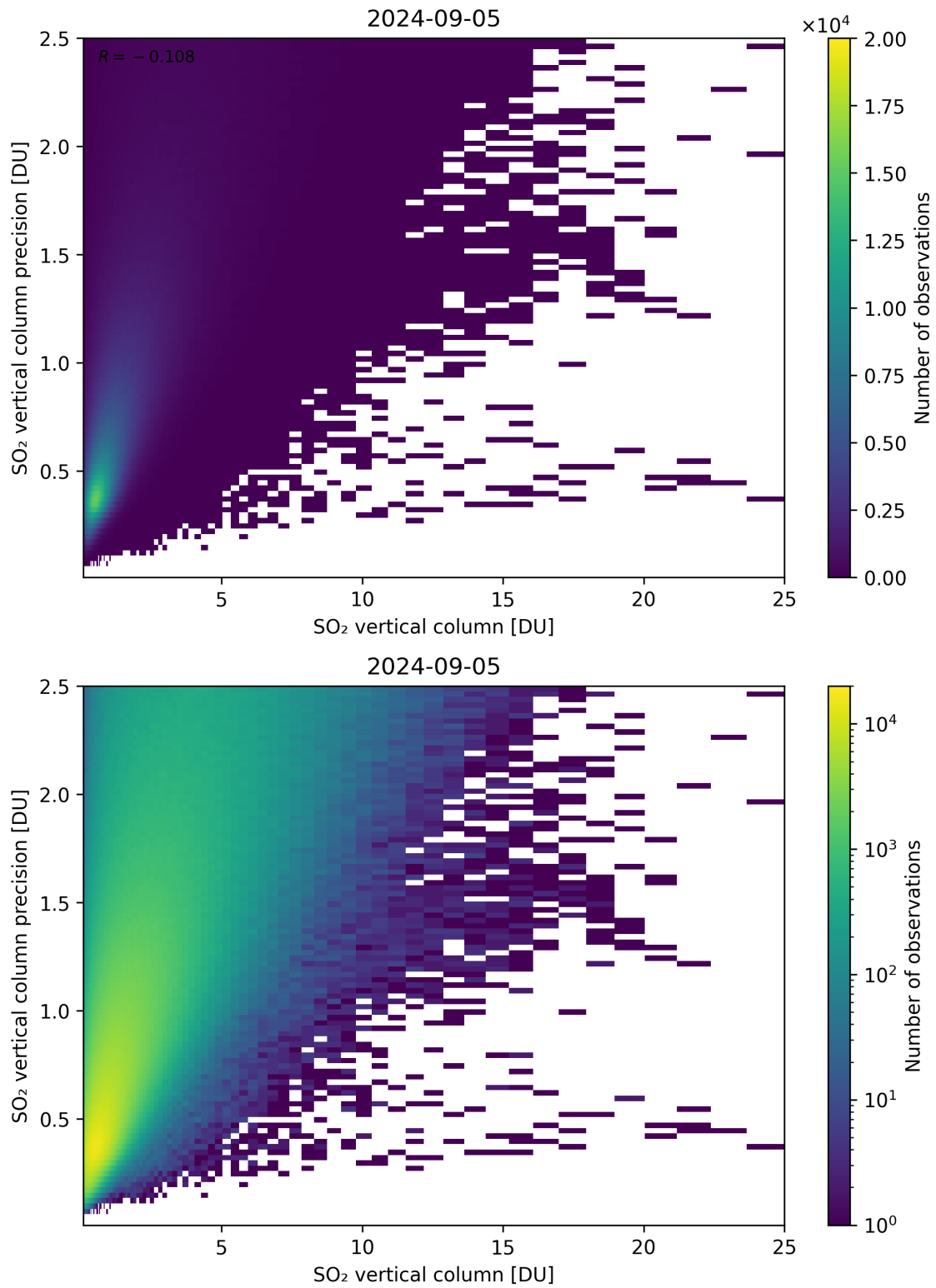
Figure 307: Scatter density plot of “SO 2 vertical column” against “SO 2 vertical column precision” for 2024-09-04 to 2024-09-06.
