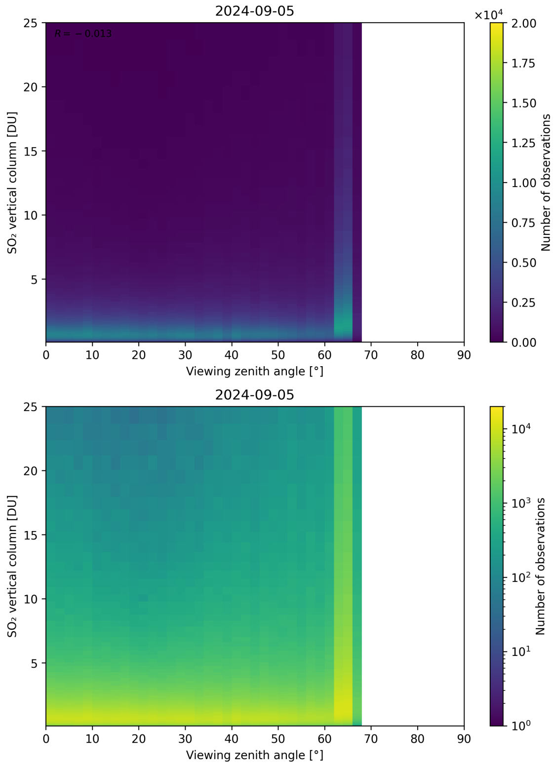
Figure 327: Scatter density plot of “Viewing zenith angle” against “SO 2 vertical column” for 2024-09-04 to 2024-09-06.
