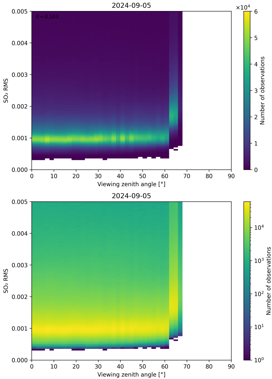
Figure 313: Scatter density plot of “Viewing zenith angle” against “SO 2 RMS” for 2024-09-04 to 2024-09-06.
