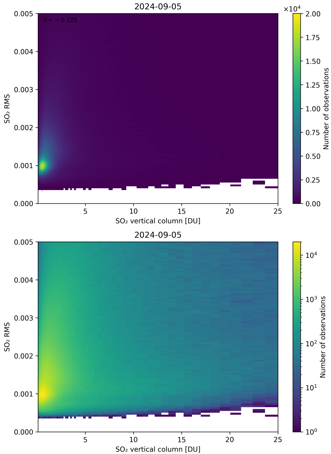
Figure 278: Scatter density plot of “SO 2 vertical column” against “SO 2 RMS” for 2024-09-04 to 2024-09-06.
