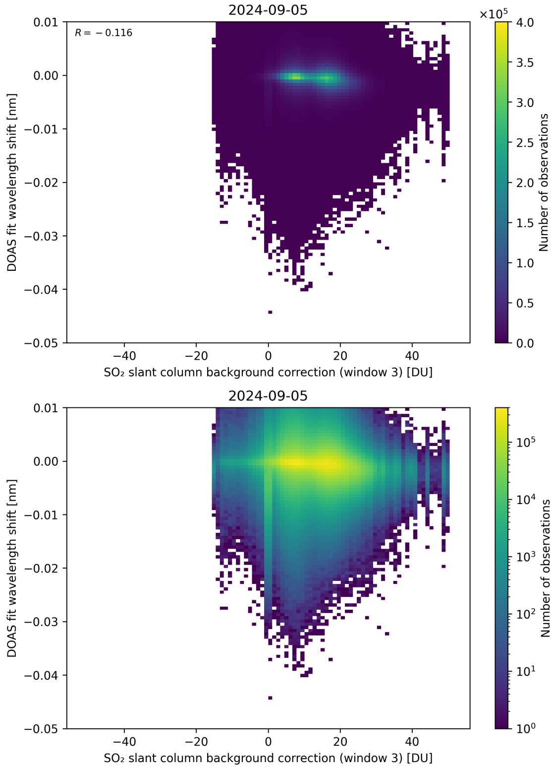
Figure 121: Scatter density plot of “SO 2 slant column background correction (window 3)” against “DOAS fit wavelength shift” for 2024-09-04 to 2024-09-06.
