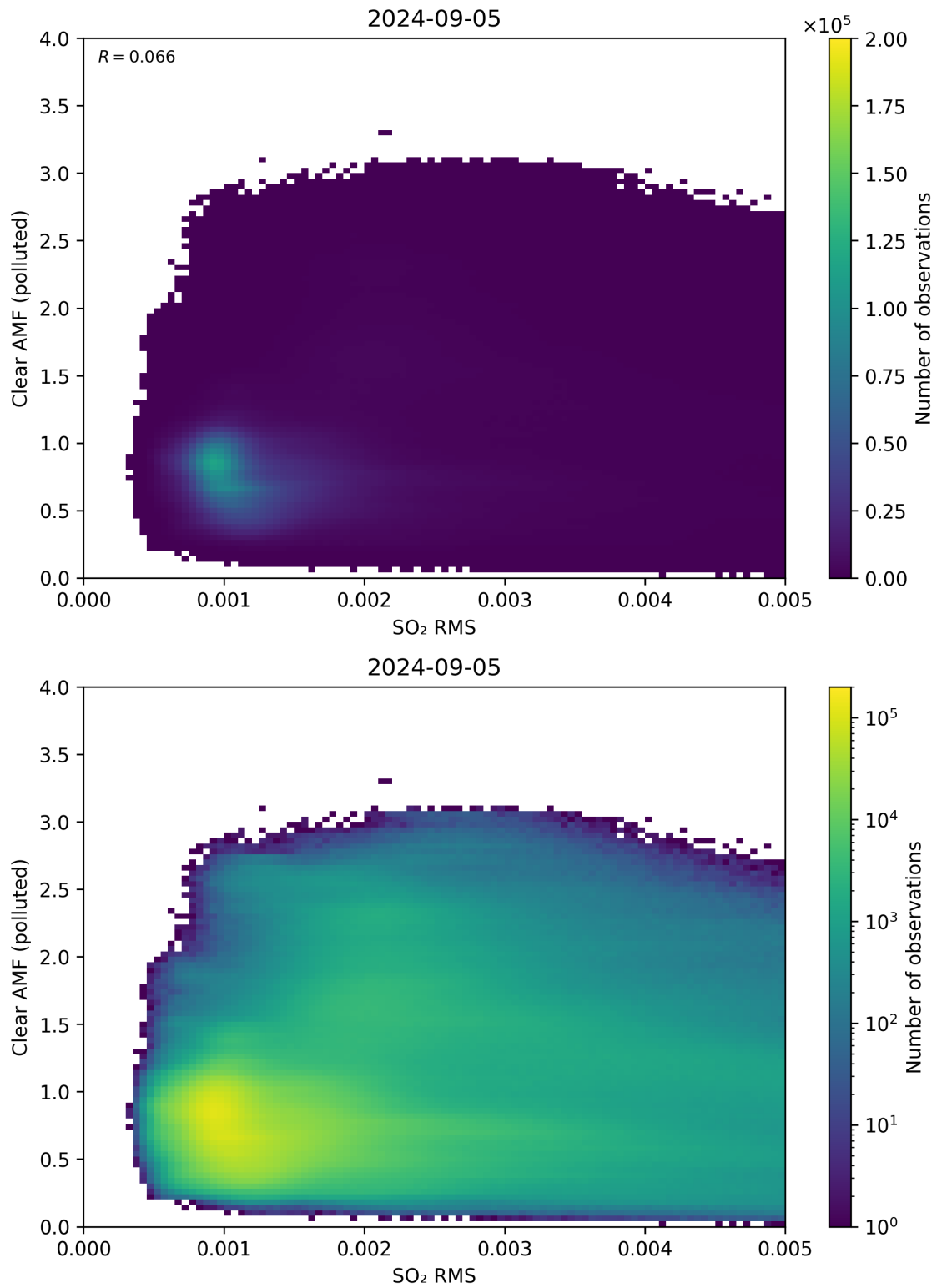
Figure 136: Scatter density plot of “SO 2 RMS” against “Clear AMF (polluted)” for 2024-09-04 to 2024-09-06.
