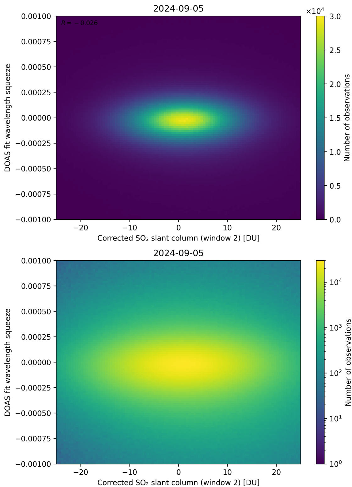
Figure 197: Scatter density plot of “Corrected SO 2 slant column (window 2)” against “DOAS fit wavelength squeeze” for 2024-09-04 to 2024-09-06.
