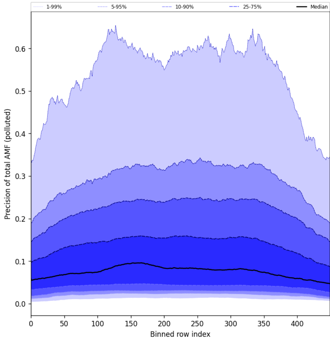
Figure 95: Along track statistics of “Precision of total AMF (polluted)” for 2024-09-04 to 2024-09-06
