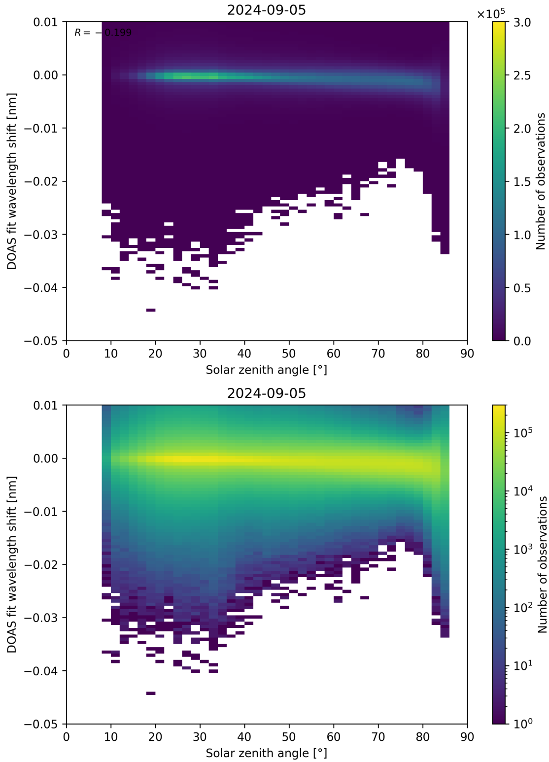
Figure 161: Scatter density plot of “Solar zenith angle” against “DOAS fit wavelength shift” for 2024-09-04 to 2024-09-06.
