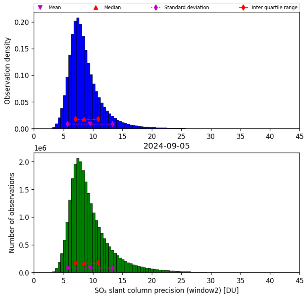
Figure 61: Histogram of “SO 2 slant column precision (window2)” for 2024-09-04 to 2024-09-06
