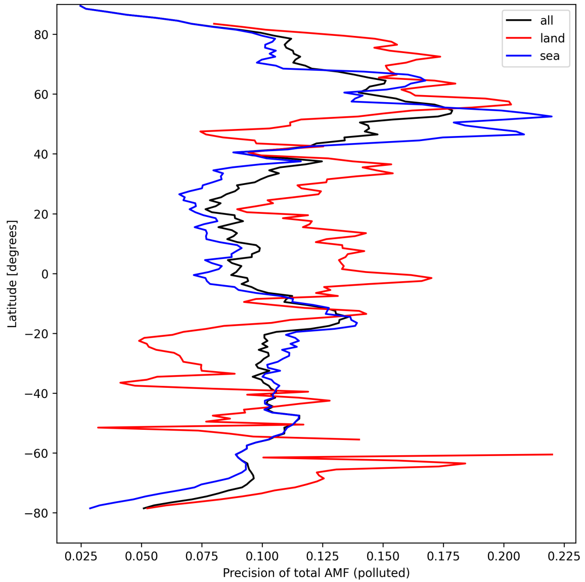
Figure 49: Zonal average of “Precision of total AMF (polluted)” for 2024-09-04 to 2024-09-06.
