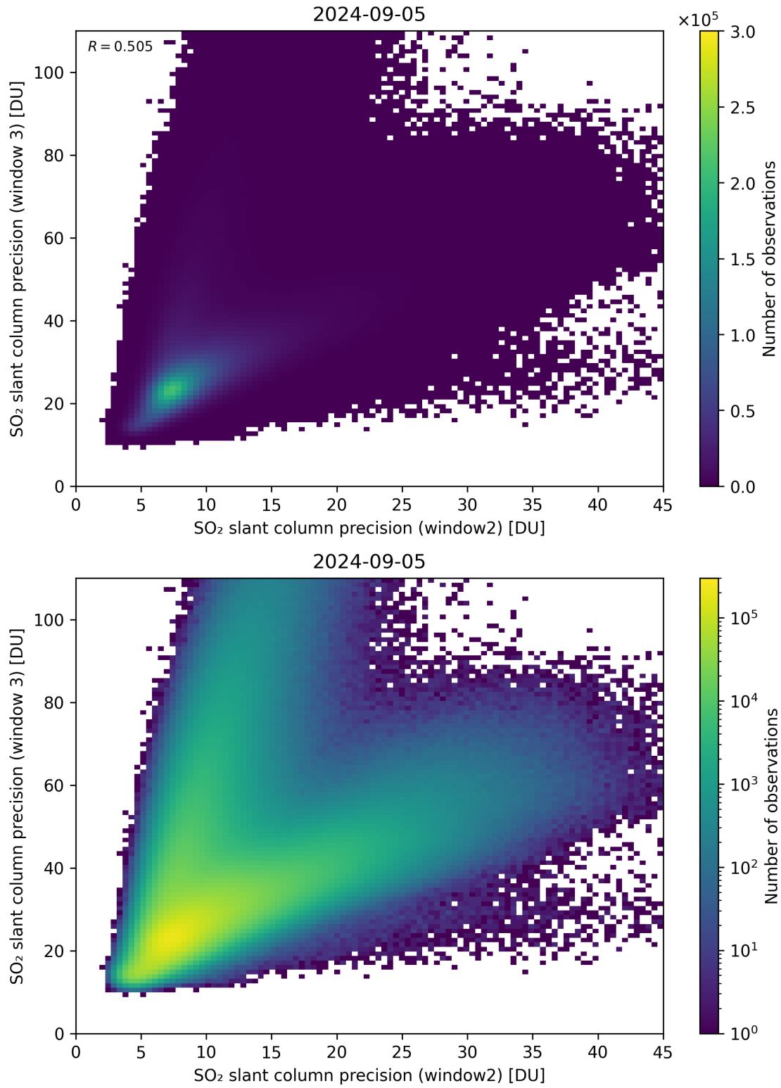
Figure 250: Scatter density plot of “SO 2 slant column precision (window2)” against “SO 2 slant column precision (window 3)” for 2024-09-04 to 2024-09-06.
