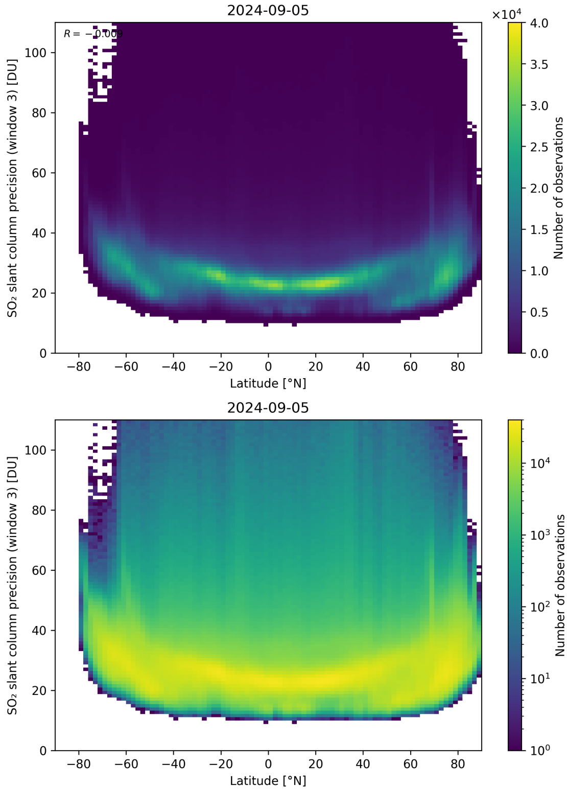
Figure 153: Scatter density plot of “Latitude” against “SO 2 slant column precision (window 3)” for 2024-09-04 to 2024-09-06.
