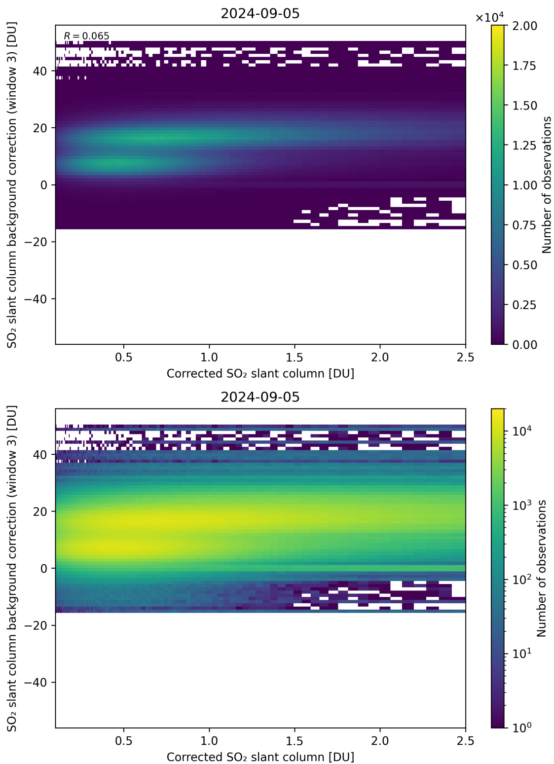
Figure 180: Scatter density plot of “Corrected SO 2 slant column” against “SO 2 slant column background correction (window 3)” for 2024-09-04 to 2024-09-06.
