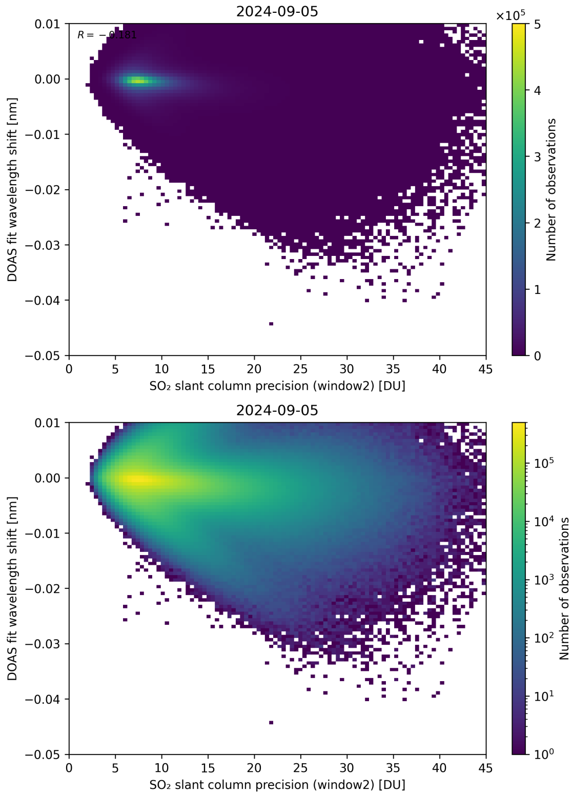
Figure 243: Scatter density plot of “SO 2 slant column precision (window2)” against “DOAS fit wavelength shift” for 2024-09-04 to 2024-09-06.
