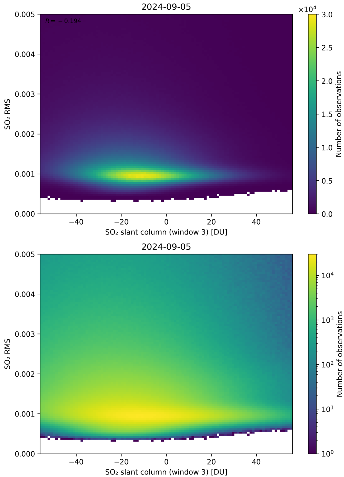
Figure 256: Scatter density plot of “SO 2 slant column (window 3)” against “SO 2 RMS” for 2024-09-04 to 2024-09-06.
