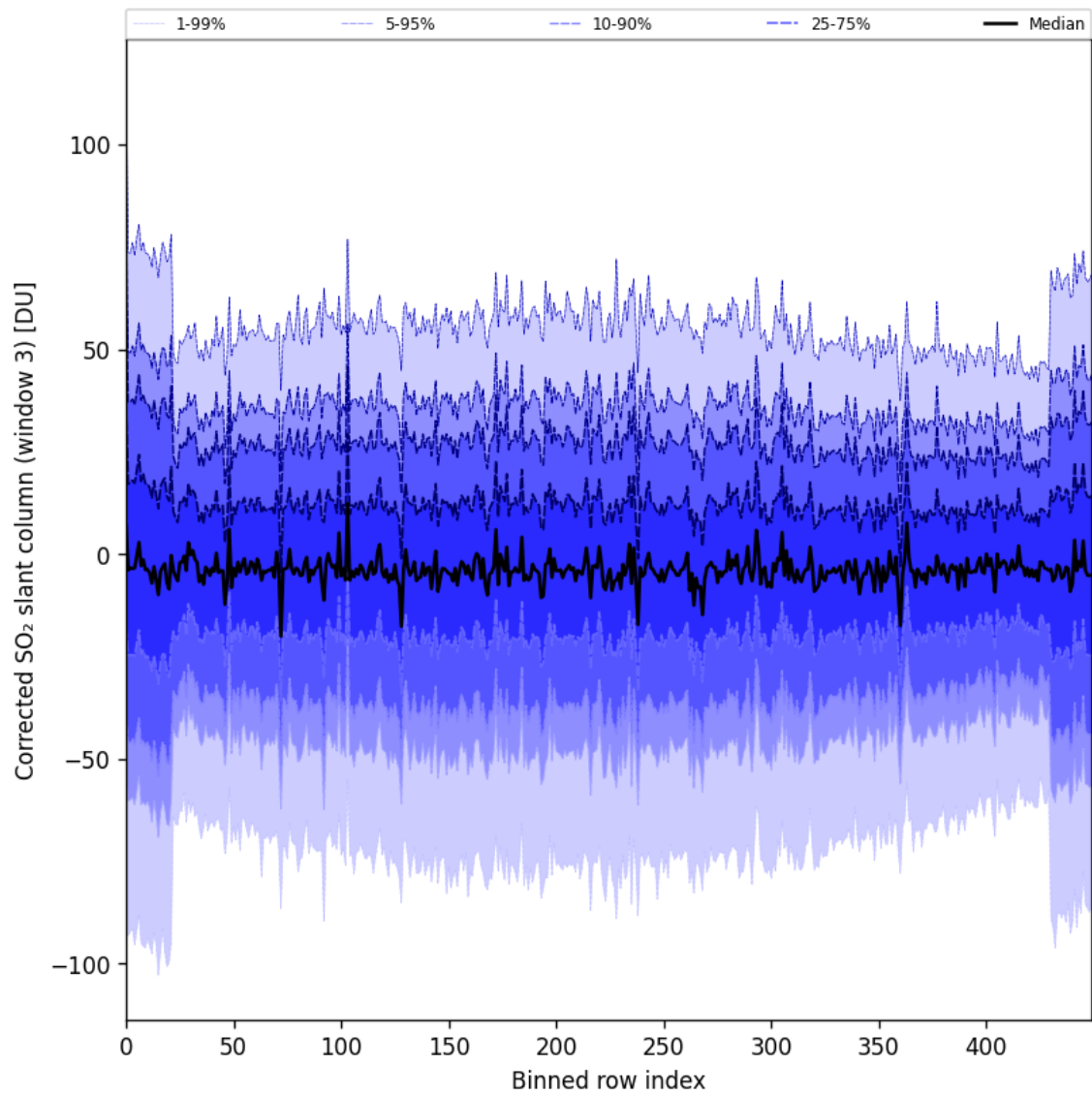
Figure 89: Along track statistics of “Corrected SO 2 slant column (window 3)” for 2024-09-04 to 2024-09-06
