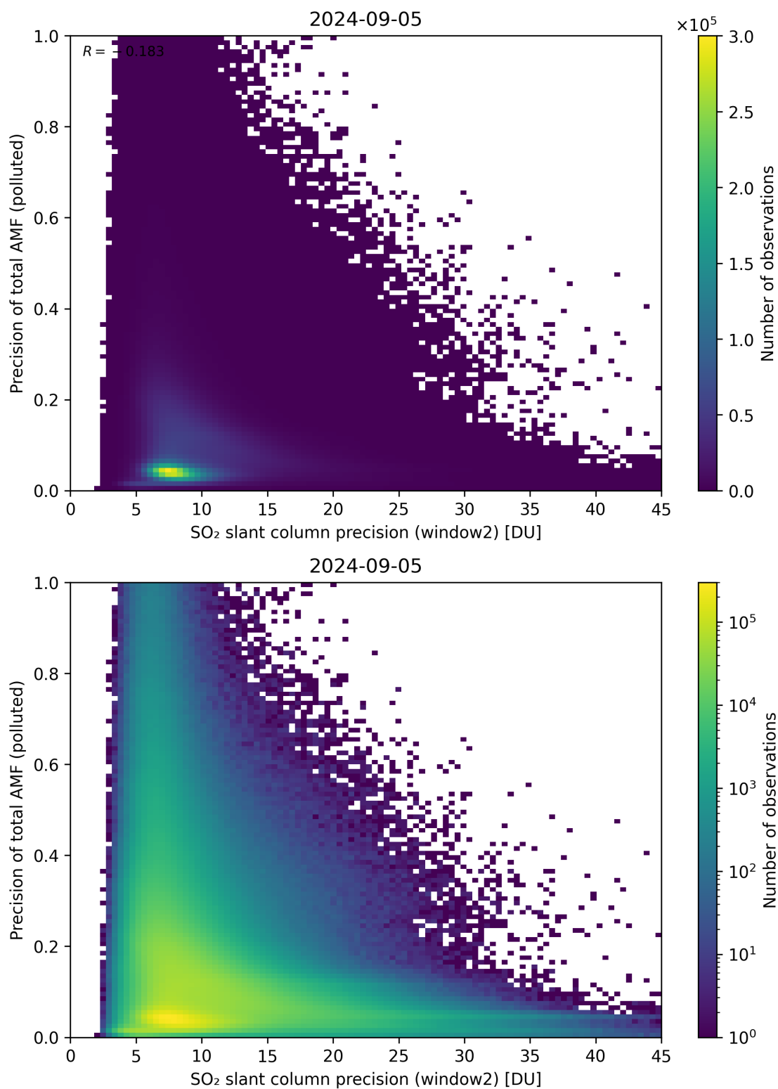
Figure 252: Scatter density plot of “SO 2 slant column precision (window2)” against “Precision of total AMF (polluted)” for 2024-09-04 to 2024-09-06.
