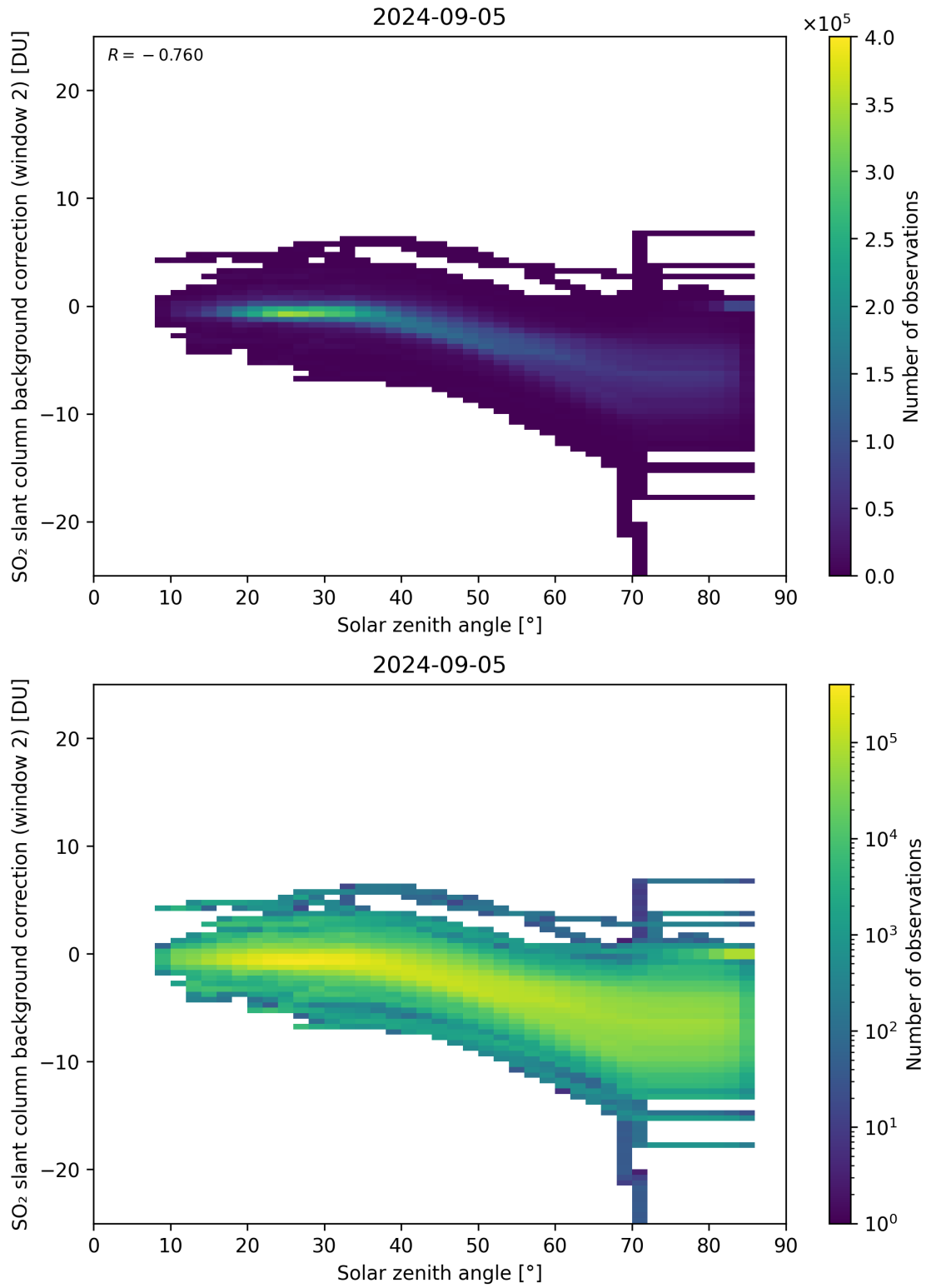
Figure 159: Scatter density plot of “Solar zenith angle” against “SO 2 slant column background correction (window 2)” for 2024-09-04 to 2024-09-06.
