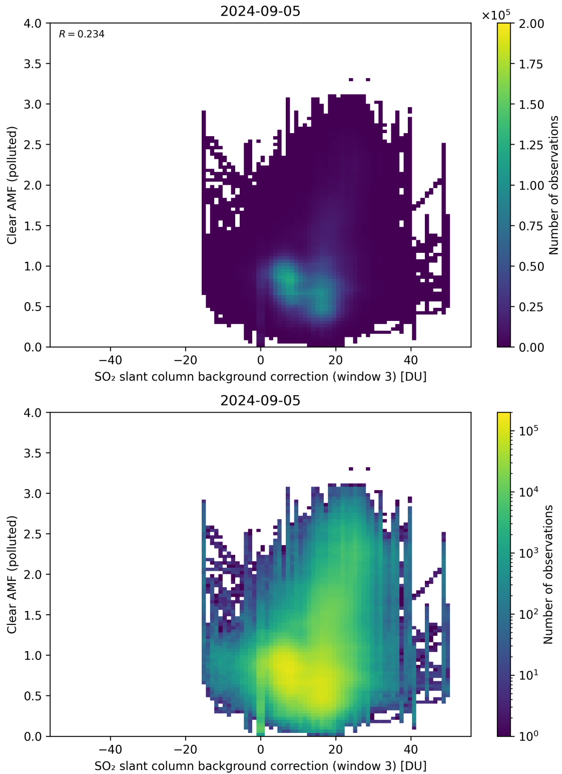
Figure 124: Scatter density plot of “SO 2 slant column background correction (window 3)” against “Clear AMF (polluted)” for 2024-09-04 to 2024-09-06.
