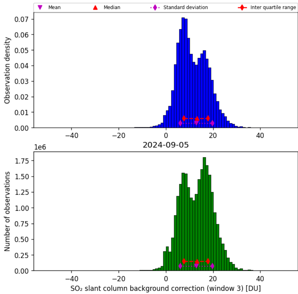
Figure 67: Histogram of “SO 2 slant column background correction (window 3)” for 2024-09-04 to 2024-09-06
