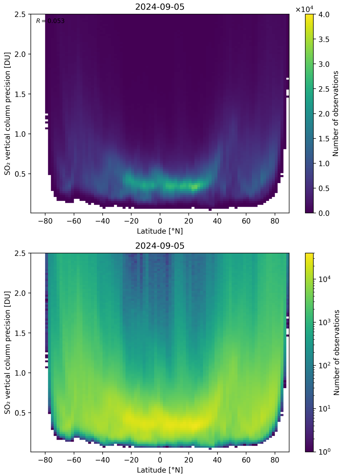
Figure 157: Scatter density plot of “Latitude” against “SO 2 vertical column precision” for 2024-09-04 to 2024-09-06.
