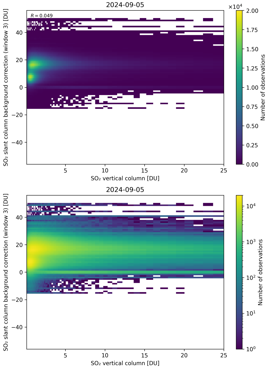
Figure 275: Scatter density plot of “SO 2 vertical column” against “SO 2 slant column background correction (window 3)” for 2024-09-04 to 2024-09-06.
