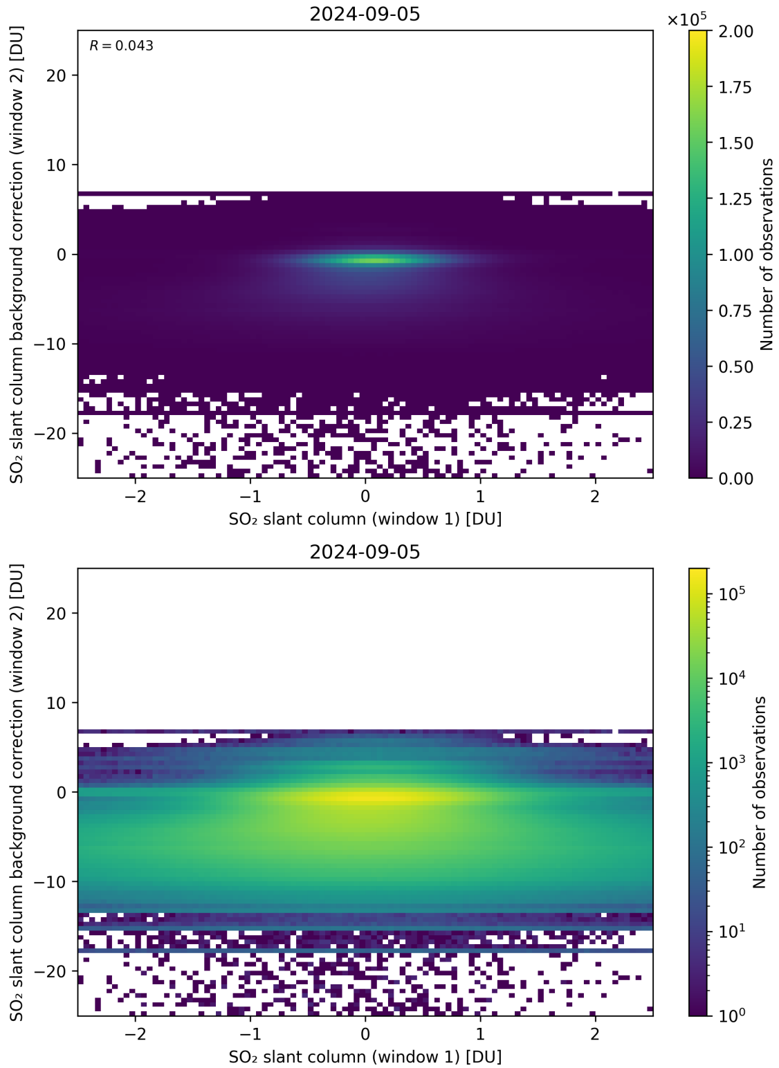
Figure 213: Scatter density plot of “SO 2 slant column (window 1)” against “SO 2 slant column background correction (window 2)” for 2024-09-04 to 2024-09-06.
