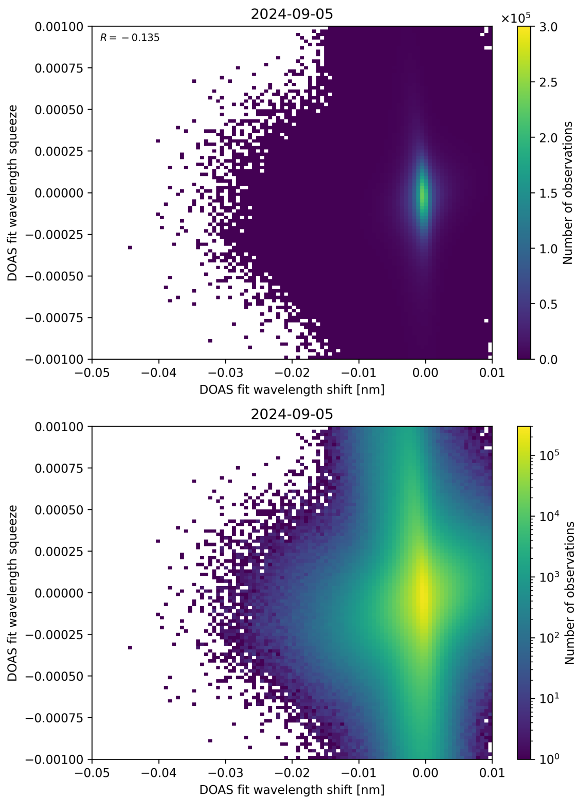
Figure 127: Scatter density plot of “DOAS fit wavelength shift” against “DOAS fit wavelength squeeze” for 2024-09-04 to 2024-09-06.
