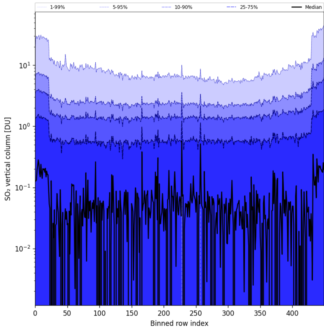
Figure 76: Along track statistics of “SO 2 vertical column” for 2024-09-04 to 2024-09-06
