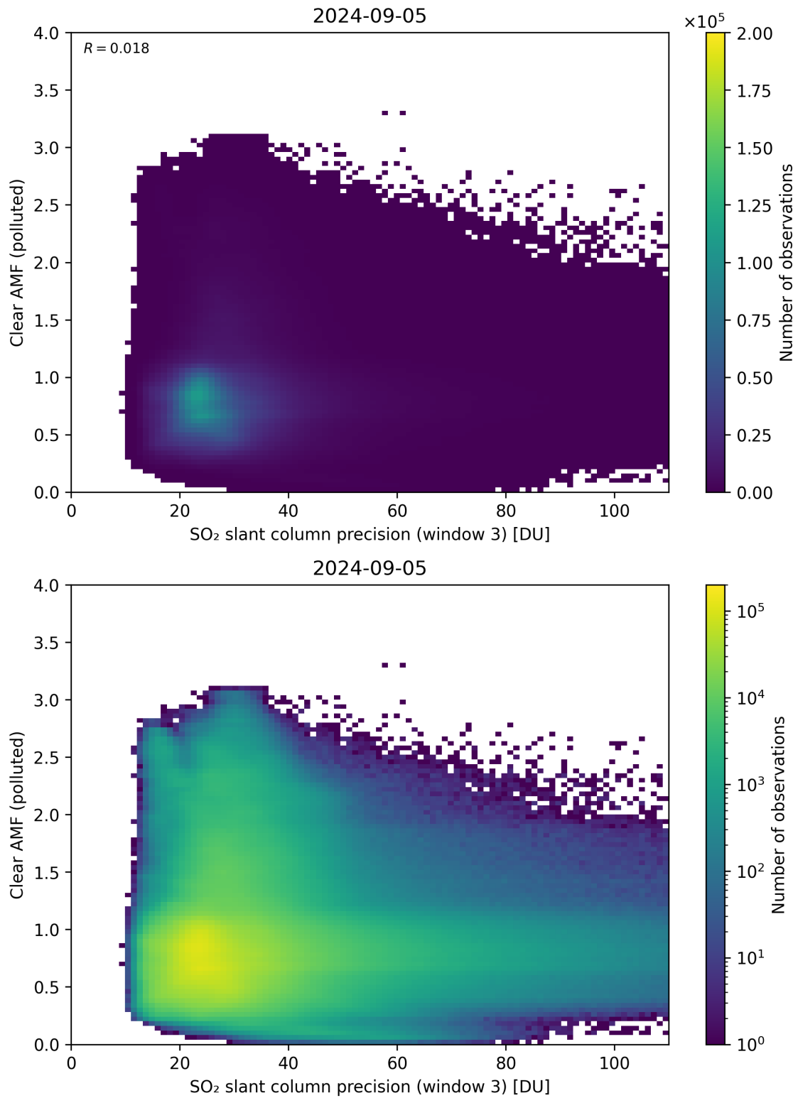
Figure 261: Scatter density plot of “SO 2 slant column precision (window 3)” against “Clear AMF (polluted)” for 2024-09-04 to 2024-09-06.
