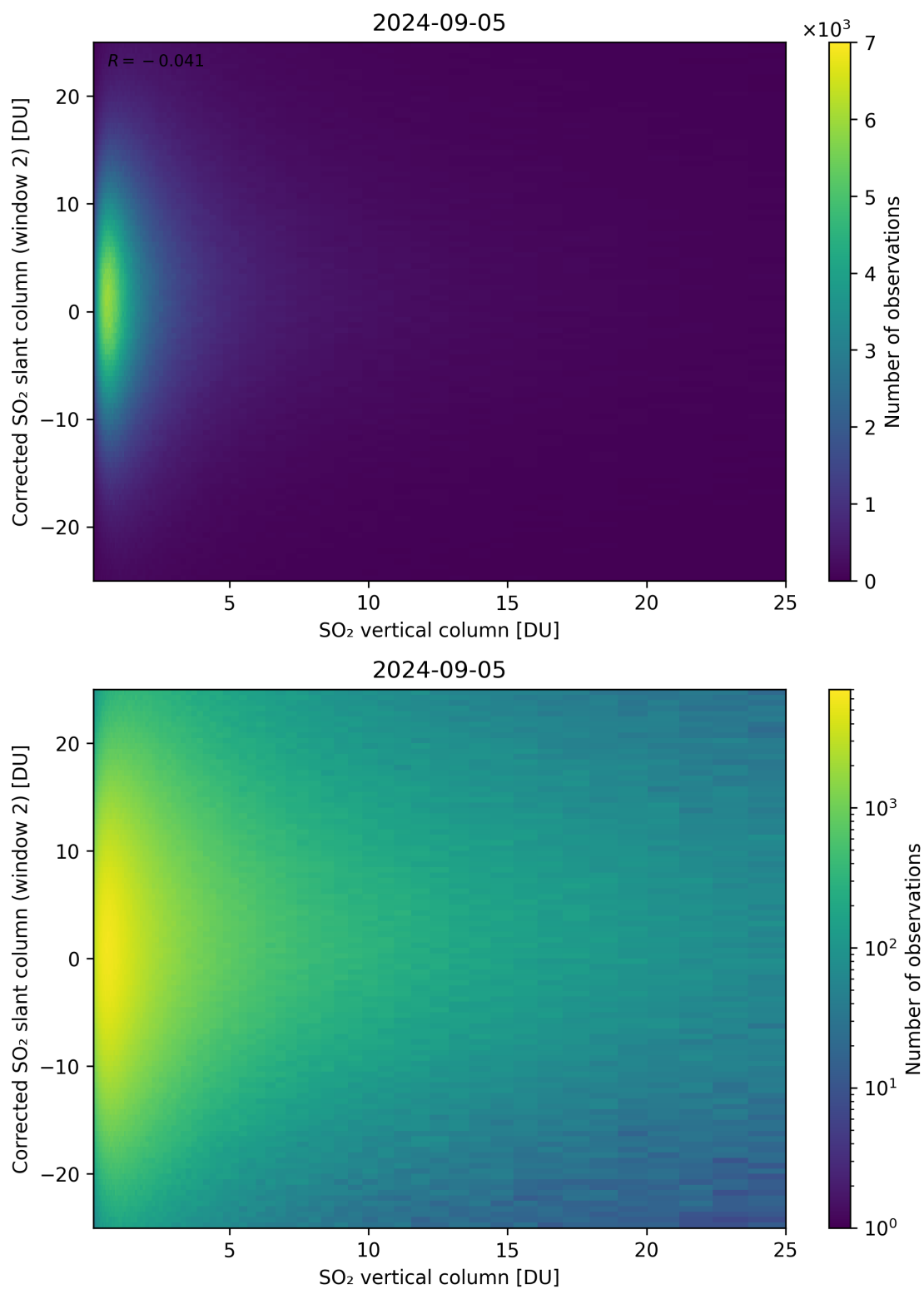
Figure 298: Scatter density plot of “SO 2 vertical column” against “Corrected SO 2 slant column (window 2)” for 2024-09-04 to 2024-09-06.
