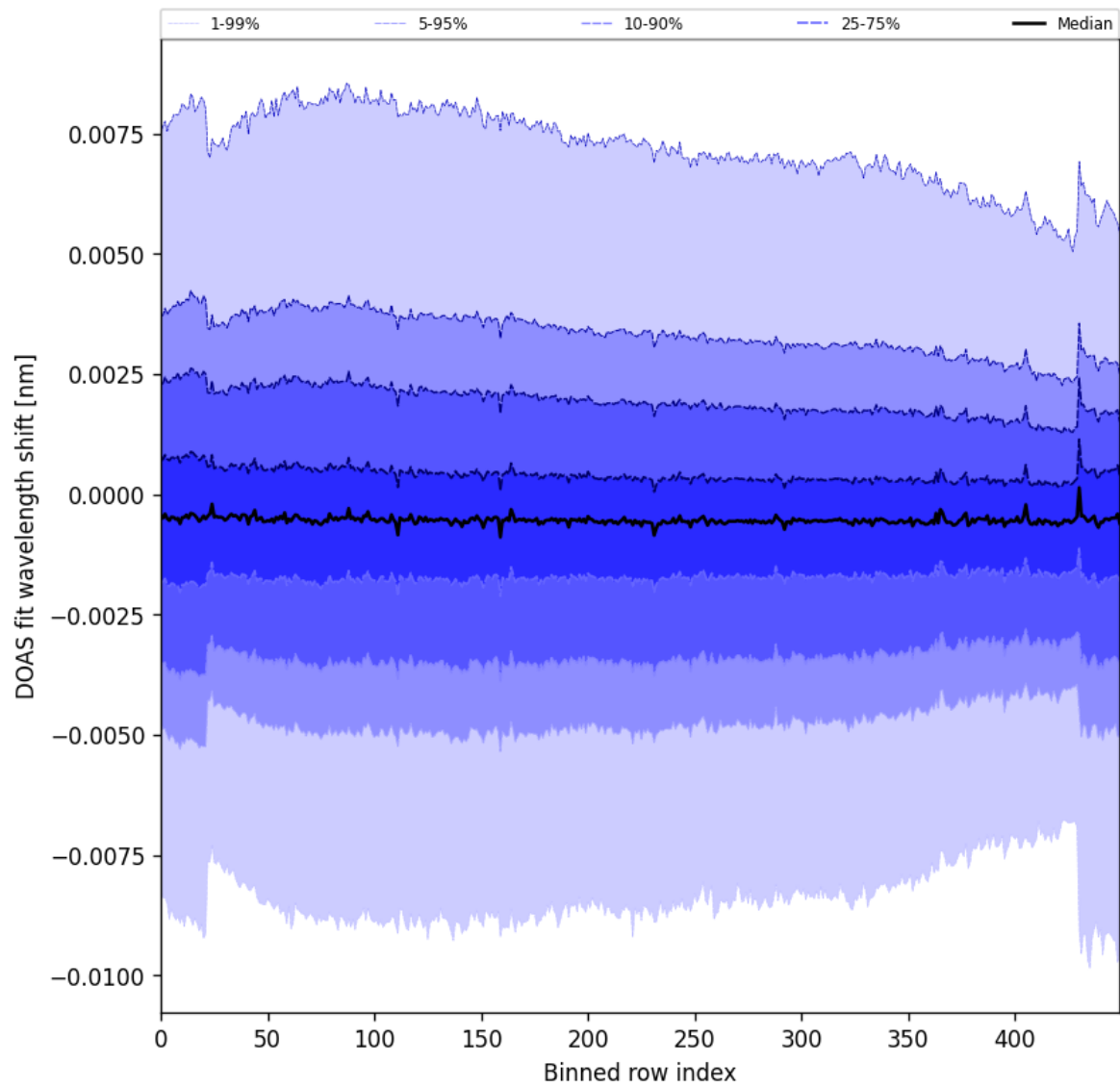
Figure 91: Along track statistics of “DOAS fit wavelength shift” for 2024-09-04 to 2024-09-06
