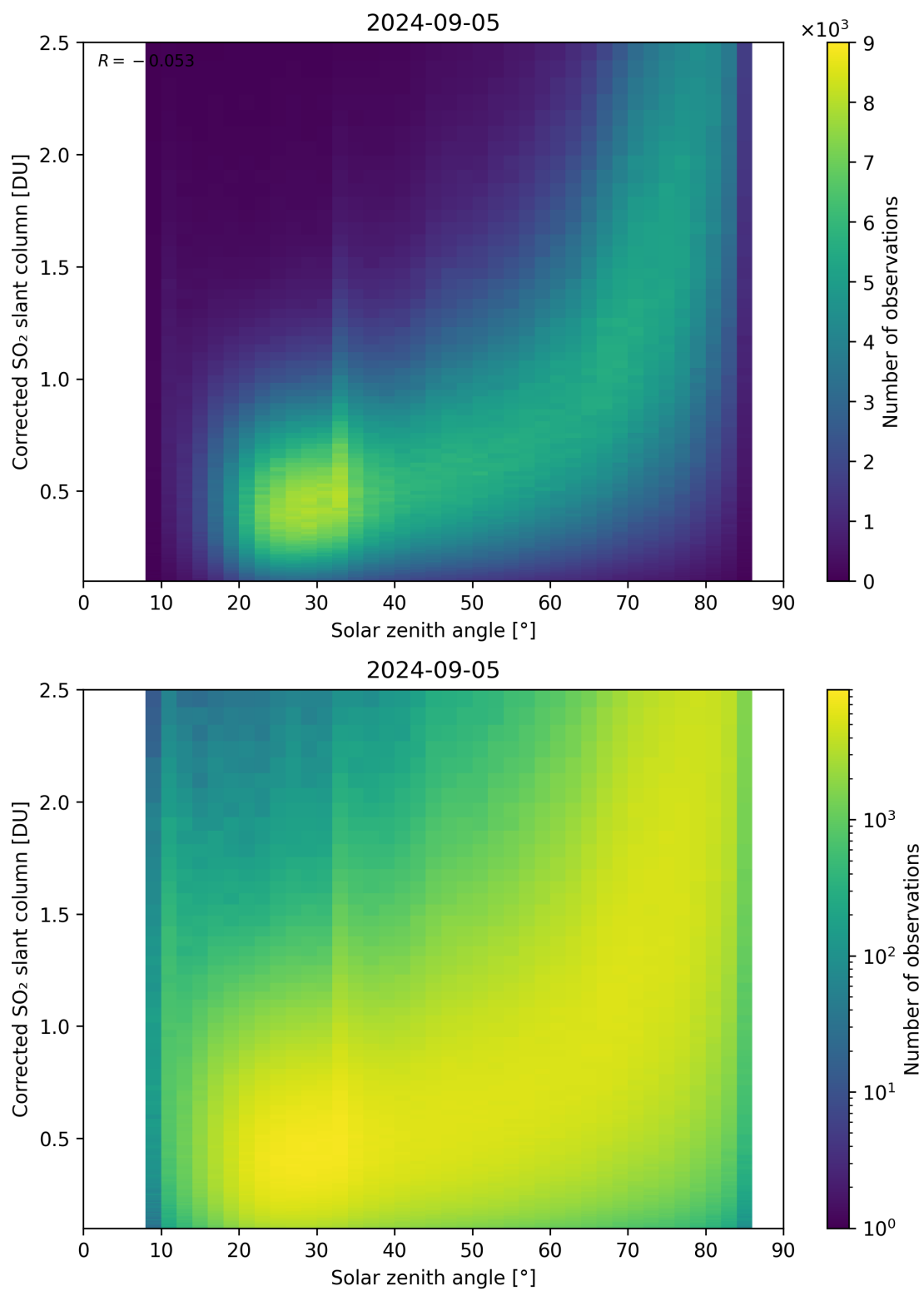
Figure 166: Scatter density plot of “Solar zenith angle” against “Corrected SO 2 slant column” for 2024-09-04 to 2024-09-06.
