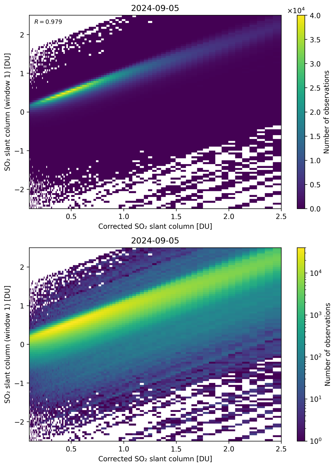
Figure 187: Scatter density plot of “Corrected SO 2 slant column” against “SO 2 slant column (window 1)” for 2024-09-04 to 2024-09-06.
