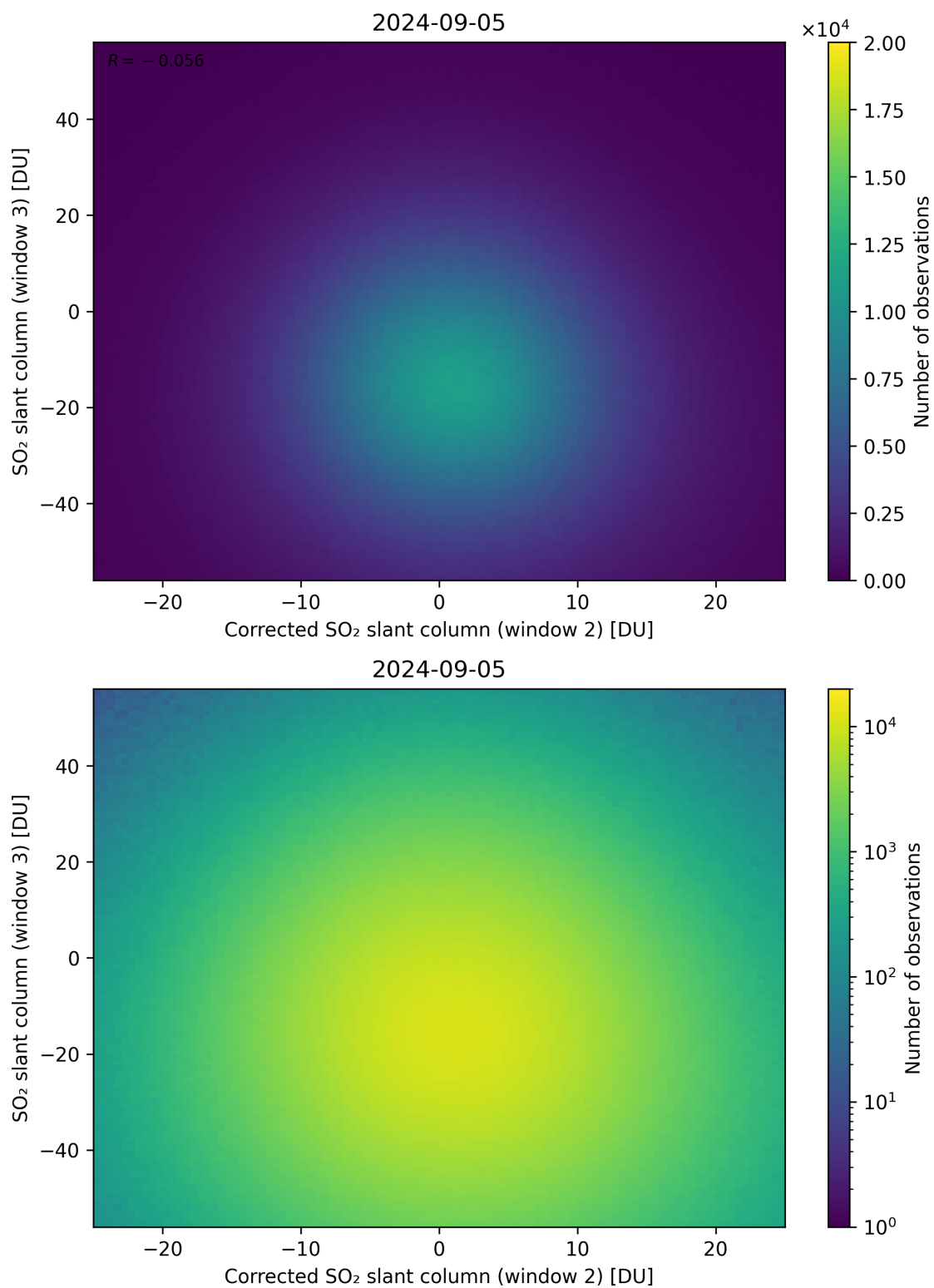
Figure 201: Scatter density plot of “Corrected SO 2 slant column (window 2)” against “SO 2 slant column (window 3)” for 2024-09-04 to 2024-09-06.
