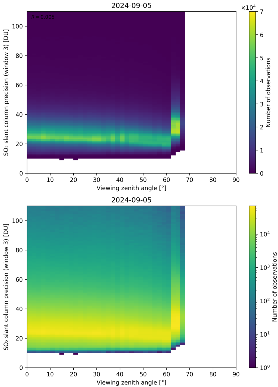
Figure 324: Scatter density plot of “Viewing zenith angle” against “SO 2 slant column precision (window 3)” for 2024-09-04 to 2024-09-06.
