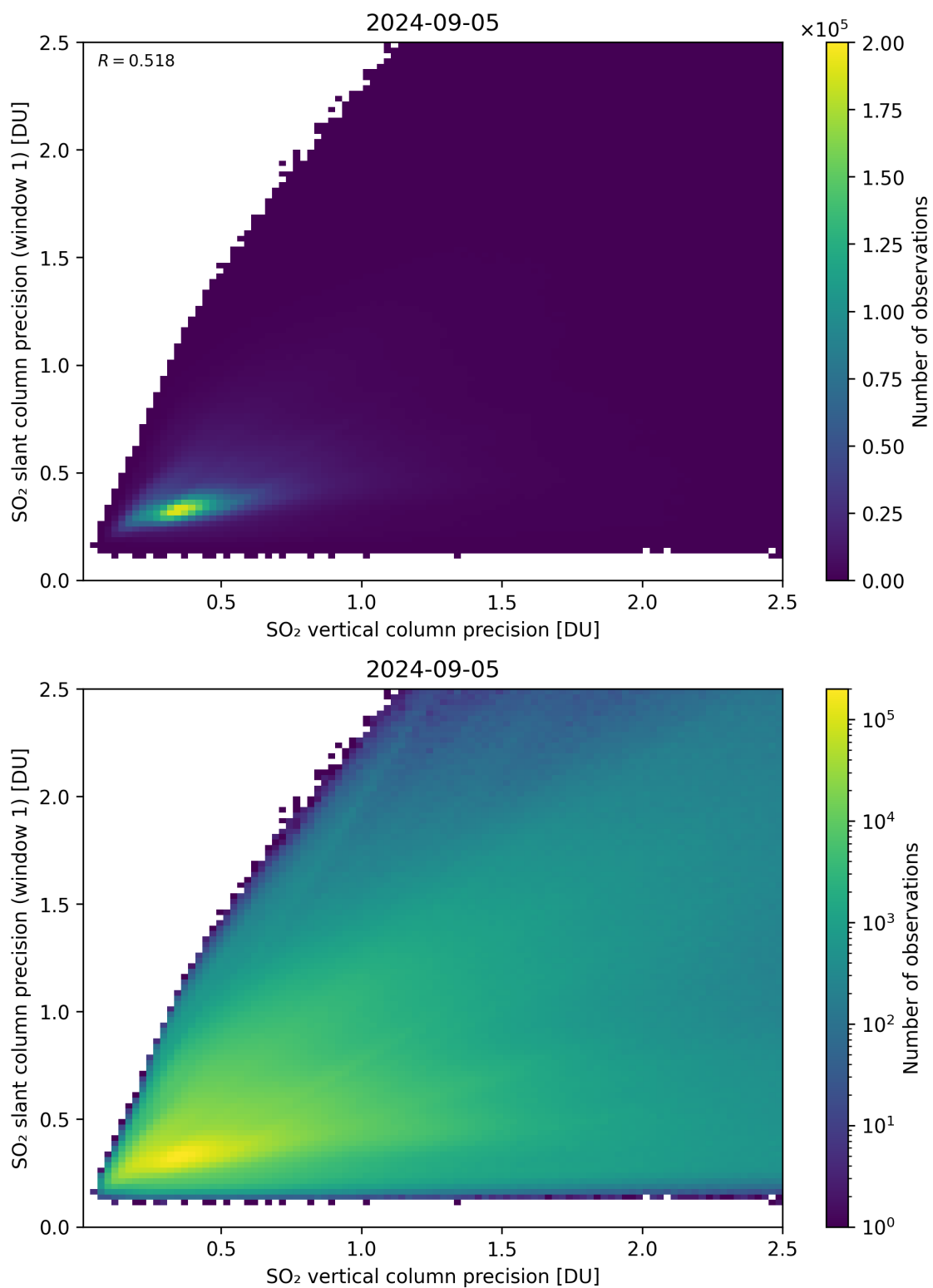
Figure 290: Scatter density plot of “SO 2 vertical column precision” against “SO 2 slant column precision (window 1)” for 2024-09-04 to 2024-09-06.
