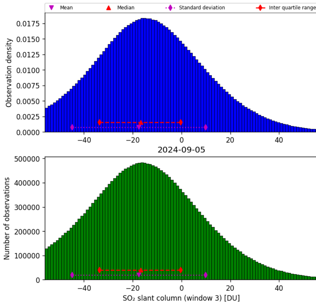
Figure 64: Histogram of “SO 2 slant column (window 3)” for 2024-09-04 to 2024-09-06
