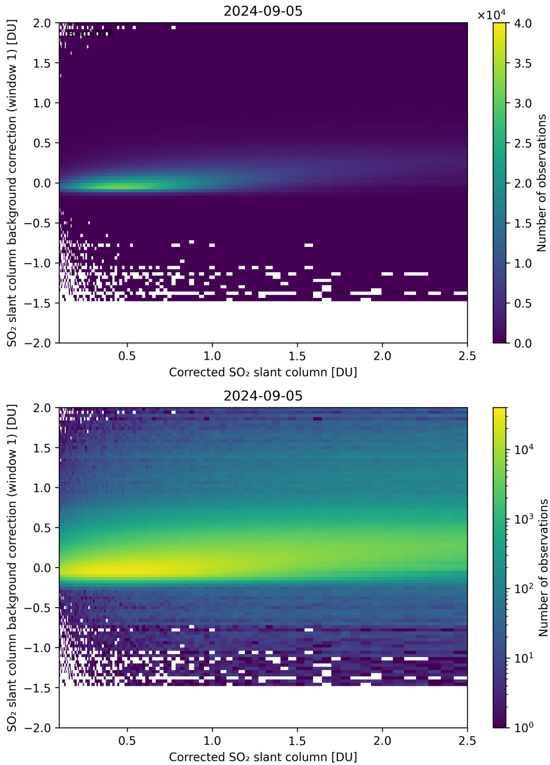
Figure 178: Scatter density plot of “Corrected SO 2 slant column” against “SO 2 slant column background correction (window 1)” for 2024-09-04 to 2024-09-06.
