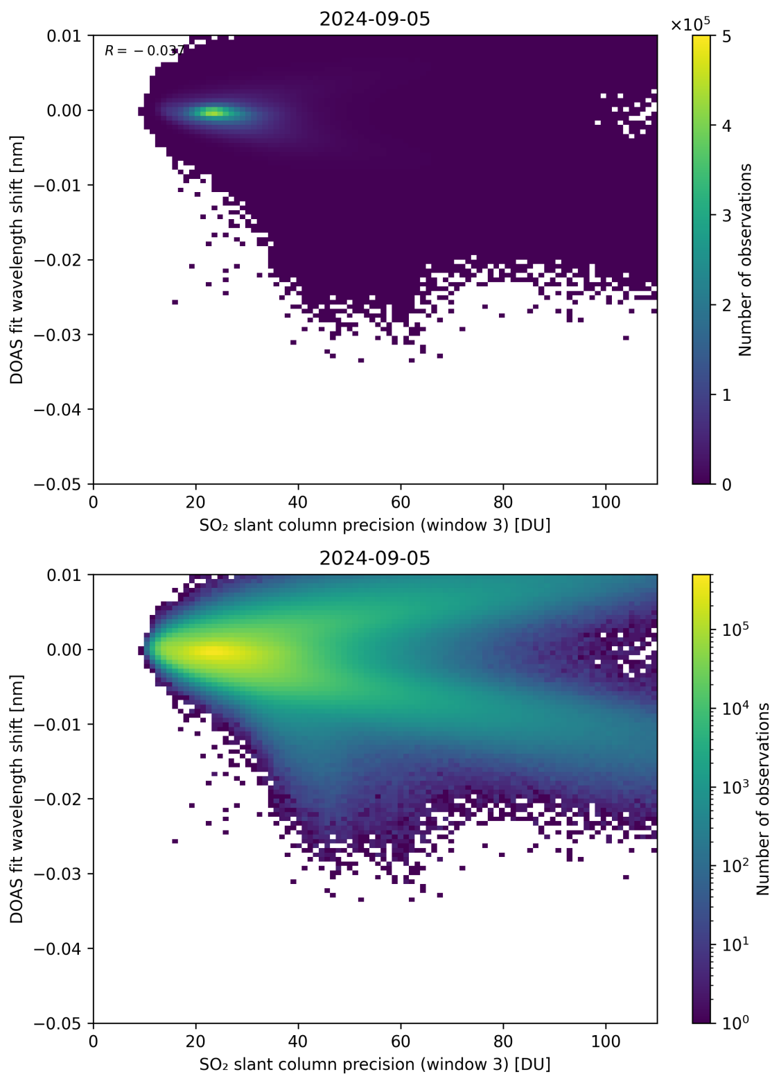
Figure 258: Scatter density plot of “SO 2 slant column precision (window 3)” against “DOAS fit wavelength shift” for 2024-09-04 to 2024-09-06.
