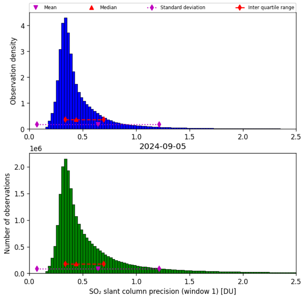
Figure 57: Histogram of “SO 2 slant column precision (window 1)” for 2024-09-04 to 2024-09-06
