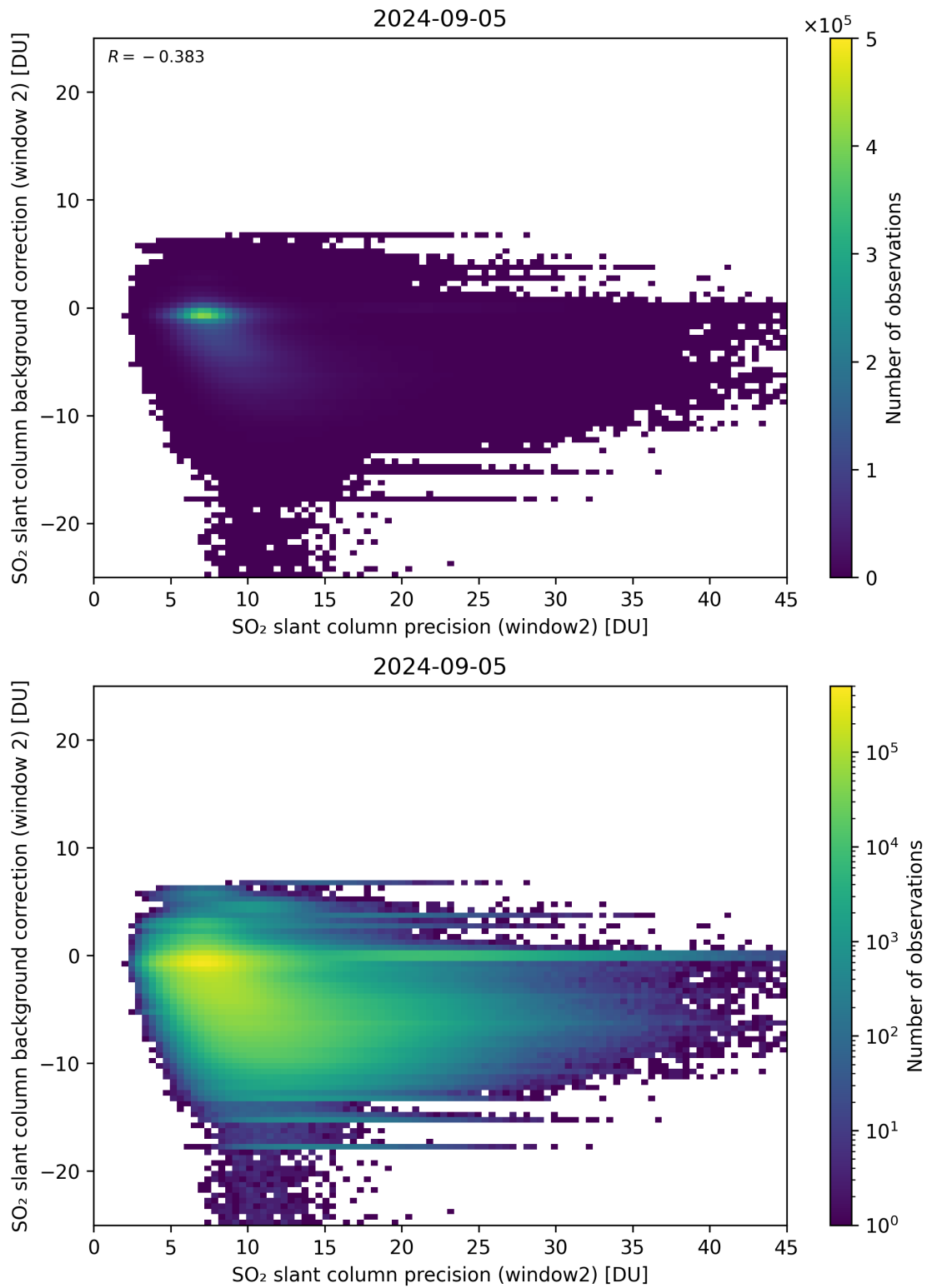
Figure 241: Scatter density plot of “SO 2 slant column precision (window2)” against “SO 2 slant column background correction (window 2)” for 2024-09-04 to 2024-09-06.
