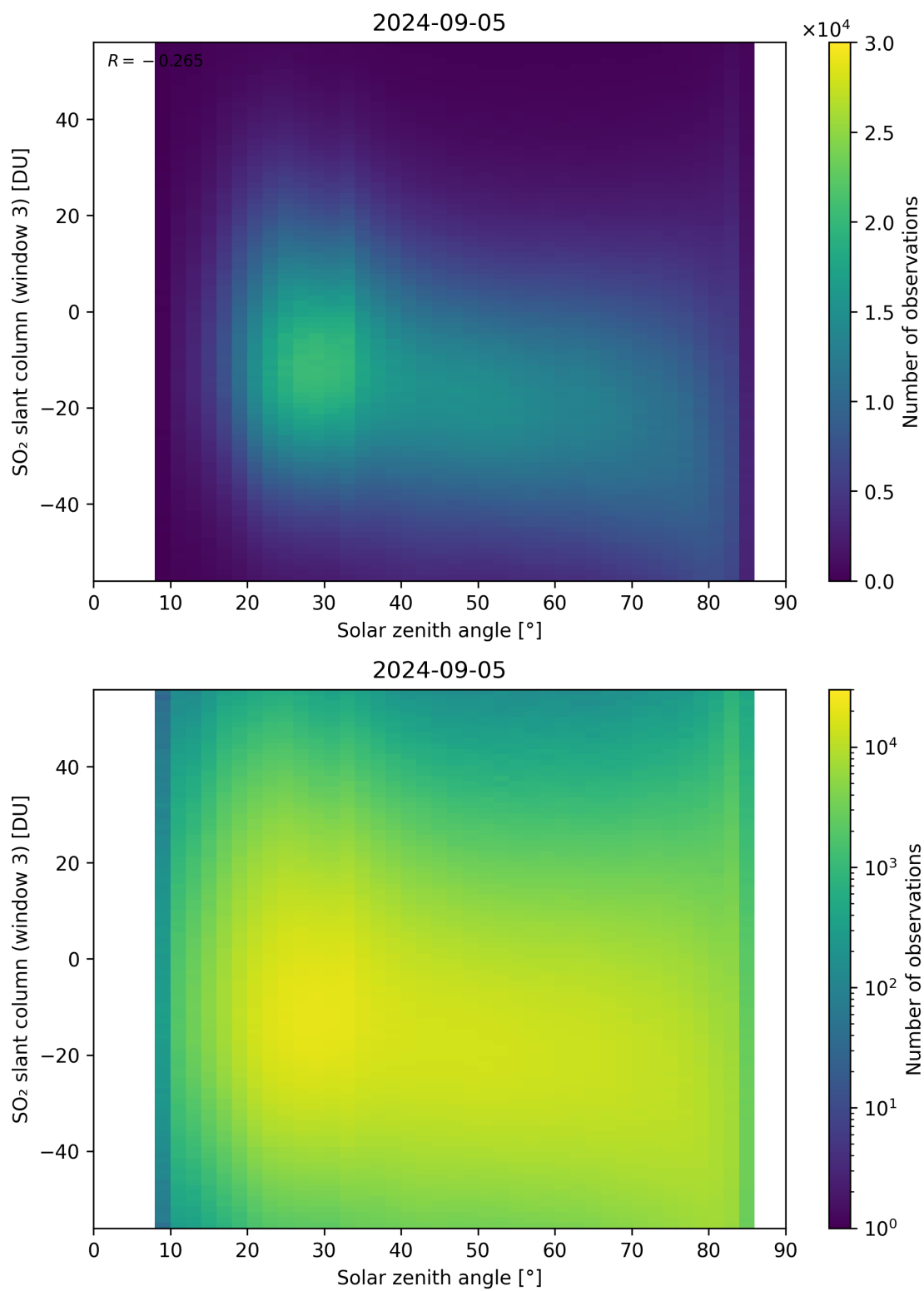
Figure 172: Scatter density plot of “Solar zenith angle” against “SO 2 slant column (window 3)” for 2024-09-04 to 2024-09-06.
