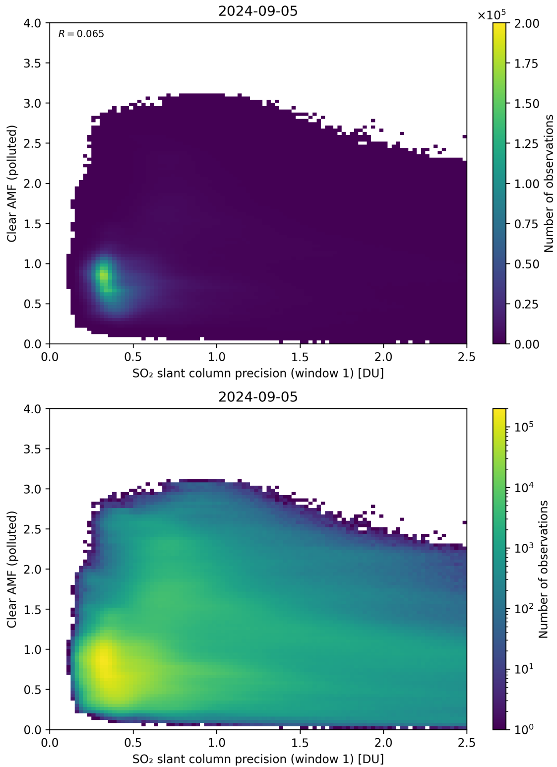
Figure 224: Scatter density plot of “SO 2 slant column precision (window 1)” against “Clear AMF (polluted)” for 2024-09-04 to 2024-09-06.
