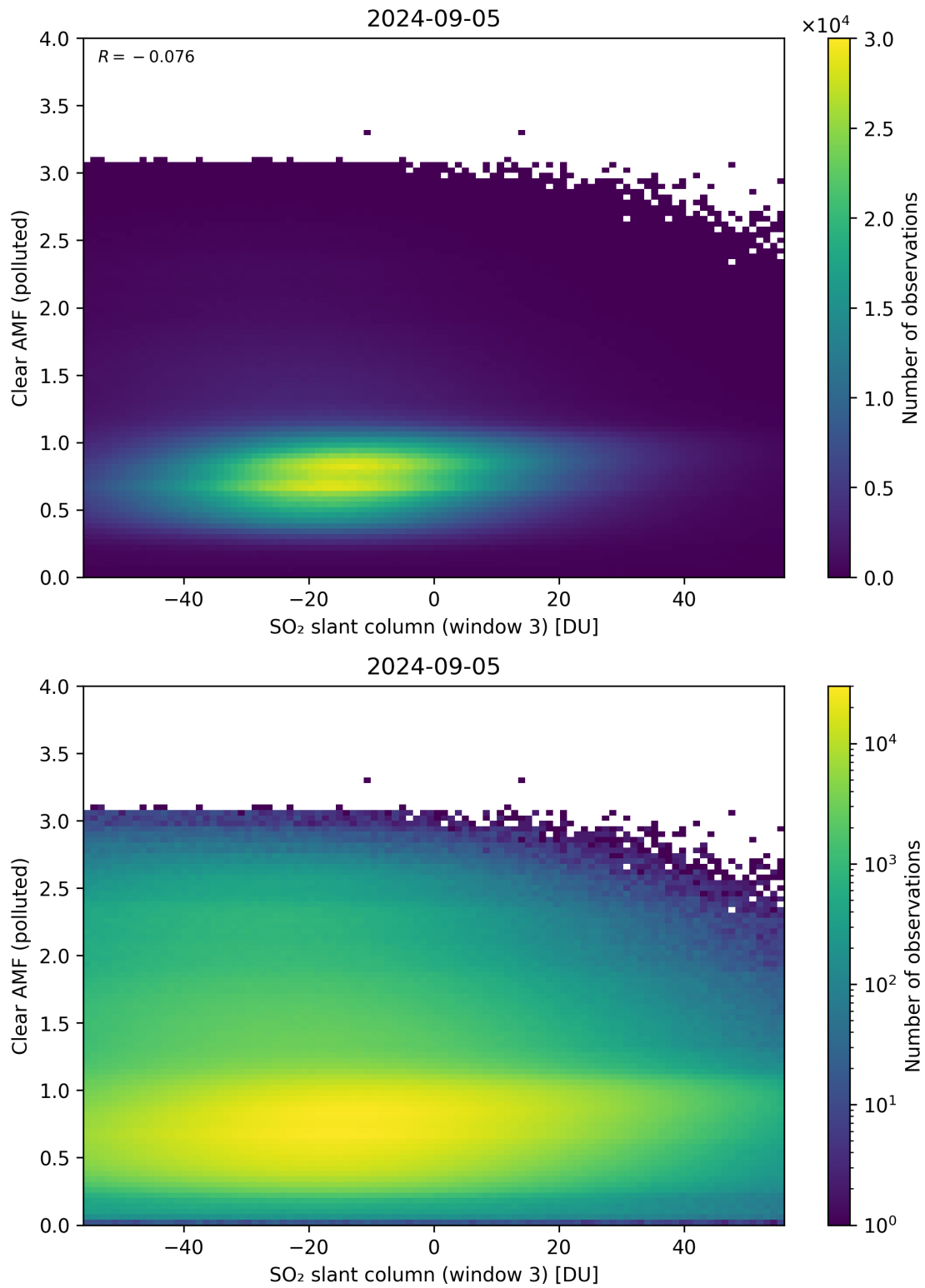
Figure 265: Scatter density plot of “SO 2 slant column (window 3)” against “Clear AMF (polluted)” for 2024-09-04 to 2024-09-06.
