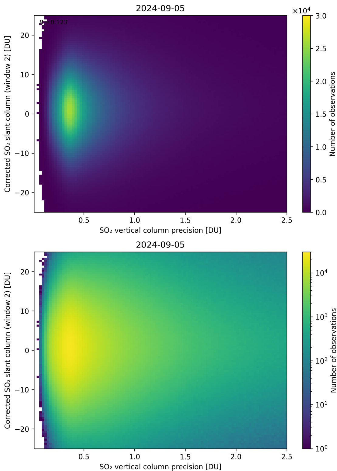
Figure 287: Scatter density plot of “SO 2 vertical column precision” against “Corrected SO 2 slant column (window 2)” for 2024-09-04 to 2024-09-06.
