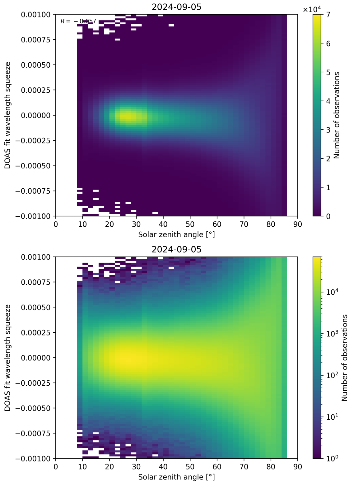
Figure 162: Scatter density plot of “Solar zenith angle” against “DOAS fit wavelength squeeze” for 2024-09-04 to 2024-09-06.
