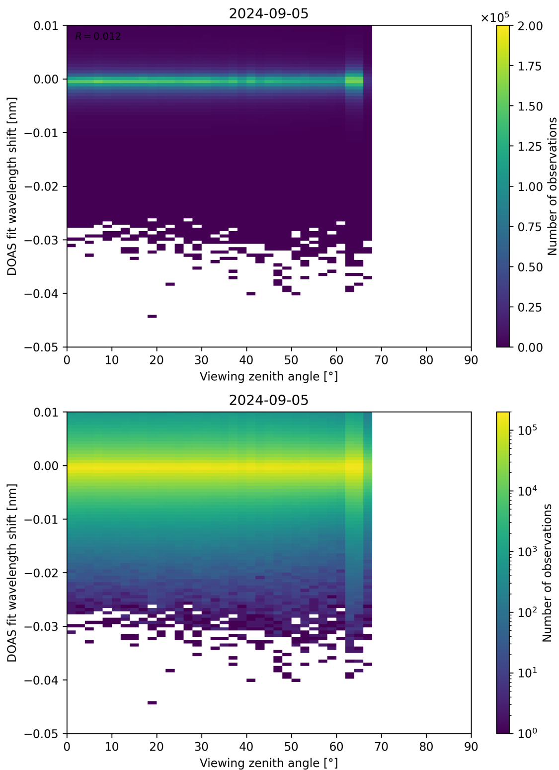
Figure 311: Scatter density plot of “Viewing zenith angle” against “DOAS fit wavelength shift” for 2024-09-04 to 2024-09-06.
