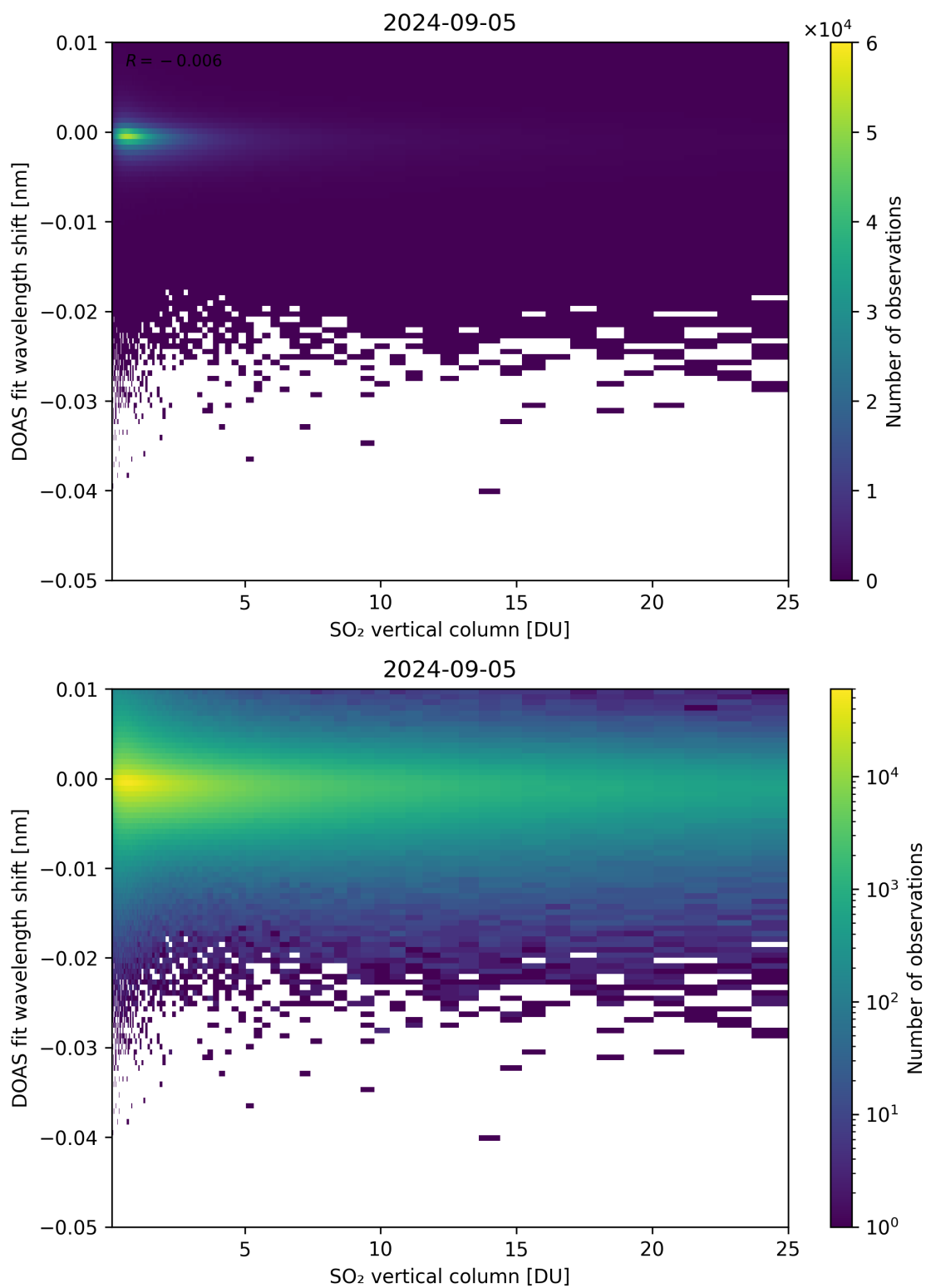
Figure 276: Scatter density plot of “SO 2 vertical column” against “DOAS fit wavelength shift” for 2024-09-04 to 2024-09-06.
