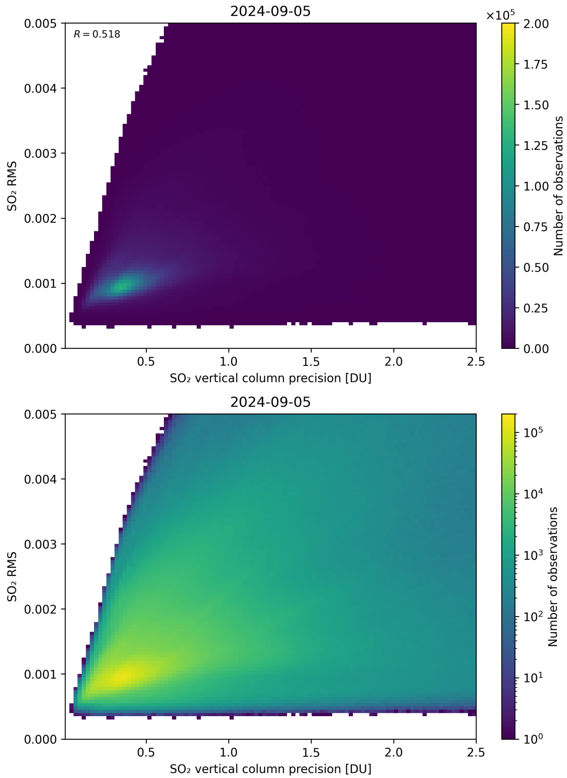
Figure 284: Scatter density plot of “SO 2 vertical column precision” against “SO 2 RMS” for 2024-09-04 to 2024-09-06.
