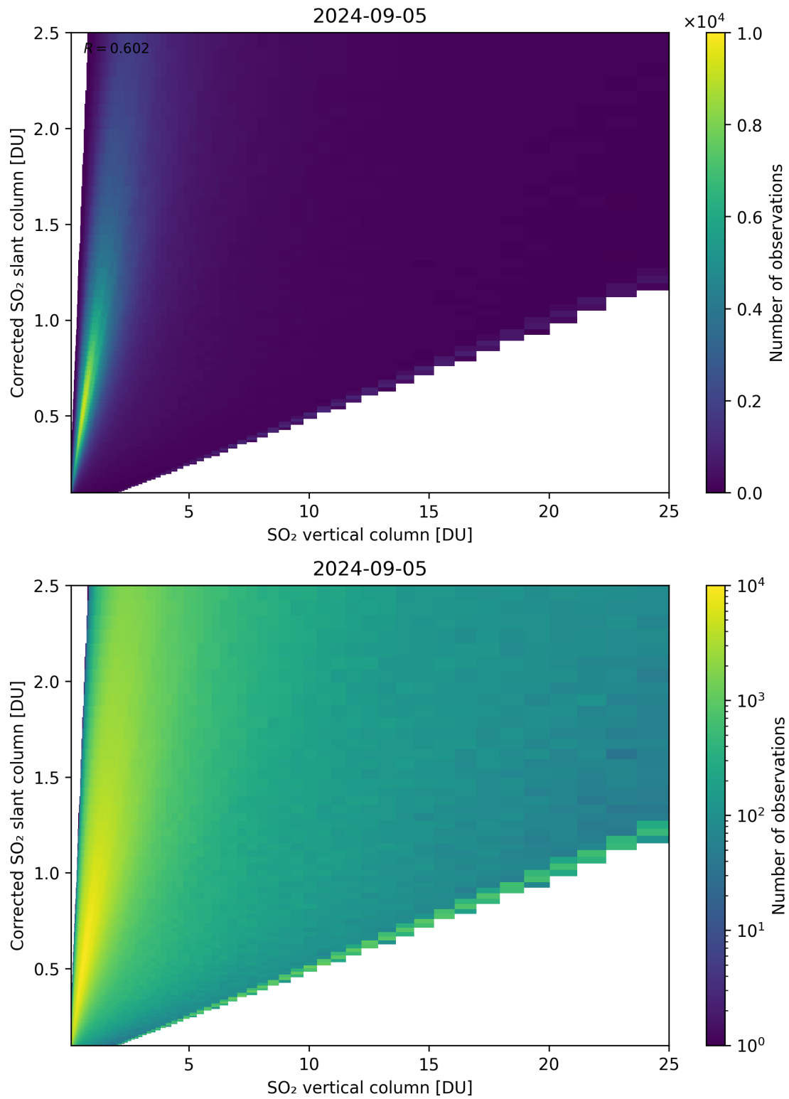
Figure 297: Scatter density plot of “SO 2 vertical column” against “Corrected SO 2 slant column” for 2024-09-04 to 2024-09-06.
