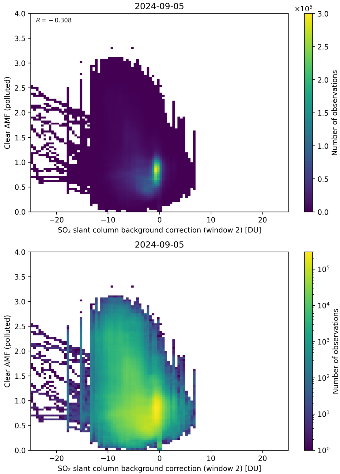
Figure 115: Scatter density plot of “SO 2 slant column background correction (window 2)” against “Clear AMF (polluted)” for 2024-09-04 to 2024-09-06.
