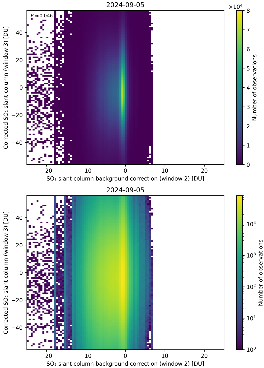
Figure 116: Scatter density plot of “SO 2 slant column background correction (window 2)” against “Corrected SO 2 slant column (window 3)” for 2024-09-04 to 2024-09-06.
