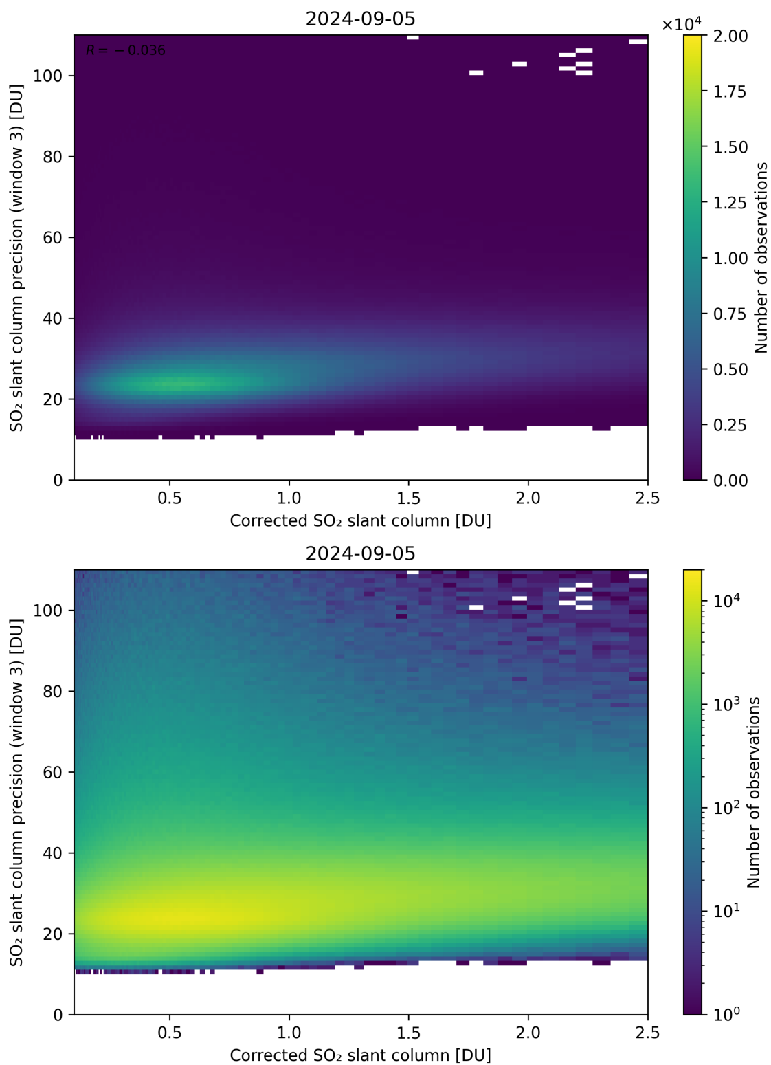
Figure 191: Scatter density plot of “Corrected SO 2 slant column” against “SO 2 slant column precision (window 3)” for 2024-09-04 to 2024-09-06.
