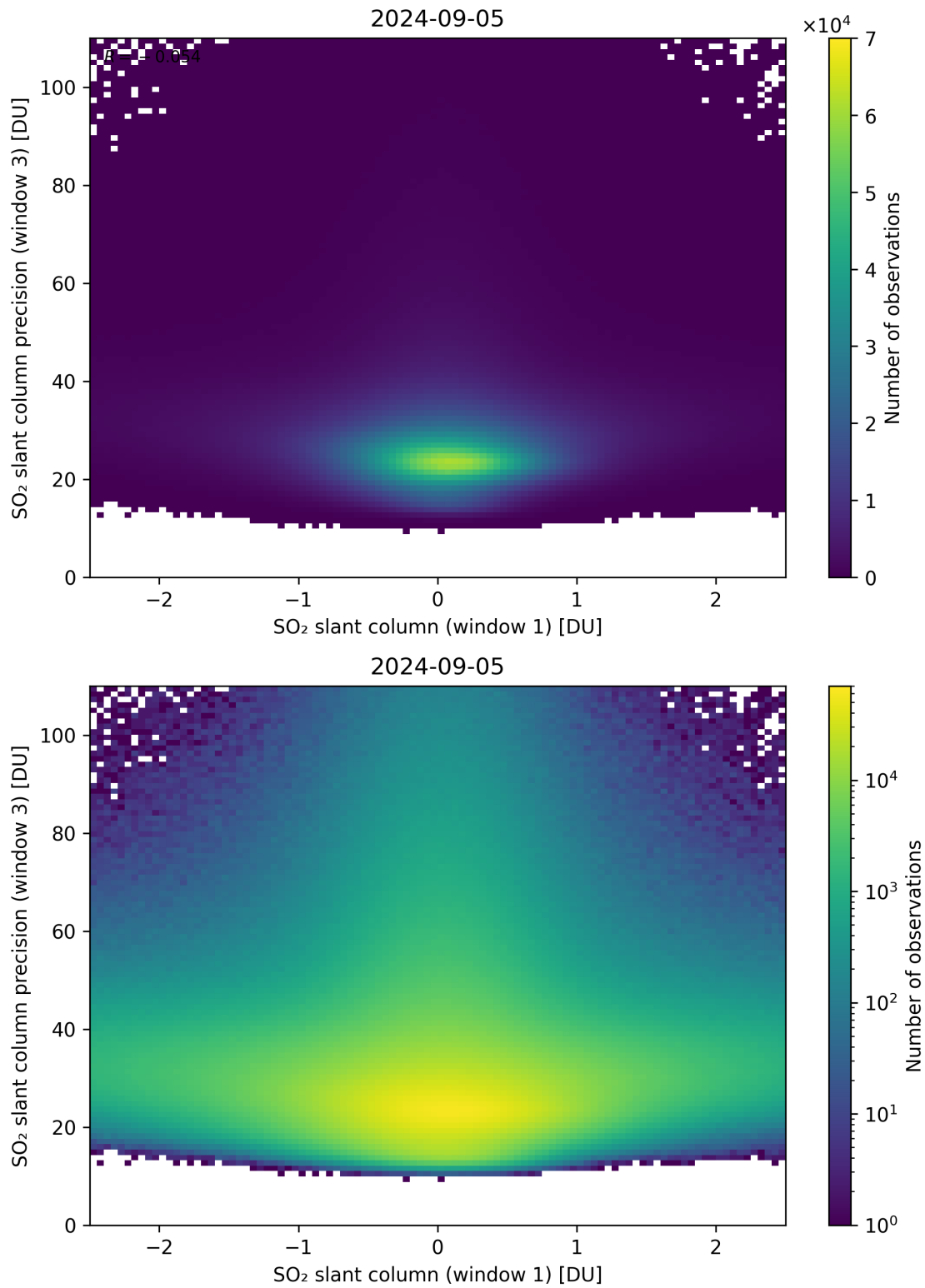
Figure 238: Scatter density plot of “SO 2 slant column (window 1)” against “SO 2 slant column precision (window 3)” for 2024-09-04 to 2024-09-06.
