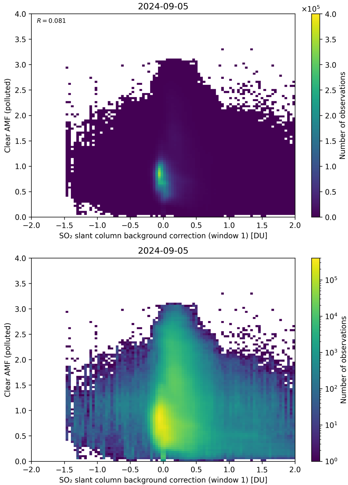
Figure 103: Scatter density plot of “SO 2 slant column background correction (window 1)” against “Clear AMF (polluted)” for 2024-09-04 to 2024-09-06.
