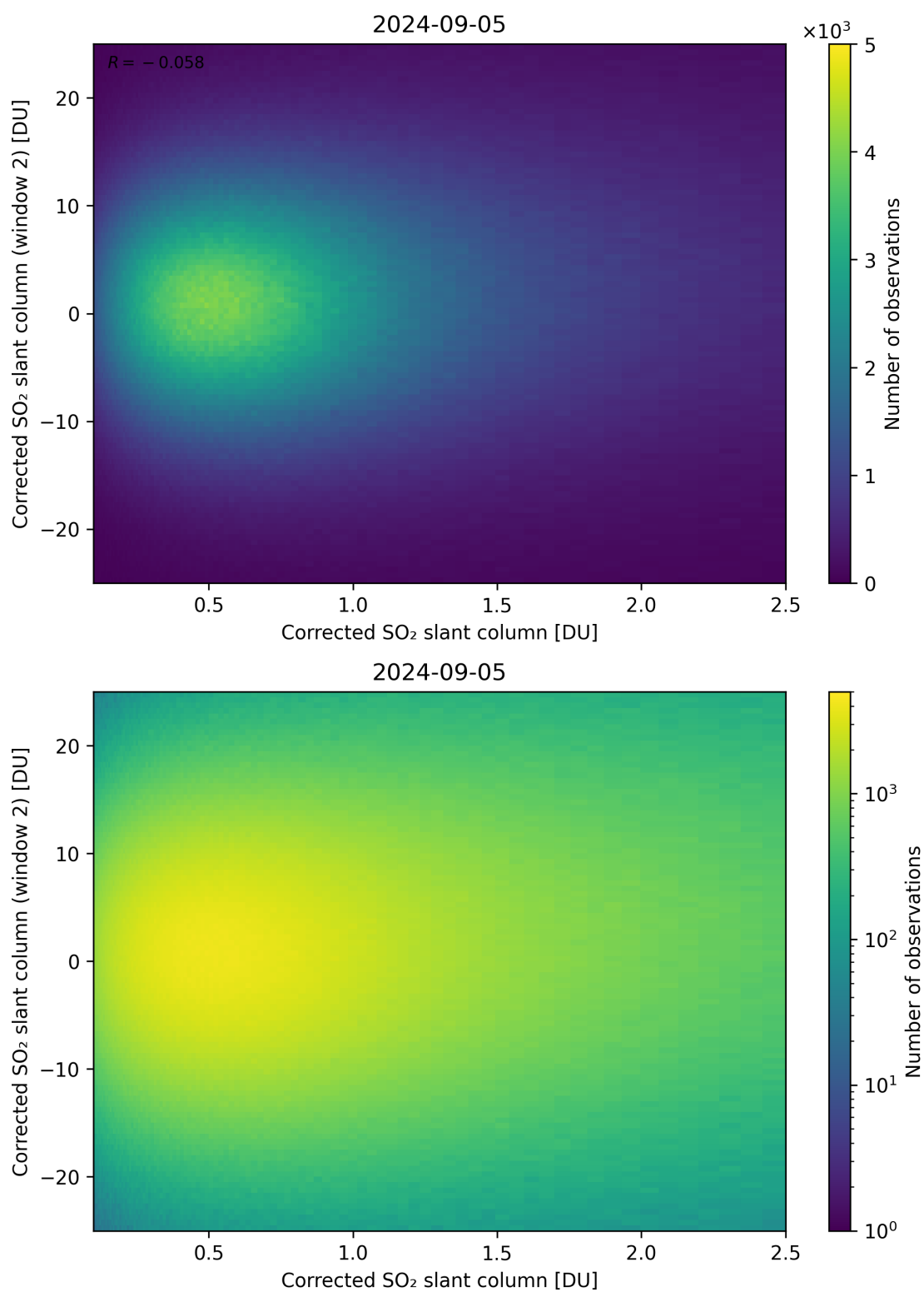
Figure 185: Scatter density plot of “Corrected SO 2 slant column” against “Corrected SO 2 slant column (window 2)” for 2024-09-04 to 2024-09-06.
