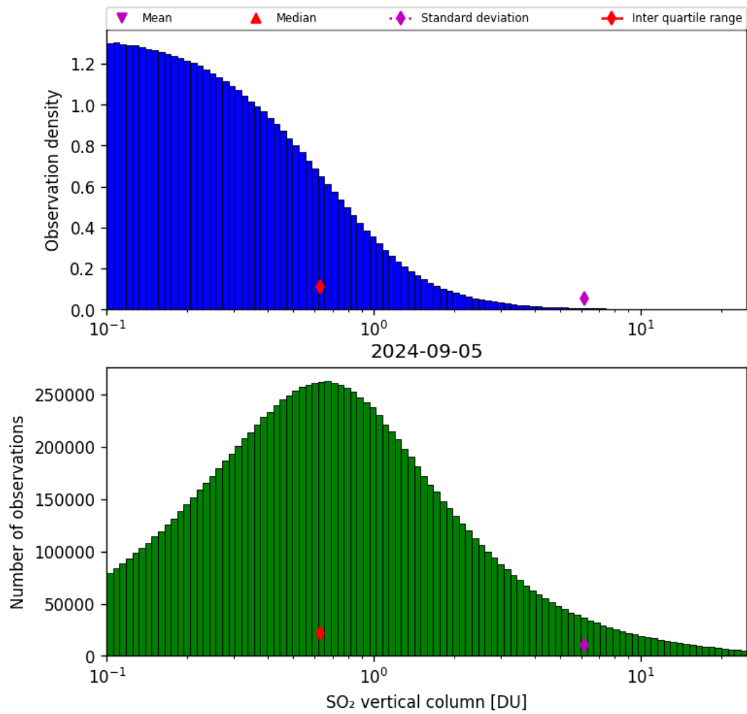
Figure 53: Histogram of “SO 2 vertical column” for 2024-09-04 to 2024-09-06
