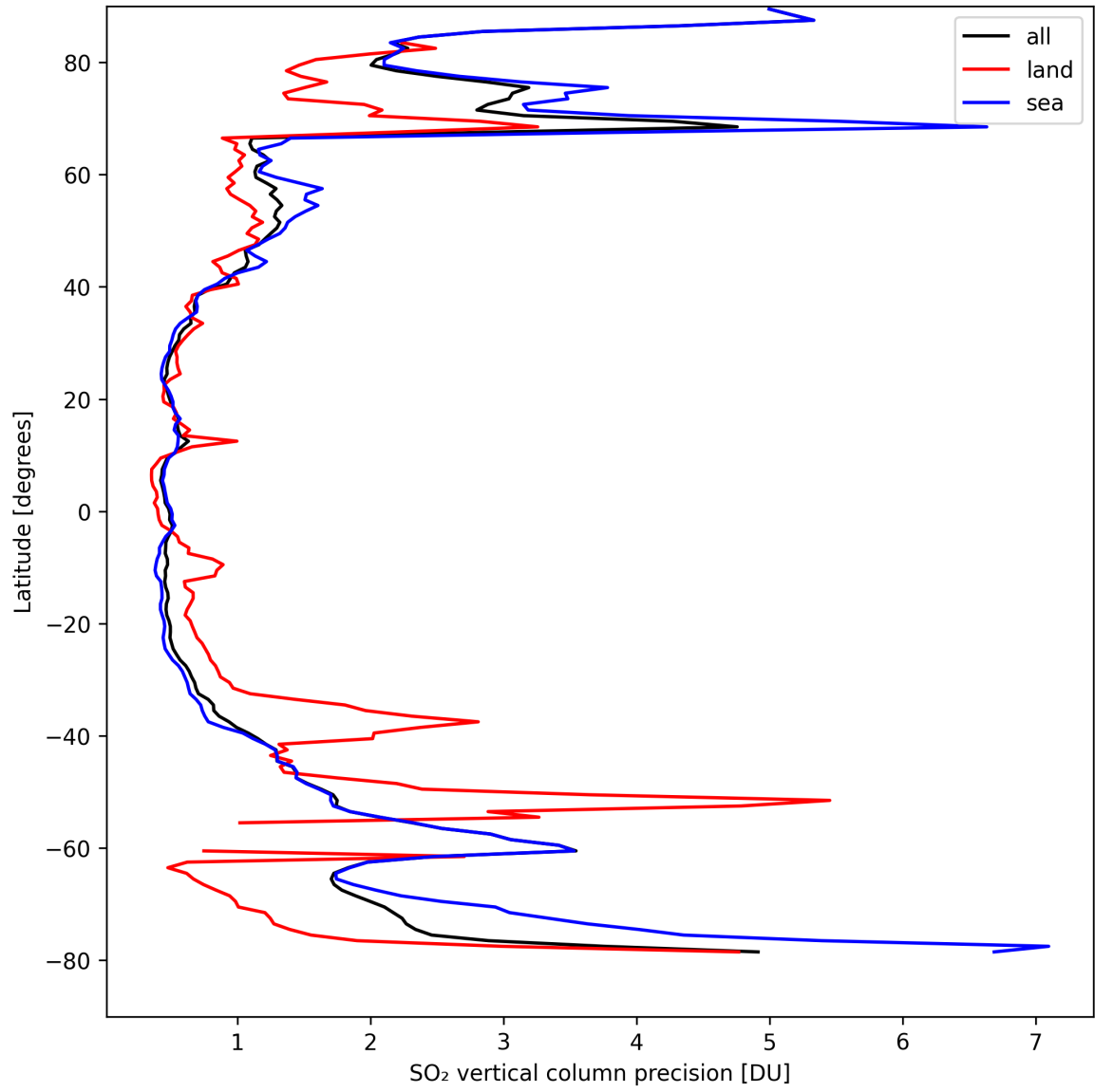
Figure 31: Zonal average of “SO 2 vertical column precision” for 2024-09-04 to 2024-09-06.
