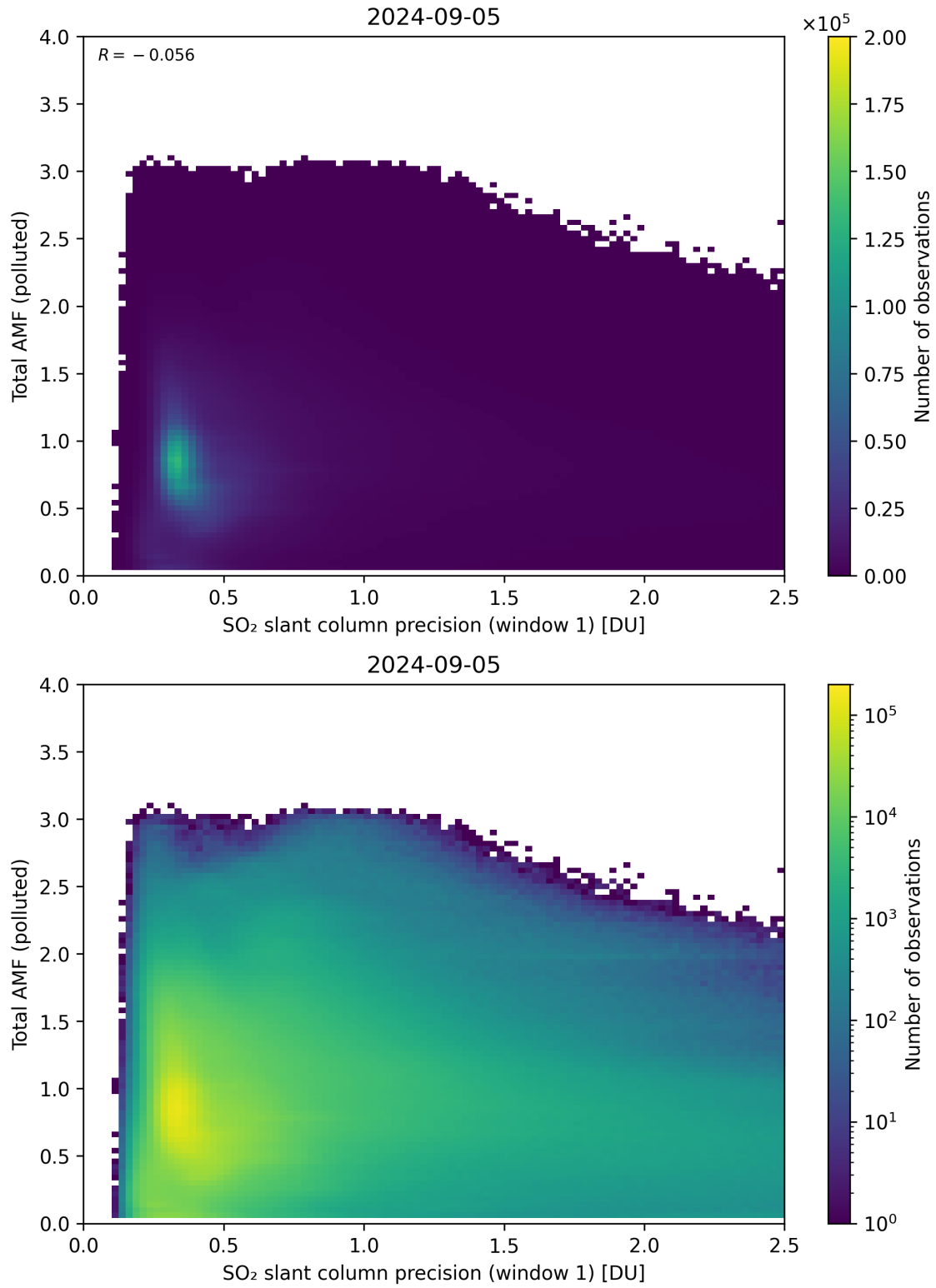
Figure 230: Scatter density plot of “SO 2 slant column precision (window 1)” against “Total AMF (polluted)” for 2024-09-04 to 2024-09-06.
