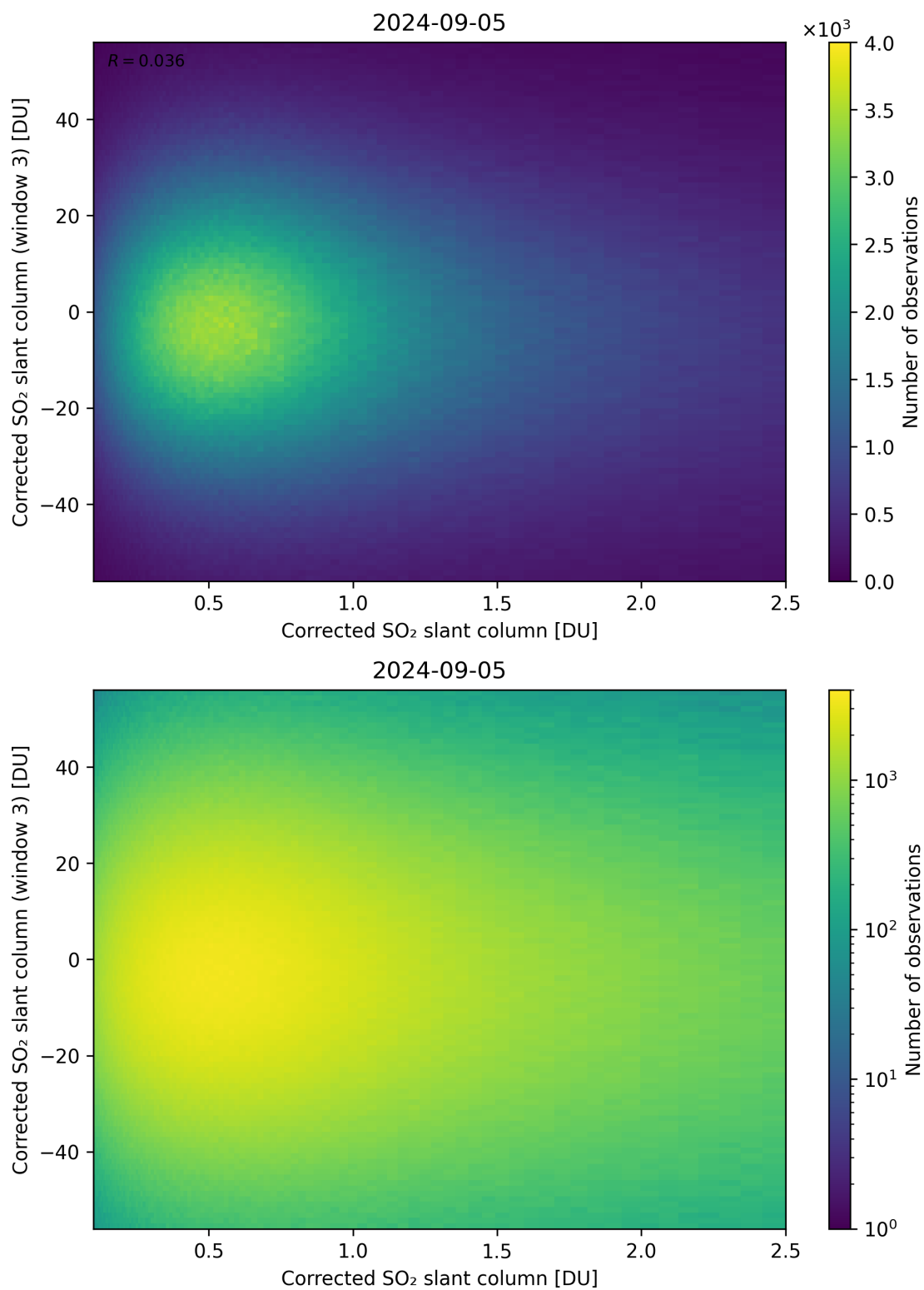
Figure 186: Scatter density plot of “Corrected SO 2 slant column” against “Corrected SO 2 slant column (window 3)” for 2024-09-04 to 2024-09-06.
