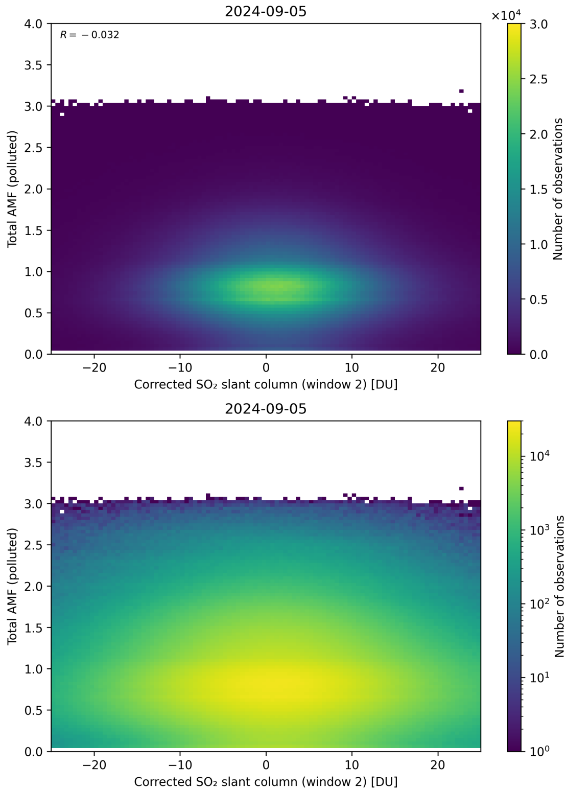
Figure 203: Scatter density plot of “Corrected SO 2 slant column (window 2)” against “Total AMF (polluted)” for 2024-09-04 to 2024-09-06.
