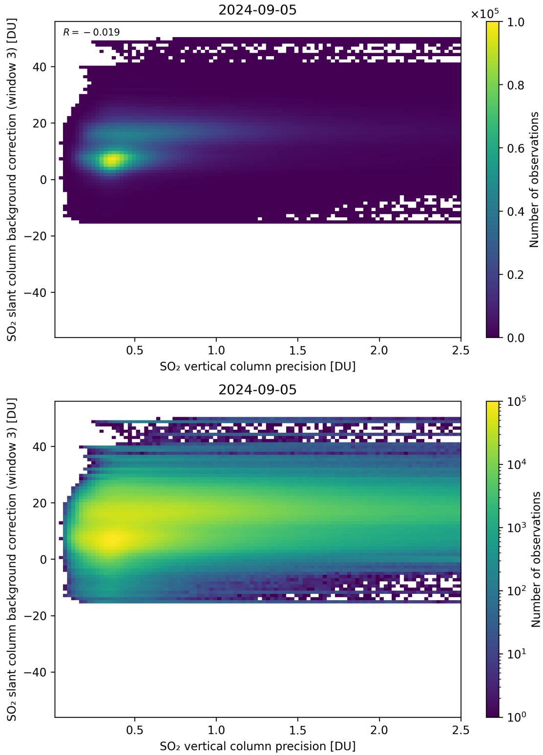
Figure 281: Scatter density plot of “SO 2 vertical column precision” against “SO 2 slant column background correction (window 3)” for 2024-09-04 to 2024-09-06.
