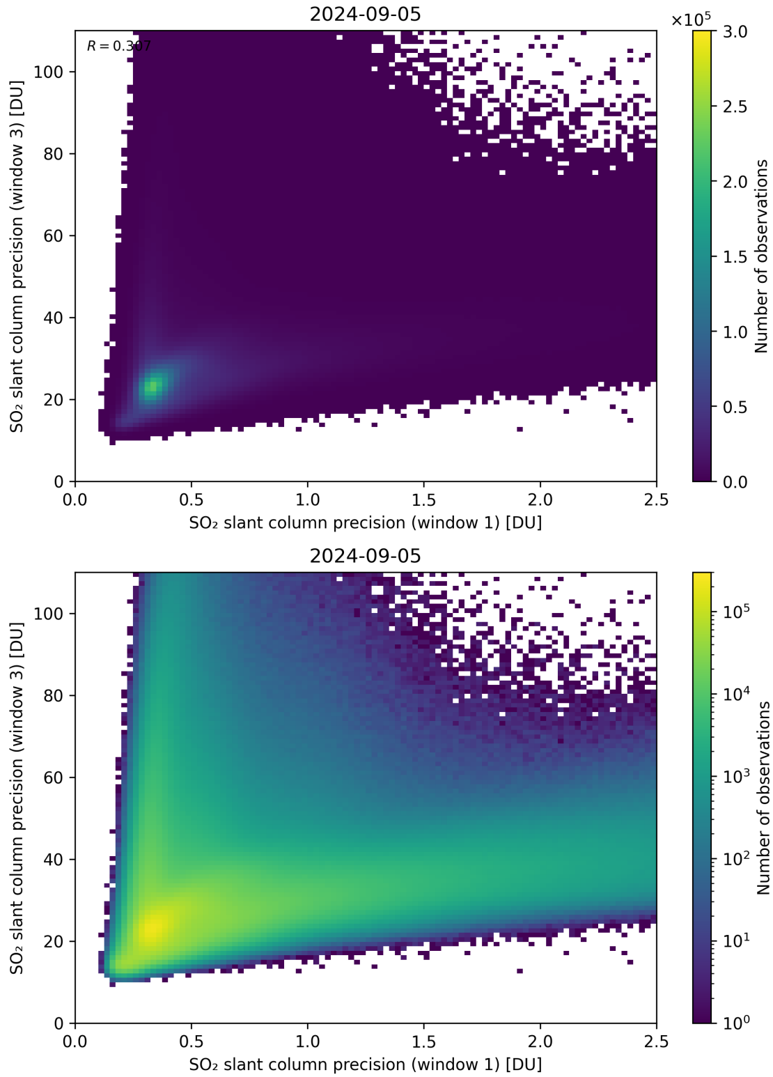
Figure 229: Scatter density plot of “SO 2 slant column precision (window 1)” against “SO 2 slant column precision (window 3)” for 2024-09-04 to 2024-09-06.
