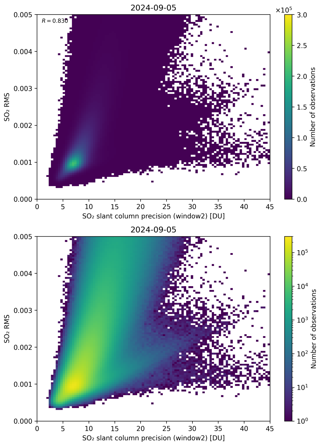
Figure 245: Scatter density plot of “SO 2 slant column precision (window2)” against “SO 2 RMS” for 2024-09-04 to 2024-09-06.
