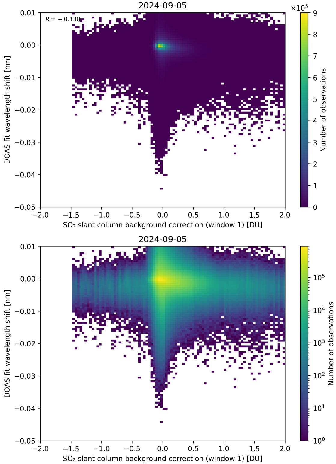
Figure 100: Scatter density plot of “SO 2 slant column background correction (window 1)” against “DOAS fit wavelength shift” for 2024-09-04 to 2024-09-06.
