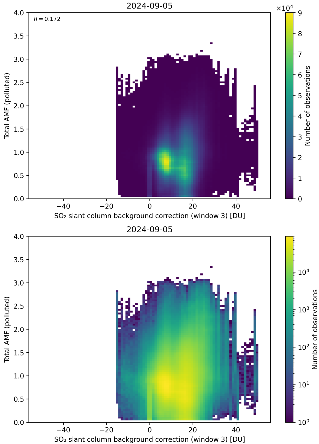
Figure 125: Scatter density plot of “SO 2 slant column background correction (window 3)” against “Total AMF (polluted)” for 2024-09-04 to 2024-09-06.
