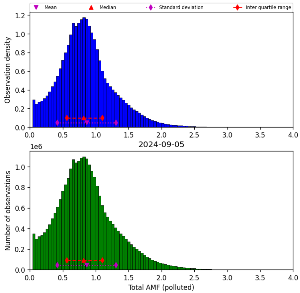
Figure 71: Histogram of “Total AMF (polluted)” for 2024-09-04 to 2024-09-06
