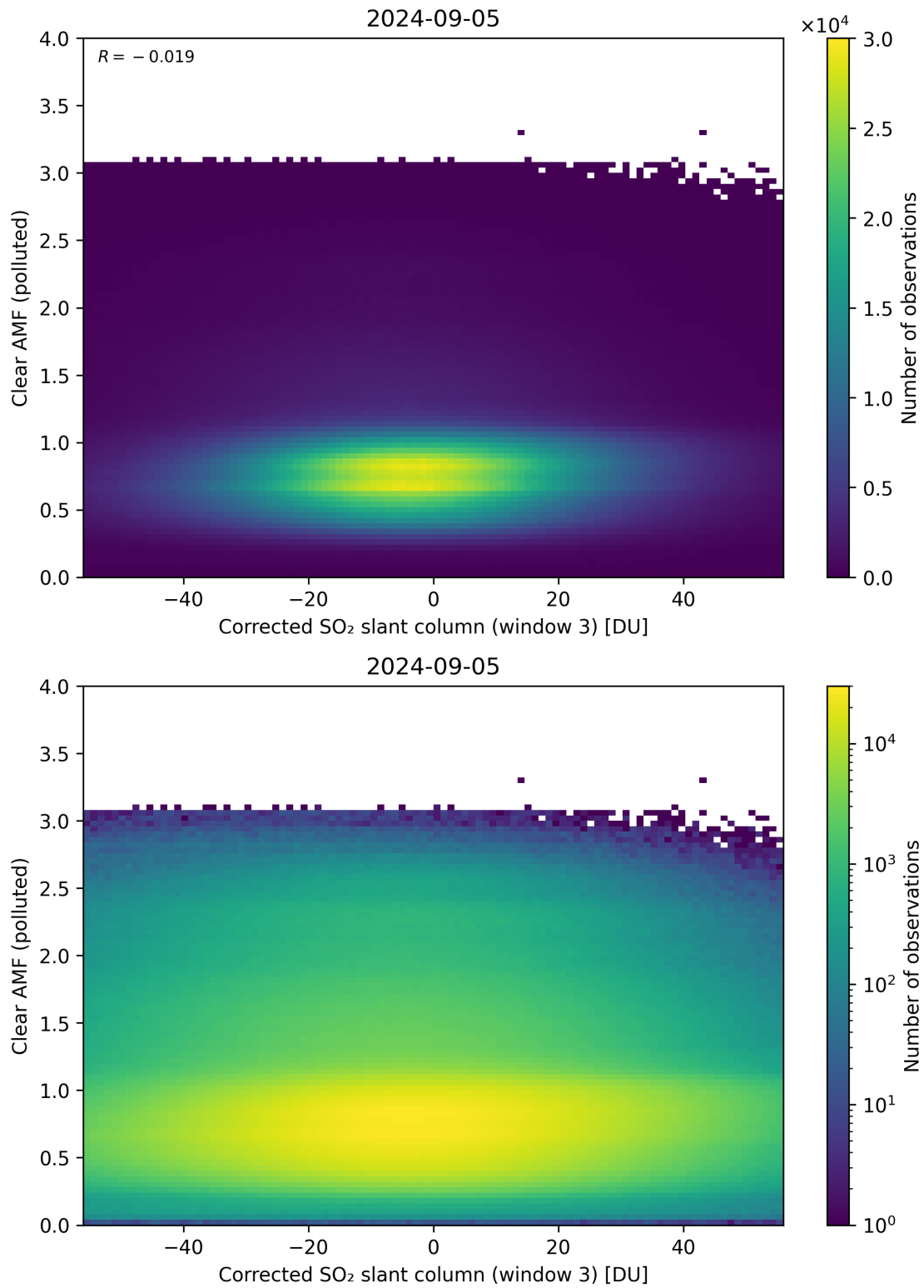
Figure 209: Scatter density plot of “Corrected SO 2 slant column (window 3)” against “Clear AMF (polluted)” for 2024-09-04 to 2024-09-06.
