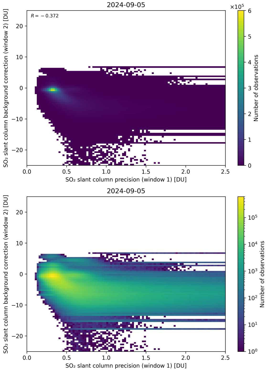
Figure 219: Scatter density plot of “SO 2 slant column precision (window 1)” against “SO 2 slant column background correction (window 2)” for 2024-09-04 to 2024-09-06.
