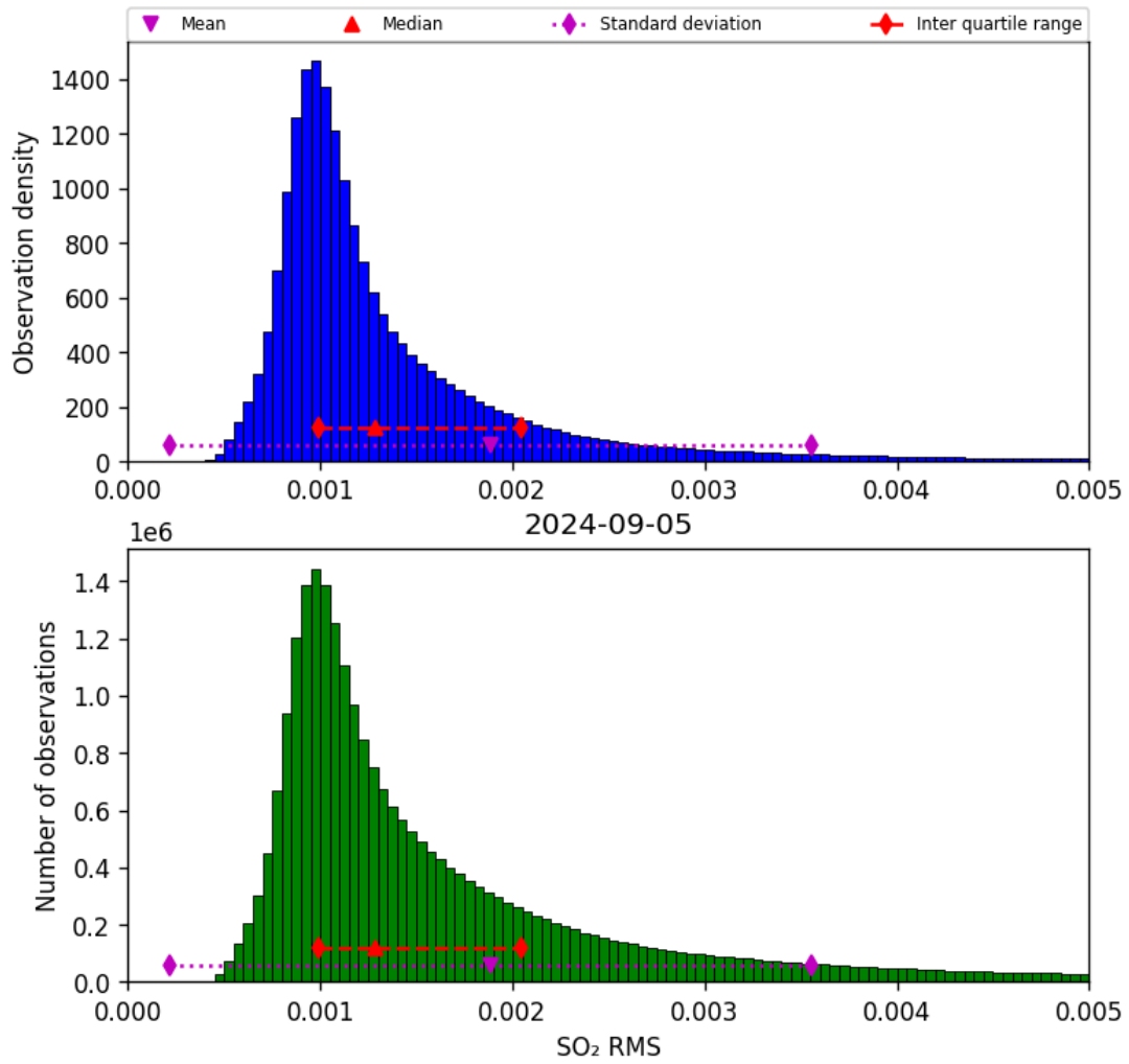
Figure 70: Histogram of “SO 2 RMS” for 2024-09-04 to 2024-09-06
