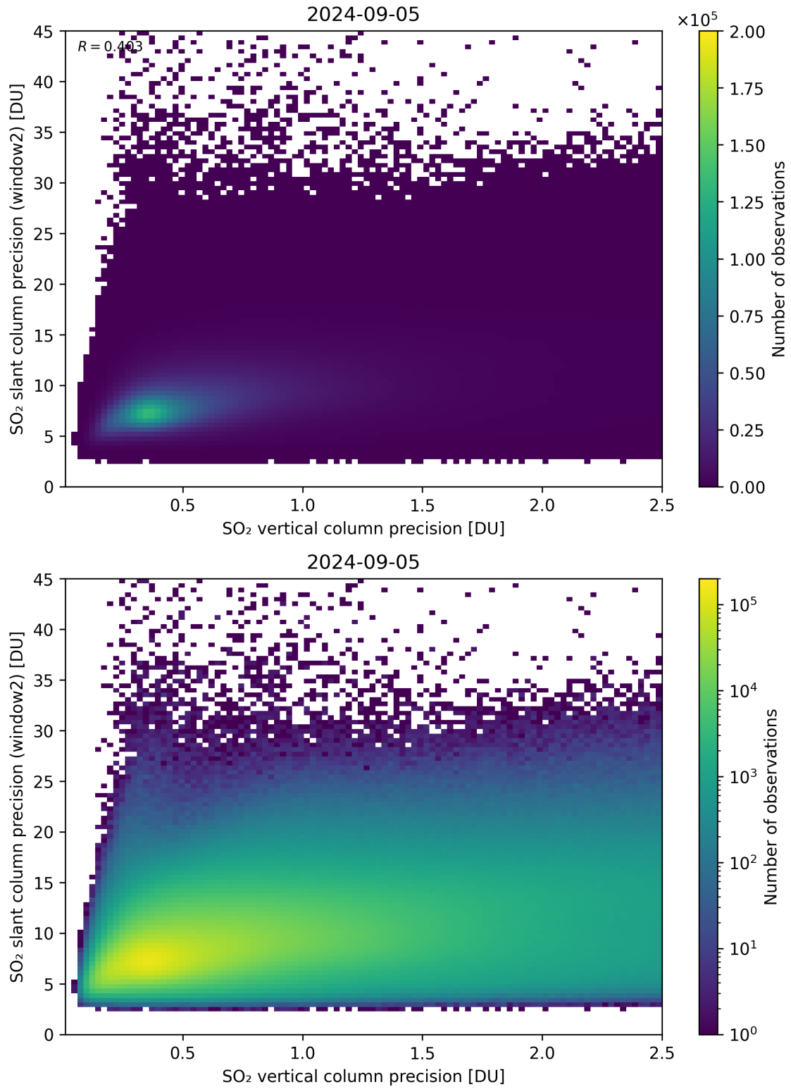
Figure 291: Scatter density plot of “SO 2 vertical column precision” against “SO 2 slant column precision (window2)” for 2024-09-04 to 2024-09-06.
