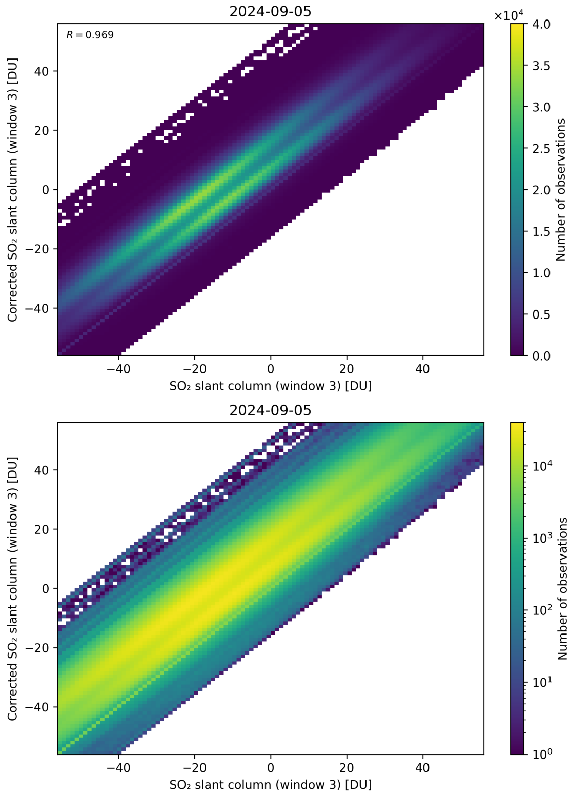
Figure 266: Scatter density plot of “SO 2 slant column (window 3)” against “Corrected SO 2 slant column (window 3)” for 2024-09-04 to 2024-09-06.
