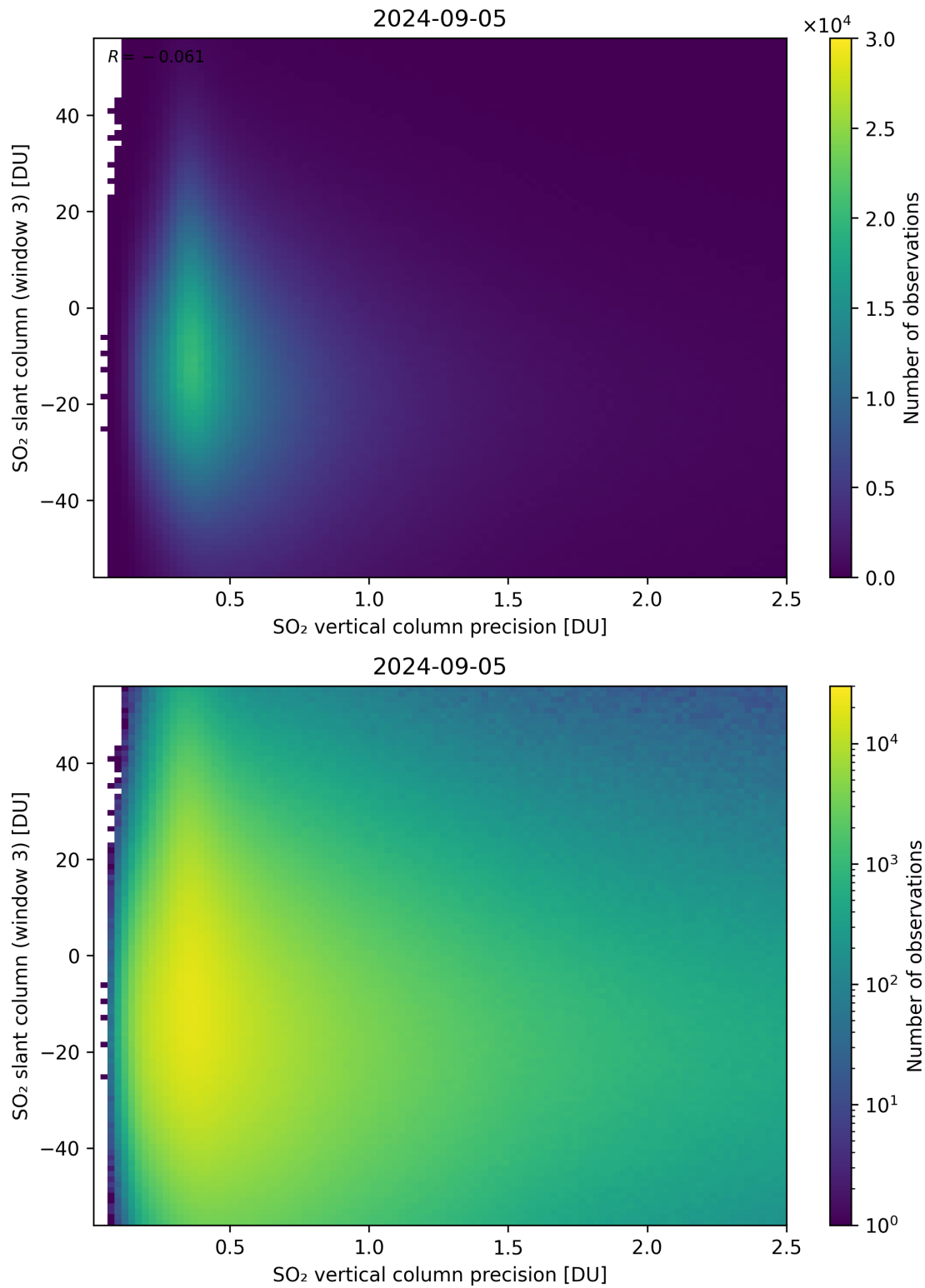
Figure 292: Scatter density plot of “SO 2 vertical column precision” against “SO 2 slant column (window 3)” for 2024-09-04 to 2024-09-06.
