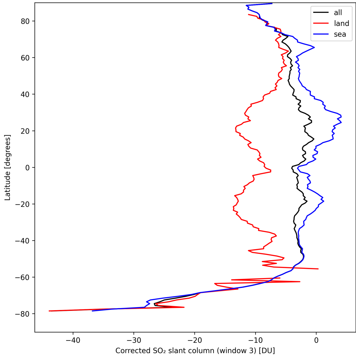
Figure 43: Zonal average of “Corrected SO 2 slant column (window 3)” for 2024-09-04 to 2024-09-06.
