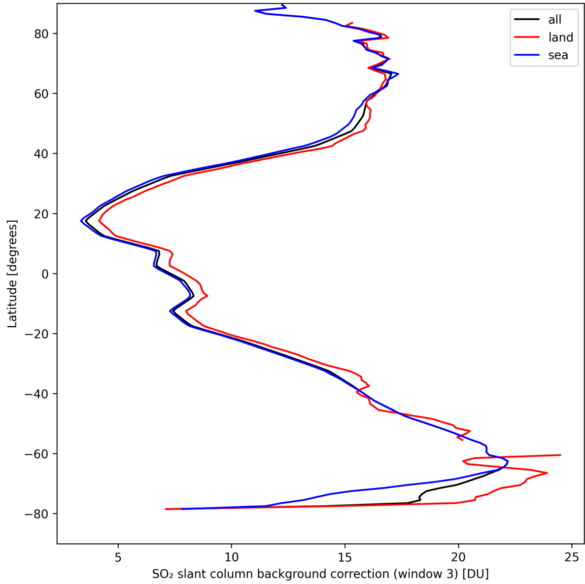
Figure 44: Zonal average of “SO 2 slant column background correction (window 3)” for 2024-09-04 to 2024-09-06.
