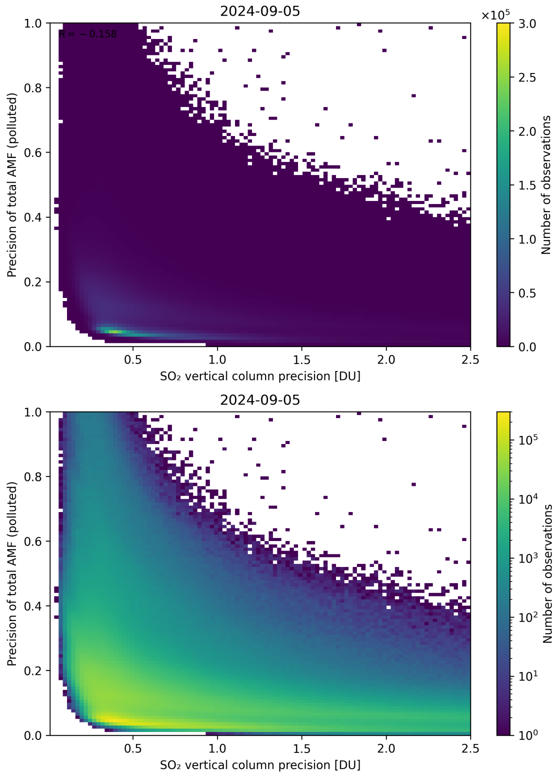
Figure 295: Scatter density plot of “SO 2 vertical column precision” against “Precision of total AMF (polluted)” for 2024-09-04 to 2024-09-06.
