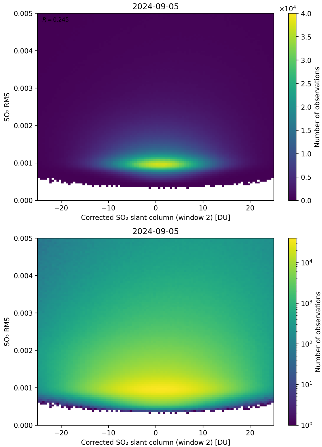
Figure 198: Scatter density plot of “Corrected SO 2 slant column (window 2)” against “SO 2 RMS” for 2024-09-04 to 2024-09-06.
