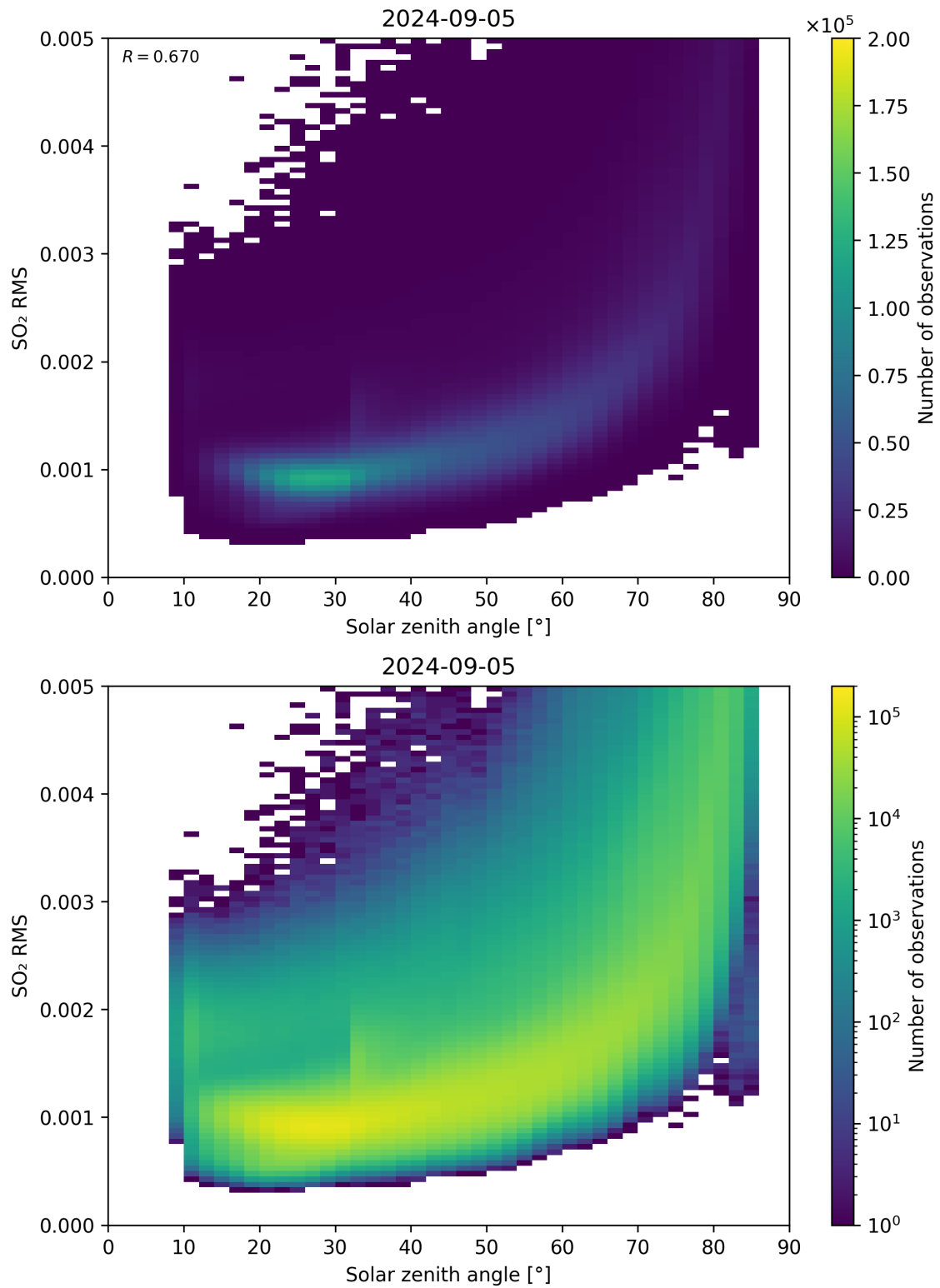
Figure 163: Scatter density plot of “Solar zenith angle” against “SO 2 RMS” for 2024-09-04 to 2024-09-06.
