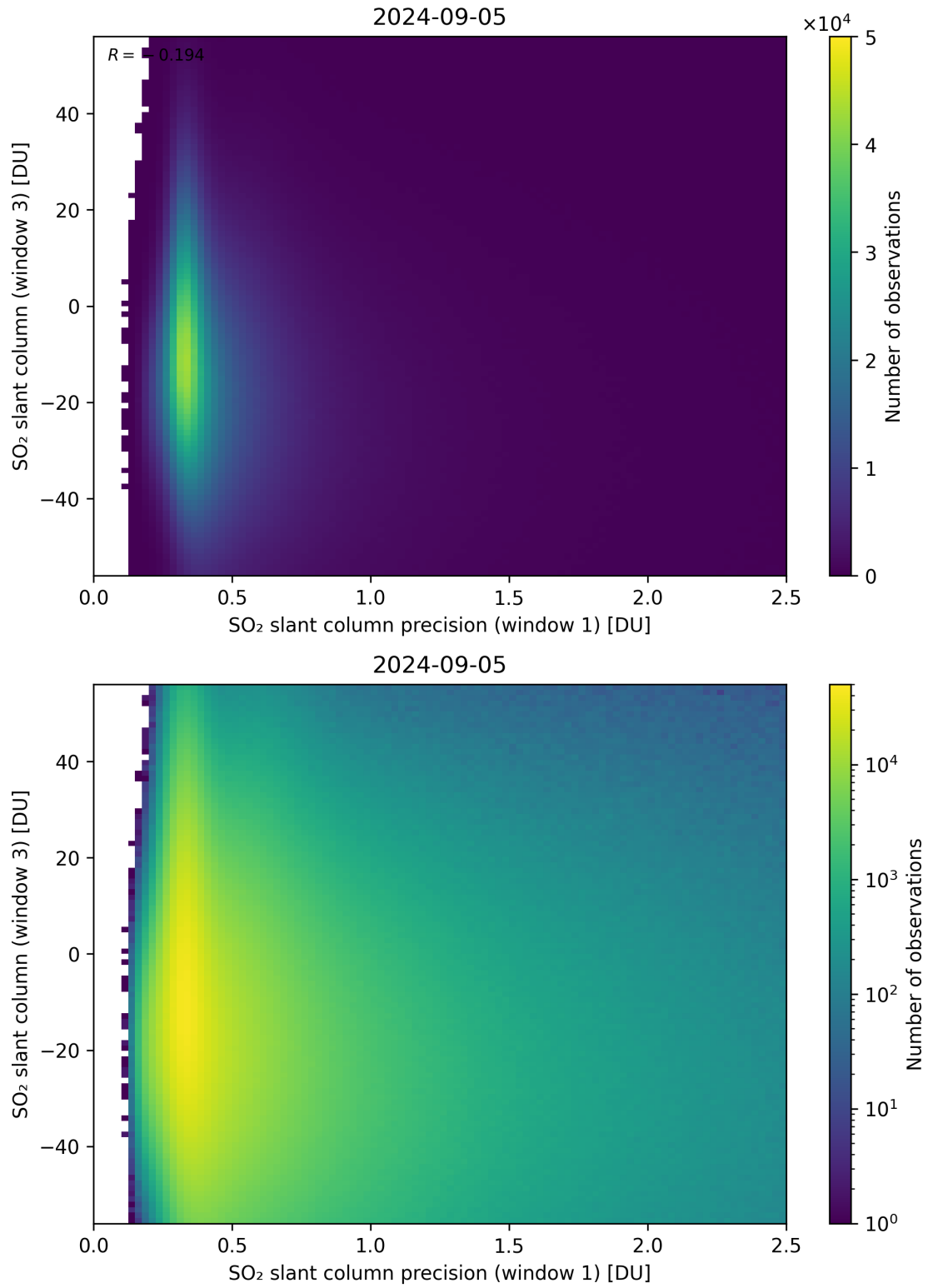
Figure 228: Scatter density plot of “SO 2 slant column precision (window 1)” against “SO 2 slant column (window 3)” for 2024-09-04 to 2024-09-06.
