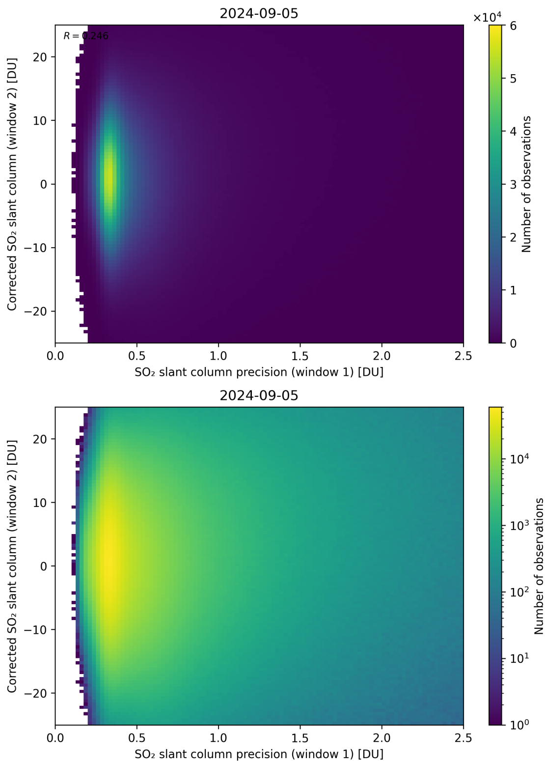
Figure 225: Scatter density plot of “SO 2 slant column precision (window 1)” against “Corrected SO 2 slant column (window 2)” for 2024-09-04 to 2024-09-06.
