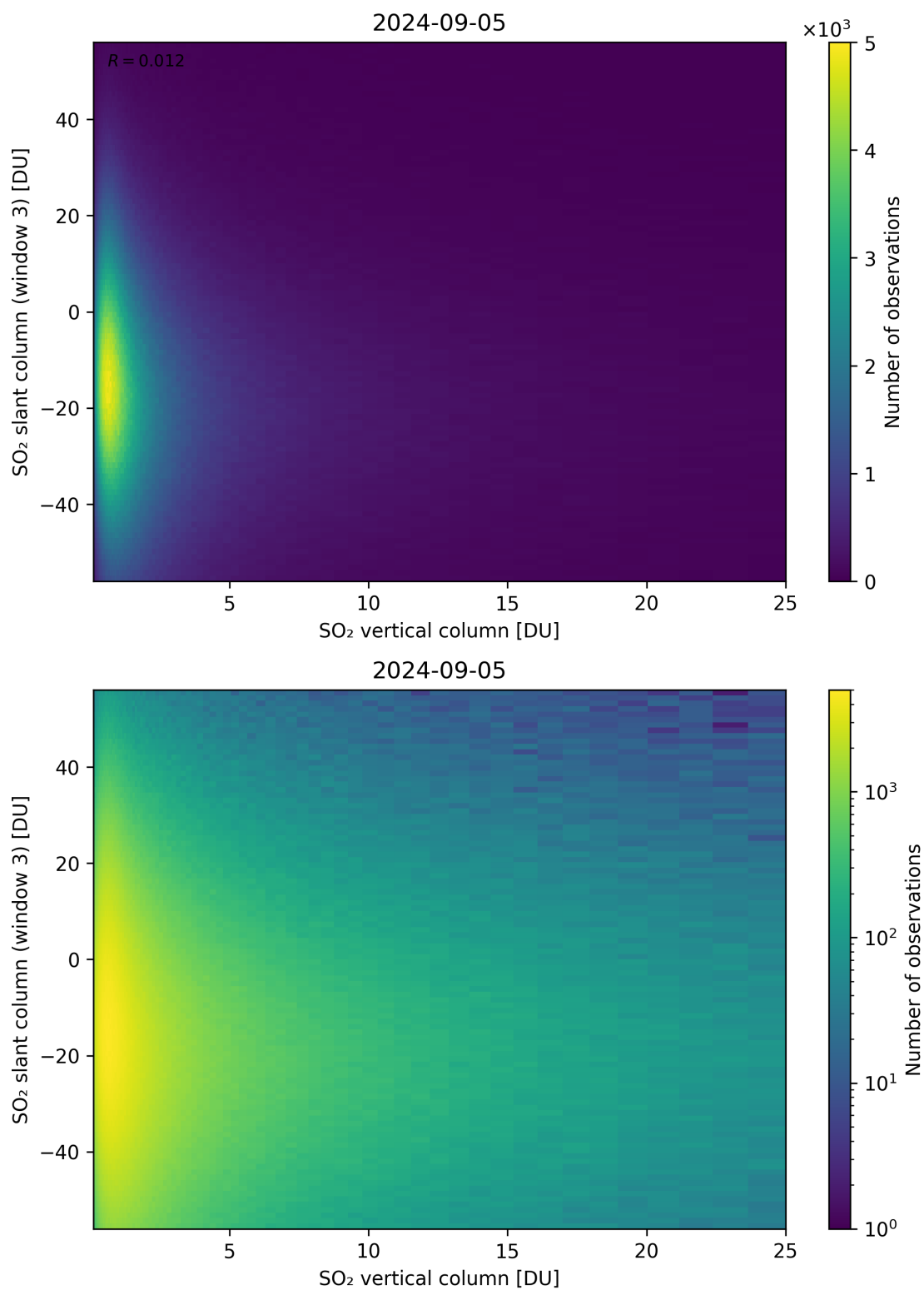
Figure 303: Scatter density plot of “SO 2 vertical column” against “SO 2 slant column (window 3)” for 2024-09-04 to 2024-09-06.
