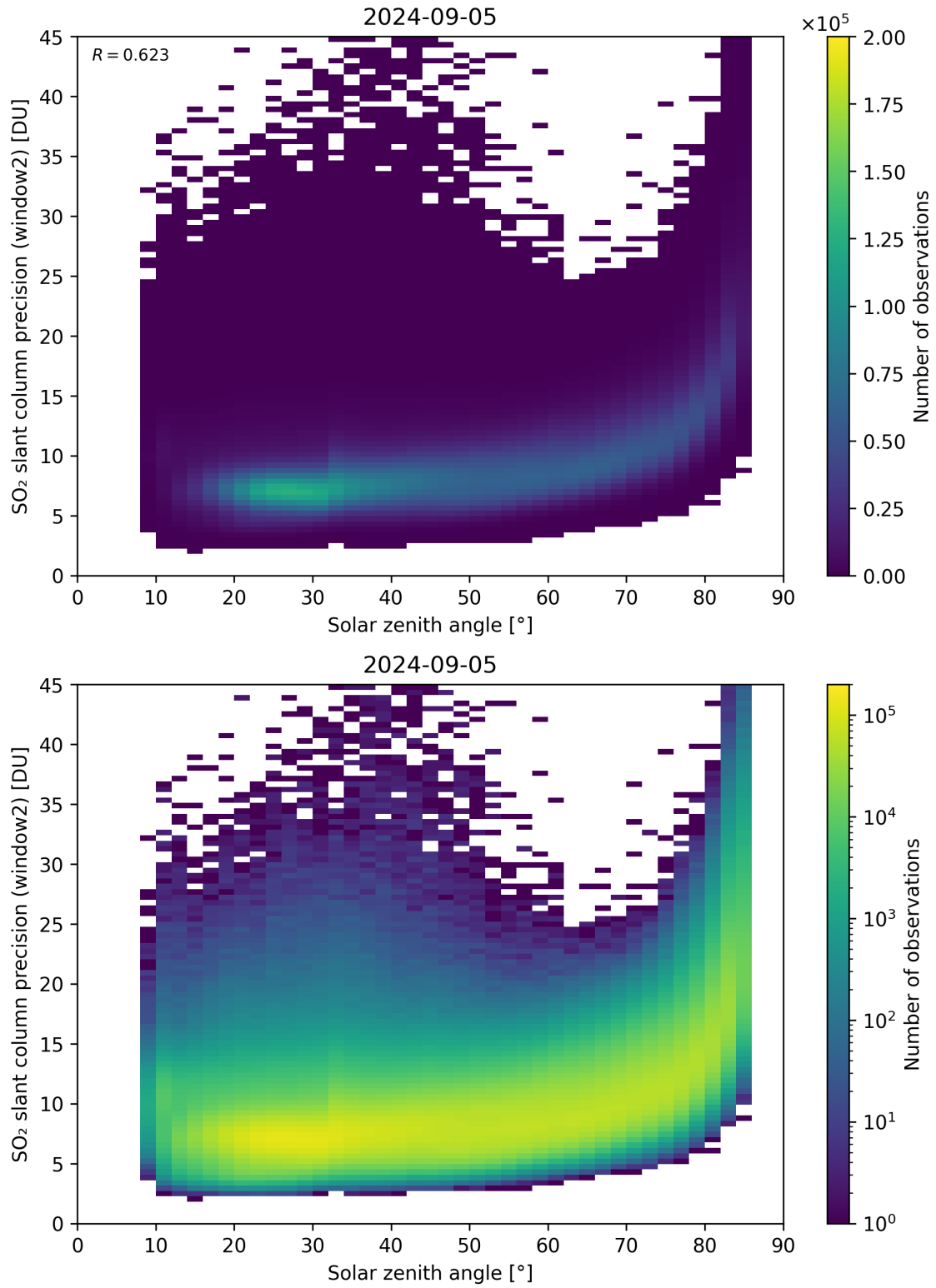
Figure 171: Scatter density plot of “Solar zenith angle” against “SO 2 slant column precision (window2)” for 2024-09-04 to 2024-09-06.
