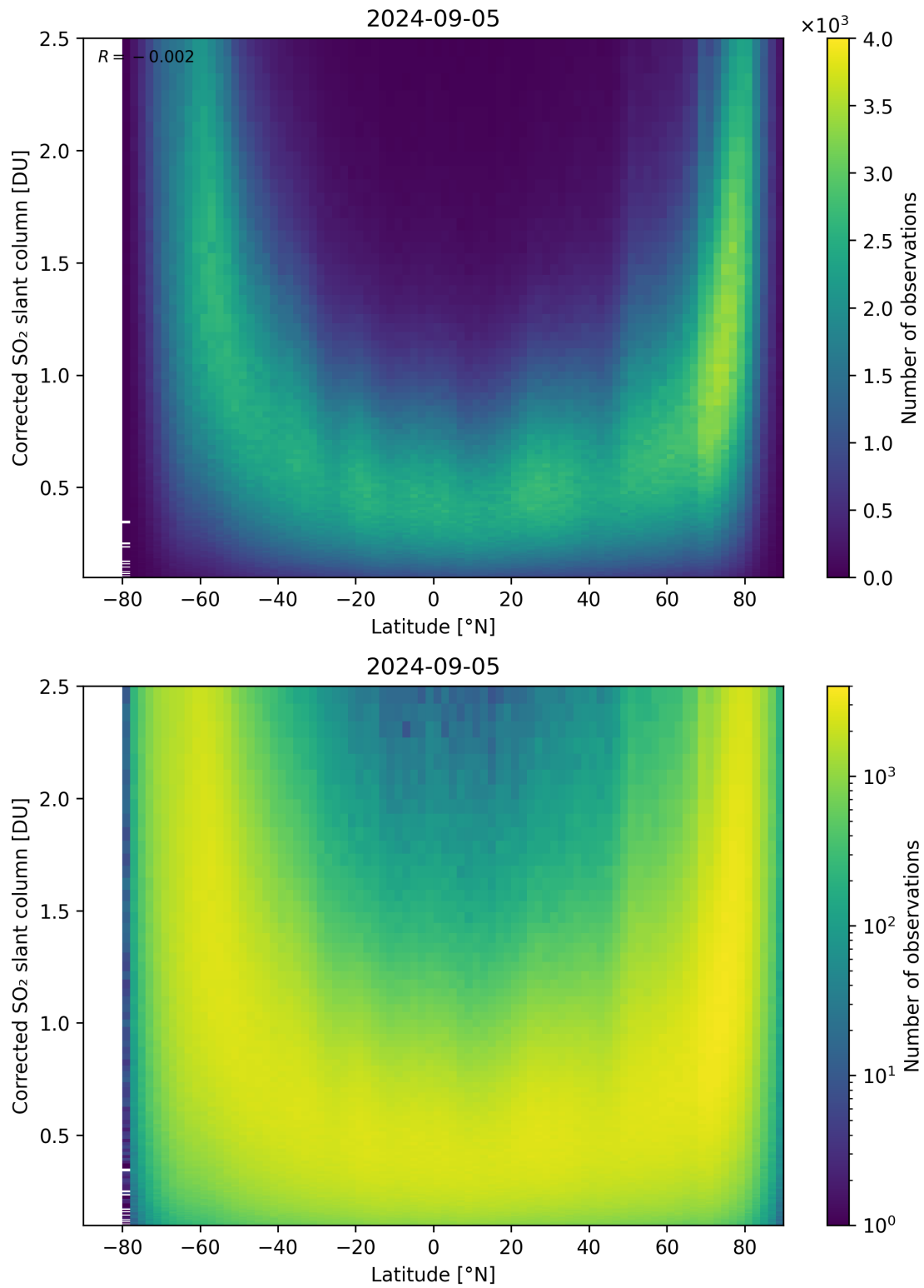
Figure 146: Scatter density plot of “Latitude” against “Corrected SO 2 slant column” for 2024-09-04 to 2024-09-06.
