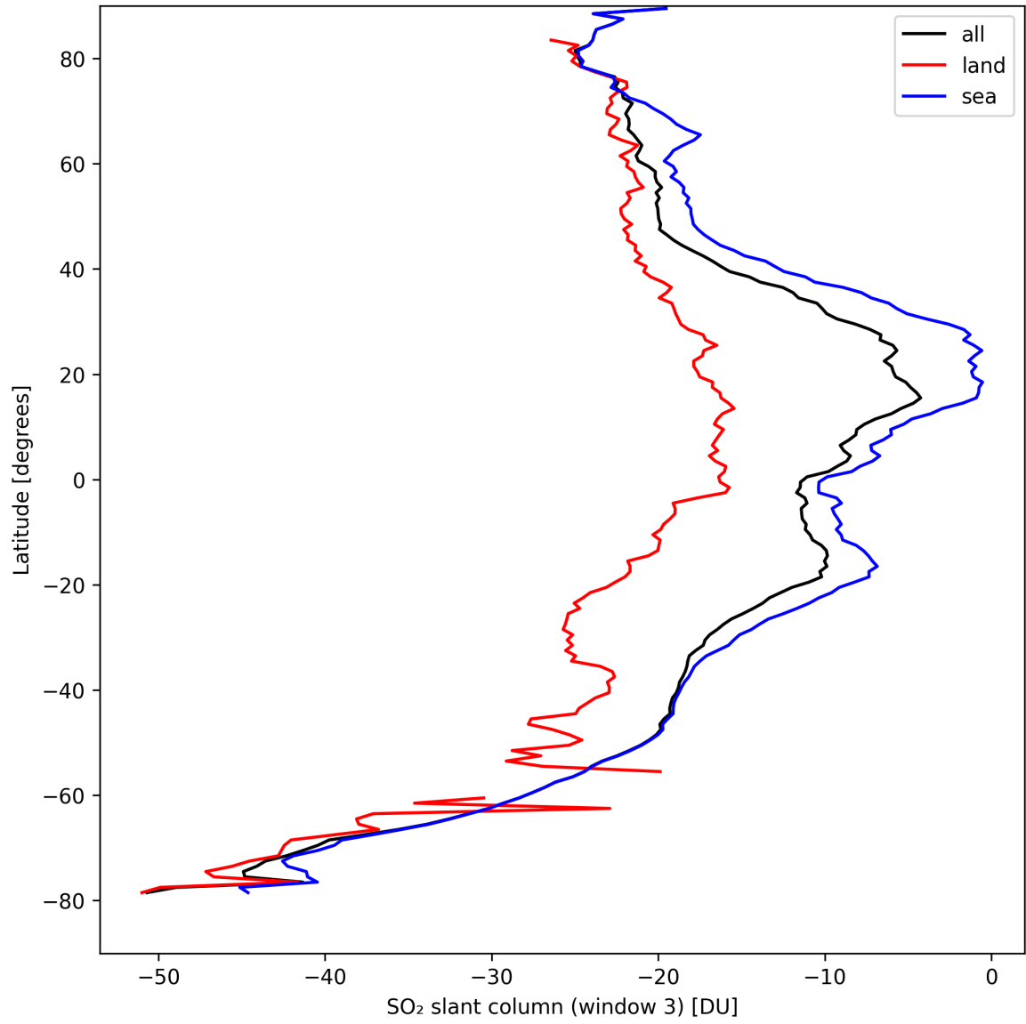
Figure 41: Zonal average of “SO 2 slant column (window 3)” for 2024-09-04 to 2024-09-06.
