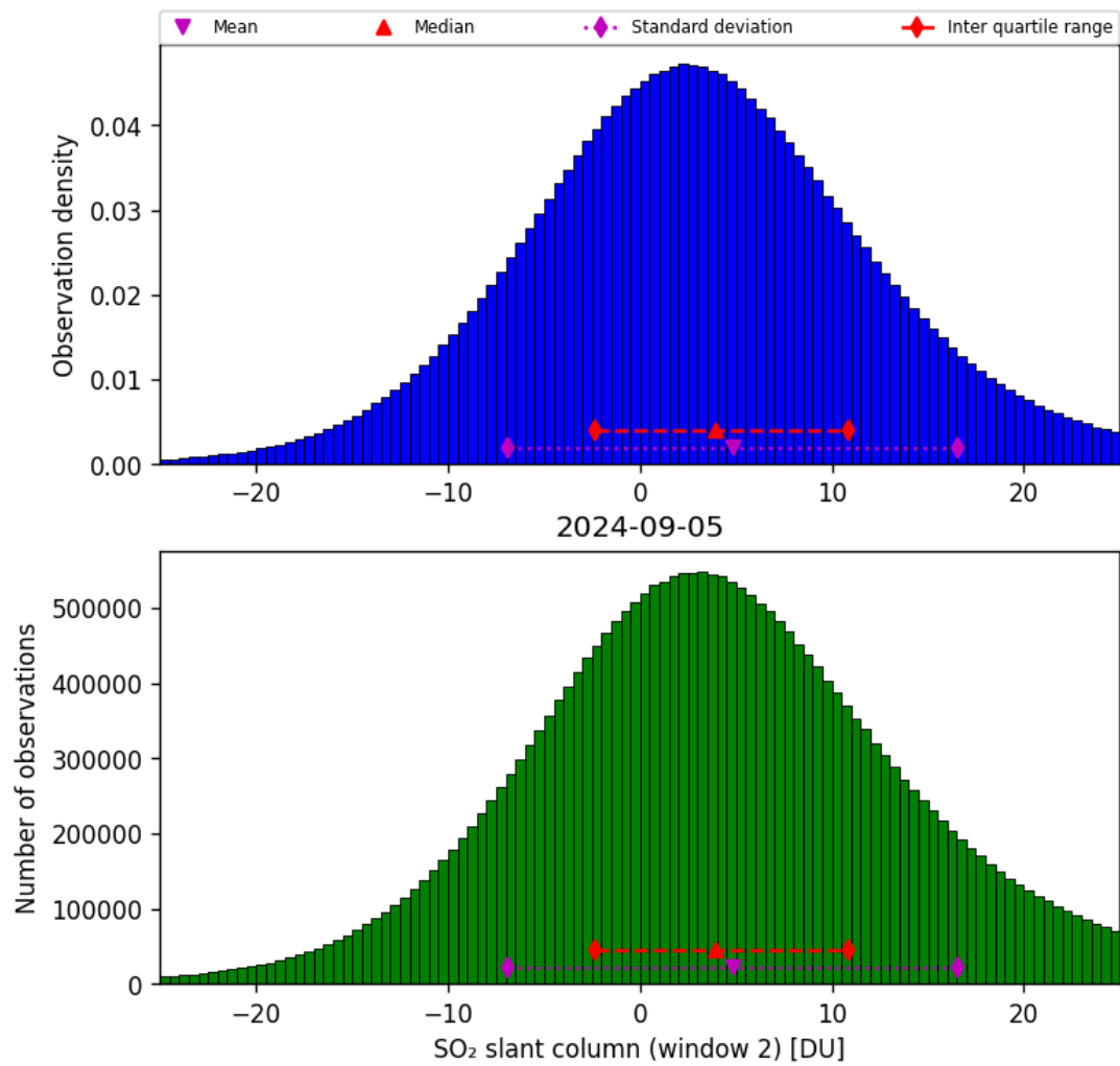
Figure 60: Histogram of “SO 2 slant column (window 2)” for 2024-09-04 to 2024-09-06
