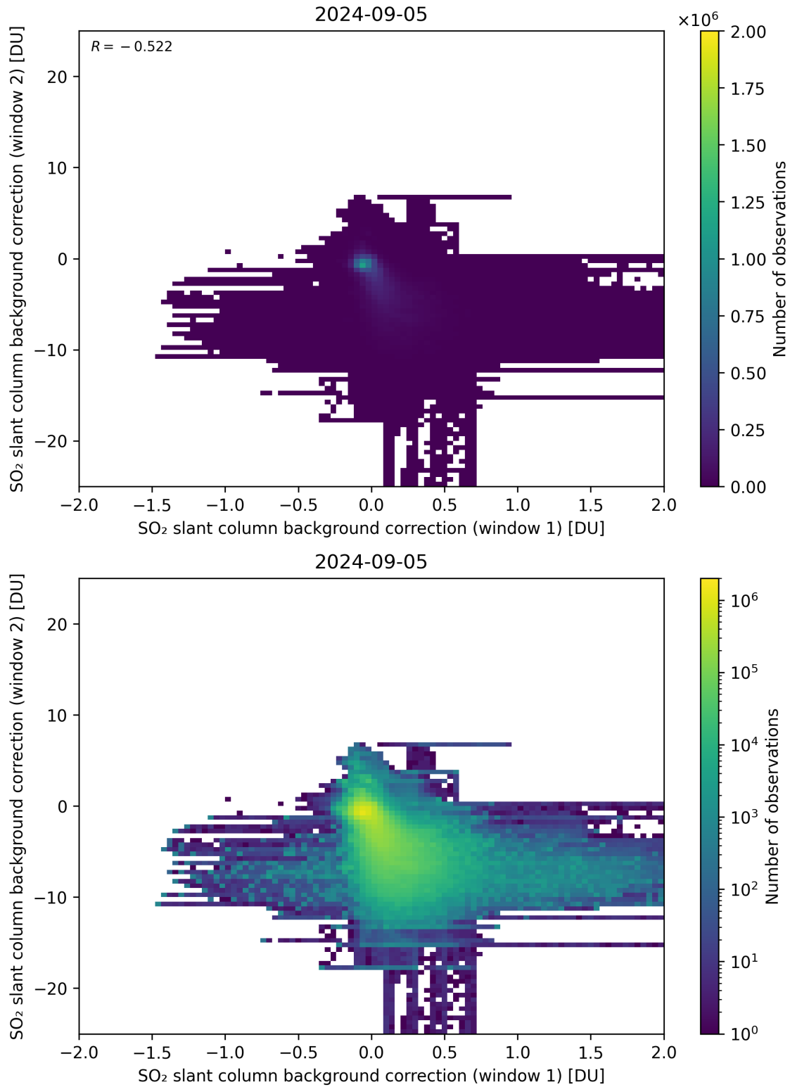
Figure 98: Scatter density plot of “SO 2 slant column background correction (window 1)” against “SO 2 slant column background correction (window 2)” for 2024-09-04 to 2024-09-06.
