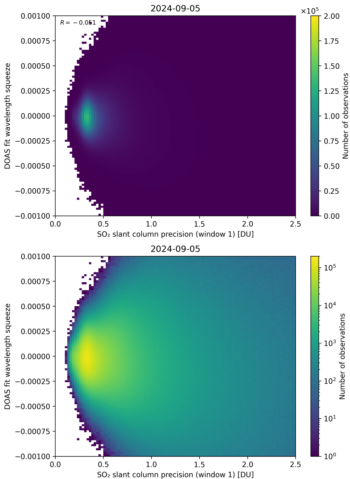
Figure 222: Scatter density plot of “SO 2 slant column precision (window 1)” against “DOAS fit wavelength squeeze” for 2024-09-04 to 2024-09-06.
