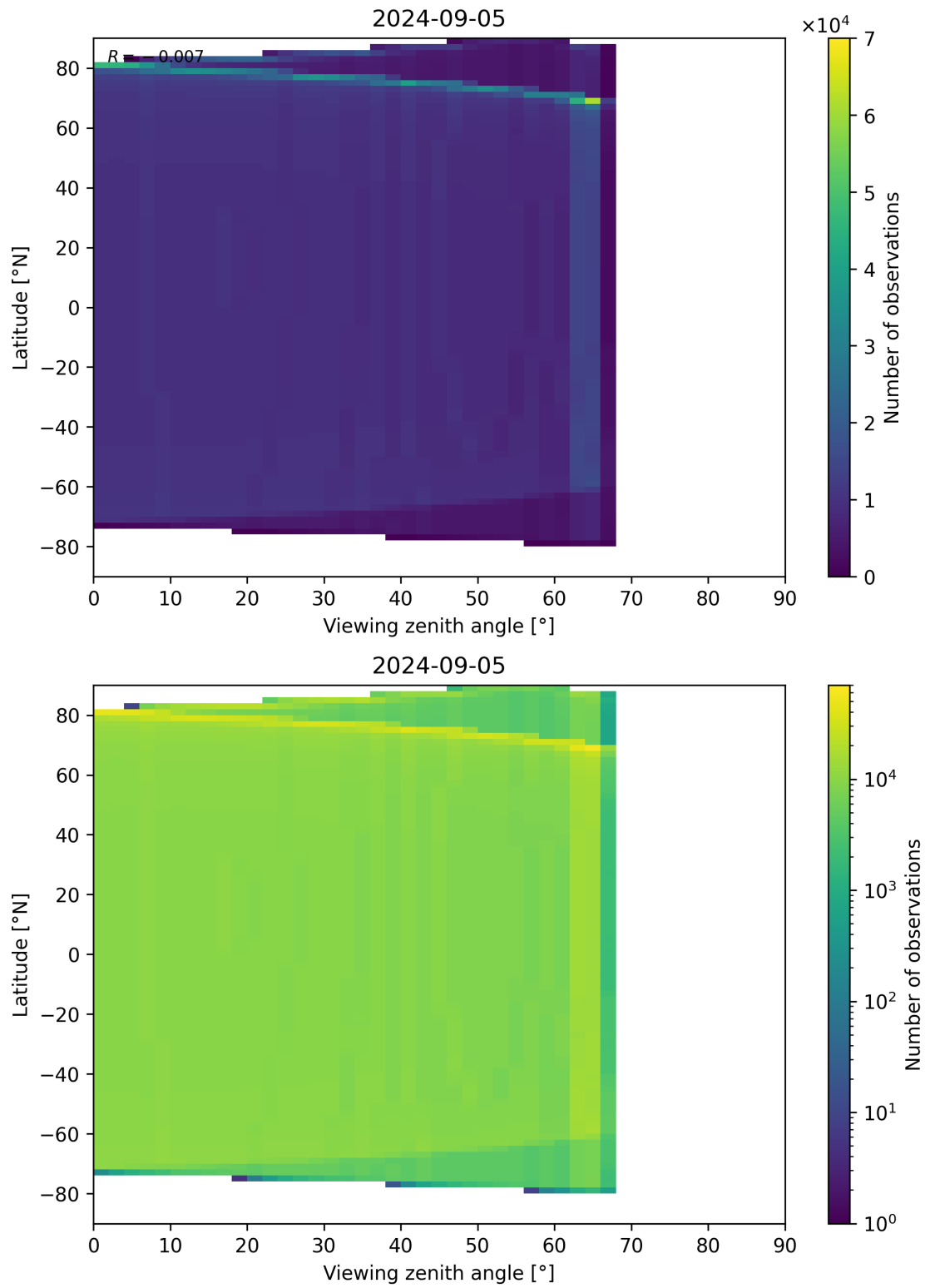
Figure 314: Scatter density plot of “Viewing zenith angle” against “Latitude” for 2024-09-04 to 2024-09-06.
