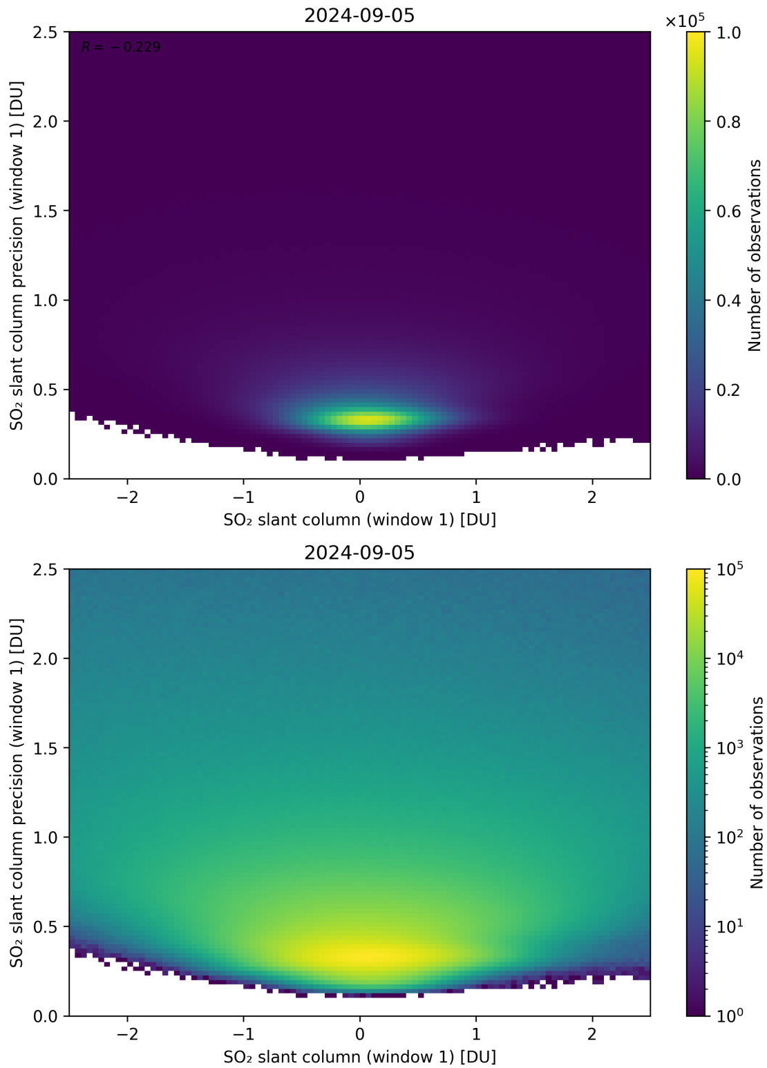
Figure 235: Scatter density plot of “SO 2 slant column (window 1)” against “SO 2 slant column precision (window 1)” for 2024-09-04 to 2024-09-06.
