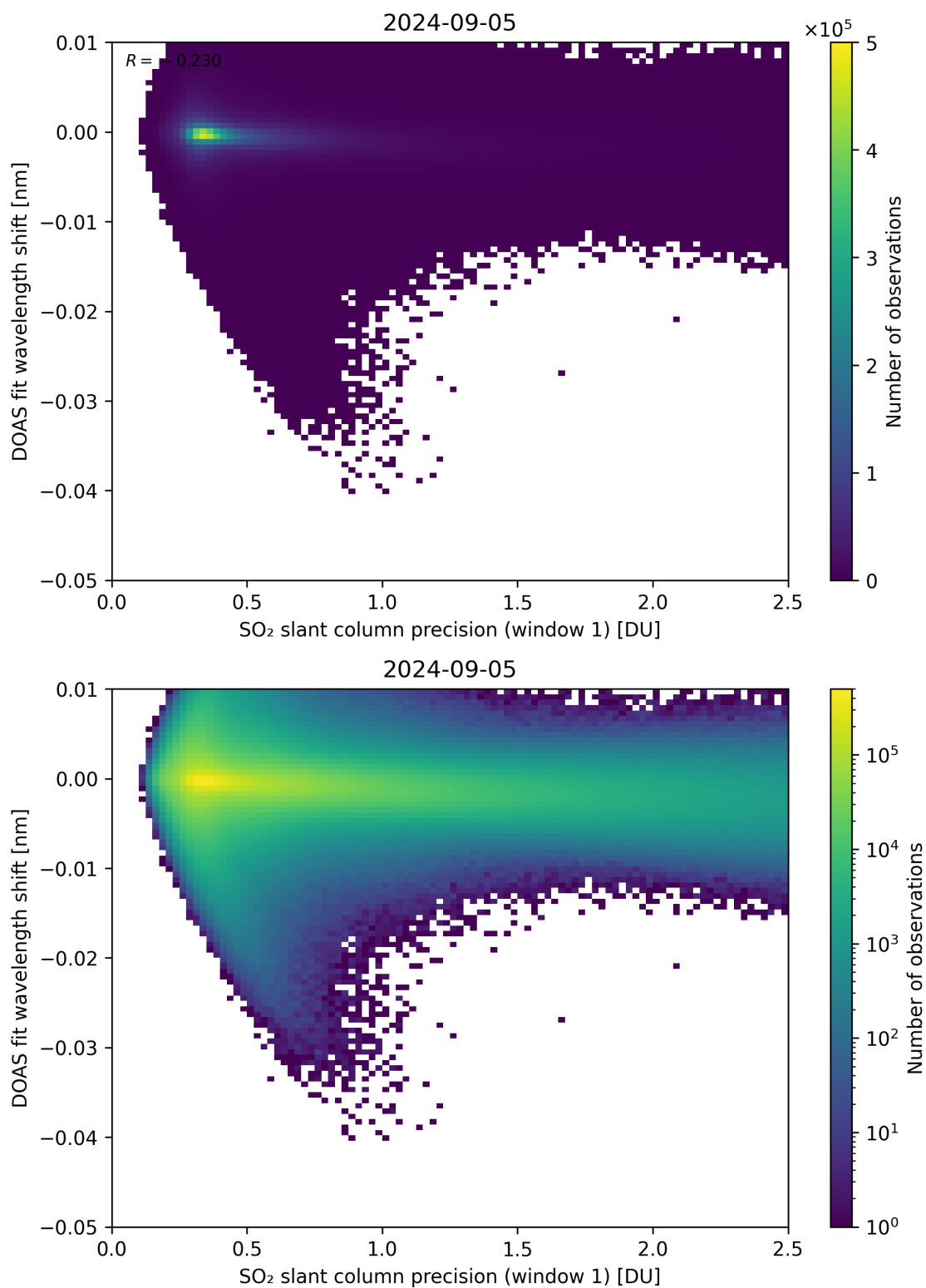
Figure 221: Scatter density plot of “SO 2 slant column precision (window 1)” against “DOAS fit wavelength shift” for 2024-09-04 to 2024-09-06.
