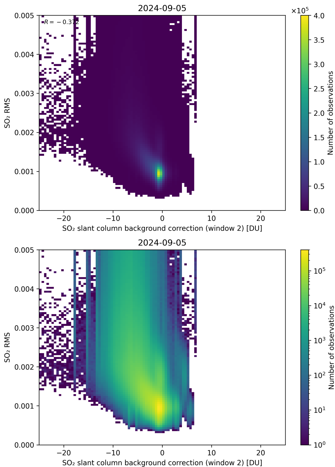
Figure 114: Scatter density plot of “SO 2 slant column background correction (window 2)” against “SO 2 RMS” for 2024-09-04 to 2024-09-06.
