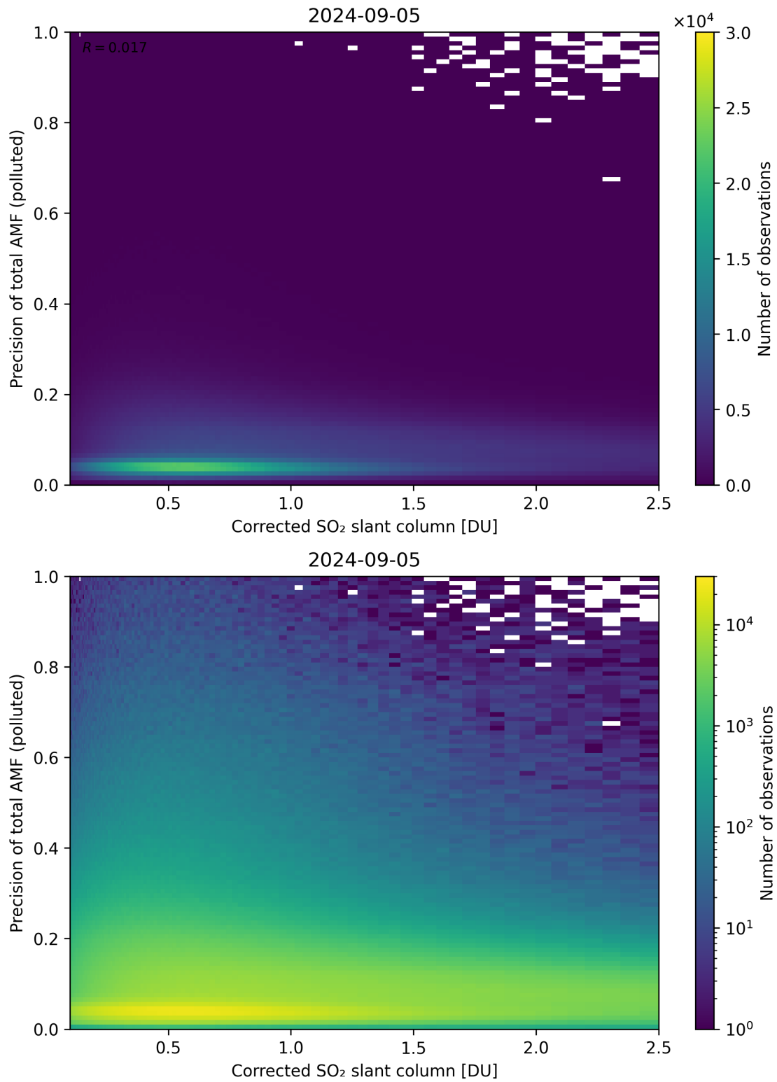
Figure 193: Scatter density plot of “Corrected SO 2 slant column” against “Precision of total AMF (polluted)” for 2024-09-04 to 2024-09-06.
