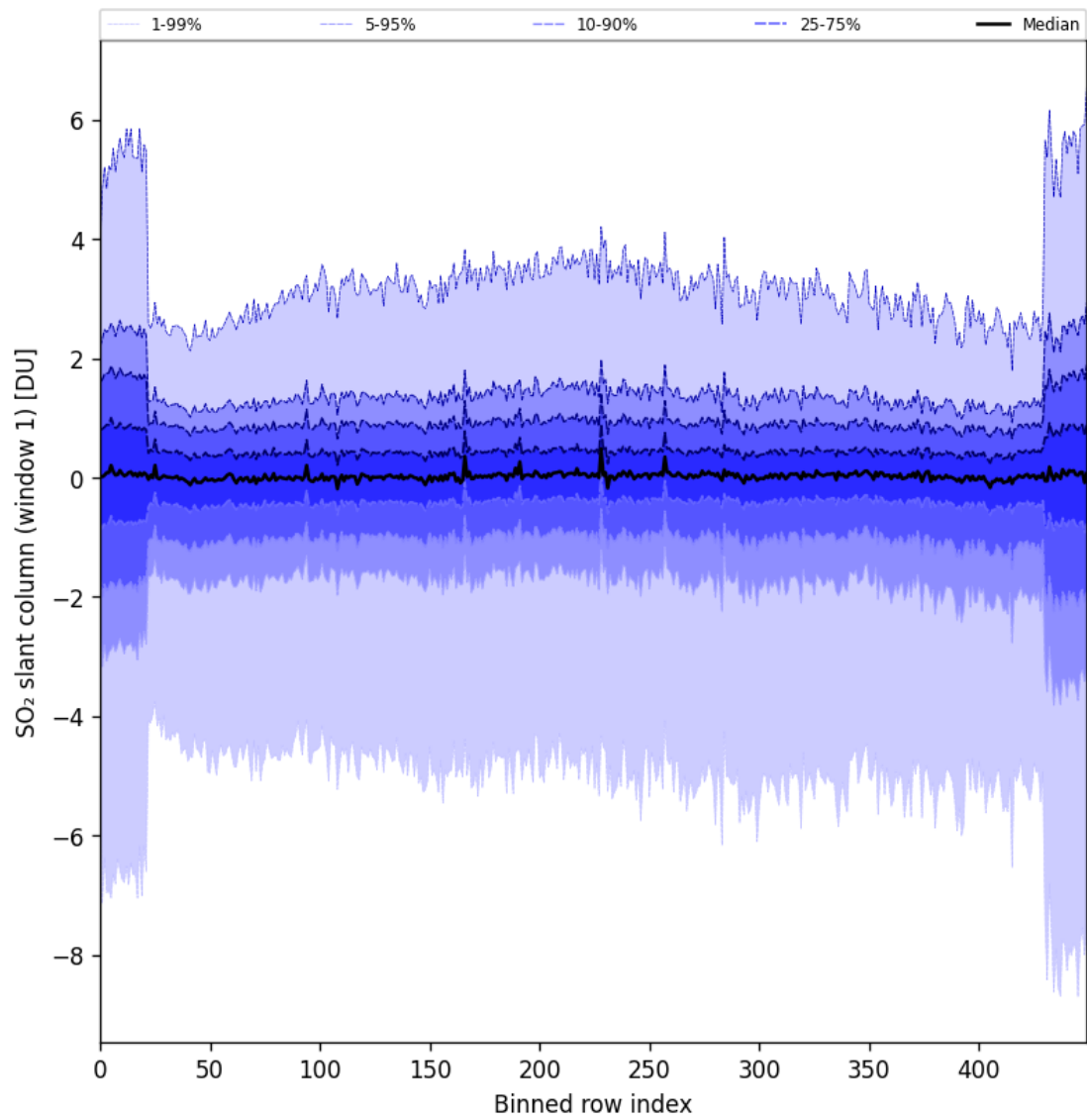
Figure 79: Along track statistics of “SO 2 slant column (window 1)” for 2024-09-04 to 2024-09-06
