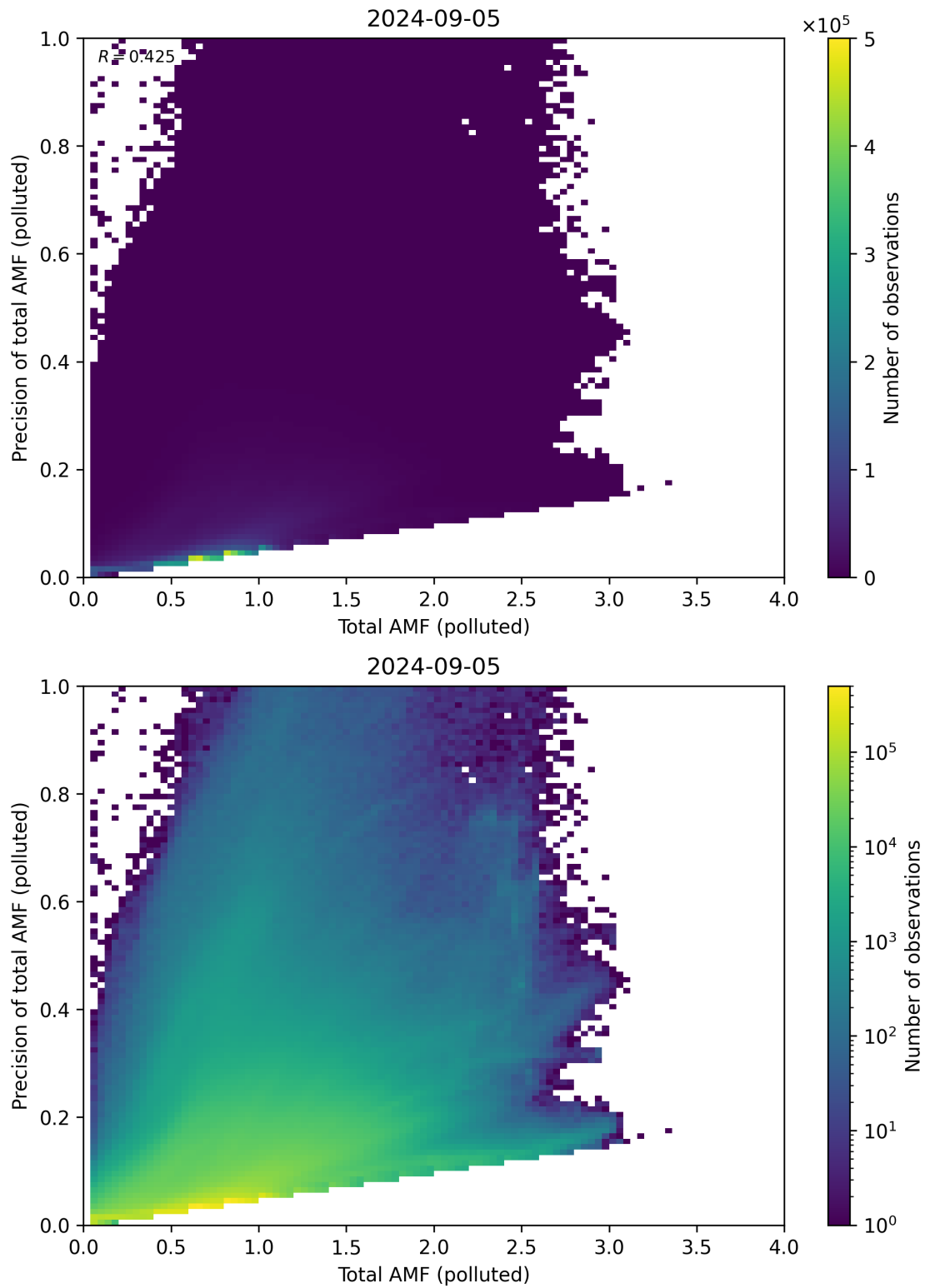
Figure 272: Scatter density plot of “Total AMF (polluted)” against “Precision of total AMF (polluted)” for 2024-09-04 to 2024-09-06.
