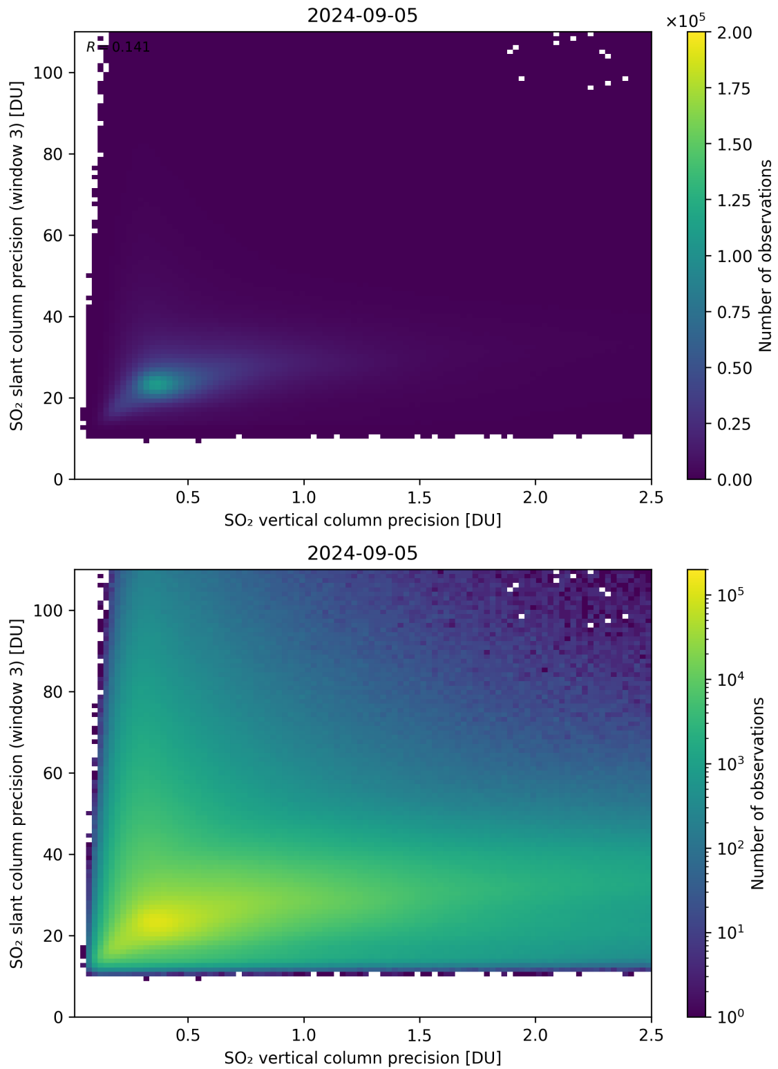
Figure 293: Scatter density plot of “SO 2 vertical column precision” against “SO 2 slant column precision (window 3)” for 2024-09-04 to 2024-09-06.
