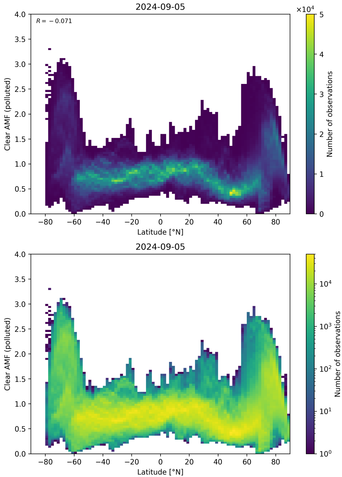
Figure 145: Scatter density plot of “Latitude” against “Clear AMF (polluted)” for 2024-09-04 to 2024-09-06.
