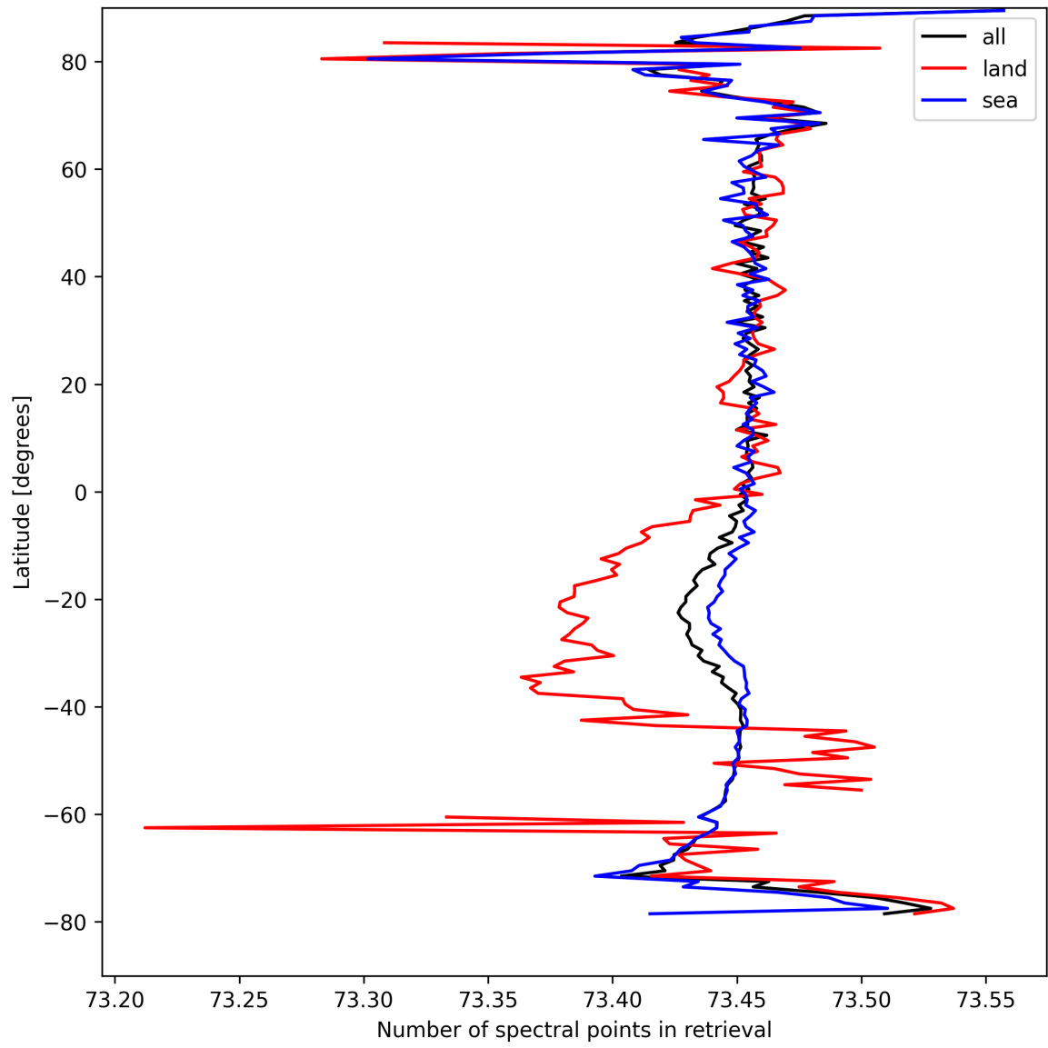
Figure 51: Zonal average of “Number of spectral points in retrieval” for 2024-09-04 to 2024-09-06.
