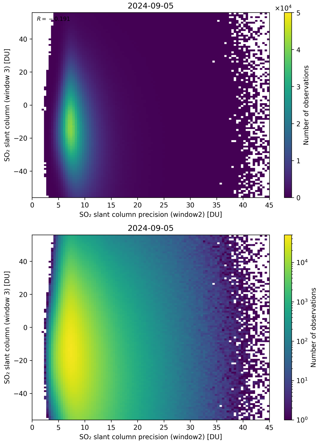
Figure 249: Scatter density plot of “SO 2 slant column precision (window2)” against “SO 2 slant column (window 3)” for 2024-09-04 to 2024-09-06.
