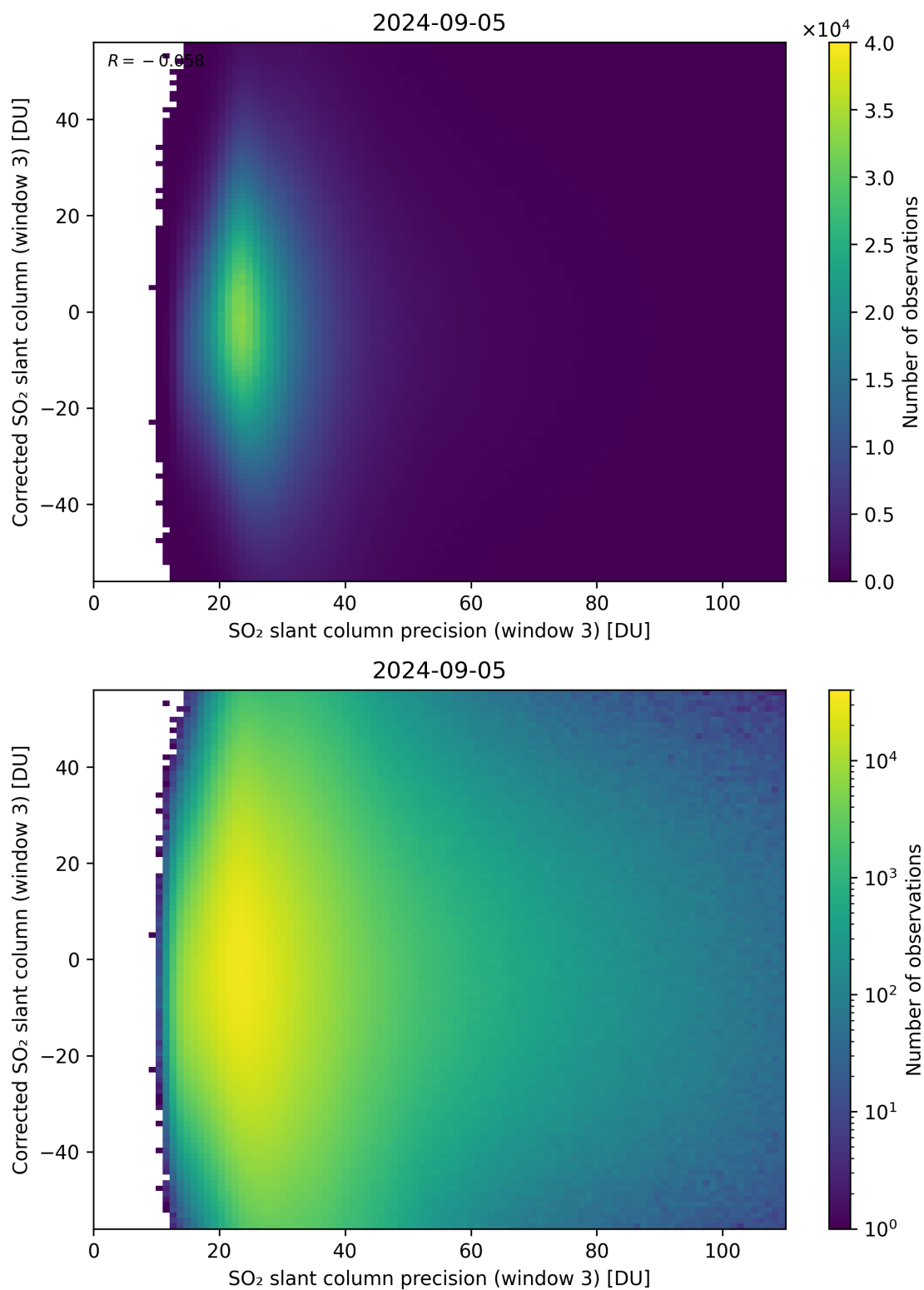
Figure 262: Scatter density plot of “SO 2 slant column precision (window 3)” against “Corrected SO 2 slant column (window 3)” for 2024-09-04 to 2024-09-06.
