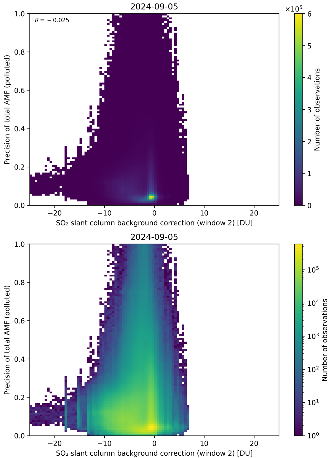
Figure 120: Scatter density plot of “SO 2 slant column background correction (window 2)” against “Precision of total AMF (polluted)” for 2024-09-04 to 2024-09-06.
