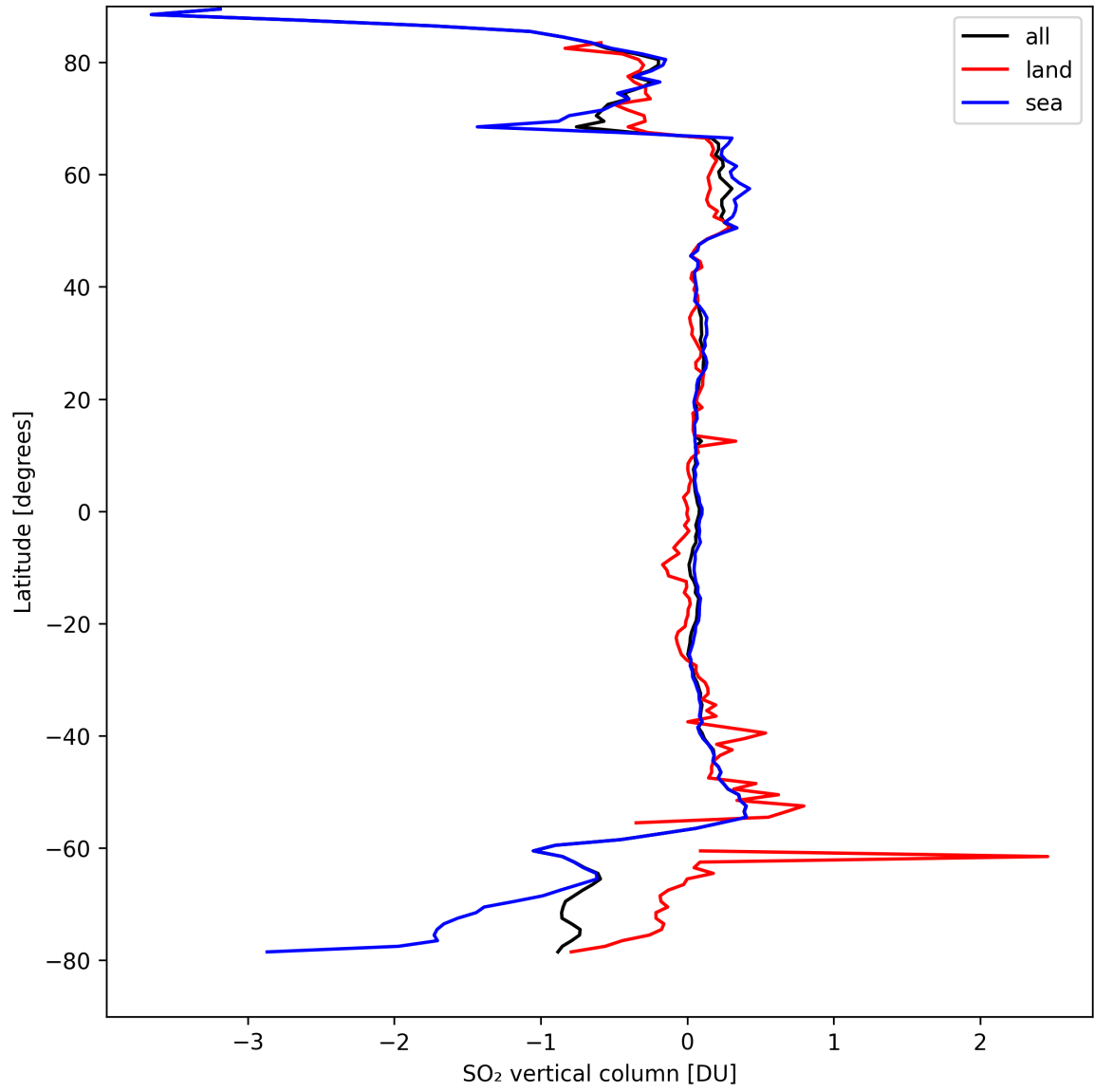
Figure 30: Zonal average of “SO 2 vertical column” for 2024-09-04 to 2024-09-06.
