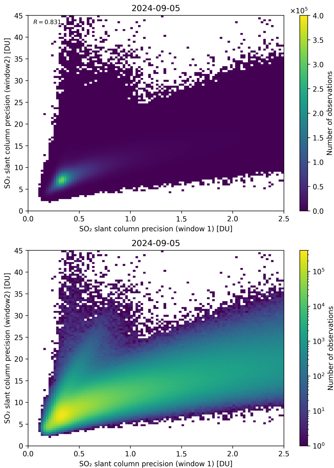
Figure 227: Scatter density plot of “SO 2 slant column precision (window 1)” against “SO 2 slant column precision (window2)” for 2024-09-04 to 2024-09-06.
