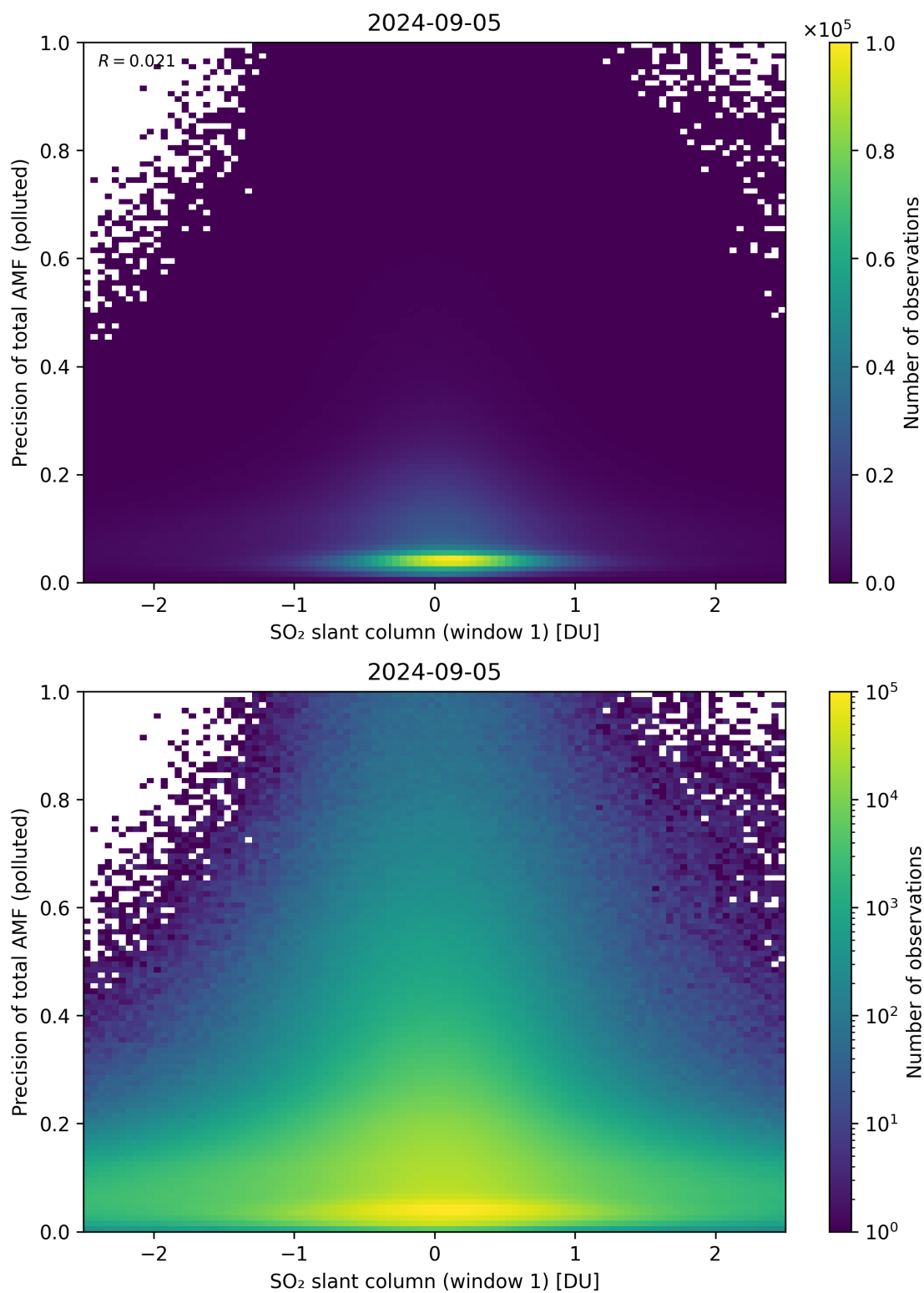
Figure 240: Scatter density plot of “SO 2 slant column (window 1)” against “Precision of total AMF (polluted)” for 2024-09-04 to 2024-09-06.
