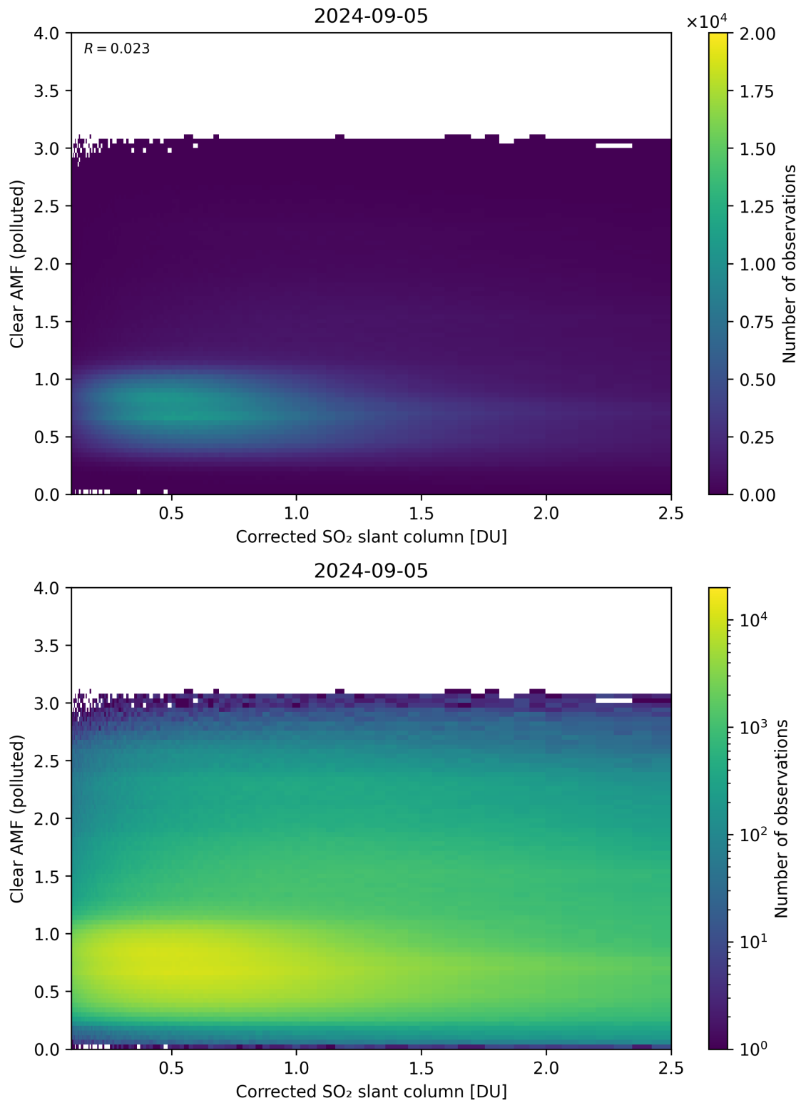
Figure 184: Scatter density plot of “Corrected SO 2 slant column” against “Clear AMF (polluted)” for 2024-09-04 to 2024-09-06.
