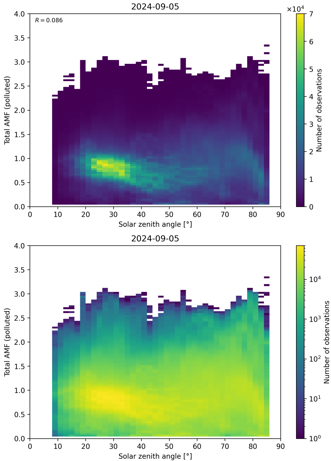
Figure 174: Scatter density plot of “Solar zenith angle” against “Total AMF (polluted)” for 2024-09-04 to 2024-09-06.
