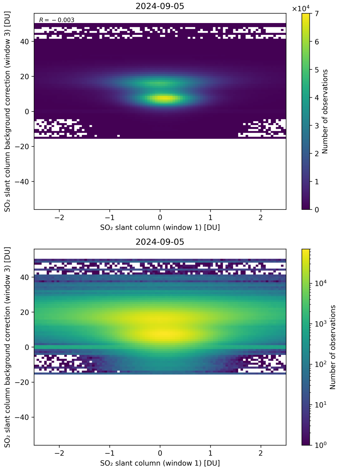
Figure 214: Scatter density plot of “SO 2 slant column (window 1)” against “SO 2 slant column background correction (window 3)” for 2024-09-04 to 2024-09-06.
