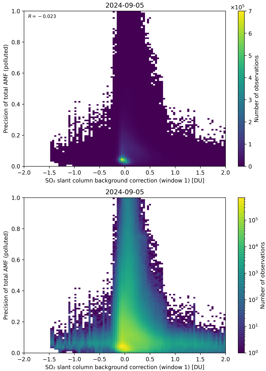
Figure 110: Scatter density plot of “SO 2 slant column background correction (window 1)” against “Precision of total AMF (polluted)” for 2024-09-04 to 2024-09-06.
