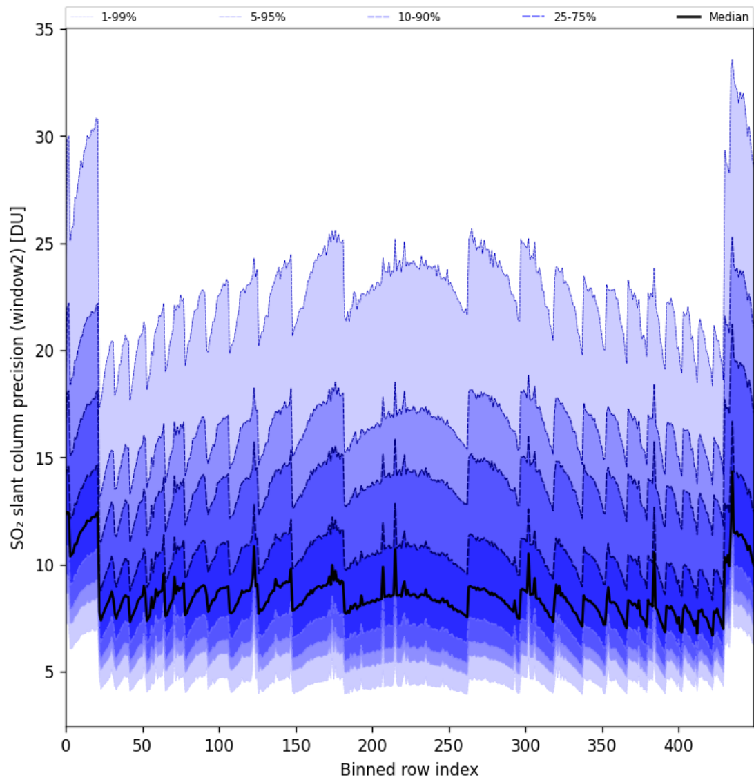
Figure 84: Along track statistics of “SO 2 slant column precision (window2)” for 2024-09-04 to 2024-09-06
