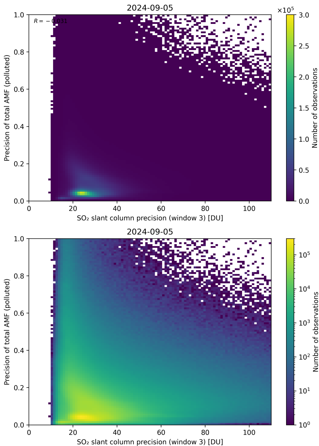
Figure 264: Scatter density plot of “SO 2 slant column precision (window 3)” against “Precision of total AMF (polluted)” for 2024-09-04 to 2024-09-06.
