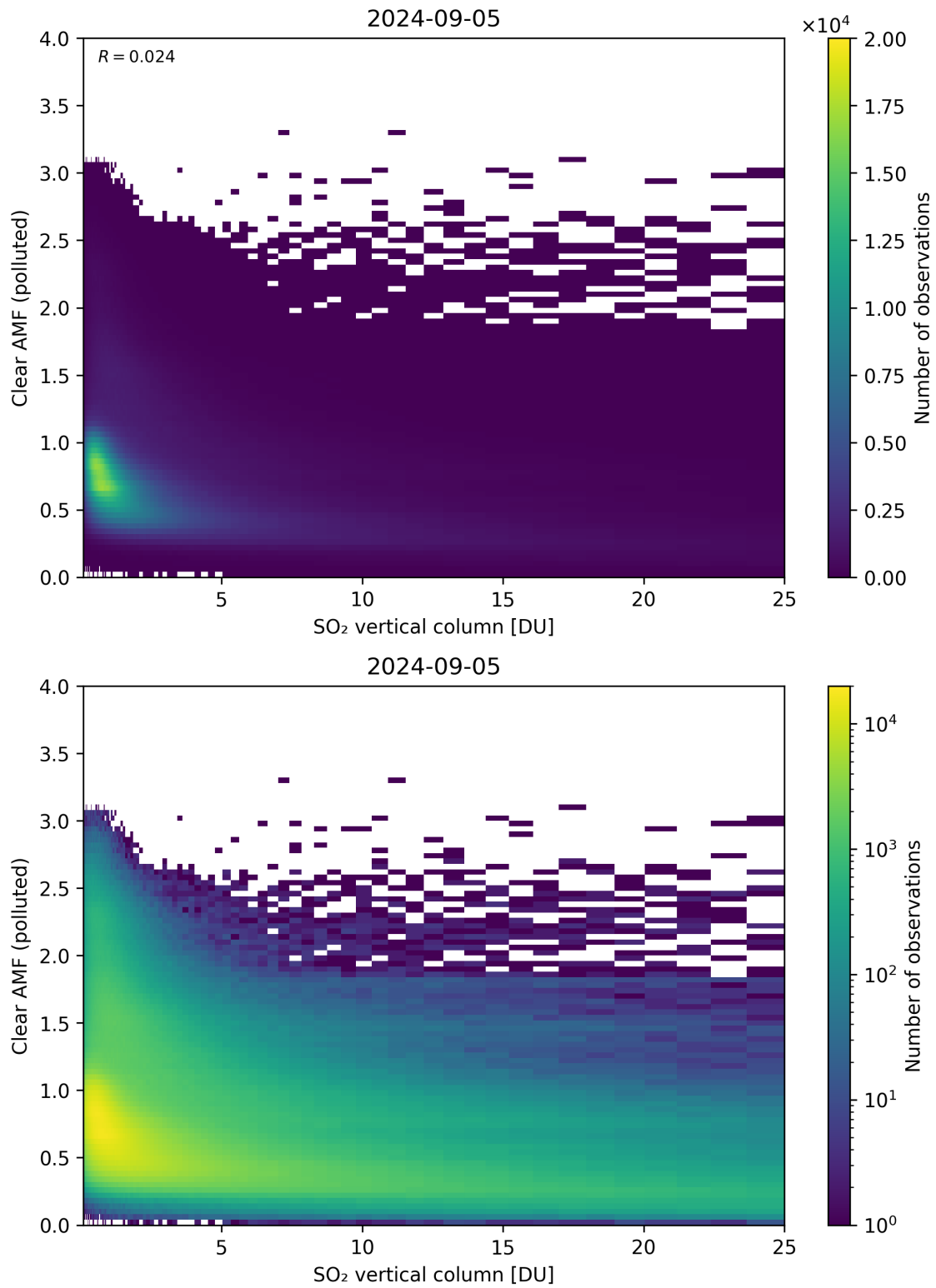
Figure 296: Scatter density plot of “SO 2 vertical column” against “Clear AMF (polluted)” for 2024-09-04 to 2024-09-06.
