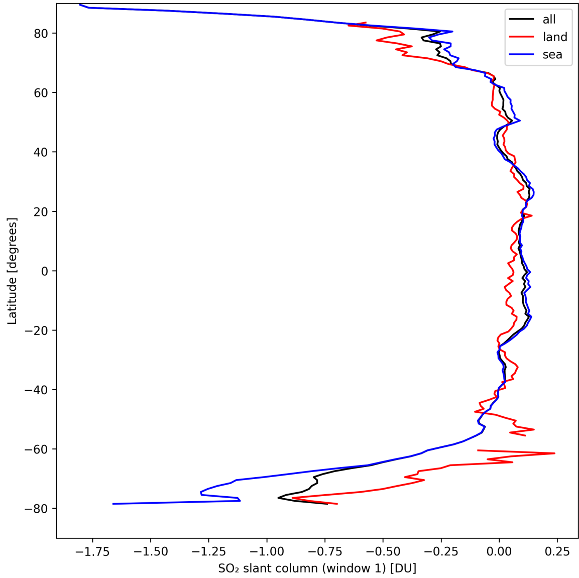
Figure 33: Zonal average of “SO 2 slant column (window 1)” for 2024-09-04 to 2024-09-06.
