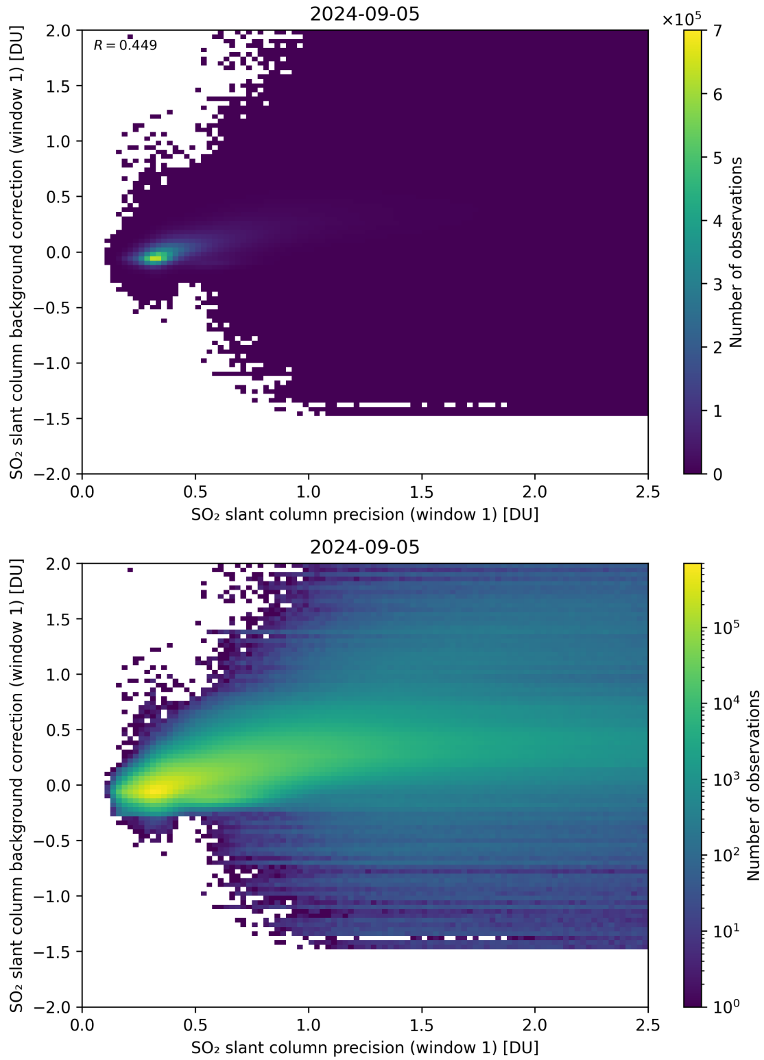
Figure 218: Scatter density plot of “SO 2 slant column precision (window 1)” against “SO 2 slant column background correction (window 1)” for 2024-09-04 to 2024-09-06.
