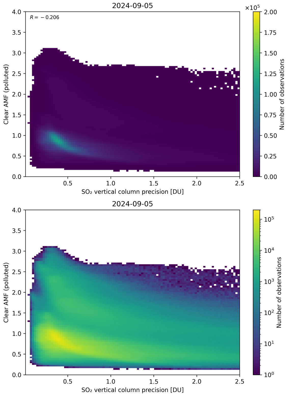
Figure 285: Scatter density plot of “SO 2 vertical column precision” against “Clear AMF (polluted)” for 2024-09-04 to 2024-09-06.
