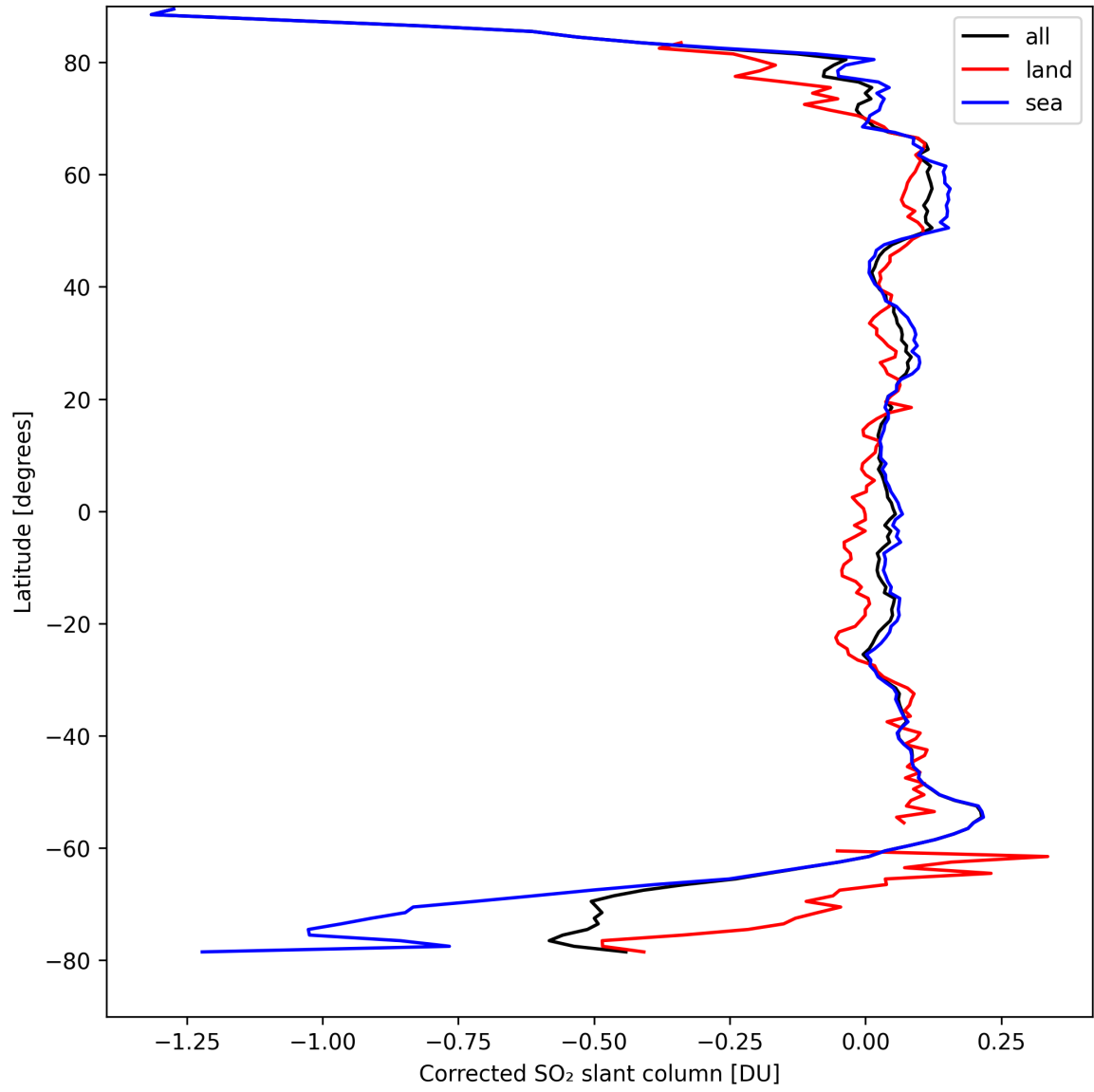
Figure 32: Zonal average of “Corrected SO 2 slant column” for 2024-09-04 to 2024-09-06.
