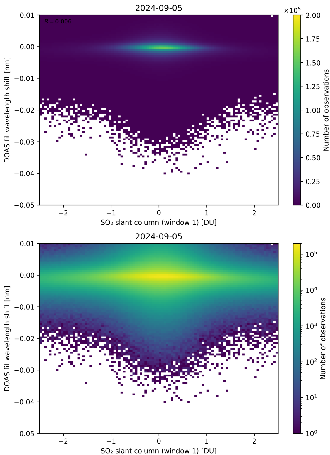
Figure 215: Scatter density plot of “SO 2 slant column (window 1)” against “DOAS fit wavelength shift” for 2024-09-04 to 2024-09-06.
