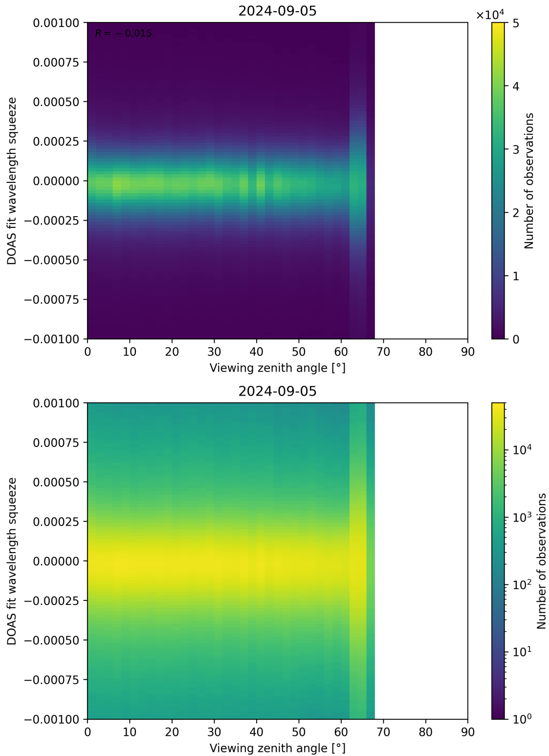
Figure 312: Scatter density plot of “Viewing zenith angle” against “DOAS fit wavelength squeeze” for 2024-09-04 to 2024-09-06.
