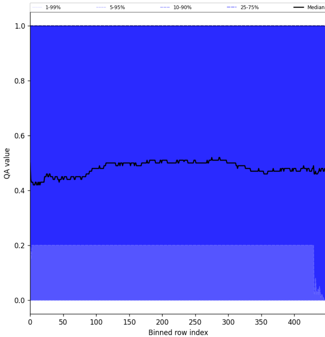
Figure 75: Along track statistics of “QA value” for 2024-09-04 to 2024-09-06
