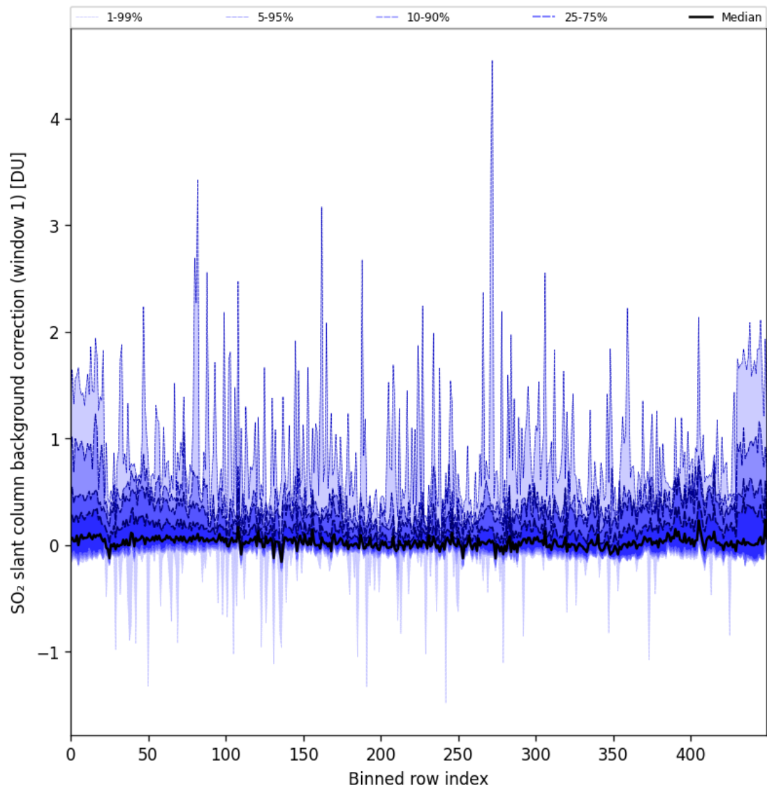
Figure 82: Along track statistics of “SO 2 slant column background correction (window 1)” for 2024-09-04 to 2024-09-06
