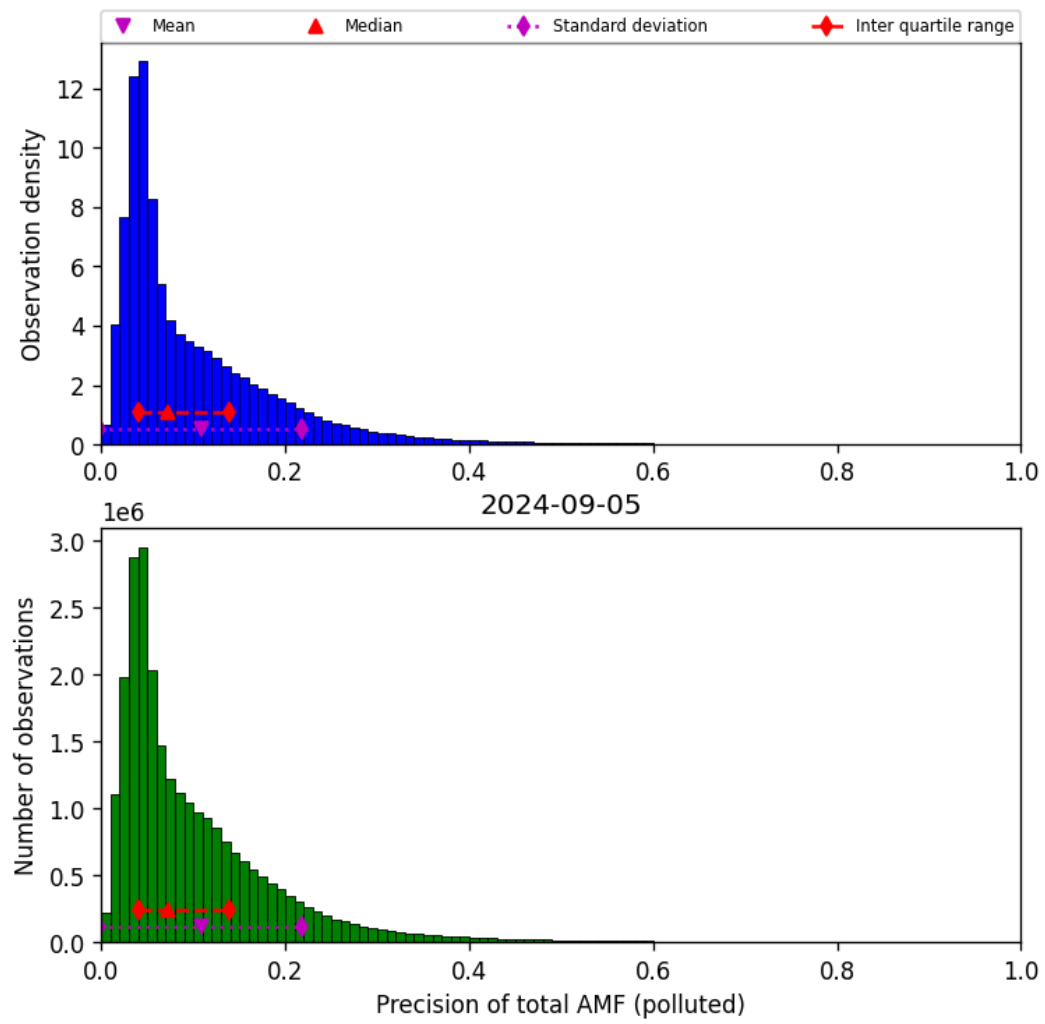
Figure 72: Histogram of “Precision of total AMF (polluted)” for 2024-09-04 to 2024-09-06
