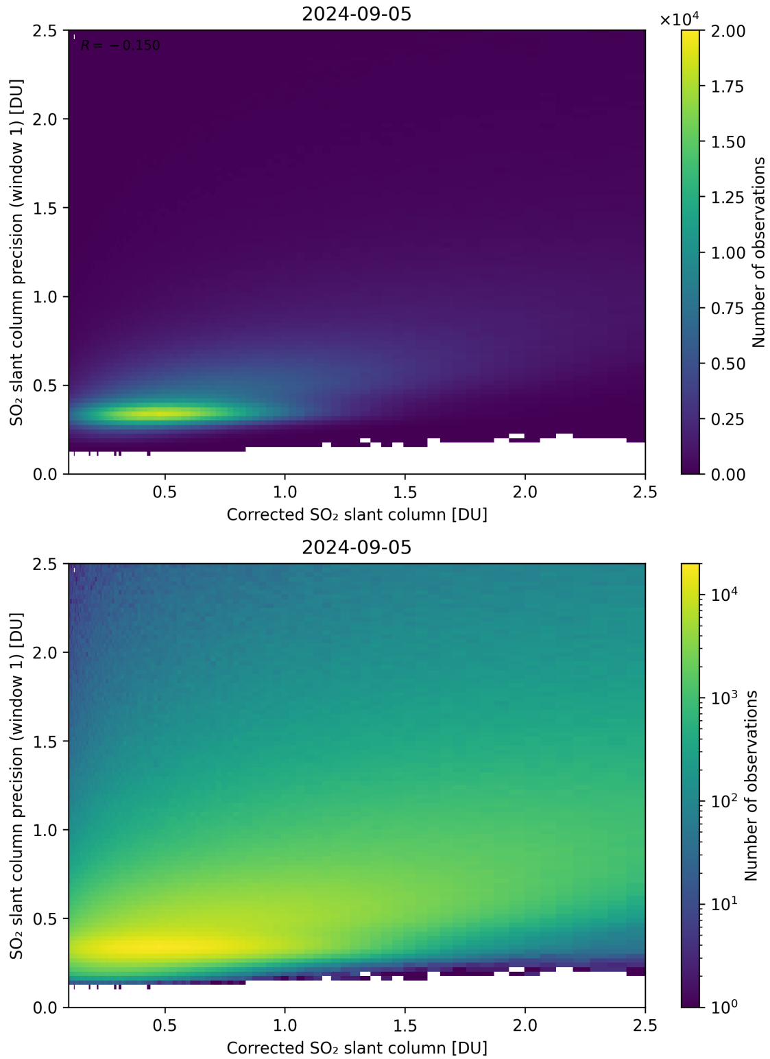
Figure 188: Scatter density plot of “Corrected SO 2 slant column” against “SO 2 slant column precision (window 1)” for 2024-09-04 to 2024-09-06.
