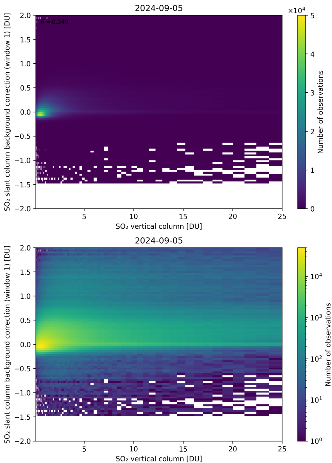
Figure 273: Scatter density plot of “SO 2 vertical column” against “SO 2 slant column background correction (window 1)” for 2024-09-04 to 2024-09-06.
