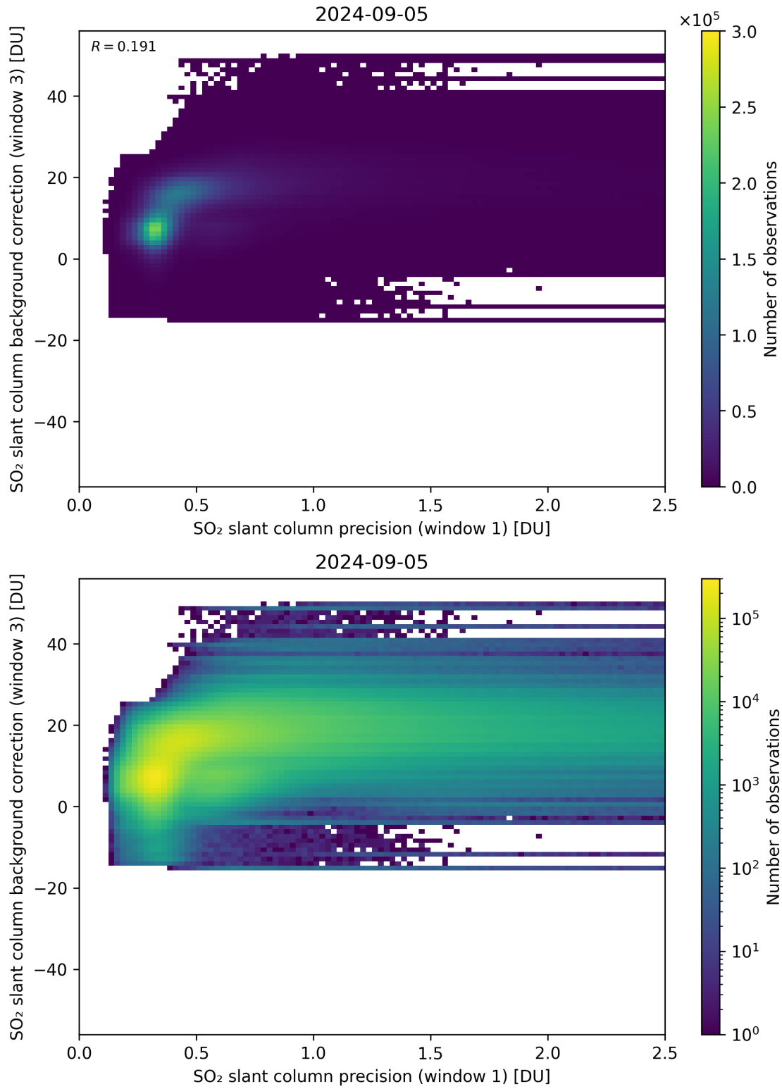
Figure 220: Scatter density plot of “SO 2 slant column precision (window 1)” against “SO 2 slant column background correction (window 3)” for 2024-09-04 to 2024-09-06.
