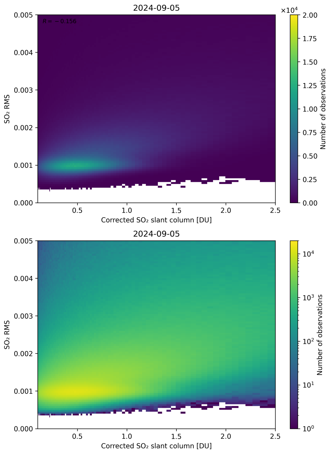
Figure 183: Scatter density plot of “Corrected SO 2 slant column” against “SO 2 RMS” for 2024-09-04 to 2024-09-06.
