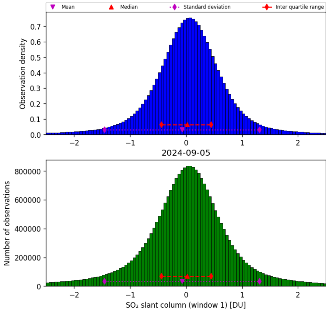
Figure 56: Histogram of “SO 2 slant column (window 1)” for 2024-09-04 to 2024-09-06
