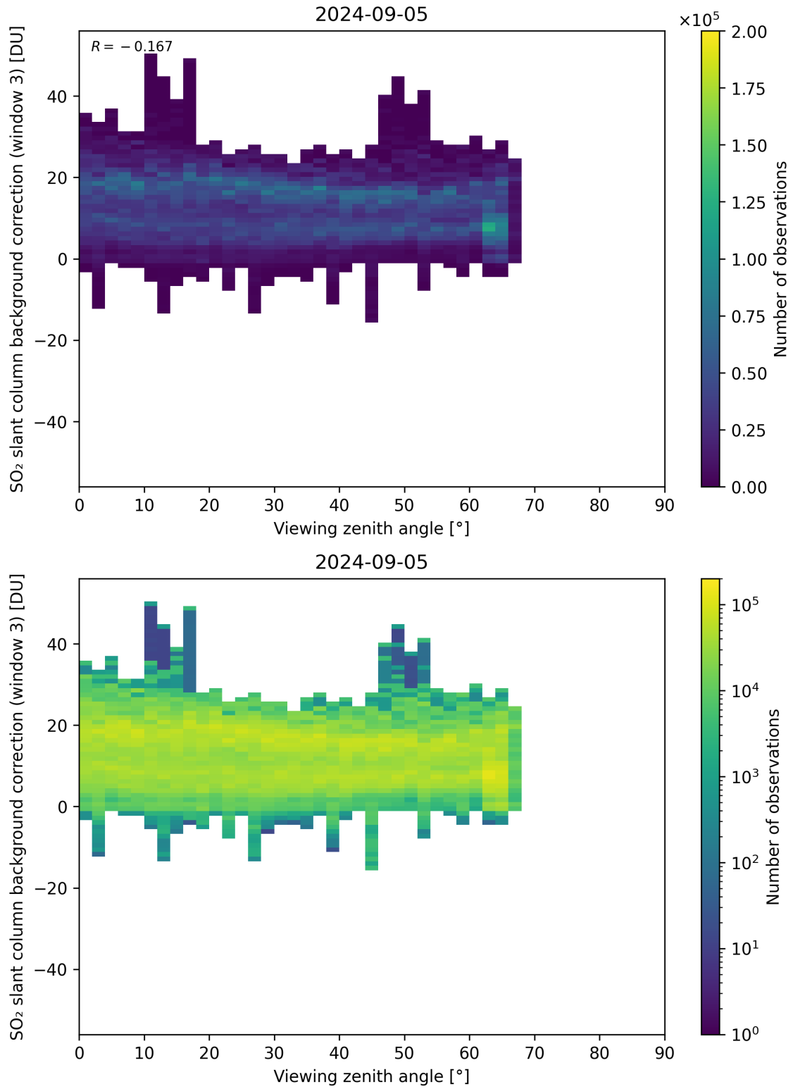
Figure 310: Scatter density plot of “Viewing zenith angle” against “SO 2 slant column background correction (window 3)” for 2024-09-04 to 2024-09-06.
