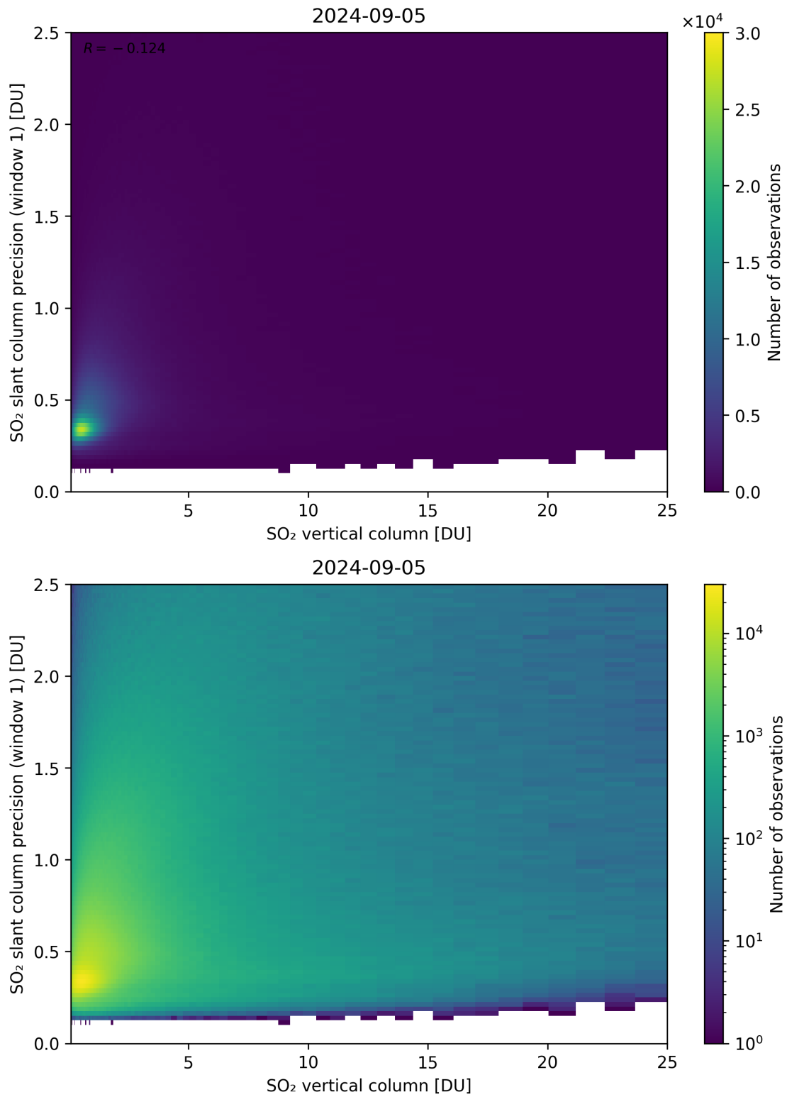
Figure 301: Scatter density plot of “SO 2 vertical column” against “SO 2 slant column precision (window 1)” for 2024-09-04 to 2024-09-06.
