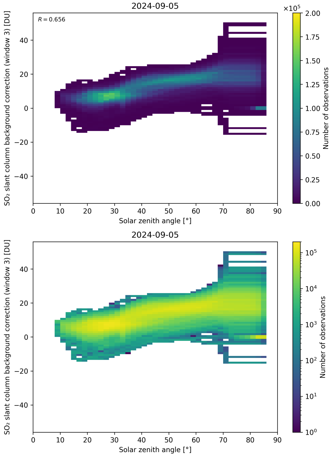
Figure 160: Scatter density plot of “Solar zenith angle” against “SO 2 slant column background correction (window 3)” for 2024-09-04 to 2024-09-06.
