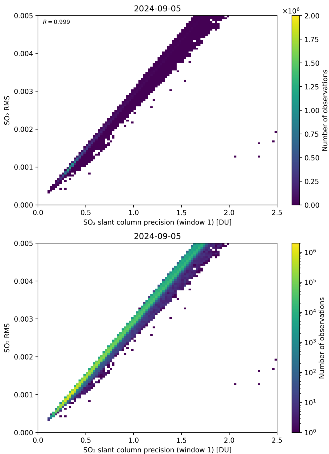
Figure 223: Scatter density plot of “SO 2 slant column precision (window 1)” against “SO 2 RMS” for 2024-09-04 to 2024-09-06.
