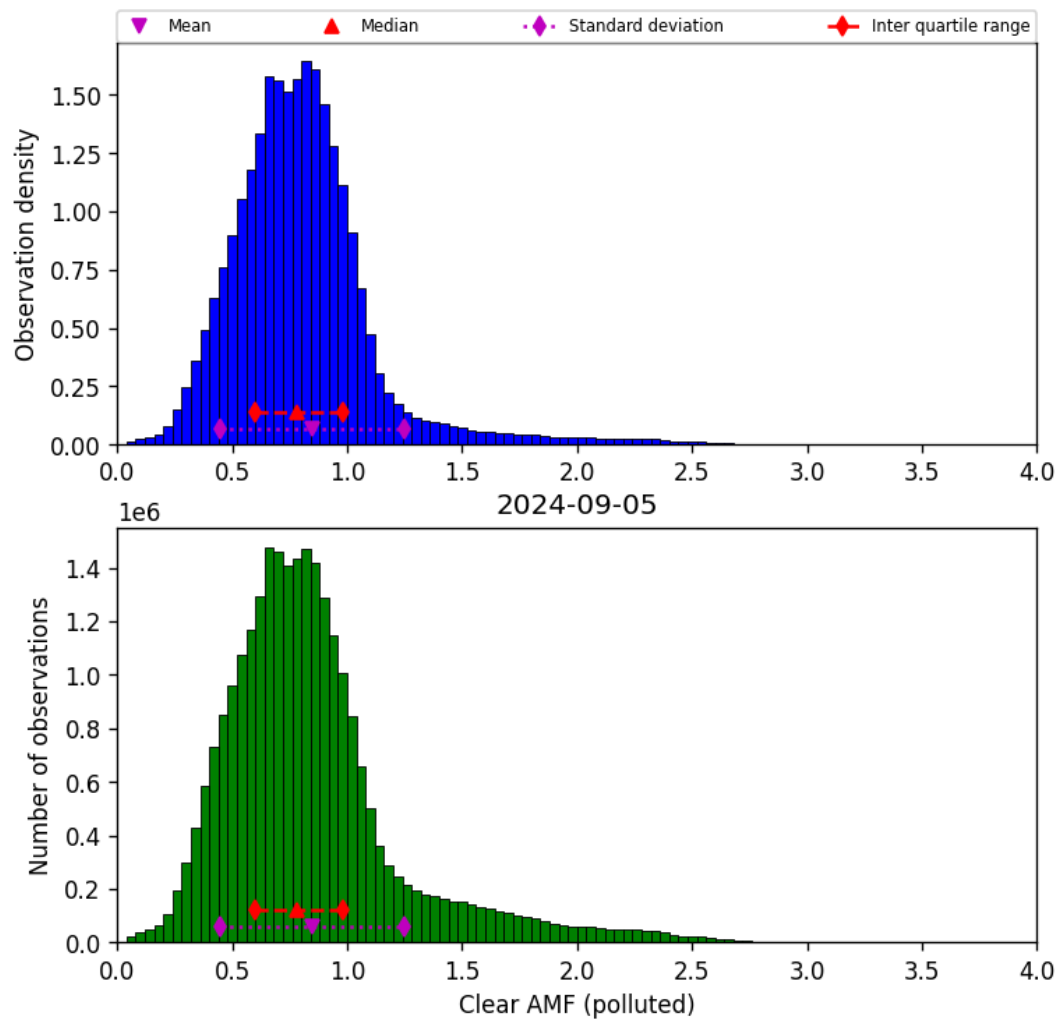
Figure 73: Histogram of “Clear AMF (polluted)” for 2024-09-04 to 2024-09-06
