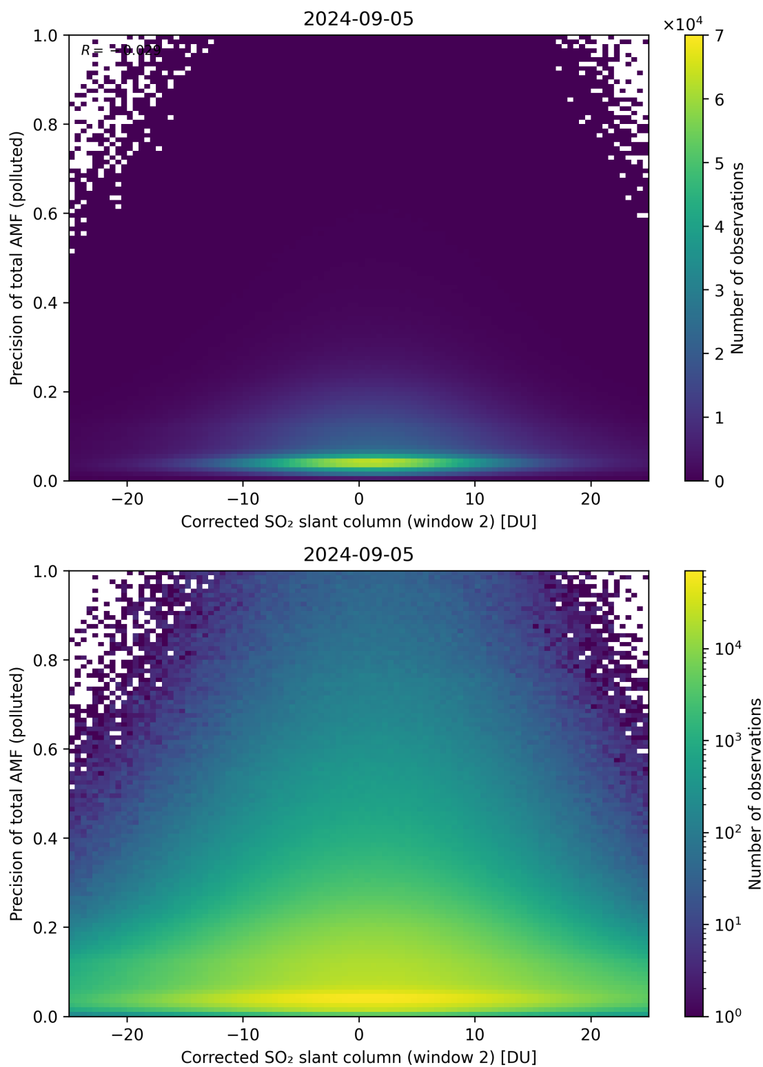
Figure 204: Scatter density plot of “Corrected SO 2 slant column (window 2)” against “Precision of total AMF (polluted)” for 2024-09-04 to 2024-09-06.
