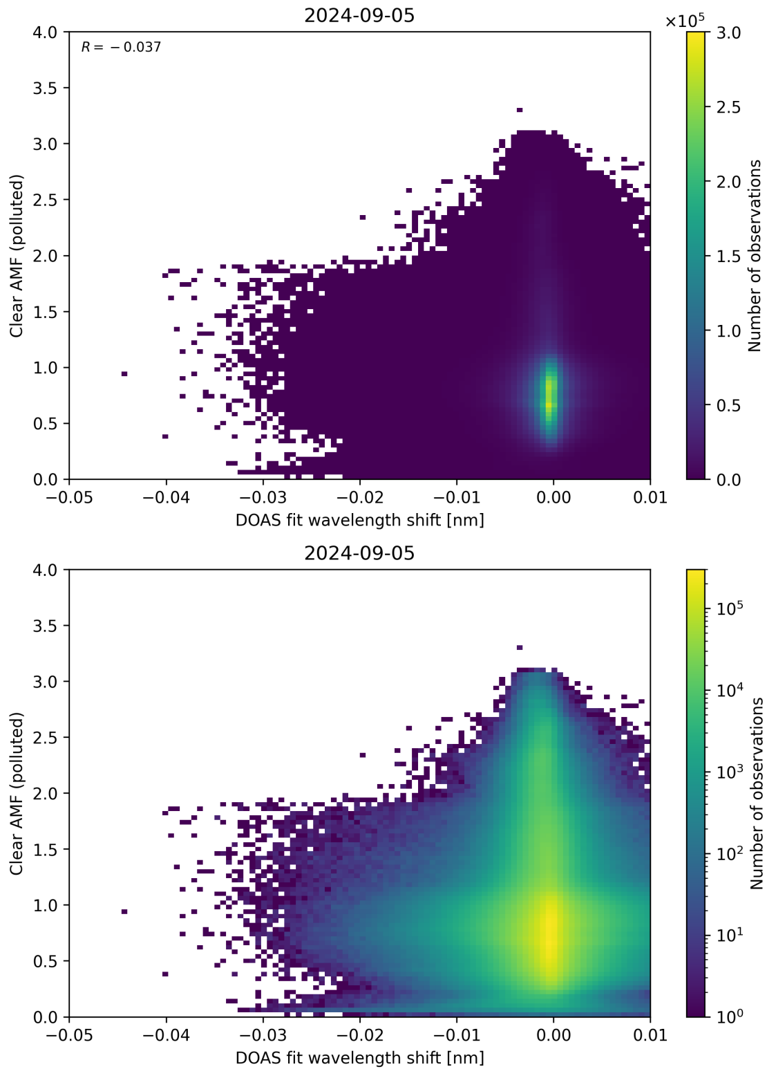
Figure 129: Scatter density plot of “DOAS fit wavelength shift” against “Clear AMF (polluted)” for 2024-09-04 to 2024-09-06.
