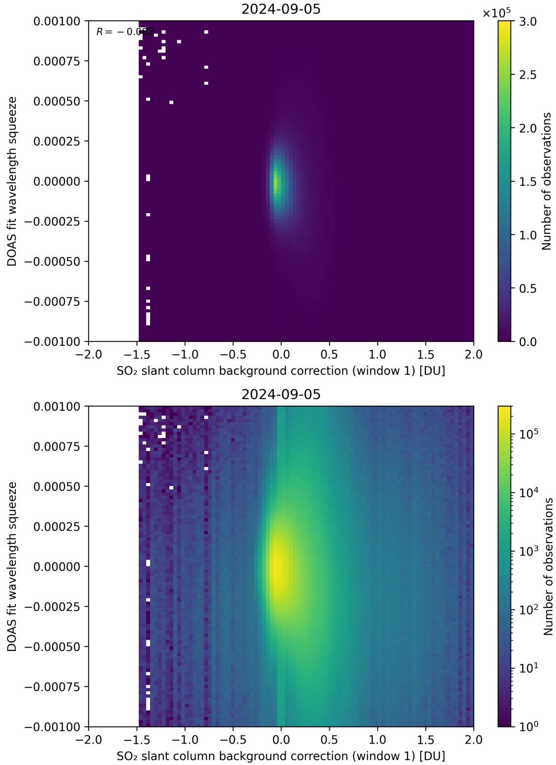
Figure 101: Scatter density plot of “SO 2 slant column background correction (window 1)” against “DOAS fit wavelength squeeze” for 2024-09-04 to 2024-09-06.
