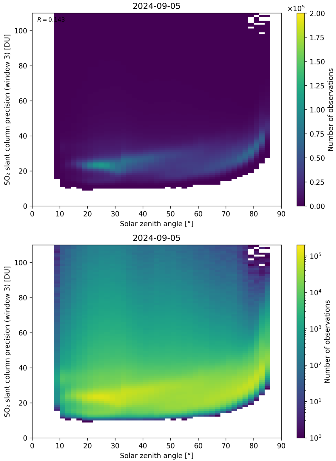
Figure 173: Scatter density plot of “Solar zenith angle” against “SO 2 slant column precision (window 3)” for 2024-09-04 to 2024-09-06.
