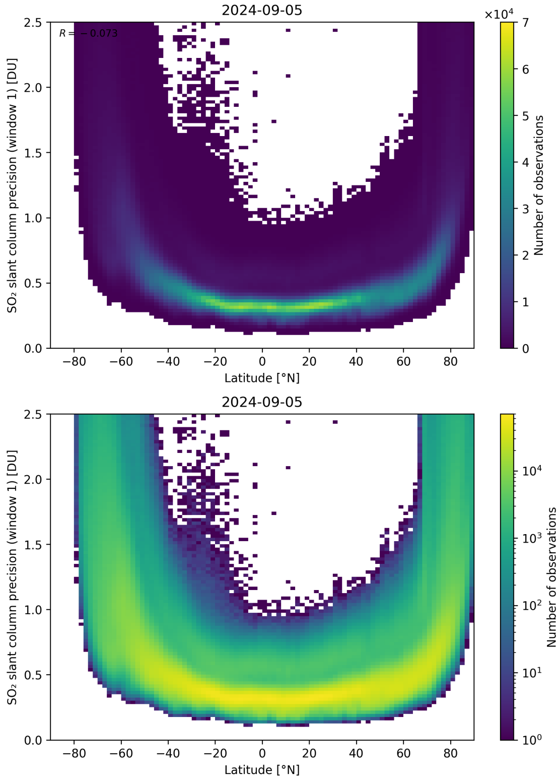
Figure 150: Scatter density plot of “Latitude” against “SO 2 slant column precision (window 1)” for 2024-09-04 to 2024-09-06.
