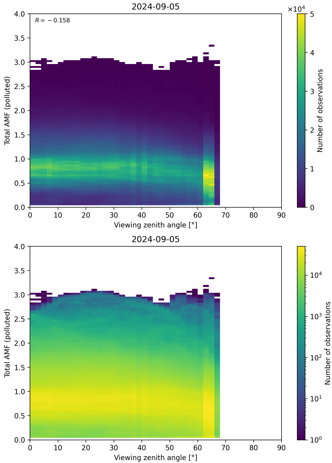
Figure 325: Scatter density plot of “Viewing zenith angle” against “Total AMF (polluted)” for 2024-09-04 to 2024-09-06.
