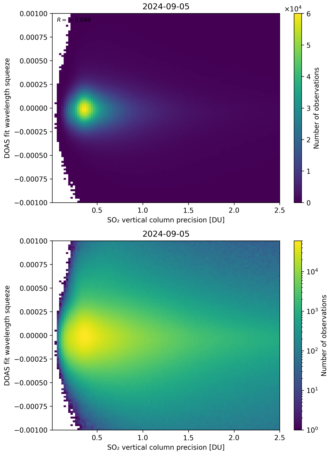
Figure 283: Scatter density plot of “SO 2 vertical column precision” against “DOAS fit wavelength squeeze” for 2024-09-04 to 2024-09-06.
