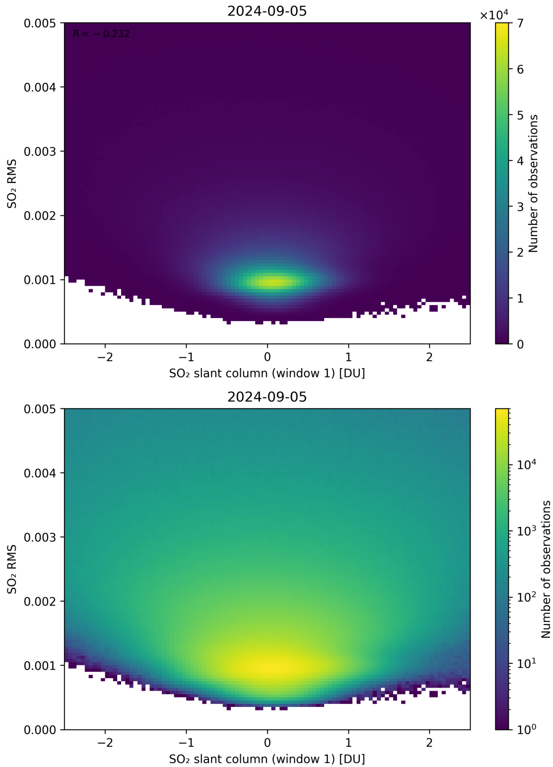
Figure 217: Scatter density plot of “SO 2 slant column (window 1)” against “SO 2 RMS” for 2024-09-04 to 2024-09-06.
