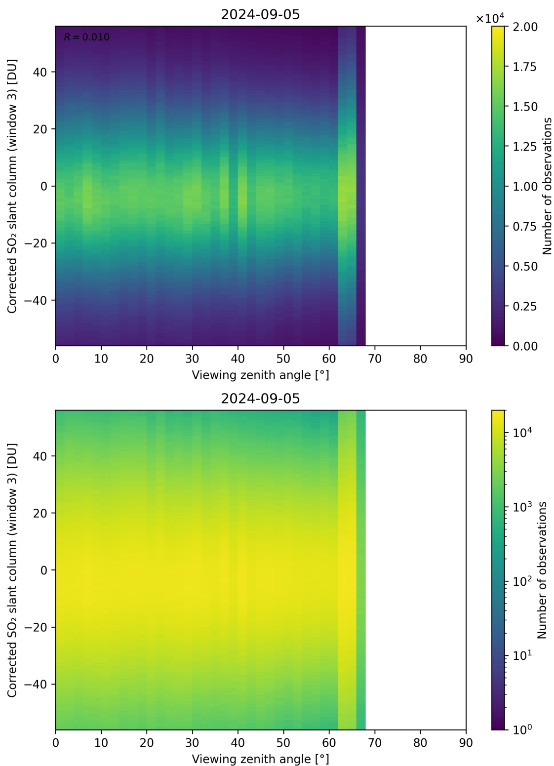
Figure 319: Scatter density plot of “Viewing zenith angle” against “Corrected SO 2 slant column (window 3)” for 2024-09-04 to 2024-09-06.
