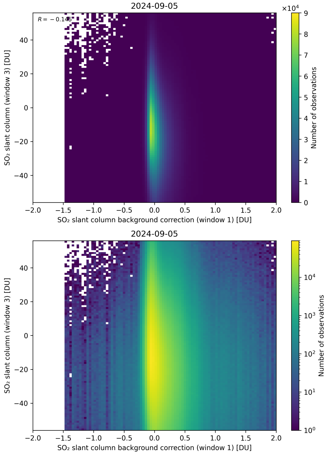
Figure 107: Scatter density plot of “SO 2 slant column background correction (window 1)” against “SO 2 slant column (window 3)” for 2024-09-04 to 2024-09-06.
