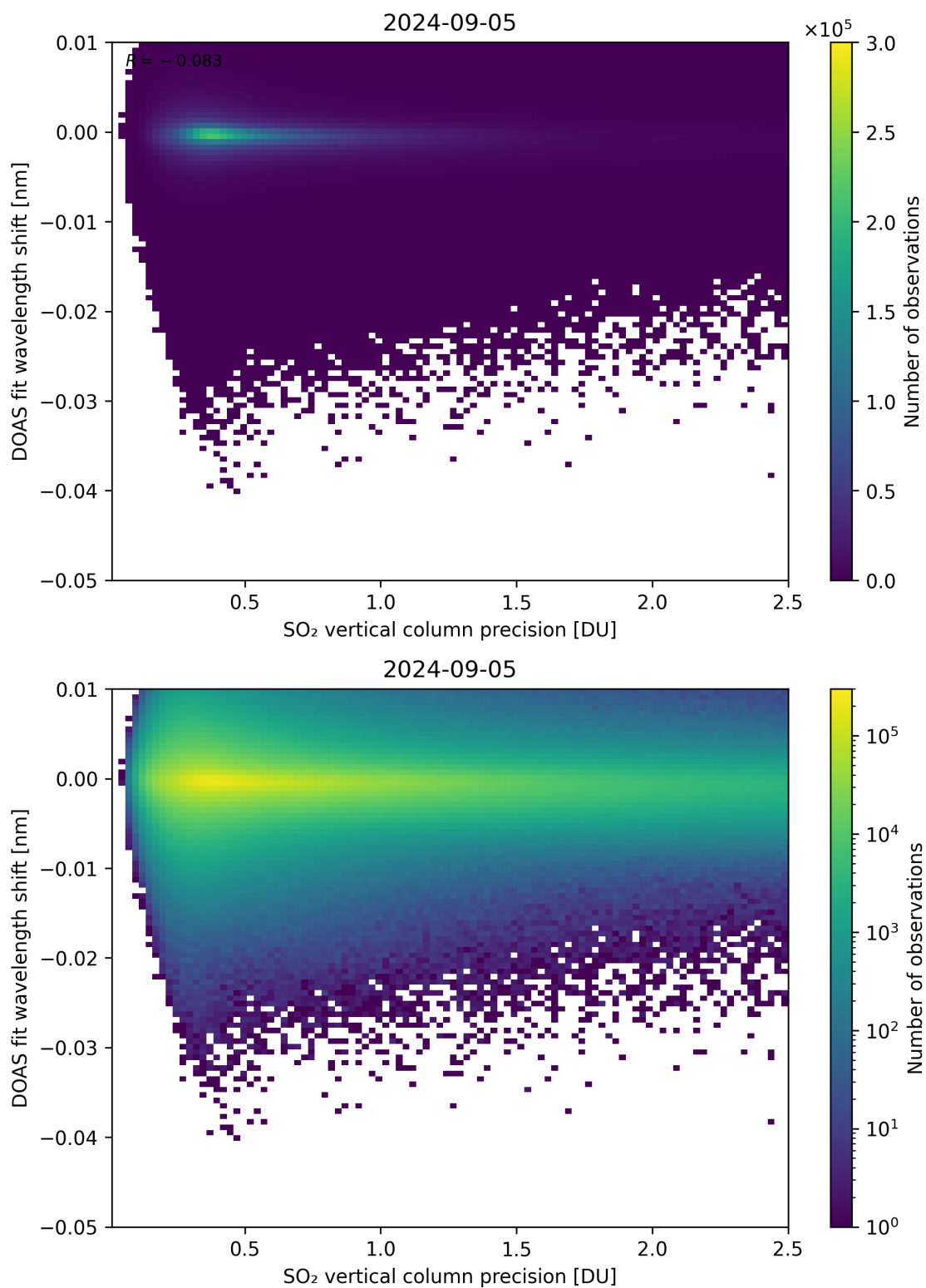
Figure 282: Scatter density plot of “SO 2 vertical column precision” against “DOAS fit wavelength shift” for 2024-09-04 to 2024-09-06.
