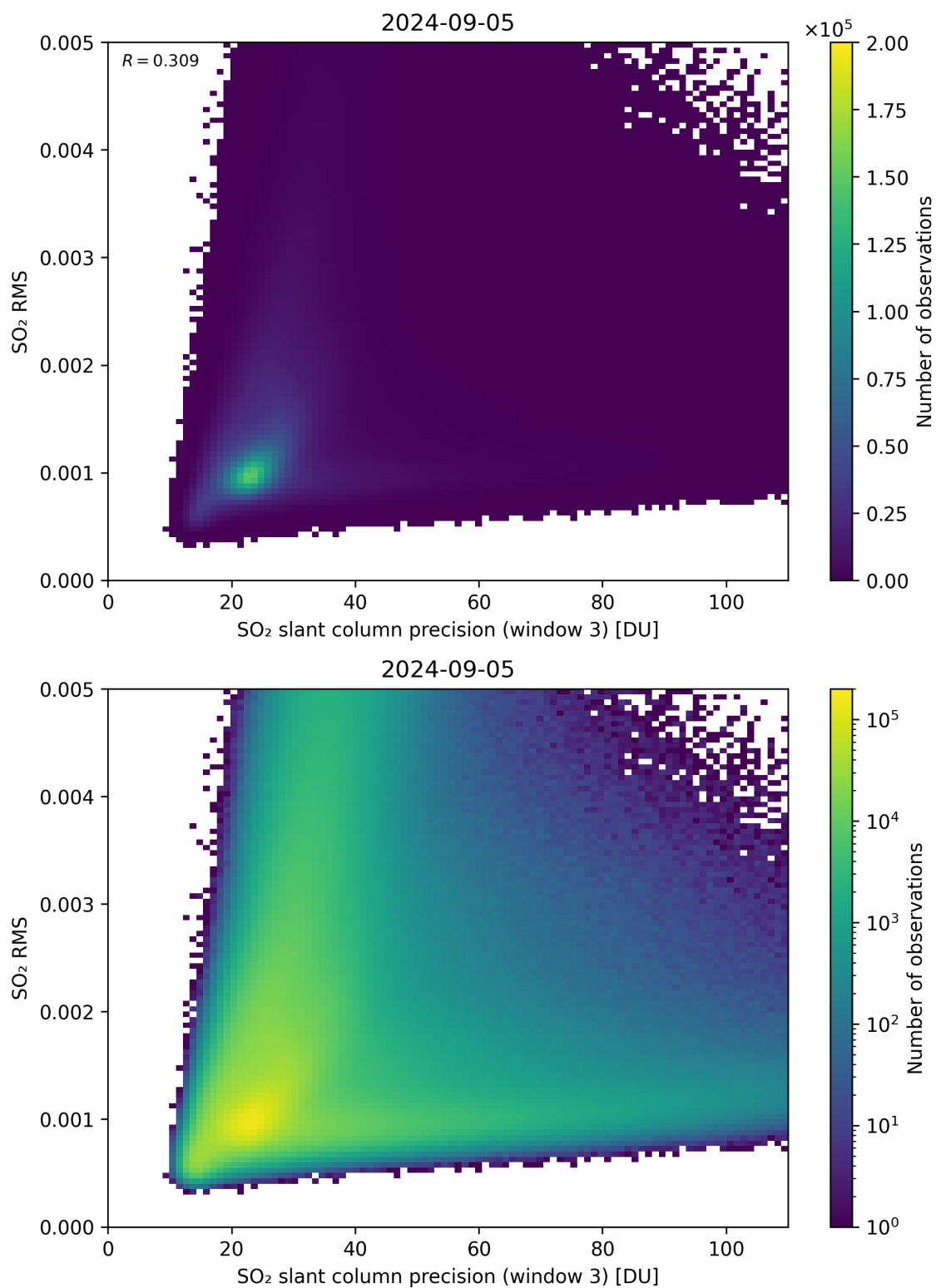
Figure 260: Scatter density plot of “SO 2 slant column precision (window 3)” against “SO 2 RMS” for 2024-09-04 to 2024-09-06.
