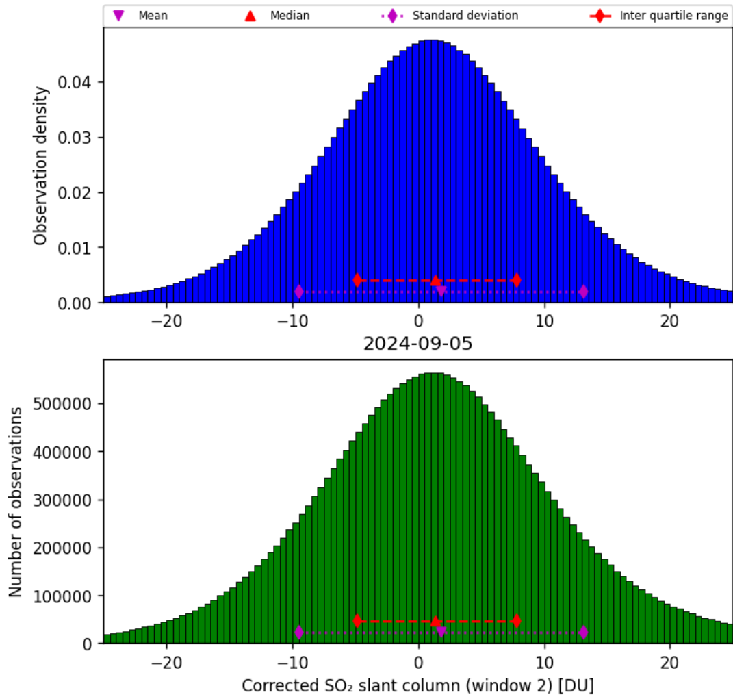
Figure 62: Histogram of “Corrected SO 2 slant column (window 2)” for 2024-09-04 to 2024-09-06
