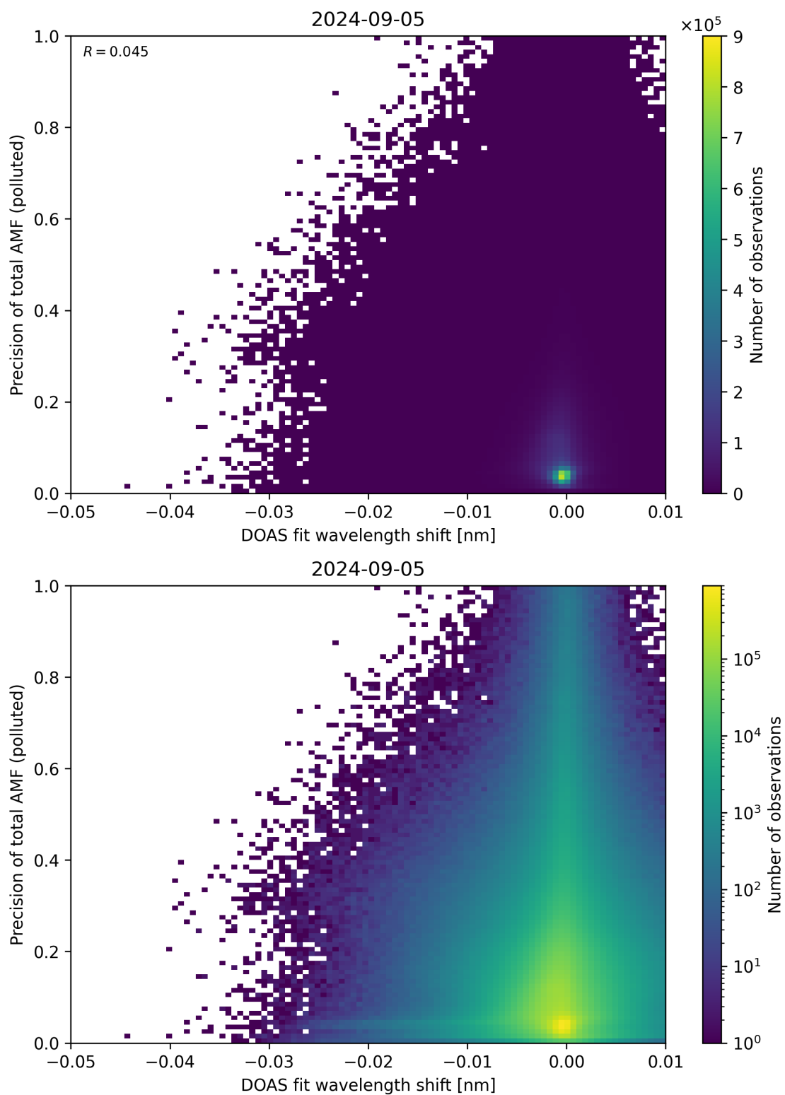
Figure 131: Scatter density plot of “DOAS fit wavelength shift” against “Precision of total AMF (polluted)” for 2024-09-04 to 2024-09-06.
