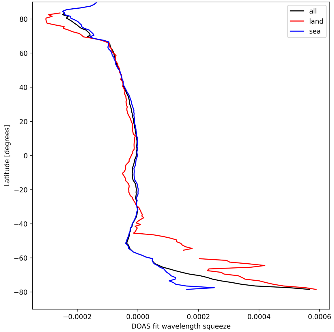
Figure 46: Zonal average of “DOAS fit wavelength squeeze” for 2024-09-04 to 2024-09-06.
