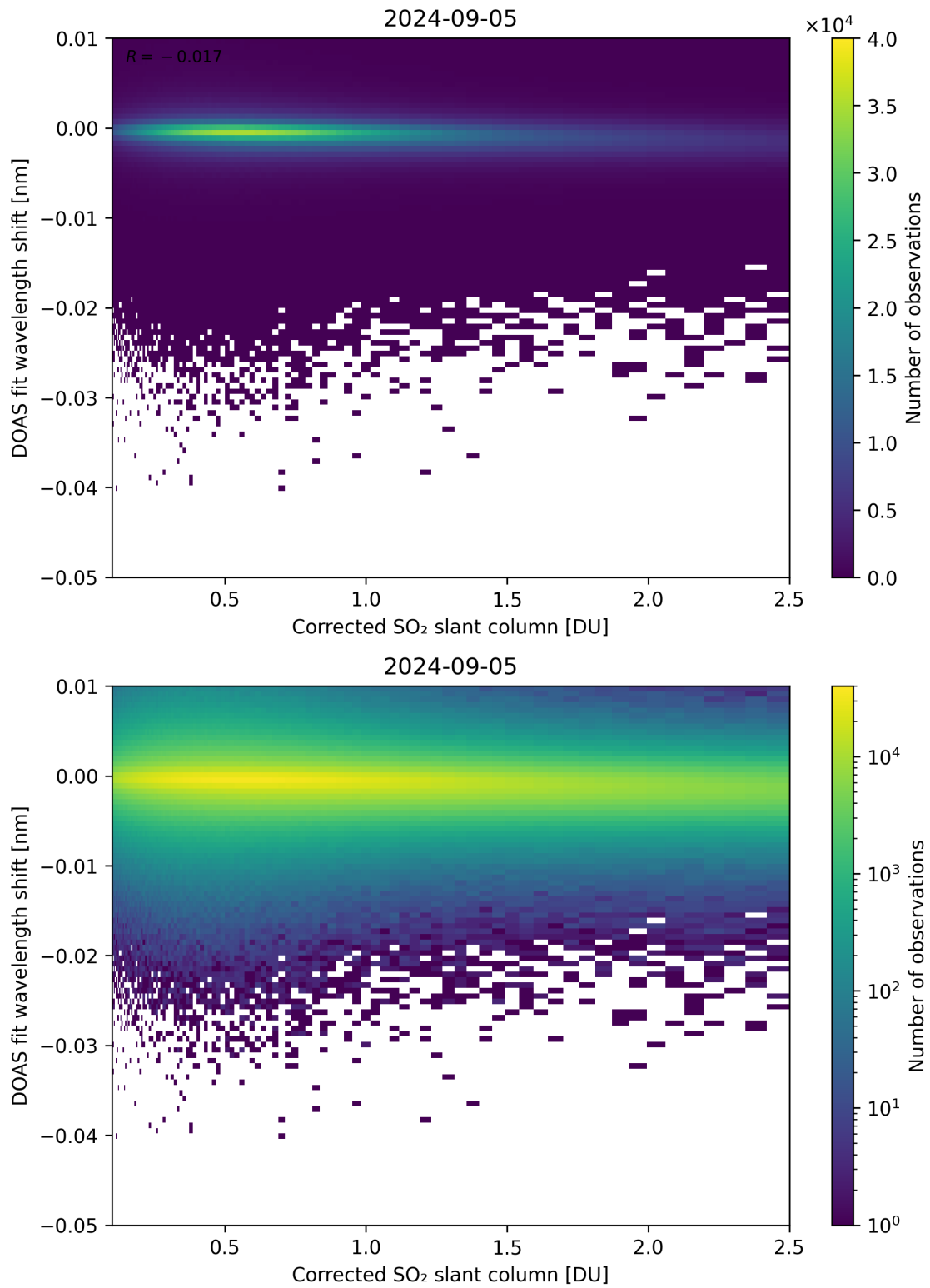
Figure 181: Scatter density plot of “Corrected SO 2 slant column” against “DOAS fit wavelength shift” for 2024-09-04 to 2024-09-06.
