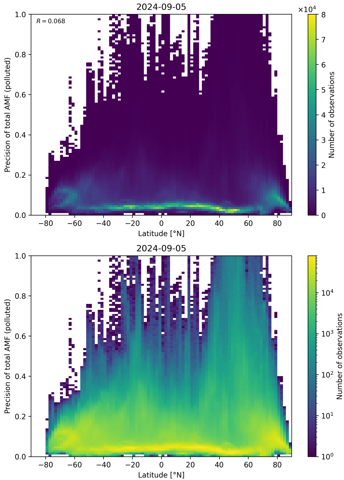
Figure 155: Scatter density plot of “Latitude” against “Precision of total AMF (polluted)” for 2024-09-04 to 2024-09-06.
