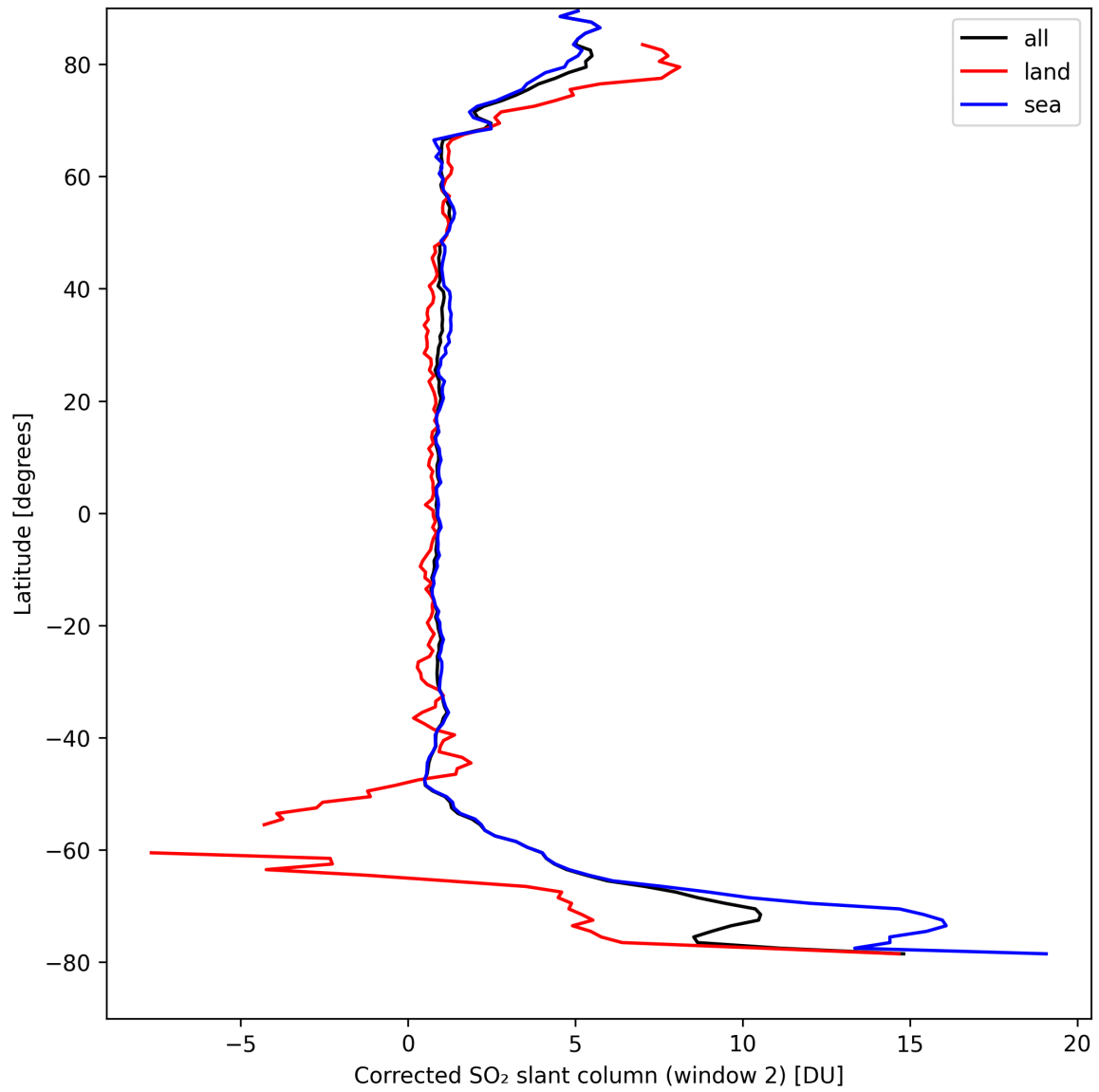
Figure 39: Zonal average of “Corrected SO 2 slant column (window 2)” for 2024-09-04 to 2024-09-06.
