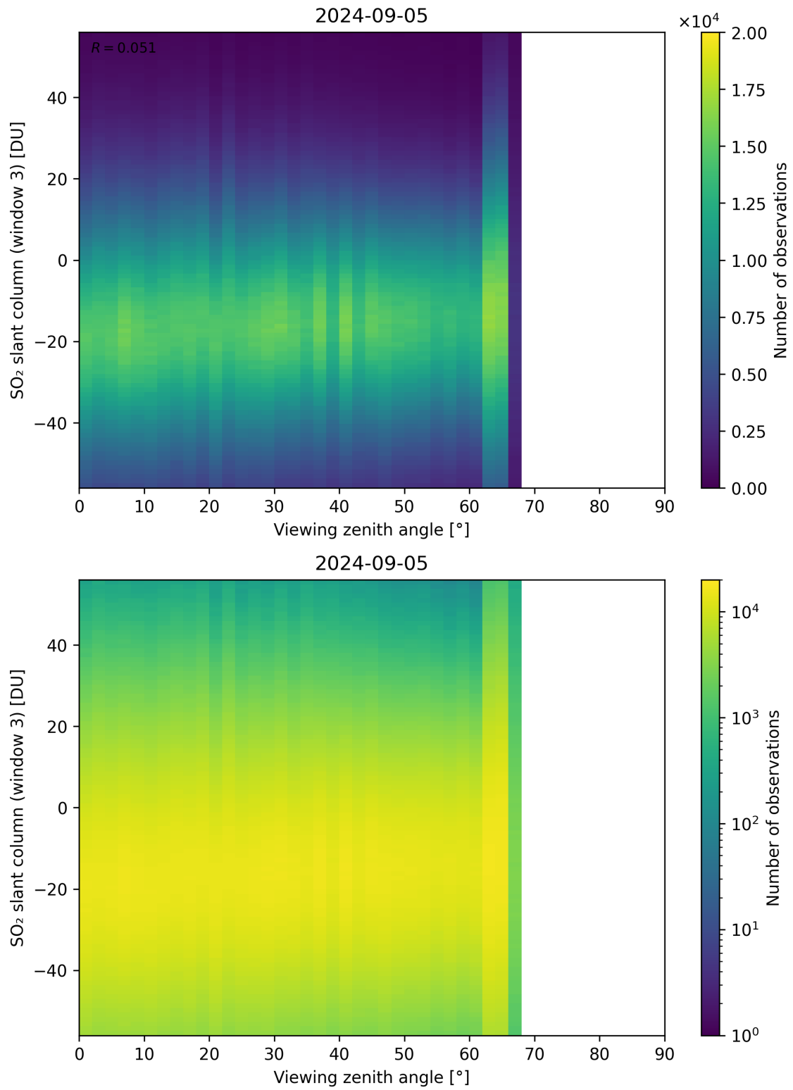
Figure 323: Scatter density plot of “Viewing zenith angle” against “SO 2 slant column (window 3)” for 2024-09-04 to 2024-09-06.
