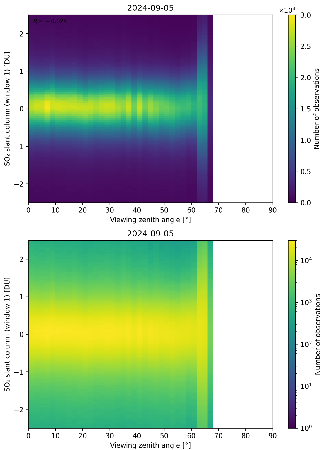
Figure 320: Scatter density plot of “Viewing zenith angle” against “SO 2 slant column (window 1)” for 2024-09-04 to 2024-09-06.
