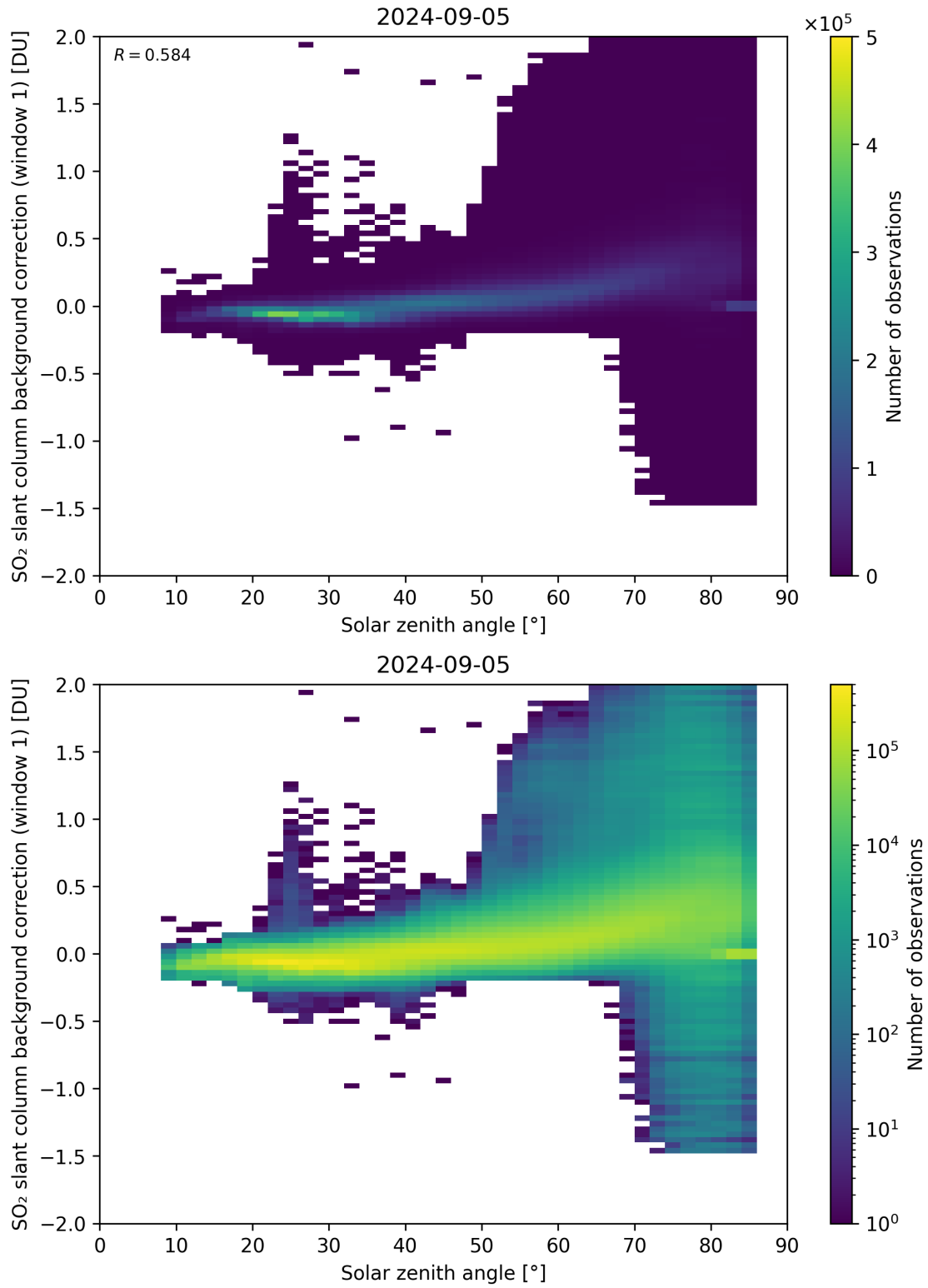
Figure 158: Scatter density plot of “Solar zenith angle” against “SO 2 slant column background correction (window 1)” for 2024-09-04 to 2024-09-06.
