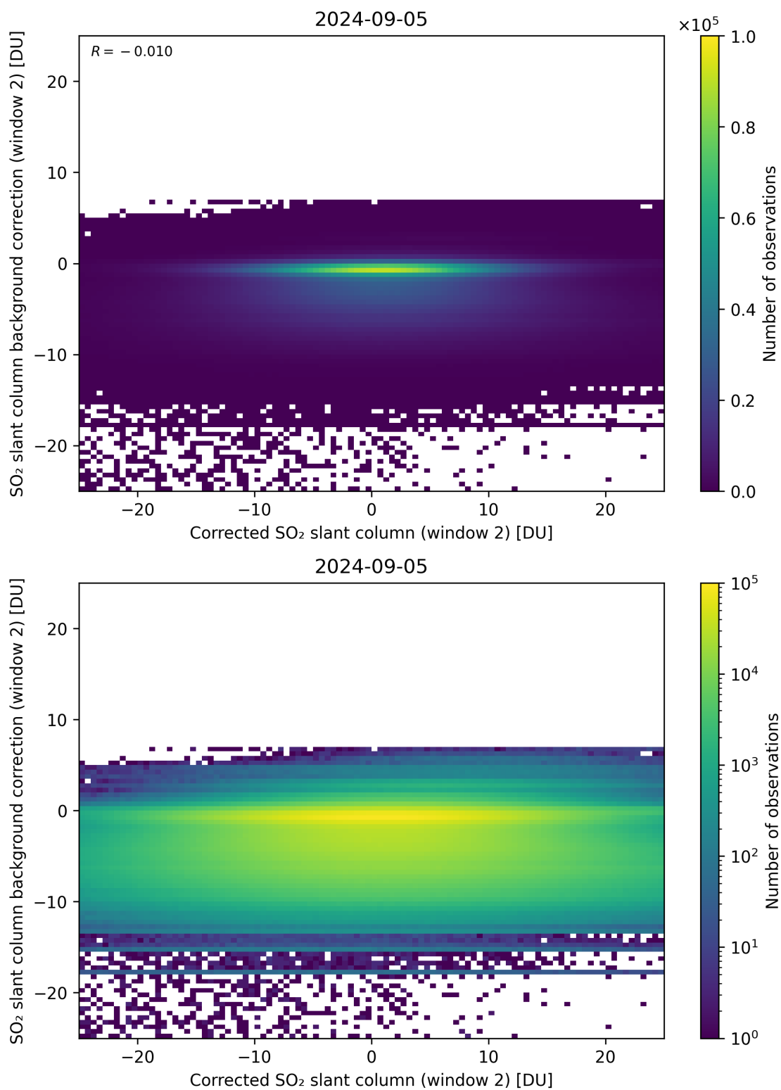
Figure 194: Scatter density plot of “Corrected SO 2 slant column (window 2)” against “SO 2 slant column background correction (window 2)” for 2024-09-04 to 2024-09-06.
