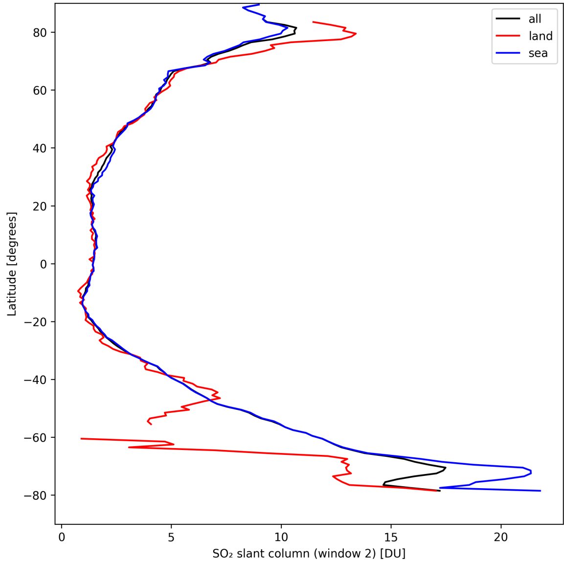
Figure 37: Zonal average of “SO 2 slant column (window 2)” for 2024-09-04 to 2024-09-06.
