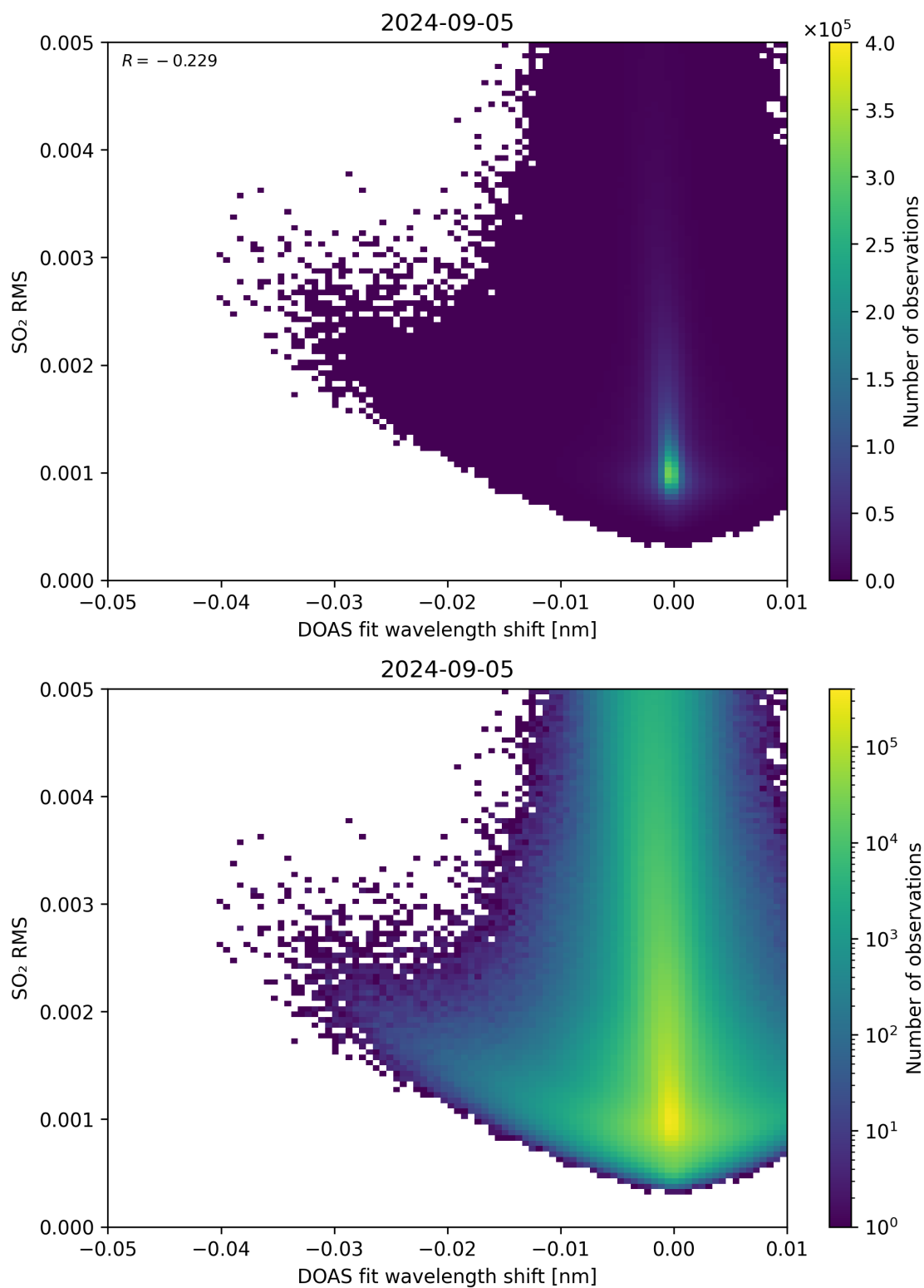
Figure 128: Scatter density plot of “DOAS fit wavelength shift” against “SO 2 RMS” for 2024-09-04 to 2024-09-06.
