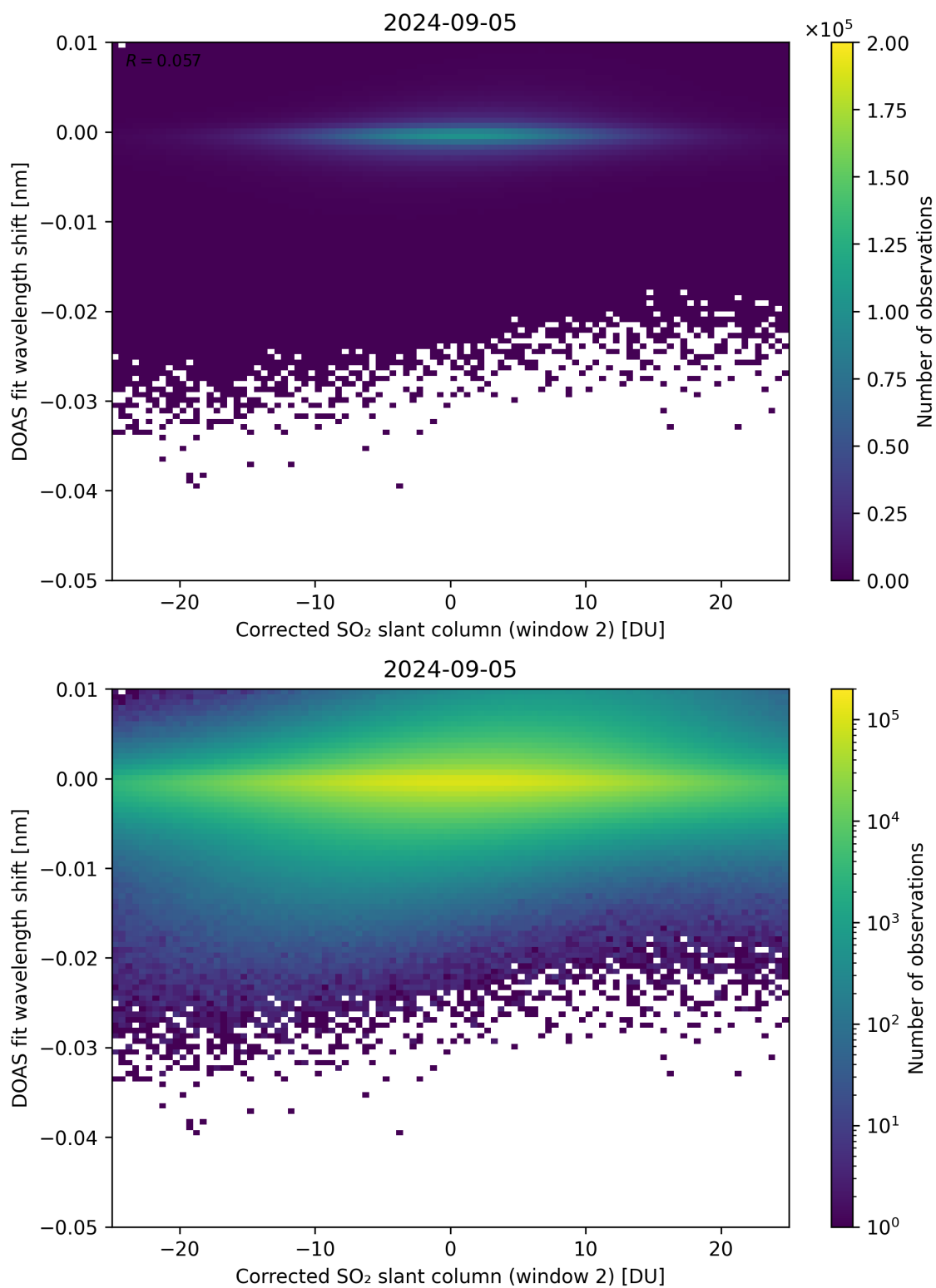
Figure 196: Scatter density plot of “Corrected SO 2 slant column (window 2)” against “DOAS fit wavelength shift” for 2024-09-04 to 2024-09-06.
