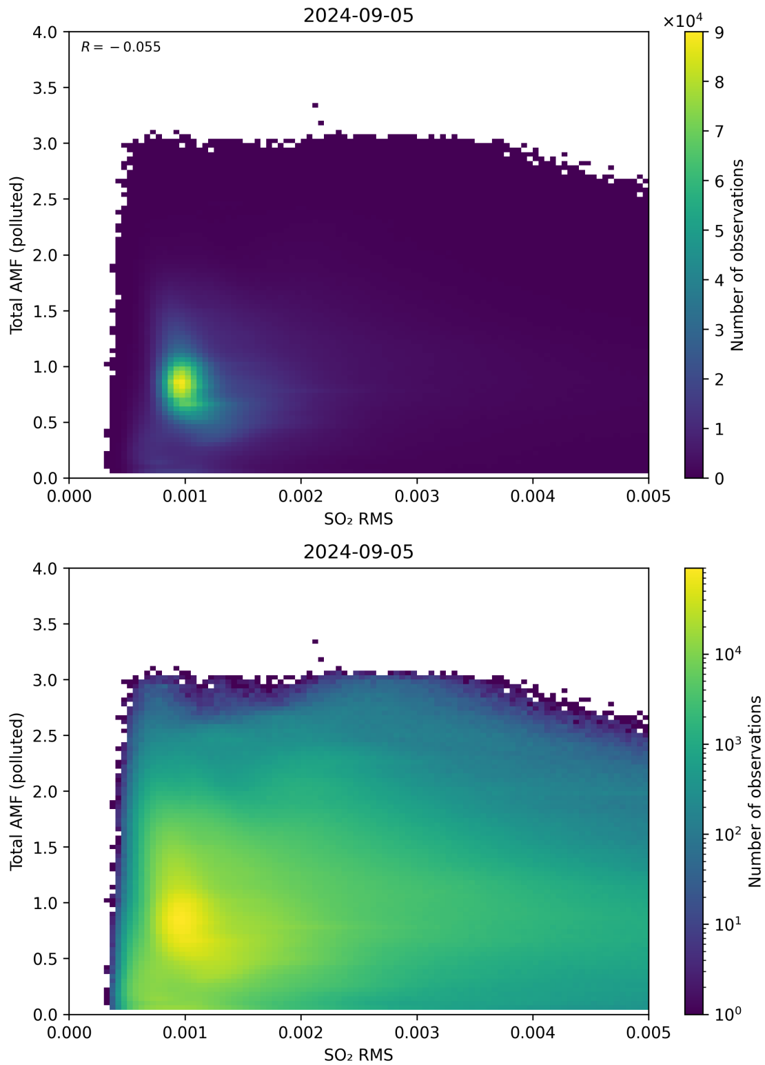
Figure 137: Scatter density plot of “SO 2 RMS” against “Total AMF (polluted)” for 2024-09-04 to 2024-09-06.
