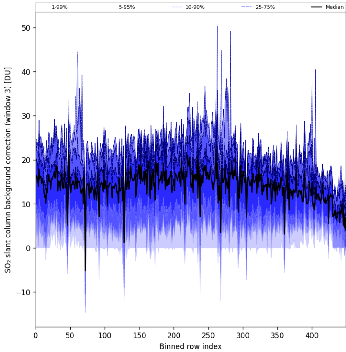
Figure 90: Along track statistics of “SO 2 slant column background correction (window 3)” for 2024-09-04 to 2024-09-06
