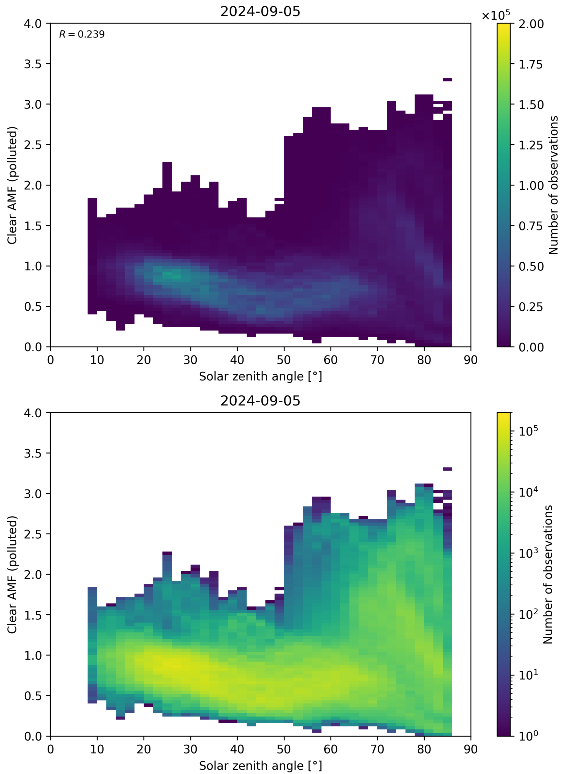
Figure 165: Scatter density plot of “Solar zenith angle” against “Clear AMF (polluted)” for 2024-09-04 to 2024-09-06.
