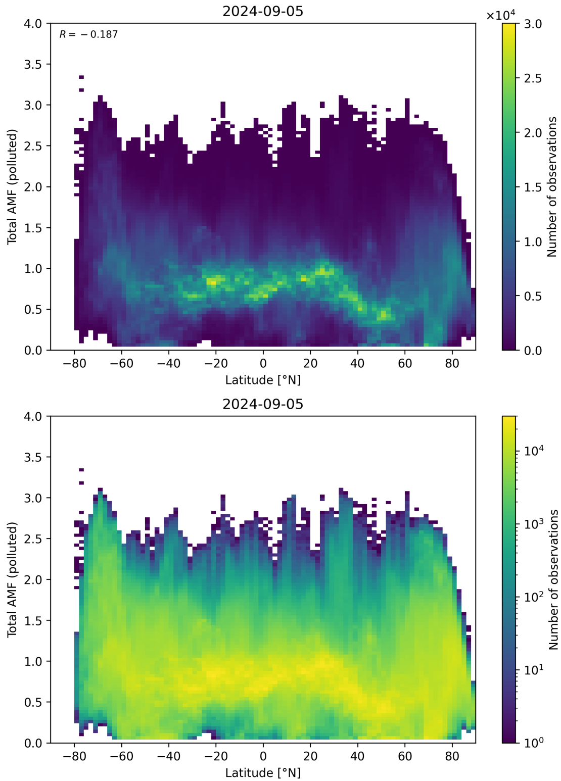
Figure 154: Scatter density plot of “Latitude” against “Total AMF (polluted)” for 2024-09-04 to 2024-09-06.
