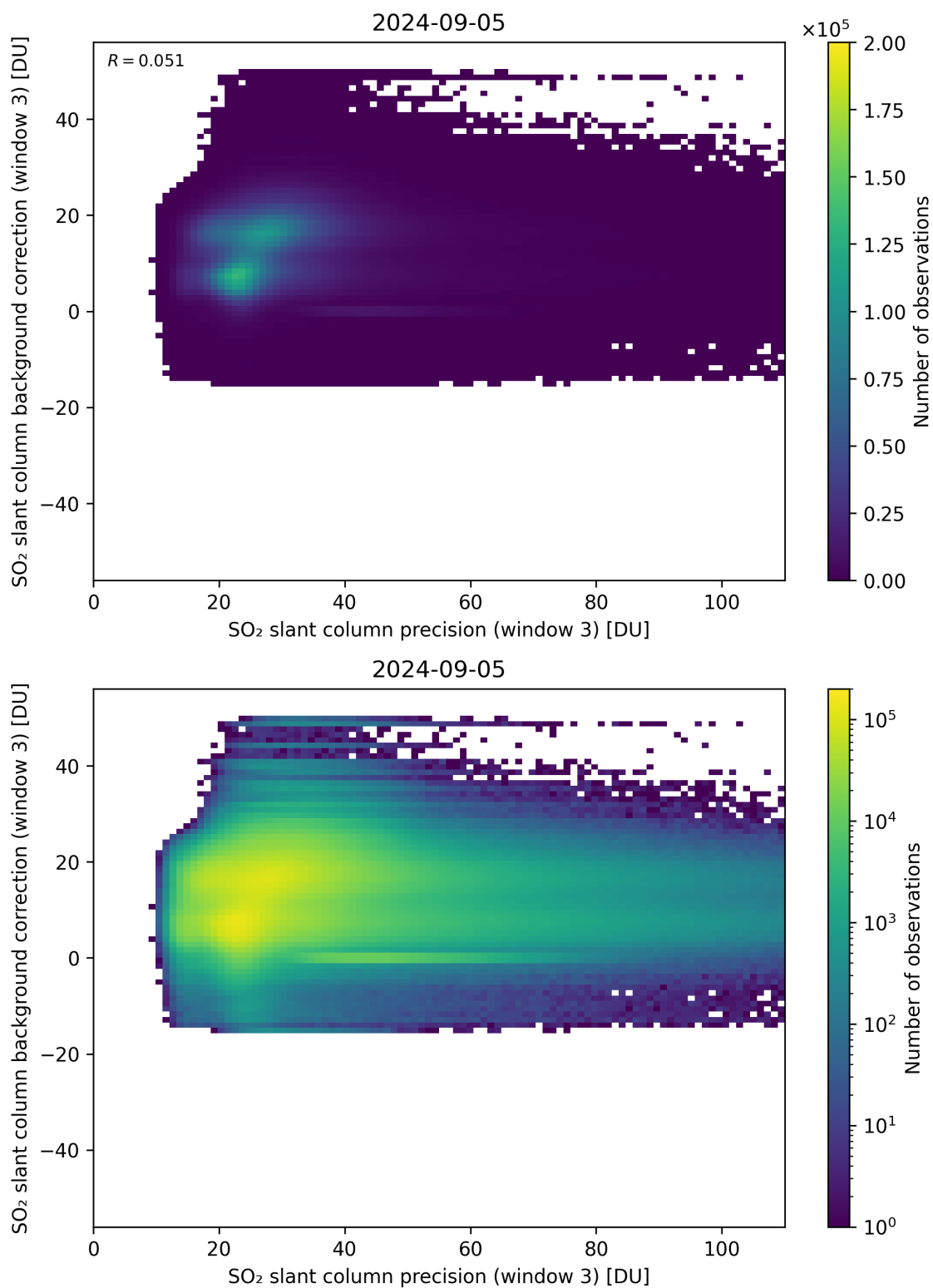
Figure 257: Scatter density plot of “SO 2 slant column precision (window 3)” against “SO 2 slant column background correction (window 3)” for 2024-09-04 to 2024-09-06.
