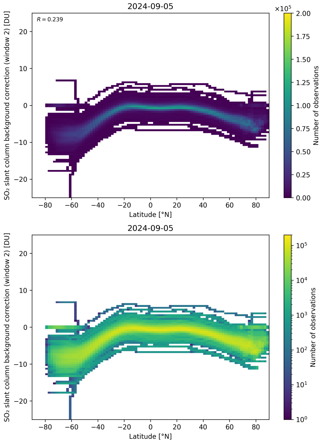
Figure 140: Scatter density plot of “Latitude” against “SO 2 slant column background correction (window 2)” for 2024-09-04 to 2024-09-06.
