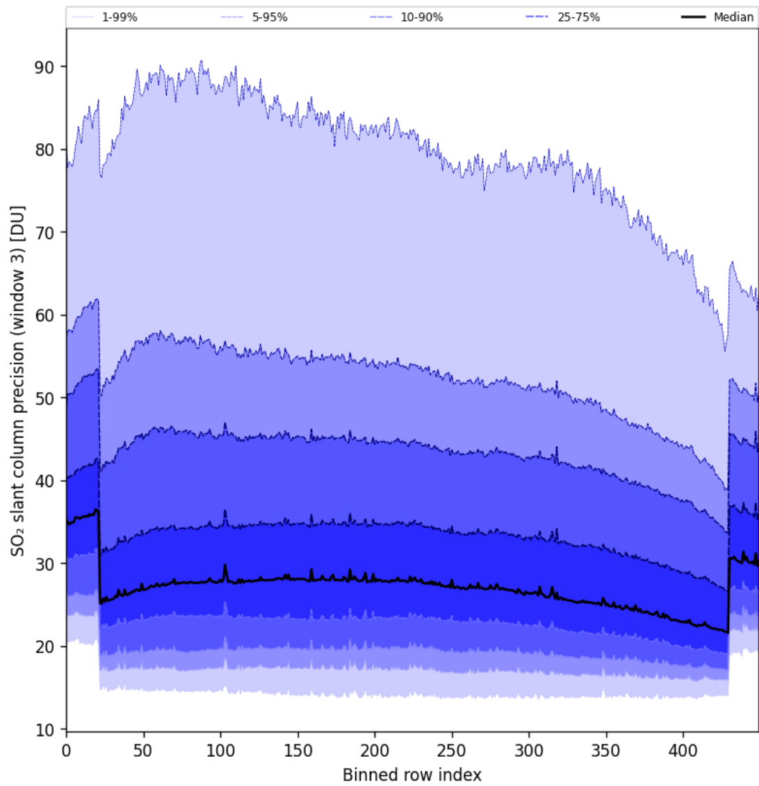
Figure 88: Along track statistics of “SO 2 slant column precision (window 3)” for 2024-09-04 to 2024-09-06
