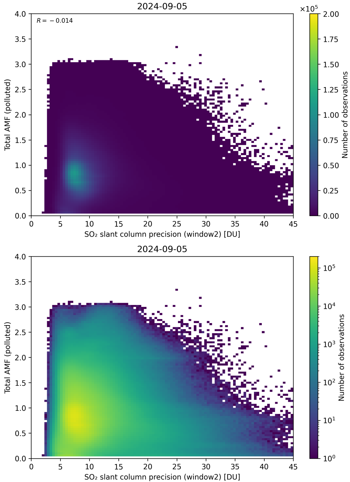
Figure 251: Scatter density plot of “SO 2 slant column precision (window2)” against “Total AMF (polluted)” for 2024-09-04 to 2024-09-06.
