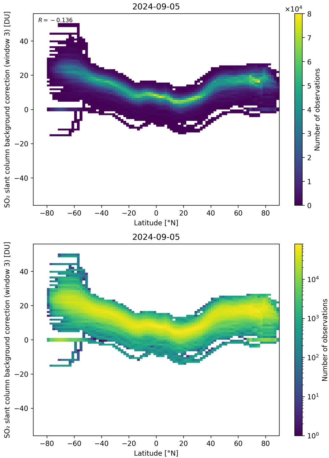
Figure 141: Scatter density plot of “Latitude” against “SO 2 slant column background correction (window 3)” for 2024-09-04 to 2024-09-06.
