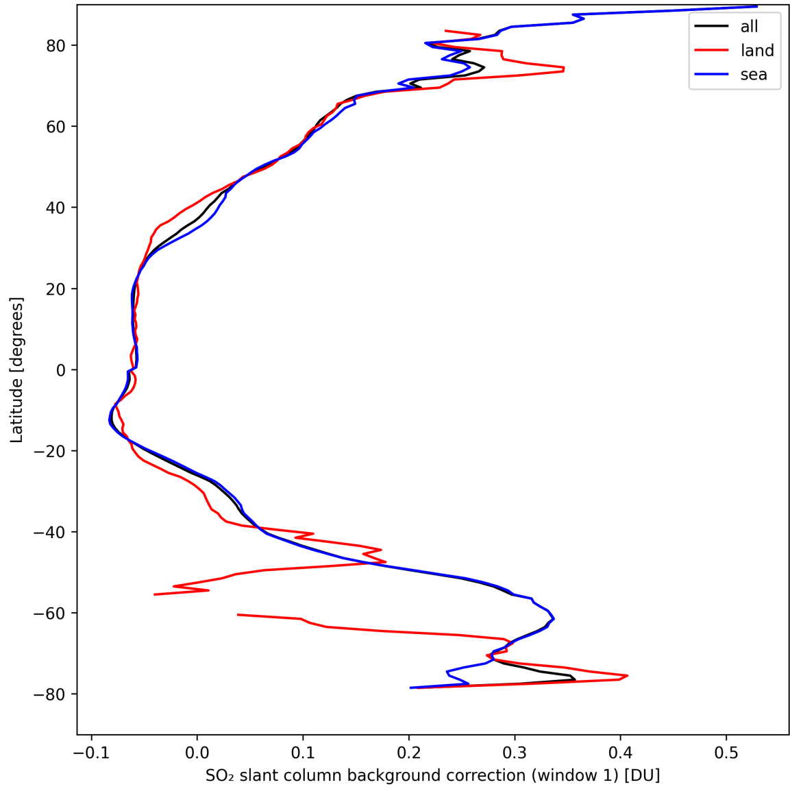
Figure 36: Zonal average of “SO 2 slant column background correction (window 1)” for 2024-09-04 to 2024-09-06.
