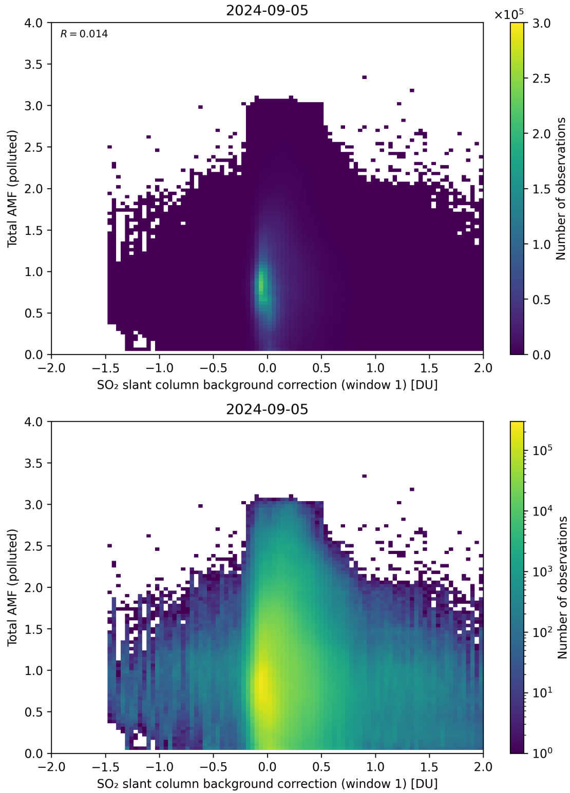
Figure 109: Scatter density plot of “SO 2 slant column background correction (window 1)” against “Total AMF (polluted)” for 2024-09-04 to 2024-09-06.
