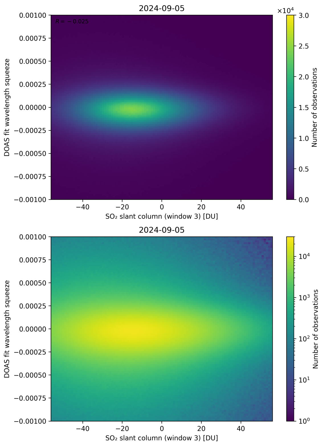
Figure 255: Scatter density plot of “SO 2 slant column (window 3)” against “DOAS fit wavelength squeeze” for 2024-09-04 to 2024-09-06.
