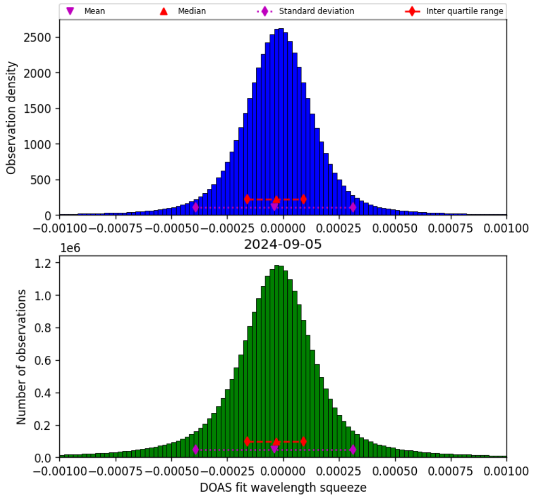
Figure 69: Histogram of “DOAS fit wavelength squeeze” for 2024-09-04 to 2024-09-06
