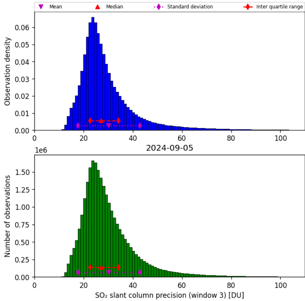
Figure 65: Histogram of “SO 2 slant column precision (window 3)” for 2024-09-04 to 2024-09-06
