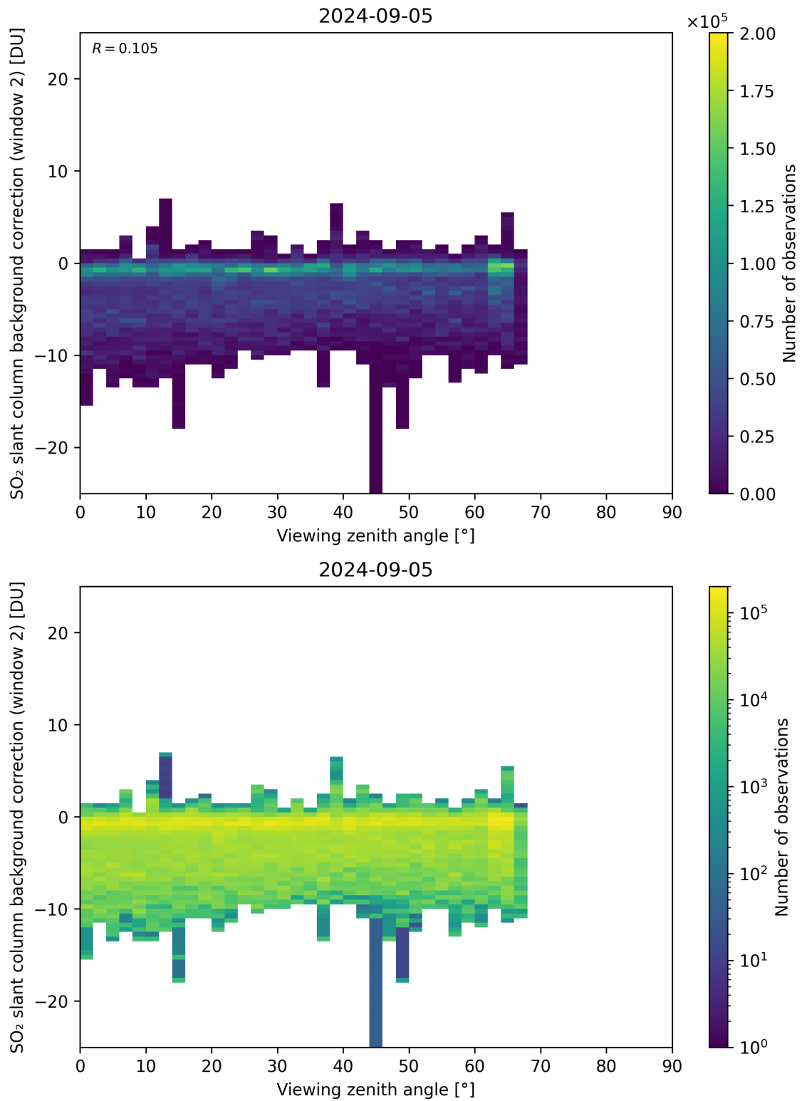
Figure 309: Scatter density plot of “Viewing zenith angle” against “SO 2 slant column background correction (window 2)” for 2024-09-04 to 2024-09-06.
