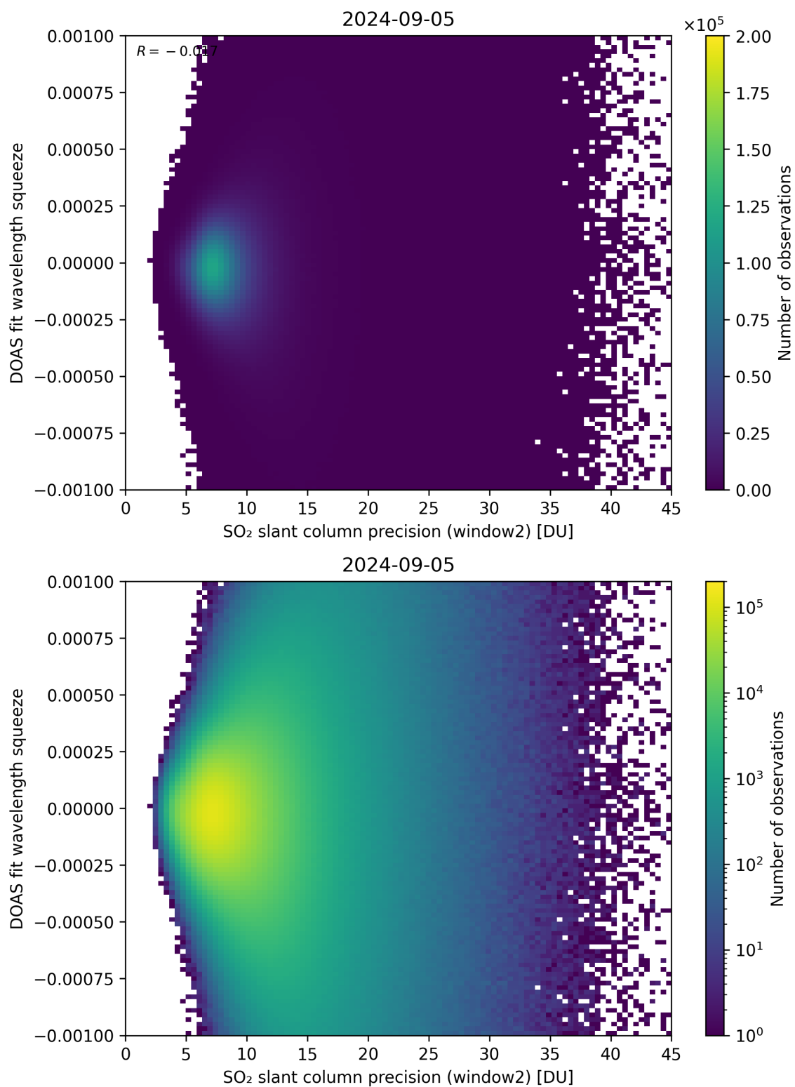
Figure 244: Scatter density plot of “SO 2 slant column precision (window2)” against “DOAS fit wavelength squeeze” for 2024-09-04 to 2024-09-06.
