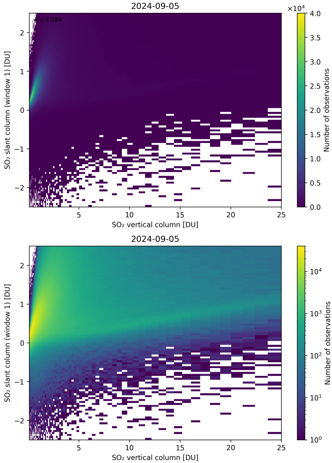
Figure 300: Scatter density plot of “SO 2 vertical column” against “SO 2 slant column (window 1)” for 2024-09-04 to 2024-09-06.
