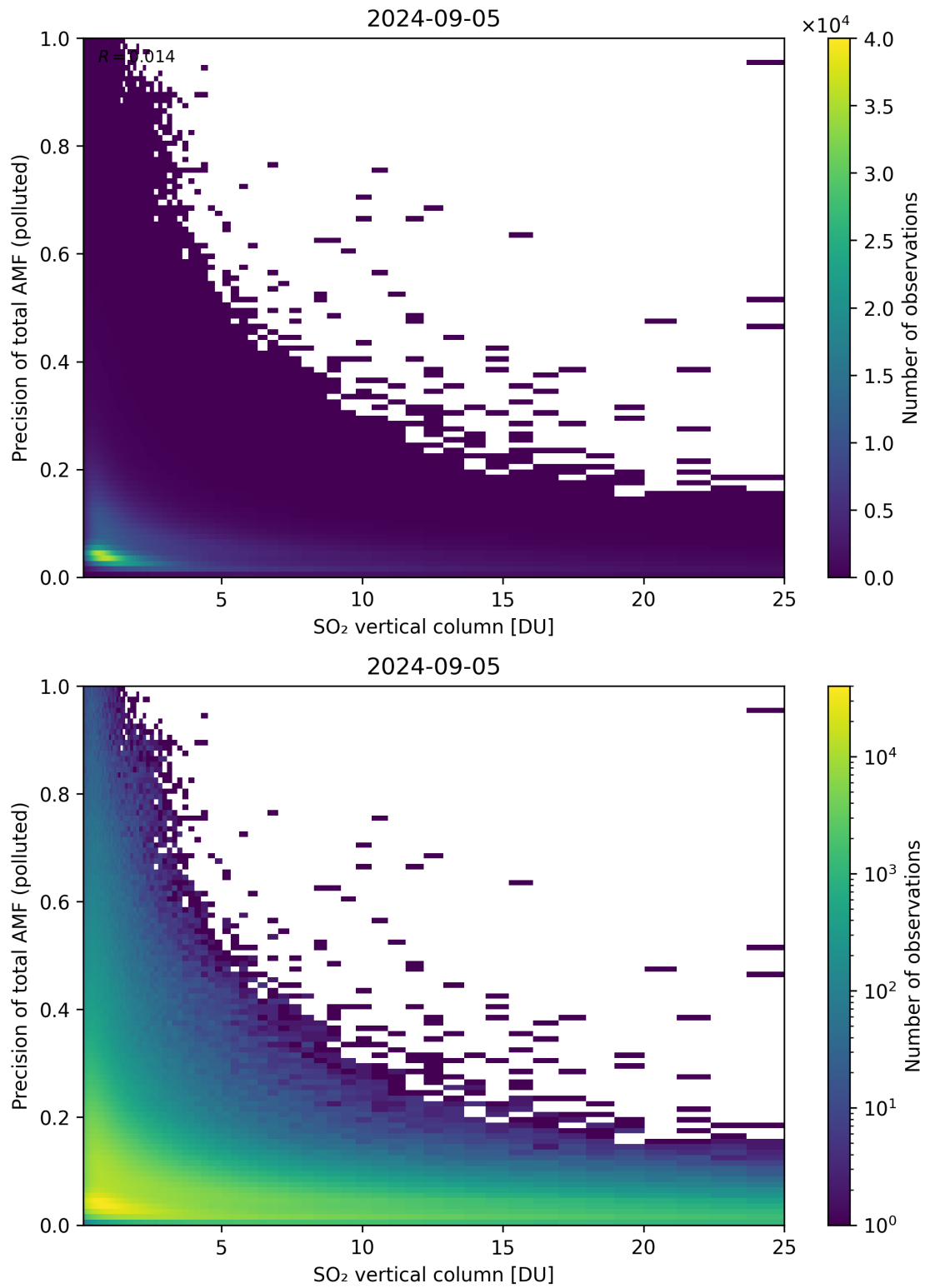
Figure 306: Scatter density plot of “SO 2 vertical column” against “Precision of total AMF (polluted)” for 2024-09-04 to 2024-09-06.
