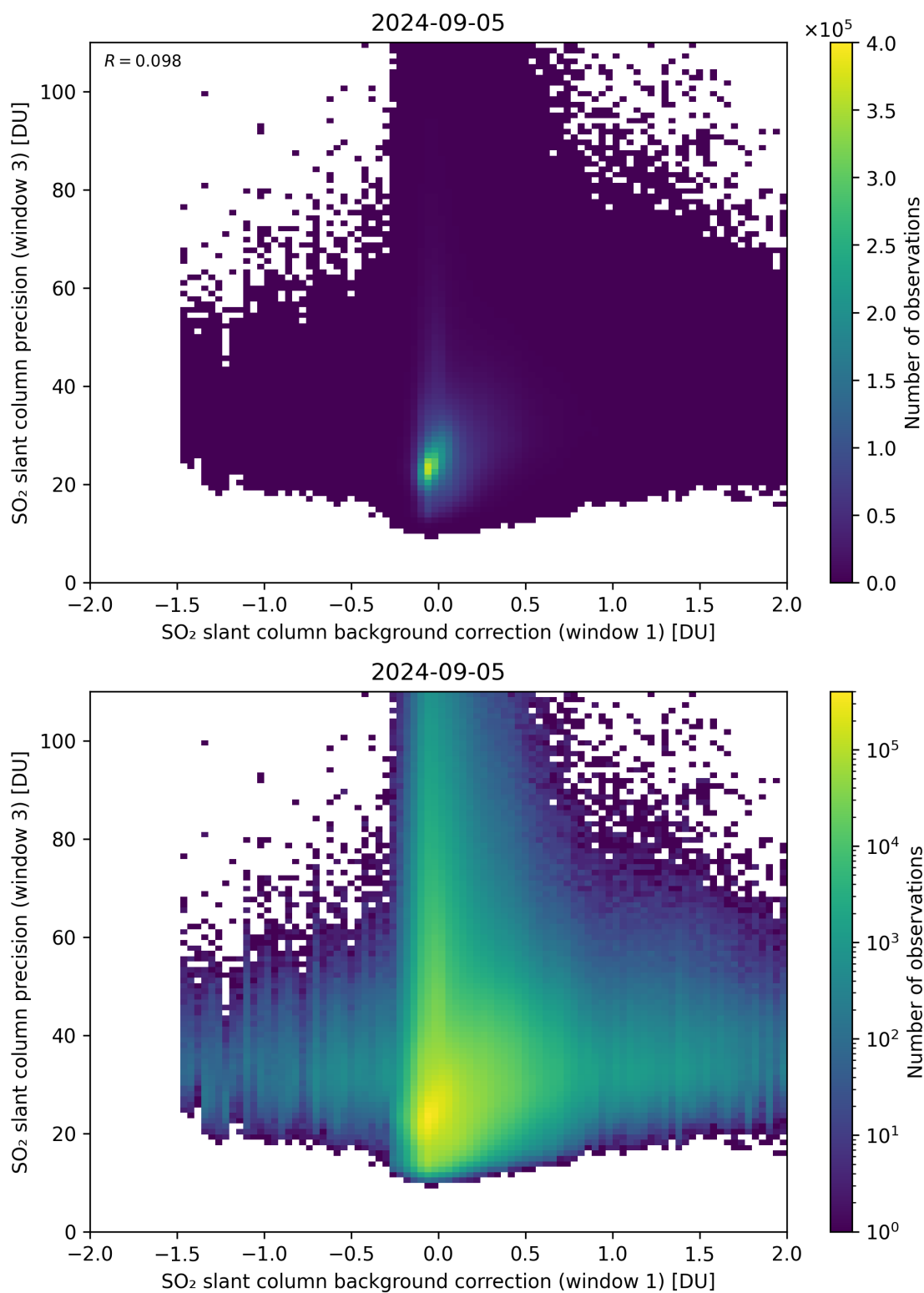
Figure 108: Scatter density plot of “SO 2 slant column background correction (window 1)” against “SO 2 slant column precision (window 3)” for 2024-09-04 to 2024-09-06.
