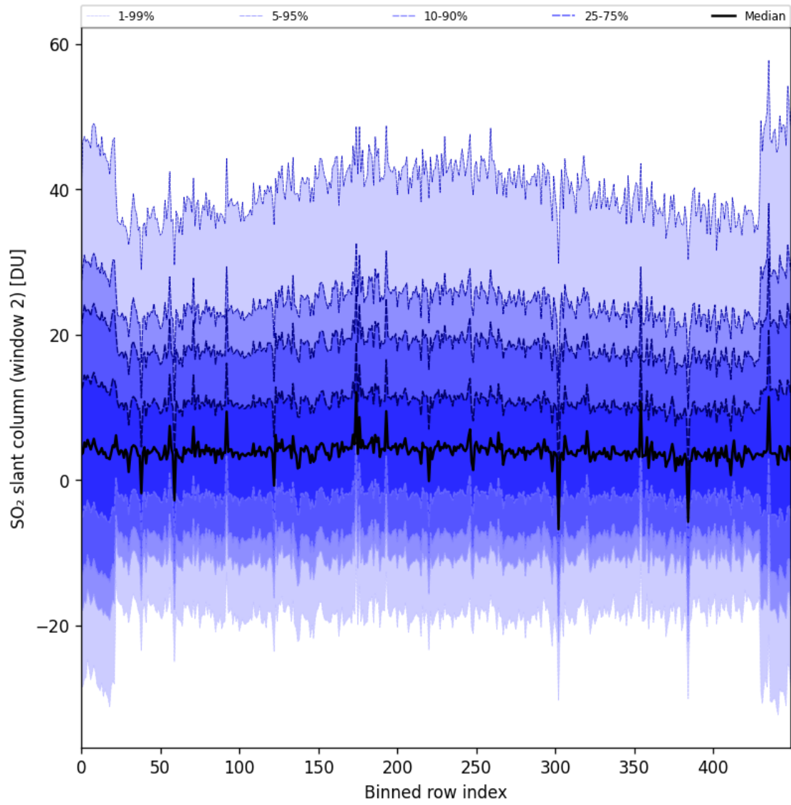
Figure 83: Along track statistics of “SO 2 slant column (window 2)” for 2024-09-04 to 2024-09-06
