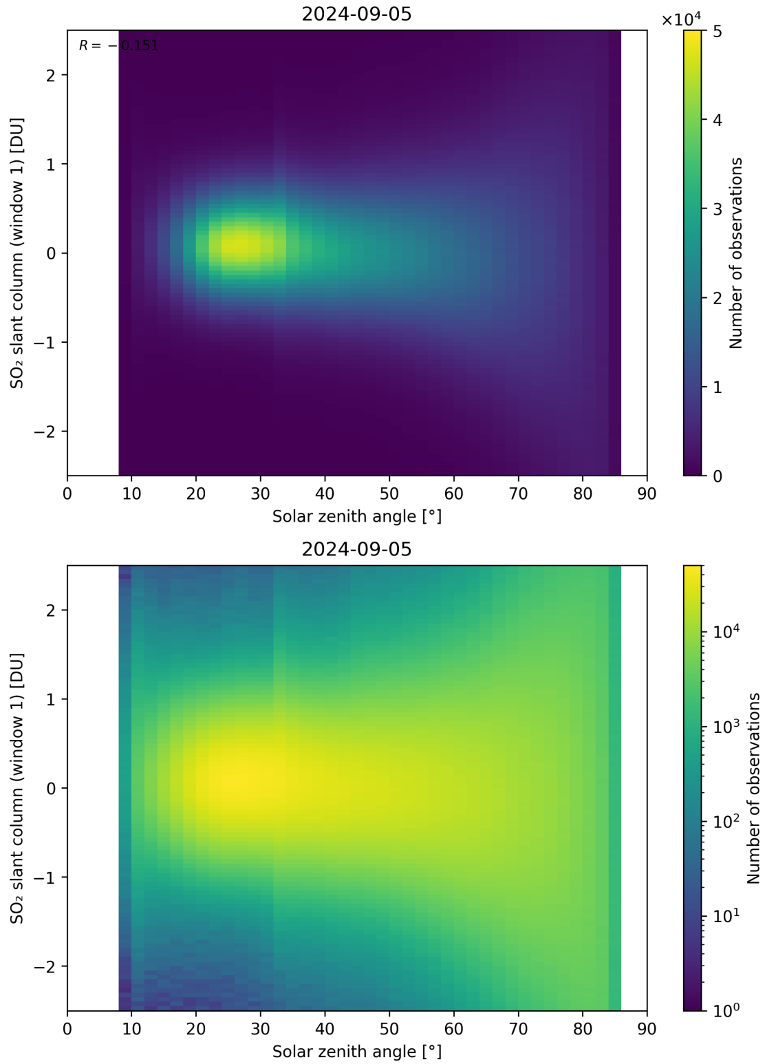
Figure 169: Scatter density plot of “Solar zenith angle” against “SO 2 slant column (window 1)” for 2024-09-04 to 2024-09-06.
