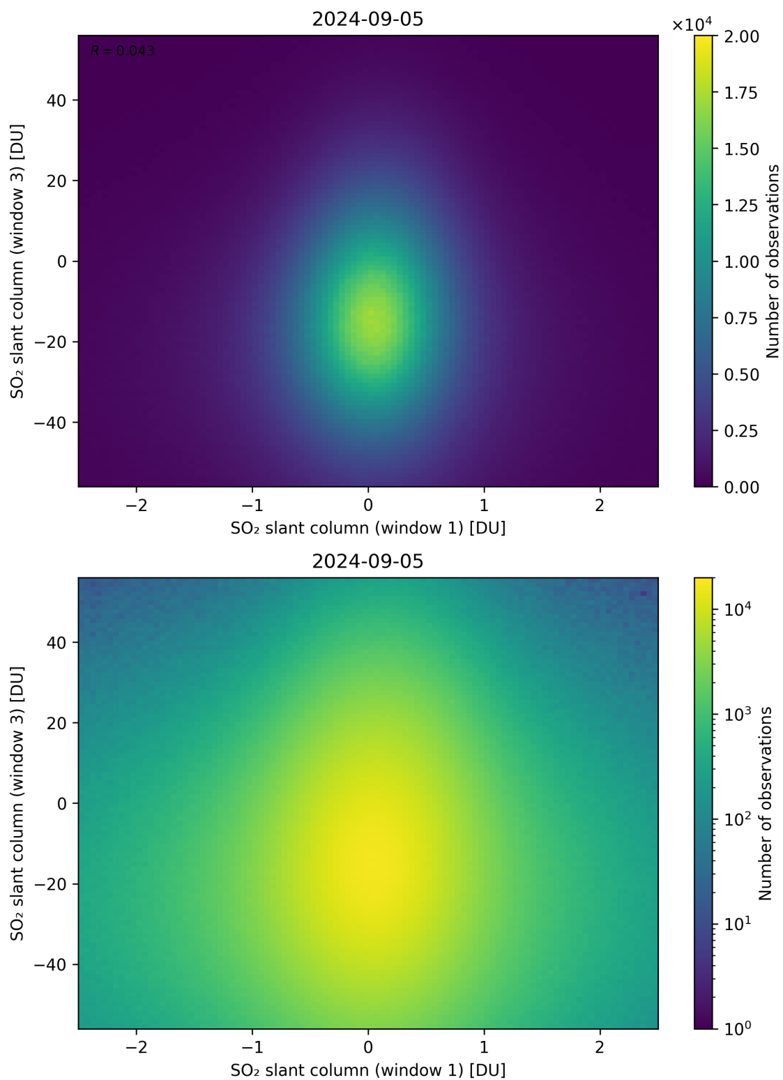
Figure 237: Scatter density plot of “SO 2 slant column (window 1)” against “SO 2 slant column (window 3)” for 2024-09-04 to 2024-09-06.
