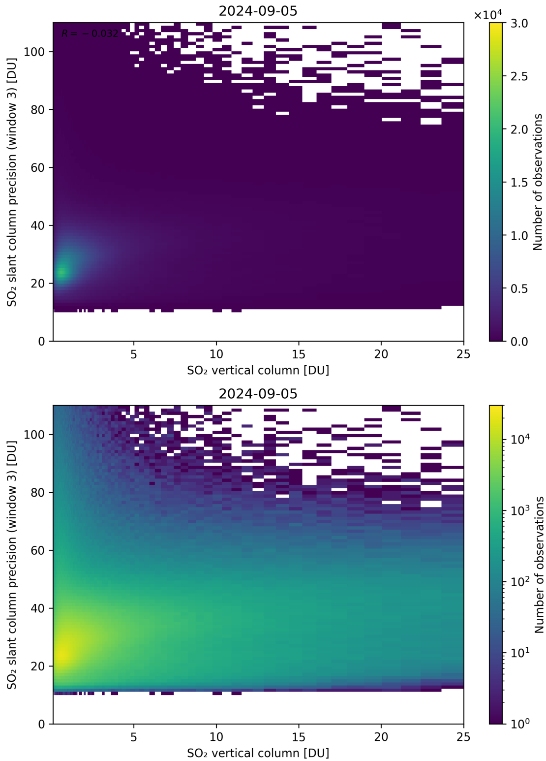
Figure 304: Scatter density plot of “SO 2 vertical column” against “SO 2 slant column precision (window 3)” for 2024-09-04 to 2024-09-06.
