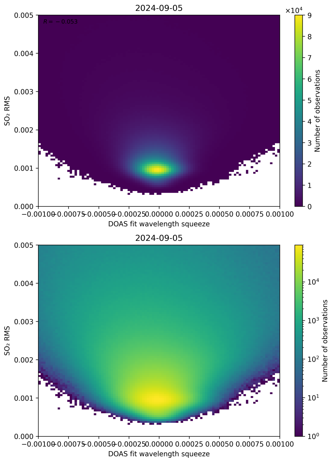
Figure 132: Scatter density plot of “DOAS fit wavelength squeeze” against “SO 2 RMS” for 2024-09-04 to 2024-09-06.
