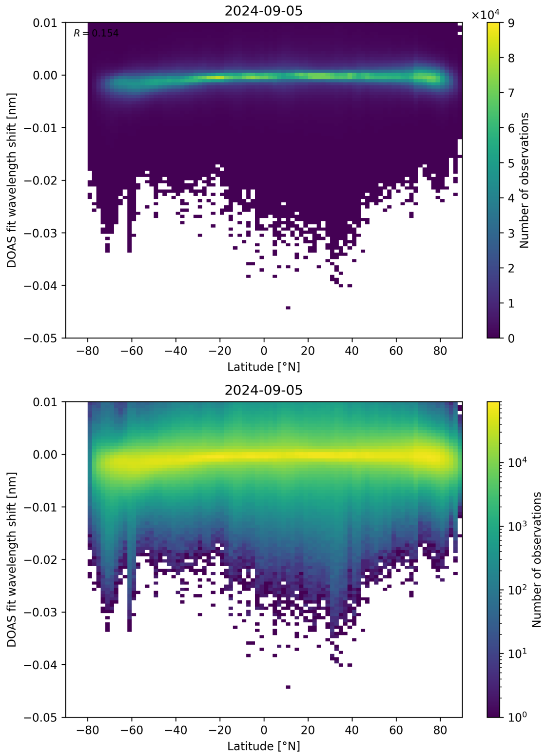
Figure 142: Scatter density plot of “Latitude” against “DOAS fit wavelength shift” for 2024-09-04 to 2024-09-06.
