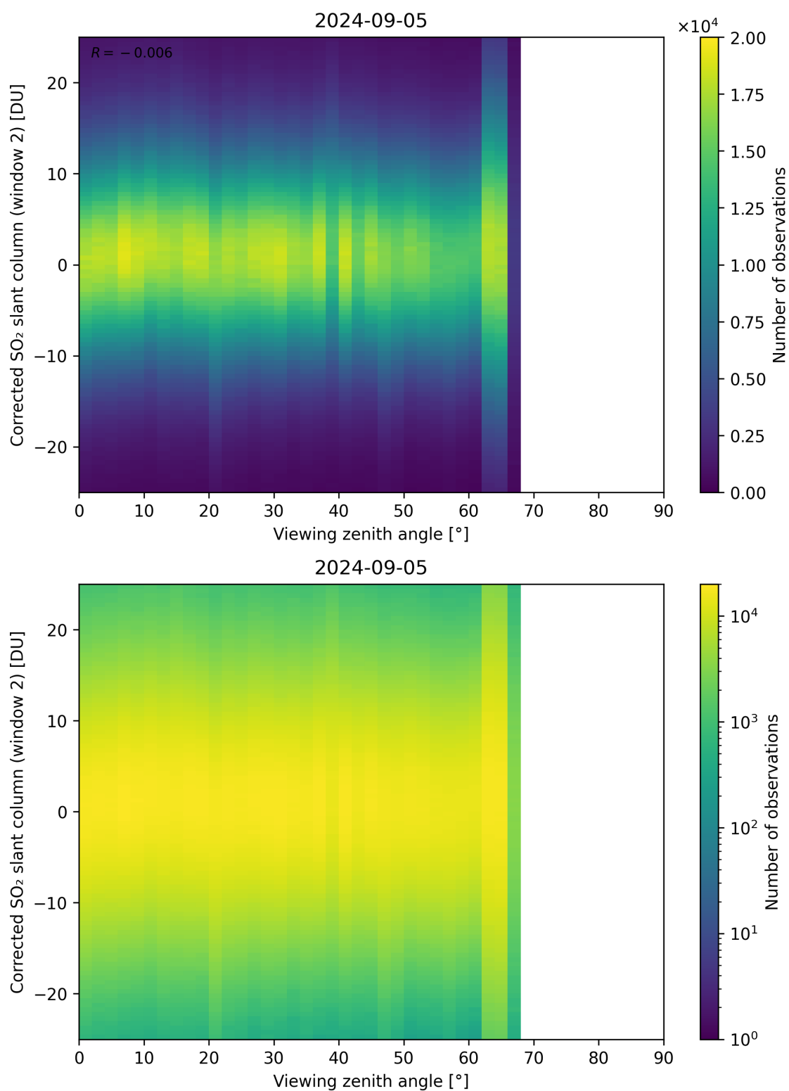
Figure 318: Scatter density plot of “Viewing zenith angle” against “Corrected SO 2 slant column (window 2)” for 2024-09-04 to 2024-09-06.
