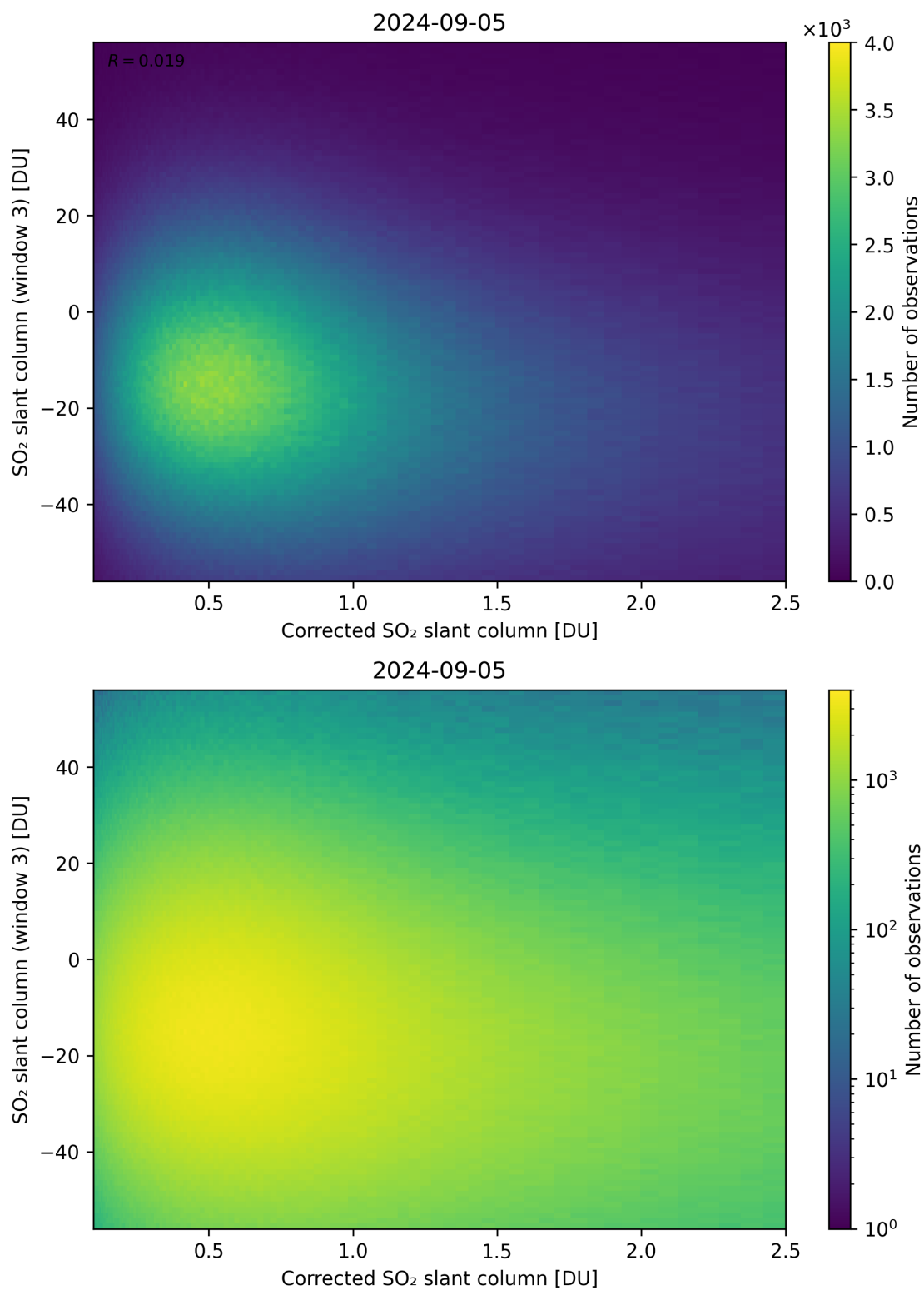
Figure 190: Scatter density plot of “Corrected SO 2 slant column” against “SO 2 slant column (window 3)” for 2024-09-04 to 2024-09-06.
