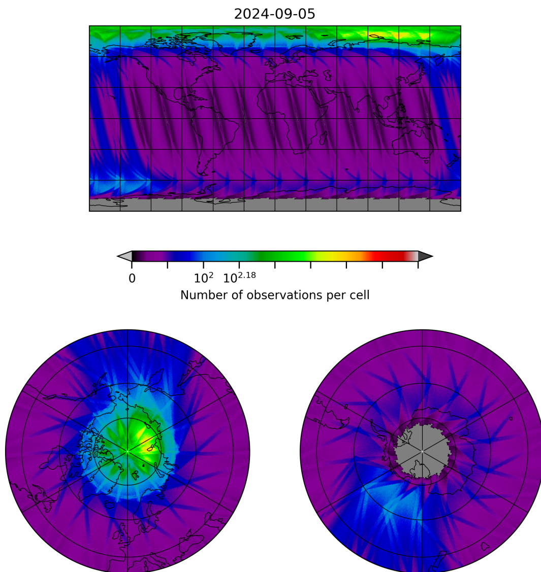
Figure 28: Map of the number of observations for 2024-09-04 to 2024-09-06
