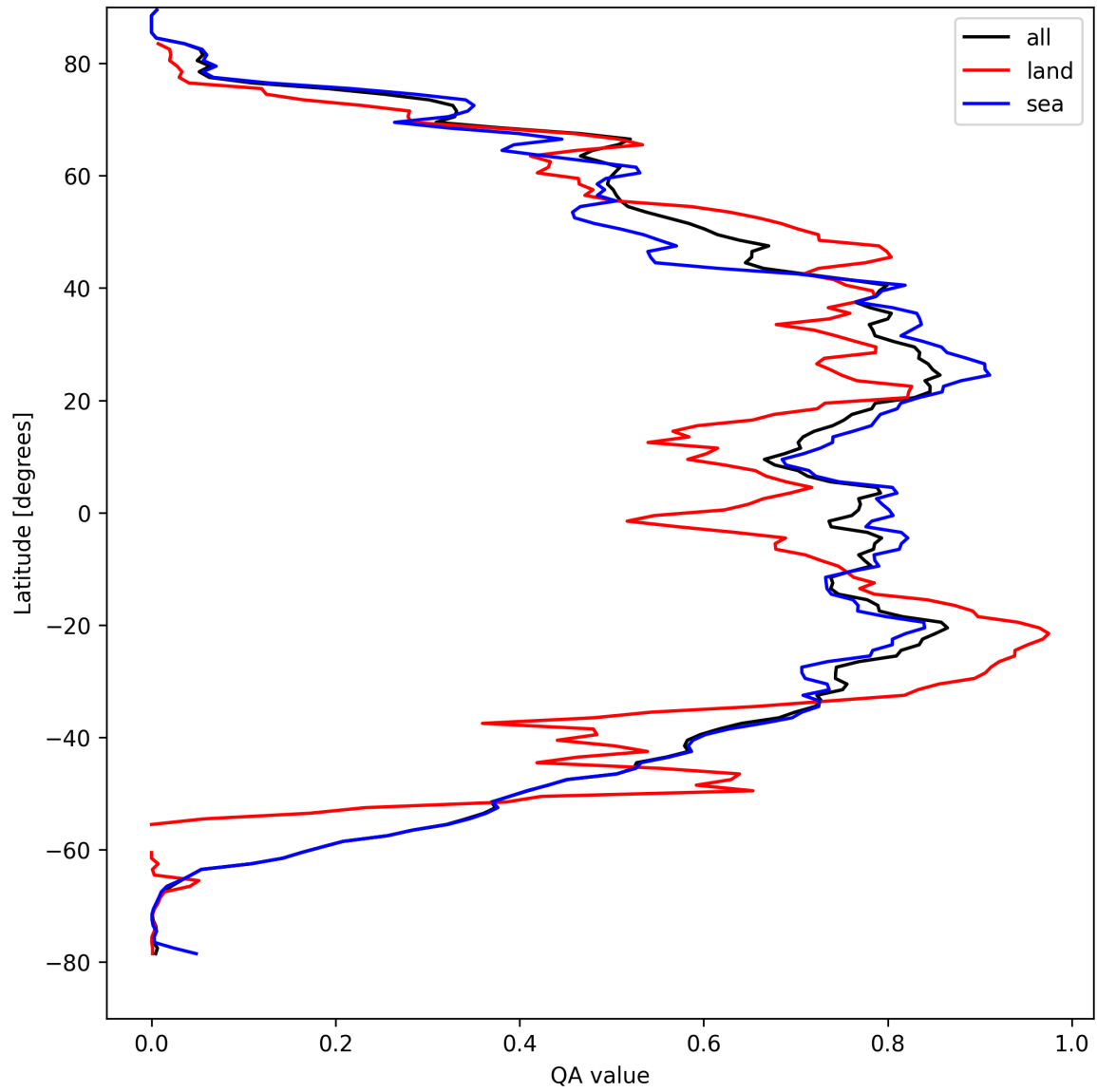
Figure 29: Zonal average of “QA value” for 2024-09-04 to 2024-09-06.
