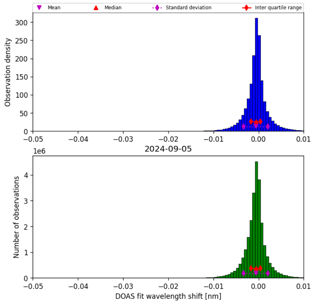
Figure 68: Histogram of “DOAS fit wavelength shift” for 2024-09-04 to 2024-09-06
