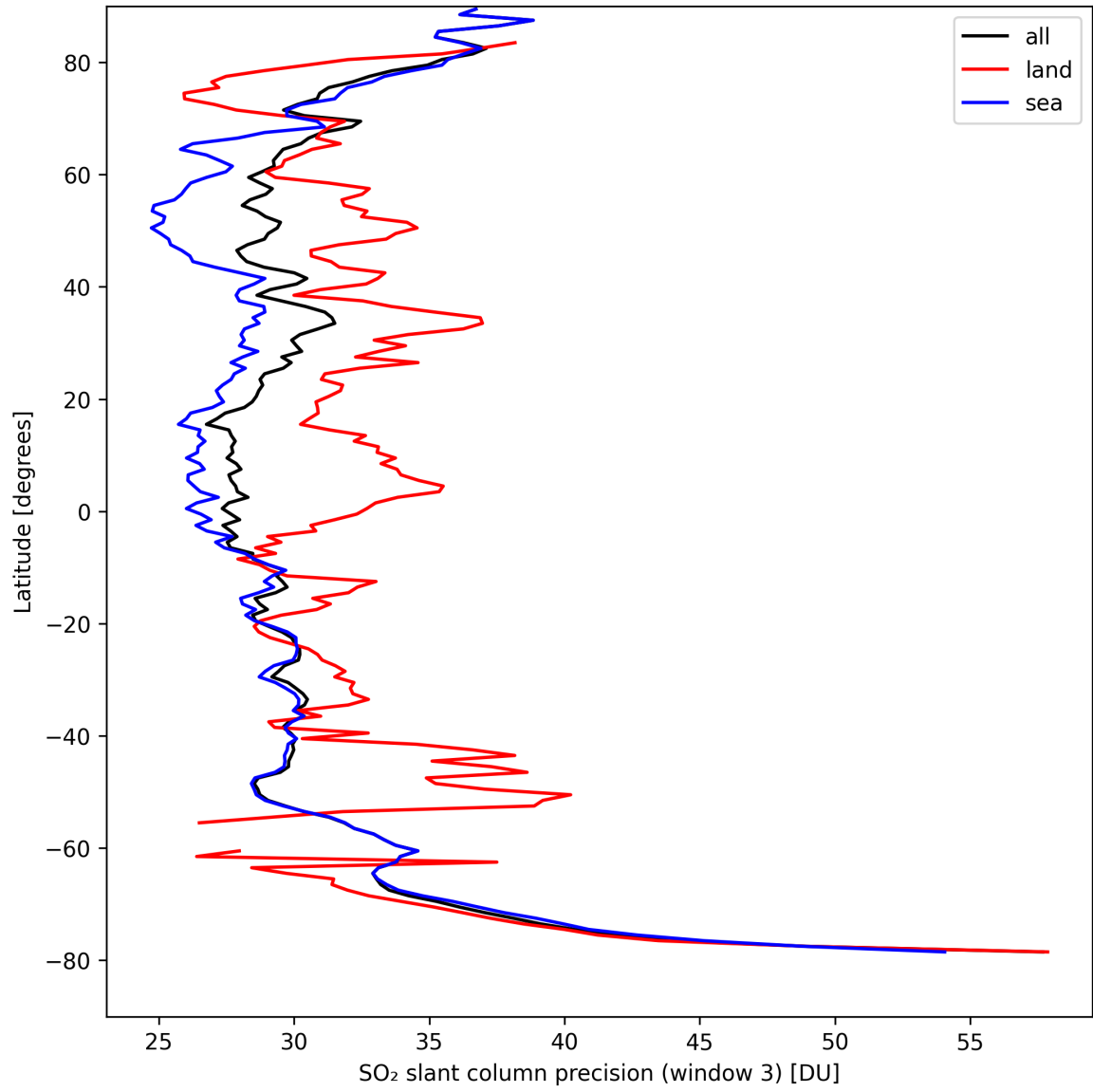
Figure 42: Zonal average of “SO 2 slant column precision (window 3)” for 2024-09-04 to 2024-09-06.
