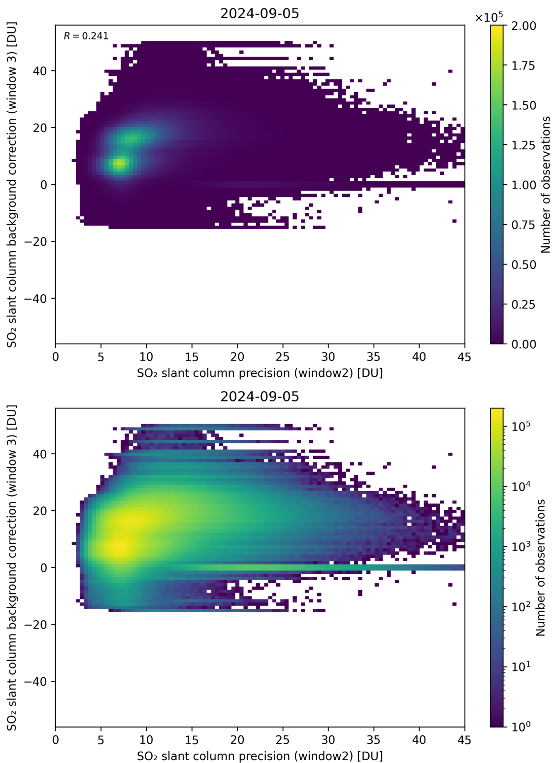
Figure 242: Scatter density plot of “SO 2 slant column precision (window2)” against “SO 2 slant column background correction (window 3)” for 2024-09-04 to 2024-09-06.
