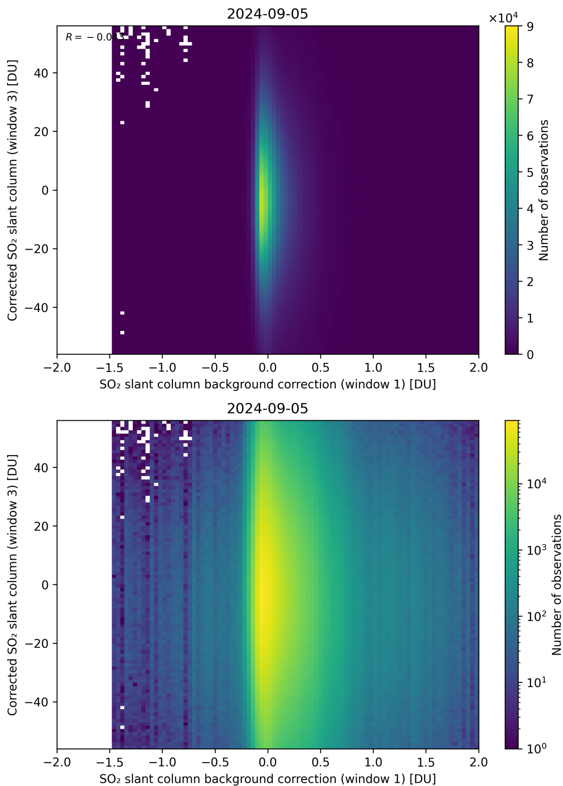
Figure 105: Scatter density plot of “SO 2 slant column background correction (window 1)” against “Corrected SO 2 slant column (window 3)” for 2024-09-04 to 2024-09-06.
