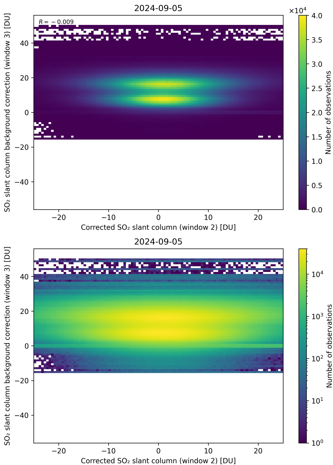
Figure 195: Scatter density plot of “Corrected SO 2 slant column (window 2)” against “SO 2 slant column background correction (window 3)” for 2024-09-04 to 2024-09-06.
