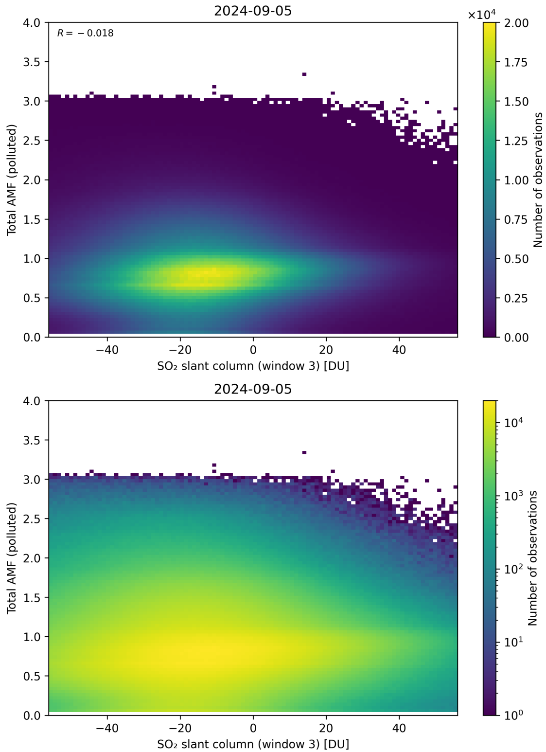
Figure 268: Scatter density plot of “SO 2 slant column (window 3)” against “Total AMF (polluted)” for 2024-09-04 to 2024-09-06.
