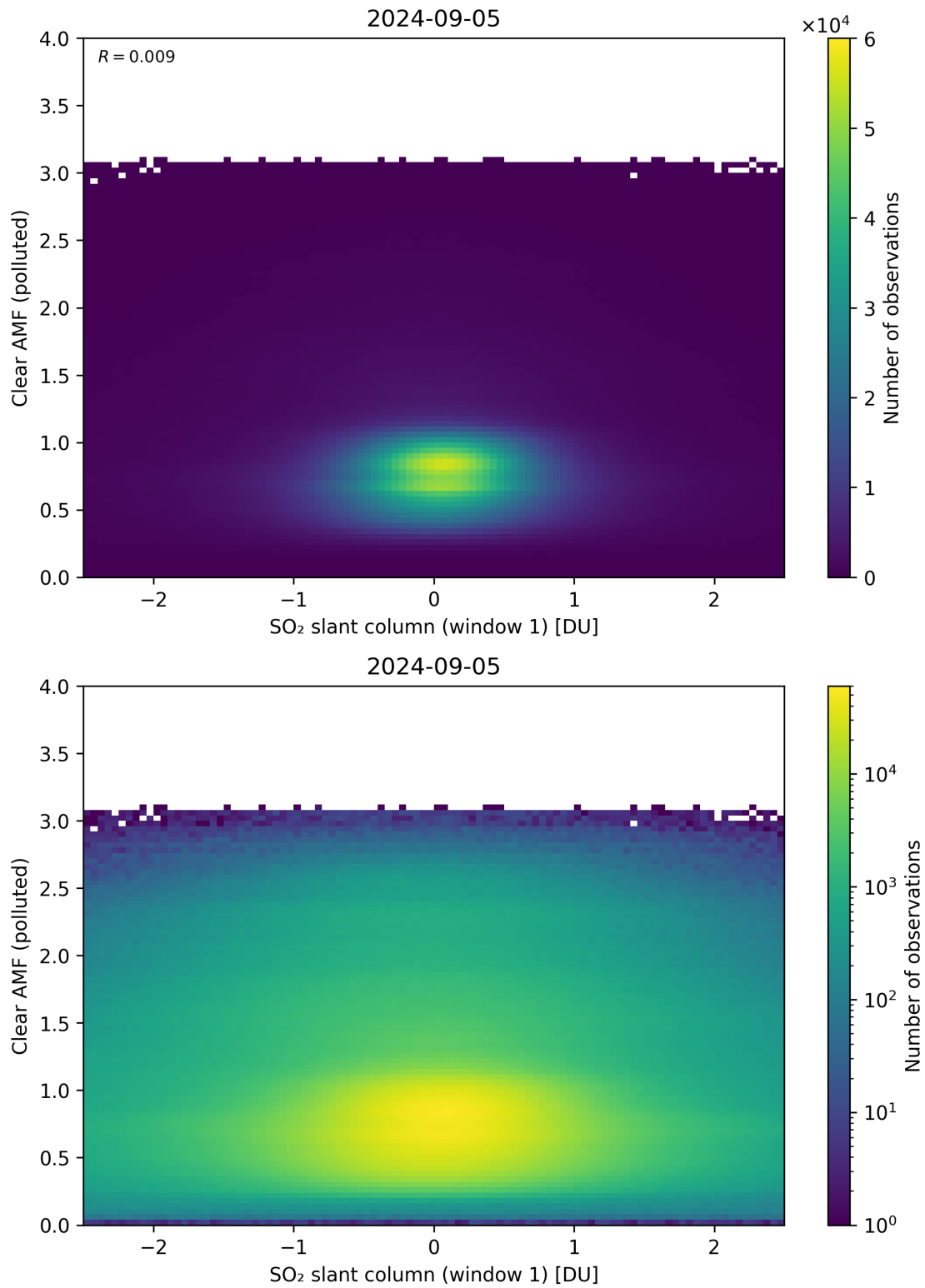
Figure 232: Scatter density plot of “SO 2 slant column (window 1)” against “Clear AMF (polluted)” for 2024-09-04 to 2024-09-06.
