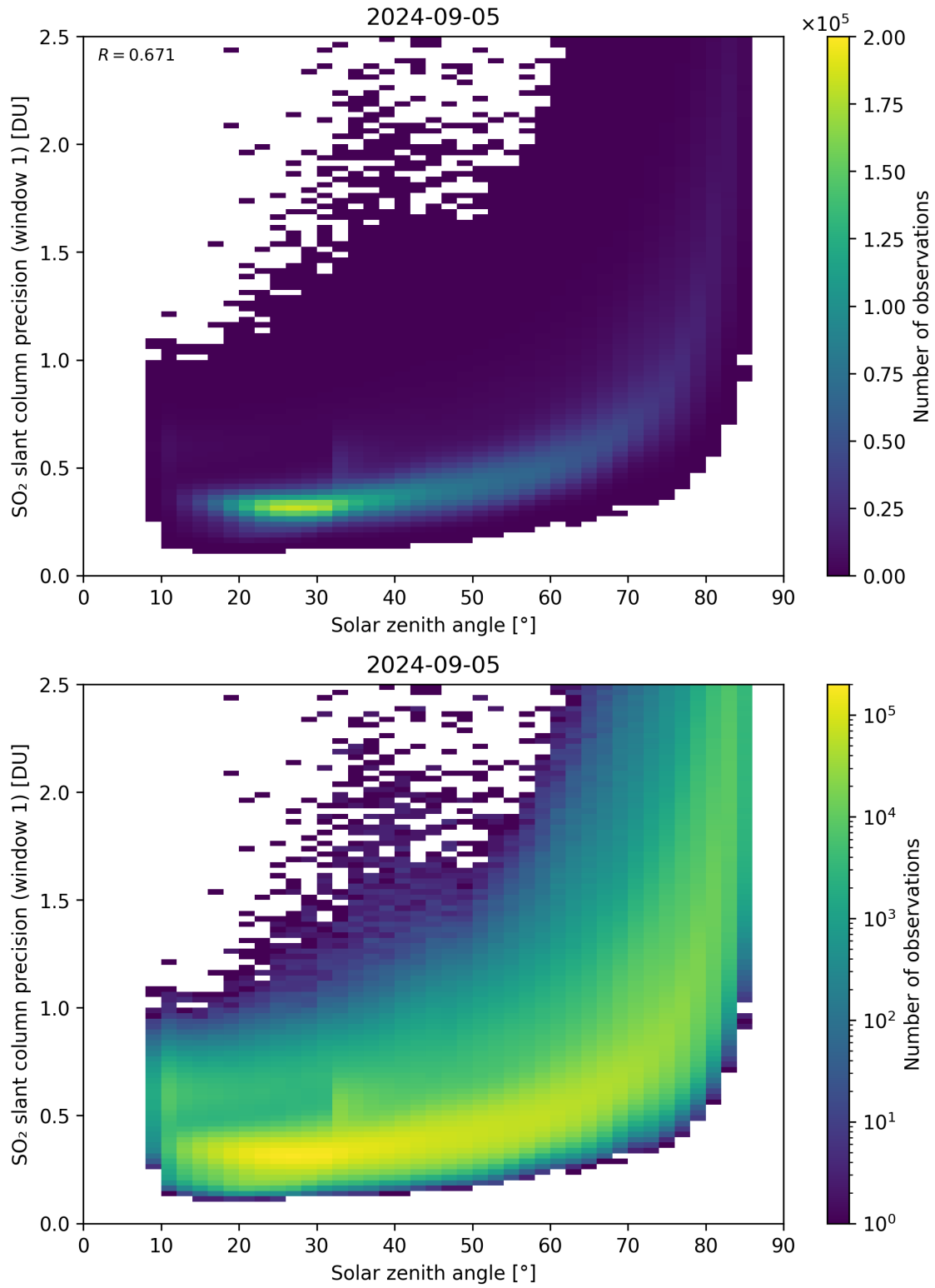
Figure 170: Scatter density plot of “Solar zenith angle” against “SO 2 slant column precision (window 1)” for 2024-09-04 to 2024-09-06.
