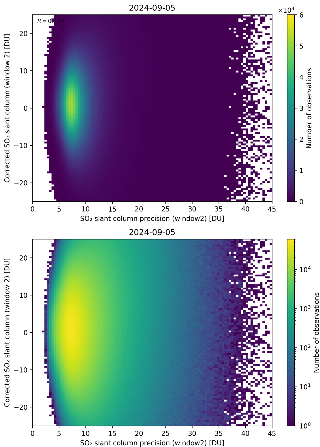
Figure 247: Scatter density plot of “SO 2 slant column precision (window2)” against “Corrected SO 2 slant column (window 2)” for 2024-09-04 to 2024-09-06.
