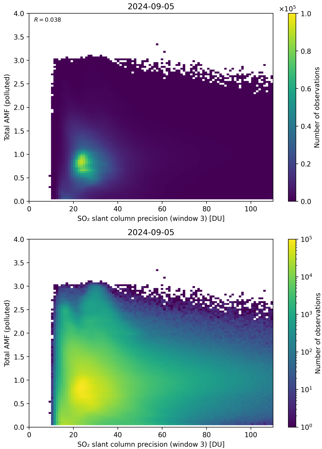
Figure 263: Scatter density plot of “SO 2 slant column precision (window 3)” against “Total AMF (polluted)” for 2024-09-04 to 2024-09-06.
