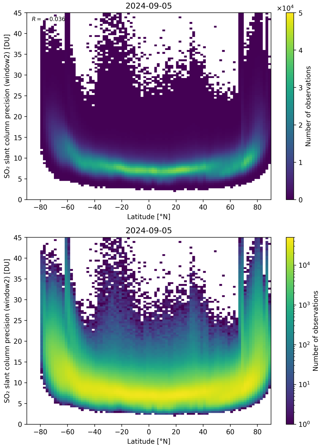
Figure 151: Scatter density plot of “Latitude” against “SO 2 slant column precision (window2)” for 2024-09-04 to 2024-09-06.
