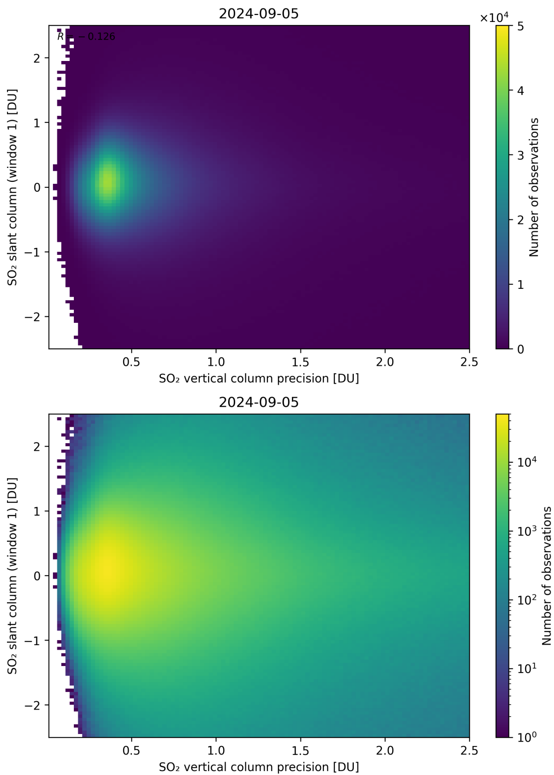
Figure 289: Scatter density plot of “SO 2 vertical column precision” against “SO 2 slant column (window 1)” for 2024-09-04 to 2024-09-06.
