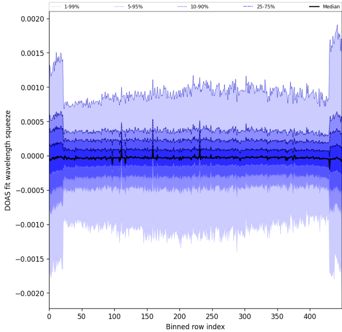
Figure 92: Along track statistics of “DOAS fit wavelength squeeze” for 2024-09-04 to 2024-09-06
