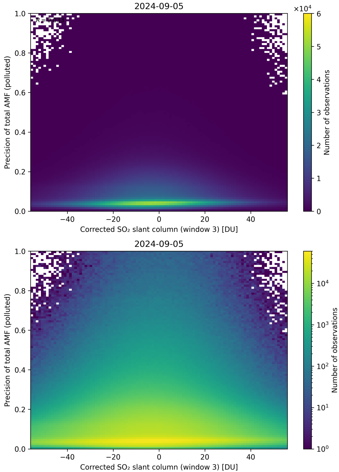
Figure 211: Scatter density plot of “Corrected SO 2 slant column (window 3)” against “Precision of total AMF (polluted)” for 2024-09-04 to 2024-09-06.
