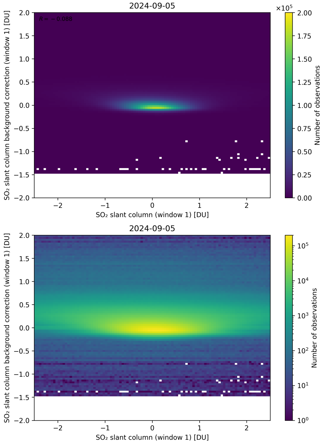
Figure 212: Scatter density plot of “SO 2 slant column (window 1)” against “SO 2 slant column background correction (window 1)” for 2024-09-04 to 2024-09-06.
