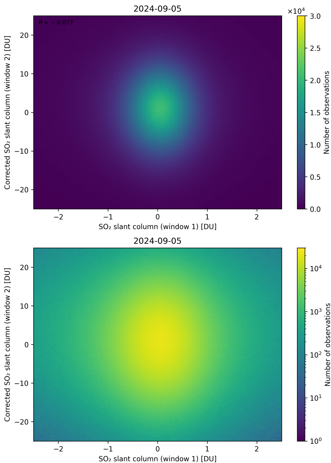
Figure 233: Scatter density plot of “SO 2 slant column (window 1)” against “Corrected SO 2 slant column (window 2)” for 2024-09-04 to 2024-09-06.
