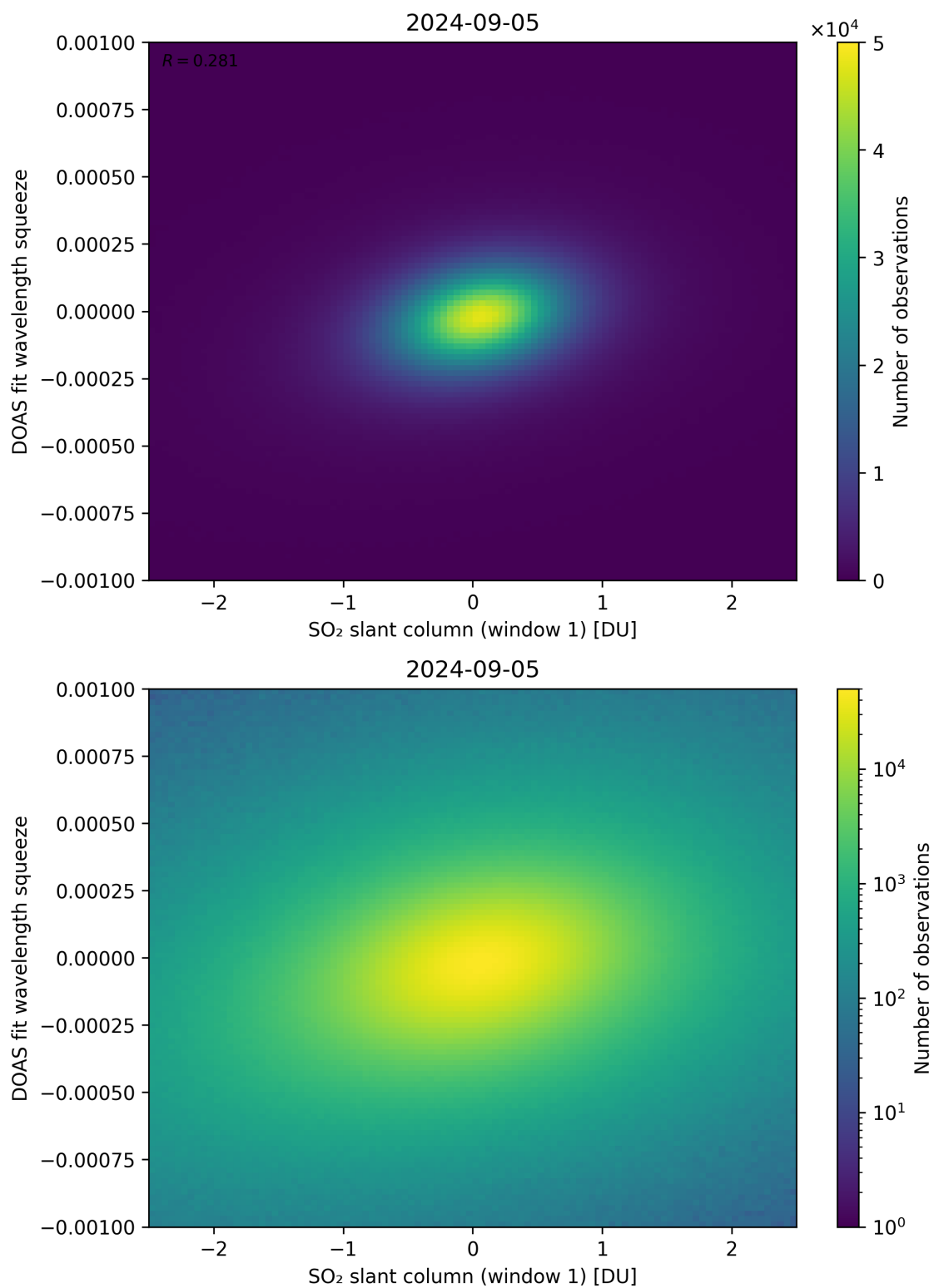
Figure 216: Scatter density plot of “SO 2 slant column (window 1)” against “DOAS fit wavelength squeeze” for 2024-09-04 to 2024-09-06.
