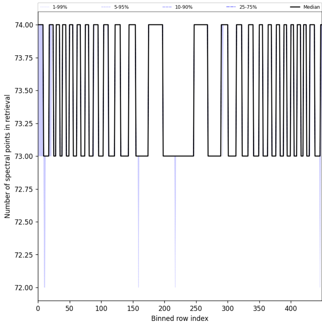
Figure 97: Along track statistics of “Number of spectral points in retrieval” for 2024-09-04 to 2024-09-06
