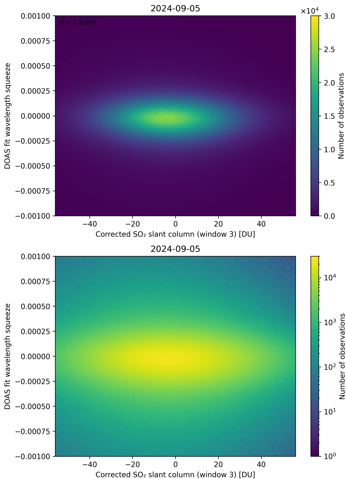
Figure 207: Scatter density plot of “Corrected SO 2 slant column (window 3)” against “DOAS fit wavelength squeeze” for 2024-09-04 to 2024-09-06.
