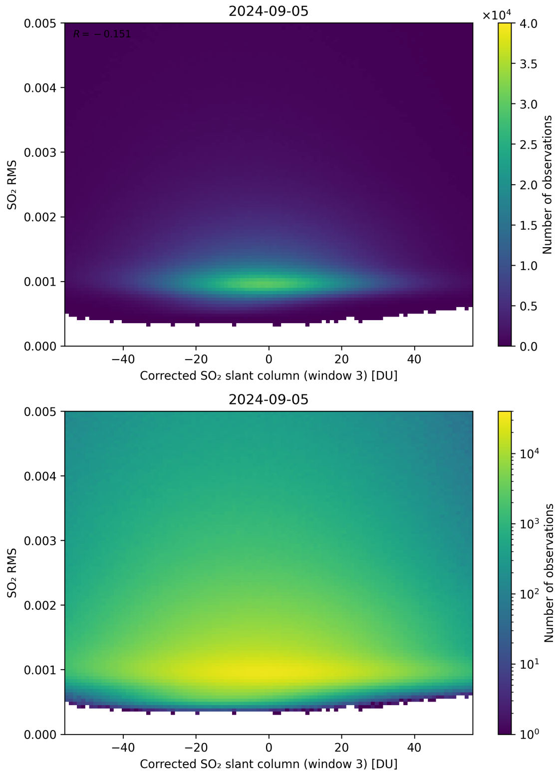
Figure 208: Scatter density plot of “Corrected SO 2 slant column (window 3)” against “SO 2 RMS” for 2024-09-04 to 2024-09-06.
