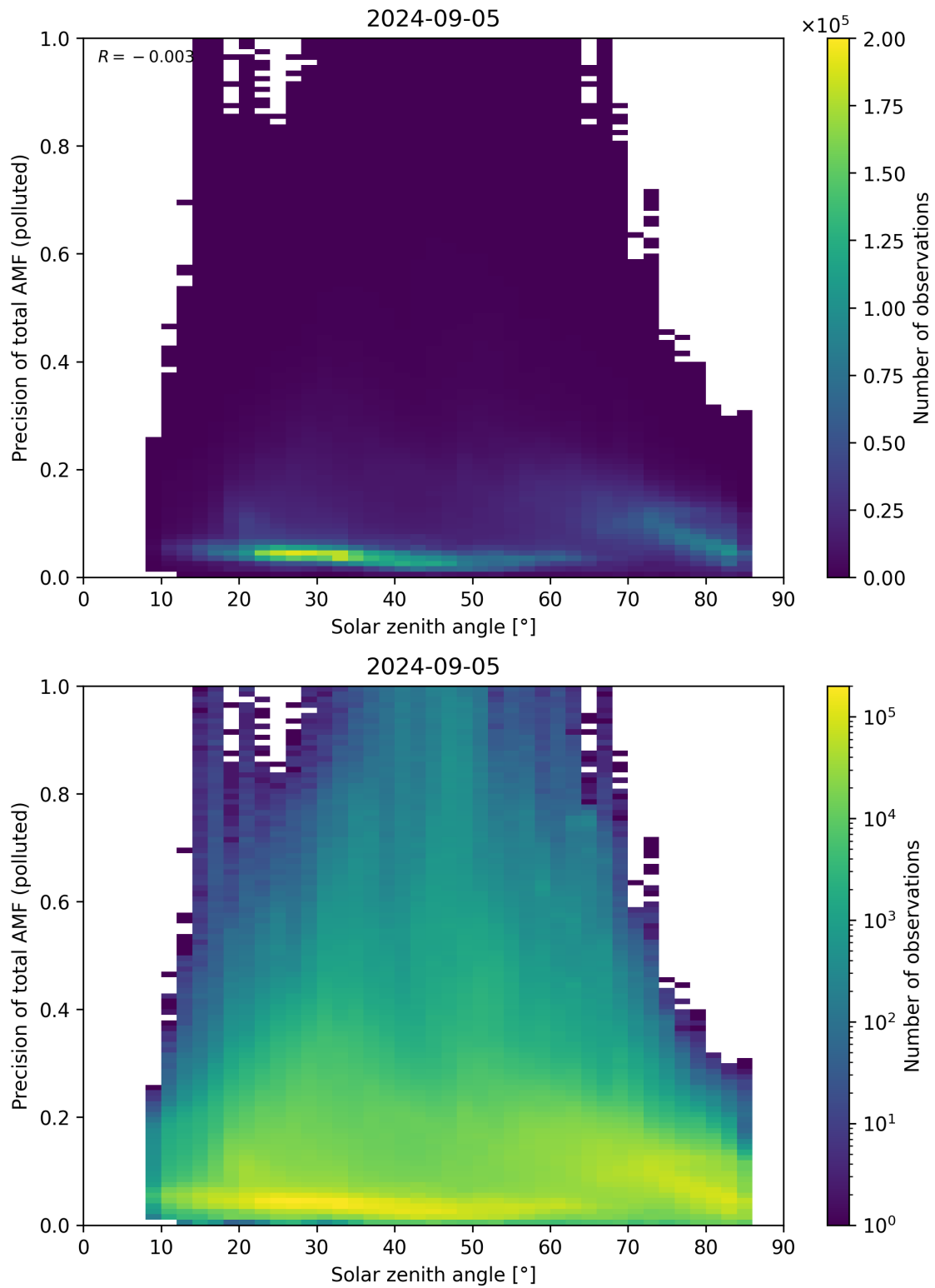
Figure 175: Scatter density plot of “Solar zenith angle” against “Precision of total AMF (polluted)” for 2024-09-04 to 2024-09-06.
