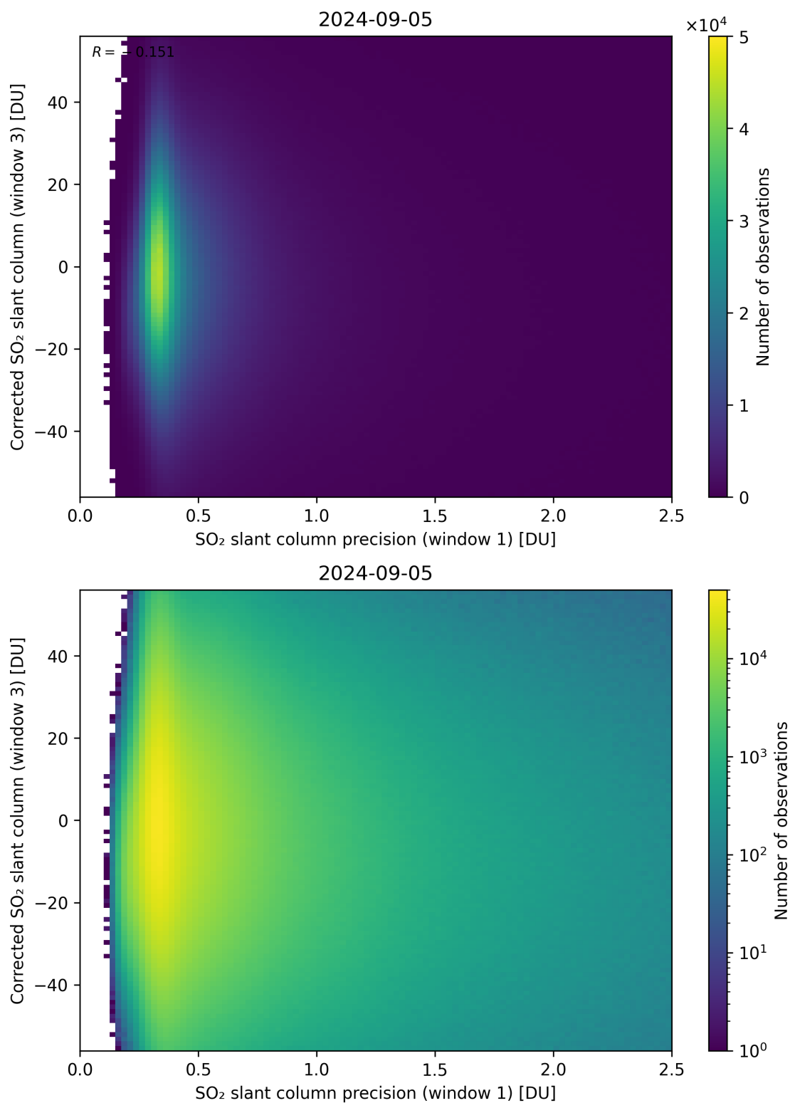
Figure 226: Scatter density plot of “SO 2 slant column precision (window 1)” against “Corrected SO 2 slant column (window 3)” for 2024-09-04 to 2024-09-06.
