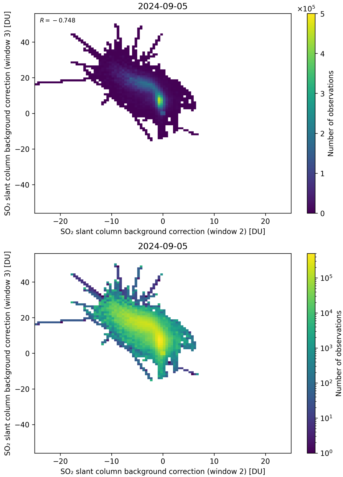
Figure 111: Scatter density plot of “SO 2 slant column background correction (window 2)” against “SO 2 slant column background correction (window 3)” for 2024-09-04 to 2024-09-06.
