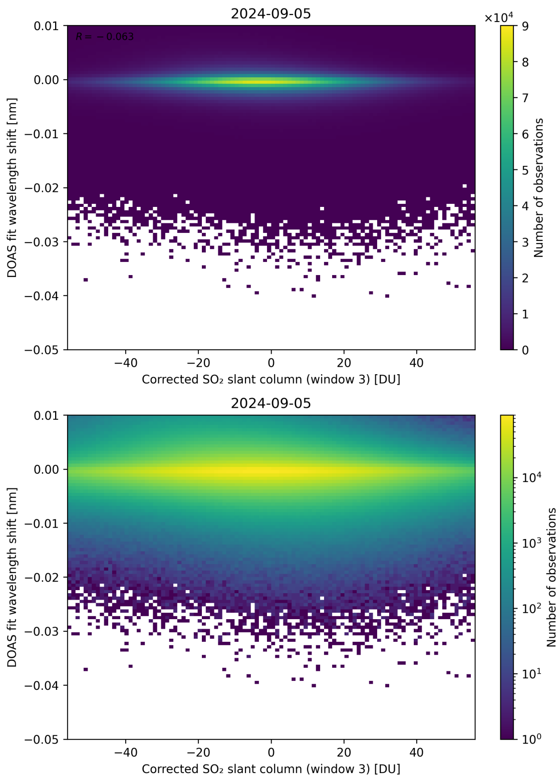
Figure 206: Scatter density plot of “Corrected SO 2 slant column (window 3)” against “DOAS fit wavelength shift” for 2024-09-04 to 2024-09-06.
