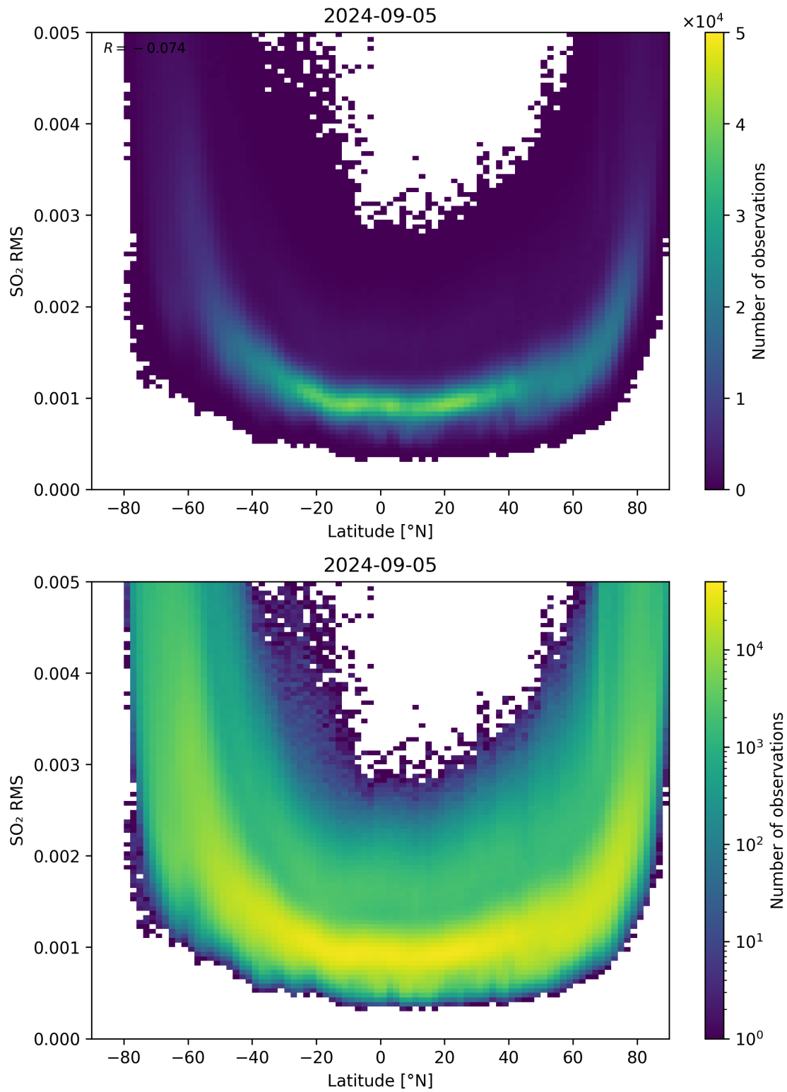
Figure 144: Scatter density plot of “Latitude” against “SO 2 RMS” for 2024-09-04 to 2024-09-06.
