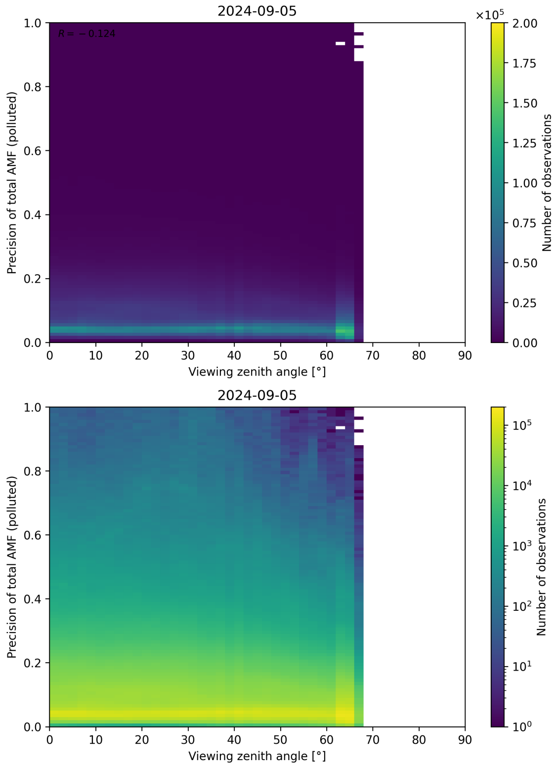
Figure 326: Scatter density plot of “Viewing zenith angle” against “Precision of total AMF (polluted)” for 2024-09-04 to 2024-09-06.
