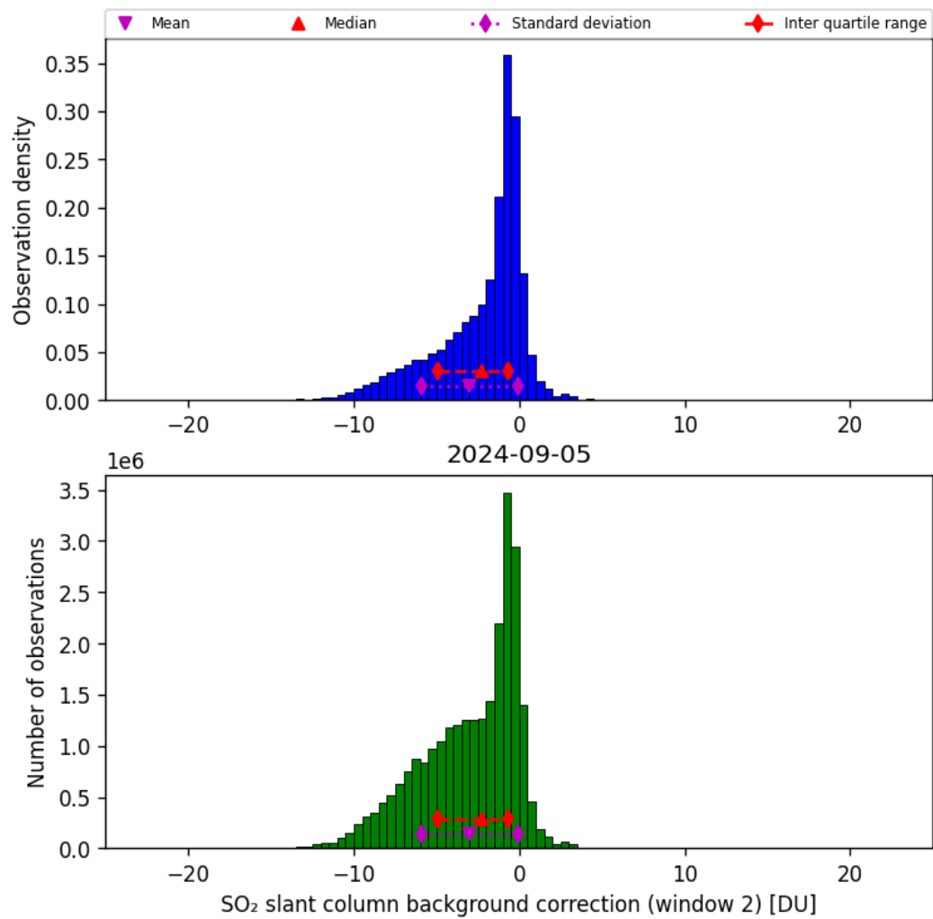
Figure 63: Histogram of “SO 2 slant column background correction (window 2)” for 2024-09-04 to 2024-09-06
