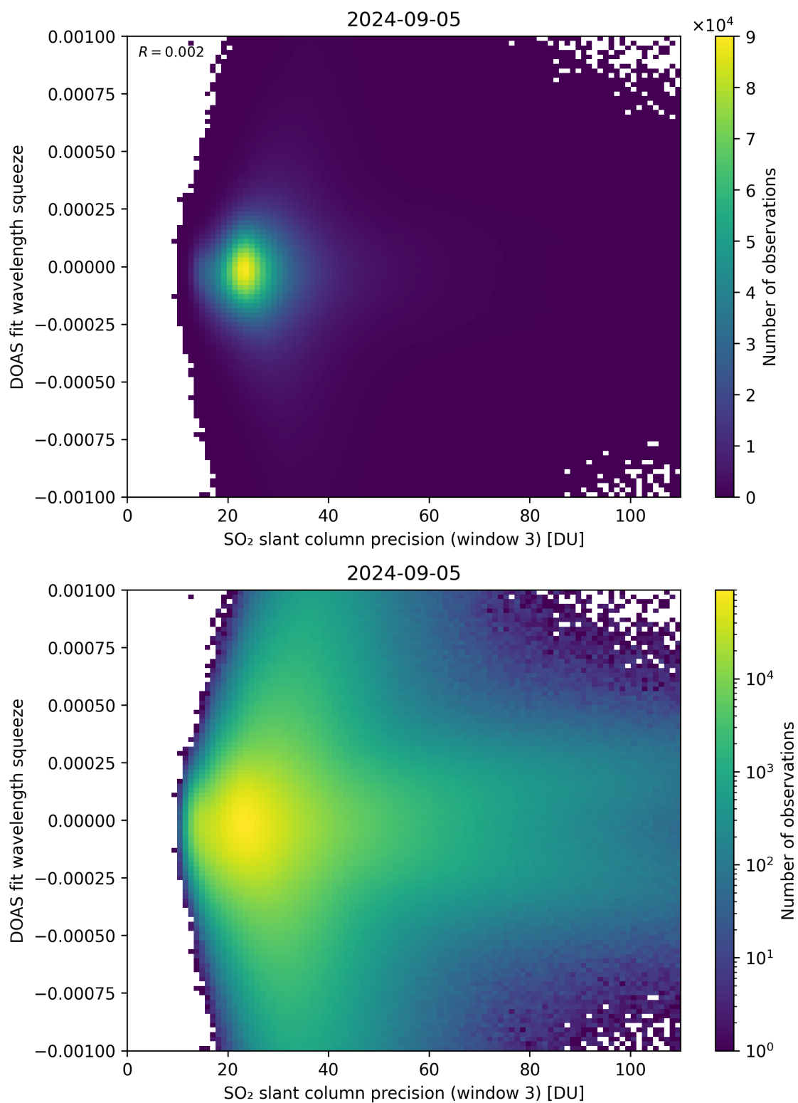
Figure 259: Scatter density plot of “SO 2 slant column precision (window 3)” against “DOAS fit wavelength squeeze” for 2024-09-04 to 2024-09-06.
