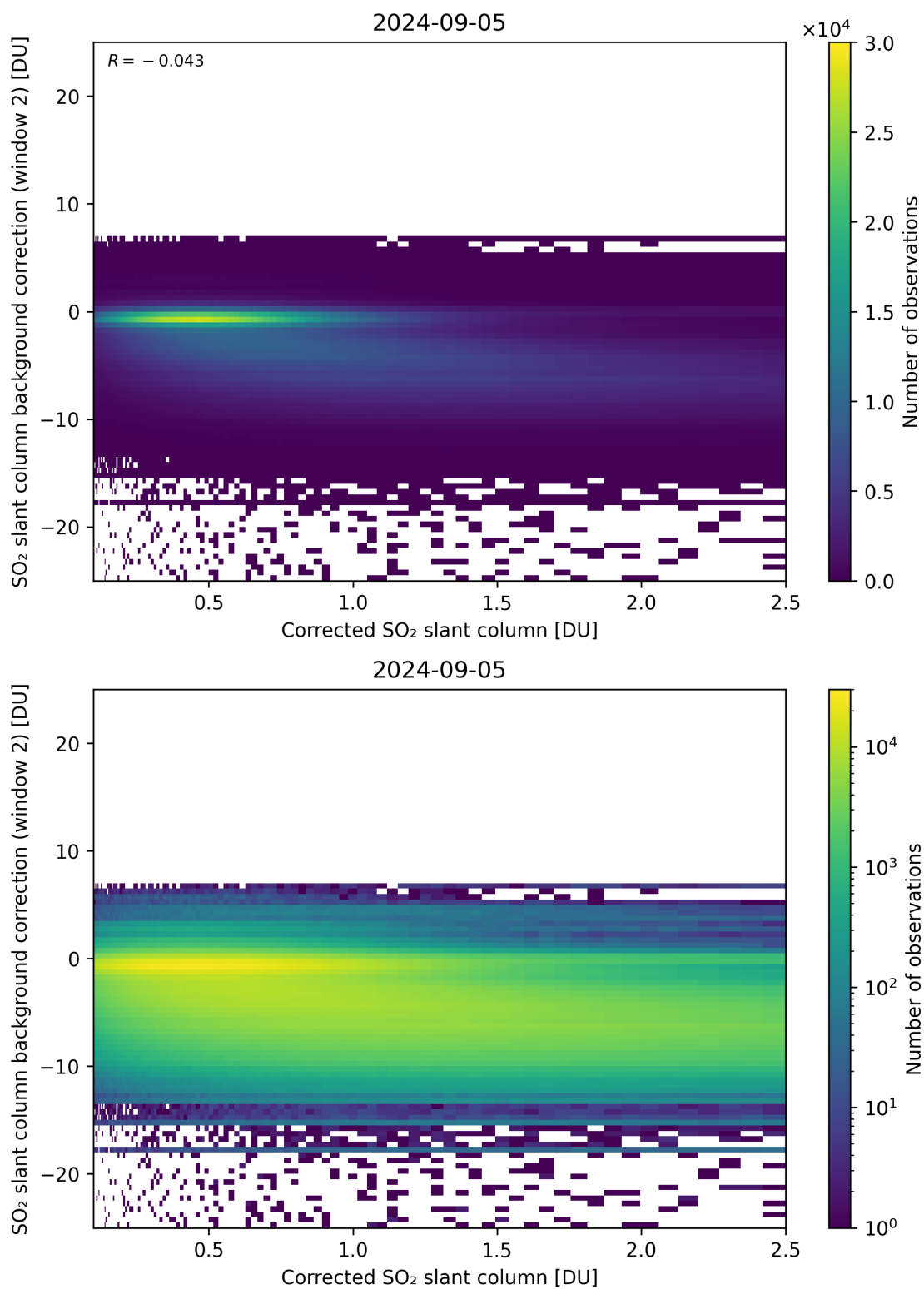
Figure 179: Scatter density plot of “Corrected SO 2 slant column” against “SO 2 slant column background correction (window 2)” for 2024-09-04 to 2024-09-06.
