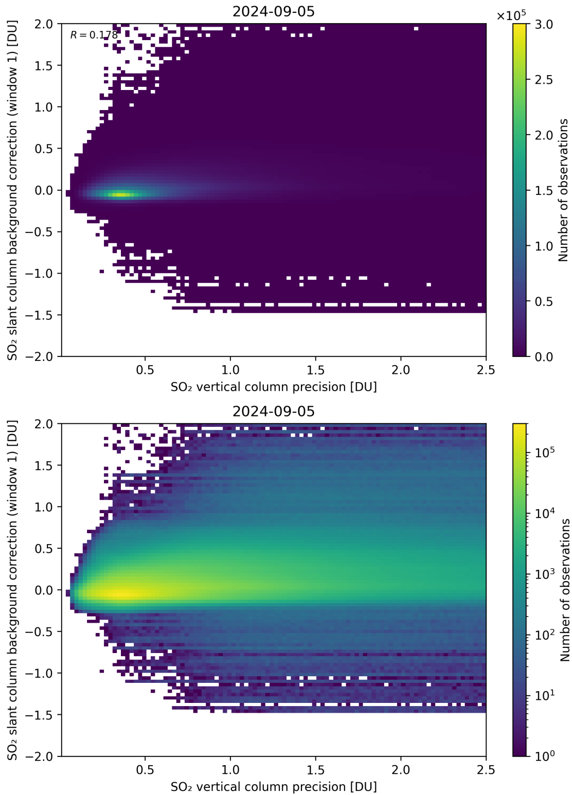
Figure 279: Scatter density plot of “SO 2 vertical column precision” against “SO 2 slant column background correction (window 1)” for 2024-09-04 to 2024-09-06.
