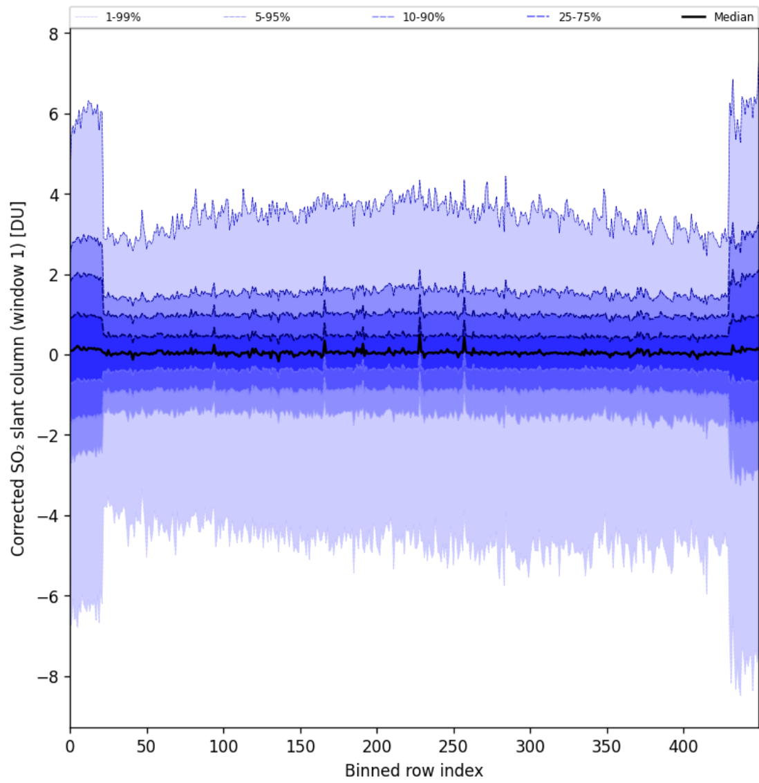
Figure 81: Along track statistics of “Corrected SO 2 slant column (window 1)” for 2024-09-04 to 2024-09-06
