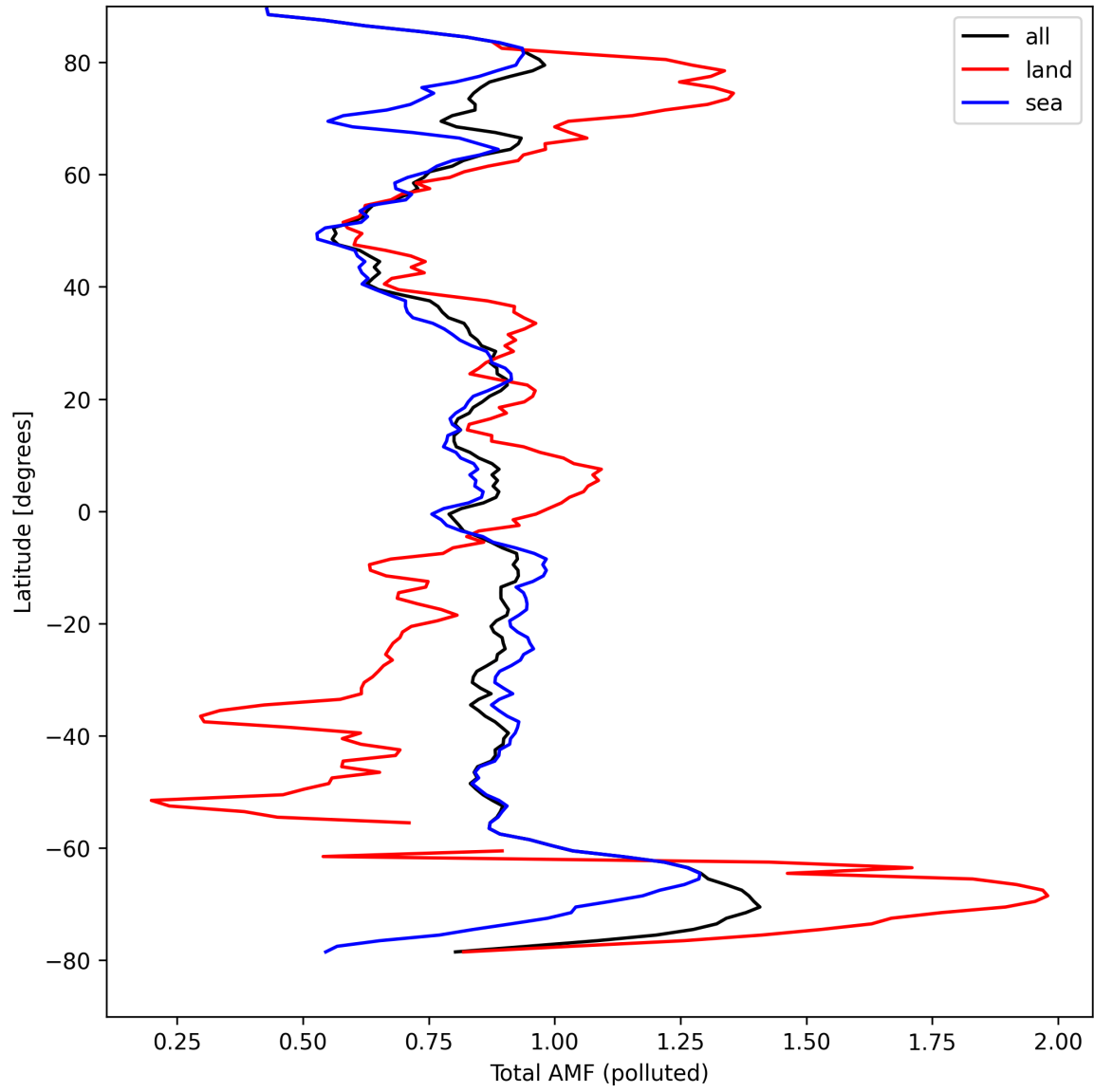
Figure 48: Zonal average of “Total AMF (polluted)” for 2024-09-04 to 2024-09-06.
