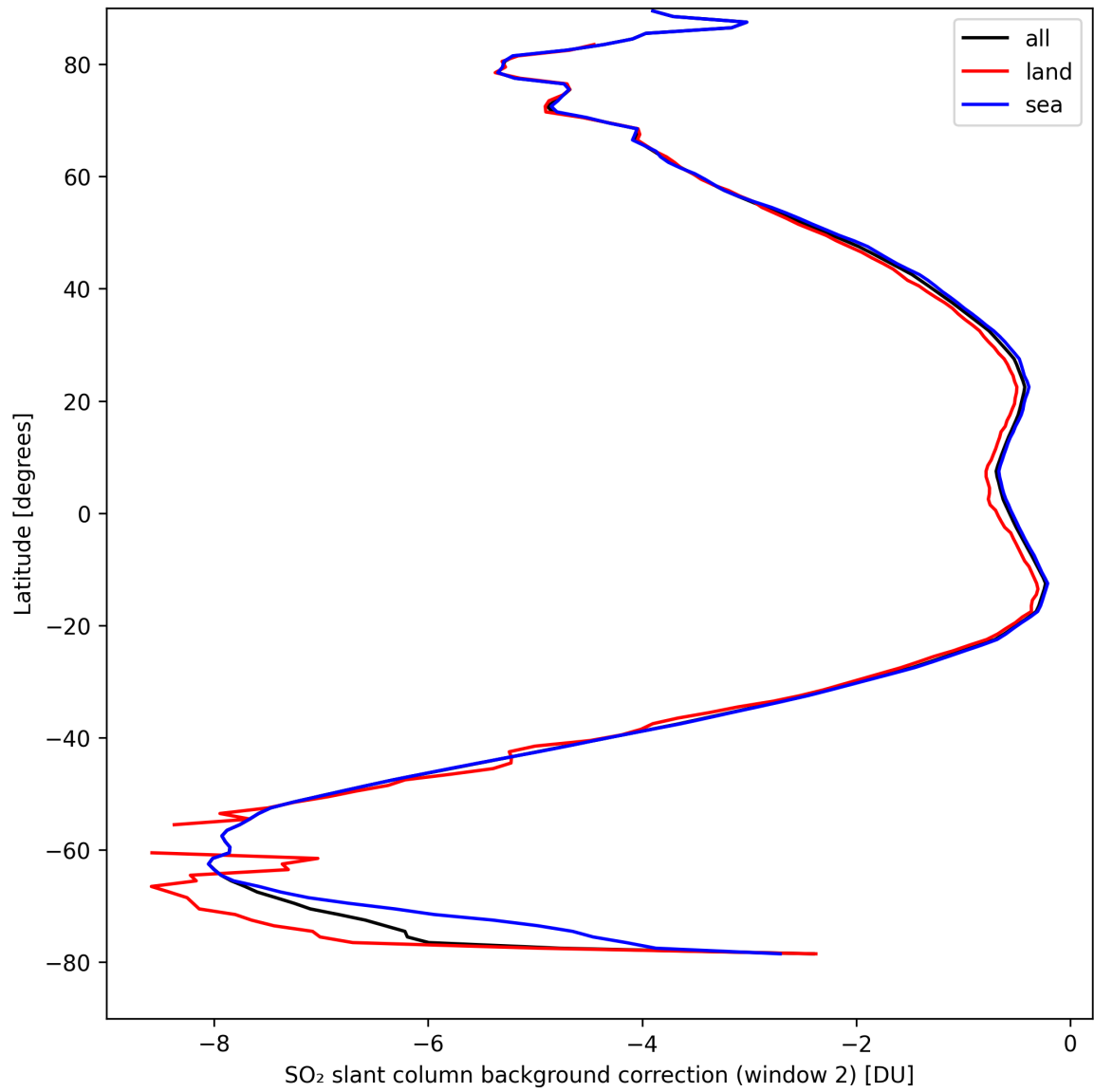
Figure 40: Zonal average of "SO 2 slant column background correction (window 2)" for 2024-09-04 to 2024-09-06.
