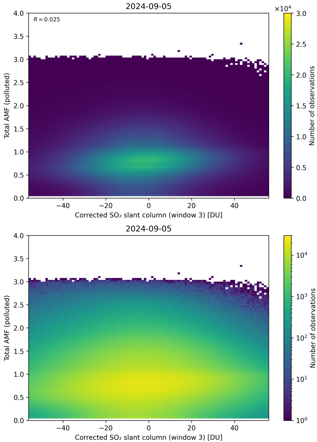
Figure 210: Scatter density plot of “Corrected SO 2 slant column (window 3)” against “Total AMF (polluted)” for 2024-09-04 to 2024-09-06.
