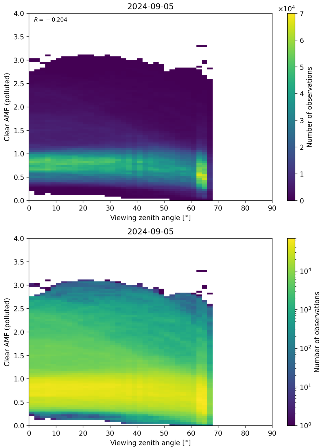
Figure 316: Scatter density plot of “Viewing zenith angle” against “Clear AMF (polluted)” for 2024-09-04 to 2024-09-06.
