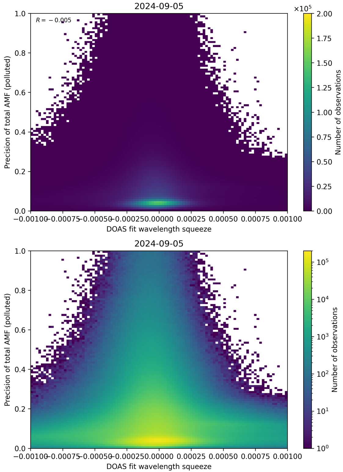
Figure 135: Scatter density plot of “DOAS fit wavelength squeeze” against “Precision of total AMF (polluted)” for 2024-09-04 to 2024-09-06.
