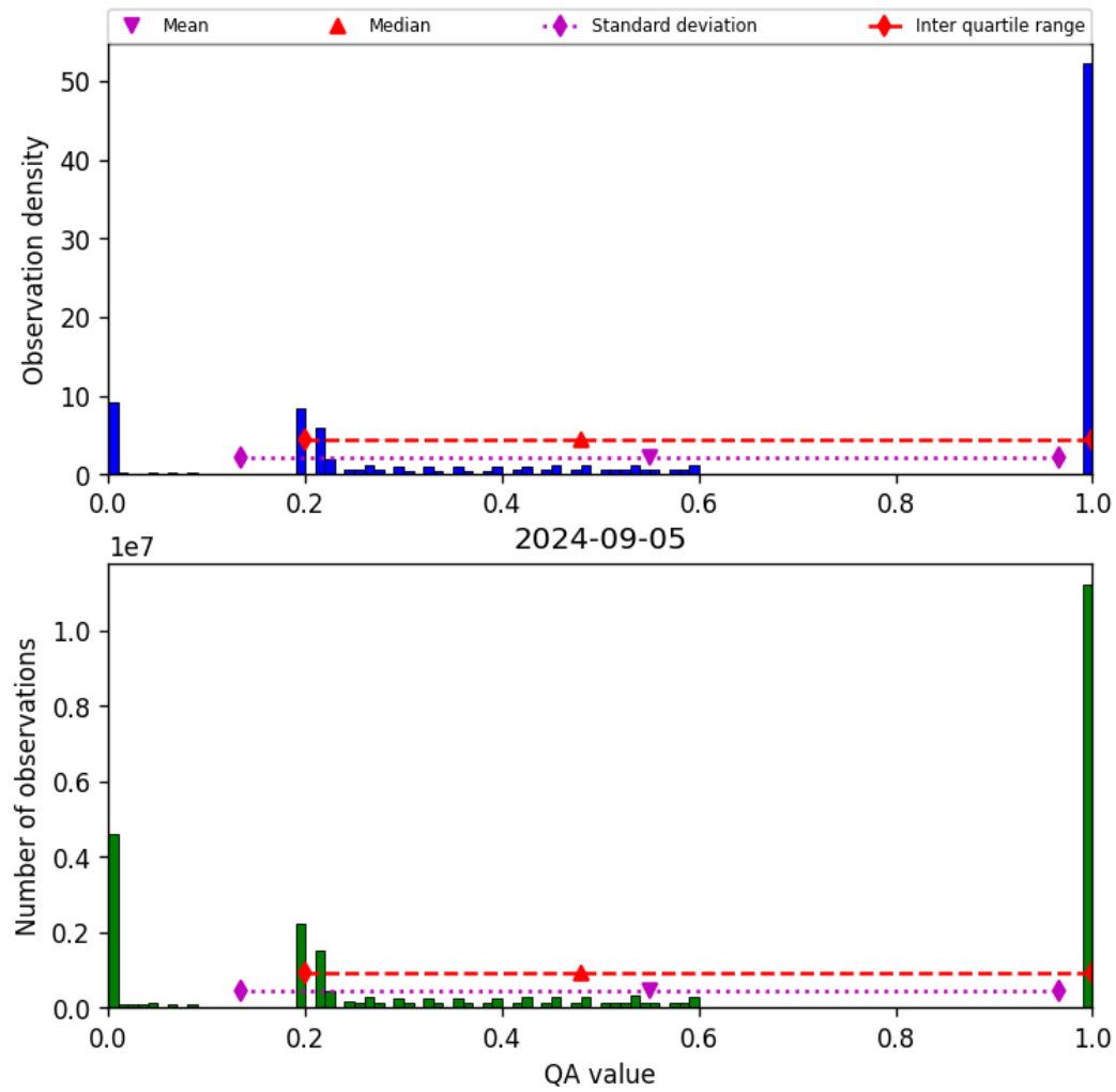
Figure 52: Histogram of “QA value” for 2024-09-04 to 2024-09-06
