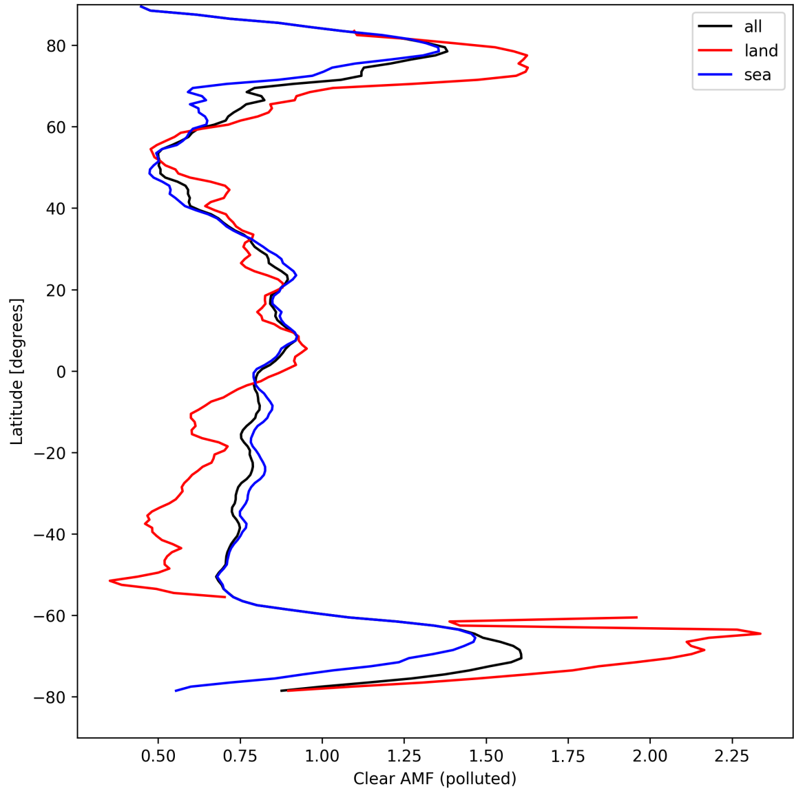
Figure 50: Zonal average of “Clear AMF (polluted)” for 2024-09-04 to 2024-09-06.
