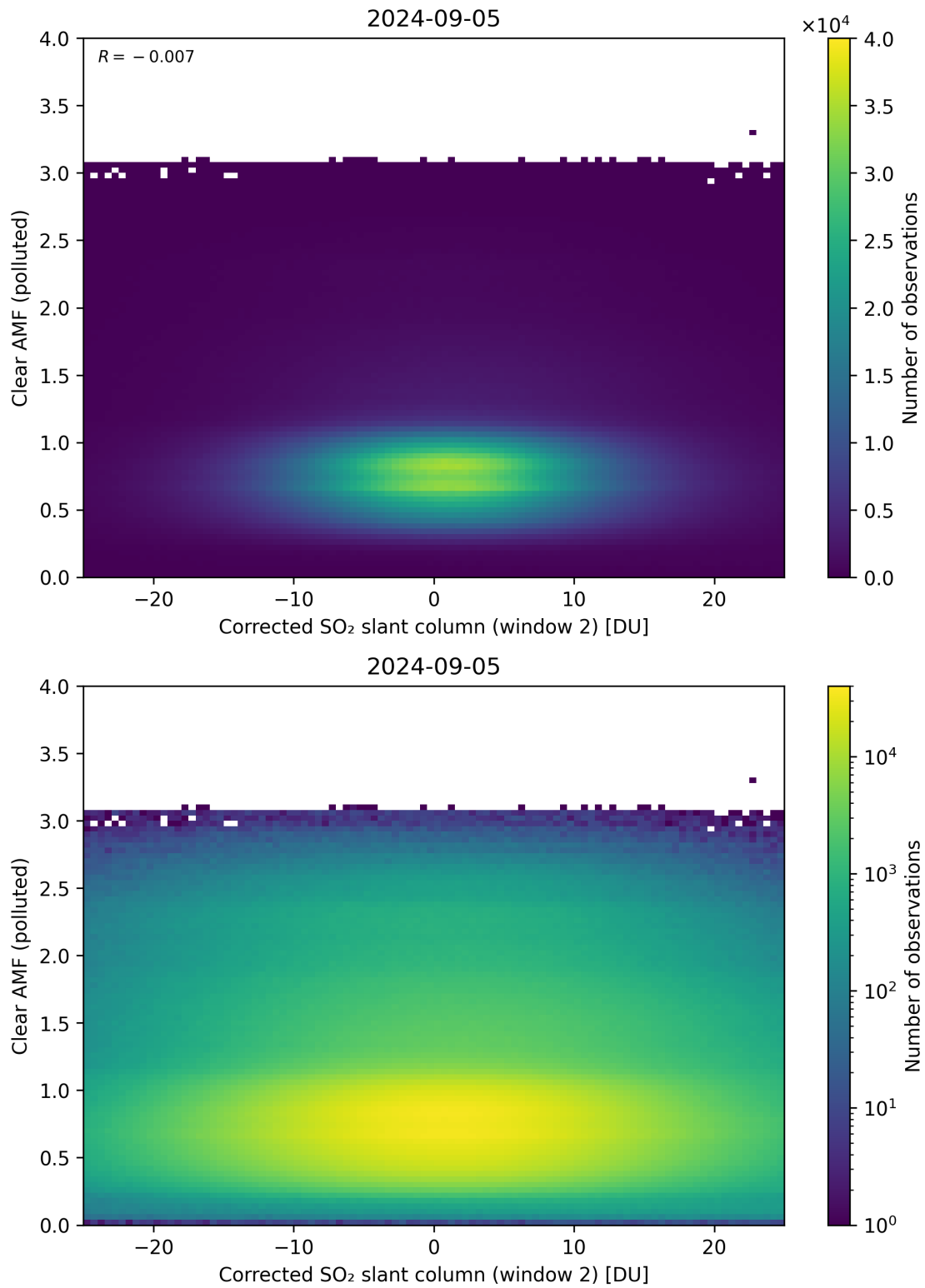
Figure 199: Scatter density plot of “Corrected SO 2 slant column (window 2)” against “Clear AMF (polluted)” for 2024-09-04 to 2024-09-06.
