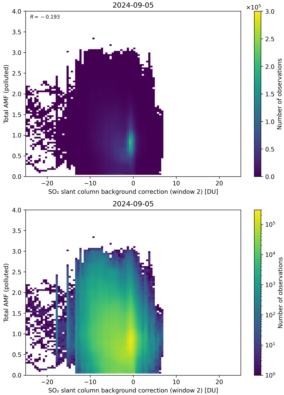
Figure 119: Scatter density plot of “SO 2 slant column background correction (window 2)” against “Total AMF (polluted)” for 2024-09-04 to 2024-09-06.
