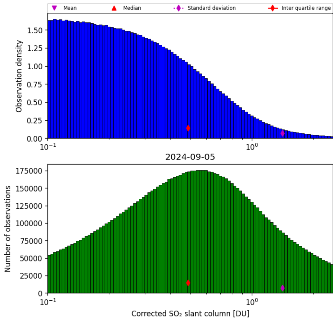
Figure 55: Histogram of "Corrected SO 2 slant column" for 2024-09-04 to 2024-09-06
