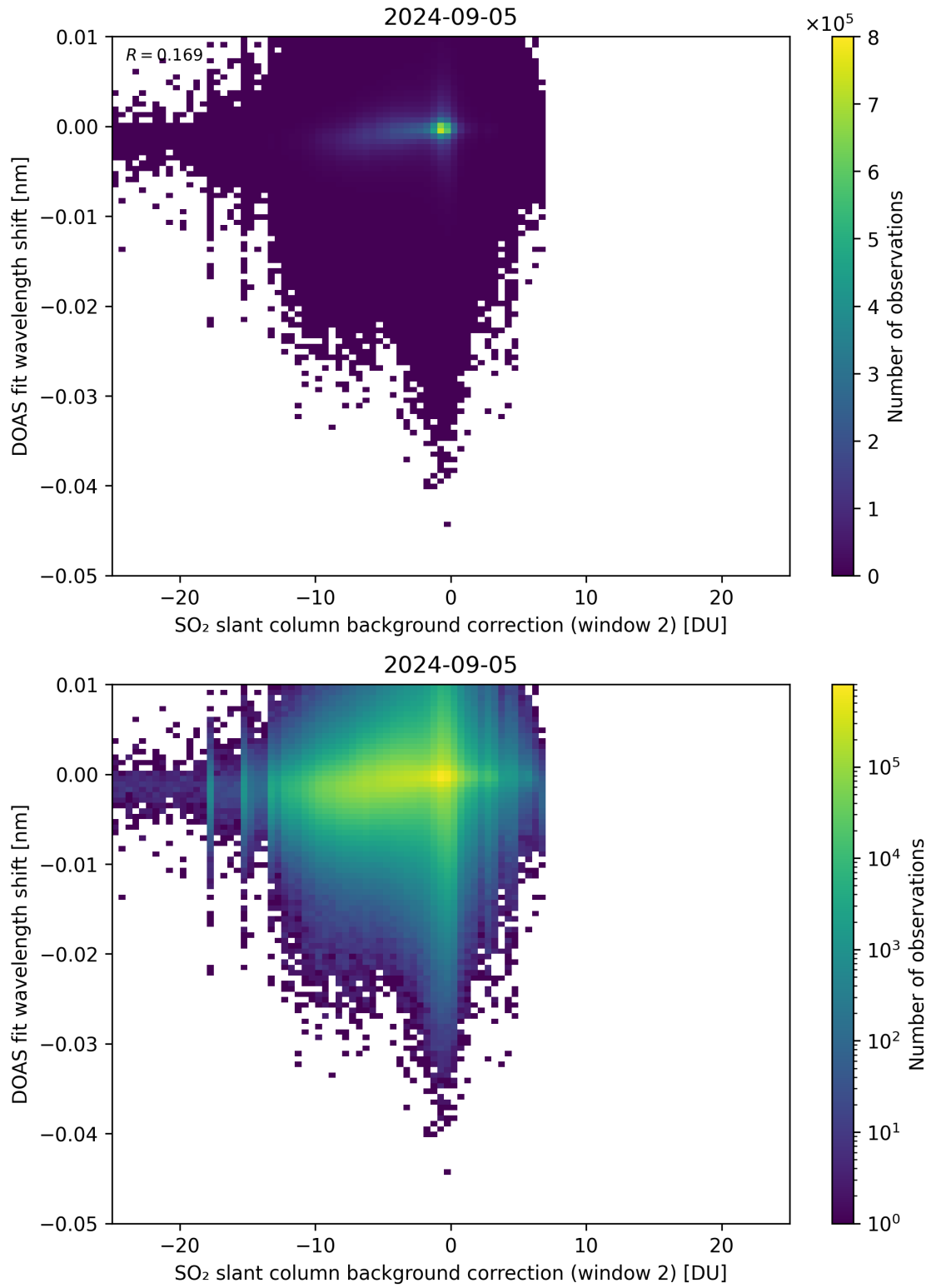
Figure 112: Scatter density plot of “SO 2 slant column background correction (window 2)” against “DOAS fit wavelength shift” for 2024-09-04 to 2024-09-06.
