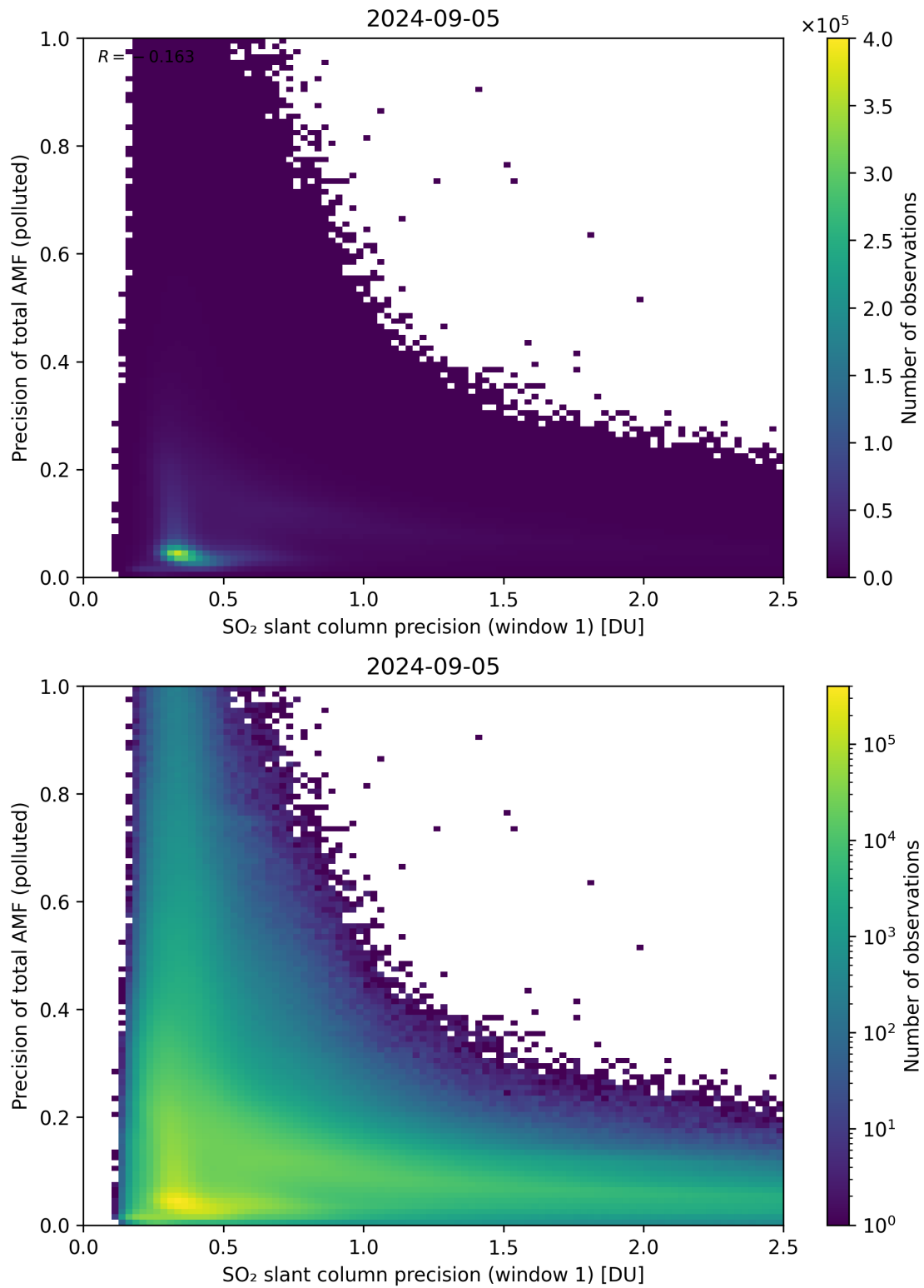
Figure 231: Scatter density plot of “SO 2 slant column precision (window 1)” against “Precision of total AMF (polluted)” for 2024-09-04 to 2024-09-06.
