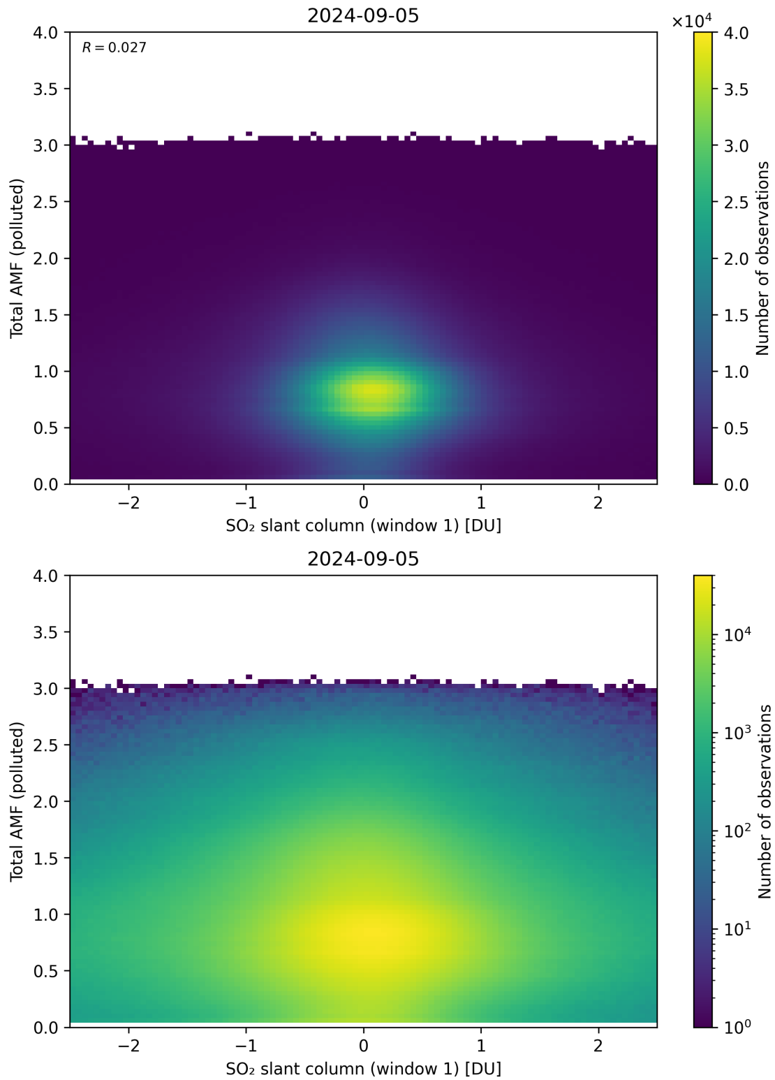
Figure 239: Scatter density plot of “SO 2 slant column (window 1)” against “Total AMF (polluted)” for 2024-09-04 to 2024-09-06.
