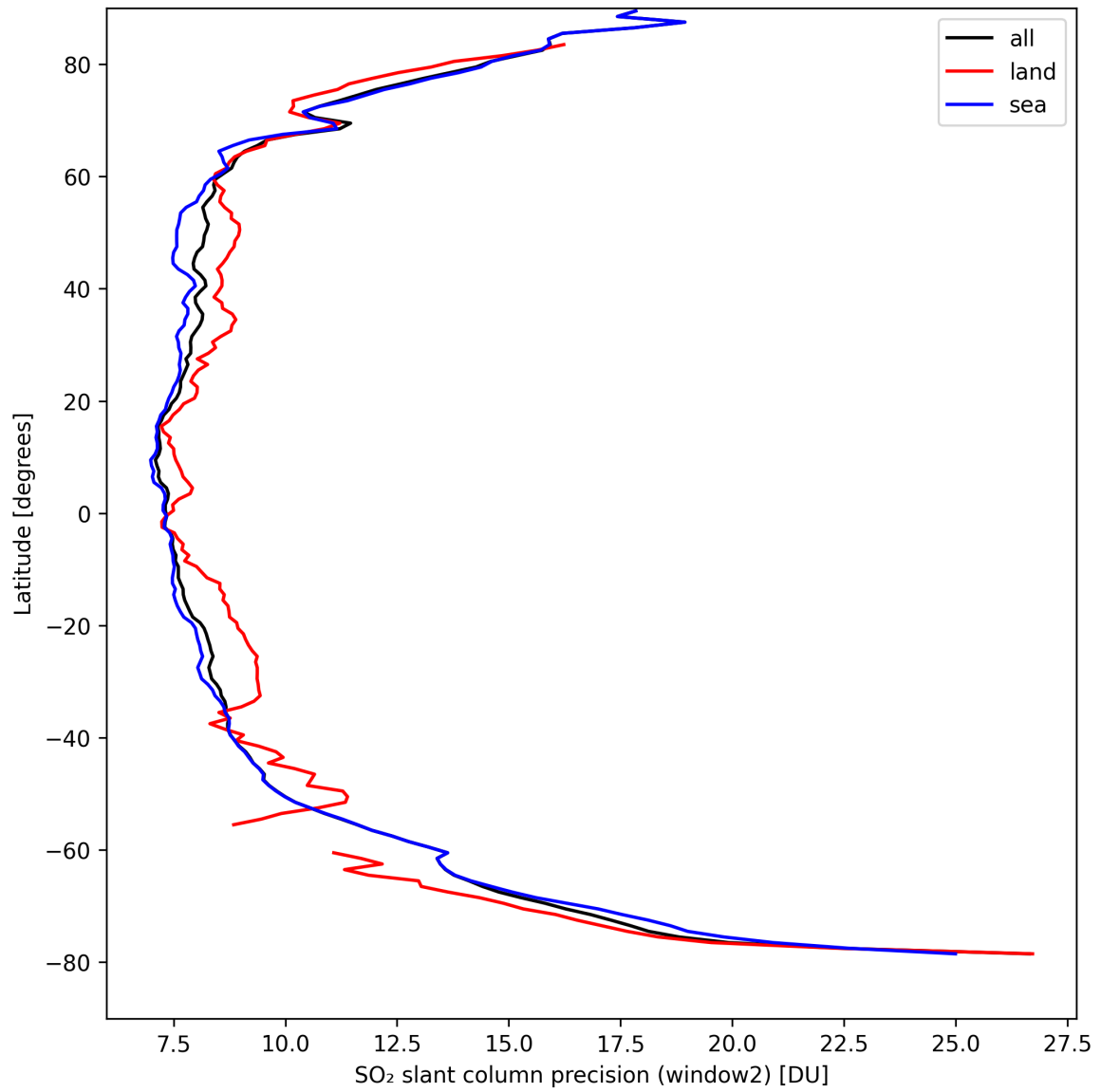
Figure 38: Zonal average of “SO 2 slant column precision (window2)” for 2024-09-04 to 2024-09-06.
