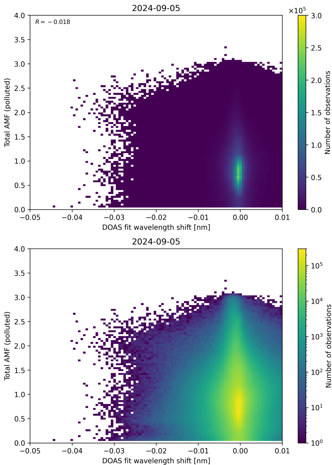
Figure 130: Scatter density plot of “DOAS fit wavelength shift” against “Total AMF (polluted)” for 2024-09-04 to 2024-09-06.
