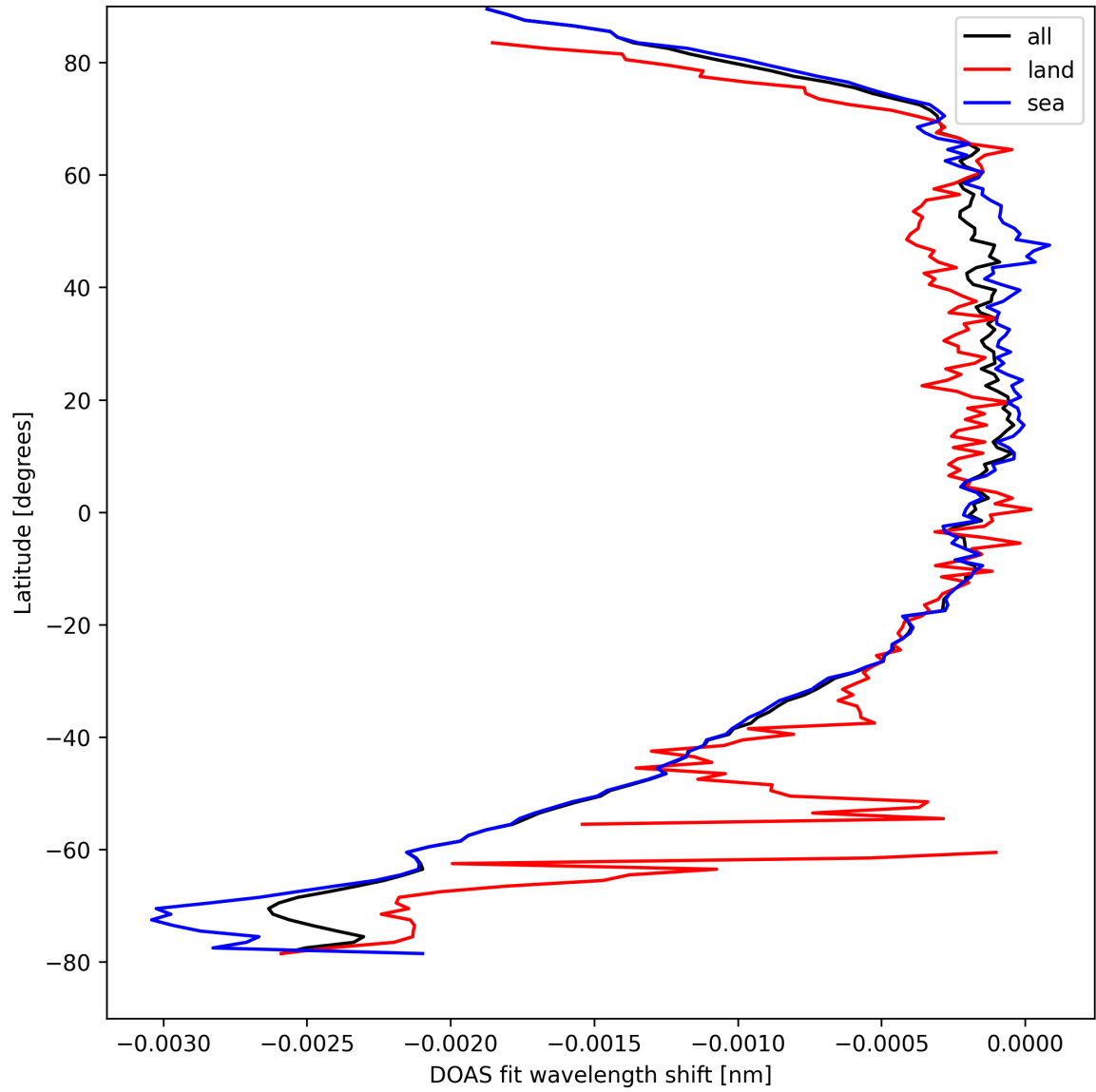
Figure 45: Zonal average of “DOAS fit wavelength shift” for 2024-09-04 to 2024-09-06.
