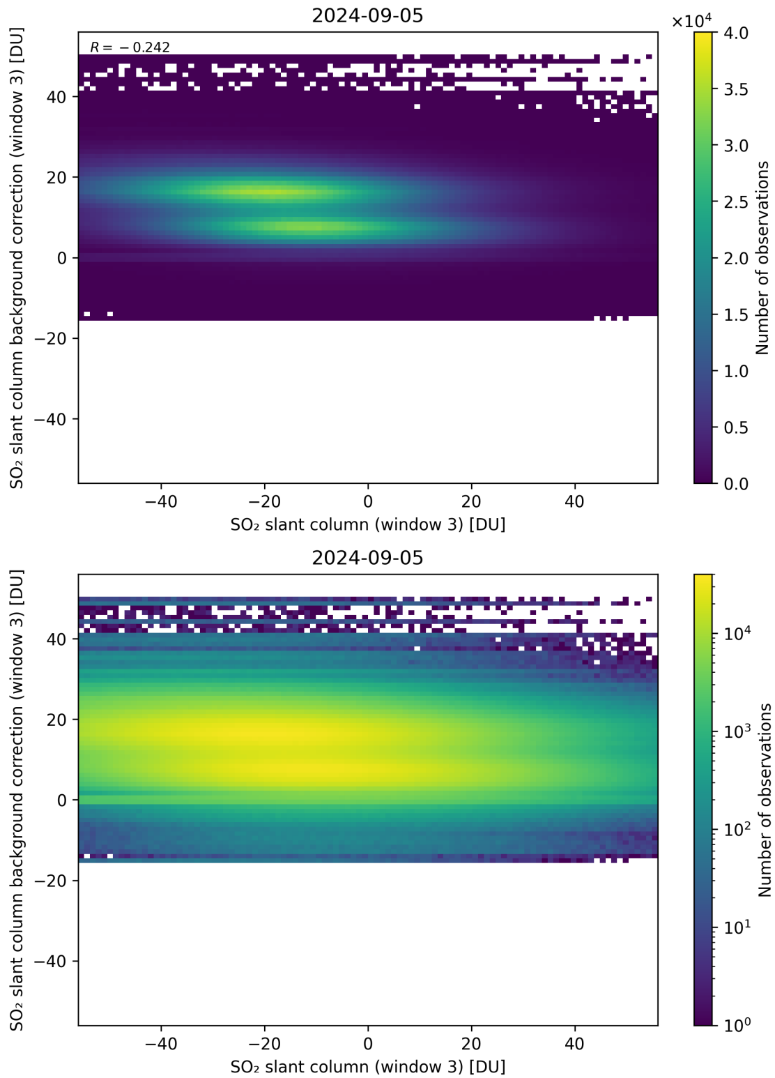
Figure 253: Scatter density plot of “SO 2 slant column (window 3)” against “SO 2 slant column background correction (window 3)” for 2024-09-04 to 2024-09-06.
