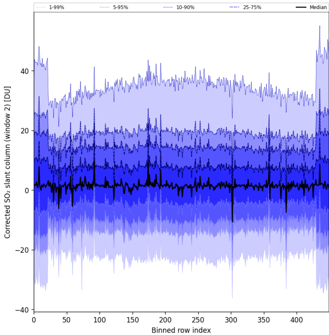
Figure 85: Along track statistics of “Corrected SO 2 slant column (window 2)” for 2024-09-04 to 2024-09-06
