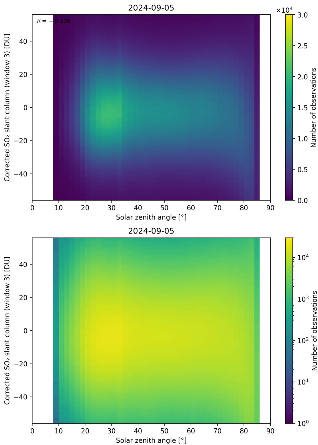
Figure 168: Scatter density plot of “Solar zenith angle” against “Corrected SO 2 slant column (window 3)” for 2024-09-04 to 2024-09-06.
