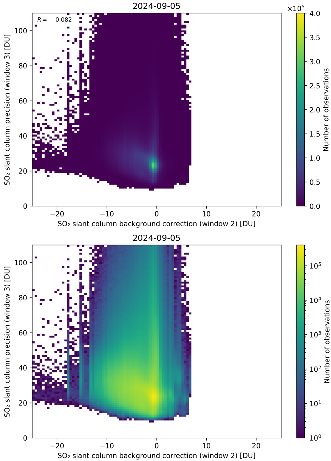
Figure 118: Scatter density plot of “SO 2 slant column background correction (window 2)” against “SO 2 slant column precision (window 3)” for 2024-09-04 to 2024-09-06.
