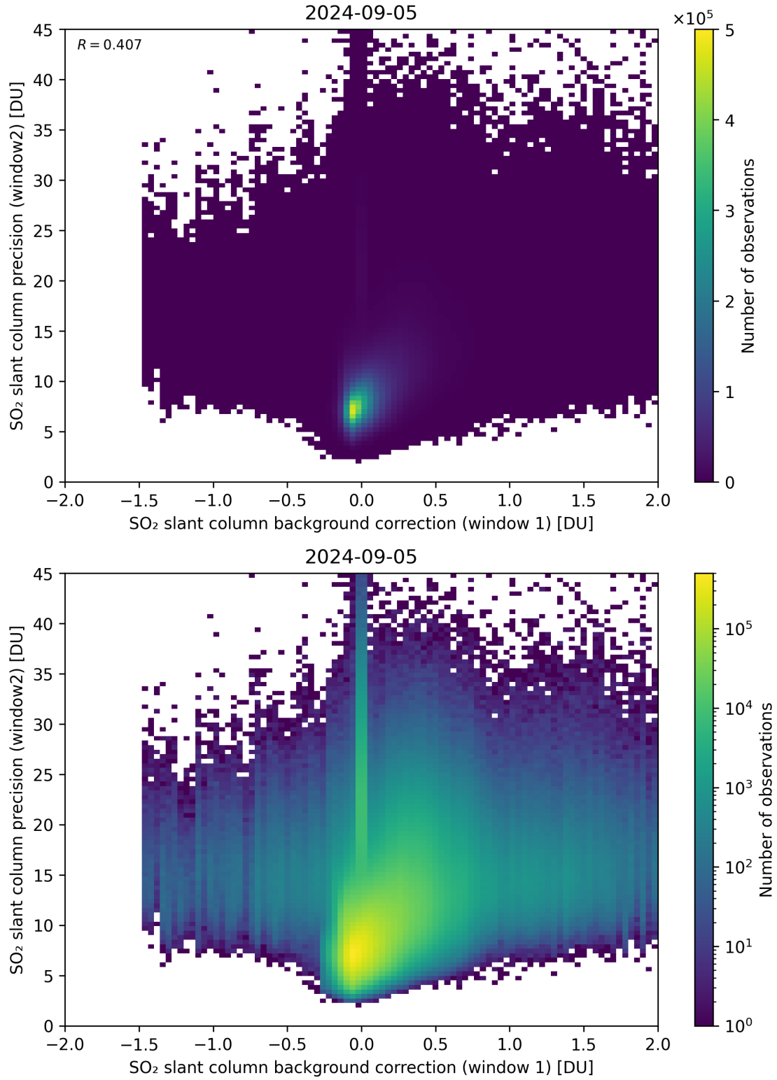
Figure 106: Scatter density plot of “SO 2 slant column background correction (window 1)” against “SO 2 slant column precision (window2)” for 2024-09-04 to 2024-09-06.
