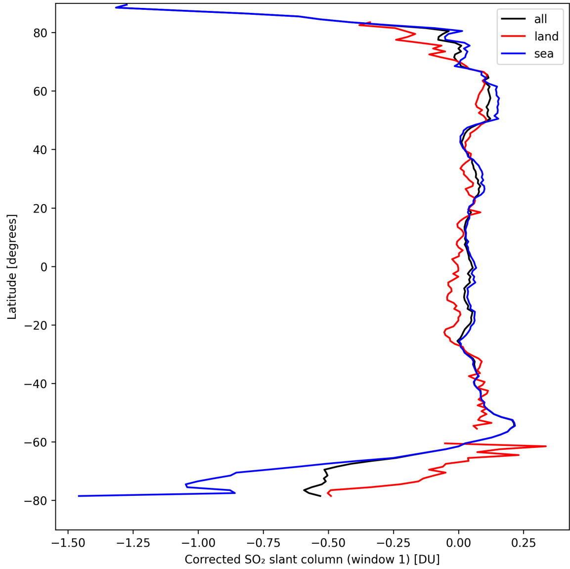
Figure 35: Zonal average of “Corrected SO 2 slant column (window 1)” for 2024-09-04 to 2024-09-06.
