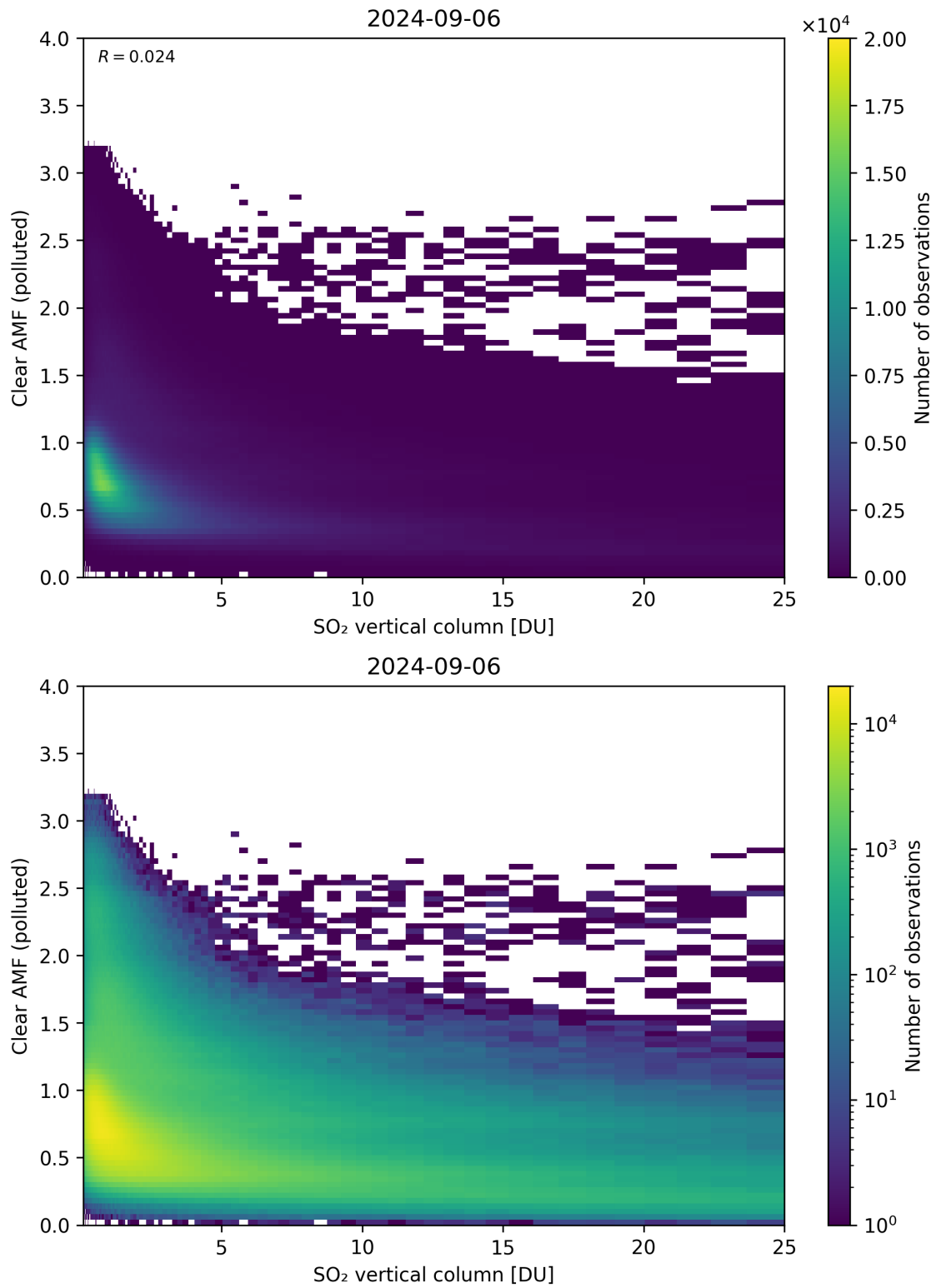
Figure 296: Scatter density plot of “SO 2 vertical column” against “Clear AMF (polluted)” for 2024-09-06 to 2024-09-07.
