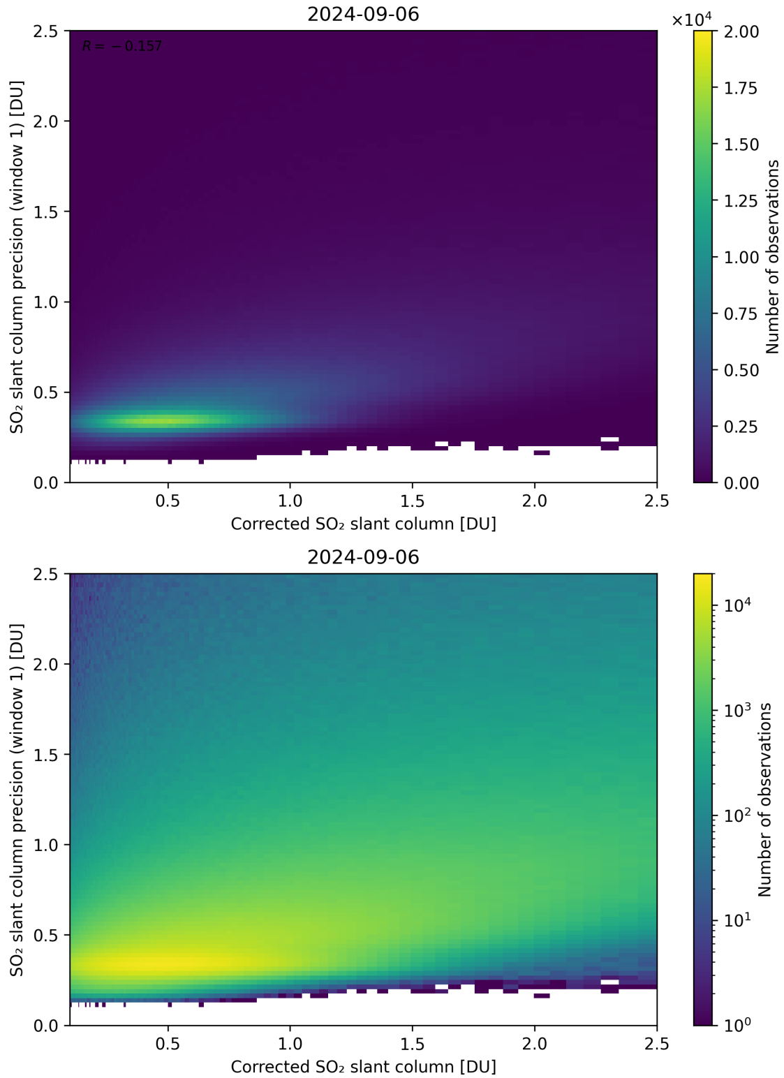
Figure 188: Scatter density plot of “Corrected SO 2 slant column” against “SO 2 slant column precision (window 1)” for 2024-09-06 to 2024-09-07.
