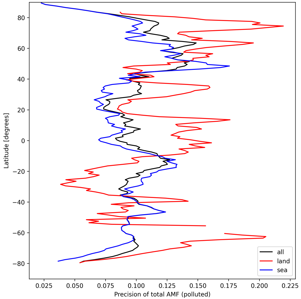
Figure 49: Zonal average of “Precision of total AMF (polluted)” for 2024-09-06 to 2024-09-07.
