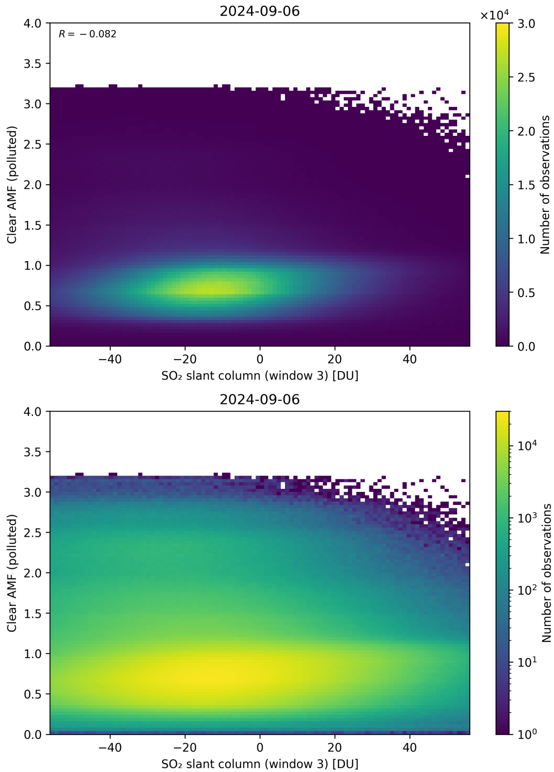
Figure 265: Scatter density plot of “SO 2 slant column (window 3)” against “Clear AMF (polluted)” for 2024-09-06 to 2024-09-07.
