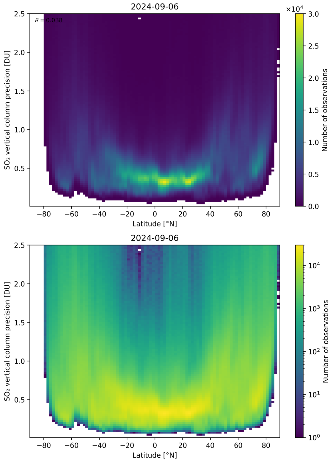
Figure 157: Scatter density plot of “Latitude” against “SO 2 vertical column precision” for 2024-09-06 to 2024-09-07.
