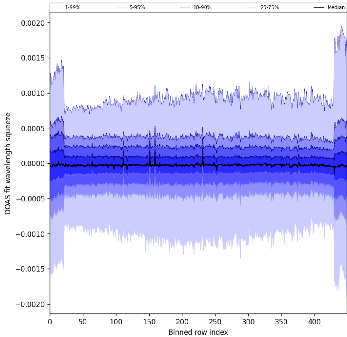
Figure 92: Along track statistics of “DOAS fit wavelength squeeze” for 2024-09-06 to 2024-09-07
