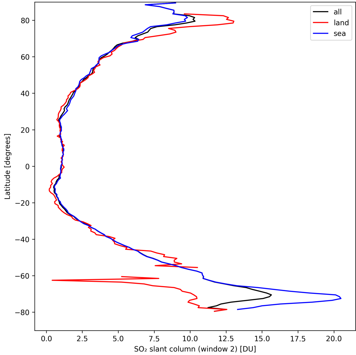
Figure 37: Zonal average of “SO 2 slant column (window 2)” for 2024-09-06 to 2024-09-07.
