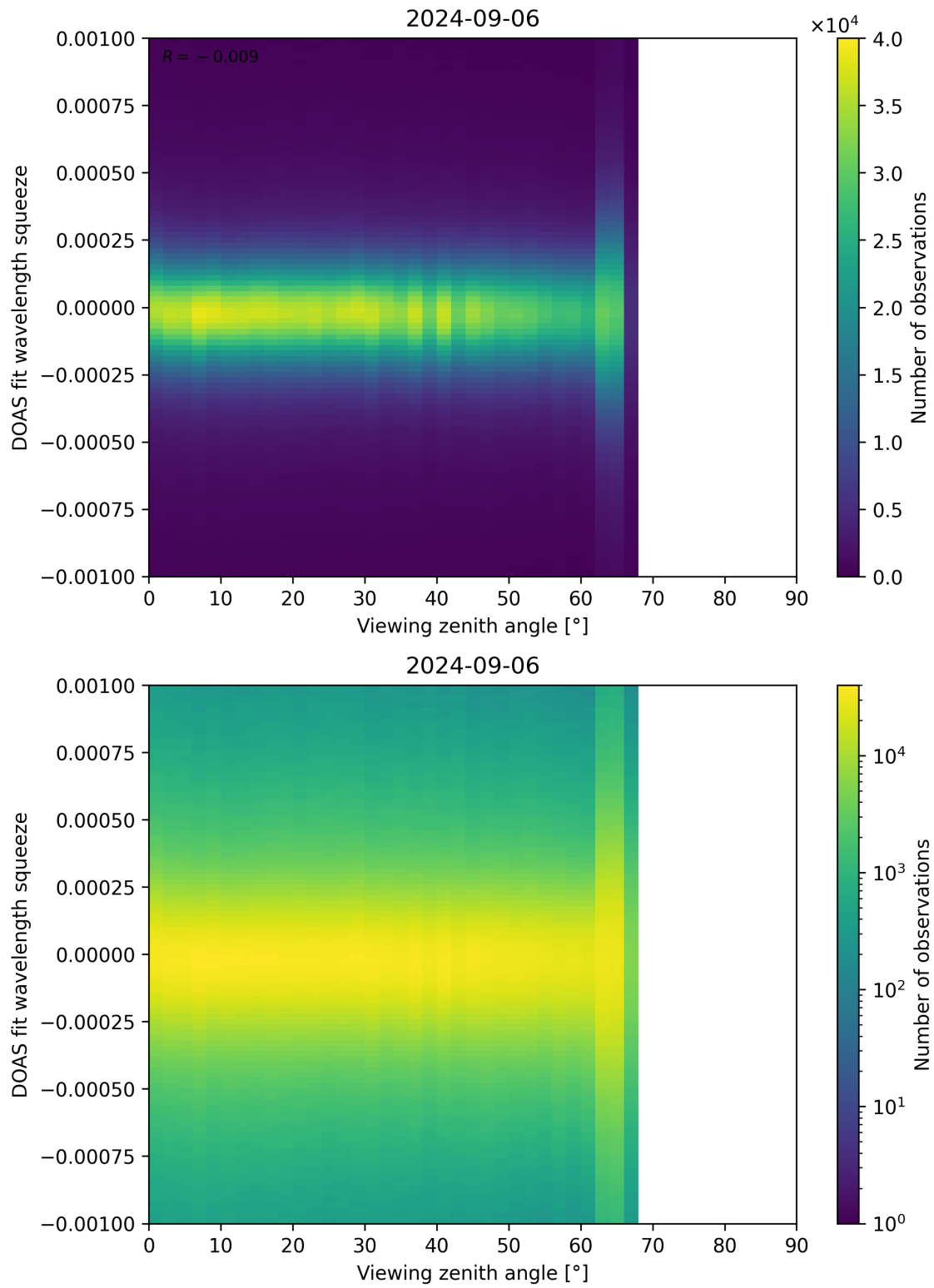
Figure 312: Scatter density plot of “Viewing zenith angle” against “DOAS fit wavelength squeeze” for 2024-09-06 to 2024-09-07.
