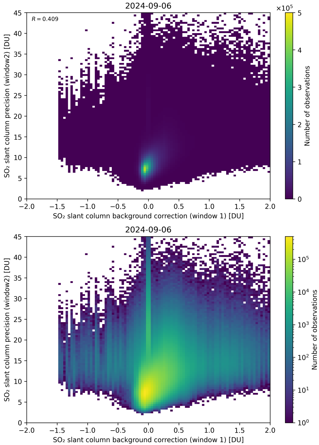
Figure 106: Scatter density plot of “SO 2 slant column background correction (window 1)” against “SO 2 slant column precision (window2)” for 2024-09-06 to 2024-09-07.
