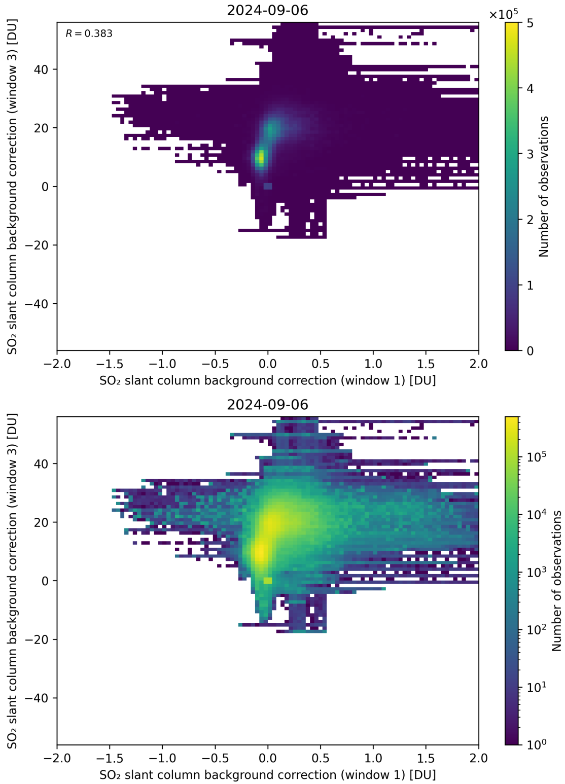
Figure 99: Scatter density plot of “SO 2 slant column background correction (window 1)” against “SO 2 slant column background correction (window 3)” for 2024-09-06 to 2024-09-07.
