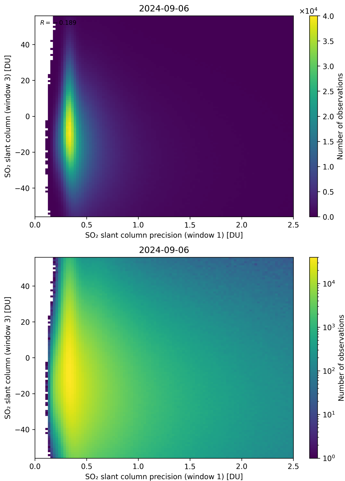
Figure 228: Scatter density plot of “SO 2 slant column precision (window 1)” against “SO 2 slant column (window 3)” for 2024-09-06 to 2024-09-07.
