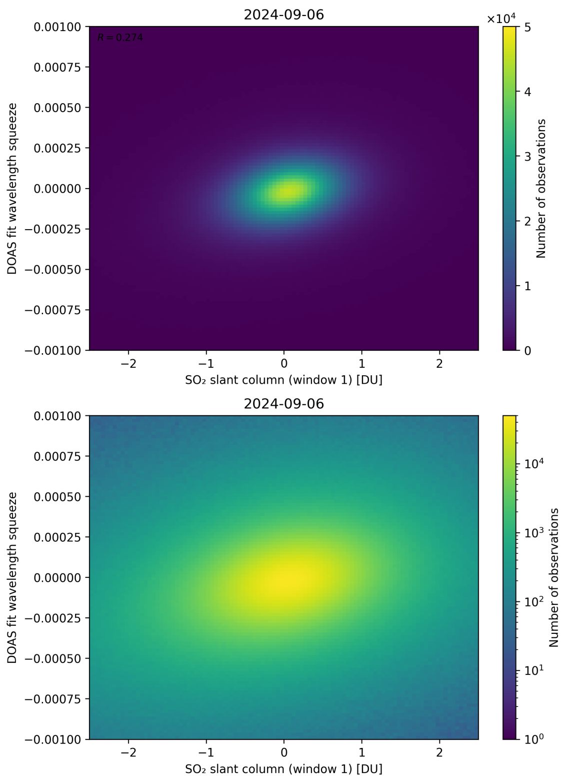
Figure 216: Scatter density plot of “SO 2 slant column (window 1)” against “DOAS fit wavelength squeeze” for 2024-09-06 to 2024-09-07.
