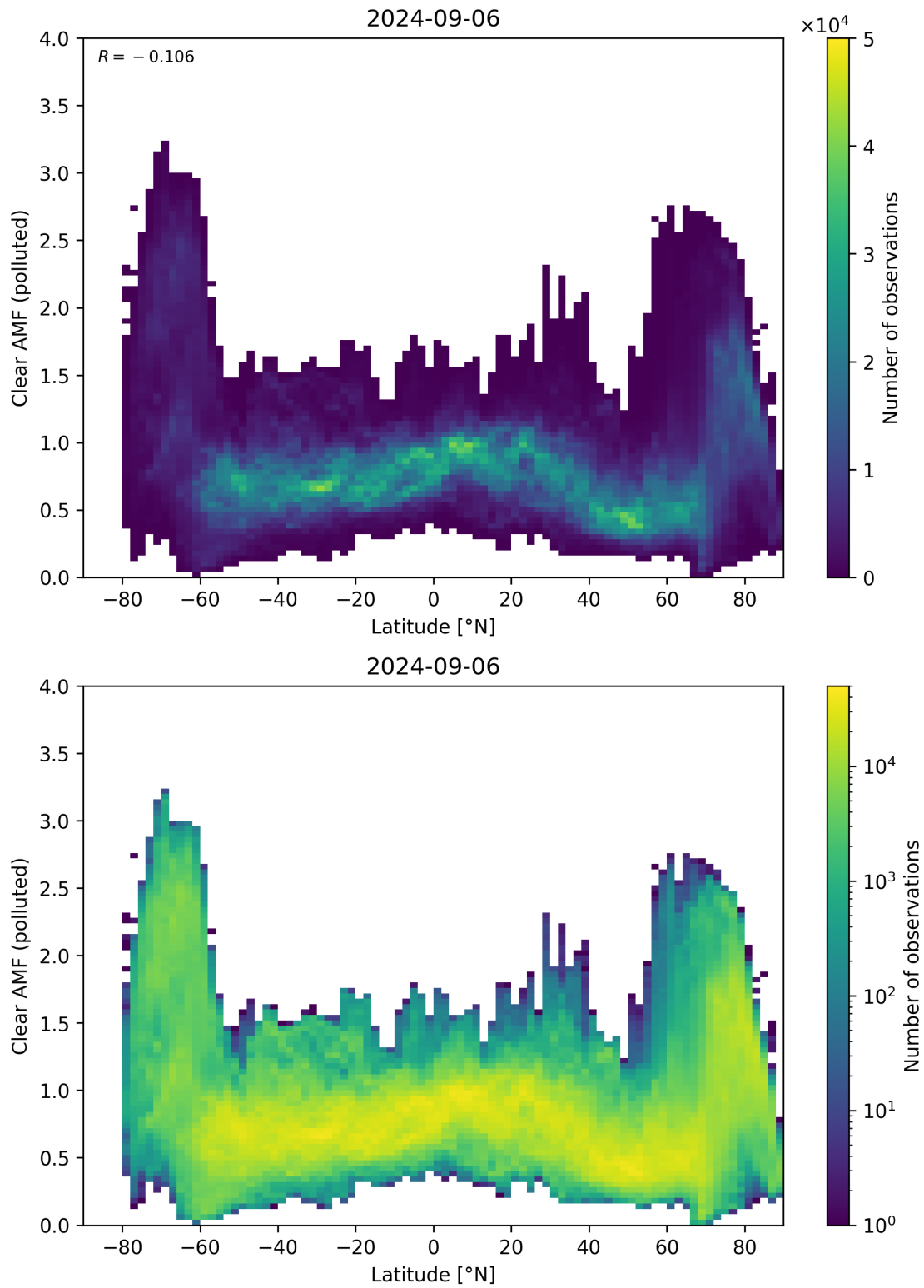
Figure 145: Scatter density plot of “Latitude” against “Clear AMF (polluted)” for 2024-09-06 to 2024-09-07.
