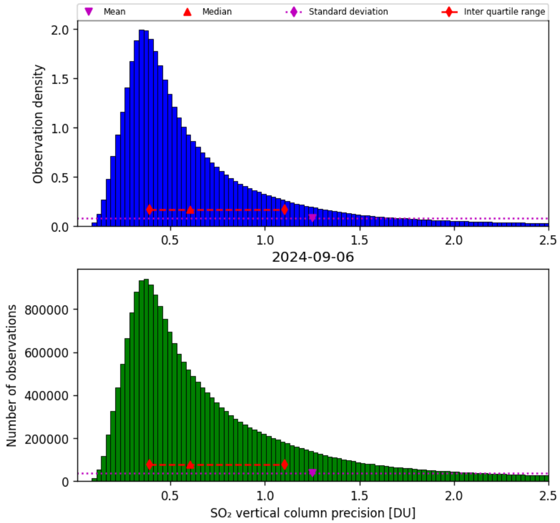
Figure 54: Histogram of “SO 2 vertical column precision” for 2024-09-06 to 2024-09-07
