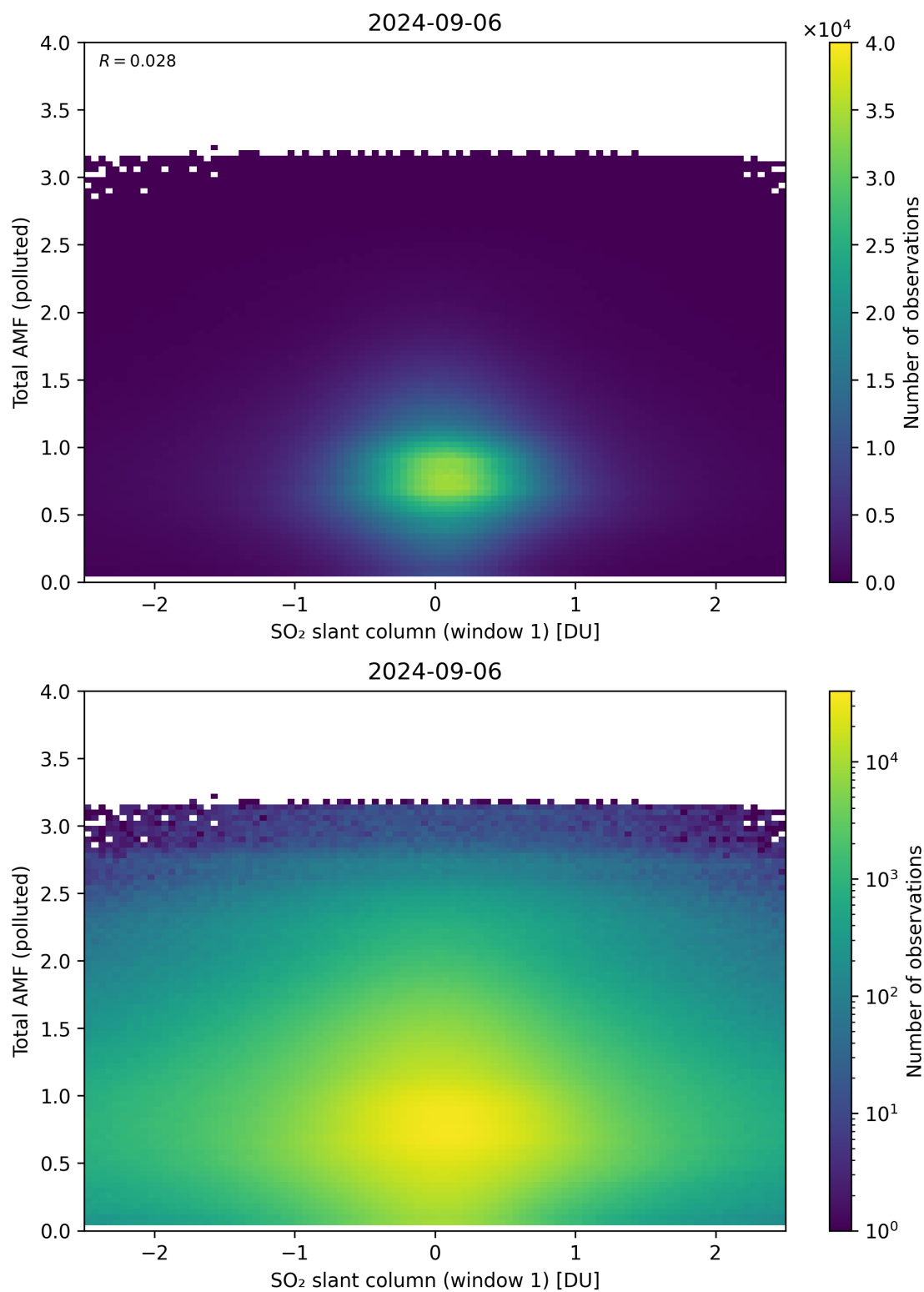
Figure 239: Scatter density plot of “SO 2 slant column (window 1)” against “Total AMF (polluted)” for 2024-09-06 to 2024-09-07.
