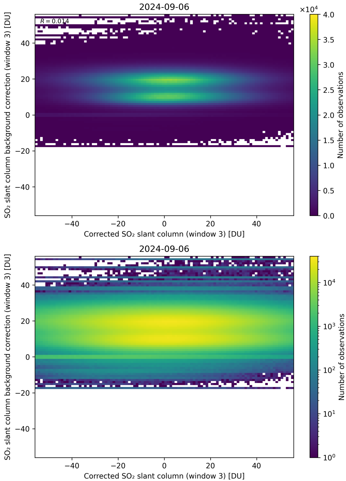
Figure 205: Scatter density plot of “Corrected SO 2 slant column (window 3)” against “SO 2 slant column background correction (window 3)” for 2024-09-06 to 2024-09-07.
