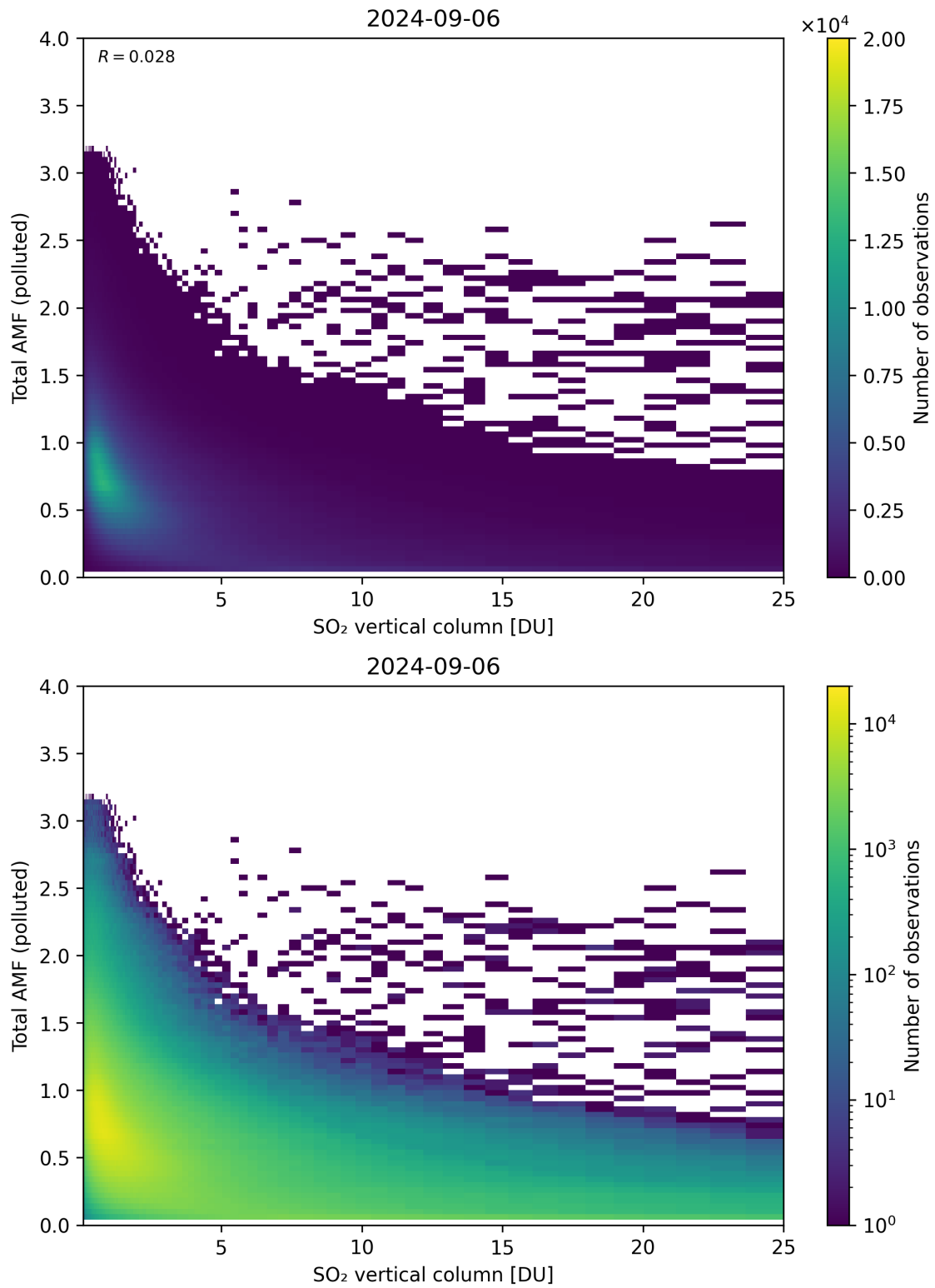
Figure 305: Scatter density plot of “SO 2 vertical column” against “Total AMF (polluted)” for 2024-09-06 to 2024-09-07.
