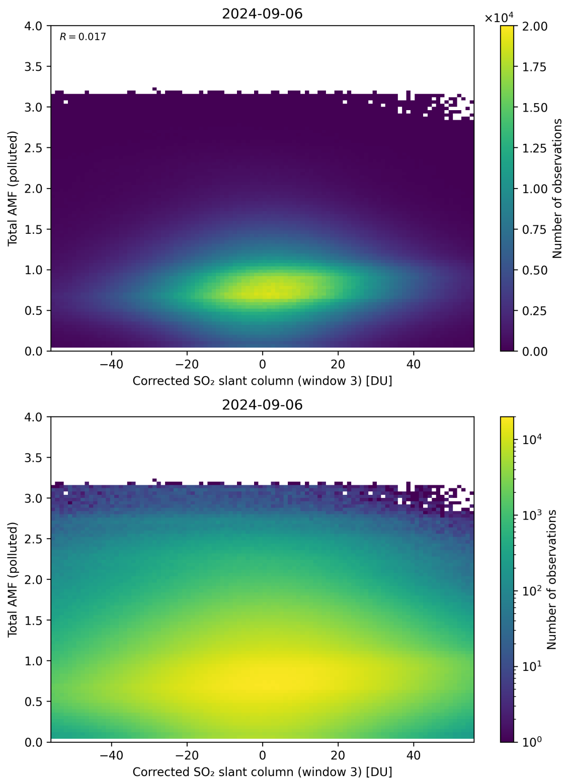
Figure 210: Scatter density plot of “Corrected SO 2 slant column (window 3)” against “Total AMF (polluted)” for 2024-09-06 to 2024-09-07.
