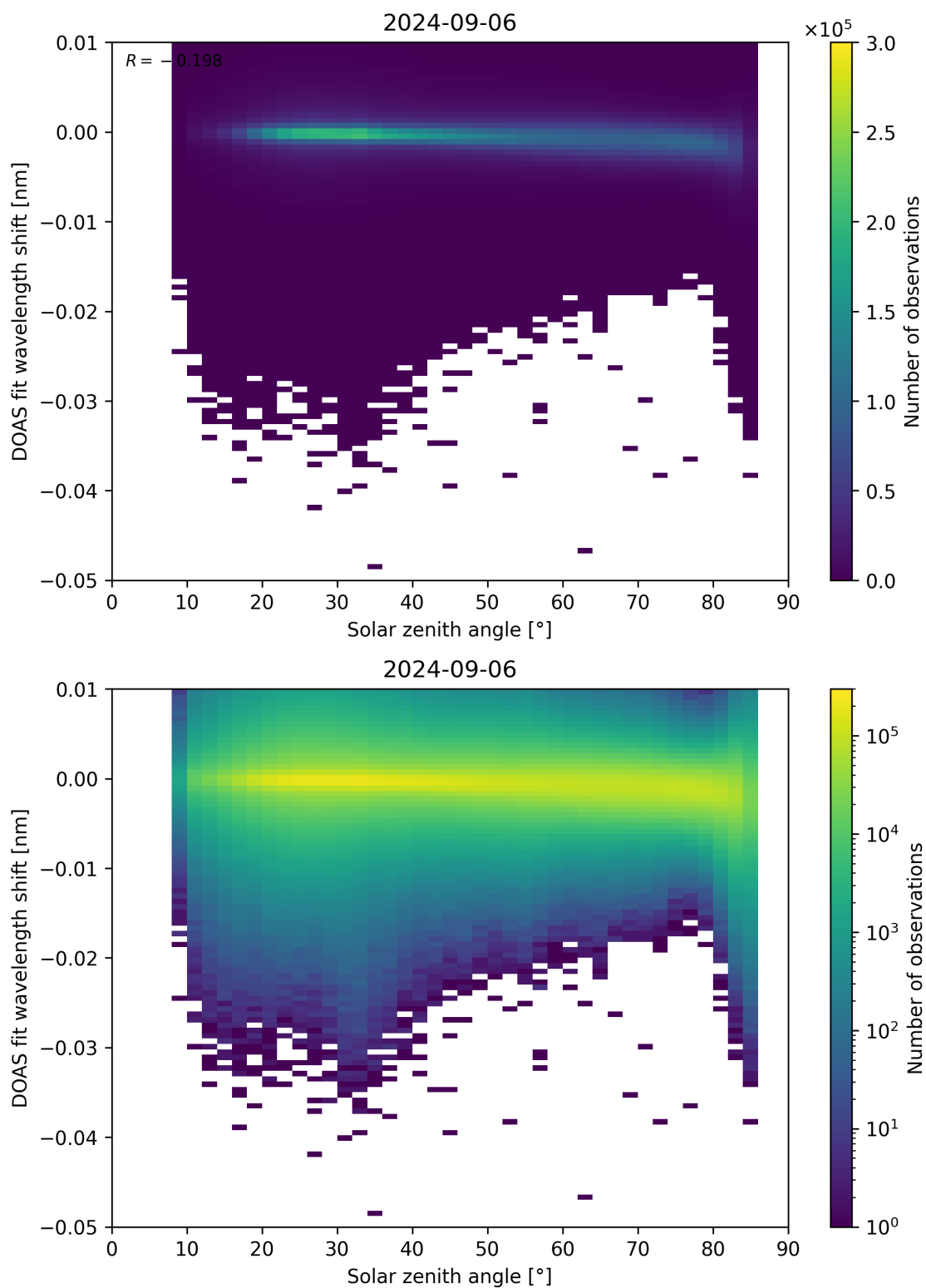
Figure 161: Scatter density plot of “Solar zenith angle” against “DOAS fit wavelength shift” for 2024-09-06 to 2024-09-07.
