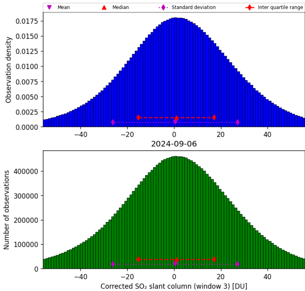
Figure 66: Histogram of “Corrected SO 2 slant column (window 3)” for 2024-09-06 to 2024-09-07
