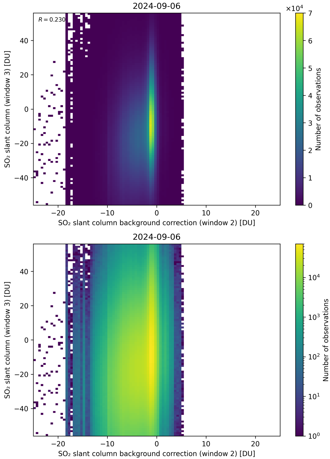
Figure 117: Scatter density plot of “SO 2 slant column background correction (window 2)” against “SO 2 slant column (window 3)” for 2024-09-06 to 2024-09-07.
