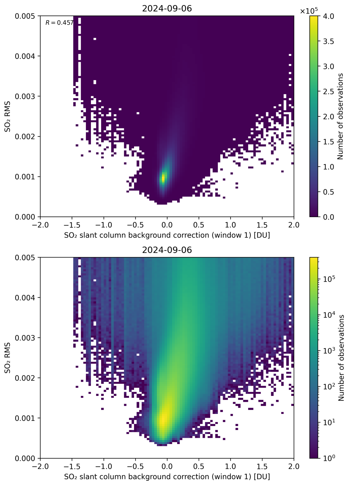
Figure 102: Scatter density plot of “SO 2 slant column background correction (window 1)” against “SO 2 RMS” for 2024-09-06 to 2024-09-07.
