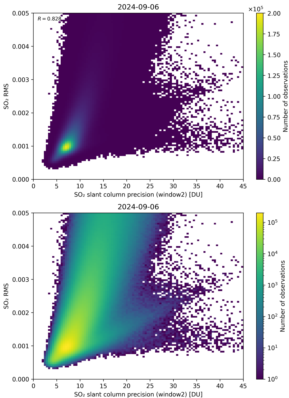
Figure 245: Scatter density plot of “SO 2 slant column precision (window2)” against “SO 2 RMS” for 2024-09-06 to 2024-09-07.
