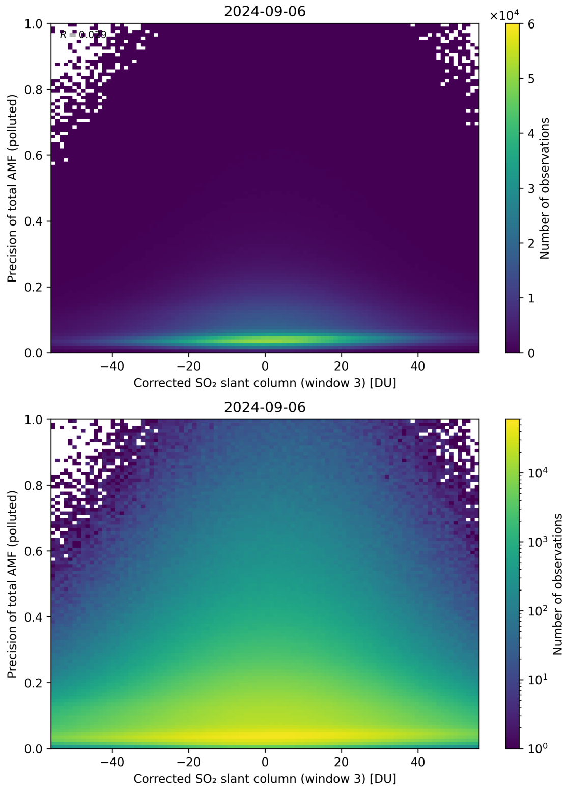
Figure 211: Scatter density plot of “Corrected SO 2 slant column (window 3)” against “Precision of total AMF (polluted)” for 2024-09-06 to 2024-09-07.
