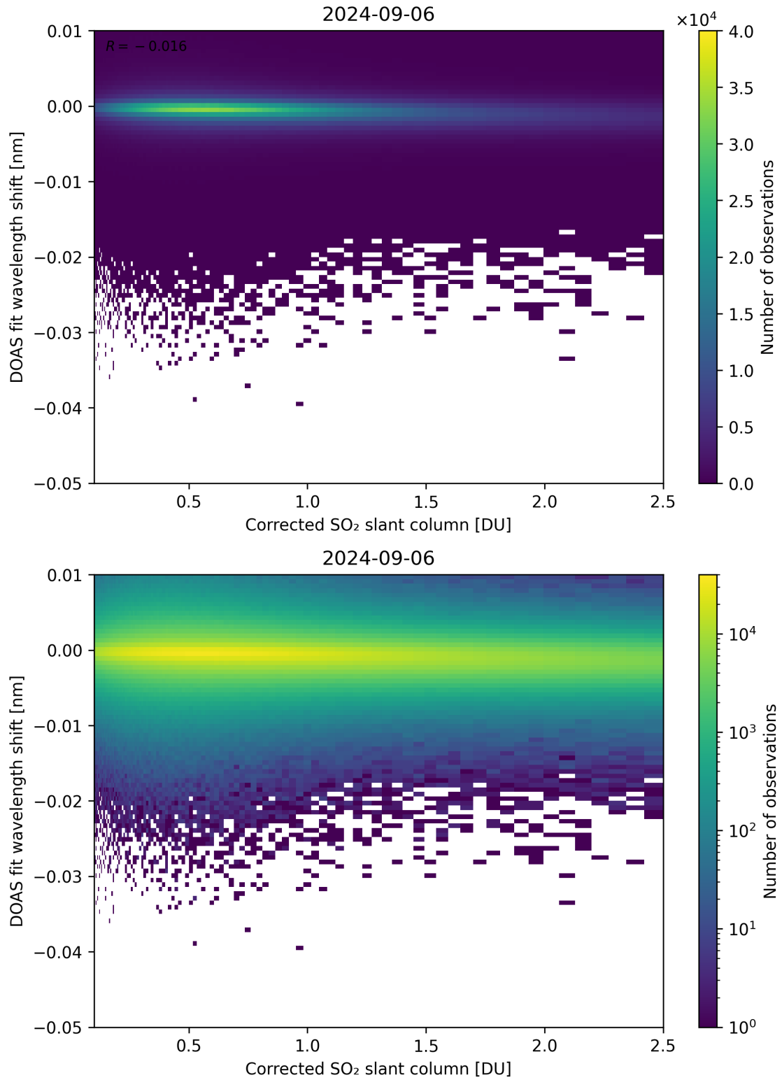
Figure 181: Scatter density plot of “Corrected SO 2 slant column” against “DOAS fit wavelength shift” for 2024-09-06 to 2024-09-07.
