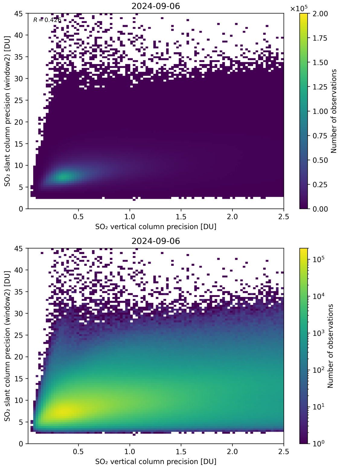
Figure 291: Scatter density plot of “SO 2 vertical column precision” against “SO 2 slant column precision (window2)” for 2024-09-06 to 2024-09-07.
