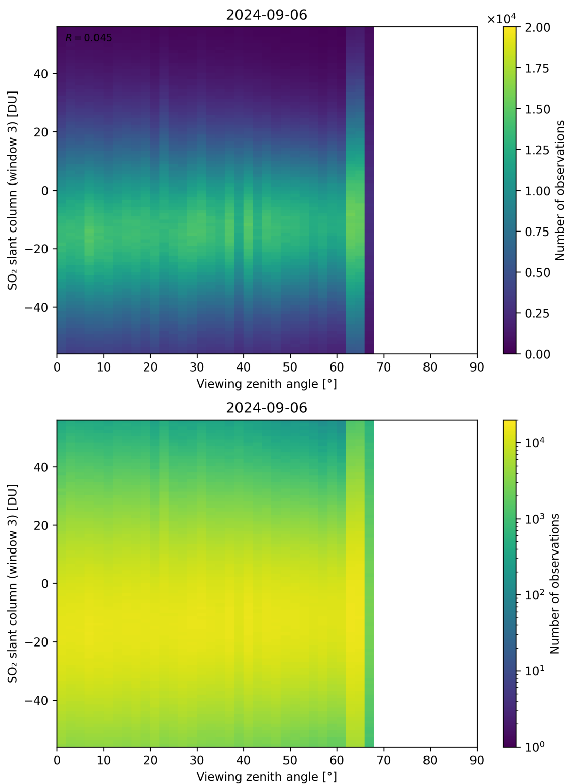
Figure 323: Scatter density plot of “Viewing zenith angle” against “SO 2 slant column (window 3)” for 2024-09-06 to 2024-09-07.
