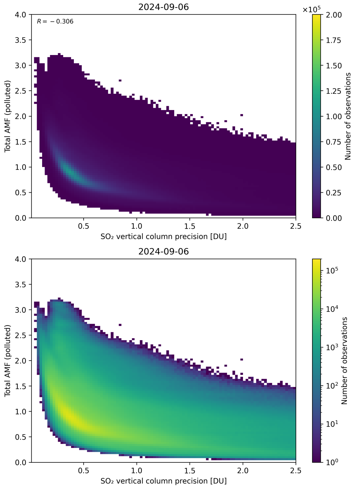
Figure 294: Scatter density plot of “SO 2 vertical column precision” against “Total AMF (polluted)” for 2024-09-06 to 2024-09-07.
