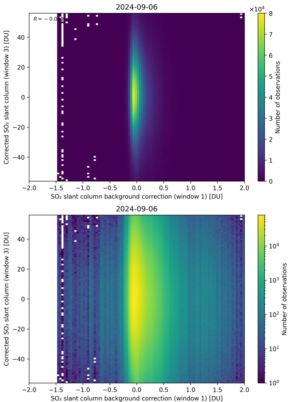
Figure 105: Scatter density plot of “SO 2 slant column background correction (window 1)” against “Corrected SO 2 slant column (window 3)” for 2024-09-06 to 2024-09-07.
