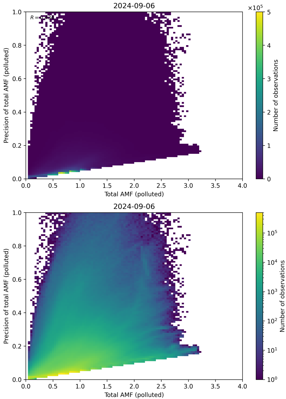
Figure 272: Scatter density plot of “Total AMF (polluted)” against “Precision of total AMF (polluted)” for 2024-09-06 to 2024-09-07.
