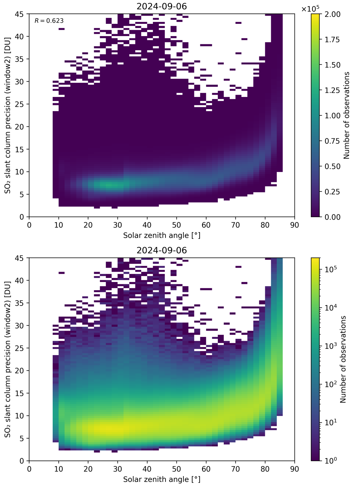
Figure 171: Scatter density plot of “Solar zenith angle” against “SO 2 slant column precision (window2)” for 2024-09-06 to 2024-09-07.
