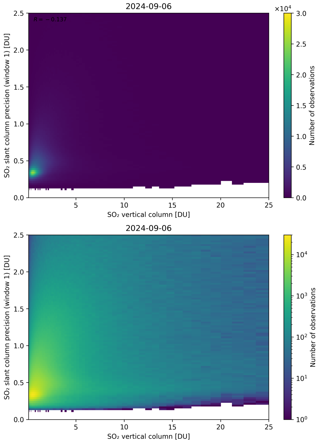
Figure 301: Scatter density plot of “SO 2 vertical column” against “SO 2 slant column precision (window 1)” for 2024-09-06 to 2024-09-07.
