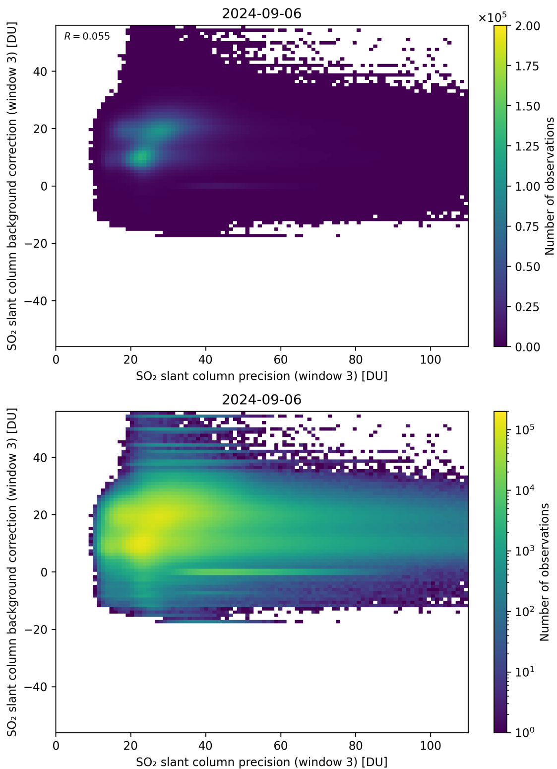
Figure 257: Scatter density plot of “SO 2 slant column precision (window 3)” against “SO 2 slant column background correction (window 3)” for 2024-09-06 to 2024-09-07.
