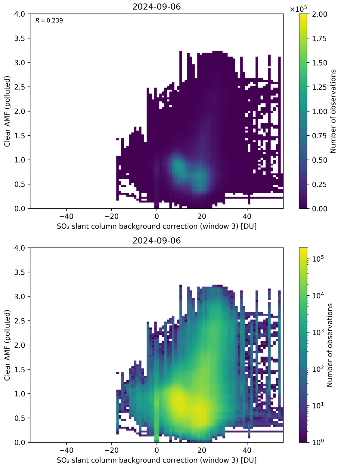
Figure 124: Scatter density plot of “SO 2 slant column background correction (window 3)” against “Clear AMF (polluted)” for 2024-09-06 to 2024-09-07.
