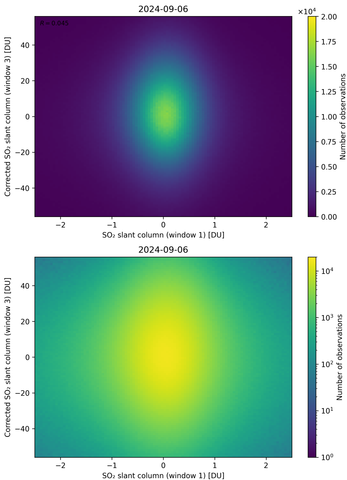
Figure 234: Scatter density plot of “SO 2 slant column (window 1)” against “Corrected SO 2 slant column (window 3)” for 2024-09-06 to 2024-09-07.
