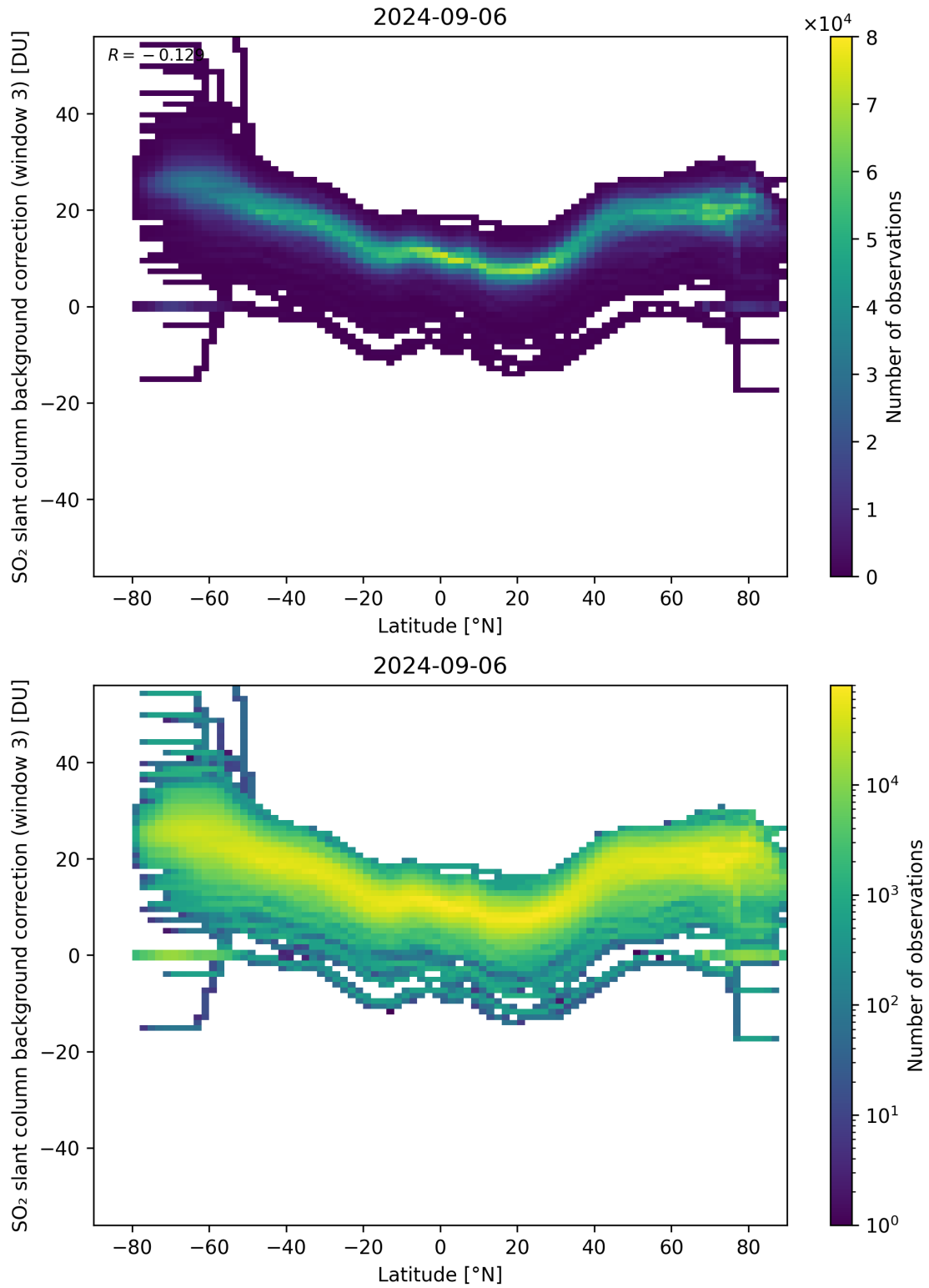
Figure 141: Scatter density plot of “Latitude” against “SO 2 slant column background correction (window 3)” for 2024-09-06 to 2024-09-07.
