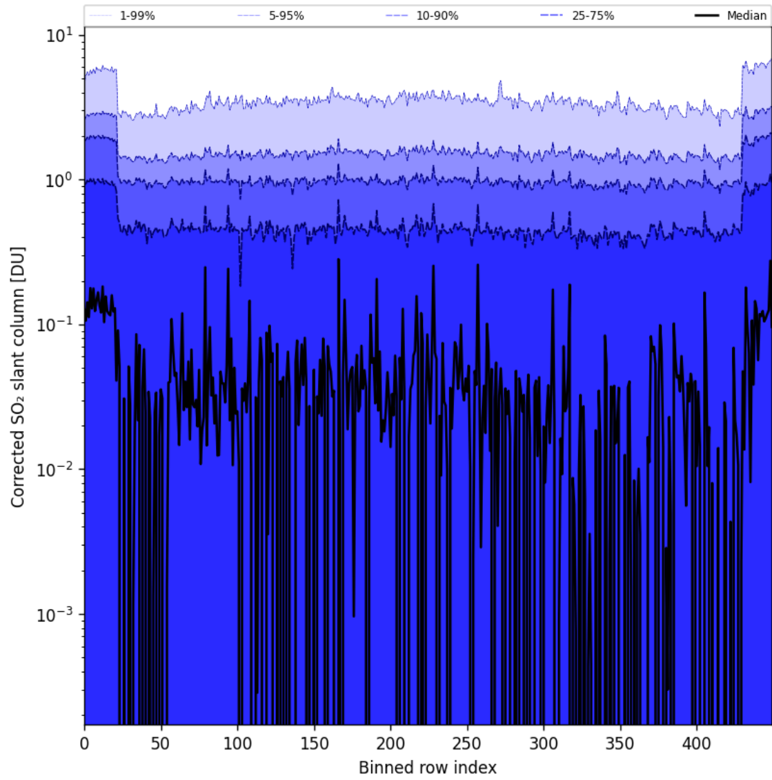
Figure 78: Along track statistics of “Corrected SO 2 slant column” for 2024-09-06 to 2024-09-07
