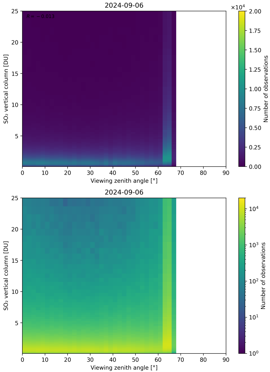
Figure 327: Scatter density plot of “Viewing zenith angle” against “SO 2 vertical column” for 2024-09-06 to 2024-09-07.
