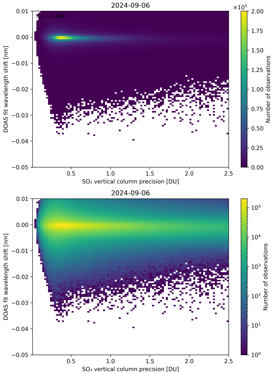
Figure 282: Scatter density plot of “SO 2 vertical column precision” against “DOAS fit wavelength shift” for 2024-09-06 to 2024-09-07.
