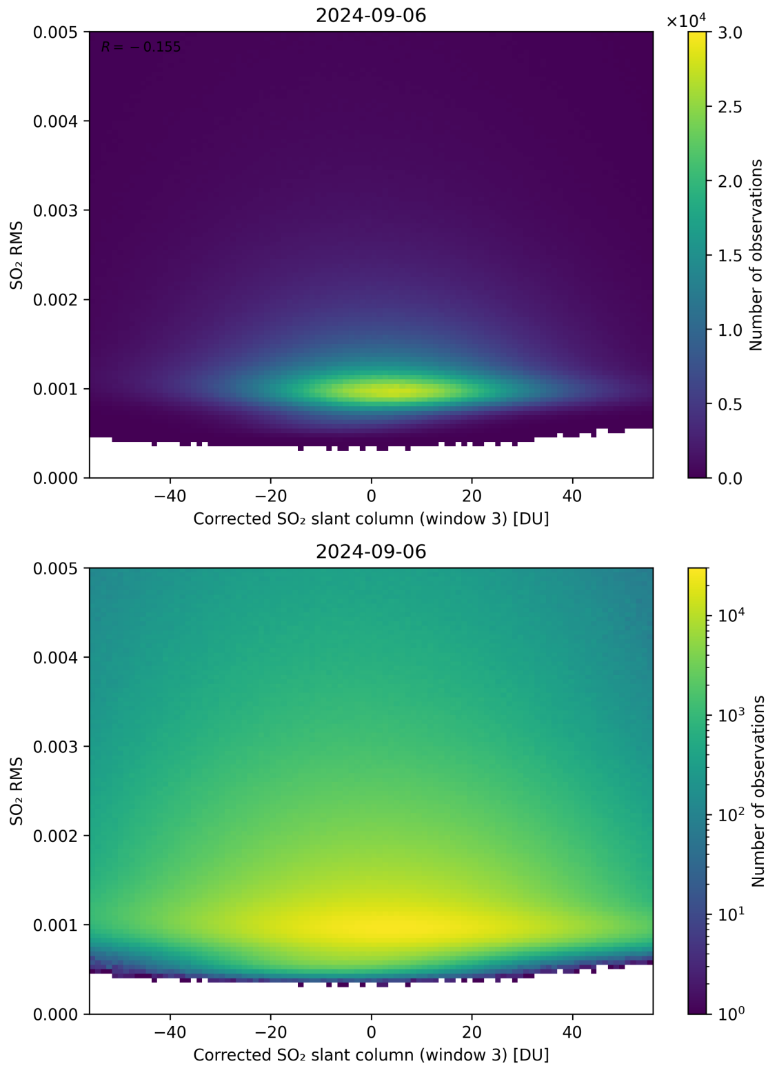
Figure 208: Scatter density plot of “Corrected SO 2 slant column (window 3)” against “SO 2 RMS” for 2024-09-06 to 2024-09-07.
