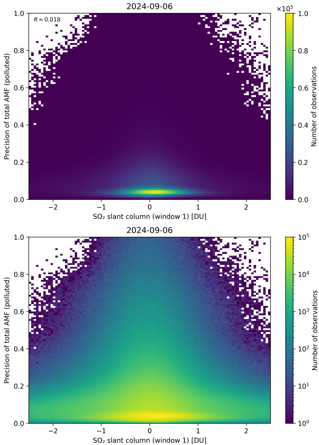
Figure 240: Scatter density plot of “SO 2 slant column (window 1)” against “Precision of total AMF (polluted)” for 2024-09-06 to 2024-09-07.
