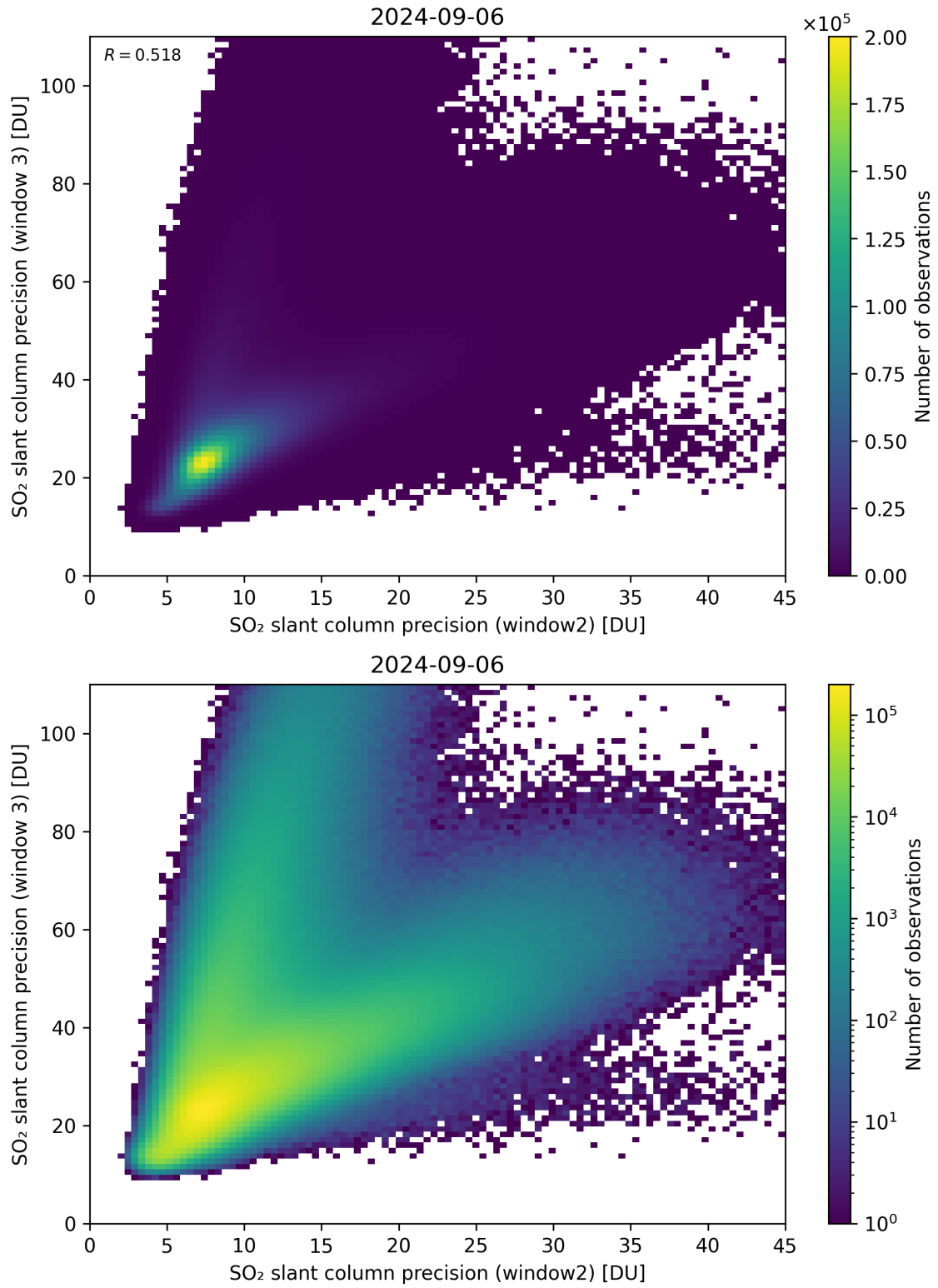
Figure 250: Scatter density plot of “SO 2 slant column precision (window2)” against “SO 2 slant column precision (window 3)” for 2024-09-06 to 2024-09-07.
