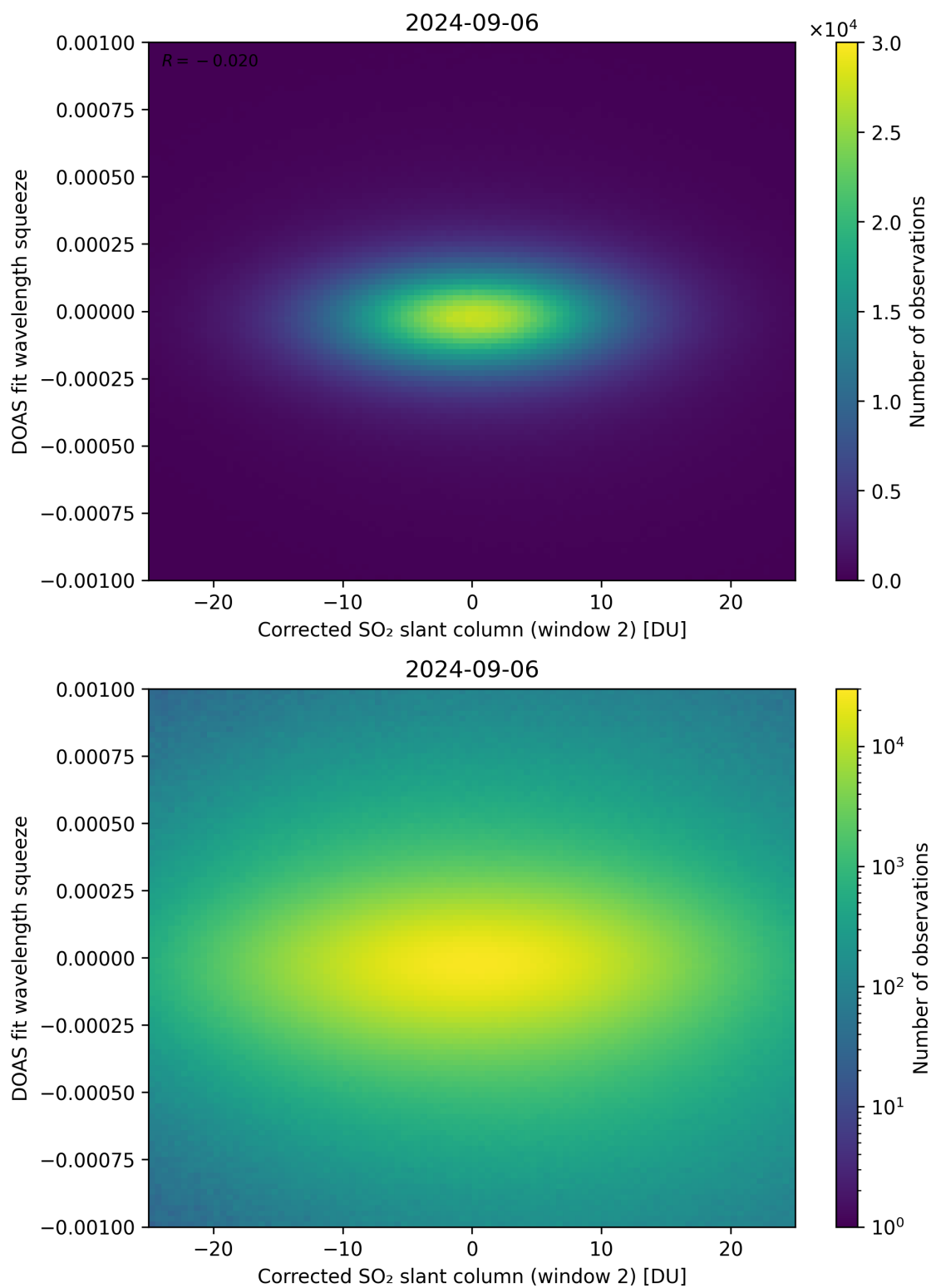
Figure 197: Scatter density plot of “Corrected SO 2 slant column (window 2)” against “DOAS fit wavelength squeeze” for 2024-09-06 to 2024-09-07.
