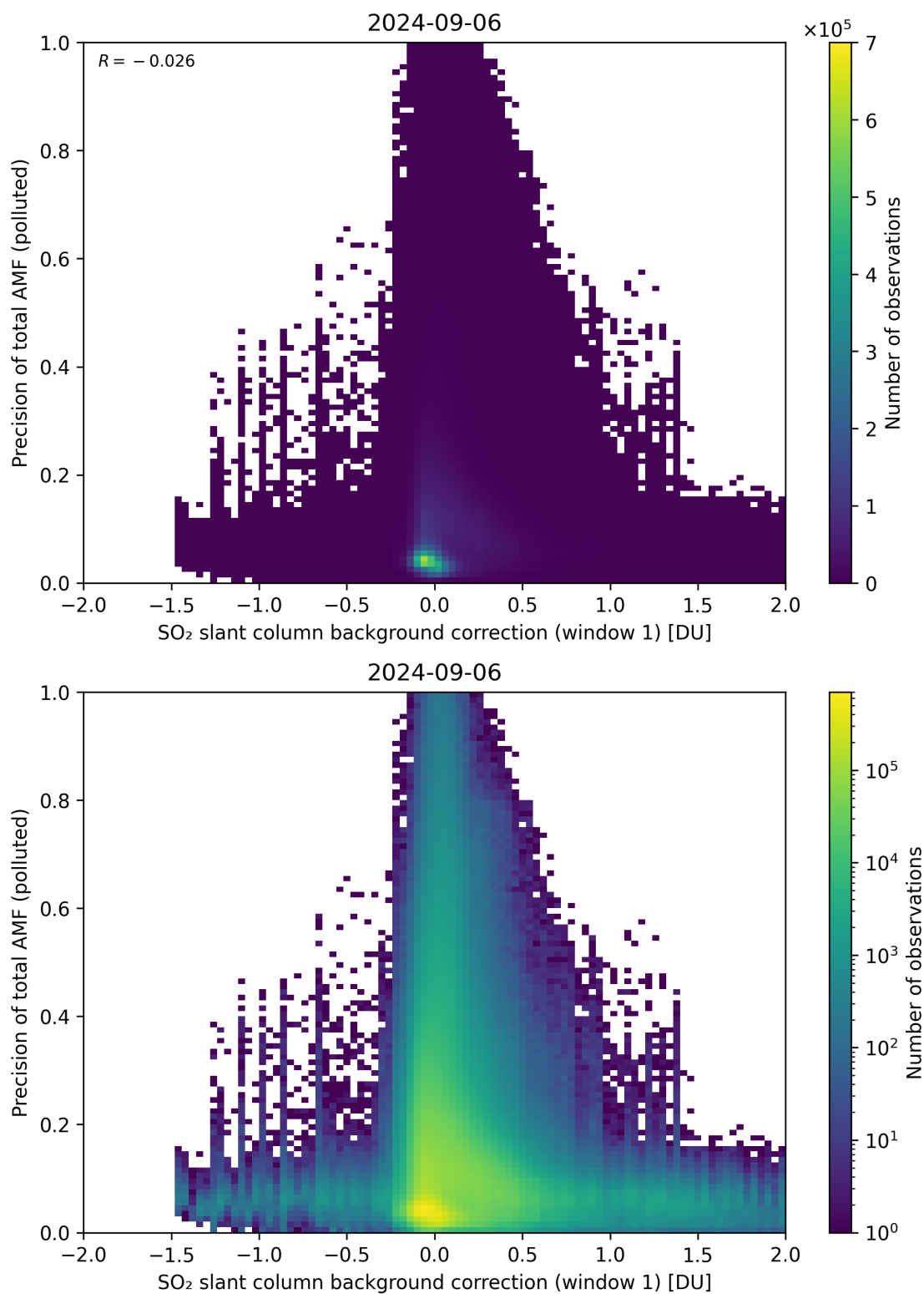
Figure 110: Scatter density plot of “SO 2 slant column background correction (window 1)” against “Precision of total AMF (polluted)” for 2024-09-06 to 2024-09-07.
