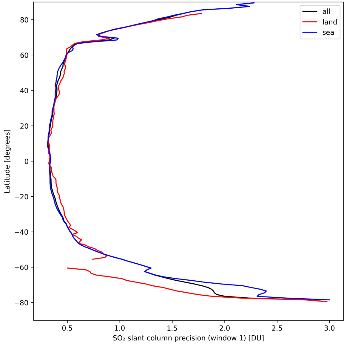
Figure 34: Zonal average of “SO 2 slant column precision (window 1)” for 2024-09-06 to 2024-09-07.
