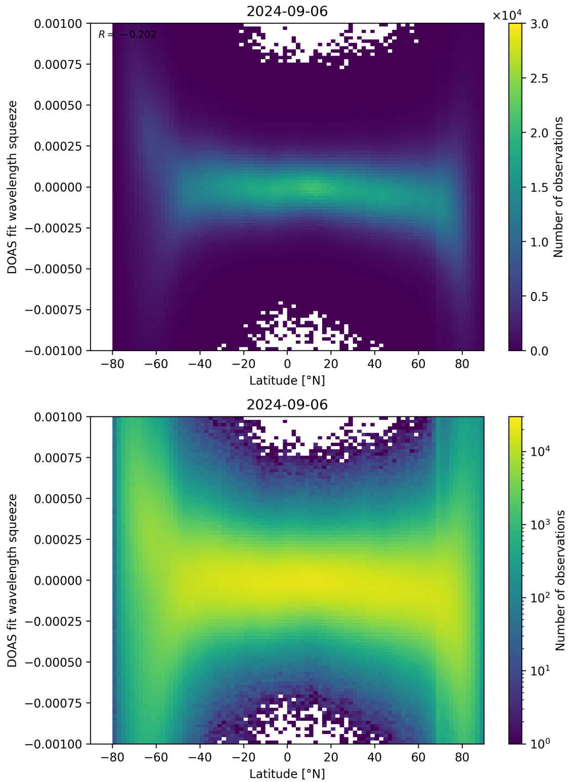
Figure 143: Scatter density plot of “Latitude” against “DOAS fit wavelength squeeze” for 2024-09-06 to 2024-09-07.
