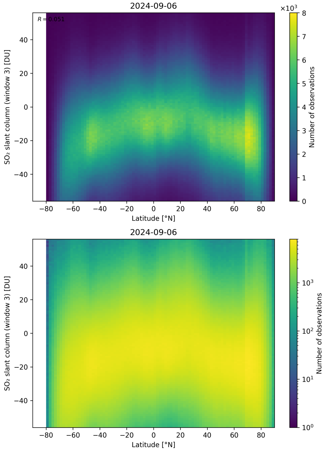
Figure 152: Scatter density plot of “Latitude” against “SO 2 slant column (window 3)” for 2024-09-06 to 2024-09-07.
