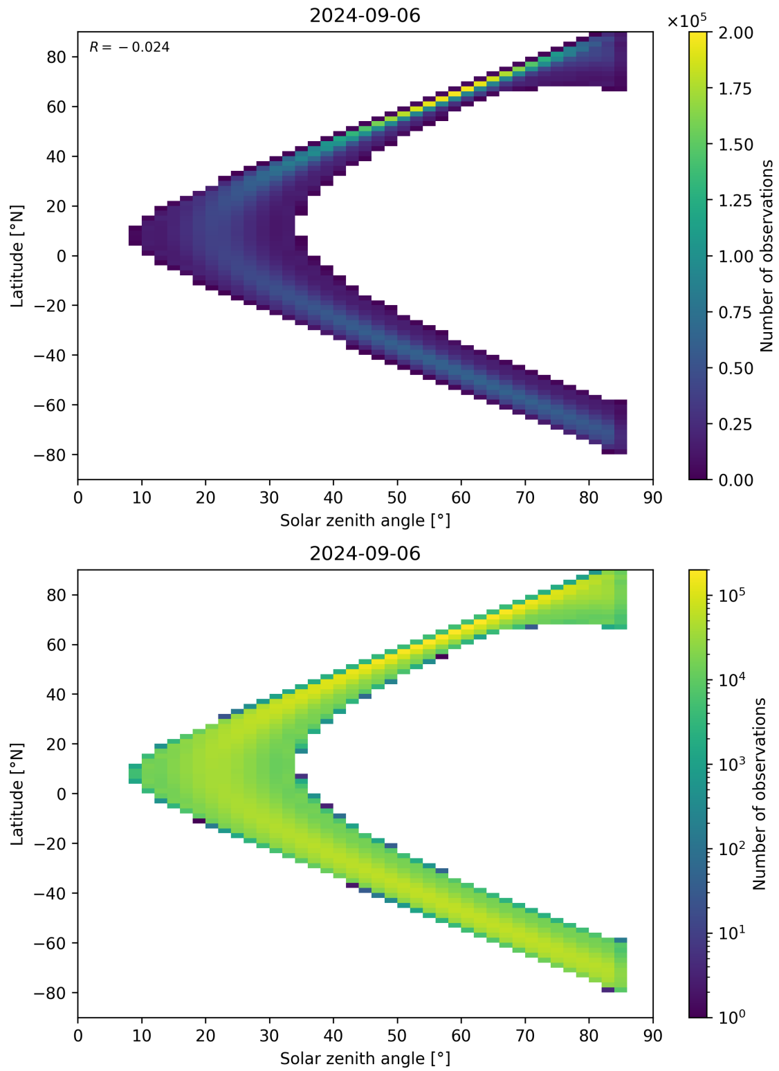
Figure 164: Scatter density plot of “Solar zenith angle” against “Latitude” for 2024-09-06 to 2024-09-07.
