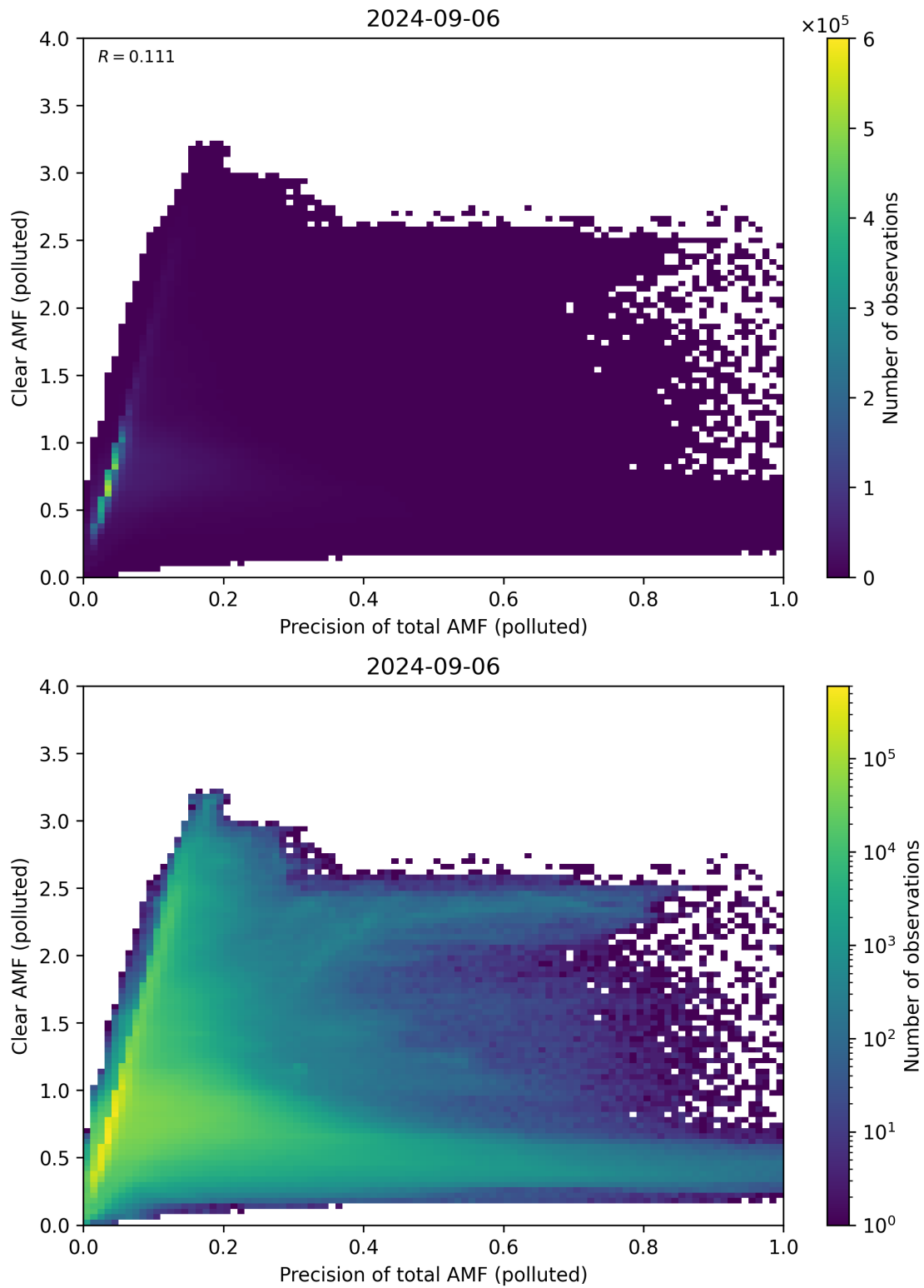
Figure 270: Scatter density plot of “Precision of total AMF (polluted)” against “Clear AMF (polluted)” for 2024-09-06 to 2024-09-07.
