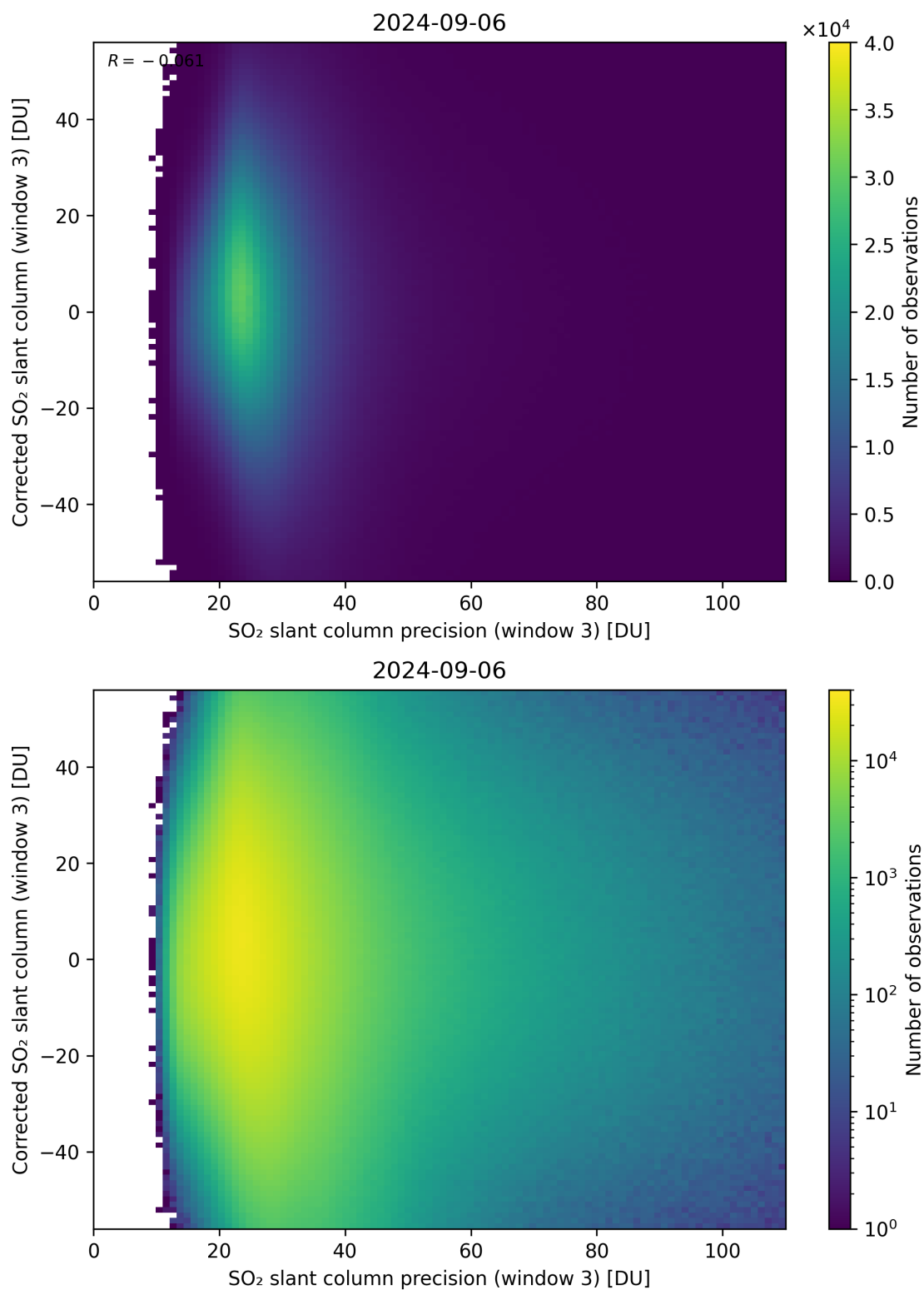
Figure 262: Scatter density plot of “SO 2 slant column precision (window 3)” against “Corrected SO 2 slant column (window 3)” for 2024-09-06 to 2024-09-07.
