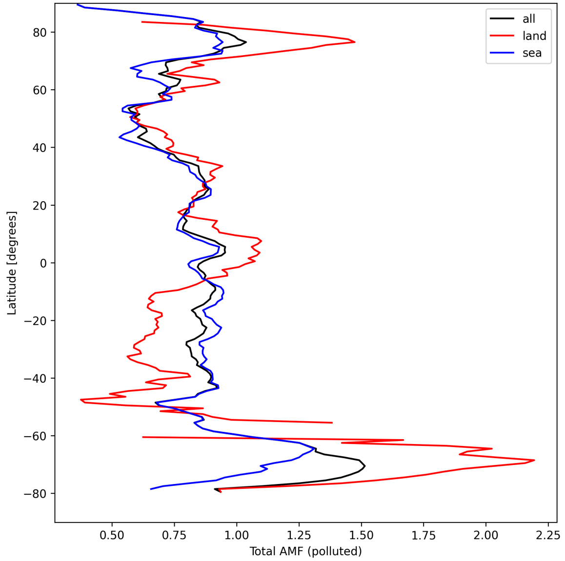
Figure 48: Zonal average of “Total AMF (polluted)” for 2024-09-06 to 2024-09-07.
