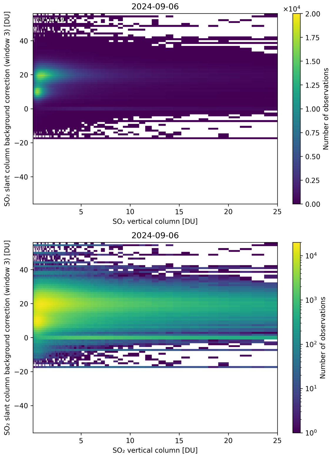
Figure 275: Scatter density plot of “SO 2 vertical column” against “SO 2 slant column background correction (window 3)” for 2024-09-06 to 2024-09-07.
