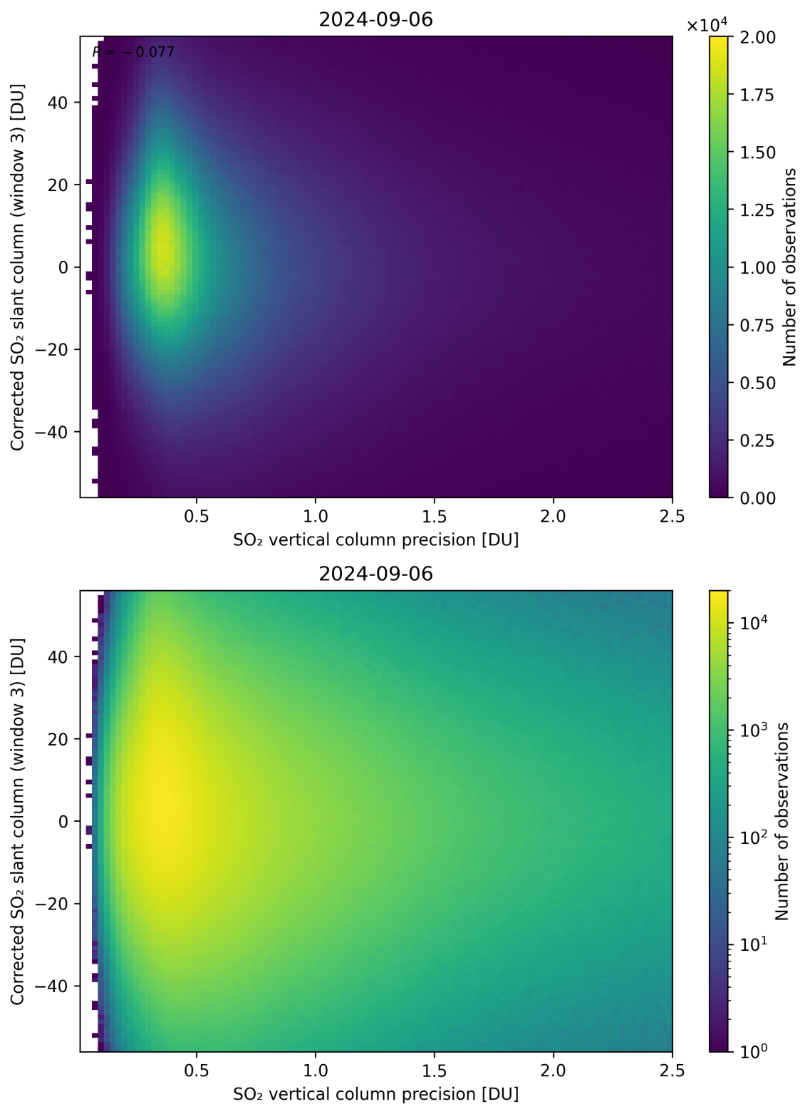
Figure 288: Scatter density plot of “SO 2 vertical column precision” against “Corrected SO 2 slant column (window 3)” for 2024-09-06 to 2024-09-07.
