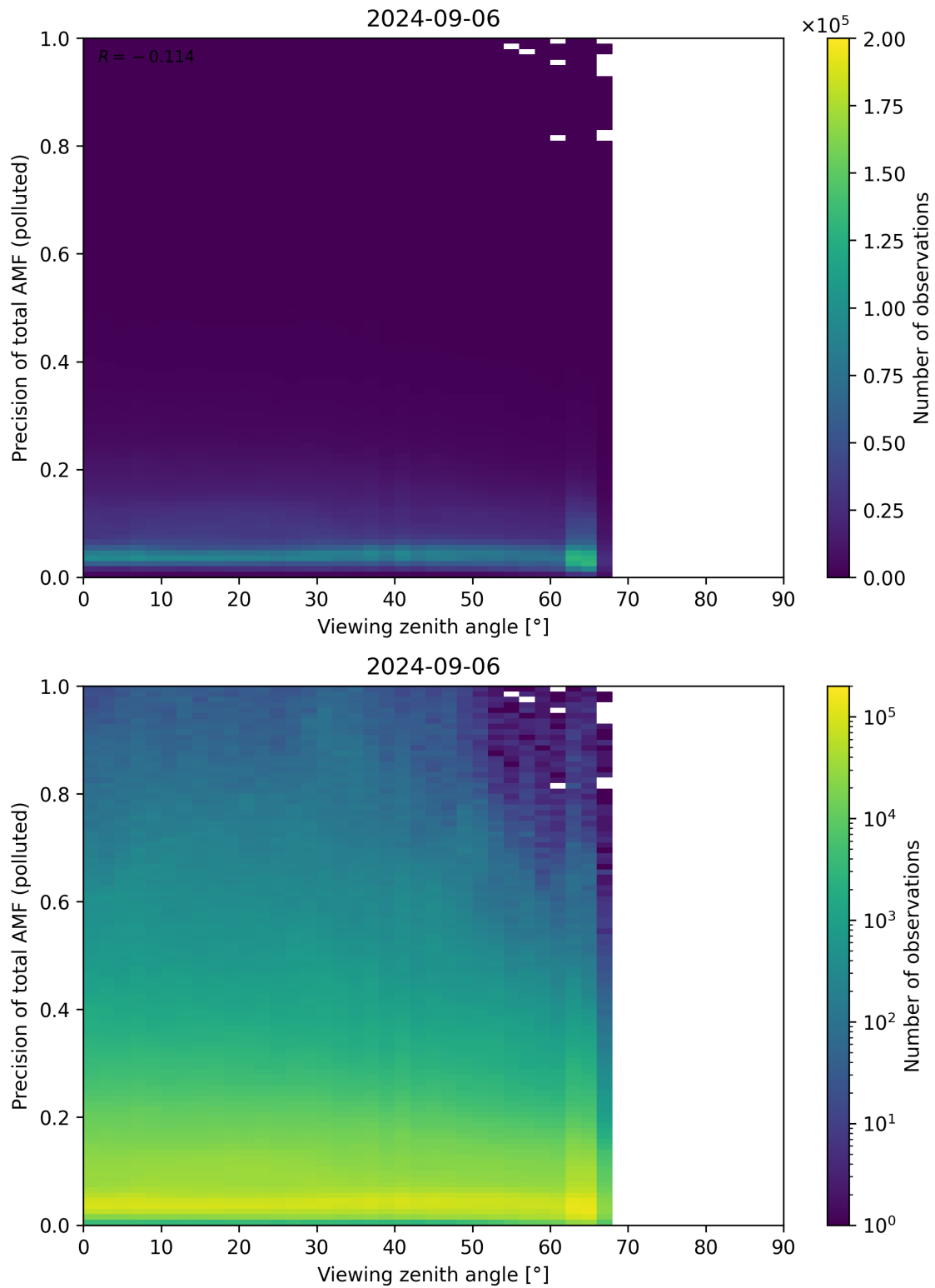
Figure 326: Scatter density plot of “Viewing zenith angle” against “Precision of total AMF (polluted)” for 2024-09-06 to 2024-09-07.
