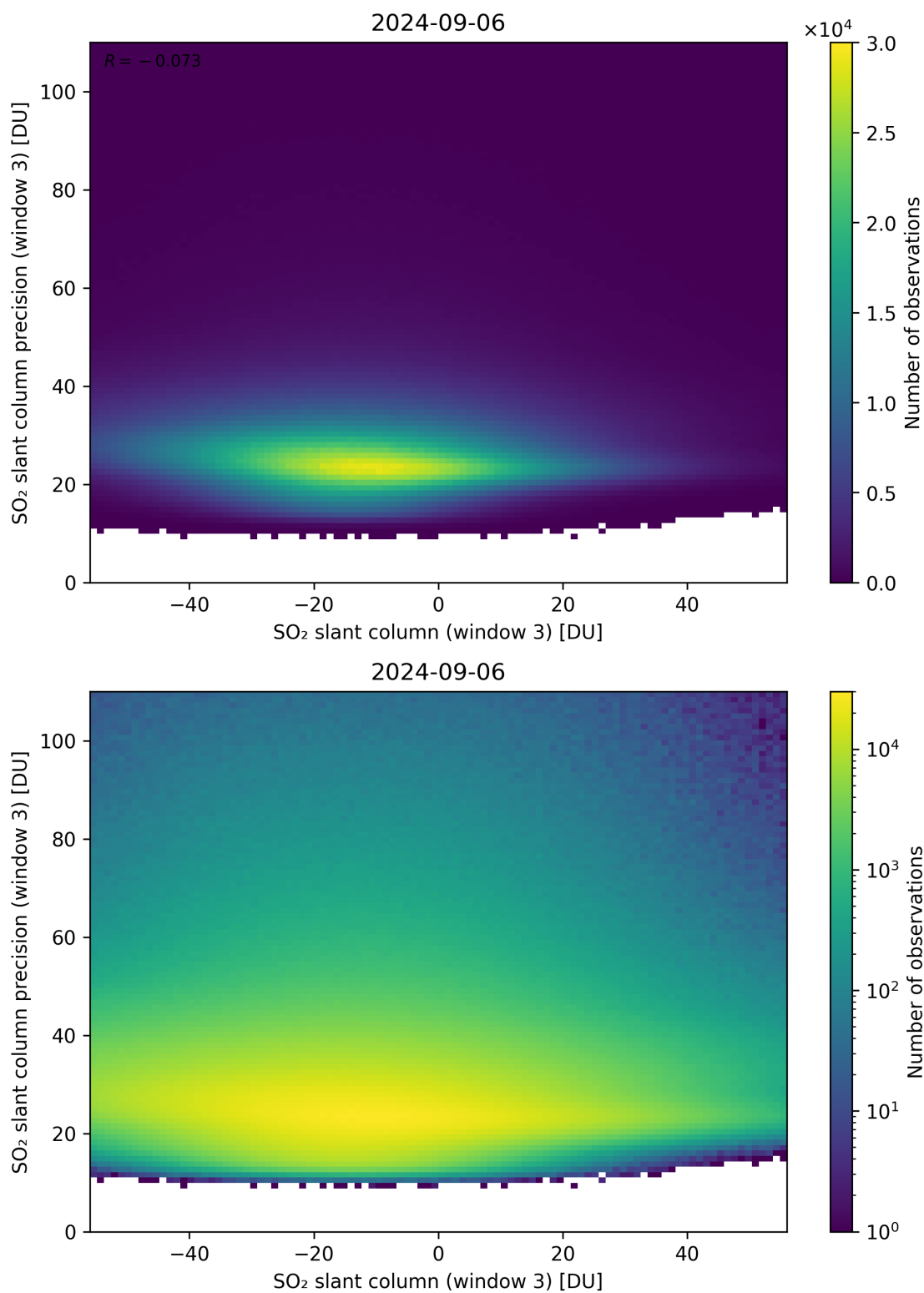
Figure 267: Scatter density plot of “SO 2 slant column (window 3)” against “SO 2 slant column precision (window 3)” for 2024-09-06 to 2024-09-07.
