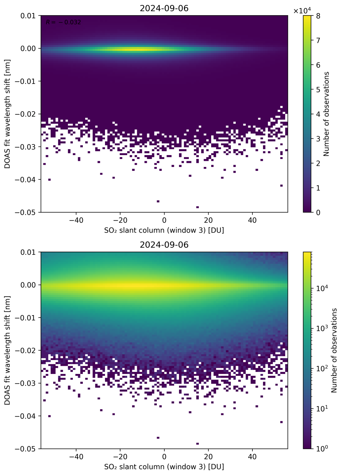
Figure 254: Scatter density plot of “SO 2 slant column (window 3)” against “DOAS fit wavelength shift” for 2024-09-06 to 2024-09-07.
