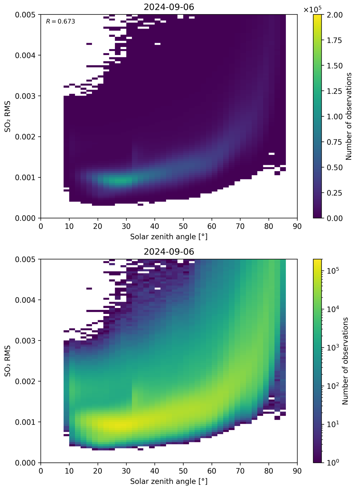
Figure 163: Scatter density plot of “Solar zenith angle” against “SO 2 RMS” for 2024-09-06 to 2024-09-07.
