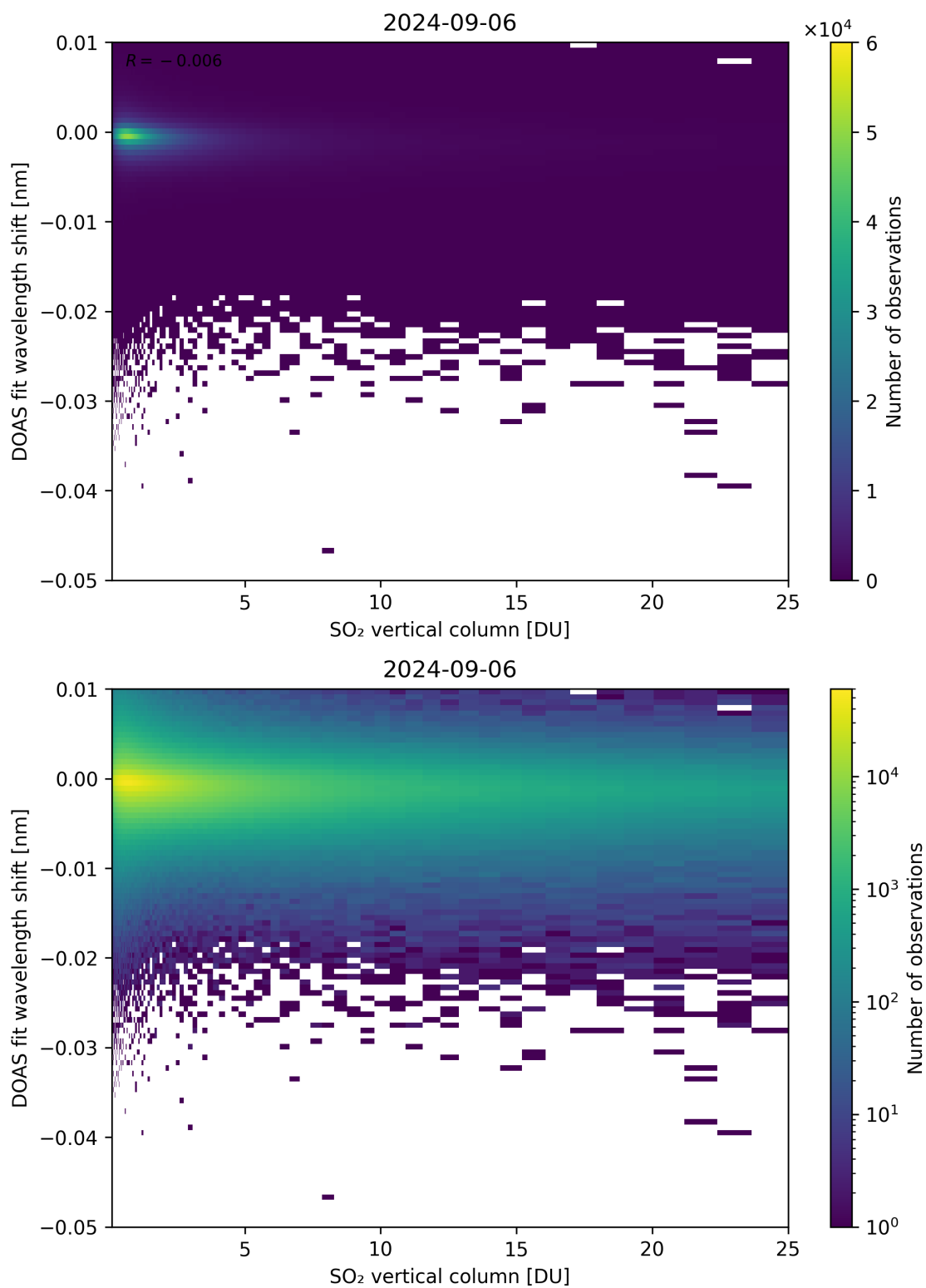
Figure 276: Scatter density plot of “SO 2 vertical column” against “DOAS fit wavelength shift” for 2024-09-06 to 2024-09-07.
