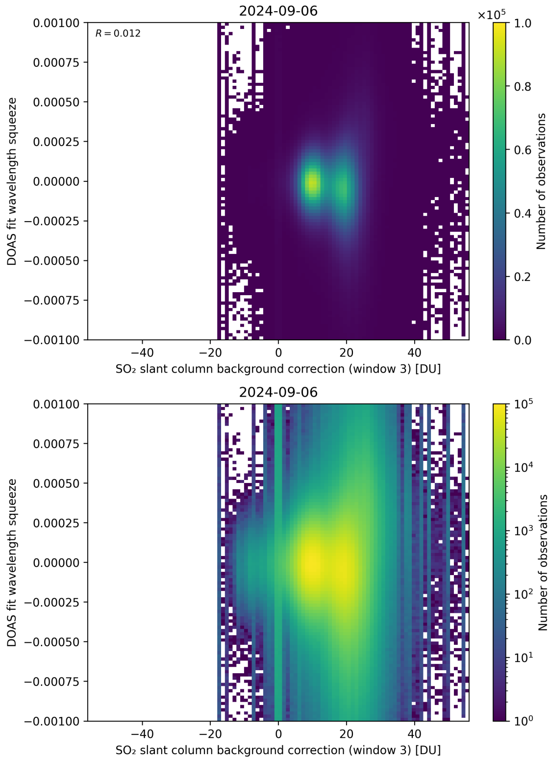
Figure 122: Scatter density plot of “SO 2 slant column background correction (window 3)” against “DOAS fit wavelength squeeze” for 2024-09-06 to 2024-09-07.
