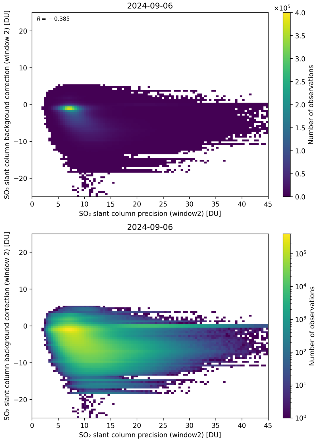
Figure 241: Scatter density plot of “SO 2 slant column precision (window2)” against “SO 2 slant column background correction (window 2)” for 2024-09-06 to 2024-09-07.
