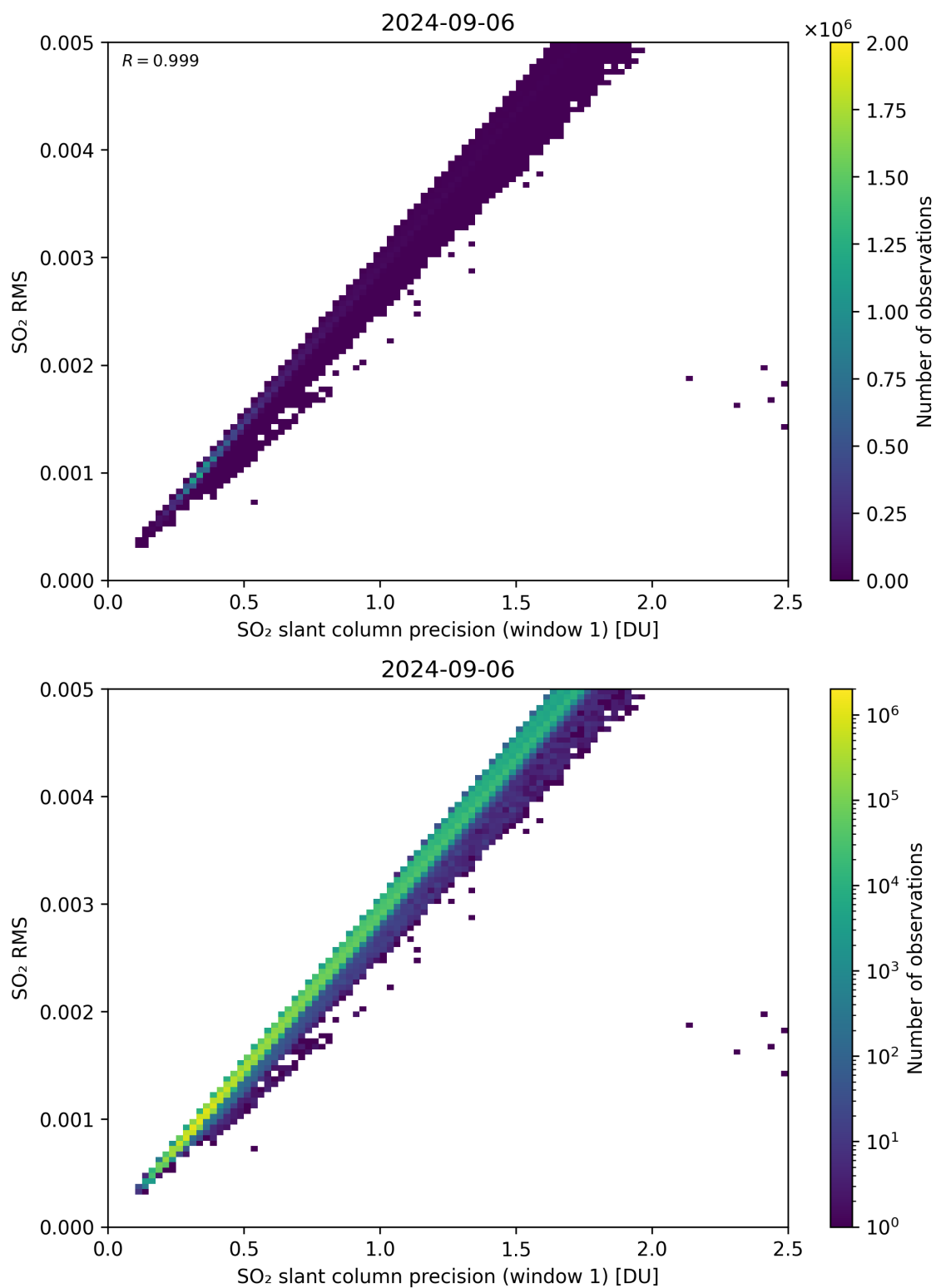
Figure 223: Scatter density plot of “SO 2 slant column precision (window 1)” against “SO 2 RMS” for 2024-09-06 to 2024-09-07.
