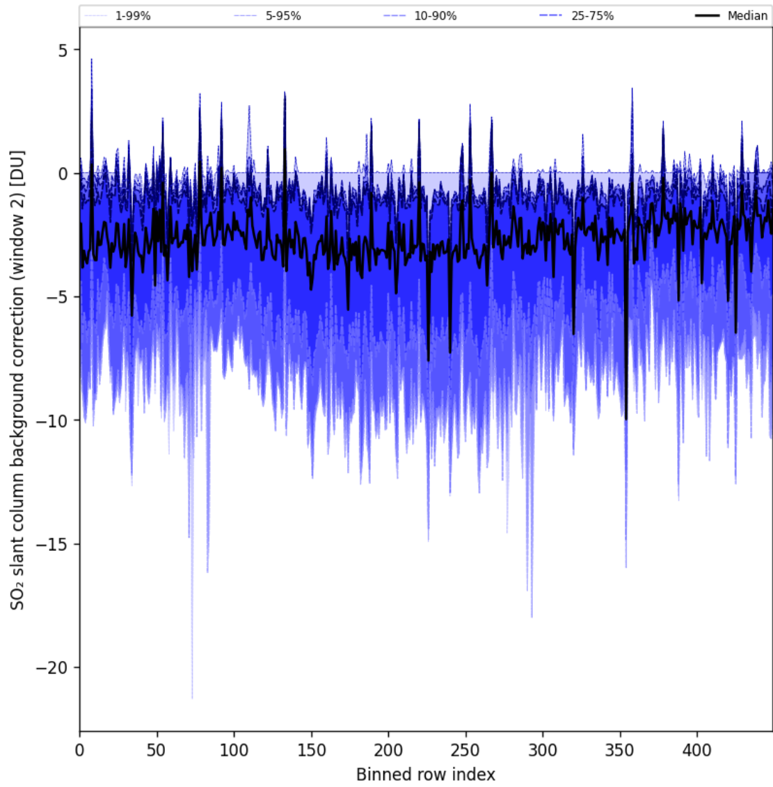
Figure 86: Along track statistics of “SO 2 slant column background correction (window 2)” for 2024-09-06 to 2024-09-07
