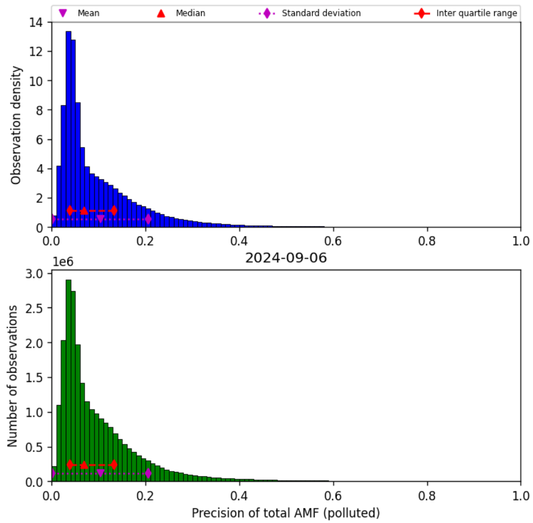
Figure 72: Histogram of “Precision of total AMF (polluted)” for 2024-09-06 to 2024-09-07
