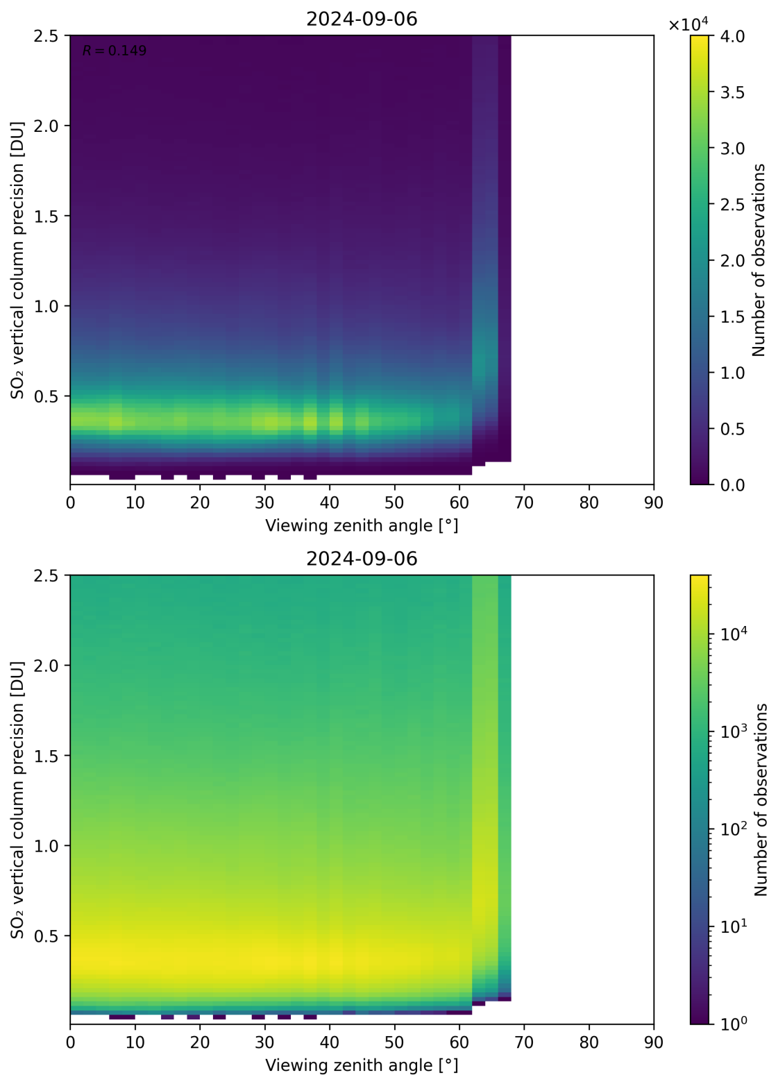
Figure 328: Scatter density plot of “Viewing zenith angle” against “SO 2 vertical column precision” for 2024-09-06 to 2024-09-07.
