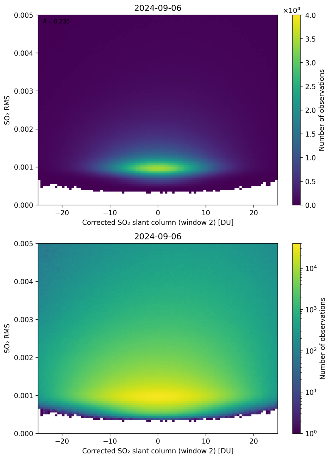
Figure 198: Scatter density plot of “Corrected SO 2 slant column (window 2)” against “SO 2 RMS” for 2024-09-06 to 2024-09-07.
