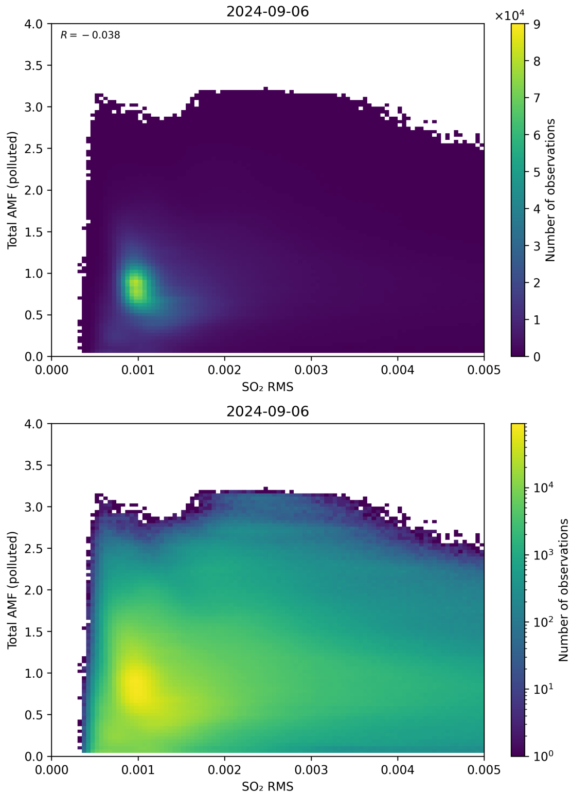
Figure 137: Scatter density plot of “SO 2 RMS” against “Total AMF (polluted)” for 2024-09-06 to 2024-09-07.
