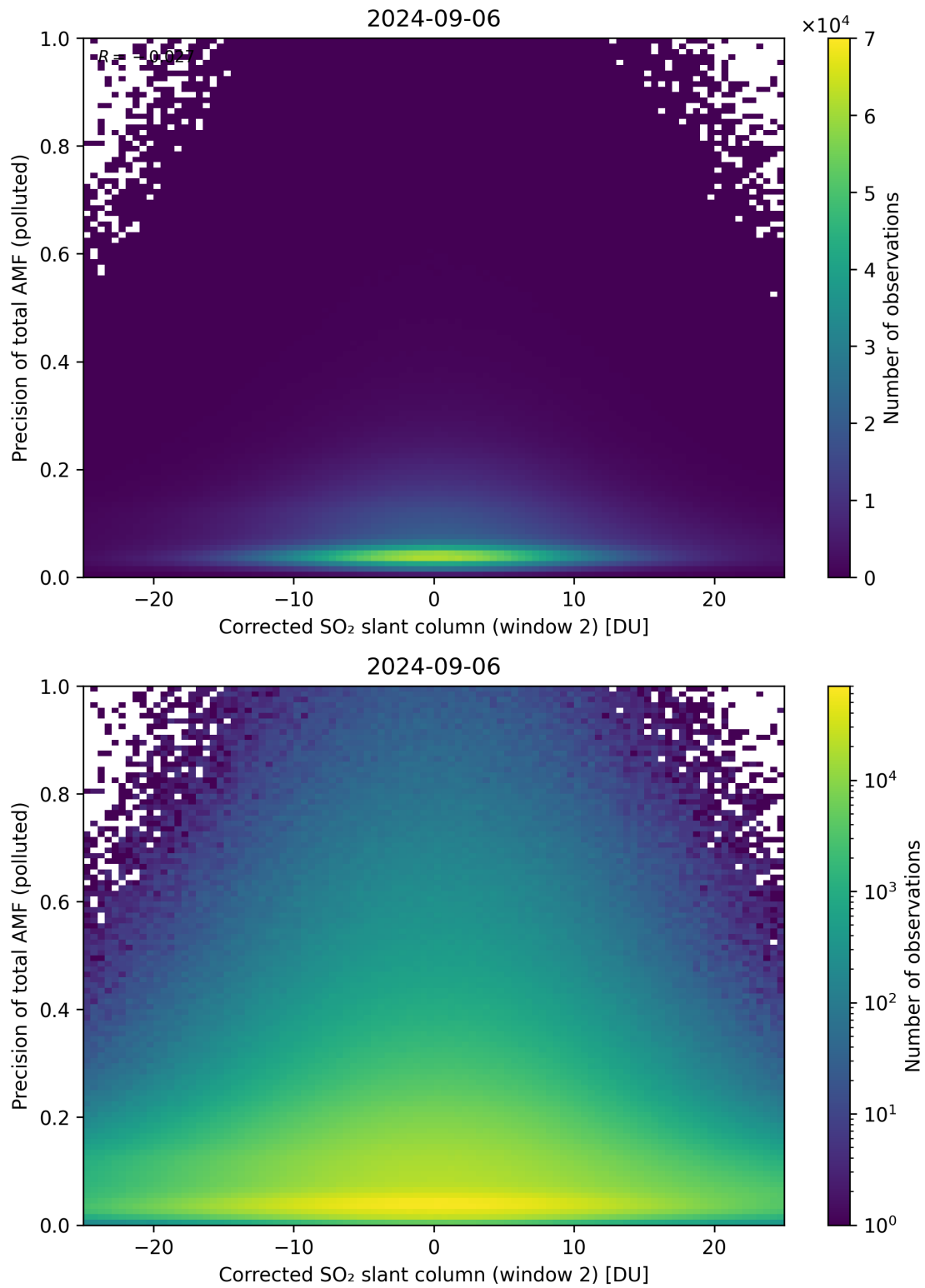
Figure 204: Scatter density plot of “Corrected SO 2 slant column (window 2)” against “Precision of total AMF (polluted)” for 2024-09-06 to 2024-09-07.
