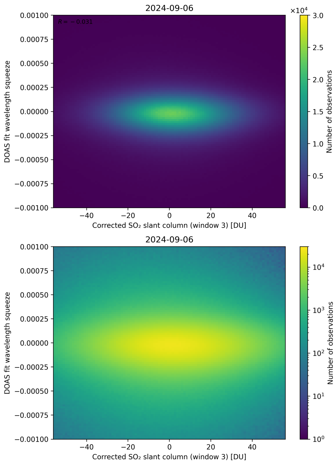
Figure 207: Scatter density plot of “Corrected SO 2 slant column (window 3)” against “DOAS fit wavelength squeeze” for 2024-09-06 to 2024-09-07.
