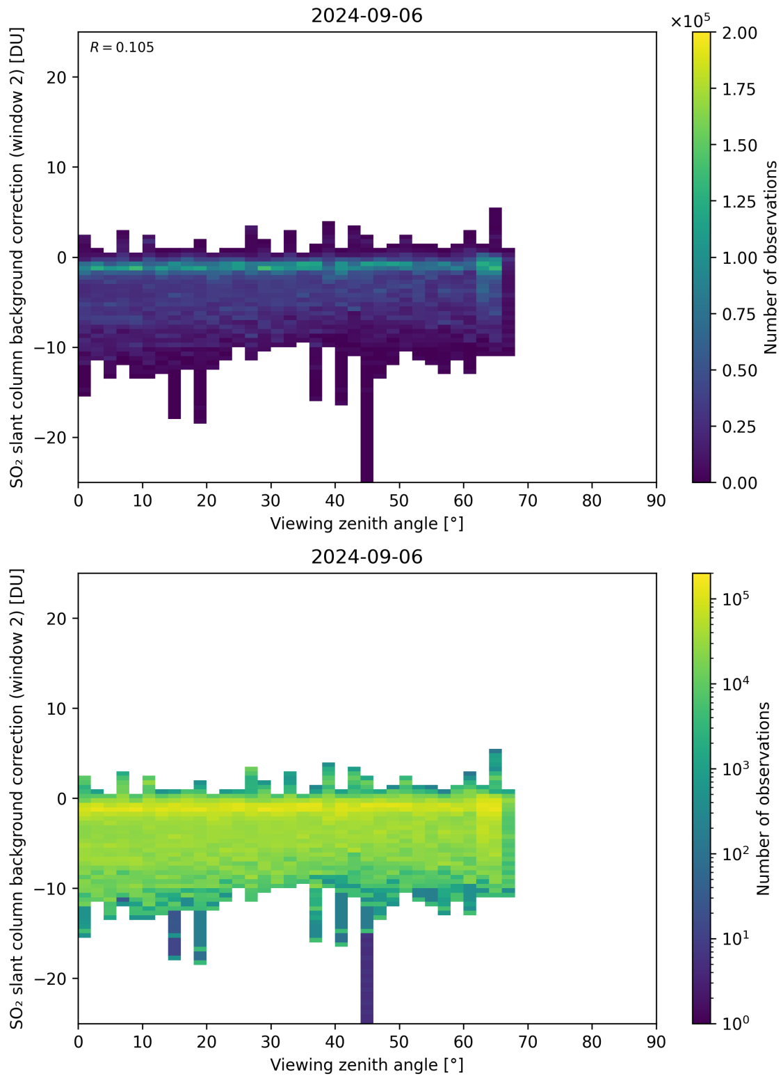
Figure 309: Scatter density plot of “Viewing zenith angle” against “SO 2 slant column background correction (window 2)” for 2024-09-06 to 2024-09-07.
