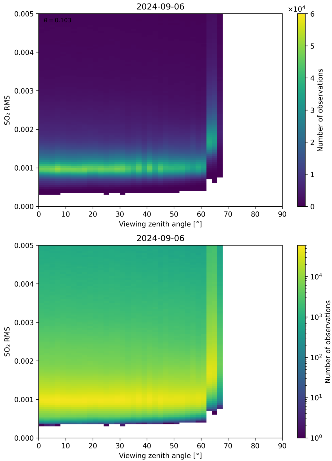
Figure 313: Scatter density plot of “Viewing zenith angle” against “SO 2 RMS” for 2024-09-06 to 2024-09-07.
