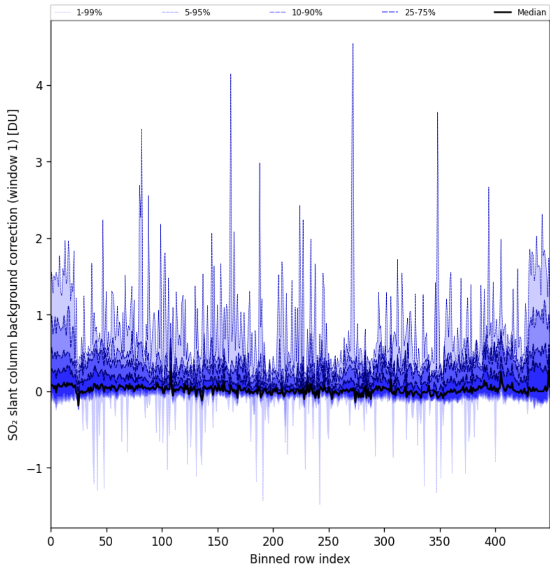
Figure 82: Along track statistics of “SO 2 slant column background correction (window 1)” for 2024-09-06 to 2024-09-07
