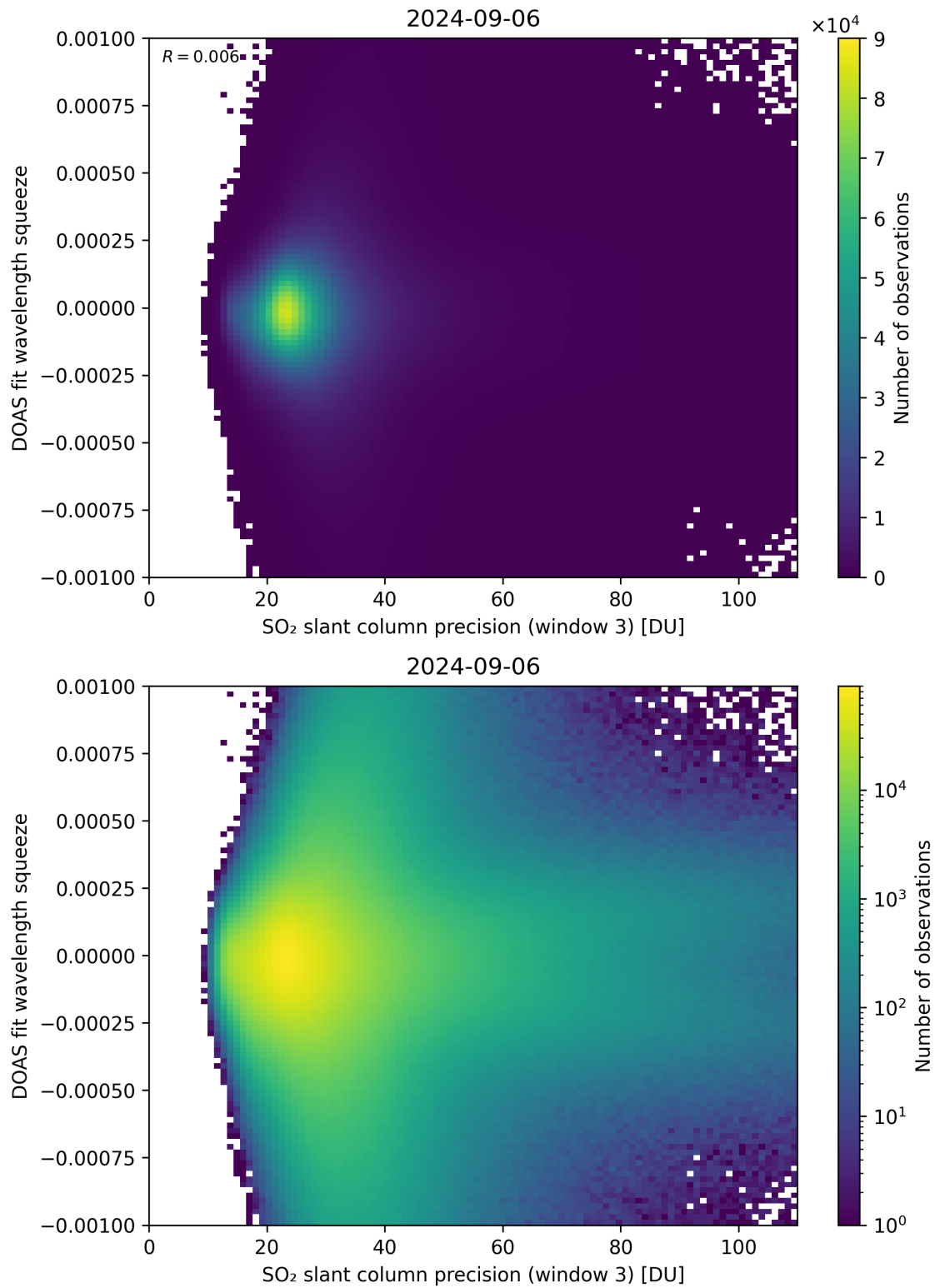
Figure 259: Scatter density plot of “SO 2 slant column precision (window 3)” against “DOAS fit wavelength squeeze” for 2024-09-06 to 2024-09-07.
