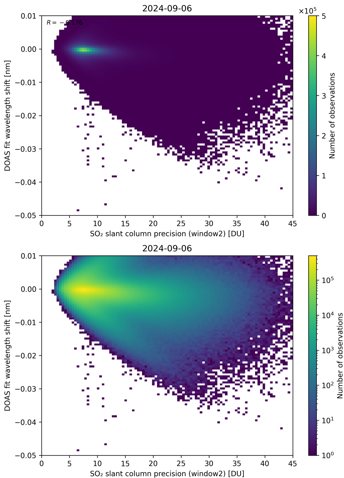
Figure 243: Scatter density plot of “SO 2 slant column precision (window2)” against “DOAS fit wavelength shift” for 2024-09-06 to 2024-09-07.
