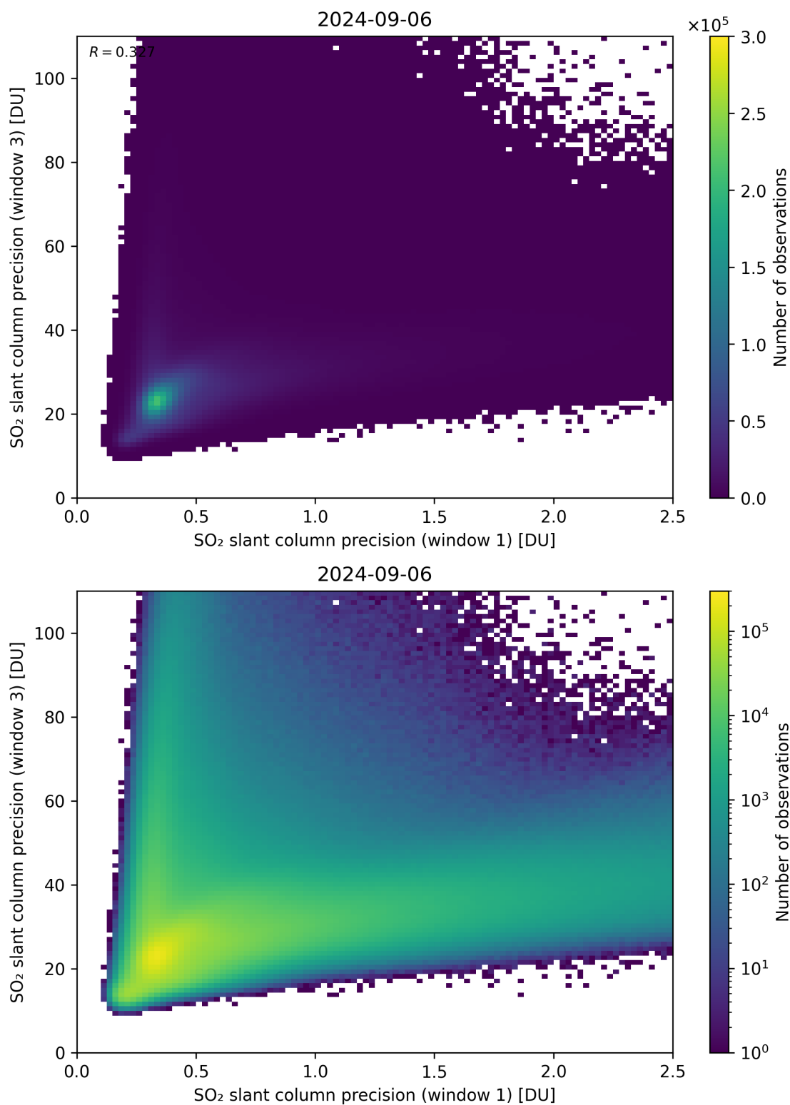
Figure 229: Scatter density plot of “SO 2 slant column precision (window 1)” against “SO 2 slant column precision (window 3)” for 2024-09-06 to 2024-09-07.
