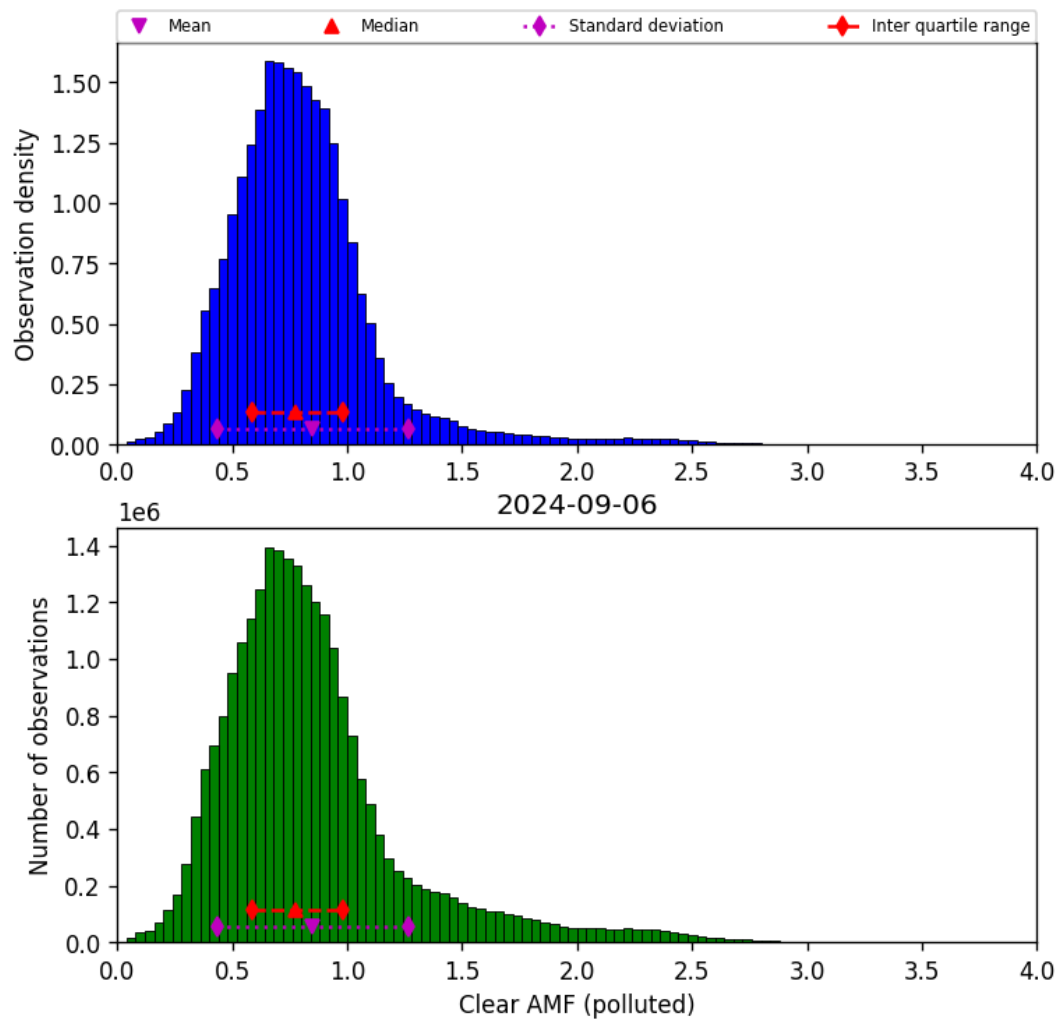
Figure 73: Histogram of “Clear AMF (polluted)” for 2024-09-06 to 2024-09-07
