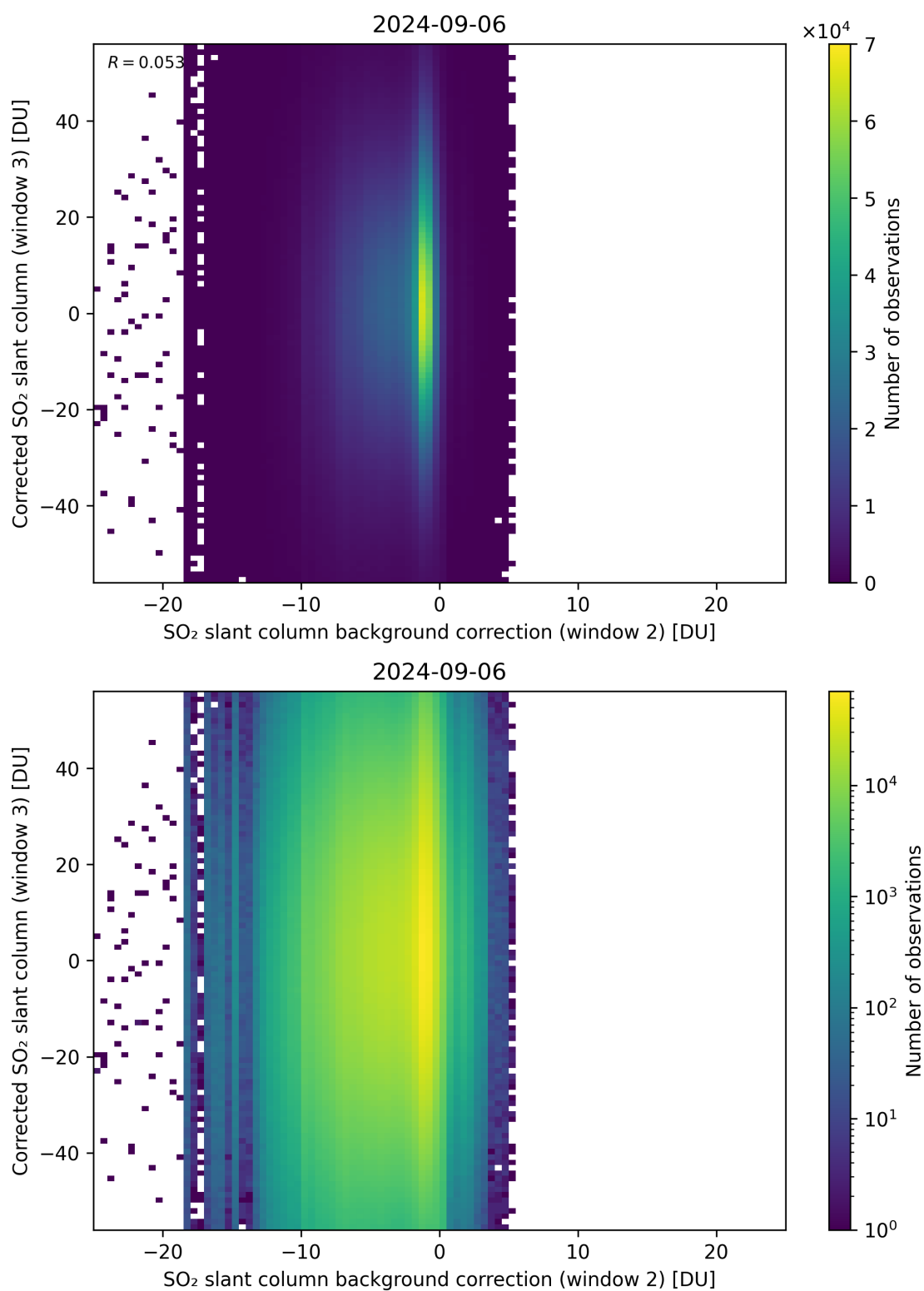
Figure 116: Scatter density plot of “SO 2 slant column background correction (window 2)” against “Corrected SO 2 slant column (window 3)” for 2024-09-06 to 2024-09-07.
