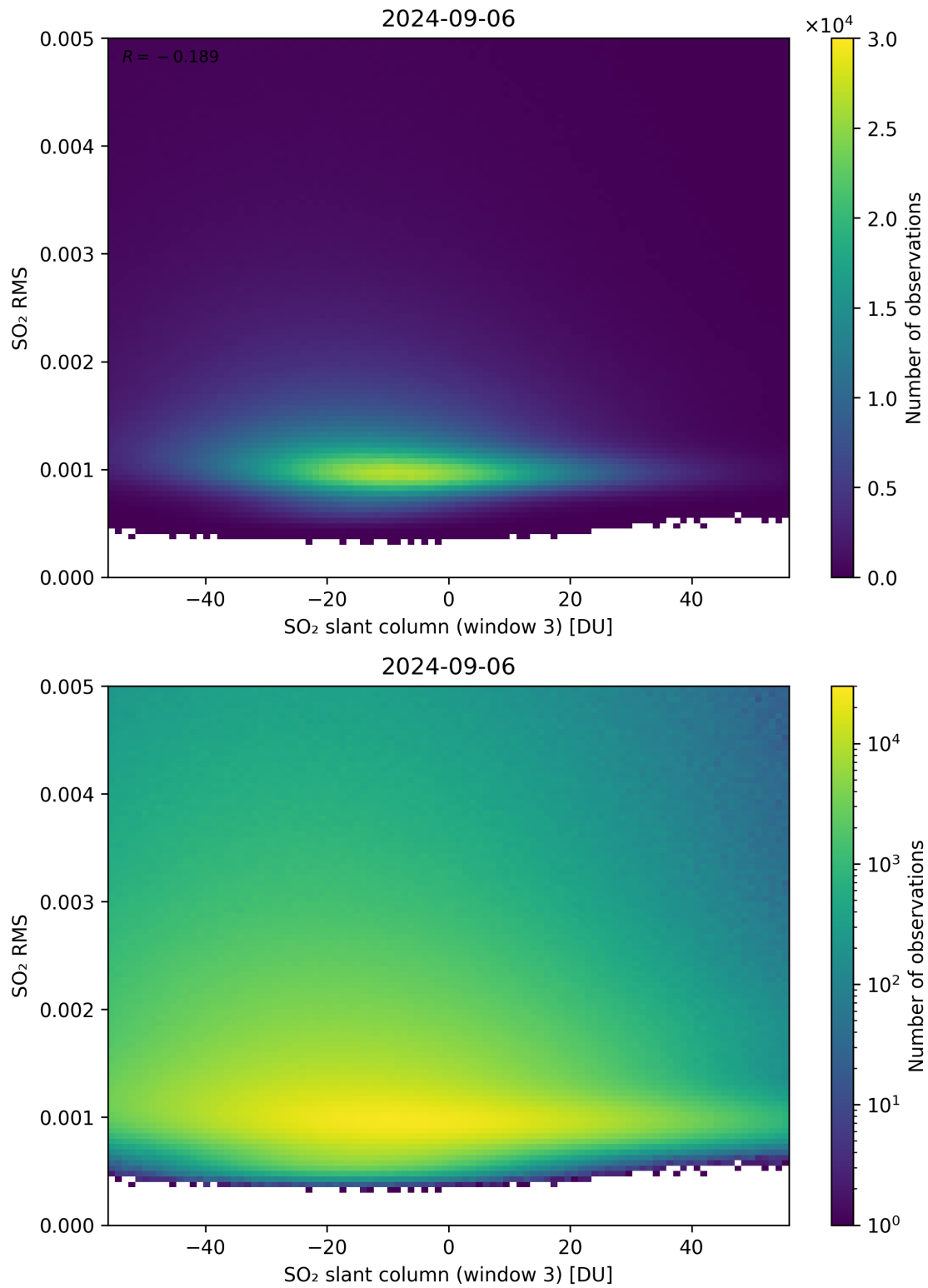
Figure 256: Scatter density plot of “SO 2 slant column (window 3)” against “SO 2 RMS” for 2024-09-06 to 2024-09-07.
