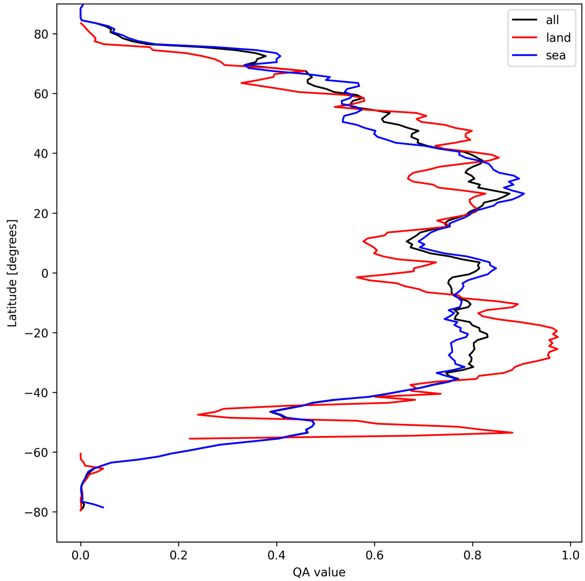
Figure 29: Zonal average of “QA value” for 2024-09-06 to 2024-09-07.
