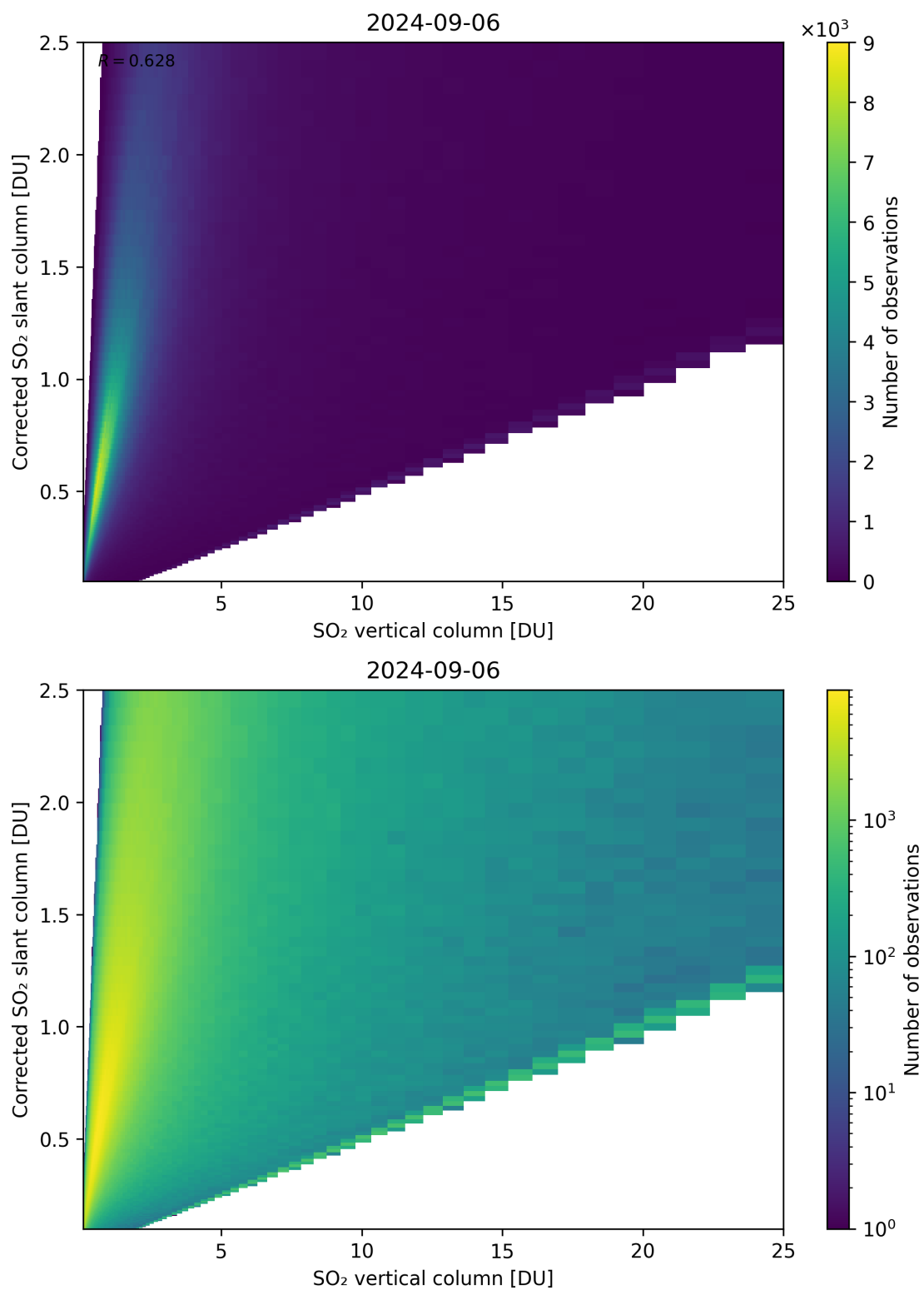
Figure 297: Scatter density plot of “SO 2 vertical column” against “Corrected SO 2 slant column” for 2024-09-06 to 2024-09-07.
