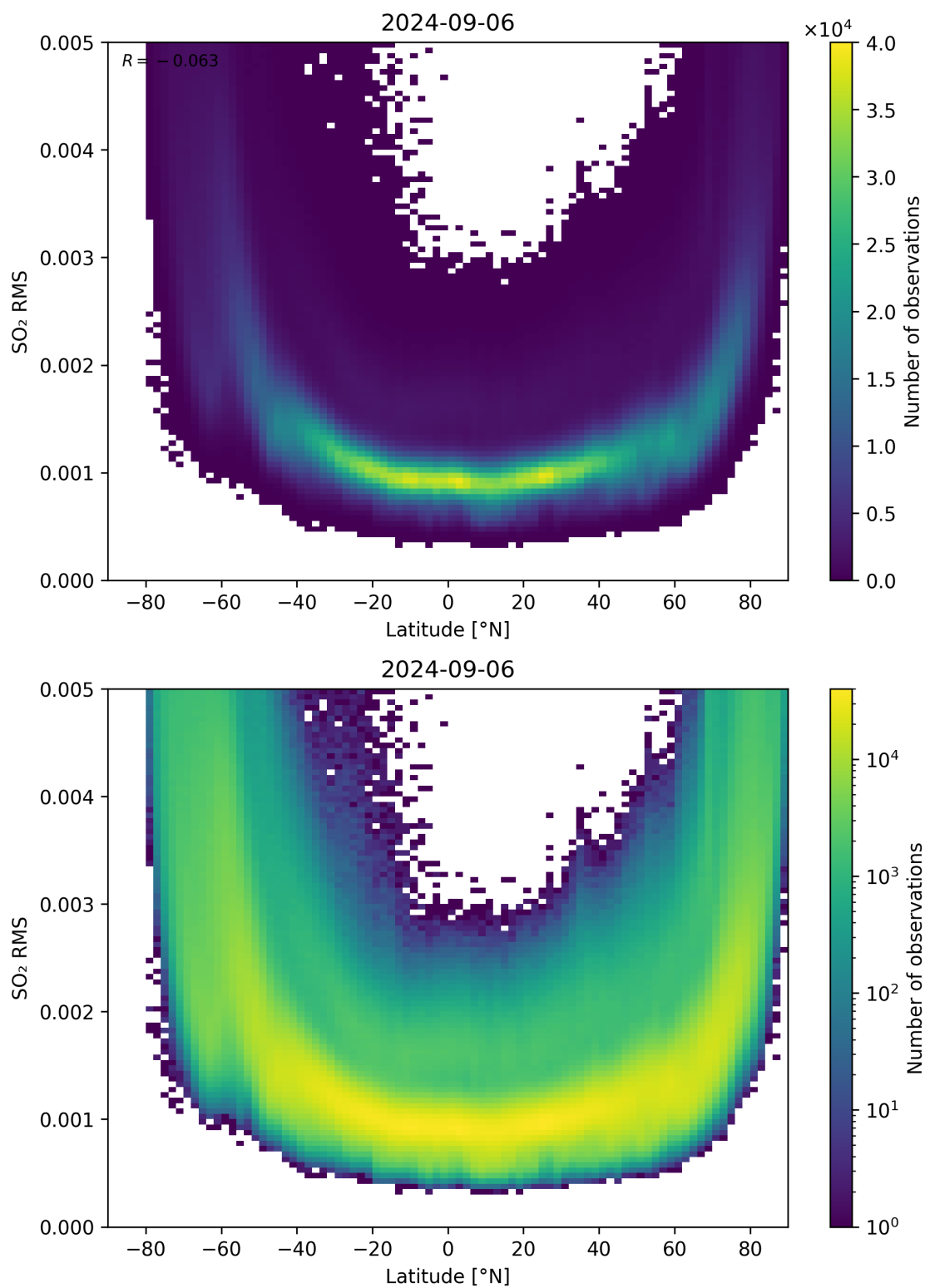
Figure 144: Scatter density plot of “Latitude” against “SO 2 RMS” for 2024-09-06 to 2024-09-07.
