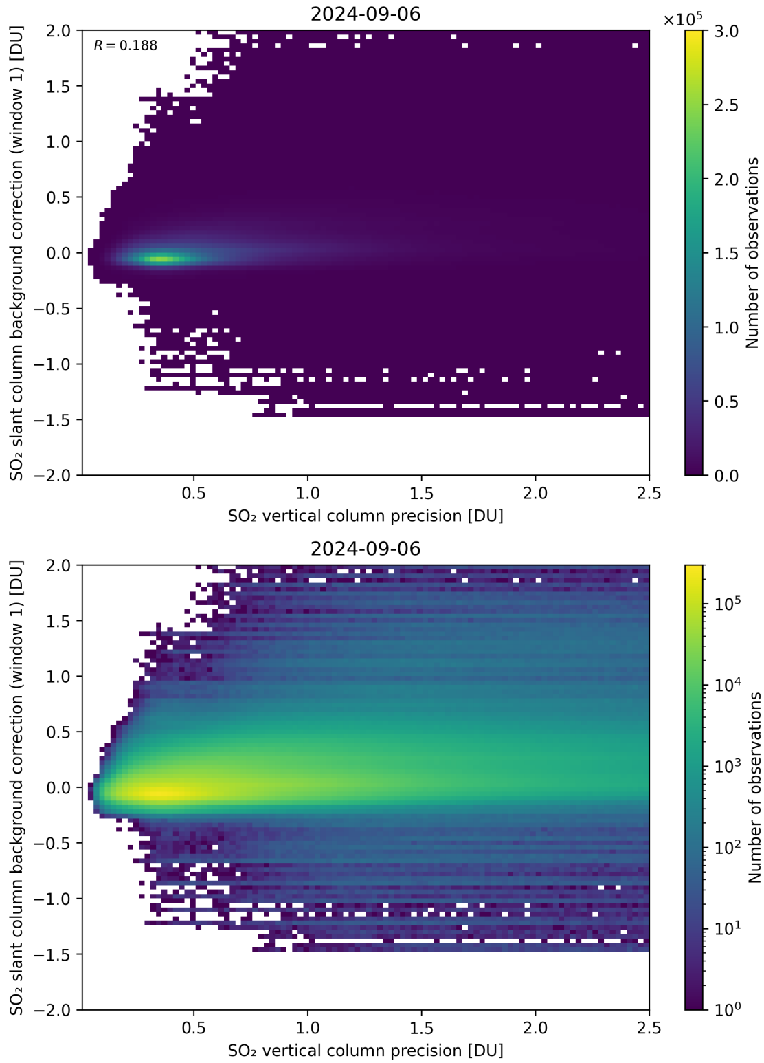
Figure 279: Scatter density plot of “SO 2 vertical column precision” against “SO 2 slant column background correction (window 1)” for 2024-09-06 to 2024-09-07.
