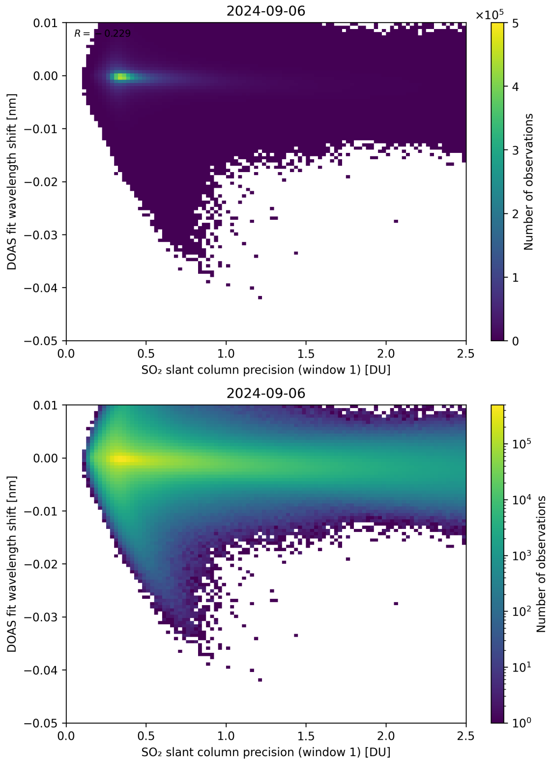
Figure 221: Scatter density plot of “SO 2 slant column precision (window 1)” against “DOAS fit wavelength shift” for 2024-09-06 to 2024-09-07.
