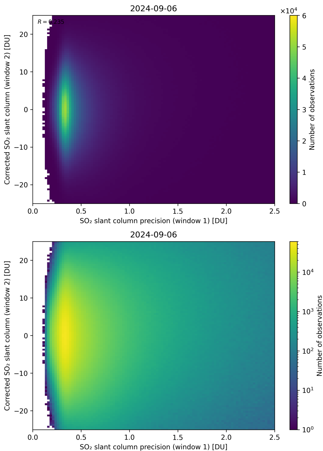
Figure 225: Scatter density plot of “SO 2 slant column precision (window 1)” against “Corrected SO 2 slant column (window 2)” for 2024-09-06 to 2024-09-07.
