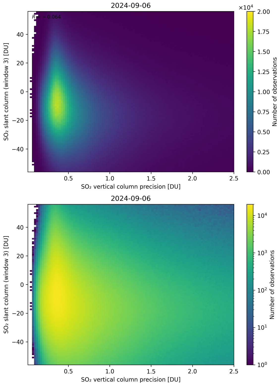
Figure 292: Scatter density plot of “SO 2 vertical column precision” against “SO 2 slant column (window 3)” for 2024-09-06 to 2024-09-07.
