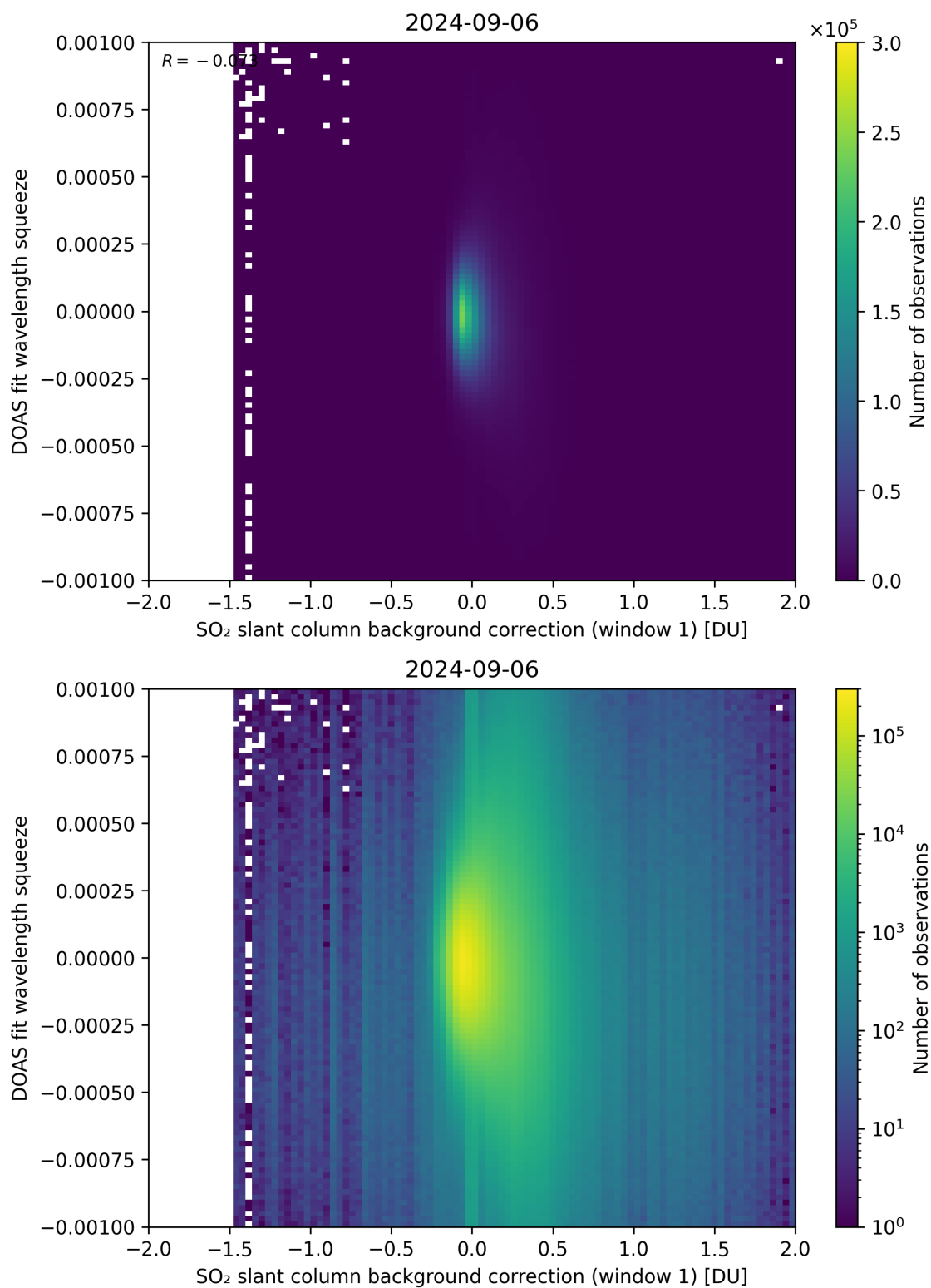
Figure 101: Scatter density plot of “SO 2 slant column background correction (window 1)” against “DOAS fit wavelength squeeze” for 2024-09-06 to 2024-09-07.
