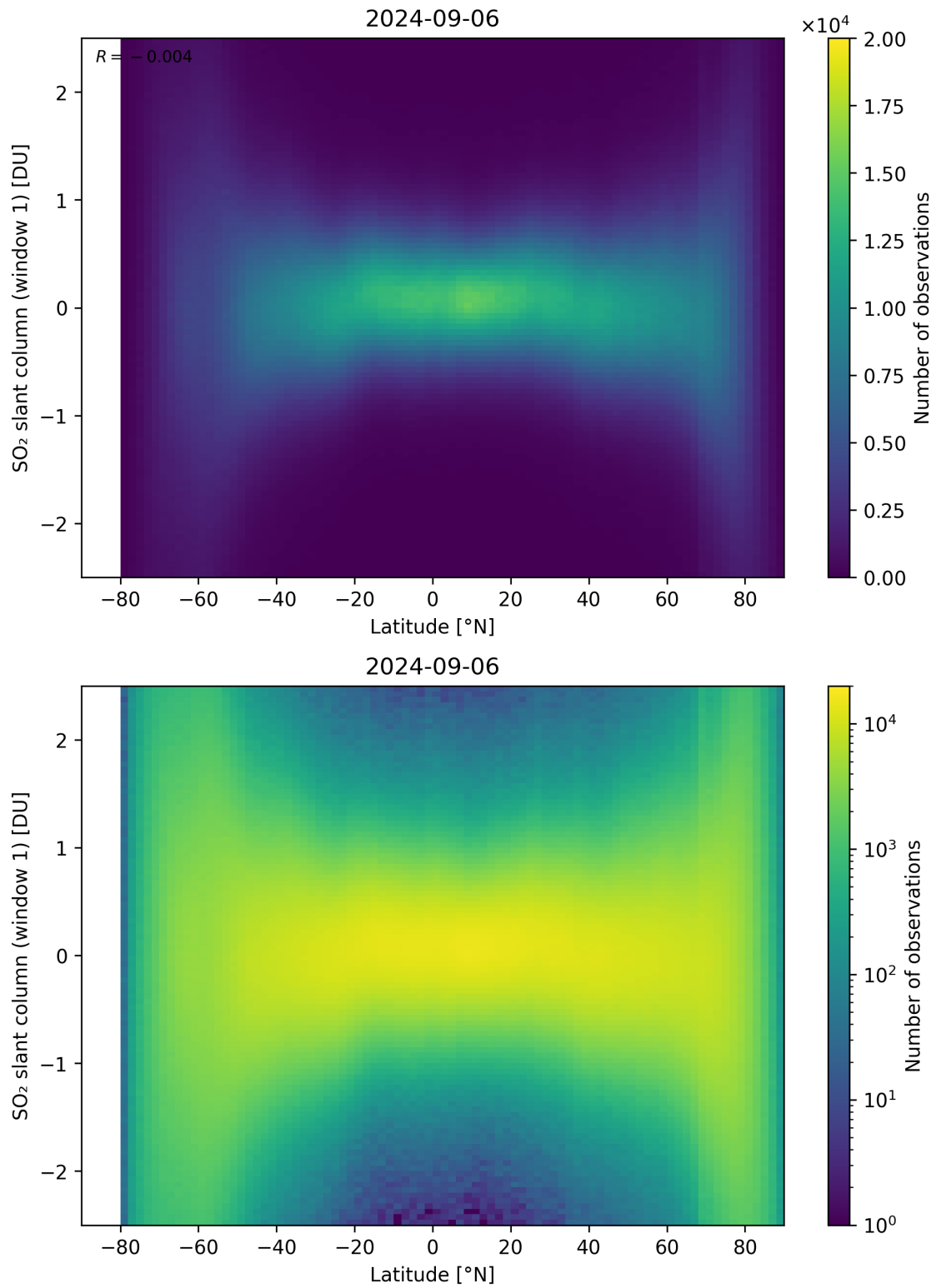
Figure 149: Scatter density plot of “Latitude” against “SO 2 slant column (window 1)” for 2024-09-06 to 2024-09-07.
