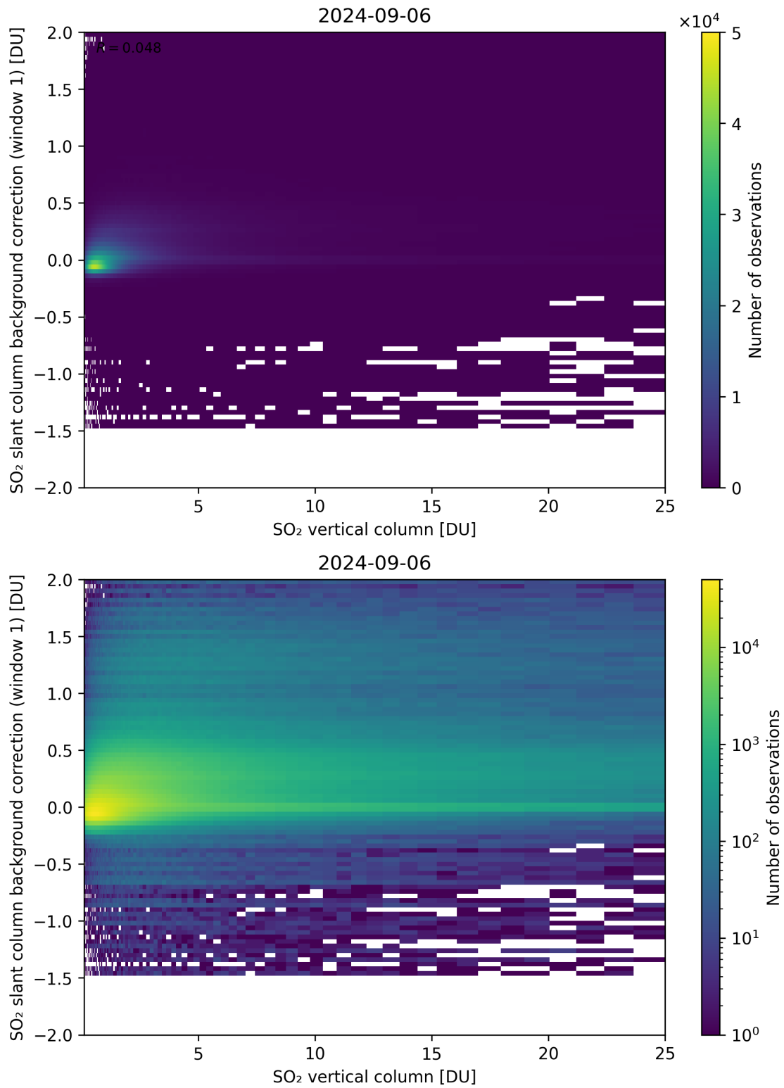
Figure 273: Scatter density plot of “SO 2 vertical column” against “SO 2 slant column background correction (window 1)” for 2024-09-06 to 2024-09-07.
