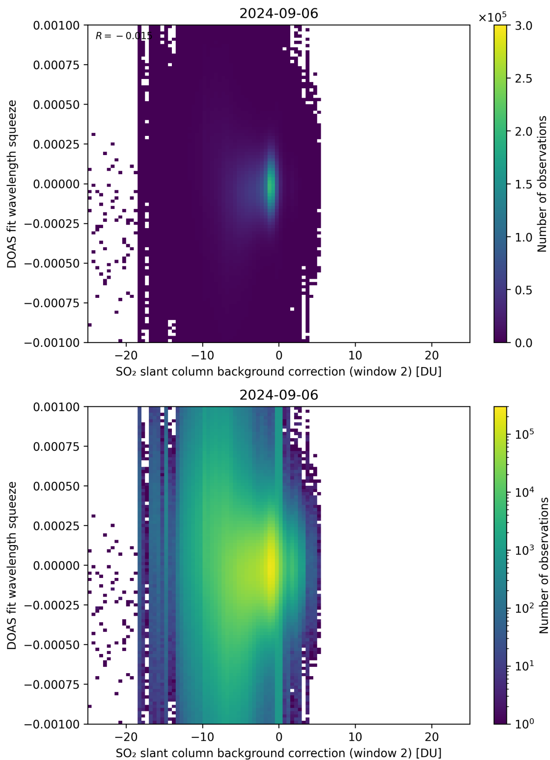
Figure 113: Scatter density plot of “SO 2 slant column background correction (window 2)” against “DOAS fit wavelength squeeze” for 2024-09-06 to 2024-09-07.
