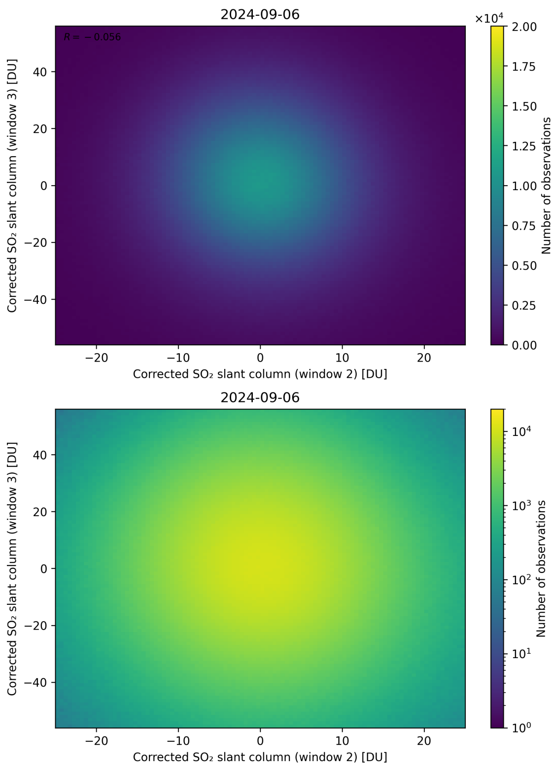
Figure 200: Scatter density plot of “Corrected SO 2 slant column (window 2)” against “Corrected SO 2 slant column (window 3)” for 2024-09-06 to 2024-09-07.
