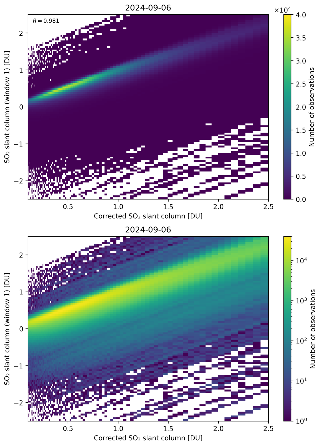
Figure 187: Scatter density plot of “Corrected SO 2 slant column” against “SO 2 slant column (window 1)” for 2024-09-06 to 2024-09-07.
