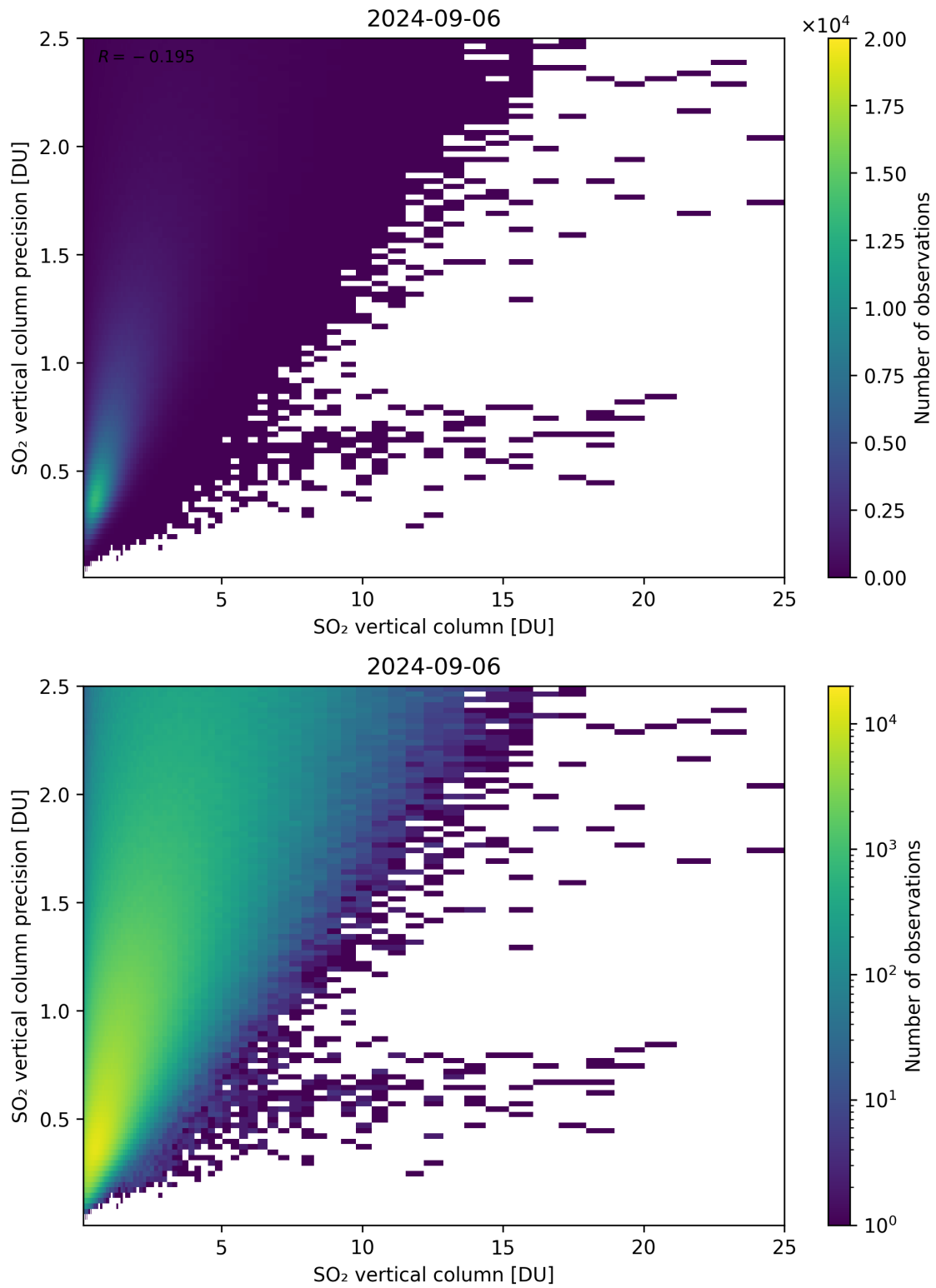
Figure 307: Scatter density plot of “SO 2 vertical column” against “SO 2 vertical column precision” for 2024-09-06 to 2024-09-07.
