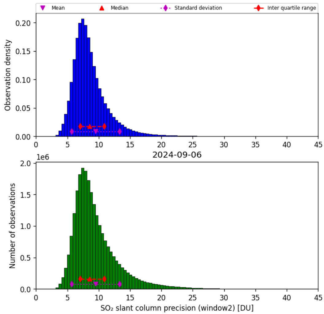
Figure 61: Histogram of “SO 2 slant column precision (window2)” for 2024-09-06 to 2024-09-07
