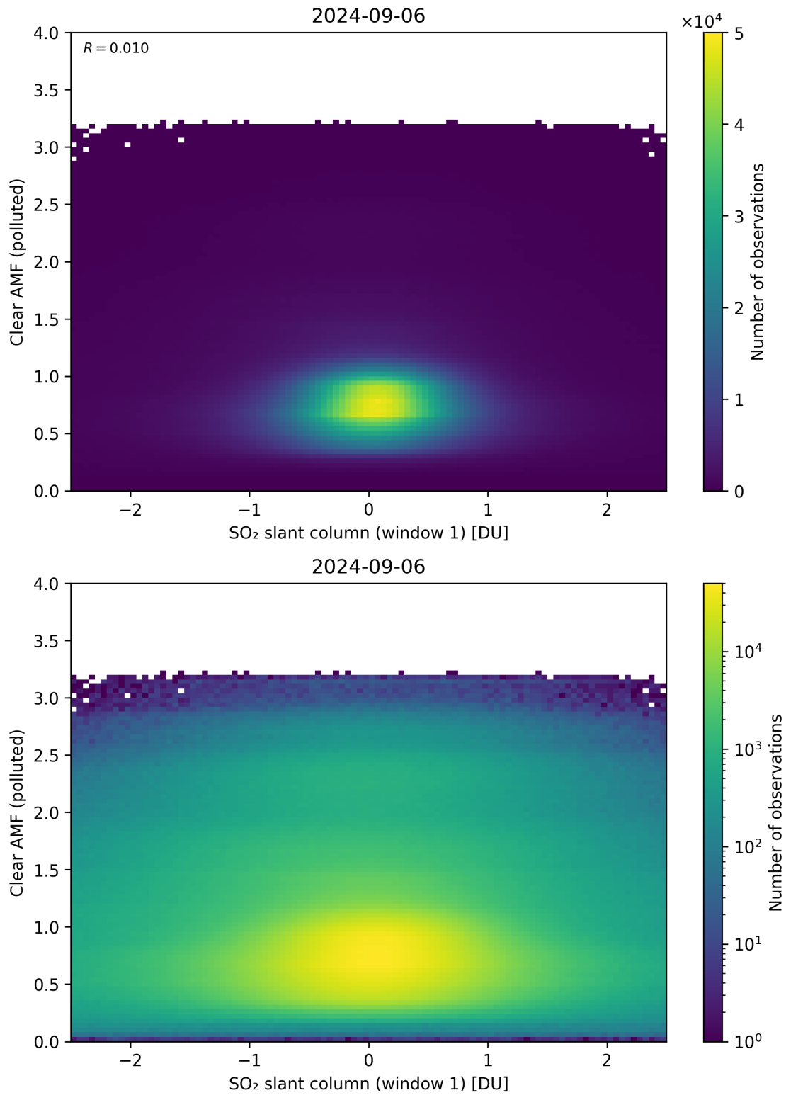
Figure 232: Scatter density plot of “SO 2 slant column (window 1)” against “Clear AMF (polluted)” for 2024-09-06 to 2024-09-07.
