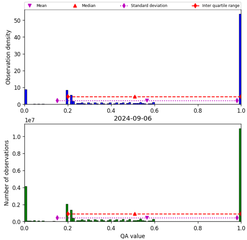
Figure 52: Histogram of “QA value” for 2024-09-06 to 2024-09-07
