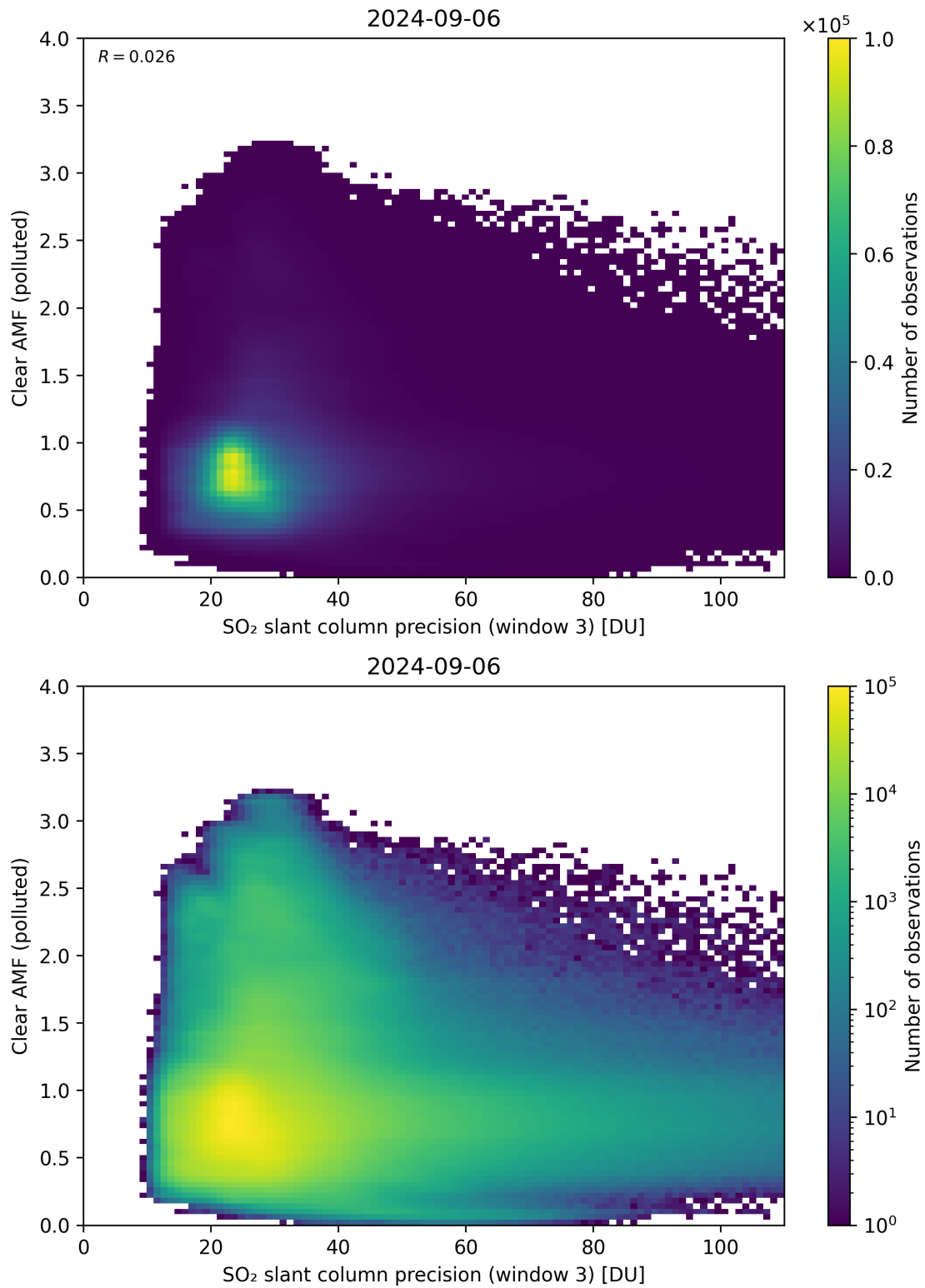
Figure 261: Scatter density plot of “SO 2 slant column precision (window 3)” against “Clear AMF (polluted)” for 2024-09-06 to 2024-09-07.
