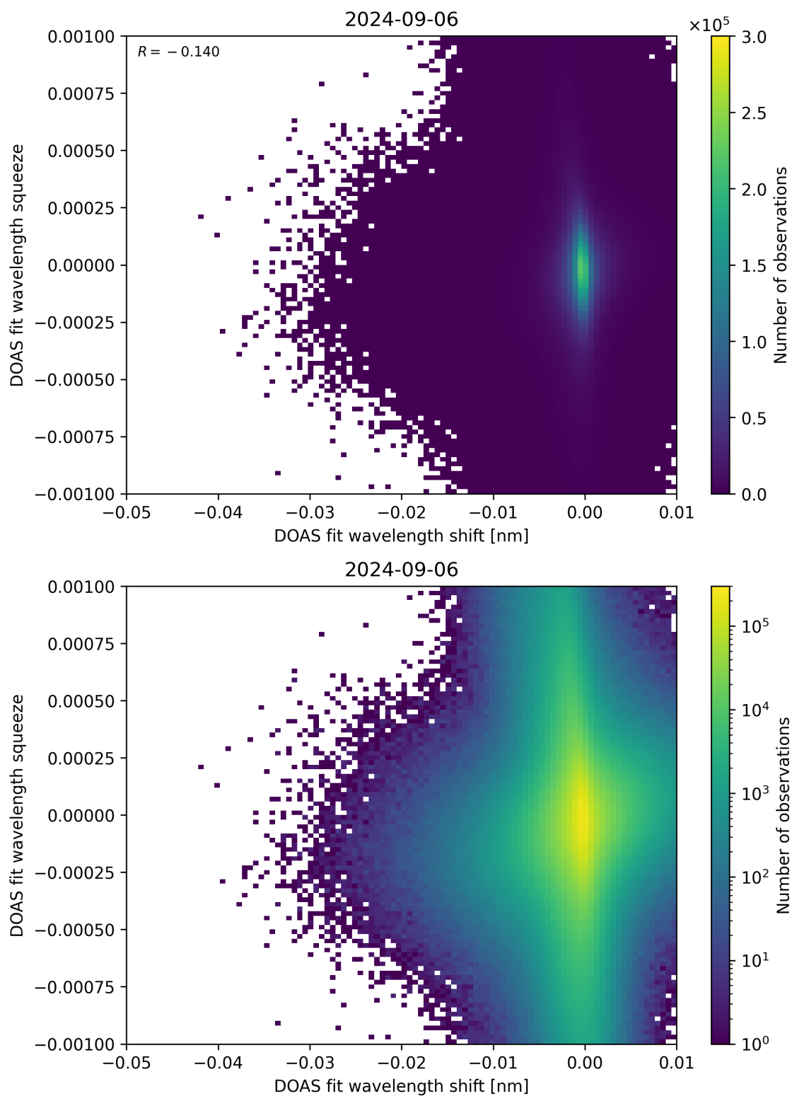
Figure 127: Scatter density plot of “DOAS fit wavelength shift” against “DOAS fit wavelength squeeze” for 2024-09-06 to 2024-09-07.
