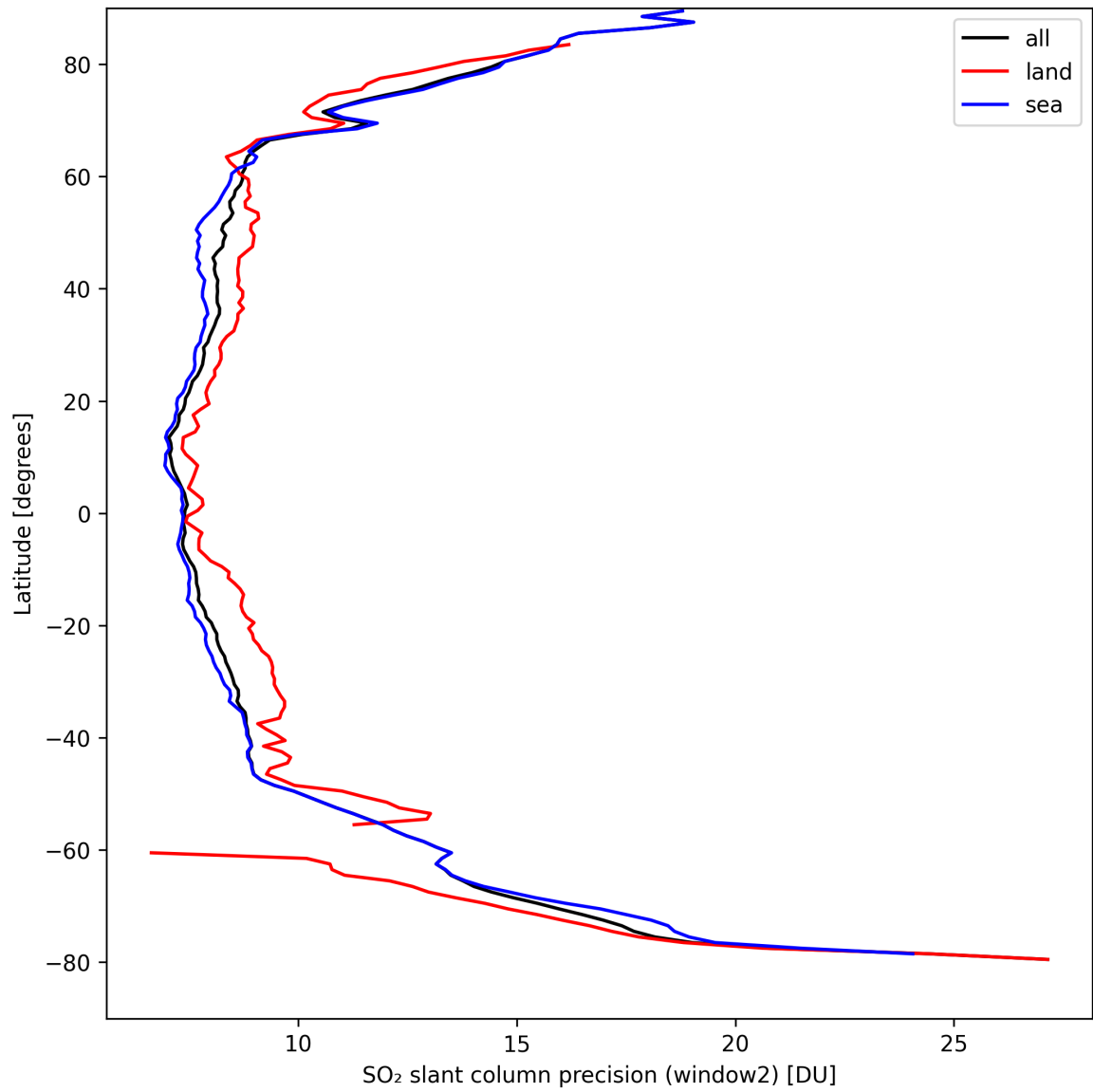
Figure 38: Zonal average of “SO 2 slant column precision (window2)” for 2024-09-06 to 2024-09-07.
