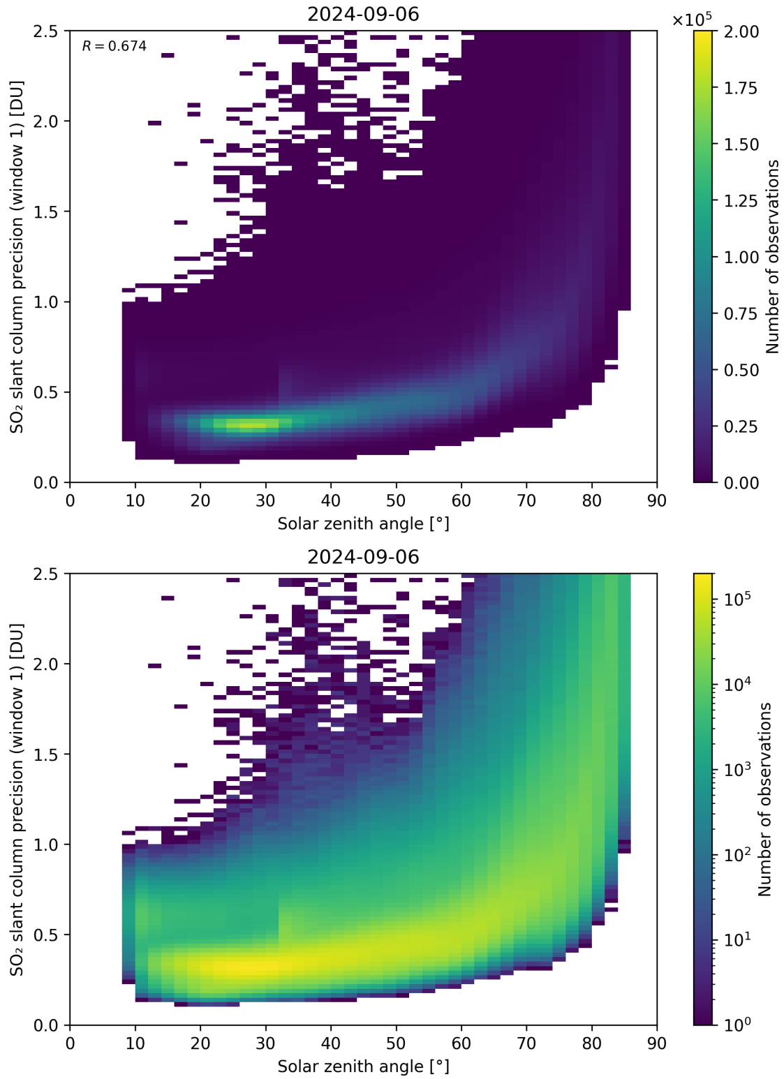
Figure 170: Scatter density plot of “Solar zenith angle” against “SO 2 slant column precision (window 1)” for 2024-09-06 to 2024-09-07.
