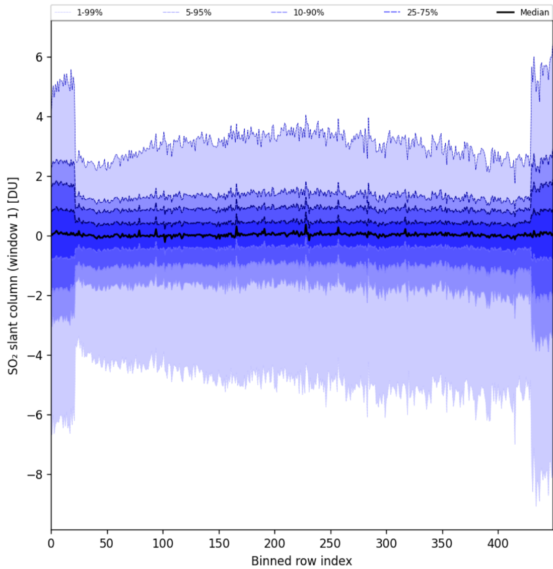
Figure 79: Along track statistics of “SO 2 slant column (window 1)” for 2024-09-06 to 2024-09-07
