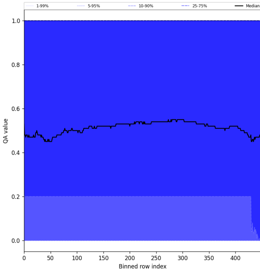
Figure 75: Along track statistics of “QA value” for 2024-09-06 to 2024-09-07
