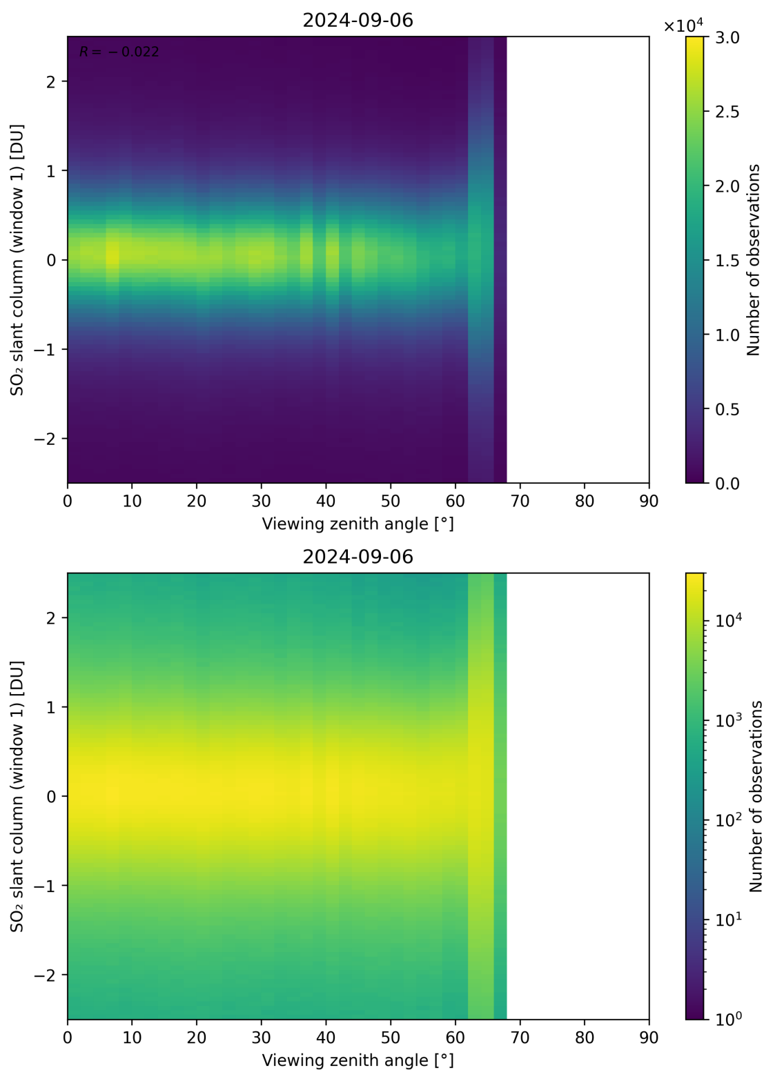
Figure 320: Scatter density plot of “Viewing zenith angle” against “SO 2 slant column (window 1)” for 2024-09-06 to 2024-09-07.
