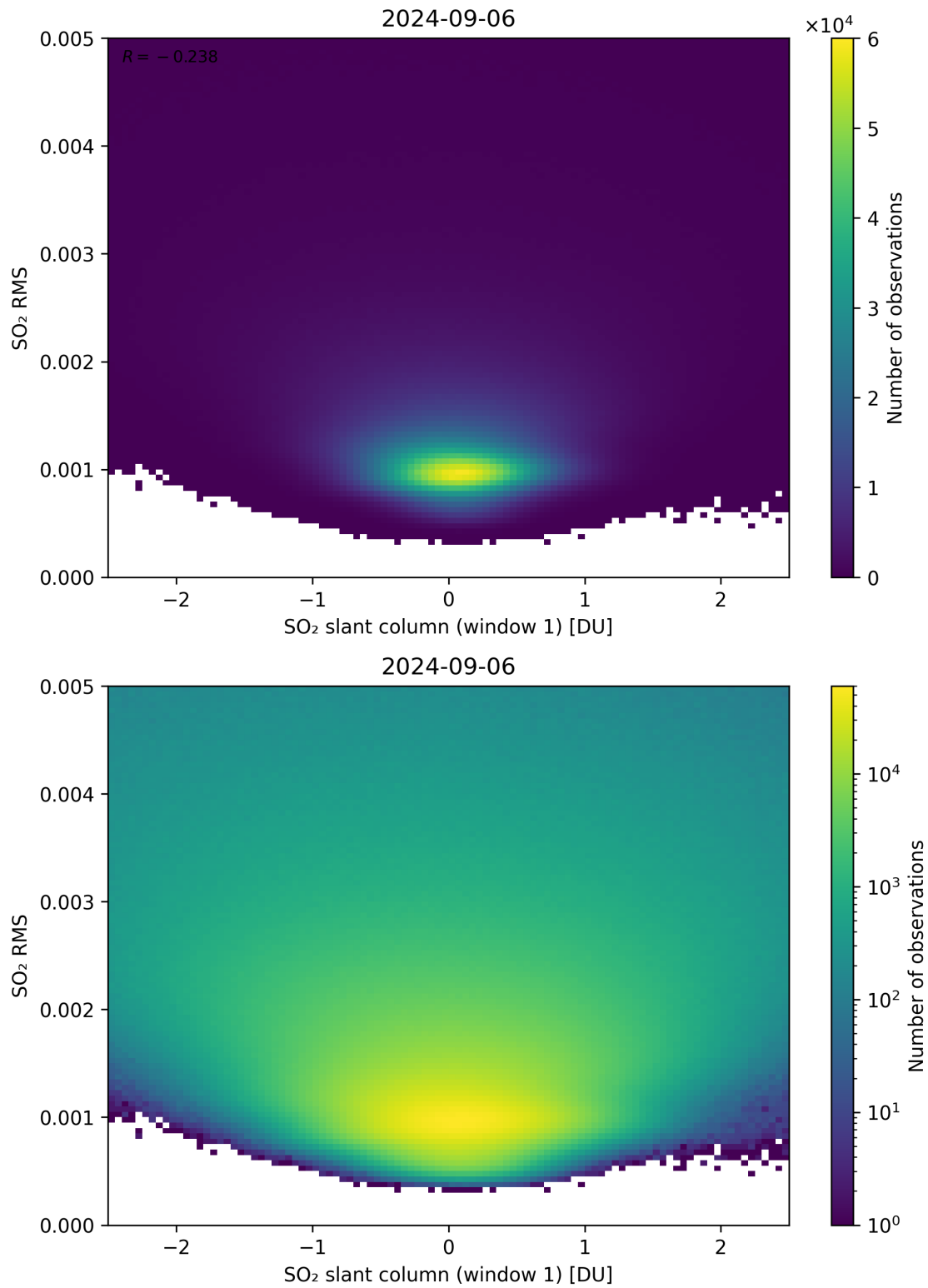
Figure 217: Scatter density plot of “SO 2 slant column (window 1)” against “SO 2 RMS” for 2024-09-06 to 2024-09-07.
