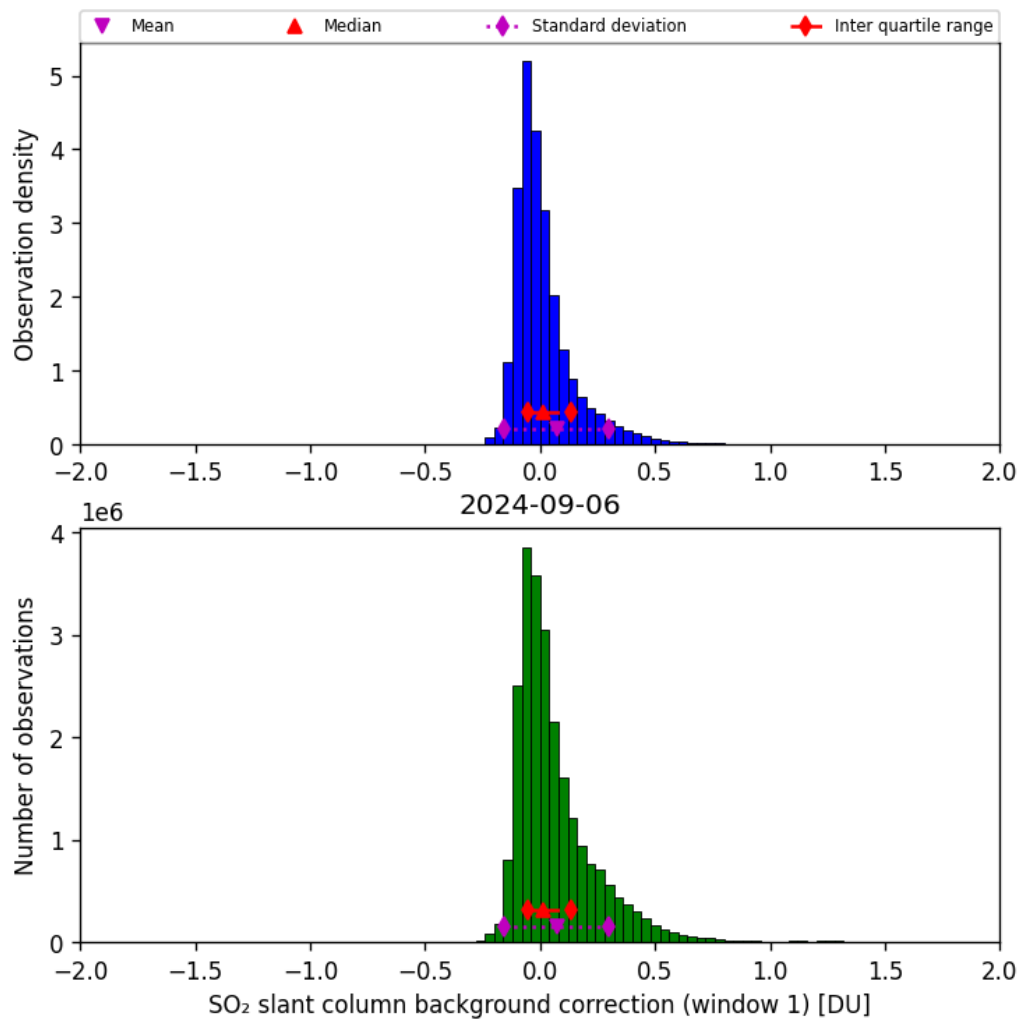
Figure 59: Histogram of “SO 2 slant column background correction (window 1)” for 2024-09-06 to 2024-09-07
