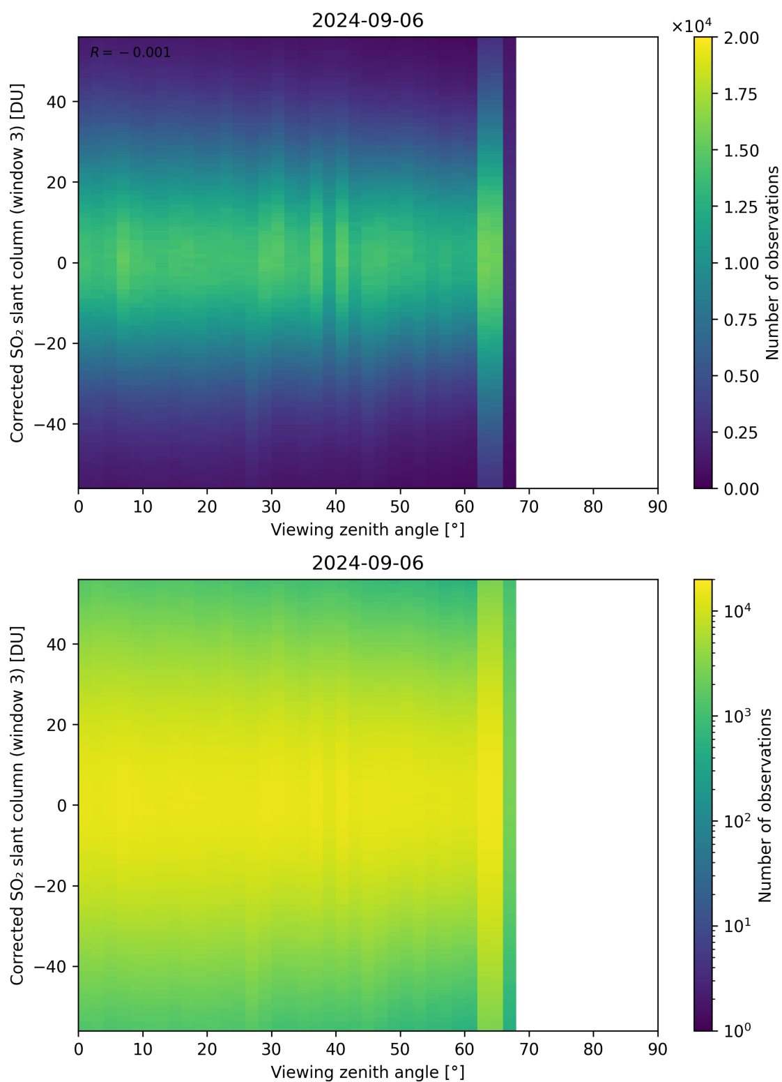
Figure 319: Scatter density plot of “Viewing zenith angle” against “Corrected SO 2 slant column (window 3)” for 2024-09-06 to 2024-09-07.
