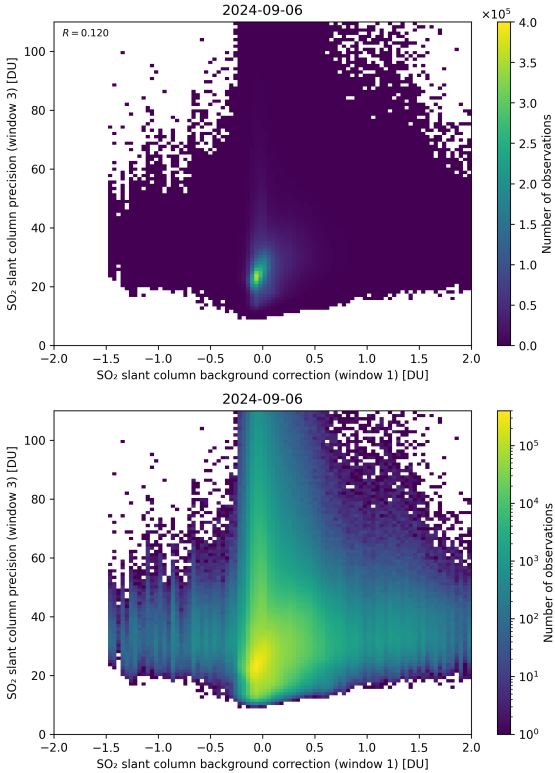
Figure 108: Scatter density plot of “SO 2 slant column background correction (window 1)” against “SO 2 slant column precision (window 3)” for 2024-09-06 to 2024-09-07.
