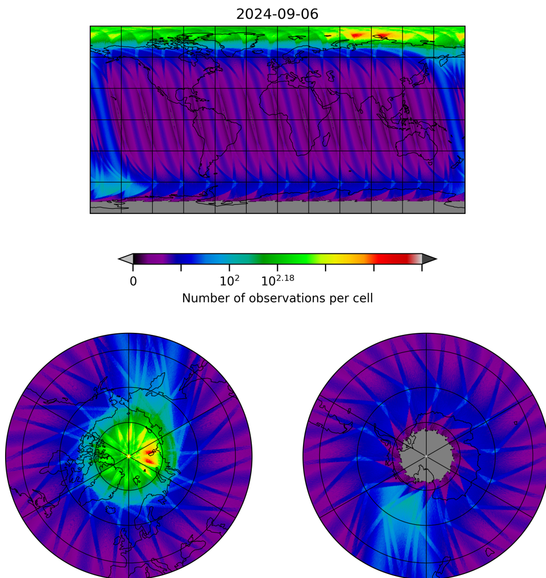
Figure 28: Map of the number of observations for 2024-09-06 to 2024-09-07
