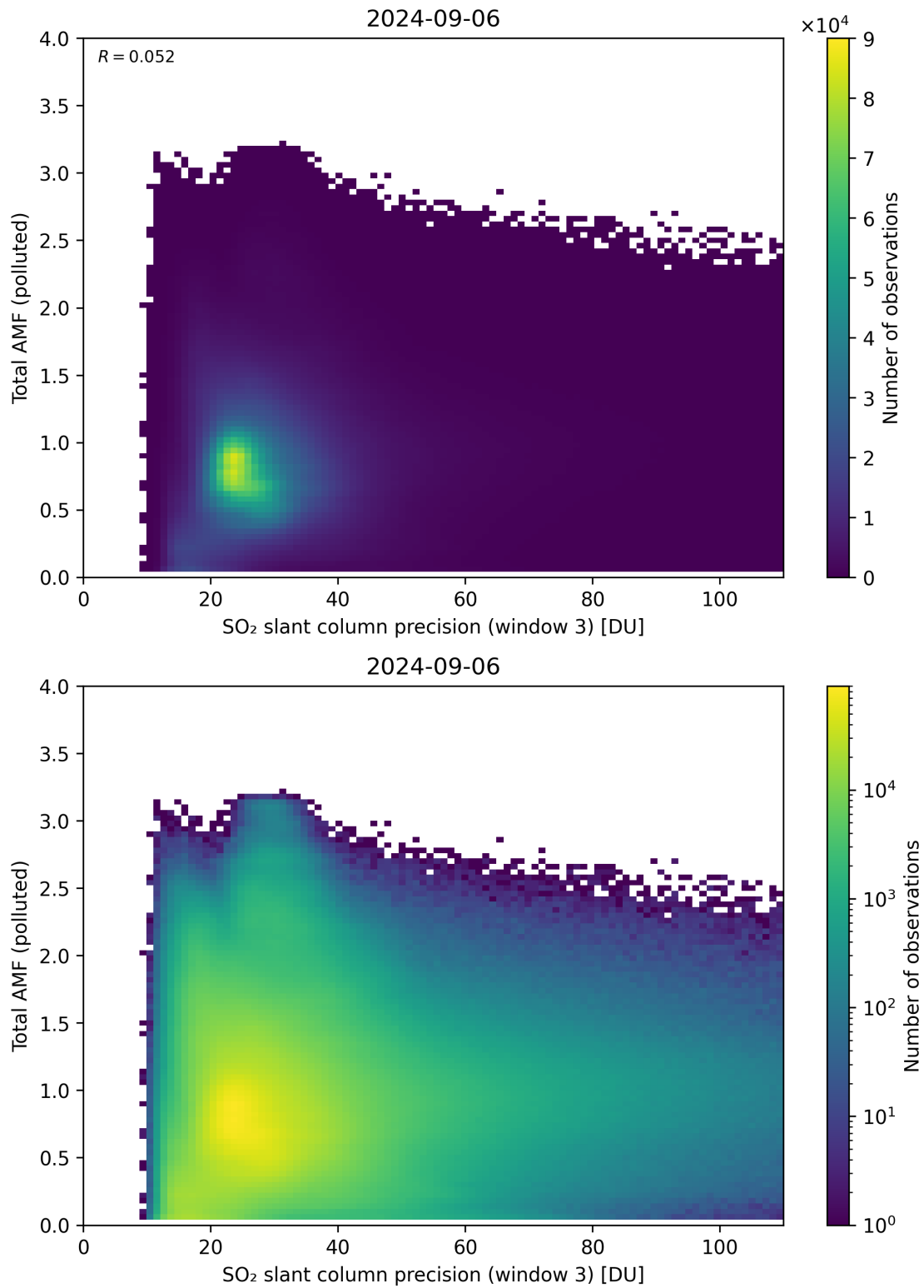
Figure 263: Scatter density plot of “SO 2 slant column precision (window 3)” against “Total AMF (polluted)” for 2024-09-06 to 2024-09-07.
