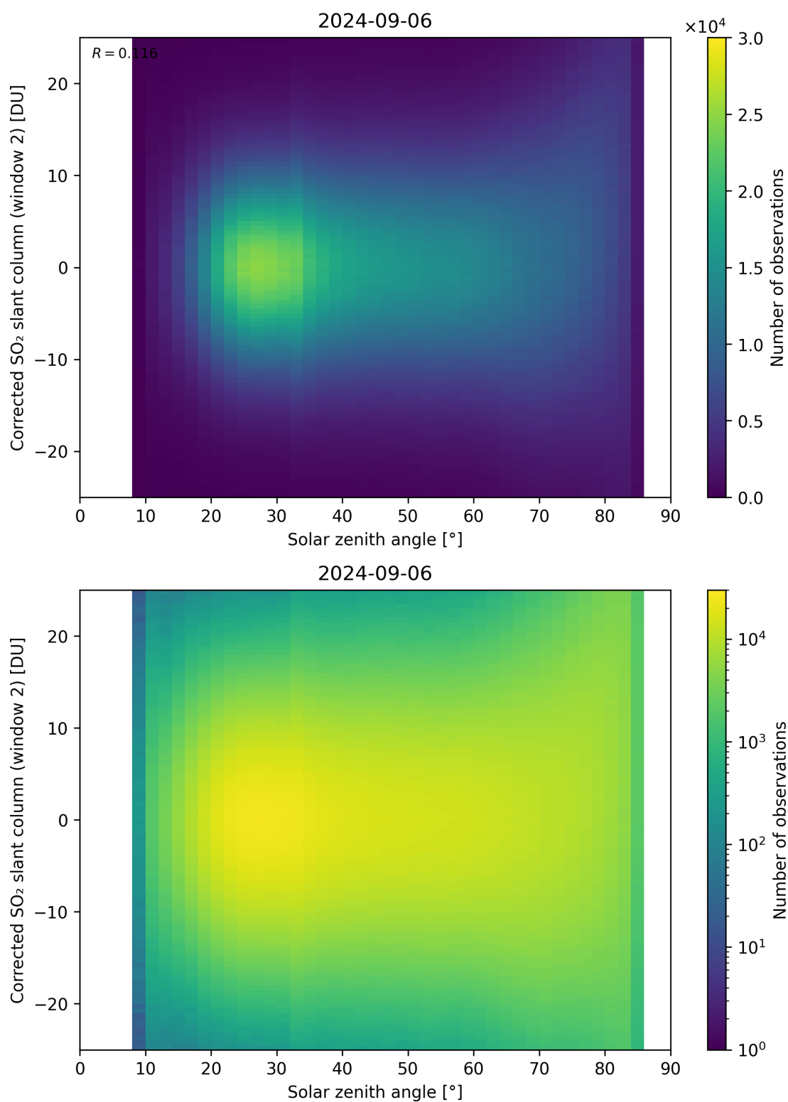
Figure 167: Scatter density plot of “Solar zenith angle” against “Corrected SO 2 slant column (window 2)” for 2024-09-06 to 2024-09-07.
