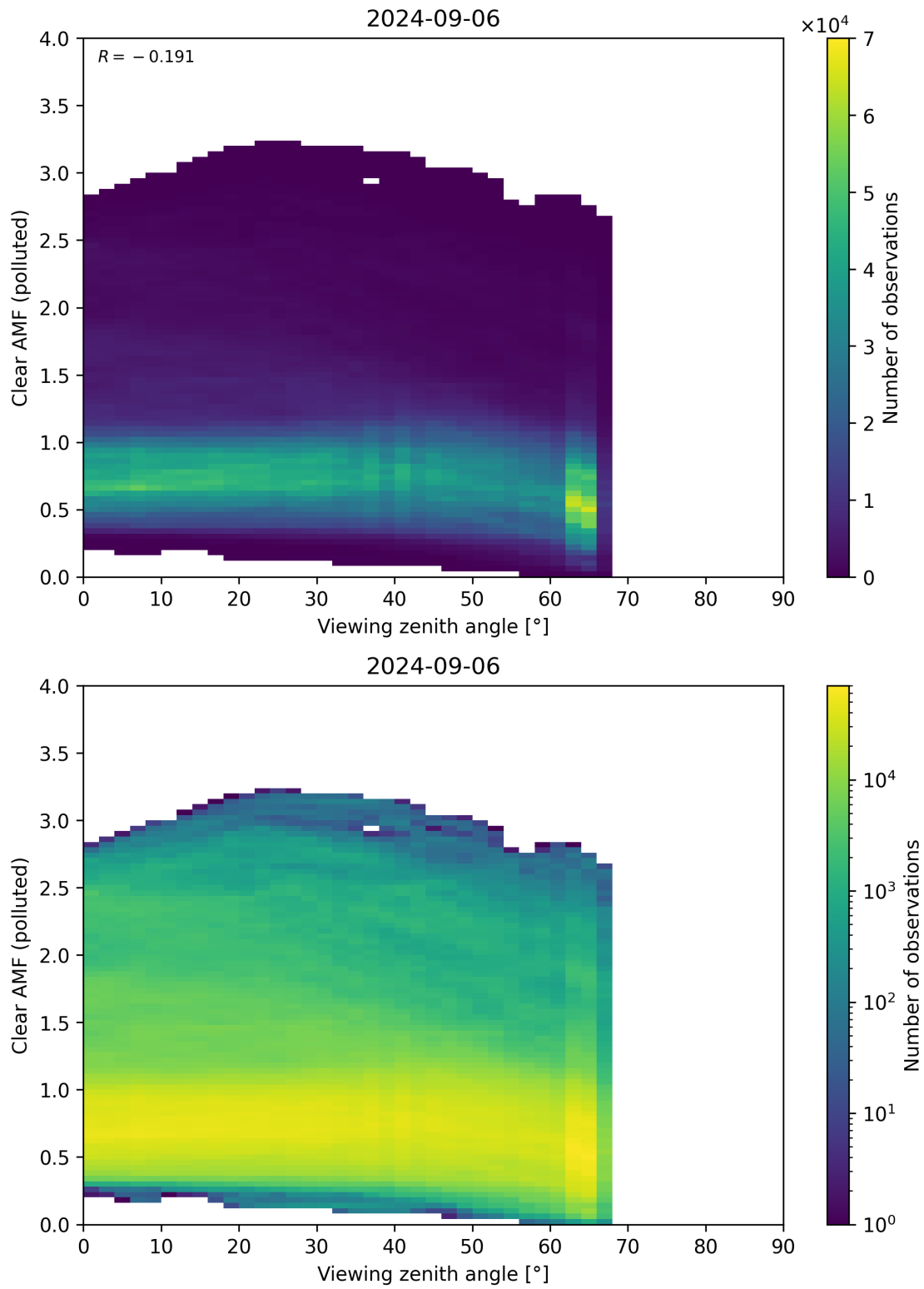
Figure 316: Scatter density plot of “Viewing zenith angle” against “Clear AMF (polluted)” for 2024-09-06 to 2024-09-07.
