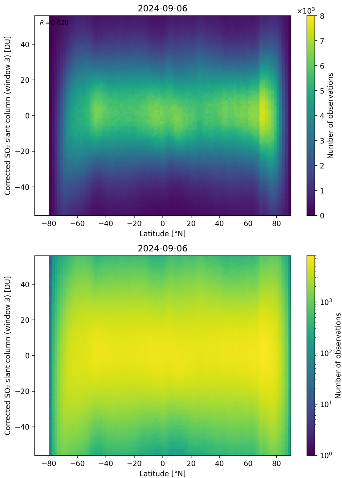
Figure 148: Scatter density plot of “Latitude” against “Corrected SO 2 slant column (window 3)” for 2024-09-06 to 2024-09-07.
