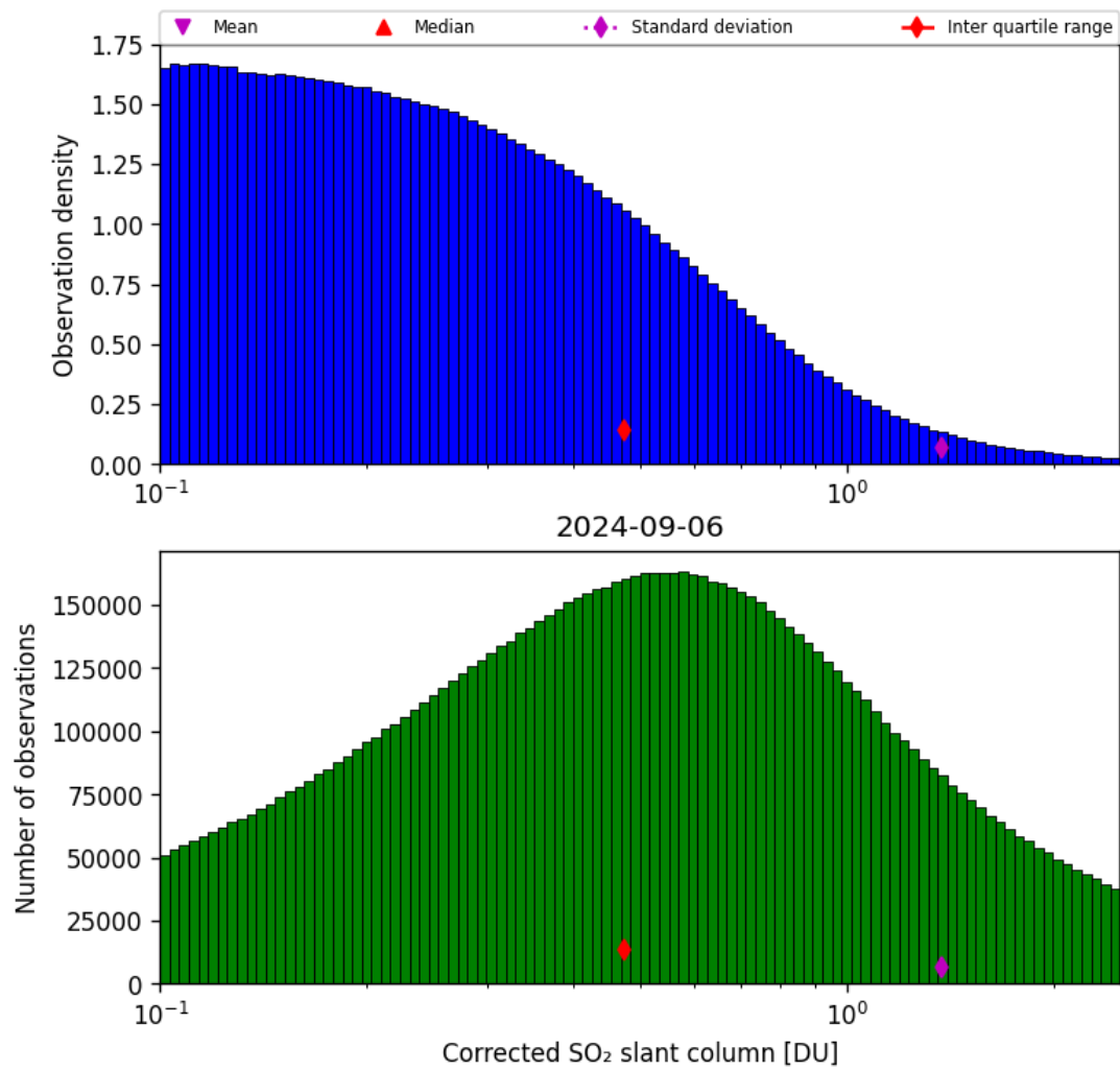
Figure 55: Histogram of “Corrected SO 2 slant column” for 2024-09-06 to 2024-09-07
