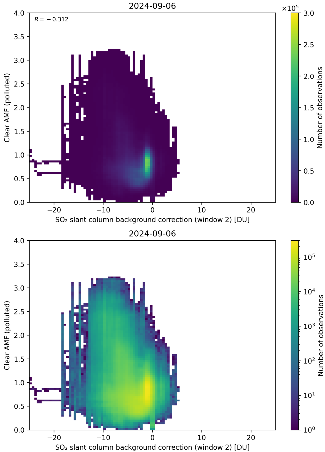
Figure 115: Scatter density plot of “SO 2 slant column background correction (window 2)” against “Clear AMF (polluted)” for 2024-09-06 to 2024-09-07.
