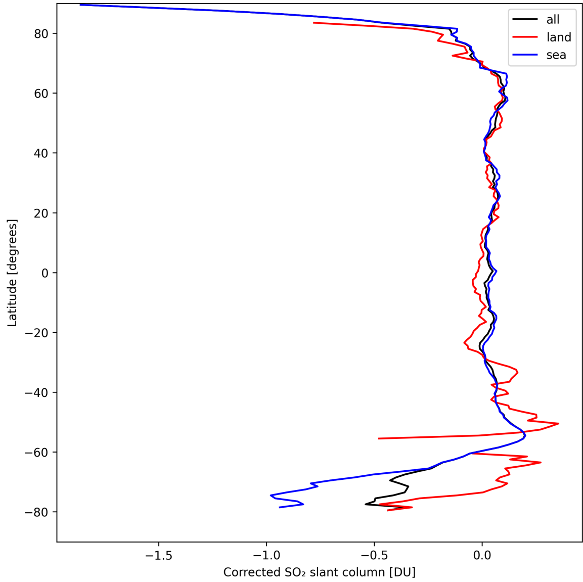
Figure 32: Zonal average of “Corrected SO 2 slant column” for 2024-09-06 to 2024-09-07.
