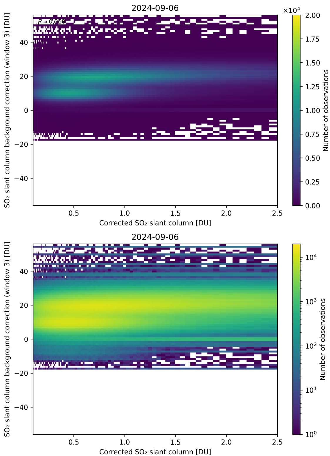
Figure 180: Scatter density plot of “Corrected SO 2 slant column” against “SO 2 slant column background correction (window 3)” for 2024-09-06 to 2024-09-07.
