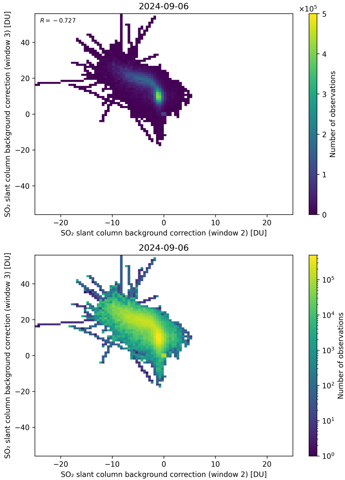
Figure 111: Scatter density plot of “SO 2 slant column background correction (window 2)” against “SO 2 slant column background correction (window 3)” for 2024-09-06 to 2024-09-07.
