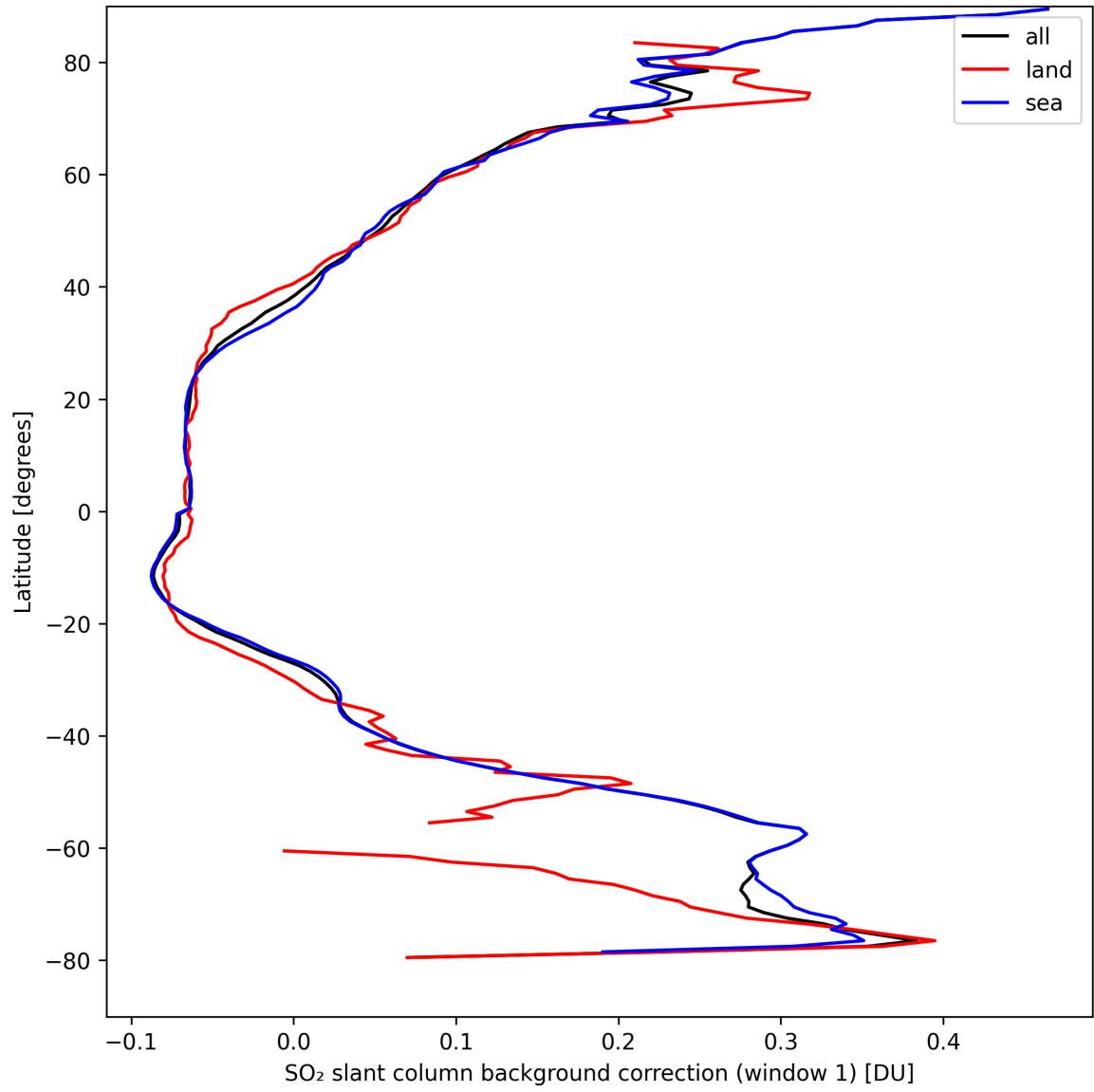
Figure 36: Zonal average of “SO 2 slant column background correction (window 1)” for 2024-09-06 to 2024-09-07.
