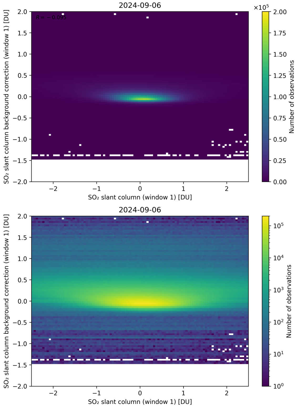
Figure 212: Scatter density plot of “SO 2 slant column (window 1)” against “SO 2 slant column background correction (window 1)” for 2024-09-06 to 2024-09-07.
