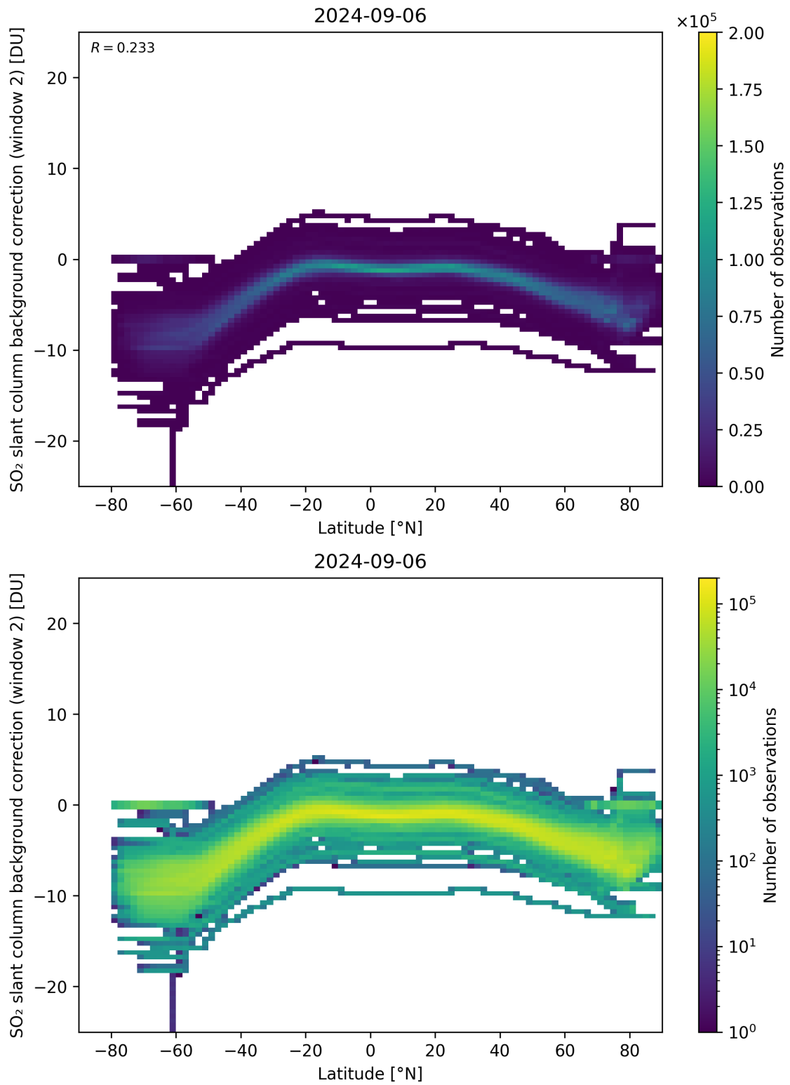
Figure 140: Scatter density plot of “Latitude” against “SO 2 slant column background correction (window 2)” for 2024-09-06 to 2024-09-07.
