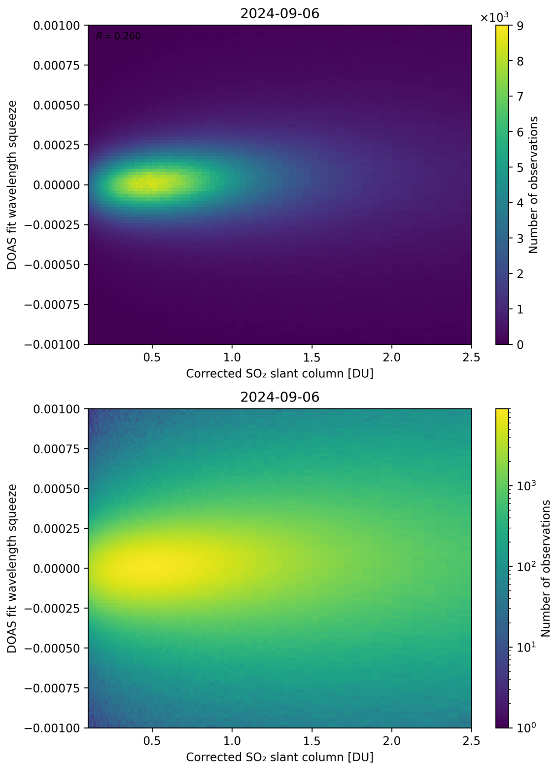
Figure 182: Scatter density plot of “Corrected SO 2 slant column” against “DOAS fit wavelength squeeze” for 2024-09-06 to 2024-09-07.
