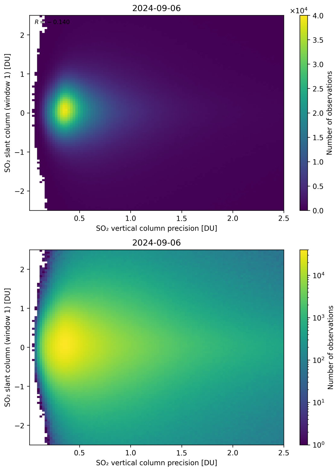
Figure 289: Scatter density plot of “SO 2 vertical column precision” against “SO 2 slant column (window 1)” for 2024-09-06 to 2024-09-07.
