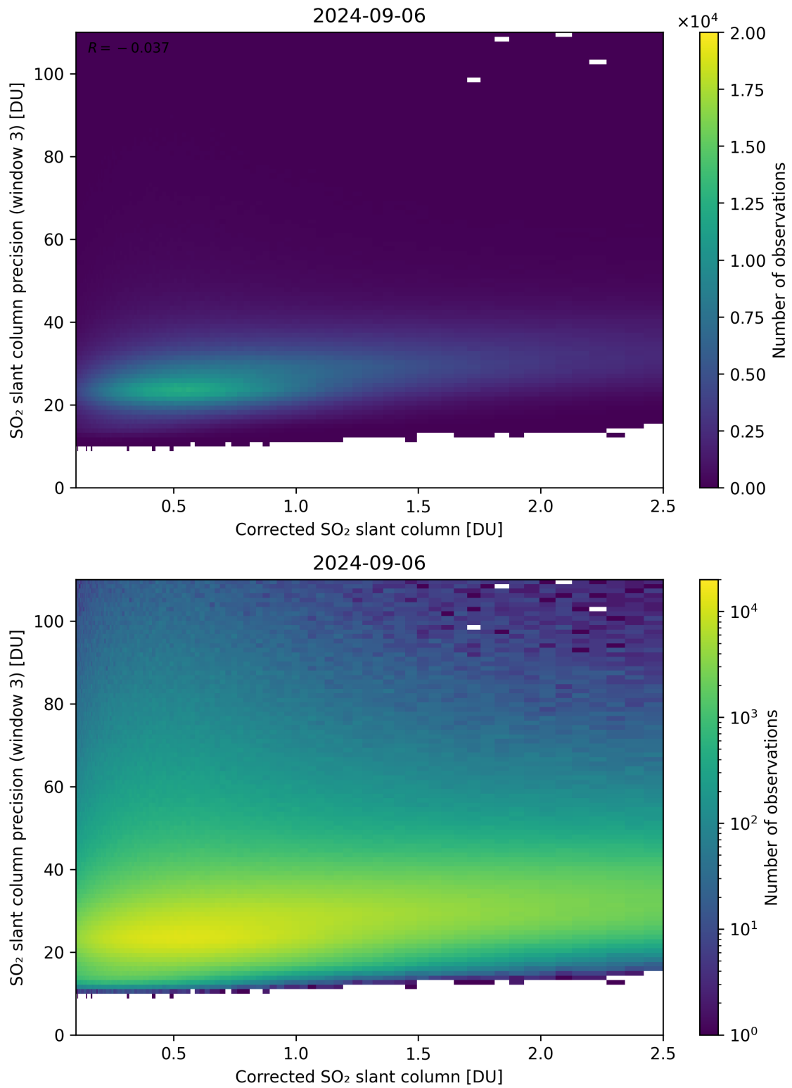
Figure 191: Scatter density plot of “Corrected SO 2 slant column” against “SO 2 slant column precision (window 3)” for 2024-09-06 to 2024-09-07.
