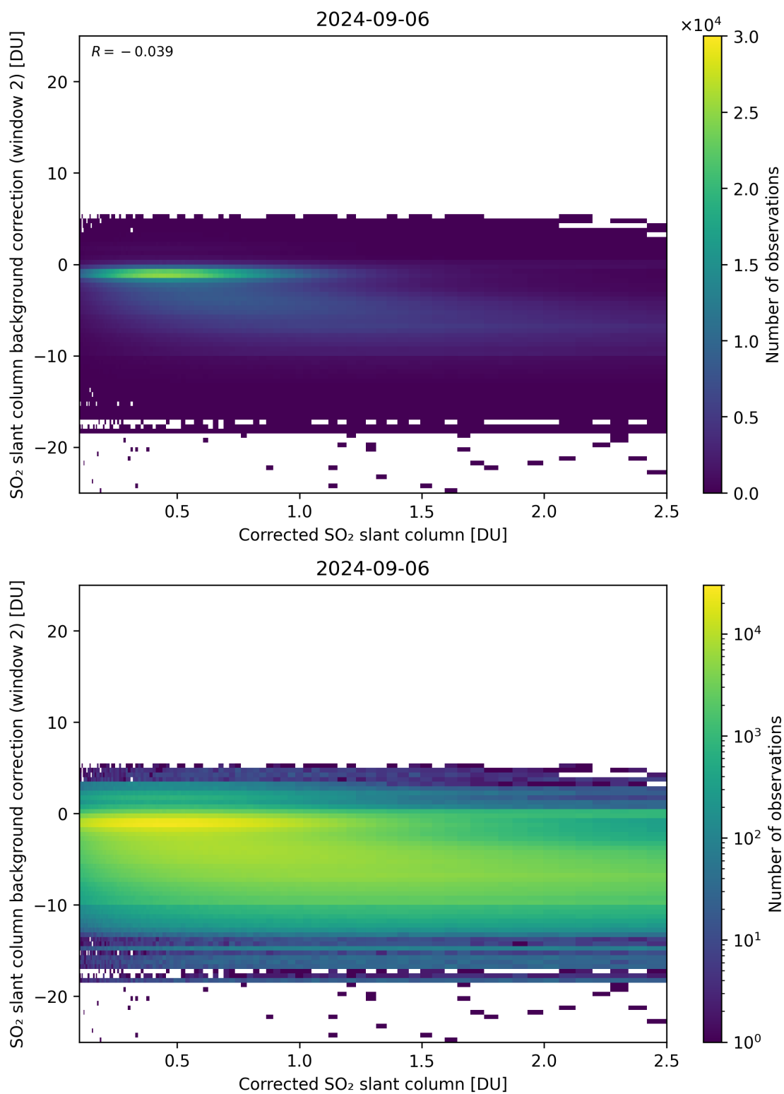
Figure 179: Scatter density plot of “Corrected SO 2 slant column” against “SO 2 slant column background correction (window 2)” for 2024-09-06 to 2024-09-07.
