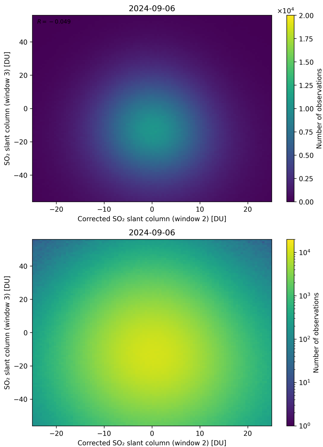
Figure 201: Scatter density plot of “Corrected SO 2 slant column (window 2)” against “SO 2 slant column (window 3)” for 2024-09-06 to 2024-09-07.
