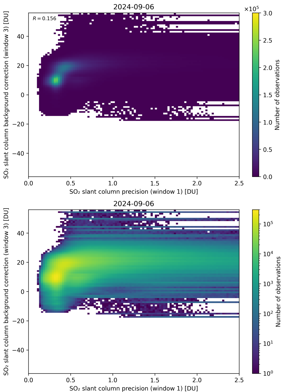
Figure 220: Scatter density plot of “SO 2 slant column precision (window 1)” against “SO 2 slant column background correction (window 3)” for 2024-09-06 to 2024-09-07.
