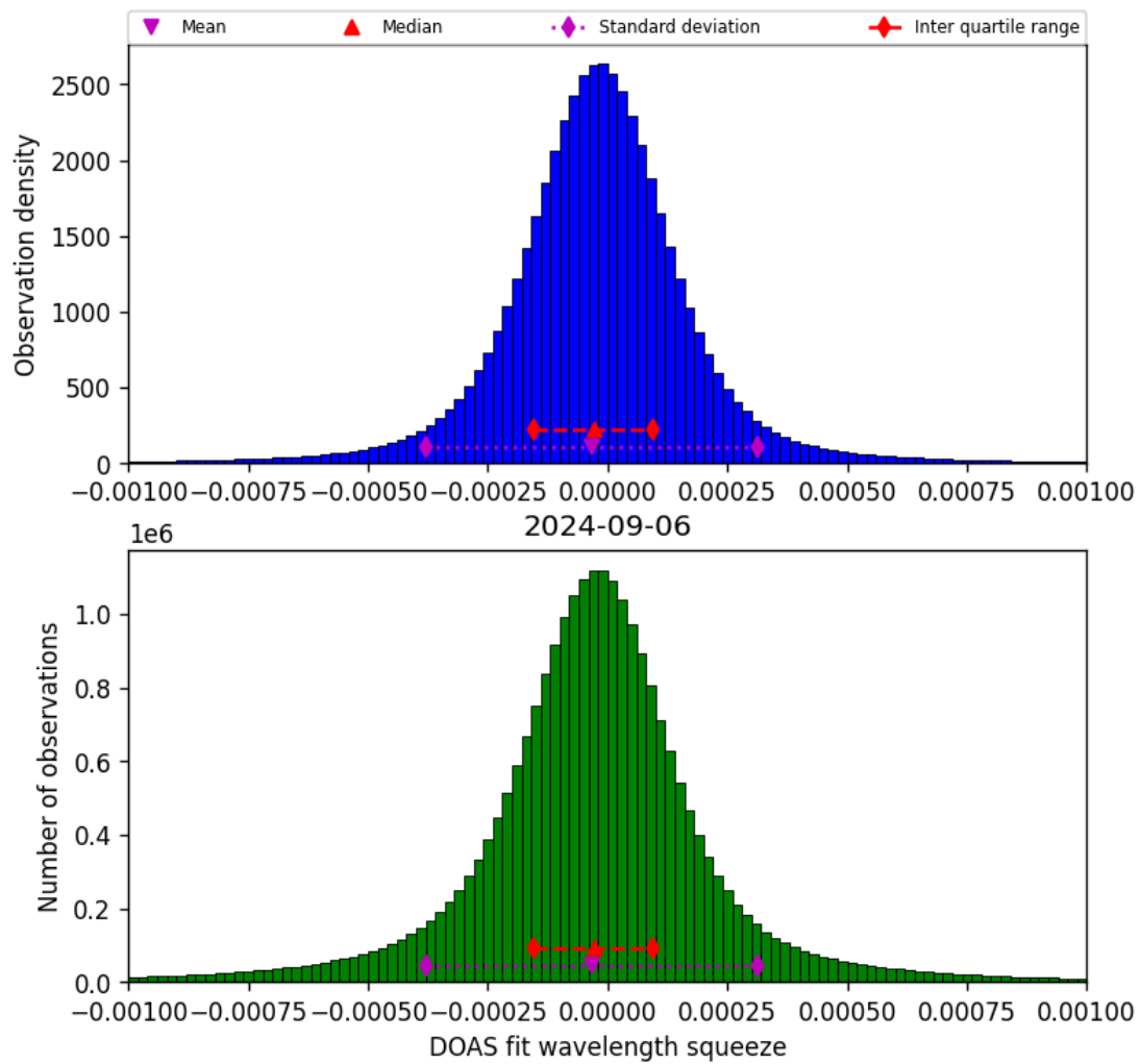
Figure 69: Histogram of “DOAS fit wavelength squeeze” for 2024-09-06 to 2024-09-07
