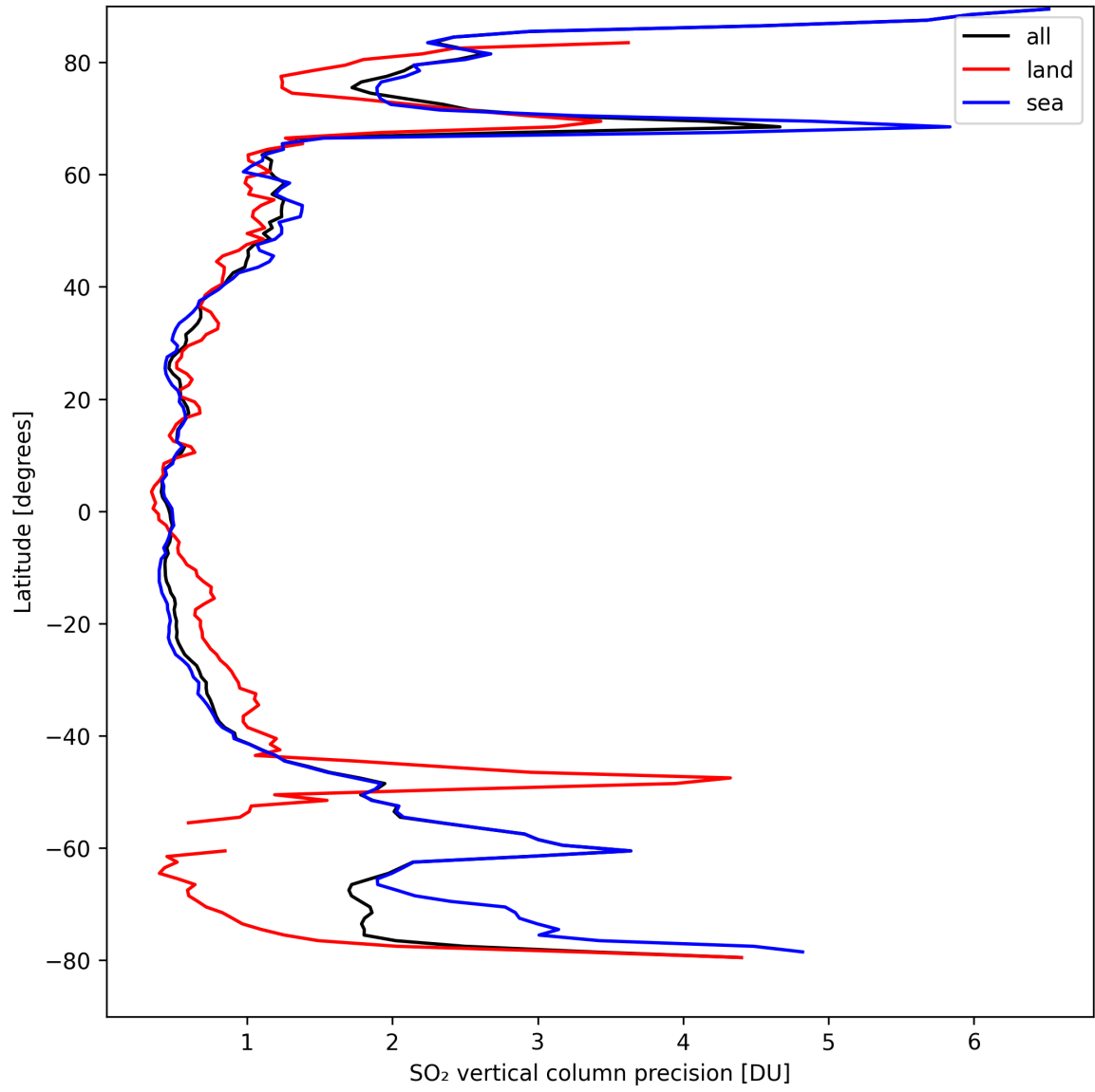
Figure 31: Zonal average of “SO 2 vertical column precision” for 2024-09-06 to 2024-09-07.
