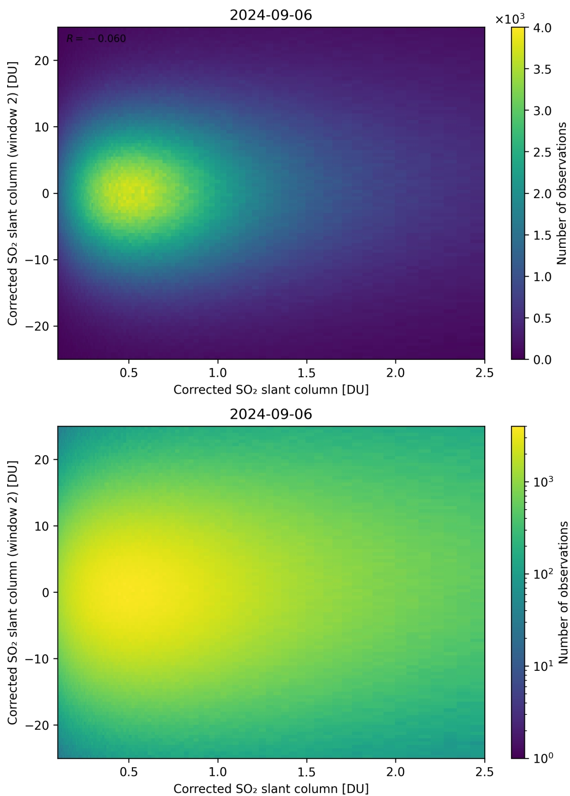
Figure 185: Scatter density plot of “Corrected SO 2 slant column” against “Corrected SO 2 slant column (window 2)” for 2024-09-06 to 2024-09-07.
