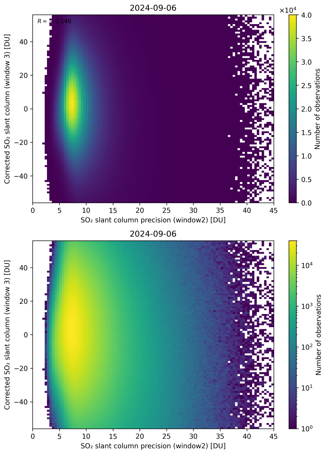
Figure 248: Scatter density plot of “SO 2 slant column precision (window2)” against “Corrected SO 2 slant column (window 3)” for 2024-09-06 to 2024-09-07.
