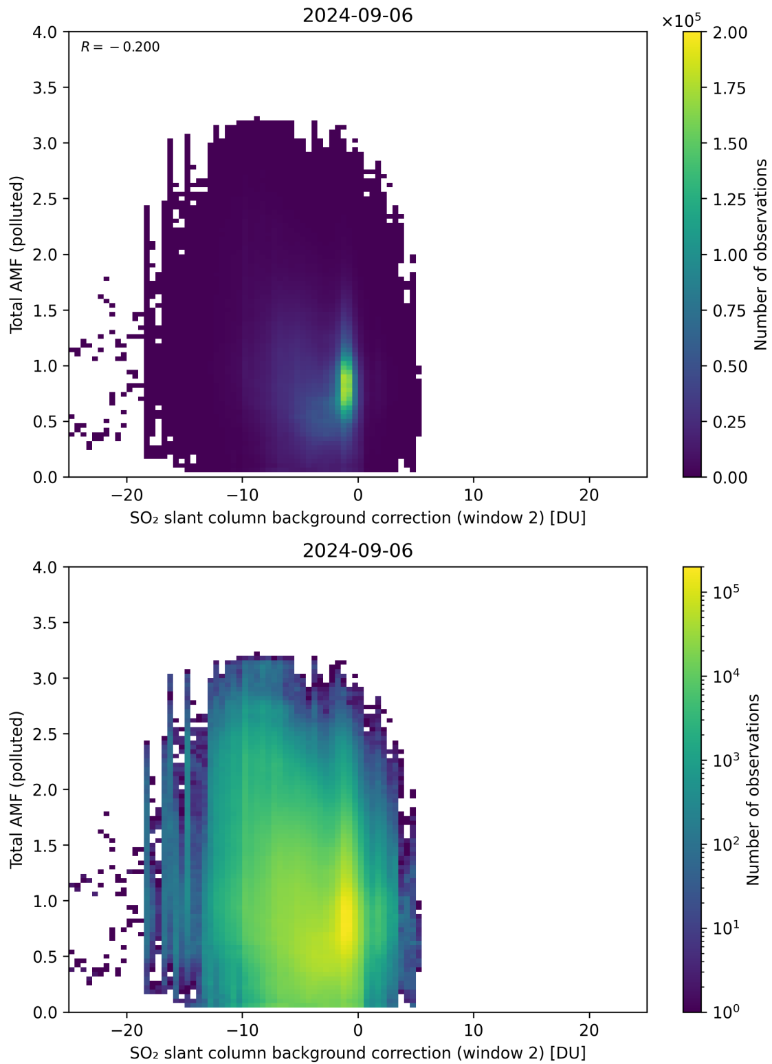
Figure 119: Scatter density plot of “SO 2 slant column background correction (window 2)” against “Total AMF (polluted)” for 2024-09-06 to 2024-09-07.
