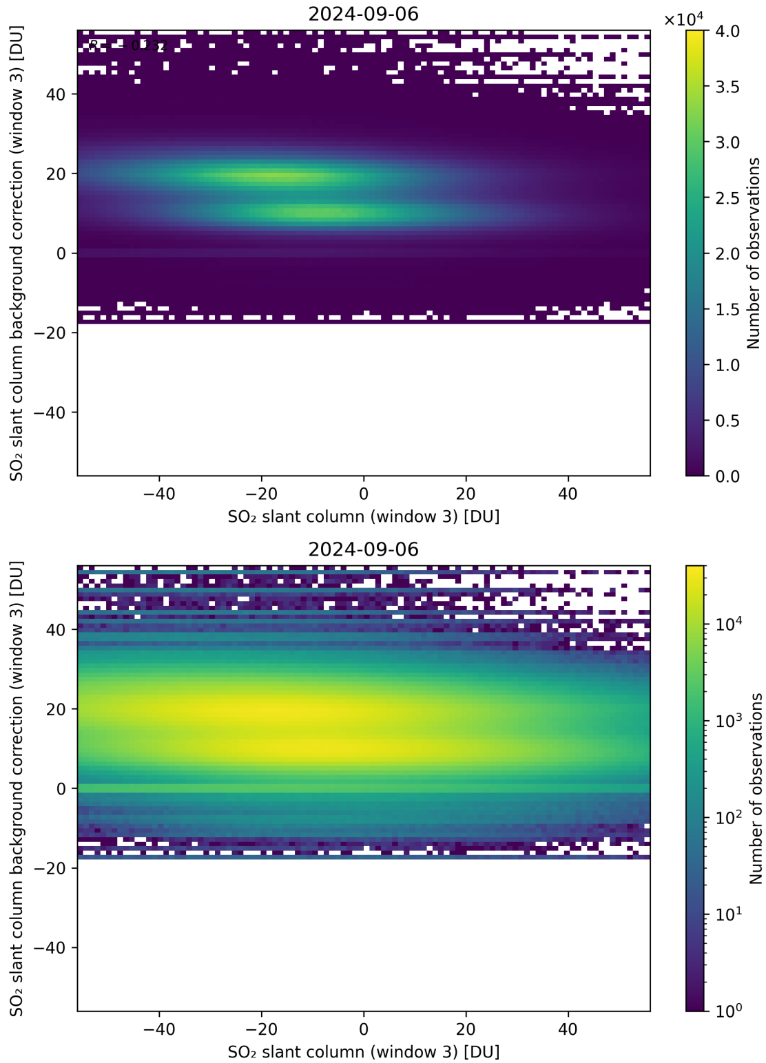
Figure 253: Scatter density plot of “SO 2 slant column (window 3)” against “SO 2 slant column background correction (window 3)” for 2024-09-06 to 2024-09-07.
