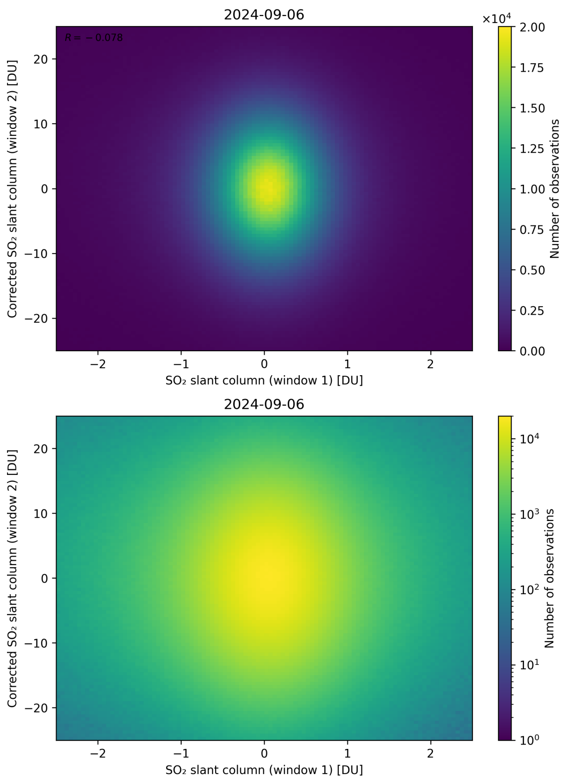
Figure 233: Scatter density plot of “SO 2 slant column (window 1)” against “Corrected SO 2 slant column (window 2)” for 2024-09-06 to 2024-09-07.
