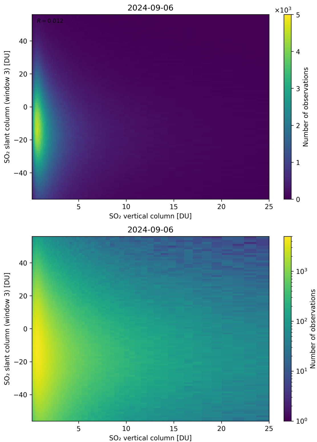
Figure 303: Scatter density plot of “SO 2 vertical column” against “SO 2 slant column (window 3)” for 2024-09-06 to 2024-09-07.
