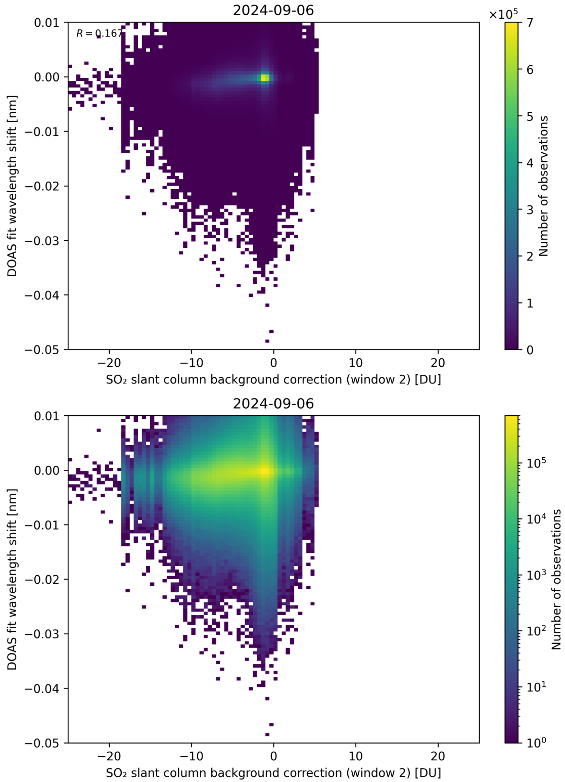
Figure 112: Scatter density plot of “SO 2 slant column background correction (window 2)” against “DOAS fit wavelength shift” for 2024-09-06 to 2024-09-07.
