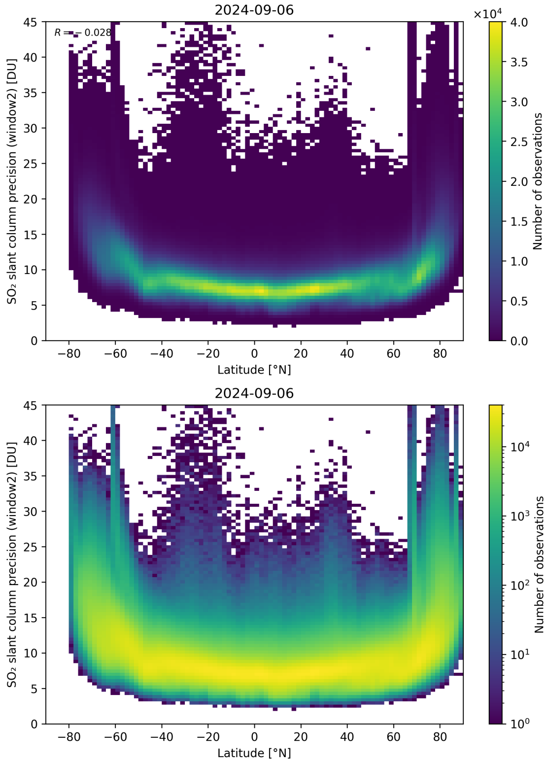
Figure 151: Scatter density plot of “Latitude” against “SO 2 slant column precision (window2)” for 2024-09-06 to 2024-09-07.
