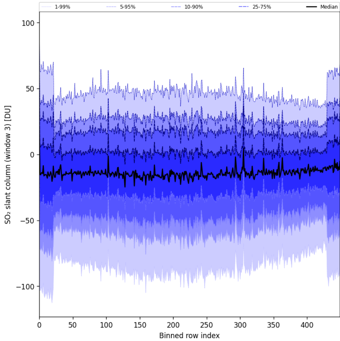
Figure 87: Along track statistics of “SO 2 slant column (window 3)” for 2024-09-06 to 2024-09-07
