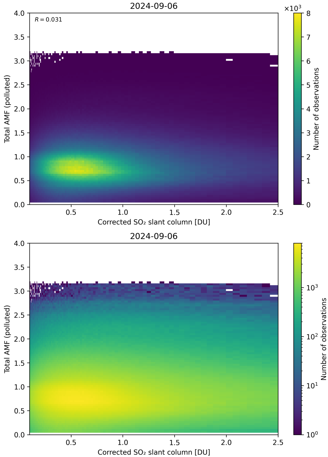
Figure 192: Scatter density plot of “Corrected SO 2 slant column” against “Total AMF (polluted)” for 2024-09-06 to 2024-09-07.
