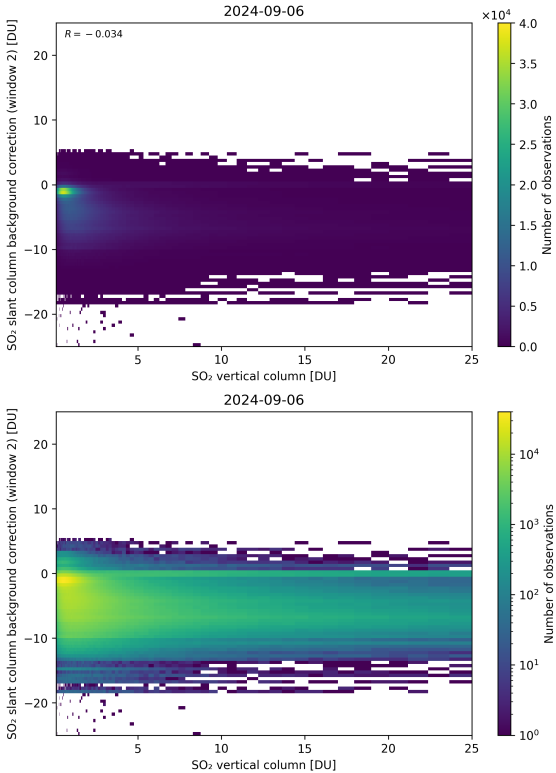
Figure 274: Scatter density plot of “SO 2 vertical column” against “SO 2 slant column background correction (window 2)” for 2024-09-06 to 2024-09-07.
