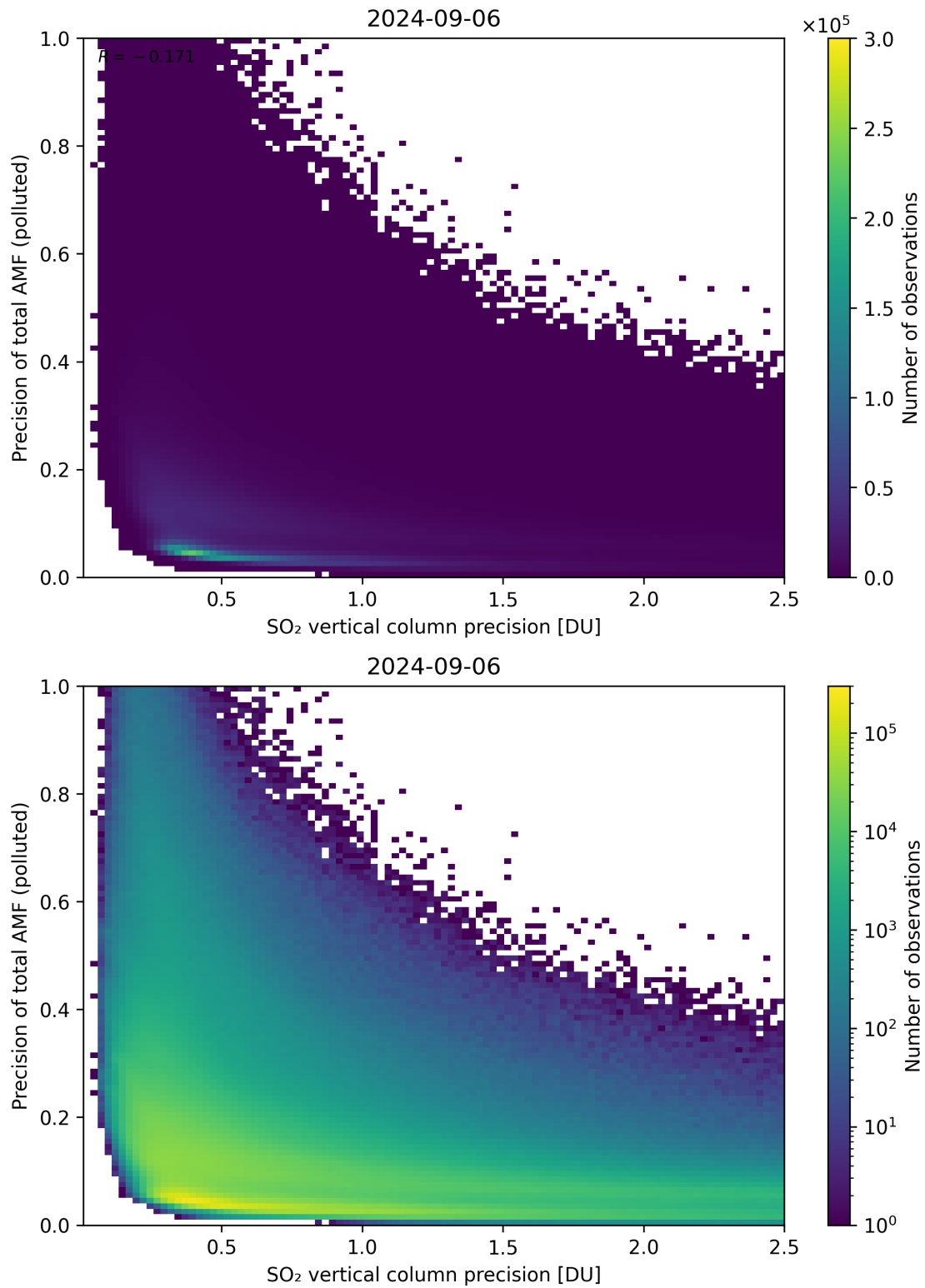
Figure 295: Scatter density plot of “SO 2 vertical column precision” against “Precision of total AMF (polluted)” for 2024-09-06 to 2024-09-07.
