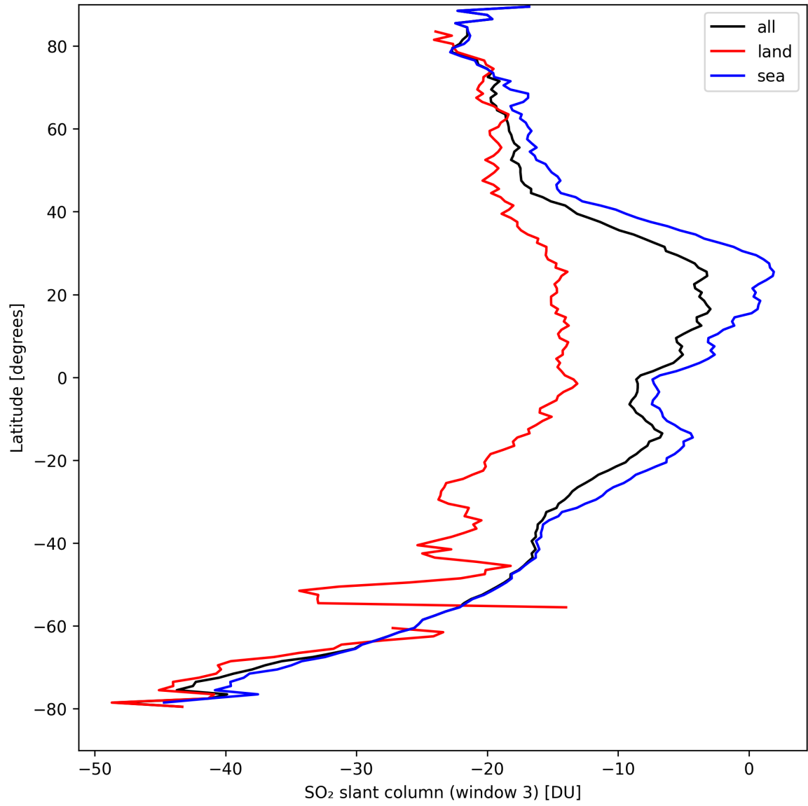
Figure 41: Zonal average of “SO 2 slant column (window 3)” for 2024-09-06 to 2024-09-07.
