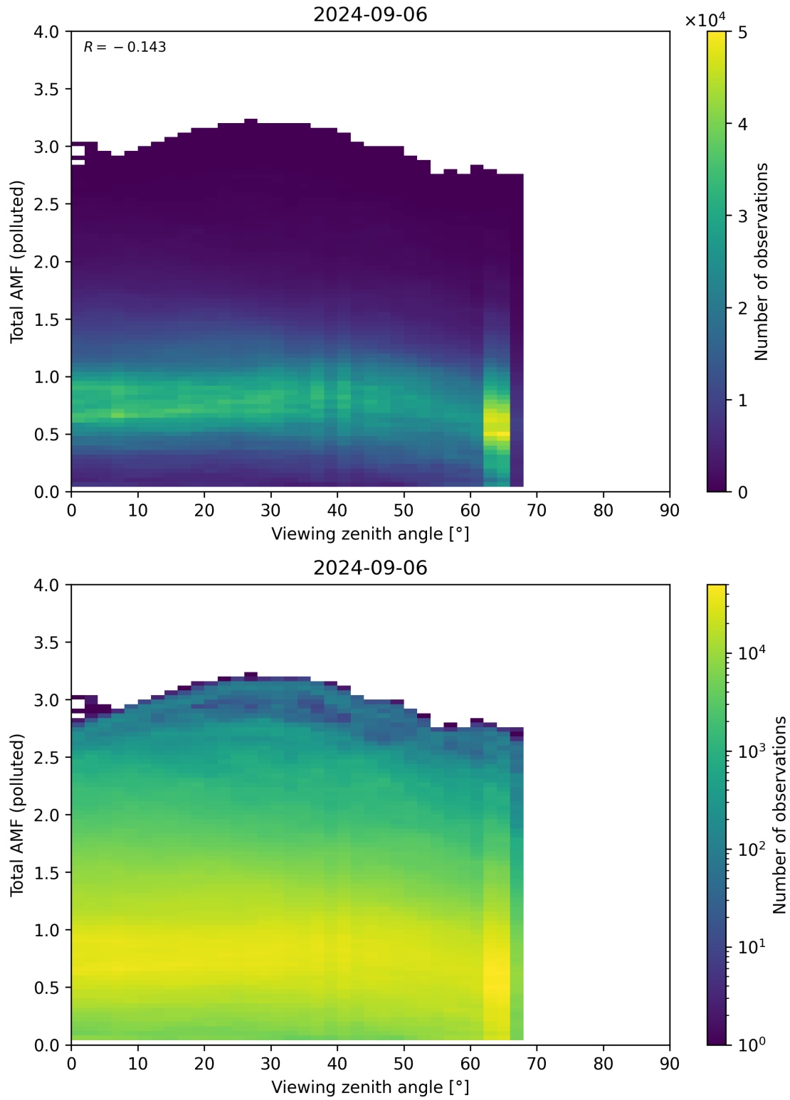
Figure 325: Scatter density plot of “Viewing zenith angle” against “Total AMF (polluted)” for 2024-09-06 to 2024-09-07.
