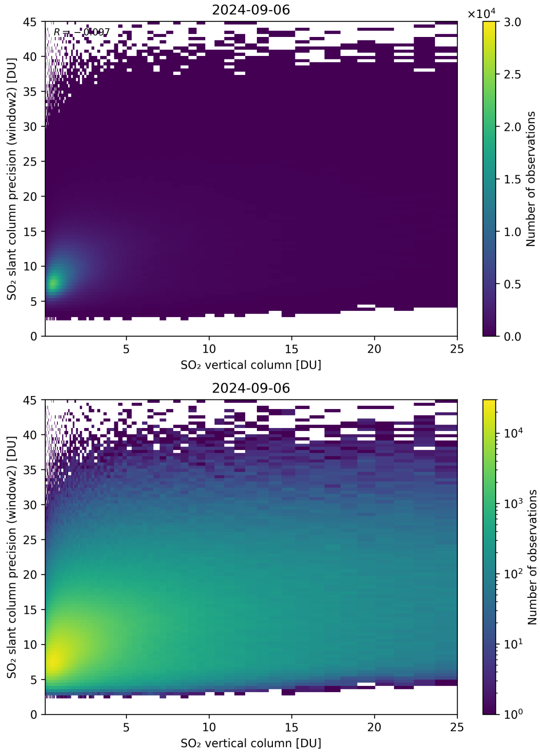
Figure 302: Scatter density plot of “SO 2 vertical column” against “SO 2 slant column precision (window2)” for 2024-09-06 to 2024-09-07.
