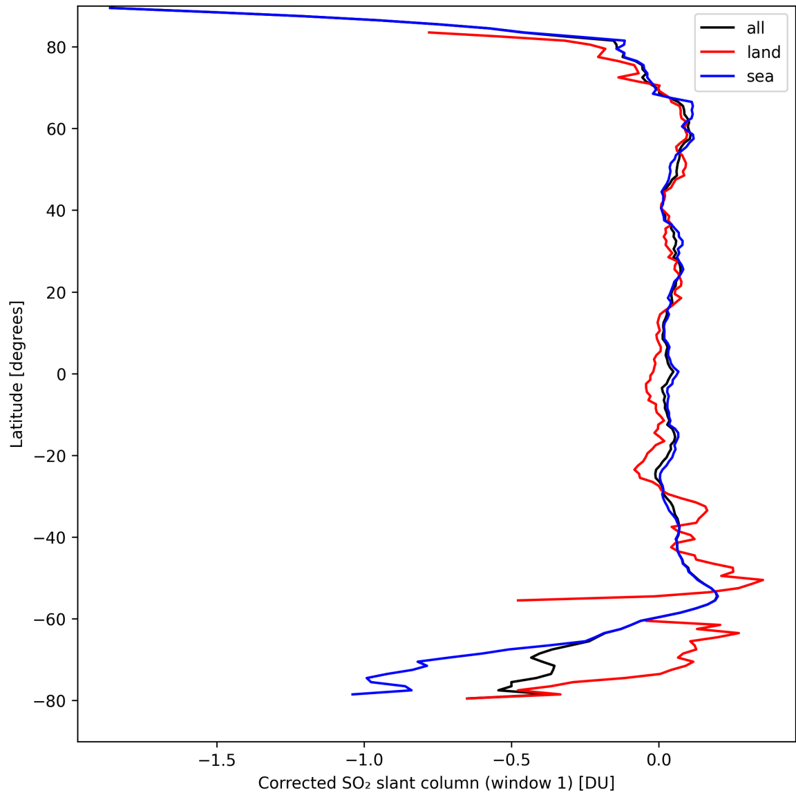
Figure 35: Zonal average of “Corrected SO 2 slant column (window 1)” for 2024-09-06 to 2024-09-07.
