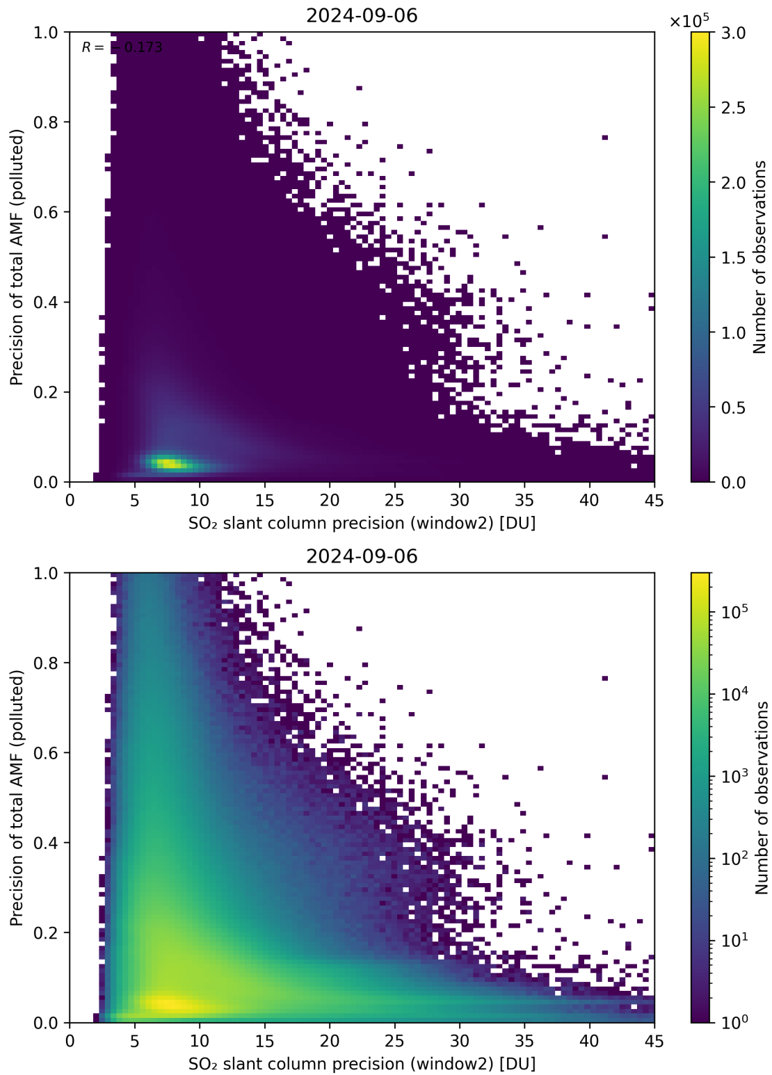
Figure 252: Scatter density plot of “SO 2 slant column precision (window2)” against “Precision of total AMF (polluted)” for 2024-09-06 to 2024-09-07.
