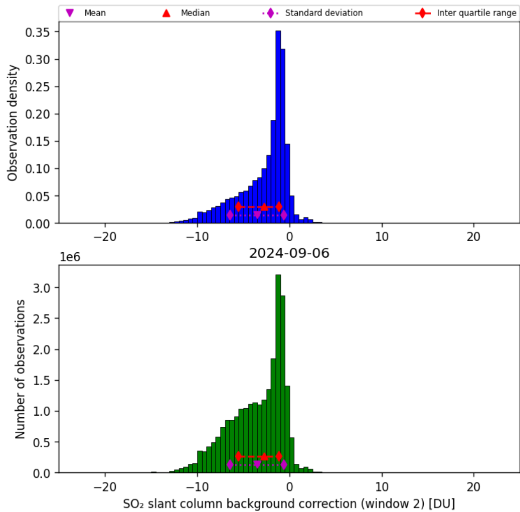
Figure 63: Histogram of “SO 2 slant column background correction (window 2)” for 2024-09-06 to 2024-09-07
