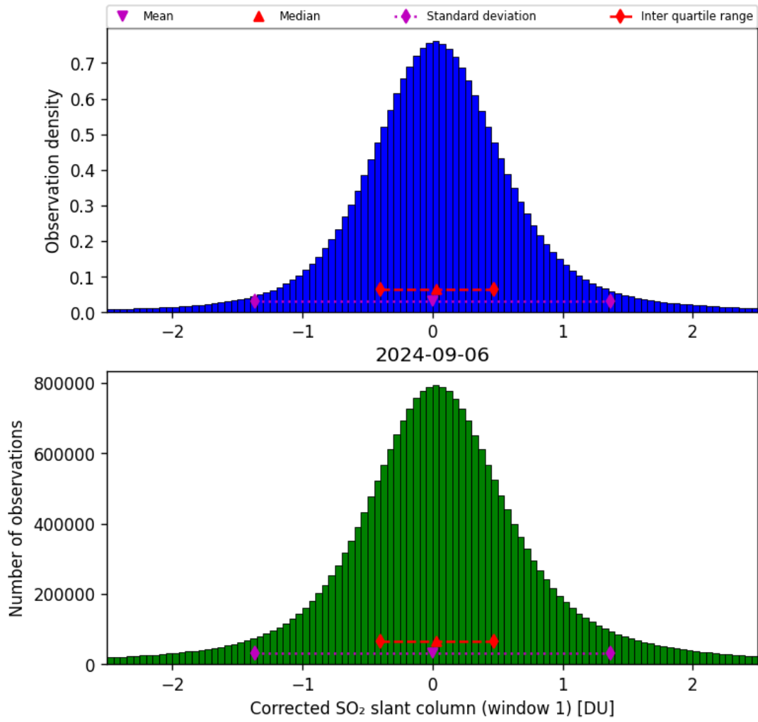
Figure 58: Histogram of “Corrected SO 2 slant column (window 1)” for 2024-09-06 to 2024-09-07
