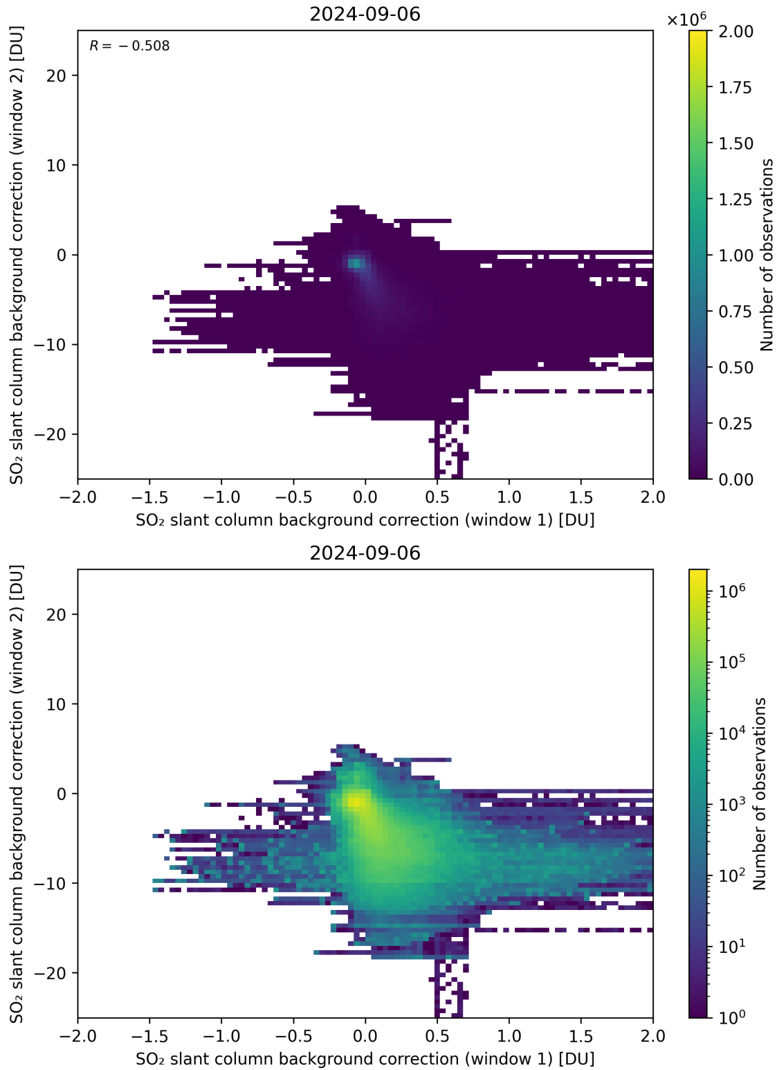
Figure 98: Scatter density plot of “SO 2 slant column background correction (window 1)” against “SO 2 slant column background correction (window 2)” for 2024-09-06 to 2024-09-07.
