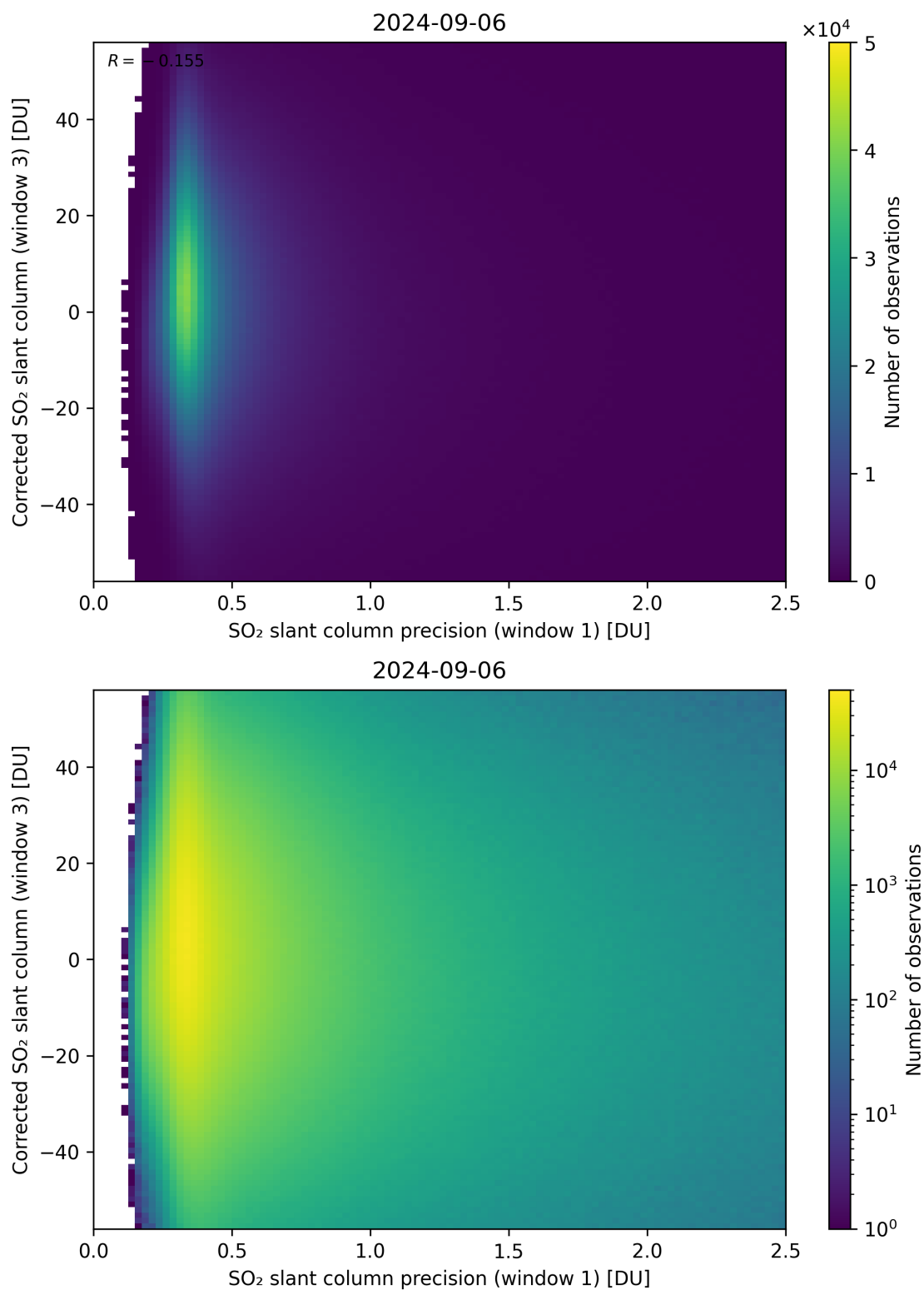
Figure 226: Scatter density plot of “SO 2 slant column precision (window 1)” against “Corrected SO 2 slant column (window 3)” for 2024-09-06 to 2024-09-07.
