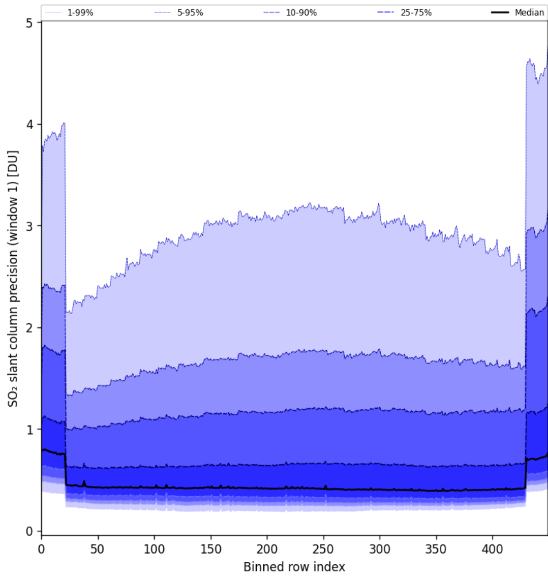
Figure 80: Along track statistics of “SO 2 slant column precision (window 1)” for 2024-09-06 to 2024-09-07
