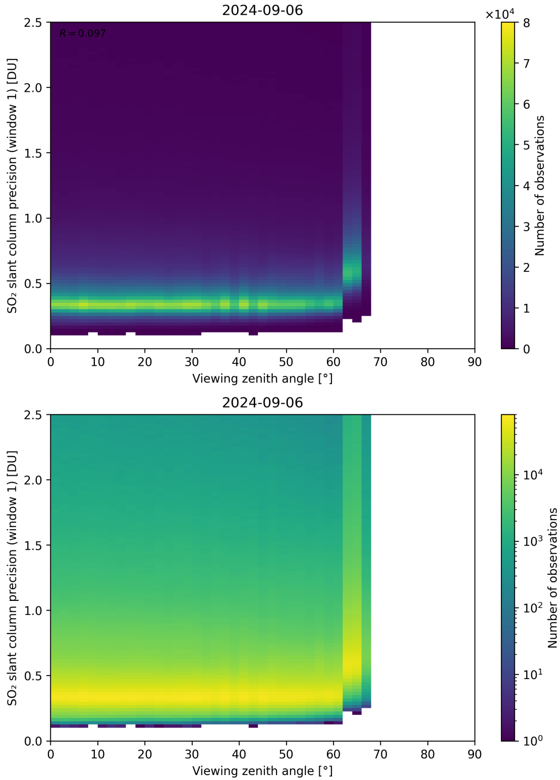
Figure 321: Scatter density plot of “Viewing zenith angle” against “SO 2 slant column precision (window 1)” for 2024-09-06 to 2024-09-07.
