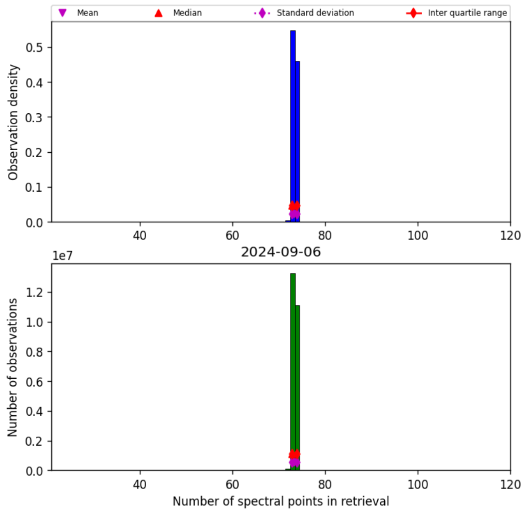
Figure 74: Histogram of “Number of spectral points in retrieval” for 2024-09-06 to 2024-09-07
