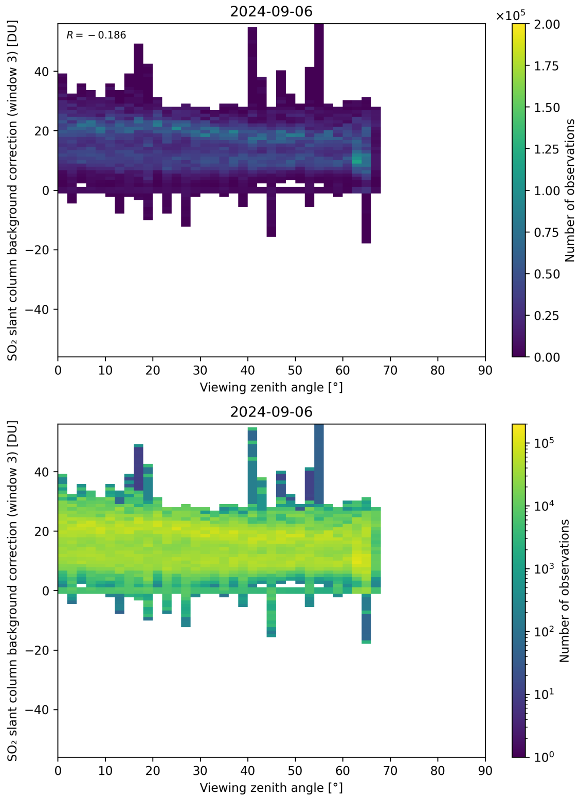
Figure 310: Scatter density plot of “Viewing zenith angle” against “SO 2 slant column background correction (window 3)” for 2024-09-06 to 2024-09-07.
