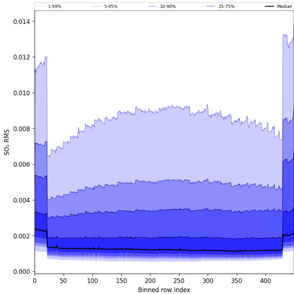
Figure 93: Along track statistics of “SO 2 RMS” for 2024-09-06 to 2024-09-07
