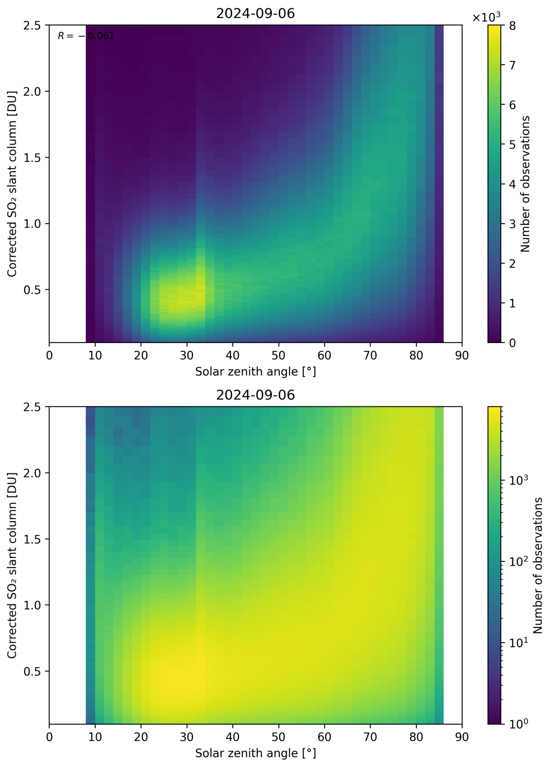
Figure 166: Scatter density plot of “Solar zenith angle” against “Corrected SO 2 slant column” for 2024-09-06 to 2024-09-07.
