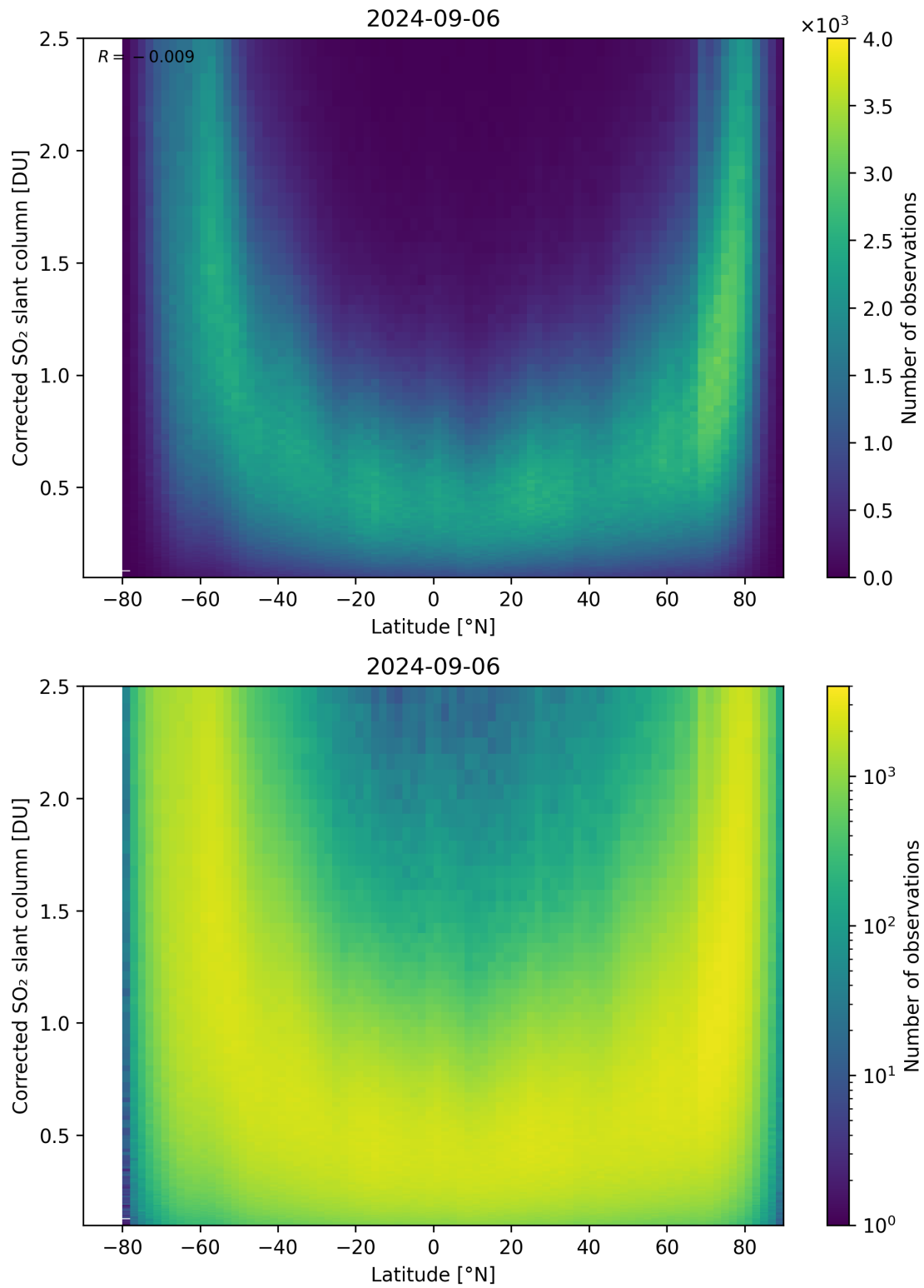
Figure 146: Scatter density plot of “Latitude” against “Corrected SO 2 slant column” for 2024-09-06 to 2024-09-07.
