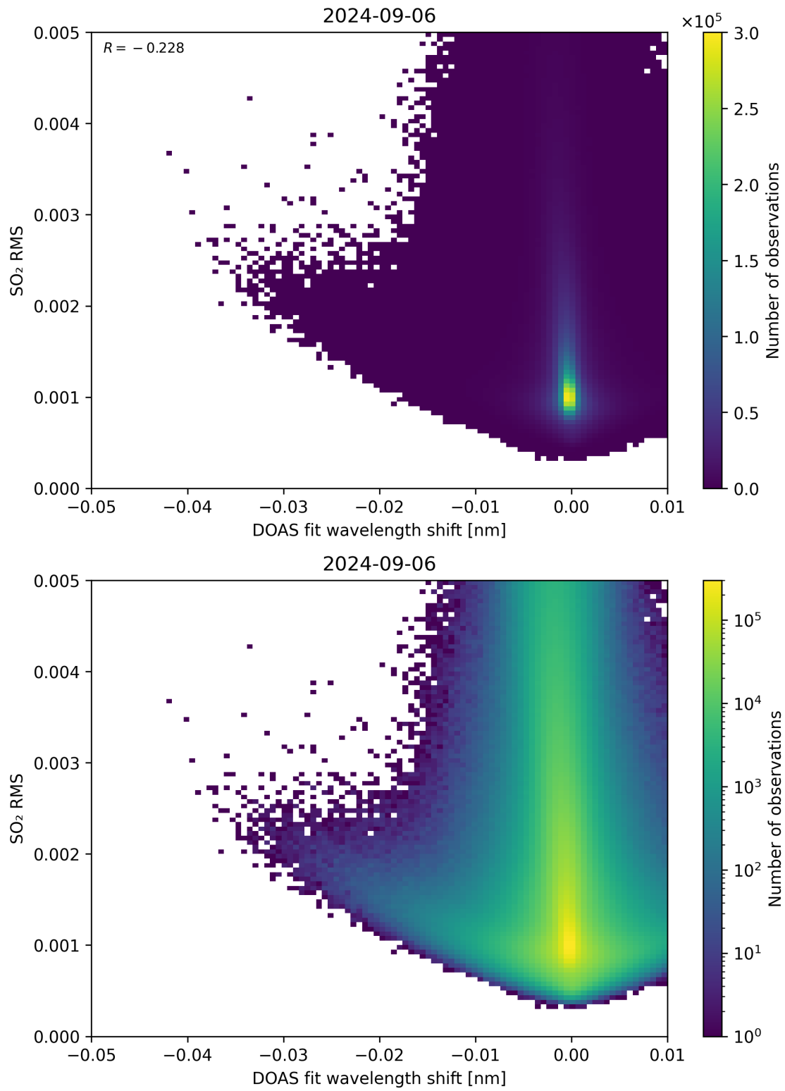
Figure 128: Scatter density plot of “DOAS fit wavelength shift” against “SO 2 RMS” for 2024-09-06 to 2024-09-07.
