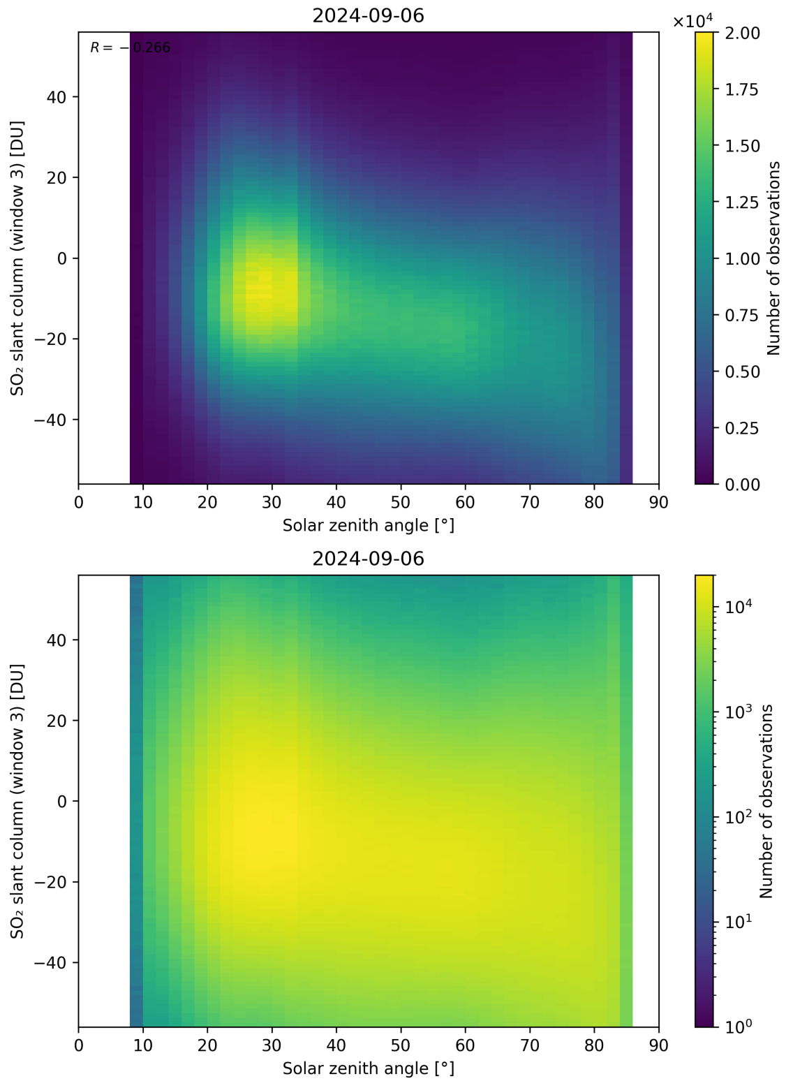
Figure 172: Scatter density plot of “Solar zenith angle” against “SO 2 slant column (window 3)” for 2024-09-06 to 2024-09-07.
