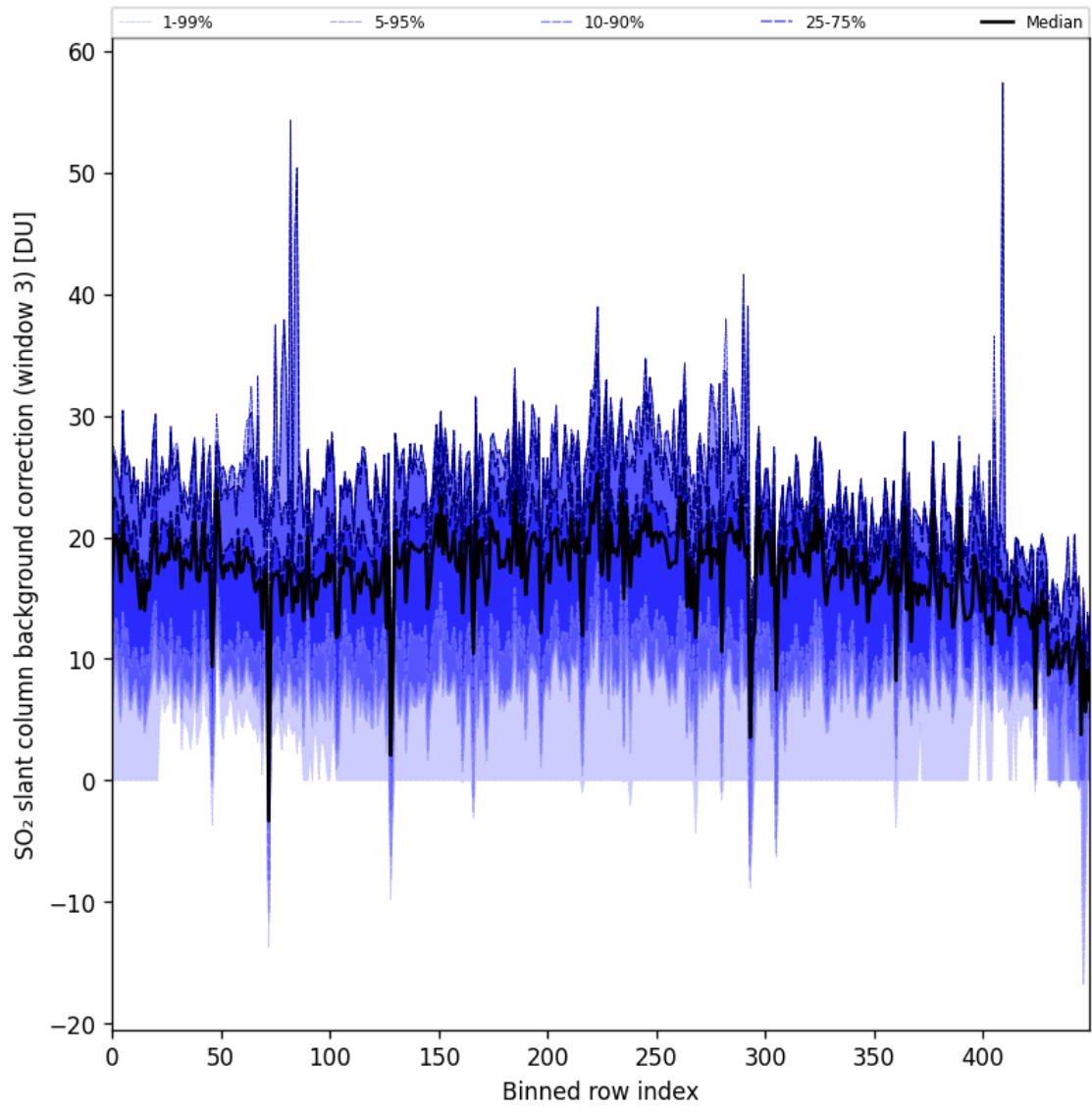
Figure 90: Along track statistics of “SO 2 slant column background correction (window 3)” for 2024-09-06 to 2024-09-07
