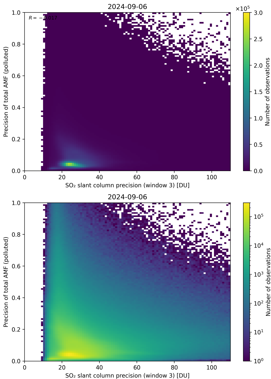
Figure 264: Scatter density plot of “SO 2 slant column precision (window 3)” against “Precision of total AMF (polluted)” for 2024-09-06 to 2024-09-07.
