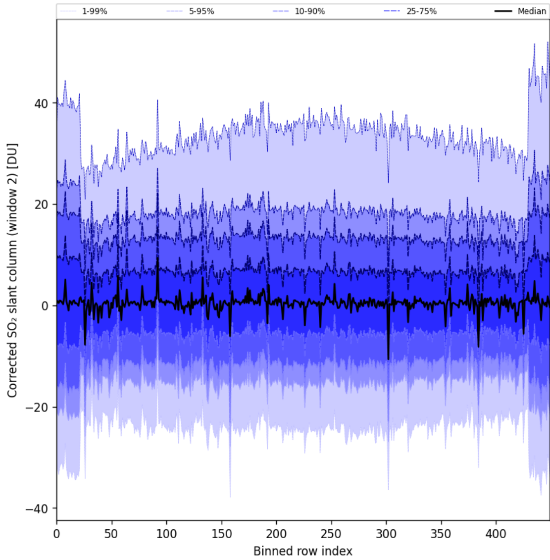
Figure 85: Along track statistics of “Corrected SO 2 slant column (window 2)” for 2024-09-06 to 2024-09-07
