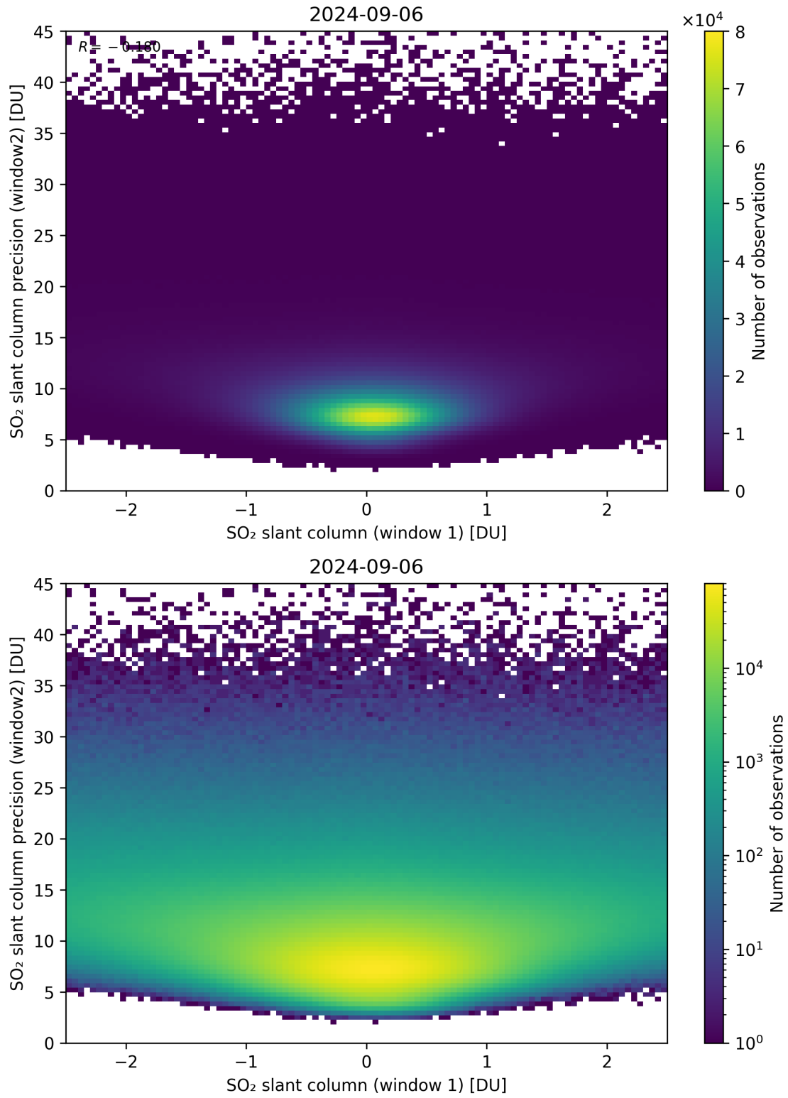
Figure 236: Scatter density plot of “SO 2 slant column (window 1)” against “SO 2 slant column precision (window2)” for 2024-09-06 to 2024-09-07.
