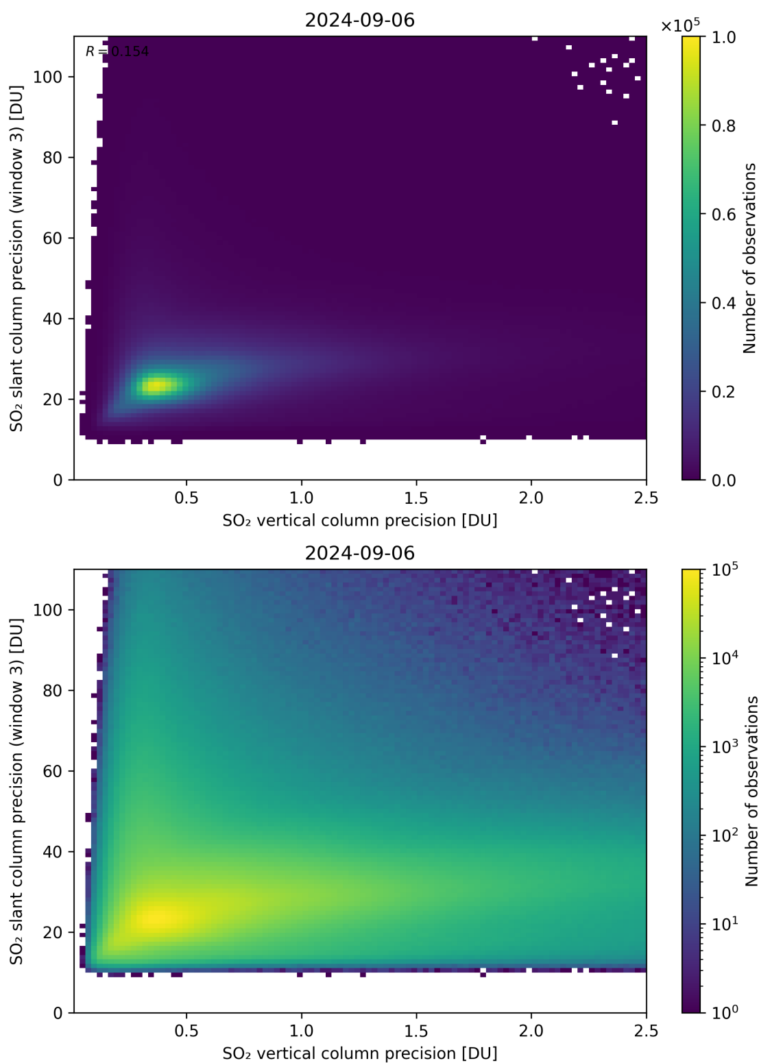
Figure 293: Scatter density plot of “SO 2 vertical column precision” against “SO 2 slant column precision (window 3)” for 2024-09-06 to 2024-09-07.
