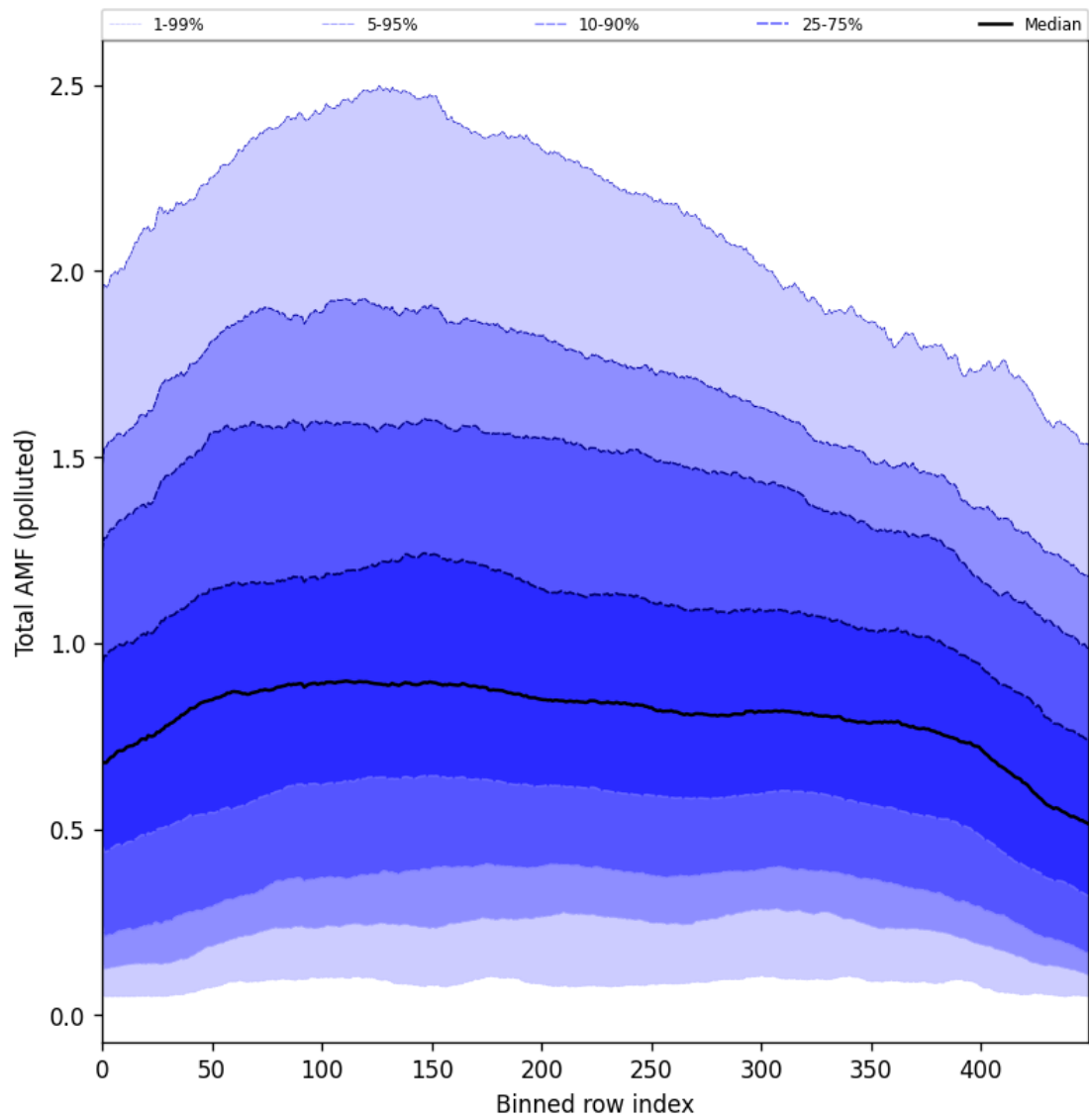
Figure 94: Along track statistics of “Total AMF (polluted)” for 2024-09-06 to 2024-09-07
