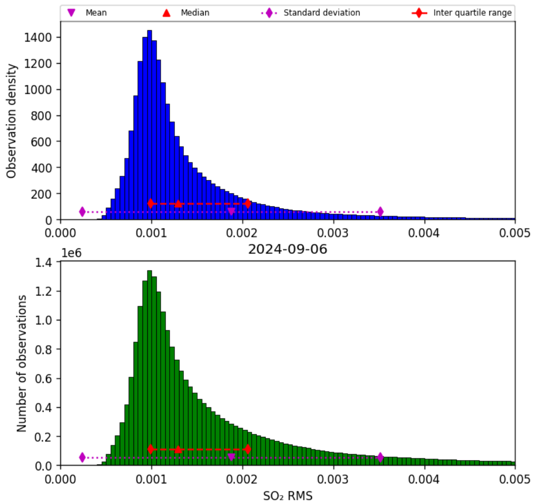
Figure 70: Histogram of “SO 2 RMS” for 2024-09-06 to 2024-09-07
