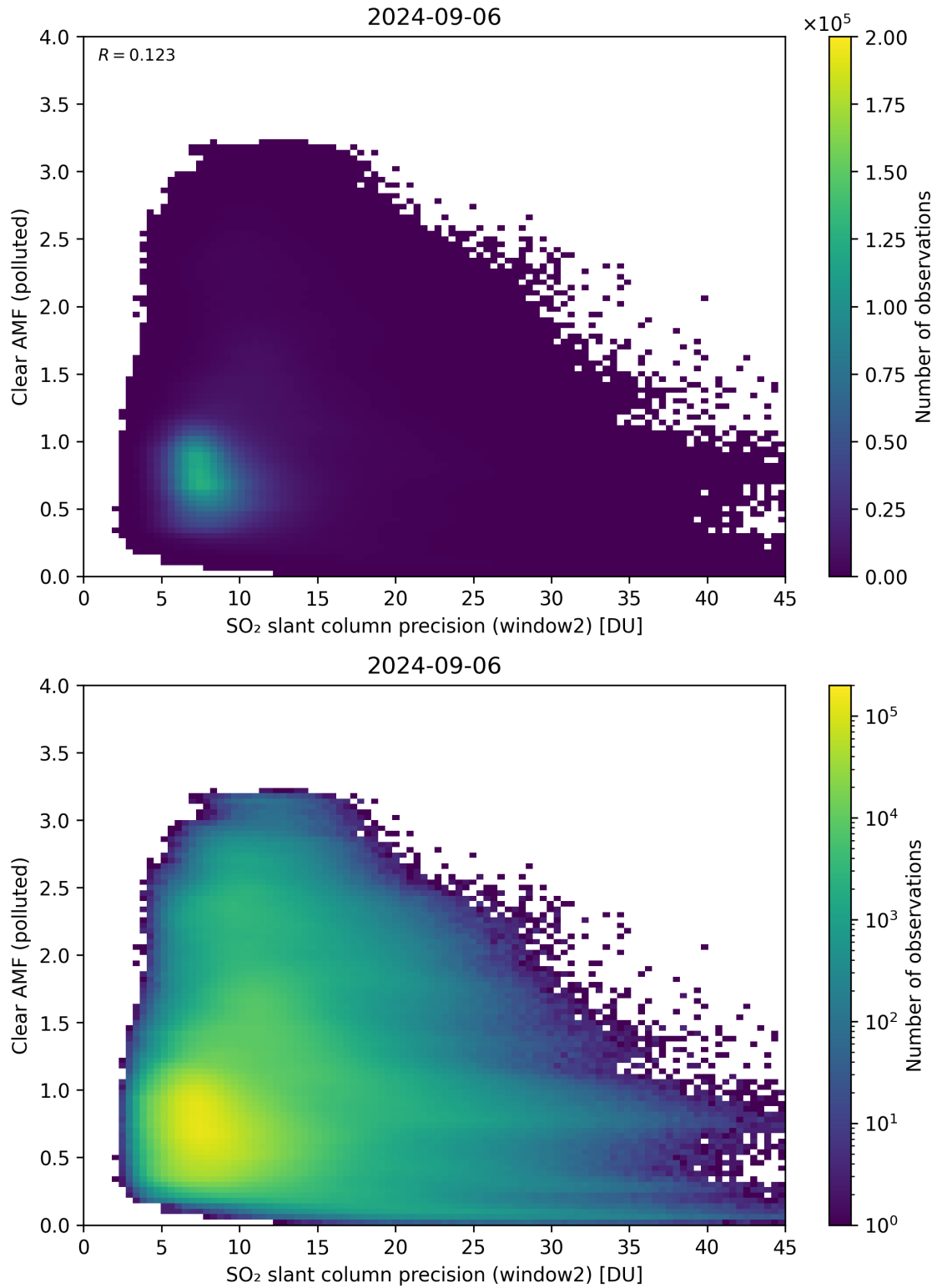
Figure 246: Scatter density plot of “SO 2 slant column precision (window2)” against “Clear AMF (polluted)” for 2024-09-06 to 2024-09-07.
