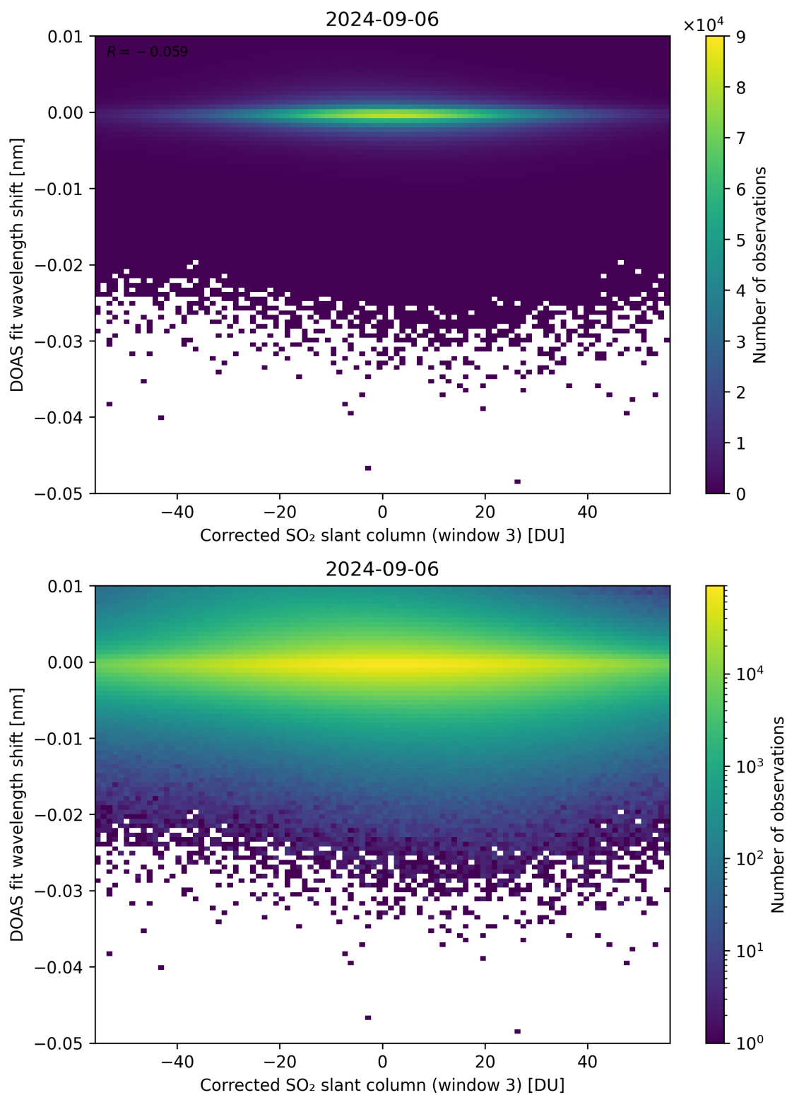
Figure 206: Scatter density plot of “Corrected SO 2 slant column (window 3)” against “DOAS fit wavelength shift” for 2024-09-06 to 2024-09-07.
