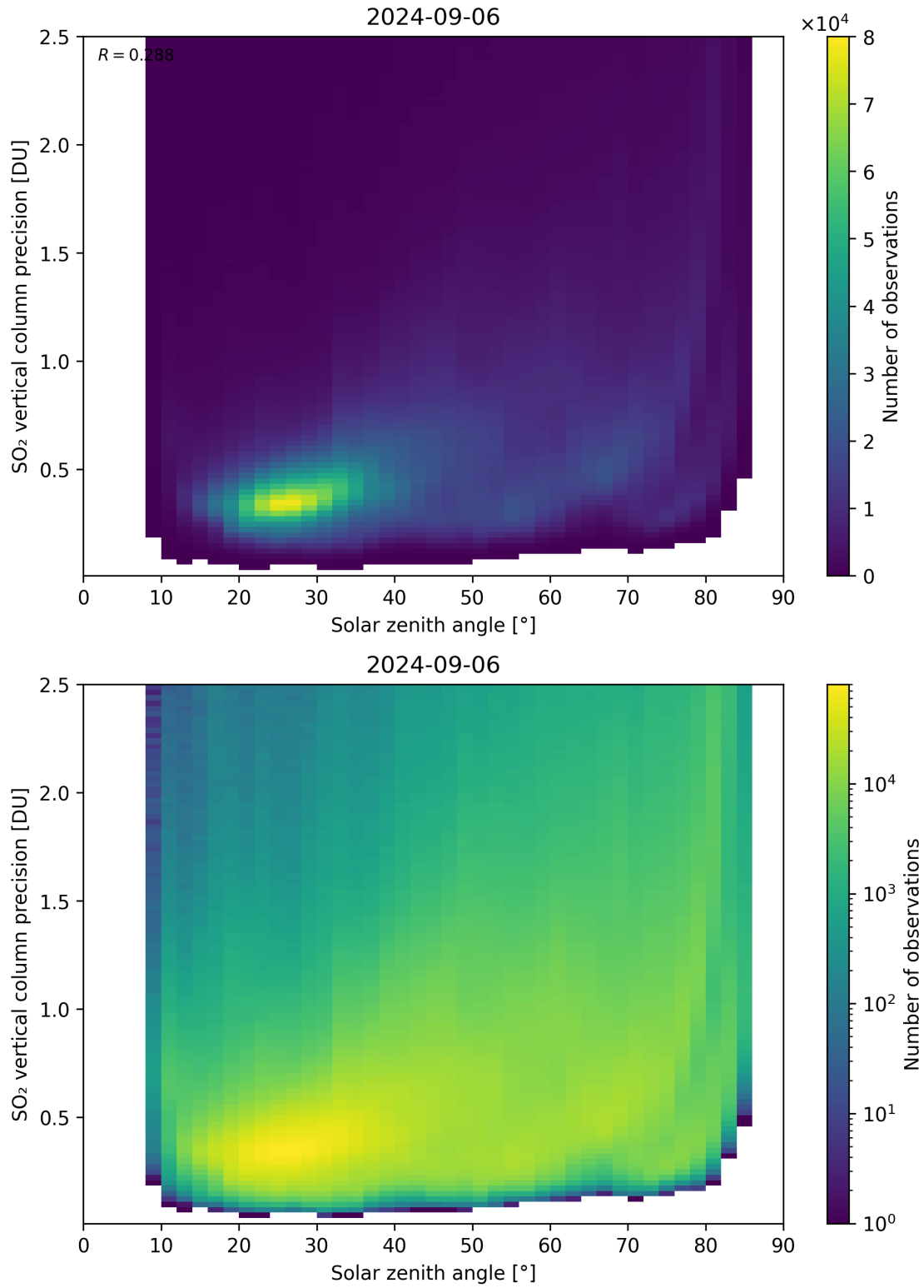
Figure 177: Scatter density plot of “Solar zenith angle” against “SO 2 vertical column precision” for 2024-09-06 to 2024-09-07.
