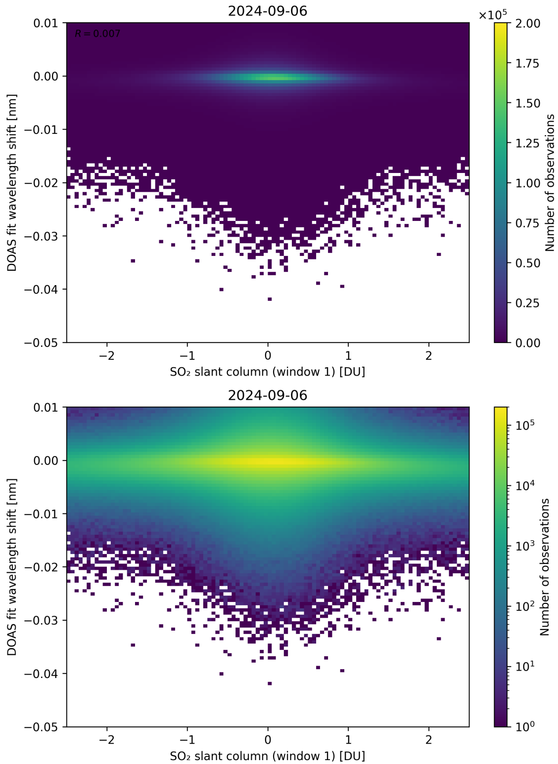
Figure 215: Scatter density plot of “SO 2 slant column (window 1)” against “DOAS fit wavelength shift” for 2024-09-06 to 2024-09-07.
