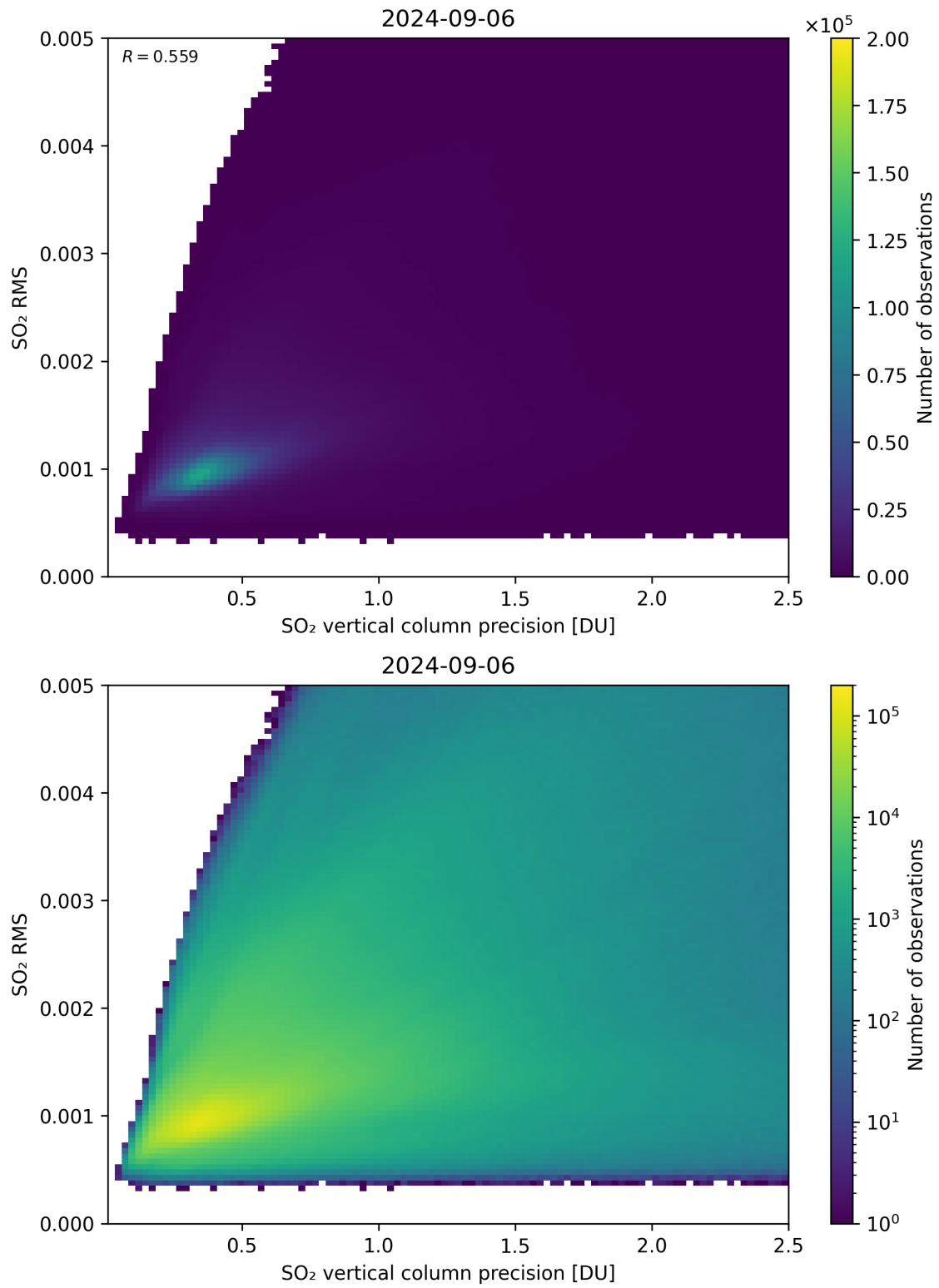
Figure 284: Scatter density plot of “SO 2 vertical column precision” against “SO 2 RMS” for 2024-09-06 to 2024-09-07.
