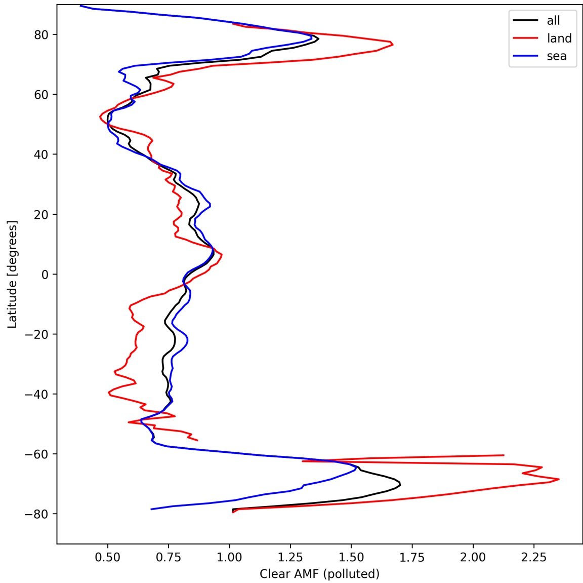
Figure 50: Zonal average of “Clear AMF (polluted)” for 2024-09-06 to 2024-09-07.
