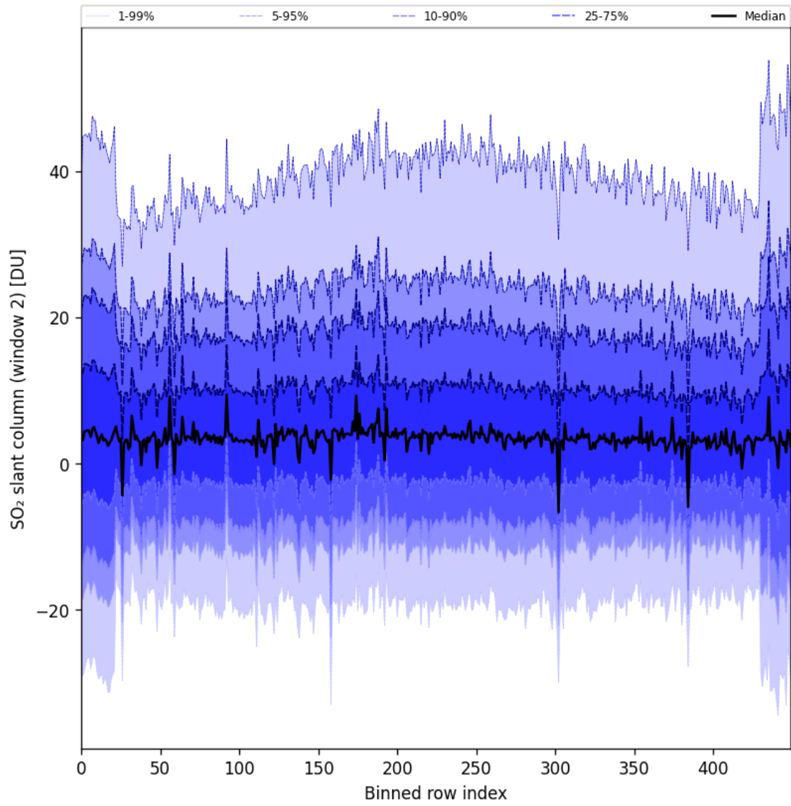
Figure 83: Along track statistics of “SO 2 slant column (window 2)” for 2024-09-06 to 2024-09-07
