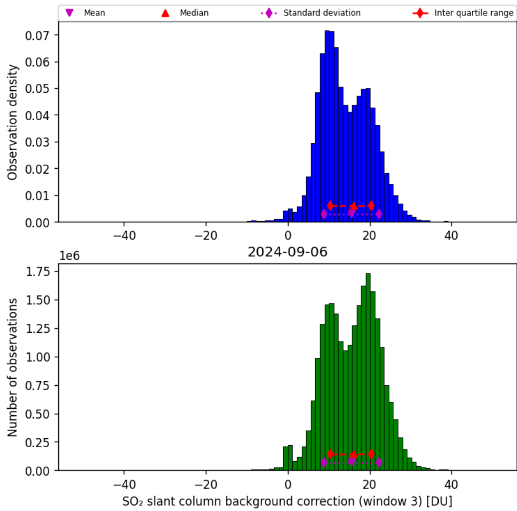
Figure 67: Histogram of “SO 2 slant column background correction (window 3)” for 2024-09-06 to 2024-09-07
