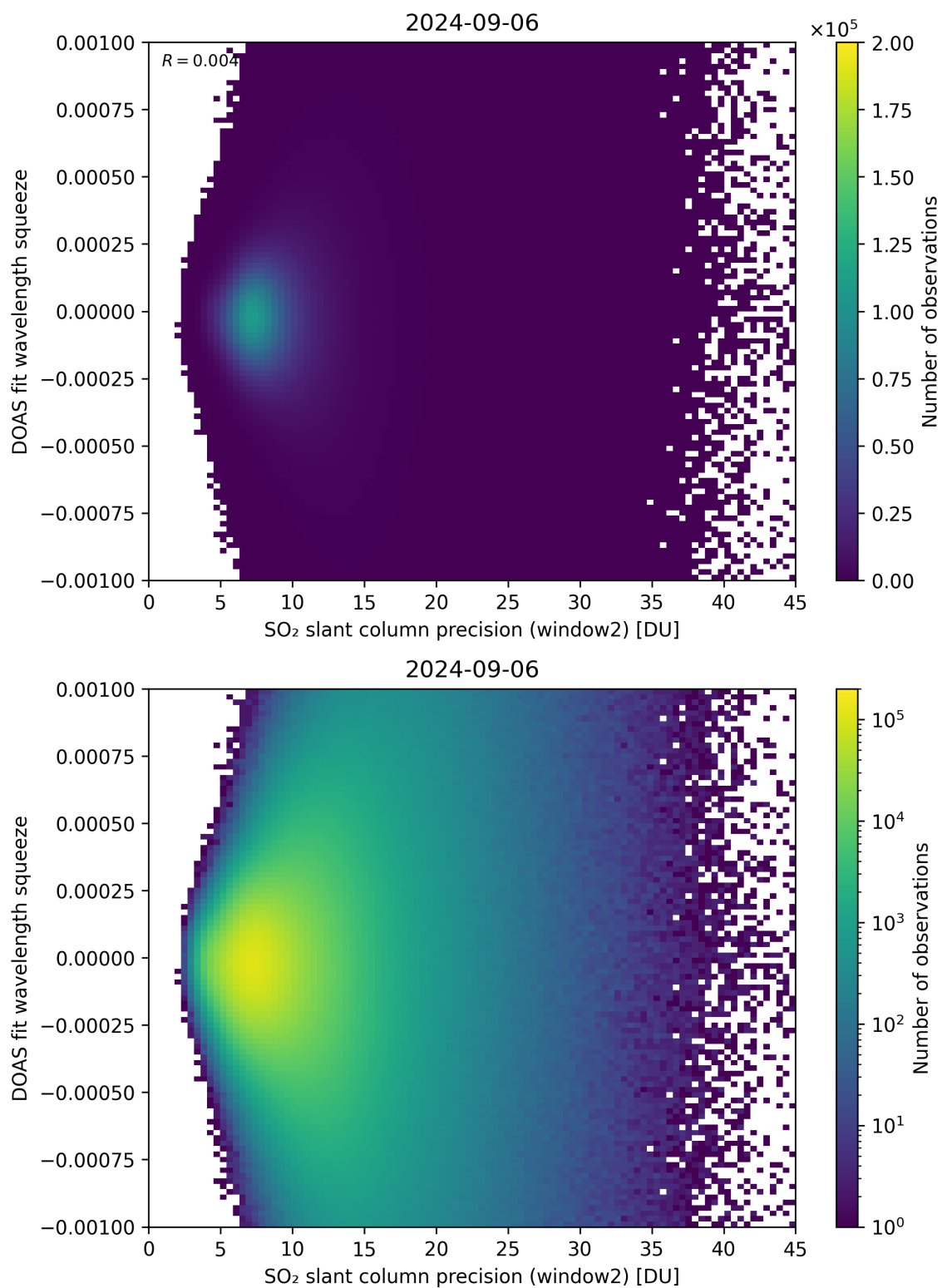
Figure 244: Scatter density plot of “SO 2 slant column precision (window2)” against “DOAS fit wavelength squeeze” for 2024-09-06 to 2024-09-07.
