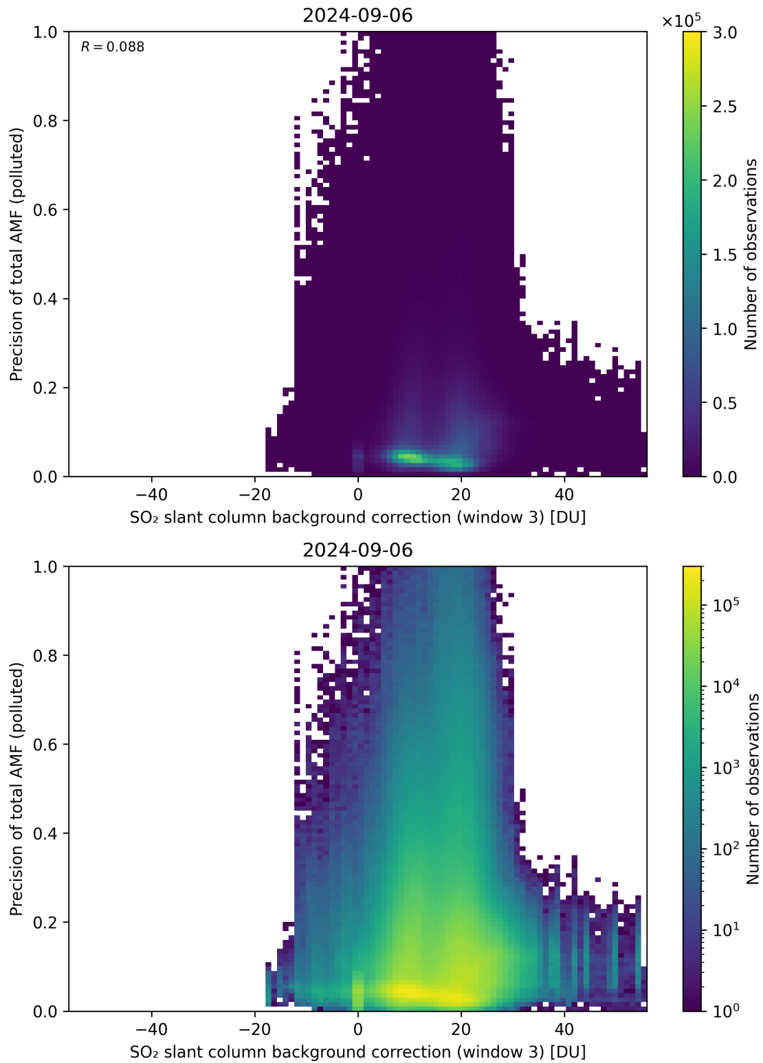
Figure 126: Scatter density plot of “SO 2 slant column background correction (window 3)” against “Precision of total AMF (polluted)” for 2024-09-06 to 2024-09-07.
