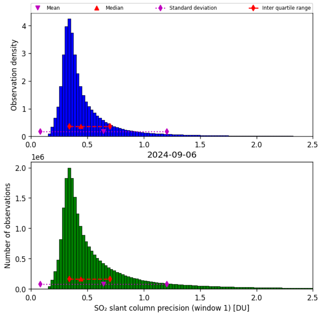
Figure 57: Histogram of “SO 2 slant column precision (window 1)” for 2024-09-06 to 2024-09-07
