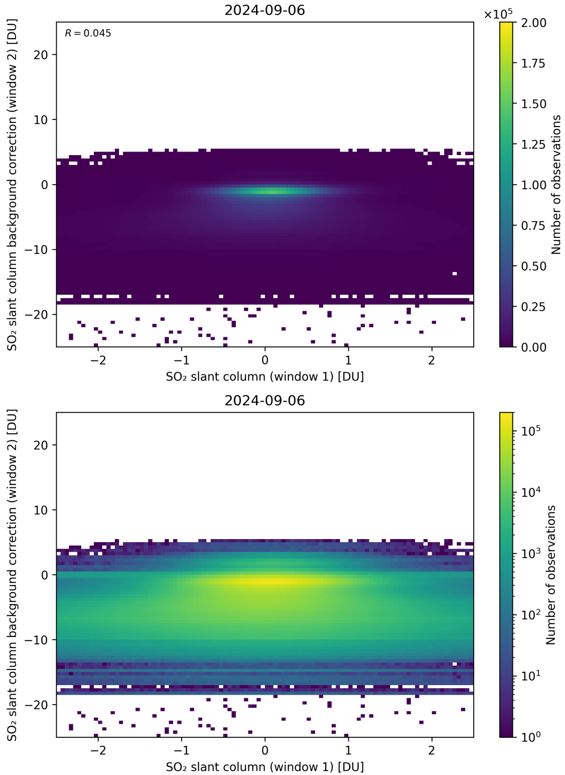
Figure 213: Scatter density plot of “SO 2 slant column (window 1)” against “SO 2 slant column background correction (window 2)” for 2024-09-06 to 2024-09-07.
