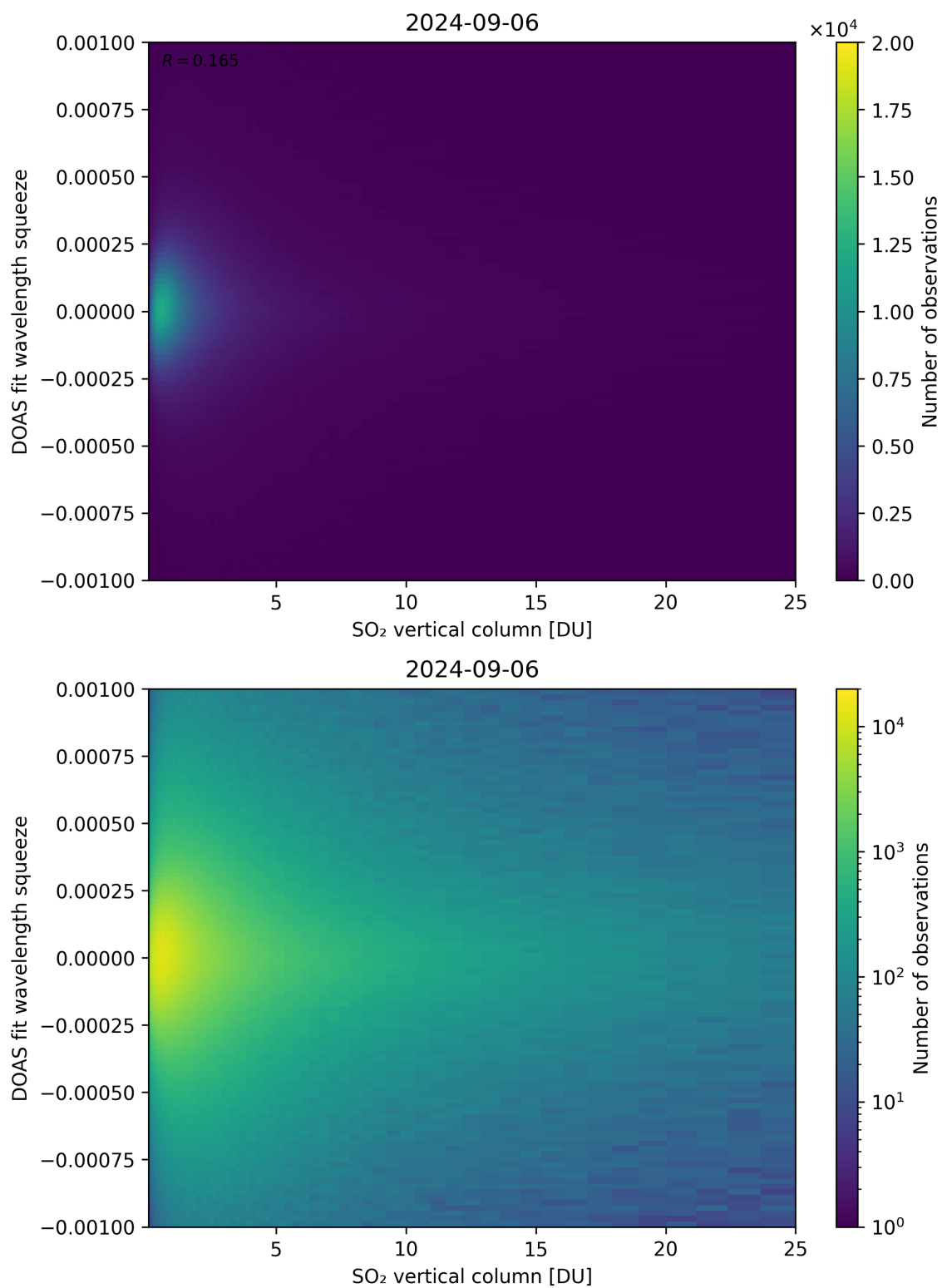
Figure 277: Scatter density plot of “SO 2 vertical column” against “DOAS fit wavelength squeeze” for 2024-09-06 to 2024-09-07.
