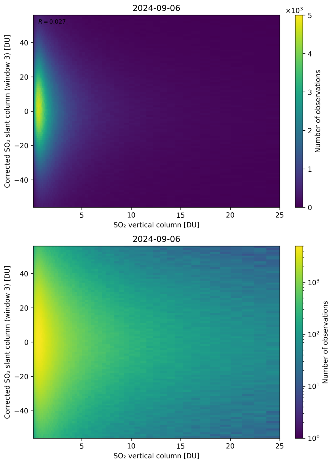
Figure 299: Scatter density plot of “SO 2 vertical column” against “Corrected SO 2 slant column (window 3)” for 2024-09-06 to 2024-09-07.
