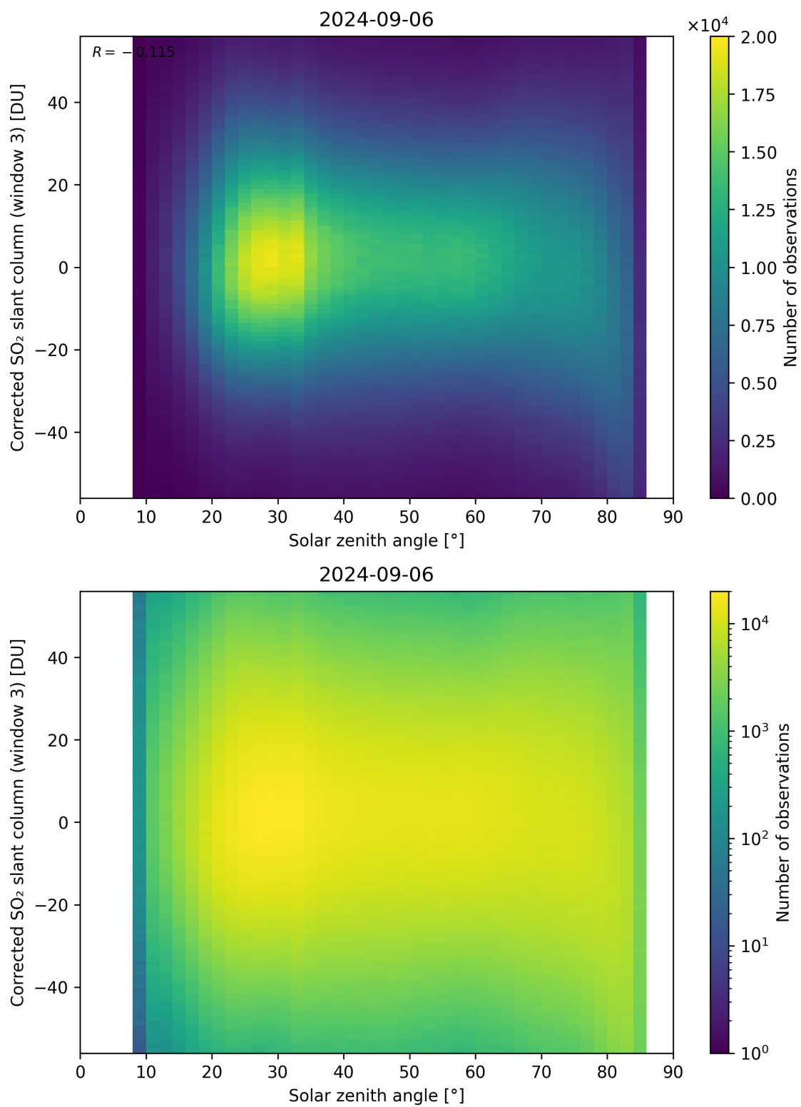
Figure 168: Scatter density plot of “Solar zenith angle” against “Corrected SO 2 slant column (window 3)” for 2024-09-06 to 2024-09-07.
