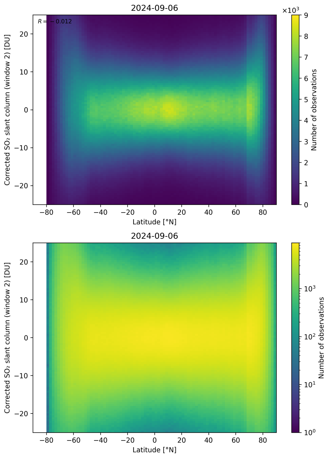
Figure 147: Scatter density plot of “Latitude” against “Corrected SO 2 slant column (window 2)” for 2024-09-06 to 2024-09-07.
