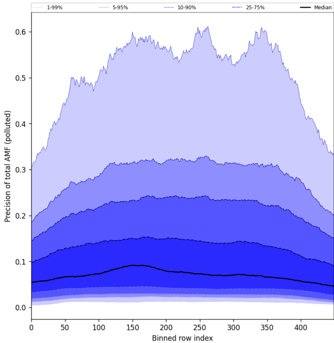
Figure 95: Along track statistics of “Precision of total AMF (polluted)” for 2024-09-06 to 2024-09-07
