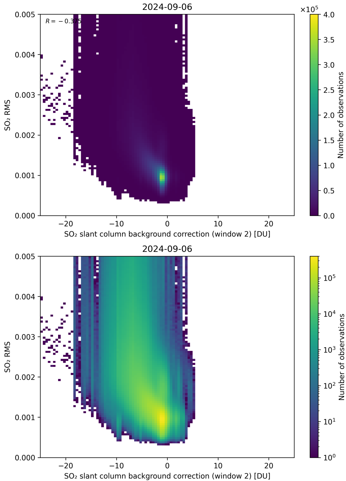
Figure 114: Scatter density plot of “SO 2 slant column background correction (window 2)” against “SO 2 RMS” for 2024-09-06 to 2024-09-07.
