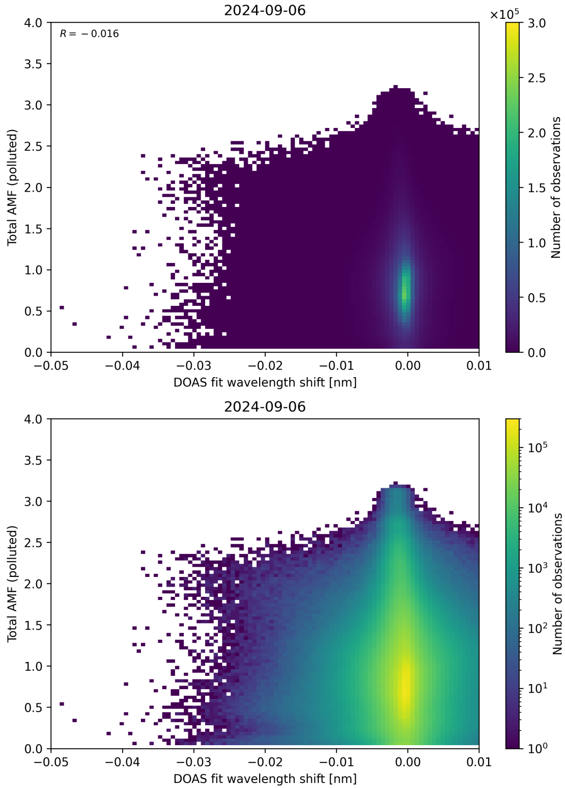
Figure 130: Scatter density plot of “DOAS fit wavelength shift” against “Total AMF (polluted)” for 2024-09-06 to 2024-09-07.
