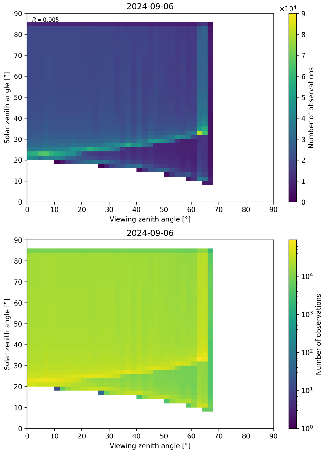
Figure 315: Scatter density plot of “Viewing zenith angle” against “Solar zenith angle” for 2024-09-06 to 2024-09-07.
