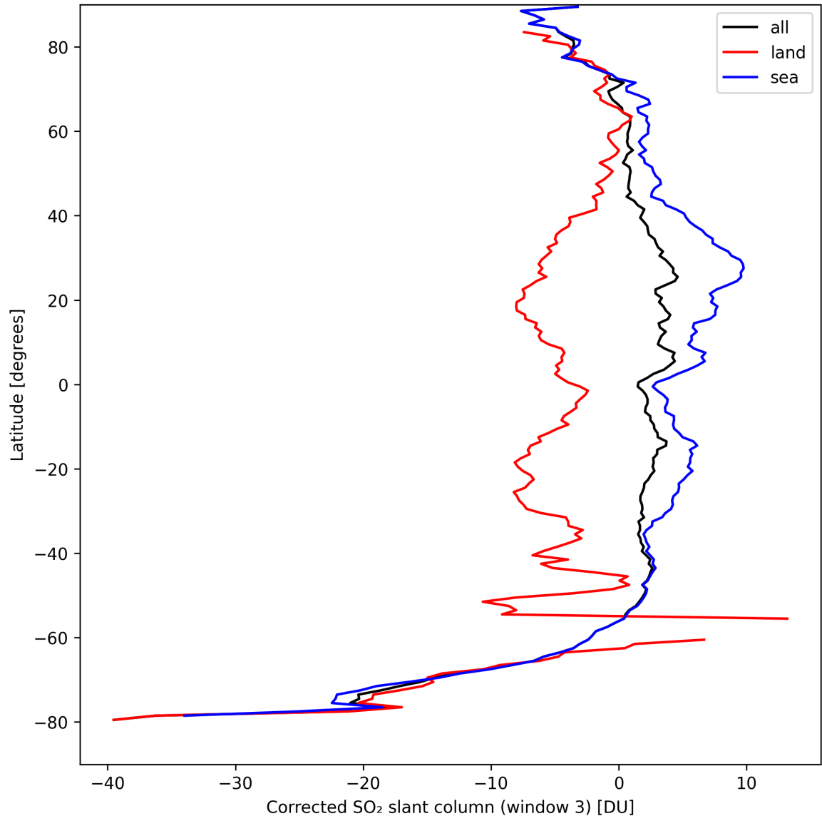
Figure 43: Zonal average of “Corrected SO 2 slant column (window 3)” for 2024-09-06 to 2024-09-07.
