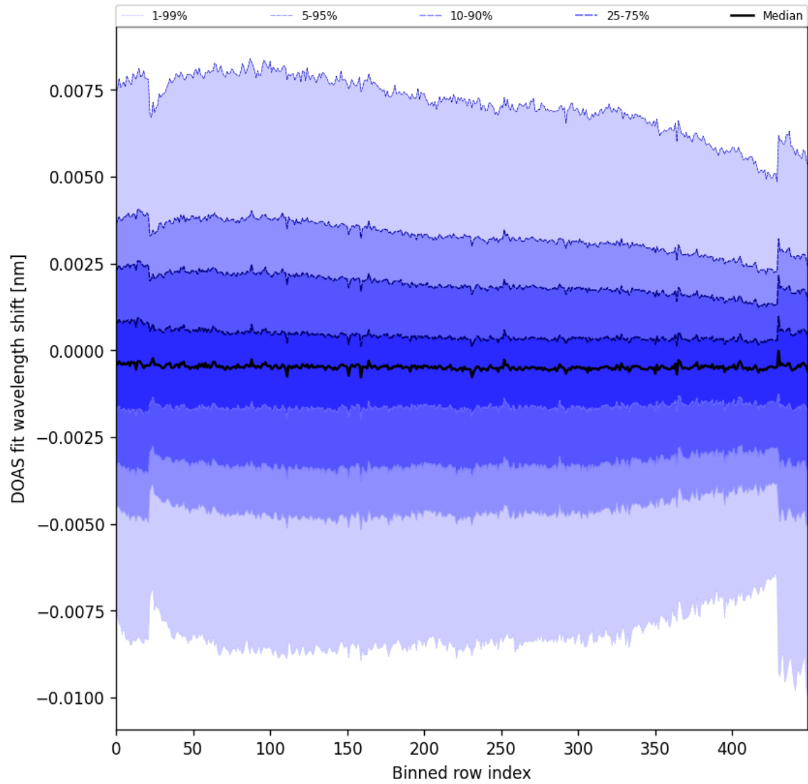
Figure 91: Along track statistics of “DOAS fit wavelength shift” for 2024-09-06 to 2024-09-07
