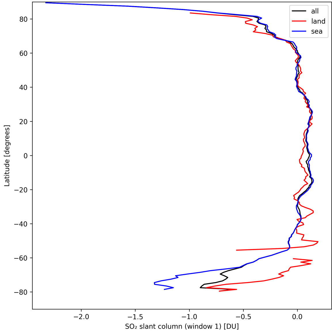
Figure 33: Zonal average of “SO 2 slant column (window 1)” for 2024-09-06 to 2024-09-07.
