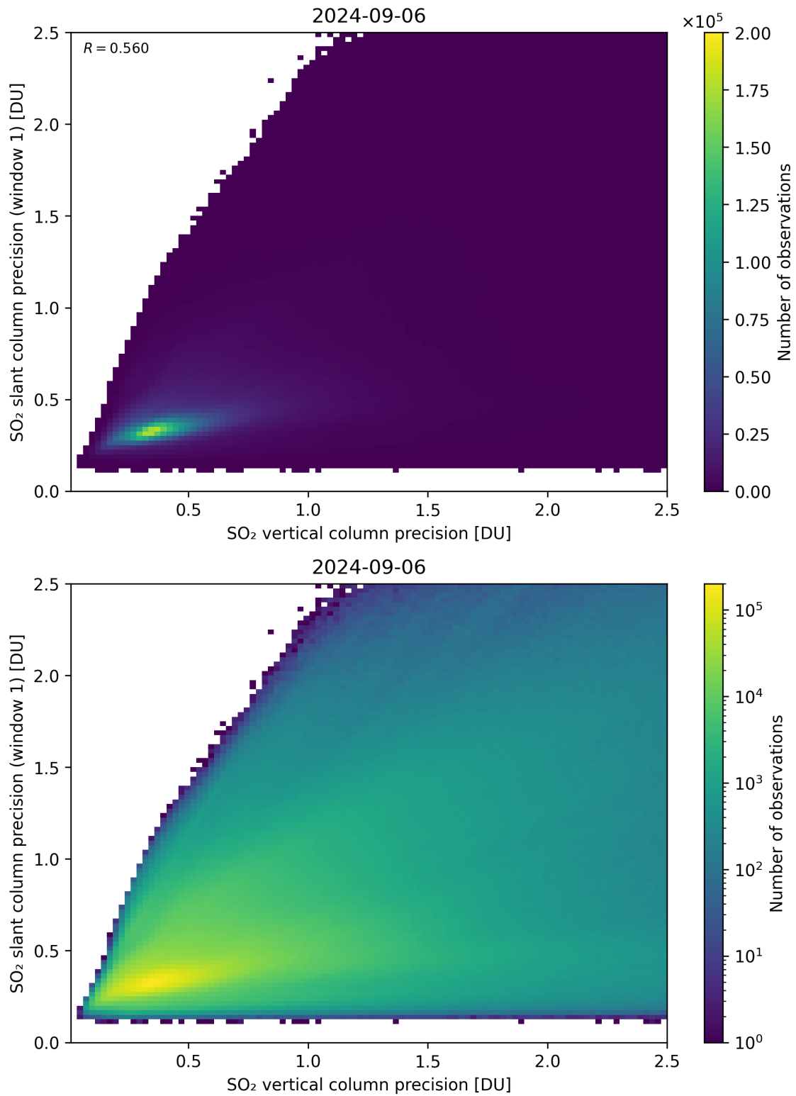
Figure 290: Scatter density plot of “SO 2 vertical column precision” against “SO 2 slant column precision (window 1)” for 2024-09-06 to 2024-09-07.
