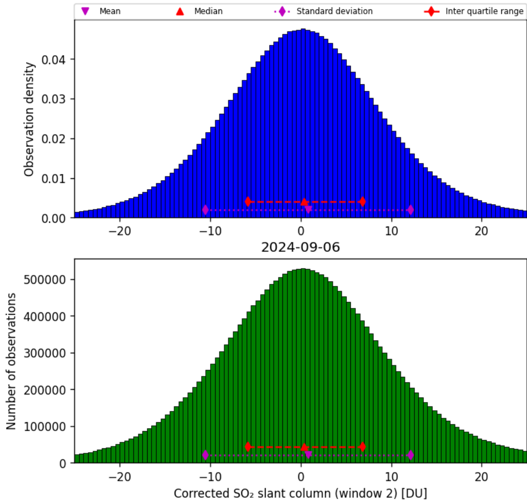
Figure 62: Histogram of “Corrected SO 2 slant column (window 2)” for 2024-09-06 to 2024-09-07
