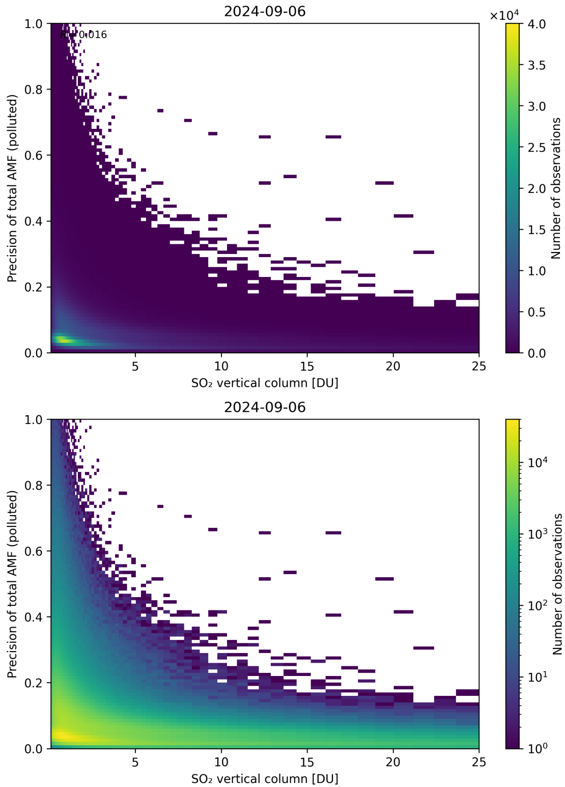
Figure 306: Scatter density plot of “SO 2 vertical column” against “Precision of total AMF (polluted)” for 2024-09-06 to 2024-09-07.
