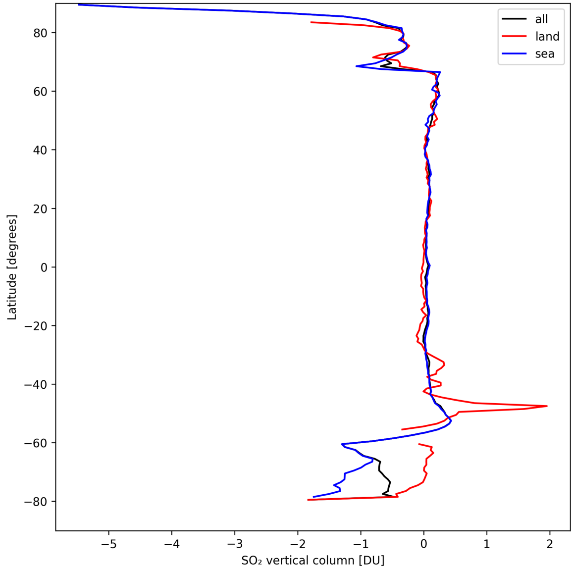
Figure 30: Zonal average of “SO 2 vertical column” for 2024-09-06 to 2024-09-07.
