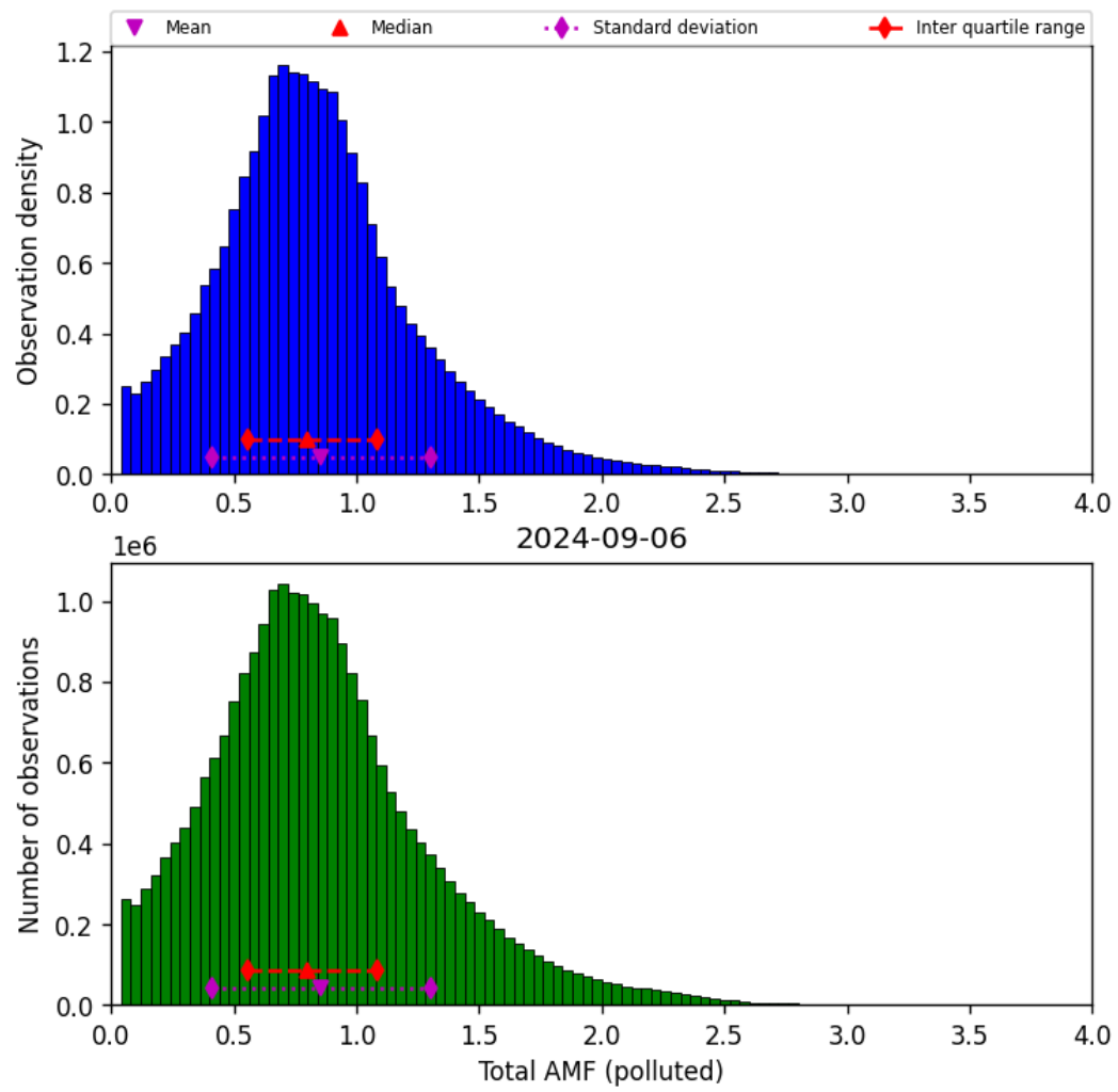
Figure 71: Histogram of “Total AMF (polluted)” for 2024-09-06 to 2024-09-07
