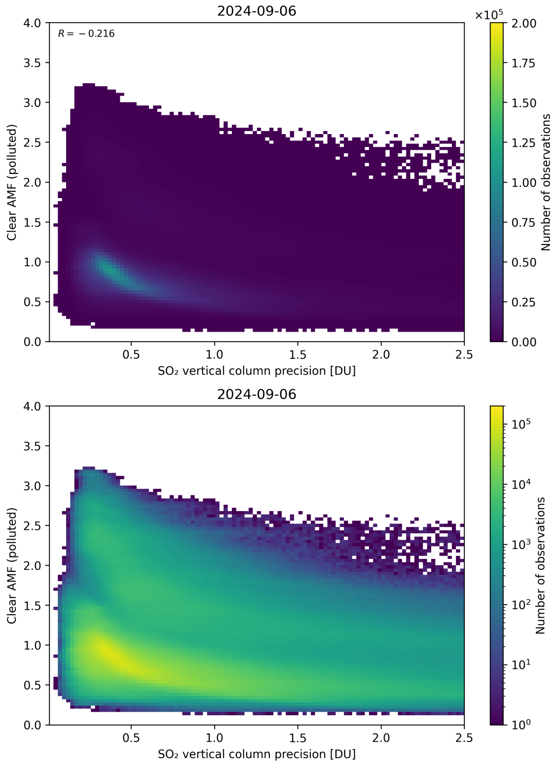
Figure 285: Scatter density plot of “SO 2 vertical column precision” against “Clear AMF (polluted)” for 2024-09-06 to 2024-09-07.
