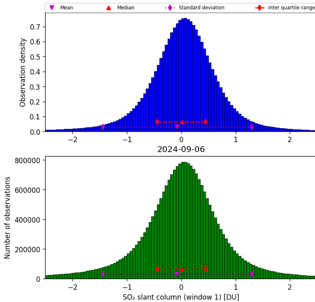
Figure 56: Histogram of “SO 2 slant column (window 1)” for 2024-09-06 to 2024-09-07
