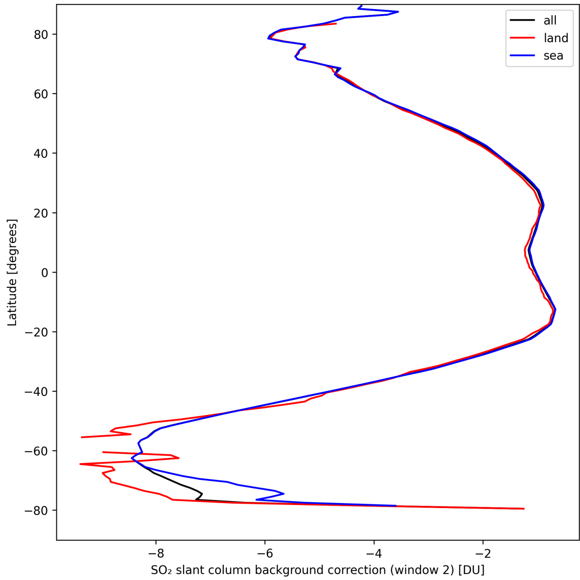
Figure 40: Zonal average of “SO 2 slant column background correction (window 2)” for 2024-09-06 to 2024-09-07.
