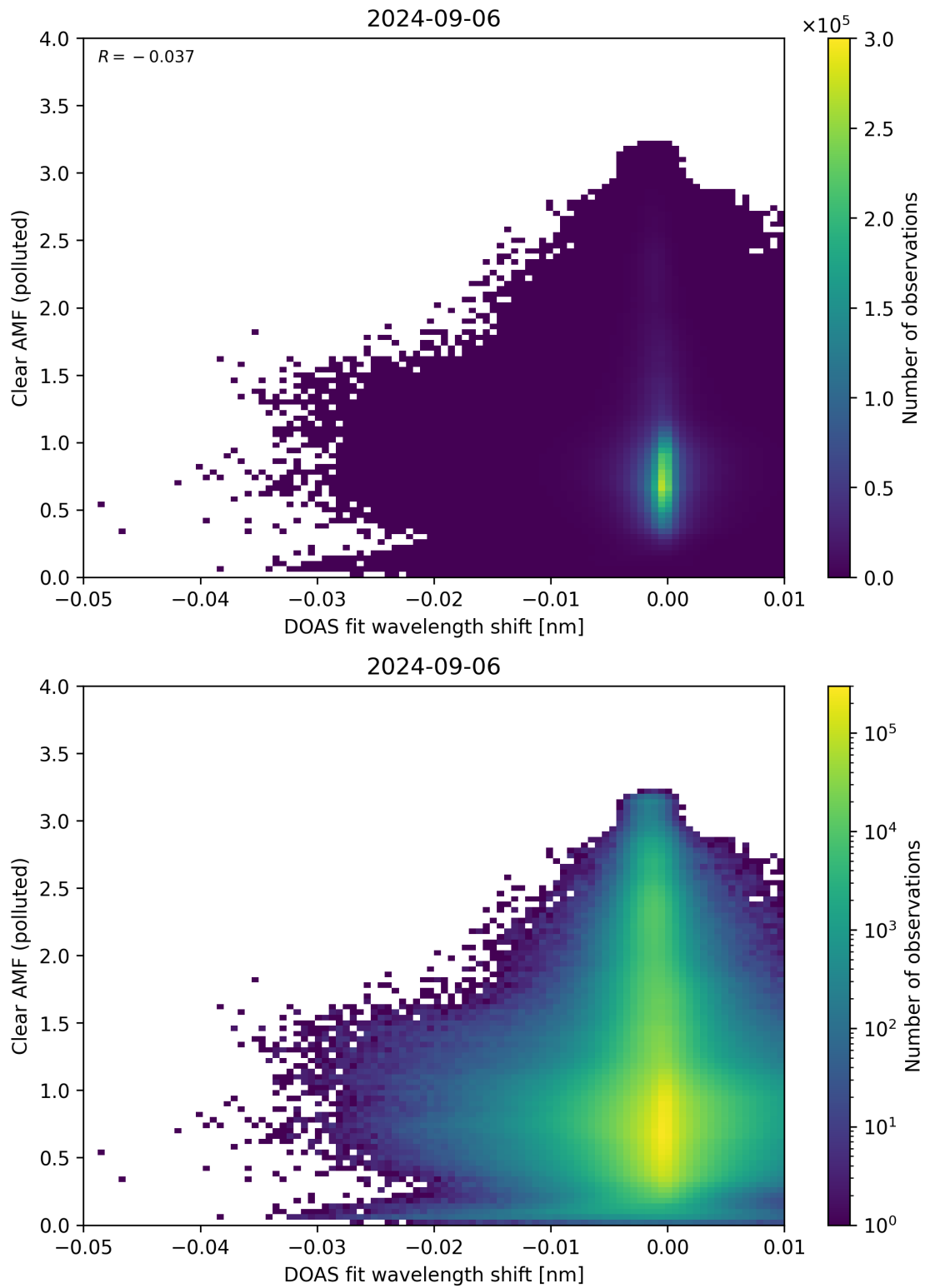
Figure 129: Scatter density plot of “DOAS fit wavelength shift” against “Clear AMF (polluted)” for 2024-09-06 to 2024-09-07.
