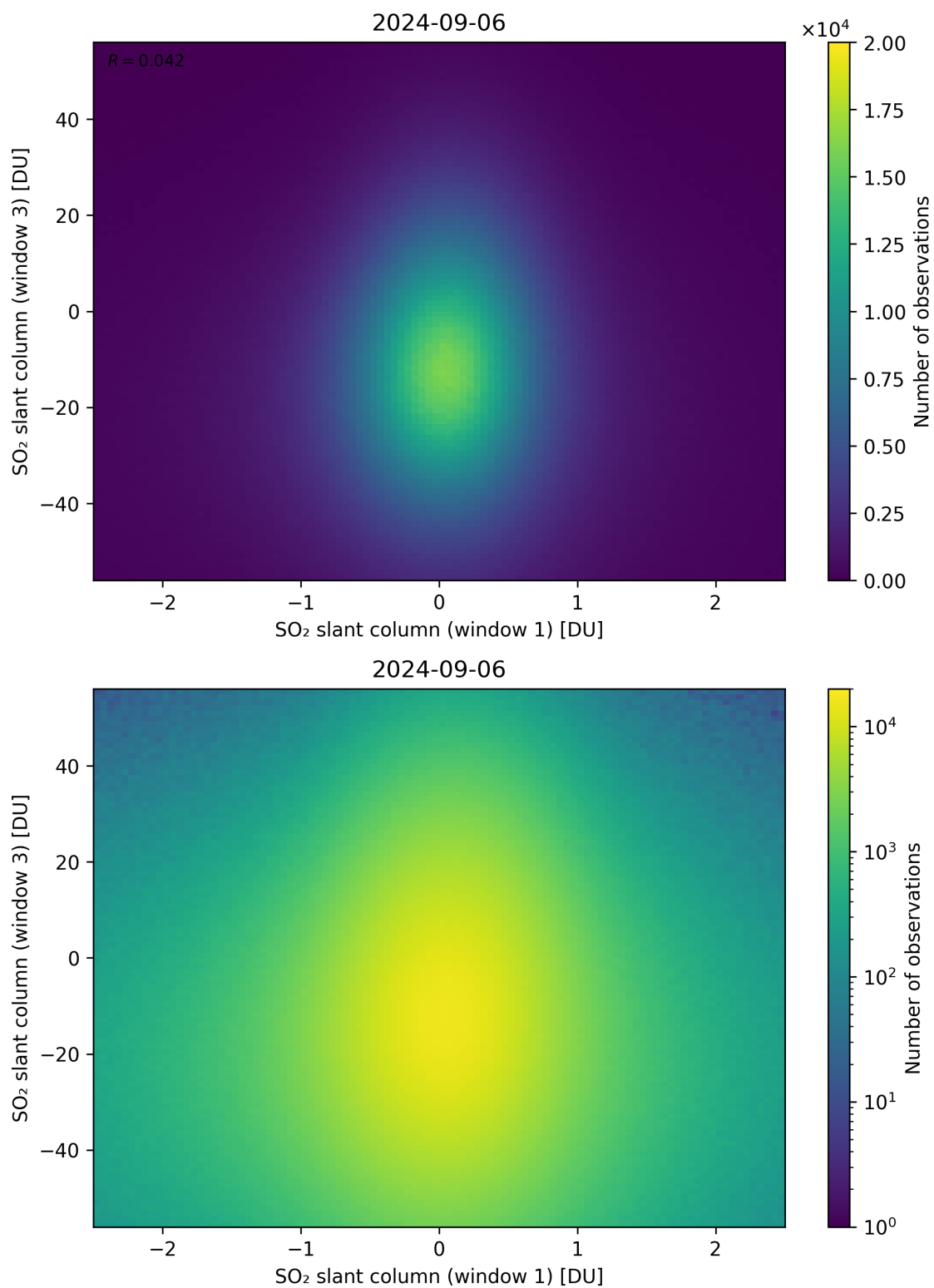
Figure 237: Scatter density plot of “SO 2 slant column (window 1)” against “SO 2 slant column (window 3)” for 2024-09-06 to 2024-09-07.
