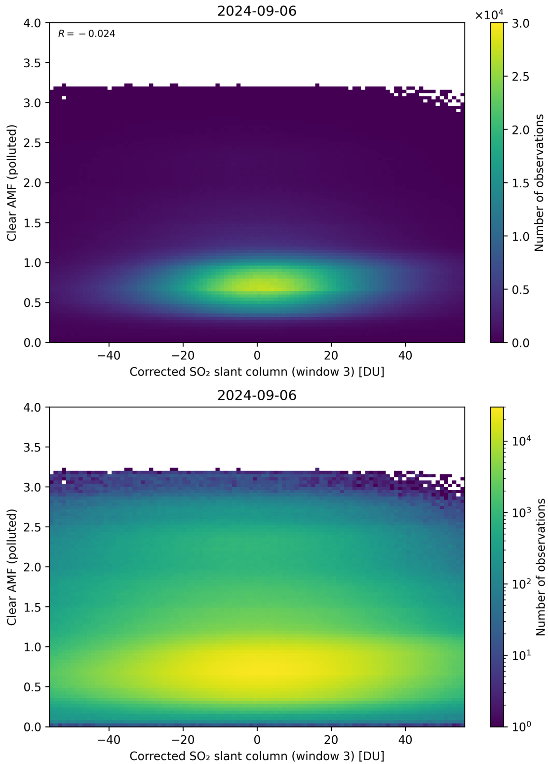
Figure 209: Scatter density plot of “Corrected SO 2 slant column (window 3)” against “Clear AMF (polluted)” for 2024-09-06 to 2024-09-07.
