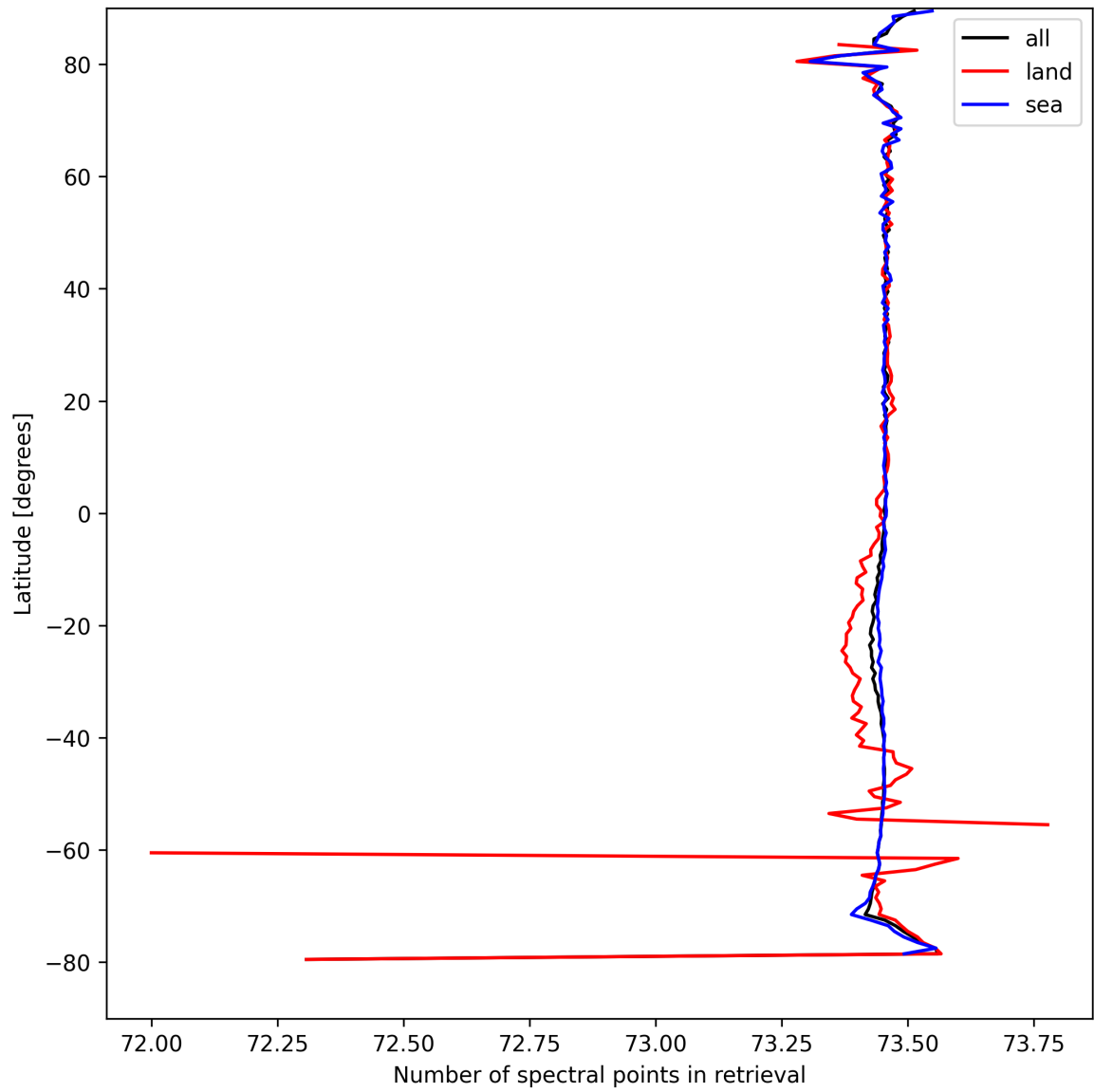
Figure 51: Zonal average of “Number of spectral points in retrieval” for 2024-09-06 to 2024-09-07.
