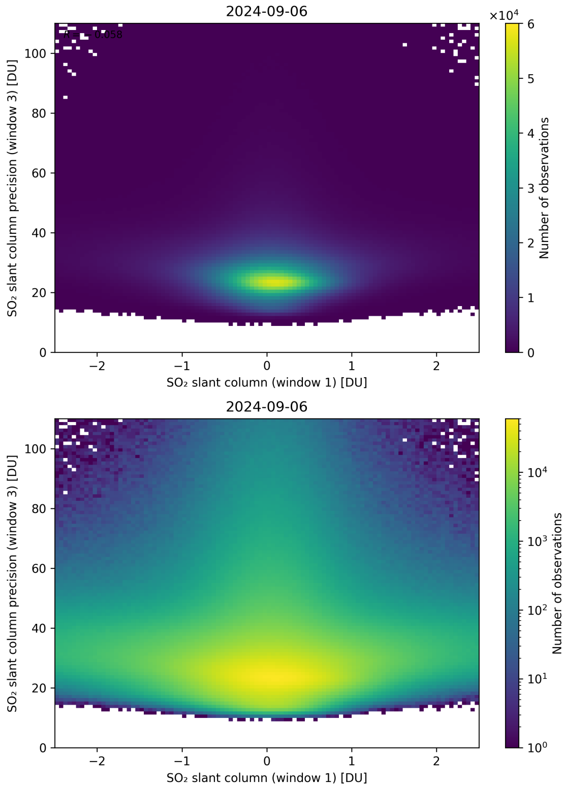
Figure 238: Scatter density plot of “SO 2 slant column (window 1)” against “SO 2 slant column precision (window 3)” for 2024-09-06 to 2024-09-07.
