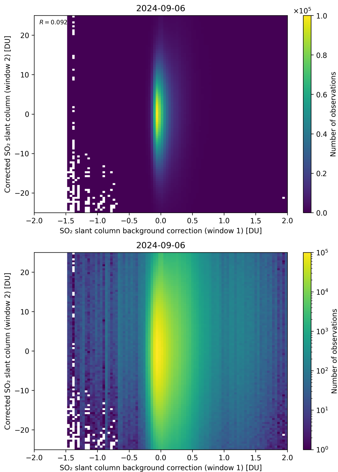
Figure 104: Scatter density plot of “SO 2 slant column background correction (window 1)” against “Corrected SO 2 slant column (window 2)” for 2024-09-06 to 2024-09-07.
