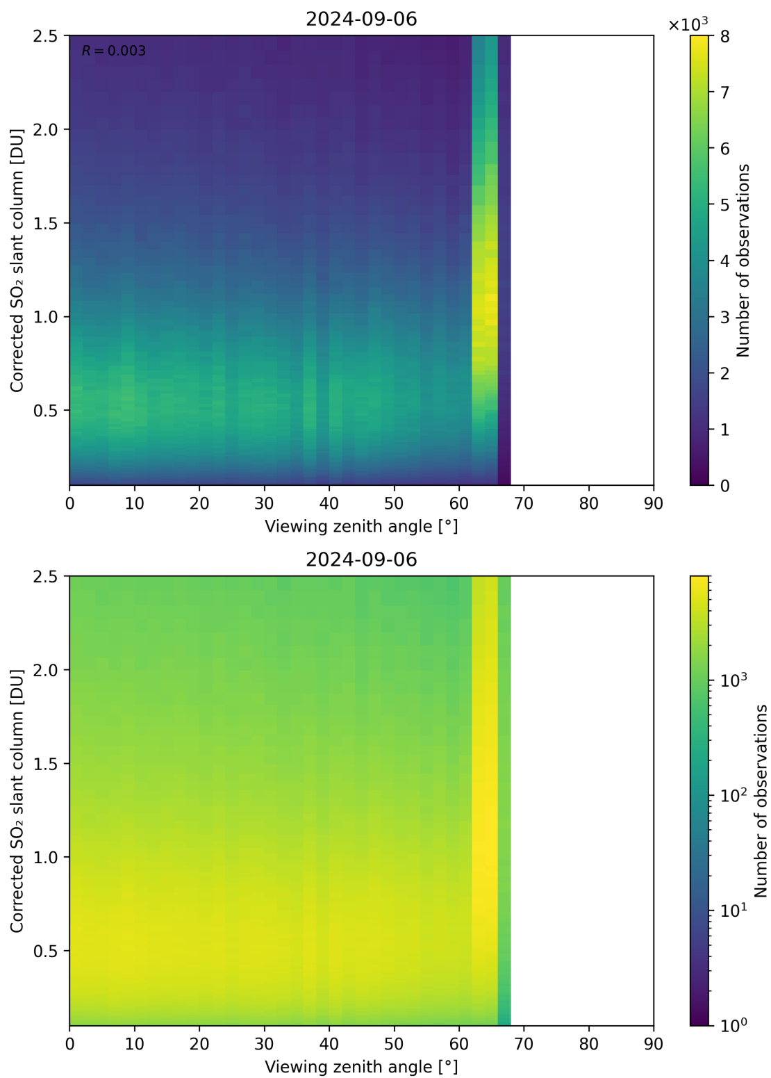
Figure 317: Scatter density plot of “Viewing zenith angle” against “Corrected SO 2 slant column” for 2024-09-06 to 2024-09-07.
