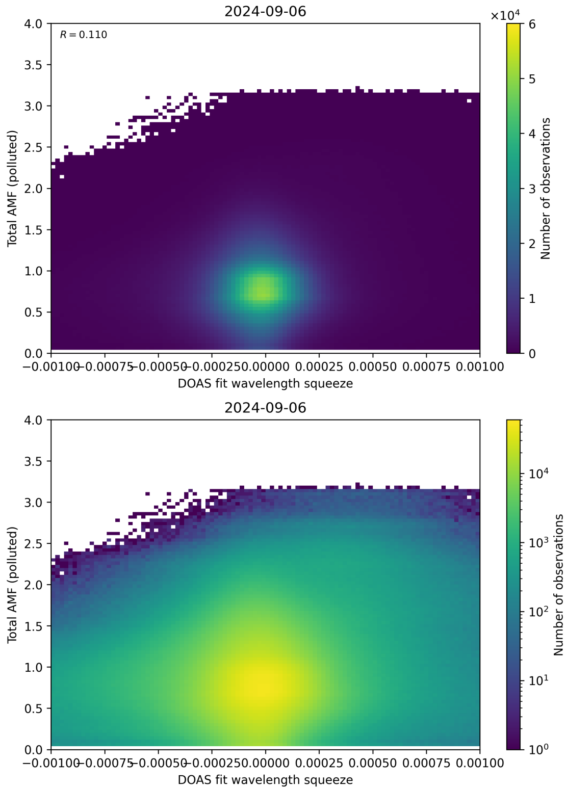
Figure 134: Scatter density plot of “DOAS fit wavelength squeeze” against “Total AMF (polluted)” for 2024-09-06 to 2024-09-07.
