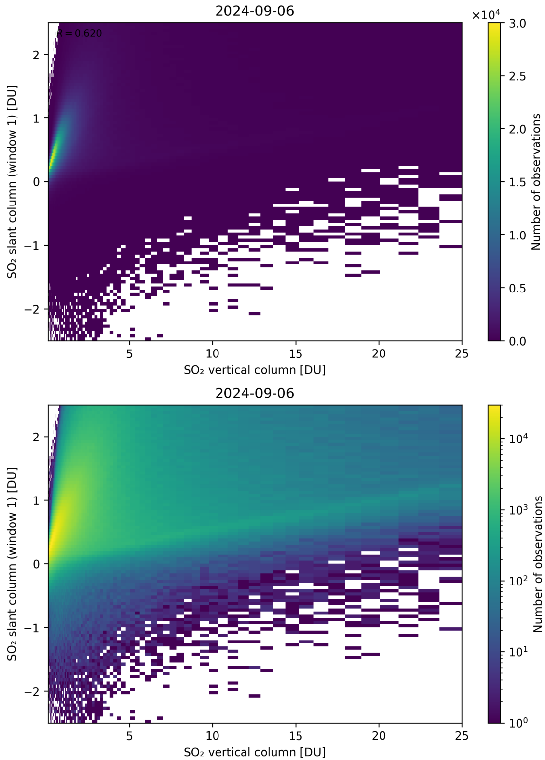
Figure 300: Scatter density plot of “SO 2 vertical column” against “SO 2 slant column (window 1)” for 2024-09-06 to 2024-09-07.
