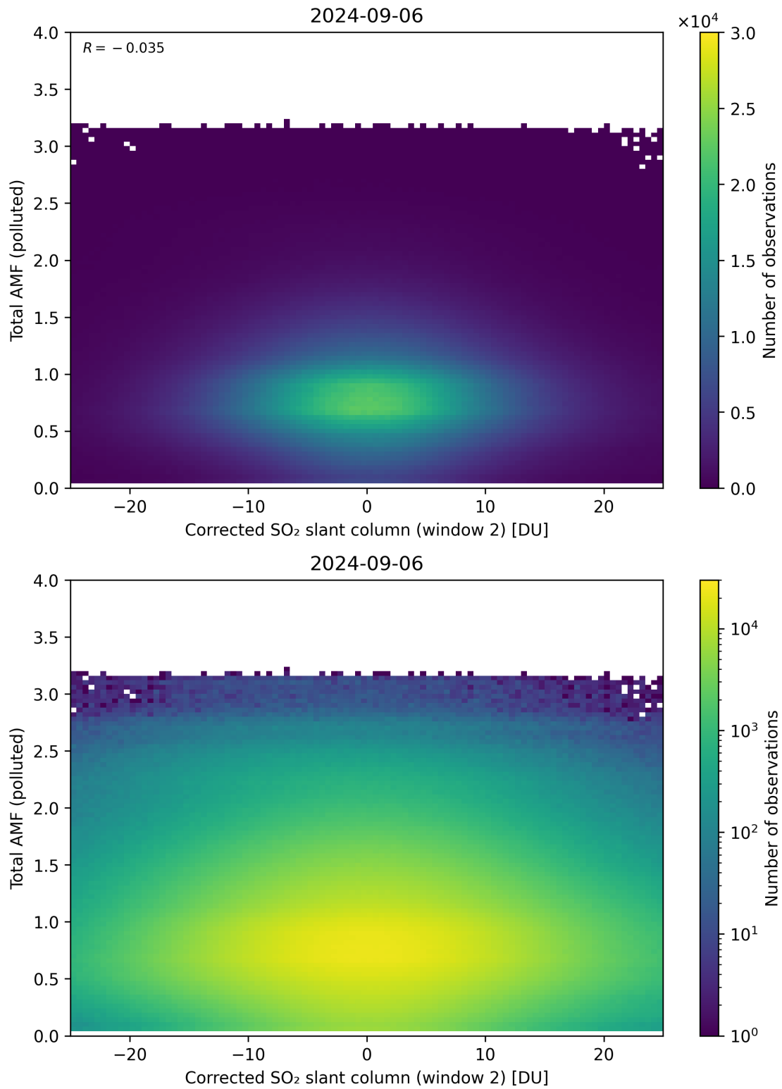
Figure 203: Scatter density plot of “Corrected SO 2 slant column (window 2)” against “Total AMF (polluted)” for 2024-09-06 to 2024-09-07.
