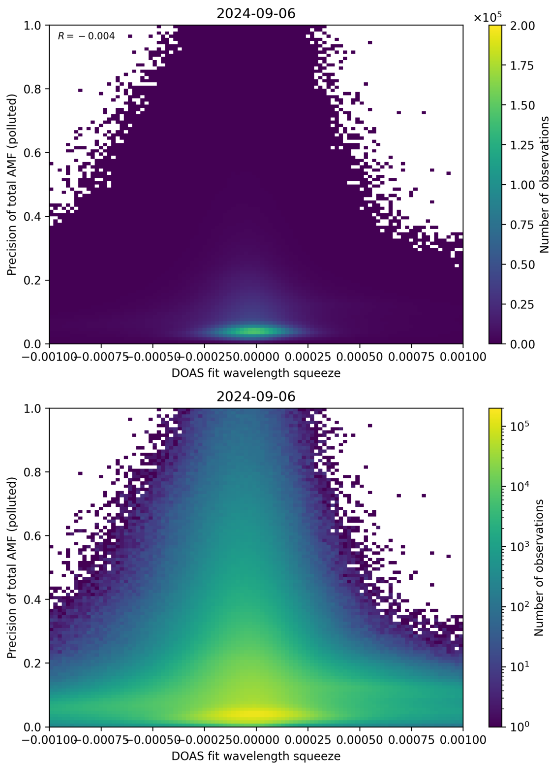
Figure 135: Scatter density plot of “DOAS fit wavelength squeeze” against “Precision of total AMF (polluted)” for 2024-09-06 to 2024-09-07.
