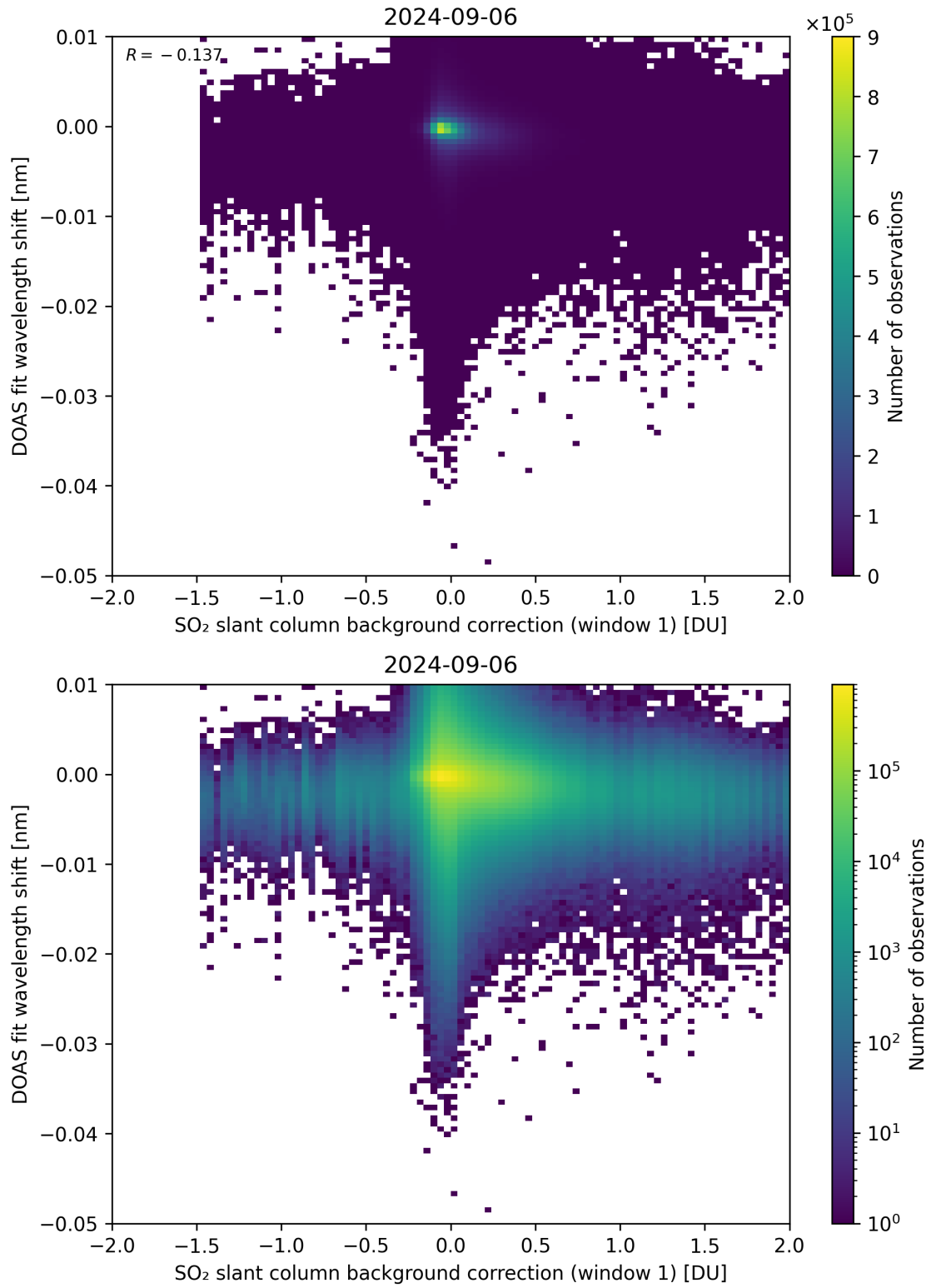
Figure 100: Scatter density plot of “SO 2 slant column background correction (window 1)” against “DOAS fit wavelength shift” for 2024-09-06 to 2024-09-07.
