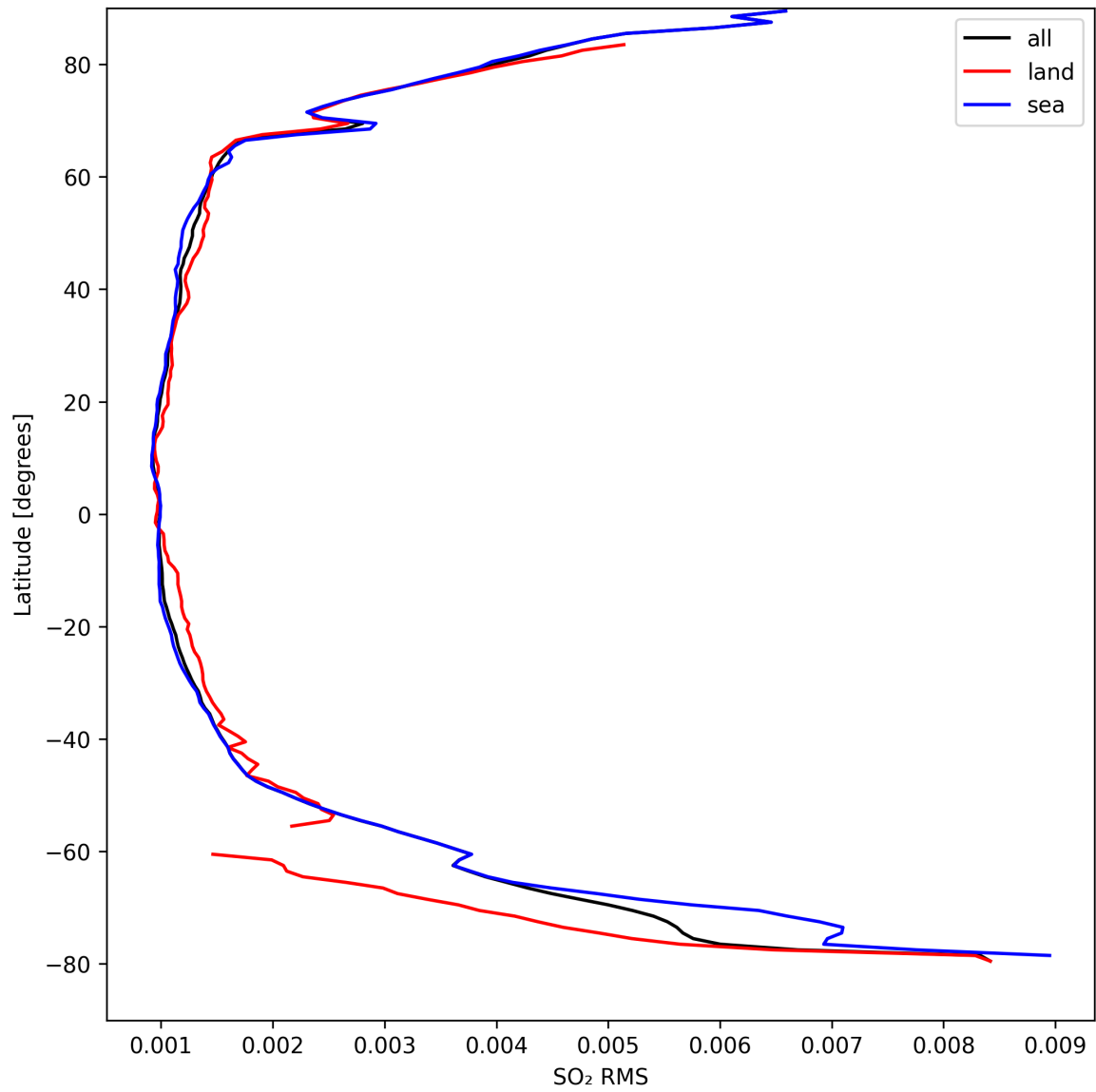
Figure 47: Zonal average of “SO 2 RMS” for 2024-09-06 to 2024-09-07.
