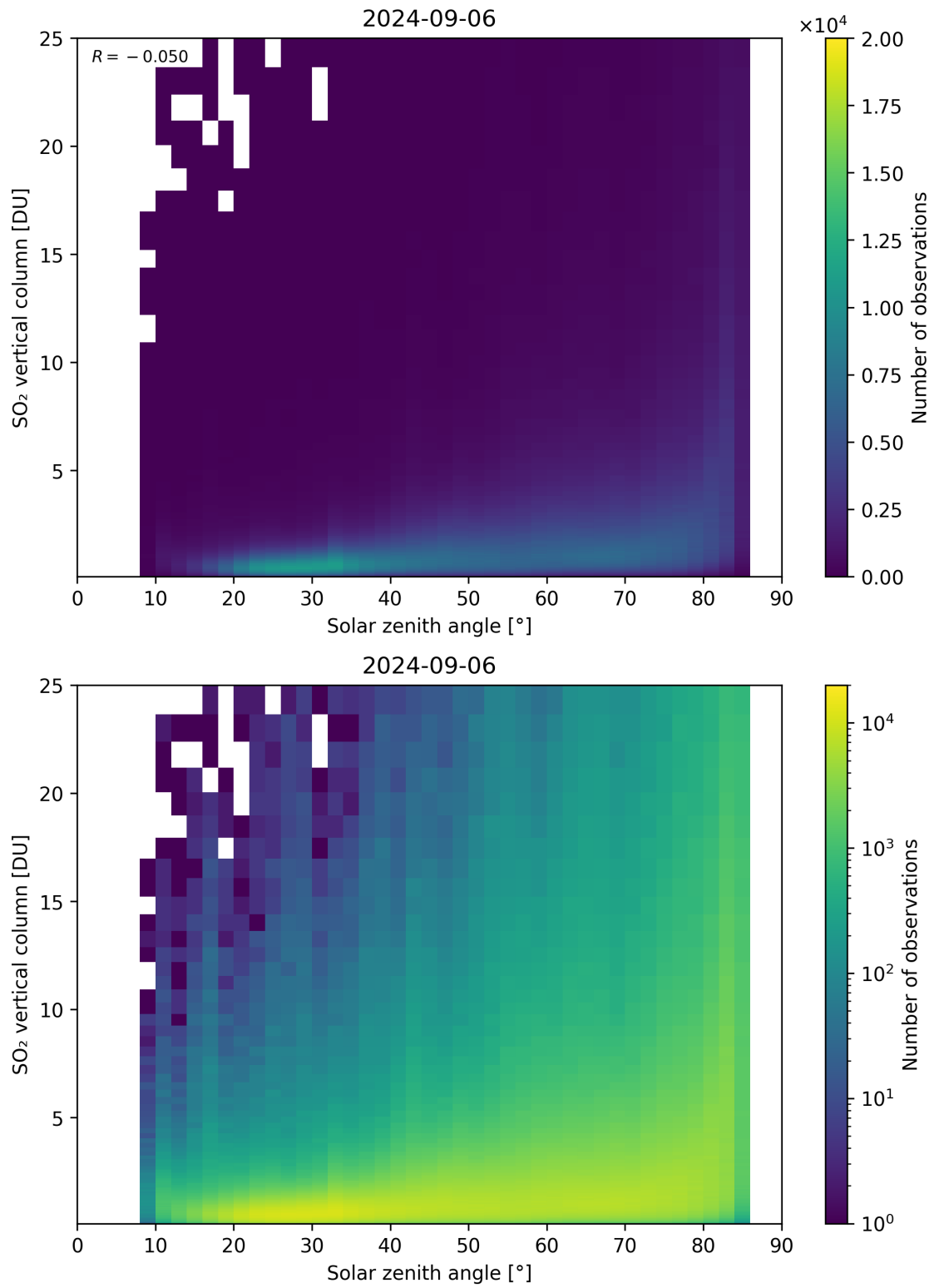
Figure 176: Scatter density plot of “Solar zenith angle” against “SO 2 vertical column” for 2024-09-06 to 2024-09-07.
