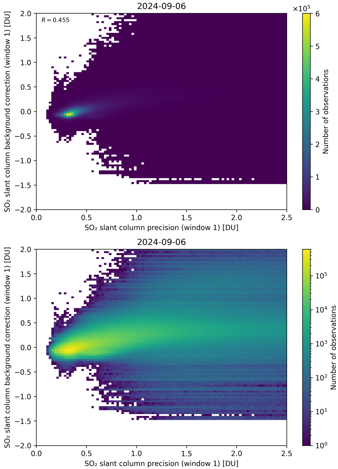
Figure 218: Scatter density plot of “SO 2 slant column precision (window 1)” against “SO 2 slant column background correction (window 1)” for 2024-09-06 to 2024-09-07.
