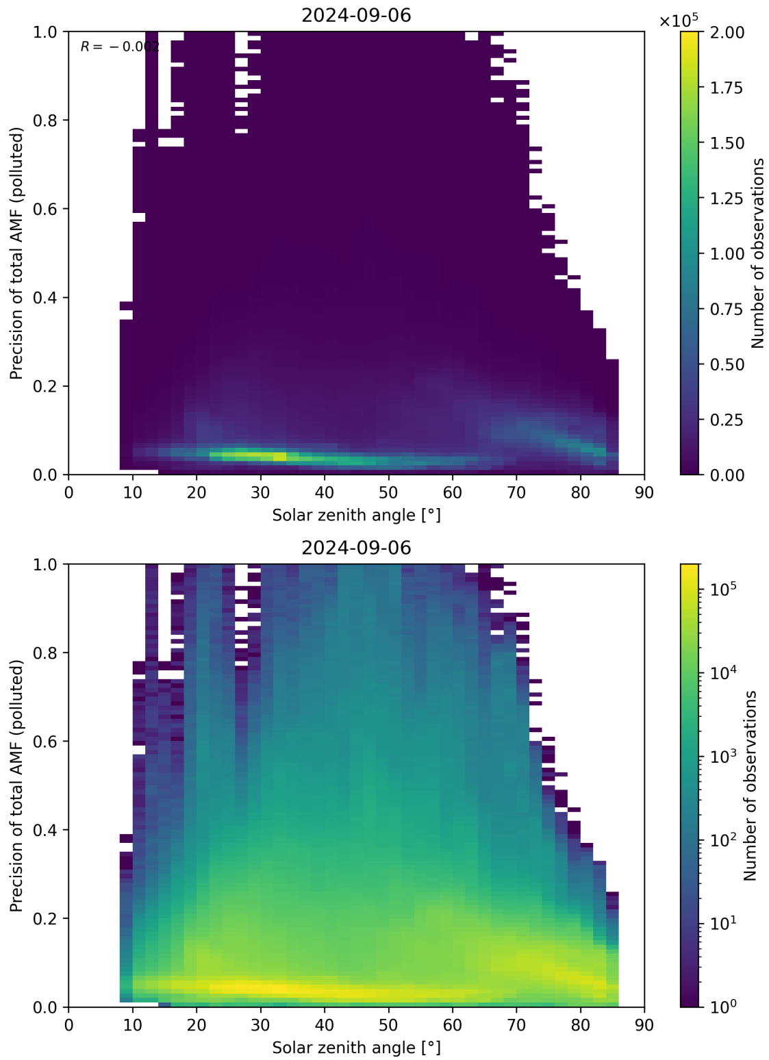
Figure 175: Scatter density plot of “Solar zenith angle” against “Precision of total AMF (polluted)” for 2024-09-06 to 2024-09-07.
