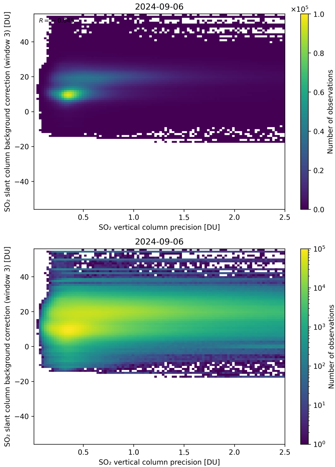
Figure 281: Scatter density plot of “SO 2 vertical column precision” against “SO 2 slant column background correction (window 3)” for 2024-09-06 to 2024-09-07.
