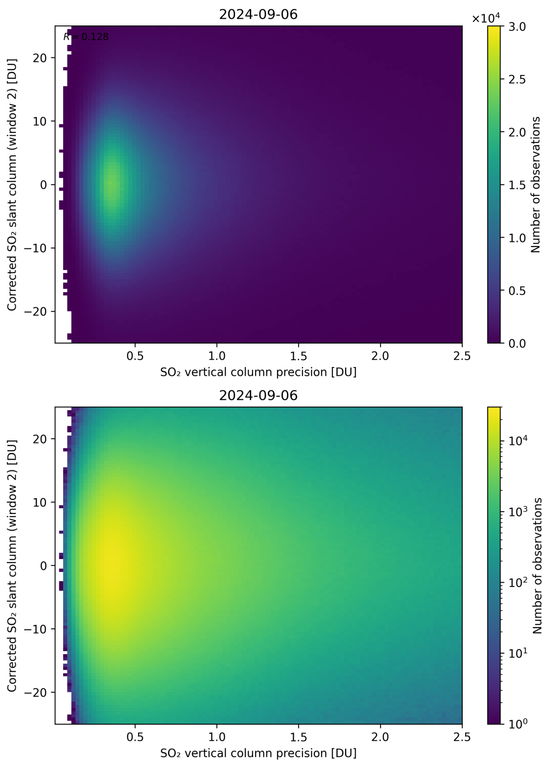
Figure 287: Scatter density plot of “SO 2 vertical column precision” against “Corrected SO 2 slant column (window 2)” for 2024-09-06 to 2024-09-07.
