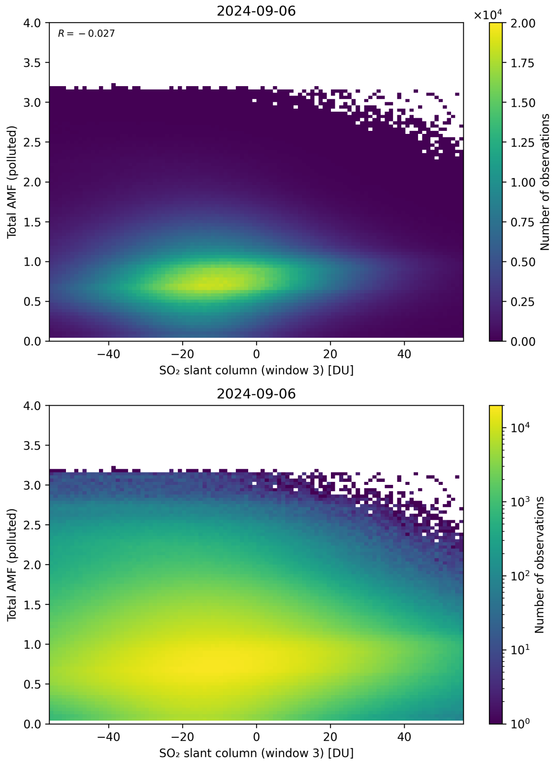
Figure 268: Scatter density plot of “SO 2 slant column (window 3)” against “Total AMF (polluted)” for 2024-09-06 to 2024-09-07.
