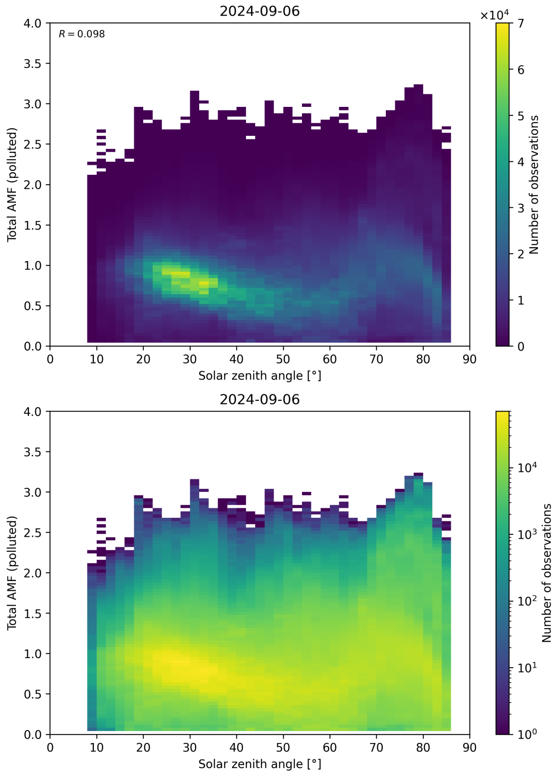
Figure 174: Scatter density plot of “Solar zenith angle” against “Total AMF (polluted)” for 2024-09-06 to 2024-09-07.
