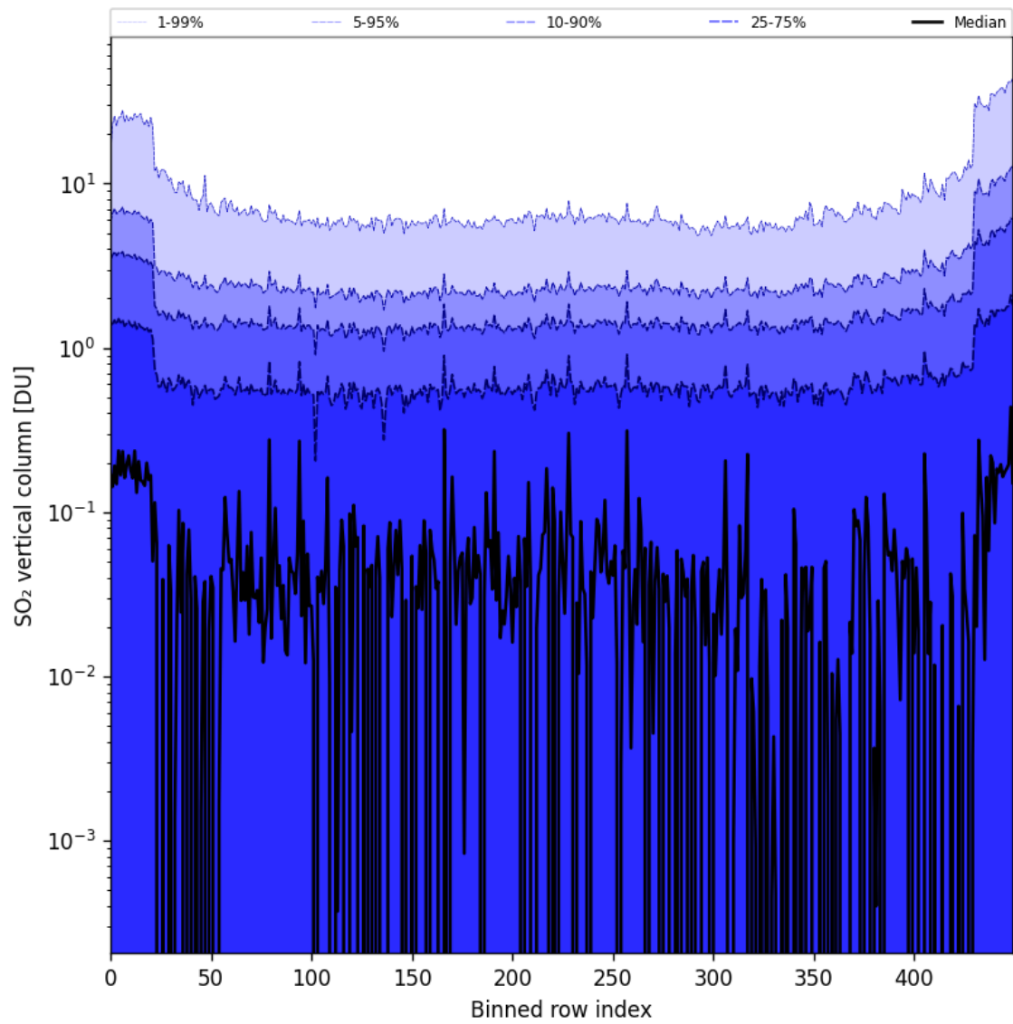
Figure 76: Along track statistics of “SO 2 vertical column” for 2024-09-06 to 2024-09-07
