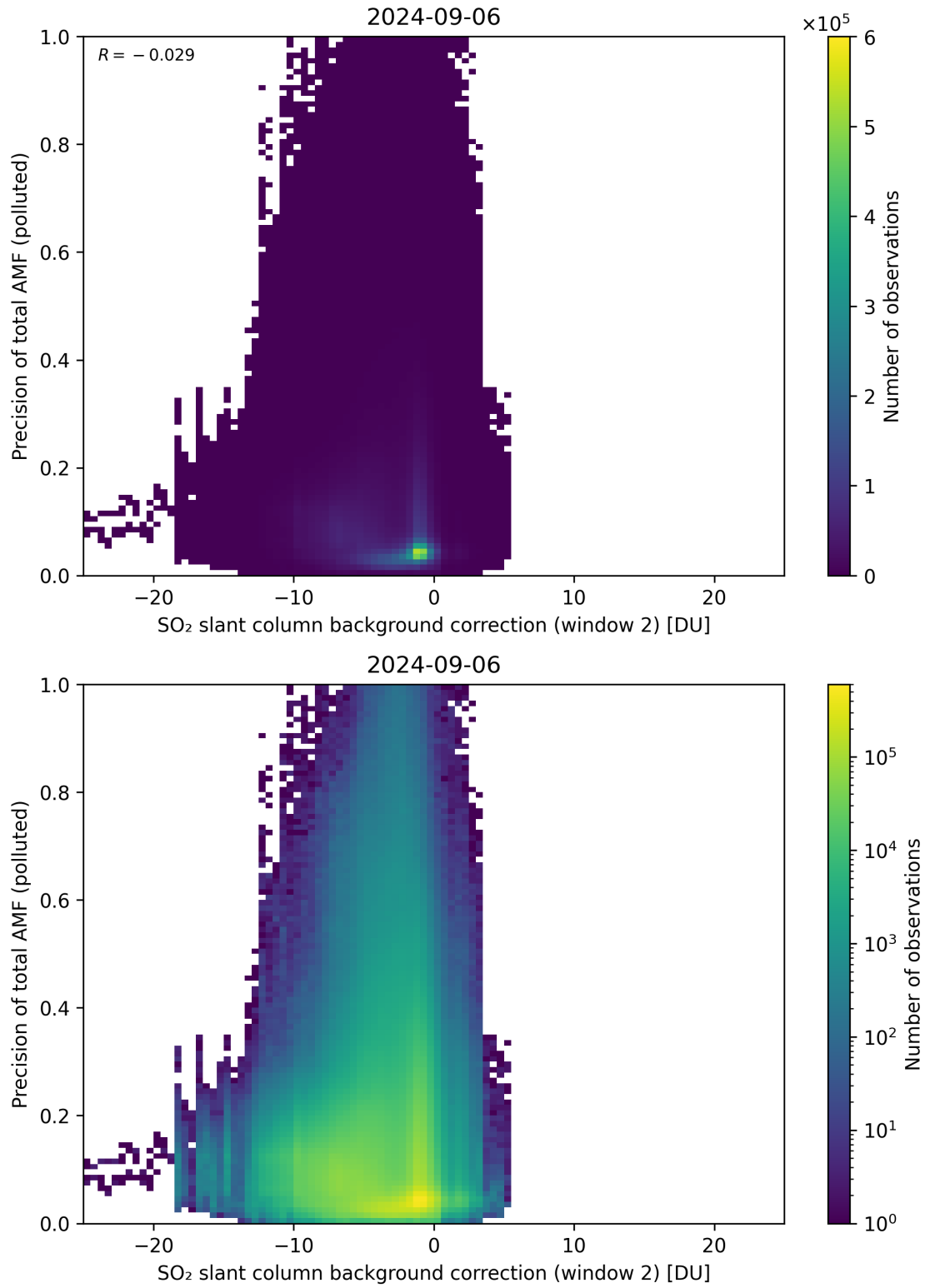
Figure 120: Scatter density plot of “SO 2 slant column background correction (window 2)” against “Precision of total AMF (polluted)” for 2024-09-06 to 2024-09-07.
