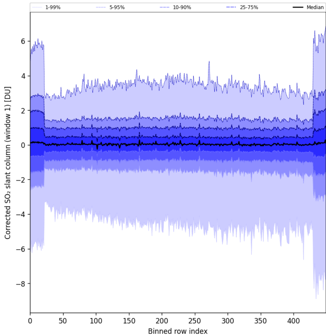
Figure 81: Along track statistics of “Corrected SO 2 slant column (window 1)” for 2024-09-06 to 2024-09-07
