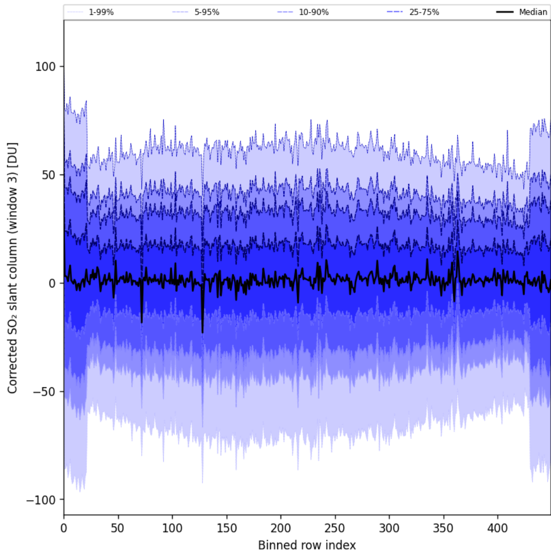
Figure 89: Along track statistics of “Corrected SO 2 slant column (window 3)” for 2024-09-06 to 2024-09-07
