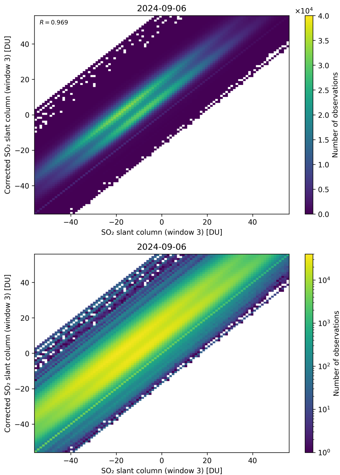
Figure 266: Scatter density plot of “SO 2 slant column (window 3)” against “Corrected SO 2 slant column (window 3)” for 2024-09-06 to 2024-09-07.
