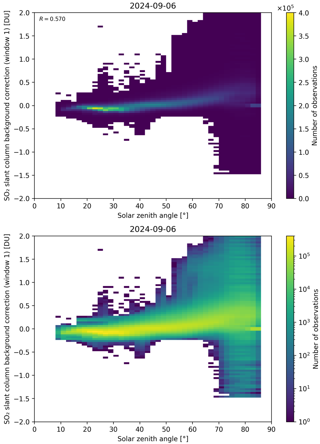
Figure 158: Scatter density plot of “Solar zenith angle” against “SO 2 slant column background correction (window 1)” for 2024-09-06 to 2024-09-07.
