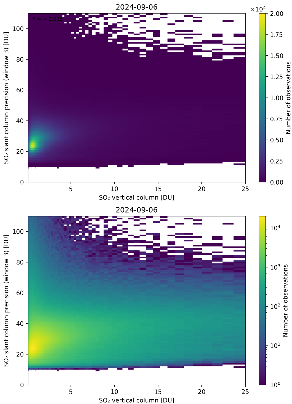
Figure 304: Scatter density plot of “SO 2 vertical column” against “SO 2 slant column precision (window 3)” for 2024-09-06 to 2024-09-07.
