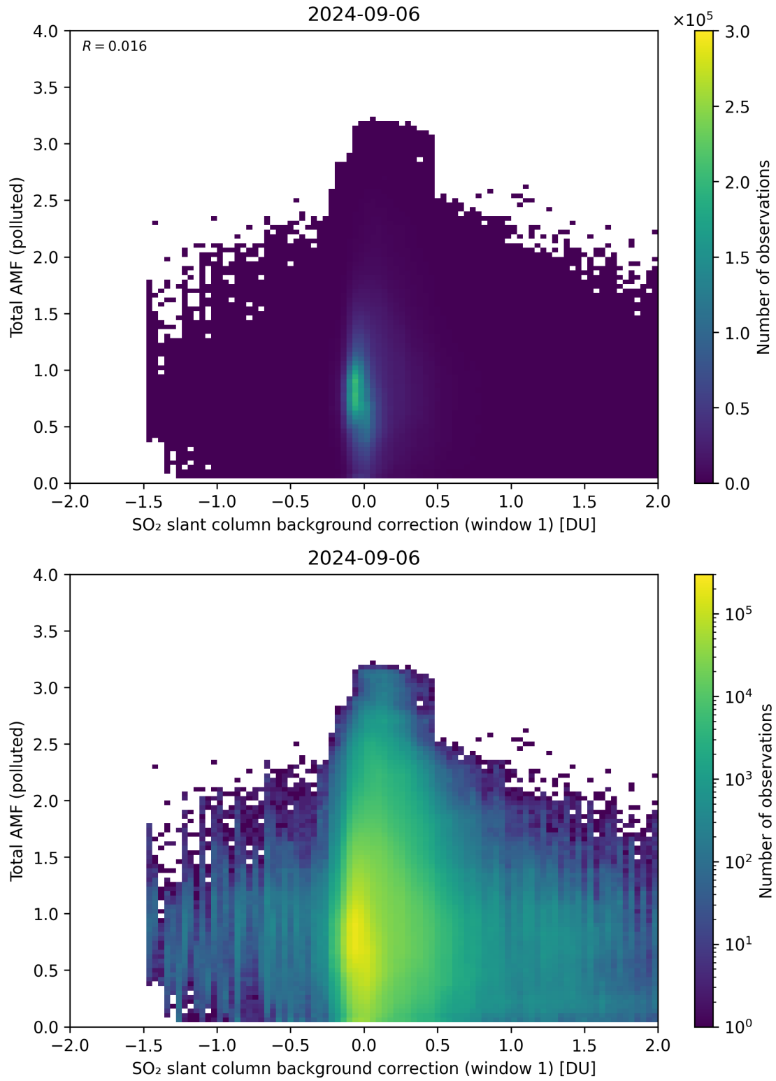
Figure 109: Scatter density plot of “SO 2 slant column background correction (window 1)” against “Total AMF (polluted)” for 2024-09-06 to 2024-09-07.
