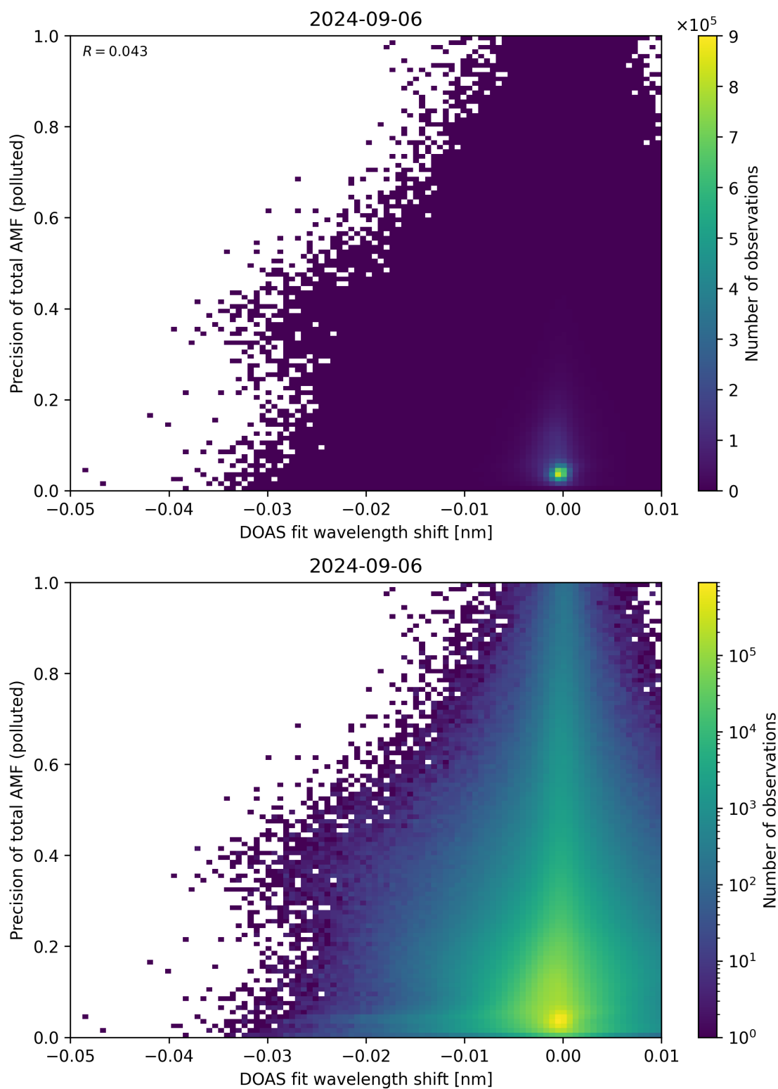
Figure 131: Scatter density plot of “DOAS fit wavelength shift” against “Precision of total AMF (polluted)” for 2024-09-06 to 2024-09-07.
