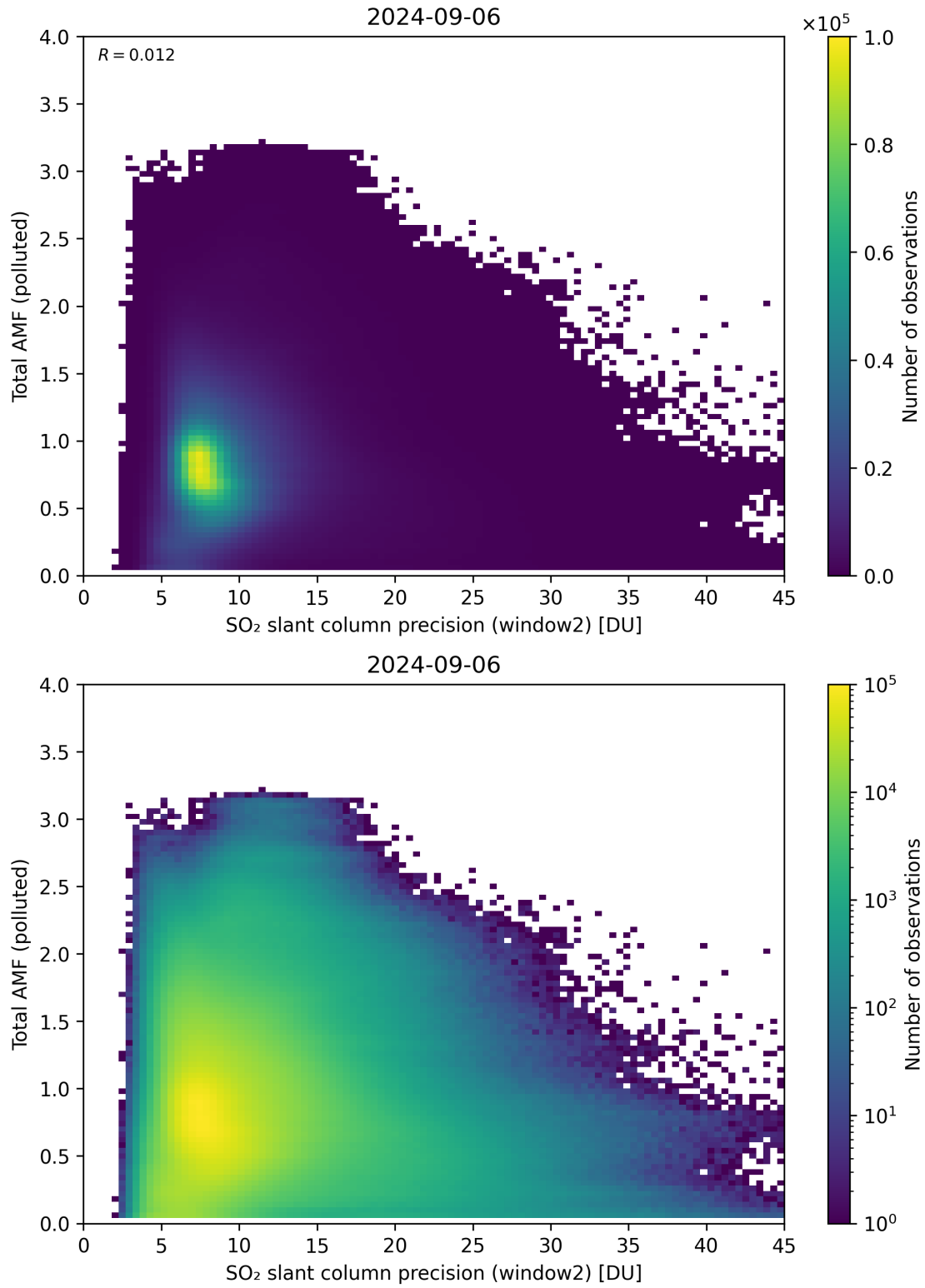
Figure 251: Scatter density plot of “SO 2 slant column precision (window2)” against “Total AMF (polluted)” for 2024-09-06 to 2024-09-07.
