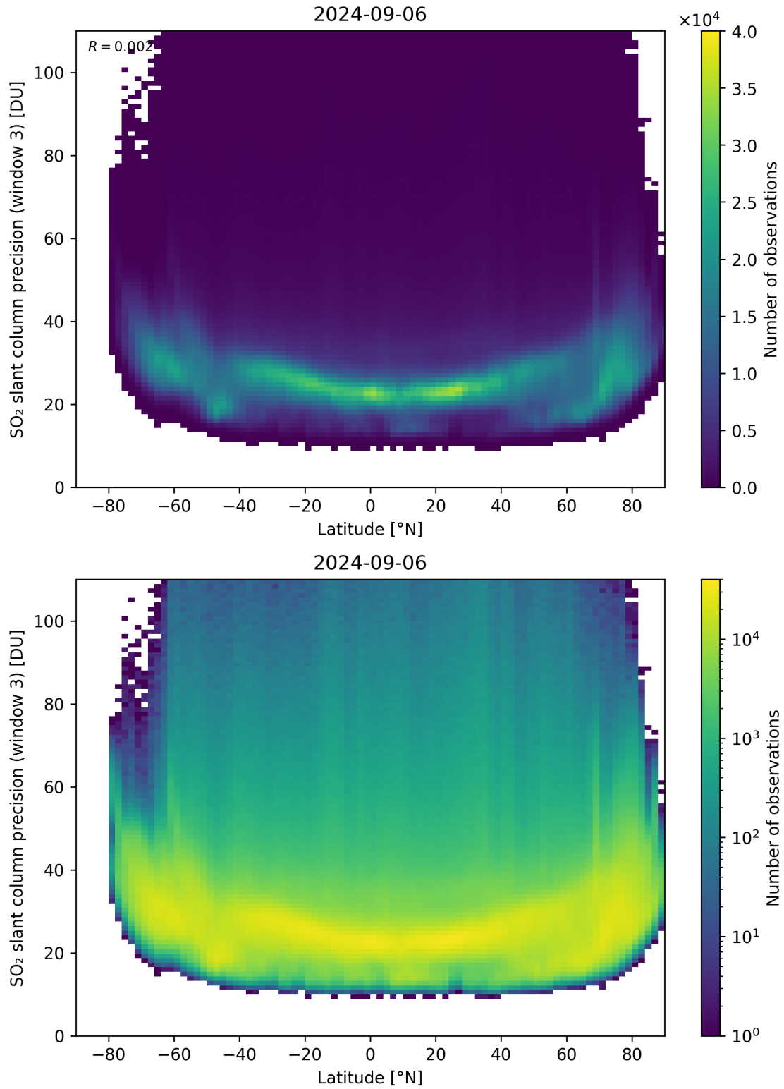
Figure 153: Scatter density plot of “Latitude” against “SO 2 slant column precision (window 3)” for 2024-09-06 to 2024-09-07.
