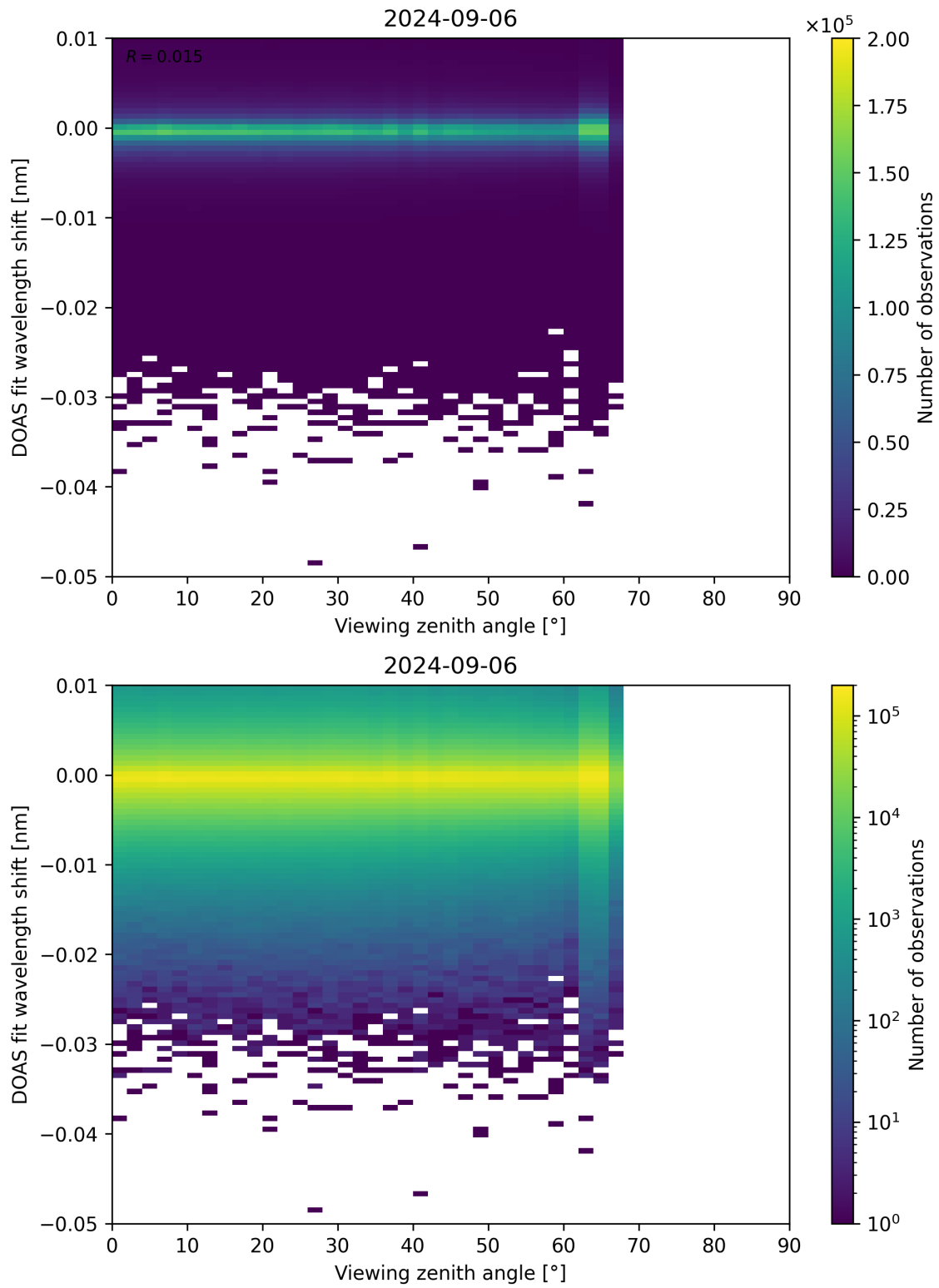
Figure 311: Scatter density plot of “Viewing zenith angle” against “DOAS fit wavelength shift” for 2024-09-06 to 2024-09-07.
