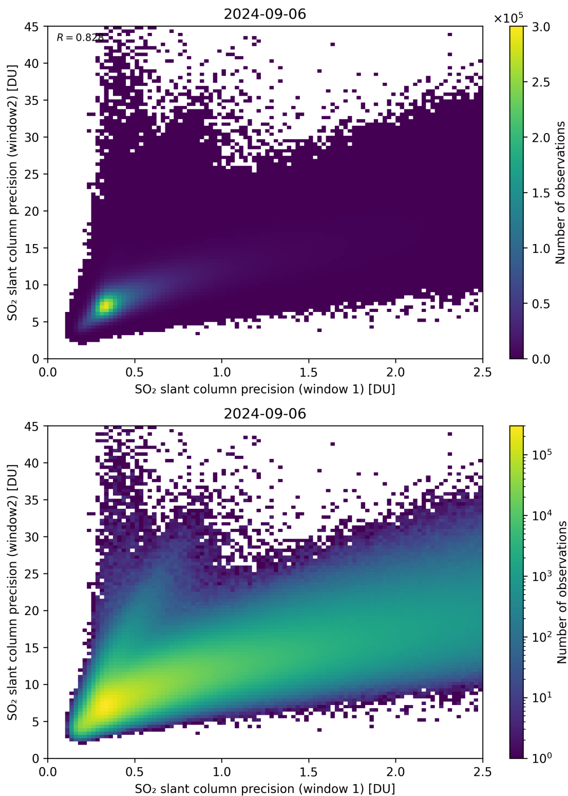
Figure 227: Scatter density plot of “SO 2 slant column precision (window 1)” against “SO 2 slant column precision (window2)” for 2024-09-06 to 2024-09-07.
