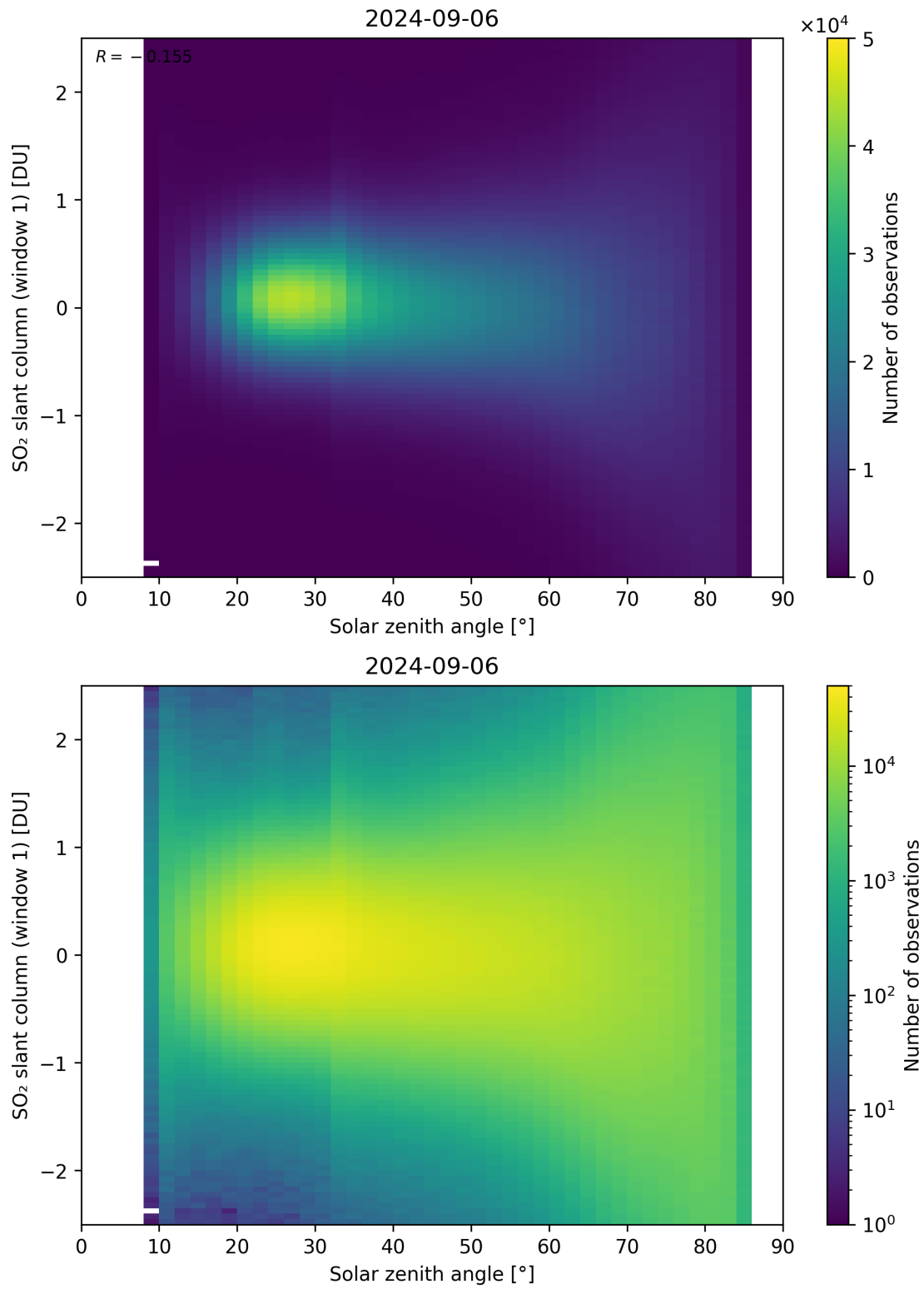
Figure 169: Scatter density plot of “Solar zenith angle” against “SO 2 slant column (window 1)” for 2024-09-06 to 2024-09-07.
