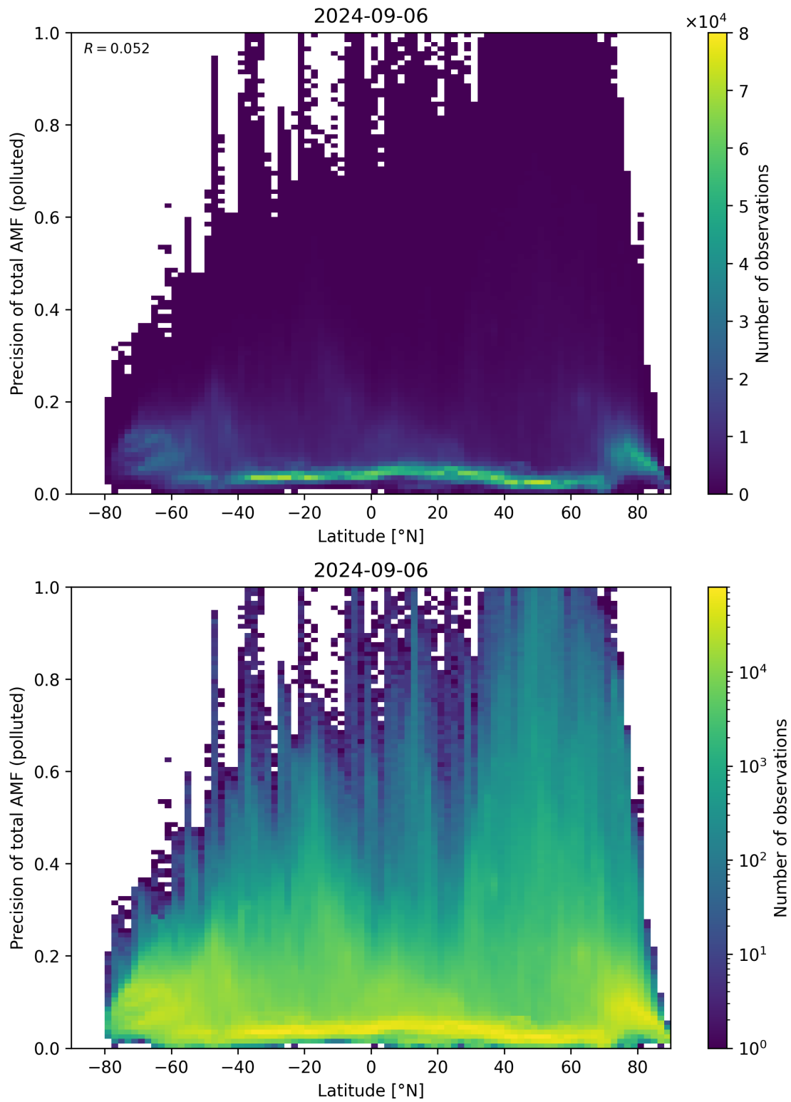
Figure 155: Scatter density plot of “Latitude” against “Precision of total AMF (polluted)” for 2024-09-06 to 2024-09-07.
