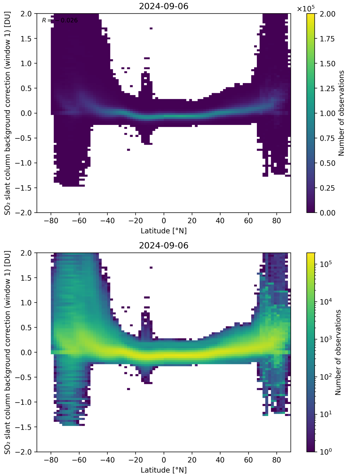
Figure 139: Scatter density plot of “Latitude” against “SO 2 slant column background correction (window 1)” for 2024-09-06 to 2024-09-07.
