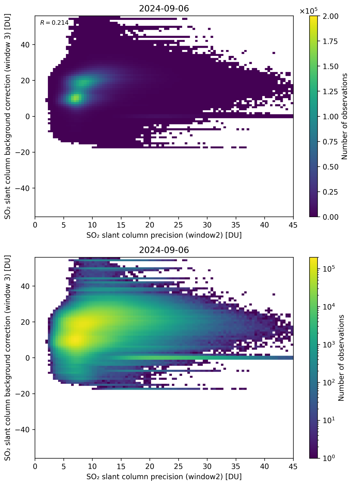
Figure 242: Scatter density plot of “SO 2 slant column precision (window2)” against “SO 2 slant column background correction (window 3)” for 2024-09-06 to 2024-09-07.
