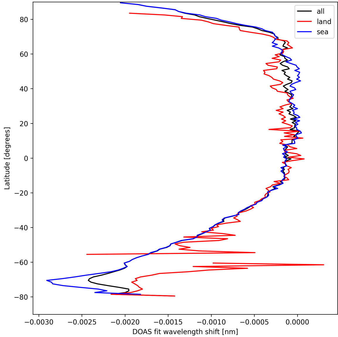
Figure 45: Zonal average of “DOAS fit wavelength shift” for 2024-09-06 to 2024-09-07.
