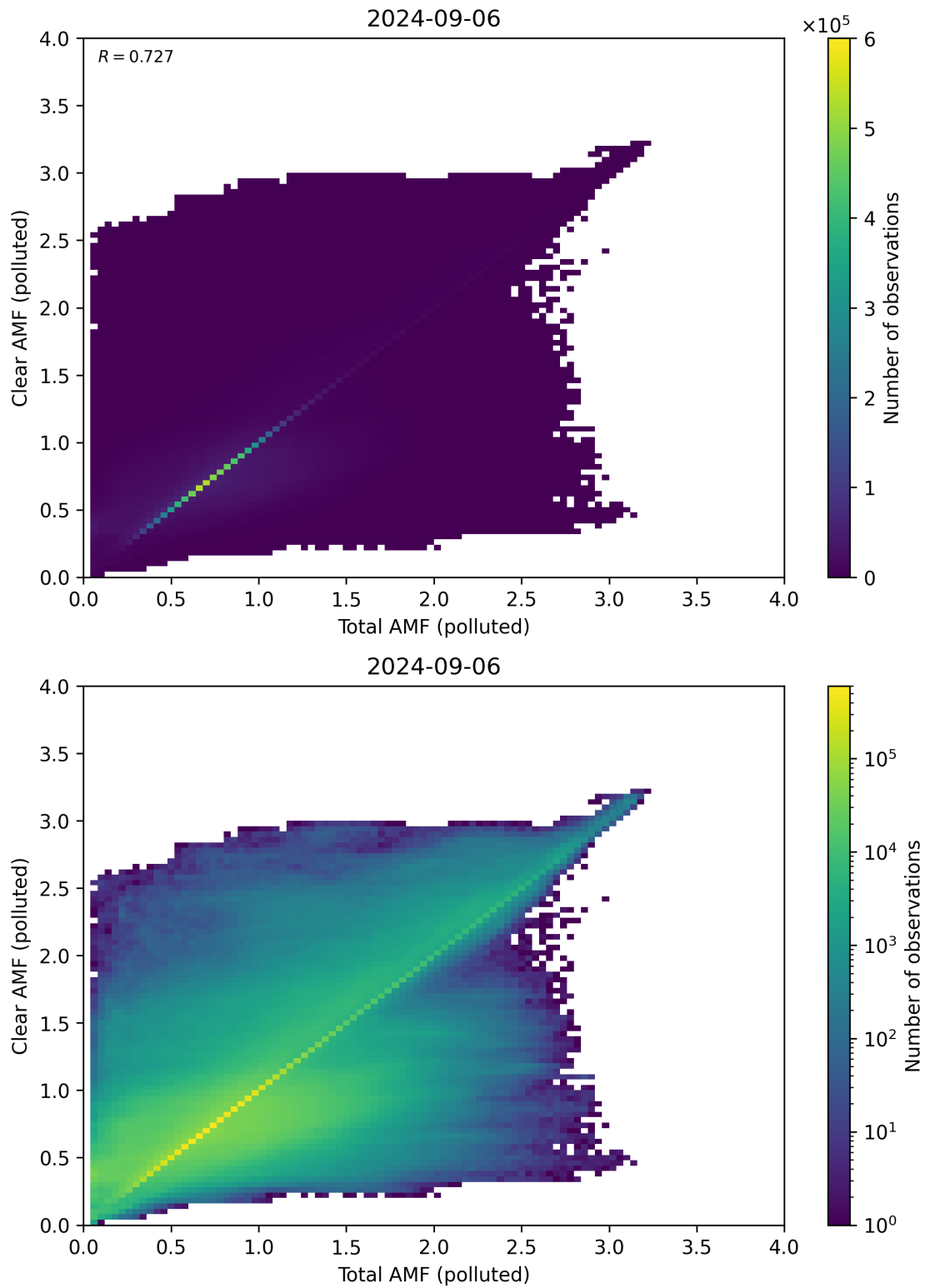
Figure 271: Scatter density plot of “Total AMF (polluted)” against “Clear AMF (polluted)” for 2024-09-06 to 2024-09-07.
