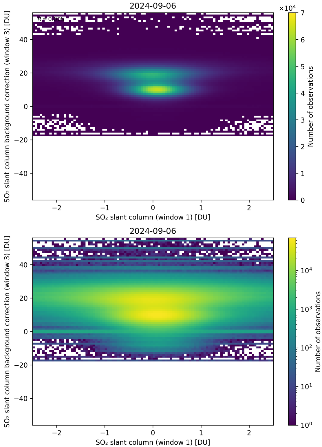
Figure 214: Scatter density plot of “SO 2 slant column (window 1)” against “SO 2 slant column background correction (window 3)” for 2024-09-06 to 2024-09-07.
