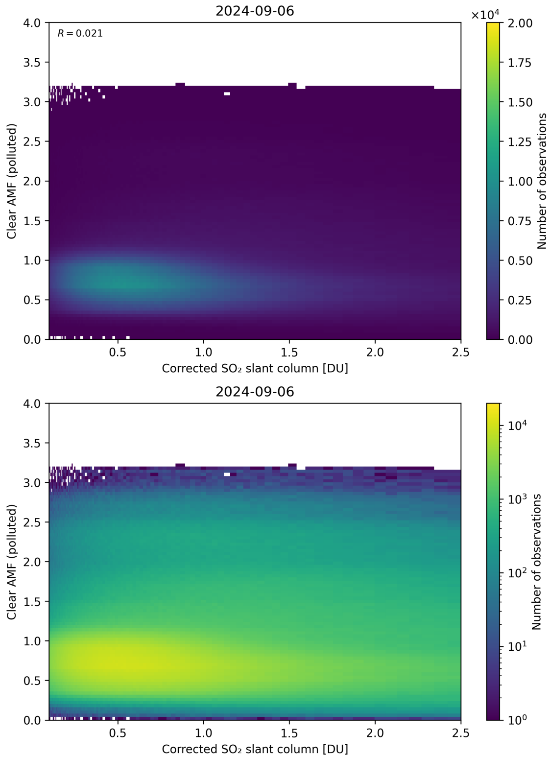
Figure 184: Scatter density plot of “Corrected SO 2 slant column” against “Clear AMF (polluted)” for 2024-09-06 to 2024-09-07.
