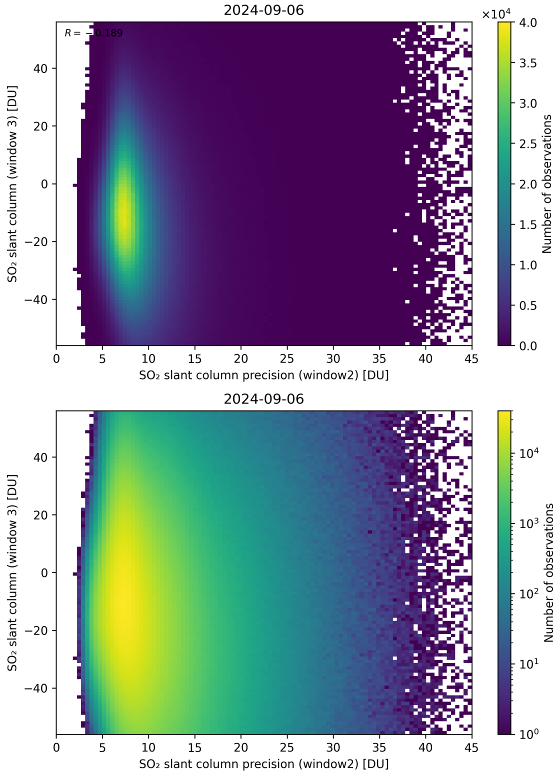
Figure 249: Scatter density plot of “SO 2 slant column precision (window2)” against “SO 2 slant column (window 3)” for 2024-09-06 to 2024-09-07.
