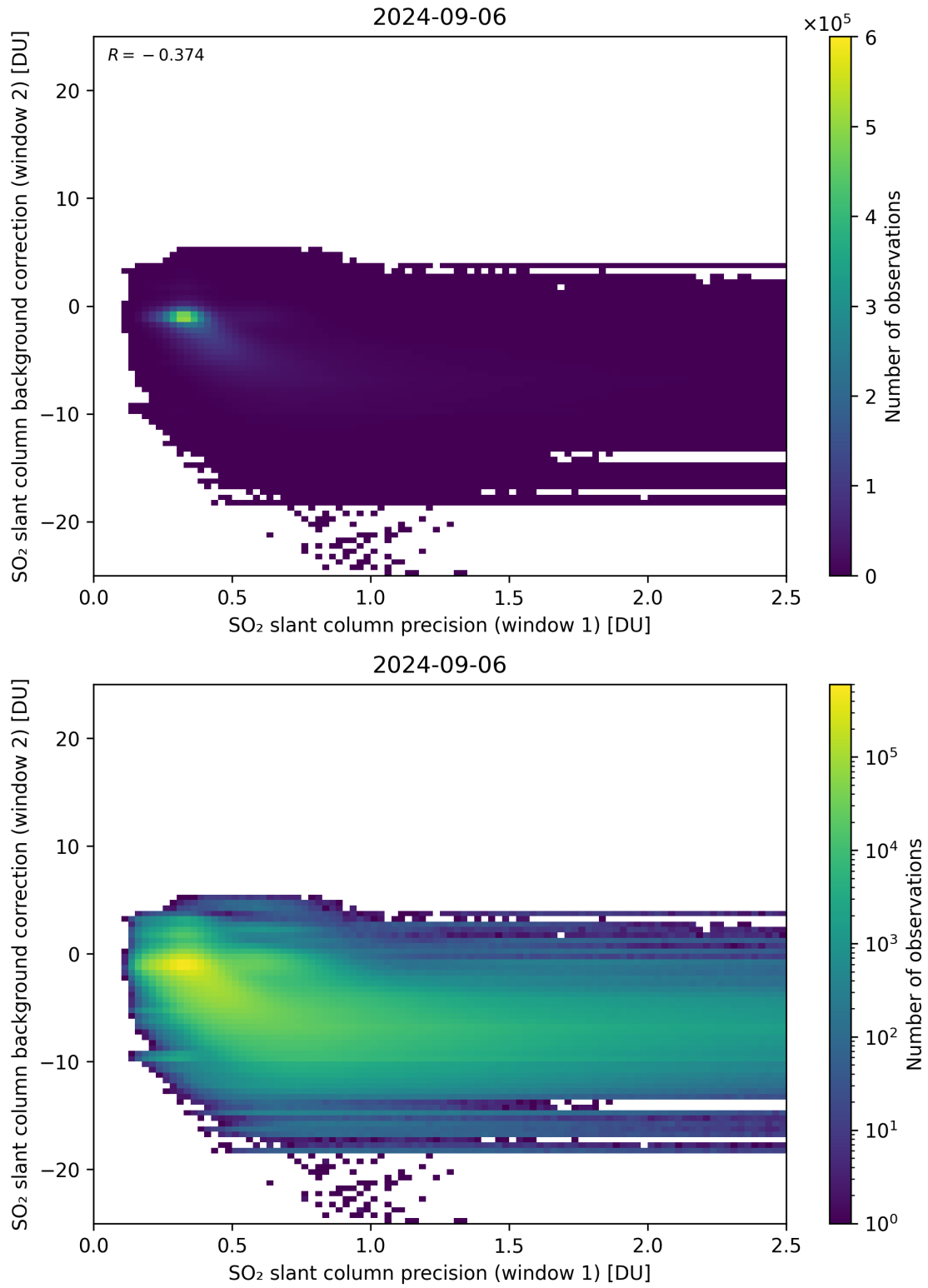
Figure 219: Scatter density plot of “SO 2 slant column precision (window 1)” against “SO 2 slant column background correction (window 2)” for 2024-09-06 to 2024-09-07.
