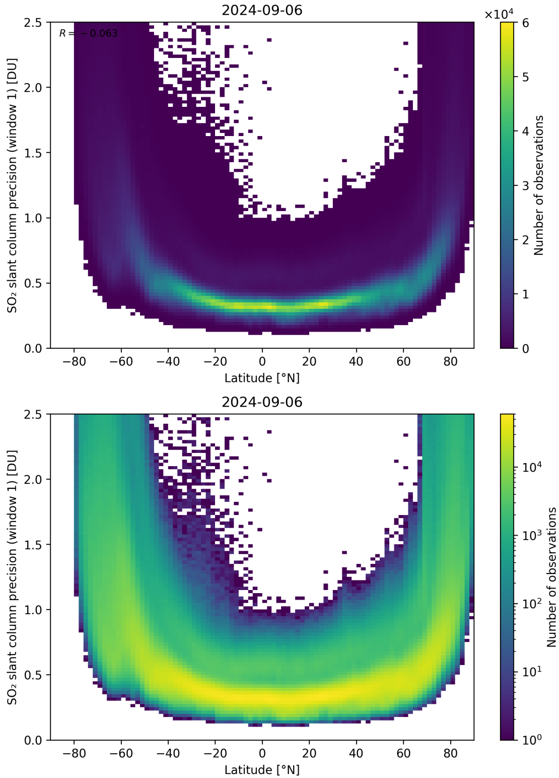
Figure 150: Scatter density plot of “Latitude” against “SO 2 slant column precision (window 1)” for 2024-09-06 to 2024-09-07.
