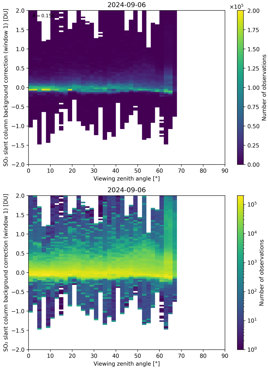
Figure 308: Scatter density plot of “Viewing zenith angle” against “SO 2 slant column background correction (window 1)” for 2024-09-06 to 2024-09-07.
