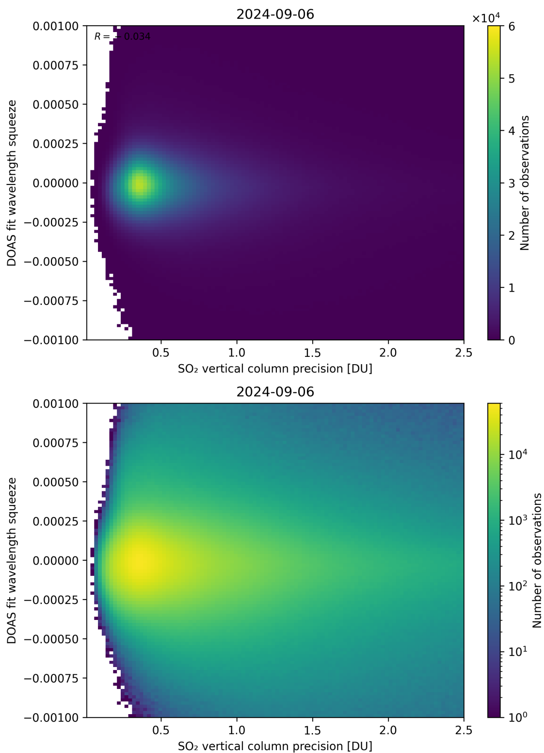
Figure 283: Scatter density plot of “SO 2 vertical column precision” against “DOAS fit wavelength squeeze” for 2024-09-06 to 2024-09-07.
