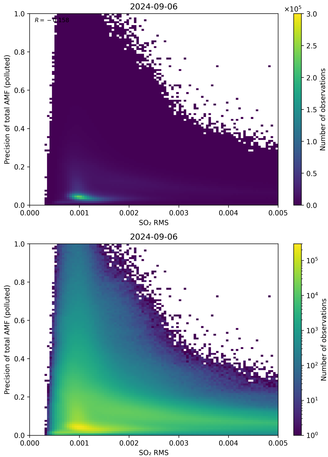
Figure 138: Scatter density plot of “SO 2 RMS” against “Precision of total AMF (polluted)” for 2024-09-06 to 2024-09-07.
