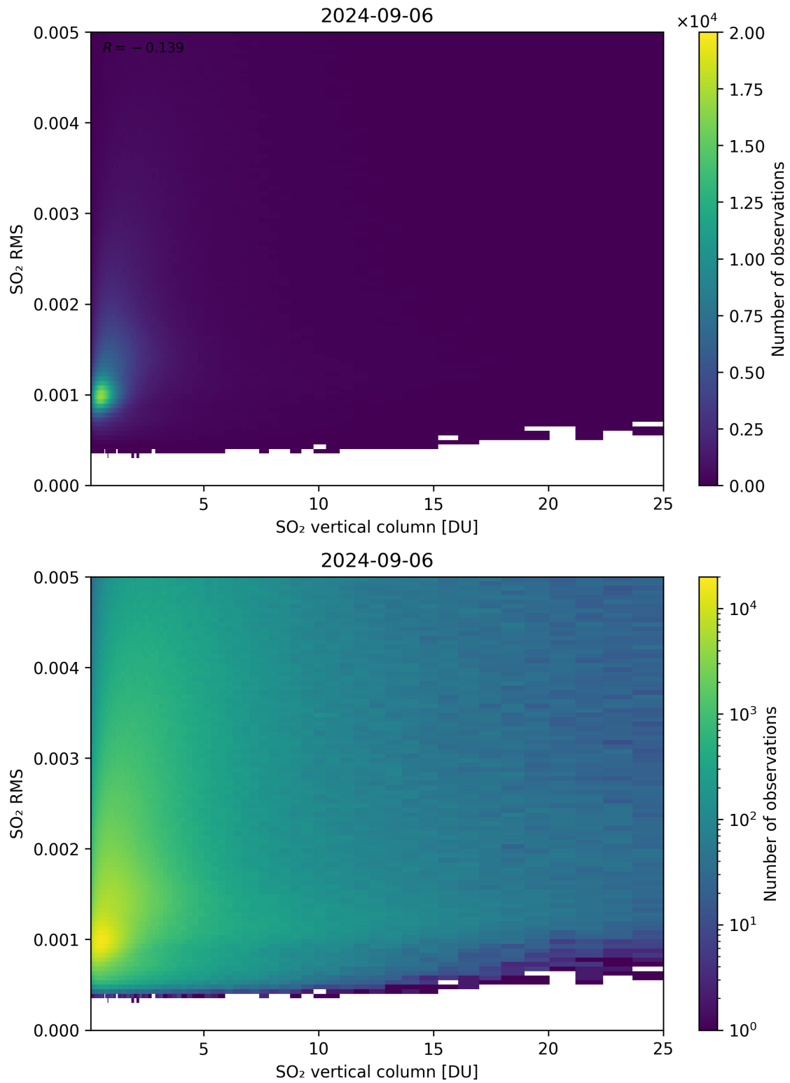
Figure 278: Scatter density plot of “SO 2 vertical column” against “SO 2 RMS” for 2024-09-06 to 2024-09-07.
