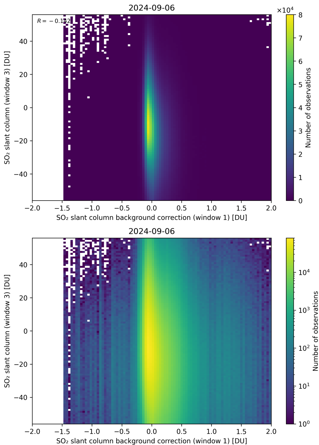
Figure 107: Scatter density plot of “SO 2 slant column background correction (window 1)” against “SO 2 slant column (window 3)” for 2024-09-06 to 2024-09-07.
