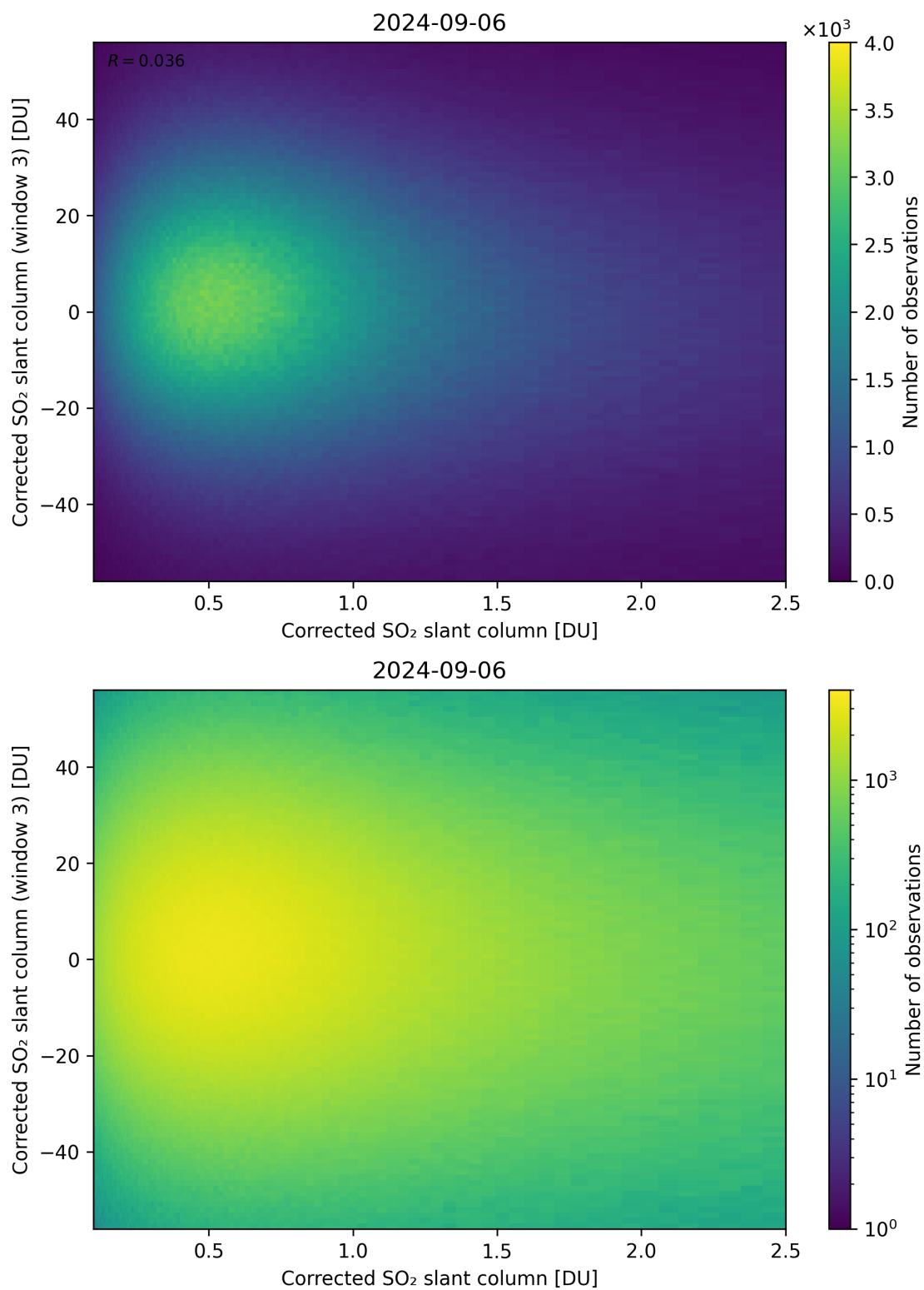
Figure 186: Scatter density plot of “Corrected SO 2 slant column” against “Corrected SO 2 slant column (window 3)” for 2024-09-06 to 2024-09-07.
