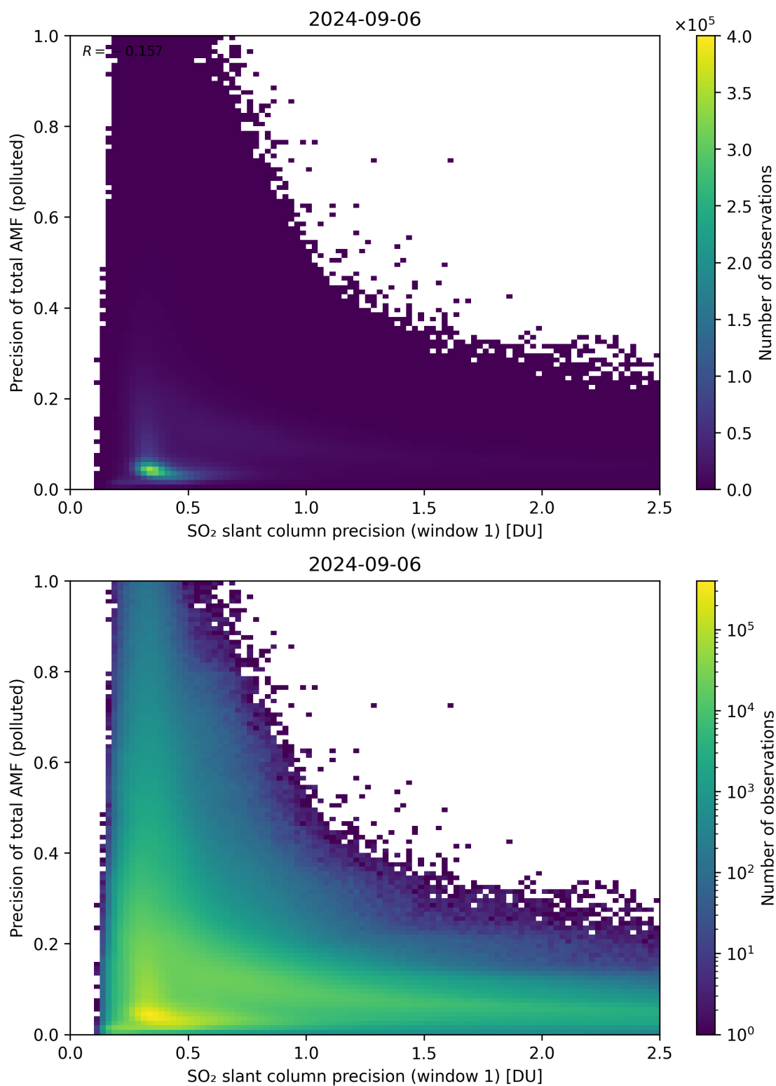
Figure 231: Scatter density plot of “SO 2 slant column precision (window 1)” against “Precision of total AMF (polluted)” for 2024-09-06 to 2024-09-07.
