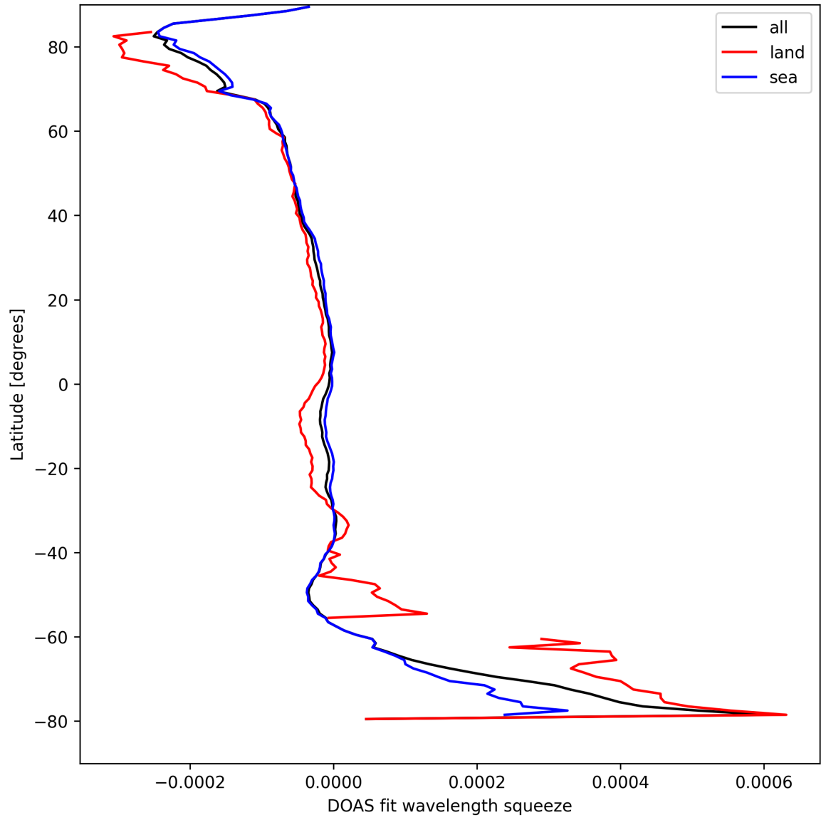
Figure 46: Zonal average of “DOAS fit wavelength squeeze” for 2024-09-06 to 2024-09-07.
