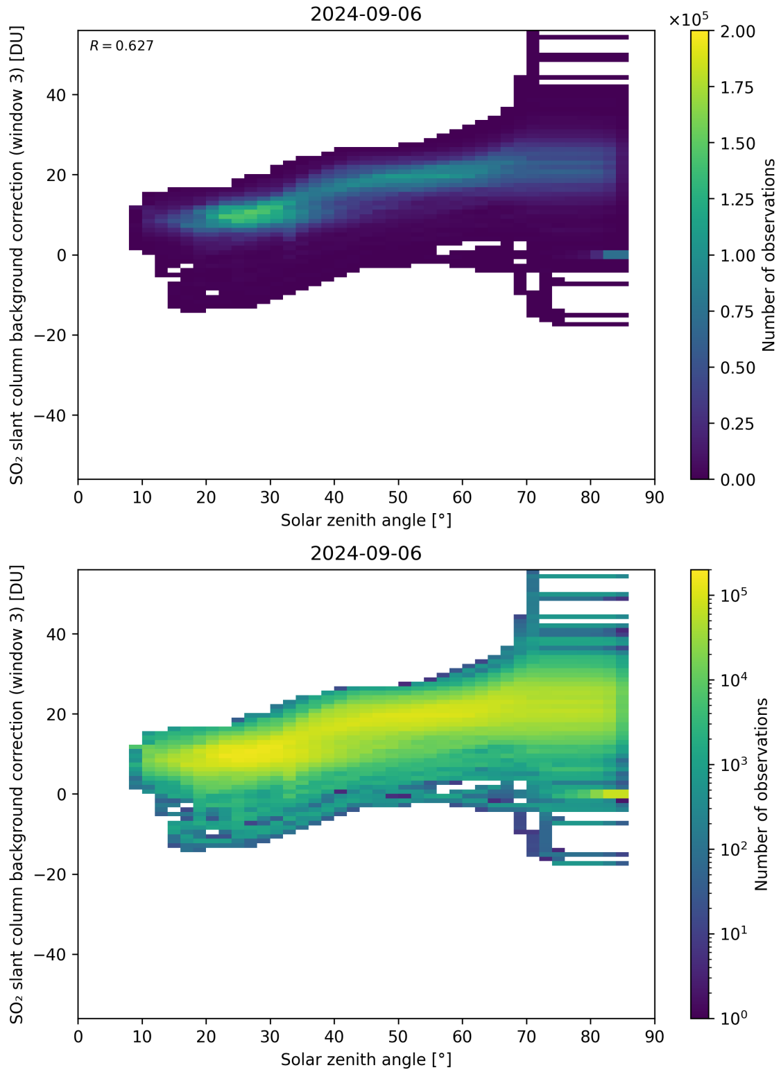
Figure 160: Scatter density plot of “Solar zenith angle” against “SO 2 slant column background correction (window 3)” for 2024-09-06 to 2024-09-07.
