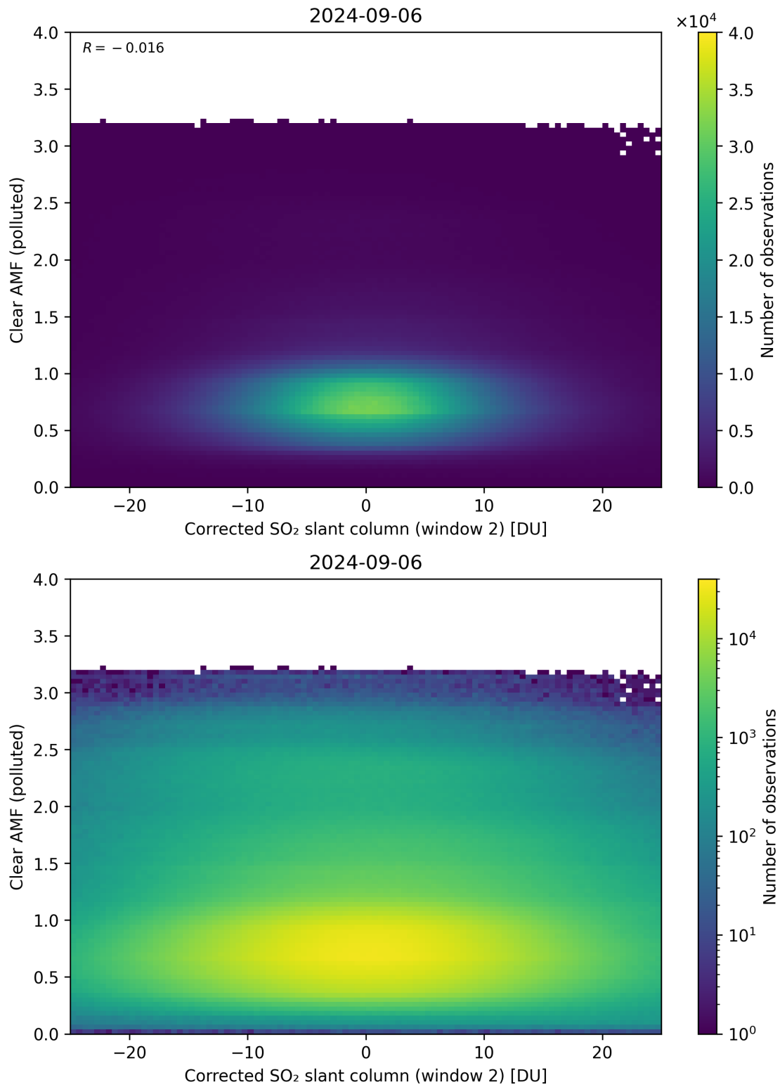
Figure 199: Scatter density plot of “Corrected SO 2 slant column (window 2)” against “Clear AMF (polluted)” for 2024-09-06 to 2024-09-07.
