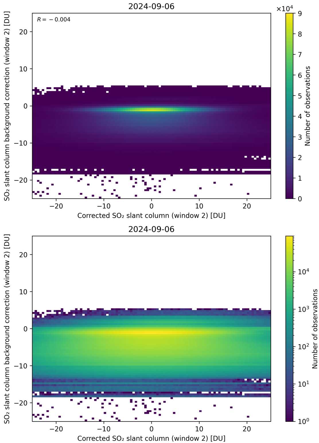
Figure 194: Scatter density plot of “Corrected SO 2 slant column (window 2)” against “SO 2 slant column background correction (window 2)” for 2024-09-06 to 2024-09-07.
