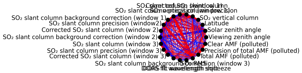
Figure 1: Map of correlation graph for 2024-09-06 to 2024-09-07.
