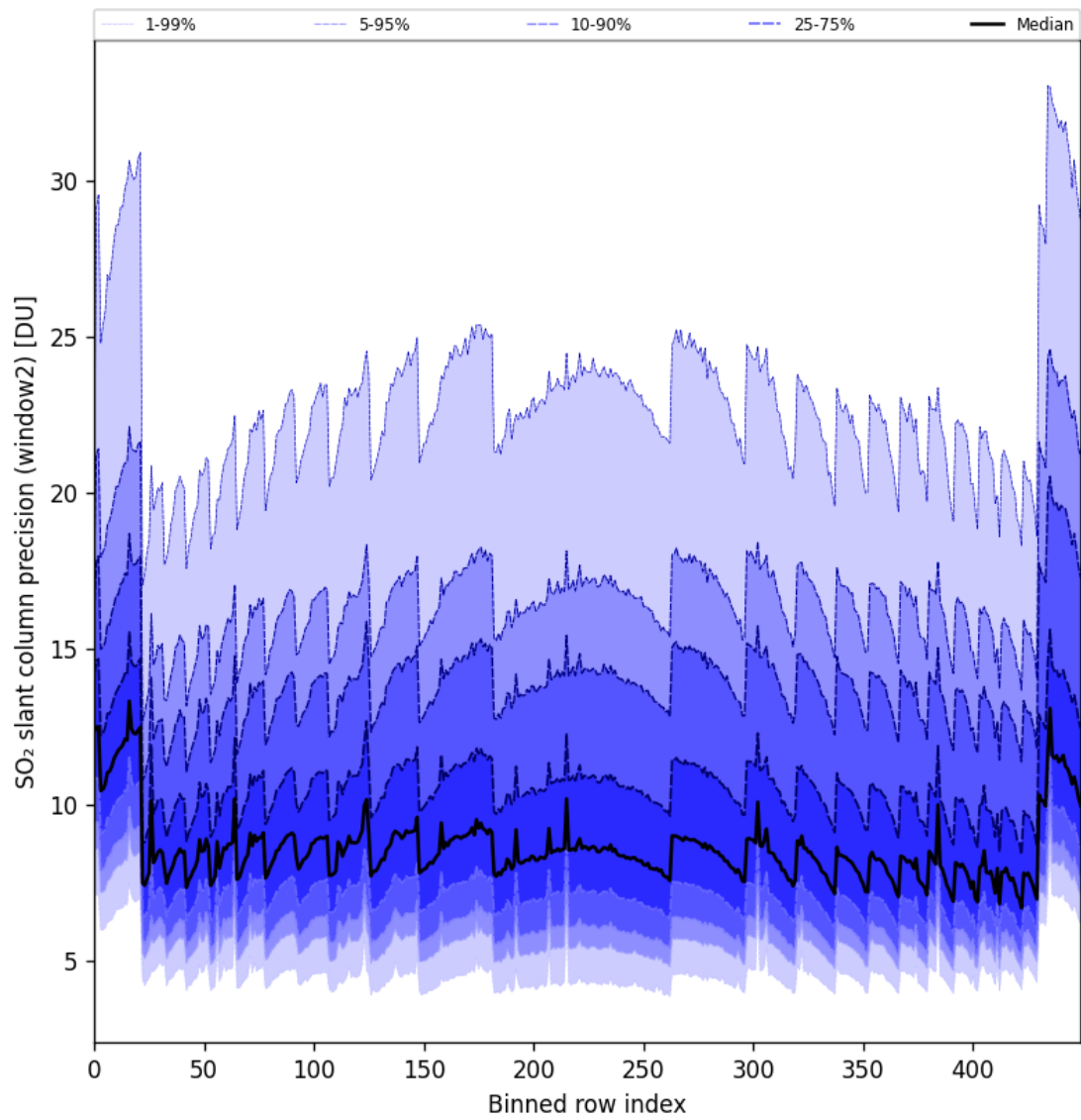
Figure 84: Along track statistics of “SO 2 slant column precision (window2)” for 2024-09-06 to 2024-09-07
