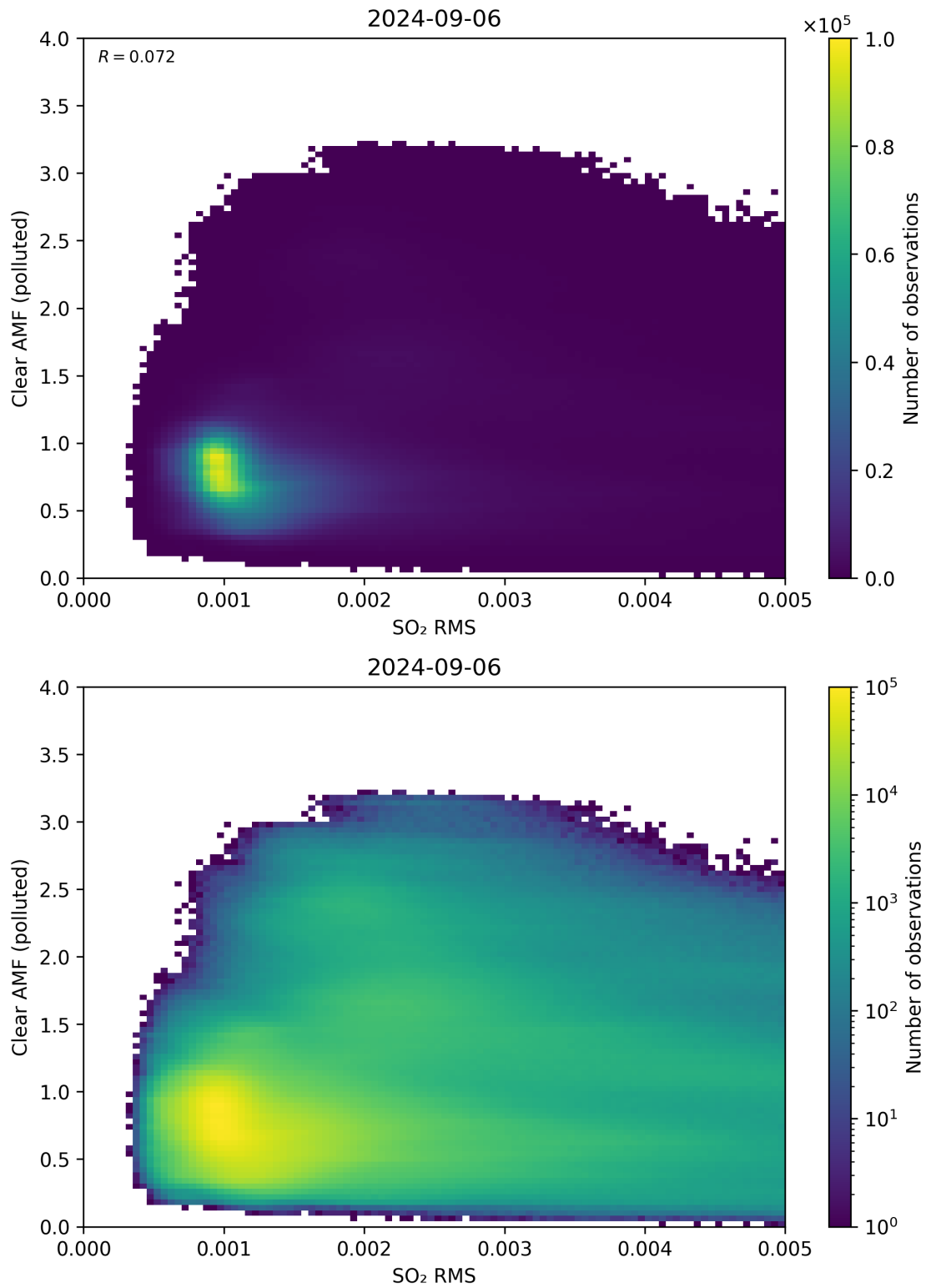
Figure 136: Scatter density plot of “SO 2 RMS” against “Clear AMF (polluted)” for 2024-09-06 to 2024-09-07.
