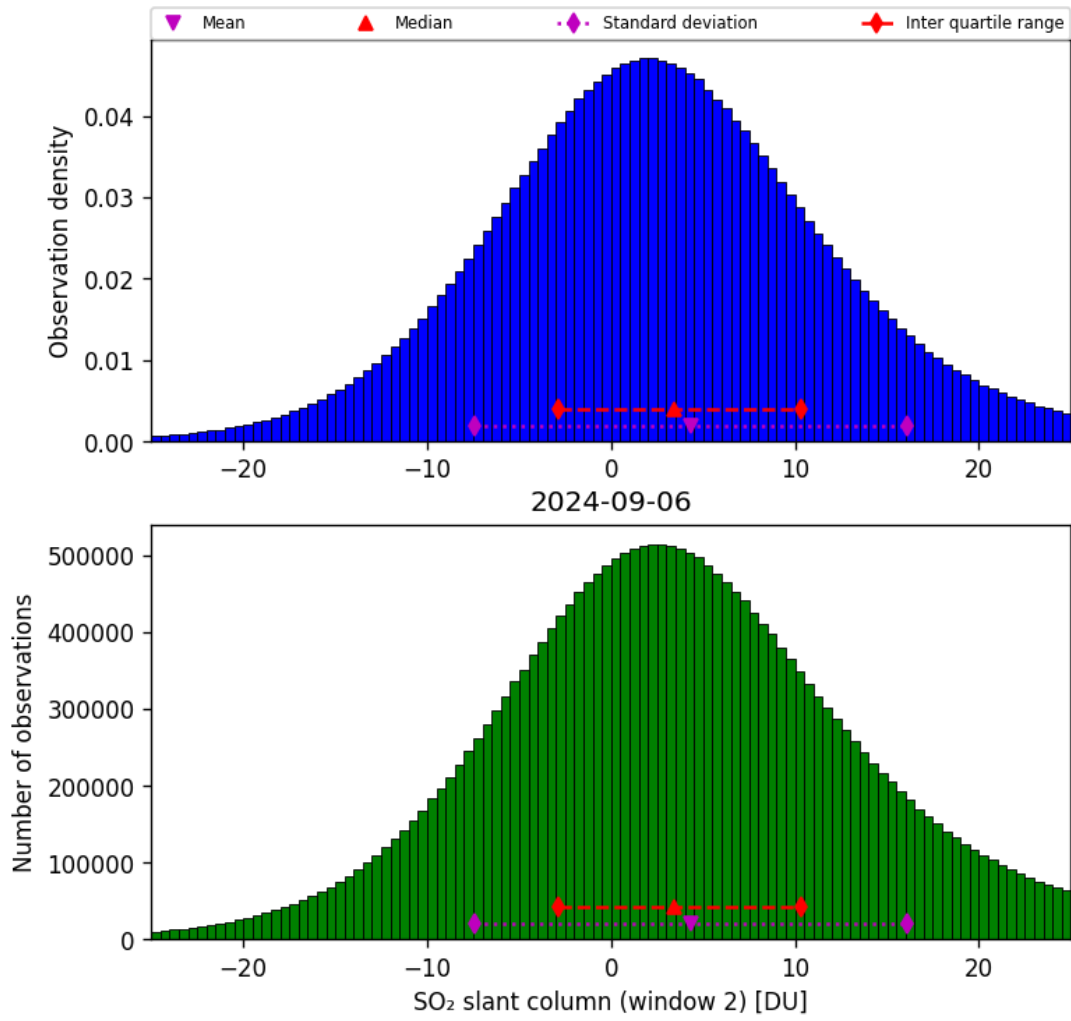
Figure 60: Histogram of “SO 2 slant column (window 2)” for 2024-09-06 to 2024-09-07
