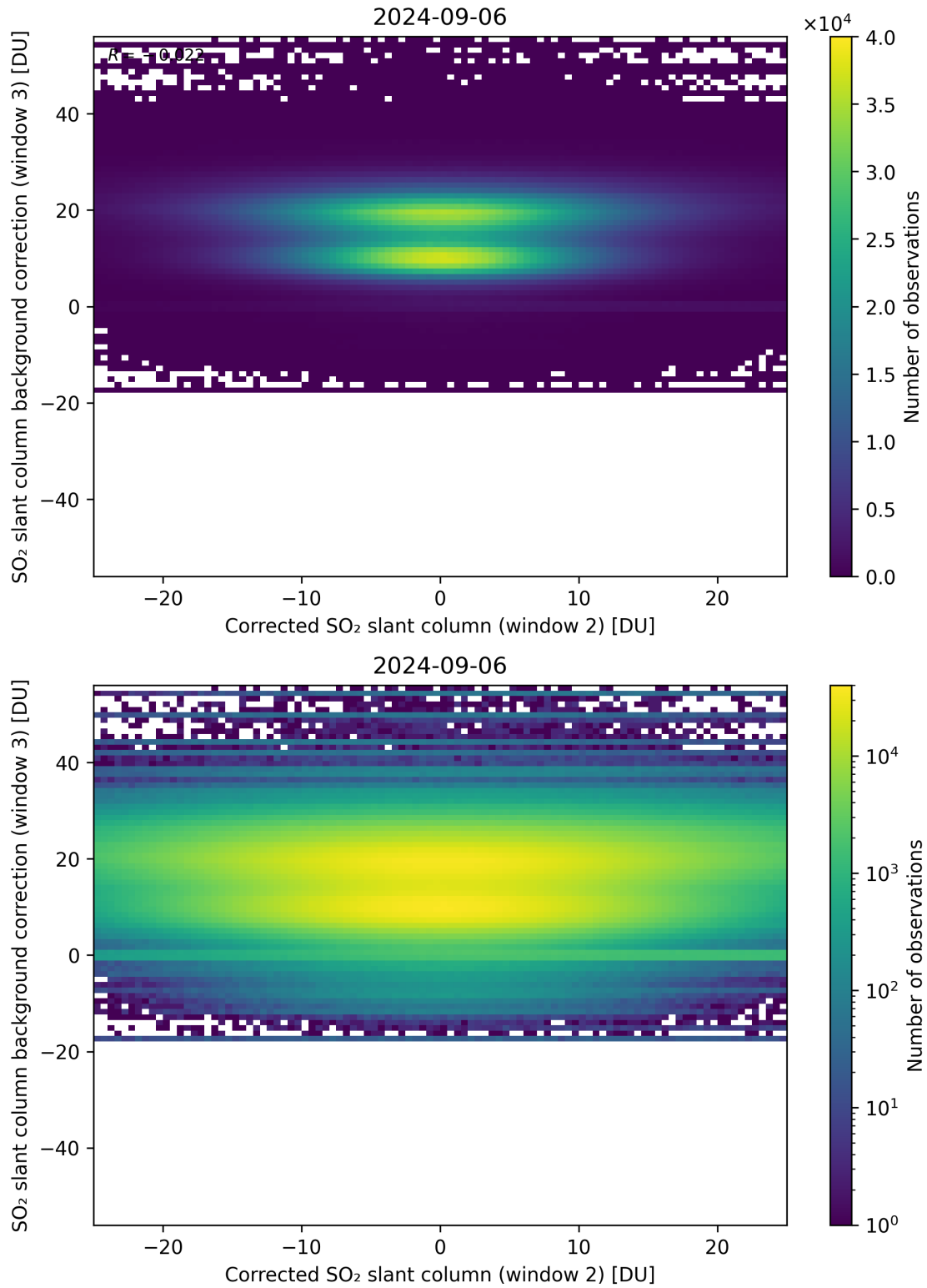
Figure 195: Scatter density plot of “Corrected SO 2 slant column (window 2)” against “SO 2 slant column background correction (window 3)” for 2024-09-06 to 2024-09-07.
