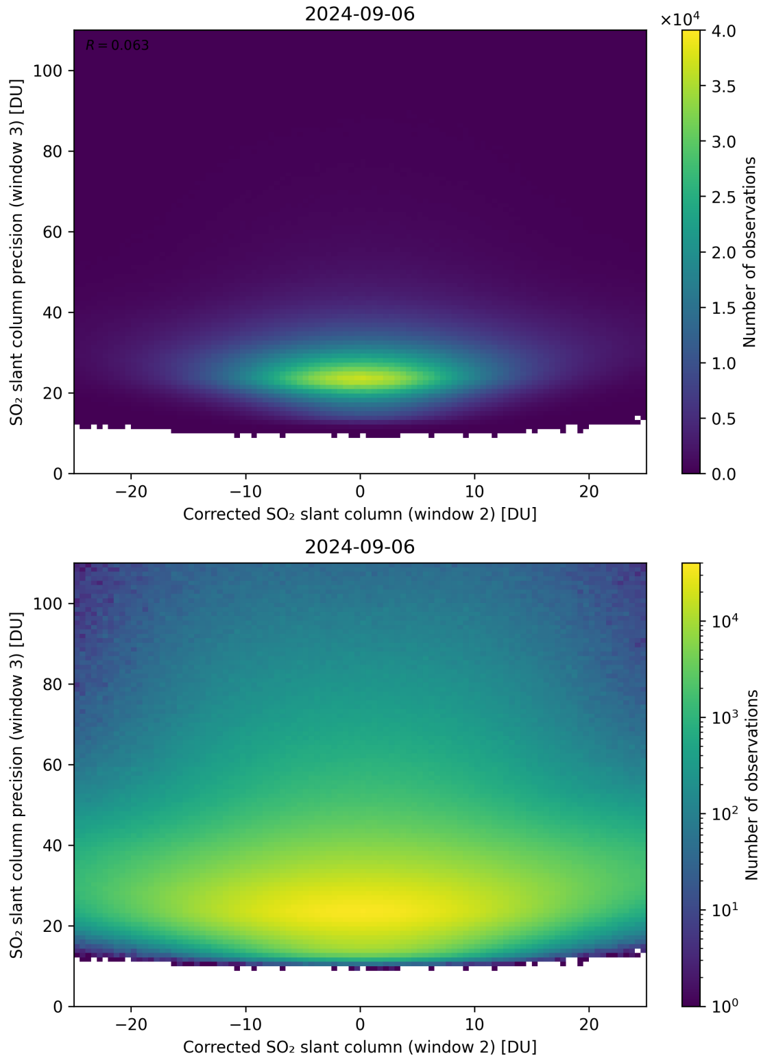
Figure 202: Scatter density plot of “Corrected SO 2 slant column (window 2)” against “SO 2 slant column precision (window 3)” for 2024-09-06 to 2024-09-07.
