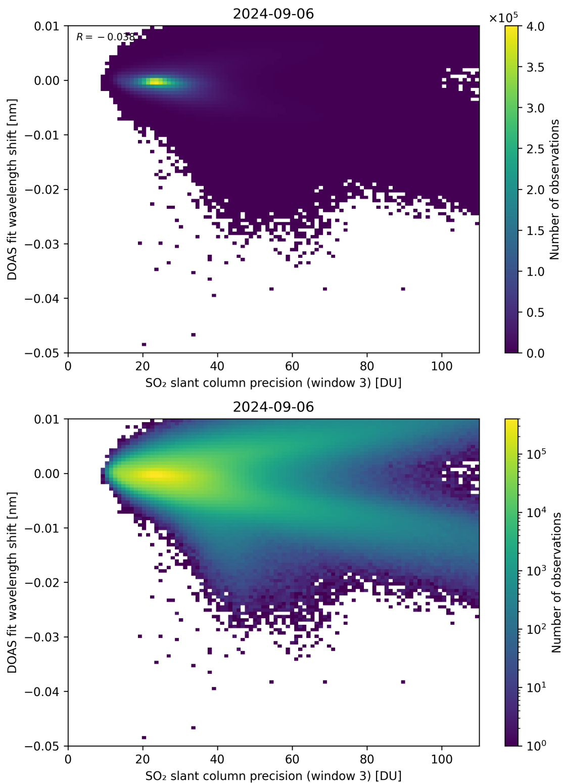
Figure 258: Scatter density plot of “SO 2 slant column precision (window 3)” against “DOAS fit wavelength shift” for 2024-09-06 to 2024-09-07.
