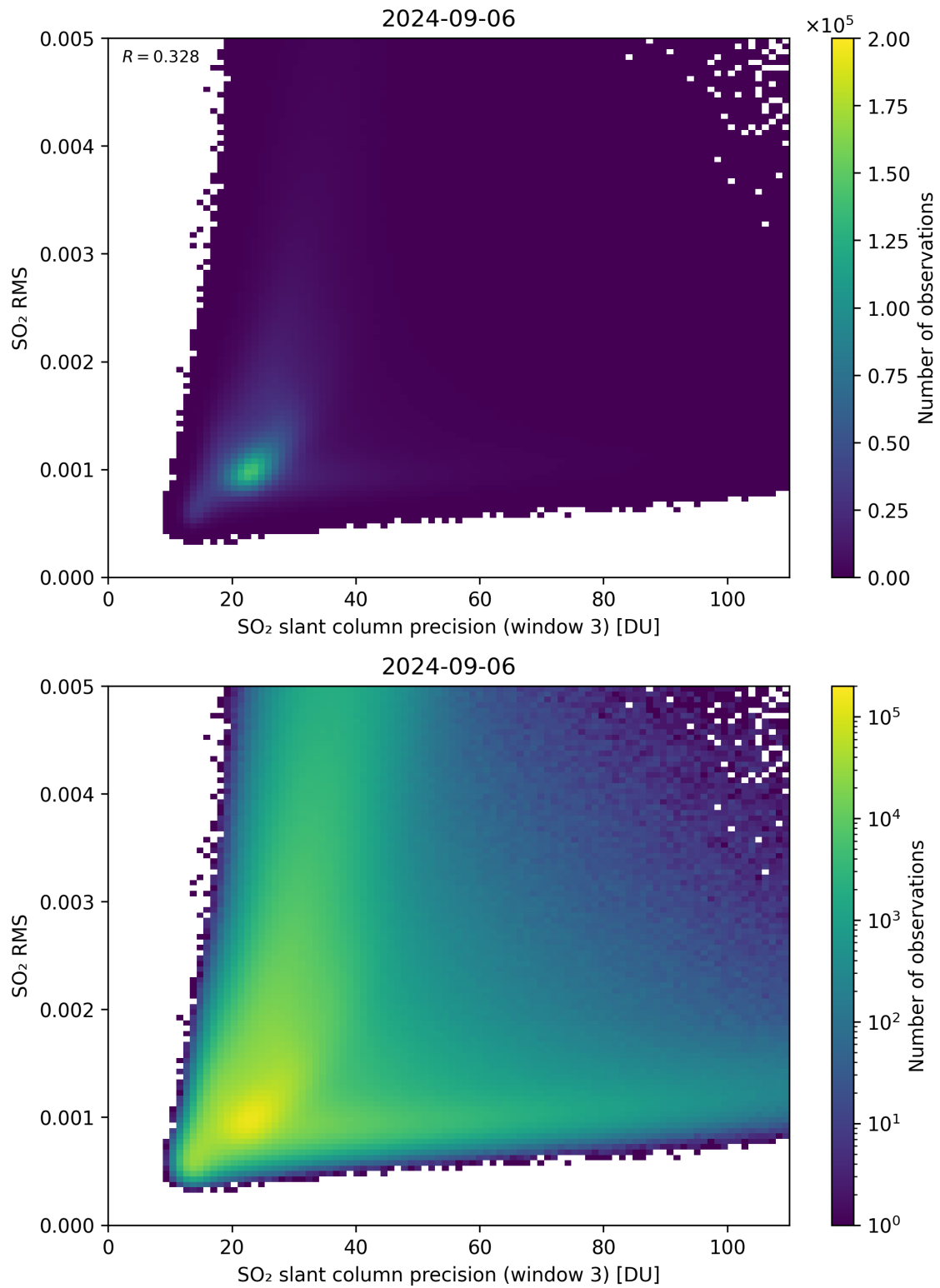
Figure 260: Scatter density plot of “SO 2 slant column precision (window 3)” against “SO 2 RMS” for 2024-09-06 to 2024-09-07.
