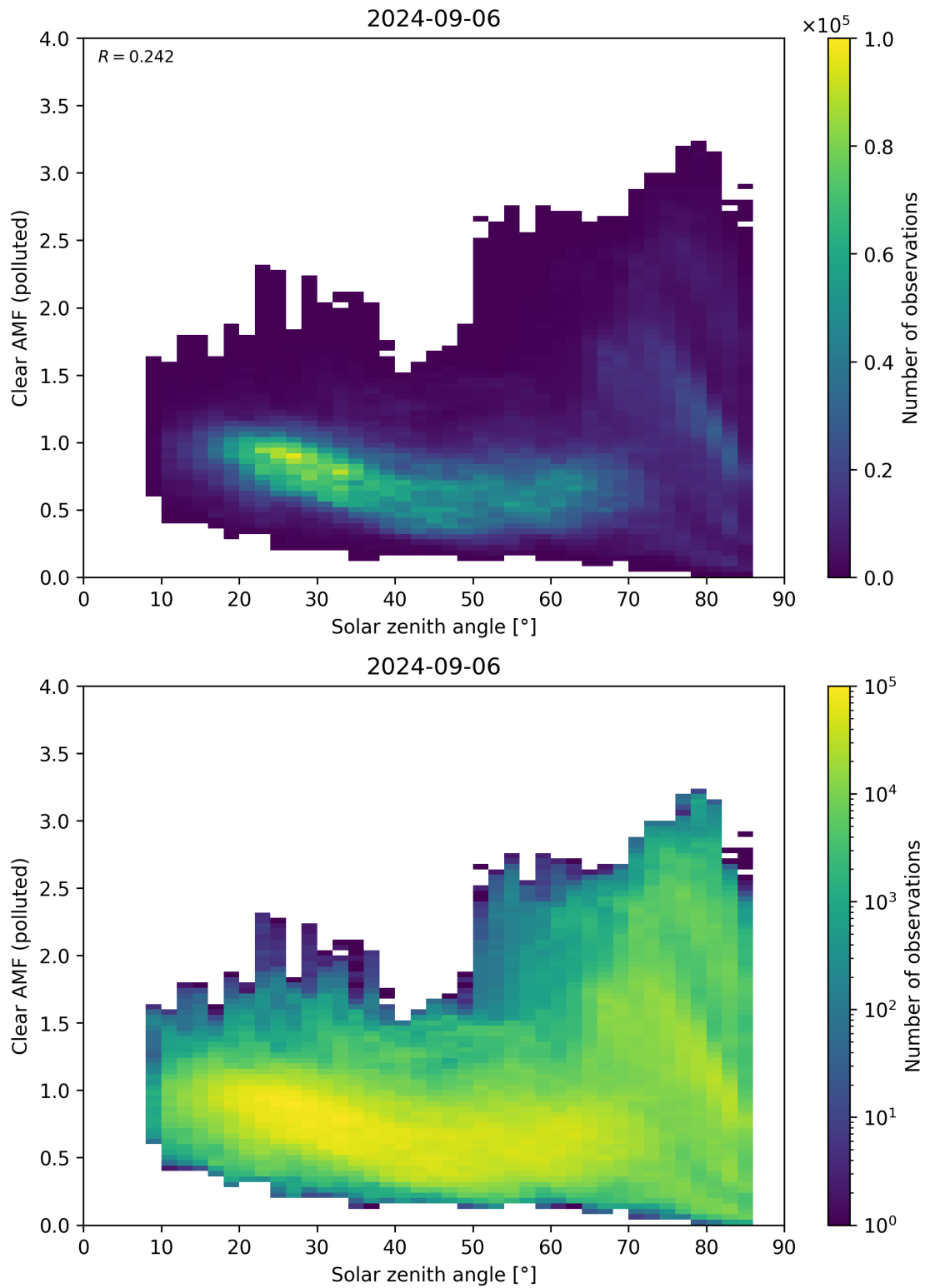
Figure 165: Scatter density plot of “Solar zenith angle” against “Clear AMF (polluted)” for 2024-09-06 to 2024-09-07.
