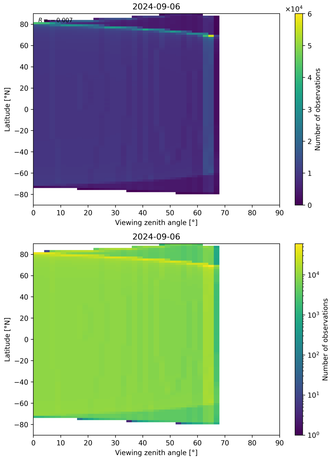
Figure 314: Scatter density plot of “Viewing zenith angle” against “Latitude” for 2024-09-06 to 2024-09-07.
