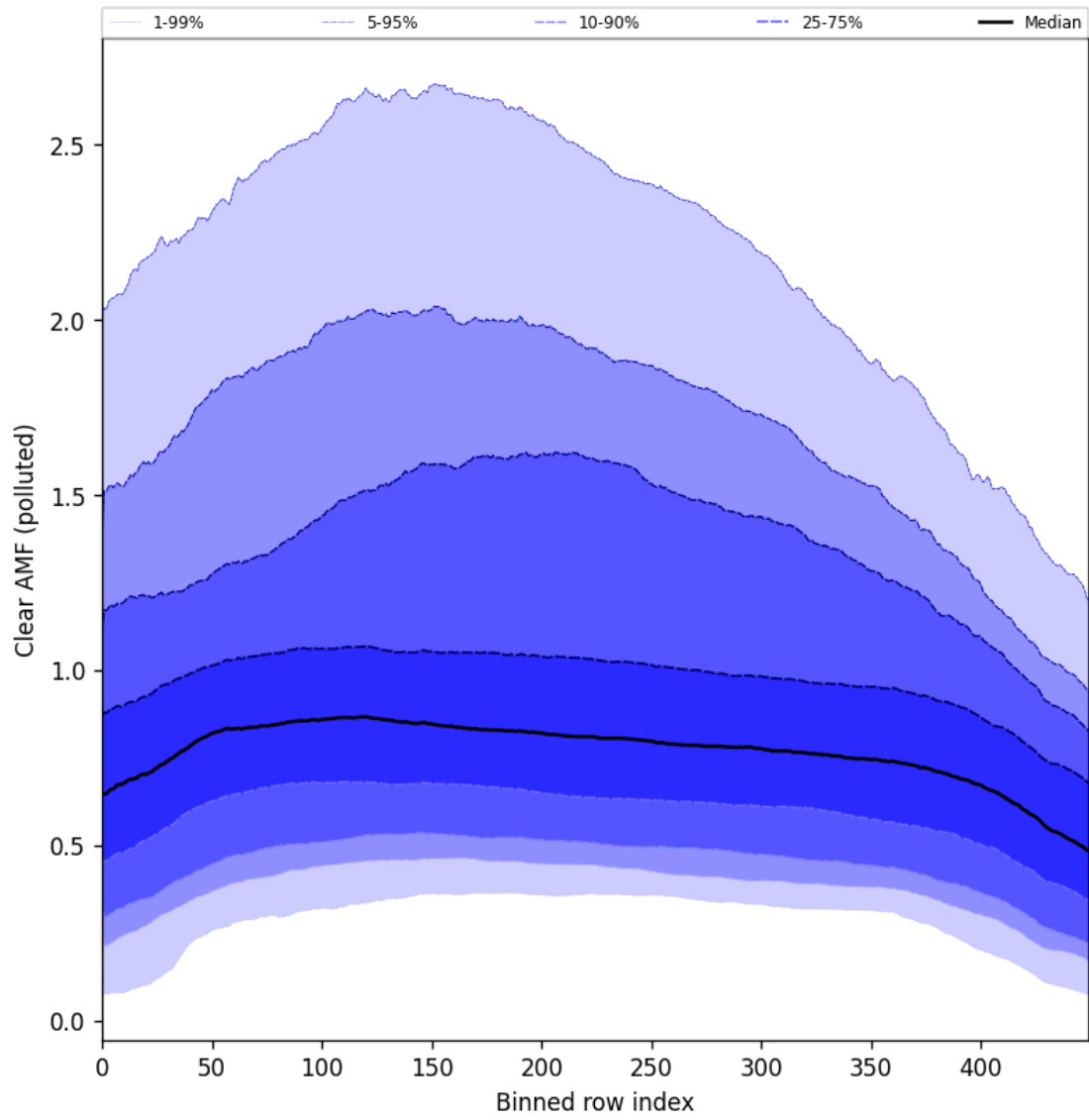
Figure 96: Along track statistics of “Clear AMF (polluted)” for 2024-09-06 to 2024-09-07
