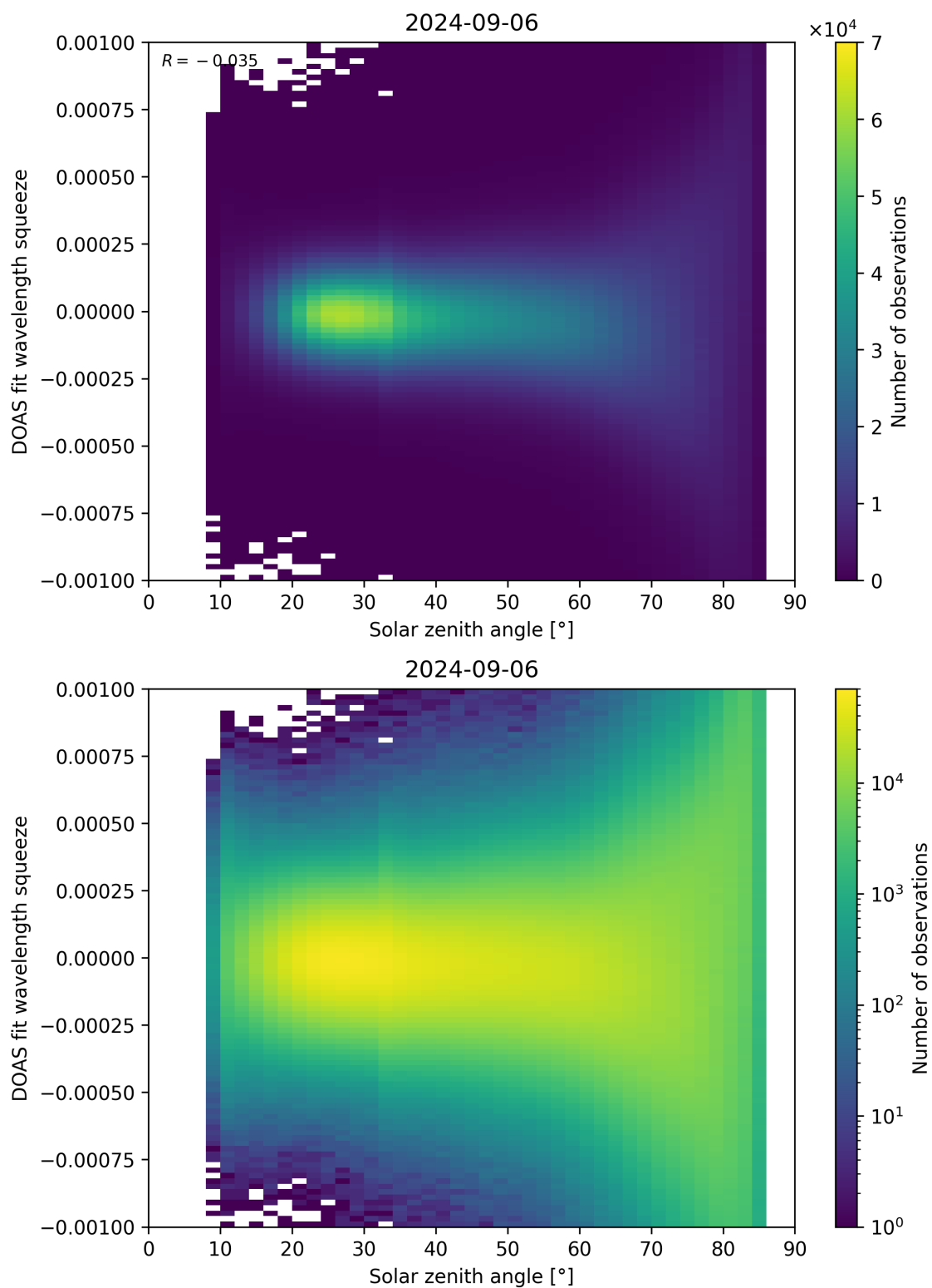
Figure 162: Scatter density plot of “Solar zenith angle” against “DOAS fit wavelength squeeze” for 2024-09-06 to 2024-09-07.
