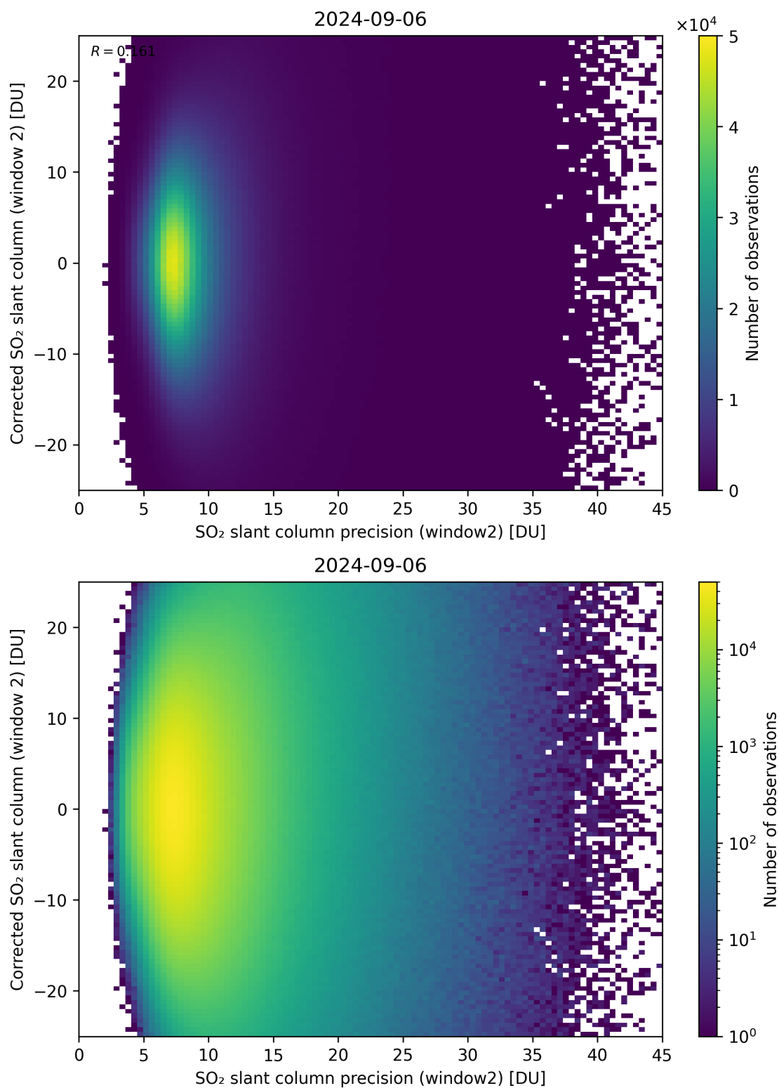
Figure 247: Scatter density plot of “SO 2 slant column precision (window2)” against “Corrected SO 2 slant column (window 2)” for 2024-09-06 to 2024-09-07.
