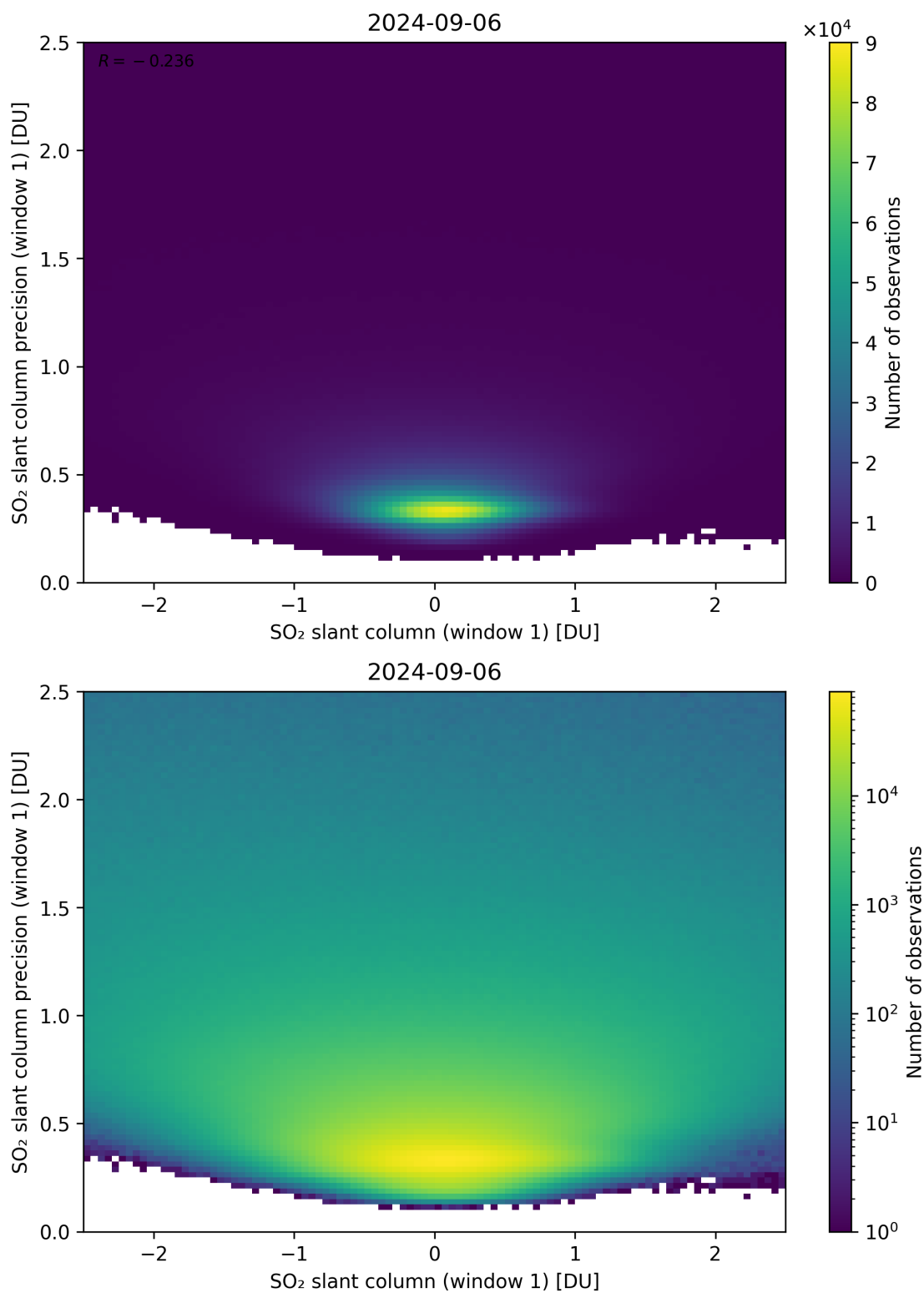
Figure 235: Scatter density plot of “SO 2 slant column (window 1)” against “SO 2 slant column precision (window 1)” for 2024-09-06 to 2024-09-07.
