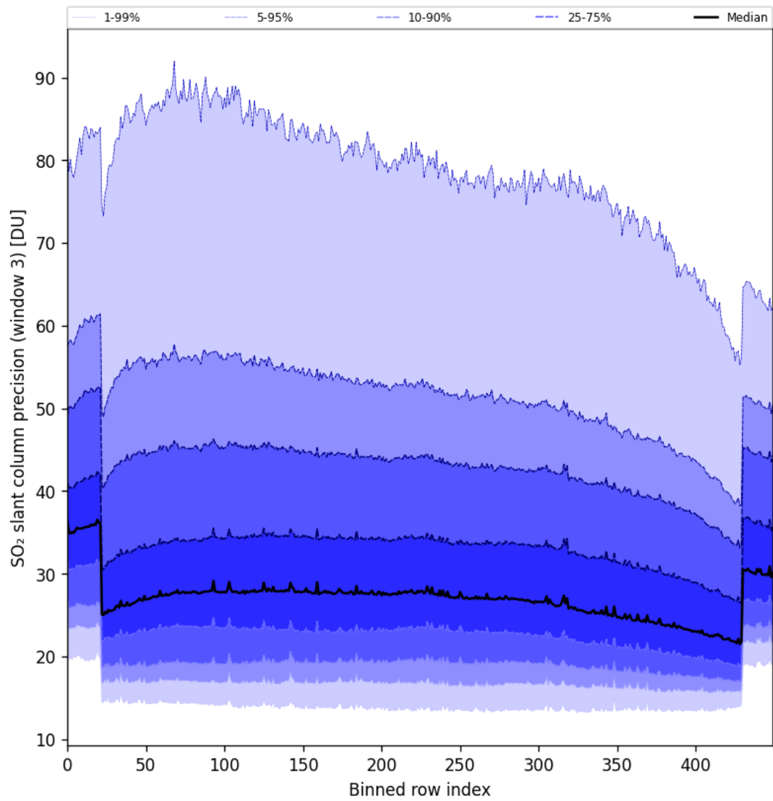
Figure 88: Along track statistics of “SO 2 slant column precision (window 3)” for 2024-09-06 to 2024-09-07
