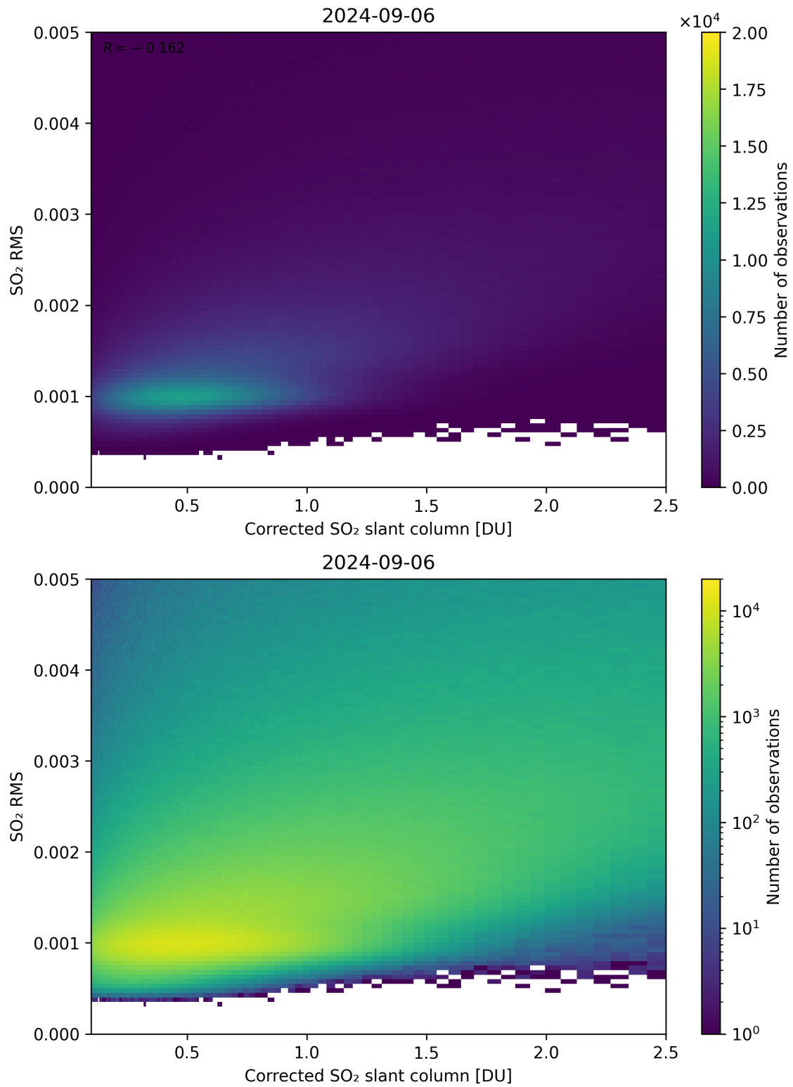
Figure 183: Scatter density plot of “Corrected SO 2 slant column” against “SO 2 RMS” for 2024-09-06 to 2024-09-07.
