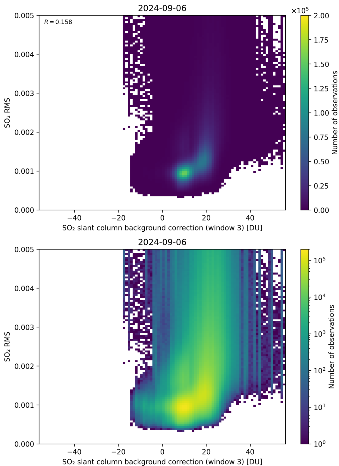
Figure 123: Scatter density plot of “SO 2 slant column background correction (window 3)” against “SO 2 RMS” for 2024-09-06 to 2024-09-07.
