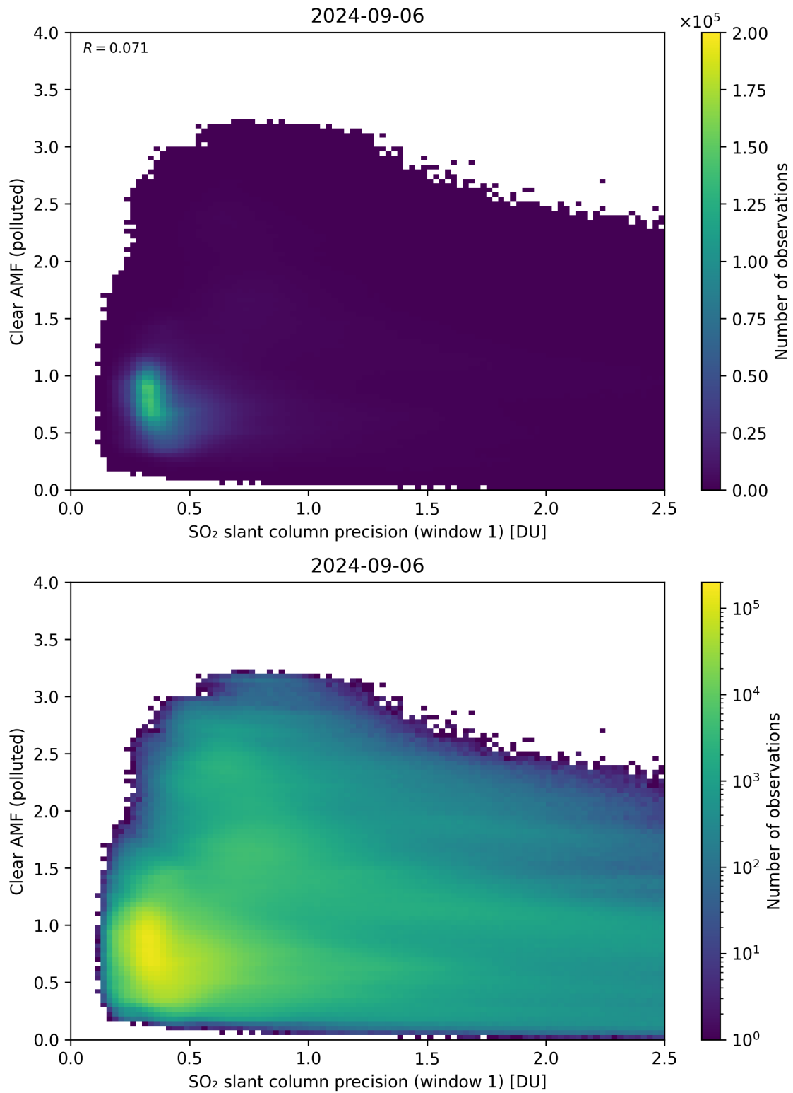
Figure 224: Scatter density plot of “SO 2 slant column precision (window 1)” against “Clear AMF (polluted)” for 2024-09-06 to 2024-09-07.
