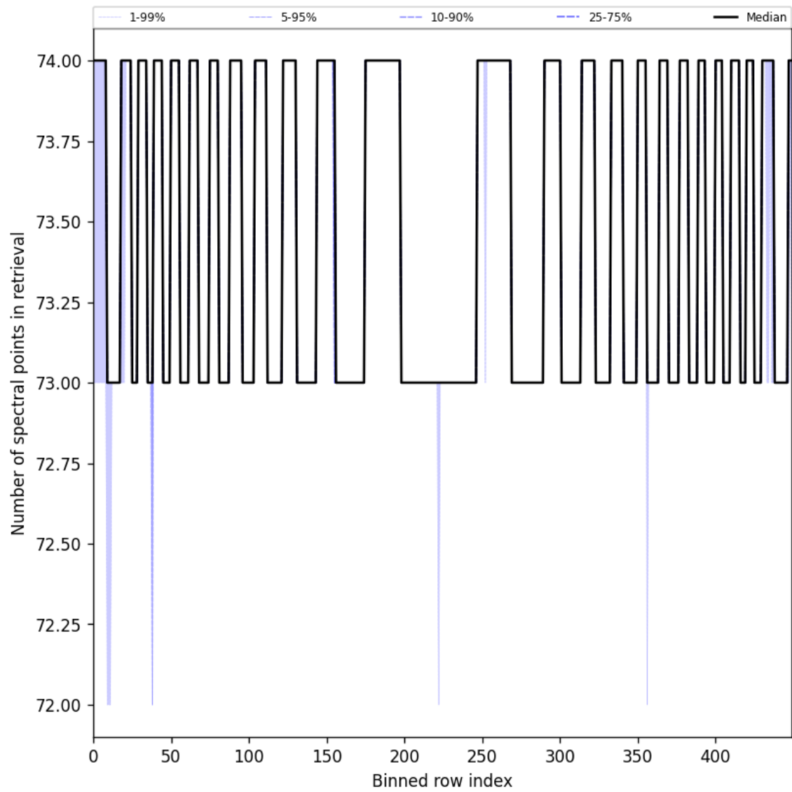
Figure 97: Along track statistics of “Number of spectral points in retrieval” for 2024-09-06 to 2024-09-07
