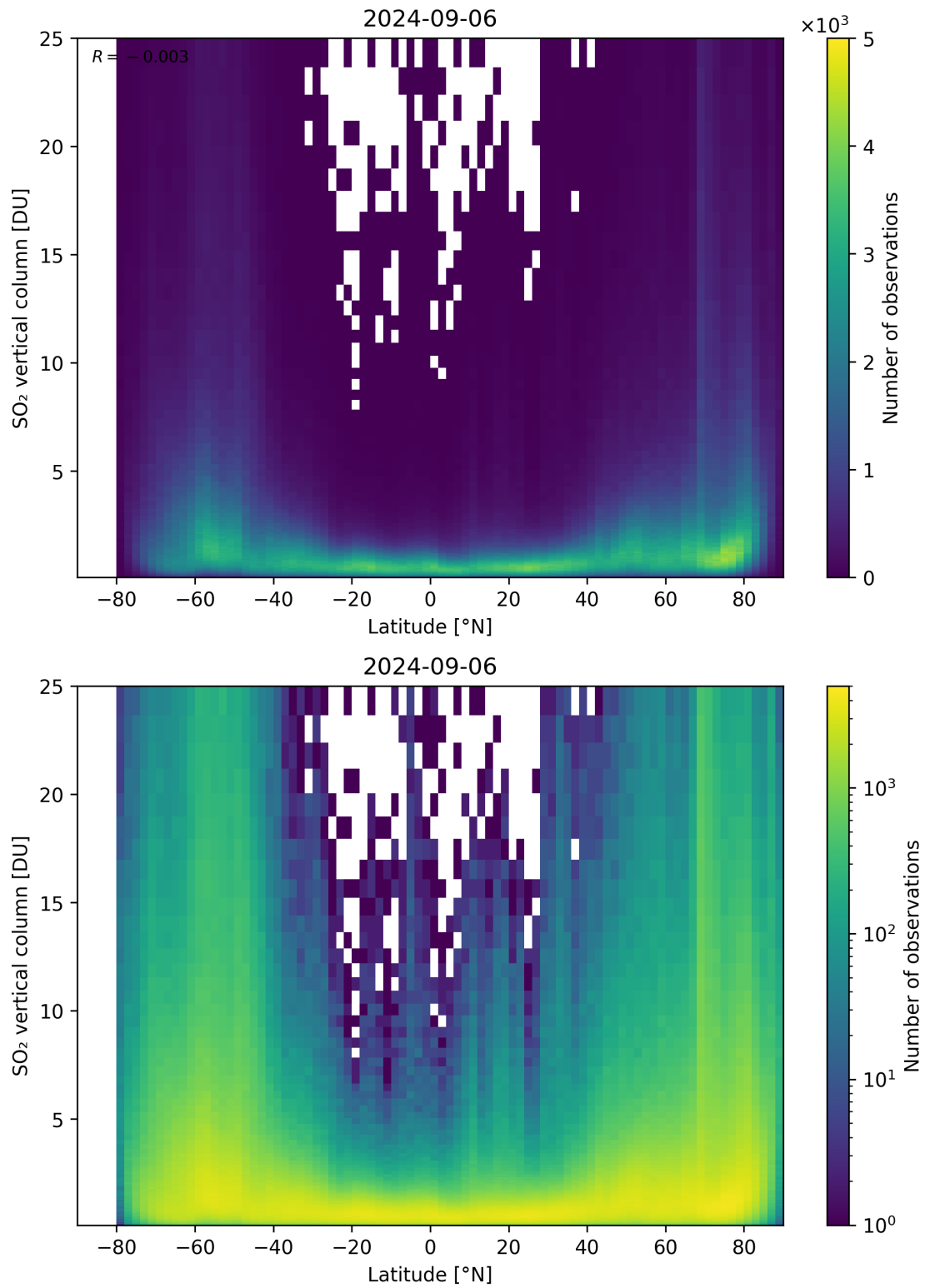
Figure 156: Scatter density plot of “Latitude” against “SO 2 vertical column” for 2024-09-06 to 2024-09-07.
