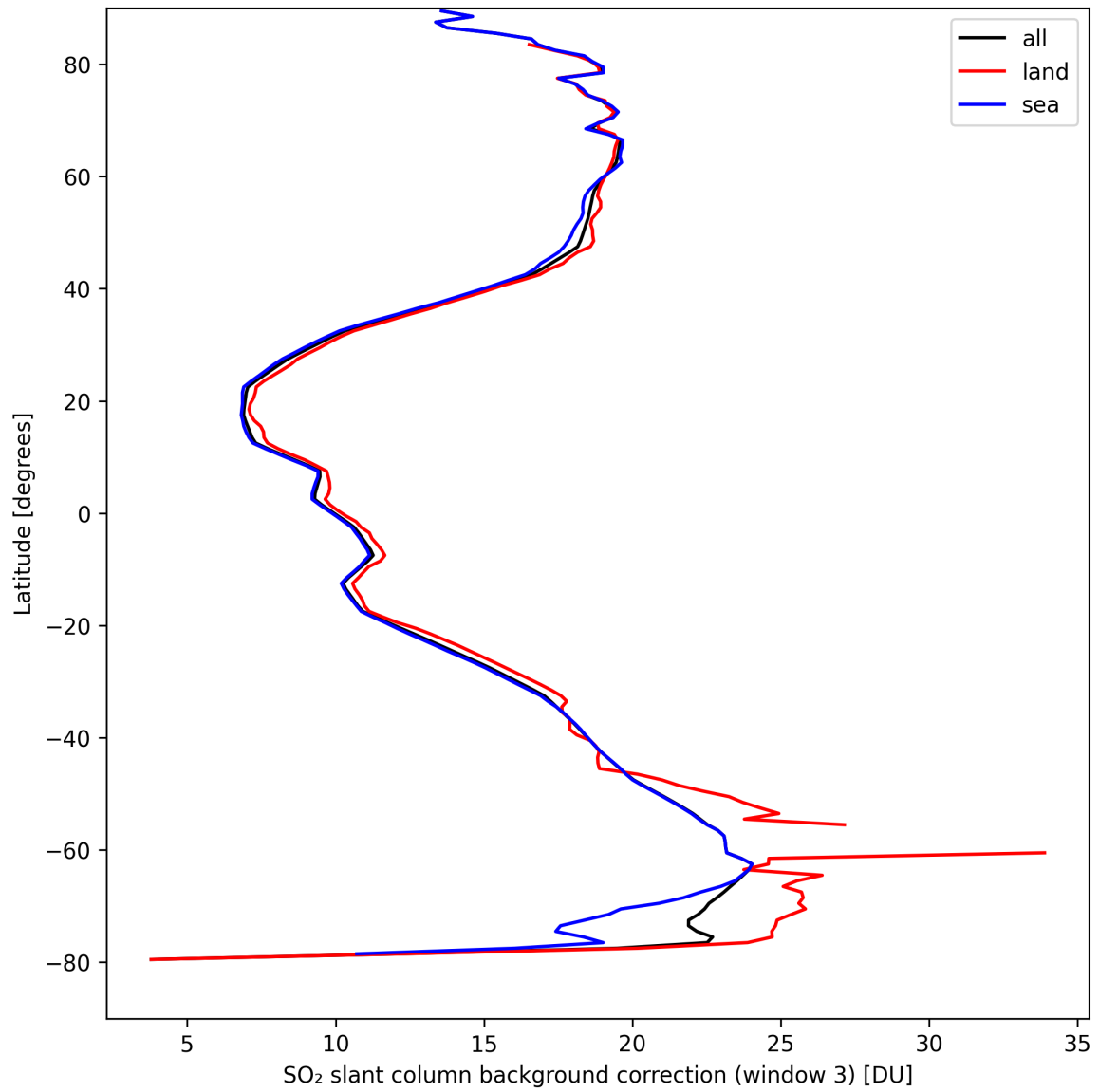
Figure 44: Zonal average of “SO 2 slant column background correction (window 3)” for 2024-09-06 to 2024-09-07.
