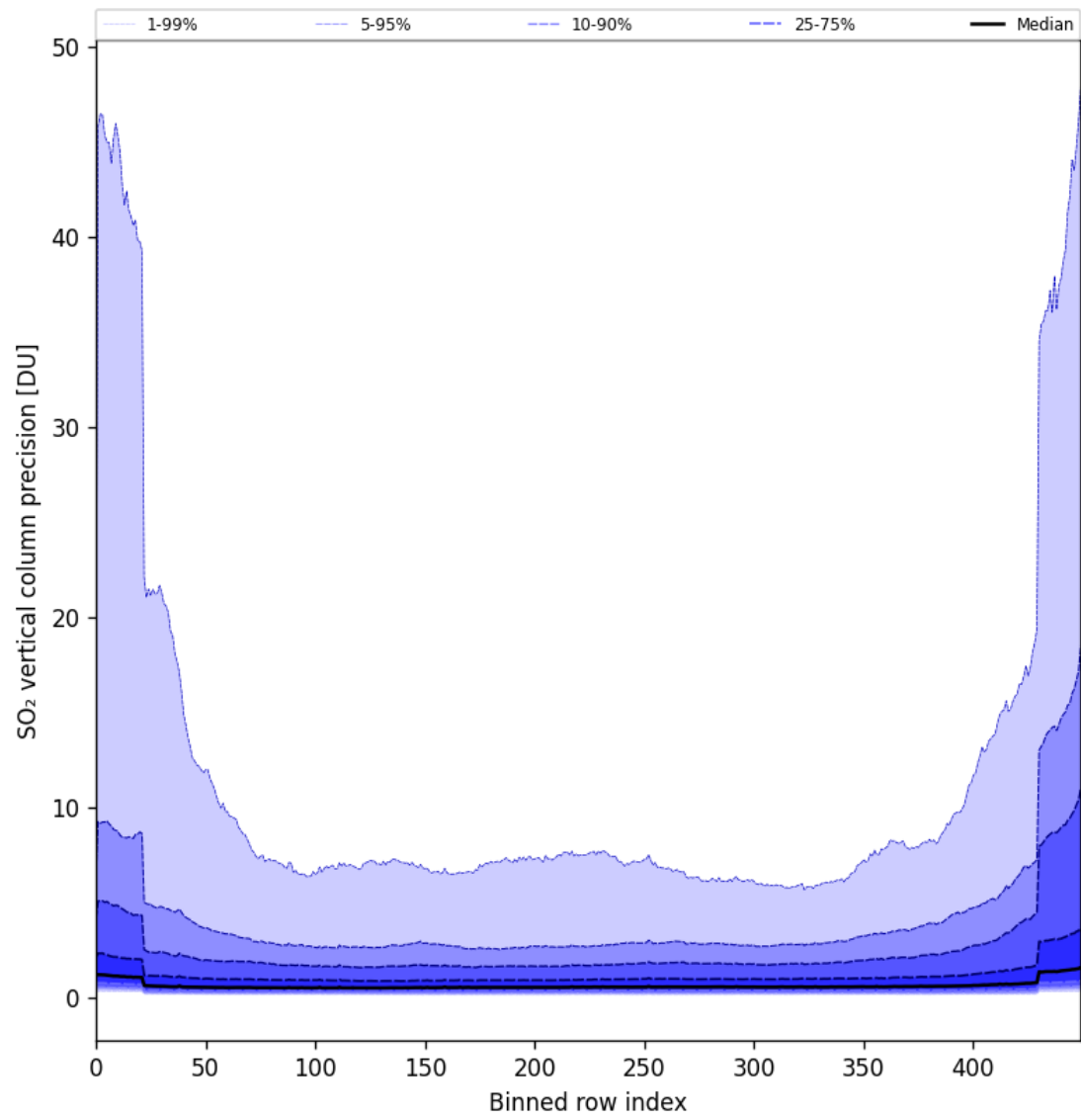
Figure 77: Along track statistics of “SO 2 vertical column precision” for 2024-09-06 to 2024-09-07
