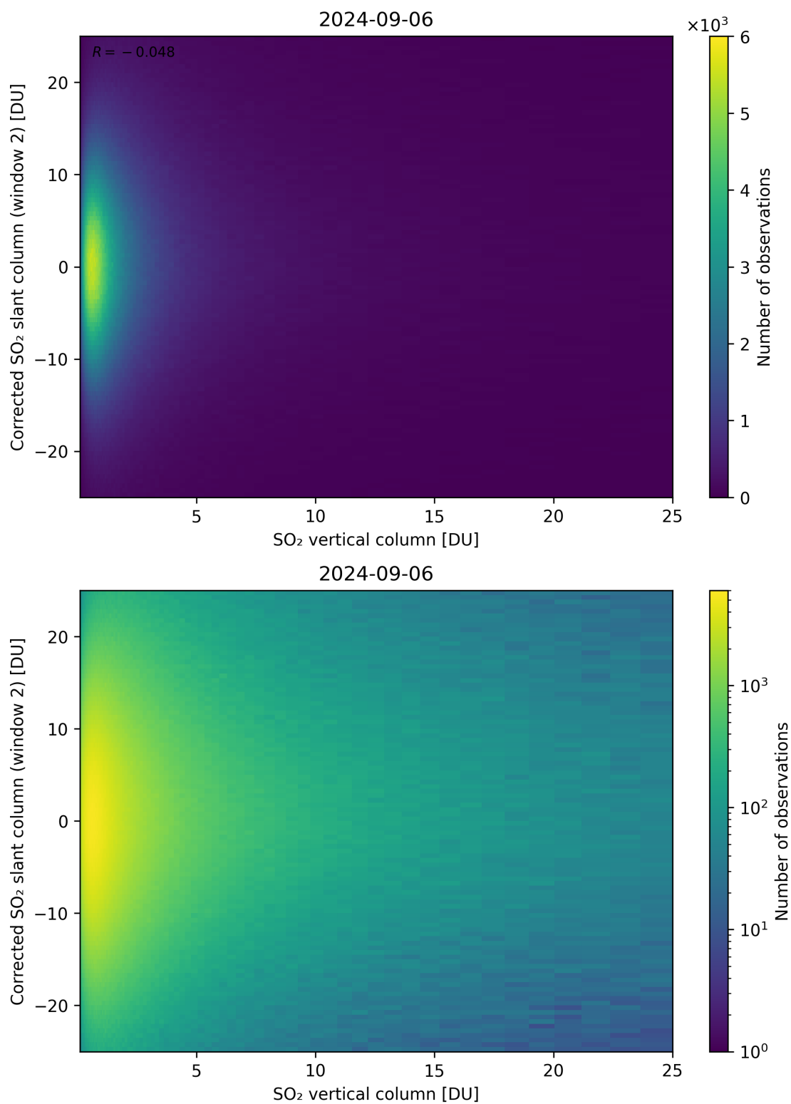
Figure 298: Scatter density plot of “SO 2 vertical column” against “Corrected SO 2 slant column (window 2)” for 2024-09-06 to 2024-09-07.
