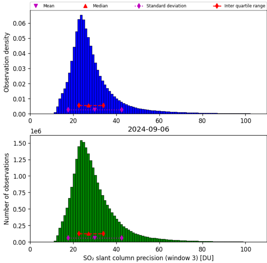
Figure 65: Histogram of “SO 2 slant column precision (window 3)” for 2024-09-06 to 2024-09-07
