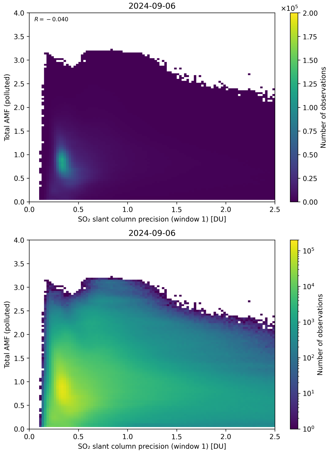
Figure 230: Scatter density plot of “SO 2 slant column precision (window 1)” against “Total AMF (polluted)” for 2024-09-06 to 2024-09-07.
