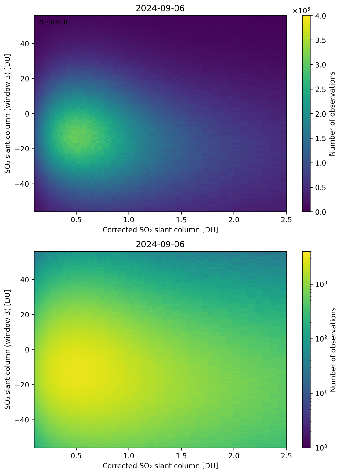
Figure 190: Scatter density plot of “Corrected SO 2 slant column” against “SO 2 slant column (window 3)” for 2024-09-06 to 2024-09-07.
