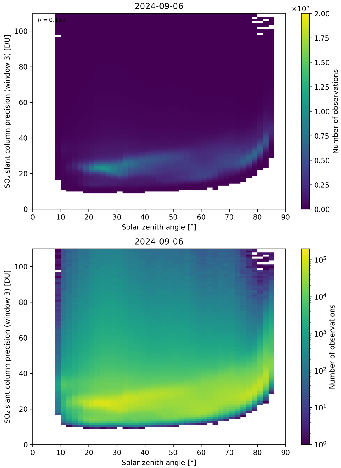
Figure 173: Scatter density plot of “Solar zenith angle” against “SO 2 slant column precision (window 3)” for 2024-09-06 to 2024-09-07.
