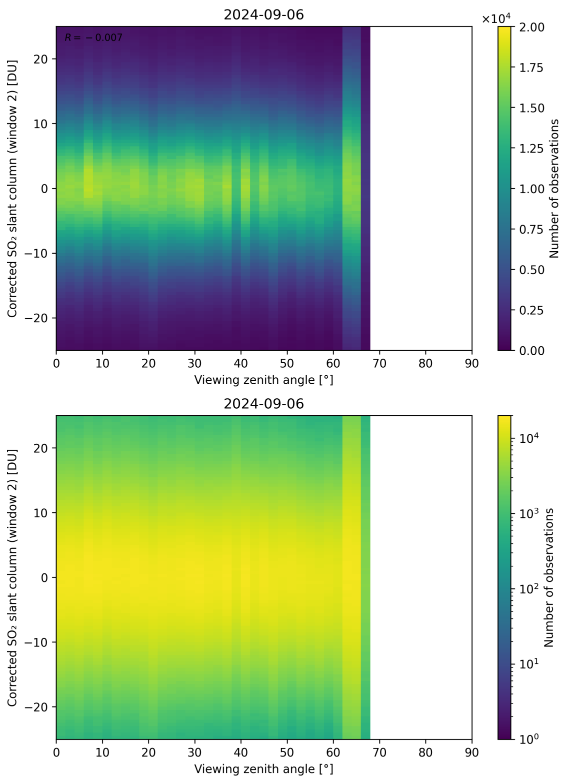
Figure 318: Scatter density plot of “Viewing zenith angle” against “Corrected SO 2 slant column (window 2)” for 2024-09-06 to 2024-09-07.
