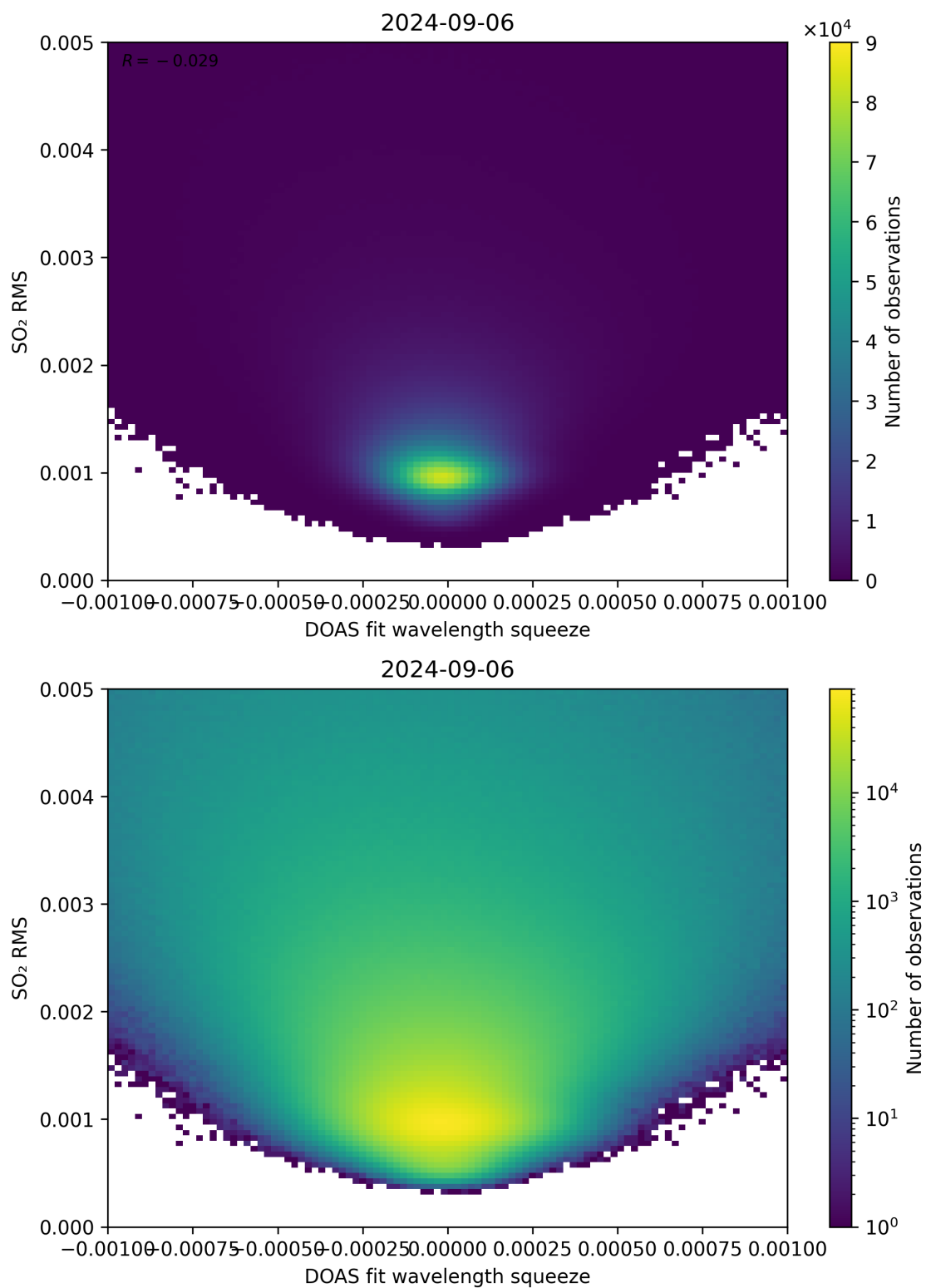
Figure 132: Scatter density plot of “DOAS fit wavelength squeeze” against “SO 2 RMS” for 2024-09-06 to 2024-09-07.
