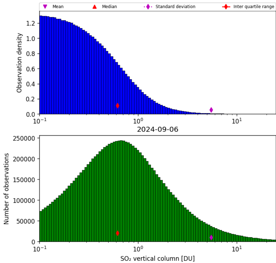
Figure 53: Histogram of “SO 2 vertical column” for 2024-09-06 to 2024-09-07
