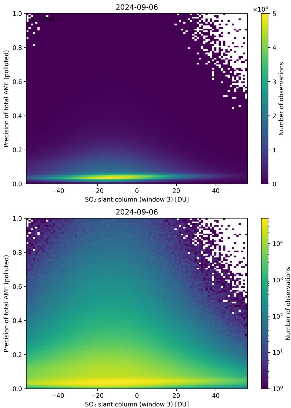
Figure 269: Scatter density plot of “SO 2 slant column (window 3)” against “Precision of total AMF (polluted)” for 2024-09-06 to 2024-09-07.
