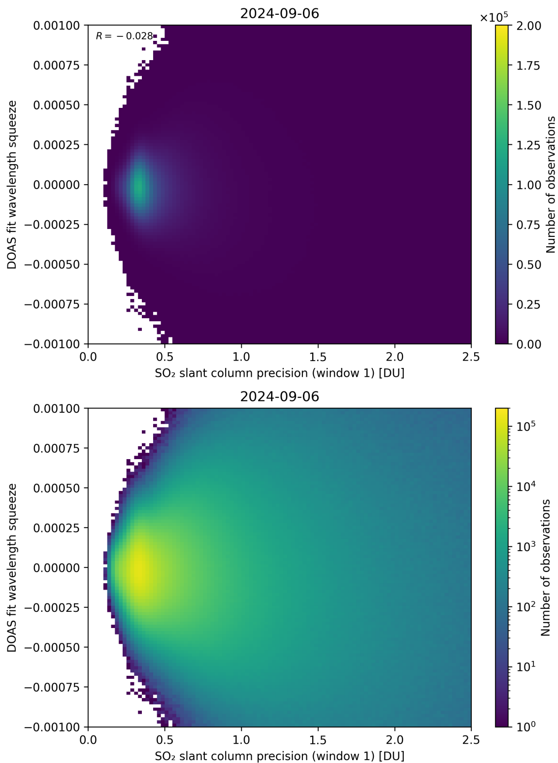
Figure 222: Scatter density plot of “SO 2 slant column precision (window 1)” against “DOAS fit wavelength squeeze” for 2024-09-06 to 2024-09-07.
