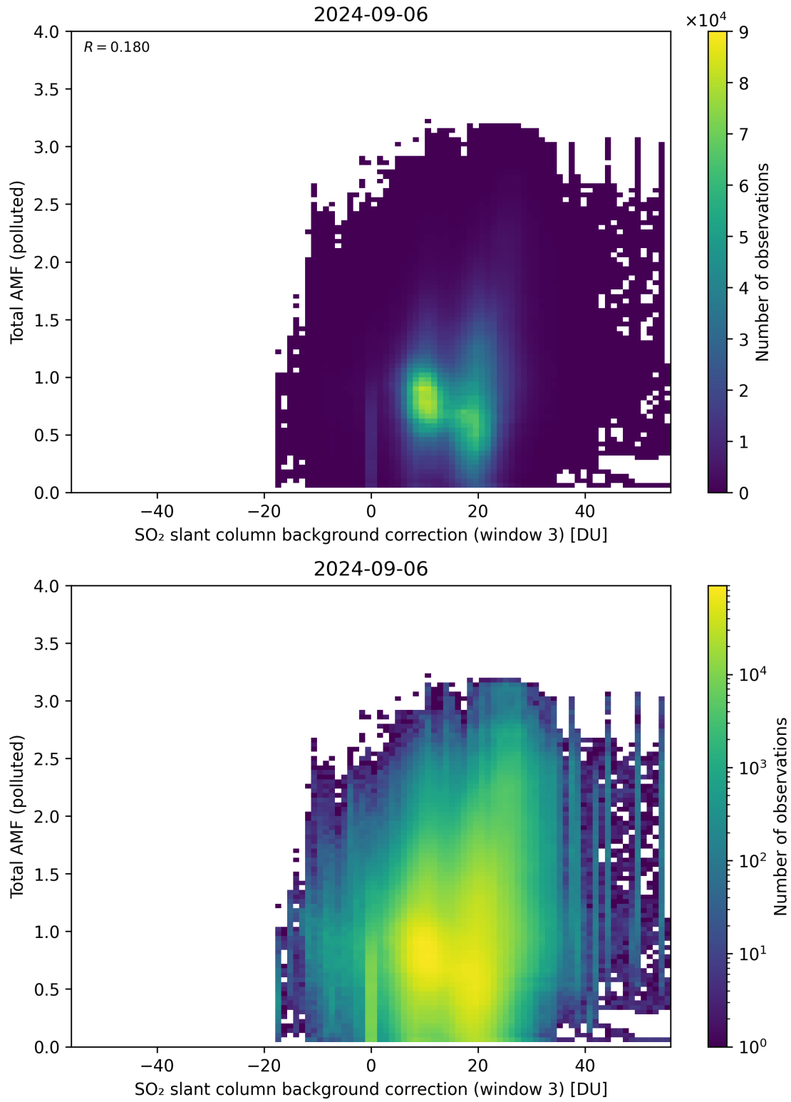
Figure 125: Scatter density plot of “SO 2 slant column background correction (window 3)” against “Total AMF (polluted)” for 2024-09-06 to 2024-09-07.
