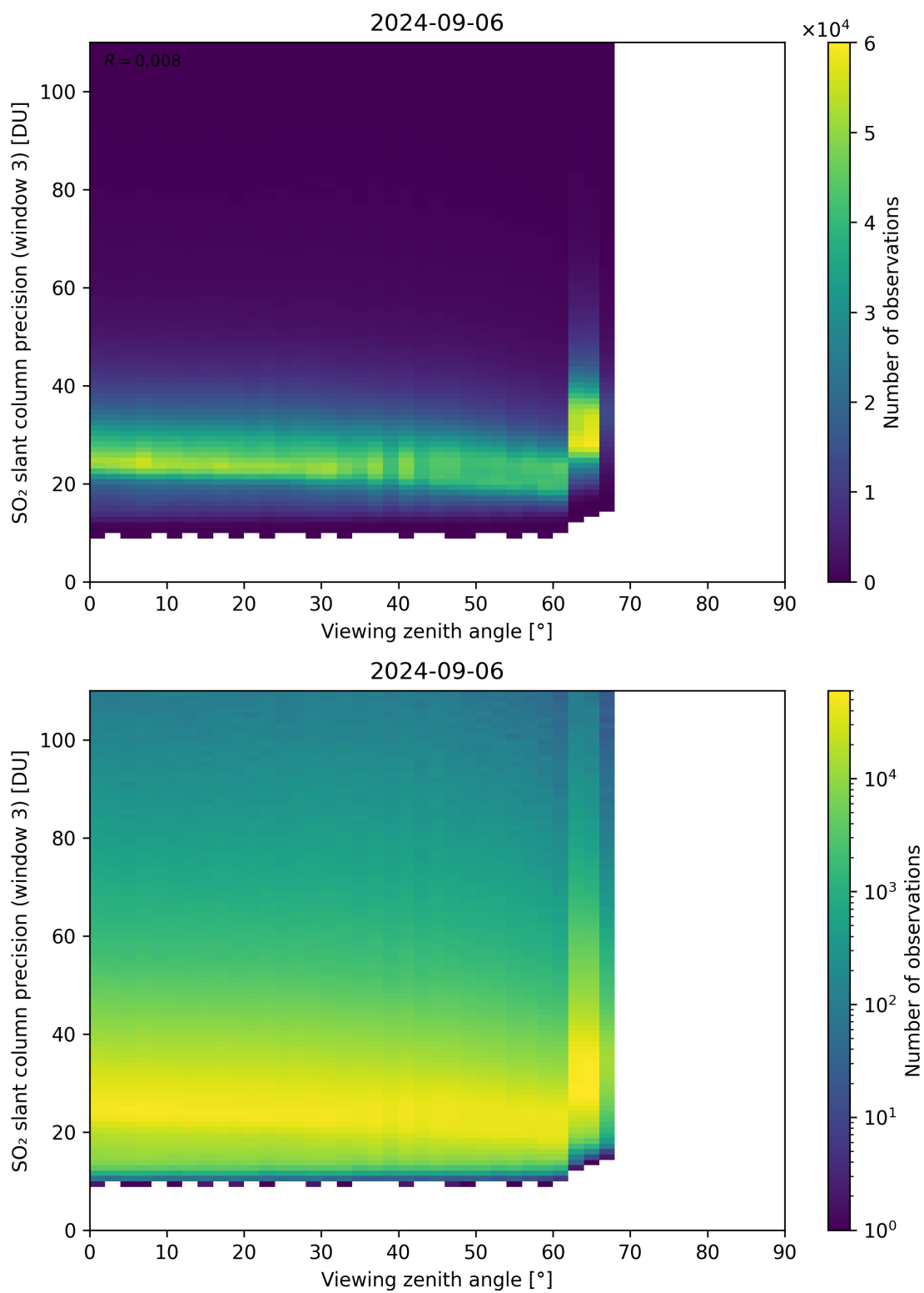
Figure 324: Scatter density plot of “Viewing zenith angle” against “SO 2 slant column precision (window 3)” for 2024-09-06 to 2024-09-07.
