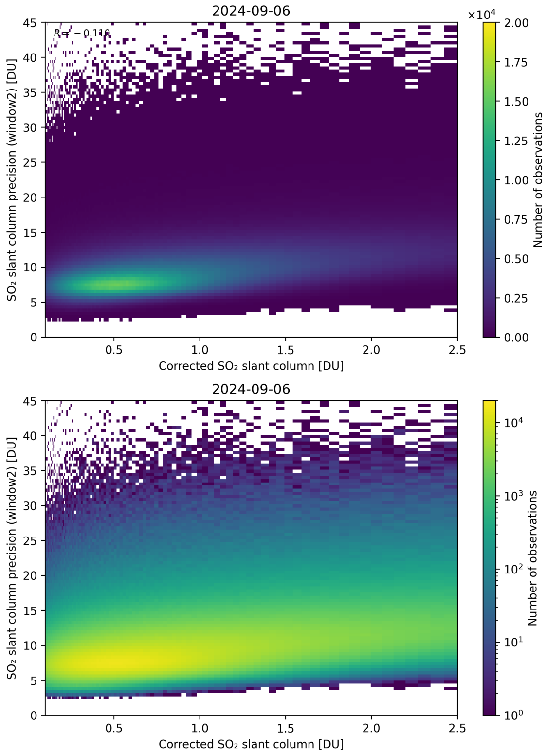
Figure 189: Scatter density plot of “Corrected SO 2 slant column” against “SO 2 slant column precision (window2)” for 2024-09-06 to 2024-09-07.
