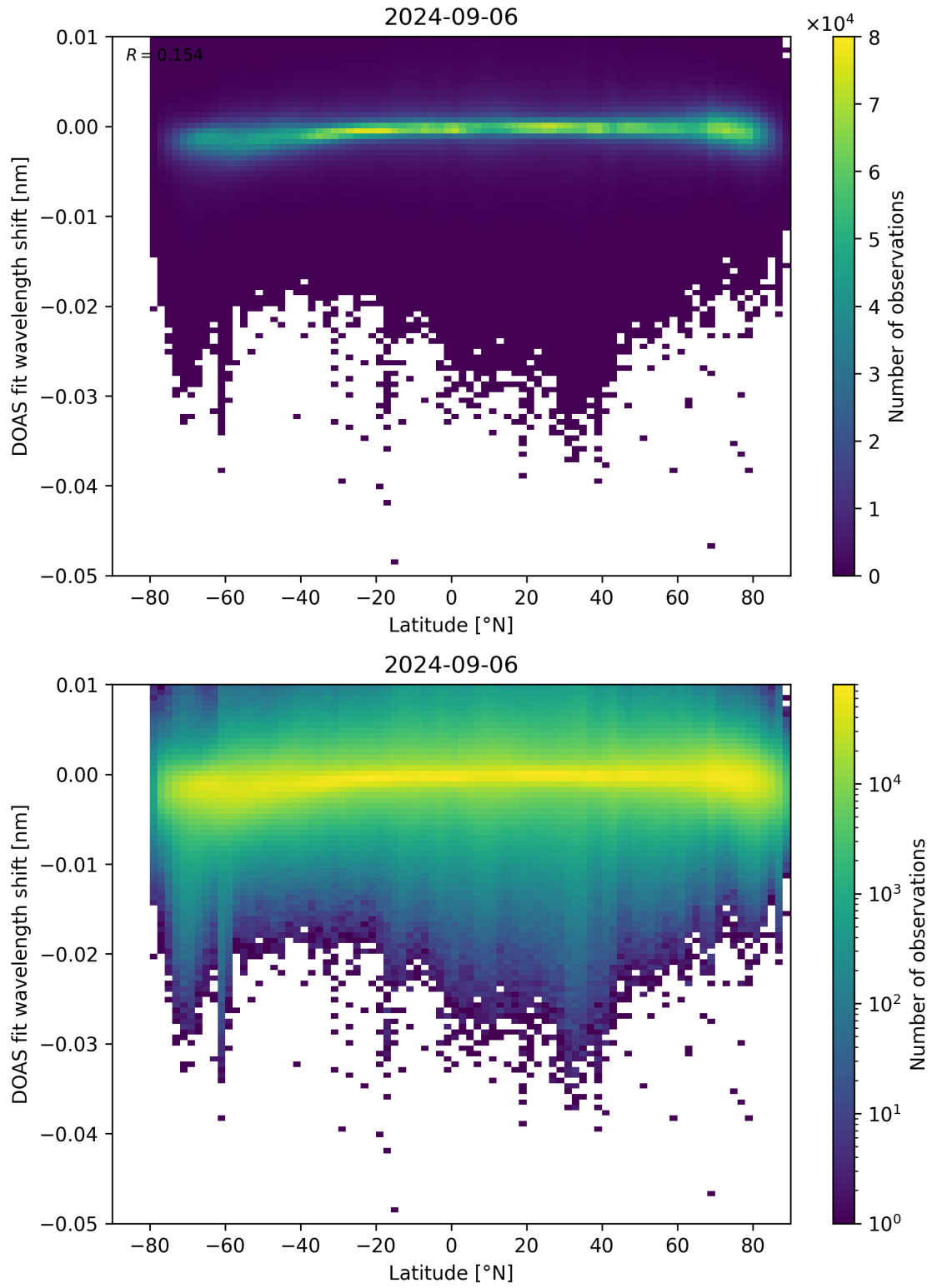
Figure 142: Scatter density plot of “Latitude” against “DOAS fit wavelength shift” for 2024-09-06 to 2024-09-07.
