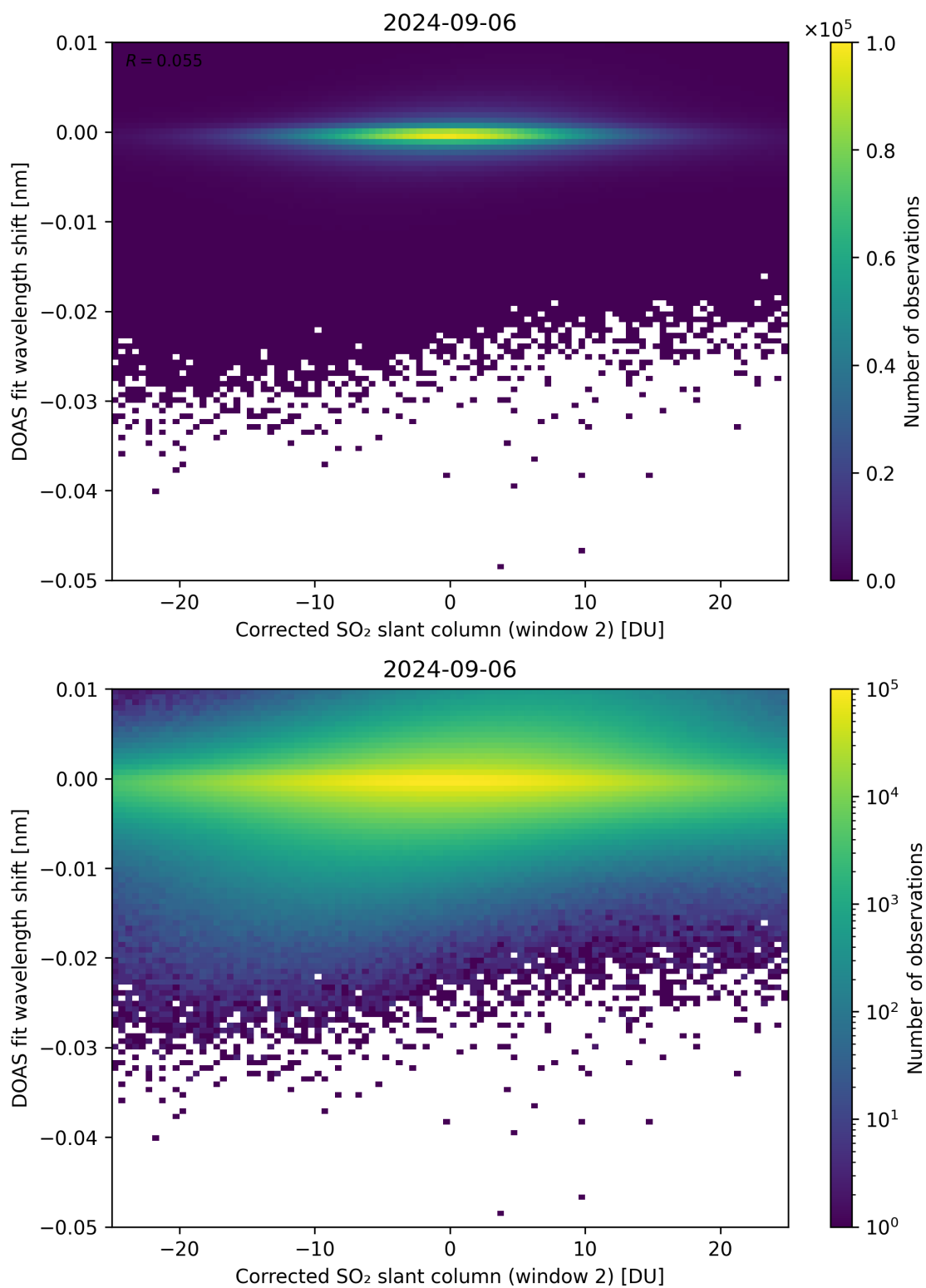
Figure 196: Scatter density plot of “Corrected SO 2 slant column (window 2)” against “DOAS fit wavelength shift” for 2024-09-06 to 2024-09-07.
