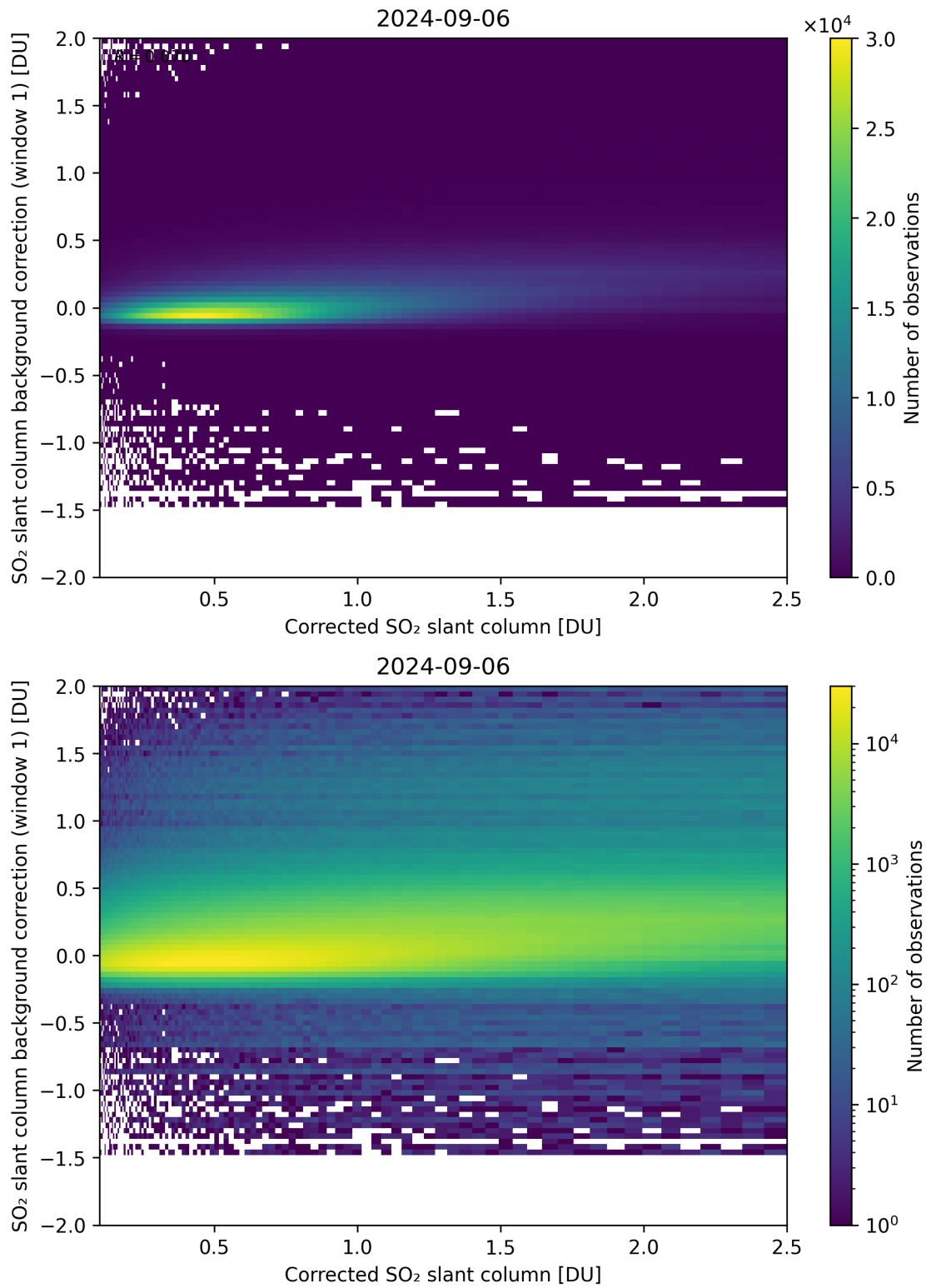
Figure 178: Scatter density plot of “Corrected SO 2 slant column” against “SO 2 slant column background correction (window 1)” for 2024-09-06 to 2024-09-07.
