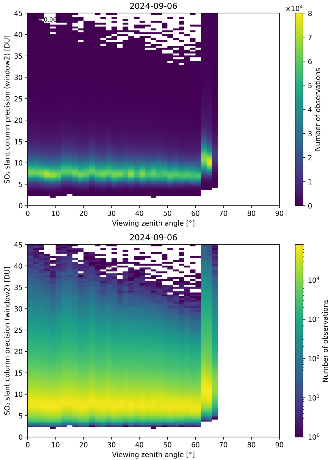
Figure 322: Scatter density plot of “Viewing zenith angle” against “SO 2 slant column precision (window2)” for 2024-09-06 to 2024-09-07.
