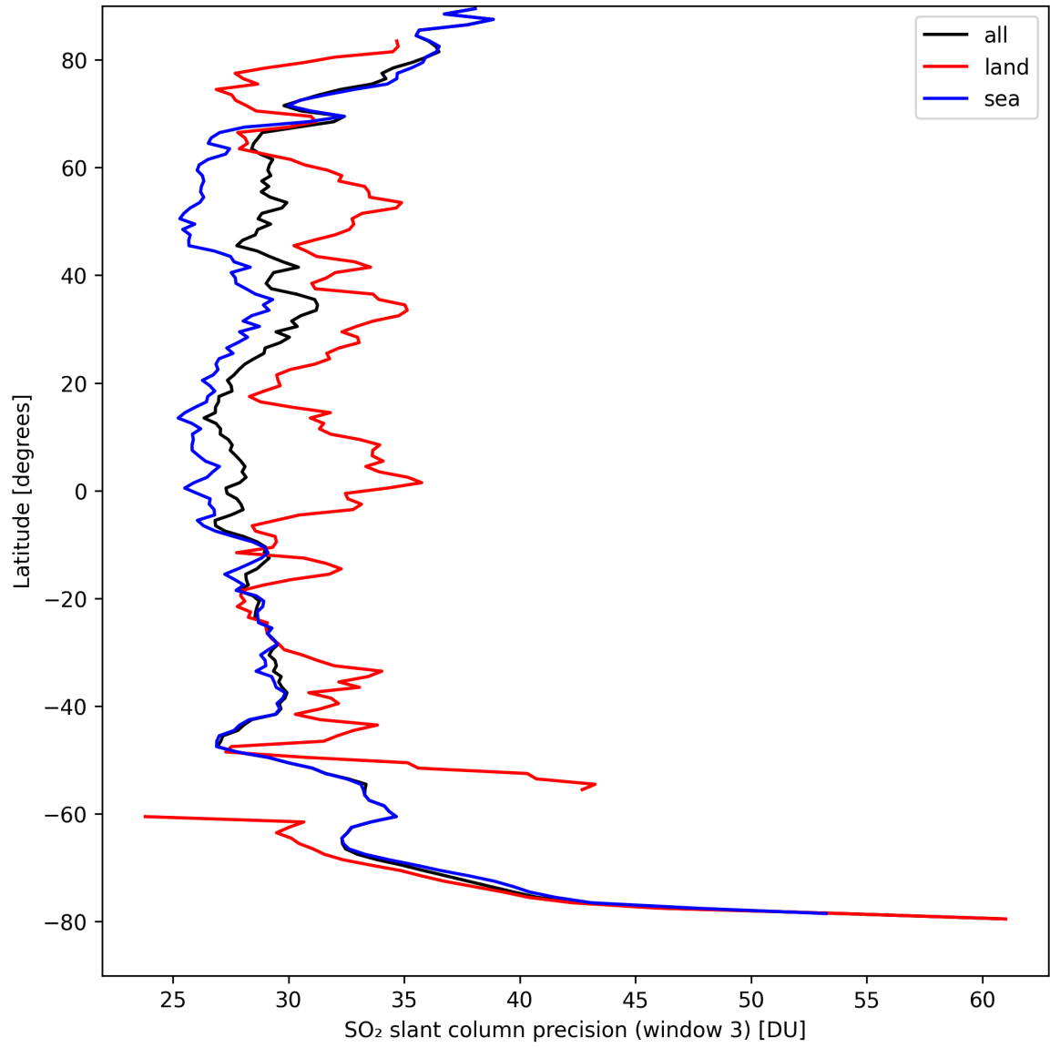
Figure 42: Zonal average of “SO 2 slant column precision (window 3)” for 2024-09-06 to 2024-09-07.
