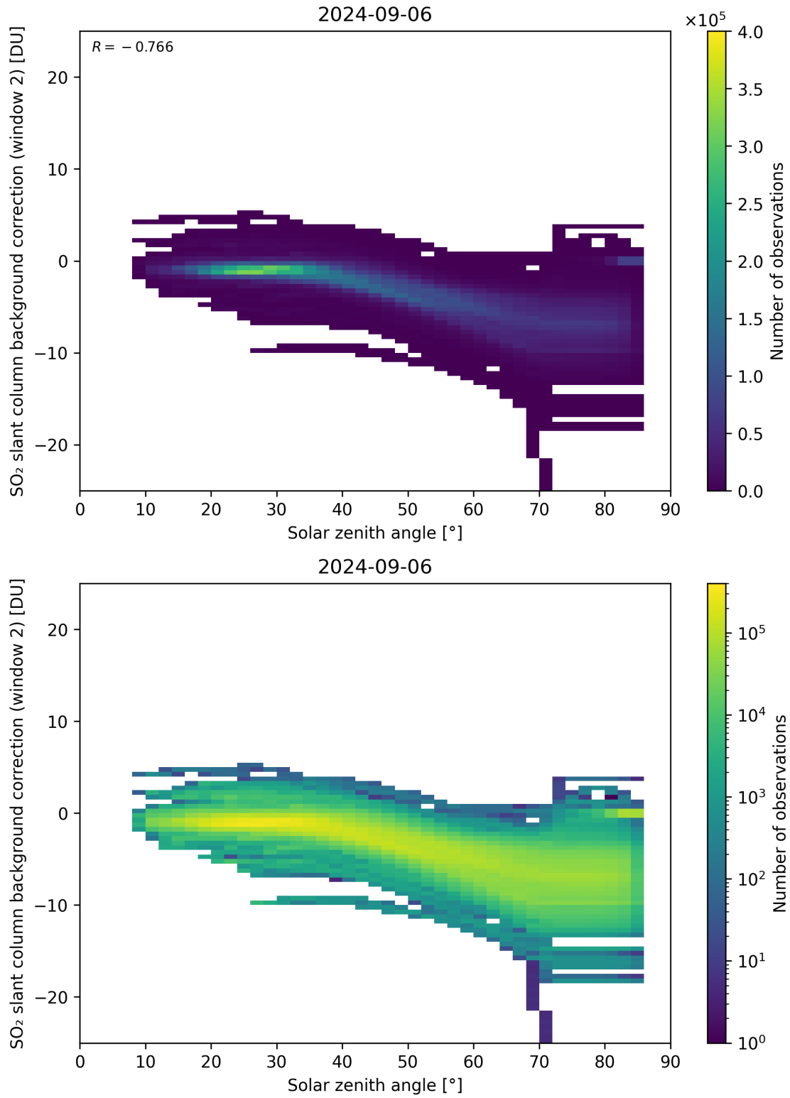
Figure 159: Scatter density plot of “Solar zenith angle” against “SO 2 slant column background correction (window 2)” for 2024-09-06 to 2024-09-07.
