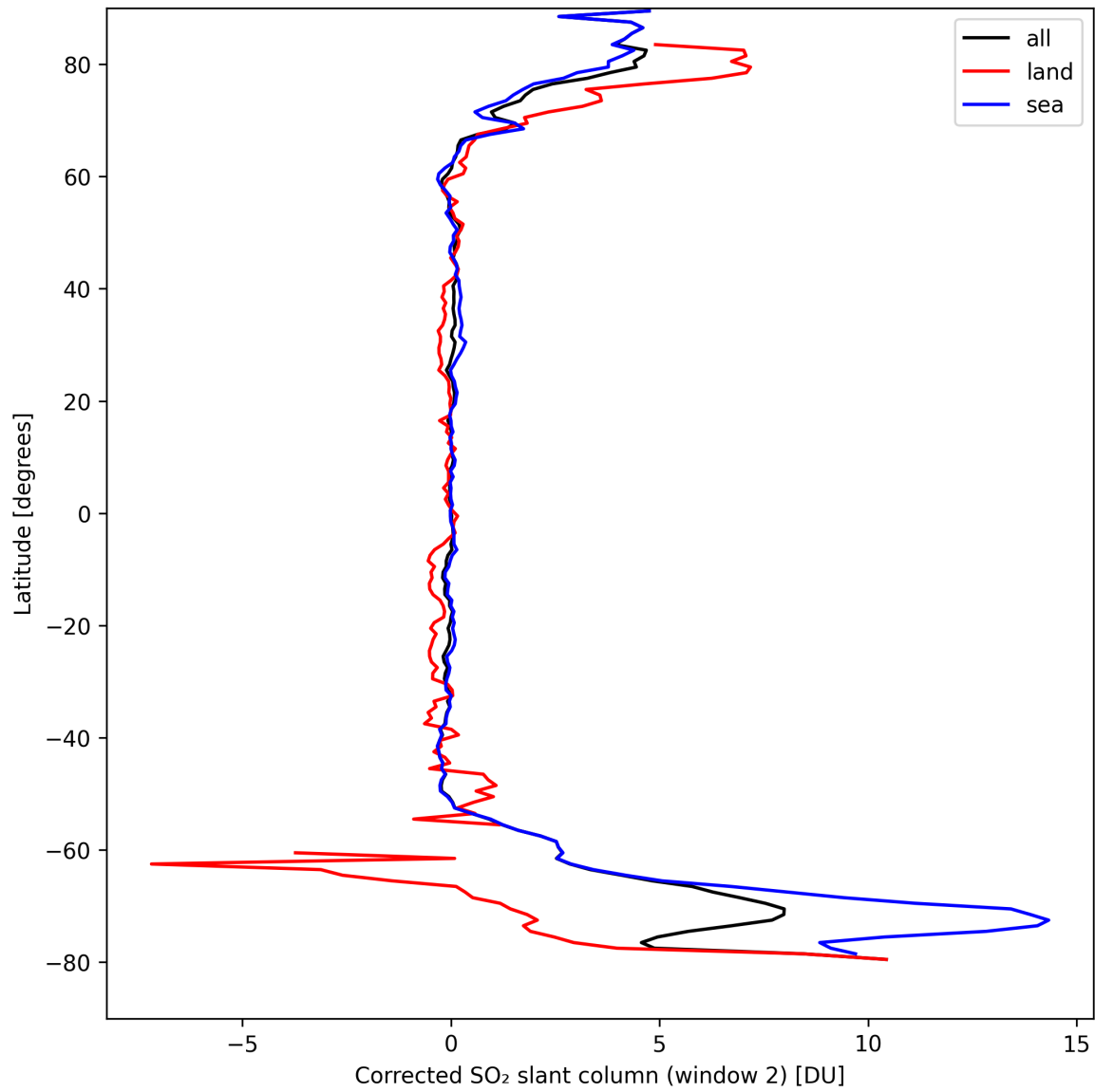
Figure 39: Zonal average of “Corrected SO 2 slant column (window 2)” for 2024-09-06 to 2024-09-07.
