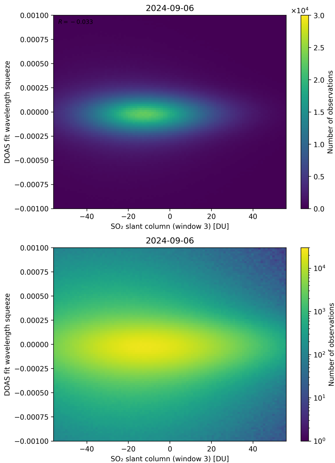
Figure 255: Scatter density plot of “SO 2 slant column (window 3)” against “DOAS fit wavelength squeeze” for 2024-09-06 to 2024-09-07.
