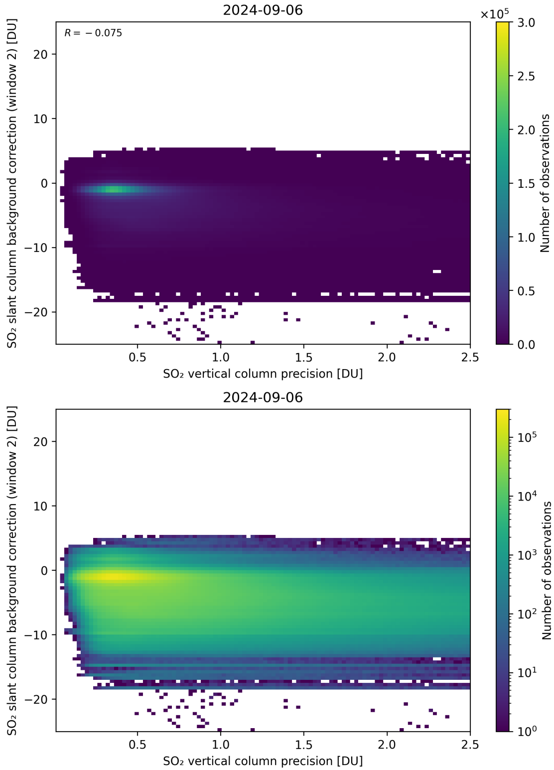
Figure 280: Scatter density plot of “SO 2 vertical column precision” against “SO 2 slant column background correction (window 2)” for 2024-09-06 to 2024-09-07.
