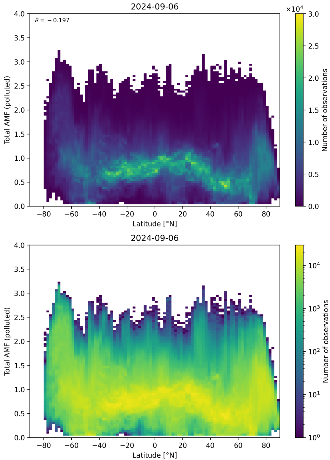
Figure 154: Scatter density plot of “Latitude” against “Total AMF (polluted)” for 2024-09-06 to 2024-09-07.
