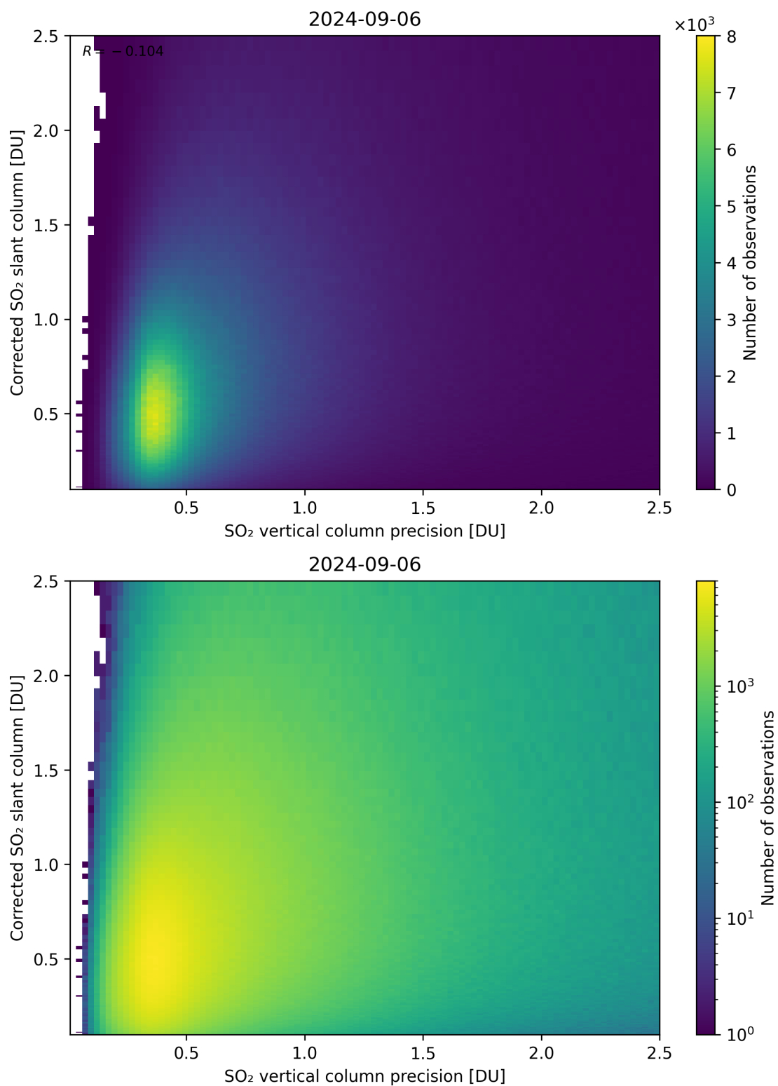
Figure 286: Scatter density plot of “SO 2 vertical column precision” against “Corrected SO 2 slant column” for 2024-09-06 to 2024-09-07.
