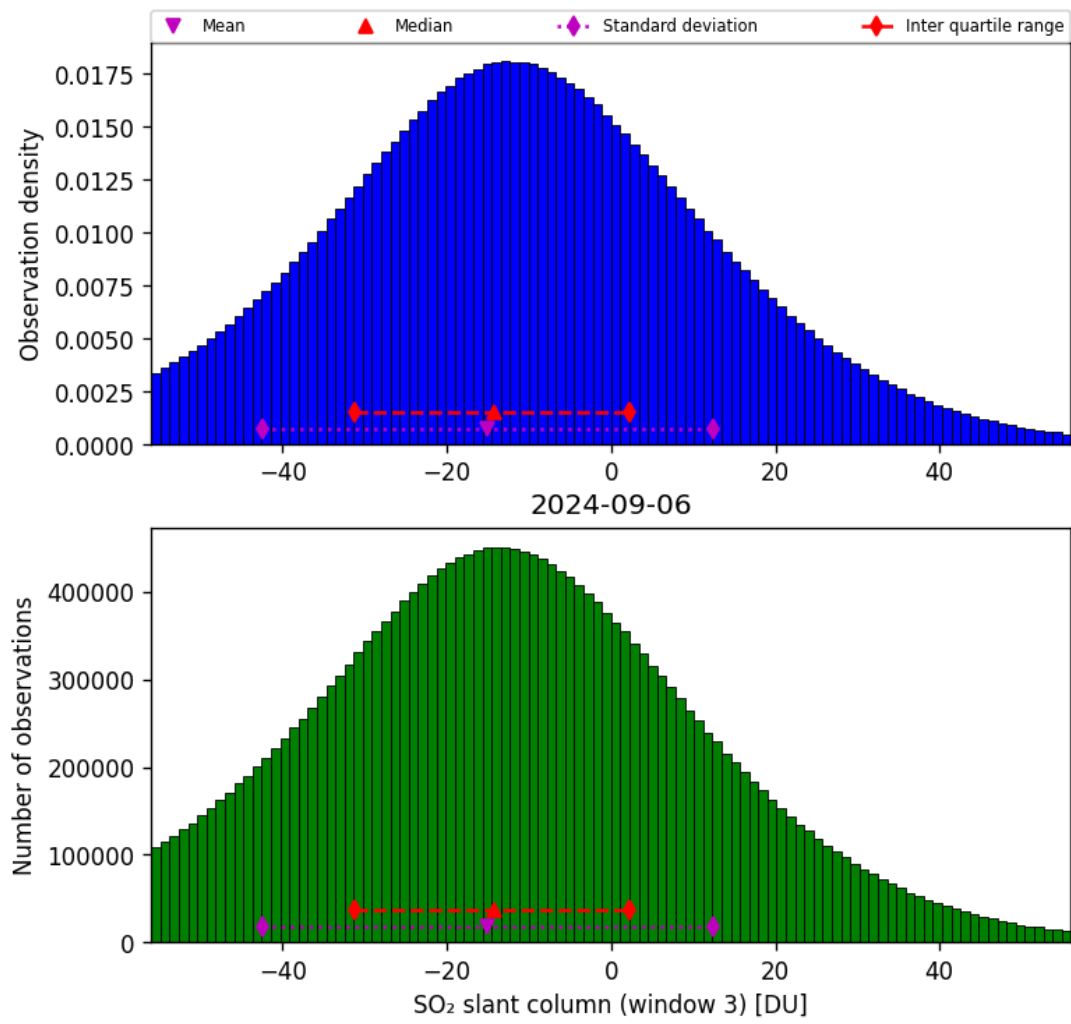
Figure 64: Histogram of “SO 2 slant column (window 3)” for 2024-09-06 to 2024-09-07
