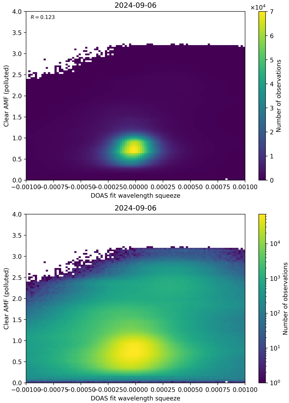
Figure 133: Scatter density plot of “DOAS fit wavelength squeeze” against “Clear AMF (polluted)” for 2024-09-06 to 2024-09-07.
