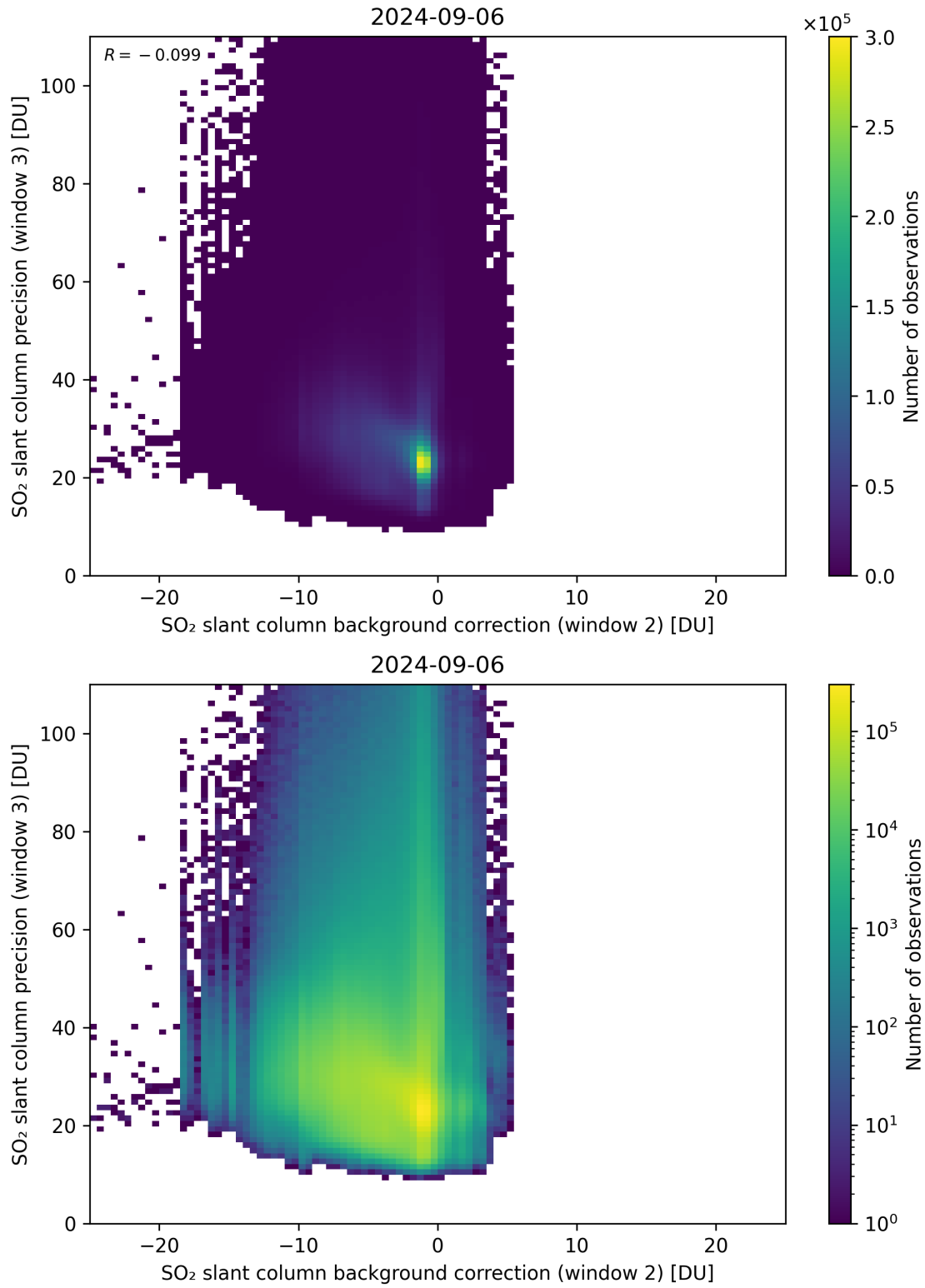
Figure 118: Scatter density plot of “SO 2 slant column background correction (window 2)” against “SO 2 slant column precision (window 3)” for 2024-09-06 to 2024-09-07.
