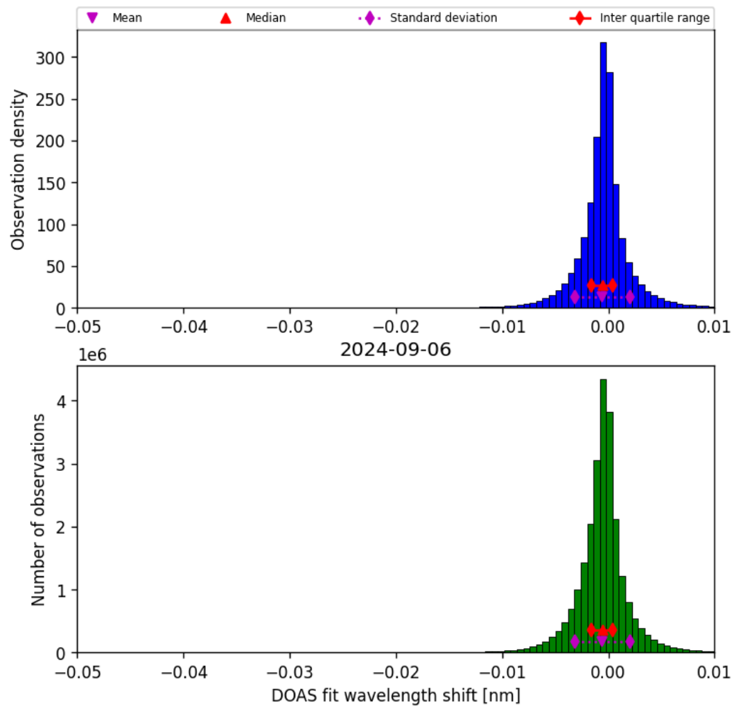
Figure 68: Histogram of “DOAS fit wavelength shift” for 2024-09-06 to 2024-09-07
