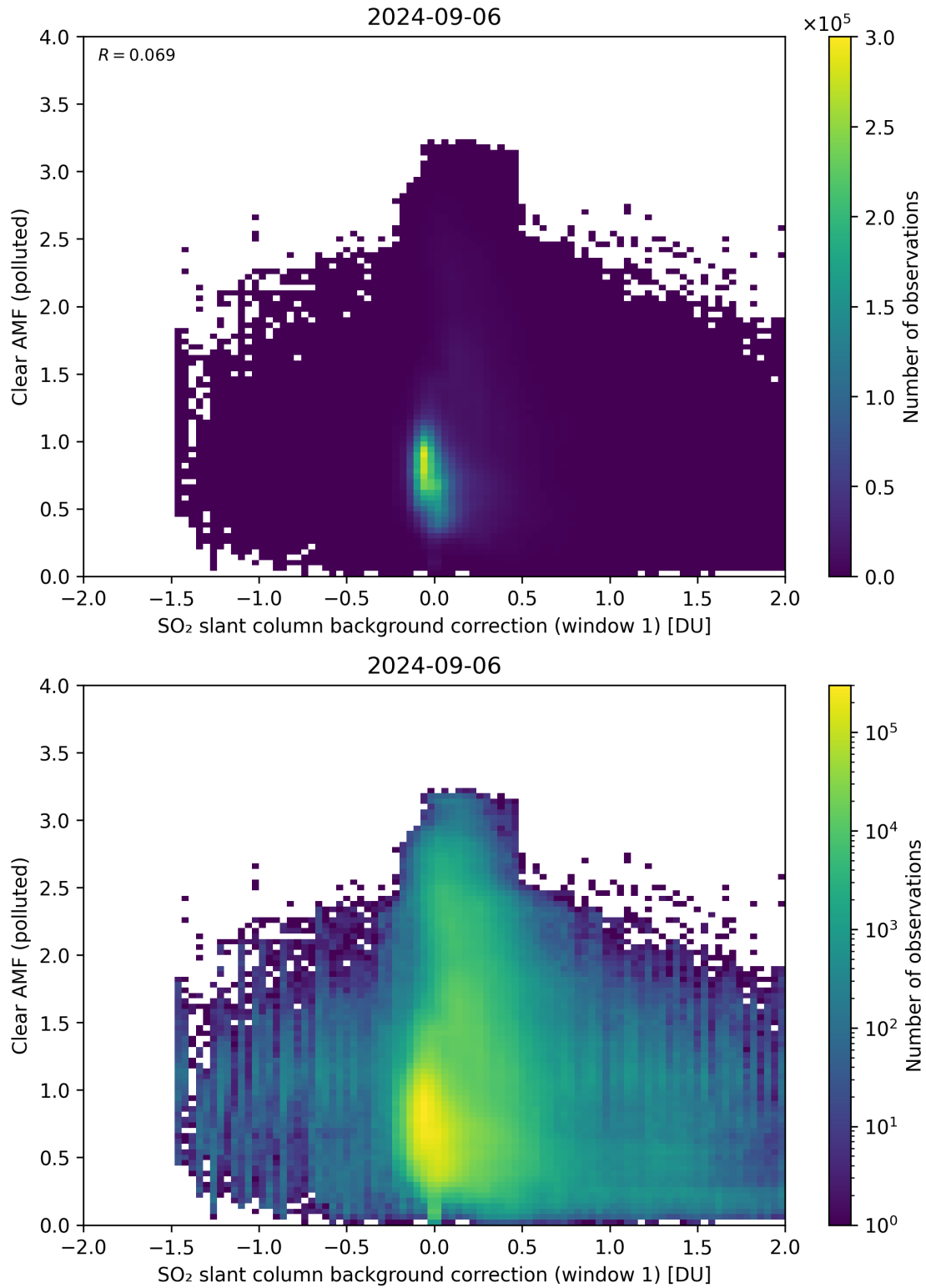
Figure 103: Scatter density plot of “SO 2 slant column background correction (window 1)” against “Clear AMF (polluted)” for 2024-09-06 to 2024-09-07.
