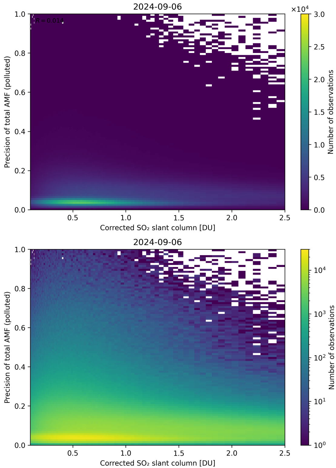
Figure 193: Scatter density plot of “Corrected SO 2 slant column” against “Precision of total AMF (polluted)” for 2024-09-06 to 2024-09-07.
