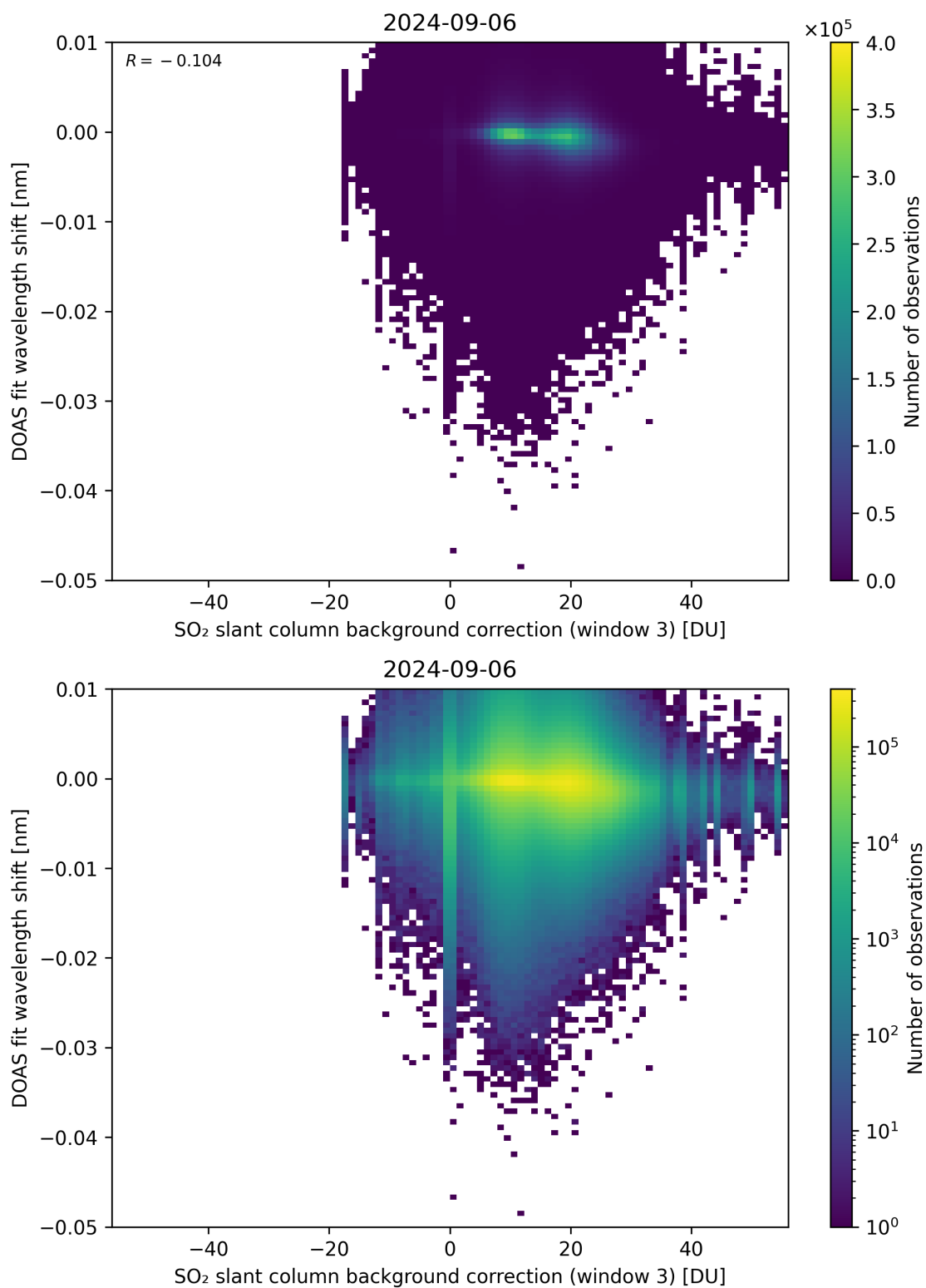
Figure 121: Scatter density plot of “SO 2 slant column background correction (window 3)” against “DOAS fit wavelength shift” for 2024-09-06 to 2024-09-07.
