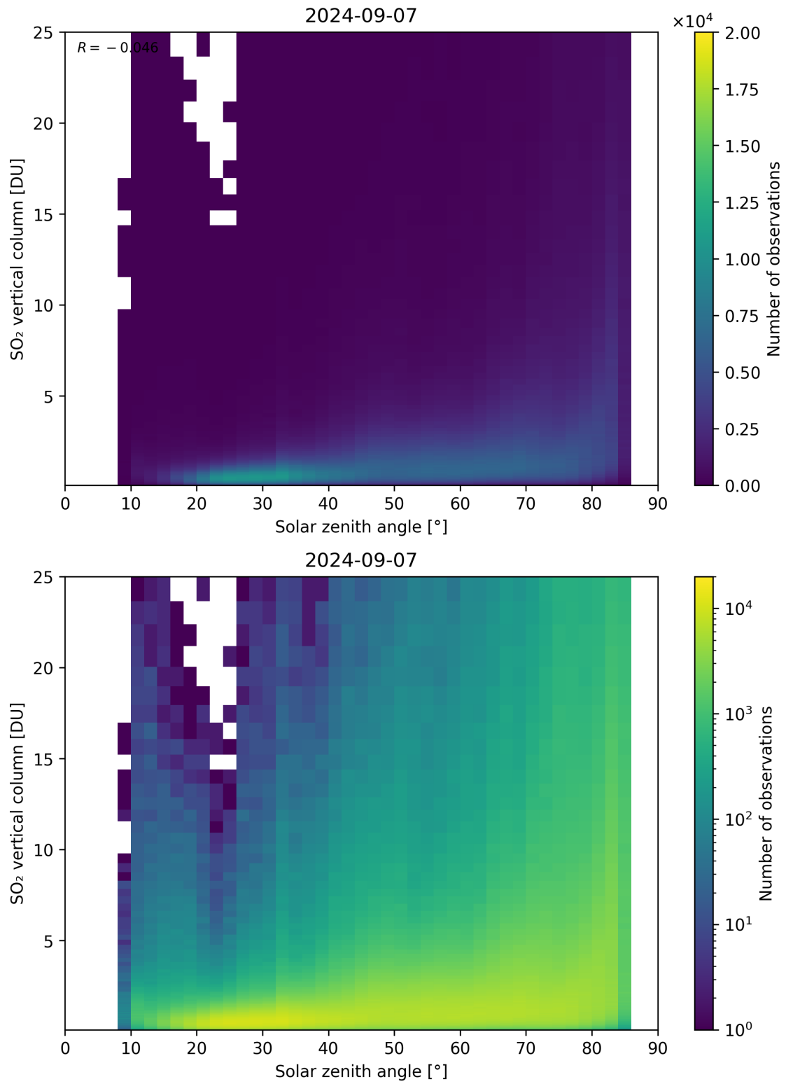
Figure 176: Scatter density plot of “Solar zenith angle” against “SO 2 vertical column” for 2024-09-06 to 2024-09-08.
