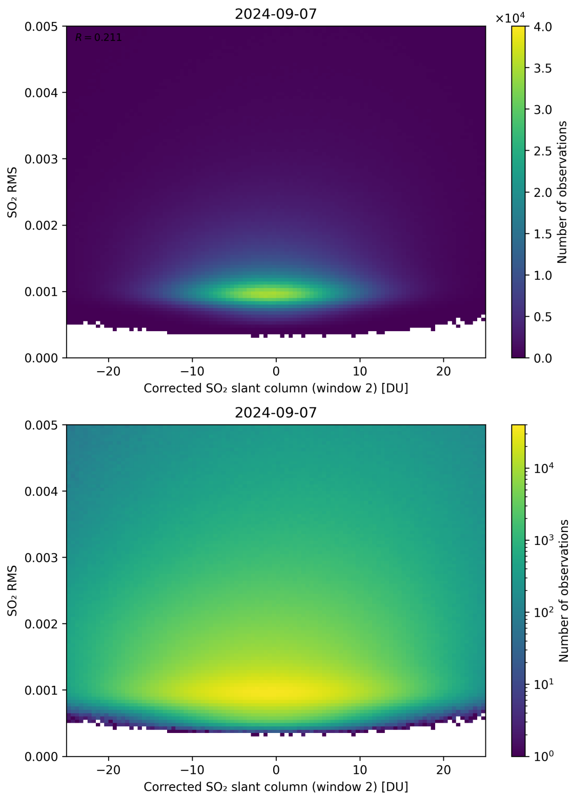
Figure 198: Scatter density plot of “Corrected SO 2 slant column (window 2)” against “SO 2 RMS” for 2024-09-06 to 2024-09-08.
