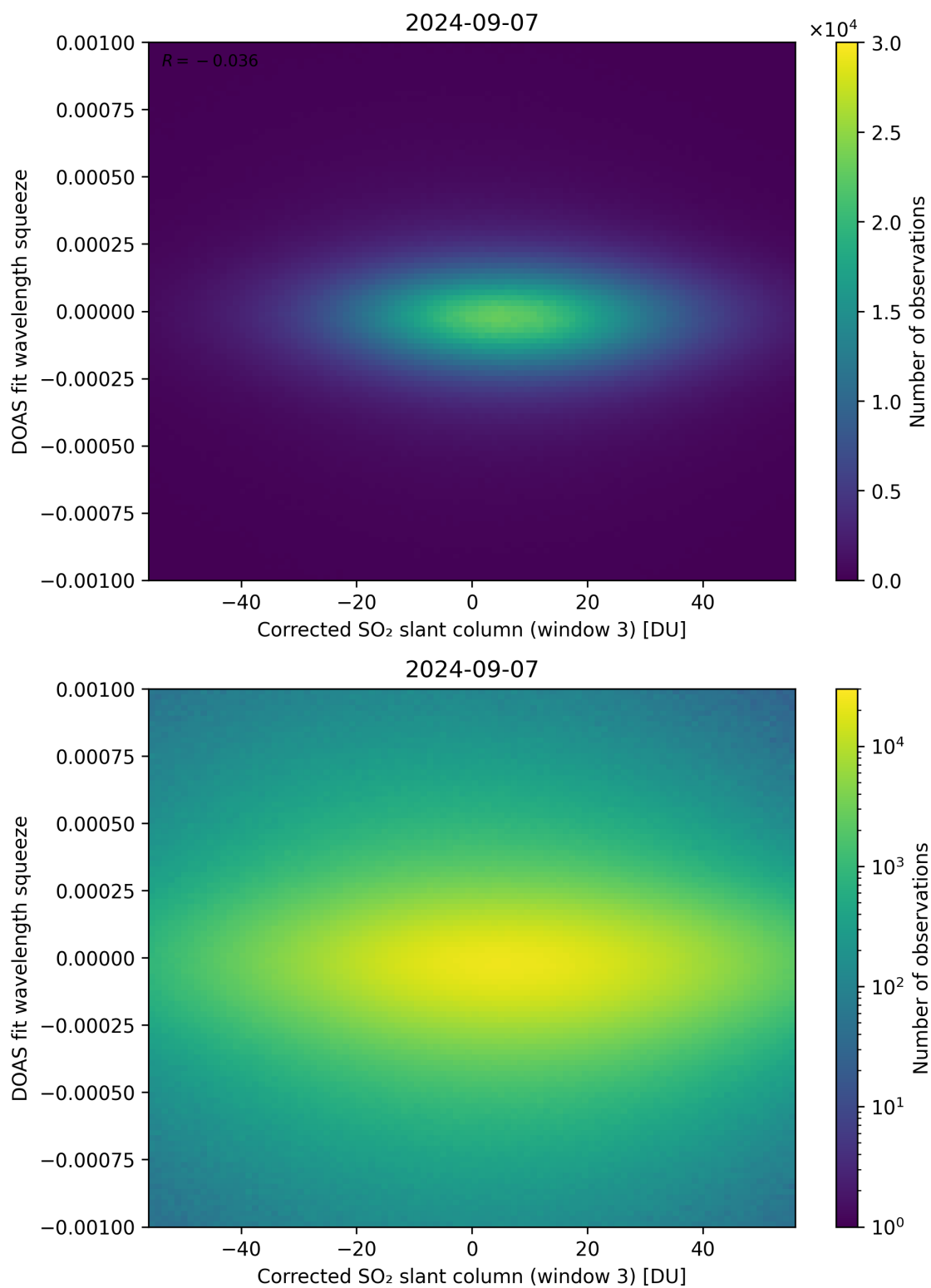
Figure 207: Scatter density plot of “Corrected SO 2 slant column (window 3)” against “DOAS fit wavelength squeeze” for 2024-09-06 to 2024-09-08.
