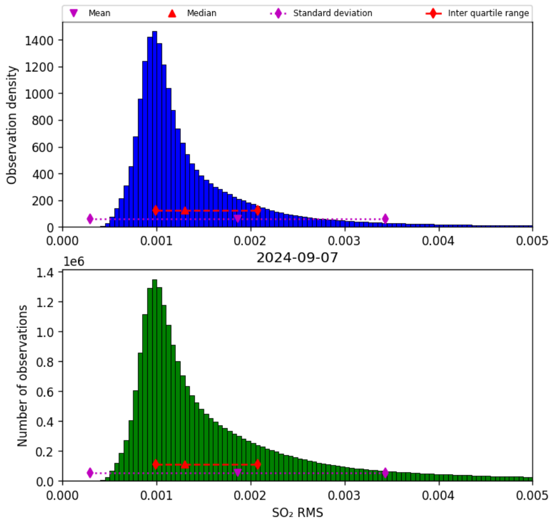
Figure 70: Histogram of “SO 2 RMS” for 2024-09-06 to 2024-09-08
