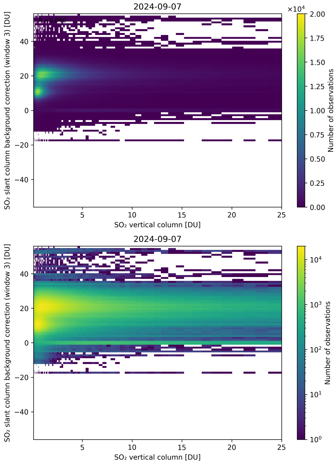
Figure 275: Scatter density plot of “SO 2 vertical column” against “SO 2 slant column background correction (window 3)” for 2024-09-06 to 2024-09-08.
