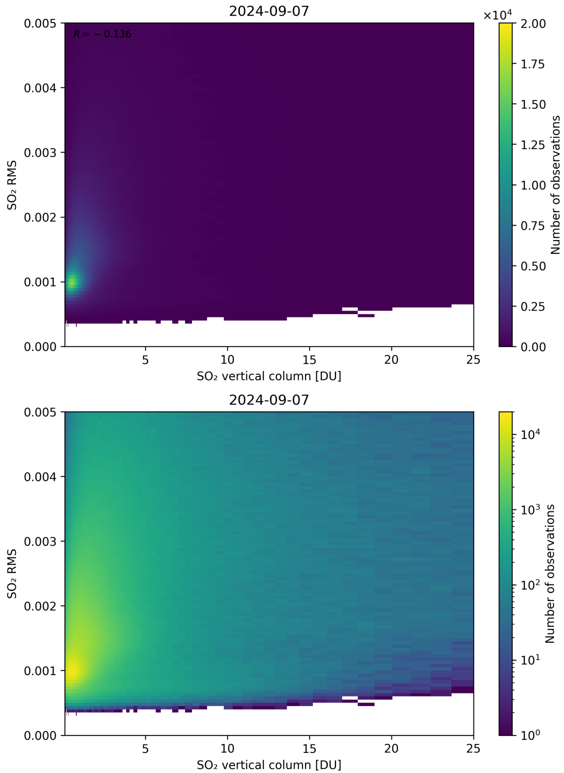
Figure 278: Scatter density plot of “SO 2 vertical column” against “SO 2 RMS” for 2024-09-06 to 2024-09-08.
