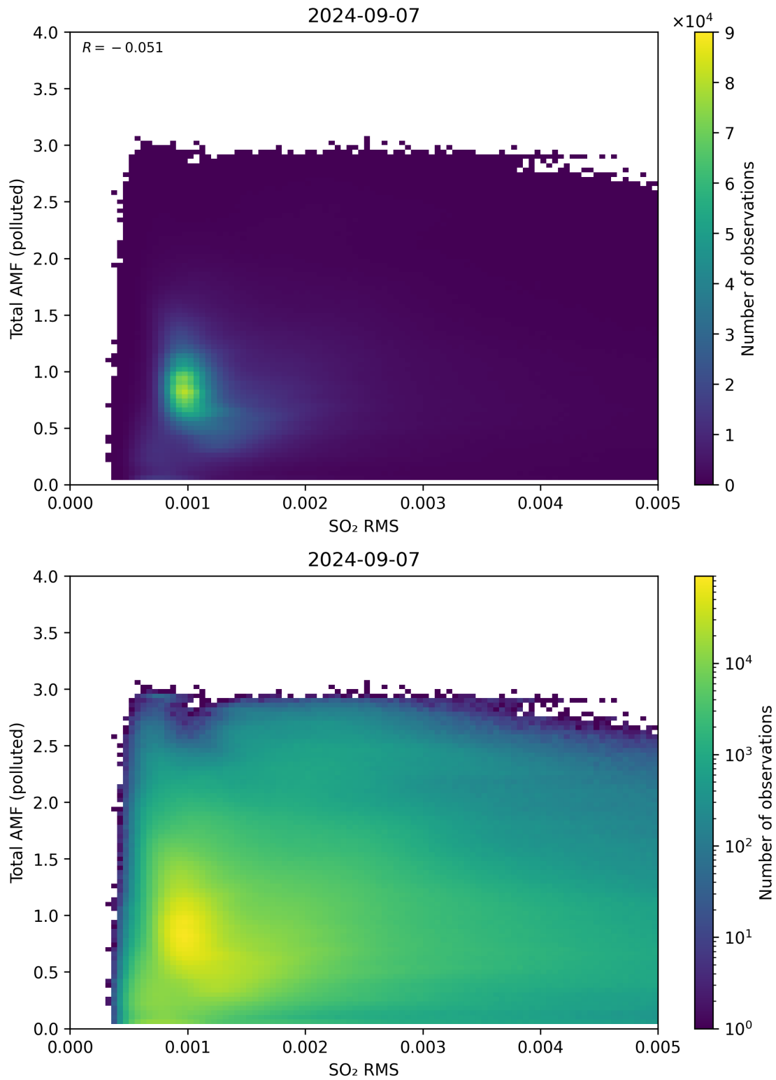
Figure 137: Scatter density plot of “SO 2 RMS” against “Total AMF (polluted)” for 2024-09-06 to 2024-09-08.
