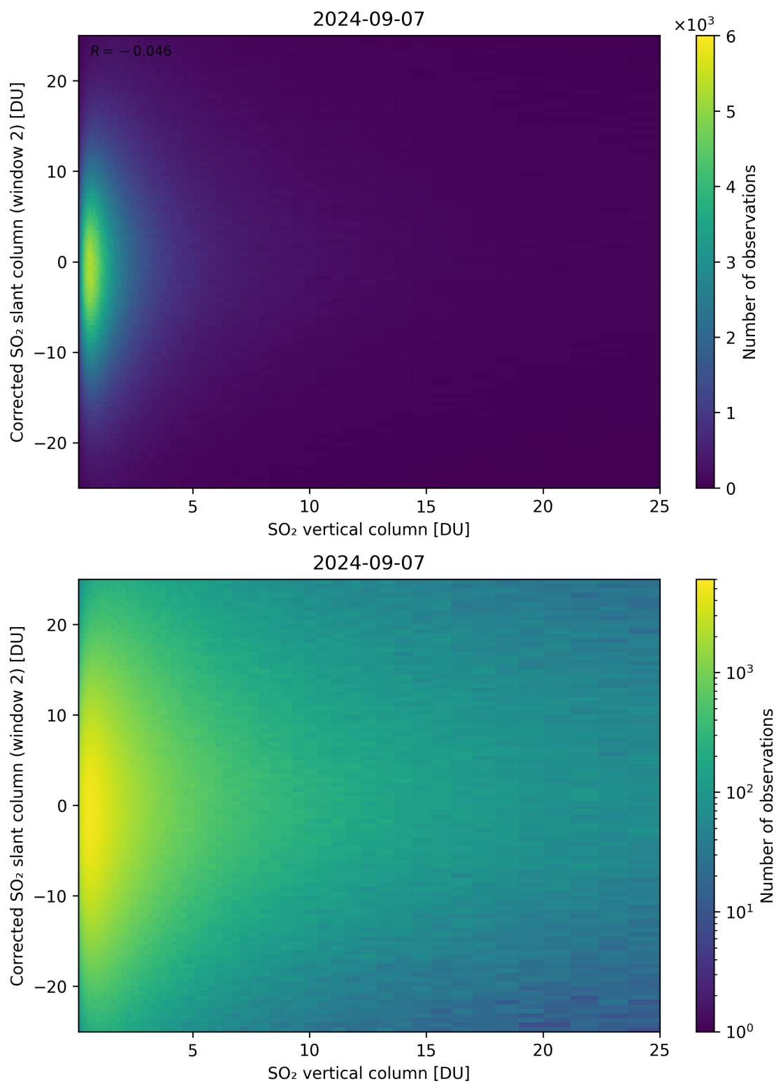
Figure 298: Scatter density plot of “SO 2 vertical column” against “Corrected SO 2 slant column (window 2)” for 2024-09-06 to 2024-09-08.
