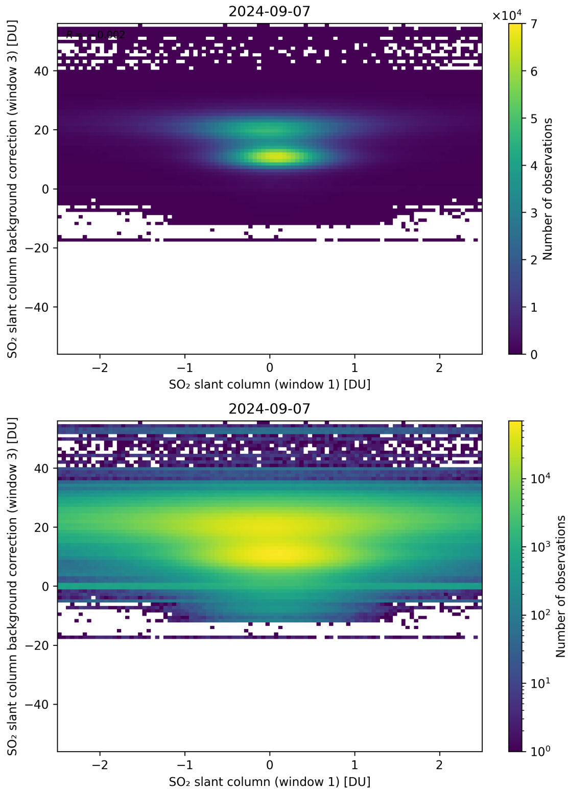
Figure 214: Scatter density plot of “SO 2 slant column (window 1)” against “SO 2 slant column background correction (window 3)” for 2024-09-06 to 2024-09-08.
