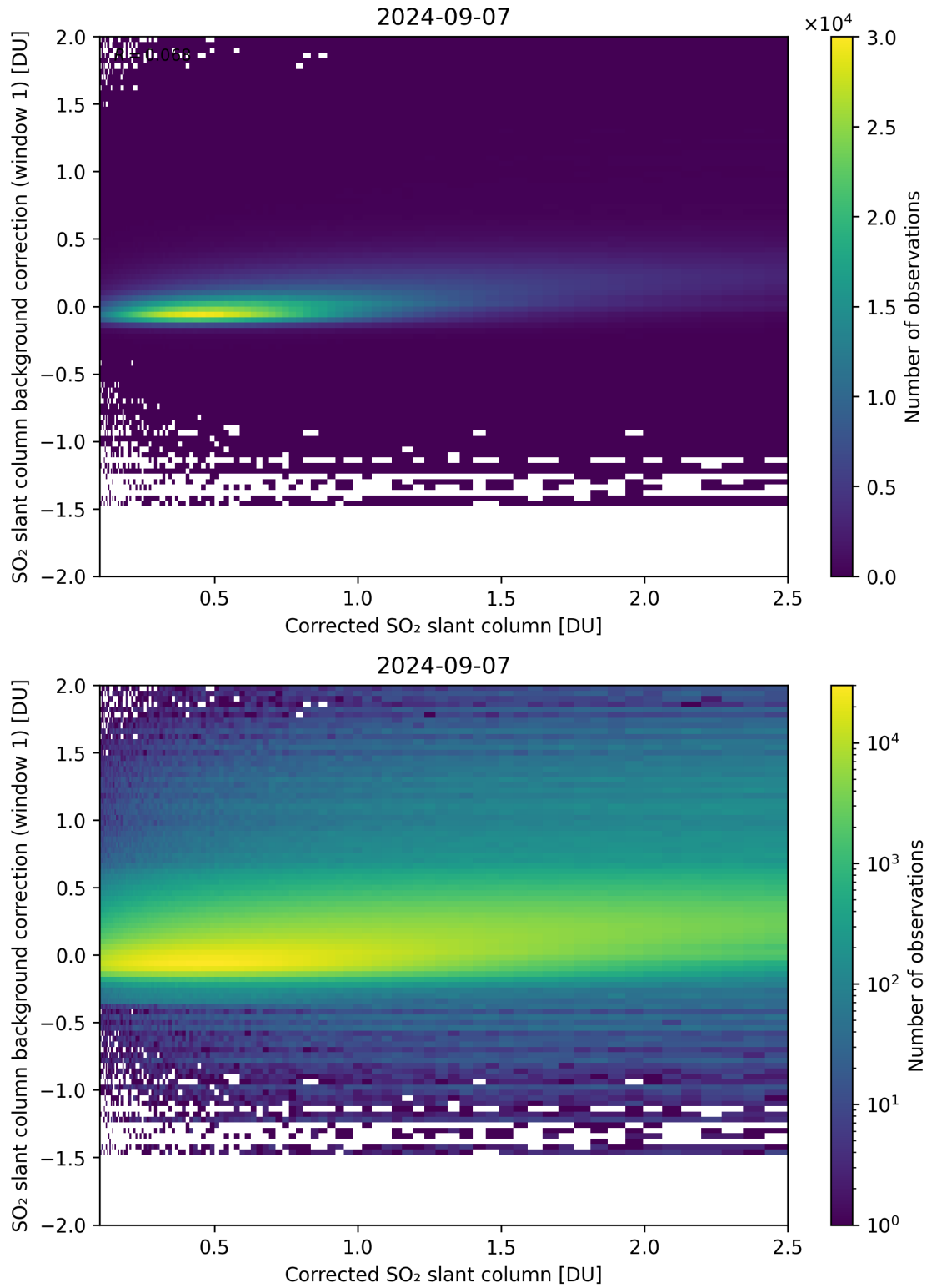
Figure 178: Scatter density plot of “Corrected SO 2 slant column” against “SO 2 slant column background correction (window 1)” for 2024-09-06 to 2024-09-08.
