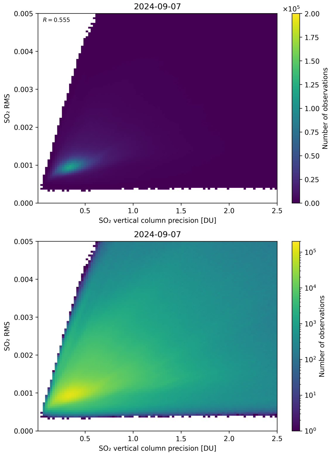
Figure 284: Scatter density plot of “SO 2 vertical column precision” against “SO 2 RMS” for 2024-09-06 to 2024-09-08.
