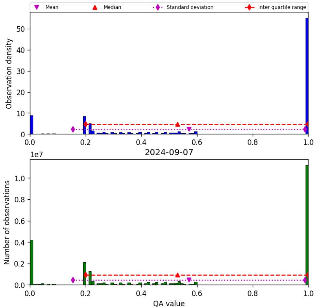
Figure 52: Histogram of “QA value” for 2024-09-06 to 2024-09-08
