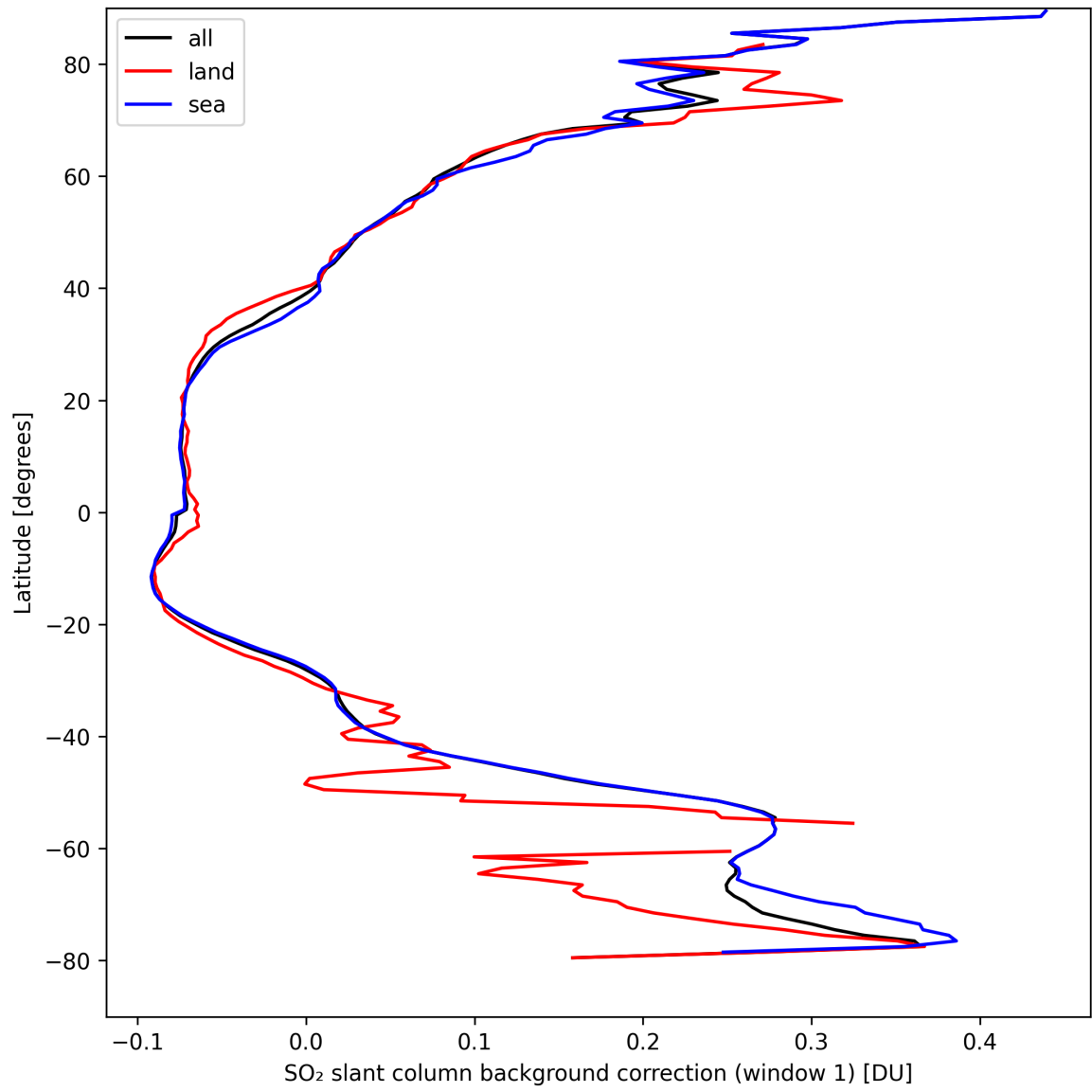
Figure 36: Zonal average of “SO 2 slant column background correction (window 1)” for 2024-09-06 to 2024-09-08.
