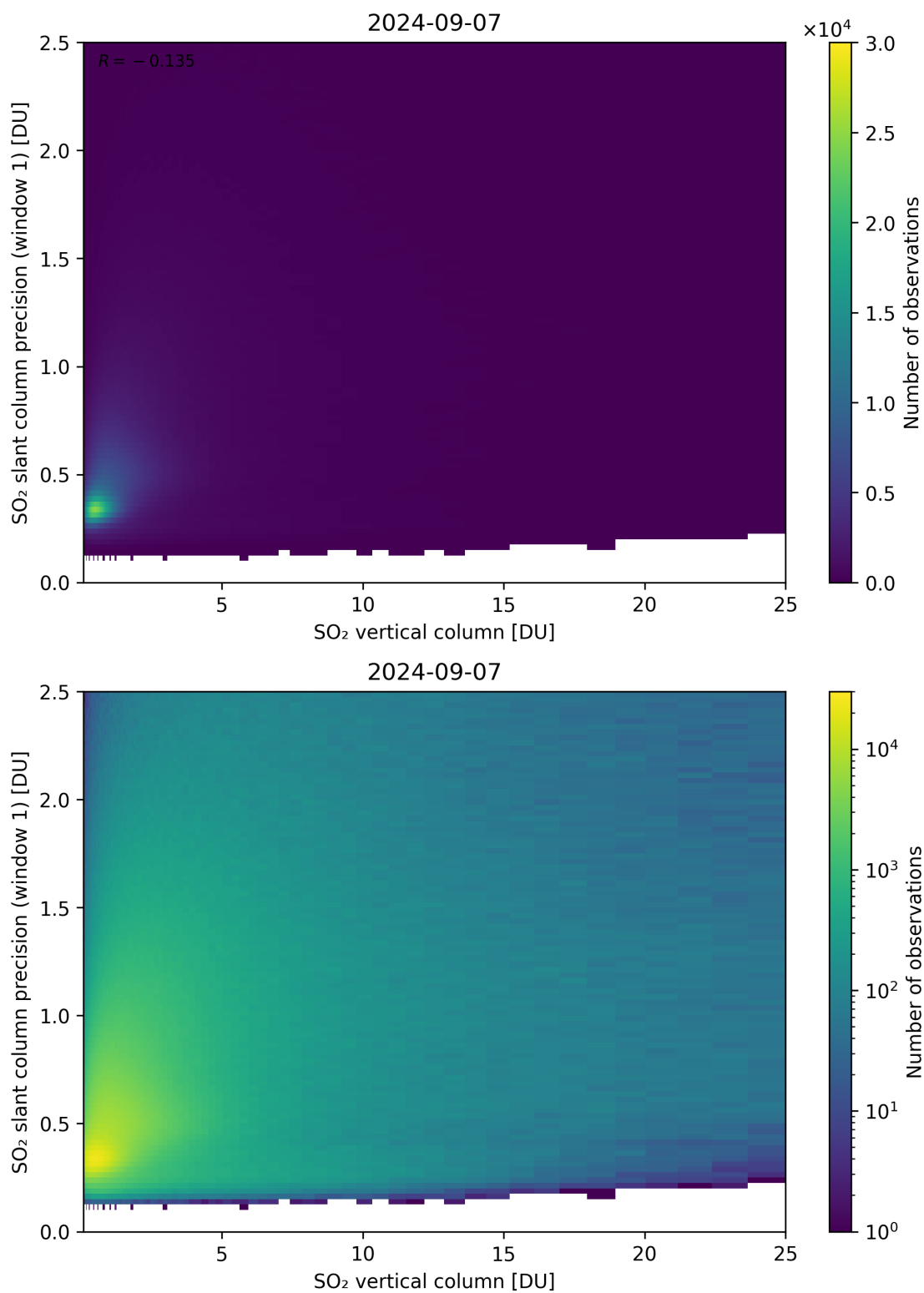
Figure 301: Scatter density plot of “SO 2 vertical column” against “SO 2 slant column precision (window 1)” for 2024-09-06 to 2024-09-08.
