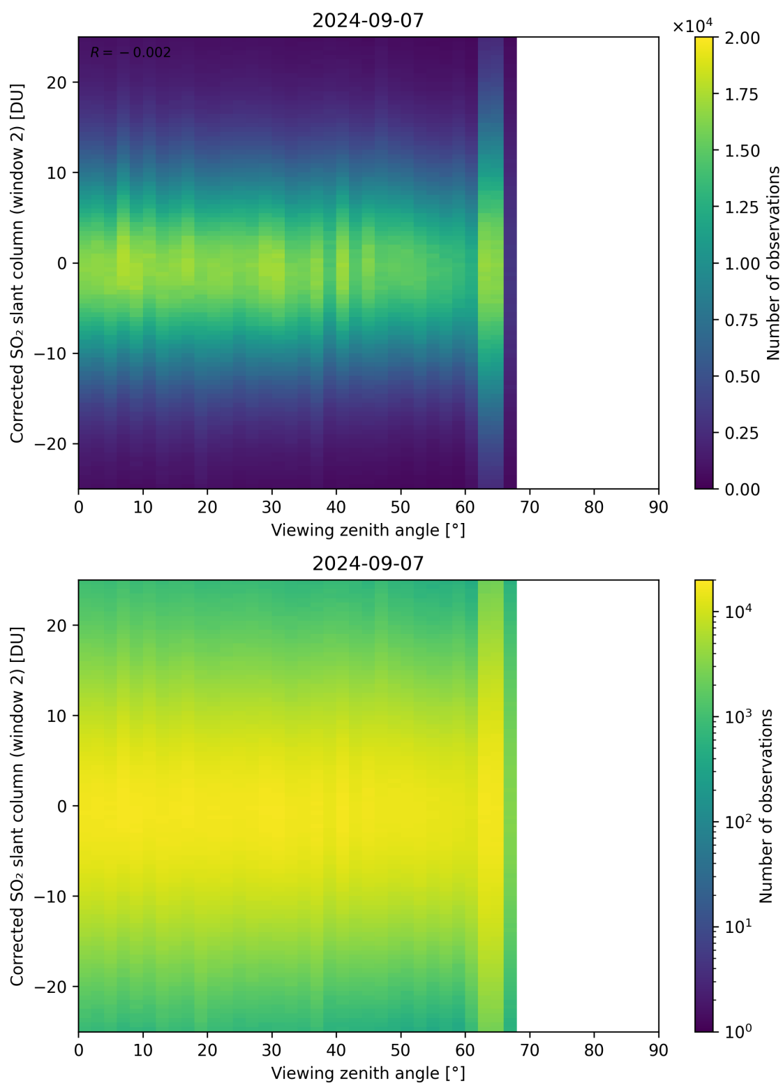
Figure 318: Scatter density plot of “Viewing zenith angle” against “Corrected SO 2 slant column (window 2)” for 2024-09-06 to 2024-09-08.
