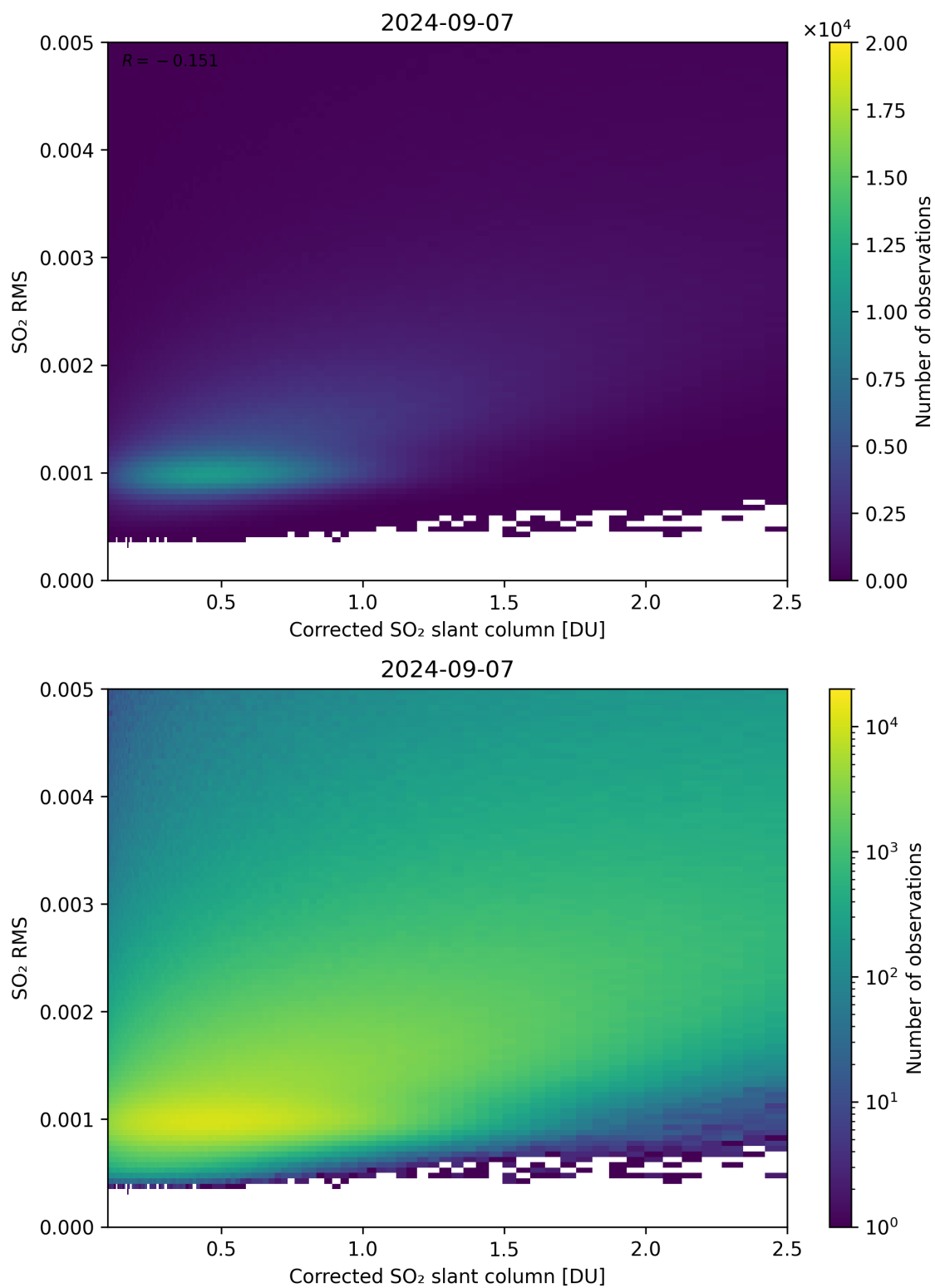
Figure 183: Scatter density plot of “Corrected SO 2 slant column” against “SO 2 RMS” for 2024-09-06 to 2024-09-08.
