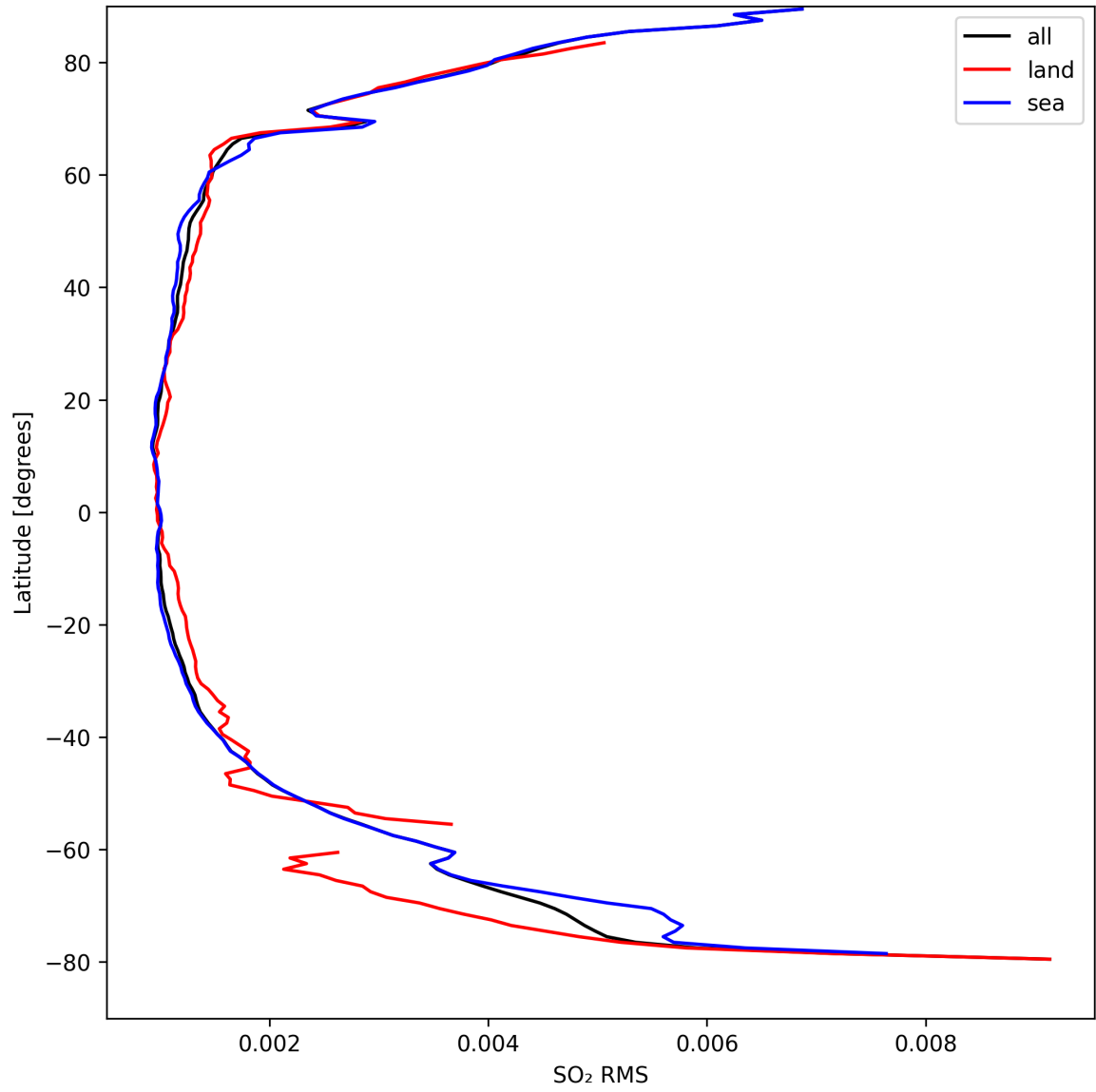
Figure 47: Zonal average of “SO 2 RMS” for 2024-09-06 to 2024-09-08.
