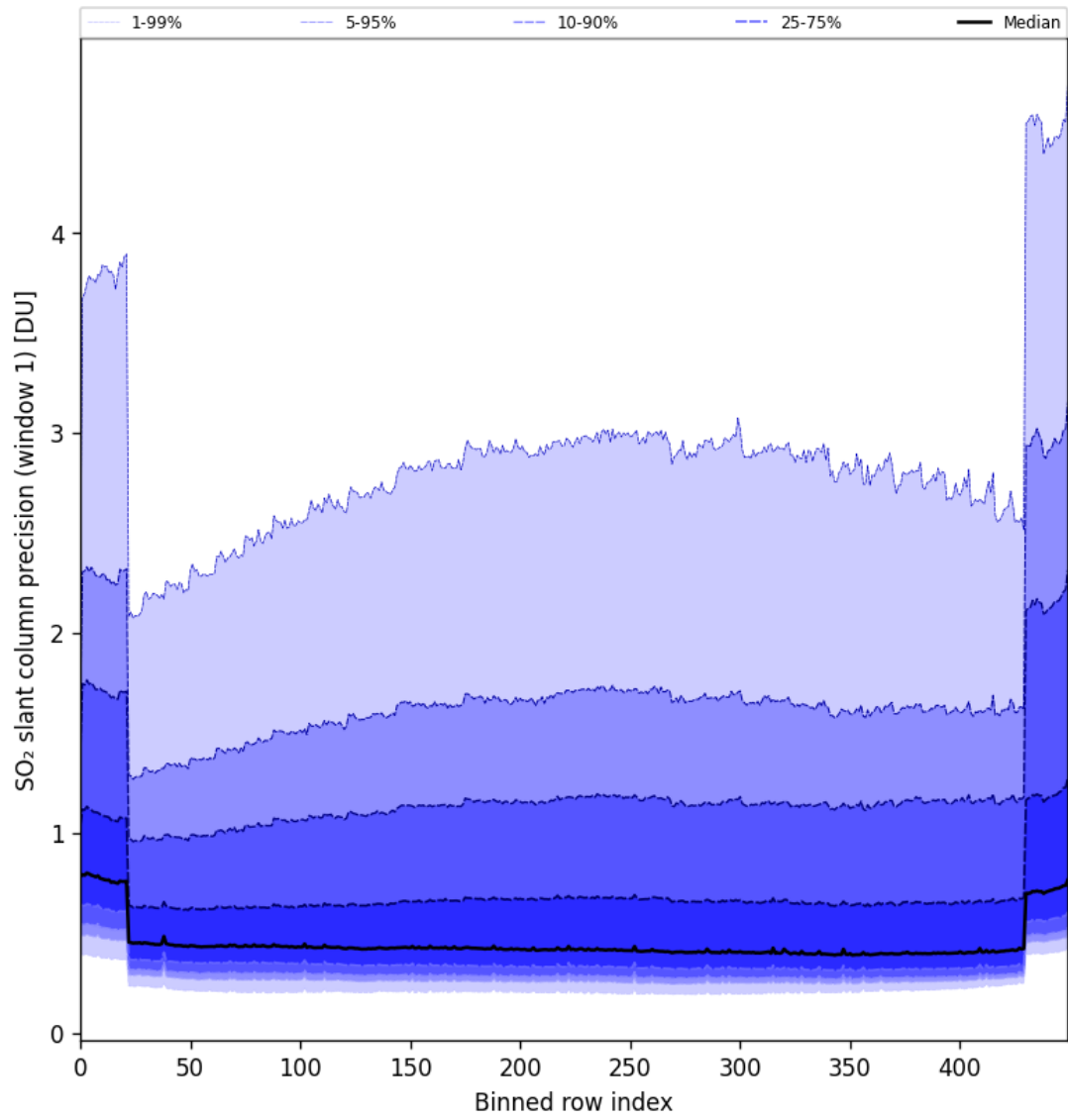
Figure 80: Along track statistics of “SO 2 slant column precision (window 1)” for 2024-09-06 to 2024-09-08
