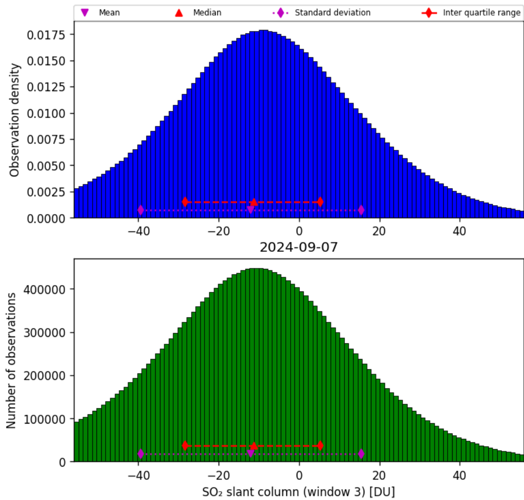
Figure 64: Histogram of “SO 2 slant column (window 3)” for 2024-09-06 to 2024-09-08
