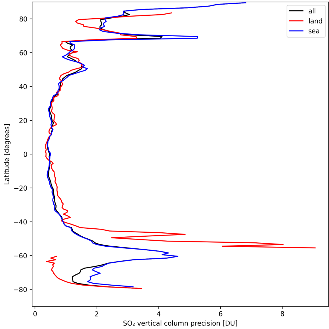
Figure 31: Zonal average of “SO 2 vertical column precision” for 2024-09-06 to 2024-09-08.
