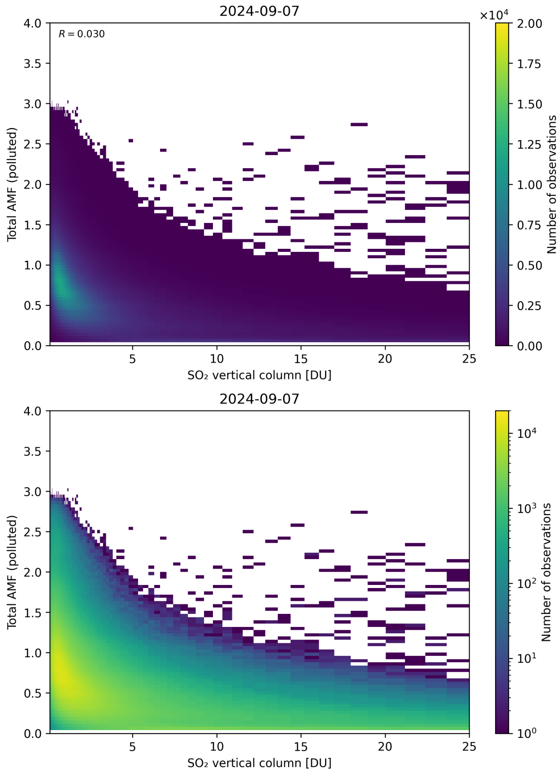
Figure 305: Scatter density plot of “SO 2 vertical column” against “Total AMF (polluted)” for 2024-09-06 to 2024-09-08.
