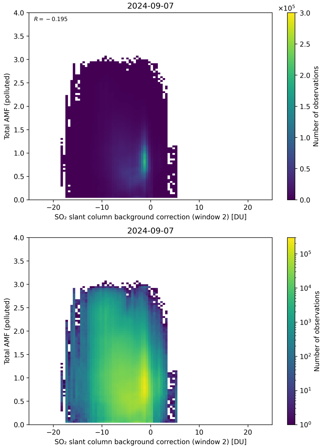
Figure 119: Scatter density plot of “SO 2 slant column background correction (window 2)” against “Total AMF (polluted)” for 2024-09-06 to 2024-09-08.
