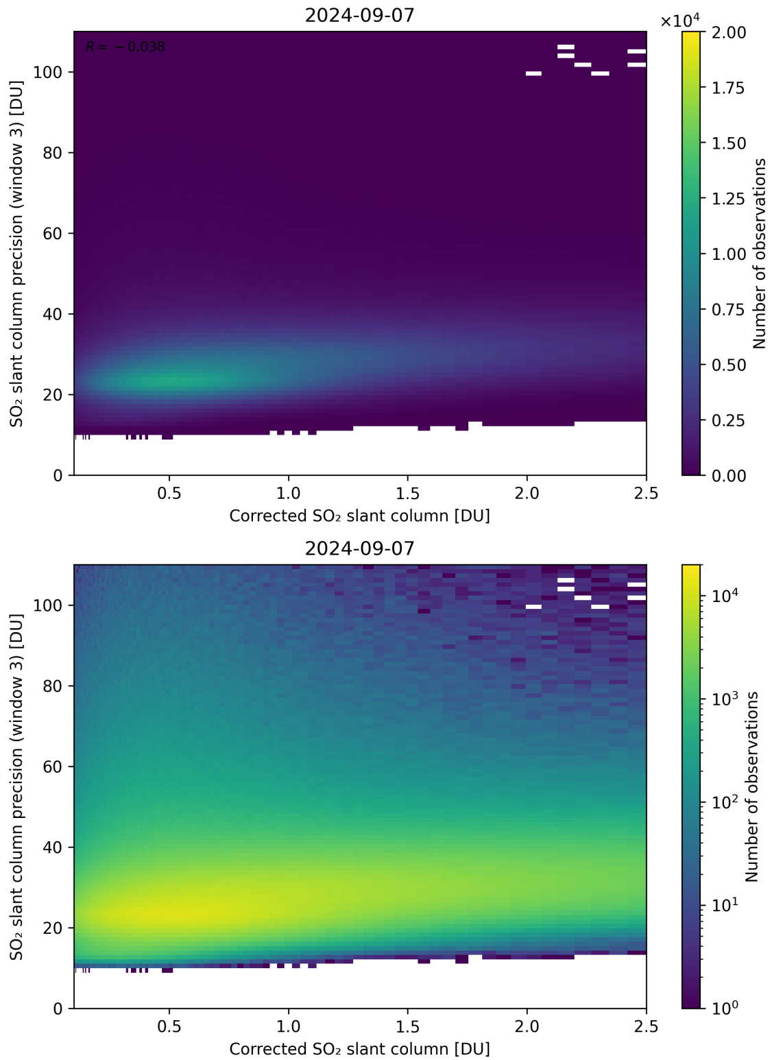
Figure 191: Scatter density plot of “Corrected SO 2 slant column” against “SO 2 slant column precision (window 3)” for 2024-09-06 to 2024-09-08.
