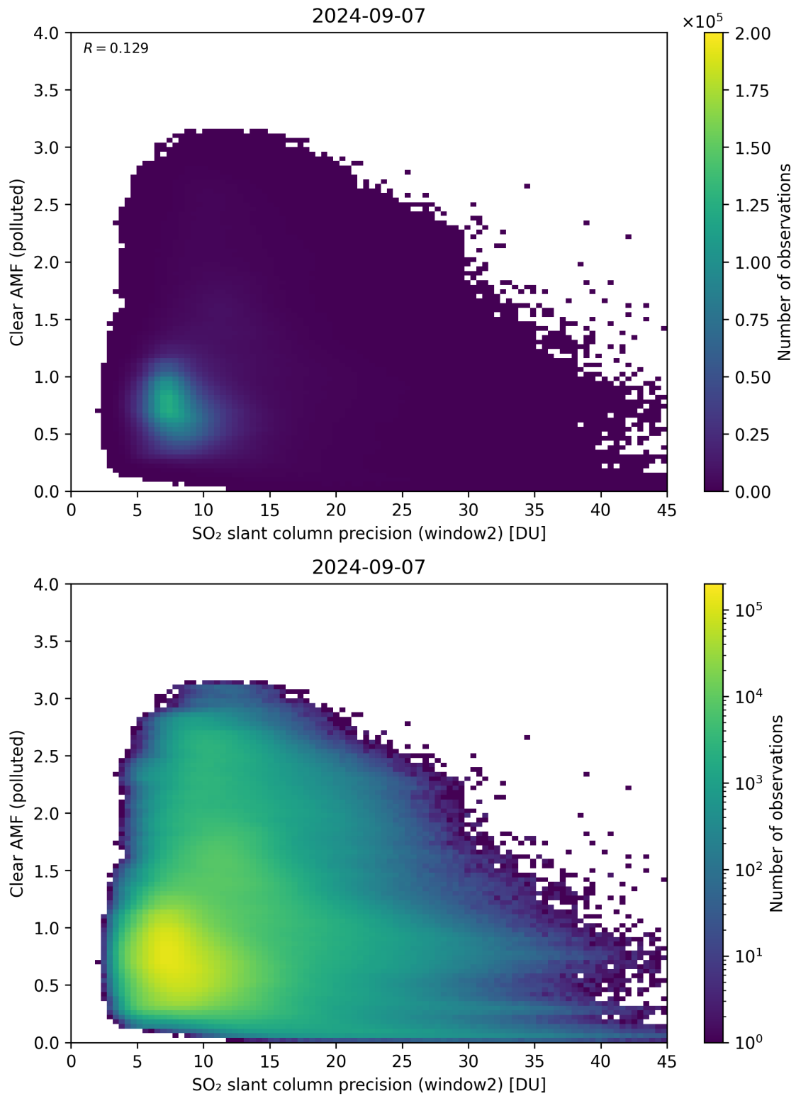
Figure 246: Scatter density plot of “SO 2 slant column precision (window2)” against “Clear AMF (polluted)” for 2024-09-06 to 2024-09-08.
