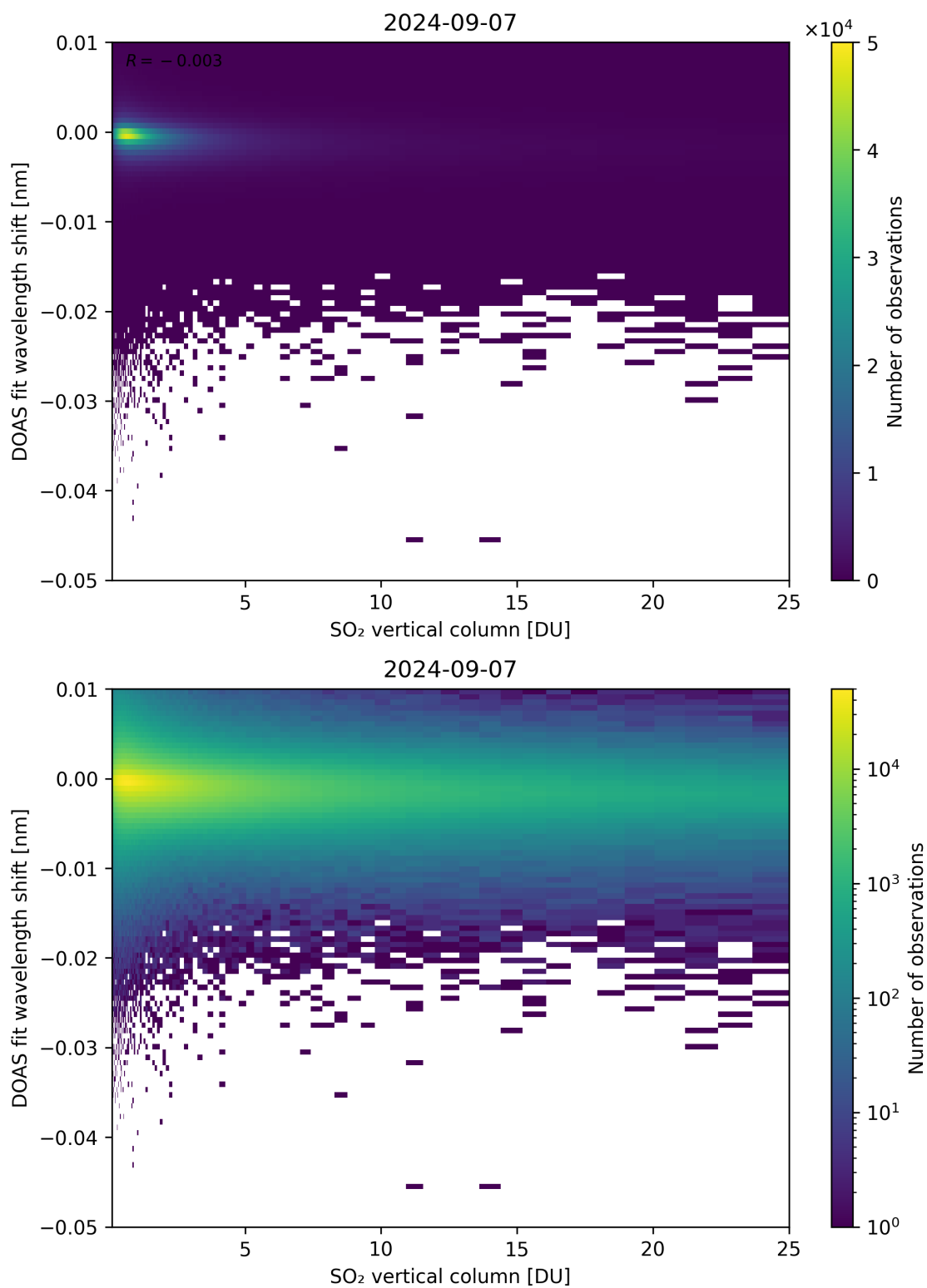
Figure 276: Scatter density plot of “SO 2 vertical column” against “DOAS fit wavelength shift” for 2024-09-06 to 2024-09-08.
