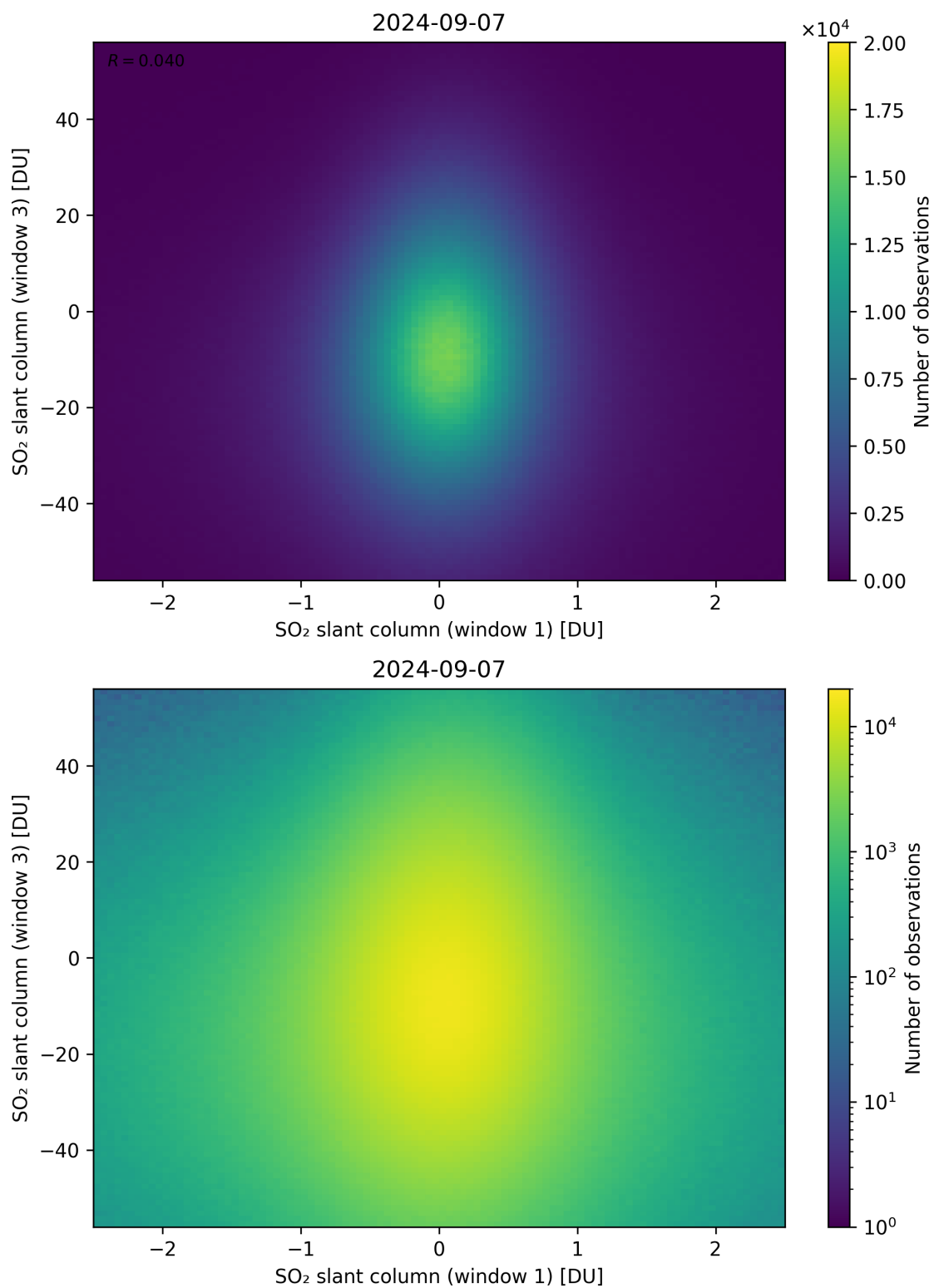
Figure 237: Scatter density plot of “SO 2 slant column (window 1)” against “SO 2 slant column (window 3)” for 2024-09-06 to 2024-09-08.
