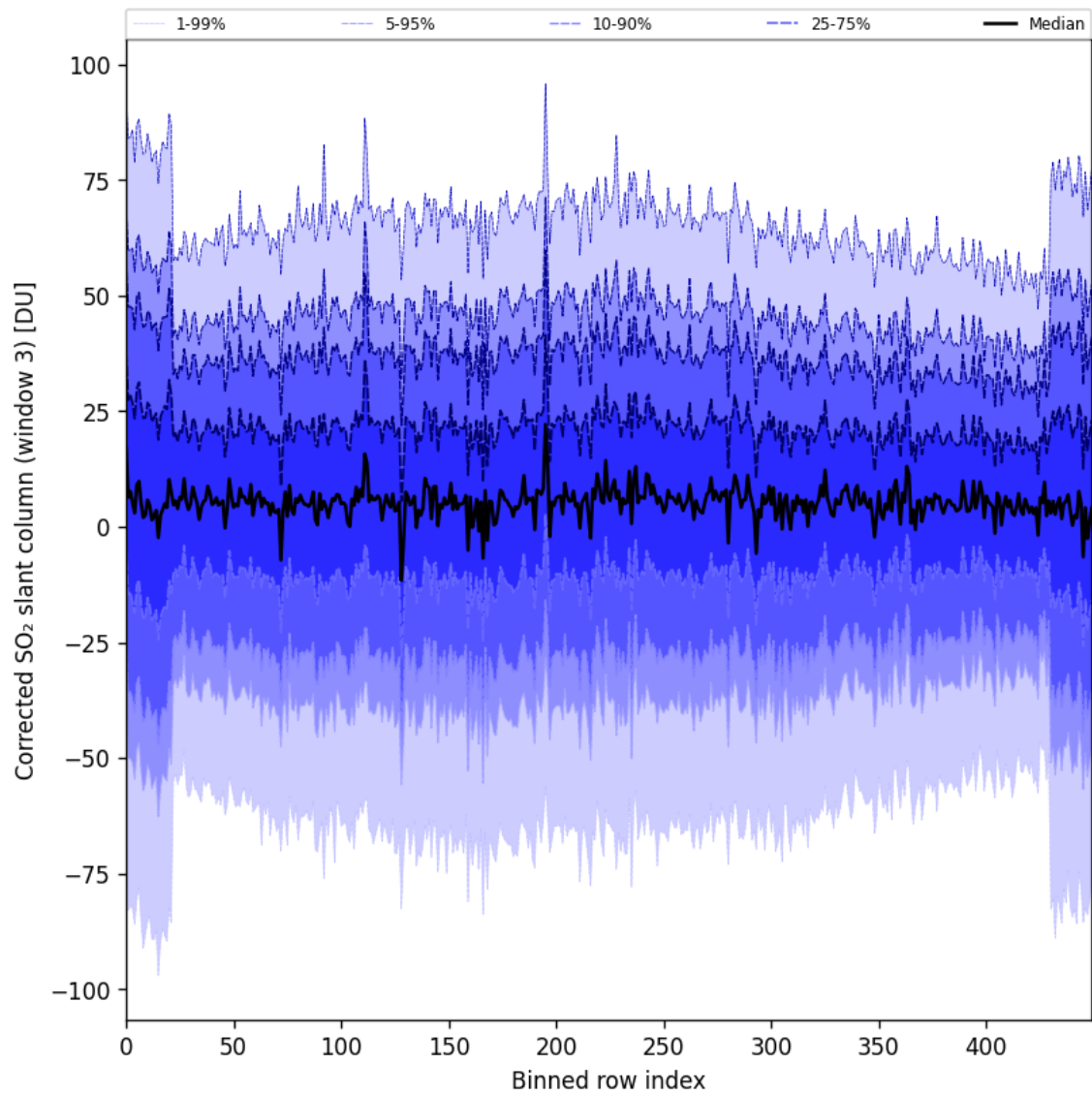
Figure 89: Along track statistics of “Corrected SO 2 slant column (window 3)” for 2024-09-06 to 2024-09-08
