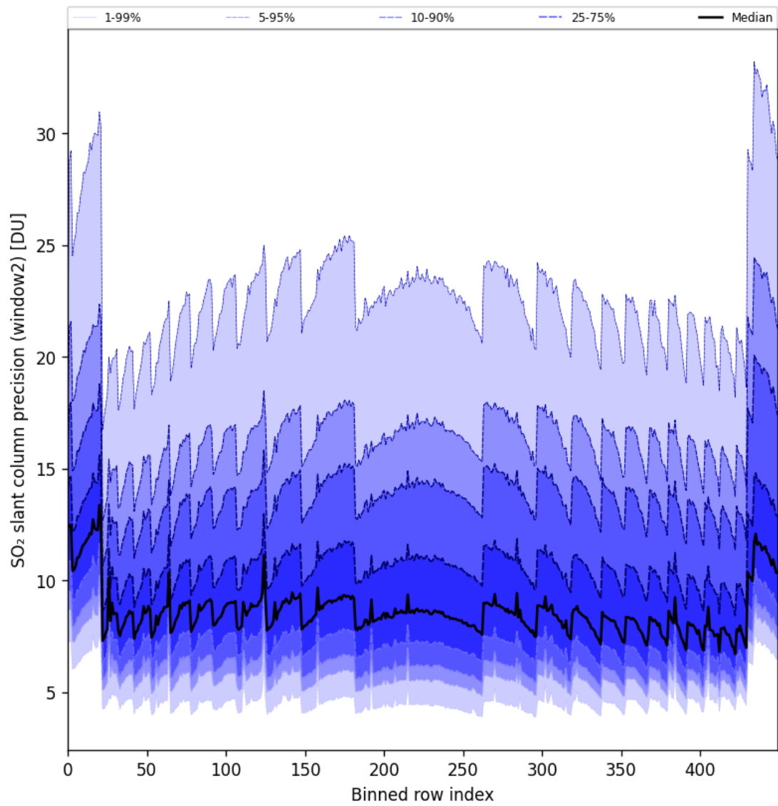
Figure 84: Along track statistics of “SO 2 slant column precision (window2)” for 2024-09-06 to 2024-09-08
