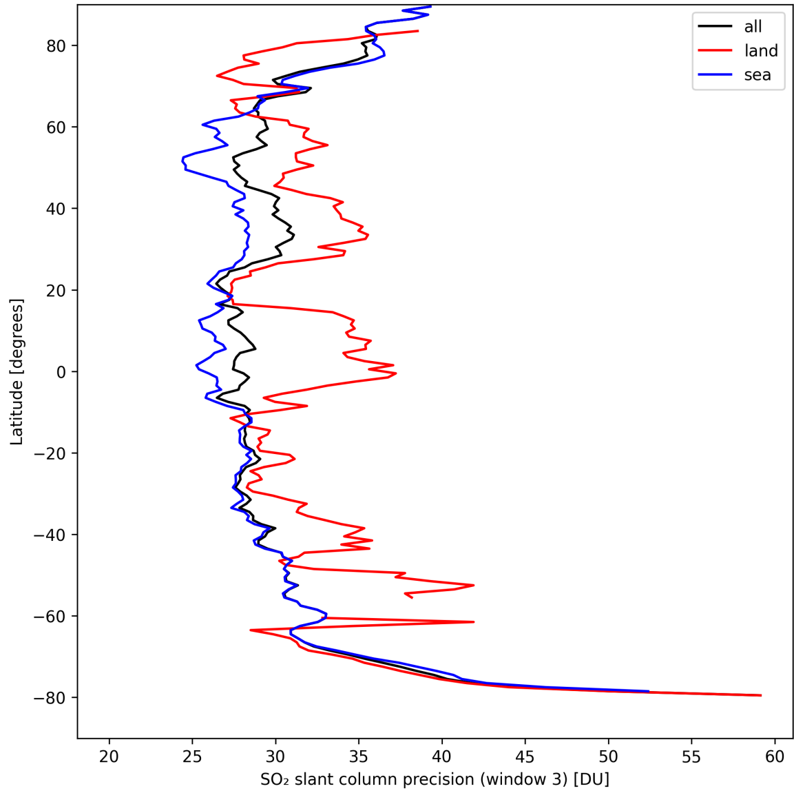
Figure 42: Zonal average of “SO 2 slant column precision (window 3)” for 2024-09-06 to 2024-09-08.
