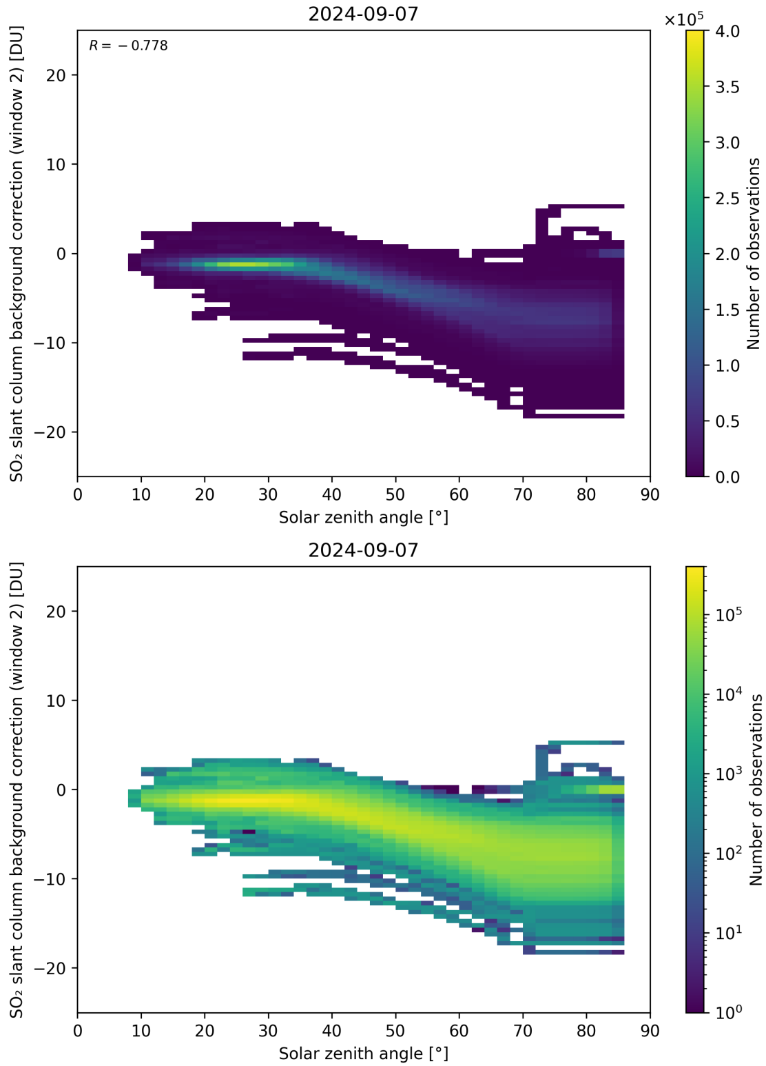
Figure 159: Scatter density plot of “Solar zenith angle” against “SO 2 slant column background correction (window 2)” for 2024-09-06 to 2024-09-08.
