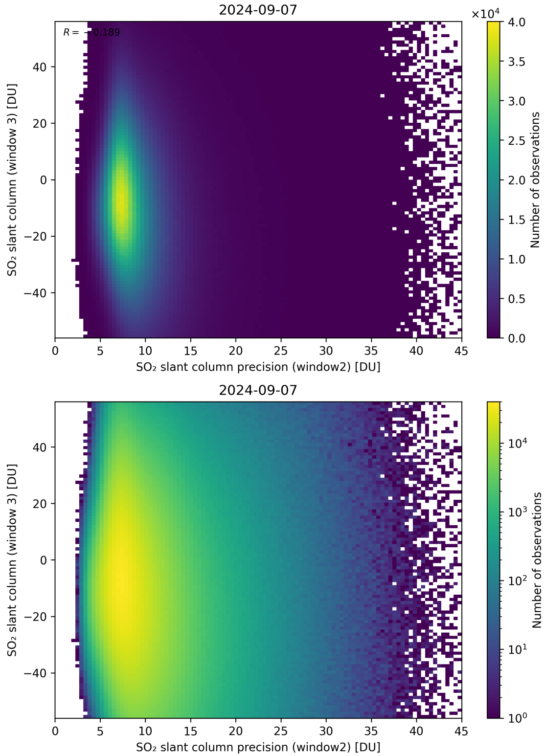
Figure 249: Scatter density plot of “SO 2 slant column precision (window2)” against “SO 2 slant column (window 3)” for 2024-09-06 to 2024-09-08.
