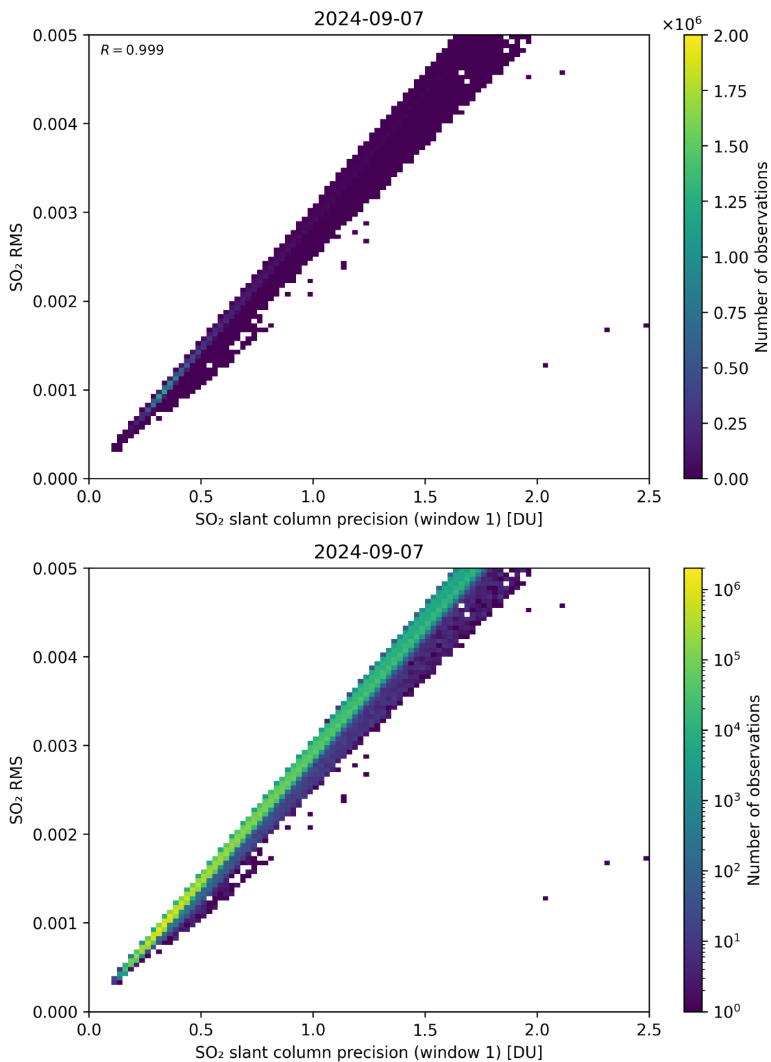
Figure 223: Scatter density plot of “SO 2 slant column precision (window 1)” against “SO 2 RMS” for 2024-09-06 to 2024-09-08.
