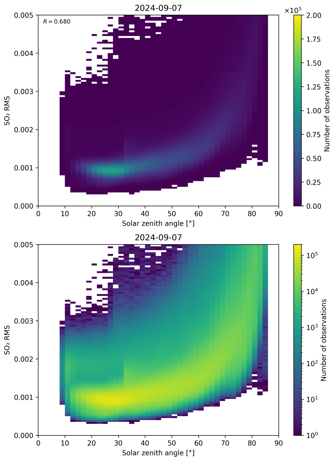
Figure 163: Scatter density plot of “Solar zenith angle” against “SO 2 RMS” for 2024-09-06 to 2024-09-08.
