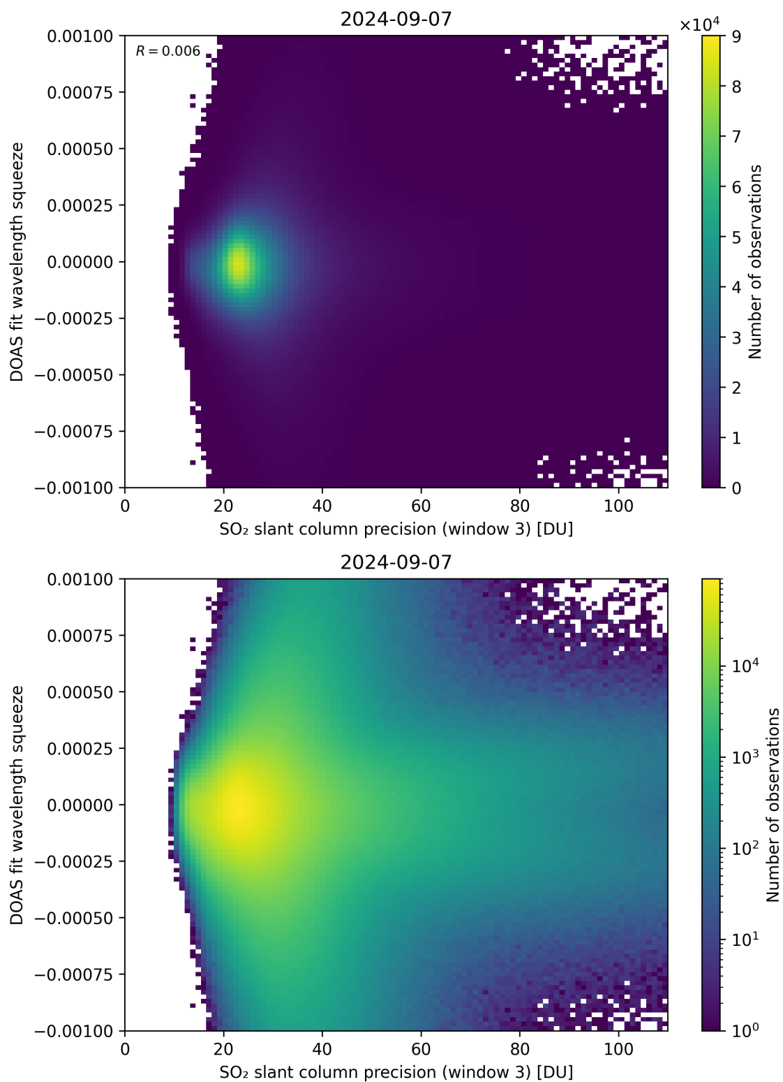
Figure 259: Scatter density plot of “SO 2 slant column precision (window 3)” against “DOAS fit wavelength squeeze” for 2024-09-06 to 2024-09-08.
