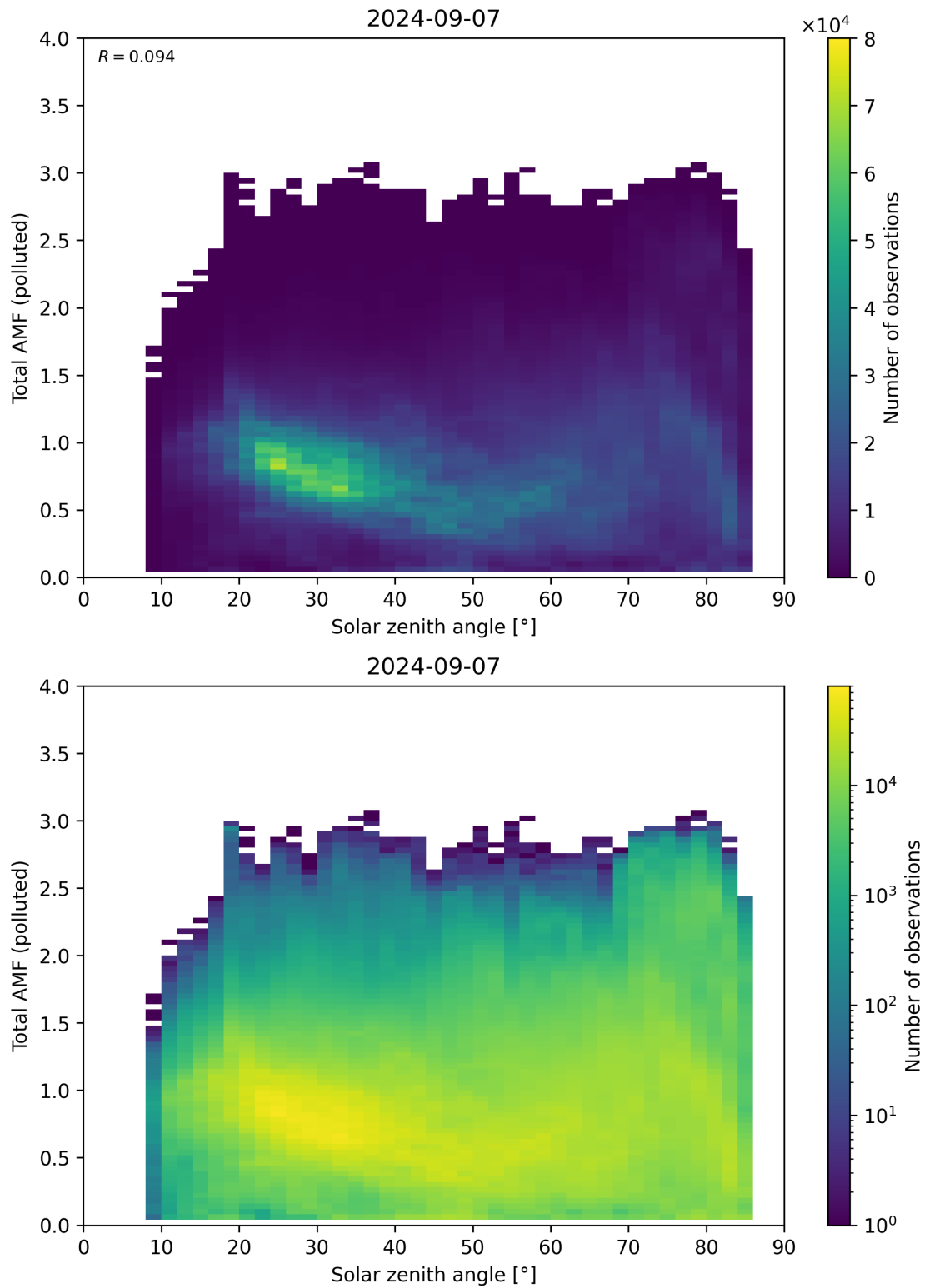
Figure 174: Scatter density plot of “Solar zenith angle” against “Total AMF (polluted)” for 2024-09-06 to 2024-09-08.
