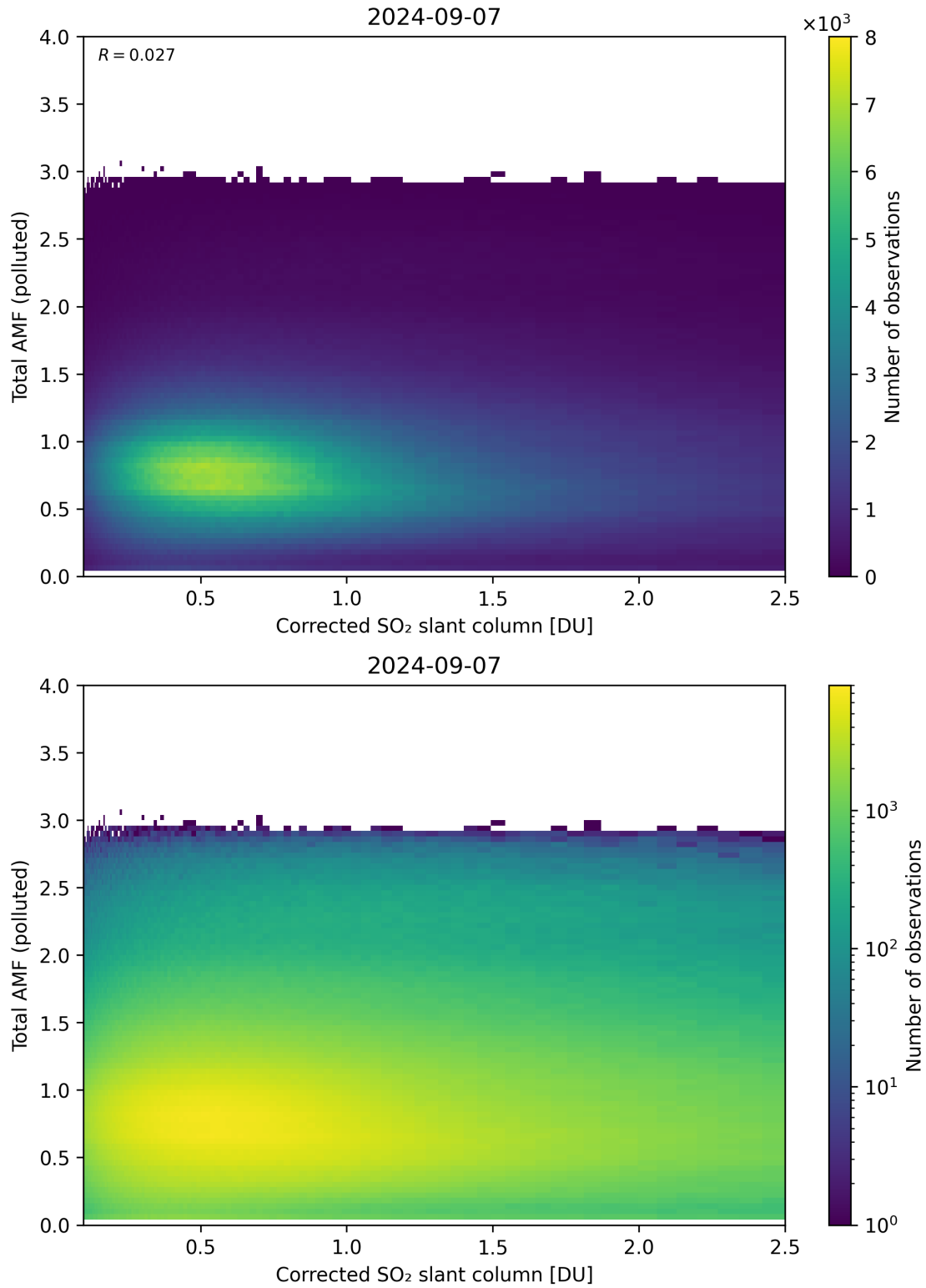
Figure 192: Scatter density plot of “Corrected SO 2 slant column” against “Total AMF (polluted)” for 2024-09-06 to 2024-09-08.
