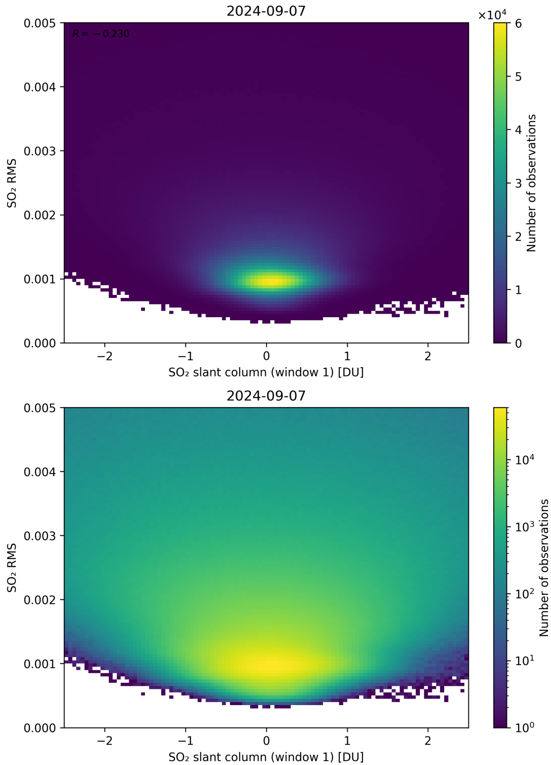
Figure 217: Scatter density plot of “SO 2 slant column (window 1)” against “SO 2 RMS” for 2024-09-06 to 2024-09-08.
