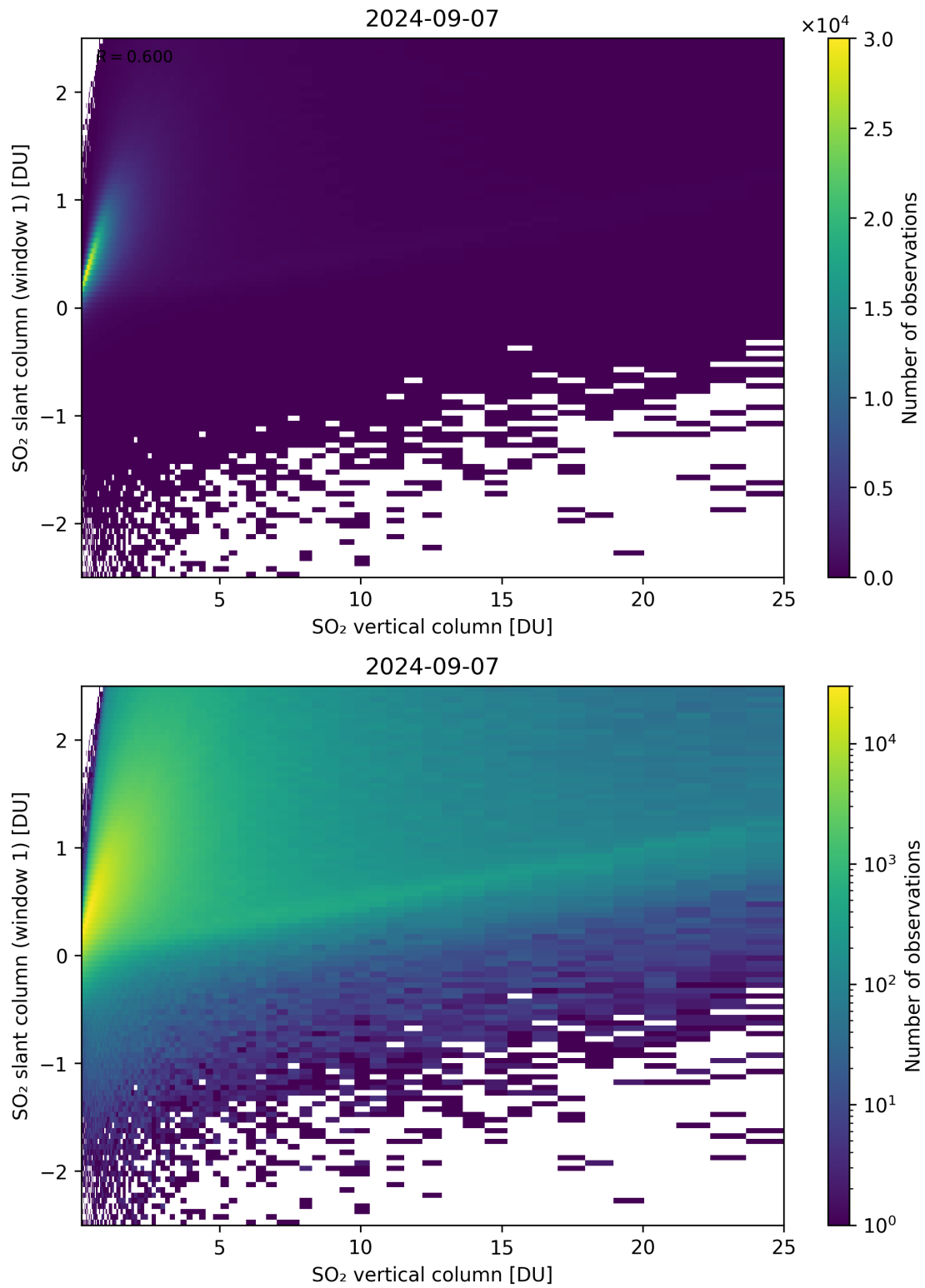
Figure 300: Scatter density plot of “SO 2 vertical column” against “SO 2 slant column (window 1)” for 2024-09-06 to 2024-09-08.
