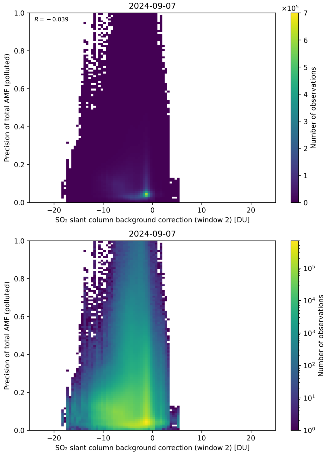
Figure 120: Scatter density plot of “SO 2 slant column background correction (window 2)” against “Precision of total AMF (polluted)” for 2024-09-06 to 2024-09-08.
