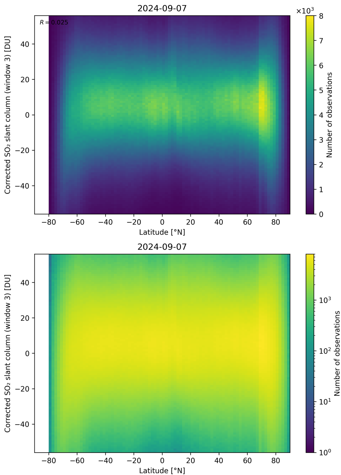
Figure 148: Scatter density plot of “Latitude” against “Corrected SO 2 slant column (window 3)” for 2024-09-06 to 2024-09-08.
