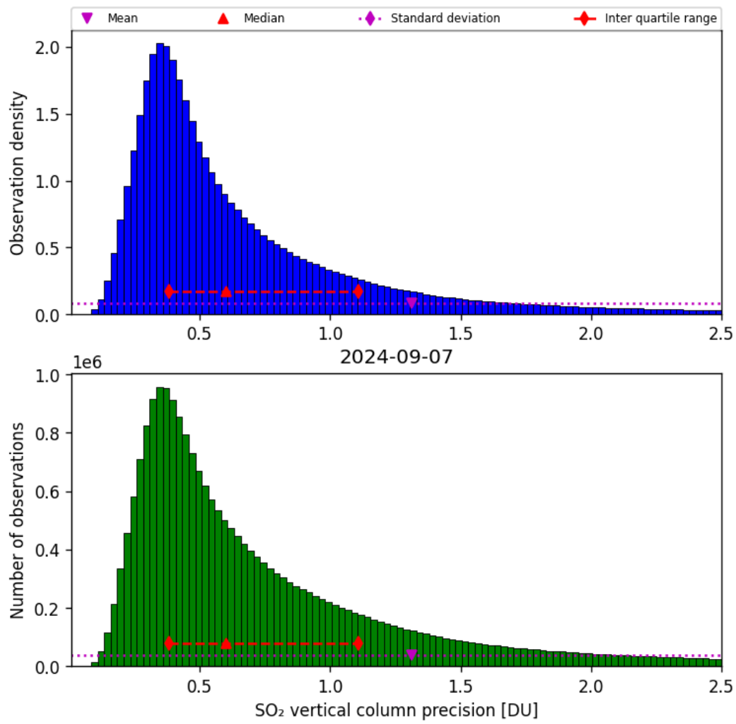
Figure 54: Histogram of “SO 2 vertical column precision” for 2024-09-06 to 2024-09-08
