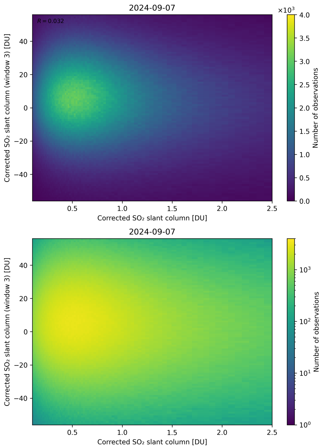
Figure 186: Scatter density plot of “Corrected SO 2 slant column” against “Corrected SO 2 slant column (window 3)” for 2024-09-06 to 2024-09-08.
