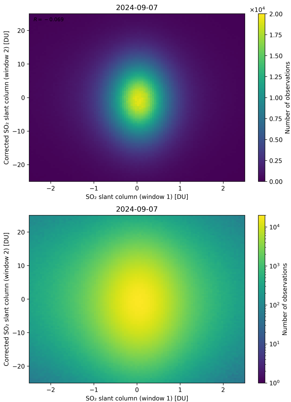
Figure 233: Scatter density plot of “SO 2 slant column (window 1)” against “Corrected SO 2 slant column (window 2)” for 2024-09-06 to 2024-09-08.
