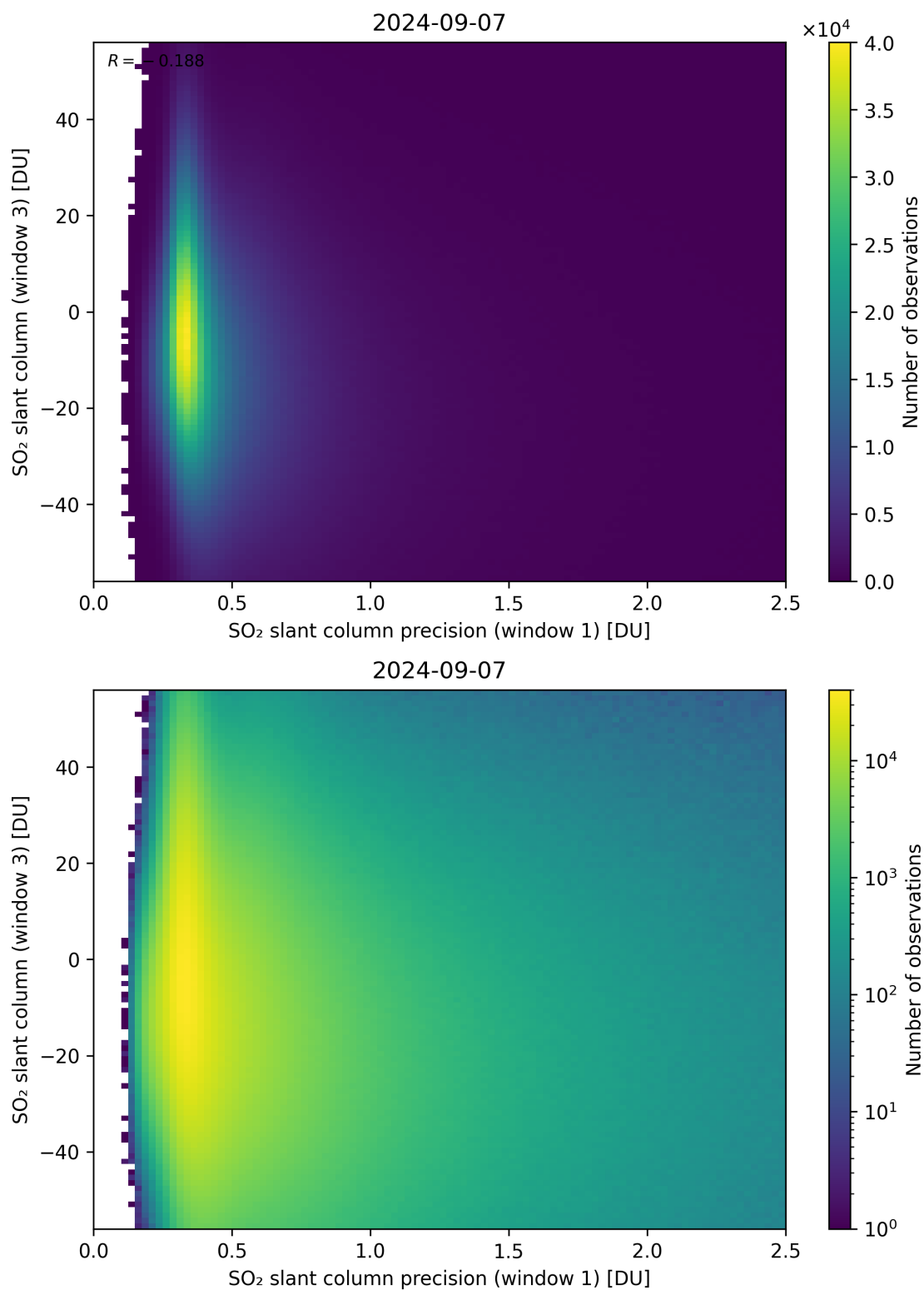
Figure 228: Scatter density plot of “SO 2 slant column precision (window 1)” against “SO 2 slant column (window 3)” for 2024-09-06 to 2024-09-08.
