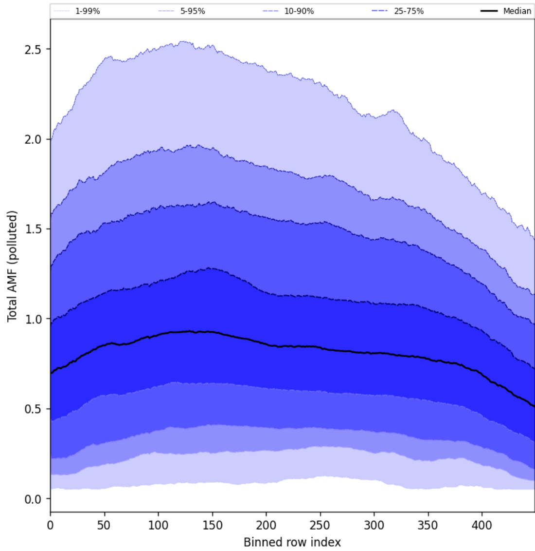
Figure 94: Along track statistics of “Total AMF (polluted)” for 2024-09-06 to 2024-09-08
