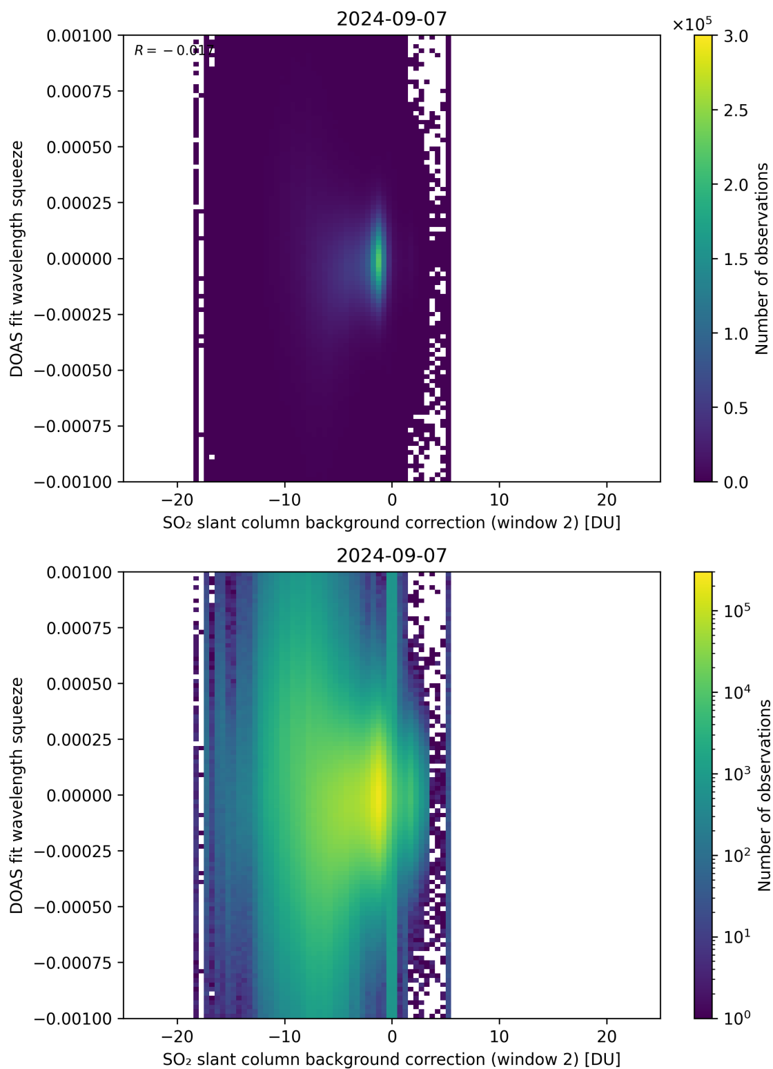
Figure 113: Scatter density plot of “SO 2 slant column background correction (window 2)” against “DOAS fit wavelength squeeze” for 2024-09-06 to 2024-09-08.
