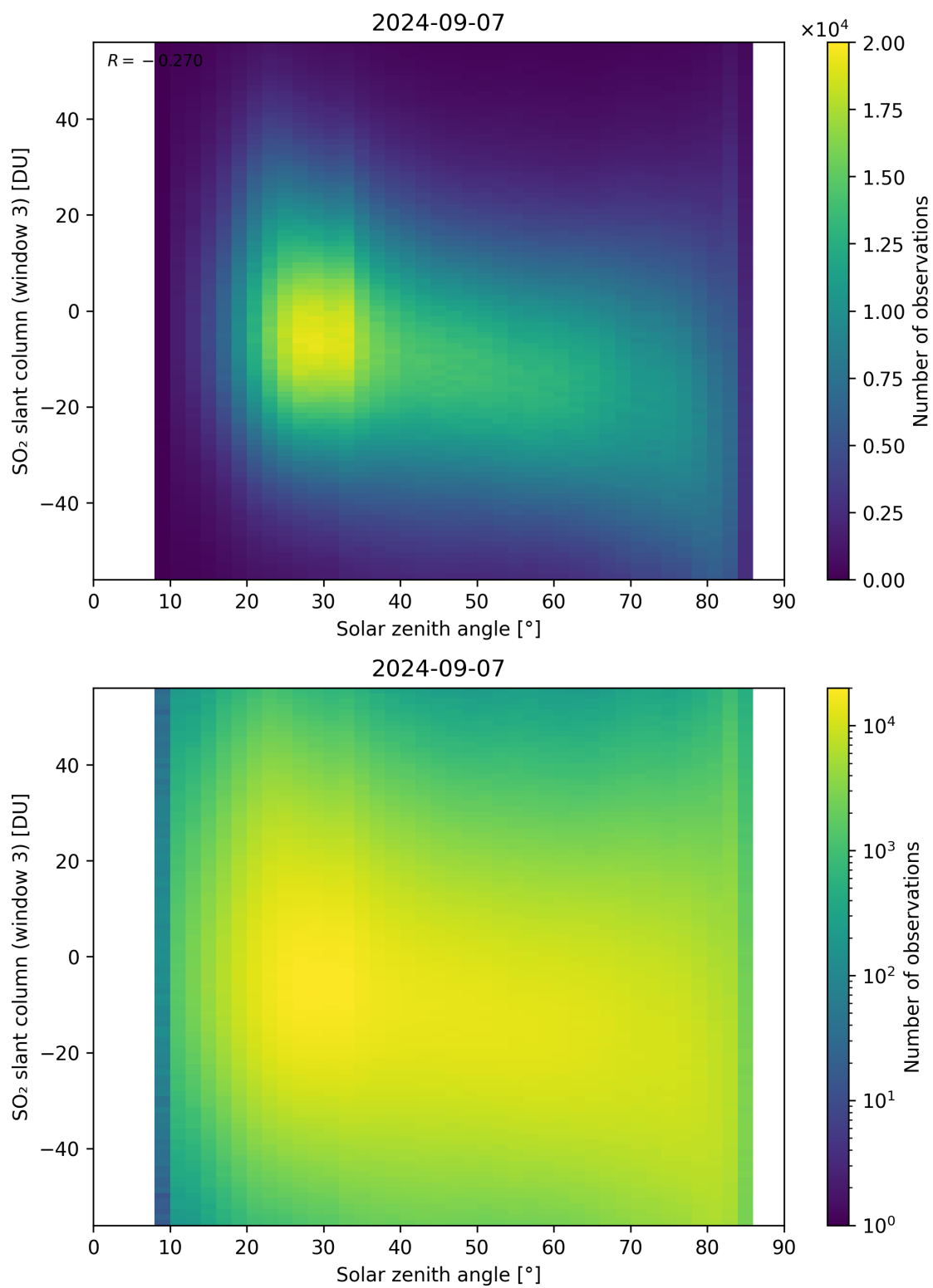
Figure 172: Scatter density plot of “Solar zenith angle” against “SO 2 slant column (window 3)” for 2024-09-06 to 2024-09-08.
