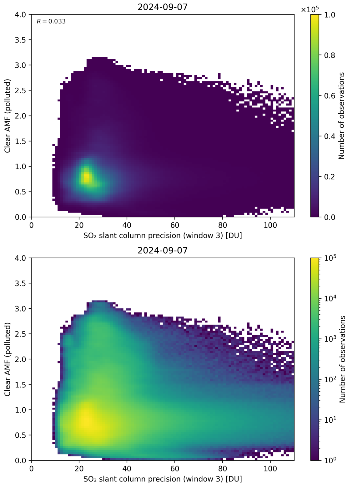
Figure 261: Scatter density plot of “SO 2 slant column precision (window 3)” against “Clear AMF (polluted)” for 2024-09-06 to 2024-09-08.
