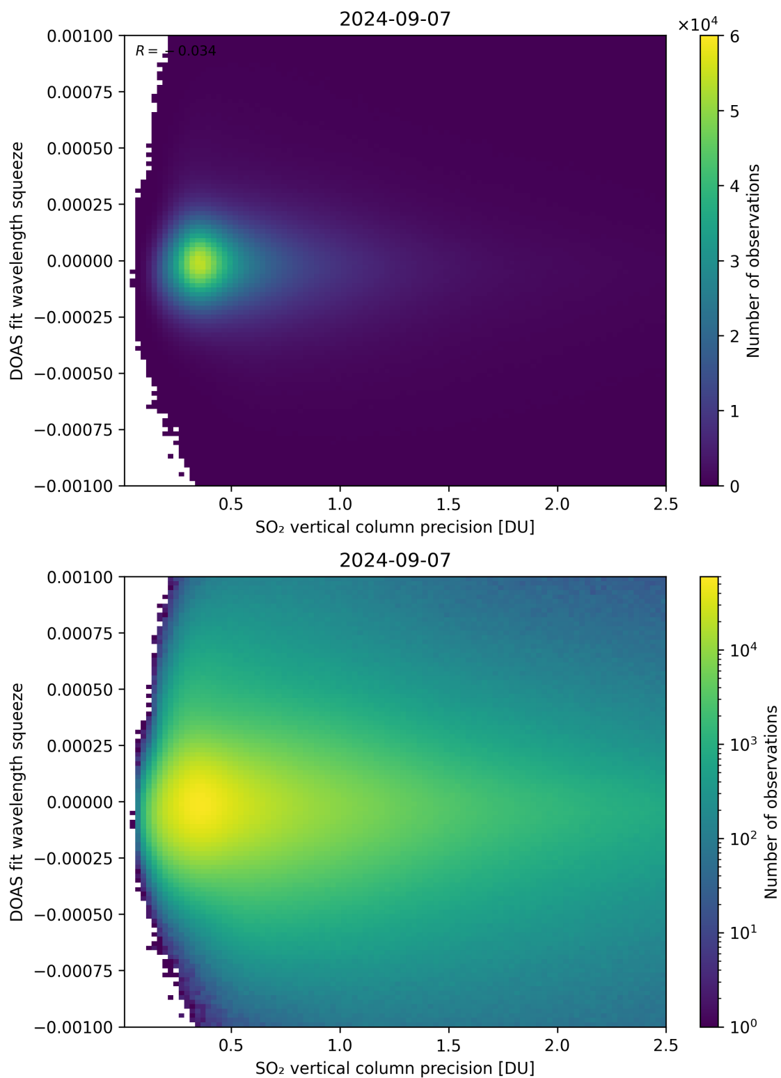
Figure 283: Scatter density plot of “SO 2 vertical column precision” against “DOAS fit wavelength squeeze” for 2024-09-06 to 2024-09-08.
