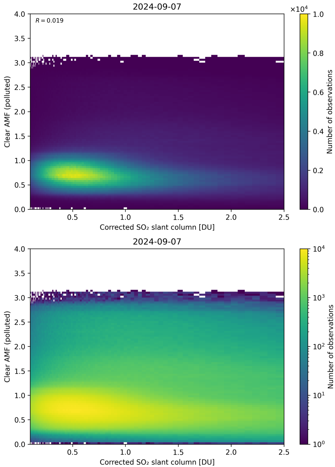
Figure 184: Scatter density plot of “Corrected SO 2 slant column” against “Clear AMF (polluted)” for 2024-09-06 to 2024-09-08.
