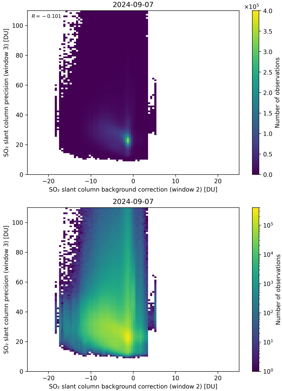
Figure 118: Scatter density plot of “SO 2 slant column background correction (window 2)” against “SO 2 slant column precision (window 3)” for 2024-09-06 to 2024-09-08.
