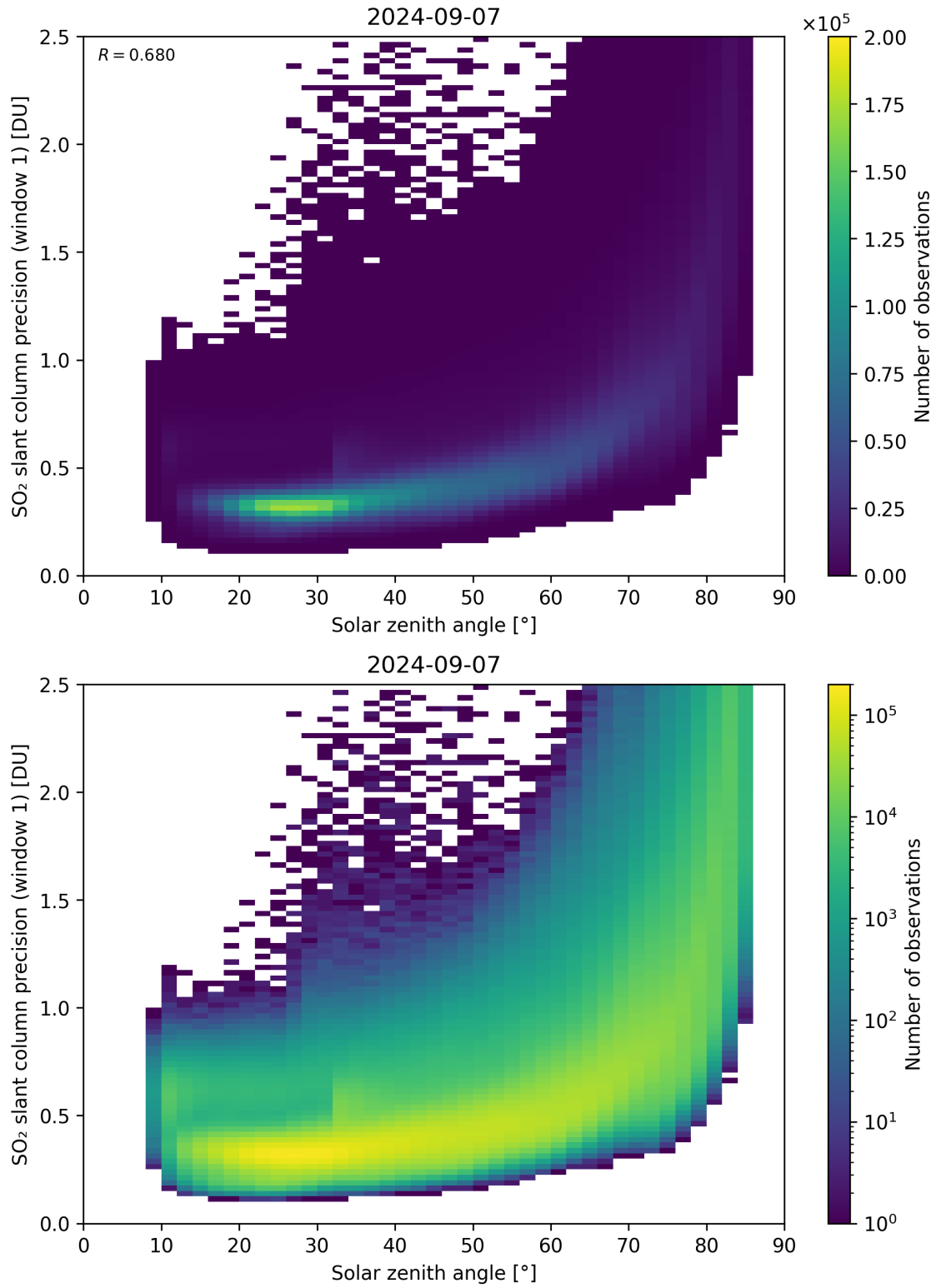
Figure 170: Scatter density plot of “Solar zenith angle” against “SO 2 slant column precision (window 1)” for 2024-09-06 to 2024-09-08.
