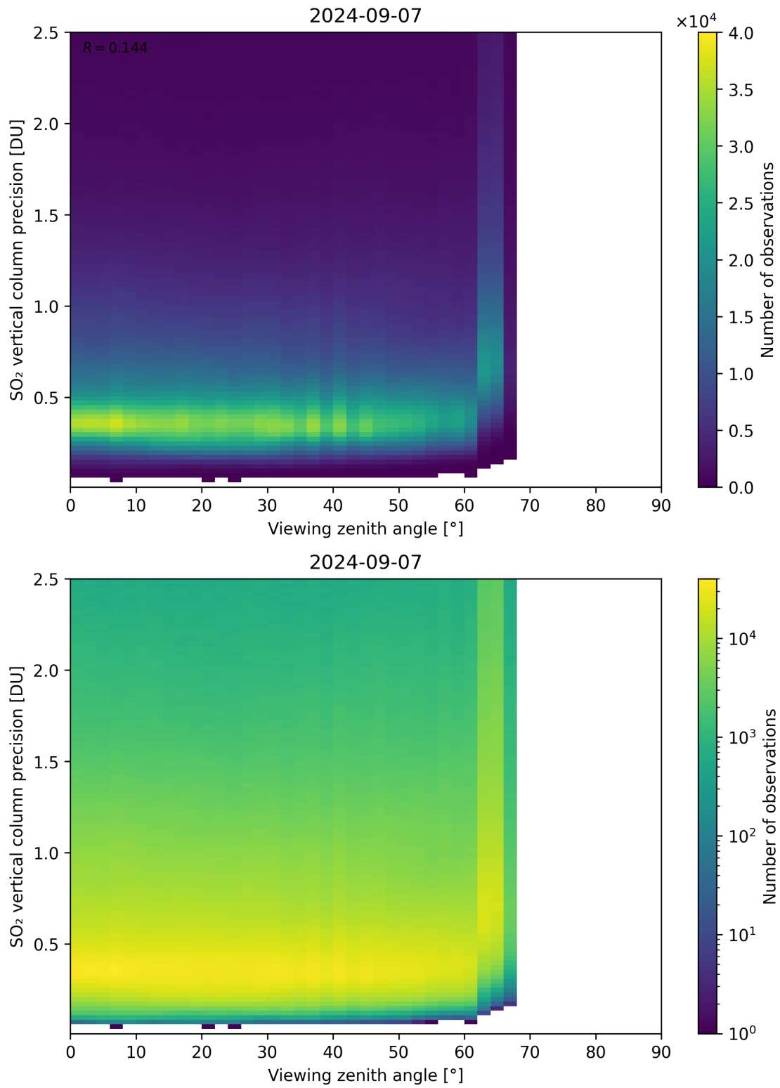
Figure 328: Scatter density plot of “Viewing zenith angle” against “SO 2 vertical column precision” for 2024-09-06 to 2024-09-08.
