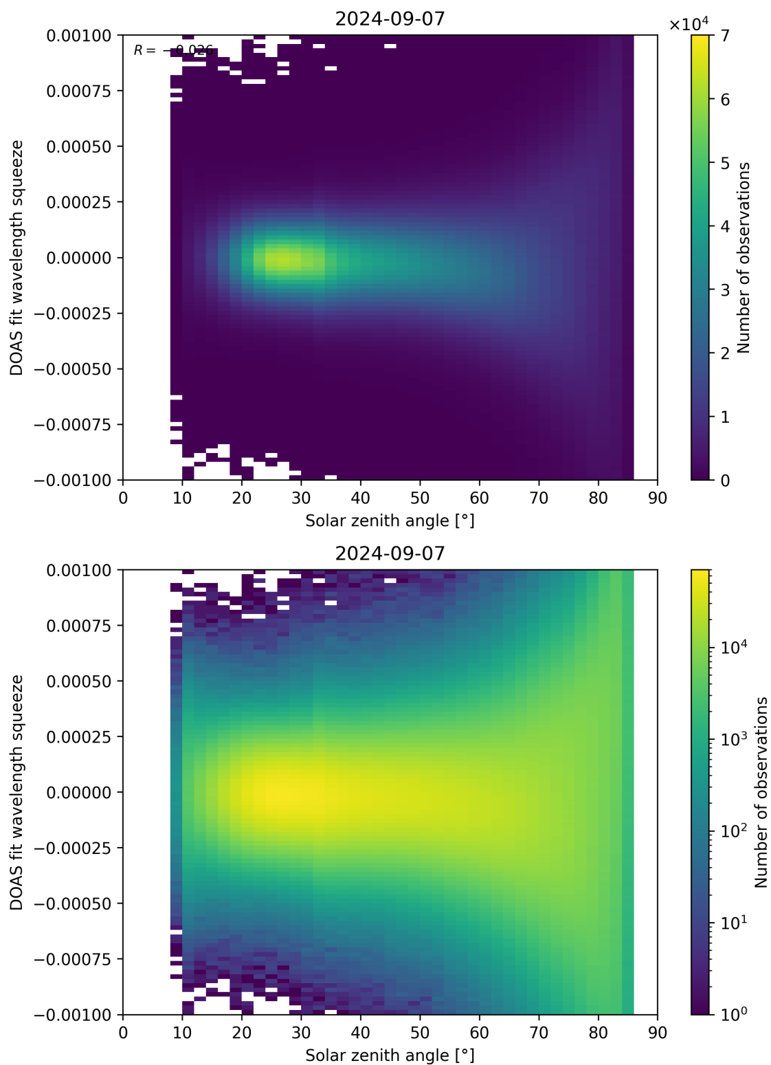
Figure 162: Scatter density plot of “Solar zenith angle” against “DOAS fit wavelength squeeze” for 2024-09-06 to 2024-09-08.
