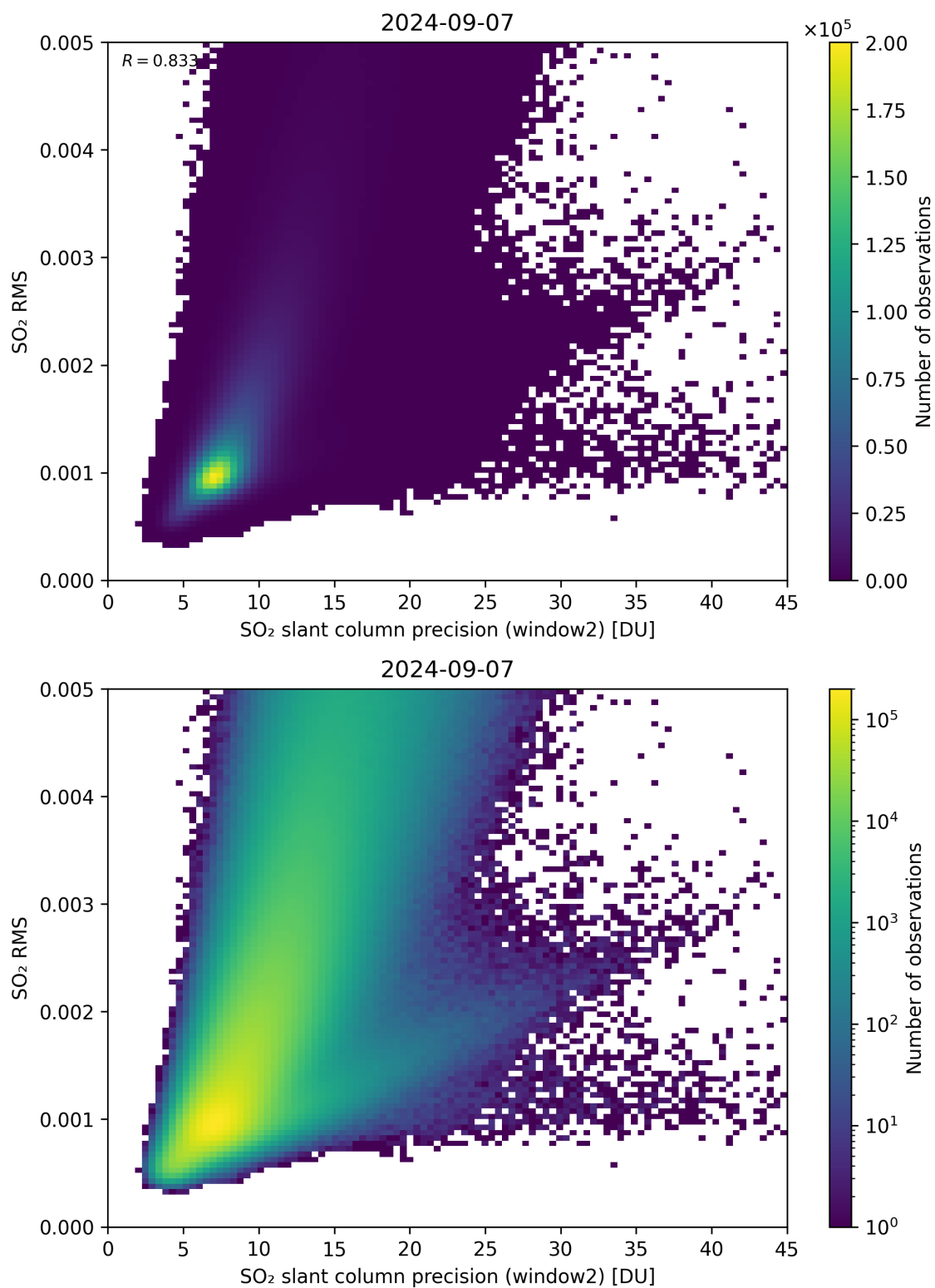
Figure 245: Scatter density plot of “SO 2 slant column precision (window2)” against “SO 2 RMS” for 2024-09-06 to 2024-09-08.
