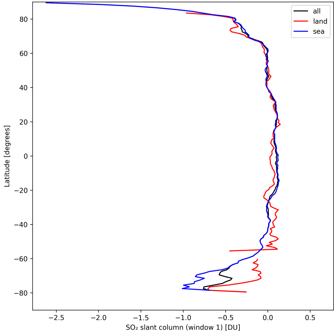
Figure 33: Zonal average of “SO 2 slant column (window 1)” for 2024-09-06 to 2024-09-08.
