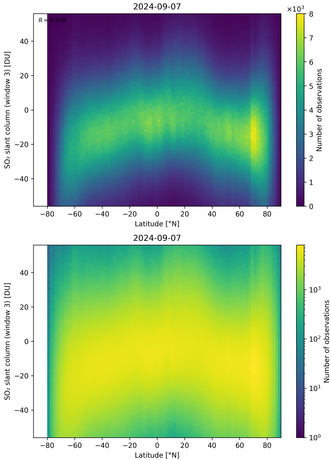
Figure 152: Scatter density plot of “Latitude” against “SO 2 slant column (window 3)” for 2024-09-06 to 2024-09-08.
