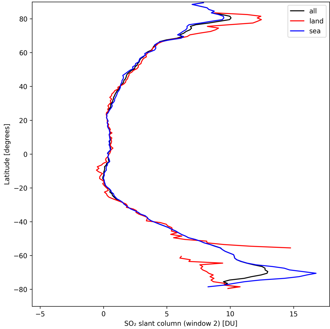
Figure 37: Zonal average of “SO 2 slant column (window 2)” for 2024-09-06 to 2024-09-08.
