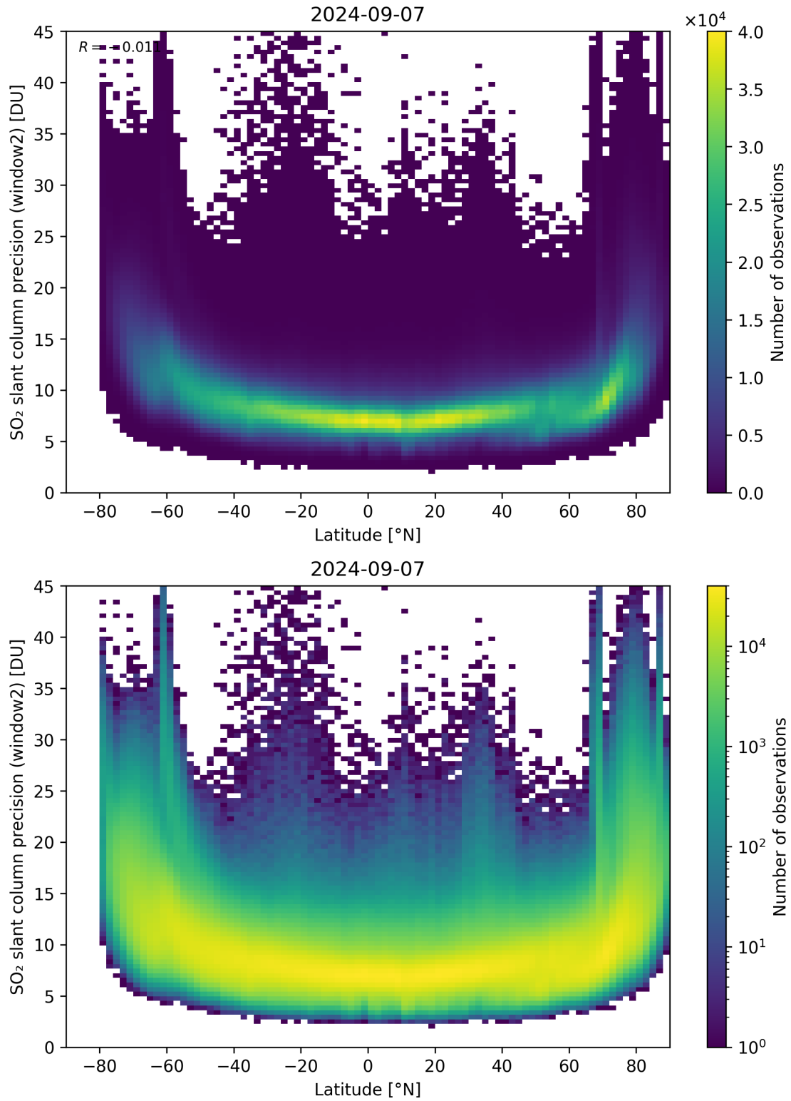
Figure 151: Scatter density plot of “Latitude” against “SO 2 slant column precision (window2)” for 2024-09-06 to 2024-09-08.
