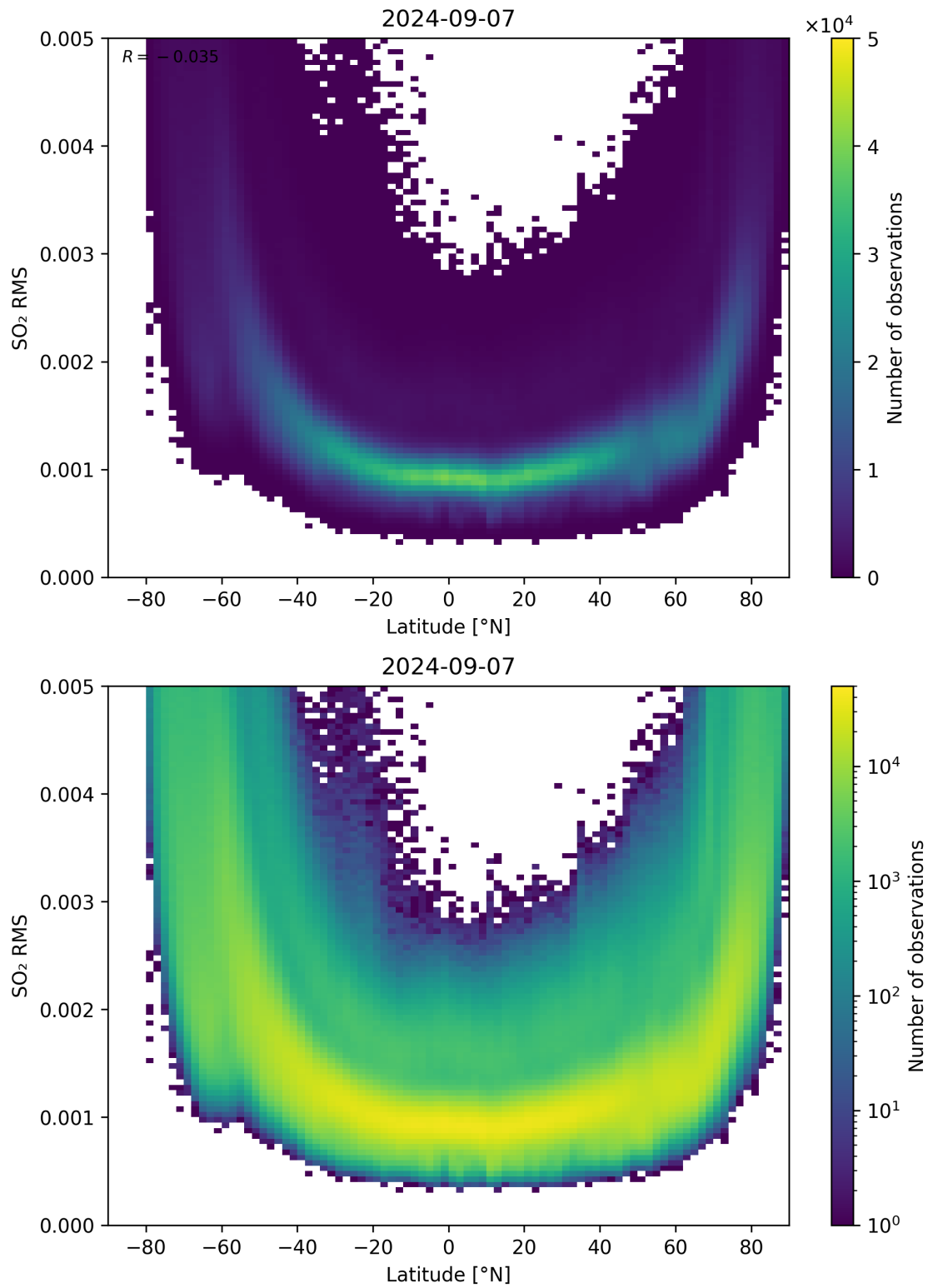
Figure 144: Scatter density plot of “Latitude” against “SO 2 RMS” for 2024-09-06 to 2024-09-08.
