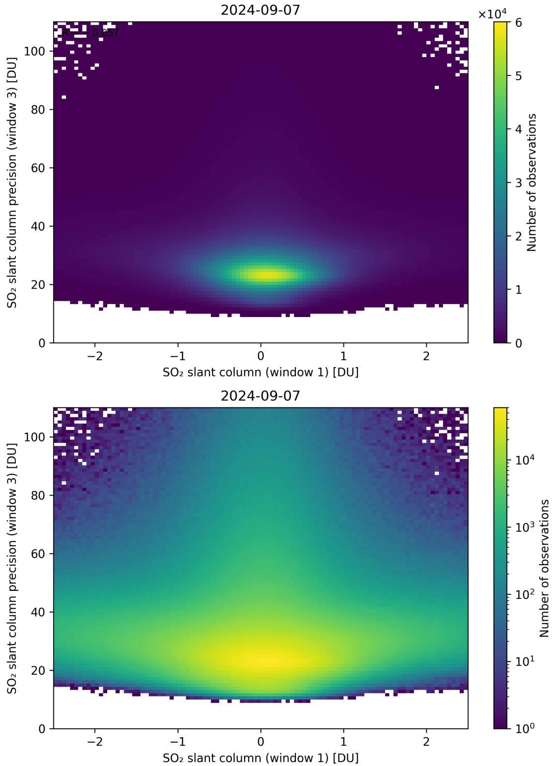
Figure 238: Scatter density plot of “SO 2 slant column (window 1)” against “SO 2 slant column precision (window 3)” for 2024-09-06 to 2024-09-08.
