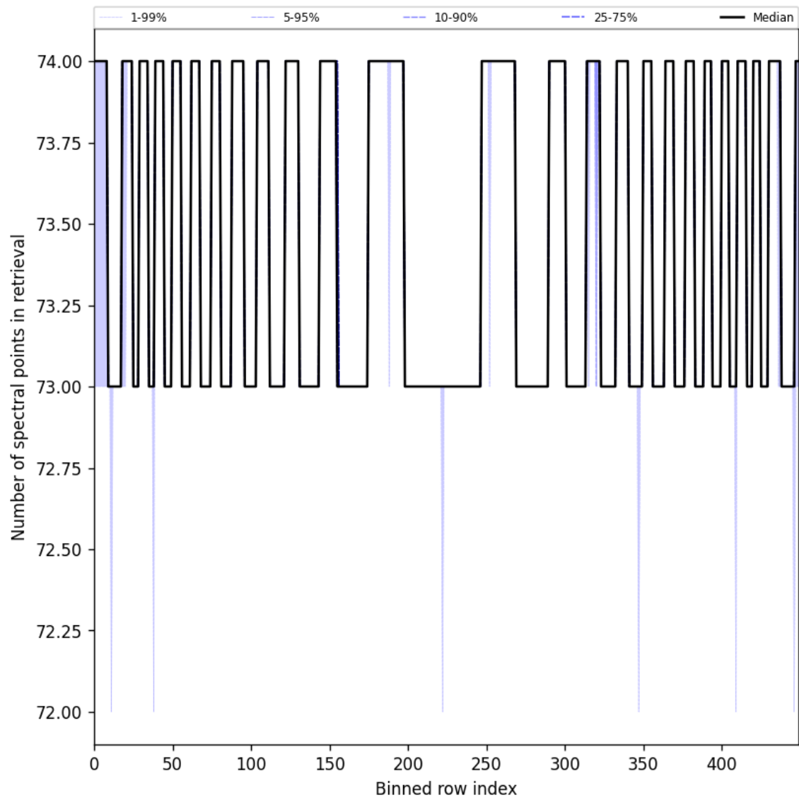
Figure 97: Along track statistics of “Number of spectral points in retrieval” for 2024-09-06 to 2024-09-08
