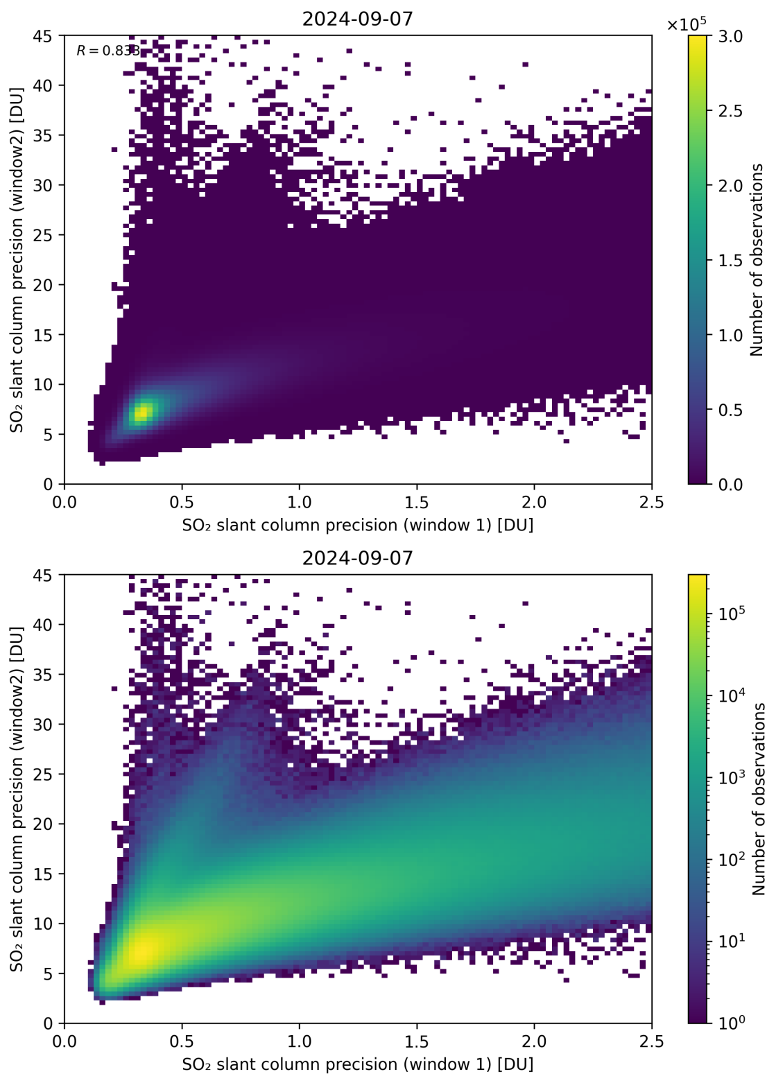
Figure 227: Scatter density plot of “SO 2 slant column precision (window 1)” against “SO 2 slant column precision (window 2)” for 2024-09-06 to 2024-09-08.
