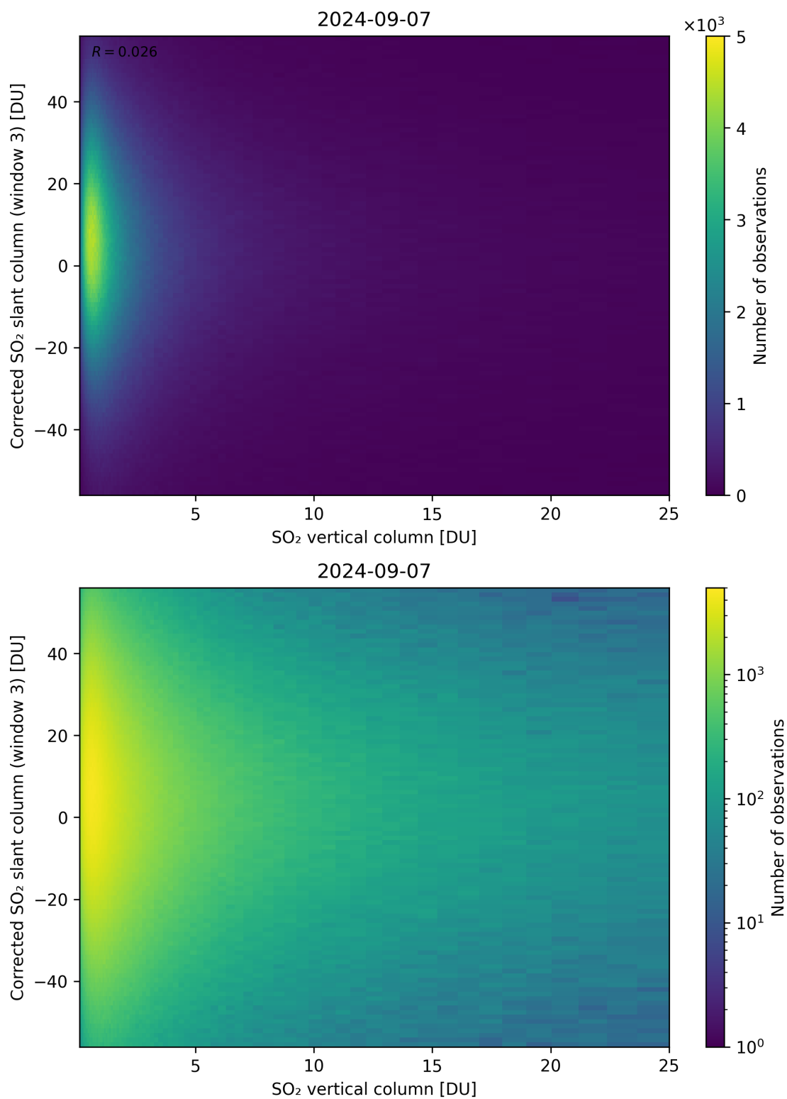
Figure 299: Scatter density plot of “SO 2 vertical column” against “Corrected SO 2 slant column (window 3)” for 2024-09-06 to 2024-09-08.
