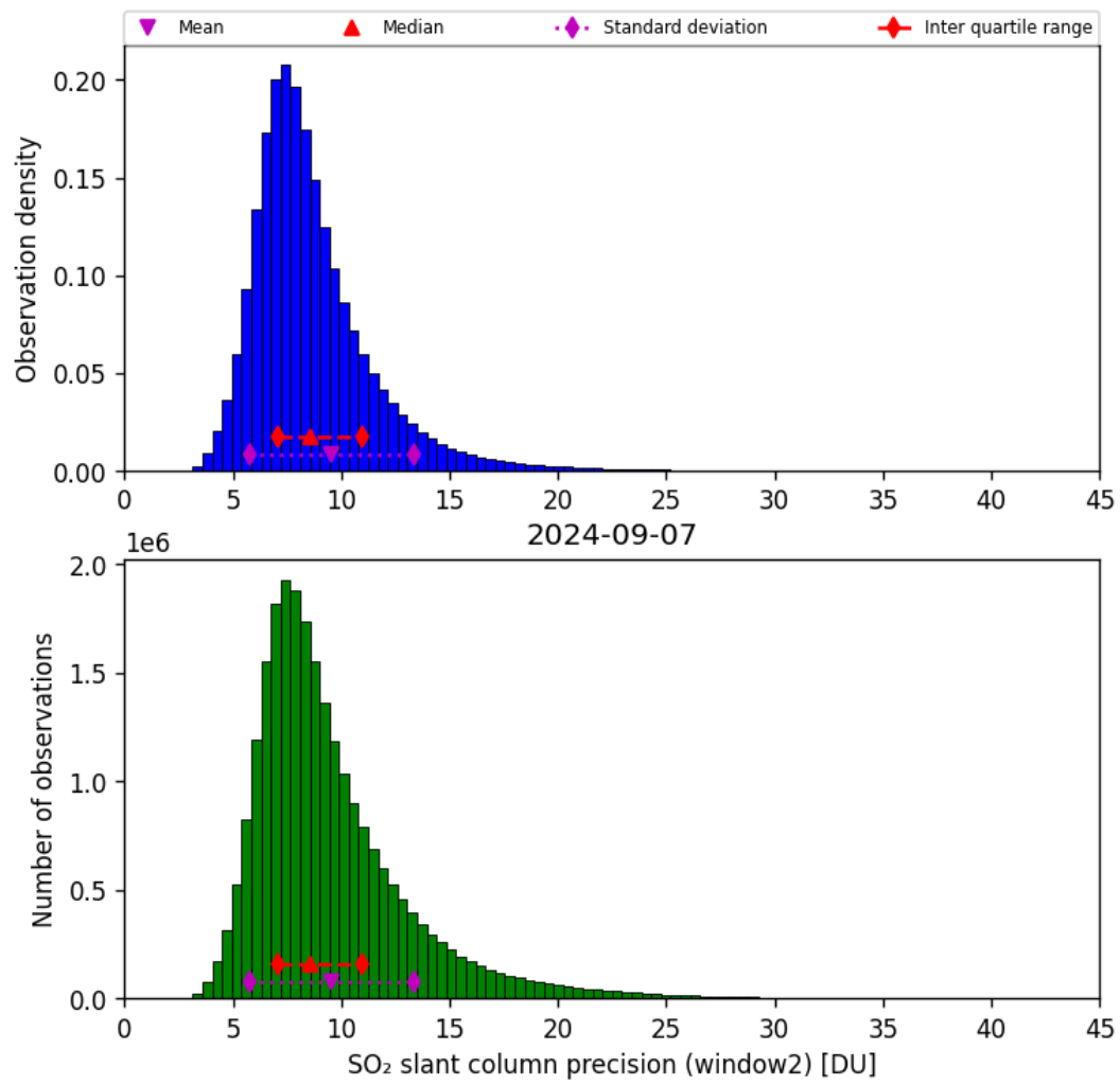
Figure 61: Histogram of “SO 2 slant column precision (window2)” for 2024-09-06 to 2024-09-08
