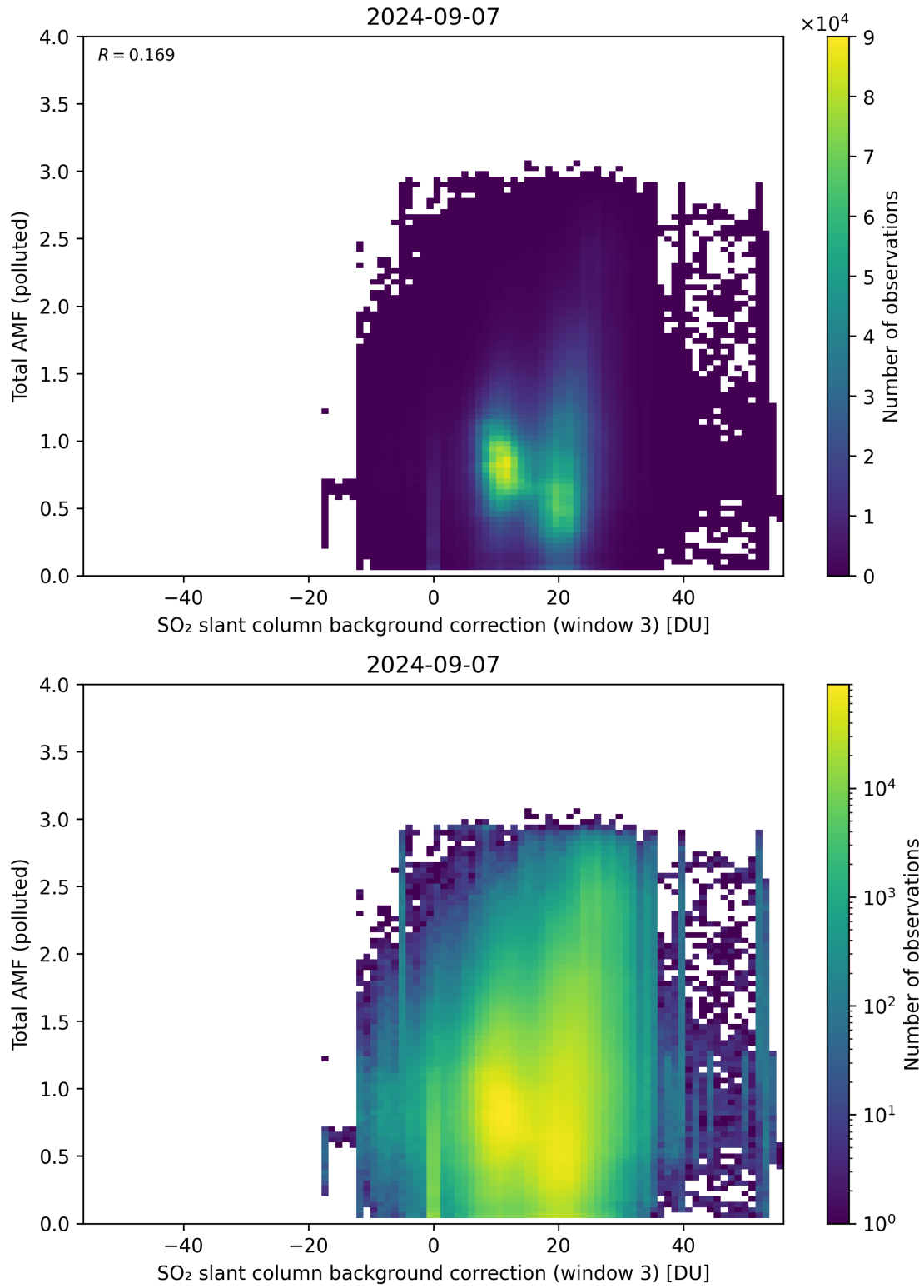
Figure 125: Scatter density plot of “SO 2 slant column background correction (window 3)” against “Total AMF (polluted)” for 2024-09-06 to 2024-09-08.
