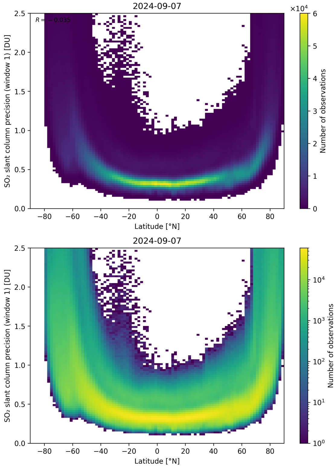
Figure 150: Scatter density plot of “Latitude” against “SO 2 slant column precision (window 1)” for 2024-09-06 to 2024-09-08.
