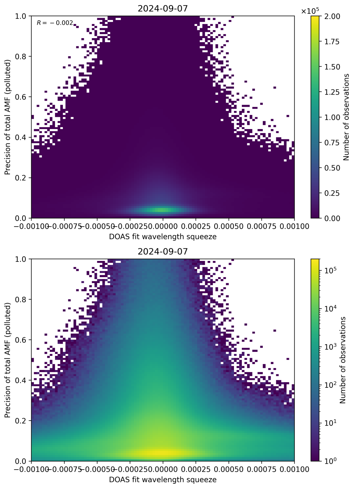
Figure 135: Scatter density plot of “DOAS fit wavelength squeeze” against “Precision of total AMF (polluted)” for 2024-09-06 to 2024-09-08.
