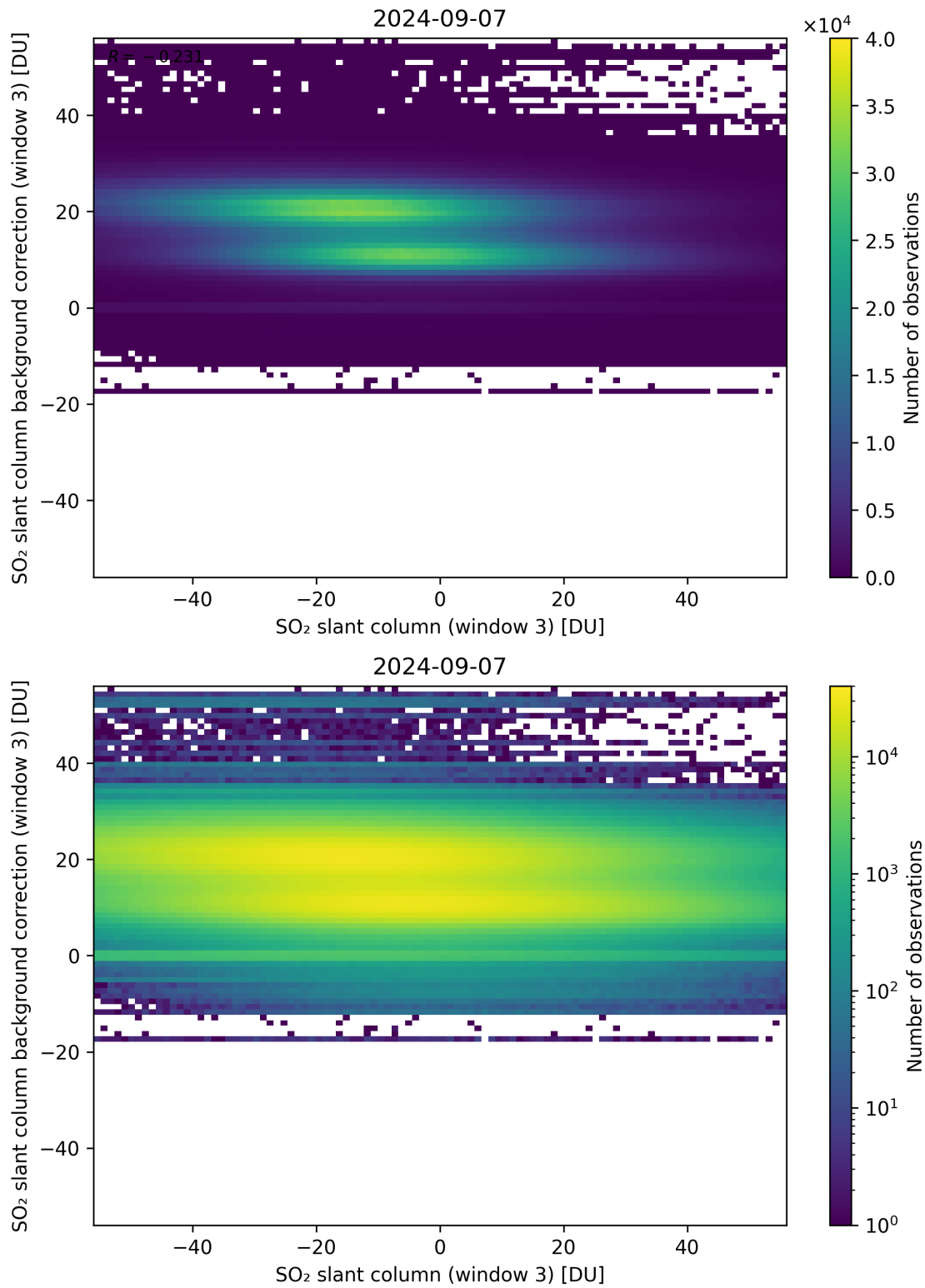
Figure 253: Scatter density plot of “SO 2 slant column (window 3)” against “SO 2 slant column background correction (window 3)” for 2024-09-06 to 2024-09-08.
