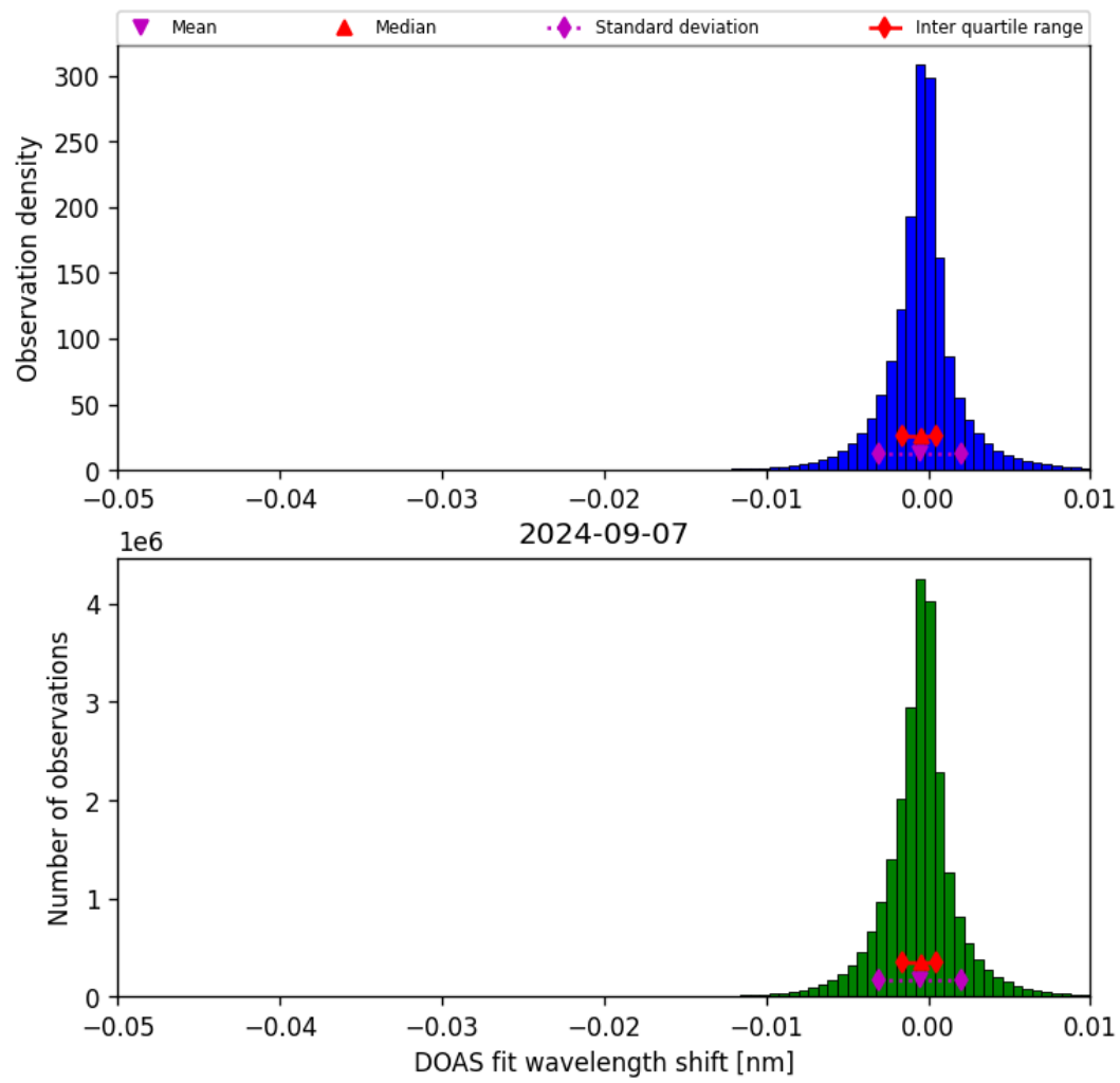
Figure 68: Histogram of “DOAS fit wavelength shift” for 2024-09-06 to 2024-09-08
