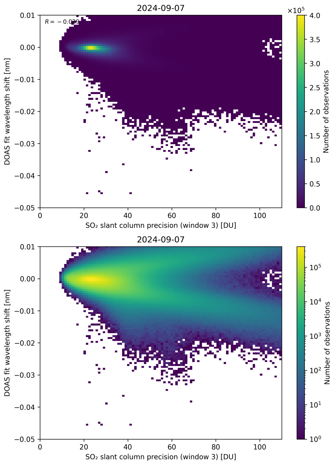
Figure 258: Scatter density plot of “SO 2 slant column precision (window 3)” against “DOAS fit wavelength shift” for 2024-09-06 to 2024-09-08.
