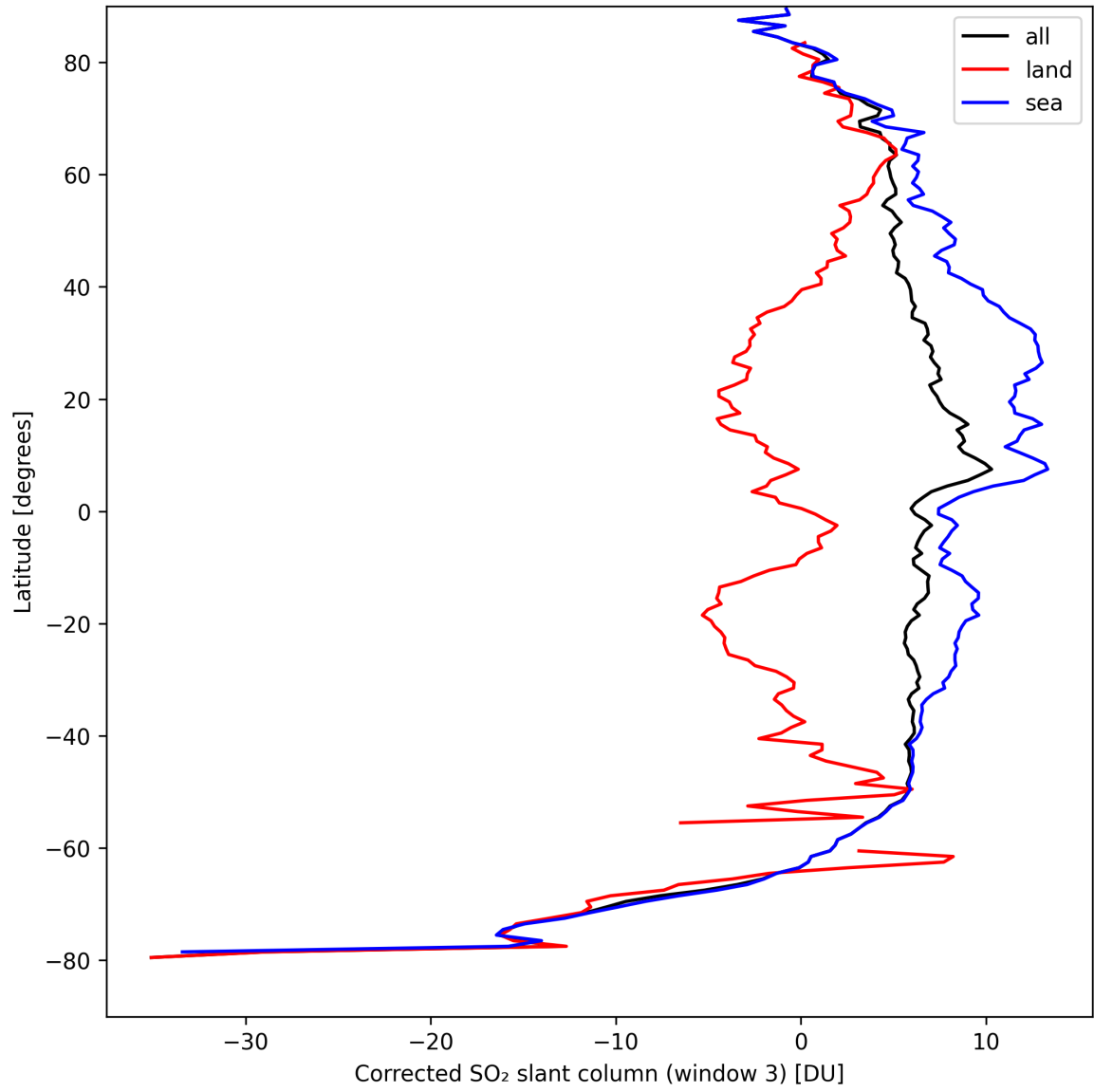
Figure 43: Zonal average of “Corrected SO 2 slant column (window 3)” for 2024-09-06 to 2024-09-08.
