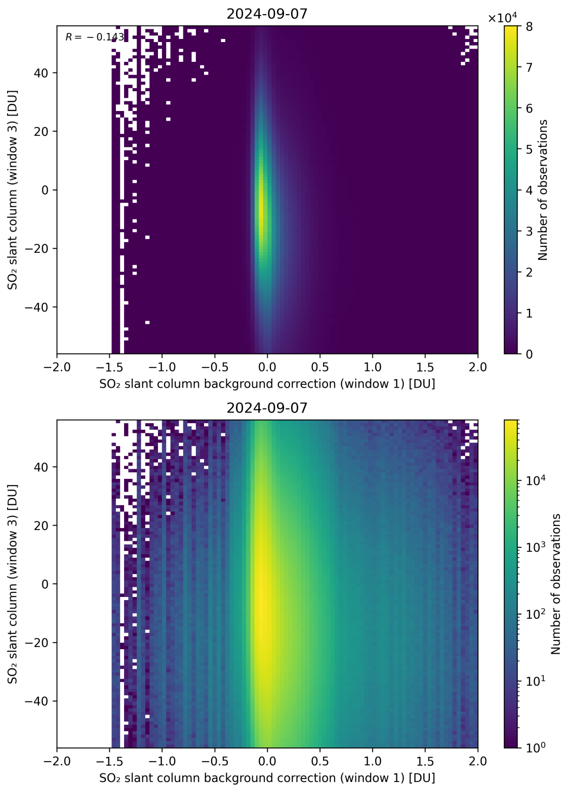
Figure 107: Scatter density plot of “SO 2 slant column background correction (window 1)” against “SO 2 slant column (window 3)” for 2024-09-06 to 2024-09-08.
