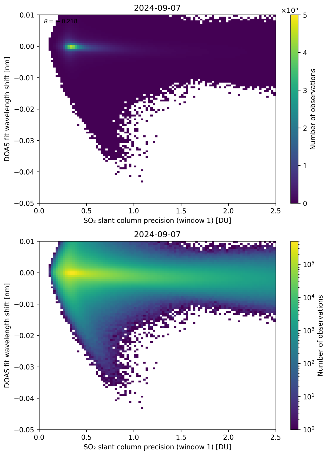
Figure 221: Scatter density plot of “SO 2 slant column precision (window 1)” against “DOAS fit wavelength shift” for 2024-09-06 to 2024-09-08.
