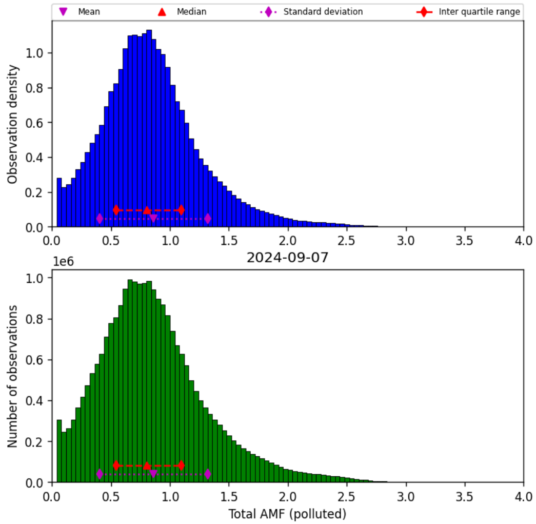
Figure 71: Histogram of “Total AMF (polluted)” for 2024-09-06 to 2024-09-08
