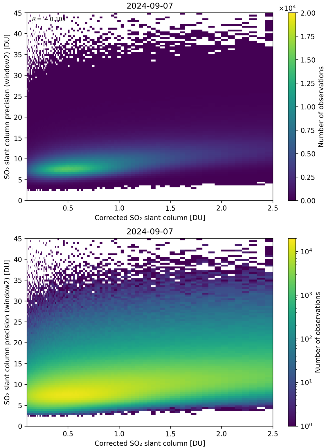
Figure 189: Scatter density plot of “Corrected SO 2 slant column” against “SO 2 slant column precision (window2)” for 2024-09-06 to 2024-09-08.
