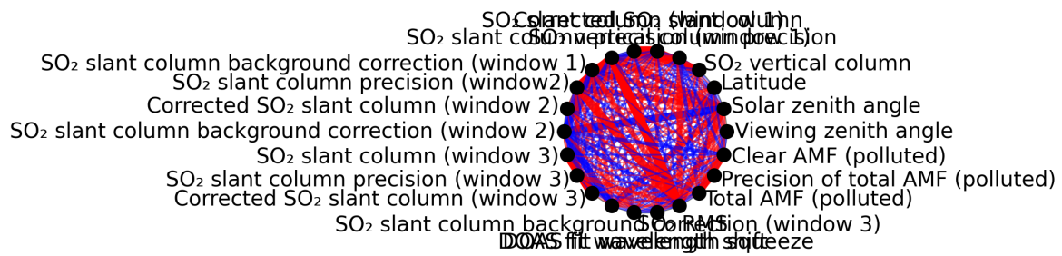
Figure 1: Map of correlation graph for 2024-09-06 to 2024-09-08.
