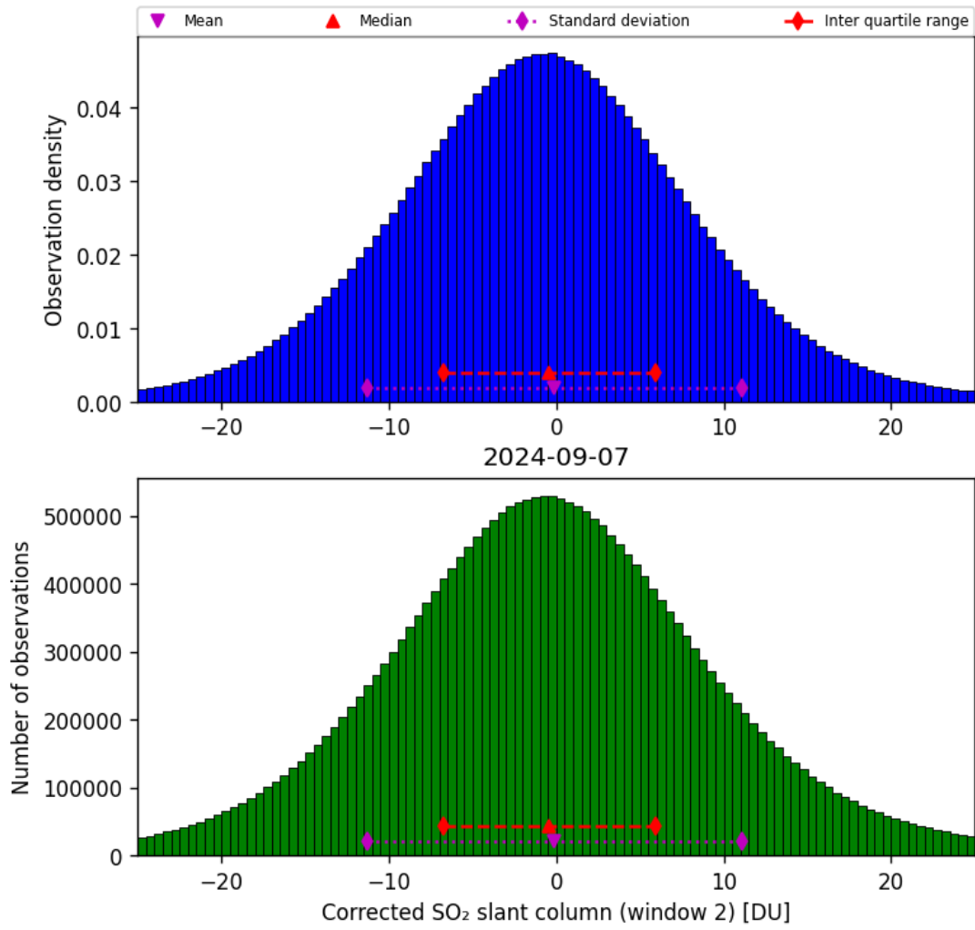
Figure 62: Histogram of “Corrected SO 2 slant column (window 2)” for 2024-09-06 to 2024-09-08
