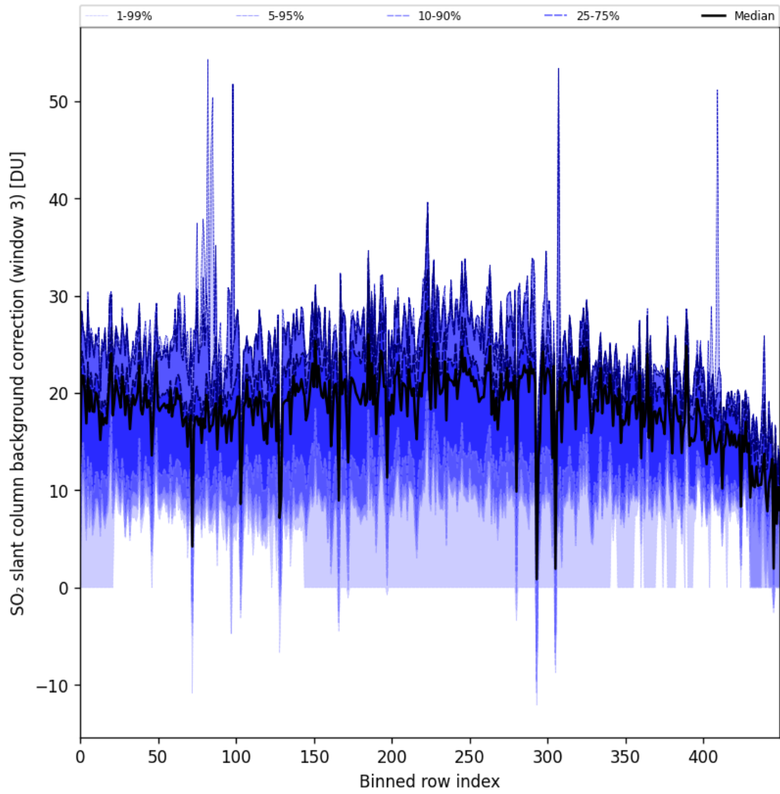
Figure 90: Along track statistics of “SO 2 slant column background correction (window 3)” for 2024-09-06 to 2024-09-08
