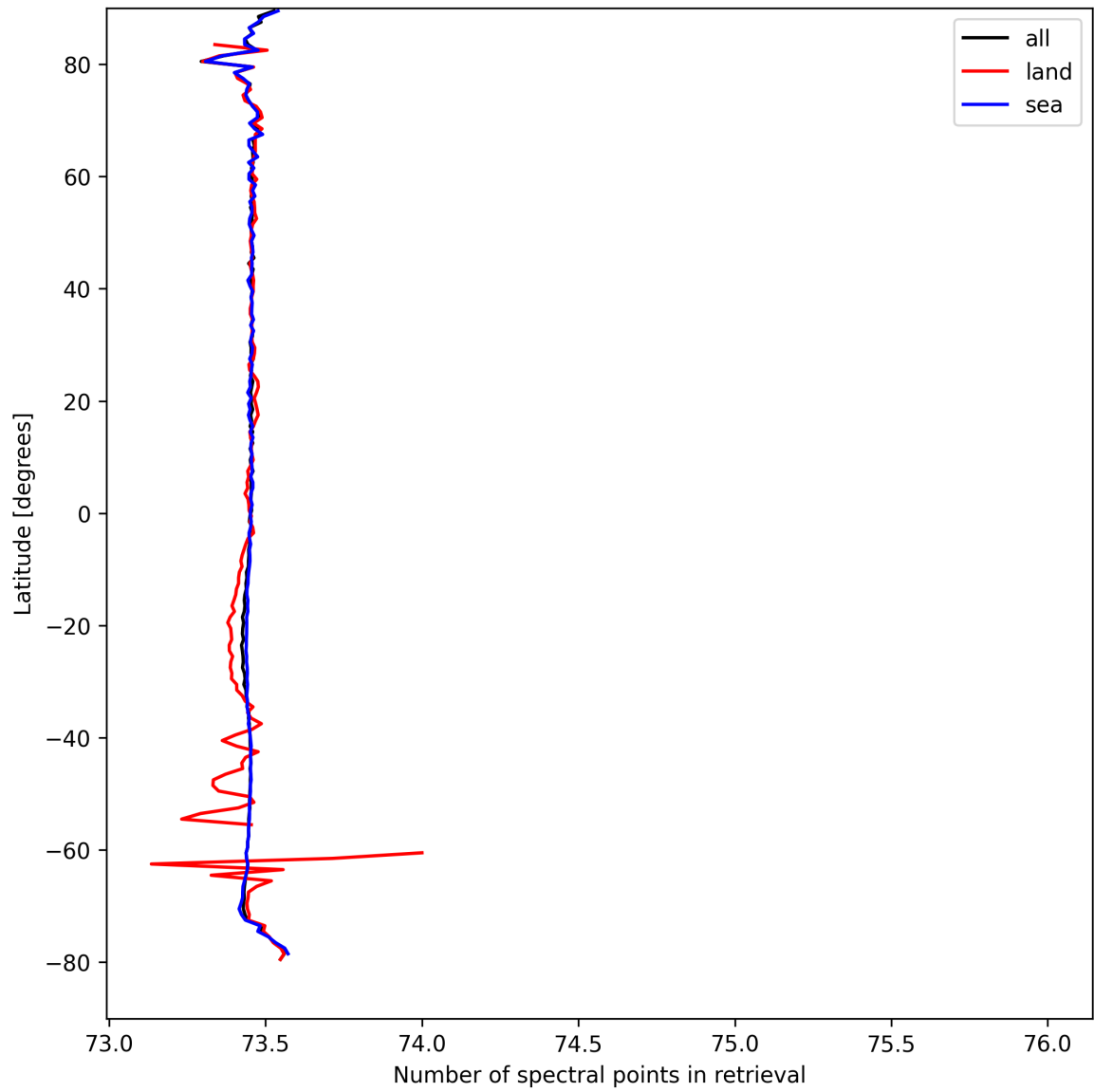
Figure 51: Zonal average of “Number of spectral points in retrieval” for 2024-09-06 to 2024-09-08.
