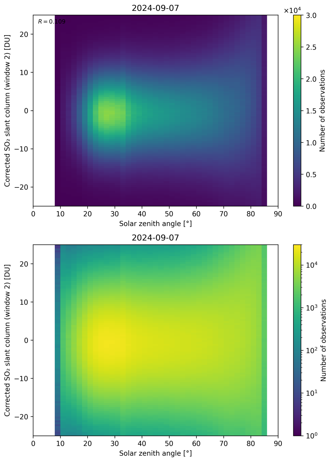
Figure 167: Scatter density plot of “Solar zenith angle” against “Corrected SO 2 slant column (window 2)” for 2024-09-06 to 2024-09-08.
