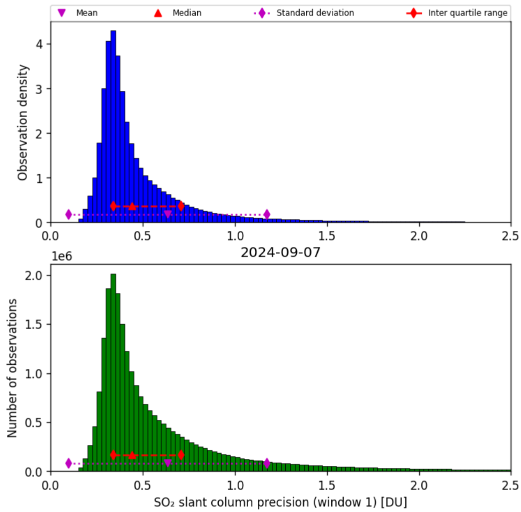
Figure 57: Histogram of “SO 2 slant column precision (window 1)” for 2024-09-06 to 2024-09-08
