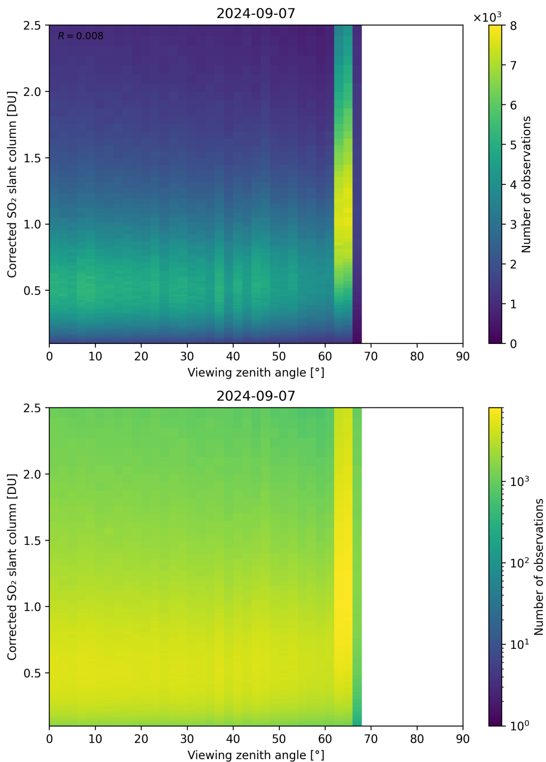
Figure 317: Scatter density plot of “Viewing zenith angle” against “Corrected SO 2 slant column” for 2024-09-06 to 2024-09-08.
