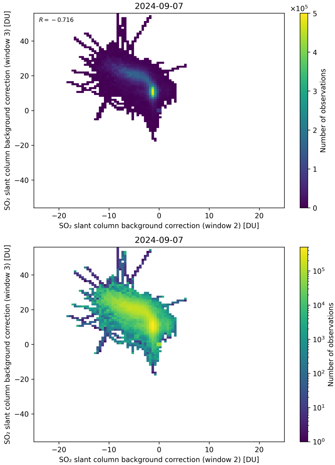
Figure 111: Scatter density plot of “SO 2 slant column background correction (window 2)” against “SO 2 slant column background correction (window 3)” for 2024-09-06 to 2024-09-08.
