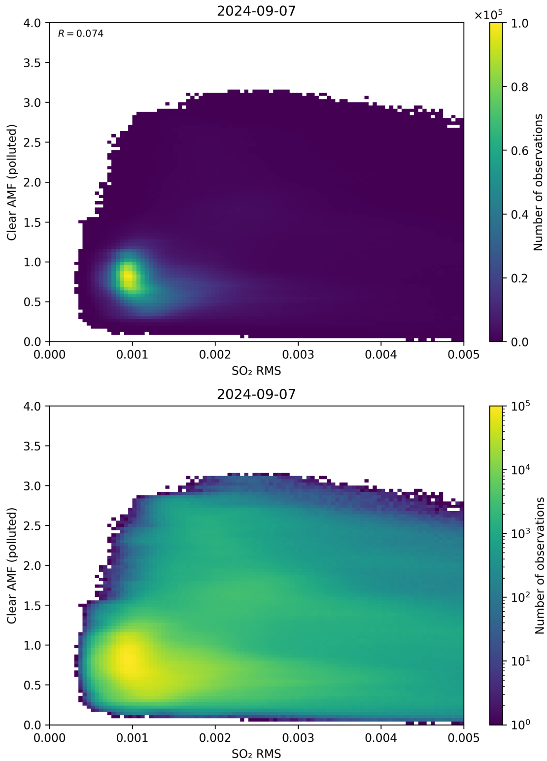
Figure 136: Scatter density plot of “SO 2 RMS” against “Clear AMF (polluted)” for 2024-09-06 to 2024-09-08.
