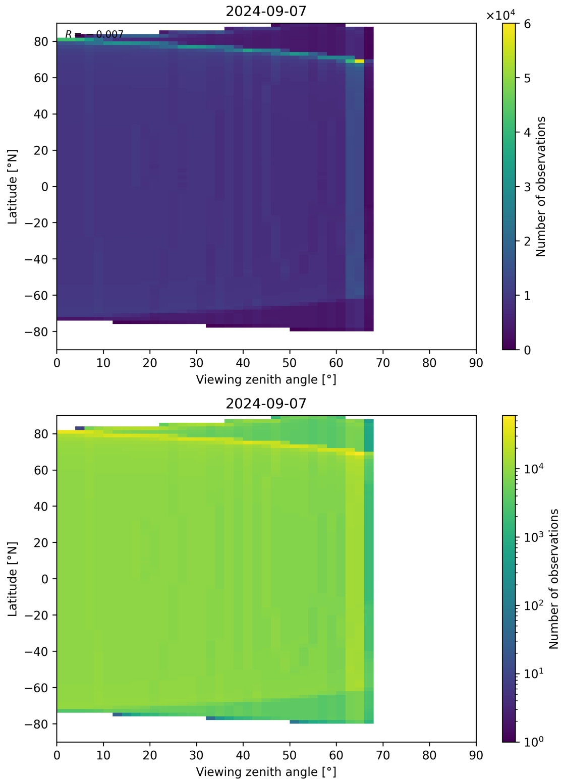
Figure 314: Scatter density plot of “Viewing zenith angle” against “Latitude” for 2024-09-06 to 2024-09-08.
