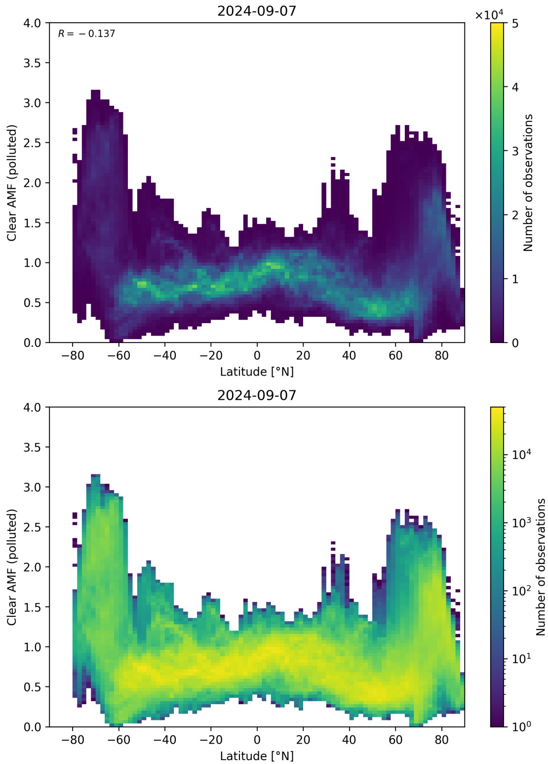
Figure 145: Scatter density plot of “Latitude” against “Clear AMF (polluted)” for 2024-09-06 to 2024-09-08.
