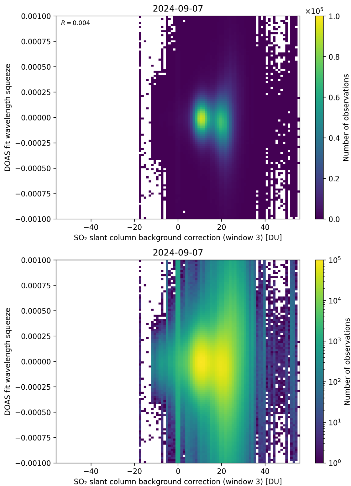
Figure 122: Scatter density plot of “SO 2 slant column background correction (window 3)” against “DOAS fit wavelength squeeze” for 2024-09-06 to 2024-09-08.
