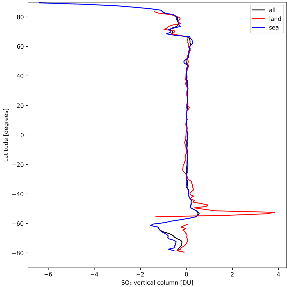
Figure 30: Zonal average of “SO 2 vertical column” for 2024-09-06 to 2024-09-08.
