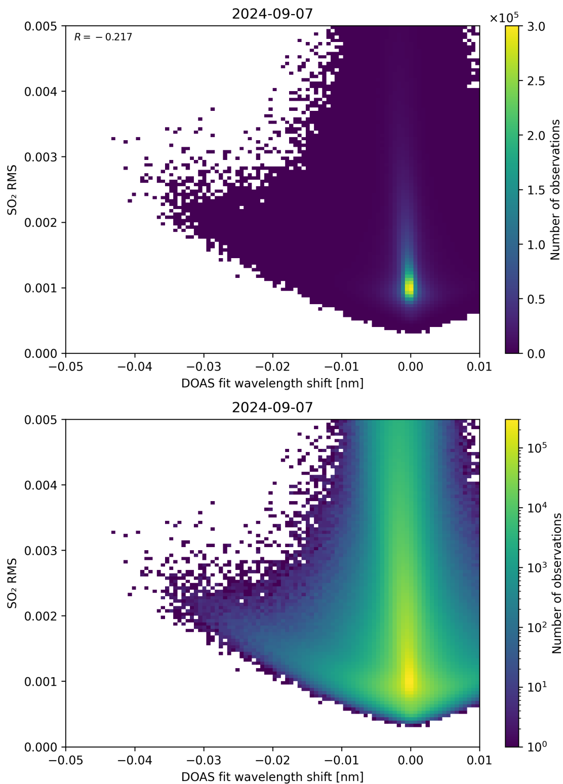
Figure 128: Scatter density plot of “DOAS fit wavelength shift” against “SO 2 RMS” for 2024-09-06 to 2024-09-08.
