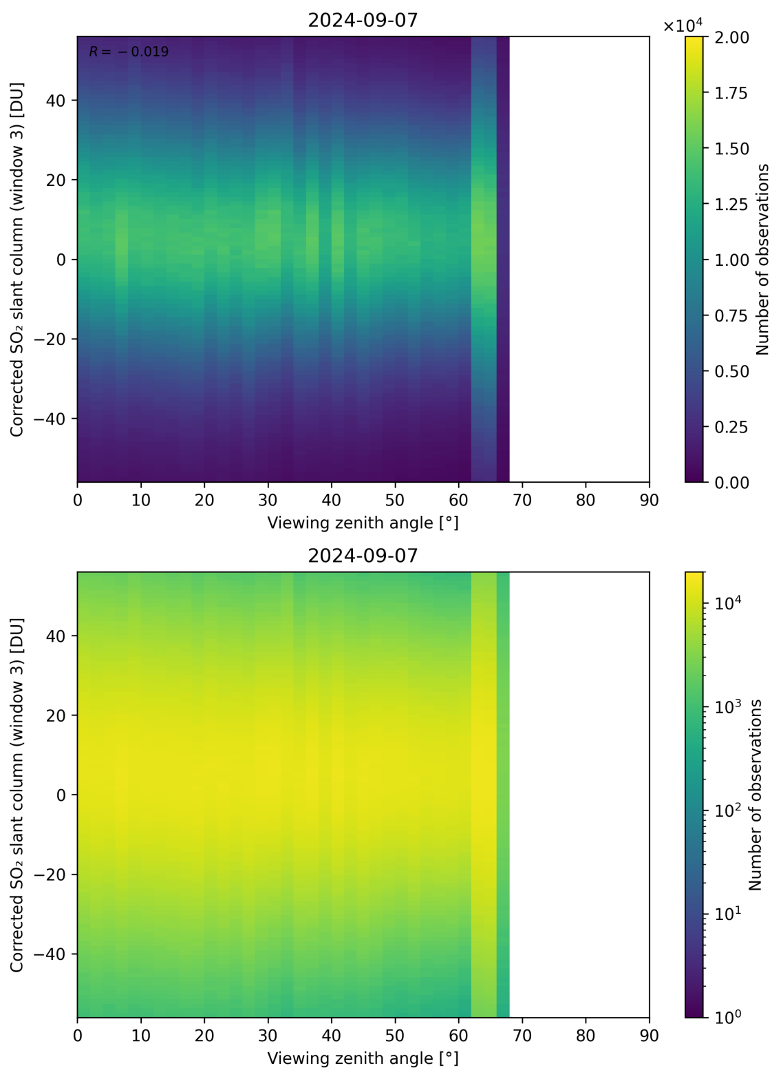
Figure 319: Scatter density plot of “Viewing zenith angle” against “Corrected SO 2 slant column (window 3)” for 2024-09-06 to 2024-09-08.
