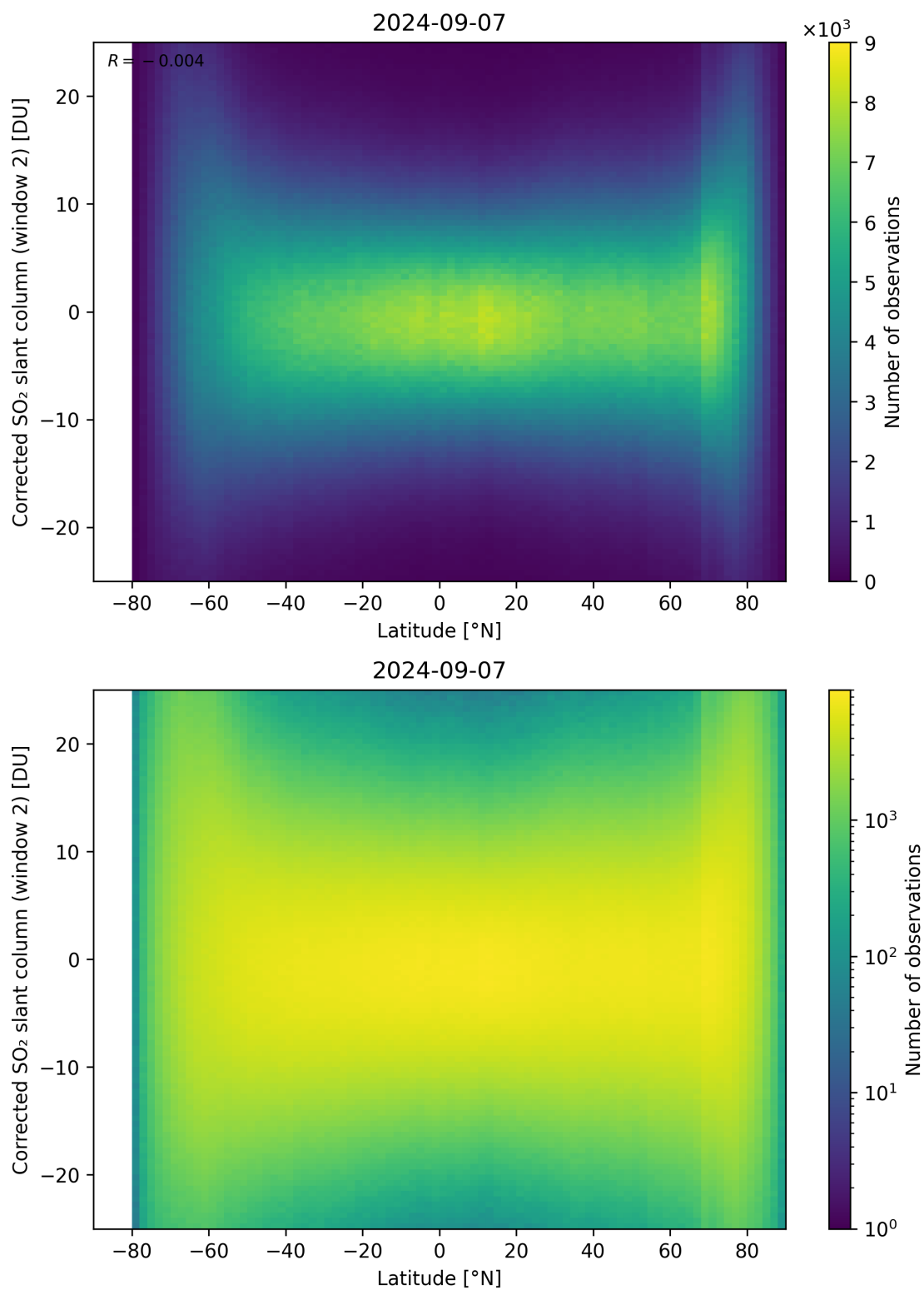
Figure 147: Scatter density plot of “Latitude” against “Corrected SO 2 slant column (window 2)” for 2024-09-06 to 2024-09-08.
