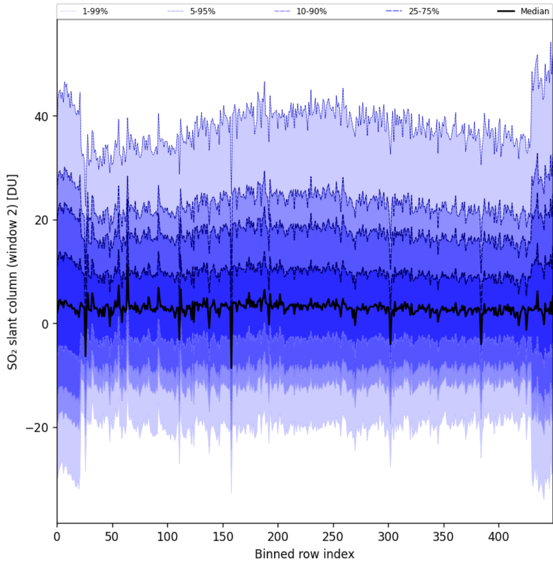
Figure 83: Along track statistics of “SO 2 slant column (window 2)” for 2024-09-06 to 2024-09-08
