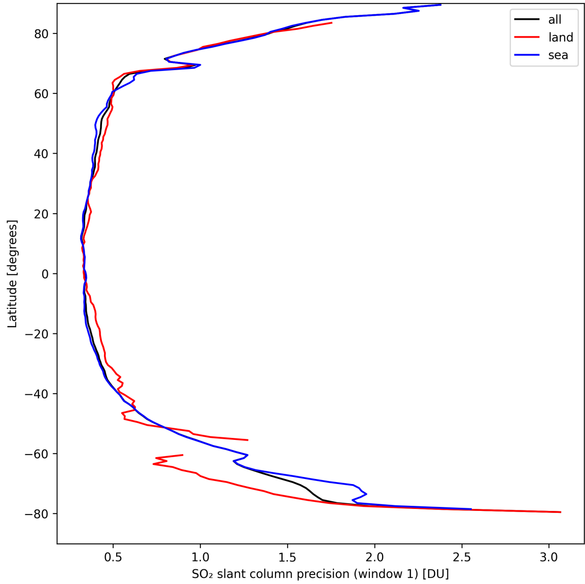
Figure 34: Zonal average of “SO 2 slant column precision (window 1)” for 2024-09-06 to 2024-09-08.
