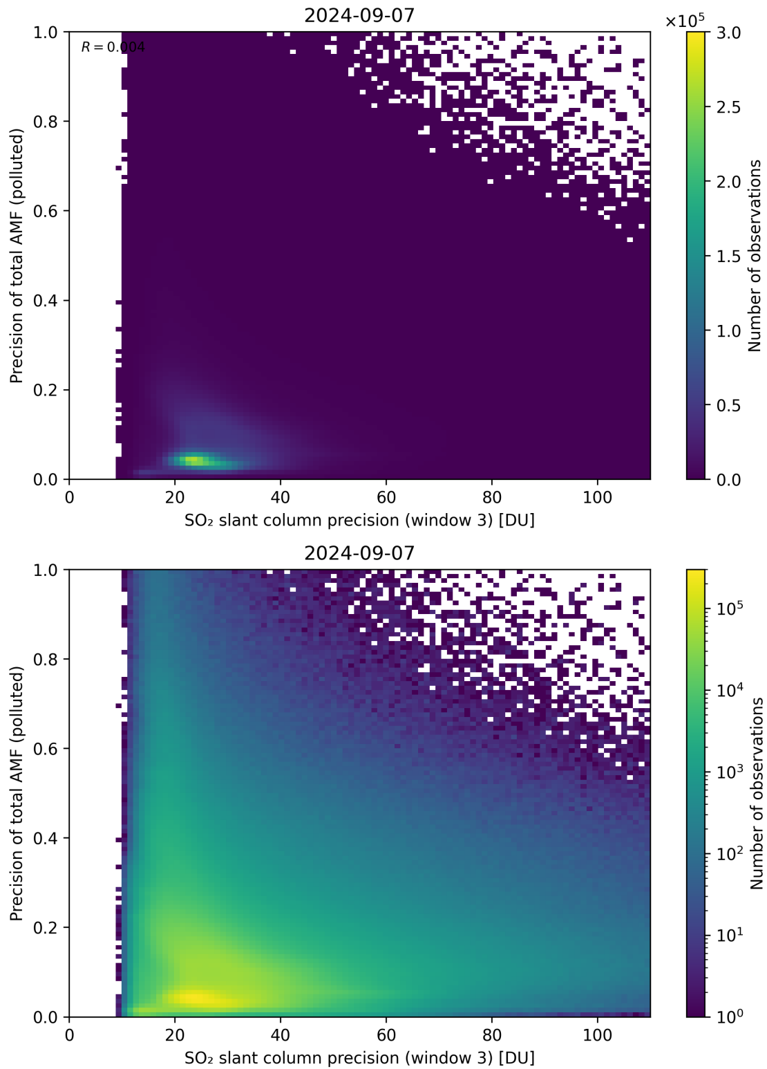
Figure 264: Scatter density plot of “SO 2 slant column precision (window 3)” against “Precision of total AMF (polluted)” for 2024-09-06 to 2024-09-08.
