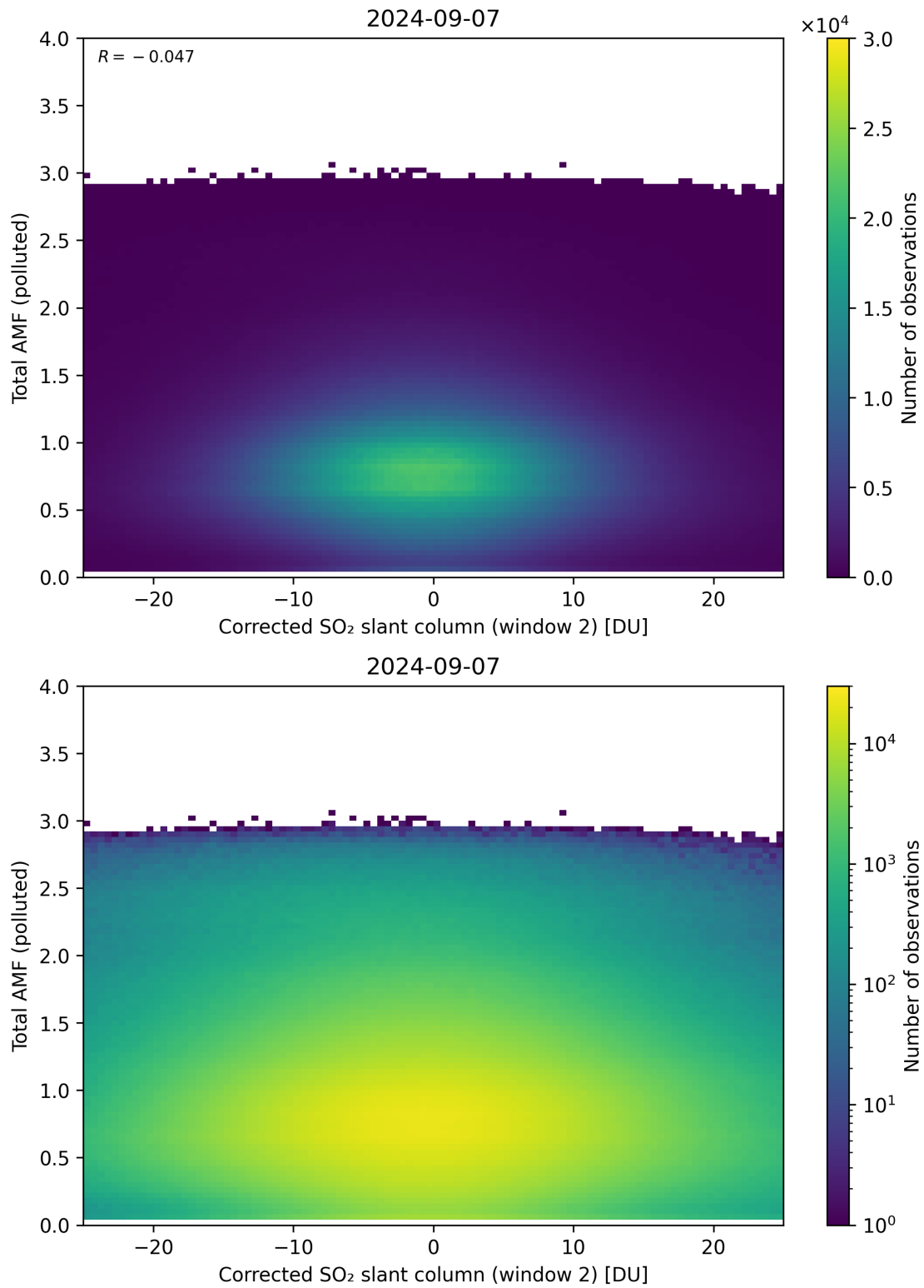
Figure 203: Scatter density plot of “Corrected SO 2 slant column (window 2)” against “Total AMF (polluted)” for 2024-09-06 to 2024-09-08.
