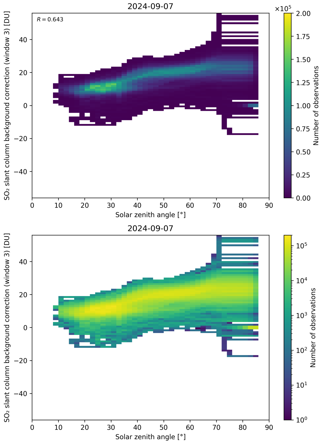
Figure 160: Scatter density plot of “Solar zenith angle” against “SO 2 slant column background correction (window 3)” for 2024-09-06 to 2024-09-08.
