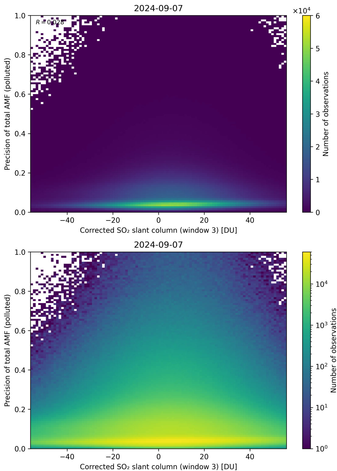
Figure 211: Scatter density plot of “Corrected SO 2 slant column (window 3)” against “Precision of total AMF (polluted)” for 2024-09-06 to 2024-09-08.
