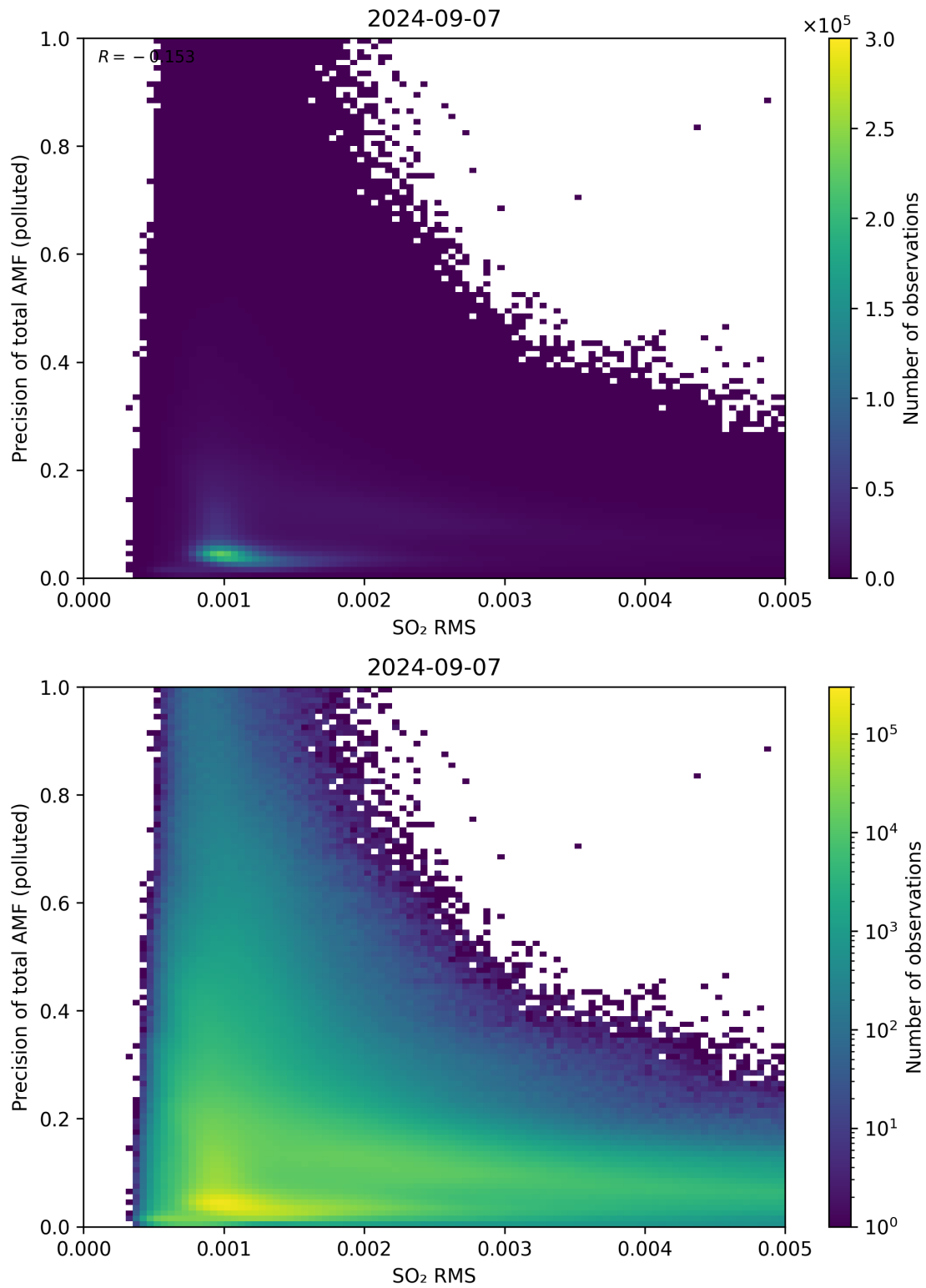
Figure 138: Scatter density plot of “SO 2 RMS” against “Precision of total AMF (polluted)” for 2024-09-06 to 2024-09-08.
