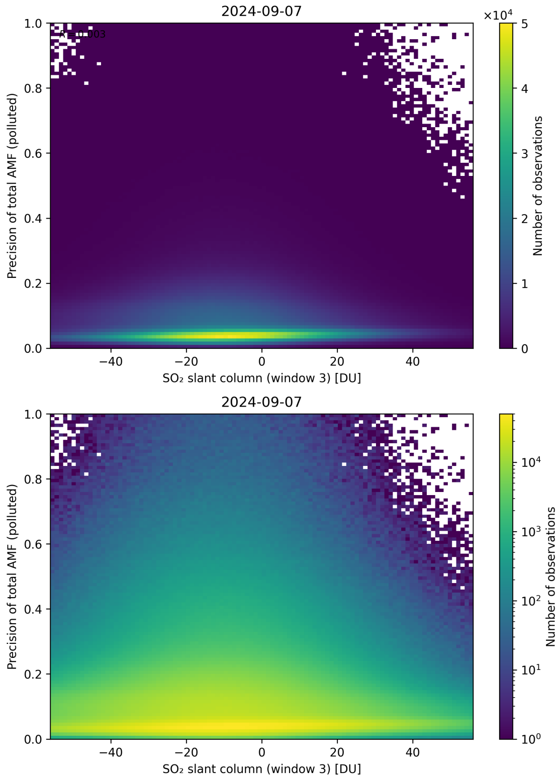
Figure 269: Scatter density plot of “SO 2 slant column (window 3)” against “Precision of total AMF (polluted)” for 2024-09-06 to 2024-09-08.
