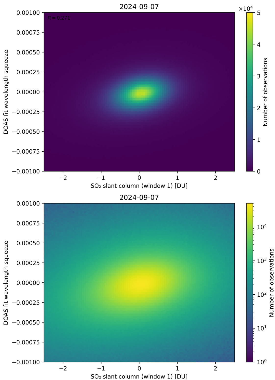
Figure 216: Scatter density plot of “SO 2 slant column (window 1)” against “DOAS fit wavelength squeeze” for 2024-09-06 to 2024-09-08.
