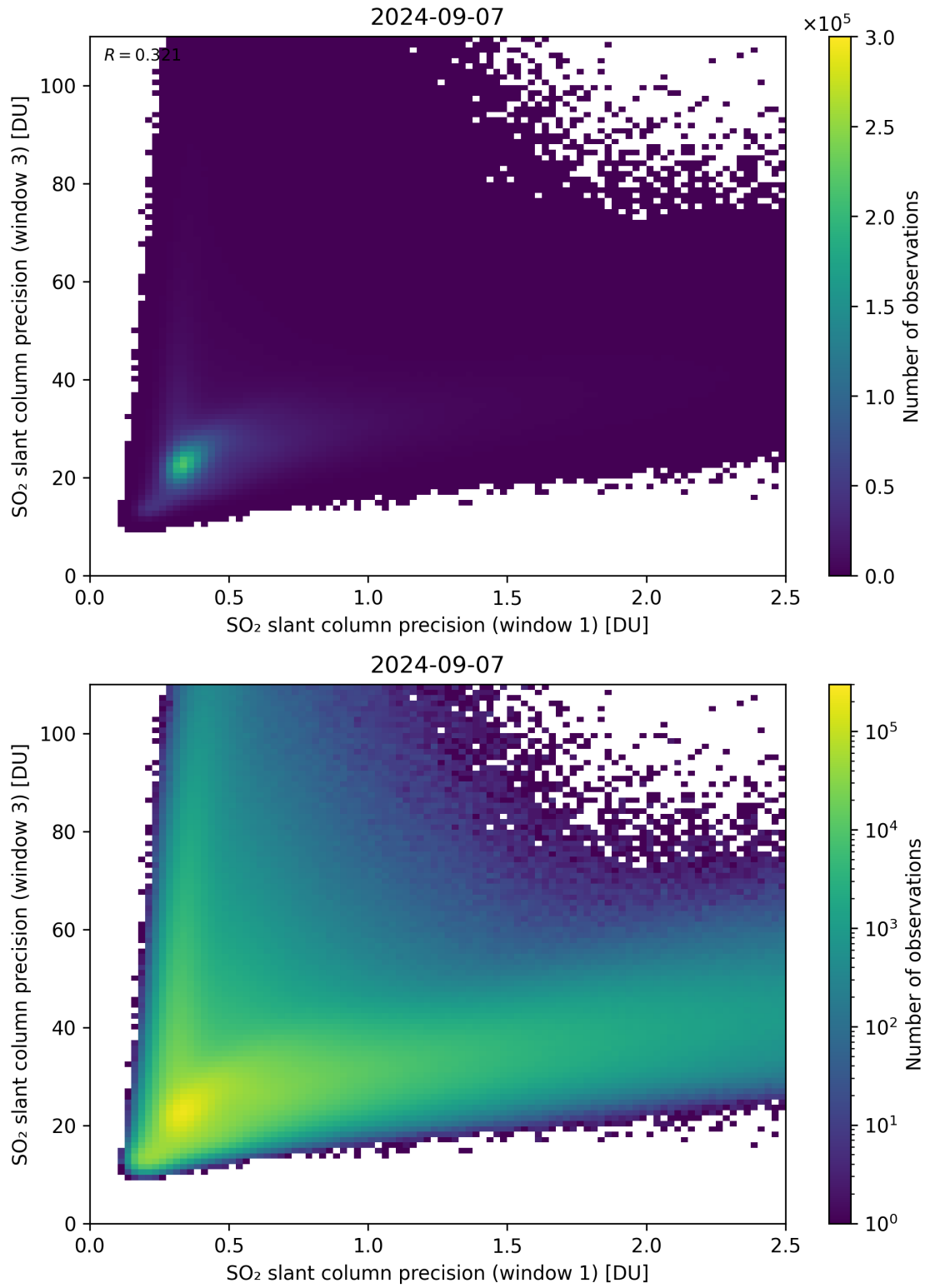
Figure 229: Scatter density plot of “SO 2 slant column precision (window 1)” against “SO 2 slant column precision (window 3)” for 2024-09-06 to 2024-09-08.
