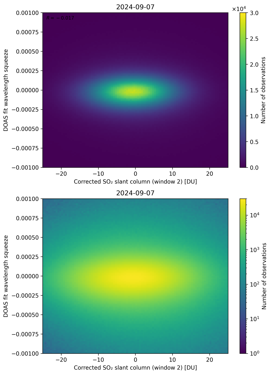
Figure 197: Scatter density plot of “Corrected SO 2 slant column (window 2)” against “DOAS fit wavelength squeeze” for 2024-09-06 to 2024-09-08.
