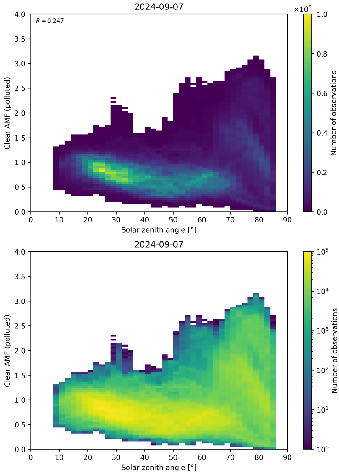
Figure 165: Scatter density plot of “Solar zenith angle” against “Clear AMF (polluted)” for 2024-09-06 to 2024-09-08.
