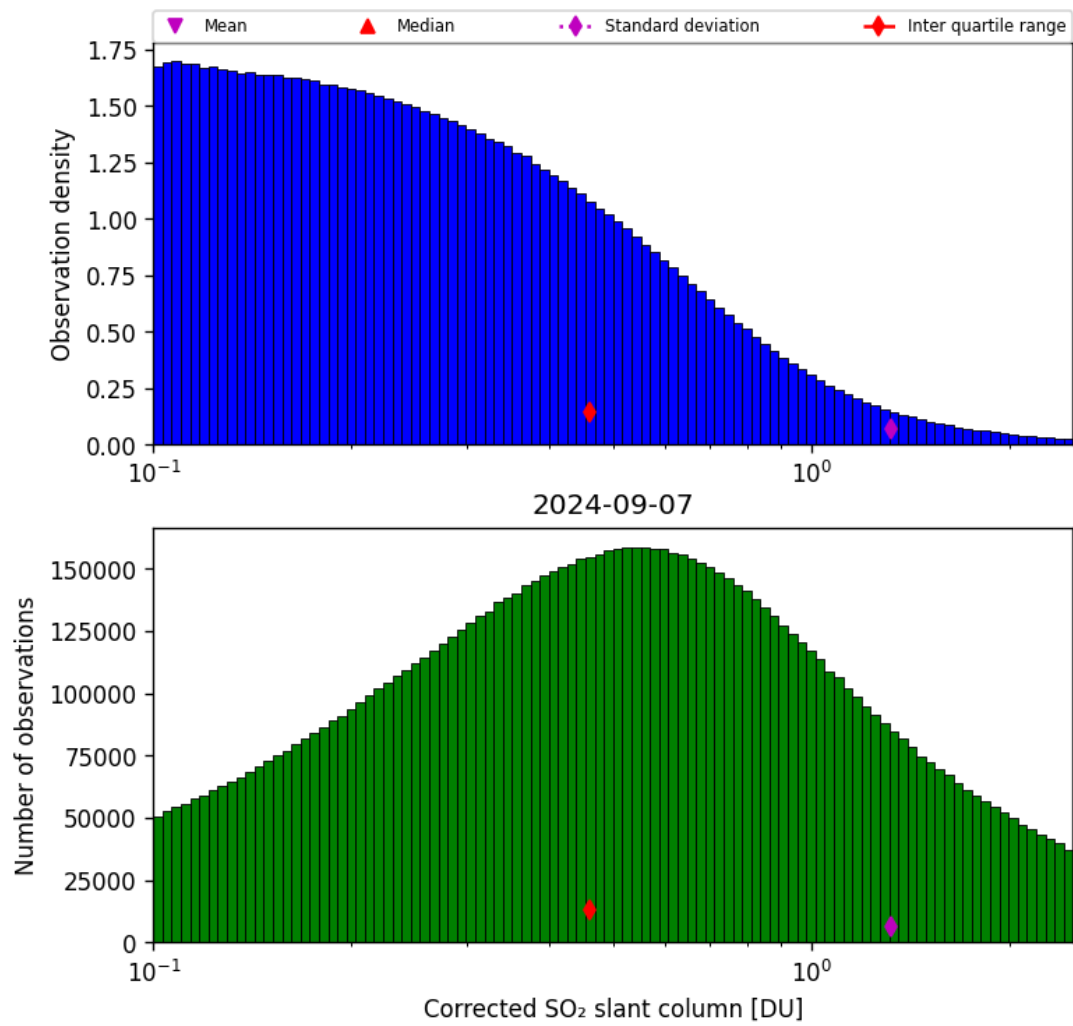
Figure 55: Histogram of “Corrected SO 2 slant column” for 2024-09-06 to 2024-09-08
