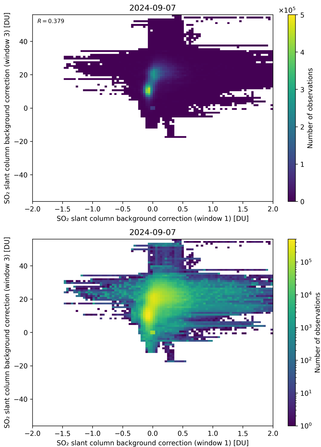
Figure 99: Scatter density plot of “SO 2 slant column background correction (window 1)” against “SO 2 slant column background correction (window 3)” for 2024-09-06 to 2024-09-08.
