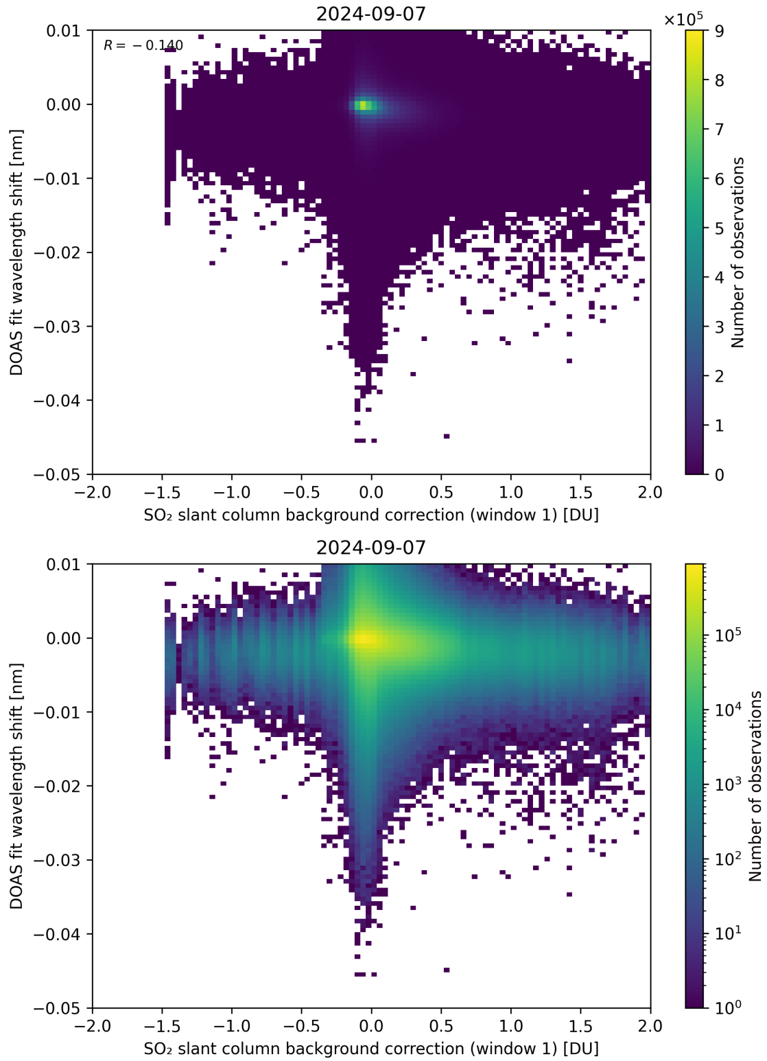
Figure 100: Scatter density plot of “SO 2 slant column background correction (window 1)” against “DOAS fit wavelength shift” for 2024-09-06 to 2024-09-08.
