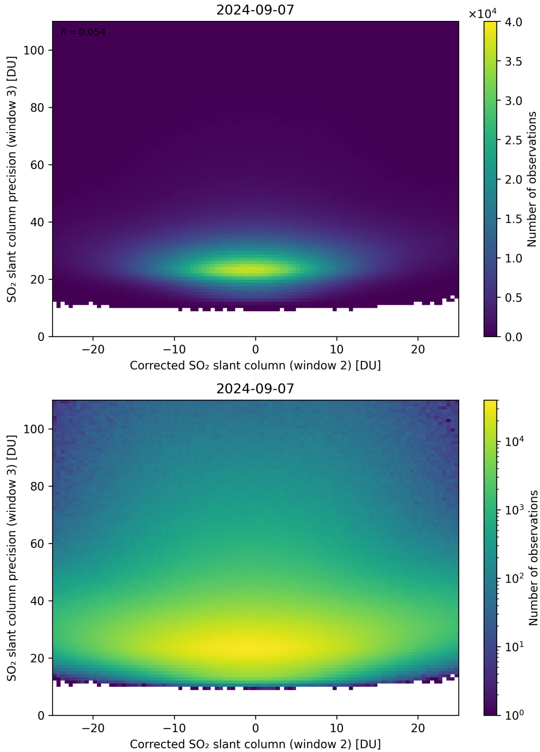
Figure 202: Scatter density plot of “Corrected SO 2 slant column (window 2)” against “SO 2 slant column precision (window 3)” for 2024-09-06 to 2024-09-08.
