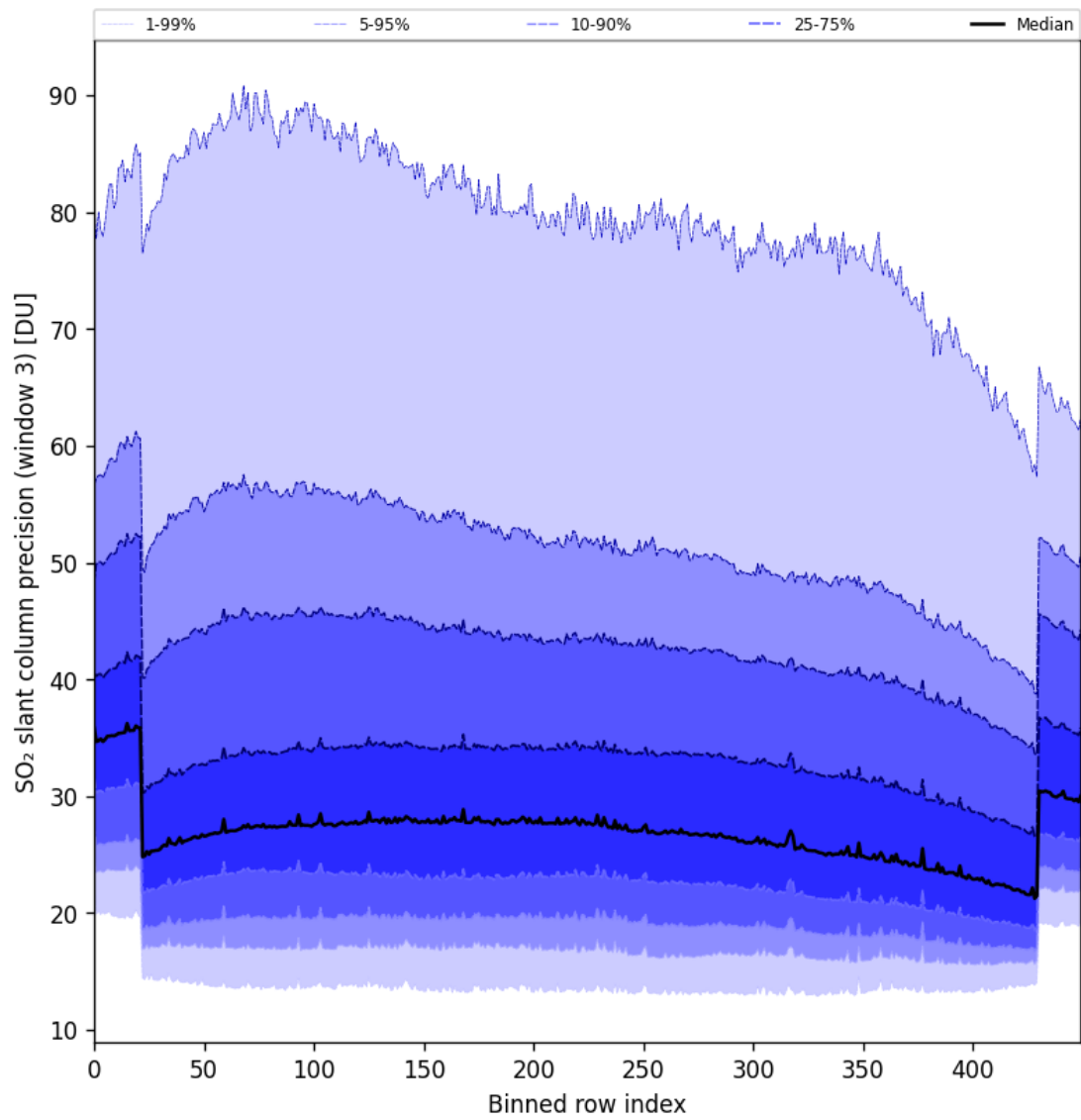
Figure 88: Along track statistics of “SO 2 slant column precision (window 3)” for 2024-09-06 to 2024-09-08
