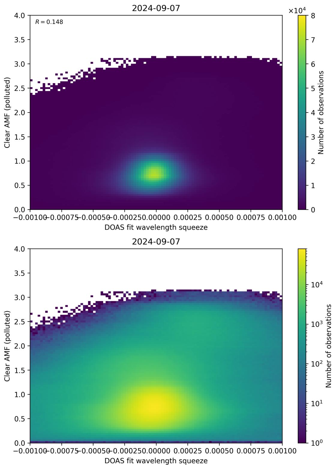
Figure 133: Scatter density plot of “DOAS fit wavelength squeeze” against “Clear AMF (polluted)” for 2024-09-06 to 2024-09-08.
