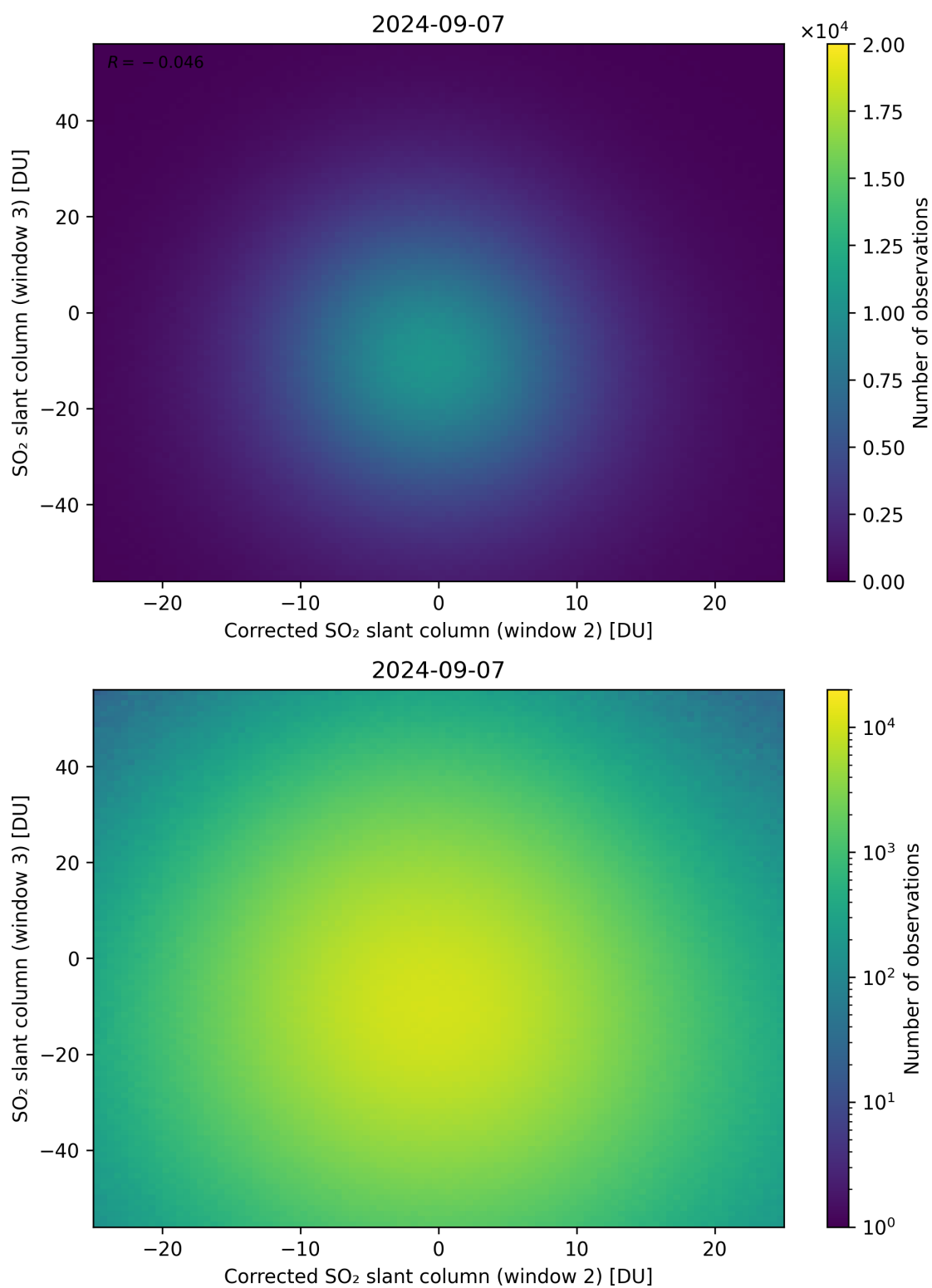
Figure 201: Scatter density plot of “Corrected SO 2 slant column (window 2)” against “SO 2 slant column (window 3)” for 2024-09-06 to 2024-09-08.
