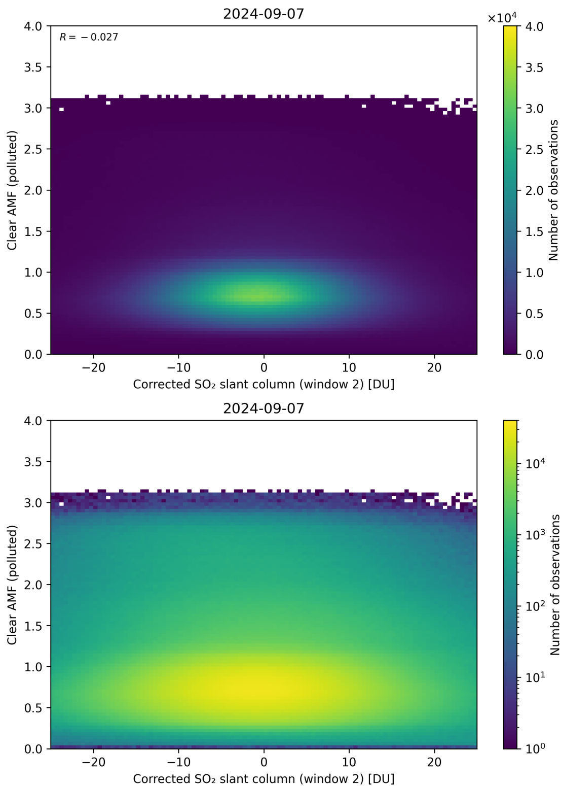
Figure 199: Scatter density plot of “Corrected SO 2 slant column (window 2)” against “Clear AMF (polluted)” for 2024-09-06 to 2024-09-08.
