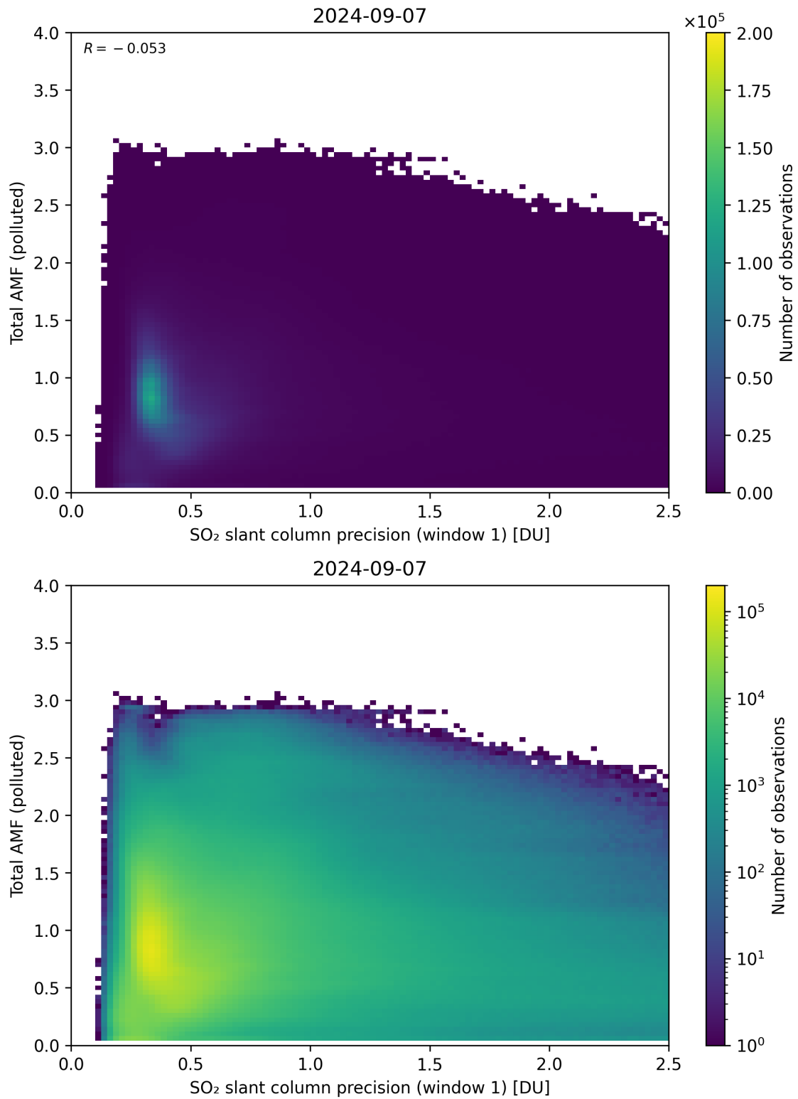
Figure 230: Scatter density plot of “SO 2 slant column precision (window 1)” against “Total AMF (polluted)” for 2024-09-06 to 2024-09-08.
