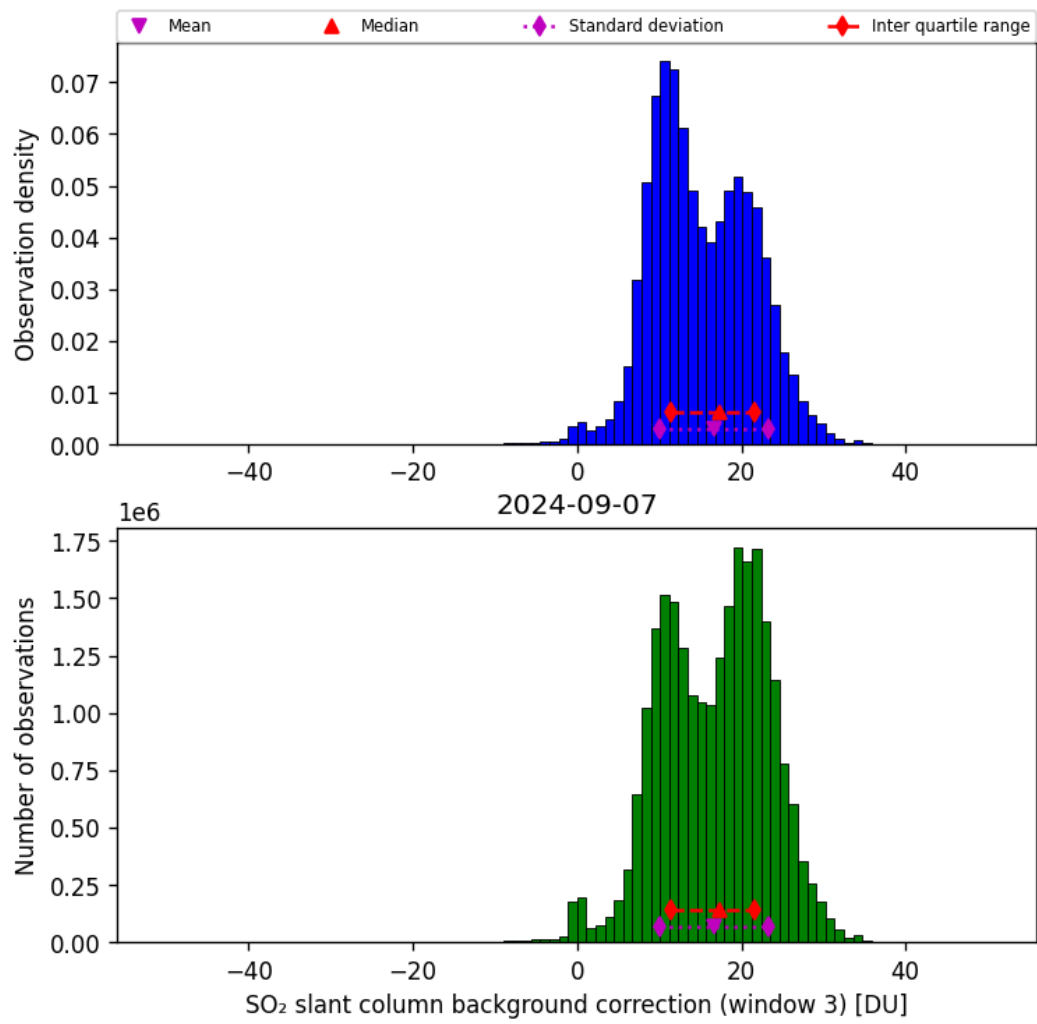
Figure 67: Histogram of “SO 2 slant column background correction (window 3)” for 2024-09-06 to 2024-09-08
