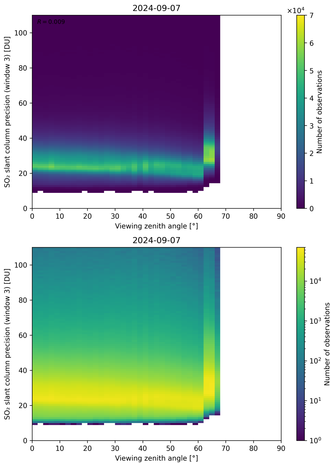
Figure 324: Scatter density plot of “Viewing zenith angle” against “SO 2 slant column precision (window 3)” for 2024-09-06 to 2024-09-08.
