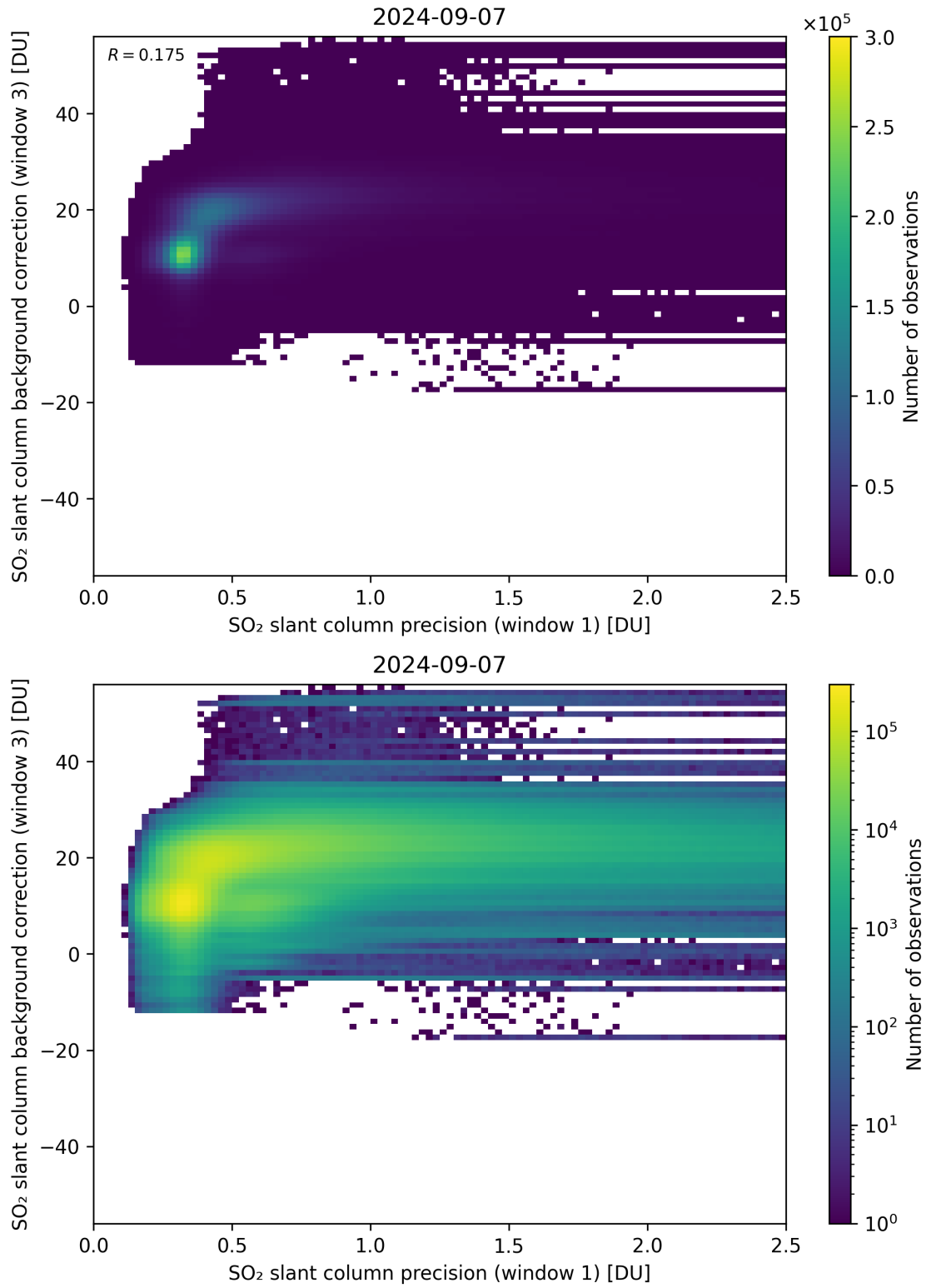
Figure 220: Scatter density plot of “SO 2 slant column precision (window 1)” against “SO 2 slant column background correction (window 3)” for 2024-09-06 to 2024-09-08.
