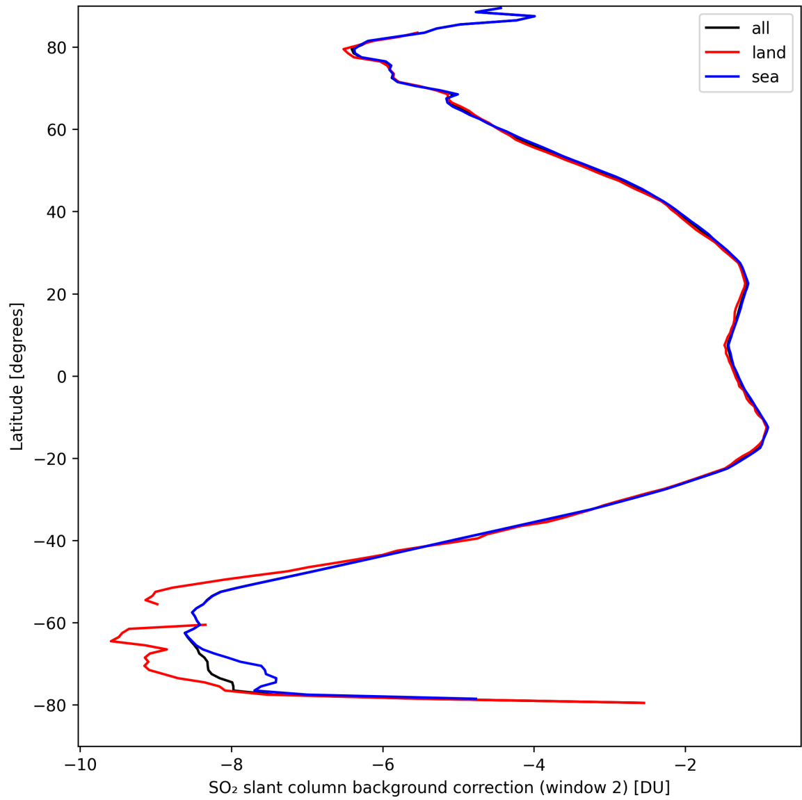
Figure 40: Zonal average of “SO 2 slant column background correction (window 2)” for 2024-09-06 to 2024-09-08.
