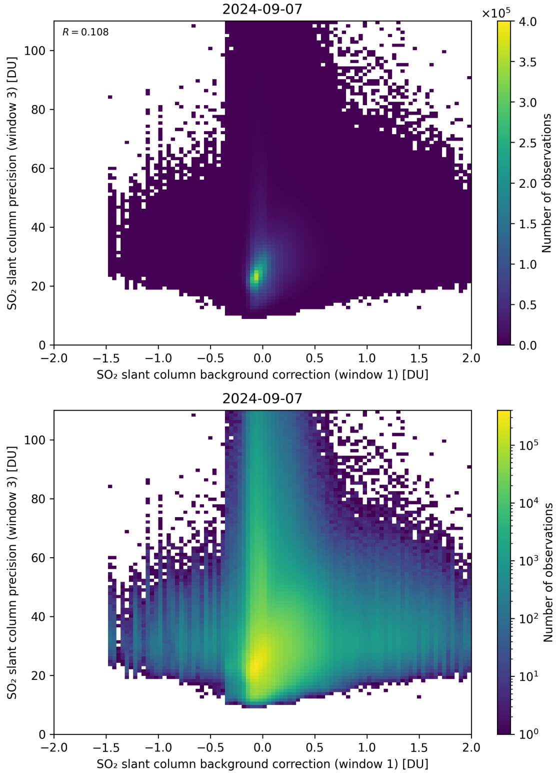
Figure 108: Scatter density plot of “SO 2 slant column background correction (window 1)” against “SO 2 slant column precision (window 3)” for 2024-09-06 to 2024-09-08.
