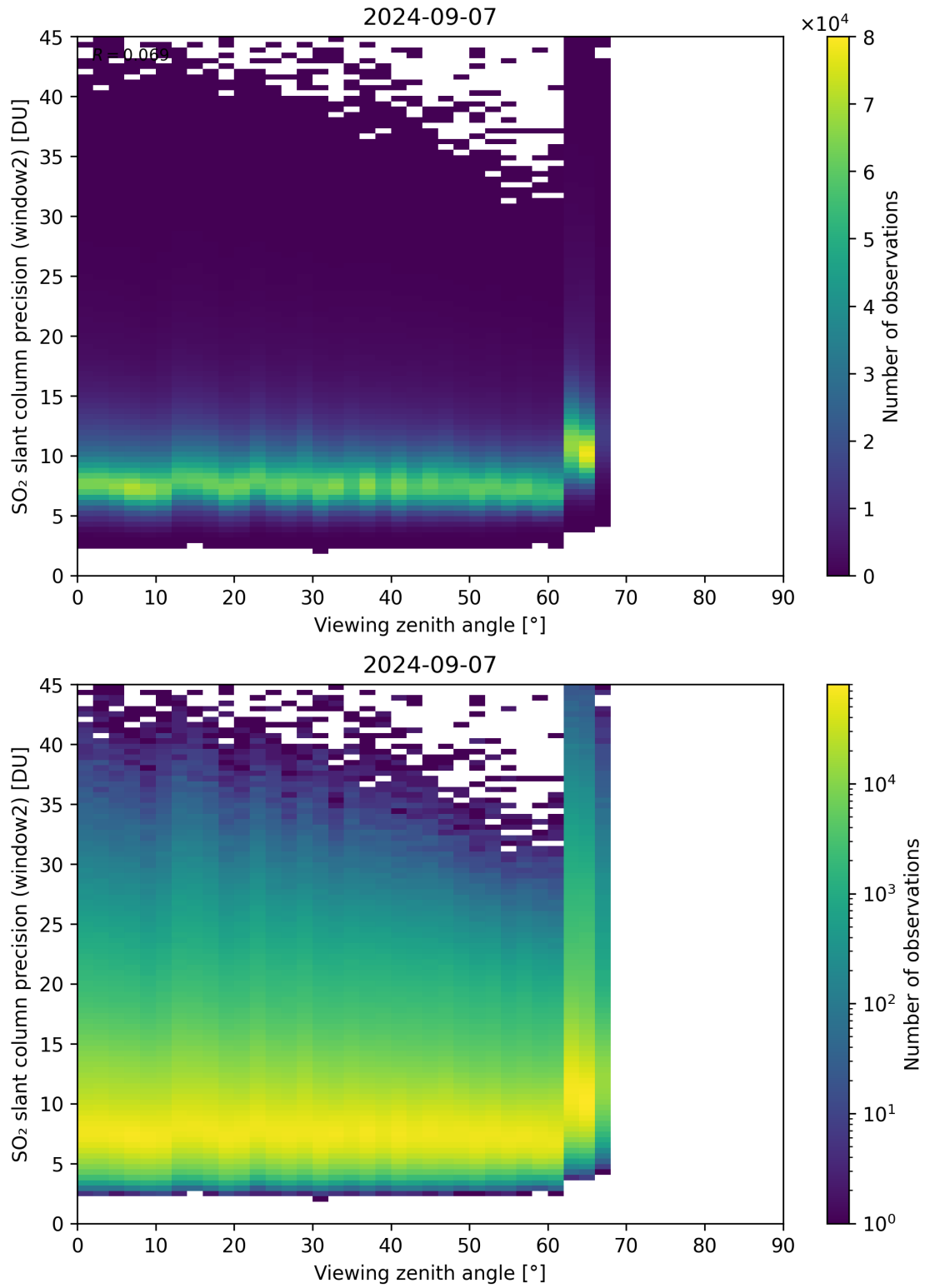
Figure 322: Scatter density plot of “Viewing zenith angle” against “SO 2 slant column precision (window2)” for 2024-09-06 to 2024-09-08.
