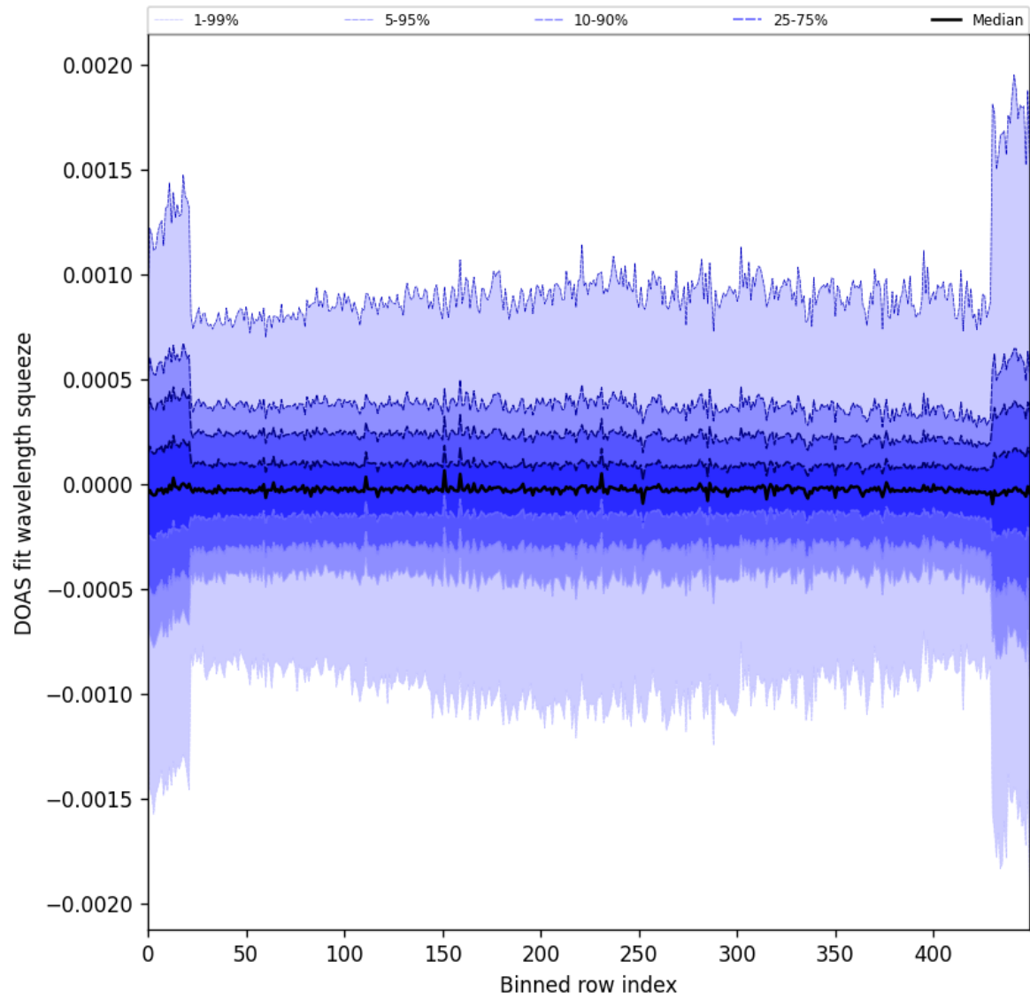
Figure 92: Along track statistics of “DOAS fit wavelength squeeze” for 2024-09-06 to 2024-09-08
