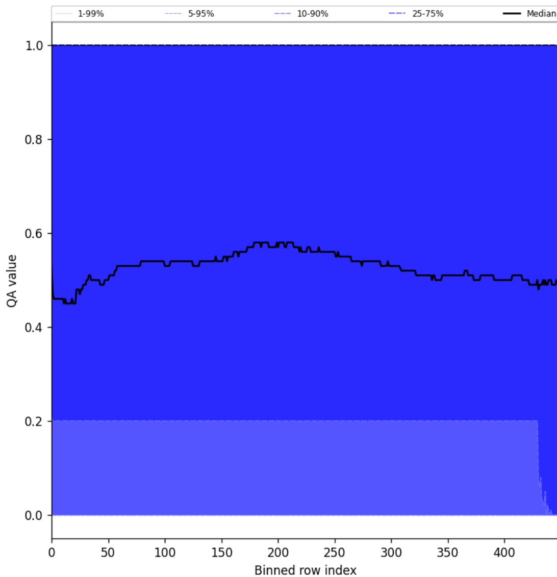
Figure 75: Along track statistics of “QA value” for 2024-09-06 to 2024-09-08
