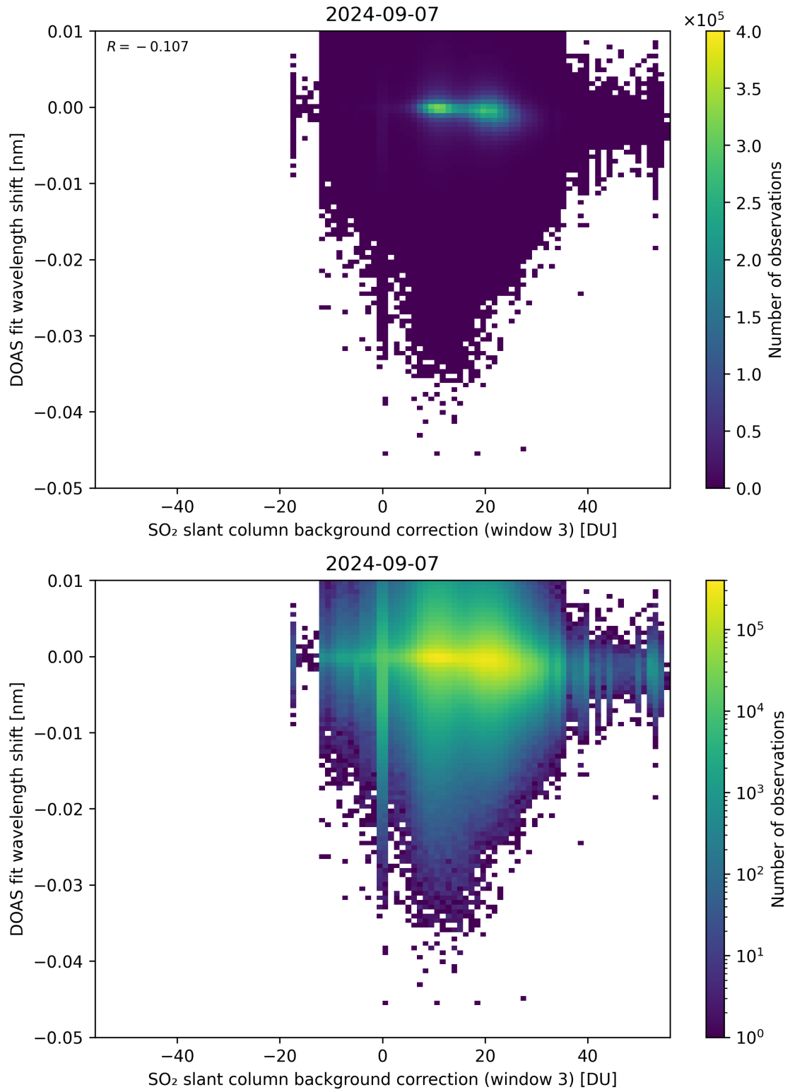
Figure 121: Scatter density plot of “SO 2 slant column background correction (window 3)” against “DOAS fit wavelength shift” for 2024-09-06 to 2024-09-08.
