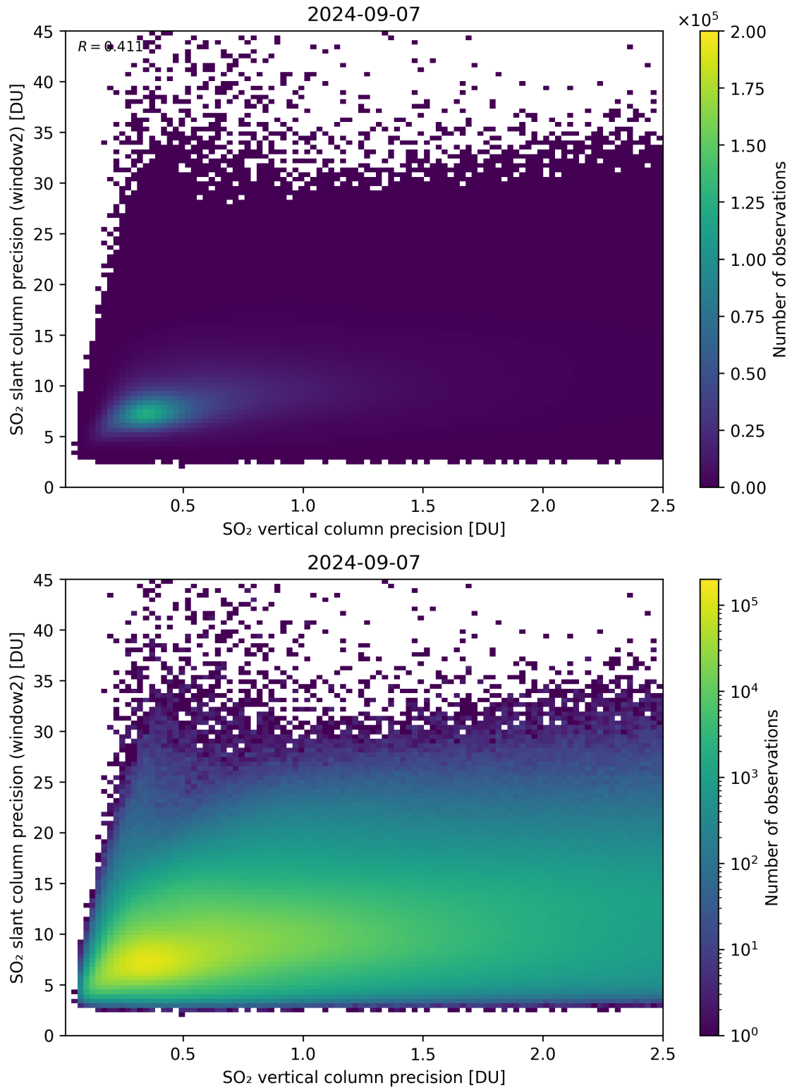
Figure 291: Scatter density plot of “SO 2 vertical column precision” against “SO 2 slant column precision (window2)” for 2024-09-06 to 2024-09-08.
