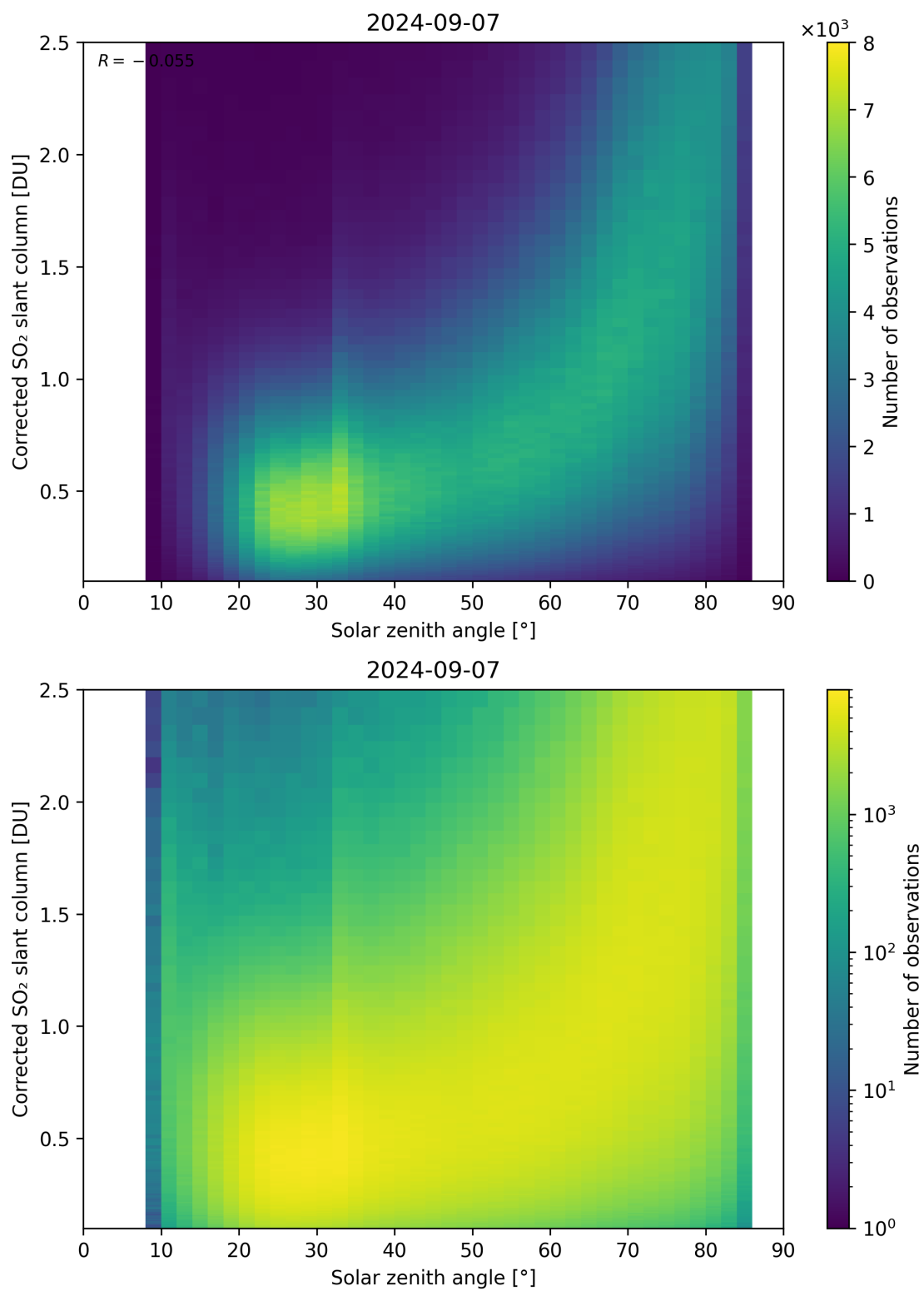
Figure 166: Scatter density plot of “Solar zenith angle” against “Corrected SO 2 slant column” for 2024-09-06 to 2024-09-08.
