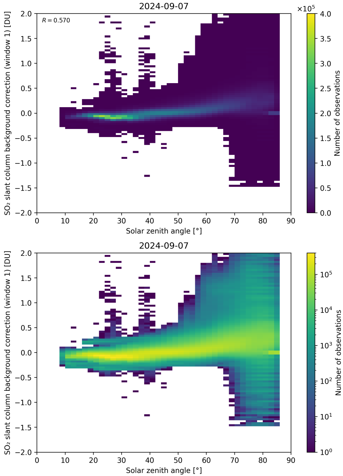
Figure 158: Scatter density plot of “Solar zenith angle” against “SO 2 slant column background correction (window 1)” for 2024-09-06 to 2024-09-08.
