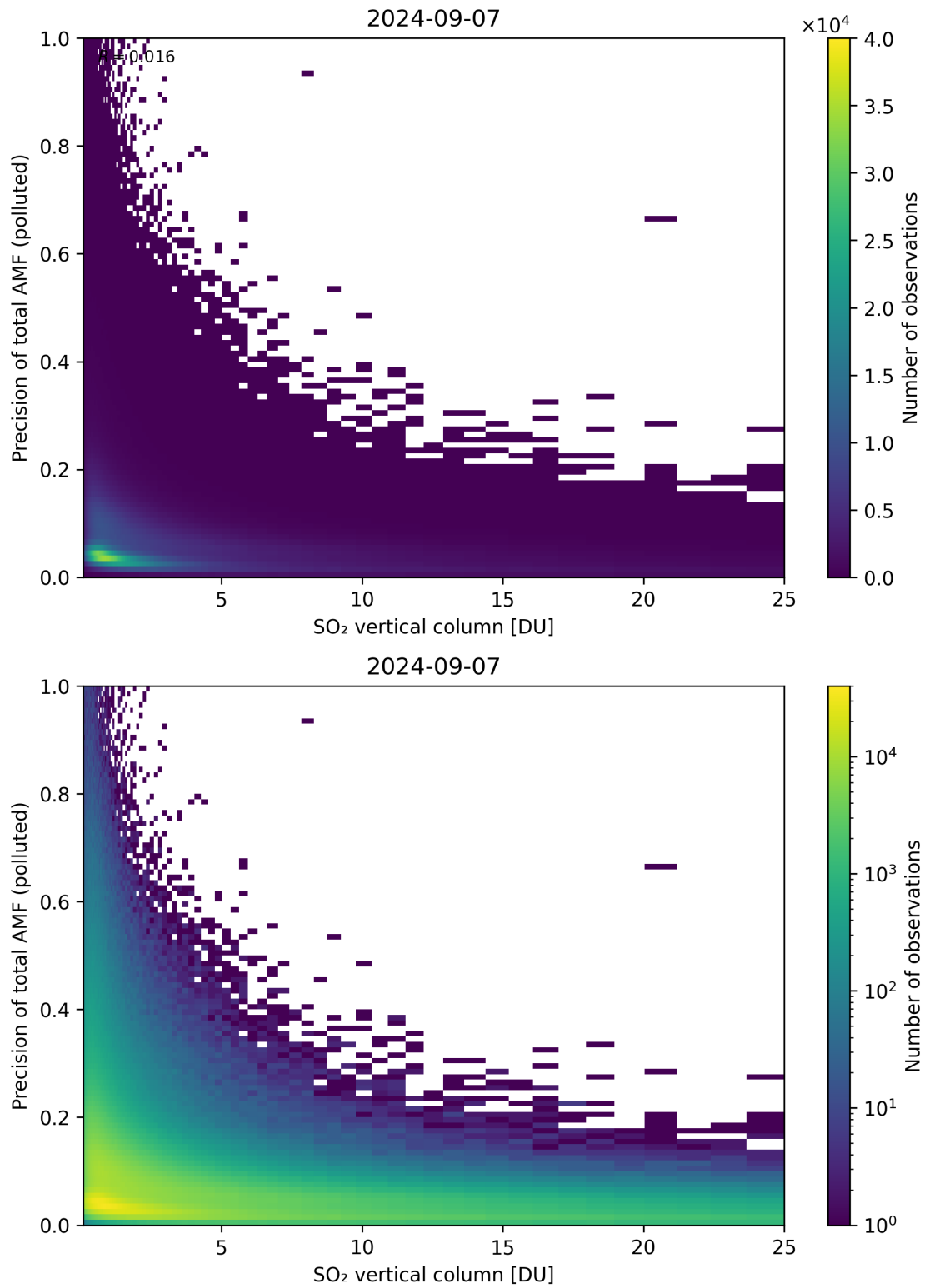
Figure 306: Scatter density plot of “SO 2 vertical column” against “Precision of total AMF (polluted)” for 2024-09-06 to 2024-09-08.
