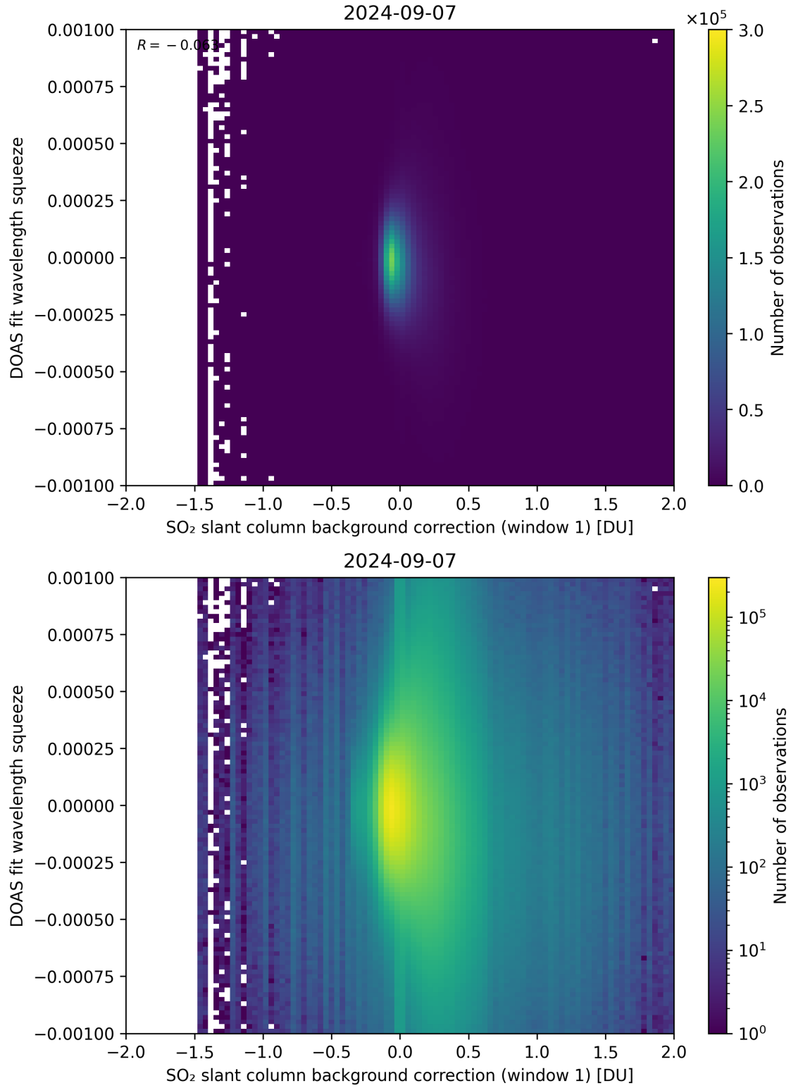
Figure 101: Scatter density plot of “SO 2 slant column background correction (window 1)” against “DOAS fit wavelength squeeze” for 2024-09-06 to 2024-09-08.
