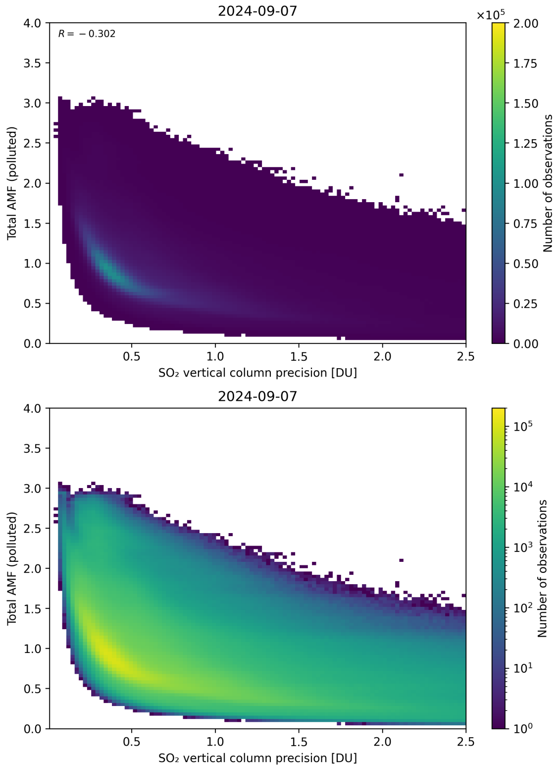
Figure 294: Scatter density plot of “SO 2 vertical column precision” against “Total AMF (polluted)” for 2024-09-06 to 2024-09-08.
