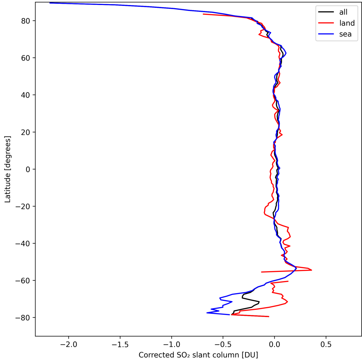
Figure 32: Zonal average of “Corrected SO 2 slant column” for 2024-09-06 to 2024-09-08.
