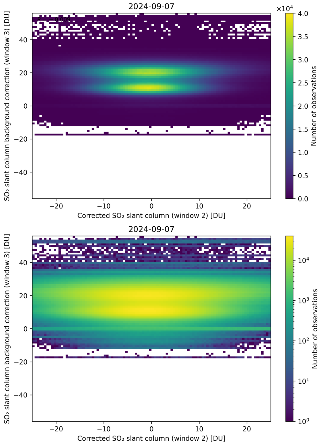
Figure 195: Scatter density plot of “Corrected SO 2 slant column (window 2)” against “SO 2 slant column background correction (window 3)” for 2024-09-06 to 2024-09-08.
