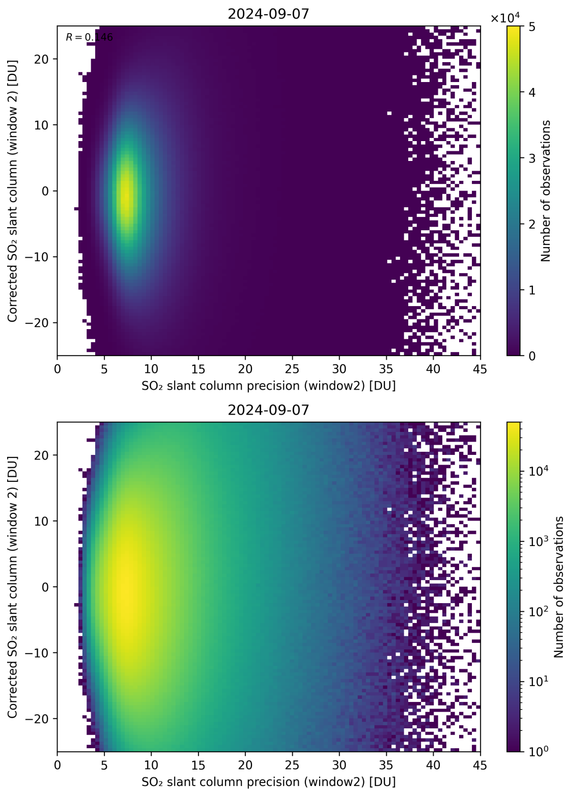
Figure 247: Scatter density plot of “SO 2 slant column precision (window2)” against “Corrected SO 2 slant column (window 2)” for 2024-09-06 to 2024-09-08.
