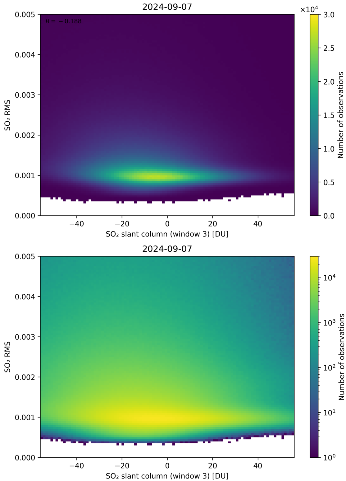
Figure 256: Scatter density plot of “SO 2 slant column (window 3)” against “SO 2 RMS” for 2024-09-06 to 2024-09-08.
