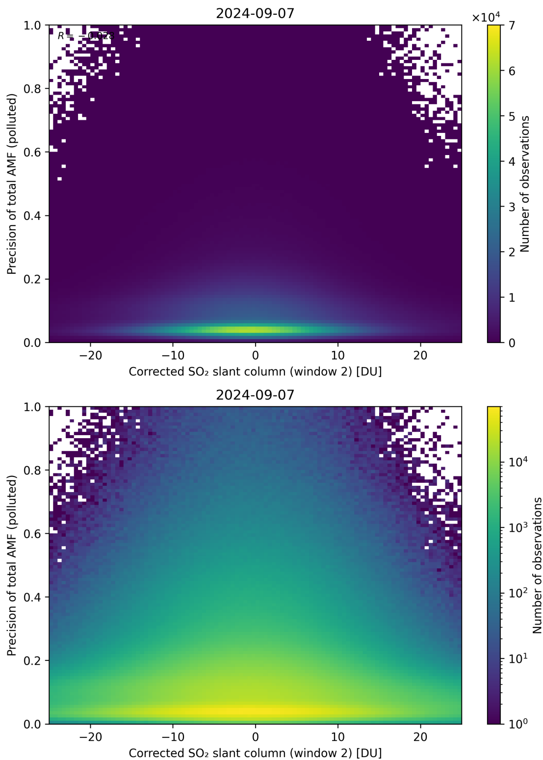
Figure 204: Scatter density plot of “Corrected SO 2 slant column (window 2)” against “Precision of total AMF (polluted)” for 2024-09-06 to 2024-09-08.
