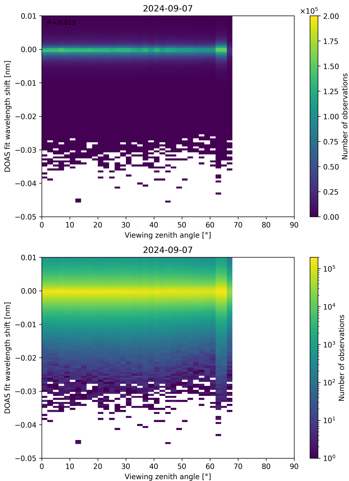
Figure 311: Scatter density plot of “Viewing zenith angle” against “DOAS fit wavelength shift” for 2024-09-06 to 2024-09-08.
