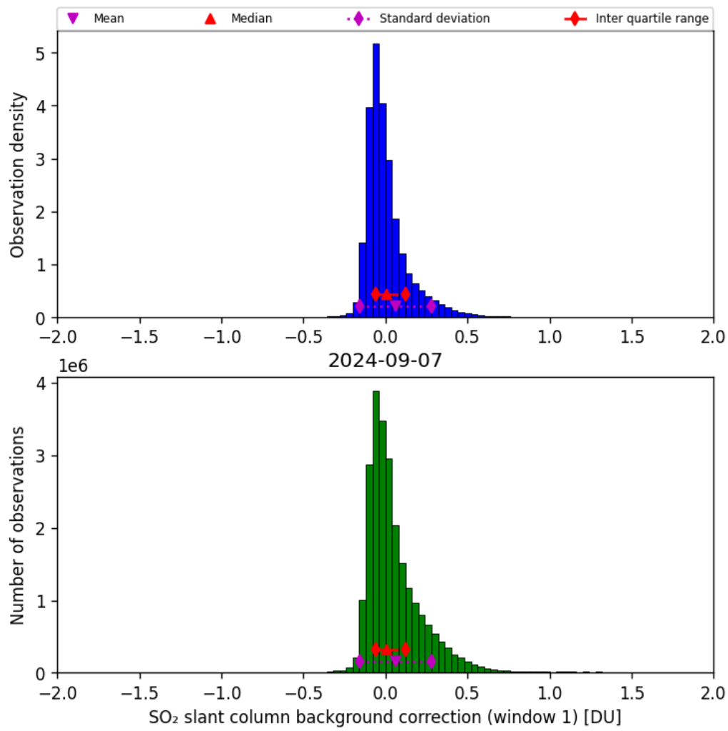
Figure 59: Histogram of “SO 2 slant column background correction (window 1)” for 2024-09-06 to 2024-09-08
