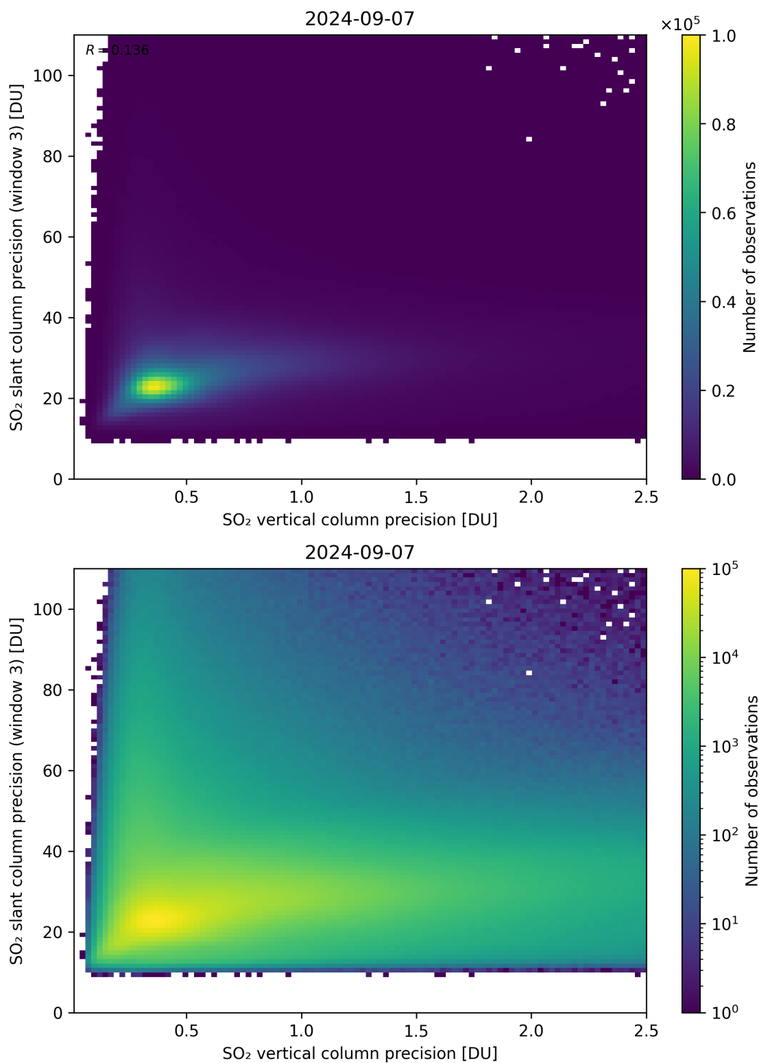
Figure 293: Scatter density plot of “SO 2 vertical column precision” against “SO 2 slant column precision (window 3)” for 2024-09-06 to 2024-09-08.
