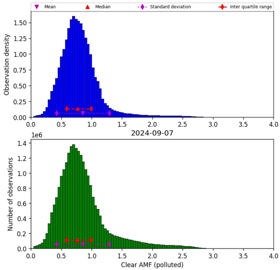
Figure 73: Histogram of “Clear AMF (polluted)” for 2024-09-06 to 2024-09-08
