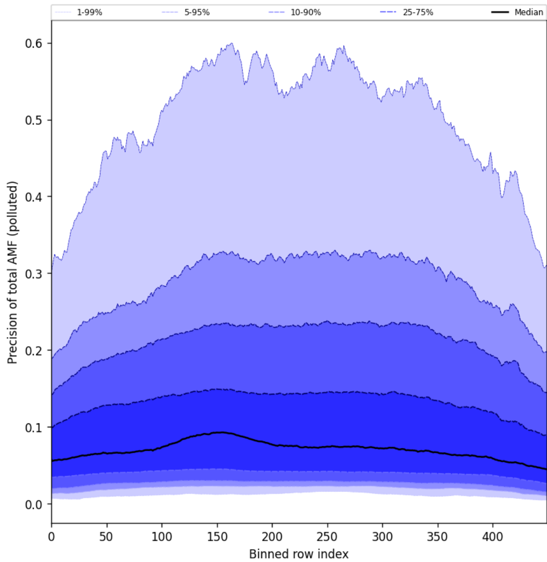
Figure 95: Along track statistics of “Precision of total AMF (polluted)” for 2024-09-06 to 2024-09-08
