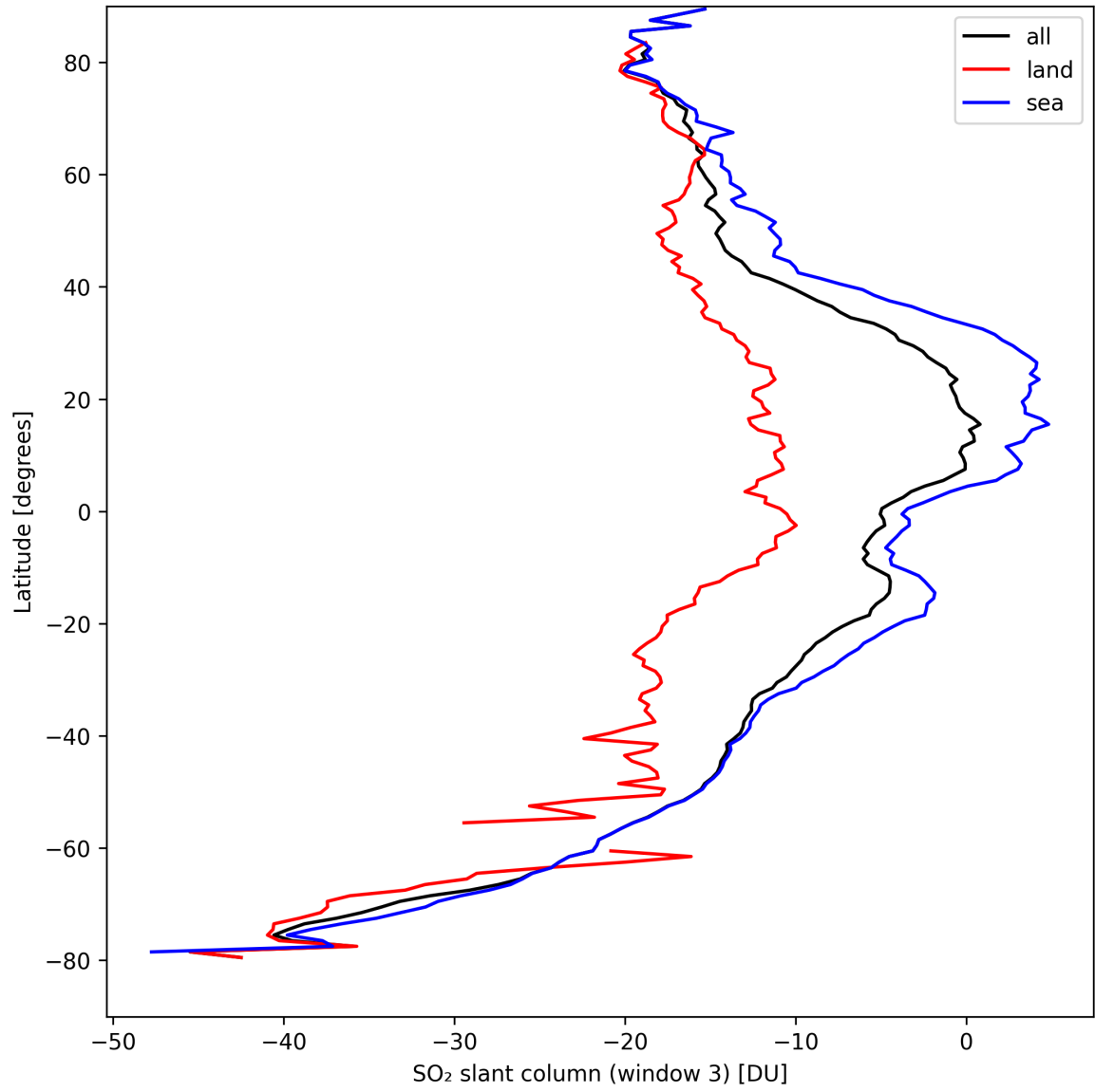
Figure 41: Zonal average of “SO 2 slant column (window 3)” for 2024-09-06 to 2024-09-08.
