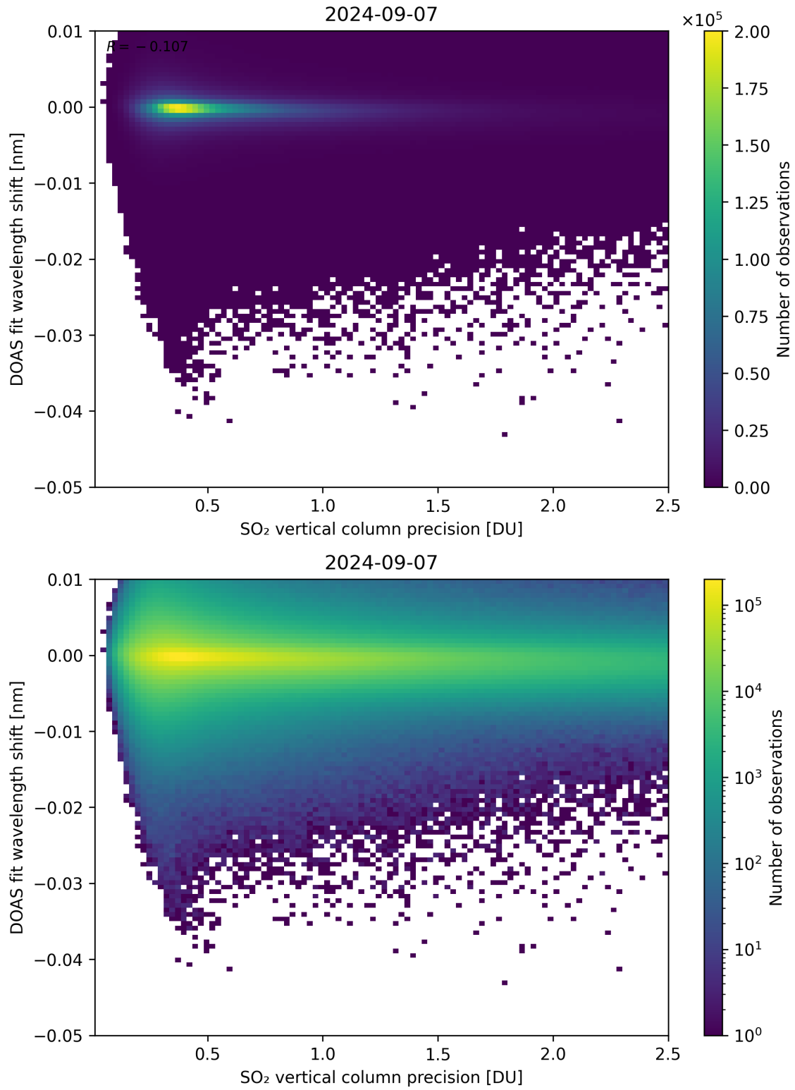
Figure 282: Scatter density plot of “SO 2 vertical column precision” against “DOAS fit wavelength shift” for 2024-09-06 to 2024-09-08.
