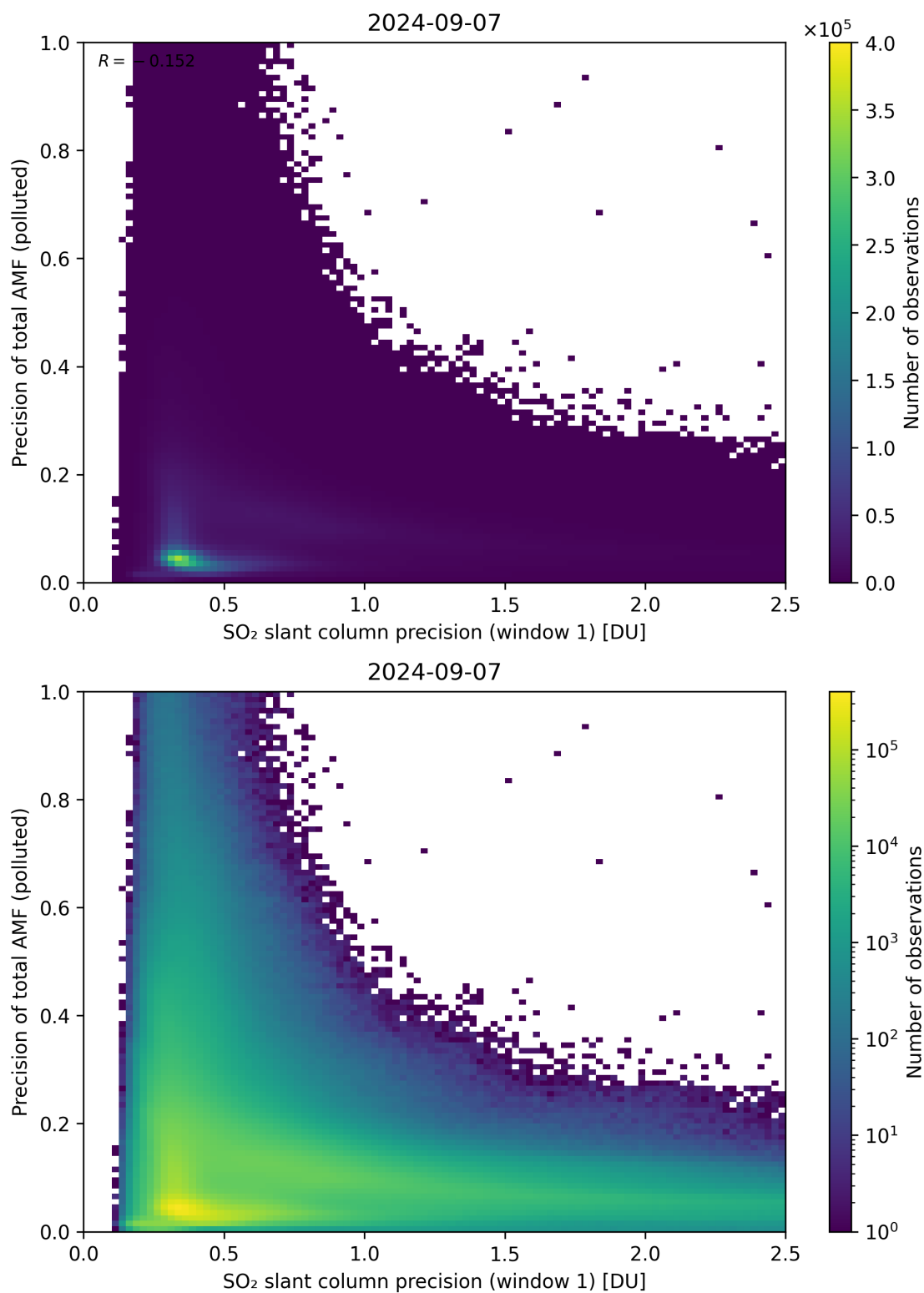
Figure 231: Scatter density plot of “SO 2 slant column precision (window 1)” against “Precision of total AMF (polluted)” for 2024-09-06 to 2024-09-08.
