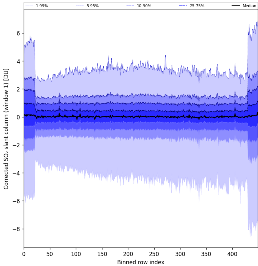
Figure 81: Along track statistics of “Corrected SO 2 slant column (window 1)” for 2024-09-06 to 2024-09-08
