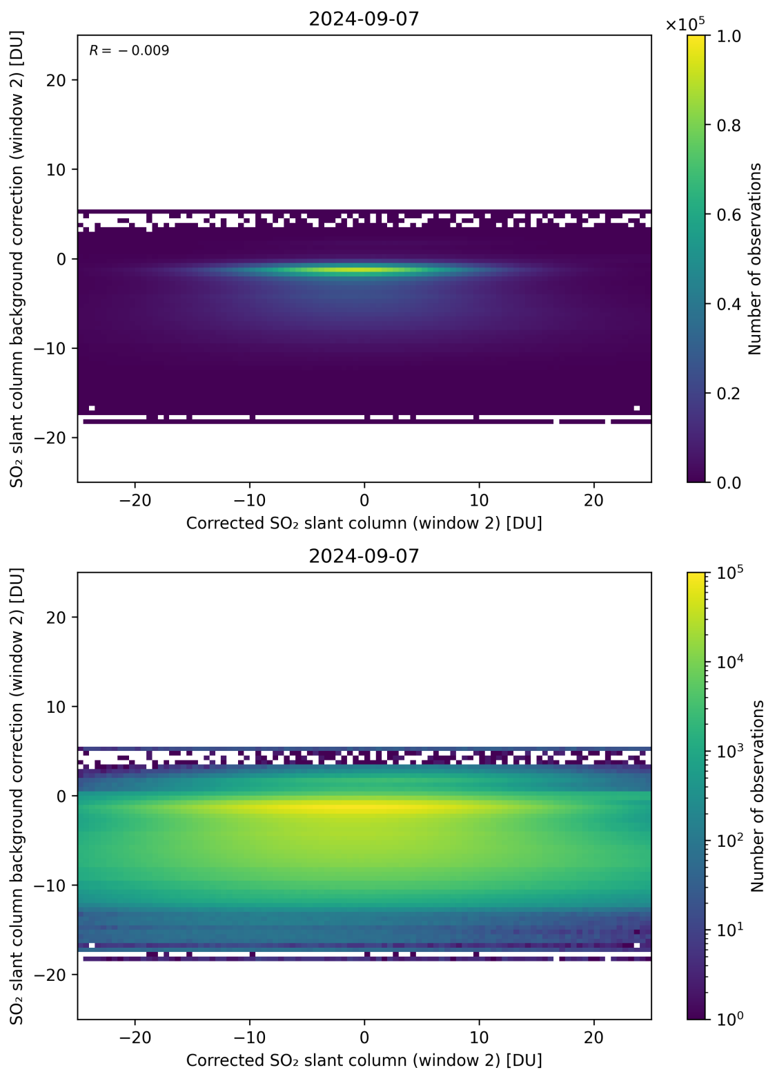
Figure 194: Scatter density plot of “Corrected SO 2 slant column (window 2)” against “SO 2 slant column background correction (window 2)” for 2024-09-06 to 2024-09-08.
