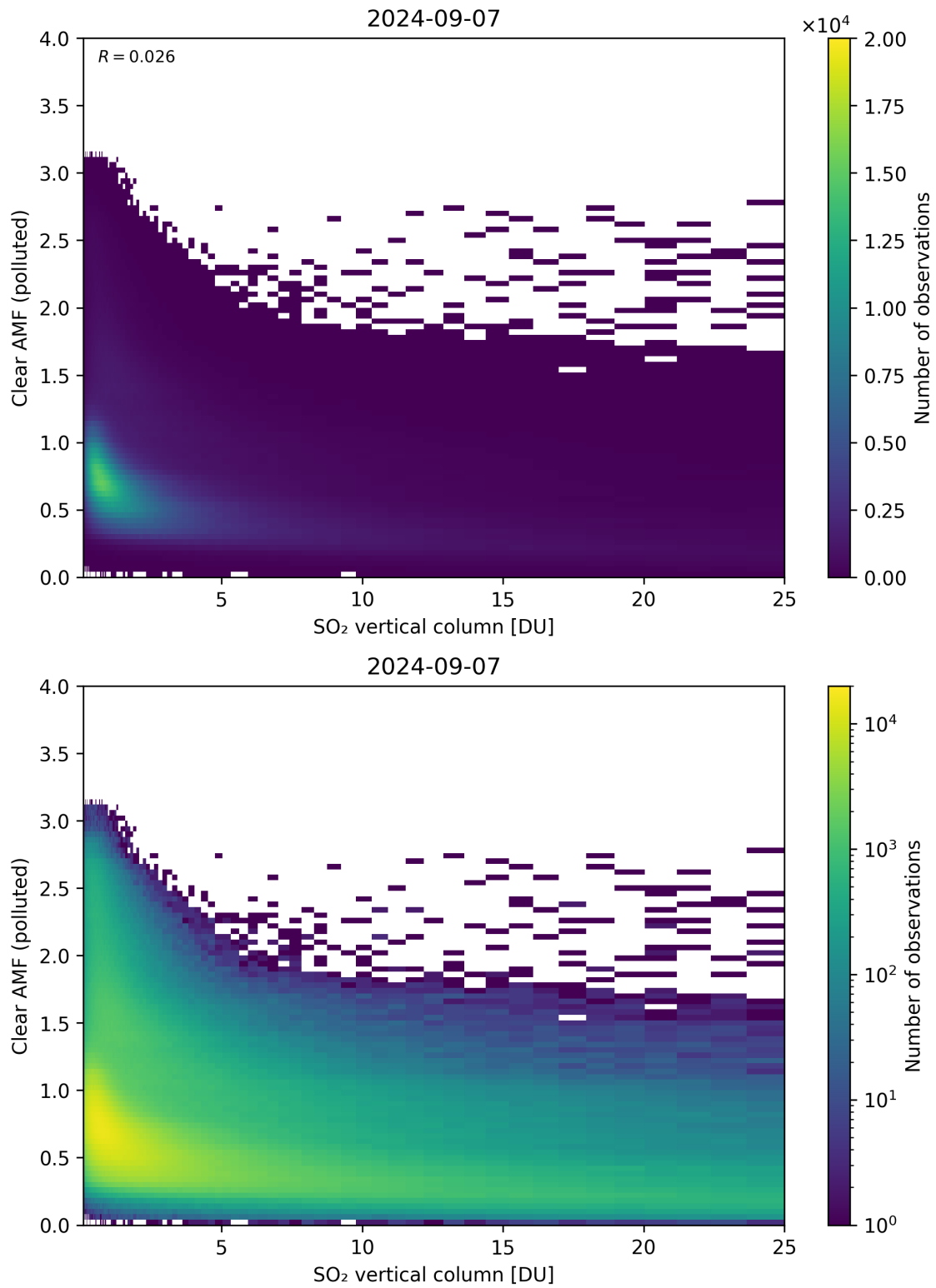
Figure 296: Scatter density plot of “SO 2 vertical column” against “Clear AMF (polluted)” for 2024-09-06 to 2024-09-08.
