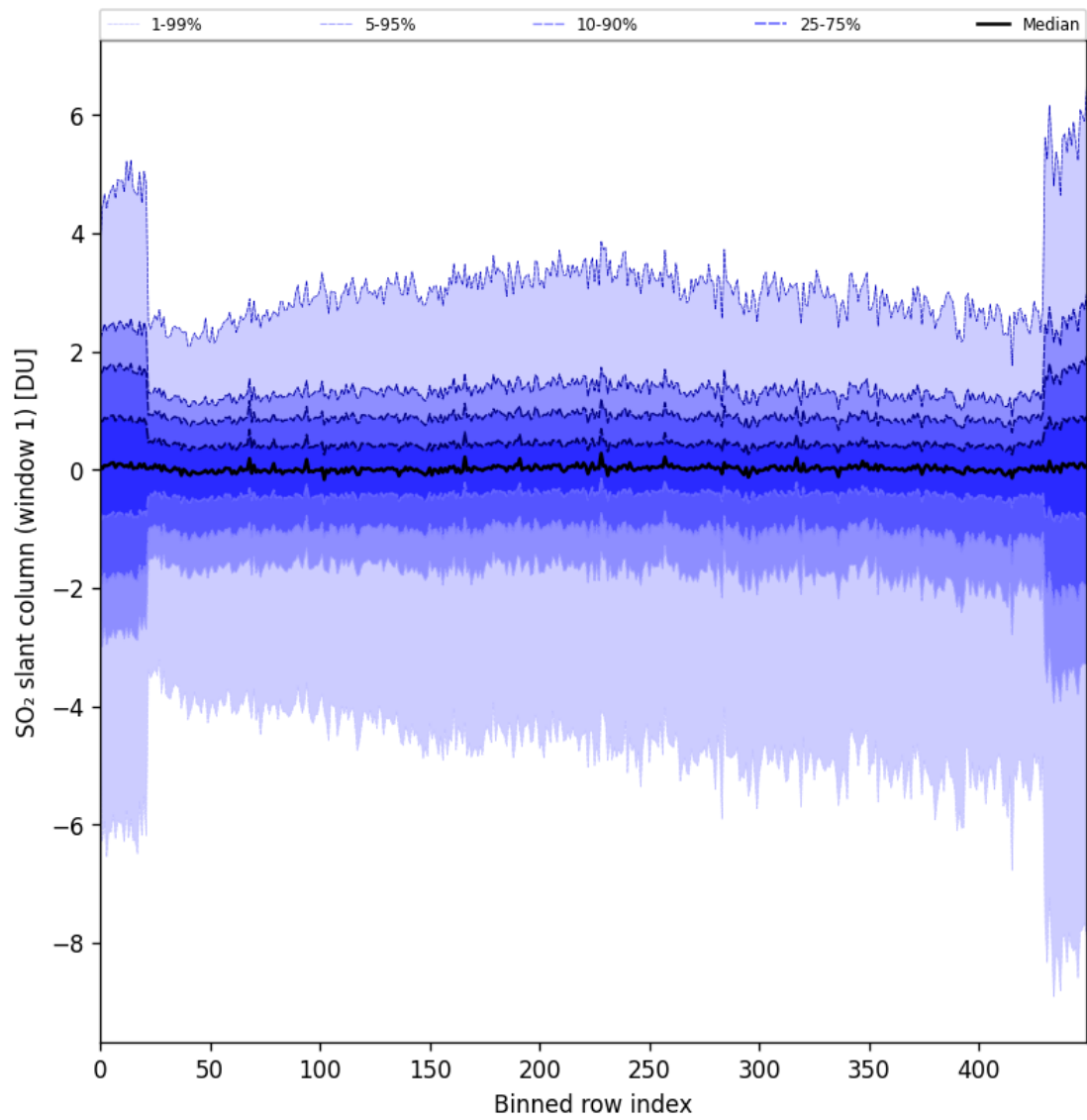
Figure 79: Along track statistics of “SO 2 slant column (window 1)” for 2024-09-06 to 2024-09-08
