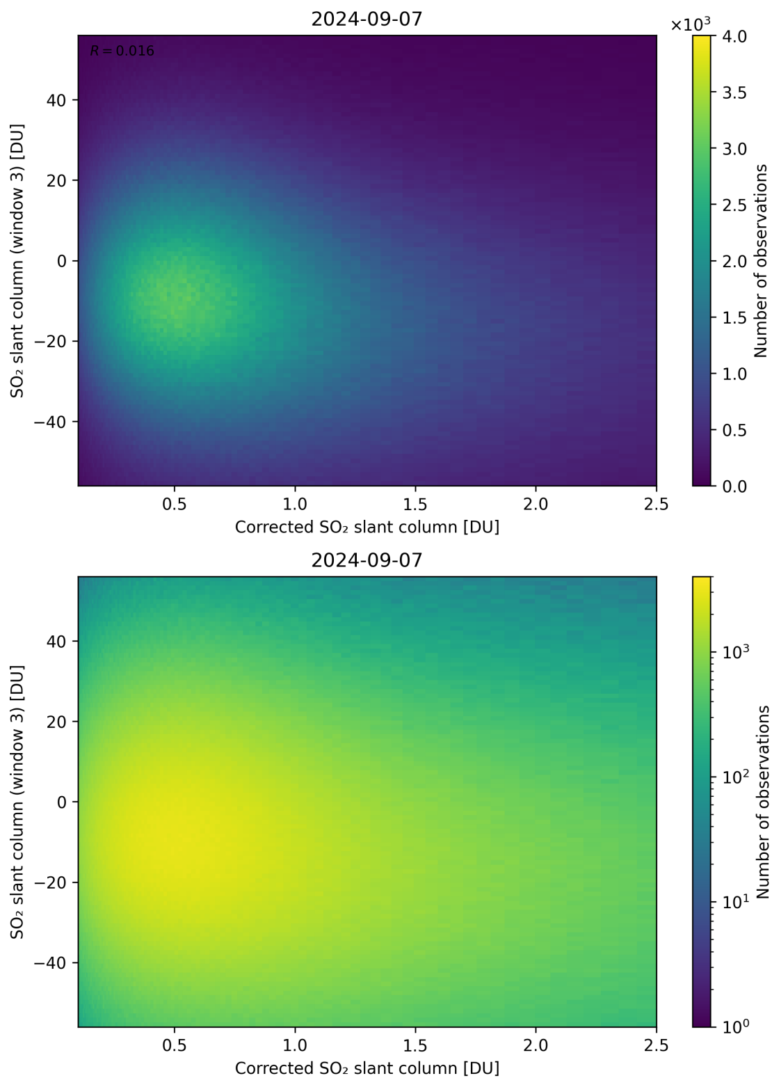
Figure 190: Scatter density plot of “Corrected SO 2 slant column” against “SO 2 slant column (window 3)” for 2024-09-06 to 2024-09-08.
