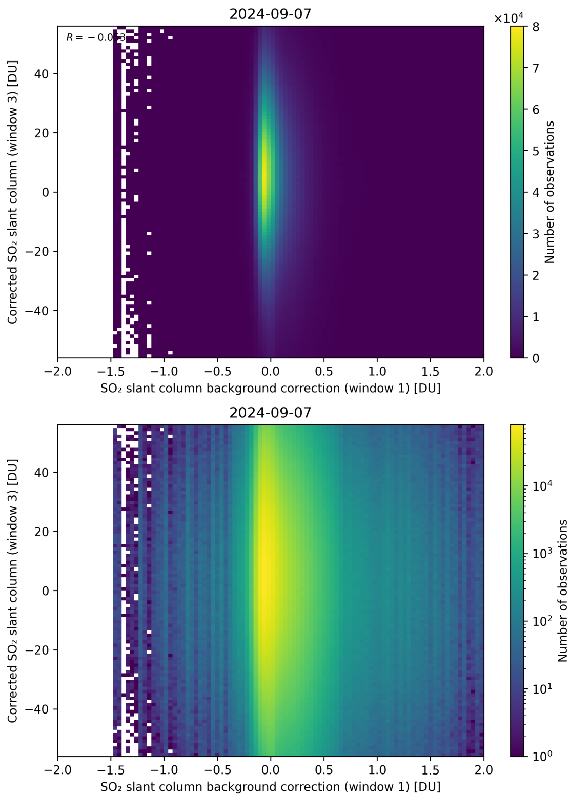
Figure 105: Scatter density plot of “SO 2 slant column background correction (window 1)” against “Corrected SO 2 slant column (window 3)” for 2024-09-06 to 2024-09-08.
