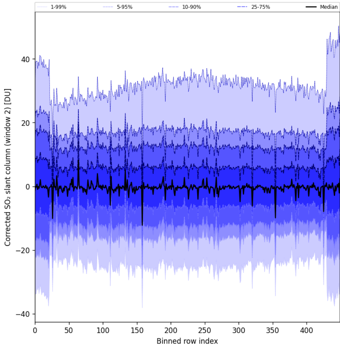
Figure 85: Along track statistics of “Corrected SO 2 slant column (window 2)” for 2024-09-06 to 2024-09-08
