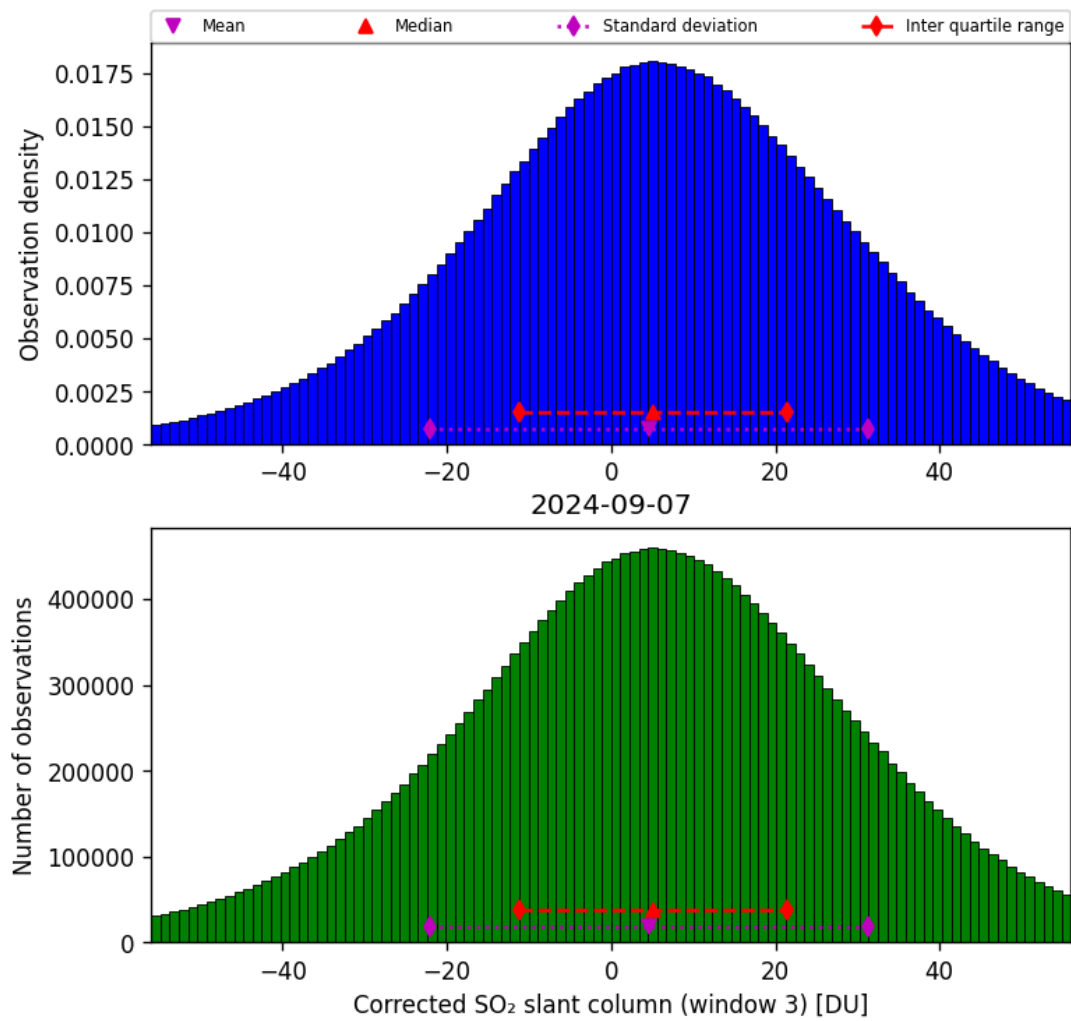
Figure 66: Histogram of “Corrected SO 2 slant column (window 3)” for 2024-09-06 to 2024-09-08
