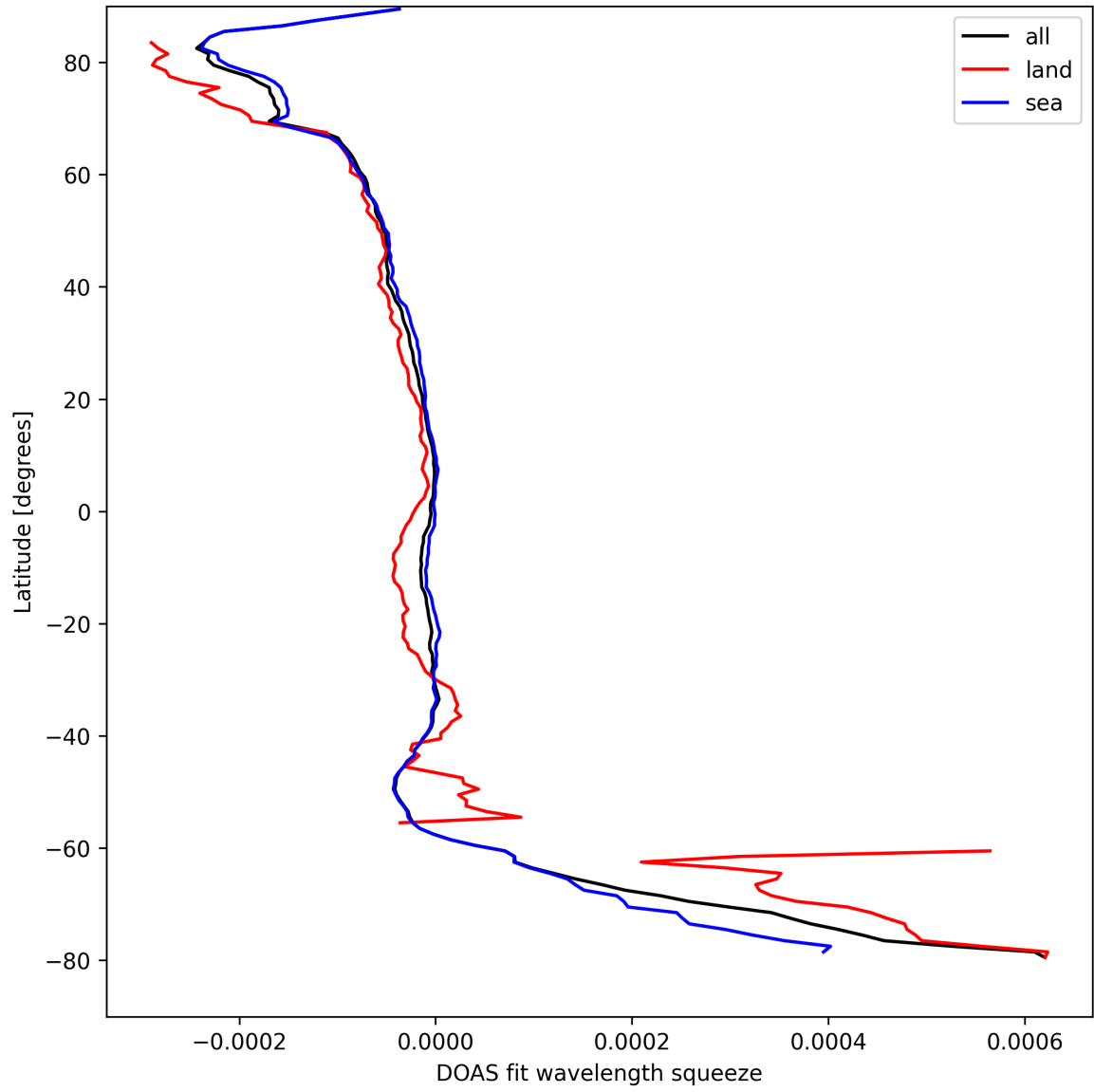
Figure 46: Zonal average of “DOAS fit wavelength squeeze” for 2024-09-06 to 2024-09-08.
