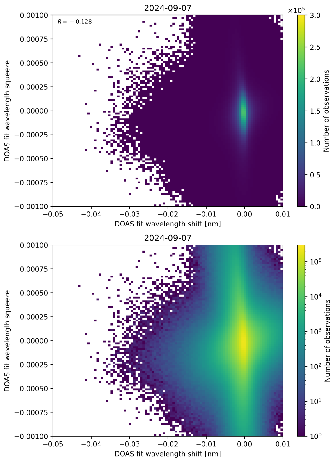
Figure 127: Scatter density plot of “DOAS fit wavelength shift” against “DOAS fit wavelength squeeze” for 2024-09-06 to 2024-09-08.
