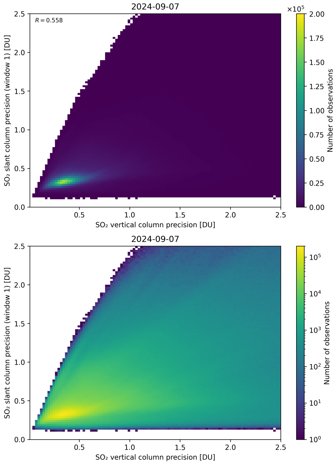
Figure 290: Scatter density plot of “SO 2 vertical column precision” against “SO 2 slant column precision (window 1)” for 2024-09-06 to 2024-09-08.
