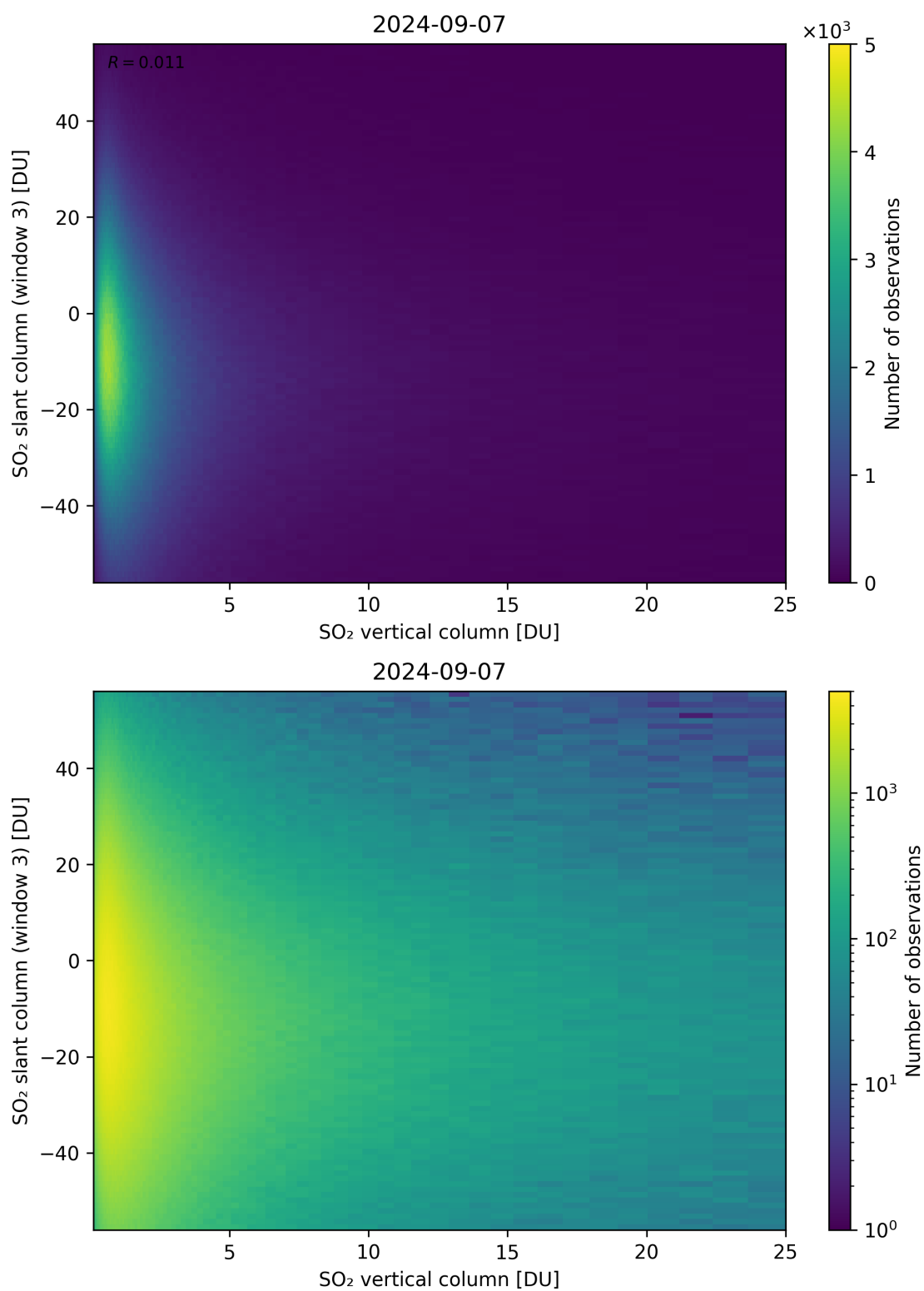
Figure 303: Scatter density plot of “SO 2 vertical column” against “SO 2 slant column (window 3)” for 2024-09-06 to 2024-09-08.
