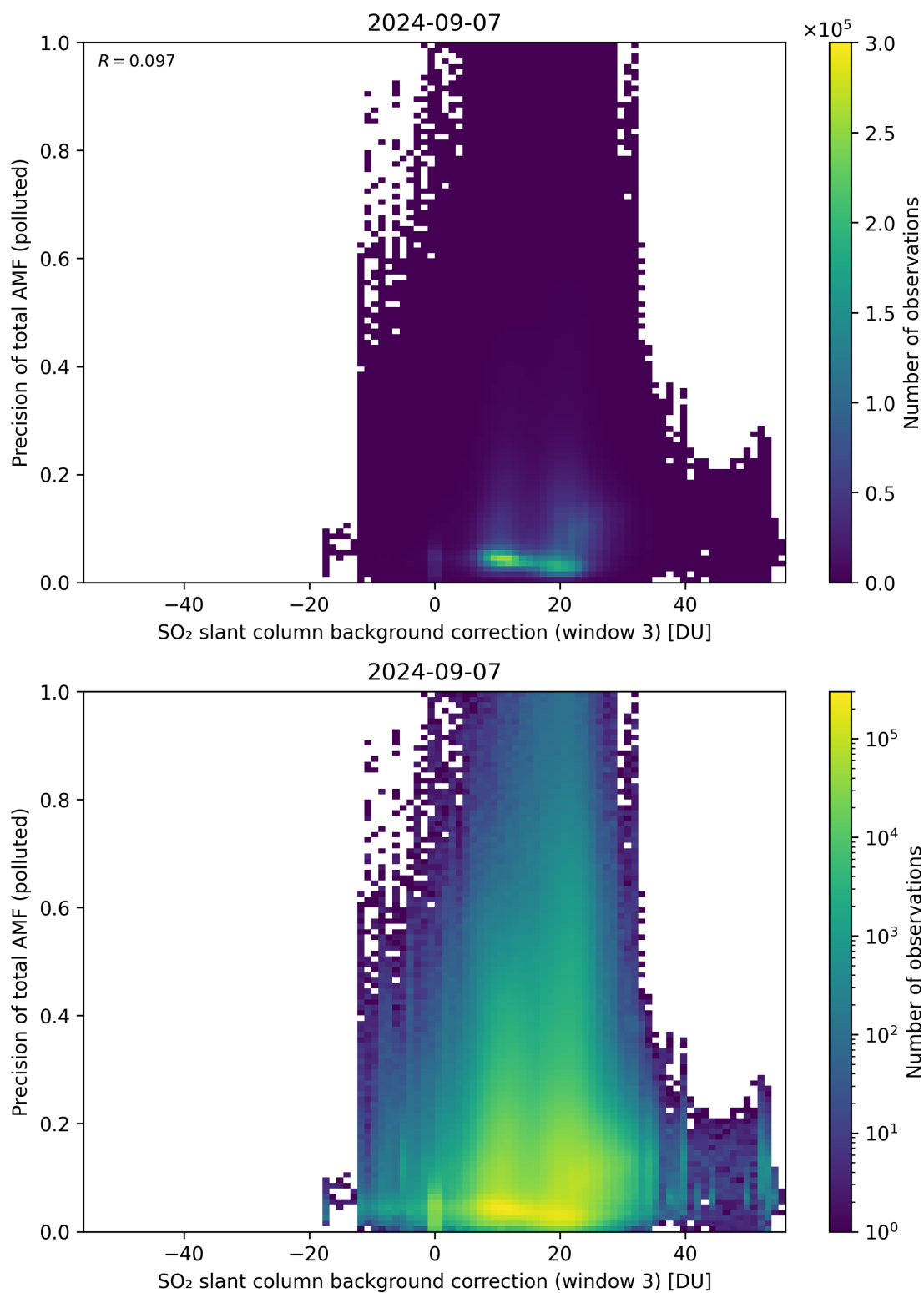
Figure 126: Scatter density plot of “SO 2 slant column background correction (window 3)” against “Precision of total AMF (polluted)” for 2024-09-06 to 2024-09-08.
