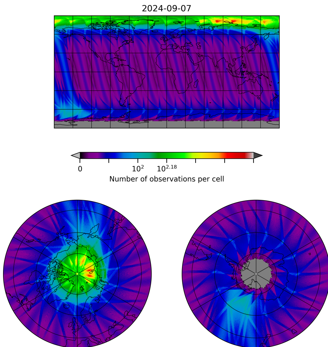
Figure 28: Map of the number of observations for 2024-09-06 to 2024-09-08
