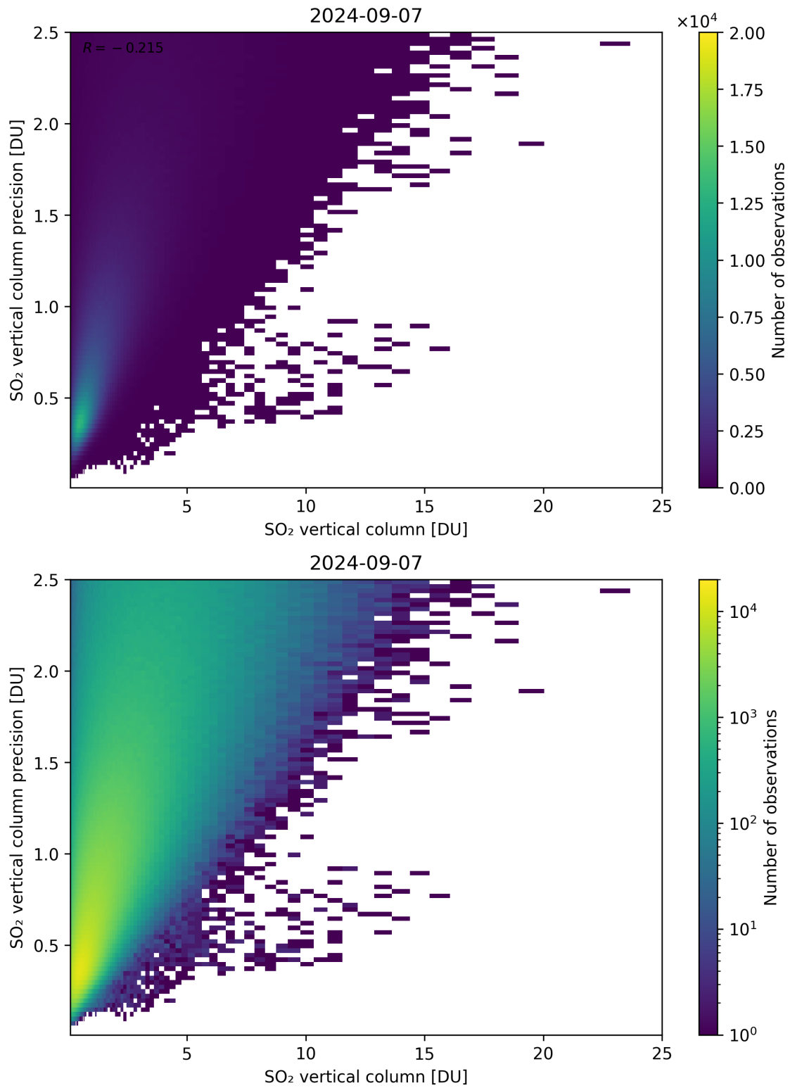
Figure 307: Scatter density plot of “SO 2 vertical column” against “SO 2 vertical column precision” for 2024-09-06 to 2024-09-08.
