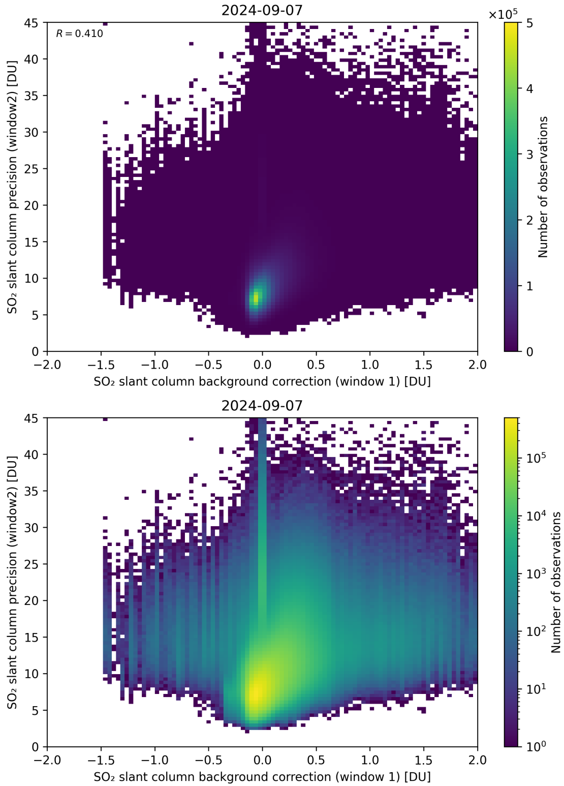
Figure 106: Scatter density plot of “SO 2 slant column background correction (window 1)” against “SO 2 slant column precision (window2)” for 2024-09-06 to 2024-09-08.
