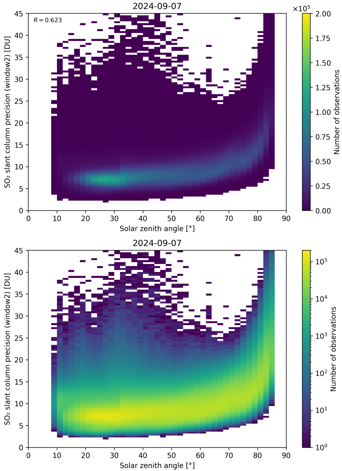
Figure 171: Scatter density plot of “Solar zenith angle” against “SO 2 slant column precision (window2)” for 2024-09-06 to 2024-09-08.
