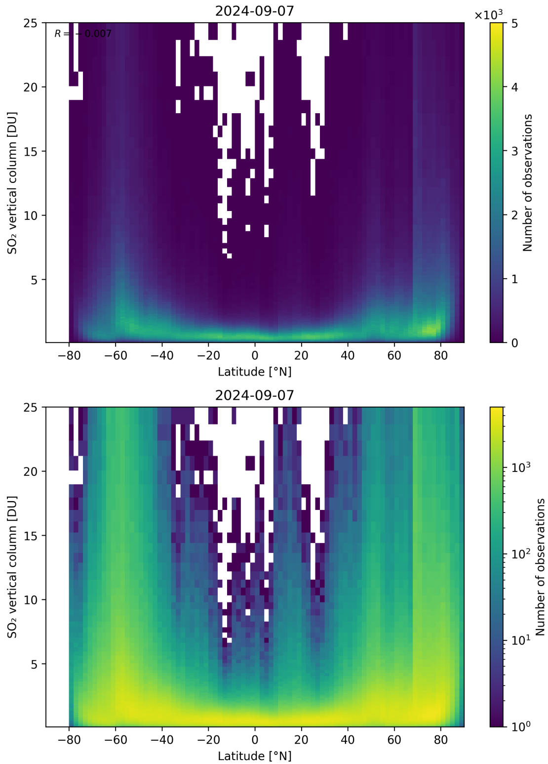
Figure 156: Scatter density plot of “Latitude” against “SO 2 vertical column” for 2024-09-06 to 2024-09-08.
