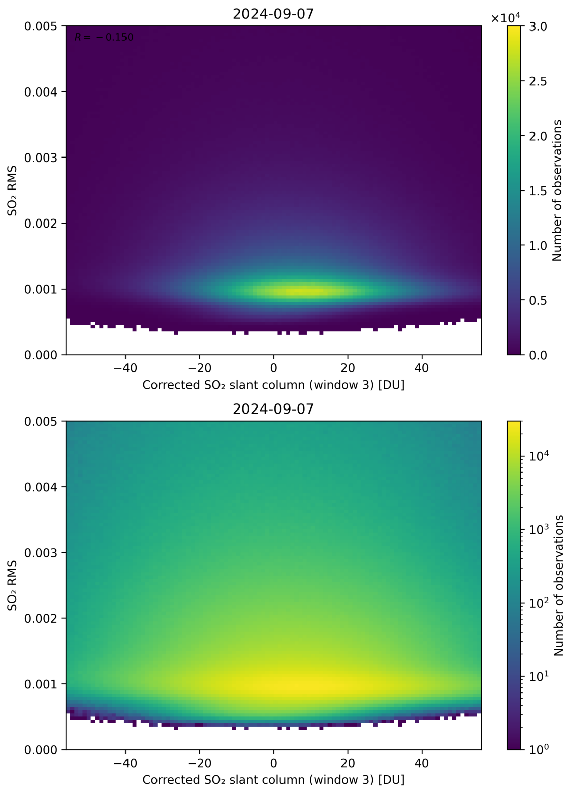
Figure 208: Scatter density plot of “Corrected SO 2 slant column (window 3)” against “SO 2 RMS” for 2024-09-06 to 2024-09-08.
