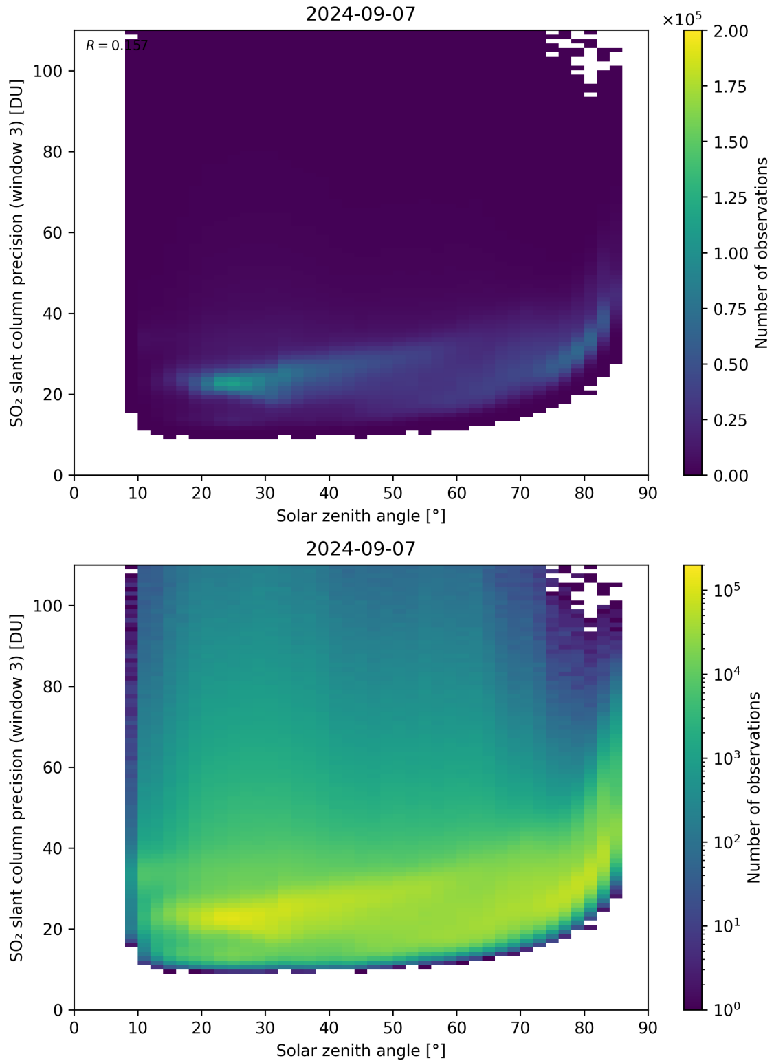
Figure 173: Scatter density plot of “Solar zenith angle” against “SO 2 slant column precision (window 3)” for 2024-09-06 to 2024-09-08.
