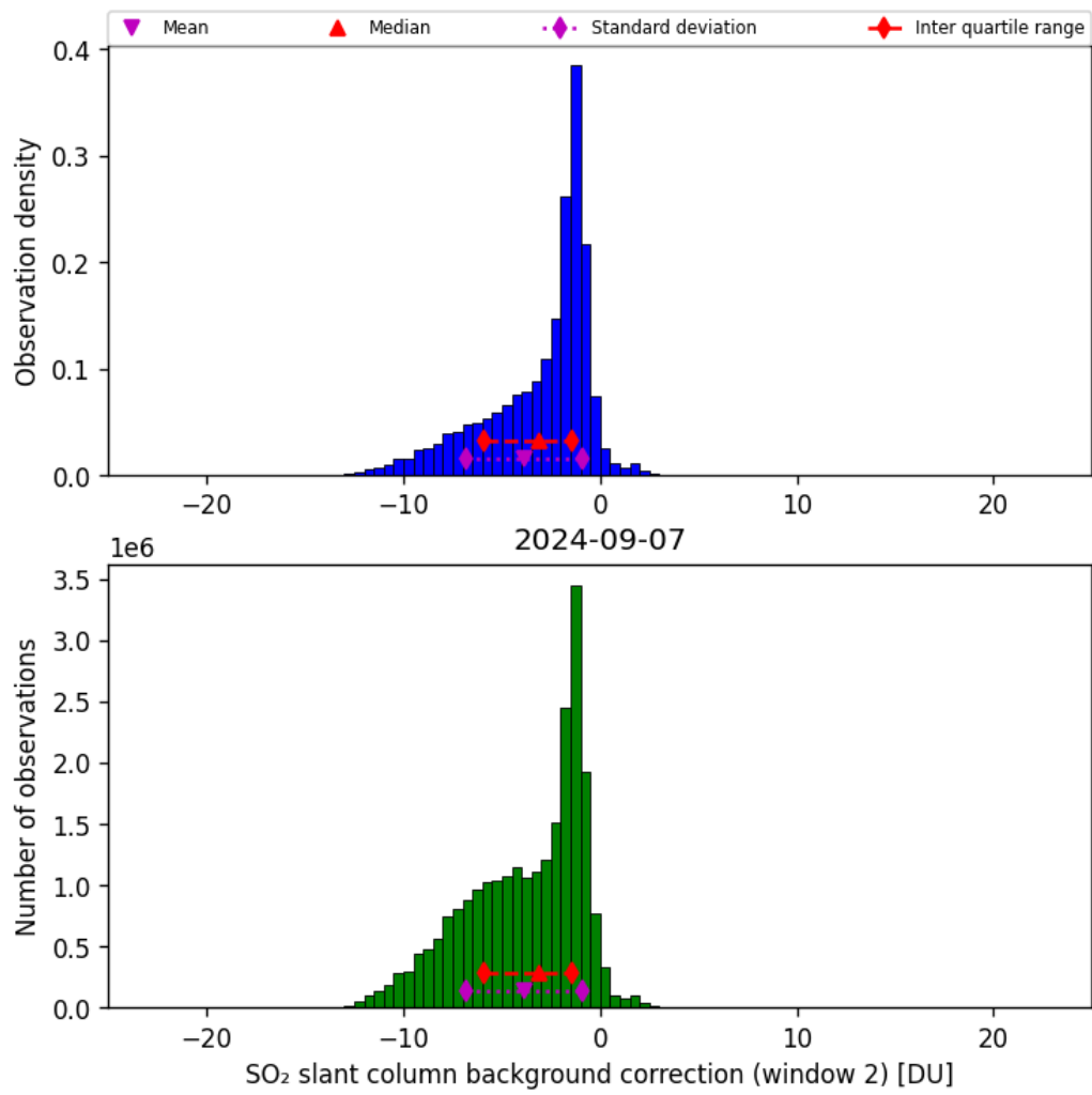
Figure 63: Histogram of “SO 2 slant column background correction (window 2)” for 2024-09-06 to 2024-09-08
