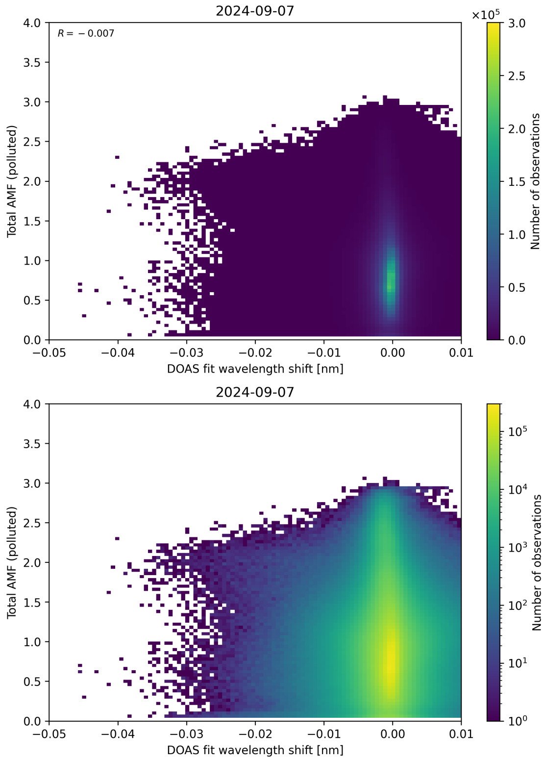
Figure 130: Scatter density plot of “DOAS fit wavelength shift” against “Total AMF (polluted)” for 2024-09-06 to 2024-09-08.
