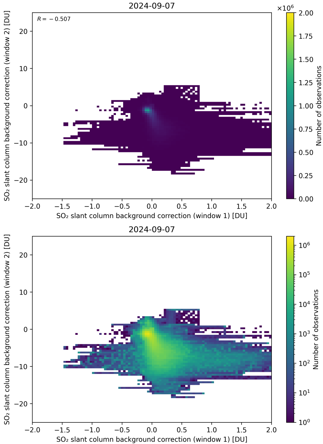
Figure 98: Scatter density plot of “SO 2 slant column background correction (window 1)” against “SO 2 slant column background correction (window 2)” for 2024-09-06 to 2024-09-08.
