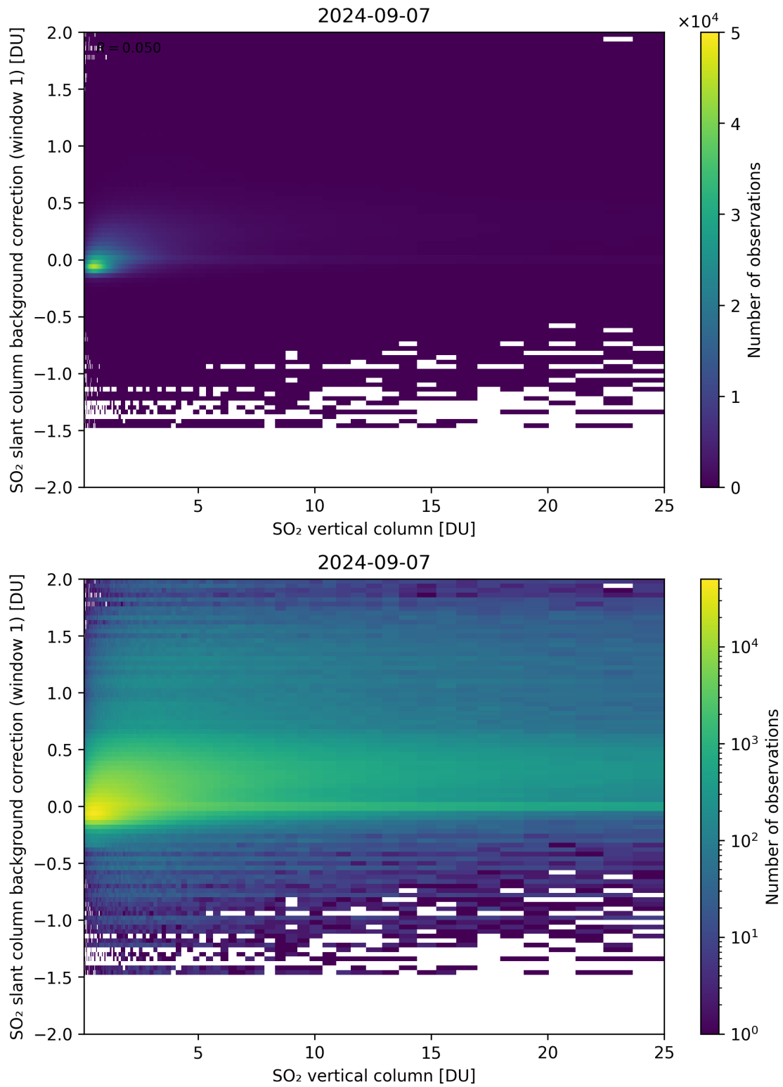
Figure 273: Scatter density plot of “SO 2 vertical column” against “SO 2 slant column background correction (window 1)” for 2024-09-06 to 2024-09-08.
