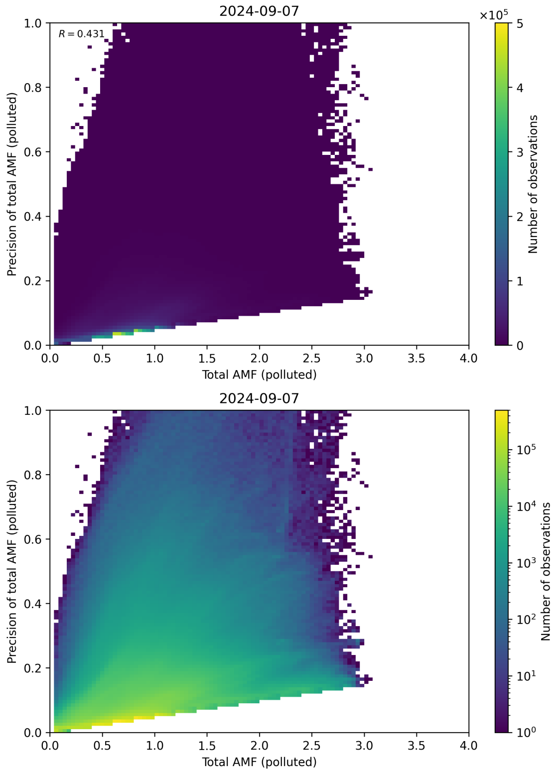
Figure 272: Scatter density plot of “Total AMF (polluted)” against “Precision of total AMF (polluted)” for 2024-09-06 to 2024-09-08.
