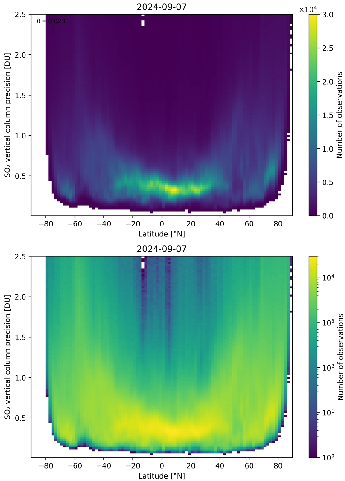
Figure 157: Scatter density plot of “Latitude” against “SO 2 vertical column precision” for 2024-09-06 to 2024-09-08.
