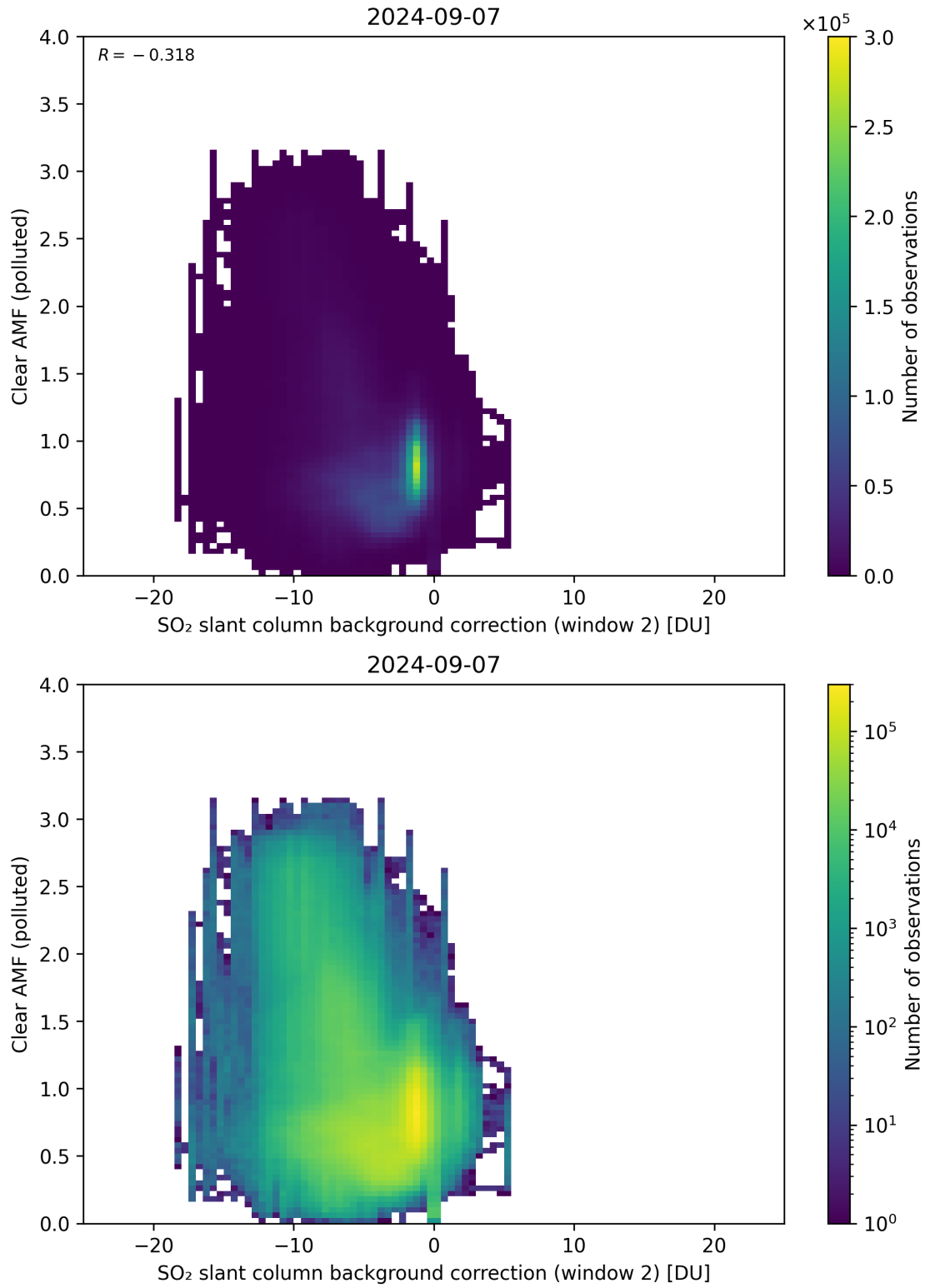
Figure 115: Scatter density plot of “SO 2 slant column background correction (window 2)” against “Clear AMF (polluted)” for 2024-09-06 to 2024-09-08.
