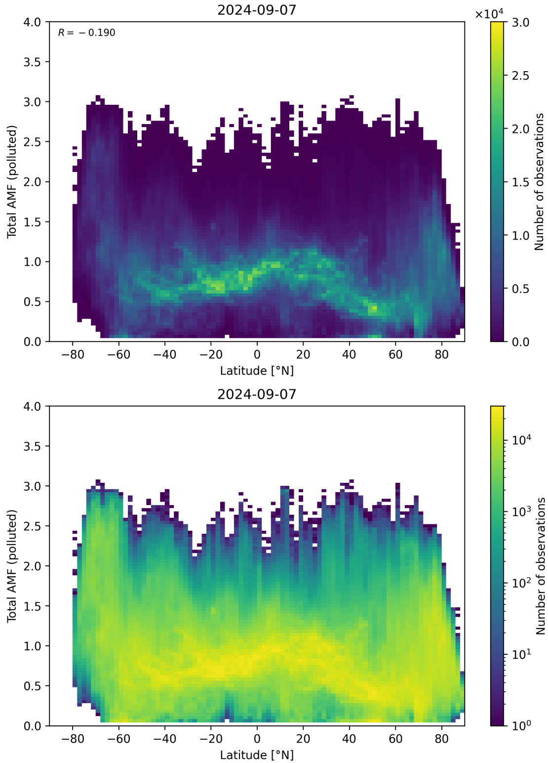
Figure 154: Scatter density plot of “Latitude” against “Total AMF (polluted)” for 2024-09-06 to 2024-09-08.
