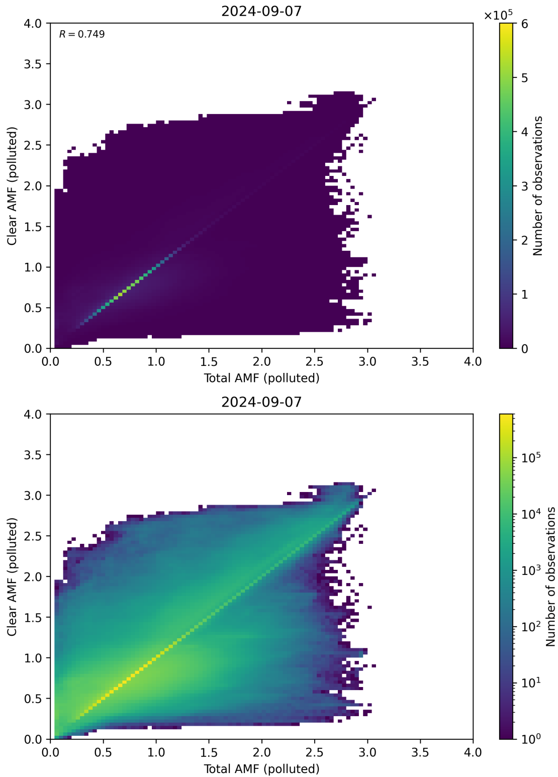
Figure 271: Scatter density plot of “Total AMF (polluted)” against “Clear AMF (polluted)” for 2024-09-06 to 2024-09-08.
