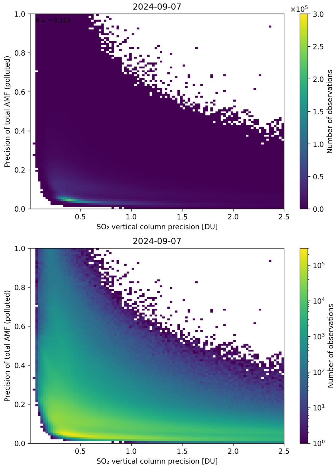
Figure 295: Scatter density plot of “SO 2 vertical column precision” against “Precision of total AMF (polluted)” for 2024-09-06 to 2024-09-08.
