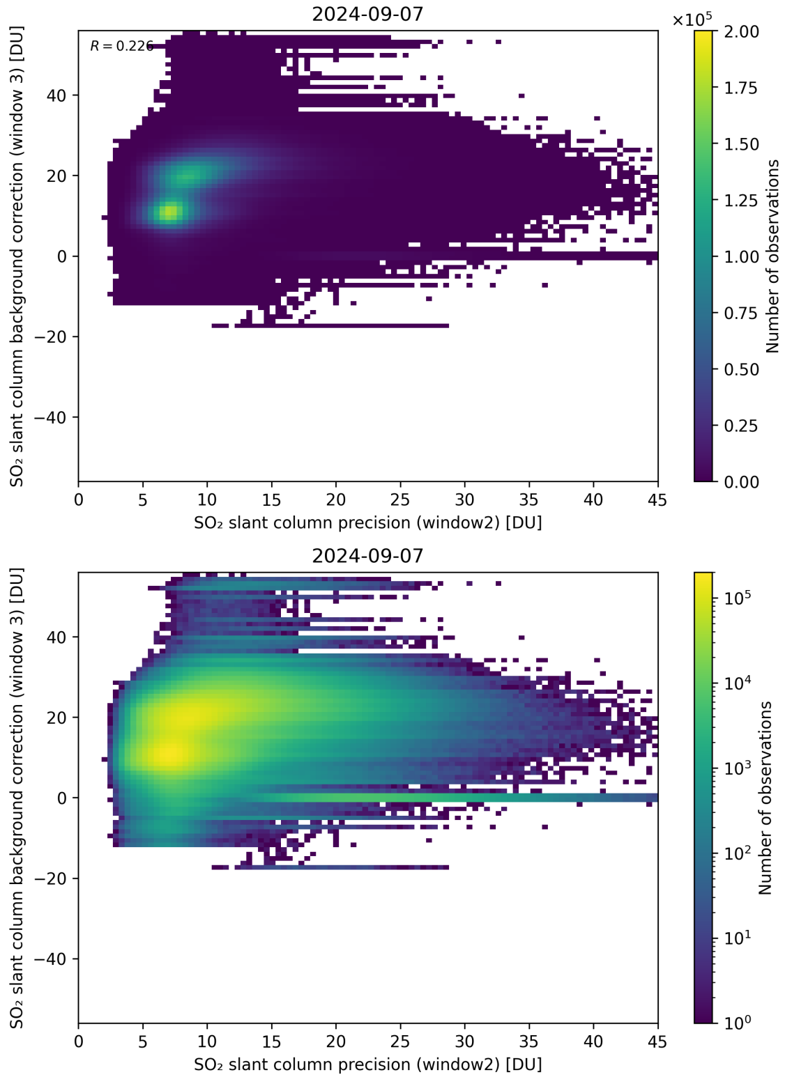
Figure 242: Scatter density plot of “SO 2 slant column precision (window2)” against “SO 2 slant column background correction (window 3)” for 2024-09-06 to 2024-09-08.
