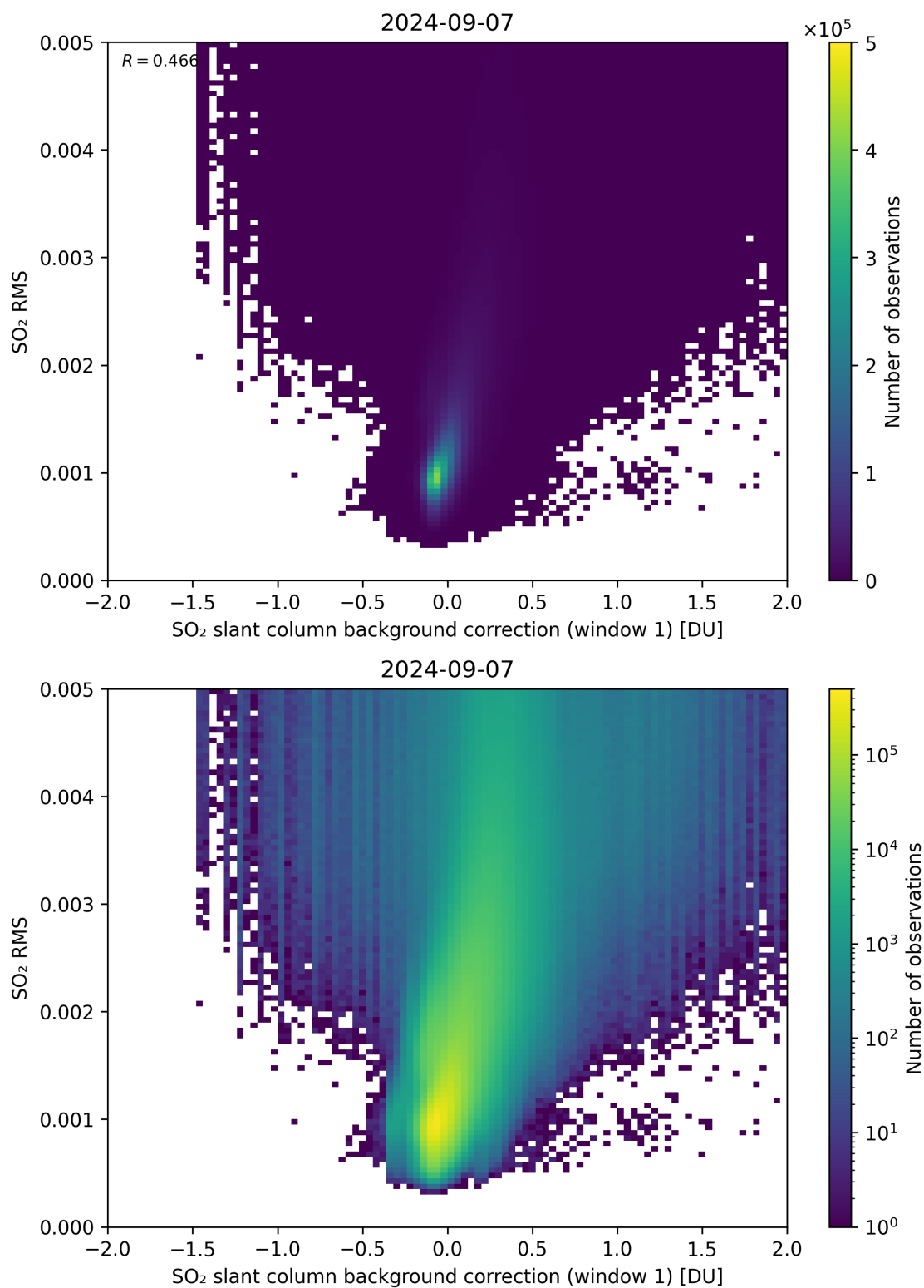
Figure 102: Scatter density plot of “SO 2 slant column background correction (window 1)” against “SO 2 RMS” for 2024-09-06 to 2024-09-08.
