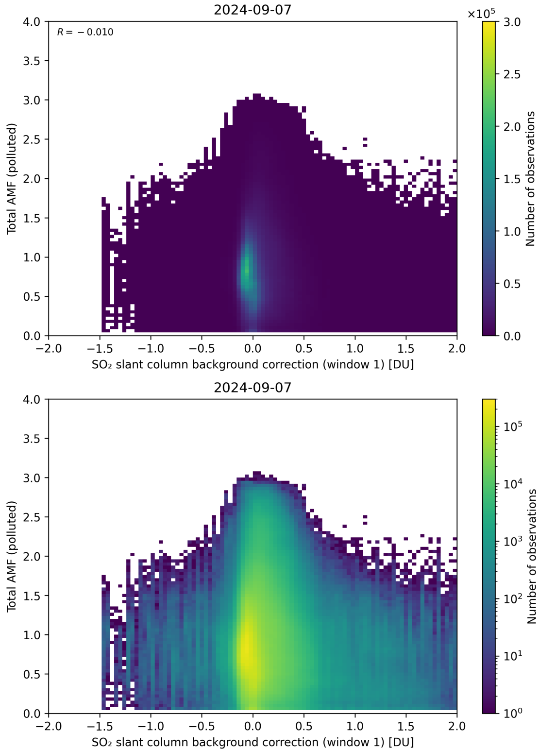
Figure 109: Scatter density plot of “SO 2 slant column background correction (window 1)” against “Total AMF (polluted)” for 2024-09-06 to 2024-09-08.
