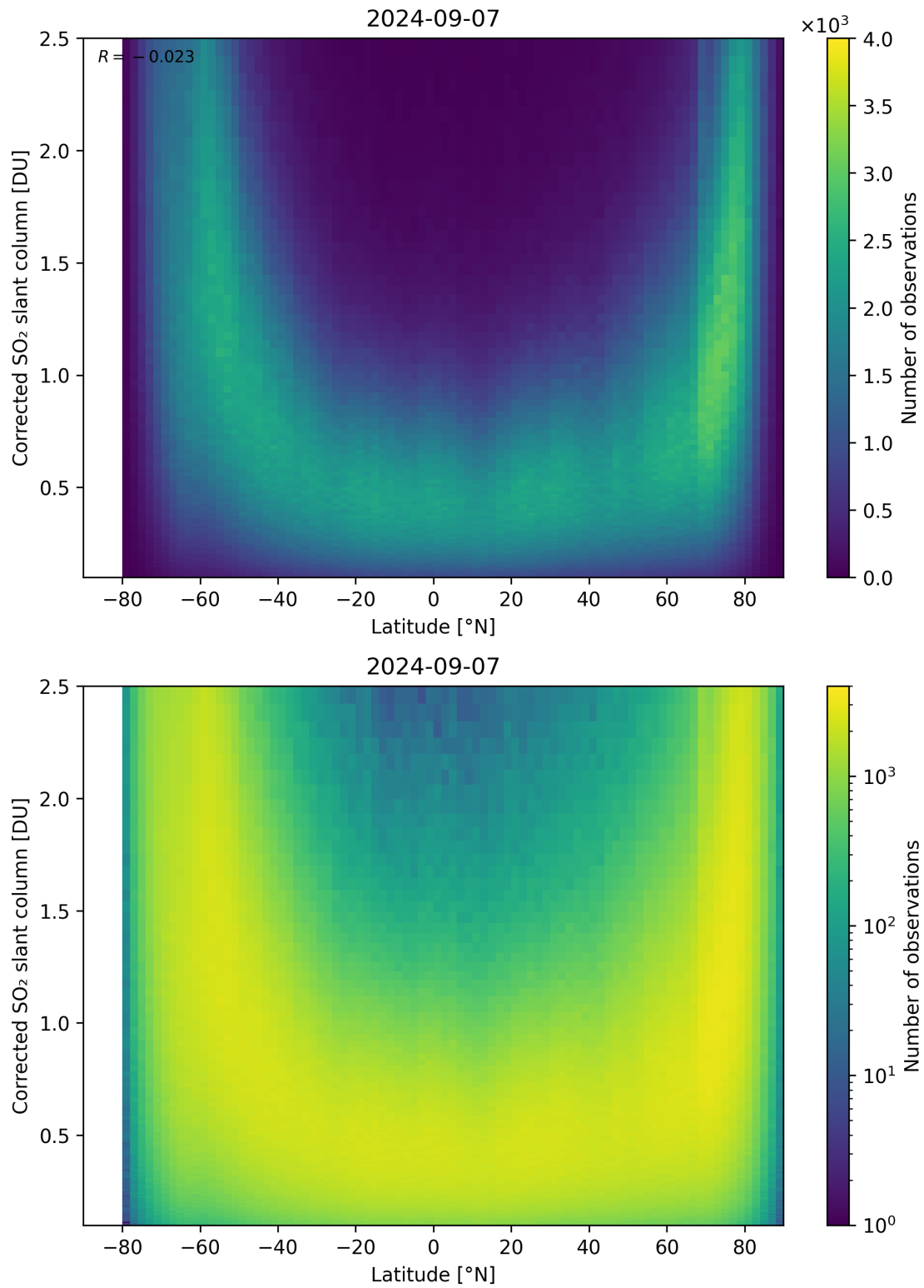
Figure 146: Scatter density plot of “Latitude” against “Corrected SO 2 slant column” for 2024-09-06 to 2024-09-08.
