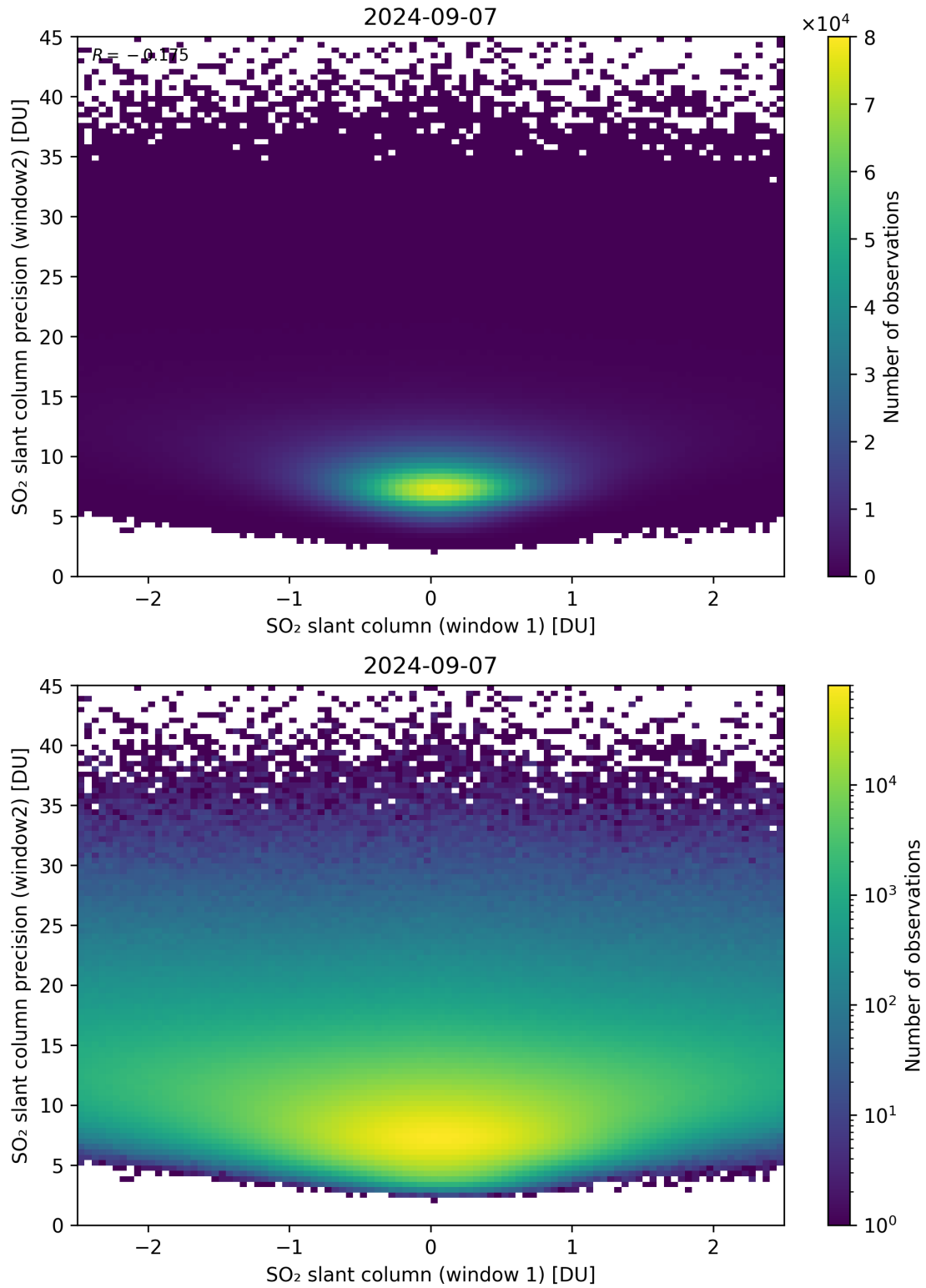
Figure 236: Scatter density plot of “SO 2 slant column (window 1)” against “SO 2 slant column precision (window2)” for 2024-09-06 to 2024-09-08.
