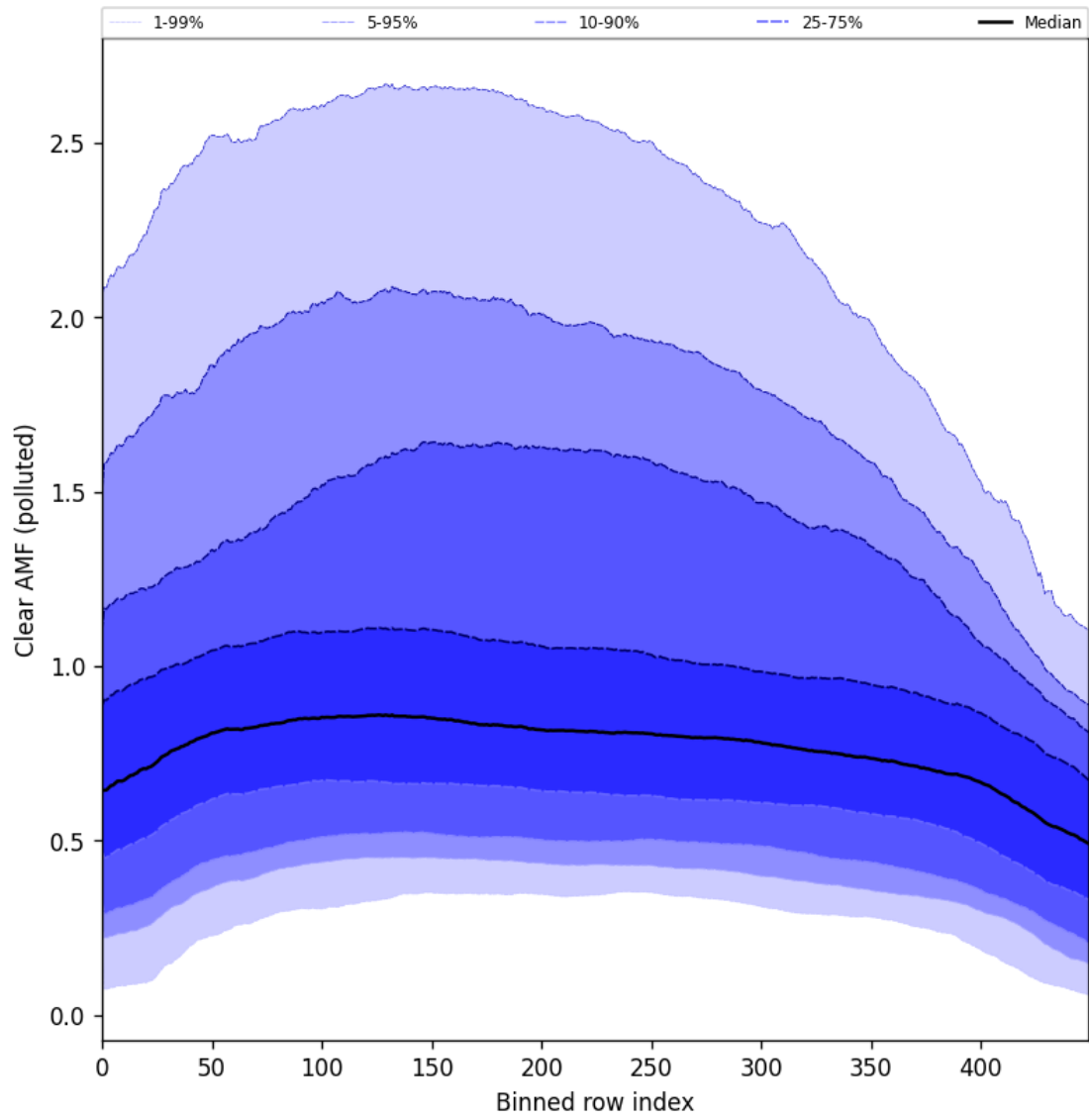
Figure 96: Along track statistics of “Clear AMF (polluted)” for 2024-09-06 to 2024-09-08
