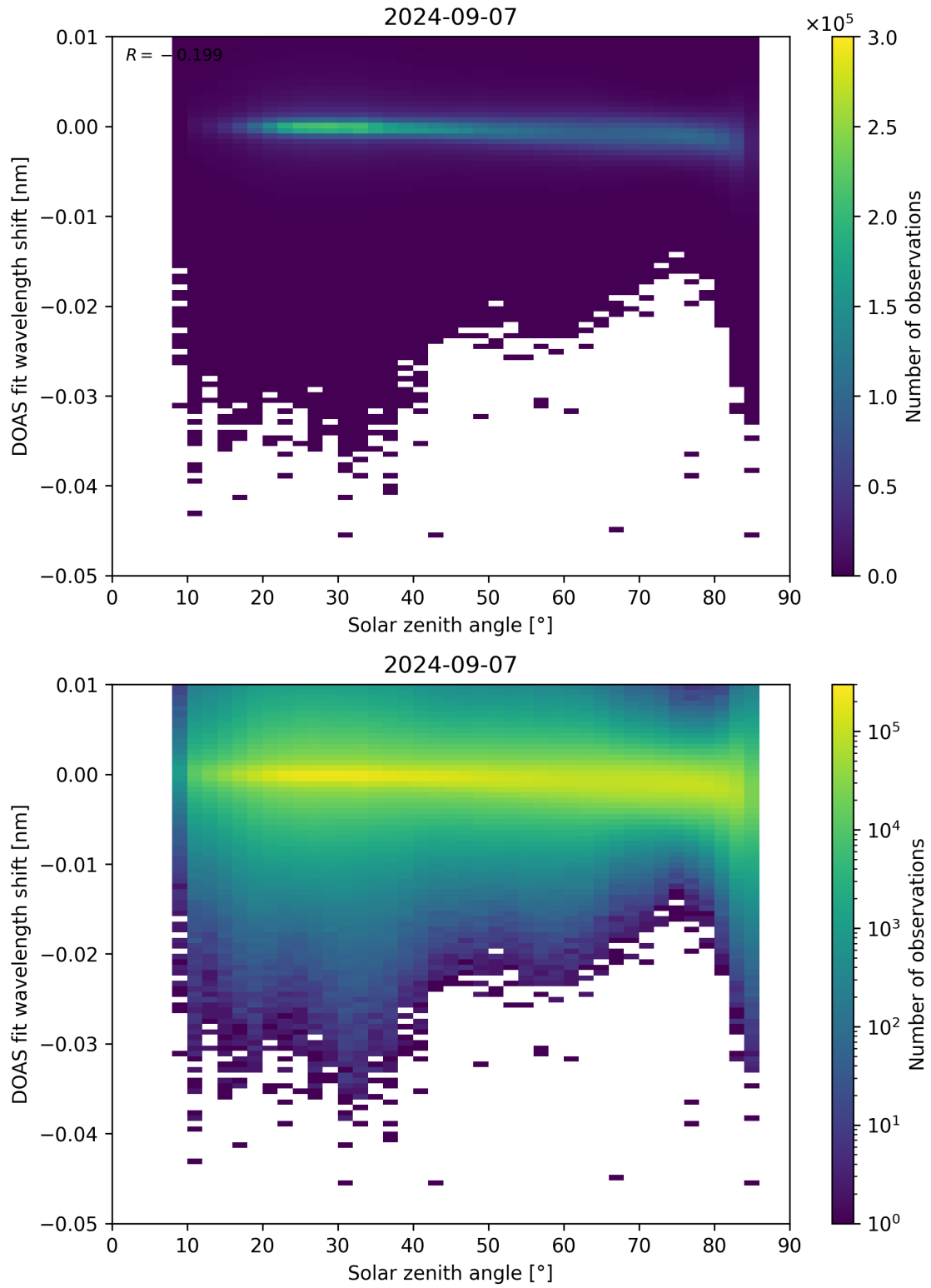
Figure 161: Scatter density plot of “Solar zenith angle” against “DOAS fit wavelength shift” for 2024-09-06 to 2024-09-08.
