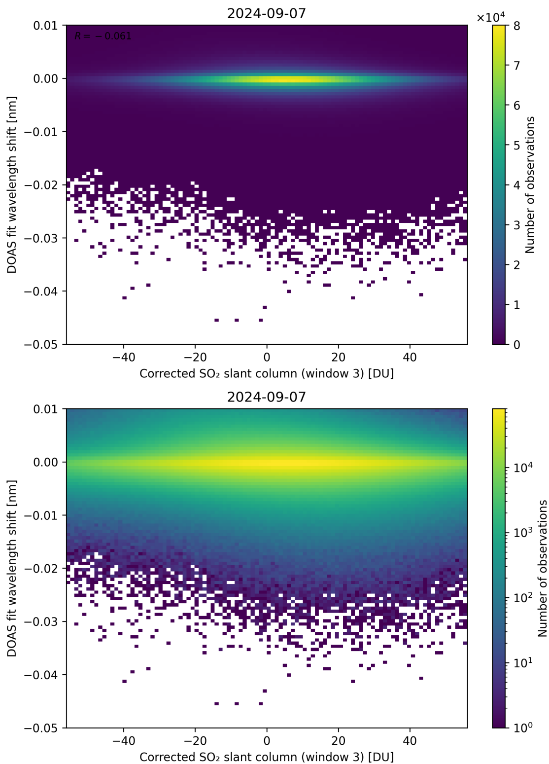
Figure 206: Scatter density plot of “Corrected SO 2 slant column (window 3)” against “DOAS fit wavelength shift” for 2024-09-06 to 2024-09-08.
