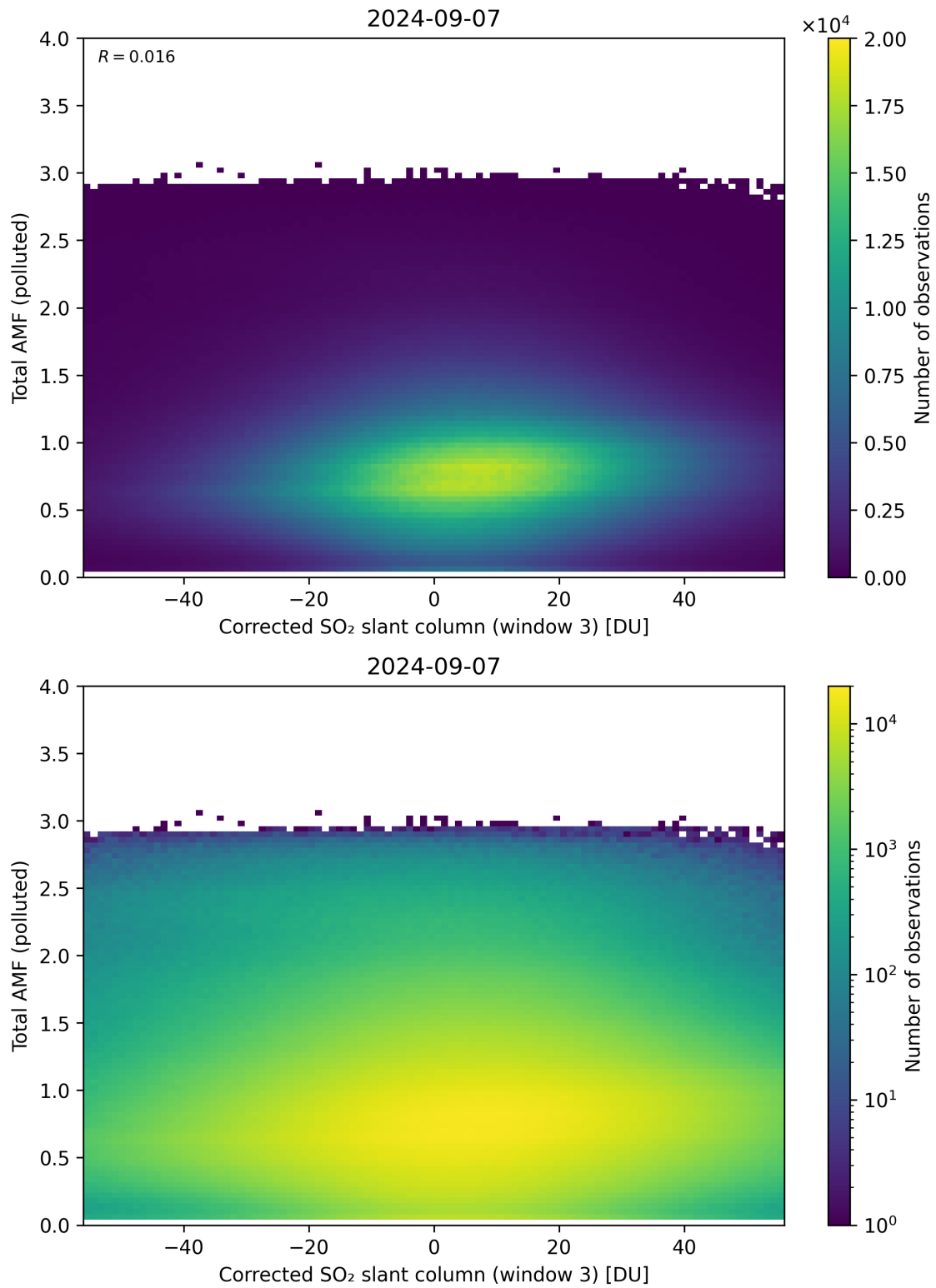
Figure 210: Scatter density plot of “Corrected SO 2 slant column (window 3)” against “Total AMF (polluted)” for 2024-09-06 to 2024-09-08.
