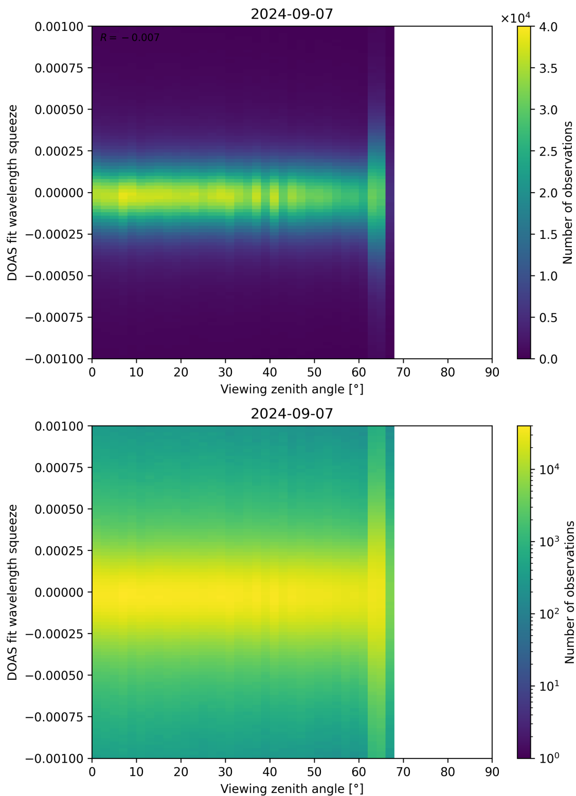
Figure 312: Scatter density plot of “Viewing zenith angle” against “DOAS fit wavelength squeeze” for 2024-09-06 to 2024-09-08.
