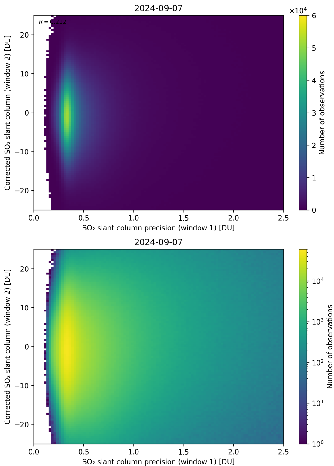
Figure 225: Scatter density plot of “SO 2 slant column precision (window 1)” against “Corrected SO 2 slant column (window 2)” for 2024-09-06 to 2024-09-08.
