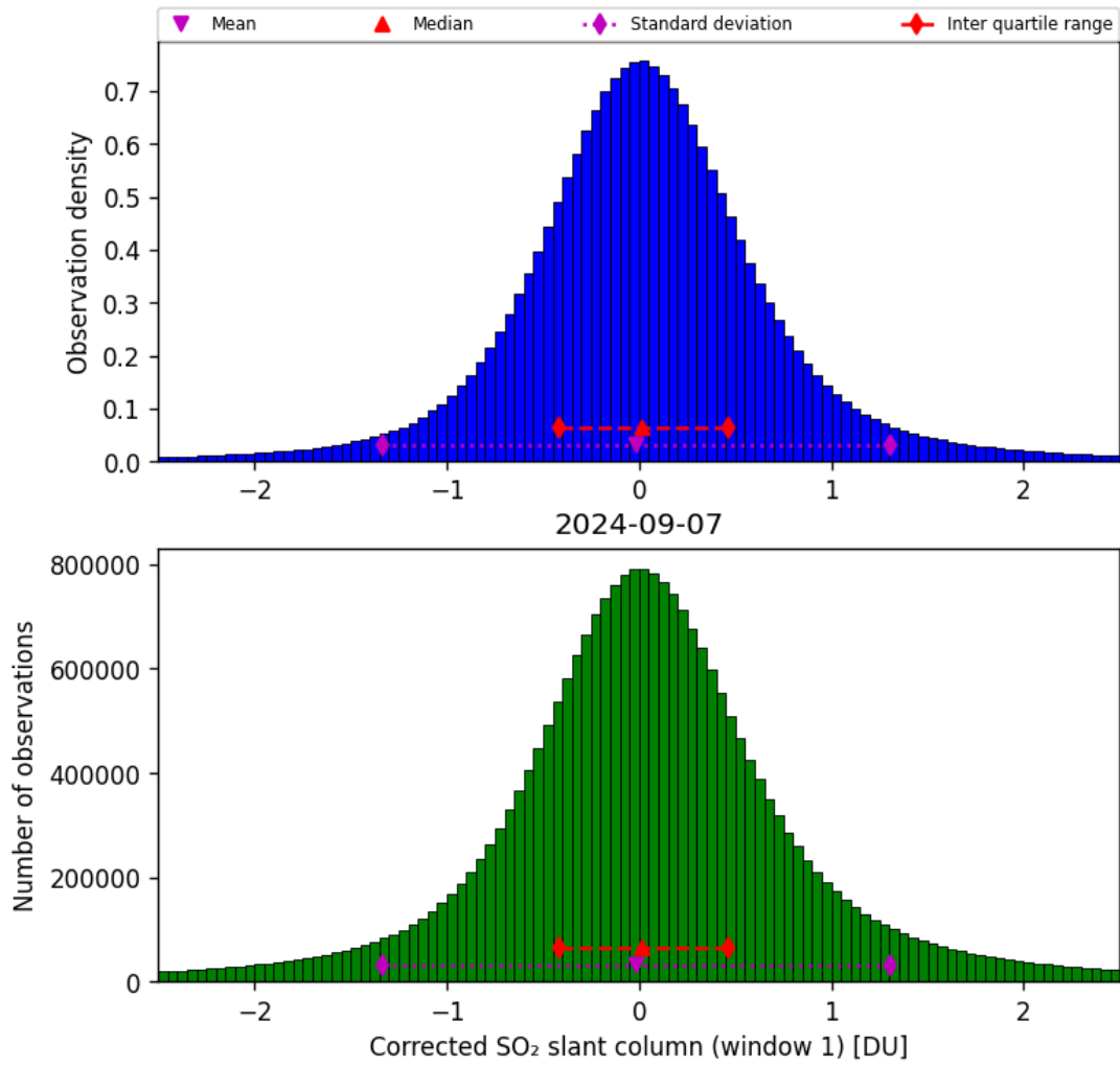
Figure 58: Histogram of “Corrected SO 2 slant column (window 1)” for 2024-09-06 to 2024-09-08
