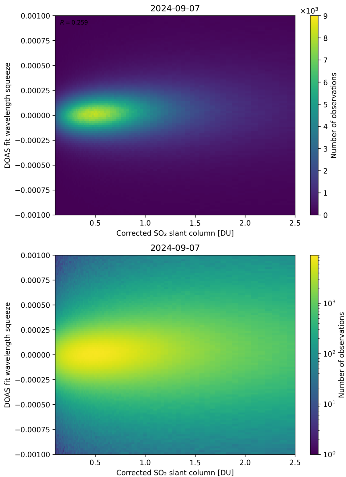
Figure 182: Scatter density plot of “Corrected SO 2 slant column” against “DOAS fit wavelength squeeze” for 2024-09-06 to 2024-09-08.
