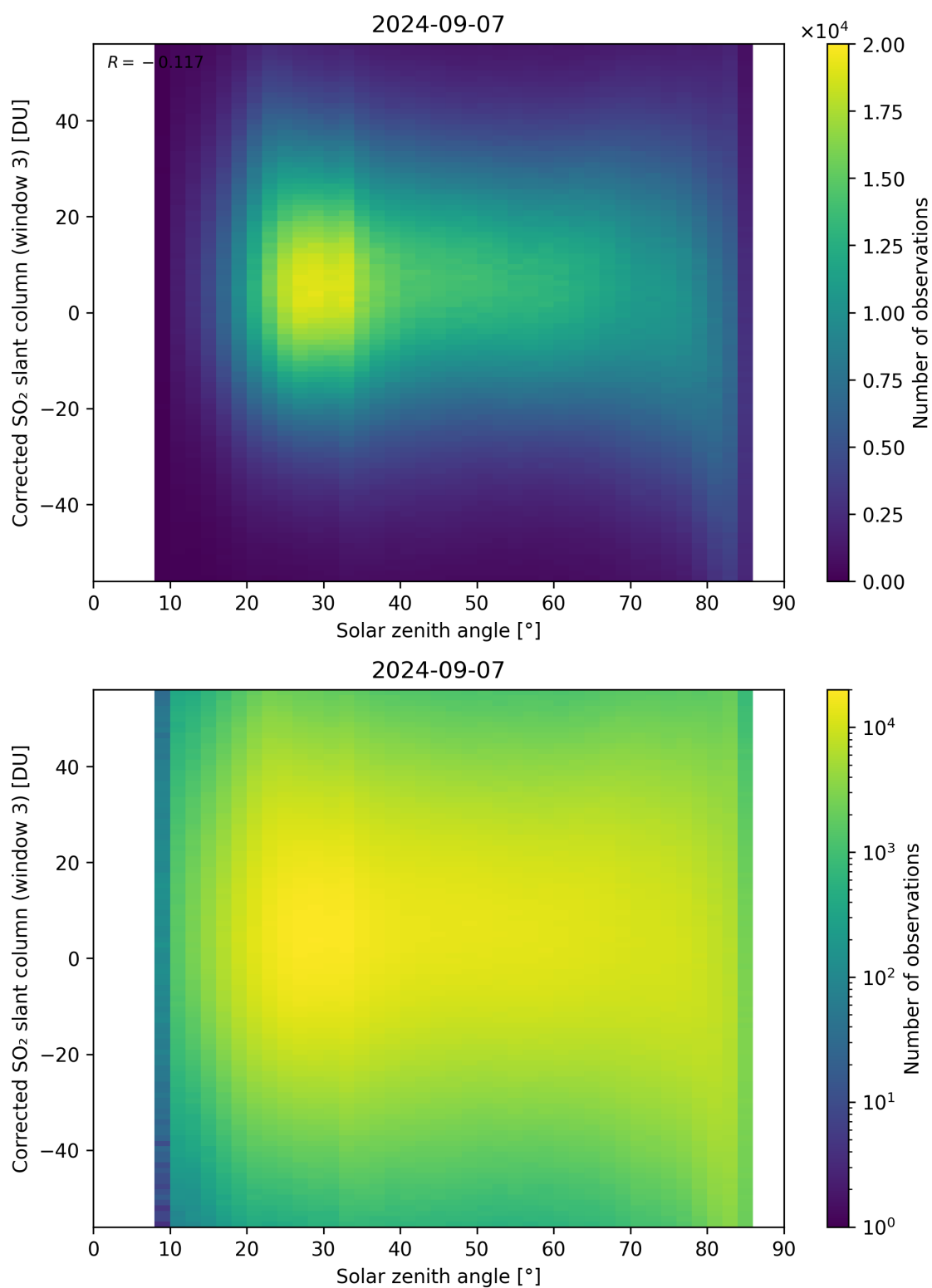
Figure 168: Scatter density plot of “Solar zenith angle” against “Corrected SO 2 slant column (window 3)” for 2024-09-06 to 2024-09-08.
