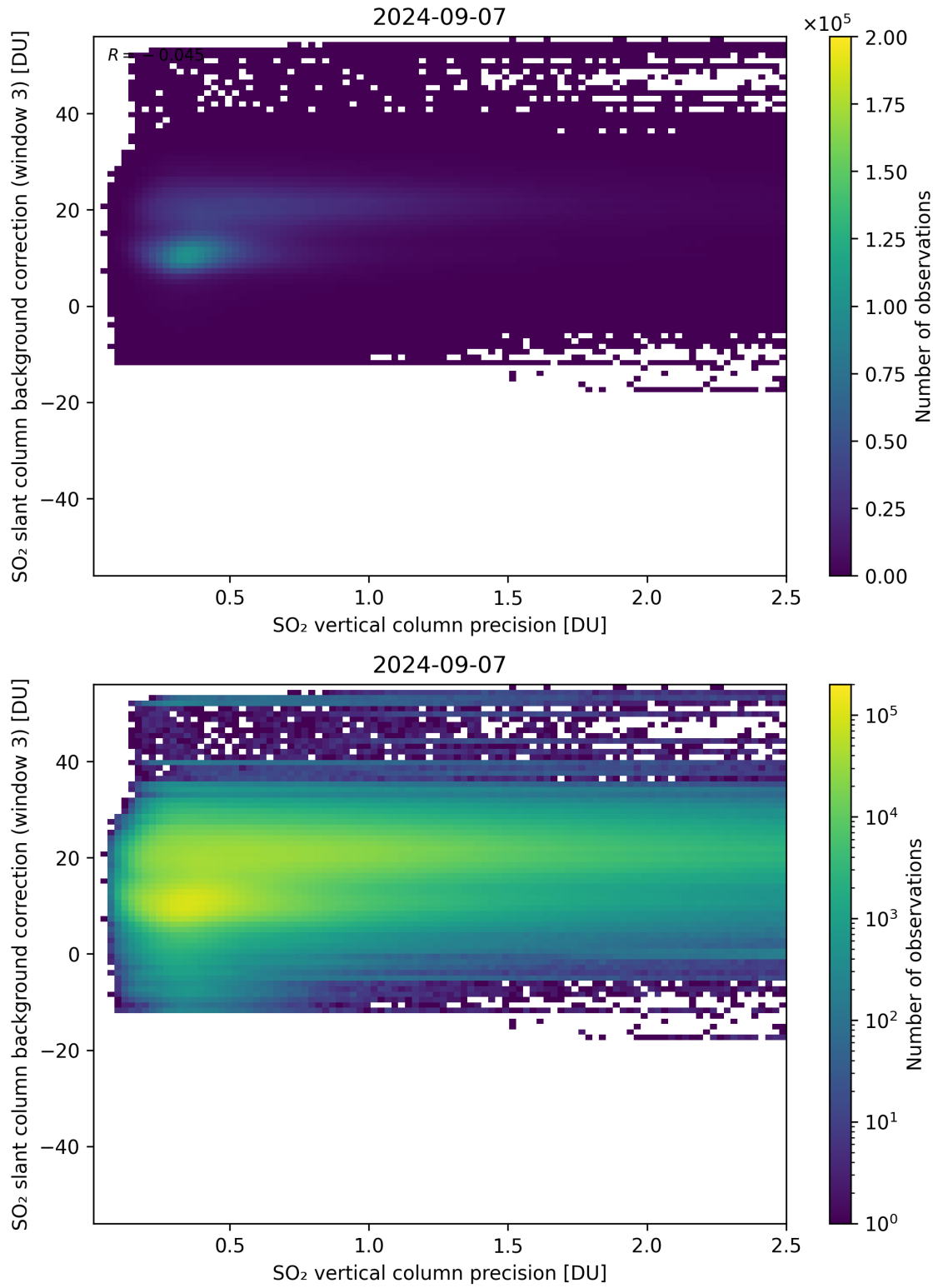
Figure 281: Scatter density plot of “SO 2 vertical column precision” against “SO 2 slant column background correction (window 3)” for 2024-09-06 to 2024-09-08.
