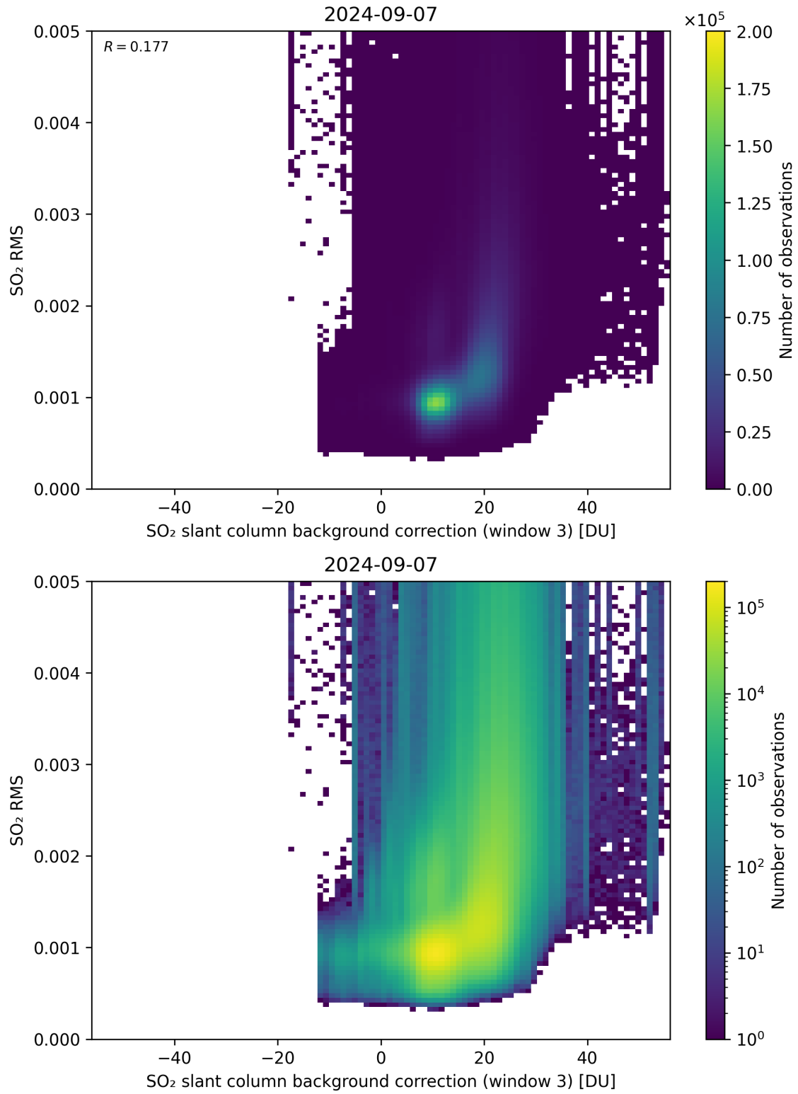
Figure 123: Scatter density plot of “SO 2 slant column background correction (window 3)” against “SO 2 RMS” for 2024-09-06 to 2024-09-08.
