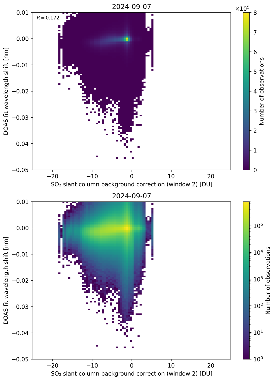
Figure 112: Scatter density plot of “SO 2 slant column background correction (window 2)” against “DOAS fit wavelength shift” for 2024-09-06 to 2024-09-08.
