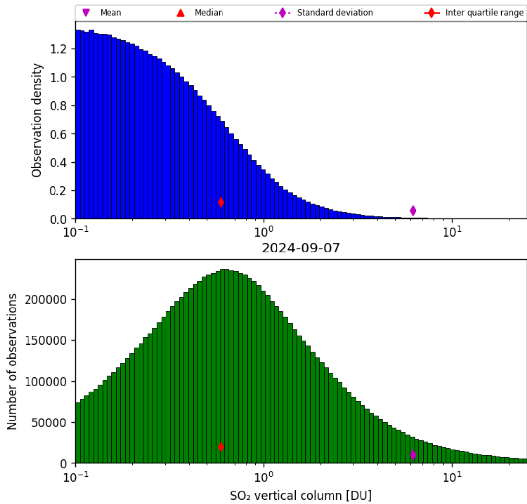
Figure 53: Histogram of “SO 2 vertical column” for 2024-09-06 to 2024-09-08
