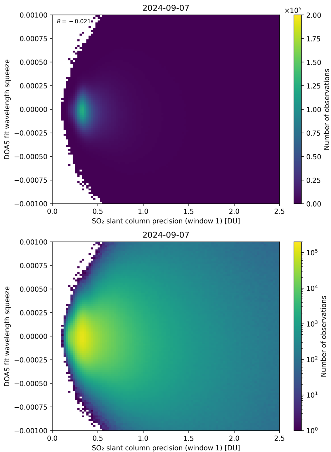
Figure 222: Scatter density plot of “SO 2 slant column precision (window 1)” against “DOAS fit wavelength squeeze” for 2024-09-06 to 2024-09-08.
