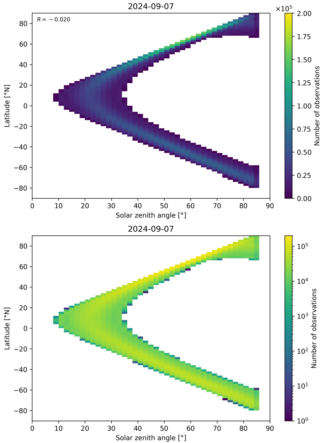
Figure 164: Scatter density plot of “Solar zenith angle” against “Latitude” for 2024-09-06 to 2024-09-08.
