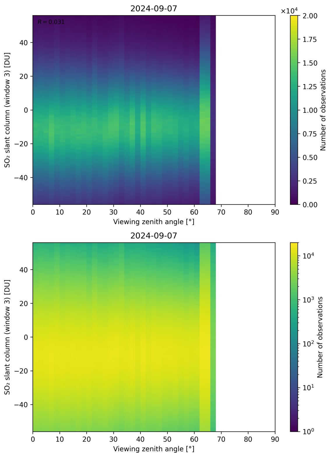
Figure 323: Scatter density plot of “Viewing zenith angle” against “SO 2 slant column (window 3)” for 2024-09-06 to 2024-09-08.
