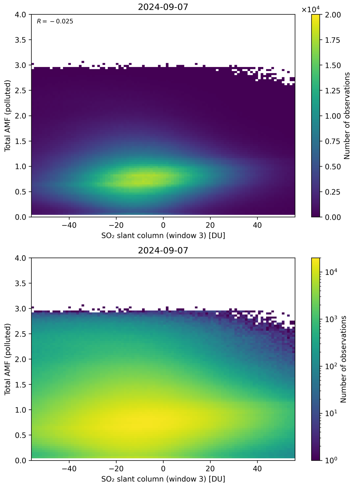
Figure 268: Scatter density plot of “SO 2 slant column (window 3)” against “Total AMF (polluted)” for 2024-09-06 to 2024-09-08.
