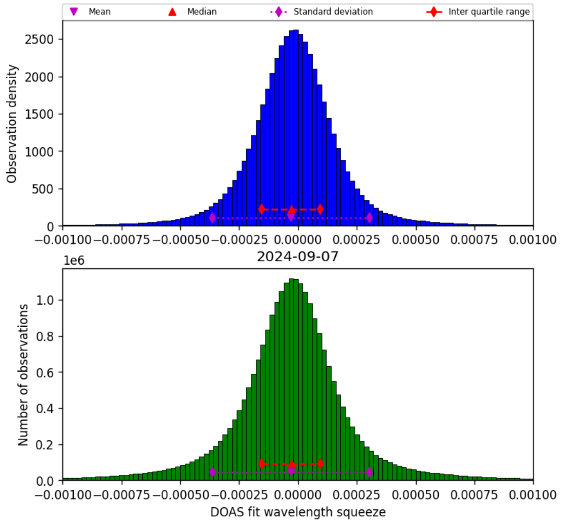
Figure 69: Histogram of “DOAS fit wavelength squeeze” for 2024-09-06 to 2024-09-08
