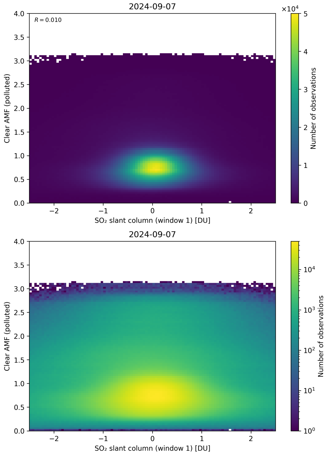
Figure 232: Scatter density plot of “SO 2 slant column (window 1)” against “Clear AMF (polluted)” for 2024-09-06 to 2024-09-08.
