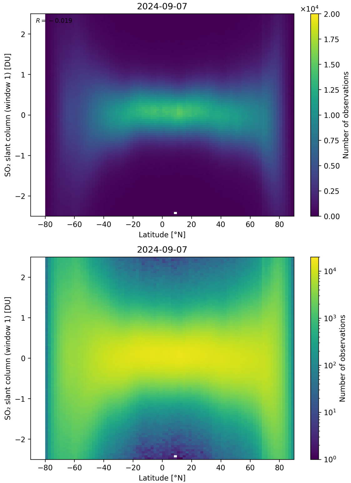
Figure 149: Scatter density plot of “Latitude” against “SO 2 slant column (window 1)” for 2024-09-06 to 2024-09-08.
