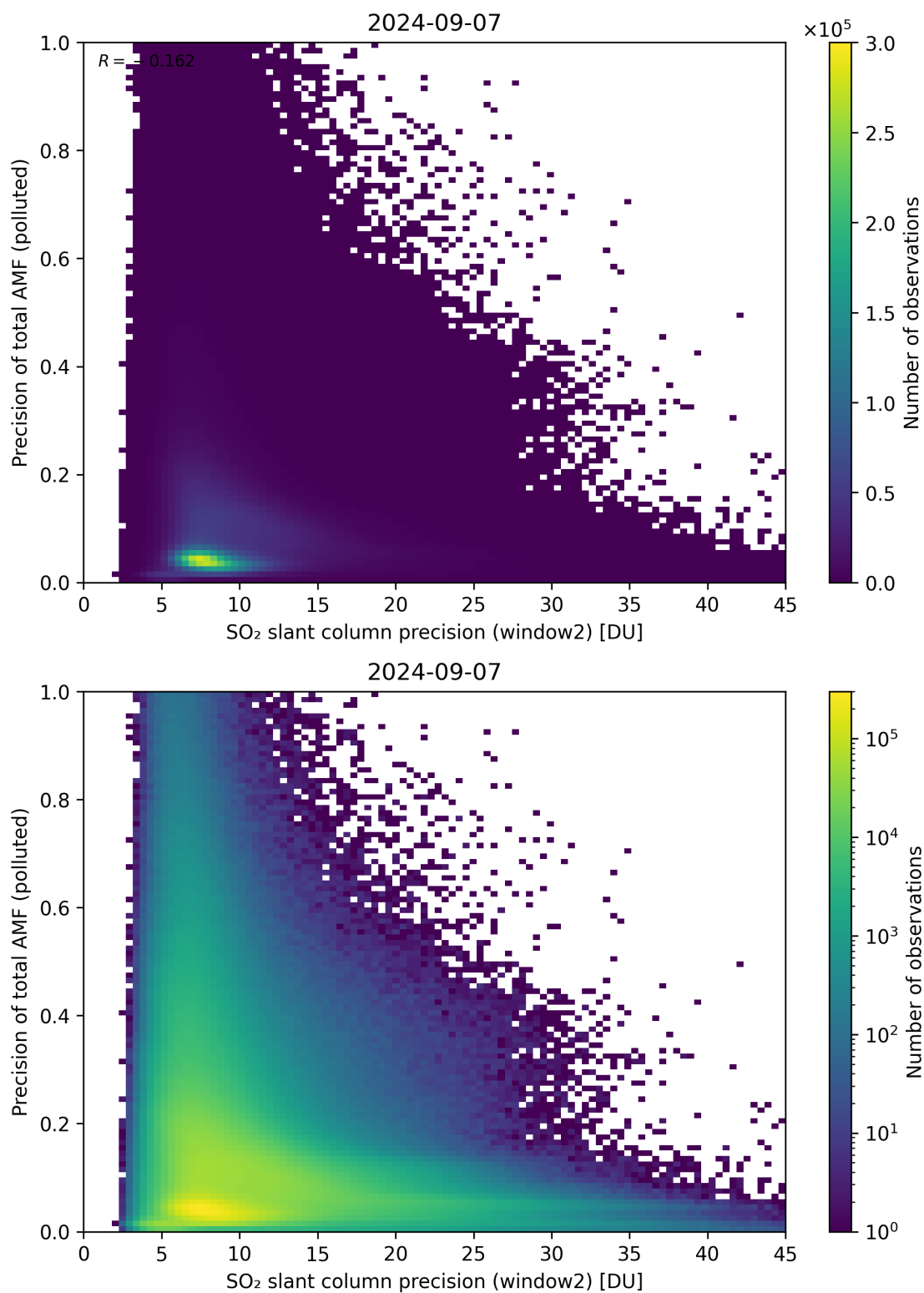
Figure 252: Scatter density plot of “SO 2 slant column precision (window2)” against “Precision of total AMF (polluted)” for 2024-09-06 to 2024-09-08.
