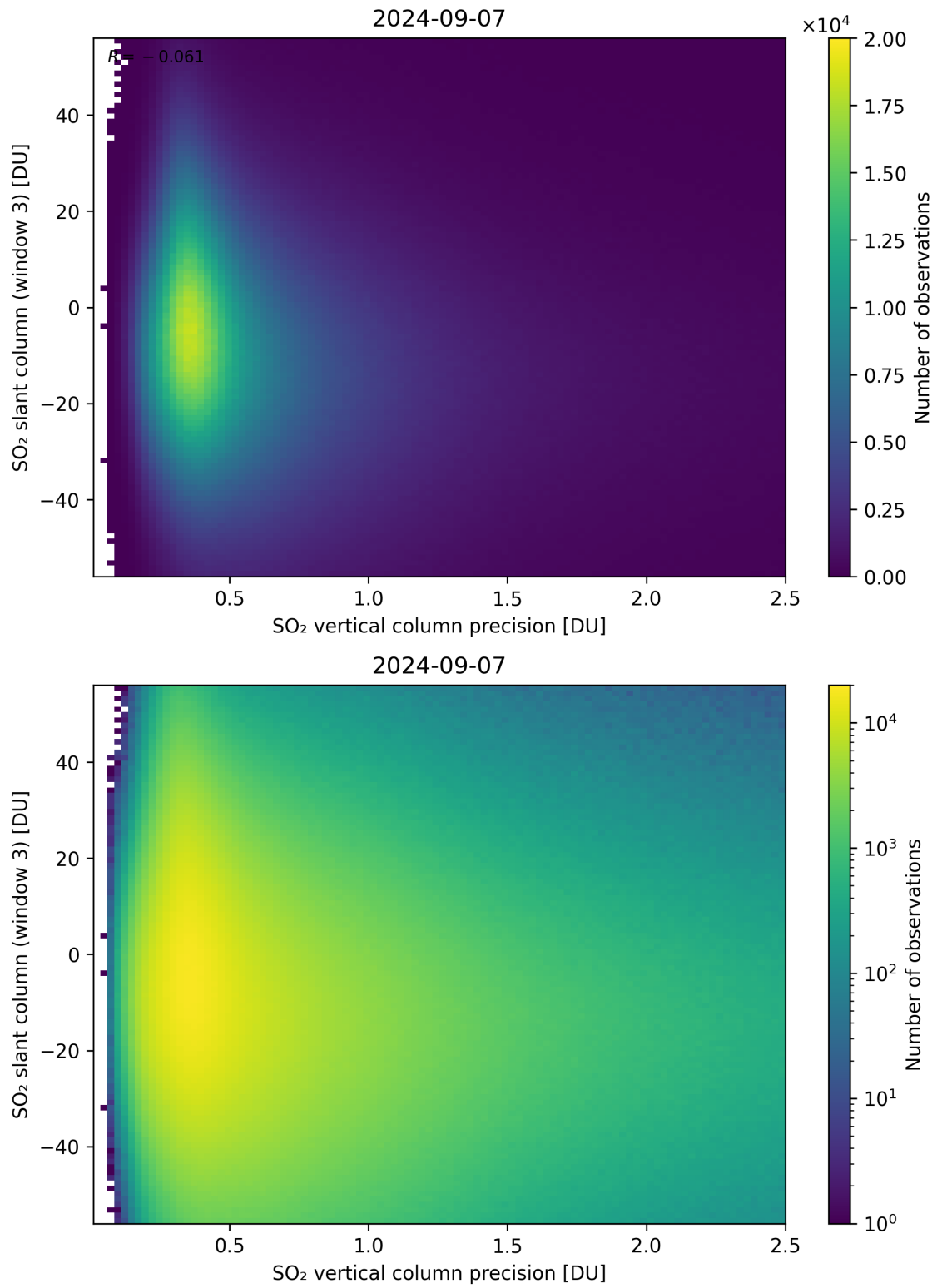
Figure 292: Scatter density plot of “SO 2 vertical column precision” against “SO 2 slant column (window 3)” for 2024-09-06 to 2024-09-08.
