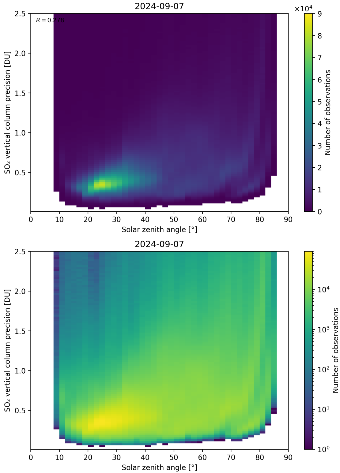
Figure 177: Scatter density plot of “Solar zenith angle” against “SO 2 vertical column precision” for 2024-09-06 to 2024-09-08.
