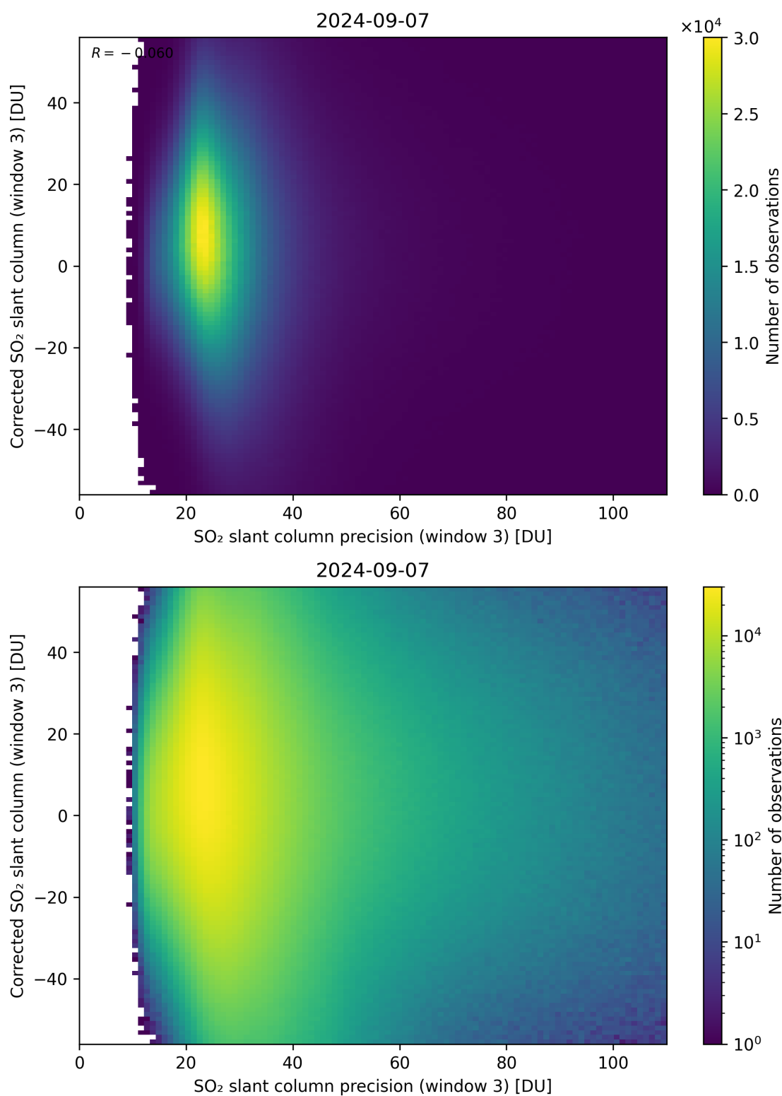
Figure 262: Scatter density plot of “SO 2 slant column precision (window 3)” against “Corrected SO 2 slant column (window 3)” for 2024-09-06 to 2024-09-08.
