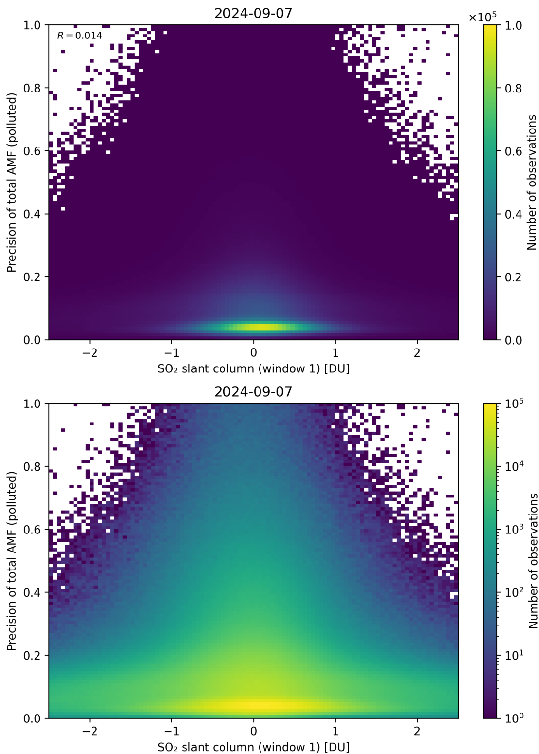
Figure 240: Scatter density plot of “SO 2 slant column (window 1)” against “Precision of total AMF (polluted)” for 2024-09-06 to 2024-09-08.
