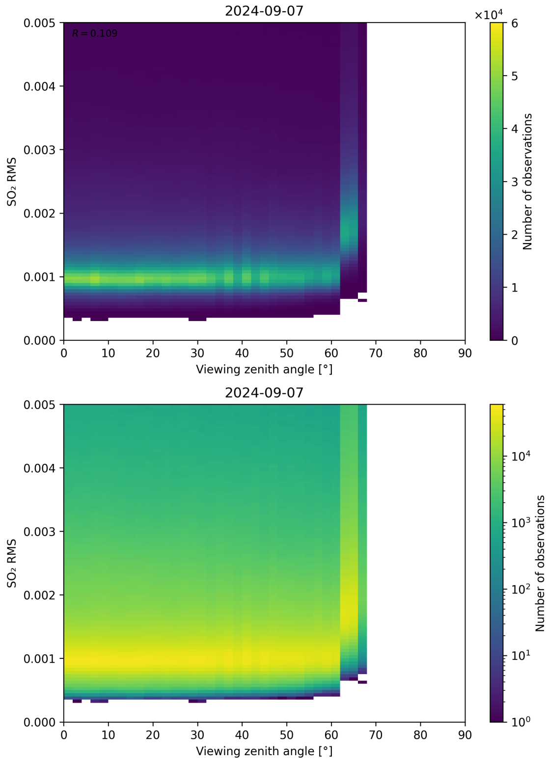
Figure 313: Scatter density plot of “Viewing zenith angle” against “SO 2 RMS” for 2024-09-06 to 2024-09-08.
