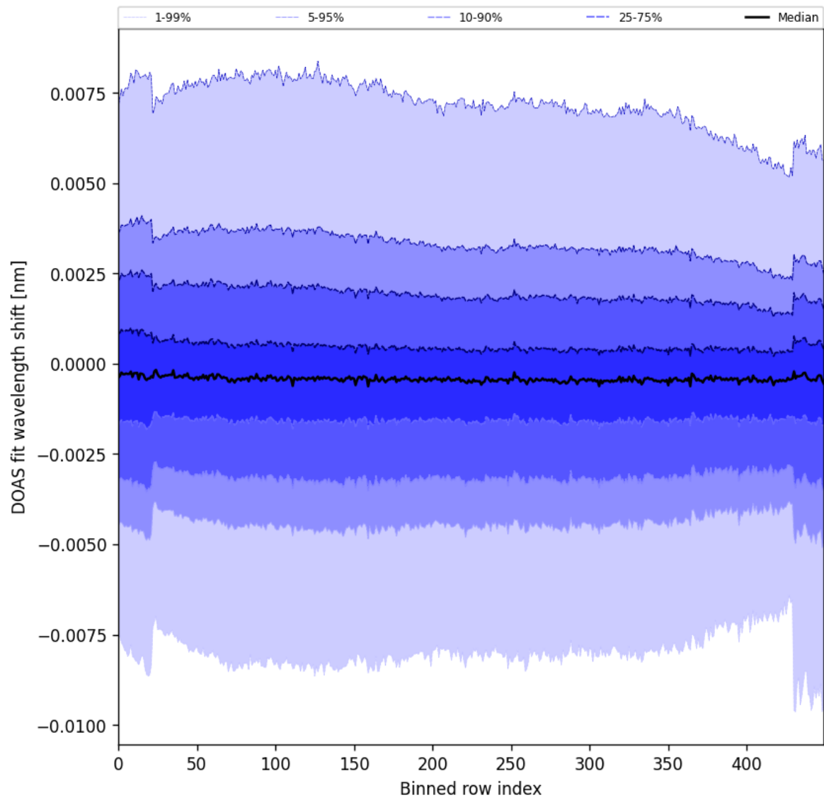
Figure 91: Along track statistics of “DOAS fit wavelength shift” for 2024-09-06 to 2024-09-08
