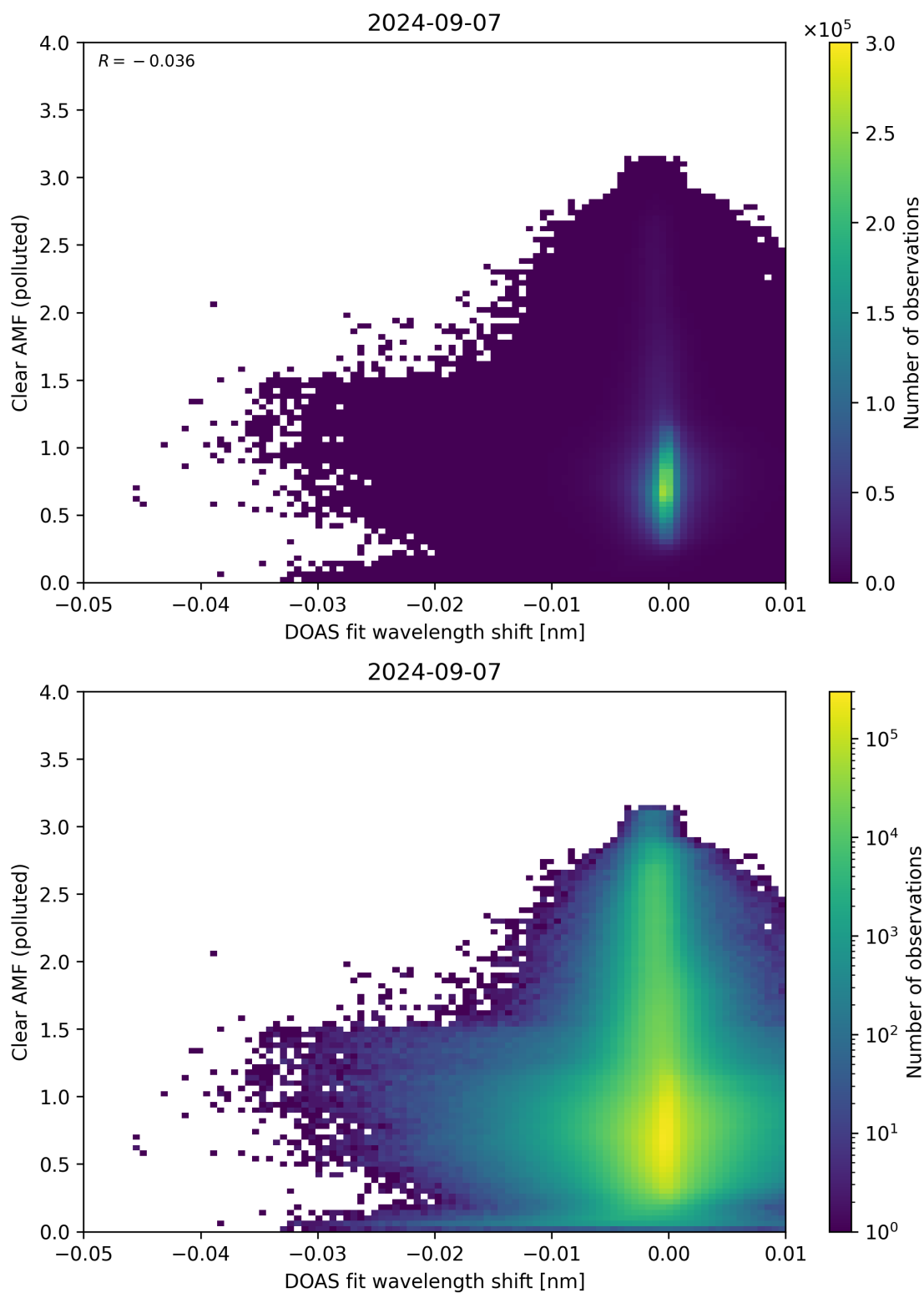
Figure 129: Scatter density plot of “DOAS fit wavelength shift” against “Clear AMF (polluted)” for 2024-09-06 to 2024-09-08.
