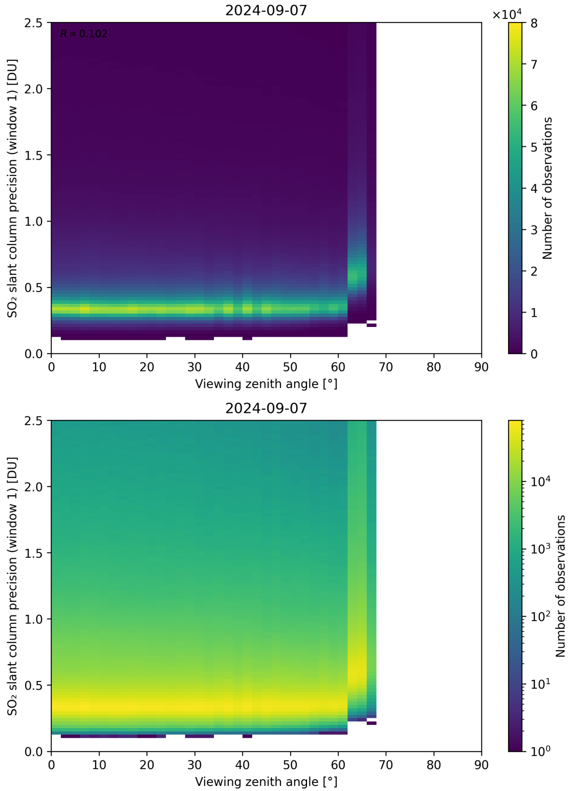
Figure 321: Scatter density plot of “Viewing zenith angle” against “SO 2 slant column precision (window 1)” for 2024-09-06 to 2024-09-08.
