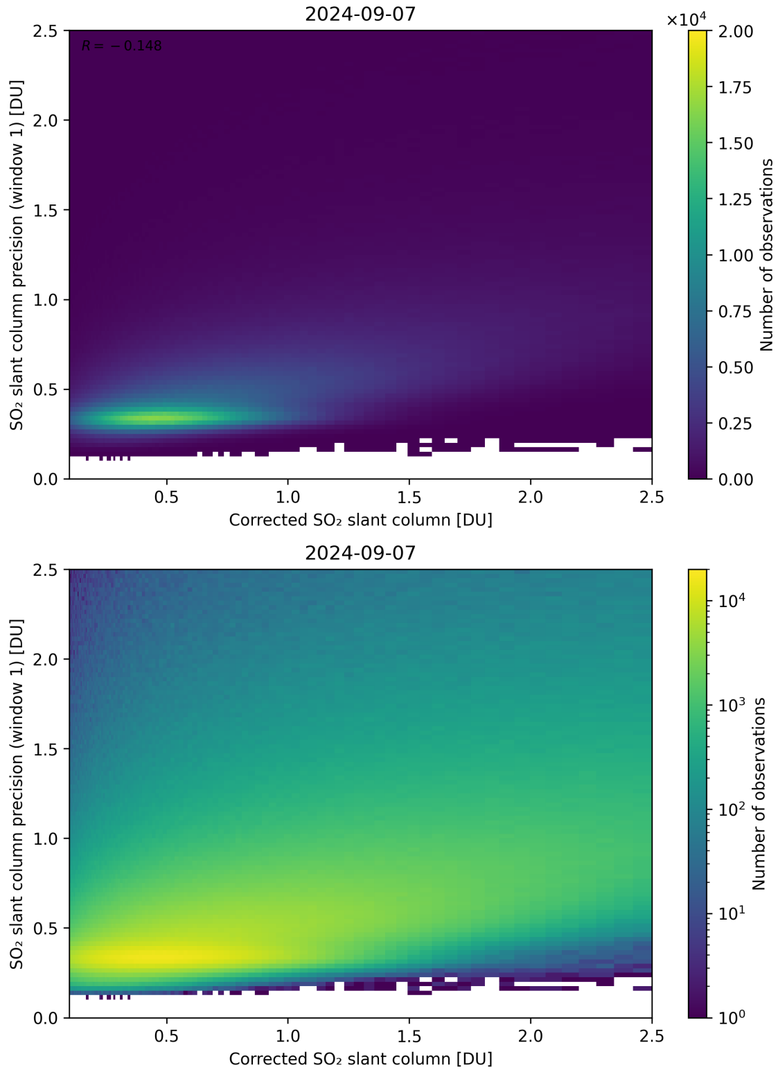
Figure 188: Scatter density plot of “Corrected SO 2 slant column” against “SO 2 slant column precision (window 1)” for 2024-09-06 to 2024-09-08.
