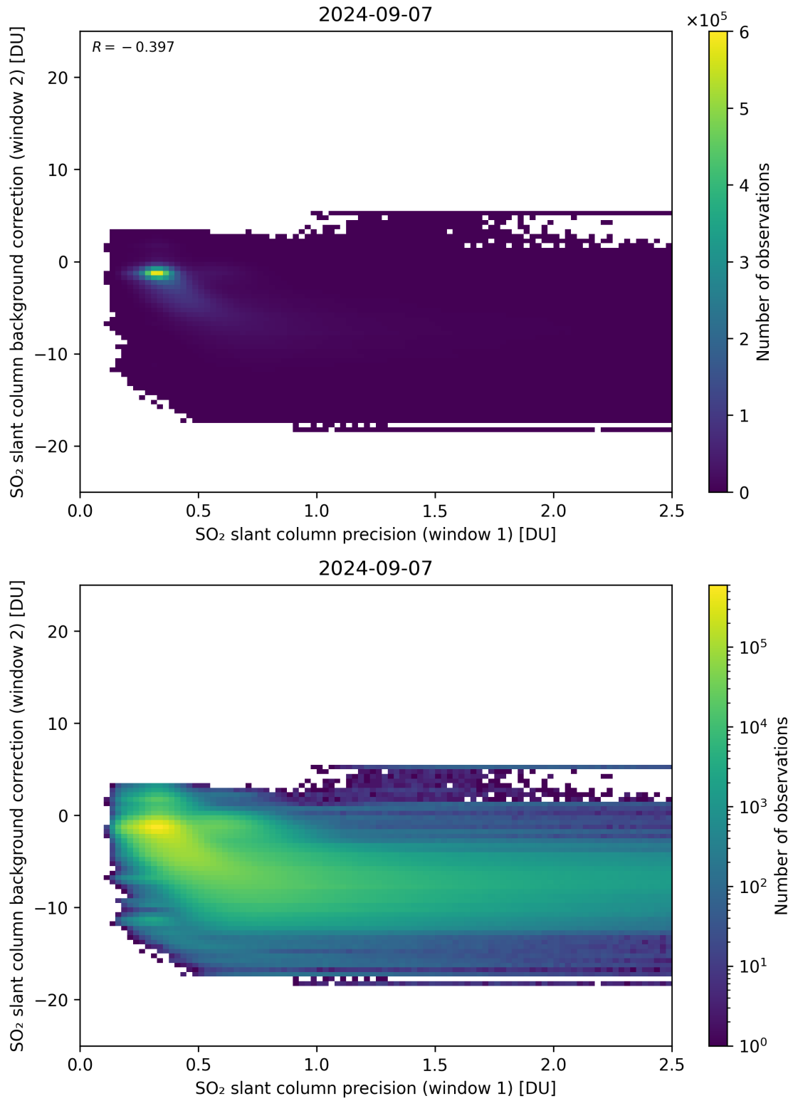
Figure 219: Scatter density plot of “SO 2 slant column precision (window 1)” against “SO 2 slant column background correction (window 2)” for 2024-09-06 to 2024-09-08.
