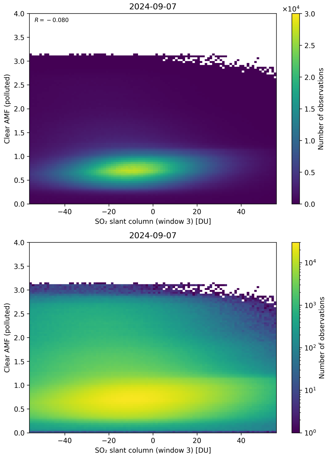
Figure 265: Scatter density plot of “SO 2 slant column (window 3)” against “Clear AMF (polluted)” for 2024-09-06 to 2024-09-08.
