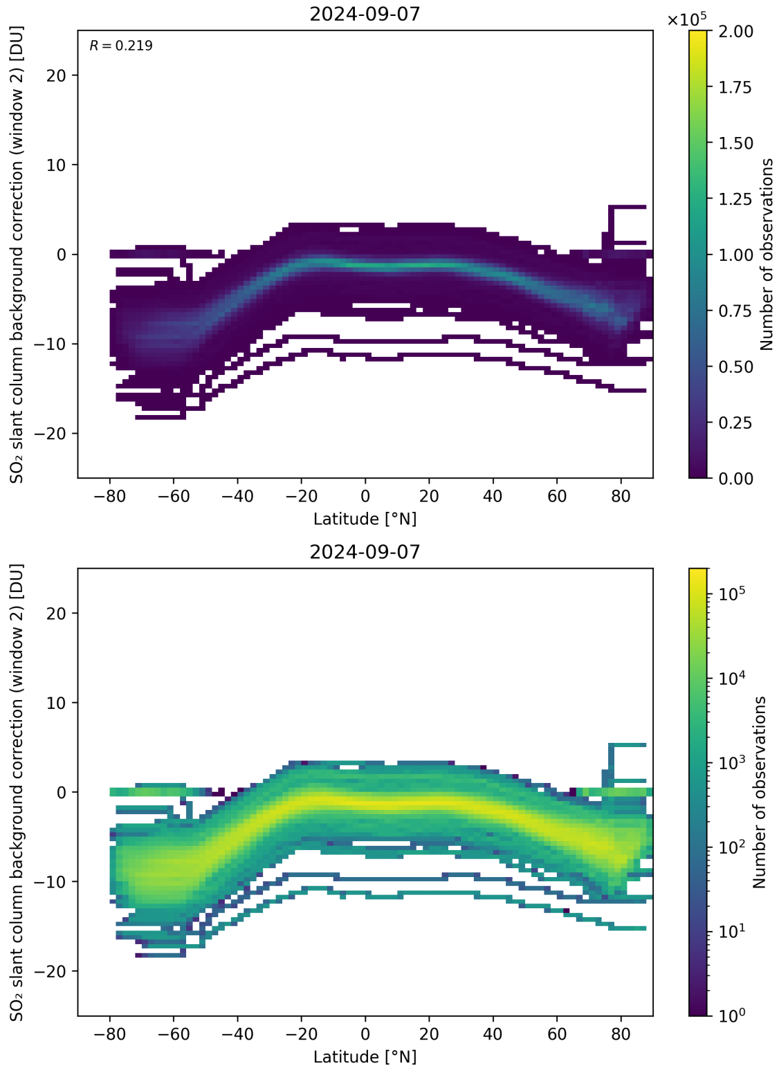
Figure 140: Scatter density plot of “Latitude” against “SO 2 slant column background correction (window 2)” for 2024-09-06 to 2024-09-08.
