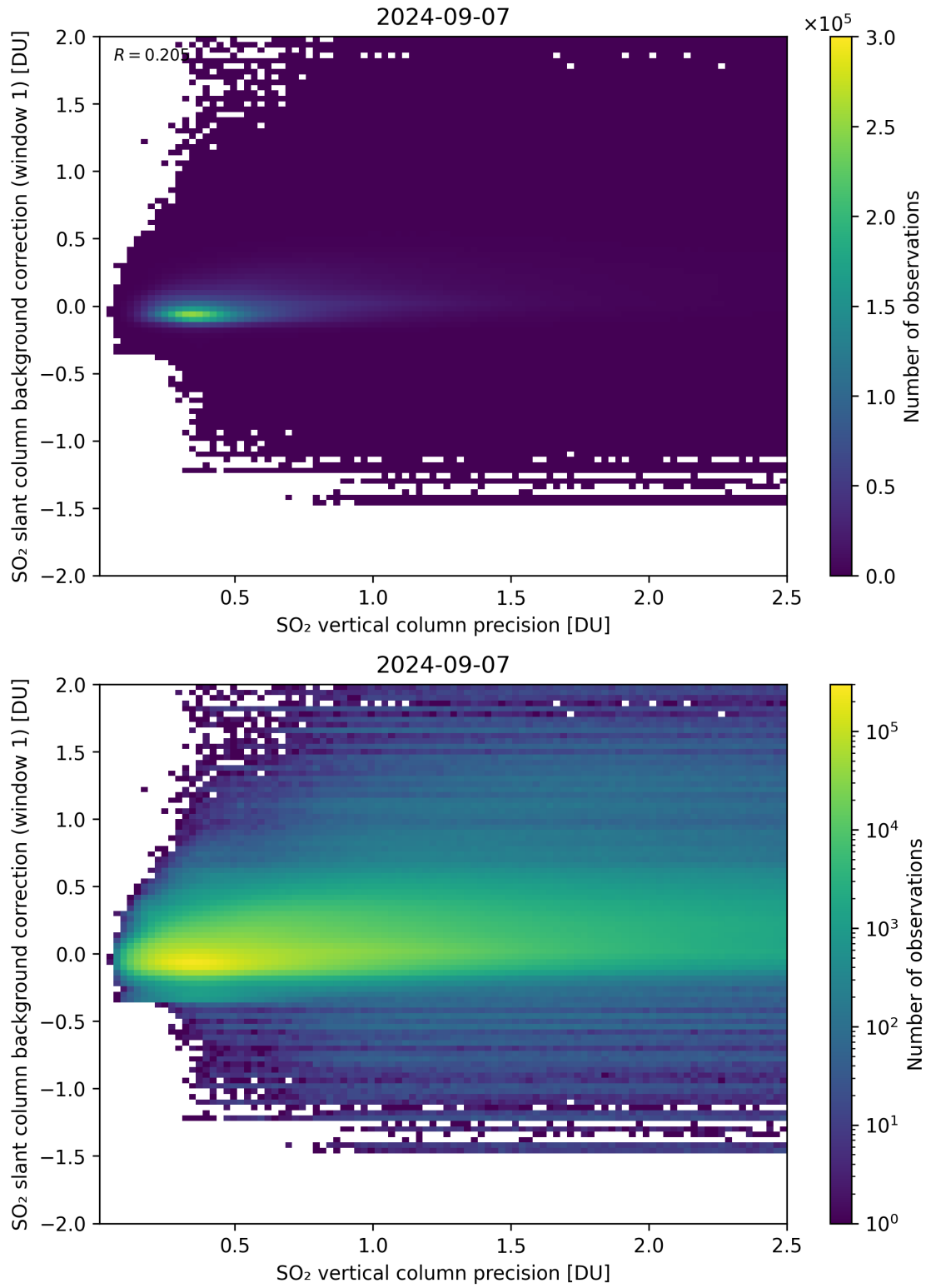
Figure 279: Scatter density plot of “SO 2 vertical column precision” against “SO 2 slant column background correction (window 1)” for 2024-09-06 to 2024-09-08.
