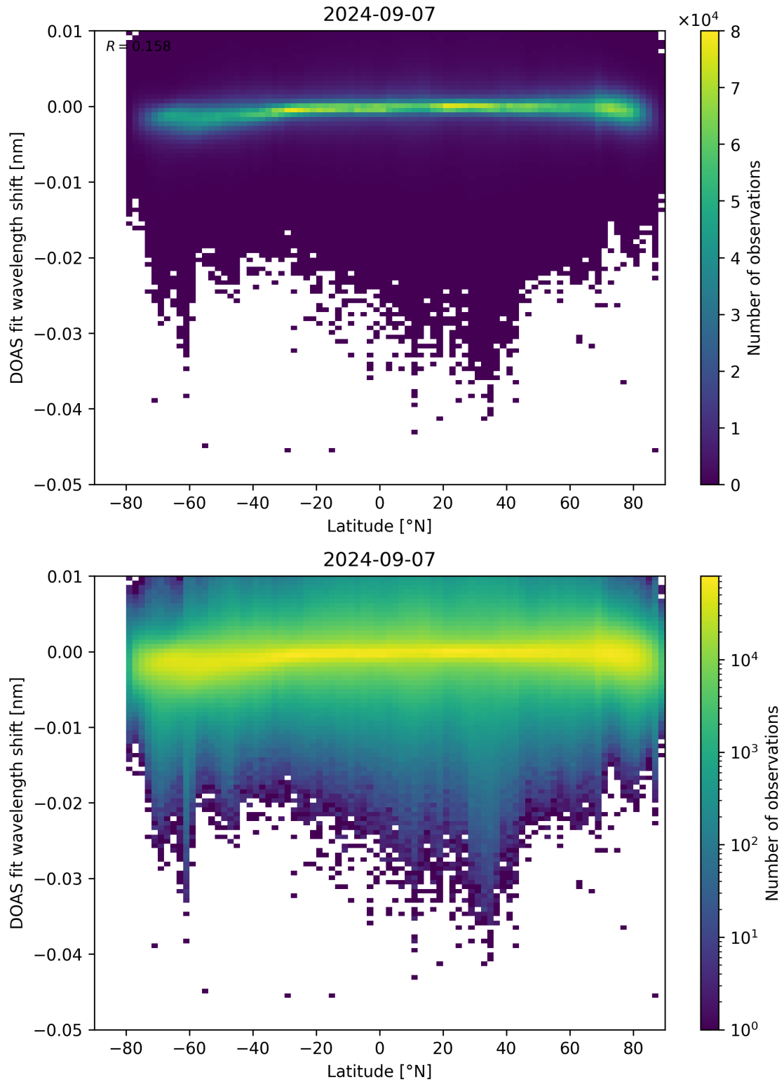
Figure 142: Scatter density plot of “Latitude” against “DOAS fit wavelength shift” for 2024-09-06 to 2024-09-08.
