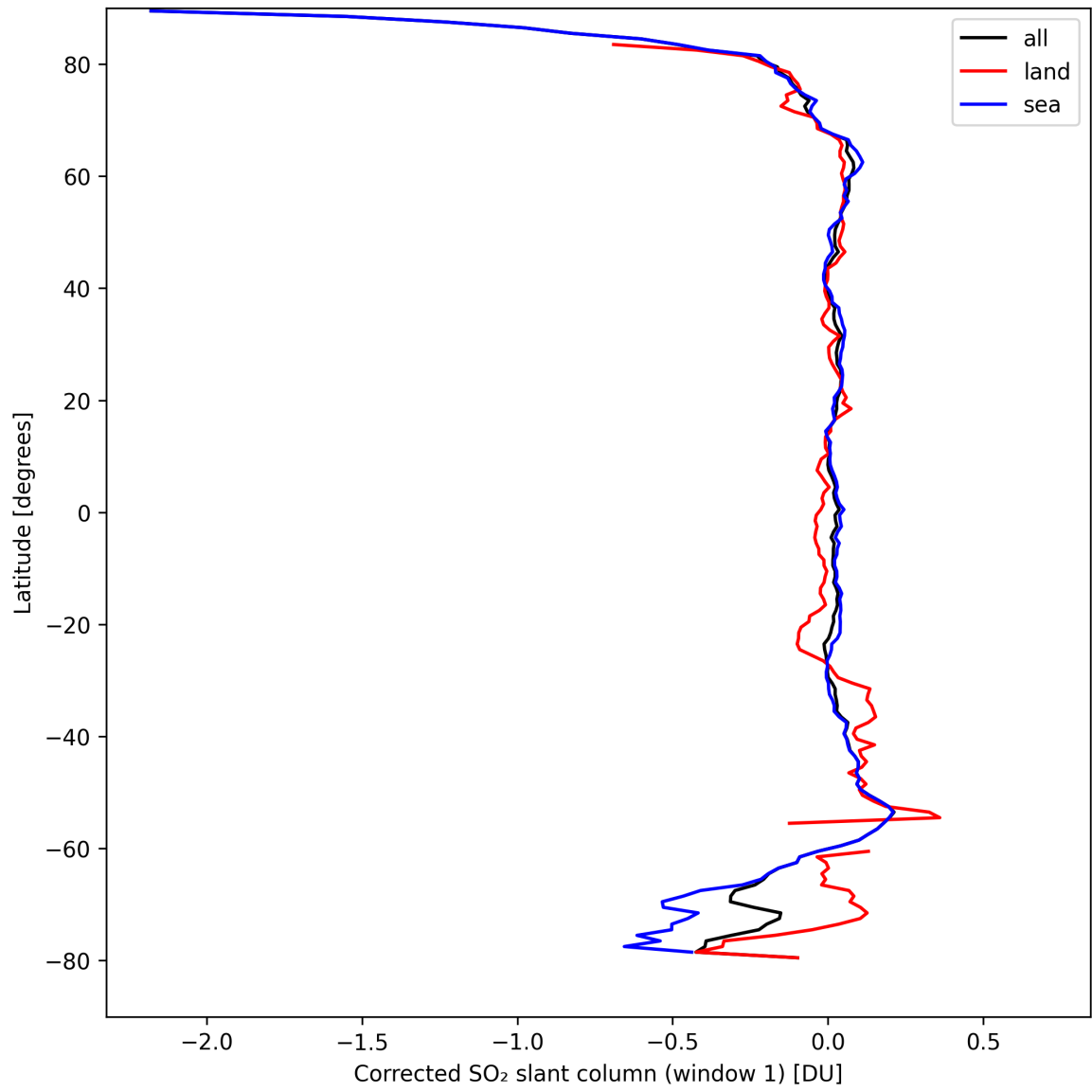
Figure 35: Zonal average of “Corrected SO 2 slant column (window 1)” for 2024-09-06 to 2024-09-08.
