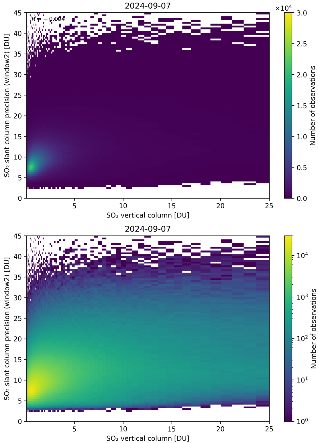
Figure 302: Scatter density plot of “SO 2 vertical column” against “SO 2 slant column precision (window2)” for 2024-09-06 to 2024-09-08.
