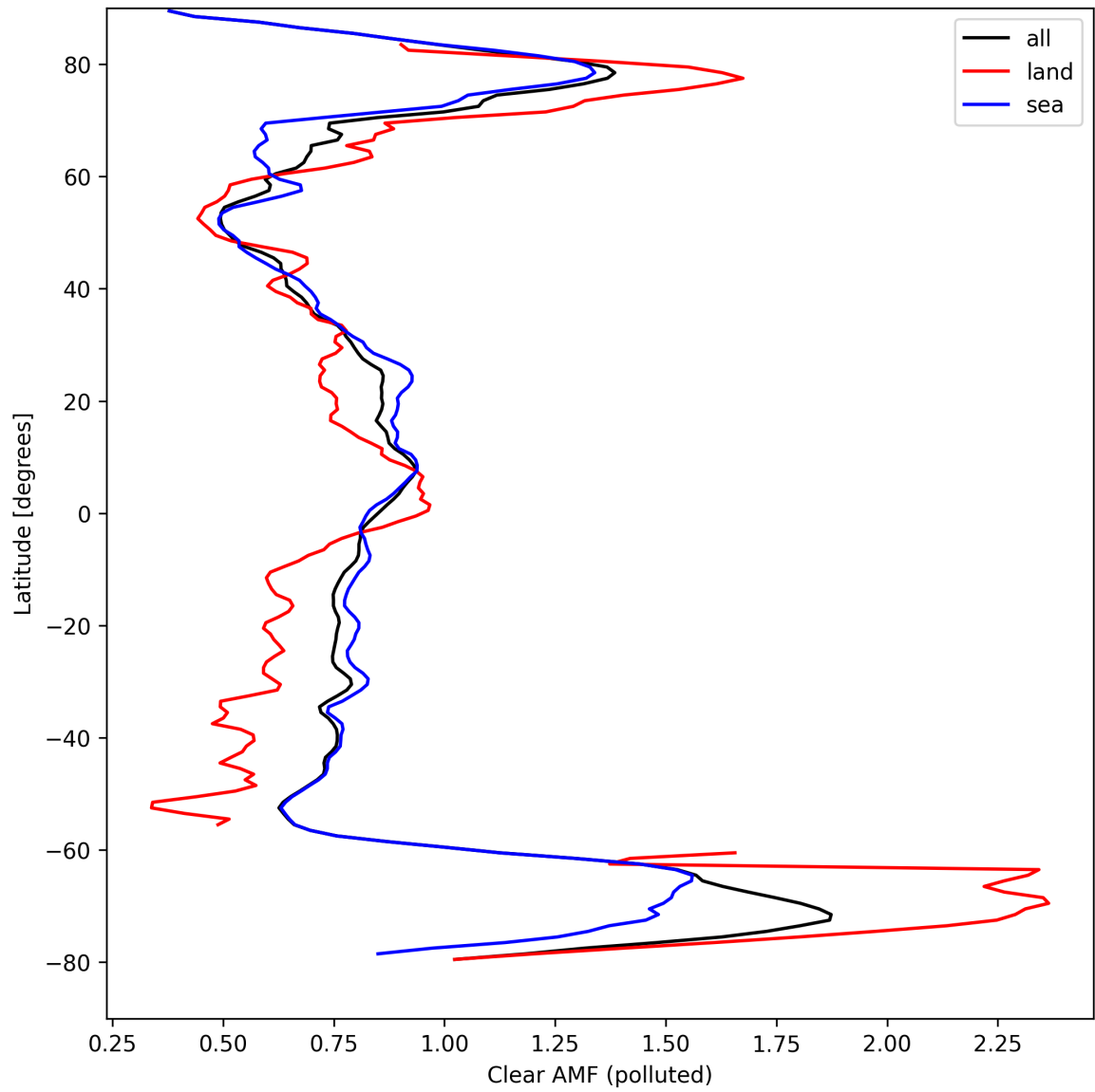
Figure 50: Zonal average of “Clear AMF (polluted)” for 2024-09-06 to 2024-09-08.
