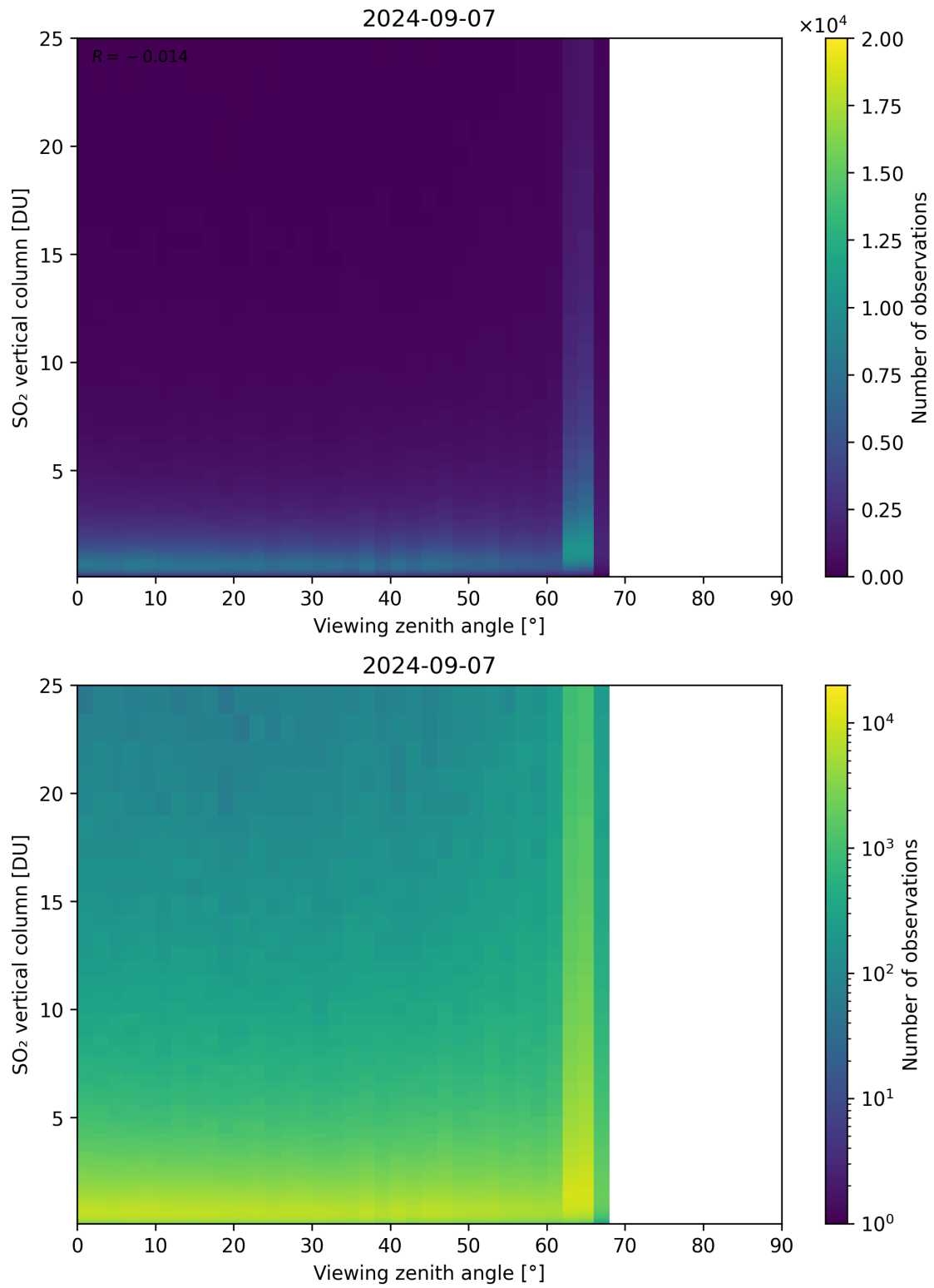
Figure 327: Scatter density plot of “Viewing zenith angle” against “SO 2 vertical column” for 2024-09-06 to 2024-09-08.
