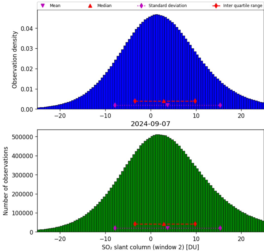
Figure 60: Histogram of “SO 2 slant column (window 2)” for 2024-09-06 to 2024-09-08
