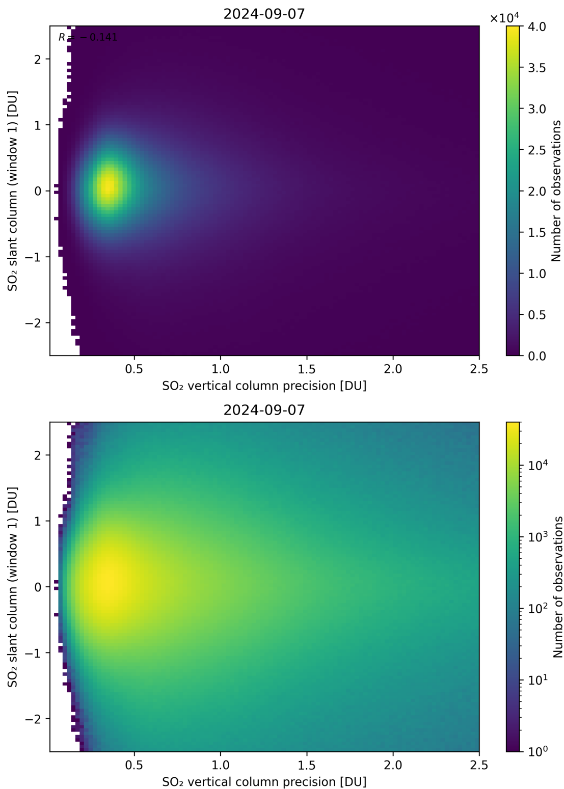
Figure 289: Scatter density plot of “SO 2 vertical column precision” against “SO 2 slant column (window 1)” for 2024-09-06 to 2024-09-08.
