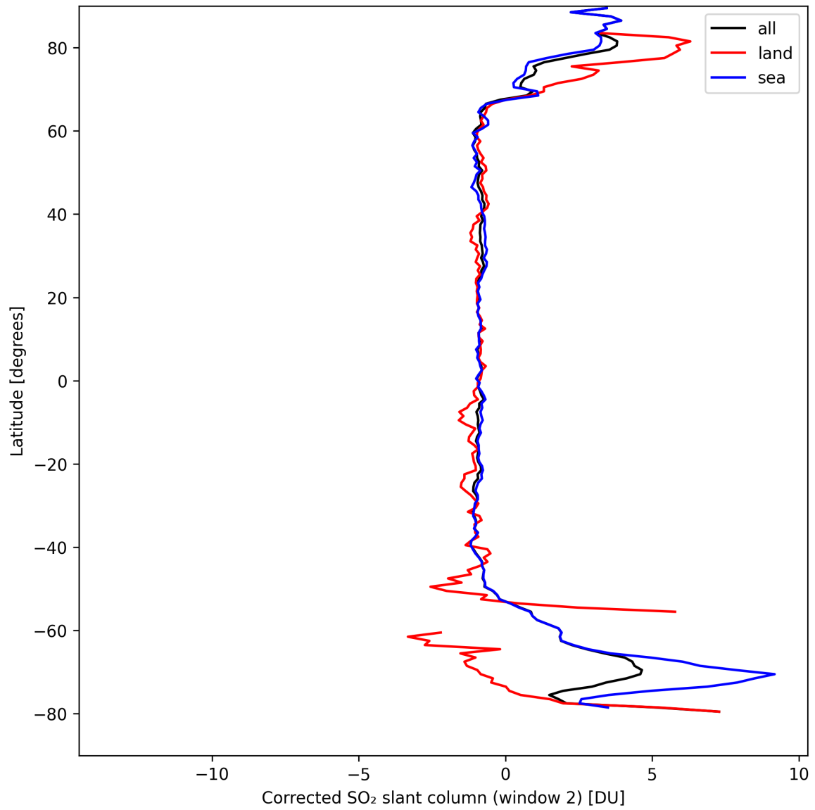
Figure 39: Zonal average of “Corrected SO 2 slant column (window 2)” for 2024-09-06 to 2024-09-08.
