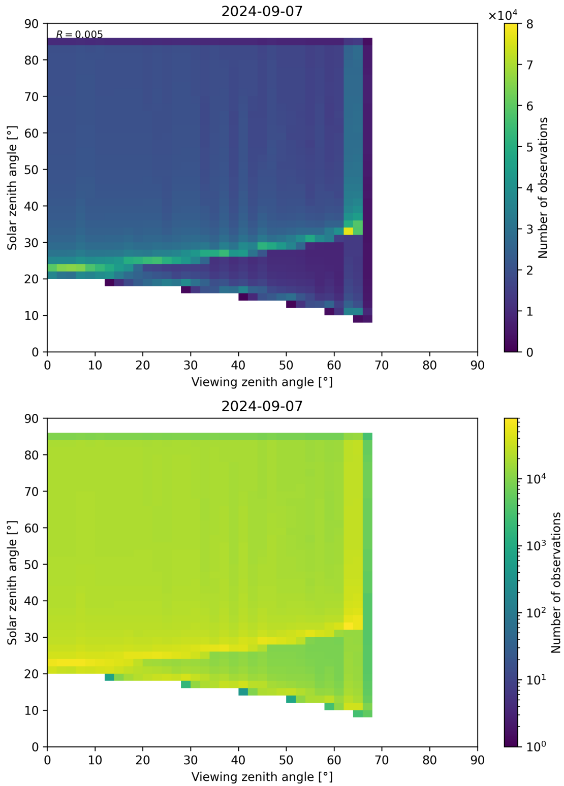
Figure 315: Scatter density plot of “Viewing zenith angle” against “Solar zenith angle” for 2024-09-06 to 2024-09-08.
