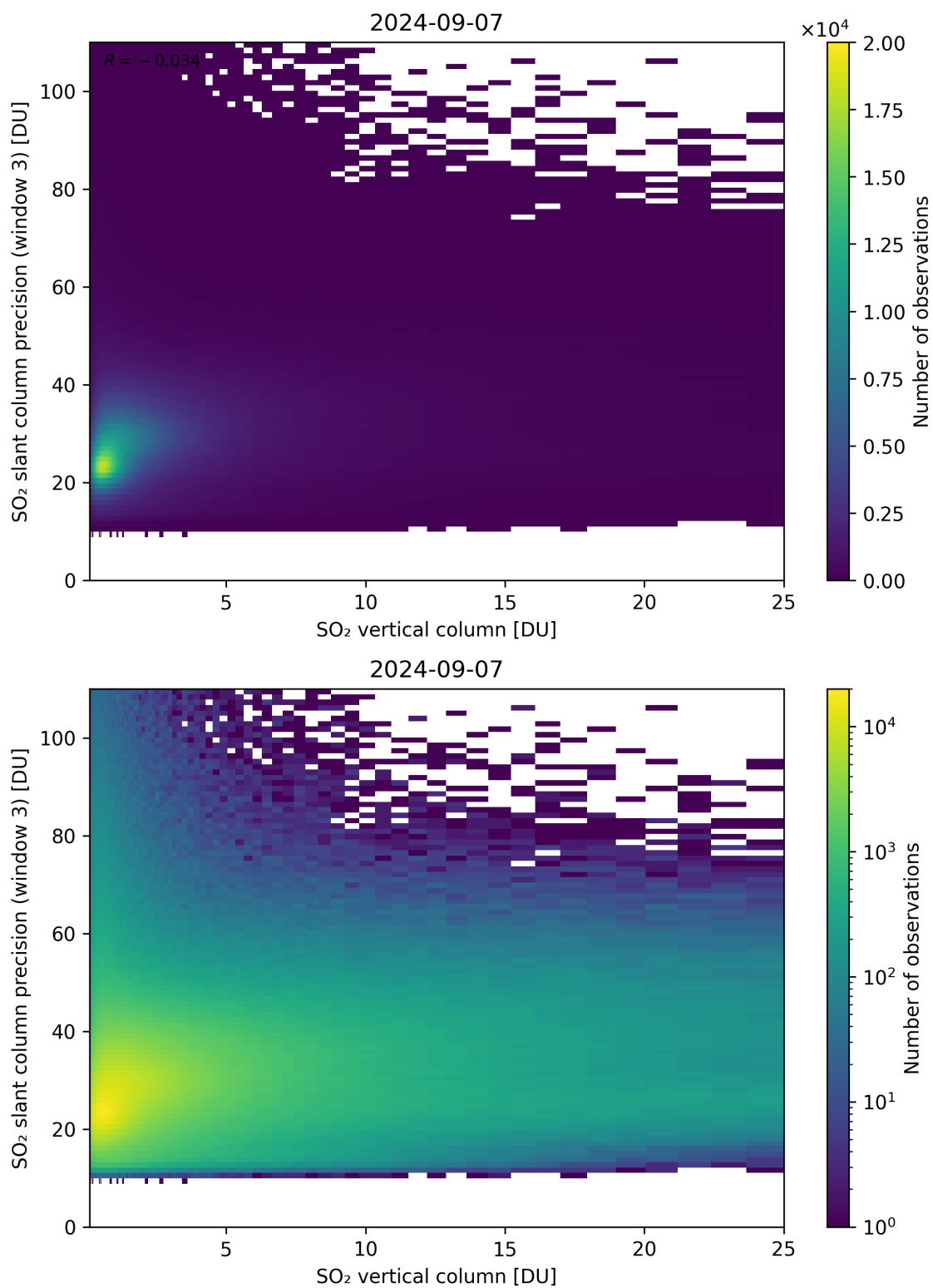
Figure 304: Scatter density plot of “SO 2 vertical column” against “SO 2 slant column precision (window 3)” for 2024-09-06 to 2024-09-08.
