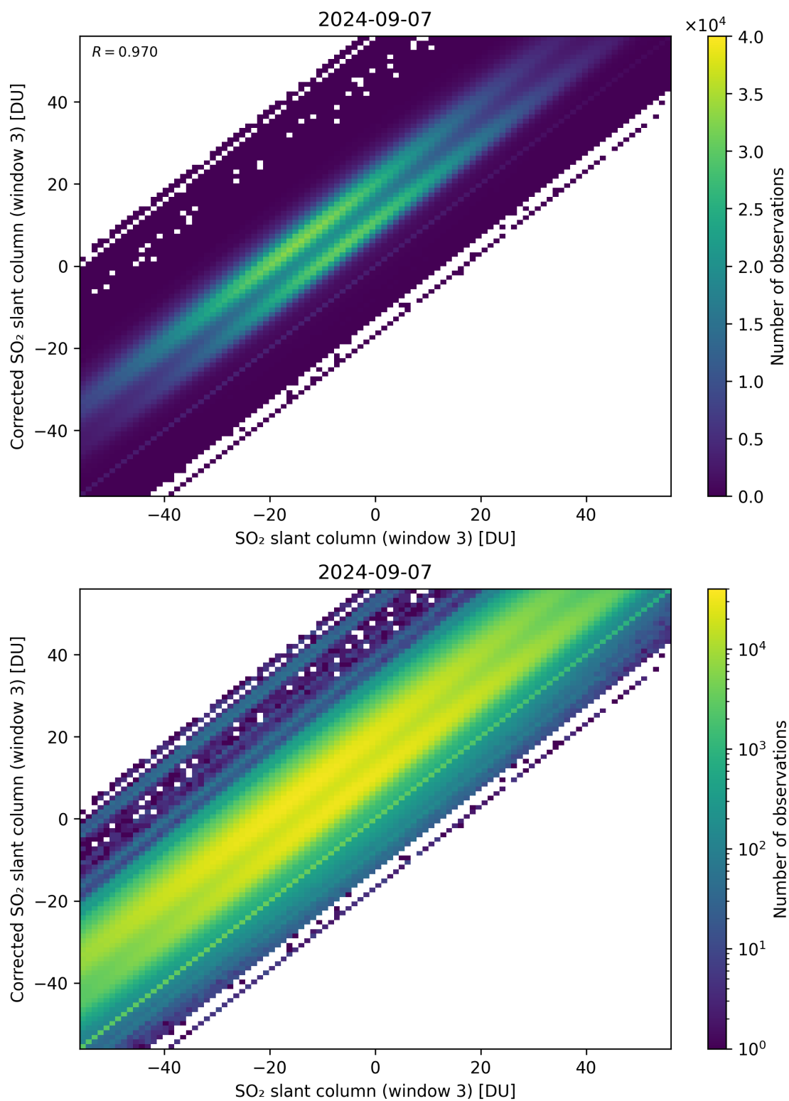
Figure 266: Scatter density plot of “SO 2 slant column (window 3)” against “Corrected SO 2 slant column (window 3)” for 2024-09-06 to 2024-09-08.
