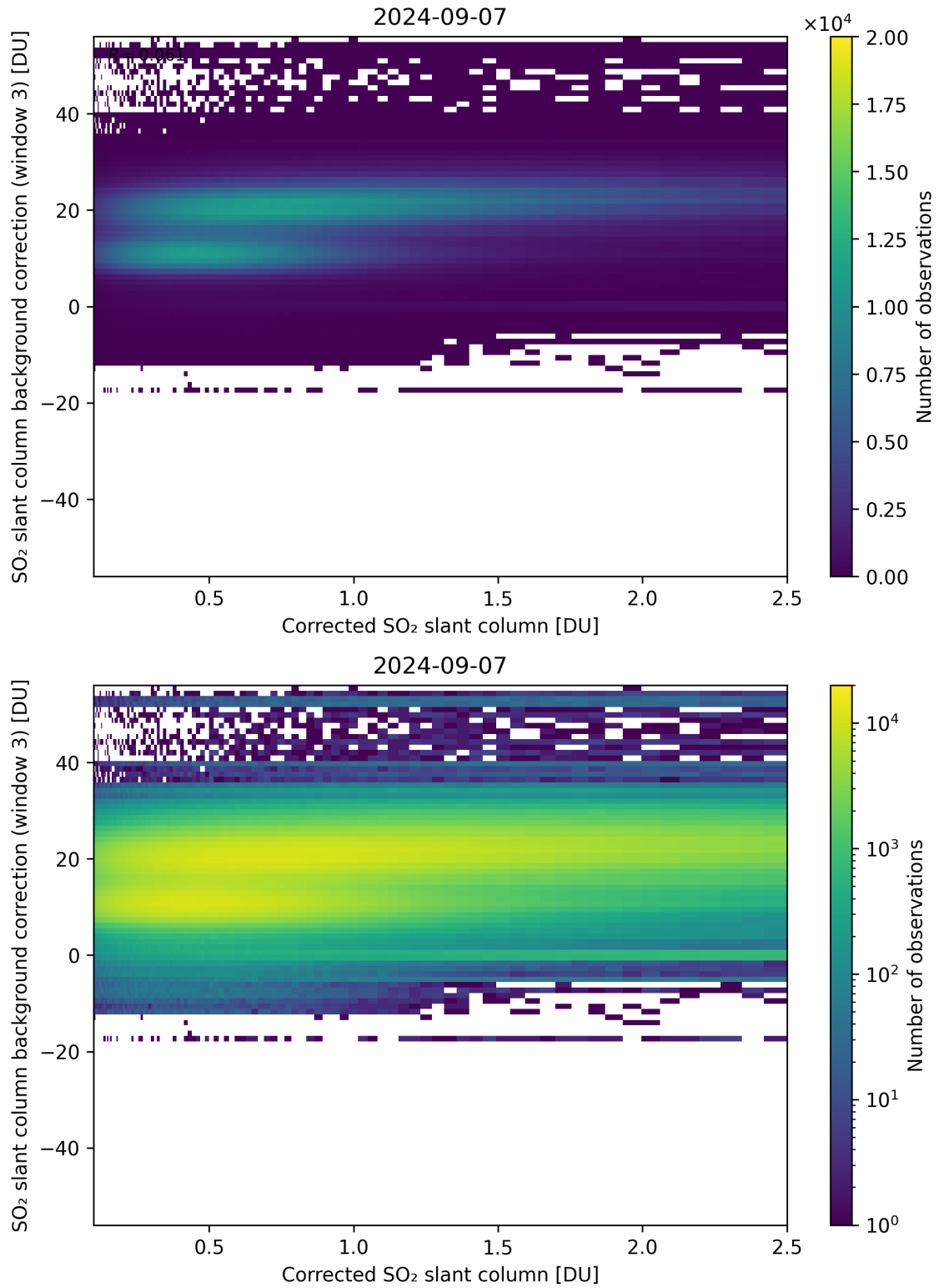
Figure 180: Scatter density plot of “Corrected SO 2 slant column” against “SO 2 slant column background correction (window 3)” for 2024-09-06 to 2024-09-08.
