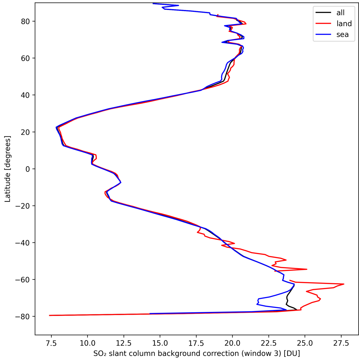
Figure 44: Zonal average of “SO 2 slant column background correction (window 3)” for 2024-09-06 to 2024-09-08.
