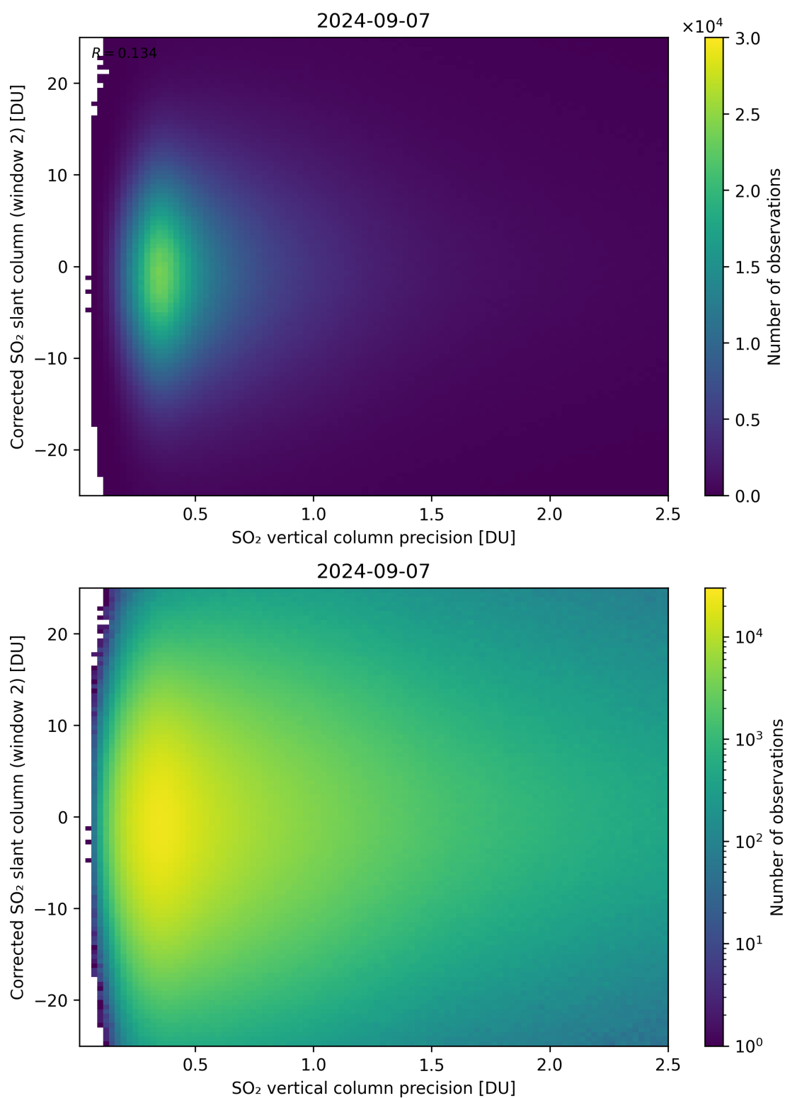
Figure 287: Scatter density plot of “SO 2 vertical column precision” against “Corrected SO 2 slant column (window 2)” for 2024-09-06 to 2024-09-08.
