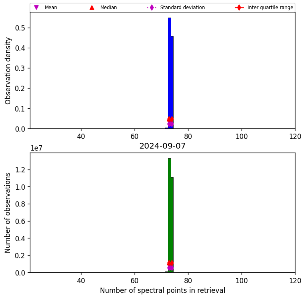
Figure 74: Histogram of “Number of spectral points in retrieval” for 2024-09-06 to 2024-09-08
