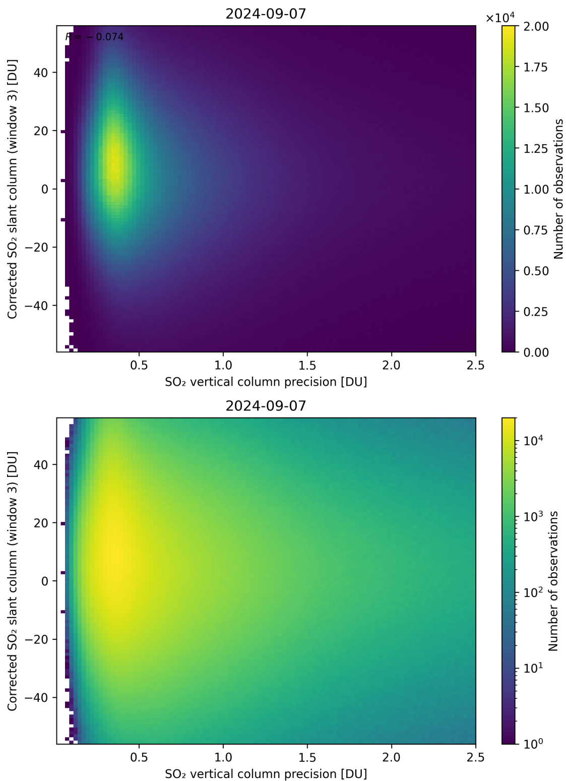
Figure 288: Scatter density plot of “SO 2 vertical column precision” against “Corrected SO 2 slant column (window 3)” for 2024-09-06 to 2024-09-08.
