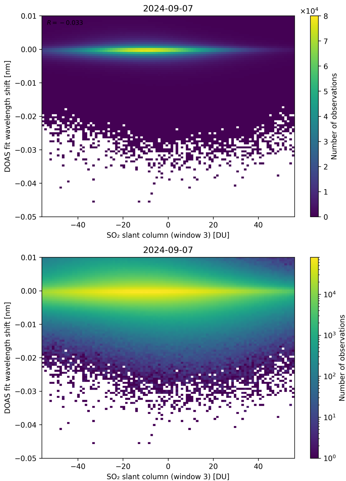
Figure 254: Scatter density plot of “SO 2 slant column (window 3)” against “DOAS fit wavelength shift” for 2024-09-06 to 2024-09-08.
