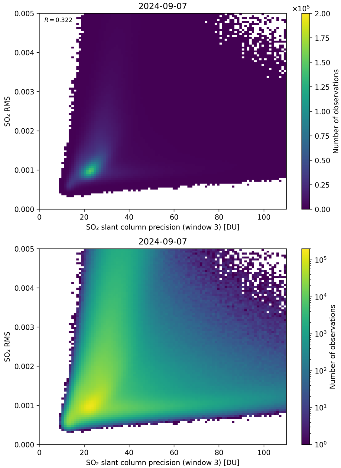
Figure 260: Scatter density plot of “SO 2 slant column precision (window 3)” against “SO 2 RMS” for 2024-09-06 to 2024-09-08.
