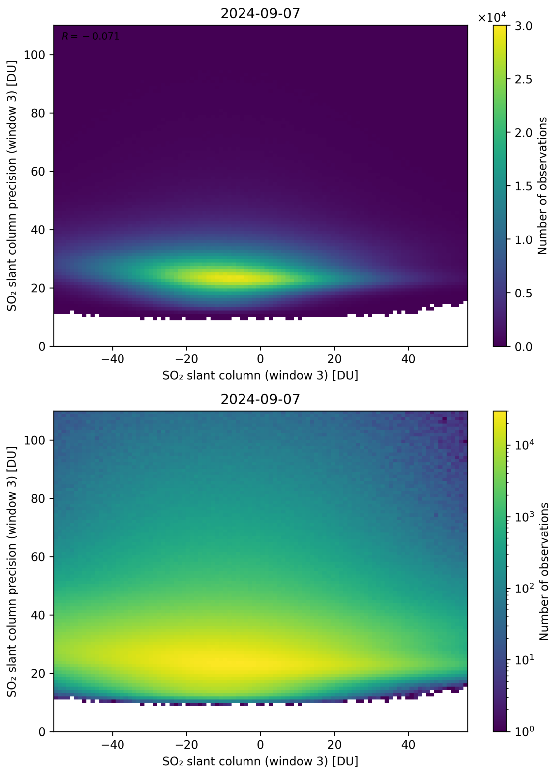
Figure 267: Scatter density plot of “SO 2 slant column (window 3)” against “SO 2 slant column precision (window 3)” for 2024-09-06 to 2024-09-08.
