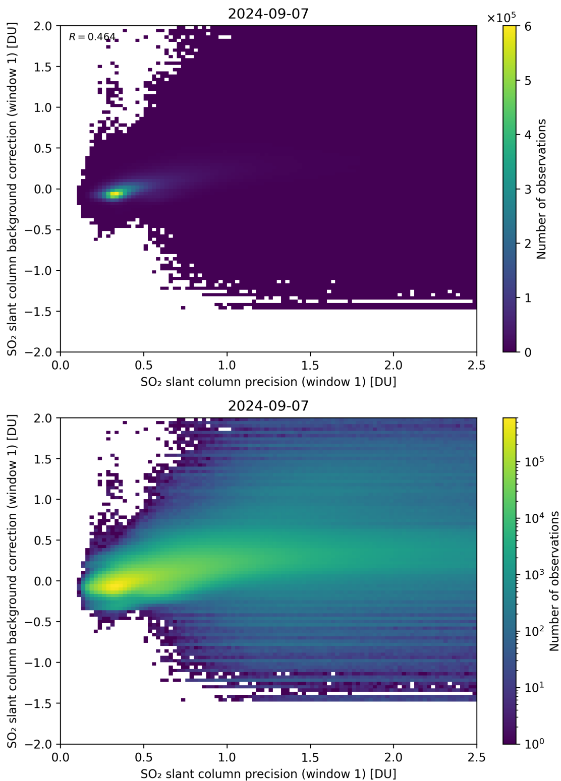
Figure 218: Scatter density plot of “SO 2 slant column precision (window 1)” against “SO 2 slant column background correction (window 1)” for 2024-09-06 to 2024-09-08.
