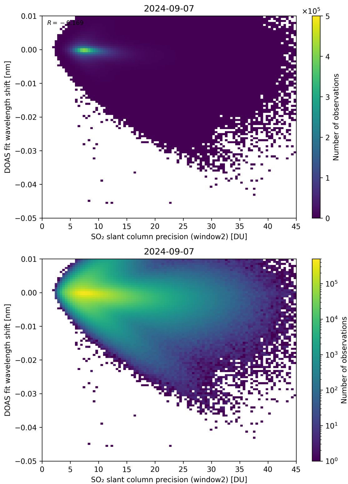
Figure 243: Scatter density plot of “SO 2 slant column precision (window2)” against “DOAS fit wavelength shift” for 2024-09-06 to 2024-09-08.
