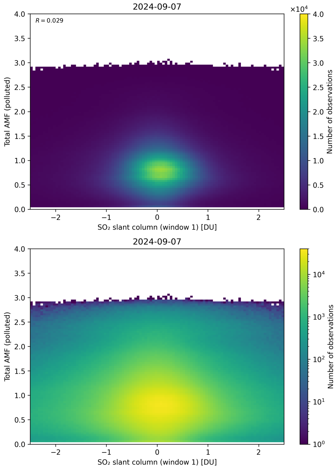
Figure 239: Scatter density plot of “SO 2 slant column (window 1)” against “Total AMF (polluted)” for 2024-09-06 to 2024-09-08.
