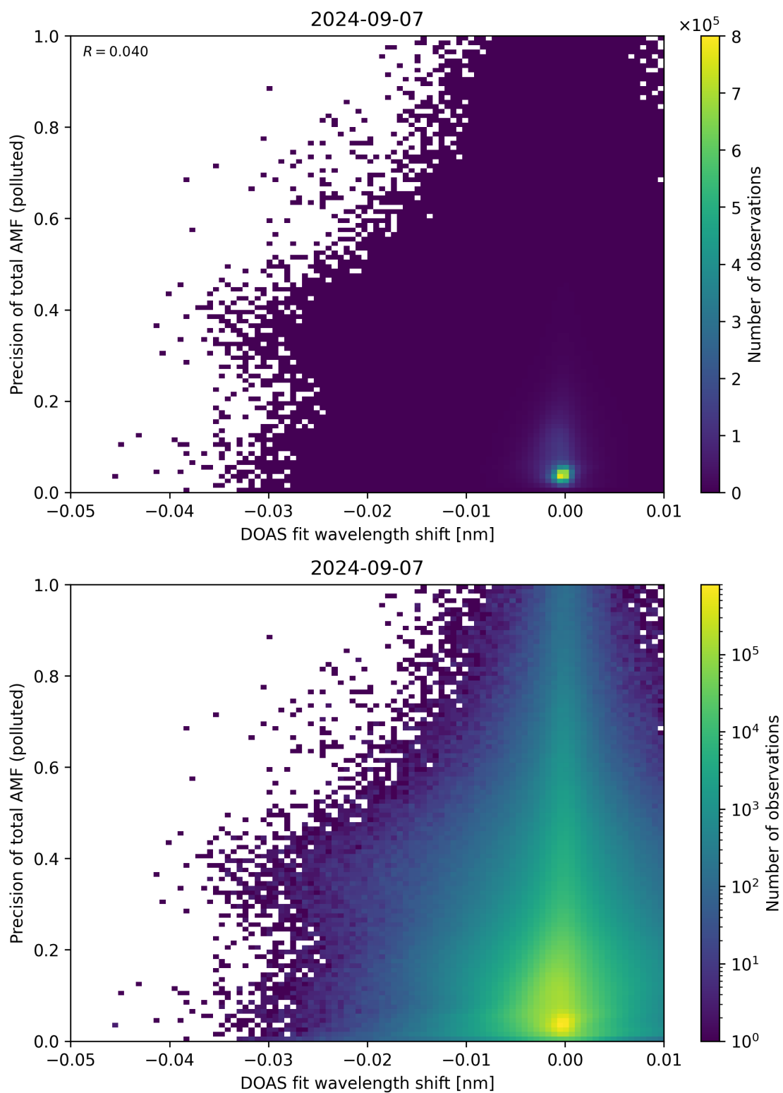
Figure 131: Scatter density plot of “DOAS fit wavelength shift” against “Precision of total AMF (polluted)” for 2024-09-06 to 2024-09-08.
