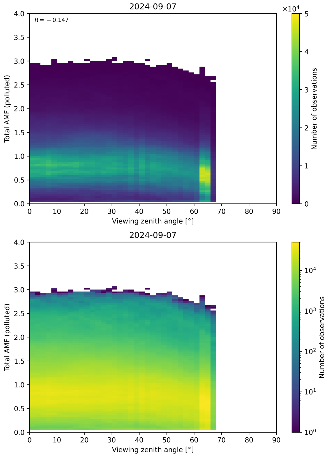
Figure 325: Scatter density plot of “Viewing zenith angle” against “Total AMF (polluted)” for 2024-09-06 to 2024-09-08.
