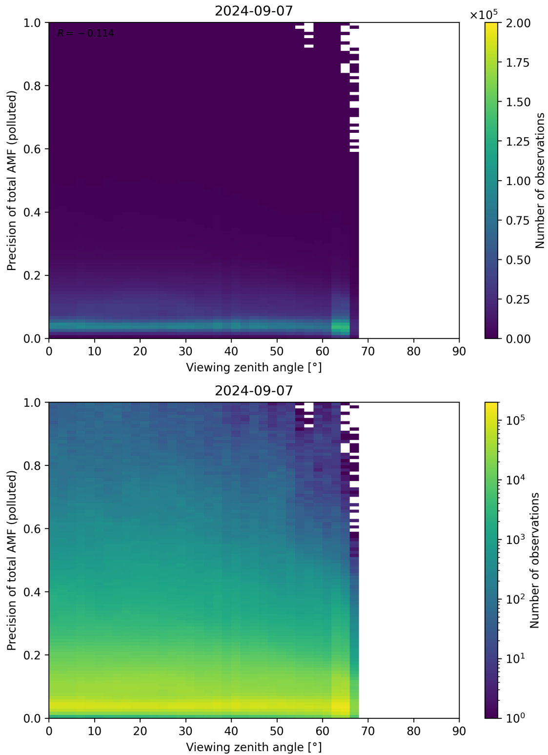
Figure 326: Scatter density plot of “Viewing zenith angle” against “Precision of total AMF (polluted)” for 2024-09-06 to 2024-09-08.
