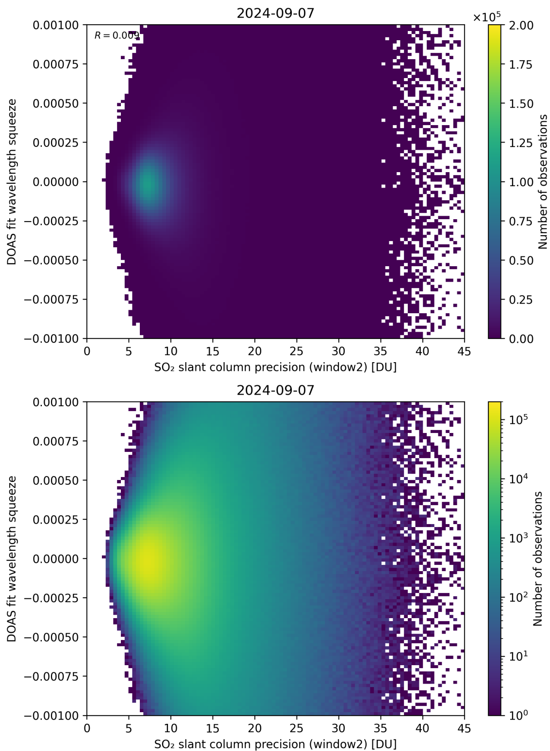
Figure 244: Scatter density plot of “SO 2 slant column precision (window2)” against “DOAS fit wavelength squeeze” for 2024-09-06 to 2024-09-08.
