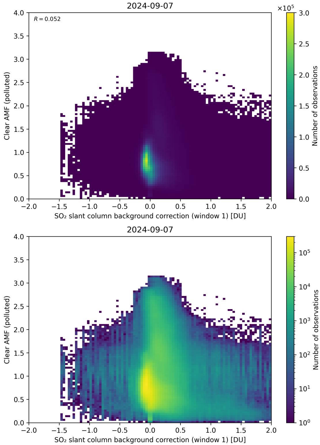
Figure 103: Scatter density plot of “SO 2 slant column background correction (window 1)” against “Clear AMF (polluted)” for 2024-09-06 to 2024-09-08.
