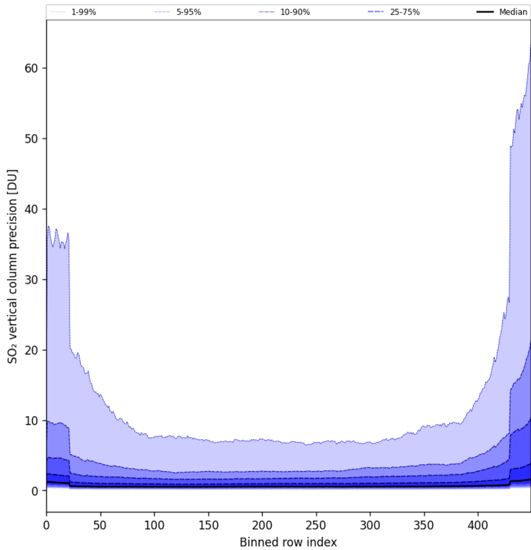
Figure 77: Along track statistics of “SO 2 vertical column precision” for 2024-09-06 to 2024-09-08
