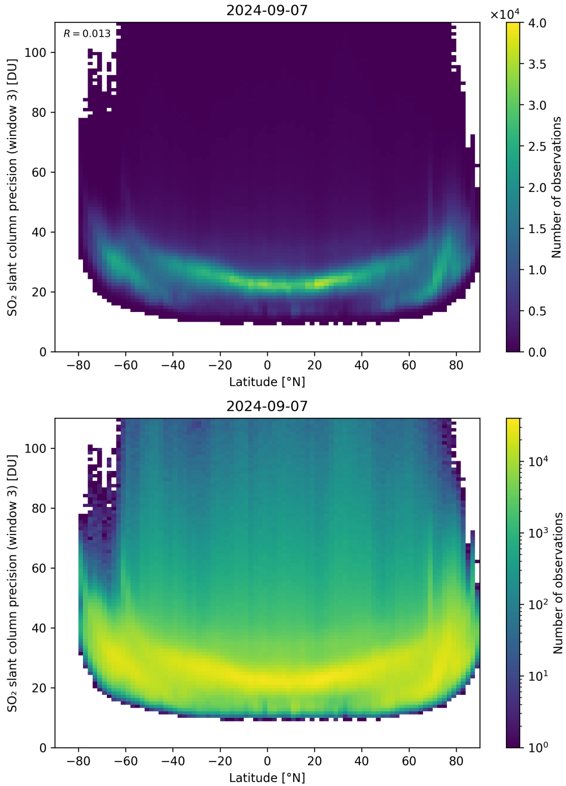
Figure 153: Scatter density plot of “Latitude” against “SO 2 slant column precision (window 3)” for 2024-09-06 to 2024-09-08.
