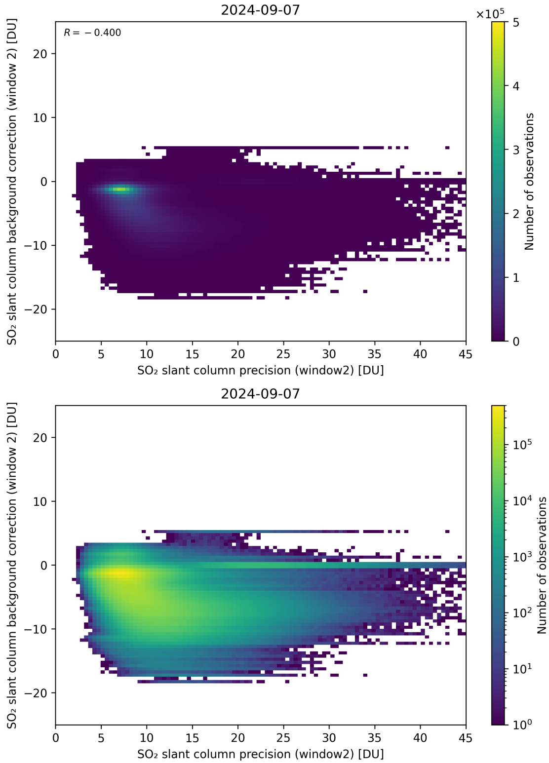
Figure 241: Scatter density plot of “SO 2 slant column precision (window2)” against “SO 2 slant column background correction (window 2)” for 2024-09-06 to 2024-09-08.
