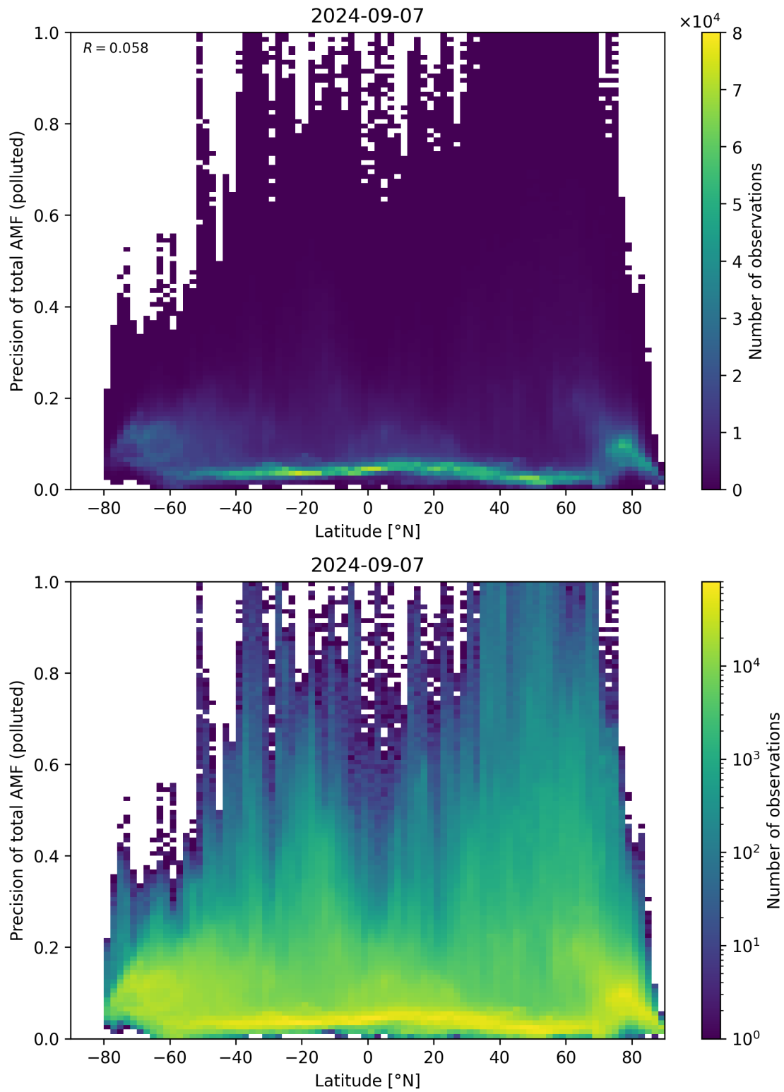
Figure 155: Scatter density plot of “Latitude” against “Precision of total AMF (polluted)” for 2024-09-06 to 2024-09-08.
