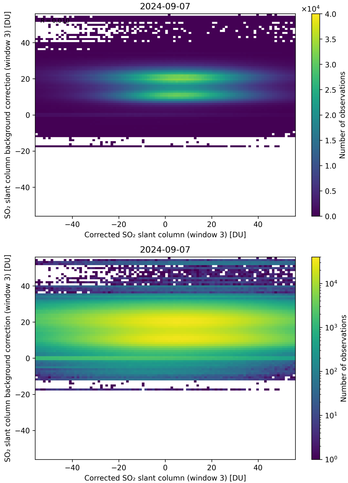
Figure 205: Scatter density plot of “Corrected SO 2 slant column (window 3)” against “SO 2 slant column background correction (window 3)” for 2024-09-06 to 2024-09-08.
