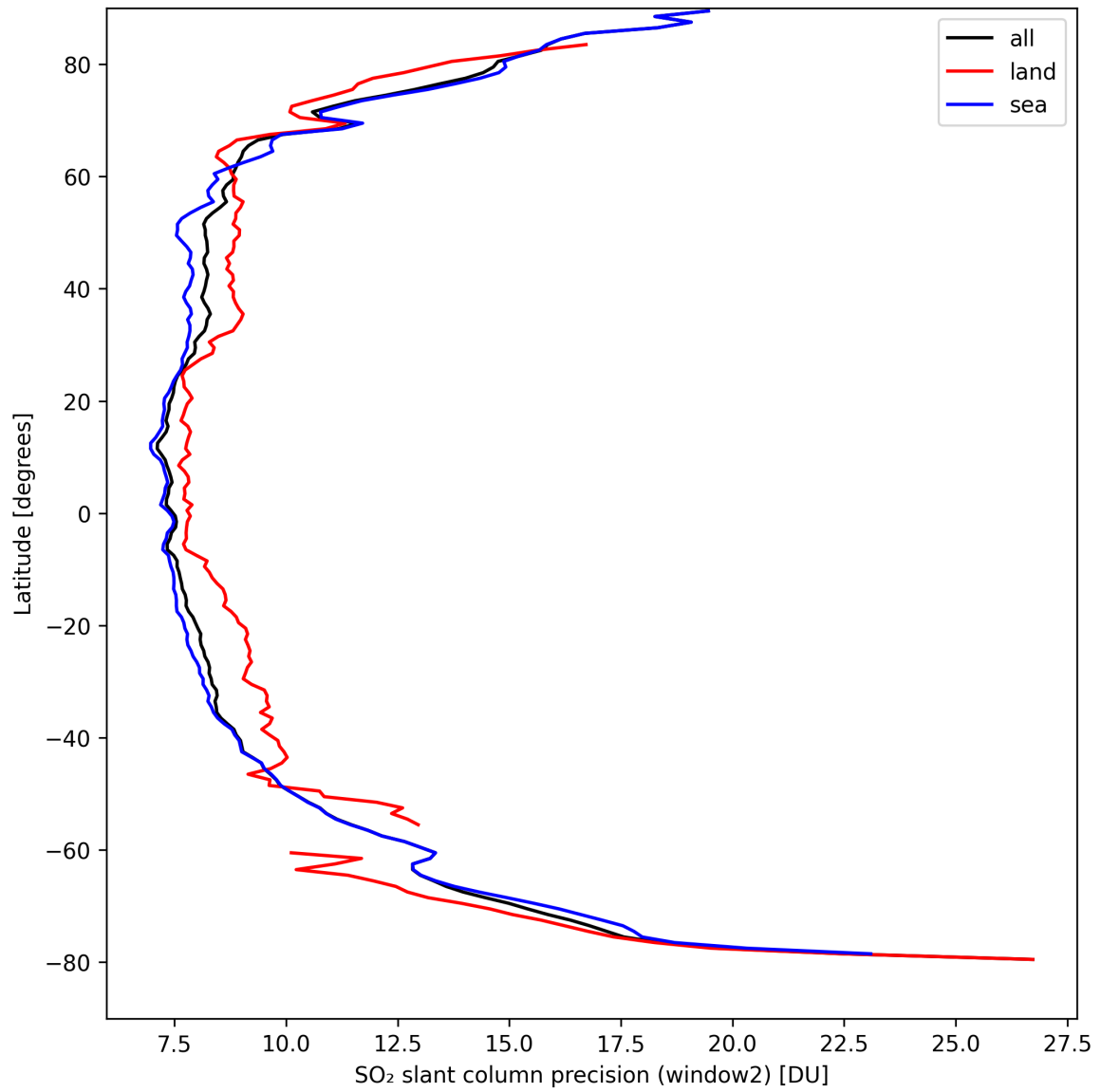
Figure 38: Zonal average of “SO 2 slant column precision (window2)” for 2024-09-06 to 2024-09-08.
