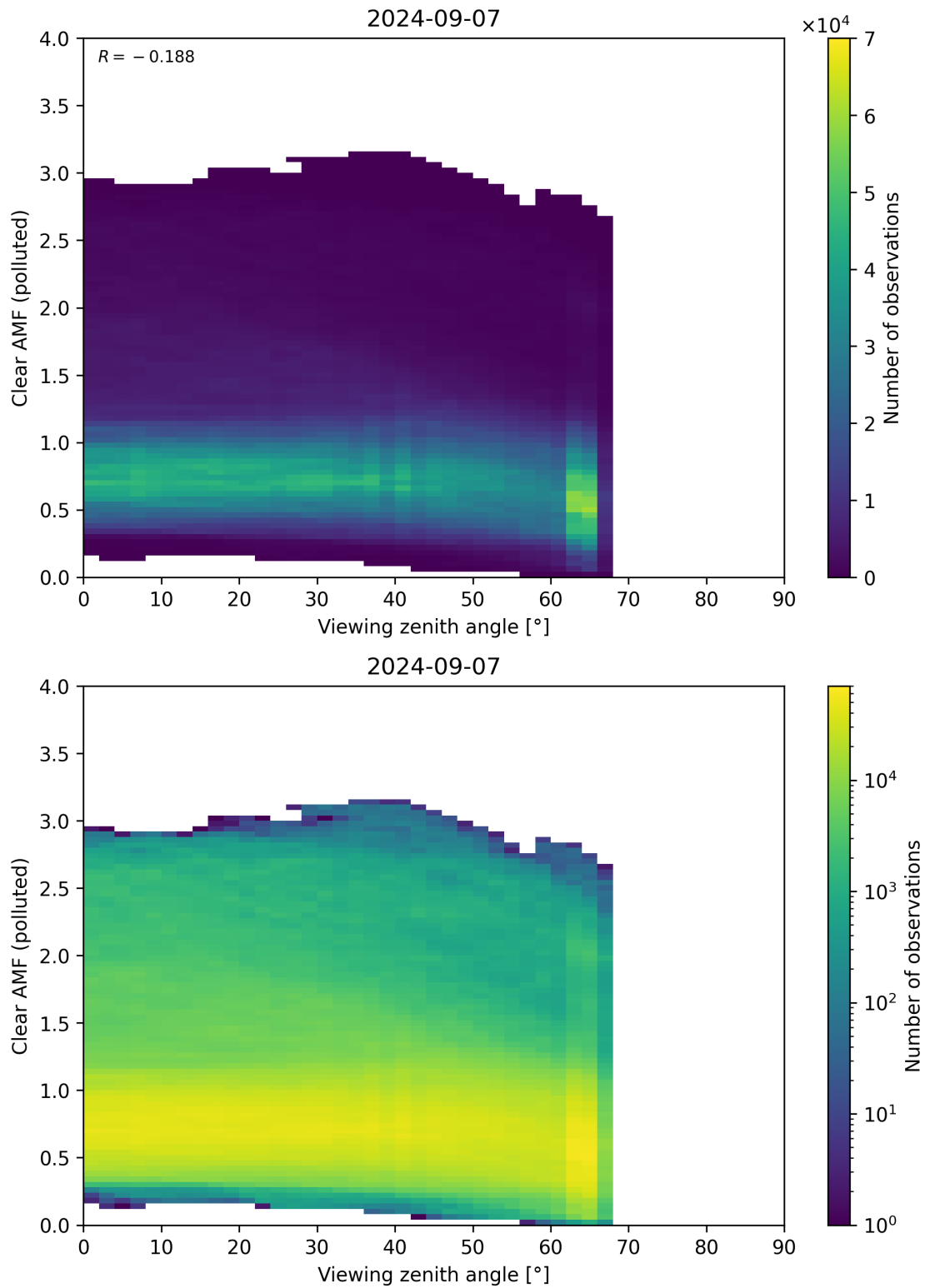
Figure 316: Scatter density plot of “Viewing zenith angle” against “Clear AMF (polluted)” for 2024-09-06 to 2024-09-08.
