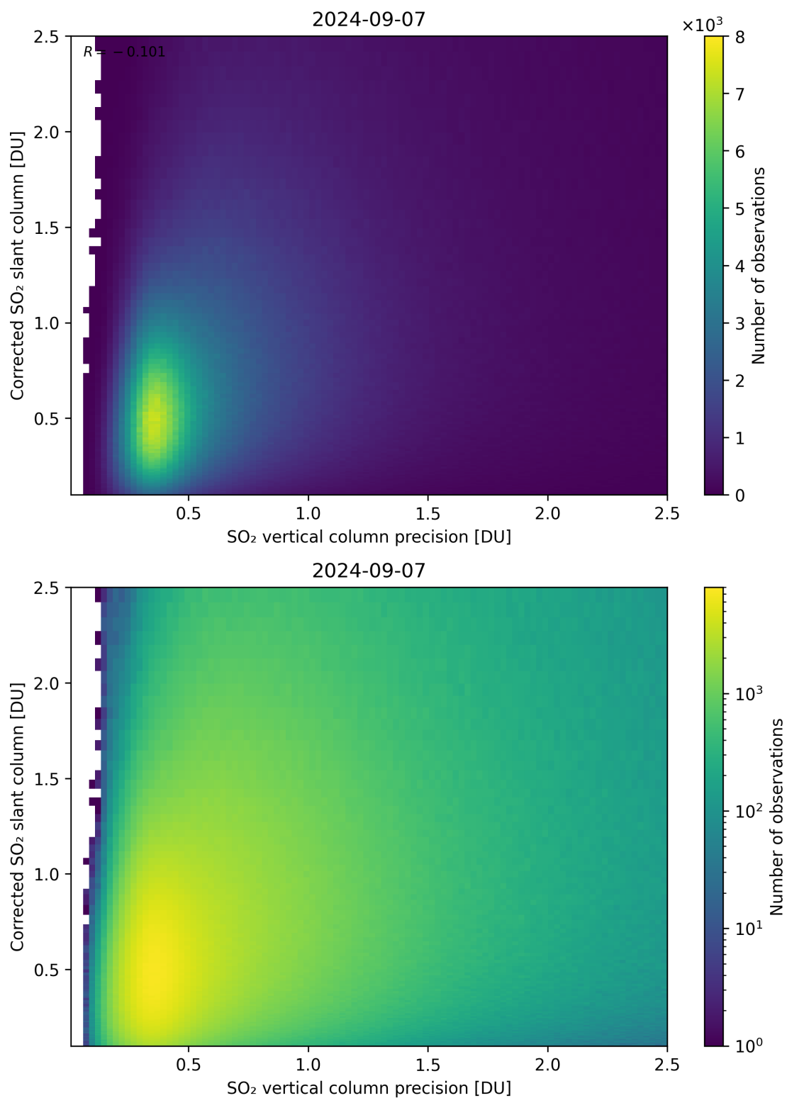
Figure 286: Scatter density plot of “SO 2 vertical column precision” against “Corrected SO 2 slant column” for 2024-09-06 to 2024-09-08.
