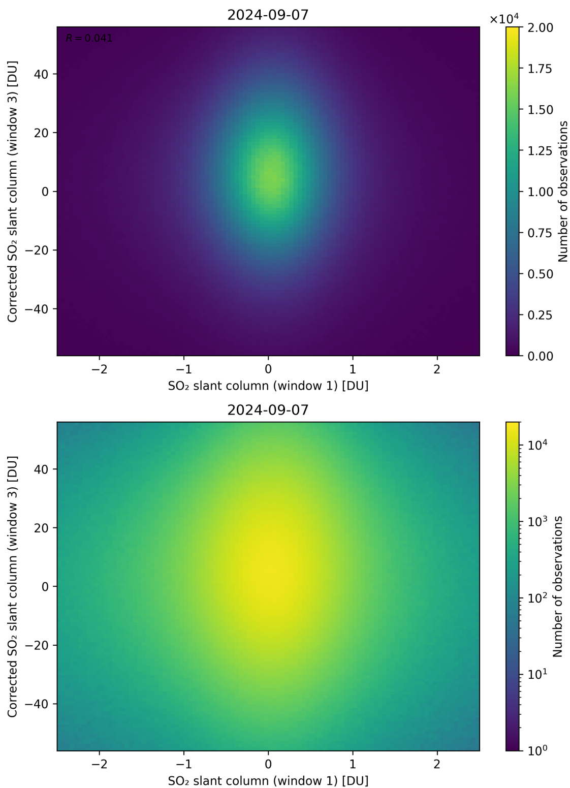
Figure 234: Scatter density plot of “SO 2 slant column (window 1)” against “Corrected SO 2 slant column (window 3)” for 2024-09-06 to 2024-09-08.
