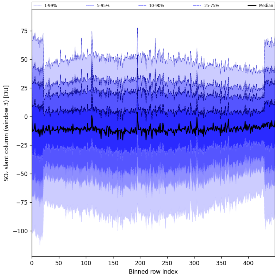
Figure 87: Along track statistics of “SO 2 slant column (window 3)” for 2024-09-06 to 2024-09-08
