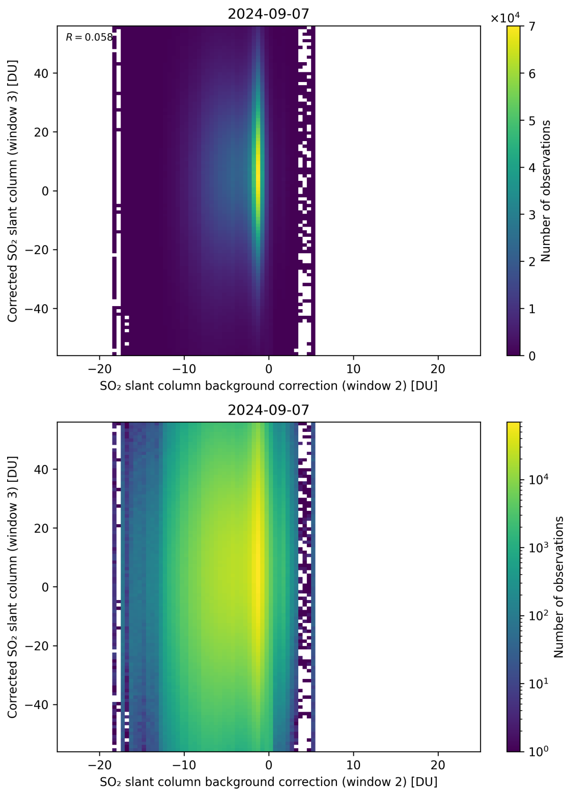
Figure 116: Scatter density plot of “SO 2 slant column background correction (window 2)” against “Corrected SO 2 slant column (window 3)” for 2024-09-06 to 2024-09-08.
