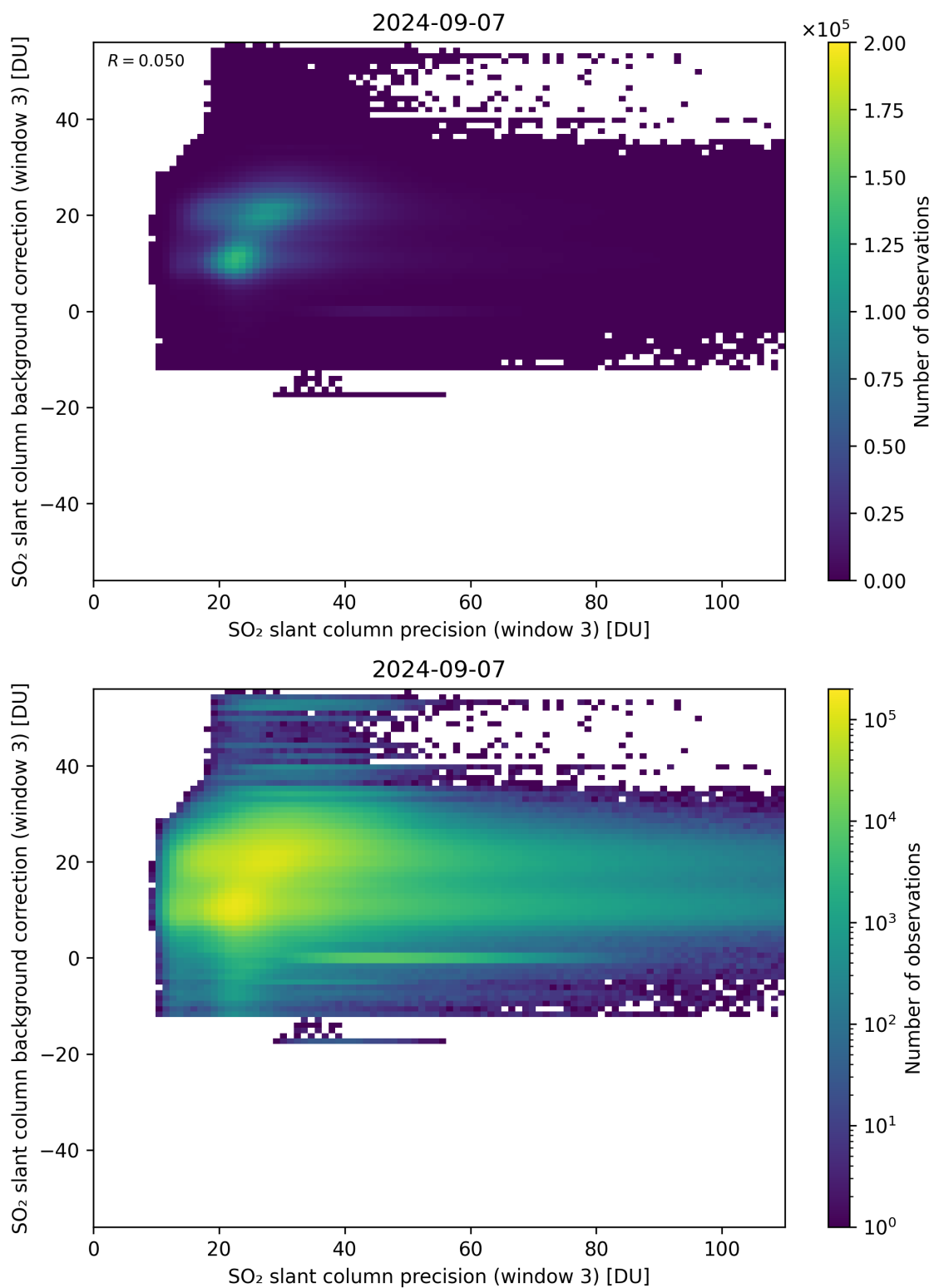
Figure 257: Scatter density plot of “SO 2 slant column precision (window 3)” against “SO 2 slant column background correction (window 3)” for 2024-09-06 to 2024-09-08.
