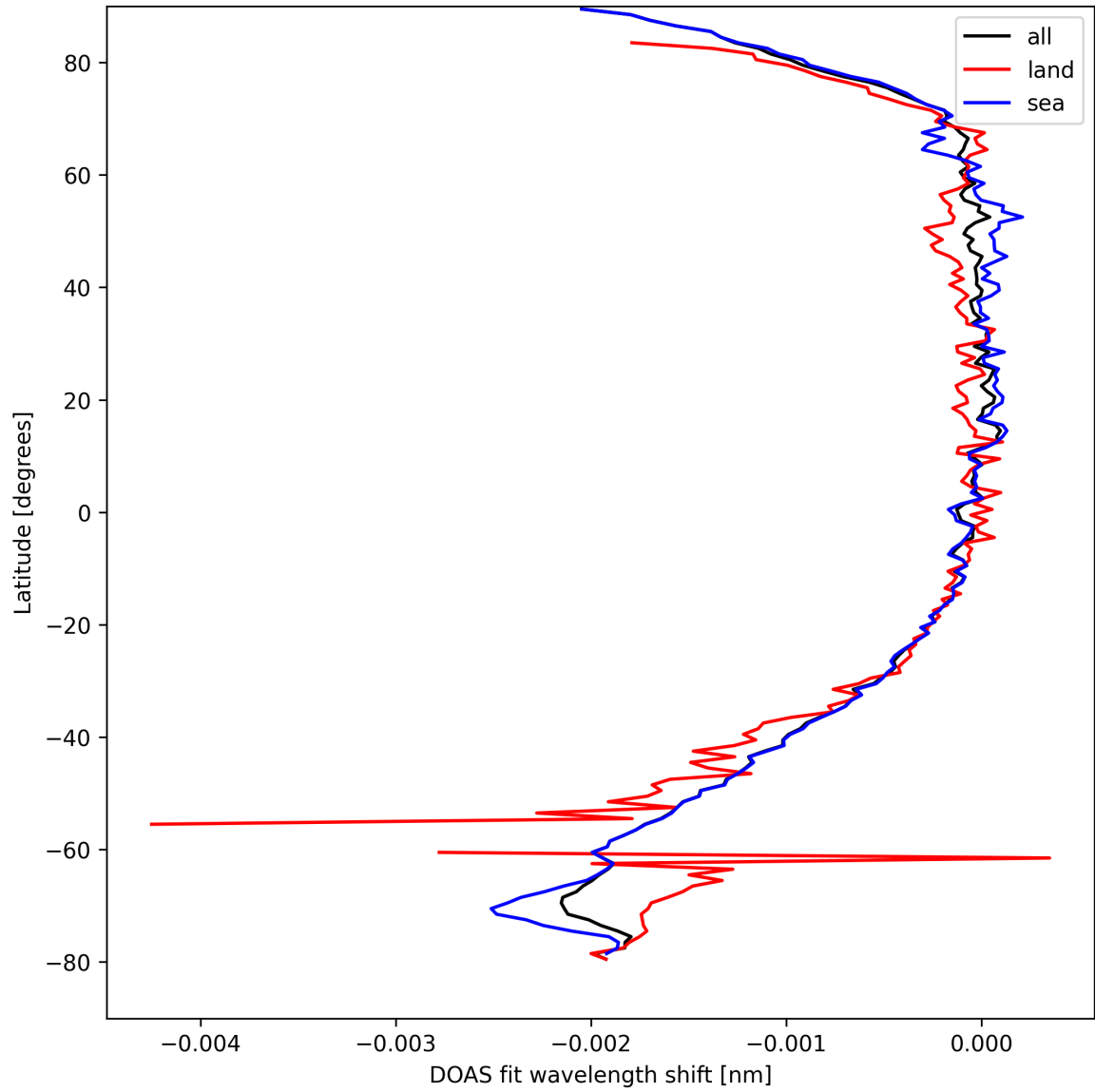
Figure 45: Zonal average of “DOAS fit wavelength shift” for 2024-09-06 to 2024-09-08.
