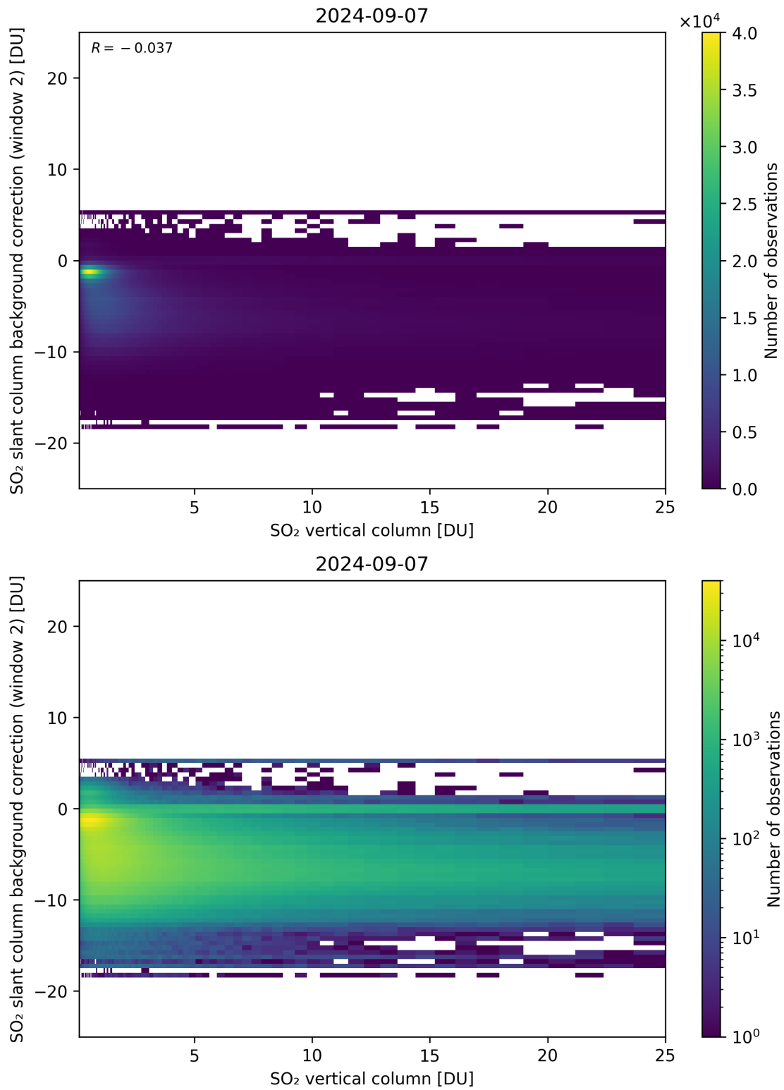
Figure 274: Scatter density plot of “SO 2 vertical column” against “SO 2 slant column background correction (window 2)” for 2024-09-06 to 2024-09-08.
