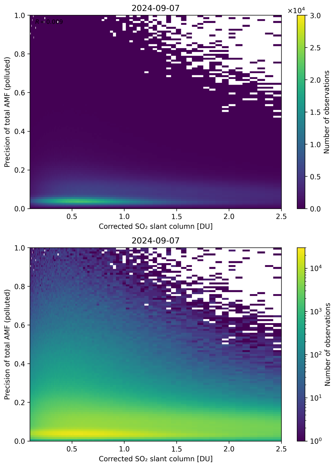
Figure 193: Scatter density plot of “Corrected SO 2 slant column” against “Precision of total AMF (polluted)” for 2024-09-06 to 2024-09-08.
