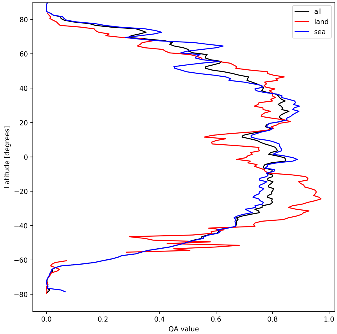
Figure 29: Zonal average of “QA value” for 2024-09-06 to 2024-09-08.
