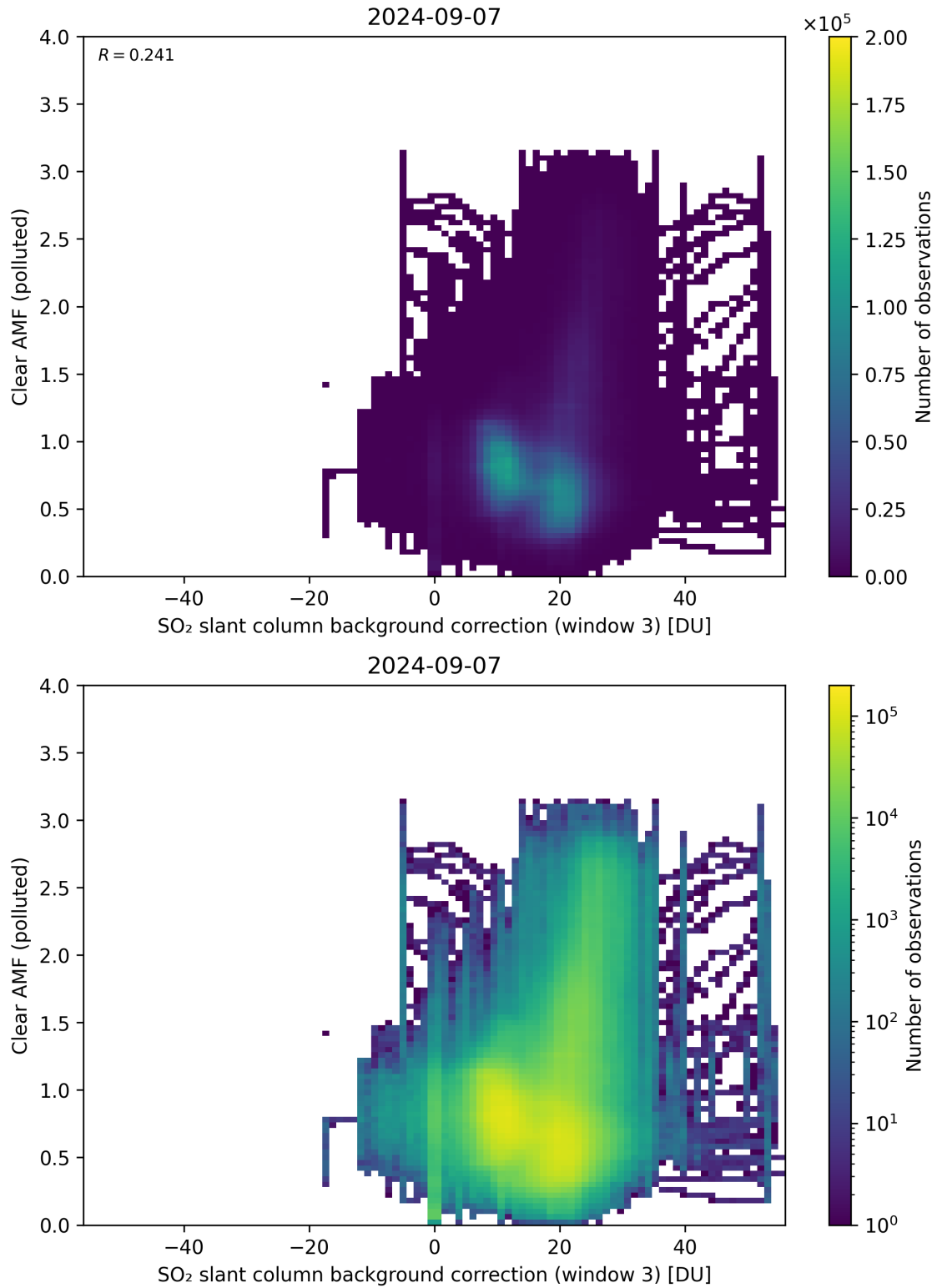
Figure 124: Scatter density plot of “SO 2 slant column background correction (window 3)” against “Clear AMF (polluted)” for 2024-09-06 to 2024-09-08.
