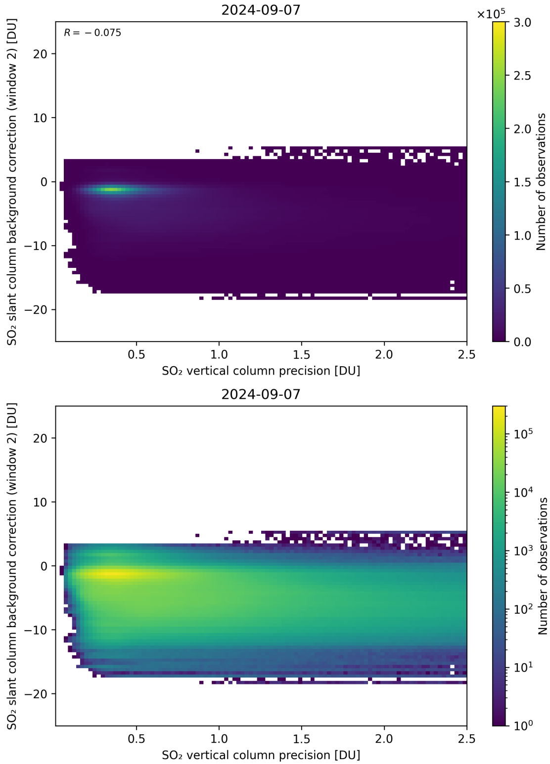
Figure 280: Scatter density plot of “SO 2 vertical column precision” against “SO 2 slant column background correction (window 2)” for 2024-09-06 to 2024-09-08.
