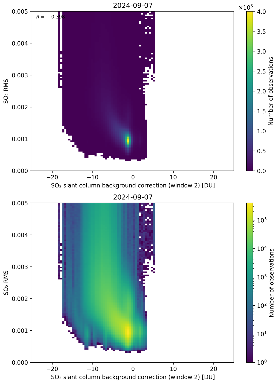
Figure 114: Scatter density plot of “SO 2 slant column background correction (window 2)” against “SO 2 RMS” for 2024-09-06 to 2024-09-08.
