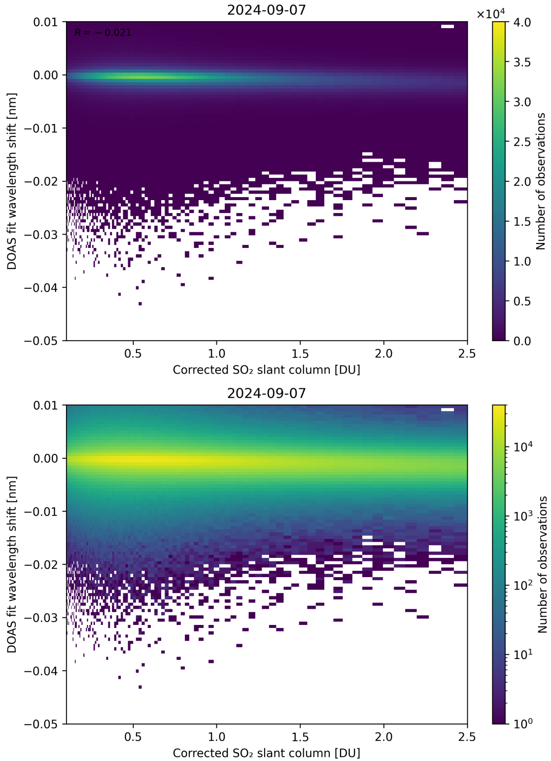
Figure 181: Scatter density plot of “Corrected SO 2 slant column” against “DOAS fit wavelength shift” for 2024-09-06 to 2024-09-08.
