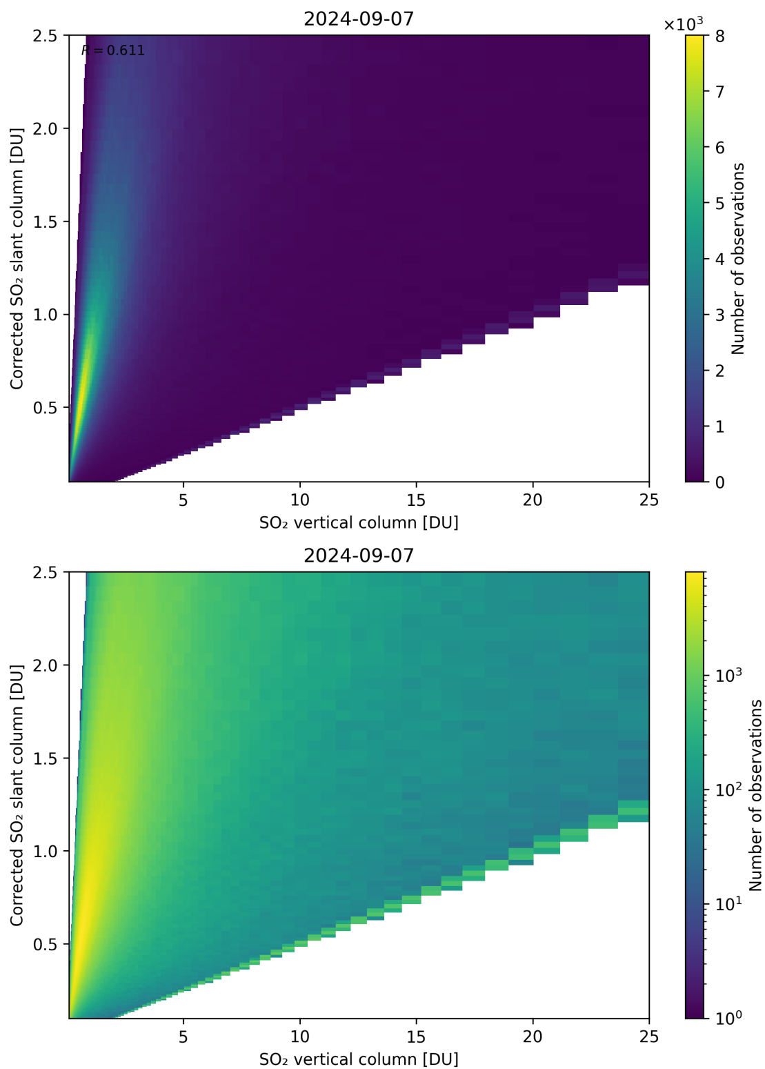
Figure 297: Scatter density plot of “SO 2 vertical column” against “Corrected SO 2 slant column” for 2024-09-06 to 2024-09-08.
