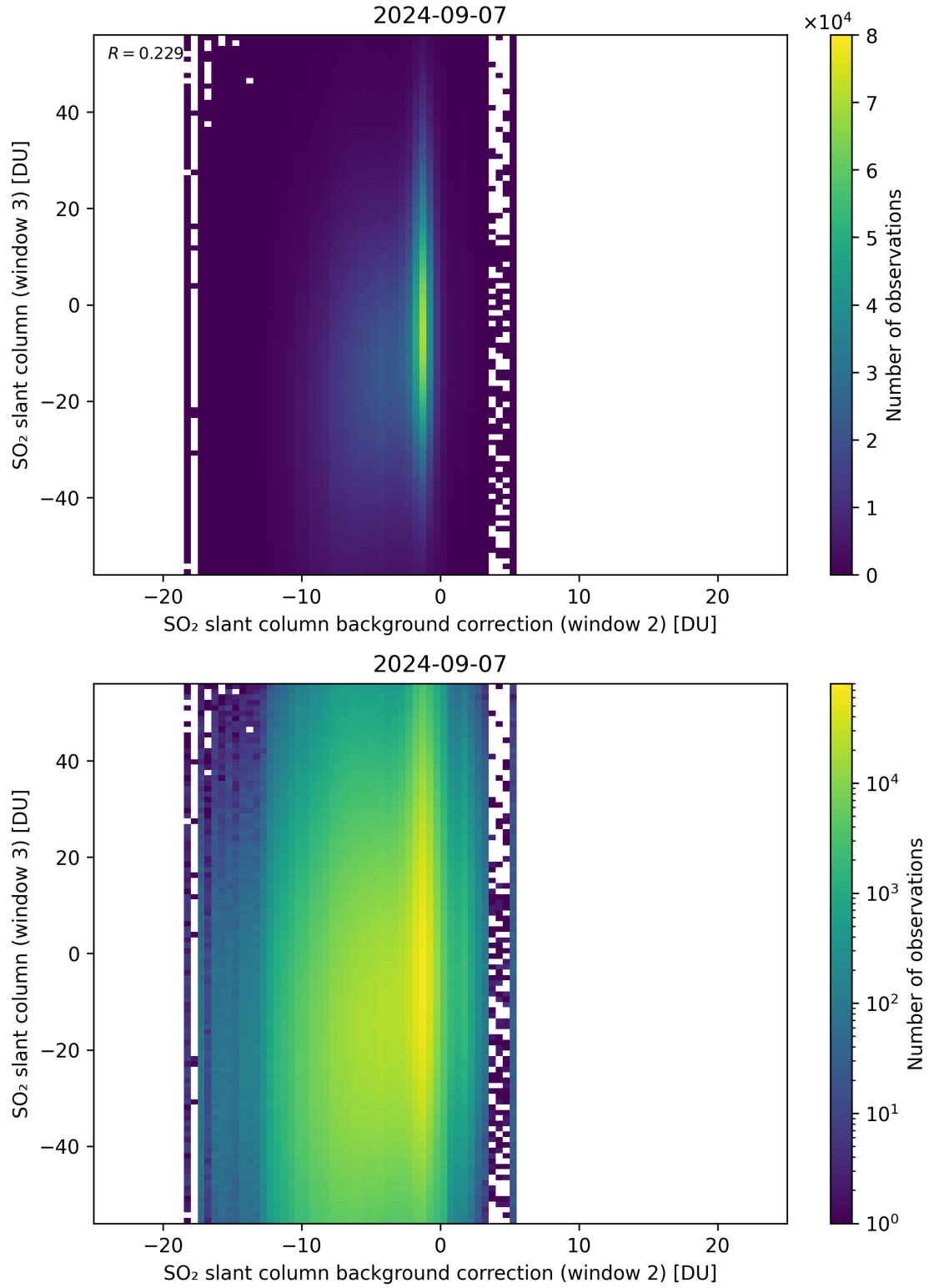
Figure 117: Scatter density plot of “SO 2 slant column background correction (window 2)” against “SO 2 slant column (window 3)” for 2024-09-06 to 2024-09-08.
