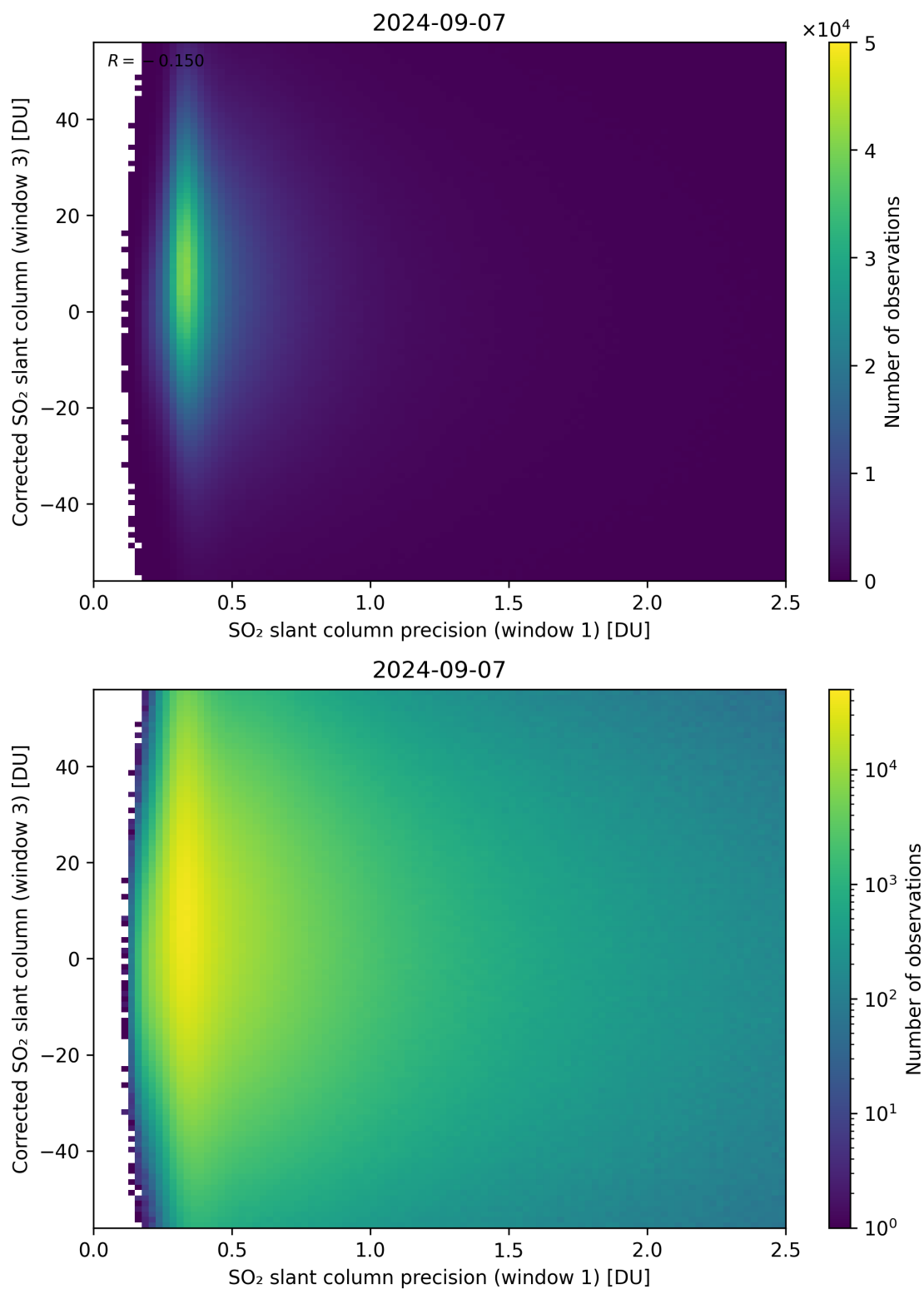
Figure 226: Scatter density plot of “SO 2 slant column precision (window 1)” against “Corrected SO 2 slant column (window 3)” for 2024-09-06 to 2024-09-08.
