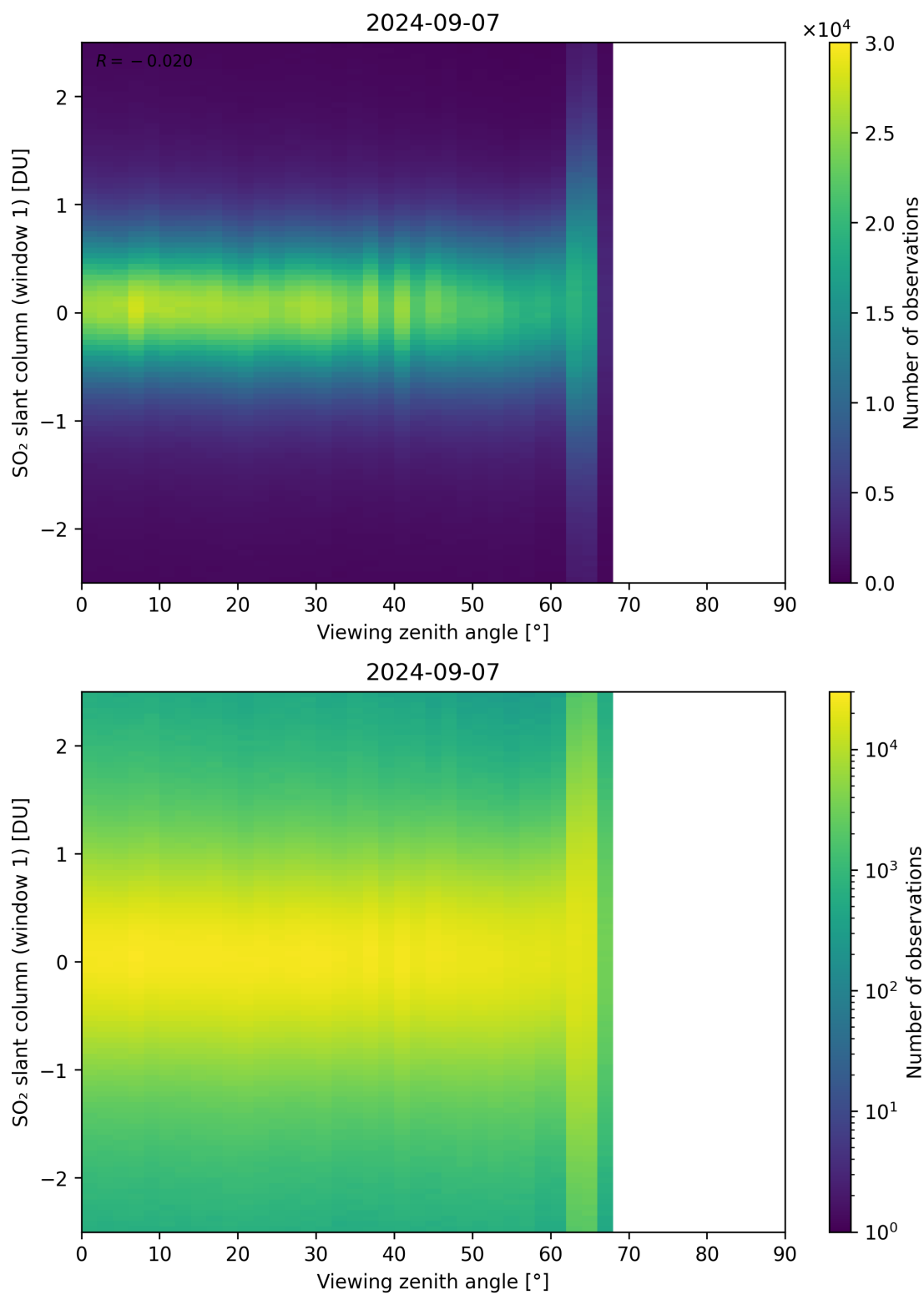
Figure 320: Scatter density plot of “Viewing zenith angle” against “SO 2 slant column (window 1)” for 2024-09-06 to 2024-09-08.
