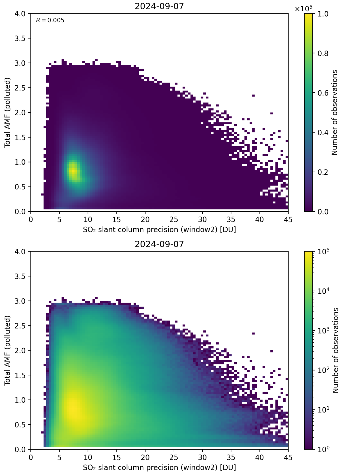
Figure 251: Scatter density plot of “SO 2 slant column precision (window2)” against “Total AMF (polluted)” for 2024-09-06 to 2024-09-08.
