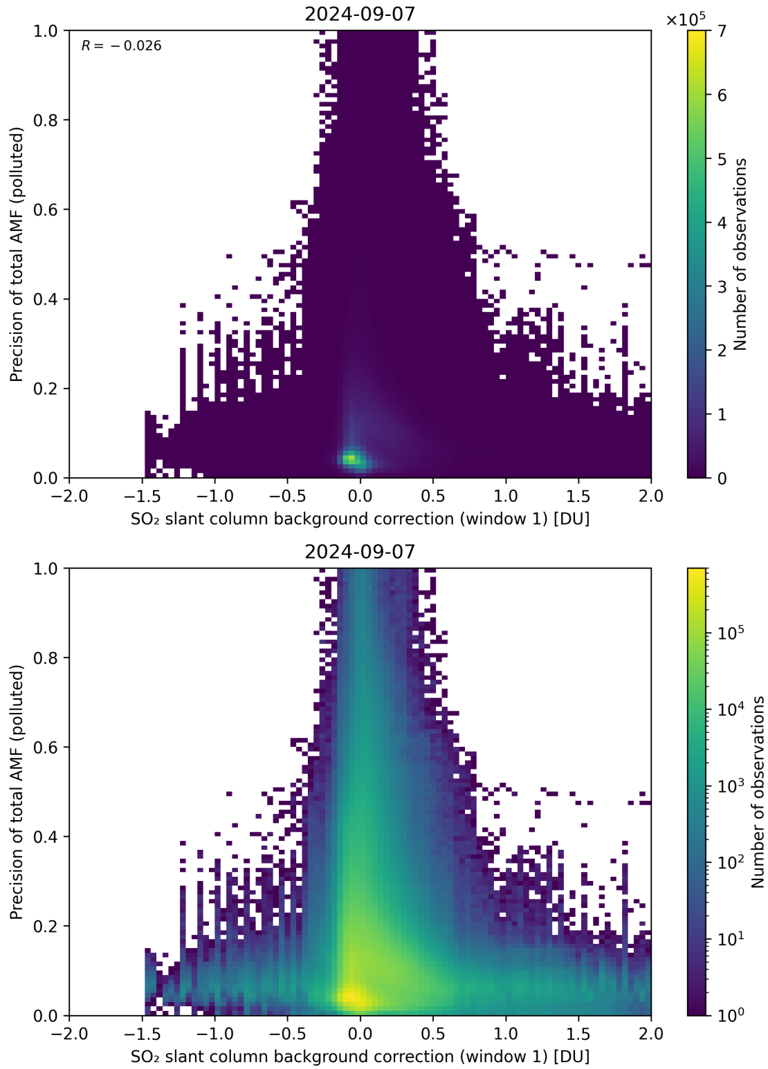
Figure 110: Scatter density plot of “SO 2 slant column background correction (window 1)” against “Precision of total AMF (polluted)” for 2024-09-06 to 2024-09-08.
