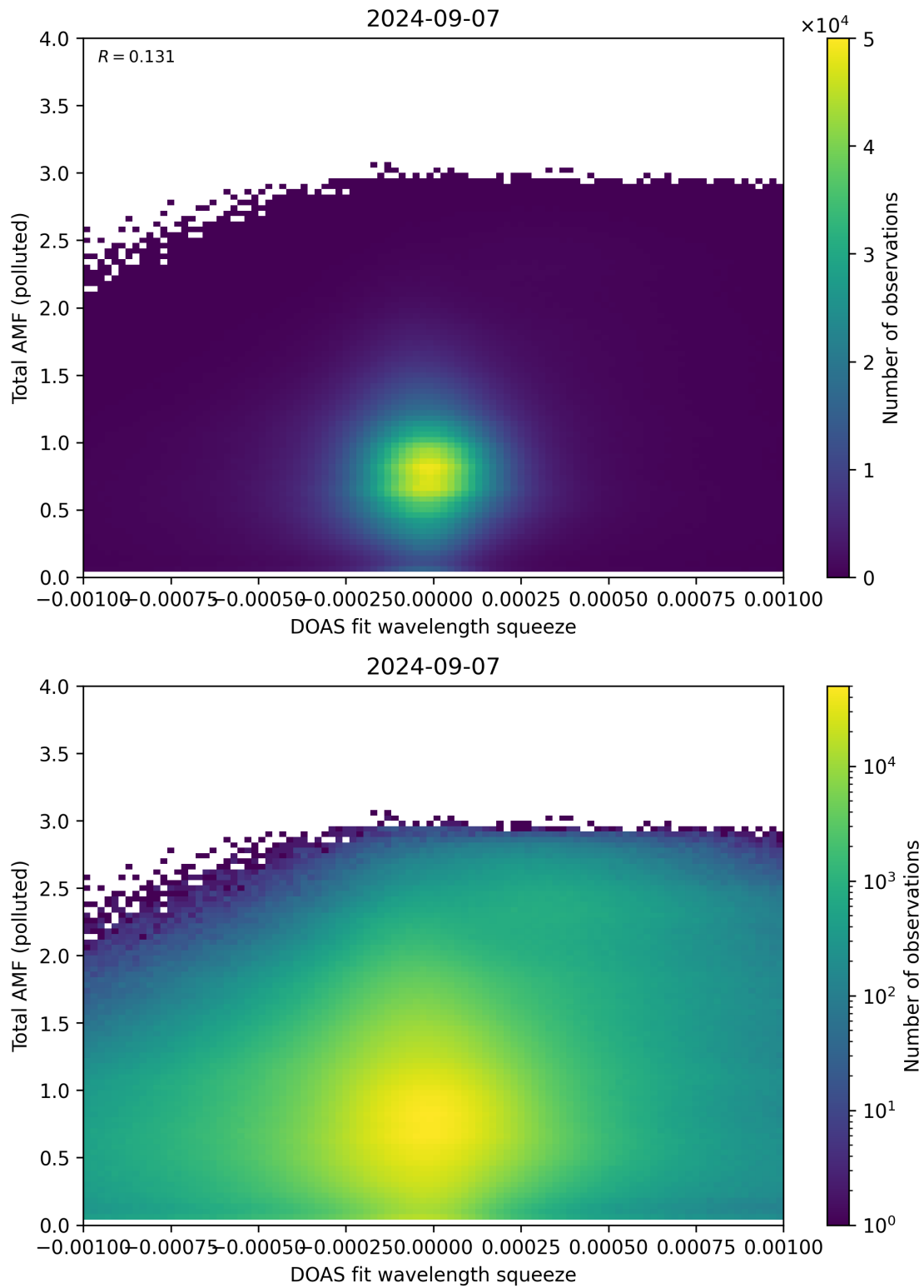
Figure 134: Scatter density plot of “DOAS fit wavelength squeeze” against “Total AMF (polluted)” for 2024-09-06 to 2024-09-08.
