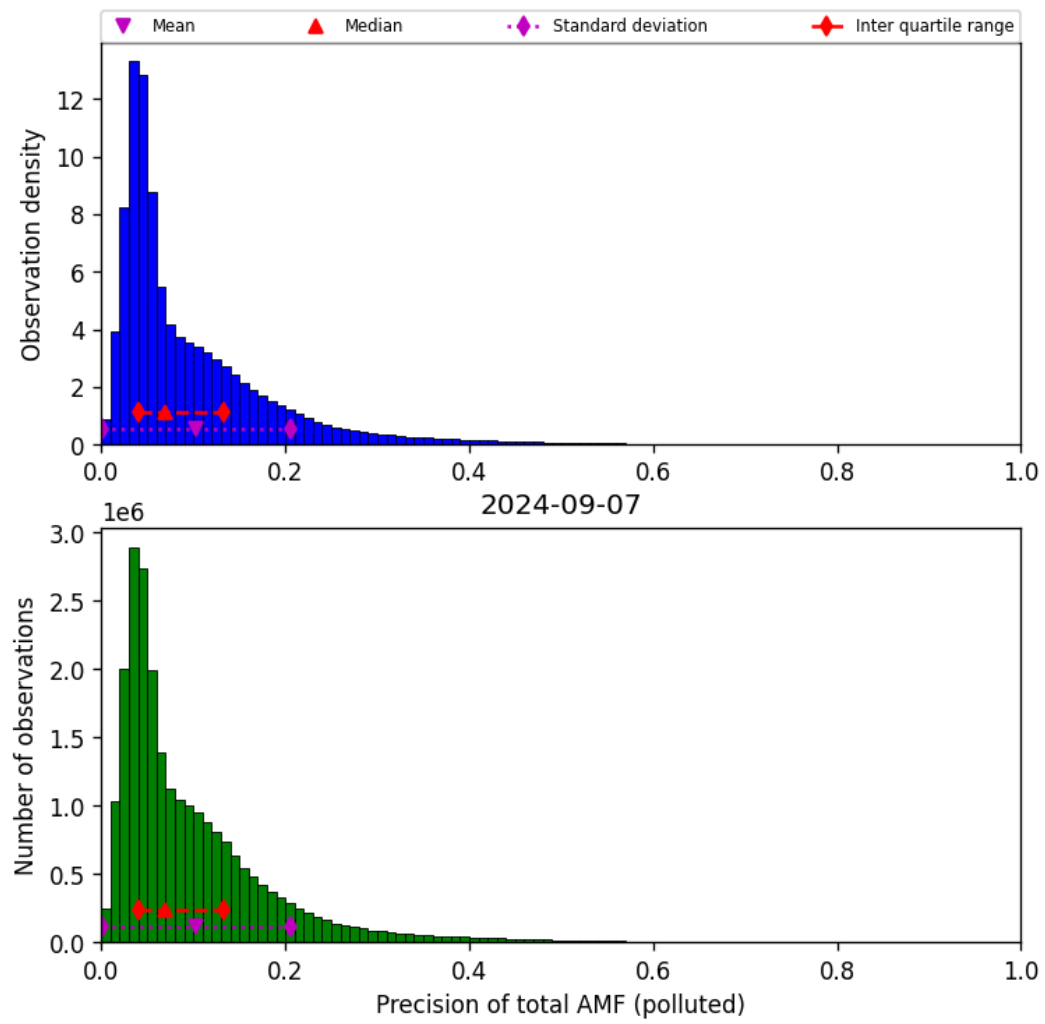
Figure 72: Histogram of “Precision of total AMF (polluted)” for 2024-09-06 to 2024-09-08
