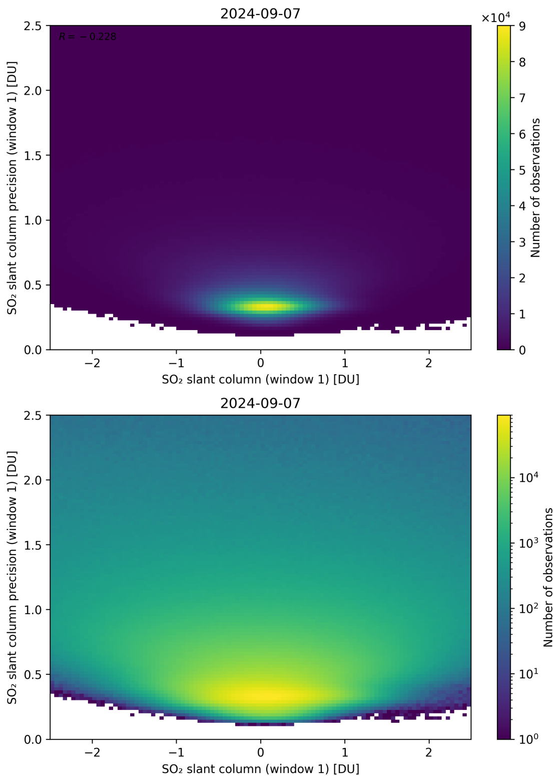
Figure 235: Scatter density plot of “SO 2 slant column (window 1)” against “SO 2 slant column precision (window 1)” for 2024-09-06 to 2024-09-08.
