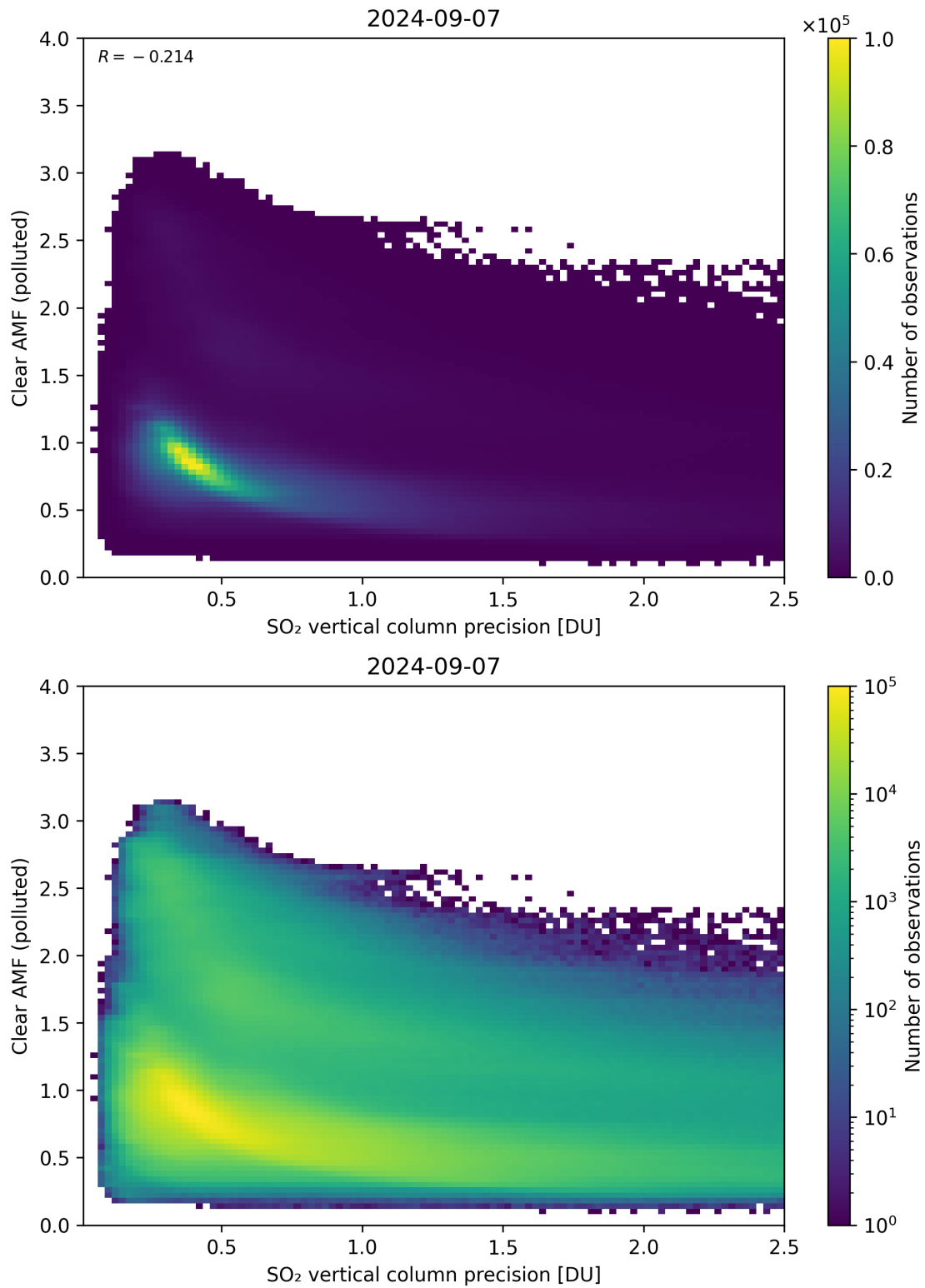
Figure 285: Scatter density plot of “SO 2 vertical column precision” against “Clear AMF (polluted)” for 2024-09-06 to 2024-09-08.
