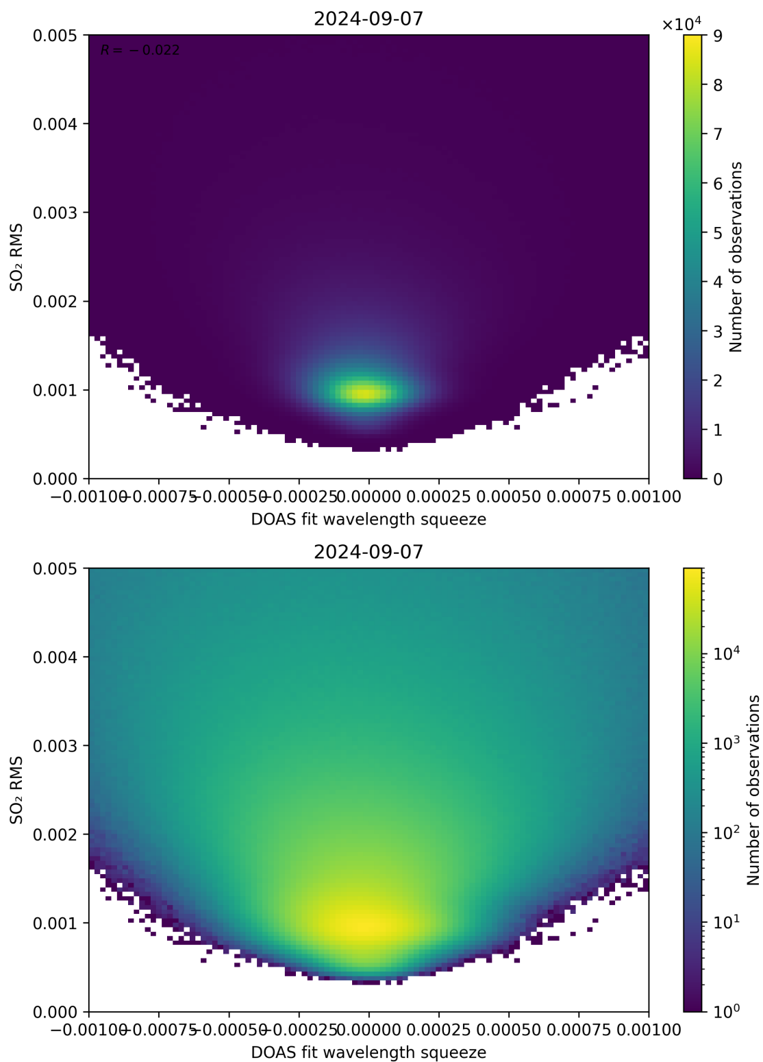
Figure 132: Scatter density plot of “DOAS fit wavelength squeeze” against “SO 2 RMS” for 2024-09-06 to 2024-09-08.
