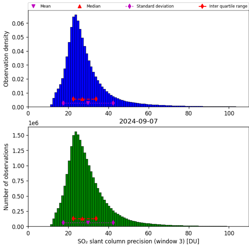
Figure 65: Histogram of “SO 2 slant column precision (window 3)” for 2024-09-06 to 2024-09-08
