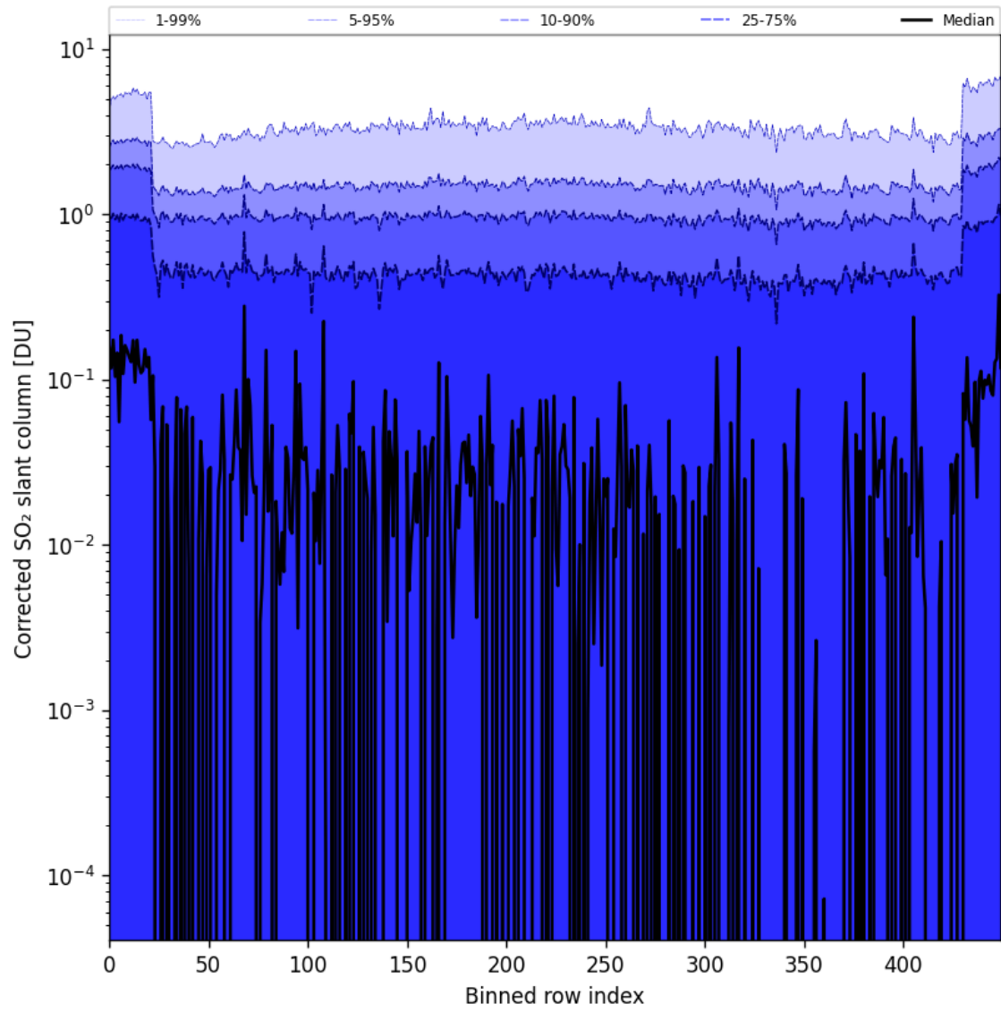
Figure 78: Along track statistics of “Corrected SO 2 slant column” for 2024-09-06 to 2024-09-08
