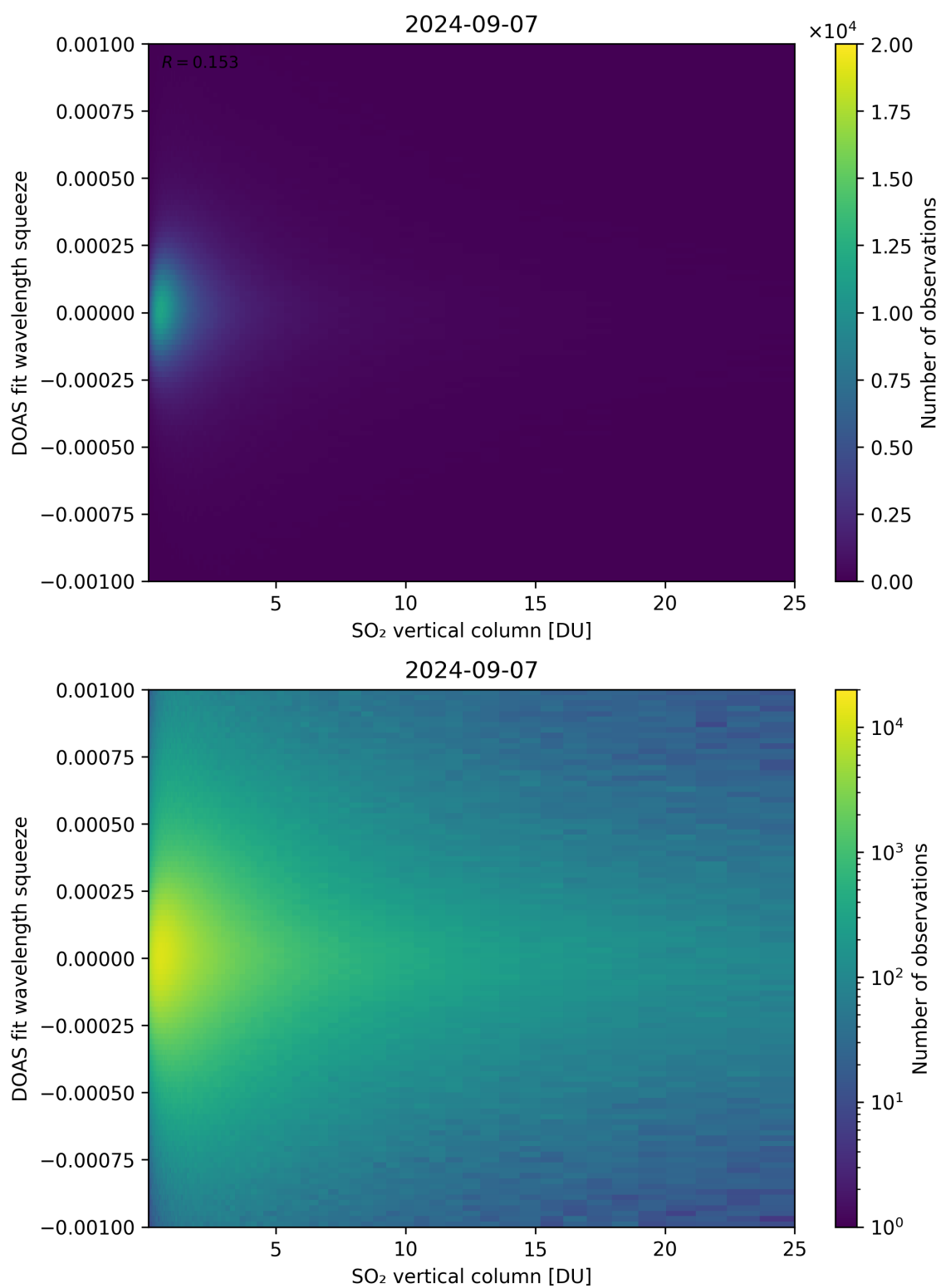
Figure 277: Scatter density plot of “SO 2 vertical column” against “DOAS fit wavelength squeeze” for 2024-09-06 to 2024-09-08.
