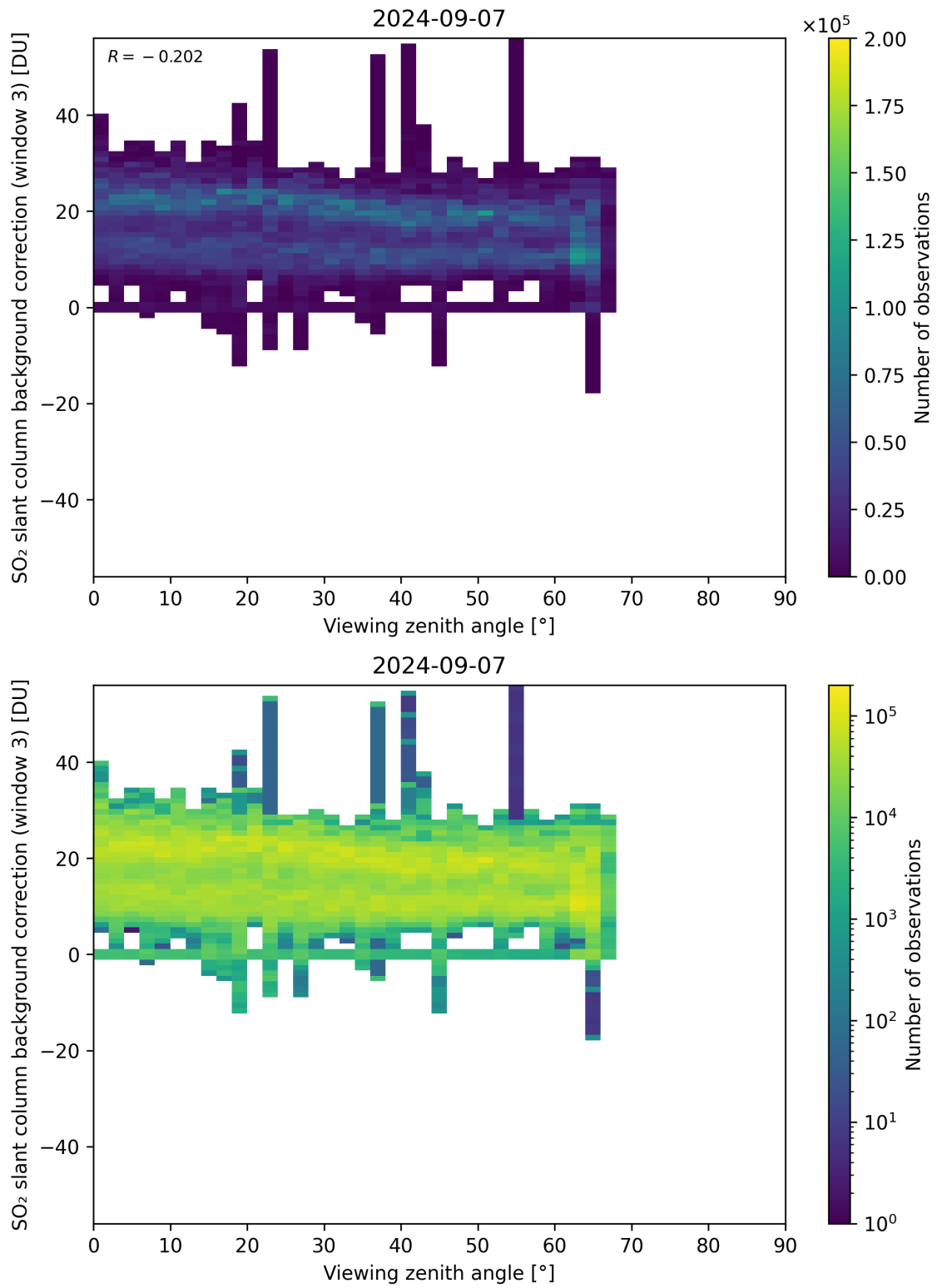
Figure 310: Scatter density plot of “Viewing zenith angle” against “SO 2 slant column background correction (window 3)” for 2024-09-06 to 2024-09-08.
