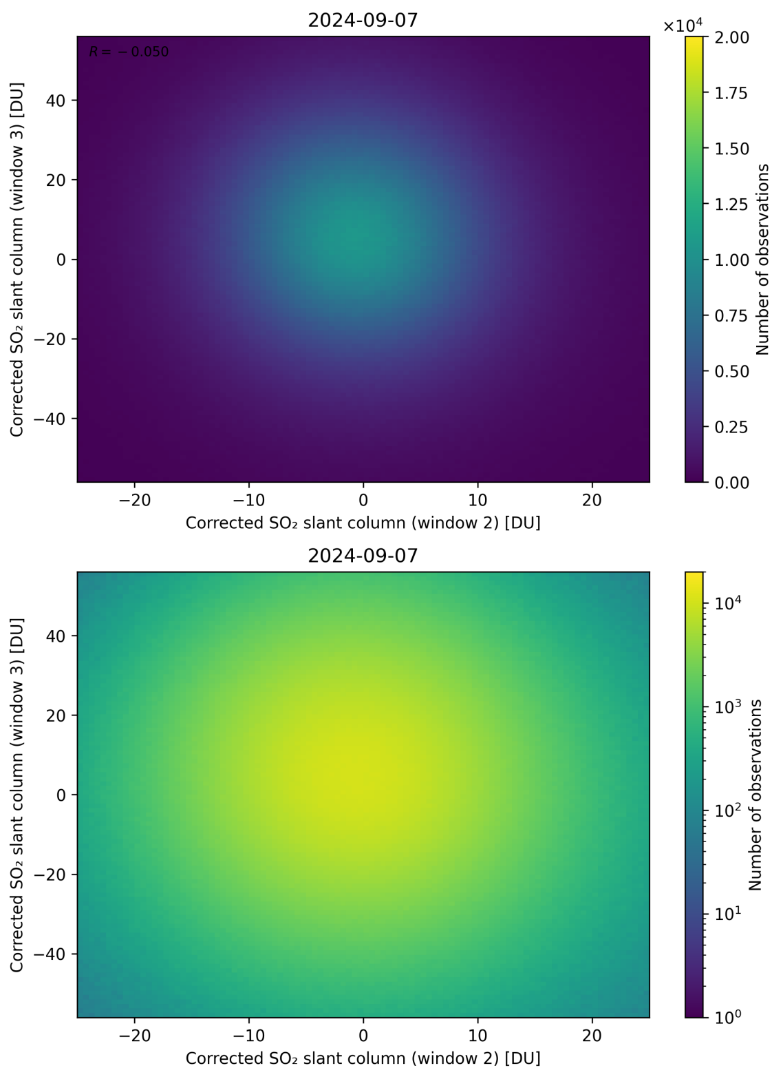
Figure 200: Scatter density plot of “Corrected SO 2 slant column (window 2)” against “Corrected SO 2 slant column (window 3)” for 2024-09-06 to 2024-09-08.
