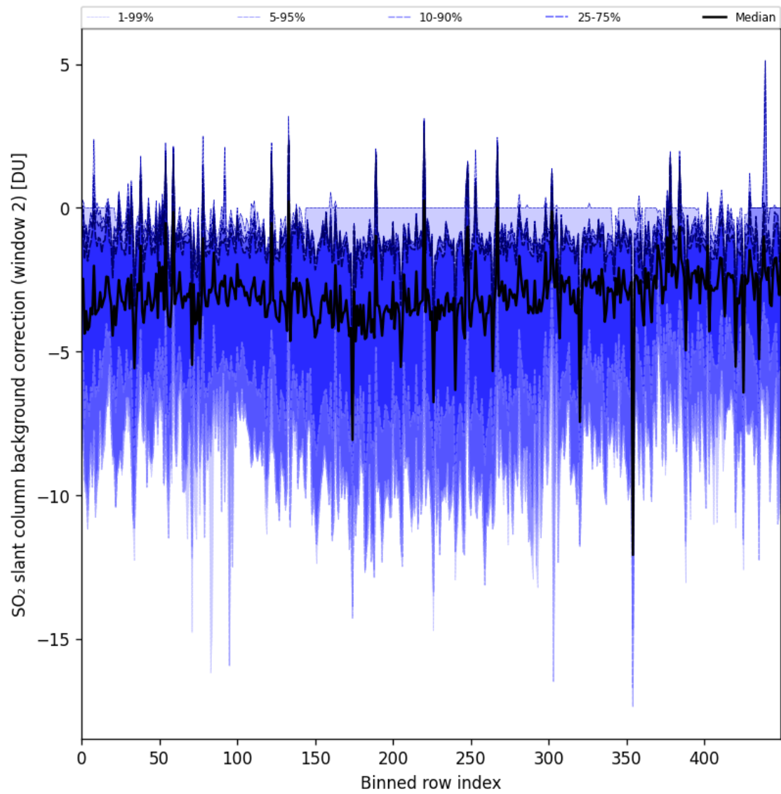
Figure 86: Along track statistics of “SO 2 slant column background correction (window 2)” for 2024-09-06 to 2024-09-08
