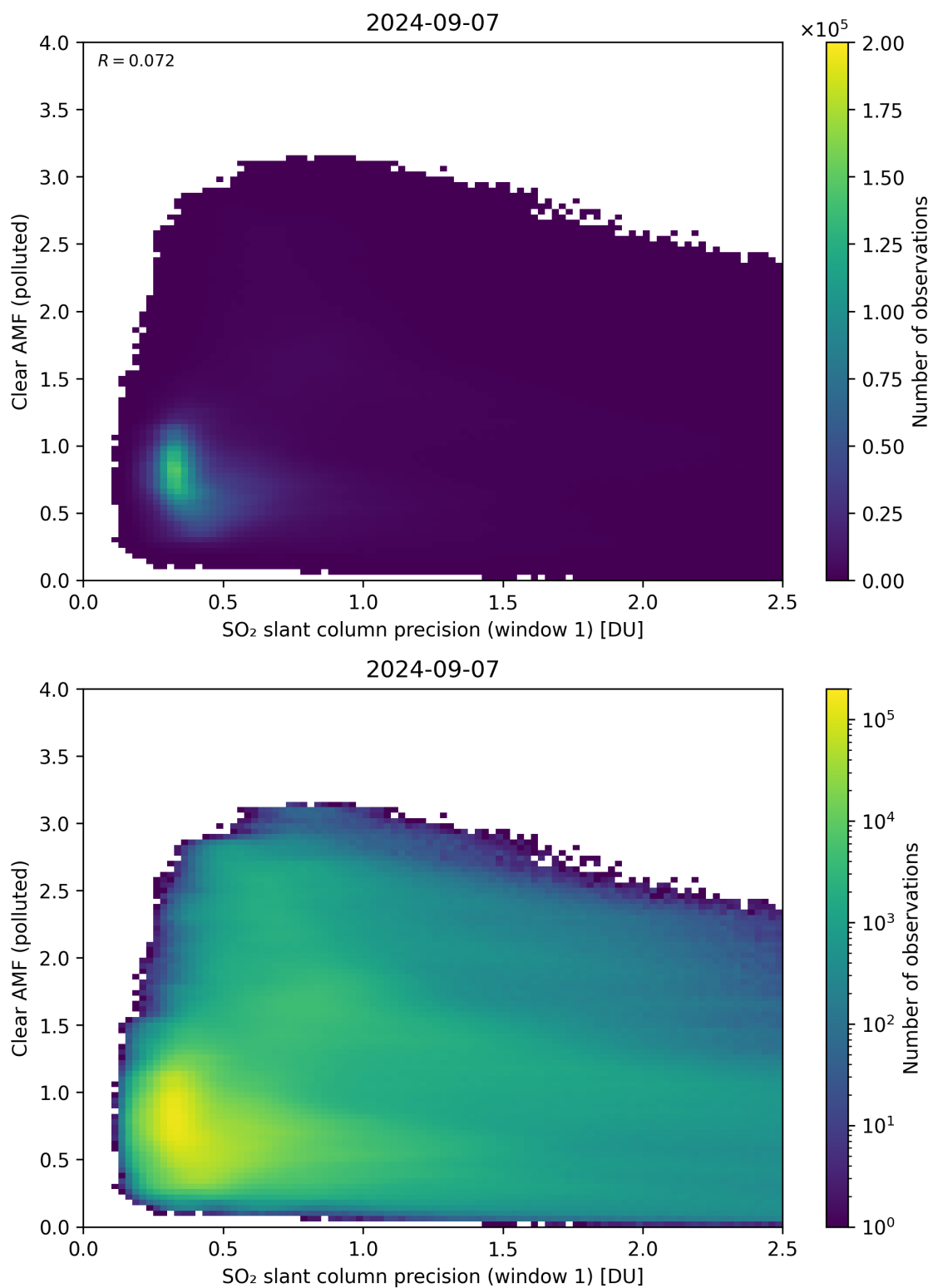
Figure 224: Scatter density plot of “SO 2 slant column precision (window 1)” against “Clear AMF (polluted)” for 2024-09-06 to 2024-09-08.
