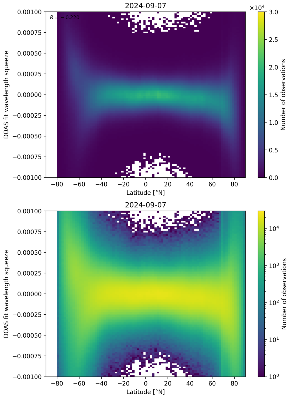
Figure 143: Scatter density plot of “Latitude” against “DOAS fit wavelength squeeze” for 2024-09-06 to 2024-09-08.
