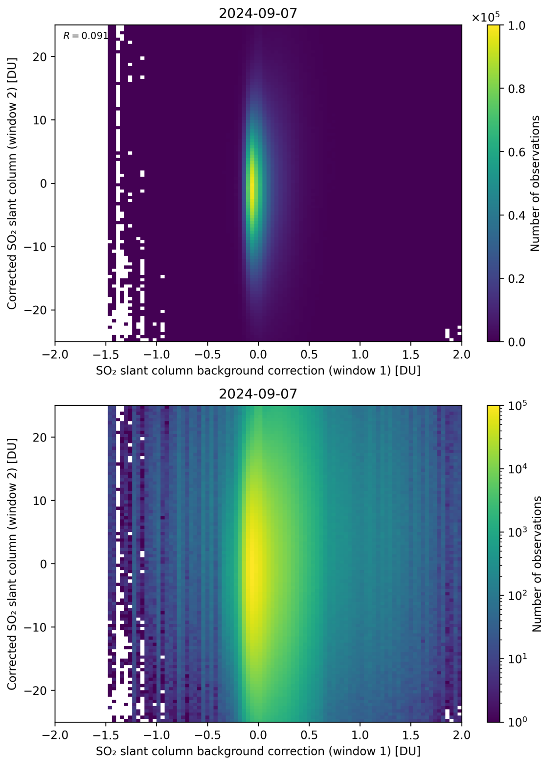
Figure 104: Scatter density plot of “SO 2 slant column background correction (window 1)” against “Corrected SO 2 slant column (window 2)” for 2024-09-06 to 2024-09-08.
