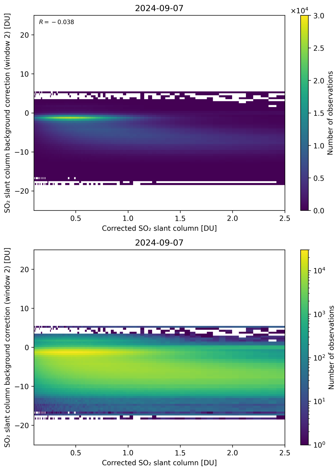
Figure 179: Scatter density plot of “Corrected SO 2 slant column” against “SO 2 slant column background correction (window 2)” for 2024-09-06 to 2024-09-08.
