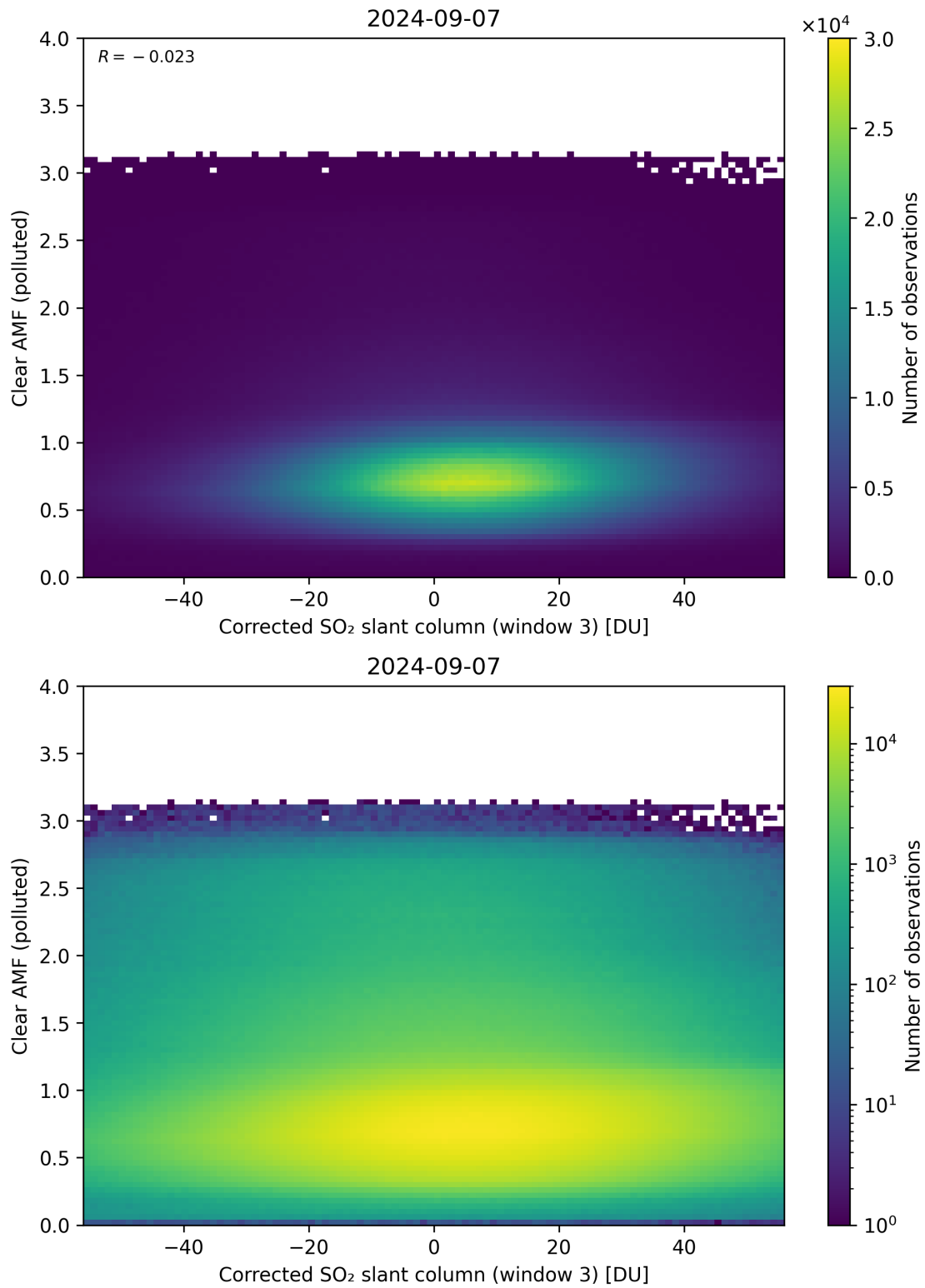
Figure 209: Scatter density plot of “Corrected SO 2 slant column (window 3)” against “Clear AMF (polluted)” for 2024-09-06 to 2024-09-08.
