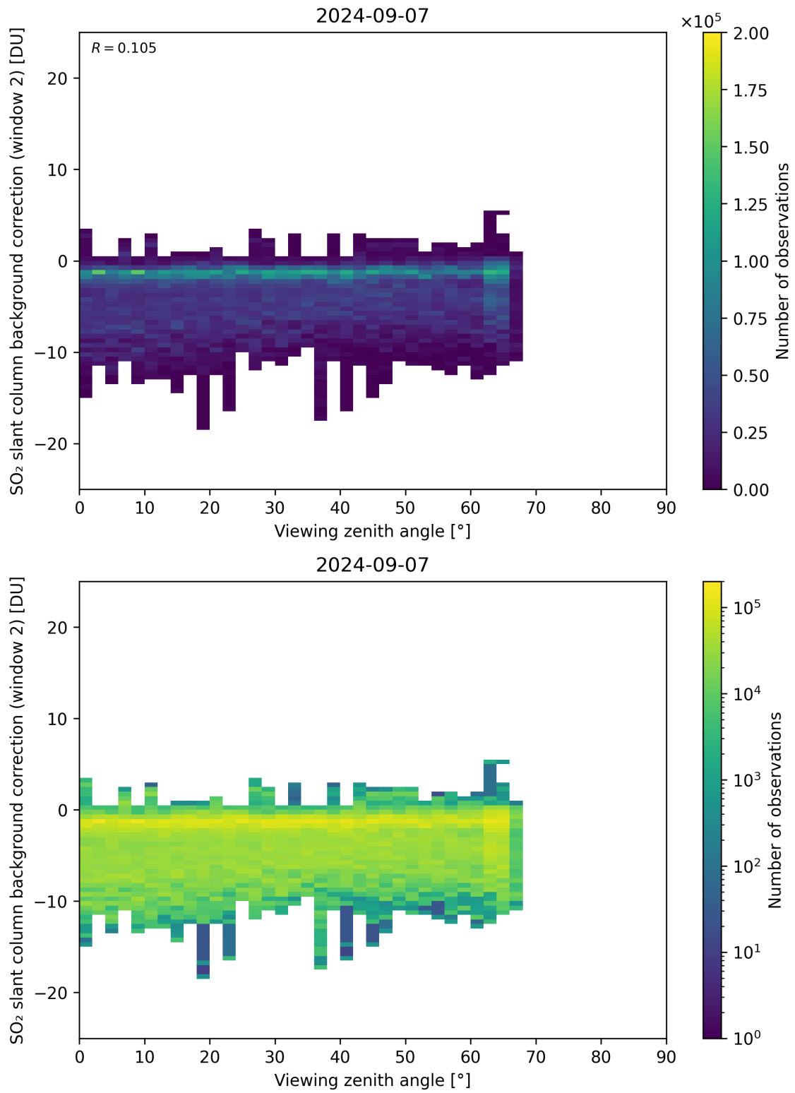
Figure 309: Scatter density plot of “Viewing zenith angle” against “SO 2 slant column background correction (window 2)” for 2024-09-06 to 2024-09-08.
