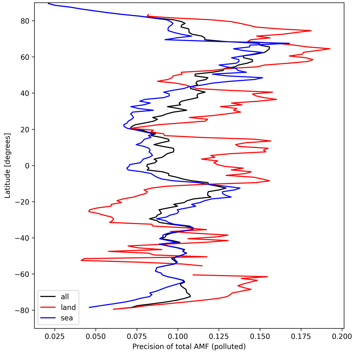
Figure 49: Zonal average of “Precision of total AMF (polluted)” for 2024-09-06 to 2024-09-08.
