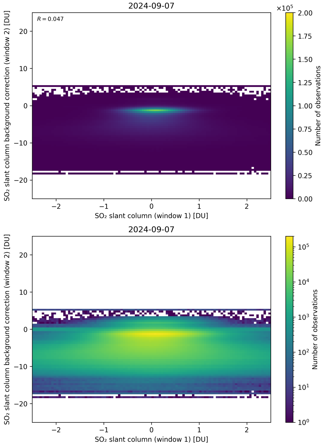
Figure 213: Scatter density plot of “SO 2 slant column (window 1)” against “SO 2 slant column background correction (window 2)” for 2024-09-06 to 2024-09-08.
