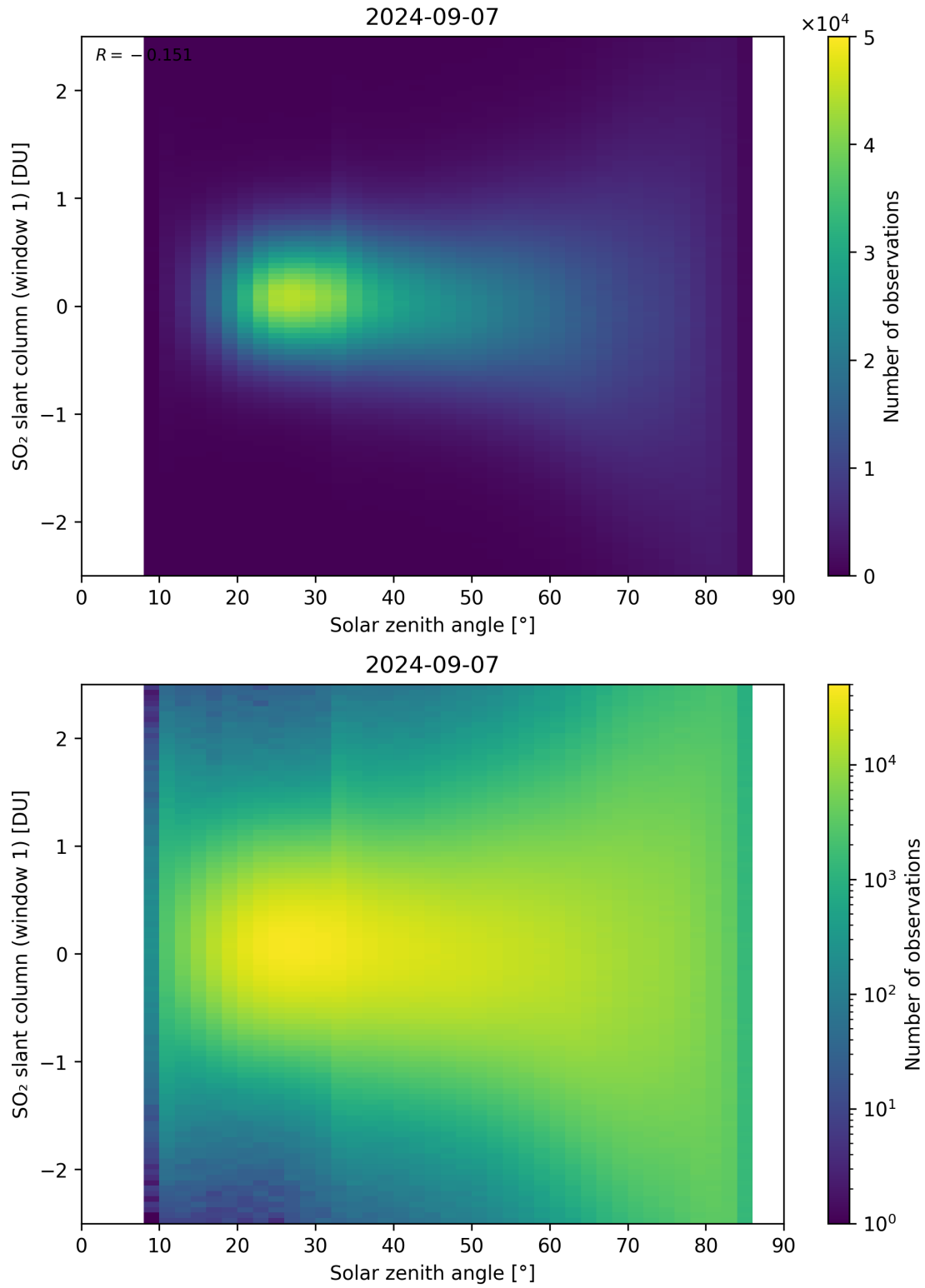
Figure 169: Scatter density plot of “Solar zenith angle” against “SO 2 slant column (window 1)” for 2024-09-06 to 2024-09-08.
