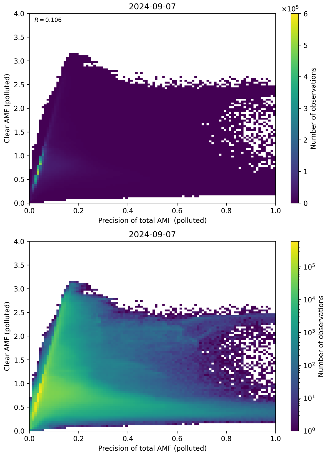
Figure 270: Scatter density plot of “Precision of total AMF (polluted)” against “Clear AMF (polluted)” for 2024-09-06 to 2024-09-08.
