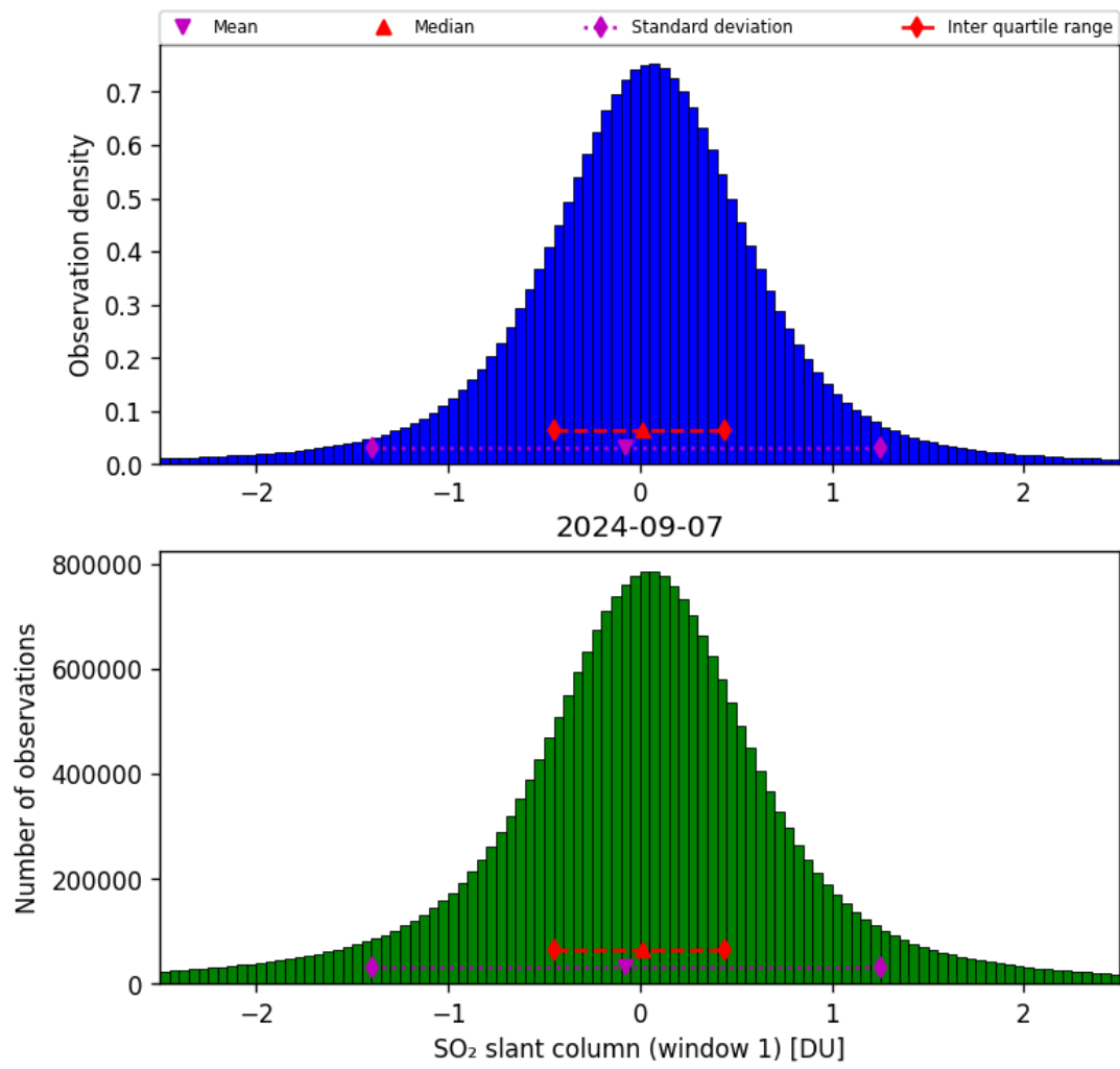
Figure 56: Histogram of “SO 2 slant column (window 1)” for 2024-09-06 to 2024-09-08
