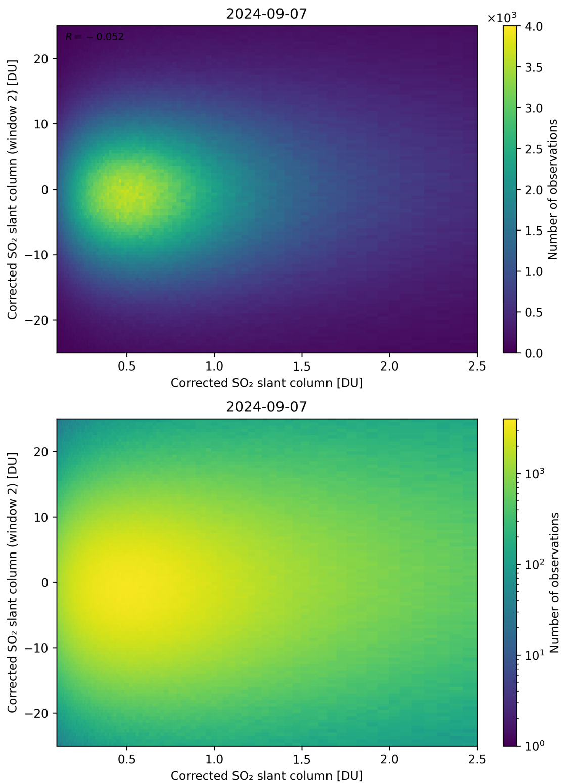
Figure 185: Scatter density plot of “Corrected SO 2 slant column” against “Corrected SO 2 slant column (window 2)” for 2024-09-06 to 2024-09-08.
