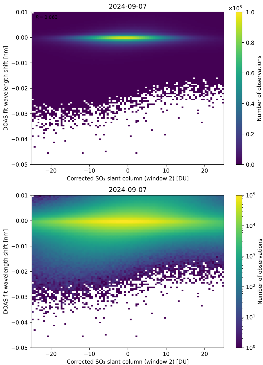
Figure 196: Scatter density plot of “Corrected SO 2 slant column (window 2)” against “DOAS fit wavelength shift” for 2024-09-06 to 2024-09-08.
