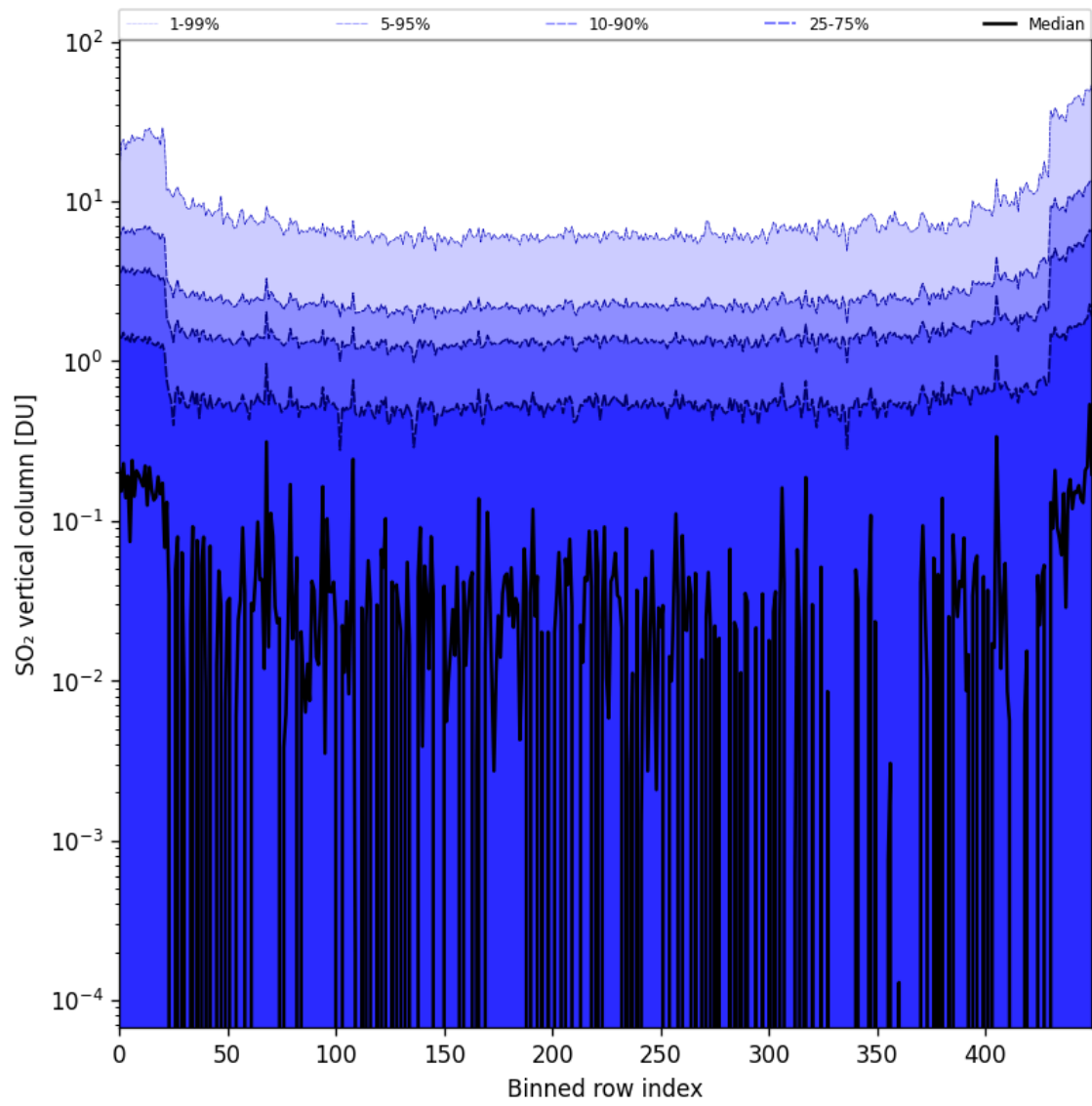
Figure 76: Along track statistics of “SO 2 vertical column” for 2024-09-06 to 2024-09-08
