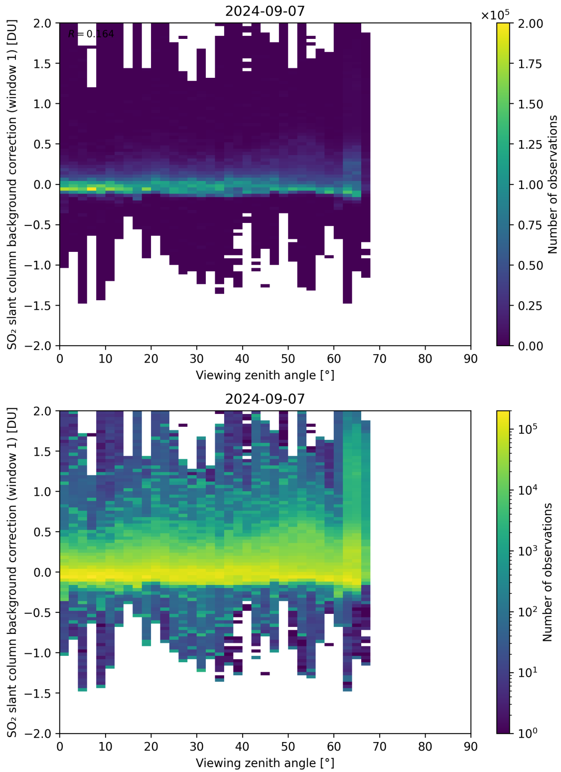
Figure 308: Scatter density plot of “Viewing zenith angle” against “SO 2 slant column background correction (window 1)” for 2024-09-06 to 2024-09-08.
