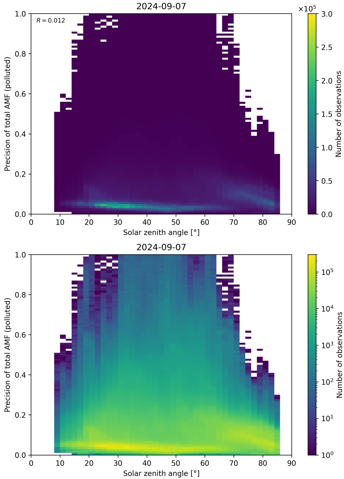
Figure 175: Scatter density plot of “Solar zenith angle” against “Precision of total AMF (polluted)” for 2024-09-06 to 2024-09-08.
