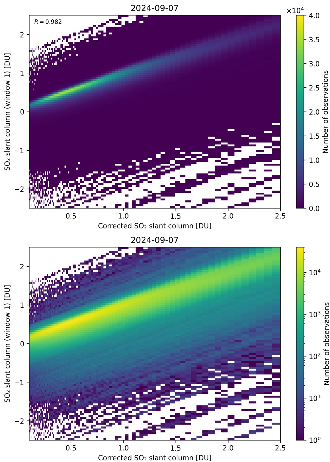
Figure 187: Scatter density plot of “Corrected SO 2 slant column” against “SO 2 slant column (window 1)” for 2024-09-06 to 2024-09-08.
