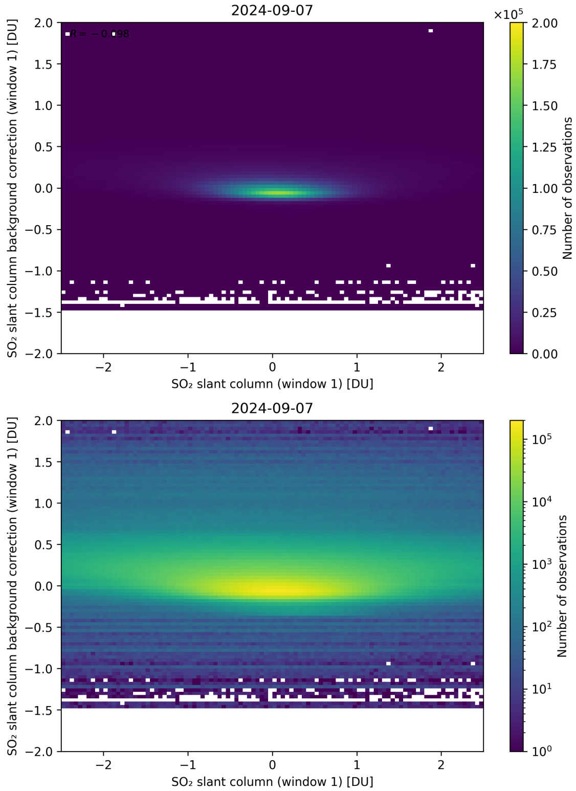
Figure 212: Scatter density plot of “SO 2 slant column (window 1)” against “SO 2 slant column background correction (window 1)” for 2024-09-06 to 2024-09-08.
