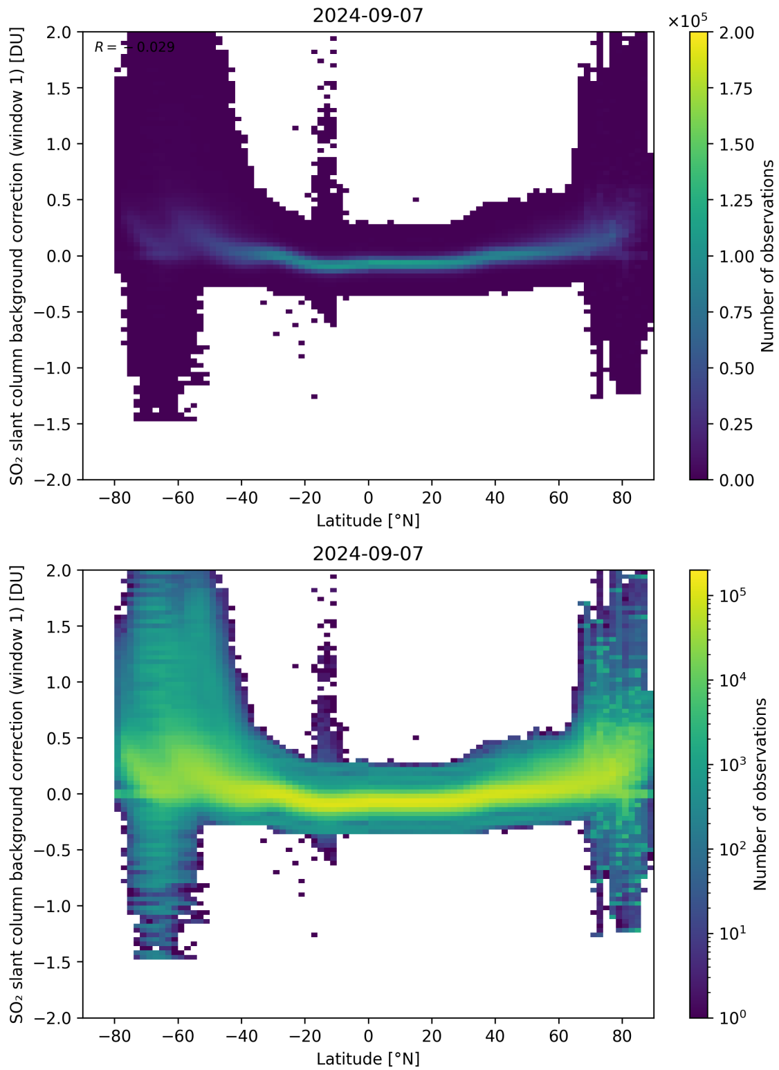
Figure 139: Scatter density plot of “Latitude” against “SO 2 slant column background correction (window 1)” for 2024-09-06 to 2024-09-08.
