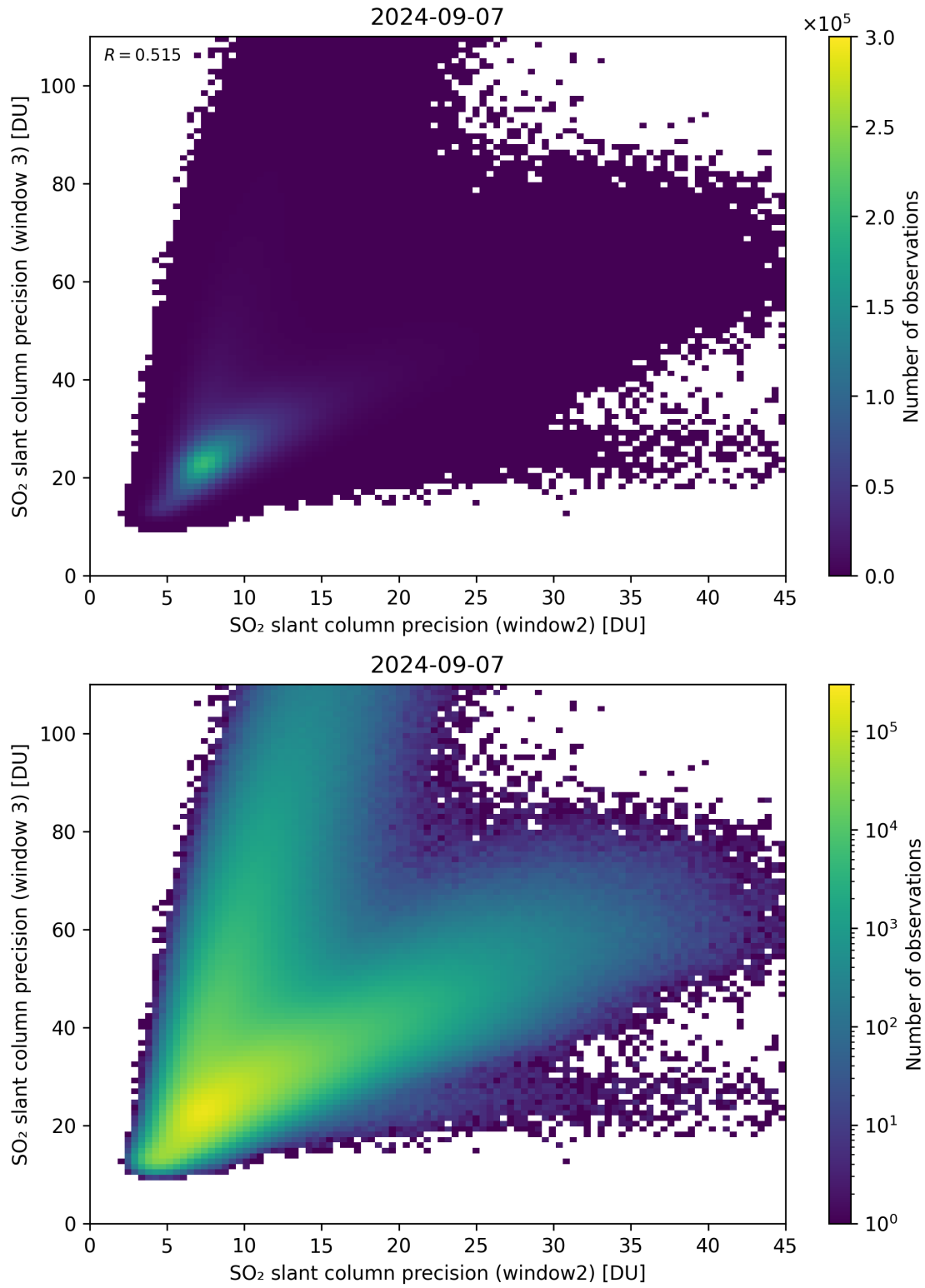
Figure 250: Scatter density plot of “SO 2 slant column precision (window2)” against “SO 2 slant column precision (window 3)” for 2024-09-06 to 2024-09-08.
