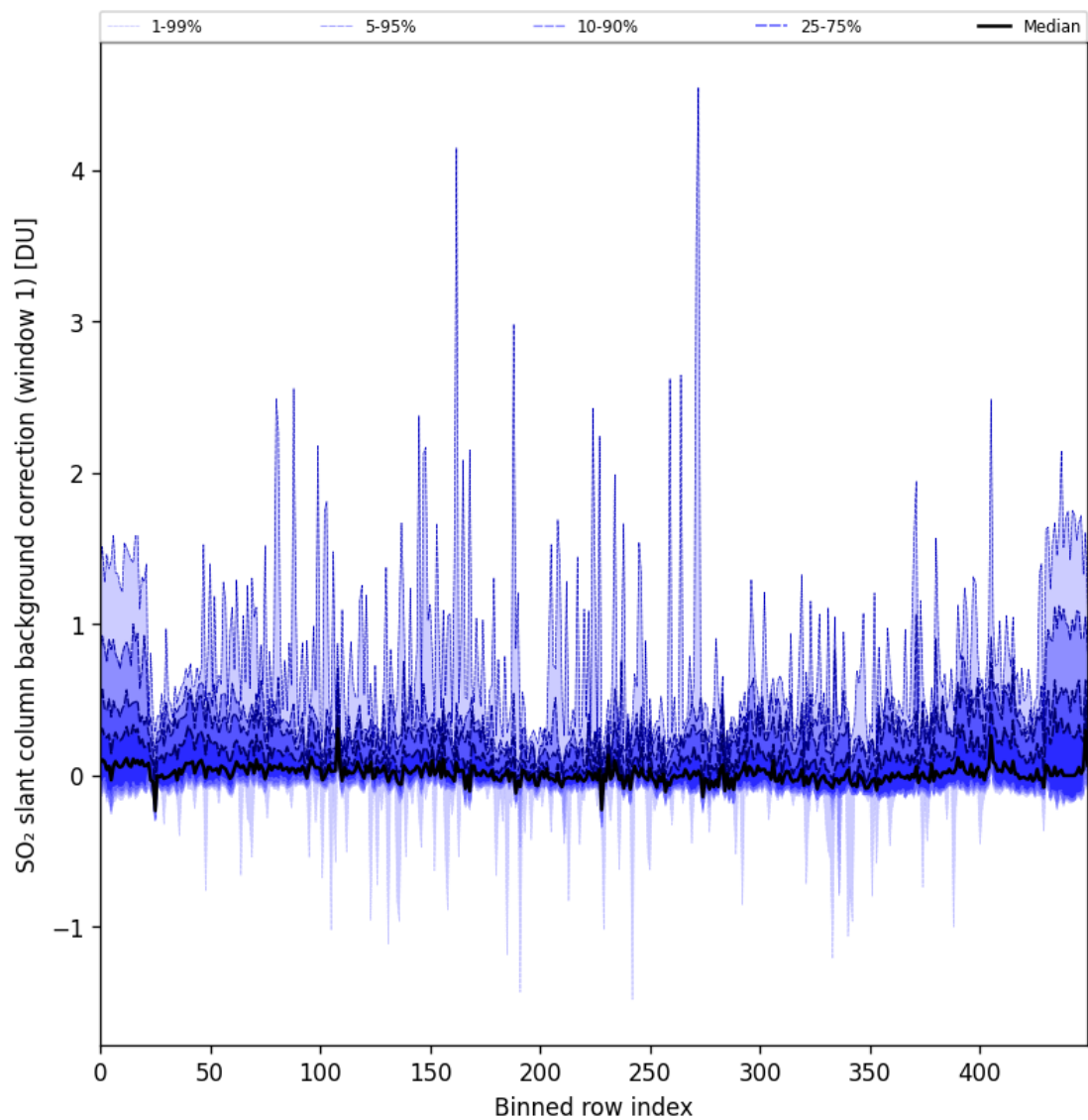
Figure 82: Along track statistics of “SO 2 slant column background correction (window 1)” for 2024-09-06 to 2024-09-08
