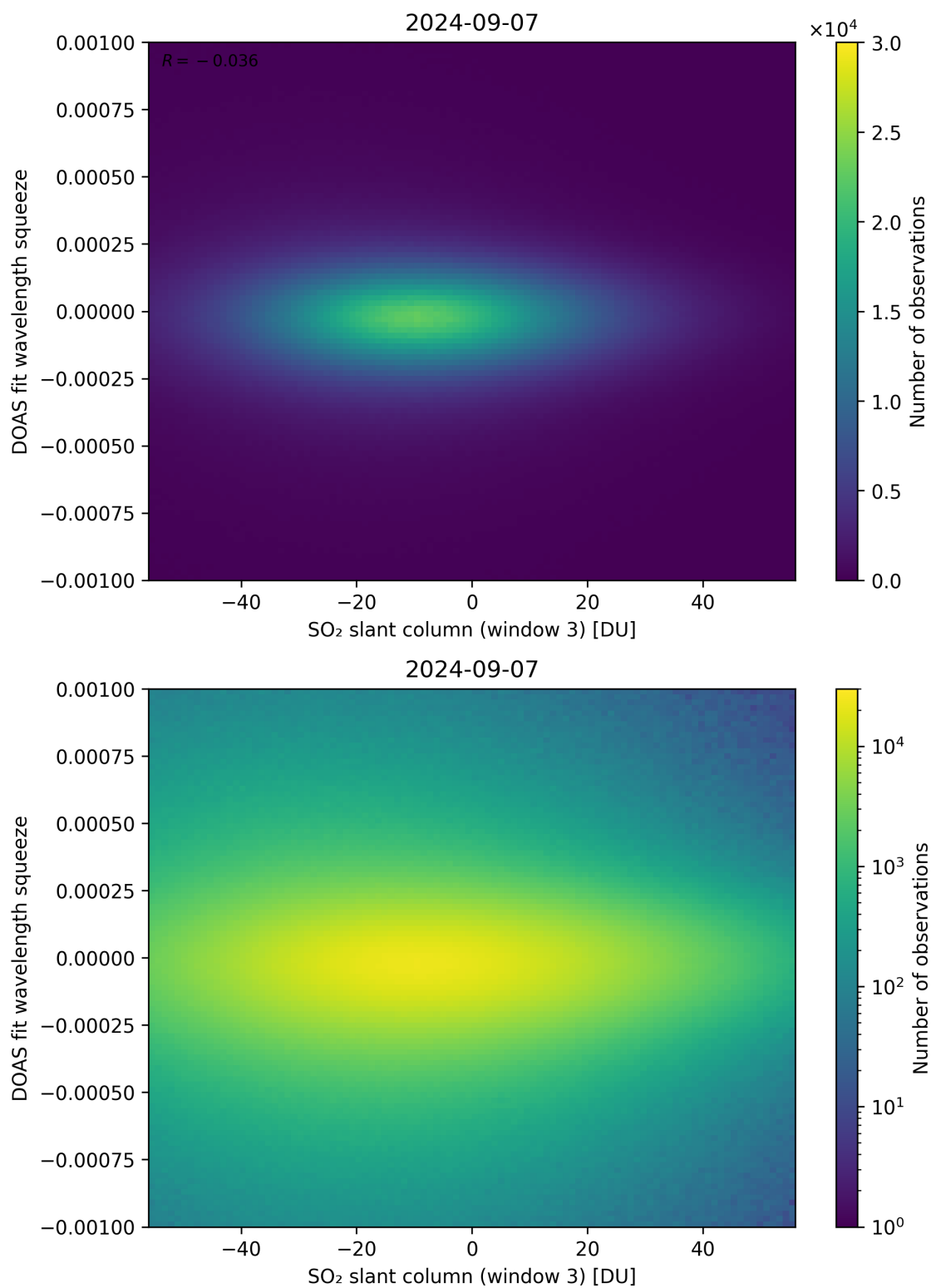
Figure 255: Scatter density plot of “SO 2 slant column (window 3)” against “DOAS fit wavelength squeeze” for 2024-09-06 to 2024-09-08.
