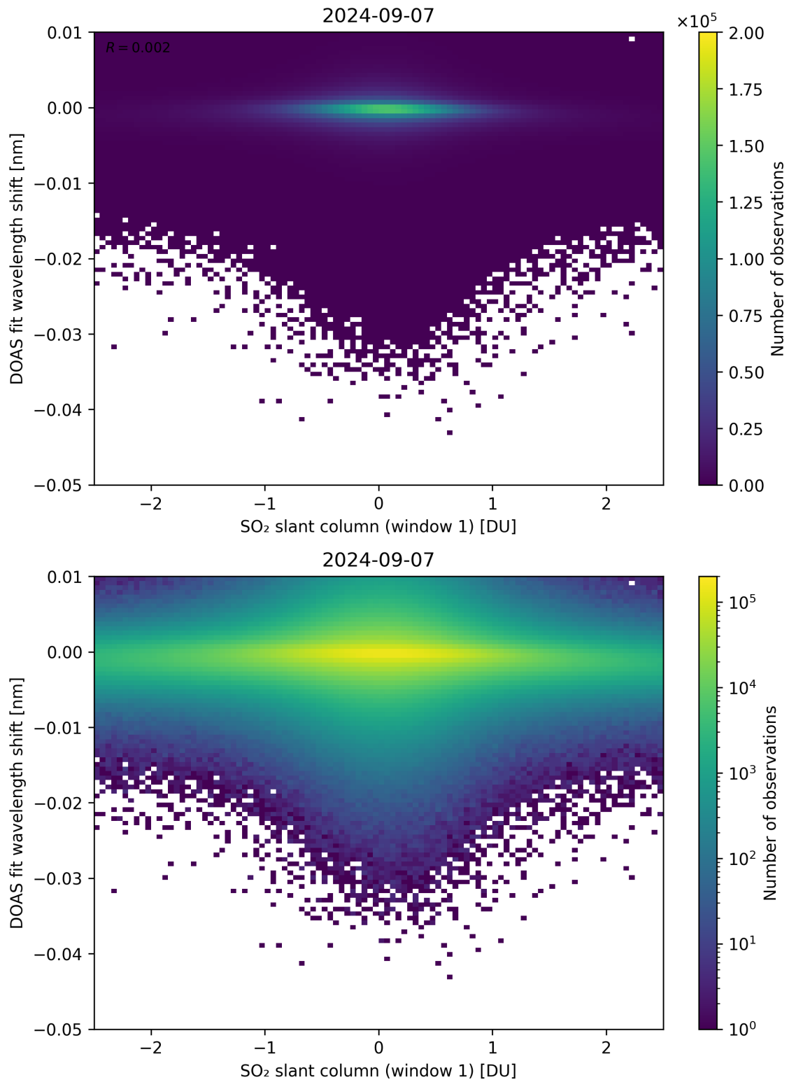
Figure 215: Scatter density plot of “SO 2 slant column (window 1)” against “DOAS fit wavelength shift” for 2024-09-06 to 2024-09-08.
