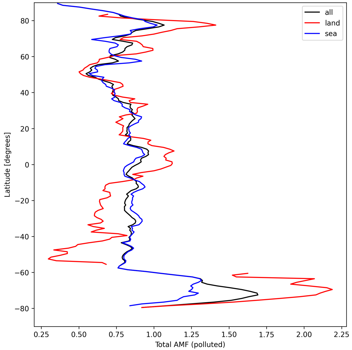
Figure 48: Zonal average of “Total AMF (polluted)” for 2024-09-06 to 2024-09-08.
