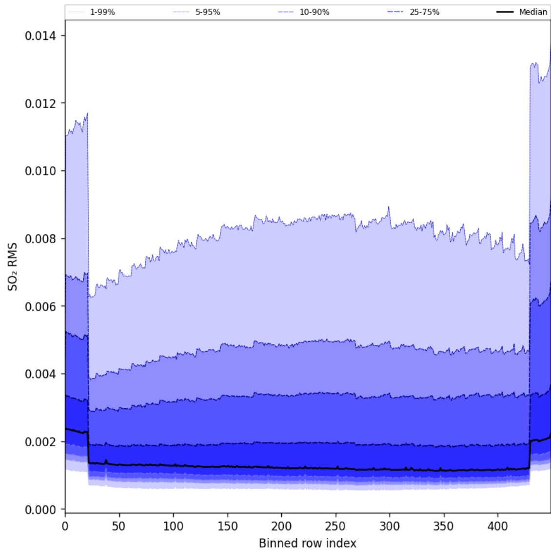
Figure 93: Along track statistics of “SO 2 RMS” for 2024-09-06 to 2024-09-08
