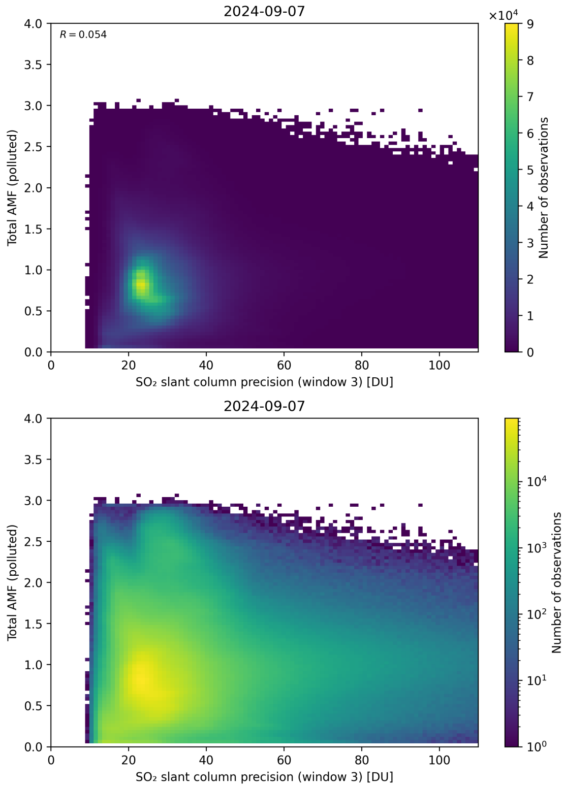
Figure 263: Scatter density plot of “SO 2 slant column precision (window 3)” against “Total AMF (polluted)” for 2024-09-06 to 2024-09-08.
