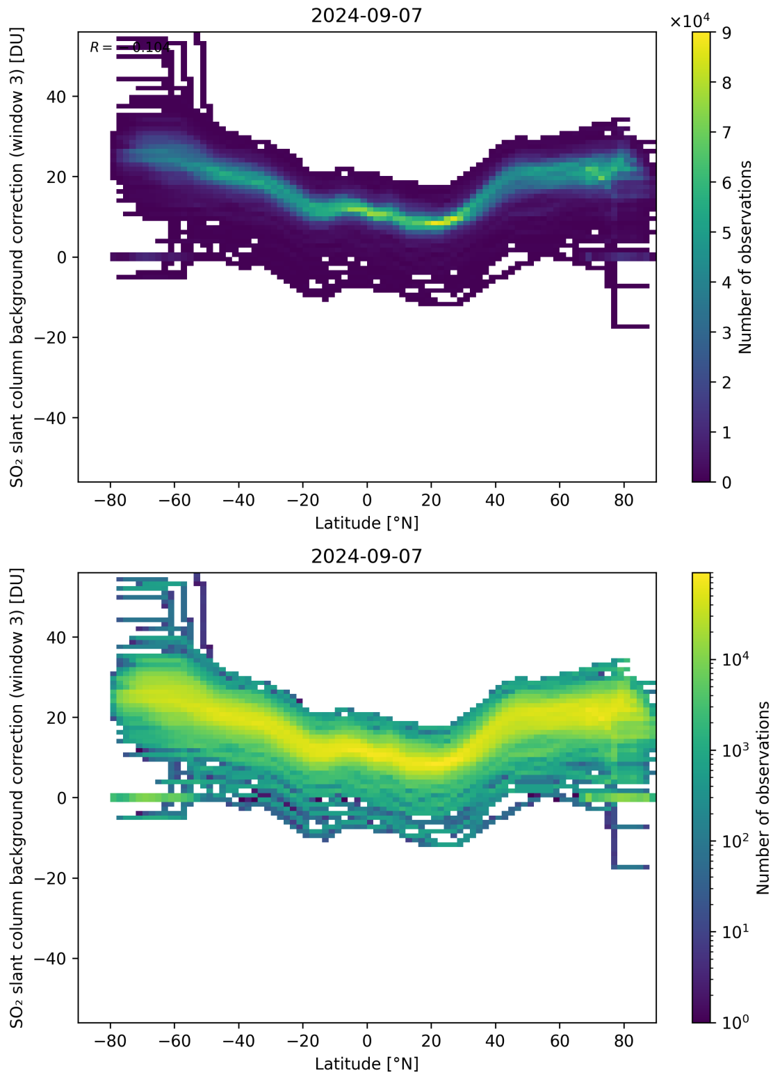
Figure 141: Scatter density plot of “Latitude” against “SO 2 slant column background correction (window 3)” for 2024-09-06 to 2024-09-08.
