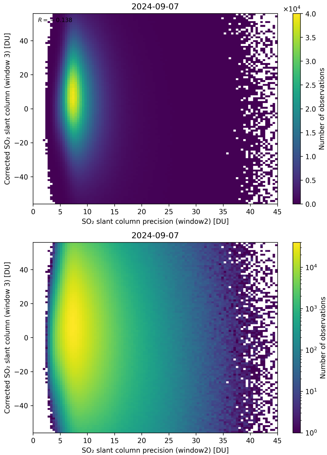
Figure 248: Scatter density plot of “SO 2 slant column precision (window2)” against “Corrected SO 2 slant column (window 3)” for 2024-09-06 to 2024-09-08.
