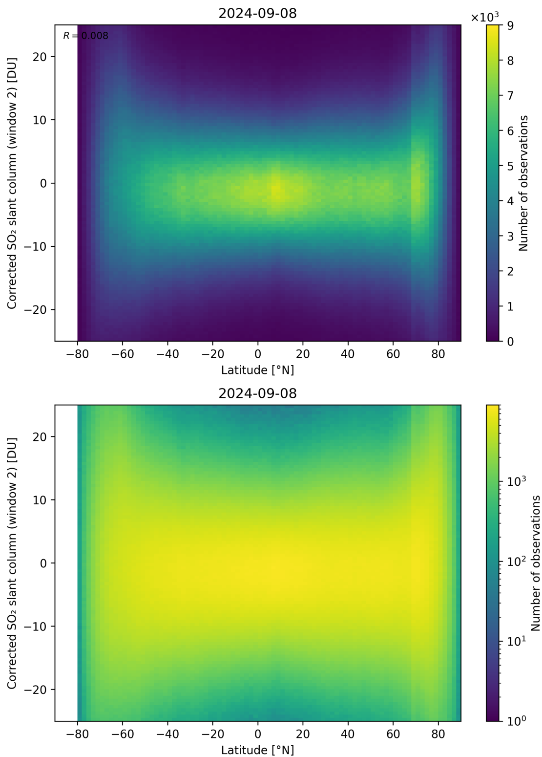
Figure 147: Scatter density plot of “Latitude” against “Corrected SO 2 slant column (window 2)” for 2024-09-07 to 2024-09-09.
