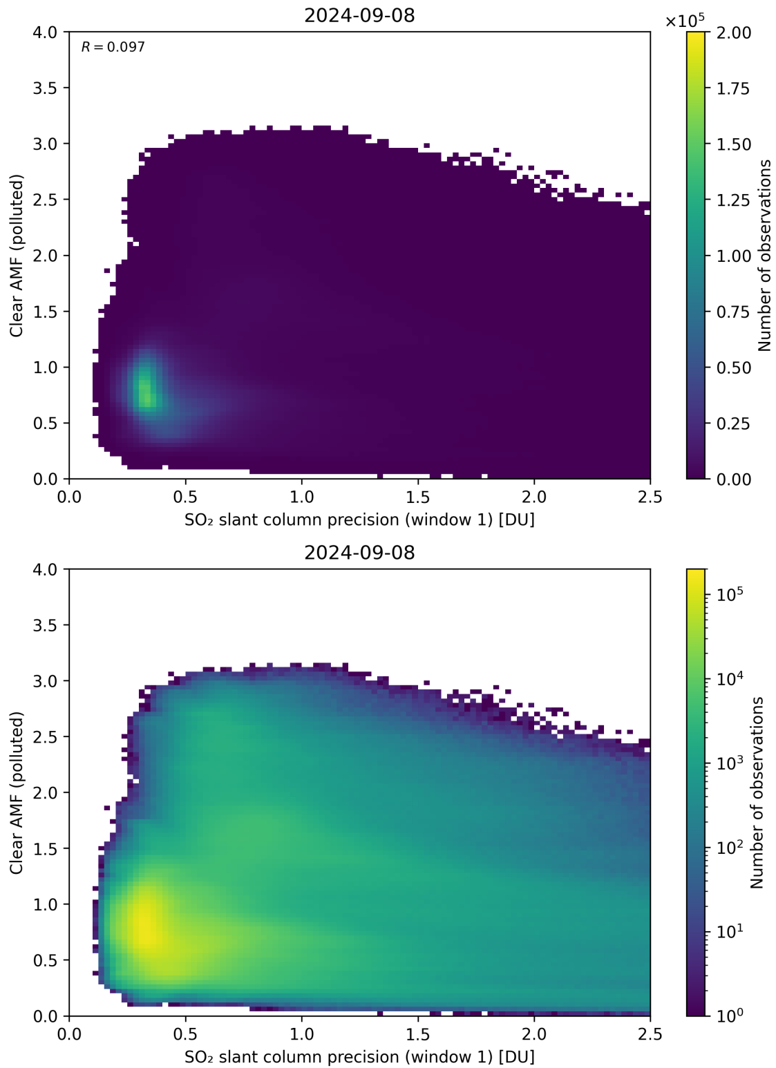
Figure 224: Scatter density plot of “SO 2 slant column precision (window 1)” against “Clear AMF (polluted)” for 2024-09-07 to 2024-09-09.
