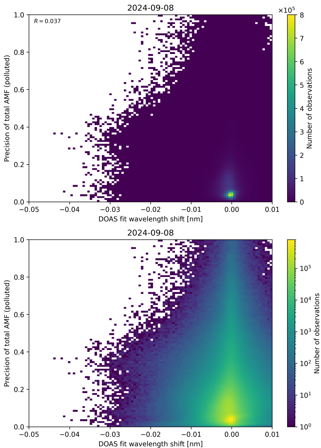
Figure 131: Scatter density plot of “DOAS fit wavelength shift” against “Precision of total AMF (polluted)” for 2024-09-07 to 2024-09-09.
