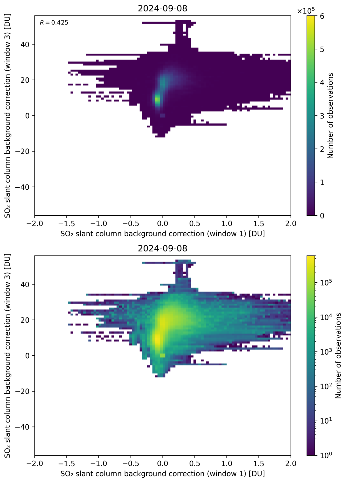
Figure 99: Scatter density plot of “SO 2 slant column background correction (window 1)” against “SO 2 slant column background correction (window 3)” for 2024-09-07 to 2024-09-09.
