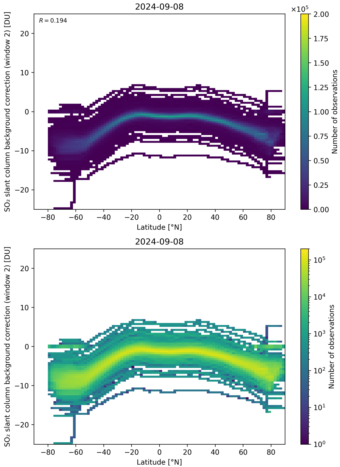
Figure 140: Scatter density plot of “Latitude” against “SO 2 slant column background correction (window 2)” for 2024-09-07 to 2024-09-09.
