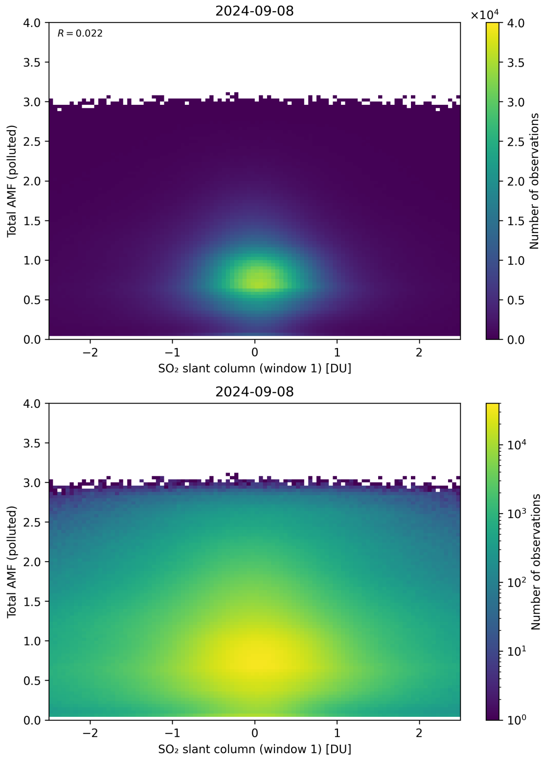
Figure 239: Scatter density plot of “SO 2 slant column (window 1)” against “Total AMF (polluted)” for 2024-09-07 to 2024-09-09.
