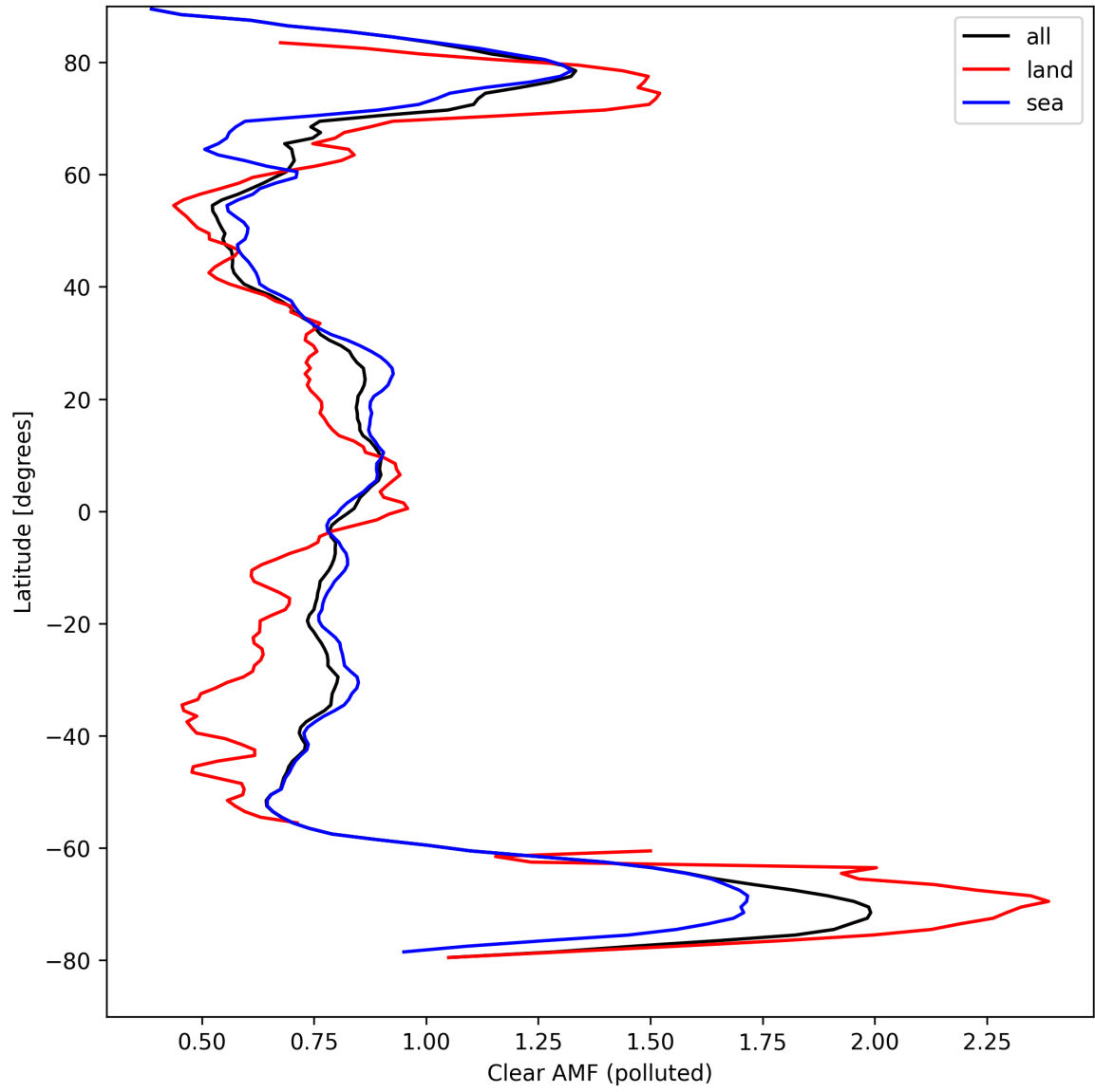
Figure 50: Zonal average of “Clear AMF (polluted)” for 2024-09-07 to 2024-09-09.
