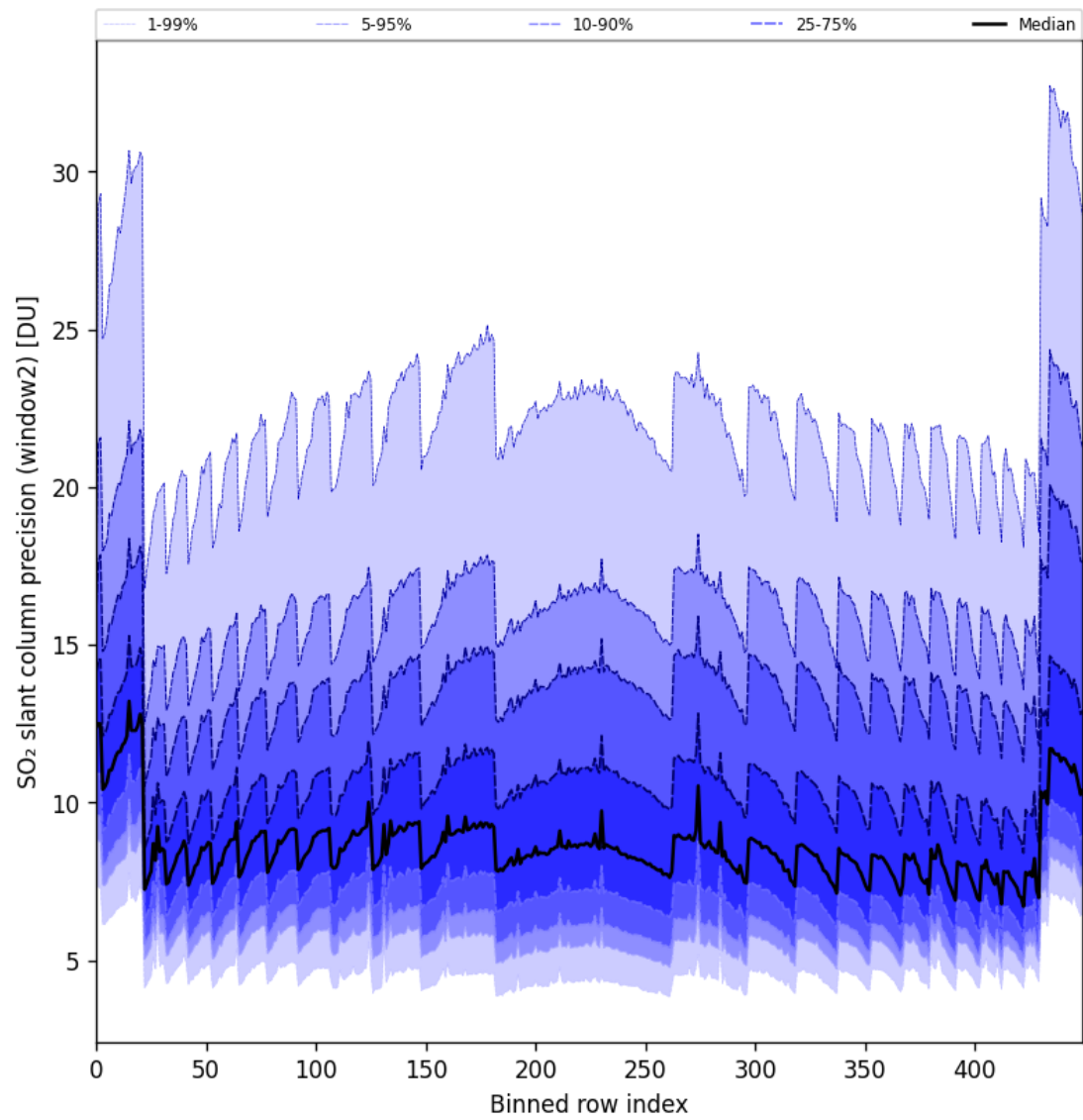
Figure 84: Along track statistics of “SO 2 slant column precision (window2)” for 2024-09-07 to 2024-09-09
