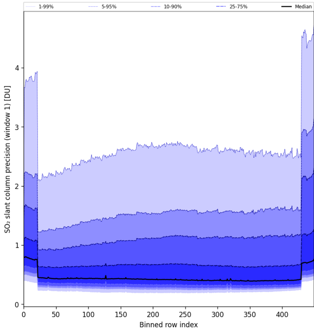
Figure 80: Along track statistics of “SO 2 slant column precision (window 1)” for 2024-09-07 to 2024-09-09
