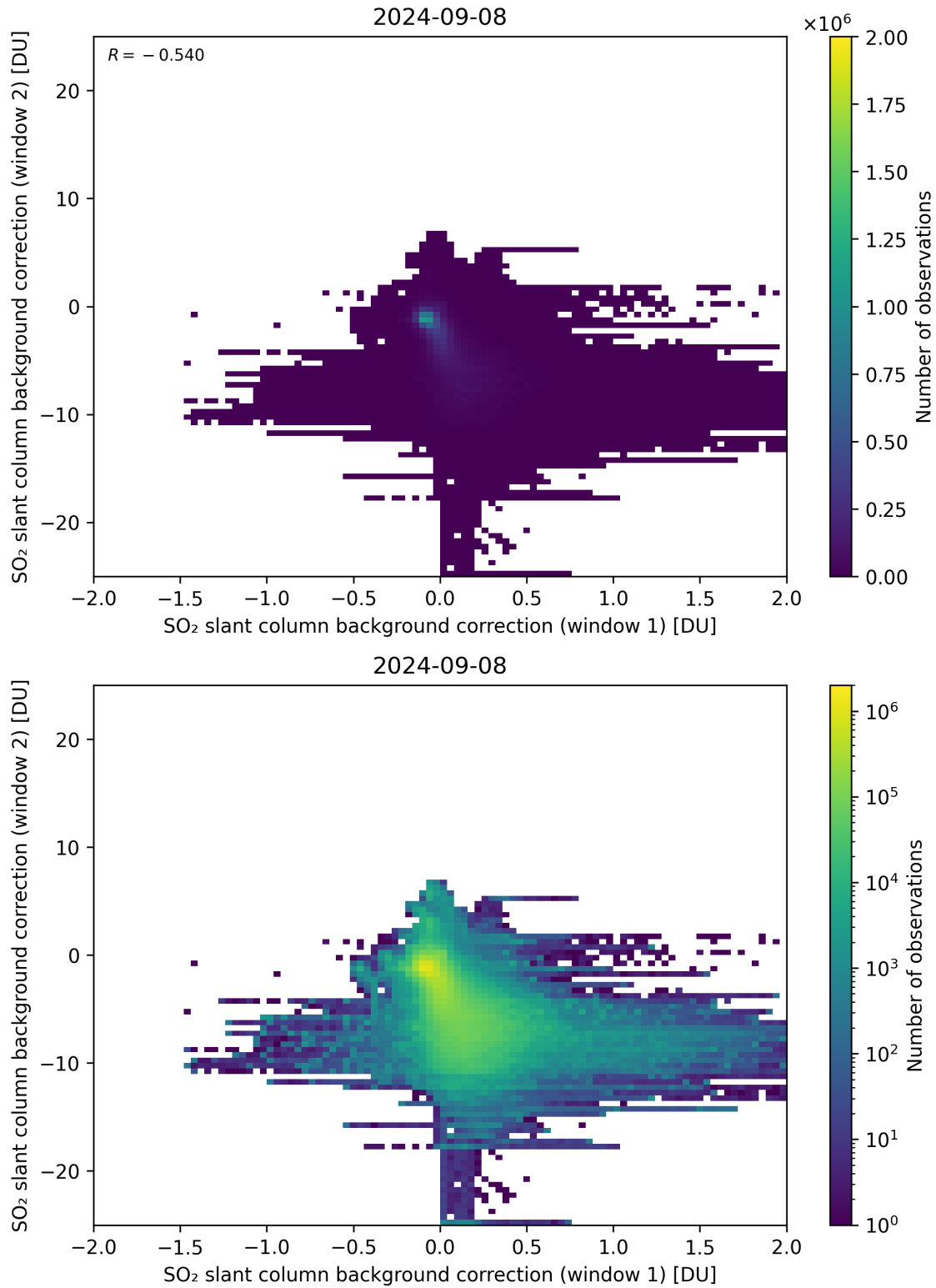
Figure 98: Scatter density plot of “SO 2 slant column background correction (window 1)” against “SO 2 slant column background correction (window 2)” for 2024-09-07 to 2024-09-09.
