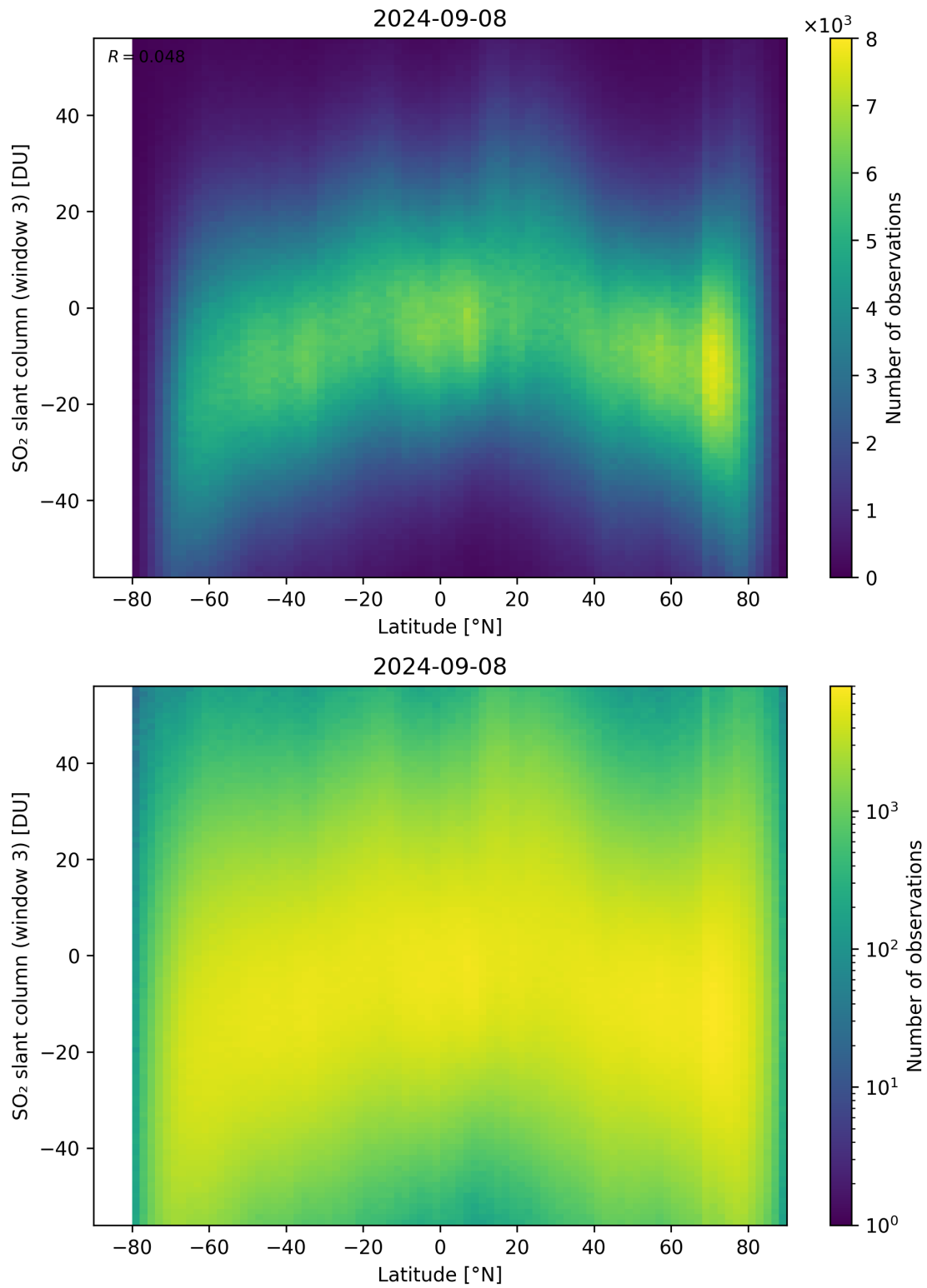
Figure 152: Scatter density plot of “Latitude” against “SO 2 slant column (window 3)” for 2024-09-07 to 2024-09-09.
