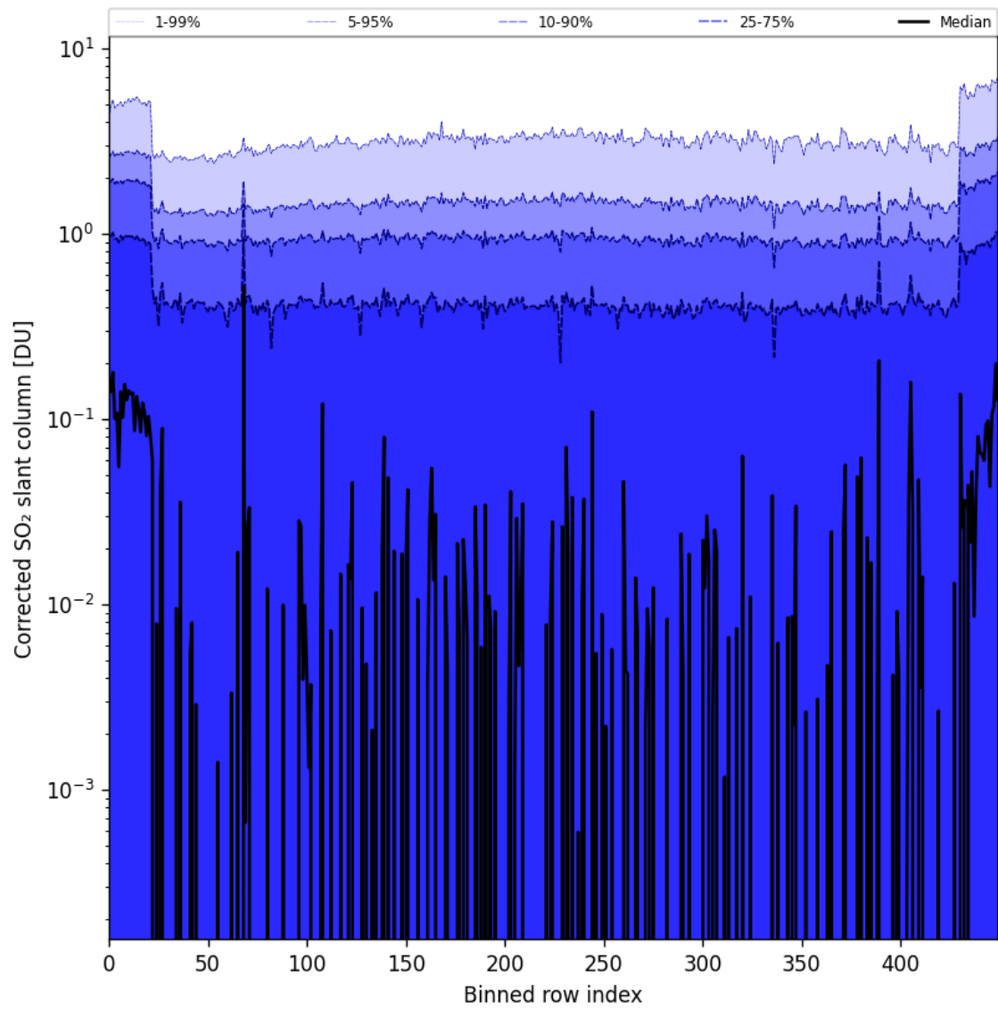
Figure 78: Along track statistics of “Corrected SO 2 slant column” for 2024-09-07 to 2024-09-09
