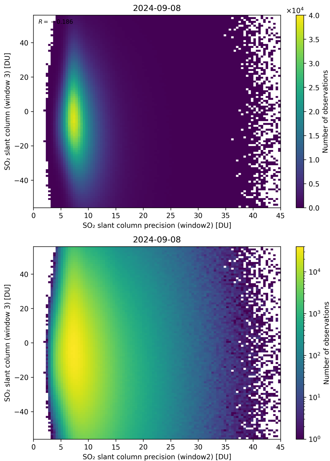
Figure 249: Scatter density plot of “SO 2 slant column precision (window2)” against “SO 2 slant column (window 3)” for 2024-09-07 to 2024-09-09.
