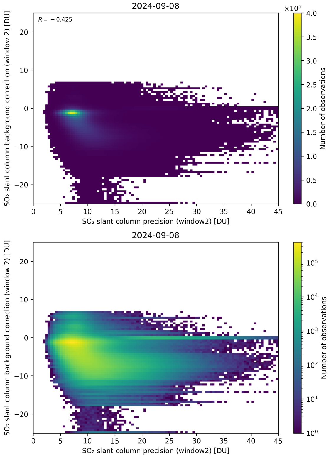
Figure 241: Scatter density plot of “SO 2 slant column precision (window2)” against “SO 2 slant column background correction (window 2)” for 2024-09-07 to 2024-09-09.
