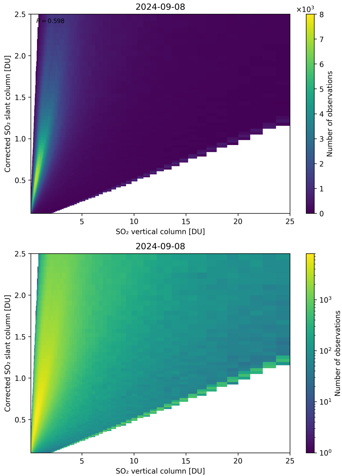
Figure 297: Scatter density plot of “SO 2 vertical column” against “Corrected SO 2 slant column” for 2024-09-07 to 2024-09-09.
