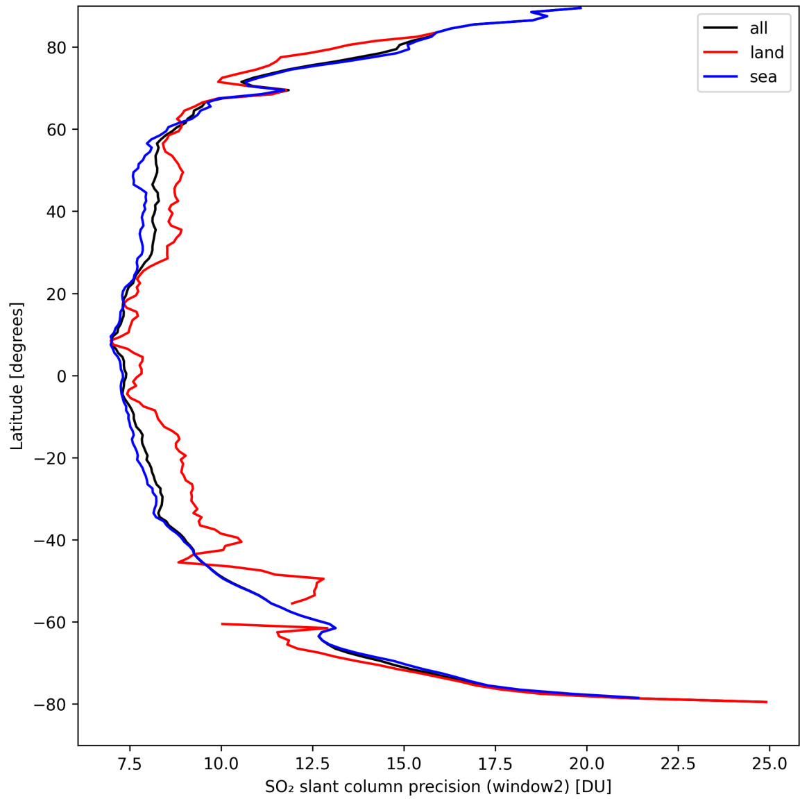
Figure 38: Zonal average of “SO 2 slant column precision (window2)” for 2024-09-07 to 2024-09-09.
