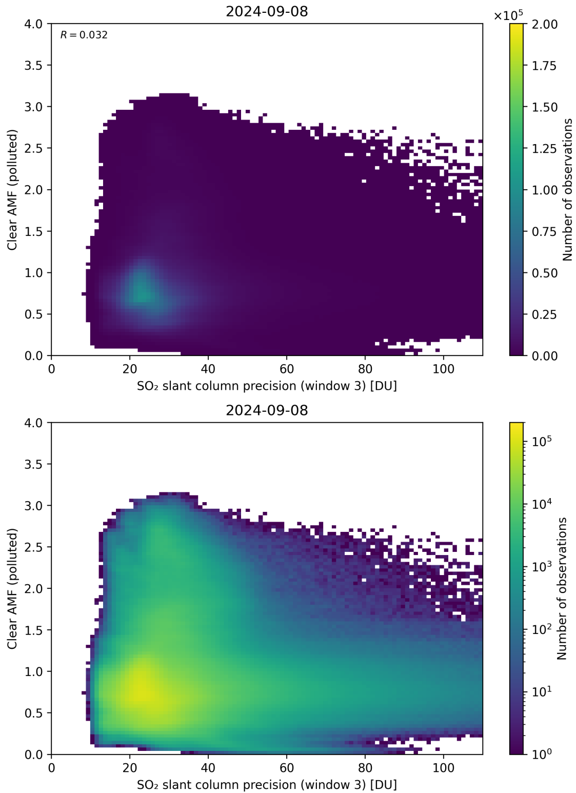
Figure 261: Scatter density plot of “SO 2 slant column precision (window 3)” against “Clear AMF (polluted)” for 2024-09-07 to 2024-09-09.
