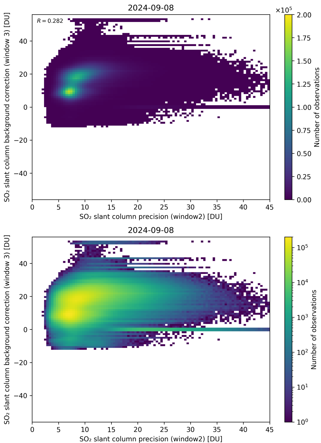
Figure 242: Scatter density plot of “SO 2 slant column precision (window2)” against “SO 2 slant column background correction (window 3)” for 2024-09-07 to 2024-09-09.
