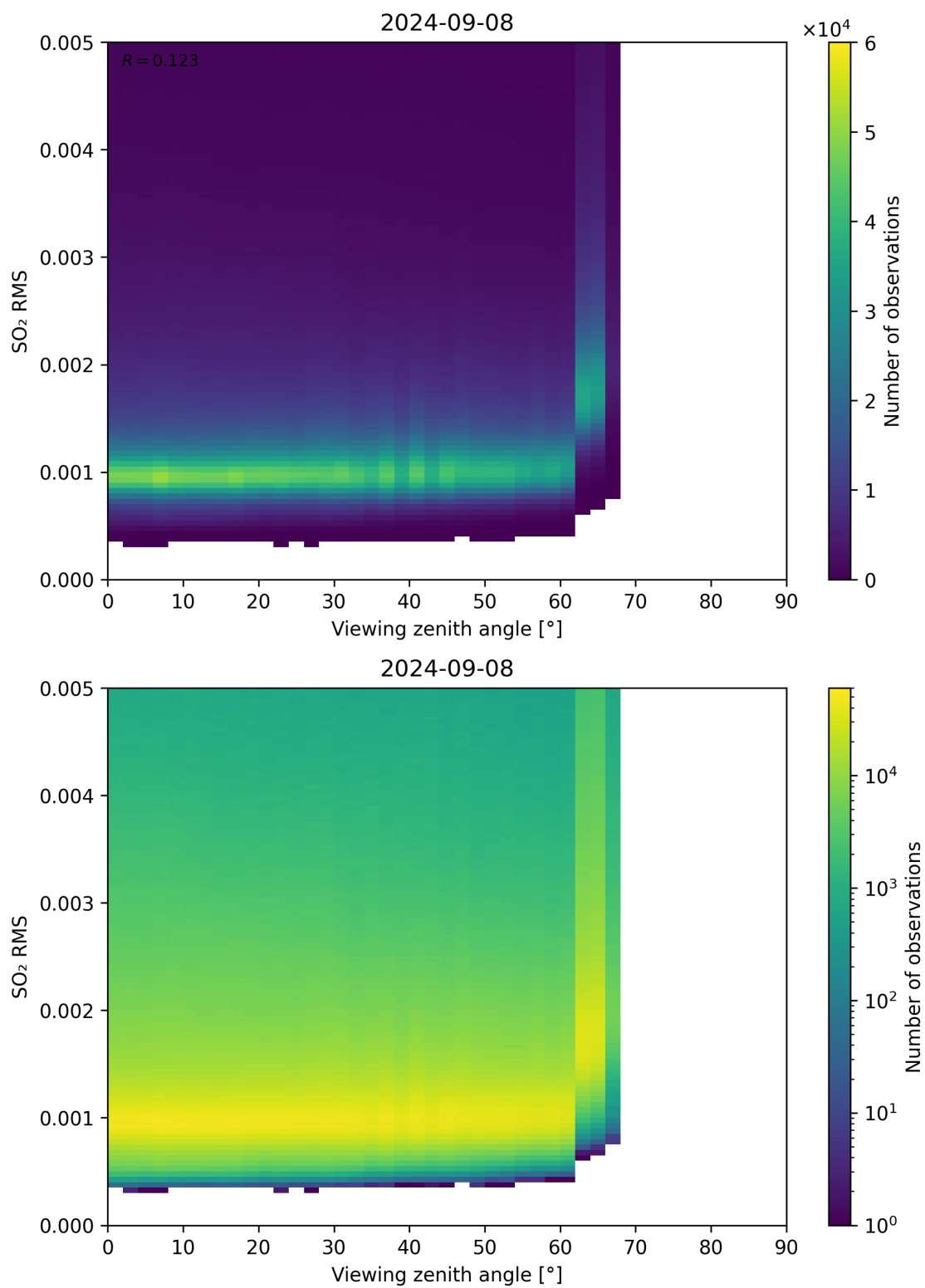
Figure 313: Scatter density plot of “Viewing zenith angle” against “SO 2 RMS” for 2024-09-07 to 2024-09-09.
