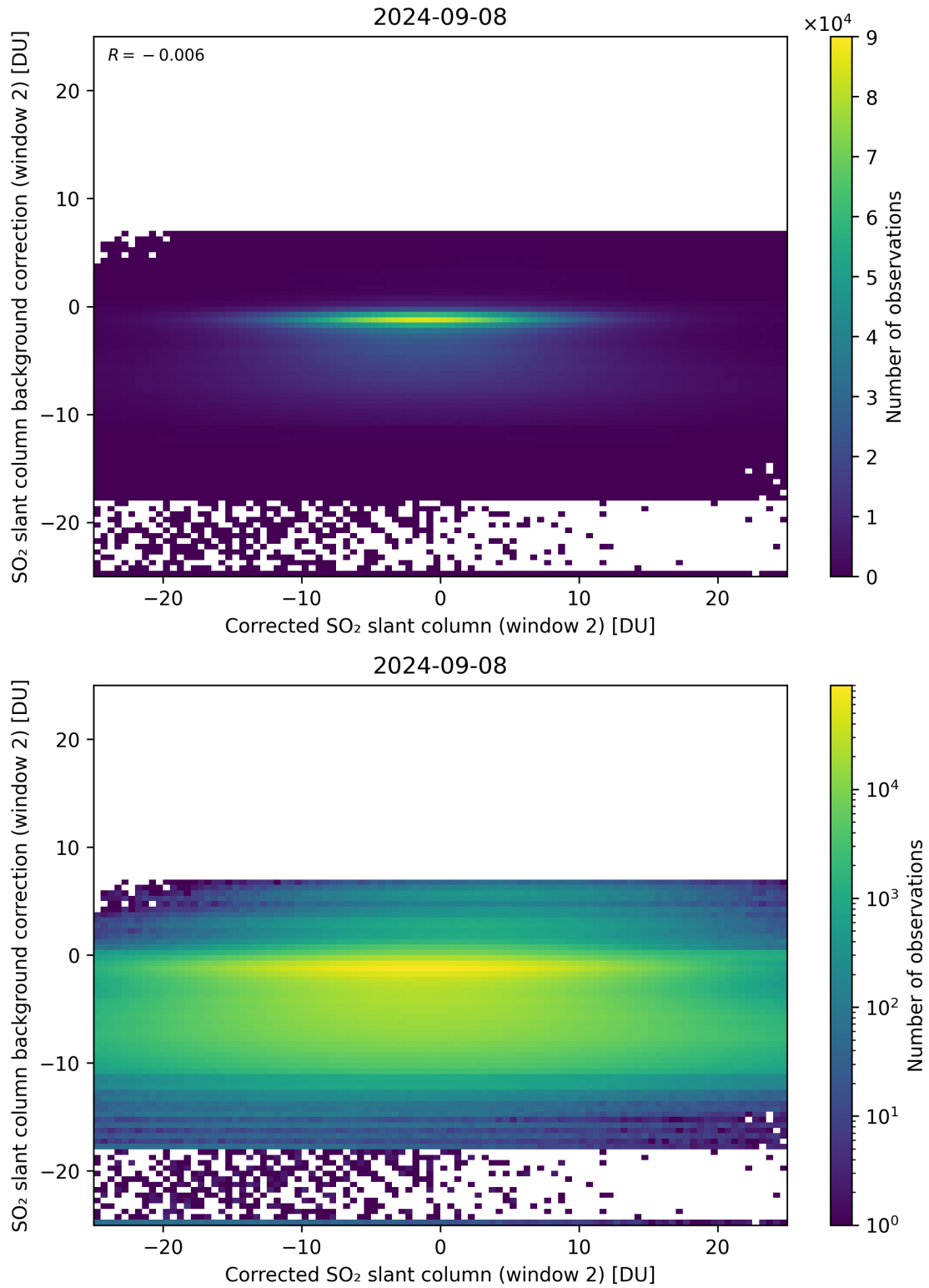
Figure 194: Scatter density plot of “Corrected SO 2 slant column (window 2)” against “SO 2 slant column background correction (window 2)” for 2024-09-07 to 2024-09-09.
