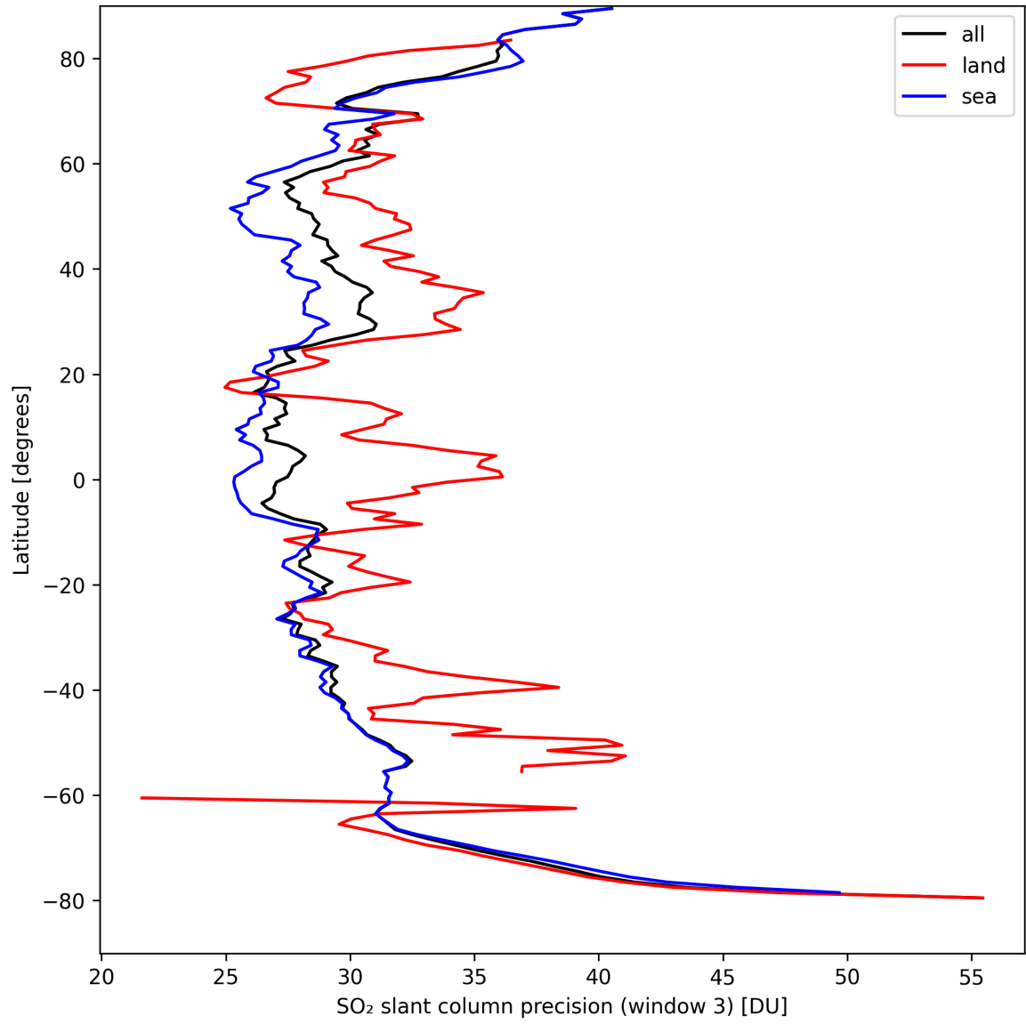
Figure 42: Zonal average of “SO 2 slant column precision (window 3)” for 2024-09-07 to 2024-09-09.
