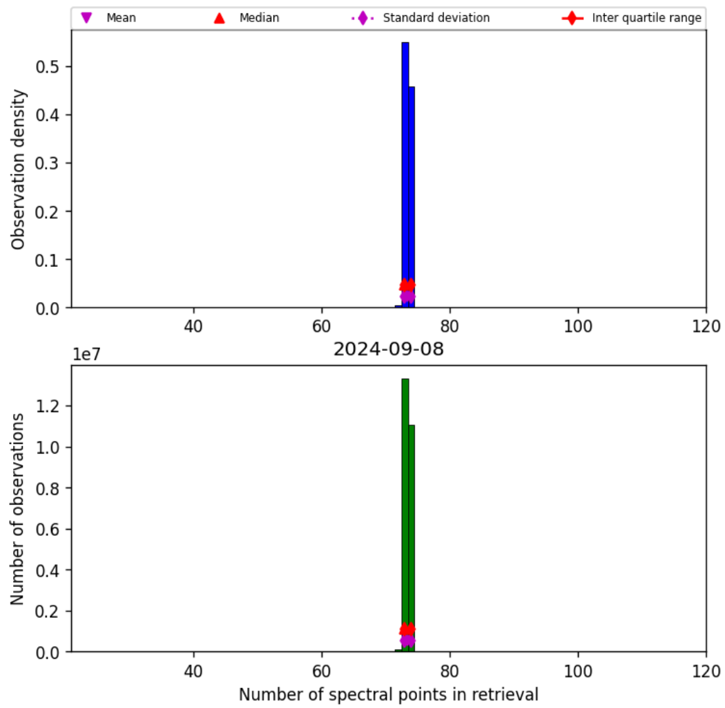
Figure 74: Histogram of “Number of spectral points in retrieval” for 2024-09-07 to 2024-09-09
