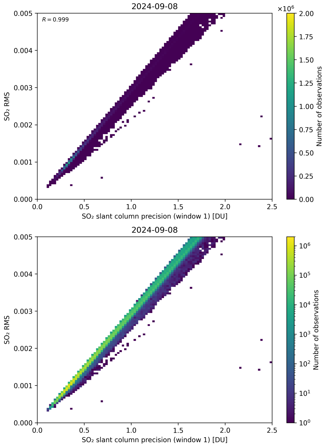
Figure 223: Scatter density plot of “SO 2 slant column precision (window 1)” against “SO 2 RMS” for 2024-09-07 to 2024-09-09.
