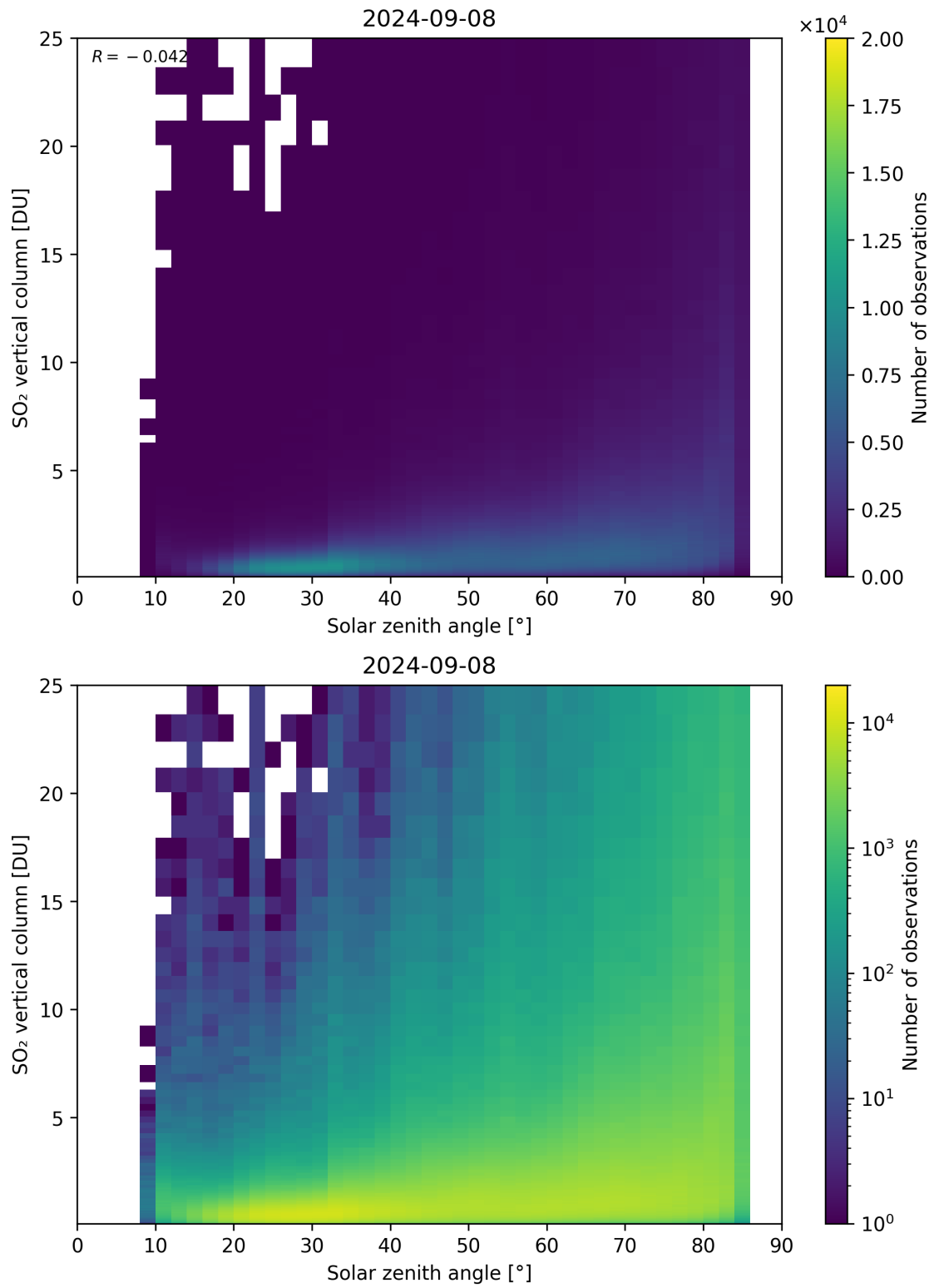
Figure 176: Scatter density plot of “Solar zenith angle” against “SO 2 vertical column” for 2024-09-07 to 2024-09-09.
