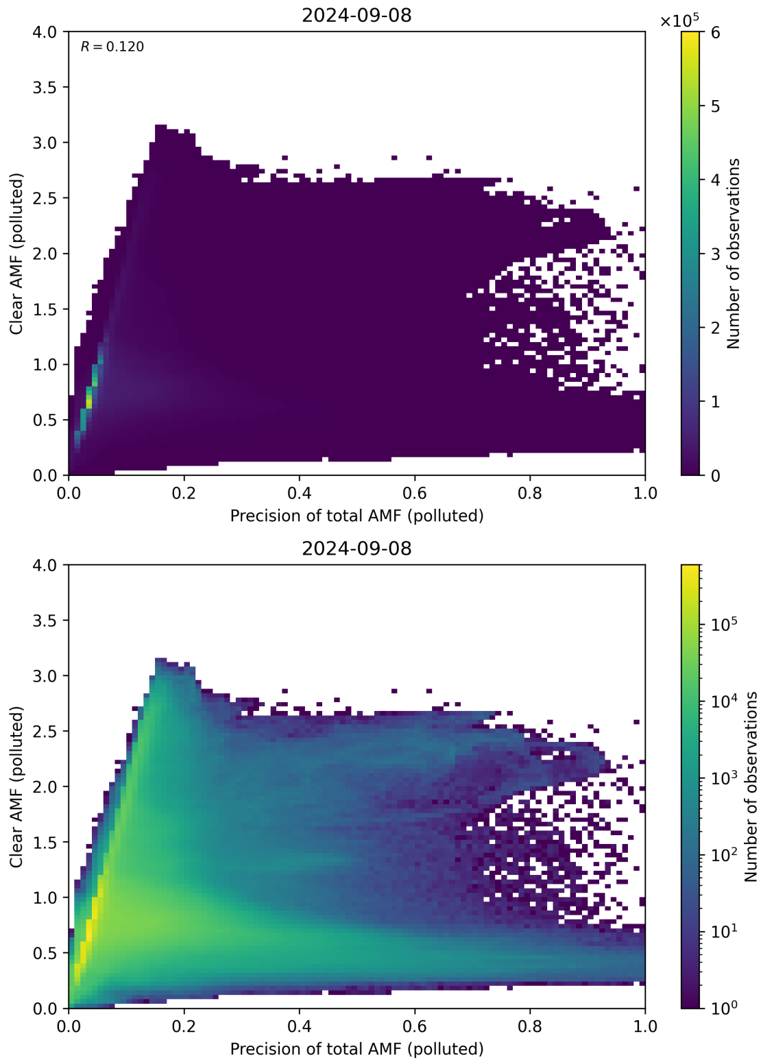
Figure 270: Scatter density plot of “Precision of total AMF (polluted)” against “Clear AMF (polluted)” for 2024-09-07 to 2024-09-09.
