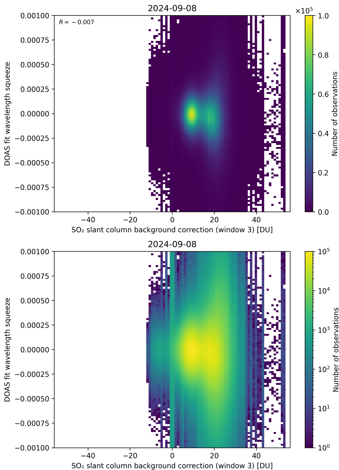
Figure 122: Scatter density plot of “SO 2 slant column background correction (window 3)” against “DOAS fit wavelength squeeze” for 2024-09-07 to 2024-09-09.
