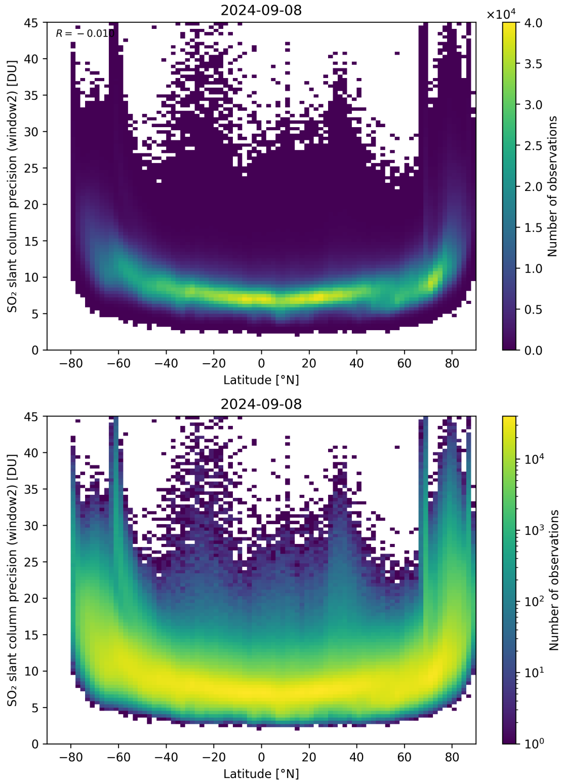
Figure 151: Scatter density plot of “Latitude” against “SO 2 slant column precision (window2)” for 2024-09-07 to 2024-09-09.
