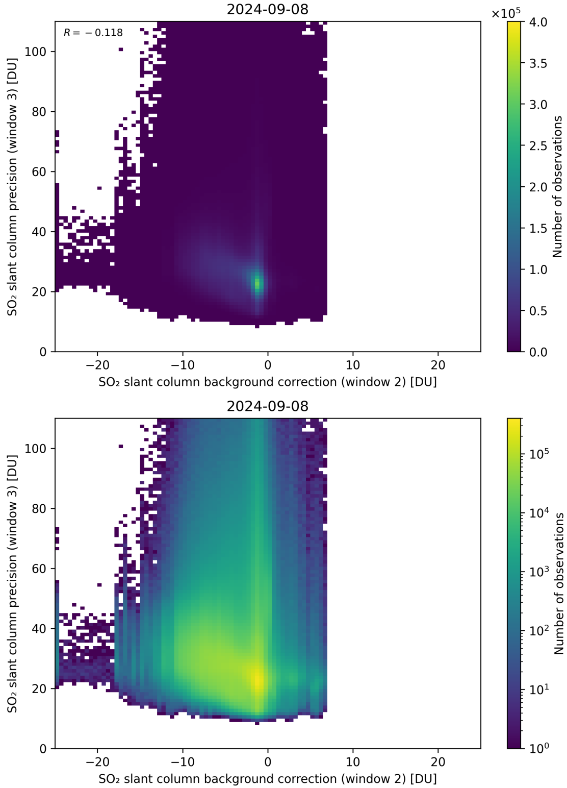
Figure 118: Scatter density plot of “SO 2 slant column background correction (window 2)” against “SO 2 slant column precision (window 3)” for 2024-09-07 to 2024-09-09.
