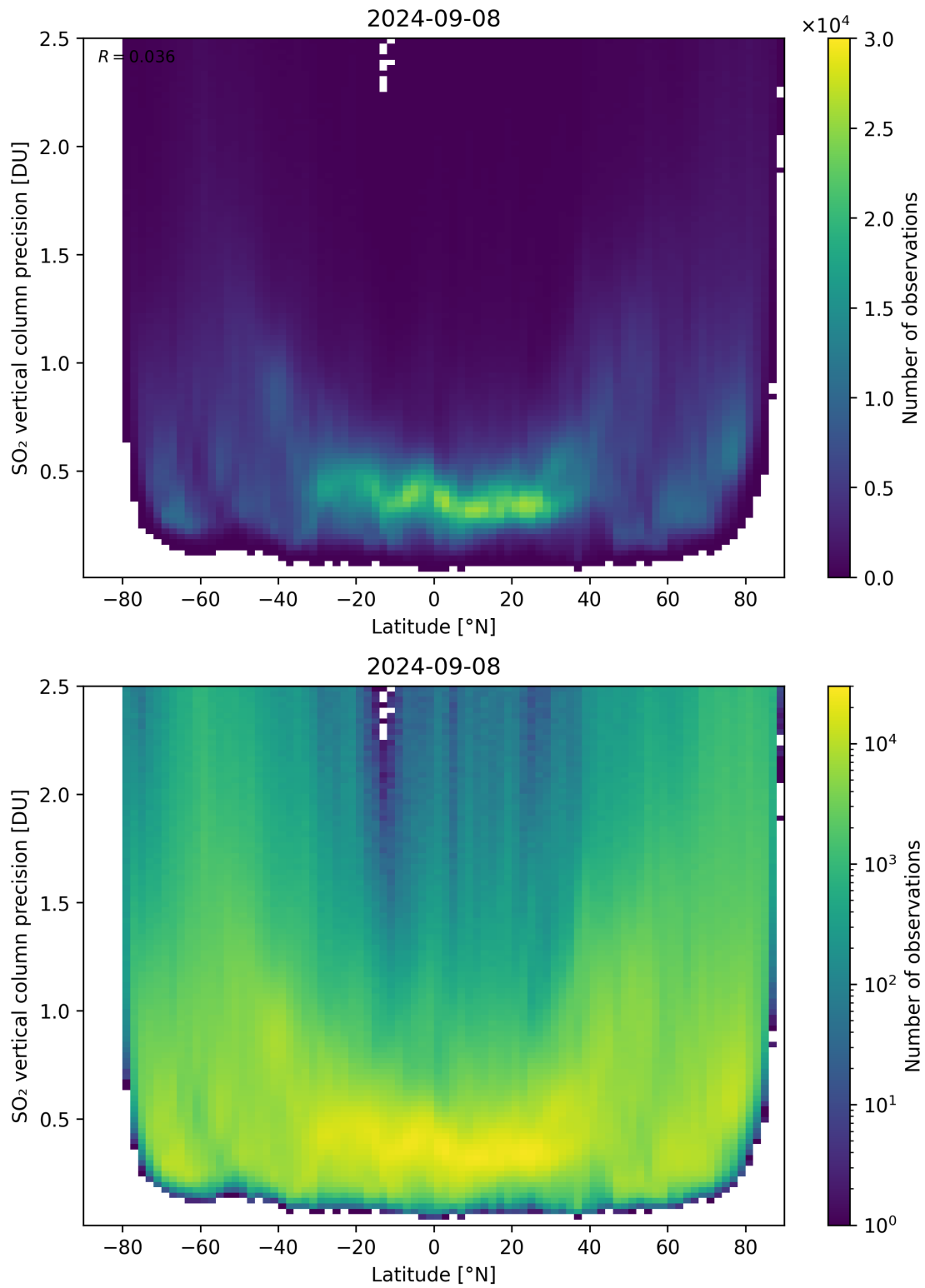
Figure 157: Scatter density plot of “Latitude” against “SO 2 vertical column precision” for 2024-09-07 to 2024-09-09.
