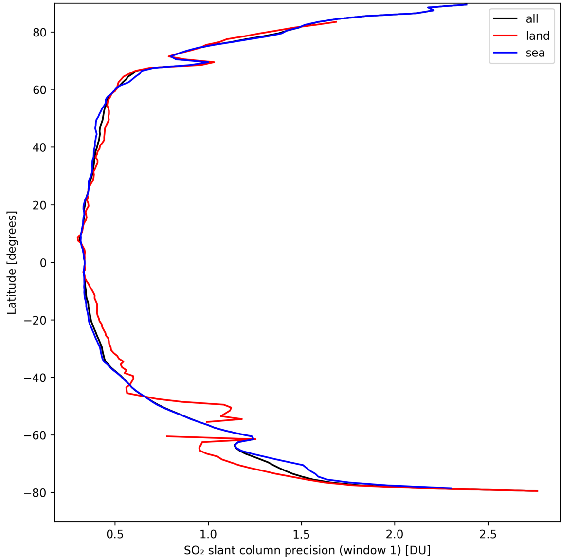
Figure 34: Zonal average of “SO 2 slant column precision (window 1)” for 2024-09-07 to 2024-09-09.
