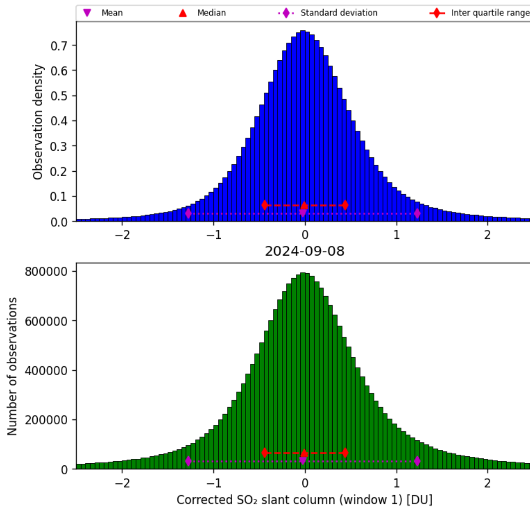
Figure 58: Histogram of “Corrected SO 2 slant column (window 1)” for 2024-09-07 to 2024-09-09
