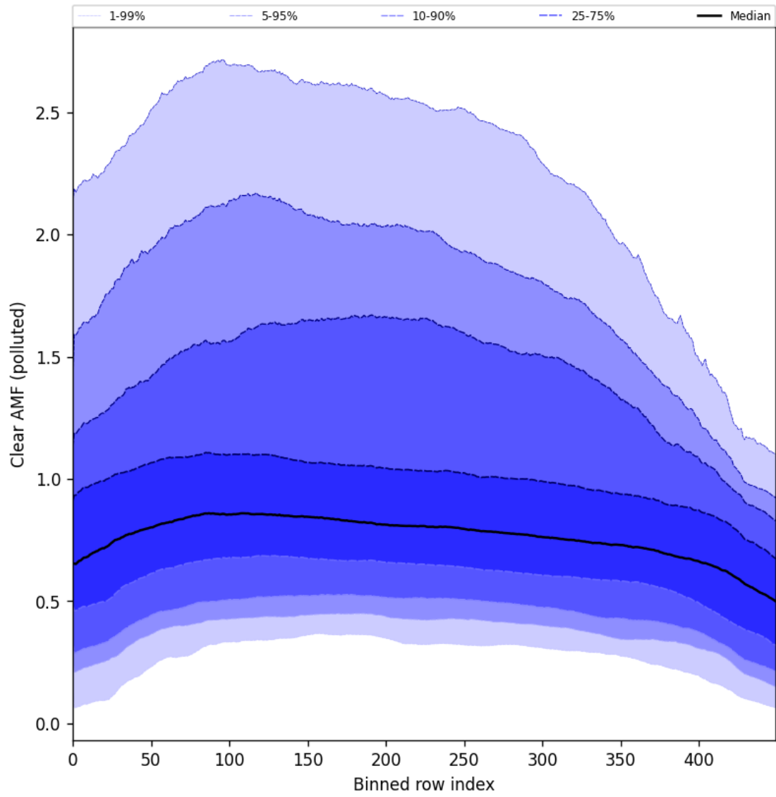
Figure 96: Along track statistics of “Clear AMF (polluted)” for 2024-09-07 to 2024-09-09
