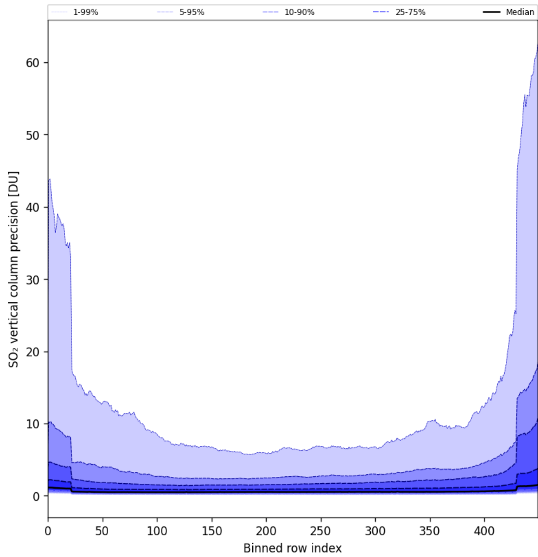
Figure 77: Along track statistics of “SO 2 vertical column precision” for 2024-09-07 to 2024-09-09
