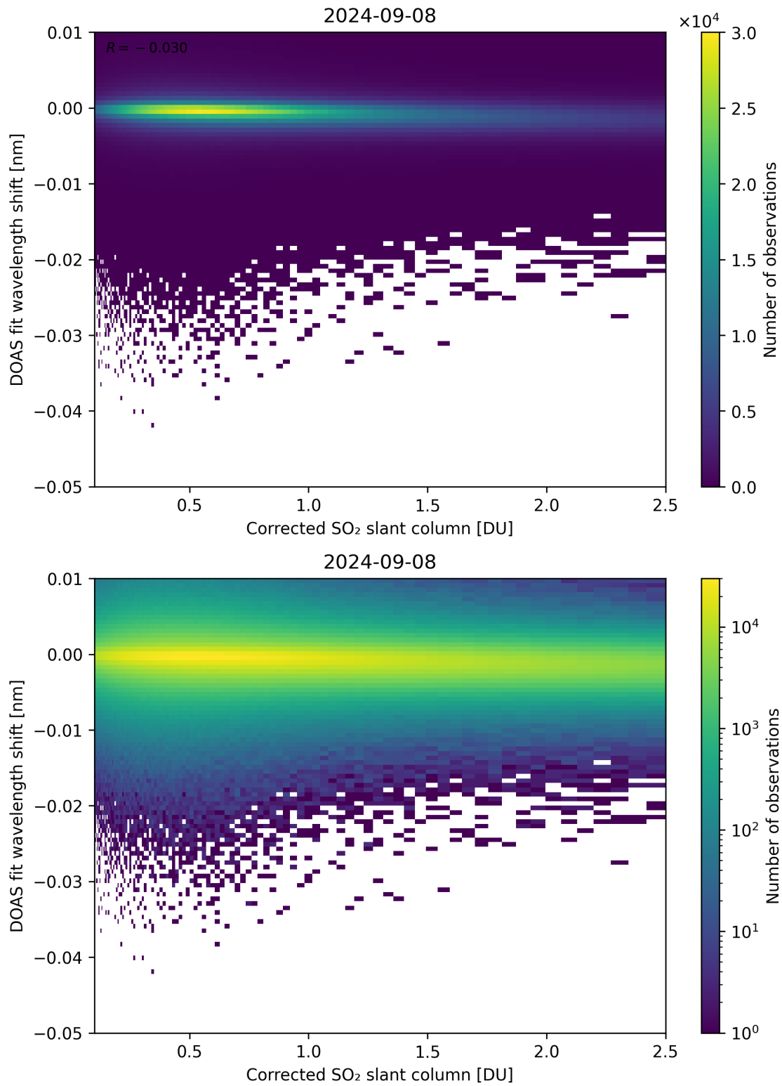
Figure 181: Scatter density plot of “Corrected SO 2 slant column” against “DOAS fit wavelength shift” for 2024-09-07 to 2024-09-09.
