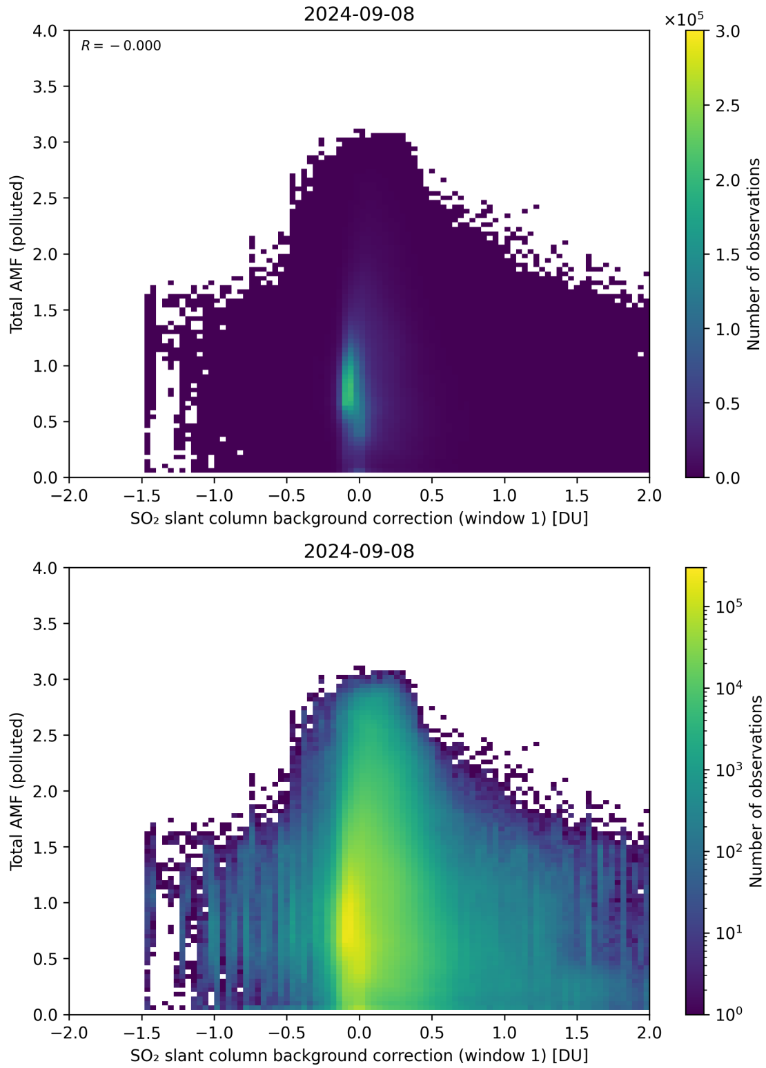
Figure 109: Scatter density plot of “SO 2 slant column background correction (window 1)” against “Total AMF (polluted)” for 2024-09-07 to 2024-09-09.
