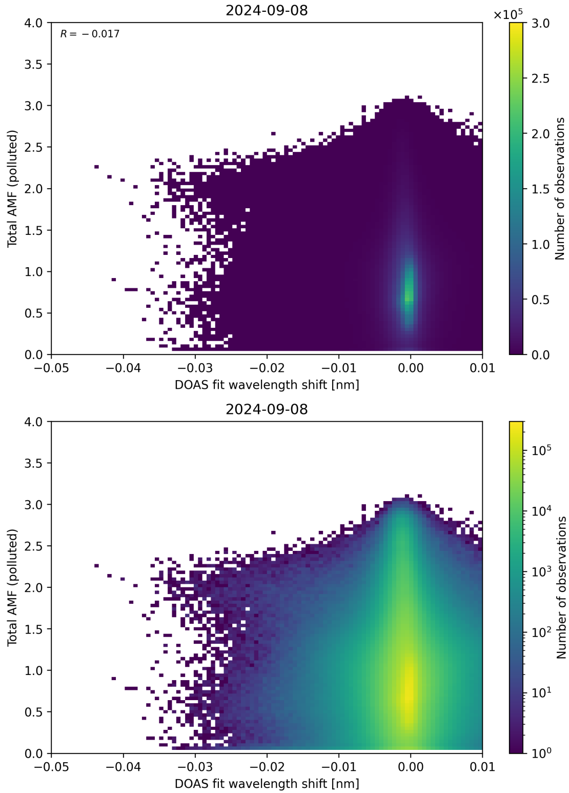
Figure 130: Scatter density plot of “DOAS fit wavelength shift” against “Total AMF (polluted)” for 2024-09-07 to 2024-09-09.
