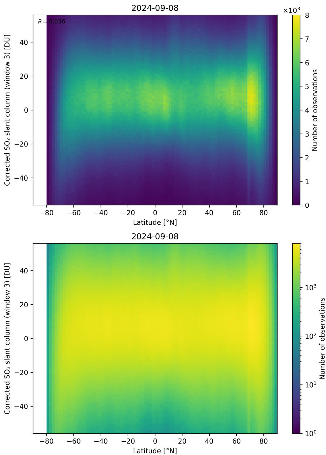
Figure 148: Scatter density plot of “Latitude” against “Corrected SO 2 slant column (window 3)” for 2024-09-07 to 2024-09-09.
