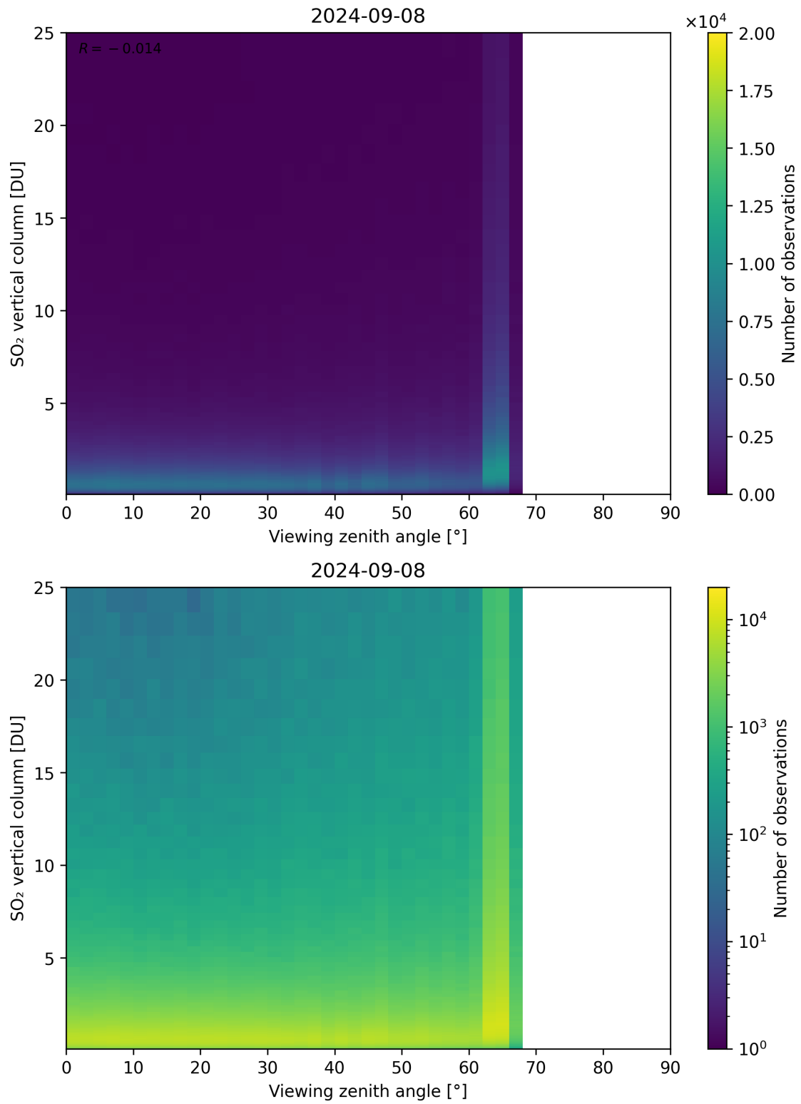
Figure 327: Scatter density plot of “Viewing zenith angle” against “SO 2 vertical column” for 2024-09-07 to 2024-09-09.
