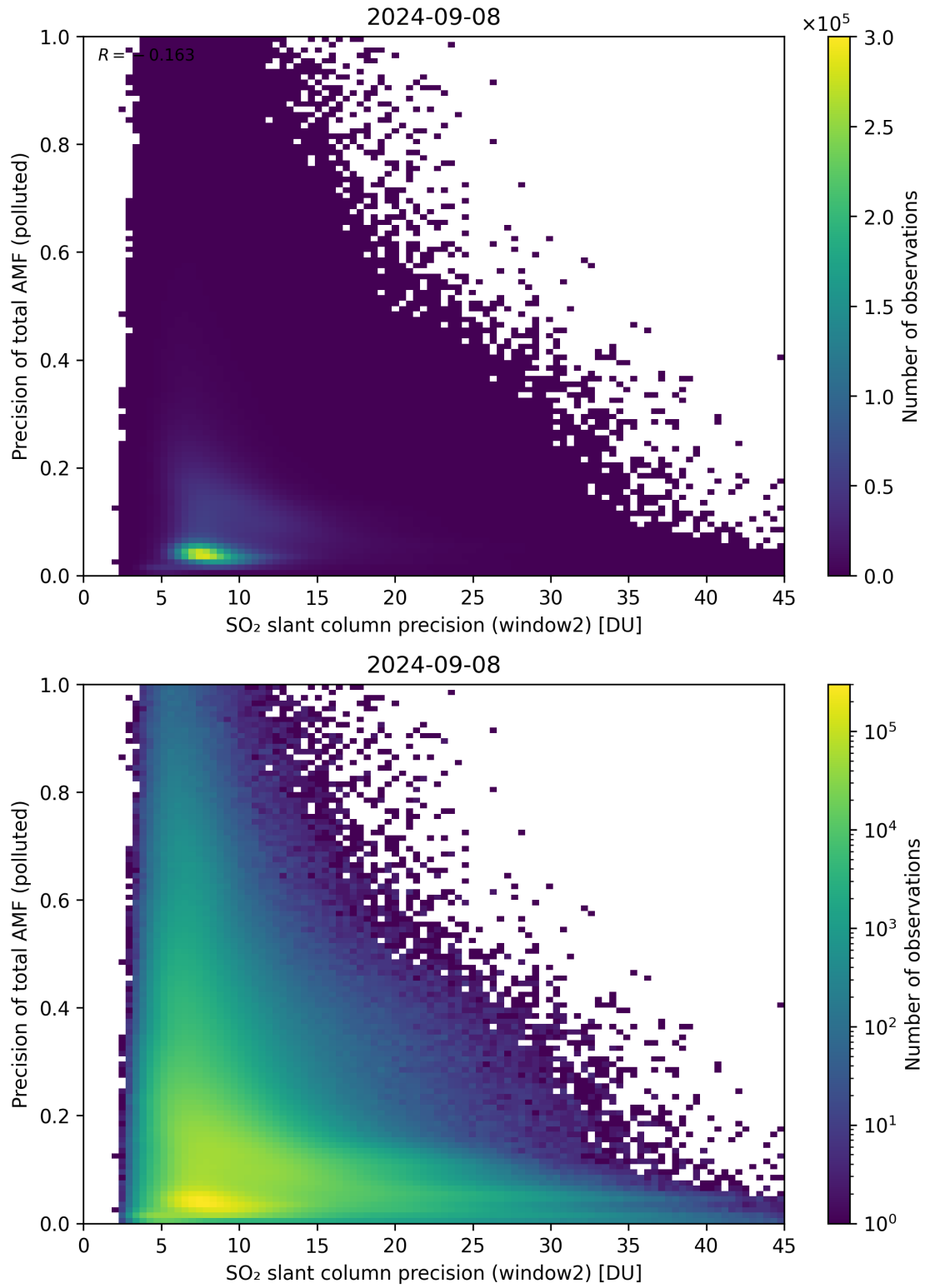
Figure 252: Scatter density plot of “SO 2 slant column precision (window2)” against “Precision of total AMF (polluted)” for 2024-09-07 to 2024-09-09.
