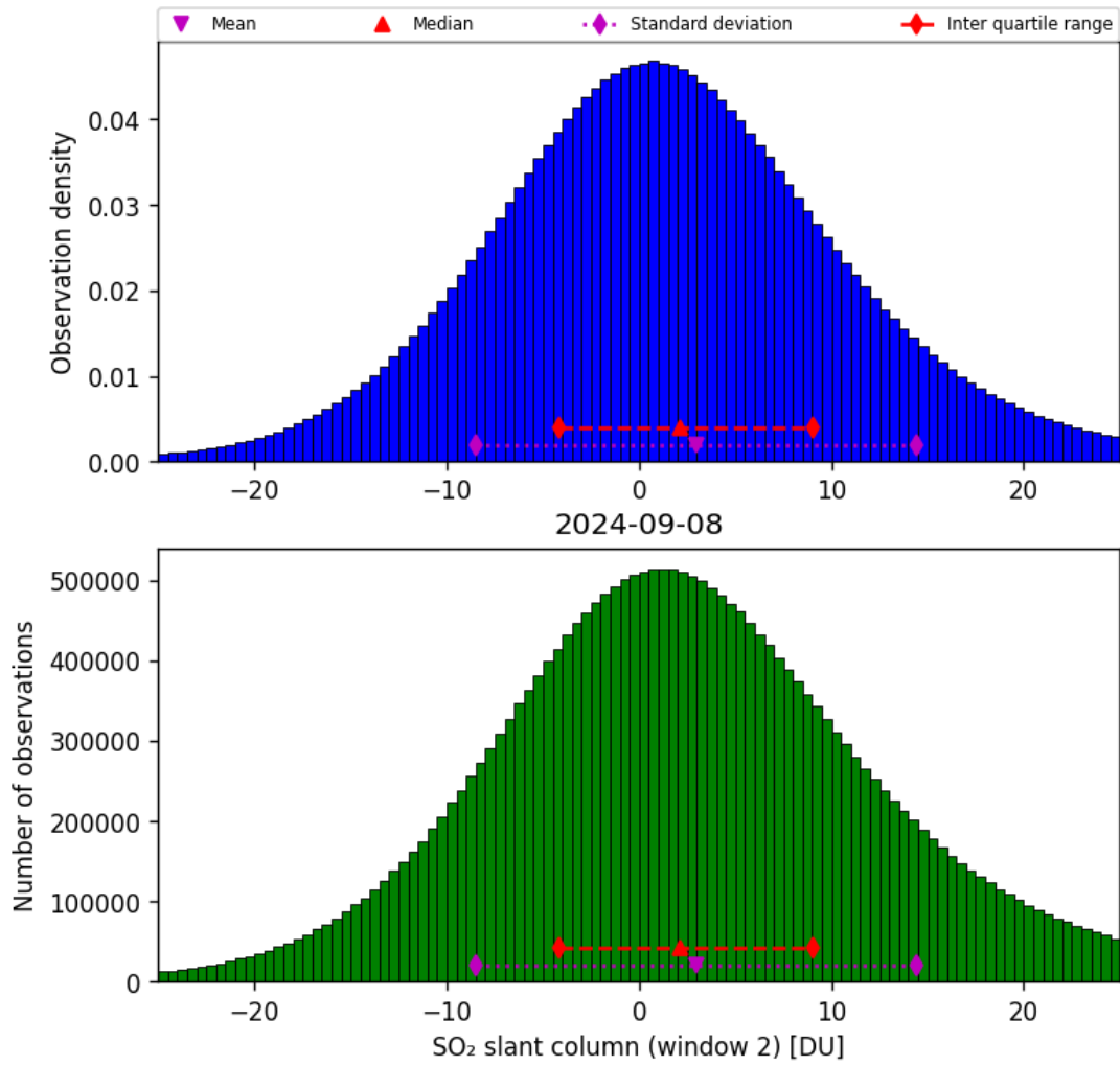
Figure 60: Histogram of “SO 2 slant column (window 2)” for 2024-09-07 to 2024-09-09
