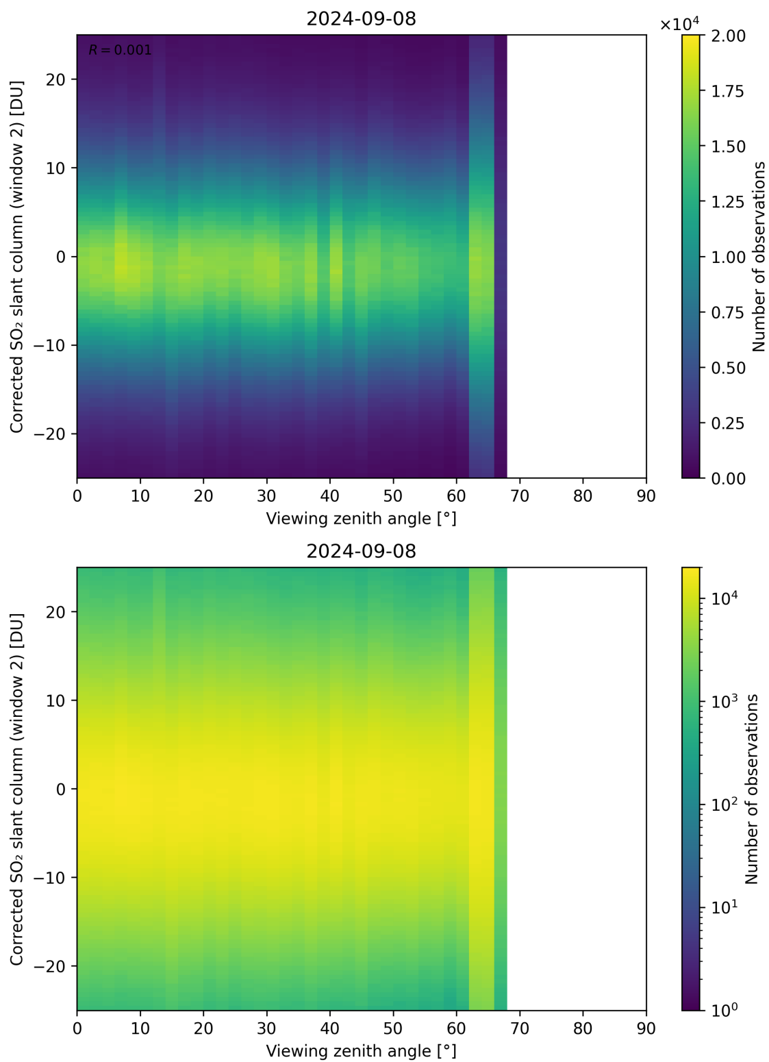
Figure 318: Scatter density plot of “Viewing zenith angle” against “Corrected SO 2 slant column (window 2)” for 2024-09-07 to 2024-09-09.
