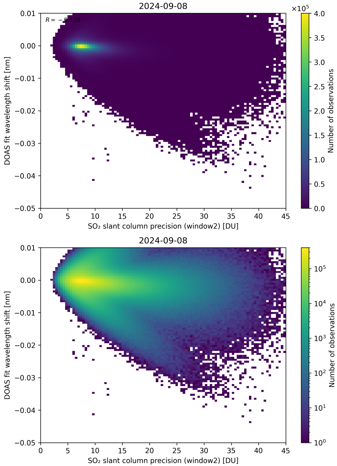
Figure 243: Scatter density plot of “SO 2 slant column precision (window2)” against “DOAS fit wavelength shift” for 2024-09-07 to 2024-09-09.
