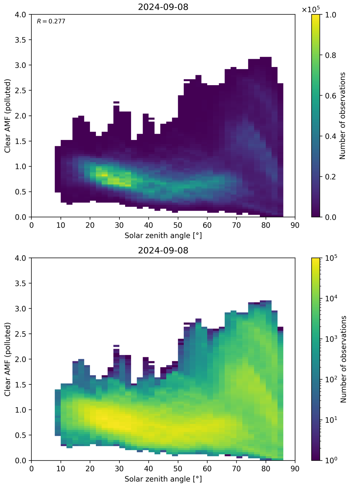
Figure 165: Scatter density plot of “Solar zenith angle” against “Clear AMF (polluted)” for 2024-09-07 to 2024-09-09.
