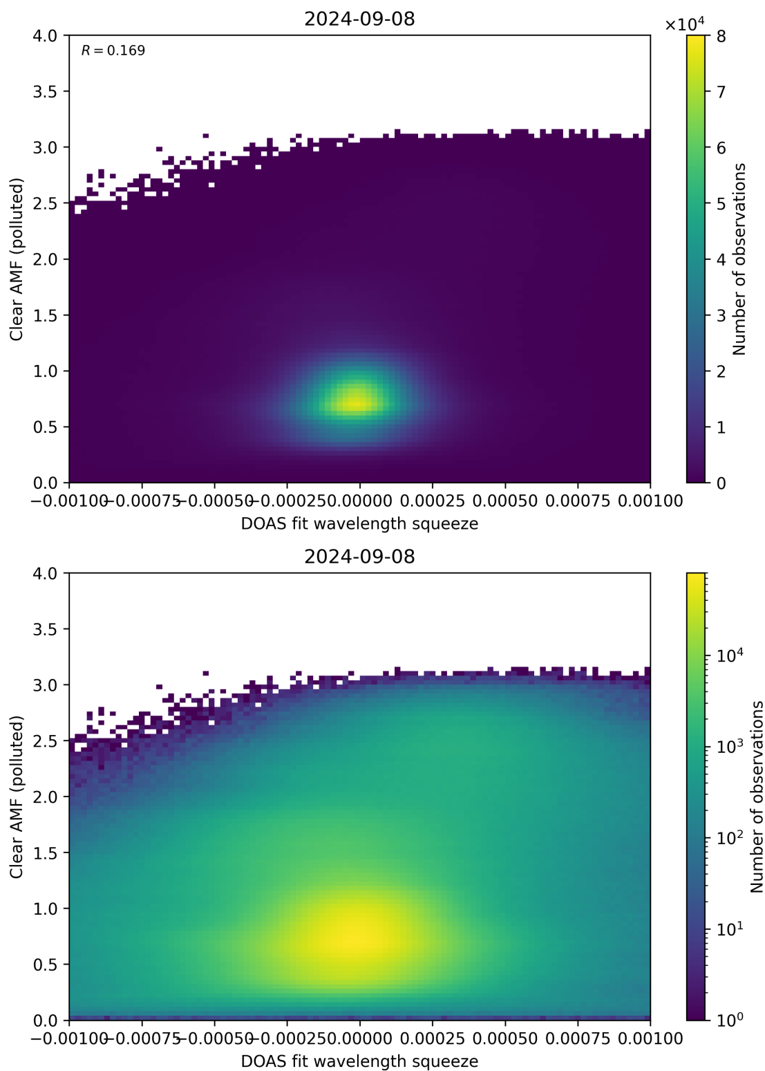
Figure 133: Scatter density plot of “DOAS fit wavelength squeeze” against “Clear AMF (polluted)” for 2024-09-07 to 2024-09-09.
