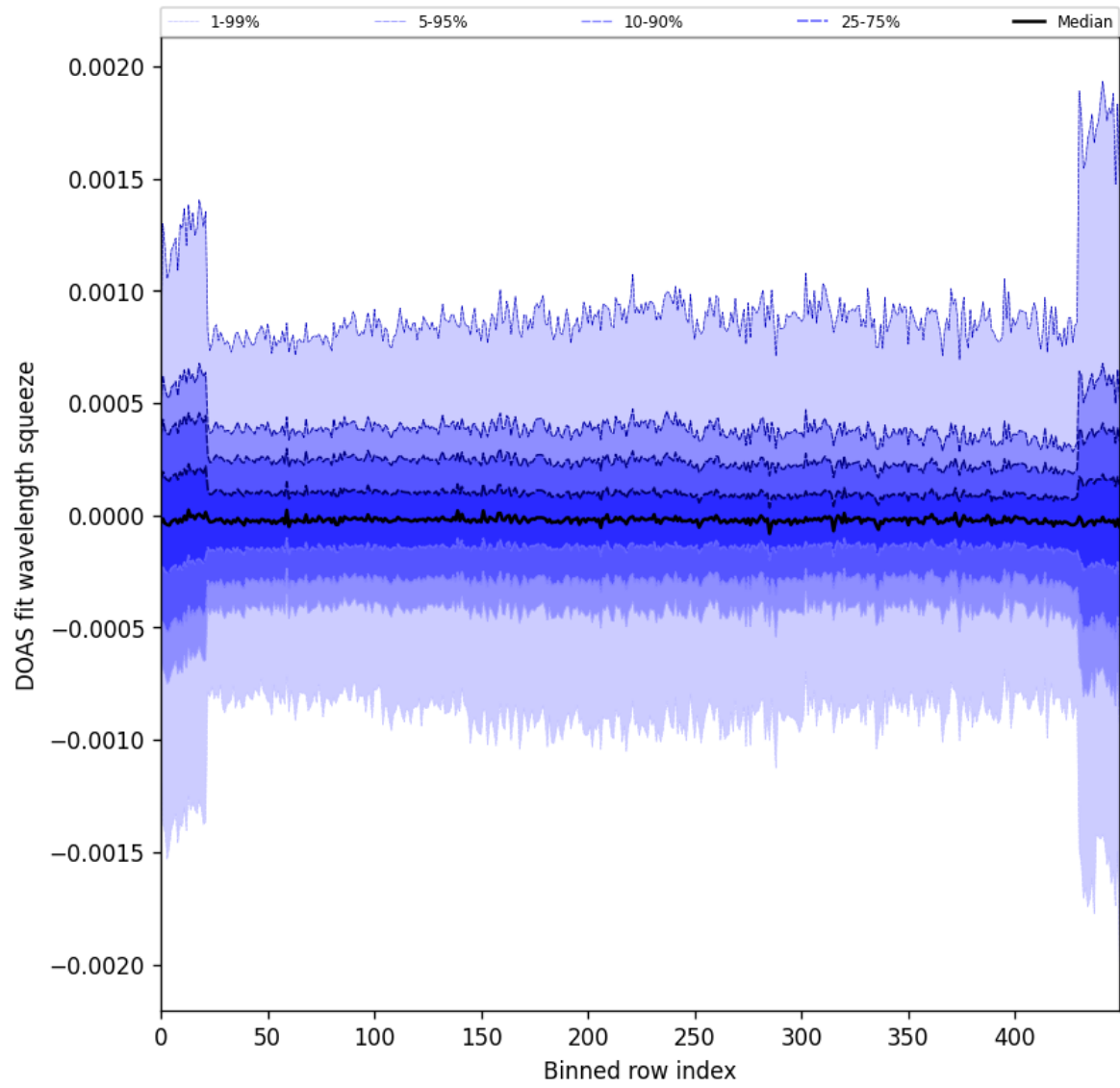
Figure 92: Along track statistics of “DOAS fit wavelength squeeze” for 2024-09-07 to 2024-09-09
