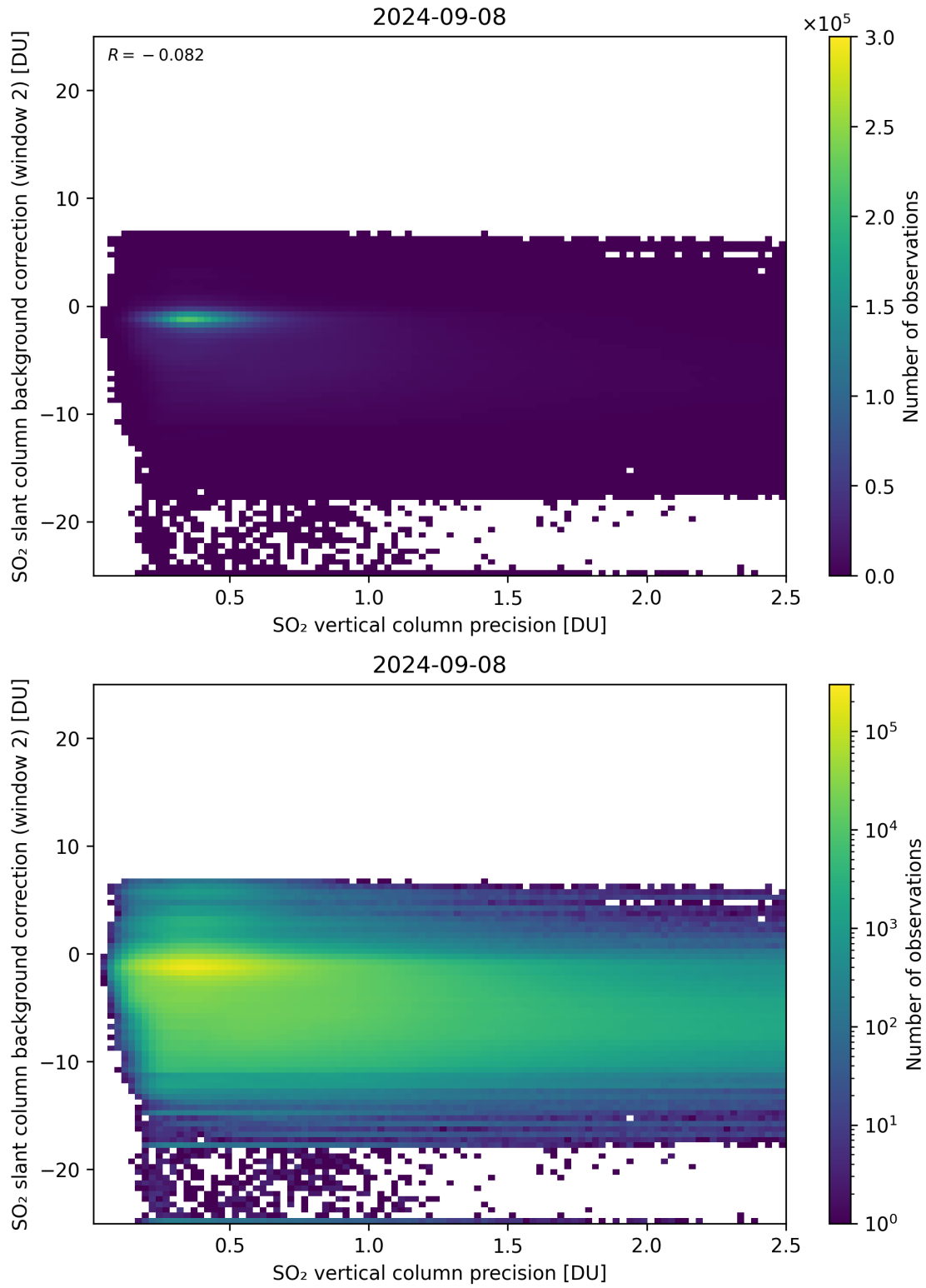
Figure 280: Scatter density plot of “SO 2 vertical column precision” against “SO 2 slant column background correction (window 2)” for 2024-09-07 to 2024-09-09.
