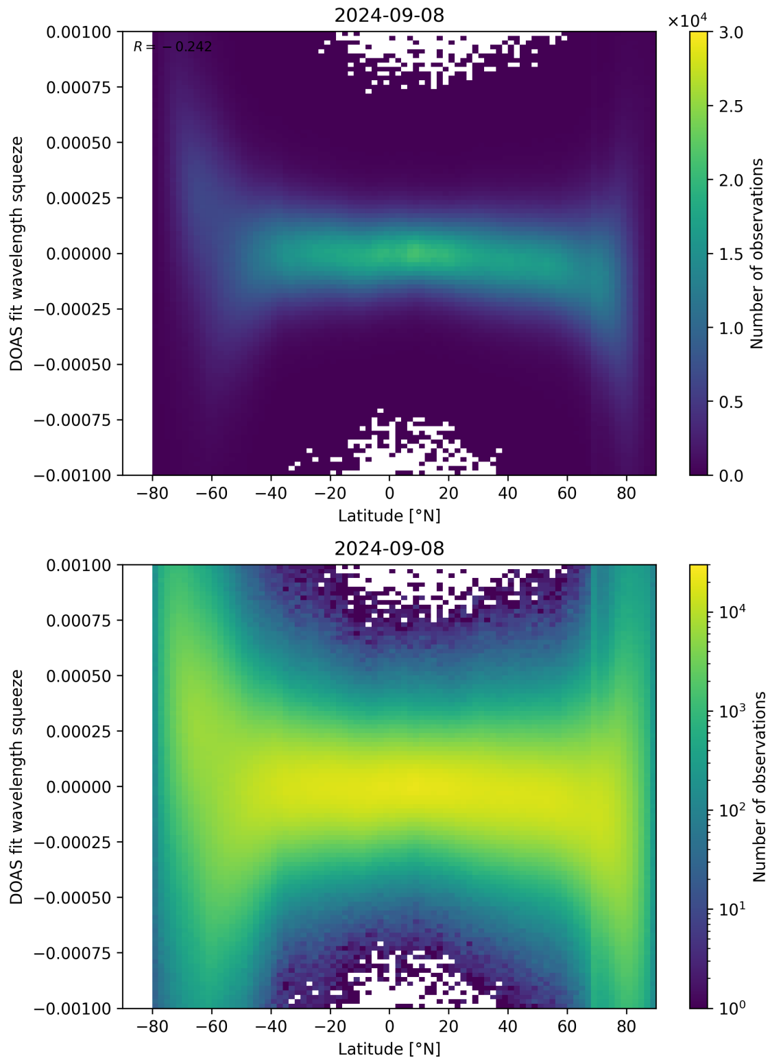
Figure 143: Scatter density plot of “Latitude” against “DOAS fit wavelength squeeze” for 2024-09-07 to 2024-09-09.
