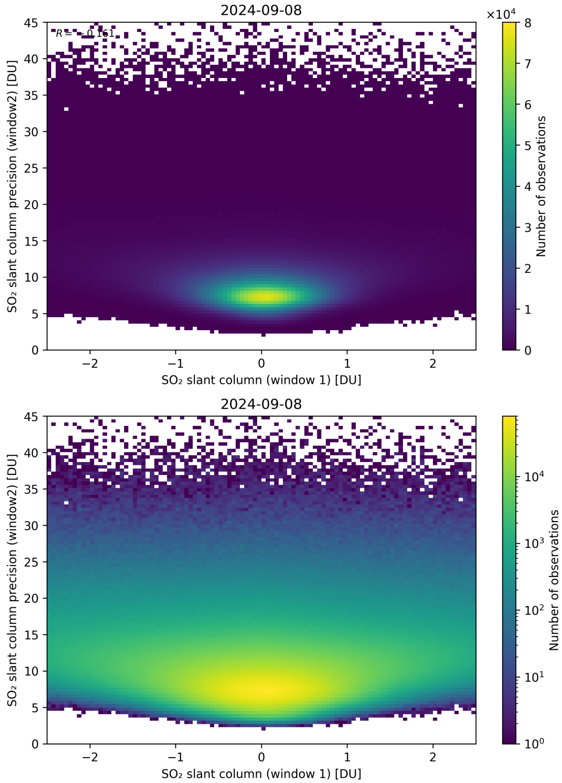
Figure 236: Scatter density plot of “SO 2 slant column (window 1)” against “SO 2 slant column precision (window2)” for 2024-09-07 to 2024-09-09.
