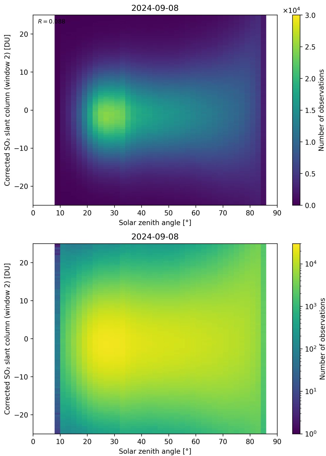
Figure 167: Scatter density plot of “Solar zenith angle” against “Corrected SO 2 slant column (window 2)” for 2024-09-07 to 2024-09-09.
