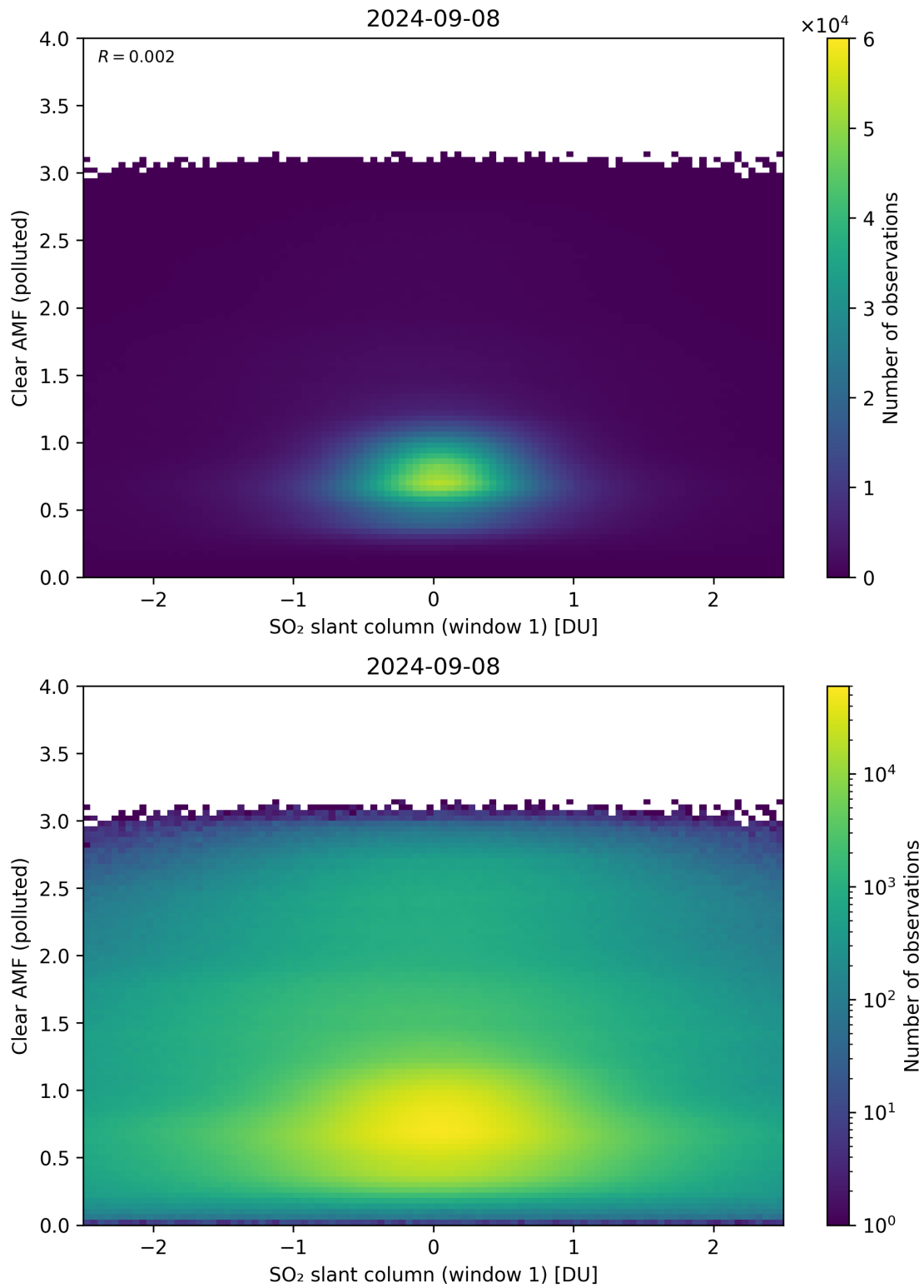
Figure 232: Scatter density plot of “SO 2 slant column (window 1)” against “Clear AMF (polluted)” for 2024-09-07 to 2024-09-09.
