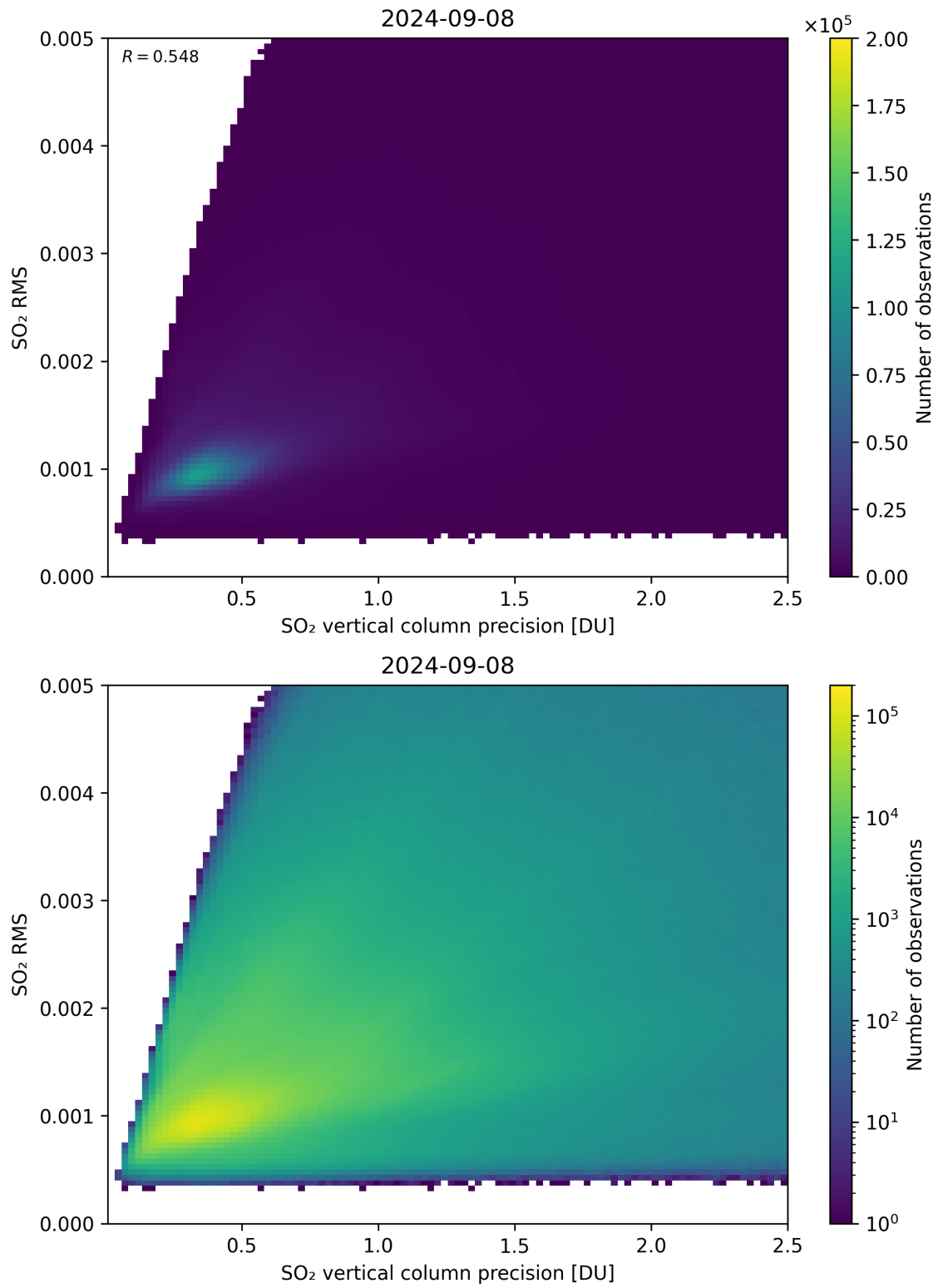
Figure 284: Scatter density plot of “SO 2 vertical column precision” against “SO 2 RMS” for 2024-09-07 to 2024-09-09.
