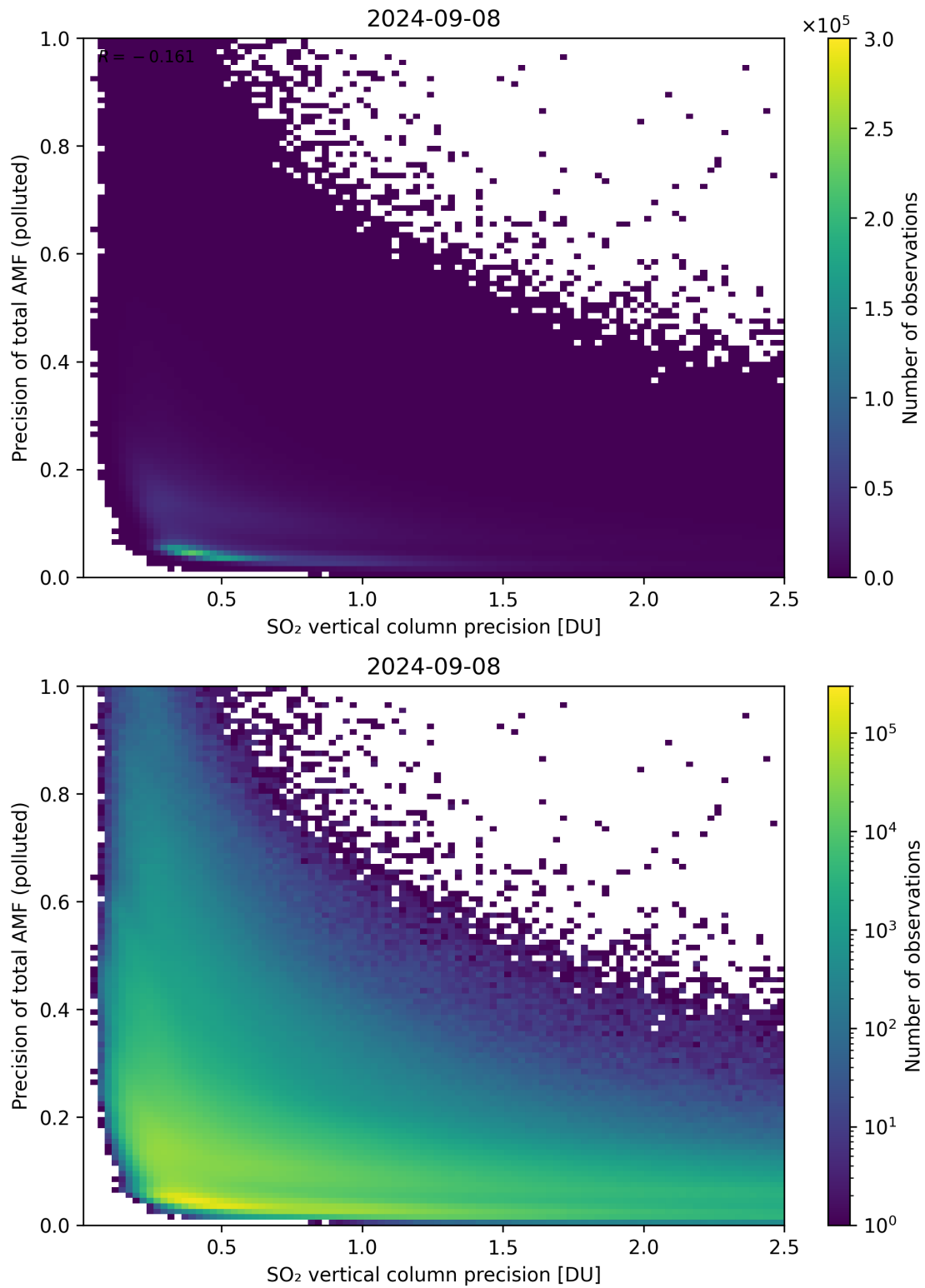
Figure 295: Scatter density plot of “SO 2 vertical column precision” against “Precision of total AMF (polluted)” for 2024-09-07 to 2024-09-09.
