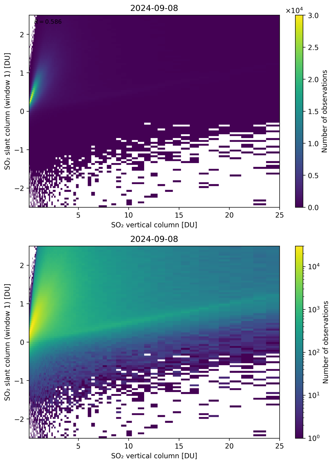
Figure 300: Scatter density plot of “SO 2 vertical column” against “SO 2 slant column (window 1)” for 2024-09-07 to 2024-09-09.
