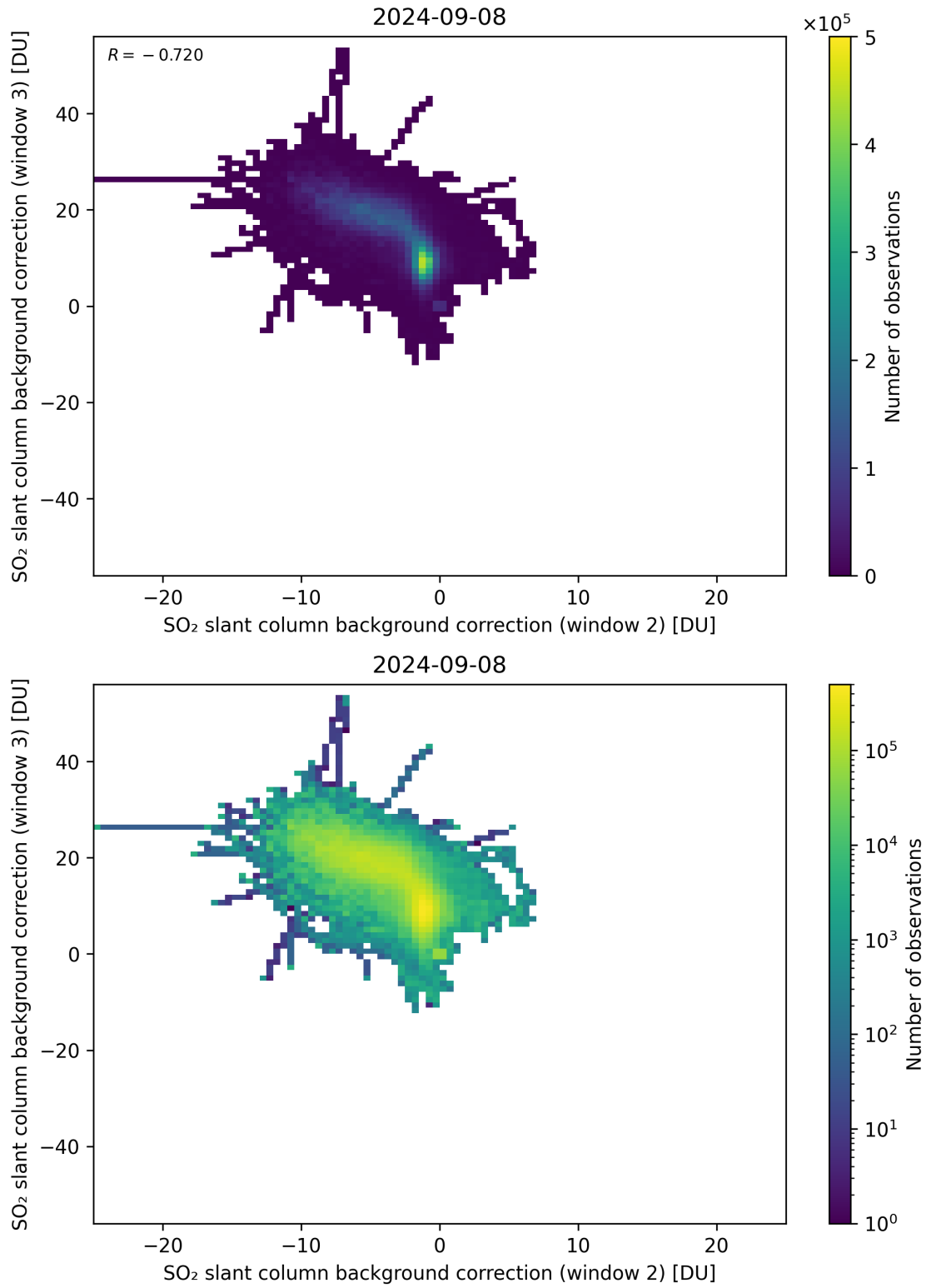
Figure 111: Scatter density plot of “SO 2 slant column background correction (window 2)” against “SO 2 slant column background correction (window 3)” for 2024-09-07 to 2024-09-09.
