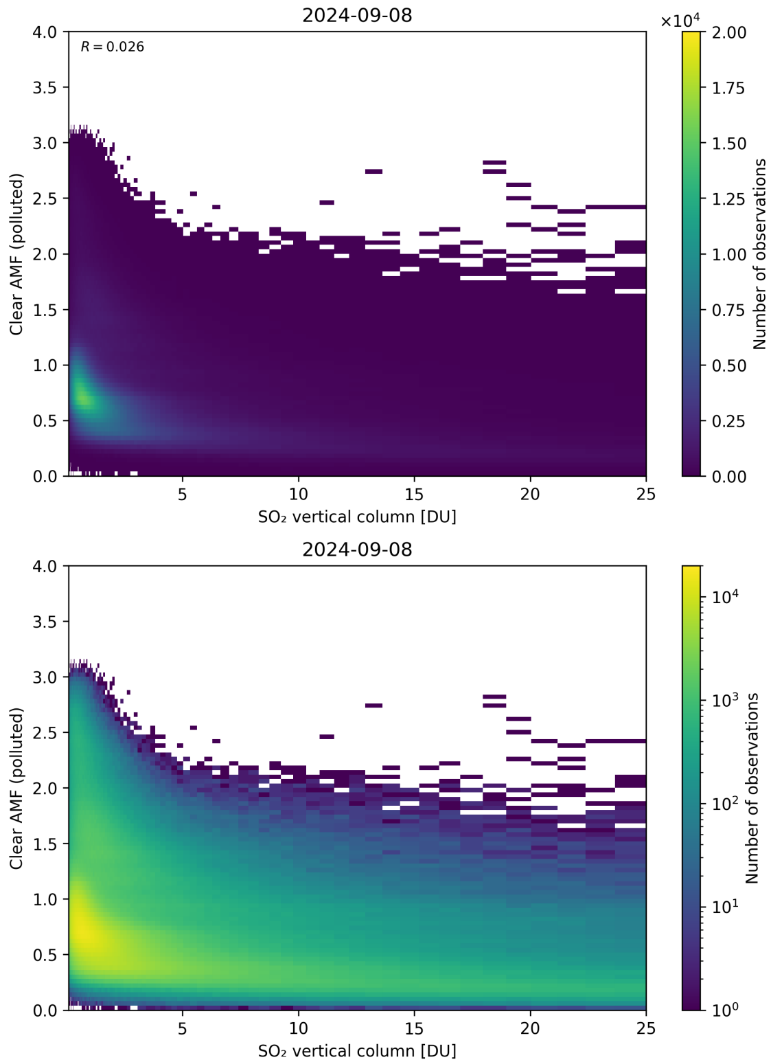
Figure 296: Scatter density plot of “SO 2 vertical column” against “Clear AMF (polluted)” for 2024-09-07 to 2024-09-09.
