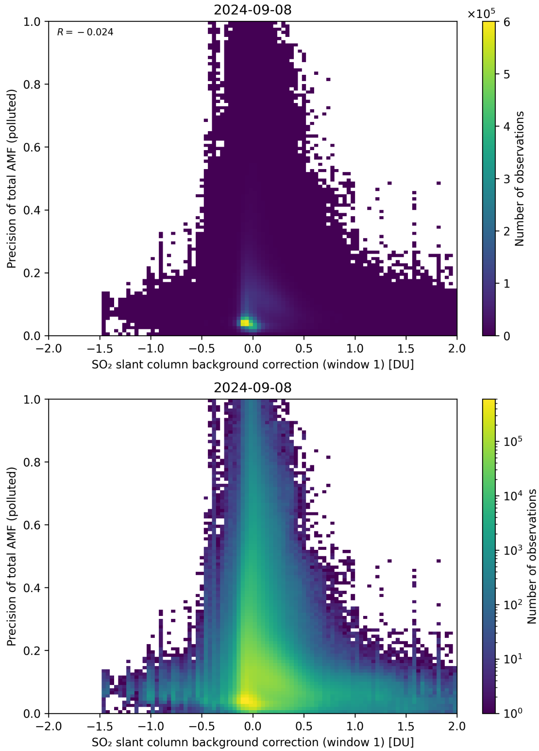
Figure 110: Scatter density plot of “SO 2 slant column background correction (window 1)” against “Precision of total AMF (polluted)” for 2024-09-07 to 2024-09-09.
