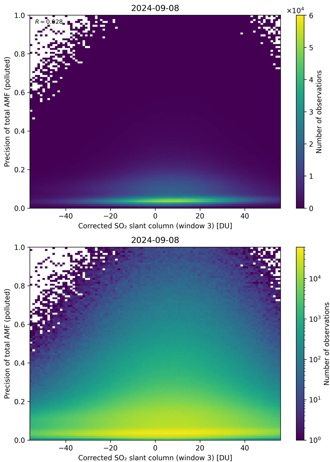
Figure 211: Scatter density plot of “Corrected SO 2 slant column (window 3)” against “Precision of total AMF (polluted)” for 2024-09-07 to 2024-09-09.
