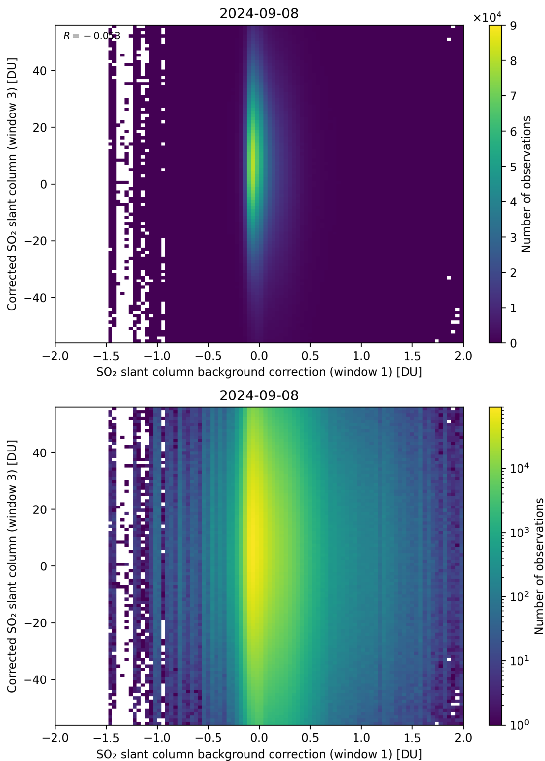
Figure 105: Scatter density plot of “SO 2 slant column background correction (window 1)” against “Corrected SO 2 slant column (window 3)” for 2024-09-07 to 2024-09-09.
