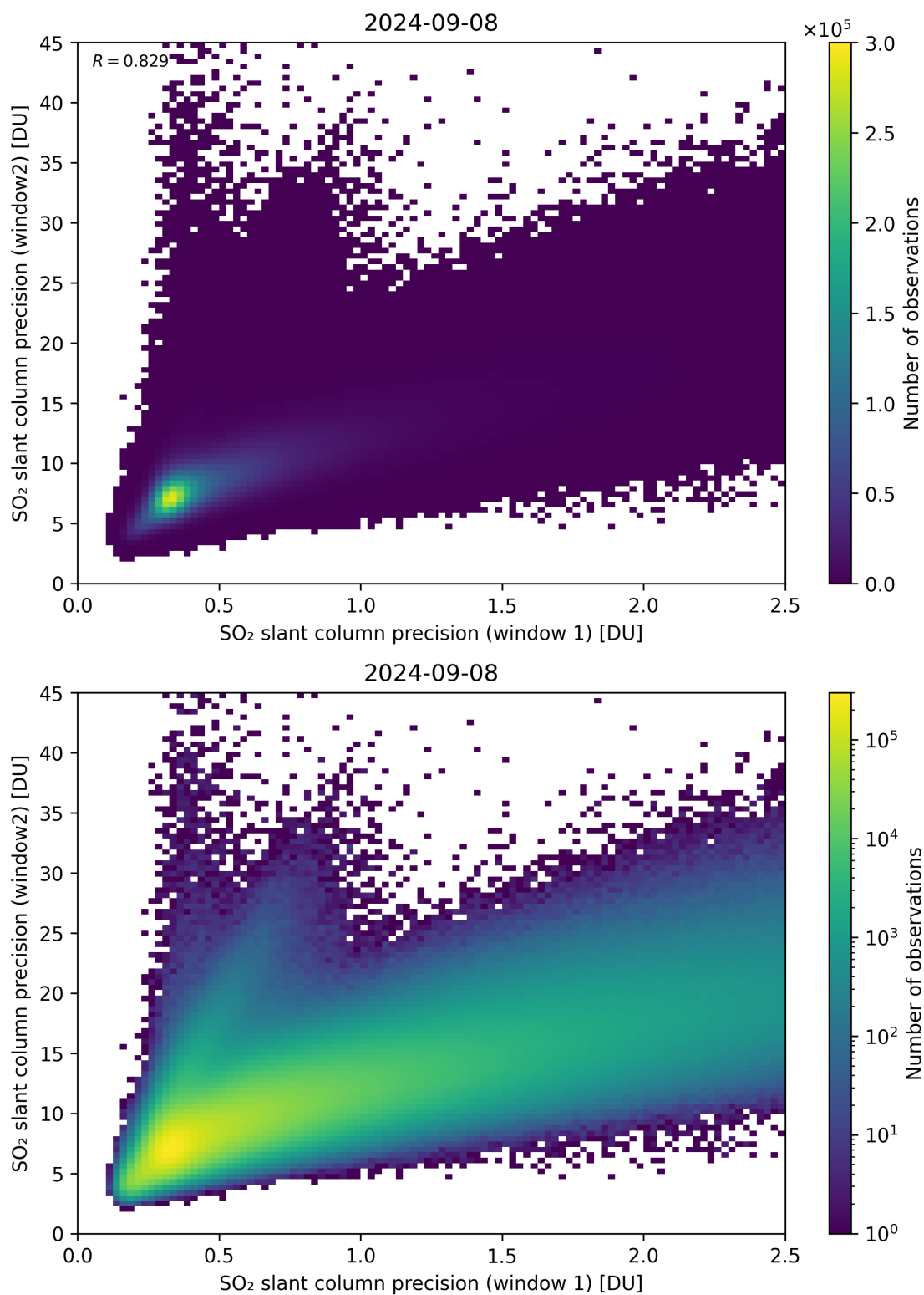
Figure 227: Scatter density plot of “SO 2 slant column precision (window 1)” against “SO 2 slant column precision (window2)” for 2024-09-07 to 2024-09-09.
