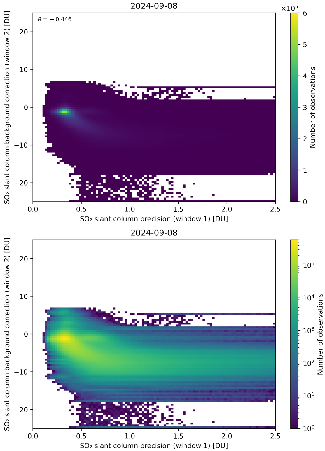
Figure 219: Scatter density plot of “SO 2 slant column precision (window 1)” against “SO 2 slant column background correction (window 2)” for 2024-09-07 to 2024-09-09.
