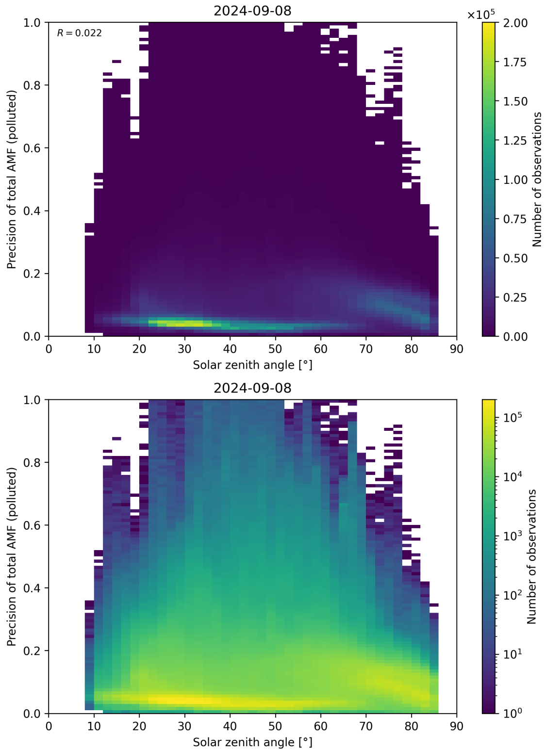
Figure 175: Scatter density plot of “Solar zenith angle” against “Precision of total AMF (polluted)” for 2024-09-07 to 2024-09-09.
