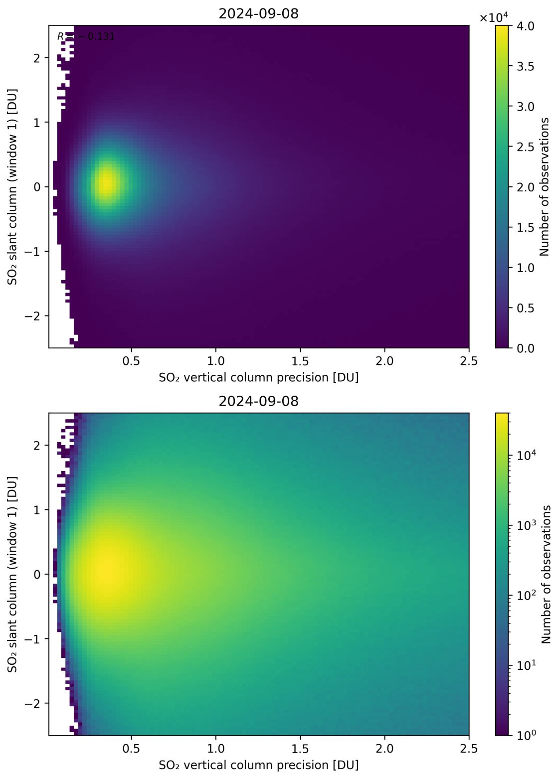
Figure 289: Scatter density plot of “SO 2 vertical column precision” against “SO 2 slant column (window 1)” for 2024-09-07 to 2024-09-09.
