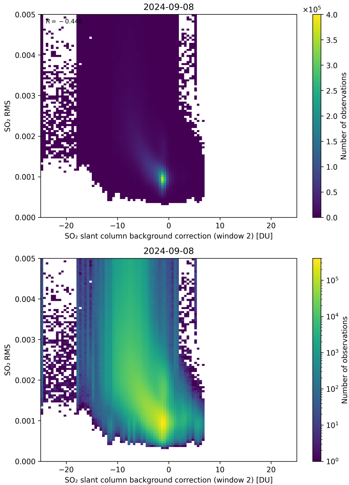
Figure 114: Scatter density plot of “SO 2 slant column background correction (window 2)” against “SO 2 RMS” for 2024-09-07 to 2024-09-09.
