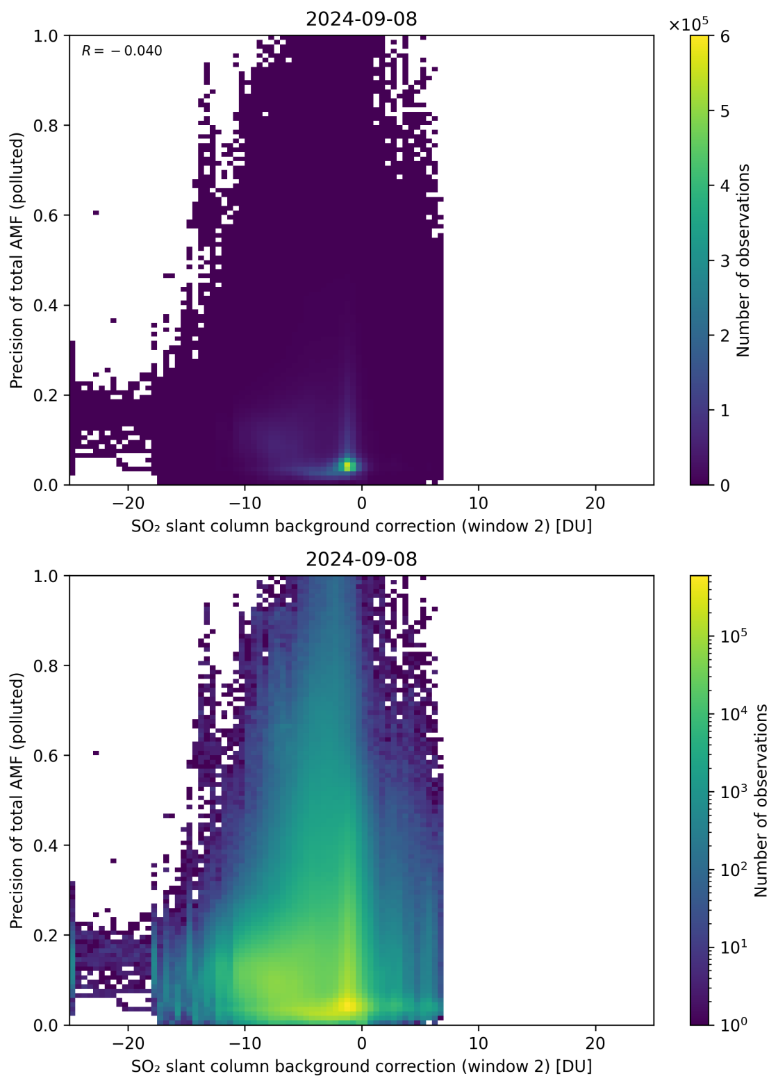
Figure 120: Scatter density plot of “SO 2 slant column background correction (window 2)” against “Precision of total AMF (polluted)” for 2024-09-07 to 2024-09-09.
