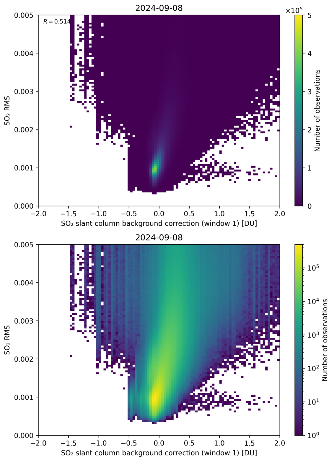
Figure 102: Scatter density plot of “SO 2 slant column background correction (window 1)” against “SO 2 RMS” for 2024-09-07 to 2024-09-09.
