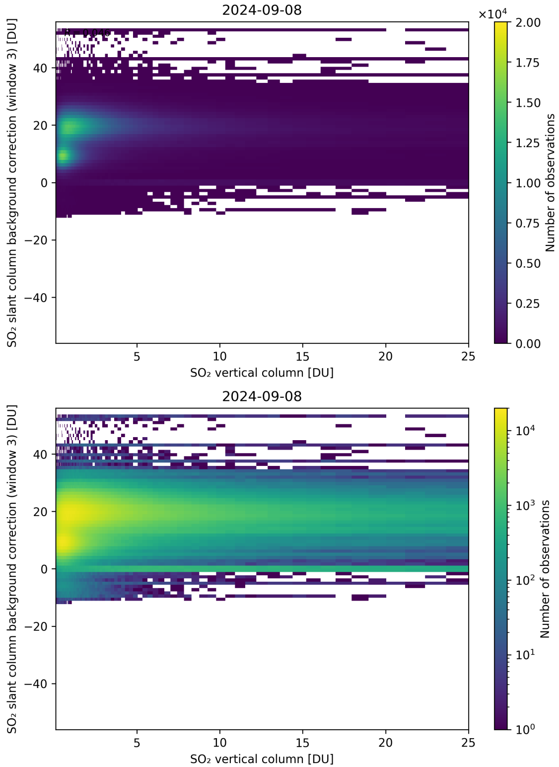
Figure 275: Scatter density plot of “SO 2 vertical column” against “SO 2 slant column background correction (window 3)” for 2024-09-07 to 2024-09-09.
