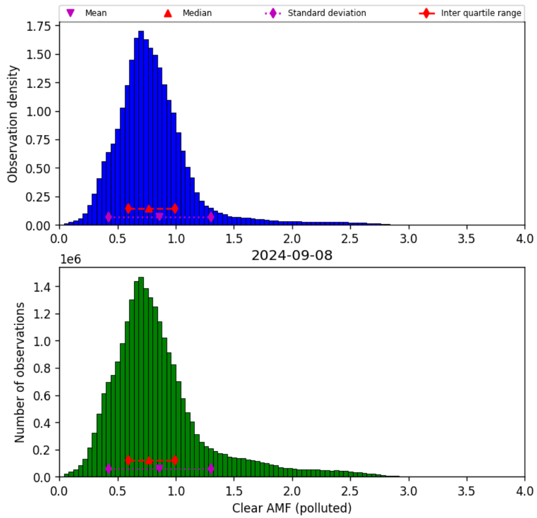
Figure 73: Histogram of “Clear AMF (polluted)” for 2024-09-07 to 2024-09-09
