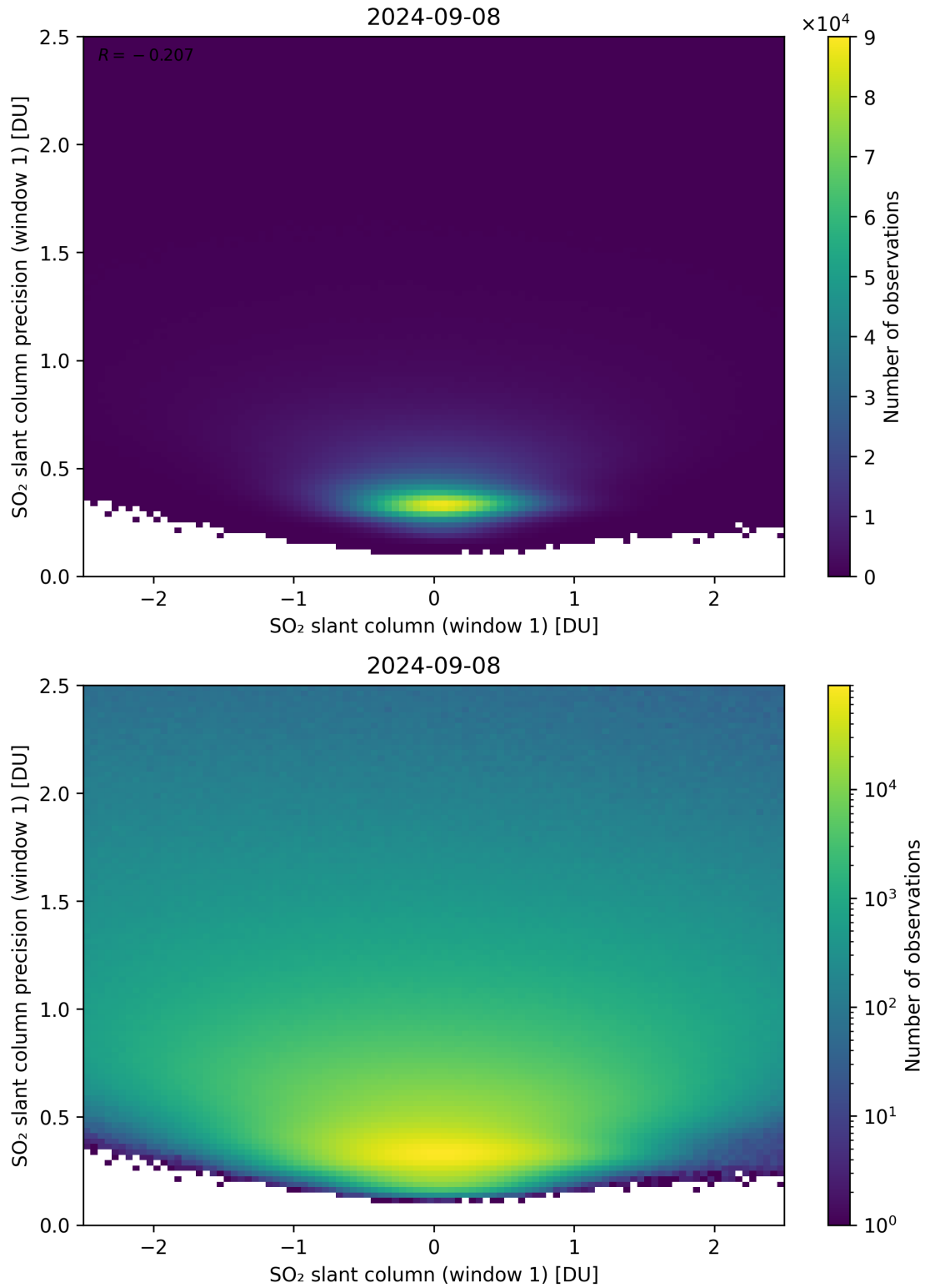
Figure 235: Scatter density plot of “SO 2 slant column (window 1)” against “SO 2 slant column precision (window 1)” for 2024-09-07 to 2024-09-09.
