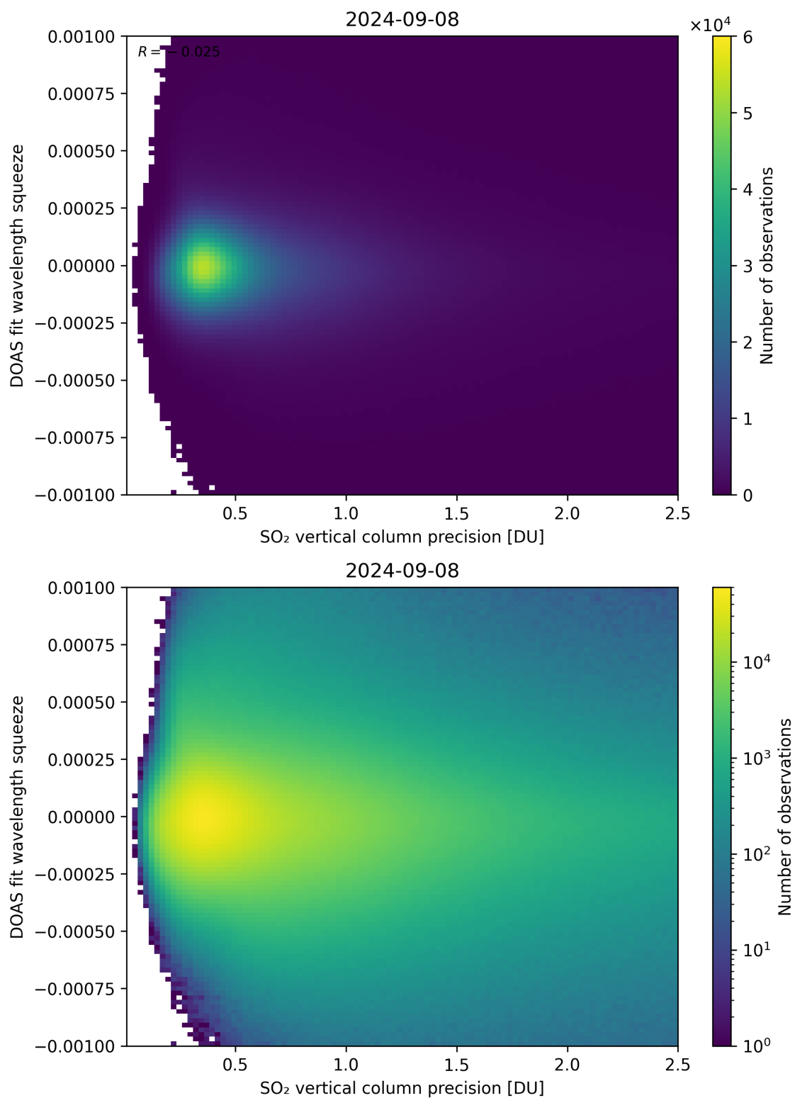
Figure 283: Scatter density plot of “SO 2 vertical column precision” against “DOAS fit wavelength squeeze” for 2024-09-07 to 2024-09-09.
