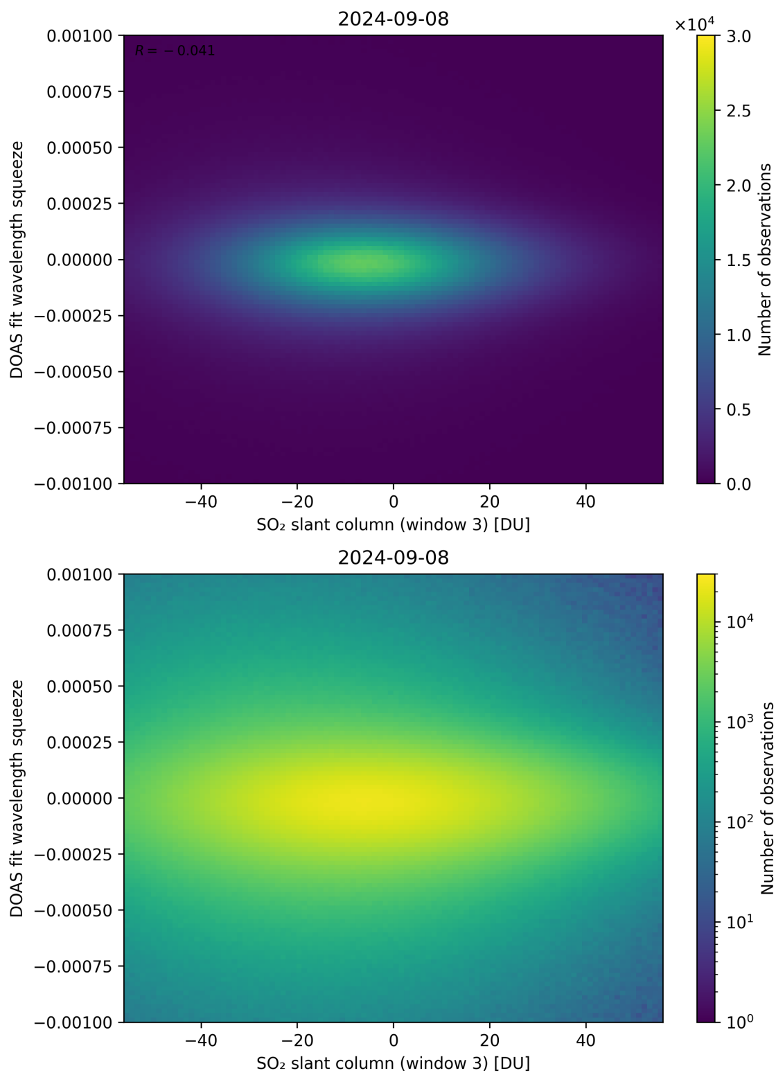
Figure 255: Scatter density plot of “SO 2 slant column (window 3)” against “DOAS fit wavelength squeeze” for 2024-09-07 to 2024-09-09.
