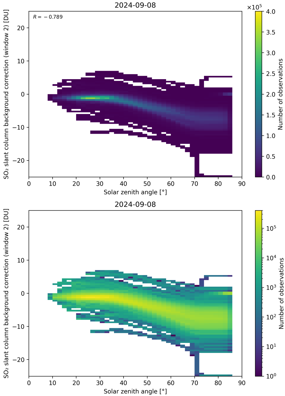
Figure 159: Scatter density plot of “Solar zenith angle” against “SO 2 slant column background correction (window 2)” for 2024-09-07 to 2024-09-09.
