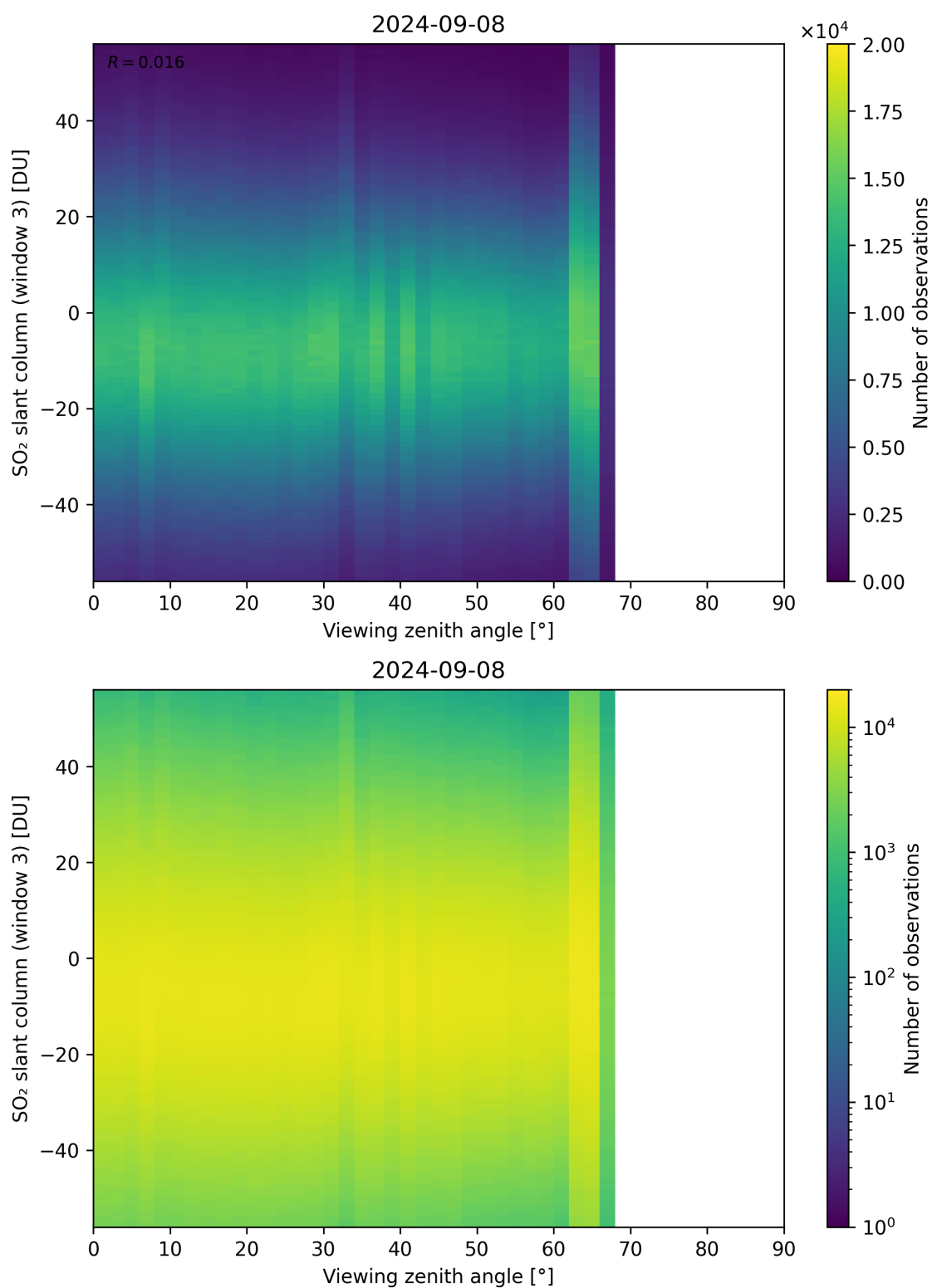
Figure 323: Scatter density plot of “Viewing zenith angle” against “SO 2 slant column (window 3)” for 2024-09-07 to 2024-09-09.
