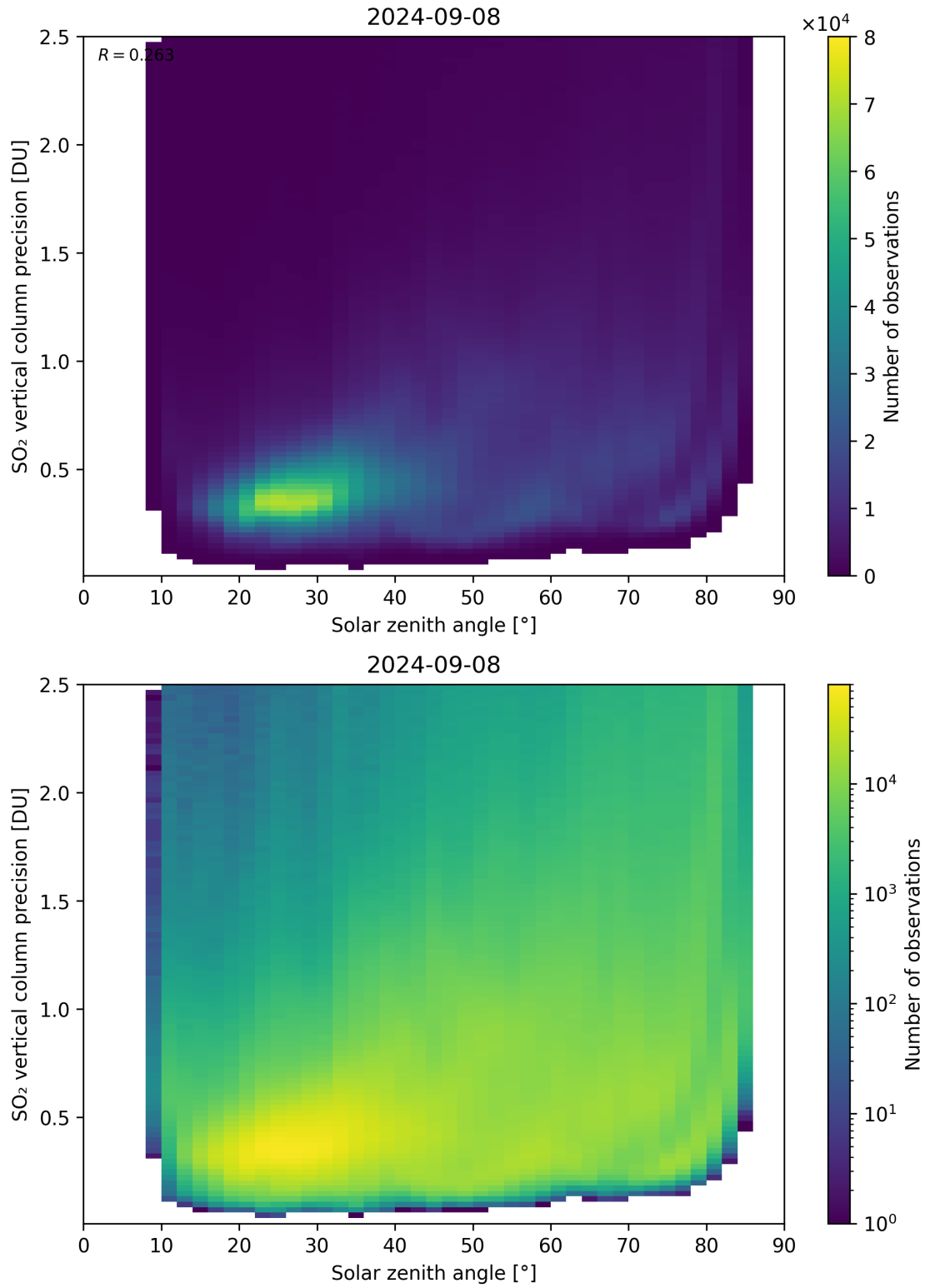
Figure 177: Scatter density plot of “Solar zenith angle” against “SO 2 vertical column precision” for 2024-09-07 to 2024-09-09.
