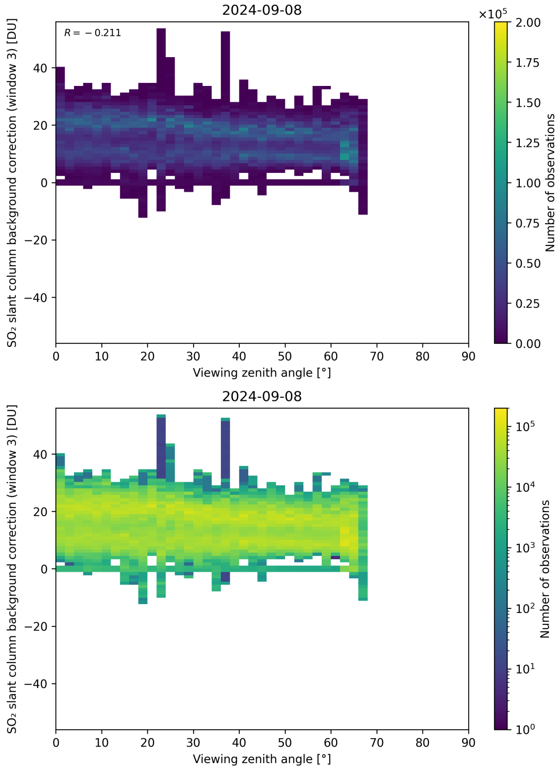
Figure 310: Scatter density plot of “Viewing zenith angle” against “SO 2 slant column background correction (window 3)” for 2024-09-07 to 2024-09-09.
