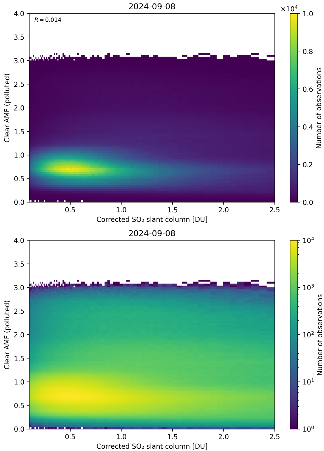
Figure 184: Scatter density plot of “Corrected SO 2 slant column” against “Clear AMF (polluted)” for 2024-09-07 to 2024-09-09.
