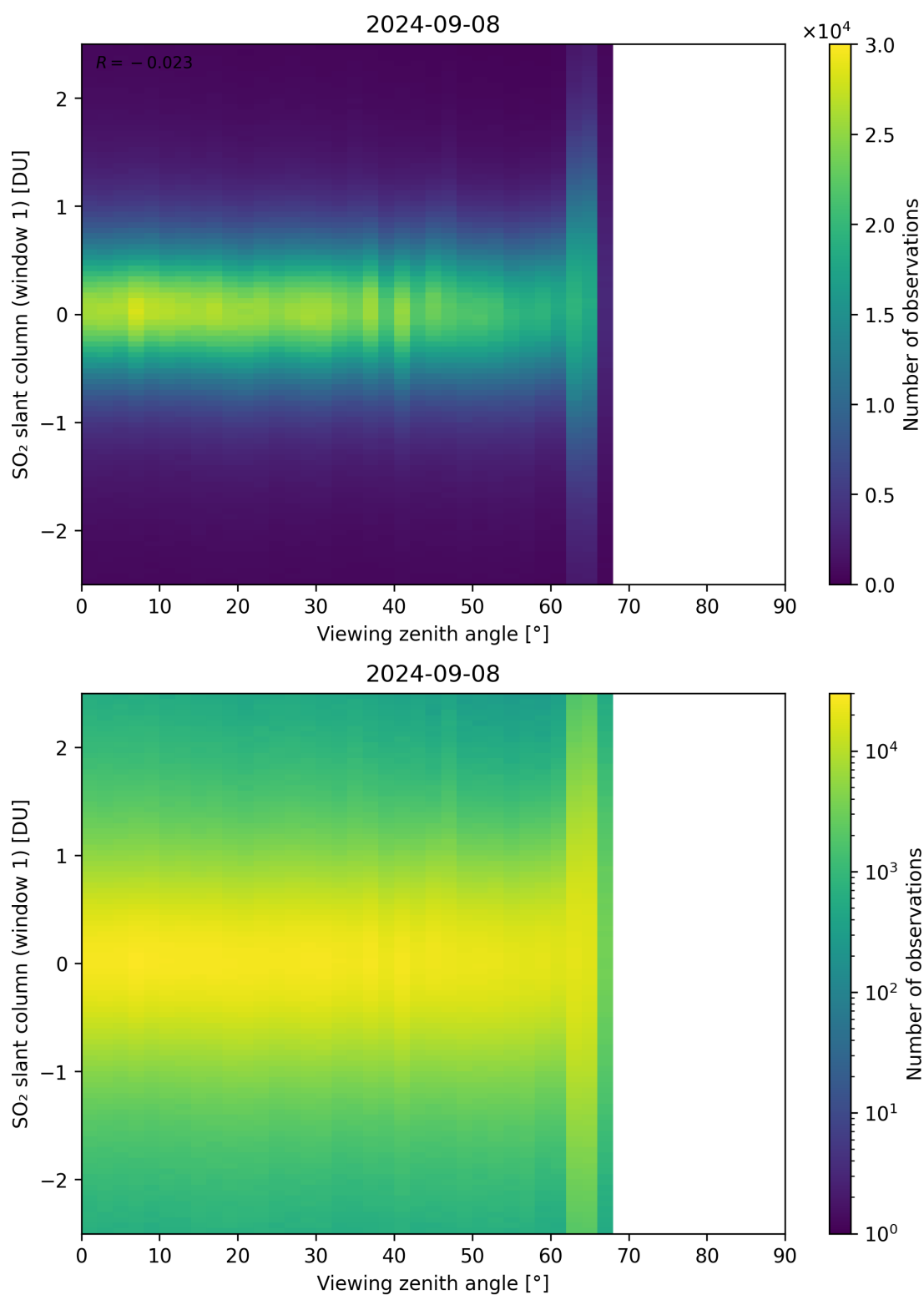
Figure 320: Scatter density plot of “Viewing zenith angle” against “SO 2 slant column (window 1)” for 2024-09-07 to 2024-09-09.
