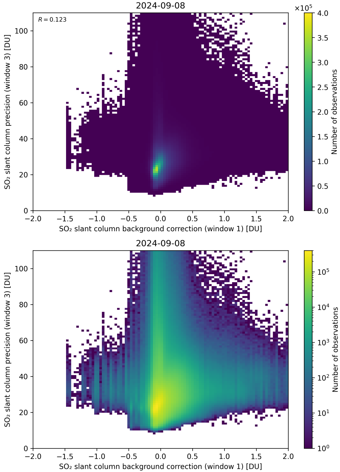
Figure 108: Scatter density plot of “SO 2 slant column background correction (window 1)” against “SO 2 slant column precision (window 3)” for 2024-09-07 to 2024-09-09.
