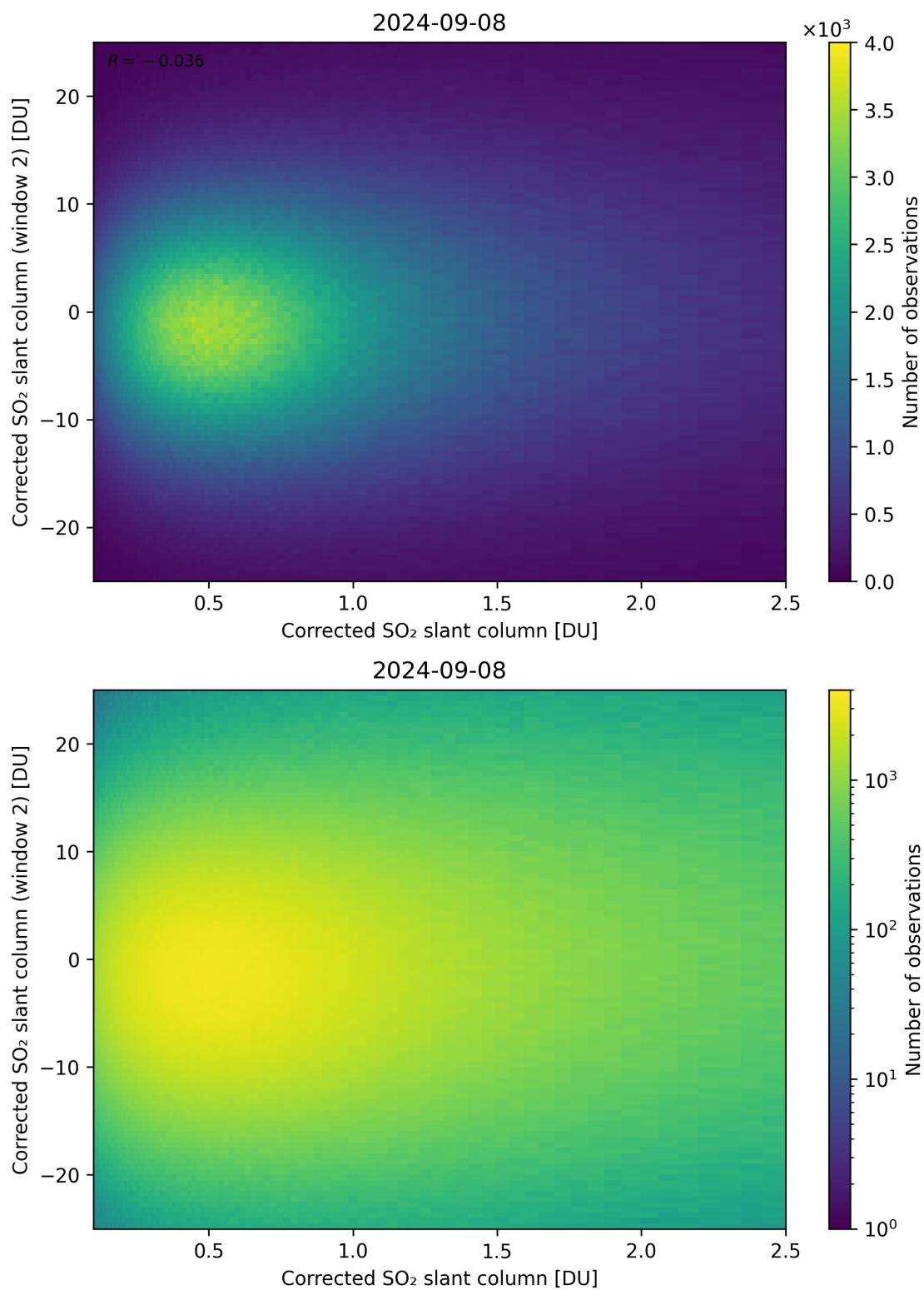
Figure 185: Scatter density plot of “Corrected SO 2 slant column” against “Corrected SO 2 slant column (window 2)” for 2024-09-07 to 2024-09-09.
