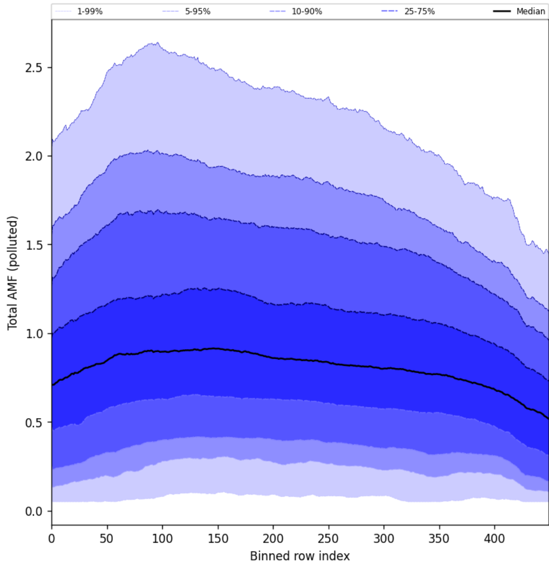
Figure 94: Along track statistics of “Total AMF (polluted)” for 2024-09-07 to 2024-09-09
