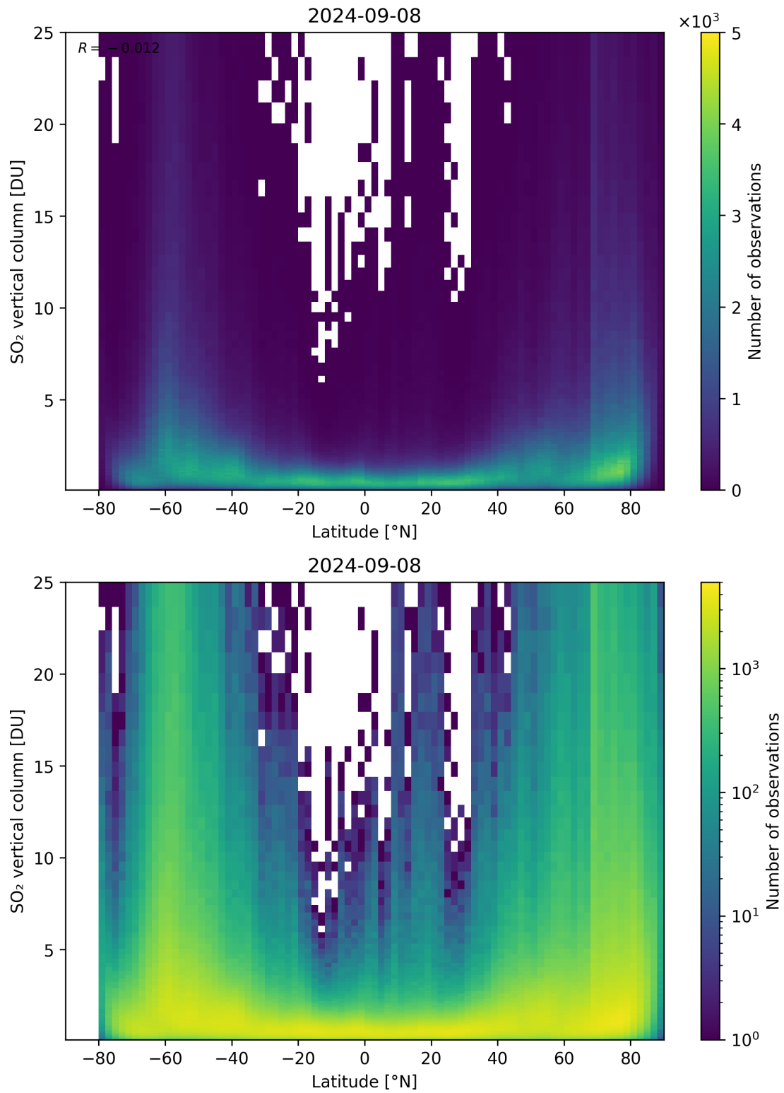
Figure 156: Scatter density plot of “Latitude” against “SO 2 vertical column” for 2024-09-07 to 2024-09-09.
