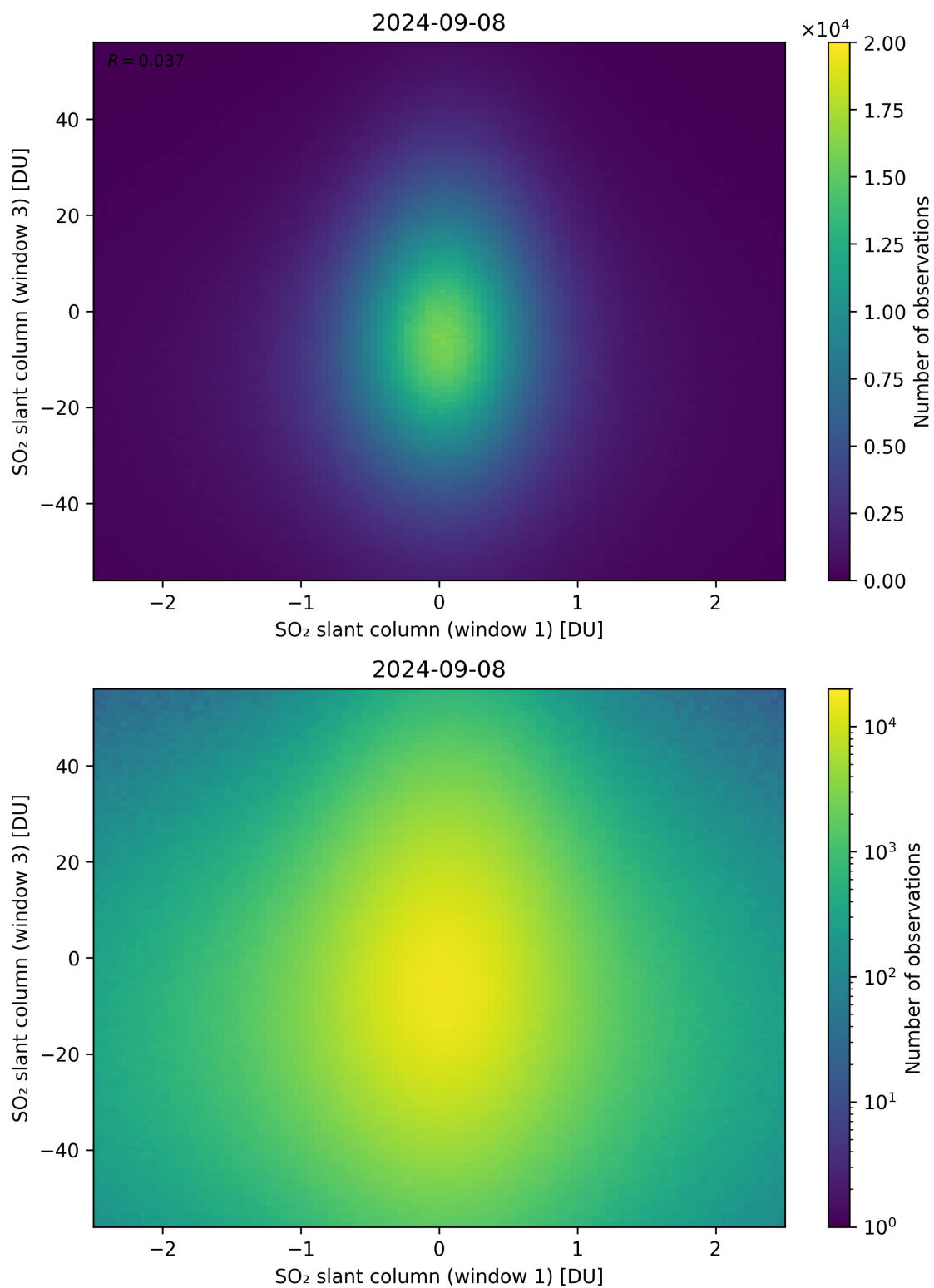
Figure 237: Scatter density plot of “SO 2 slant column (window 1)” against “SO 2 slant column (window 3)” for 2024-09-07 to 2024-09-09.
