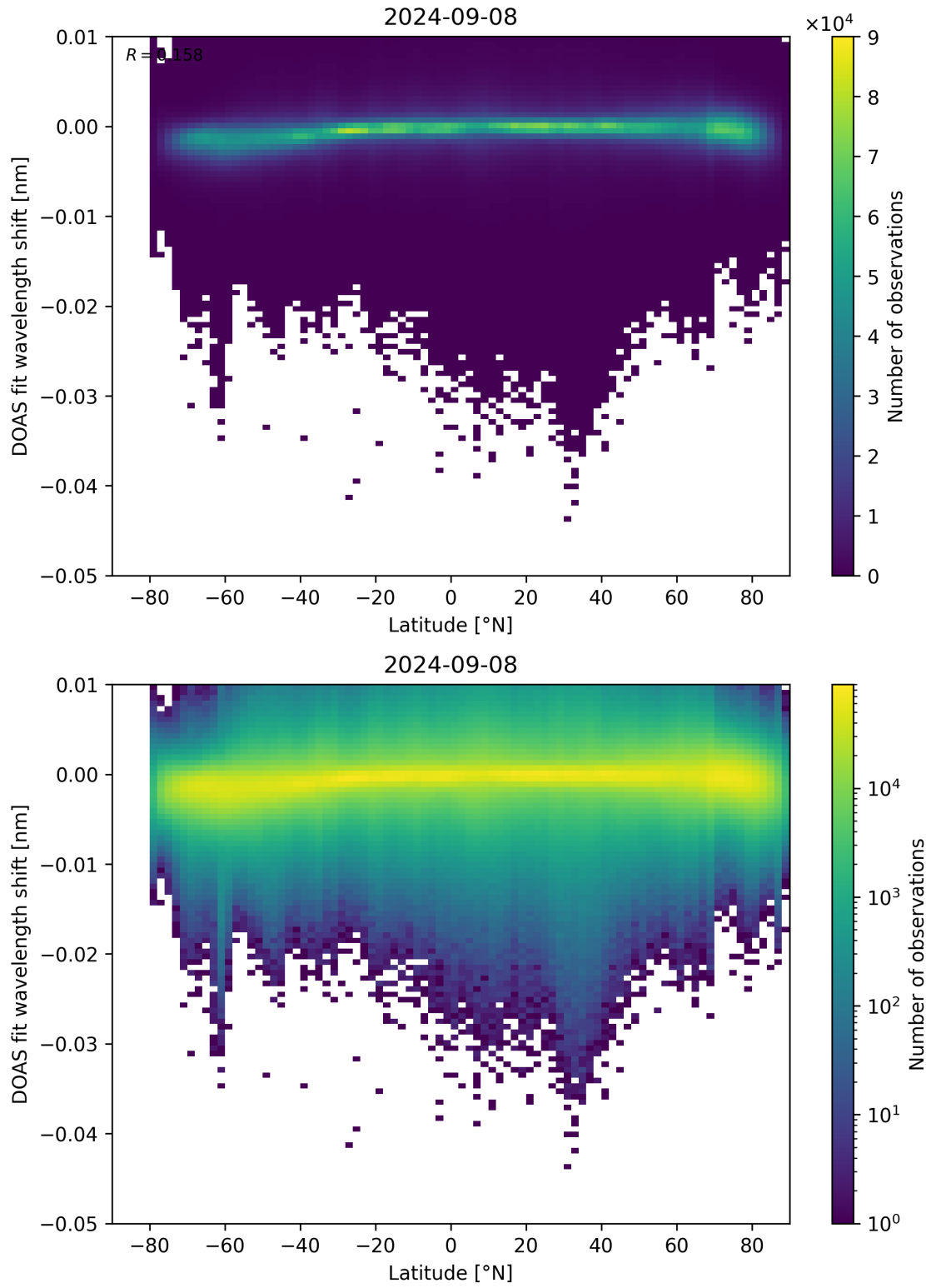
Figure 142: Scatter density plot of “Latitude” against “DOAS fit wavelength shift” for 2024-09-07 to 2024-09-09.
