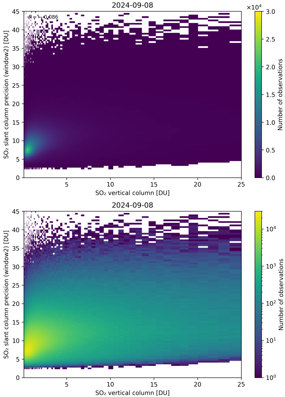
Figure 302: Scatter density plot of “SO 2 vertical column” against “SO 2 slant column precision (window2)” for 2024-09-07 to 2024-09-09.
