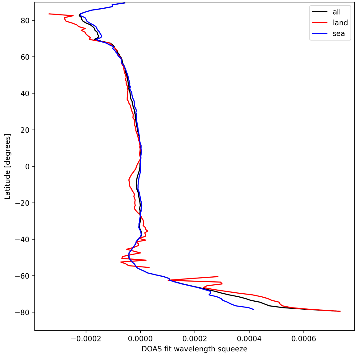
Figure 46: Zonal average of “DOAS fit wavelength squeeze” for 2024-09-07 to 2024-09-09.
