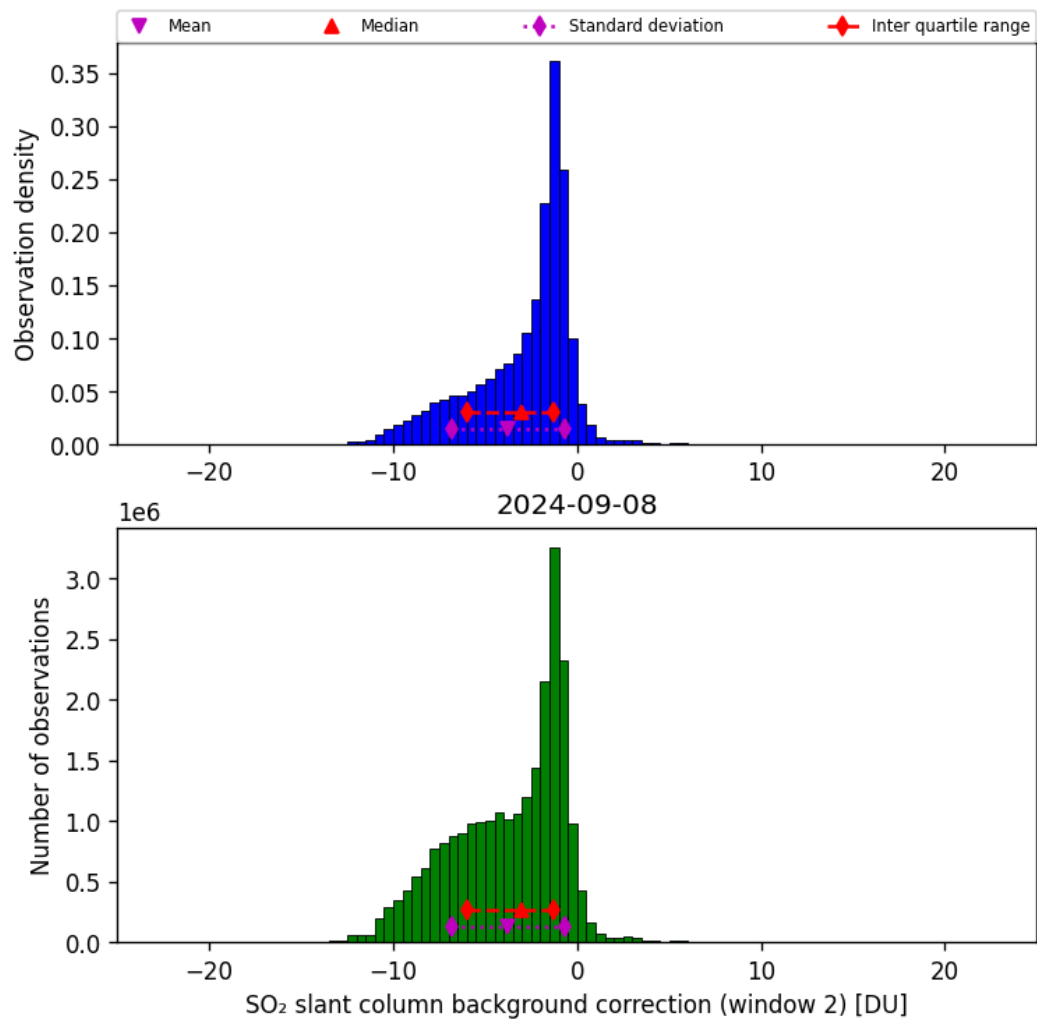
Figure 63: Histogram of “SO 2 slant column background correction (window 2)” for 2024-09-07 to 2024-09-09
