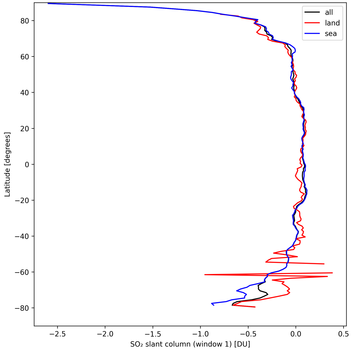
Figure 33: Zonal average of “SO 2 slant column (window 1)” for 2024-09-07 to 2024-09-09.
