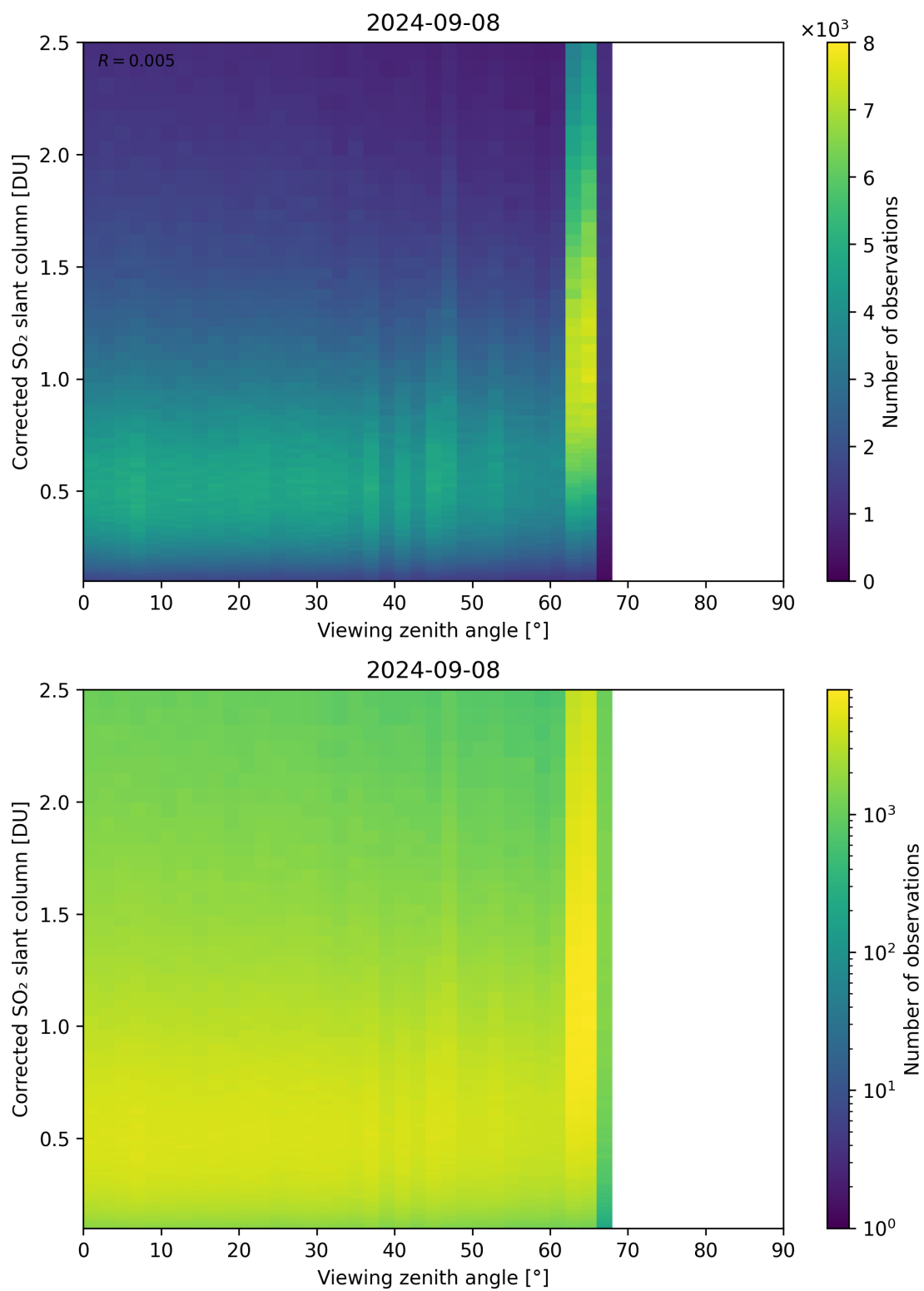
Figure 317: Scatter density plot of “Viewing zenith angle” against “Corrected SO 2 slant column” for 2024-09-07 to 2024-09-09.
