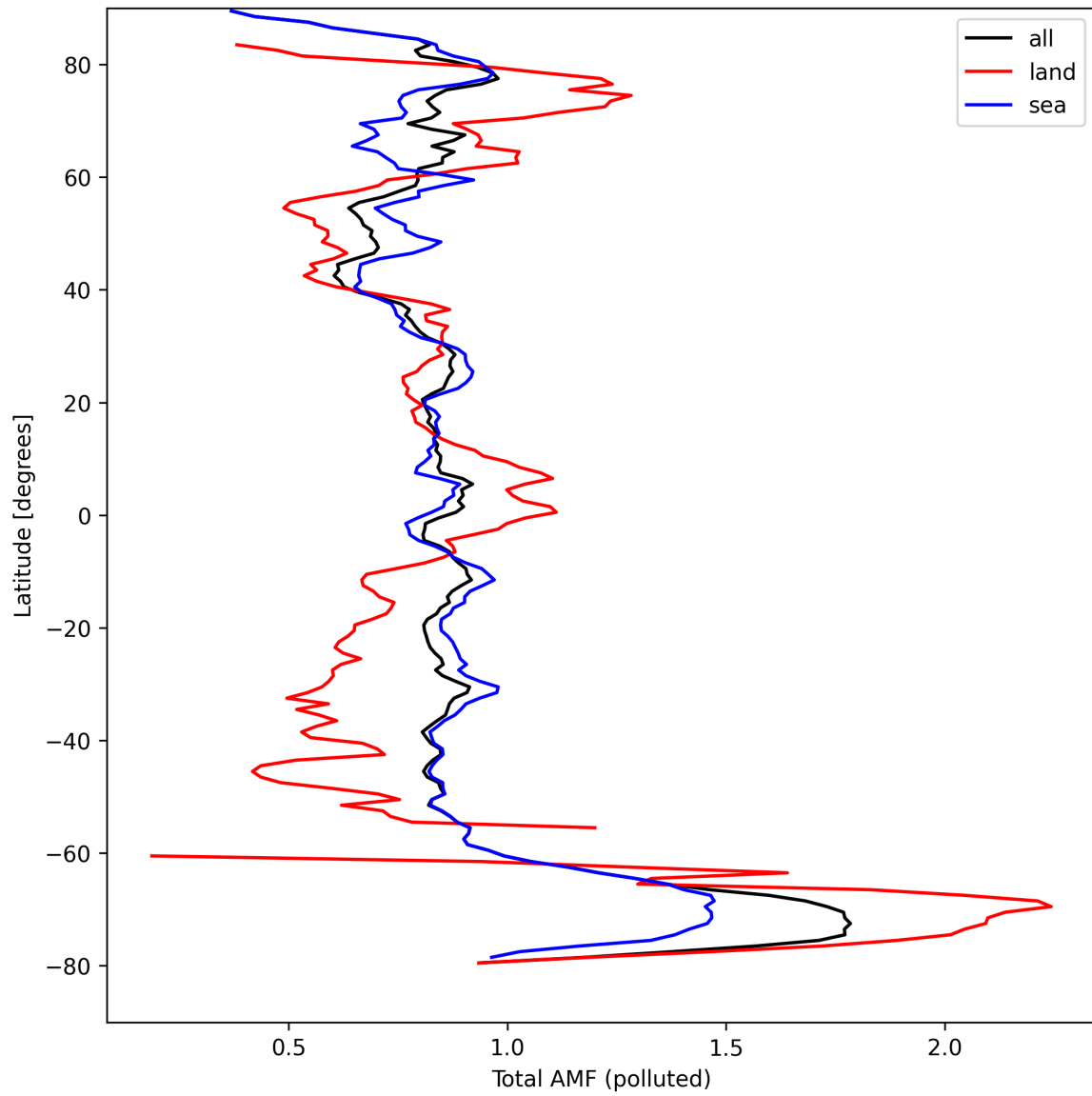
Figure 48: Zonal average of “Total AMF (polluted)” for 2024-09-07 to 2024-09-09.
