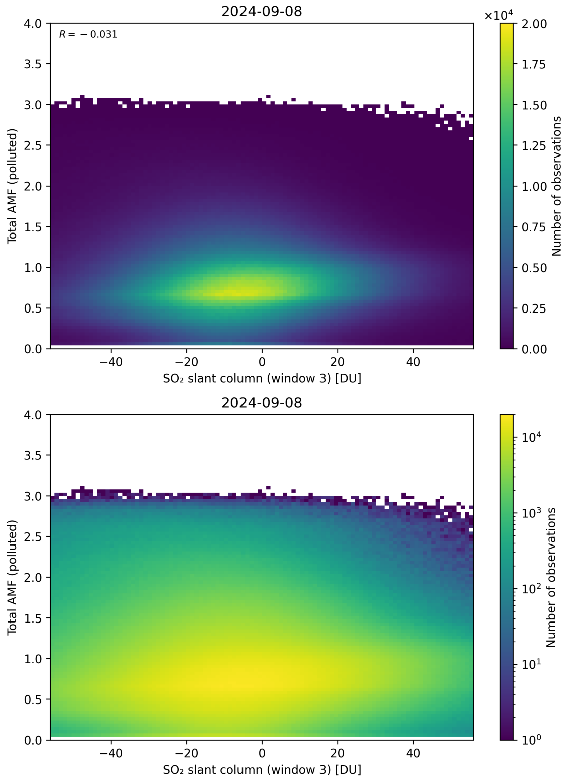
Figure 268: Scatter density plot of “SO 2 slant column (window 3)” against “Total AMF (polluted)” for 2024-09-07 to 2024-09-09.
