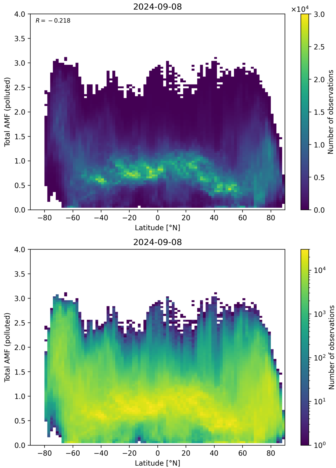
Figure 154: Scatter density plot of “Latitude” against “Total AMF (polluted)” for 2024-09-07 to 2024-09-09.
