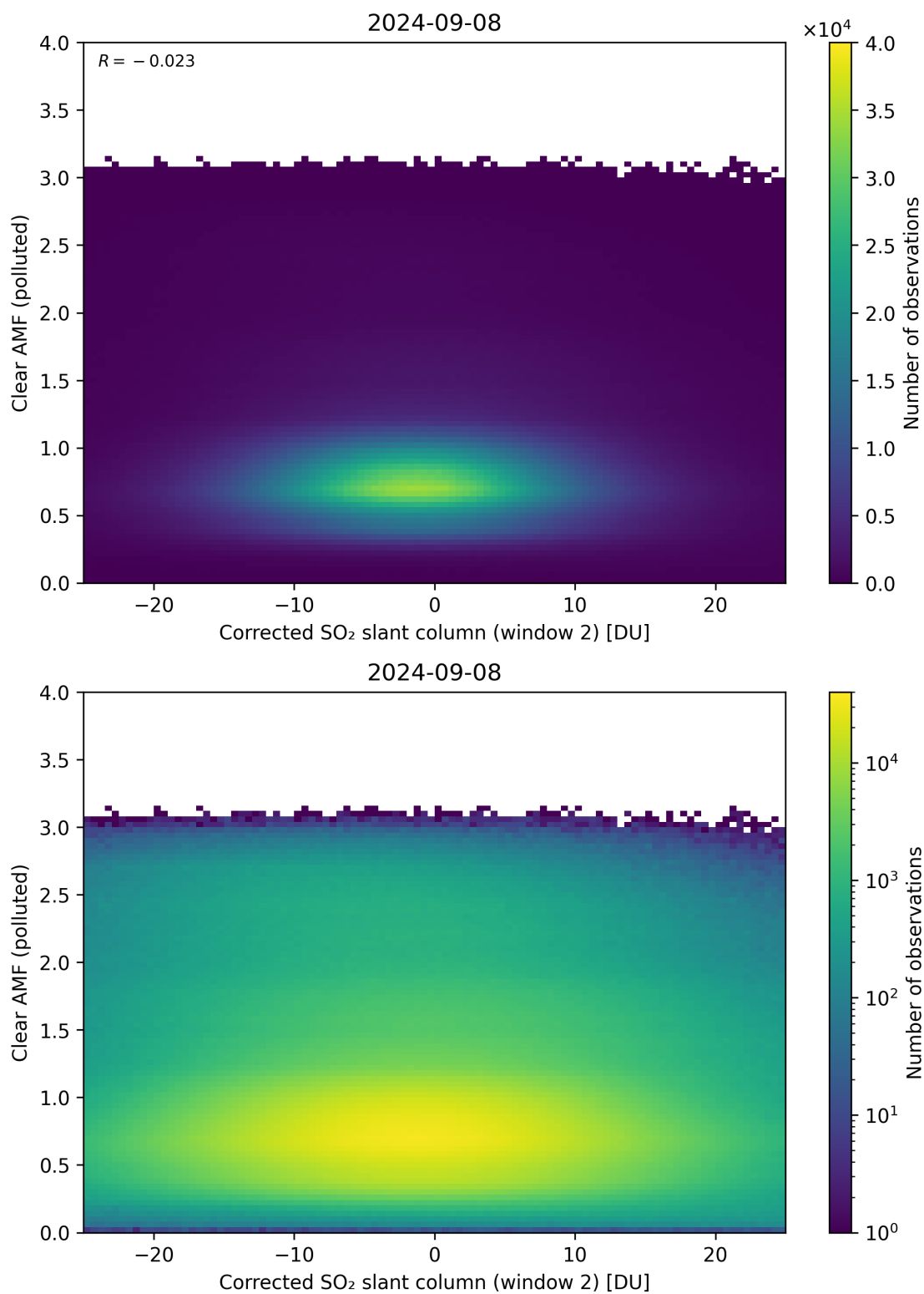
Figure 199: Scatter density plot of “Corrected SO 2 slant column (window 2)” against “Clear AMF (polluted)” for 2024-09-07 to 2024-09-09.
