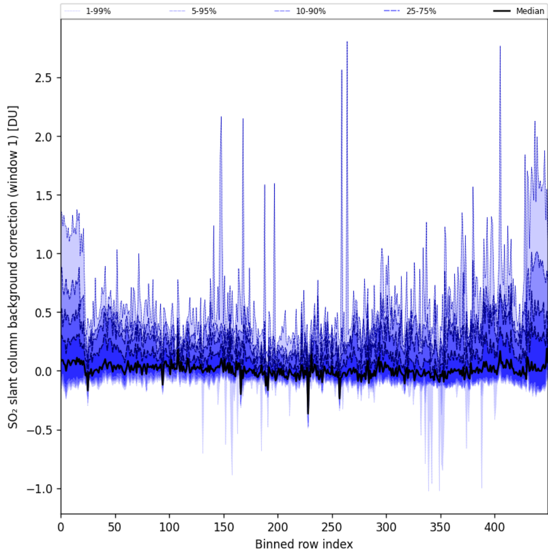
Figure 82: Along track statistics of “SO 2 slant column background correction (window 1)” for 2024-09-07 to 2024-09-09
