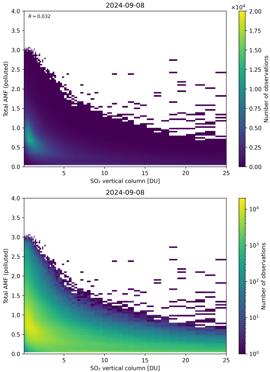
Figure 305: Scatter density plot of “SO 2 vertical column” against “Total AMF (polluted)” for 2024-09-07 to 2024-09-09.
