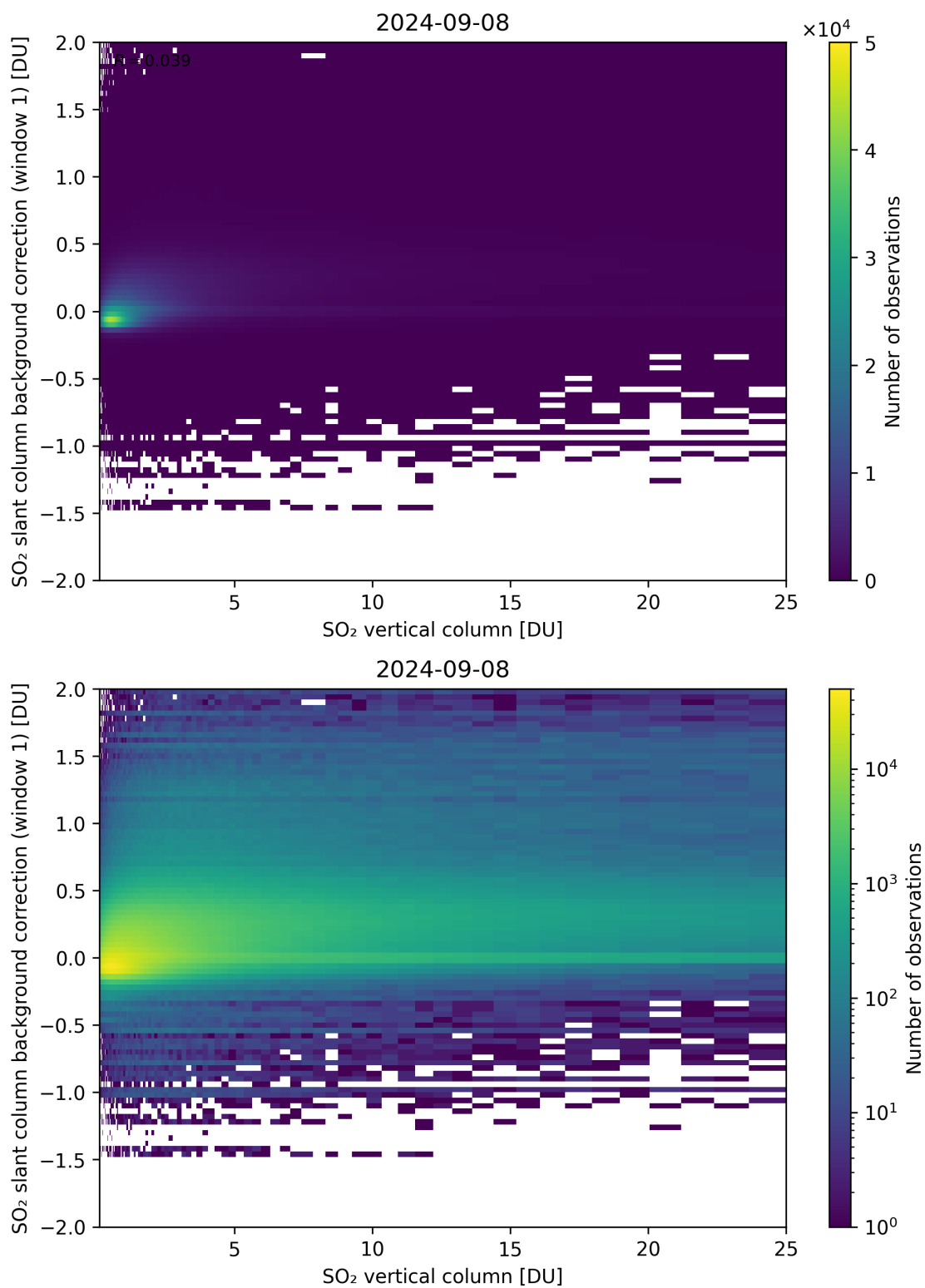
Figure 273: Scatter density plot of “SO 2 vertical column” against “SO 2 slant column background correction (window 1)” for 2024-09-07 to 2024-09-09.
