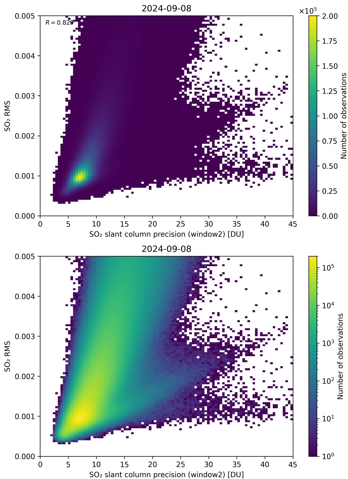
Figure 245: Scatter density plot of “SO 2 slant column precision (window2)” against “SO 2 RMS” for 2024-09-07 to 2024-09-09.
