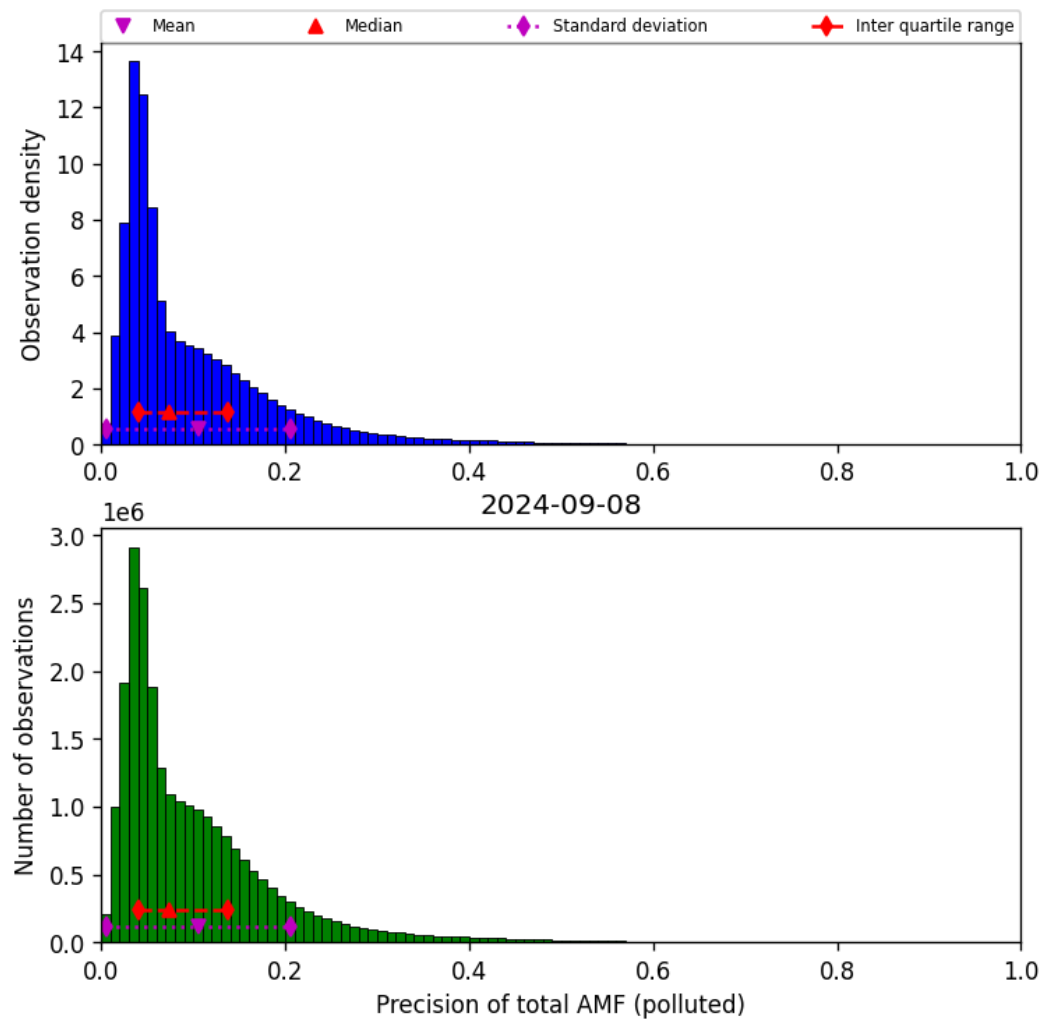
Figure 72: Histogram of “Precision of total AMF (polluted)” for 2024-09-07 to 2024-09-09
