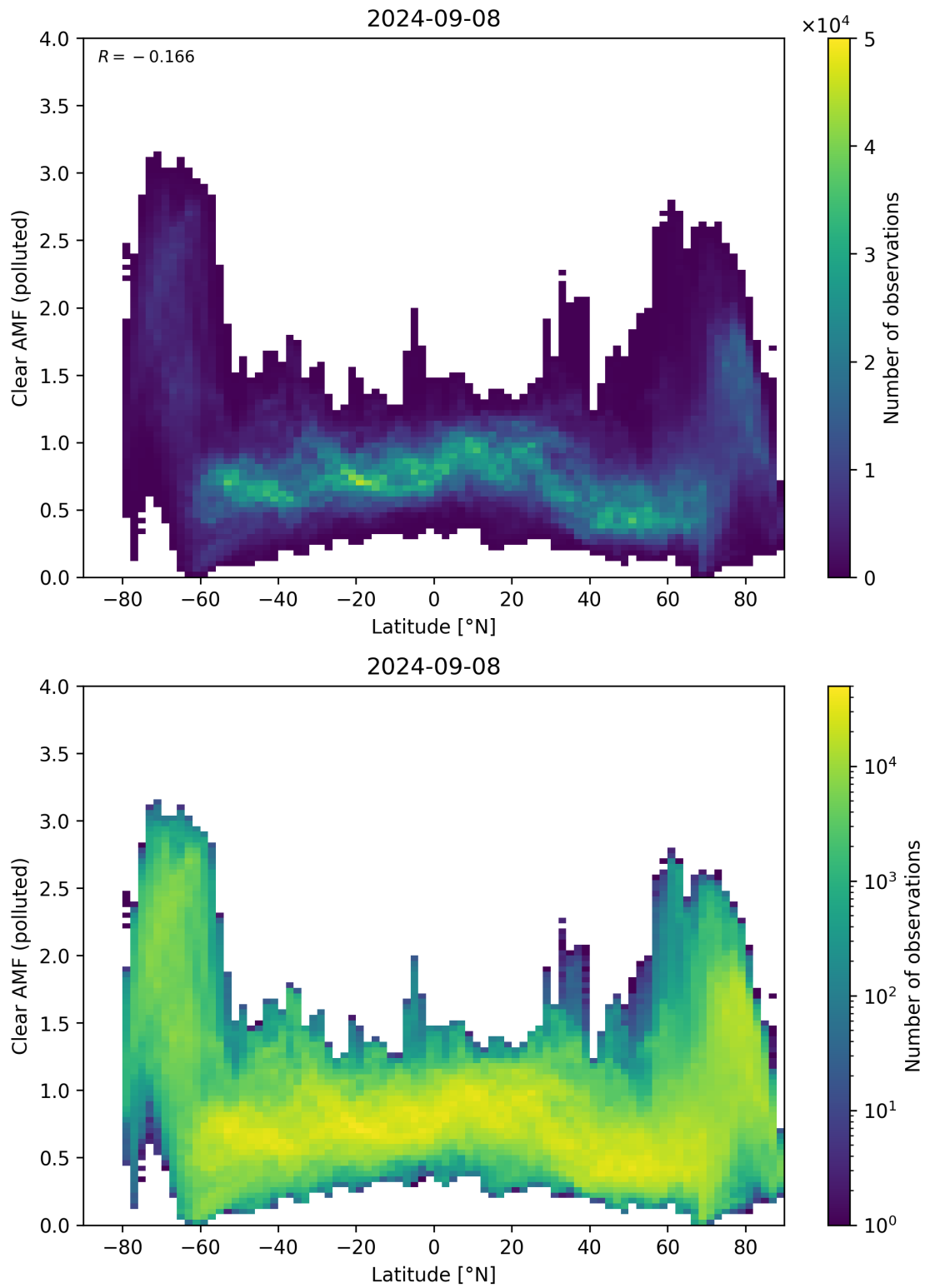
Figure 145: Scatter density plot of “Latitude” against “Clear AMF (polluted)” for 2024-09-07 to 2024-09-09.
