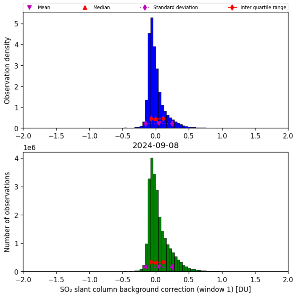
Figure 59: Histogram of “SO 2 slant column background correction (window 1)” for 2024-09-07 to 2024-09-09
