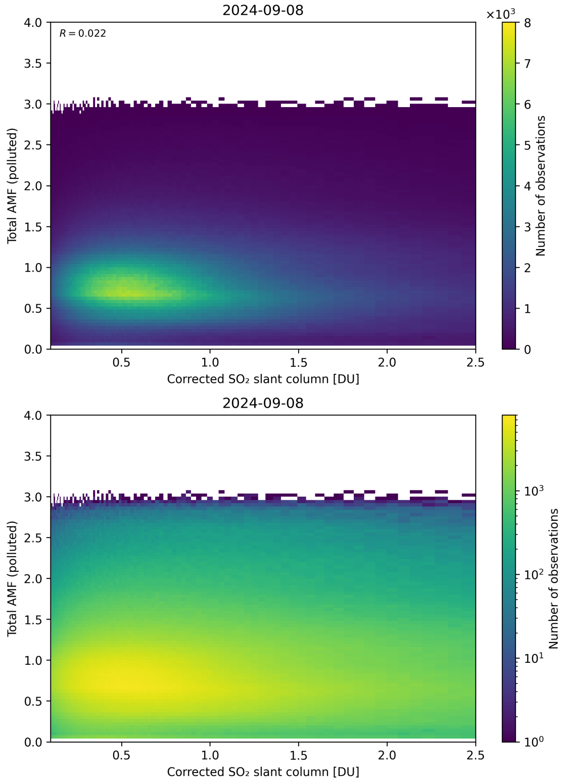
Figure 192: Scatter density plot of “Corrected SO 2 slant column” against “Total AMF (polluted)” for 2024-09-07 to 2024-09-09.
