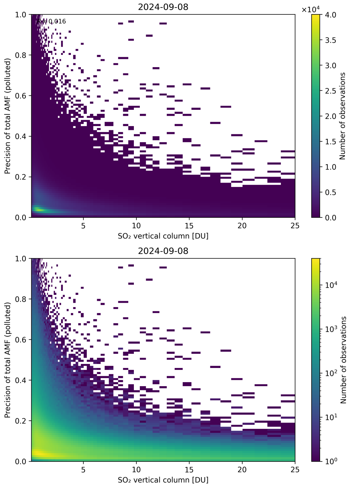
Figure 306: Scatter density plot of “SO 2 vertical column” against “Precision of total AMF (polluted)” for 2024-09-07 to 2024-09-09.
