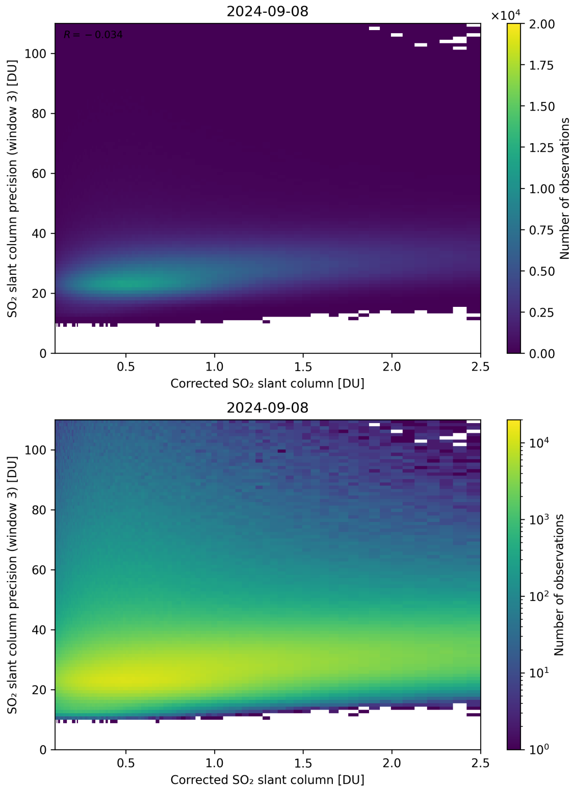
Figure 191: Scatter density plot of “Corrected SO 2 slant column” against “SO 2 slant column precision (window 3)” for 2024-09-07 to 2024-09-09.
