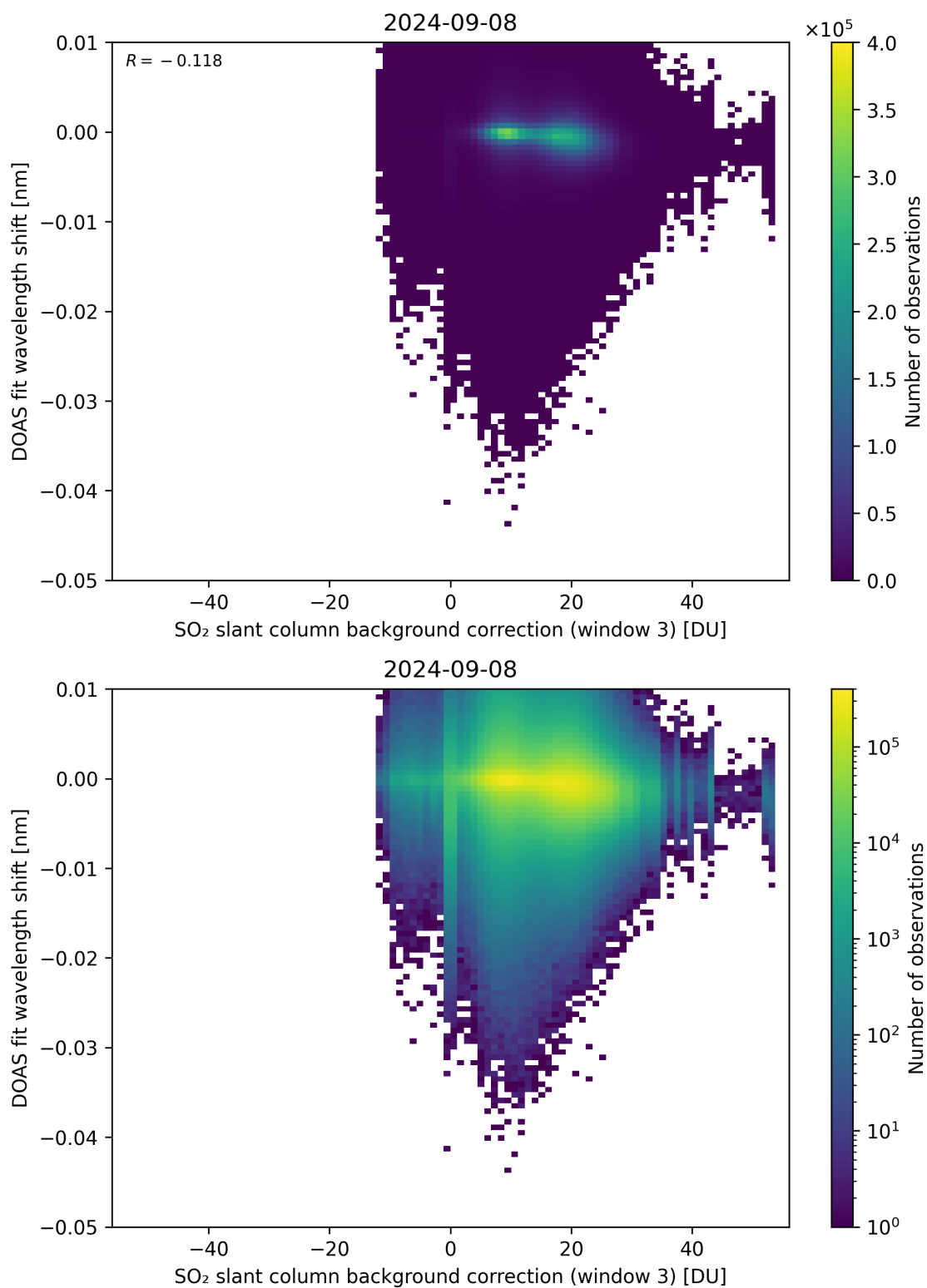
Figure 121: Scatter density plot of “SO 2 slant column background correction (window 3)” against “DOAS fit wavelength shift” for 2024-09-07 to 2024-09-09.
