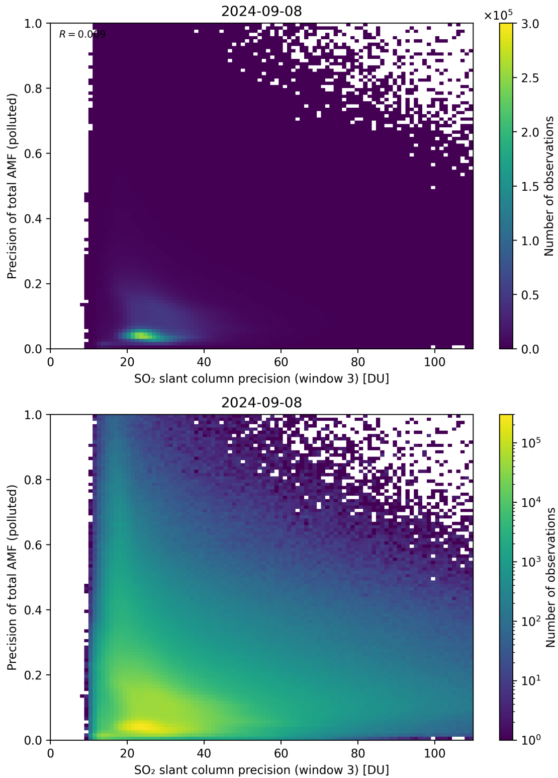
Figure 264: Scatter density plot of “SO 2 slant column precision (window 3)” against “Precision of total AMF (polluted)” for 2024-09-07 to 2024-09-09.
