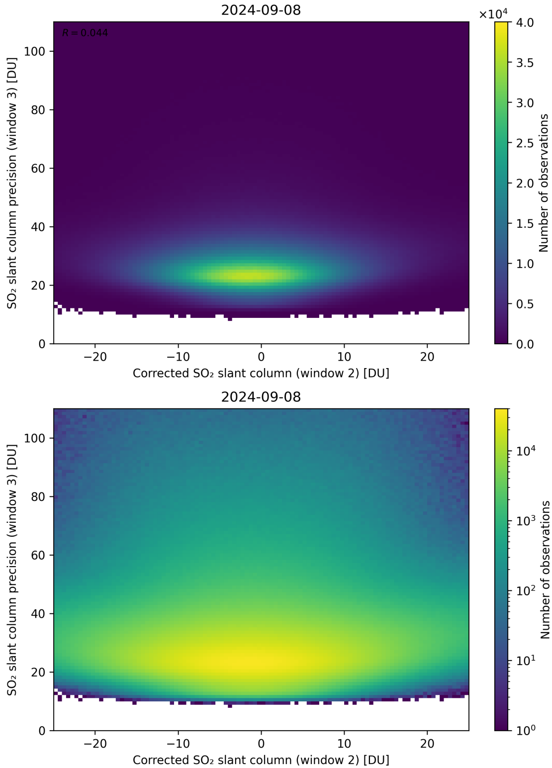
Figure 202: Scatter density plot of “Corrected SO 2 slant column (window 2)” against “SO 2 slant column precision (window 3)” for 2024-09-07 to 2024-09-09.
