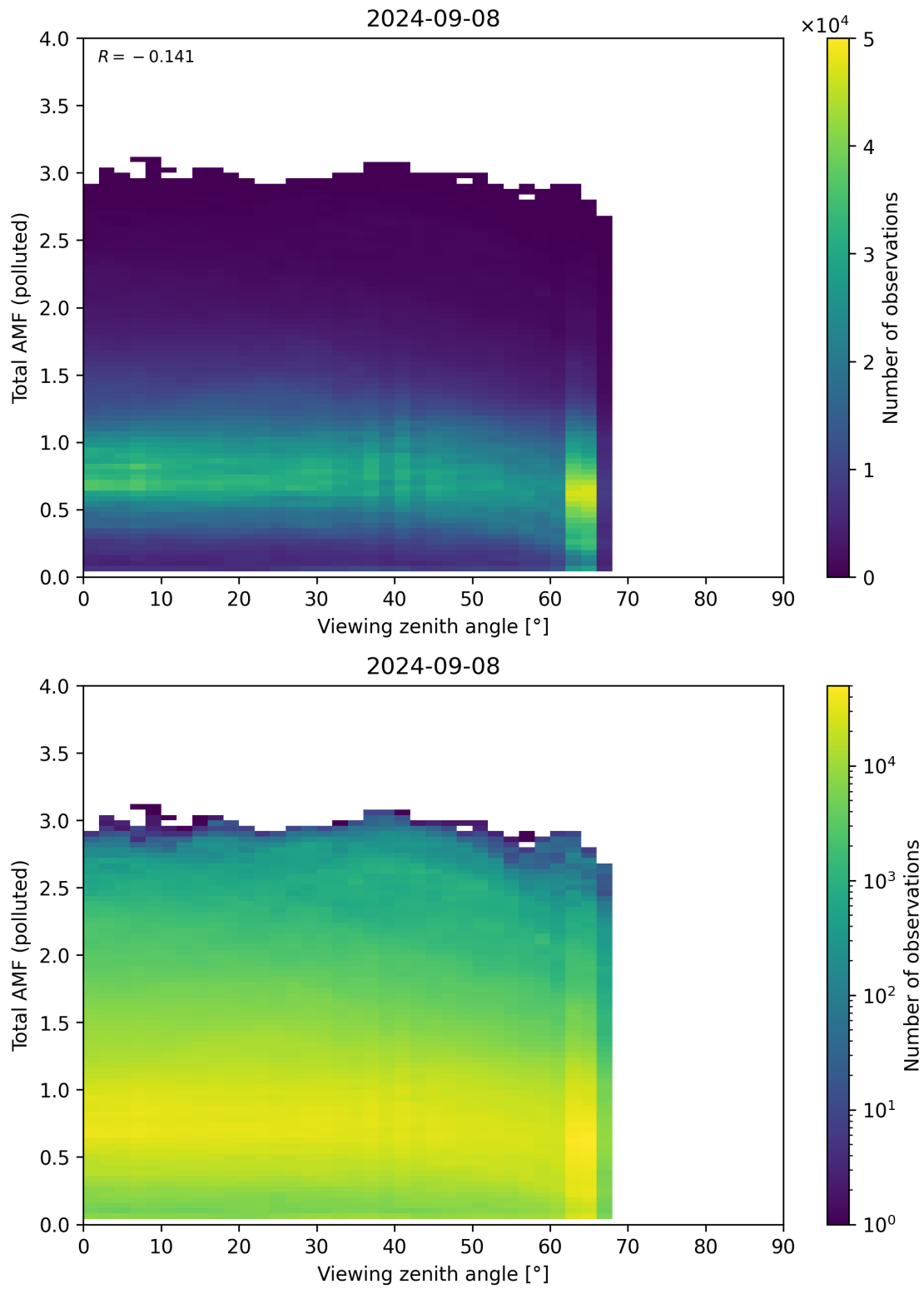
Figure 325: Scatter density plot of “Viewing zenith angle” against “Total AMF (polluted)” for 2024-09-07 to 2024-09-09.
