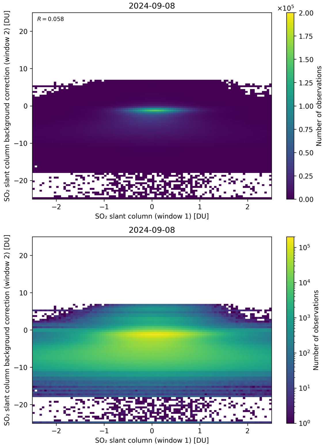
Figure 213: Scatter density plot of “SO 2 slant column (window 1)” against “SO 2 slant column background correction (window 2)” for 2024-09-07 to 2024-09-09.
