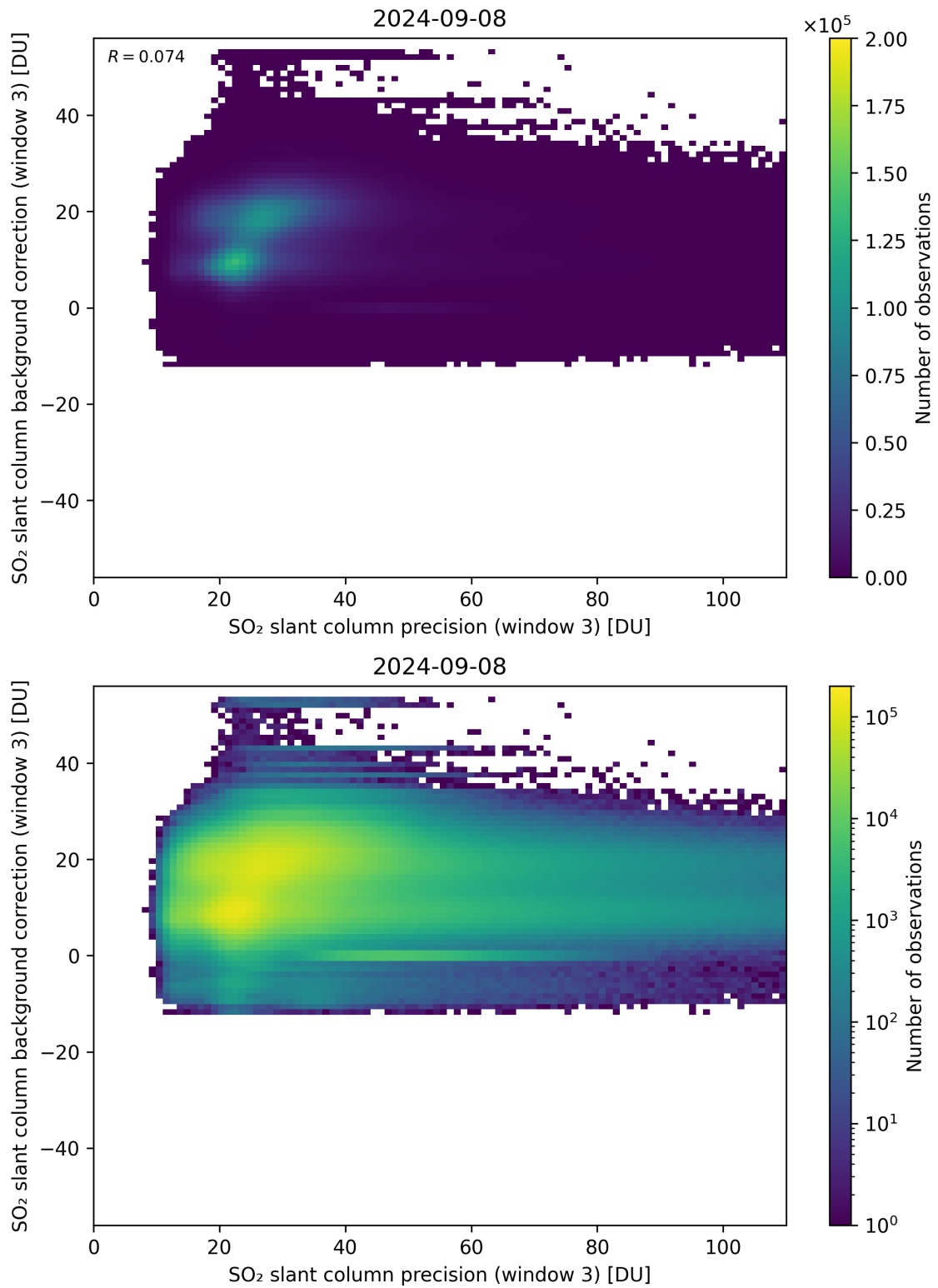
Figure 257: Scatter density plot of “SO 2 slant column precision (window 3)” against “SO 2 slant column background correction (window 3)” for 2024-09-07 to 2024-09-09.
