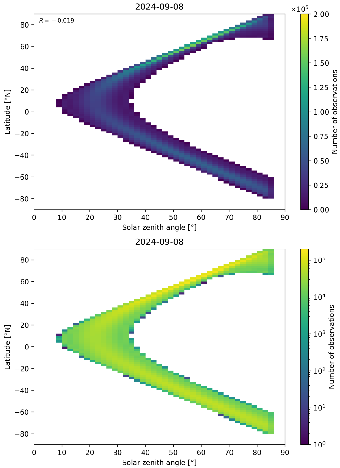
Figure 164: Scatter density plot of “Solar zenith angle” against “Latitude” for 2024-09-07 to 2024-09-09.
