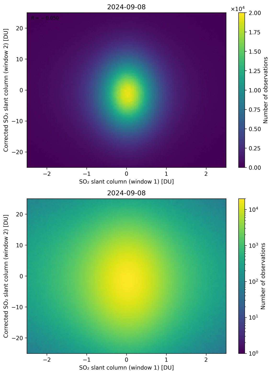
Figure 233: Scatter density plot of “SO 2 slant column (window 1)” against “Corrected SO 2 slant column (window 2)” for 2024-09-07 to 2024-09-09.
