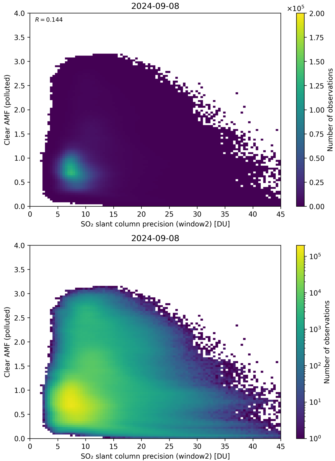
Figure 246: Scatter density plot of “SO 2 slant column precision (window2)” against “Clear AMF (polluted)” for 2024-09-07 to 2024-09-09.
