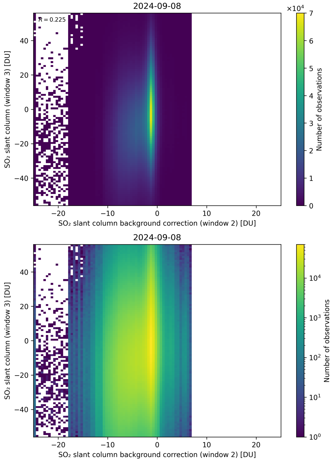
Figure 117: Scatter density plot of “SO 2 slant column background correction (window 2)” against “SO 2 slant column (window 3)” for 2024-09-07 to 2024-09-09.
