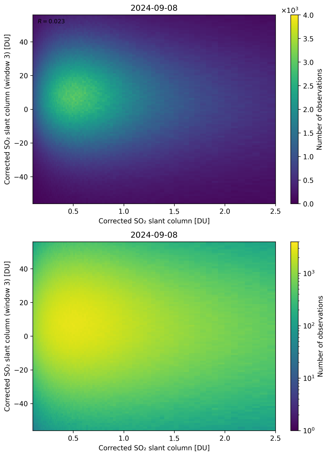
Figure 186: Scatter density plot of “Corrected SO 2 slant column” against “Corrected SO 2 slant column (window 3)” for 2024-09-07 to 2024-09-09.
