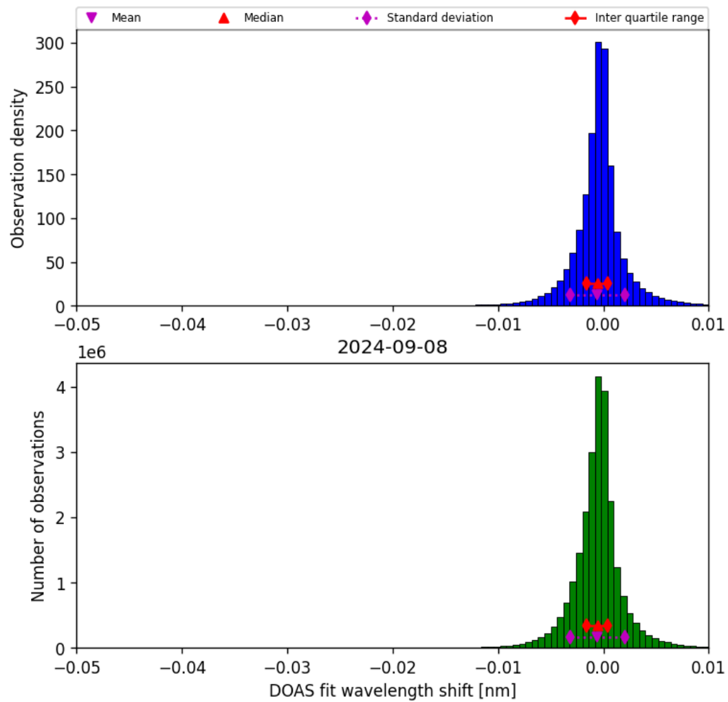
Figure 68: Histogram of “DOAS fit wavelength shift” for 2024-09-07 to 2024-09-09
