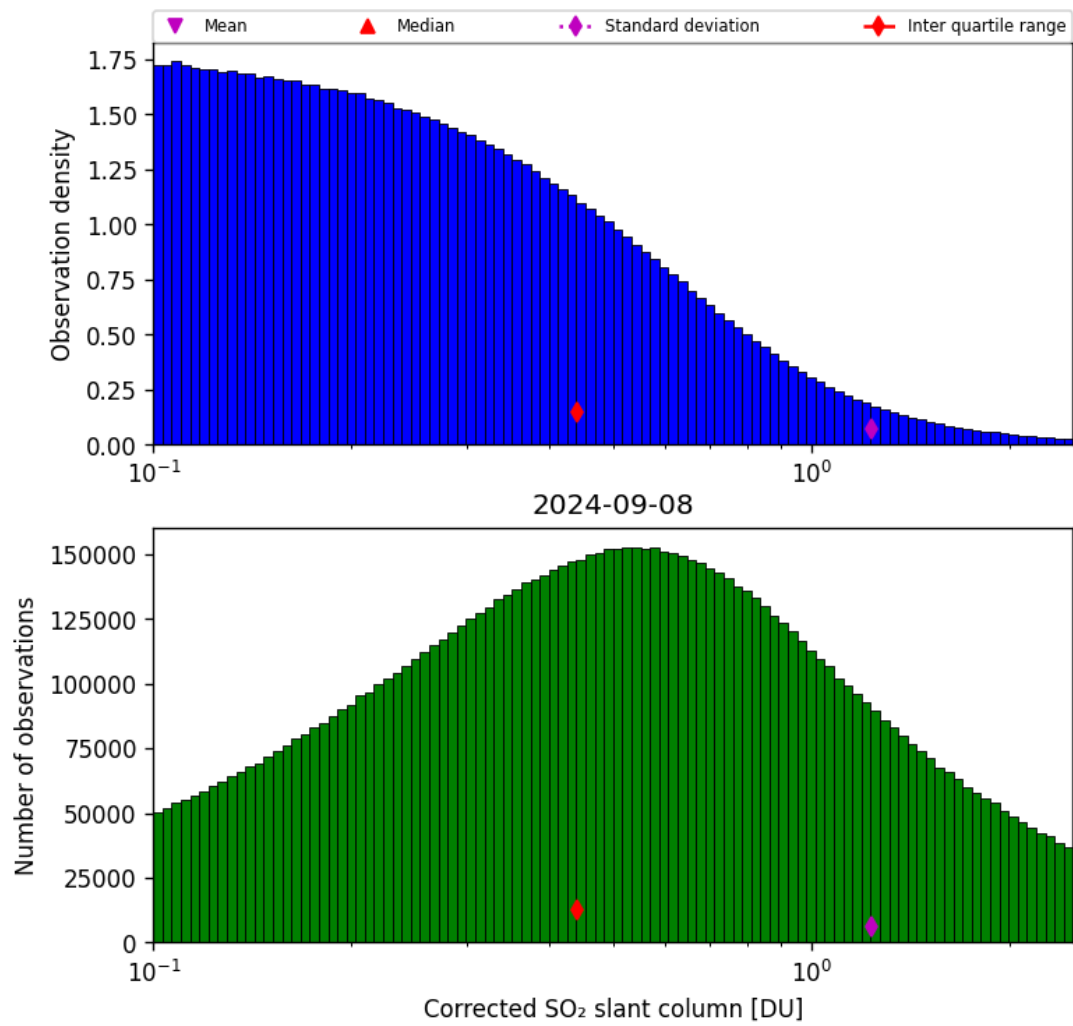
Figure 55: Histogram of “Corrected SO 2 slant column” for 2024-09-07 to 2024-09-09
