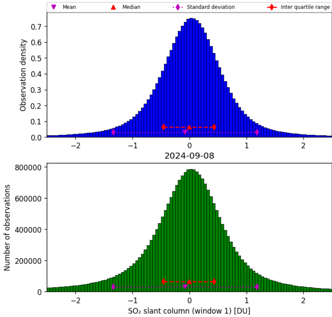
Figure 56: Histogram of “SO 2 slant column (window 1)” for 2024-09-07 to 2024-09-09
