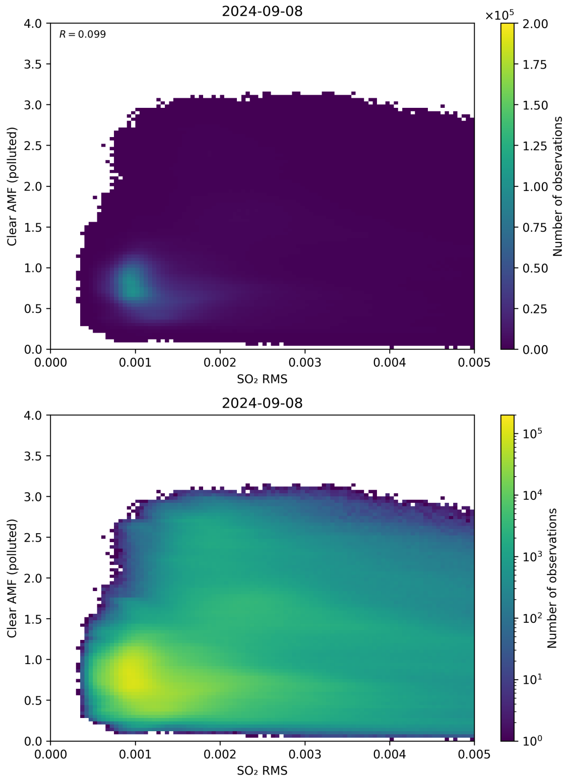
Figure 136: Scatter density plot of “SO 2 RMS” against “Clear AMF (polluted)” for 2024-09-07 to 2024-09-09.
