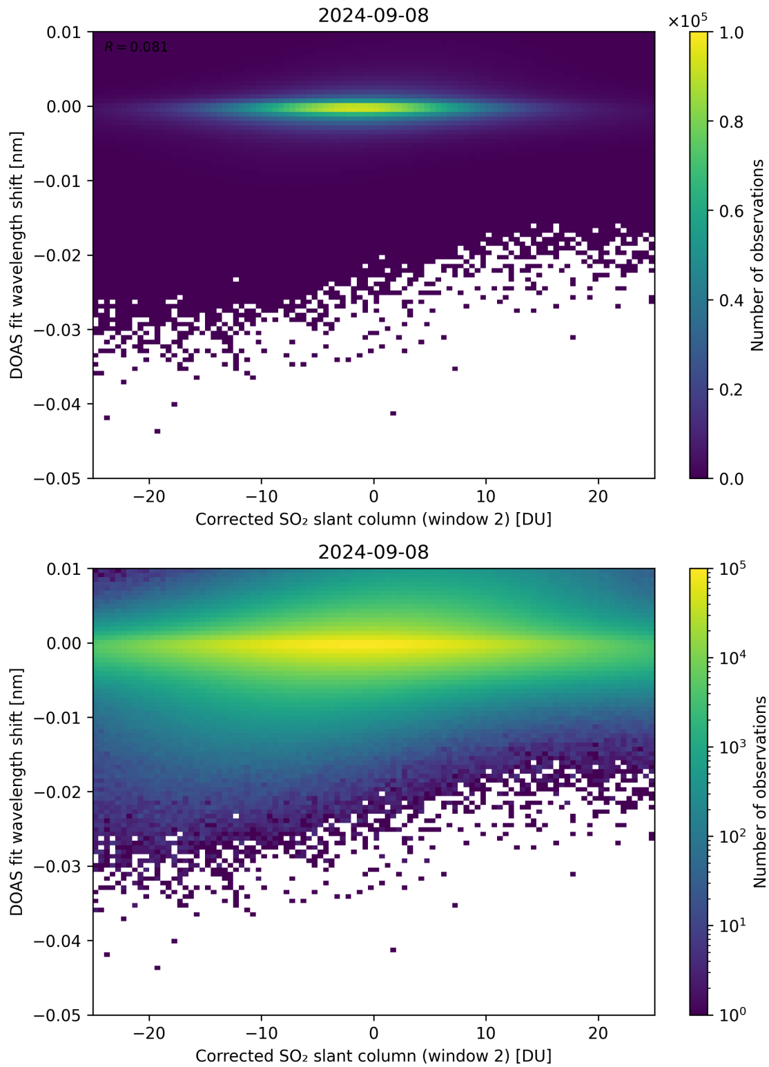
Figure 196: Scatter density plot of “Corrected SO 2 slant column (window 2)” against “DOAS fit wavelength shift” for 2024-09-07 to 2024-09-09.
