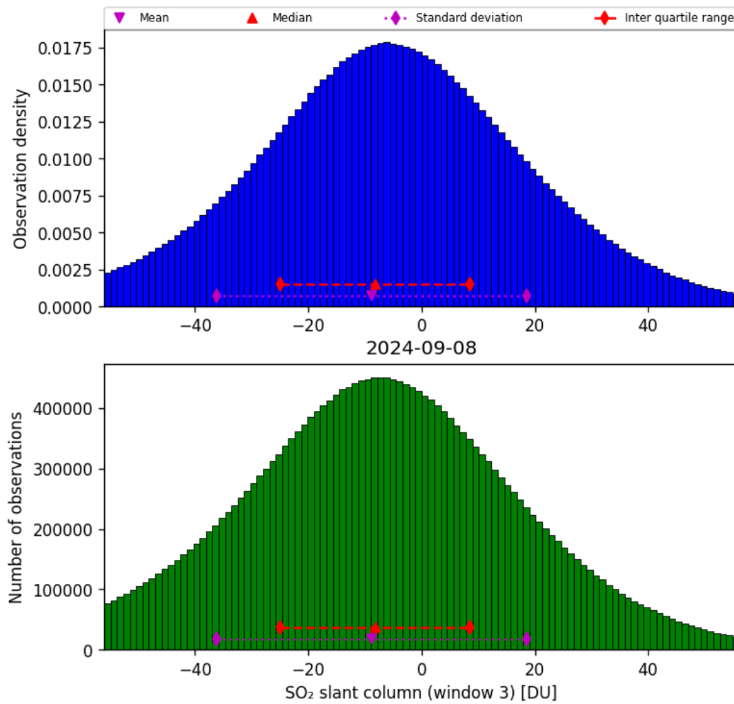
Figure 64: Histogram of “SO 2 slant column (window 3)” for 2024-09-07 to 2024-09-09
