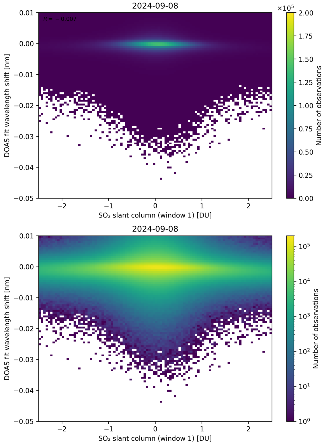
Figure 215: Scatter density plot of “SO 2 slant column (window 1)” against “DOAS fit wavelength shift” for 2024-09-07 to 2024-09-09.
