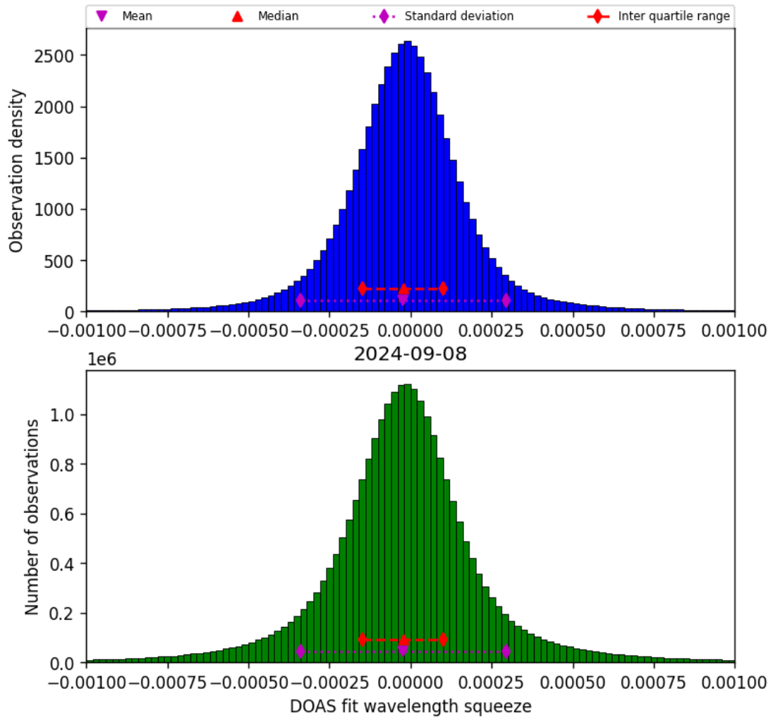
Figure 69: Histogram of “DOAS fit wavelength squeeze” for 2024-09-07 to 2024-09-09
