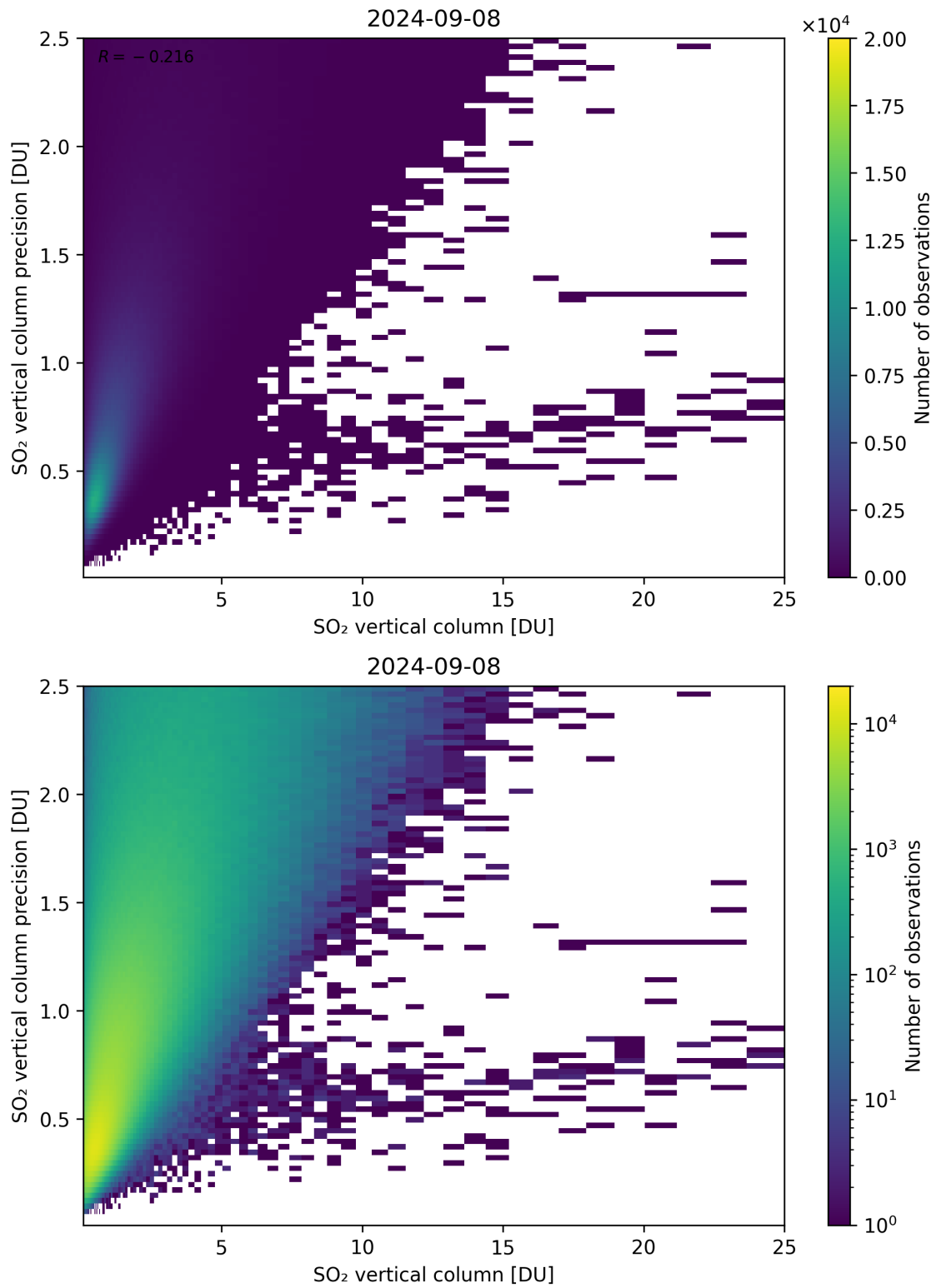
Figure 307: Scatter density plot of “SO 2 vertical column” against “SO 2 vertical column precision” for 2024-09-07 to 2024-09-09.
