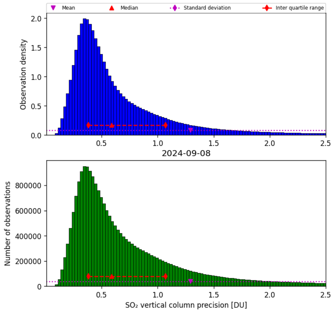
Figure 54: Histogram of “SO 2 vertical column precision” for 2024-09-07 to 2024-09-09
