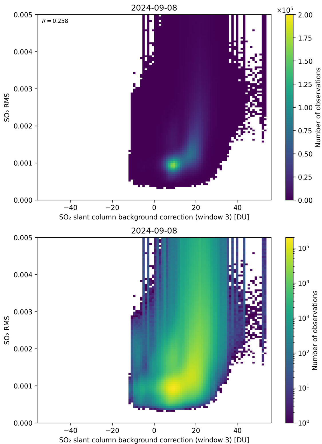
Figure 123: Scatter density plot of “SO 2 slant column background correction (window 3)” against “SO 2 RMS” for 2024-09-07 to 2024-09-09.
