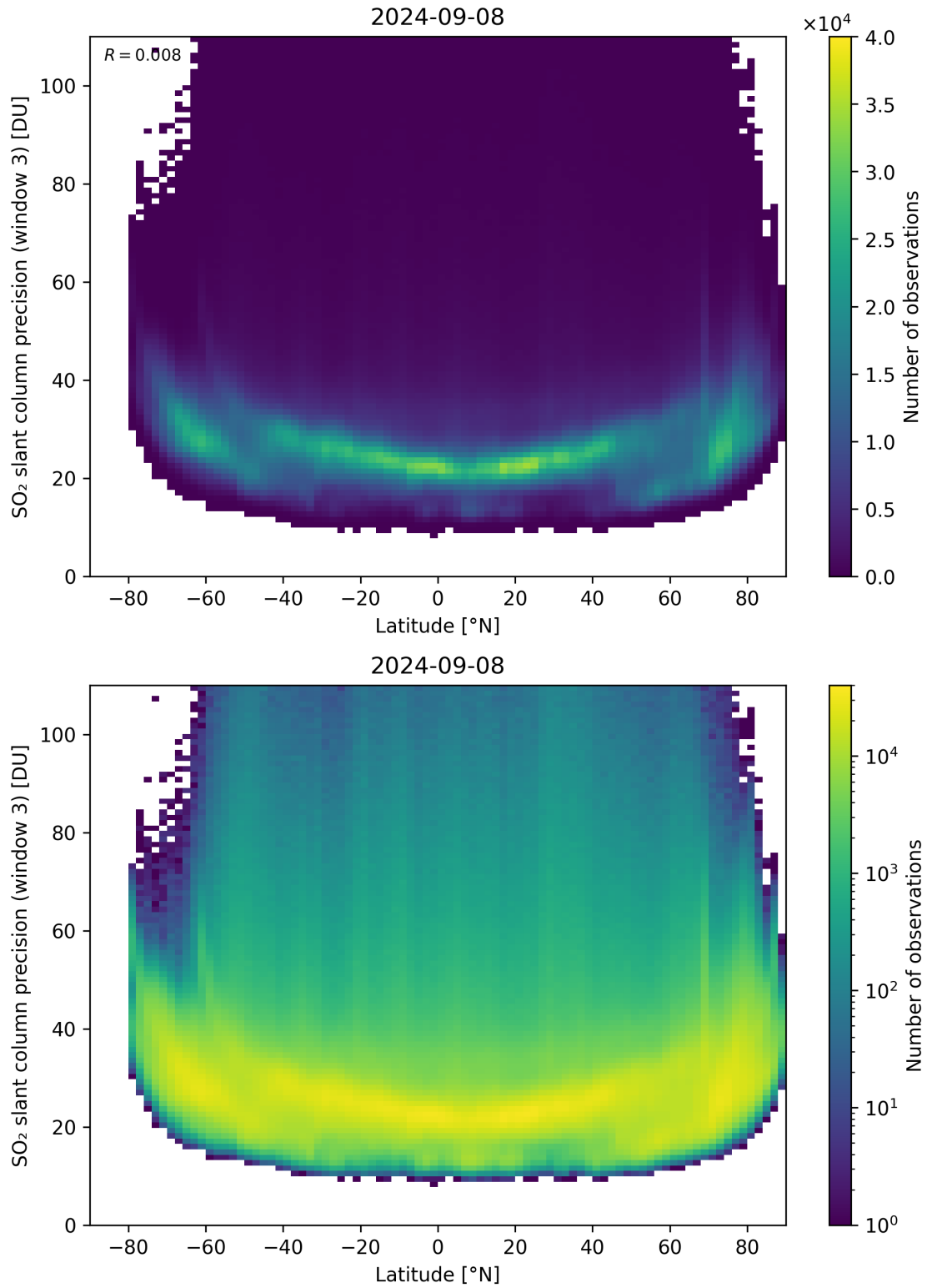
Figure 153: Scatter density plot of “Latitude” against “SO 2 slant column precision (window 3)” for 2024-09-07 to 2024-09-09.
