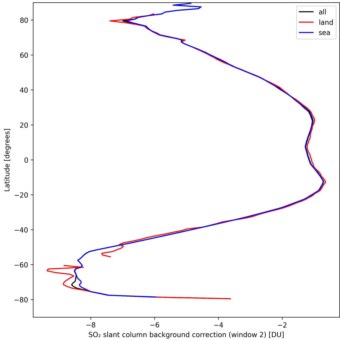
Figure 40: Zonal average of “SO 2 slant column background correction (window 2)” for 2024-09-07 to 2024-09-09.
