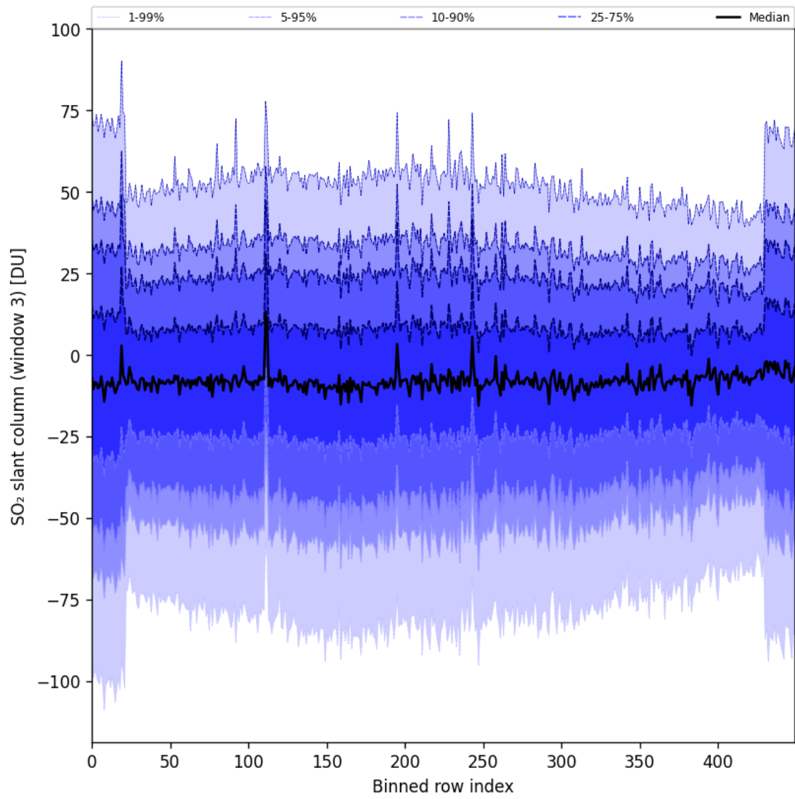
Figure 87: Along track statistics of “SO 2 slant column (window 3)” for 2024-09-07 to 2024-09-09
