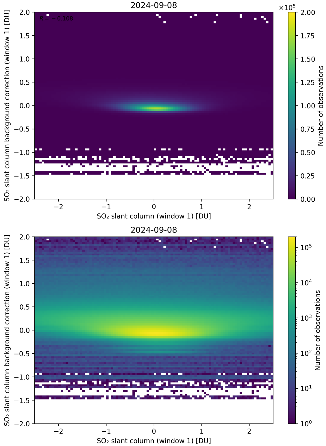
Figure 212: Scatter density plot of “SO 2 slant column (window 1)” against “SO 2 slant column background correction (window 1)” for 2024-09-07 to 2024-09-09.
