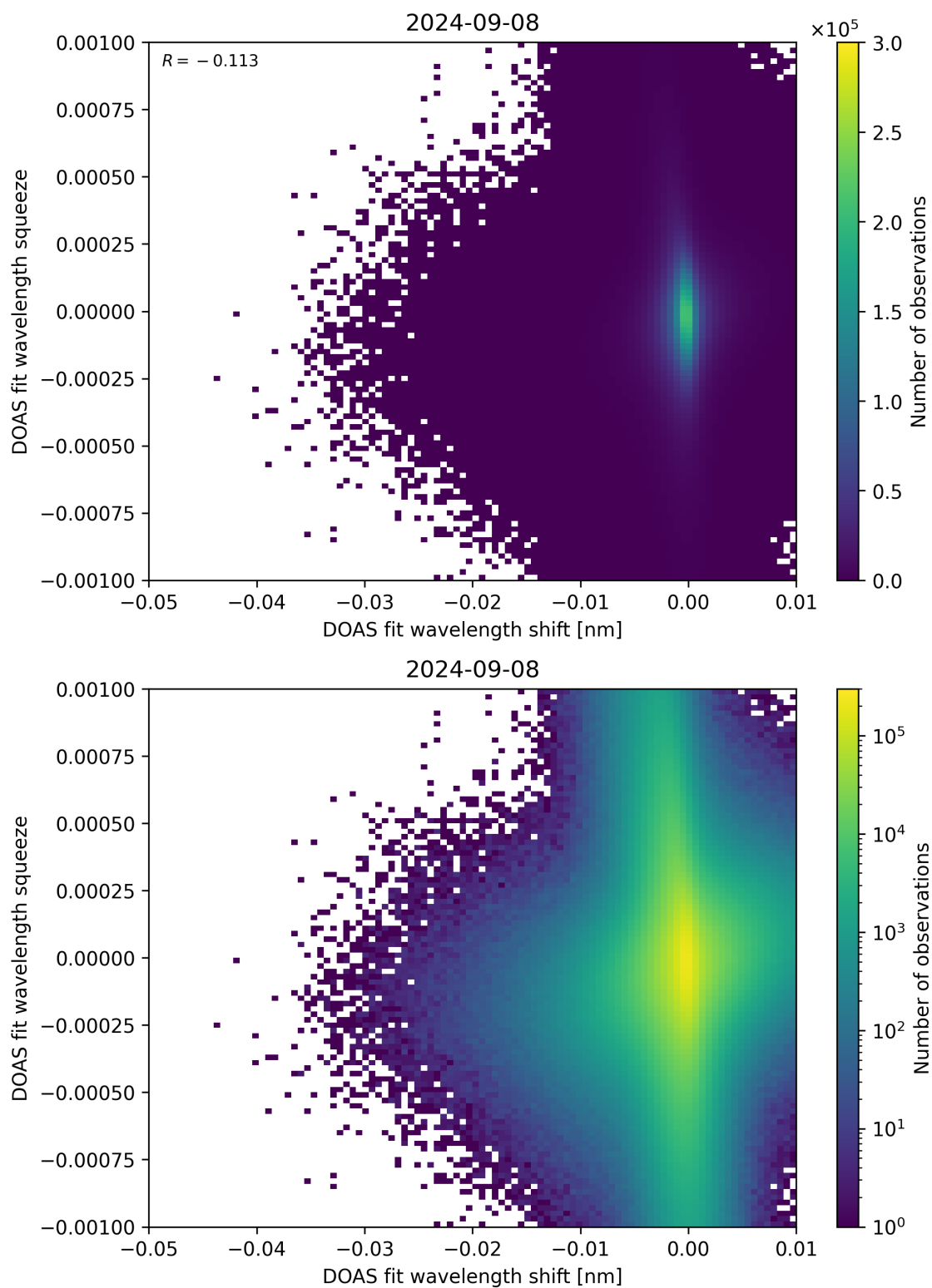
Figure 127: Scatter density plot of “DOAS fit wavelength shift” against “DOAS fit wavelength squeeze” for 2024-09-07 to 2024-09-09.
