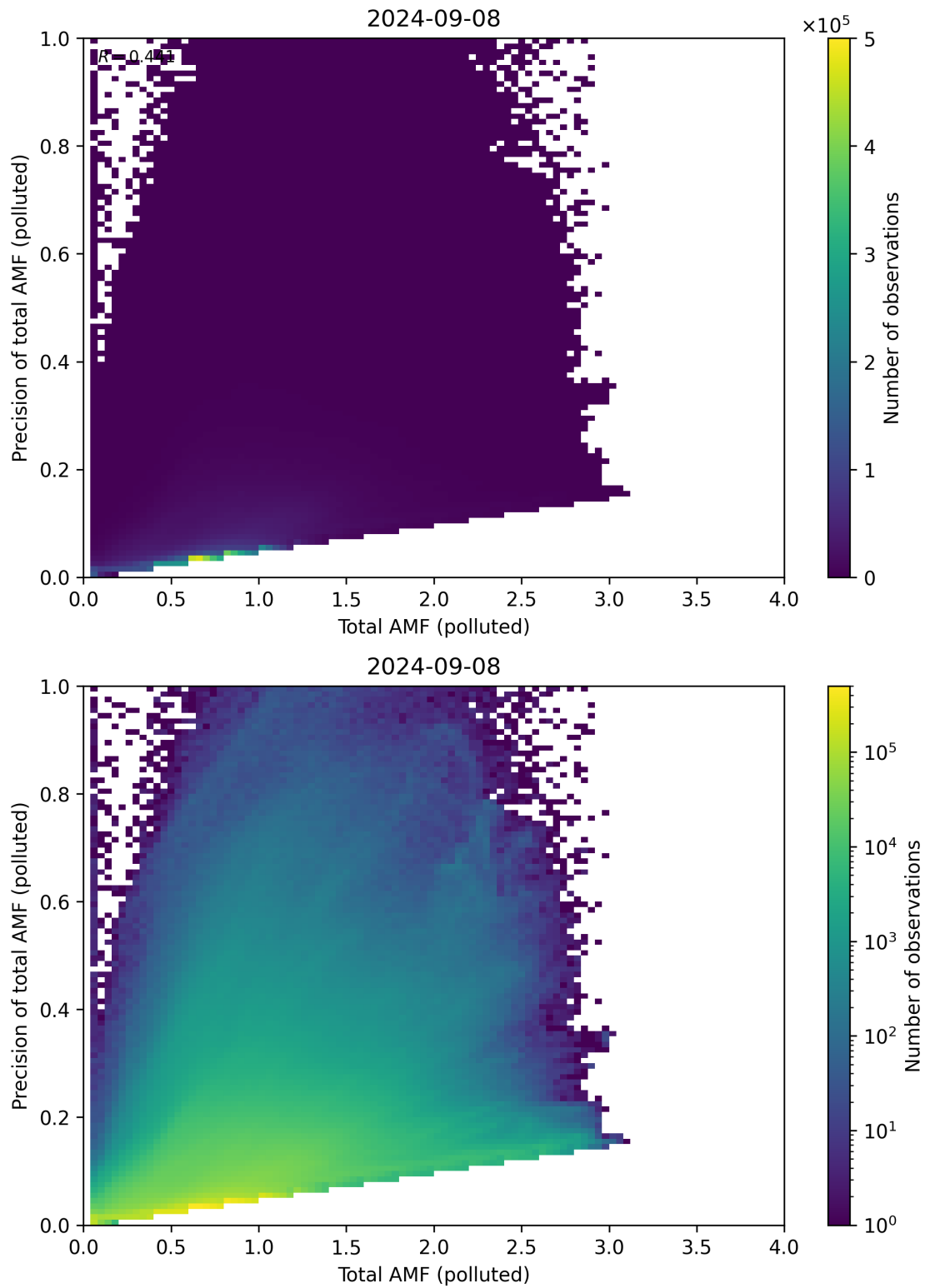
Figure 272: Scatter density plot of “Total AMF (polluted)” against “Precision of total AMF (polluted)” for 2024-09-07 to 2024-09-09.
