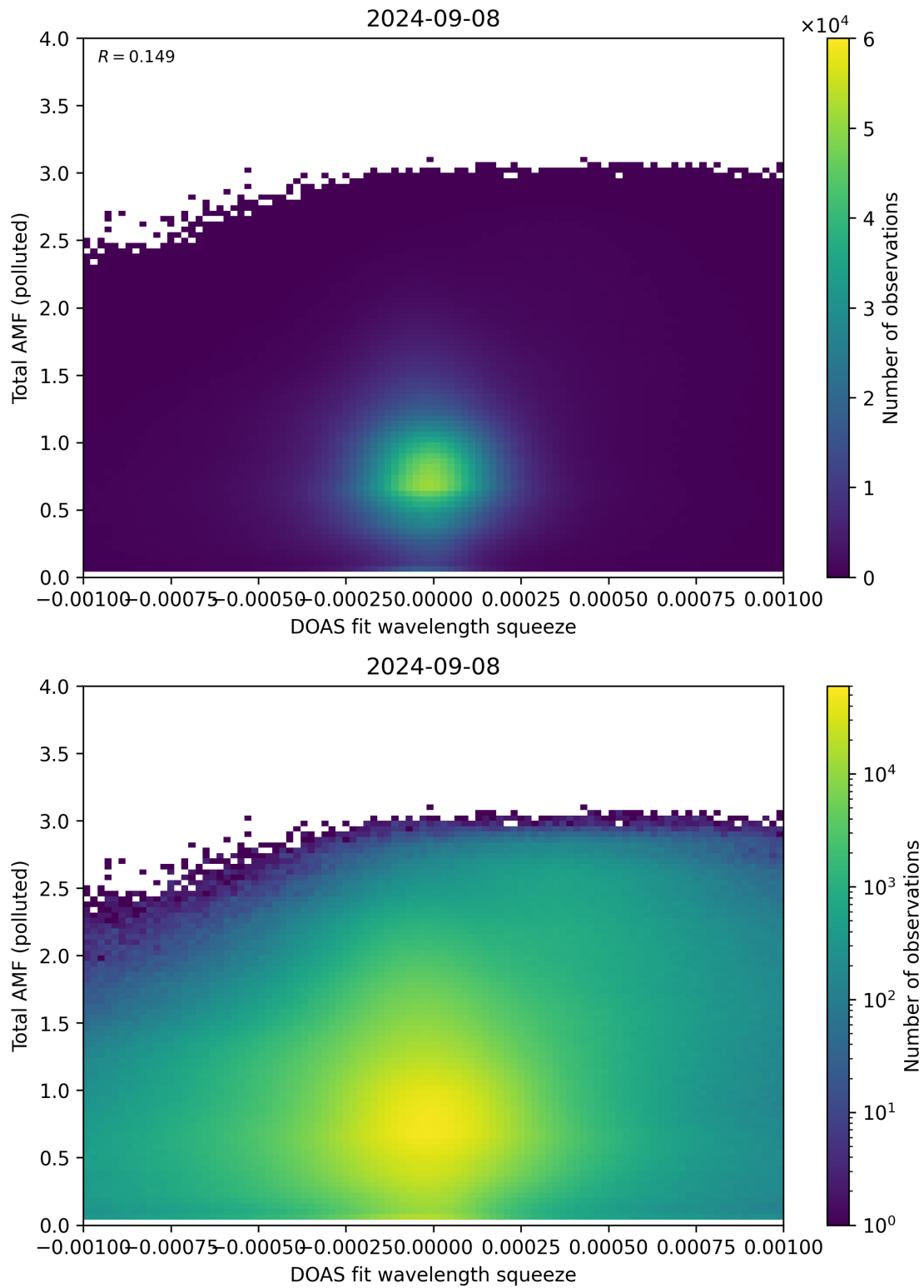
Figure 134: Scatter density plot of “DOAS fit wavelength squeeze” against “Total AMF (polluted)” for 2024-09-07 to 2024-09-09.
