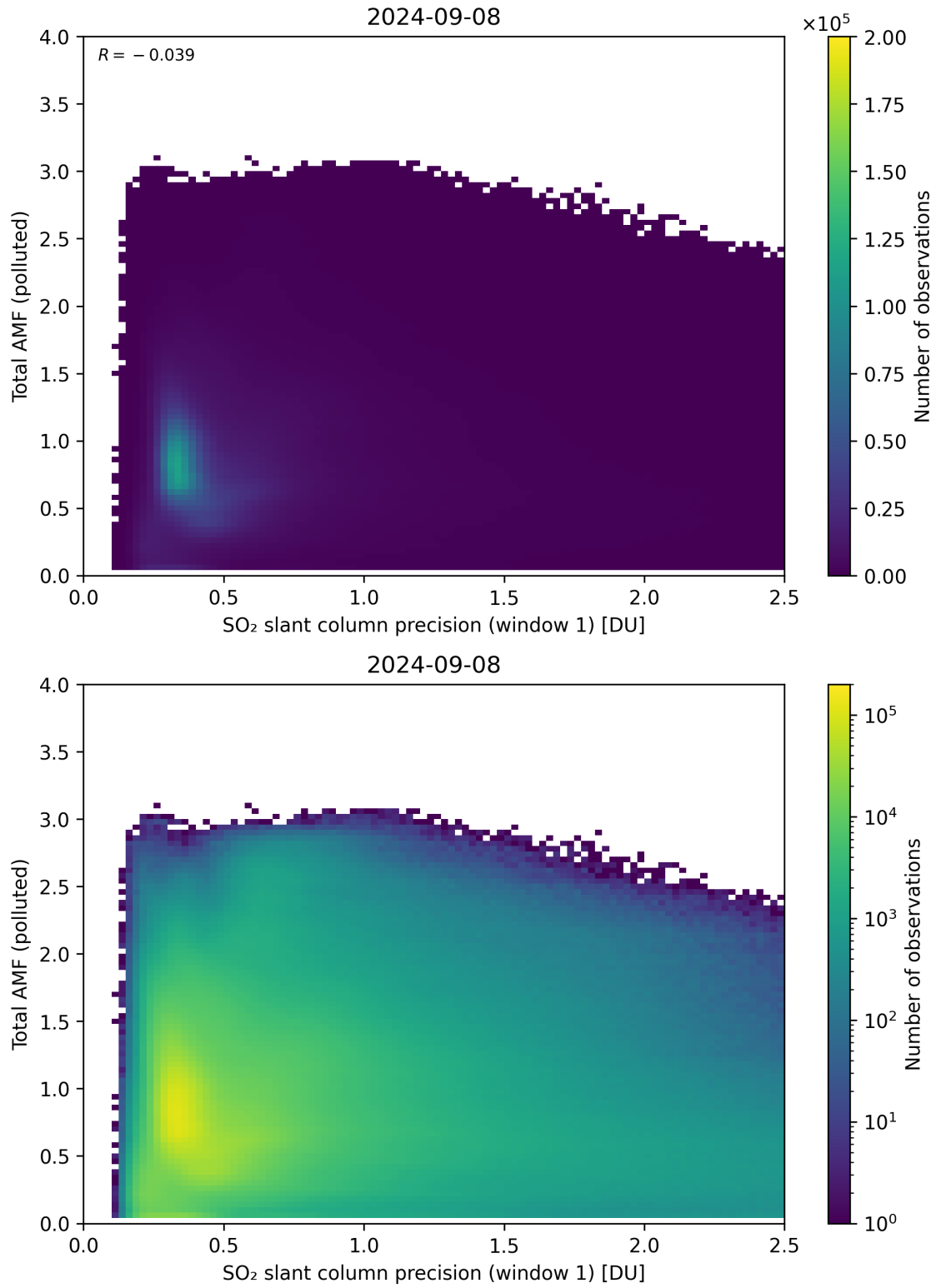
Figure 230: Scatter density plot of “SO 2 slant column precision (window 1)” against “Total AMF (polluted)” for 2024-09-07 to 2024-09-09.
