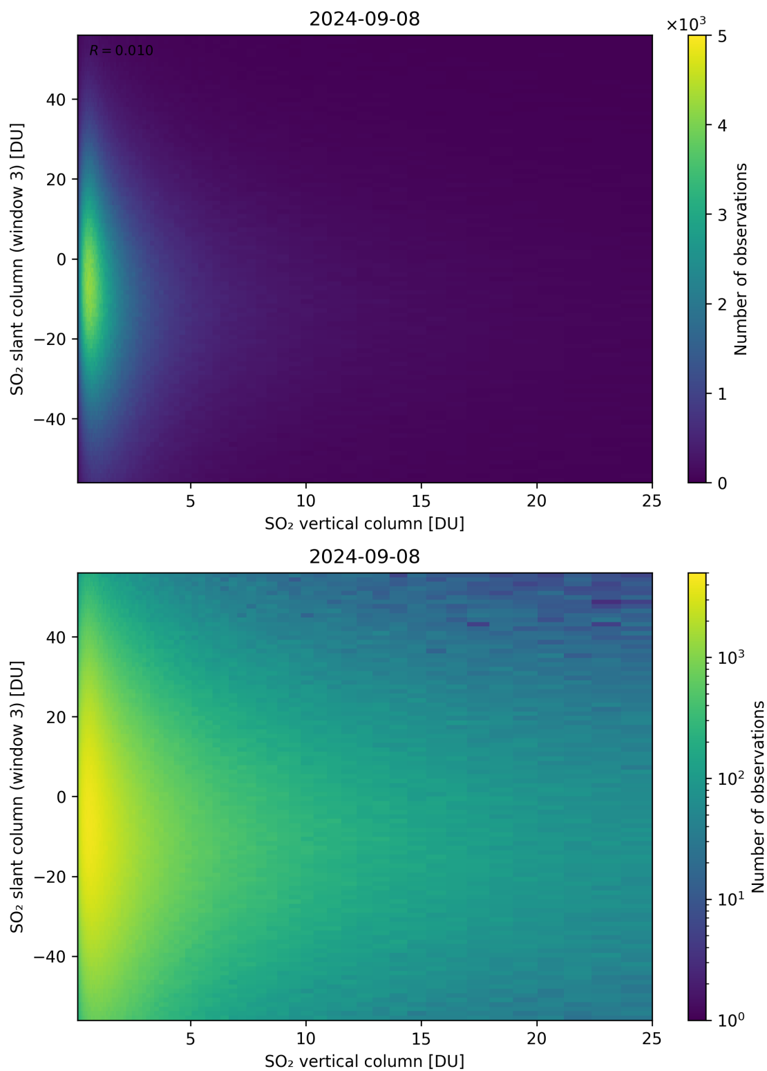
Figure 303: Scatter density plot of “SO 2 vertical column” against “SO 2 slant column (window 3)” for 2024-09-07 to 2024-09-09.
