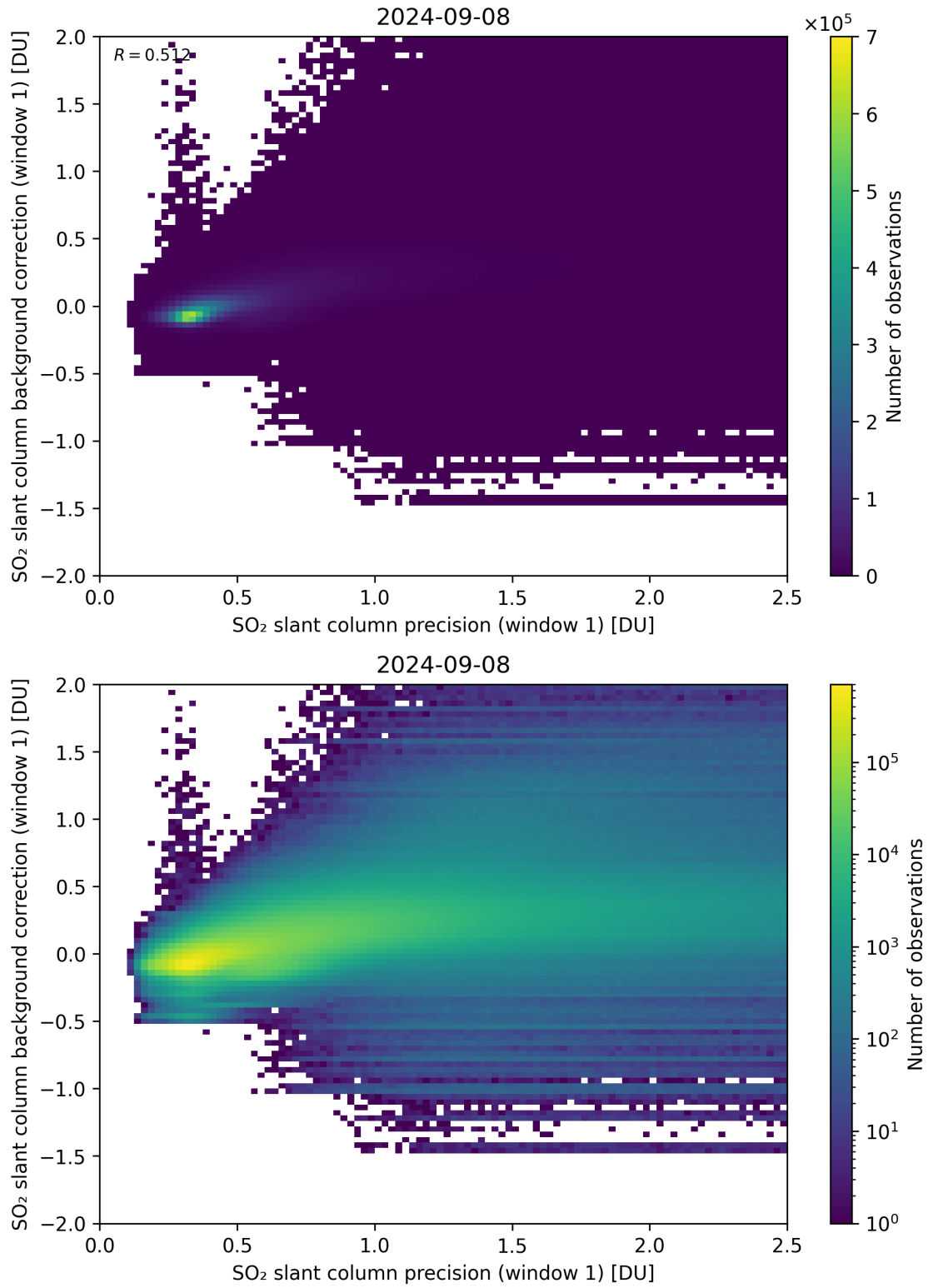
Figure 218: Scatter density plot of “SO 2 slant column precision (window 1)” against “SO 2 slant column background correction (window 1)” for 2024-09-07 to 2024-09-09.
