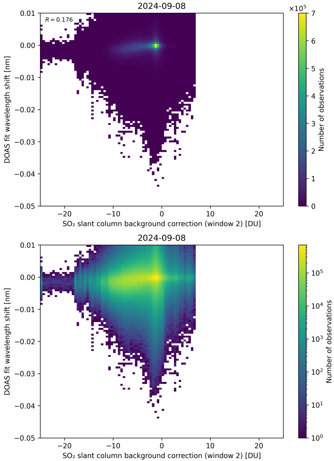
Figure 112: Scatter density plot of “SO 2 slant column background correction (window 2)” against “DOAS fit wavelength shift” for 2024-09-07 to 2024-09-09.
