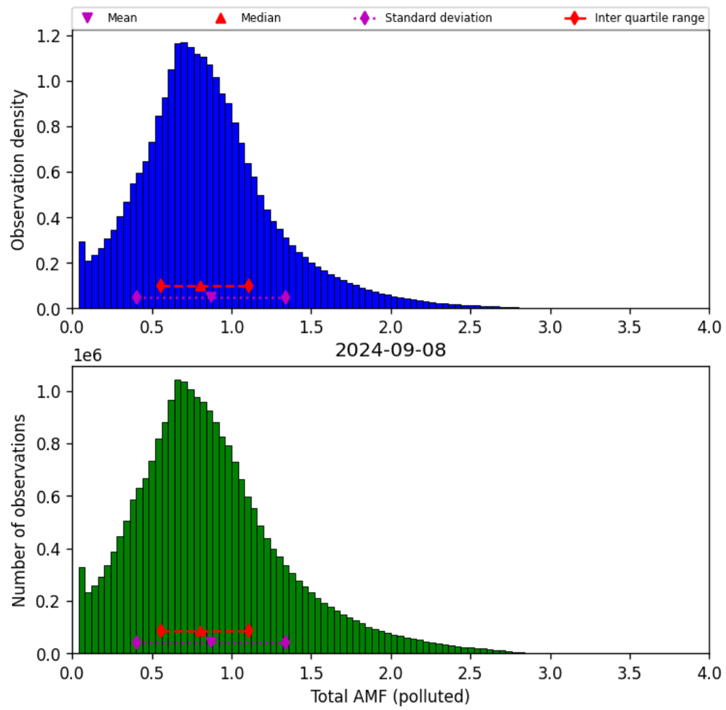
Figure 71: Histogram of “Total AMF (polluted)” for 2024-09-07 to 2024-09-09
