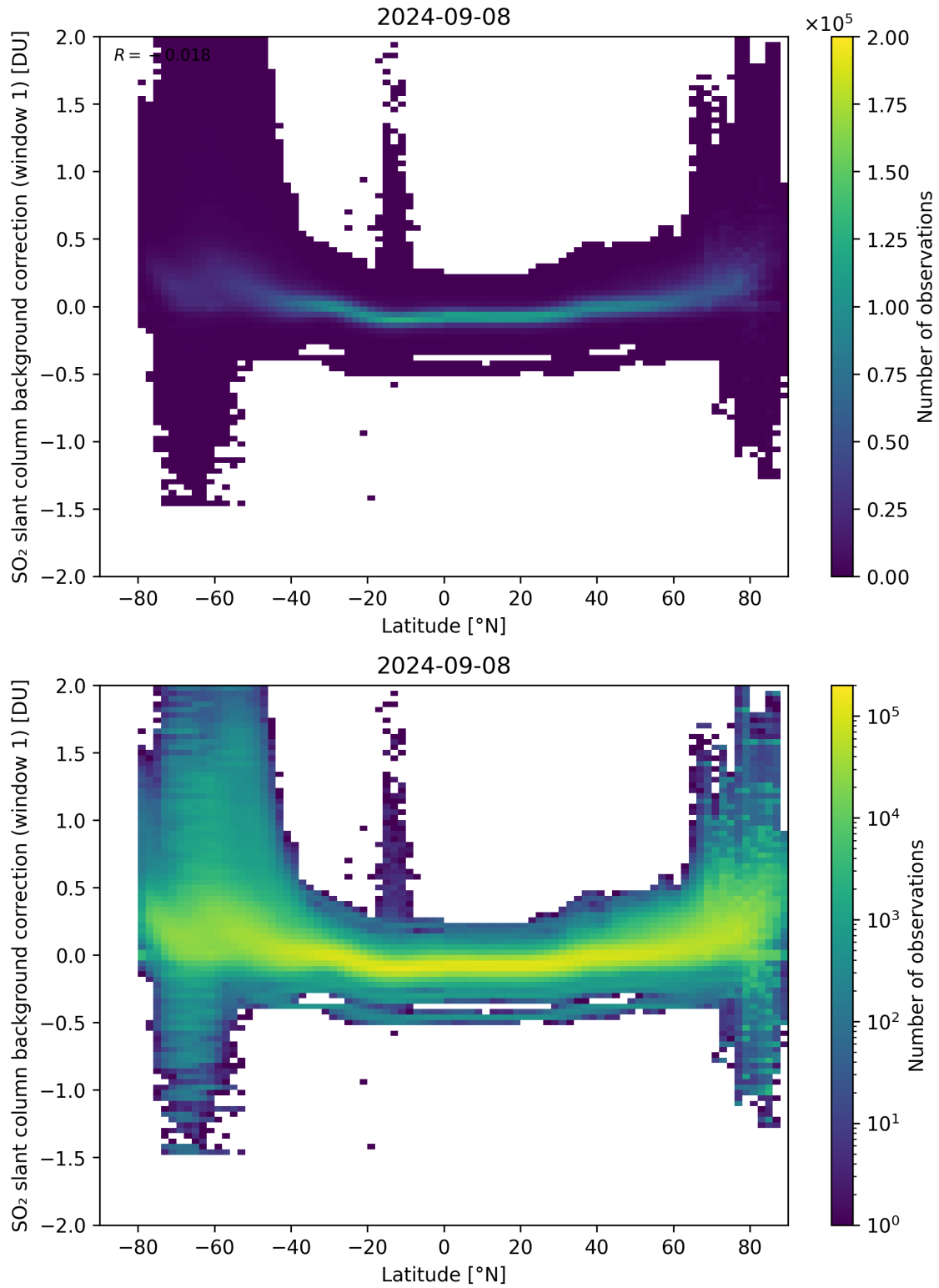
Figure 139: Scatter density plot of “Latitude” against “SO 2 slant column background correction (window 1)” for 2024-09-07 to 2024-09-09.
