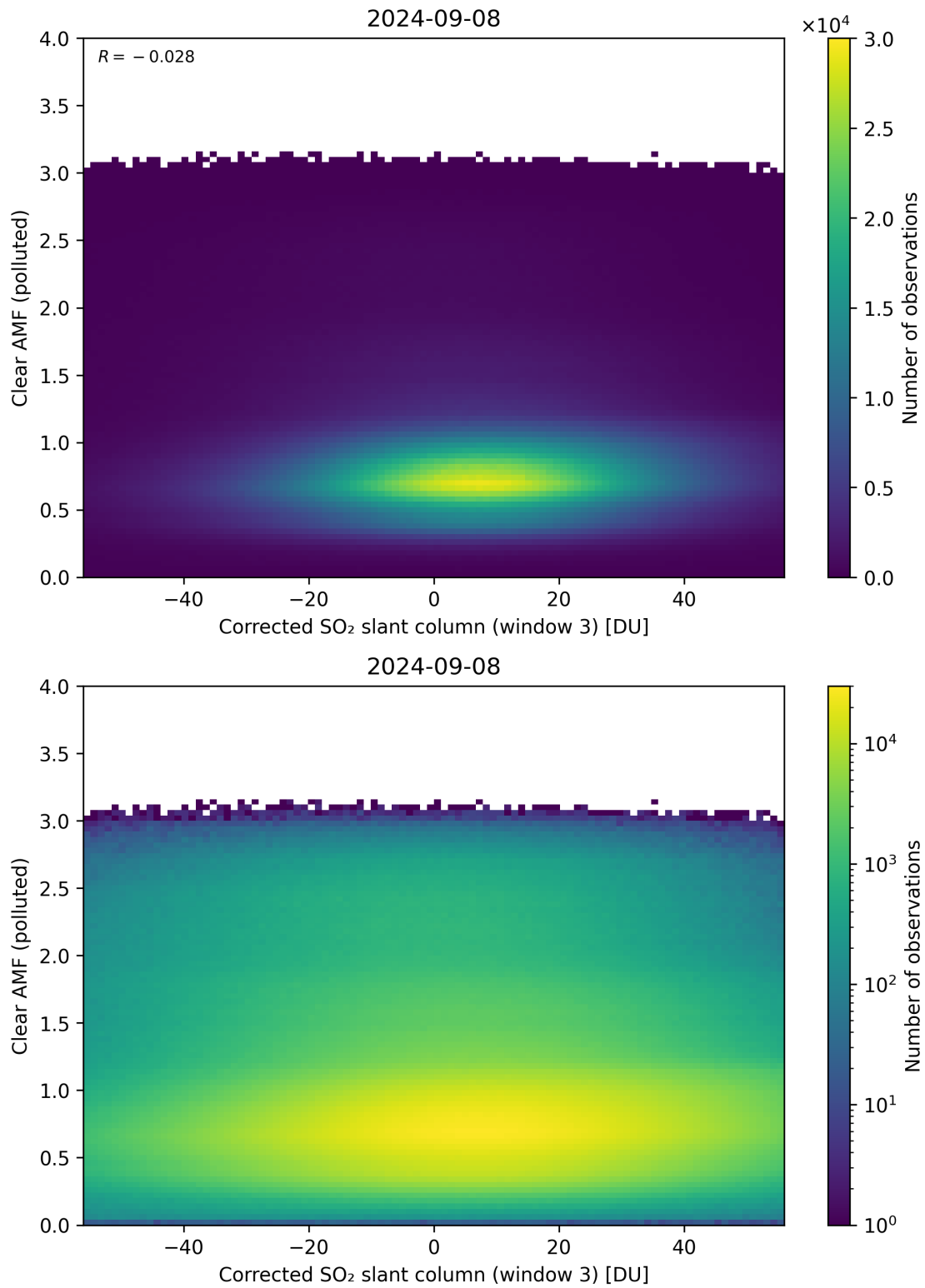
Figure 209: Scatter density plot of “Corrected SO 2 slant column (window 3)” against “Clear AMF (polluted)” for 2024-09-07 to 2024-09-09.
