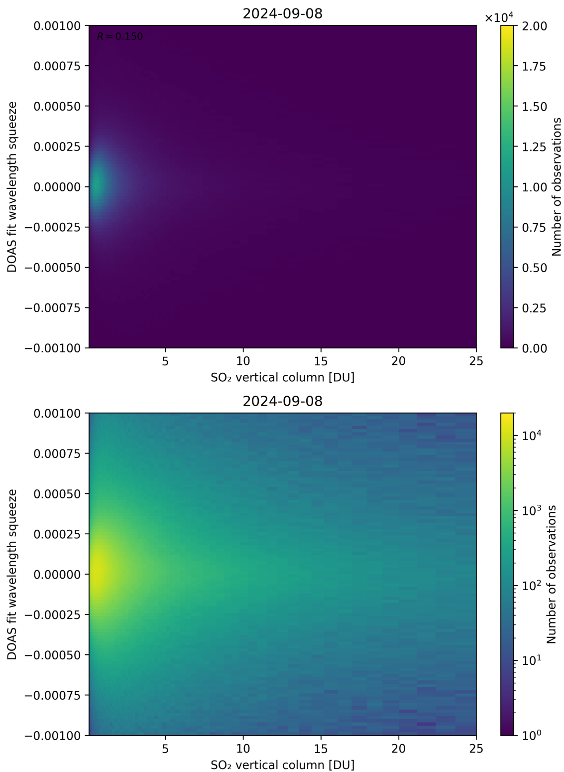
Figure 277: Scatter density plot of “SO 2 vertical column” against “DOAS fit wavelength squeeze” for 2024-09-07 to 2024-09-09.
