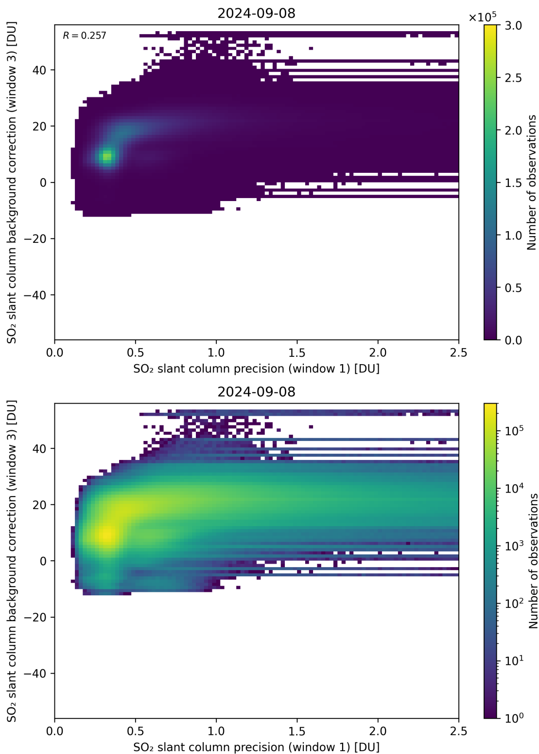
Figure 220: Scatter density plot of “SO 2 slant column precision (window 1)” against “SO 2 slant column background correction (window 3)” for 2024-09-07 to 2024-09-09.
