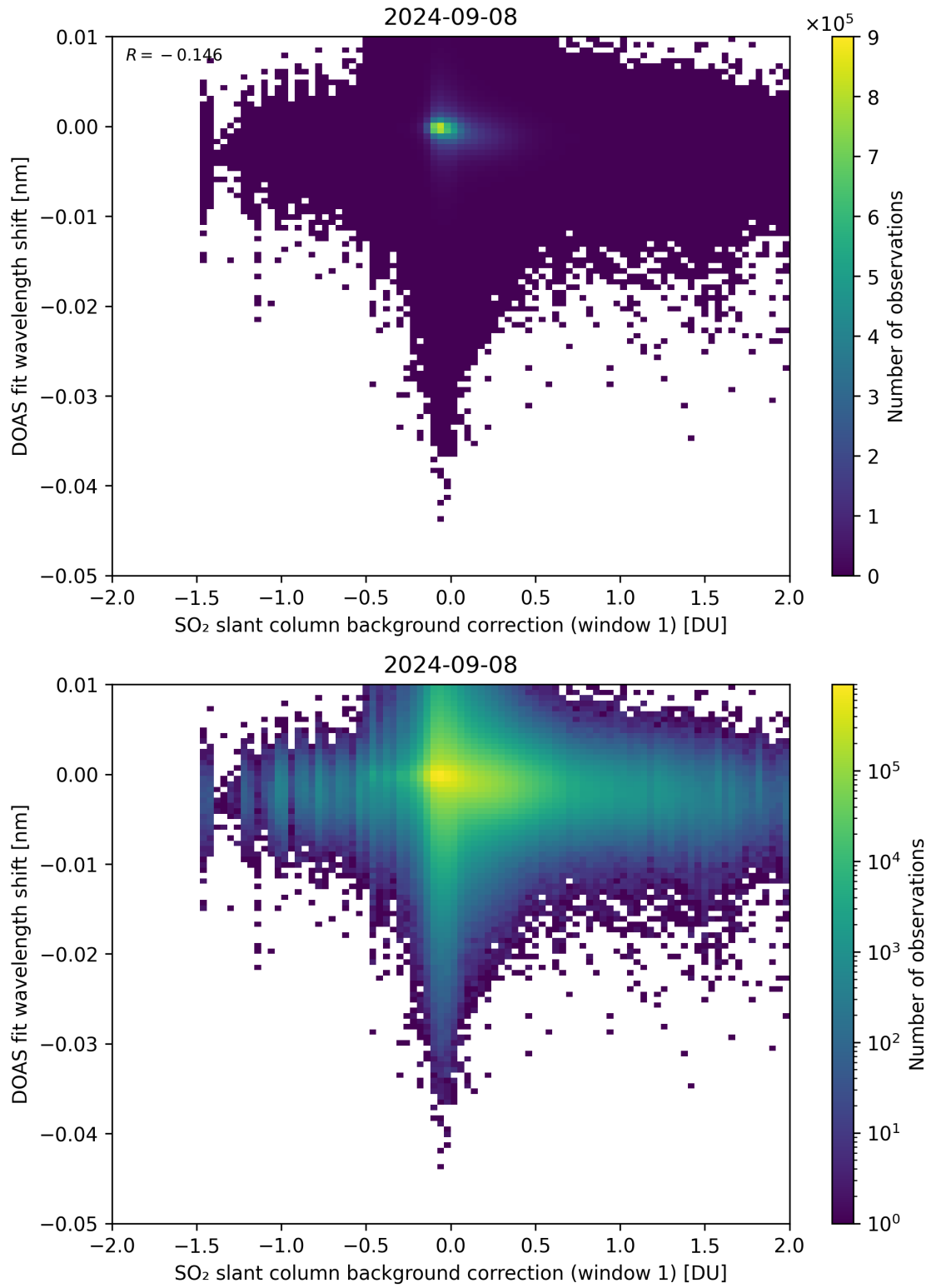
Figure 100: Scatter density plot of “SO 2 slant column background correction (window 1)” against “DOAS fit wavelength shift” for 2024-09-07 to 2024-09-09.
