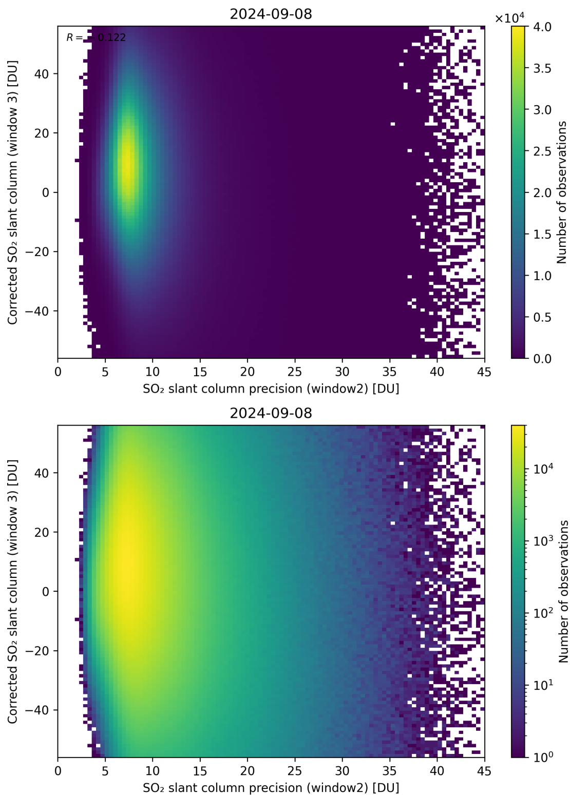
Figure 248: Scatter density plot of “SO 2 slant column precision (window2)” against “Corrected SO 2 slant column (window 3)” for 2024-09-07 to 2024-09-09.
