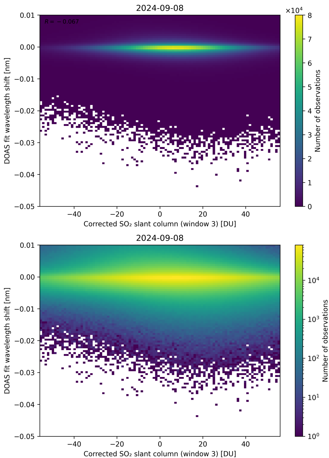
Figure 206: Scatter density plot of “Corrected SO 2 slant column (window 3)” against “DOAS fit wavelength shift” for 2024-09-07 to 2024-09-09.
