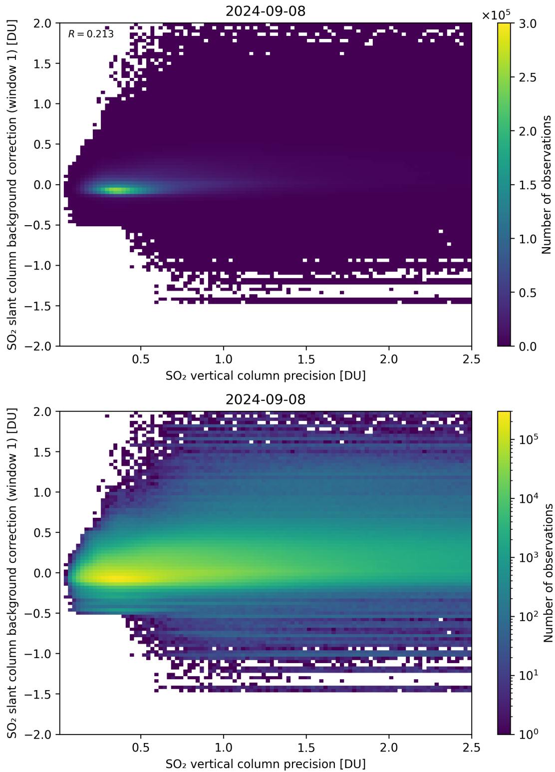
Figure 279: Scatter density plot of “SO 2 vertical column precision” against “SO 2 slant column background correction (window 1)” for 2024-09-07 to 2024-09-09.
