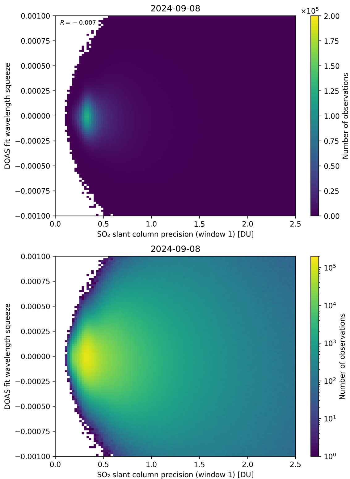
Figure 222: Scatter density plot of “SO 2 slant column precision (window 1)” against “DOAS fit wavelength squeeze” for 2024-09-07 to 2024-09-09.
