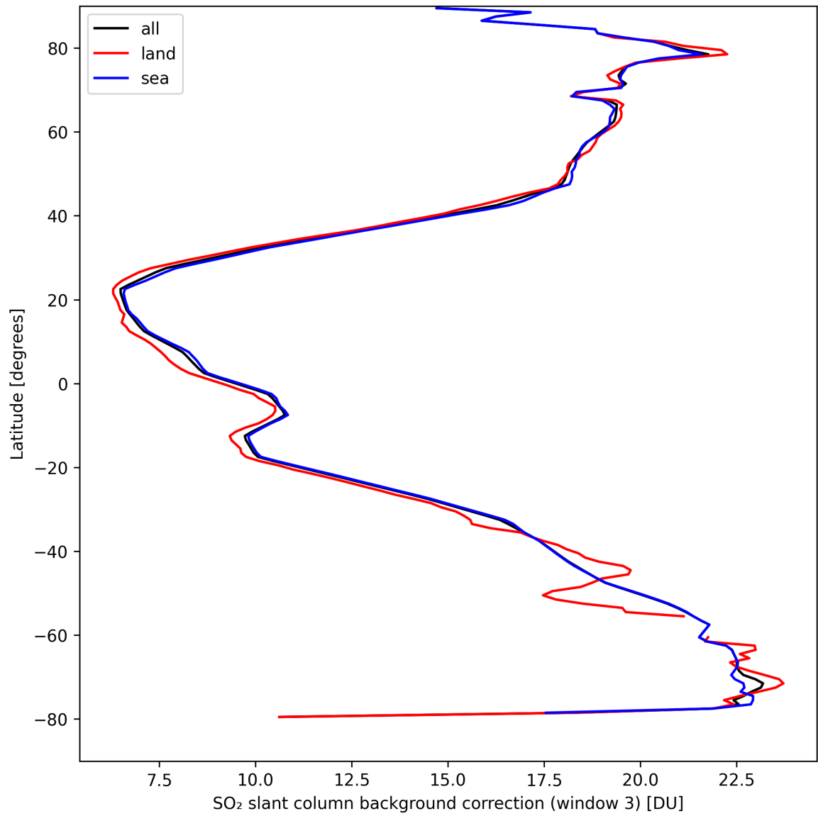
Figure 44: Zonal average of "SO 2 slant column background correction (window 3)" for 2024-09-07 to 2024-09-09.
