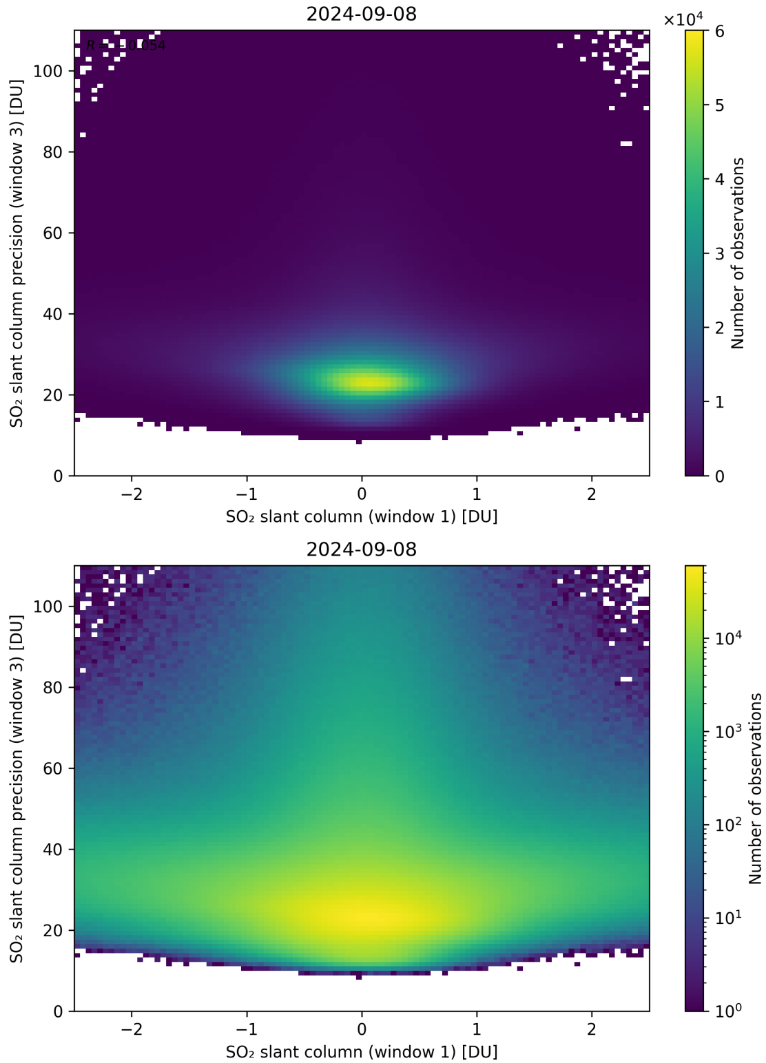
Figure 238: Scatter density plot of “SO 2 slant column (window 1)” against “SO 2 slant column precision (window 3)” for 2024-09-07 to 2024-09-09.
