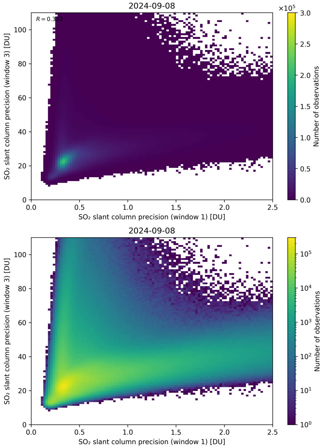
Figure 229: Scatter density plot of “SO 2 slant column precision (window 1)” against “SO 2 slant column precision (window 3)” for 2024-09-07 to 2024-09-09.
