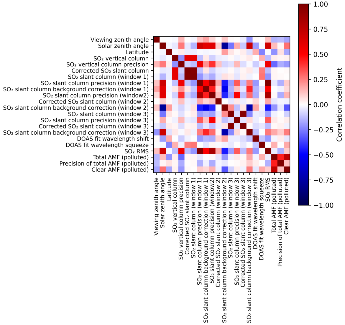
Figure 2: Map of correlation matrix for 2024-09-07 to 2024-09-09.
