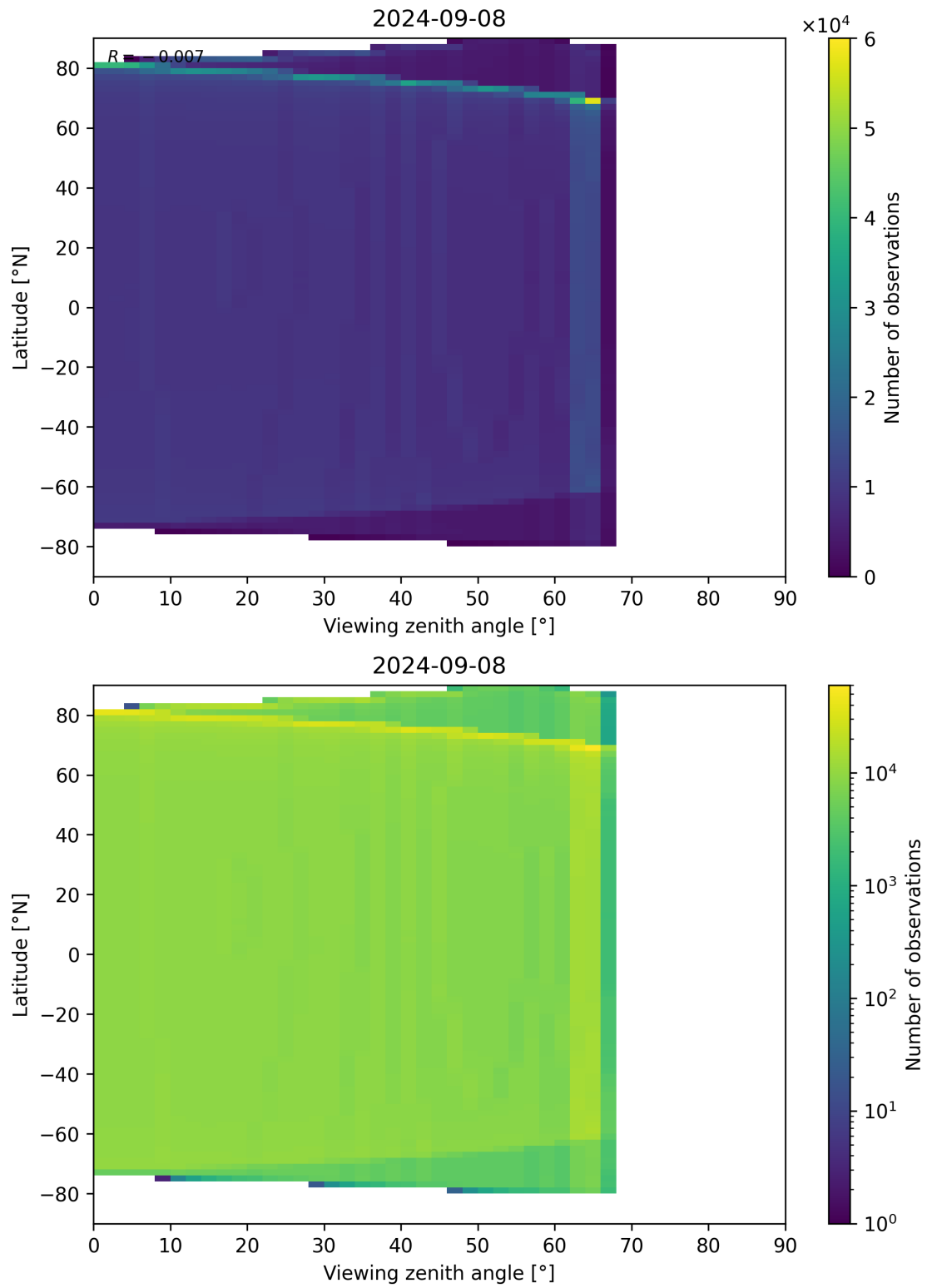
Figure 314: Scatter density plot of “Viewing zenith angle” against “Latitude” for 2024-09-07 to 2024-09-09.
