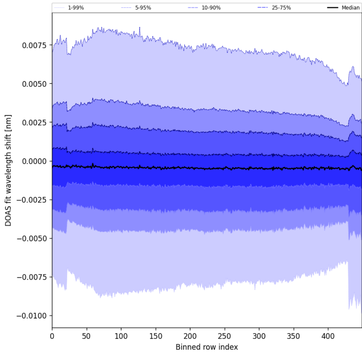
Figure 91: Along track statistics of “DOAS fit wavelength shift” for 2024-09-07 to 2024-09-09
