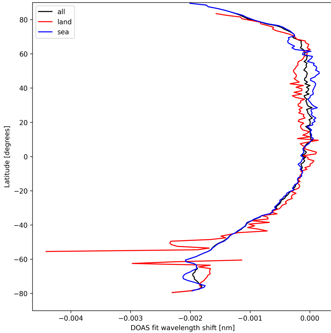
Figure 45: Zonal average of “DOAS fit wavelength shift” for 2024-09-07 to 2024-09-09.
