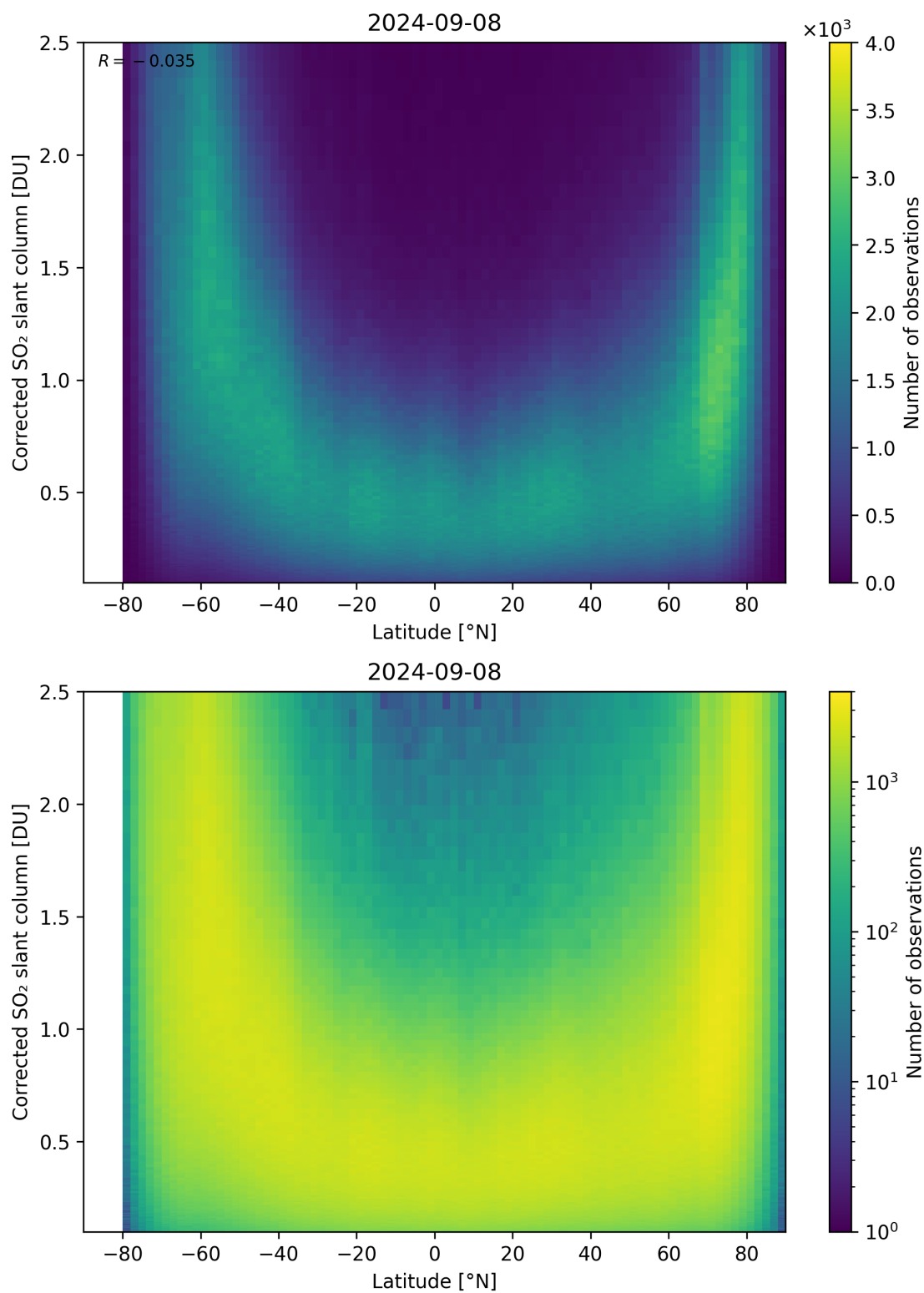
Figure 146: Scatter density plot of “Latitude” against “Corrected SO 2 slant column” for 2024-09-07 to 2024-09-09.
