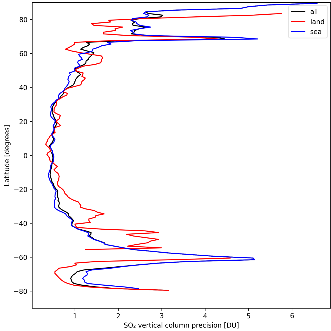
Figure 31: Zonal average of “SO 2 vertical column precision” for 2024-09-07 to 2024-09-09.
