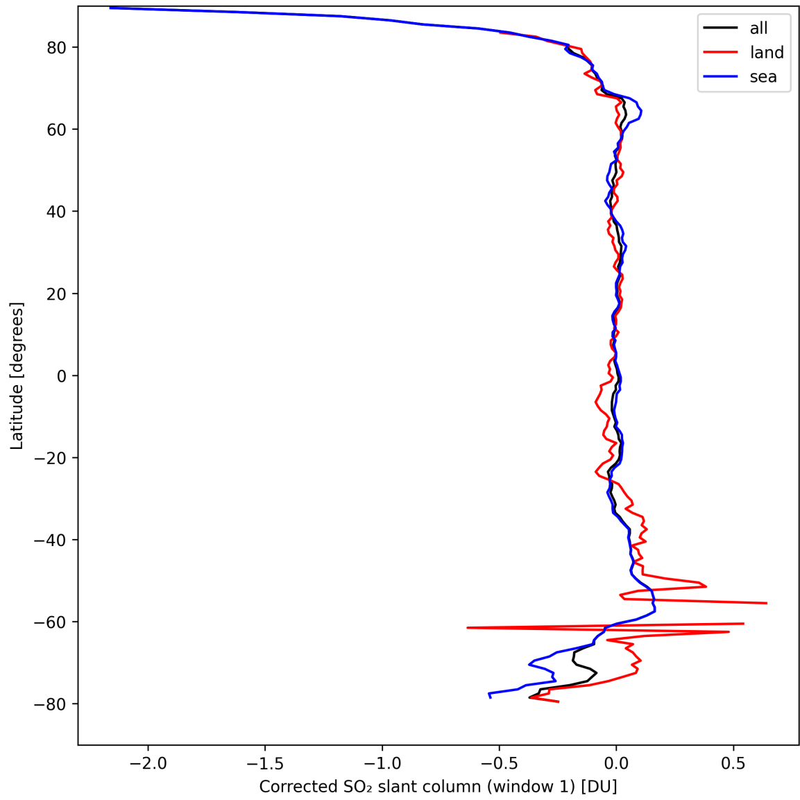
Figure 35: Zonal average of “Corrected SO 2 slant column (window 1)” for 2024-09-07 to 2024-09-09.
