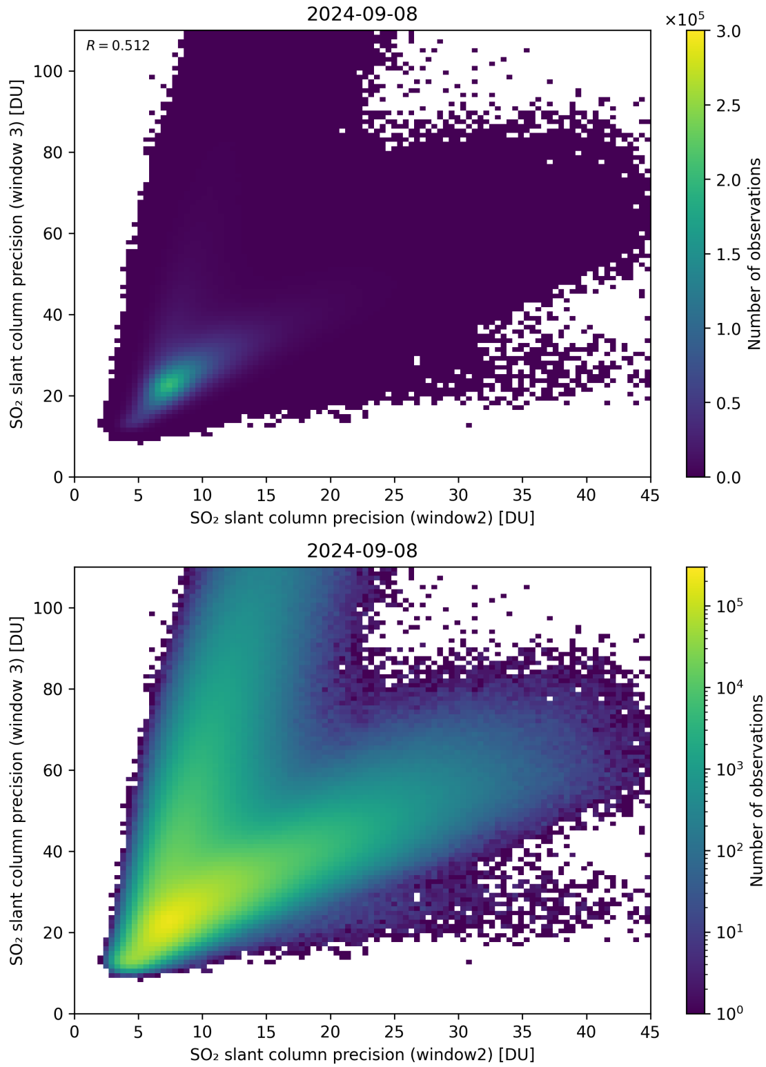
Figure 250: Scatter density plot of “SO 2 slant column precision (window2)” against “SO 2 slant column precision (window 3)” for 2024-09-07 to 2024-09-09.
