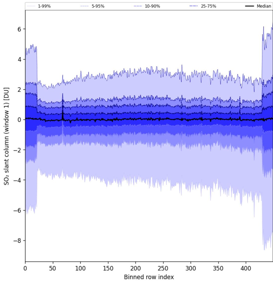
Figure 79: Along track statistics of “SO 2 slant column (window 1)” for 2024-09-07 to 2024-09-09
