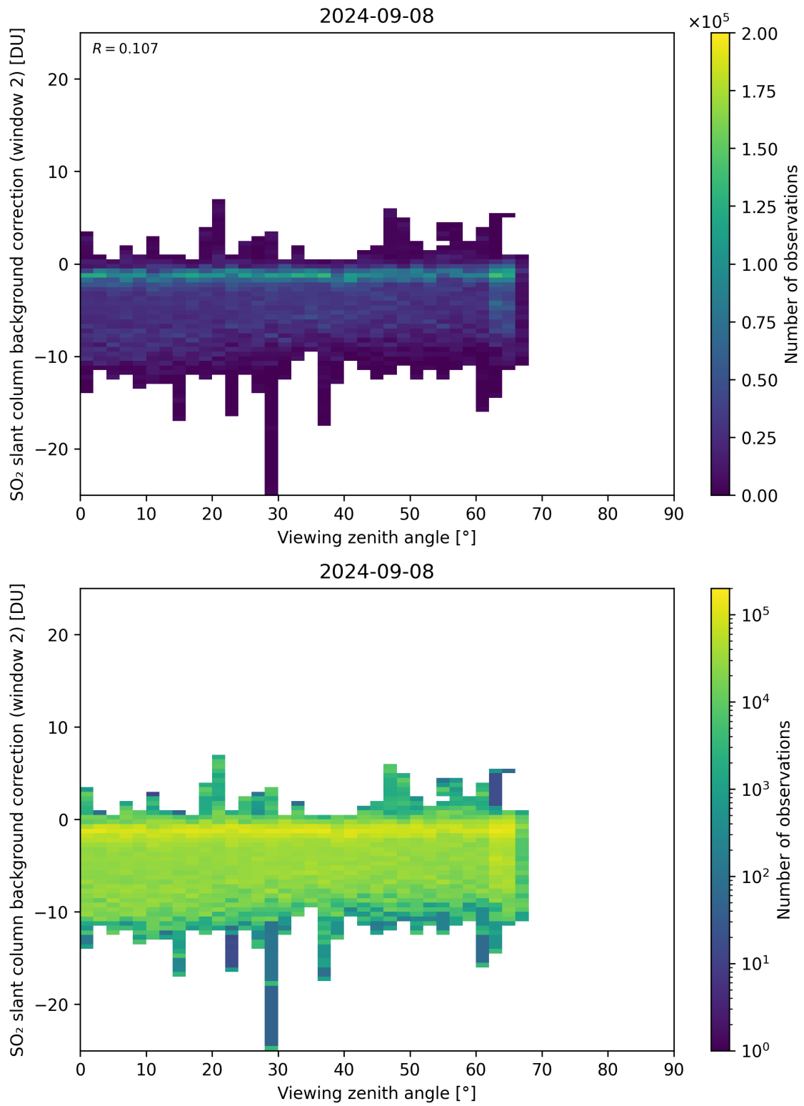
Figure 309: Scatter density plot of “Viewing zenith angle” against “SO 2 slant column background correction (window 2)” for 2024-09-07 to 2024-09-09.
