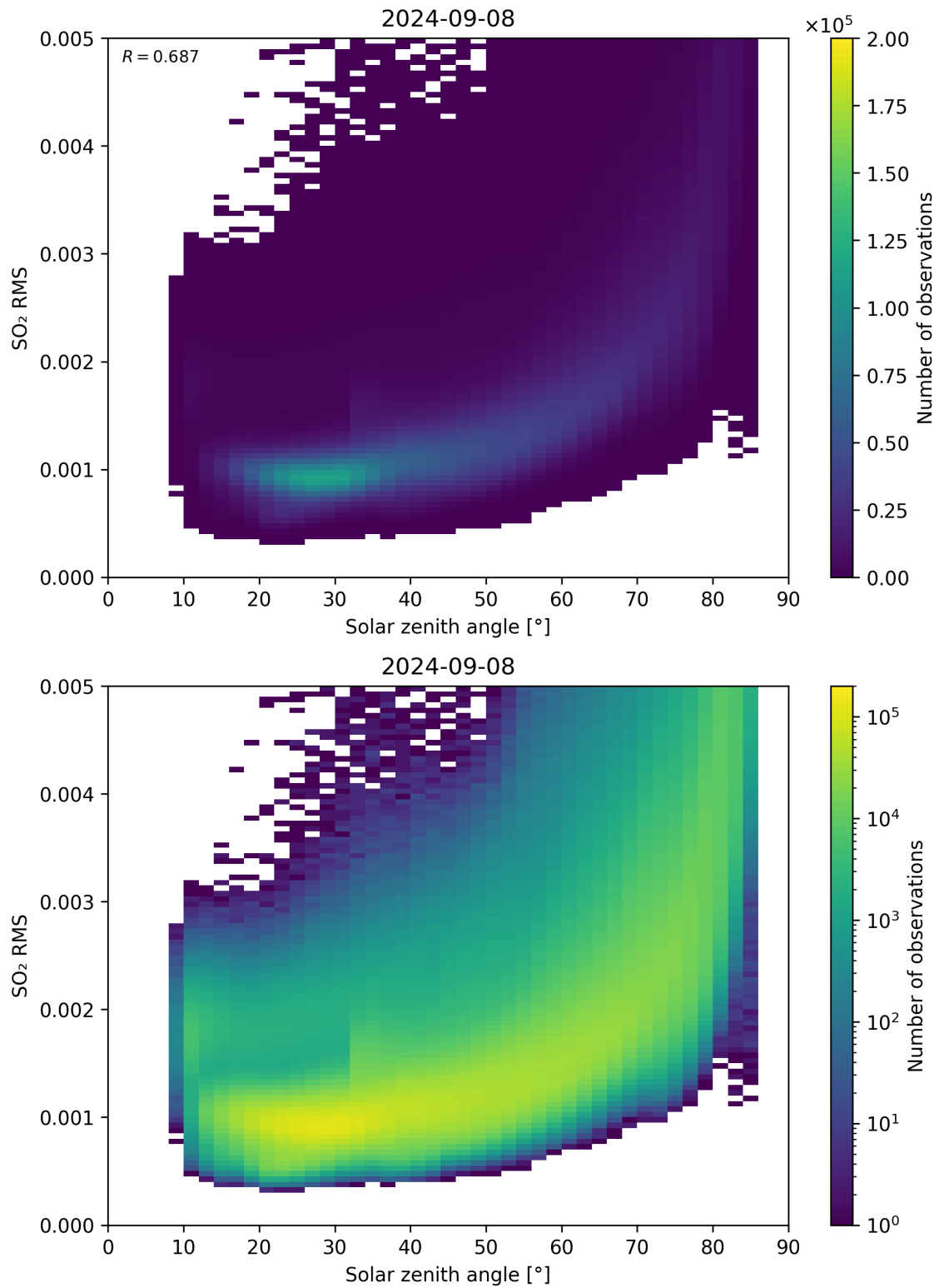
Figure 163: Scatter density plot of “Solar zenith angle” against “SO 2 RMS” for 2024-09-07 to 2024-09-09.
