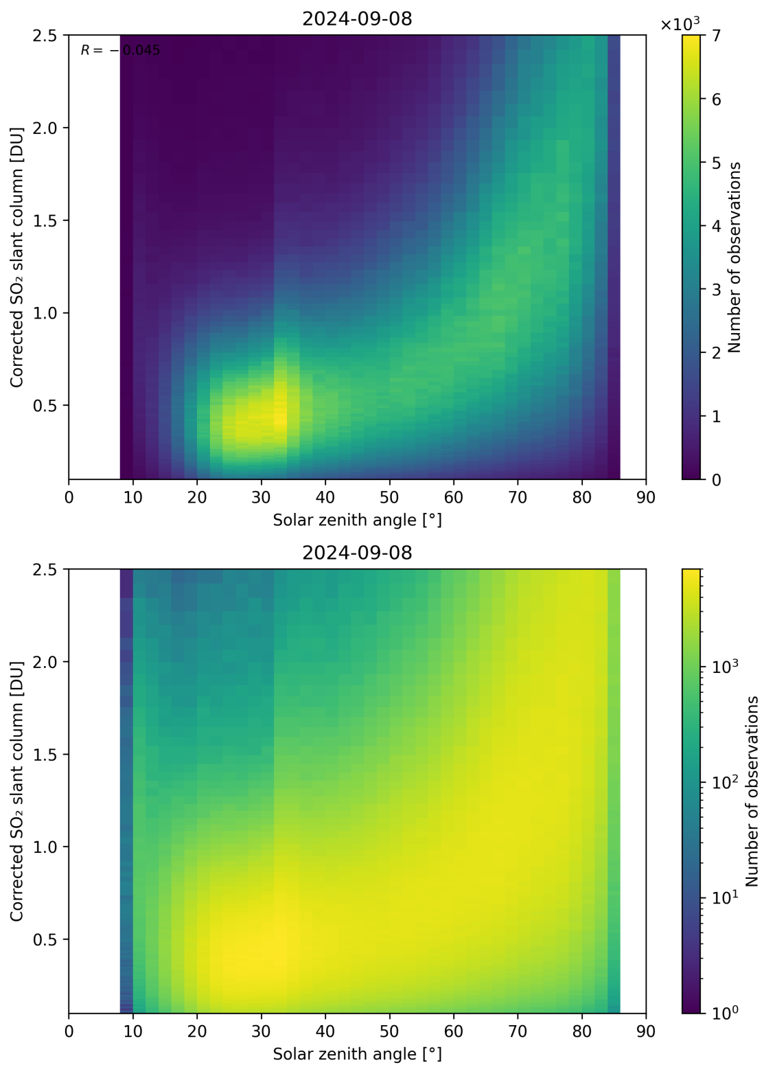
Figure 166: Scatter density plot of “Solar zenith angle” against “Corrected SO 2 slant column” for 2024-09-07 to 2024-09-09.
