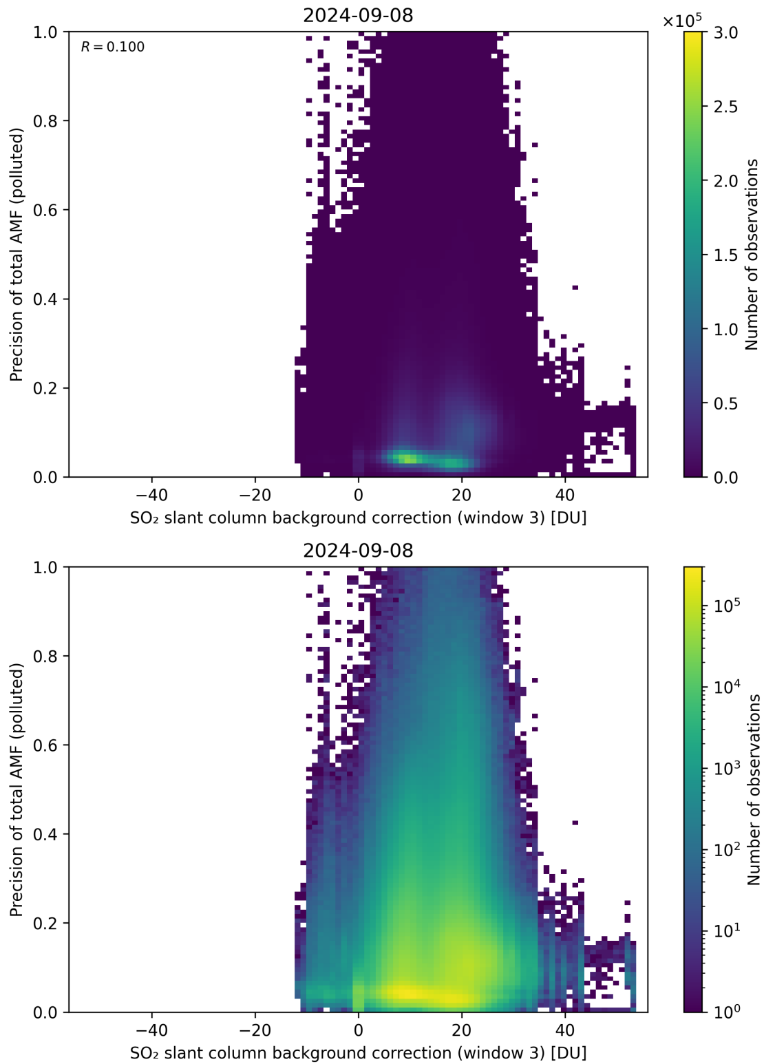
Figure 126: Scatter density plot of “SO 2 slant column background correction (window 3)” against “Precision of total AMF (polluted)” for 2024-09-07 to 2024-09-09.
