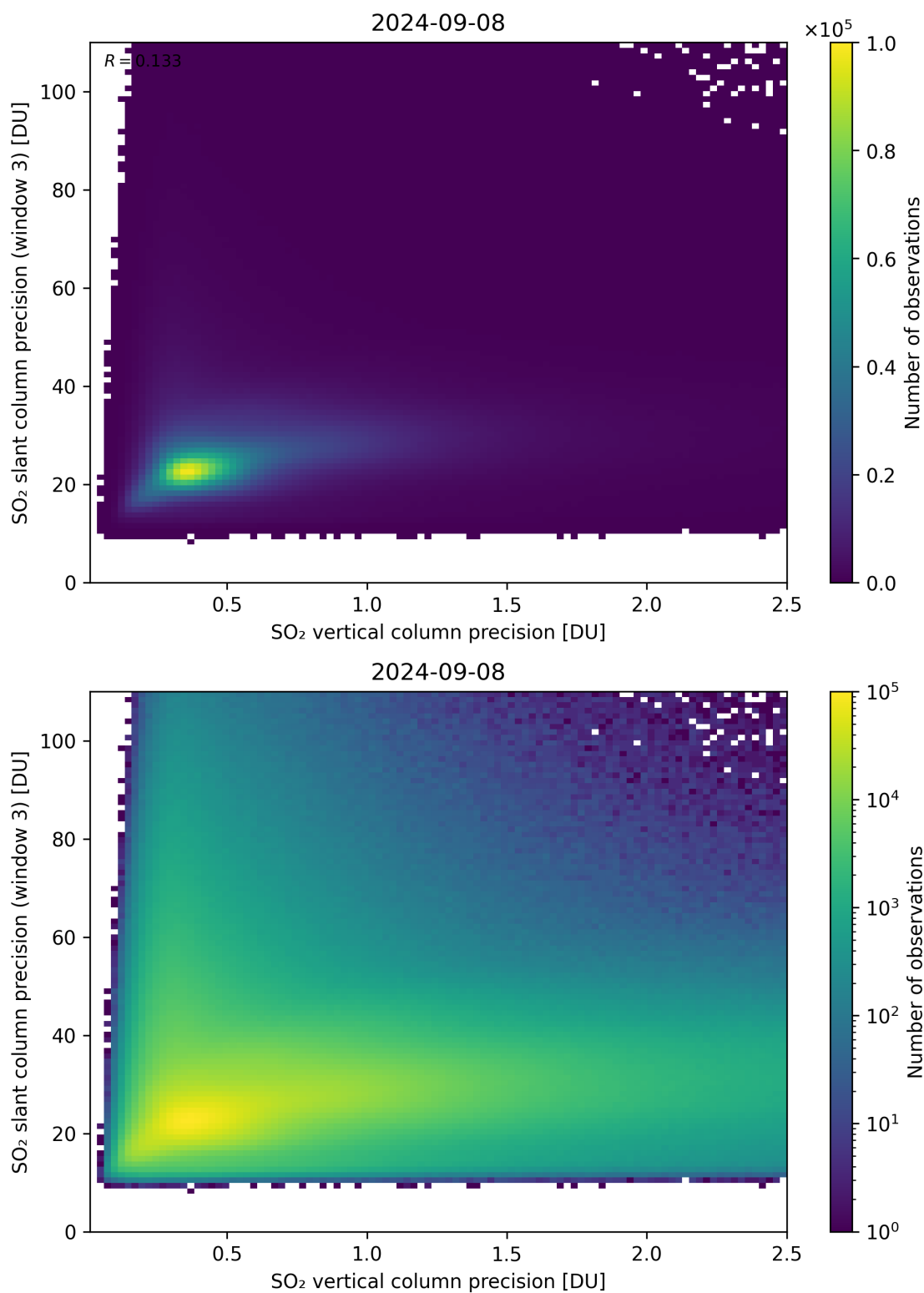
Figure 293: Scatter density plot of “SO 2 vertical column precision” against “SO 2 slant column precision (window 3)” for 2024-09-07 to 2024-09-09.
