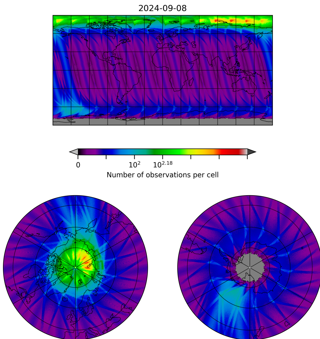
Figure 28: Map of the number of observations for 2024-09-07 to 2024-09-09
