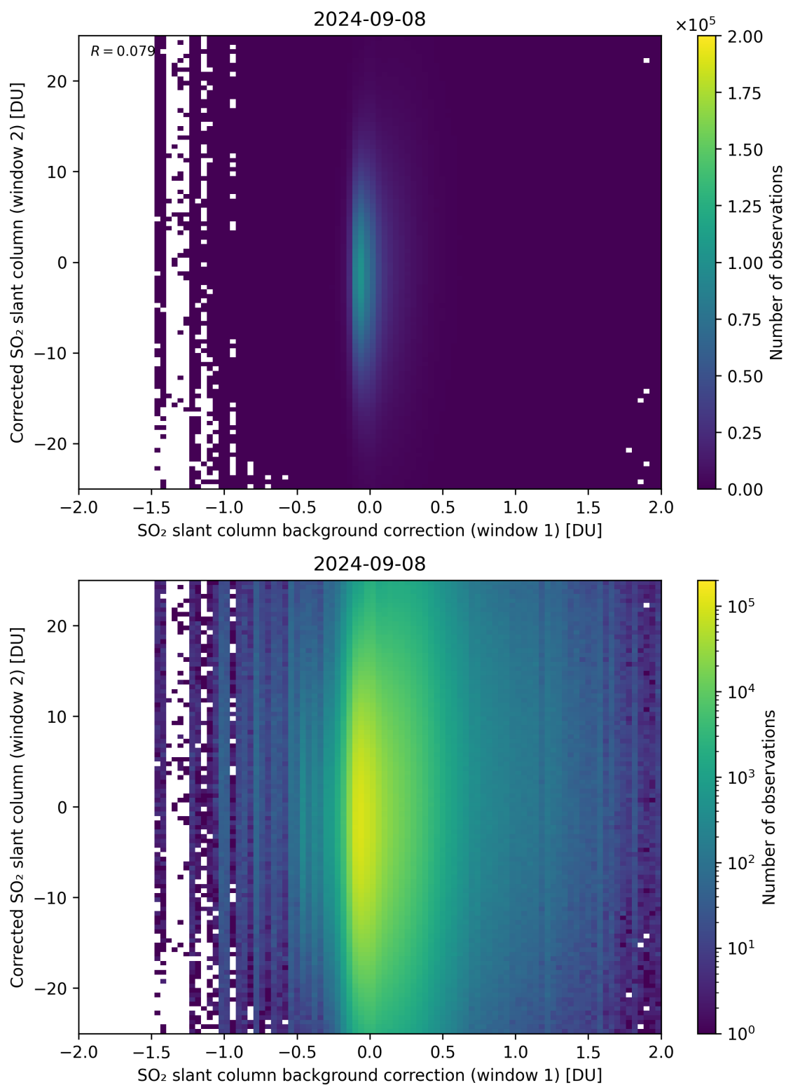
Figure 104: Scatter density plot of “SO 2 slant column background correction (window 1)” against “Corrected SO 2 slant column (window 2)” for 2024-09-07 to 2024-09-09.
