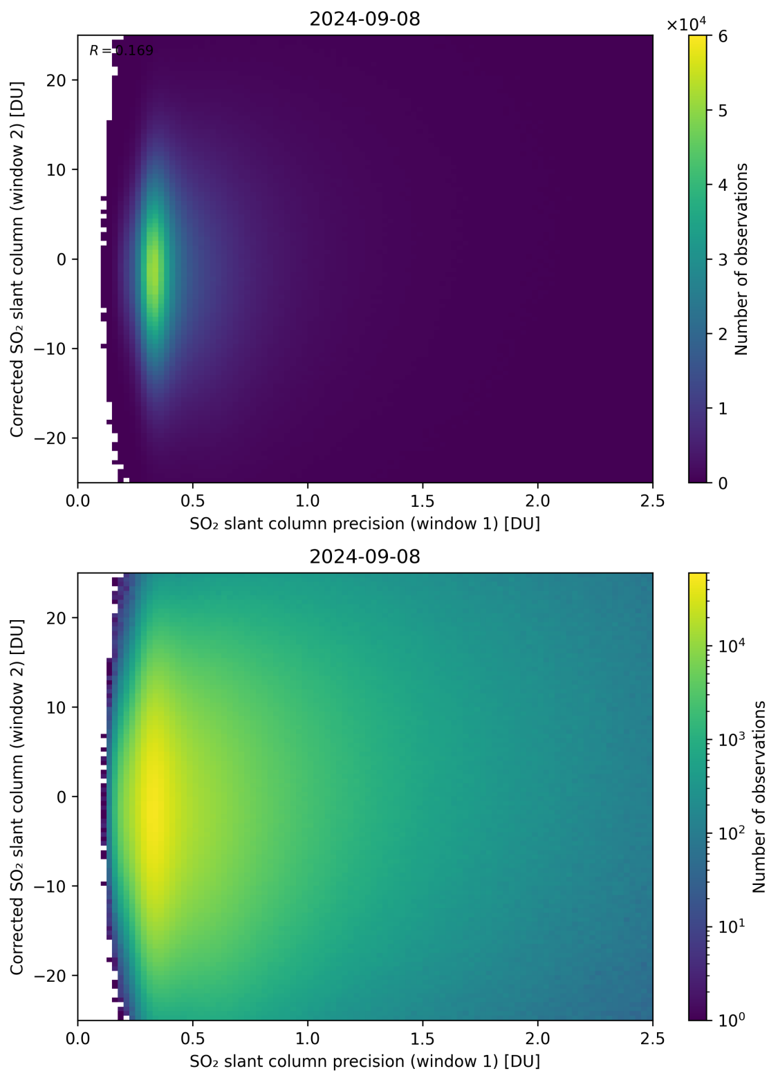
Figure 225: Scatter density plot of “SO 2 slant column precision (window 1)” against “Corrected SO 2 slant column (window 2)” for 2024-09-07 to 2024-09-09.
