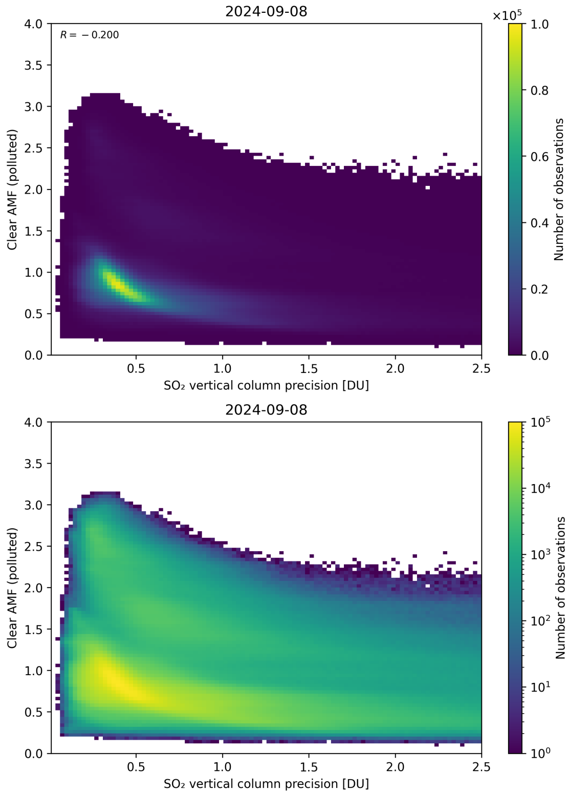
Figure 285: Scatter density plot of “SO 2 vertical column precision” against “Clear AMF (polluted)” for 2024-09-07 to 2024-09-09.
