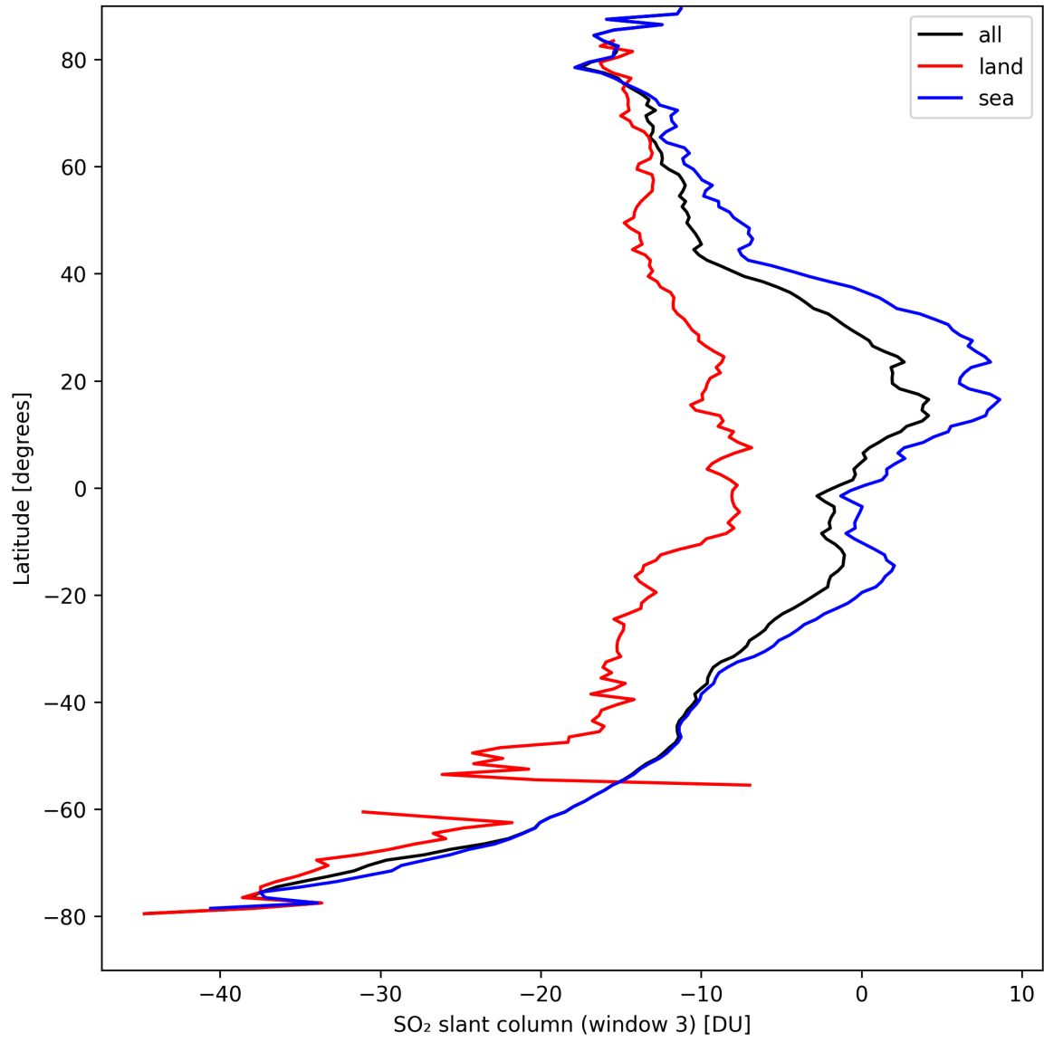
Figure 41: Zonal average of “SO 2 slant column (window 3)” for 2024-09-07 to 2024-09-09.
