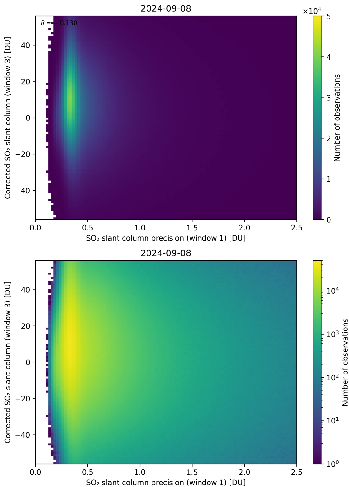
Figure 226: Scatter density plot of “SO 2 slant column precision (window 1)” against “Corrected SO 2 slant column (window 3)” for 2024-09-07 to 2024-09-09.
