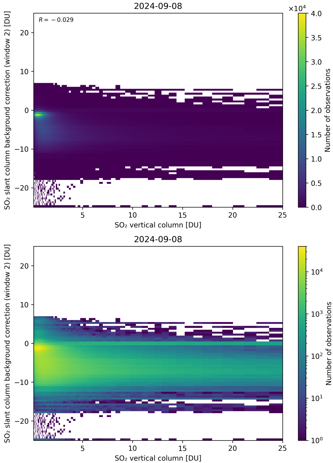
Figure 274: Scatter density plot of “SO 2 vertical column” against “SO 2 slant column background correction (window 2)” for 2024-09-07 to 2024-09-09.
