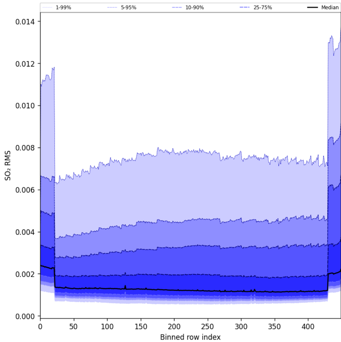
Figure 93: Along track statistics of “SO 2 RMS” for 2024-09-07 to 2024-09-09
