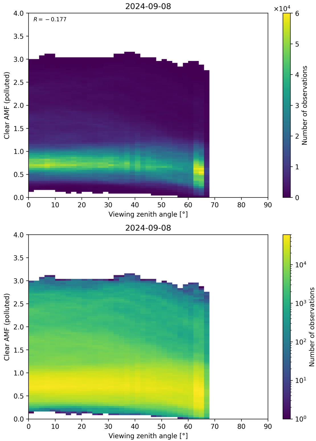
Figure 316: Scatter density plot of “Viewing zenith angle” against “Clear AMF (polluted)” for 2024-09-07 to 2024-09-09.
