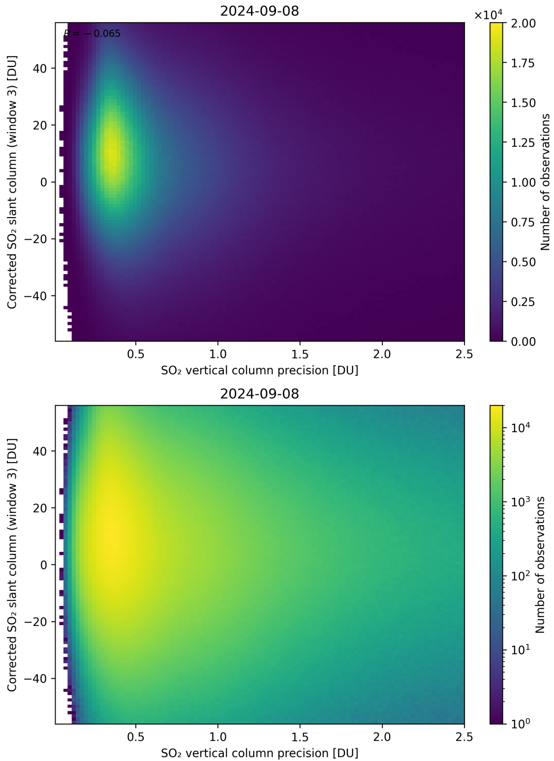
Figure 288: Scatter density plot of “SO 2 vertical column precision” against “Corrected SO 2 slant column (window 3)” for 2024-09-07 to 2024-09-09.
