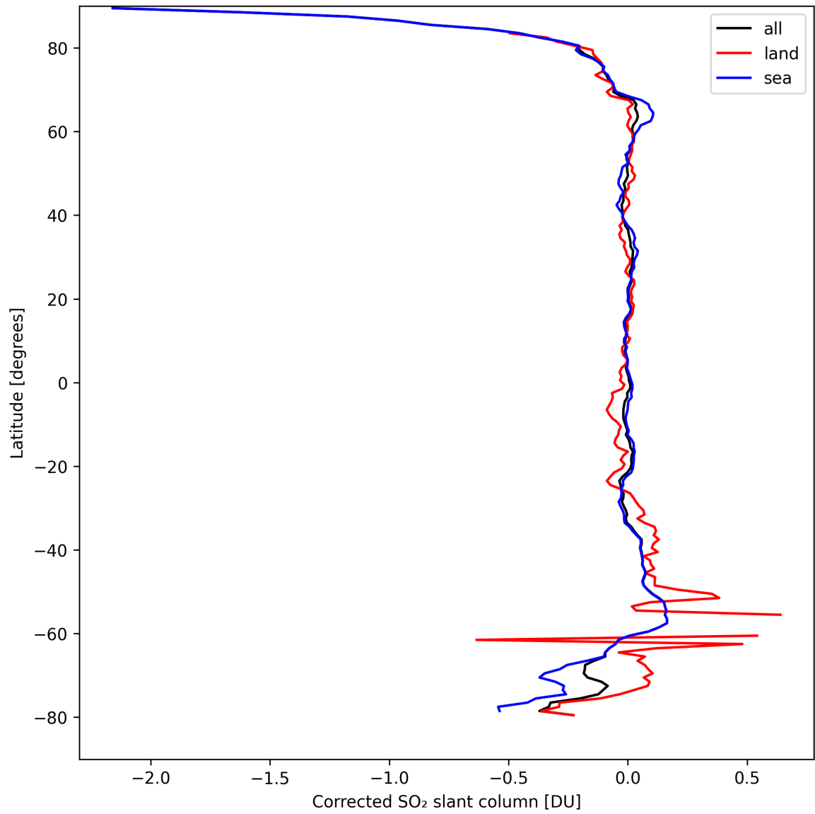
Figure 32: Zonal average of “Corrected SO 2 slant column” for 2024-09-07 to 2024-09-09.
