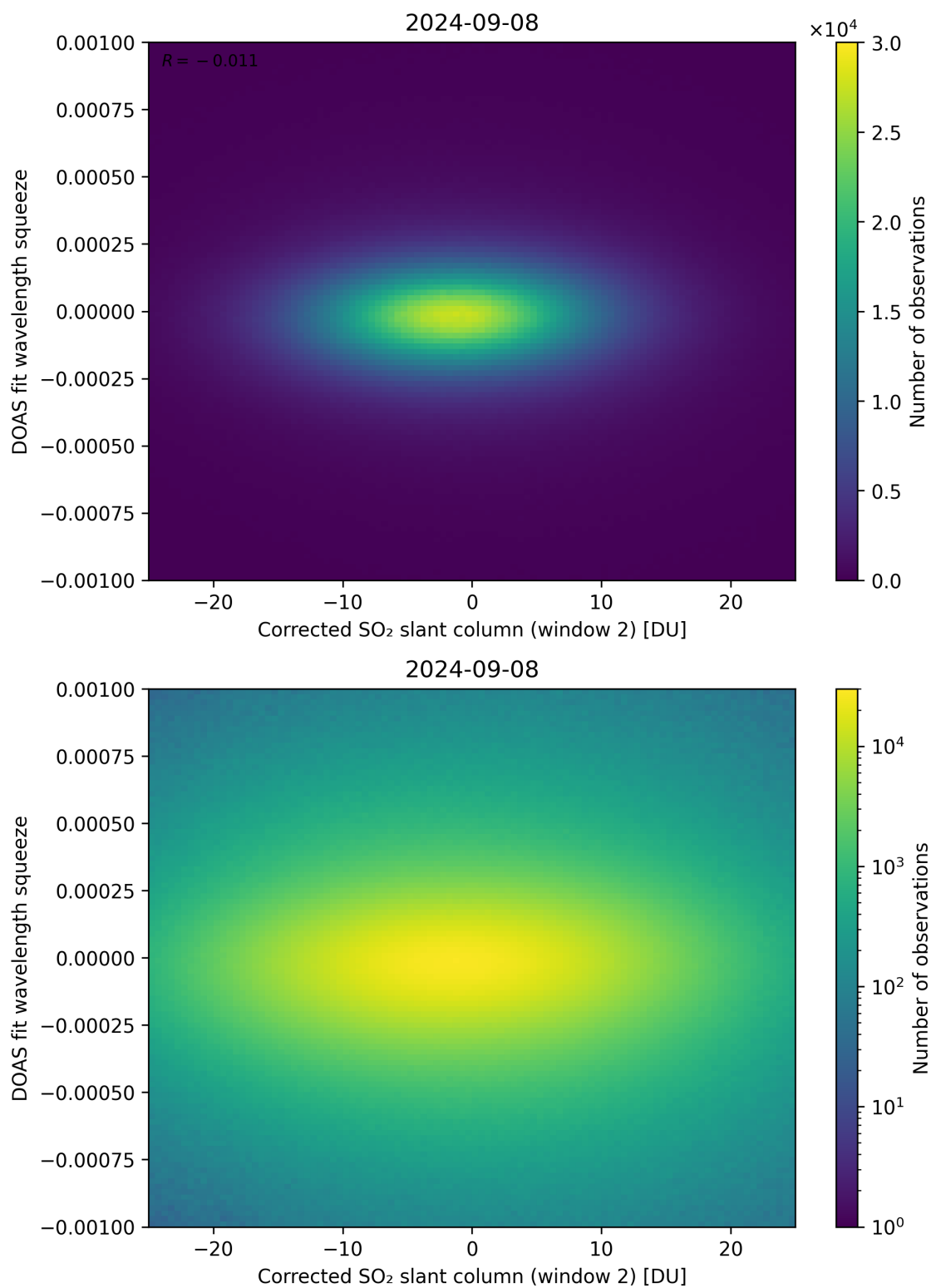
Figure 197: Scatter density plot of “Corrected SO 2 slant column (window 2)” against “DOAS fit wavelength squeeze” for 2024-09-07 to 2024-09-09.
