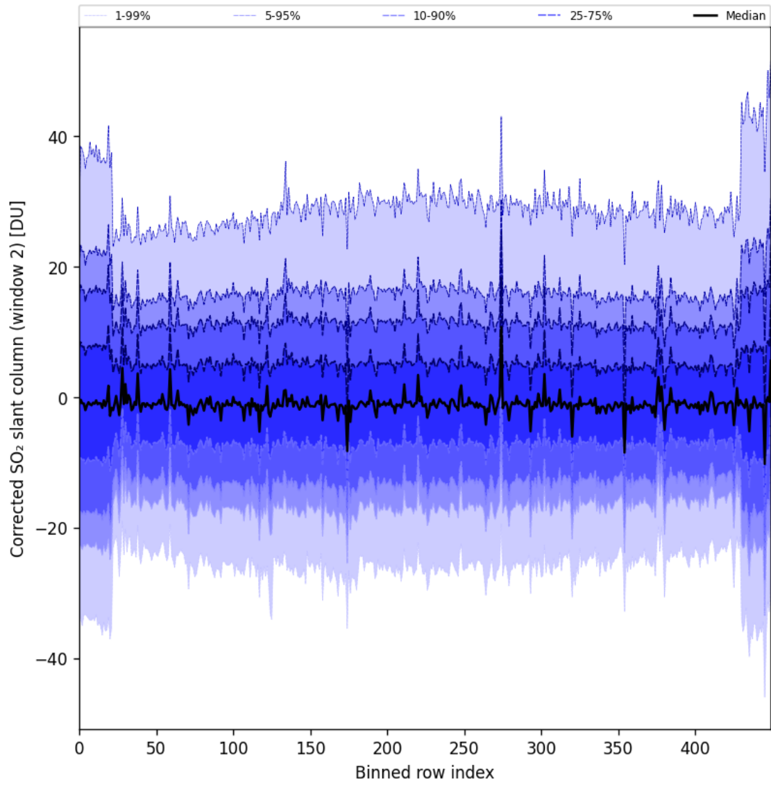
Figure 85: Along track statistics of “Corrected SO 2 slant column (window 2)” for 2024-09-07 to 2024-09-09
