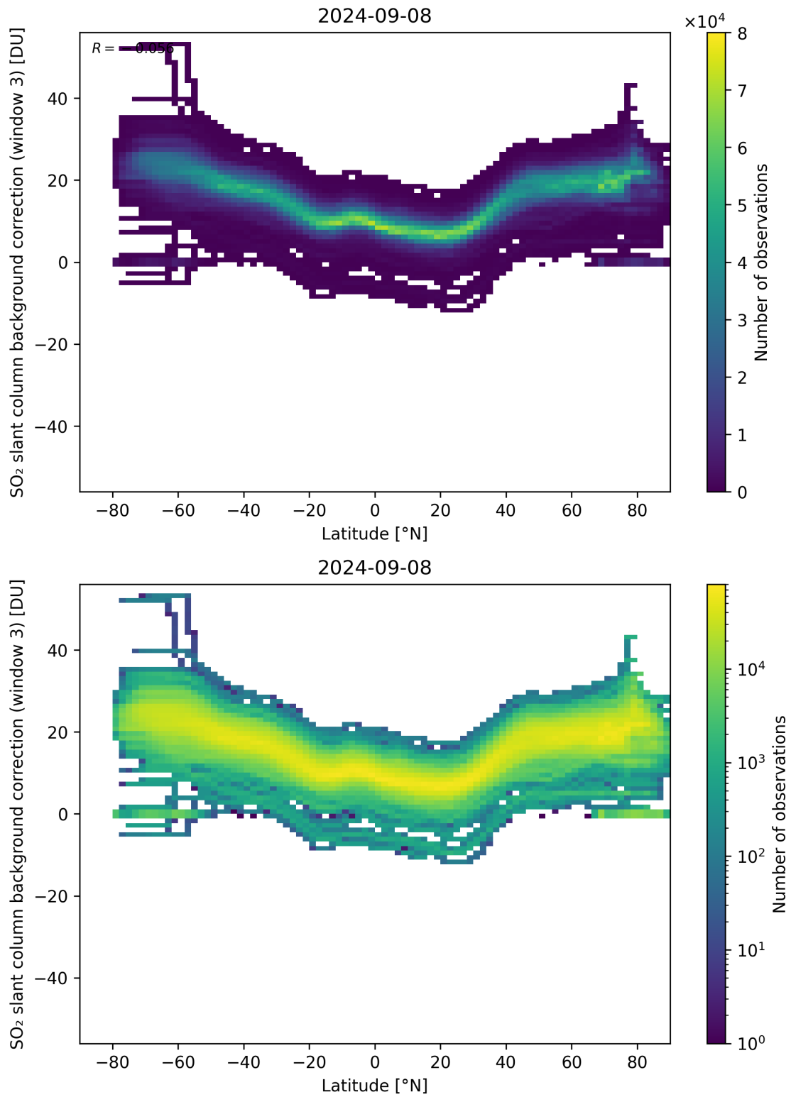
Figure 141: Scatter density plot of “Latitude” against “SO 2 slant column background correction (window 3)” for 2024-09-07 to 2024-09-09.
