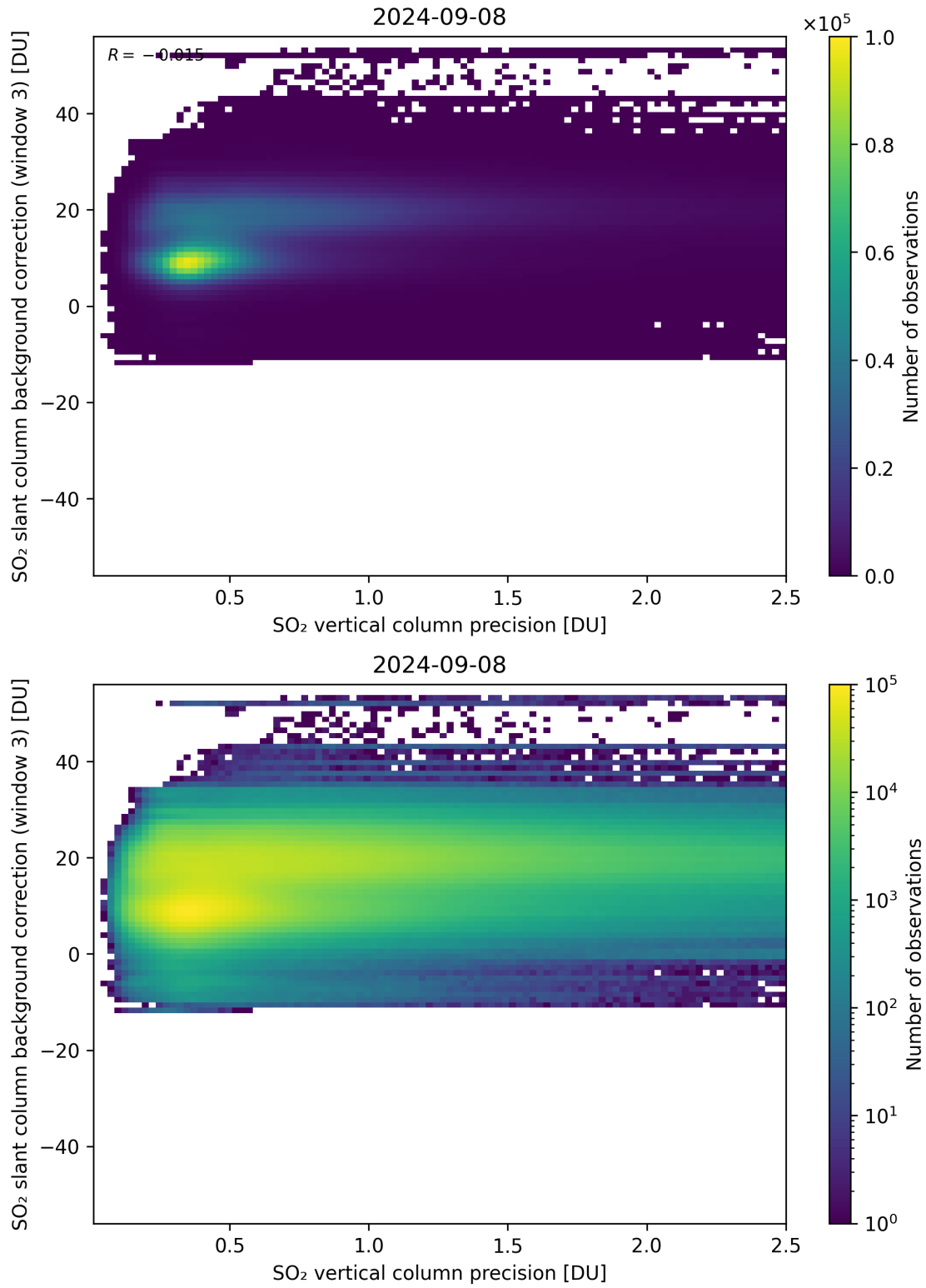
Figure 281: Scatter density plot of “SO 2 vertical column precision” against “SO 2 slant column background correction (window 3)” for 2024-09-07 to 2024-09-09.
