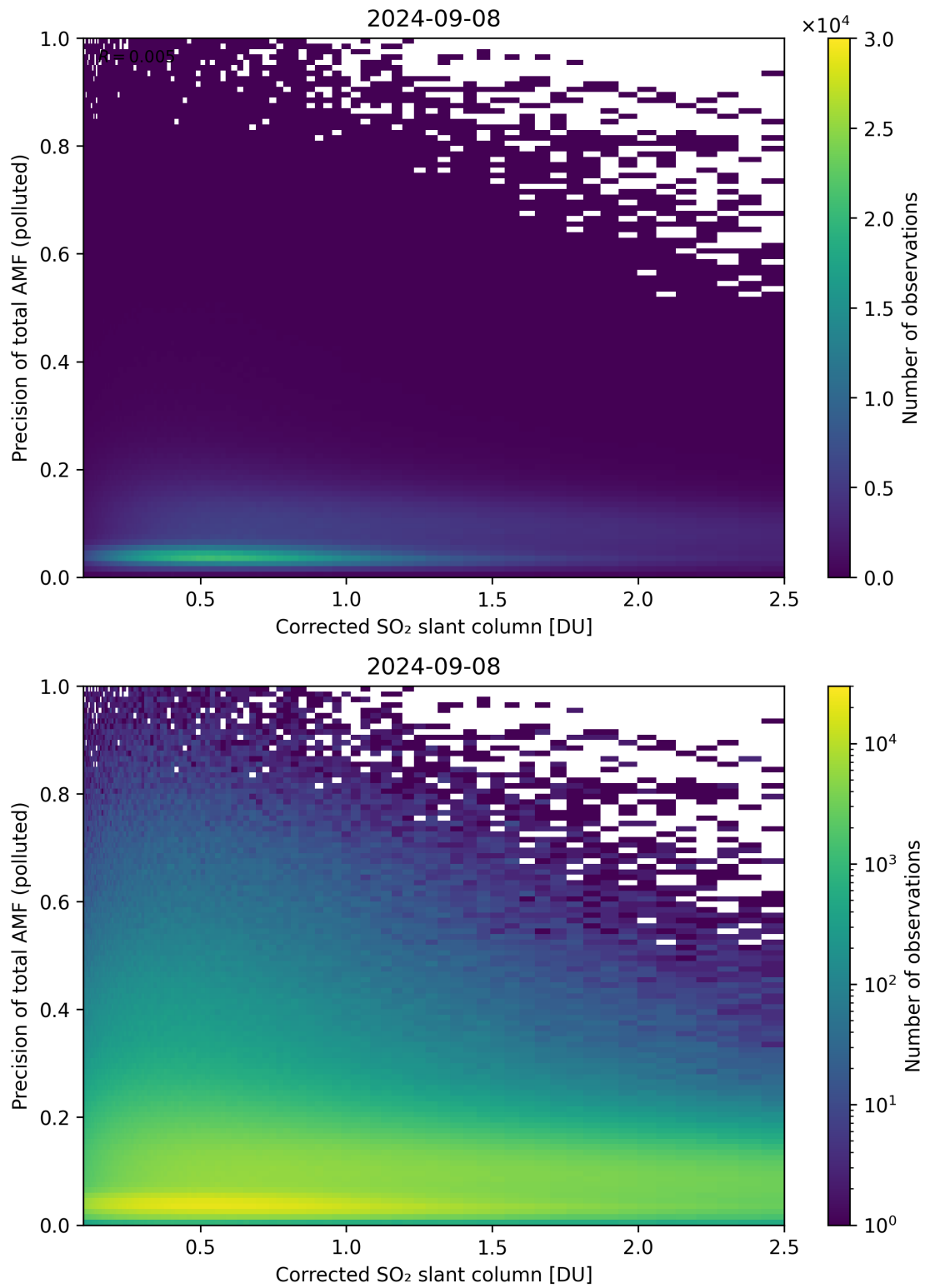
Figure 193: Scatter density plot of “Corrected SO 2 slant column” against “Precision of total AMF (polluted)” for 2024-09-07 to 2024-09-09.
