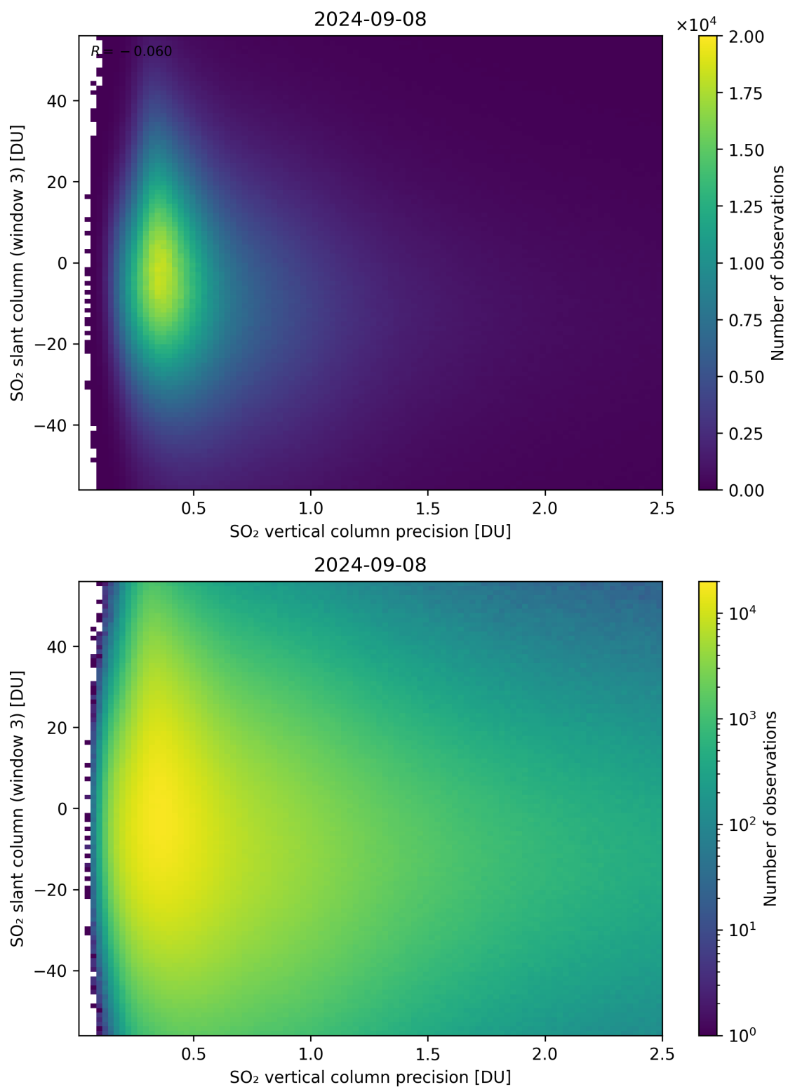
Figure 292: Scatter density plot of “SO 2 vertical column precision” against “SO 2 slant column (window 3)” for 2024-09-07 to 2024-09-09.
