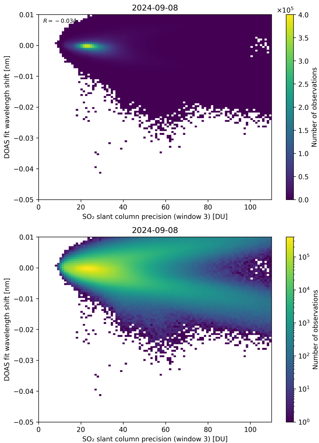
Figure 258: Scatter density plot of “SO 2 slant column precision (window 3)” against “DOAS fit wavelength shift” for 2024-09-07 to 2024-09-09.
