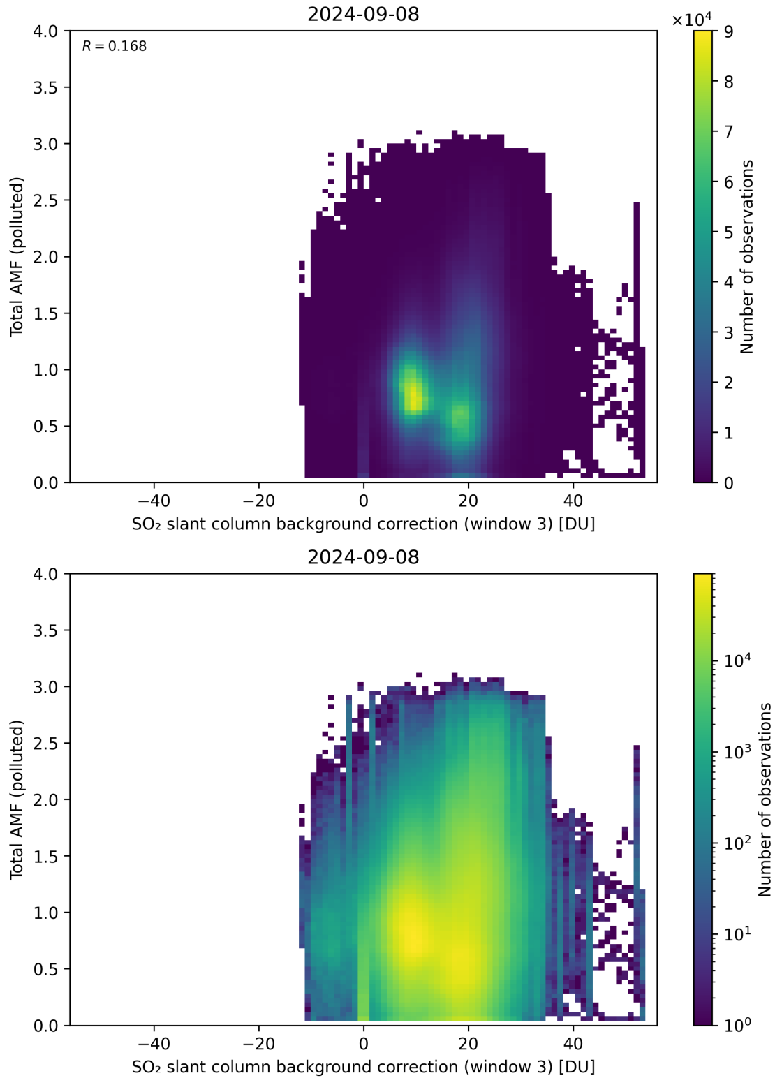
Figure 125: Scatter density plot of “SO 2 slant column background correction (window 3)” against “Total AMF (polluted)” for 2024-09-07 to 2024-09-09.
