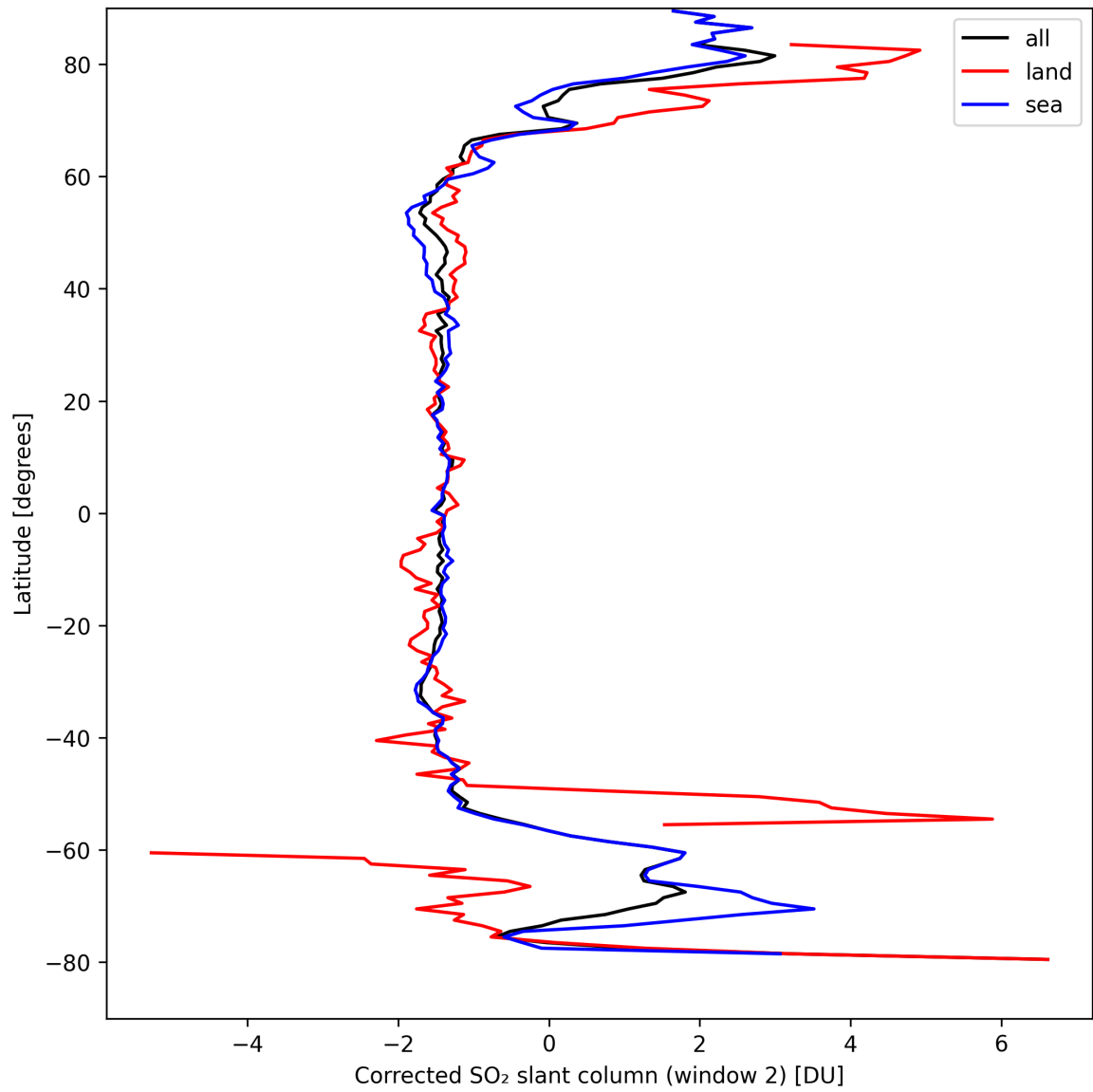
Figure 39: Zonal average of “Corrected SO 2 slant column (window 2)” for 2024-09-07 to 2024-09-09.
