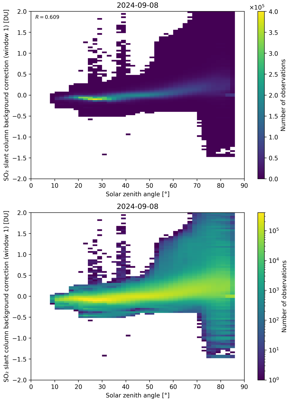
Figure 158: Scatter density plot of “Solar zenith angle” against “SO 2 slant column background correction (window 1)” for 2024-09-07 to 2024-09-09.
