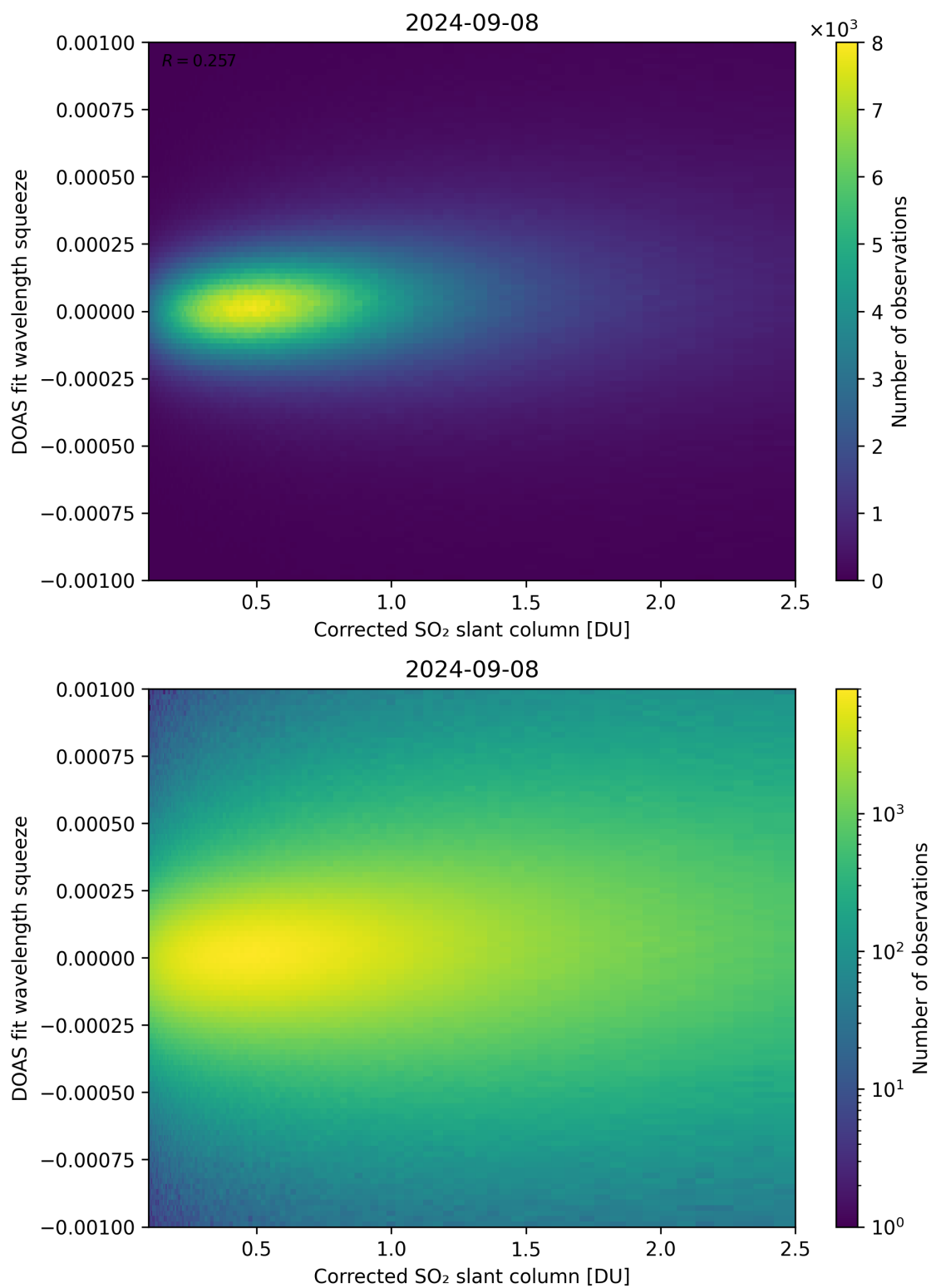
Figure 182: Scatter density plot of "Corrected SO 2 slant column" against "DOAS fit wavelength squeeze" for 2024-09-07 to 2024-09-09.
