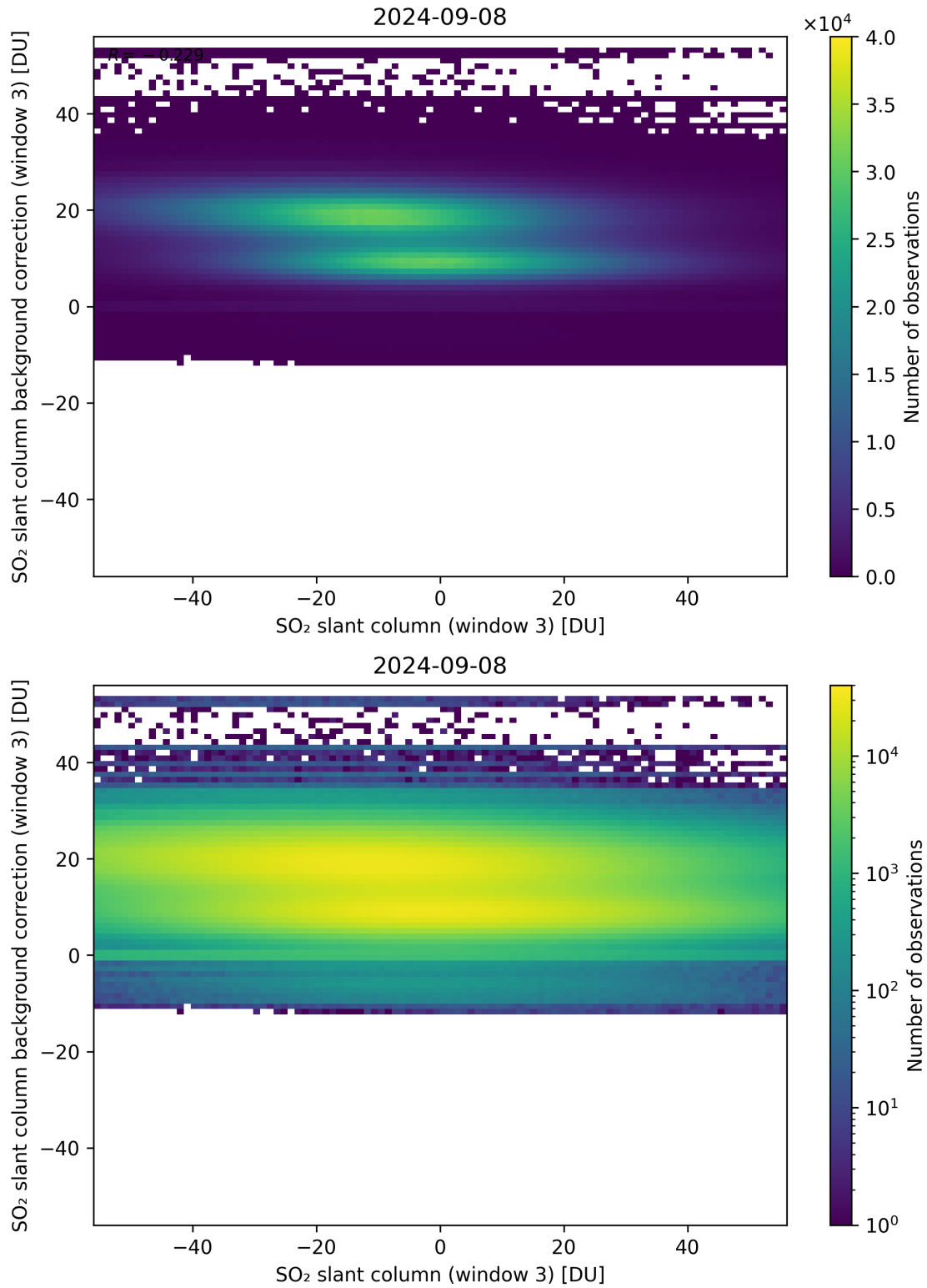
Figure 253: Scatter density plot of “SO 2 slant column (window 3)” against “SO 2 slant column background correction (window 3)” for 2024-09-07 to 2024-09-09.
