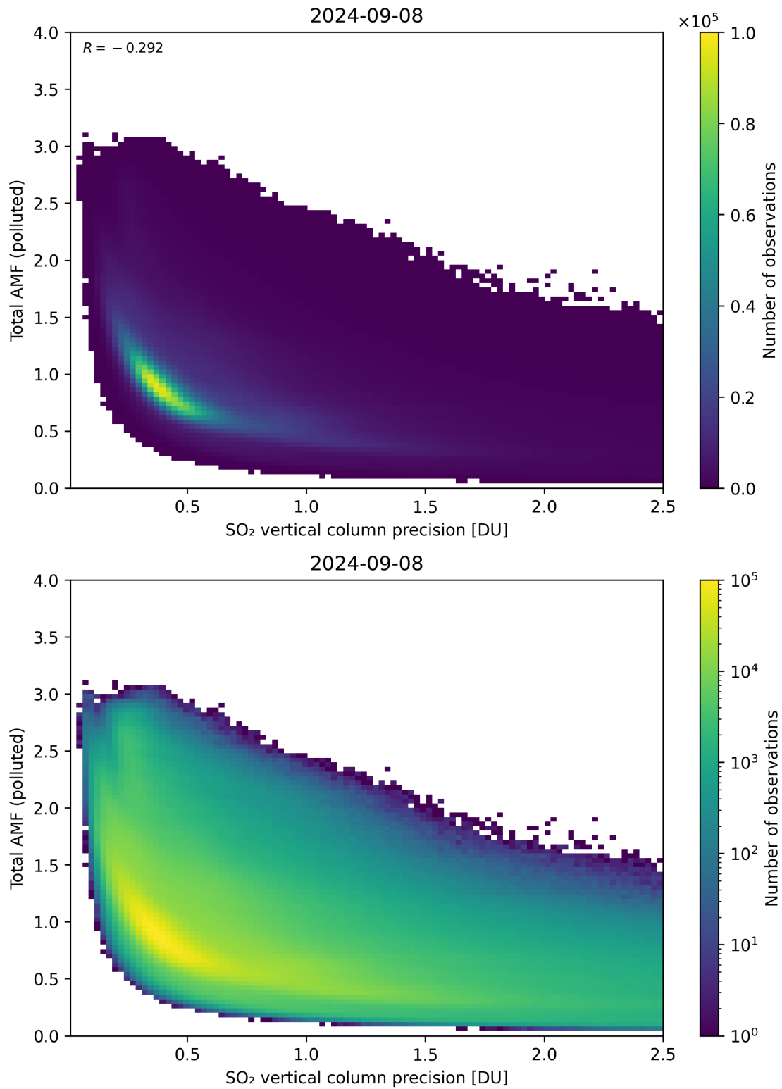
Figure 294: Scatter density plot of “SO 2 vertical column precision” against “Total AMF (polluted)” for 2024-09-07 to 2024-09-09.
