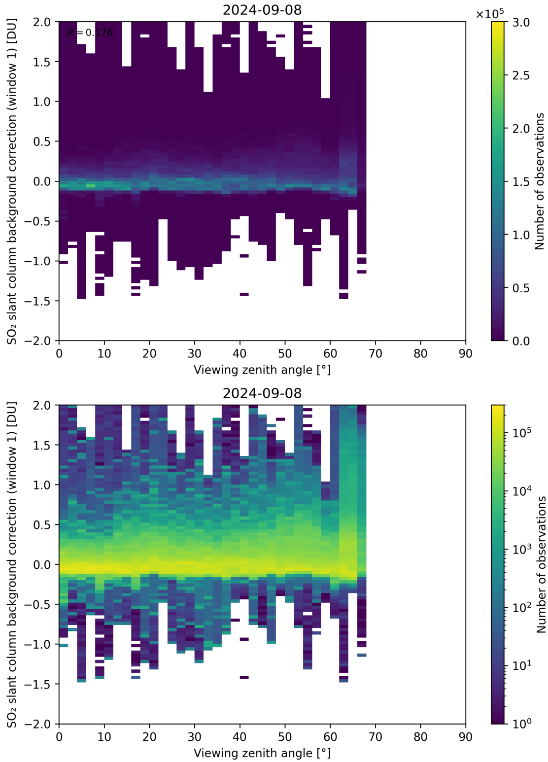
Figure 308: Scatter density plot of “Viewing zenith angle” against “SO 2 slant column background correction (window 1)” for 2024-09-07 to 2024-09-09.
