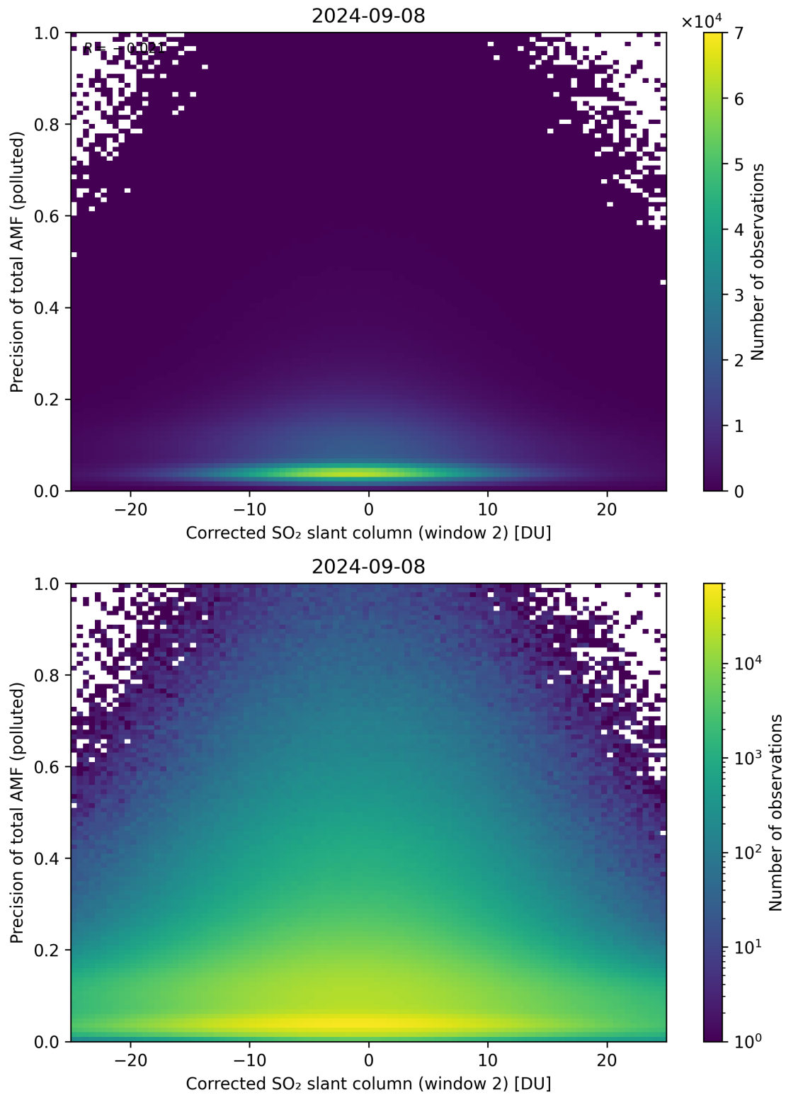
Figure 204: Scatter density plot of “Corrected SO 2 slant column (window 2)” against “Precision of total AMF (polluted)” for 2024-09-07 to 2024-09-09.
