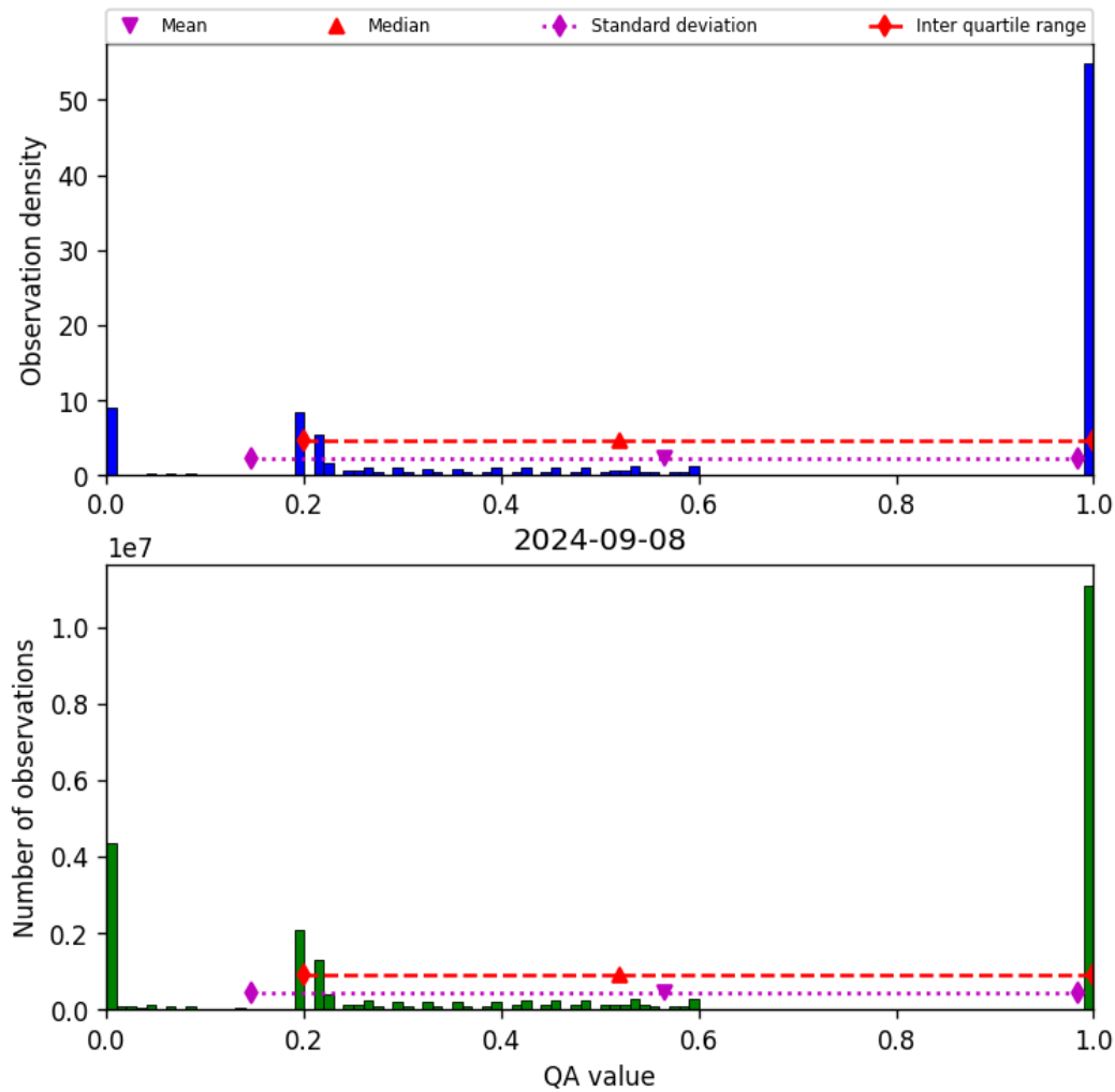
Figure 52: Histogram of “QA value” for 2024-09-07 to 2024-09-09
