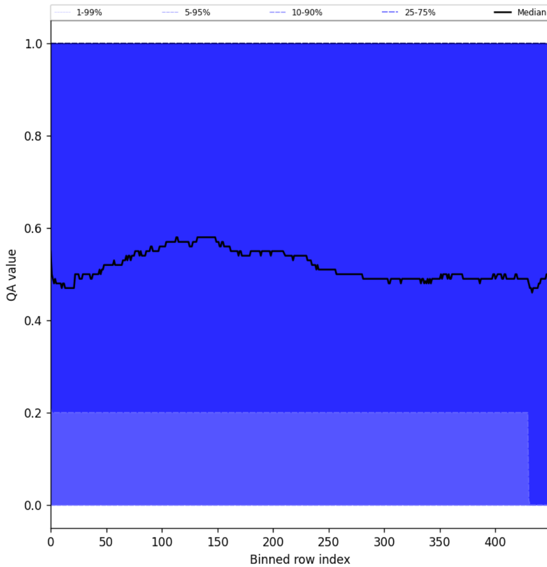
Figure 75: Along track statistics of “QA value” for 2024-09-07 to 2024-09-09
