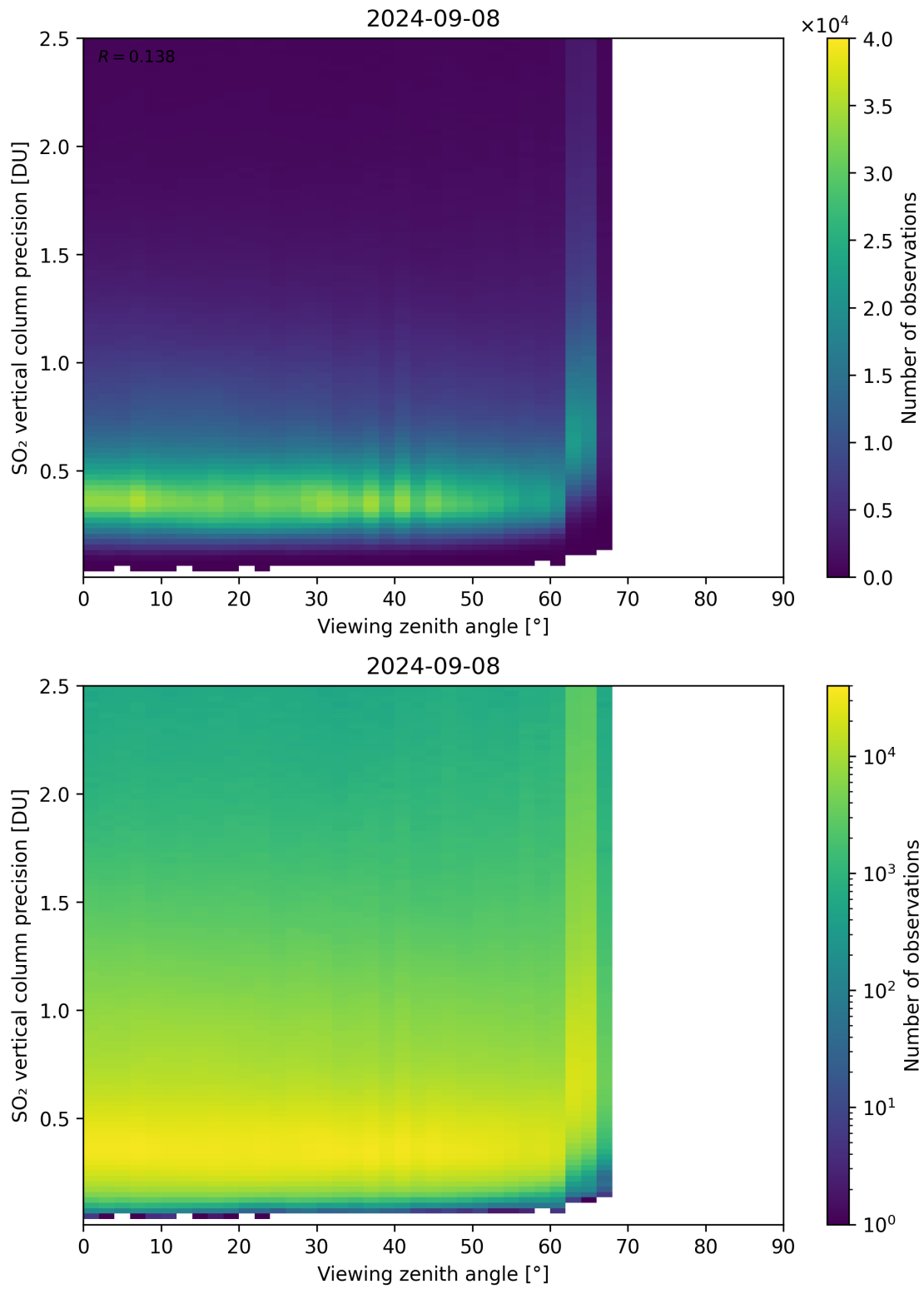
Figure 328: Scatter density plot of “Viewing zenith angle” against “SO 2 vertical column precision” for 2024-09-07 to 2024-09-09.
