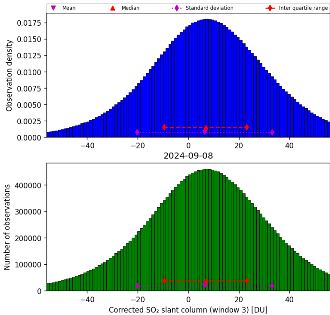
Figure 66: Histogram of “Corrected SO 2 slant column (window 3)” for 2024-09-07 to 2024-09-09
