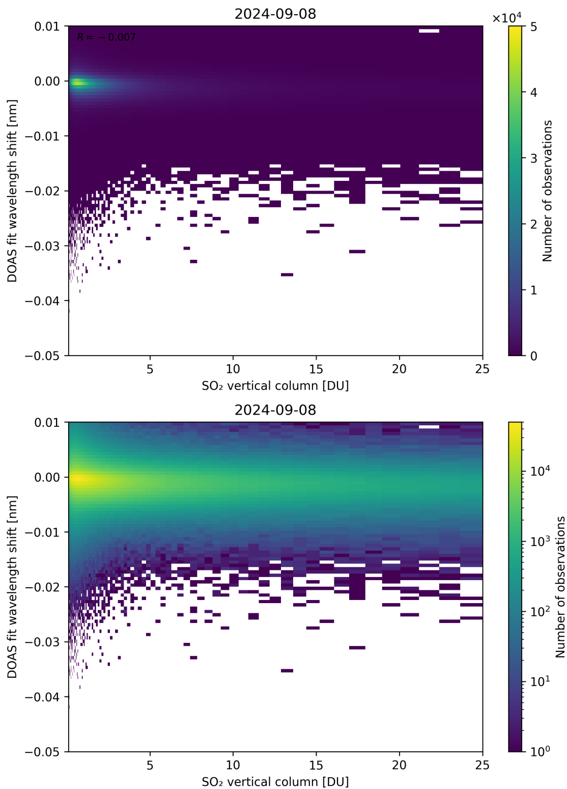
Figure 276: Scatter density plot of “SO 2 vertical column” against “DOAS fit wavelength shift” for 2024-09-07 to 2024-09-09.
