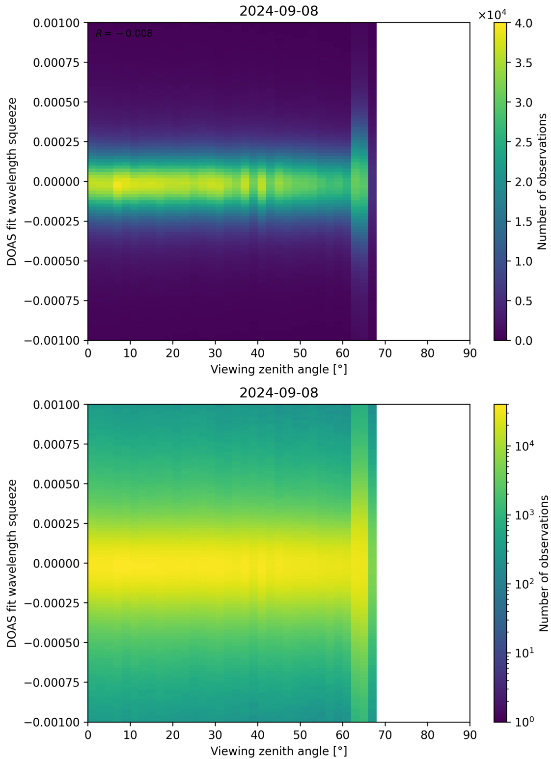
Figure 312: Scatter density plot of “Viewing zenith angle” against “DOAS fit wavelength squeeze” for 2024-09-07 to 2024-09-09.
