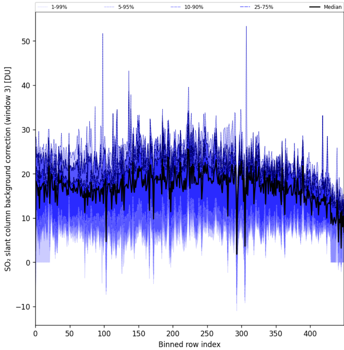
Figure 90: Along track statistics of “SO 2 slant column background correction (window 3)” for 2024-09-07 to 2024-09-09
