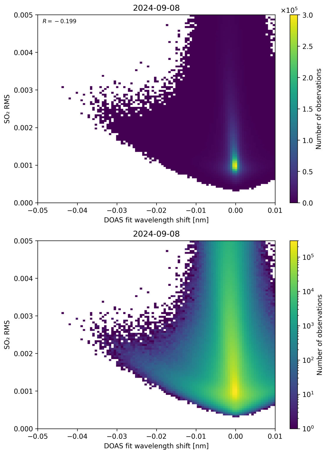
Figure 128: Scatter density plot of “DOAS fit wavelength shift” against “SO 2 RMS” for 2024-09-07 to 2024-09-09.
