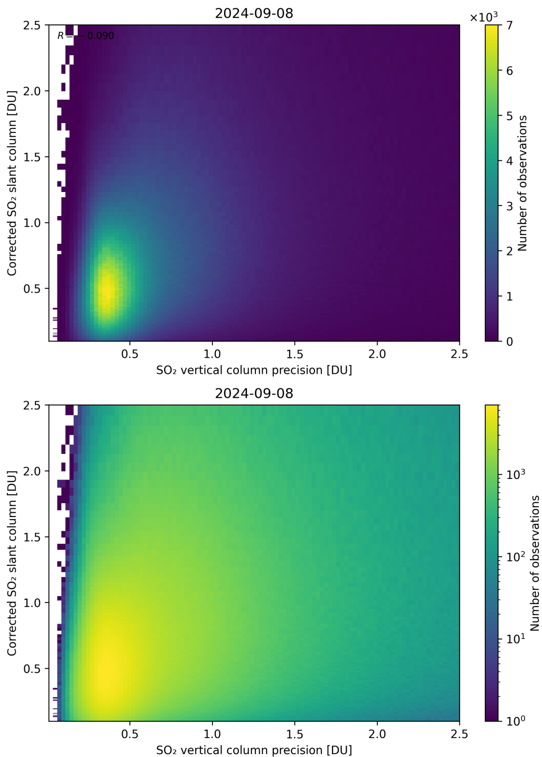
Figure 286: Scatter density plot of “SO 2 vertical column precision” against “Corrected SO 2 slant column” for 2024-09-07 to 2024-09-09.
