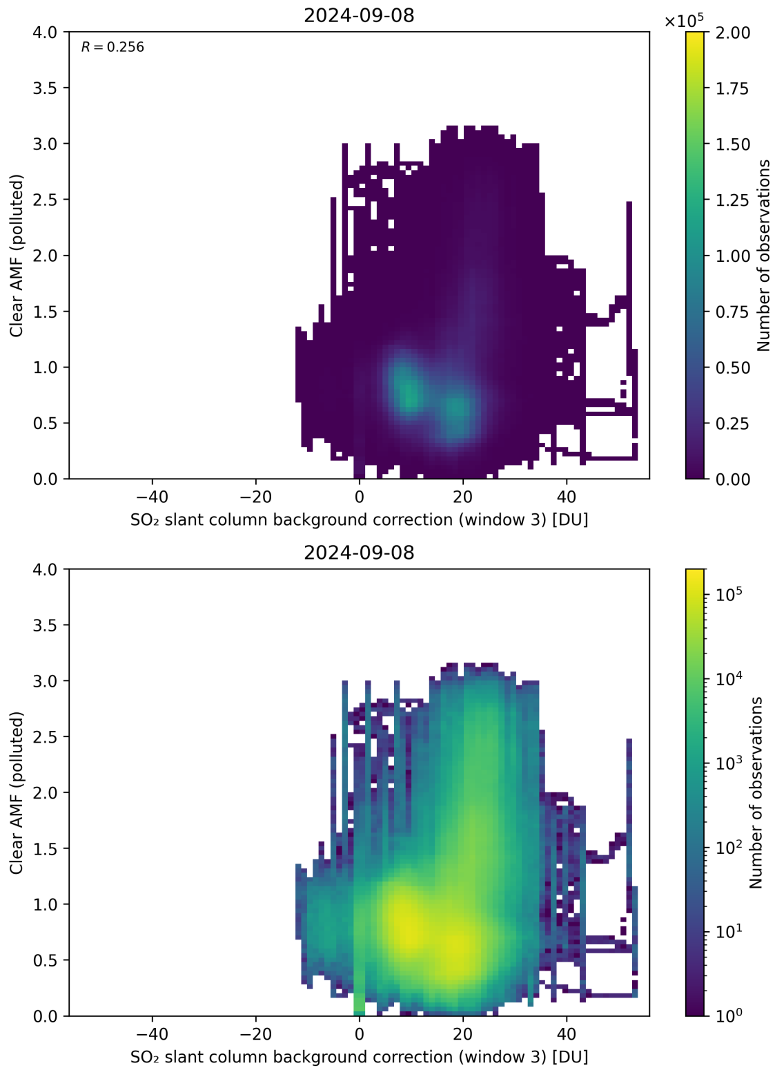
Figure 124: Scatter density plot of “SO 2 slant column background correction (window 3)” against “Clear AMF (polluted)” for 2024-09-07 to 2024-09-09.
