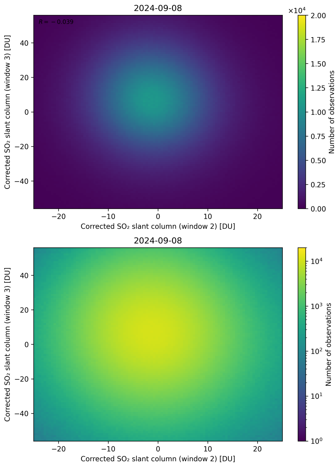
Figure 200: Scatter density plot of “Corrected SO 2 slant column (window 2)” against “Corrected SO 2 slant column (window 3)” for 2024-09-07 to 2024-09-09.
