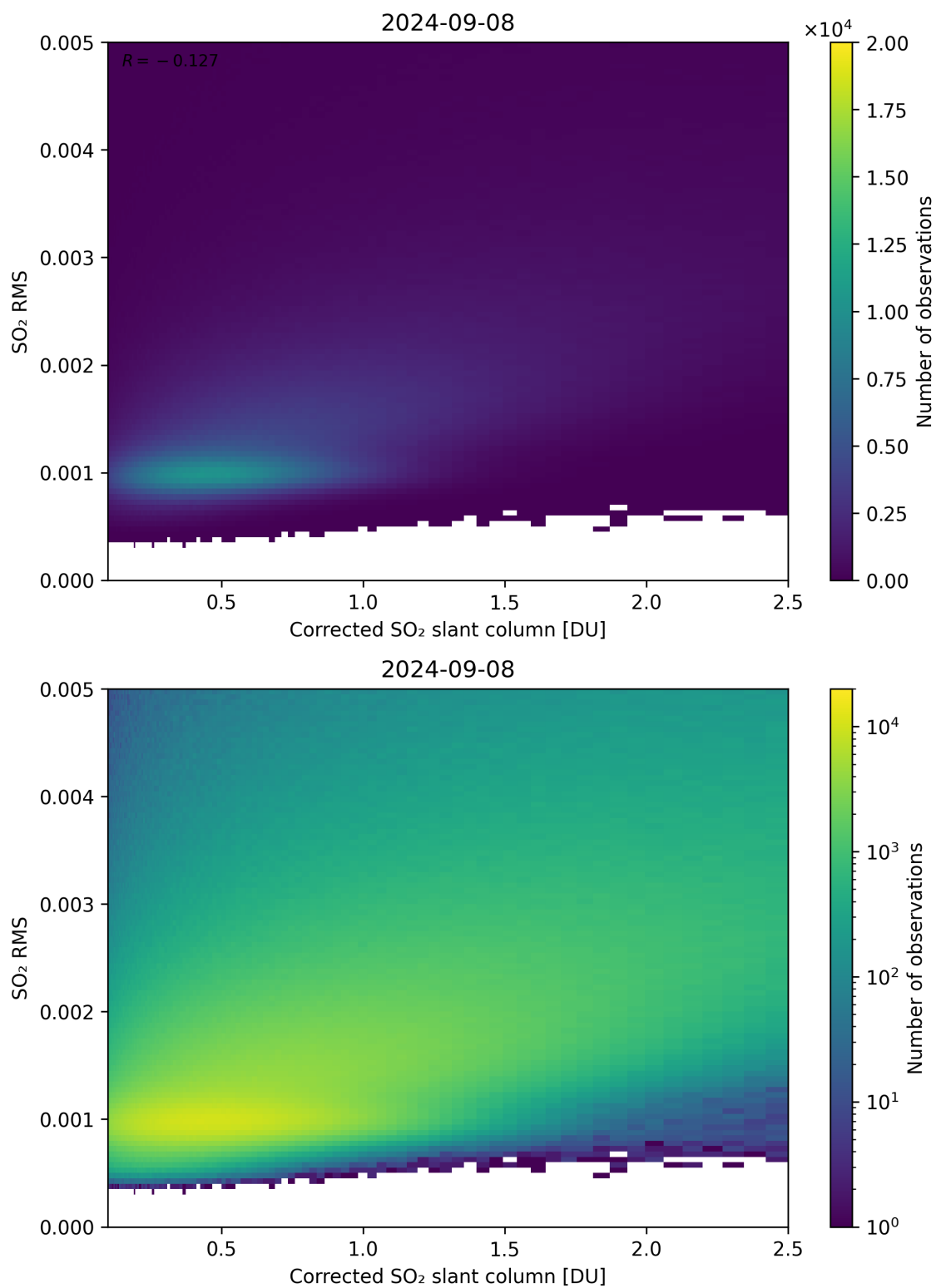
Figure 183: Scatter density plot of “Corrected SO 2 slant column” against “SO 2 RMS” for 2024-09-07 to 2024-09-09.
