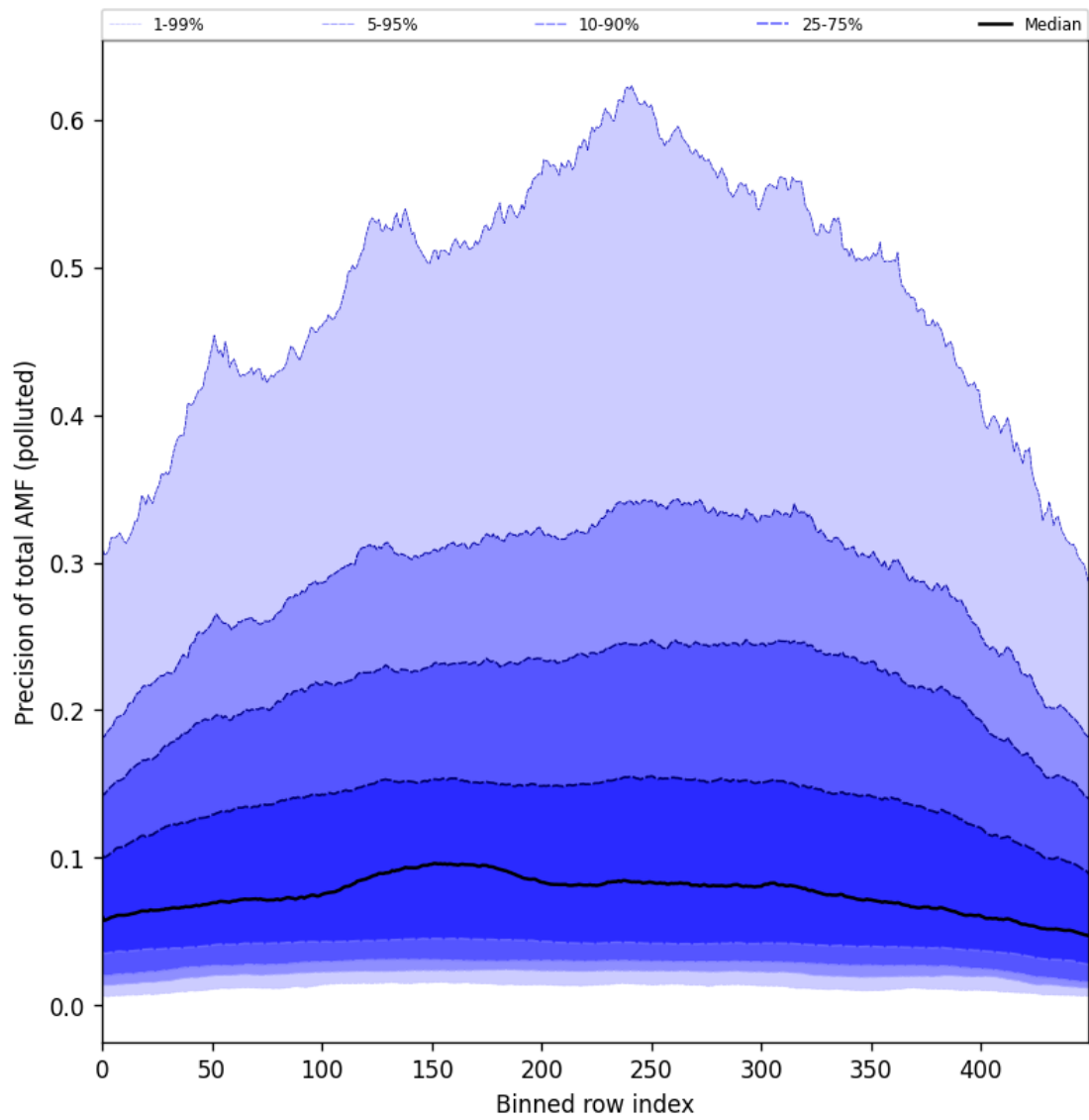
Figure 95: Along track statistics of “Precision of total AMF (polluted)” for 2024-09-07 to 2024-09-09
