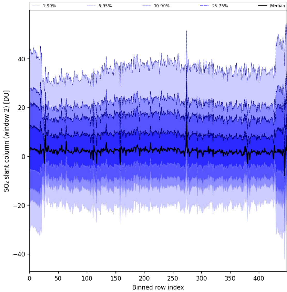
Figure 83: Along track statistics of “SO 2 slant column (window 2)” for 2024-09-07 to 2024-09-09
