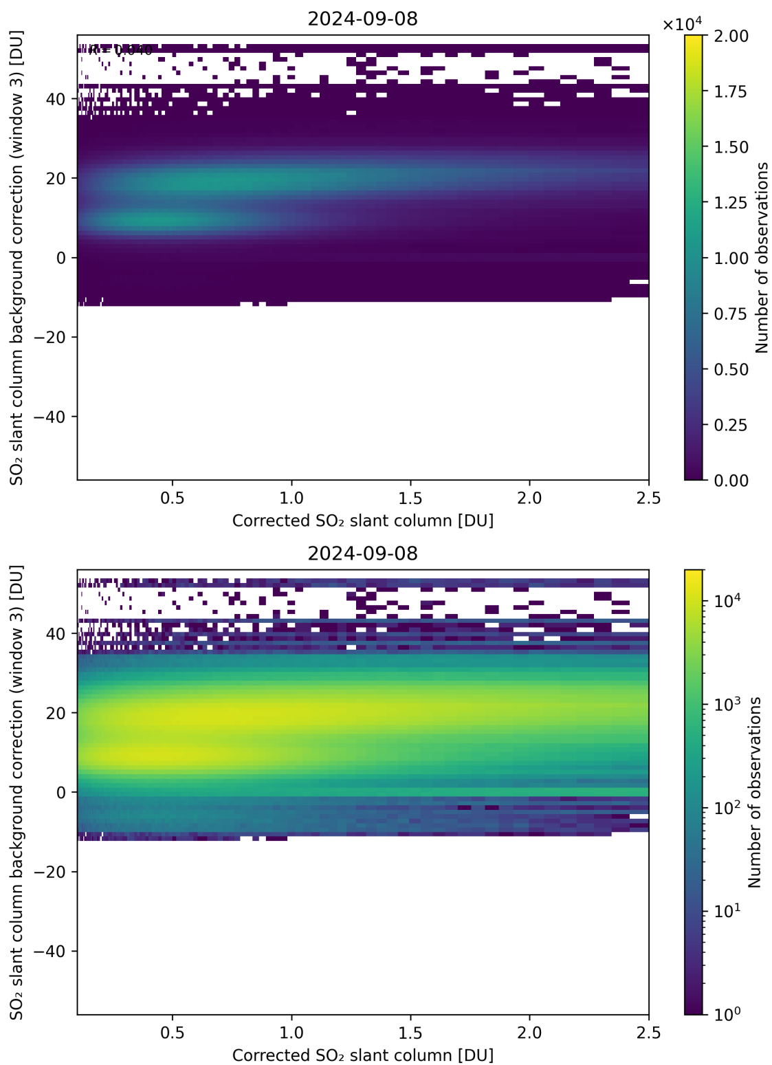
Figure 180: Scatter density plot of “Corrected SO 2 slant column” against “SO 2 slant column background correction (window 3)” for 2024-09-07 to 2024-09-09.
