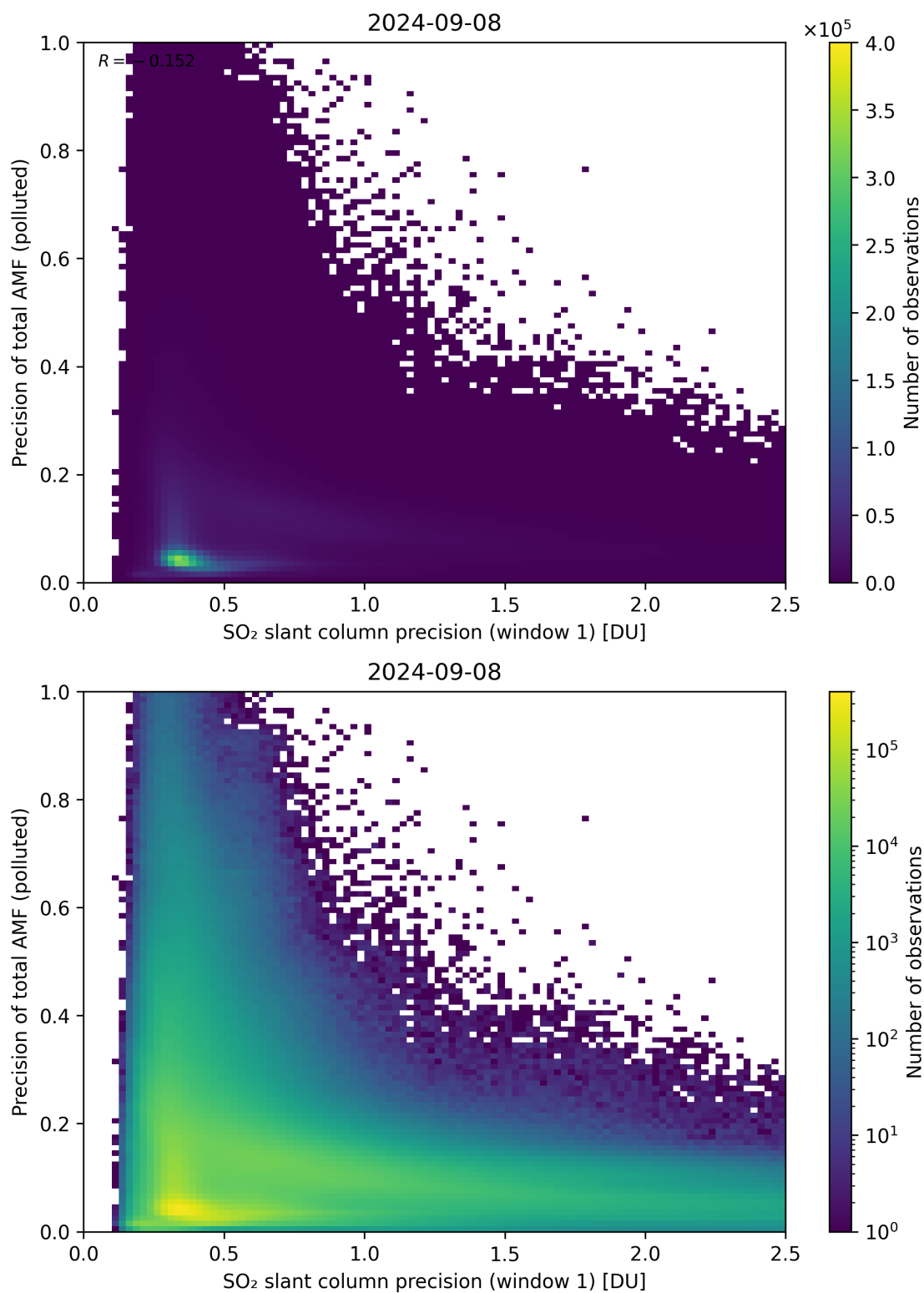
Figure 231: Scatter density plot of “SO 2 slant column precision (window 1)” against “Precision of total AMF (polluted)” for 2024-09-07 to 2024-09-09.
