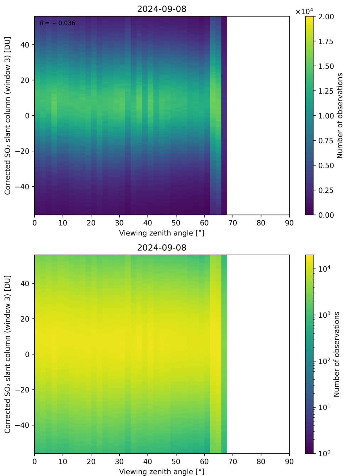
Figure 319: Scatter density plot of “Viewing zenith angle” against “Corrected SO 2 slant column (window 3)” for 2024-09-07 to 2024-09-09.
