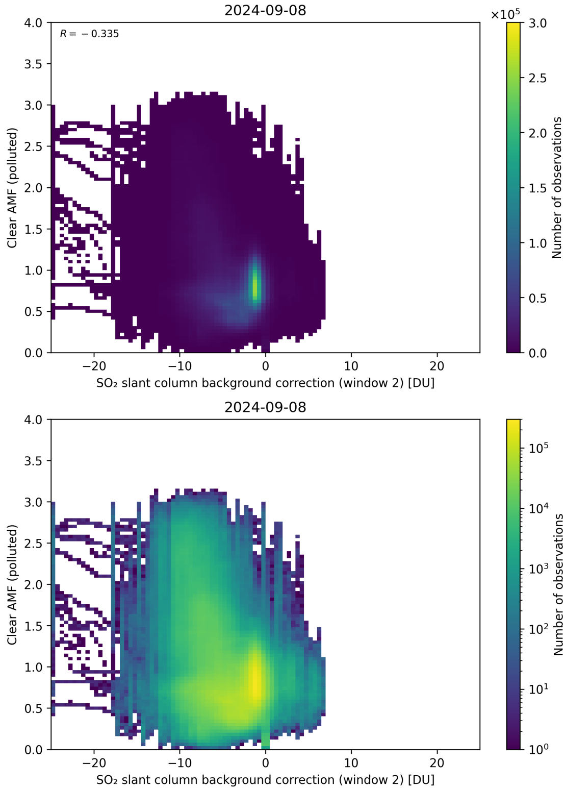
Figure 115: Scatter density plot of “SO 2 slant column background correction (window 2)” against “Clear AMF (polluted)” for 2024-09-07 to 2024-09-09.
