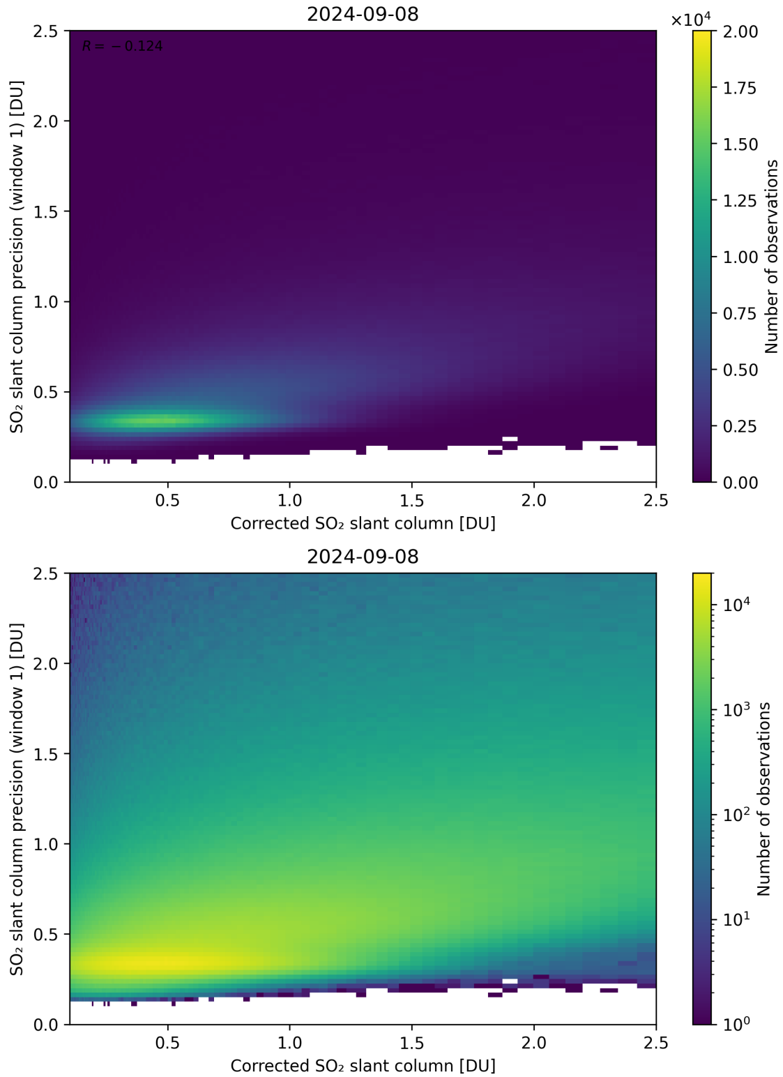
Figure 188: Scatter density plot of “Corrected SO 2 slant column” against “SO 2 slant column precision (window 1)” for 2024-09-07 to 2024-09-09.
