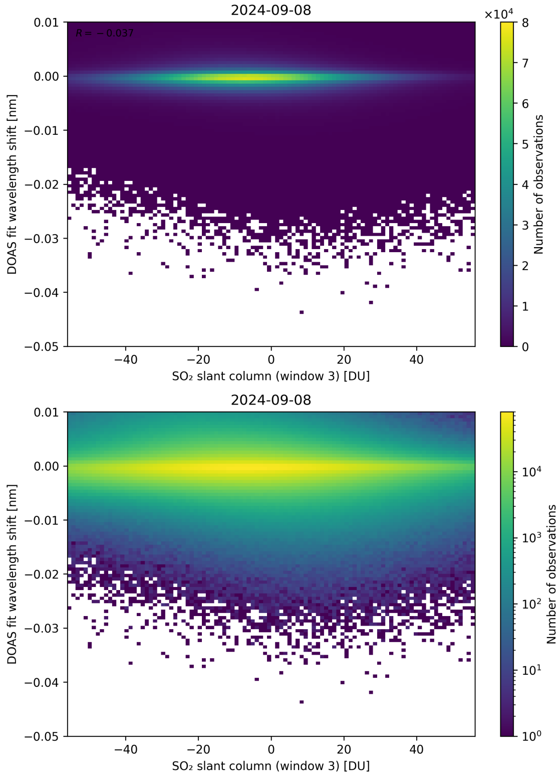
Figure 254: Scatter density plot of “SO 2 slant column (window 3)” against “DOAS fit wavelength shift” for 2024-09-07 to 2024-09-09.
