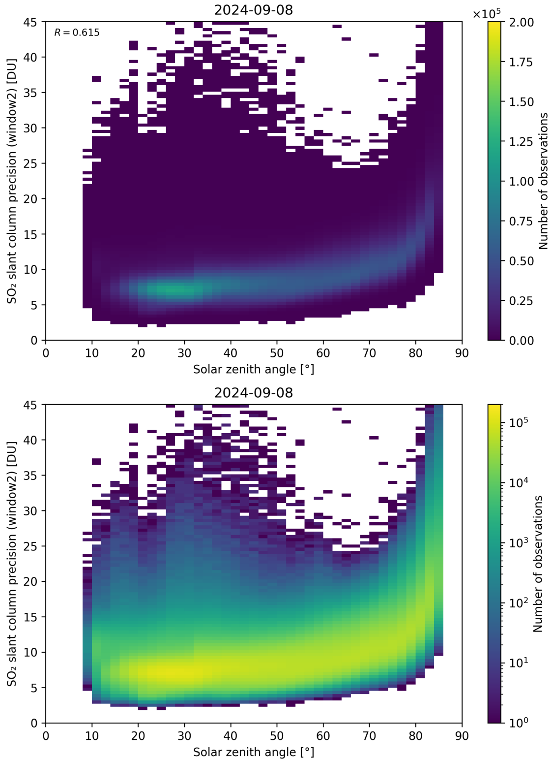
Figure 171: Scatter density plot of “Solar zenith angle” against “SO 2 slant column precision (window2)” for 2024-09-07 to 2024-09-09.
