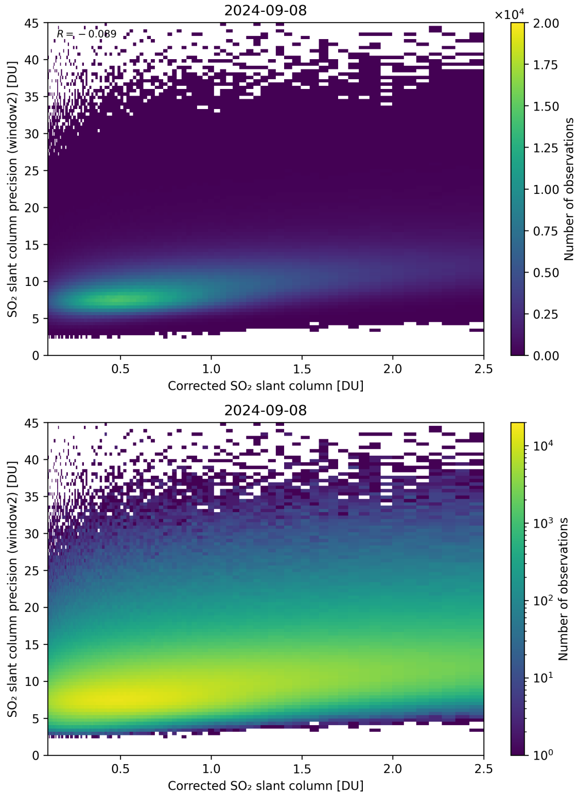
Figure 189: Scatter density plot of “Corrected SO 2 slant column” against “SO 2 slant column precision (window2)” for 2024-09-07 to 2024-09-09.
