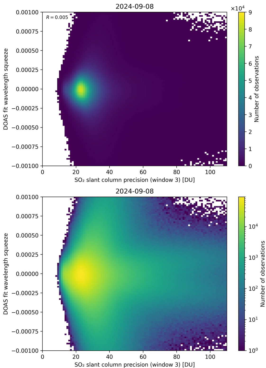
Figure 259: Scatter density plot of “SO 2 slant column precision (window 3)” against “DOAS fit wavelength squeeze” for 2024-09-07 to 2024-09-09.
