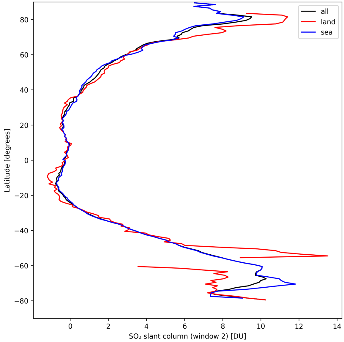
Figure 37: Zonal average of “SO 2 slant column (window 2)” for 2024-09-07 to 2024-09-09.
