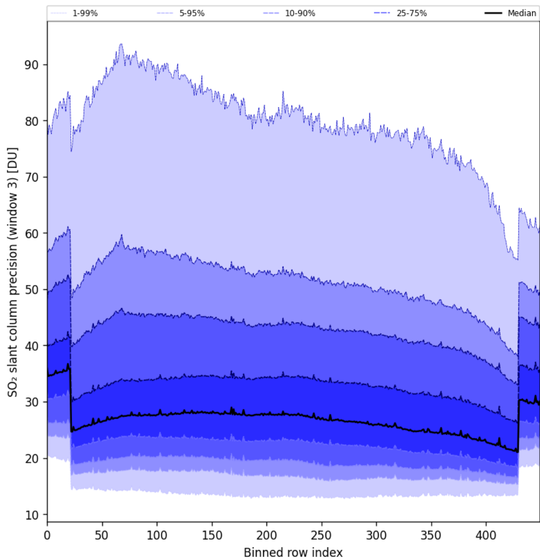
Figure 88: Along track statistics of “SO 2 slant column precision (window 3)” for 2024-09-07 to 2024-09-09
