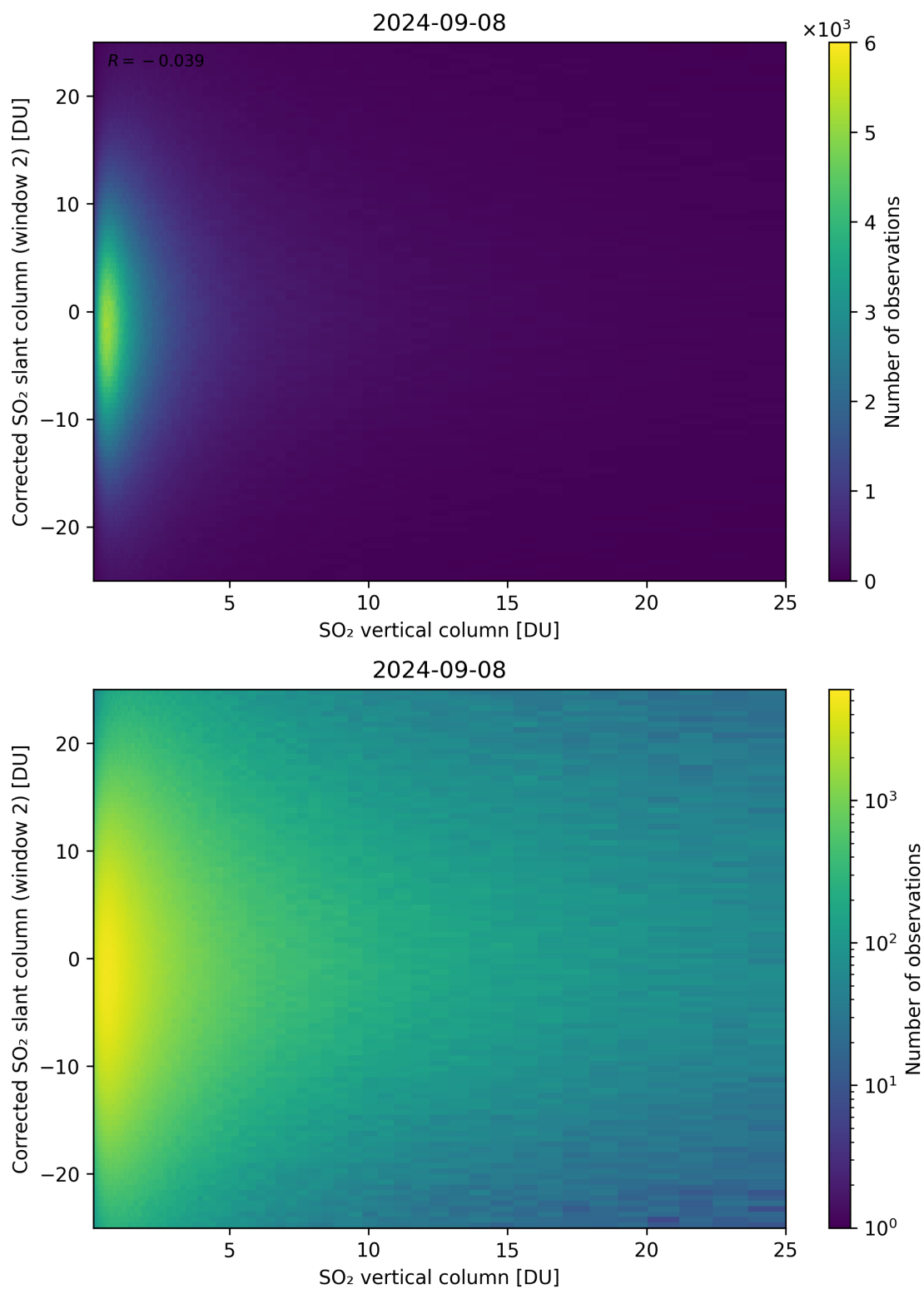
Figure 298: Scatter density plot of “SO 2 vertical column” against “Corrected SO 2 slant column (window 2)” for 2024-09-07 to 2024-09-09.
