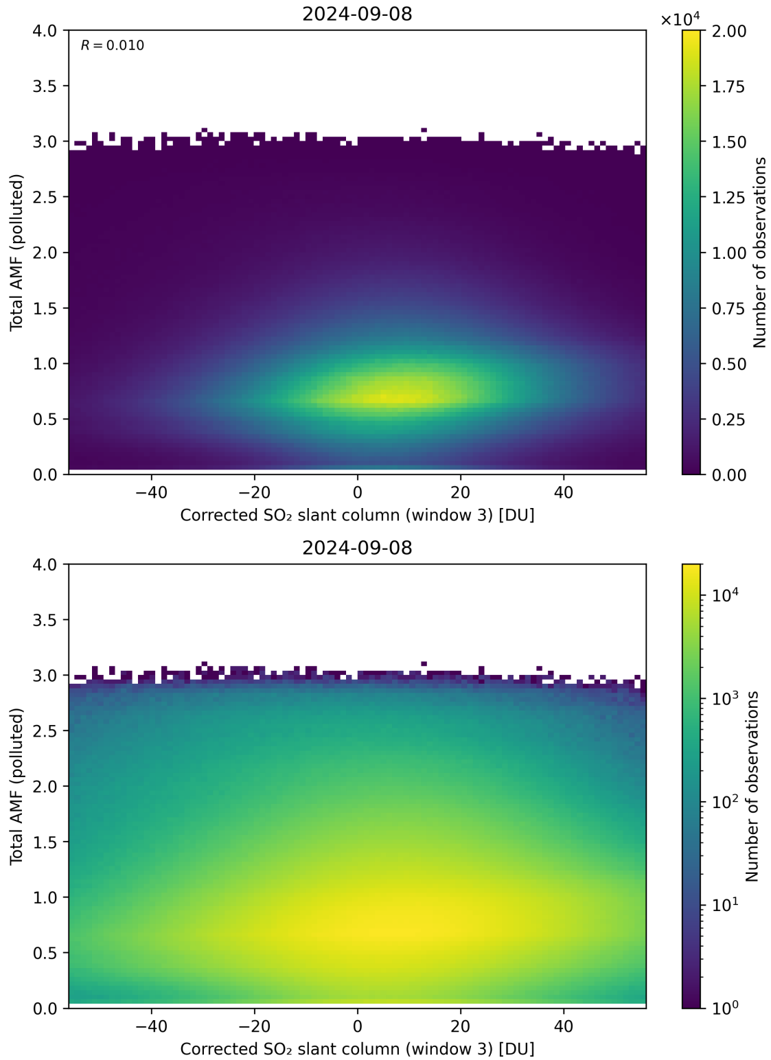
Figure 210: Scatter density plot of “Corrected SO 2 slant column (window 3)” against “Total AMF (polluted)” for 2024-09-07 to 2024-09-09.
