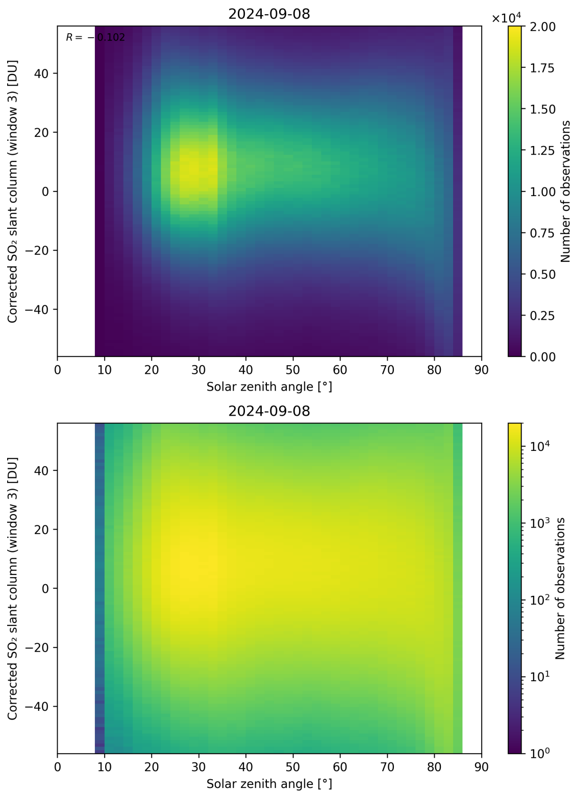
Figure 168: Scatter density plot of “Solar zenith angle” against “Corrected SO 2 slant column (window 3)” for 2024-09-07 to 2024-09-09.
