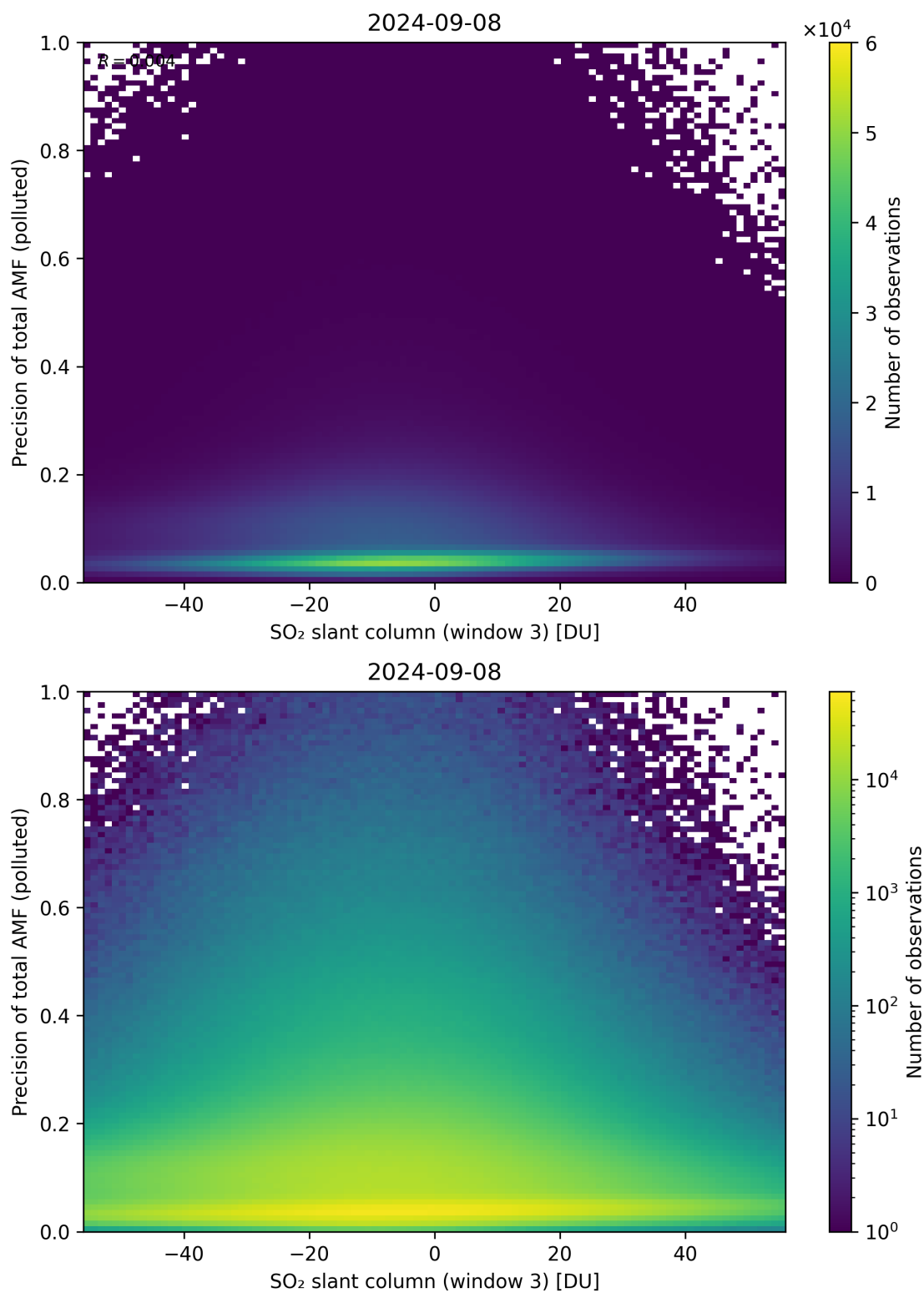
Figure 269: Scatter density plot of “SO 2 slant column (window 3)” against “Precision of total AMF (polluted)” for 2024-09-07 to 2024-09-09.
