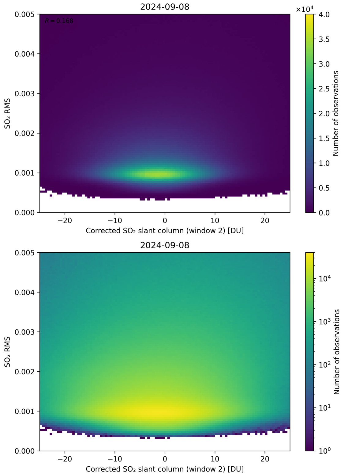
Figure 198: Scatter density plot of “Corrected SO 2 slant column (window 2)” against “SO 2 RMS” for 2024-09-07 to 2024-09-09.
