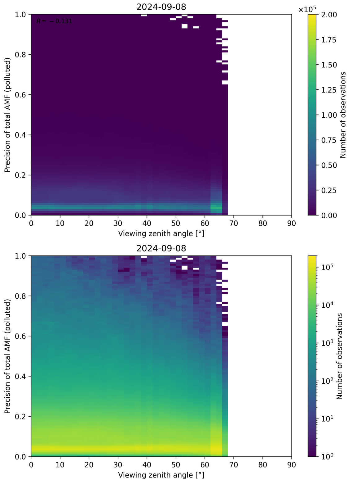
Figure 326: Scatter density plot of “Viewing zenith angle” against “Precision of total AMF (polluted)” for 2024-09-07 to 2024-09-09.
