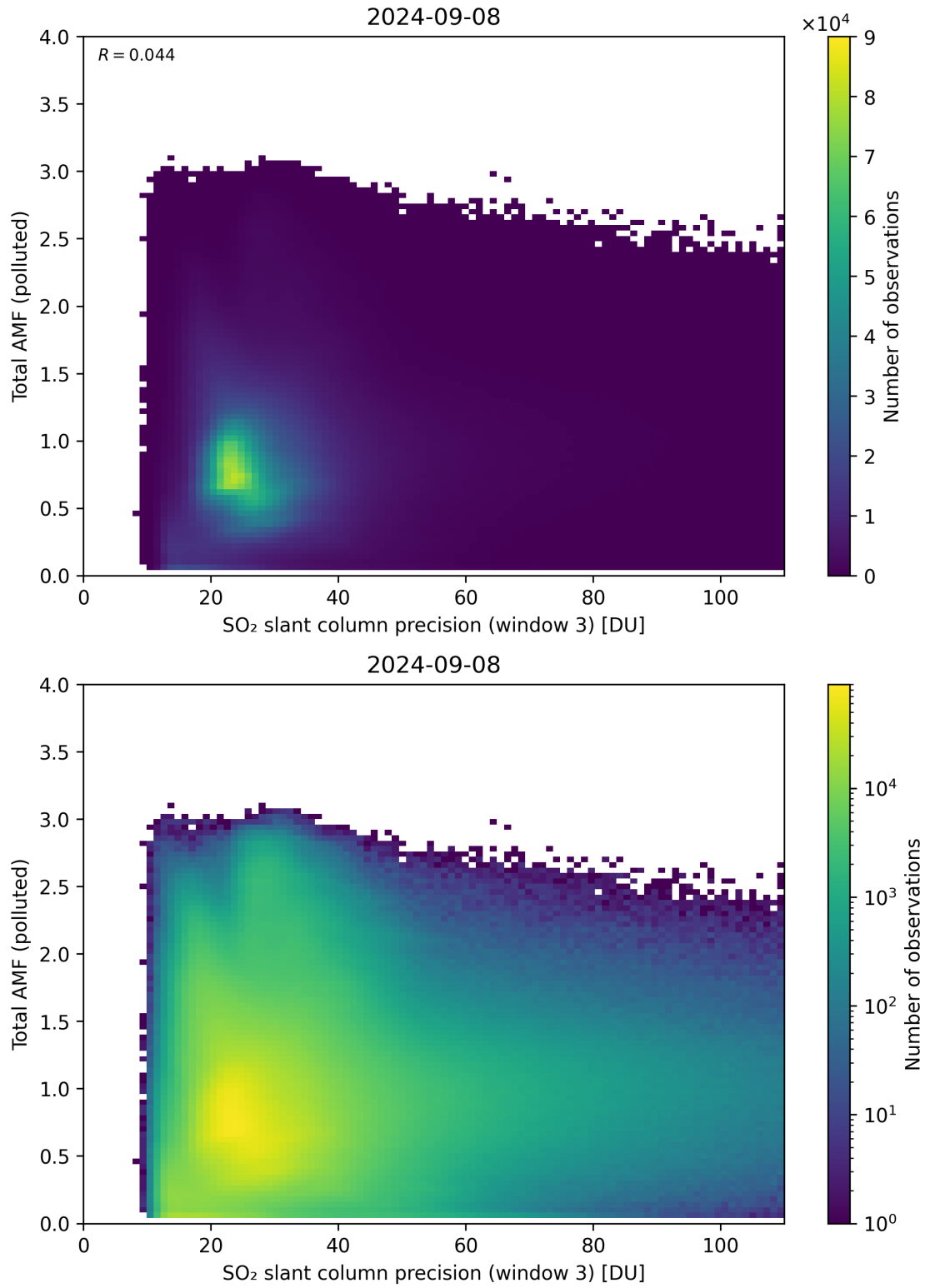
Figure 263: Scatter density plot of “SO 2 slant column precision (window 3)” against “Total AMF (polluted)” for 2024-09-07 to 2024-09-09.
