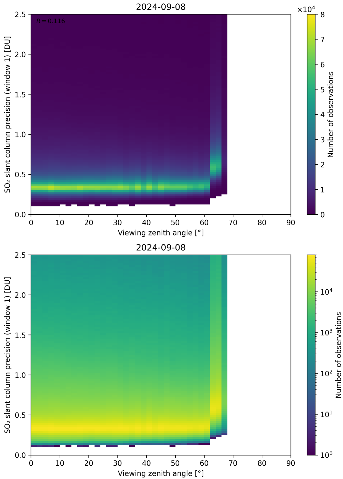
Figure 321: Scatter density plot of “Viewing zenith angle” against “SO 2 slant column precision (window 1)” for 2024-09-07 to 2024-09-09.
