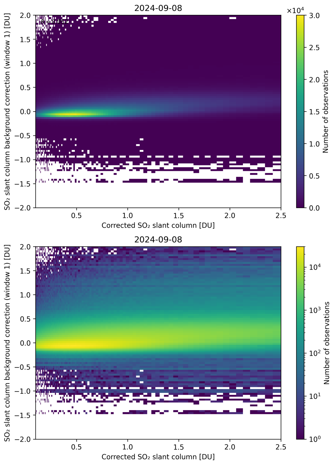
Figure 178: Scatter density plot of “Corrected SO 2 slant column” against “SO 2 slant column background correction (window 1)” for 2024-09-07 to 2024-09-09.
