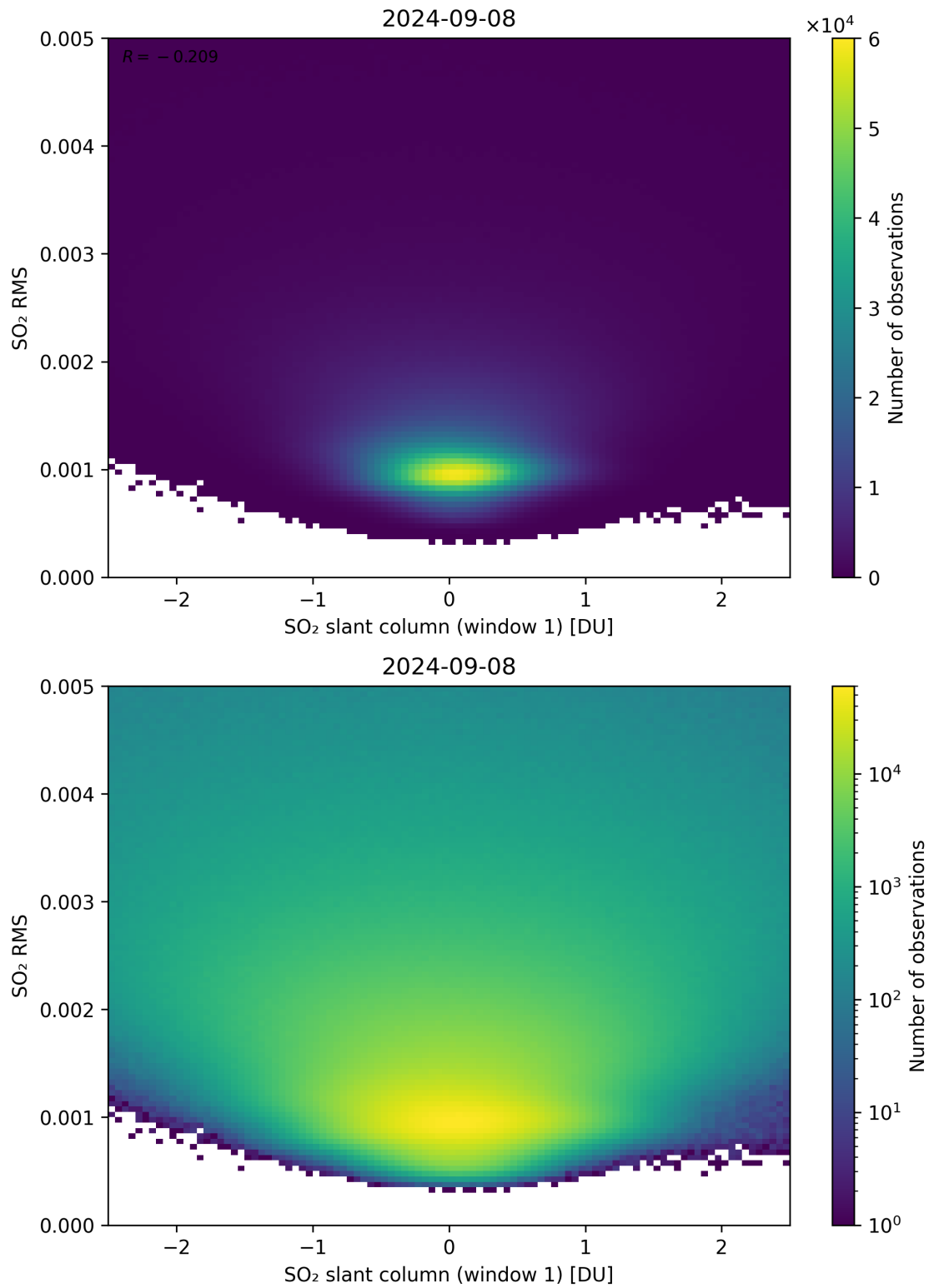
Figure 217: Scatter density plot of “SO 2 slant column (window 1)” against “SO 2 RMS” for 2024-09-07 to 2024-09-09.
