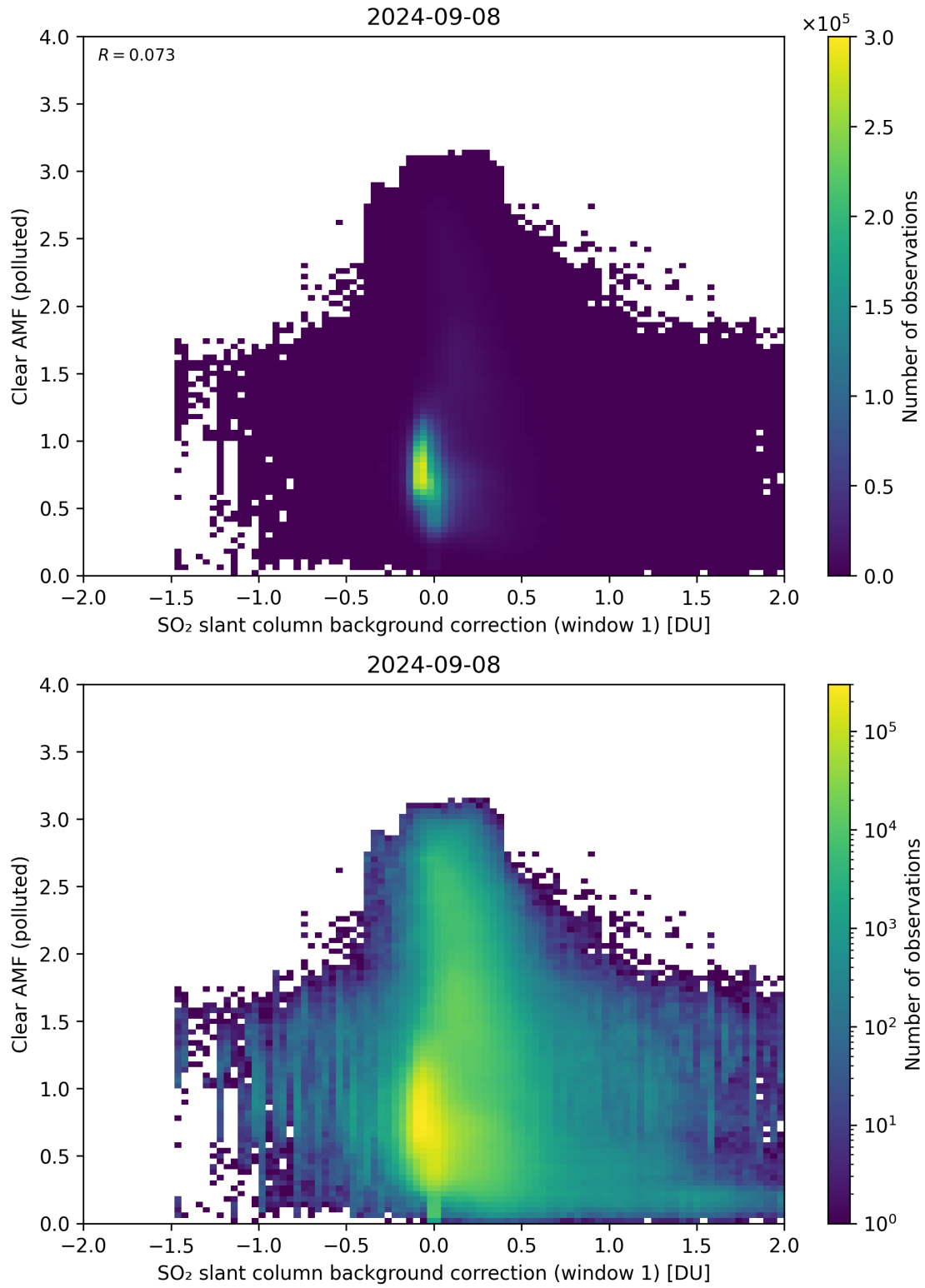
Figure 103: Scatter density plot of “SO 2 slant column background correction (window 1)” against “Clear AMF (polluted)” for 2024-09-07 to 2024-09-09.
