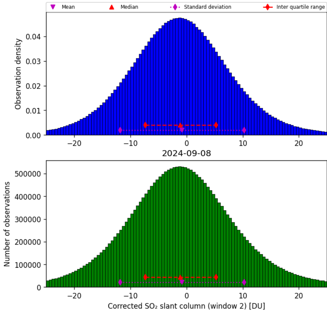
Figure 62: Histogram of “Corrected SO 2 slant column (window 2)” for 2024-09-07 to 2024-09-09
