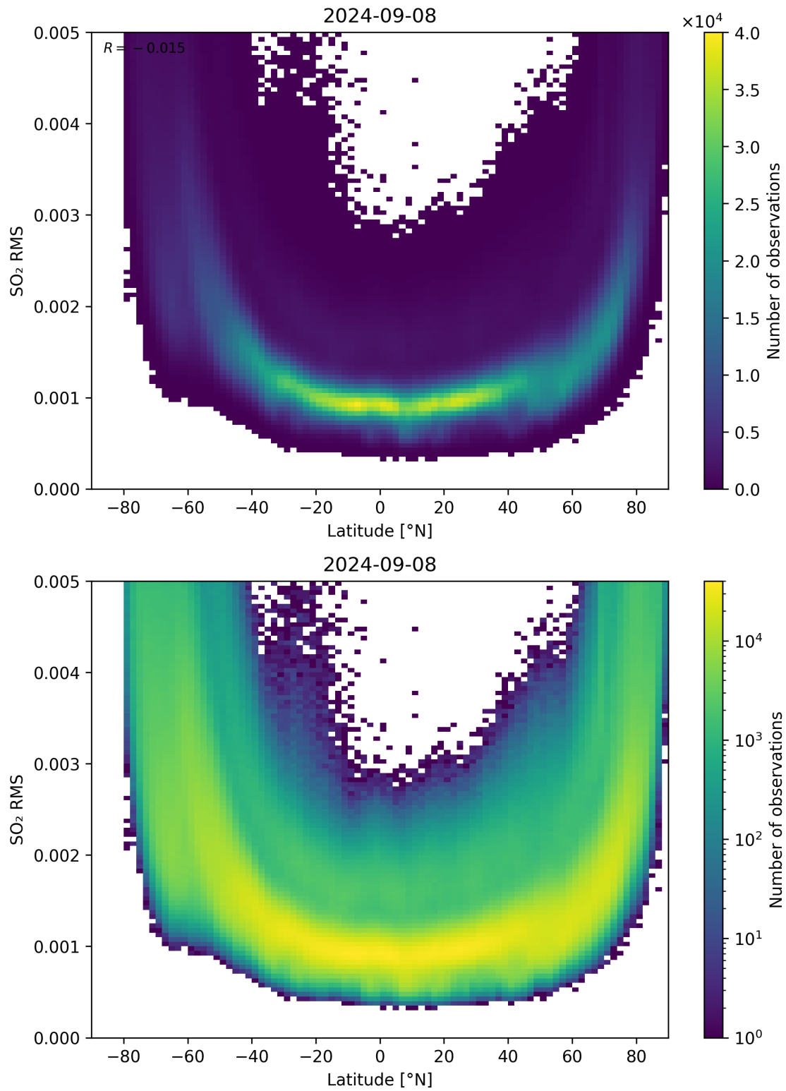
Figure 144: Scatter density plot of “Latitude” against “SO 2 RMS” for 2024-09-07 to 2024-09-09.
