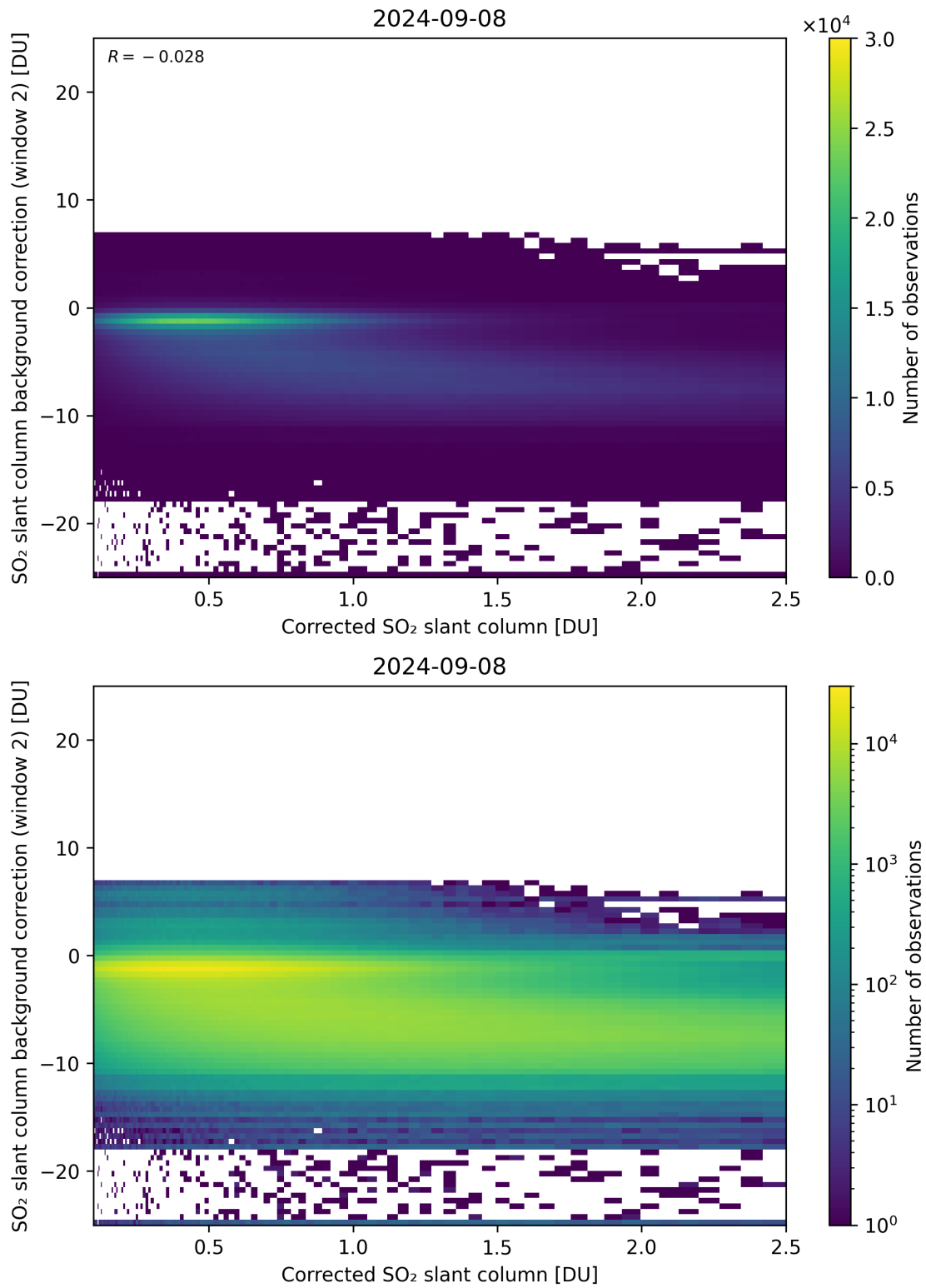
Figure 179: Scatter density plot of “Corrected SO 2 slant column” against “SO 2 slant column background correction (window 2)” for 2024-09-07 to 2024-09-09.
