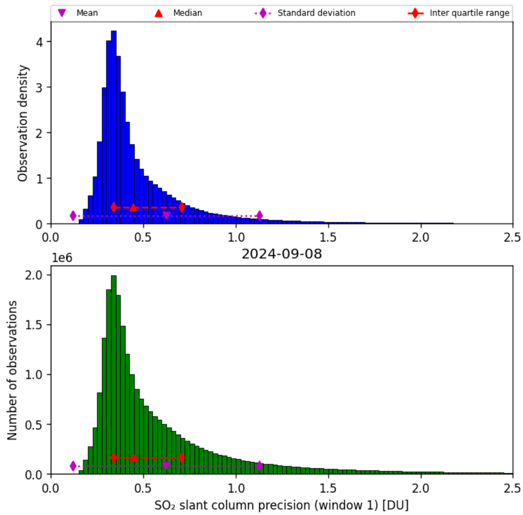
Figure 57: Histogram of “SO 2 slant column precision (window 1)” for 2024-09-07 to 2024-09-09
