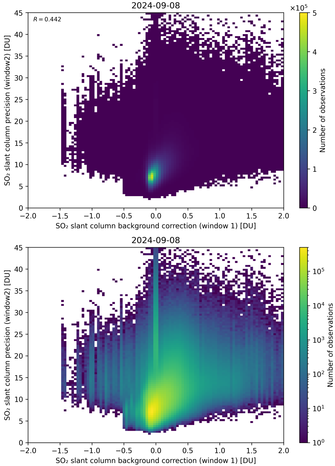
Figure 106: Scatter density plot of “SO 2 slant column background correction (window 1)” against “SO 2 slant column precision (window2)” for 2024-09-07 to 2024-09-09.
