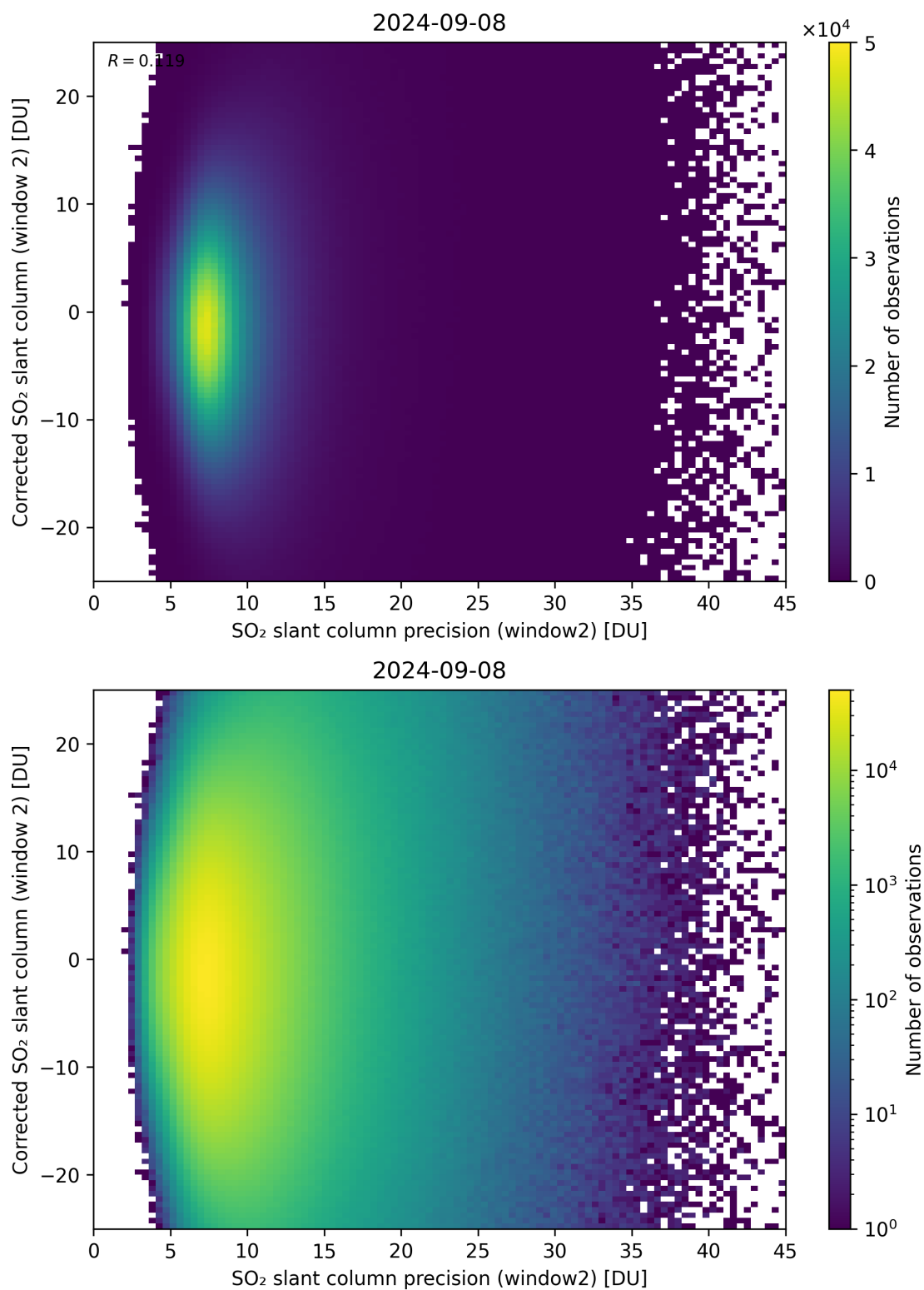
Figure 247: Scatter density plot of “SO 2 slant column precision (window2)” against “Corrected SO 2 slant column (window 2)” for 2024-09-07 to 2024-09-09.
