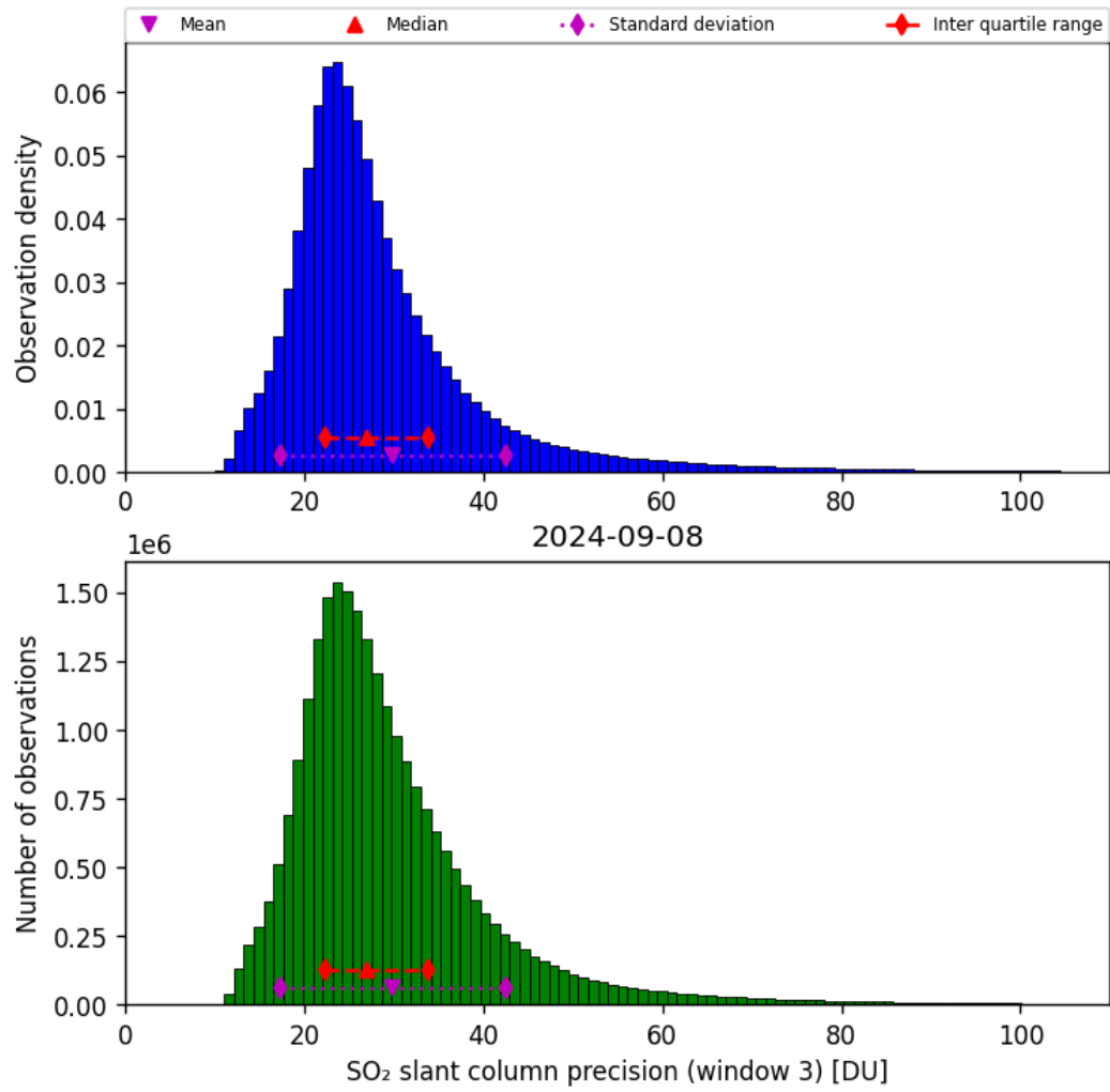
Figure 65: Histogram of “SO 2 slant column precision (window 3)” for 2024-09-07 to 2024-09-09
