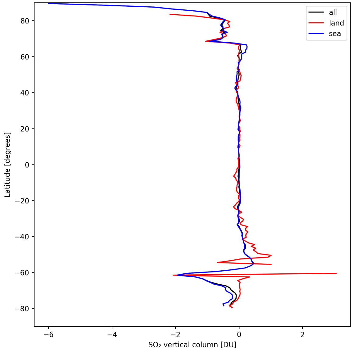
Figure 30: Zonal average of “SO 2 vertical column” for 2024-09-07 to 2024-09-09.
