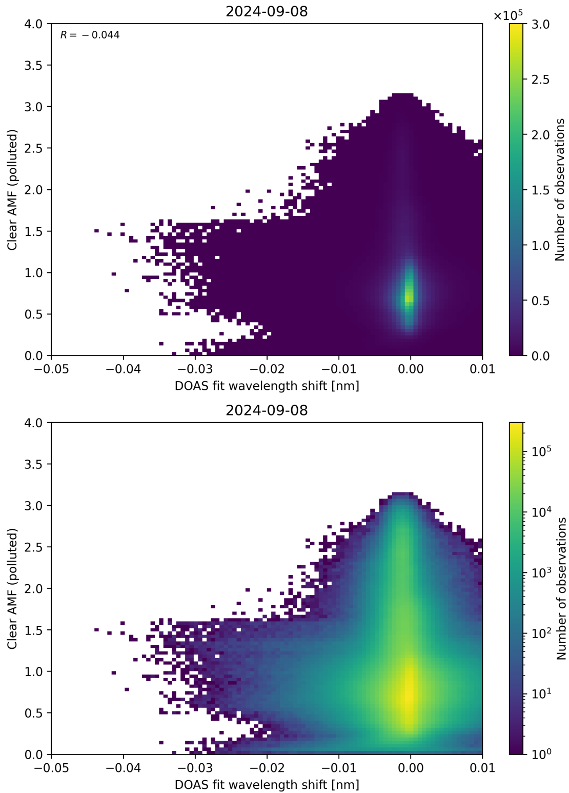
Figure 129: Scatter density plot of “DOAS fit wavelength shift” against “Clear AMF (polluted)” for 2024-09-07 to 2024-09-09.
