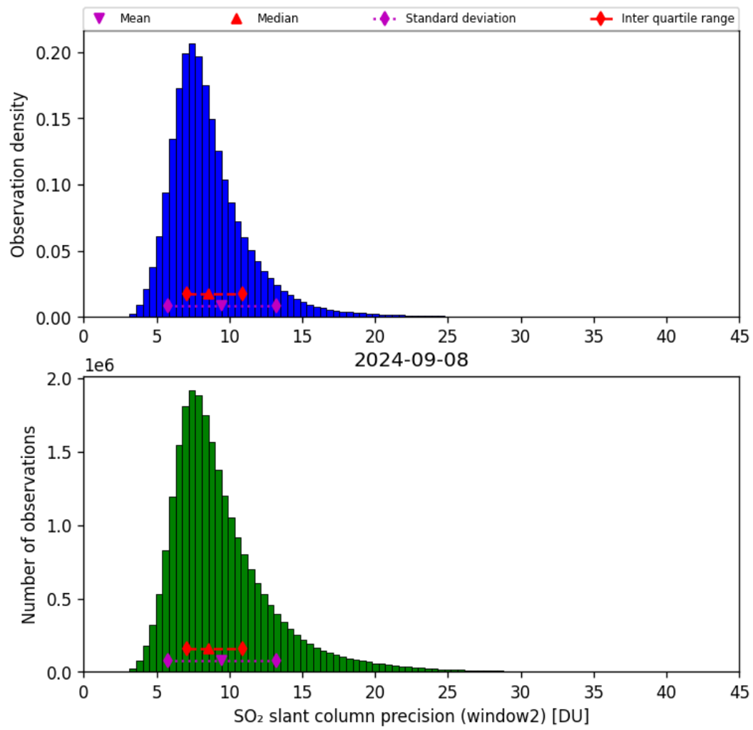
Figure 61: Histogram of “SO 2 slant column precision (window2)” for 2024-09-07 to 2024-09-09
