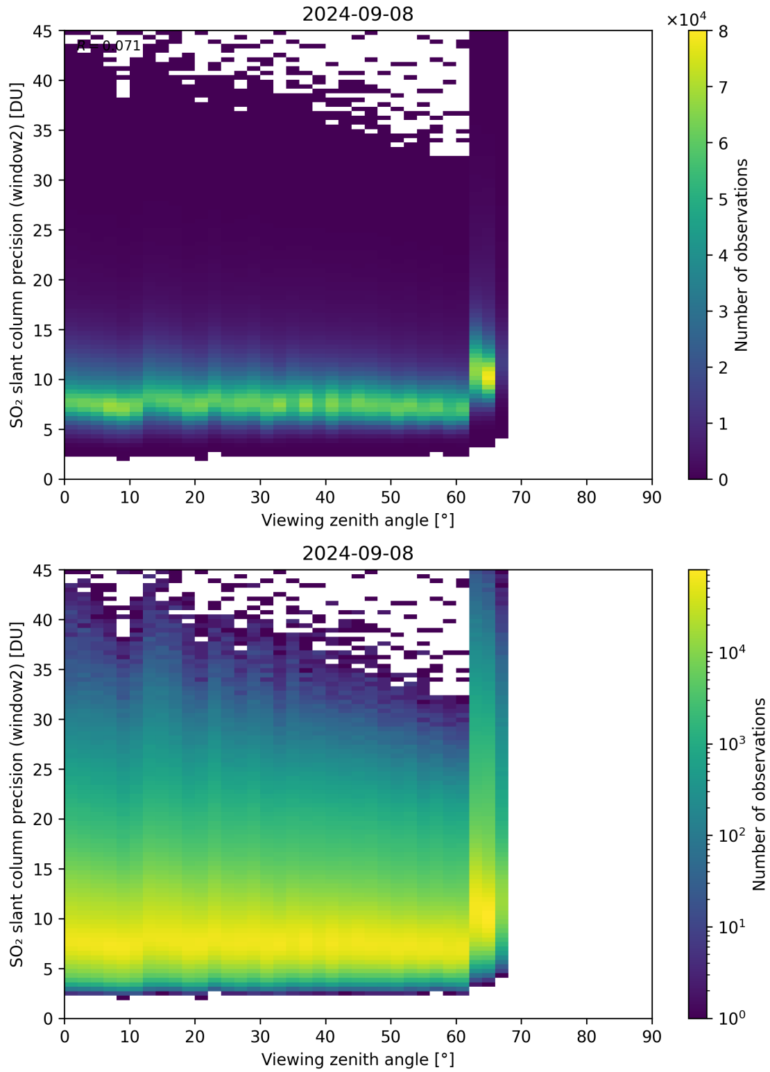
Figure 322: Scatter density plot of “Viewing zenith angle” against “SO 2 slant column precision (window2)” for 2024-09-07 to 2024-09-09.
