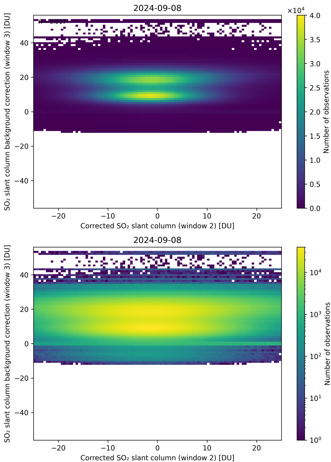
Figure 195: Scatter density plot of “Corrected SO 2 slant column (window 2)” against “SO 2 slant column background correction (window 3)” for 2024-09-07 to 2024-09-09.
