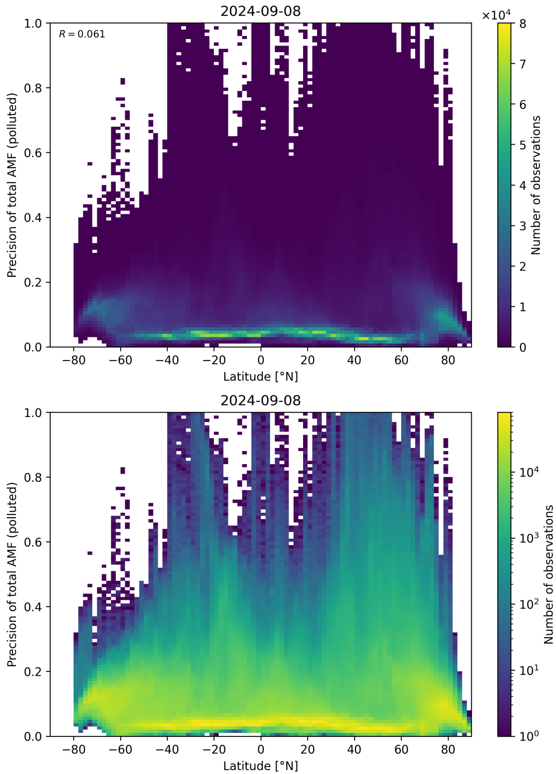
Figure 155: Scatter density plot of “Latitude” against “Precision of total AMF (polluted)” for 2024-09-07 to 2024-09-09.
