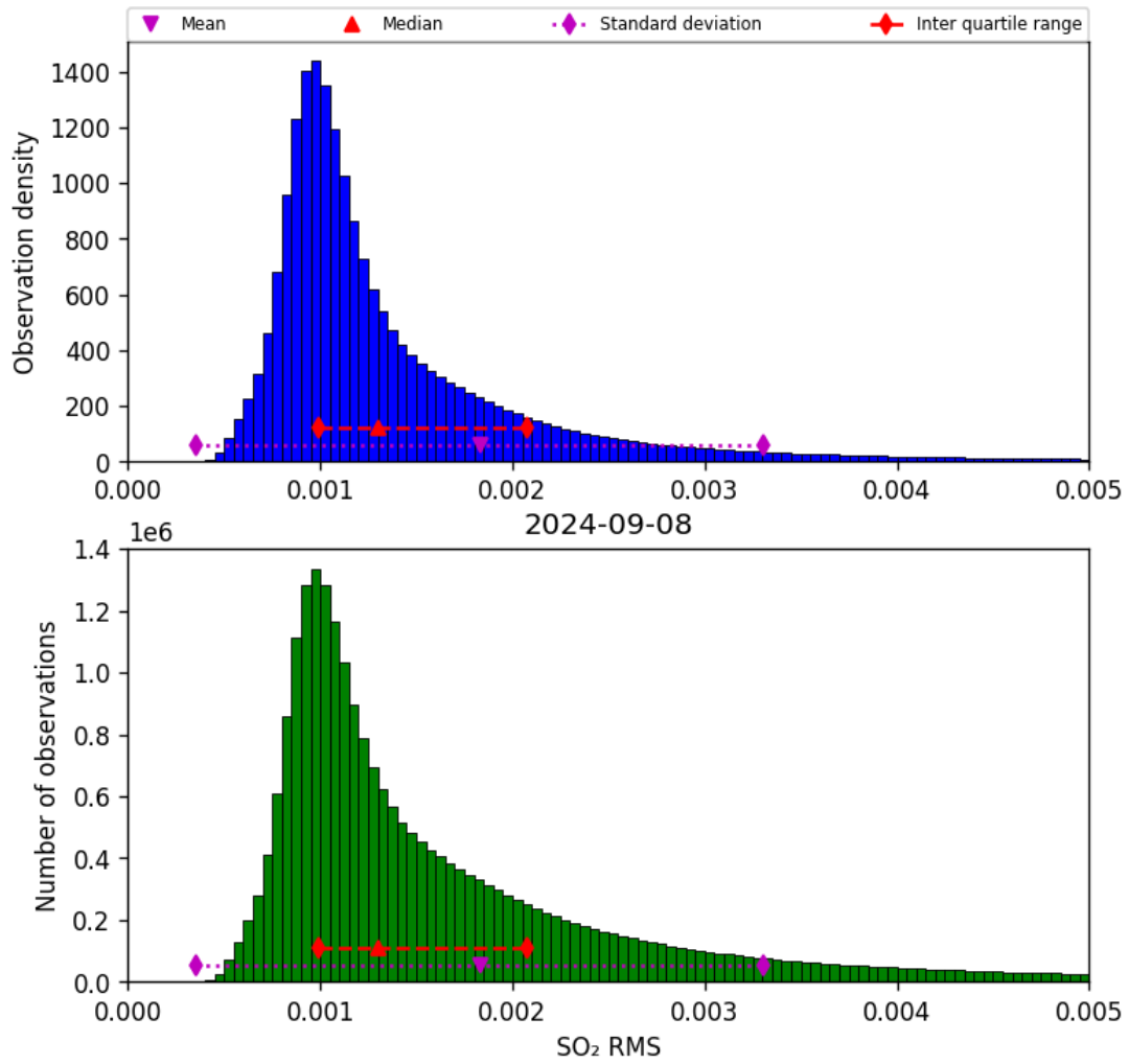
Figure 70: Histogram of “SO 2 RMS” for 2024-09-07 to 2024-09-09
