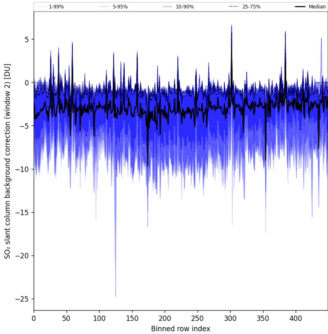
Figure 86: Along track statistics of “SO 2 slant column background correction (window 2)” for 2024-09-07 to 2024-09-09
