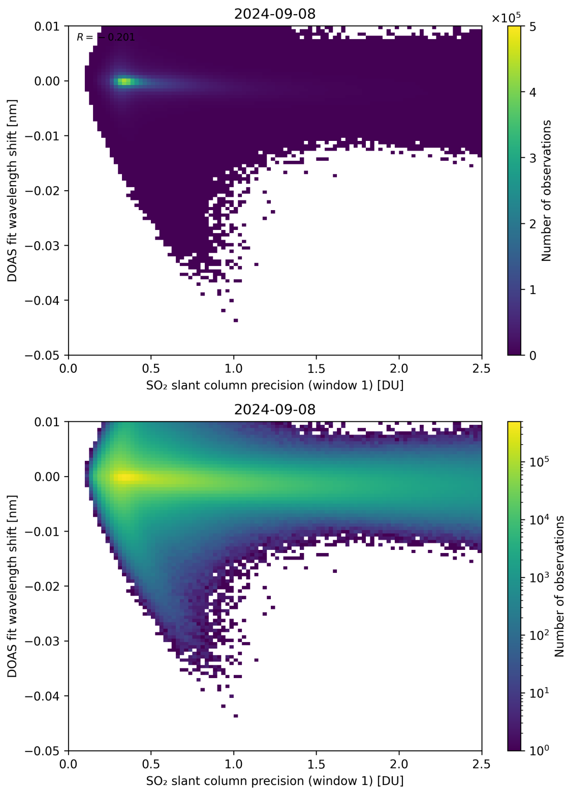
Figure 221: Scatter density plot of “SO 2 slant column precision (window 1)” against “DOAS fit wavelength shift” for 2024-09-07 to 2024-09-09.
