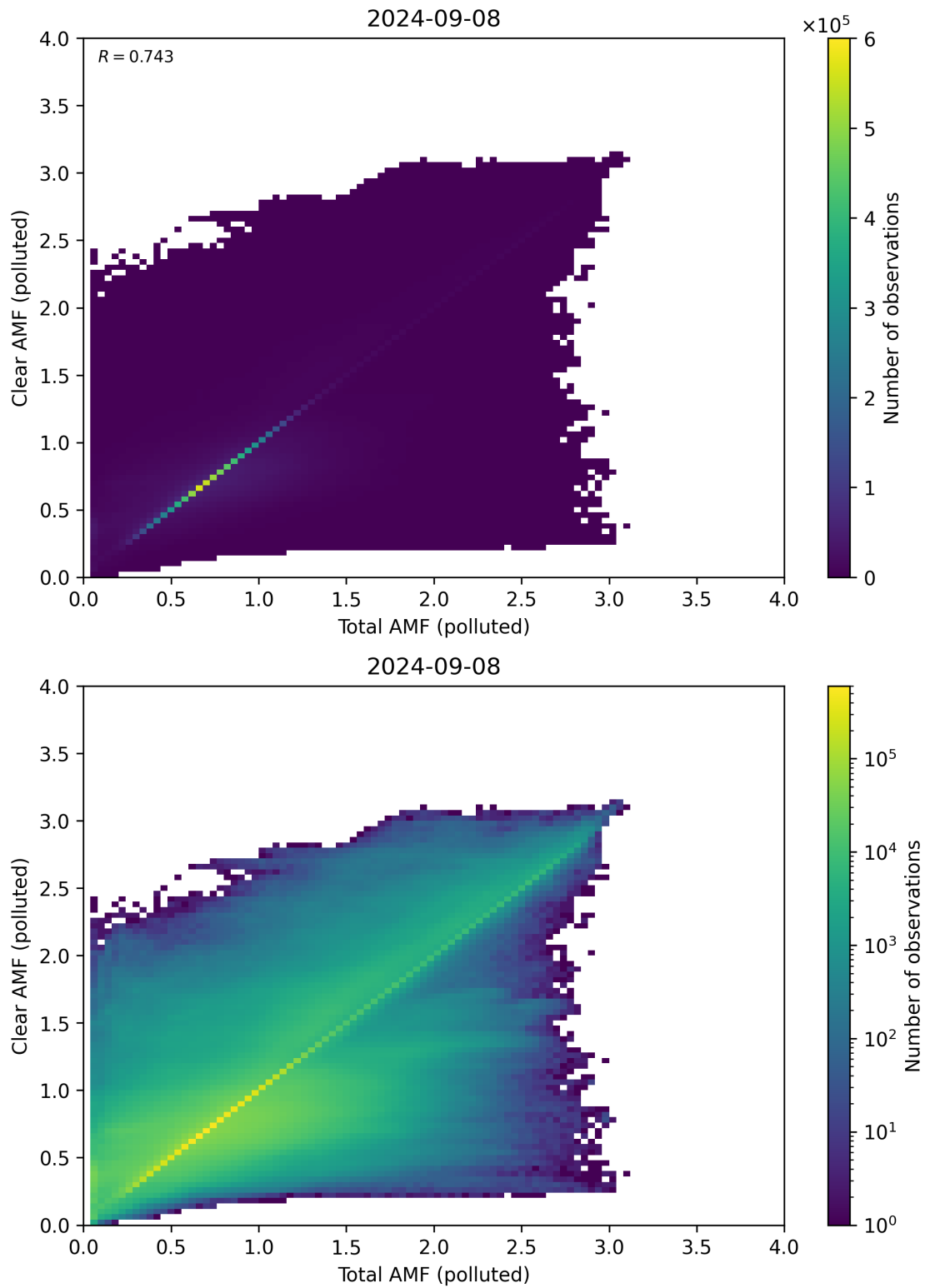
Figure 271: Scatter density plot of “Total AMF (polluted)” against “Clear AMF (polluted)” for 2024-09-07 to 2024-09-09.
