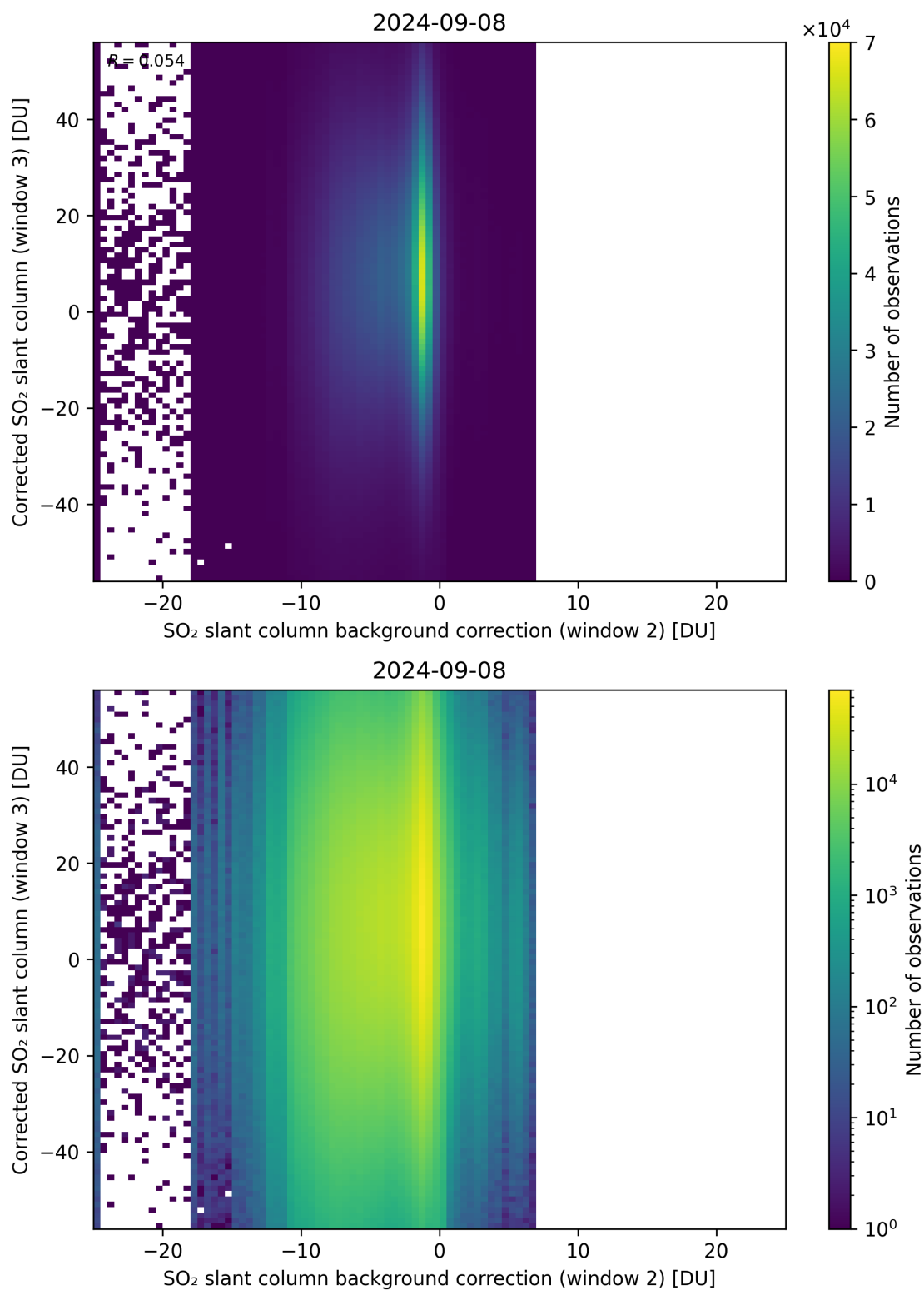
Figure 116: Scatter density plot of “SO 2 slant column background correction (window 2)” against “Corrected SO 2 slant column (window 3)” for 2024-09-07 to 2024-09-09.
