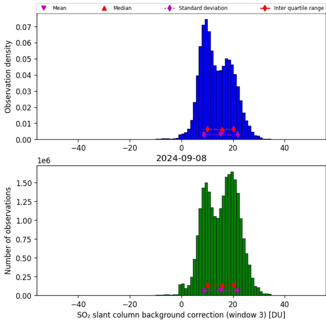
Figure 67: Histogram of “SO 2 slant column background correction (window 3)” for 2024-09-07 to 2024-09-09
