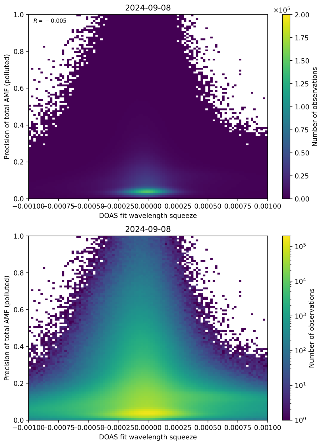
Figure 135: Scatter density plot of “DOAS fit wavelength squeeze” against “Precision of total AMF (polluted)” for 2024-09-07 to 2024-09-09.
