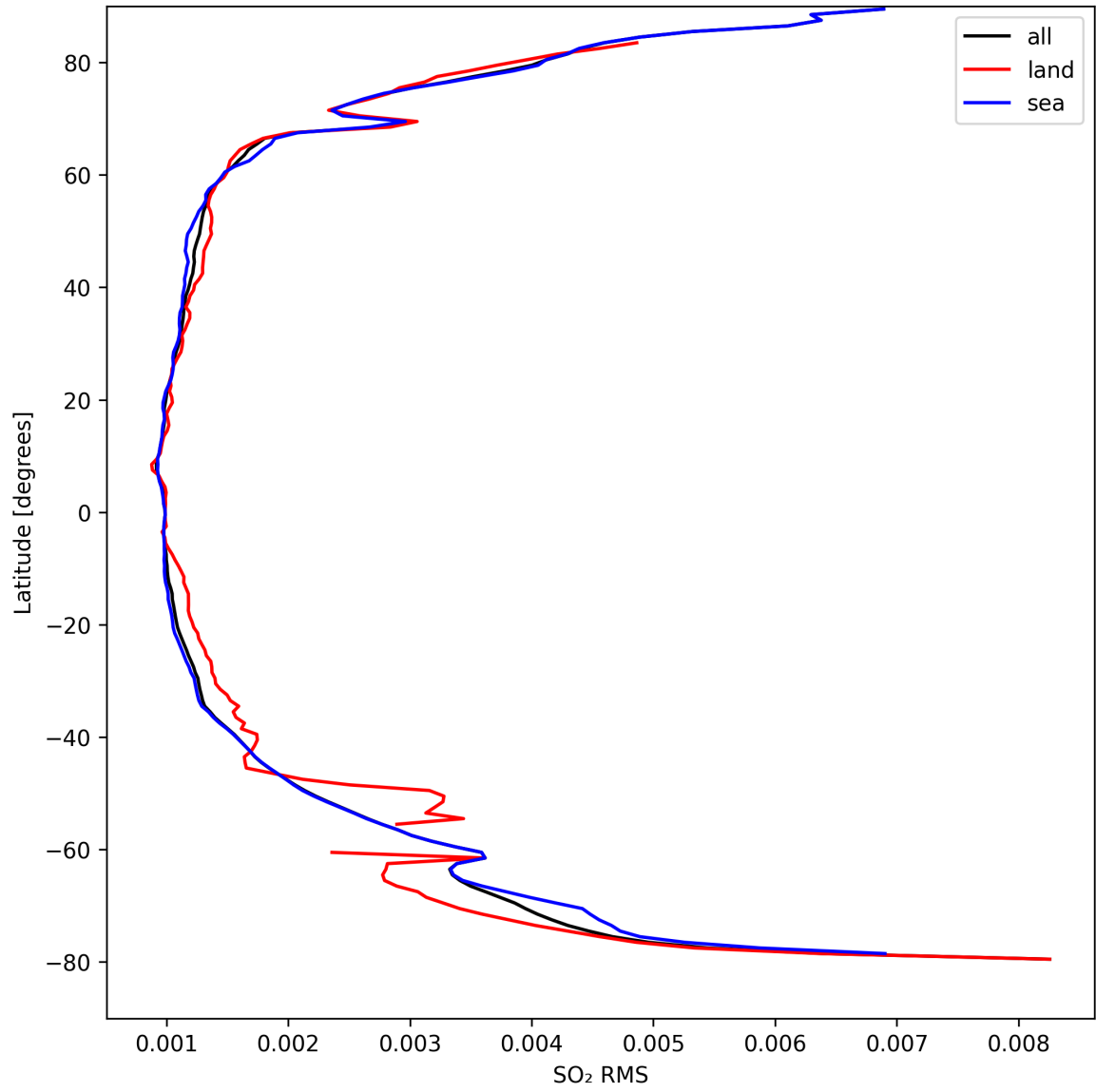
Figure 47: Zonal average of “SO 2 RMS” for 2024-09-07 to 2024-09-09.
