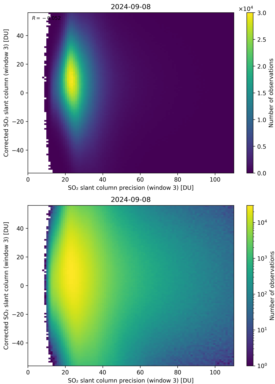
Figure 262: Scatter density plot of “SO 2 slant column precision (window 3)” against “Corrected SO 2 slant column (window 3)” for 2024-09-07 to 2024-09-09.
