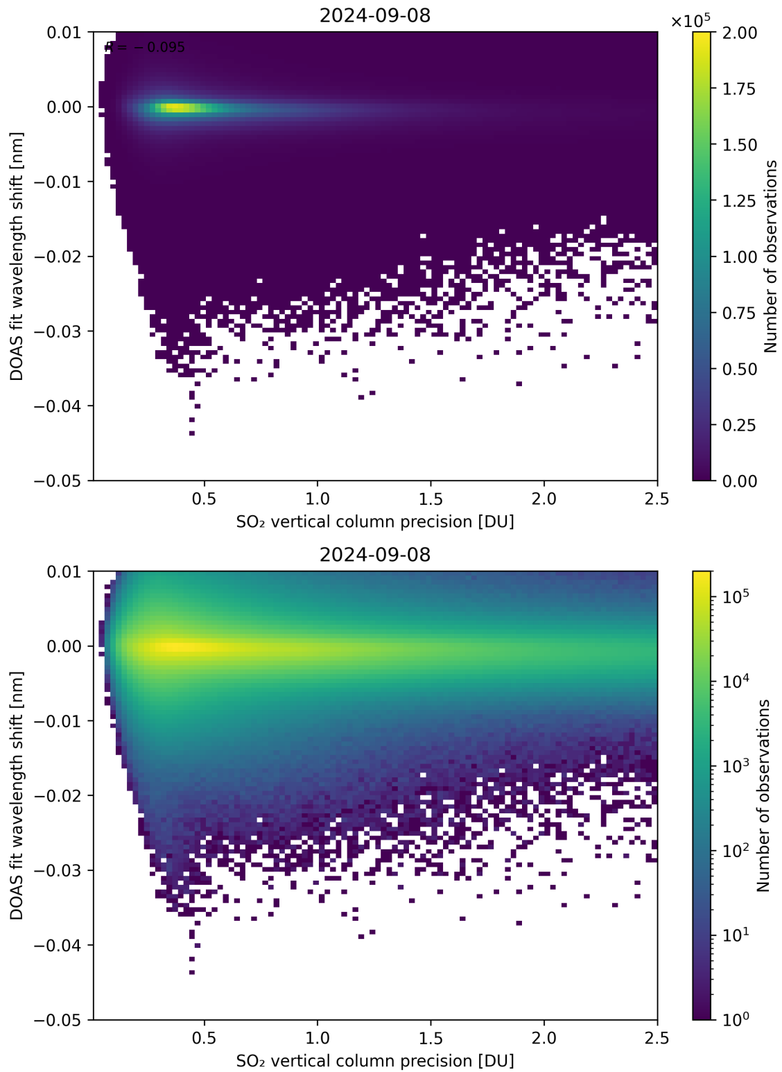
Figure 282: Scatter density plot of “SO 2 vertical column precision” against “DOAS fit wavelength shift” for 2024-09-07 to 2024-09-09.
