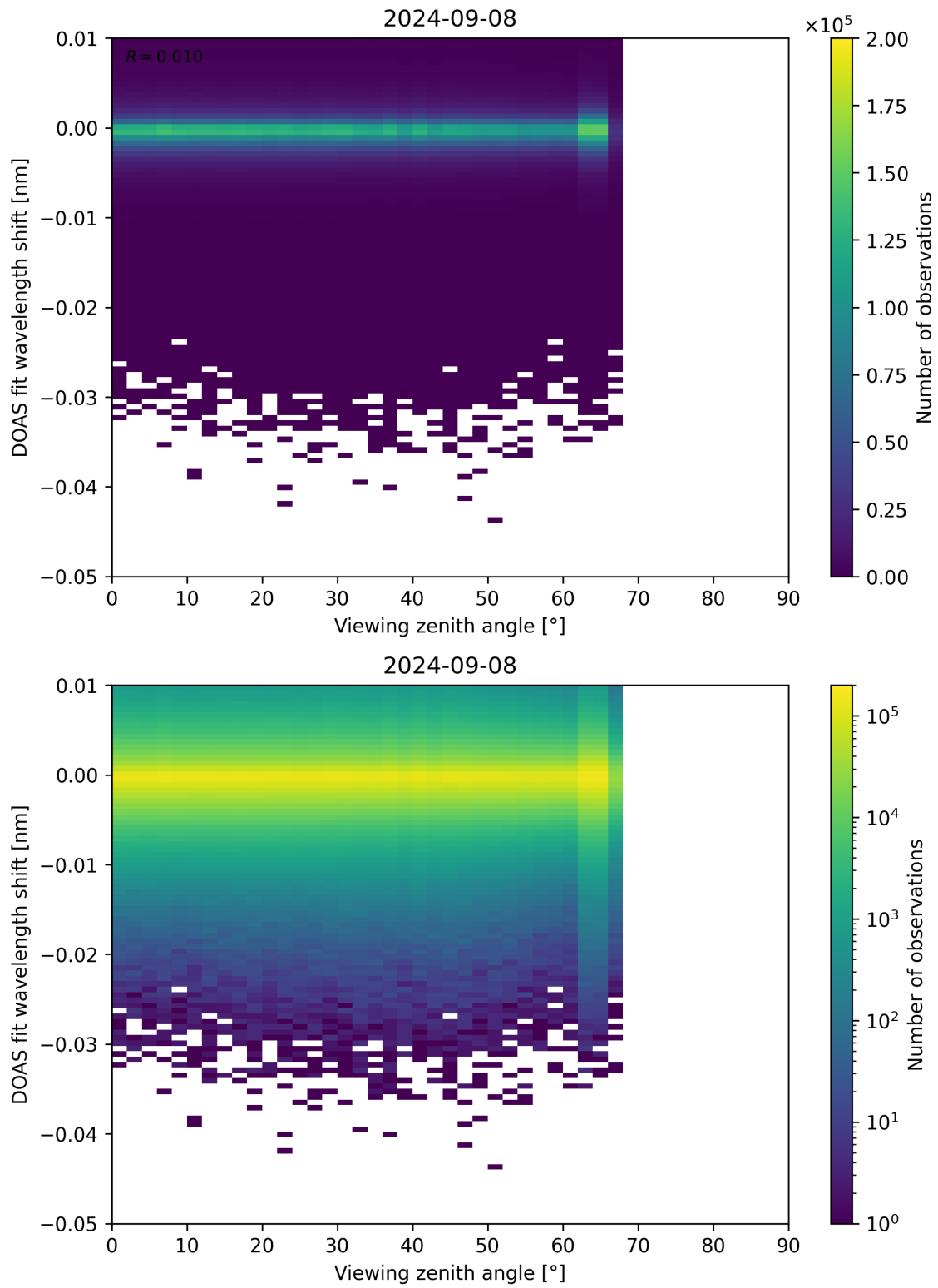
Figure 311: Scatter density plot of “Viewing zenith angle” against “DOAS fit wavelength shift” for 2024-09-07 to 2024-09-09.
