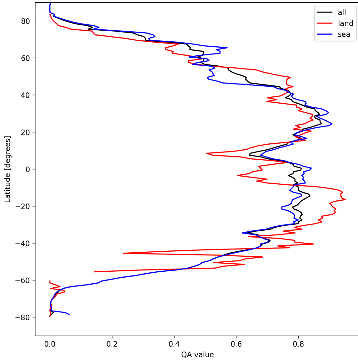
Figure 29: Zonal average of “QA value” for 2024-09-07 to 2024-09-09.
