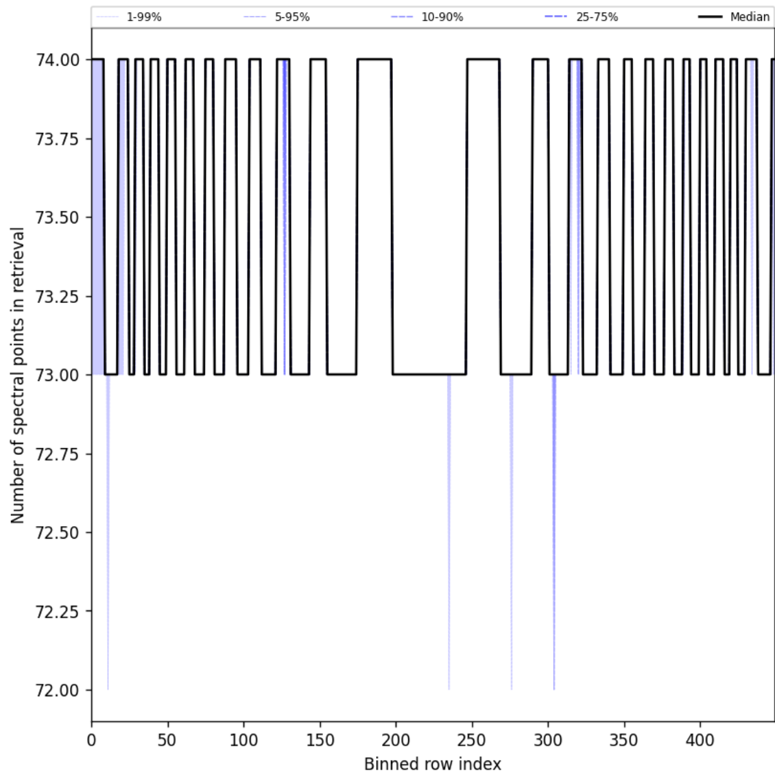
Figure 97: Along track statistics of “Number of spectral points in retrieval” for 2024-09-07 to 2024-09-09
