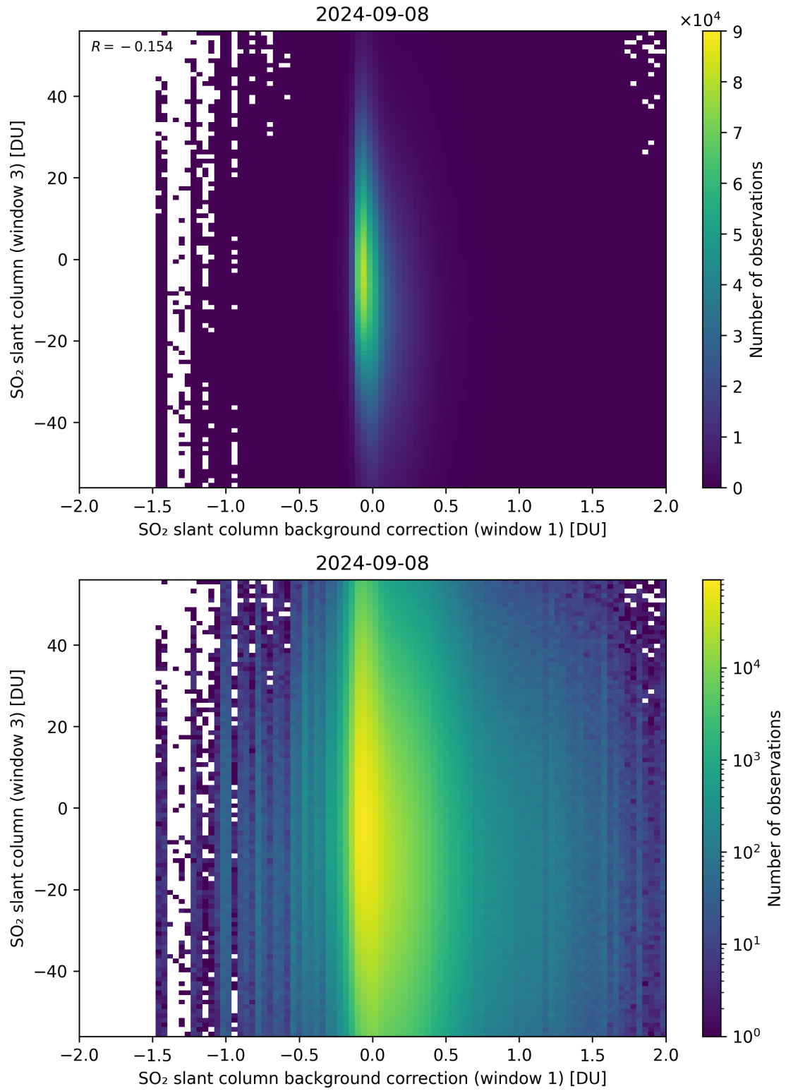
Figure 107: Scatter density plot of “SO 2 slant column background correction (window 1)” against “SO 2 slant column (window 3)” for 2024-09-07 to 2024-09-09.
