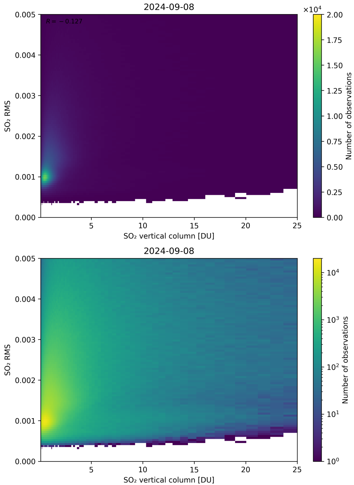
Figure 278: Scatter density plot of “SO 2 vertical column” against “SO 2 RMS” for 2024-09-07 to 2024-09-09.
