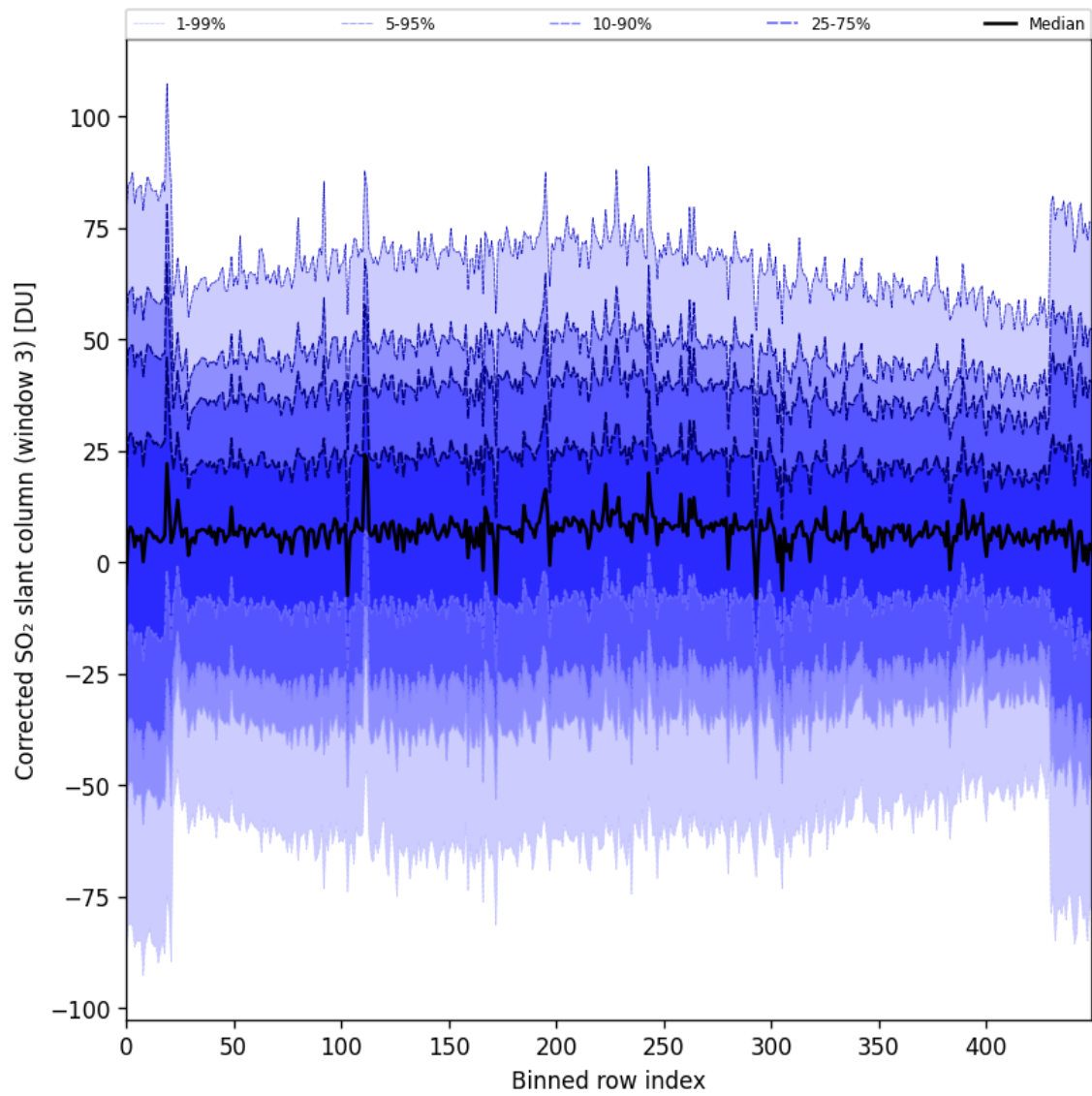
Figure 89: Along track statistics of “Corrected SO 2 slant column (window 3)” for 2024-09-07 to 2024-09-09
