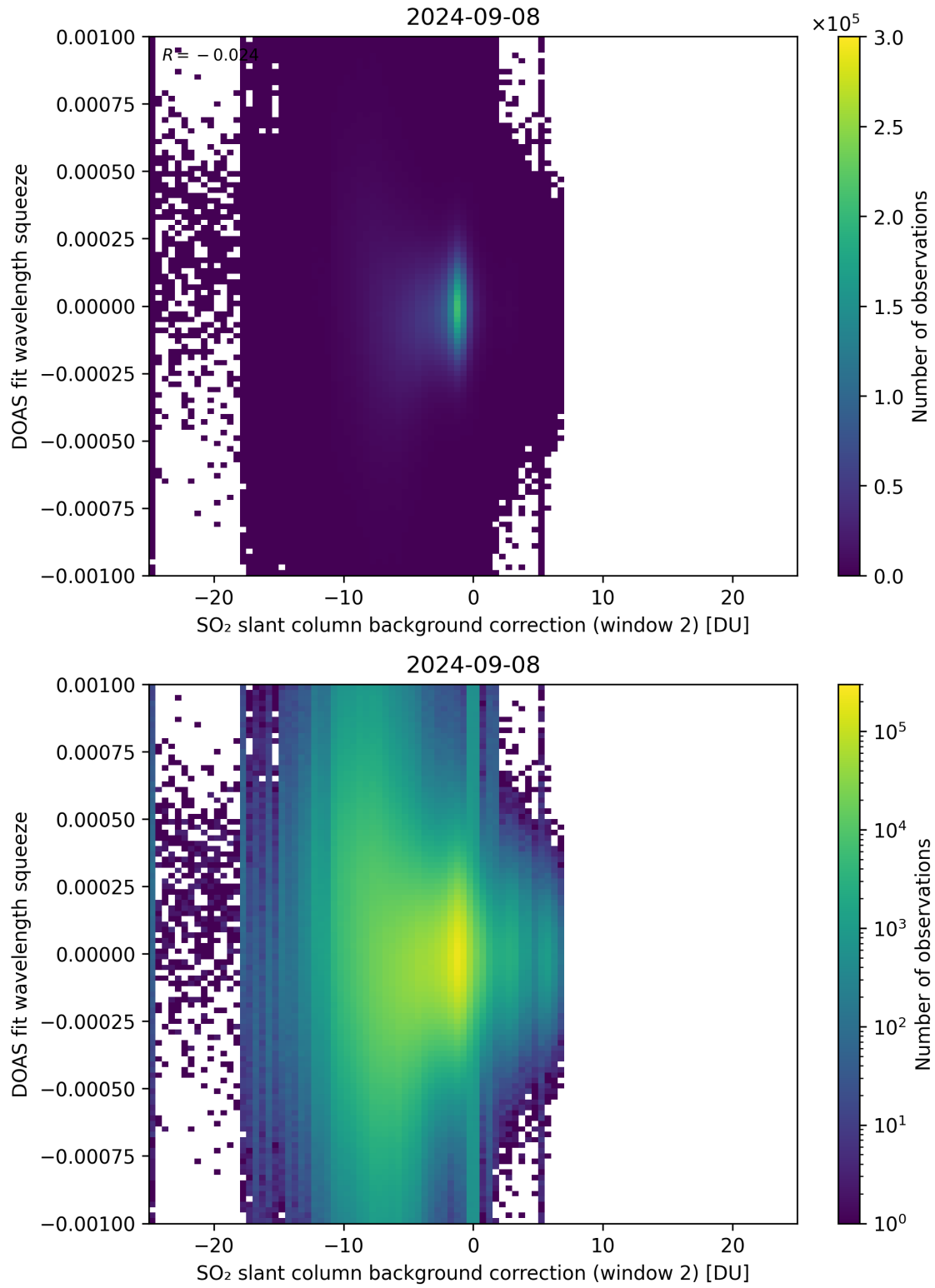
Figure 113: Scatter density plot of “SO 2 slant column background correction (window 2)” against “DOAS fit wavelength squeeze” for 2024-09-07 to 2024-09-09.
