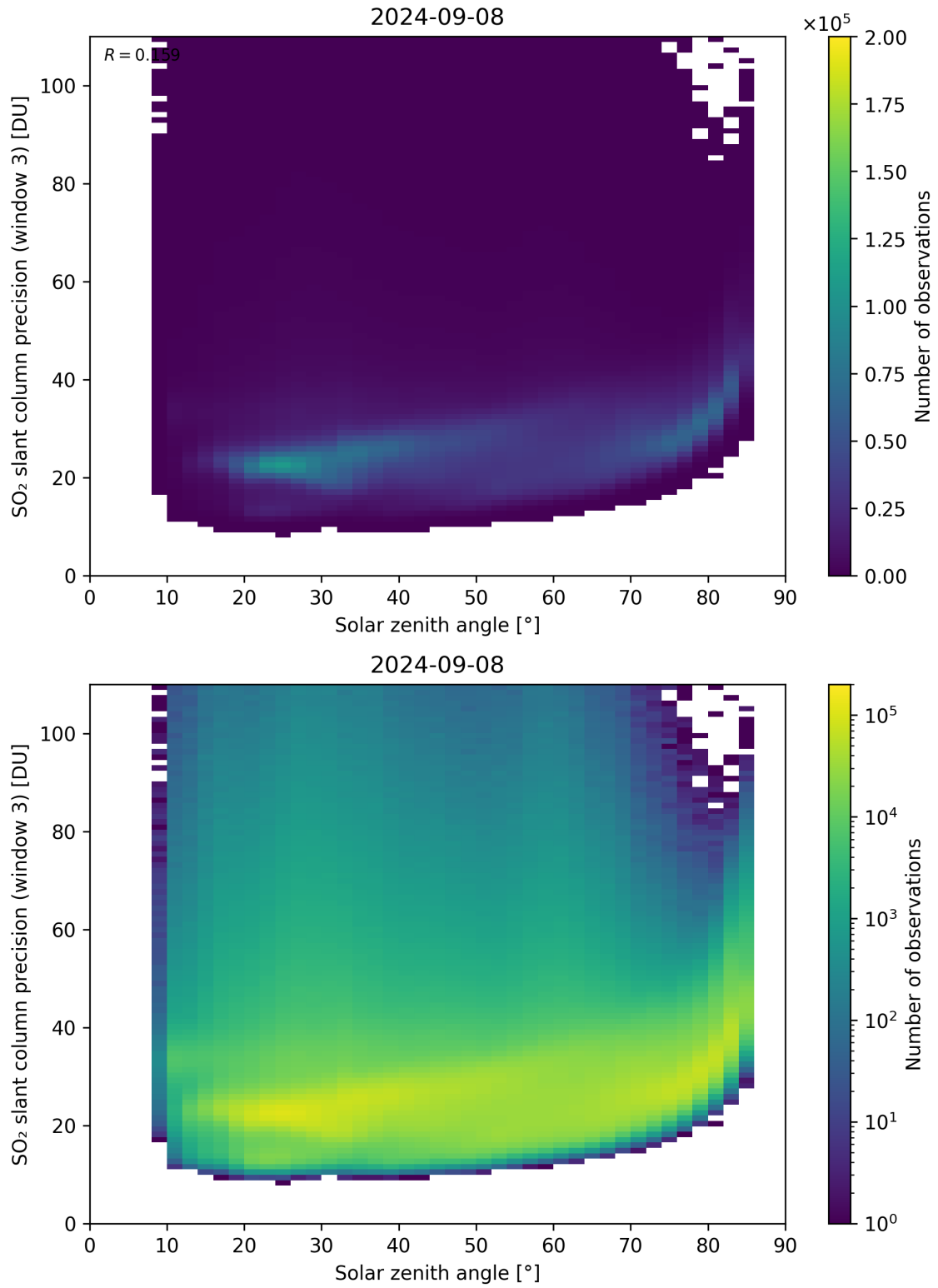
Figure 173: Scatter density plot of “Solar zenith angle” against “SO 2 slant column precision (window 3)” for 2024-09-07 to 2024-09-09.
