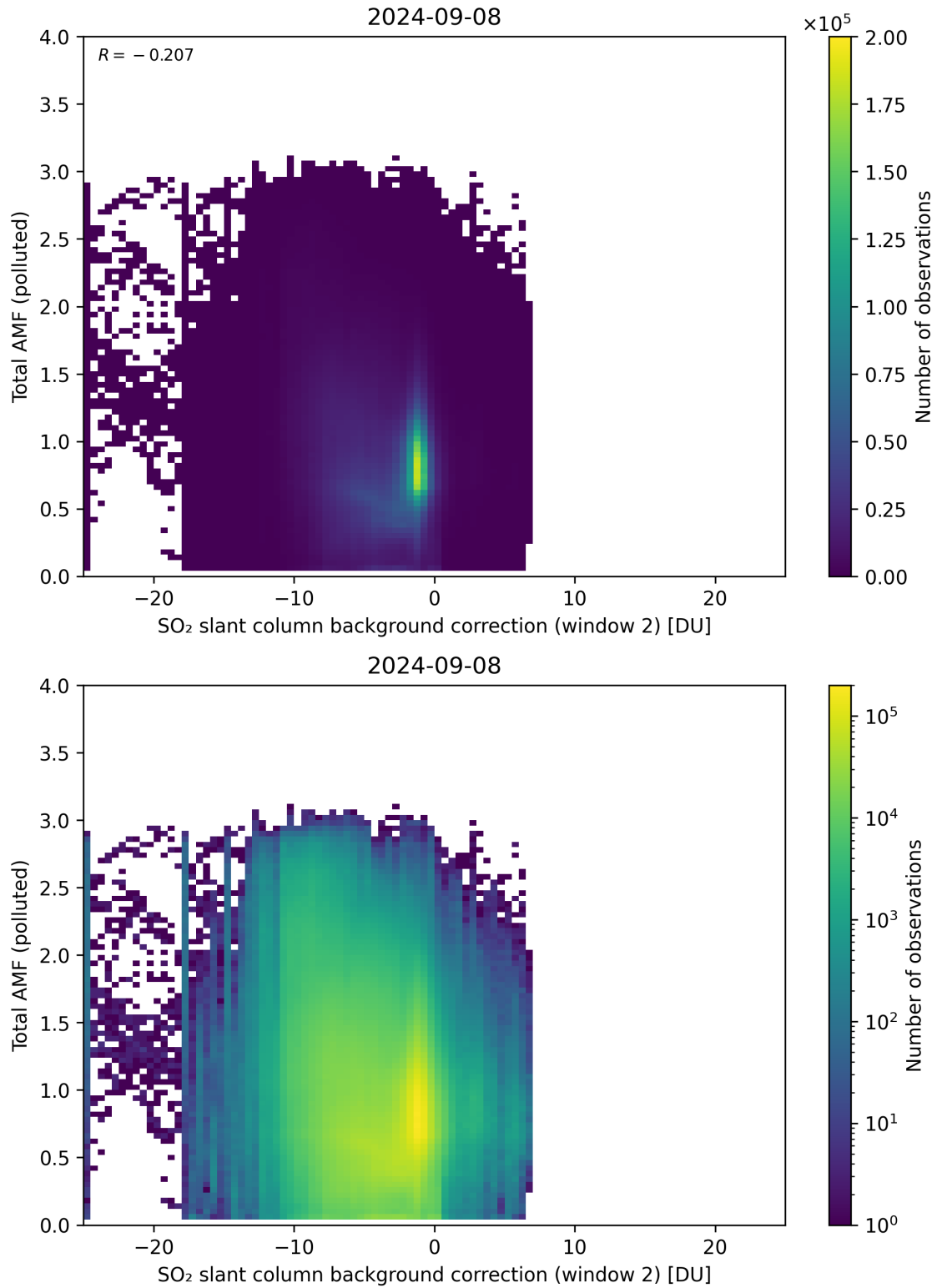
Figure 119: Scatter density plot of “SO 2 slant column background correction (window 2)” against “Total AMF (polluted)” for 2024-09-07 to 2024-09-09.
