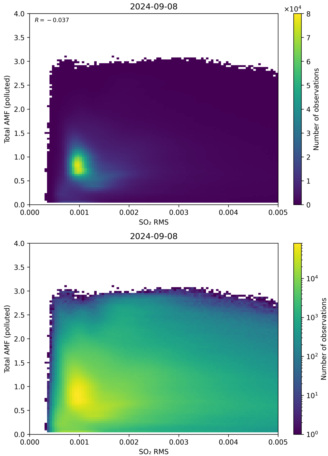
Figure 137: Scatter density plot of “SO 2 RMS” against “Total AMF (polluted)” for 2024-09-07 to 2024-09-09.
