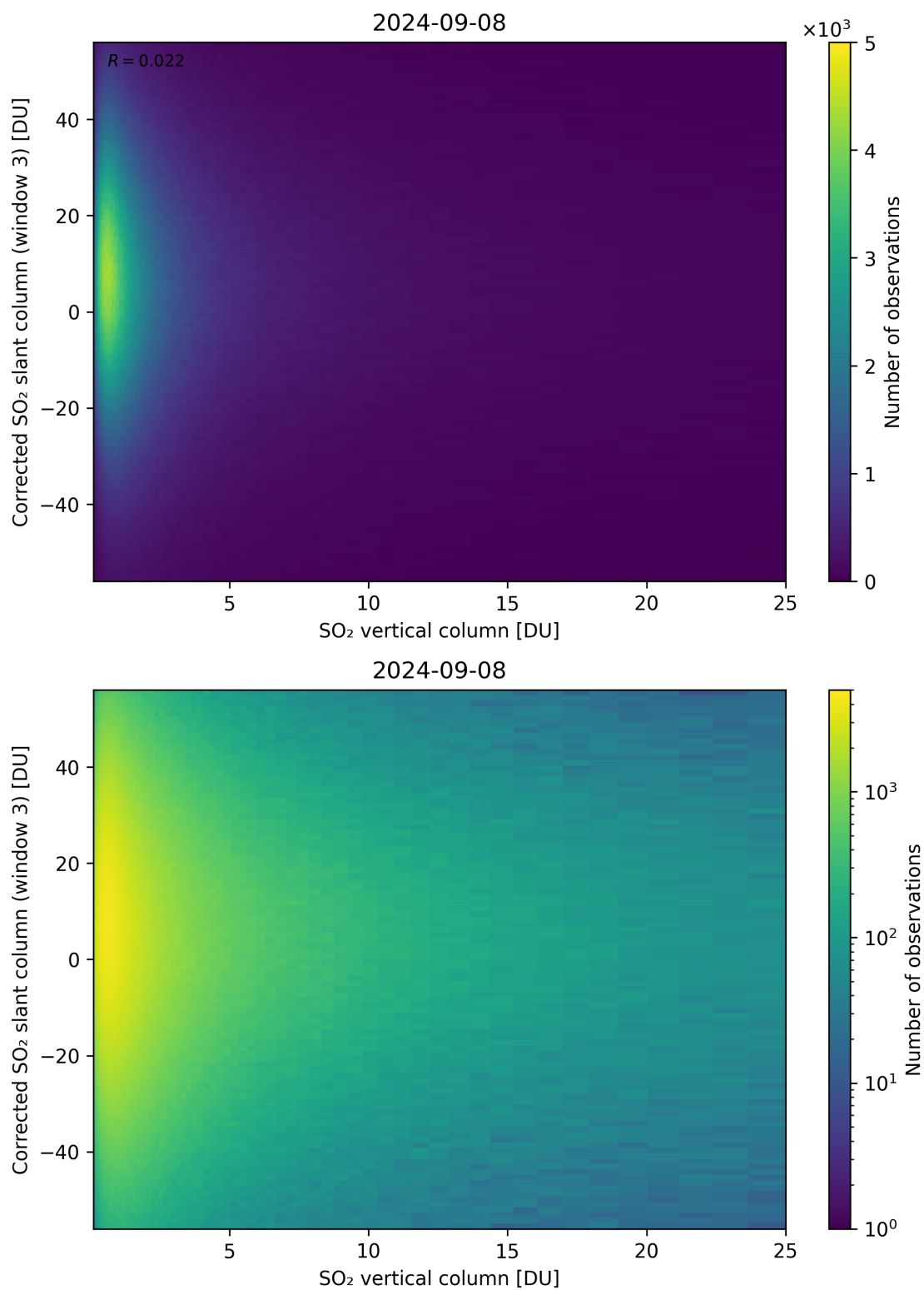
Figure 299: Scatter density plot of “SO 2 vertical column” against “Corrected SO 2 slant column (window 3)” for 2024-09-07 to 2024-09-09.
