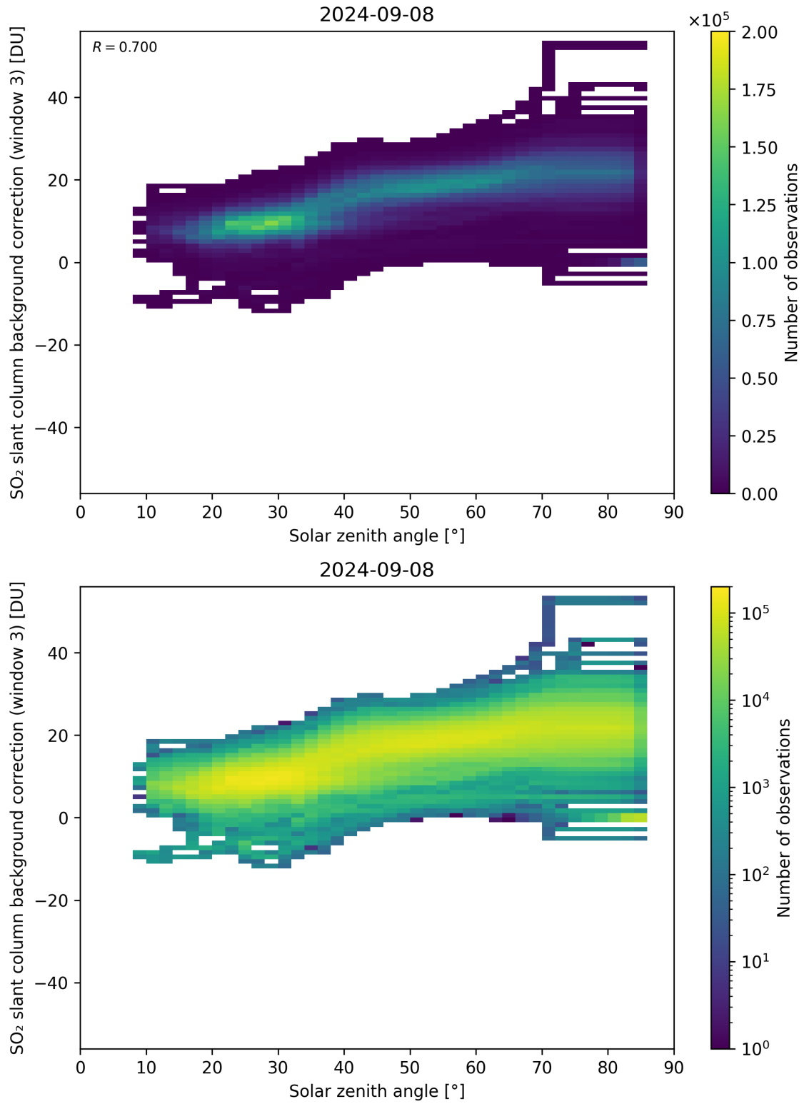
Figure 160: Scatter density plot of “Solar zenith angle” against “SO 2 slant column background correction (window 3)” for 2024-09-07 to 2024-09-09.
