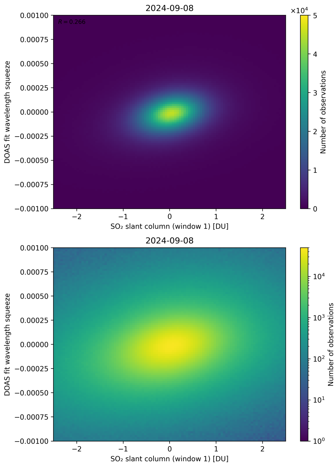
Figure 216: Scatter density plot of “SO 2 slant column (window 1)” against “DOAS fit wavelength squeeze” for 2024-09-07 to 2024-09-09.
