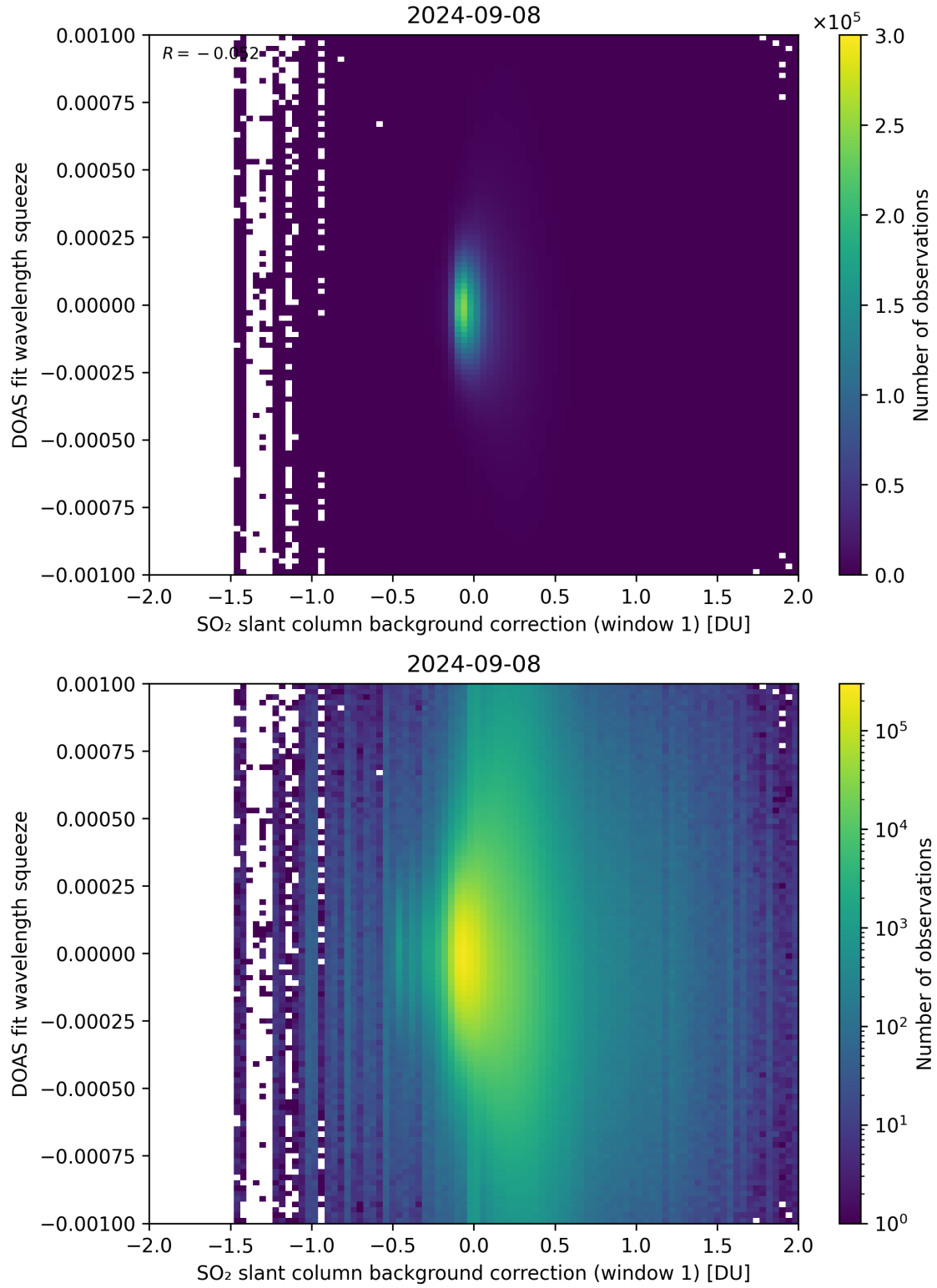
Figure 101: Scatter density plot of “SO 2 slant column background correction (window 1)” against “DOAS fit wavelength squeeze” for 2024-09-07 to 2024-09-09.
