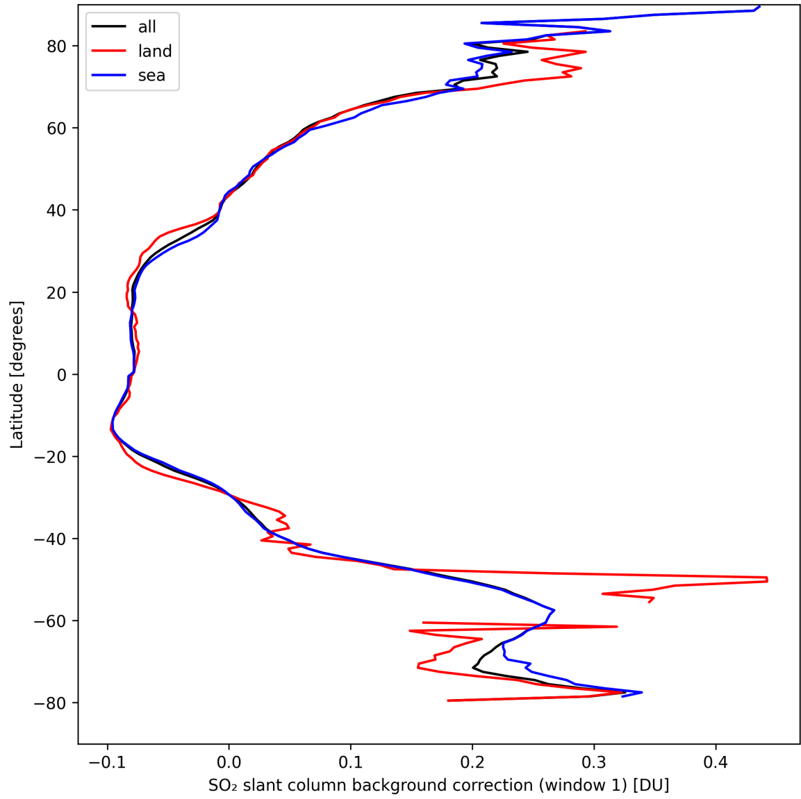
Figure 36: Zonal average of “SO 2 slant column background correction (window 1)” for 2024-09-07 to 2024-09-09.
