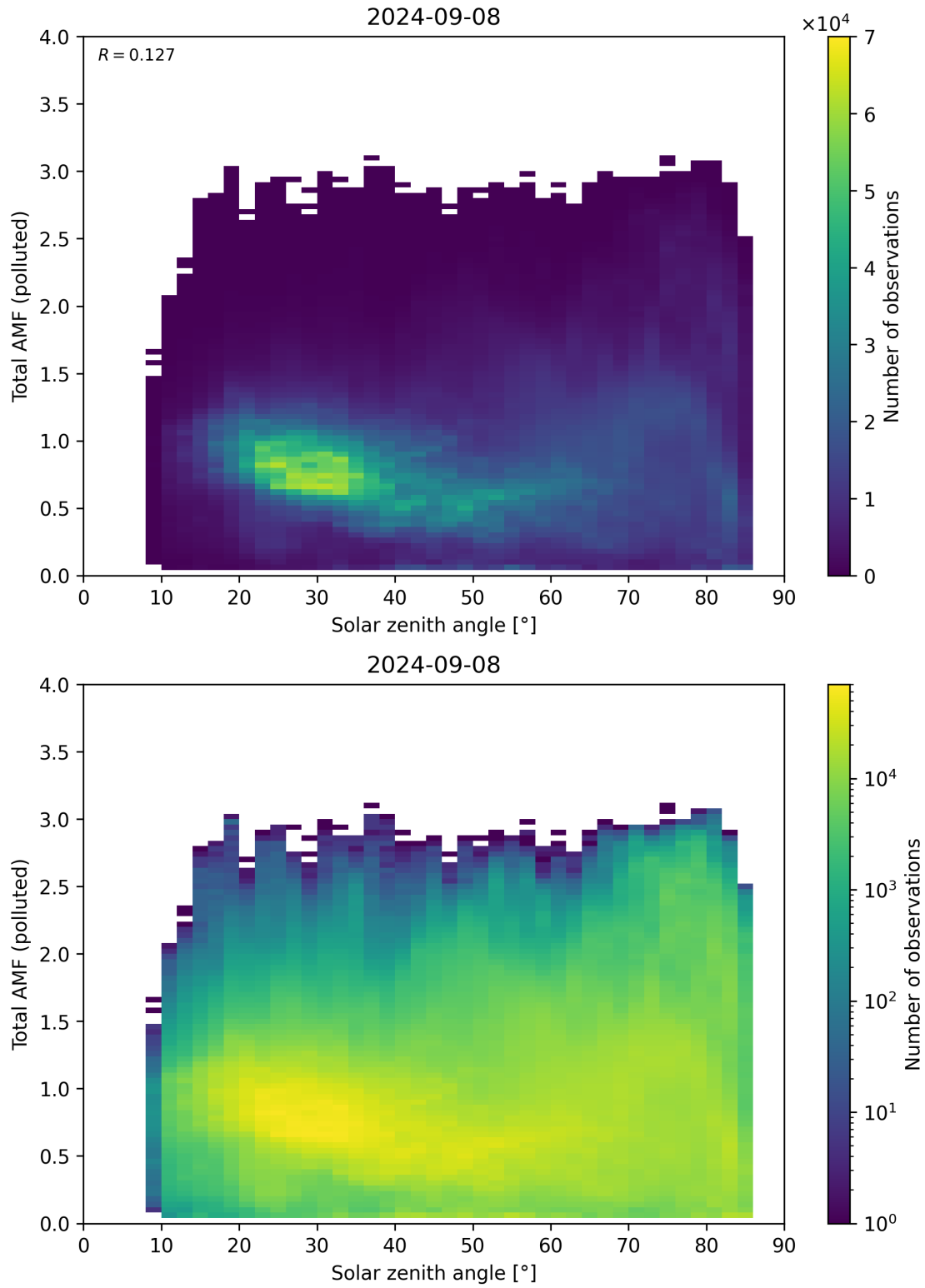
Figure 174: Scatter density plot of “Solar zenith angle” against “Total AMF (polluted)” for 2024-09-07 to 2024-09-09.
