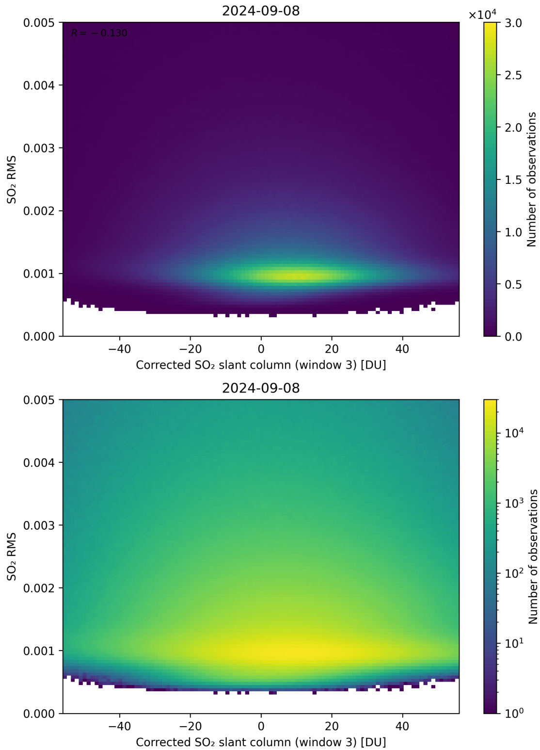
Figure 208: Scatter density plot of “Corrected SO 2 slant column (window 3)” against “SO 2 RMS” for 2024-09-07 to 2024-09-09.
