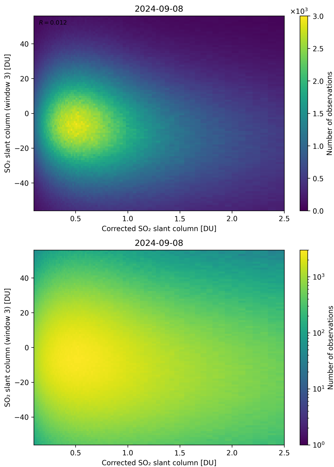
Figure 190: Scatter density plot of “Corrected SO 2 slant column” against “SO 2 slant column (window 3)” for 2024-09-07 to 2024-09-09.
