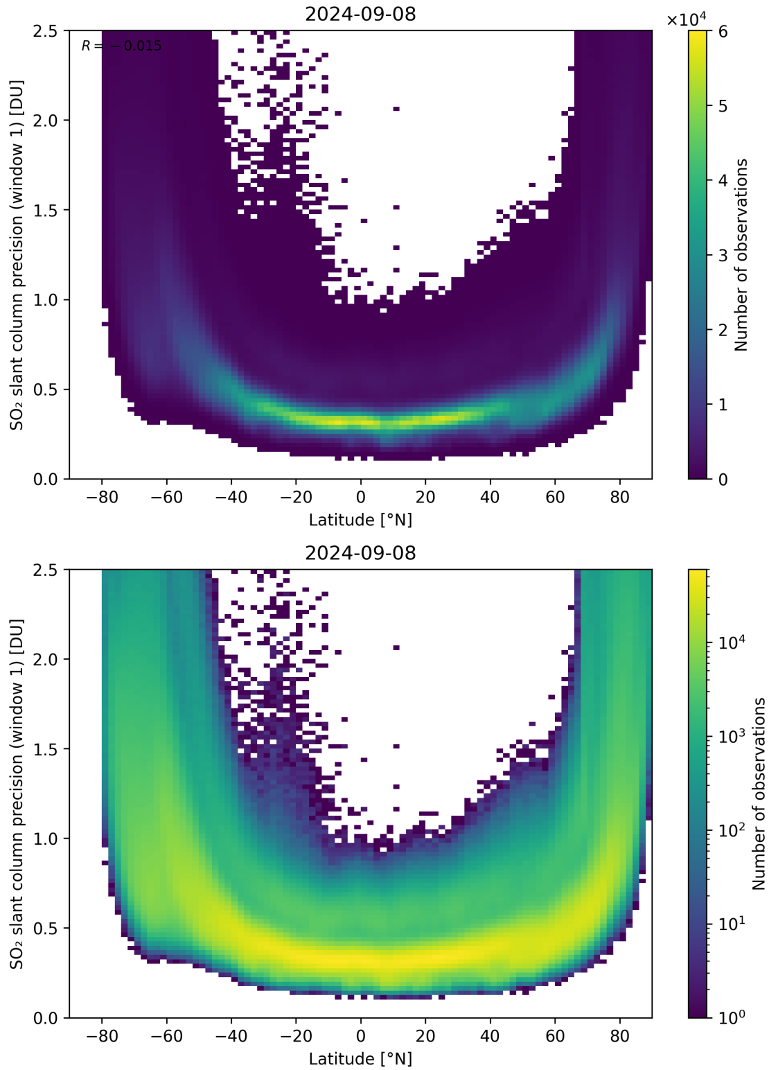
Figure 150: Scatter density plot of “Latitude” against “SO 2 slant column precision (window 1)” for 2024-09-07 to 2024-09-09.
