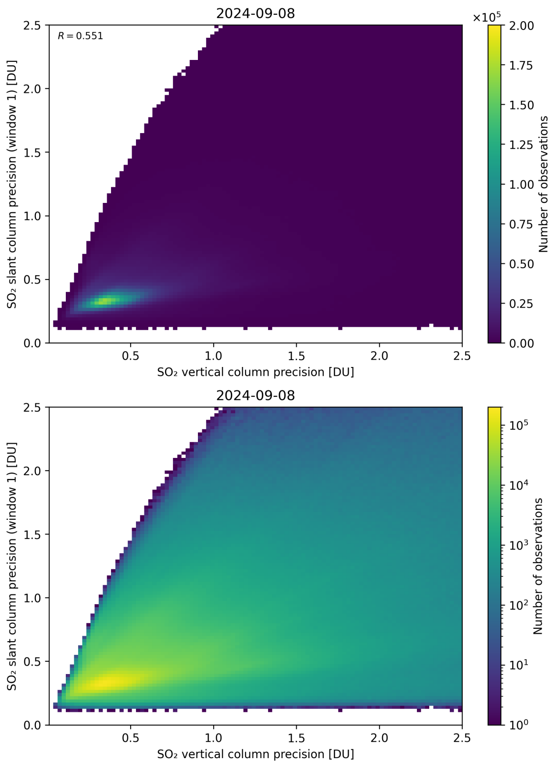
Figure 290: Scatter density plot of “SO 2 vertical column precision” against “SO 2 slant column precision (window 1)” for 2024-09-07 to 2024-09-09.
