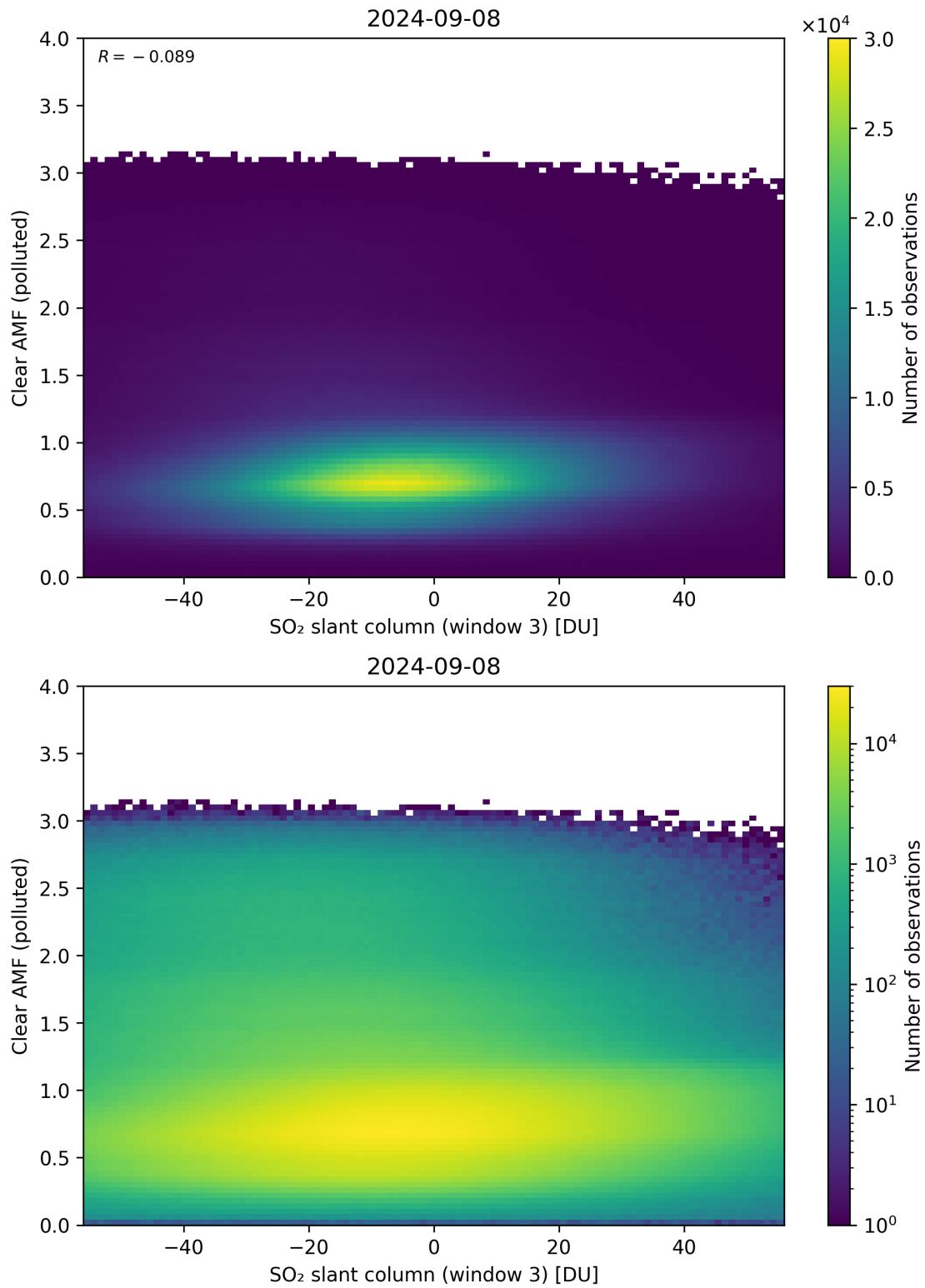
Figure 265: Scatter density plot of “SO 2 slant column (window 3)” against “Clear AMF (polluted)” for 2024-09-07 to 2024-09-09.
