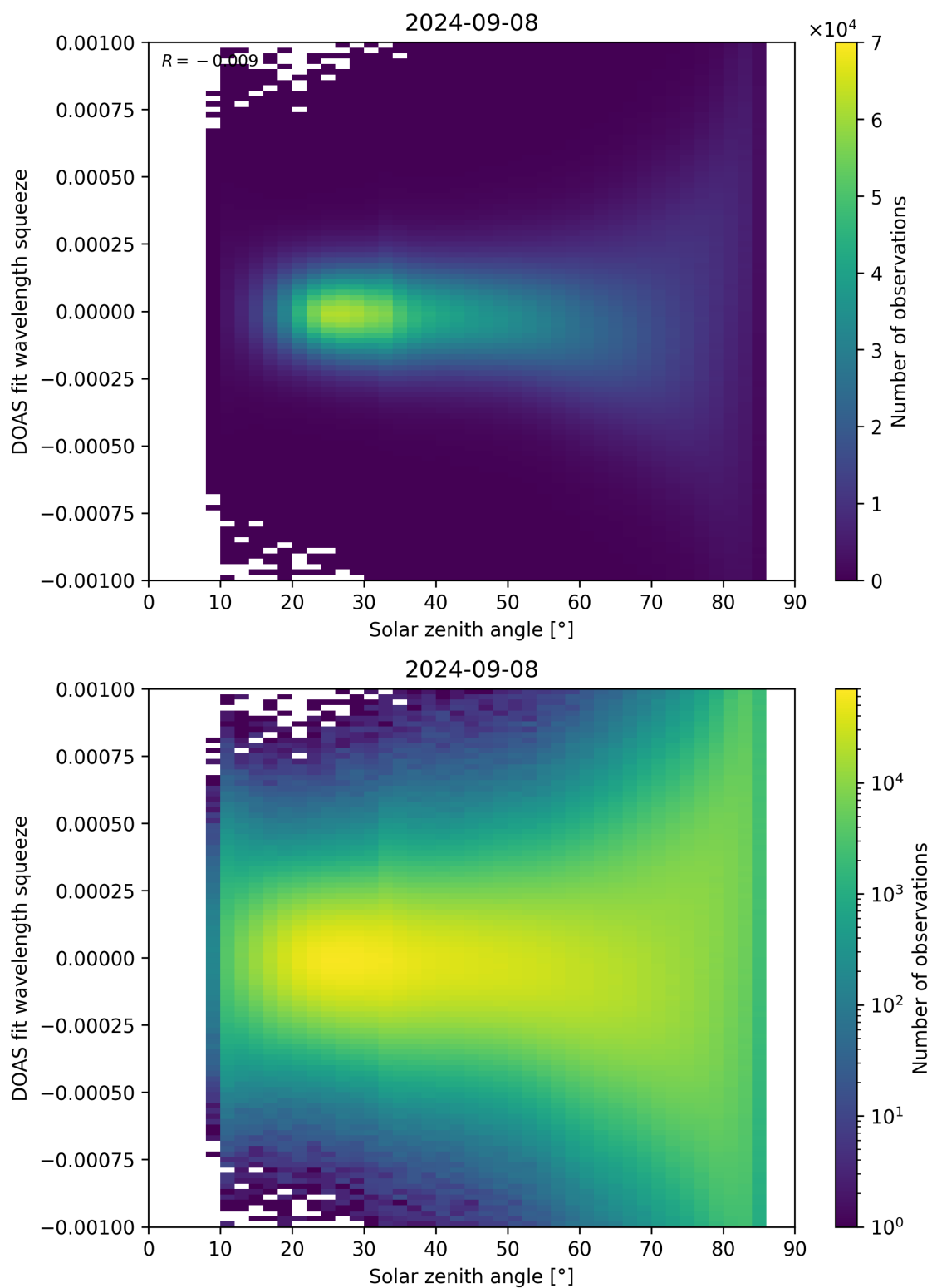
Figure 162: Scatter density plot of “Solar zenith angle” against “DOAS fit wavelength squeeze” for 2024-09-07 to 2024-09-09.
