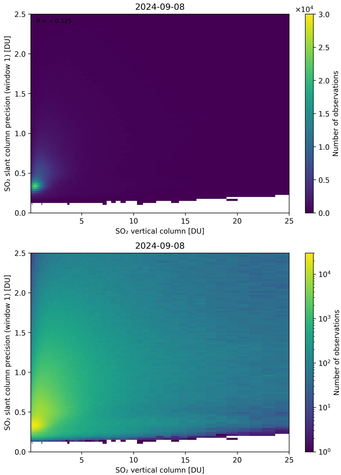
Figure 301: Scatter density plot of “SO 2 vertical column” against “SO 2 slant column precision (window 1)” for 2024-09-07 to 2024-09-09.
