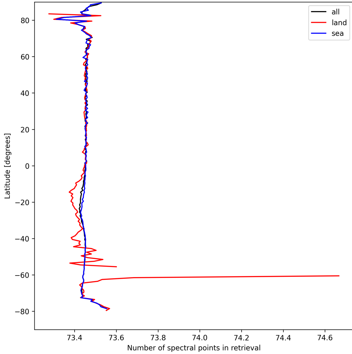
Figure 51: Zonal average of “Number of spectral points in retrieval” for 2024-09-07 to 2024-09-09.
