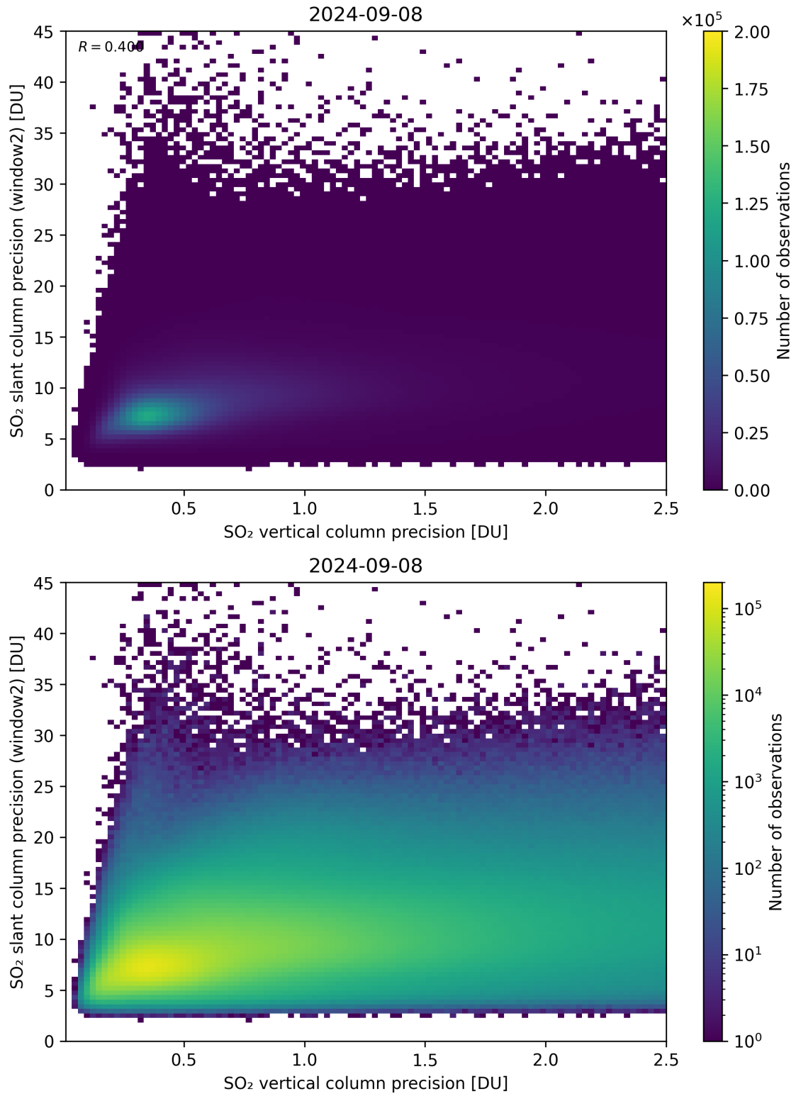
Figure 291: Scatter density plot of “SO 2 vertical column precision” against “SO 2 slant column precision (window2)” for 2024-09-07 to 2024-09-09.
