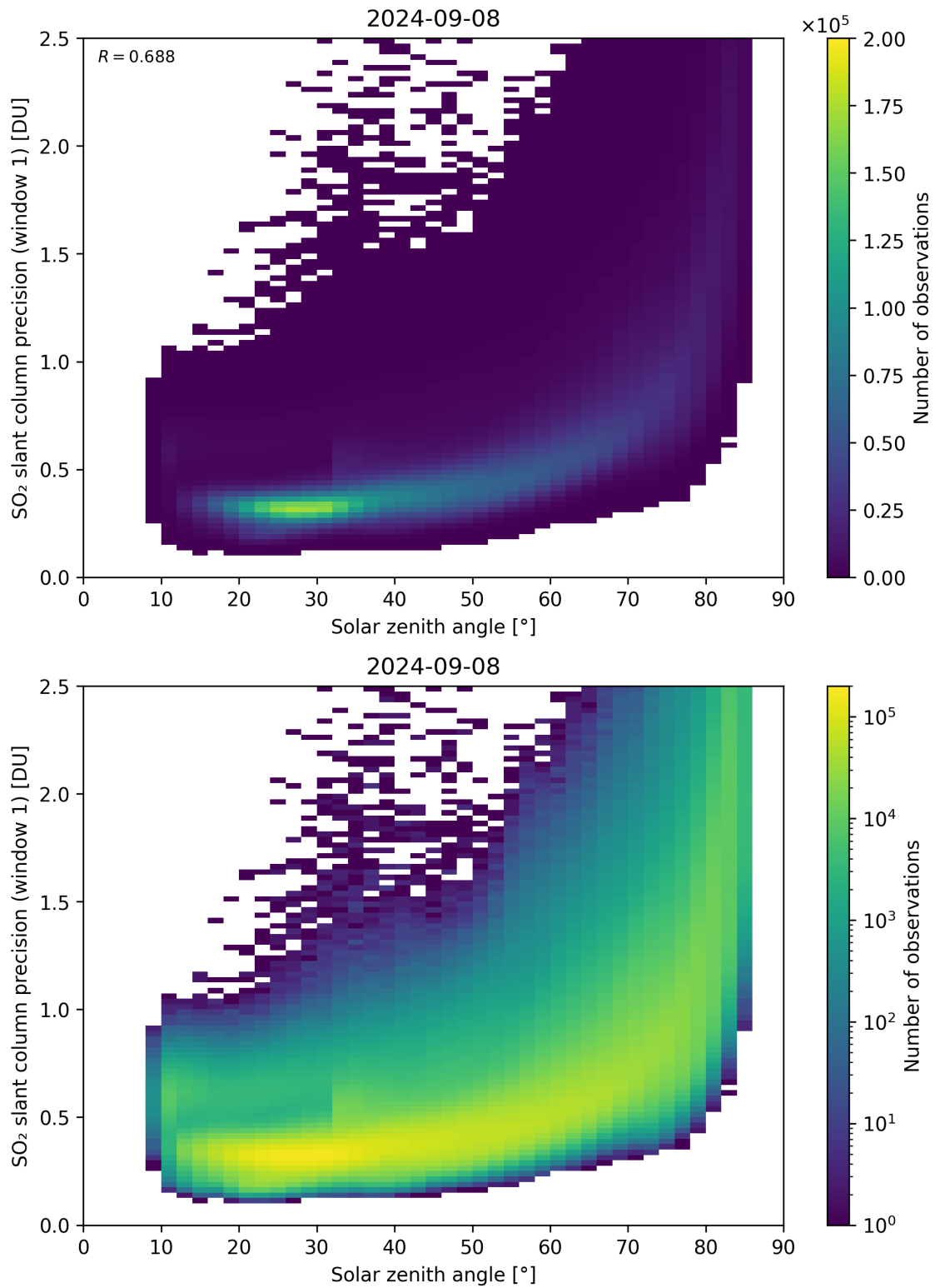
Figure 170: Scatter density plot of “Solar zenith angle” against “SO 2 slant column precision (window 1)” for 2024-09-07 to 2024-09-09.
