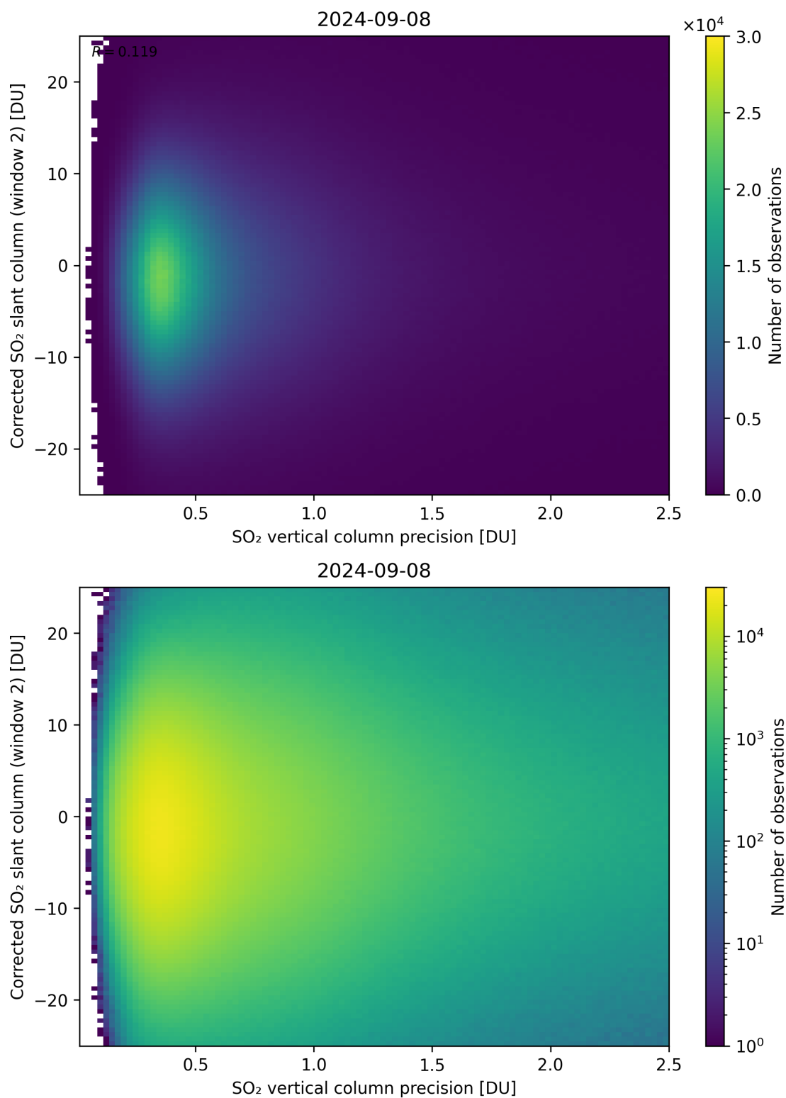
Figure 287: Scatter density plot of “SO 2 vertical column precision” against “Corrected SO 2 slant column (window 2)” for 2024-09-07 to 2024-09-09.
