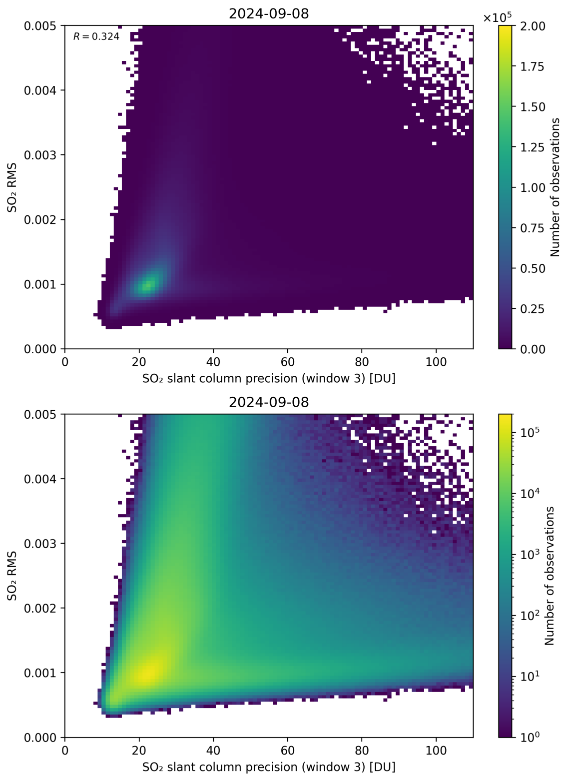
Figure 260: Scatter density plot of “SO 2 slant column precision (window 3)” against “SO 2 RMS” for 2024-09-07 to 2024-09-09.
