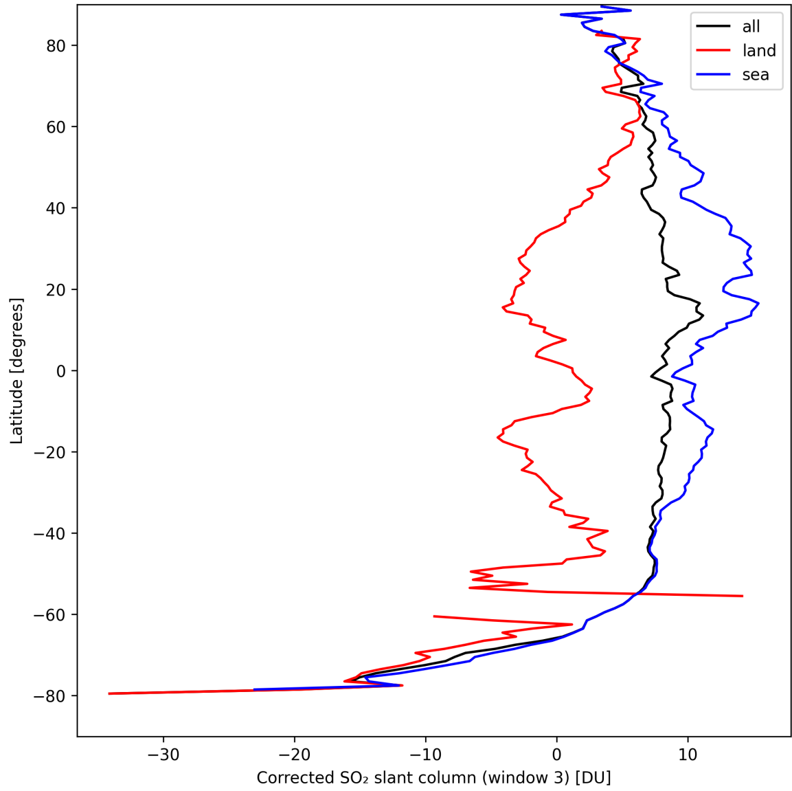
Figure 43: Zonal average of “Corrected SO 2 slant column (window 3)” for 2024-09-07 to 2024-09-09.
