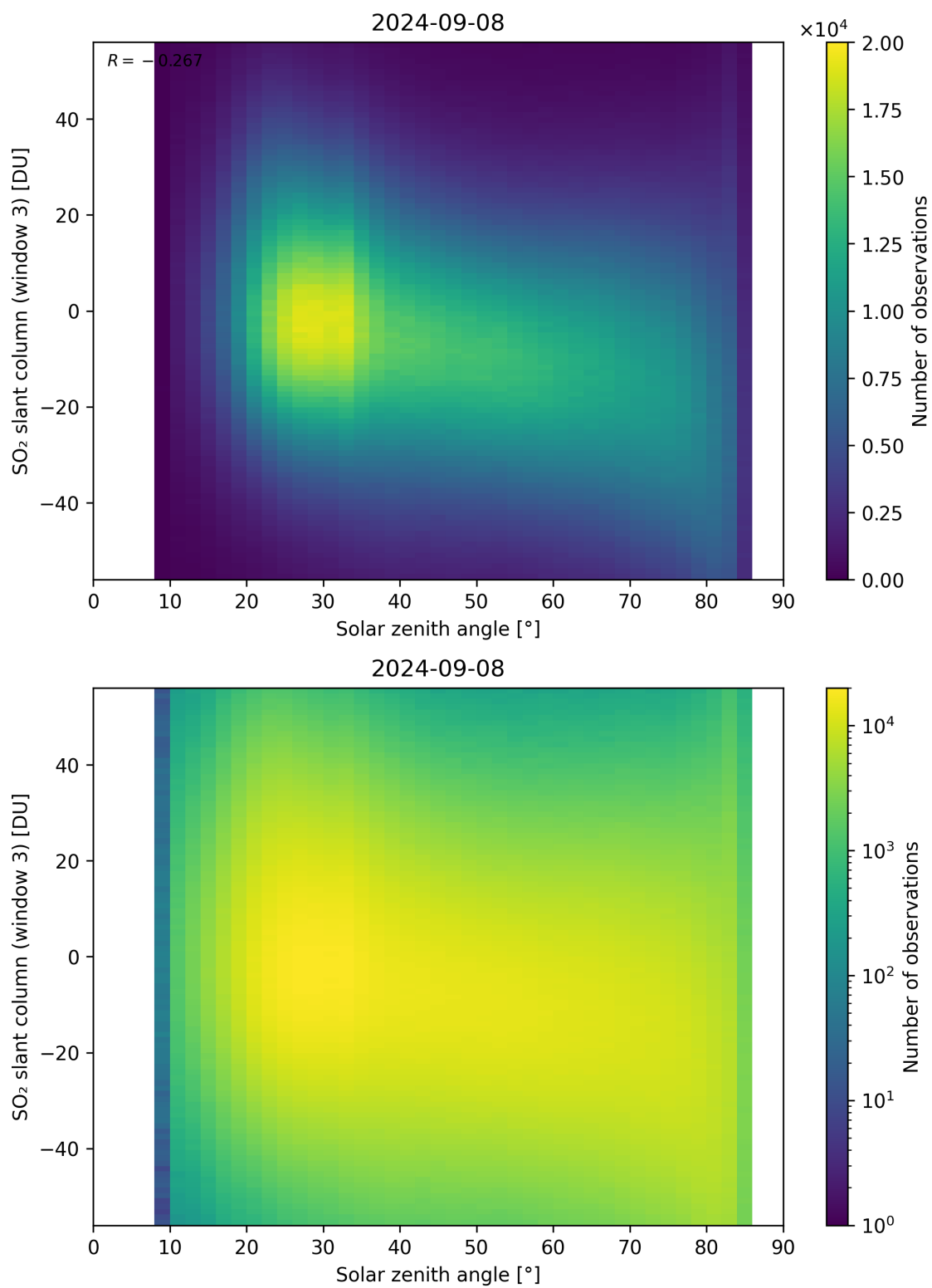
Figure 172: Scatter density plot of “Solar zenith angle” against “SO 2 slant column (window 3)” for 2024-09-07 to 2024-09-09.
