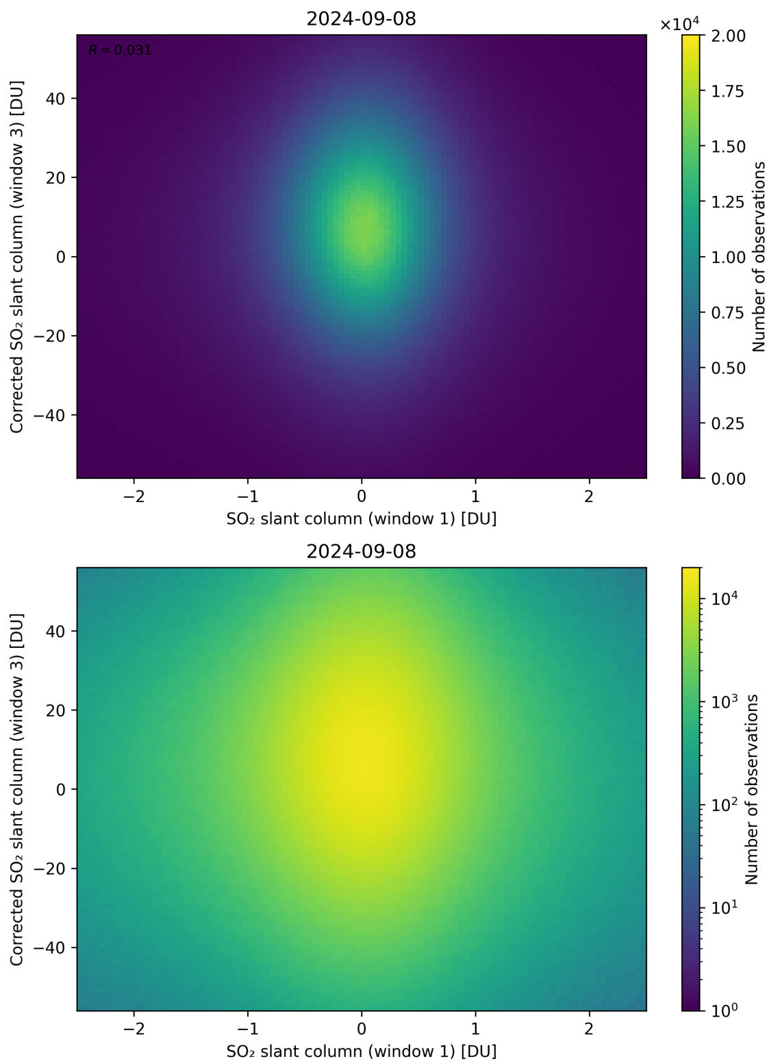
Figure 234: Scatter density plot of “SO 2 slant column (window 1)” against “Corrected SO 2 slant column (window 3)” for 2024-09-07 to 2024-09-09.
