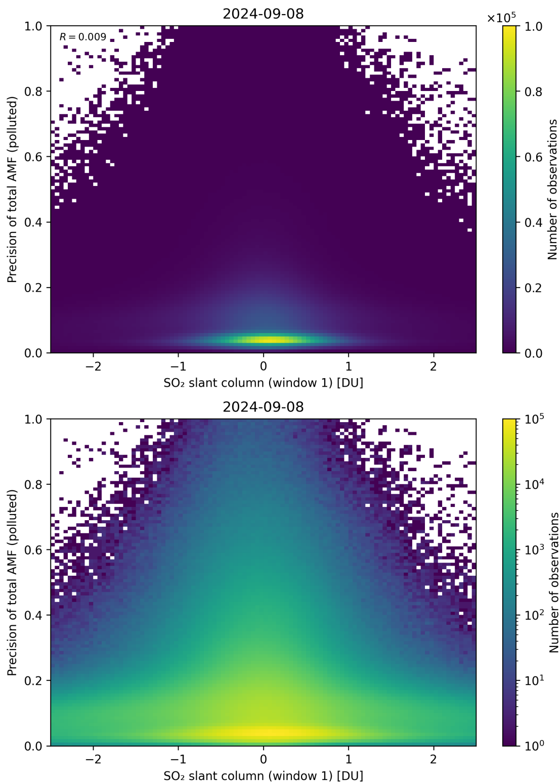
Figure 240: Scatter density plot of “SO 2 slant column (window 1)” against “Precision of total AMF (polluted)” for 2024-09-07 to 2024-09-09.
