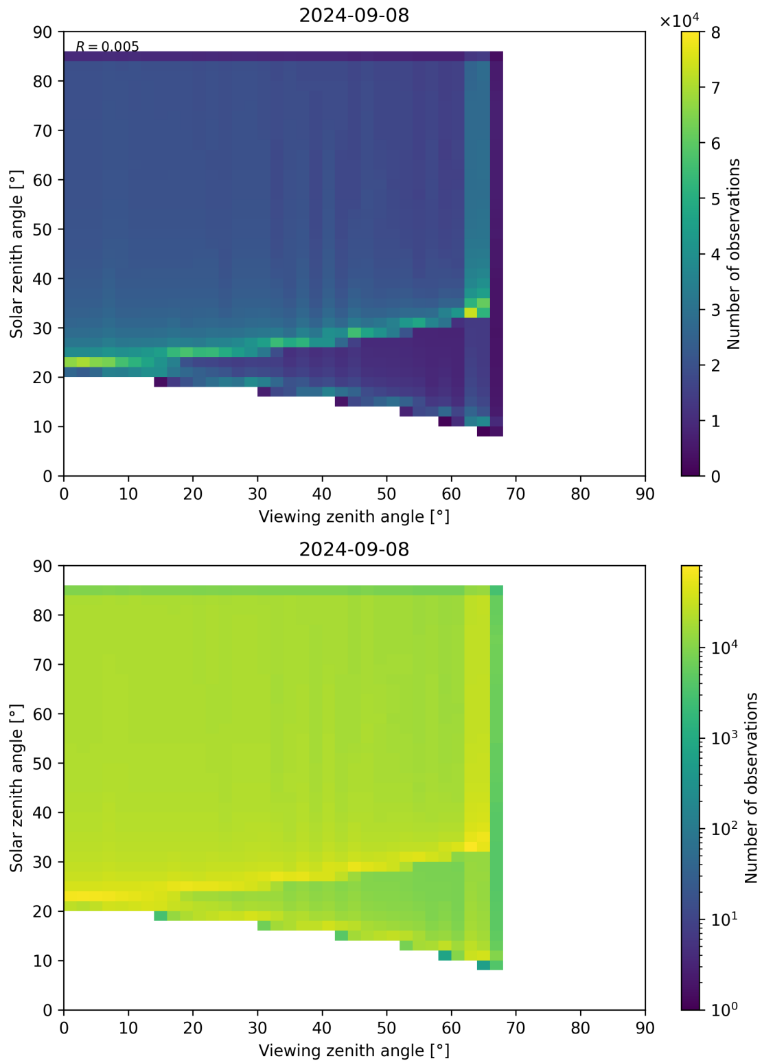
Figure 315: Scatter density plot of “Viewing zenith angle” against “Solar zenith angle” for 2024-09-07 to 2024-09-09.
