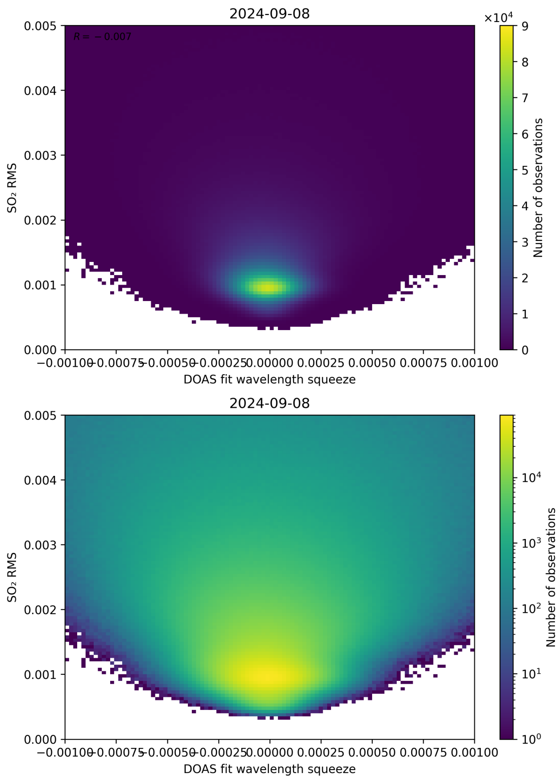
Figure 132: Scatter density plot of “DOAS fit wavelength squeeze” against “SO 2 RMS” for 2024-09-07 to 2024-09-09.
