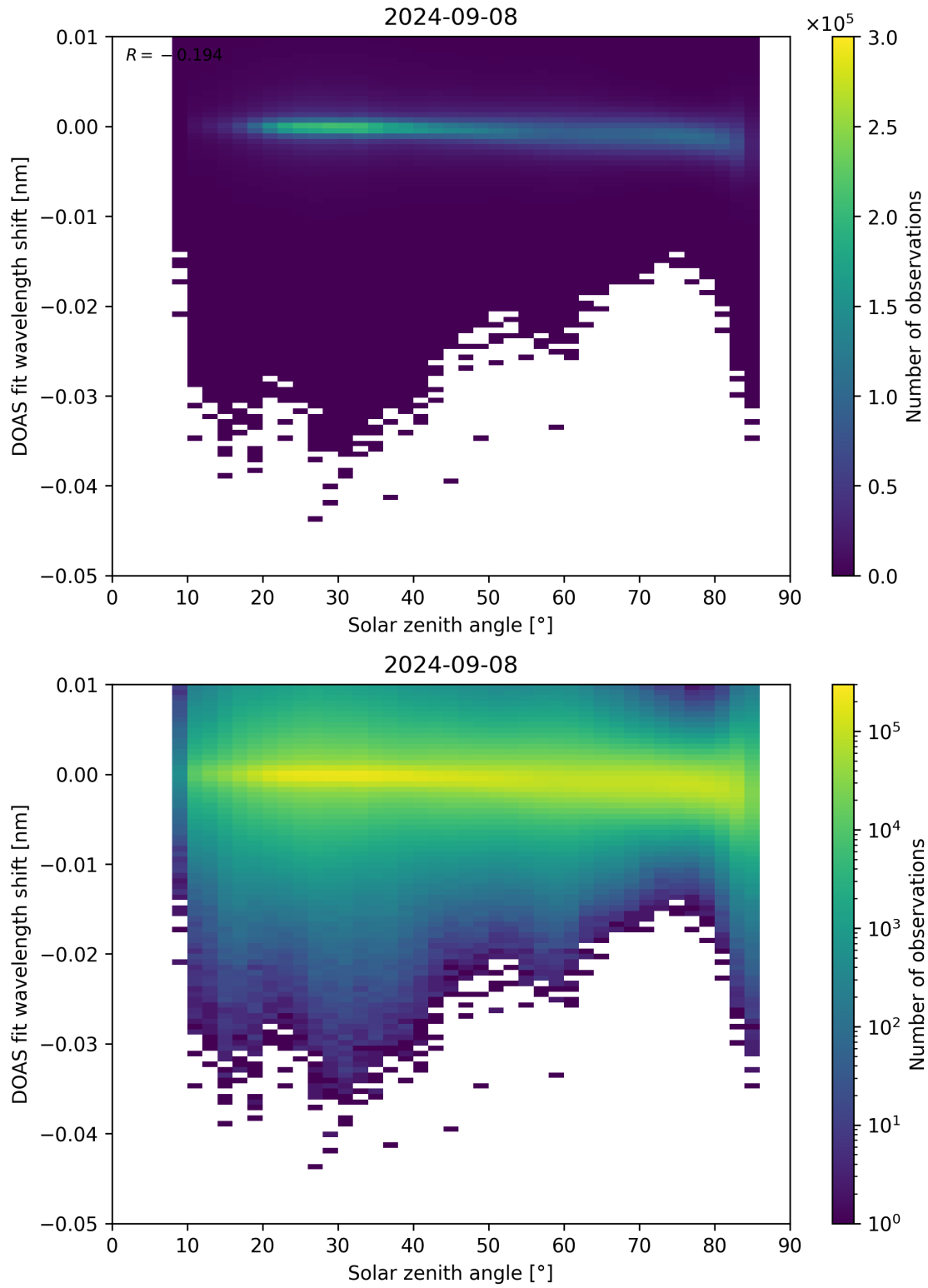
Figure 161: Scatter density plot of “Solar zenith angle” against “DOAS fit wavelength shift” for 2024-09-07 to 2024-09-09.
