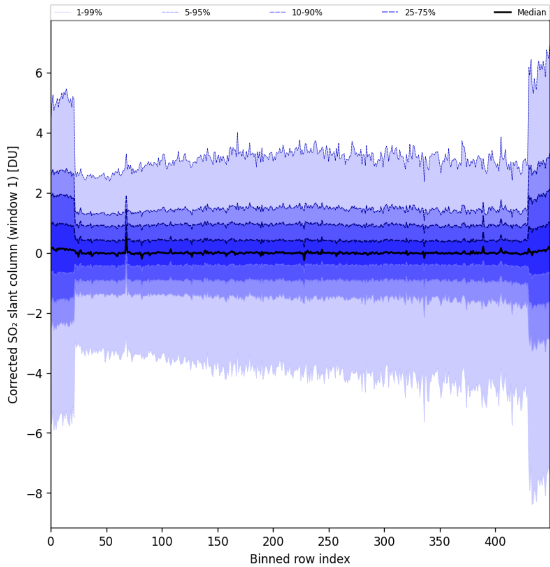
Figure 81: Along track statistics of “Corrected SO 2 slant column (window 1)” for 2024-09-07 to 2024-09-09
