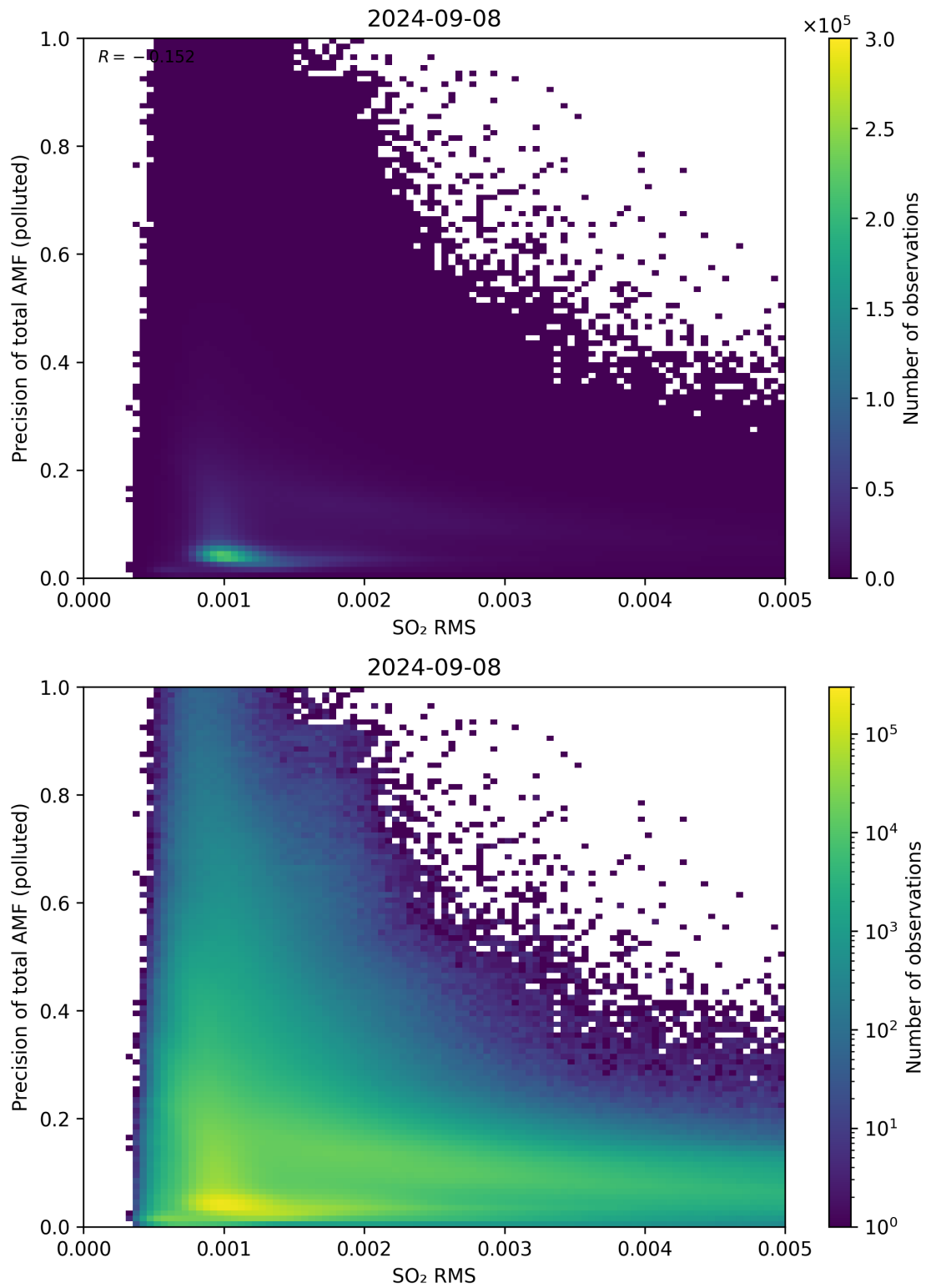
Figure 138: Scatter density plot of “SO 2 RMS” against “Precision of total AMF (polluted)” for 2024-09-07 to 2024-09-09.
