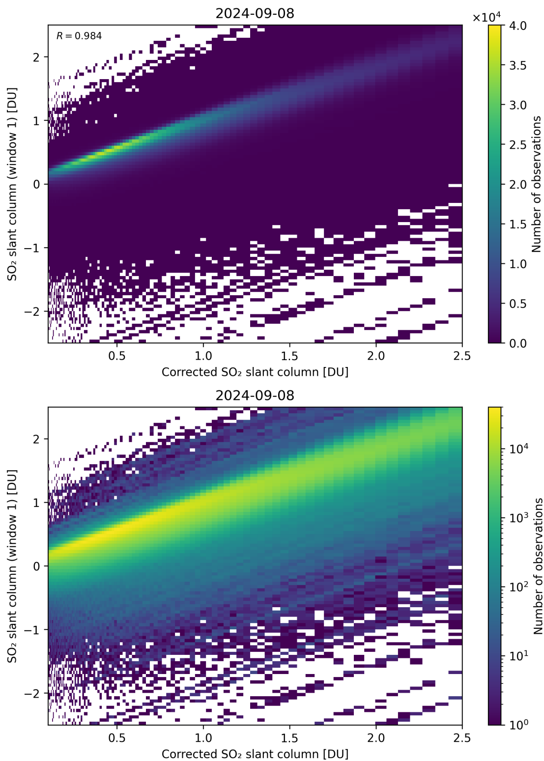
Figure 187: Scatter density plot of “Corrected SO 2 slant column” against “SO 2 slant column (window 1)” for 2024-09-07 to 2024-09-09.
