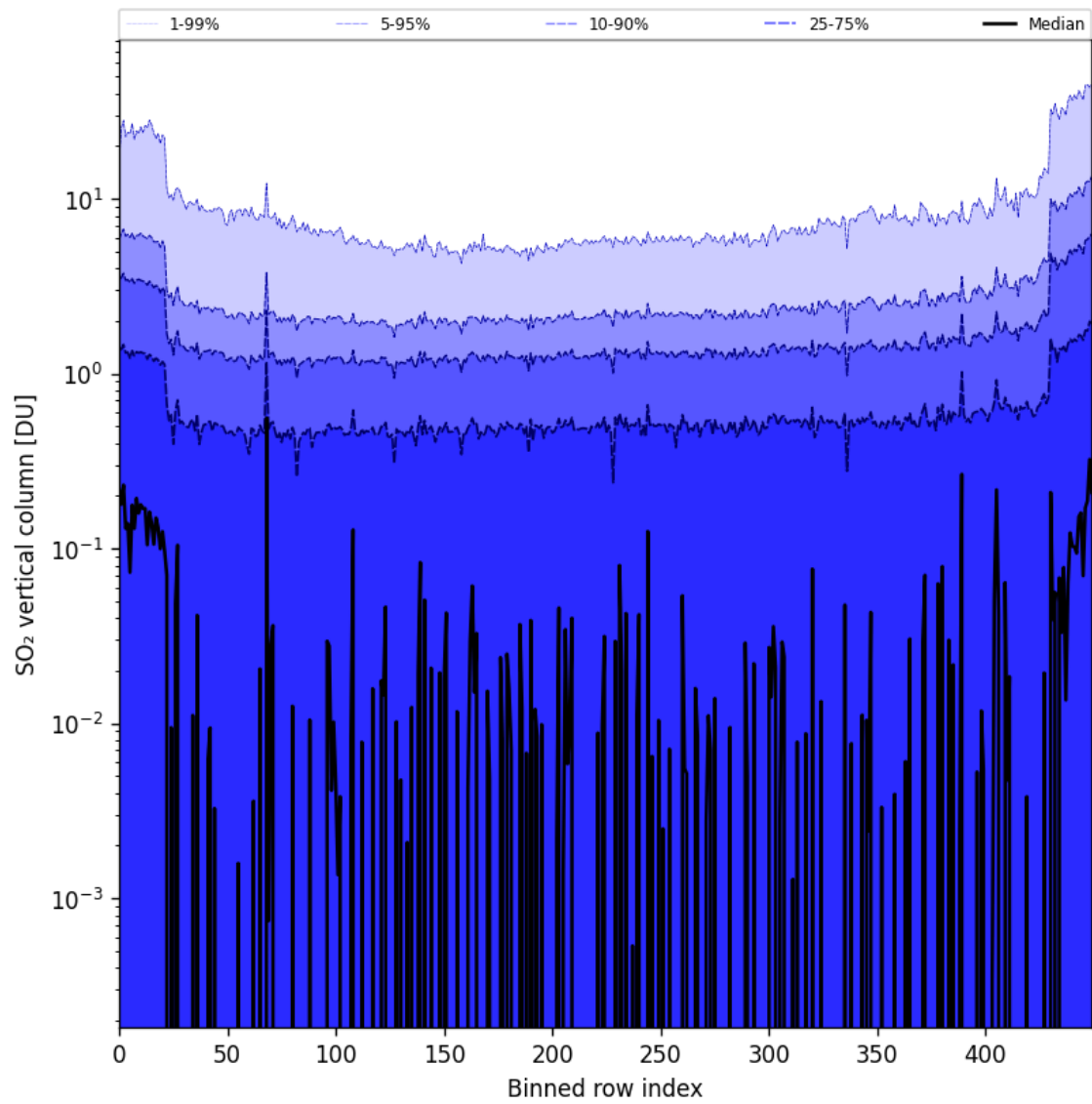
Figure 76: Along track statistics of “SO 2 vertical column” for 2024-09-07 to 2024-09-09
