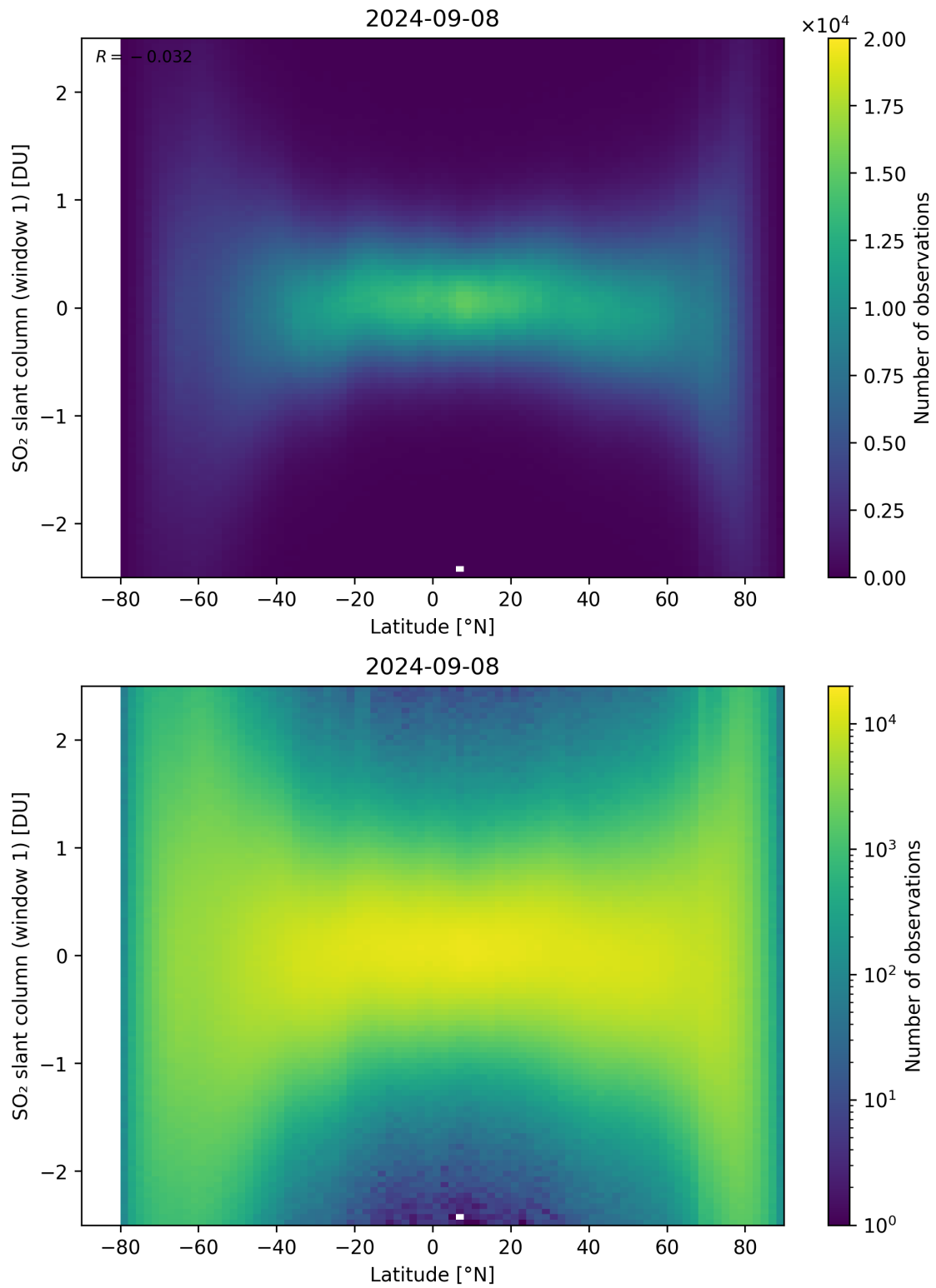
Figure 149: Scatter density plot of “Latitude” against “SO 2 slant column (window 1)” for 2024-09-07 to 2024-09-09.
