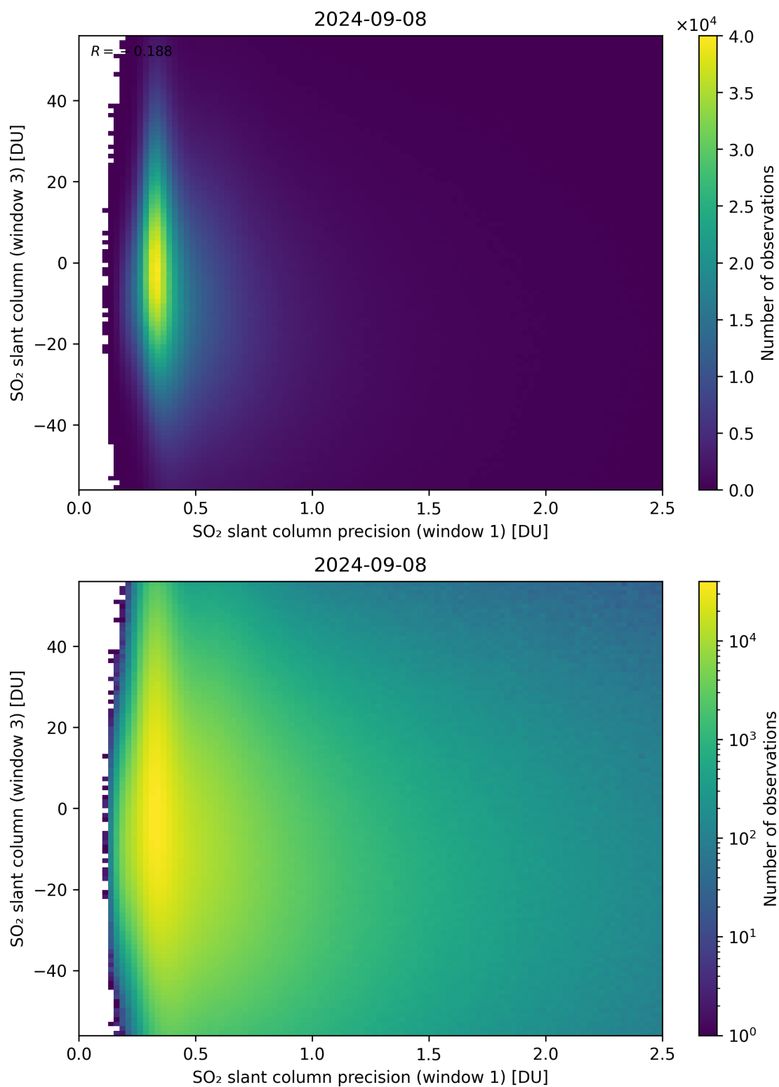
Figure 228: Scatter density plot of “SO 2 slant column precision (window 1)” against “SO 2 slant column (window 3)” for 2024-09-07 to 2024-09-09.
