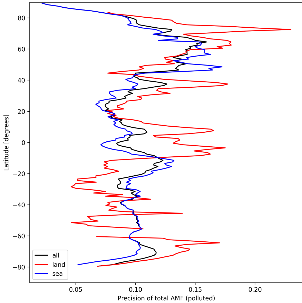
Figure 49: Zonal average of “Precision of total AMF (polluted)” for 2024-09-07 to 2024-09-09.
