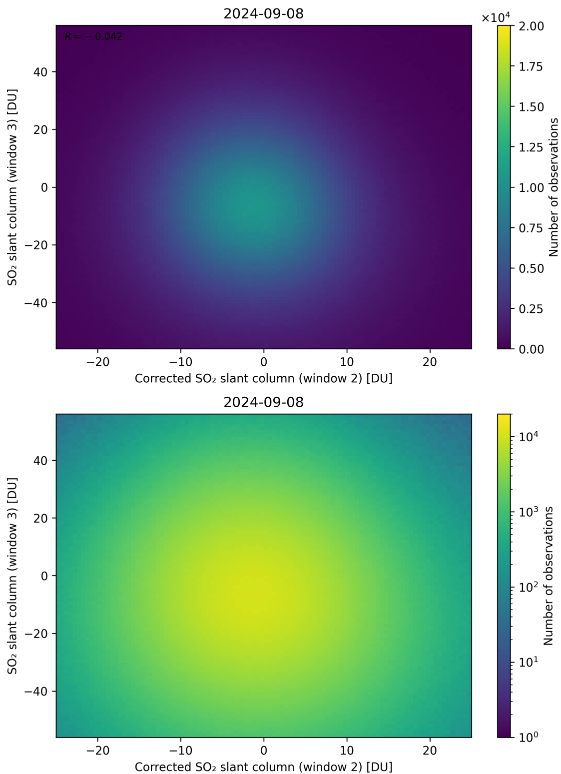
Figure 201: Scatter density plot of “Corrected SO 2 slant column (window 2)” against “SO 2 slant column (window 3)” for 2024-09-07 to 2024-09-09.
