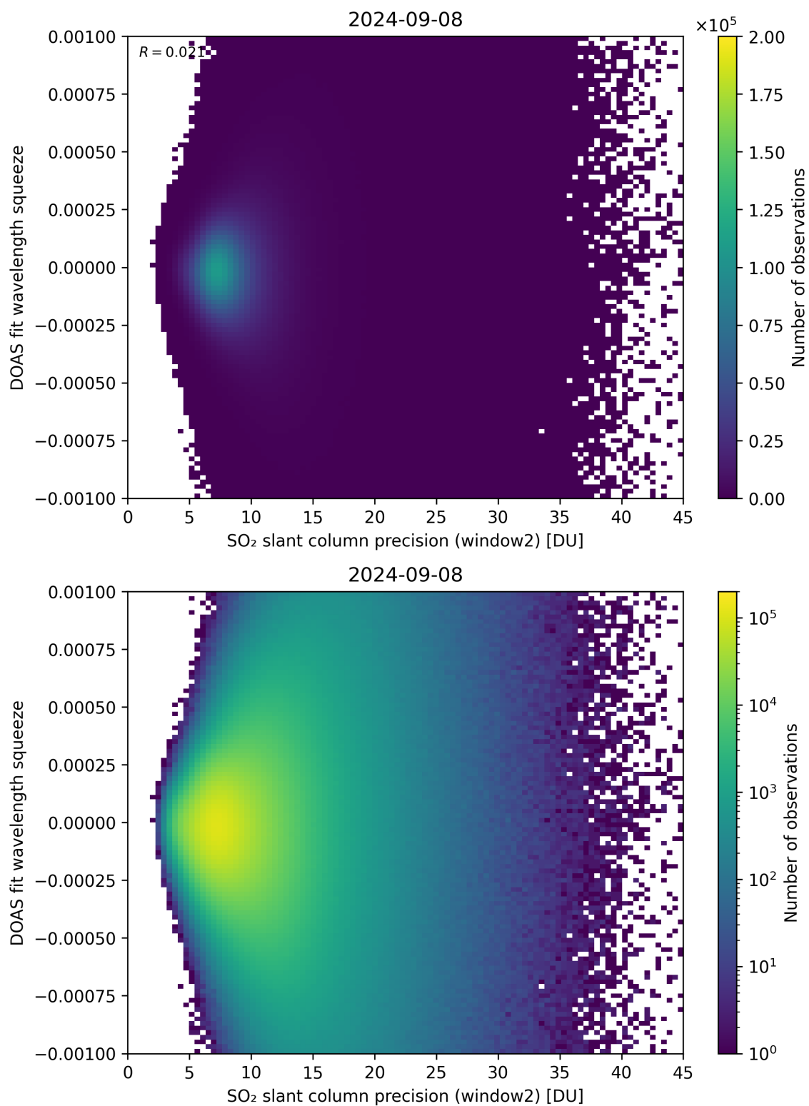
Figure 244: Scatter density plot of “SO 2 slant column precision (window2)” against “DOAS fit wavelength squeeze” for 2024-09-07 to 2024-09-09.
