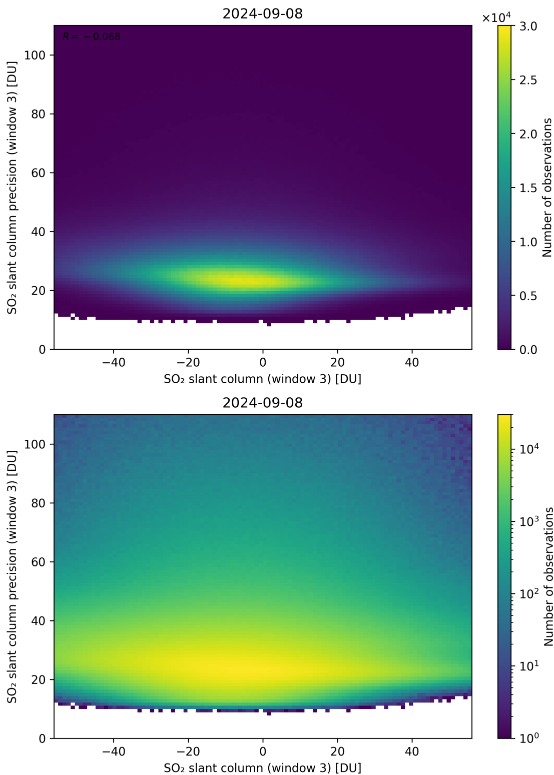
Figure 267: Scatter density plot of “SO 2 slant column (window 3)” against “SO 2 slant column precision (window 3)” for 2024-09-07 to 2024-09-09.
