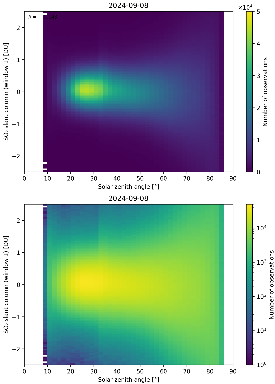
Figure 169: Scatter density plot of “Solar zenith angle” against “SO 2 slant column (window 1)” for 2024-09-07 to 2024-09-09.
