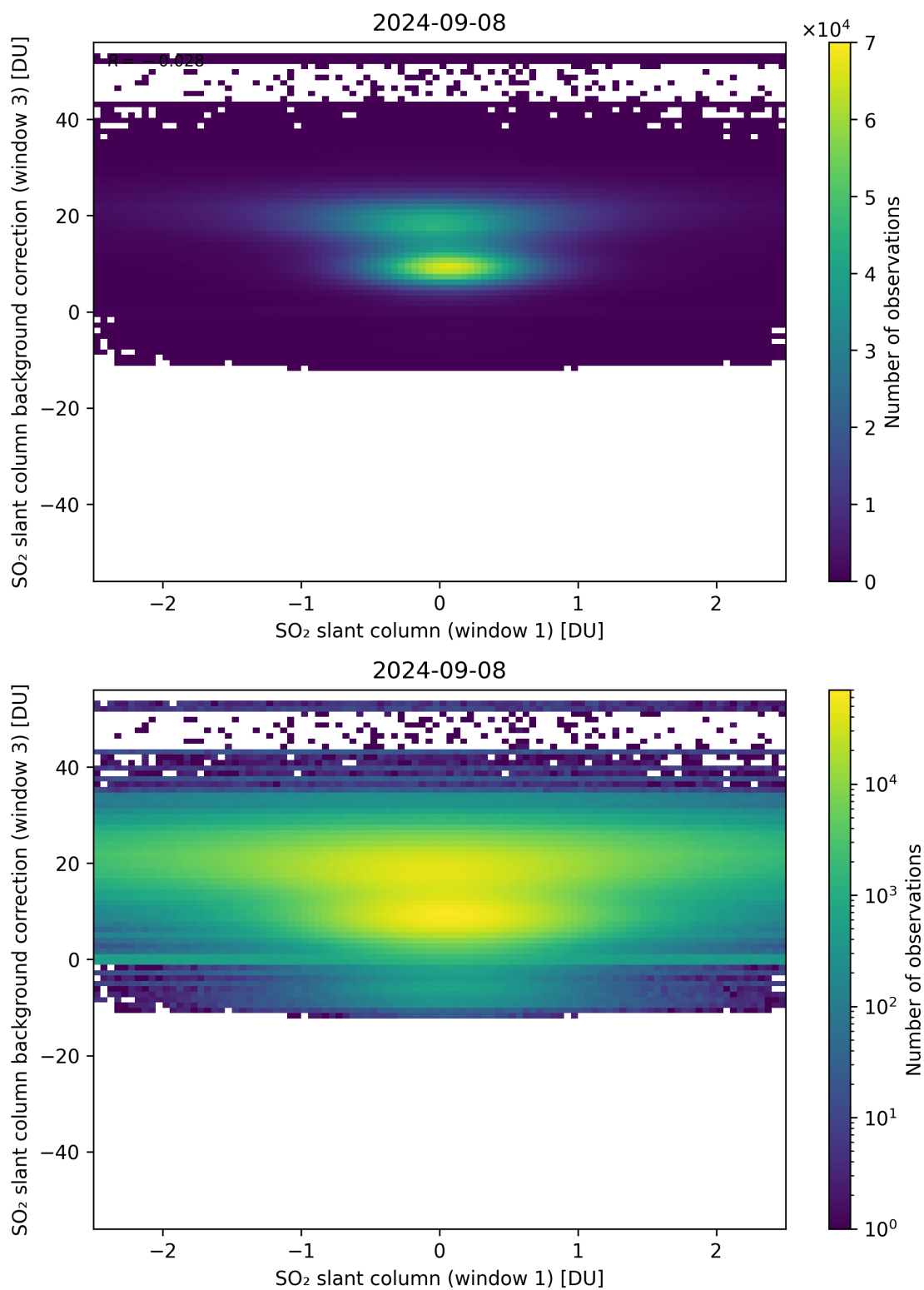
Figure 214: Scatter density plot of “SO 2 slant column (window 1)” against “SO 2 slant column background correction (window 3)” for 2024-09-07 to 2024-09-09.
