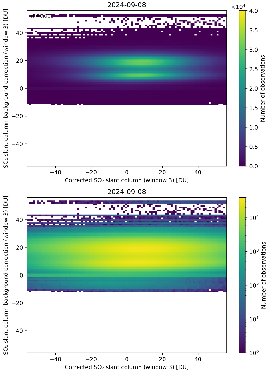
Figure 205: Scatter density plot of “Corrected SO 2 slant column (window 3)” against “SO 2 slant column background correction (window 3)” for 2024-09-07 to 2024-09-09.
