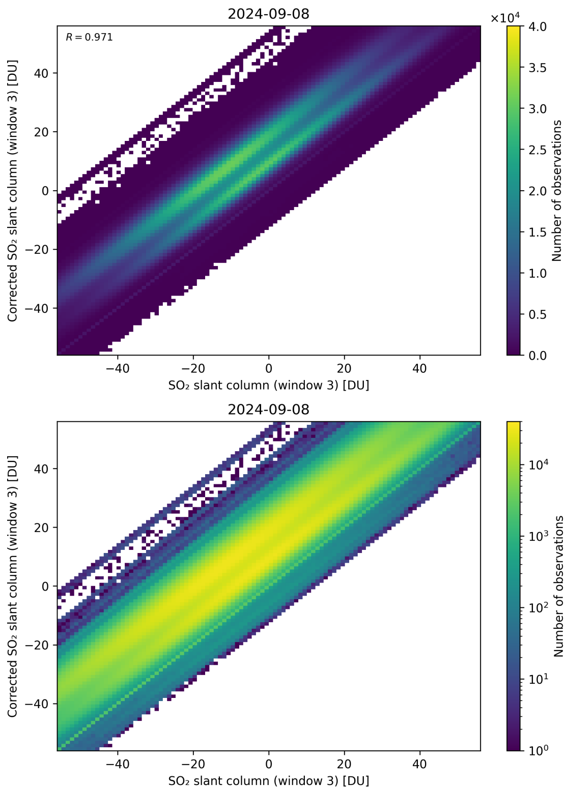
Figure 266: Scatter density plot of “SO 2 slant column (window 3)” against “Corrected SO 2 slant column (window 3)” for 2024-09-07 to 2024-09-09.
