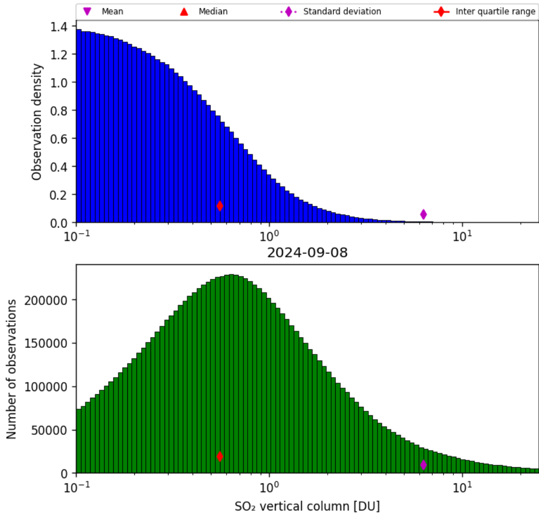
Figure 53: Histogram of “SO 2 vertical column” for 2024-09-07 to 2024-09-09
