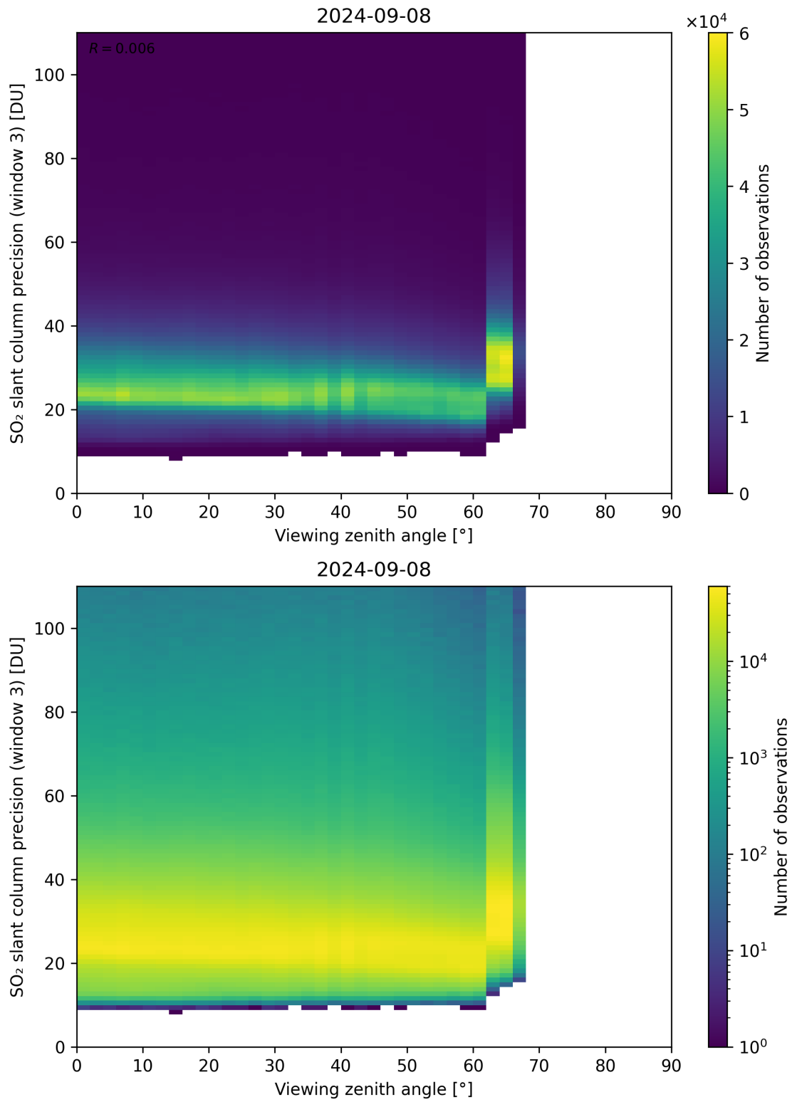
Figure 324: Scatter density plot of “Viewing zenith angle” against “SO 2 slant column precision (window 3)” for 2024-09-07 to 2024-09-09.
