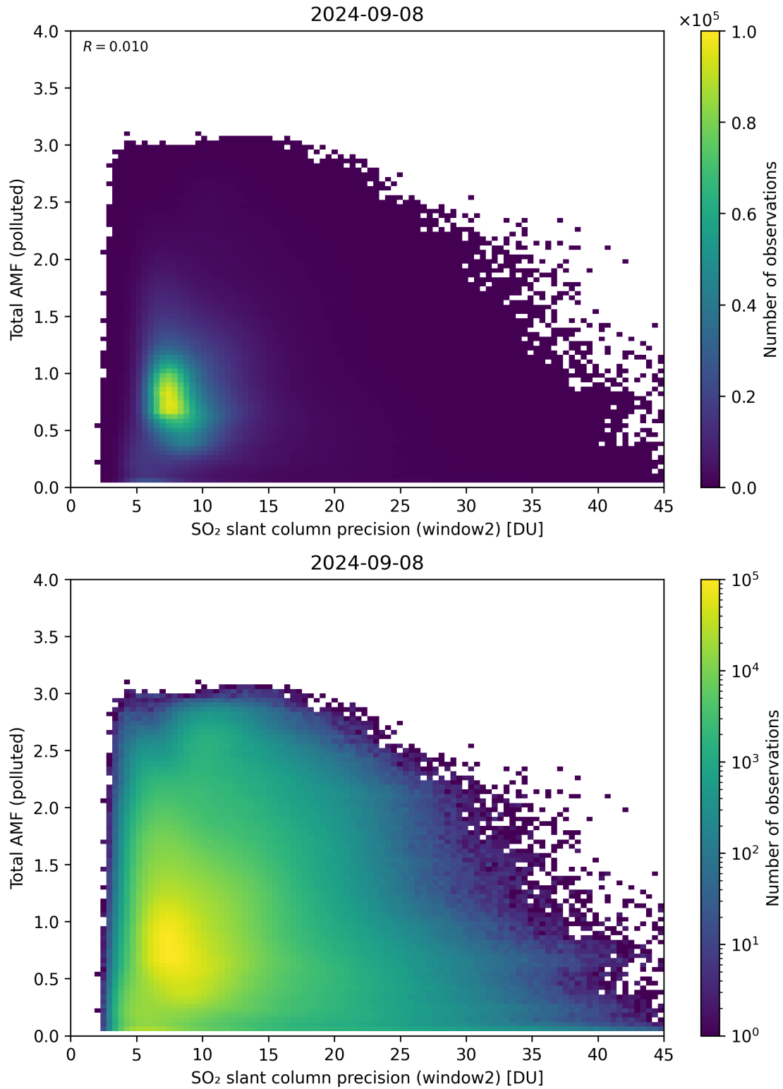
Figure 251: Scatter density plot of “SO 2 slant column precision (window2)” against “Total AMF (polluted)” for 2024-09-07 to 2024-09-09.
