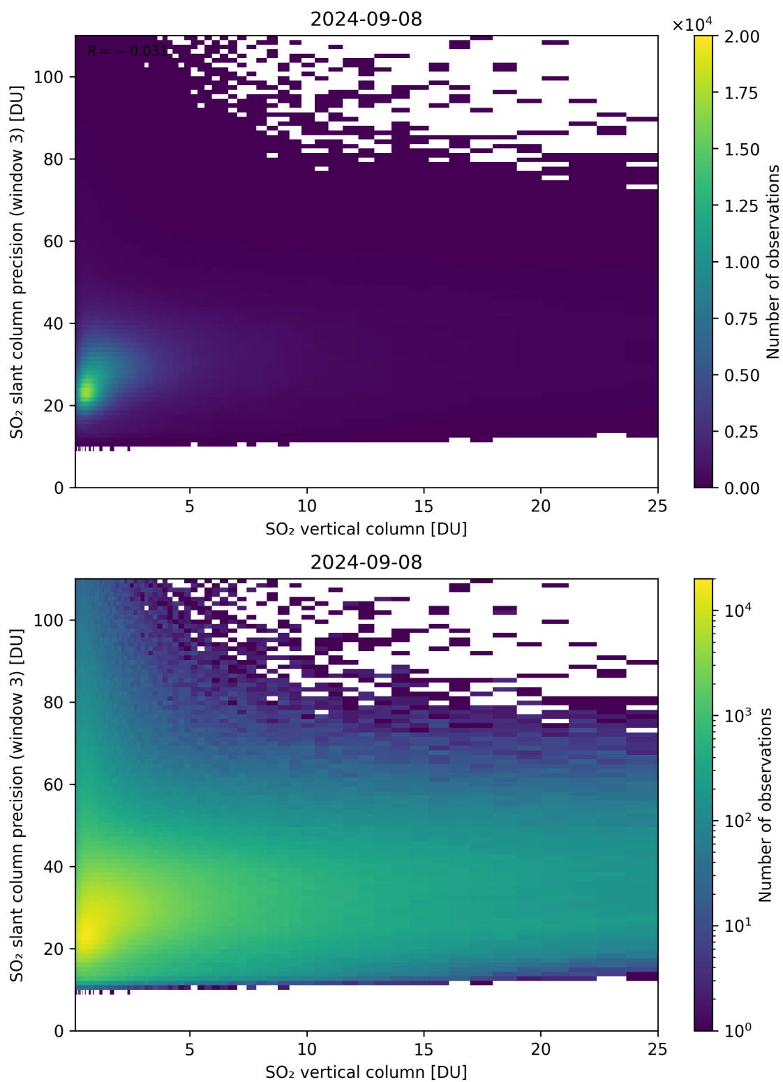
Figure 304: Scatter density plot of “SO 2 vertical column” against “SO 2 slant column precision (window 3)” for 2024-09-07 to 2024-09-09.
