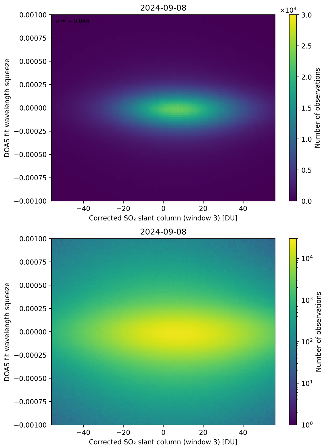
Figure 207: Scatter density plot of “Corrected SO 2 slant column (window 3)” against “DOAS fit wavelength squeeze” for 2024-09-07 to 2024-09-09.
