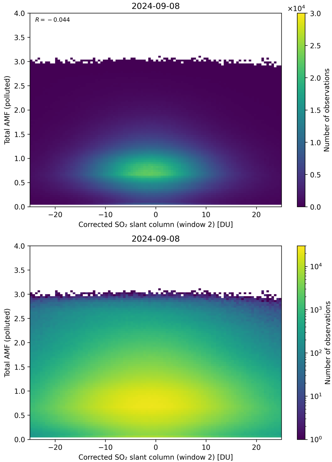
Figure 203: Scatter density plot of “Corrected SO 2 slant column (window 2)” against “Total AMF (polluted)” for 2024-09-07 to 2024-09-09.
