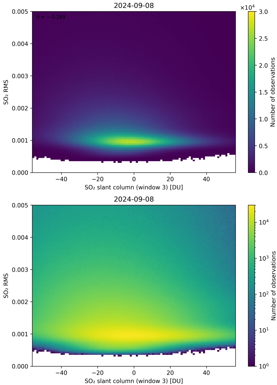
Figure 256: Scatter density plot of “SO 2 slant column (window 3)” against “SO 2 RMS” for 2024-09-07 to 2024-09-09.
