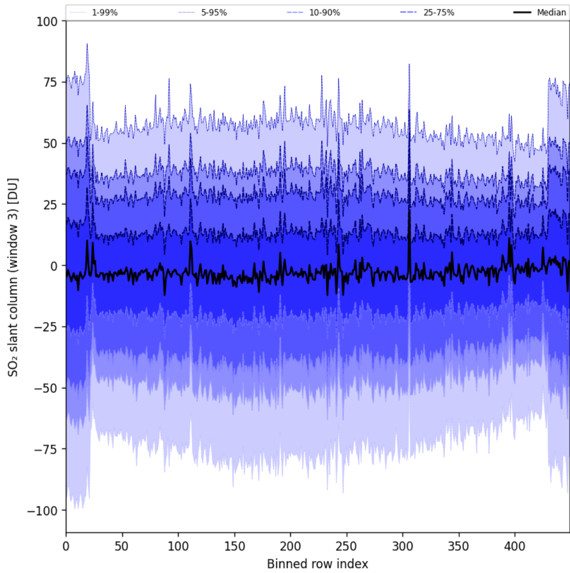
Figure 87: Along track statistics of “SO 2 slant column (window 3)” for 2024-09-09 to 2024-09-11
