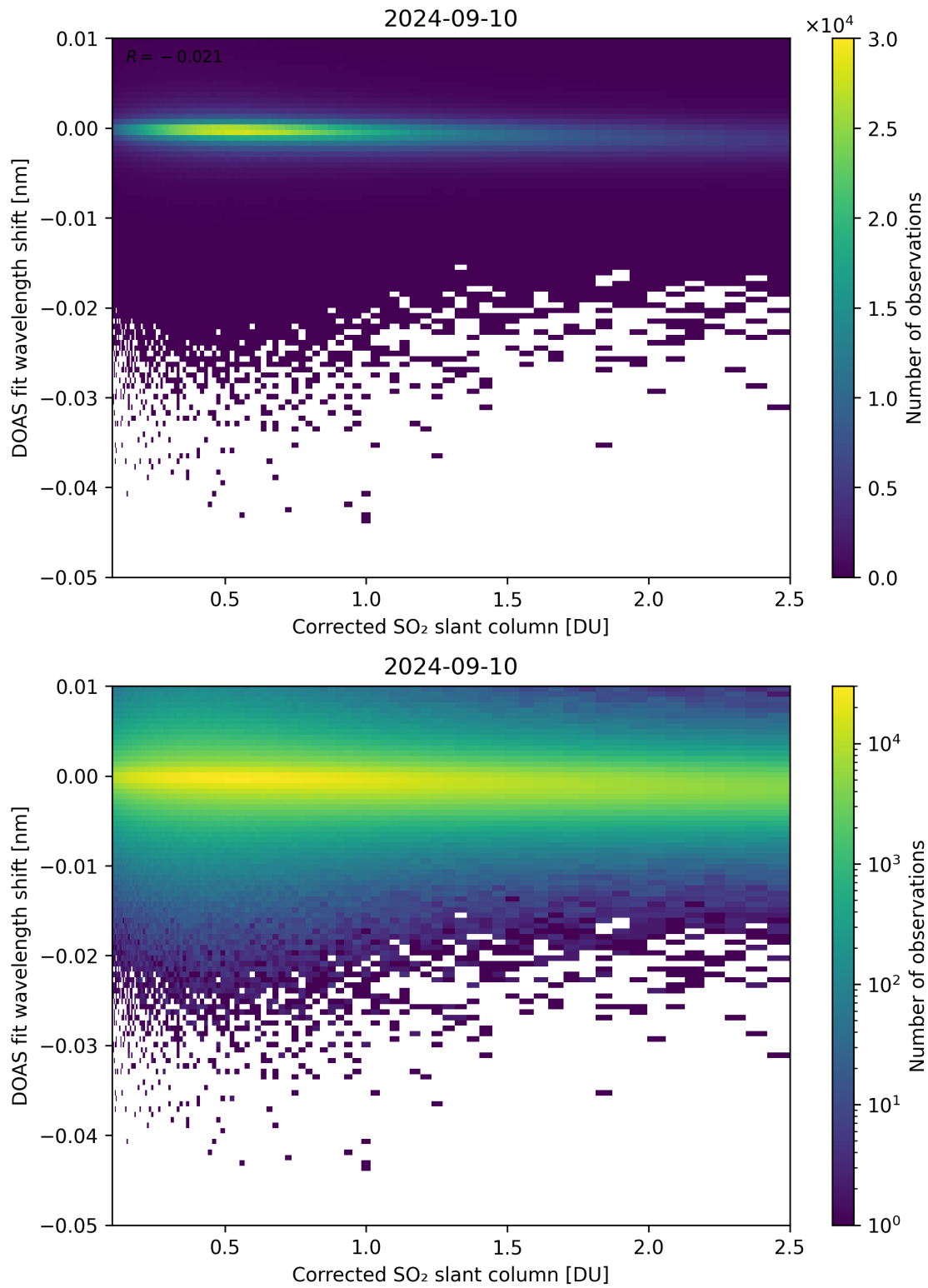
Figure 181: Scatter density plot of “Corrected SO 2 slant column” against “DOAS fit wavelength shift” for 2024-09-09 to 2024-09-11.
