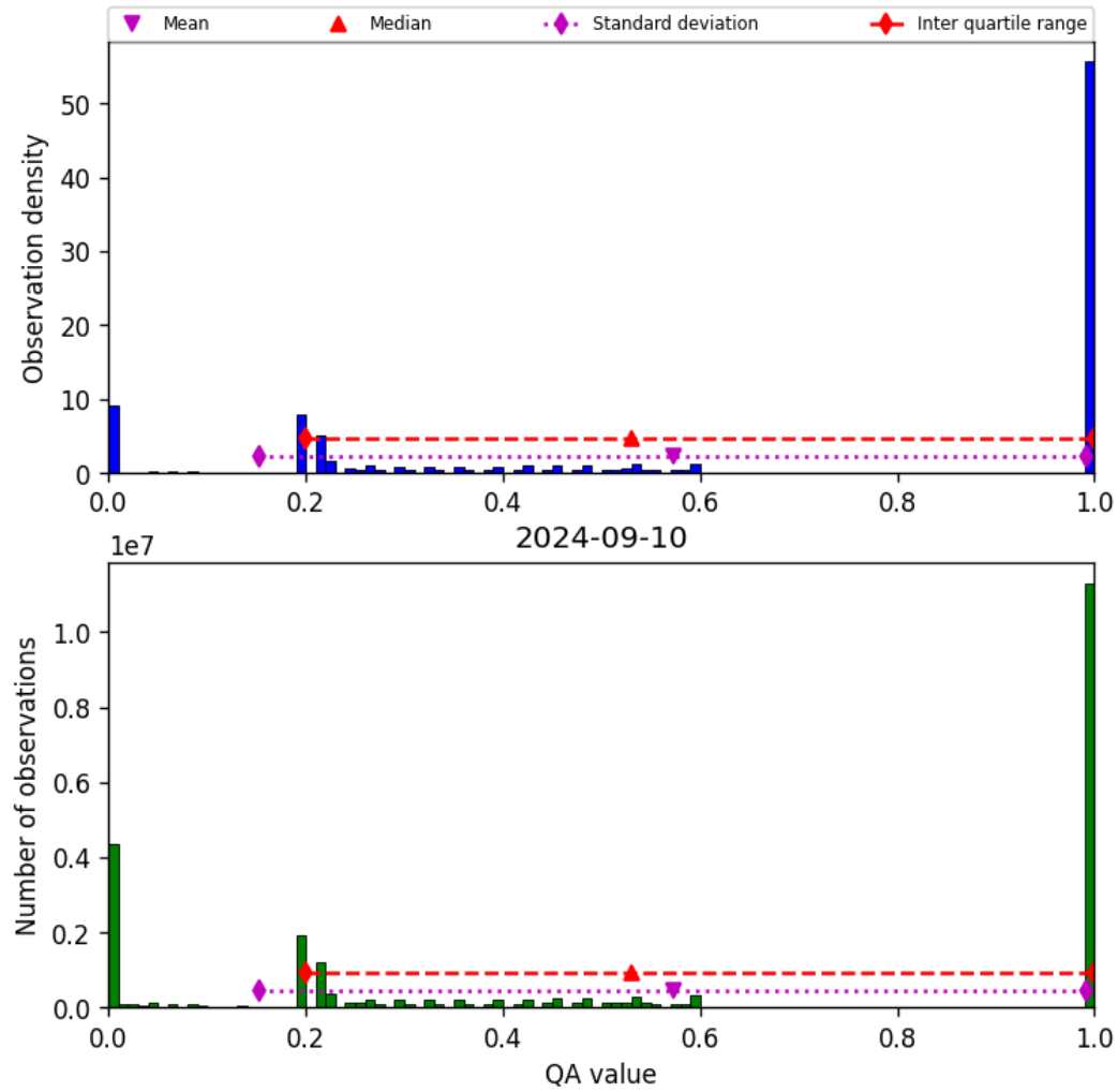
Figure 52: Histogram of “QA value” for 2024-09-09 to 2024-09-11
