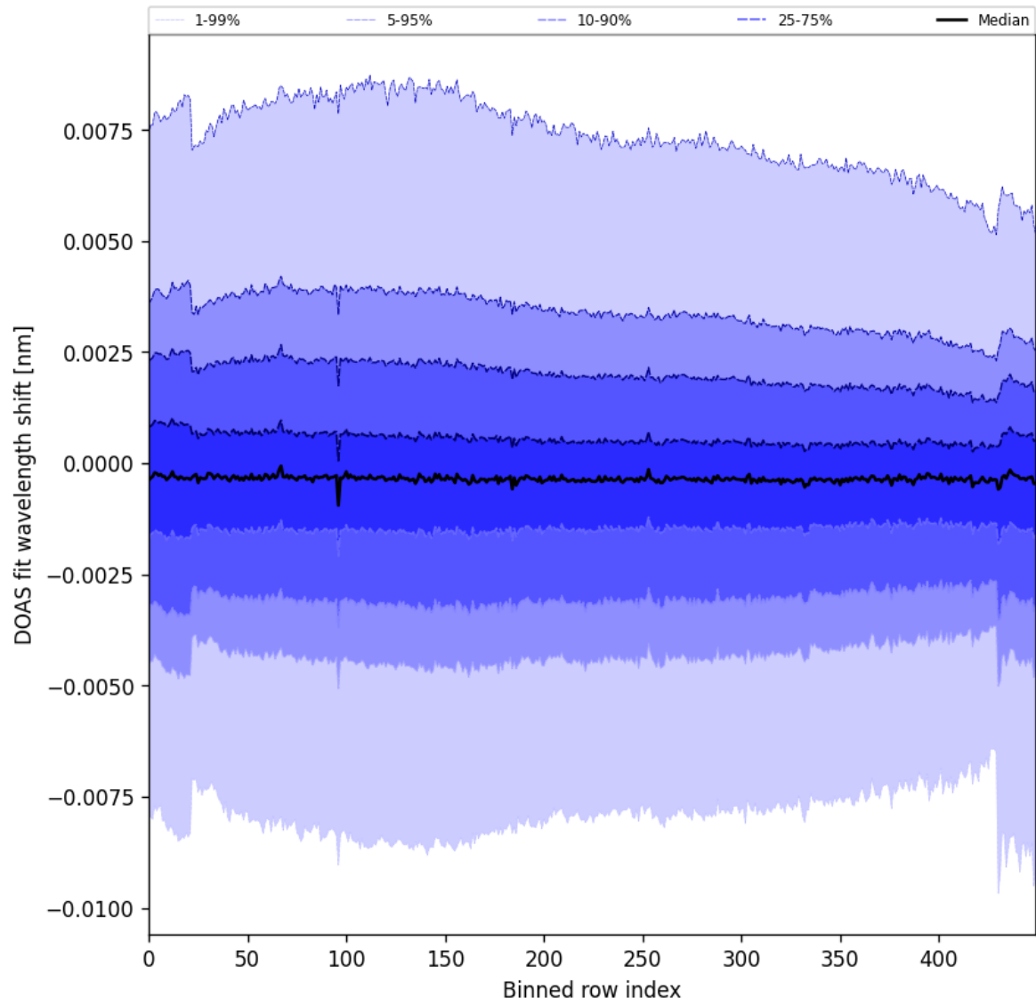
Figure 91: Along track statistics of “DOAS fit wavelength shift” for 2024-09-09 to 2024-09-11
