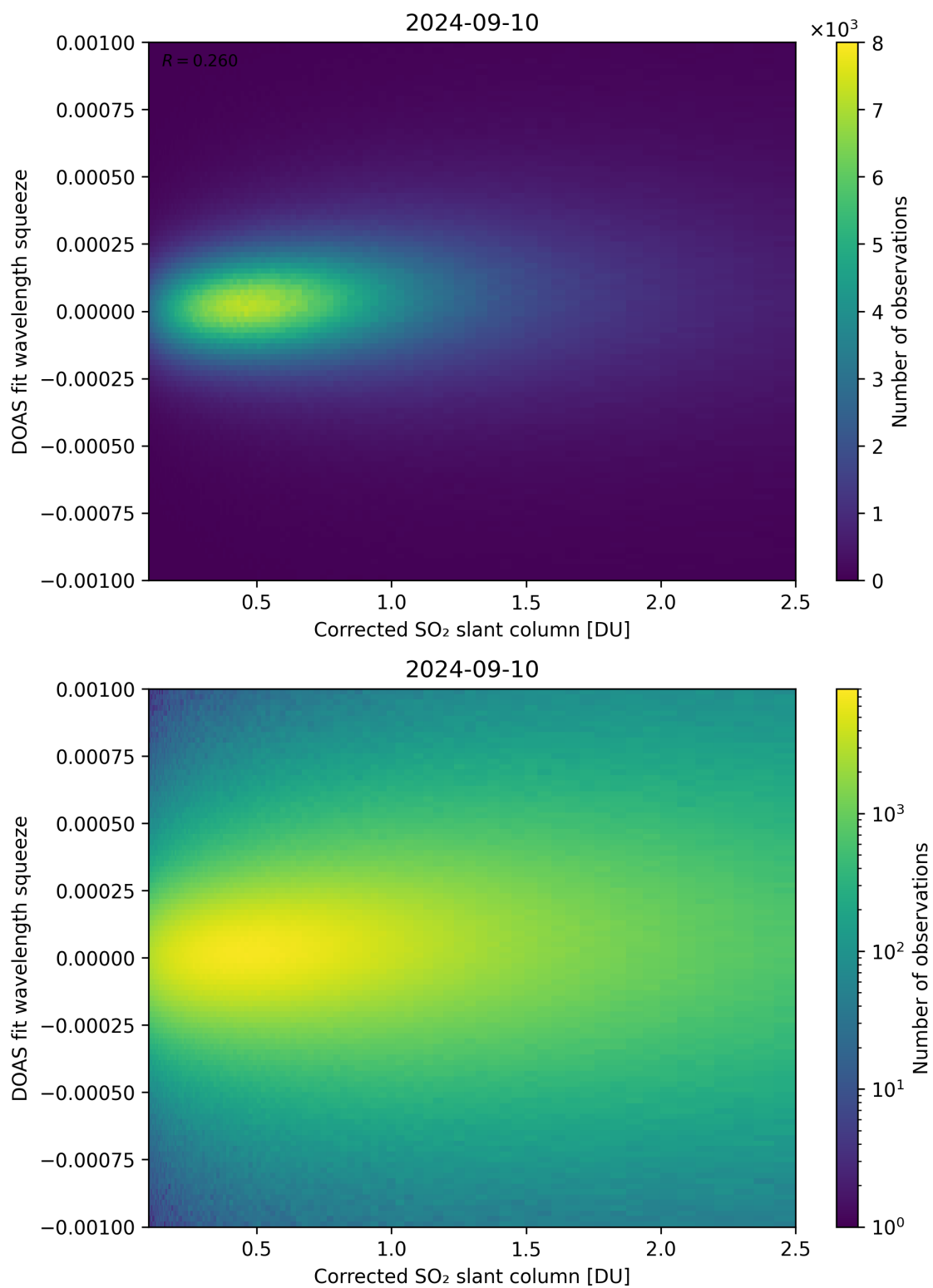
Figure 182: Scatter density plot of “Corrected SO 2 slant column” against “DOAS fit wavelength squeeze” for 2024-09-09 to 2024-09-11.
