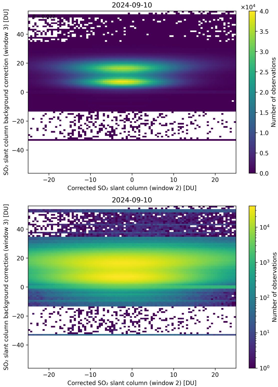
Figure 195: Scatter density plot of “Corrected SO 2 slant column (window 2)” against “SO 2 slant column background correction (window 3)” for 2024-09-09 to 2024-09-11.
