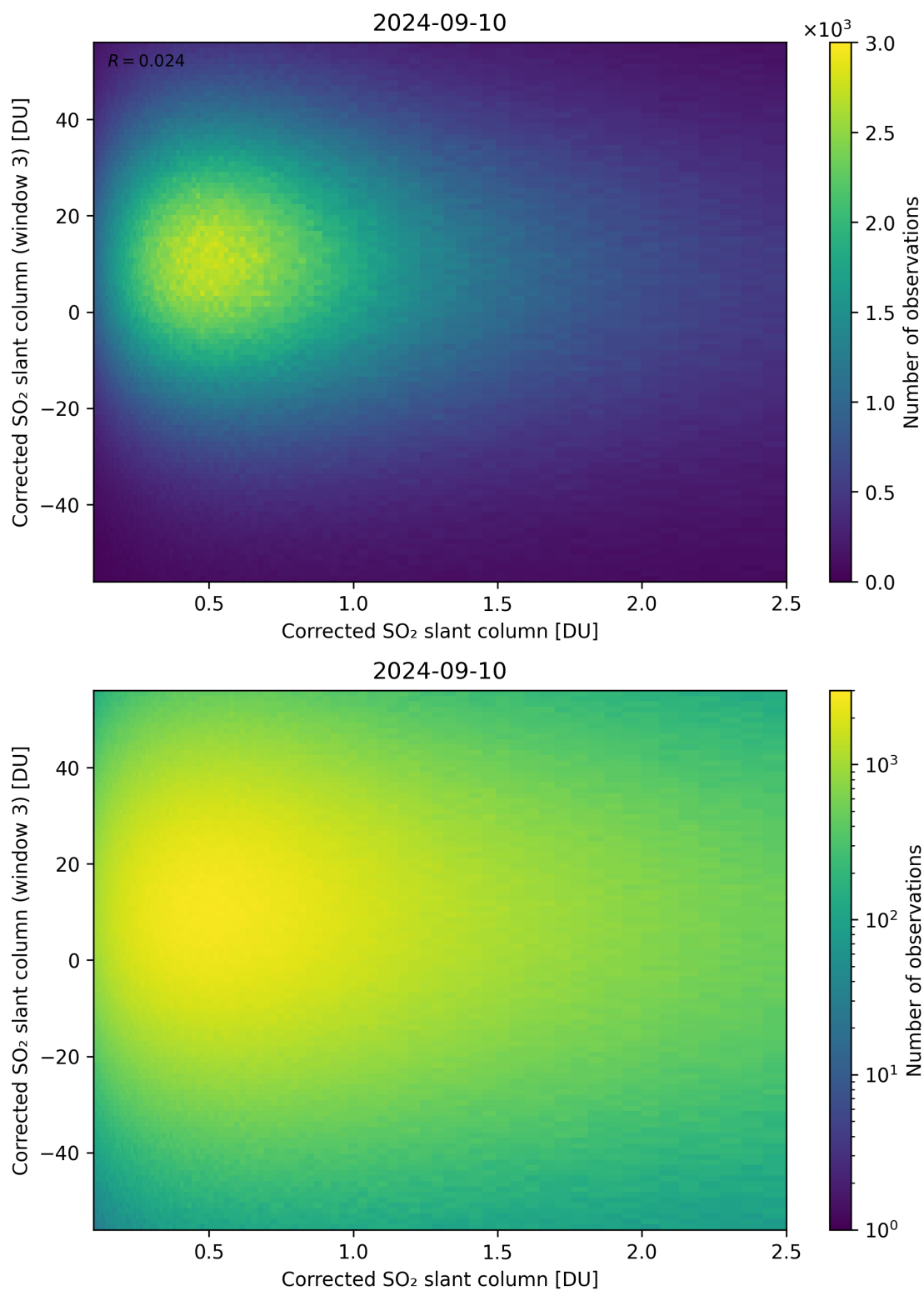
Figure 186: Scatter density plot of “Corrected SO 2 slant column” against “Corrected SO 2 slant column (window 3)” for 2024-09-09 to 2024-09-11.
