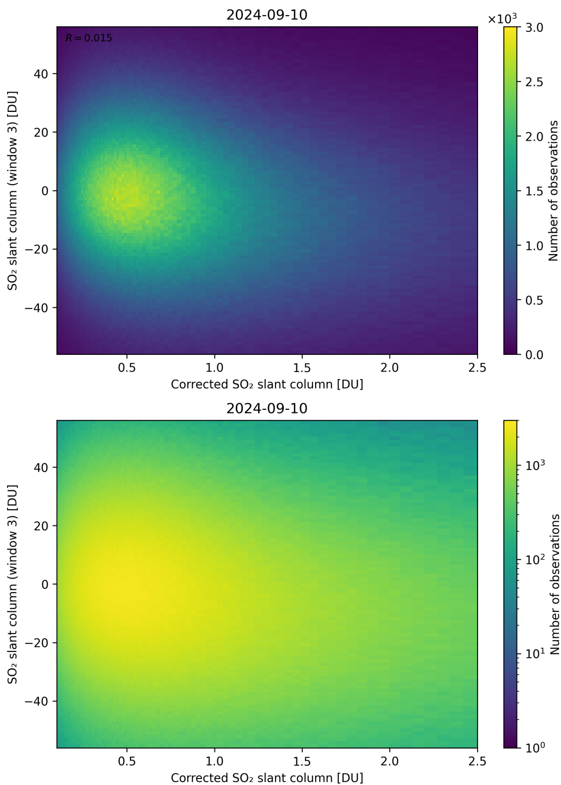
Figure 190: Scatter density plot of “Corrected SO 2 slant column” against “SO 2 slant column (window 3)” for 2024-09-09 to 2024-09-11.
