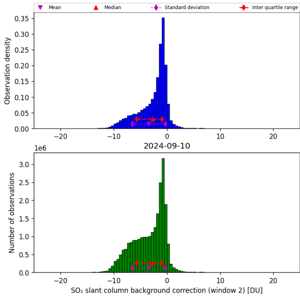
Figure 63: Histogram of “SO 2 slant column background correction (window 2)” for 2024-09-09 to 2024-09-11
