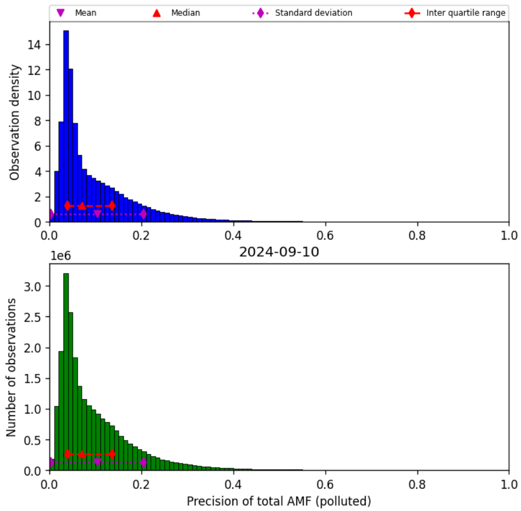
Figure 72: Histogram of “Precision of total AMF (polluted)” for 2024-09-09 to 2024-09-11
