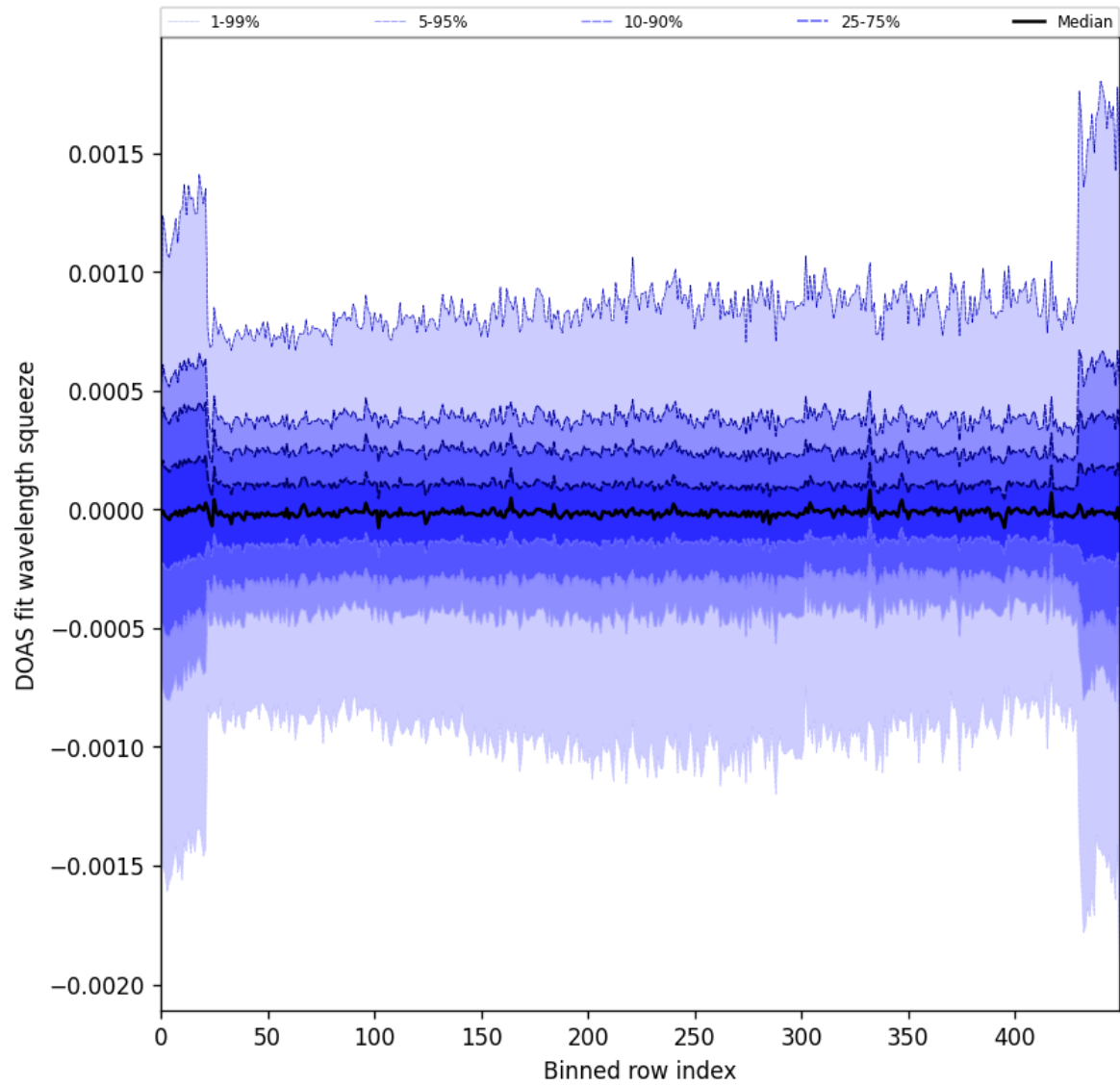
Figure 92: Along track statistics of “DOAS fit wavelength squeeze” for 2024-09-09 to 2024-09-11
