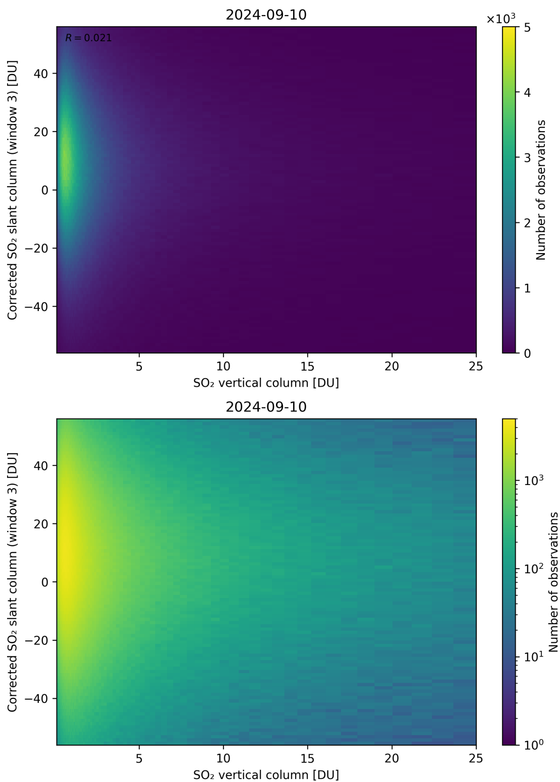
Figure 299: Scatter density plot of “SO 2 vertical column” against “Corrected SO 2 slant column (window 3)” for 2024-09-09 to 2024-09-11.
