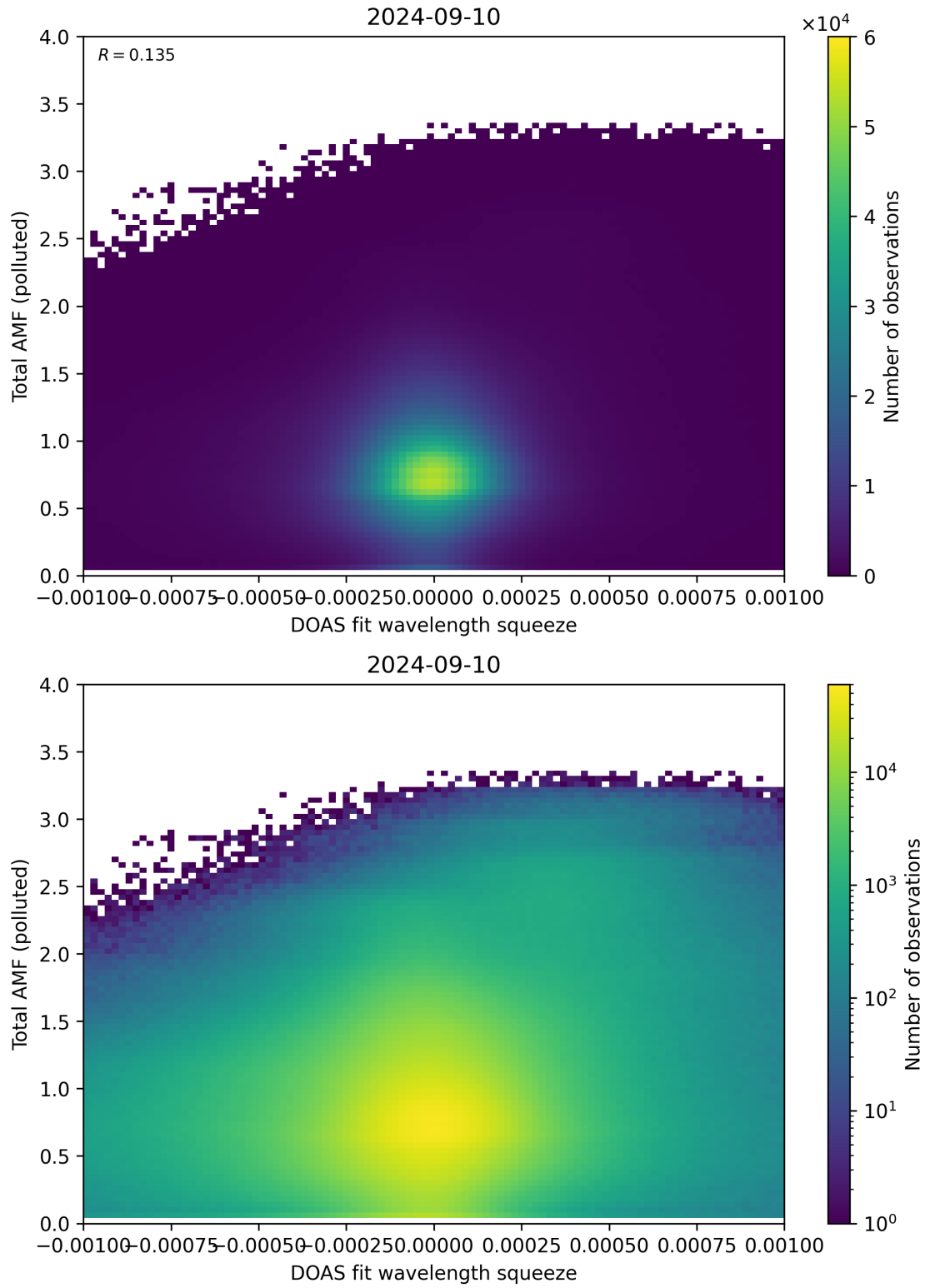
Figure 134: Scatter density plot of “DOAS fit wavelength squeeze” against “Total AMF (polluted)” for 2024-09-09 to 2024-09-11.
