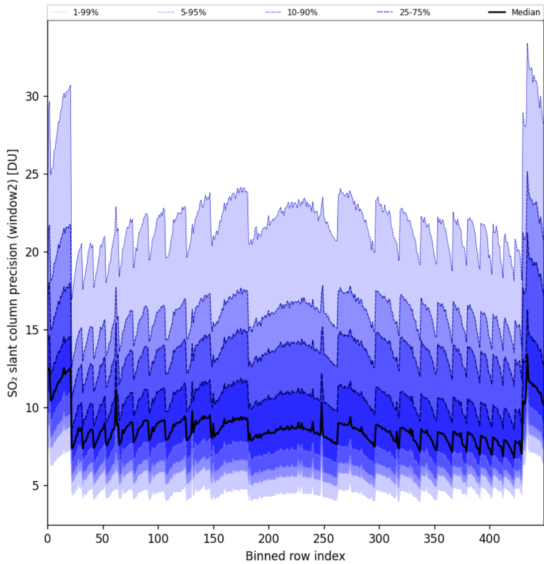
Figure 84: Along track statistics of “SO 2 slant column precision (window2)” for 2024-09-09 to 2024-09-11
