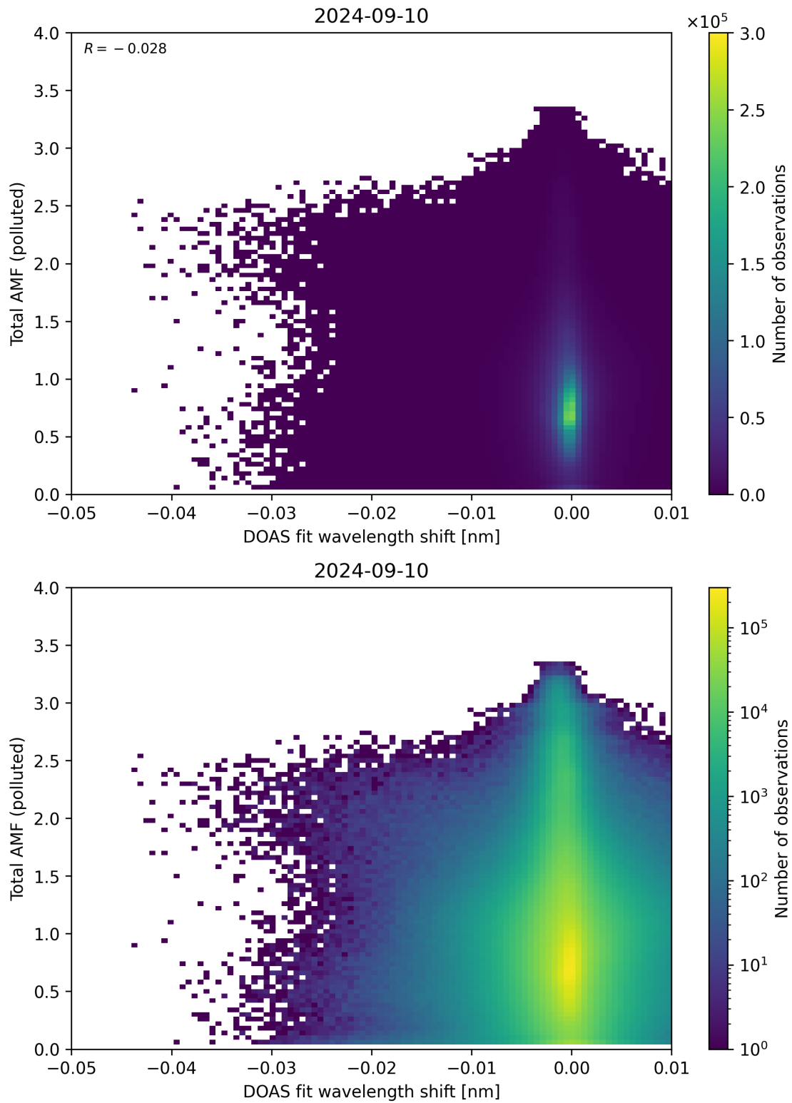
Figure 130: Scatter density plot of “DOAS fit wavelength shift” against “Total AMF (polluted)” for 2024-09-09 to 2024-09-11.
