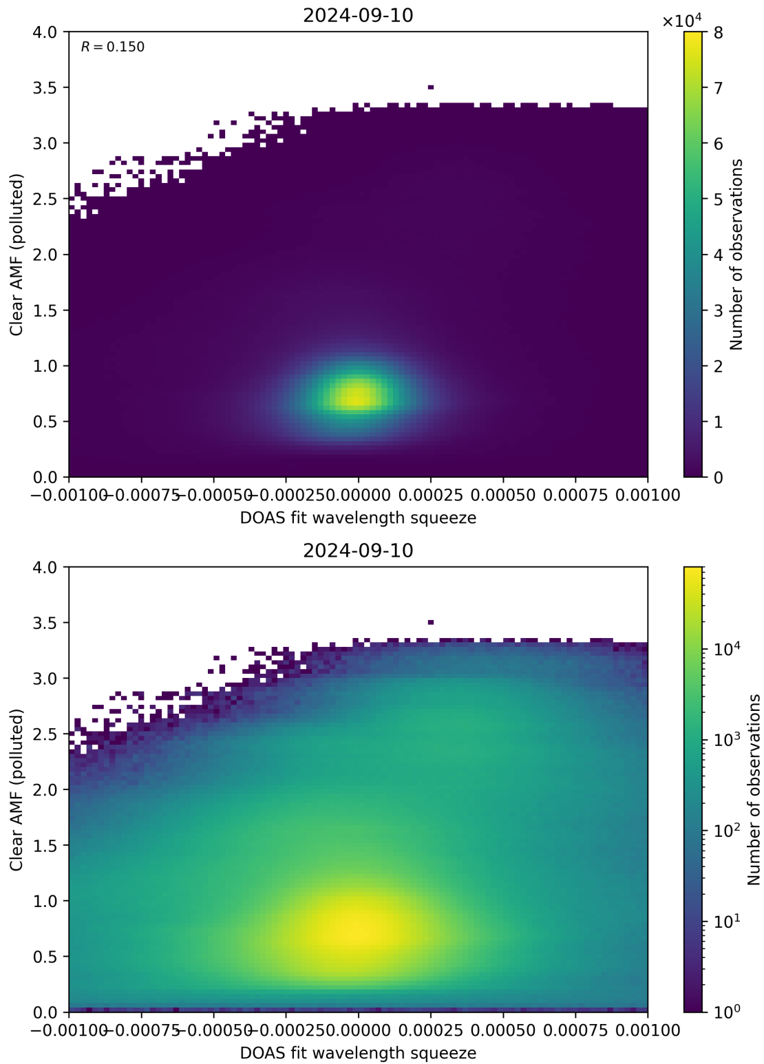
Figure 133: Scatter density plot of “DOAS fit wavelength squeeze” against “Clear AMF (polluted)” for 2024-09-09 to 2024-09-11.
