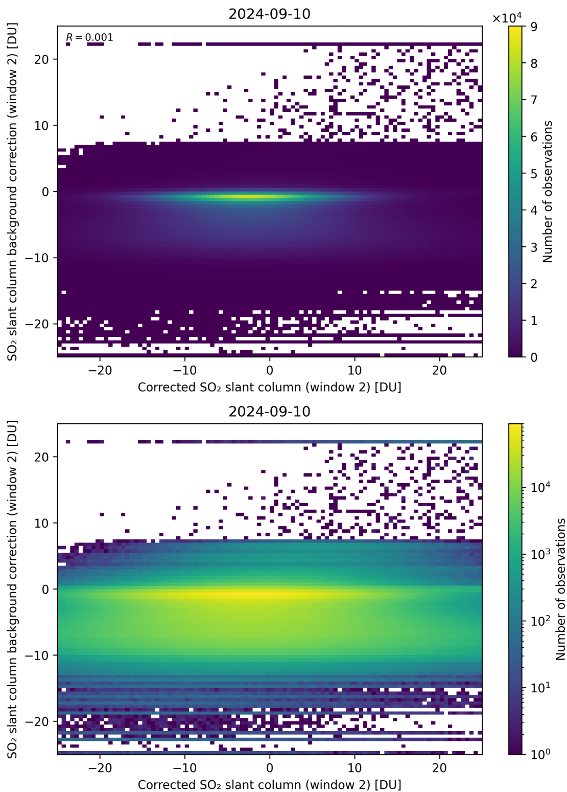
Figure 194: Scatter density plot of “Corrected SO 2 slant column (window 2)” against “SO 2 slant column background correction (window 2)” for 2024-09-09 to 2024-09-11.
