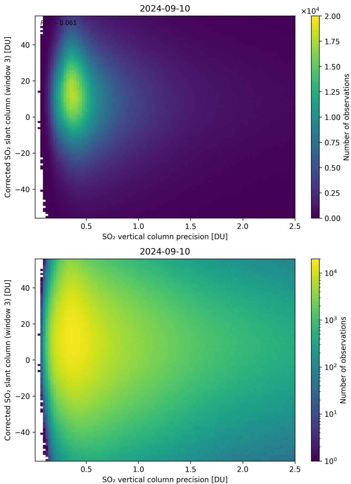
Figure 288: Scatter density plot of “SO 2 vertical column precision” against “Corrected SO 2 slant column (window 3)” for 2024-09-09 to 2024-09-11.
