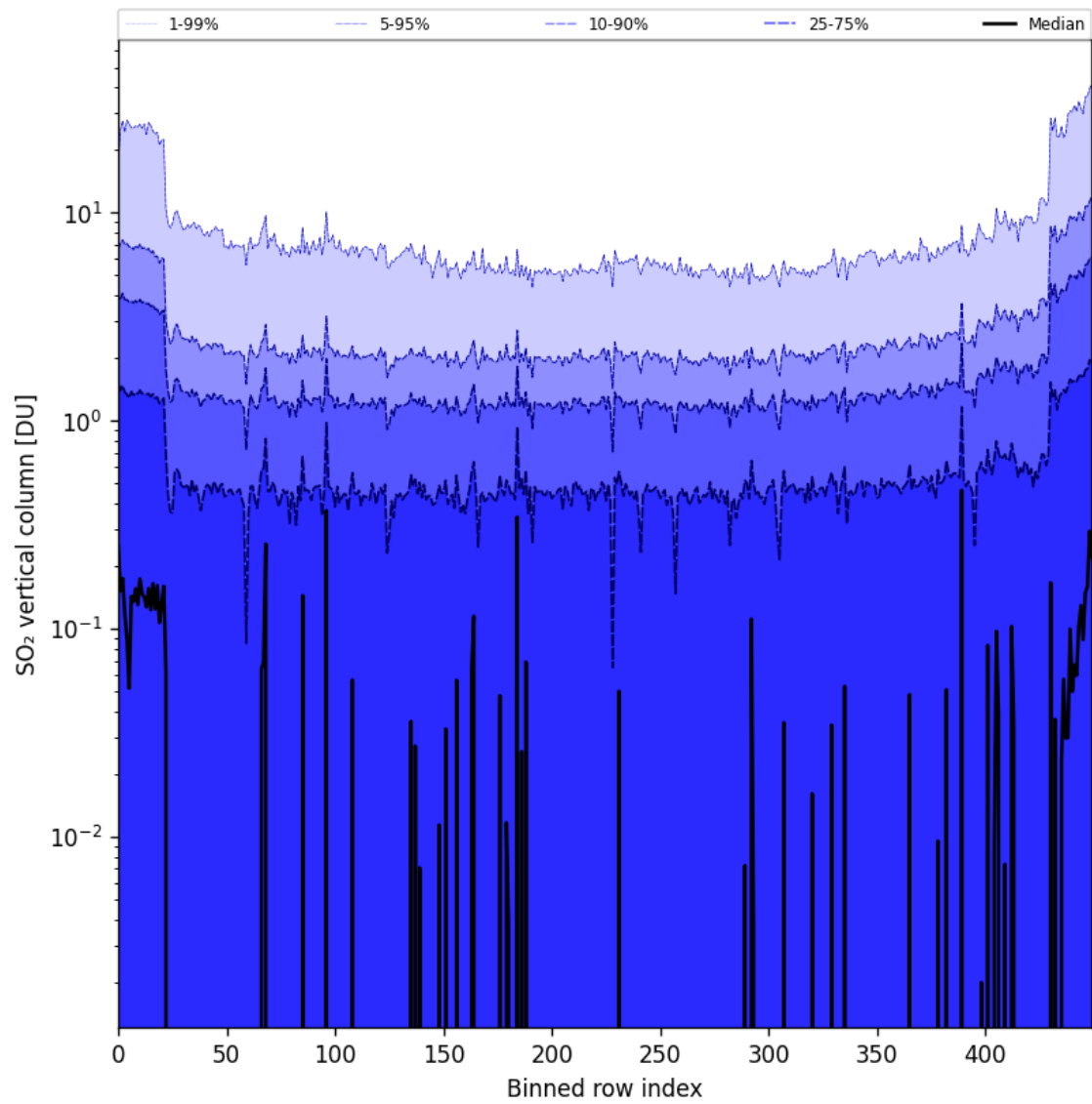
Figure 76: Along track statistics of “SO 2 vertical column” for 2024-09-09 to 2024-09-11
