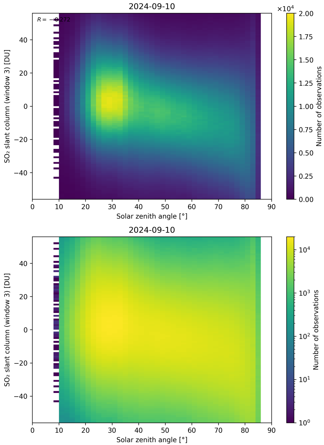
Figure 172: Scatter density plot of “Solar zenith angle” against “SO 2 slant column (window 3)” for 2024-09-09 to 2024-09-11.
