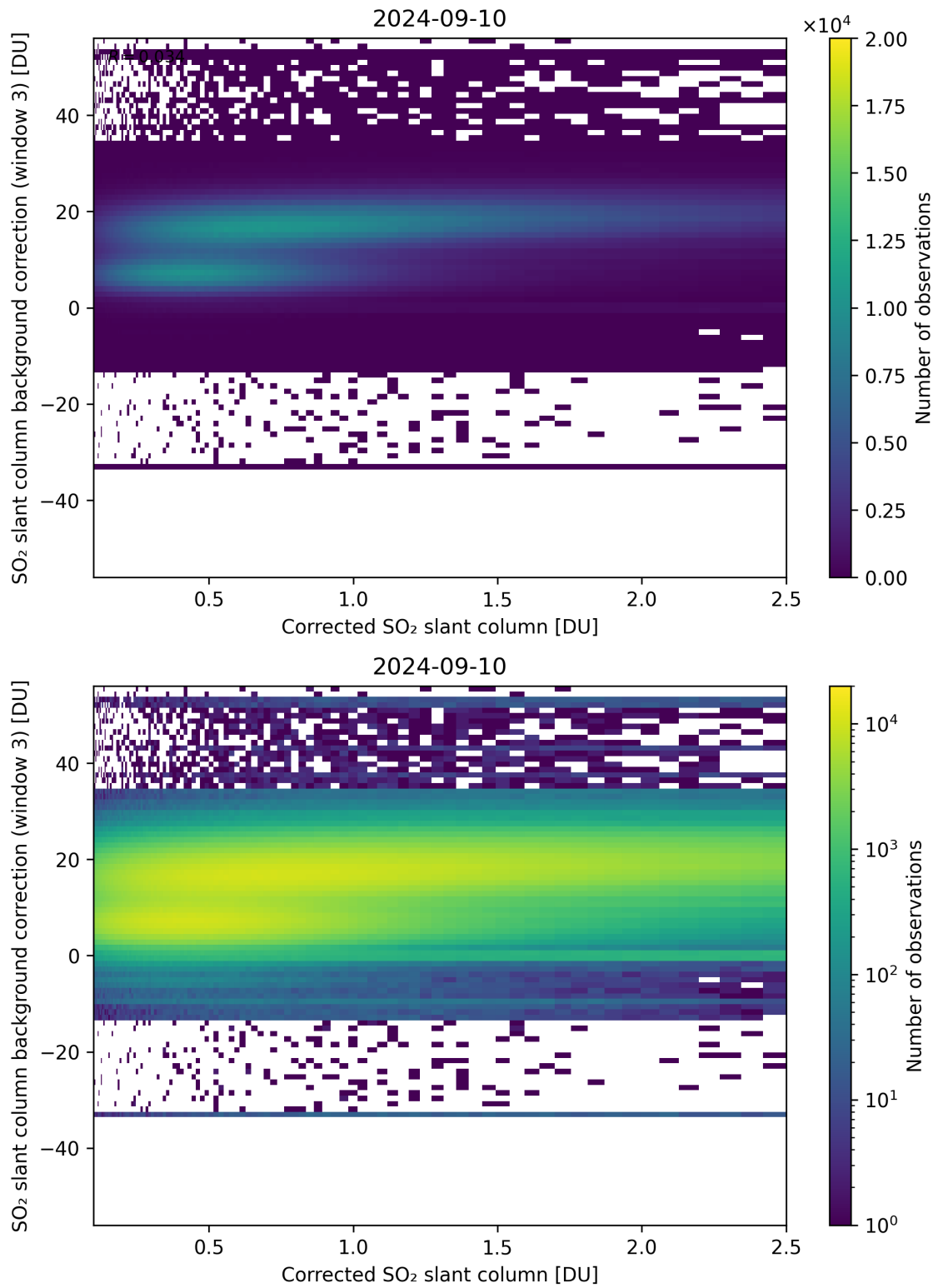
Figure 180: Scatter density plot of “Corrected SO 2 slant column” against “SO 2 slant column background correction (window 3)” for 2024-09-09 to 2024-09-11.
