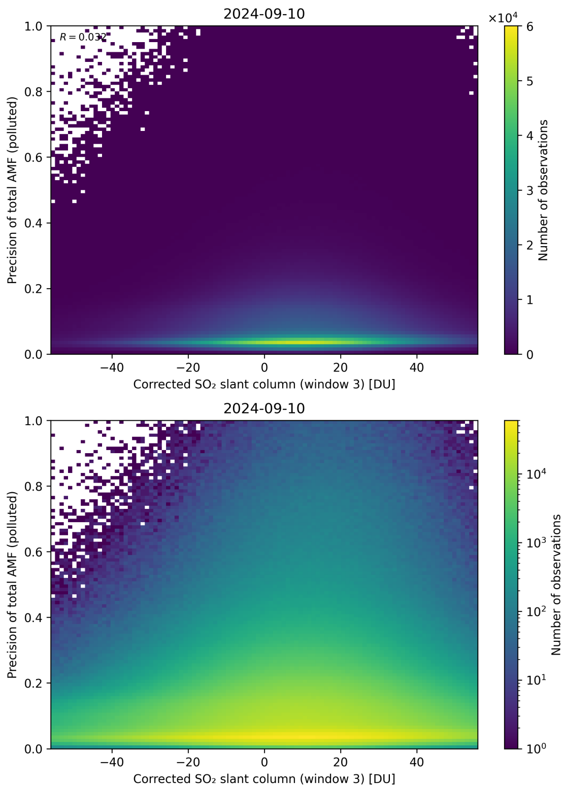
Figure 211: Scatter density plot of “Corrected SO 2 slant column (window 3)” against “Precision of total AMF (polluted)” for 2024-09-09 to 2024-09-11.
