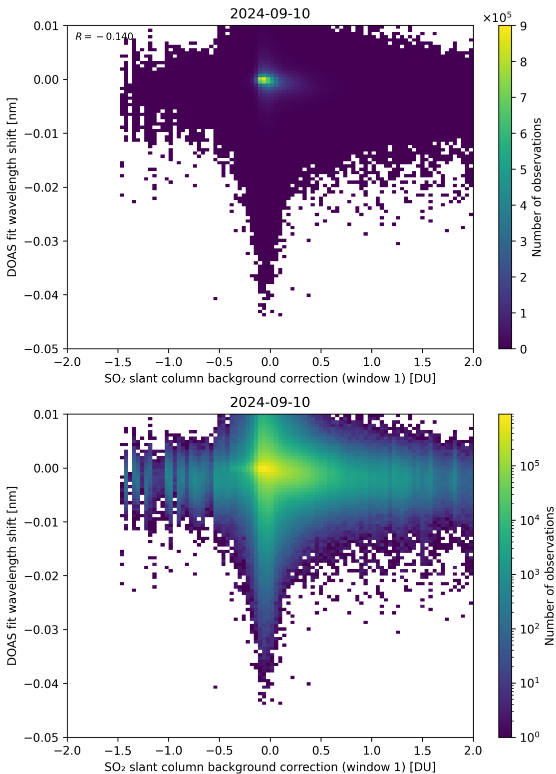
Figure 100: Scatter density plot of “SO 2 slant column background correction (window 1)” against “DOAS fit wavelength shift” for 2024-09-09 to 2024-09-11.
