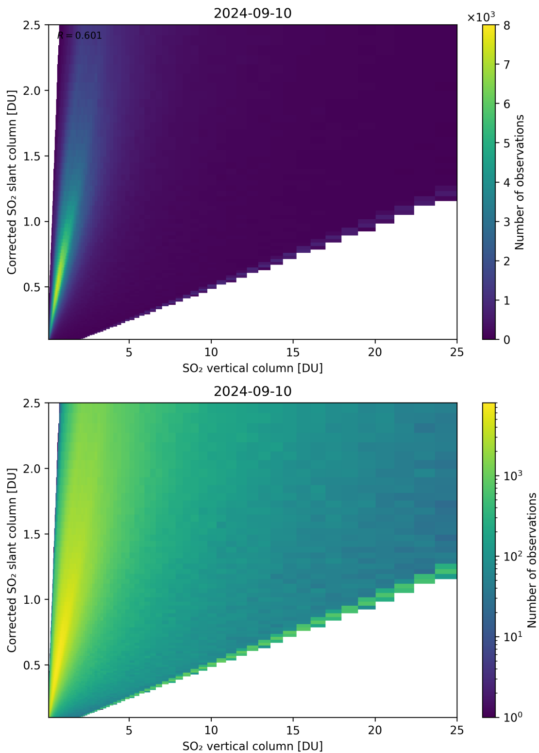
Figure 297: Scatter density plot of “SO 2 vertical column” against “Corrected SO 2 slant column” for 2024-09-09 to 2024-09-11.
