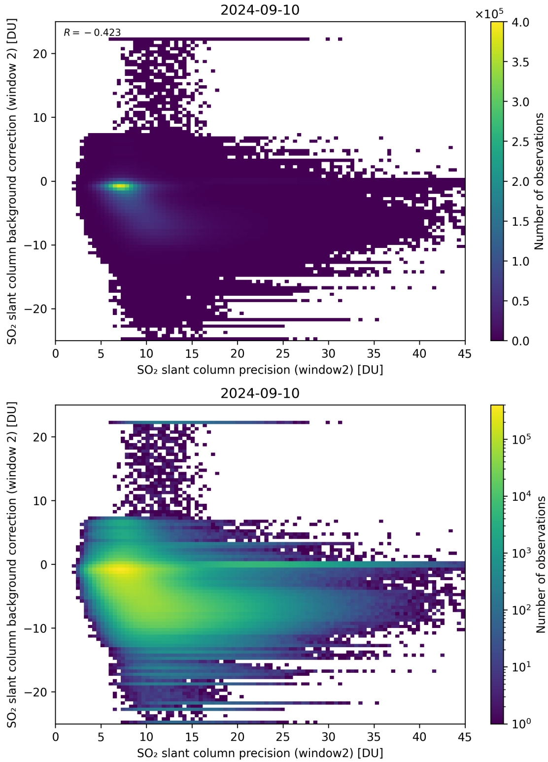
Figure 241: Scatter density plot of “SO 2 slant column precision (window2)” against “SO 2 slant column background correction (window 2)” for 2024-09-09 to 2024-09-11.
