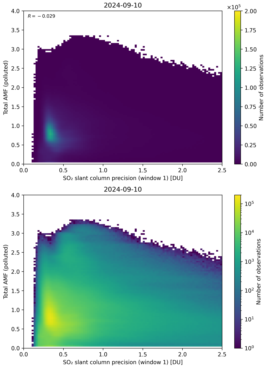
Figure 230: Scatter density plot of “SO 2 slant column precision (window 1)” against “Total AMF (polluted)” for 2024-09-09 to 2024-09-11.
