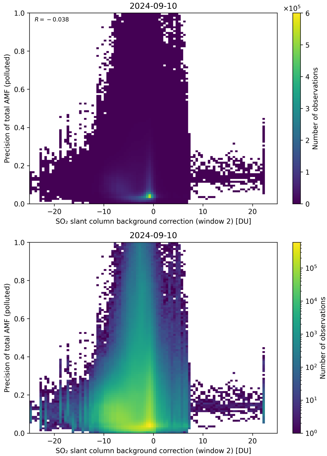
Figure 120: Scatter density plot of “SO 2 slant column background correction (window 2)” against “Precision of total AMF (polluted)” for 2024-09-09 to 2024-09-11.
