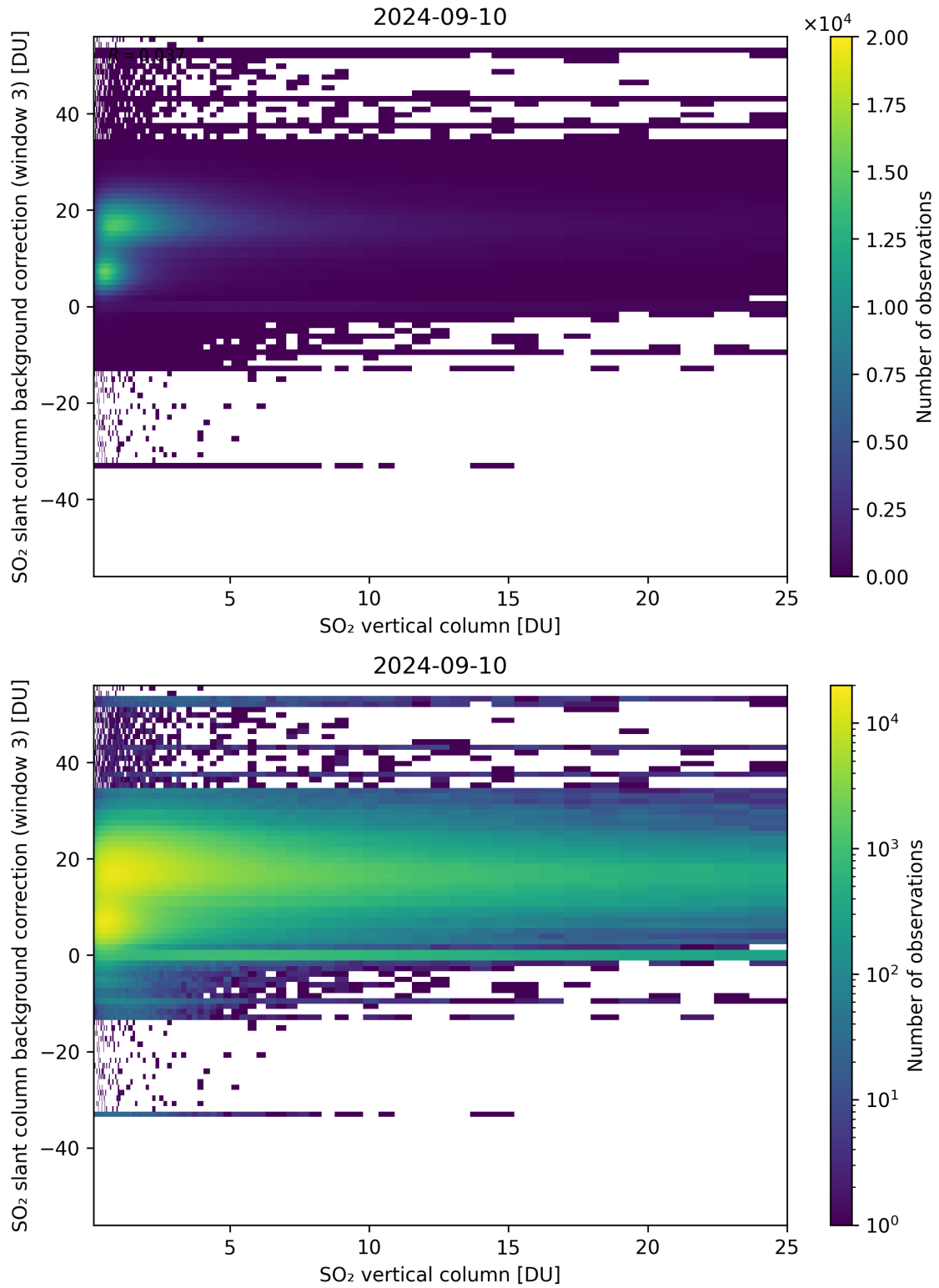
Figure 275: Scatter density plot of “SO 2 vertical column” against “SO 2 slant column background correction (window 3)” for 2024-09-09 to 2024-09-11.
