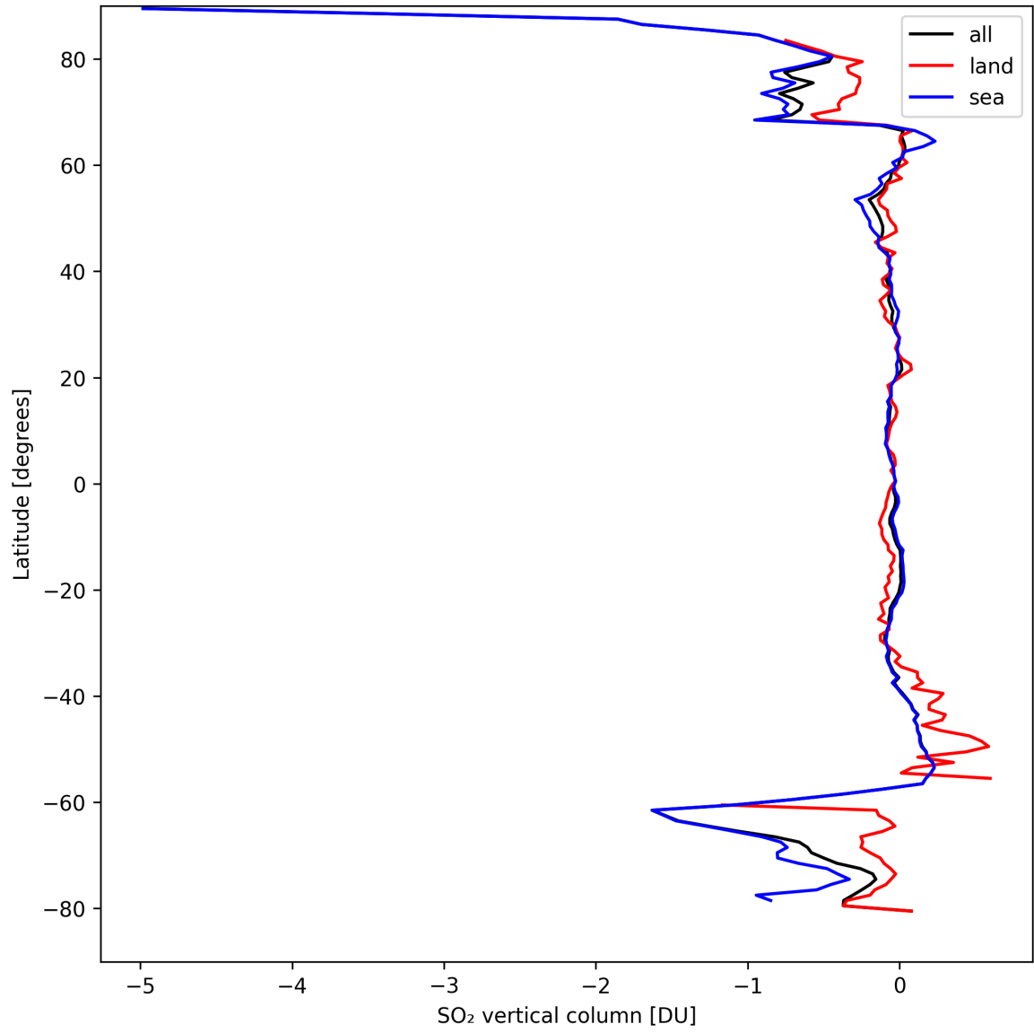
Figure 30: Zonal average of “SO 2 vertical column” for 2024-09-09 to 2024-09-11.
