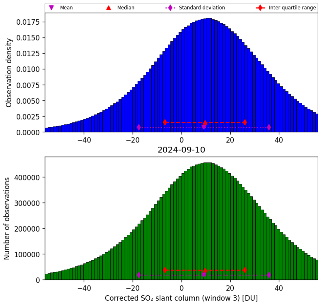
Figure 66: Histogram of “Corrected SO 2 slant column (window 3)” for 2024-09-09 to 2024-09-11
