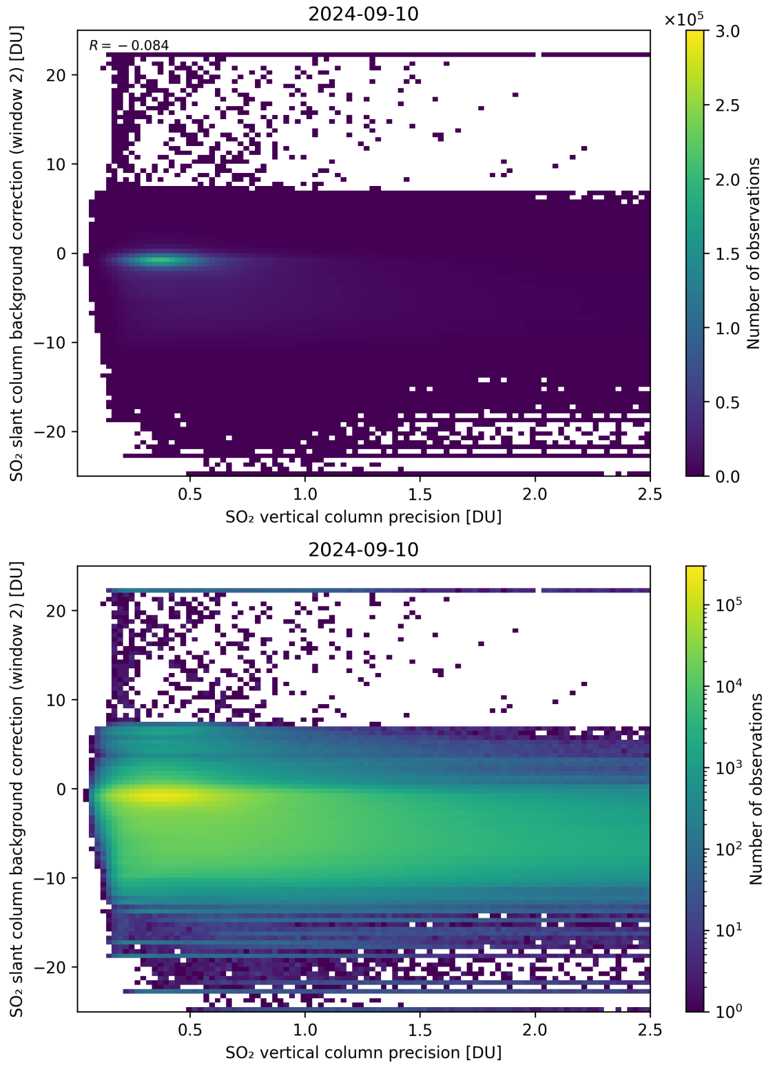
Figure 280: Scatter density plot of “SO 2 vertical column precision” against “SO 2 slant column background correction (window 2)” for 2024-09-09 to 2024-09-11.
