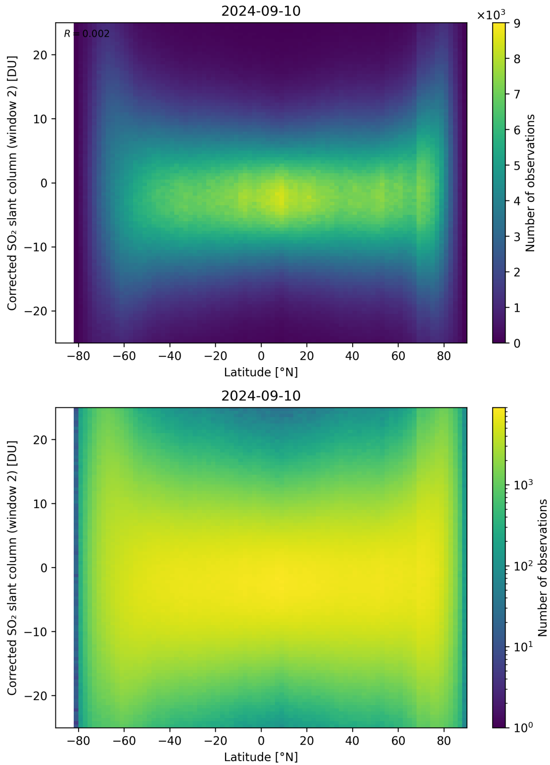
Figure 147: Scatter density plot of “Latitude” against “Corrected SO 2 slant column (window 2)” for 2024-09-09 to 2024-09-11.
