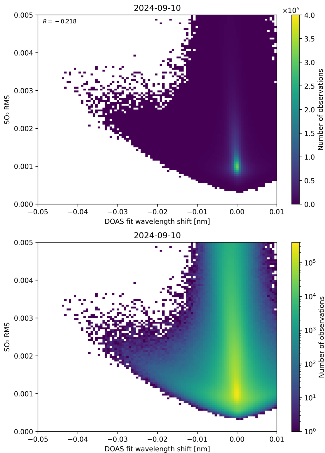
Figure 128: Scatter density plot of “DOAS fit wavelength shift” against “SO 2 RMS” for 2024-09-09 to 2024-09-11.
