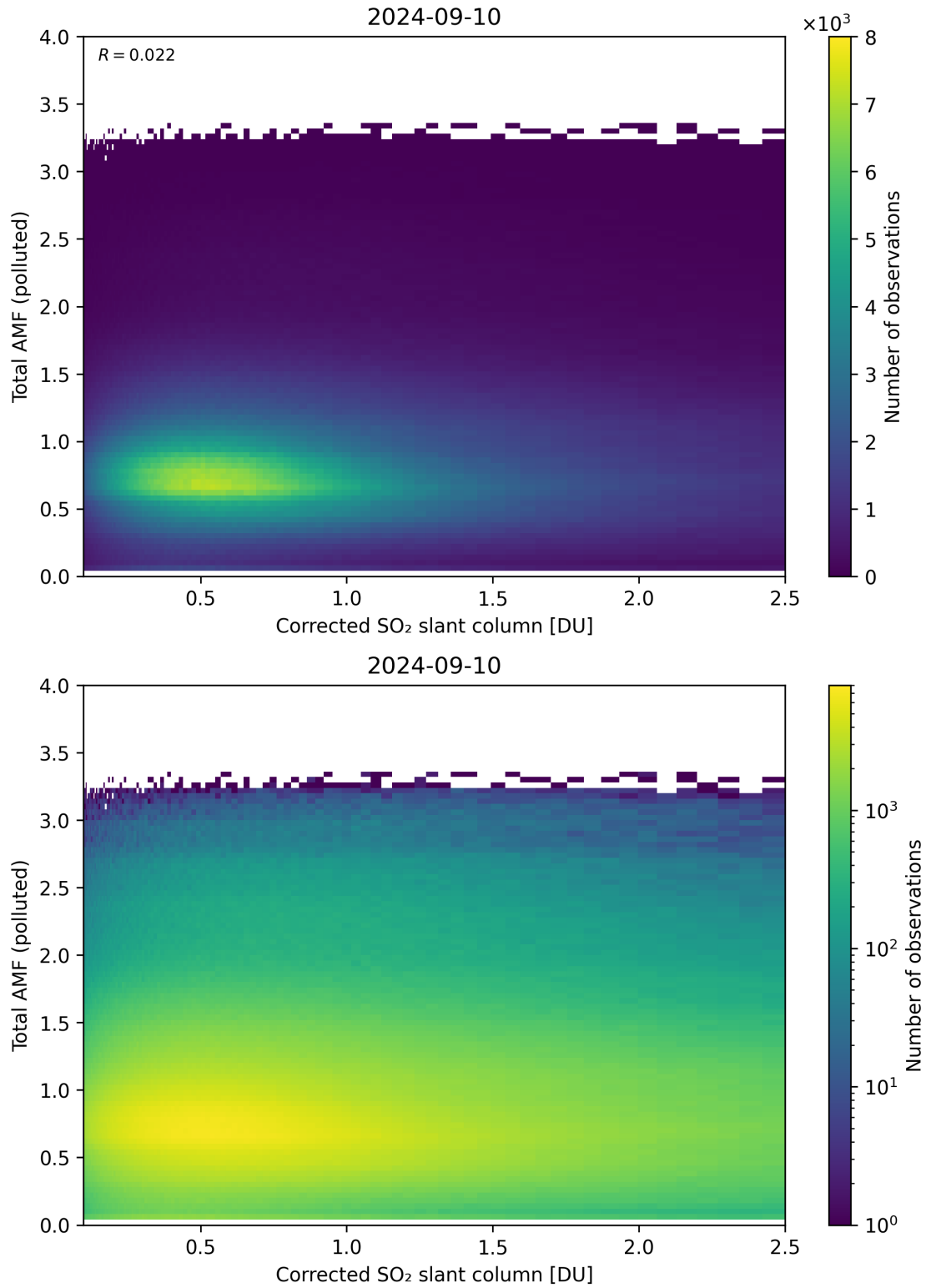
Figure 192: Scatter density plot of “Corrected SO 2 slant column” against “Total AMF (polluted)” for 2024-09-09 to 2024-09-11.
