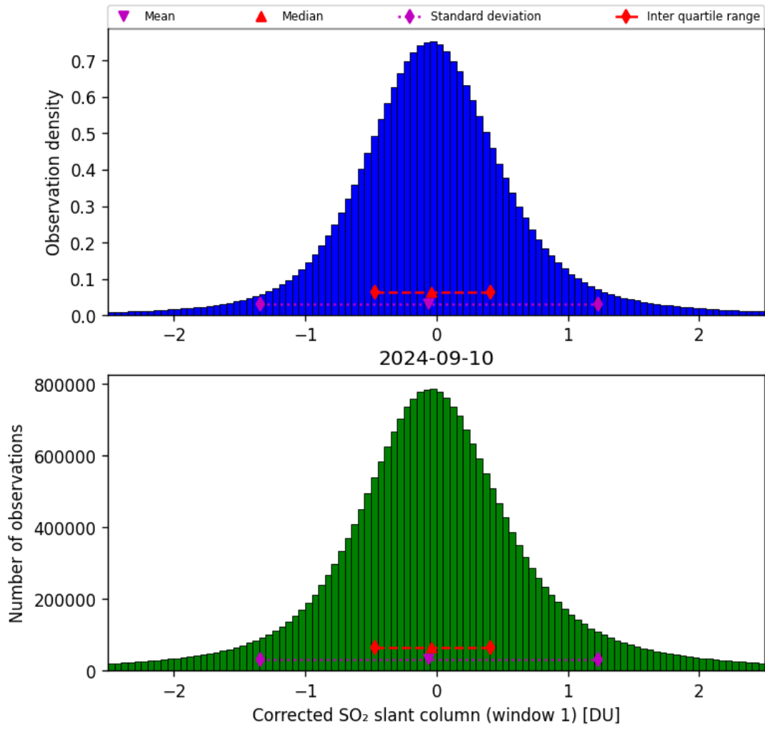
Figure 58: Histogram of “Corrected SO 2 slant column (window 1)” for 2024-09-09 to 2024-09-11
