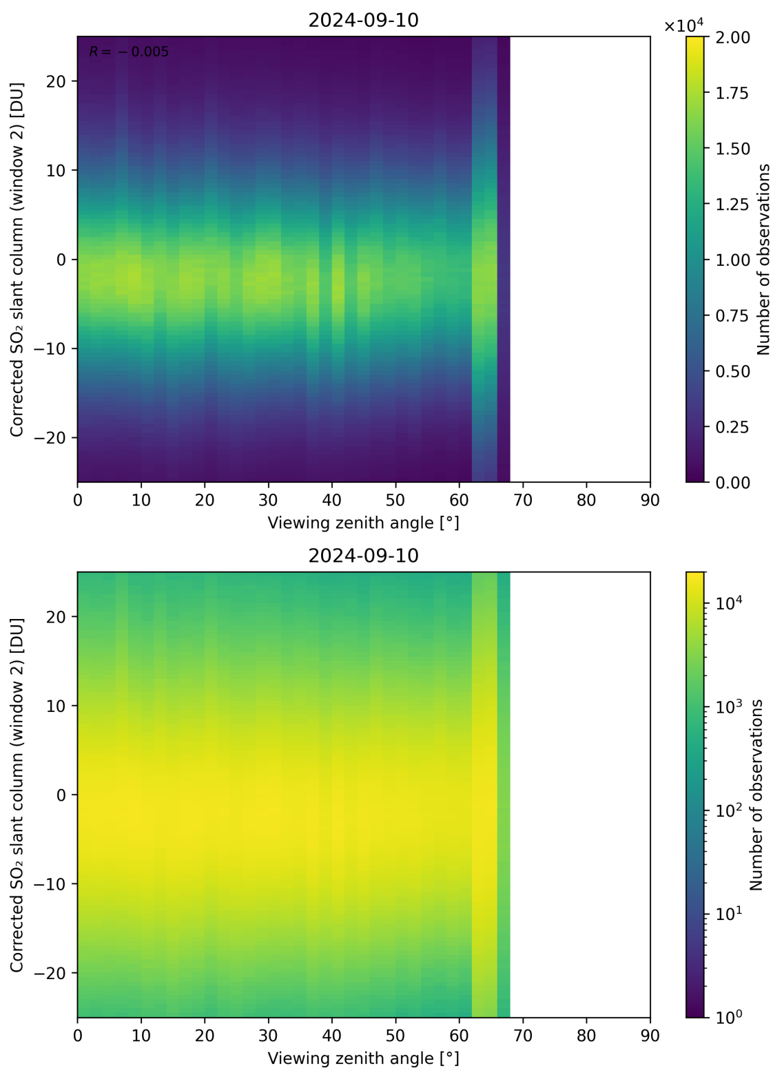
Figure 318: Scatter density plot of “Viewing zenith angle” against “Corrected SO 2 slant column (window 2)” for 2024-09-09 to 2024-09-11.
