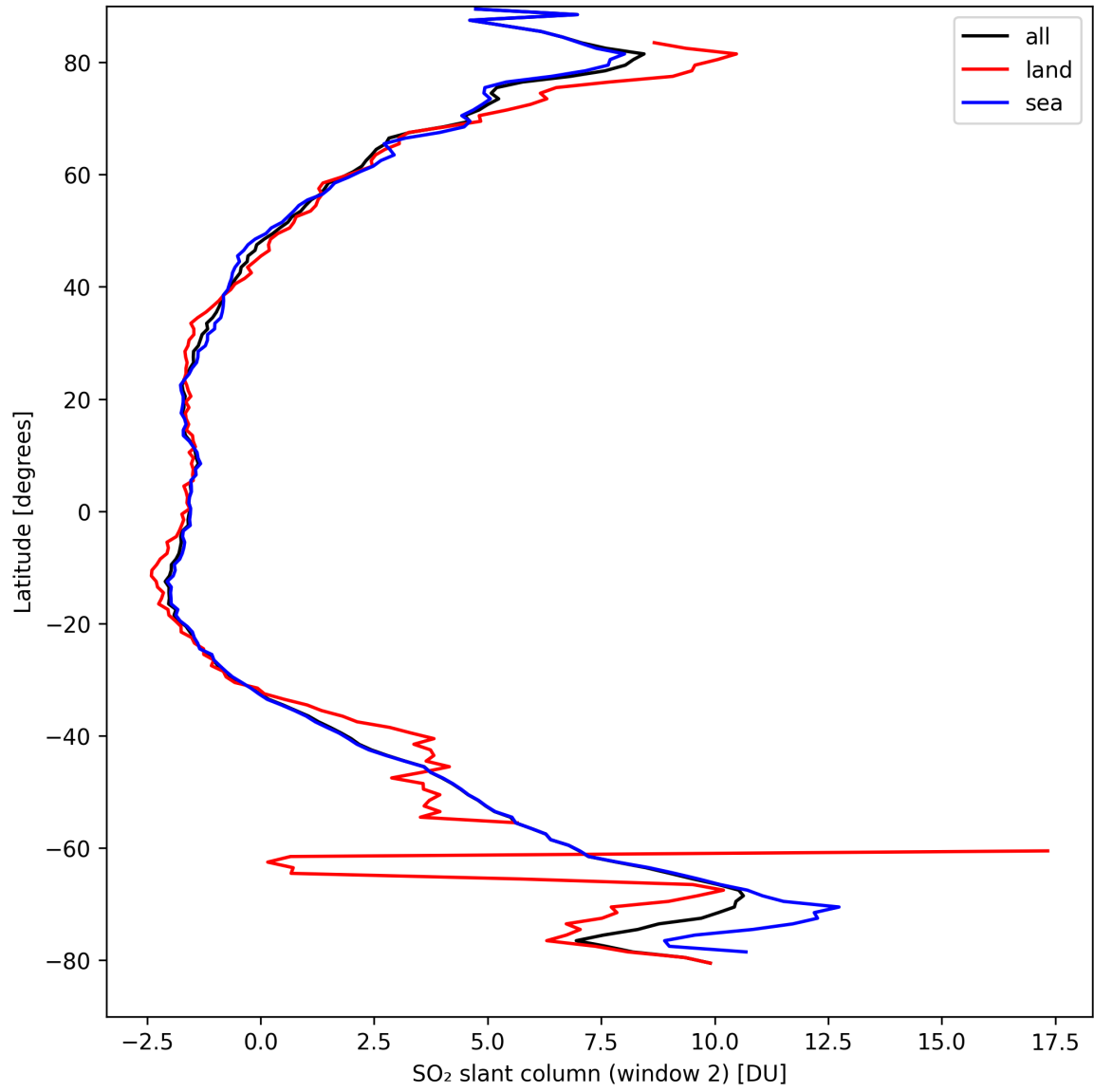
Figure 37: Zonal average of “SO 2 slant column (window 2)” for 2024-09-09 to 2024-09-11.
