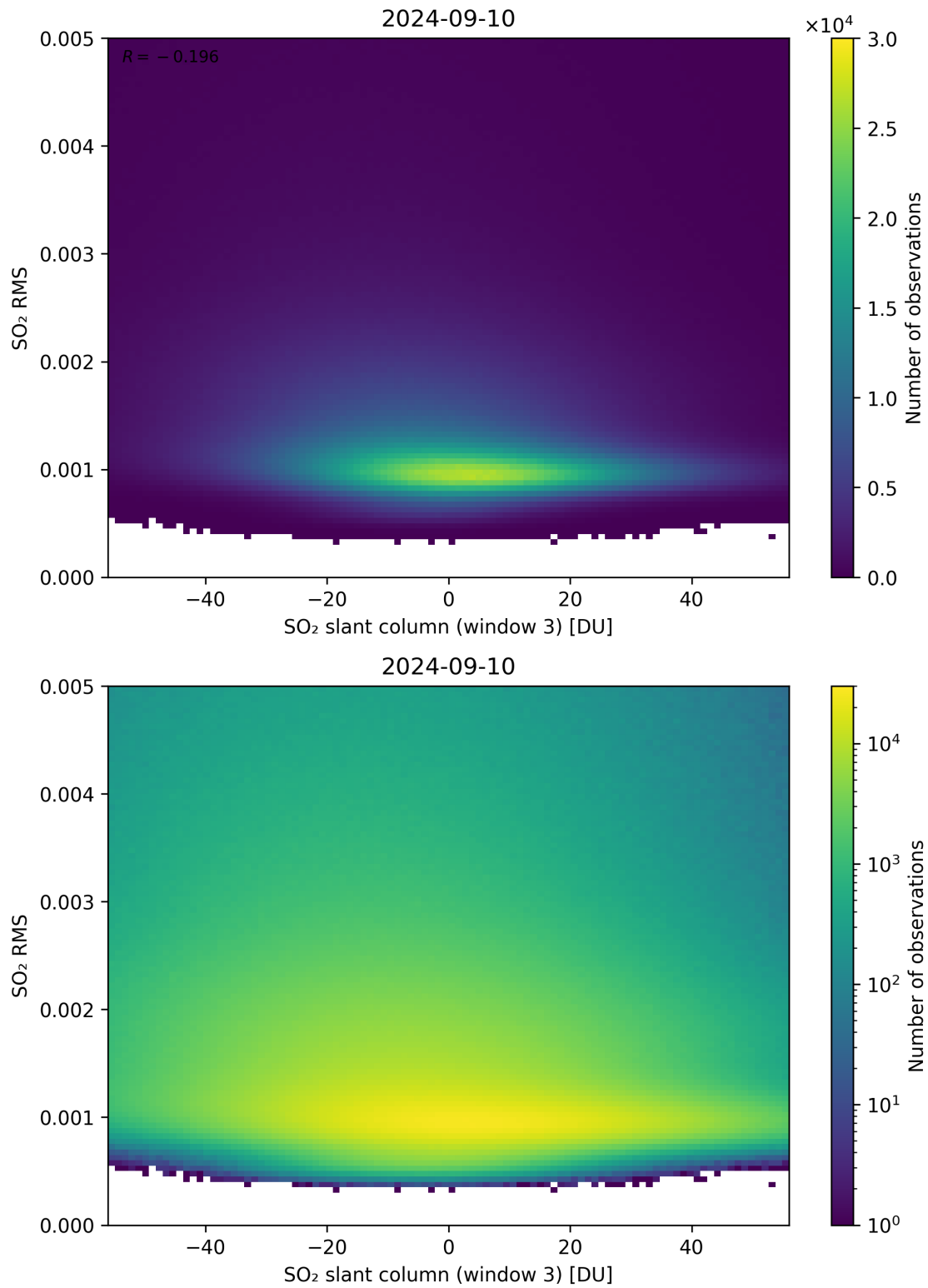
Figure 256: Scatter density plot of “SO 2 slant column (window 3)” against “SO 2 RMS” for 2024-09-09 to 2024-09-11.
