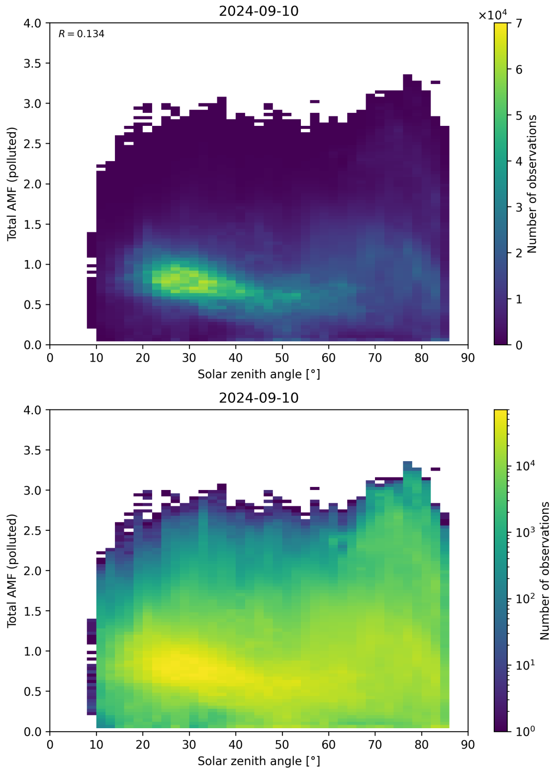
Figure 174: Scatter density plot of “Solar zenith angle” against “Total AMF (polluted)” for 2024-09-09 to 2024-09-11.
