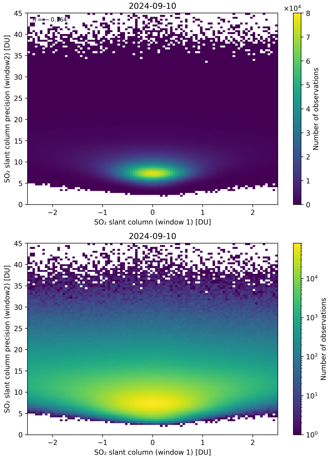
Figure 236: Scatter density plot of “SO 2 slant column (window 1)” against “SO 2 slant column precision (window2)” for 2024-09-09 to 2024-09-11.
