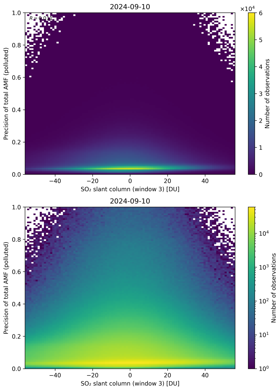
Figure 269: Scatter density plot of “SO 2 slant column (window 3)” against “Precision of total AMF (polluted)” for 2024-09-09 to 2024-09-11.
