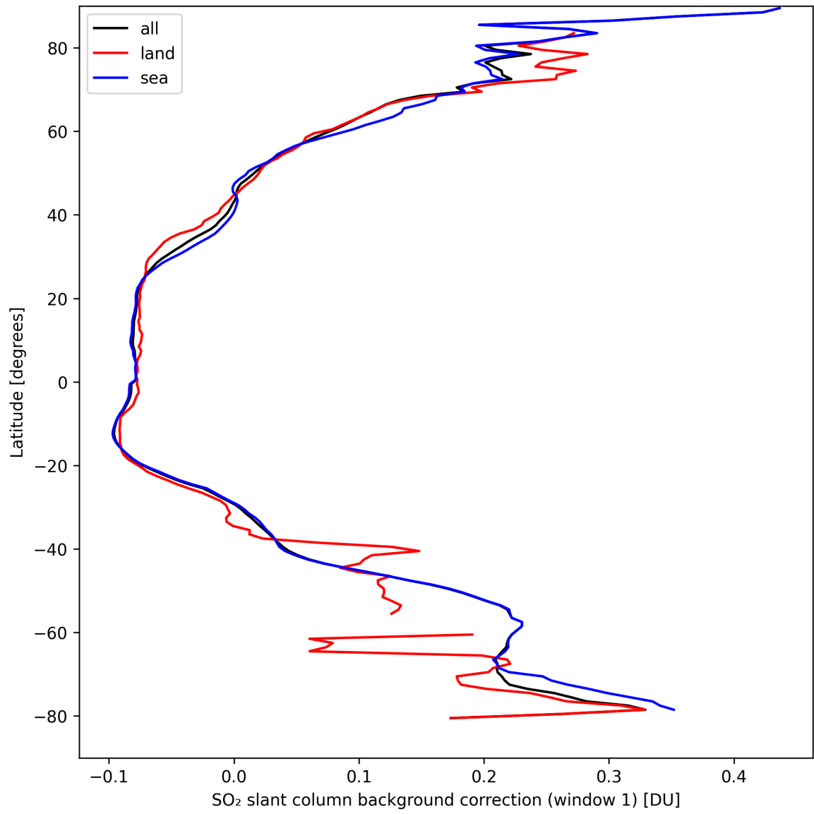
Figure 36: Zonal average of “SO 2 slant column background correction (window 1)” for 2024-09-09 to 2024-09-11.
