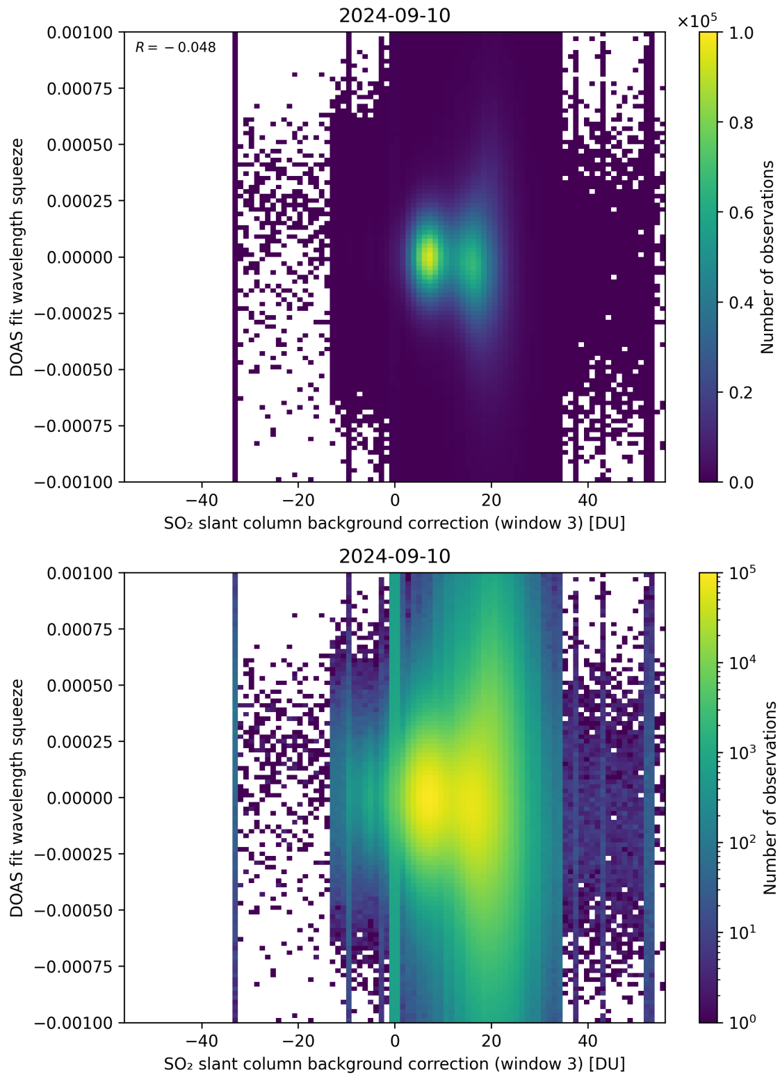
Figure 122: Scatter density plot of “SO 2 slant column background correction (window 3)” against “DOAS fit wavelength squeeze” for 2024-09-09 to 2024-09-11.
