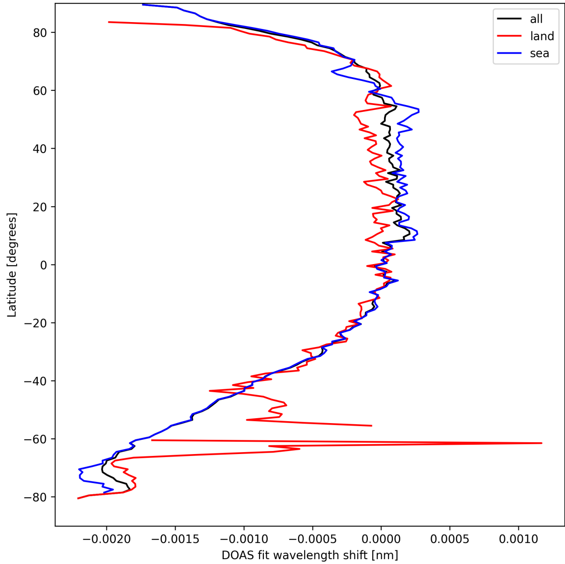
Figure 45: Zonal average of “DOAS fit wavelength shift” for 2024-09-09 to 2024-09-11.
