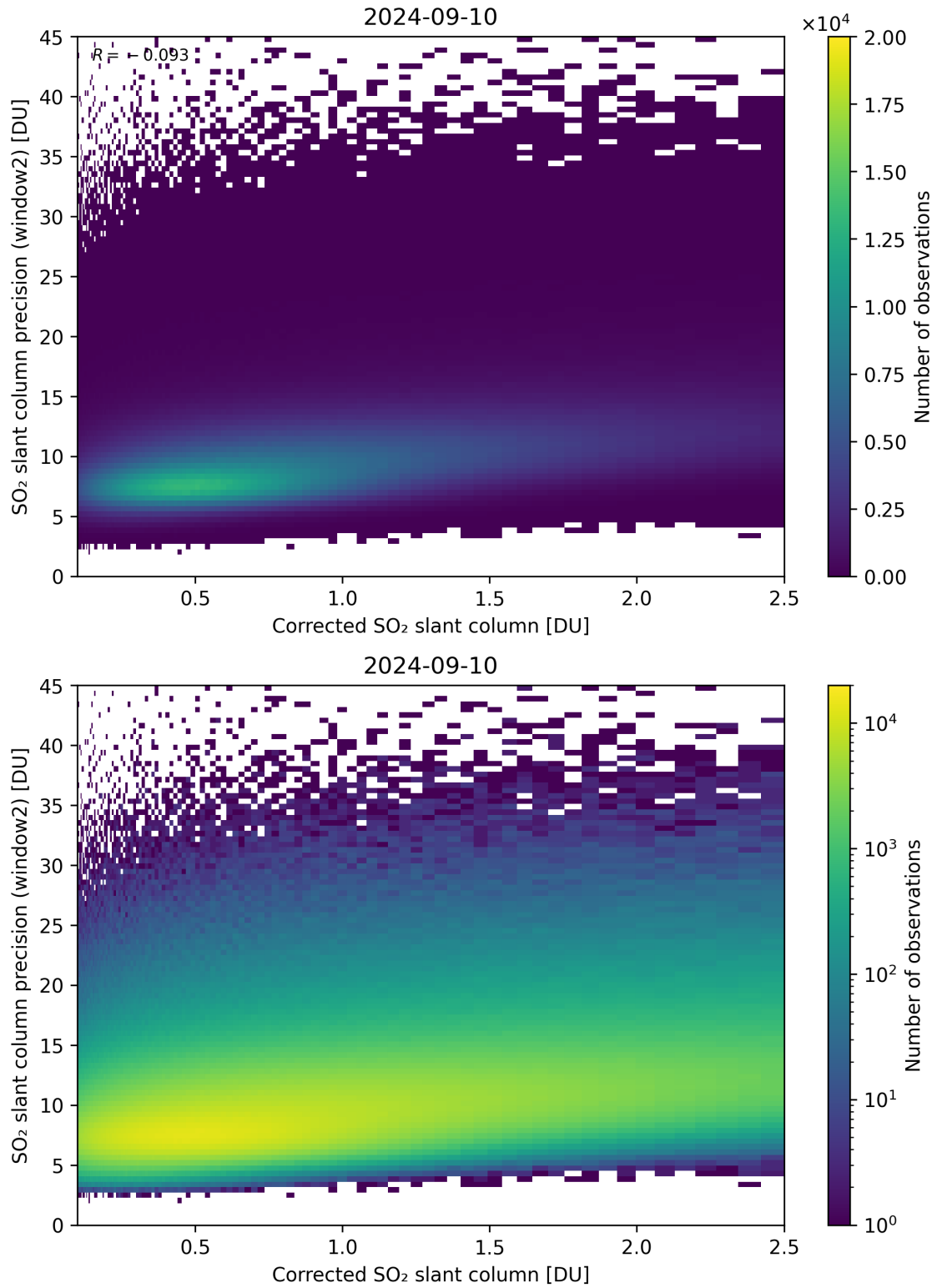
Figure 189: Scatter density plot of “Corrected SO 2 slant column” against “SO 2 slant column precision (window2)” for 2024-09-09 to 2024-09-11.
