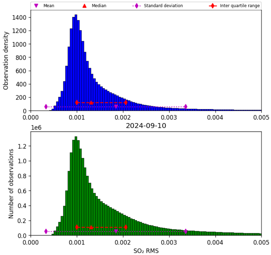
Figure 70: Histogram of “SO 2 RMS” for 2024-09-09 to 2024-09-11
