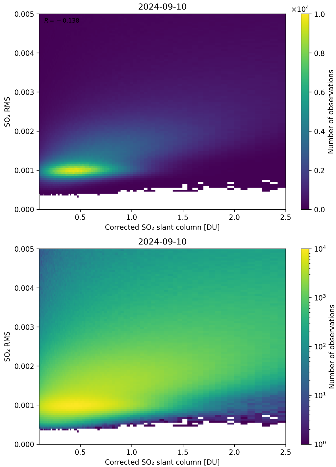
Figure 183: Scatter density plot of “Corrected SO 2 slant column” against “SO 2 RMS” for 2024-09-09 to 2024-09-11.
