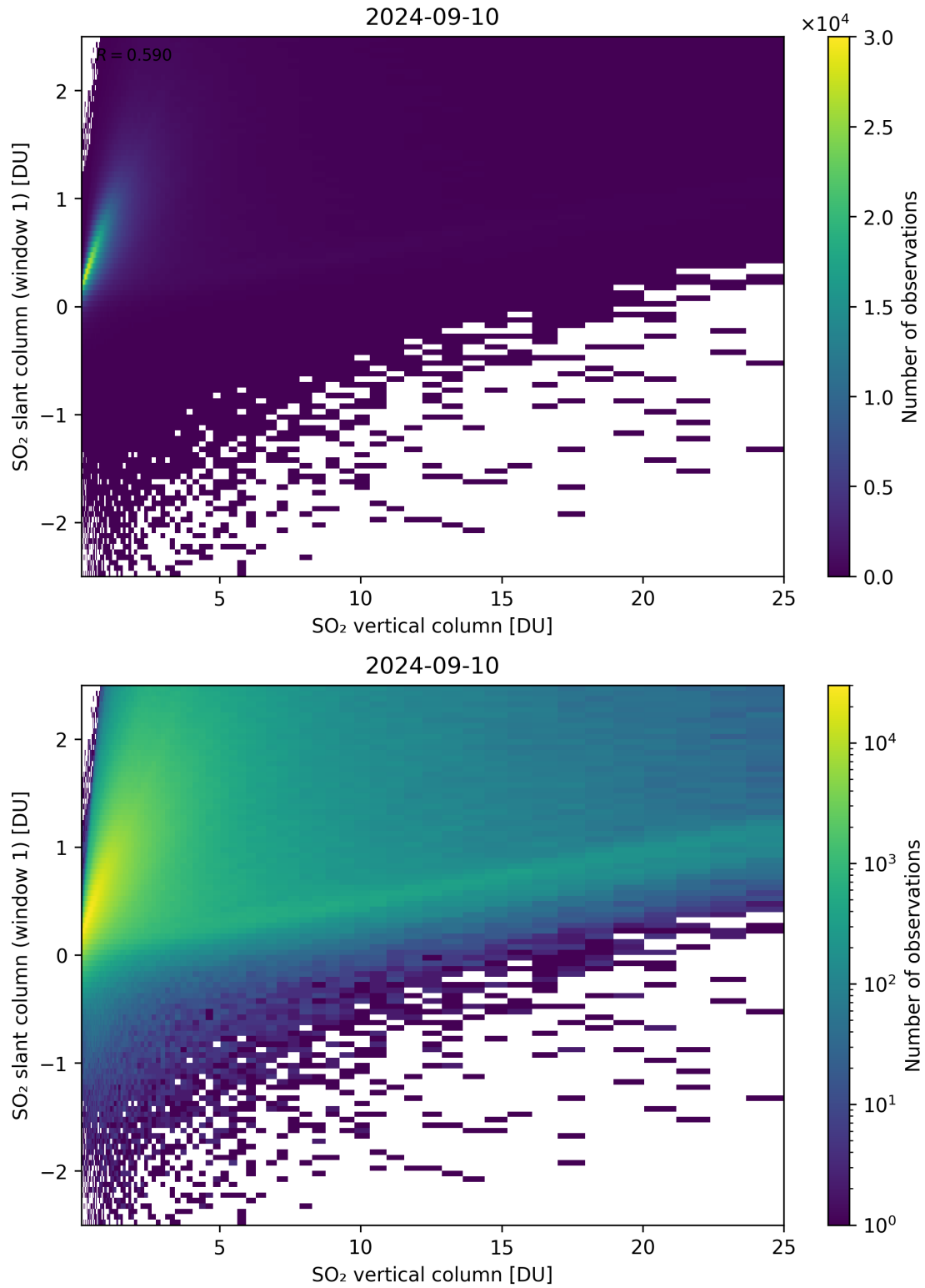
Figure 300: Scatter density plot of “SO 2 vertical column” against “SO 2 slant column (window 1)” for 2024-09-09 to 2024-09-11.
