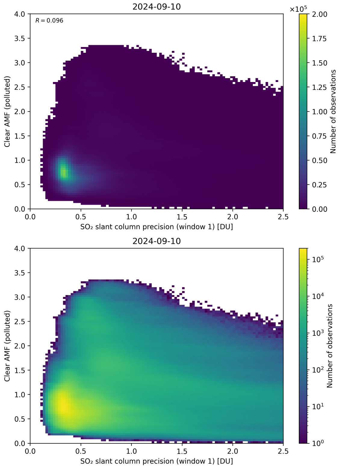
Figure 224: Scatter density plot of “SO 2 slant column precision (window 1)” against “Clear AMF (polluted)” for 2024-09-09 to 2024-09-11.
