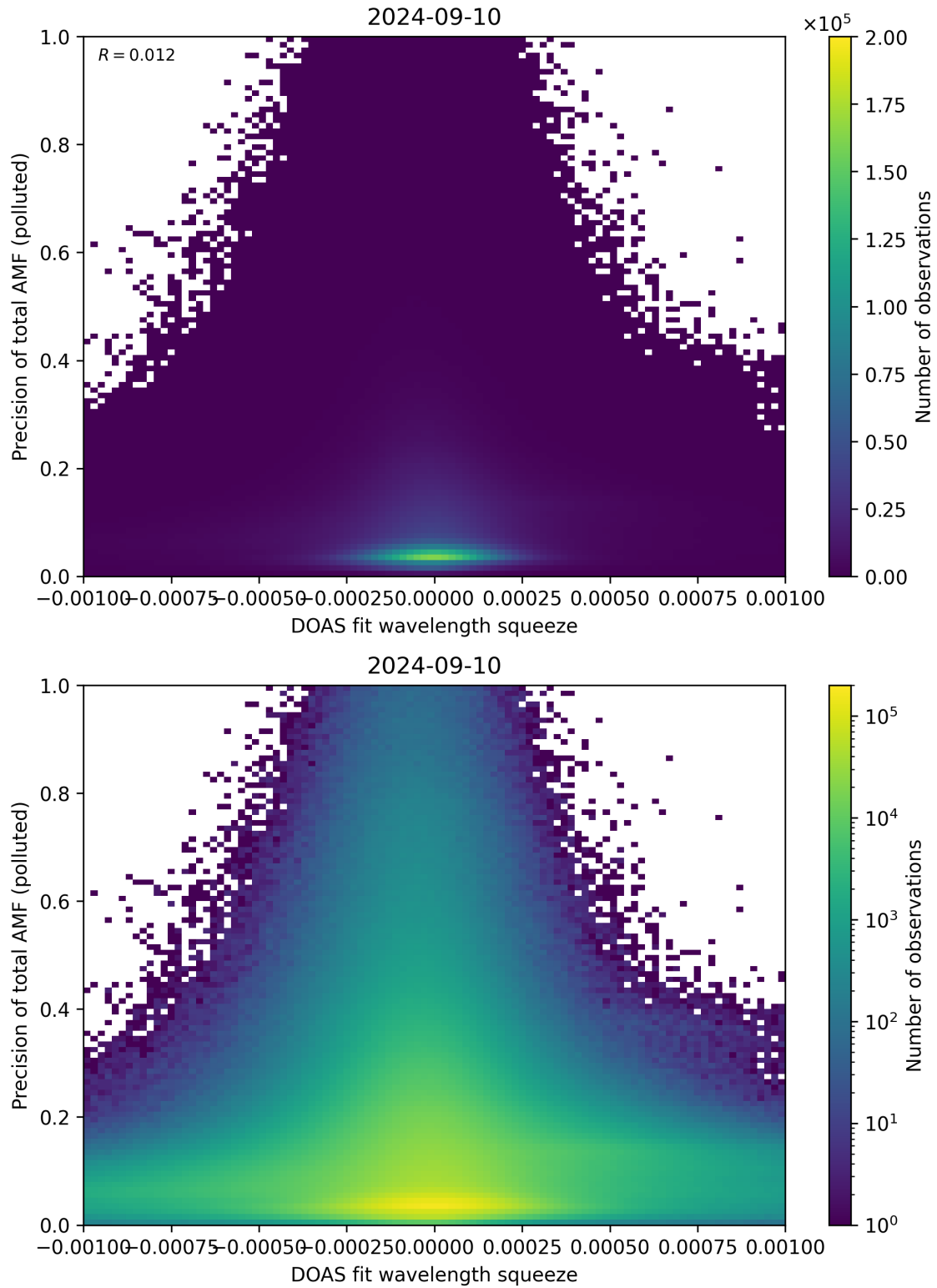
Figure 135: Scatter density plot of “DOAS fit wavelength squeeze” against “Precision of total AMF (polluted)” for 2024-09-09 to 2024-09-11.
