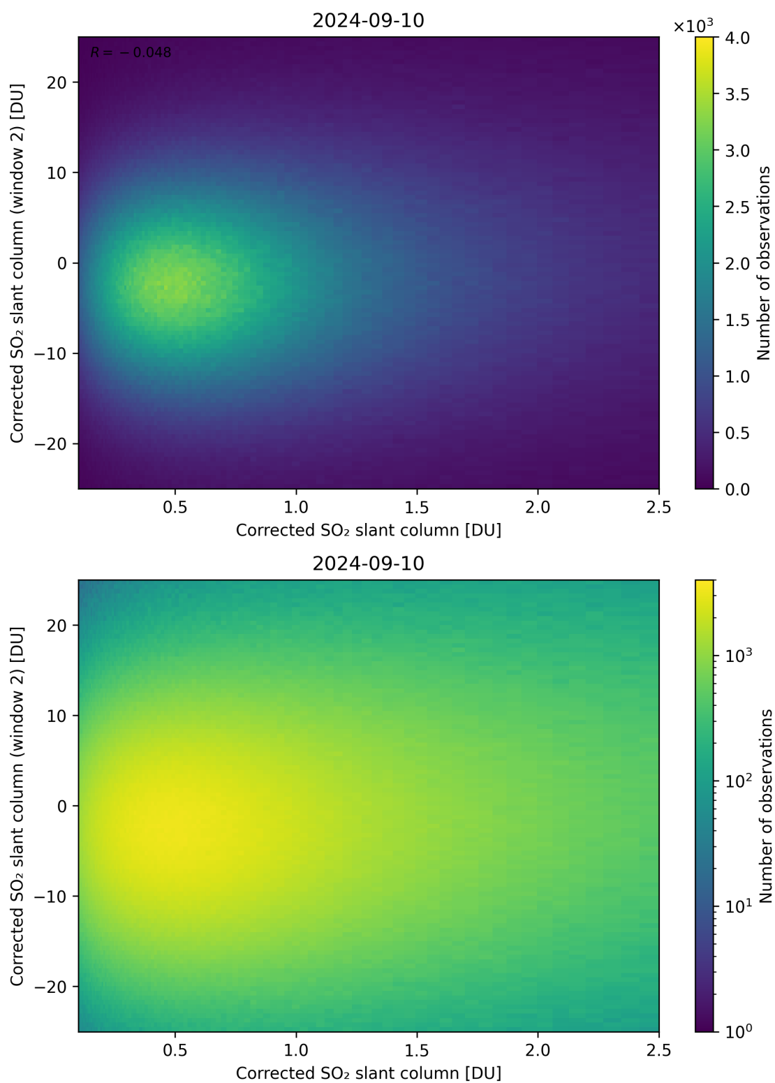
Figure 185: Scatter density plot of “Corrected SO 2 slant column” against “Corrected SO 2 slant column (window 2)” for 2024-09-09 to 2024-09-11.
