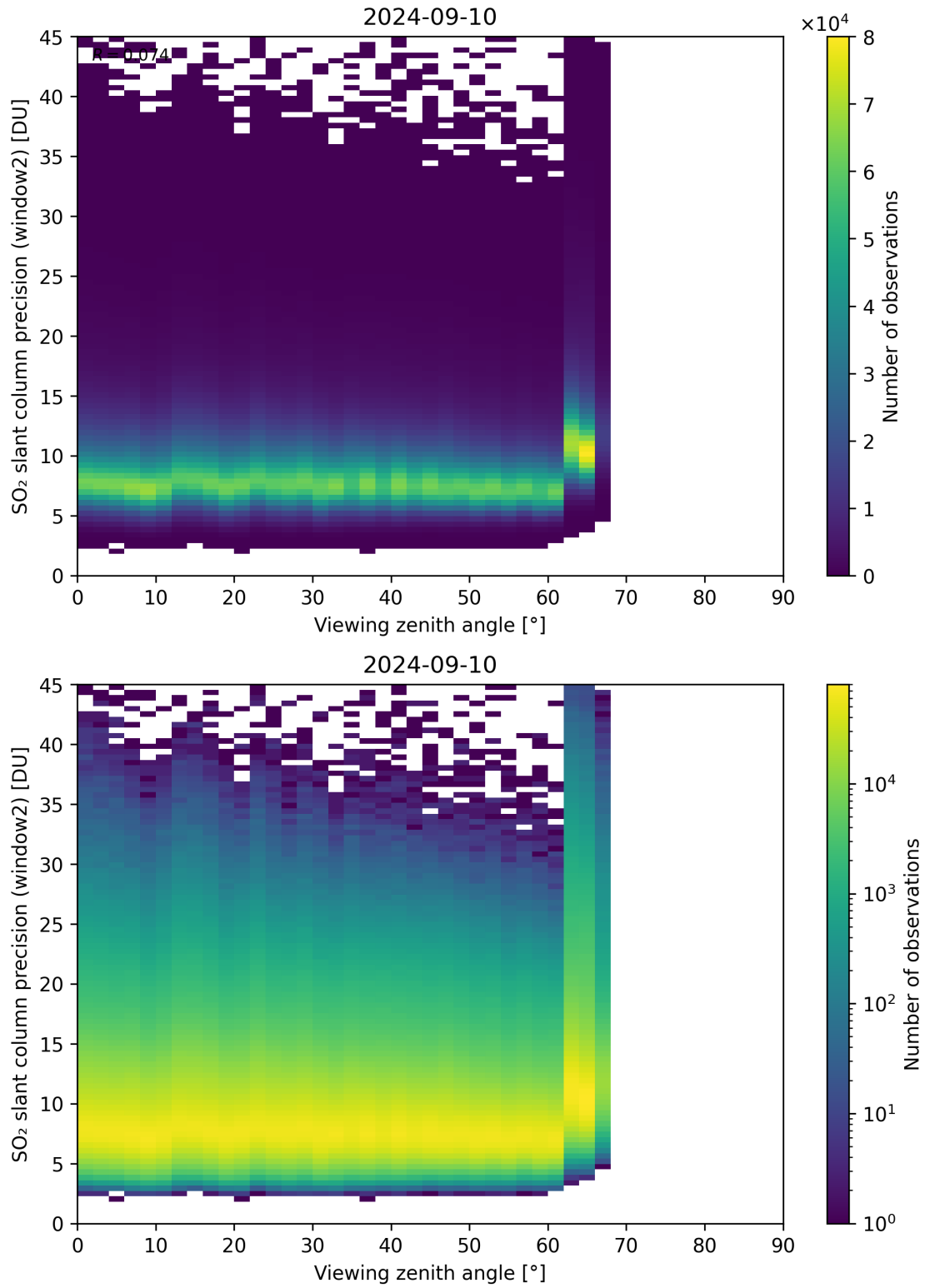
Figure 322: Scatter density plot of “Viewing zenith angle” against “SO 2 slant column precision (window2)” for 2024-09-09 to 2024-09-11.
