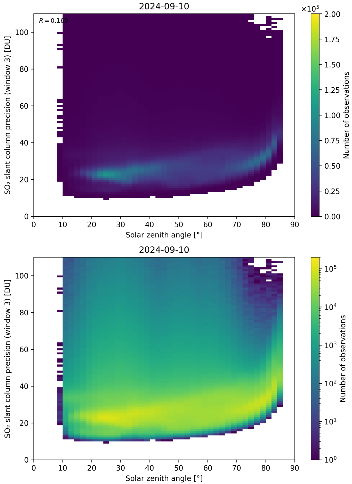
Figure 173: Scatter density plot of “Solar zenith angle” against “SO 2 slant column precision (window 3)” for 2024-09-09 to 2024-09-11.
