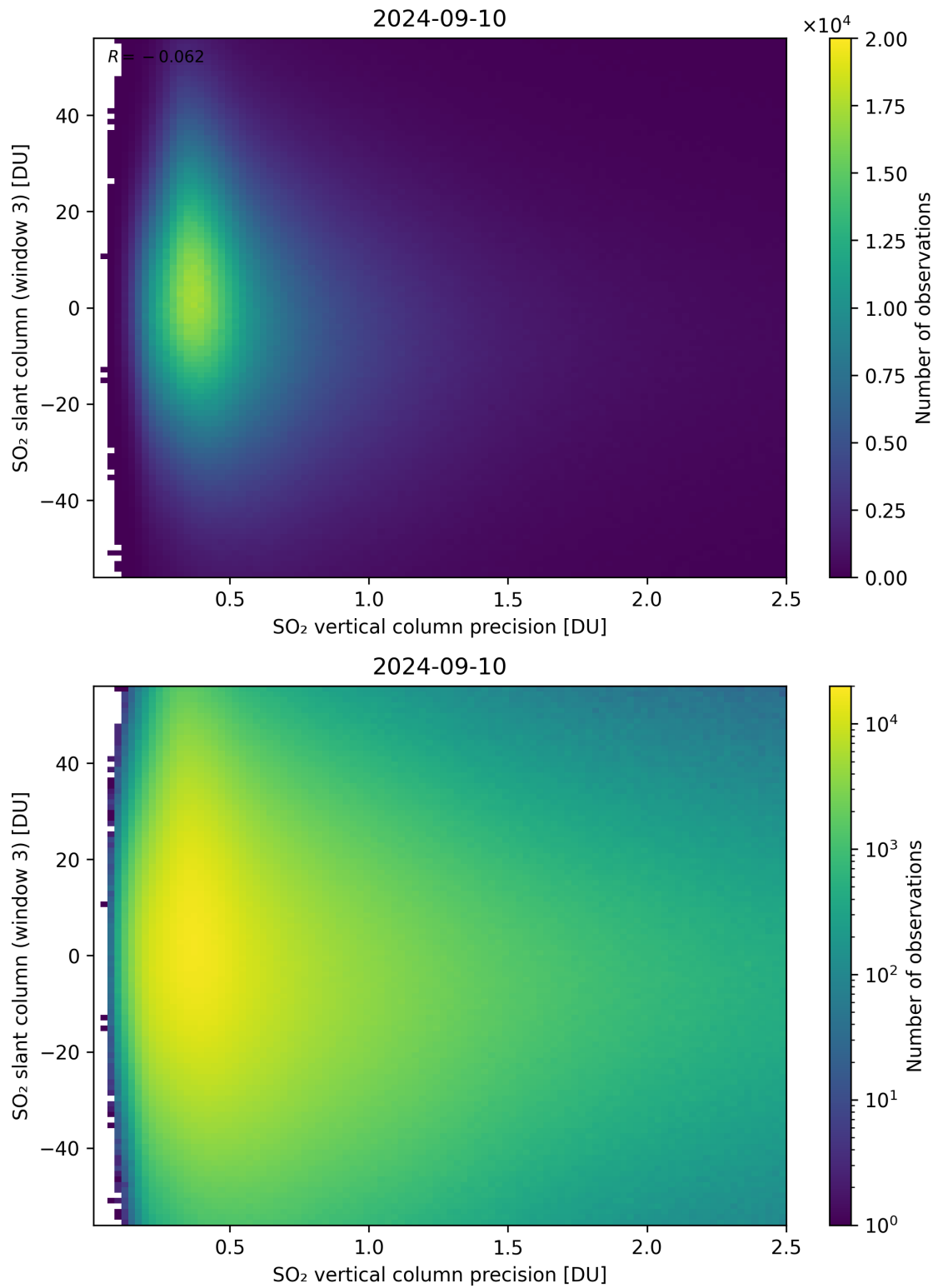
Figure 292: Scatter density plot of “SO 2 vertical column precision” against “SO 2 slant column (window 3)” for 2024-09-09 to 2024-09-11.
