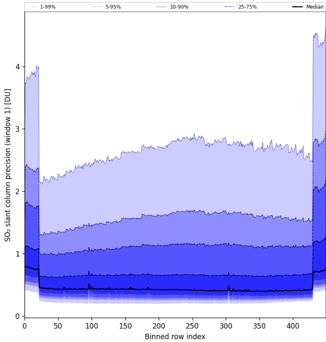
Figure 80: Along track statistics of “SO 2 slant column precision (window 1)” for 2024-09-09 to 2024-09-11
