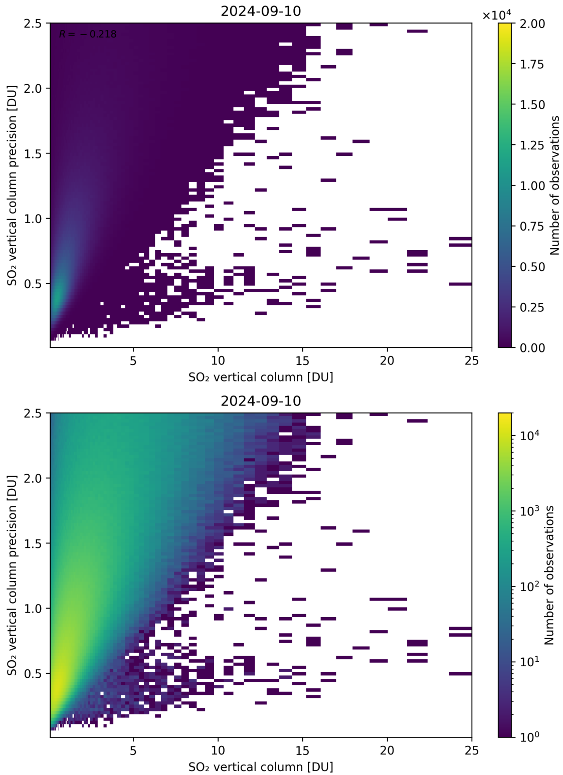
Figure 307: Scatter density plot of “SO 2 vertical column” against “SO 2 vertical column precision” for 2024-09-09 to 2024-09-11.
