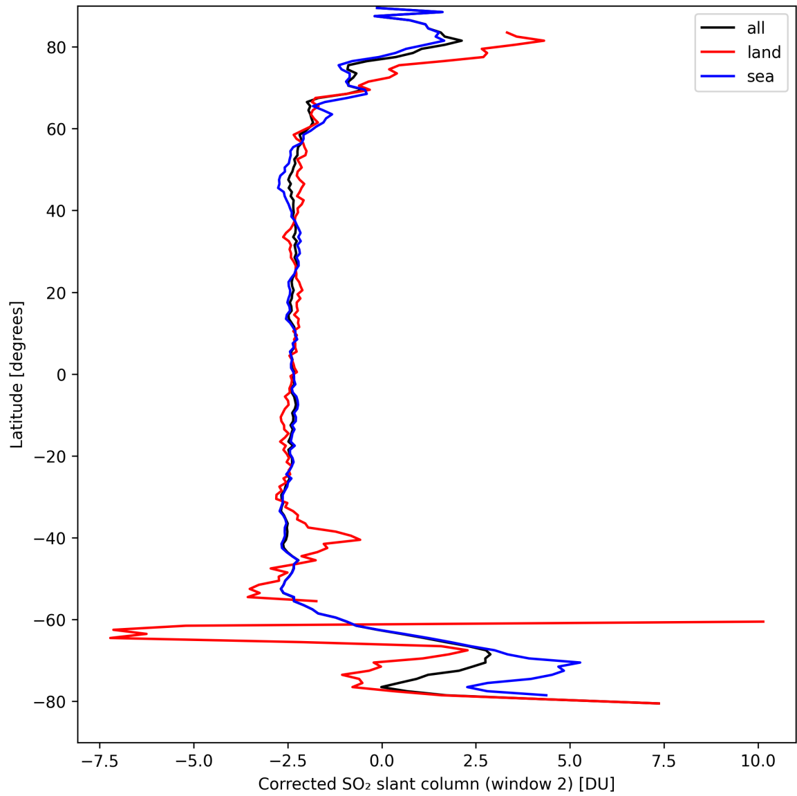
Figure 39: Zonal average of “Corrected SO 2 slant column (window 2)” for 2024-09-09 to 2024-09-11.
