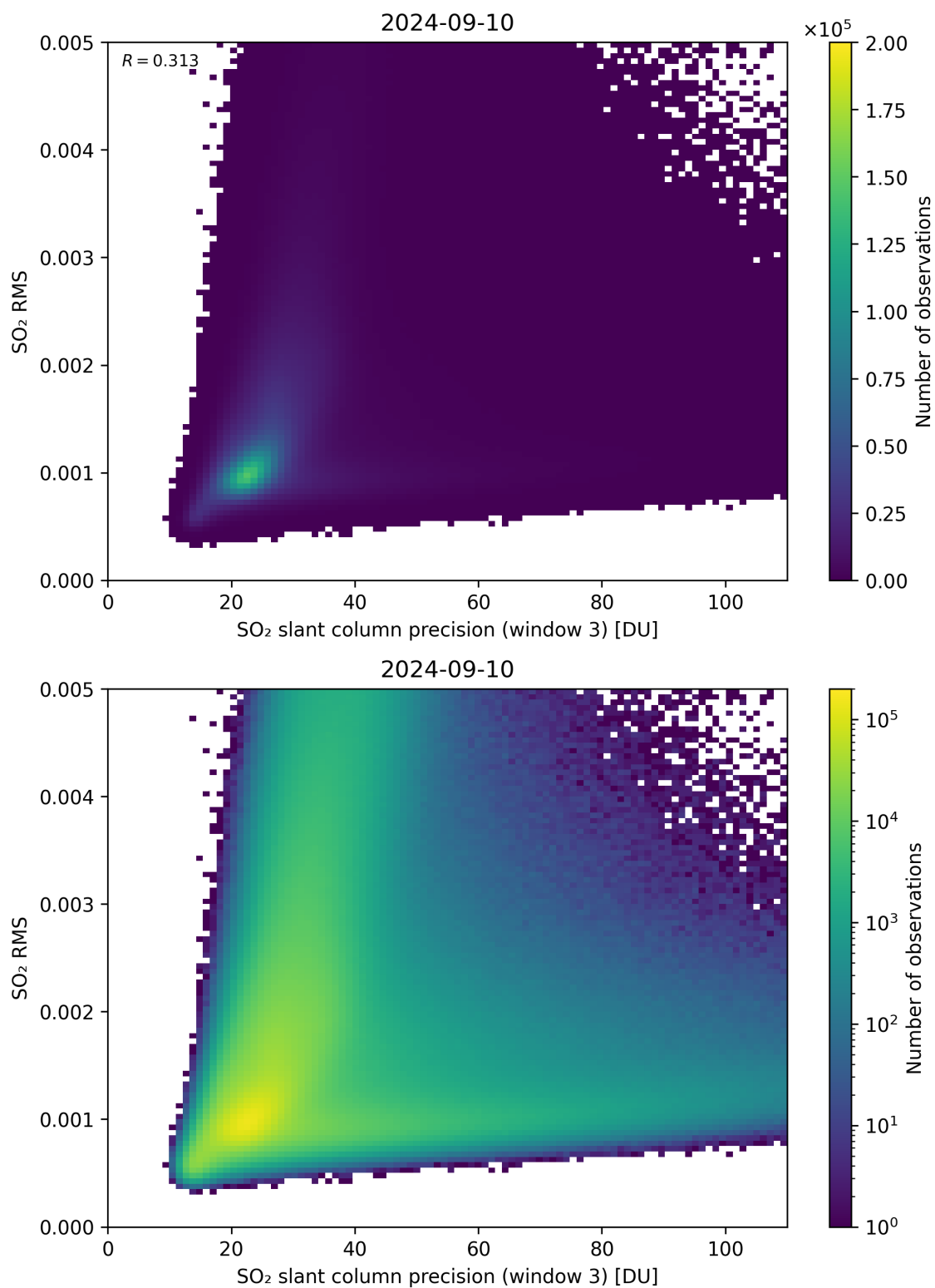
Figure 260: Scatter density plot of “SO 2 slant column precision (window 3)” against “SO 2 RMS” for 2024-09-09 to 2024-09-11.
