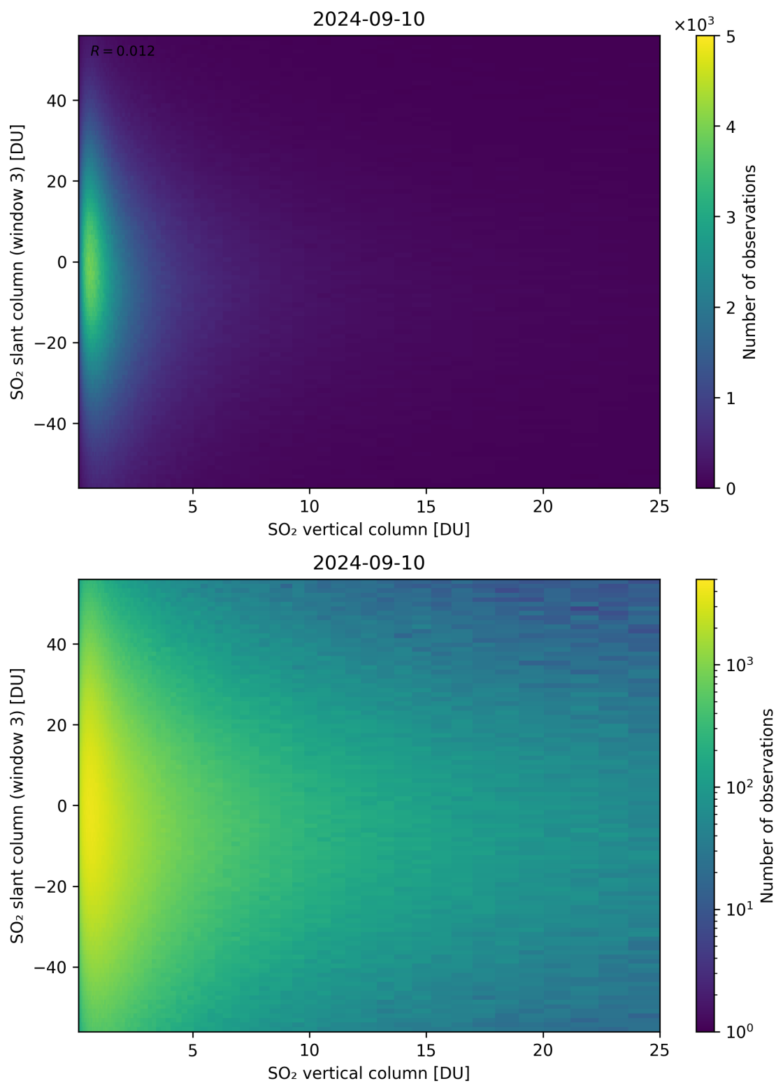
Figure 303: Scatter density plot of “SO 2 vertical column” against “SO 2 slant column (window 3)” for 2024-09-09 to 2024-09-11.
