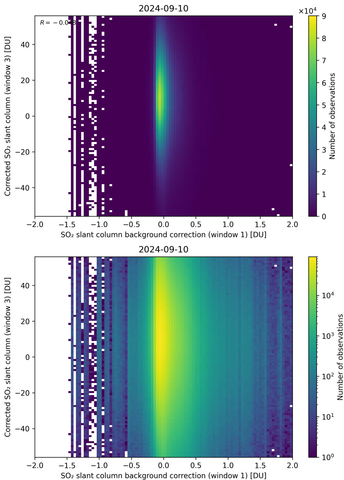
Figure 105: Scatter density plot of “SO 2 slant column background correction (window 1)” against “Corrected SO 2 slant column (window 3)” for 2024-09-09 to 2024-09-11.
