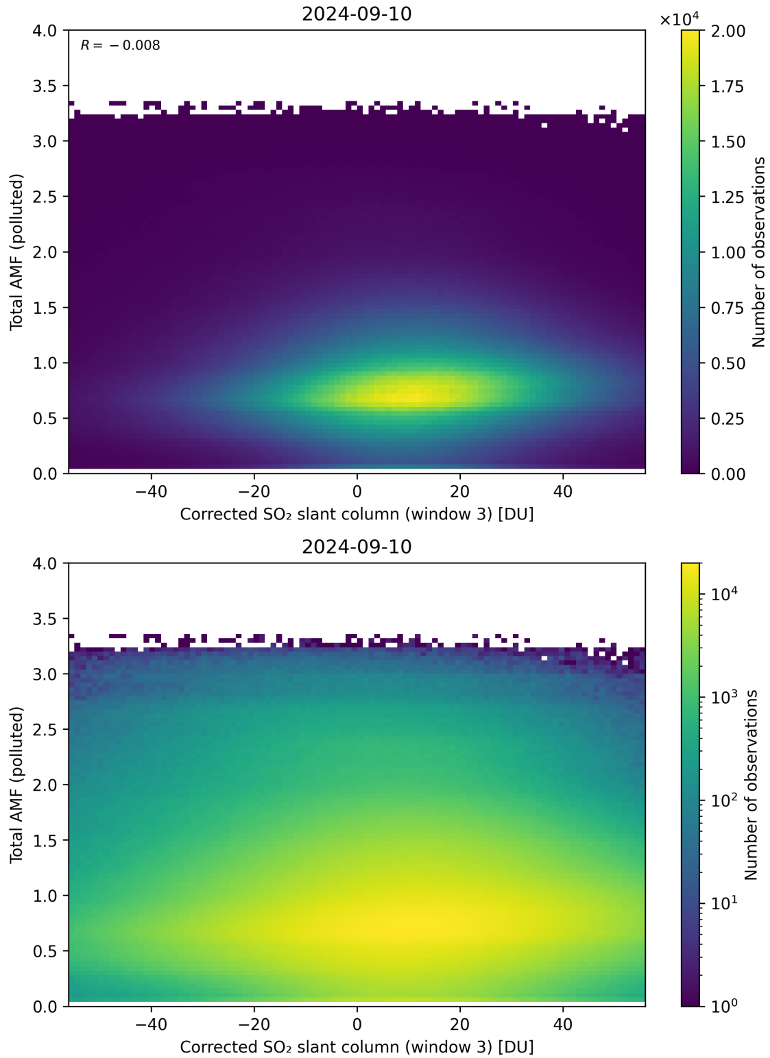
Figure 210: Scatter density plot of “Corrected SO 2 slant column (window 3)” against “Total AMF (polluted)” for 2024-09-09 to 2024-09-11.
