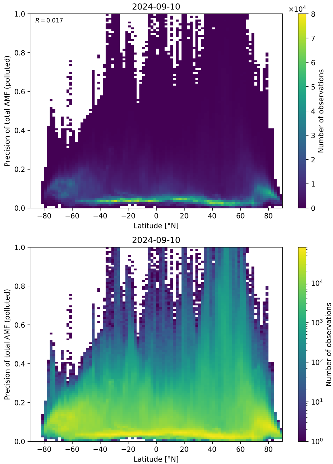
Figure 155: Scatter density plot of “Latitude” against “Precision of total AMF (polluted)” for 2024-09-09 to 2024-09-11.
