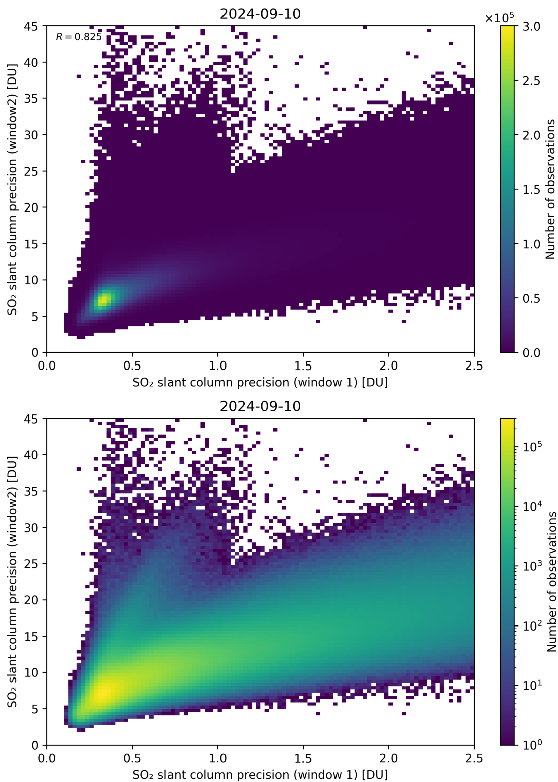
Figure 227: Scatter density plot of “SO 2 slant column precision (window 1)” against “SO 2 slant column precision (window2)” for 2024-09-09 to 2024-09-11.
