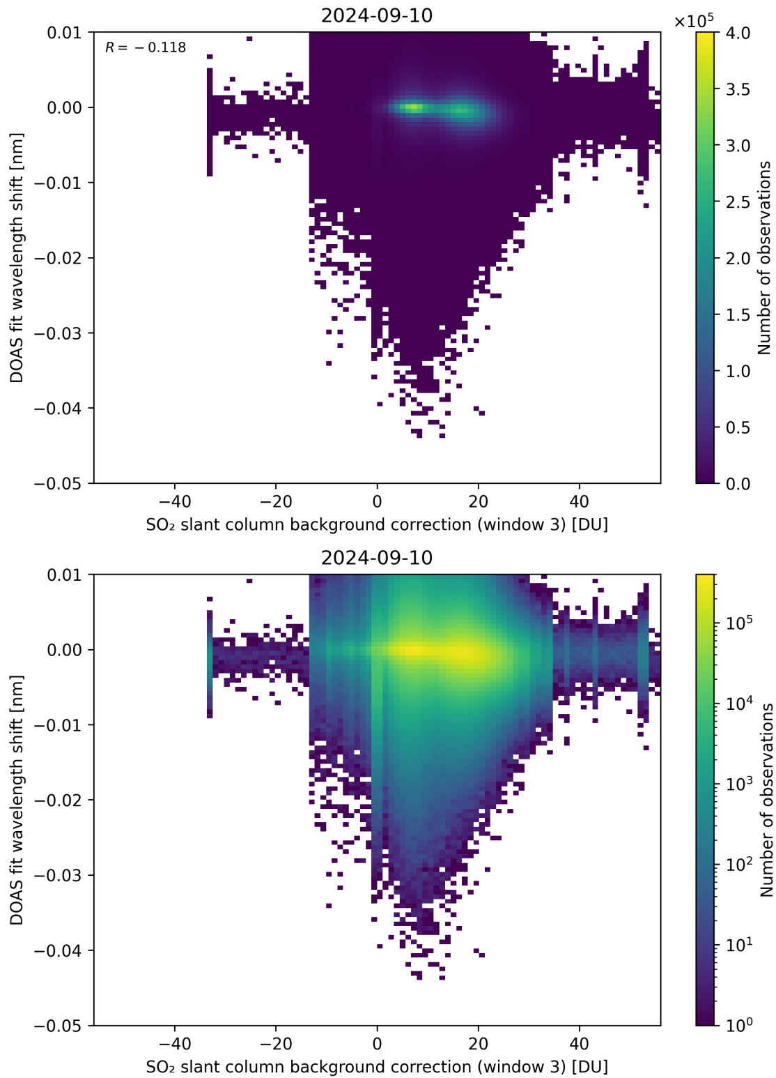
Figure 121: Scatter density plot of “SO 2 slant column background correction (window 3)” against “DOAS fit wavelength shift” for 2024-09-09 to 2024-09-11.
