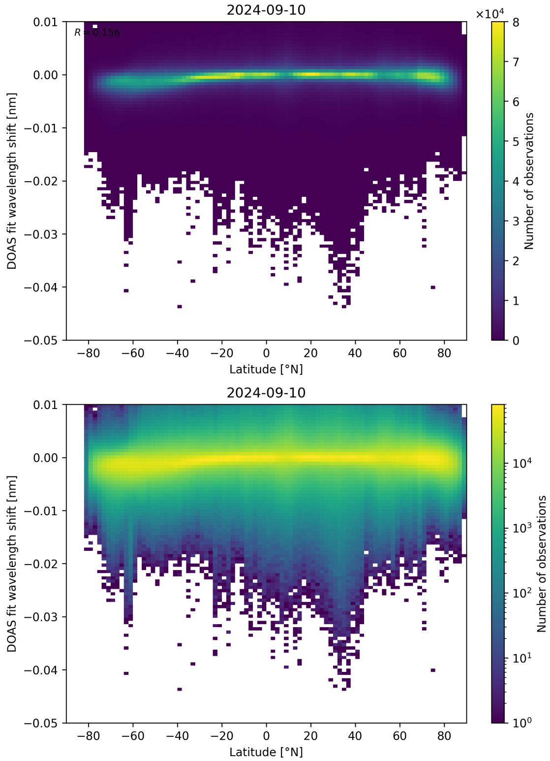
Figure 142: Scatter density plot of “Latitude” against “DOAS fit wavelength shift” for 2024-09-09 to 2024-09-11.
