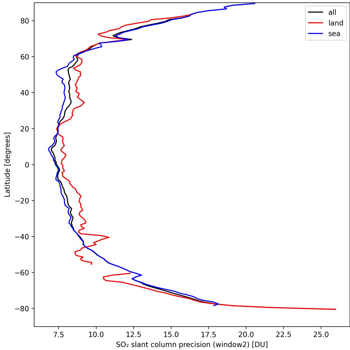
Figure 38: Zonal average of “SO 2 slant column precision (window2)” for 2024-09-09 to 2024-09-11.
