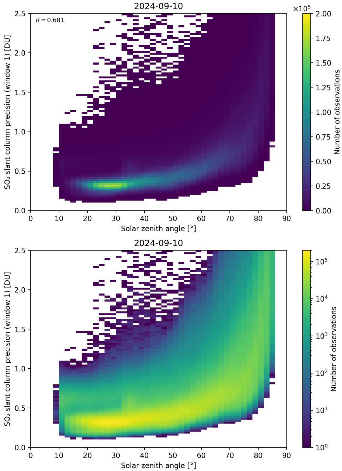
Figure 170: Scatter density plot of “Solar zenith angle” against “SO 2 slant column precision (window 1)” for 2024-09-09 to 2024-09-11.
