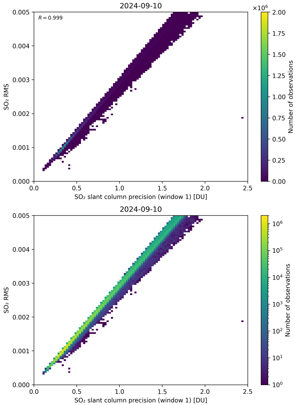
Figure 223: Scatter density plot of “SO 2 slant column precision (window 1)” against “SO 2 RMS” for 2024-09-09 to 2024-09-11.
