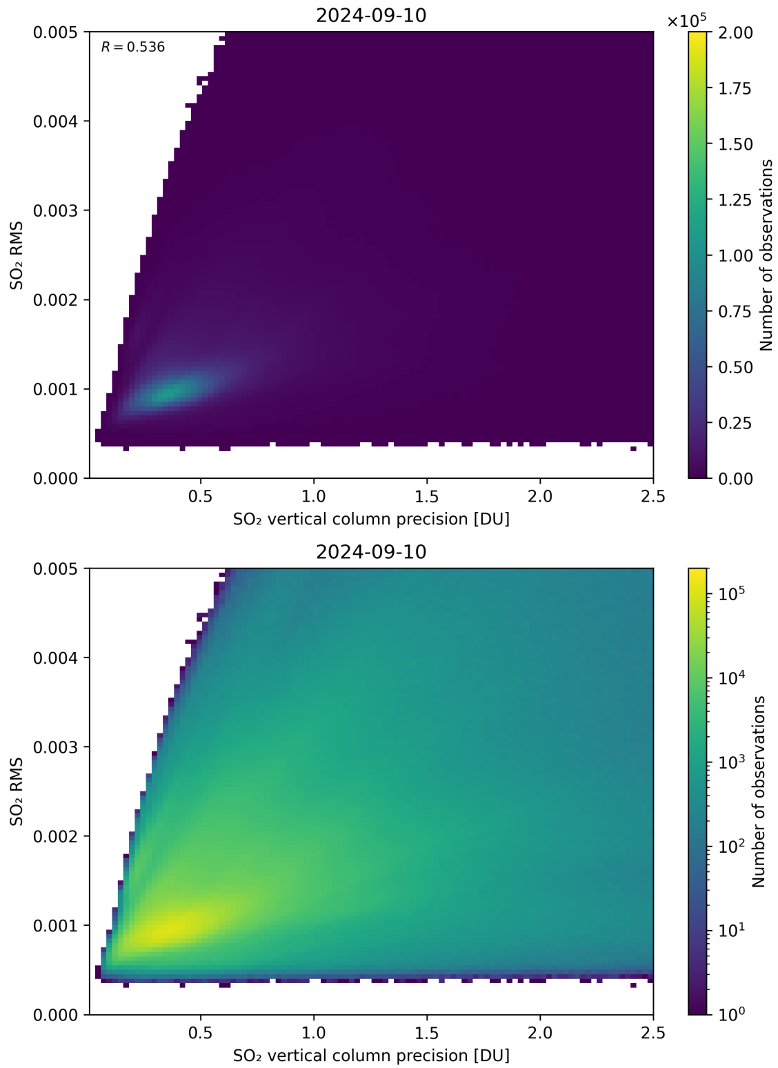
Figure 284: Scatter density plot of “SO 2 vertical column precision” against “SO 2 RMS” for 2024-09-09 to 2024-09-11.
