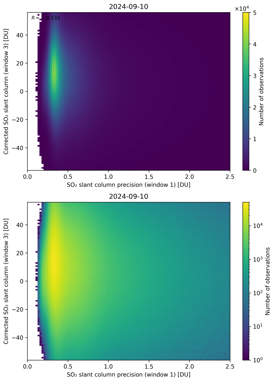
Figure 226: Scatter density plot of “SO 2 slant column precision (window 1)” against “Corrected SO 2 slant column (window 3)” for 2024-09-09 to 2024-09-11.
