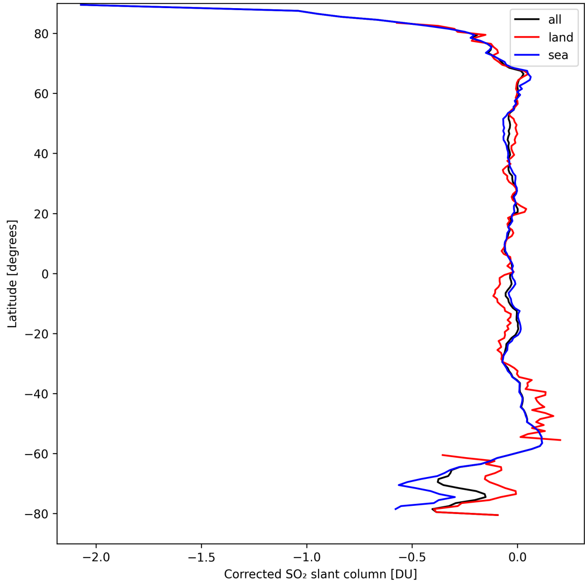
Figure 32: Zonal average of “Corrected SO 2 slant column” for 2024-09-09 to 2024-09-11.
