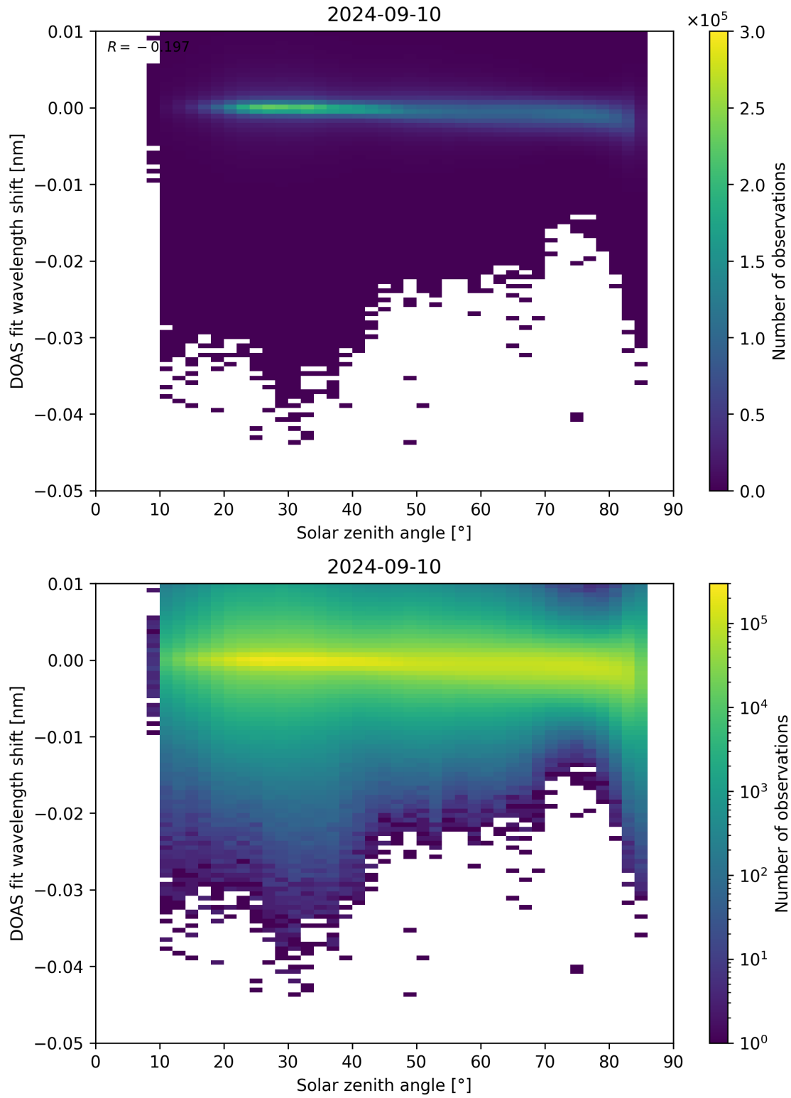
Figure 161: Scatter density plot of “Solar zenith angle” against “DOAS fit wavelength shift” for 2024-09-09 to 2024-09-11.
