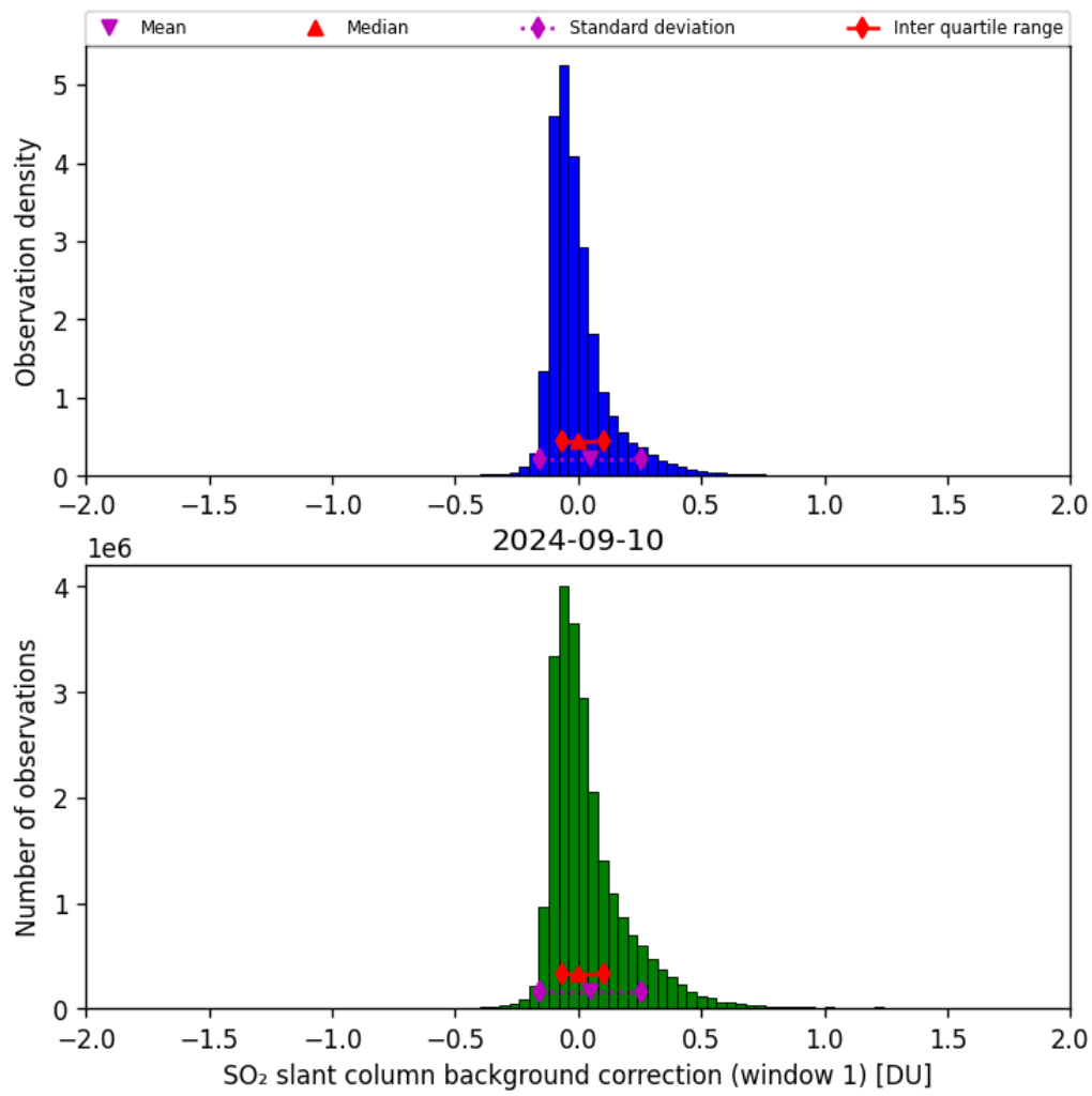
Figure 59: Histogram of “SO 2 slant column background correction (window 1)” for 2024-09-09 to 2024-09-11
