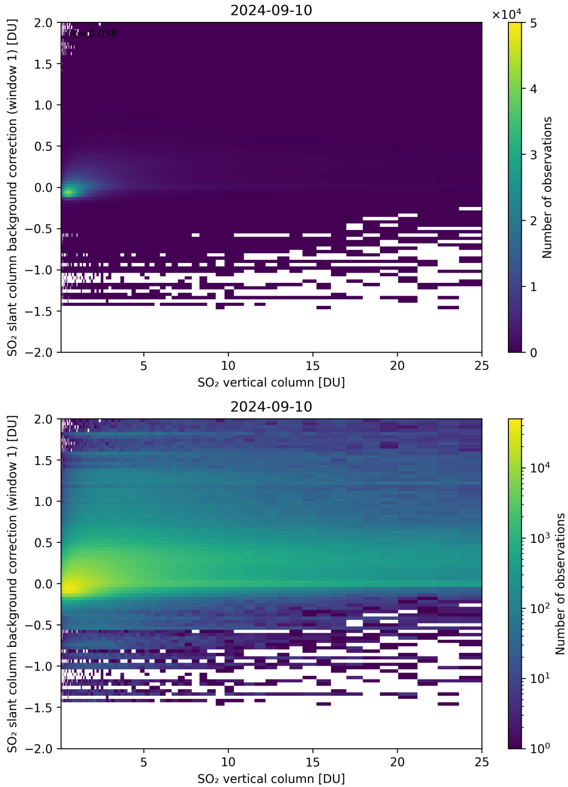
Figure 273: Scatter density plot of “SO 2 vertical column” against “SO 2 slant column background correction (window 1)” for 2024-09-09 to 2024-09-11.
