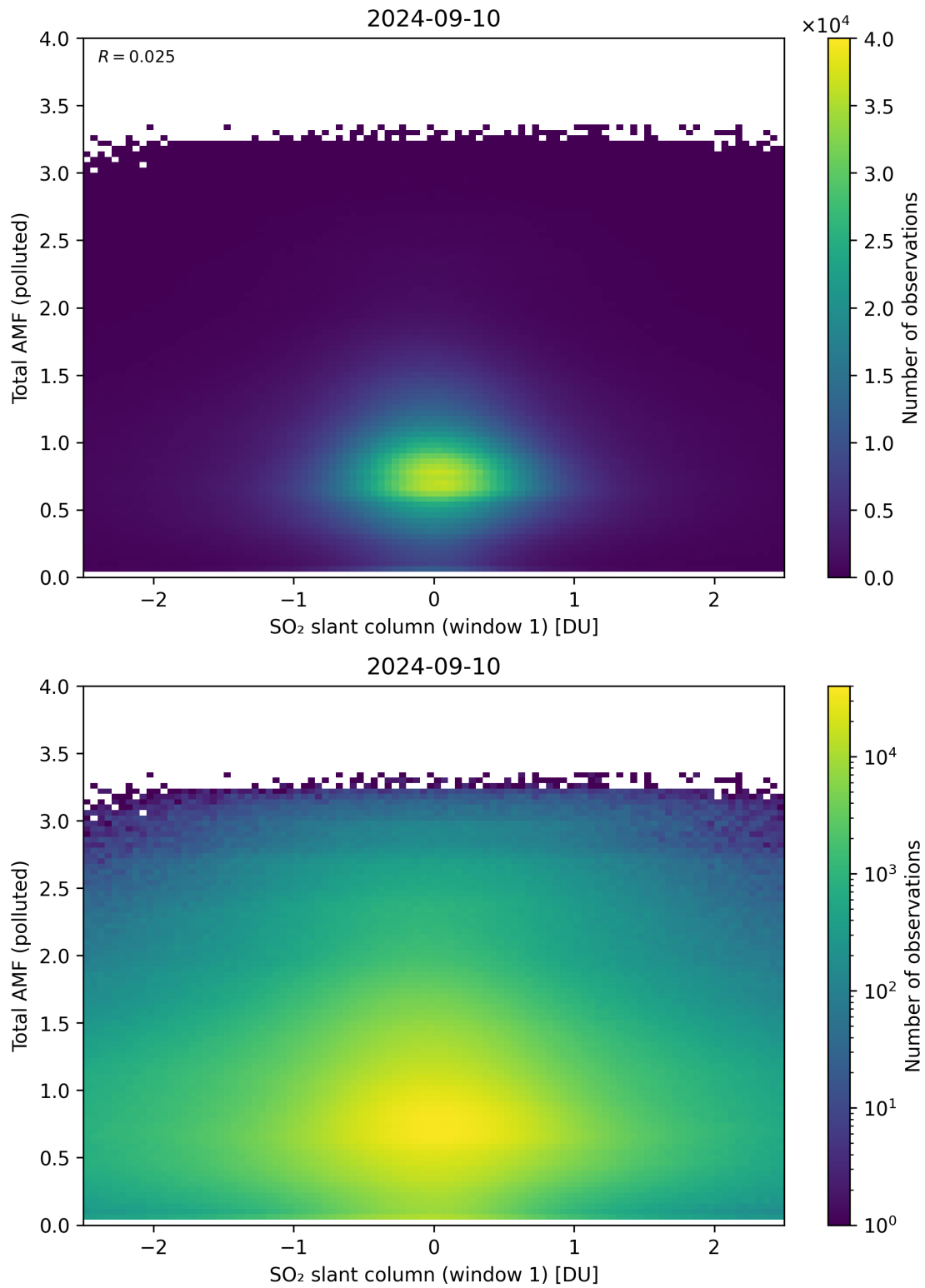
Figure 239: Scatter density plot of “SO 2 slant column (window 1)” against “Total AMF (polluted)” for 2024-09-09 to 2024-09-11.
