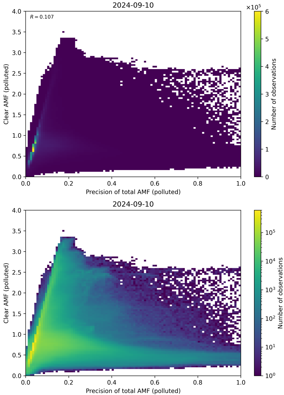
Figure 270: Scatter density plot of “Precision of total AMF (polluted)” against “Clear AMF (polluted)” for 2024-09-09 to 2024-09-11.
