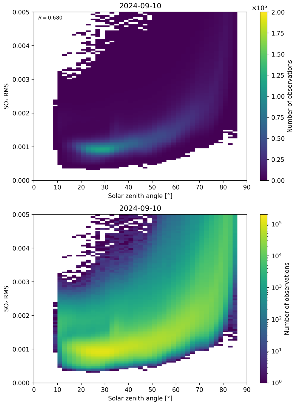
Figure 163: Scatter density plot of “Solar zenith angle” against “SO 2 RMS” for 2024-09-09 to 2024-09-11.
