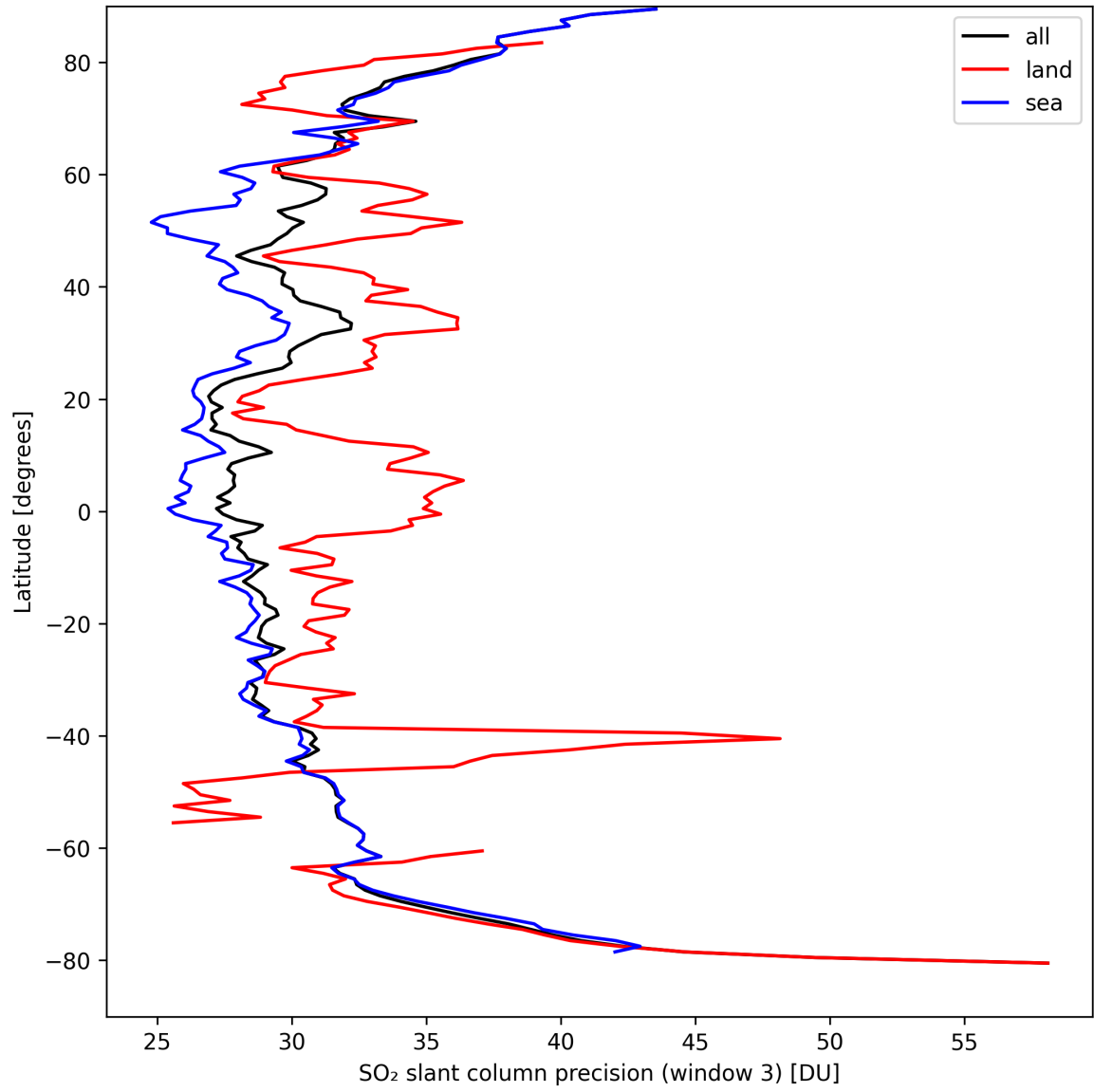
Figure 42: Zonal average of “SO 2 slant column precision (window 3)” for 2024-09-09 to 2024-09-11.
