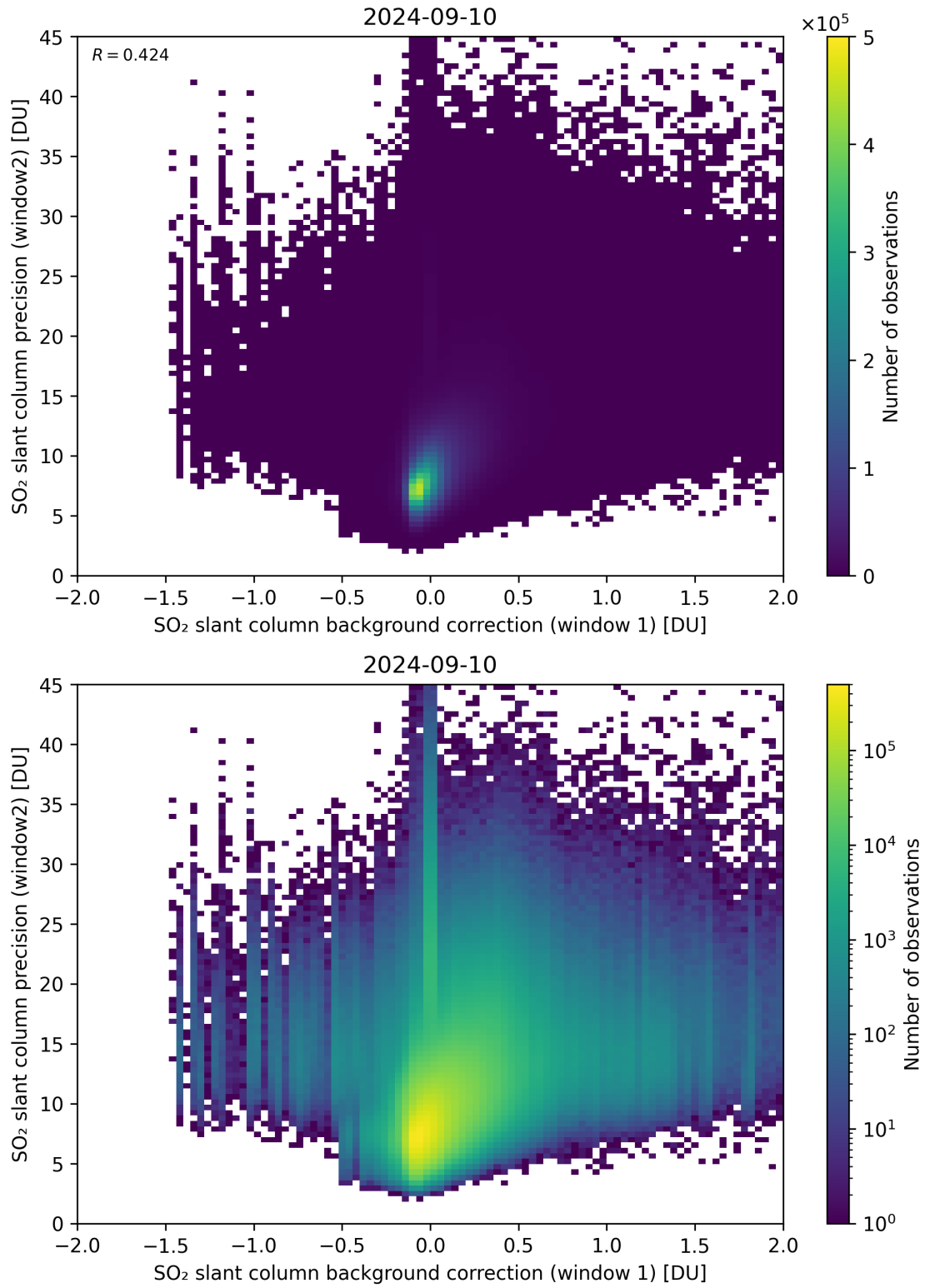
Figure 106: Scatter density plot of “SO 2 slant column background correction (window 1)” against “SO 2 slant column precision (window2)” for 2024-09-09 to 2024-09-11.
