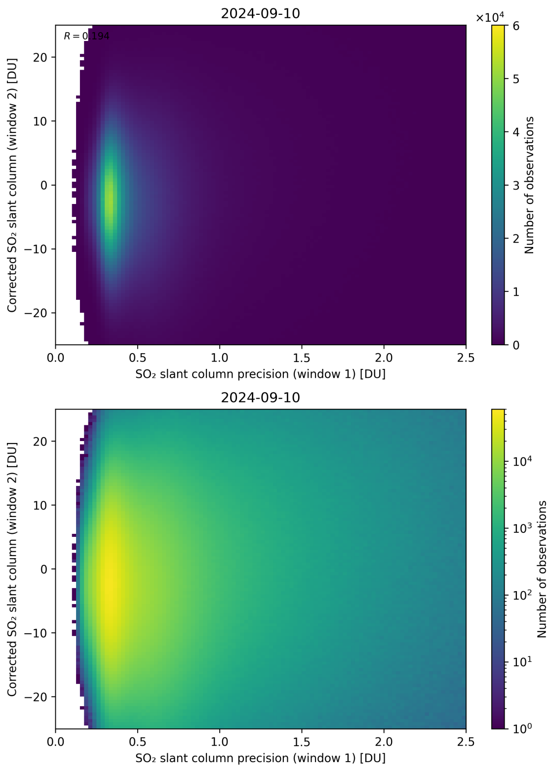
Figure 225: Scatter density plot of “SO 2 slant column precision (window 1)” against “Corrected SO 2 slant column (window 2)” for 2024-09-09 to 2024-09-11.
