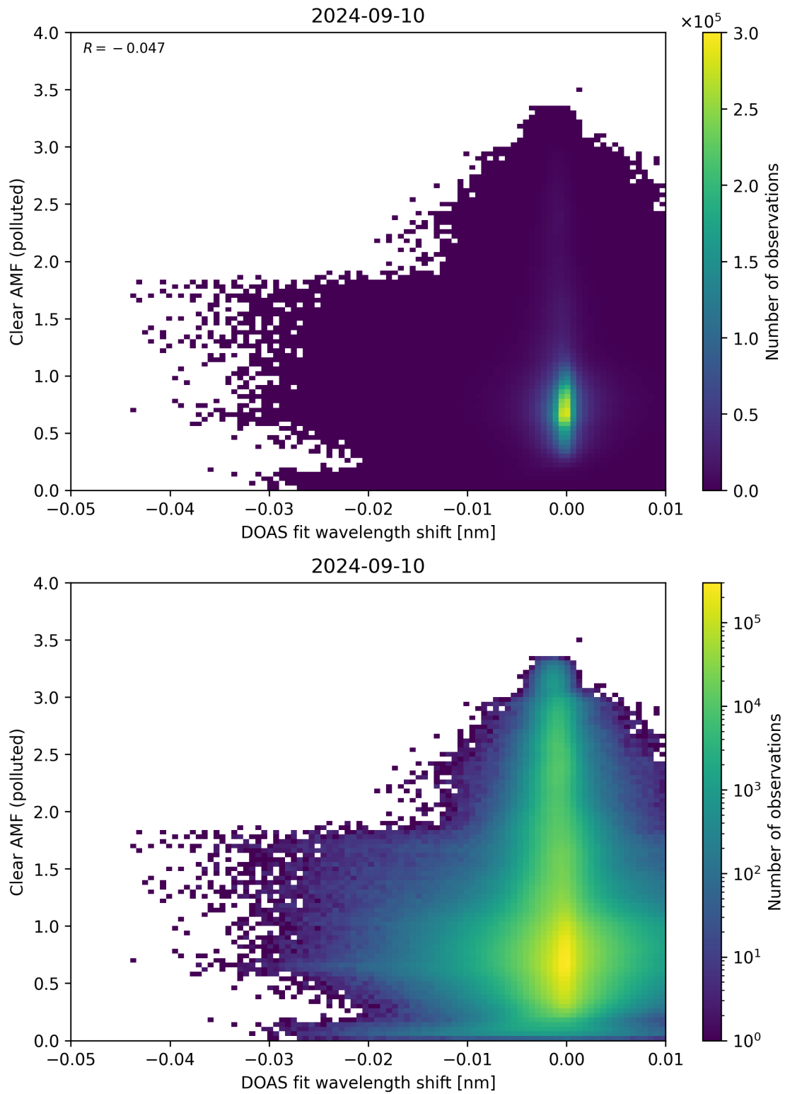
Figure 129: Scatter density plot of “DOAS fit wavelength shift” against “Clear AMF (polluted)” for 2024-09-09 to 2024-09-11.
