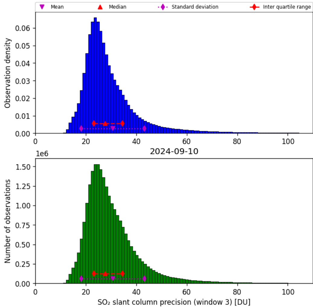
Figure 65: Histogram of “SO 2 slant column precision (window 3)” for 2024-09-09 to 2024-09-11
