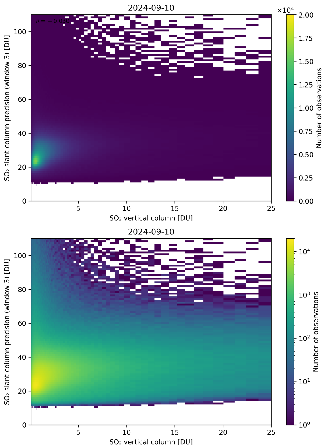
Figure 304: Scatter density plot of “SO 2 vertical column” against “SO 2 slant column precision (window 3)” for 2024-09-09 to 2024-09-11.
