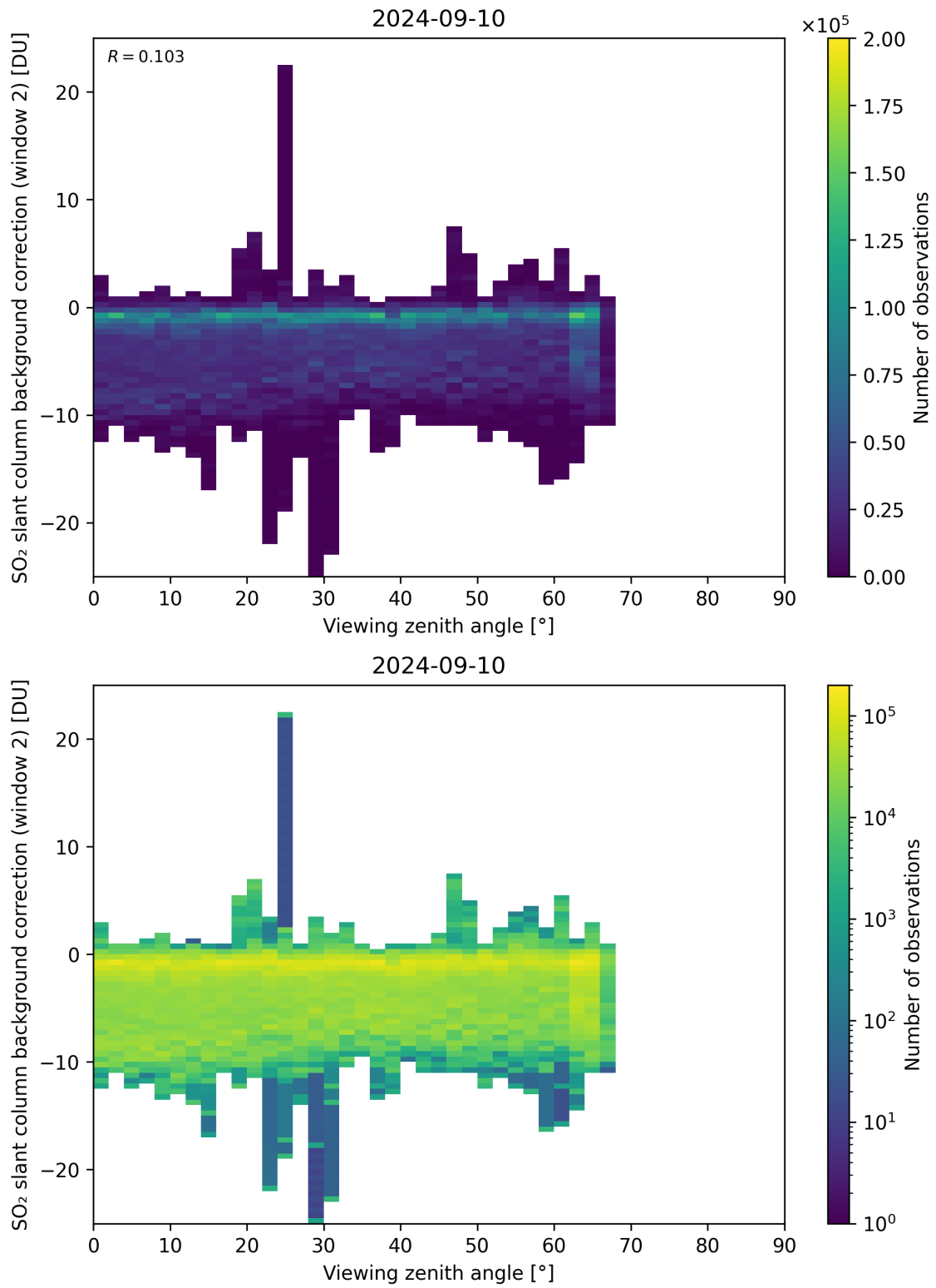
Figure 309: Scatter density plot of “Viewing zenith angle” against “SO 2 slant column background correction (window 2)” for 2024-09-09 to 2024-09-11.
