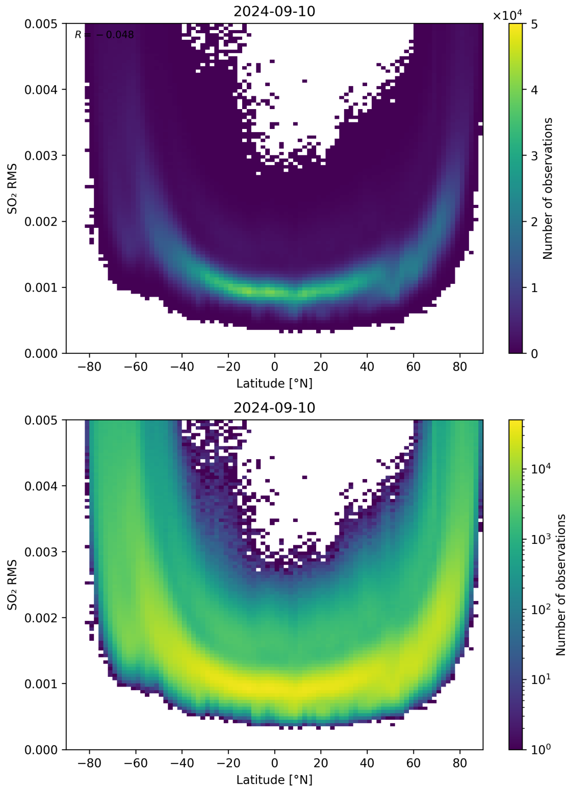
Figure 144: Scatter density plot of “Latitude” against “SO 2 RMS” for 2024-09-09 to 2024-09-11.
