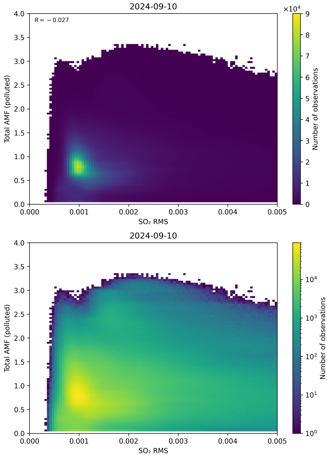
Figure 137: Scatter density plot of “SO 2 RMS” against “Total AMF (polluted)” for 2024-09-09 to 2024-09-11.
