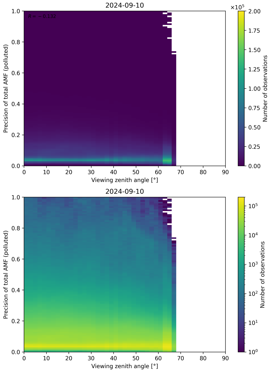
Figure 326: Scatter density plot of “Viewing zenith angle” against “Precision of total AMF (polluted)” for 2024-09-09 to 2024-09-11.
