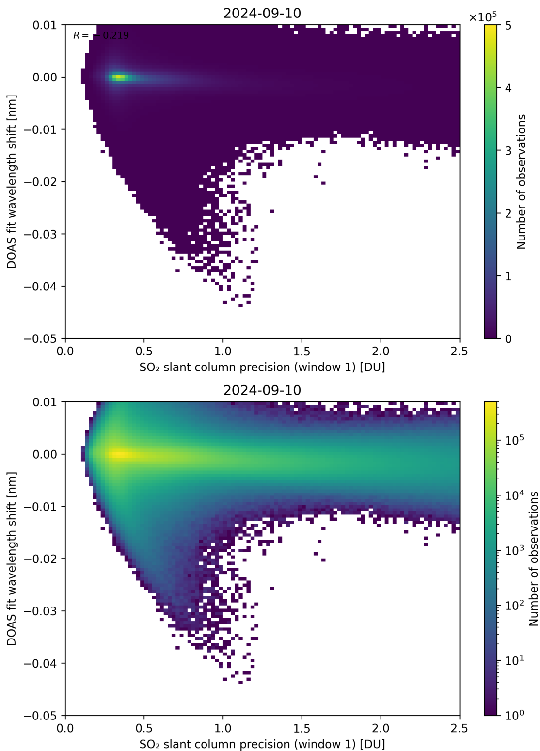
Figure 221: Scatter density plot of “SO 2 slant column precision (window 1)” against “DOAS fit wavelength shift” for 2024-09-09 to 2024-09-11.
