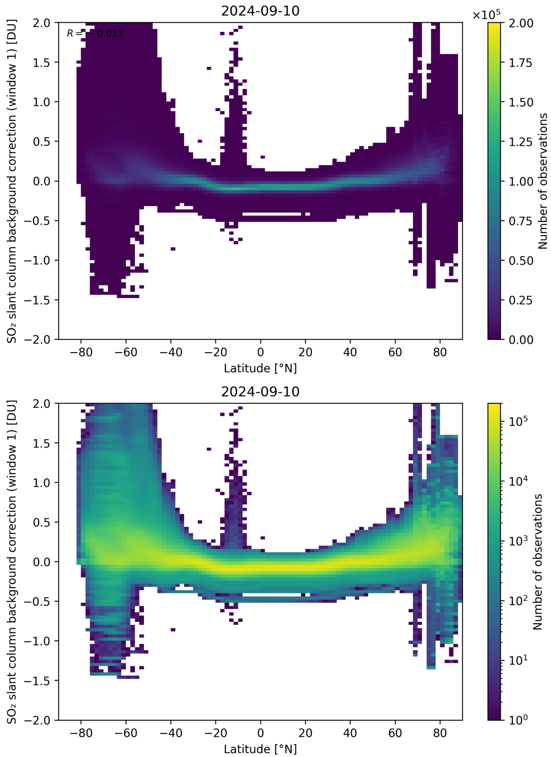
Figure 139: Scatter density plot of “Latitude” against “SO 2 slant column background correction (window 1)” for 2024-09-09 to 2024-09-11.
