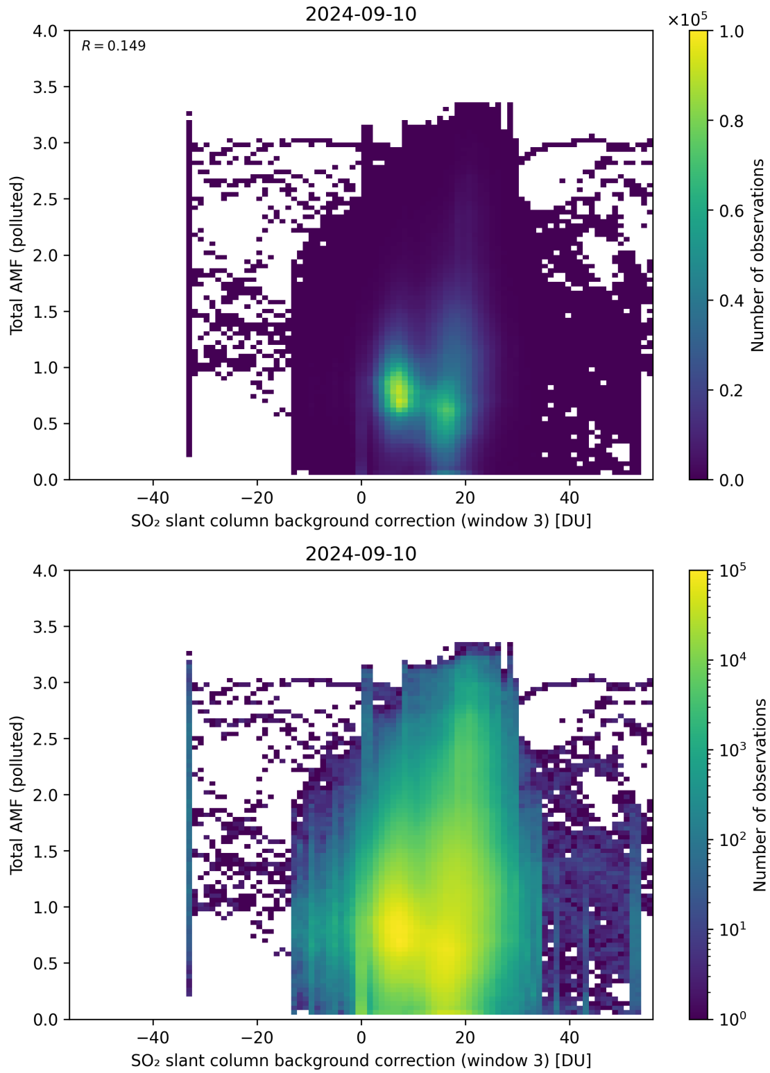
Figure 125: Scatter density plot of “SO 2 slant column background correction (window 3)” against “Total AMF (polluted)” for 2024-09-09 to 2024-09-11.
