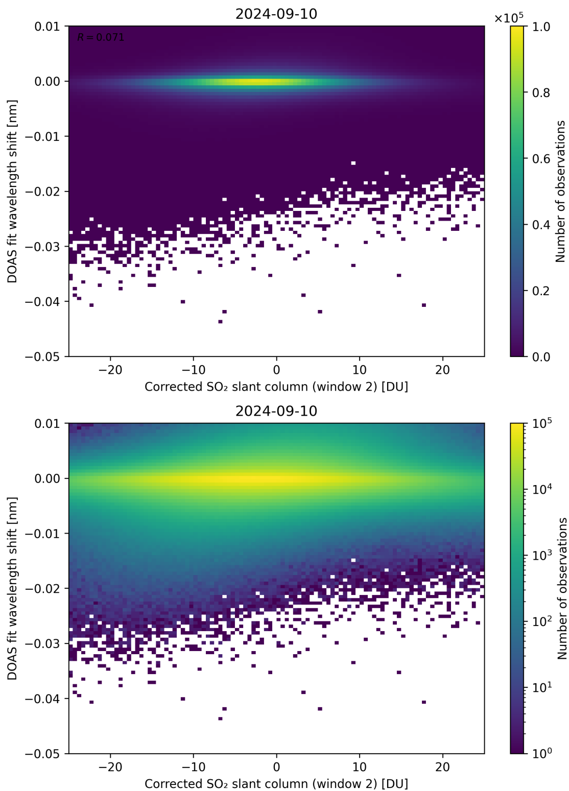
Figure 196: Scatter density plot of “Corrected SO 2 slant column (window 2)” against “DOAS fit wavelength shift” for 2024-09-09 to 2024-09-11.
