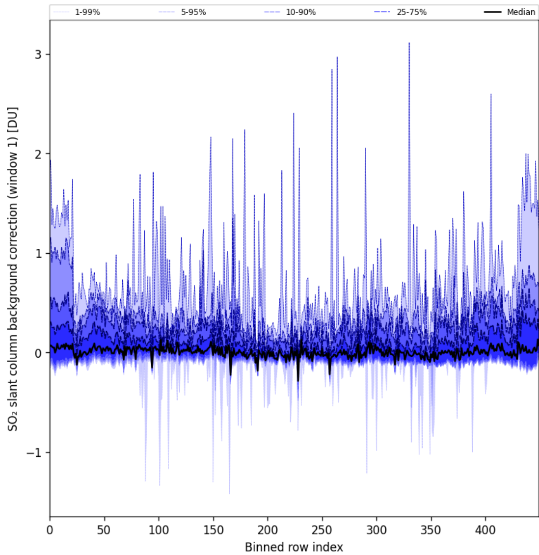
Figure 82: Along track statistics of “SO 2 slant column background correction (window 1)” for 2024-09-09 to 2024-09-11
