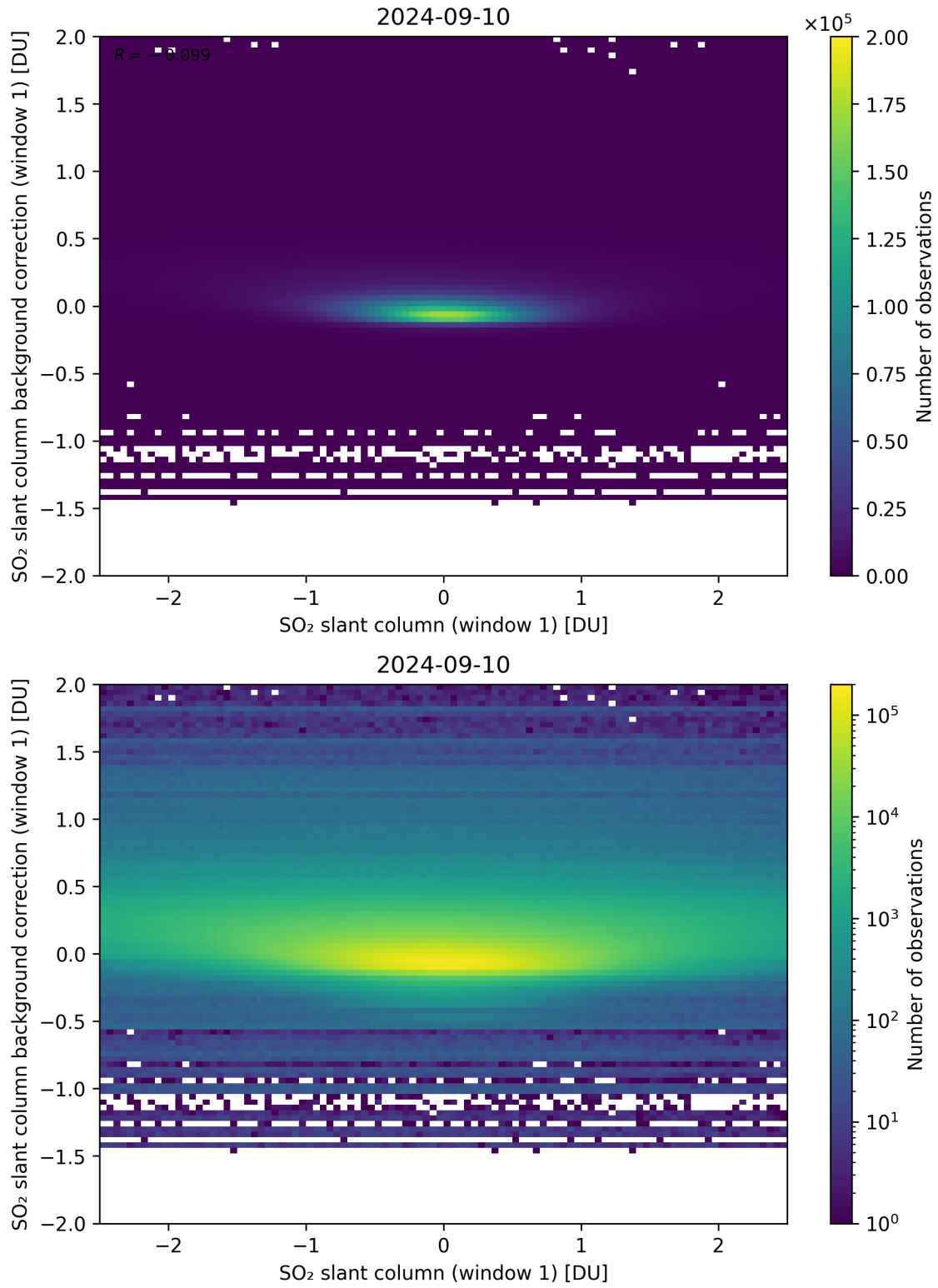
Figure 212: Scatter density plot of “SO 2 slant column (window 1)” against “SO 2 slant column background correction (window 1)” for 2024-09-09 to 2024-09-11.
