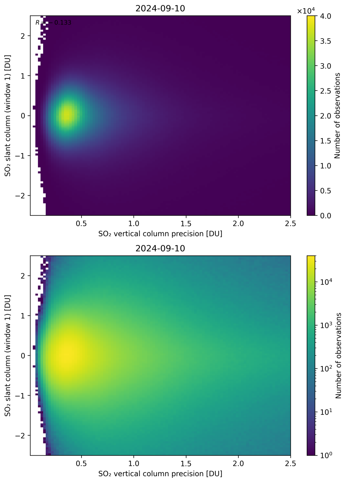
Figure 289: Scatter density plot of “SO 2 vertical column precision” against “SO 2 slant column (window 1)” for 2024-09-09 to 2024-09-11.
