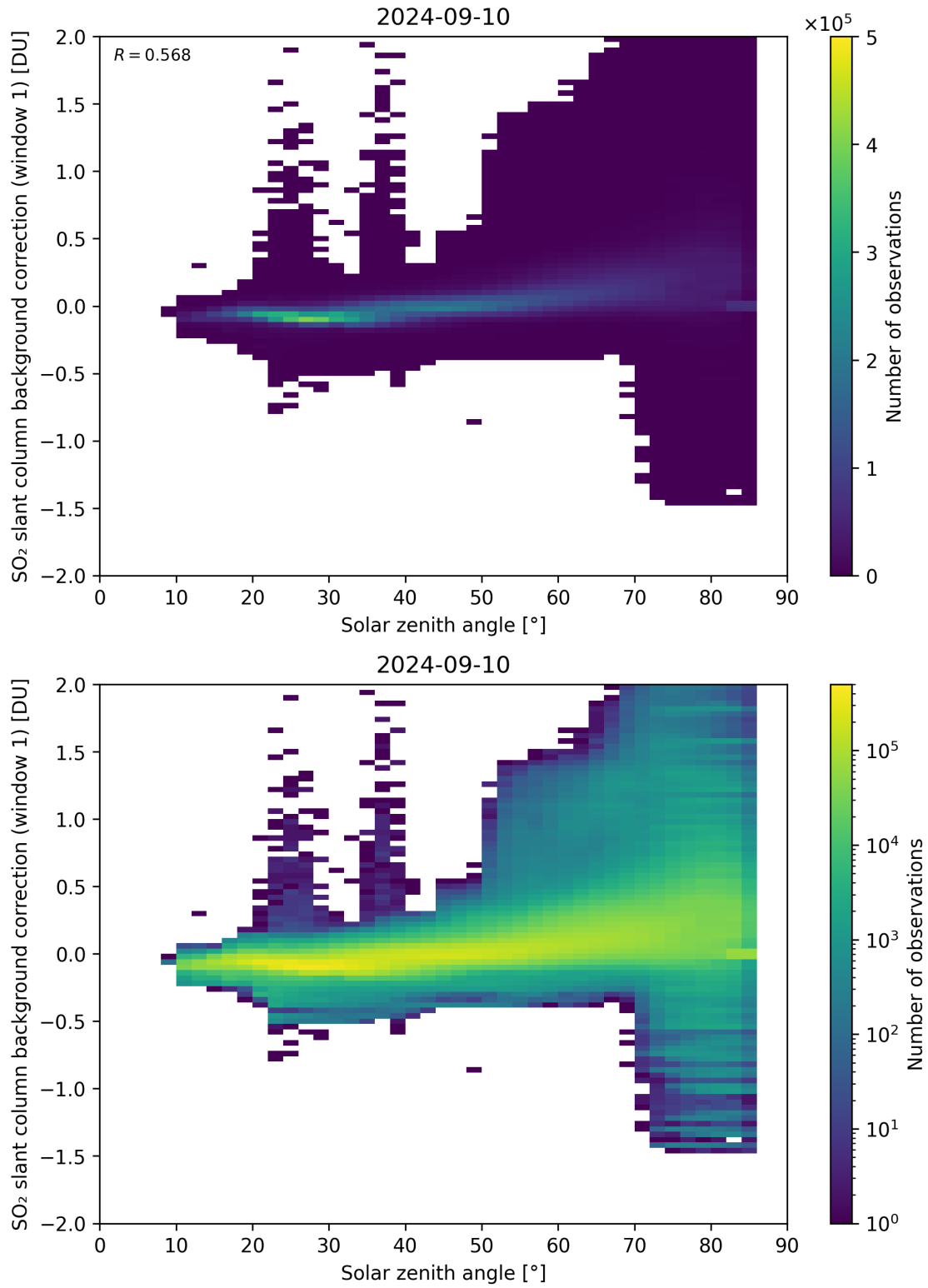
Figure 158: Scatter density plot of “Solar zenith angle” against “SO 2 slant column background correction (window 1)” for 2024-09-09 to 2024-09-11.
