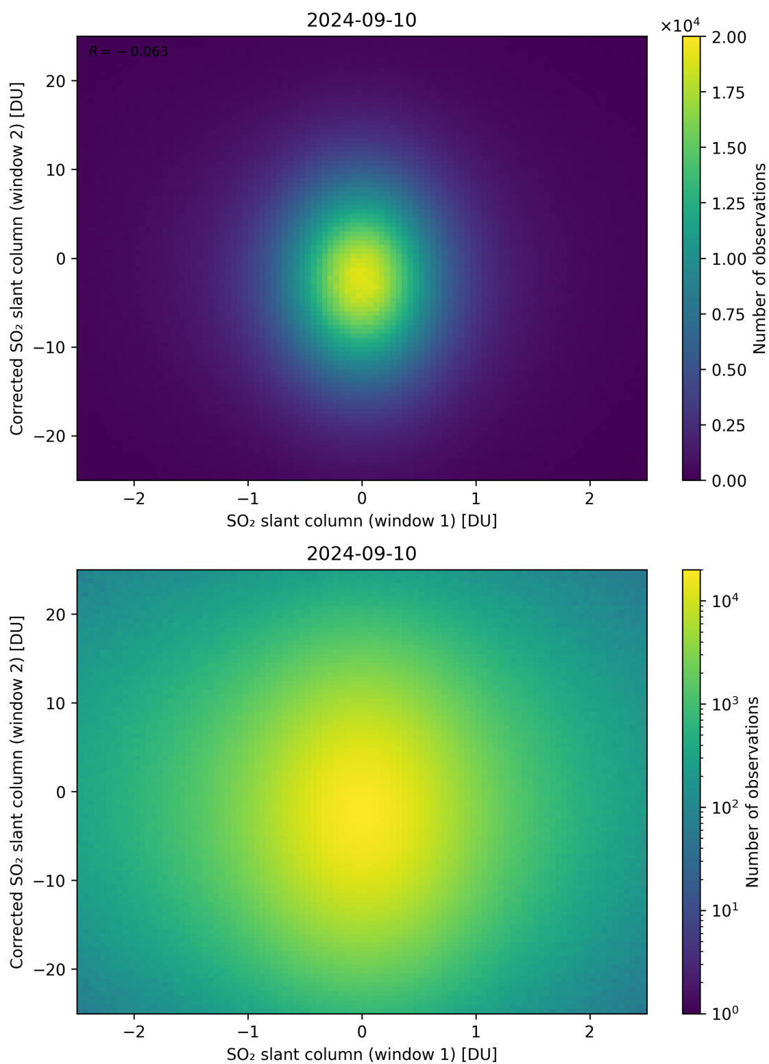
Figure 233: Scatter density plot of “SO 2 slant column (window 1)” against “Corrected SO 2 slant column (window 2)” for 2024-09-09 to 2024-09-11.
