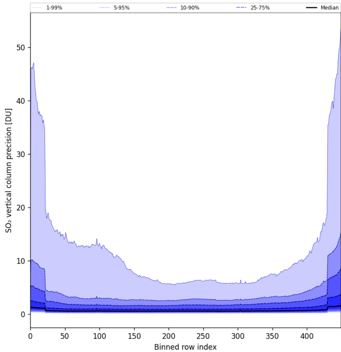
Figure 77: Along track statistics of “SO 2 vertical column precision” for 2024-09-09 to 2024-09-11
