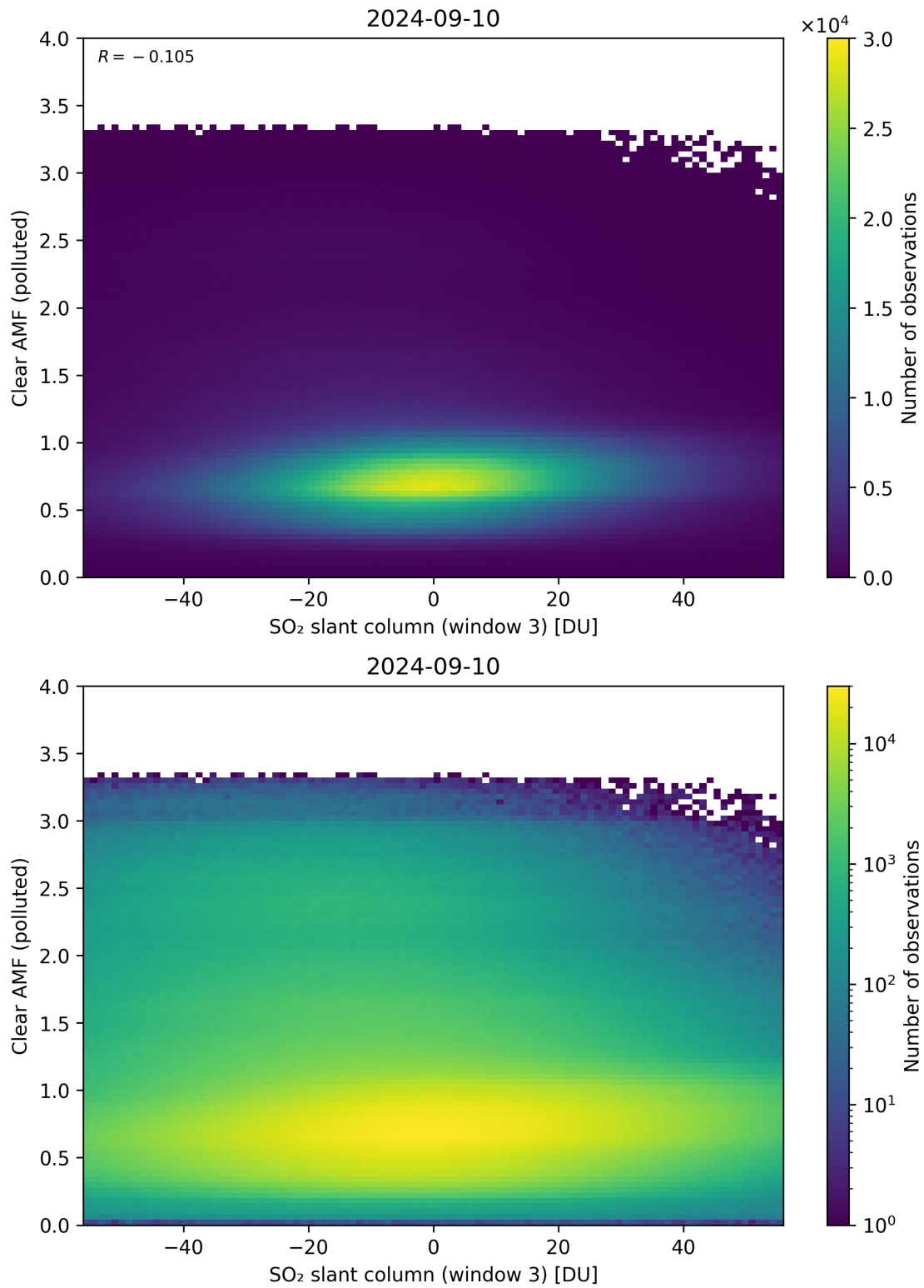
Figure 265: Scatter density plot of “SO 2 slant column (window 3)” against “Clear AMF (polluted)” for 2024-09-09 to 2024-09-11.
