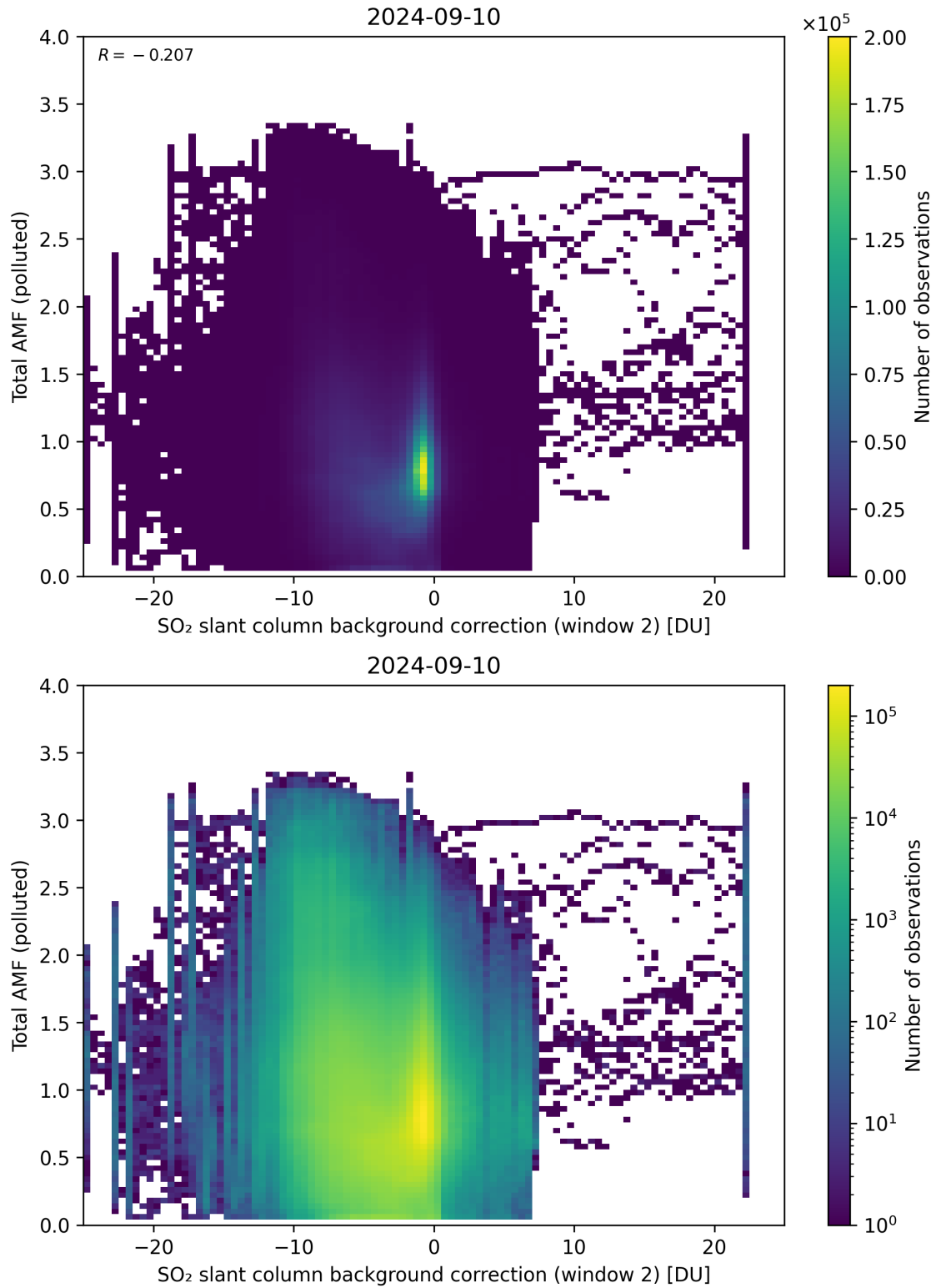
Figure 119: Scatter density plot of “SO 2 slant column background correction (window 2)” against “Total AMF (polluted)” for 2024-09-09 to 2024-09-11.
