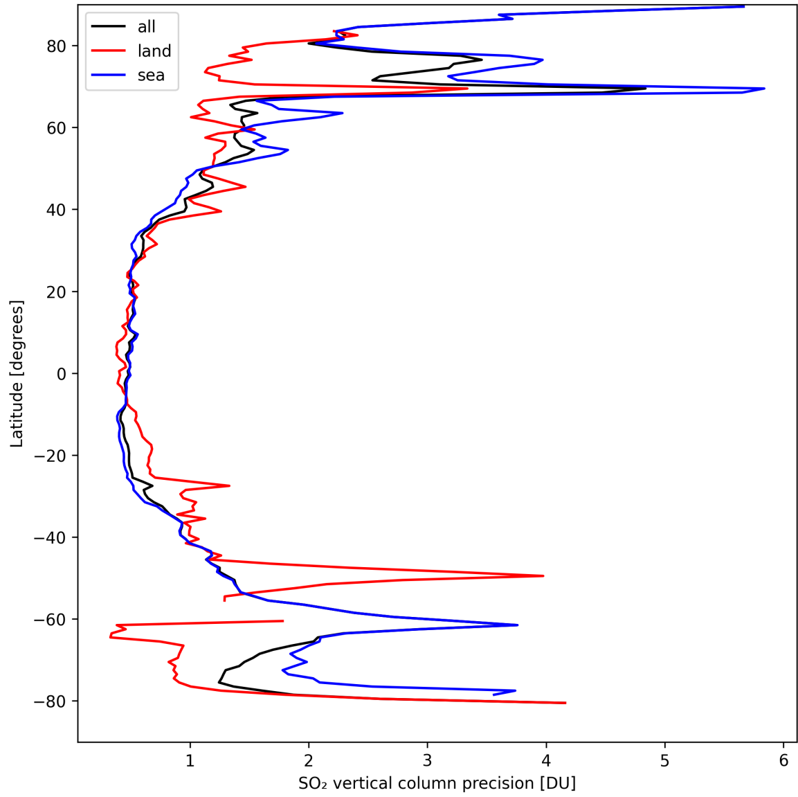
Figure 31: Zonal average of “SO 2 vertical column precision” for 2024-09-09 to 2024-09-11.
