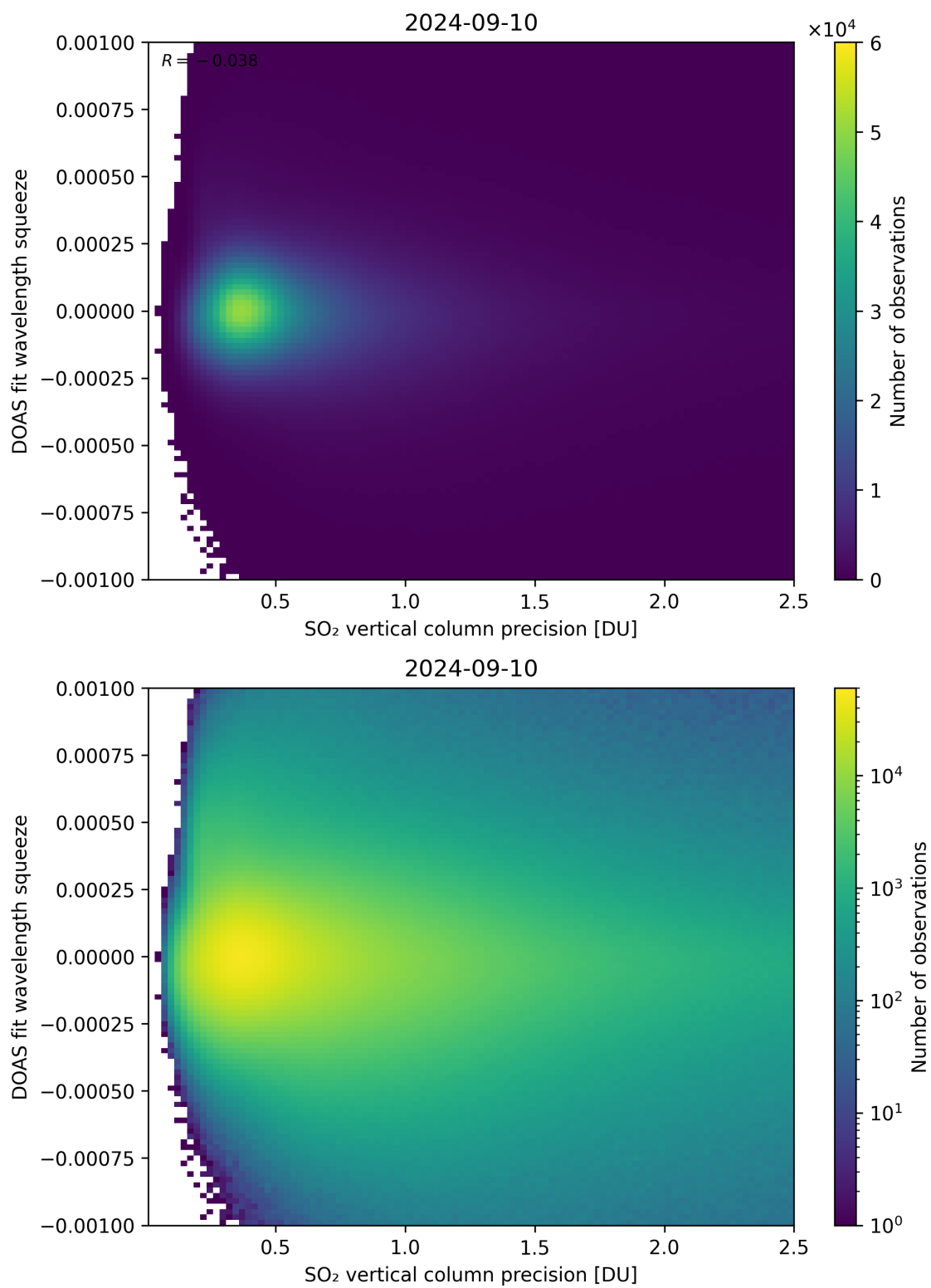
Figure 283: Scatter density plot of “SO 2 vertical column precision” against “DOAS fit wavelength squeeze” for 2024-09-09 to 2024-09-11.
