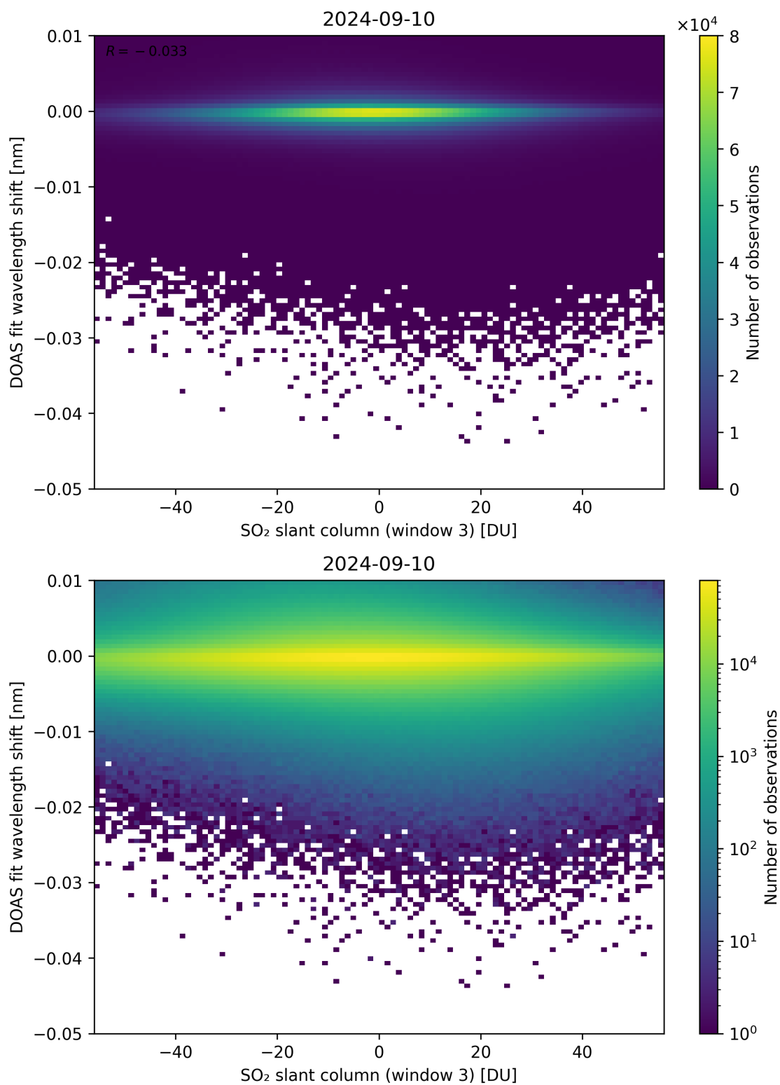
Figure 254: Scatter density plot of “SO 2 slant column (window 3)” against “DOAS fit wavelength shift” for 2024-09-09 to 2024-09-11.
