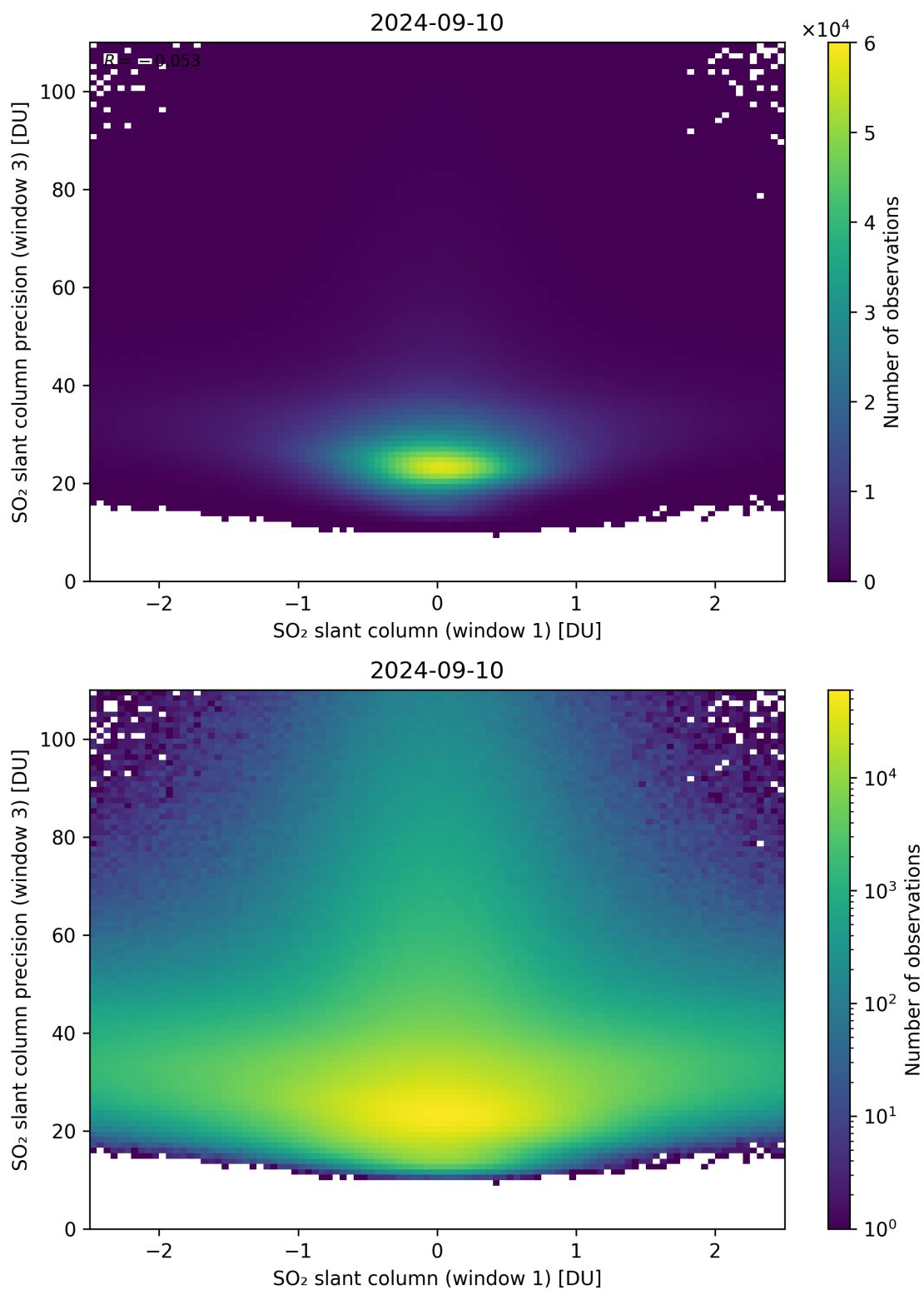
Figure 238: Scatter density plot of “SO 2 slant column (window 1)” against “SO 2 slant column precision (window 3)” for 2024-09-09 to 2024-09-11.
