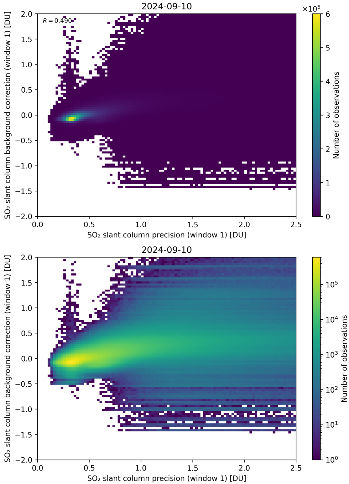
Figure 218: Scatter density plot of “SO 2 slant column precision (window 1)” against “SO 2 slant column background correction (window 1)” for 2024-09-09 to 2024-09-11.
