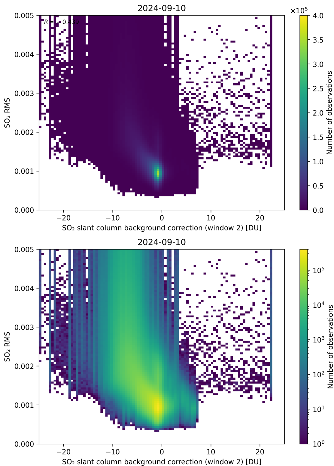
Figure 114: Scatter density plot of “SO 2 slant column background correction (window 2)” against “SO 2 RMS” for 2024-09-09 to 2024-09-11.
