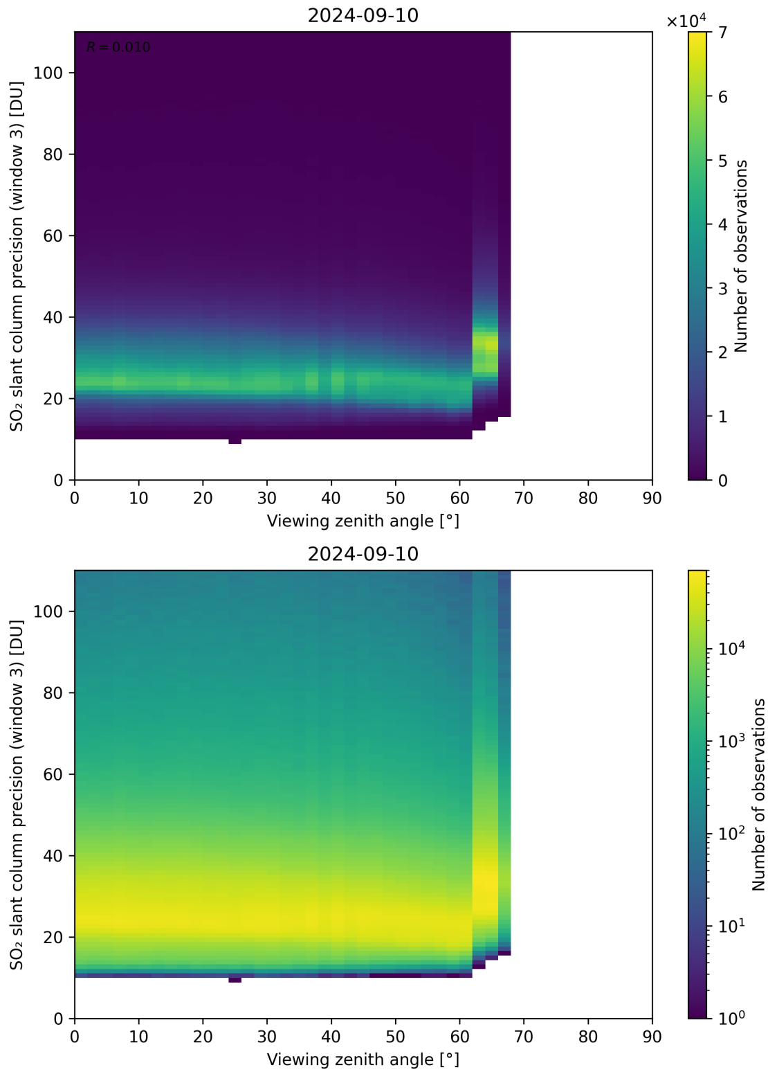
Figure 324: Scatter density plot of “Viewing zenith angle” against “SO 2 slant column precision (window 3)” for 2024-09-09 to 2024-09-11.
