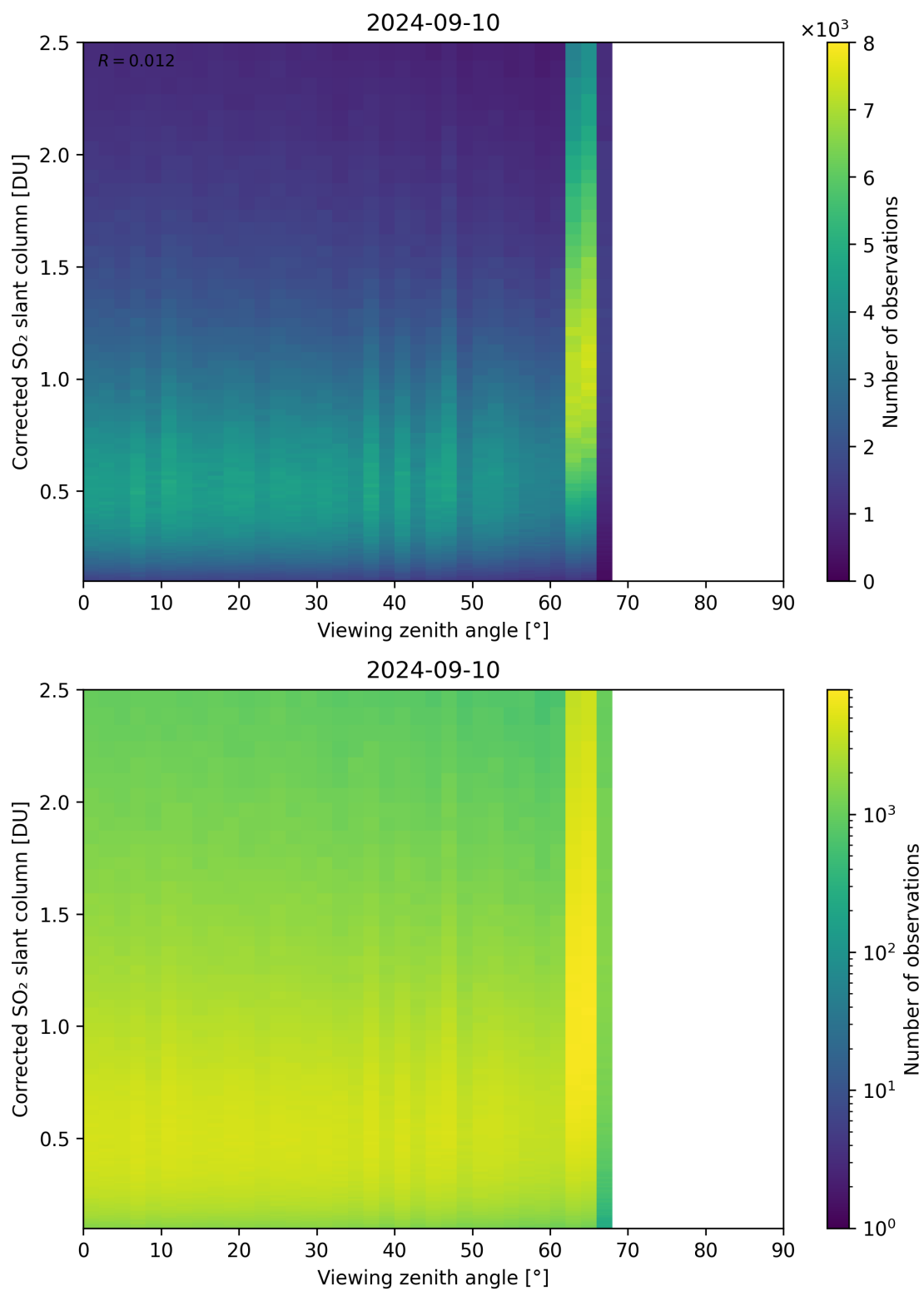
Figure 317: Scatter density plot of “Viewing zenith angle” against “Corrected SO 2 slant column” for 2024-09-09 to 2024-09-11.
