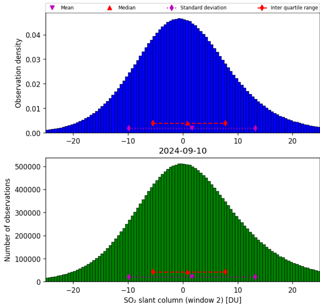
Figure 60: Histogram of “SO 2 slant column (window 2)” for 2024-09-09 to 2024-09-11
