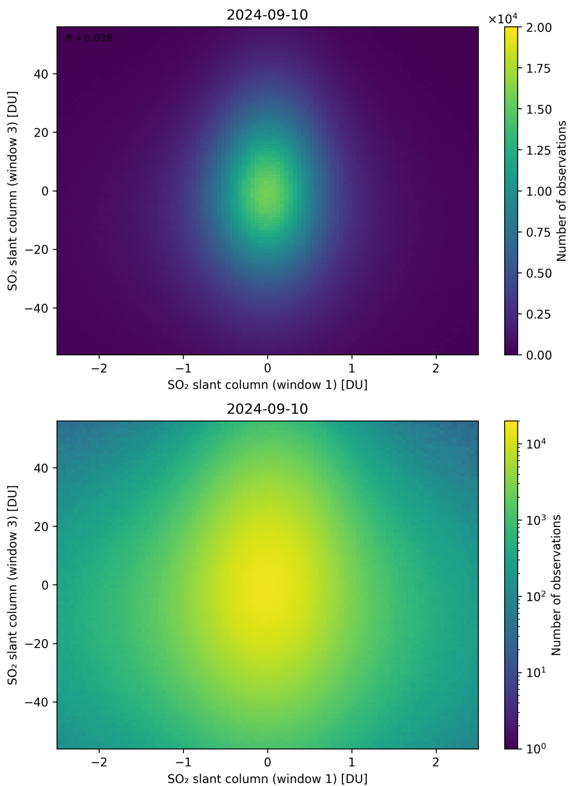
Figure 237: Scatter density plot of “SO 2 slant column (window 1)” against “SO 2 slant column (window 3)” for 2024-09-09 to 2024-09-11.
