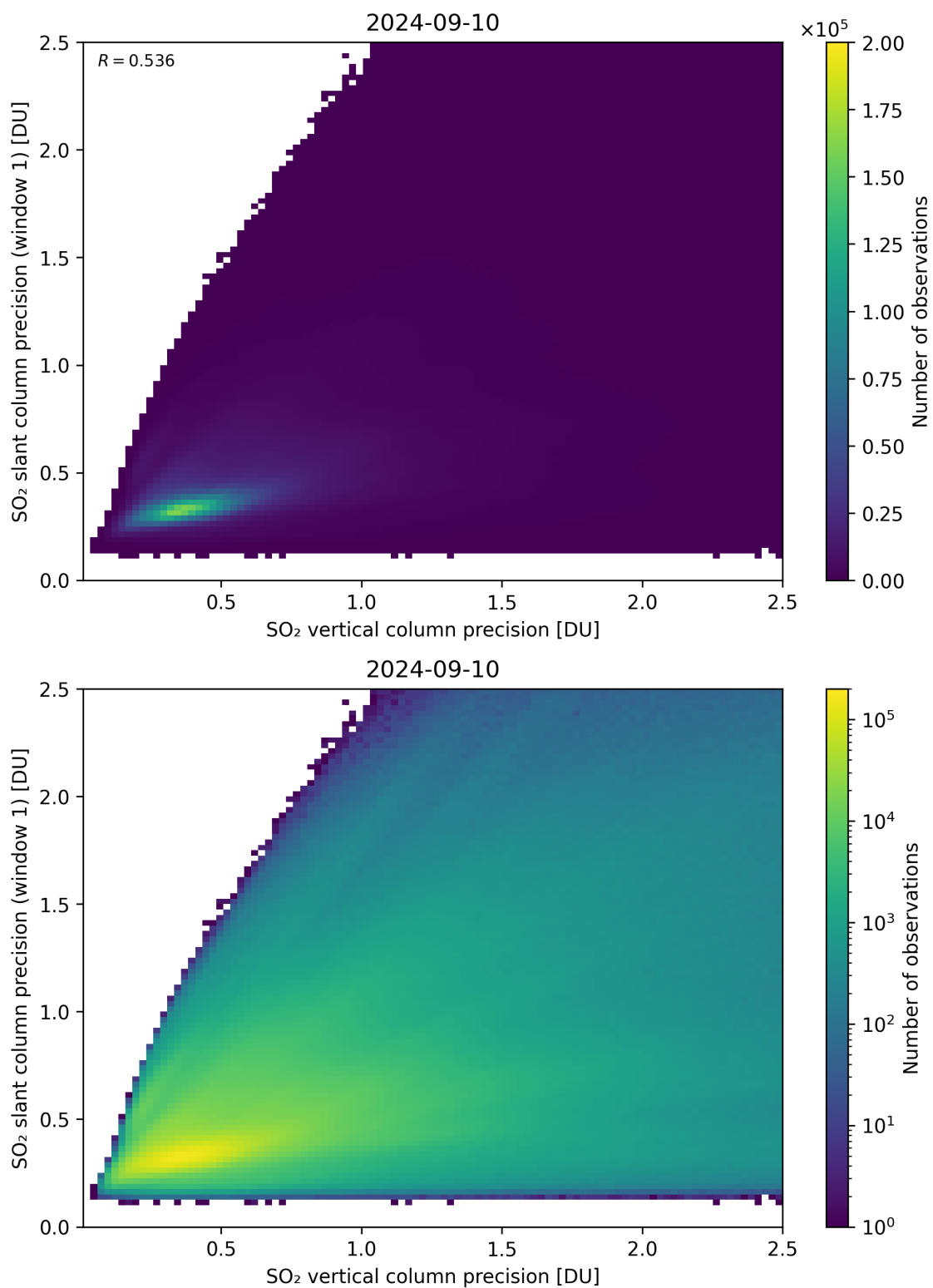
Figure 290: Scatter density plot of “SO 2 vertical column precision” against “SO 2 slant column precision (window 1)” for 2024-09-09 to 2024-09-11.
