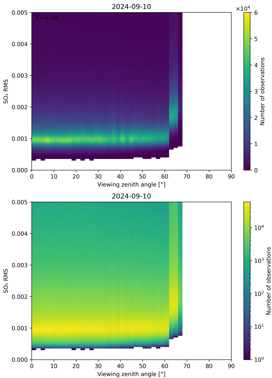
Figure 313: Scatter density plot of “Viewing zenith angle” against “SO 2 RMS” for 2024-09-09 to 2024-09-11.
