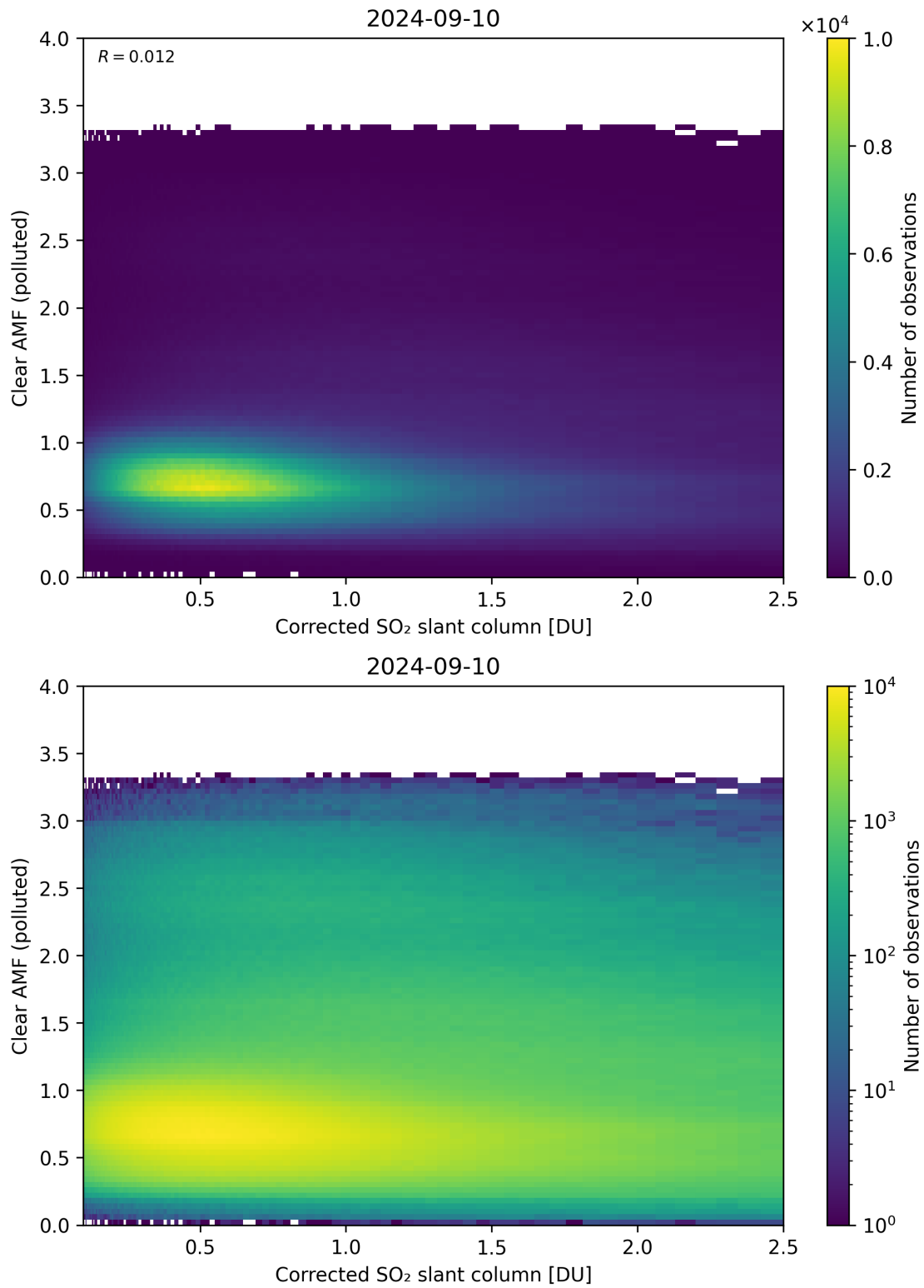
Figure 184: Scatter density plot of “Corrected SO 2 slant column” against “Clear AMF (polluted)” for 2024-09-09 to 2024-09-11.
