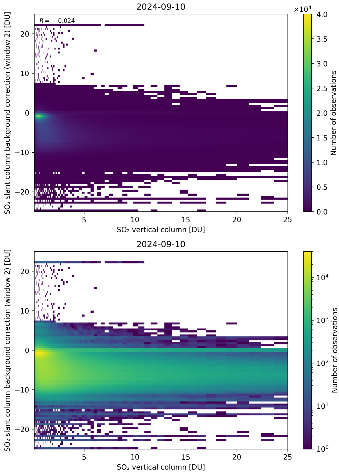
Figure 274: Scatter density plot of “SO 2 vertical column” against “SO 2 slant column background correction (window 2)” for 2024-09-09 to 2024-09-11.
