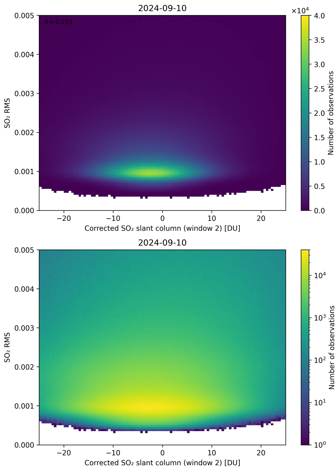
Figure 198: Scatter density plot of “Corrected SO 2 slant column (window 2)” against “SO 2 RMS” for 2024-09-09 to 2024-09-11.
