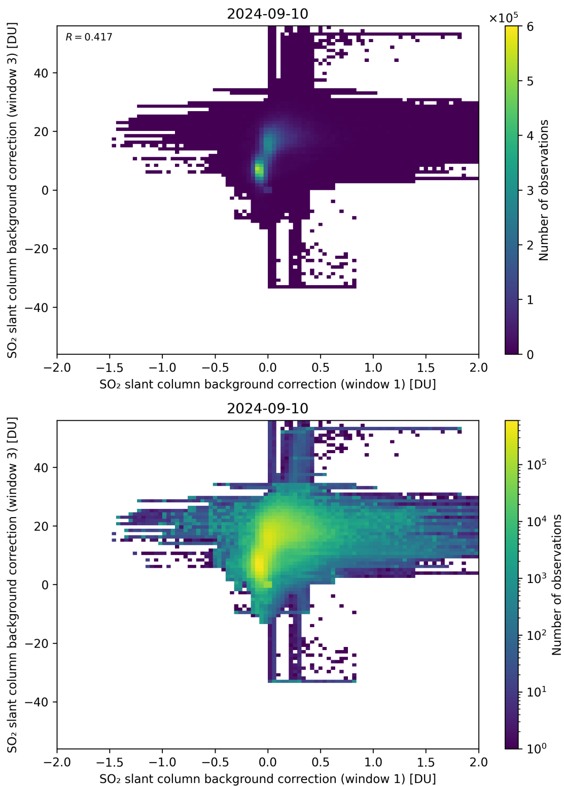
Figure 99: Scatter density plot of “SO 2 slant column background correction (window 1)” against “SO 2 slant column background correction (window 3)” for 2024-09-09 to 2024-09-11.
