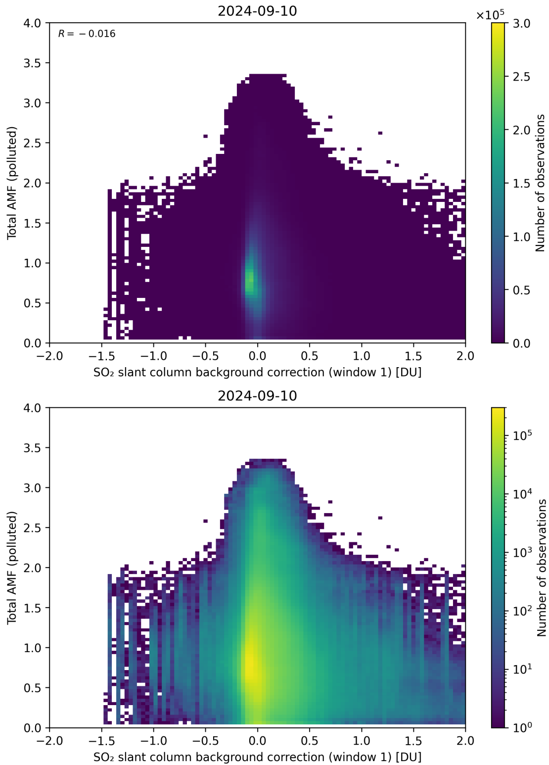
Figure 109: Scatter density plot of “SO 2 slant column background correction (window 1)” against “Total AMF (polluted)” for 2024-09-09 to 2024-09-11.
