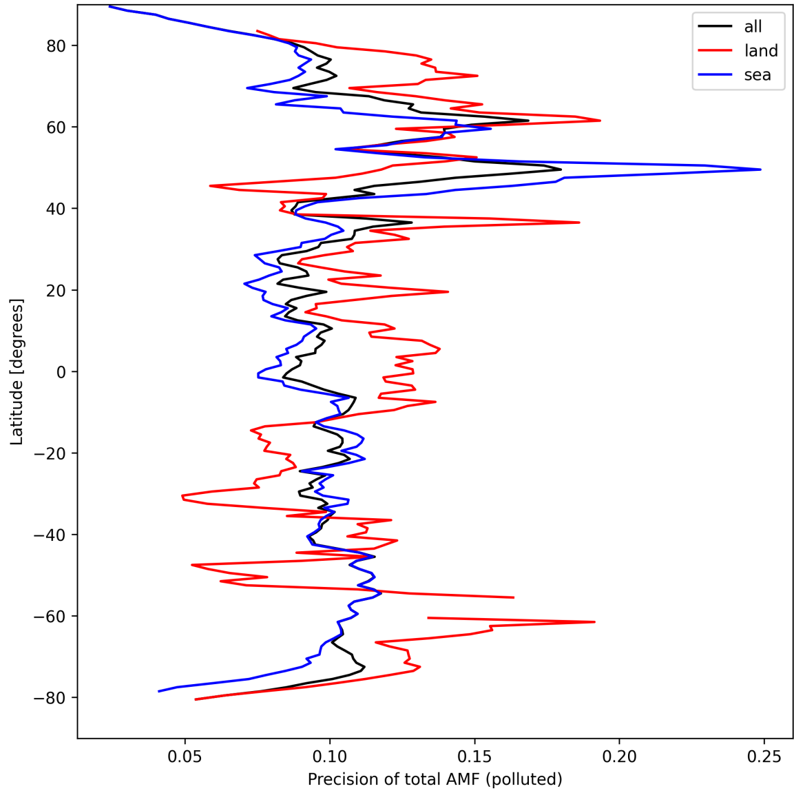
Figure 49: Zonal average of “Precision of total AMF (polluted)” for 2024-09-09 to 2024-09-11.
