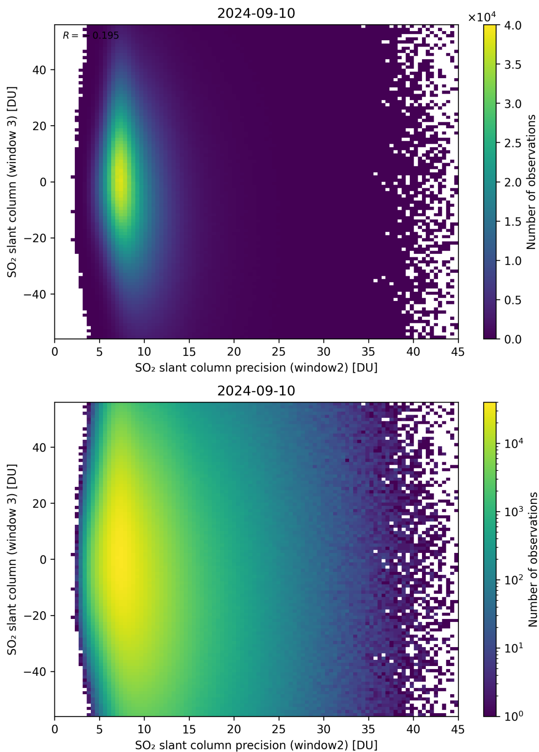
Figure 249: Scatter density plot of “SO 2 slant column precision (window2)” against “SO 2 slant column (window 3)” for 2024-09-09 to 2024-09-11.
