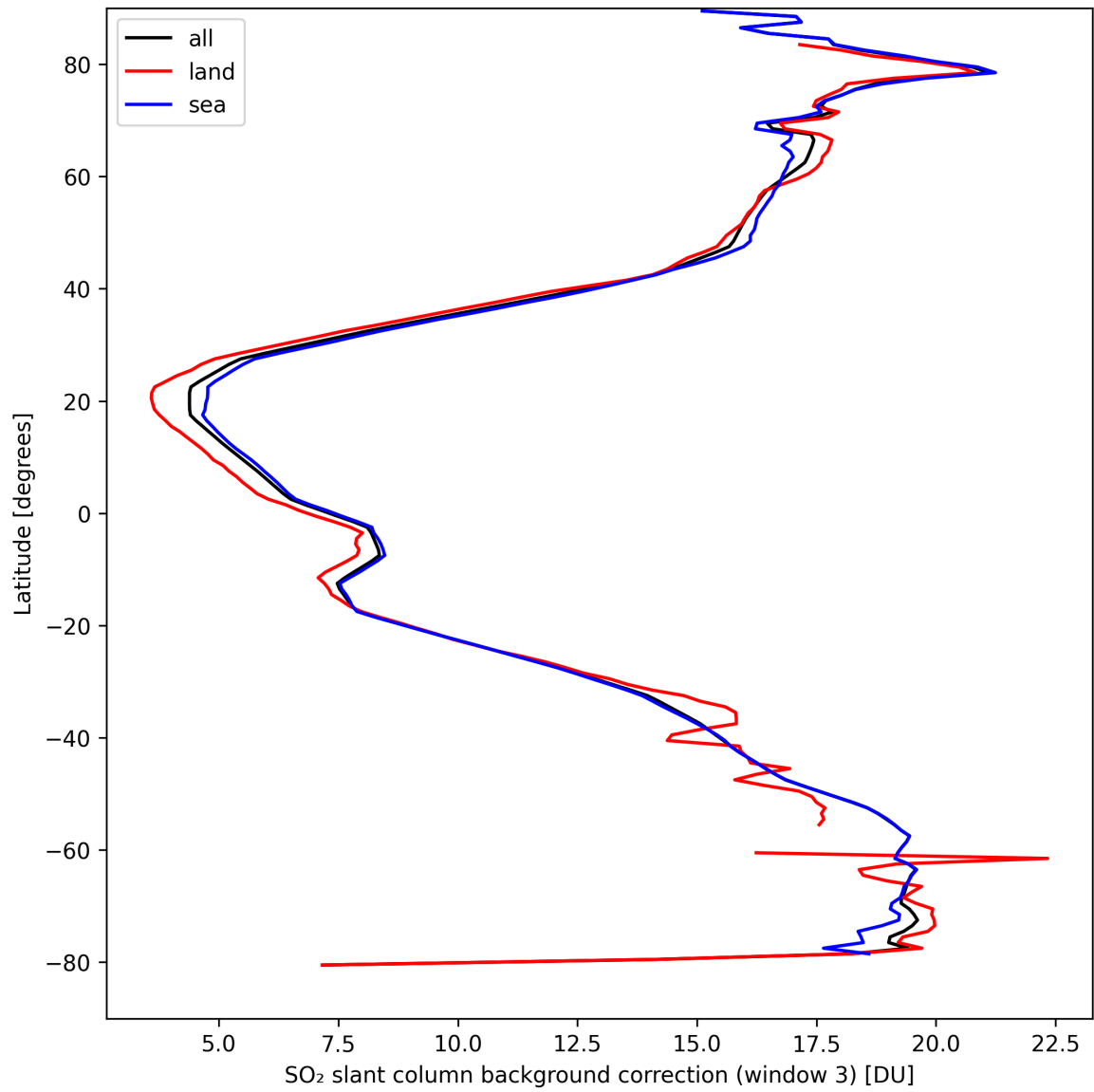
Figure 44: Zonal average of “SO 2 slant column background correction (window 3)” for 2024-09-09 to 2024-09-11.
