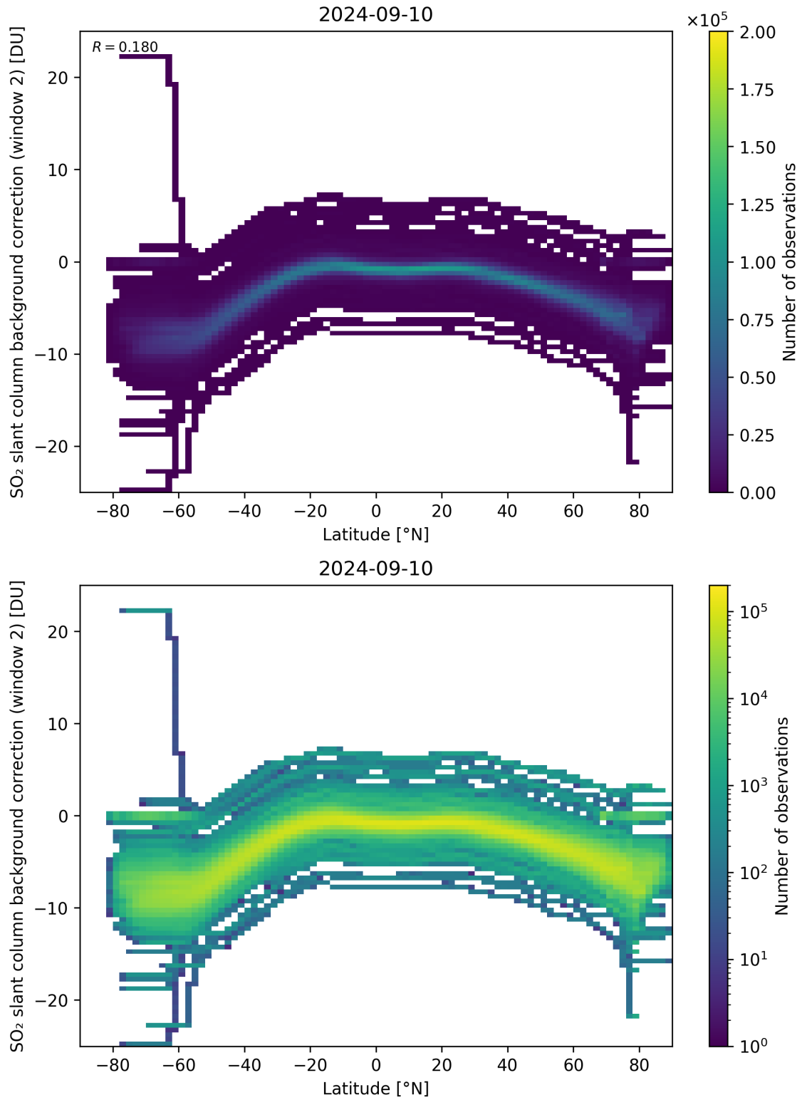
Figure 140: Scatter density plot of “Latitude” against “SO 2 slant column background correction (window 2)” for 2024-09-09 to 2024-09-11.
