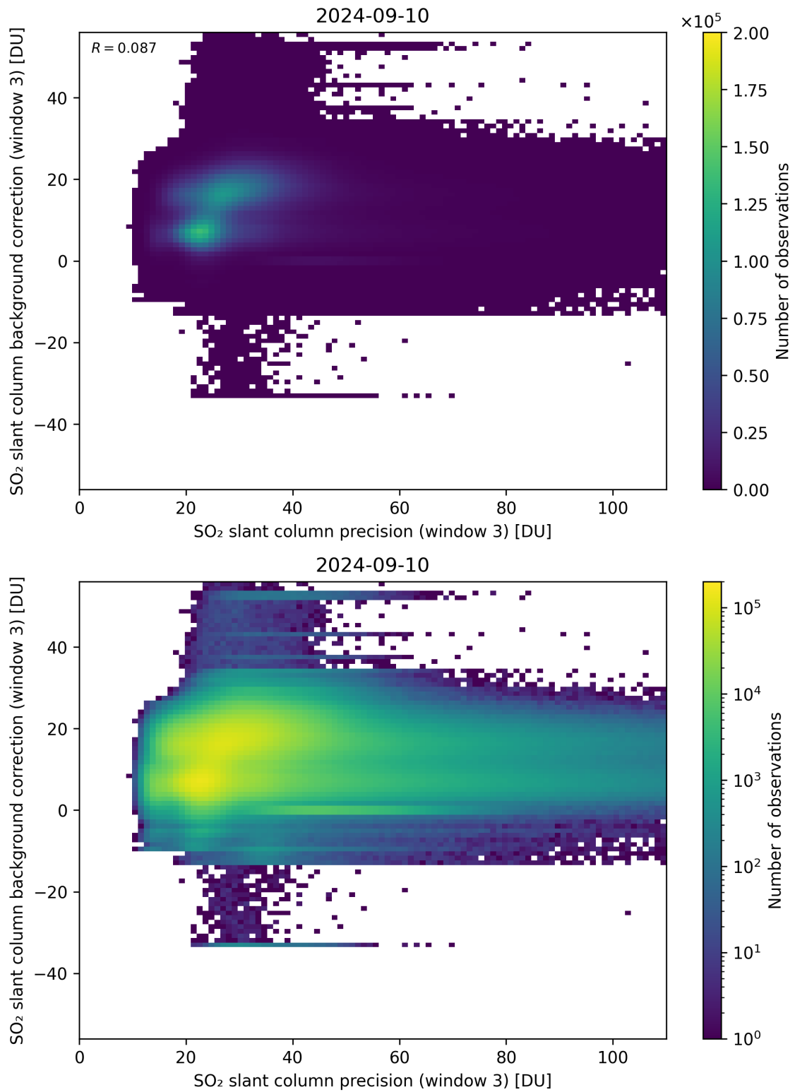
Figure 257: Scatter density plot of “SO 2 slant column precision (window 3)” against “SO 2 slant column background correction (window 3)” for 2024-09-09 to 2024-09-11.
