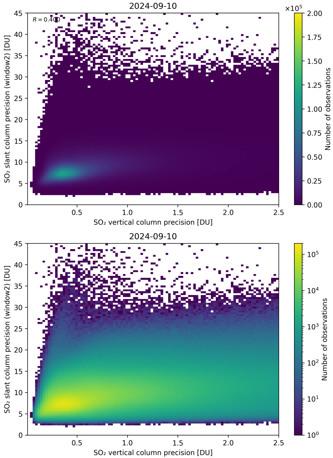
Figure 291: Scatter density plot of “SO 2 vertical column precision” against “SO 2 slant column precision (window2)” for 2024-09-09 to 2024-09-11.
