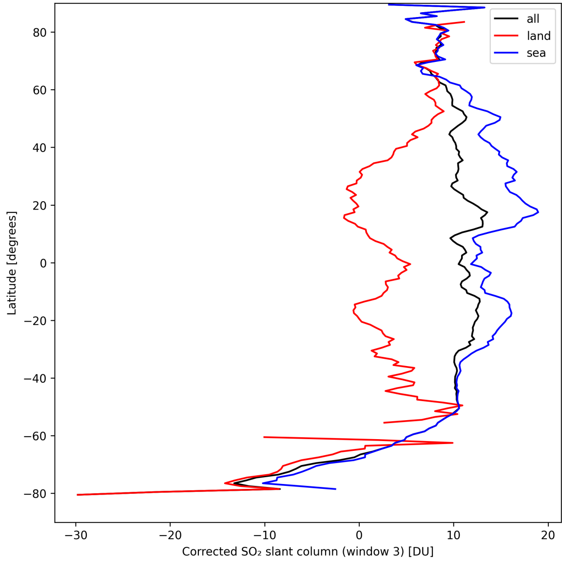
Figure 43: Zonal average of “Corrected SO 2 slant column (window 3)” for 2024-09-09 to 2024-09-11.
