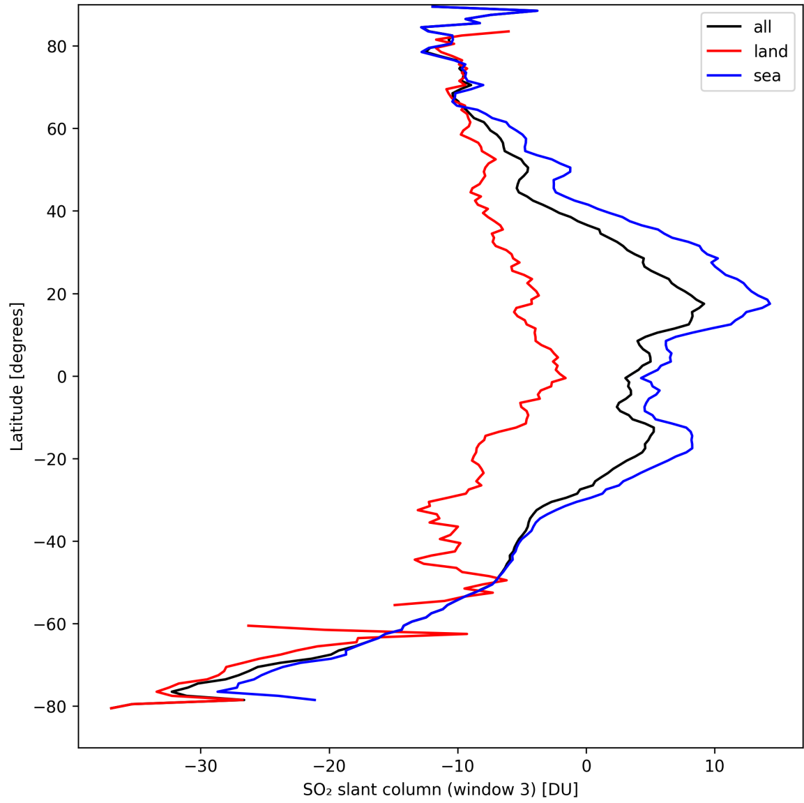
Figure 41: Zonal average of “SO 2 slant column (window 3)” for 2024-09-09 to 2024-09-11.
