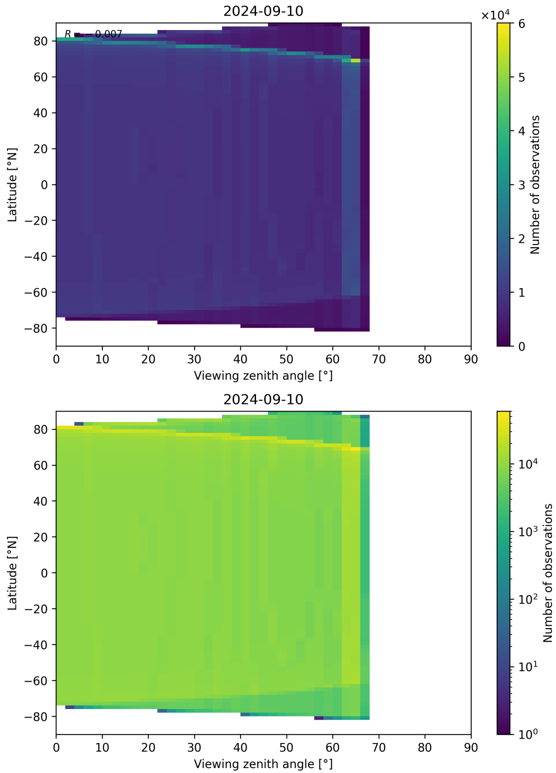
Figure 314: Scatter density plot of “Viewing zenith angle” against “Latitude” for 2024-09-09 to 2024-09-11.
