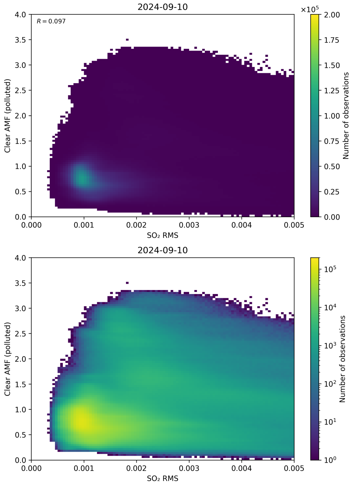
Figure 136: Scatter density plot of “SO 2 RMS” against “Clear AMF (polluted)” for 2024-09-09 to 2024-09-11.
