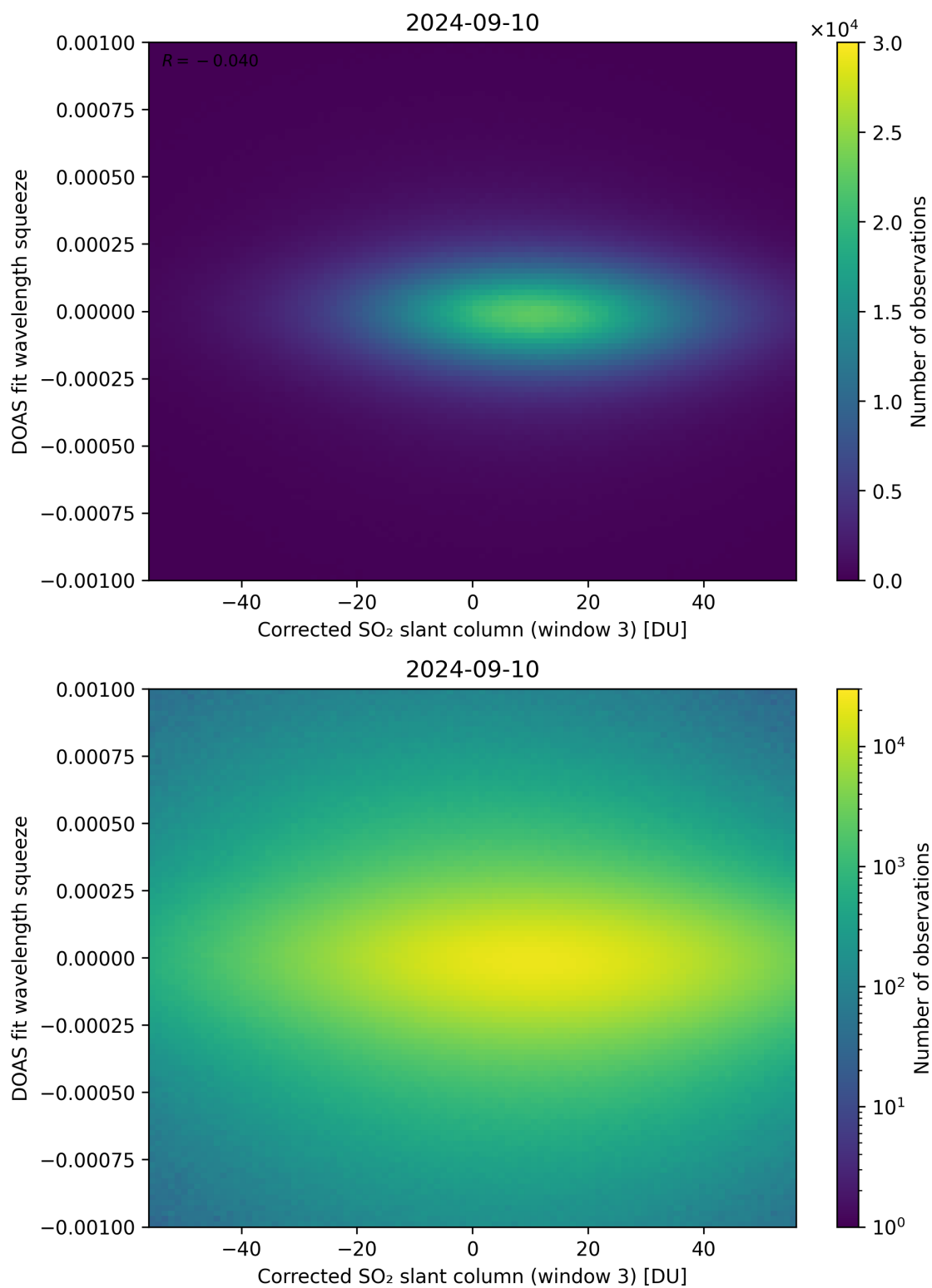
Figure 207: Scatter density plot of “Corrected SO 2 slant column (window 3)” against “DOAS fit wavelength squeeze” for 2024-09-09 to 2024-09-11.
