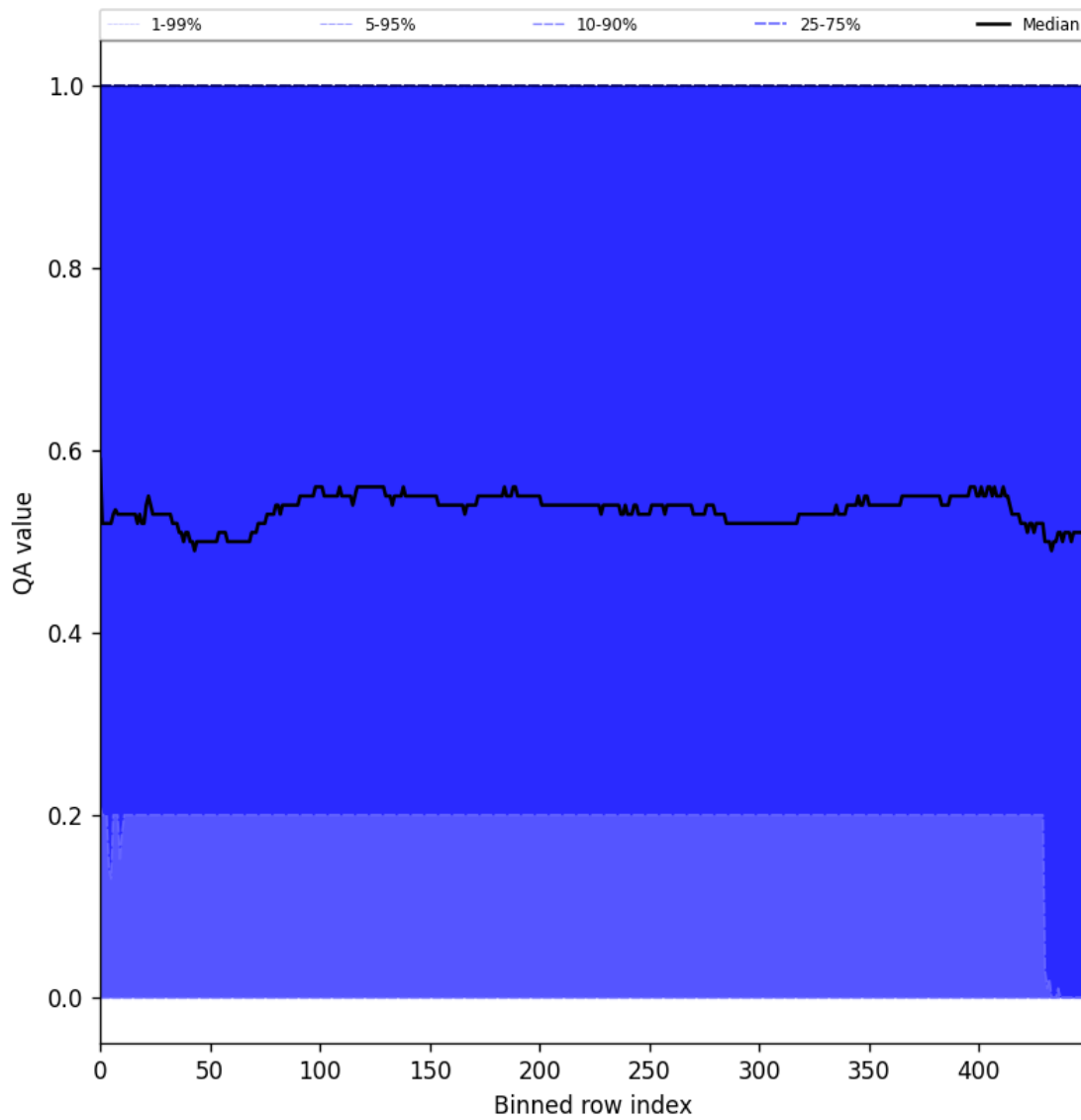
Figure 75: Along track statistics of “QA value” for 2024-09-09 to 2024-09-11
