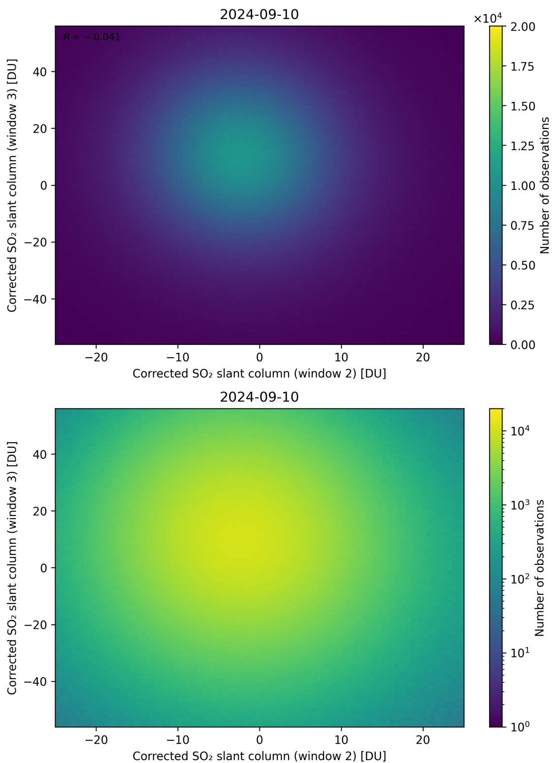
Figure 200: Scatter density plot of “Corrected SO 2 slant column (window 2)” against “Corrected SO 2 slant column (window 3)” for 2024-09-09 to 2024-09-11.
