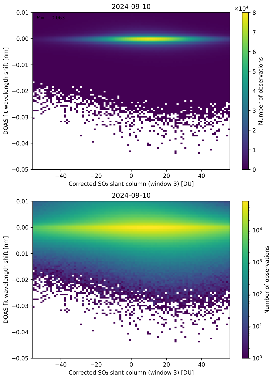
Figure 206: Scatter density plot of “Corrected SO 2 slant column (window 3)” against “DOAS fit wavelength shift” for 2024-09-09 to 2024-09-11.
