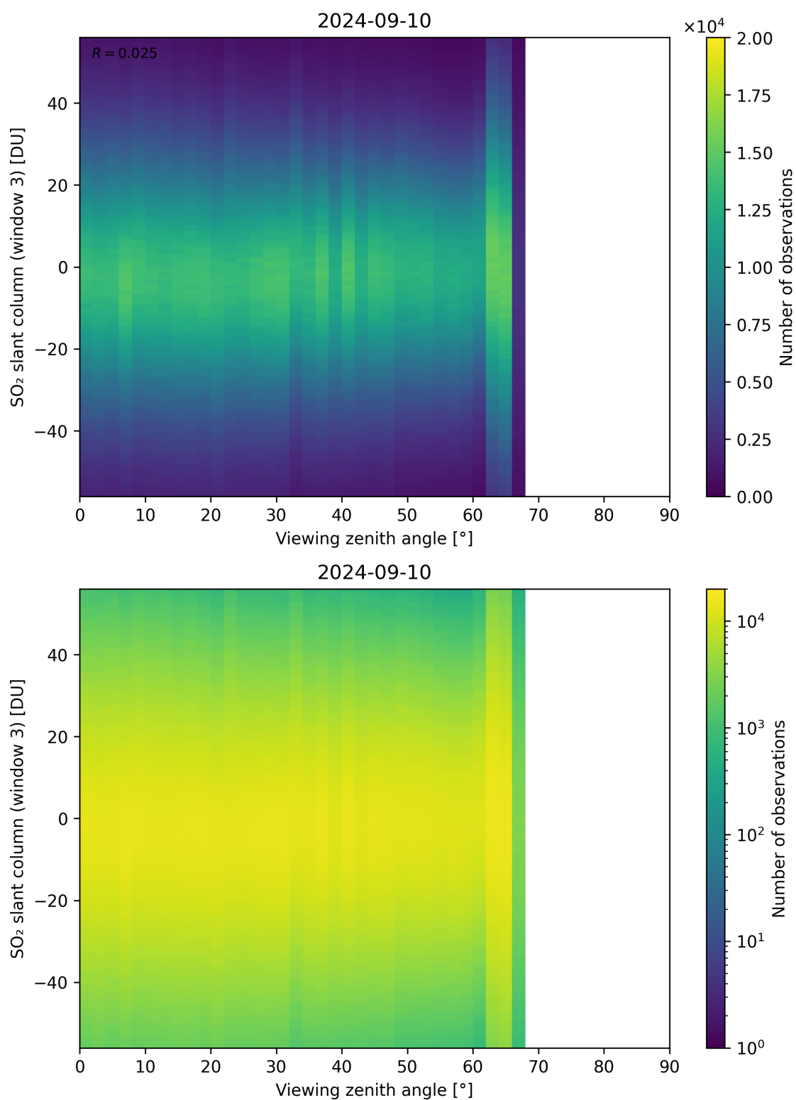
Figure 323: Scatter density plot of “Viewing zenith angle” against “SO 2 slant column (window 3)” for 2024-09-09 to 2024-09-11.
