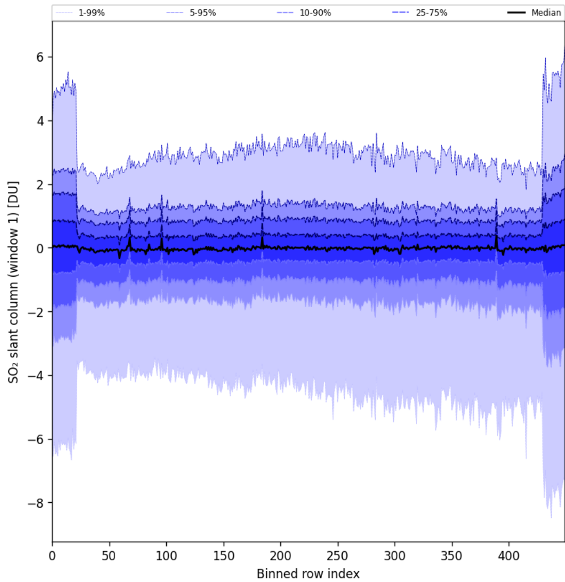
Figure 79: Along track statistics of “SO 2 slant column (window 1)” for 2024-09-09 to 2024-09-11
