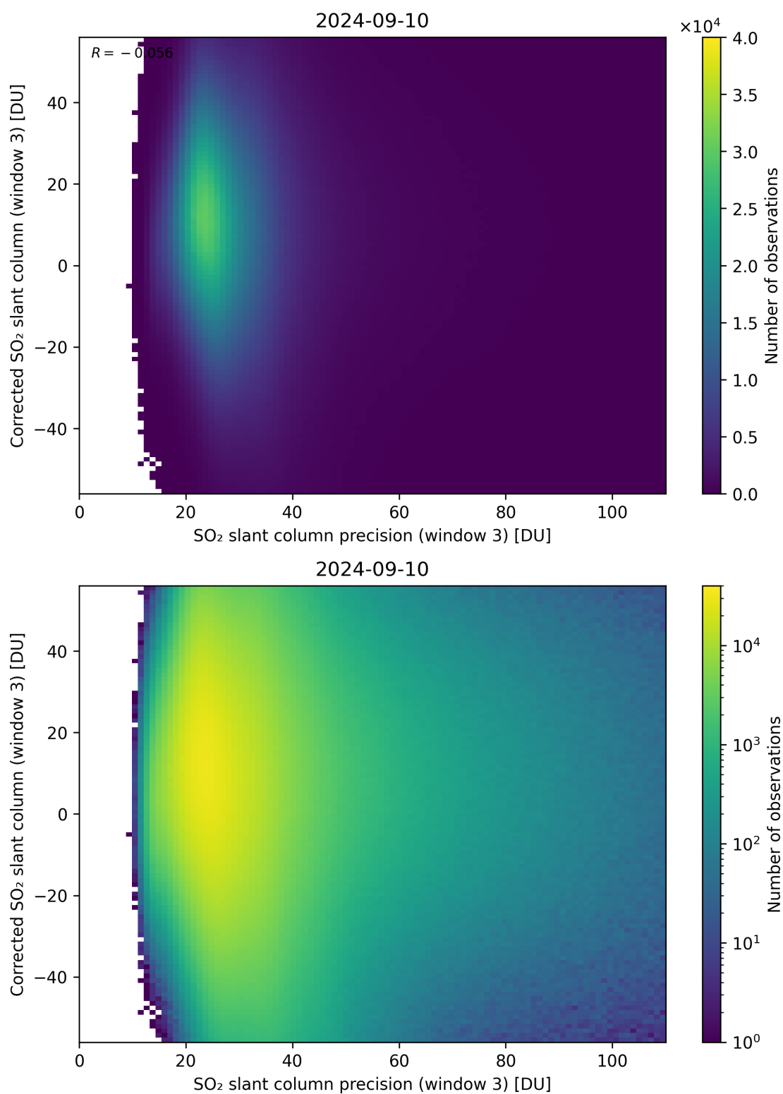
Figure 262: Scatter density plot of “SO 2 slant column precision (window 3)” against “Corrected SO 2 slant column (window 3)” for 2024-09-09 to 2024-09-11.
