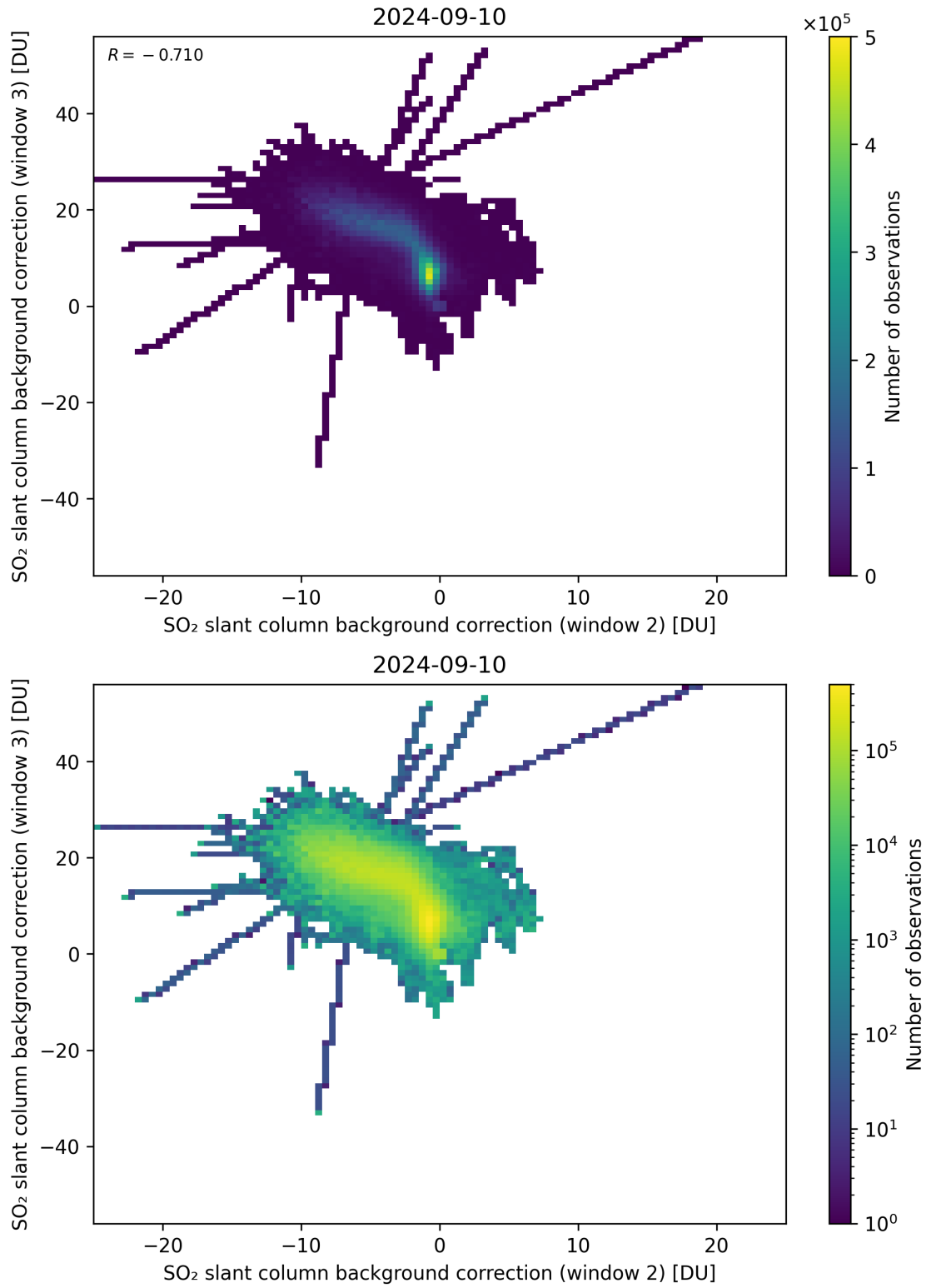
Figure 111: Scatter density plot of “SO 2 slant column background correction (window 2)” against “SO 2 slant column background correction (window 3)” for 2024-09-09 to 2024-09-11.
