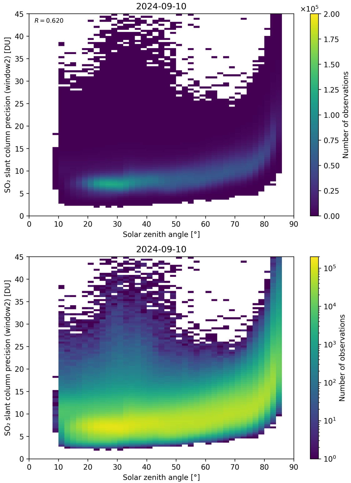
Figure 171: Scatter density plot of “Solar zenith angle” against “SO 2 slant column precision (window2)” for 2024-09-09 to 2024-09-11.
