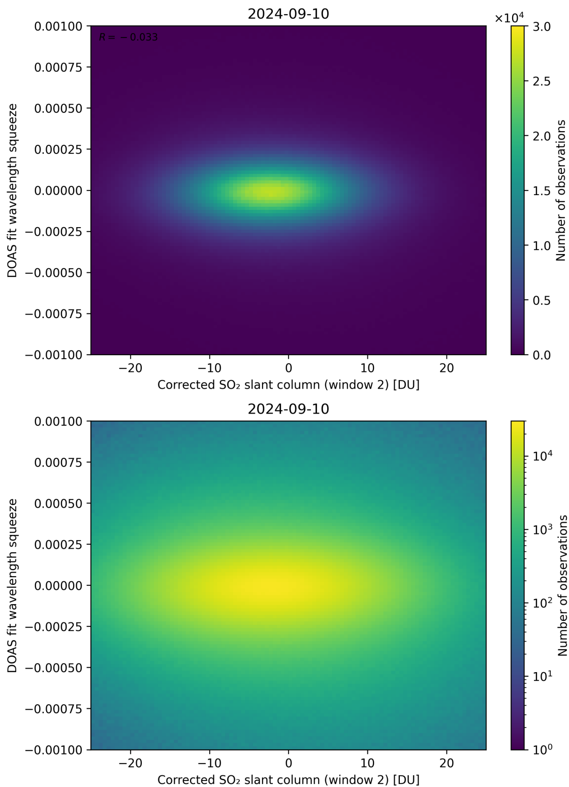
Figure 197: Scatter density plot of “Corrected SO 2 slant column (window 2)” against “DOAS fit wavelength squeeze” for 2024-09-09 to 2024-09-11.
