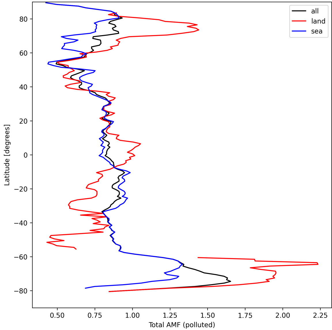
Figure 48: Zonal average of “Total AMF (polluted)” for 2024-09-09 to 2024-09-11.
