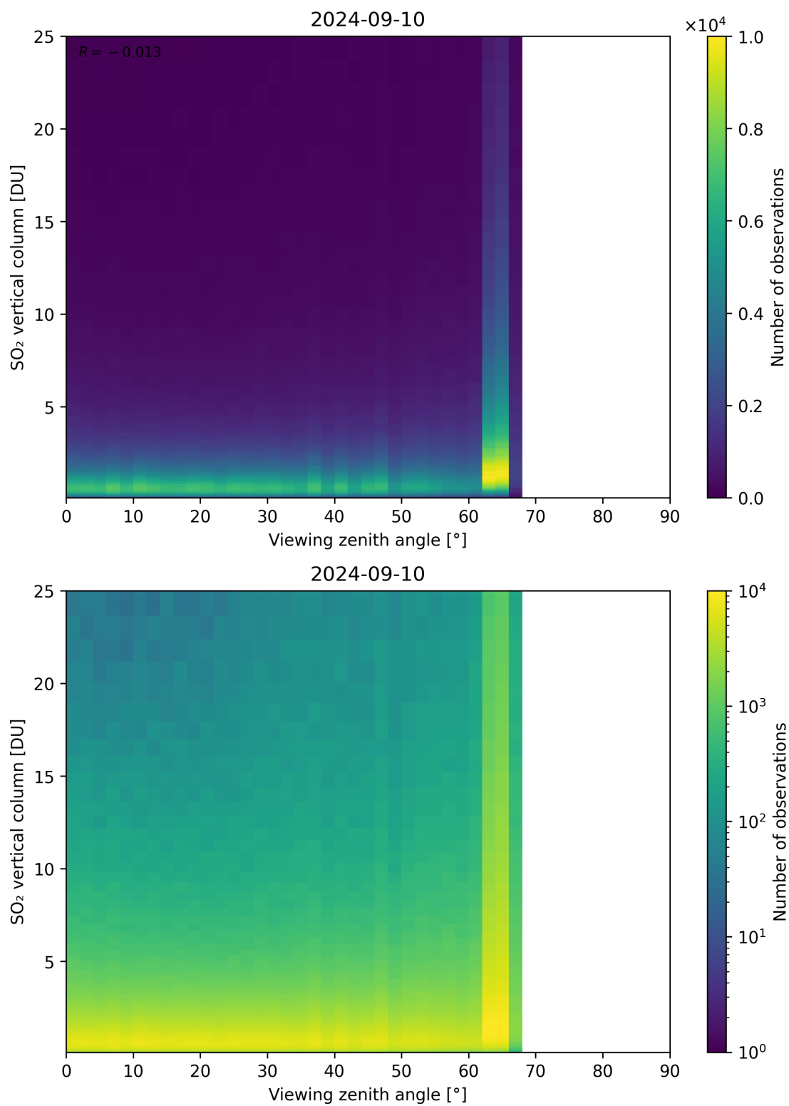
Figure 327: Scatter density plot of “Viewing zenith angle” against “SO 2 vertical column” for 2024-09-09 to 2024-09-11.
