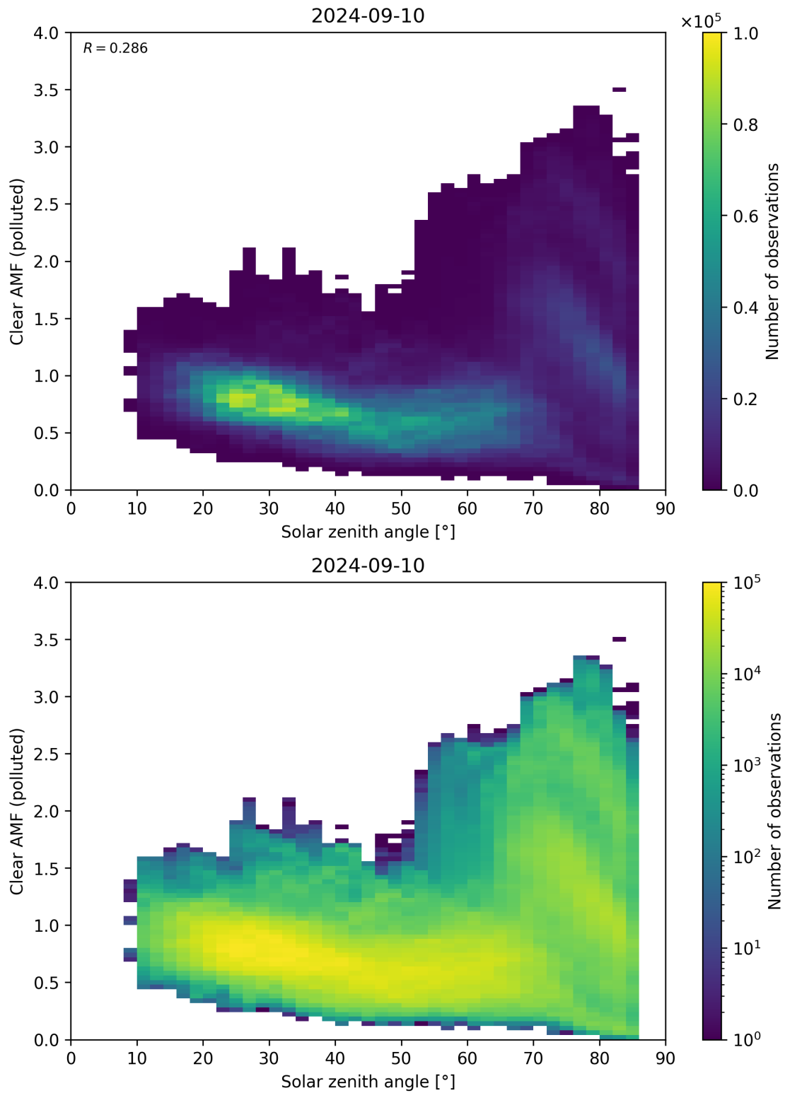
Figure 165: Scatter density plot of “Solar zenith angle” against “Clear AMF (polluted)” for 2024-09-09 to 2024-09-11.
