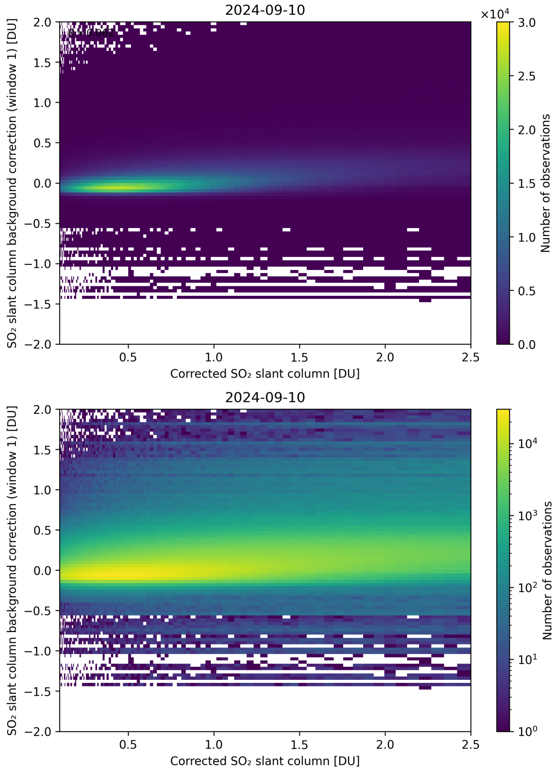
Figure 178: Scatter density plot of “Corrected SO 2 slant column” against “SO 2 slant column background correction (window 1)” for 2024-09-09 to 2024-09-11.
