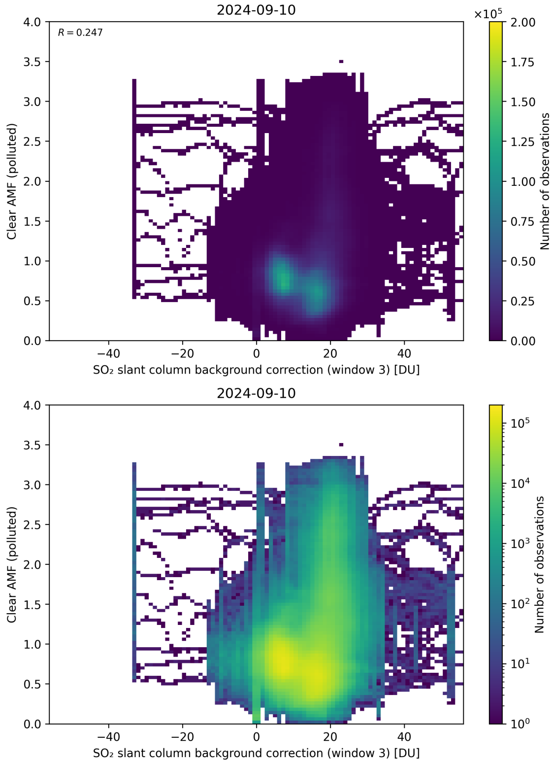
Figure 124: Scatter density plot of “SO 2 slant column background correction (window 3)” against “Clear AMF (polluted)” for 2024-09-09 to 2024-09-11.
