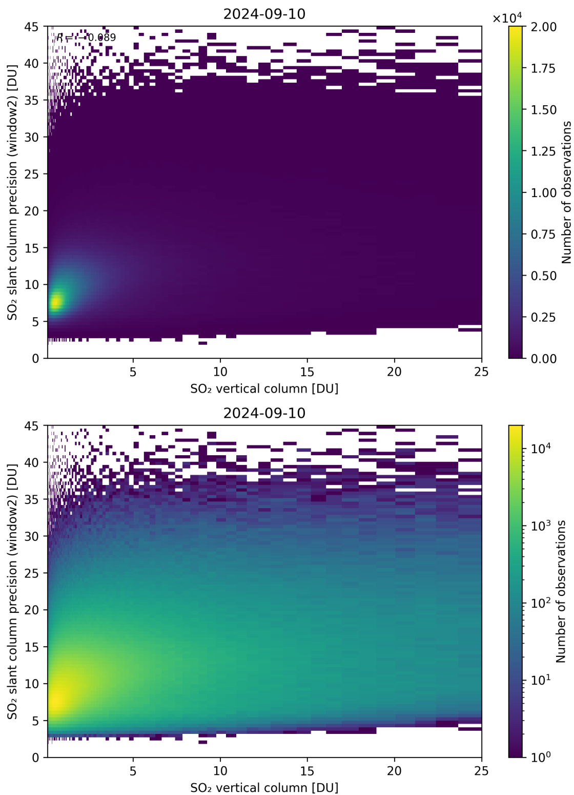
Figure 302: Scatter density plot of “SO 2 vertical column” against “SO 2 slant column precision (window2)” for 2024-09-09 to 2024-09-11.
