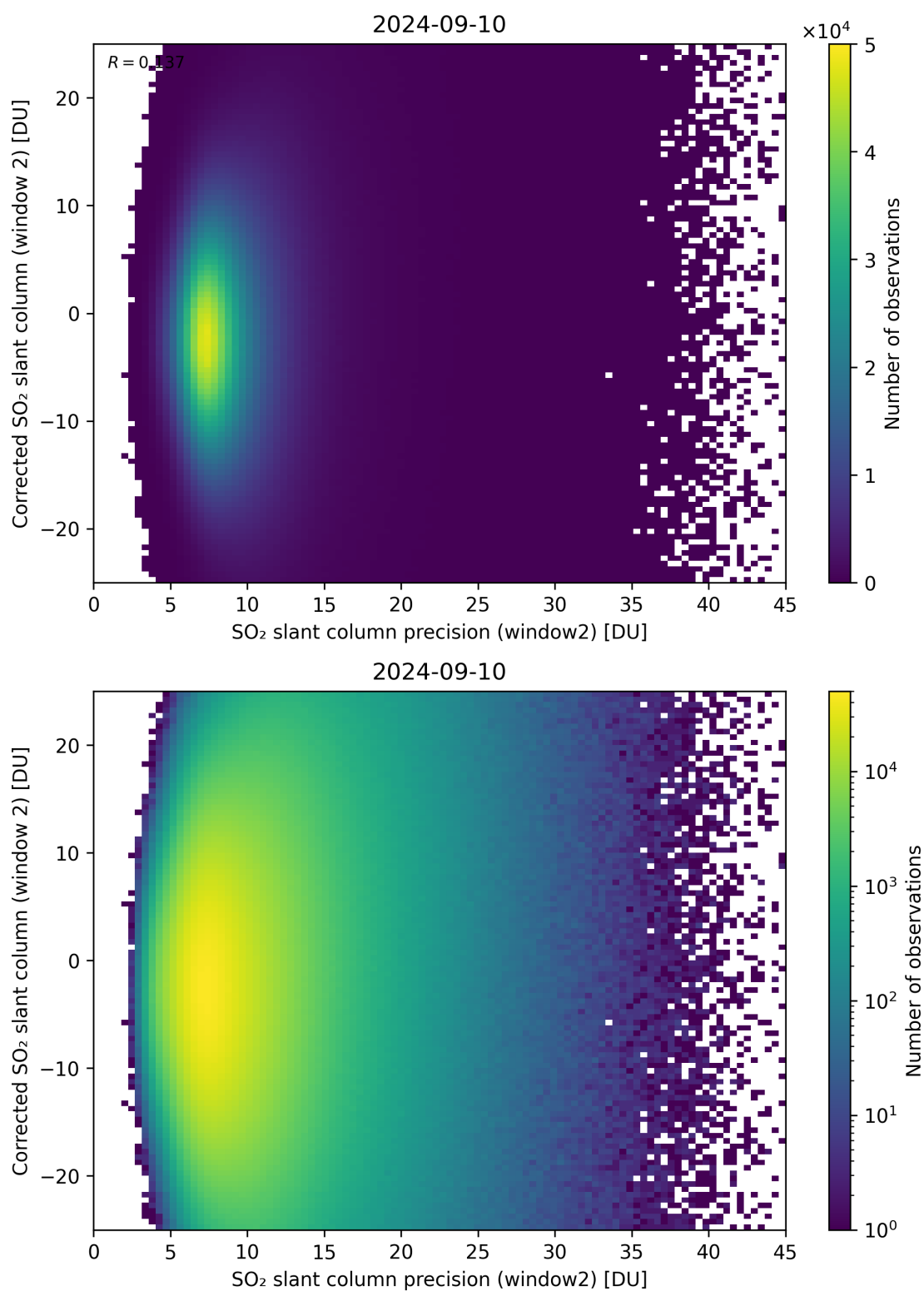
Figure 247: Scatter density plot of “SO 2 slant column precision (window2)” against “Corrected SO 2 slant column (window 2)” for 2024-09-09 to 2024-09-11.
