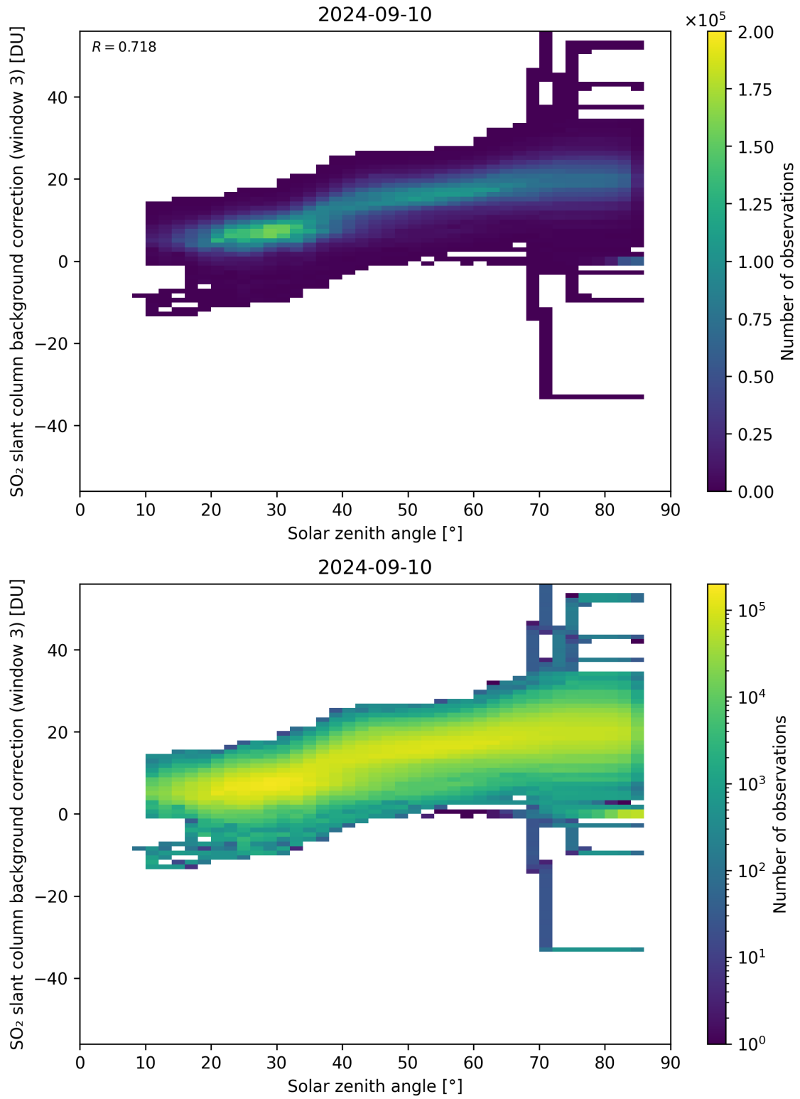
Figure 160: Scatter density plot of “Solar zenith angle” against “SO 2 slant column background correction (window 3)” for 2024-09-09 to 2024-09-11.
