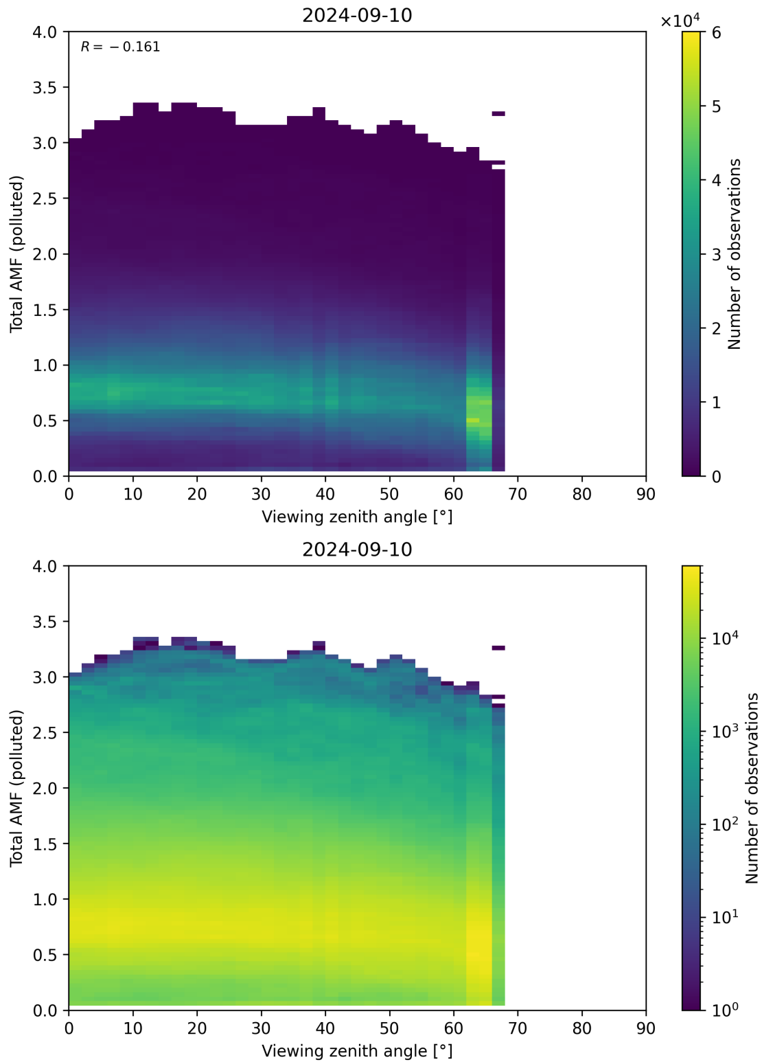
Figure 325: Scatter density plot of “Viewing zenith angle” against “Total AMF (polluted)” for 2024-09-09 to 2024-09-11.
