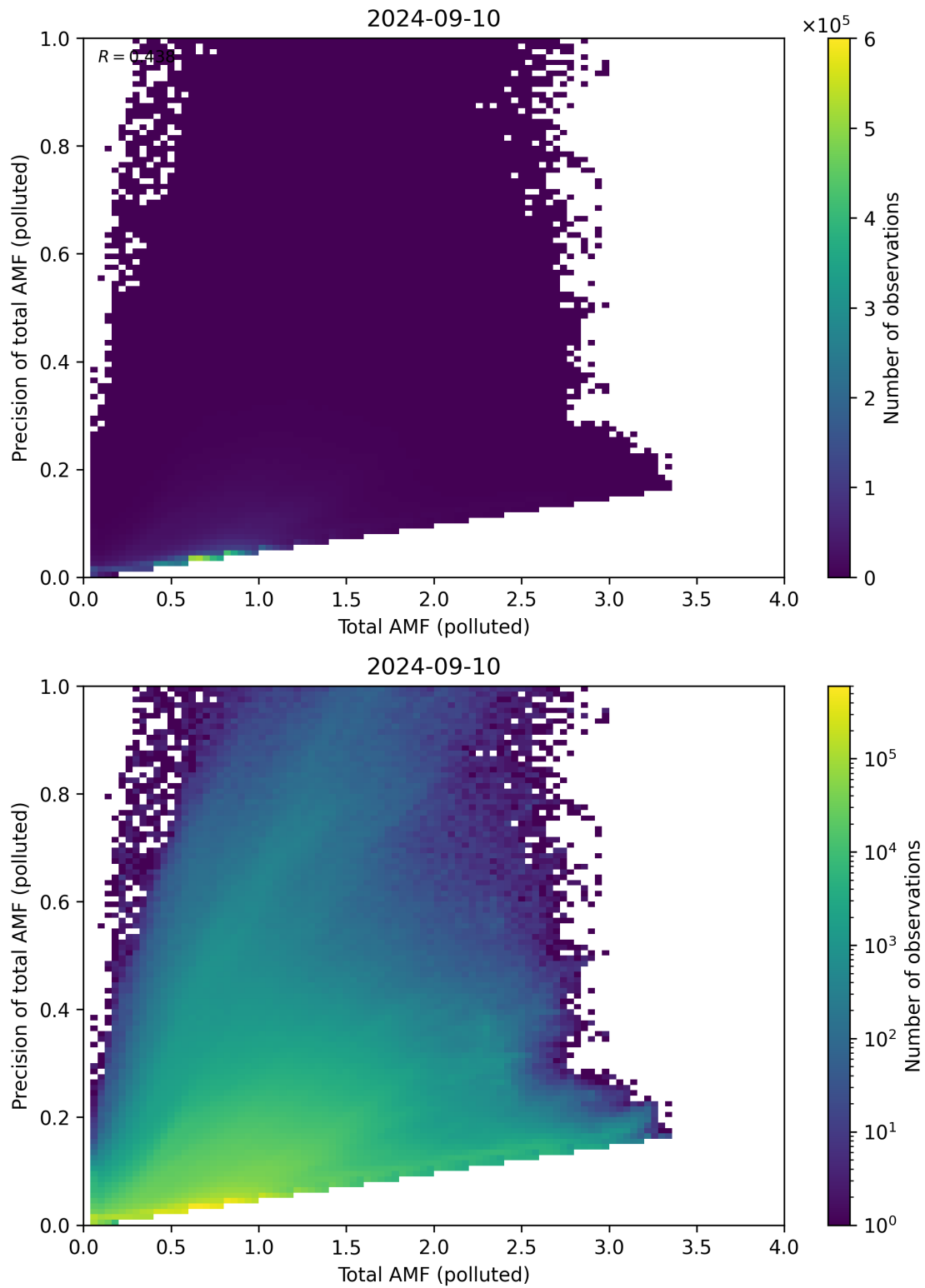
Figure 272: Scatter density plot of “Total AMF (polluted)” against “Precision of total AMF (polluted)” for 2024-09-09 to 2024-09-11.
