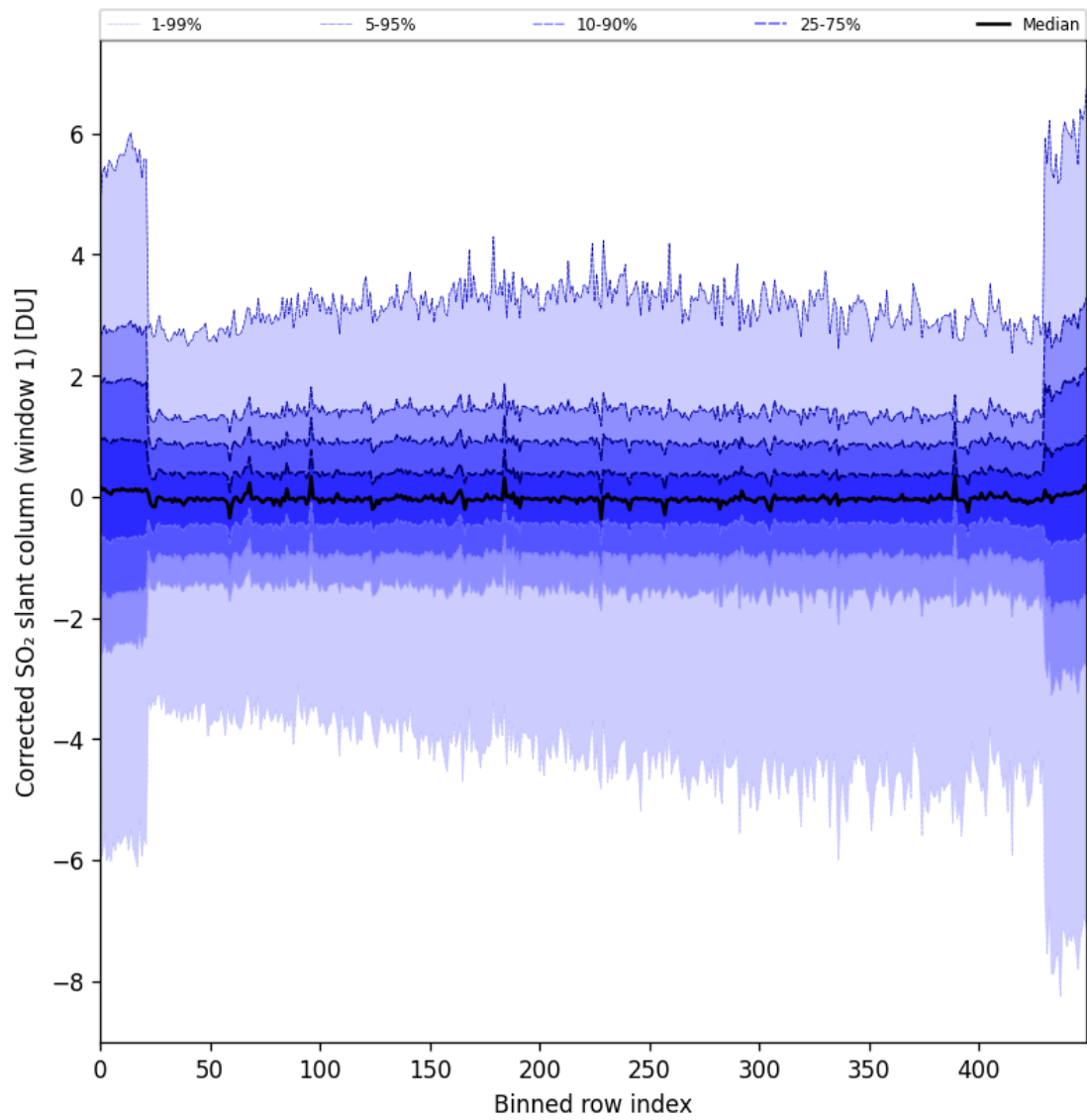
Figure 81: Along track statistics of “Corrected SO 2 slant column (window 1)” for 2024-09-09 to 2024-09-11
