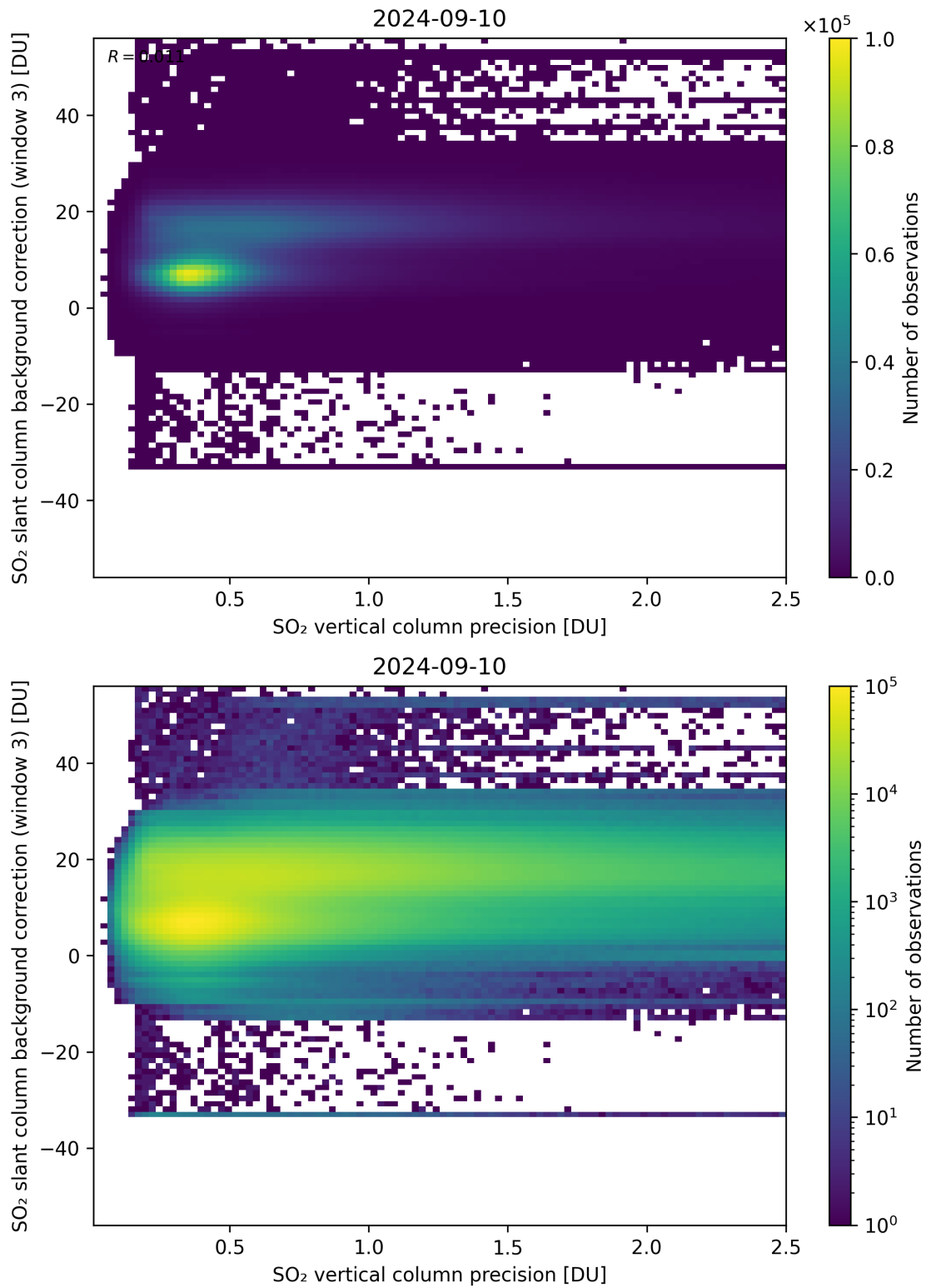
Figure 281: Scatter density plot of “SO 2 vertical column precision” against “SO 2 slant column background correction (window 3)” for 2024-09-09 to 2024-09-11.
