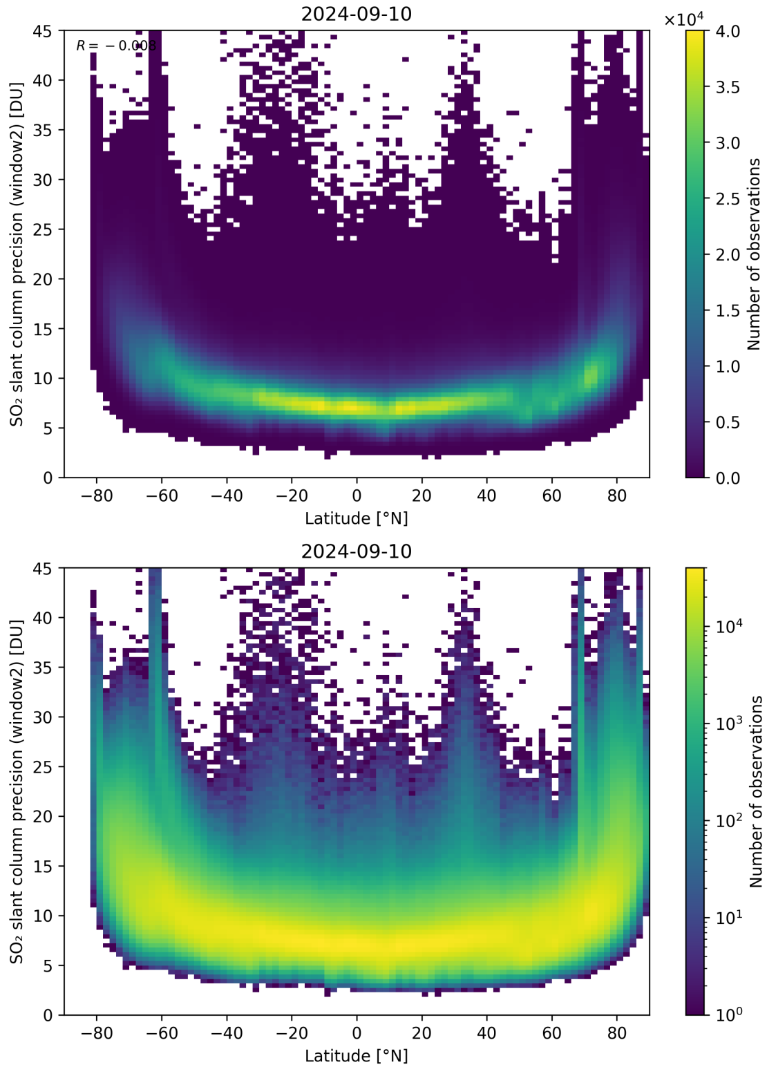
Figure 151: Scatter density plot of “Latitude” against “SO 2 slant column precision (window2)” for 2024-09-09 to 2024-09-11.
