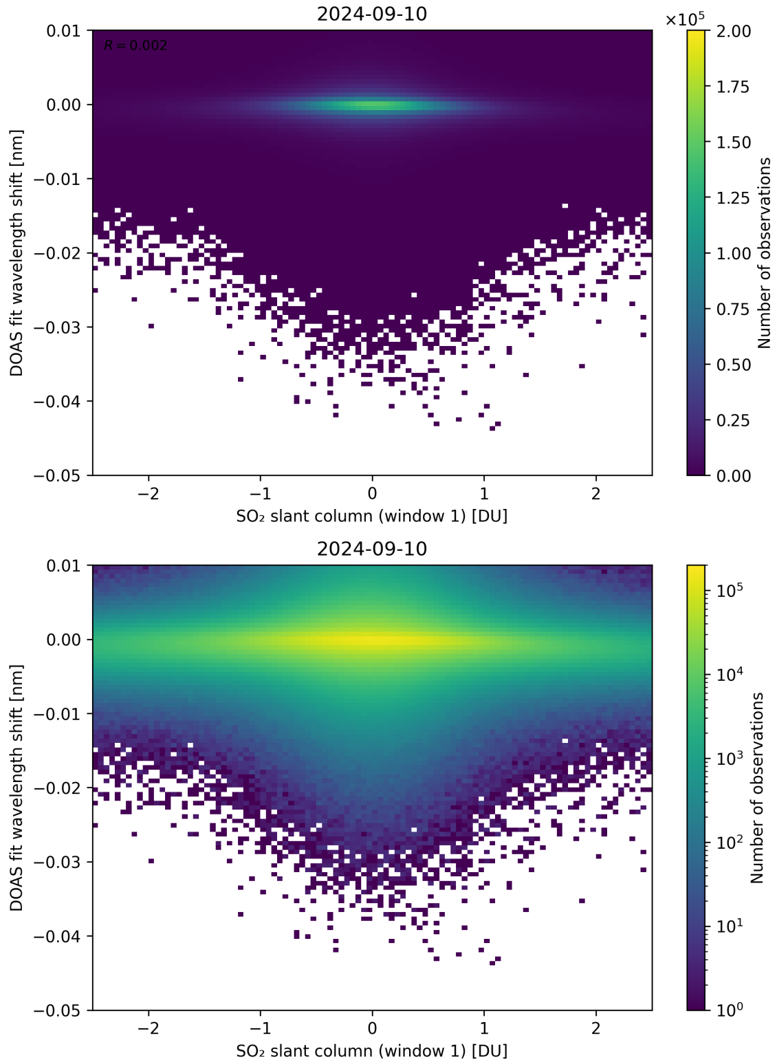
Figure 215: Scatter density plot of “SO 2 slant column (window 1)” against “DOAS fit wavelength shift” for 2024-09-09 to 2024-09-11.
