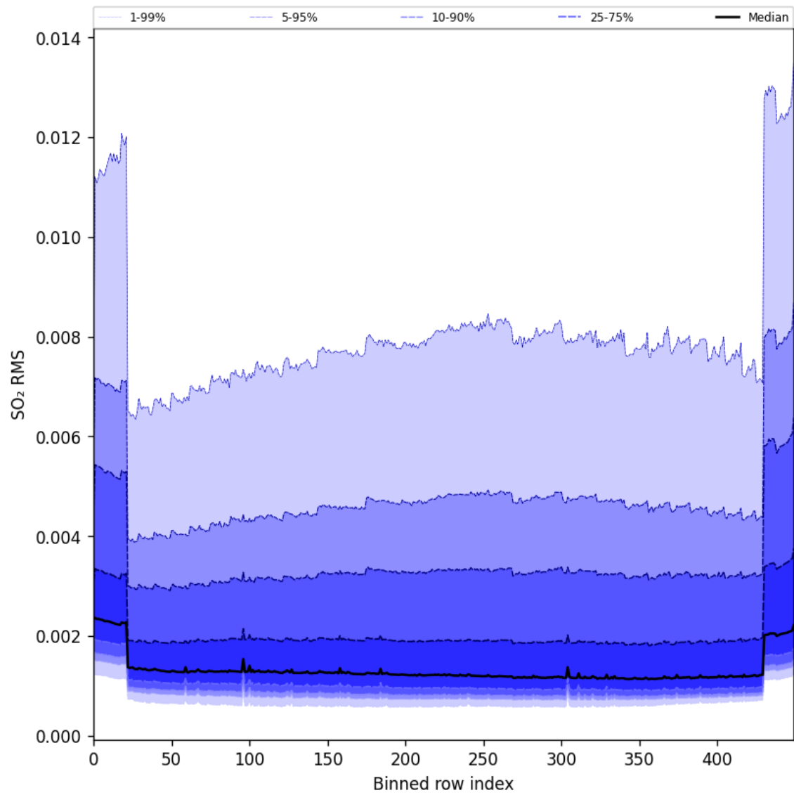
Figure 93: Along track statistics of “SO 2 RMS” for 2024-09-09 to 2024-09-11
