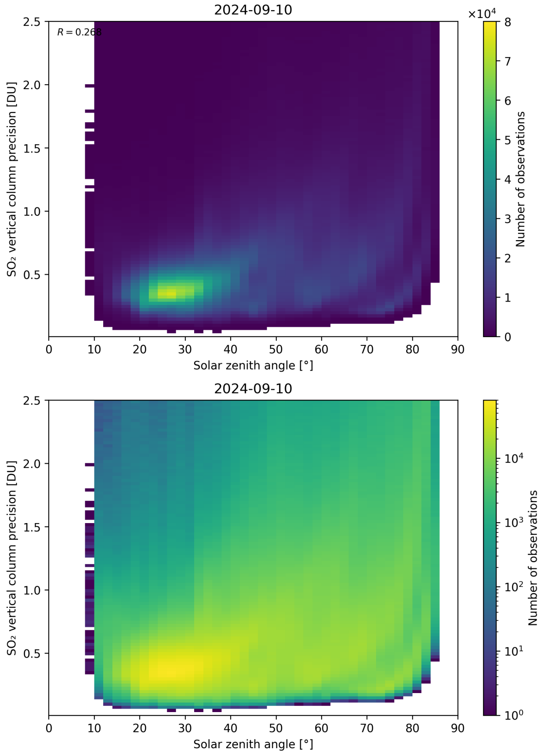
Figure 177: Scatter density plot of “Solar zenith angle” against “SO 2 vertical column precision” for 2024-09-09 to 2024-09-11.
