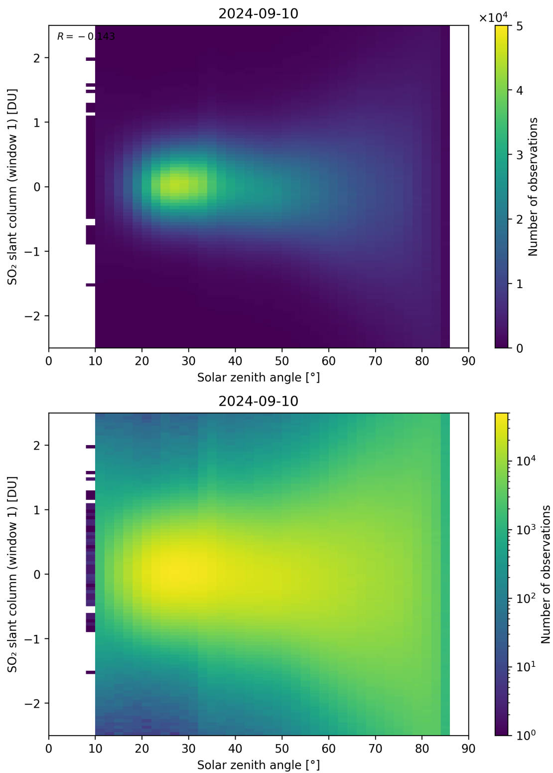
Figure 169: Scatter density plot of “Solar zenith angle” against “SO 2 slant column (window 1)” for 2024-09-09 to 2024-09-11.
