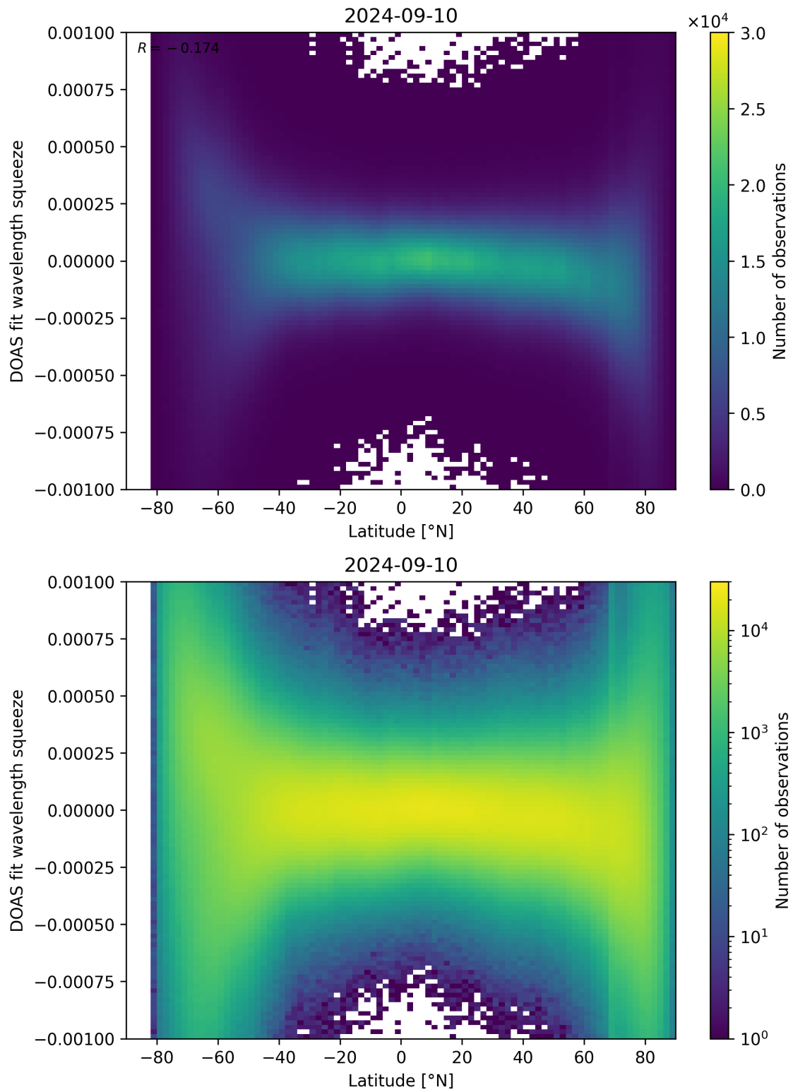
Figure 143: Scatter density plot of “Latitude” against “DOAS fit wavelength squeeze” for 2024-09-09 to 2024-09-11.
