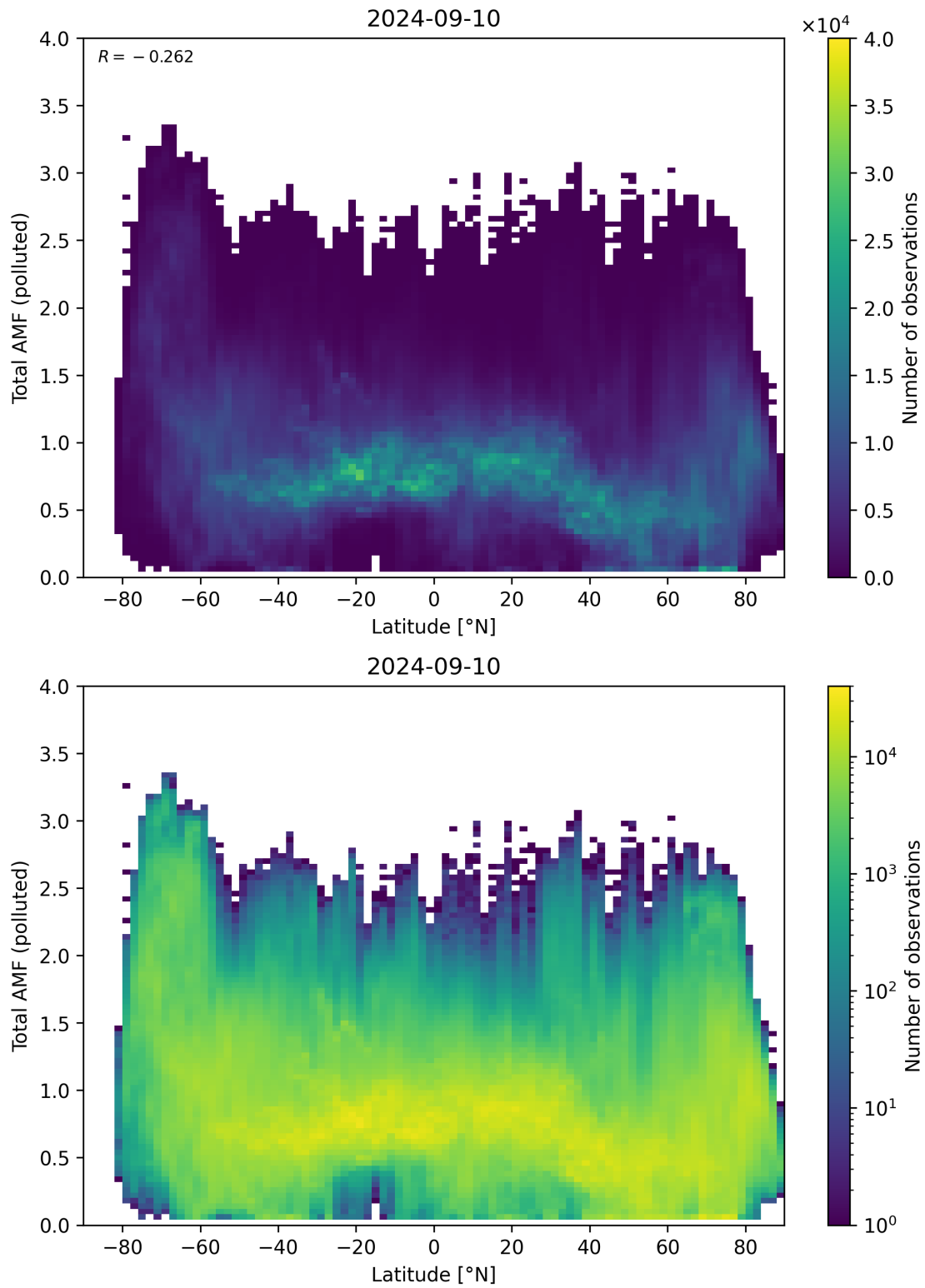
Figure 154: Scatter density plot of “Latitude” against “Total AMF (polluted)” for 2024-09-09 to 2024-09-11.
