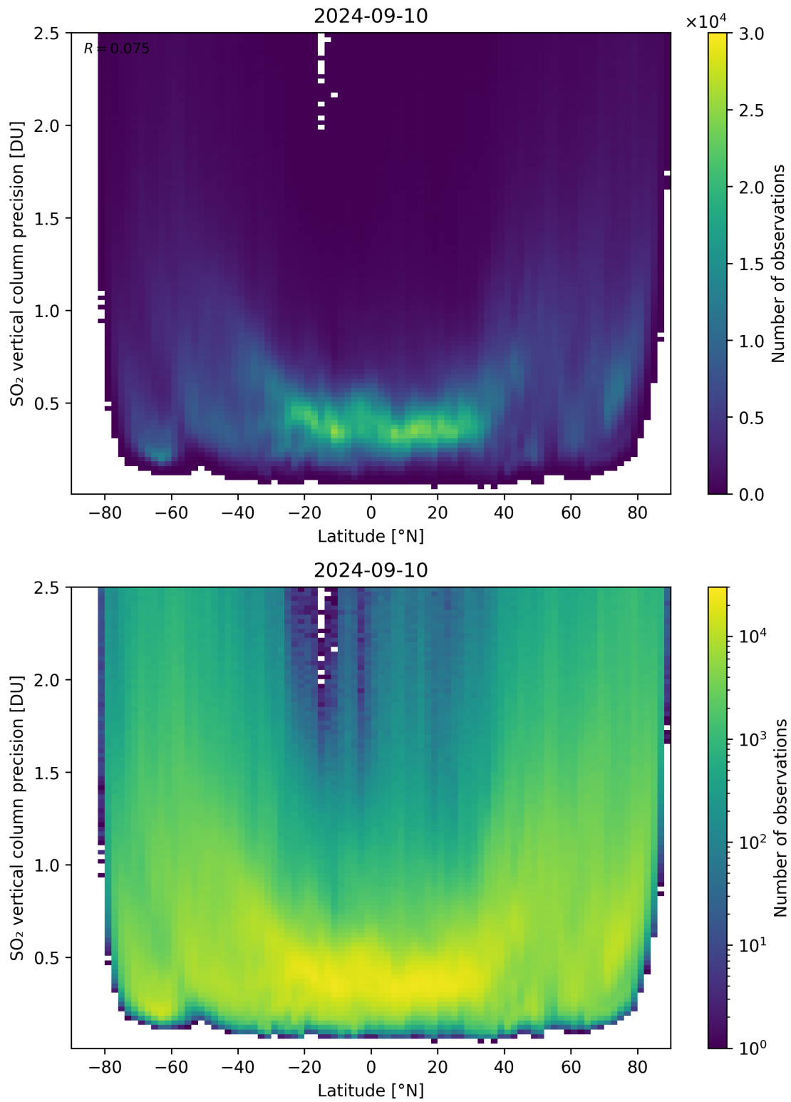
Figure 157: Scatter density plot of “Latitude” against “SO 2 vertical column precision” for 2024-09-09 to 2024-09-11.
