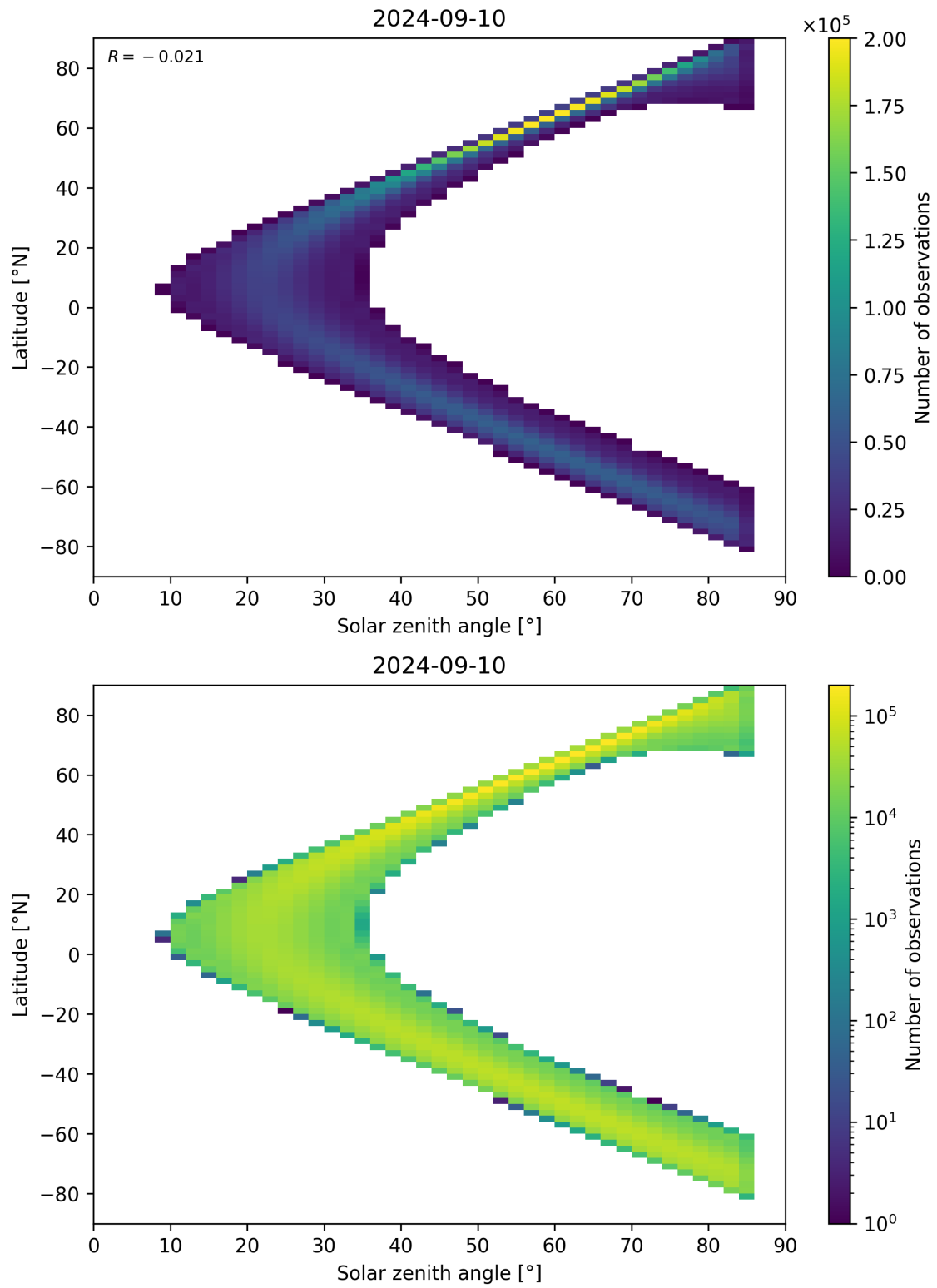
Figure 164: Scatter density plot of “Solar zenith angle” against “Latitude” for 2024-09-09 to 2024-09-11.
