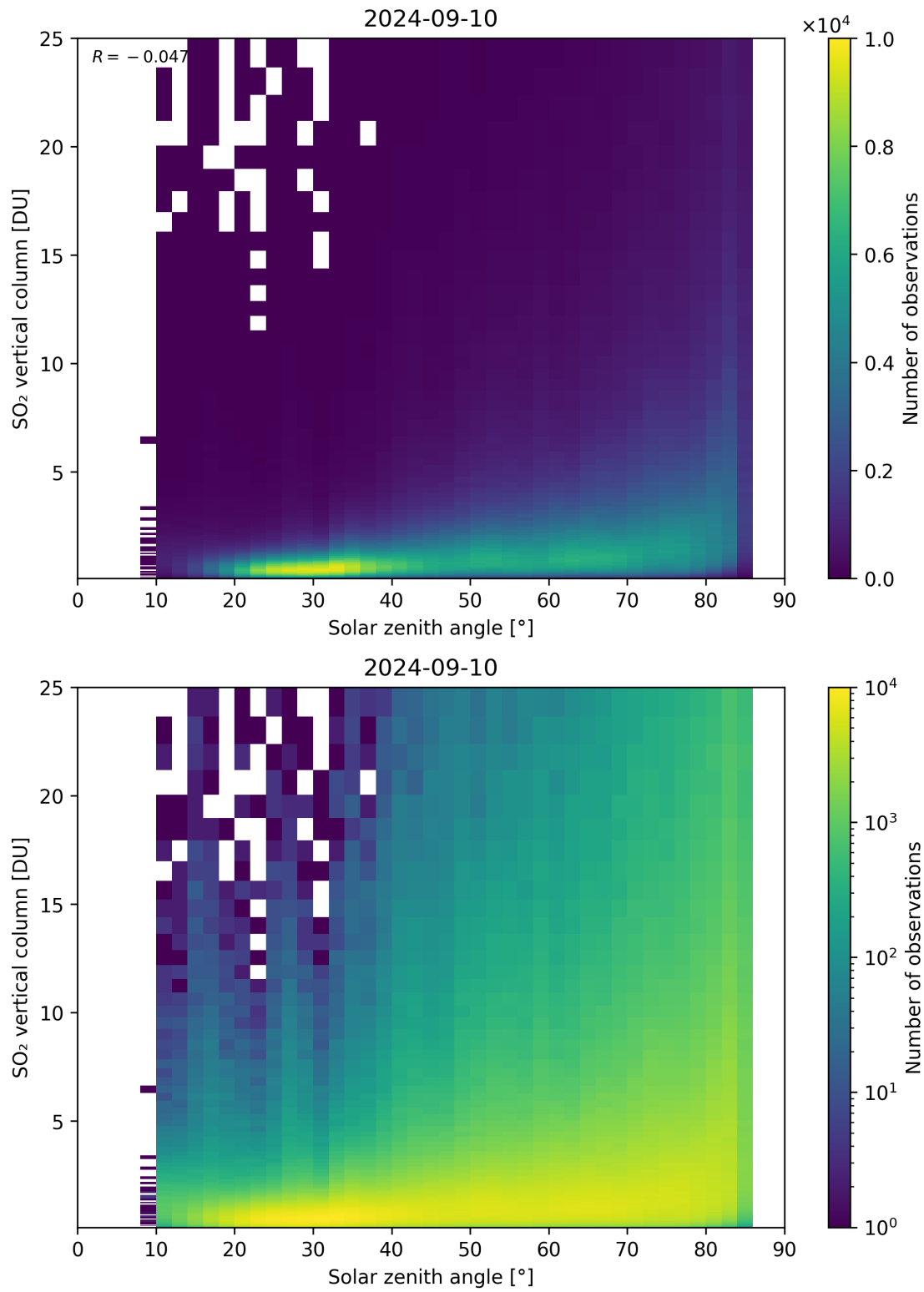
Figure 176: Scatter density plot of “Solar zenith angle” against “SO 2 vertical column” for 2024-09-09 to 2024-09-11.
