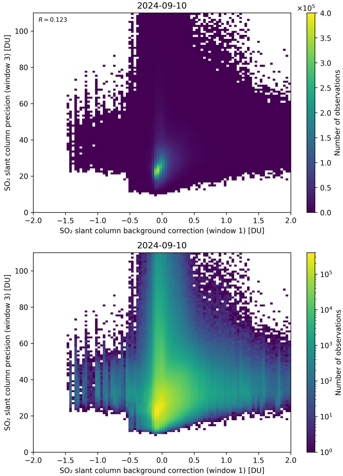
Figure 108: Scatter density plot of “SO 2 slant column background correction (window 1)” against “SO 2 slant column precision (window 3)” for 2024-09-09 to 2024-09-11.
