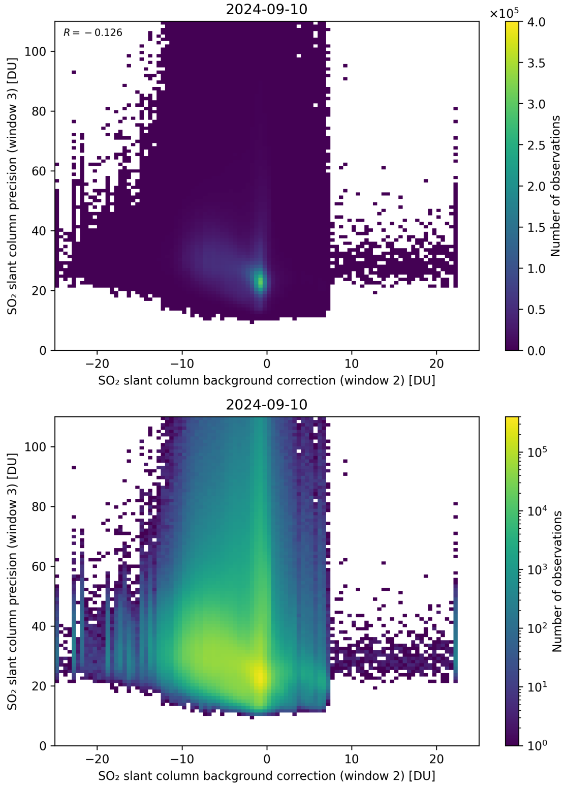
Figure 118: Scatter density plot of “SO 2 slant column background correction (window 2)” against “SO 2 slant column precision (window 3)” for 2024-09-09 to 2024-09-11.
