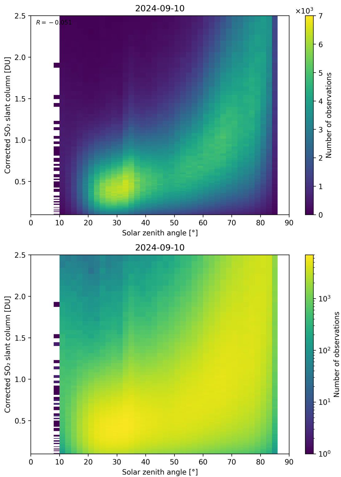
Figure 166: Scatter density plot of “Solar zenith angle” against “Corrected SO 2 slant column” for 2024-09-09 to 2024-09-11.
