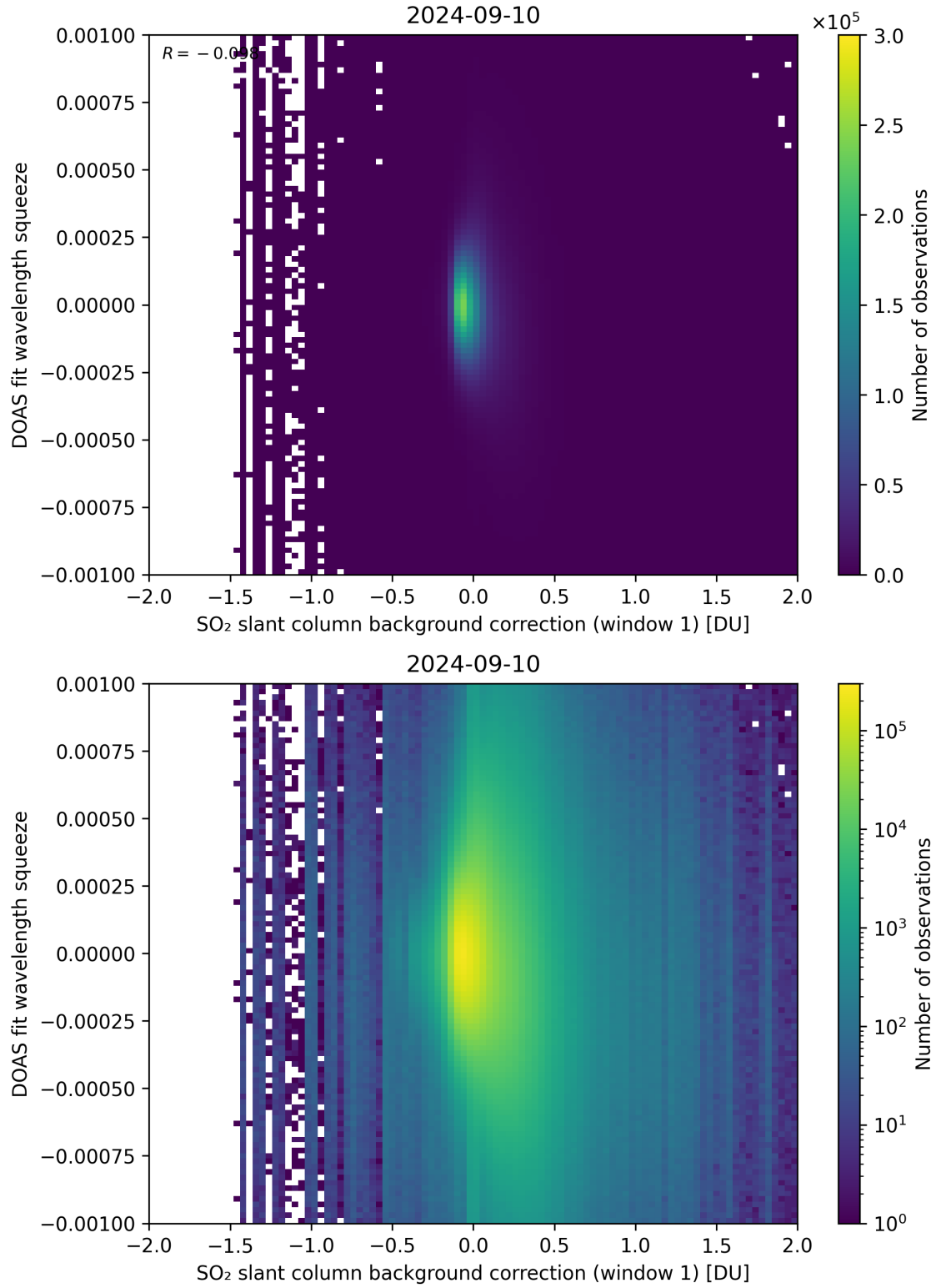
Figure 101: Scatter density plot of “SO 2 slant column background correction (window 1)” against “DOAS fit wavelength squeeze” for 2024-09-09 to 2024-09-11.
