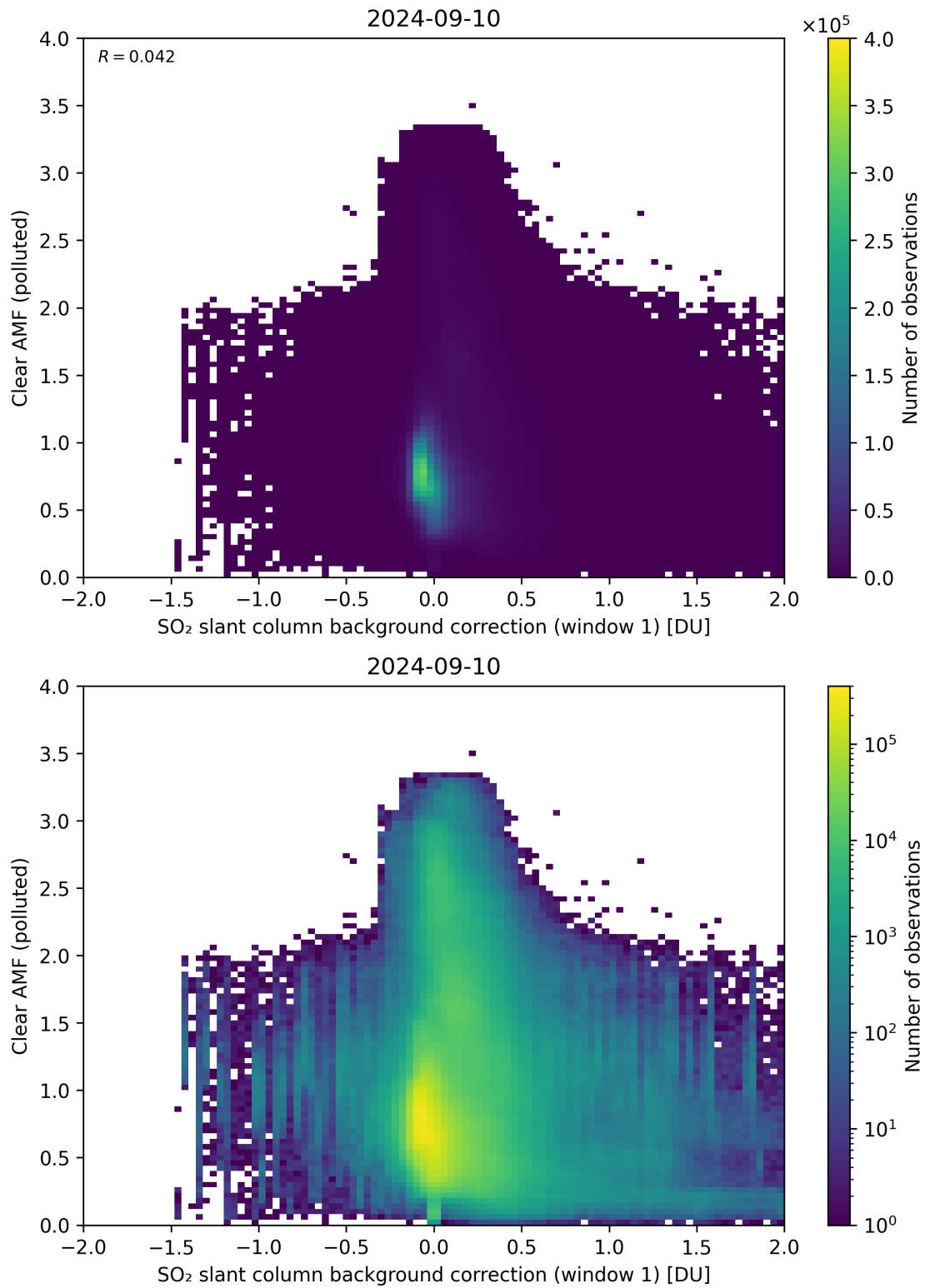
Figure 103: Scatter density plot of “SO 2 slant column background correction (window 1)” against “Clear AMF (polluted)” for 2024-09-09 to 2024-09-11.
