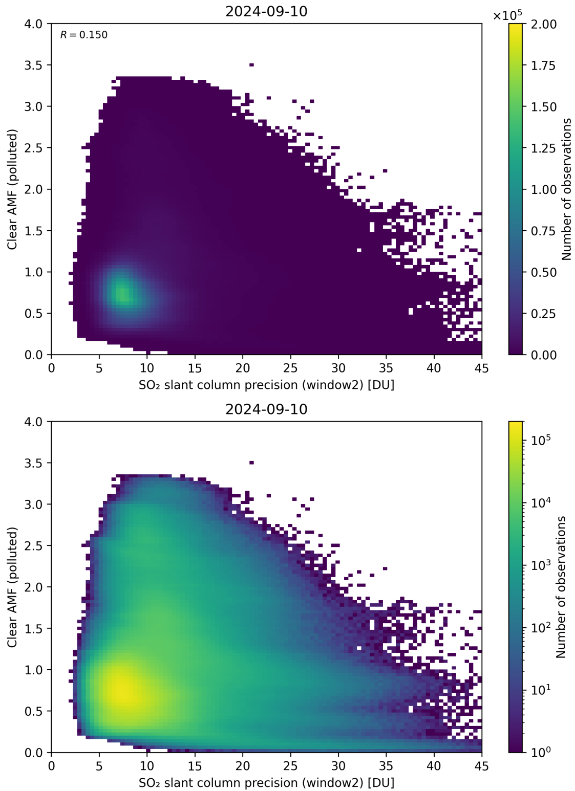
Figure 246: Scatter density plot of “SO 2 slant column precision (window2)” against “Clear AMF (polluted)” for 2024-09-09 to 2024-09-11.
