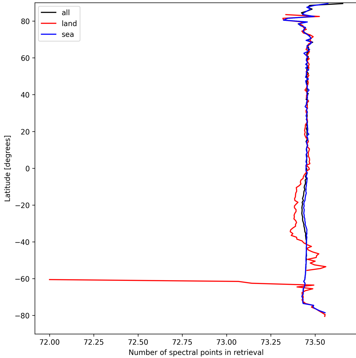
Figure 51: Zonal average of “Number of spectral points in retrieval” for 2024-09-09 to 2024-09-11.
