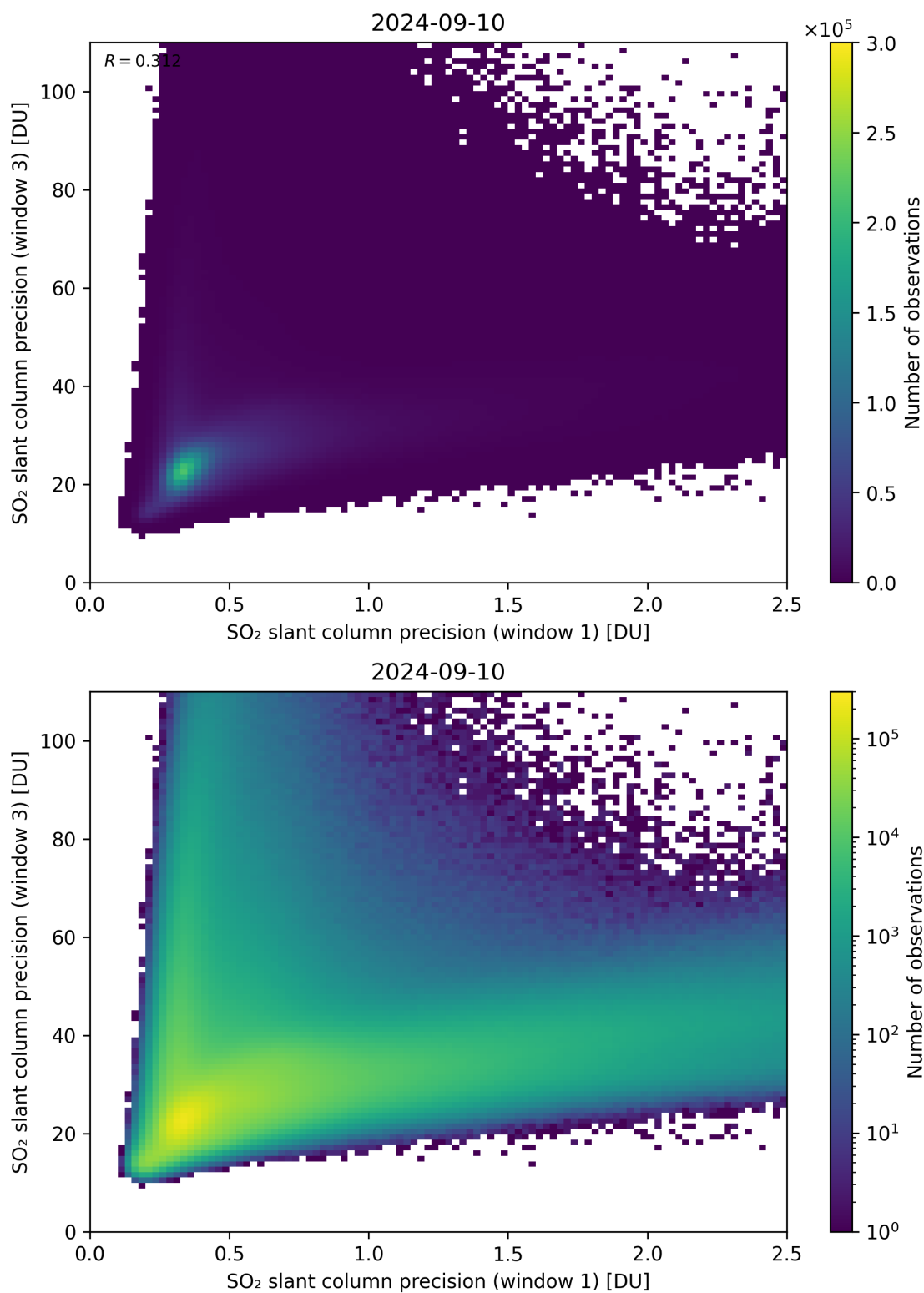
Figure 229: Scatter density plot of “SO 2 slant column precision (window 1)” against “SO 2 slant column precision (window 3)” for 2024-09-09 to 2024-09-11.
