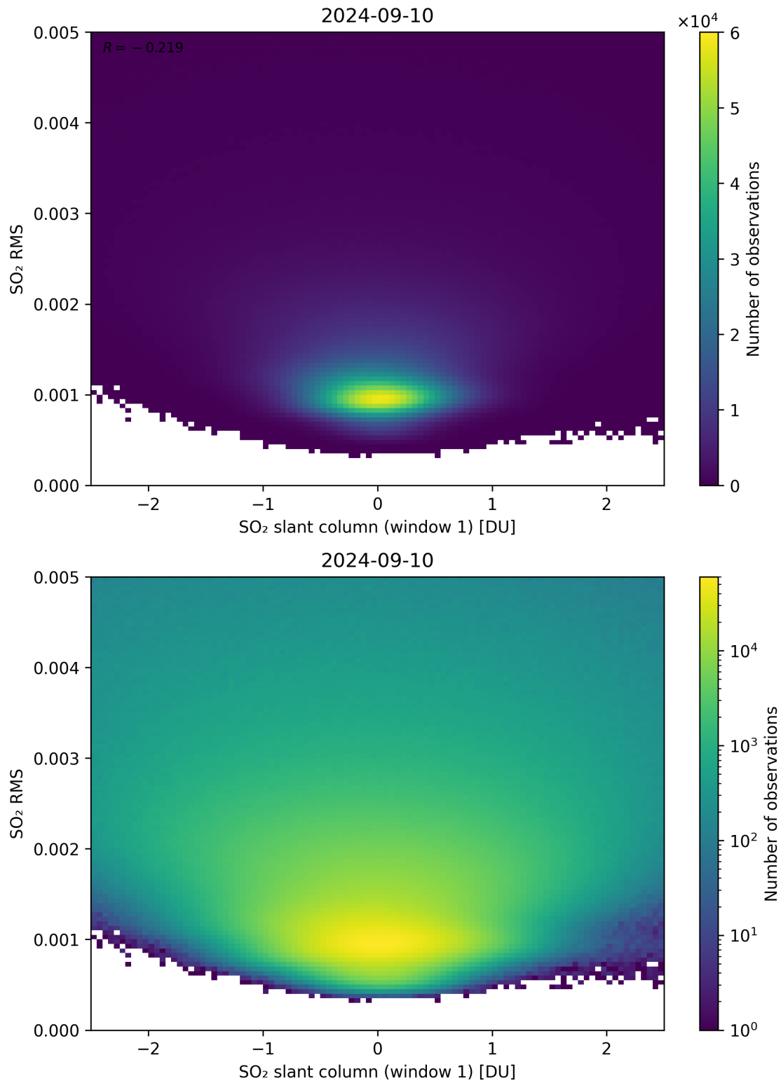
Figure 217: Scatter density plot of “SO 2 slant column (window 1)” against “SO 2 RMS” for 2024-09-09 to 2024-09-11.
