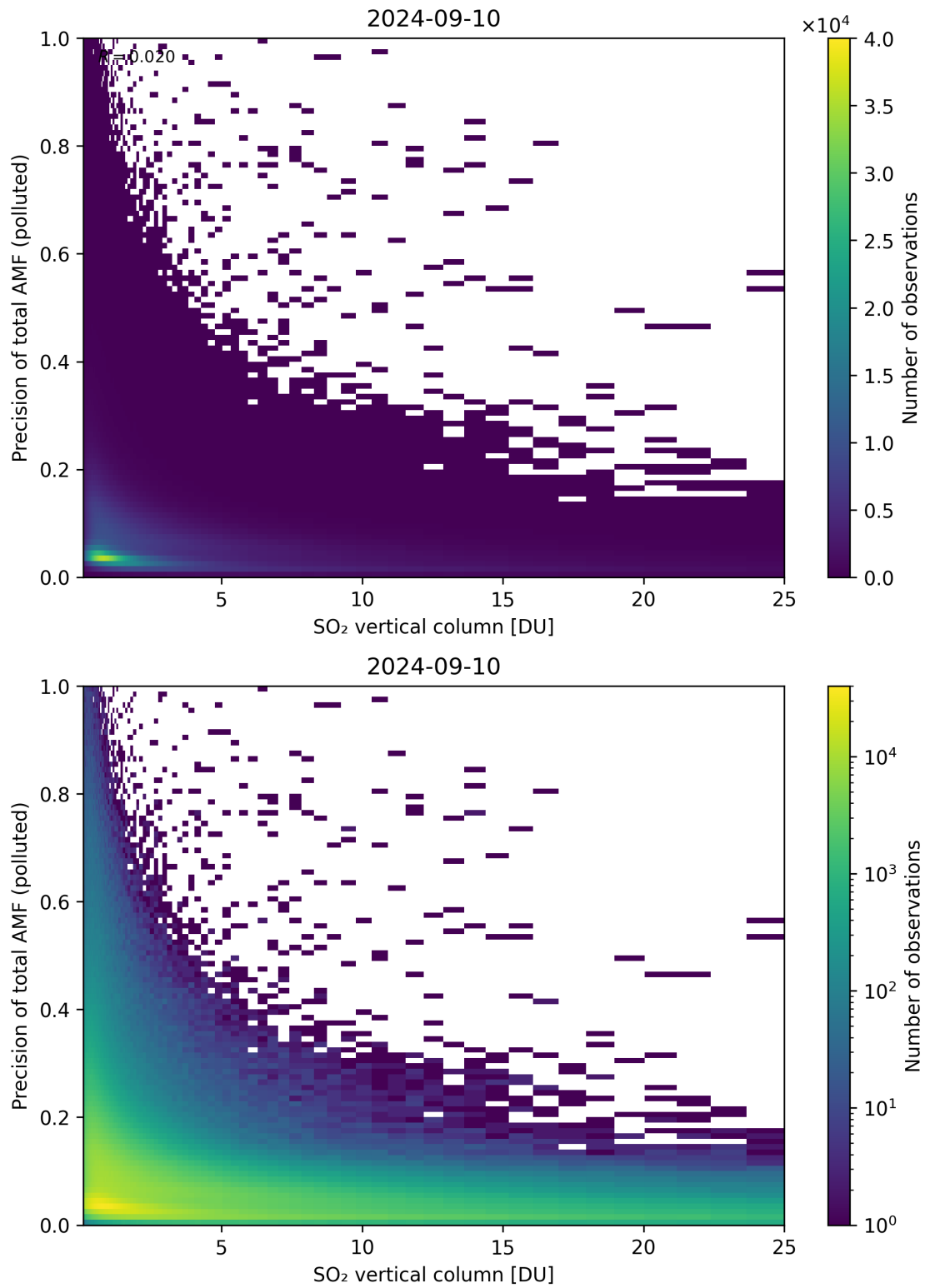
Figure 306: Scatter density plot of “SO 2 vertical column” against “Precision of total AMF (polluted)” for 2024-09-09 to 2024-09-11.
