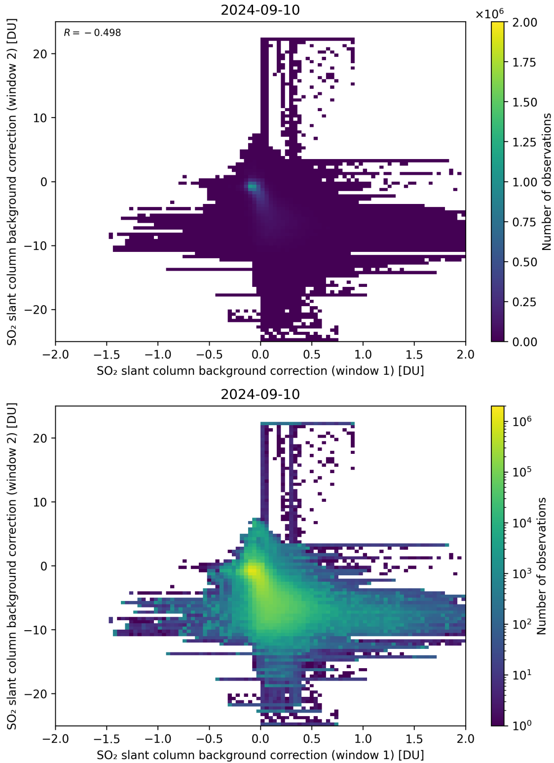
Figure 98: Scatter density plot of “SO 2 slant column background correction (window 1)” against “SO 2 slant column background correction (window 2)” for 2024-09-09 to 2024-09-11.
