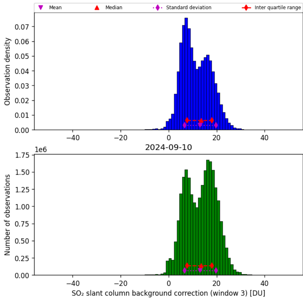
Figure 67: Histogram of “SO 2 slant column background correction (window 3)” for 2024-09-09 to 2024-09-11
