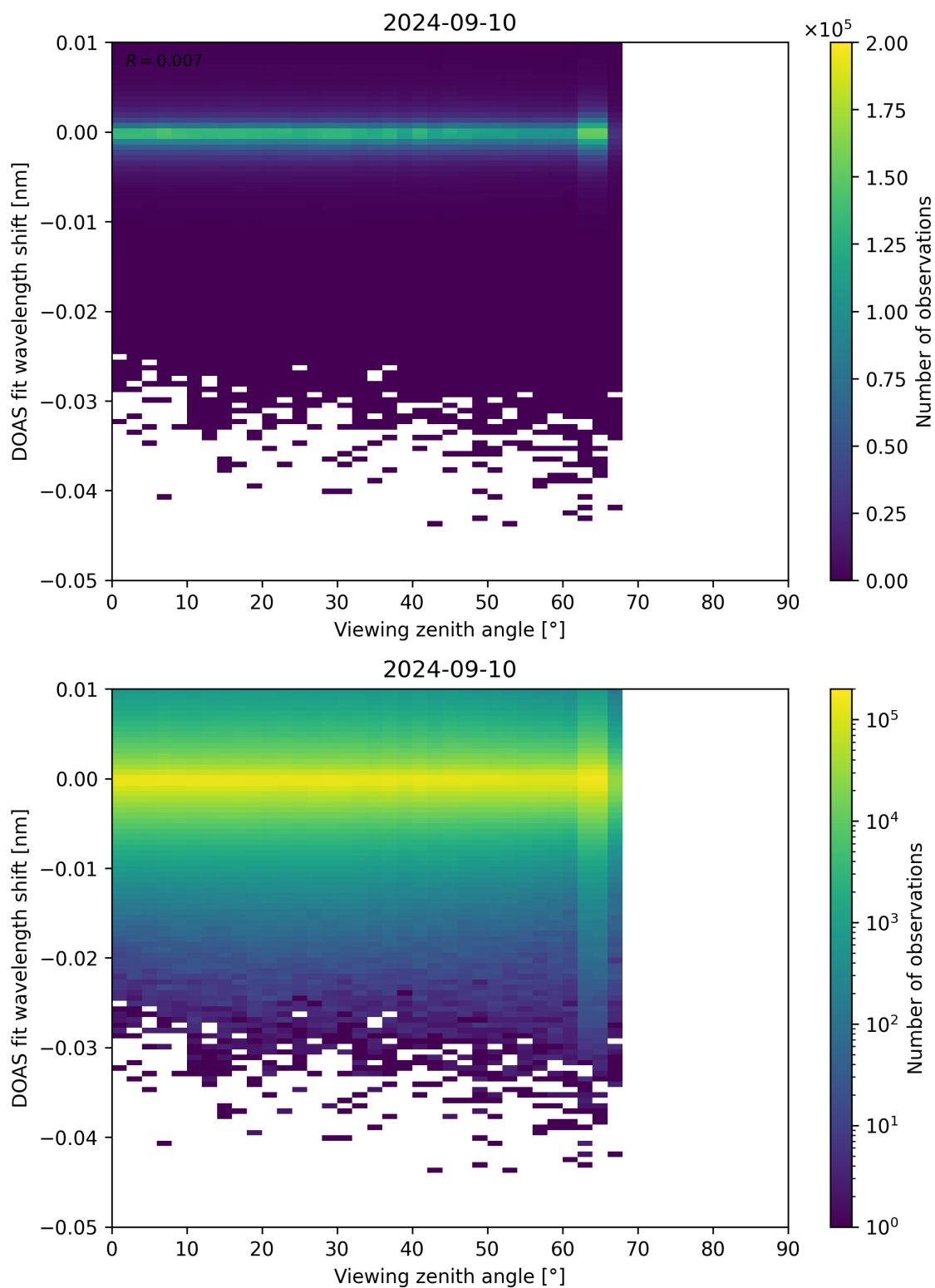
Figure 311: Scatter density plot of “Viewing zenith angle” against “DOAS fit wavelength shift” for 2024-09-09 to 2024-09-11.
