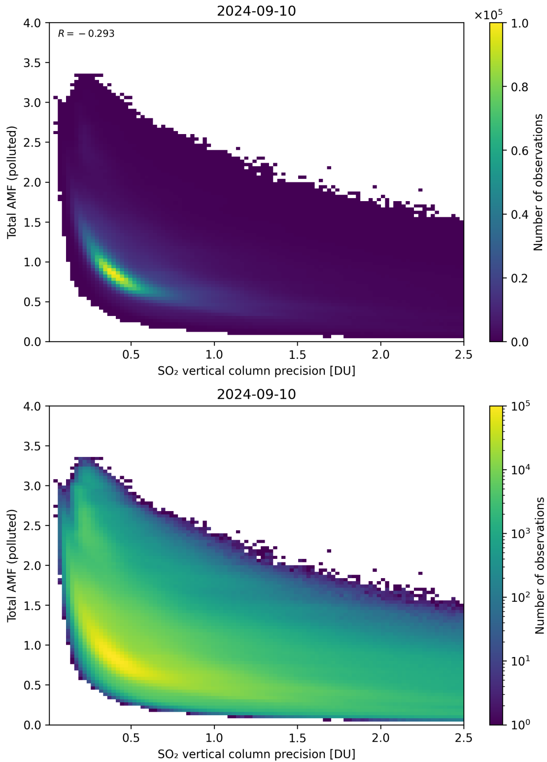
Figure 294: Scatter density plot of “SO 2 vertical column precision” against “Total AMF (polluted)” for 2024-09-09 to 2024-09-11.
