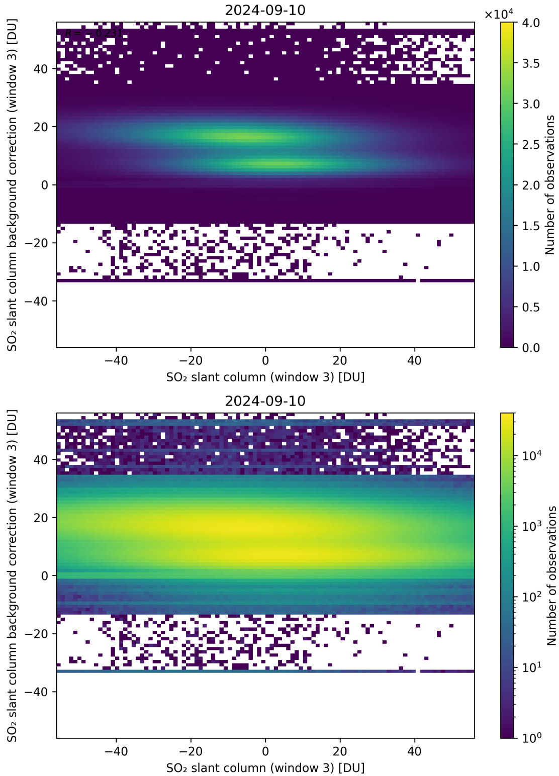
Figure 253: Scatter density plot of “SO 2 slant column (window 3)” against “SO 2 slant column background correction (window 3)” for 2024-09-09 to 2024-09-11.
