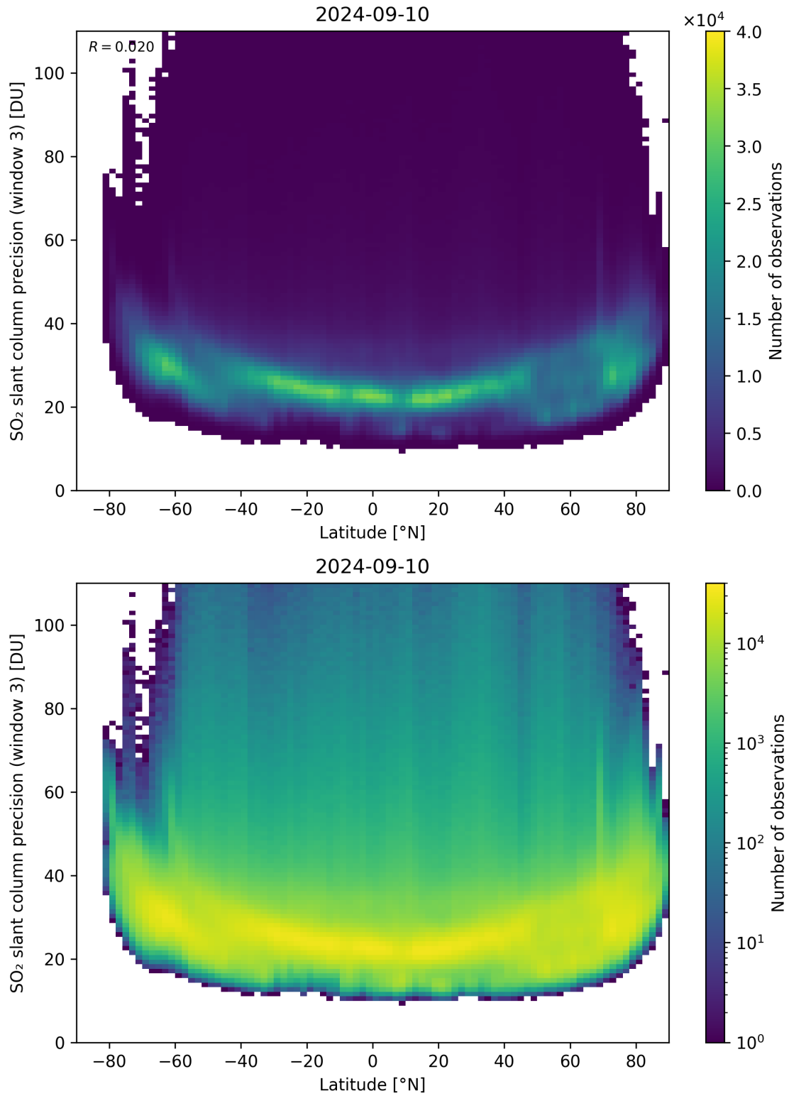
Figure 153: Scatter density plot of “Latitude” against “SO 2 slant column precision (window 3)” for 2024-09-09 to 2024-09-11.
