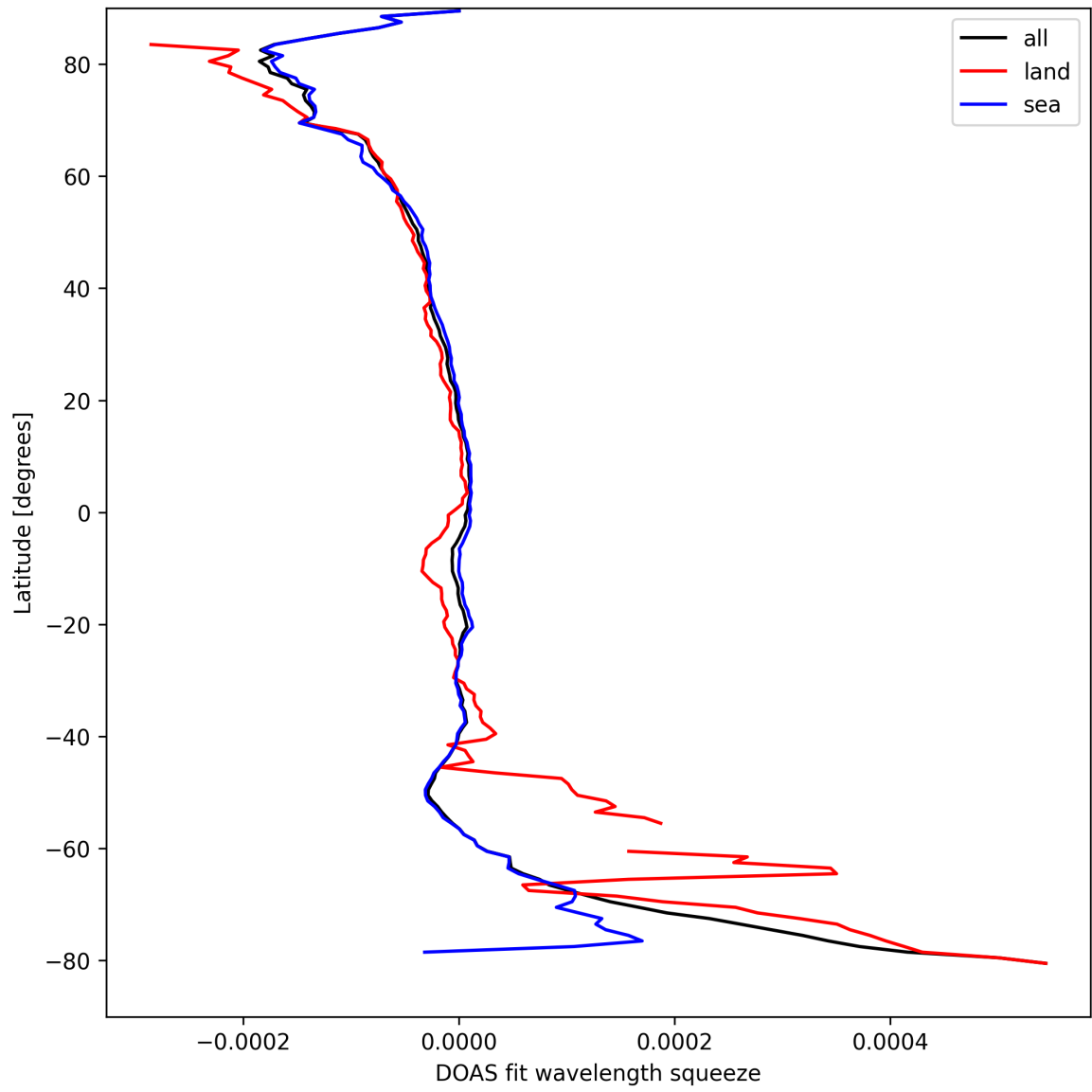
Figure 46: Zonal average of “DOAS fit wavelength squeeze” for 2024-09-09 to 2024-09-11.
