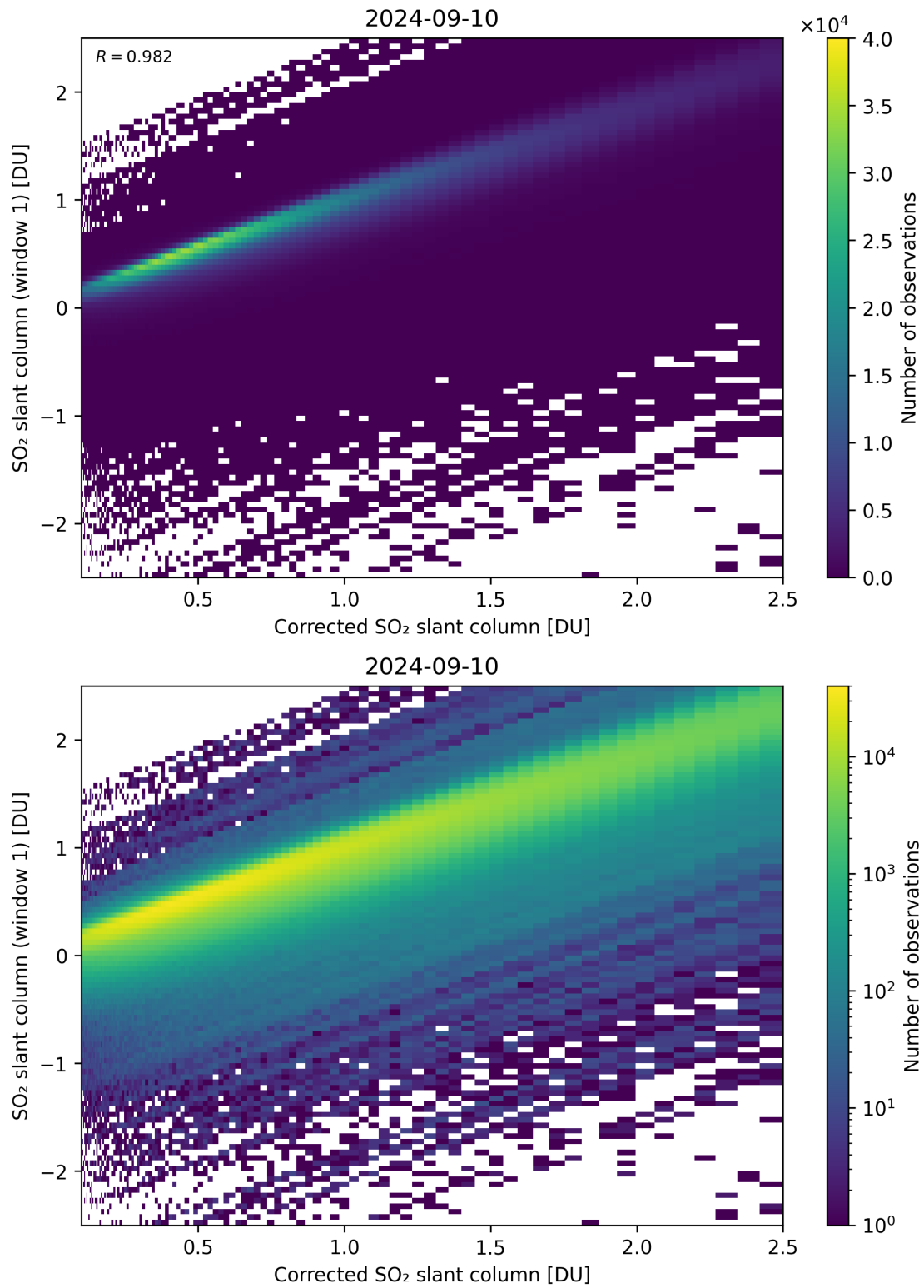
Figure 187: Scatter density plot of “Corrected SO 2 slant column” against “SO 2 slant column (window 1)” for 2024-09-09 to 2024-09-11.
