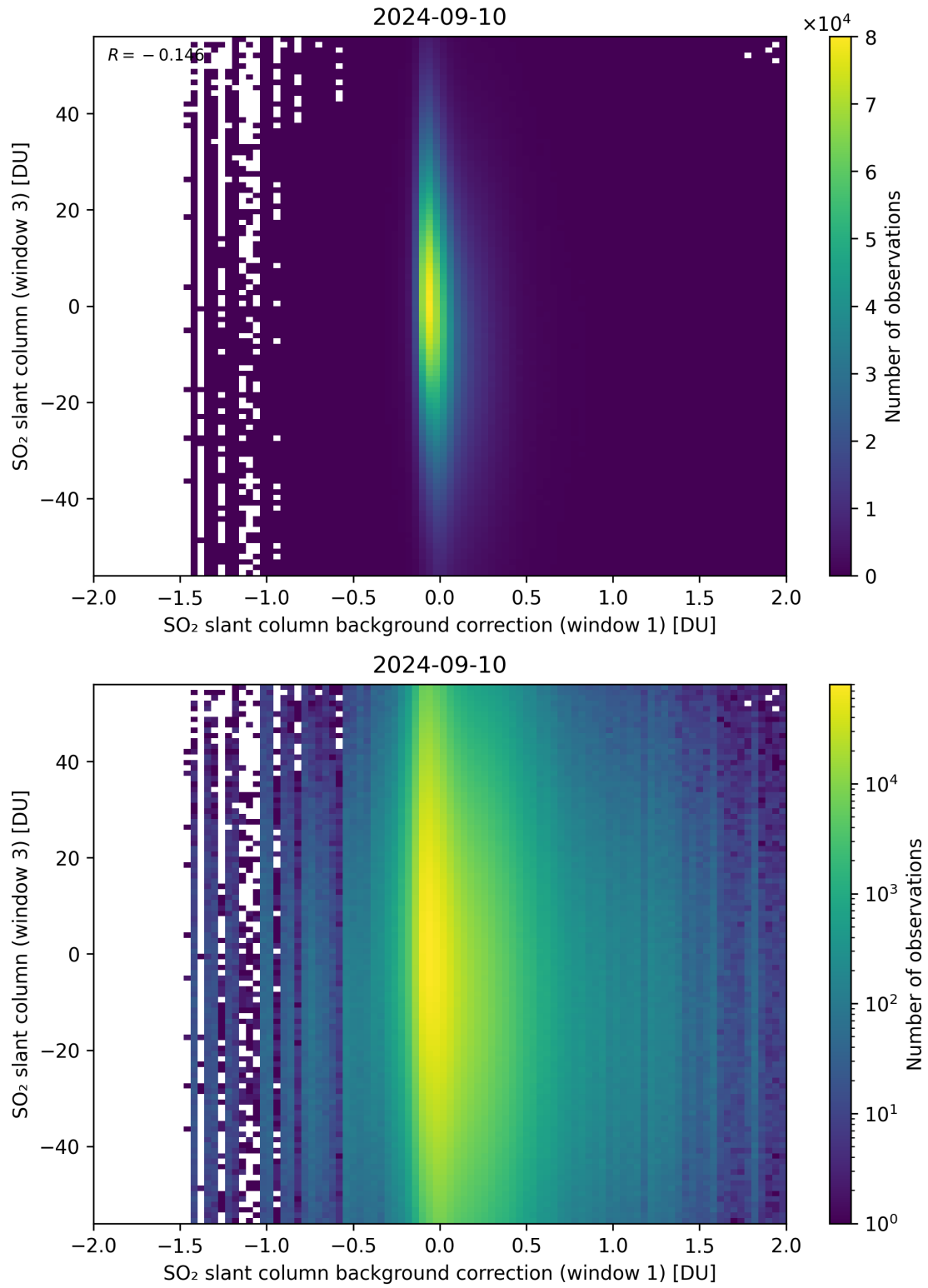
Figure 107: Scatter density plot of “SO 2 slant column background correction (window 1)” against “SO 2 slant column (window 3)” for 2024-09-09 to 2024-09-11.
