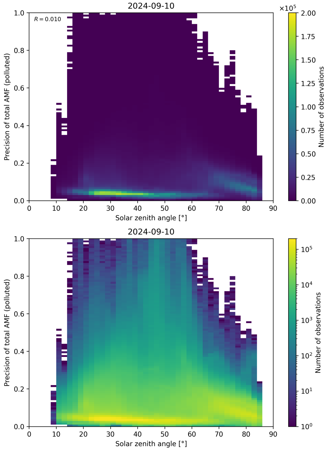
Figure 175: Scatter density plot of “Solar zenith angle” against “Precision of total AMF (polluted)” for 2024-09-09 to 2024-09-11.
