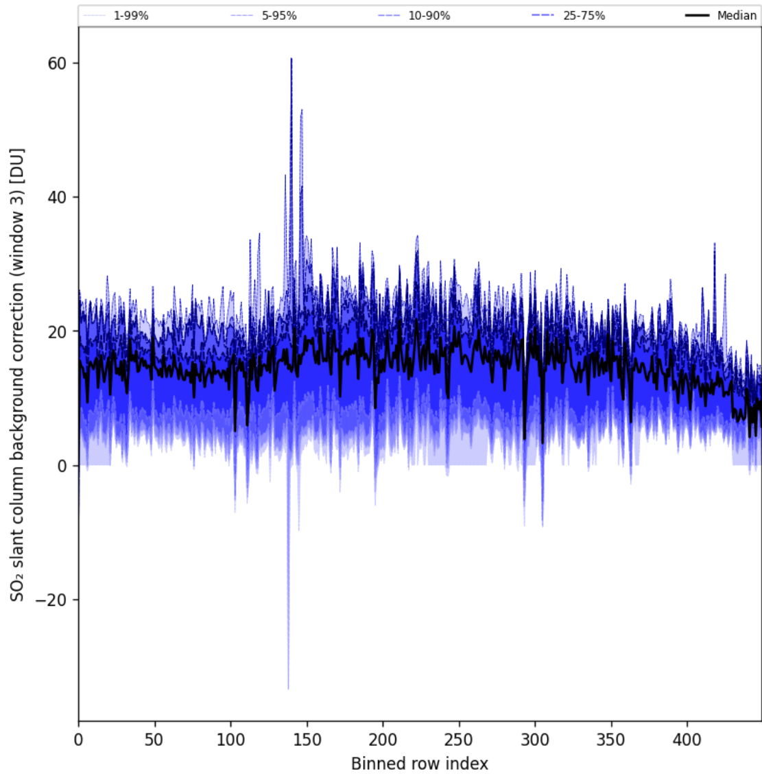
Figure 90: Along track statistics of “SO 2 slant column background correction (window 3)” for 2024-09-09 to 2024-09-11
