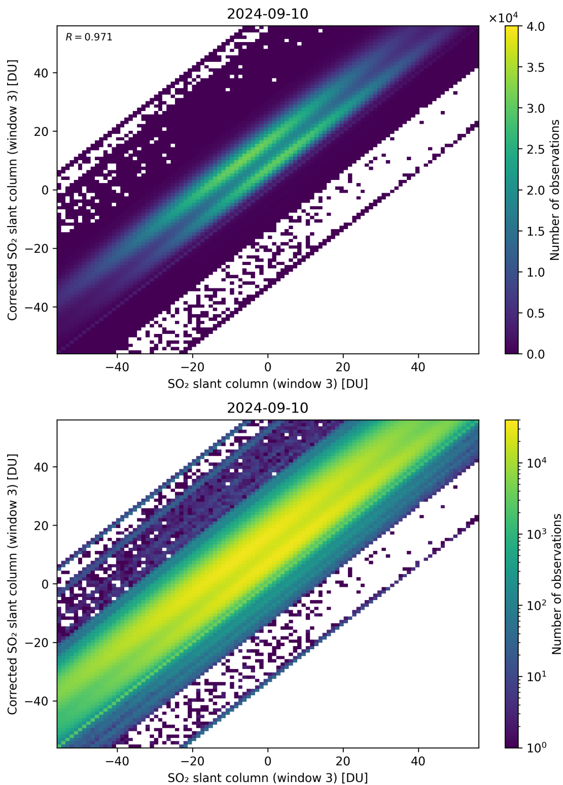
Figure 266: Scatter density plot of “SO 2 slant column (window 3)” against “Corrected SO 2 slant column (window 3)” for 2024-09-09 to 2024-09-11.
