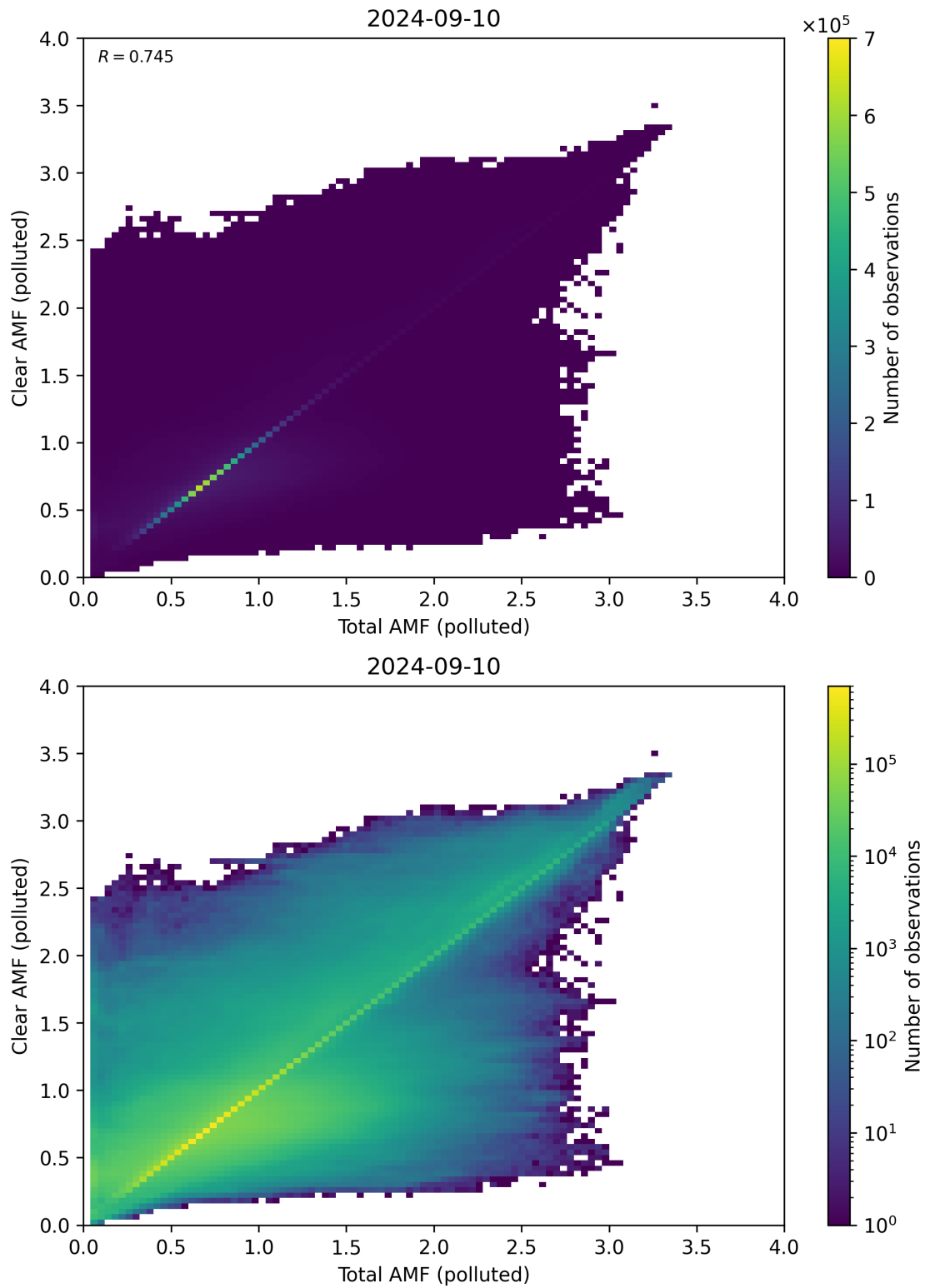
Figure 271: Scatter density plot of “Total AMF (polluted)” against “Clear AMF (polluted)” for 2024-09-09 to 2024-09-11.
