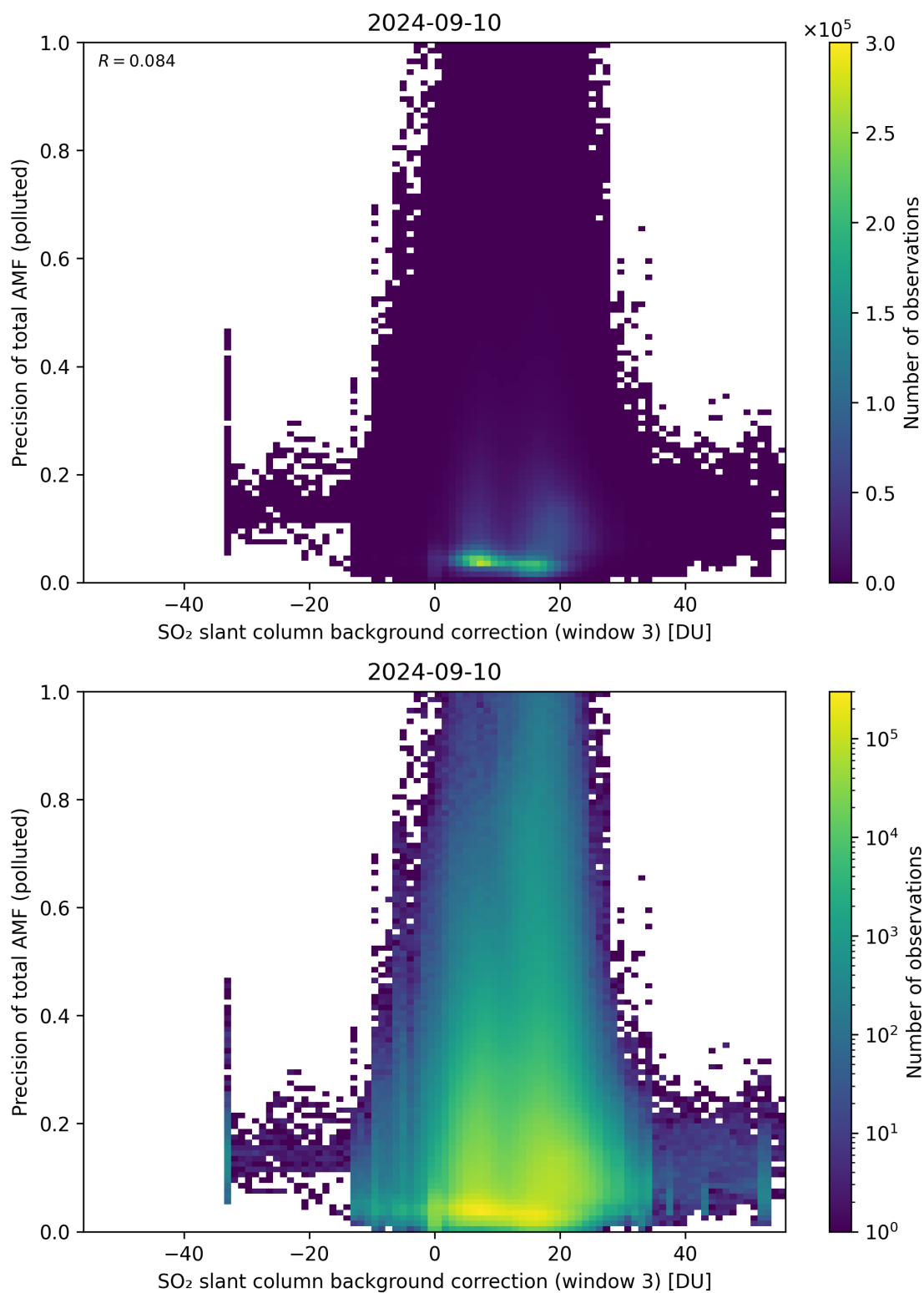
Figure 126: Scatter density plot of “SO 2 slant column background correction (window 3)” against “Precision of total AMF (polluted)” for 2024-09-09 to 2024-09-11.
