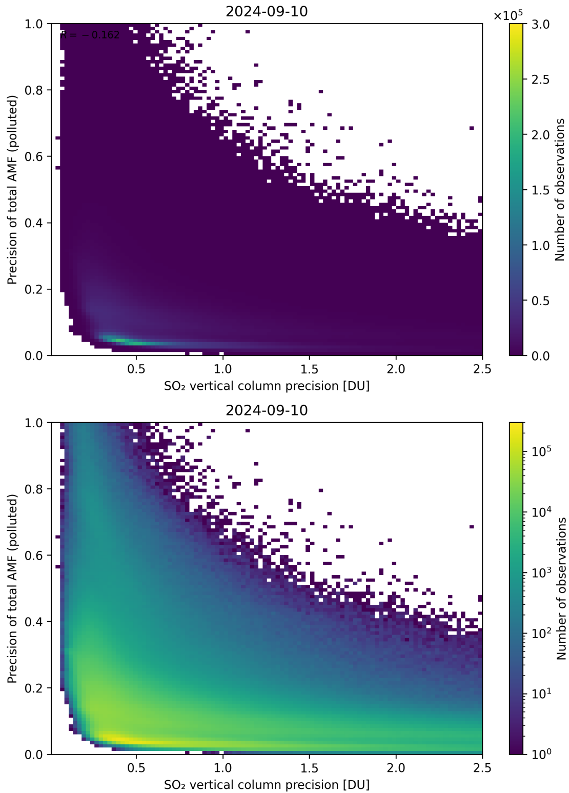
Figure 295: Scatter density plot of “SO 2 vertical column precision” against “Precision of total AMF (polluted)” for 2024-09-09 to 2024-09-11.
