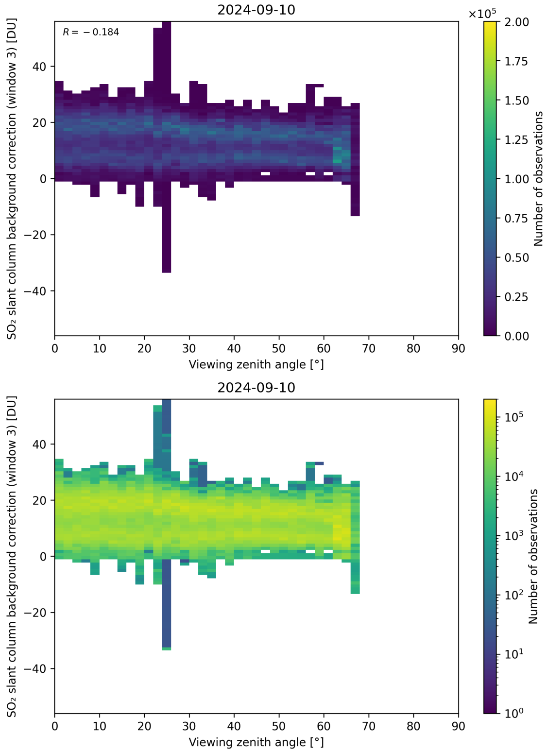
Figure 310: Scatter density plot of “Viewing zenith angle” against “SO 2 slant column background correction (window 3)” for 2024-09-09 to 2024-09-11.
