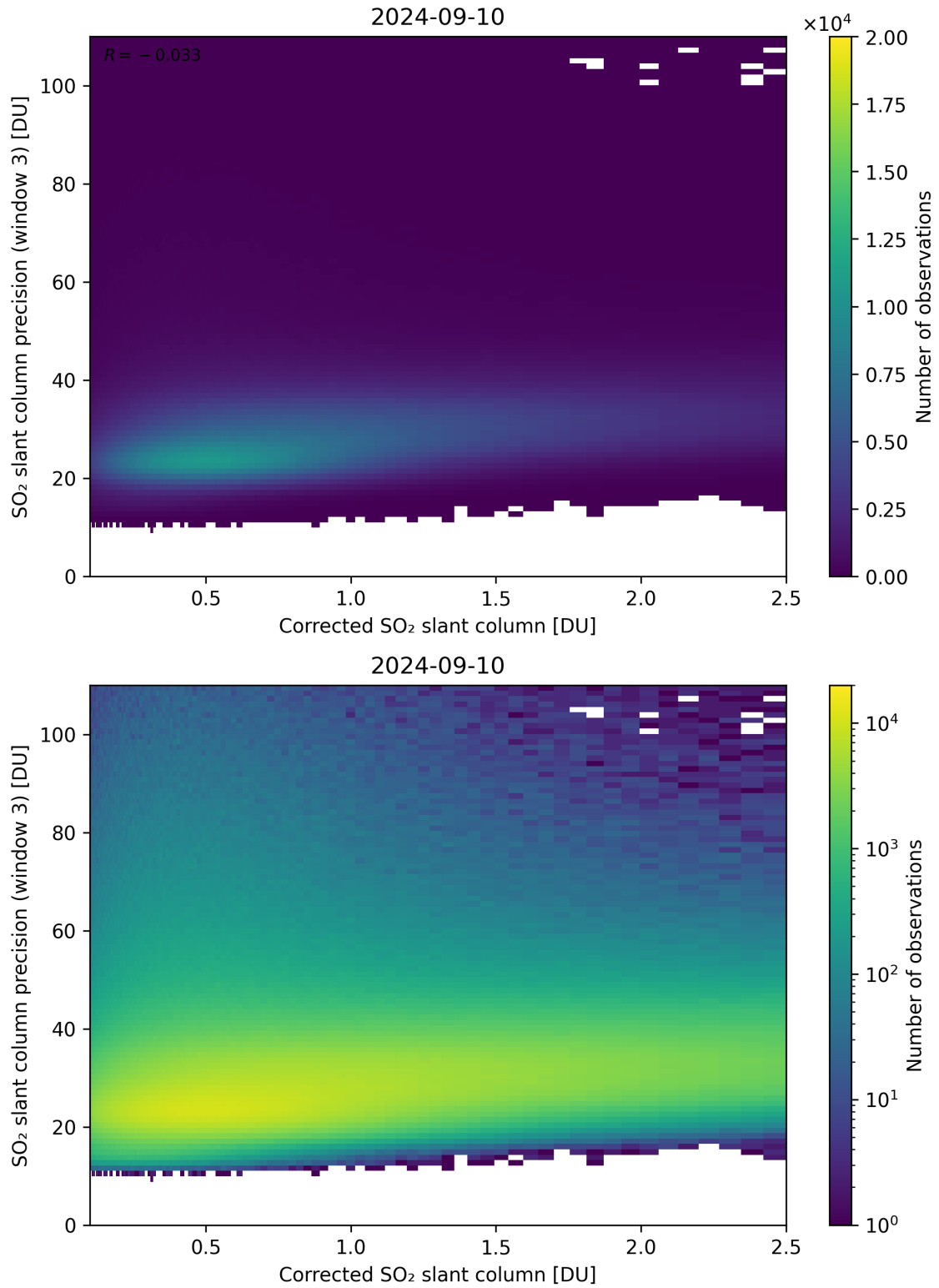
Figure 191: Scatter density plot of “Corrected SO 2 slant column” against “SO 2 slant column precision (window 3)” for 2024-09-09 to 2024-09-11.
