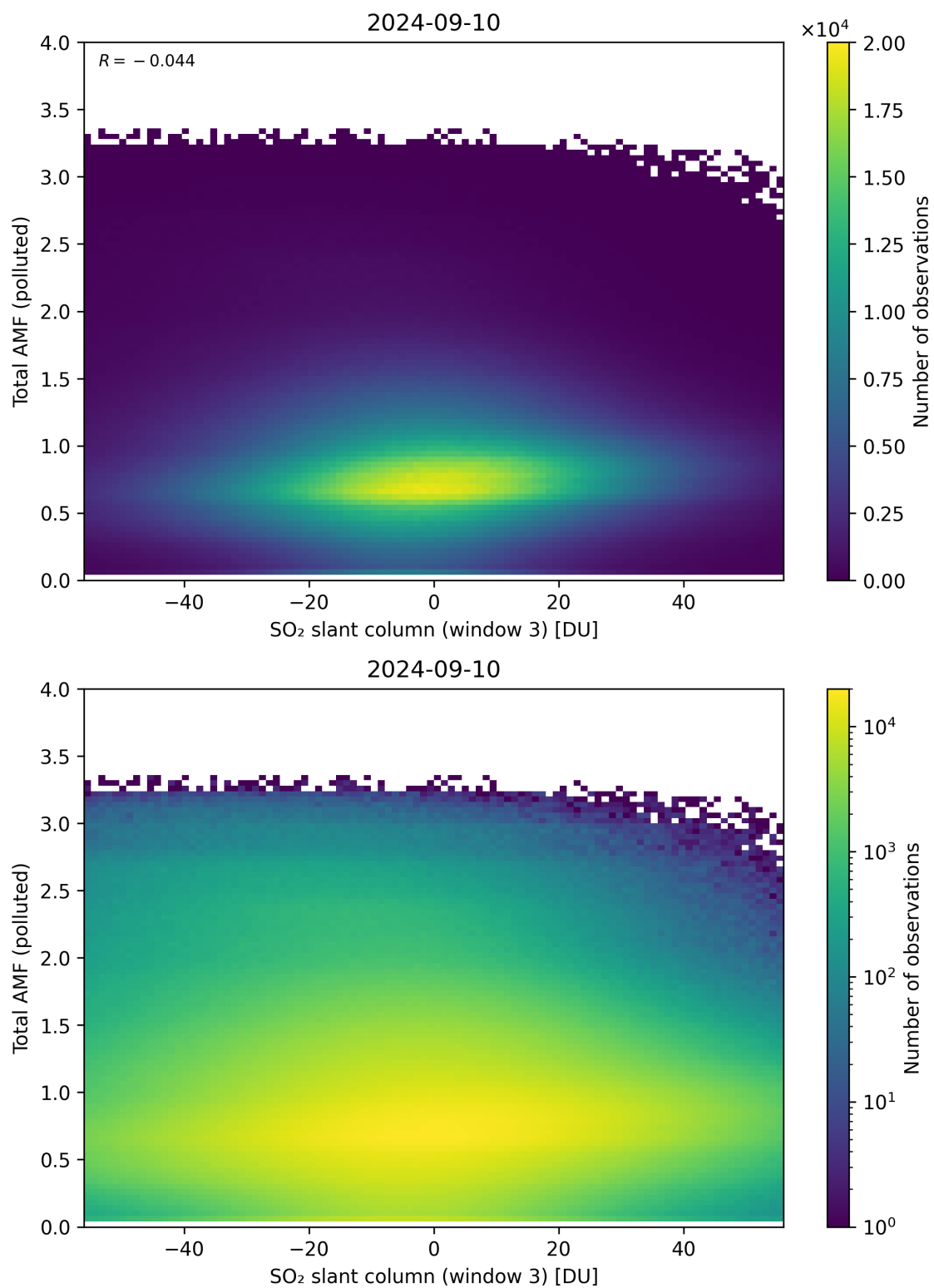
Figure 268: Scatter density plot of “SO 2 slant column (window 3)” against “Total AMF (polluted)” for 2024-09-09 to 2024-09-11.
