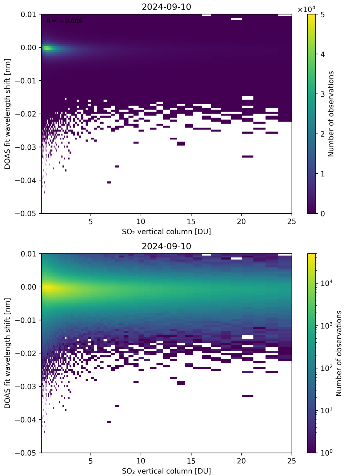
Figure 276: Scatter density plot of “SO 2 vertical column” against “DOAS fit wavelength shift” for 2024-09-09 to 2024-09-11.
