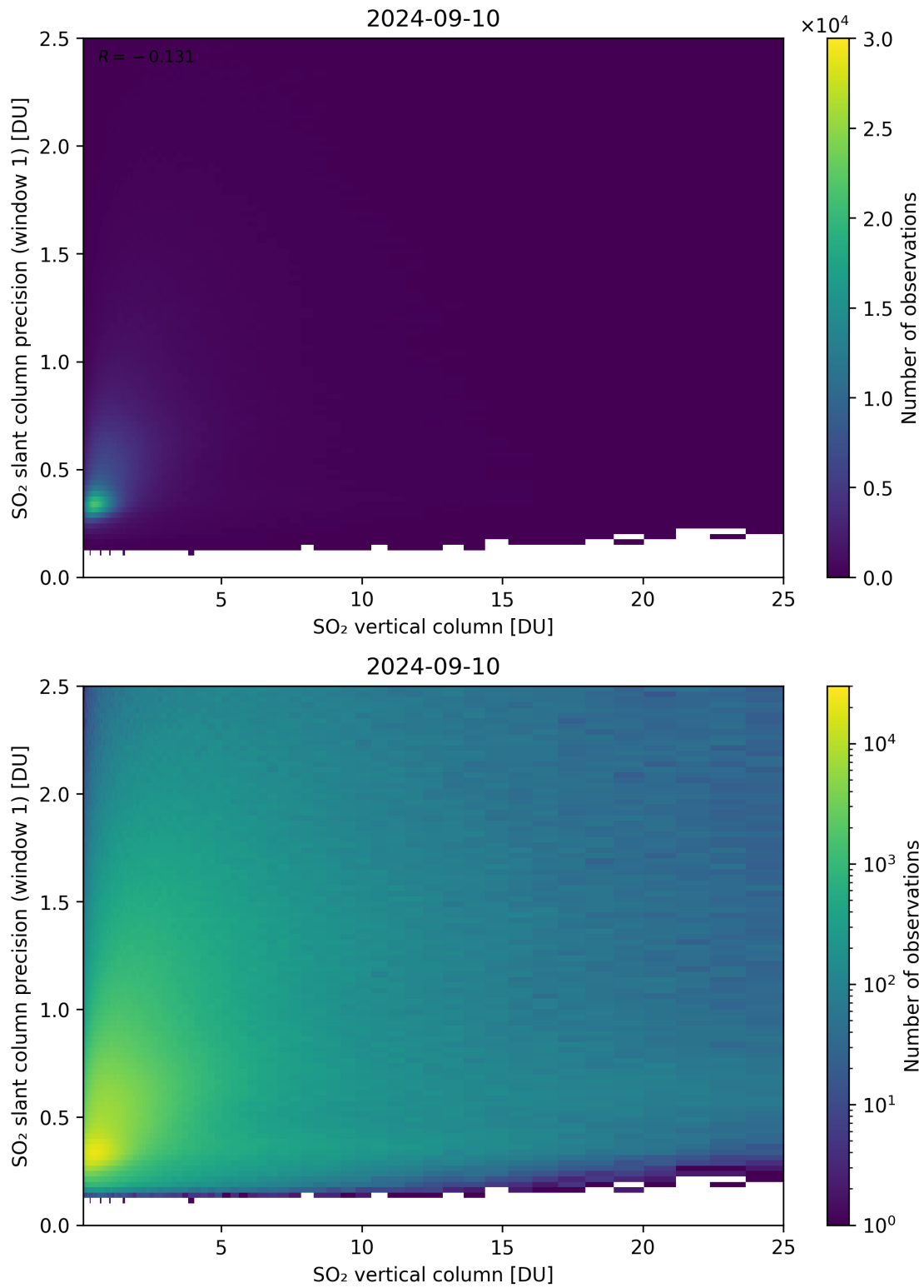
Figure 301: Scatter density plot of “SO 2 vertical column” against “SO 2 slant column precision (window 1)” for 2024-09-09 to 2024-09-11.
