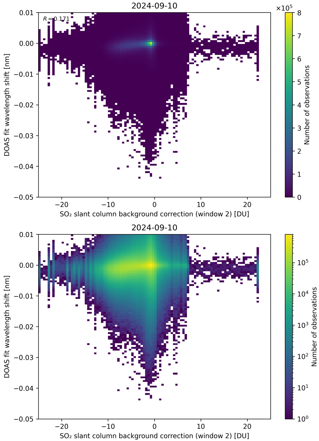
Figure 112: Scatter density plot of “SO 2 slant column background correction (window 2)” against “DOAS fit wavelength shift” for 2024-09-09 to 2024-09-11.
