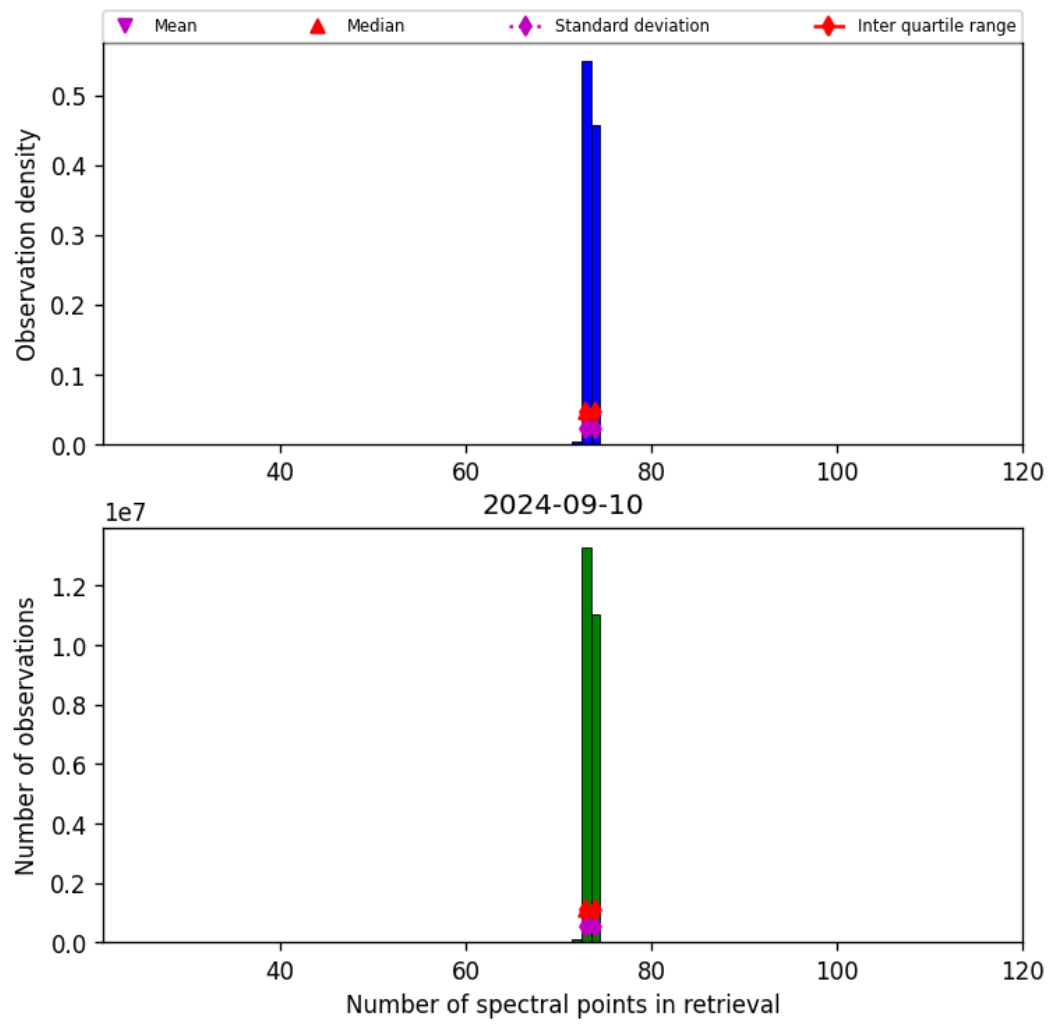
Figure 74: Histogram of “Number of spectral points in retrieval” for 2024-09-09 to 2024-09-11
