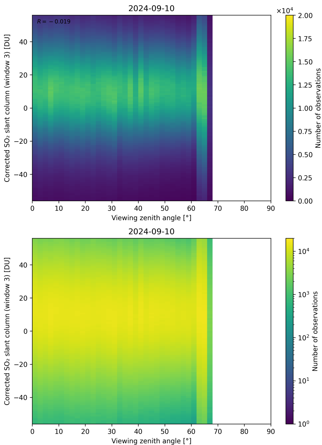
Figure 319: Scatter density plot of “Viewing zenith angle” against “Corrected SO 2 slant column (window 3)” for 2024-09-09 to 2024-09-11.
