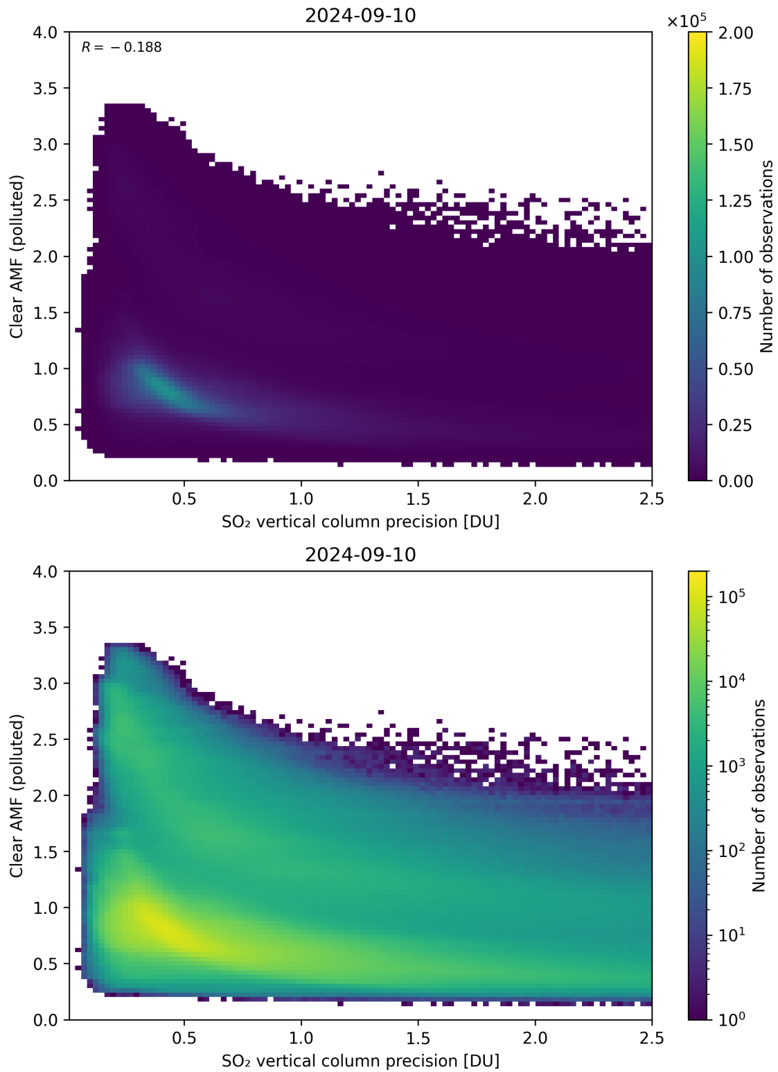
Figure 285: Scatter density plot of “SO 2 vertical column precision” against “Clear AMF (polluted)” for 2024-09-09 to 2024-09-11.
