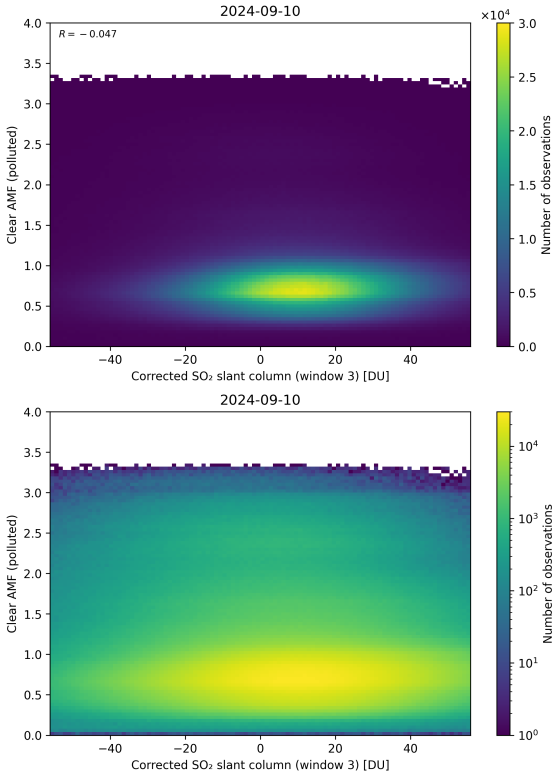
Figure 209: Scatter density plot of “Corrected SO 2 slant column (window 3)” against “Clear AMF (polluted)” for 2024-09-09 to 2024-09-11.
