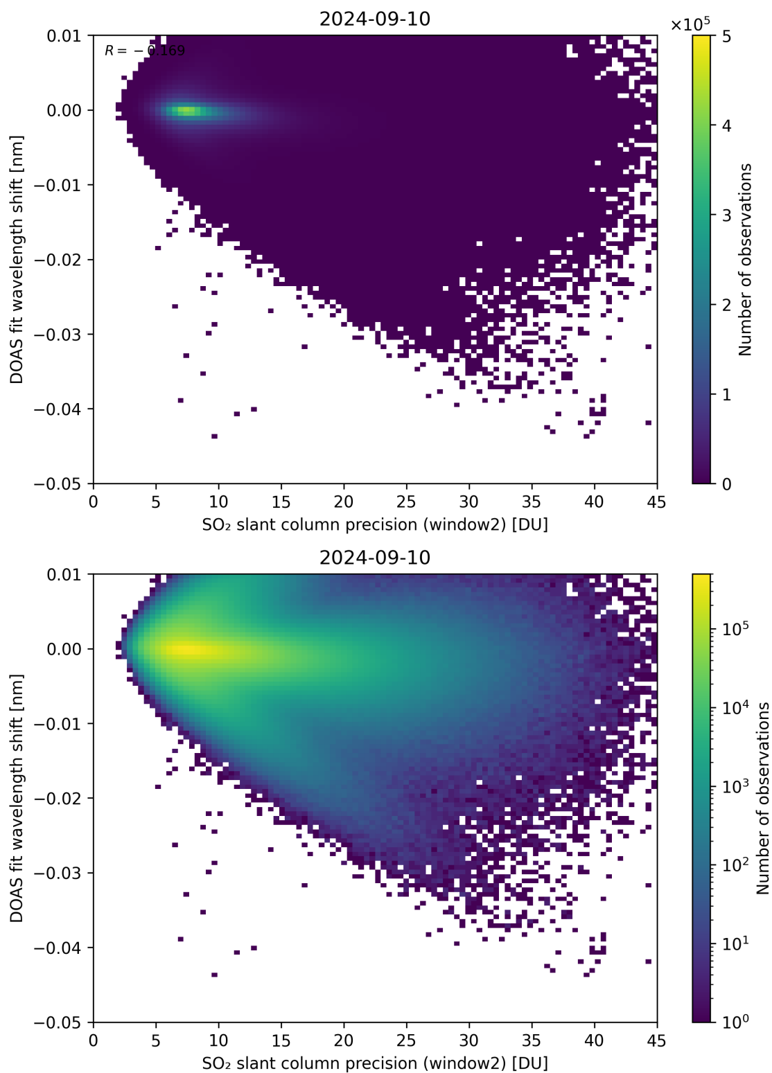
Figure 243: Scatter density plot of “SO 2 slant column precision (window2)” against “DOAS fit wavelength shift” for 2024-09-09 to 2024-09-11.
