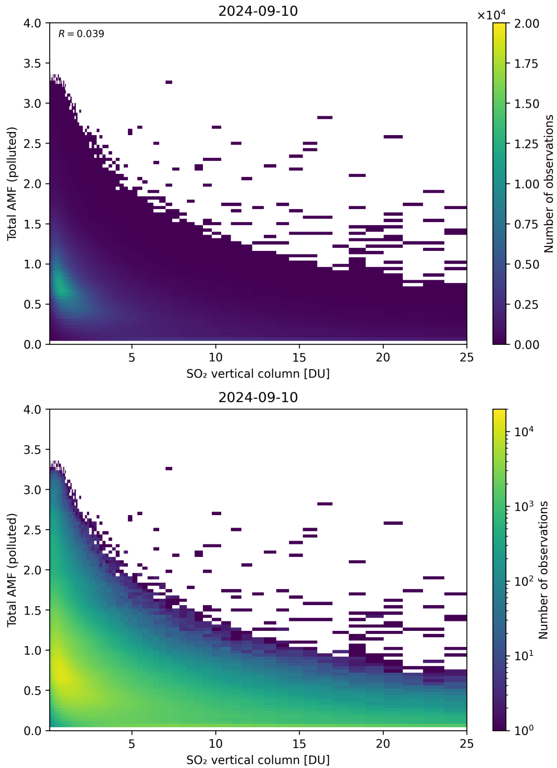
Figure 305: Scatter density plot of “SO 2 vertical column” against “Total AMF (polluted)” for 2024-09-09 to 2024-09-11.
