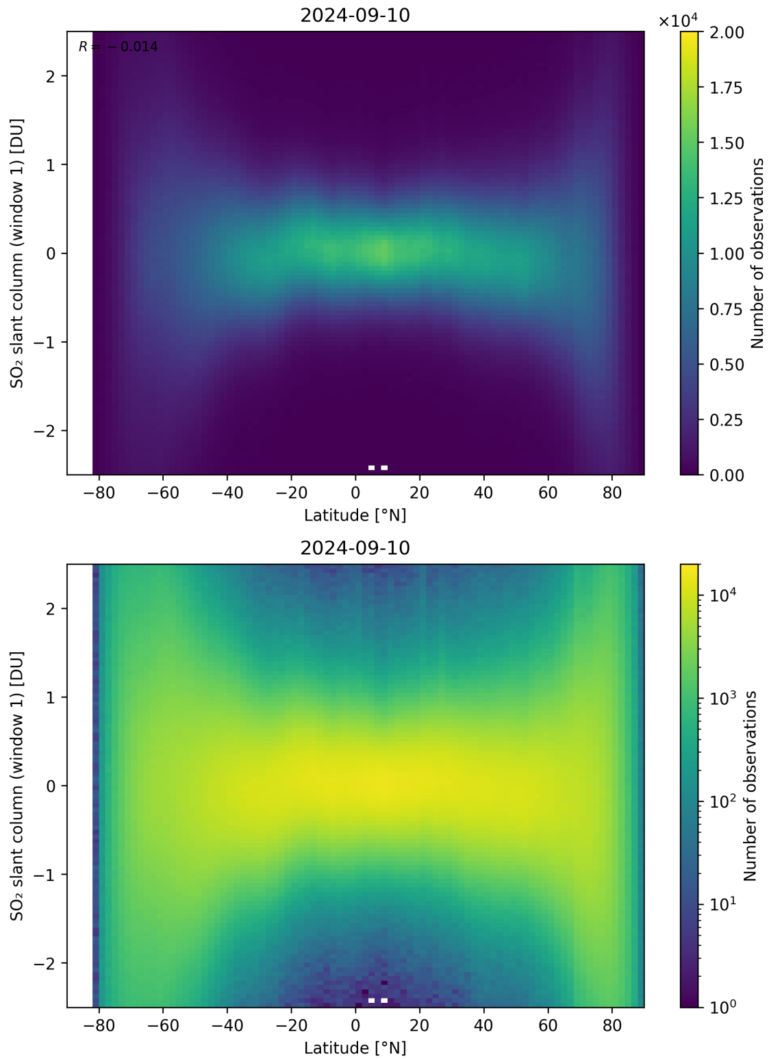
Figure 149: Scatter density plot of “Latitude” against “SO 2 slant column (window 1)” for 2024-09-09 to 2024-09-11.
