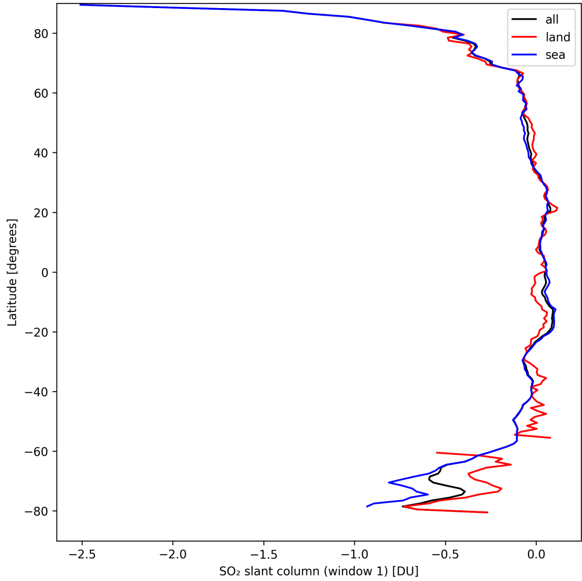
Figure 33: Zonal average of “SO 2 slant column (window 1)” for 2024-09-09 to 2024-09-11.
