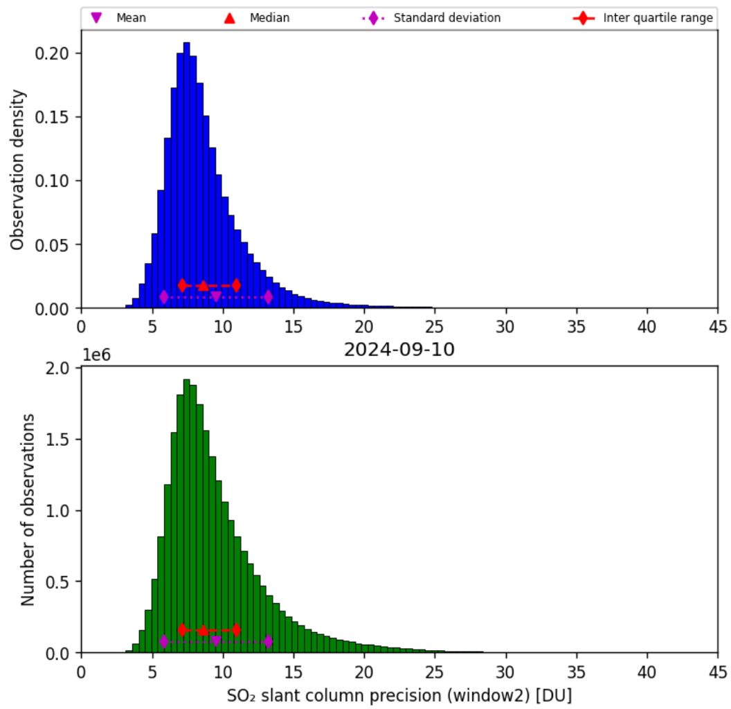
Figure 61: Histogram of “SO 2 slant column precision (window2)” for 2024-09-09 to 2024-09-11
