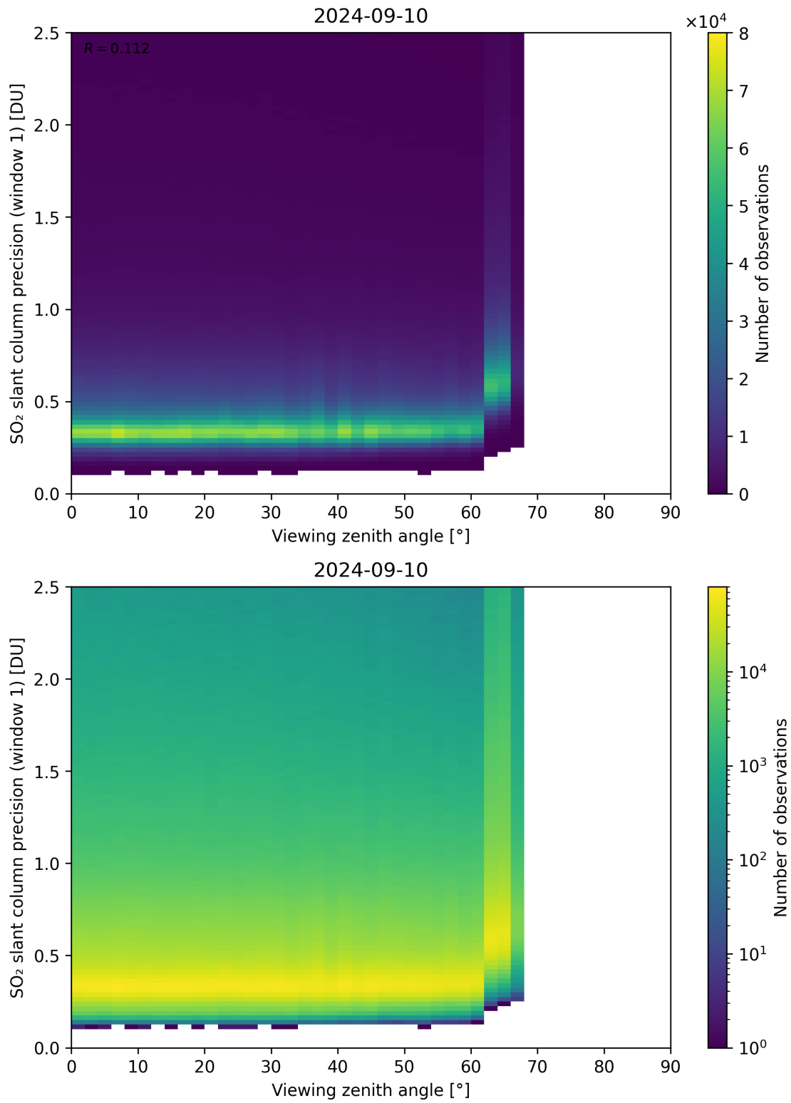
Figure 321: Scatter density plot of “Viewing zenith angle” against “SO 2 slant column precision (window 1)” for 2024-09-09 to 2024-09-11.
