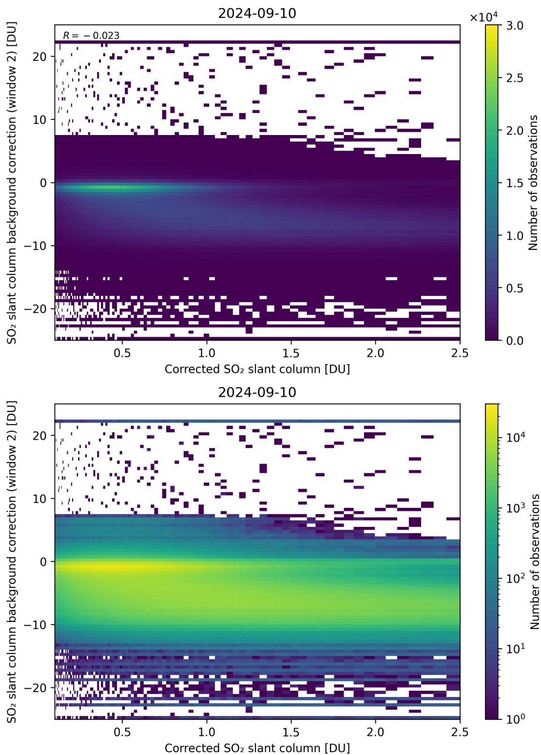
Figure 179: Scatter density plot of “Corrected SO 2 slant column” against “SO 2 slant column background correction (window 2)” for 2024-09-09 to 2024-09-11.
