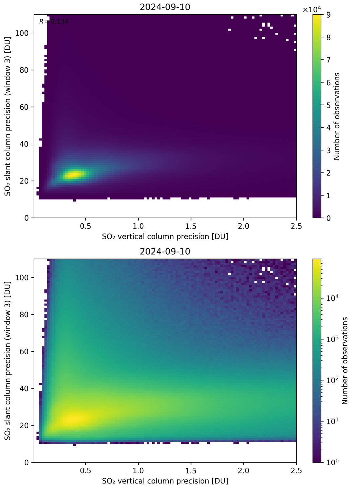
Figure 293: Scatter density plot of “SO 2 vertical column precision” against “SO 2 slant column precision (window 3)” for 2024-09-09 to 2024-09-11.
