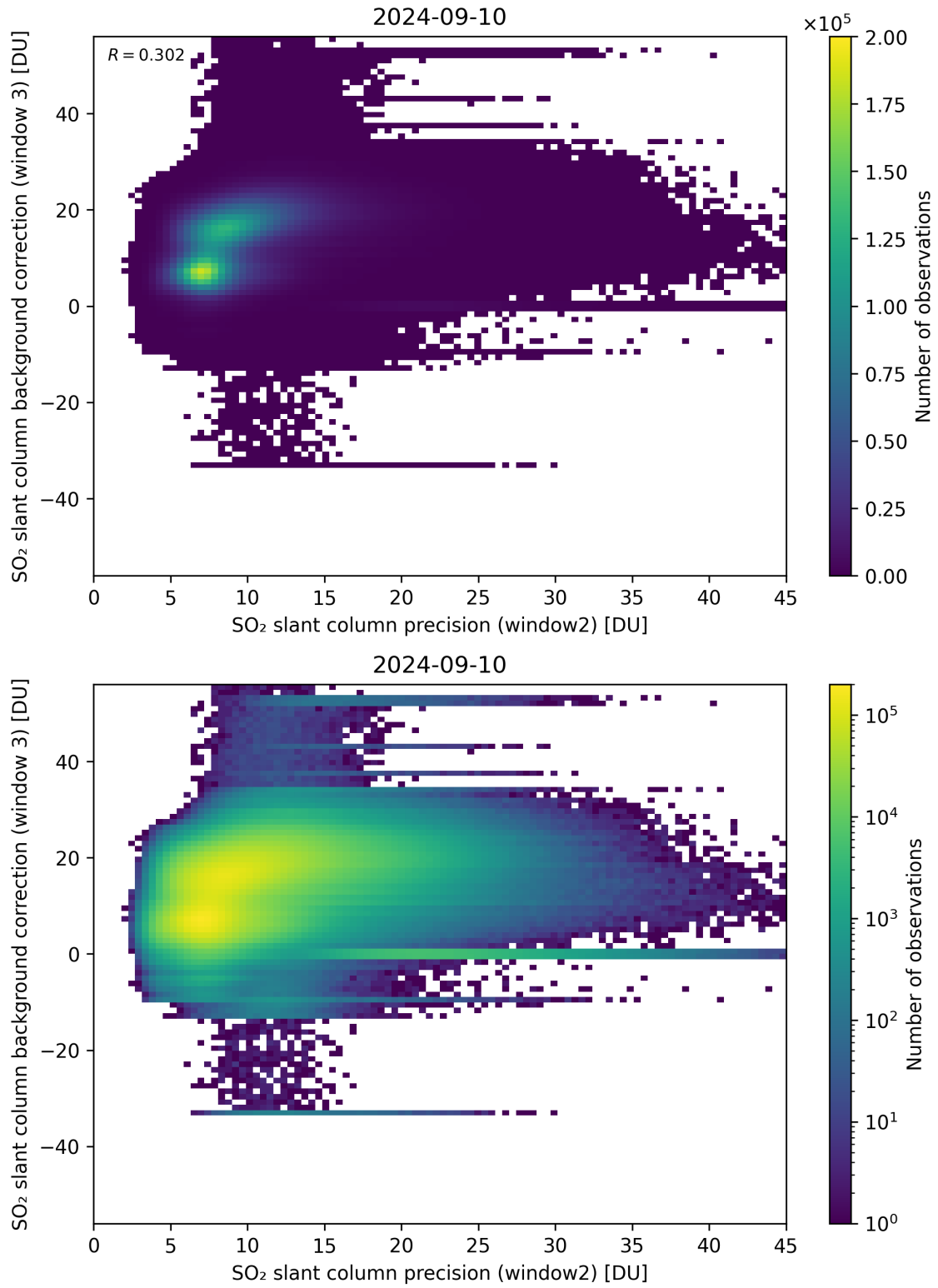
Figure 242: Scatter density plot of “SO 2 slant column precision (window2)” against “SO 2 slant column background correction (window 3)” for 2024-09-09 to 2024-09-11.
