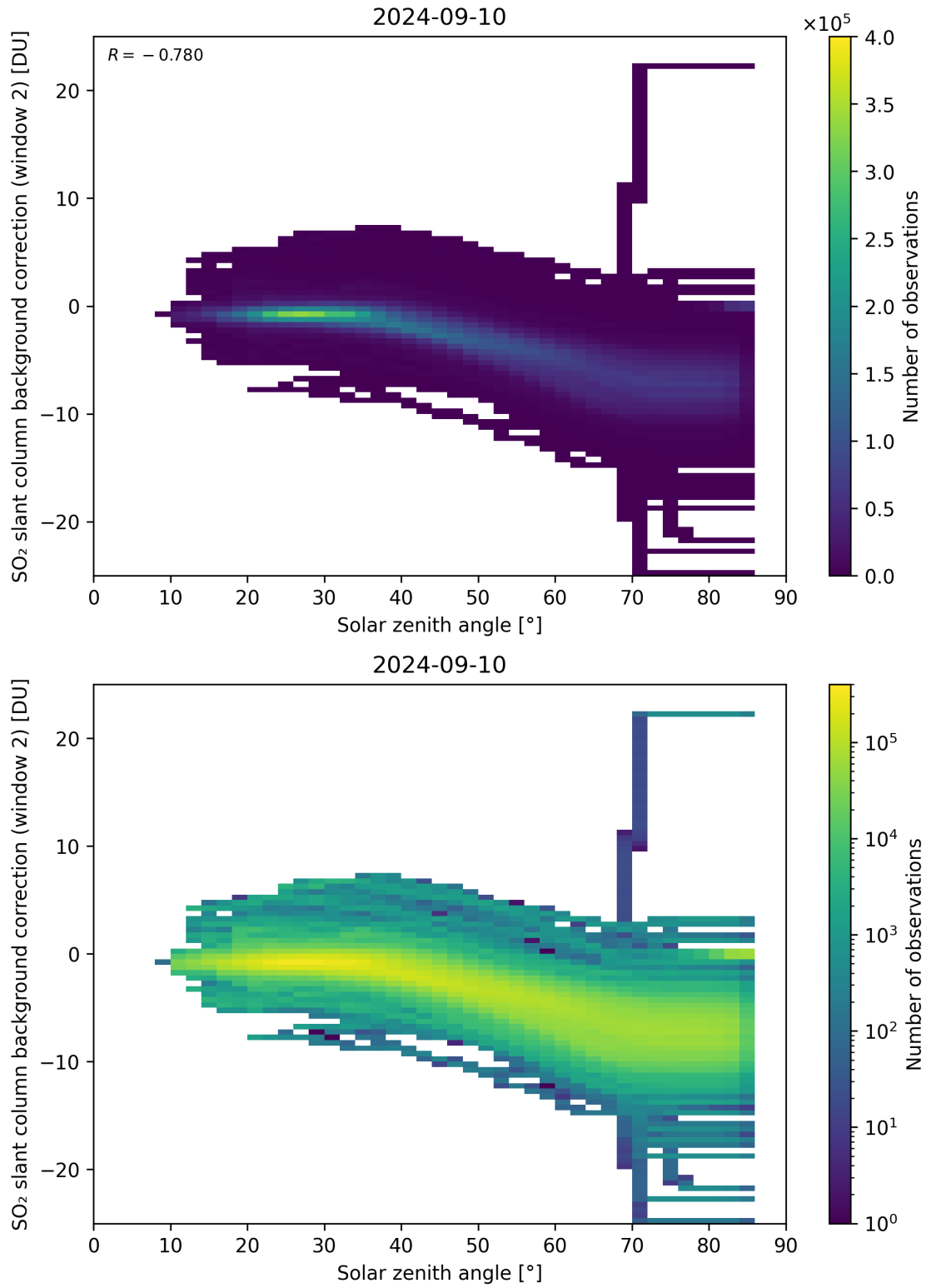
Figure 159: Scatter density plot of “Solar zenith angle” against “SO 2 slant column background correction (window 2)” for 2024-09-09 to 2024-09-11.
