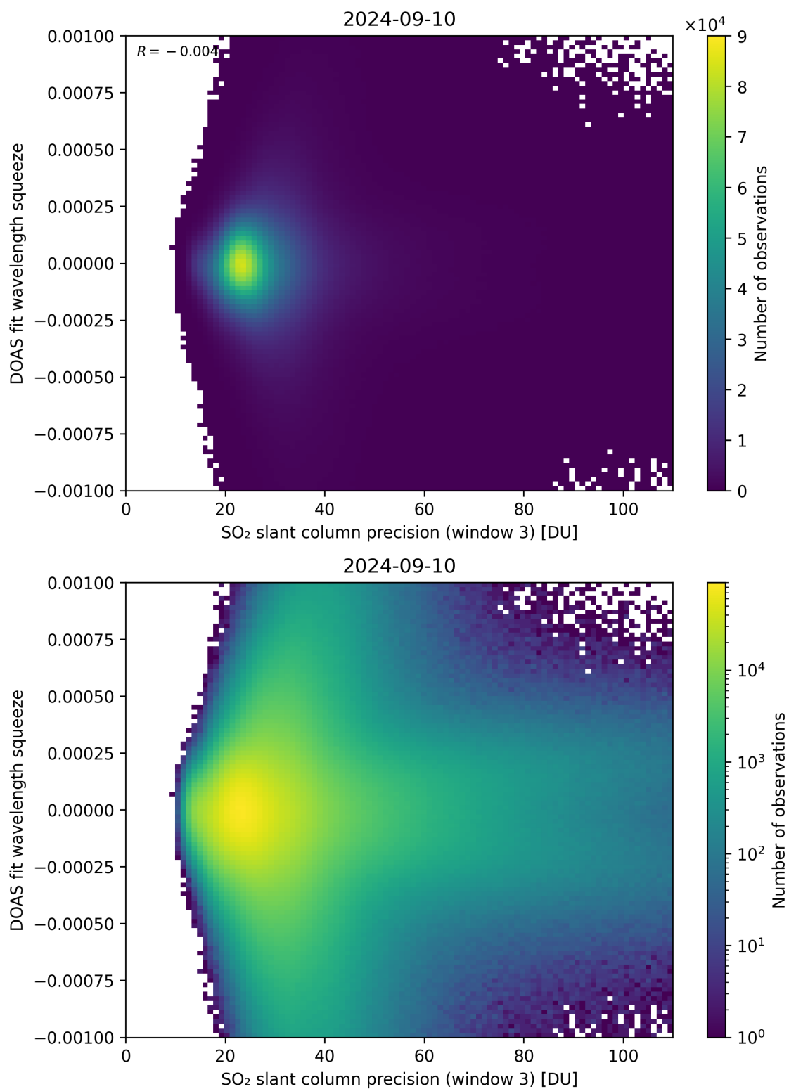
Figure 259: Scatter density plot of “SO 2 slant column precision (window 3)” against “DOAS fit wavelength squeeze” for 2024-09-09 to 2024-09-11.
