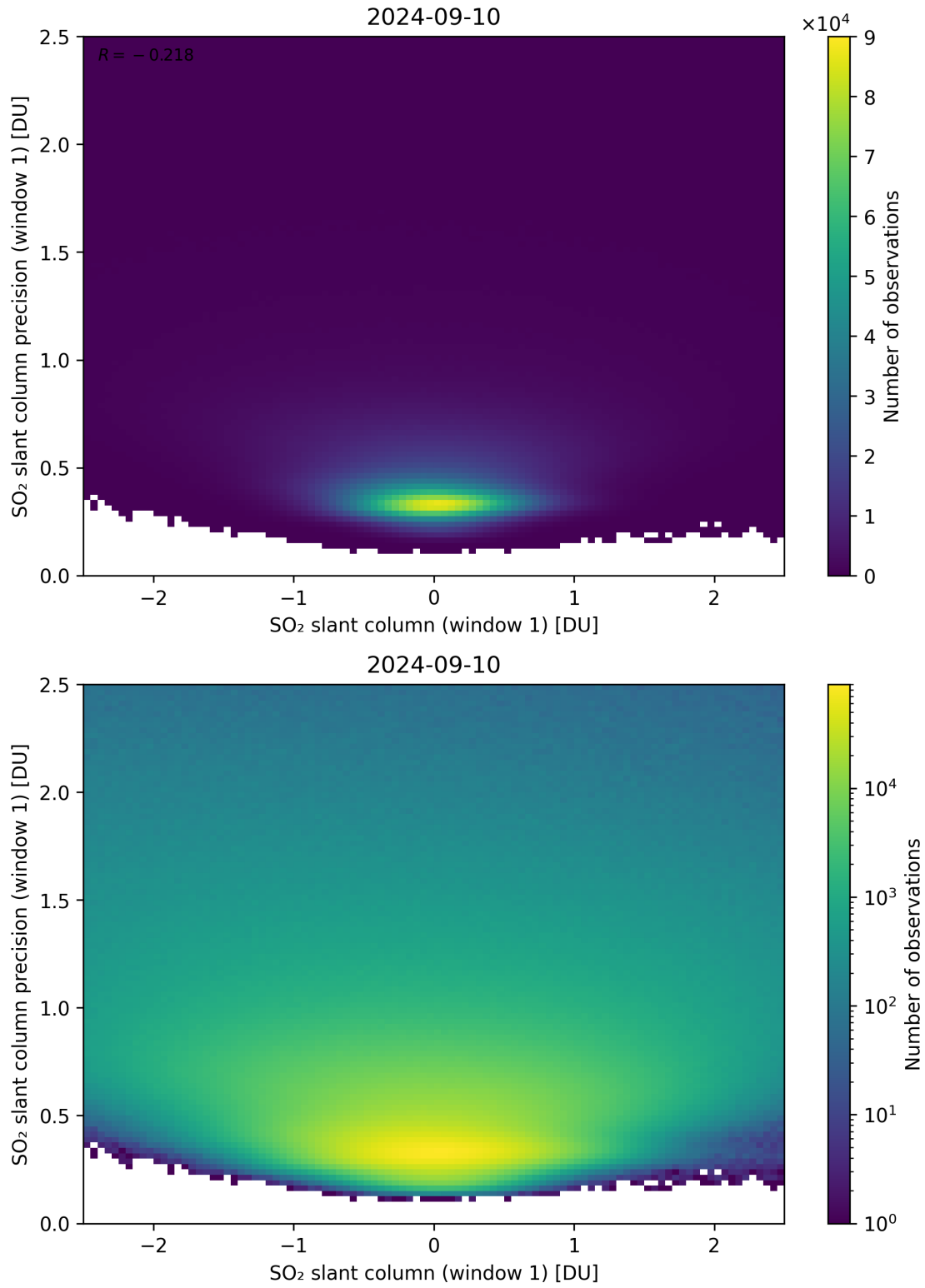
Figure 235: Scatter density plot of “SO 2 slant column (window 1)” against “SO 2 slant column precision (window 1)” for 2024-09-09 to 2024-09-11.
