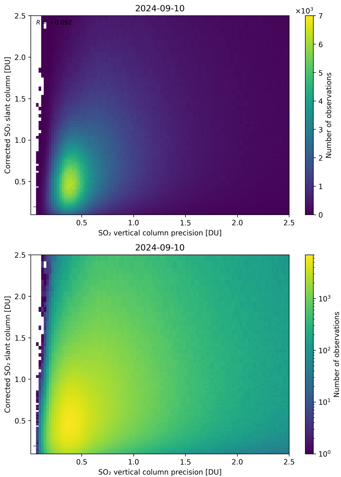
Figure 286: Scatter density plot of “SO 2 vertical column precision” against “Corrected SO 2 slant column” for 2024-09-09 to 2024-09-11.
