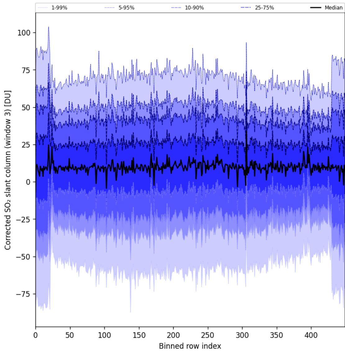
Figure 89: Along track statistics of “Corrected SO 2 slant column (window 3)” for 2024-09-09 to 2024-09-11
