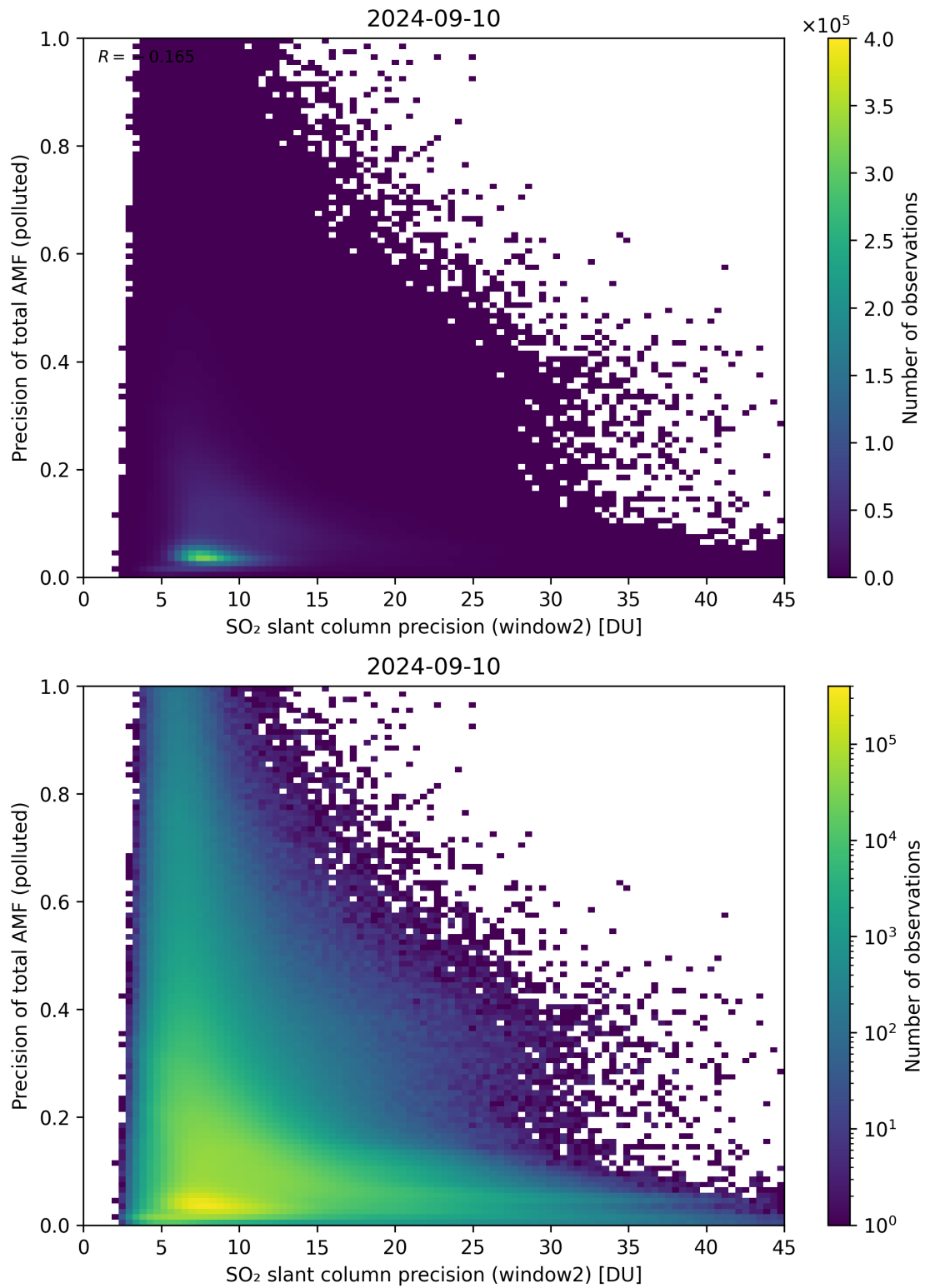
Figure 252: Scatter density plot of “SO 2 slant column precision (window2)” against “Precision of total AMF (polluted)” for 2024-09-09 to 2024-09-11.
