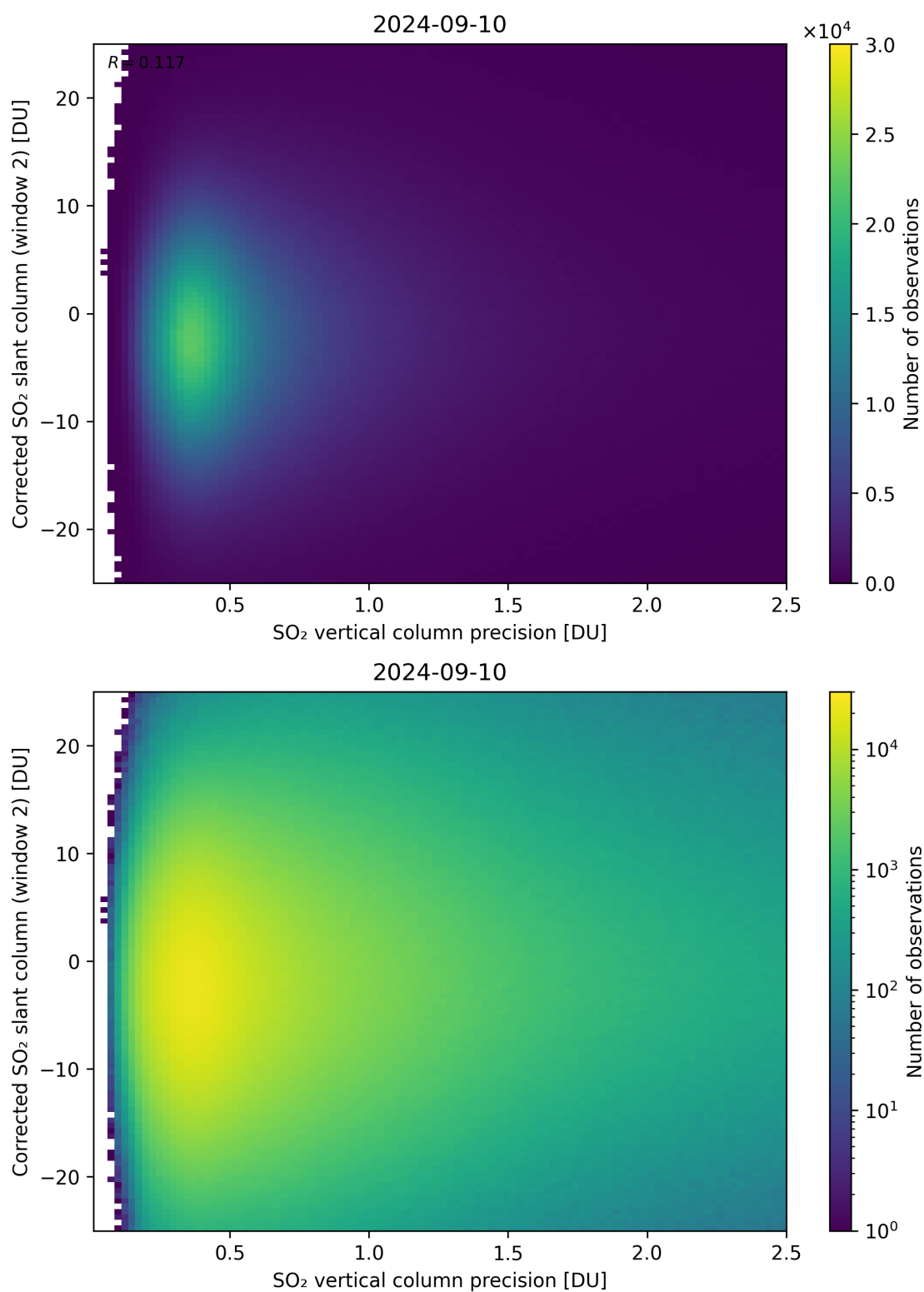
Figure 287: Scatter density plot of “SO 2 vertical column precision” against “Corrected SO 2 slant column (window 2)” for 2024-09-09 to 2024-09-11.
