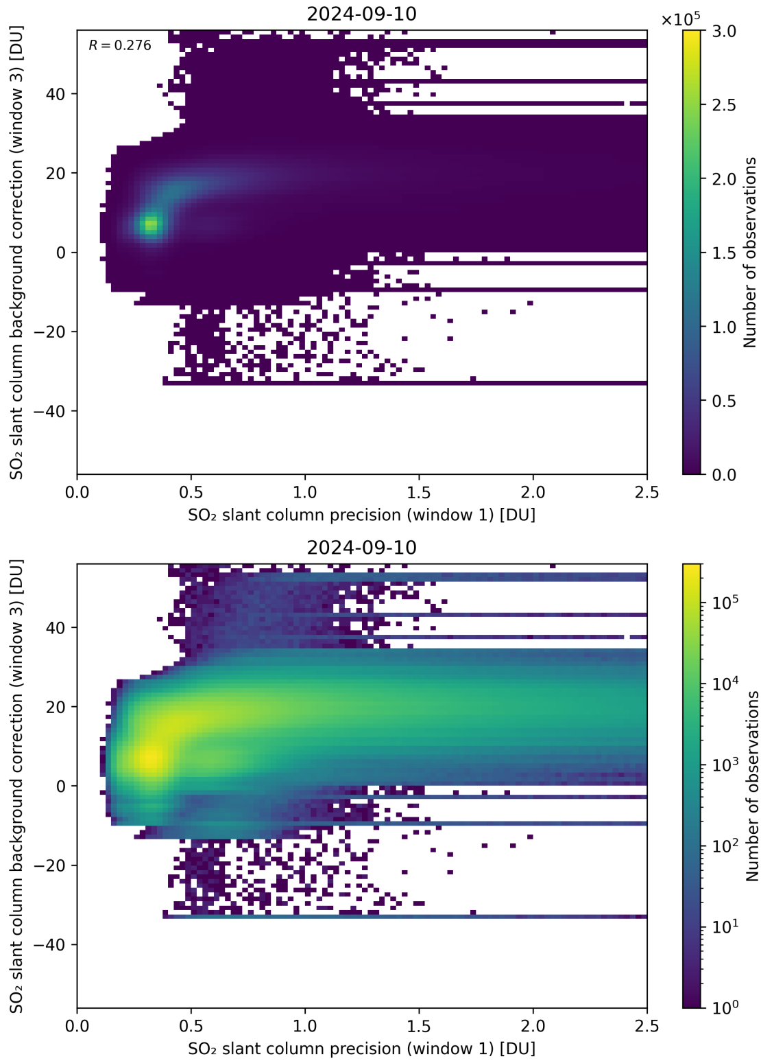
Figure 220: Scatter density plot of “SO 2 slant column precision (window 1)” against “SO 2 slant column background correction (window 3)” for 2024-09-09 to 2024-09-11.
