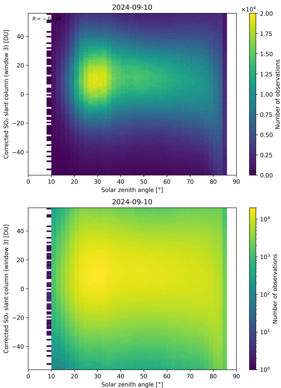
Figure 168: Scatter density plot of “Solar zenith angle” against “Corrected SO 2 slant column (window 3)” for 2024-09-09 to 2024-09-11.
