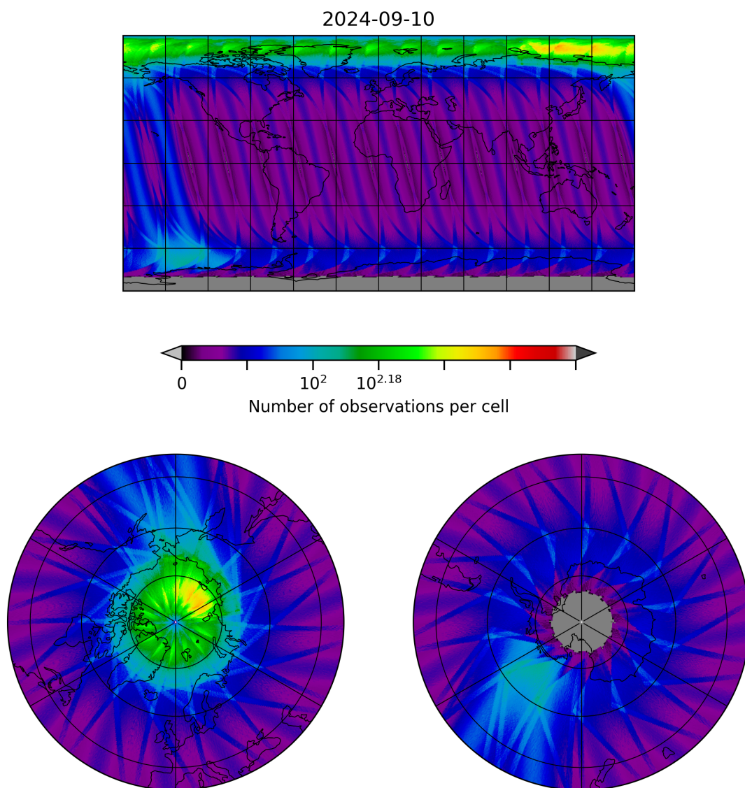
Figure 28: Map of the number of observations for 2024-09-09 to 2024-09-11
