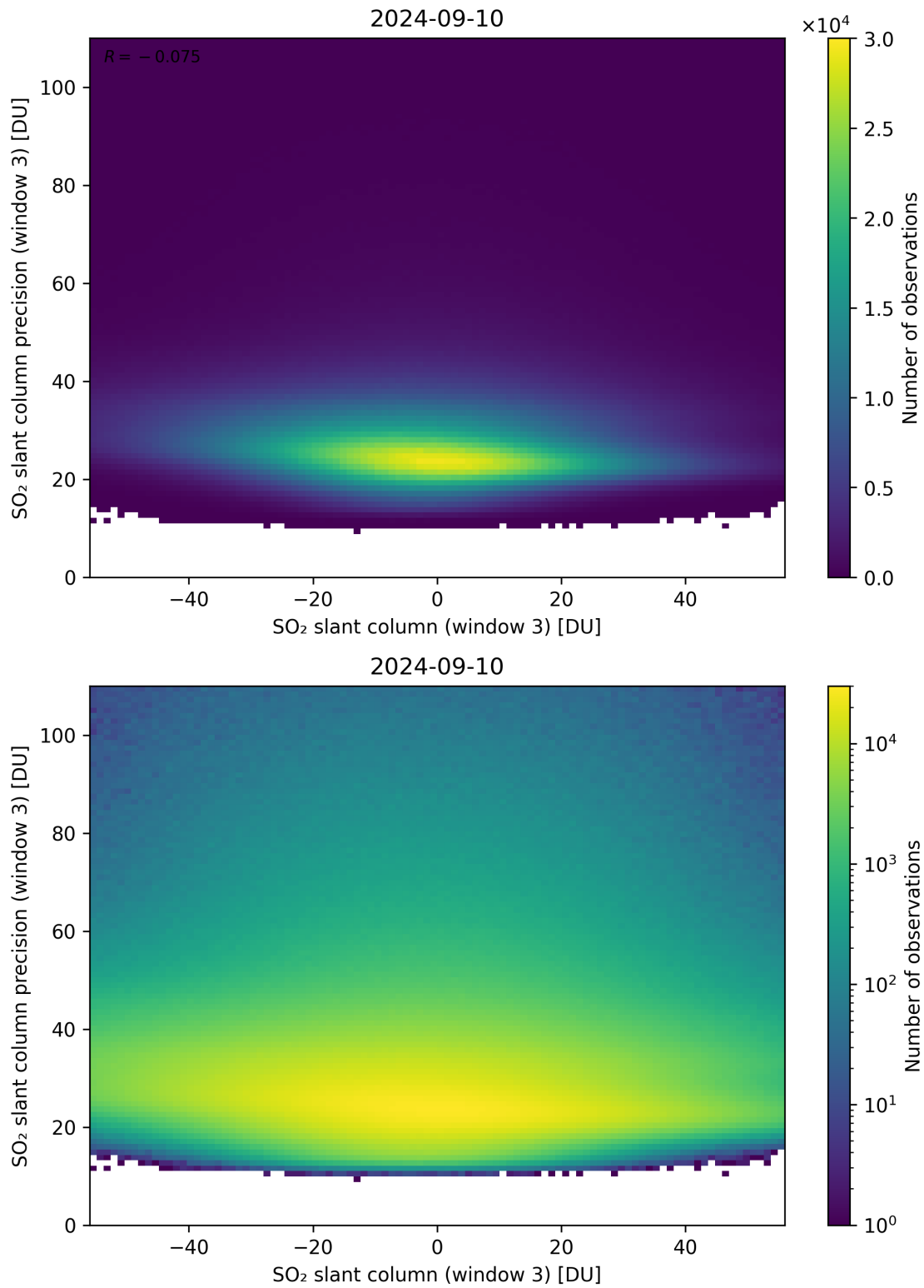
Figure 267: Scatter density plot of “SO 2 slant column (window 3)” against “SO 2 slant column precision (window 3)” for 2024-09-09 to 2024-09-11.
