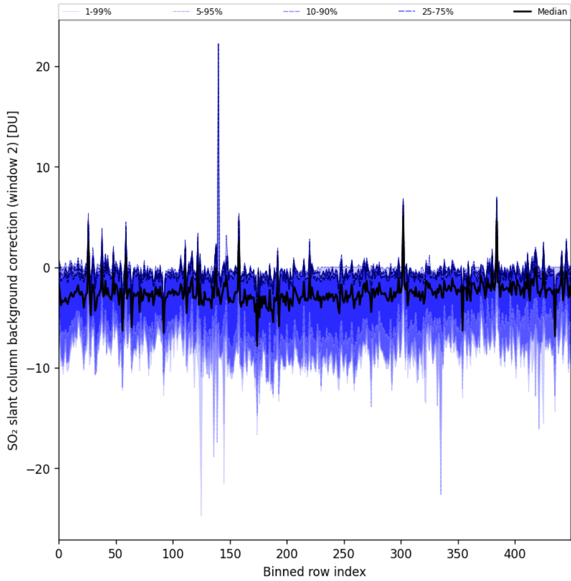
Figure 86: Along track statistics of “SO 2 slant column background correction (window 2)” for 2024-09-09 to 2024-09-11
