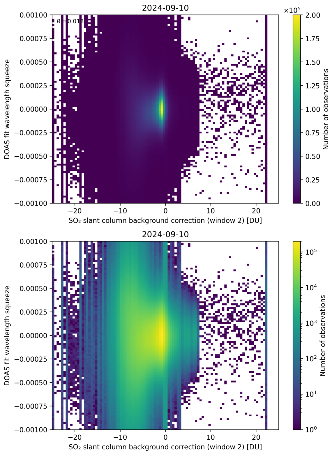
Figure 113: Scatter density plot of “SO 2 slant column background correction (window 2)” against “DOAS fit wavelength squeeze” for 2024-09-09 to 2024-09-11.
