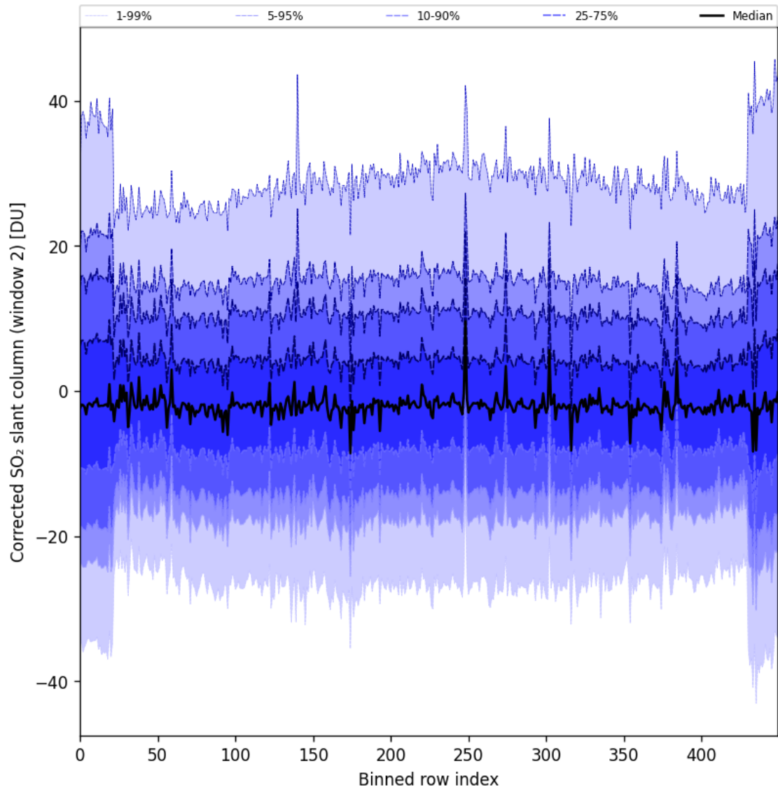
Figure 85: Along track statistics of “Corrected SO 2 slant column (window 2)” for 2024-09-09 to 2024-09-11
