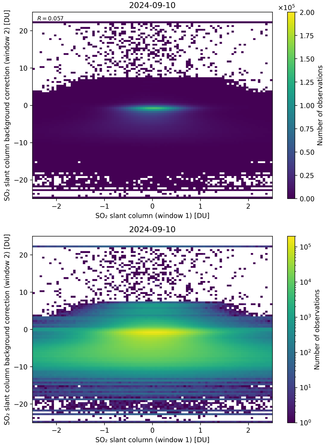
Figure 213: Scatter density plot of “SO 2 slant column (window 1)” against “SO 2 slant column background correction (window 2)” for 2024-09-09 to 2024-09-11.
