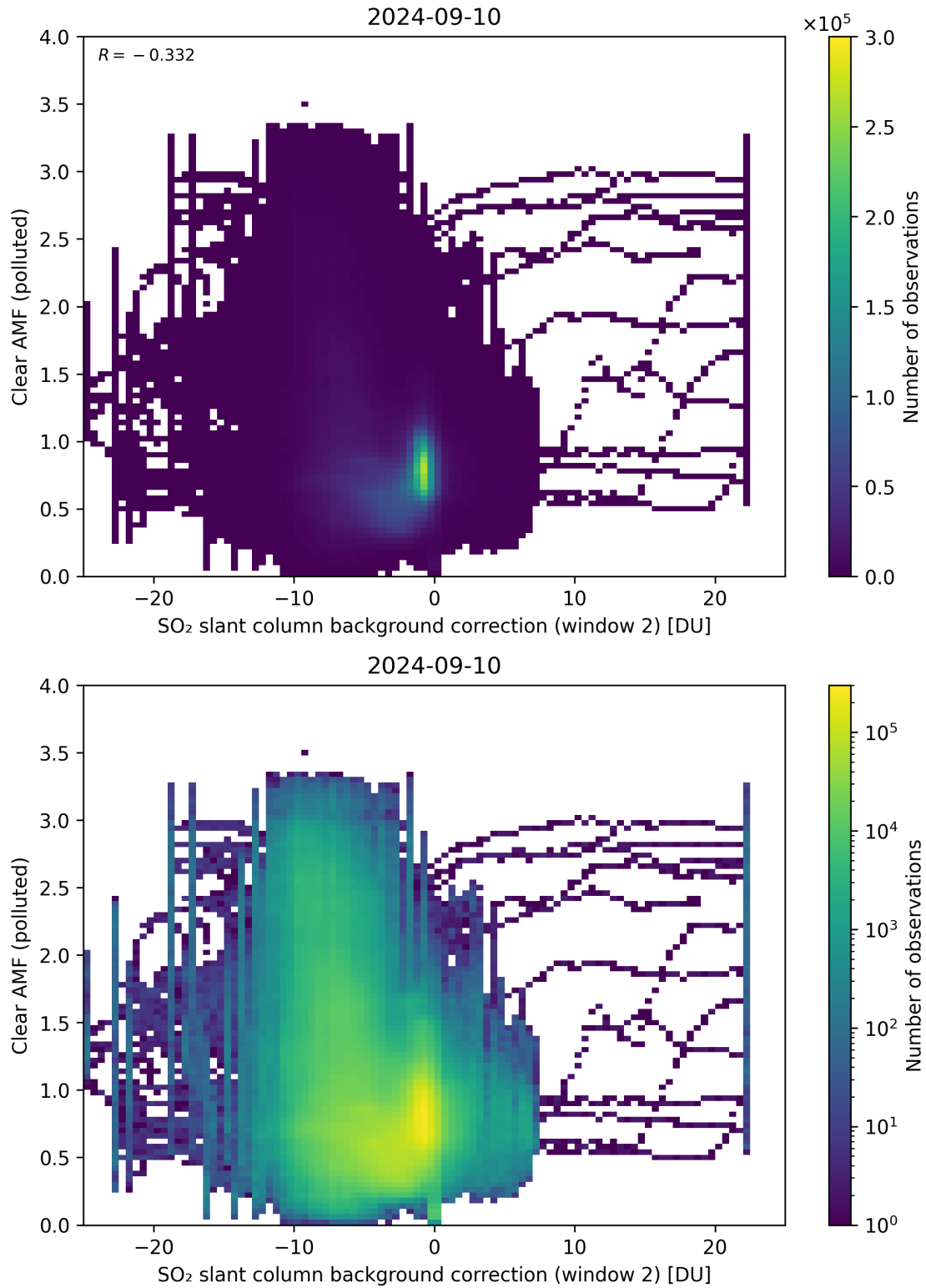
Figure 115: Scatter density plot of “SO 2 slant column background correction (window 2)” against “Clear AMF (polluted)” for 2024-09-09 to 2024-09-11.
