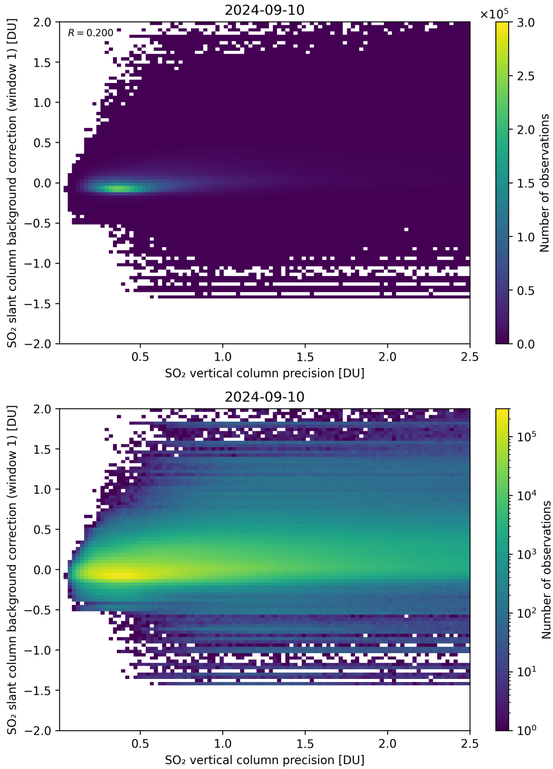
Figure 279: Scatter density plot of “SO 2 vertical column precision” against “SO 2 slant column background correction (window 1)” for 2024-09-09 to 2024-09-11.
