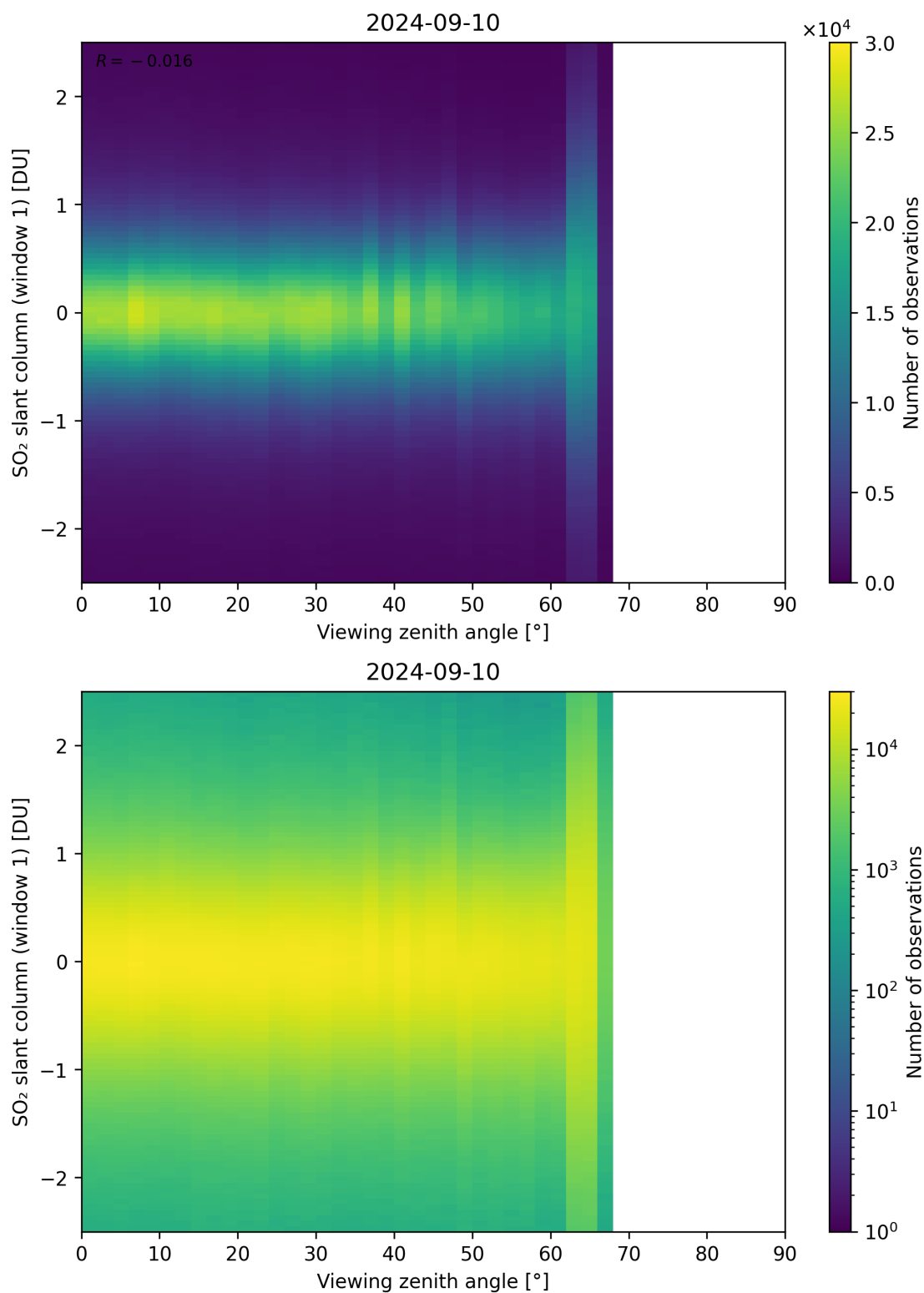
Figure 320: Scatter density plot of “Viewing zenith angle” against “SO 2 slant column (window 1)” for 2024-09-09 to 2024-09-11.
