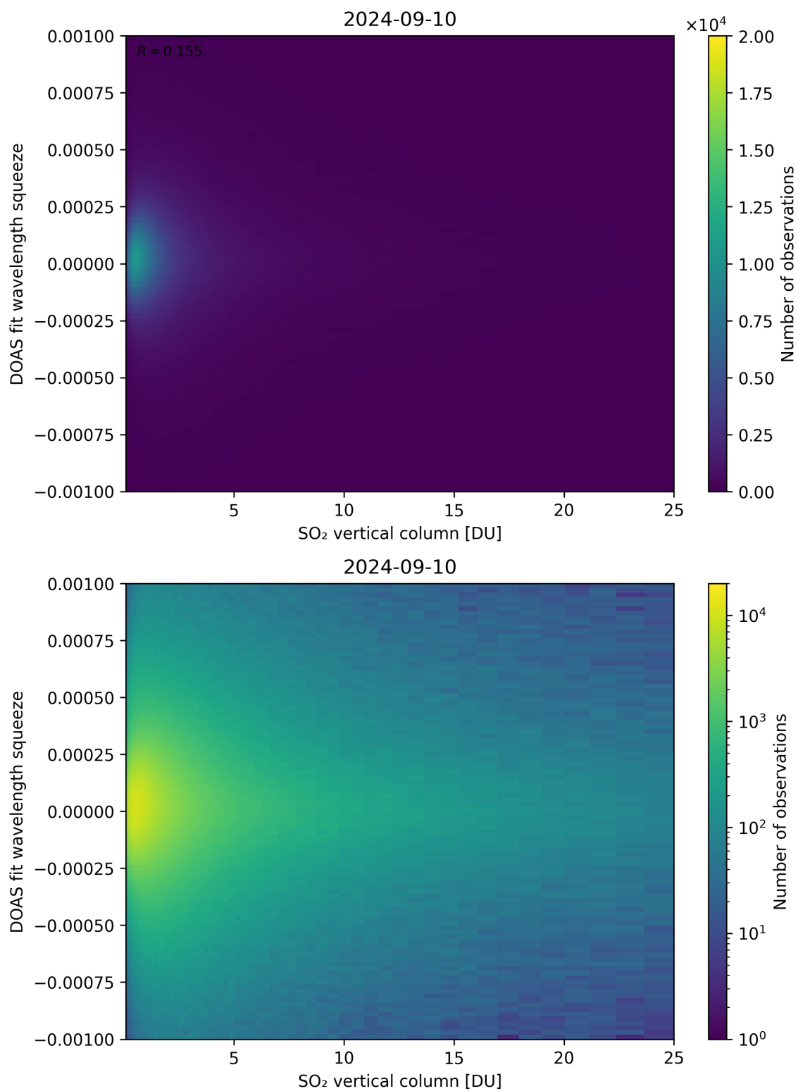
Figure 277: Scatter density plot of “SO 2 vertical column” against “DOAS fit wavelength squeeze” for 2024-09-09 to 2024-09-11.
