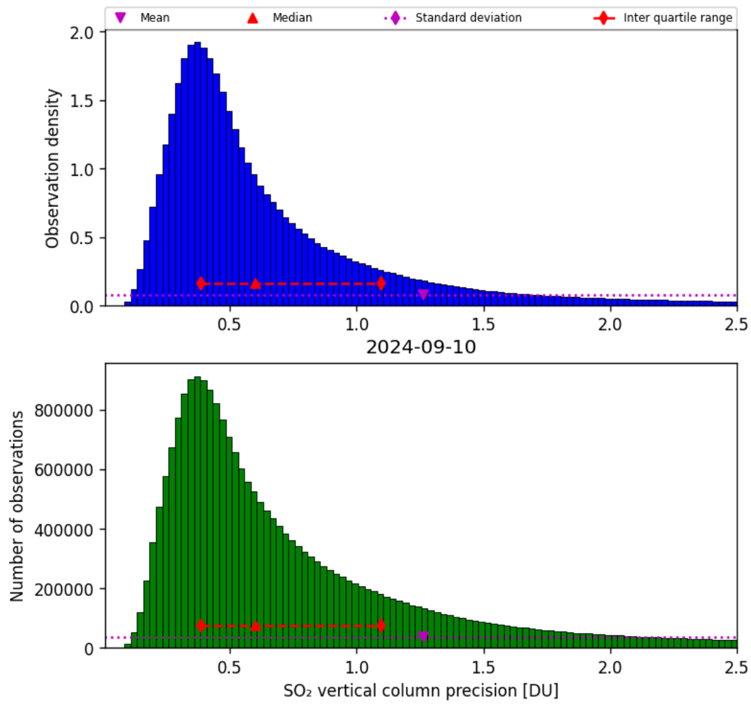
Figure 54: Histogram of “SO 2 vertical column precision” for 2024-09-09 to 2024-09-11
