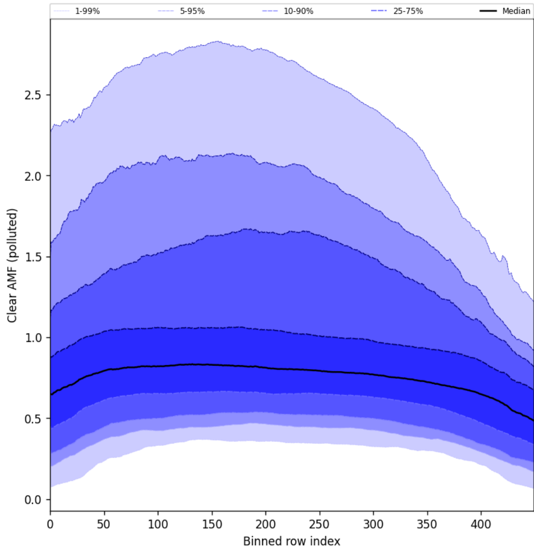
Figure 96: Along track statistics of “Clear AMF (polluted)” for 2024-09-09 to 2024-09-11
