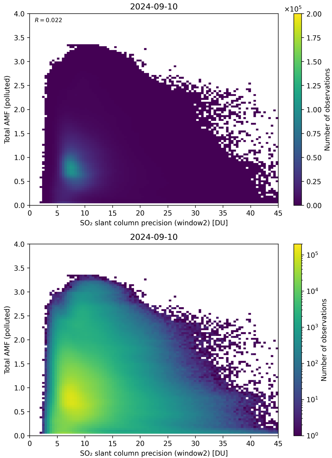
Figure 251: Scatter density plot of “SO 2 slant column precision (window2)” against “Total AMF (polluted)” for 2024-09-09 to 2024-09-11.
