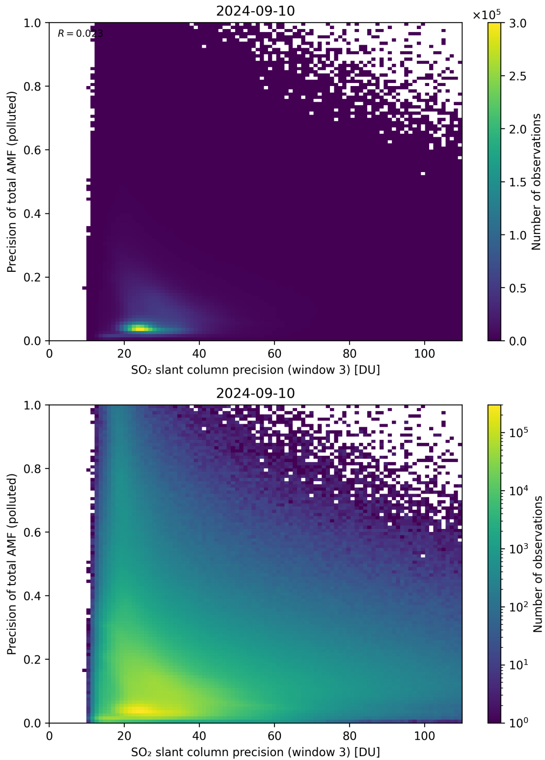
Figure 264: Scatter density plot of “SO 2 slant column precision (window 3)” against “Precision of total AMF (polluted)” for 2024-09-09 to 2024-09-11.
