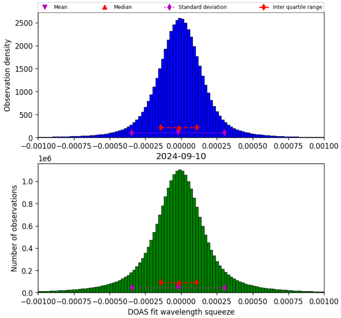
Figure 69: Histogram of “DOAS fit wavelength squeeze” for 2024-09-09 to 2024-09-11
