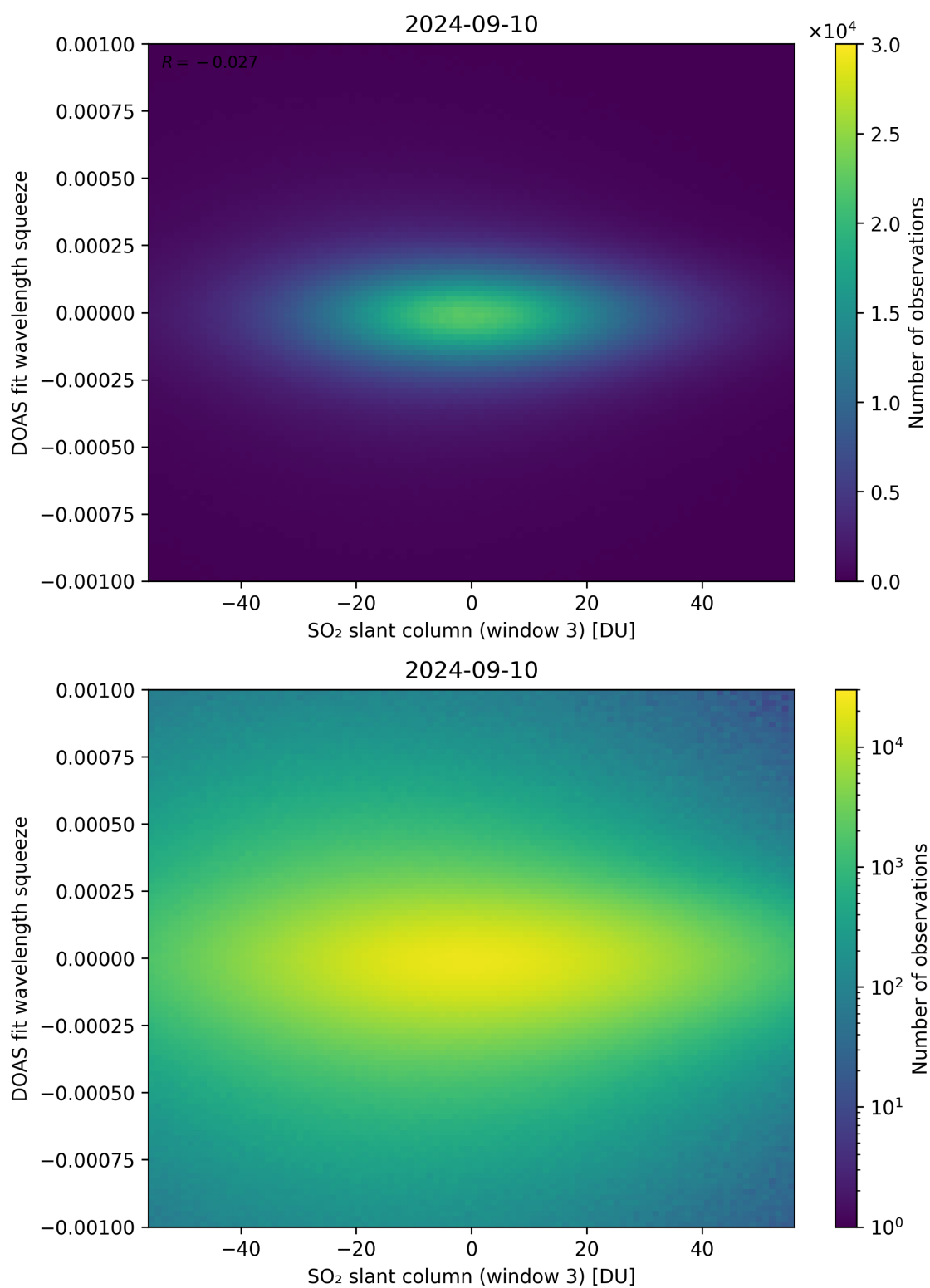
Figure 255: Scatter density plot of “SO 2 slant column (window 3)” against “DOAS fit wavelength squeeze” for 2024-09-09 to 2024-09-11.
