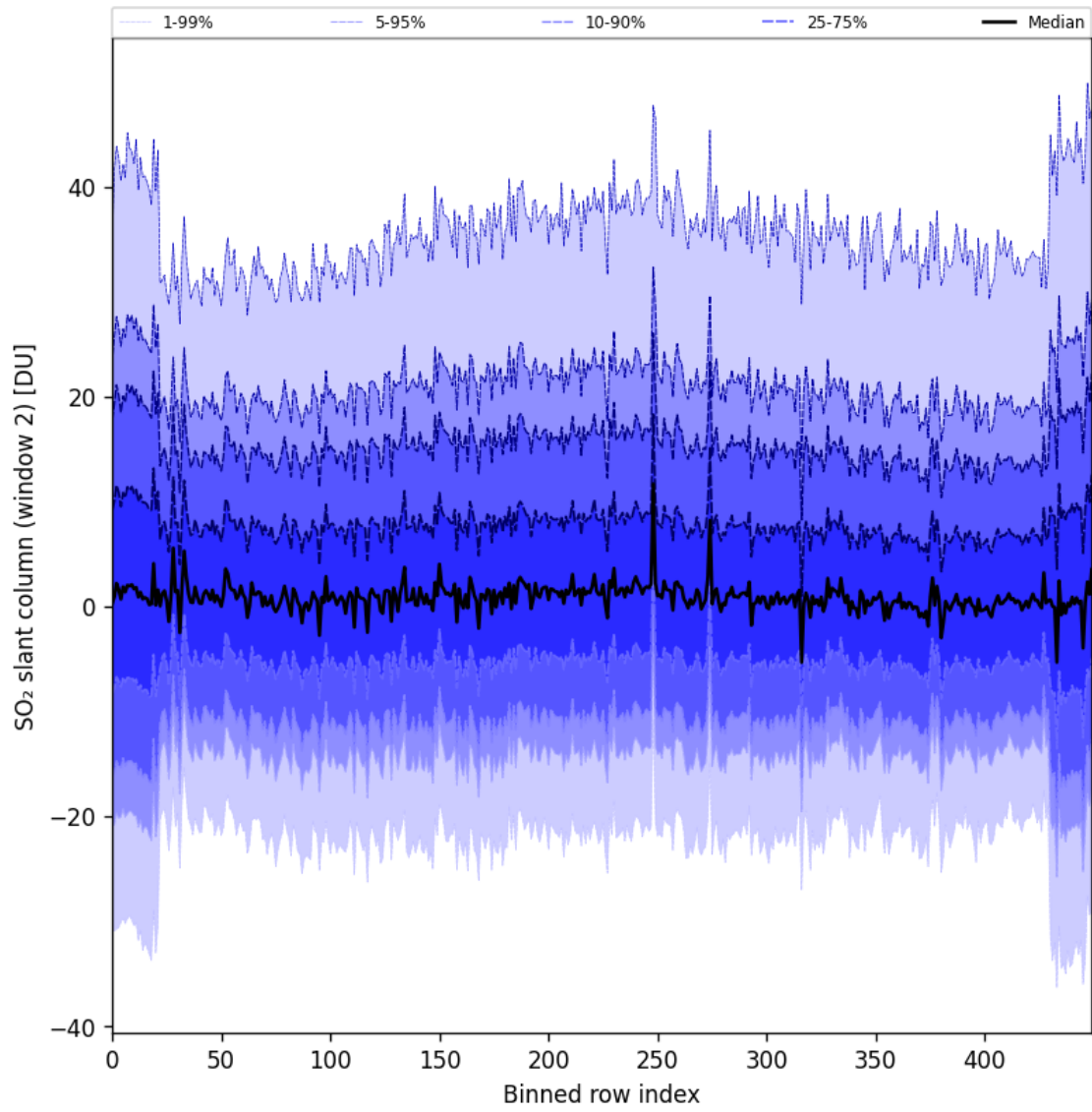
Figure 83: Along track statistics of “SO 2 slant column (window 2)” for 2024-09-09 to 2024-09-11
