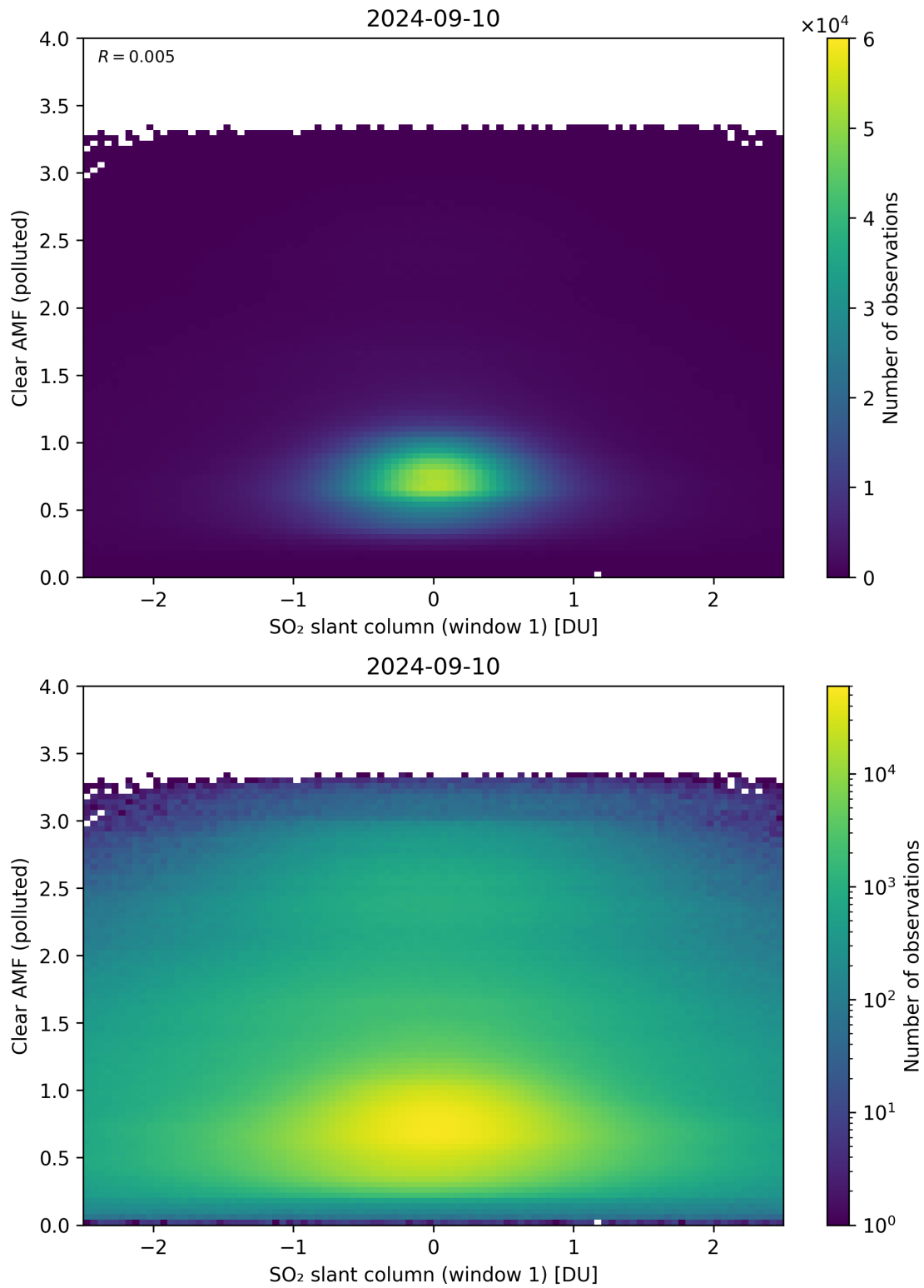
Figure 232: Scatter density plot of “SO 2 slant column (window 1)” against “Clear AMF (polluted)” for 2024-09-09 to 2024-09-11.
