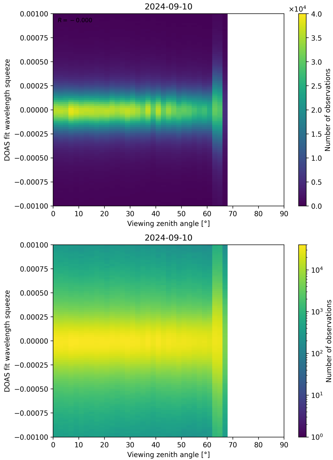
Figure 312: Scatter density plot of “Viewing zenith angle” against “DOAS fit wavelength squeeze” for 2024-09-09 to 2024-09-11.
