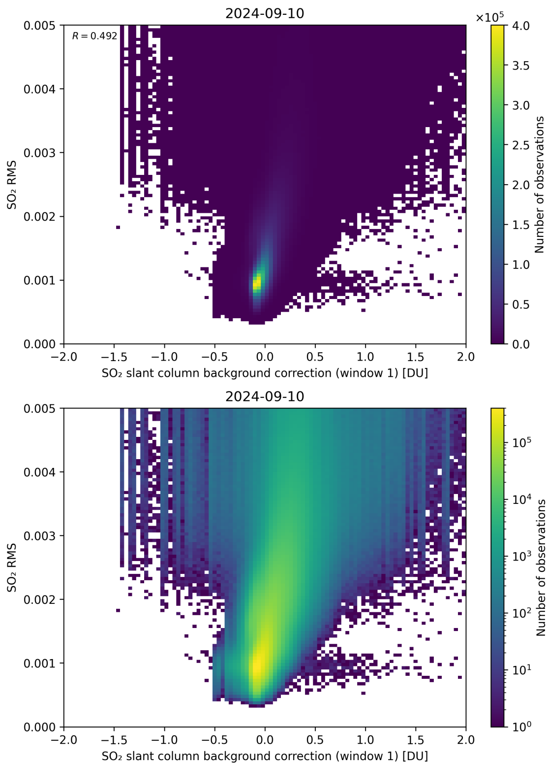
Figure 102: Scatter density plot of “SO 2 slant column background correction (window 1)” against “SO 2 RMS” for 2024-09-09 to 2024-09-11.
