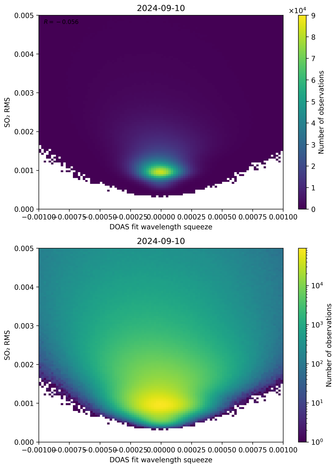
Figure 132: Scatter density plot of “DOAS fit wavelength squeeze” against “SO 2 RMS” for 2024-09-09 to 2024-09-11.
