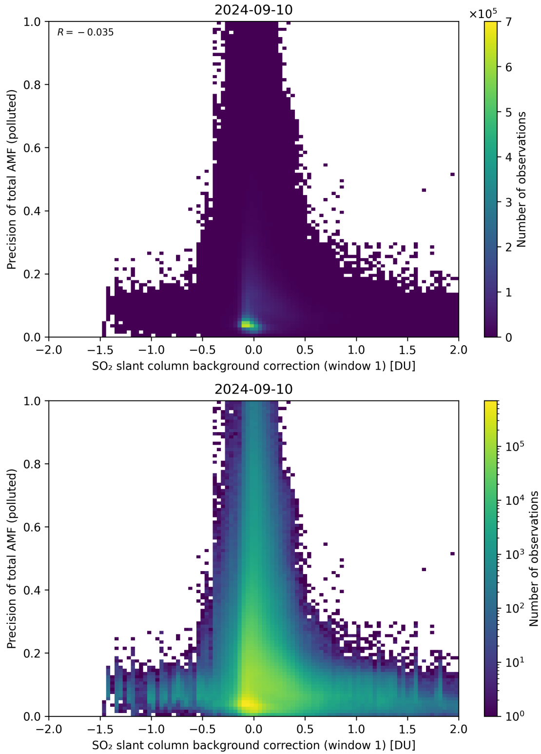
Figure 110: Scatter density plot of “SO 2 slant column background correction (window 1)” against “Precision of total AMF (polluted)” for 2024-09-09 to 2024-09-11.
