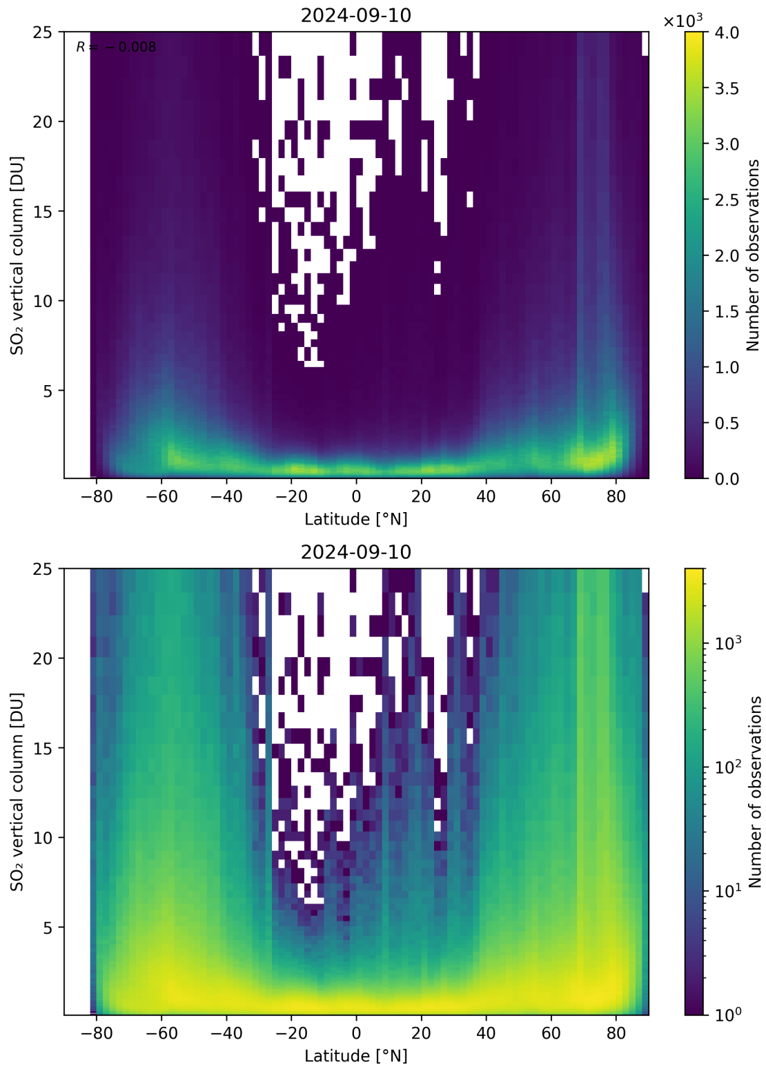
Figure 156: Scatter density plot of “Latitude” against “SO 2 vertical column” for 2024-09-09 to 2024-09-11.
