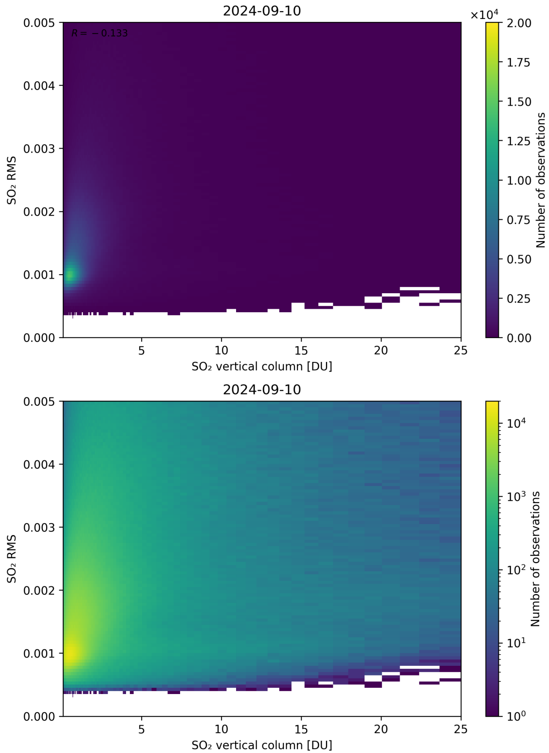
Figure 278: Scatter density plot of “SO 2 vertical column” against “SO 2 RMS” for 2024-09-09 to 2024-09-11.
