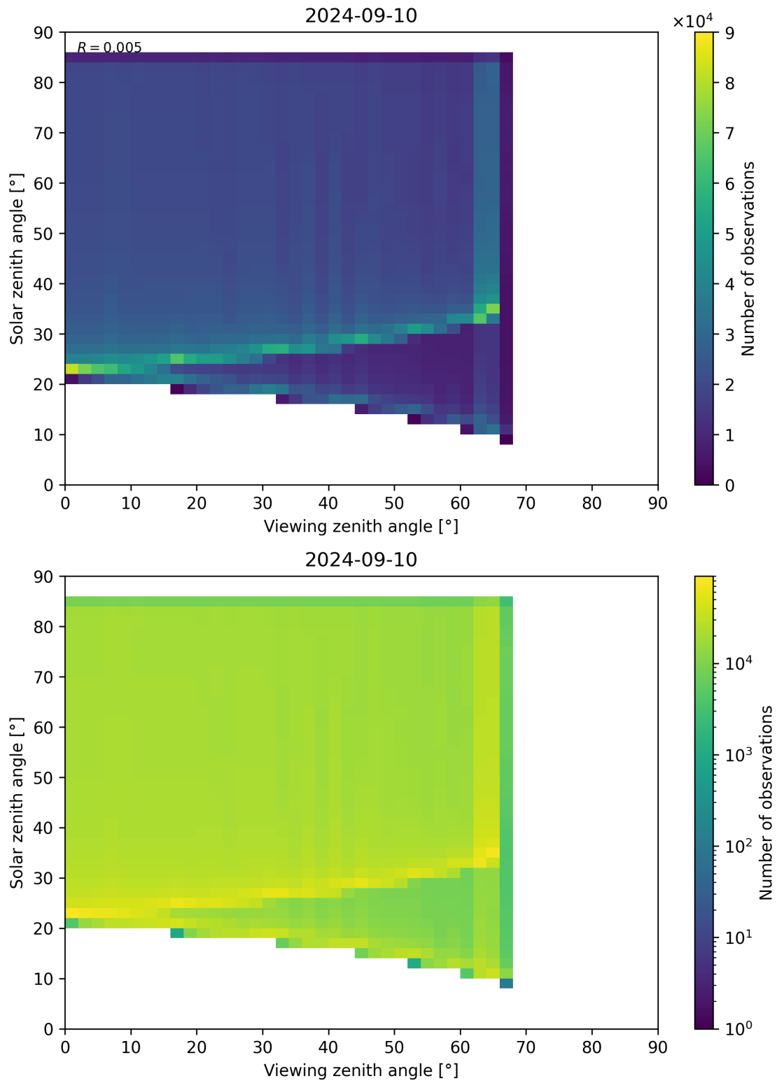
Figure 315: Scatter density plot of “Viewing zenith angle” against “Solar zenith angle” for 2024-09-09 to 2024-09-11.
