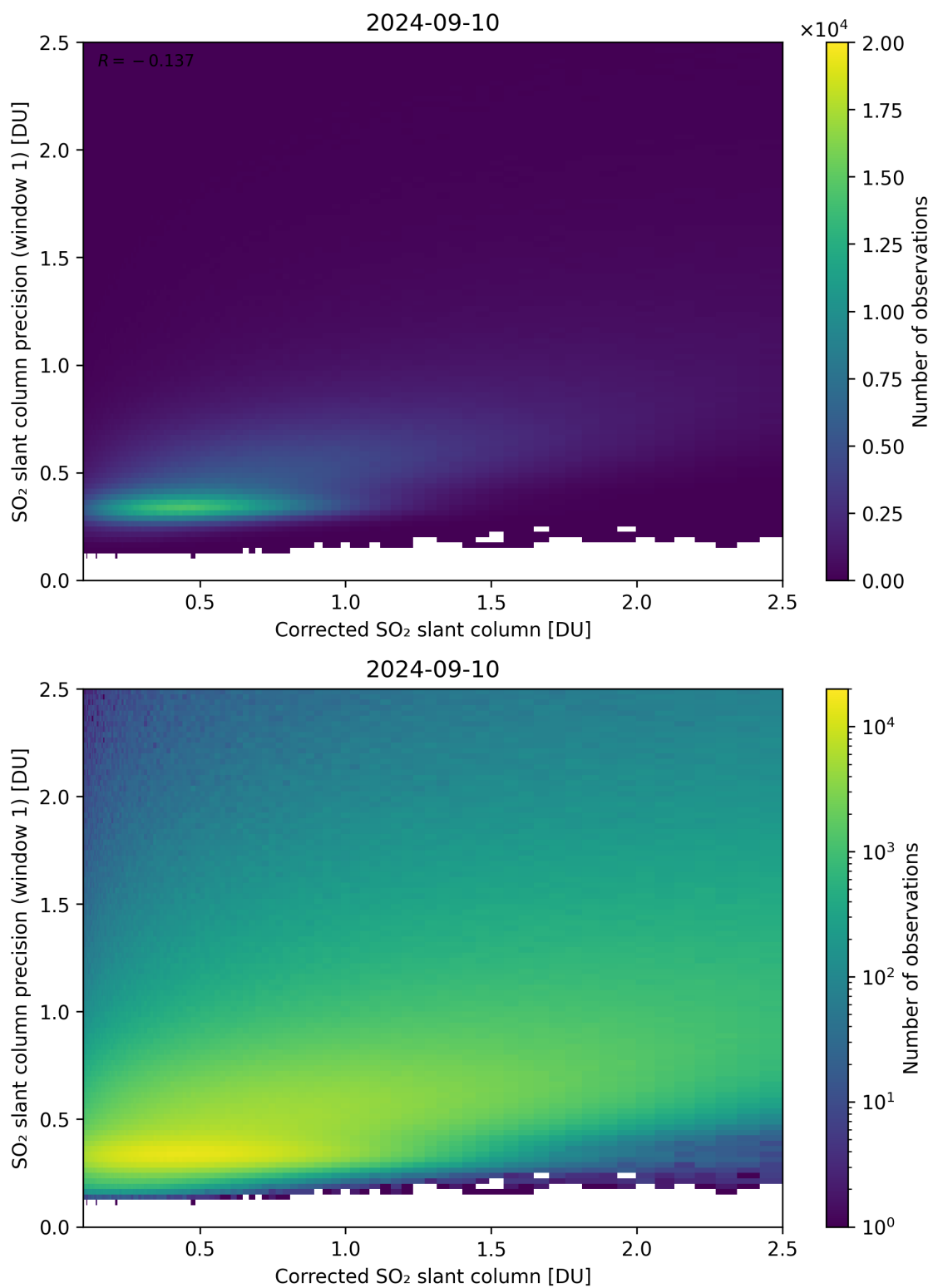
Figure 188: Scatter density plot of “Corrected SO 2 slant column” against “SO 2 slant column precision (window 1)” for 2024-09-09 to 2024-09-11.
