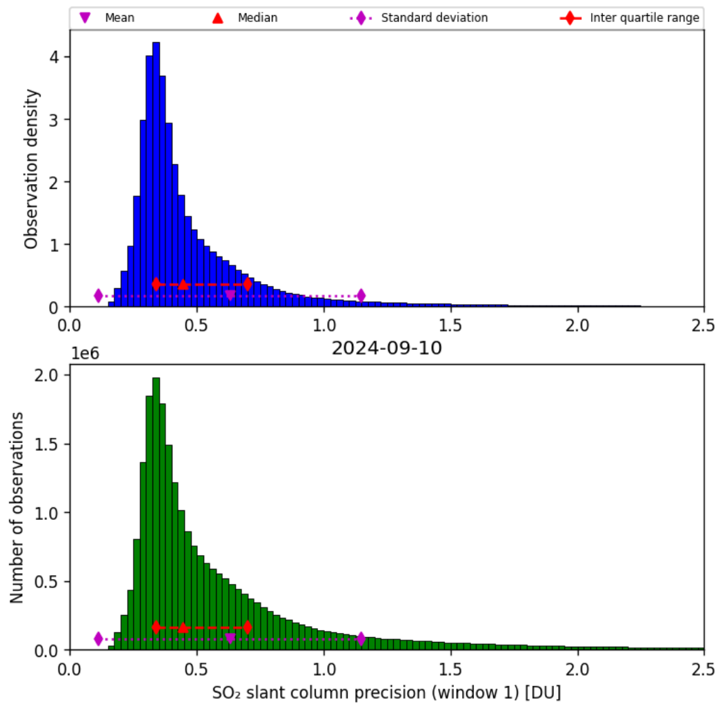
Figure 57: Histogram of “SO 2 slant column precision (window 1)” for 2024-09-09 to 2024-09-11
