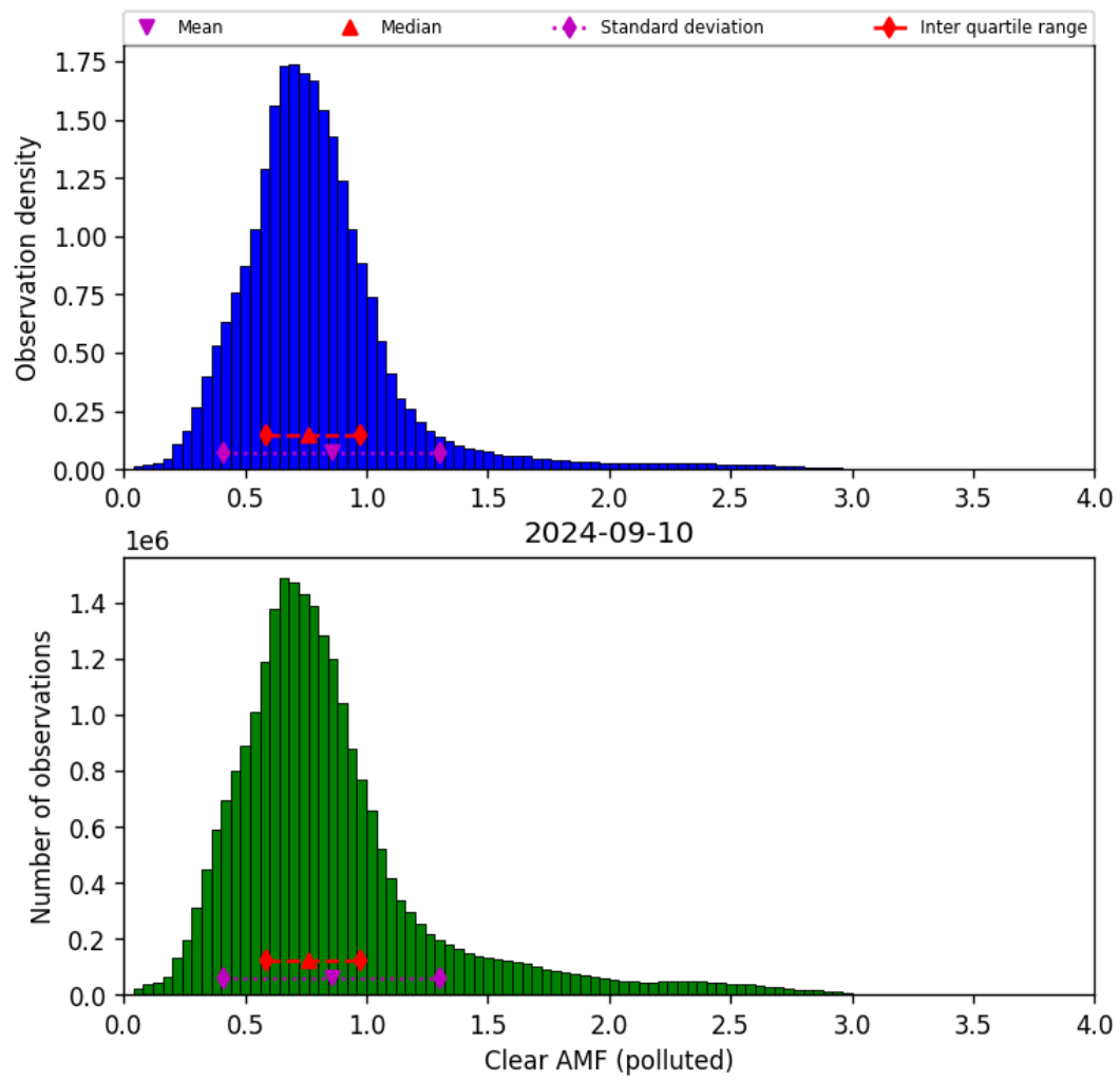
Figure 73: Histogram of “Clear AMF (polluted)” for 2024-09-09 to 2024-09-11
