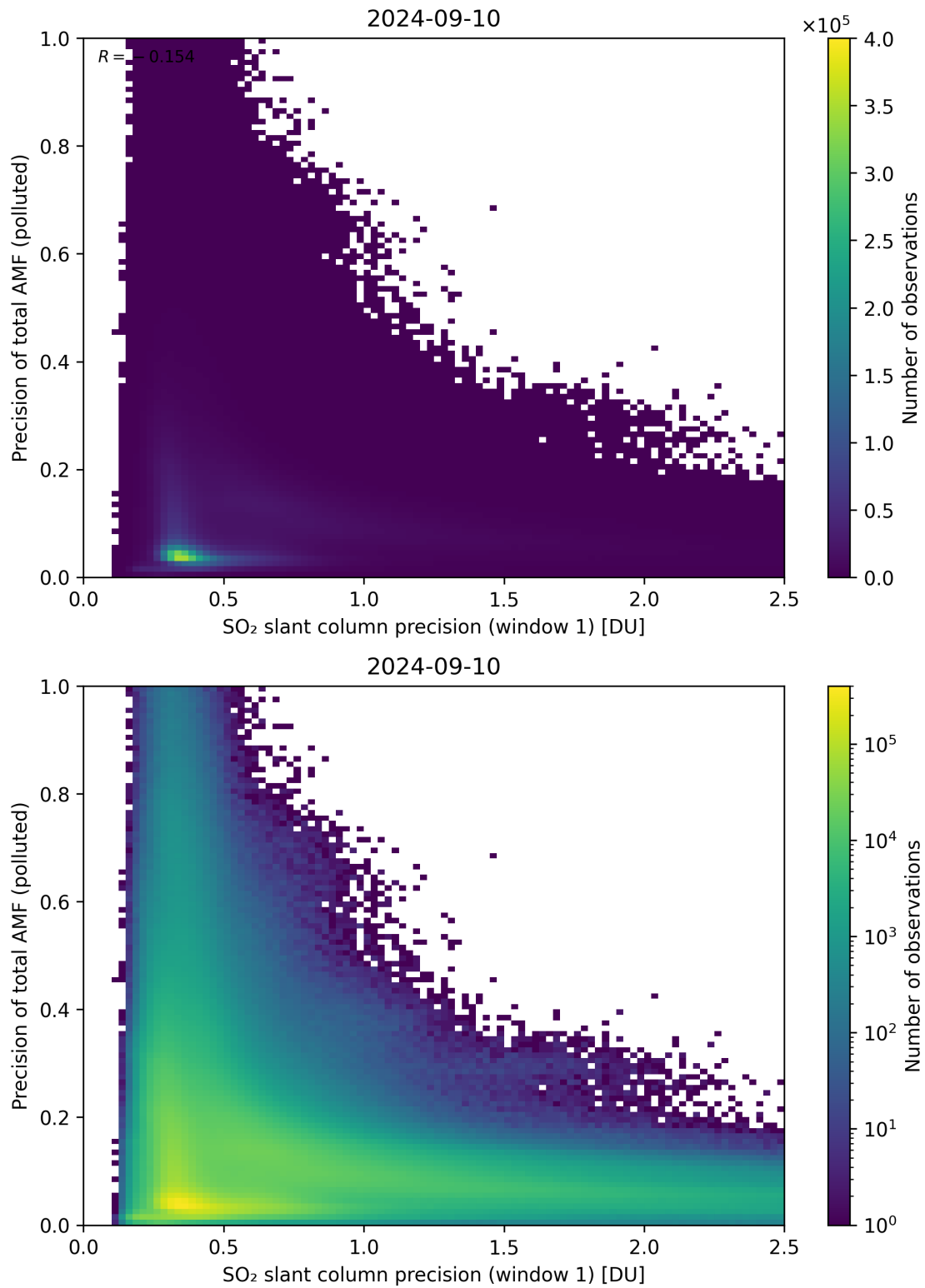
Figure 231: Scatter density plot of “SO 2 slant column precision (window 1)” against “Precision of total AMF (polluted)” for 2024-09-09 to 2024-09-11.
