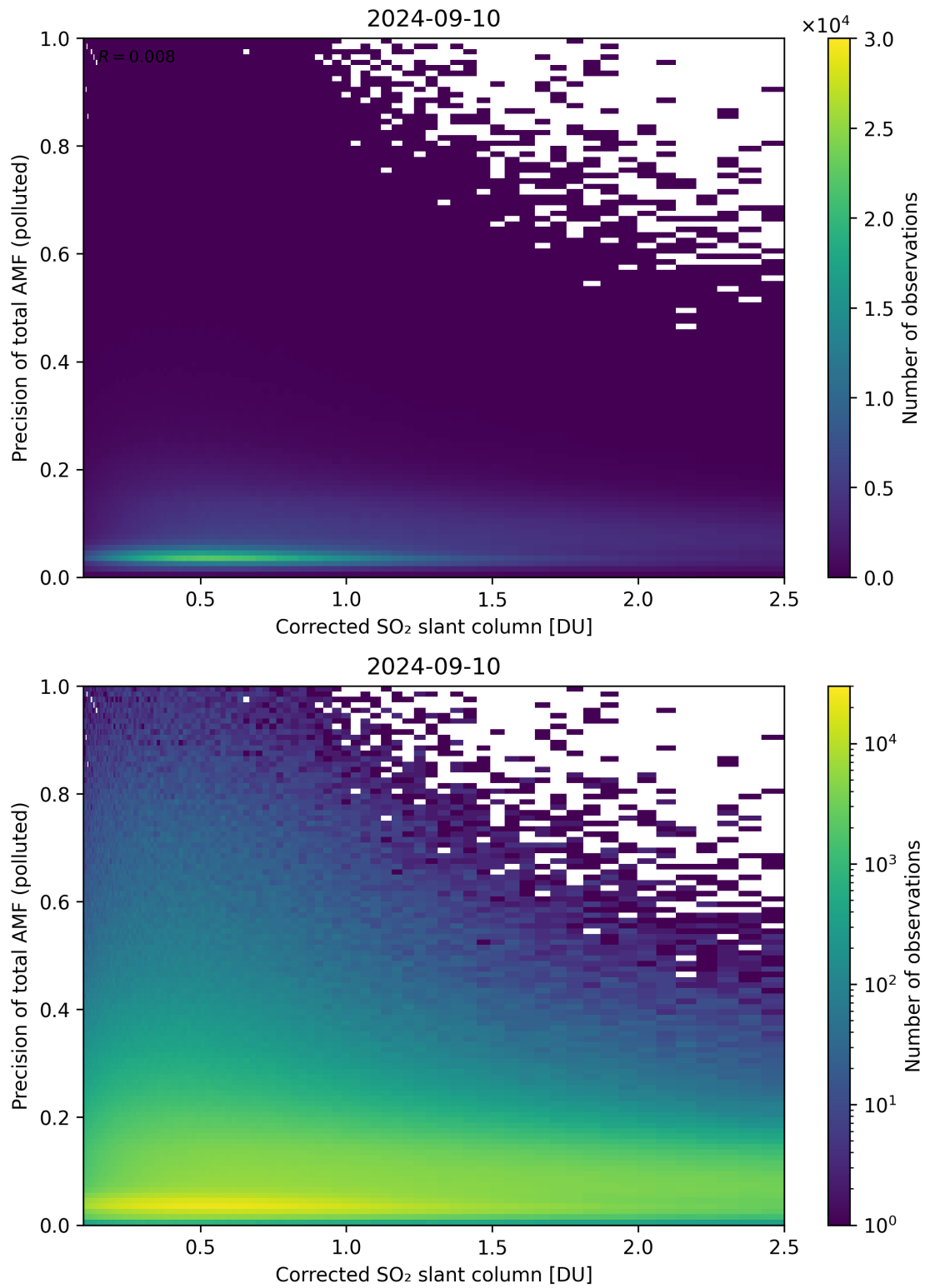
Figure 193: Scatter density plot of “Corrected SO 2 slant column” against “Precision of total AMF (polluted)” for 2024-09-09 to 2024-09-11.
