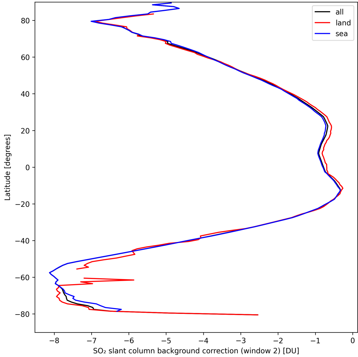
Figure 40: Zonal average of “SO 2 slant column background correction (window 2)” for 2024-09-09 to 2024-09-11.
