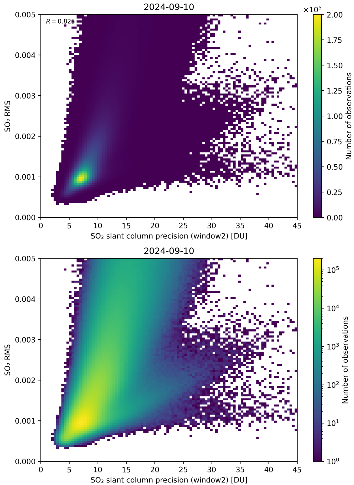
Figure 245: Scatter density plot of “SO 2 slant column precision (window2)” against “SO 2 RMS” for 2024-09-09 to 2024-09-11.
