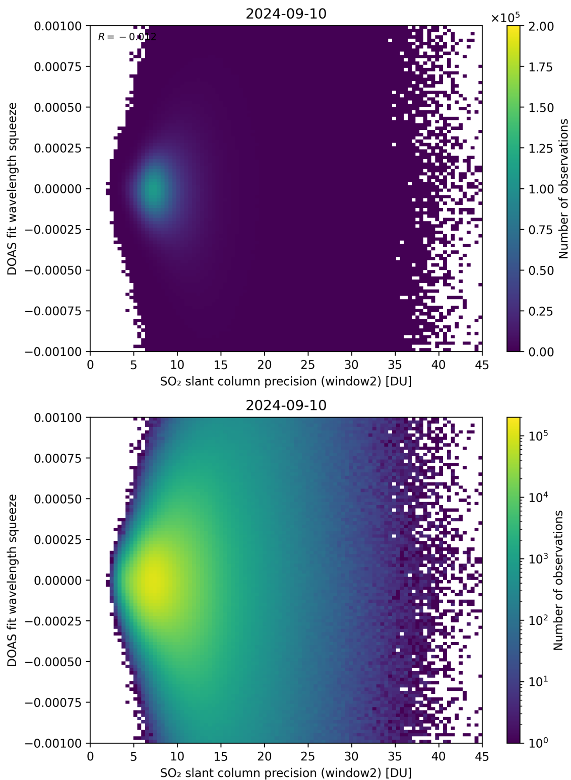
Figure 244: Scatter density plot of “SO 2 slant column precision (window2)” against “DOAS fit wavelength squeeze” for 2024-09-09 to 2024-09-11.
