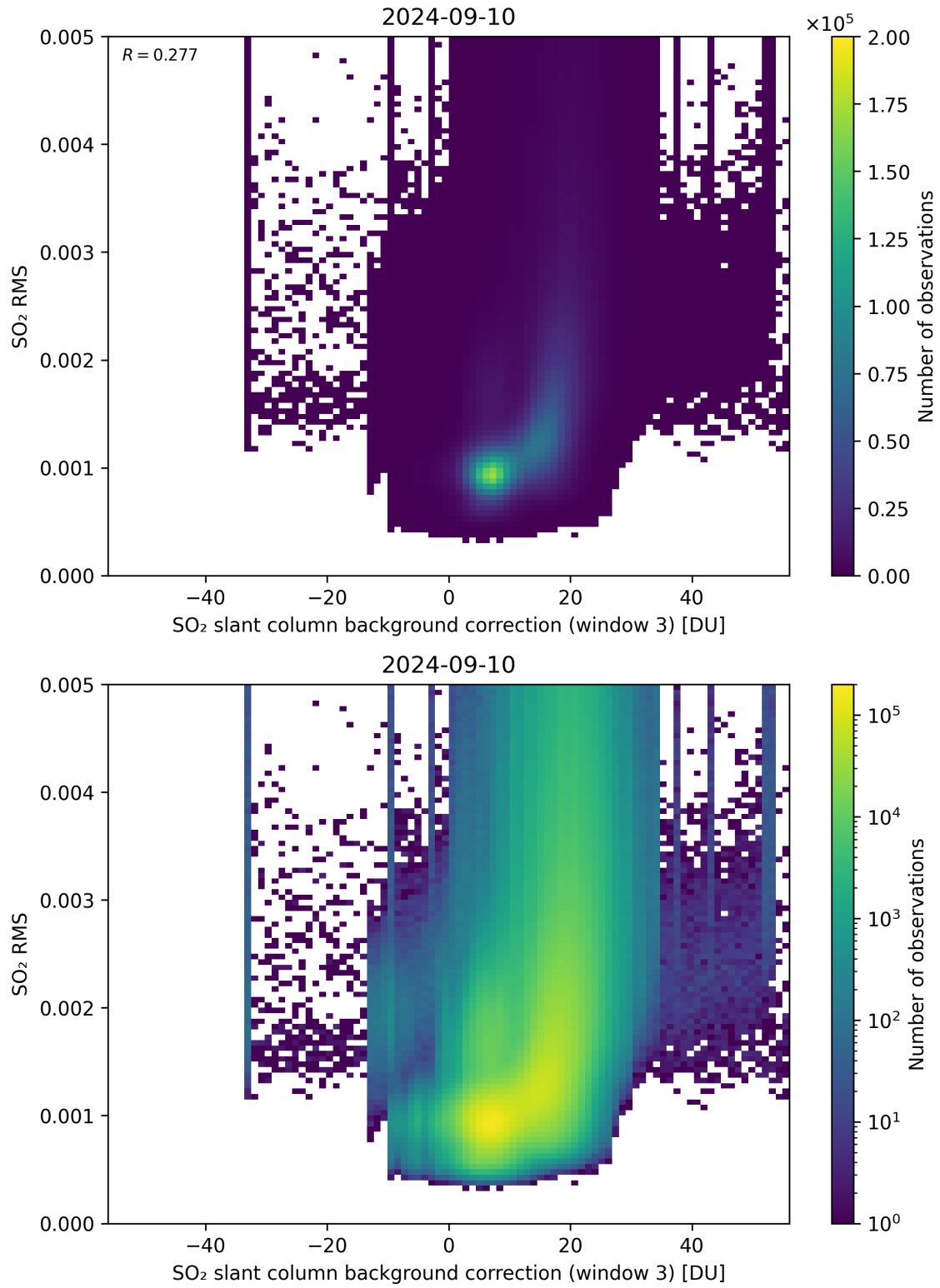
Figure 123: Scatter density plot of “SO 2 slant column background correction (window 3)” against “SO 2 RMS” for 2024-09-09 to 2024-09-11.
