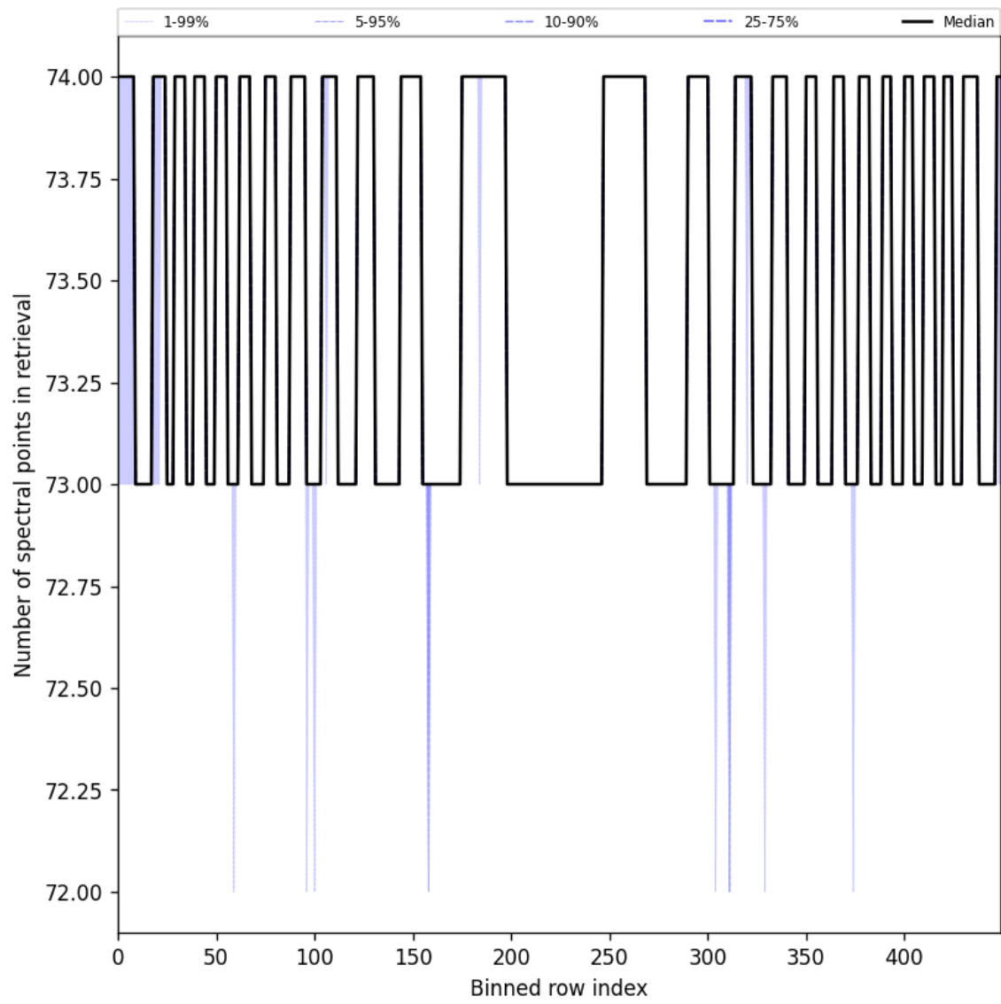
Figure 97: Along track statistics of “Number of spectral points in retrieval” for 2024-09-09 to 2024-09-11
