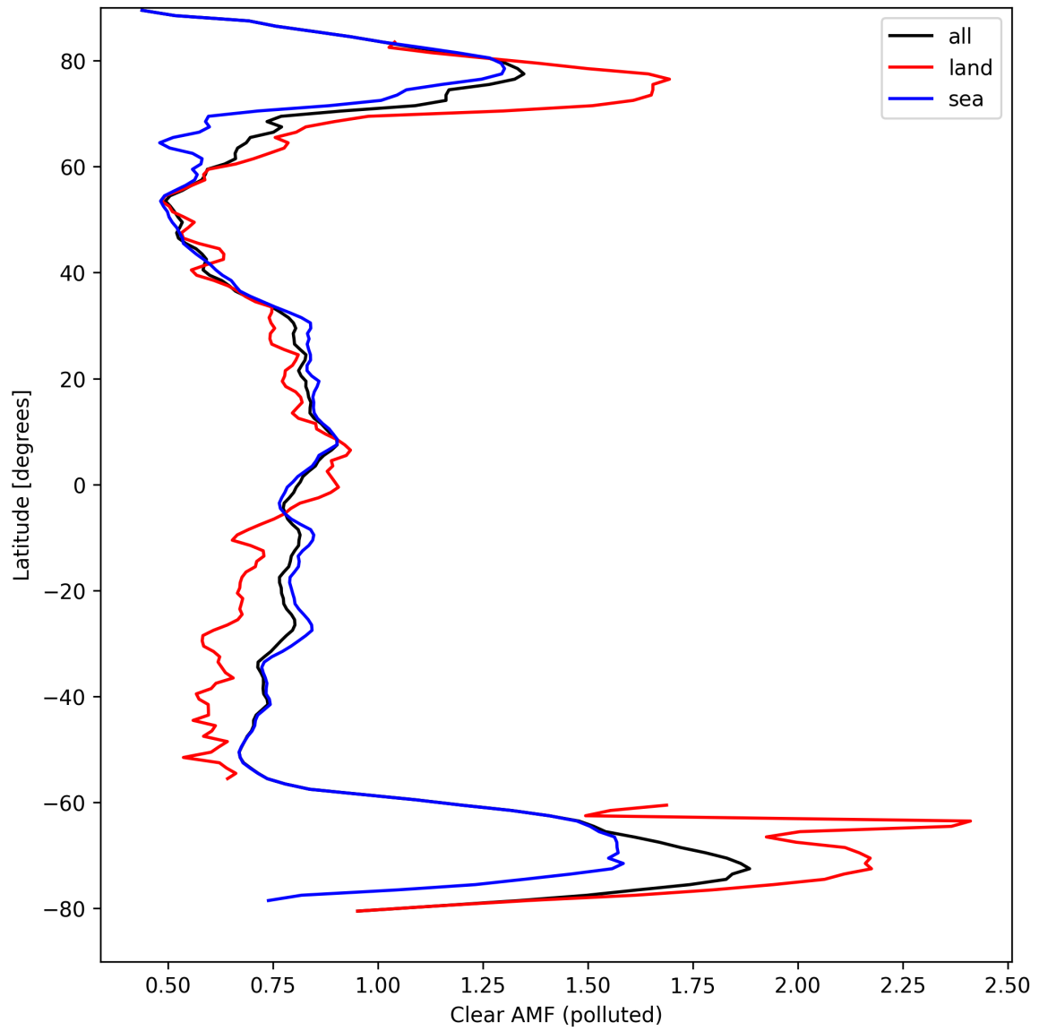
Figure 50: Zonal average of “Clear AMF (polluted)” for 2024-09-09 to 2024-09-11.
