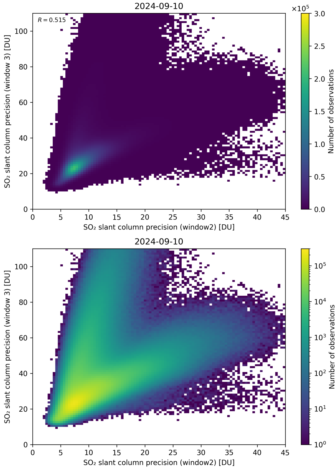
Figure 250: Scatter density plot of “SO 2 slant column precision (window2)” against “SO 2 slant column precision (window 3)” for 2024-09-09 to 2024-09-11.
