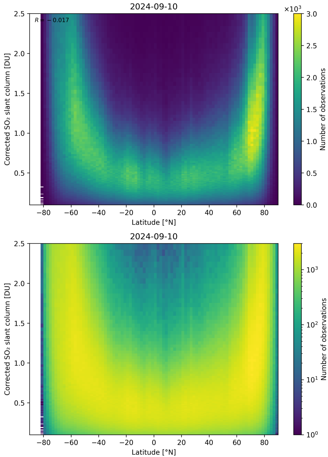
Figure 146: Scatter density plot of “Latitude” against “Corrected SO 2 slant column” for 2024-09-09 to 2024-09-11.
