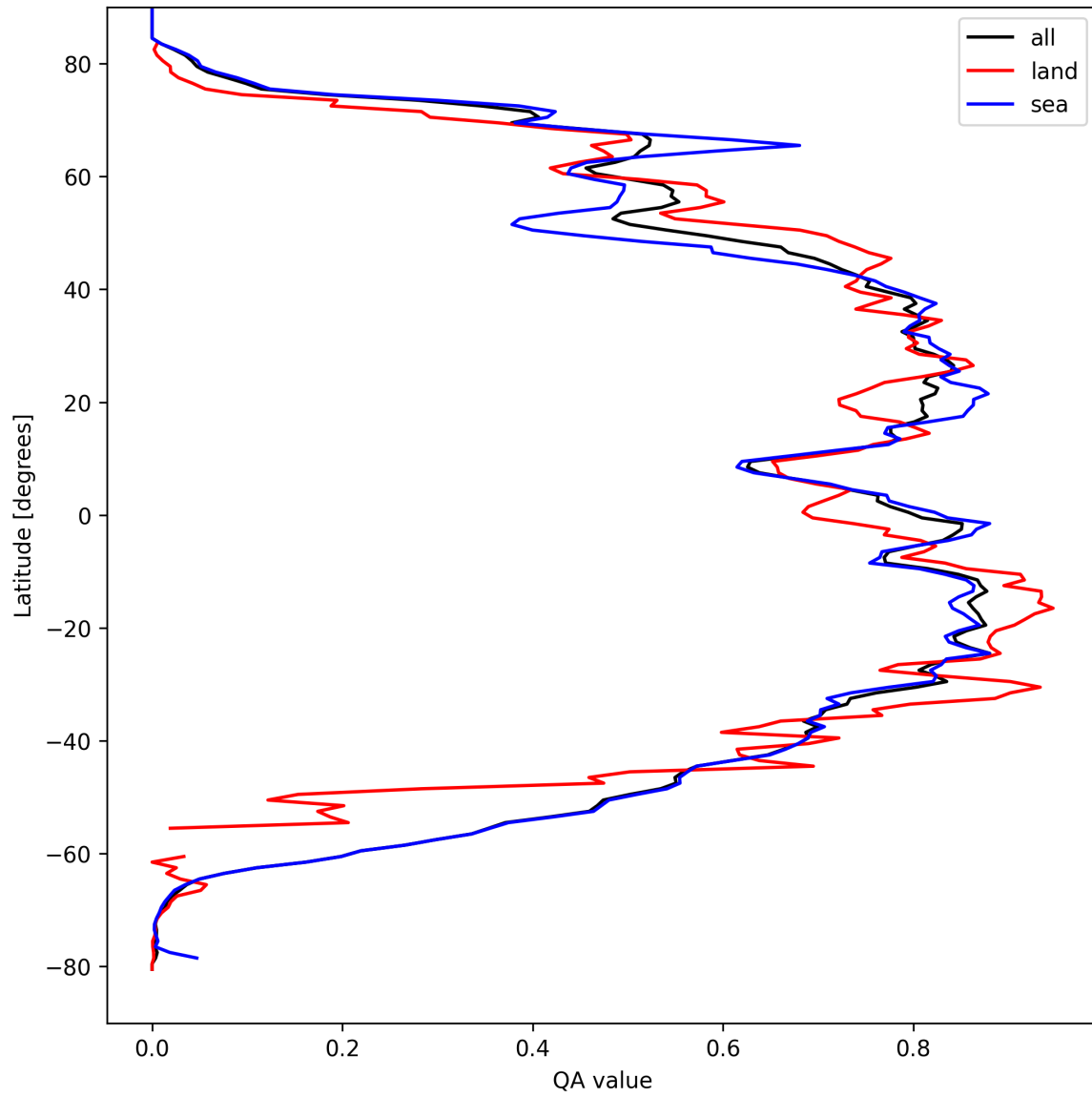
Figure 29: Zonal average of “QA value” for 2024-09-09 to 2024-09-11.
