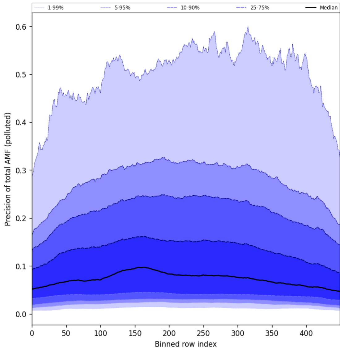
Figure 95: Along track statistics of “Precision of total AMF (polluted)” for 2024-09-09 to 2024-09-11
