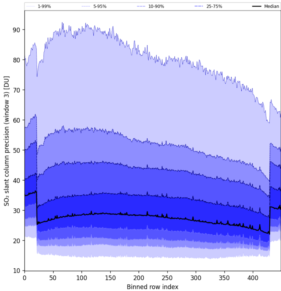
Figure 88: Along track statistics of “SO 2 slant column precision (window 3)” for 2024-09-09 to 2024-09-11
