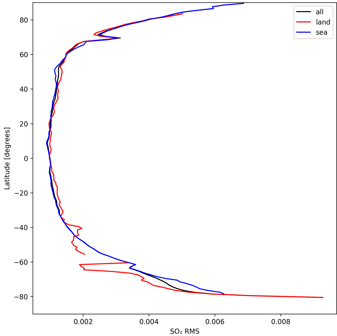
Figure 47: Zonal average of “SO 2 RMS” for 2024-09-09 to 2024-09-11.
