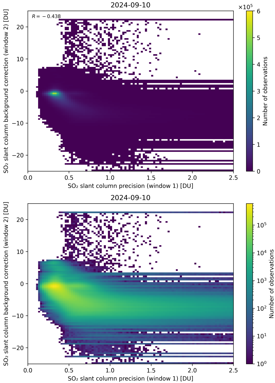
Figure 219: Scatter density plot of “SO 2 slant column precision (window 1)” against “SO 2 slant column background correction (window 2)” for 2024-09-09 to 2024-09-11.
