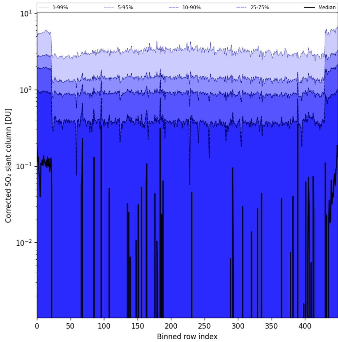
Figure 78: Along track statistics of "Corrected SO 2 slant column" for 2024-09-09 to 2024-09-11
