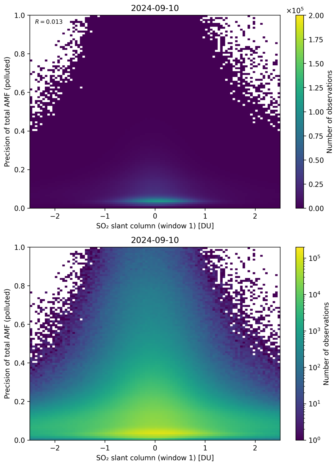
Figure 240: Scatter density plot of “SO 2 slant column (window 1)” against “Precision of total AMF (polluted)” for 2024-09-09 to 2024-09-11.
