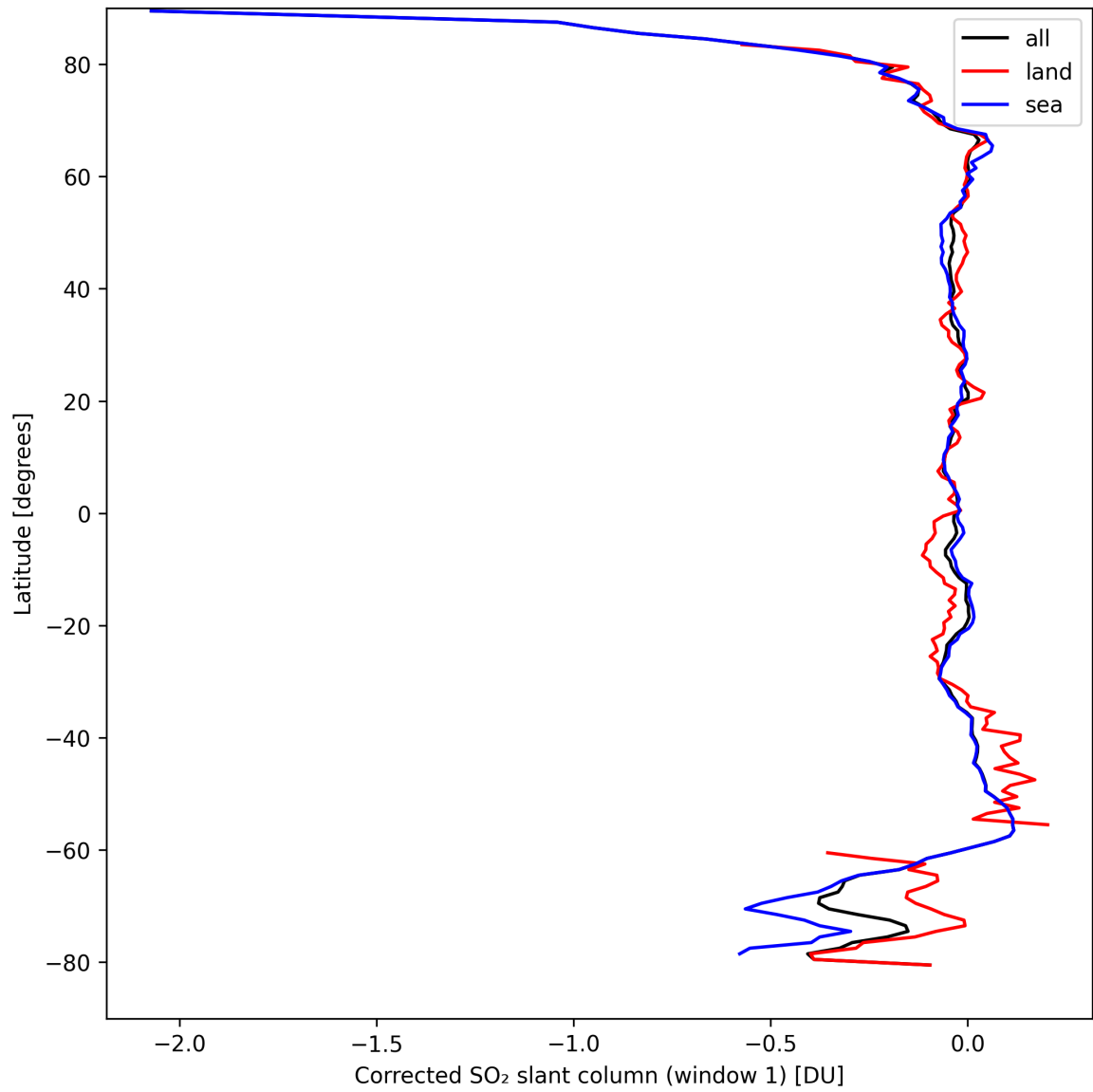
Figure 35: Zonal average of “Corrected SO 2 slant column (window 1)” for 2024-09-09 to 2024-09-11.
