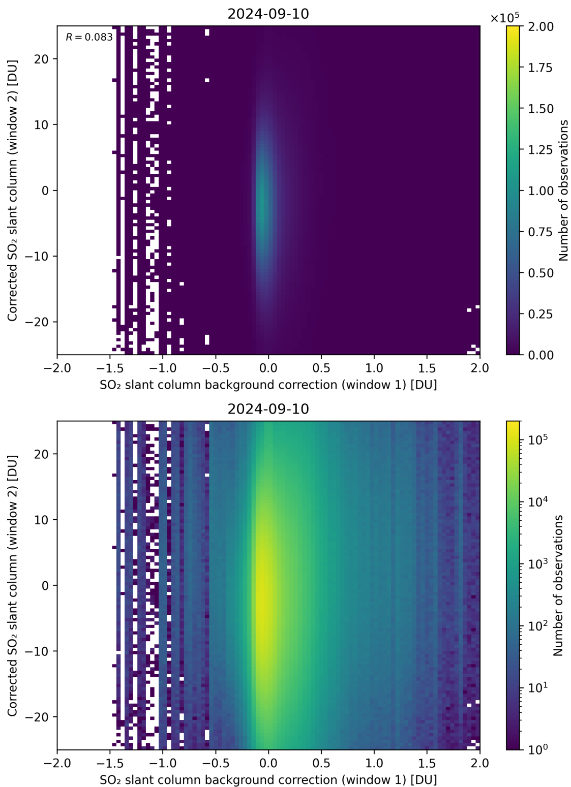
Figure 104: Scatter density plot of “SO 2 slant column background correction (window 1)” against “Corrected SO 2 slant column (window 2)” for 2024-09-09 to 2024-09-11.
