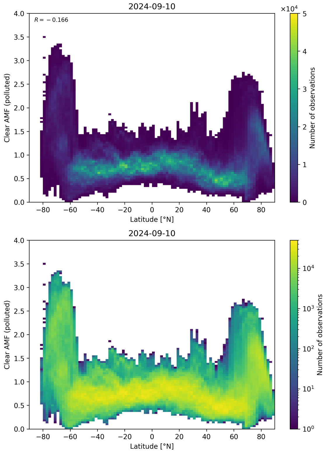
Figure 145: Scatter density plot of “Latitude” against “Clear AMF (polluted)” for 2024-09-09 to 2024-09-11.
