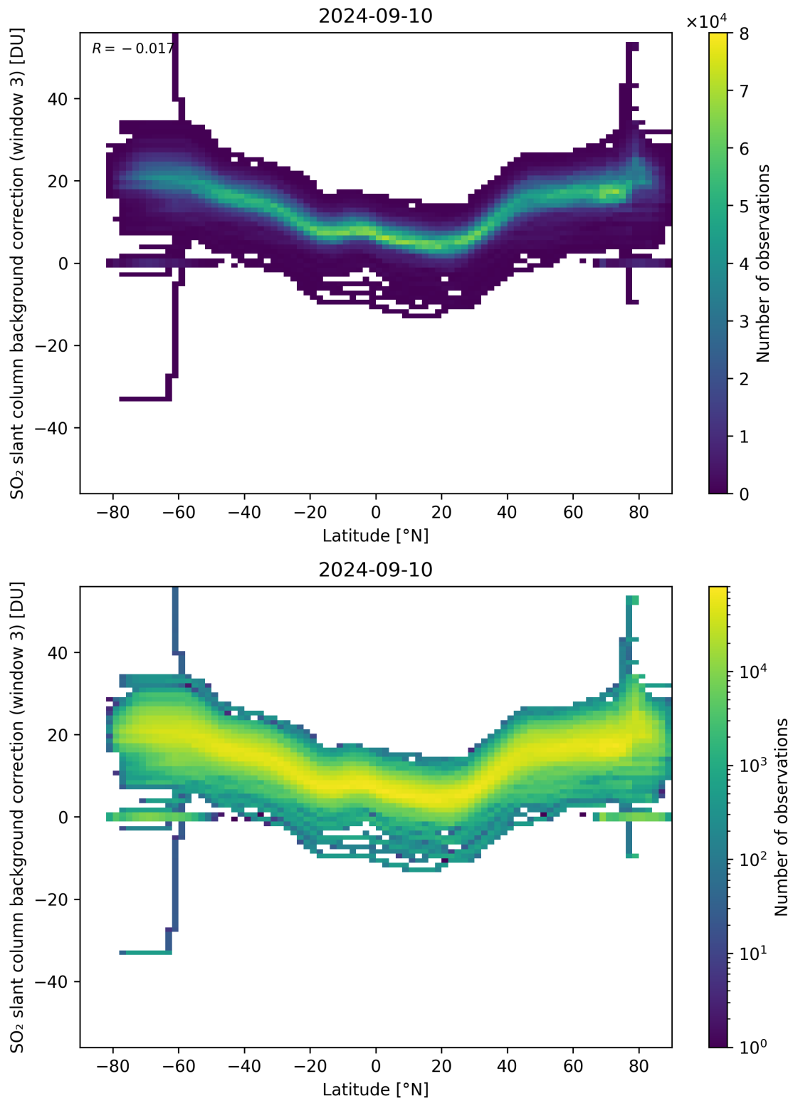
Figure 141: Scatter density plot of “Latitude” against “SO 2 slant column background correction (window 3)” for 2024-09-09 to 2024-09-11.
