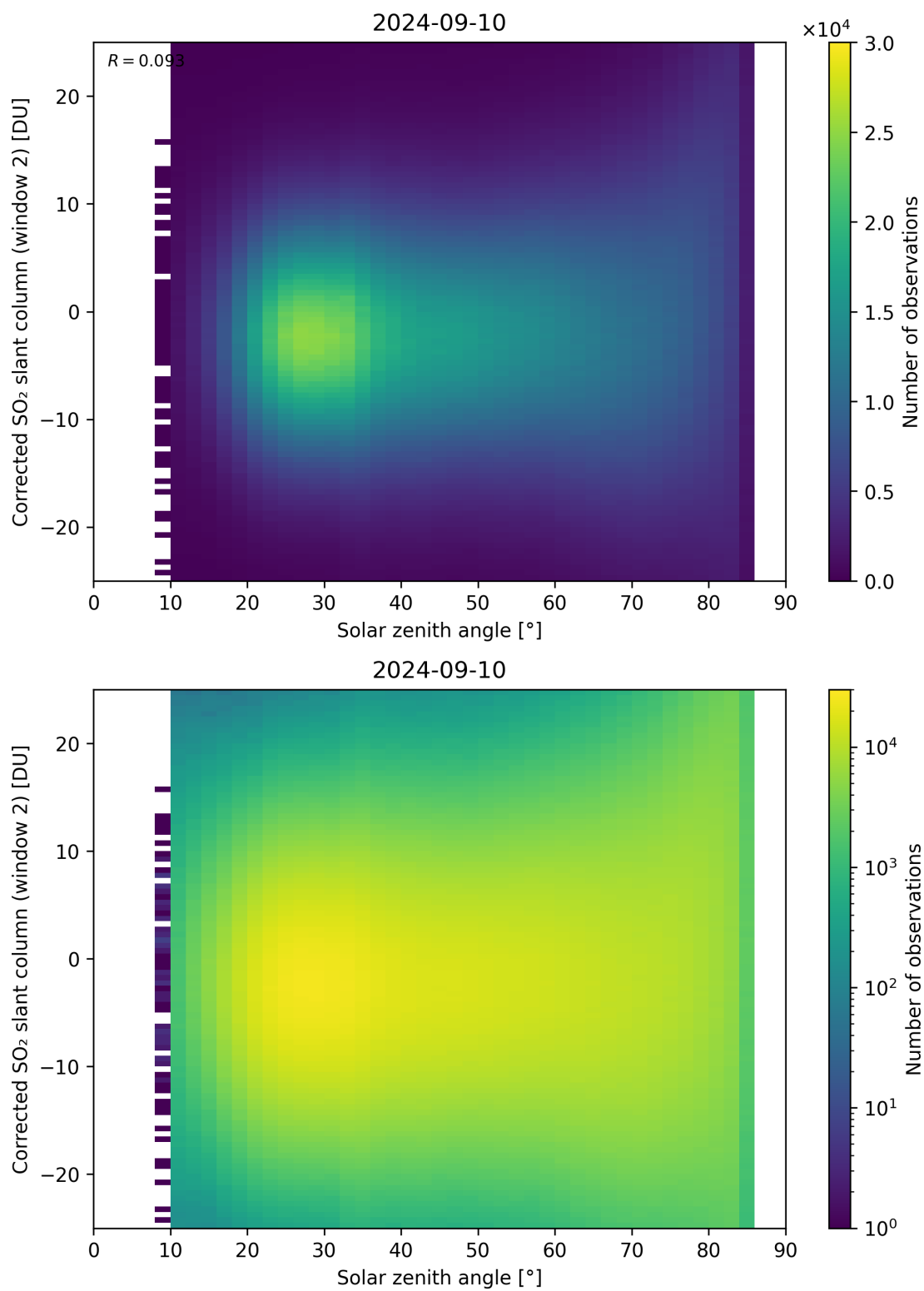
Figure 167: Scatter density plot of “Solar zenith angle” against “Corrected SO 2 slant column (window 2)” for 2024-09-09 to 2024-09-11.
