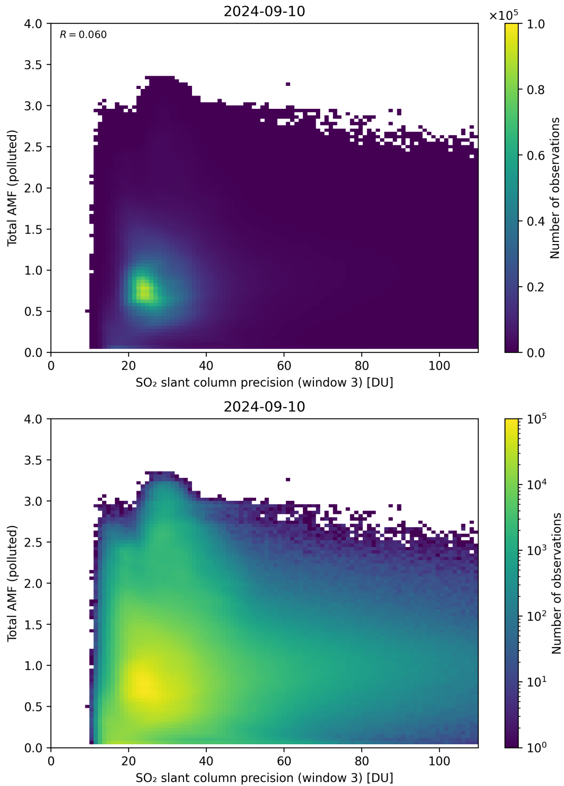
Figure 263: Scatter density plot of “SO 2 slant column precision (window 3)” against “Total AMF (polluted)” for 2024-09-09 to 2024-09-11.
