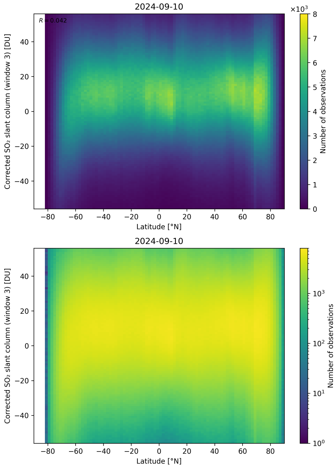
Figure 148: Scatter density plot of “Latitude” against “Corrected SO 2 slant column (window 3)” for 2024-09-09 to 2024-09-11.
