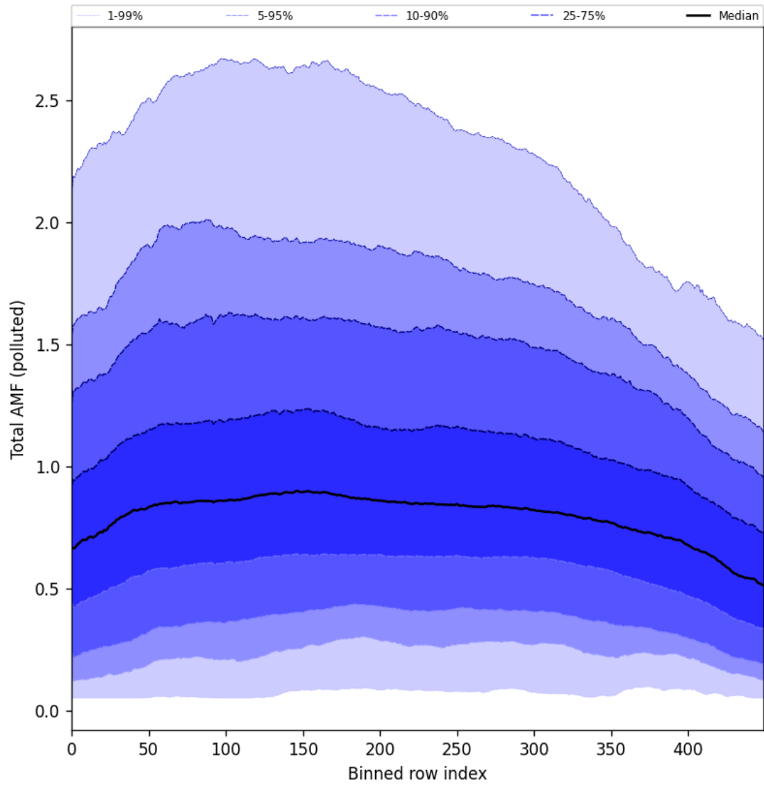
Figure 94: Along track statistics of “Total AMF (polluted)” for 2024-09-09 to 2024-09-11
