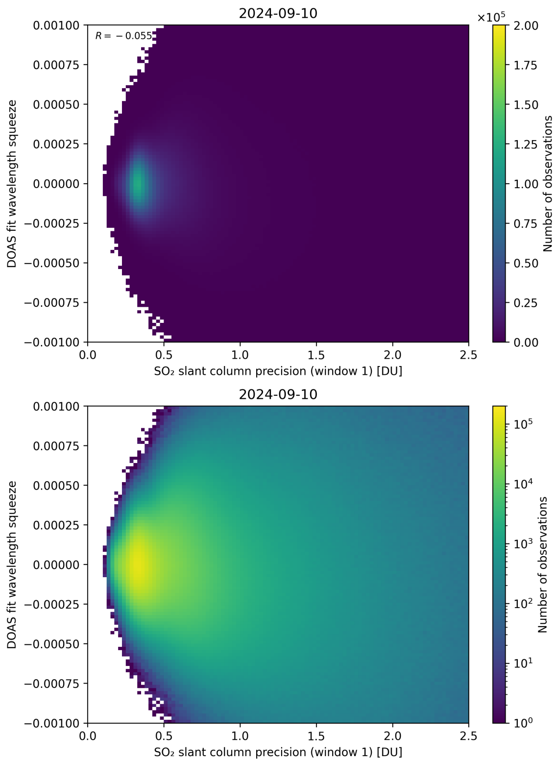
Figure 222: Scatter density plot of “SO 2 slant column precision (window 1)” against “DOAS fit wavelength squeeze” for 2024-09-09 to 2024-09-11.
