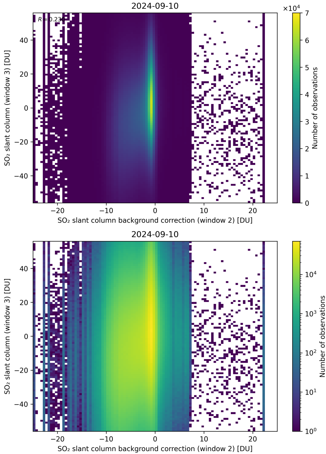
Figure 117: Scatter density plot of “SO 2 slant column background correction (window 2)” against “SO 2 slant column (window 3)” for 2024-09-09 to 2024-09-11.
