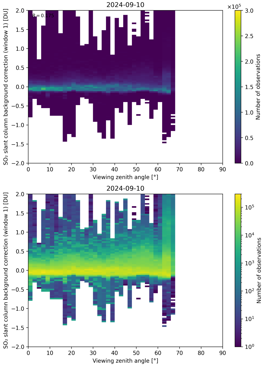
Figure 308: Scatter density plot of “Viewing zenith angle” against “SO 2 slant column background correction (window 1)” for 2024-09-09 to 2024-09-11.
