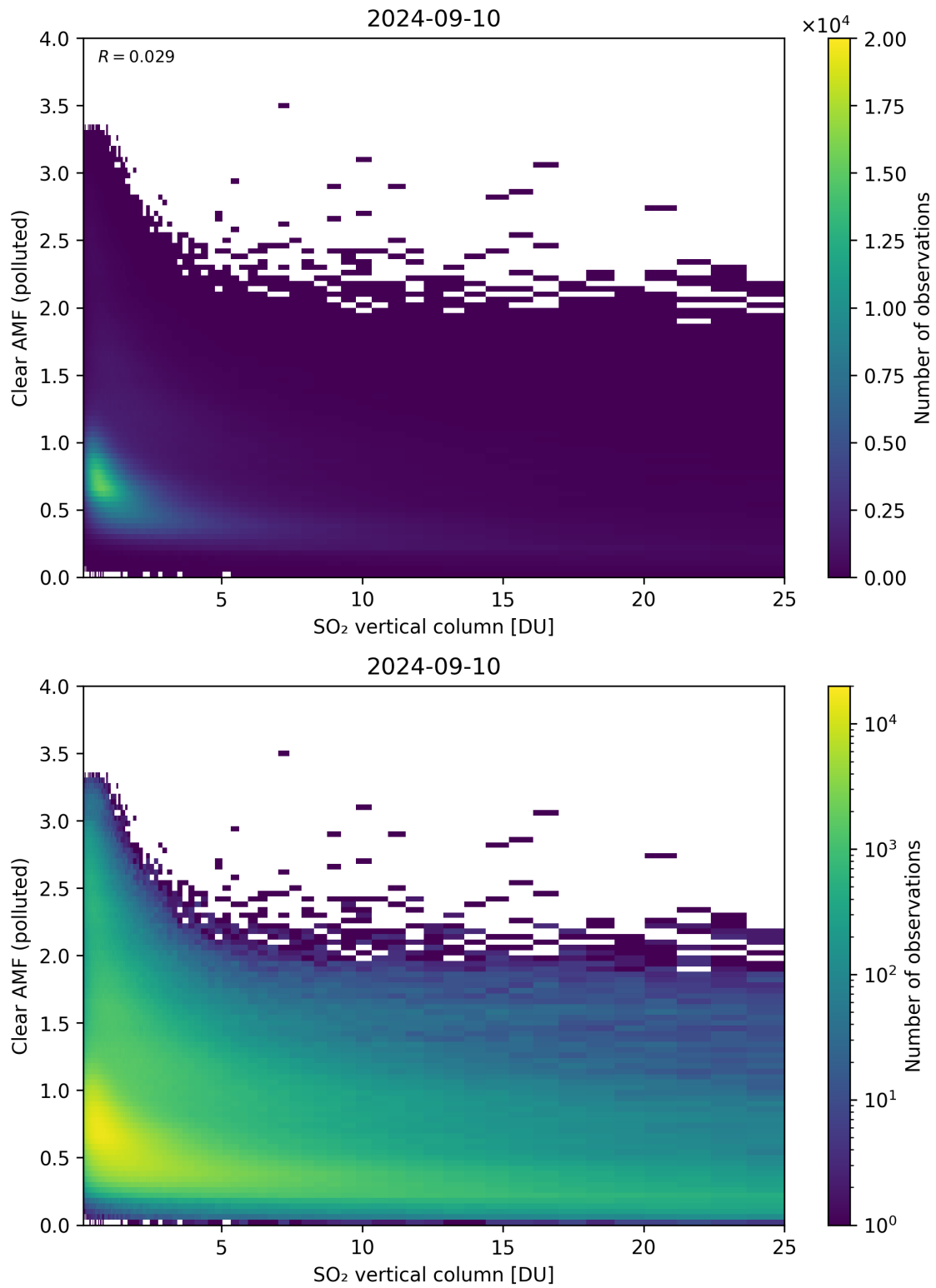
Figure 296: Scatter density plot of “SO 2 vertical column” against “Clear AMF (polluted)” for 2024-09-09 to 2024-09-11.
