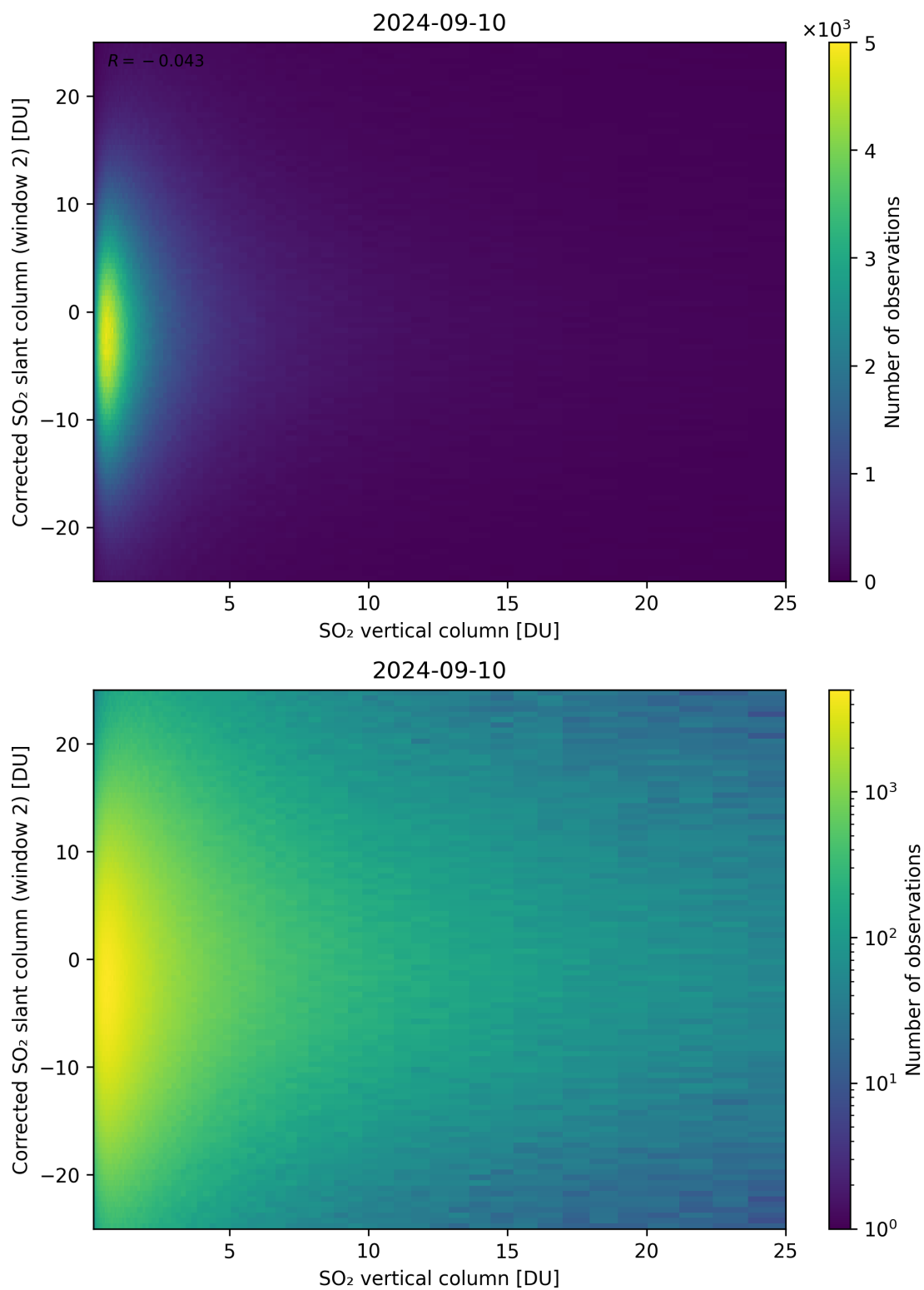
Figure 298: Scatter density plot of “SO 2 vertical column” against “Corrected SO 2 slant column (window 2)” for 2024-09-09 to 2024-09-11.
