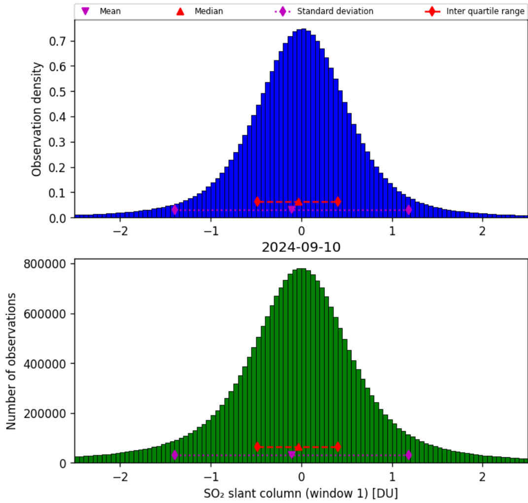
Figure 56: Histogram of “SO 2 slant column (window 1)” for 2024-09-09 to 2024-09-11
