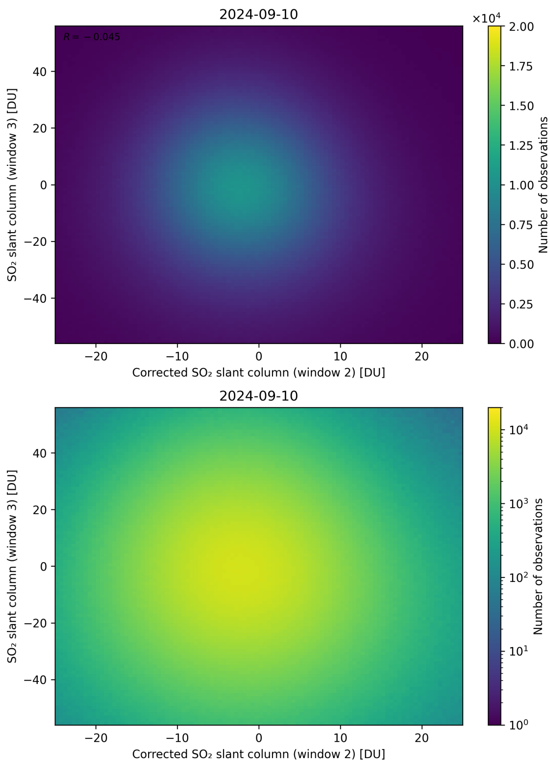
Figure 201: Scatter density plot of “Corrected SO 2 slant column (window 2)” against “SO 2 slant column (window 3)” for 2024-09-09 to 2024-09-11.
