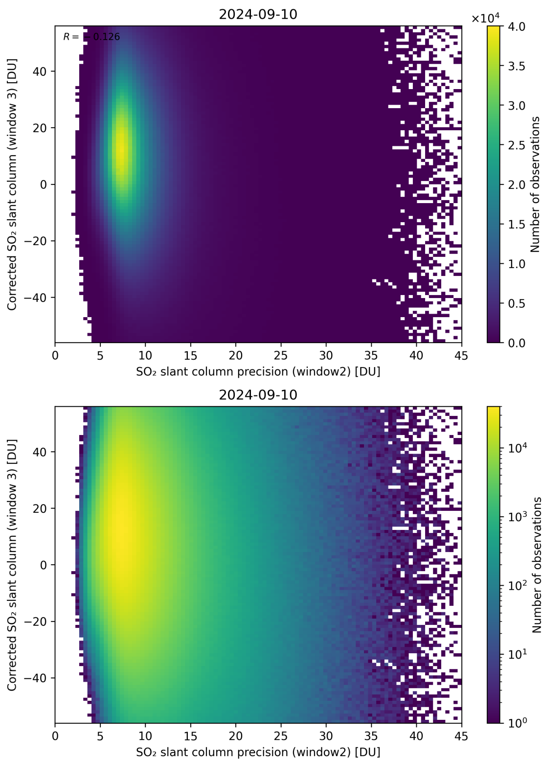
Figure 248: Scatter density plot of “SO 2 slant column precision (window2)” against “Corrected SO 2 slant column (window 3)” for 2024-09-09 to 2024-09-11.
