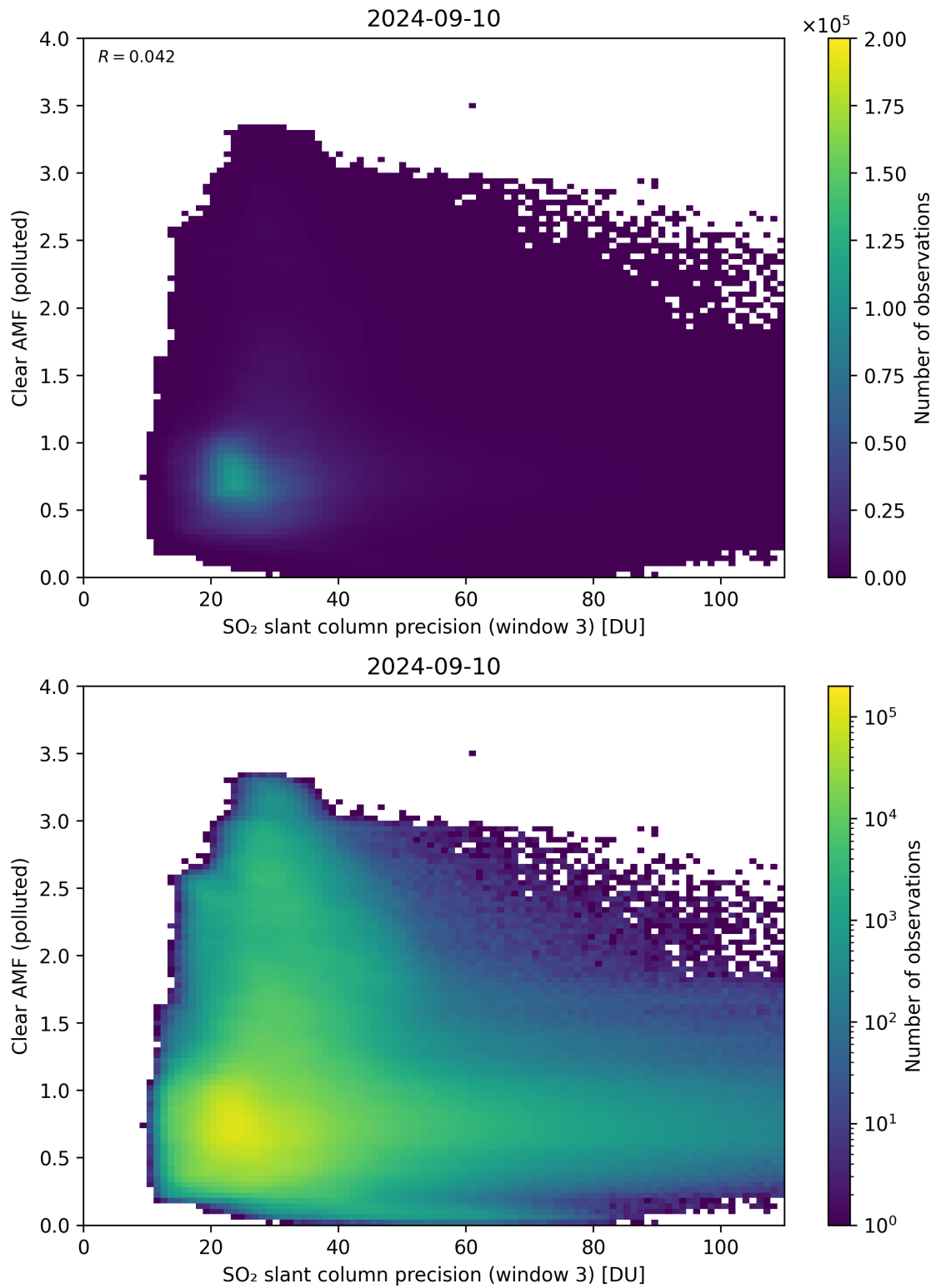
Figure 261: Scatter density plot of “SO 2 slant column precision (window 3)” against “Clear AMF (polluted)” for 2024-09-09 to 2024-09-11.
