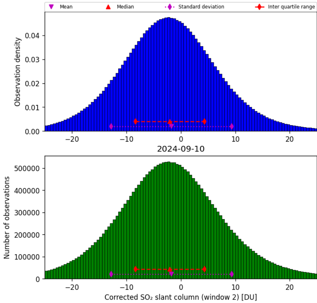
Figure 62: Histogram of “Corrected SO 2 slant column (window 2)” for 2024-09-09 to 2024-09-11
