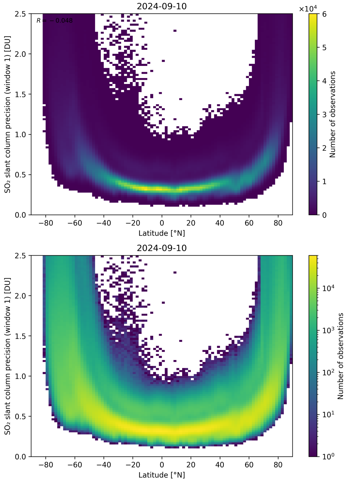
Figure 150: Scatter density plot of “Latitude” against “SO 2 slant column precision (window 1)” for 2024-09-09 to 2024-09-11.
