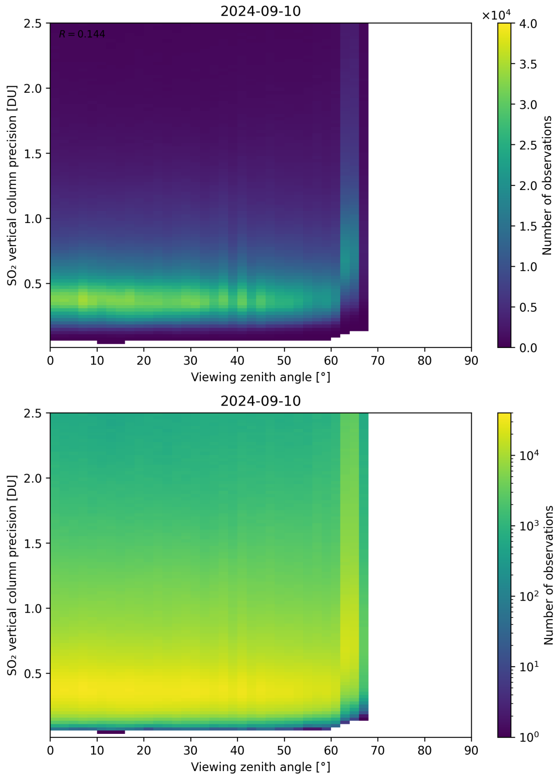
Figure 328: Scatter density plot of “Viewing zenith angle” against “SO 2 vertical column precision” for 2024-09-09 to 2024-09-11.
