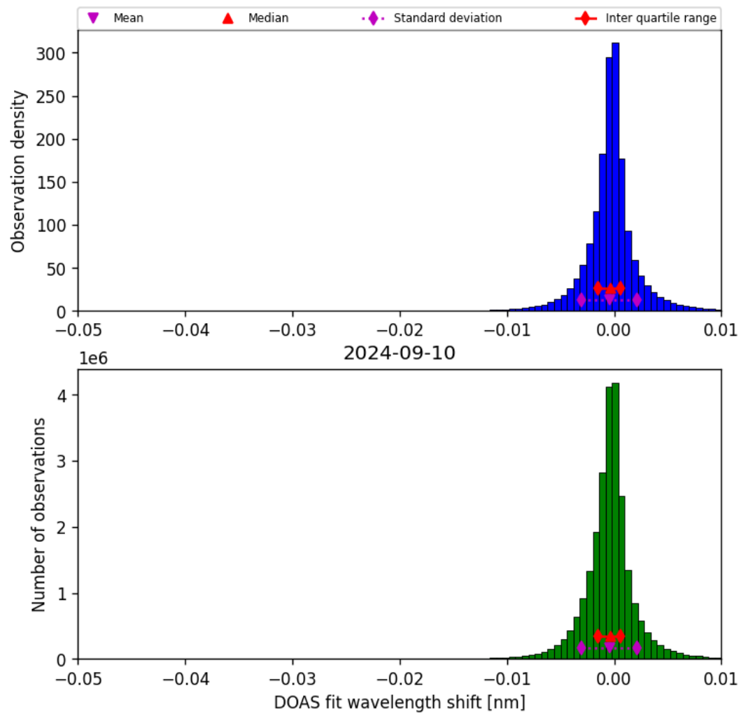
Figure 68: Histogram of “DOAS fit wavelength shift” for 2024-09-09 to 2024-09-11
