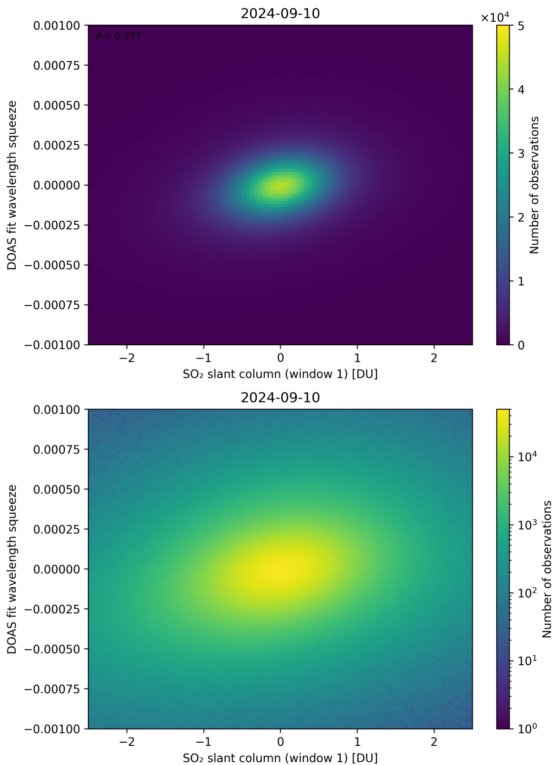
Figure 216: Scatter density plot of “SO 2 slant column (window 1)” against “DOAS fit wavelength squeeze” for 2024-09-09 to 2024-09-11.
