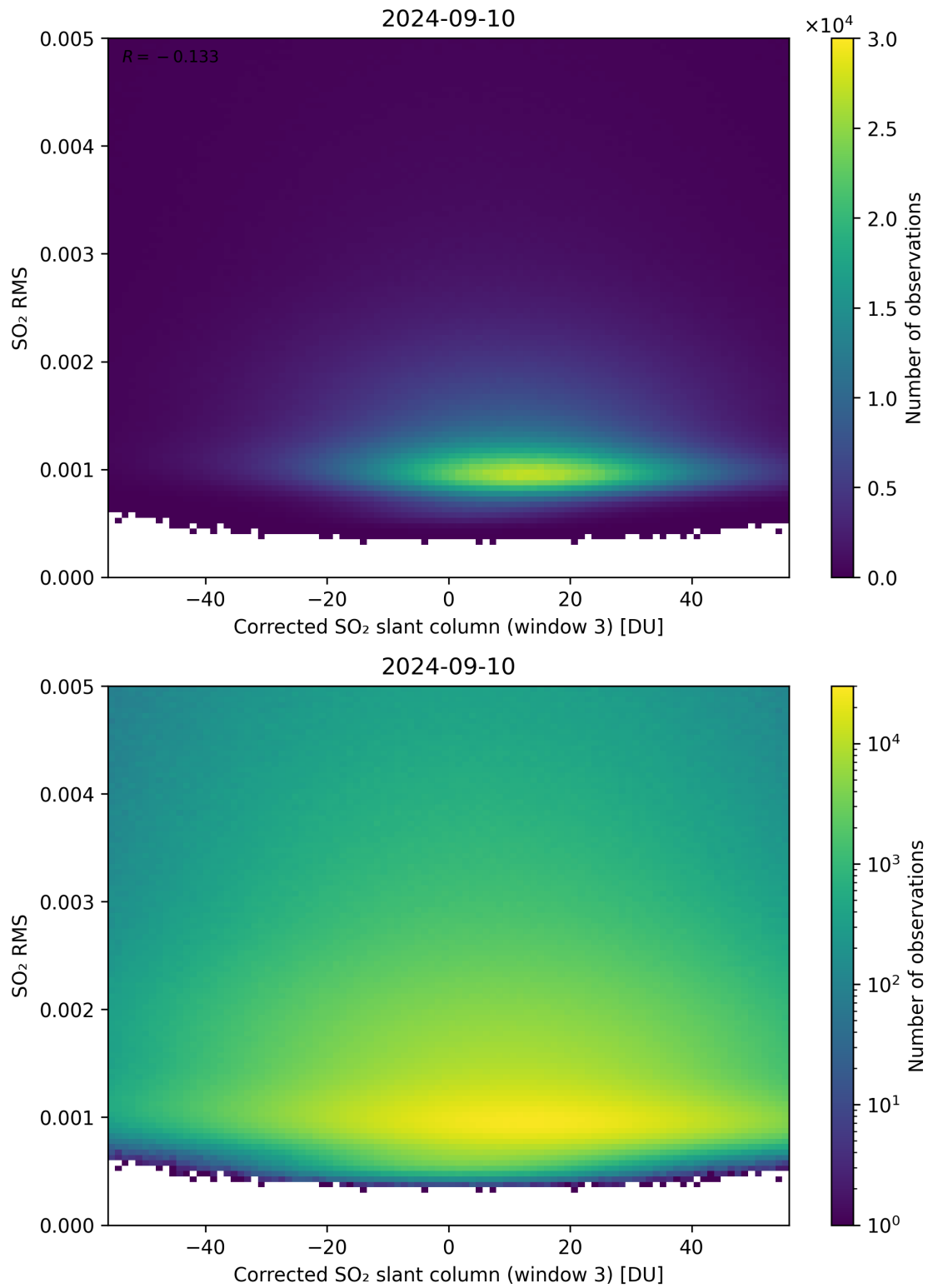
Figure 208: Scatter density plot of “Corrected SO 2 slant column (window 3)” against “SO 2 RMS” for 2024-09-09 to 2024-09-11.
