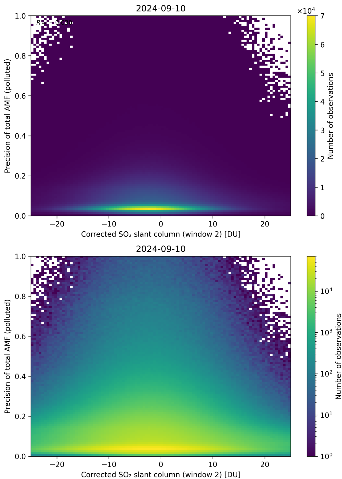
Figure 204: Scatter density plot of “Corrected SO 2 slant column (window 2)” against “Precision of total AMF (polluted)” for 2024-09-09 to 2024-09-11.
