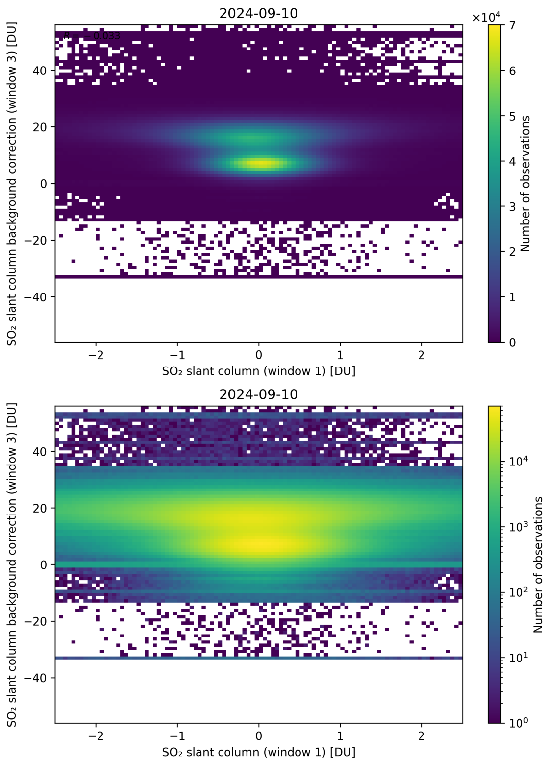
Figure 214: Scatter density plot of “SO 2 slant column (window 1)” against “SO 2 slant column background correction (window 3)” for 2024-09-09 to 2024-09-11.
