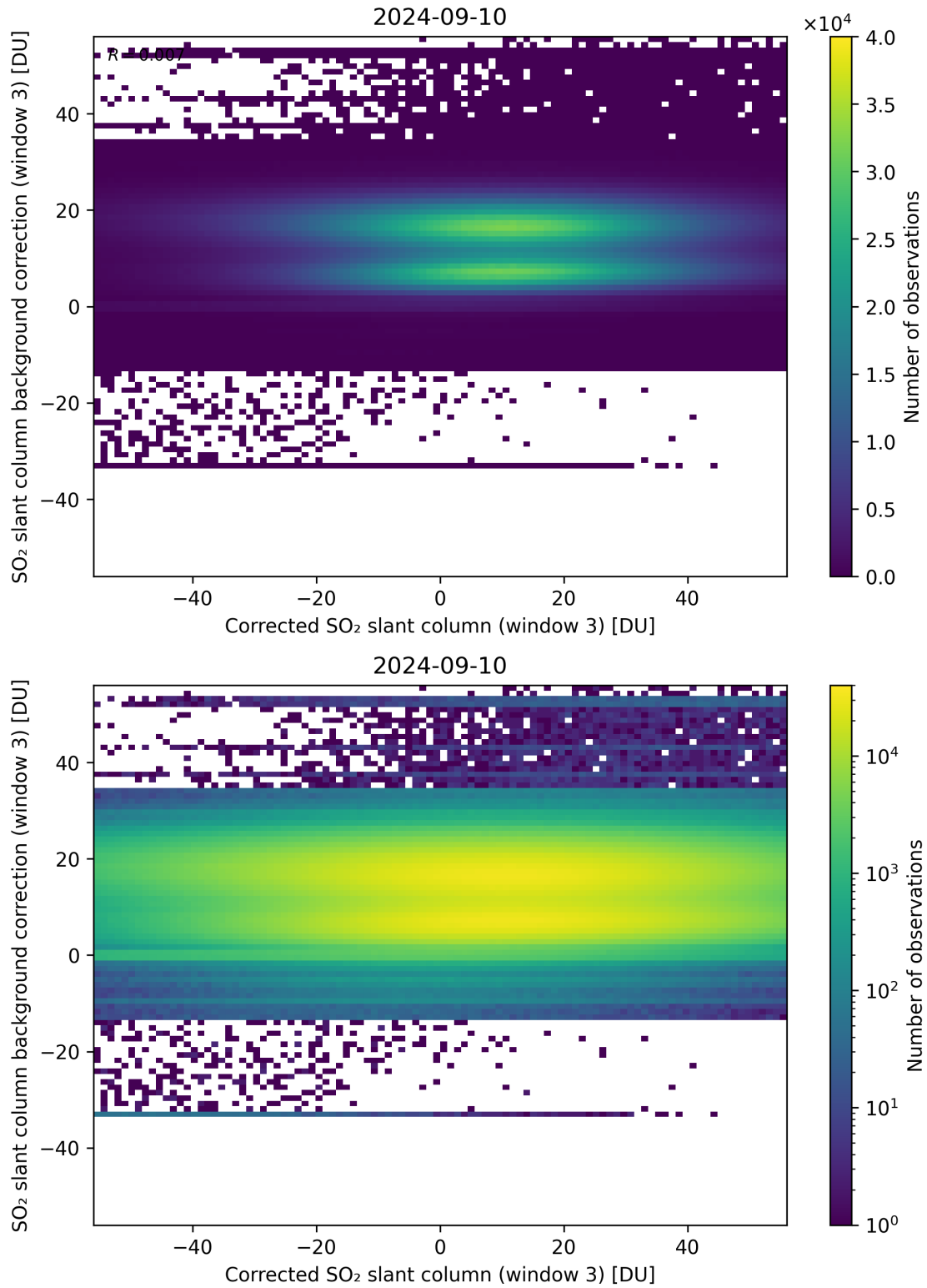
Figure 205: Scatter density plot of “Corrected SO 2 slant column (window 3)” against “SO 2 slant column background correction (window 3)” for 2024-09-09 to 2024-09-11.
