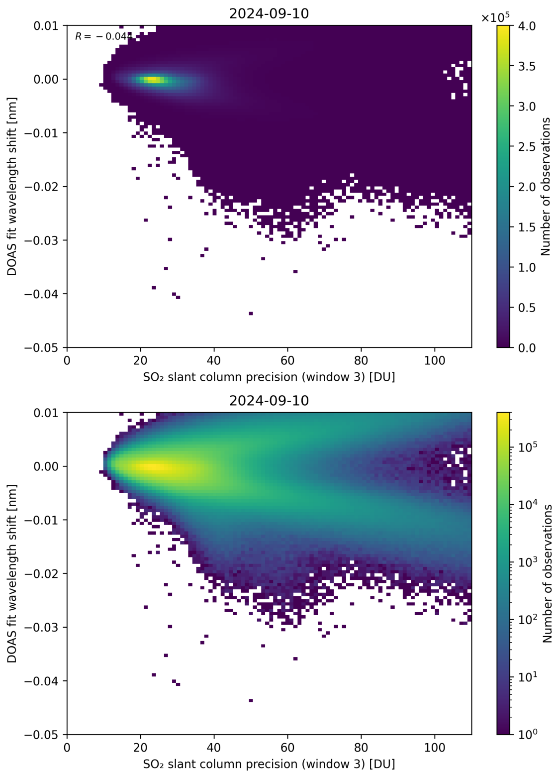
Figure 258: Scatter density plot of “SO 2 slant column precision (window 3)” against “DOAS fit wavelength shift” for 2024-09-09 to 2024-09-11.
