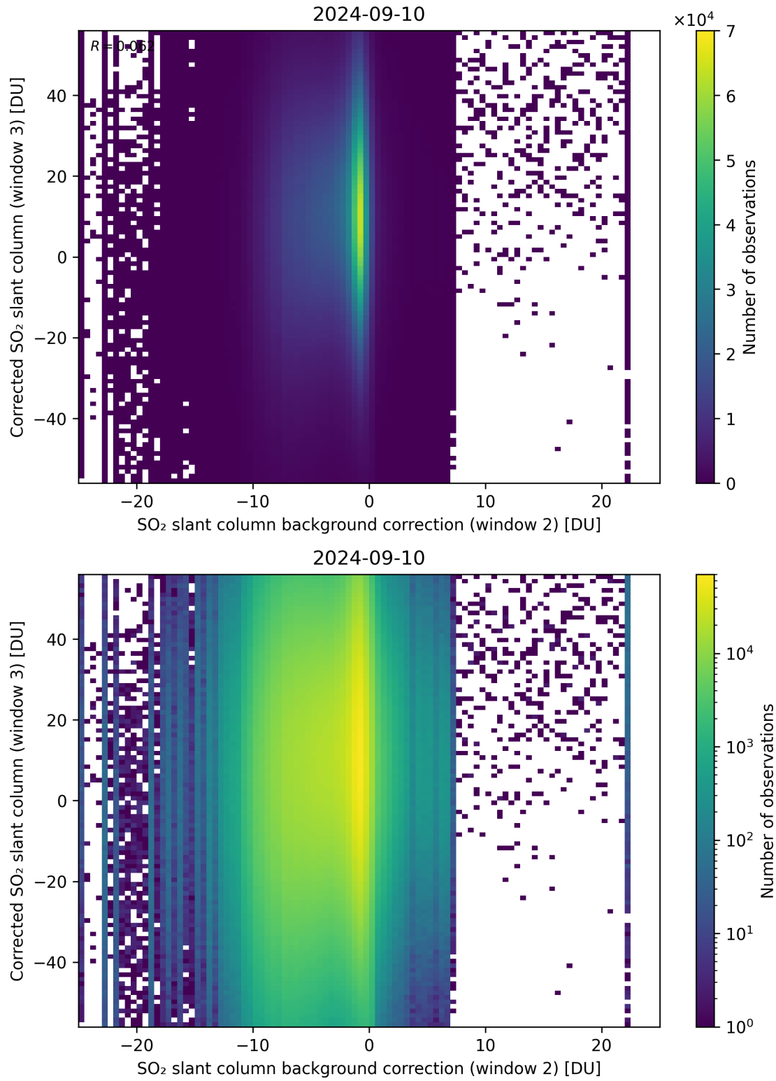
Figure 116: Scatter density plot of “SO 2 slant column background correction (window 2)” against “Corrected SO 2 slant column (window 3)” for 2024-09-09 to 2024-09-11.
