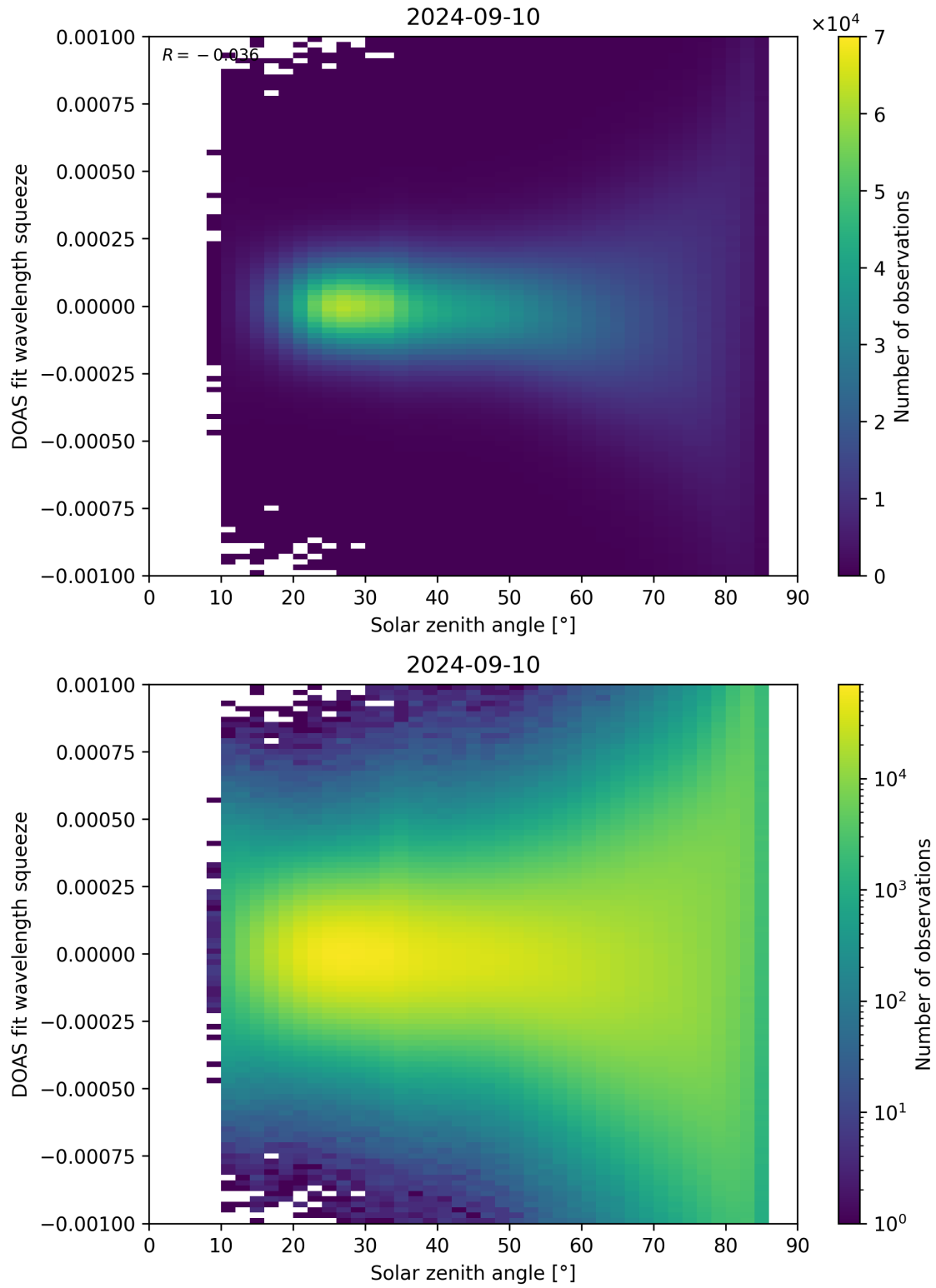
Figure 162: Scatter density plot of “Solar zenith angle” against “DOAS fit wavelength squeeze” for 2024-09-09 to 2024-09-11.
