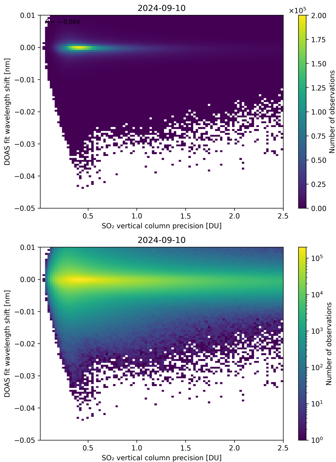
Figure 282: Scatter density plot of “SO 2 vertical column precision” against “DOAS fit wavelength shift” for 2024-09-09 to 2024-09-11.
