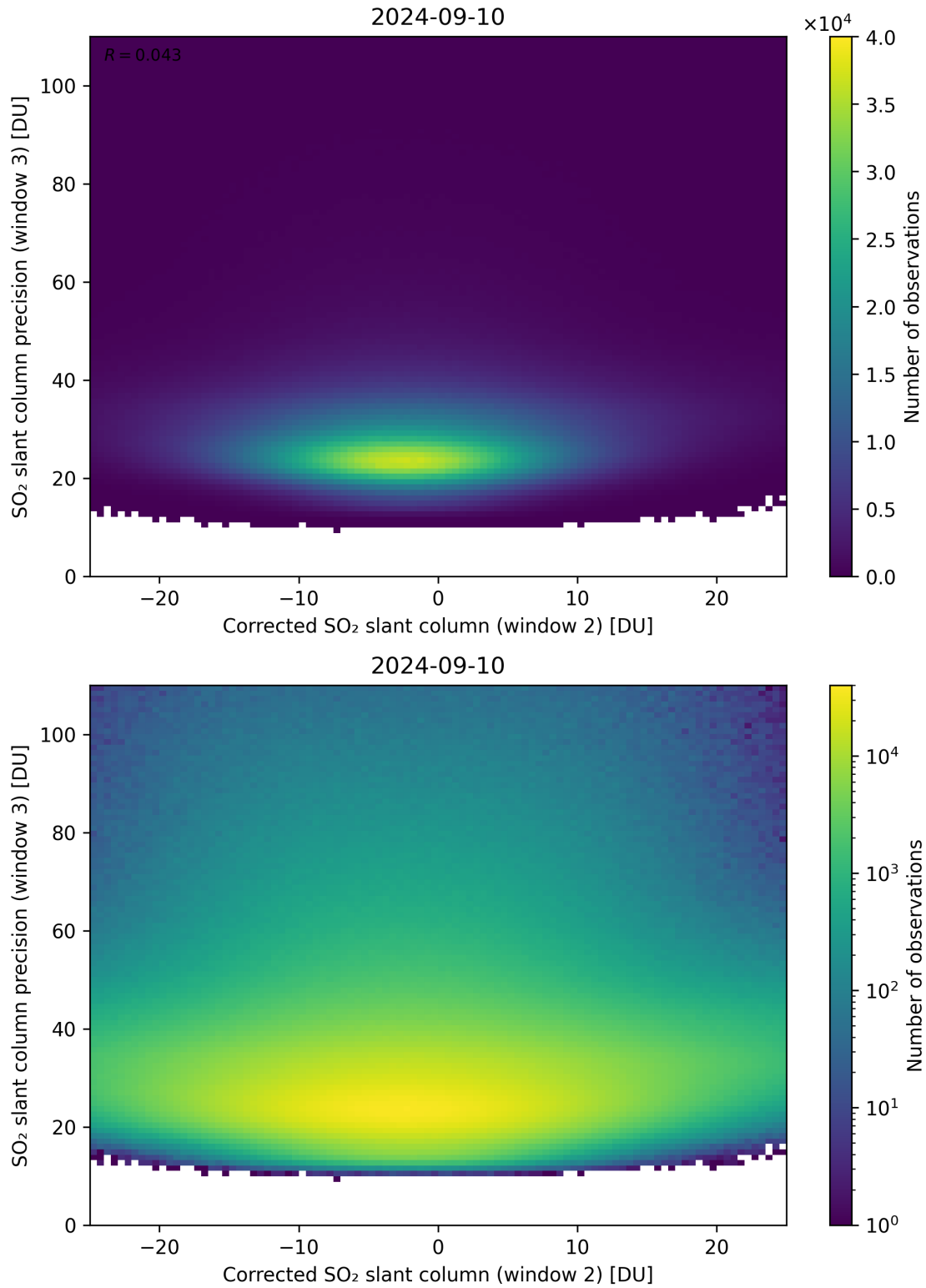
Figure 202: Scatter density plot of “Corrected SO 2 slant column (window 2)” against “SO 2 slant column precision (window 3)” for 2024-09-09 to 2024-09-11.
