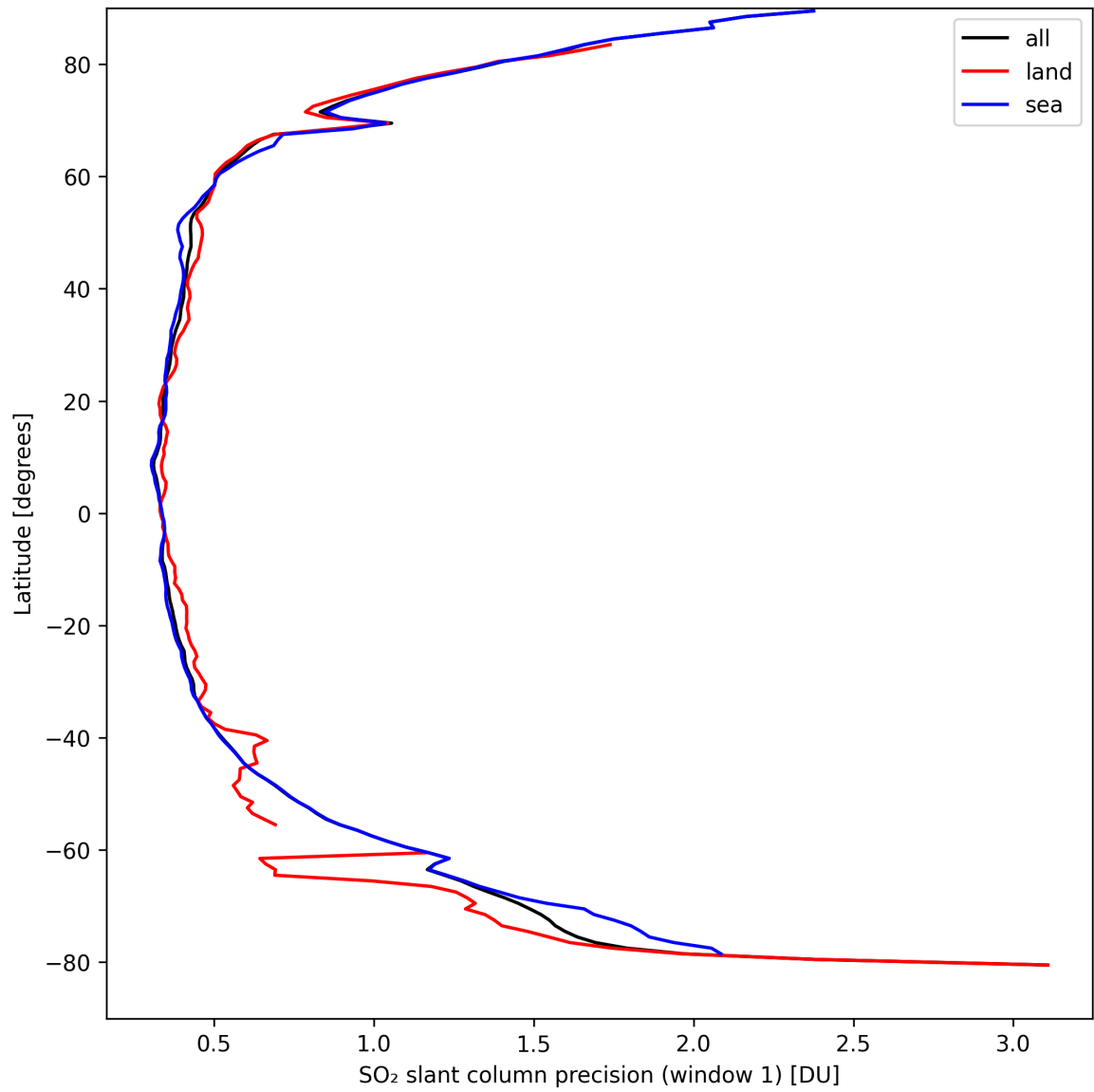
Figure 34: Zonal average of “SO 2 slant column precision (window 1)” for 2024-09-09 to 2024-09-11.
