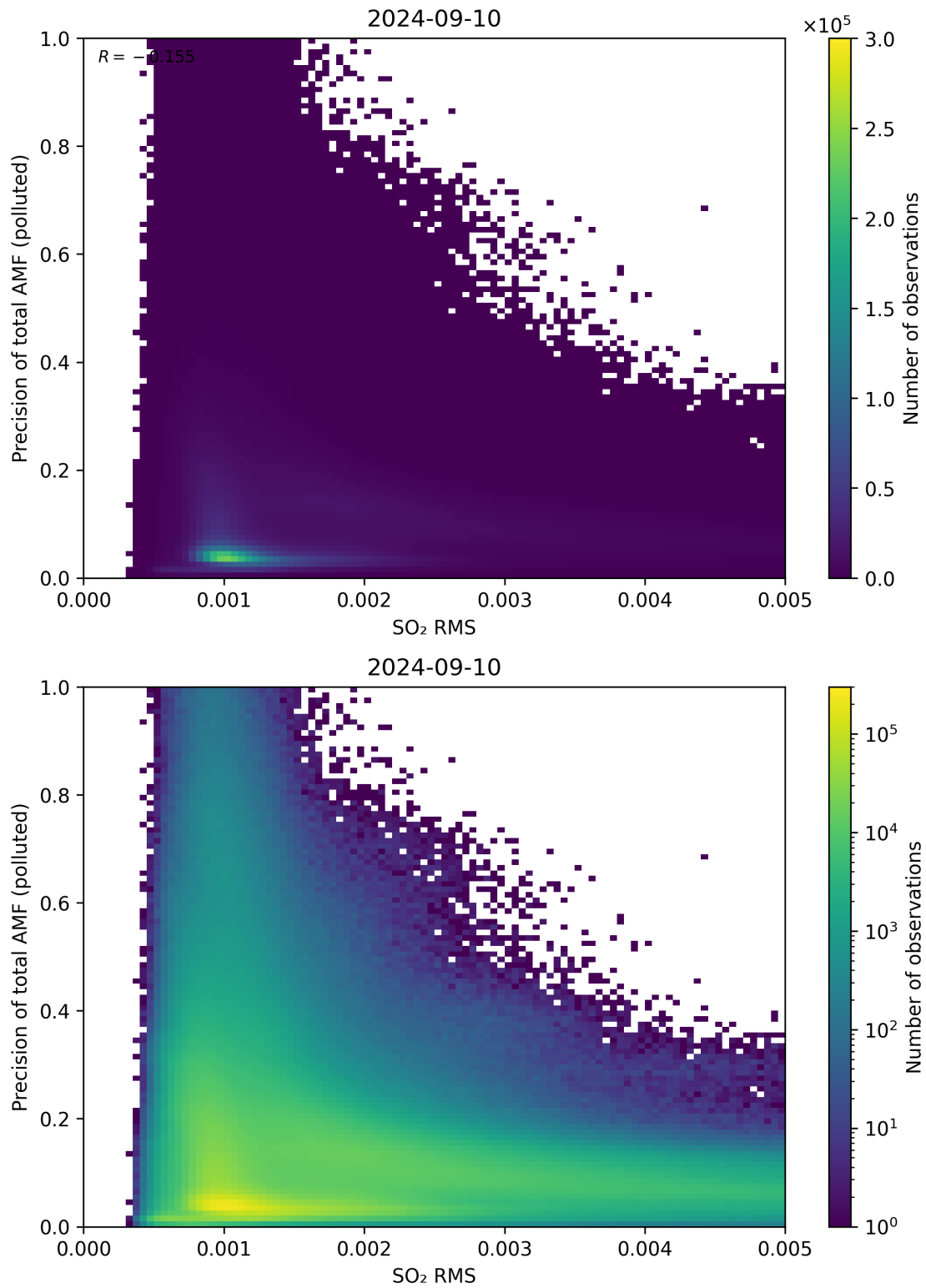
Figure 138: Scatter density plot of “SO 2 RMS” against “Precision of total AMF (polluted)” for 2024-09-09 to 2024-09-11.
