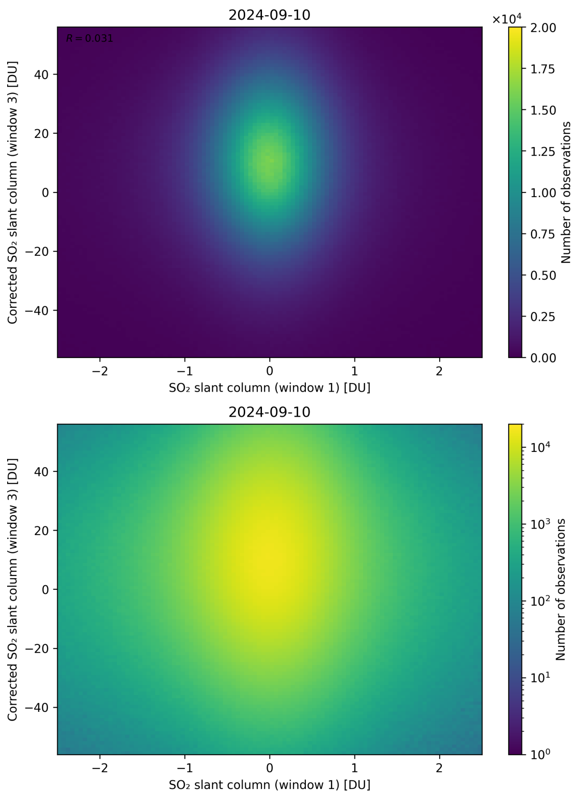
Figure 234: Scatter density plot of “SO 2 slant column (window 1)” against “Corrected SO 2 slant column (window 3)” for 2024-09-09 to 2024-09-11.
