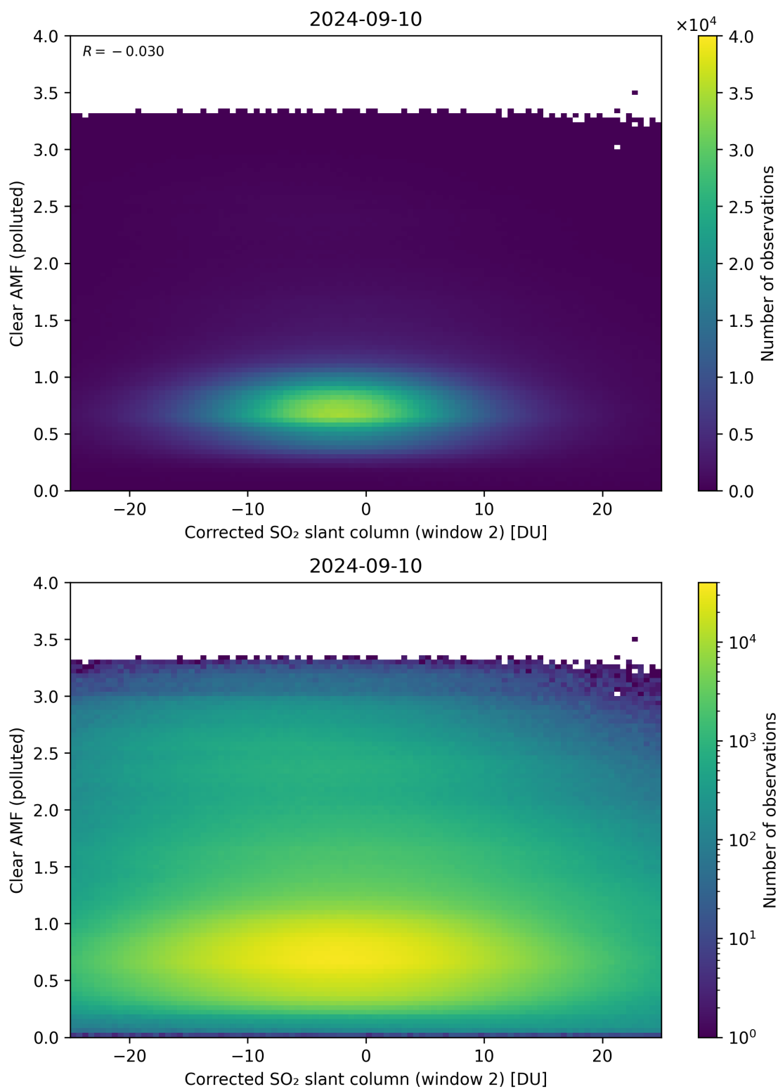
Figure 199: Scatter density plot of “Corrected SO 2 slant column (window 2)” against “Clear AMF (polluted)” for 2024-09-09 to 2024-09-11.
