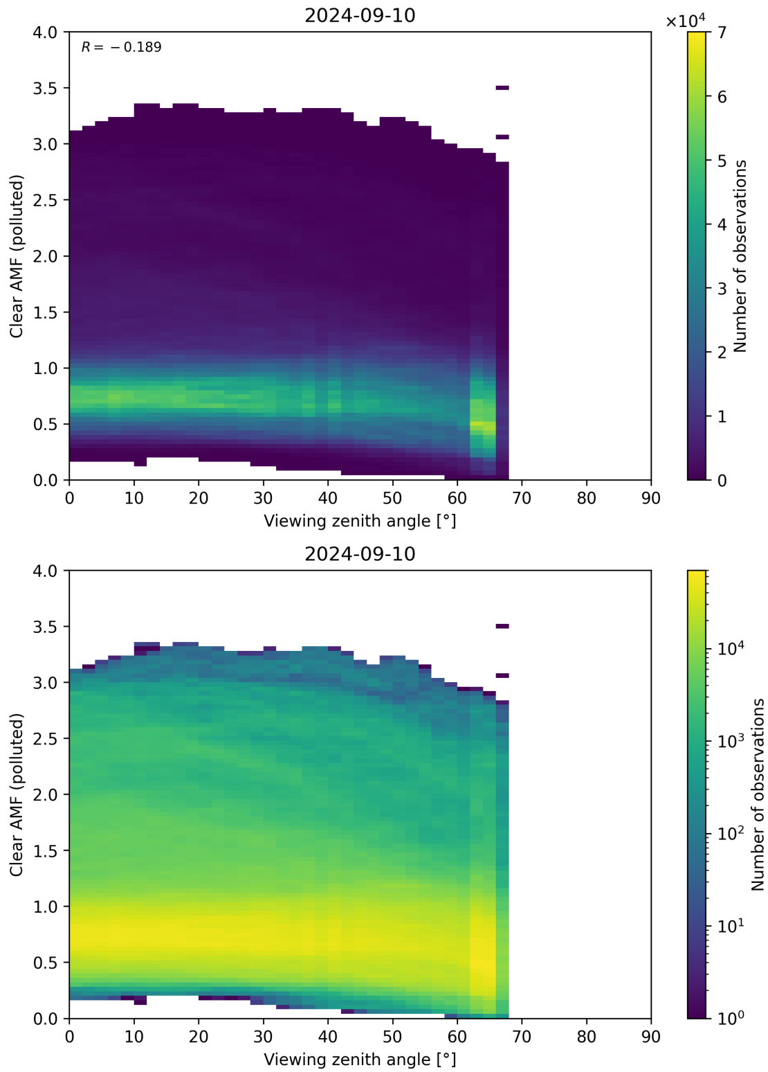
Figure 316: Scatter density plot of “Viewing zenith angle” against “Clear AMF (polluted)” for 2024-09-09 to 2024-09-11.
