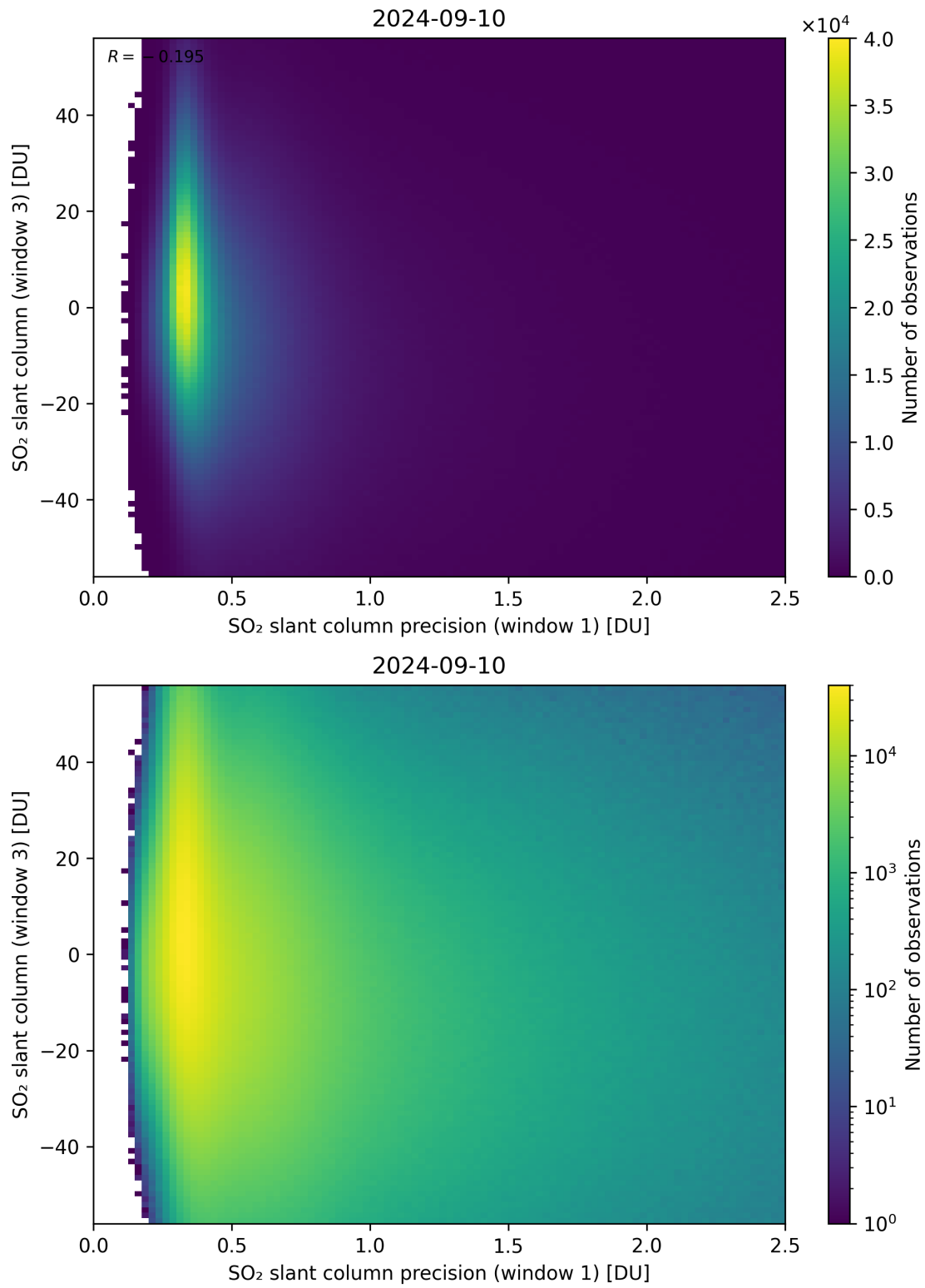
Figure 228: Scatter density plot of “SO 2 slant column precision (window 1)” against “SO 2 slant column (window 3)” for 2024-09-09 to 2024-09-11.
