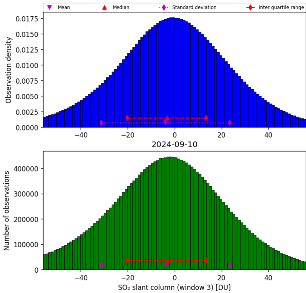
Figure 64: Histogram of “SO 2 slant column (window 3)” for 2024-09-09 to 2024-09-11
