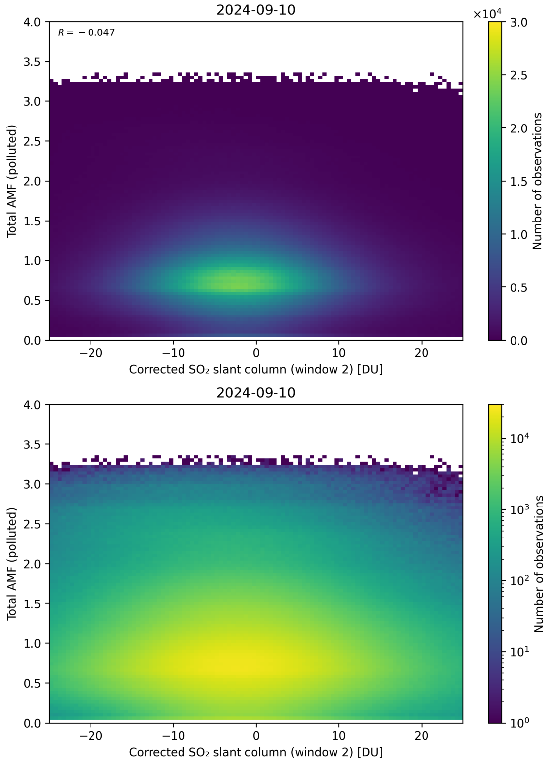
Figure 203: Scatter density plot of “Corrected SO 2 slant column (window 2)” against “Total AMF (polluted)” for 2024-09-09 to 2024-09-11.
