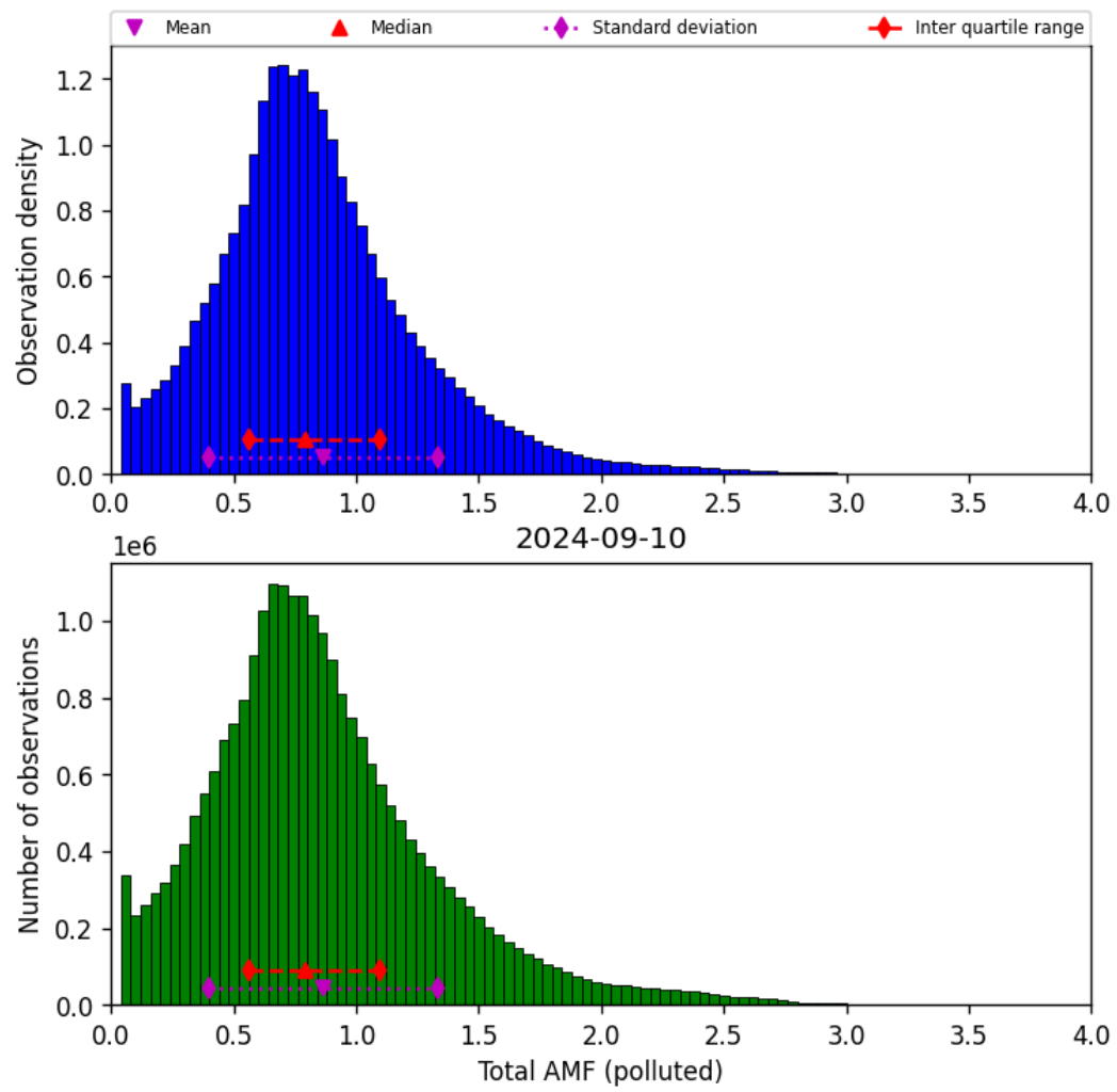
Figure 71: Histogram of “Total AMF (polluted)” for 2024-09-09 to 2024-09-11
