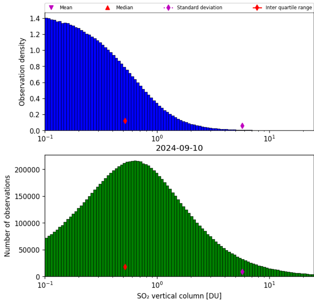
Figure 53: Histogram of “SO 2 vertical column” for 2024-09-09 to 2024-09-11
