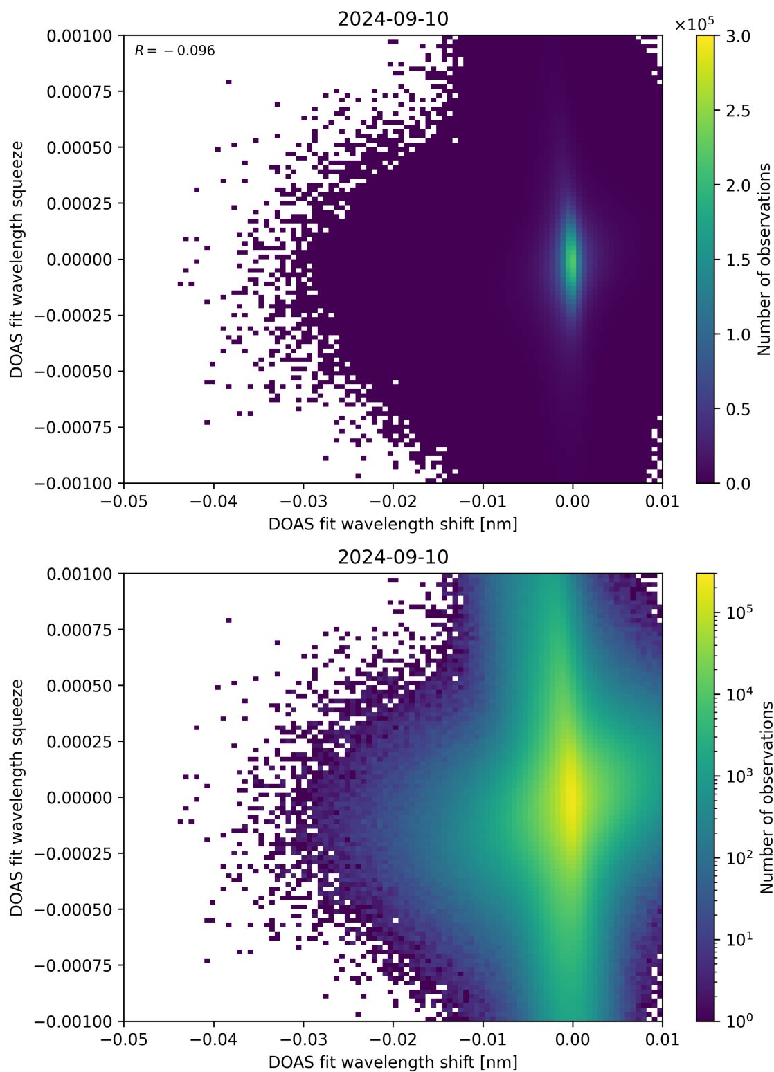
Figure 127: Scatter density plot of “DOAS fit wavelength shift” against “DOAS fit wavelength squeeze” for 2024-09-09 to 2024-09-11.
