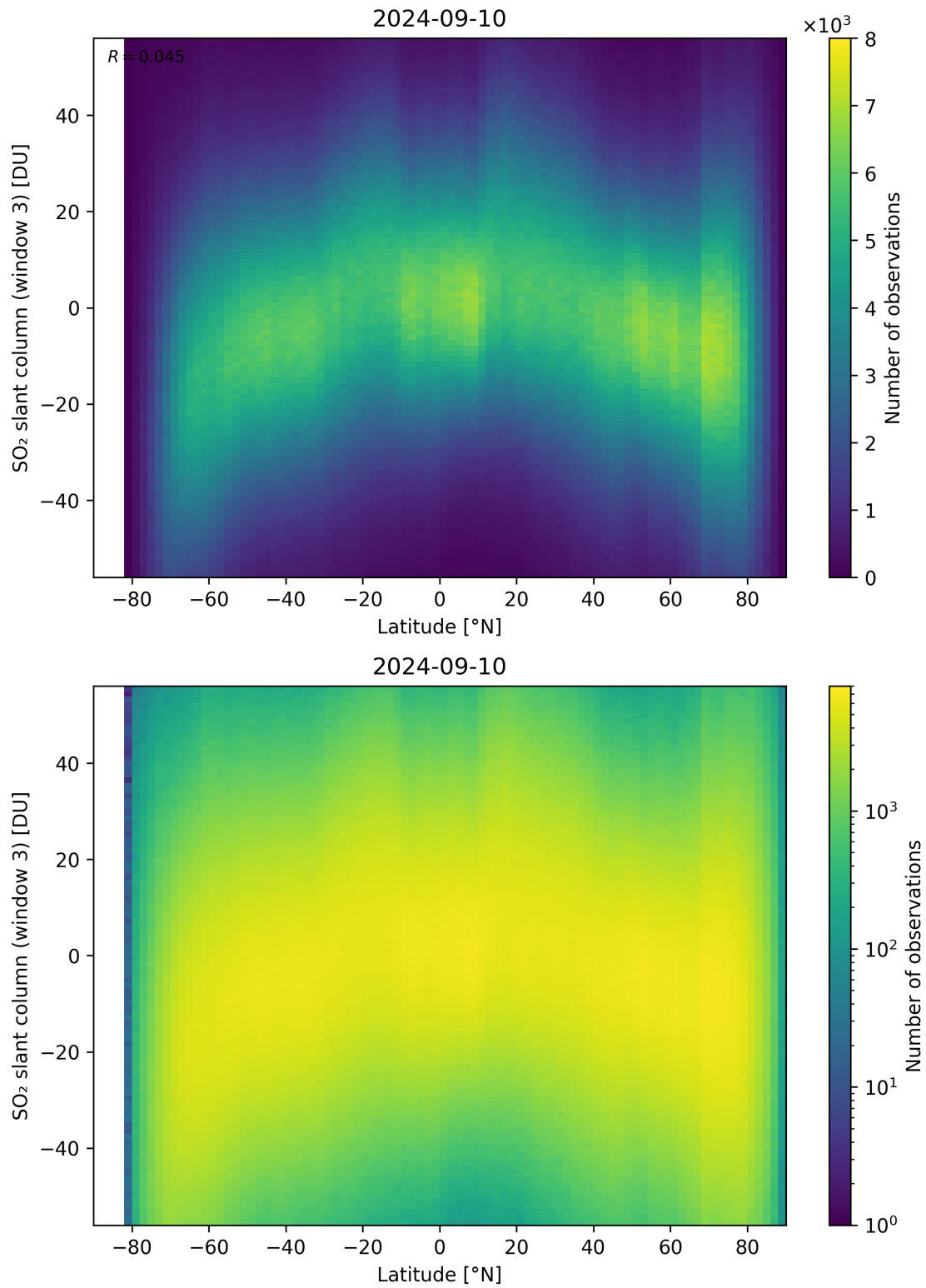
Figure 152: Scatter density plot of “Latitude” against “SO 2 slant column (window 3)” for 2024-09-09 to 2024-09-11.
