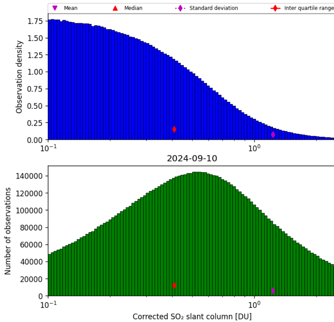
Figure 55: Histogram of “Corrected SO 2 slant column” for 2024-09-09 to 2024-09-11
