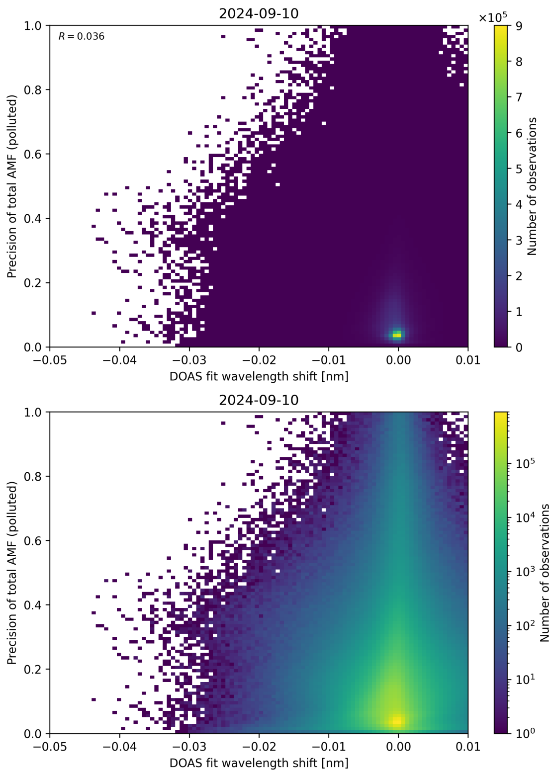
Figure 131: Scatter density plot of “DOAS fit wavelength shift” against “Precision of total AMF (polluted)” for 2024-09-09 to 2024-09-11.
