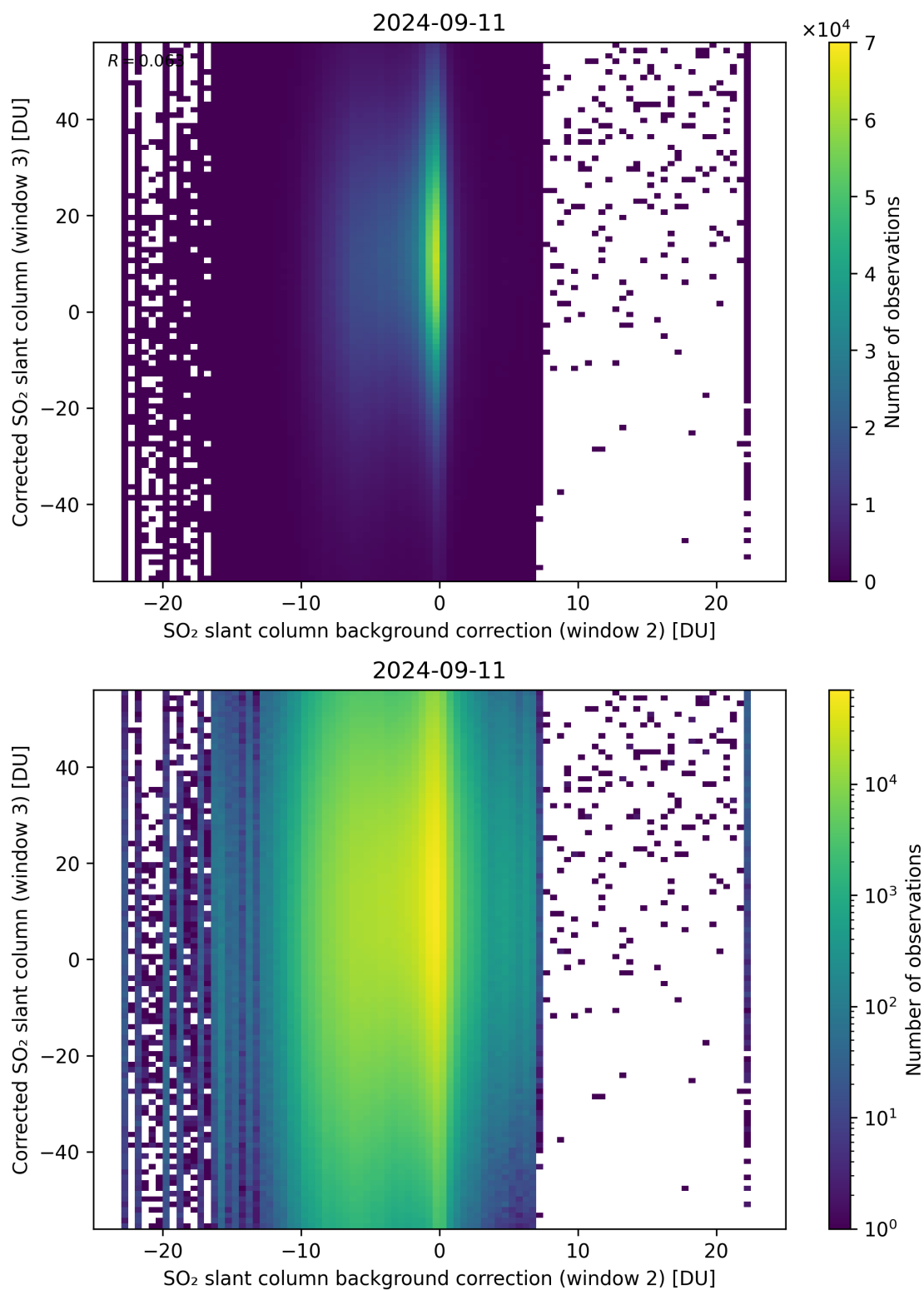
Figure 116: Scatter density plot of “SO 2 slant column background correction (window 2)” against “Corrected SO 2 slant column (window 3)” for 2024-09-10 to 2024-09-12.
