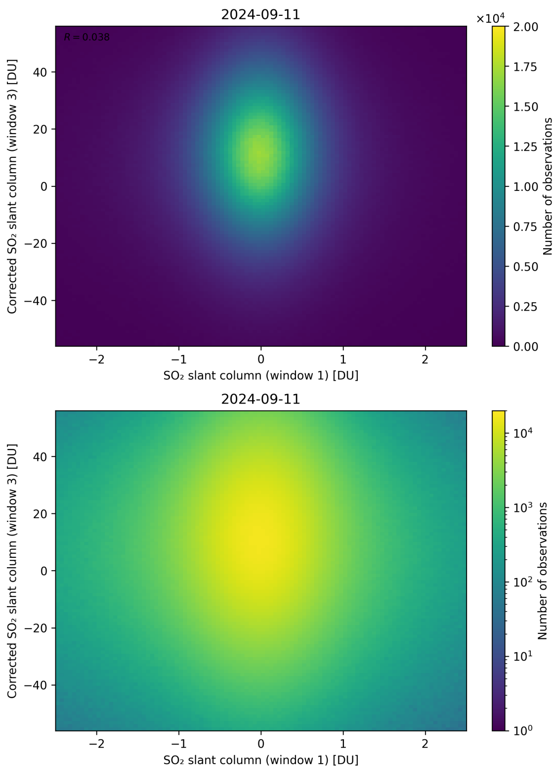
Figure 234: Scatter density plot of “SO 2 slant column (window 1)” against “Corrected SO 2 slant column (window 3)” for 2024-09-10 to 2024-09-12.
