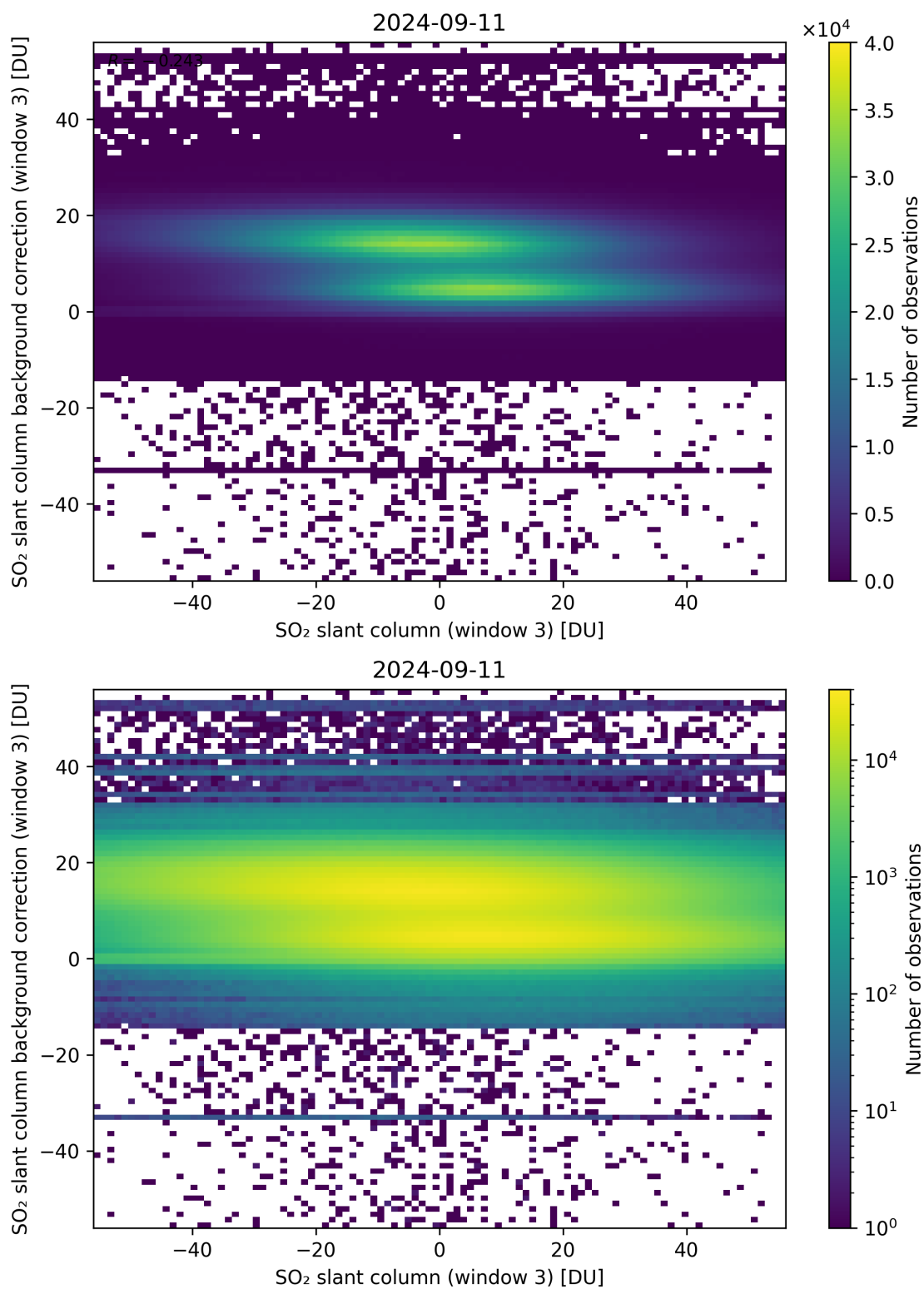
Figure 253: Scatter density plot of “SO 2 slant column (window 3)” against “SO 2 slant column background correction (window 3)” for 2024-09-10 to 2024-09-12.
