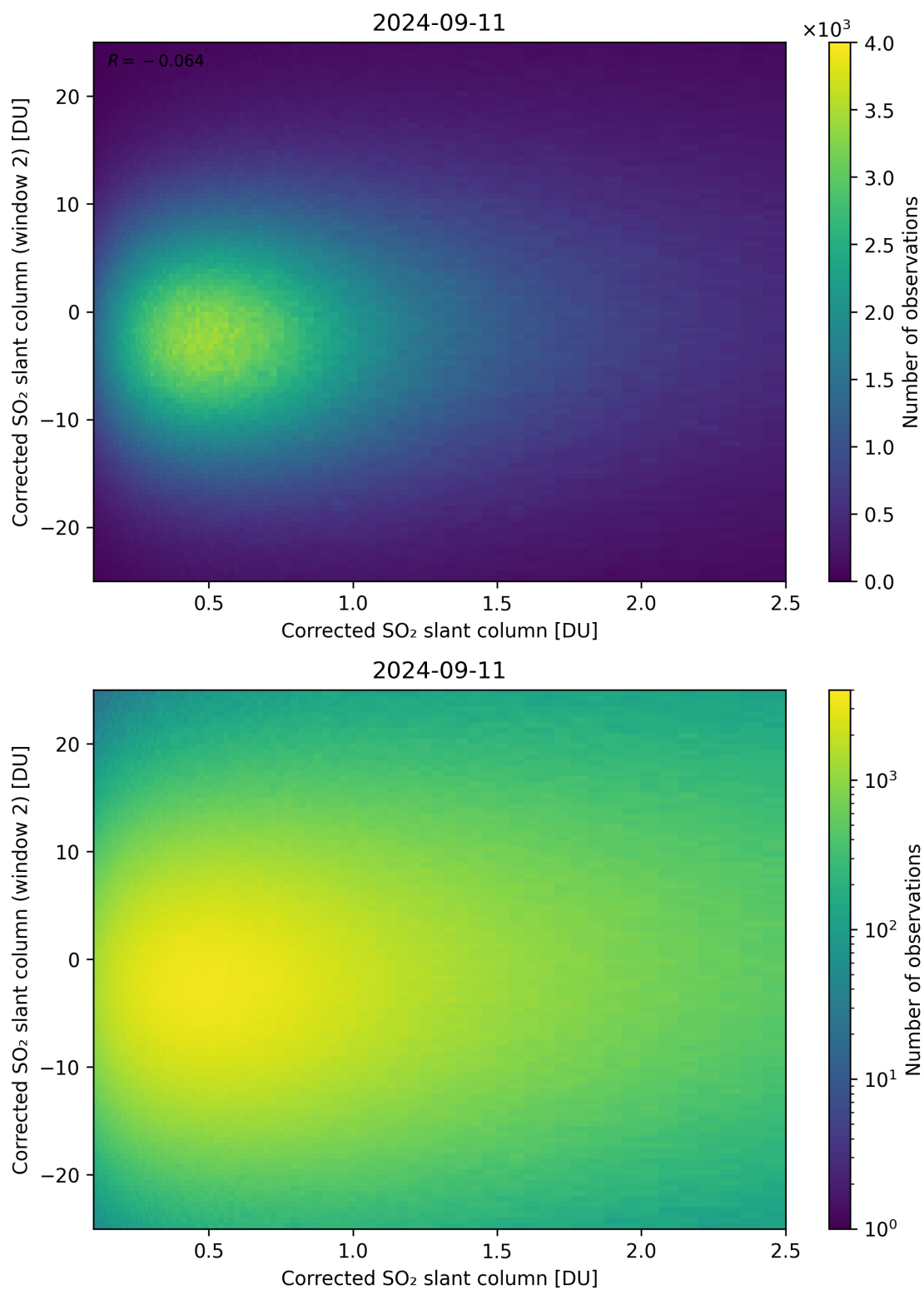
Figure 185: Scatter density plot of “Corrected SO 2 slant column” against “Corrected SO 2 slant column (window 2)” for 2024-09-10 to 2024-09-12.
