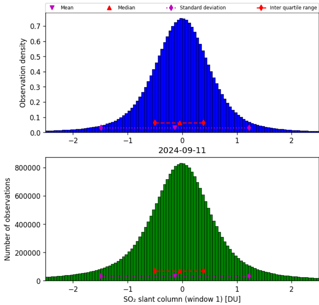
Figure 56: Histogram of “SO 2 slant column (window 1)” for 2024-09-10 to 2024-09-12
