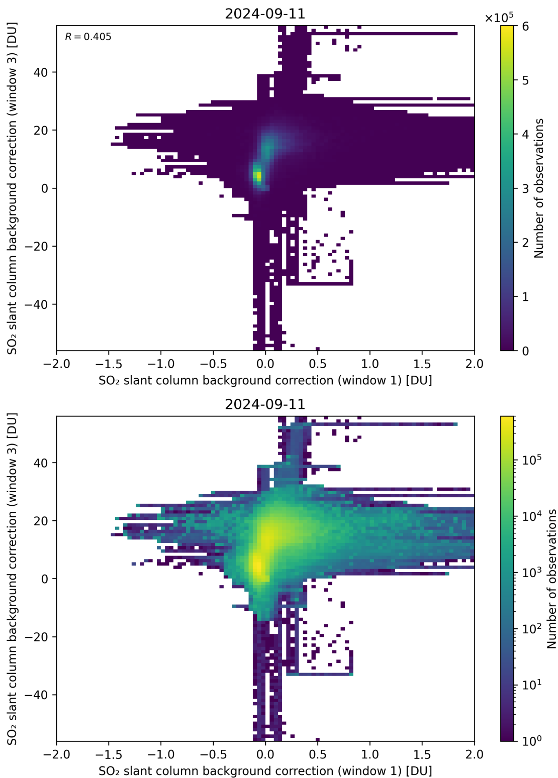
Figure 99: Scatter density plot of “SO 2 slant column background correction (window 1)” against “SO 2 slant column background correction (window 3)” for 2024-09-10 to 2024-09-12.
