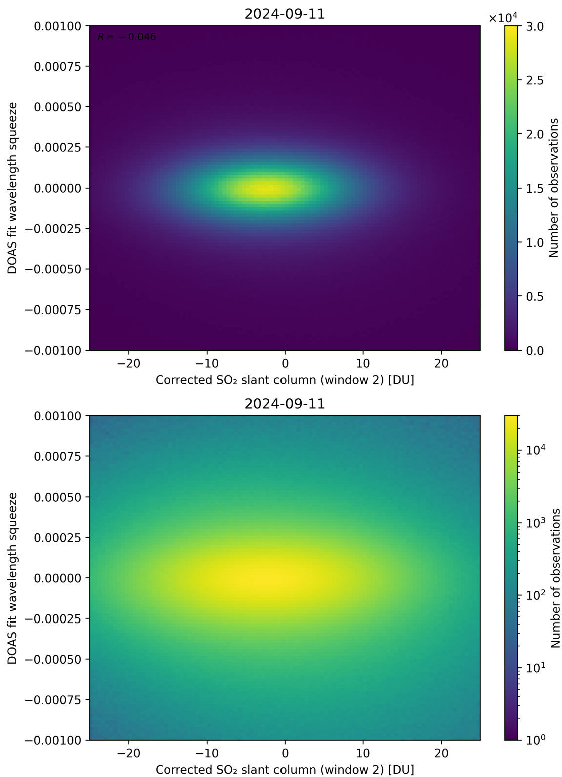
Figure 197: Scatter density plot of “Corrected SO 2 slant column (window 2)” against “DOAS fit wavelength squeeze” for 2024-09-10 to 2024-09-12.
