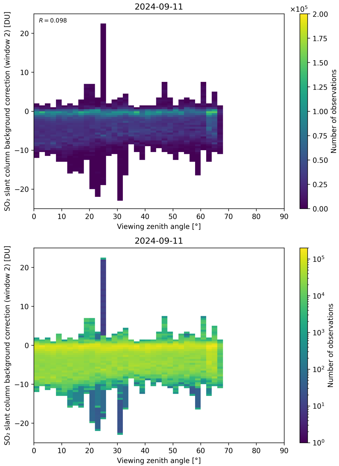
Figure 309: Scatter density plot of “Viewing zenith angle” against “SO 2 slant column background correction (window 2)” for 2024-09-10 to 2024-09-12.
