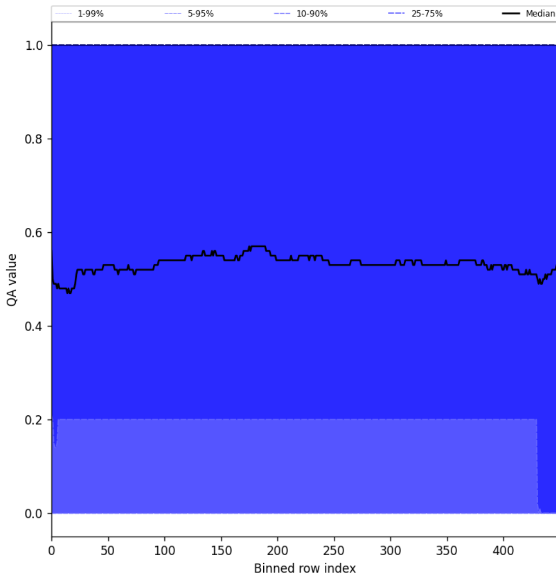
Figure 75: Along track statistics of “QA value” for 2024-09-10 to 2024-09-12
