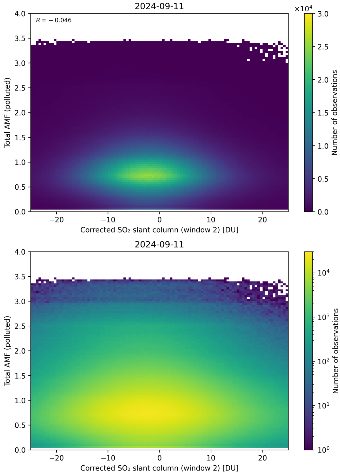
Figure 203: Scatter density plot of “Corrected SO 2 slant column (window 2)” against “Total AMF (polluted)” for 2024-09-10 to 2024-09-12.
