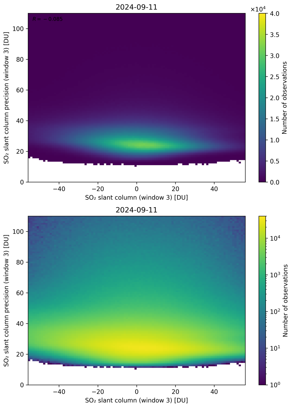
Figure 267: Scatter density plot of “SO 2 slant column (window 3)” against “SO 2 slant column precision (window 3)” for 2024-09-10 to 2024-09-12.
