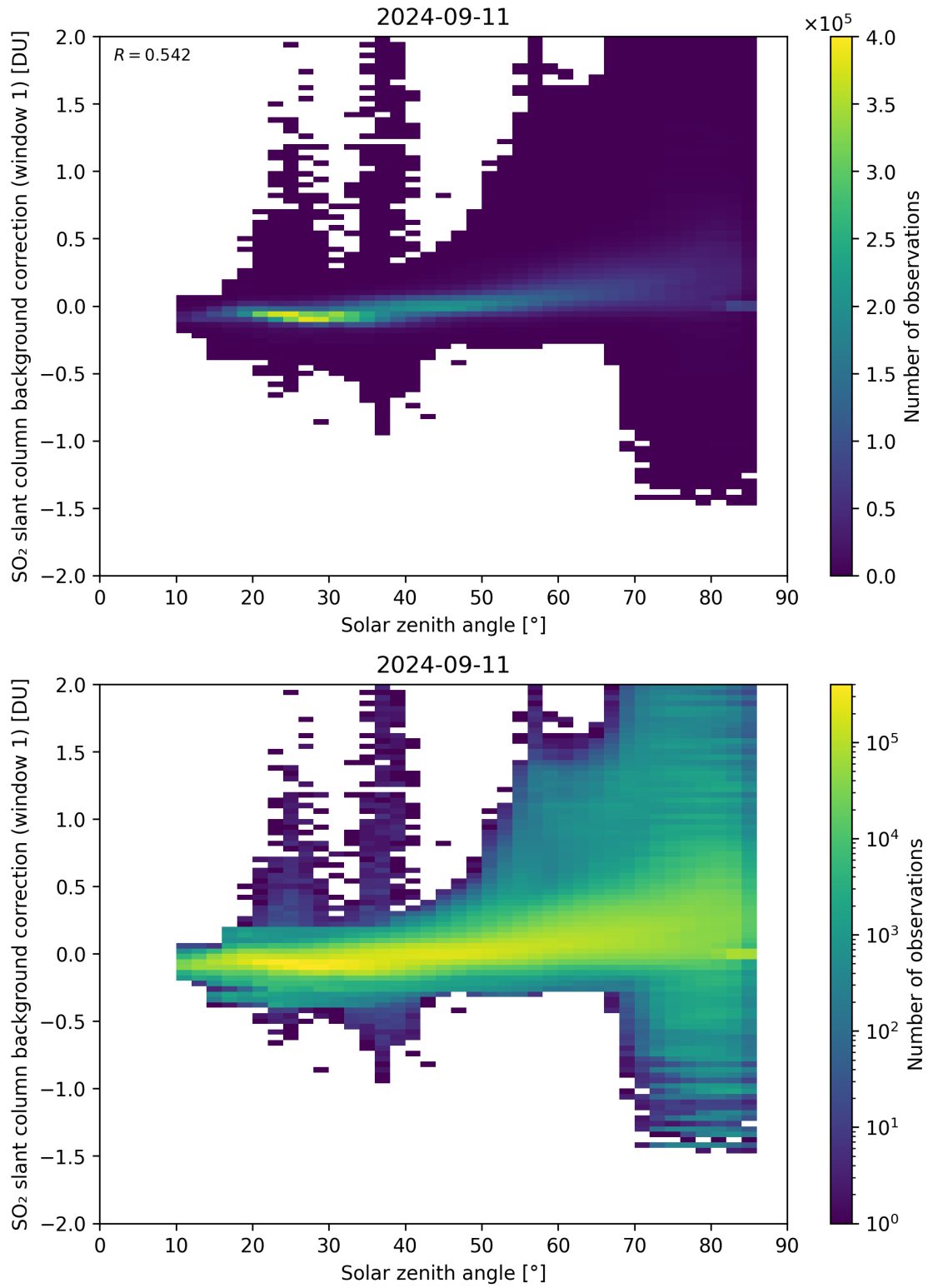
Figure 158: Scatter density plot of “Solar zenith angle” against “SO 2 slant column background correction (window 1)” for 2024-09-10 to 2024-09-12.
