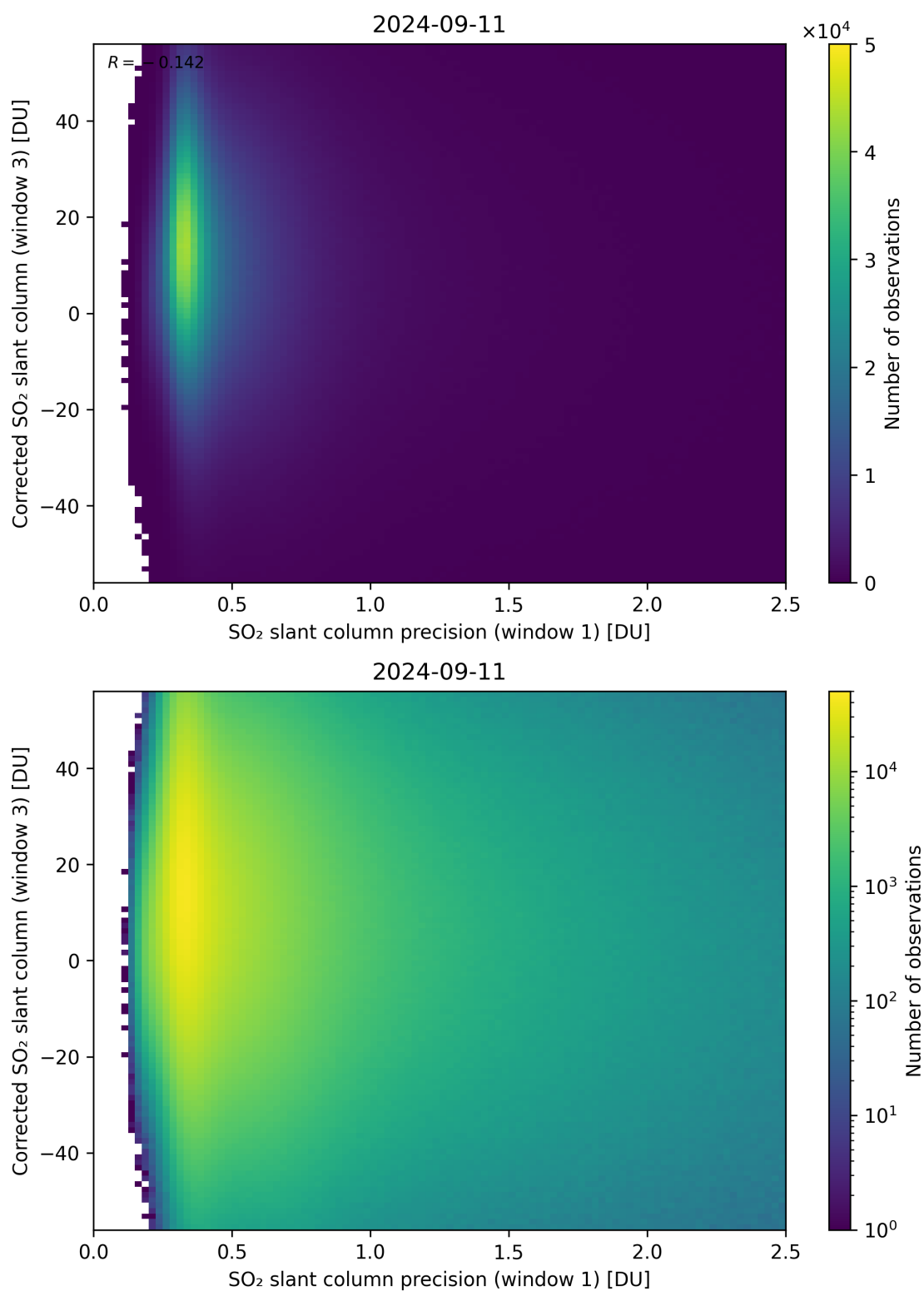
Figure 226: Scatter density plot of “SO 2 slant column precision (window 1)” against “Corrected SO 2 slant column (window 3)” for 2024-09-10 to 2024-09-12.
