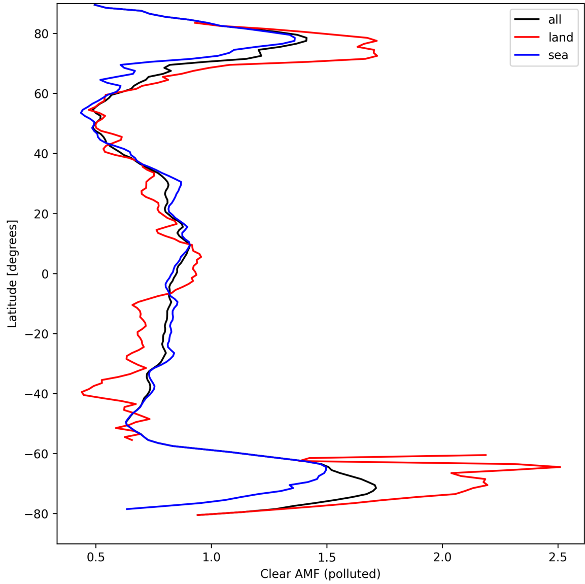
Figure 50: Zonal average of “Clear AMF (polluted)” for 2024-09-10 to 2024-09-12.
