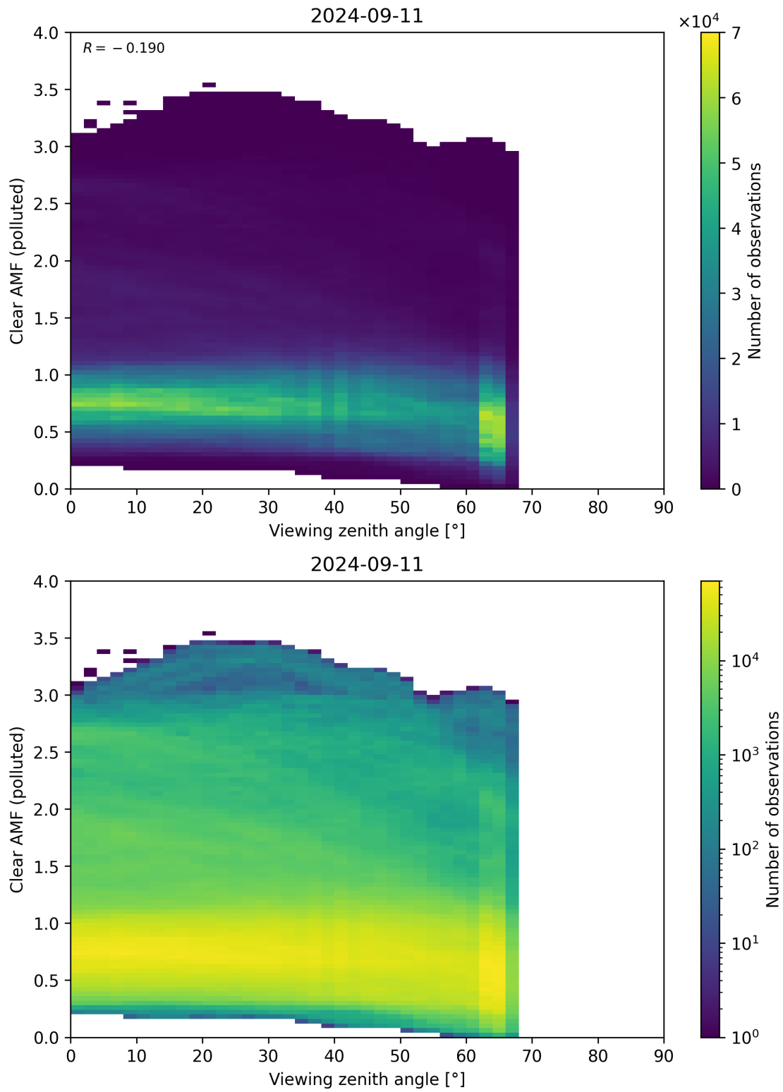
Figure 316: Scatter density plot of “Viewing zenith angle” against “Clear AMF (polluted)” for 2024-09-10 to 2024-09-12.
