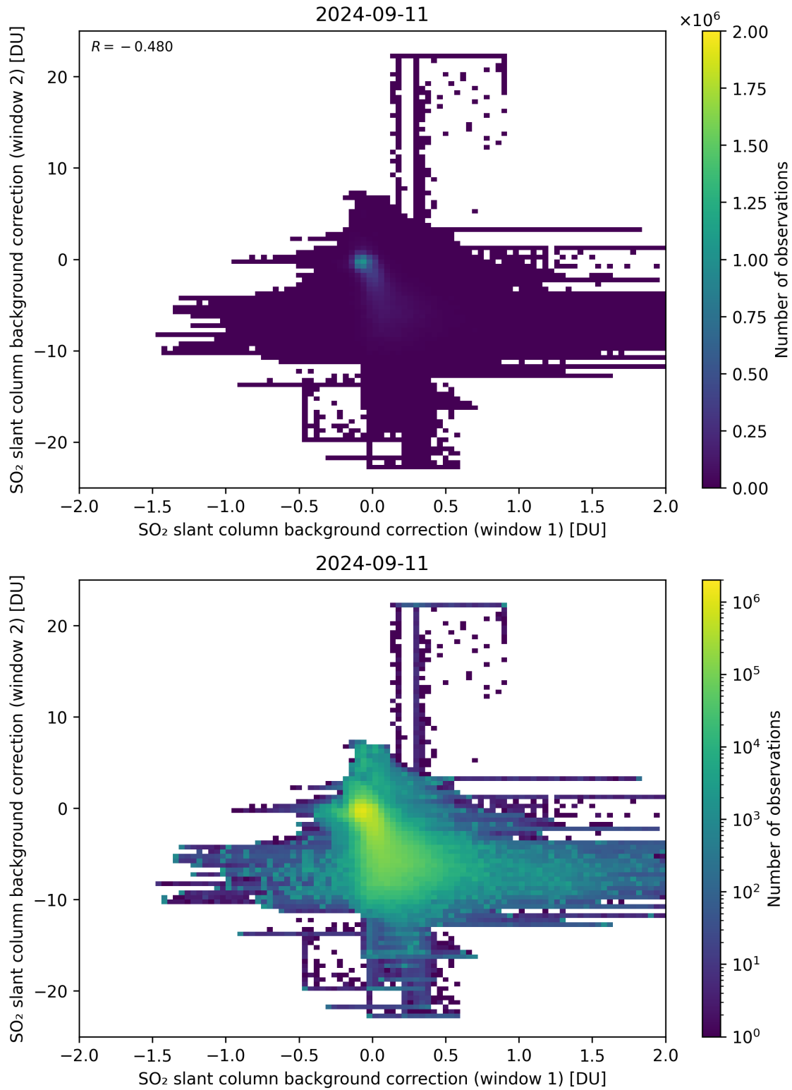
Figure 98: Scatter density plot of “SO 2 slant column background correction (window 1)” against “SO 2 slant column background correction (window 2)” for 2024-09-10 to 2024-09-12.
