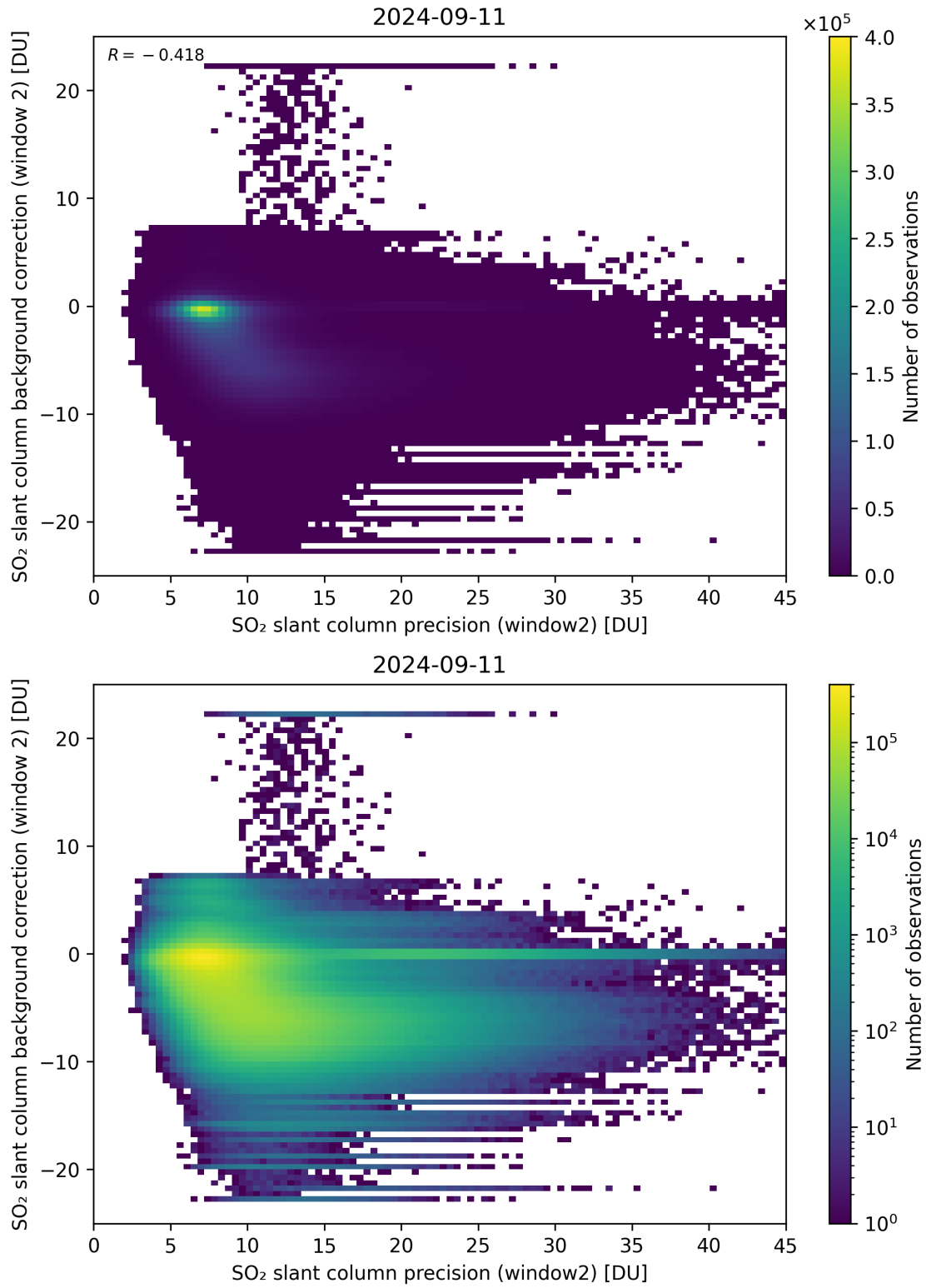
Figure 241: Scatter density plot of “SO 2 slant column precision (window2)” against “SO 2 slant column background correction (window 2)” for 2024-09-10 to 2024-09-12.
