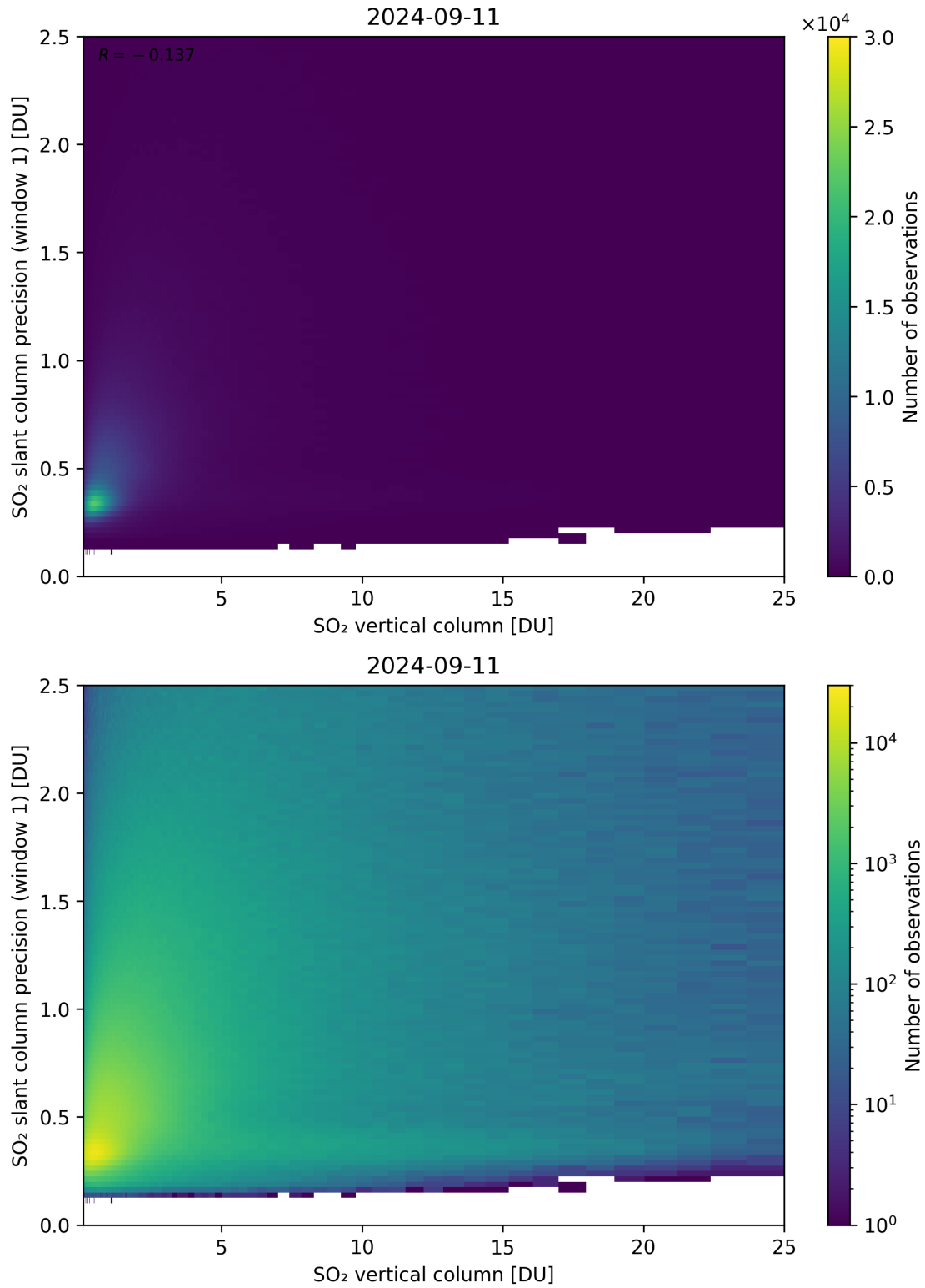
Figure 301: Scatter density plot of “SO 2 vertical column” against “SO 2 slant column precision (window 1)” for 2024-09-10 to 2024-09-12.
