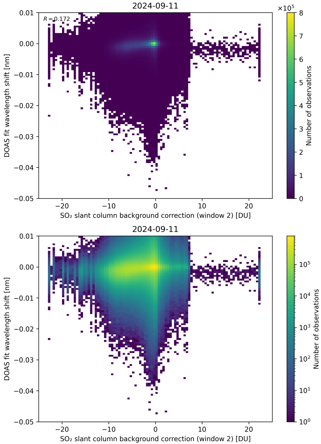
Figure 112: Scatter density plot of “SO 2 slant column background correction (window 2)” against “DOAS fit wavelength shift” for 2024-09-10 to 2024-09-12.
