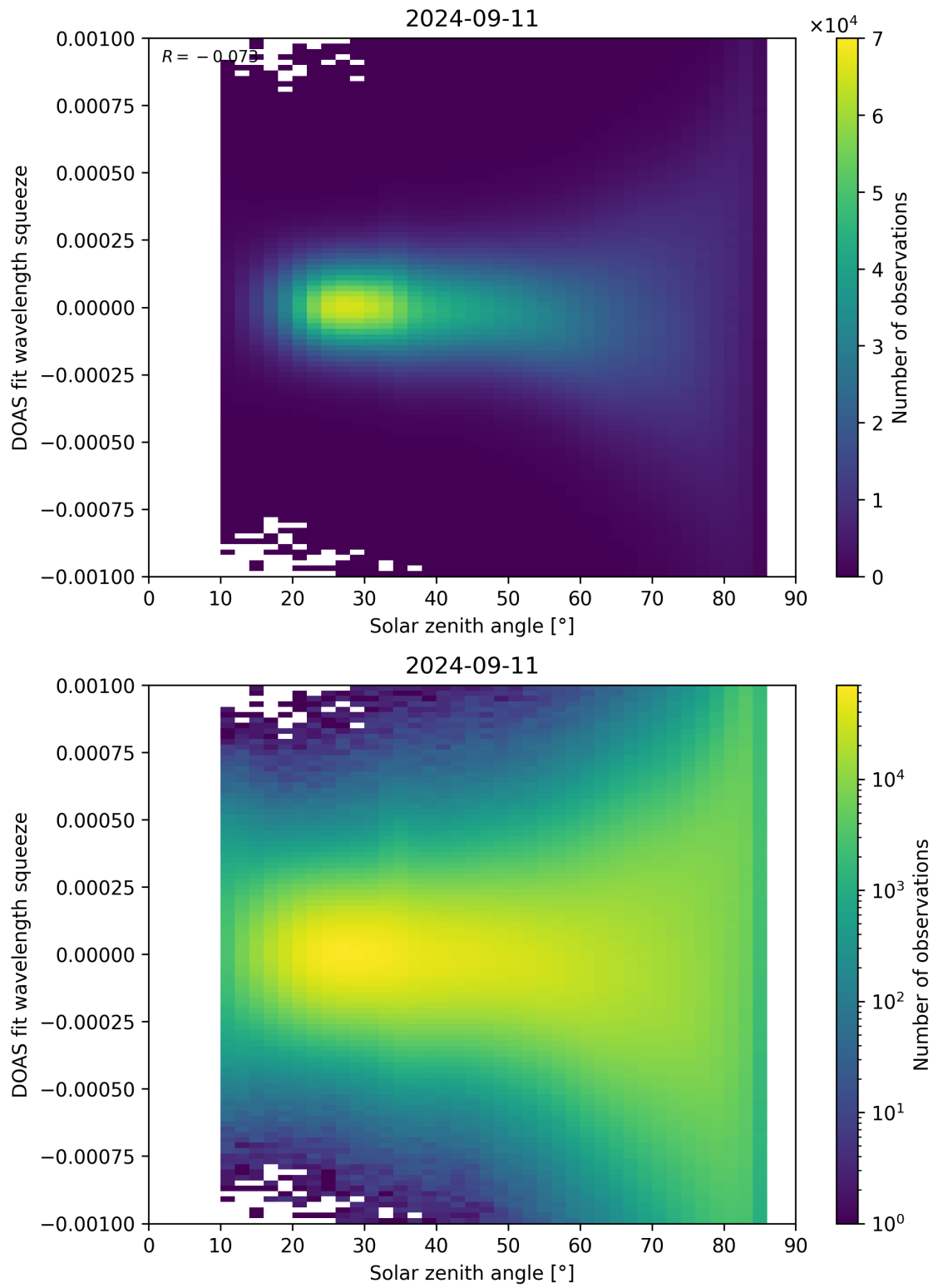
Figure 162: Scatter density plot of “Solar zenith angle” against “DOAS fit wavelength squeeze” for 2024-09-10 to 2024-09-12.
