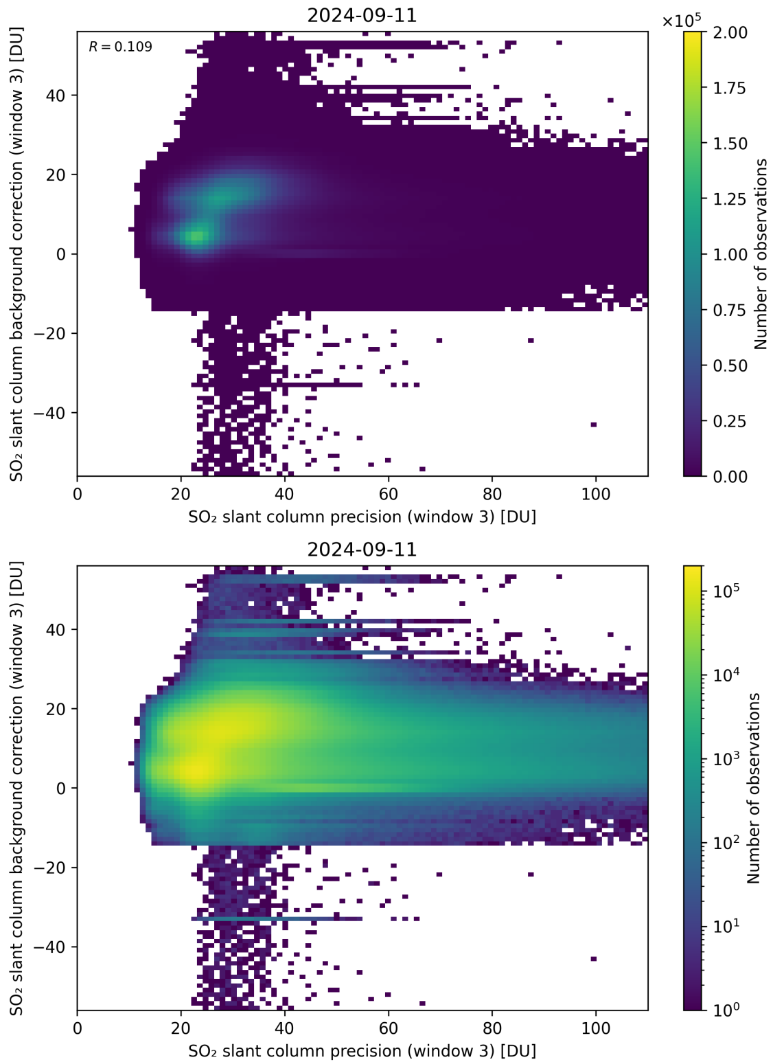
Figure 257: Scatter density plot of “SO 2 slant column precision (window 3)” against “SO 2 slant column background correction (window 3)” for 2024-09-10 to 2024-09-12.
