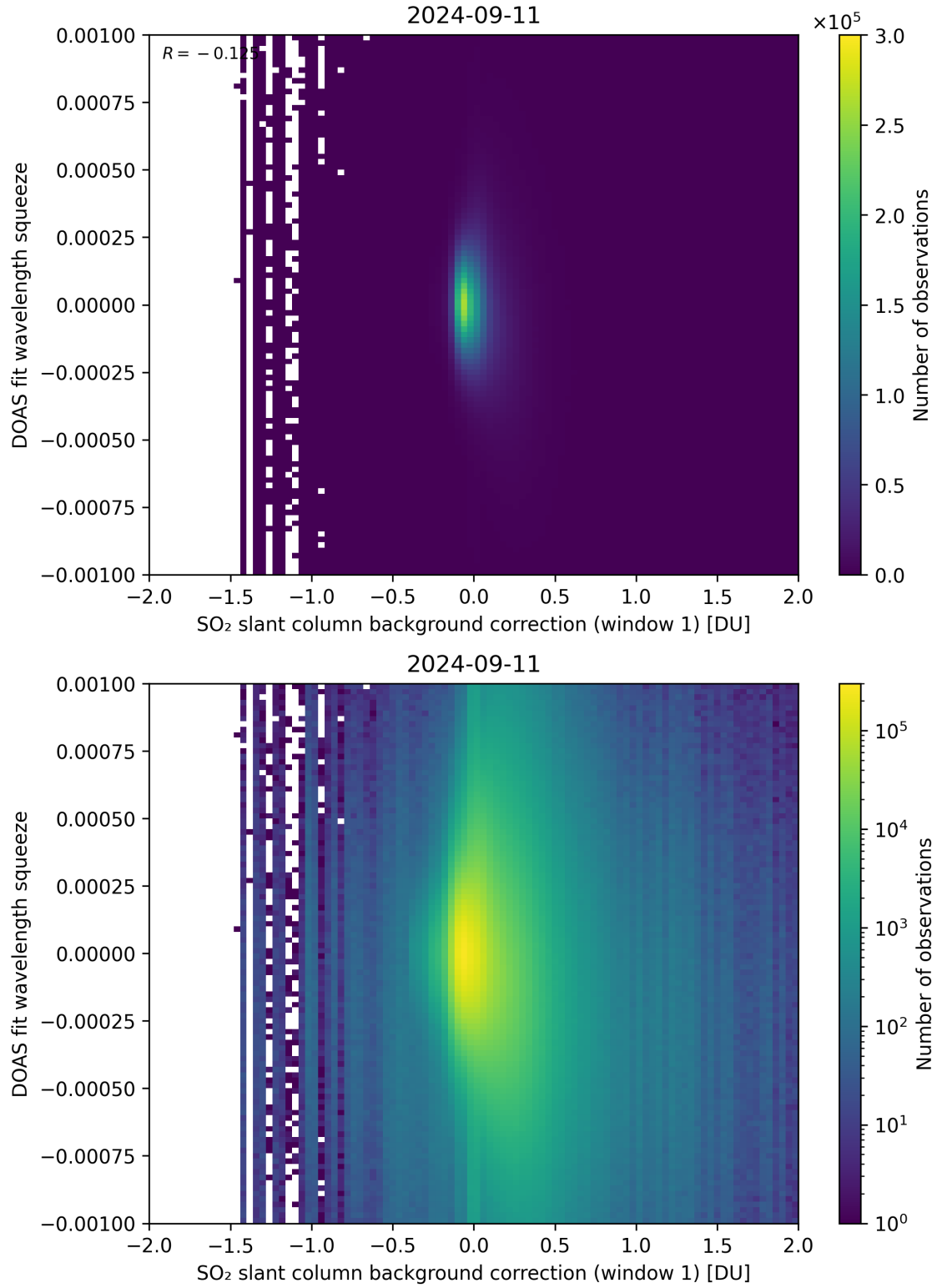
Figure 101: Scatter density plot of “SO 2 slant column background correction (window 1)” against “DOAS fit wavelength squeeze” for 2024-09-10 to 2024-09-12.
