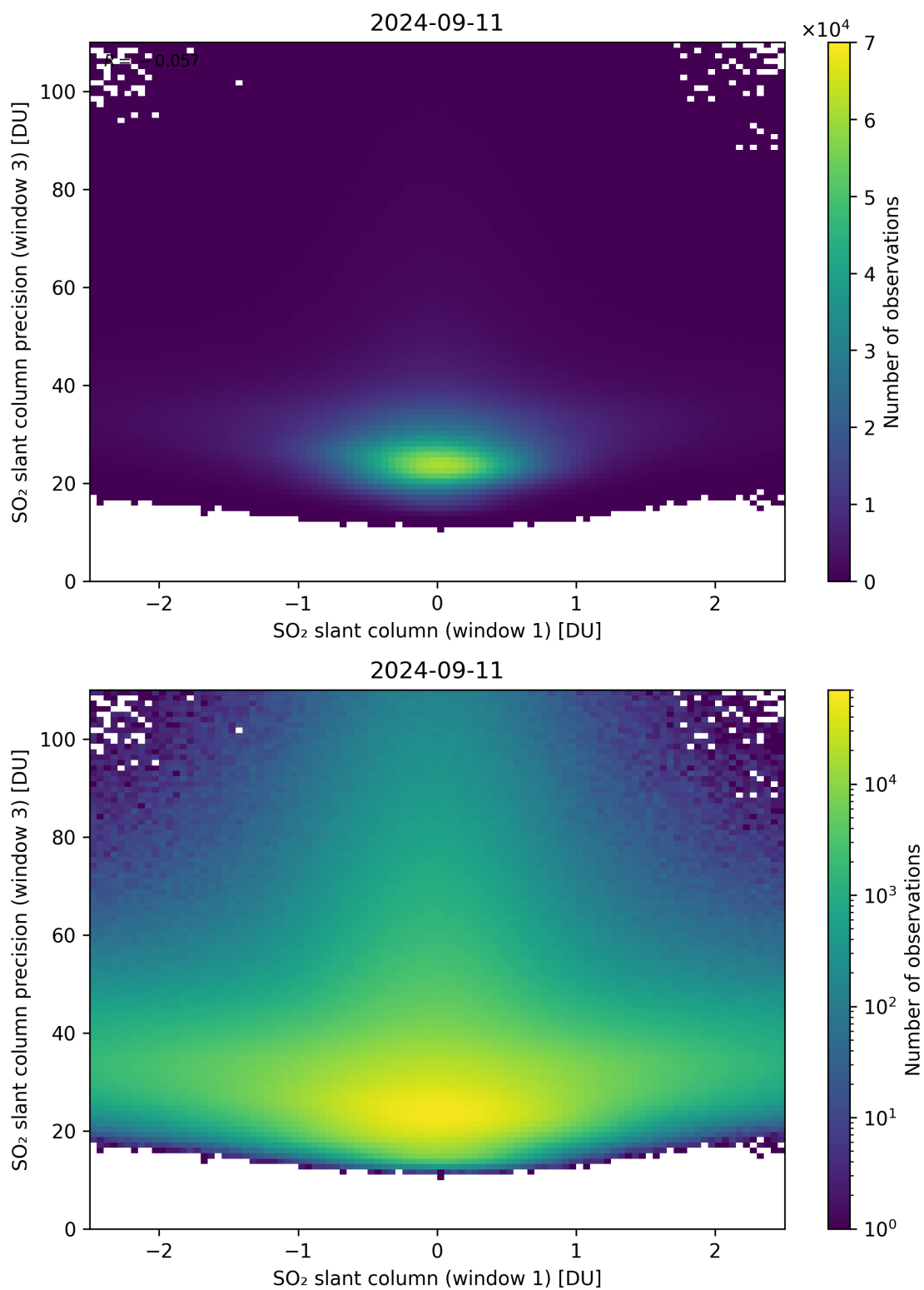
Figure 238: Scatter density plot of “SO 2 slant column (window 1)” against “SO 2 slant column precision (window 3)” for 2024-09-10 to 2024-09-12.
