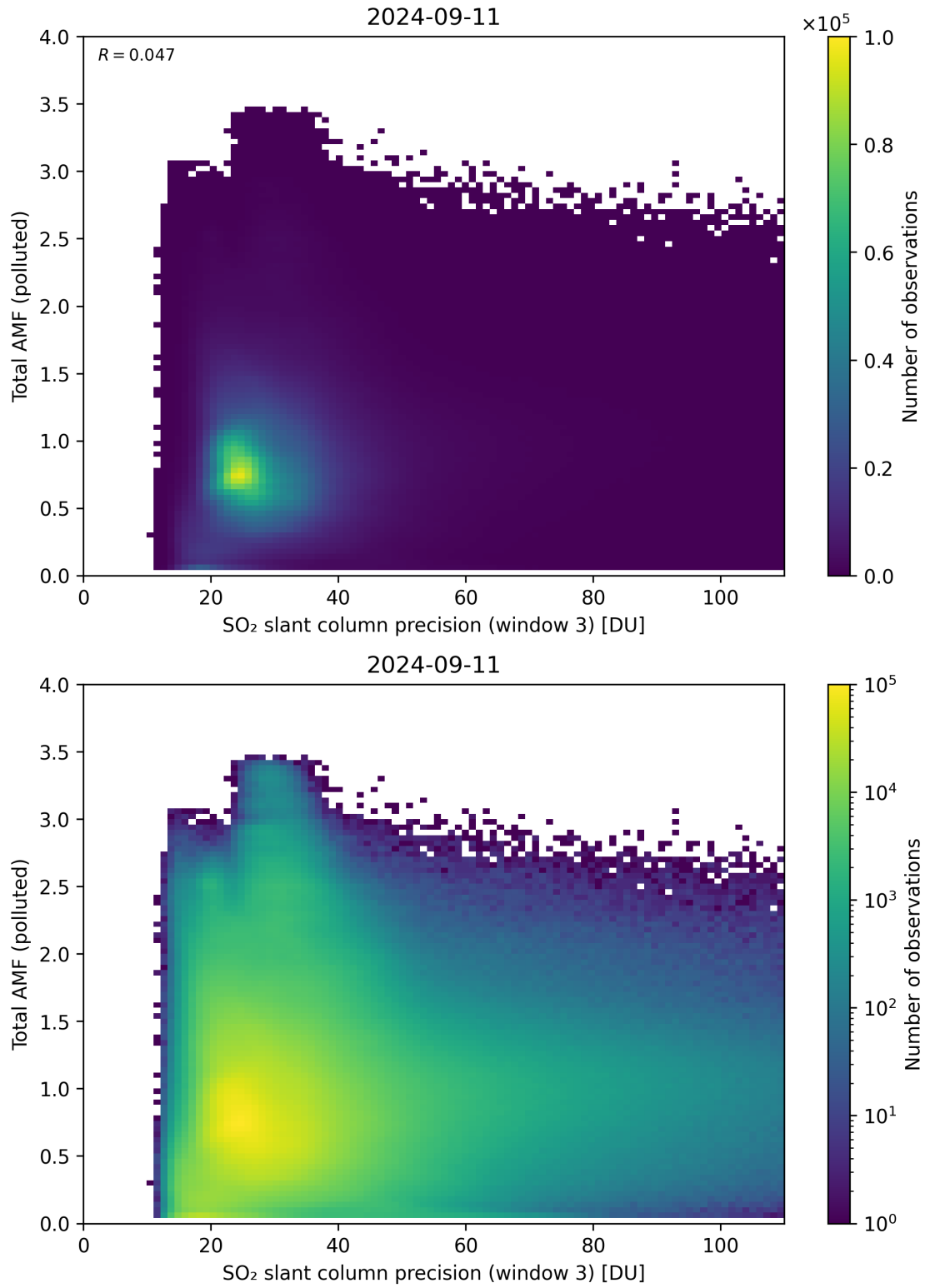
Figure 263: Scatter density plot of “SO 2 slant column precision (window 3)” against “Total AMF (polluted)” for 2024-09-10 to 2024-09-12.
