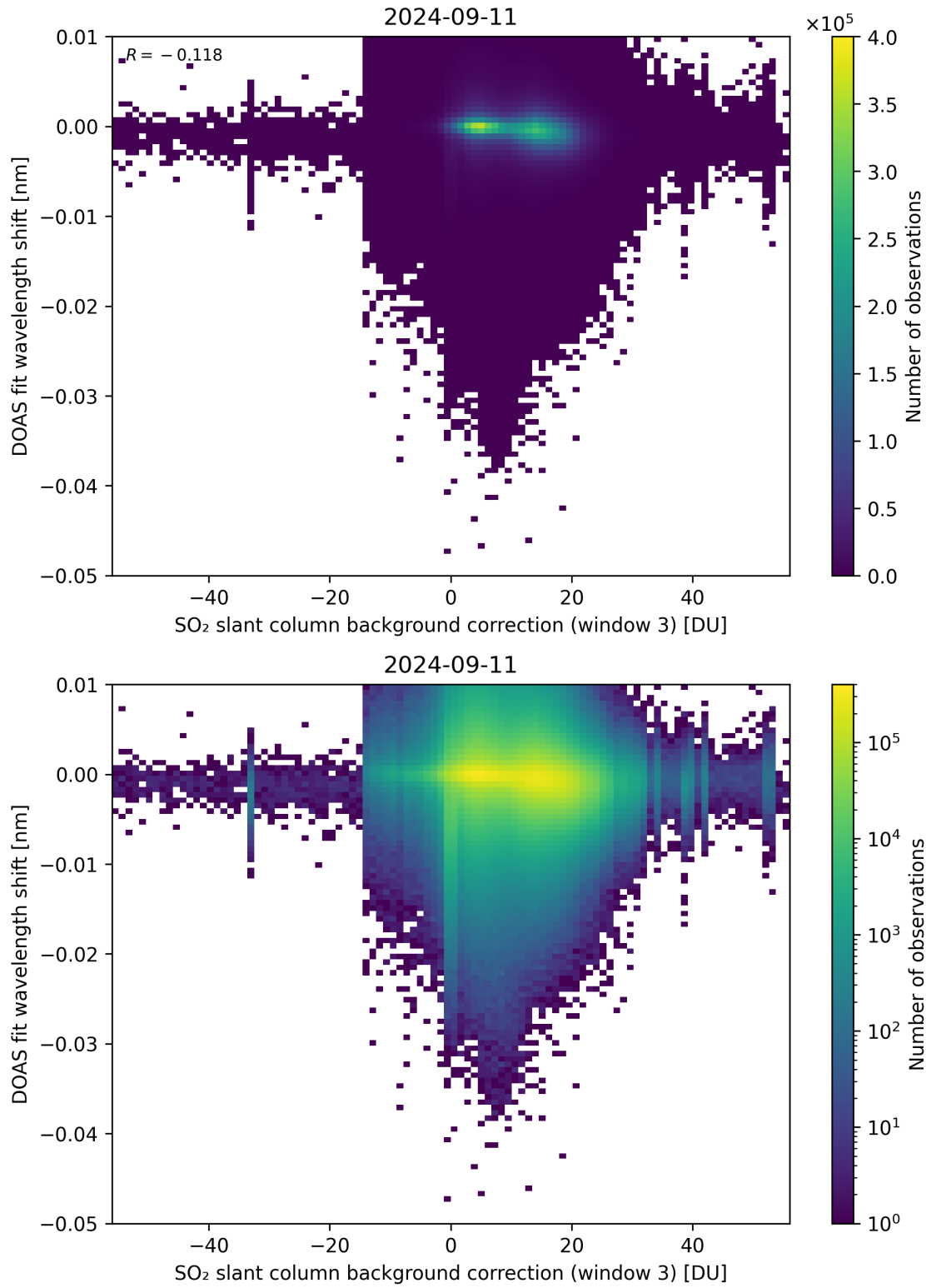
Figure 121: Scatter density plot of “SO 2 slant column background correction (window 3)” against “DOAS fit wavelength shift” for 2024-09-10 to 2024-09-12.
