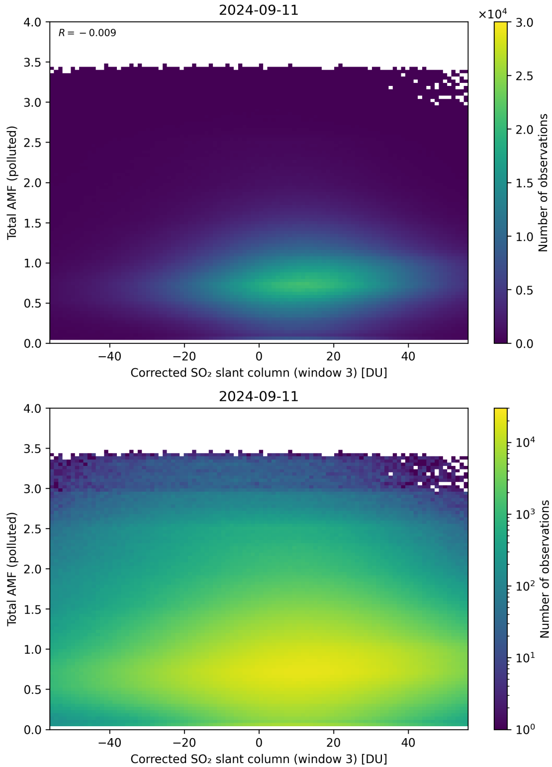
Figure 210: Scatter density plot of “Corrected SO 2 slant column (window 3)” against “Total AMF (polluted)” for 2024-09-10 to 2024-09-12.
