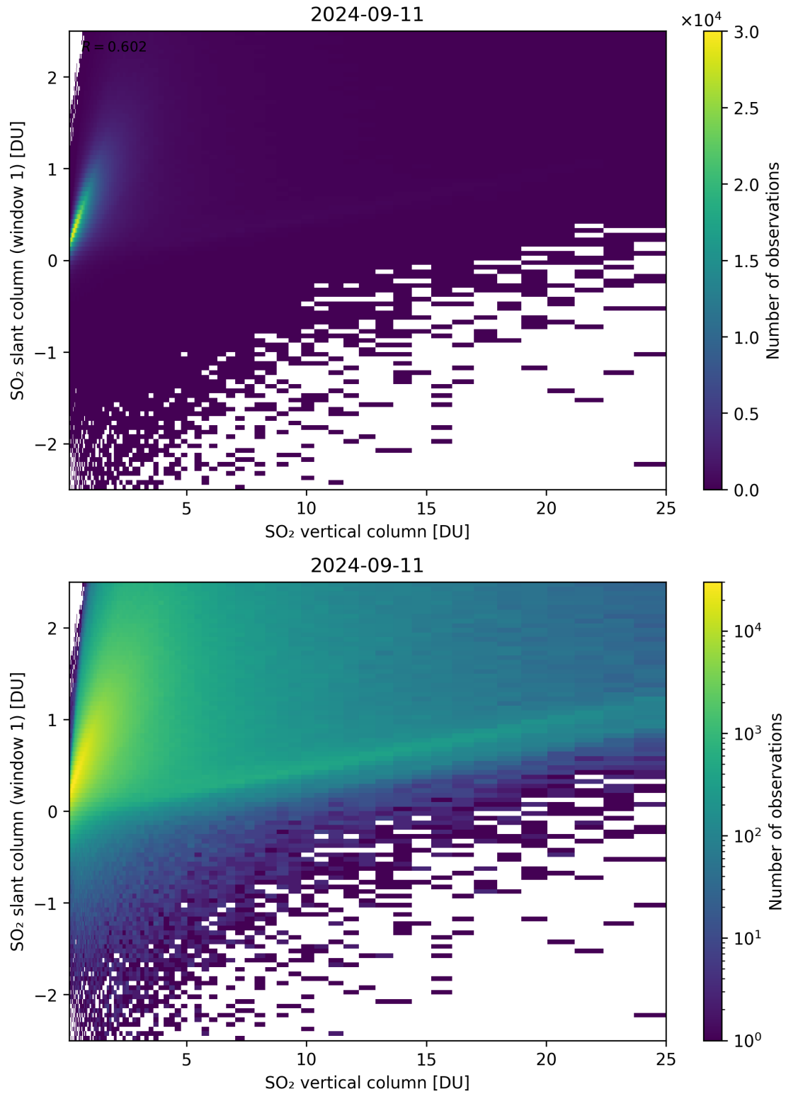
Figure 300: Scatter density plot of “SO 2 vertical column” against “SO 2 slant column (window 1)” for 2024-09-10 to 2024-09-12.
