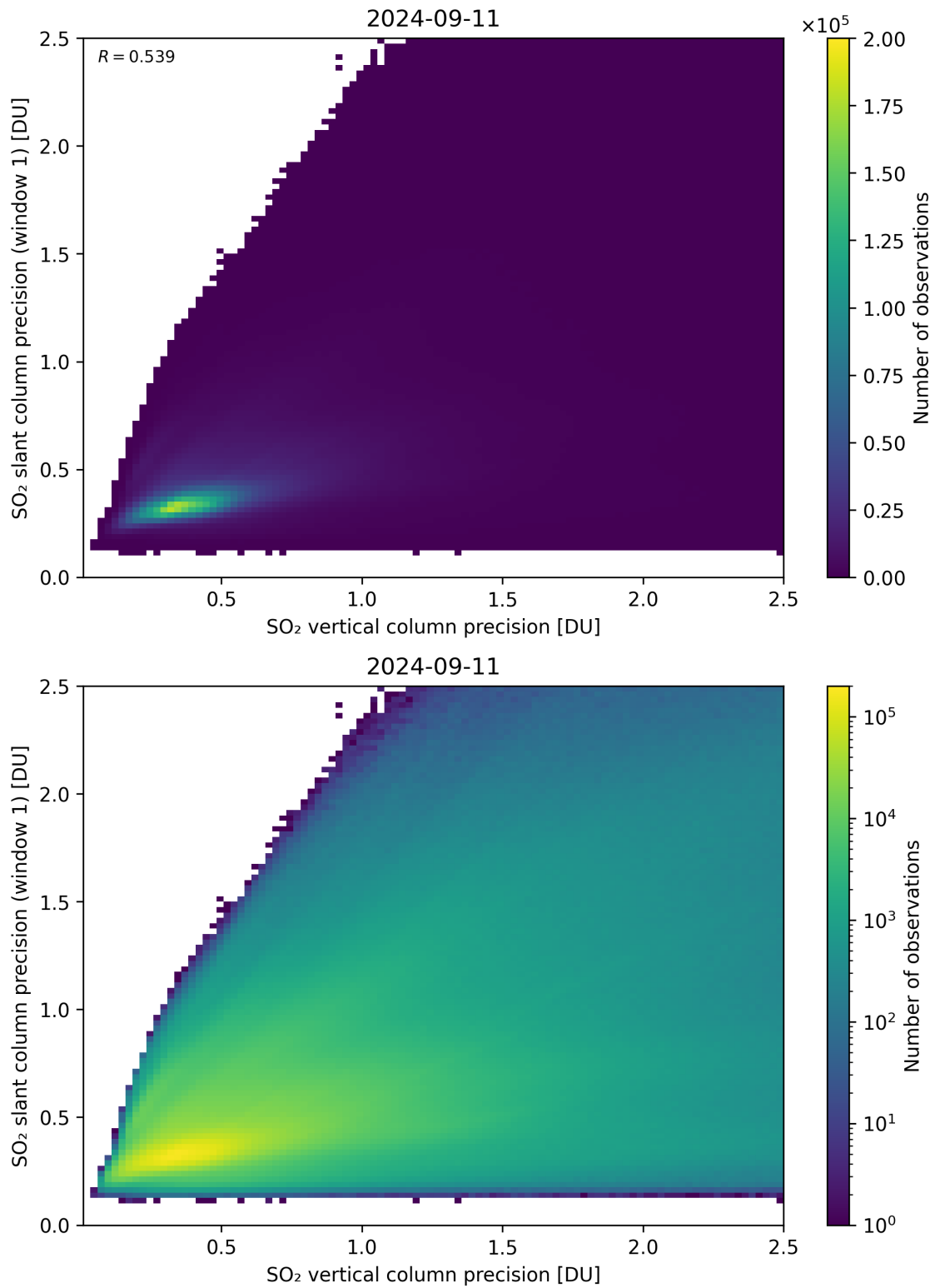
Figure 290: Scatter density plot of “SO 2 vertical column precision” against “SO 2 slant column precision (window 1)” for 2024-09-10 to 2024-09-12.
