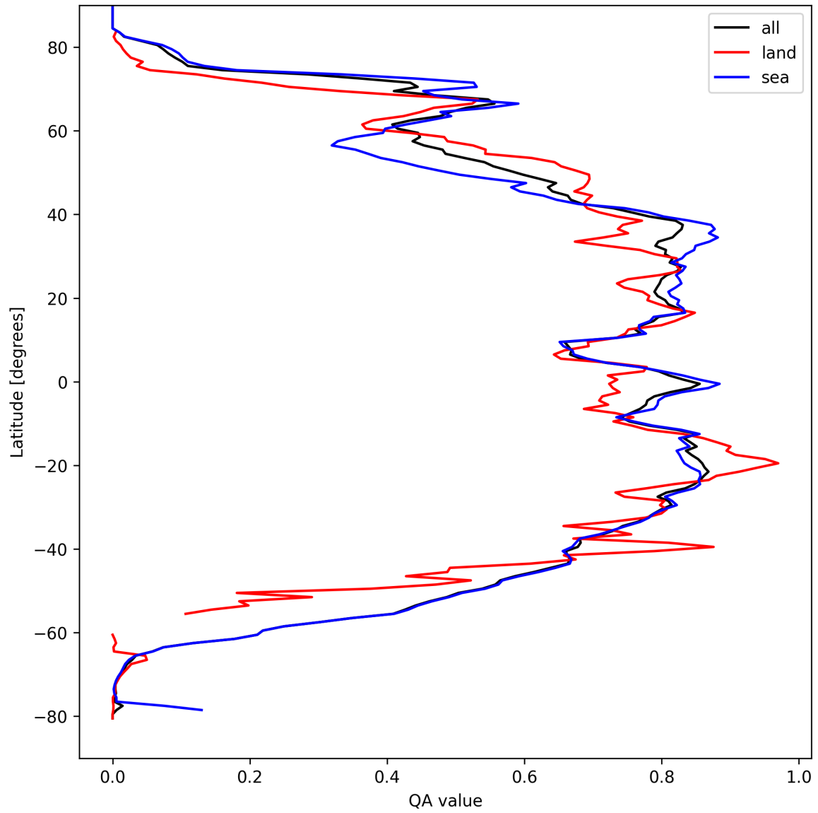
Figure 29: Zonal average of “QA value” for 2024-09-10 to 2024-09-12.
