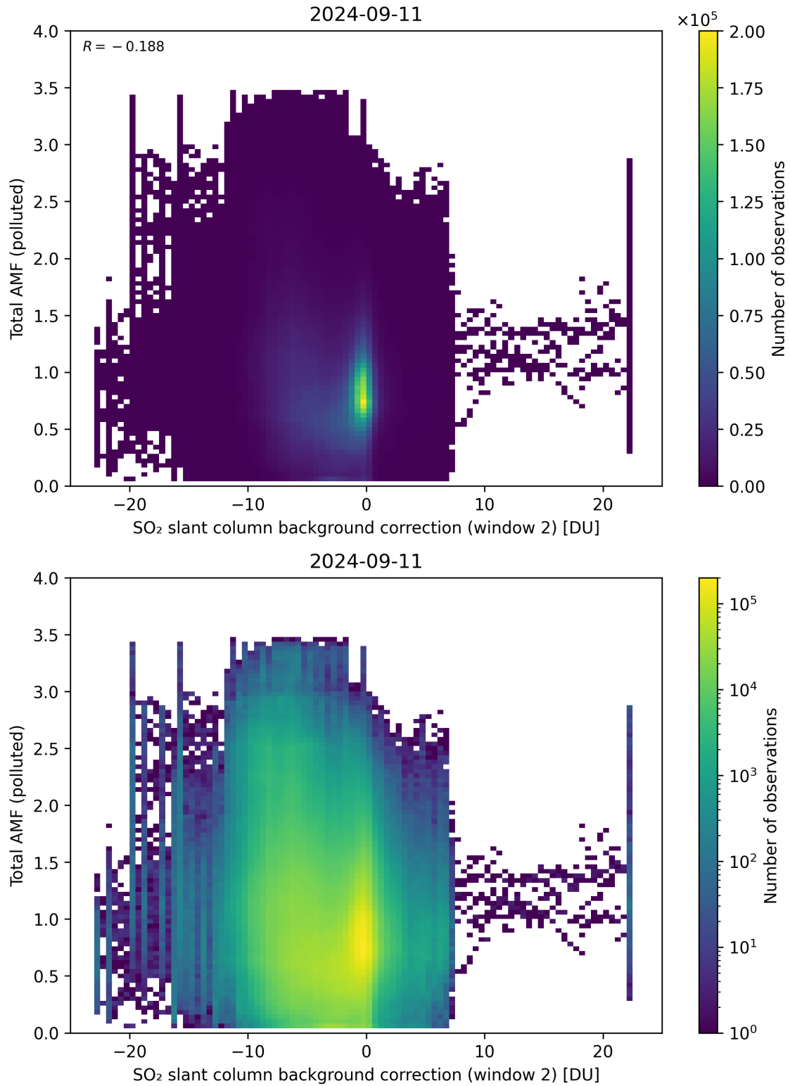
Figure 119: Scatter density plot of “SO 2 slant column background correction (window 2)” against “Total AMF (polluted)” for 2024-09-10 to 2024-09-12.
