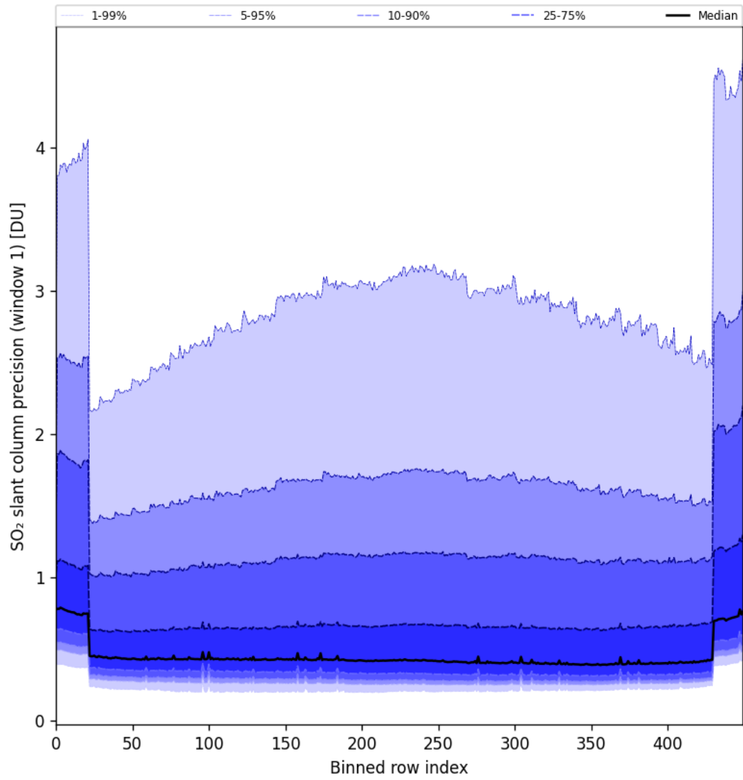
Figure 80: Along track statistics of “SO 2 slant column precision (window 1)” for 2024-09-10 to 2024-09-12
