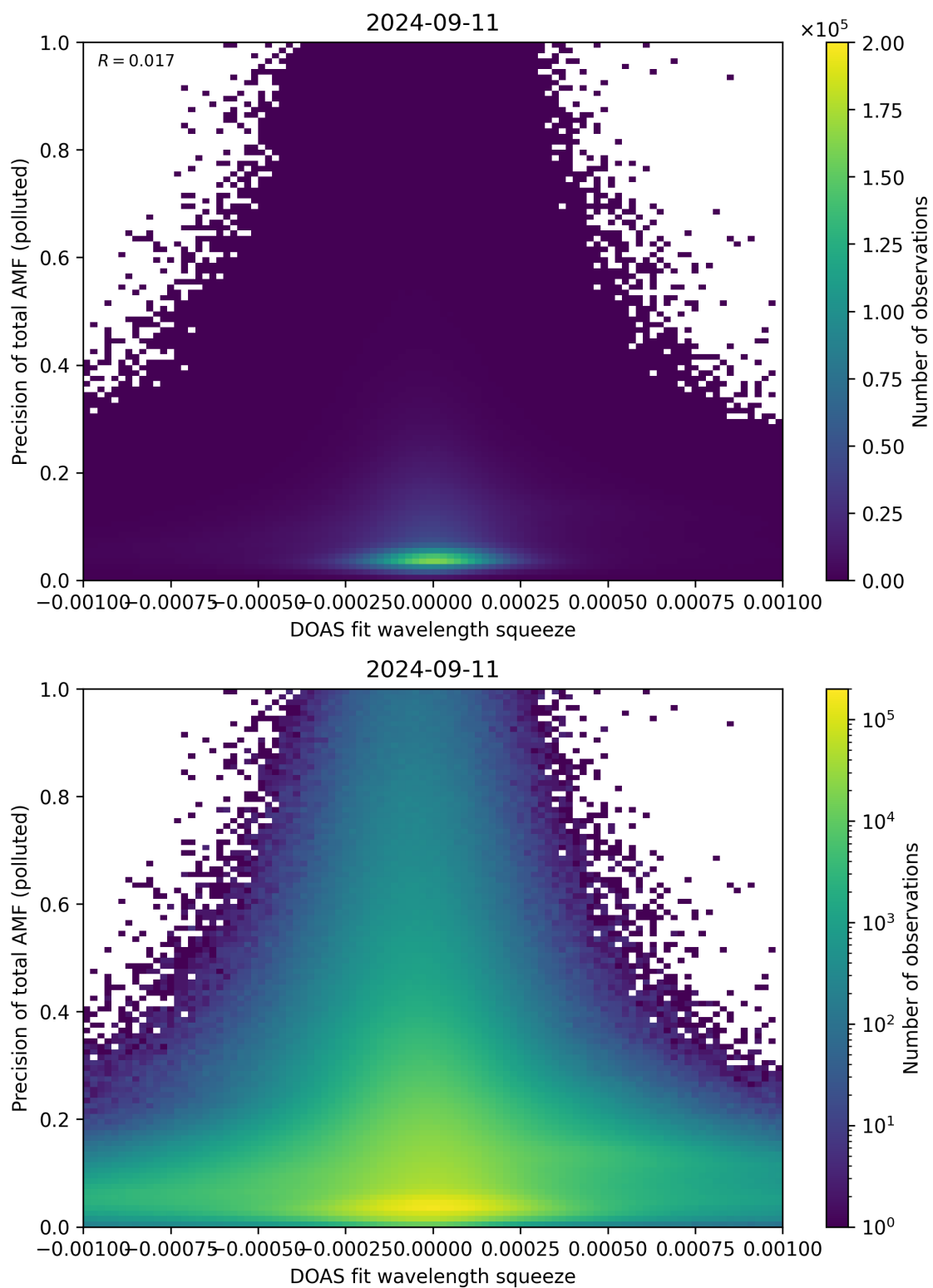
Figure 135: Scatter density plot of “DOAS fit wavelength squeeze” against “Precision of total AMF (polluted)” for 2024-09-10 to 2024-09-12.
