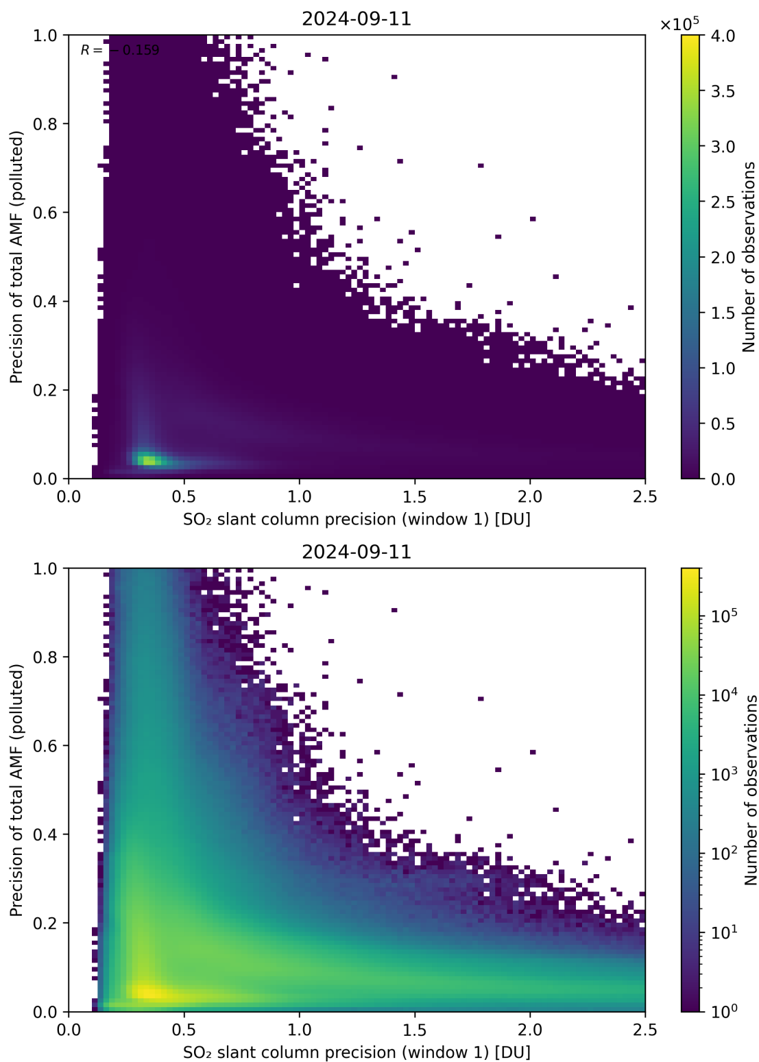
Figure 231: Scatter density plot of “SO 2 slant column precision (window 1)” against “Precision of total AMF (polluted)” for 2024-09-10 to 2024-09-12.
