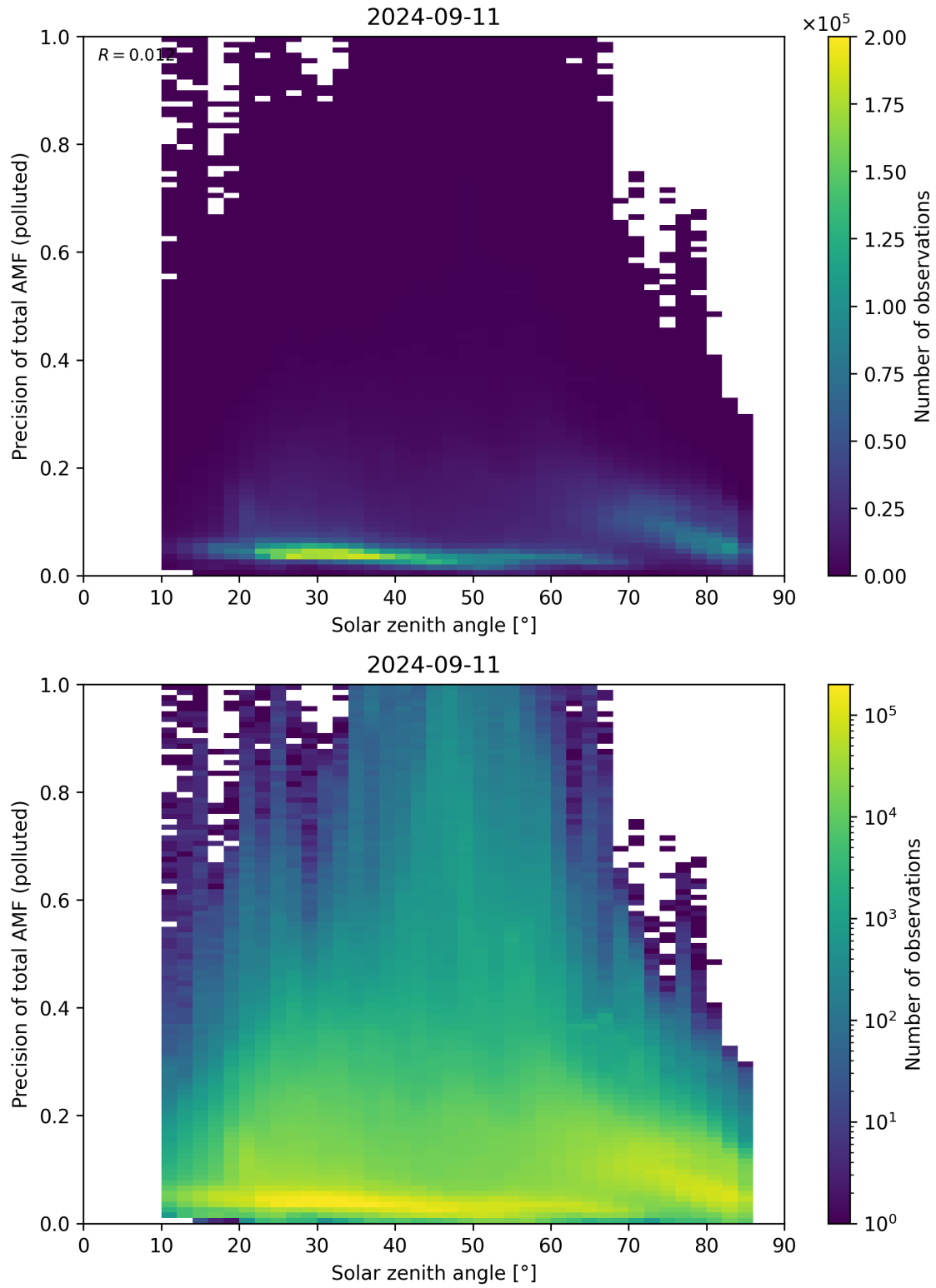
Figure 175: Scatter density plot of “Solar zenith angle” against “Precision of total AMF (polluted)” for 2024-09-10 to 2024-09-12.
