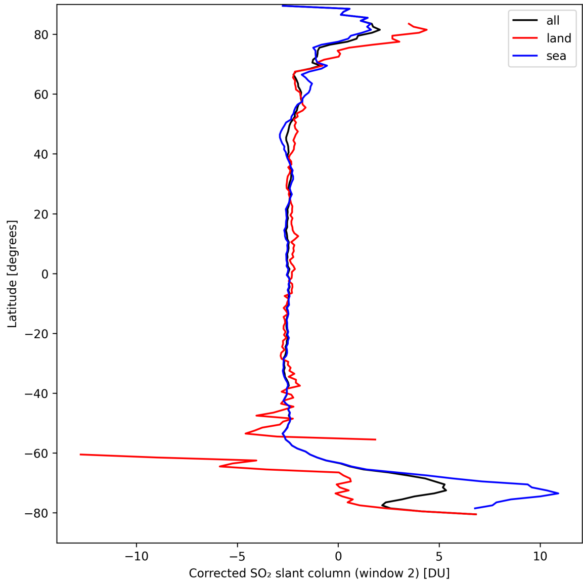
Figure 39: Zonal average of “Corrected SO 2 slant column (window 2)” for 2024-09-10 to 2024-09-12.
