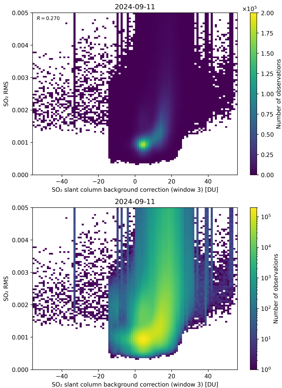
Figure 123: Scatter density plot of “SO 2 slant column background correction (window 3)” against “SO 2 RMS” for 2024-09-10 to 2024-09-12.
