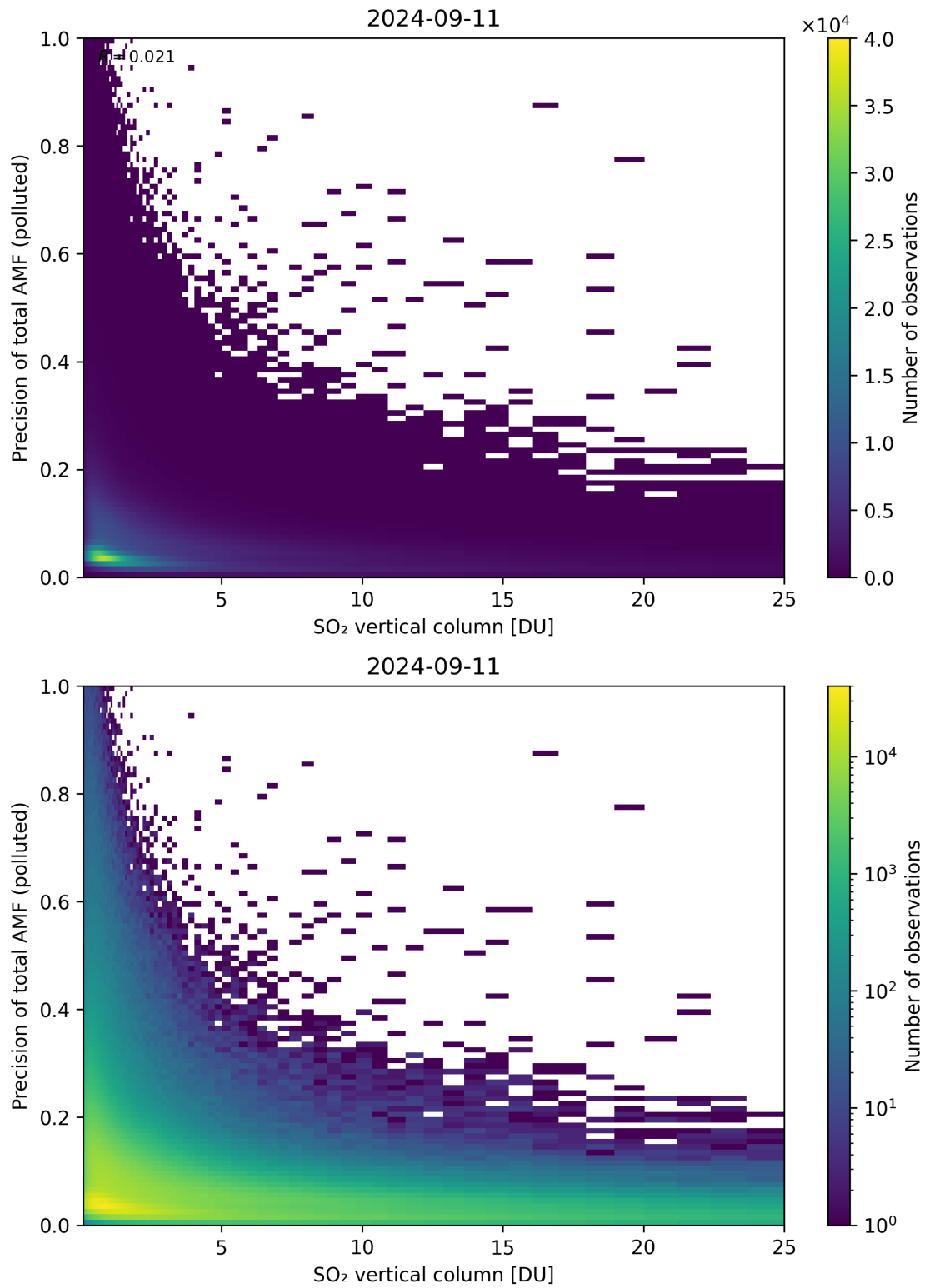
Figure 306: Scatter density plot of “SO 2 vertical column” against “Precision of total AMF (polluted)” for 2024-09-10 to 2024-09-12.
