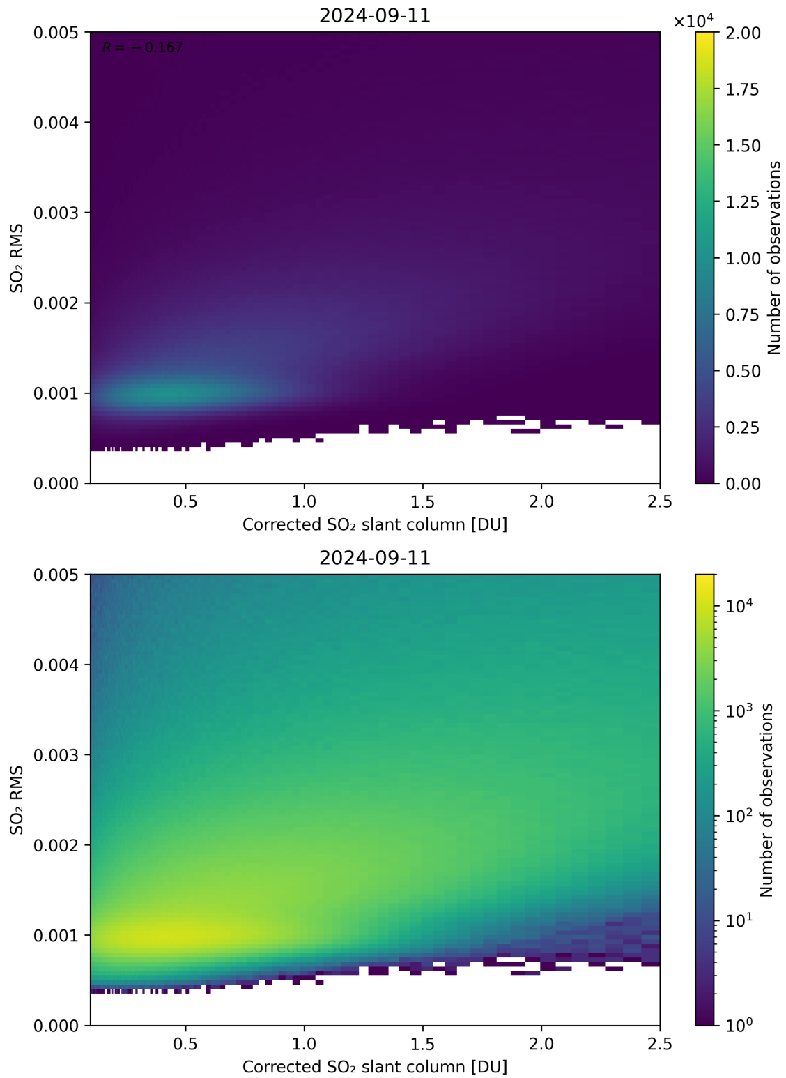
Figure 183: Scatter density plot of “Corrected SO 2 slant column” against “SO 2 RMS” for 2024-09-10 to 2024-09-12.
