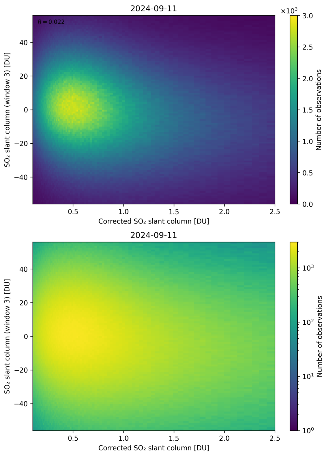
Figure 190: Scatter density plot of “Corrected SO 2 slant column” against “SO 2 slant column (window 3)” for 2024-09-10 to 2024-09-12.
