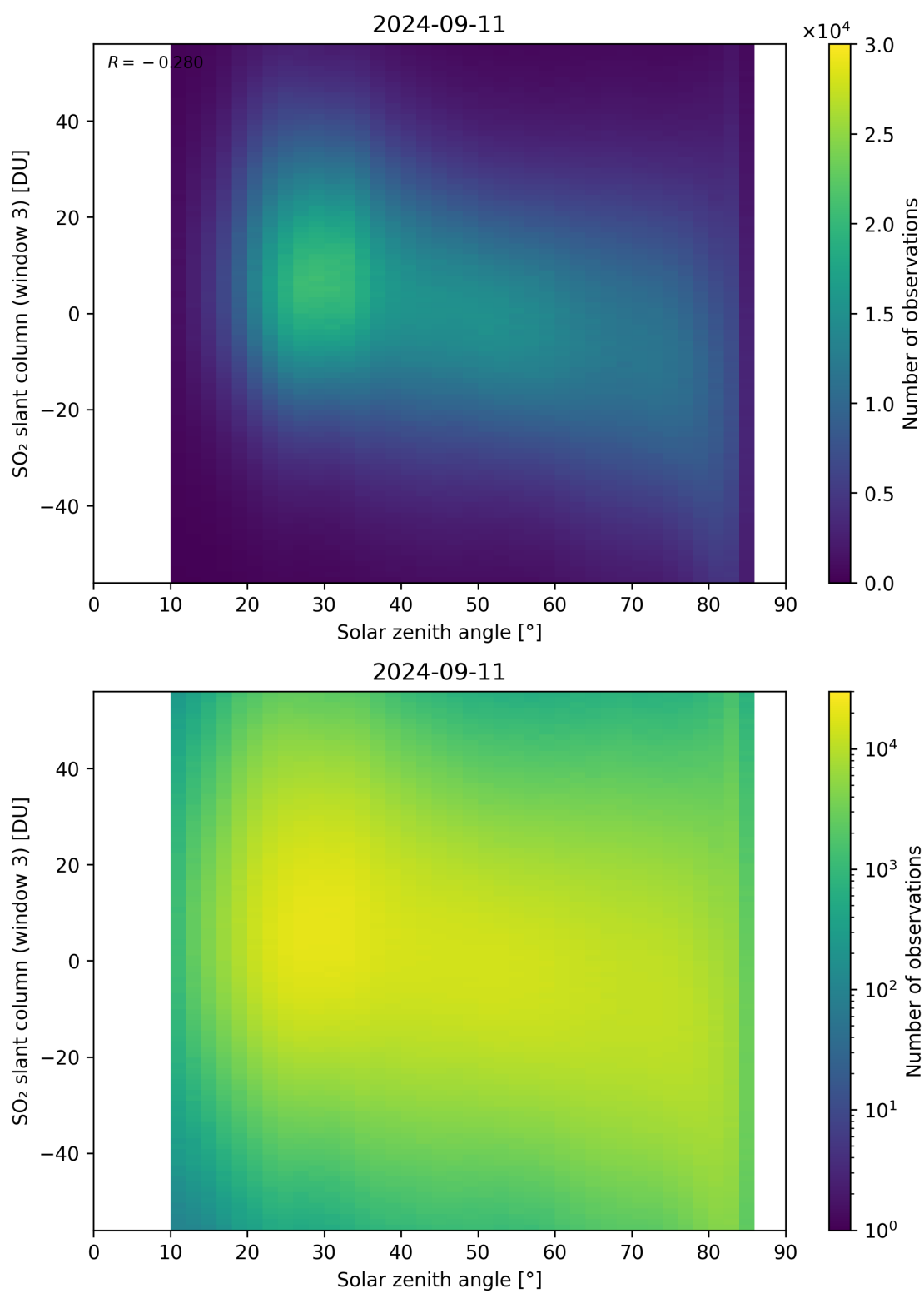
Figure 172: Scatter density plot of “Solar zenith angle” against “SO 2 slant column (window 3)” for 2024-09-10 to 2024-09-12.
