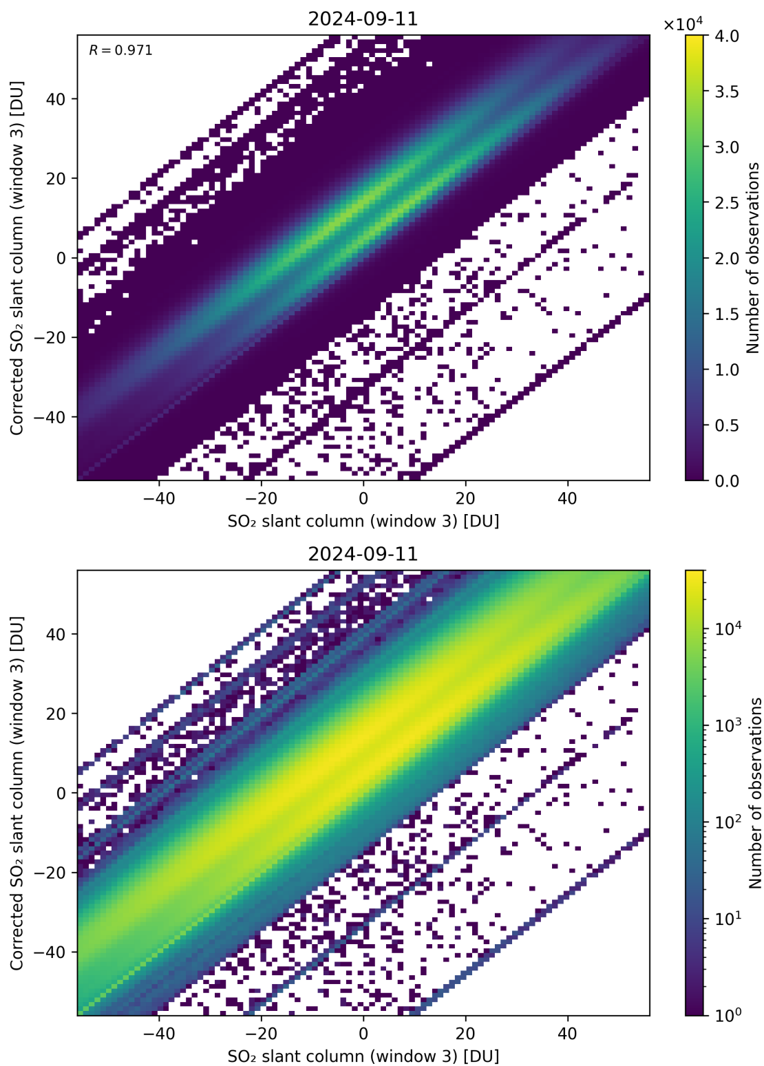
Figure 266: Scatter density plot of “SO 2 slant column (window 3)” against “Corrected SO 2 slant column (window 3)” for 2024-09-10 to 2024-09-12.
