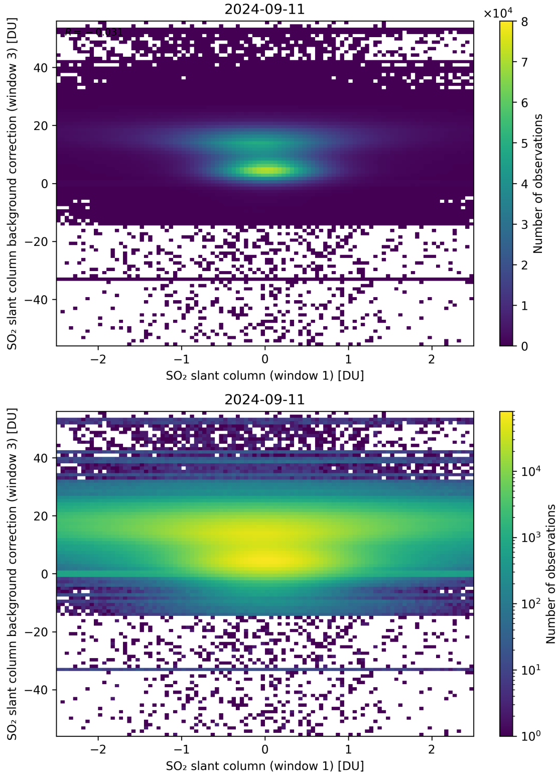
Figure 214: Scatter density plot of “SO 2 slant column (window 1)” against “SO 2 slant column background correction (window 3)” for 2024-09-10 to 2024-09-12.
