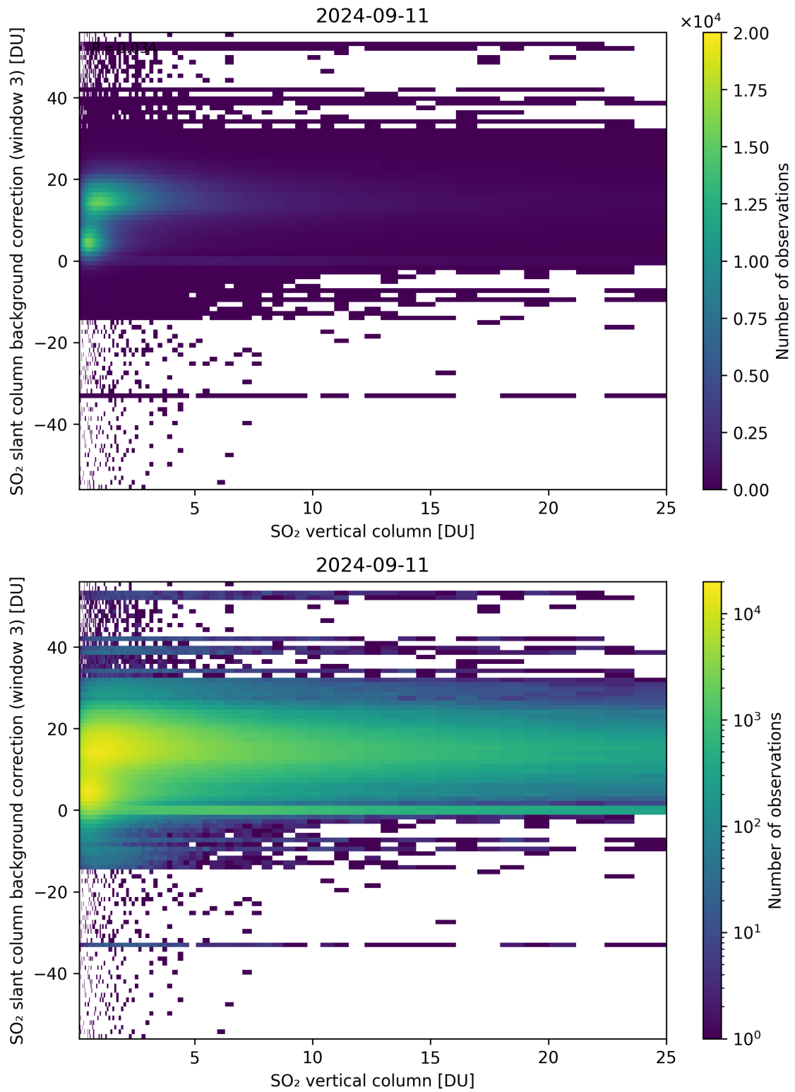
Figure 275: Scatter density plot of “SO 2 vertical column” against “SO 2 slant column background correction (window 3)” for 2024-09-10 to 2024-09-12.
