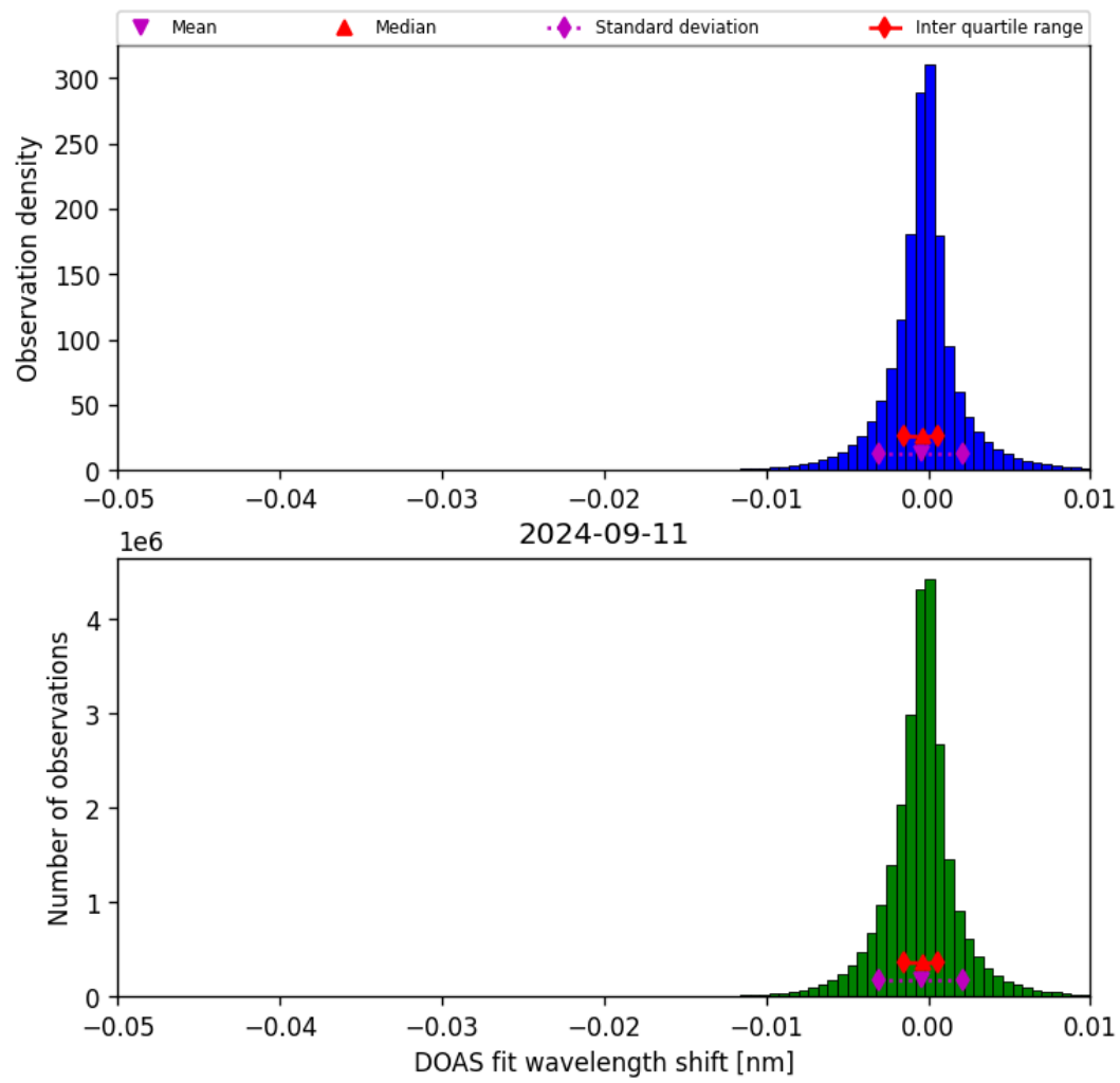
Figure 68: Histogram of “DOAS fit wavelength shift” for 2024-09-10 to 2024-09-12
