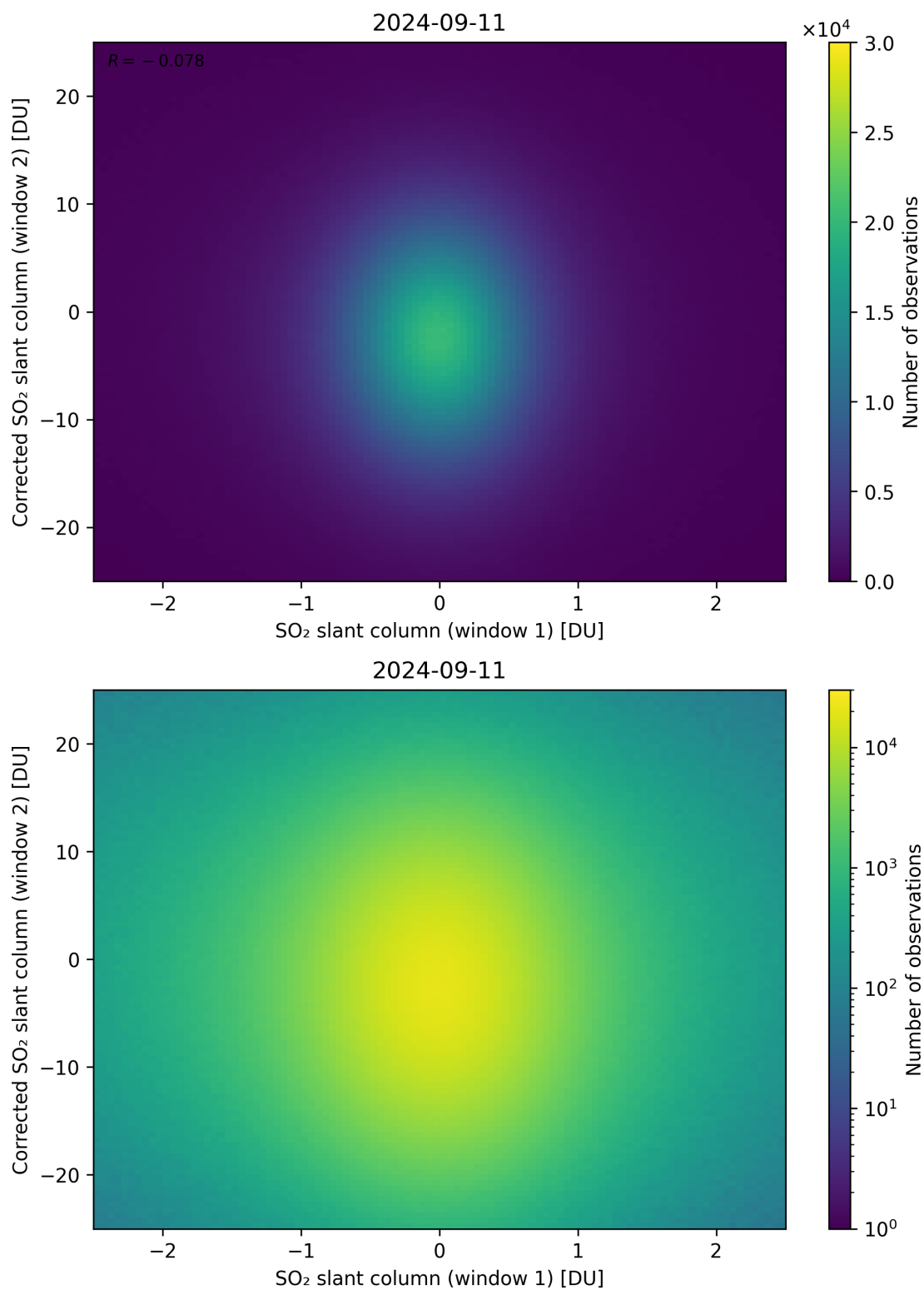
Figure 233: Scatter density plot of “SO 2 slant column (window 1)” against “Corrected SO 2 slant column (window 2)” for 2024-09-10 to 2024-09-12.
