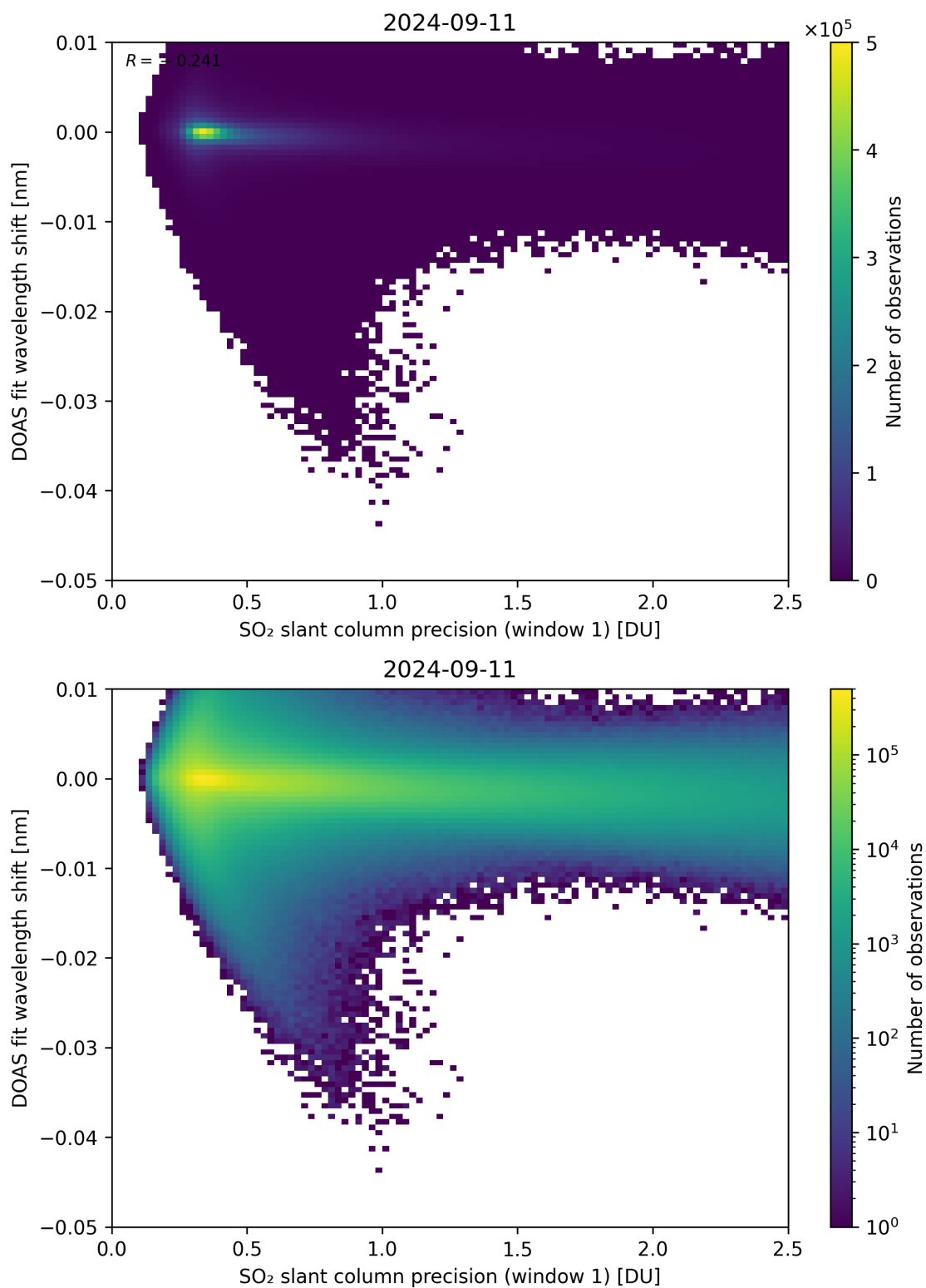
Figure 221: Scatter density plot of “SO 2 slant column precision (window 1)” against “DOAS fit wavelength shift” for 2024-09-10 to 2024-09-12.
