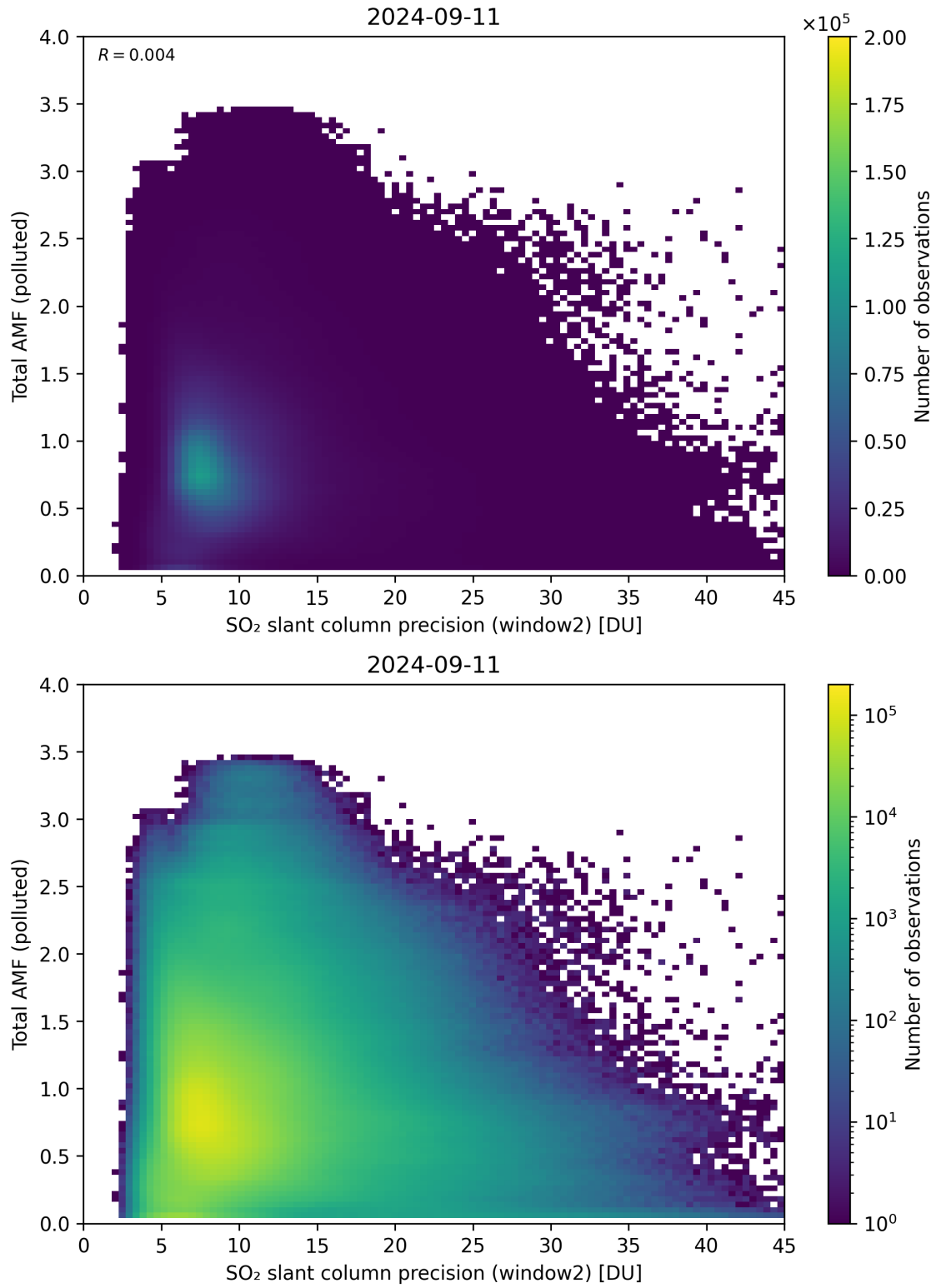
Figure 251: Scatter density plot of “SO 2 slant column precision (window2)” against “Total AMF (polluted)” for 2024-09-10 to 2024-09-12.
