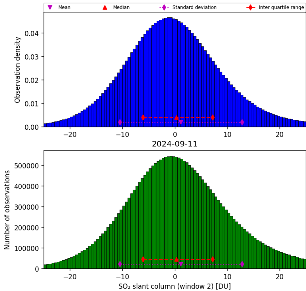
Figure 60: Histogram of “SO 2 slant column (window 2)” for 2024-09-10 to 2024-09-12
