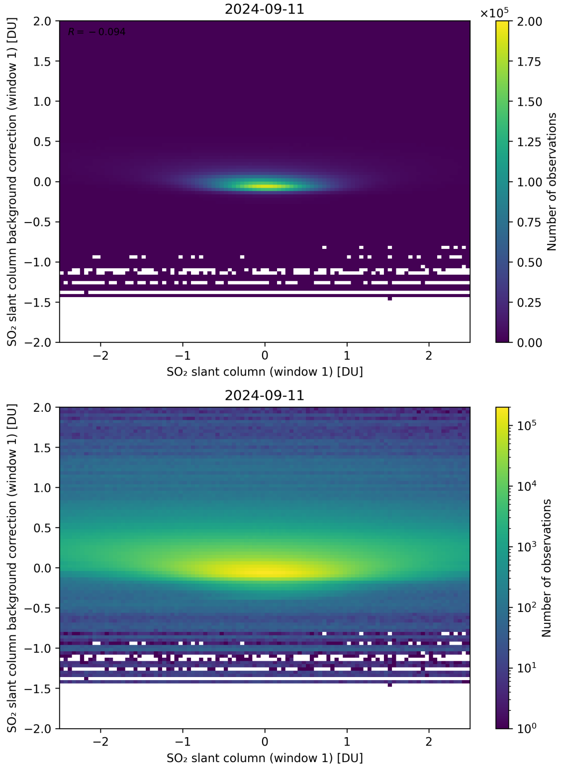
Figure 212: Scatter density plot of “SO 2 slant column (window 1)” against “SO 2 slant column background correction (window 1)” for 2024-09-10 to 2024-09-12.
