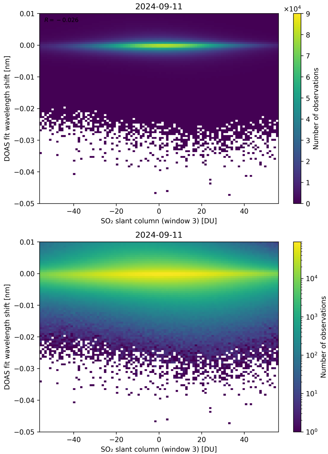
Figure 254: Scatter density plot of “SO 2 slant column (window 3)” against “DOAS fit wavelength shift” for 2024-09-10 to 2024-09-12.
