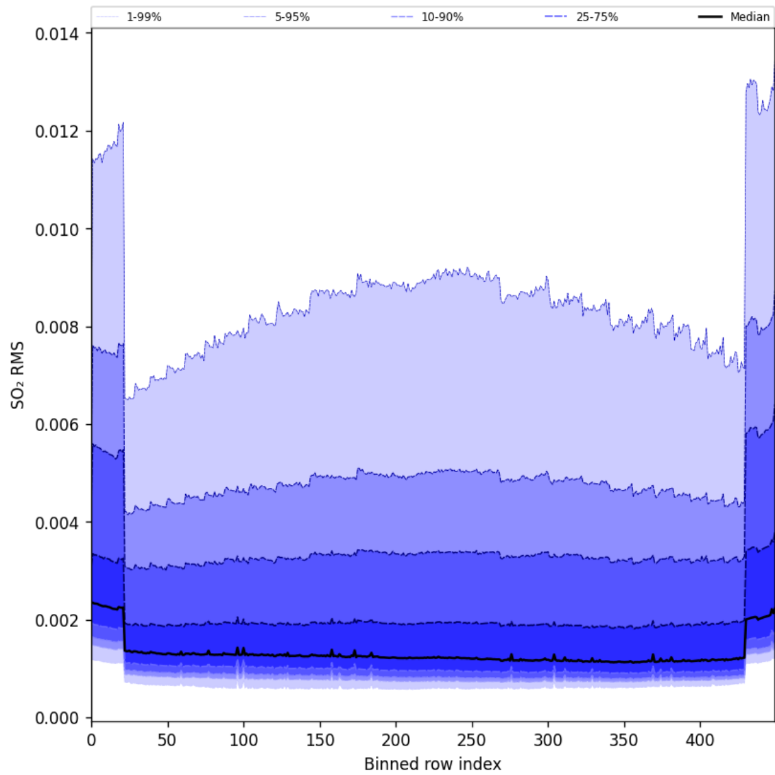
Figure 93: Along track statistics of “SO 2 RMS” for 2024-09-10 to 2024-09-12
