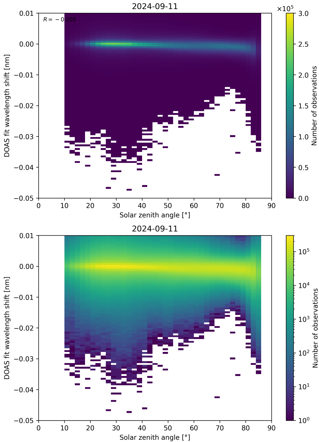
Figure 161: Scatter density plot of “Solar zenith angle” against “DOAS fit wavelength shift” for 2024-09-10 to 2024-09-12.
