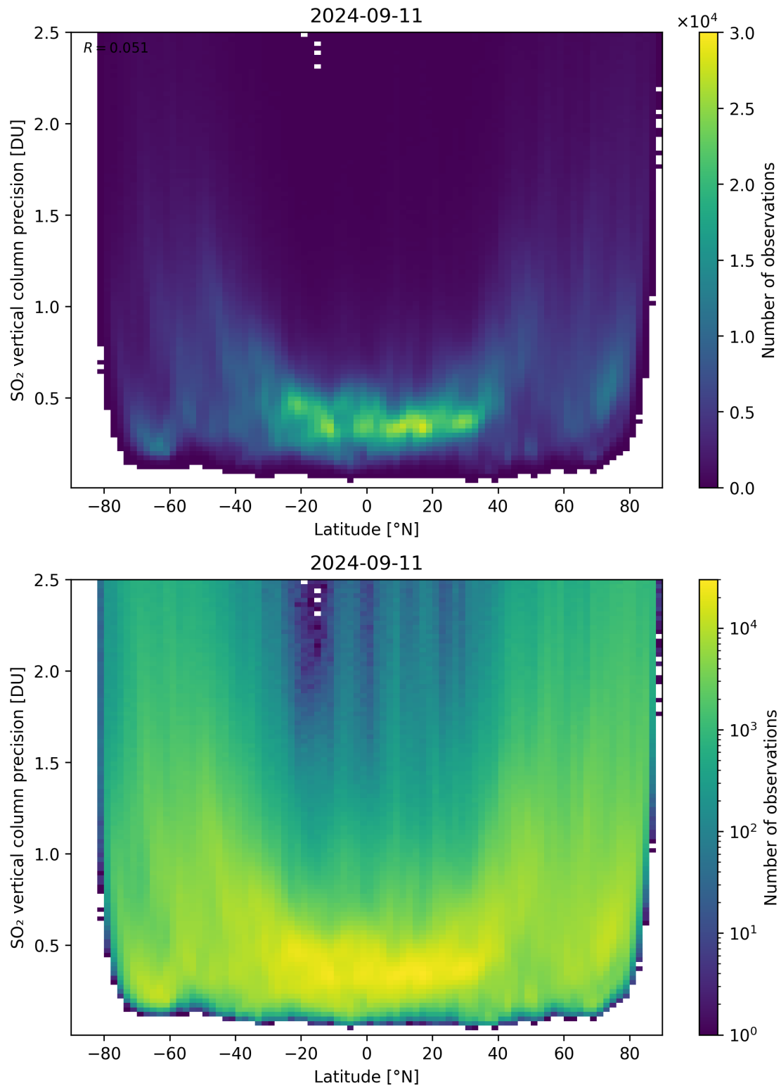
Figure 157: Scatter density plot of “Latitude” against “SO 2 vertical column precision” for 2024-09-10 to 2024-09-12.
