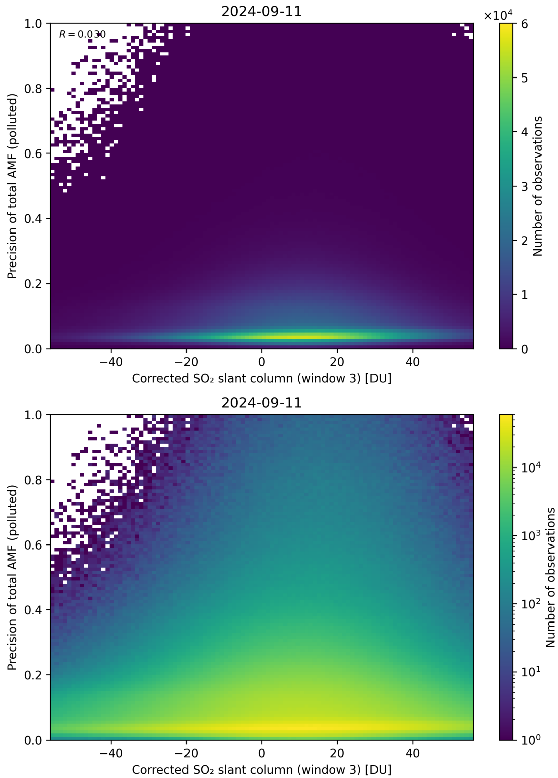
Figure 211: Scatter density plot of “Corrected SO 2 slant column (window 3)” against “Precision of total AMF (polluted)” for 2024-09-10 to 2024-09-12.
