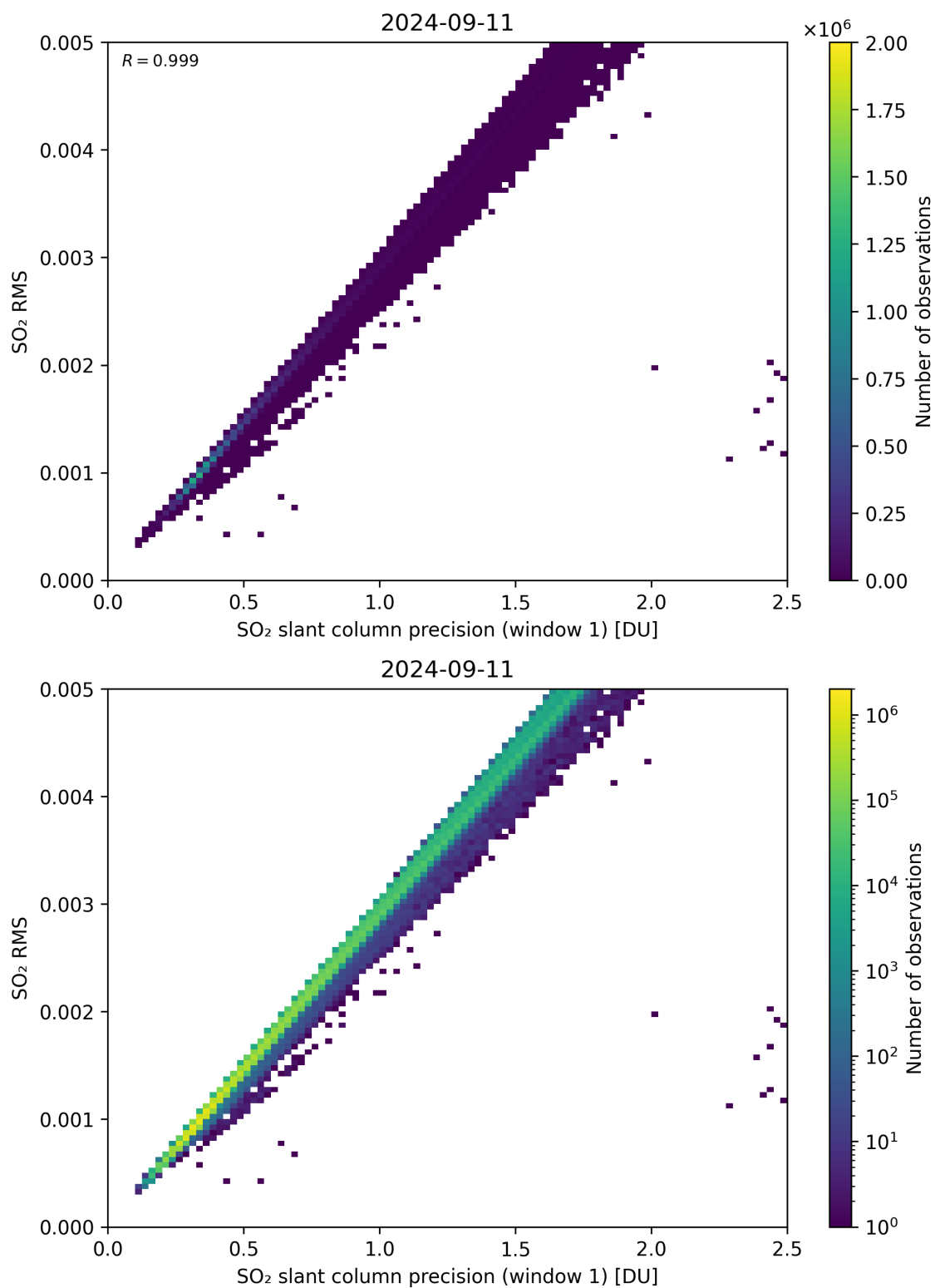
Figure 223: Scatter density plot of “SO 2 slant column precision (window 1)” against “SO 2 RMS” for 2024-09-10 to 2024-09-12.
