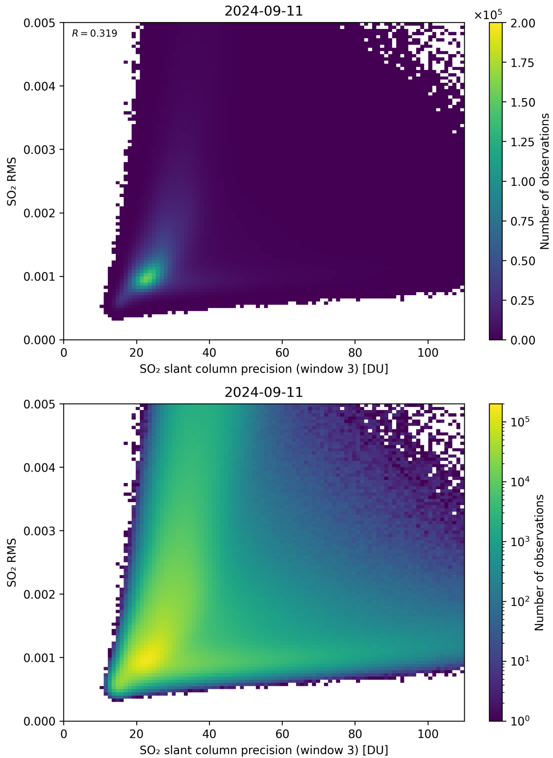
Figure 260: Scatter density plot of “SO 2 slant column precision (window 3)” against “SO 2 RMS” for 2024-09-10 to 2024-09-12.
