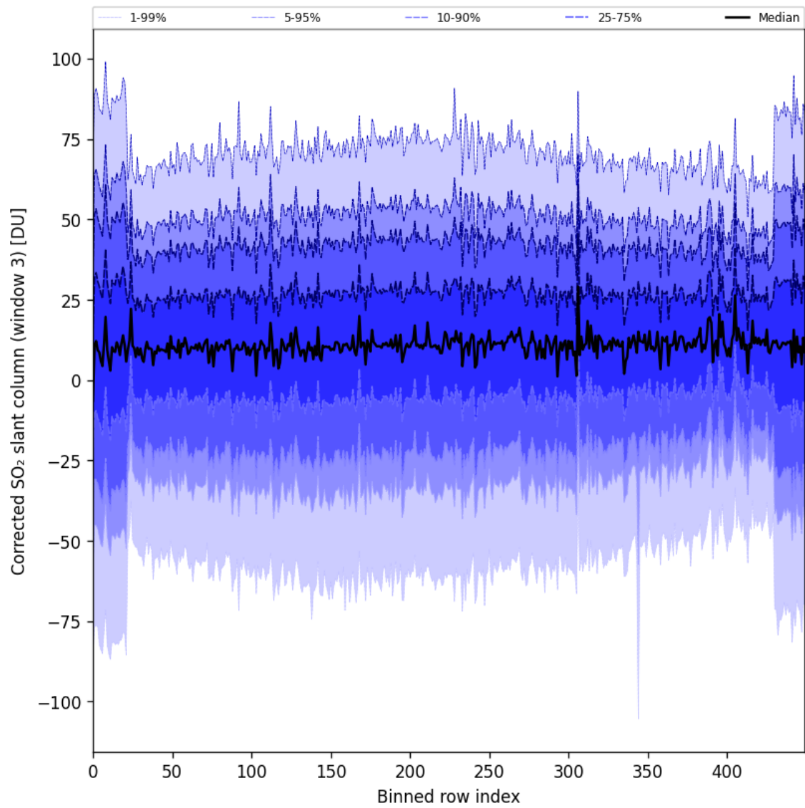
Figure 89: Along track statistics of “Corrected SO 2 slant column (window 3)” for 2024-09-10 to 2024-09-12
