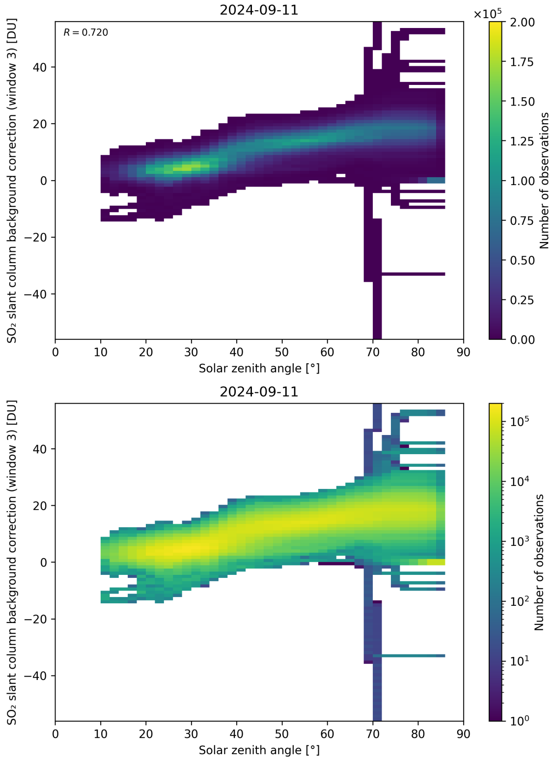
Figure 160: Scatter density plot of “Solar zenith angle” against “SO 2 slant column background correction (window 3)” for 2024-09-10 to 2024-09-12.
