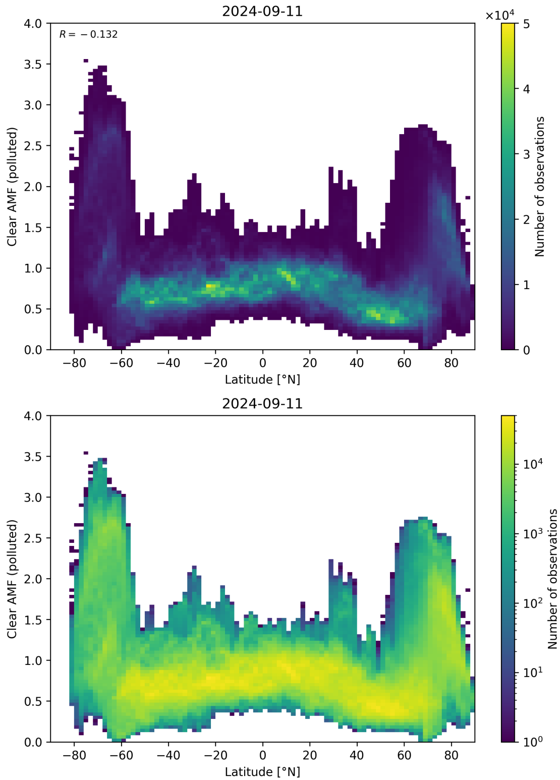
Figure 145: Scatter density plot of “Latitude” against “Clear AMF (polluted)” for 2024-09-10 to 2024-09-12.
