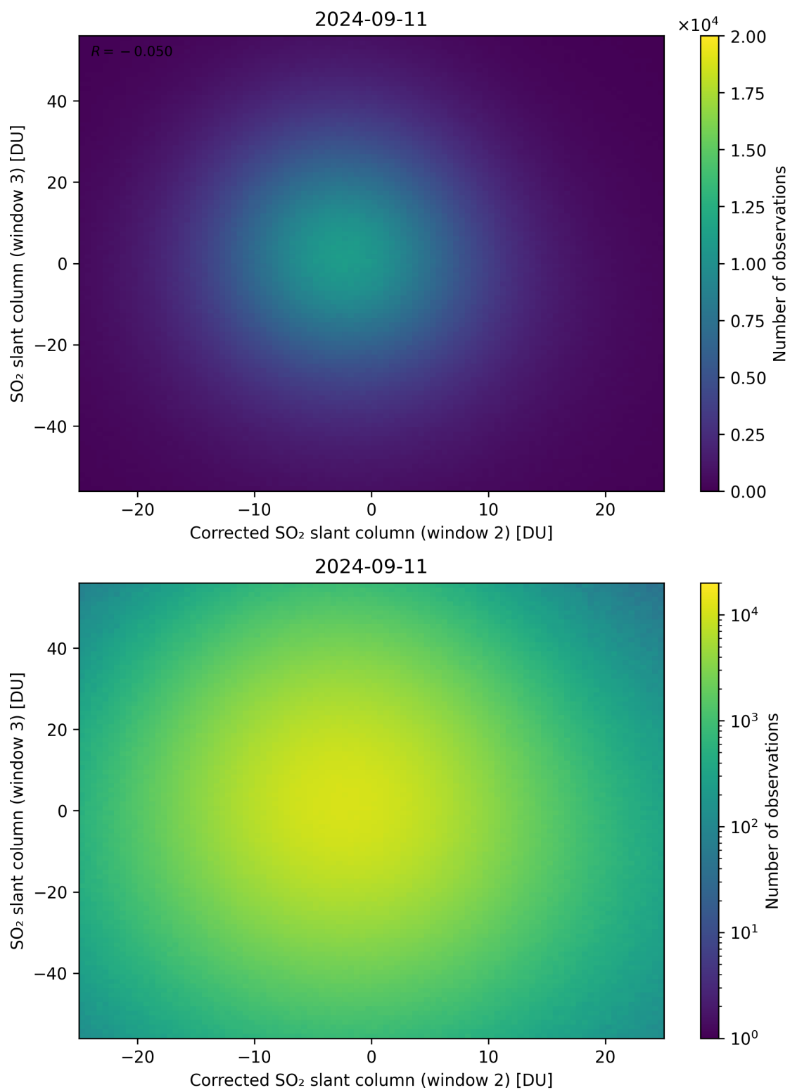
Figure 201: Scatter density plot of “Corrected SO 2 slant column (window 2)” against “SO 2 slant column (window 3)” for 2024-09-10 to 2024-09-12.
