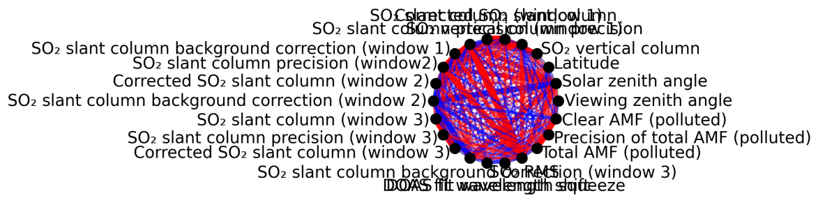
Figure 1: Map of correlation graph for 2024-09-10 to 2024-09-12.
