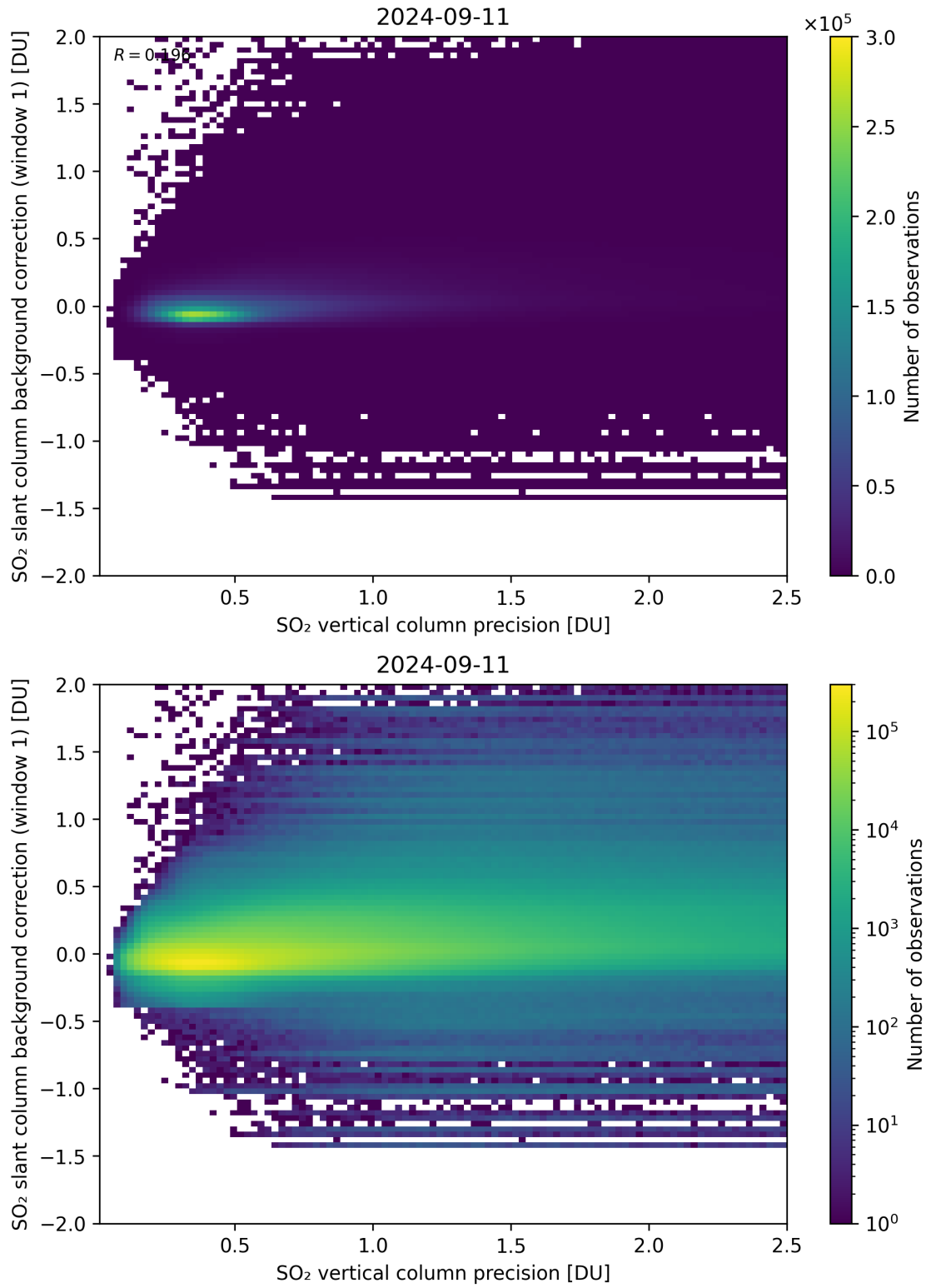
Figure 279: Scatter density plot of “SO 2 vertical column precision” against “SO 2 slant column background correction (window 1)” for 2024-09-10 to 2024-09-12.
