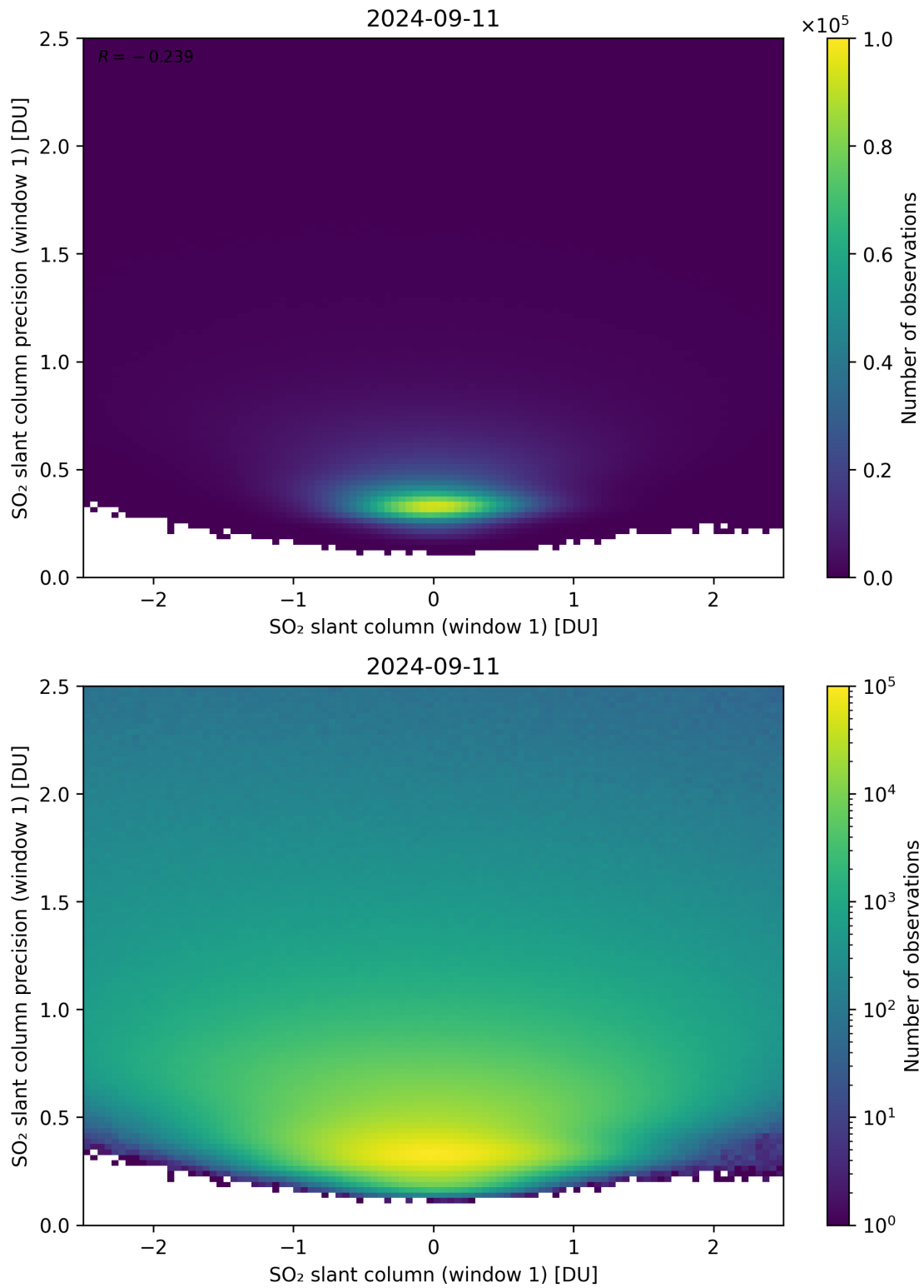
Figure 235: Scatter density plot of “SO 2 slant column (window 1)” against “SO 2 slant column precision (window 1)” for 2024-09-10 to 2024-09-12.
