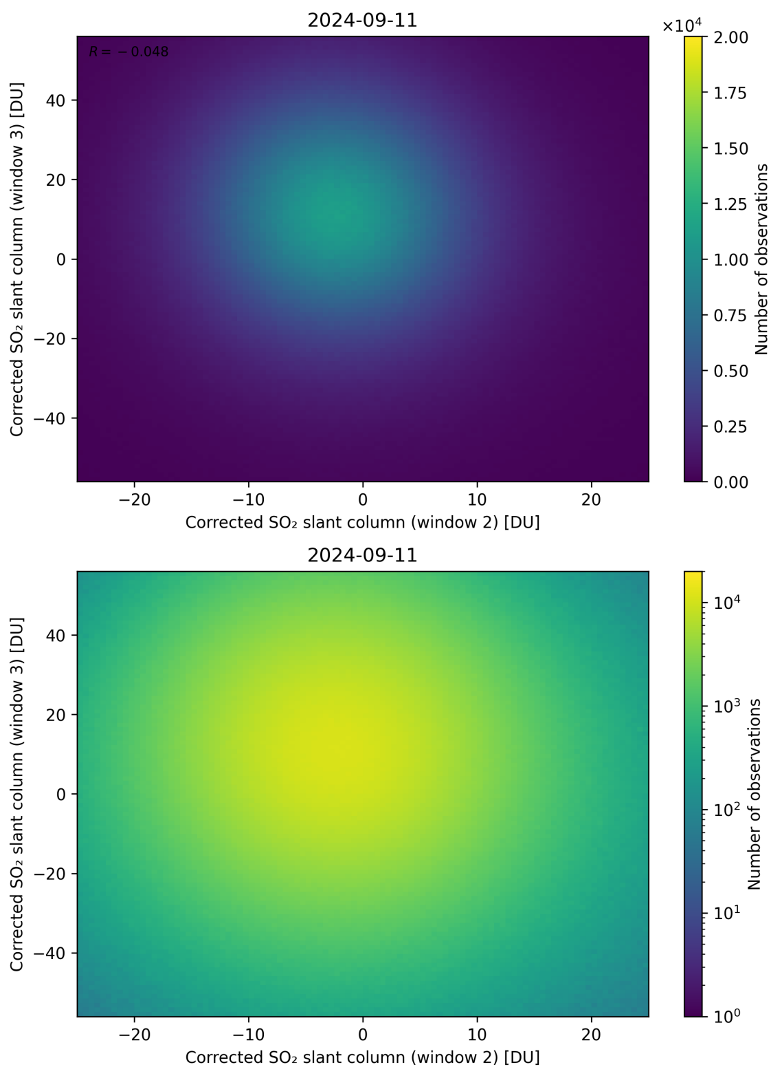
Figure 200: Scatter density plot of “Corrected SO 2 slant column (window 2)” against “Corrected SO 2 slant column (window 3)” for 2024-09-10 to 2024-09-12.
