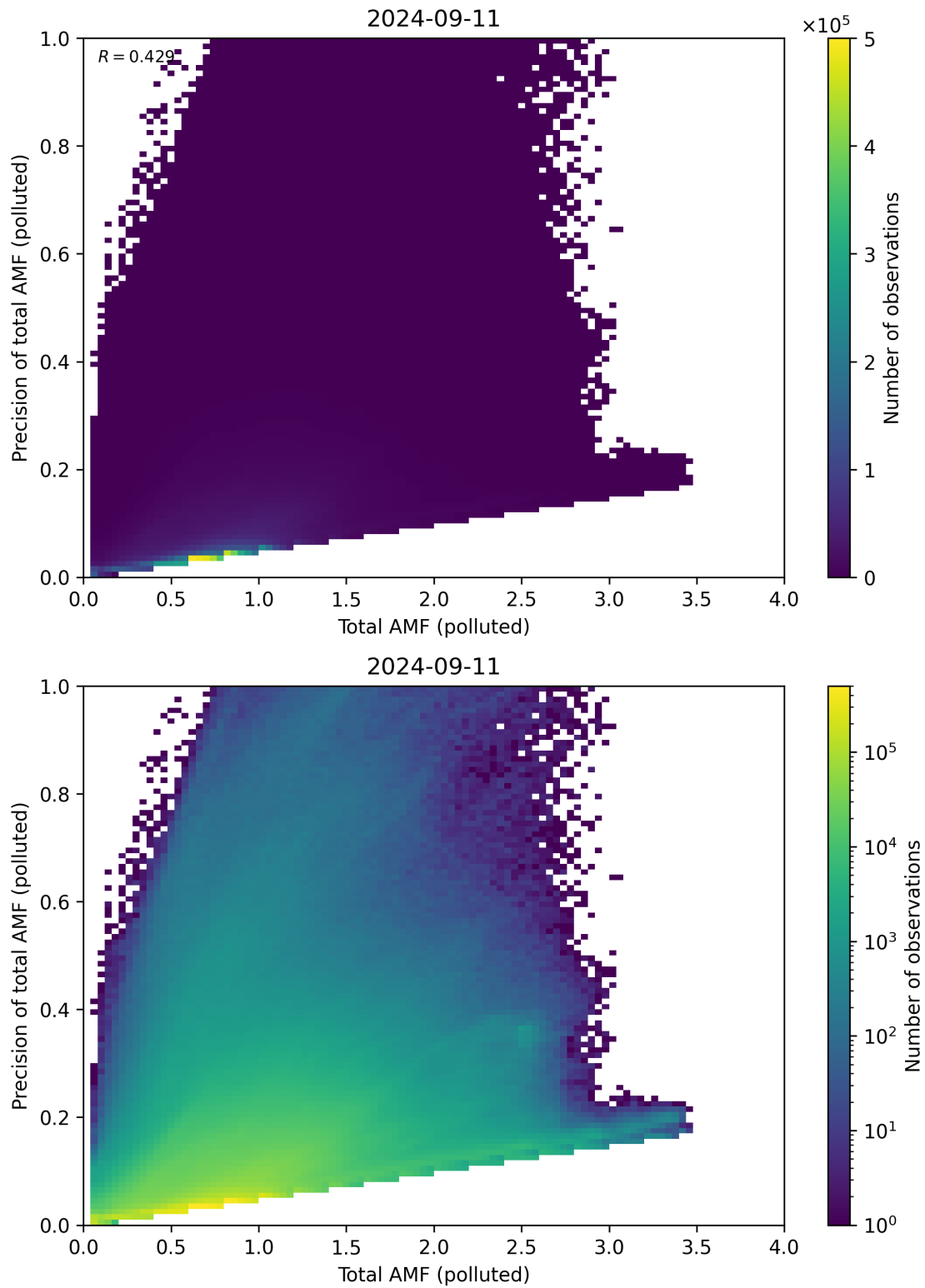
Figure 272: Scatter density plot of “Total AMF (polluted)” against “Precision of total AMF (polluted)” for 2024-09-10 to 2024-09-12.
