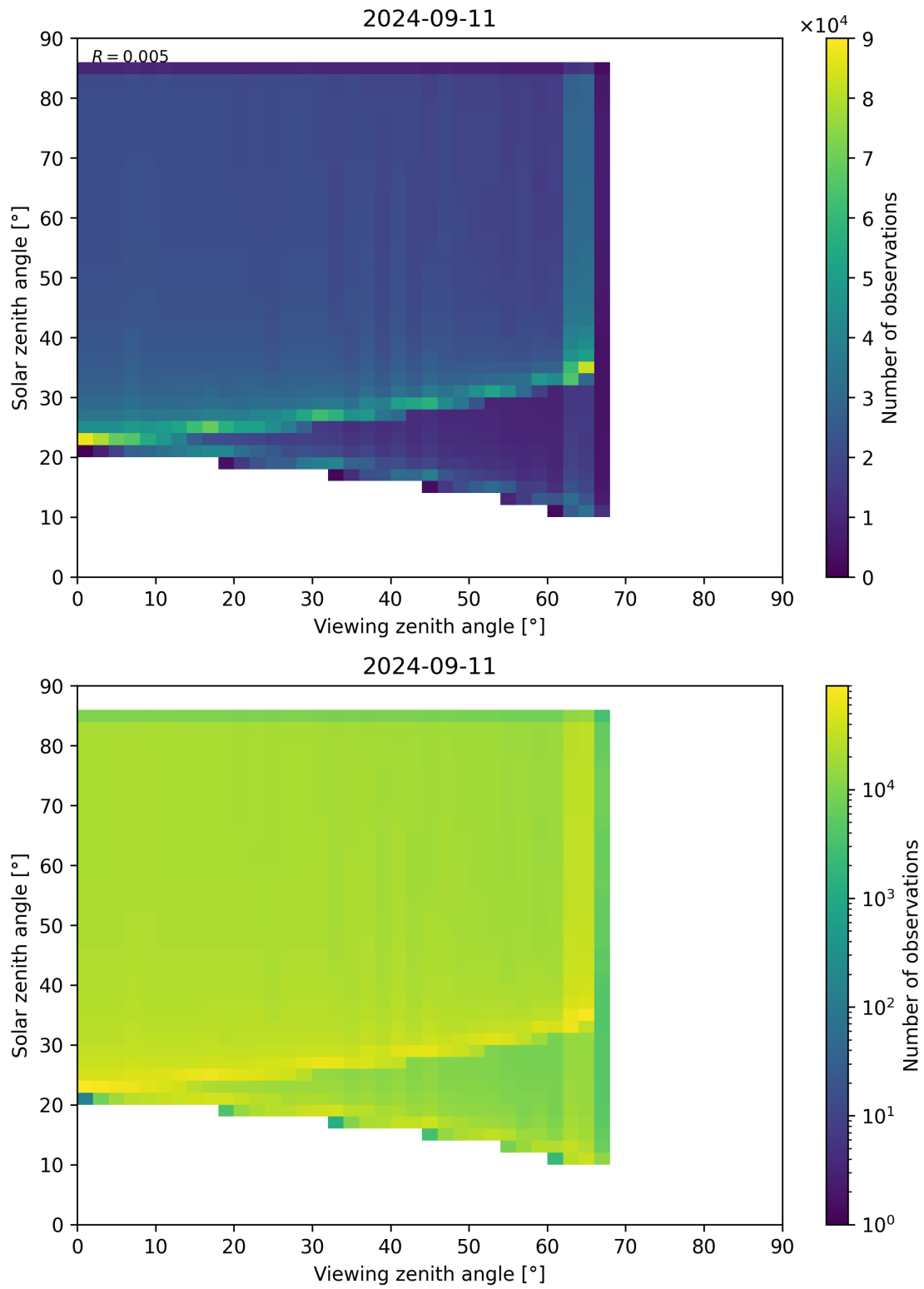
Figure 315: Scatter density plot of “Viewing zenith angle” against “Solar zenith angle” for 2024-09-10 to 2024-09-12.
