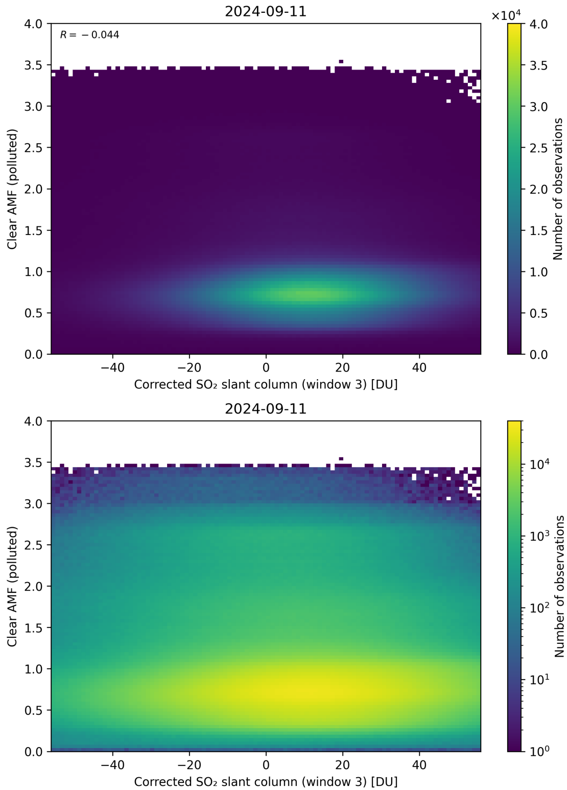
Figure 209: Scatter density plot of “Corrected SO 2 slant column (window 3)” against “Clear AMF (polluted)” for 2024-09-10 to 2024-09-12.
