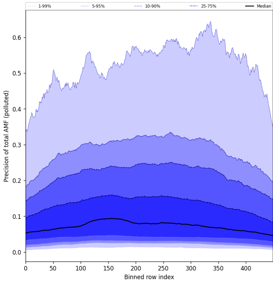
Figure 95: Along track statistics of “Precision of total AMF (polluted)” for 2024-09-10 to 2024-09-12
