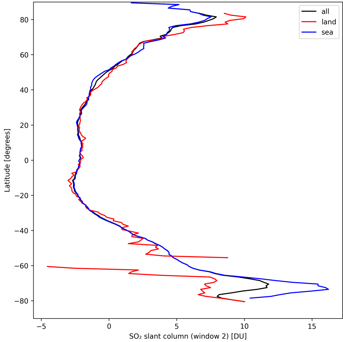
Figure 37: Zonal average of “SO 2 slant column (window 2)” for 2024-09-10 to 2024-09-12.
