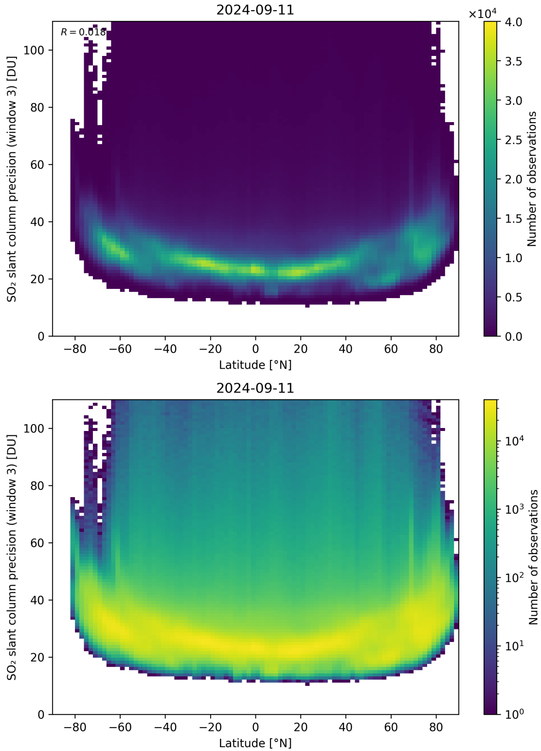
Figure 153: Scatter density plot of “Latitude” against “SO 2 slant column precision (window 3)” for 2024-09-10 to 2024-09-12.
