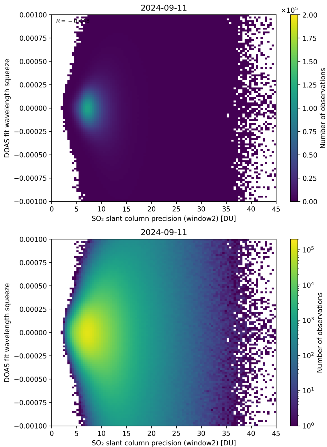
Figure 244: Scatter density plot of “SO 2 slant column precision (window2)” against “DOAS fit wavelength squeeze” for 2024-09-10 to 2024-09-12.
