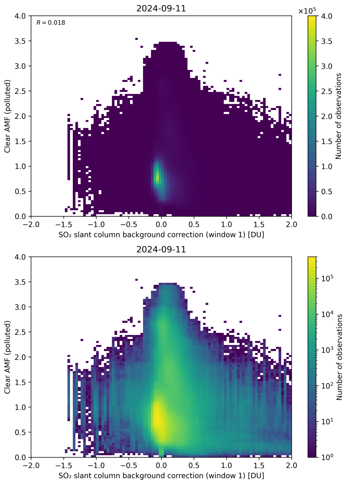
Figure 103: Scatter density plot of “SO 2 slant column background correction (window 1)” against “Clear AMF (polluted)” for 2024-09-10 to 2024-09-12.
