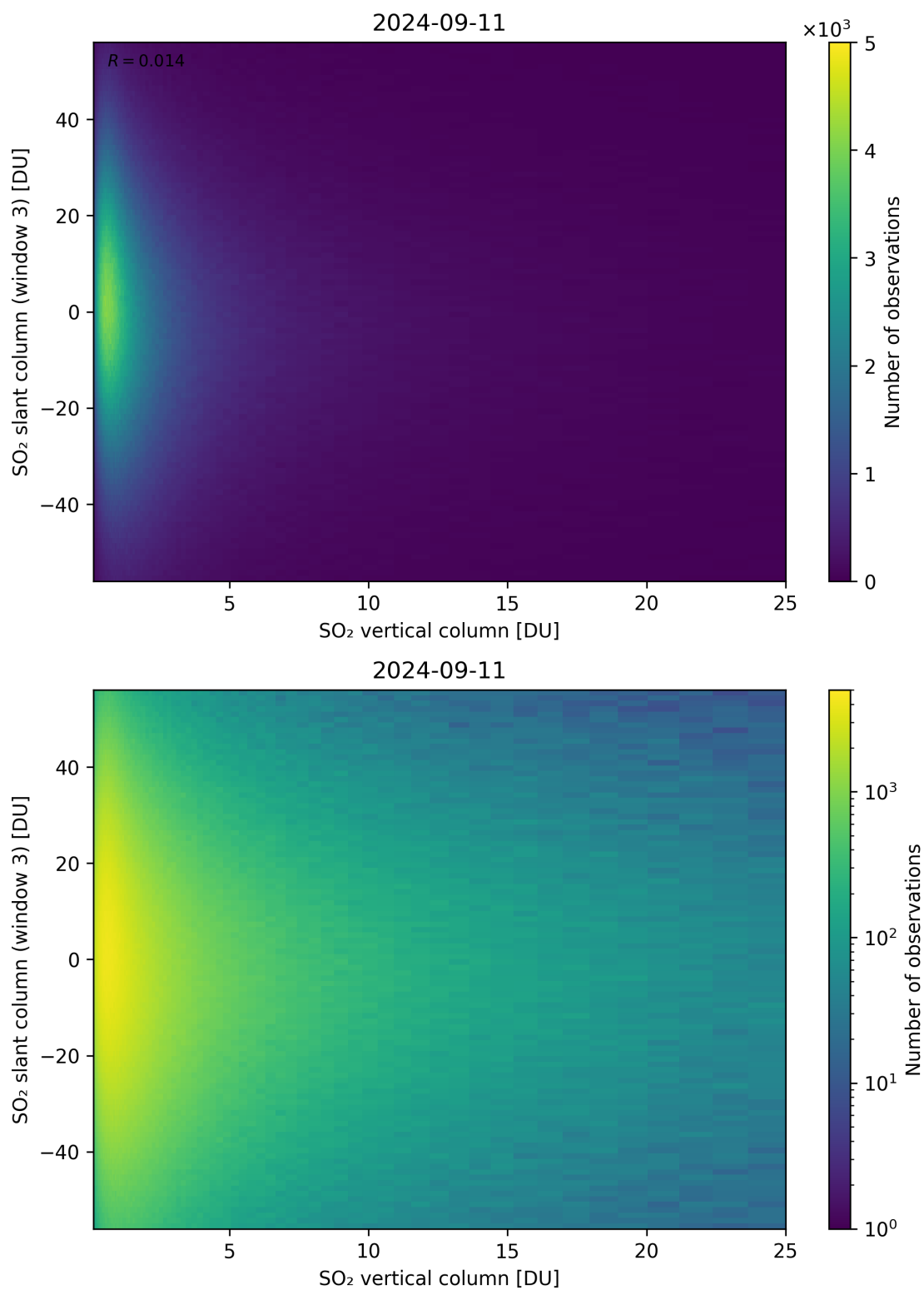
Figure 303: Scatter density plot of “SO 2 vertical column” against “SO 2 slant column (window 3)” for 2024-09-10 to 2024-09-12.
