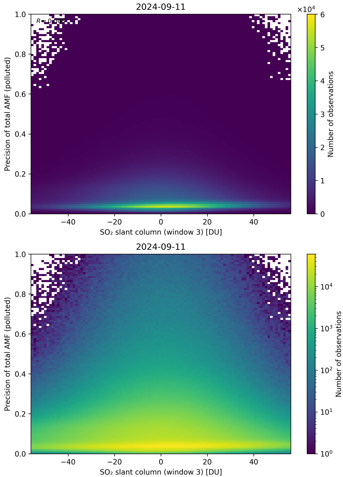
Figure 269: Scatter density plot of “SO 2 slant column (window 3)” against “Precision of total AMF (polluted)” for 2024-09-10 to 2024-09-12.
