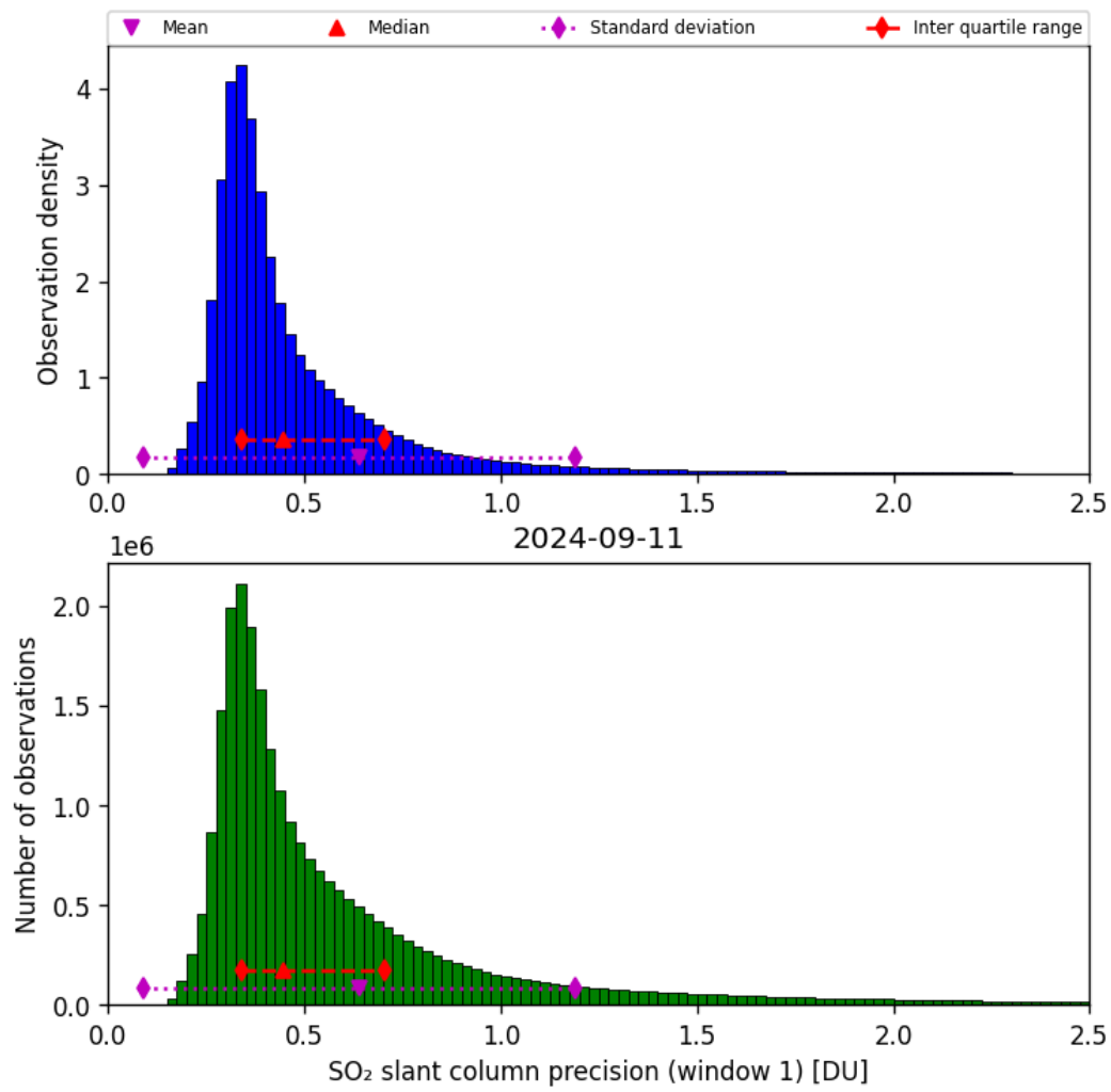
Figure 57: Histogram of “SO 2 slant column precision (window 1)” for 2024-09-10 to 2024-09-12
