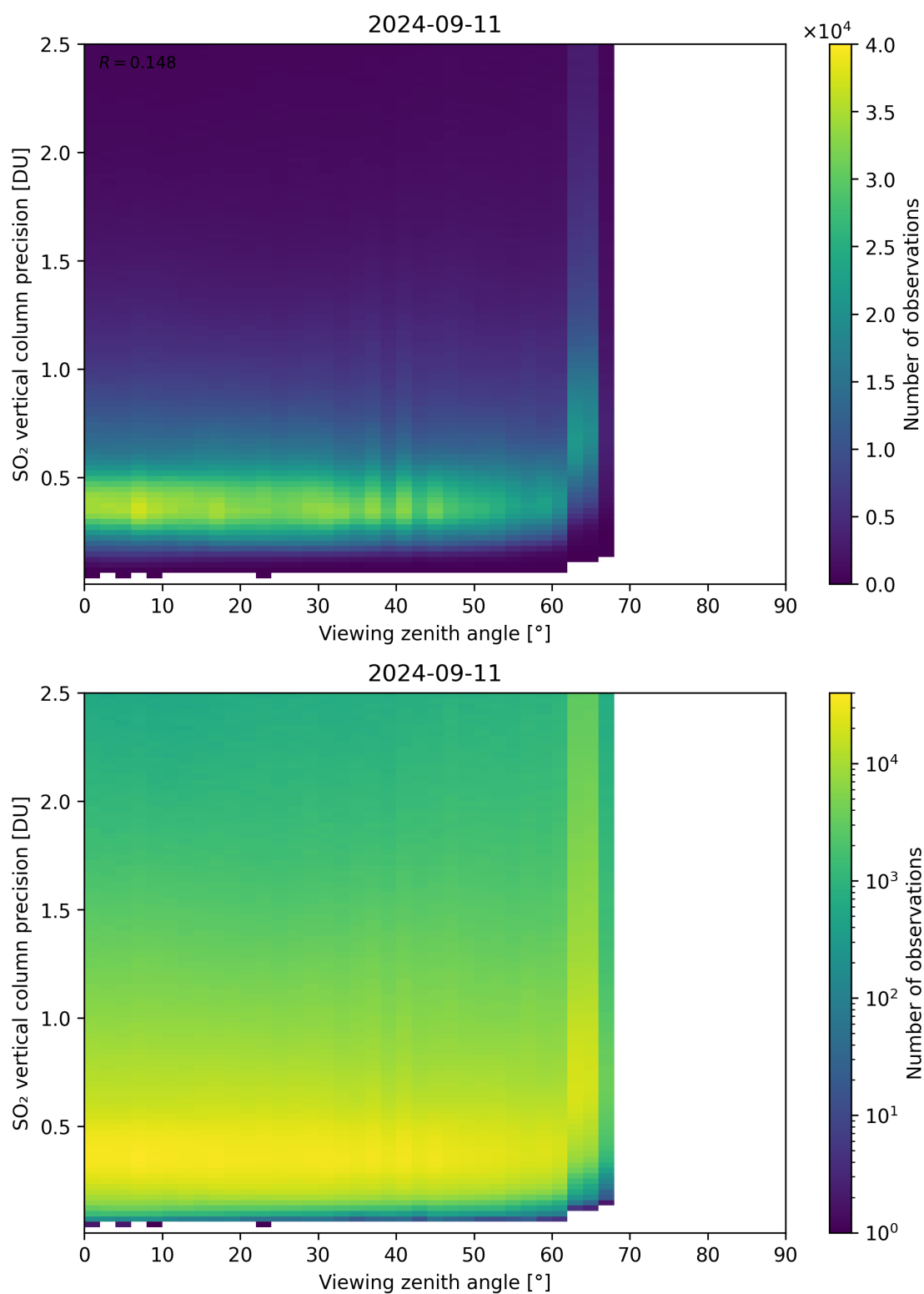
Figure 328: Scatter density plot of “Viewing zenith angle” against “SO 2 vertical column precision” for 2024-09-10 to 2024-09-12.
