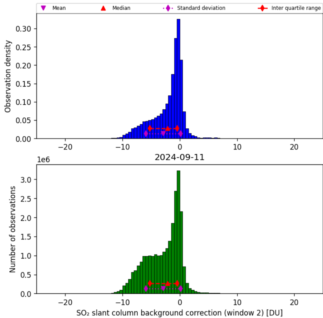
Figure 63: Histogram of “SO 2 slant column background correction (window 2)” for 2024-09-10 to 2024-09-12
