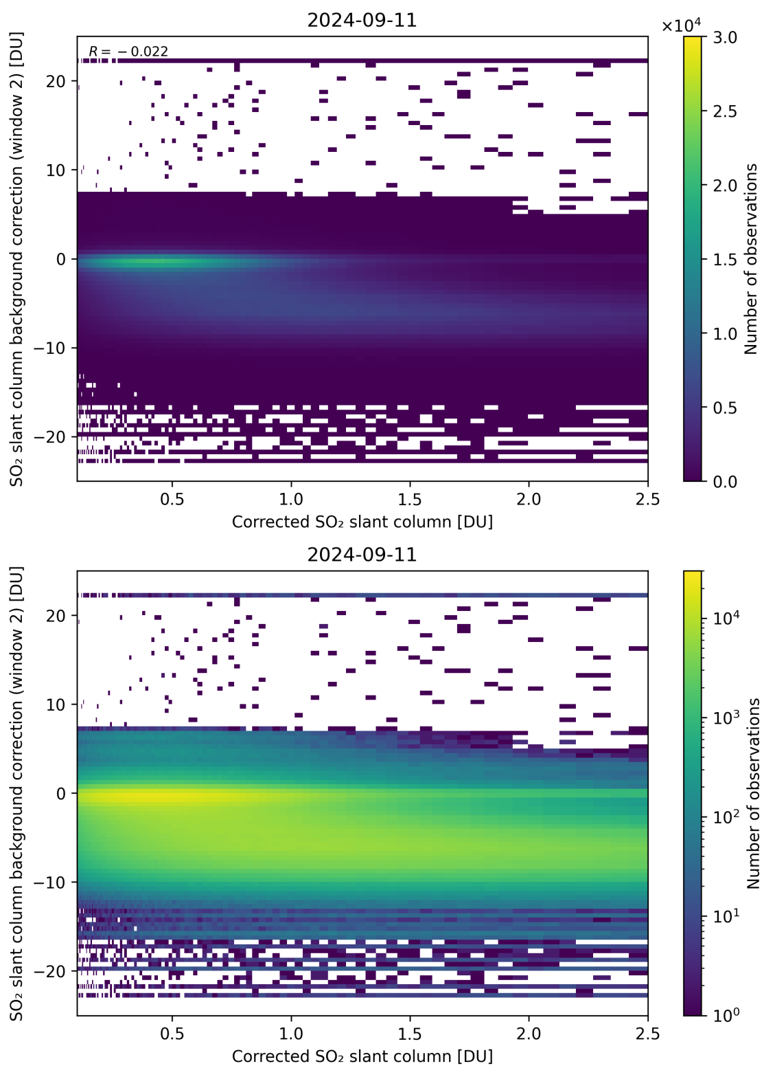
Figure 179: Scatter density plot of “Corrected SO 2 slant column” against “SO 2 slant column background correction (window 2)” for 2024-09-10 to 2024-09-12.
