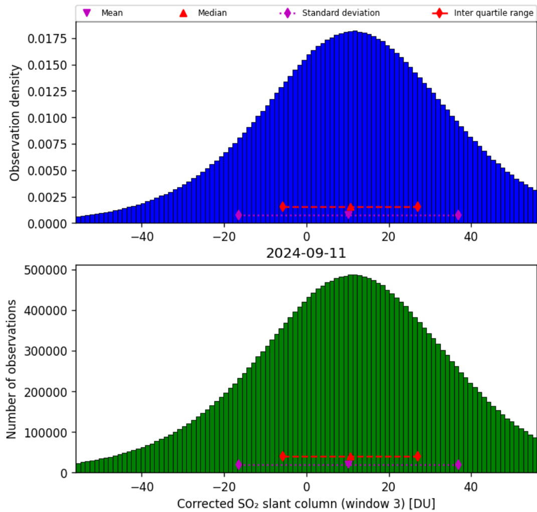
Figure 66: Histogram of “Corrected SO 2 slant column (window 3)” for 2024-09-10 to 2024-09-12
