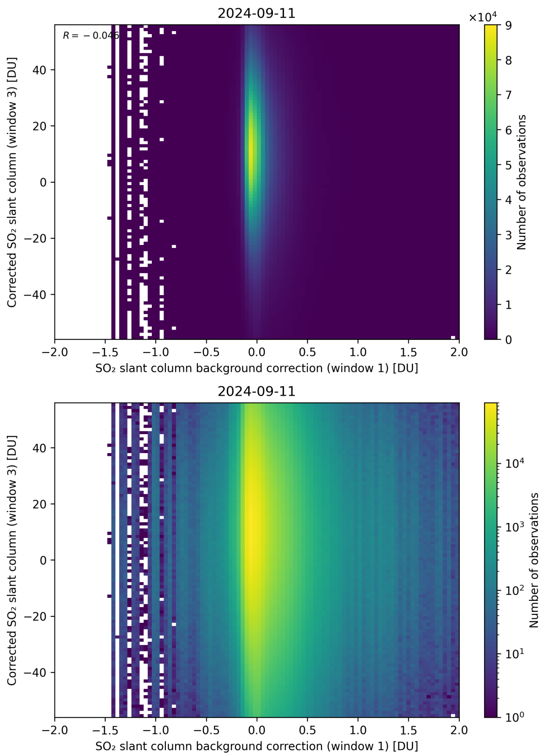
Figure 105: Scatter density plot of “SO 2 slant column background correction (window 1)” against “Corrected SO 2 slant column (window 3)” for 2024-09-10 to 2024-09-12.
