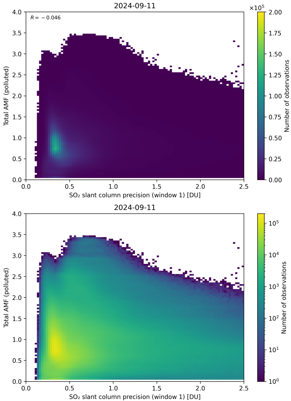
Figure 230: Scatter density plot of “SO 2 slant column precision (window 1)” against “Total AMF (polluted)” for 2024-09-10 to 2024-09-12.
