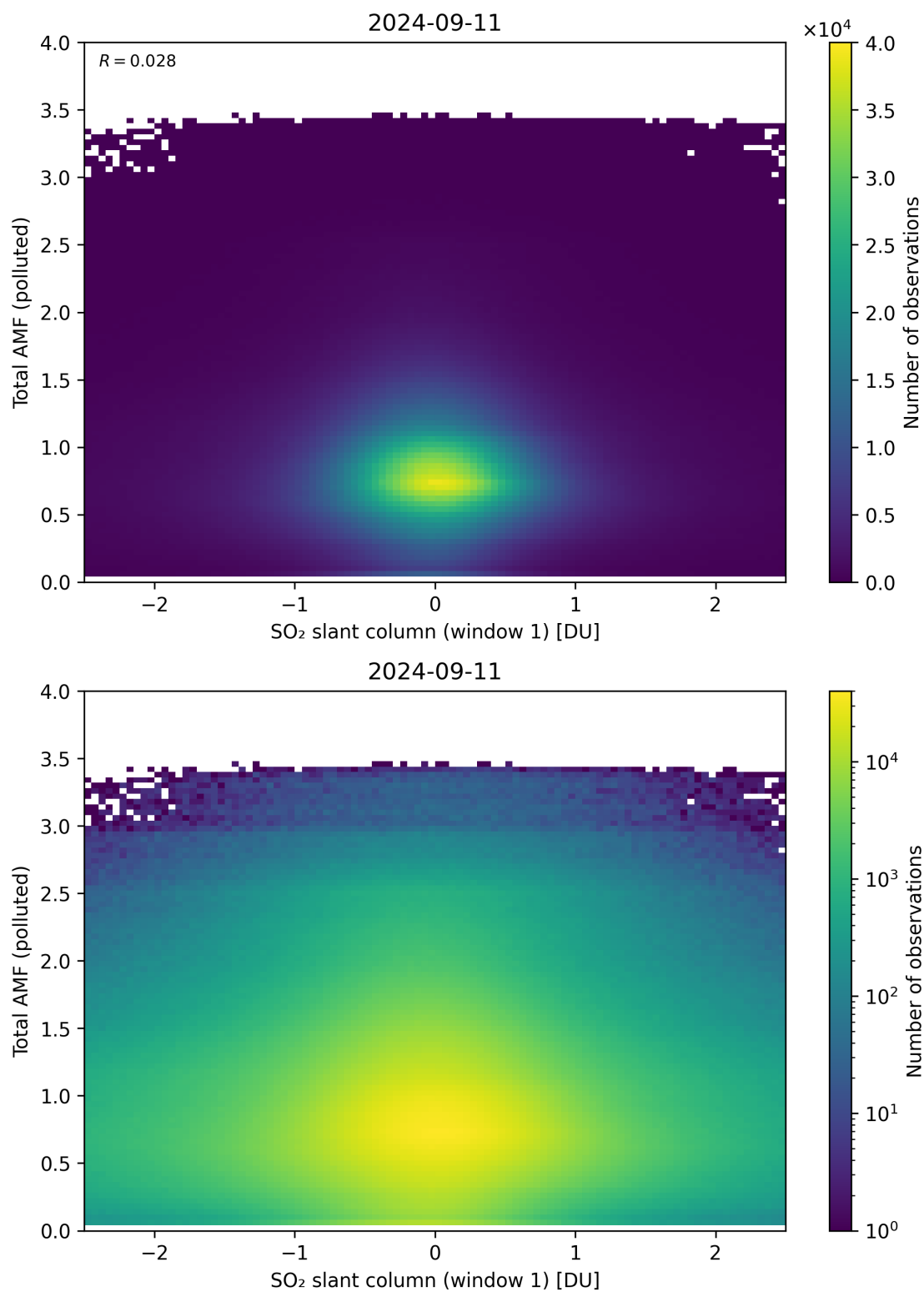
Figure 239: Scatter density plot of “SO 2 slant column (window 1)” against “Total AMF (polluted)” for 2024-09-10 to 2024-09-12.
