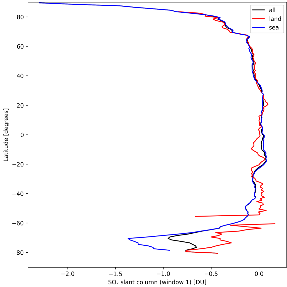
Figure 33: Zonal average of “SO 2 slant column (window 1)” for 2024-09-10 to 2024-09-12.
