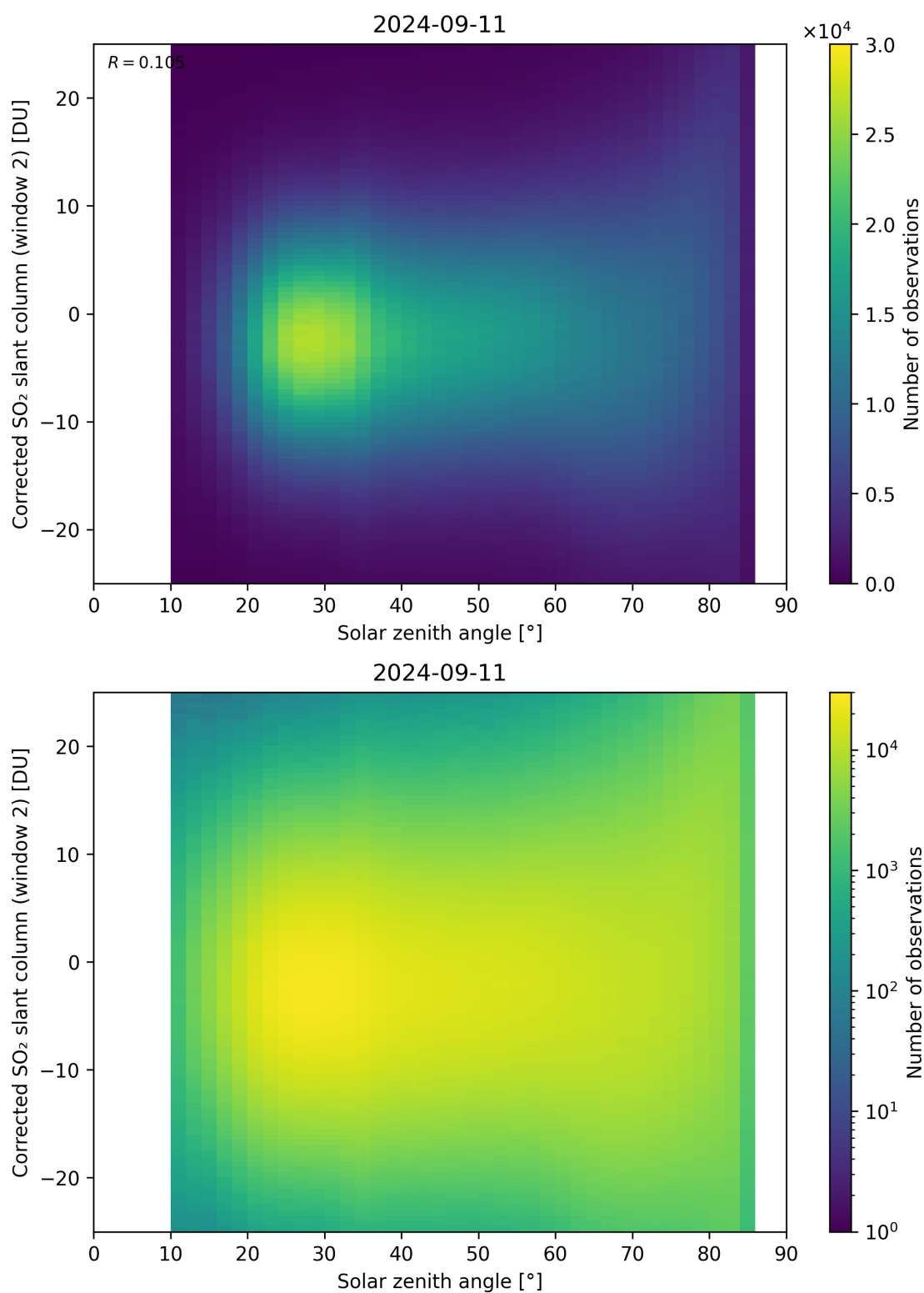
Figure 167: Scatter density plot of “Solar zenith angle” against “Corrected SO 2 slant column (window 2)” for 2024-09-10 to 2024-09-12.
