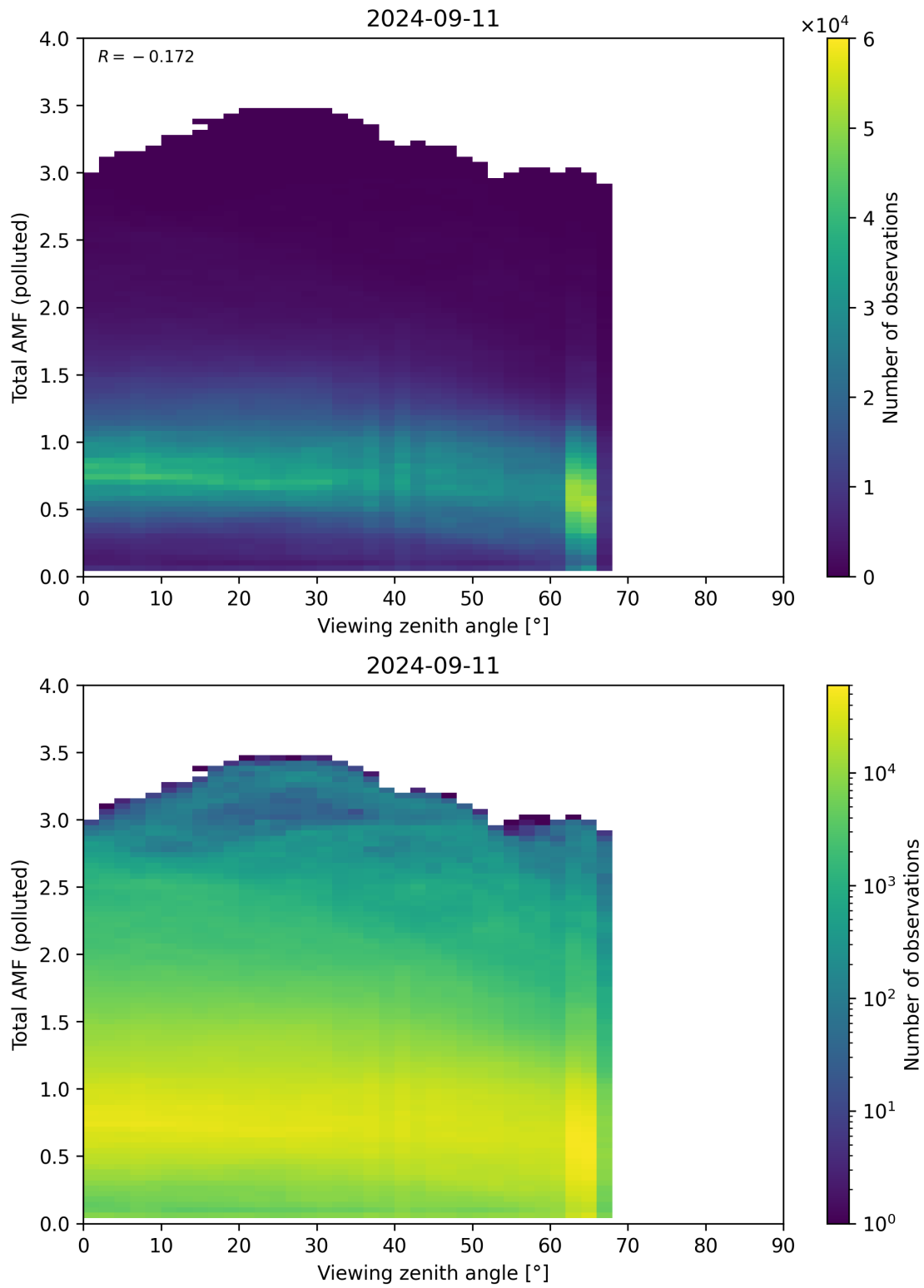
Figure 325: Scatter density plot of “Viewing zenith angle” against “Total AMF (polluted)” for 2024-09-10 to 2024-09-12.
