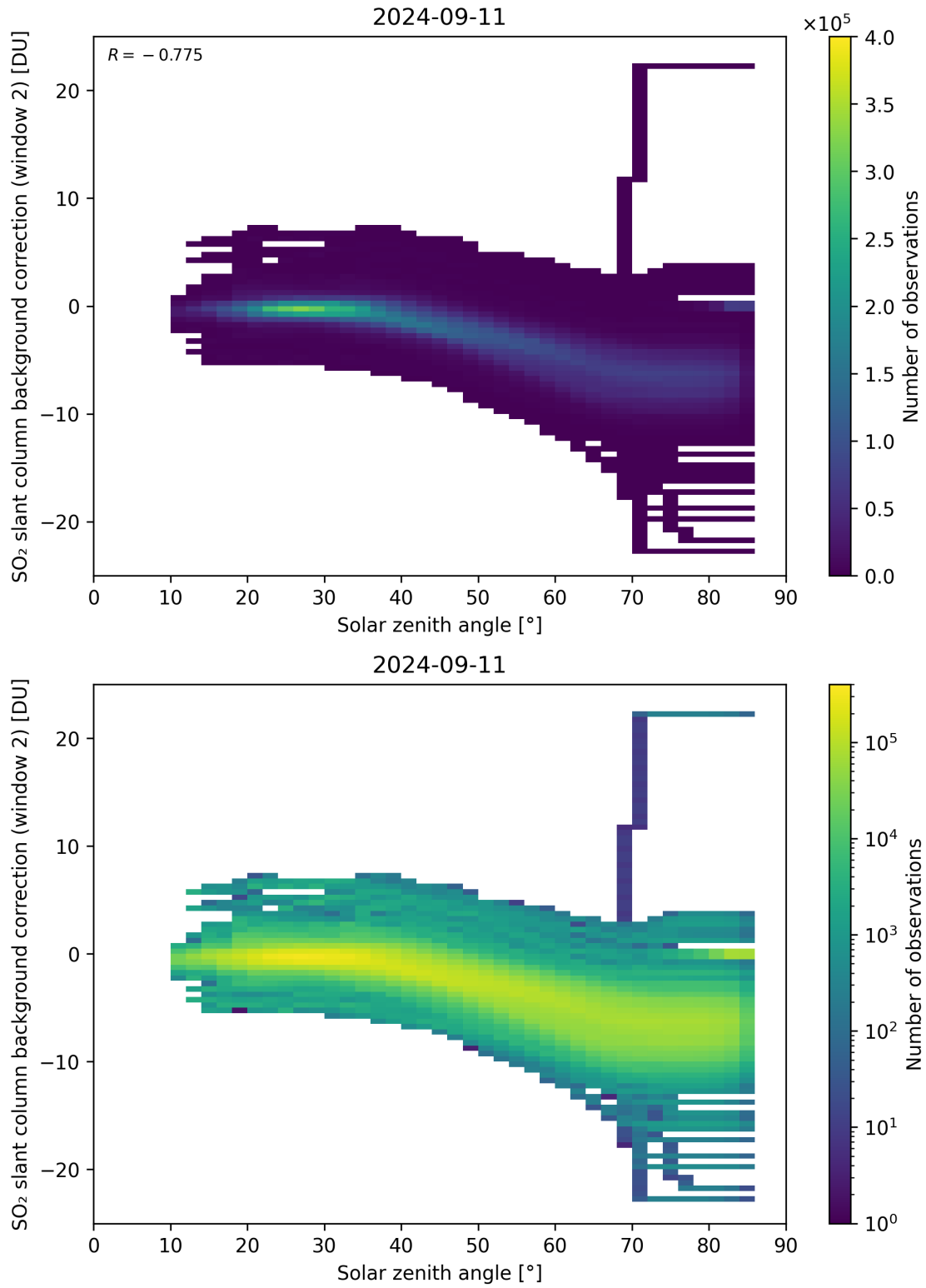
Figure 159: Scatter density plot of “Solar zenith angle” against “SO 2 slant column background correction (window 2)” for 2024-09-10 to 2024-09-12.
