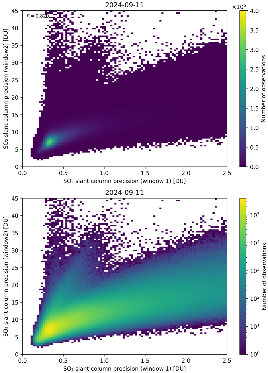
Figure 227: Scatter density plot of “SO 2 slant column precision (window 1)” against “SO 2 slant column precision (window2)” for 2024-09-10 to 2024-09-12.
