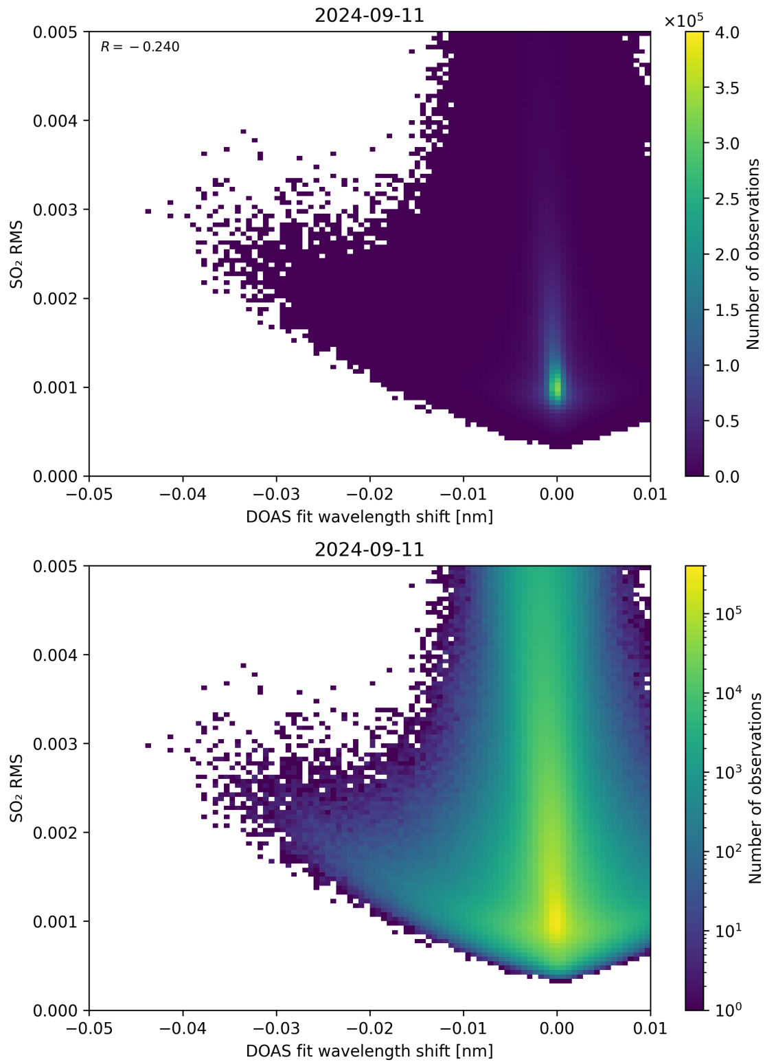
Figure 128: Scatter density plot of “DOAS fit wavelength shift” against “SO 2 RMS” for 2024-09-10 to 2024-09-12.
