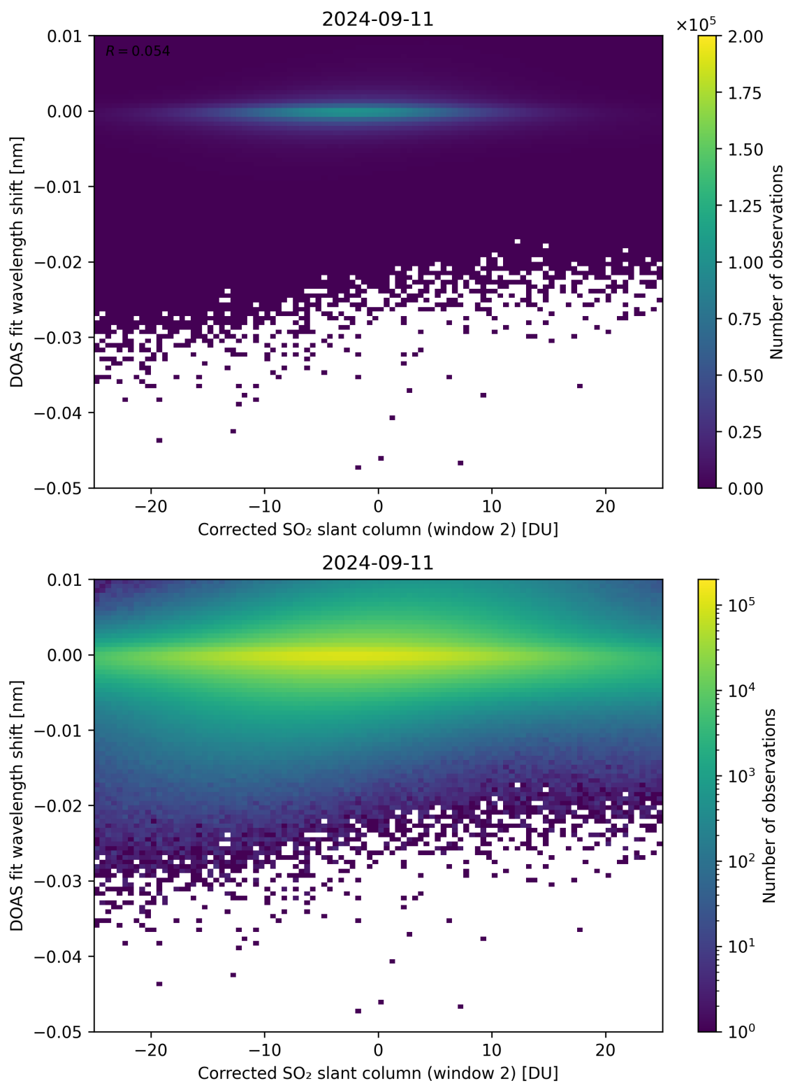
Figure 196: Scatter density plot of “Corrected SO 2 slant column (window 2)” against “DOAS fit wavelength shift” for 2024-09-10 to 2024-09-12.
