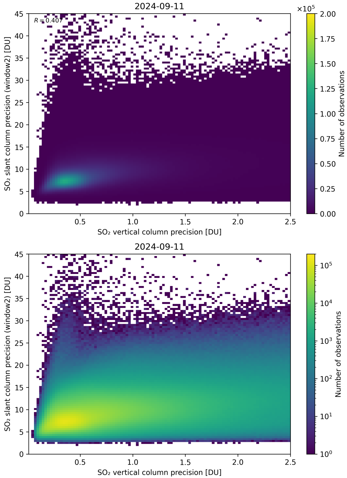
Figure 291: Scatter density plot of “SO 2 vertical column precision” against “SO 2 slant column precision (window2)” for 2024-09-10 to 2024-09-12.
