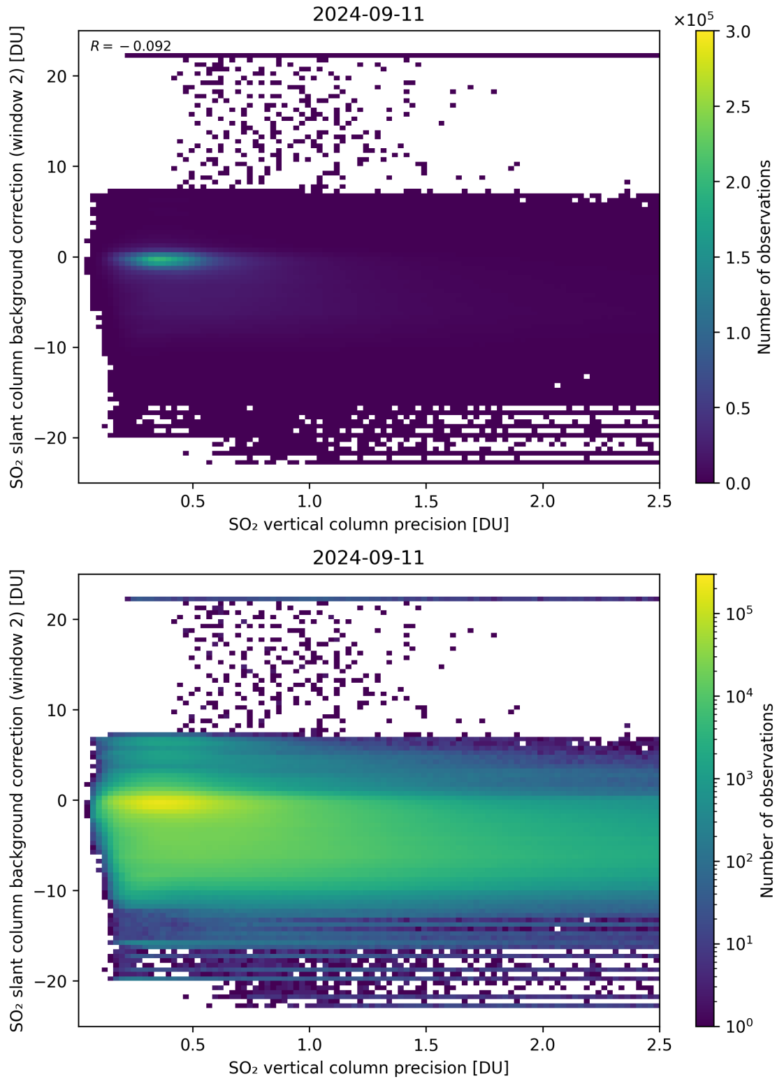
Figure 280: Scatter density plot of “SO 2 vertical column precision” against “SO 2 slant column background correction (window 2)” for 2024-09-10 to 2024-09-12.
