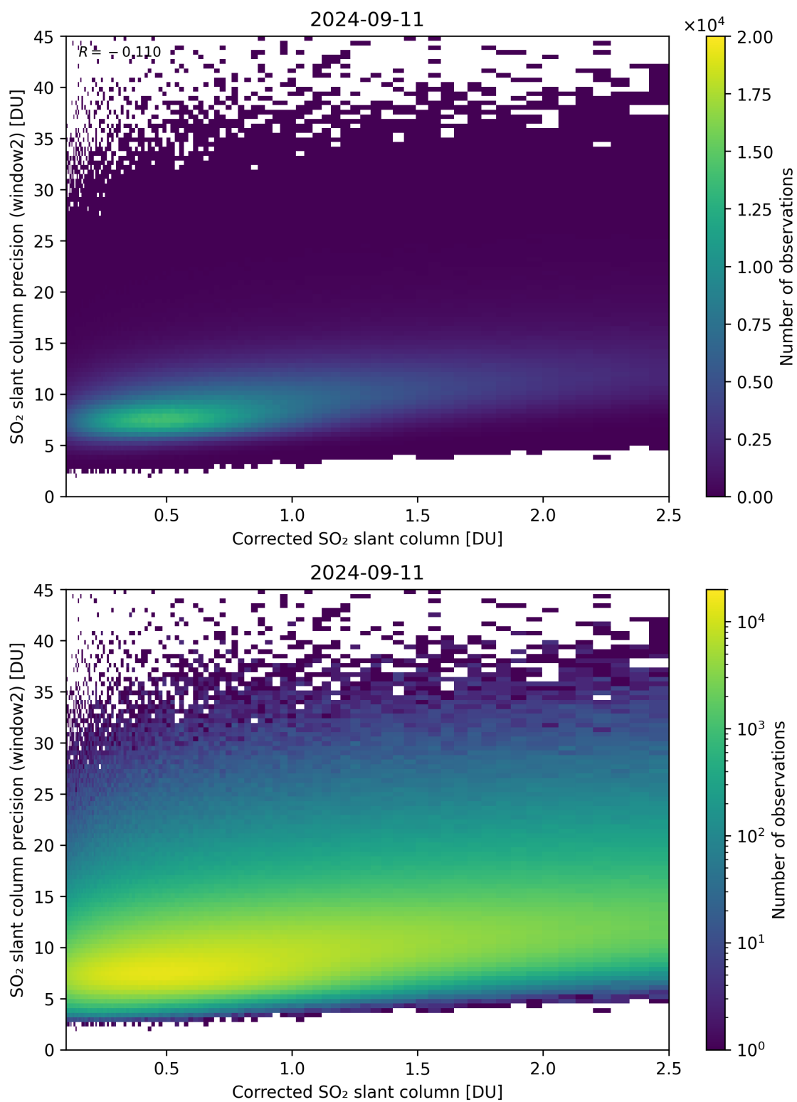
Figure 189: Scatter density plot of “Corrected SO 2 slant column” against “SO 2 slant column precision (window2)” for 2024-09-10 to 2024-09-12.
