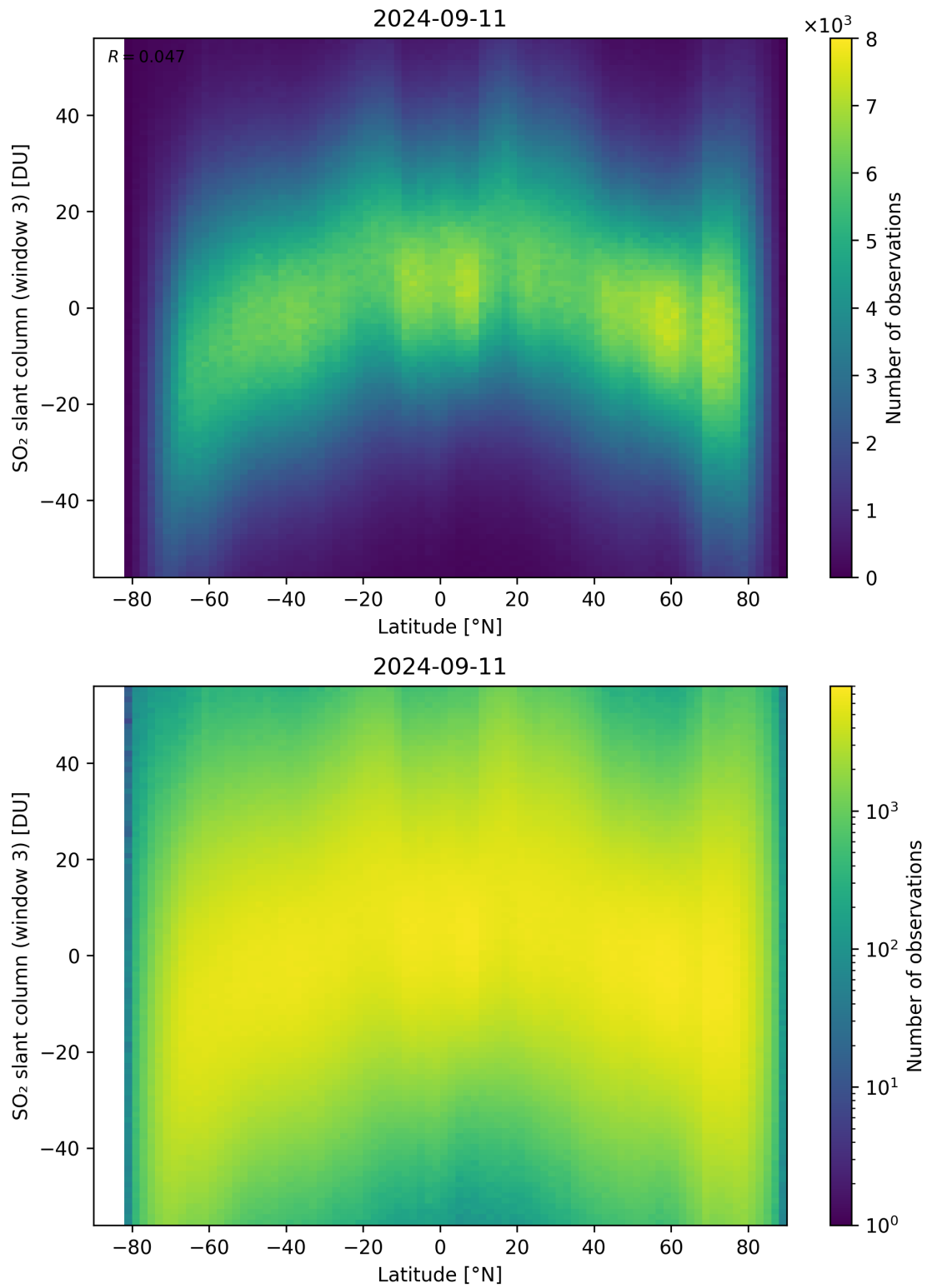
Figure 152: Scatter density plot of “Latitude” against “SO 2 slant column (window 3)” for 2024-09-10 to 2024-09-12.
