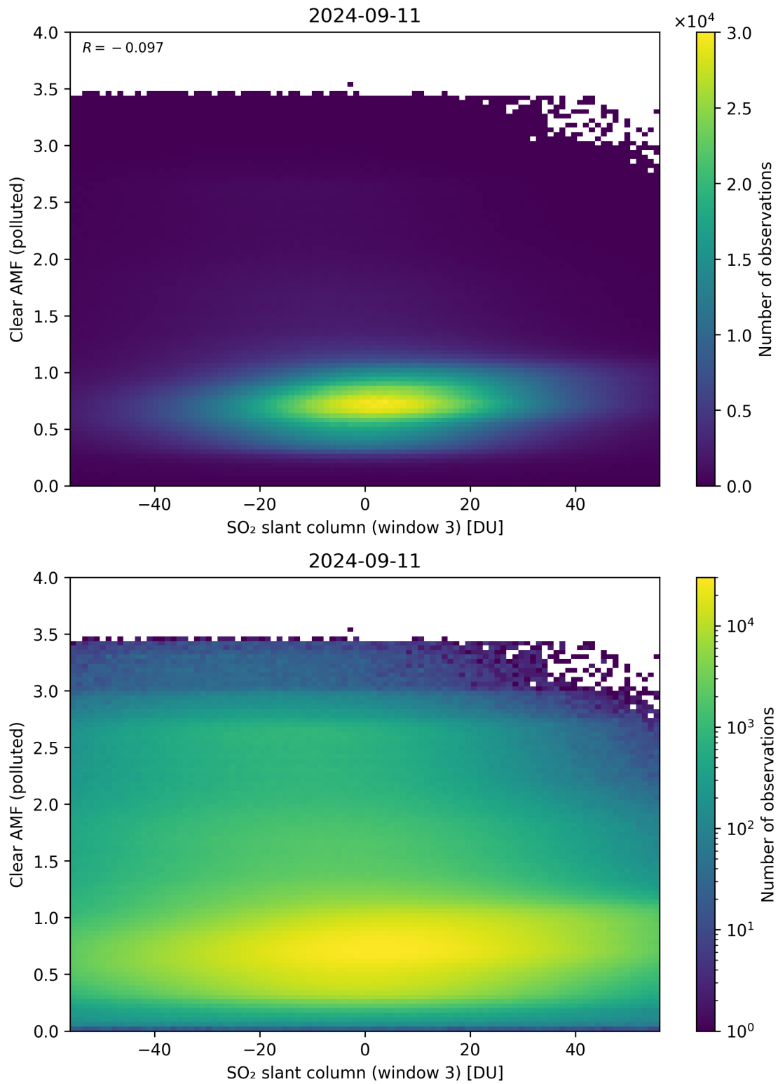
Figure 265: Scatter density plot of “SO 2 slant column (window 3)” against “Clear AMF (polluted)” for 2024-09-10 to 2024-09-12.
