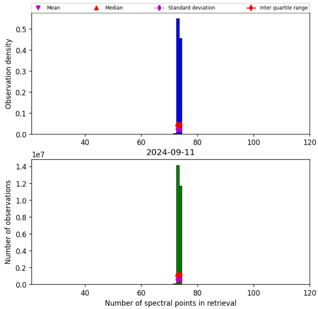
Figure 74: Histogram of “Number of spectral points in retrieval” for 2024-09-10 to 2024-09-12
