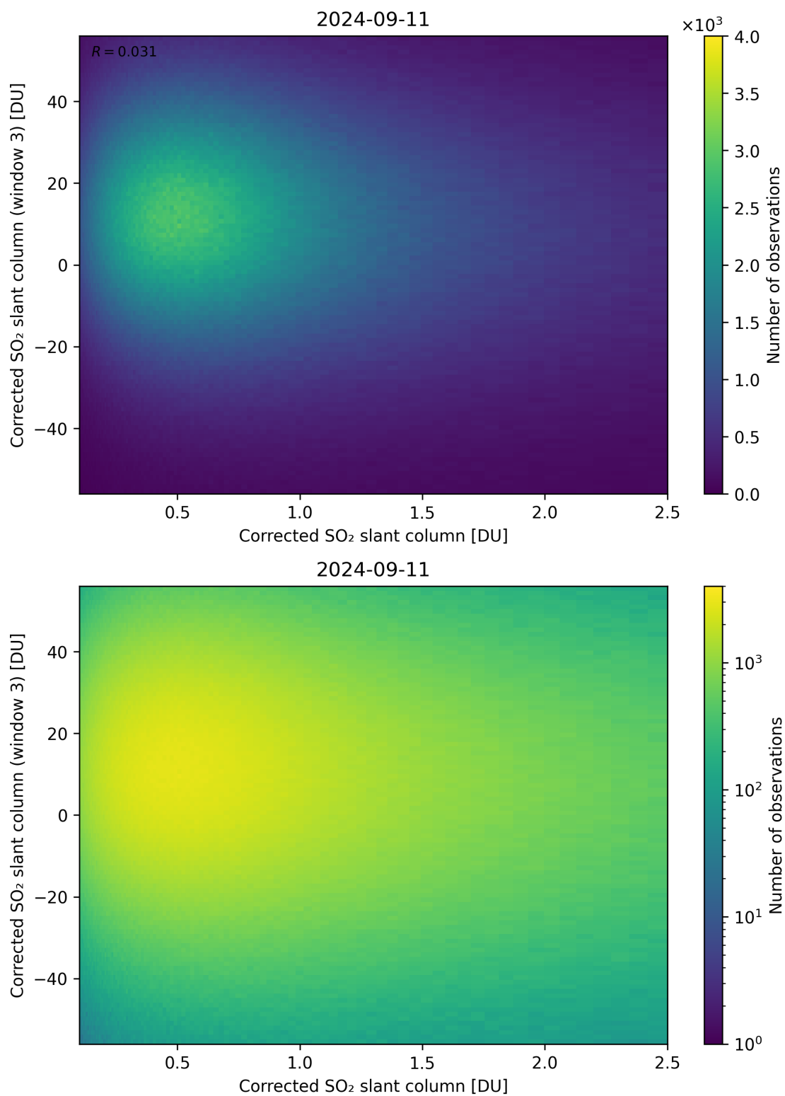
Figure 186: Scatter density plot of “Corrected SO 2 slant column” against “Corrected SO 2 slant column (window 3)” for 2024-09-10 to 2024-09-12.
