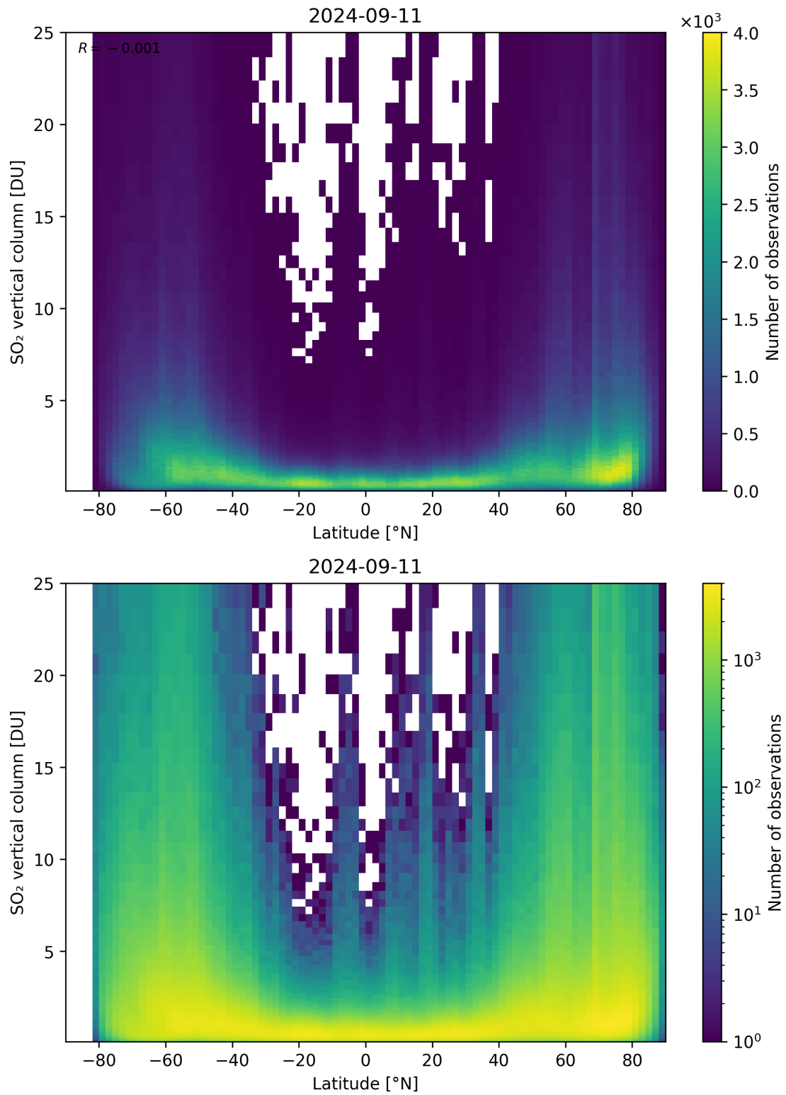
Figure 156: Scatter density plot of “Latitude” against “SO 2 vertical column” for 2024-09-10 to 2024-09-12.
