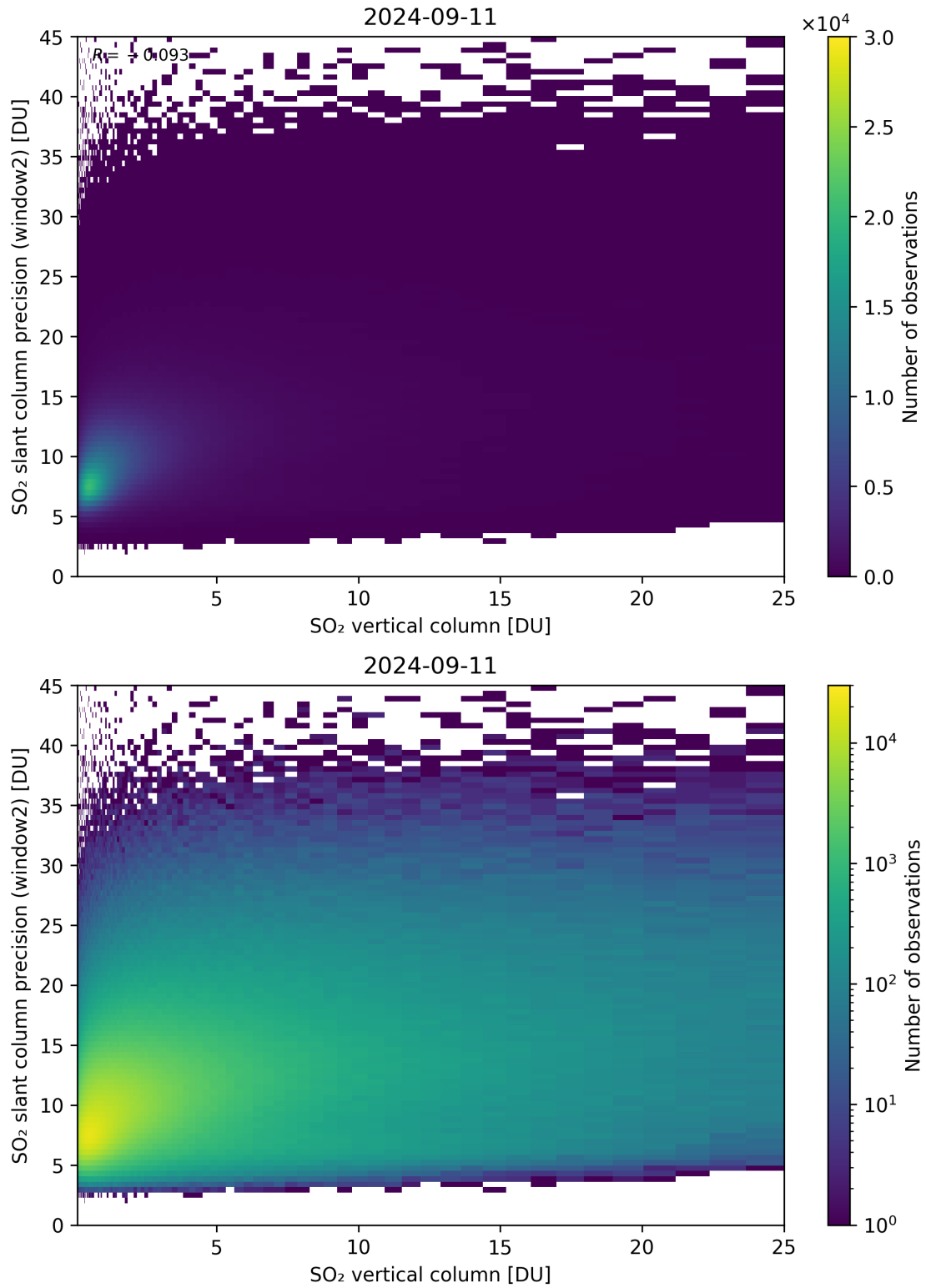
Figure 302: Scatter density plot of “SO 2 vertical column” against “SO 2 slant column precision (window2)” for 2024-09-10 to 2024-09-12.
