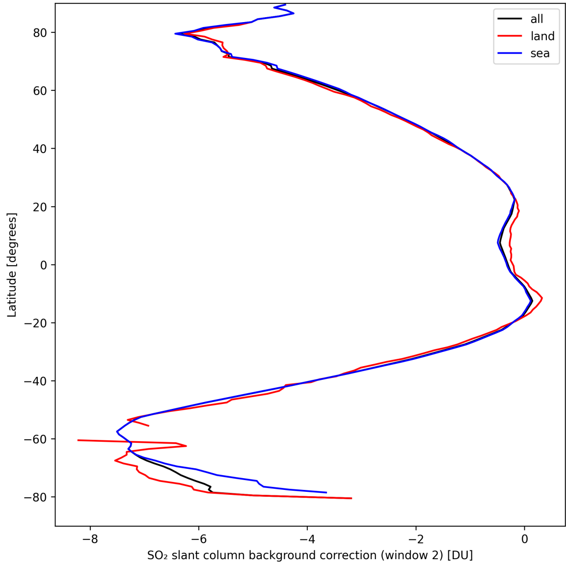
Figure 40: Zonal average of “SO 2 slant column background correction (window 2)” for 2024-09-10 to 2024-09-12.
