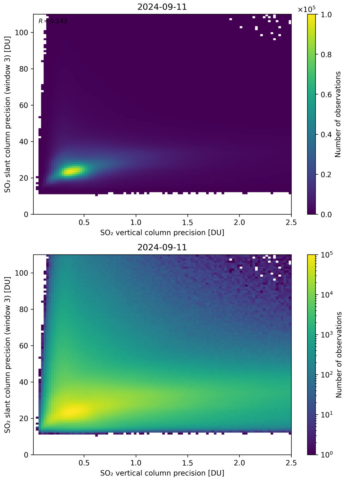
Figure 293: Scatter density plot of “SO 2 vertical column precision” against “SO 2 slant column precision (window 3)” for 2024-09-10 to 2024-09-12.
