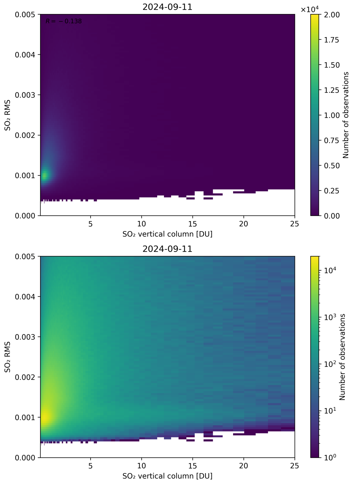
Figure 278: Scatter density plot of “SO 2 vertical column” against “SO 2 RMS” for 2024-09-10 to 2024-09-12.
