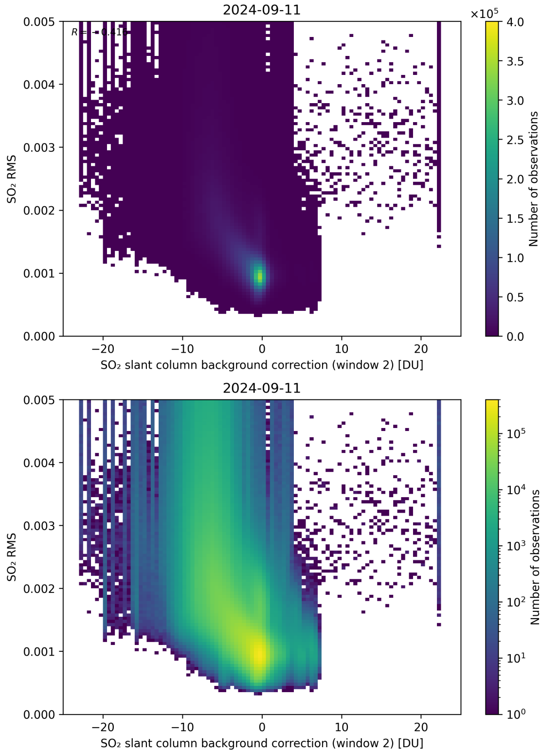
Figure 114: Scatter density plot of “SO 2 slant column background correction (window 2)” against “SO 2 RMS” for 2024-09-10 to 2024-09-12.
