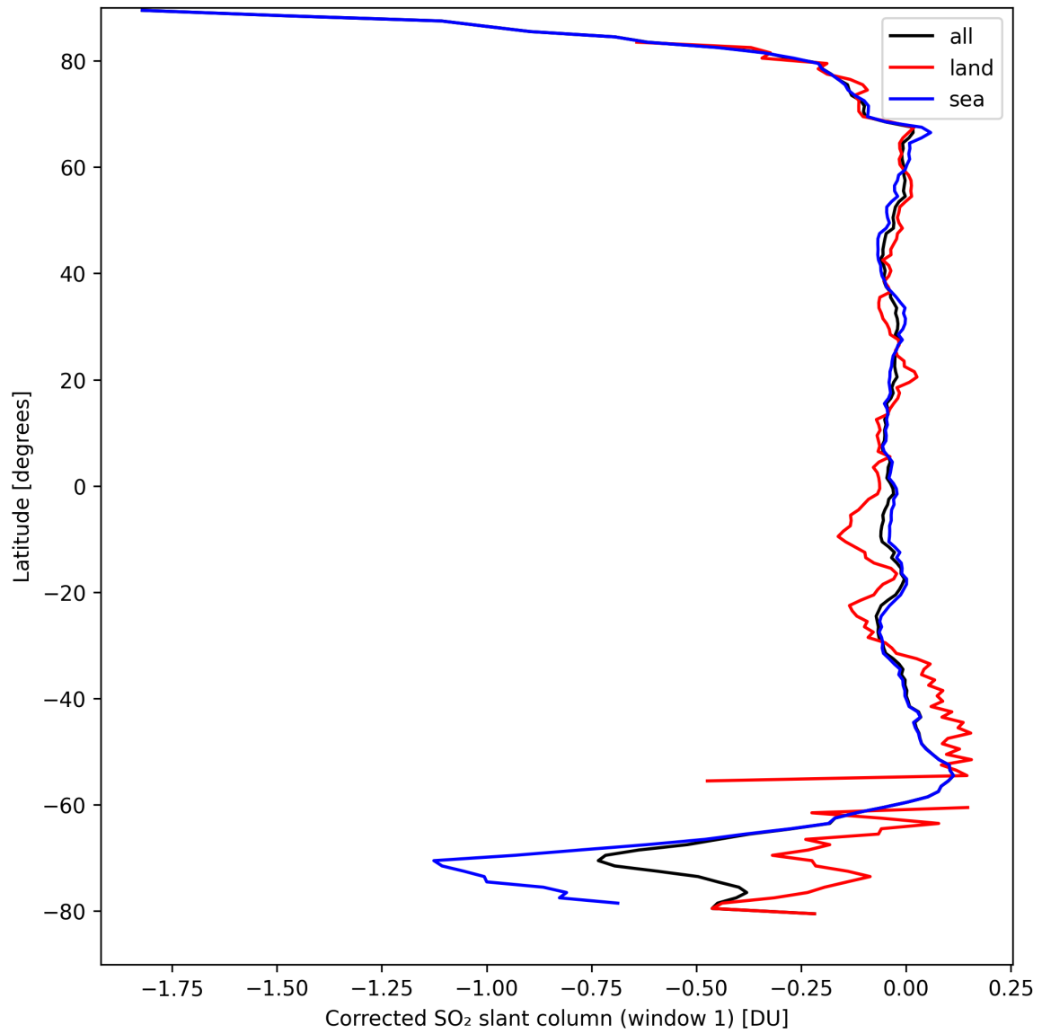
Figure 35: Zonal average of “Corrected SO 2 slant column (window 1)” for 2024-09-10 to 2024-09-12.
