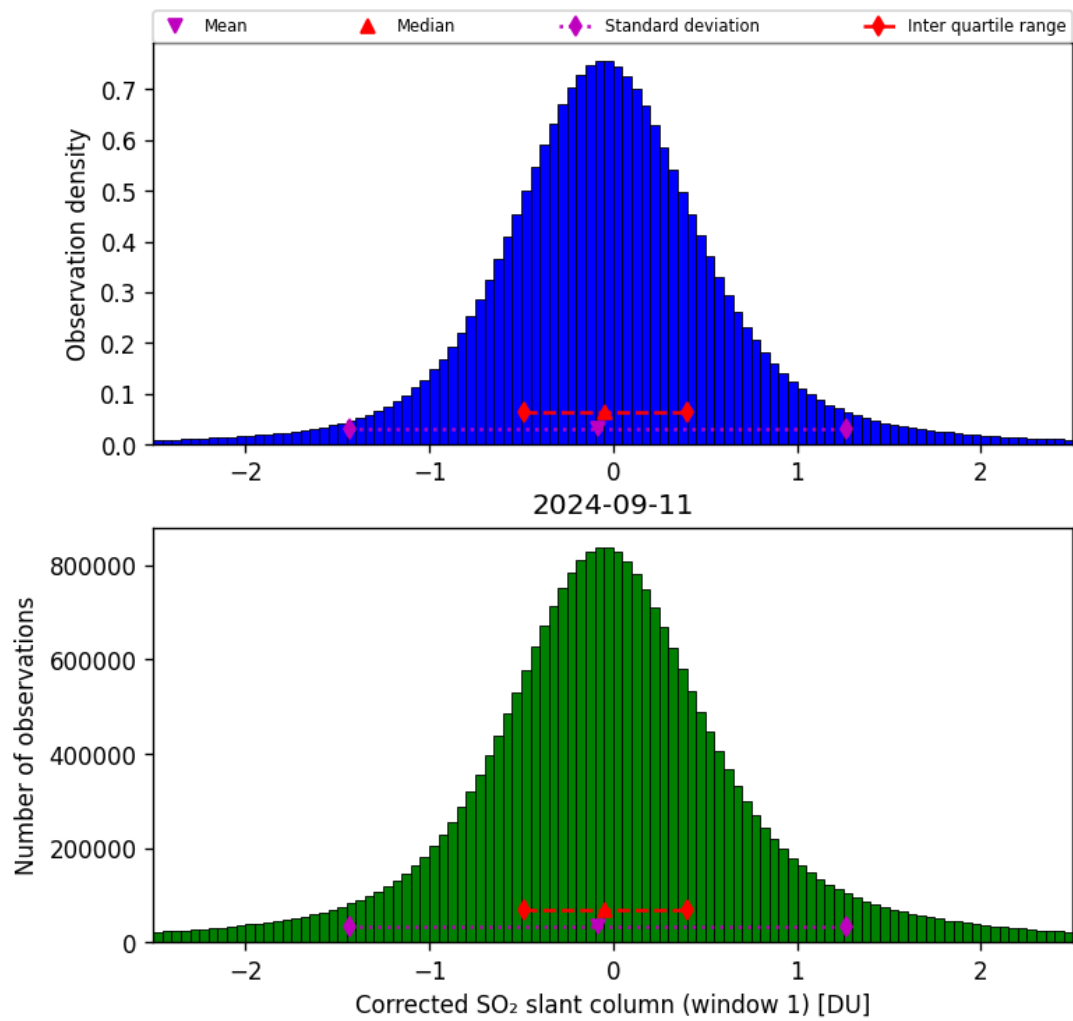
Figure 58: Histogram of “Corrected SO 2 slant column (window 1)” for 2024-09-10 to 2024-09-12
