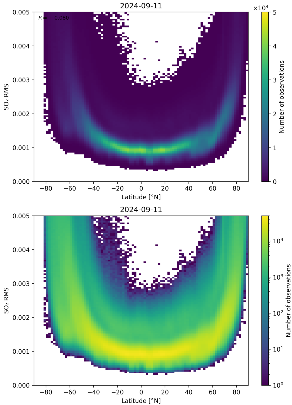
Figure 144: Scatter density plot of “Latitude” against “SO 2 RMS” for 2024-09-10 to 2024-09-12.
