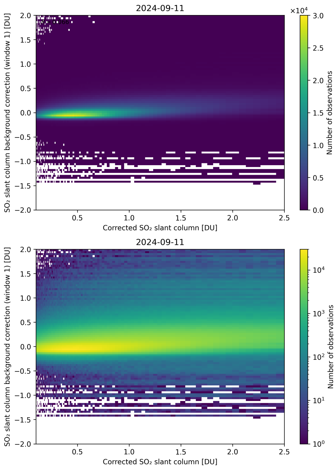
Figure 178: Scatter density plot of “Corrected SO 2 slant column” against “SO 2 slant column background correction (window 1)” for 2024-09-10 to 2024-09-12.
