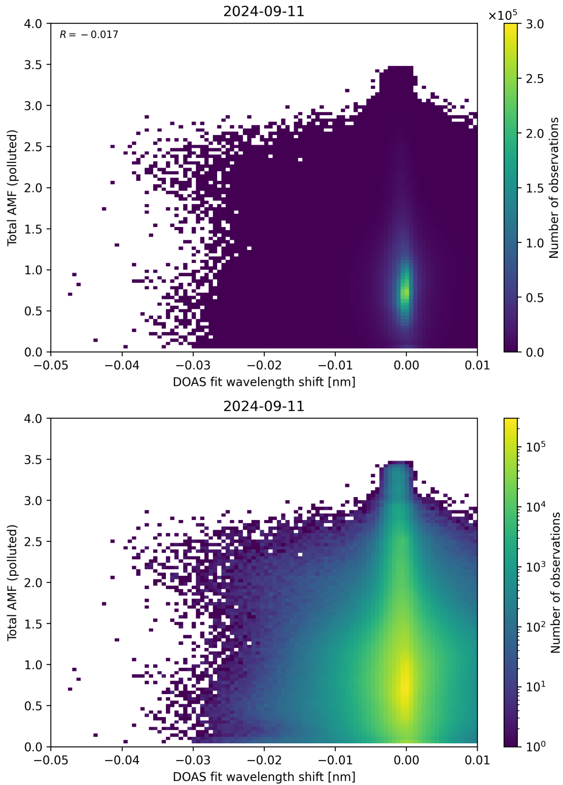
Figure 130: Scatter density plot of “DOAS fit wavelength shift” against “Total AMF (polluted)” for 2024-09-10 to 2024-09-12.
