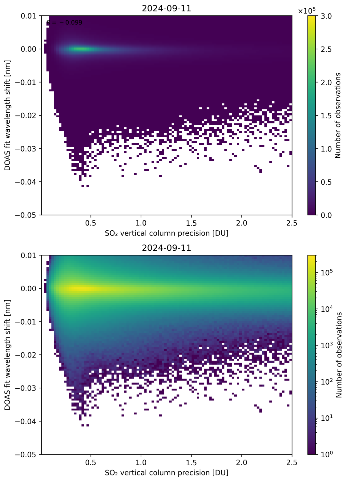
Figure 282: Scatter density plot of “SO 2 vertical column precision” against “DOAS fit wavelength shift” for 2024-09-10 to 2024-09-12.
