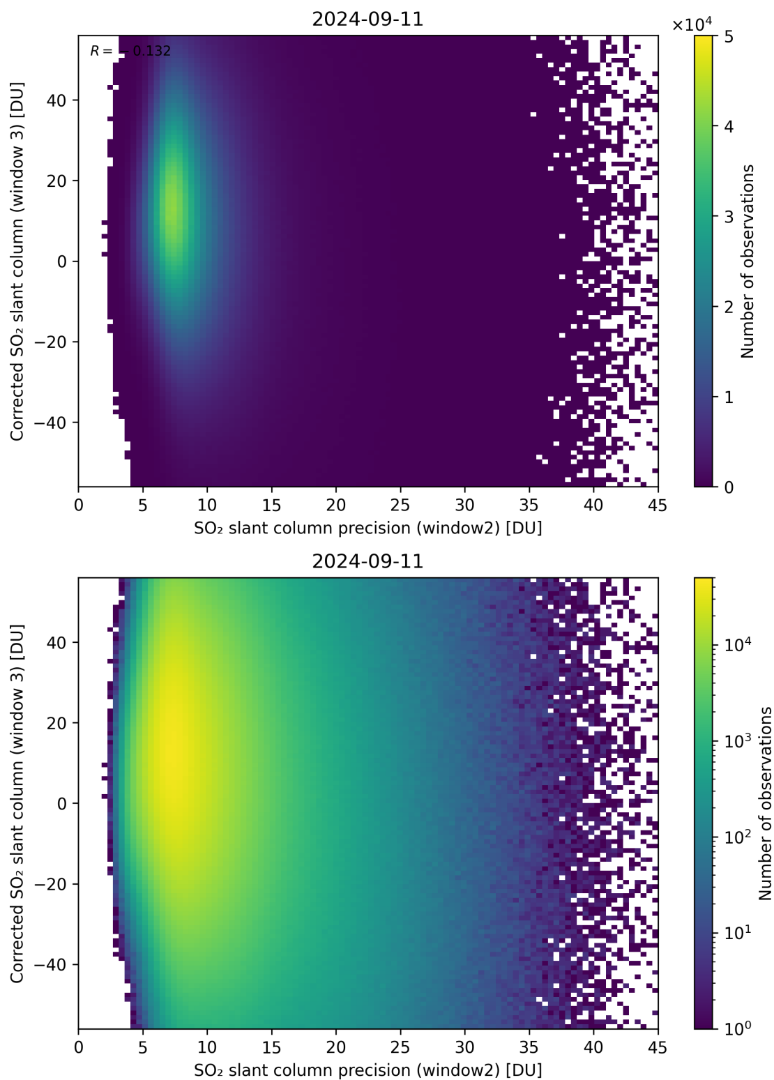
Figure 248: Scatter density plot of “SO 2 slant column precision (window2)” against “Corrected SO 2 slant column (window 3)” for 2024-09-10 to 2024-09-12.
