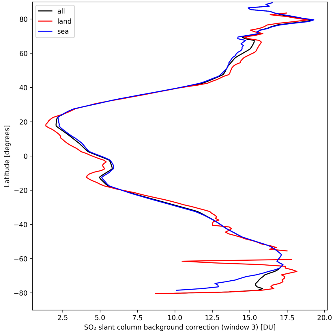
Figure 44: Zonal average of "SO 2 slant column background correction (window 3)" for 2024-09-10 to 2024-09-12.
