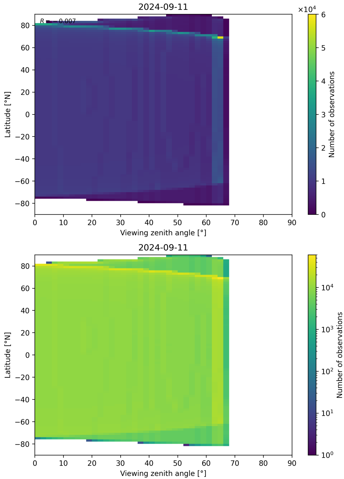
Figure 314: Scatter density plot of “Viewing zenith angle” against “Latitude” for 2024-09-10 to 2024-09-12.
