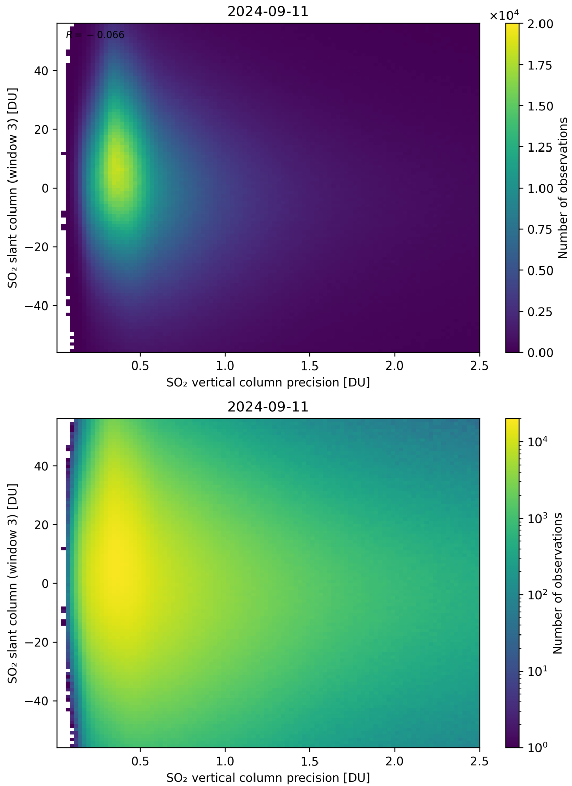
Figure 292: Scatter density plot of “SO 2 vertical column precision” against “SO 2 slant column (window 3)” for 2024-09-10 to 2024-09-12.
