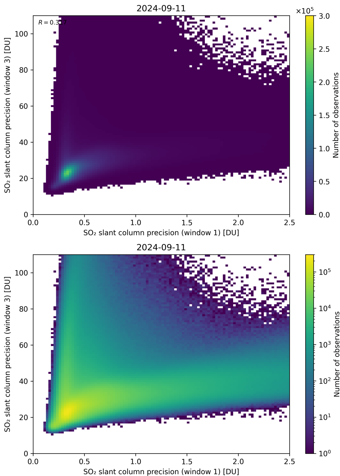
Figure 229: Scatter density plot of “SO 2 slant column precision (window 1)” against “SO 2 slant column precision (window 3)” for 2024-09-10 to 2024-09-12.
