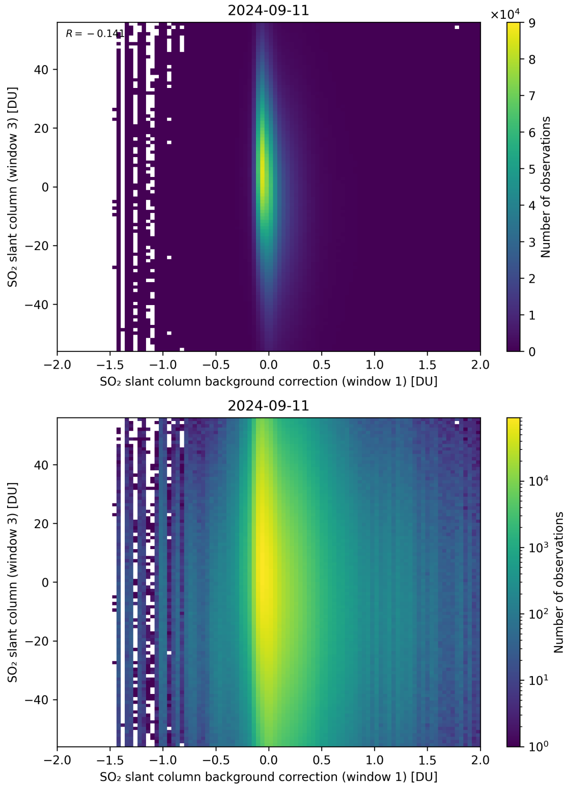
Figure 107: Scatter density plot of “SO 2 slant column background correction (window 1)” against “SO 2 slant column (window 3)” for 2024-09-10 to 2024-09-12.
