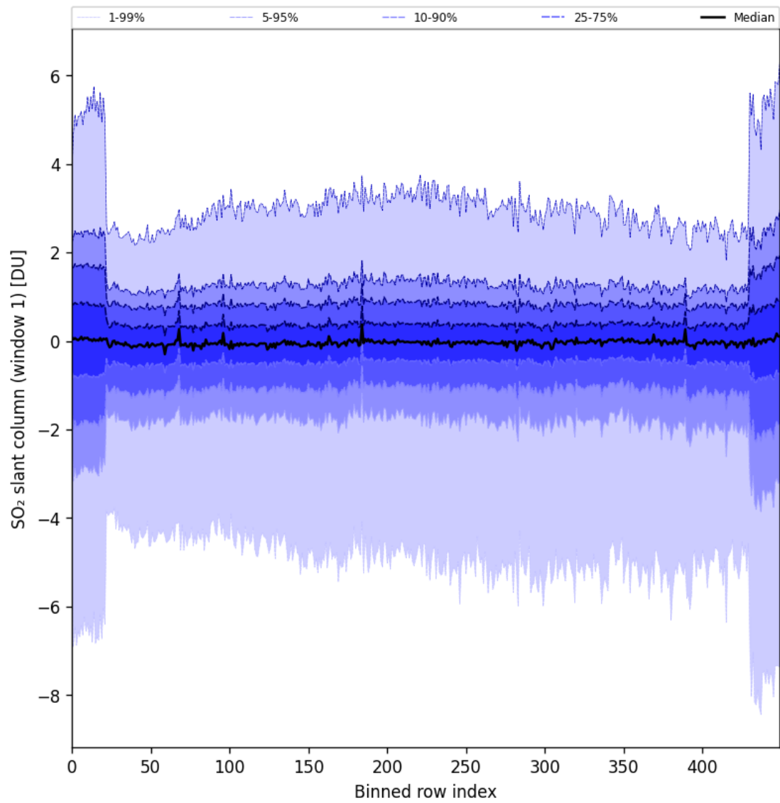
Figure 79: Along track statistics of “SO 2 slant column (window 1)” for 2024-09-10 to 2024-09-12
