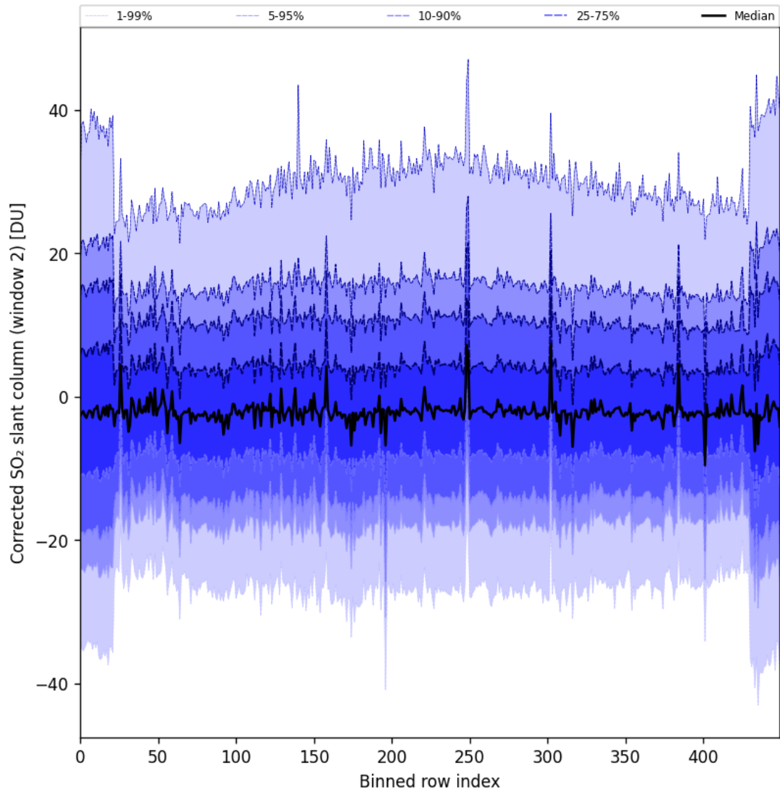
Figure 85: Along track statistics of “Corrected SO 2 slant column (window 2)” for 2024-09-10 to 2024-09-12
