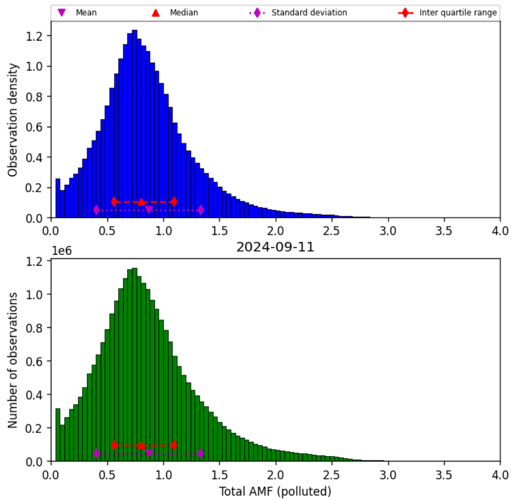
Figure 71: Histogram of “Total AMF (polluted)” for 2024-09-10 to 2024-09-12
