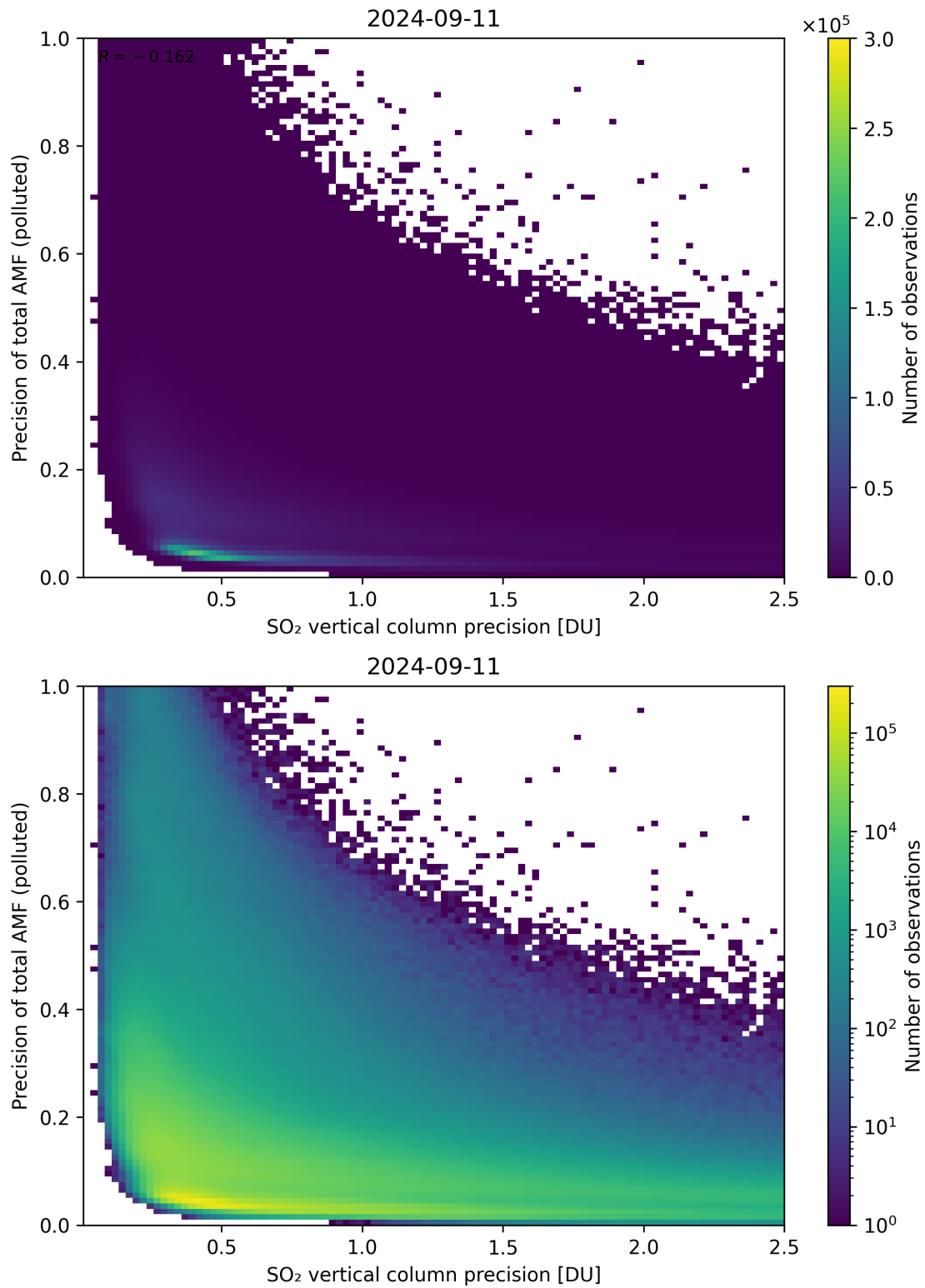
Figure 295: Scatter density plot of “SO 2 vertical column precision” against “Precision of total AMF (polluted)” for 2024-09-10 to 2024-09-12.
