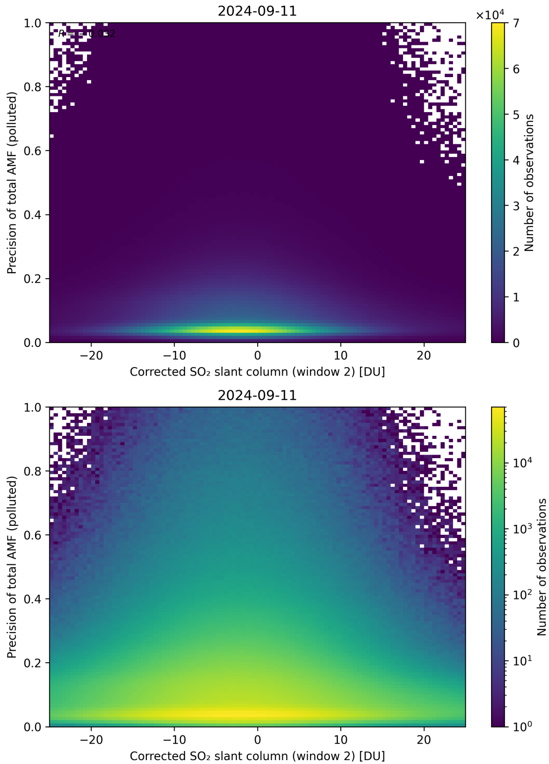
Figure 204: Scatter density plot of “Corrected SO 2 slant column (window 2)” against “Precision of total AMF (polluted)” for 2024-09-10 to 2024-09-12.
