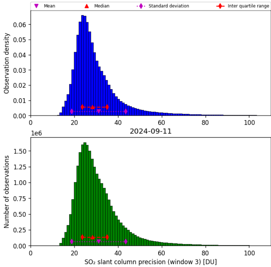
Figure 65: Histogram of “SO 2 slant column precision (window 3)” for 2024-09-10 to 2024-09-12
