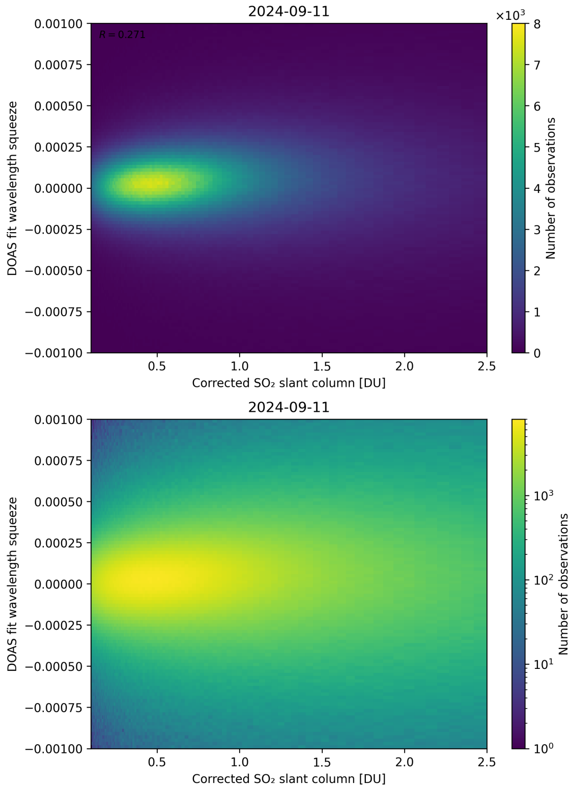
Figure 182: Scatter density plot of “Corrected SO 2 slant column” against “DOAS fit wavelength squeeze” for 2024-09-10 to 2024-09-12.
