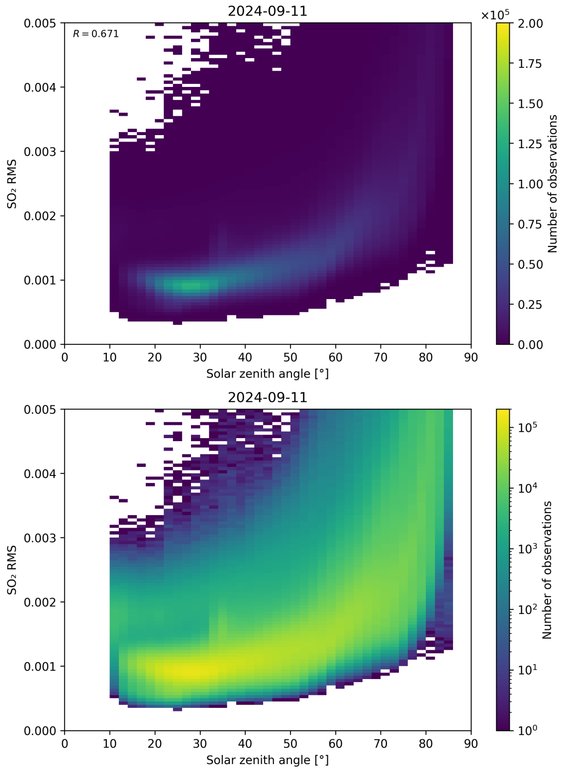
Figure 163: Scatter density plot of “Solar zenith angle” against “SO 2 RMS” for 2024-09-10 to 2024-09-12.
