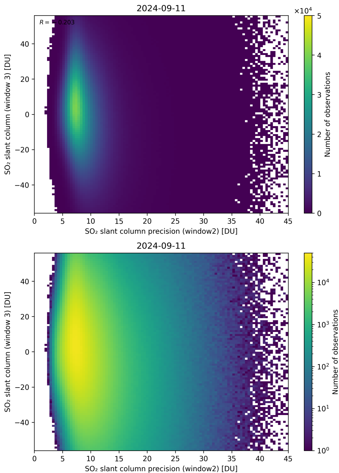
Figure 249: Scatter density plot of “SO 2 slant column precision (window2)” against “SO 2 slant column (window 3)” for 2024-09-10 to 2024-09-12.
