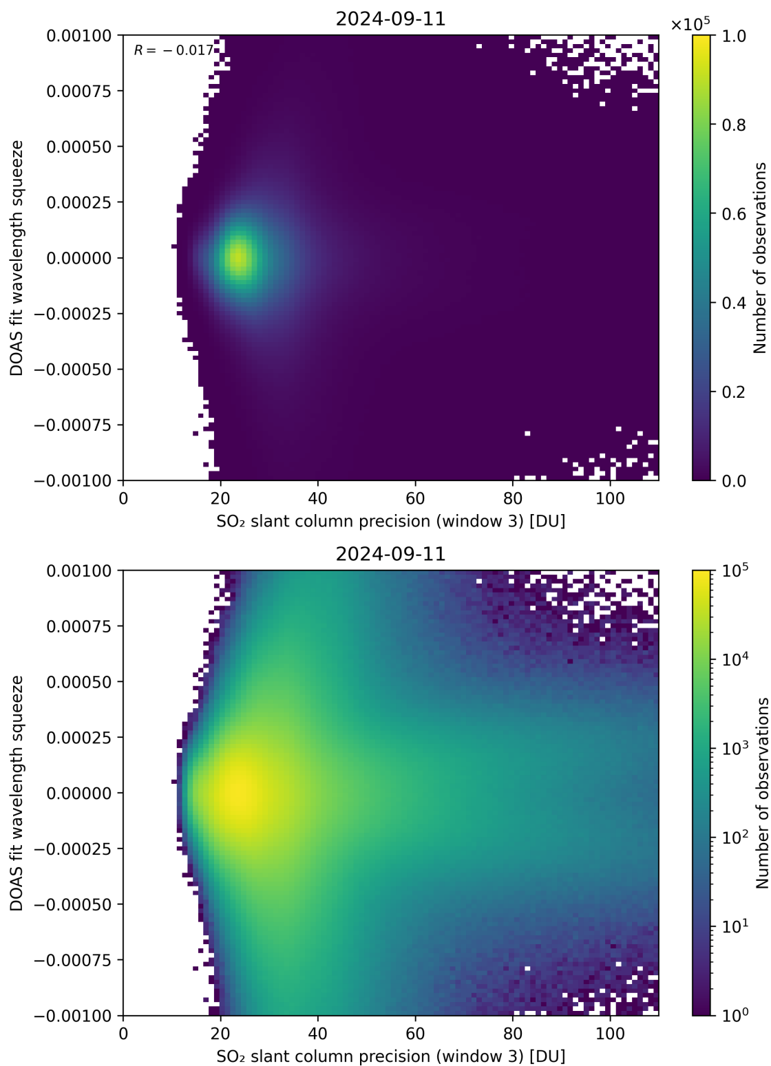
Figure 259: Scatter density plot of “SO 2 slant column precision (window 3)” against “DOAS fit wavelength squeeze” for 2024-09-10 to 2024-09-12.
