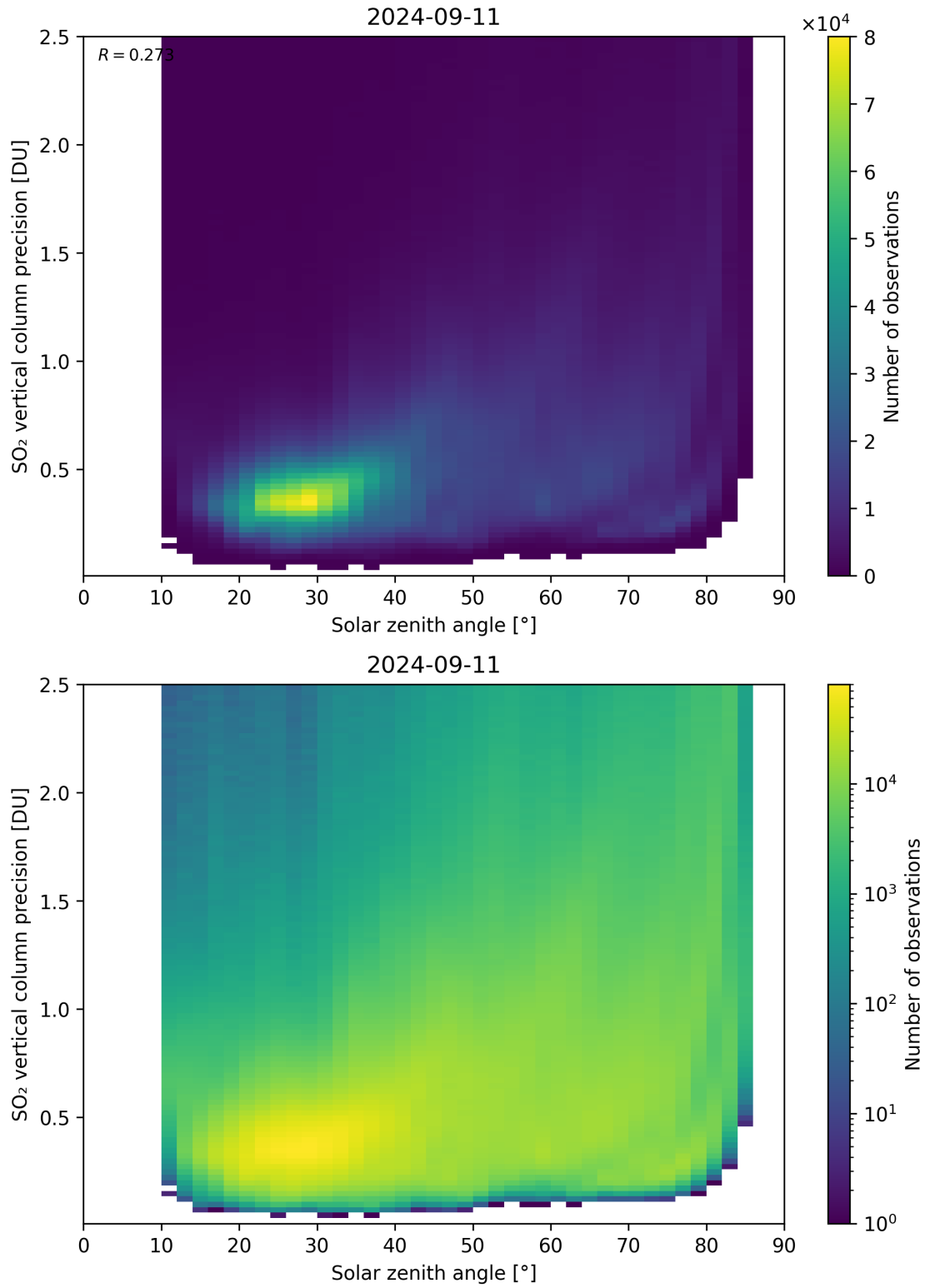
Figure 177: Scatter density plot of “Solar zenith angle” against “SO 2 vertical column precision” for 2024-09-10 to 2024-09-12.
