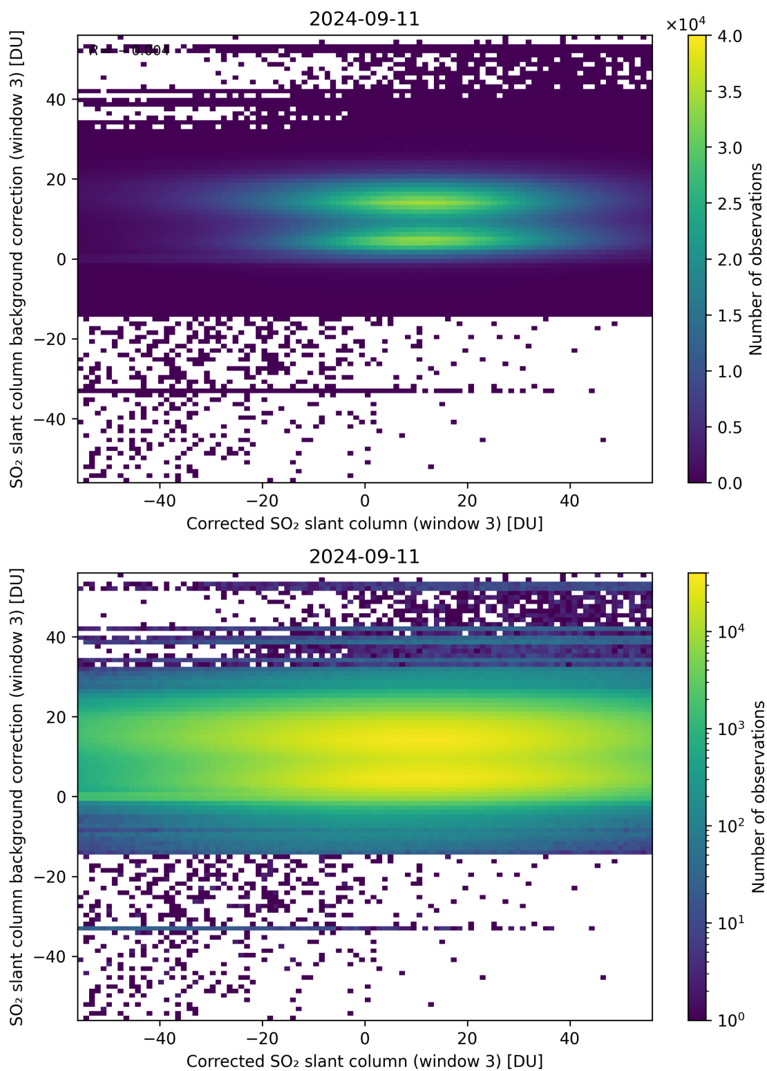
Figure 205: Scatter density plot of “Corrected SO 2 slant column (window 3)” against “SO 2 slant column background correction (window 3)” for 2024-09-10 to 2024-09-12.
