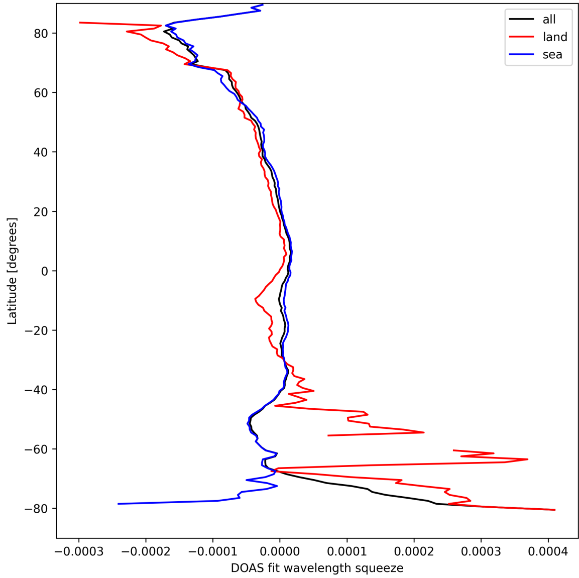
Figure 46: Zonal average of “DOAS fit wavelength squeeze” for 2024-09-10 to 2024-09-12.
