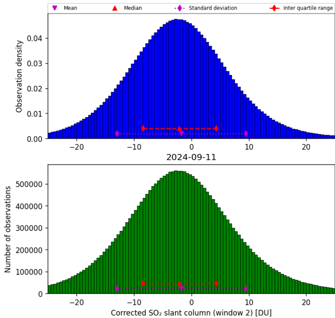
Figure 62: Histogram of “Corrected SO 2 slant column (window 2)” for 2024-09-10 to 2024-09-12
