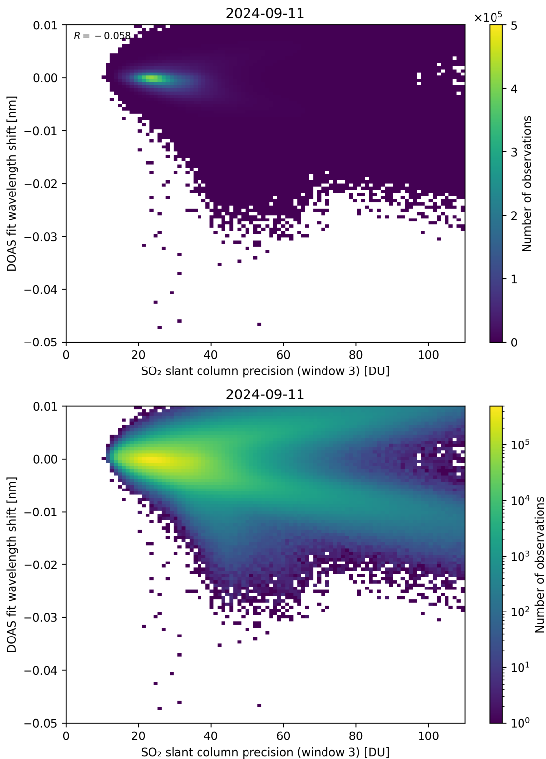
Figure 258: Scatter density plot of “SO 2 slant column precision (window 3)” against “DOAS fit wavelength shift” for 2024-09-10 to 2024-09-12.
