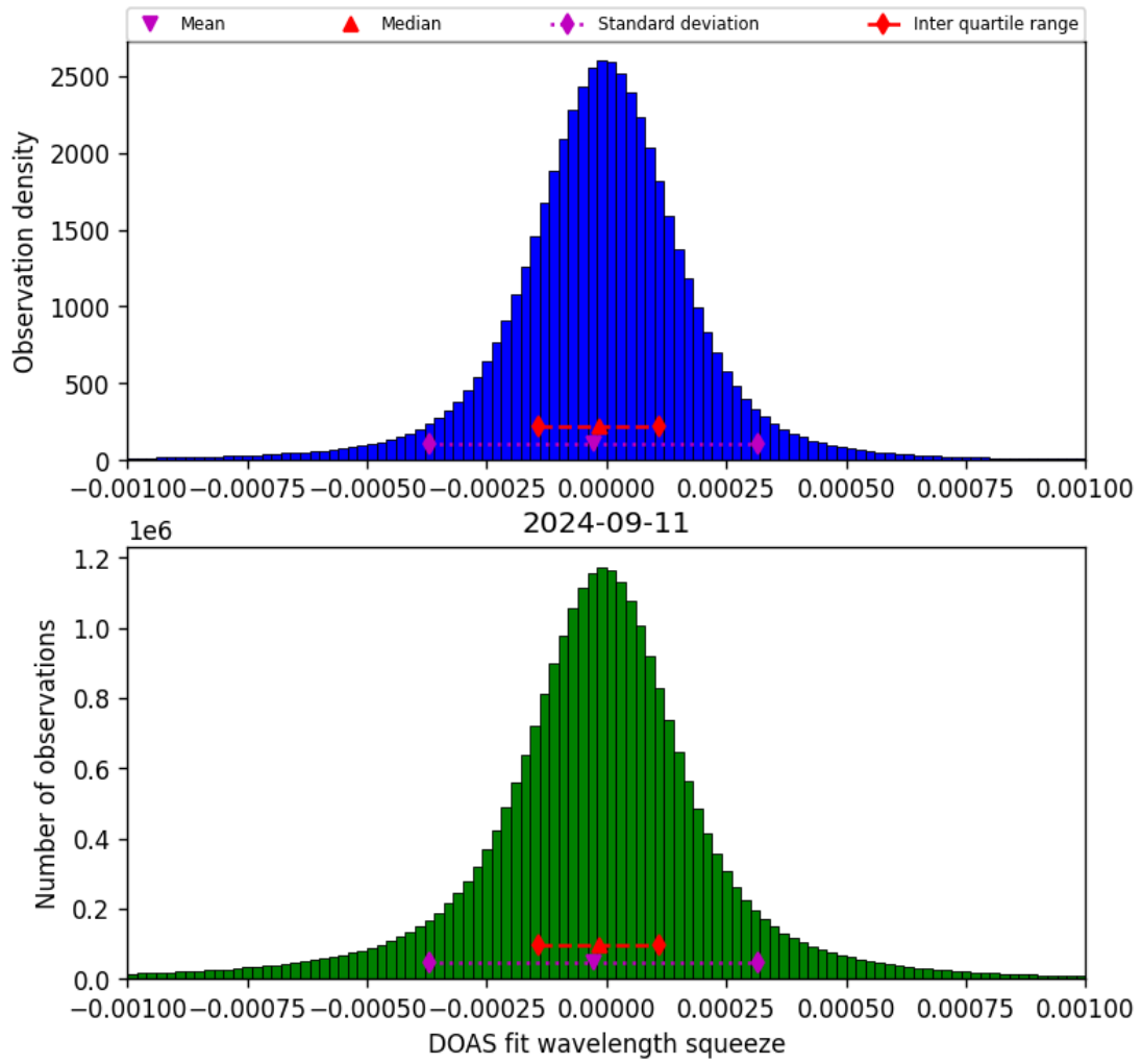
Figure 69: Histogram of “DOAS fit wavelength squeeze” for 2024-09-10 to 2024-09-12
