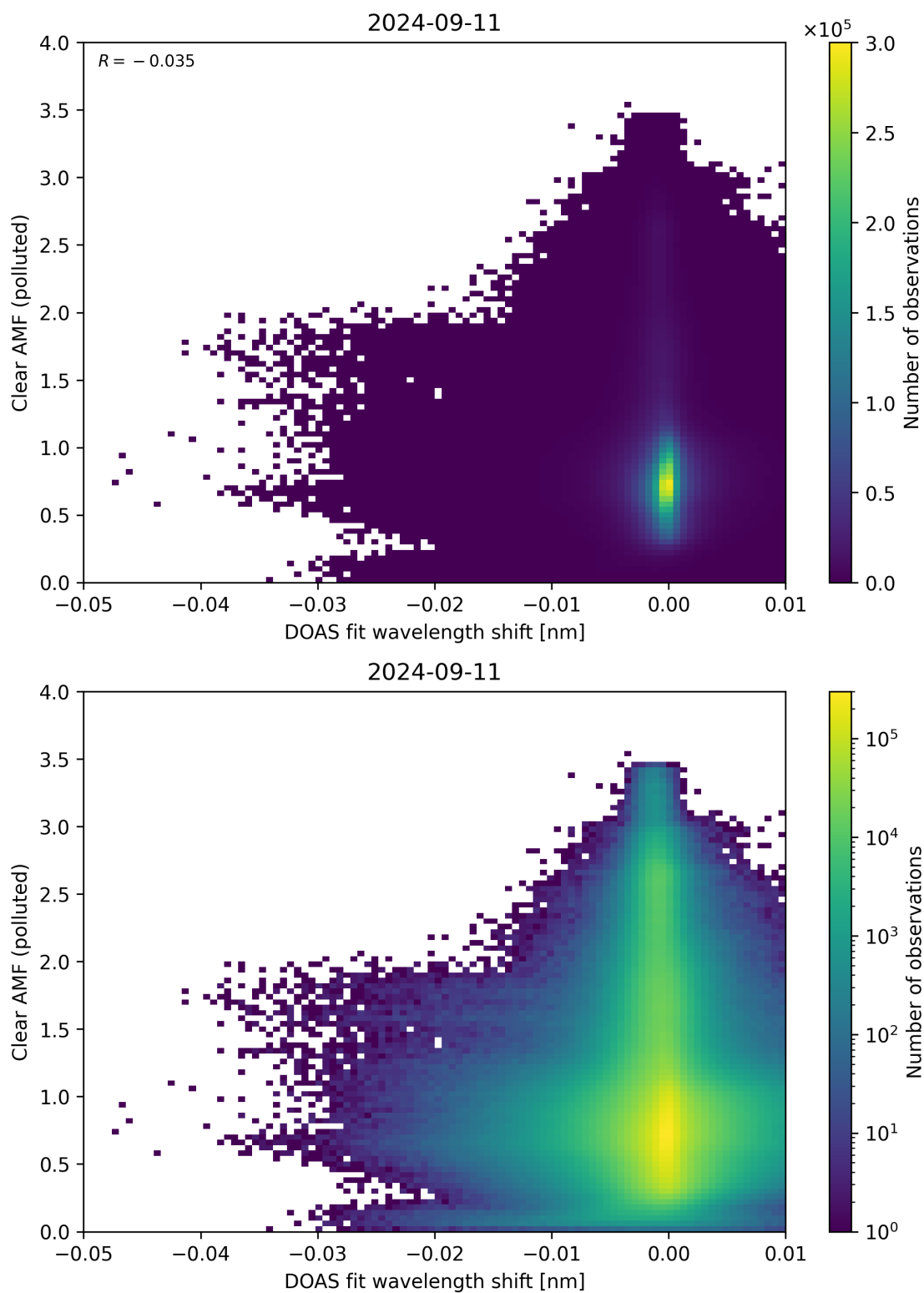
Figure 129: Scatter density plot of “DOAS fit wavelength shift” against “Clear AMF (polluted)” for 2024-09-10 to 2024-09-12.
