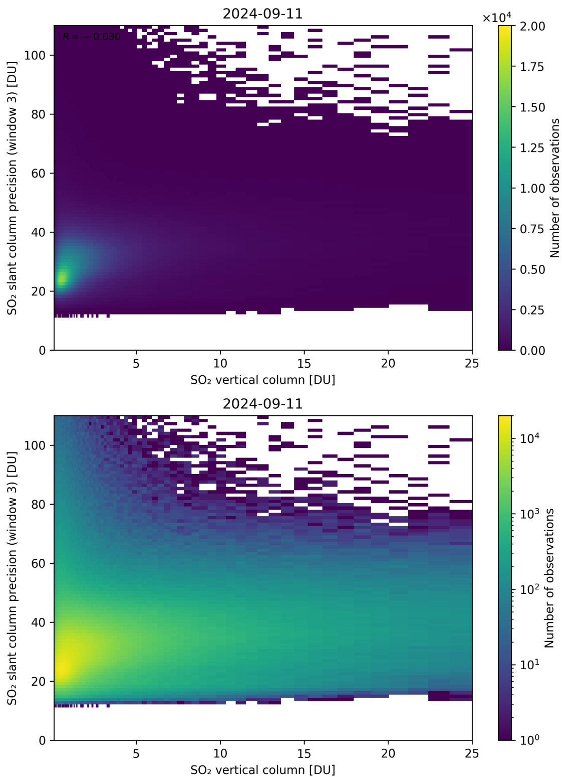
Figure 304: Scatter density plot of “SO 2 vertical column” against “SO 2 slant column precision (window 3)” for 2024-09-10 to 2024-09-12.
