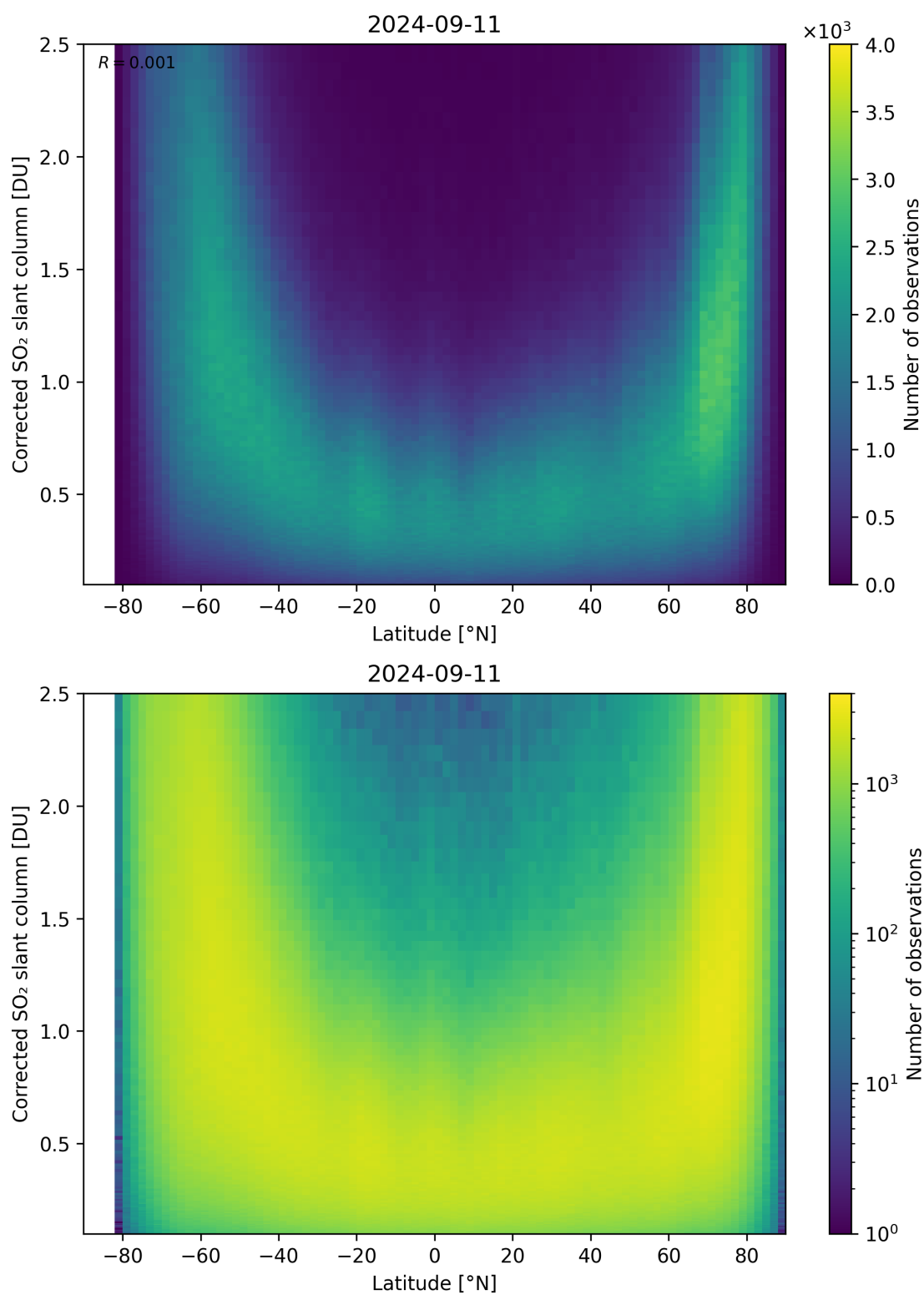
Figure 146: Scatter density plot of “Latitude” against “Corrected SO 2 slant column” for 2024-09-10 to 2024-09-12.
