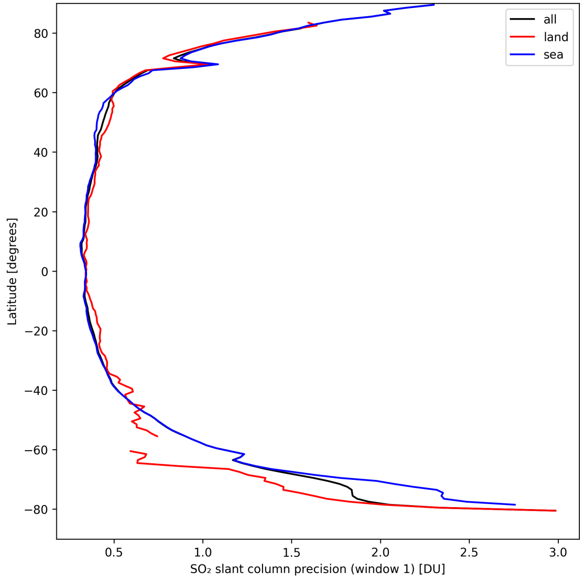
Figure 34: Zonal average of “SO 2 slant column precision (window 1)” for 2024-09-10 to 2024-09-12.
