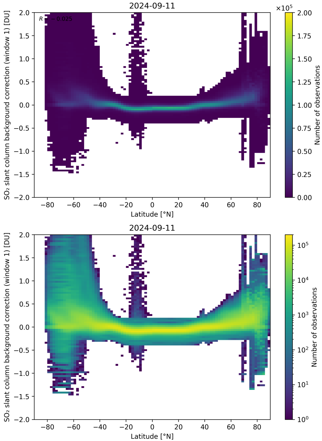
Figure 139: Scatter density plot of “Latitude” against “SO 2 slant column background correction (window 1)” for 2024-09-10 to 2024-09-12.
