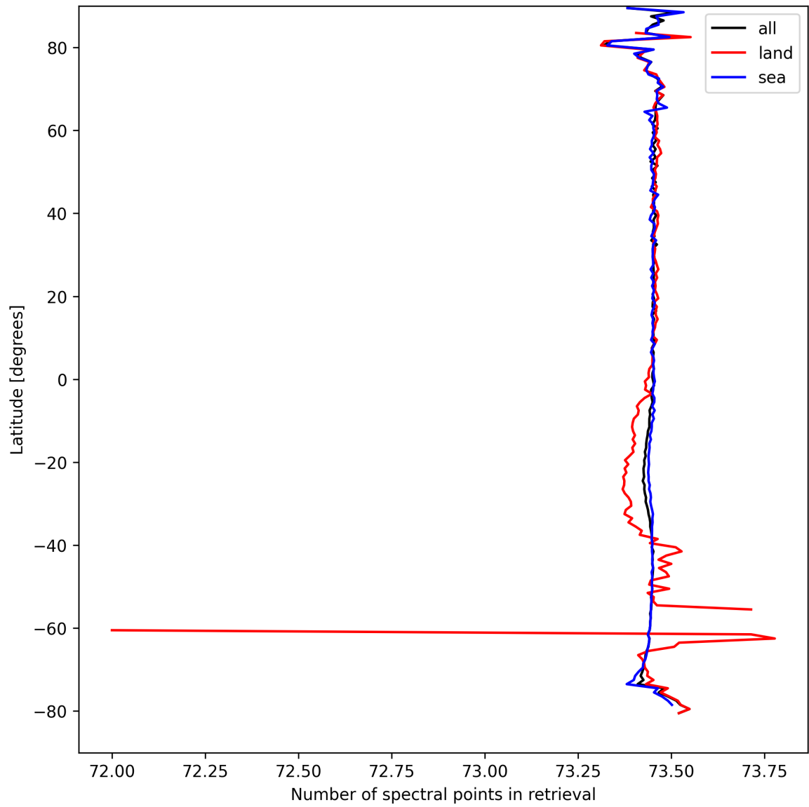
Figure 51: Zonal average of “Number of spectral points in retrieval” for 2024-09-10 to 2024-09-12.
