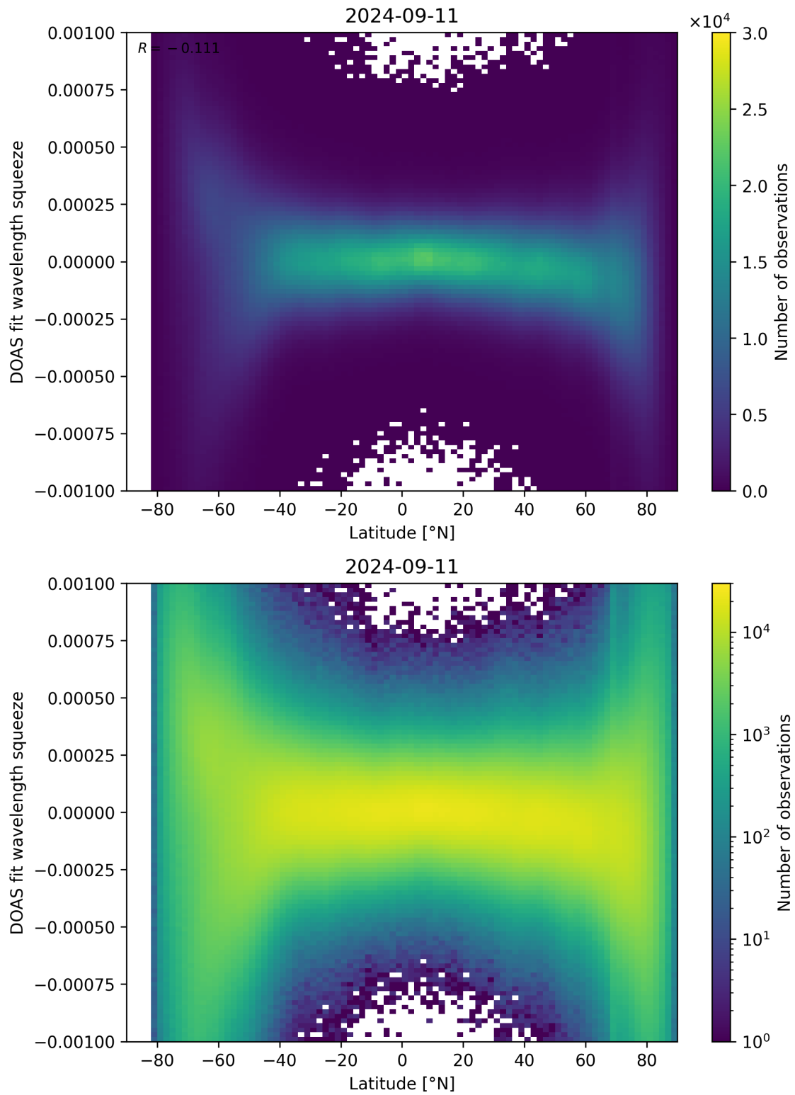
Figure 143: Scatter density plot of “Latitude” against “DOAS fit wavelength squeeze” for 2024-09-10 to 2024-09-12.
