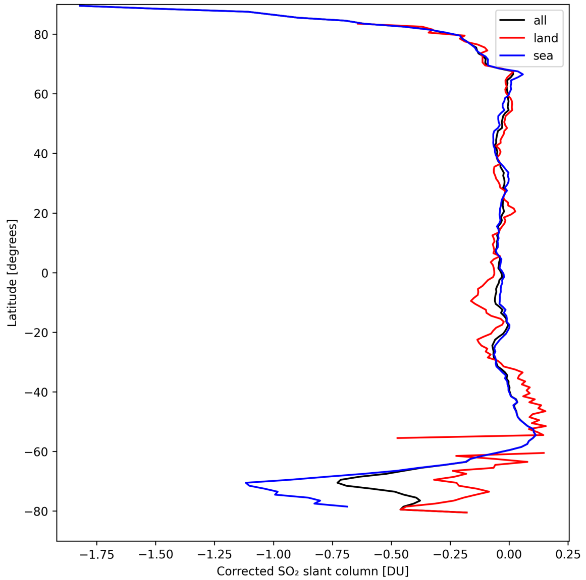
Figure 32: Zonal average of “Corrected SO 2 slant column” for 2024-09-10 to 2024-09-12.
