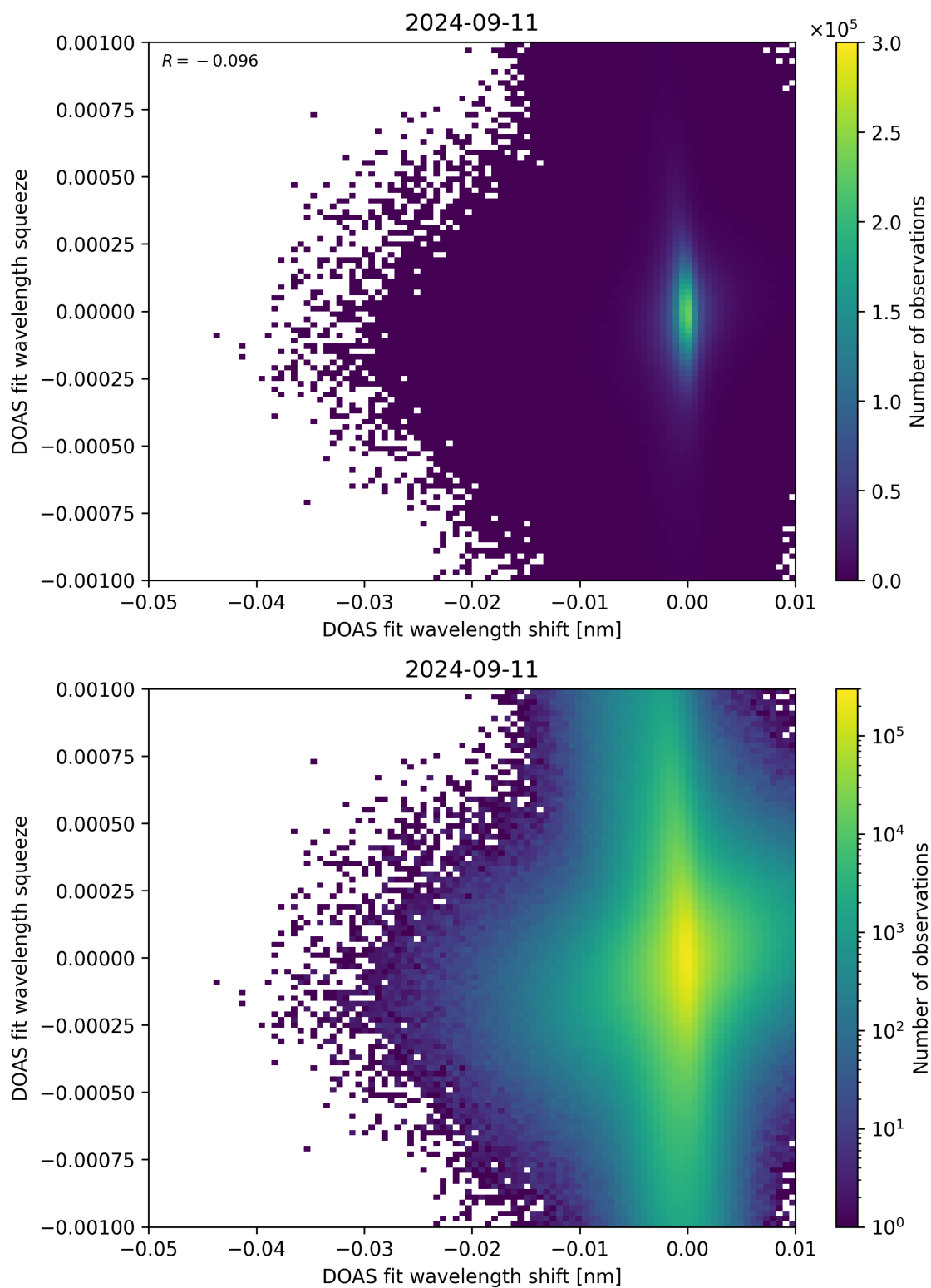
Figure 127: Scatter density plot of “DOAS fit wavelength shift” against “DOAS fit wavelength squeeze” for 2024-09-10 to 2024-09-12.
