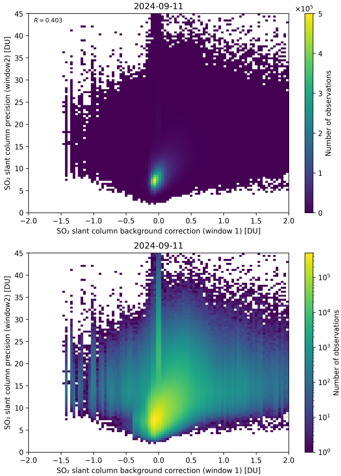
Figure 106: Scatter density plot of “SO 2 slant column background correction (window 1)” against “SO 2 slant column precision (window2)” for 2024-09-10 to 2024-09-12.
