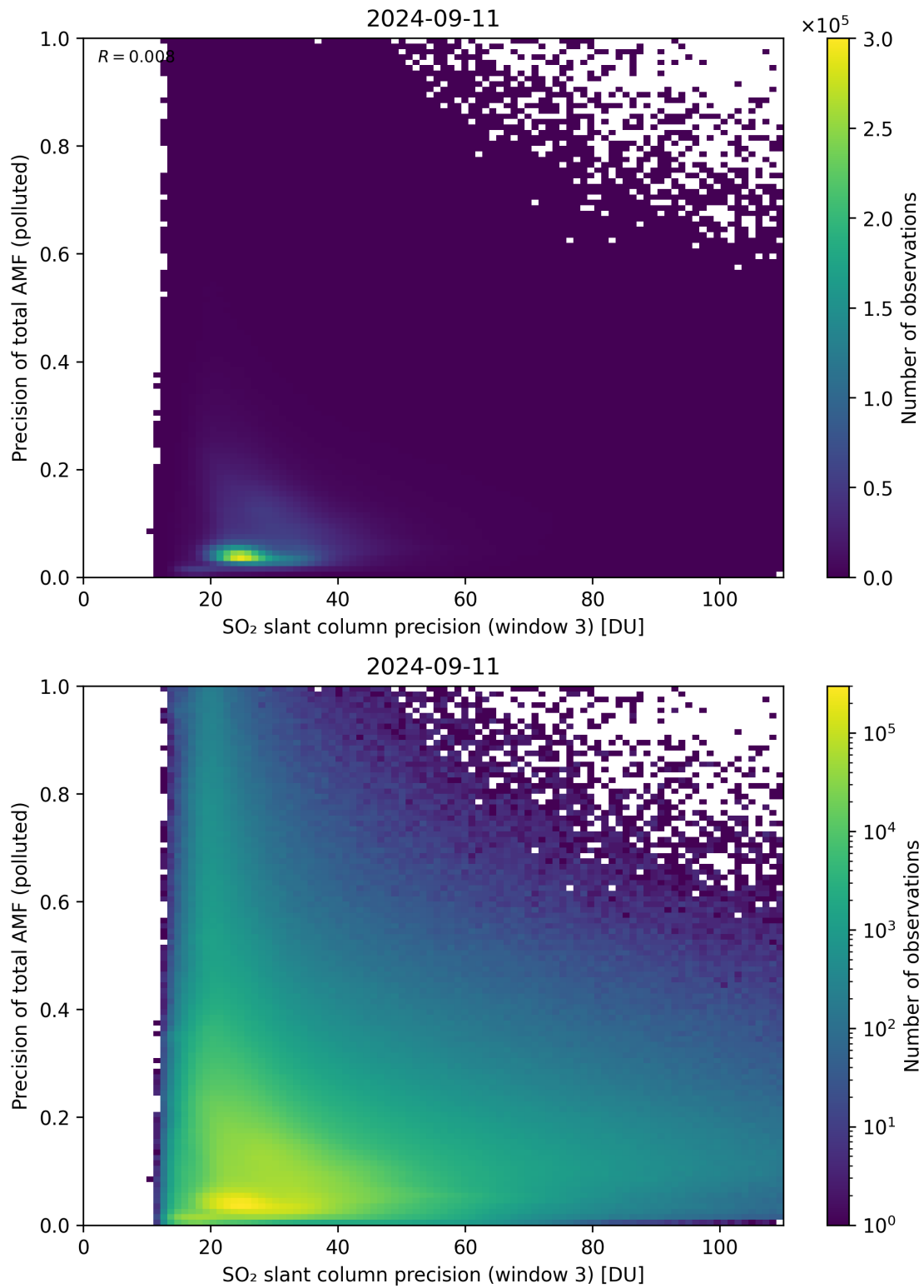
Figure 264: Scatter density plot of “SO 2 slant column precision (window 3)” against “Precision of total AMF (polluted)” for 2024-09-10 to 2024-09-12.
