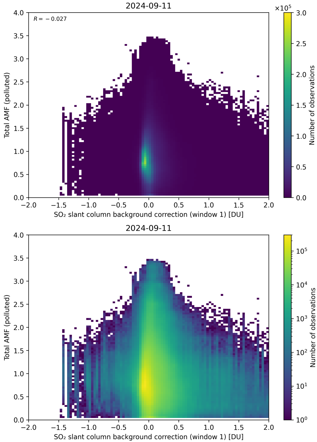
Figure 109: Scatter density plot of “SO 2 slant column background correction (window 1)” against “Total AMF (polluted)” for 2024-09-10 to 2024-09-12.
