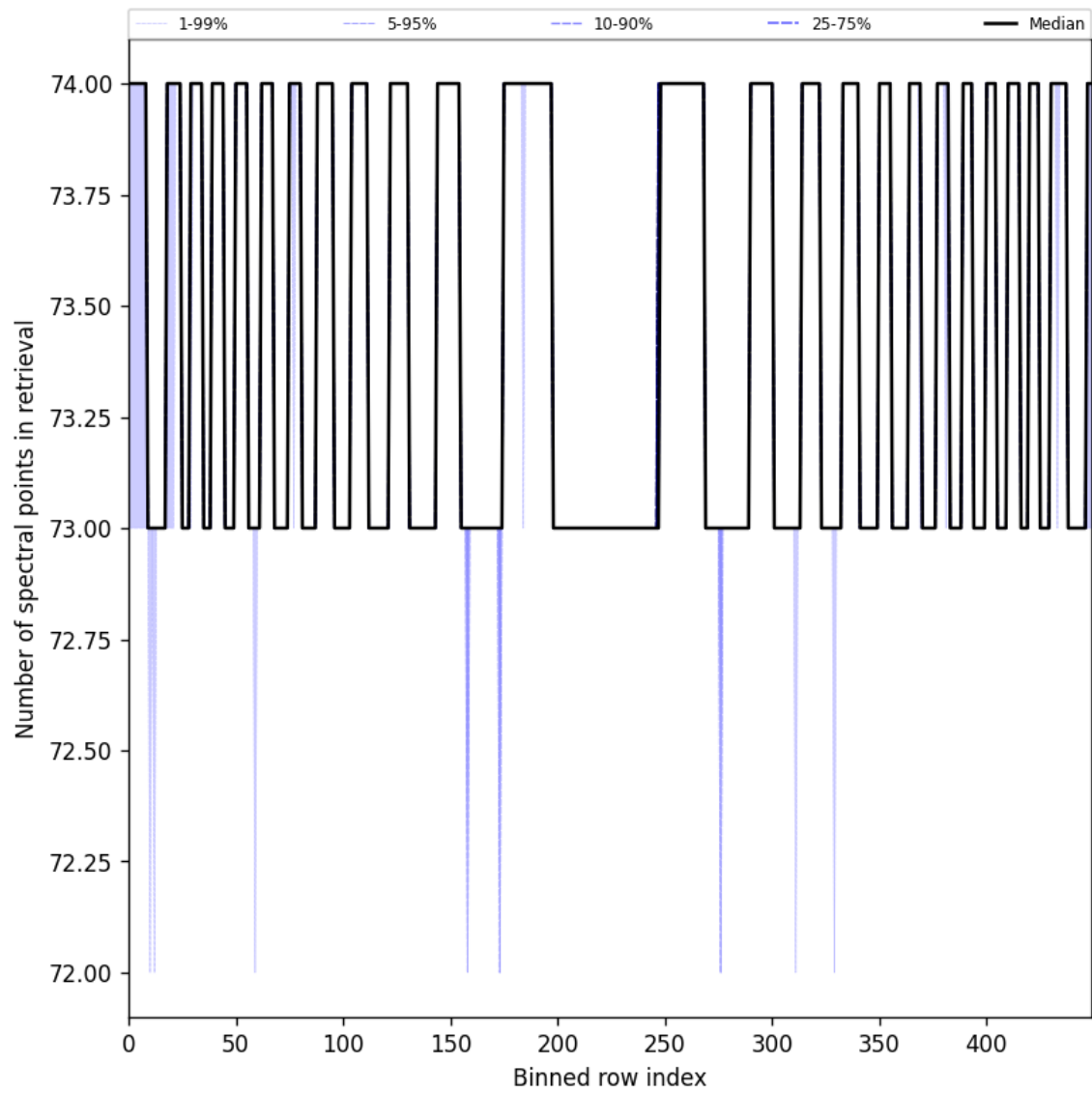
Figure 97: Along track statistics of “Number of spectral points in retrieval” for 2024-09-10 to 2024-09-12
