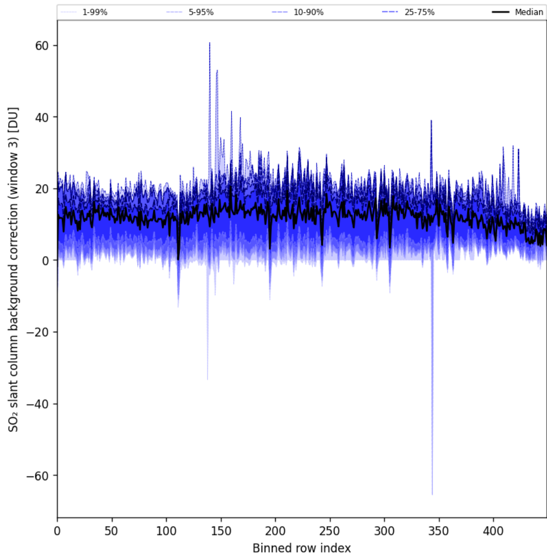
Figure 90: Along track statistics of “SO 2 slant column background correction (window 3)” for 2024-09-10 to 2024-09-12
