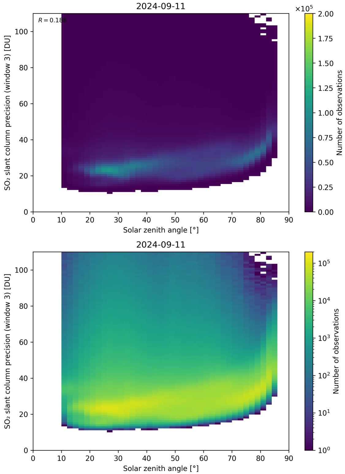
Figure 173: Scatter density plot of “Solar zenith angle” against “SO 2 slant column precision (window 3)” for 2024-09-10 to 2024-09-12.
