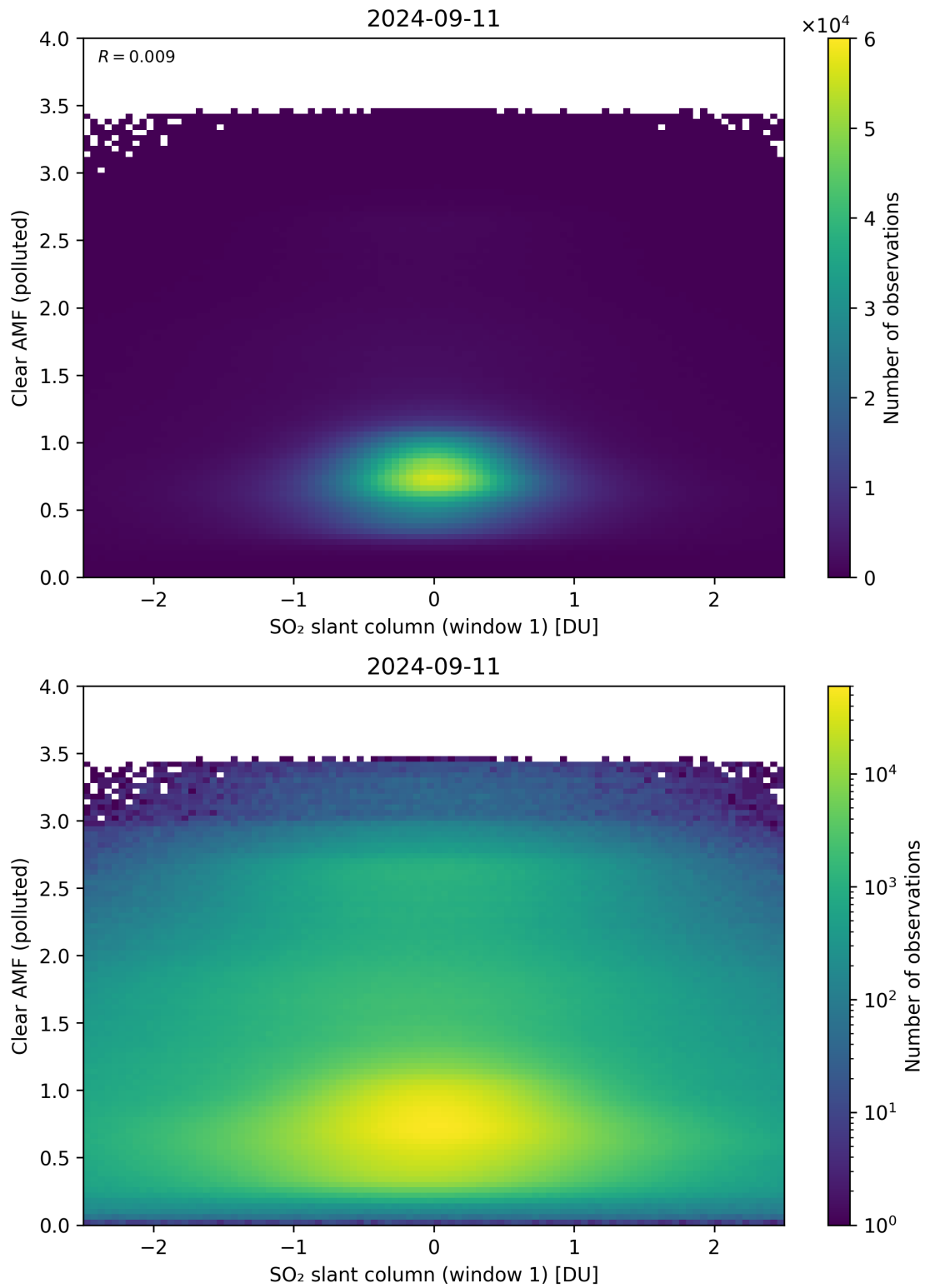
Figure 232: Scatter density plot of “SO 2 slant column (window 1)” against “Clear AMF (polluted)” for 2024-09-10 to 2024-09-12.
