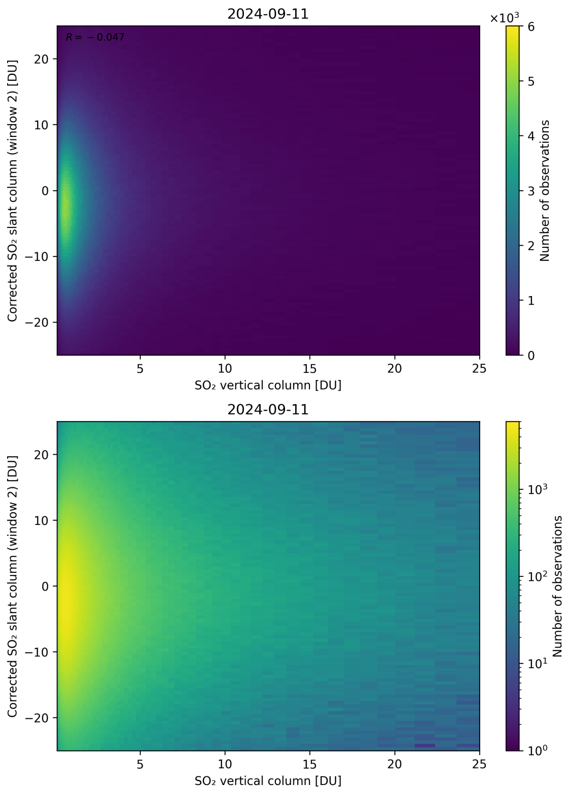
Figure 298: Scatter density plot of “SO 2 vertical column” against “Corrected SO 2 slant column (window 2)” for 2024-09-10 to 2024-09-12.
