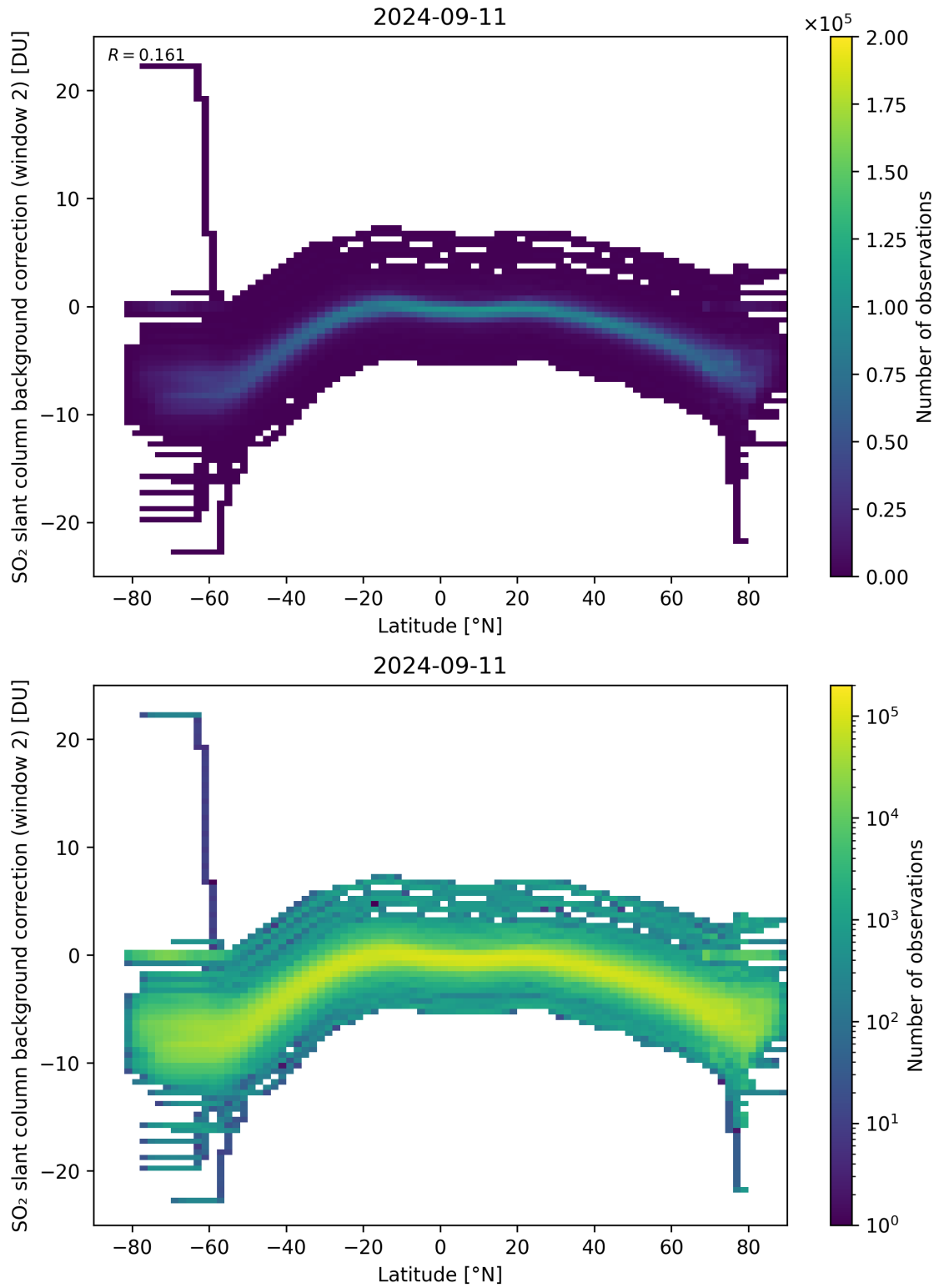
Figure 140: Scatter density plot of “Latitude” against “SO 2 slant column background correction (window 2)” for 2024-09-10 to 2024-09-12.
