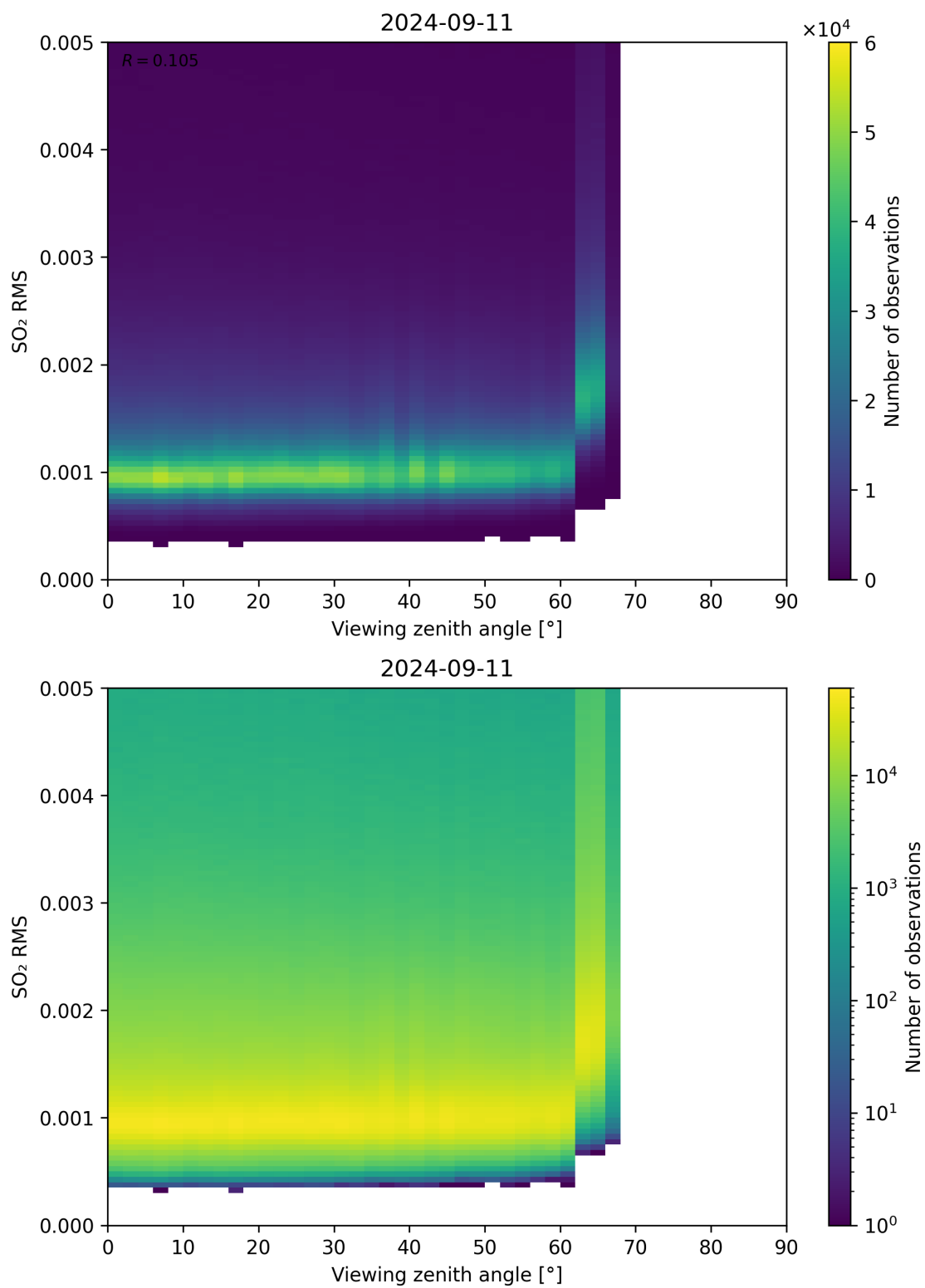
Figure 313: Scatter density plot of “Viewing zenith angle” against “SO 2 RMS” for 2024-09-10 to 2024-09-12.
