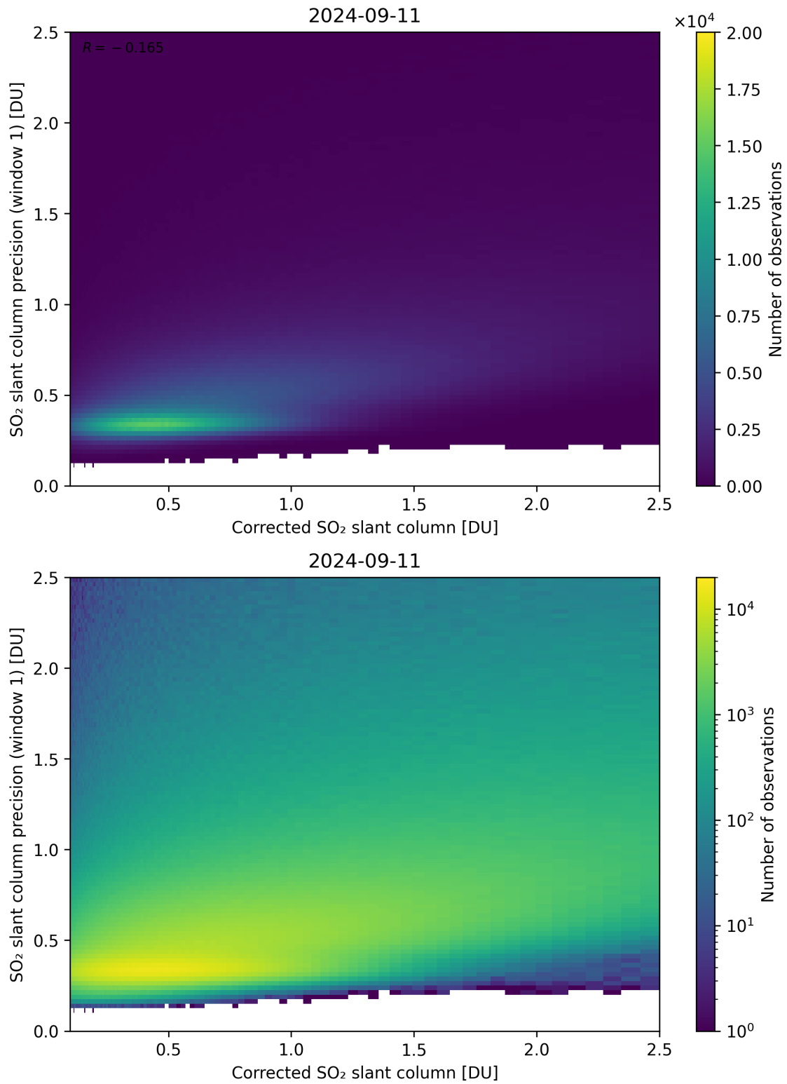
Figure 188: Scatter density plot of “Corrected SO 2 slant column” against “SO 2 slant column precision (window 1)” for 2024-09-10 to 2024-09-12.
