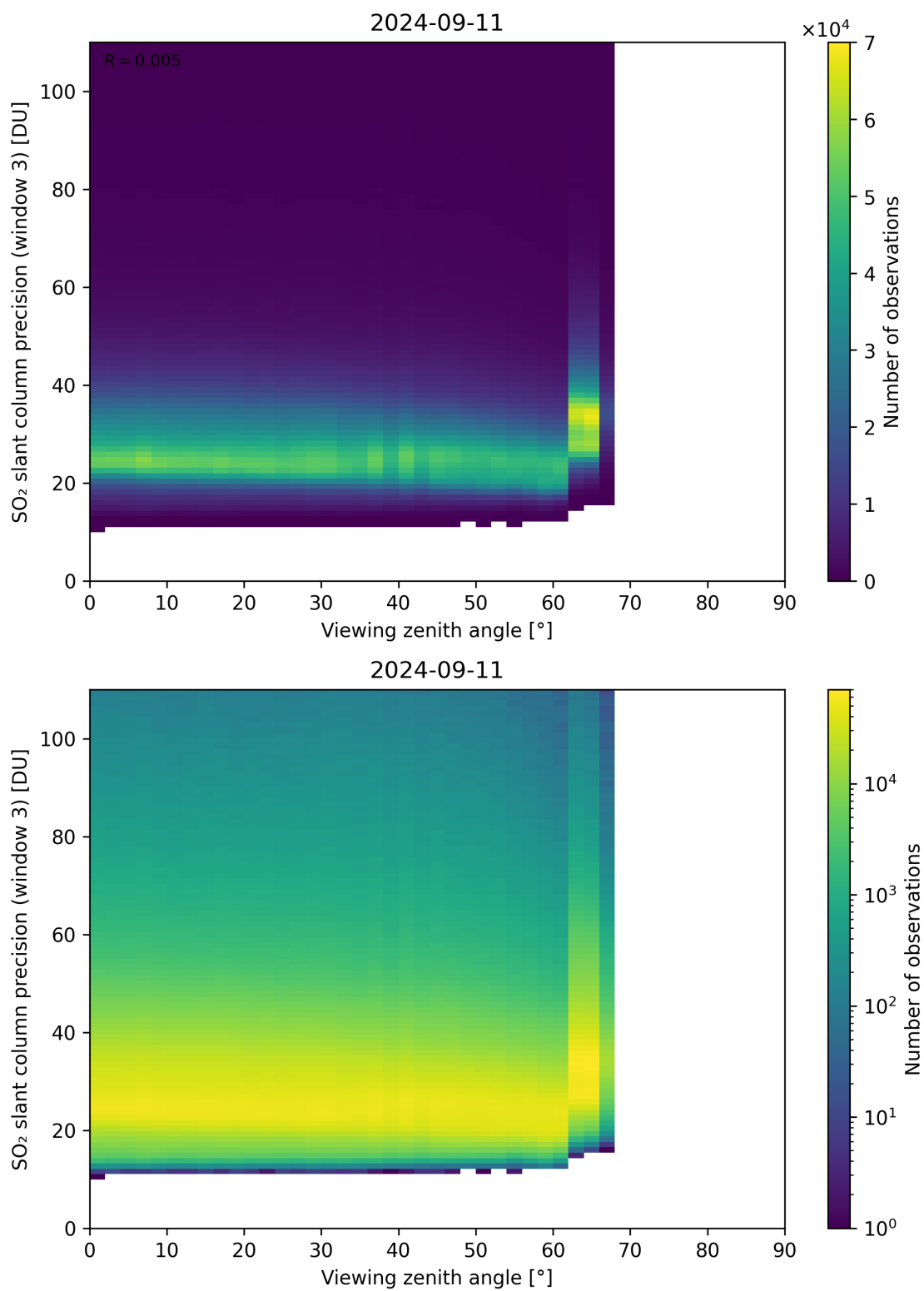
Figure 324: Scatter density plot of “Viewing zenith angle” against “SO 2 slant column precision (window 3)” for 2024-09-10 to 2024-09-12.
