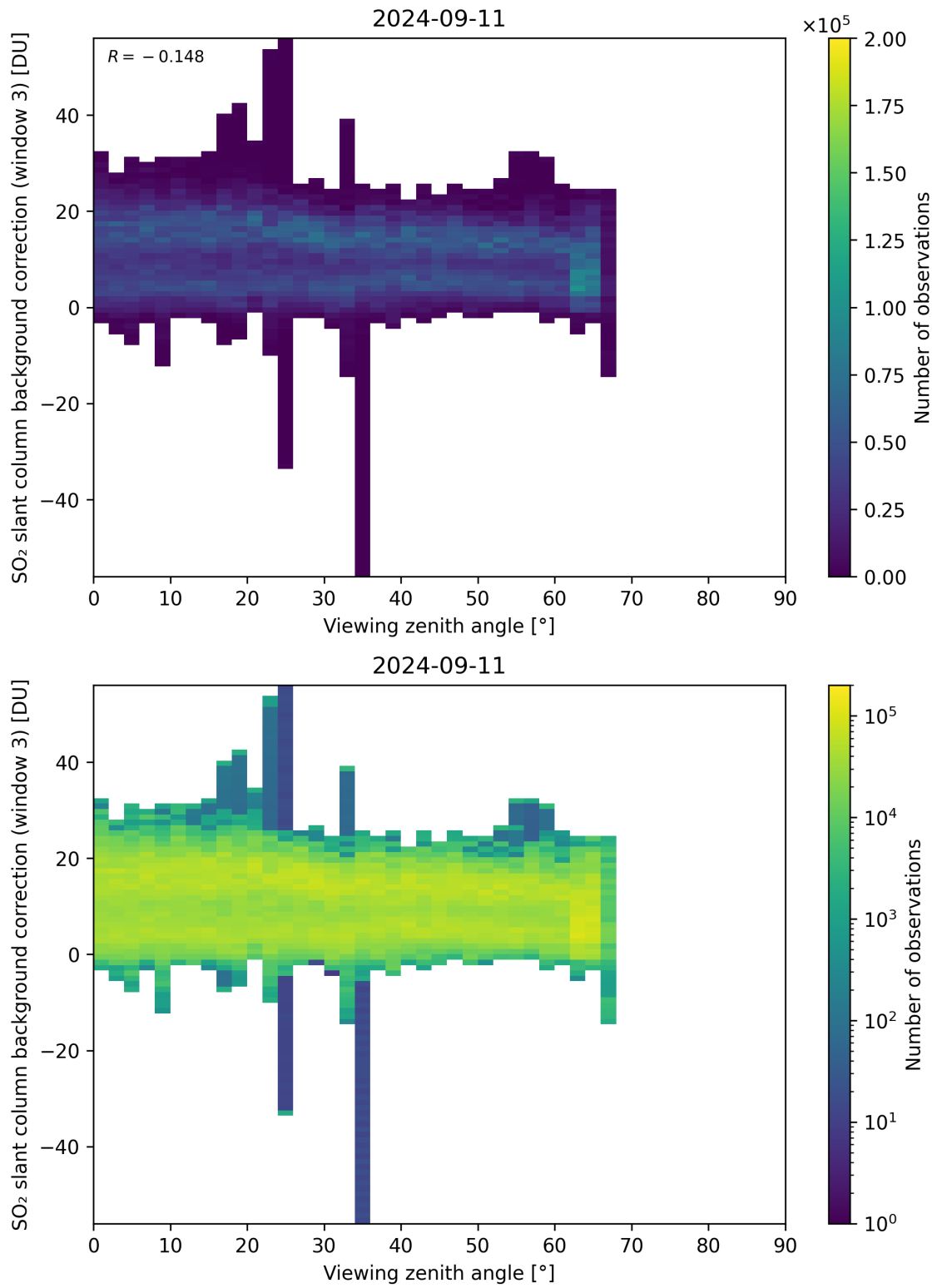
Figure 310: Scatter density plot of “Viewing zenith angle” against “SO 2 slant column background correction (window 3)” for 2024-09-10 to 2024-09-12.
