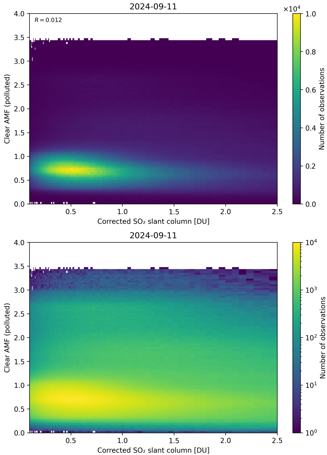
Figure 184: Scatter density plot of “Corrected SO 2 slant column” against “Clear AMF (polluted)” for 2024-09-10 to 2024-09-12.
