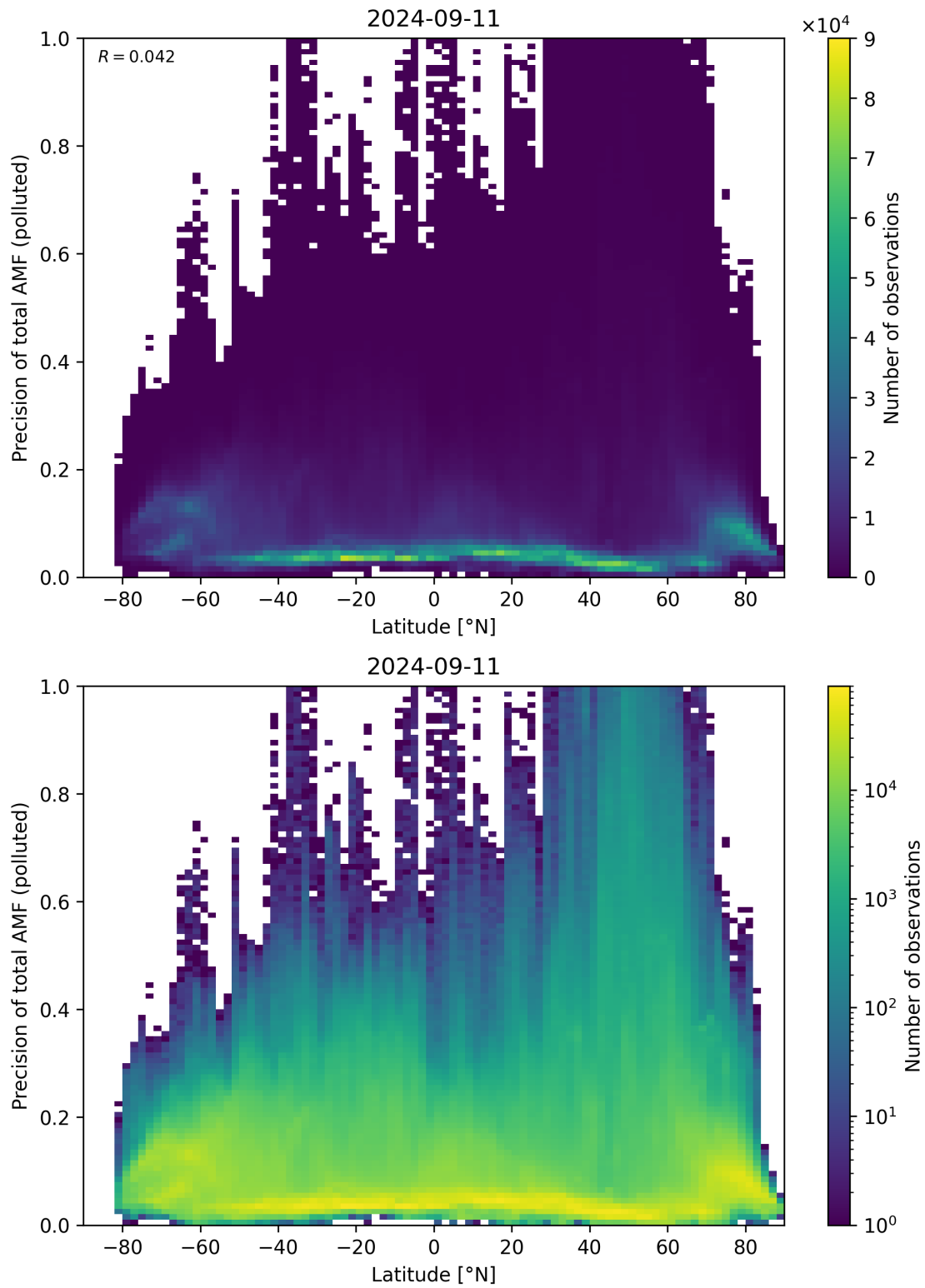
Figure 155: Scatter density plot of “Latitude” against “Precision of total AMF (polluted)” for 2024-09-10 to 2024-09-12.
