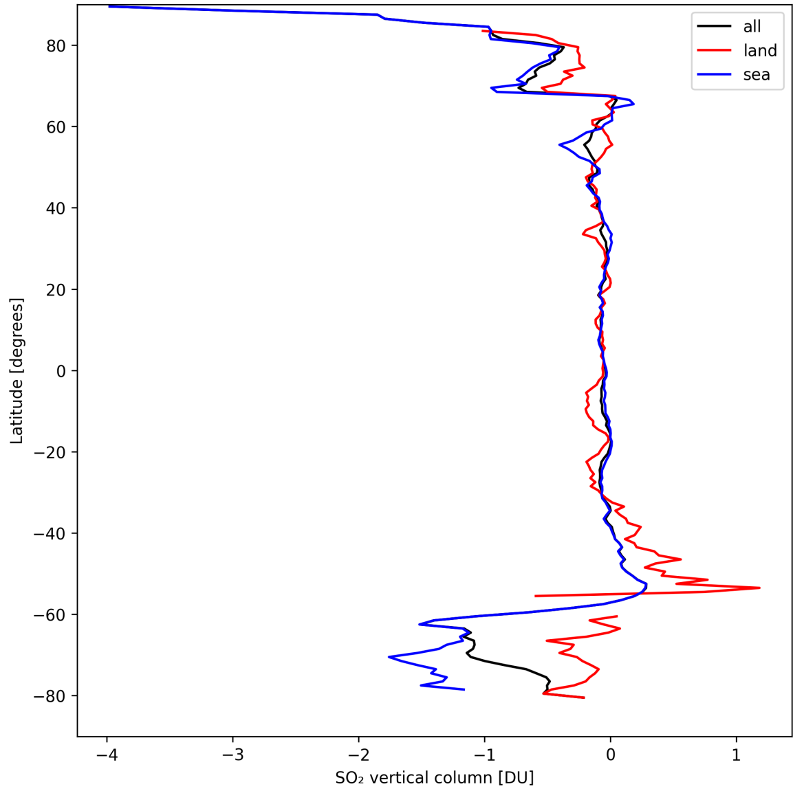
Figure 30: Zonal average of “SO 2 vertical column” for 2024-09-10 to 2024-09-12.
