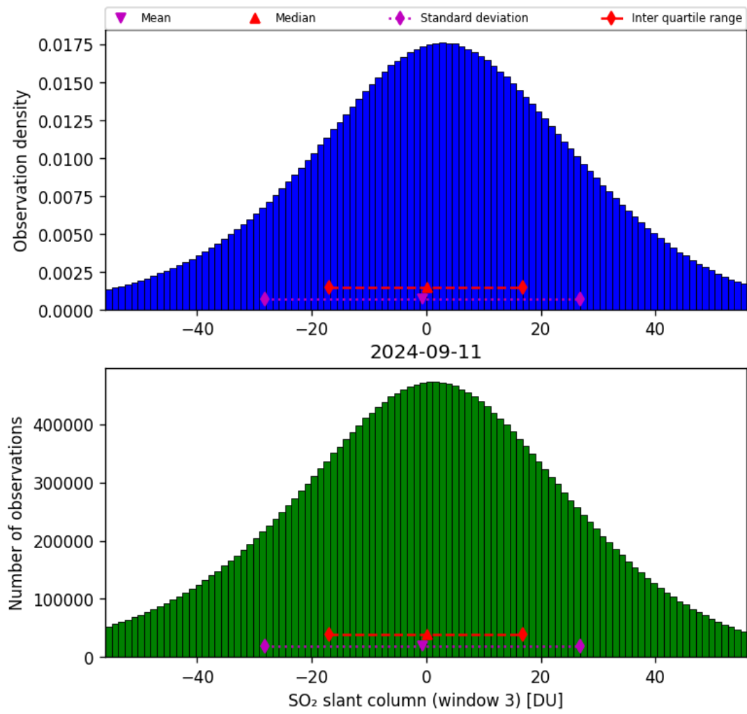
Figure 64: Histogram of “SO 2 slant column (window 3)” for 2024-09-10 to 2024-09-12
