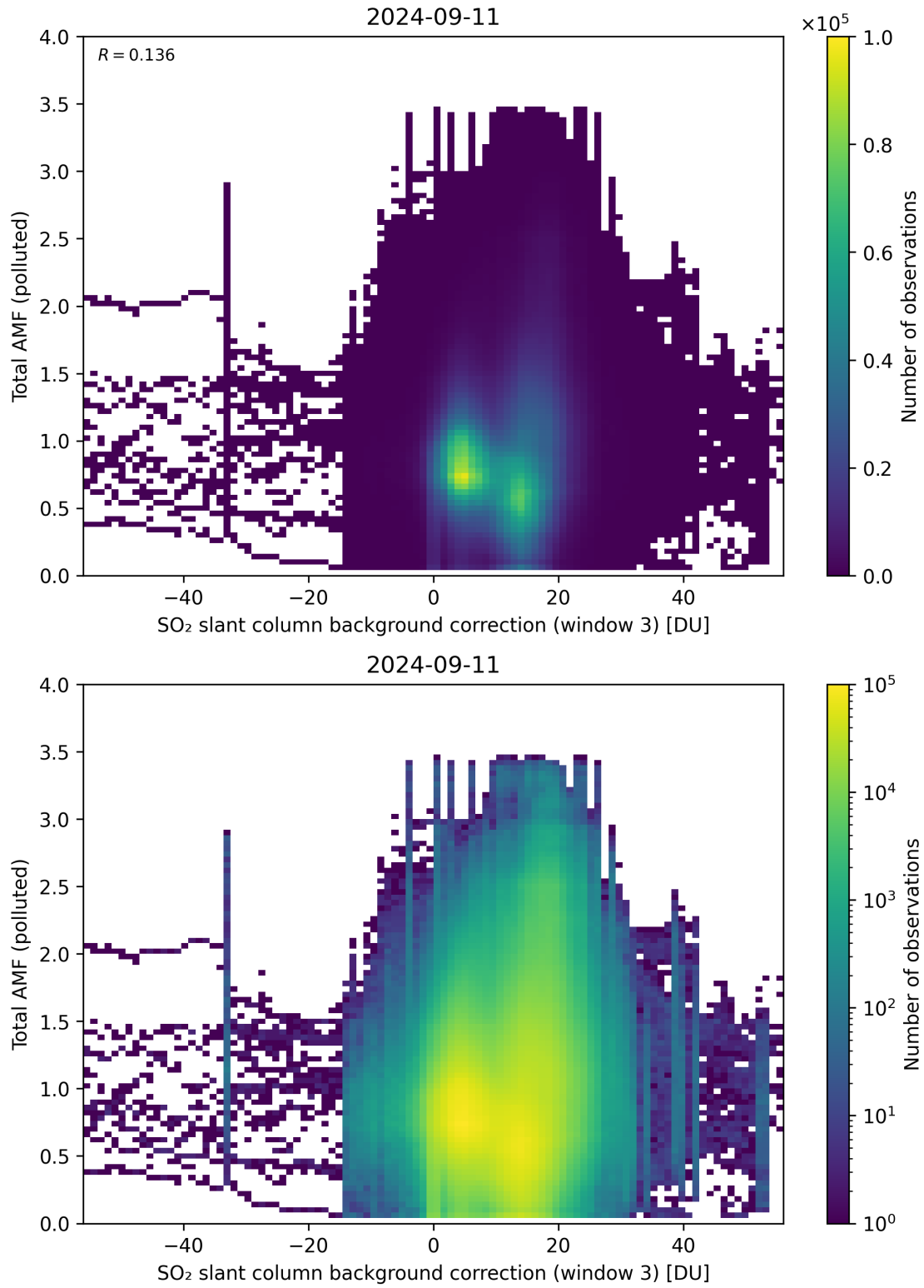
Figure 125: Scatter density plot of “SO 2 slant column background correction (window 3)” against “Total AMF (polluted)” for 2024-09-10 to 2024-09-12.
