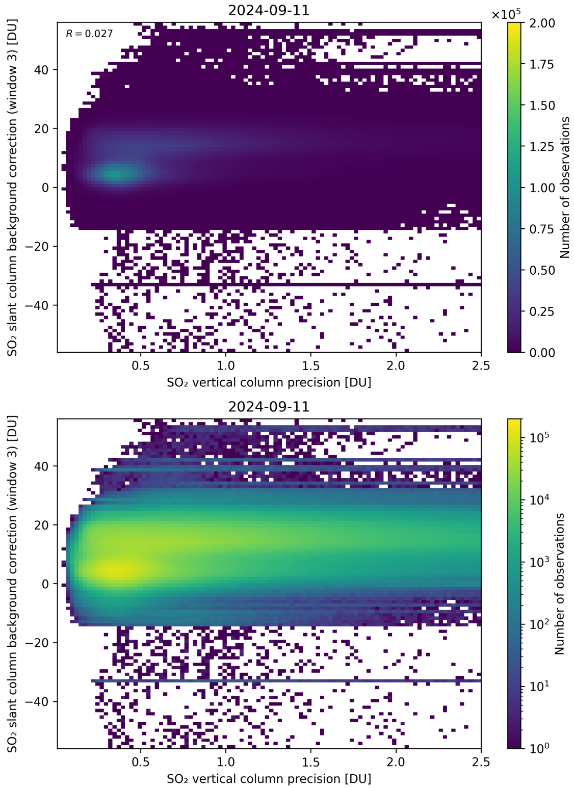
Figure 281: Scatter density plot of “SO 2 vertical column precision” against “SO 2 slant column background correction (window 3)” for 2024-09-10 to 2024-09-12.
