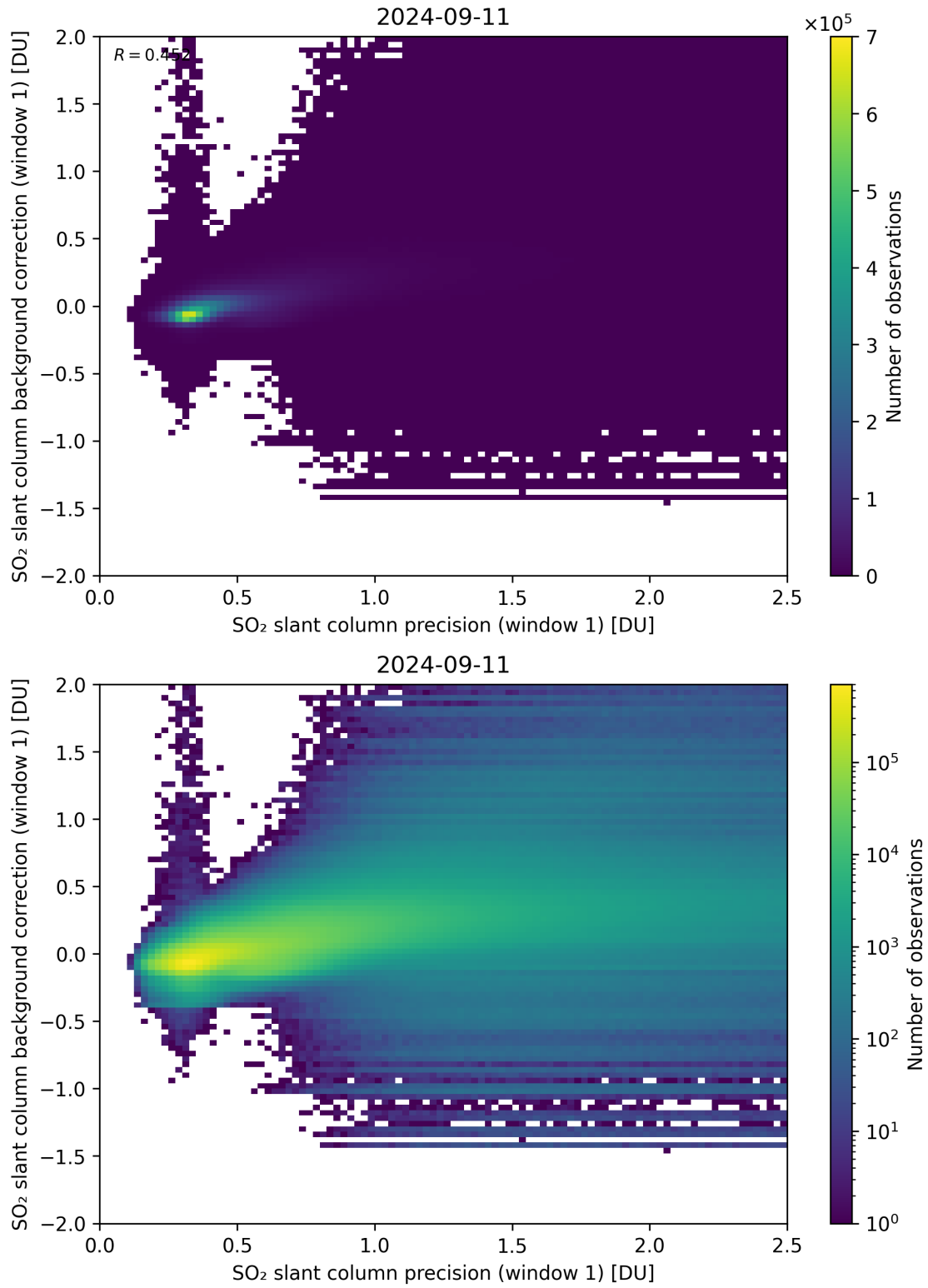
Figure 218: Scatter density plot of “SO 2 slant column precision (window 1)” against “SO 2 slant column background correction (window 1)” for 2024-09-10 to 2024-09-12.
