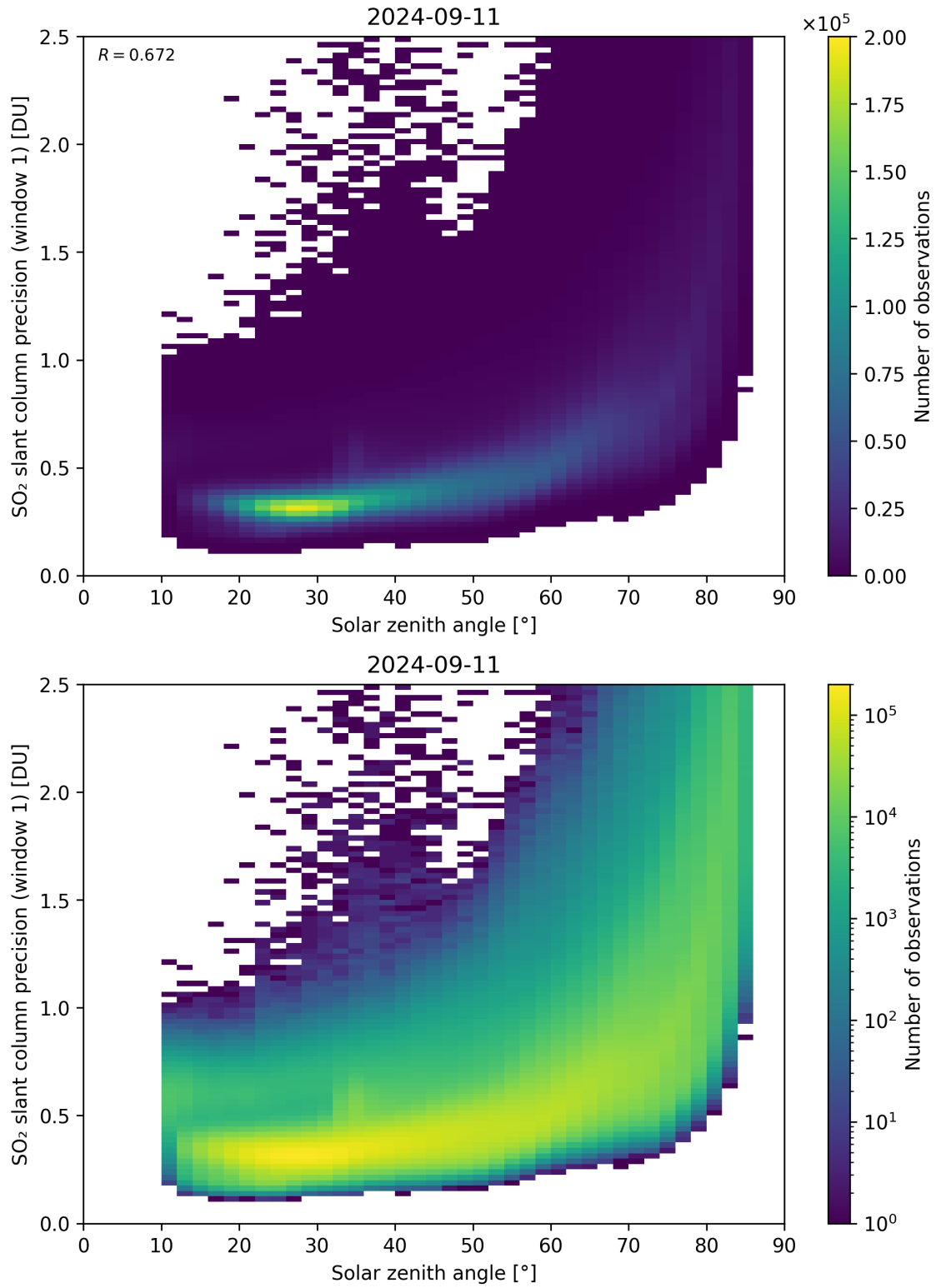
Figure 170: Scatter density plot of “Solar zenith angle” against “SO 2 slant column precision (window 1)” for 2024-09-10 to 2024-09-12.
