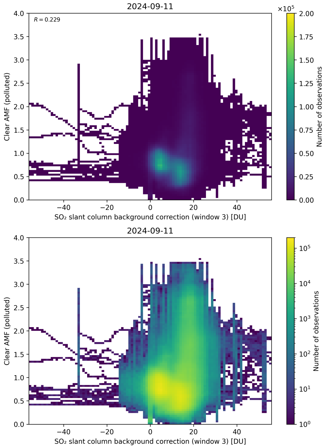
Figure 124: Scatter density plot of “SO 2 slant column background correction (window 3)” against “Clear AMF (polluted)” for 2024-09-10 to 2024-09-12.
