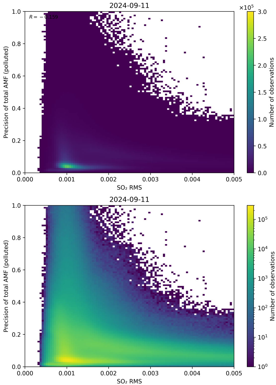
Figure 138: Scatter density plot of “SO 2 RMS” against “Precision of total AMF (polluted)” for 2024-09-10 to 2024-09-12.
