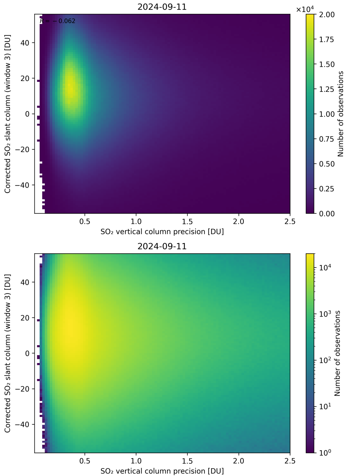
Figure 288: Scatter density plot of “SO 2 vertical column precision” against “Corrected SO 2 slant column (window 3)” for 2024-09-10 to 2024-09-12.
