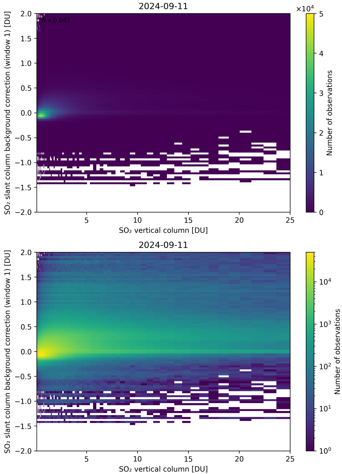
Figure 273: Scatter density plot of “SO 2 vertical column” against “SO 2 slant column background correction (window 1)” for 2024-09-10 to 2024-09-12.
