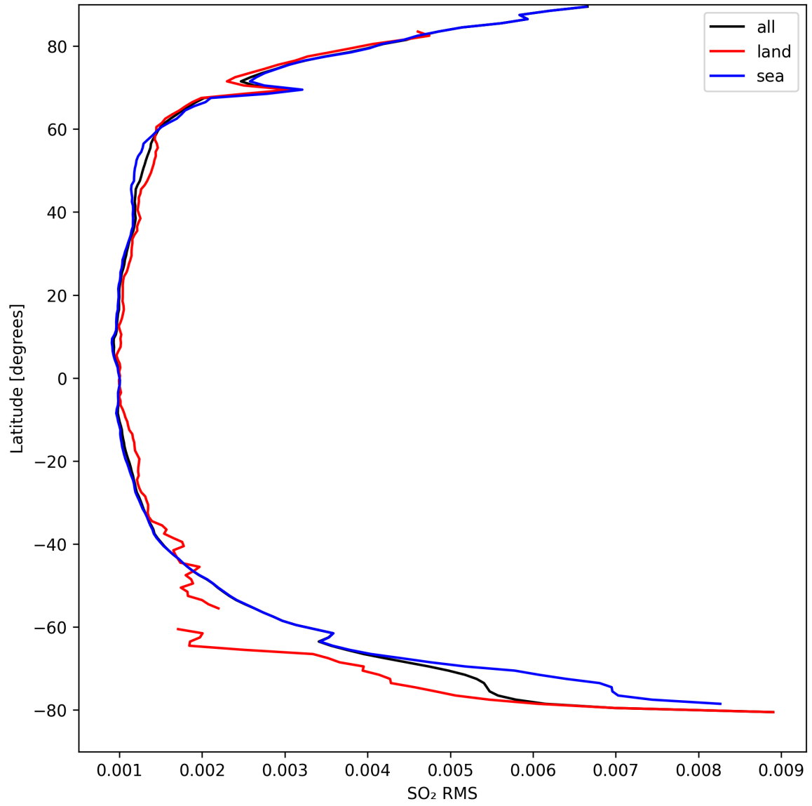
Figure 47: Zonal average of “SO 2 RMS” for 2024-09-10 to 2024-09-12.
