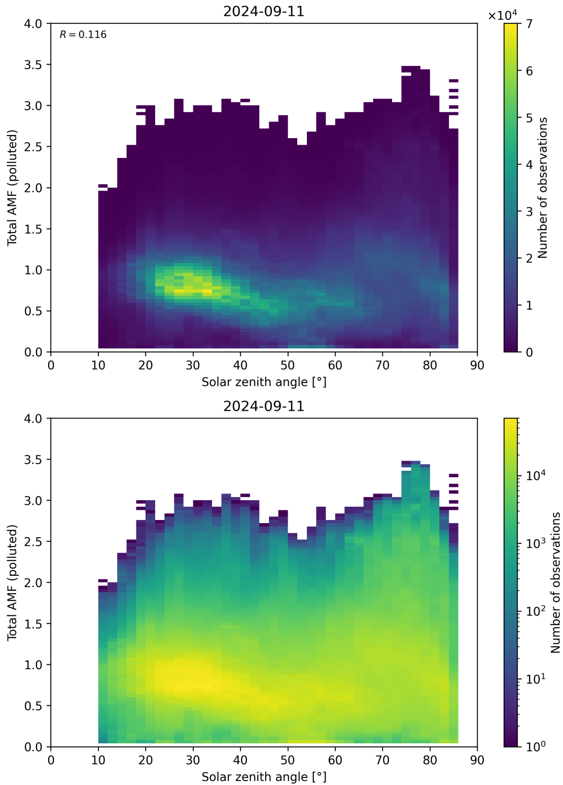
Figure 174: Scatter density plot of “Solar zenith angle” against “Total AMF (polluted)” for 2024-09-10 to 2024-09-12.
