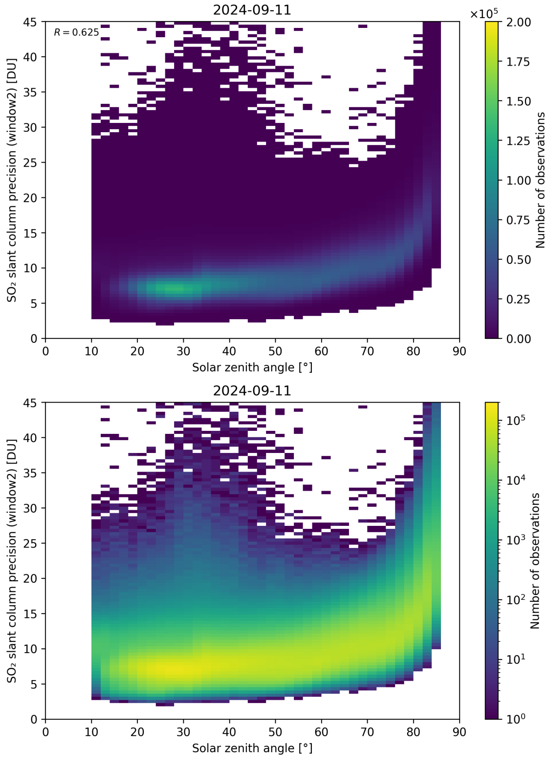
Figure 171: Scatter density plot of “Solar zenith angle” against “SO 2 slant column precision (window2)” for 2024-09-10 to 2024-09-12.
