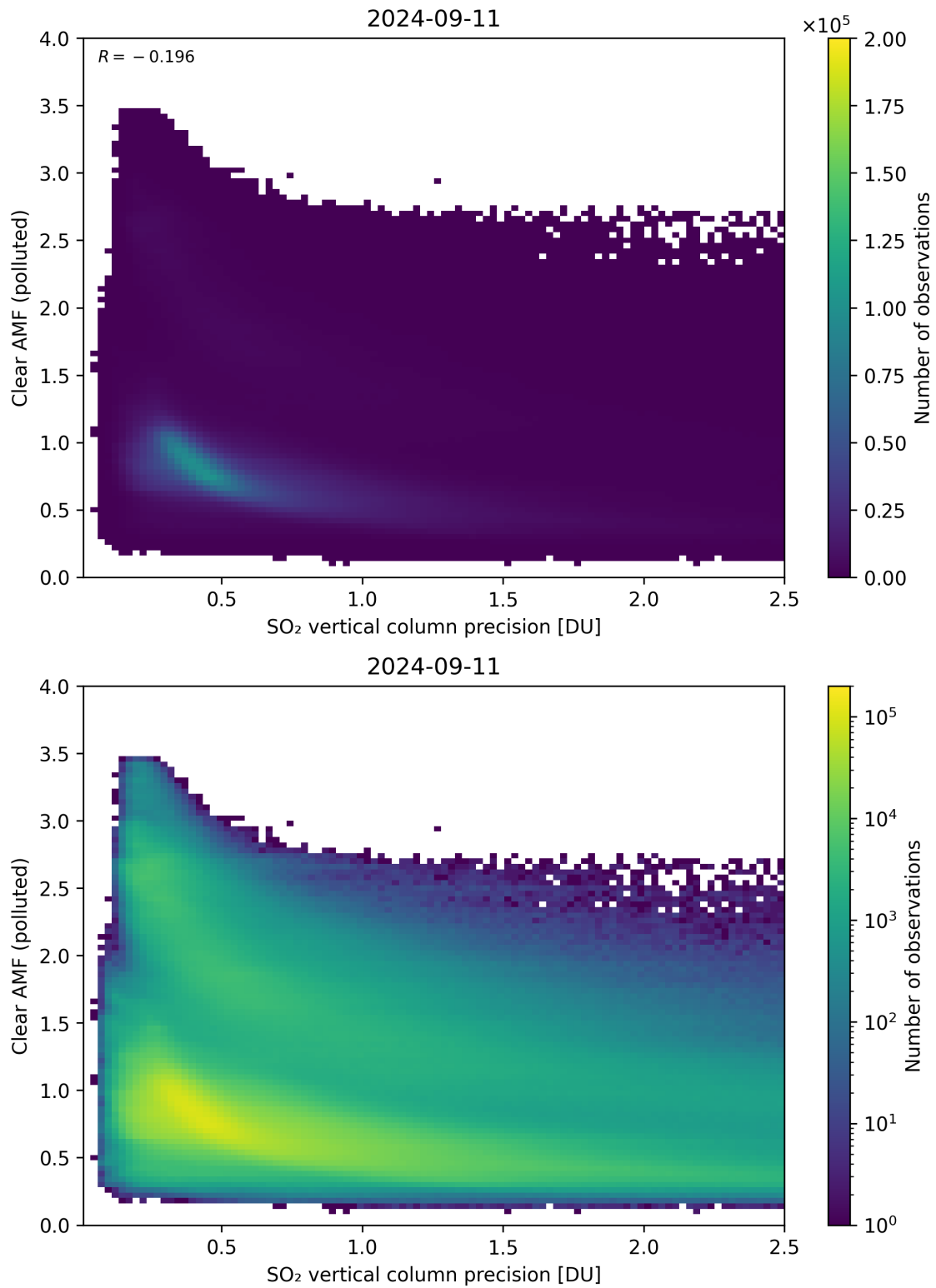
Figure 285: Scatter density plot of “SO 2 vertical column precision” against “Clear AMF (polluted)” for 2024-09-10 to 2024-09-12.
