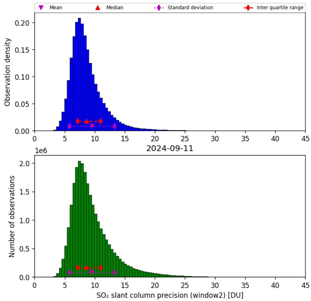
Figure 61: Histogram of “SO 2 slant column precision (window2)” for 2024-09-10 to 2024-09-12
