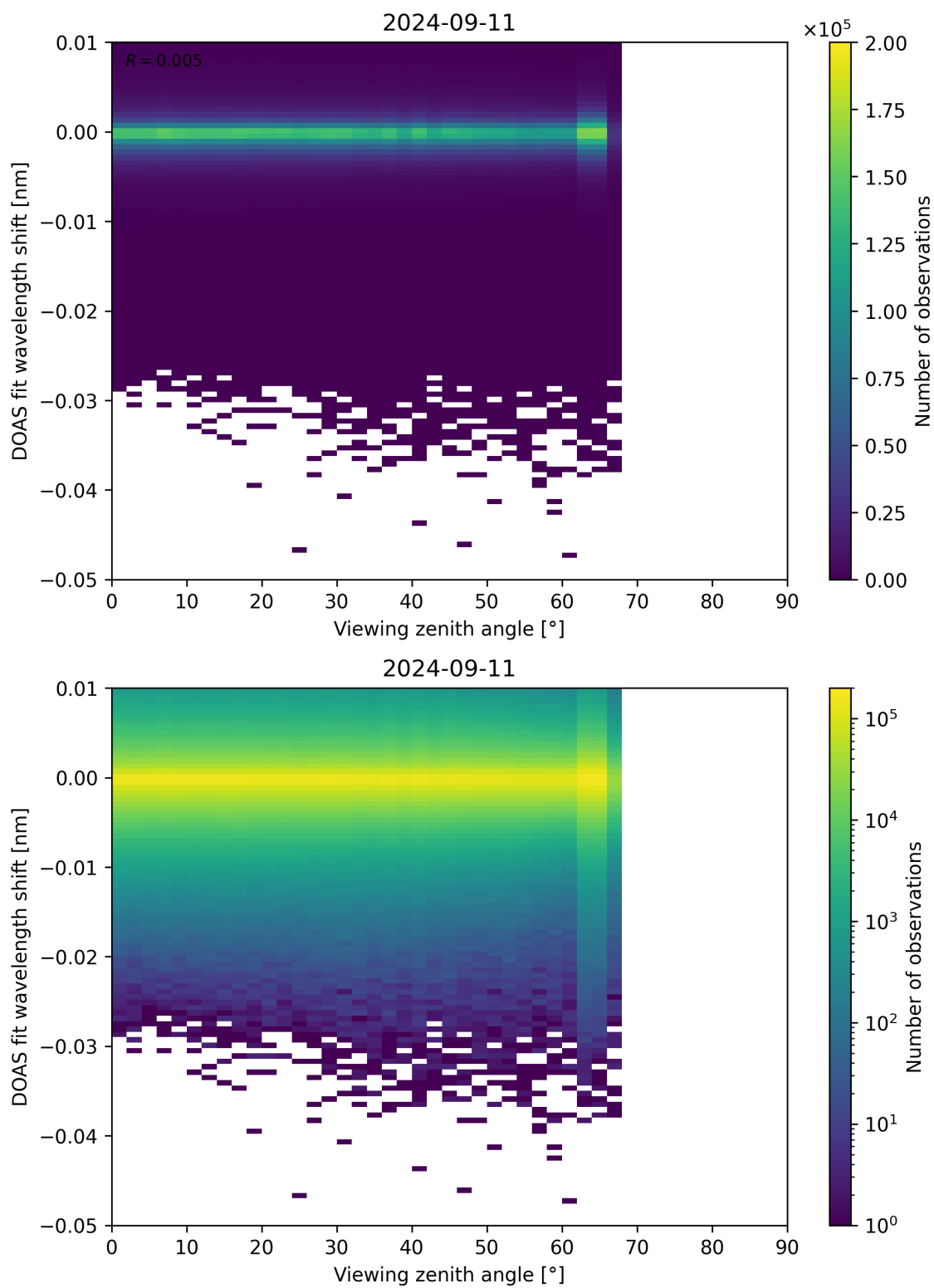
Figure 311: Scatter density plot of “Viewing zenith angle” against “DOAS fit wavelength shift” for 2024-09-10 to 2024-09-12.
