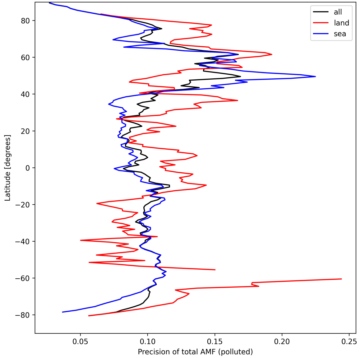
Figure 49: Zonal average of “Precision of total AMF (polluted)” for 2024-09-10 to 2024-09-12.
