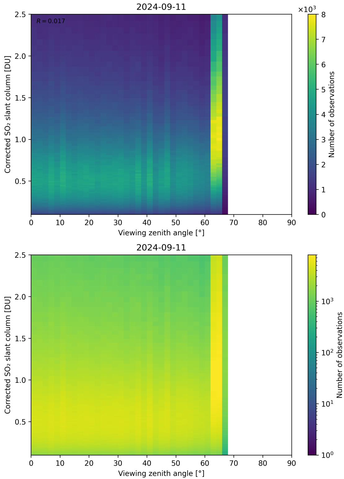
Figure 317: Scatter density plot of “Viewing zenith angle” against “Corrected SO 2 slant column” for 2024-09-10 to 2024-09-12.
