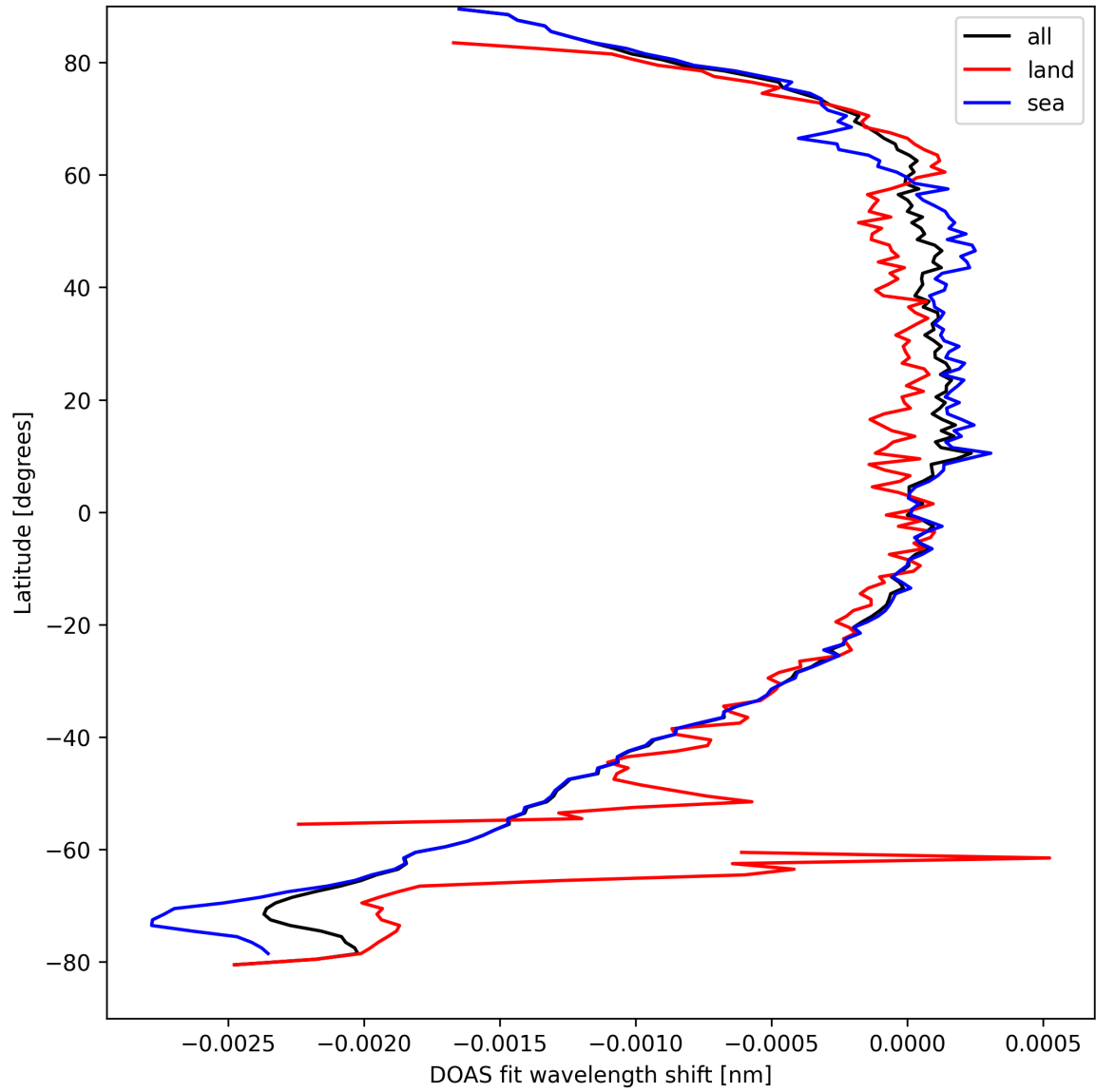
Figure 45: Zonal average of “DOAS fit wavelength shift” for 2024-09-10 to 2024-09-12.
