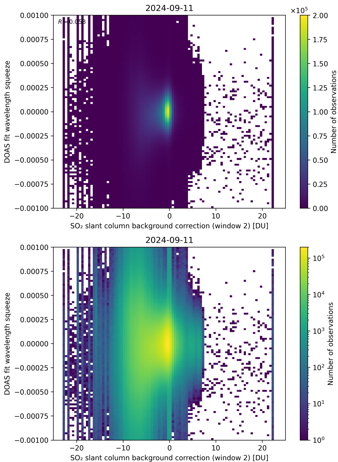
Figure 113: Scatter density plot of “SO 2 slant column background correction (window 2)” against “DOAS fit wavelength squeeze” for 2024-09-10 to 2024-09-12.
