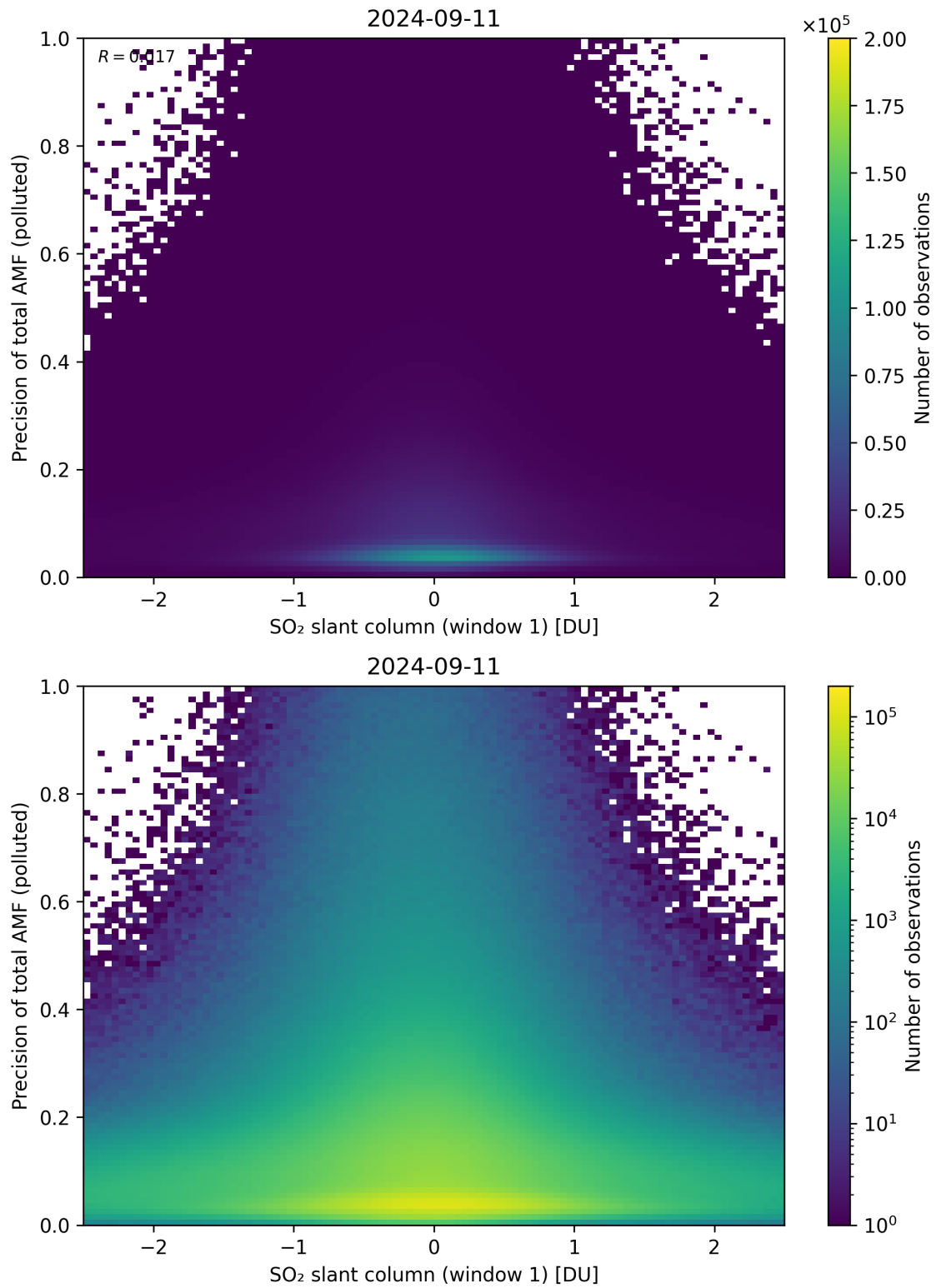
Figure 240: Scatter density plot of “SO 2 slant column (window 1)” against “Precision of total AMF (polluted)” for 2024-09-10 to 2024-09-12.
