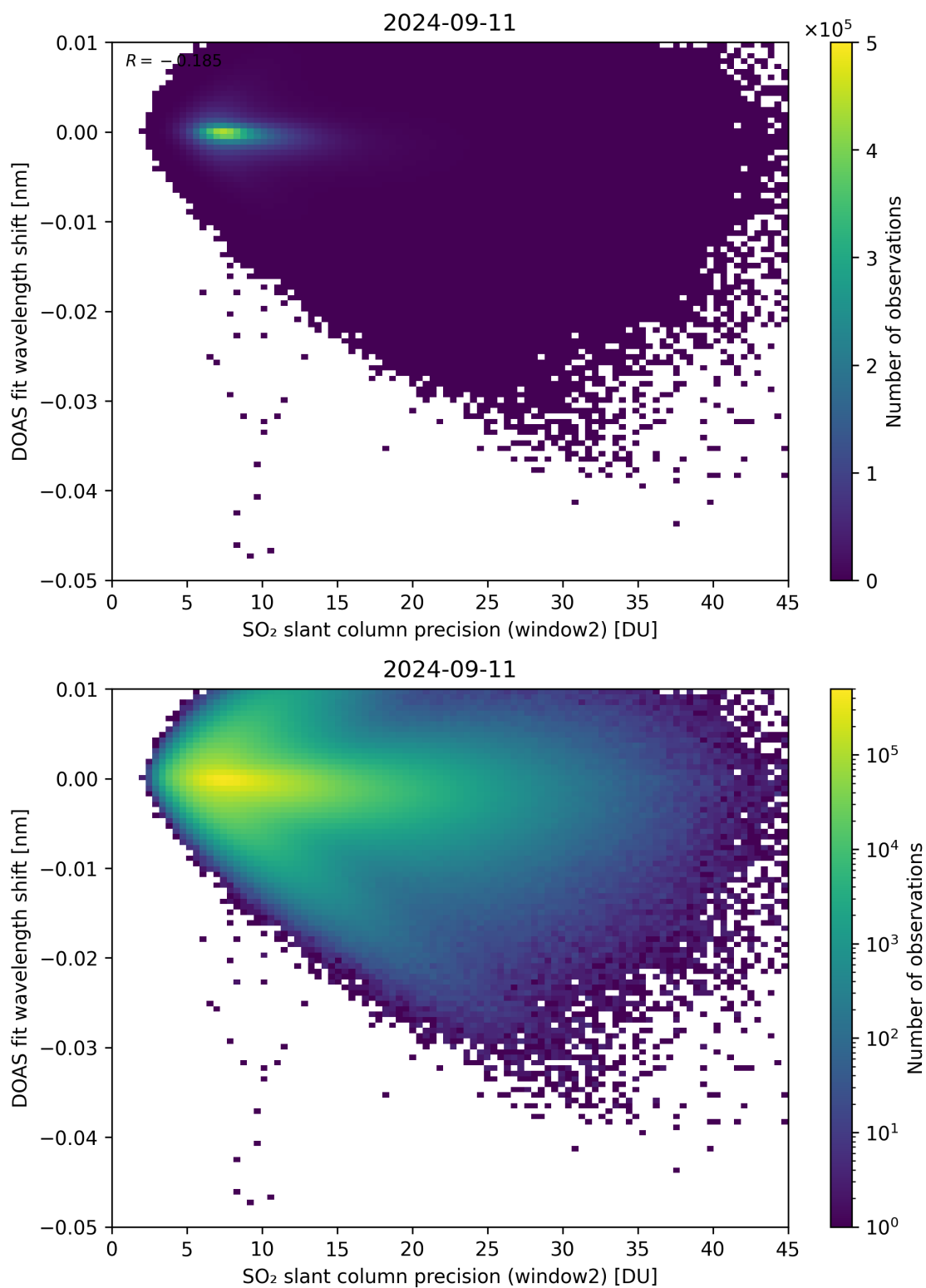
Figure 243: Scatter density plot of “SO 2 slant column precision (window2)” against “DOAS fit wavelength shift” for 2024-09-10 to 2024-09-12.
