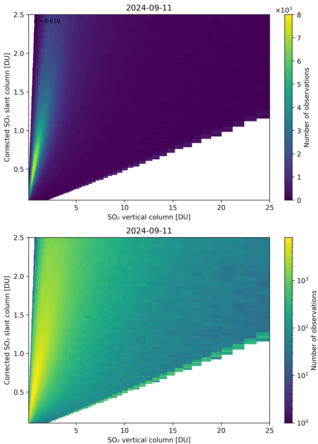
Figure 297: Scatter density plot of “SO 2 vertical column” against “Corrected SO 2 slant column” for 2024-09-10 to 2024-09-12.
