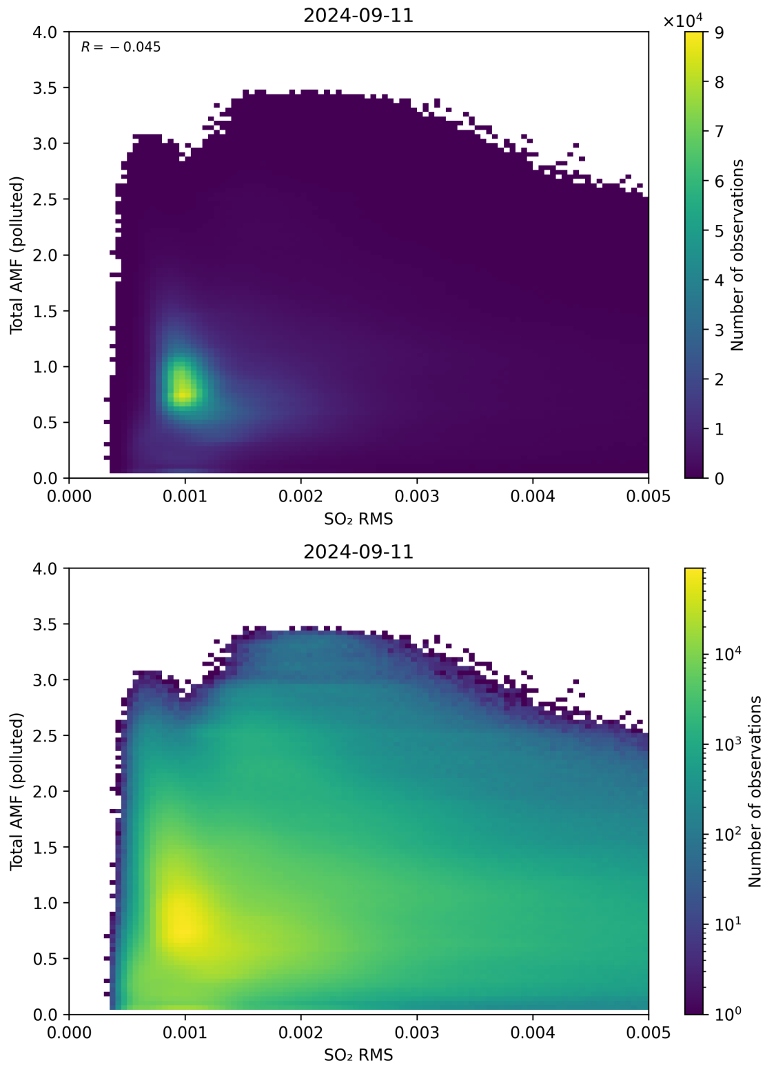
Figure 137: Scatter density plot of “SO 2 RMS” against “Total AMF (polluted)” for 2024-09-10 to 2024-09-12.
