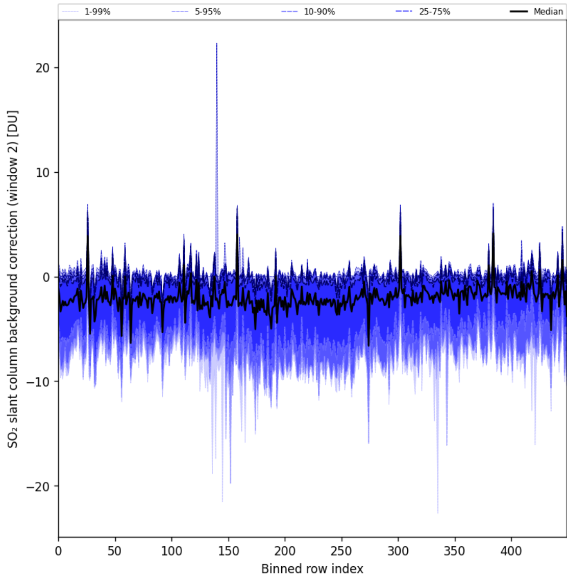
Figure 86: Along track statistics of “SO 2 slant column background correction (window 2)” for 2024-09-10 to 2024-09-12
