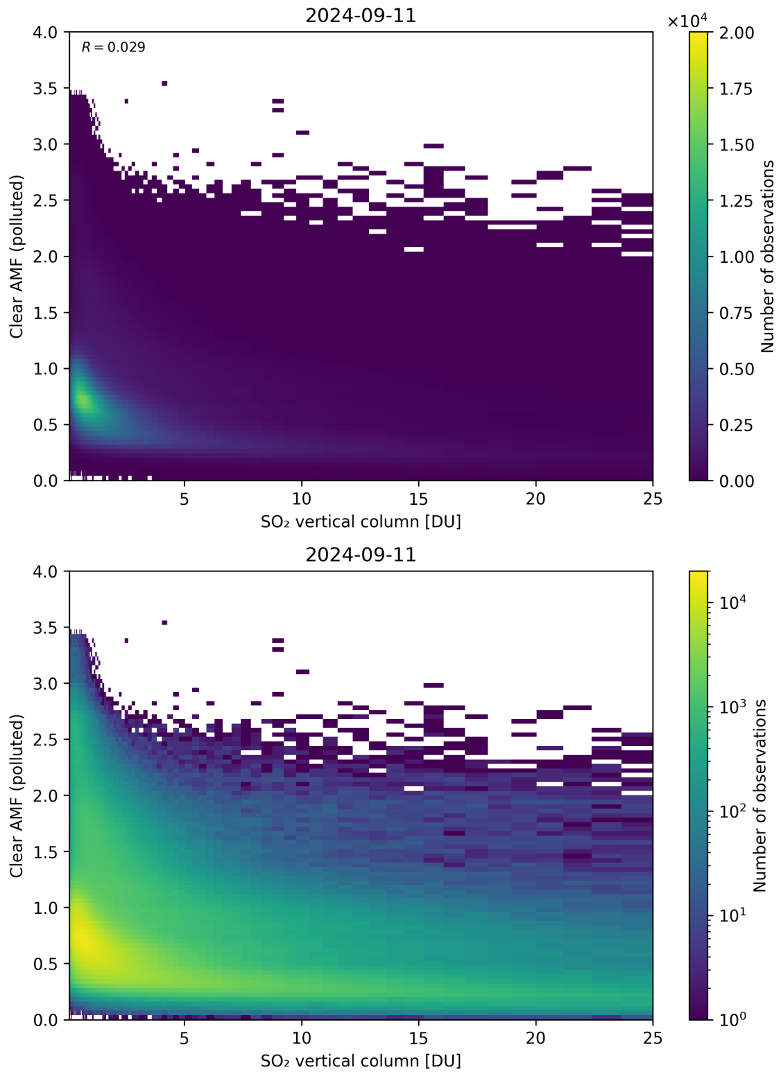
Figure 296: Scatter density plot of “SO 2 vertical column” against “Clear AMF (polluted)” for 2024-09-10 to 2024-09-12.
