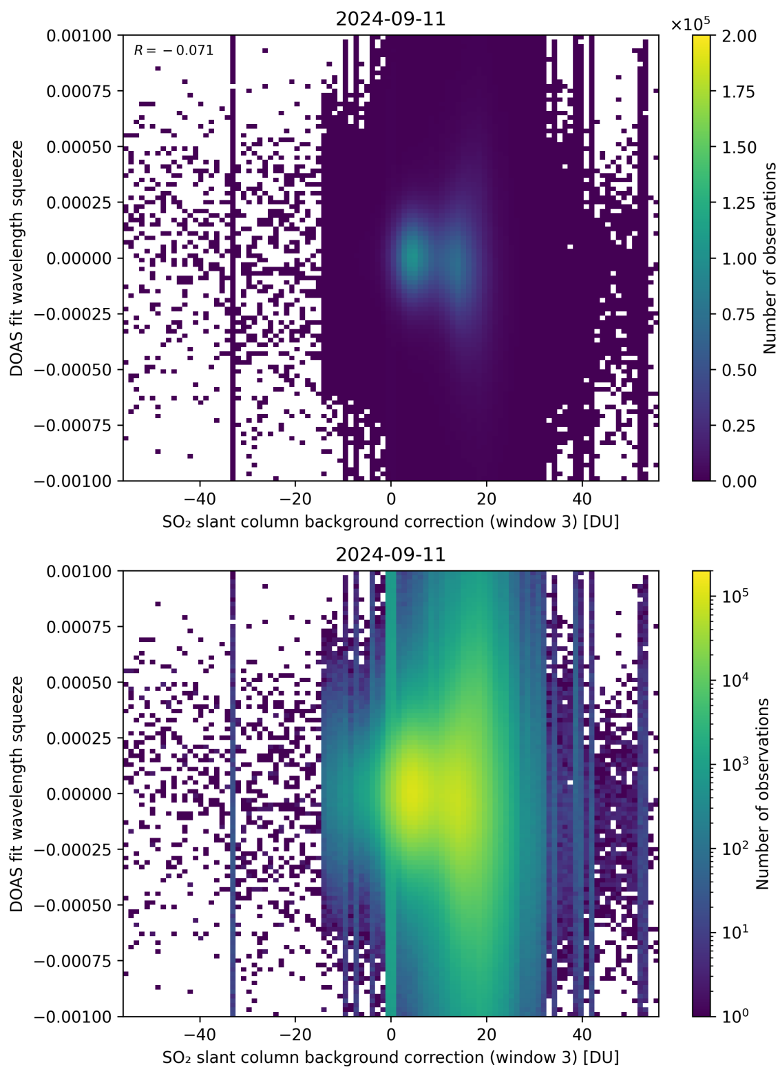
Figure 122: Scatter density plot of “SO 2 slant column background correction (window 3)” against “DOAS fit wavelength squeeze” for 2024-09-10 to 2024-09-12.
