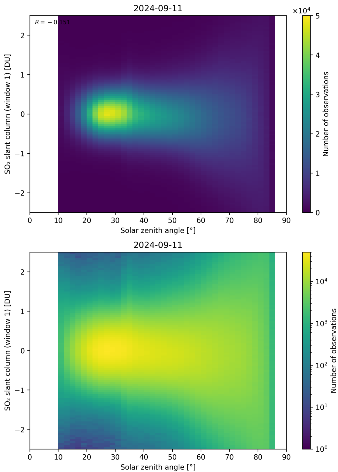
Figure 169: Scatter density plot of “Solar zenith angle” against “SO 2 slant column (window 1)” for 2024-09-10 to 2024-09-12.
