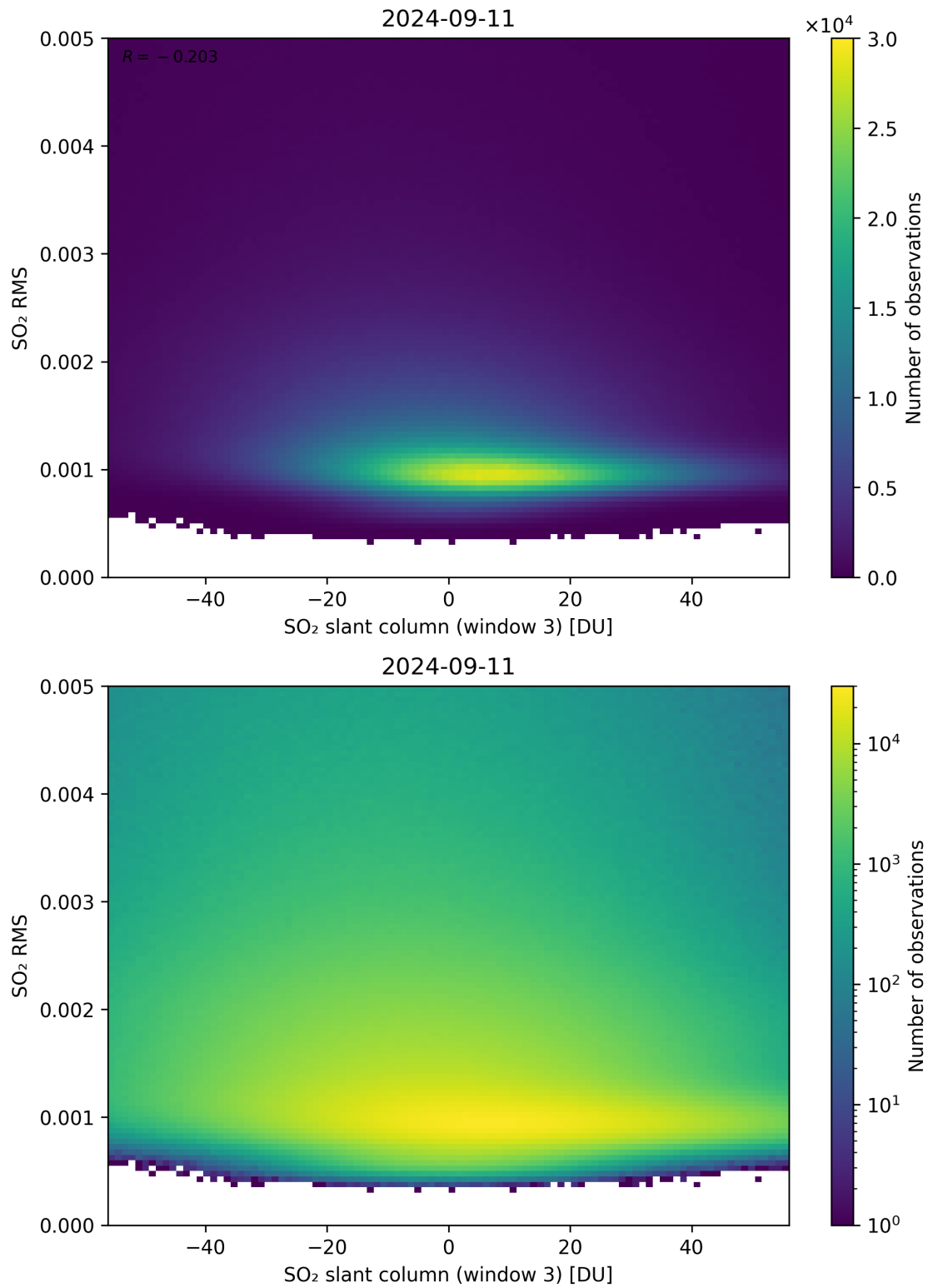
Figure 256: Scatter density plot of “SO 2 slant column (window 3)” against “SO 2 RMS” for 2024-09-10 to 2024-09-12.
