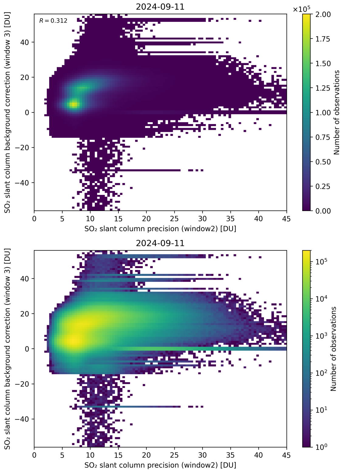
Figure 242: Scatter density plot of “SO 2 slant column precision (window2)” against “SO 2 slant column background correction (window 3)” for 2024-09-10 to 2024-09-12.
