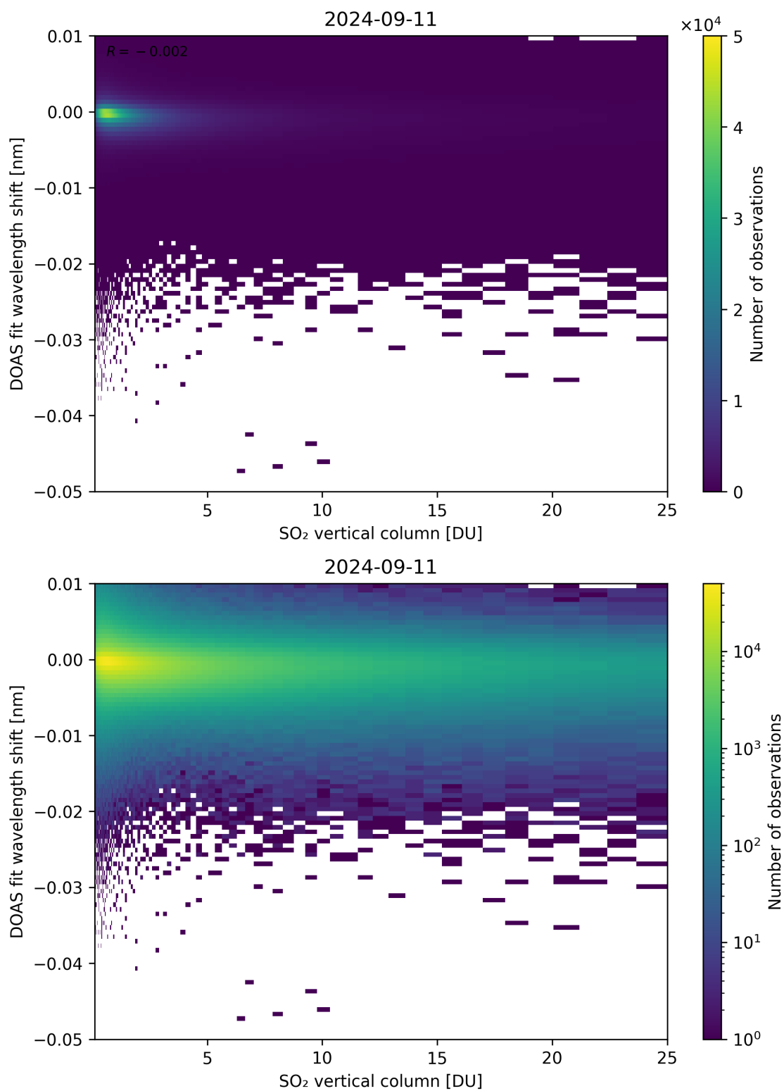
Figure 276: Scatter density plot of “SO 2 vertical column” against “DOAS fit wavelength shift” for 2024-09-10 to 2024-09-12.
