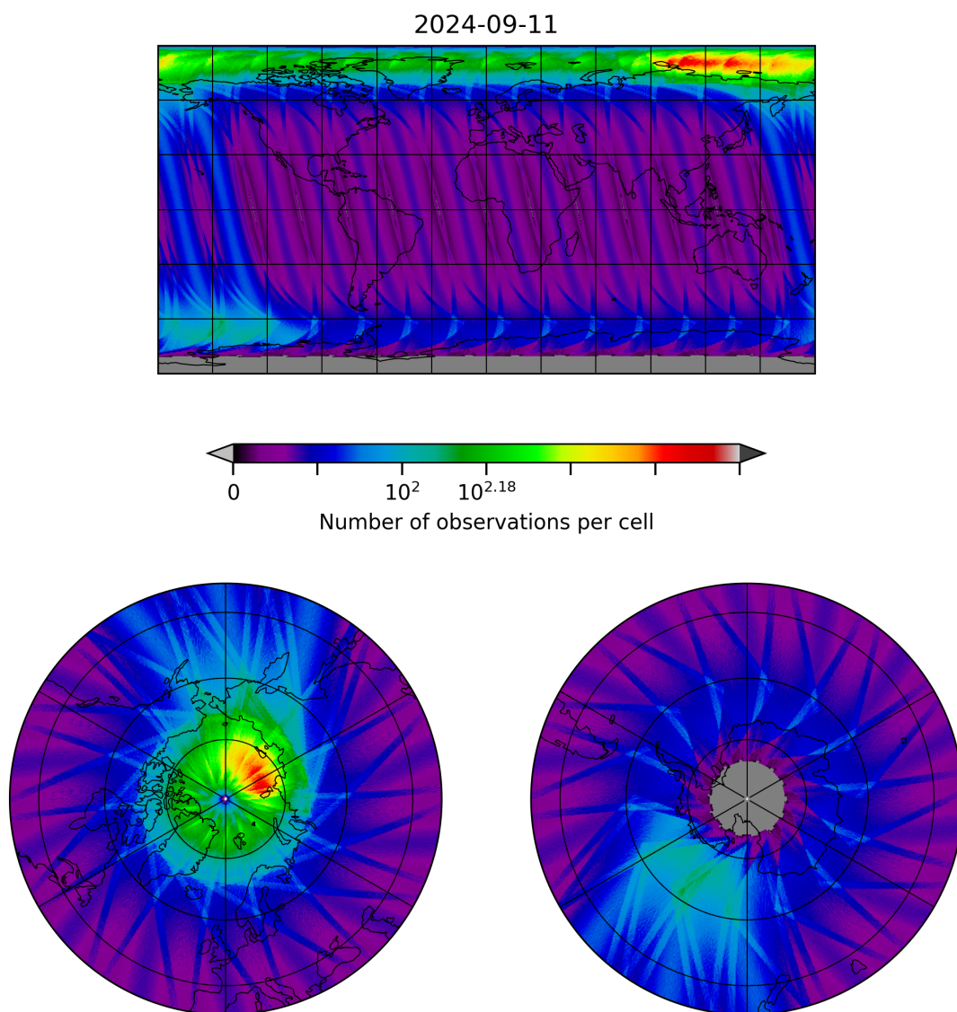
Figure 28: Map of the number of observations for 2024-09-10 to 2024-09-12
