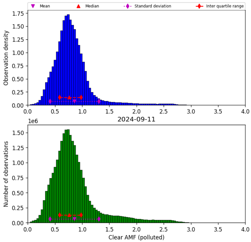
Figure 73: Histogram of “Clear AMF (polluted)” for 2024-09-10 to 2024-09-12
