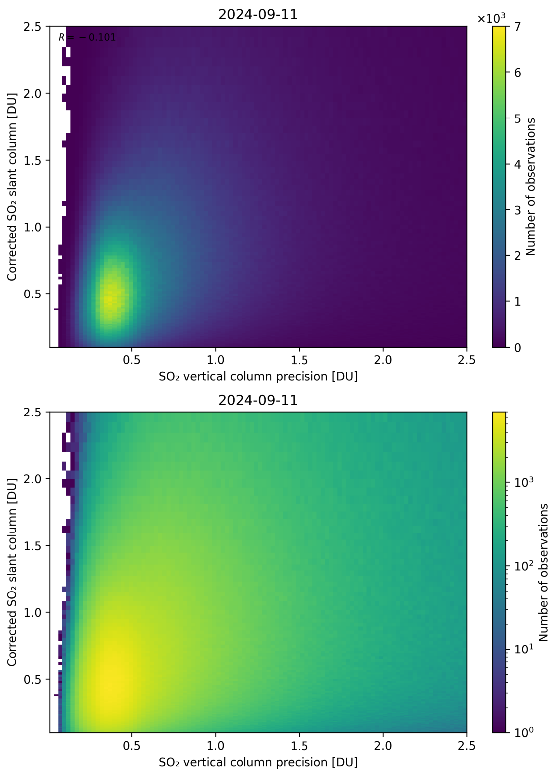
Figure 286: Scatter density plot of “SO 2 vertical column precision” against “Corrected SO 2 slant column” for 2024-09-10 to 2024-09-12.
