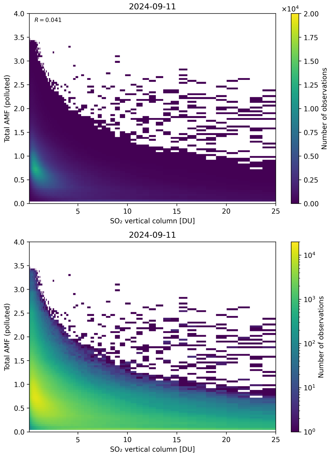
Figure 305: Scatter density plot of “SO 2 vertical column” against “Total AMF (polluted)” for 2024-09-10 to 2024-09-12.
