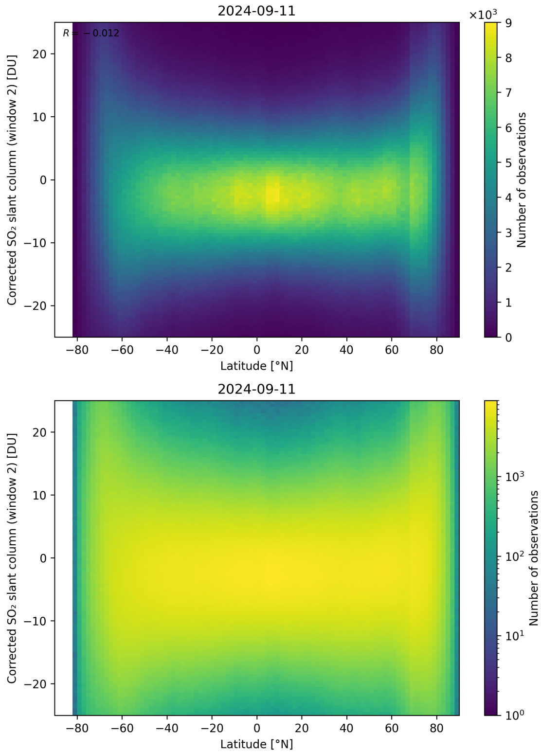
Figure 147: Scatter density plot of “Latitude” against “Corrected SO 2 slant column (window 2)” for 2024-09-10 to 2024-09-12.
