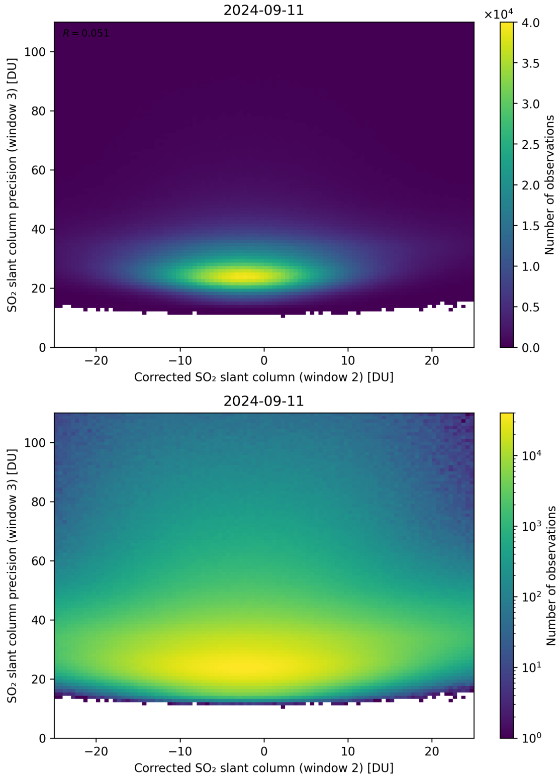
Figure 202: Scatter density plot of “Corrected SO 2 slant column (window 2)” against “SO 2 slant column precision (window 3)” for 2024-09-10 to 2024-09-12.
