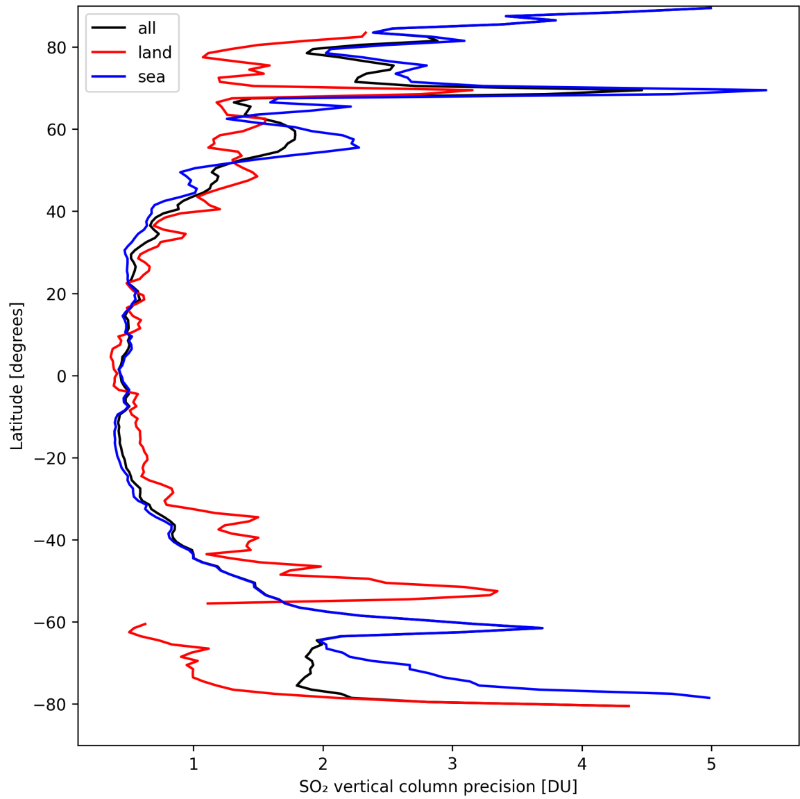
Figure 31: Zonal average of “SO 2 vertical column precision” for 2024-09-10 to 2024-09-12.
