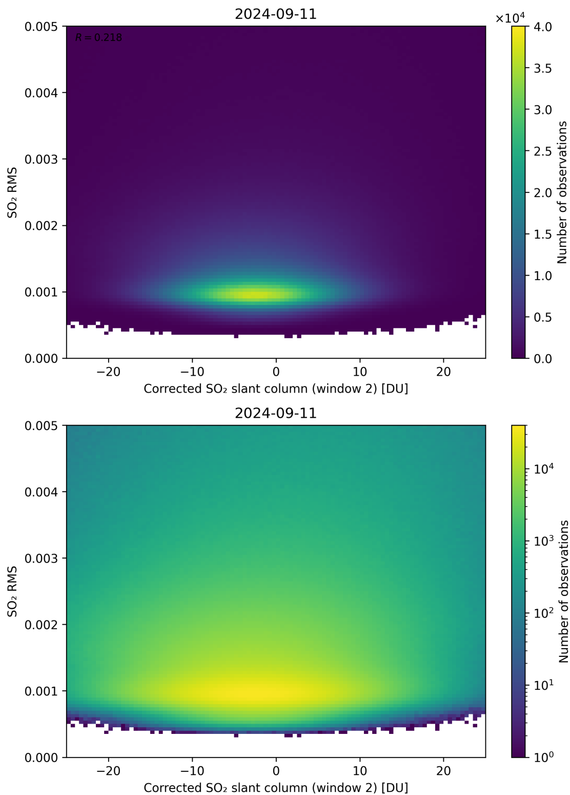
Figure 198: Scatter density plot of “Corrected SO 2 slant column (window 2)” against “SO 2 RMS” for 2024-09-10 to 2024-09-12.
