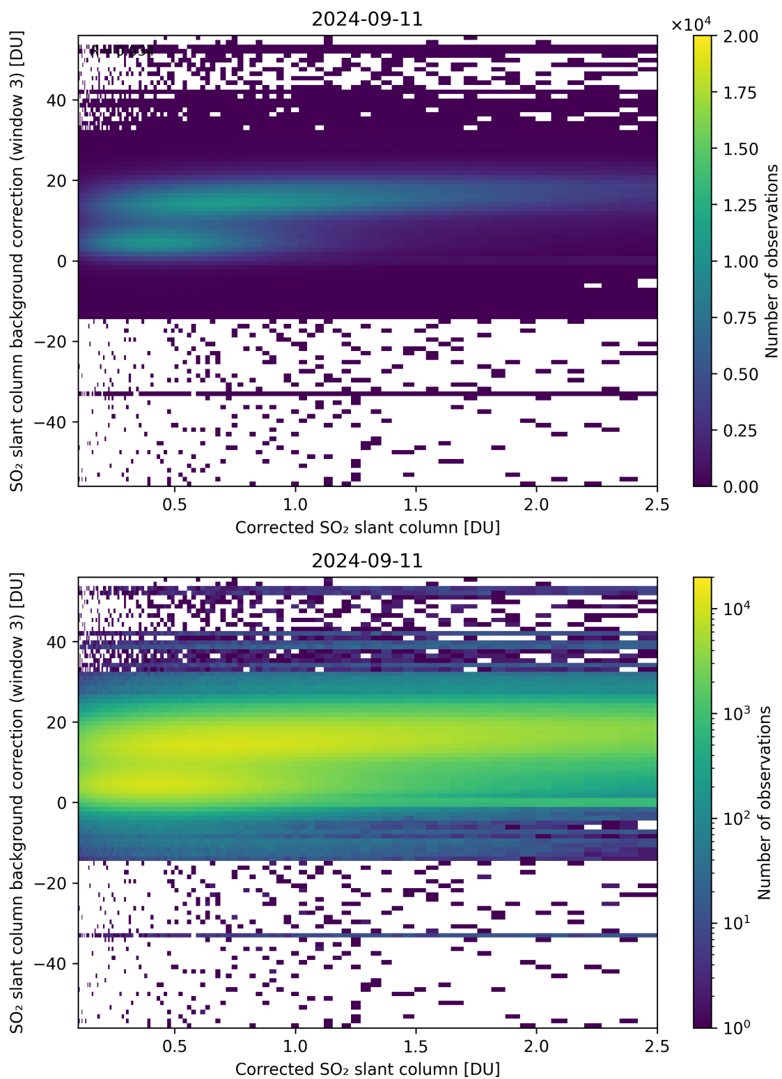
Figure 180: Scatter density plot of “Corrected SO 2 slant column” against “SO 2 slant column background correction (window 3)” for 2024-09-10 to 2024-09-12.
