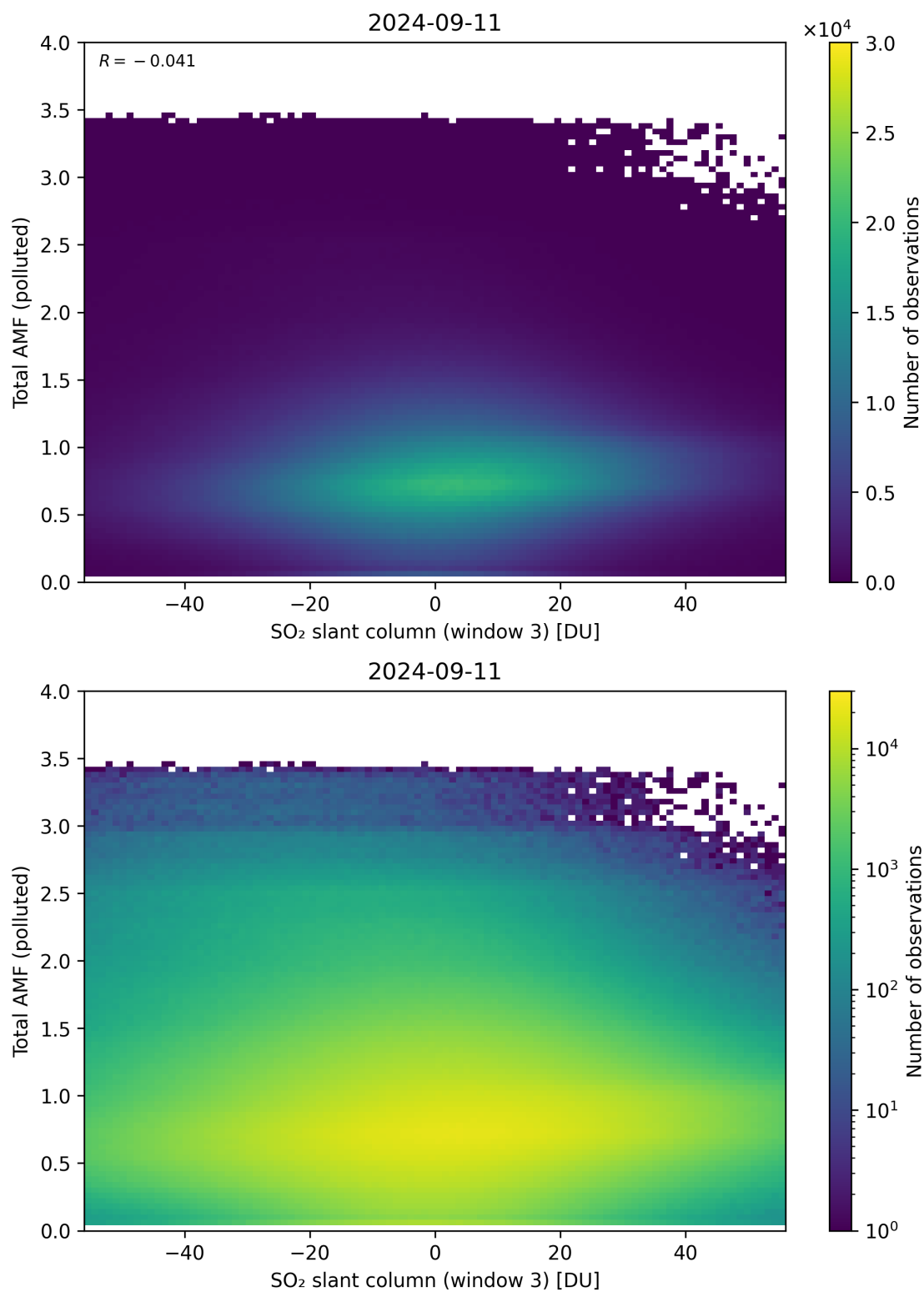
Figure 268: Scatter density plot of “SO 2 slant column (window 3)” against “Total AMF (polluted)” for 2024-09-10 to 2024-09-12.
