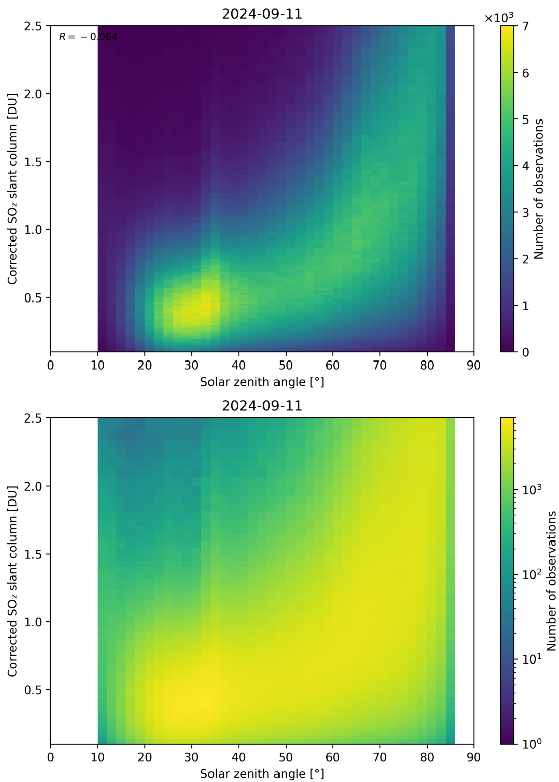
Figure 166: Scatter density plot of “Solar zenith angle” against “Corrected SO 2 slant column” for 2024-09-10 to 2024-09-12.
