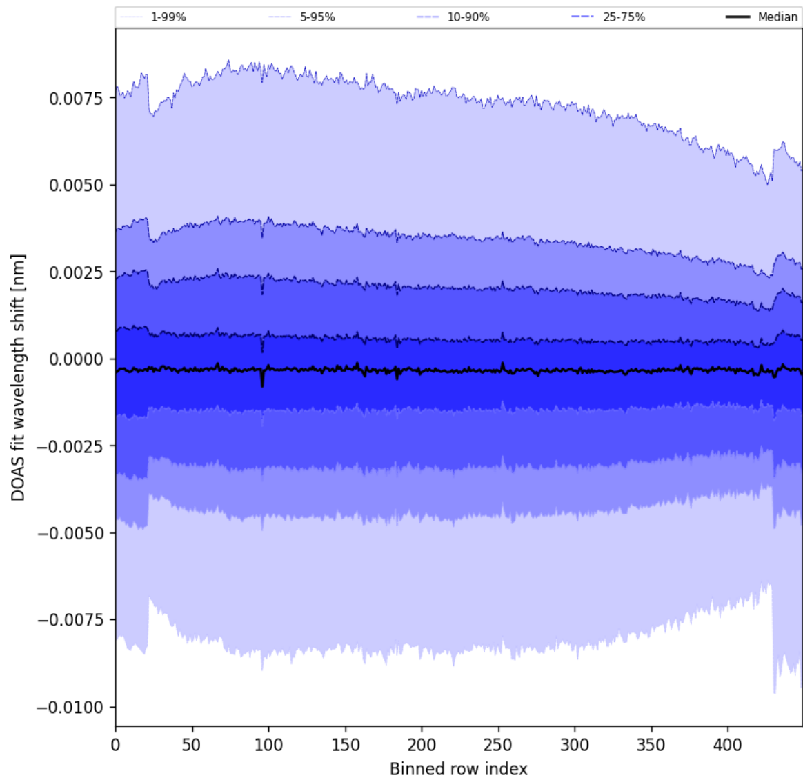
Figure 91: Along track statistics of “DOAS fit wavelength shift” for 2024-09-10 to 2024-09-12
