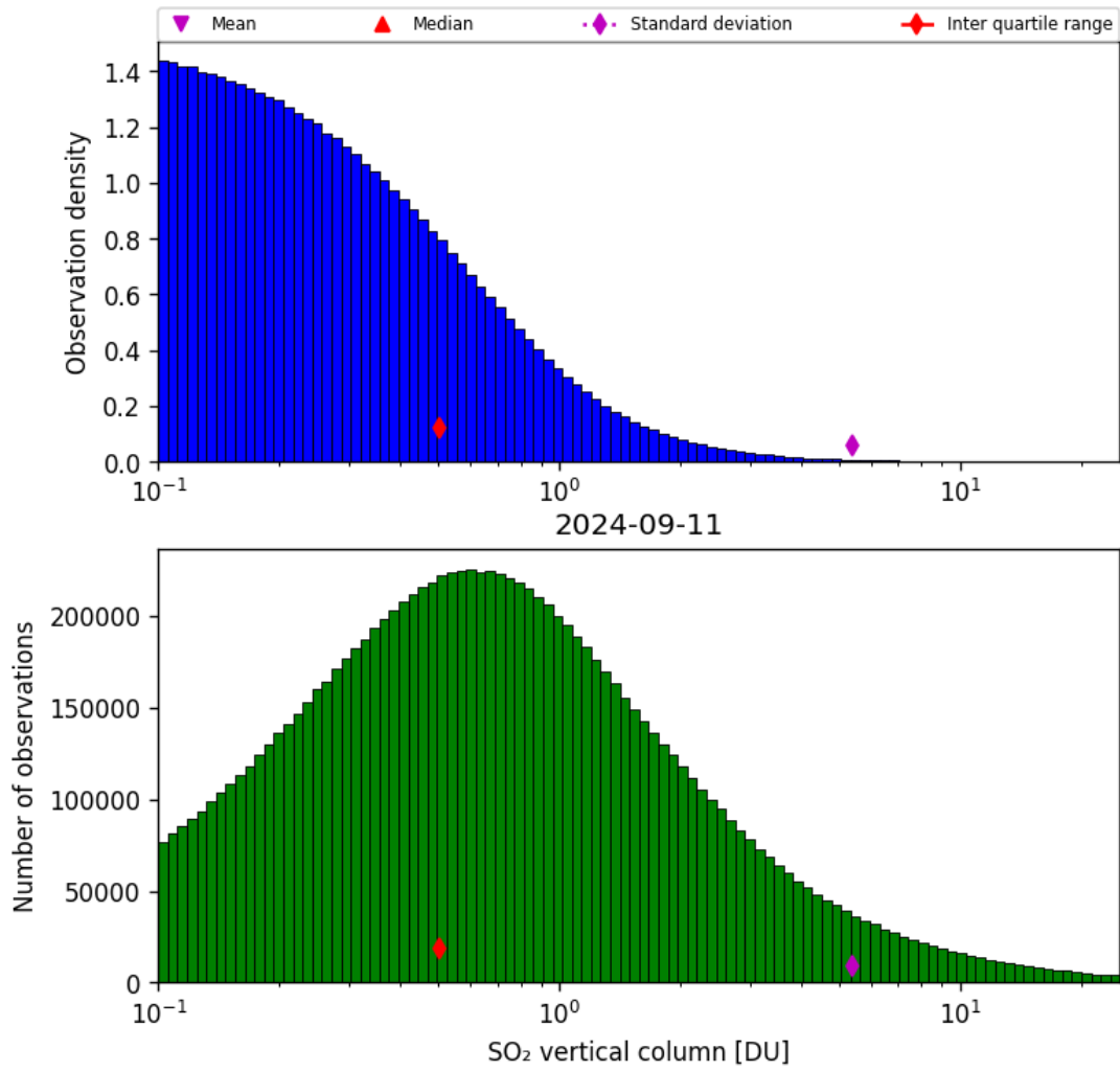
Figure 53: Histogram of “SO 2 vertical column” for 2024-09-10 to 2024-09-12
