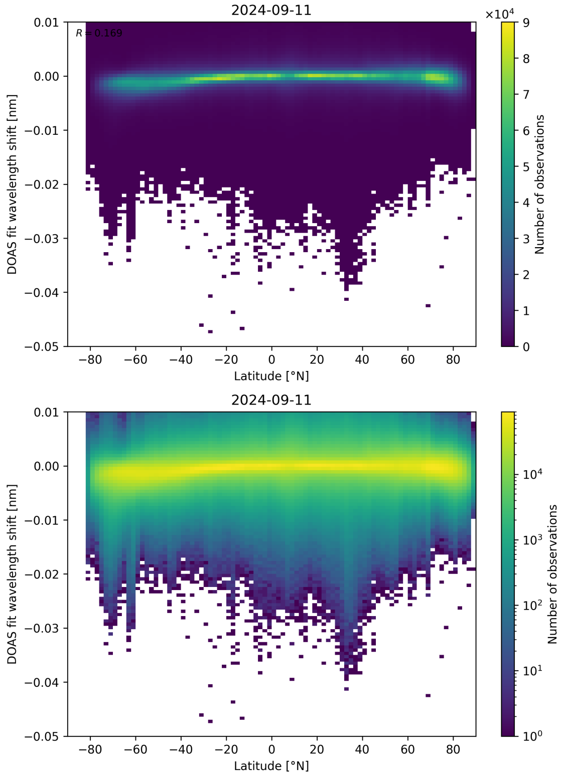
Figure 142: Scatter density plot of “Latitude” against “DOAS fit wavelength shift” for 2024-09-10 to 2024-09-12.
