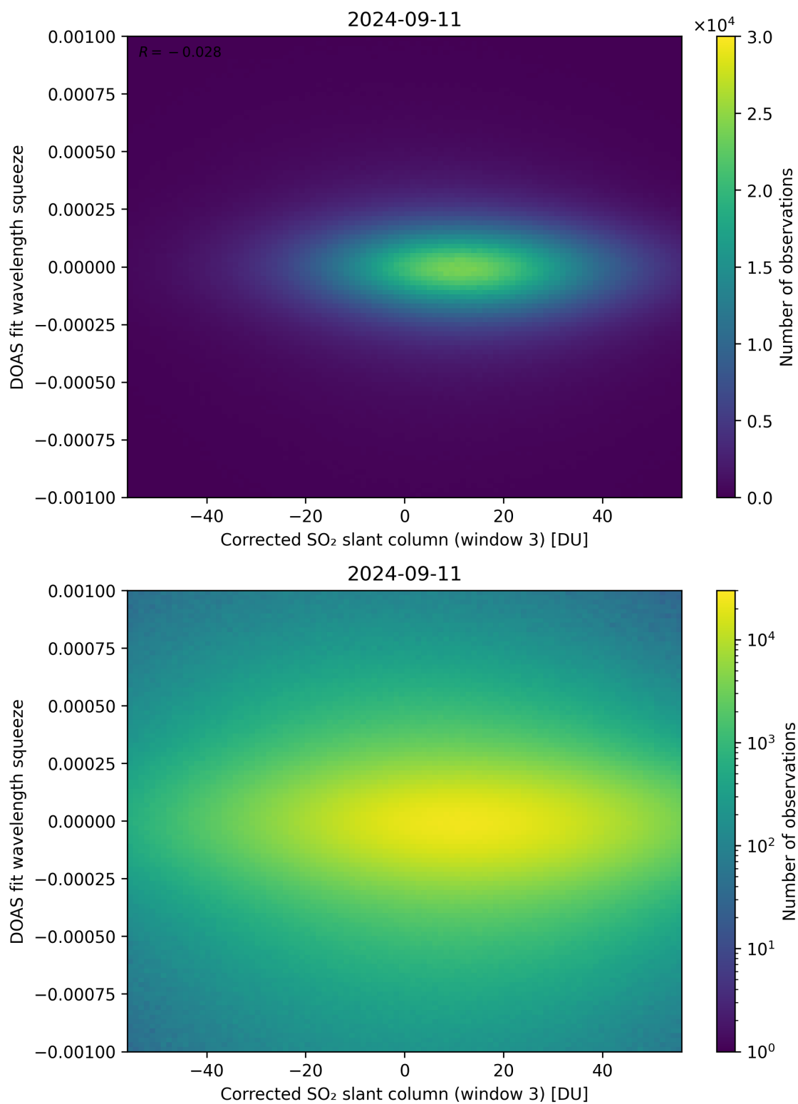
Figure 207: Scatter density plot of “Corrected SO 2 slant column (window 3)” against “DOAS fit wavelength squeeze” for 2024-09-10 to 2024-09-12.
