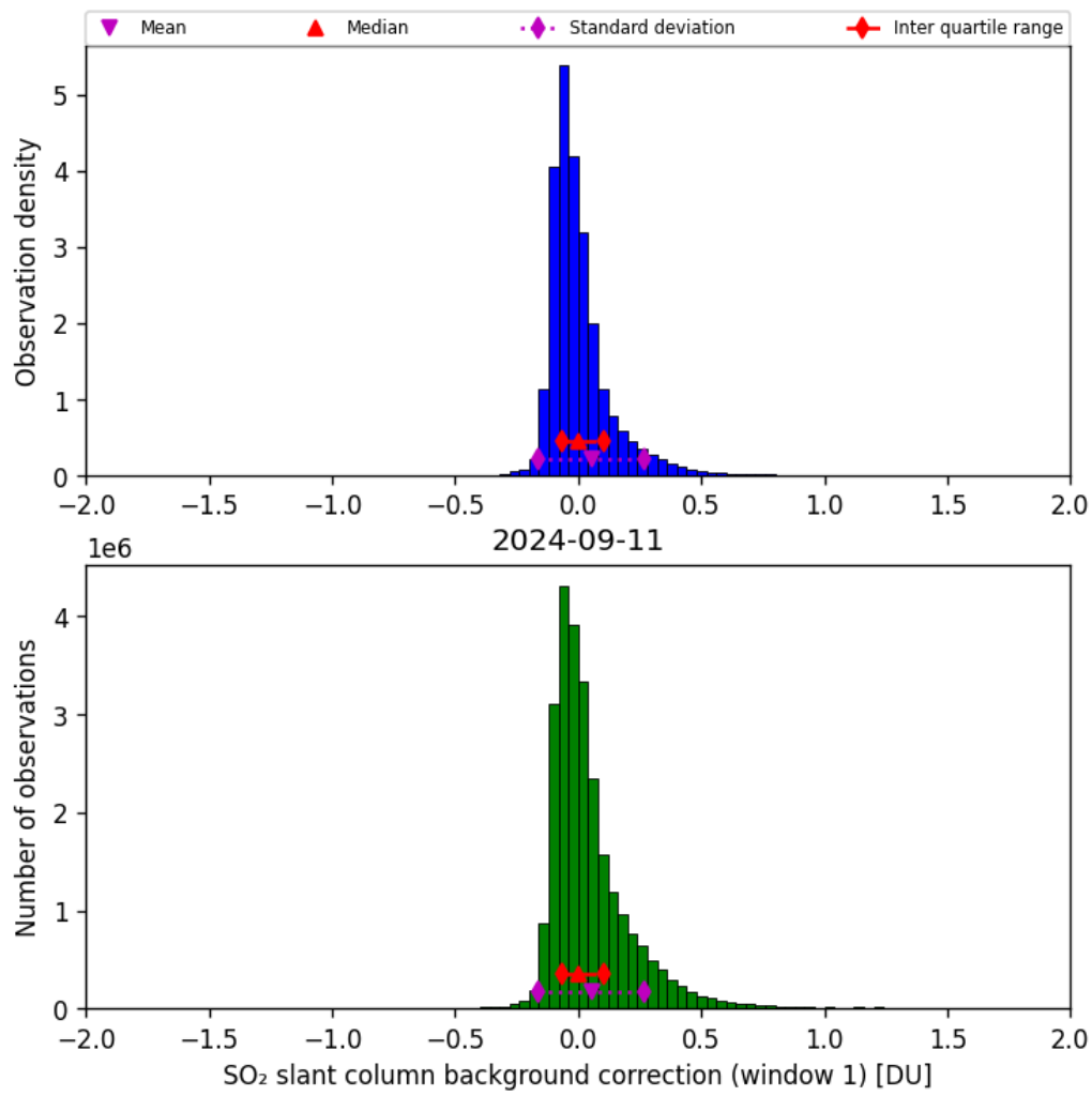
Figure 59: Histogram of “SO 2 slant column background correction (window 1)” for 2024-09-10 to 2024-09-12
