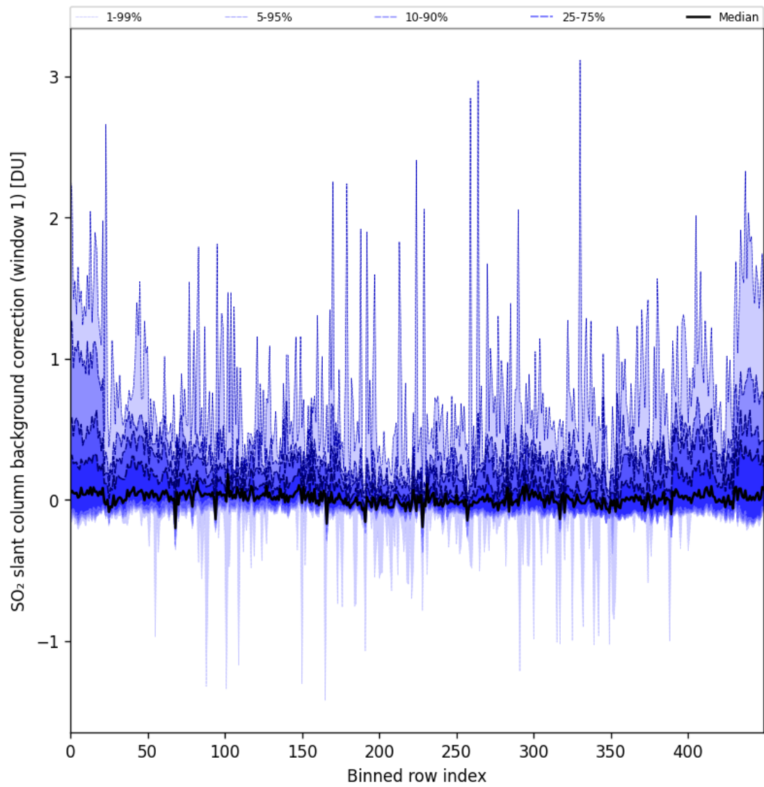
Figure 82: Along track statistics of “SO 2 slant column background correction (window 1)” for 2024-09-10 to 2024-09-12
