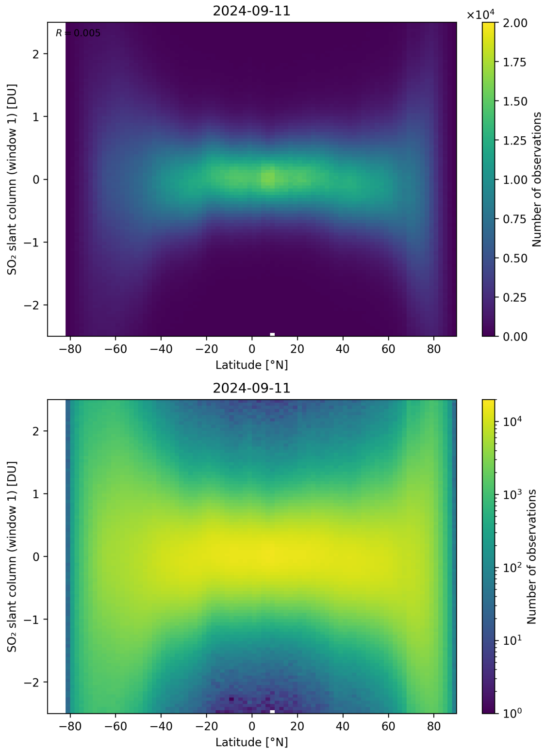
Figure 149: Scatter density plot of “Latitude” against “SO 2 slant column (window 1)” for 2024-09-10 to 2024-09-12.
