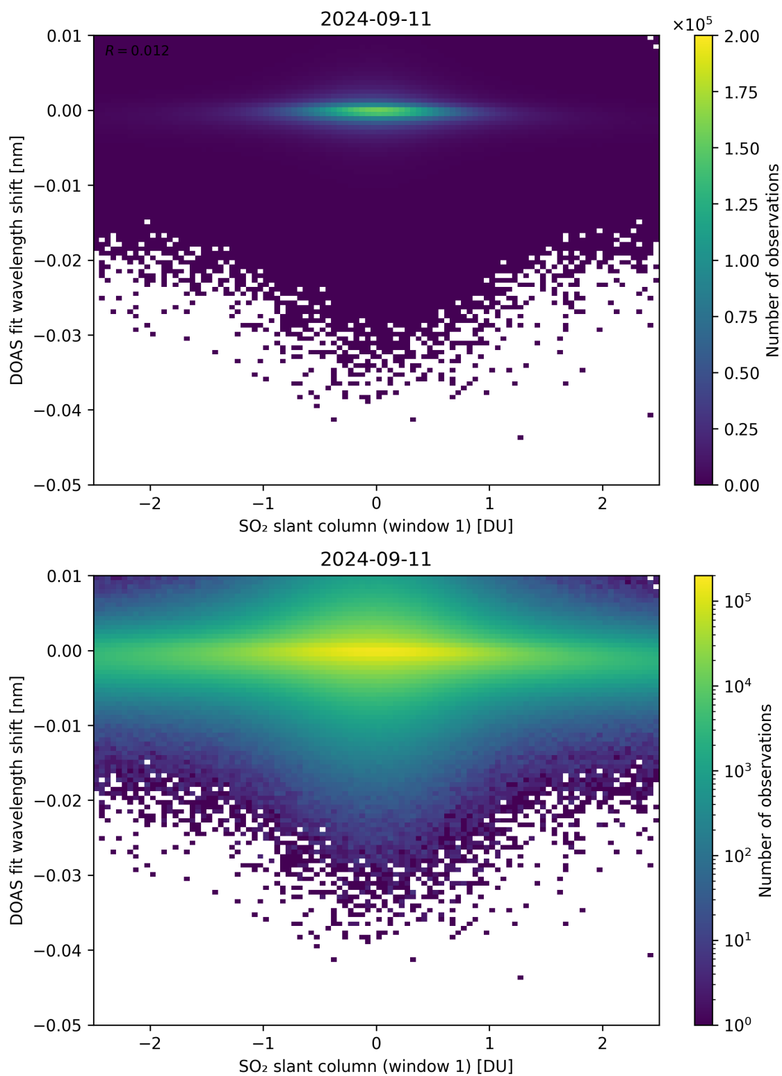
Figure 215: Scatter density plot of “SO 2 slant column (window 1)” against “DOAS fit wavelength shift” for 2024-09-10 to 2024-09-12.
