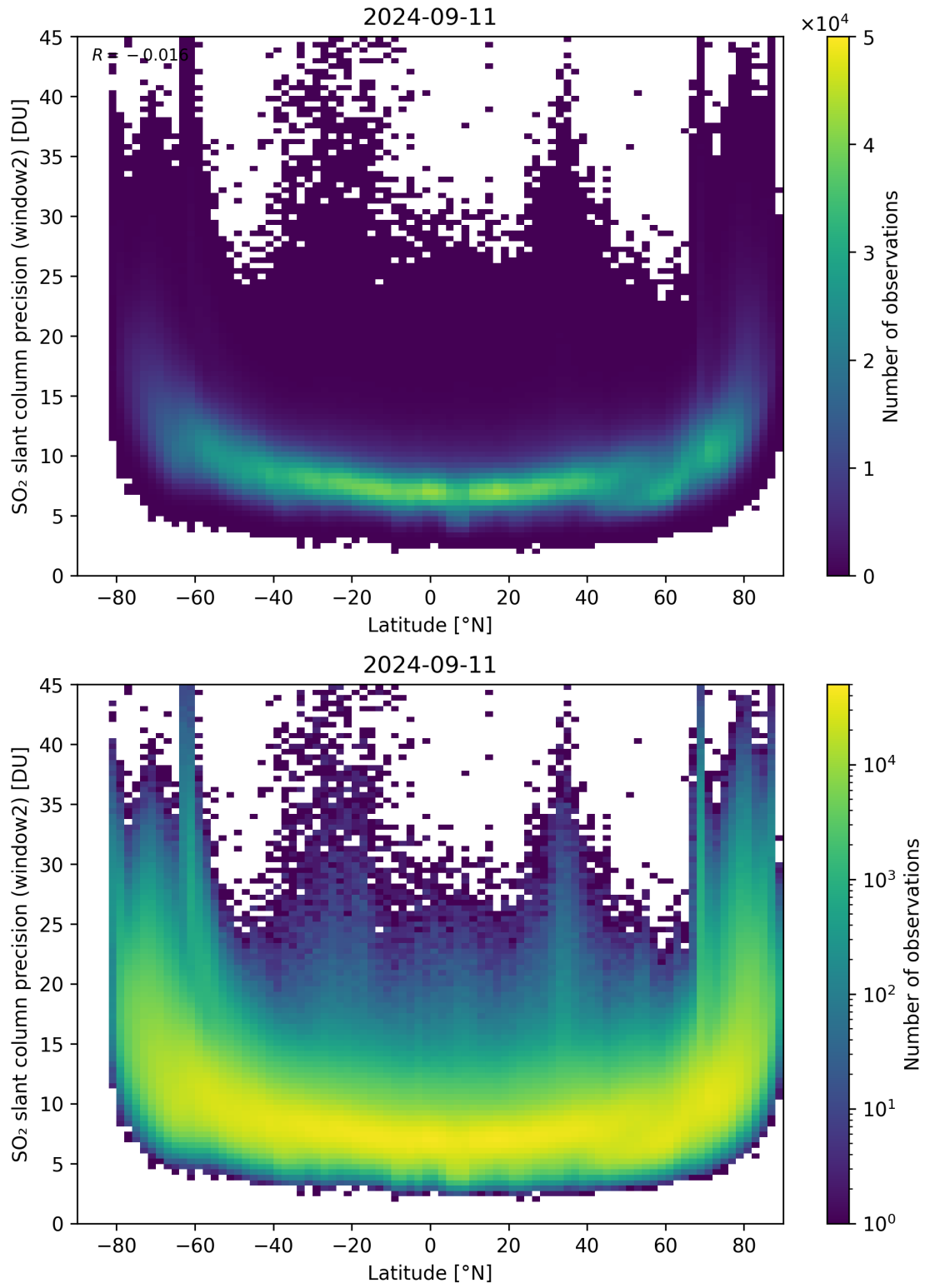
Figure 151: Scatter density plot of “Latitude” against “SO 2 slant column precision (window2)” for 2024-09-10 to 2024-09-12.
