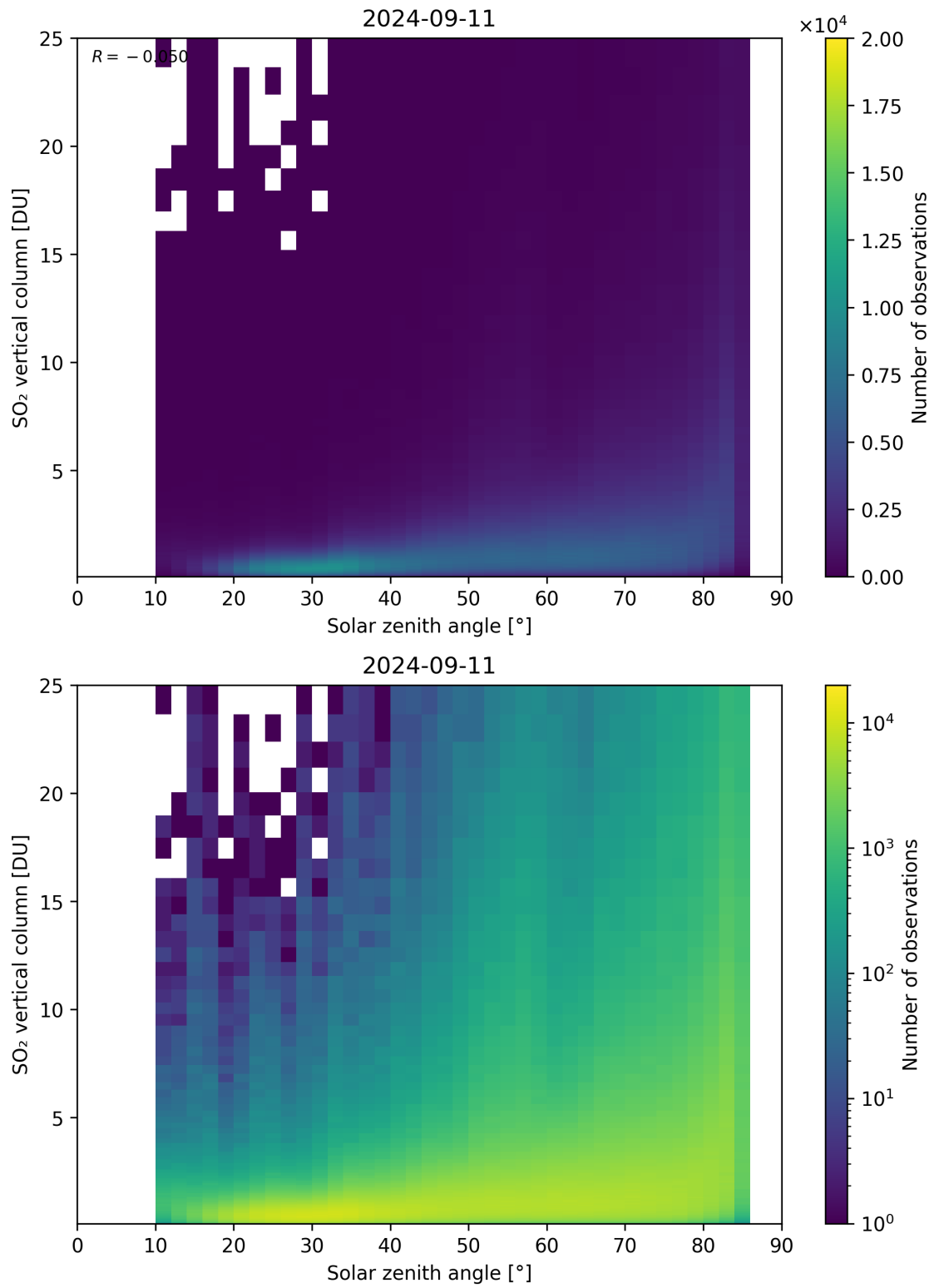
Figure 176: Scatter density plot of “Solar zenith angle” against “SO 2 vertical column” for 2024-09-10 to 2024-09-12.
