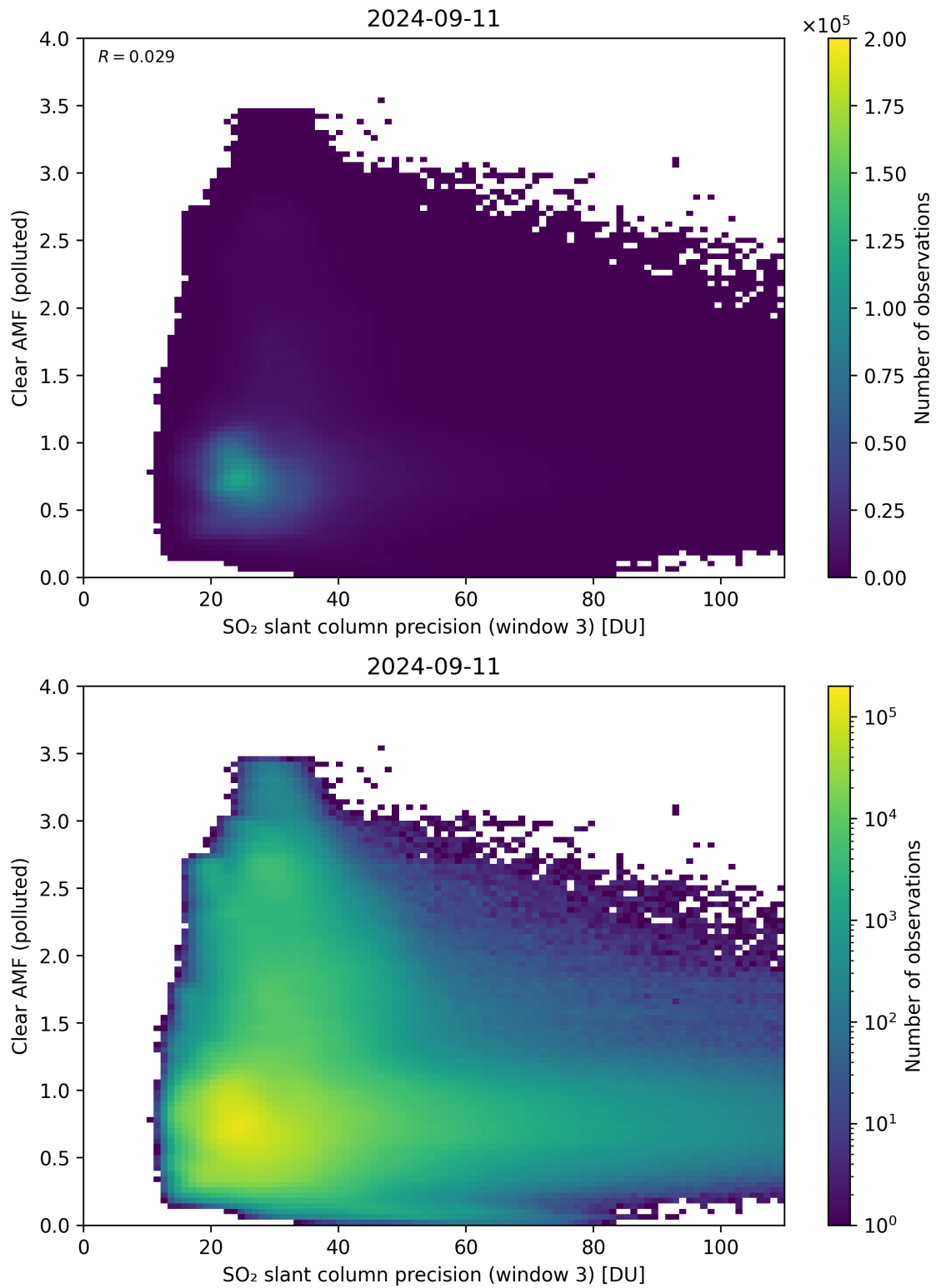
Figure 261: Scatter density plot of “SO 2 slant column precision (window 3)” against “Clear AMF (polluted)” for 2024-09-10 to 2024-09-12.
