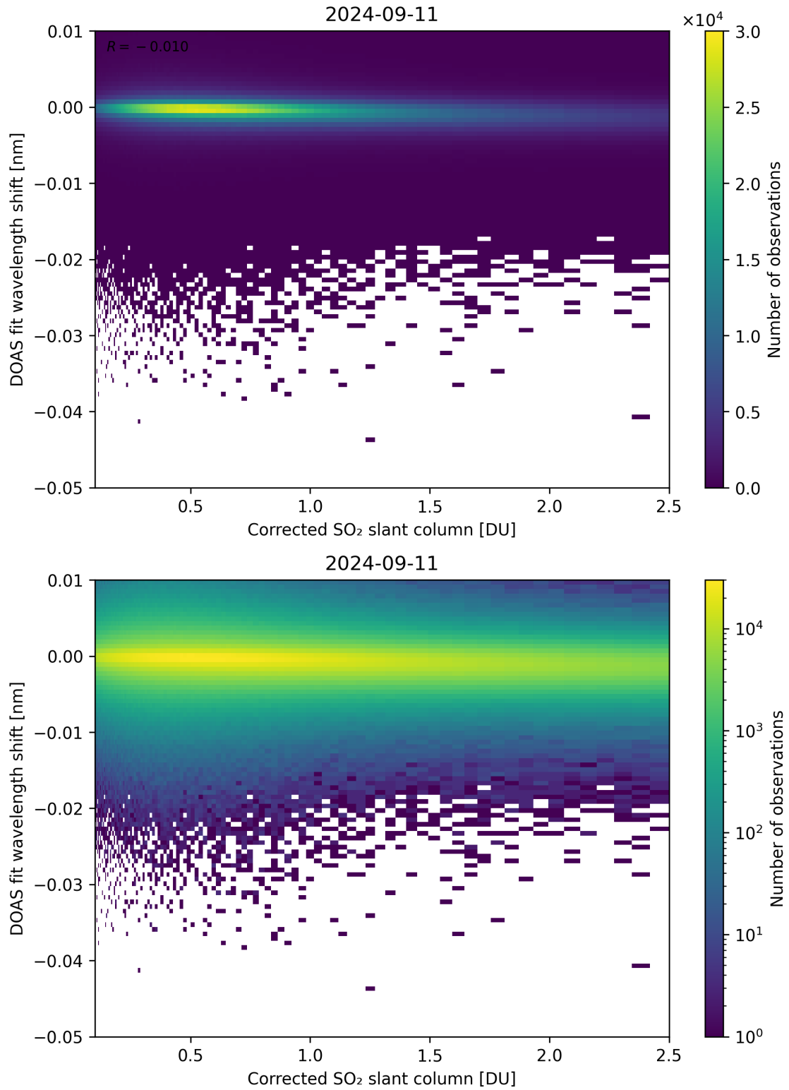
Figure 181: Scatter density plot of “Corrected SO 2 slant column” against “DOAS fit wavelength shift” for 2024-09-10 to 2024-09-12.
