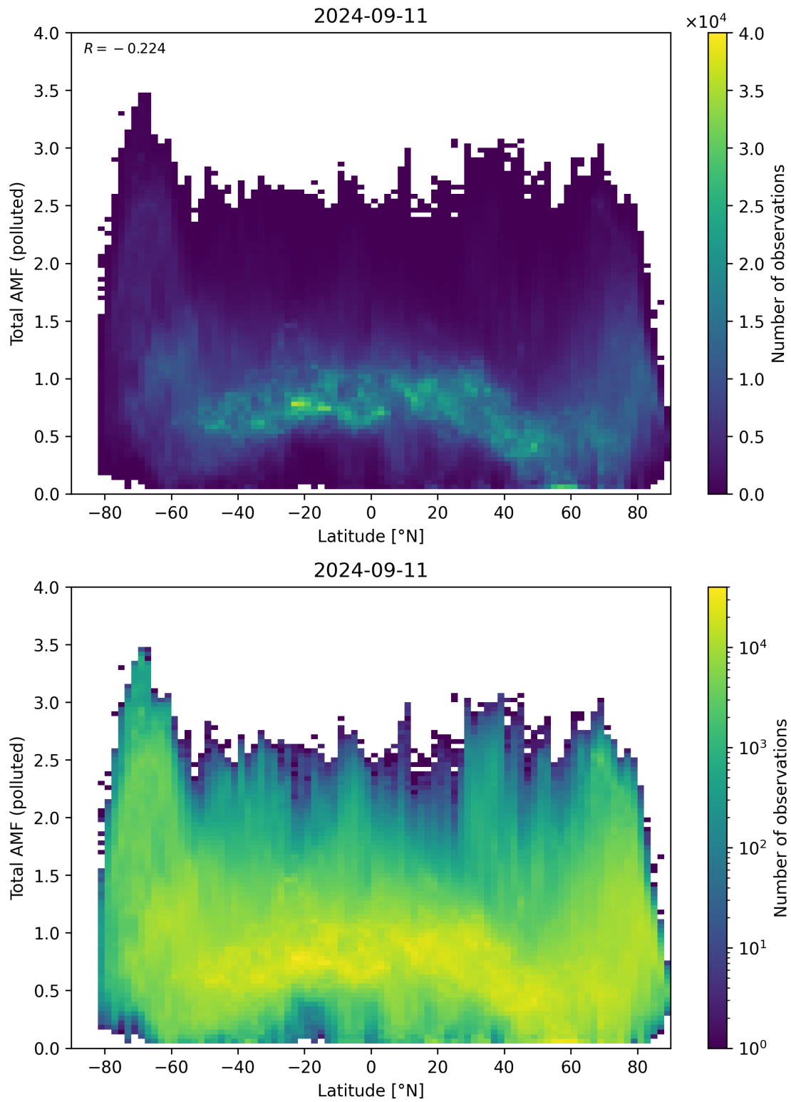
Figure 154: Scatter density plot of “Latitude” against “Total AMF (polluted)” for 2024-09-10 to 2024-09-12.
