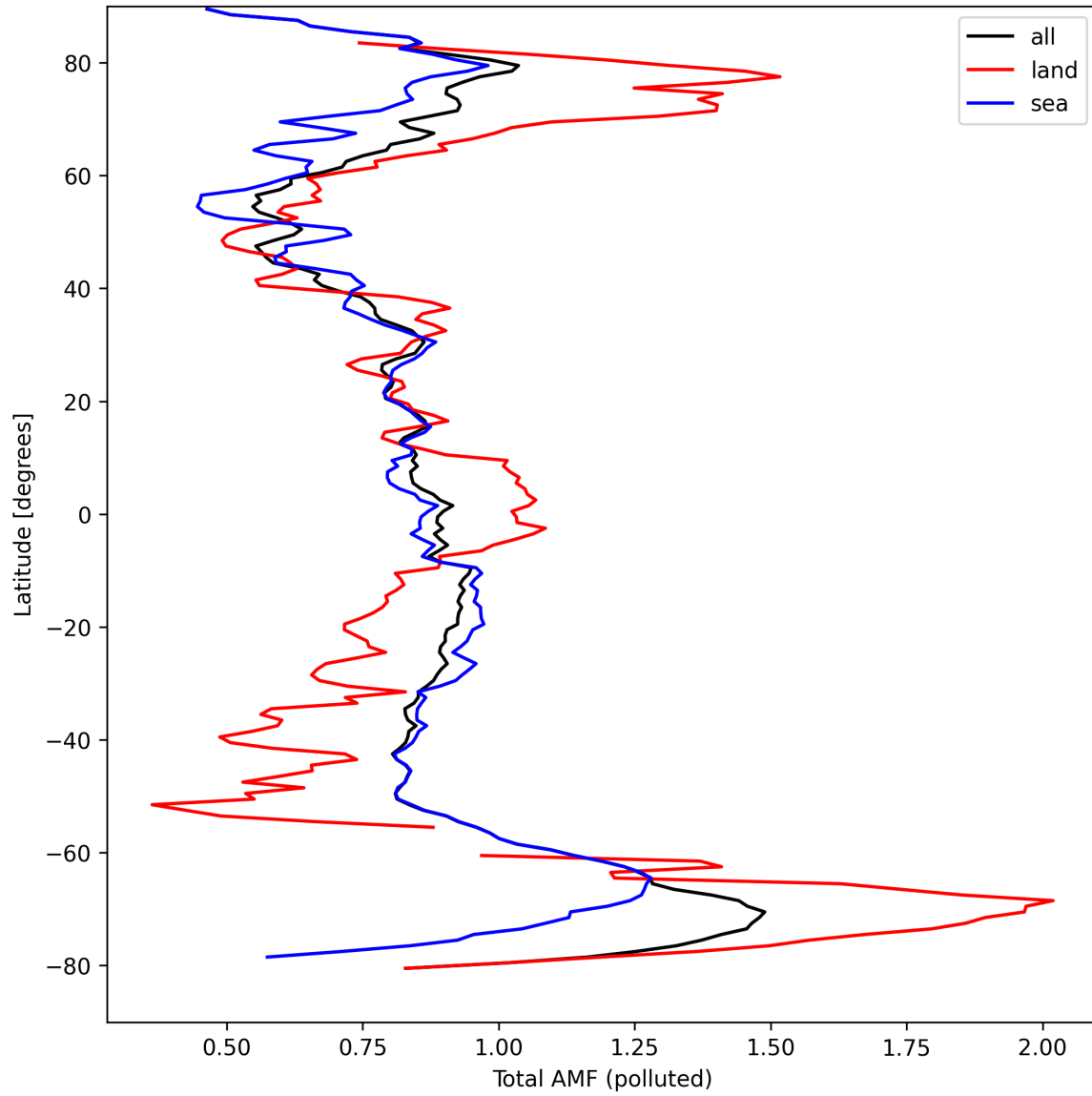
Figure 48: Zonal average of “Total AMF (polluted)” for 2024-09-10 to 2024-09-12.
