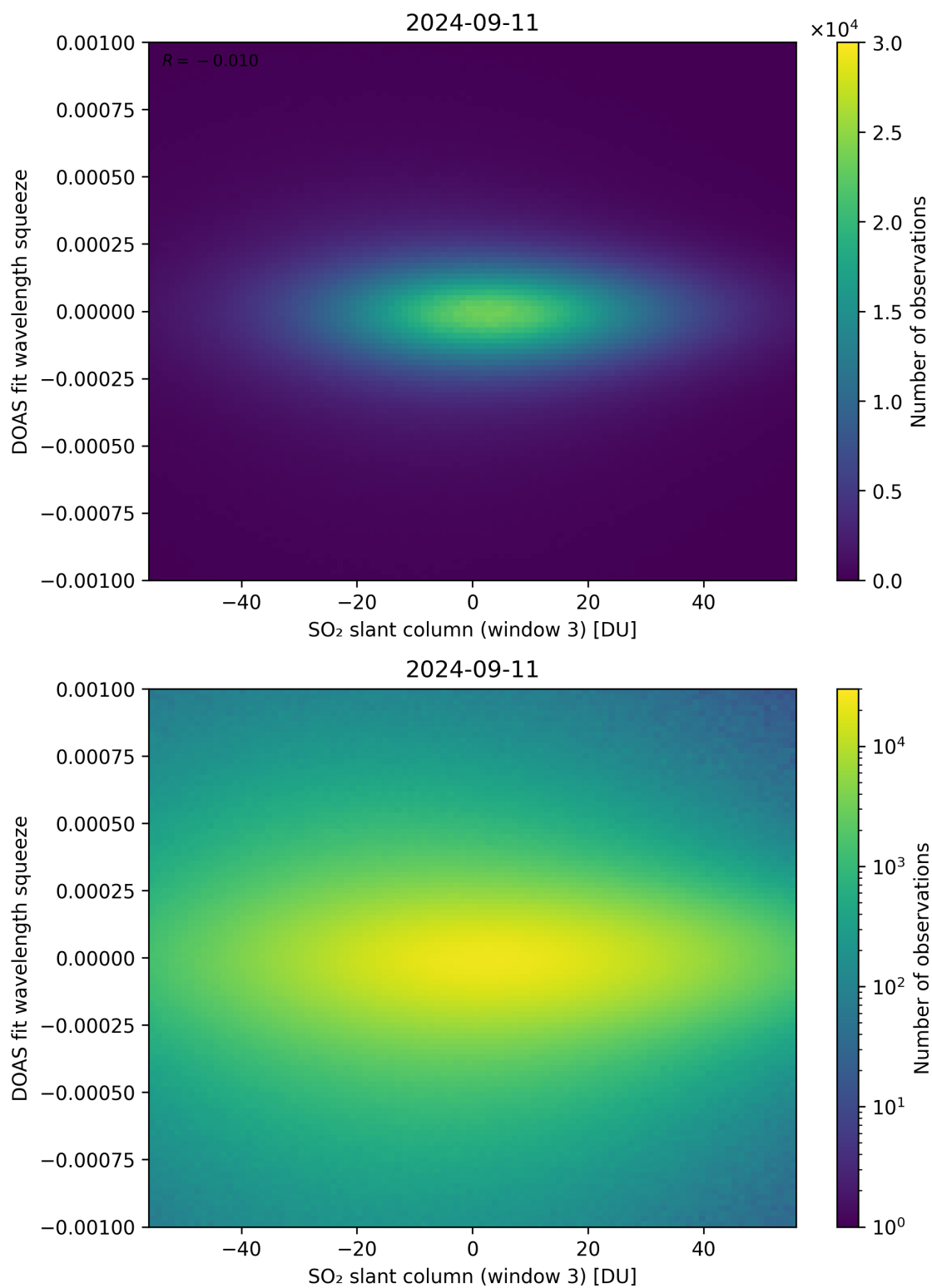
Figure 255: Scatter density plot of “SO 2 slant column (window 3)” against “DOAS fit wavelength squeeze” for 2024-09-10 to 2024-09-12.
