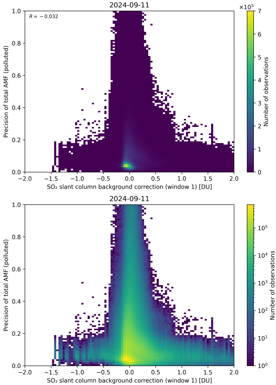
Figure 110: Scatter density plot of “SO 2 slant column background correction (window 1)” against “Precision of total AMF (polluted)” for 2024-09-10 to 2024-09-12.
