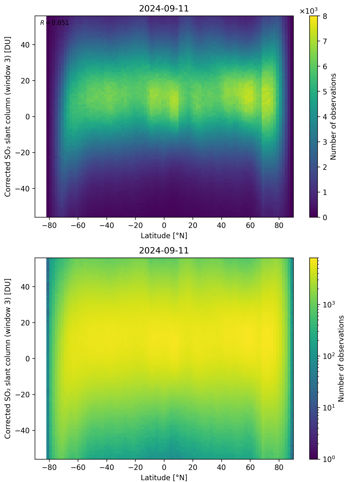
Figure 148: Scatter density plot of “Latitude” against “Corrected SO 2 slant column (window 3)” for 2024-09-10 to 2024-09-12.
