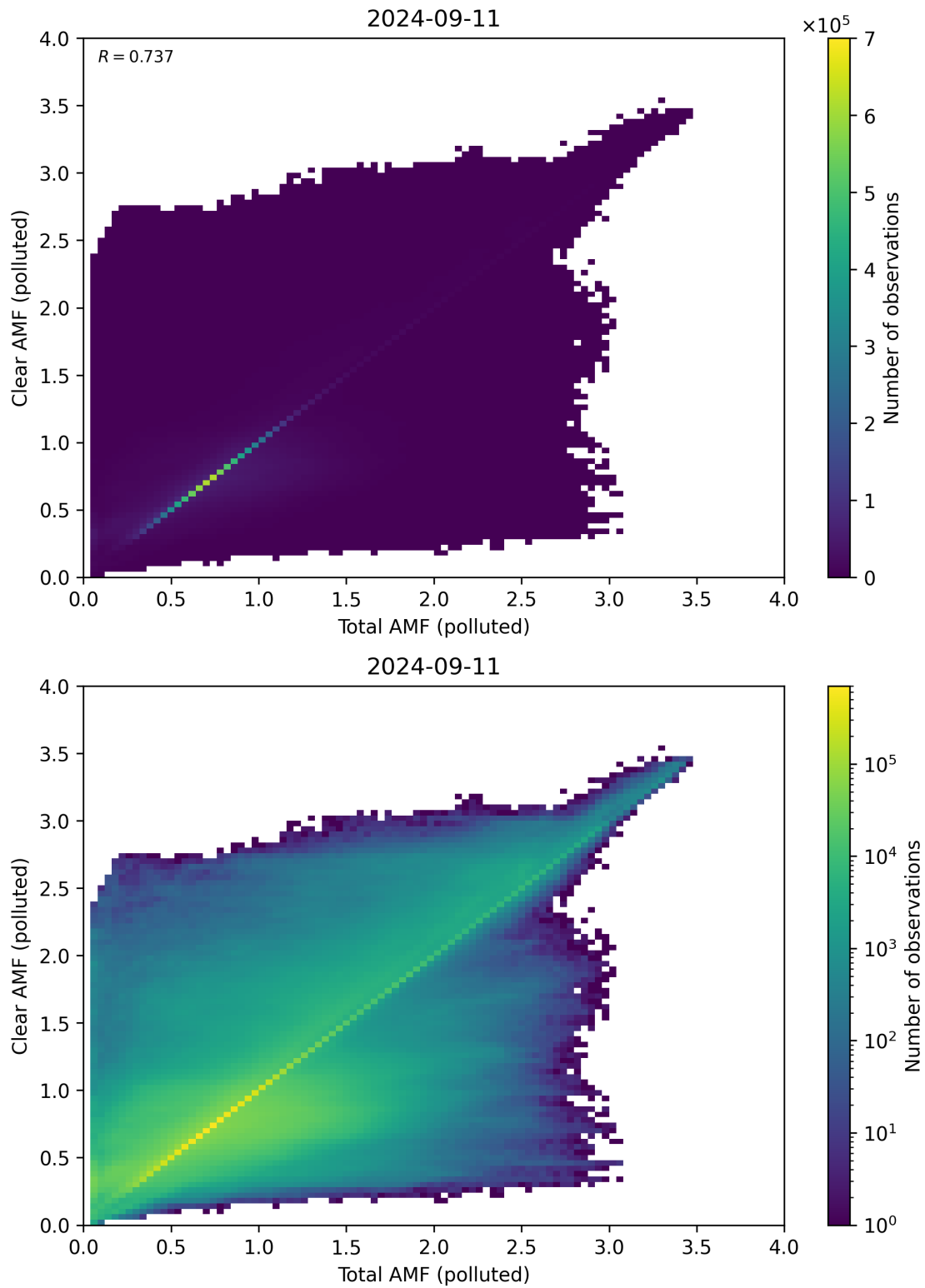
Figure 271: Scatter density plot of “Total AMF (polluted)” against “Clear AMF (polluted)” for 2024-09-10 to 2024-09-12.
