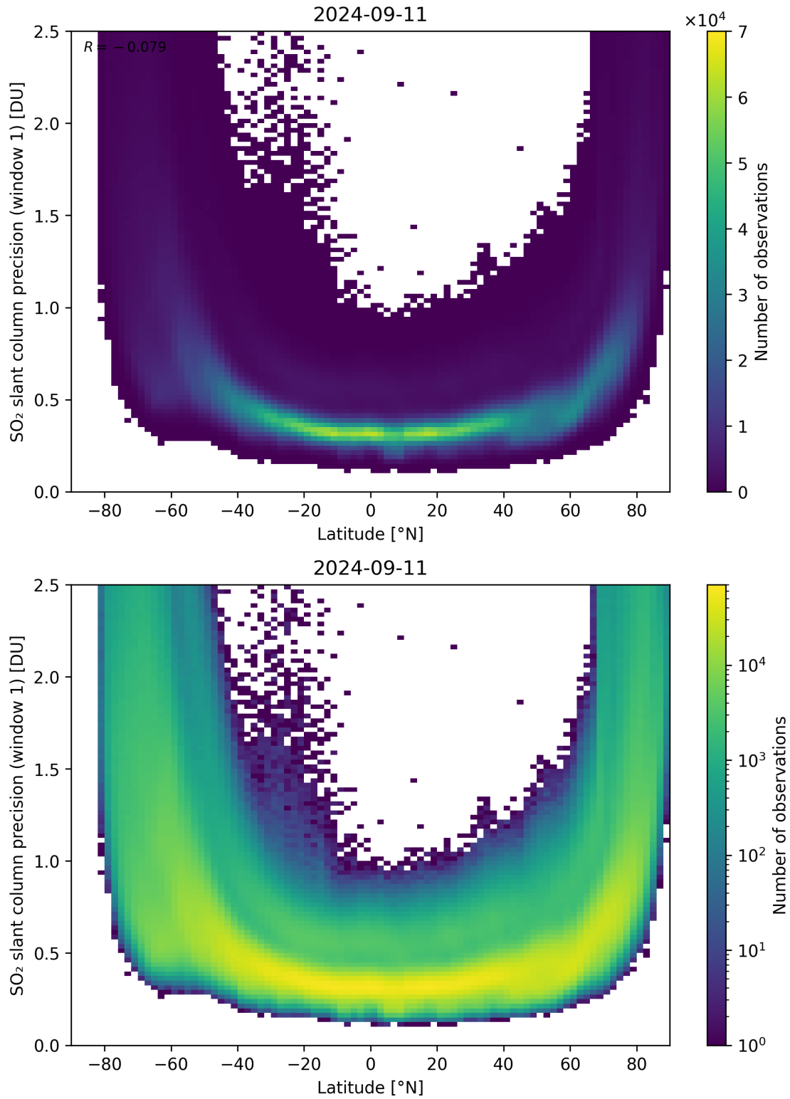
Figure 150: Scatter density plot of “Latitude” against “SO 2 slant column precision (window 1)” for 2024-09-10 to 2024-09-12.
