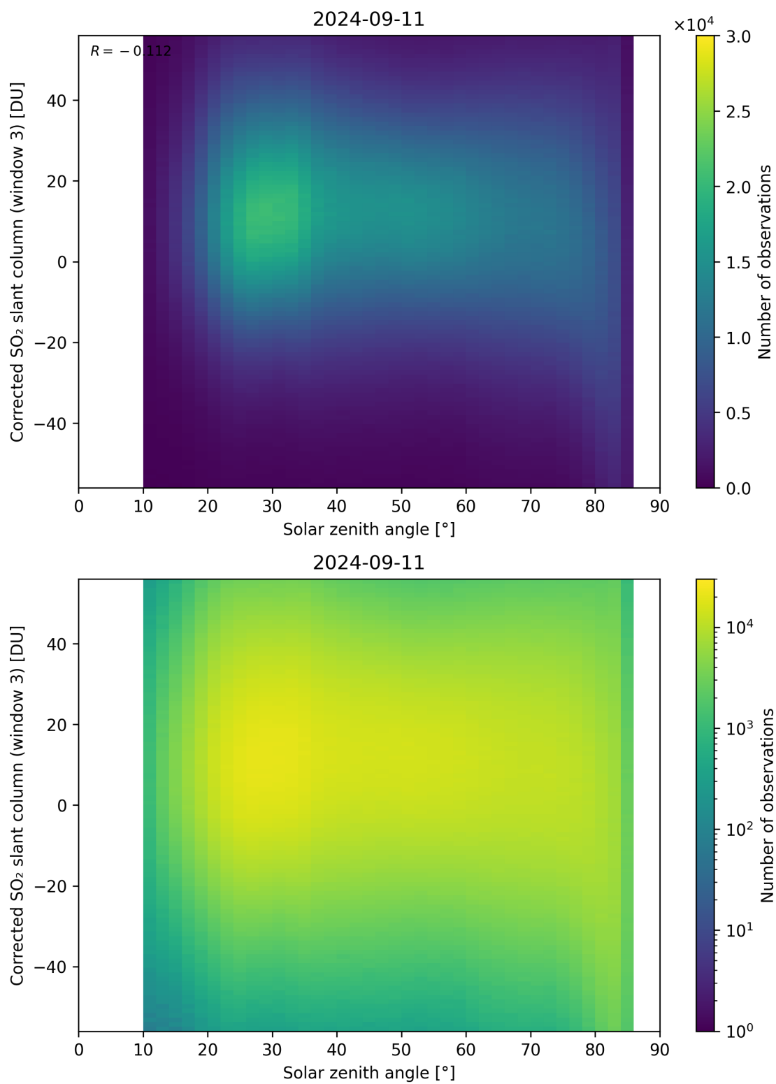
Figure 168: Scatter density plot of “Solar zenith angle” against “Corrected SO 2 slant column (window 3)” for 2024-09-10 to 2024-09-12.
