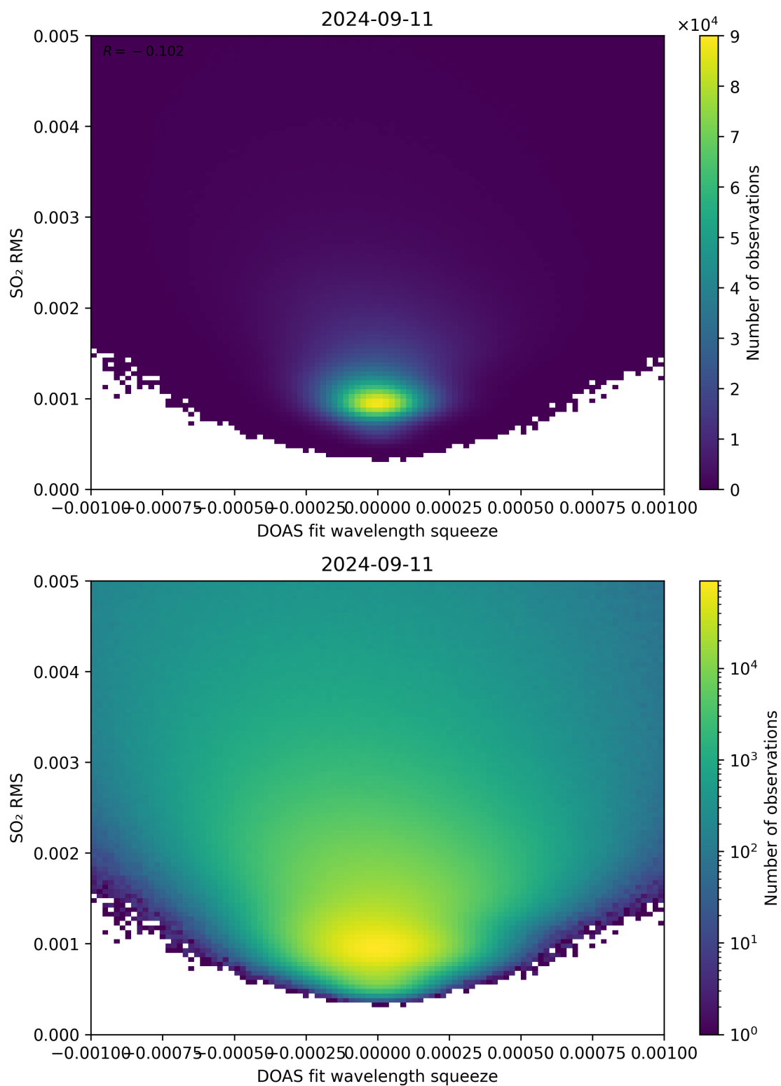
Figure 132: Scatter density plot of “DOAS fit wavelength squeeze” against “SO 2 RMS” for 2024-09-10 to 2024-09-12.
