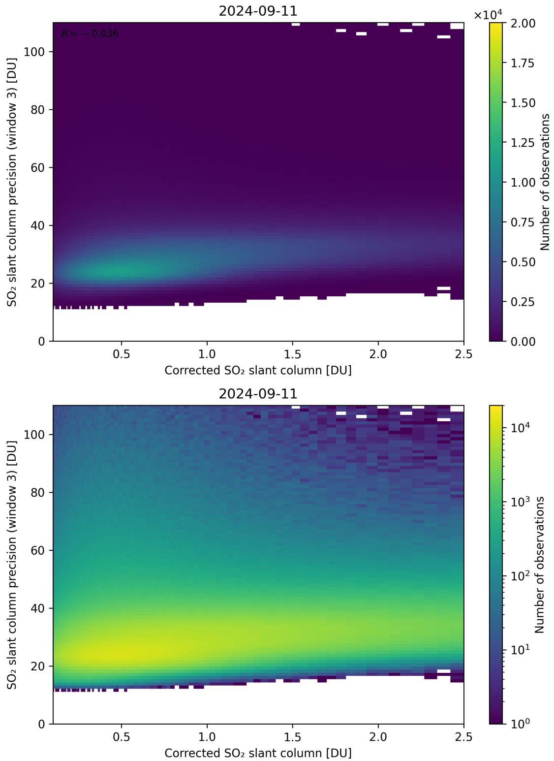
Figure 191: Scatter density plot of “Corrected SO 2 slant column” against “SO 2 slant column precision (window 3)” for 2024-09-10 to 2024-09-12.
