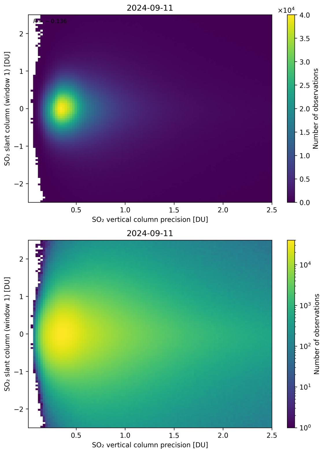
Figure 289: Scatter density plot of “SO 2 vertical column precision” against “SO 2 slant column (window 1)” for 2024-09-10 to 2024-09-12.
