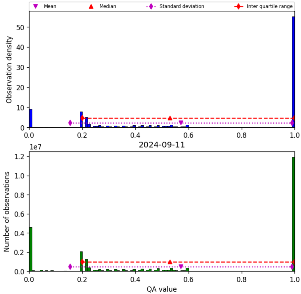
Figure 52: Histogram of “QA value” for 2024-09-10 to 2024-09-12
