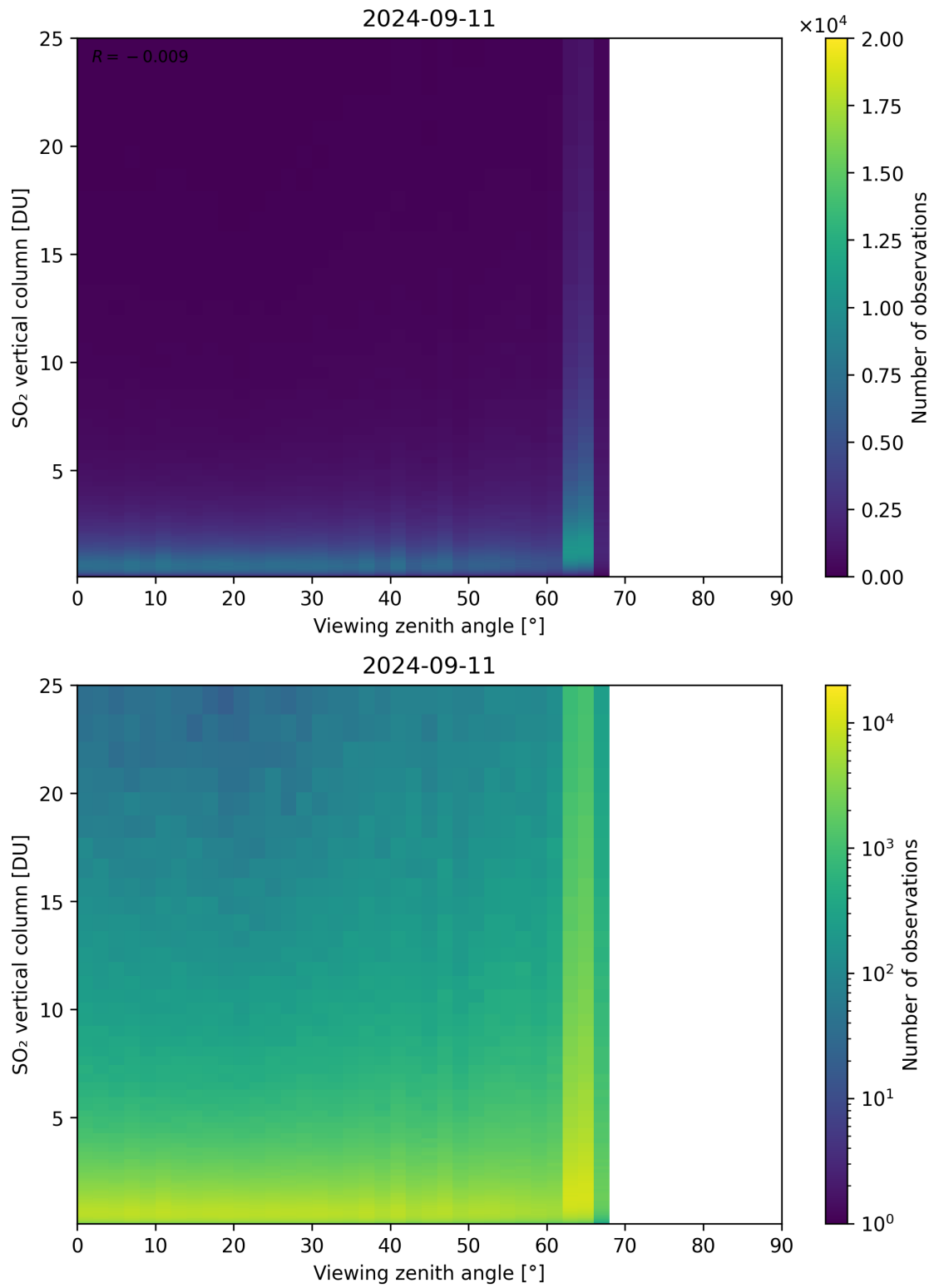
Figure 327: Scatter density plot of “Viewing zenith angle” against “SO 2 vertical column” for 2024-09-10 to 2024-09-12.
