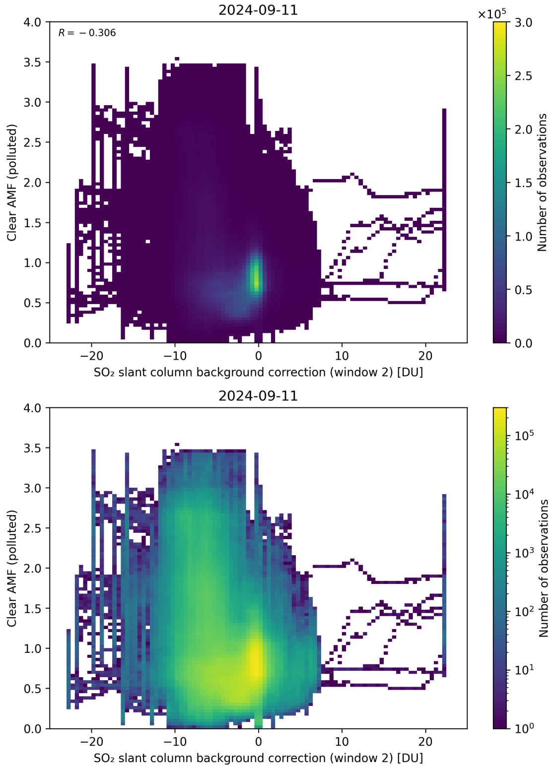
Figure 115: Scatter density plot of “SO 2 slant column background correction (window 2)” against “Clear AMF (polluted)” for 2024-09-10 to 2024-09-12.
