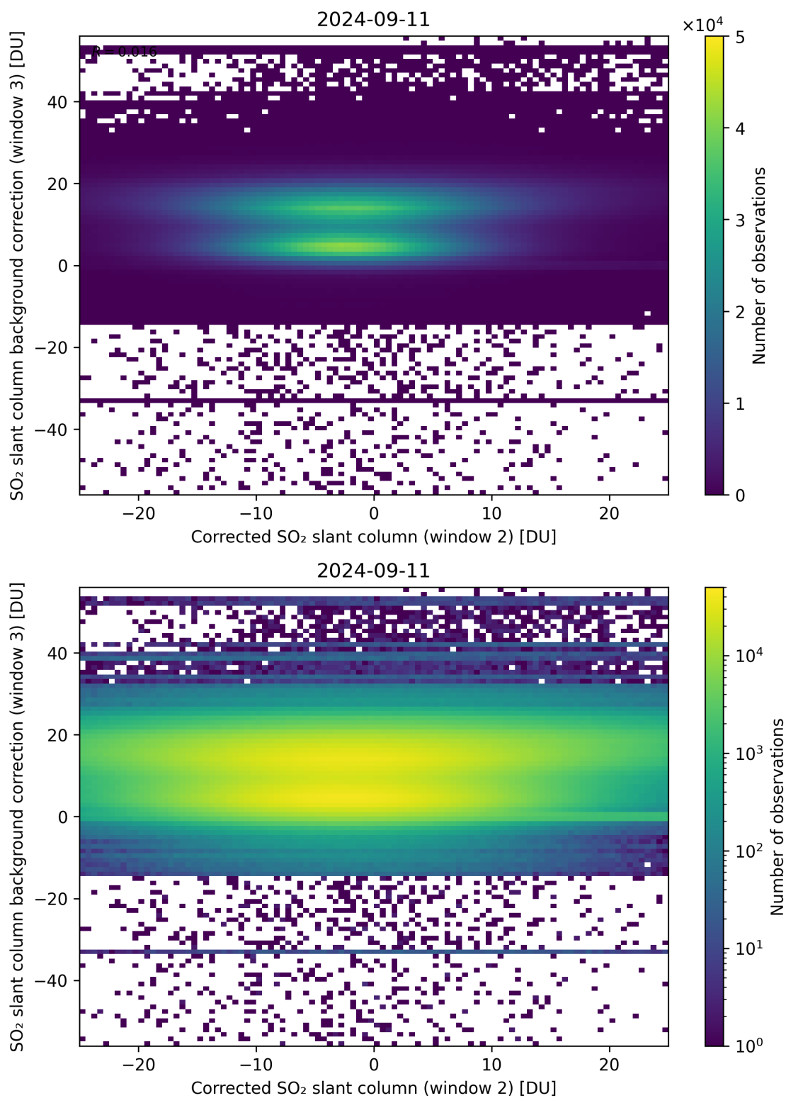
Figure 195: Scatter density plot of “Corrected SO 2 slant column (window 2)” against “SO 2 slant column background correction (window 3)” for 2024-09-10 to 2024-09-12.
