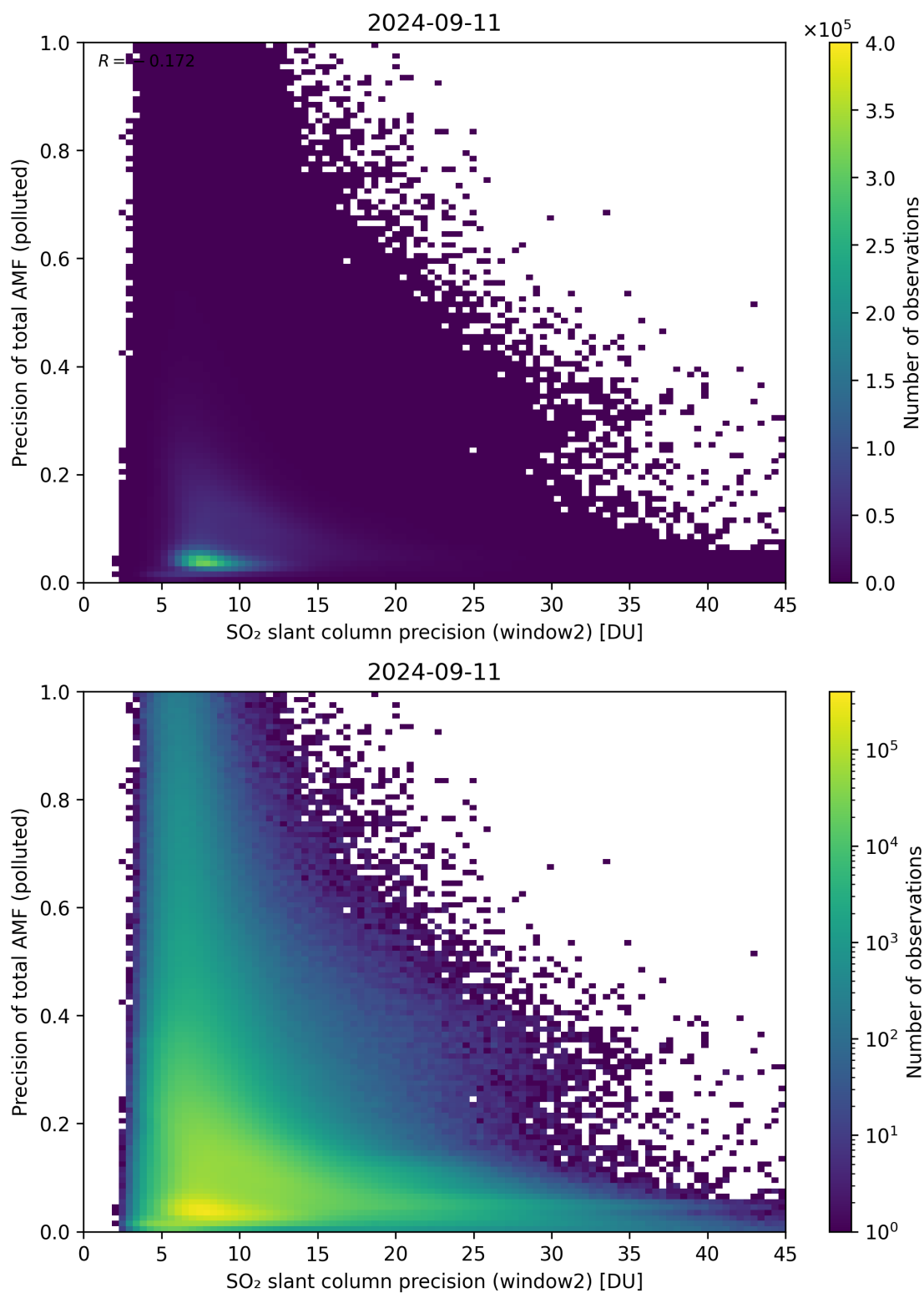
Figure 252: Scatter density plot of “SO 2 slant column precision (window2)” against “Precision of total AMF (polluted)” for 2024-09-10 to 2024-09-12.
