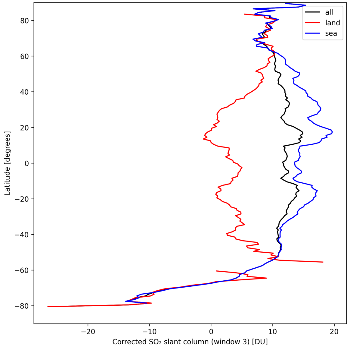
Figure 43: Zonal average of “Corrected SO 2 slant column (window 3)” for 2024-09-10 to 2024-09-12.
