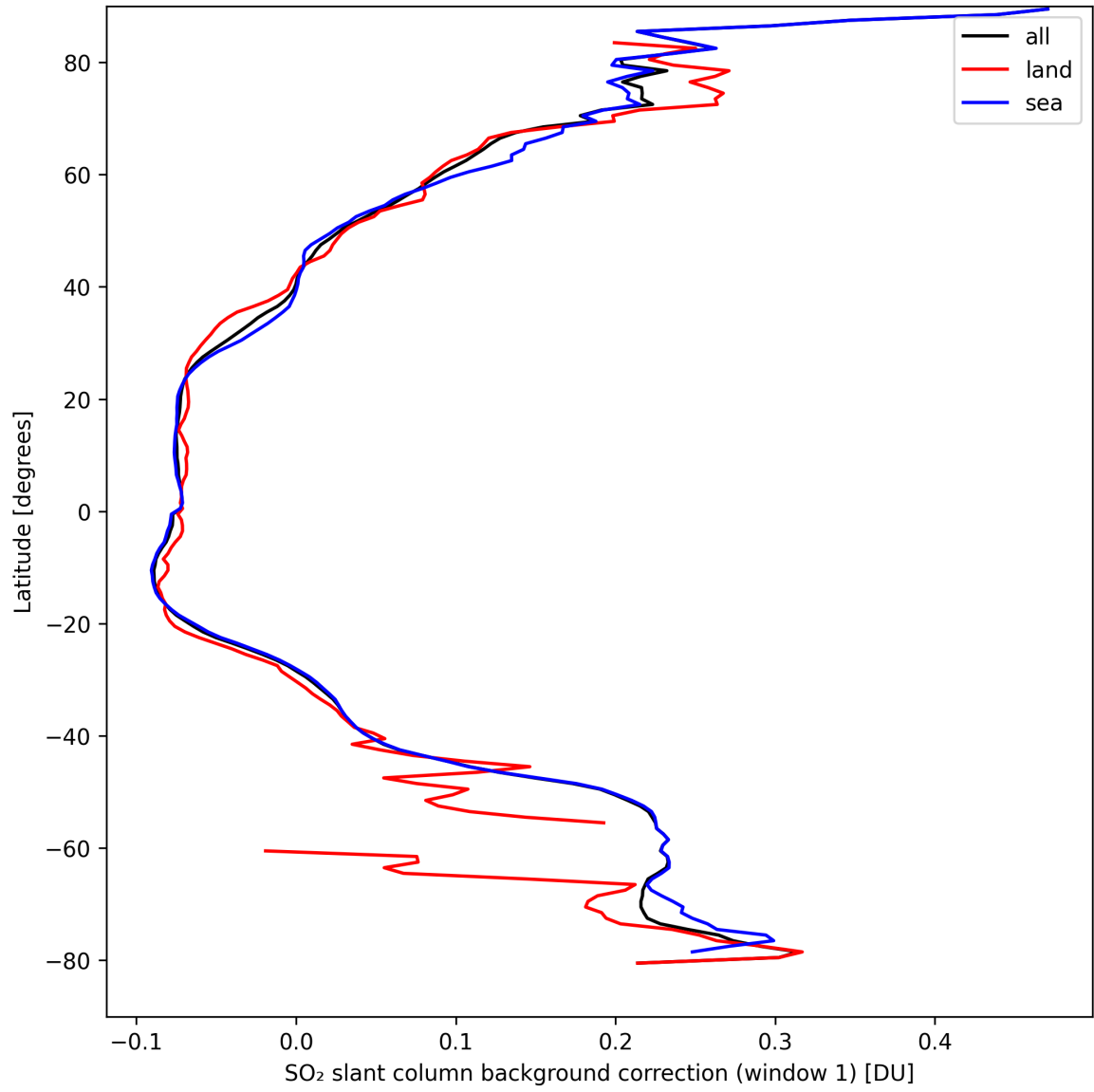
Figure 36: Zonal average of “SO 2 slant column background correction (window 1)” for 2024-09-10 to 2024-09-12.
