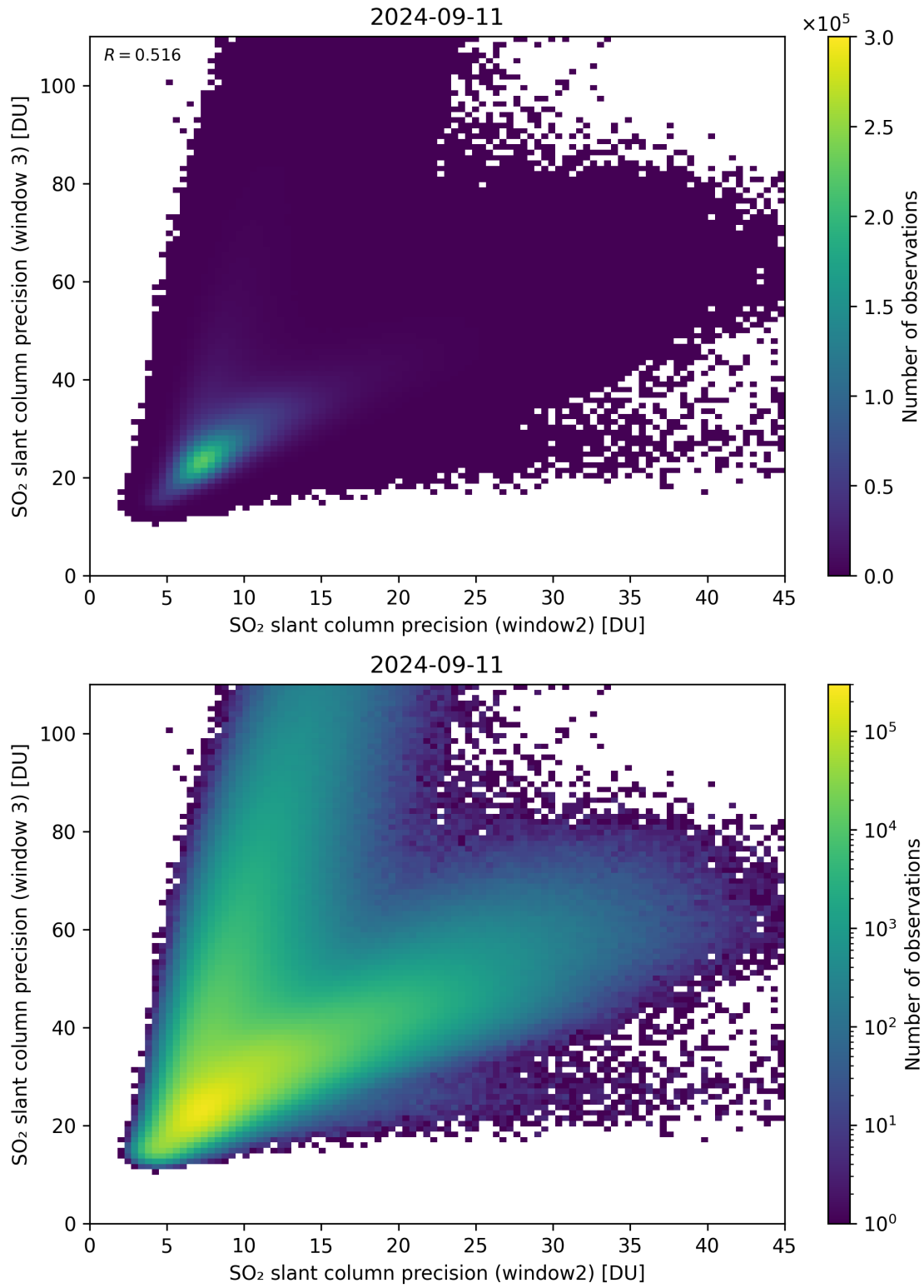
Figure 250: Scatter density plot of “SO 2 slant column precision (window2)” against “SO 2 slant column precision (window 3)” for 2024-09-10 to 2024-09-12.
