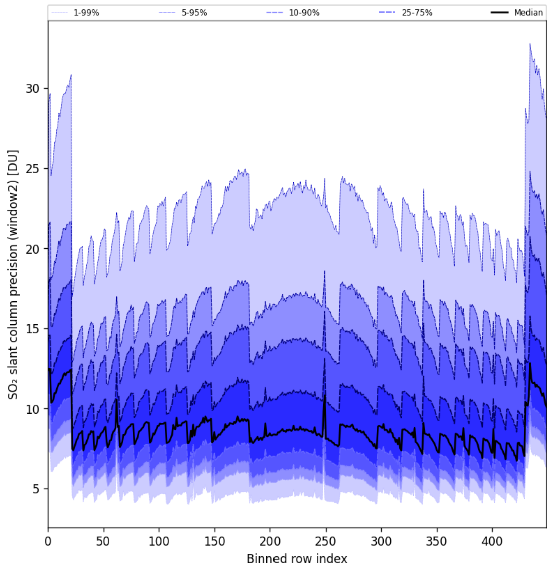
Figure 84: Along track statistics of “SO 2 slant column precision (window2)” for 2024-09-10 to 2024-09-12
