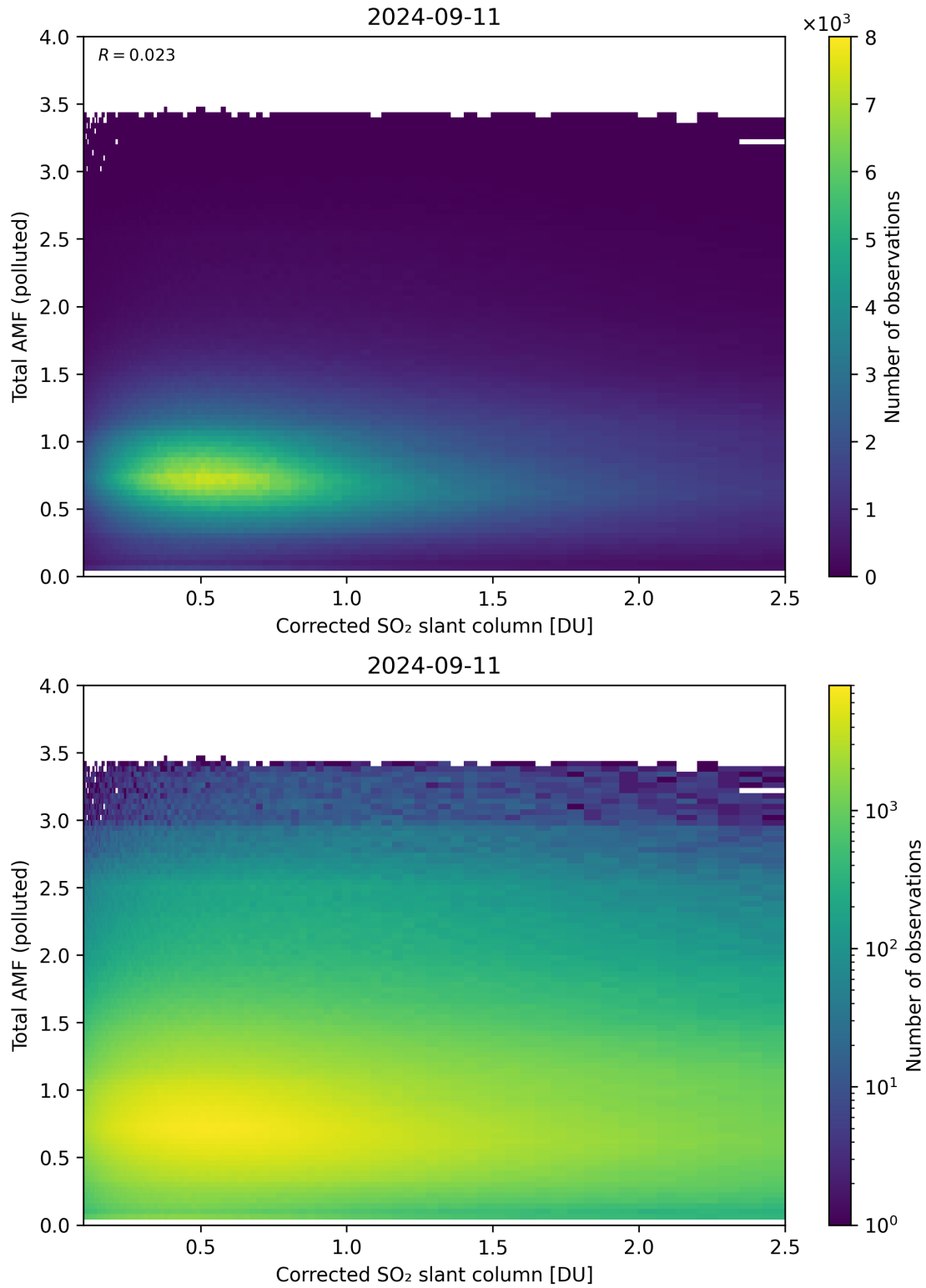
Figure 192: Scatter density plot of “Corrected SO 2 slant column” against “Total AMF (polluted)” for 2024-09-10 to 2024-09-12.
