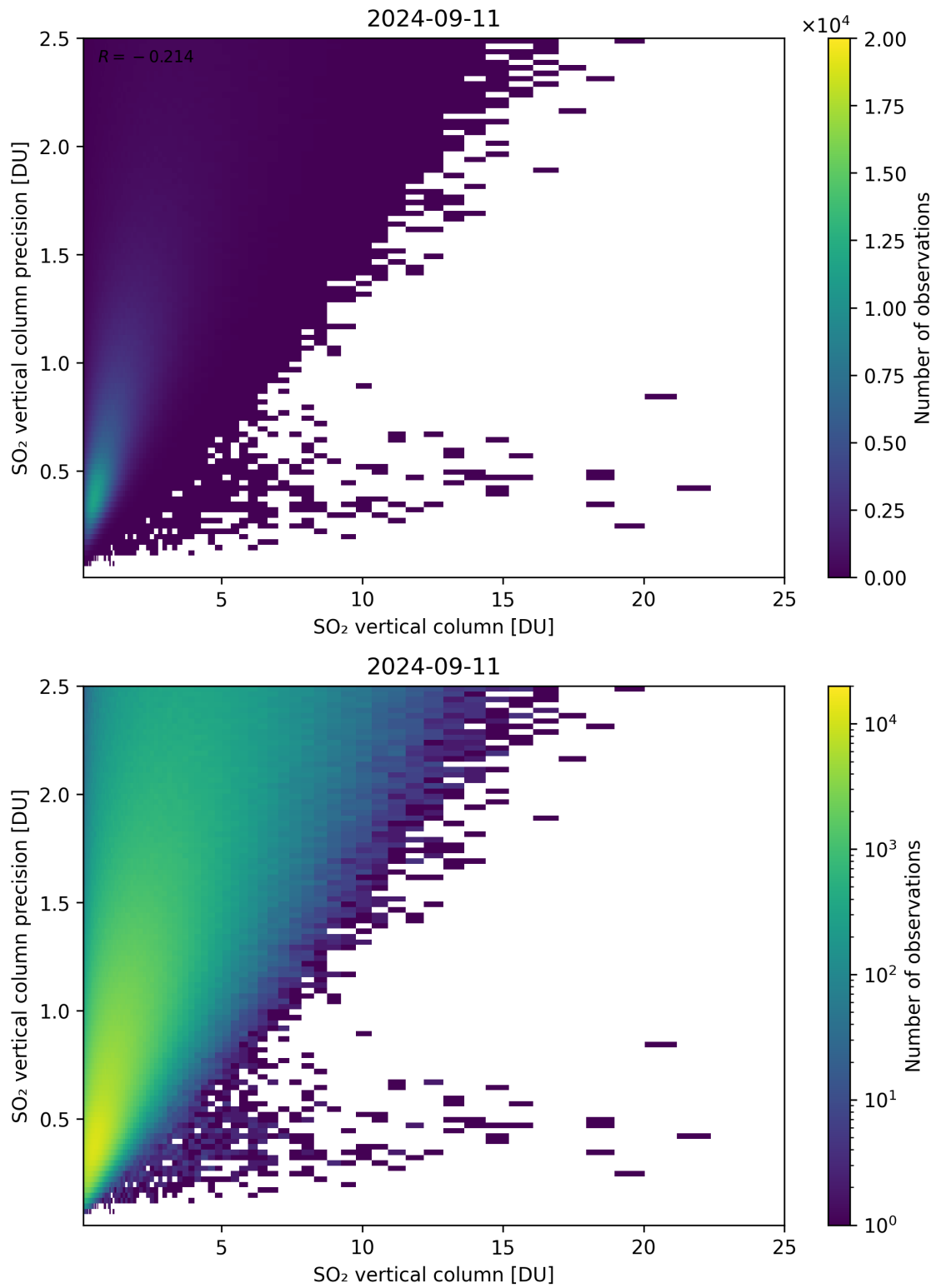
Figure 307: Scatter density plot of “SO 2 vertical column” against “SO 2 vertical column precision” for 2024-09-10 to 2024-09-12.
