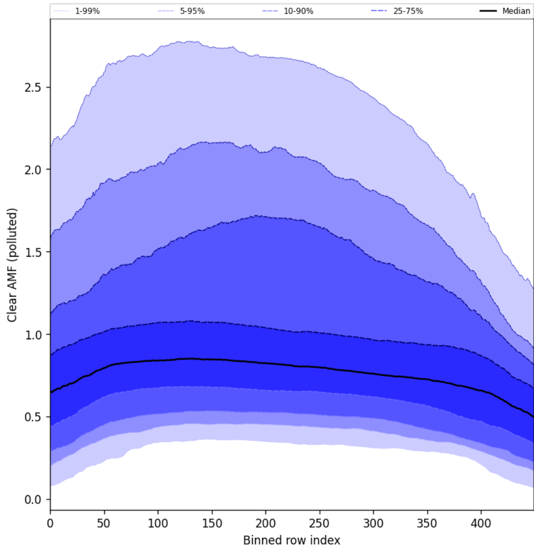
Figure 96: Along track statistics of “Clear AMF (polluted)” for 2024-09-10 to 2024-09-12
