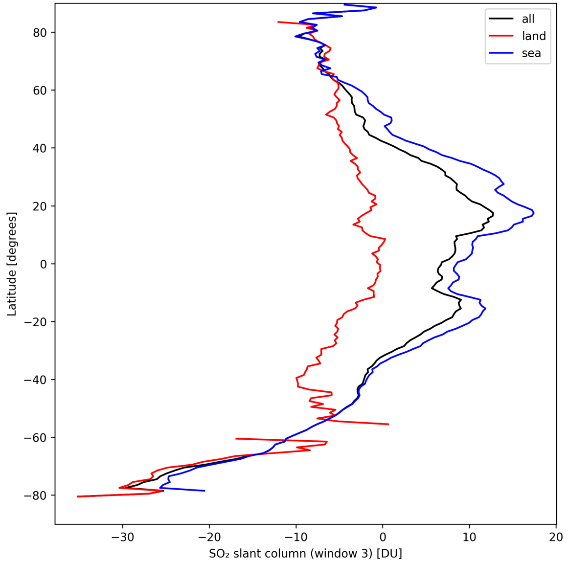
Figure 41: Zonal average of “SO 2 slant column (window 3)” for 2024-09-10 to 2024-09-12.
