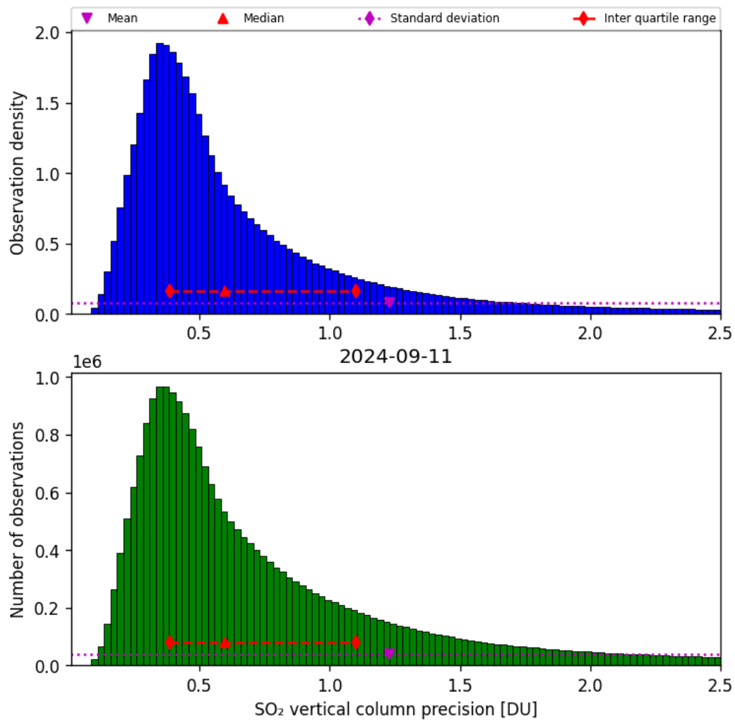
Figure 54: Histogram of “SO 2 vertical column precision” for 2024-09-10 to 2024-09-12
