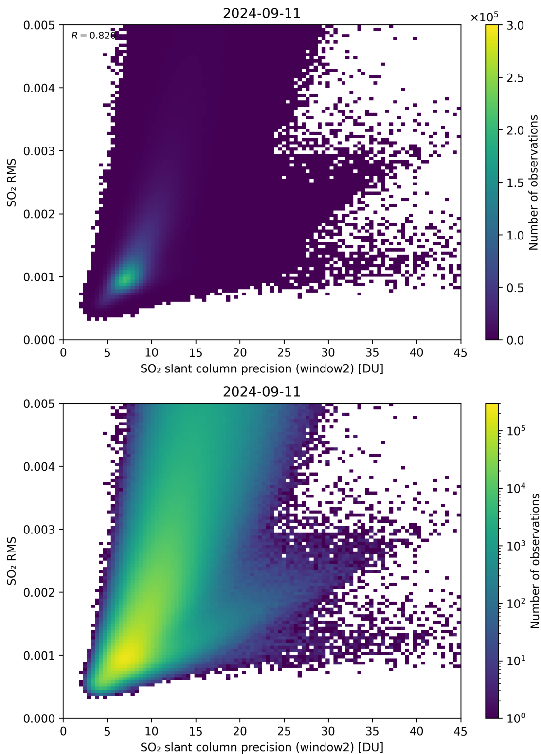
Figure 245: Scatter density plot of “SO 2 slant column precision (window2)” against “SO 2 RMS” for 2024-09-10 to 2024-09-12.
