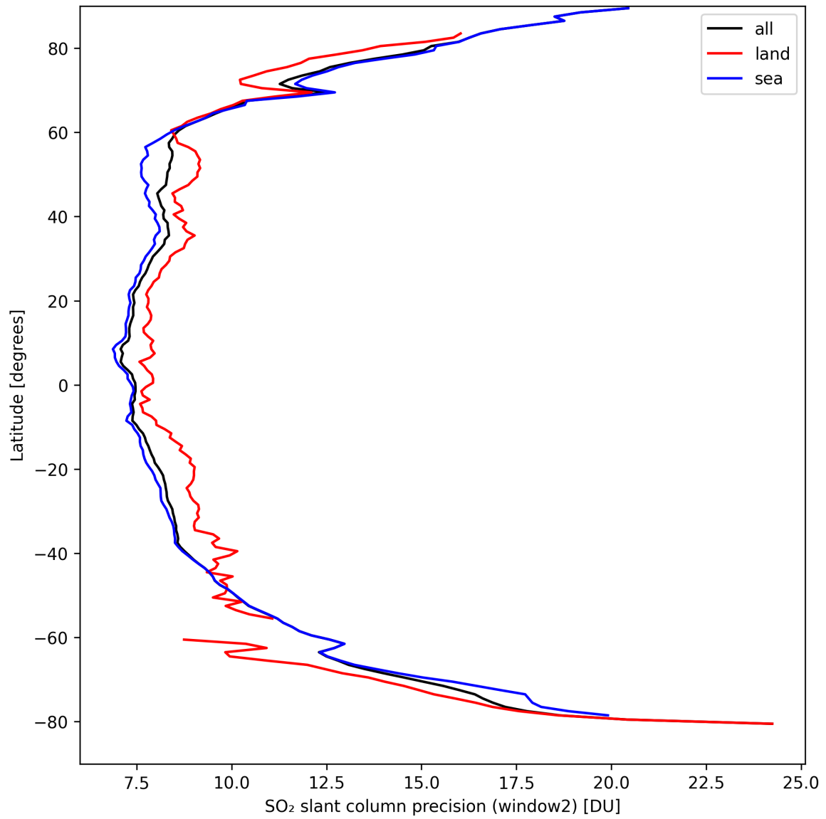
Figure 38: Zonal average of “SO 2 slant column precision (window2)” for 2024-09-10 to 2024-09-12.
