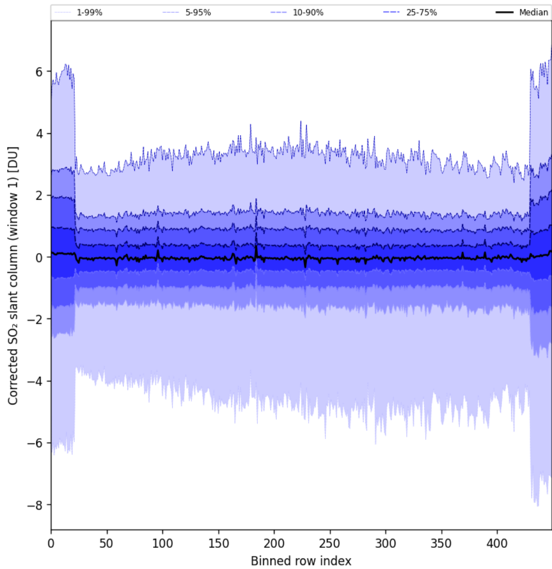
Figure 81: Along track statistics of “Corrected SO 2 slant column (window 1)” for 2024-09-10 to 2024-09-12
