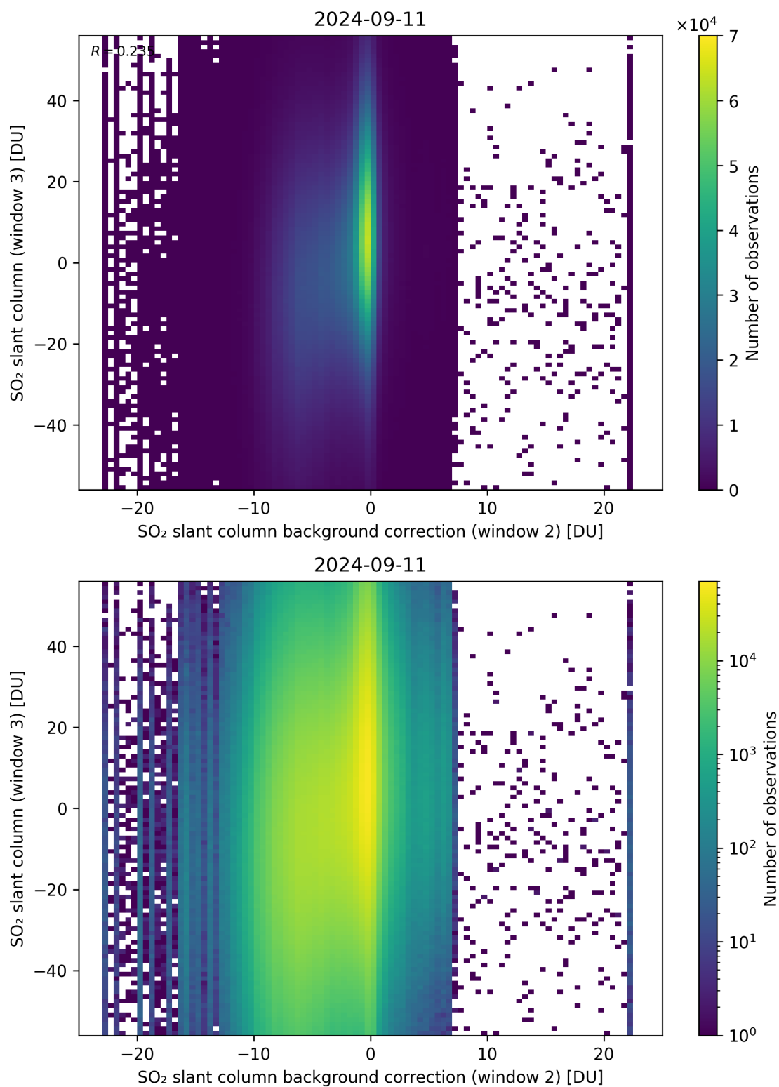
Figure 117: Scatter density plot of “SO 2 slant column background correction (window 2)” against “SO 2 slant column (window 3)” for 2024-09-10 to 2024-09-12.
