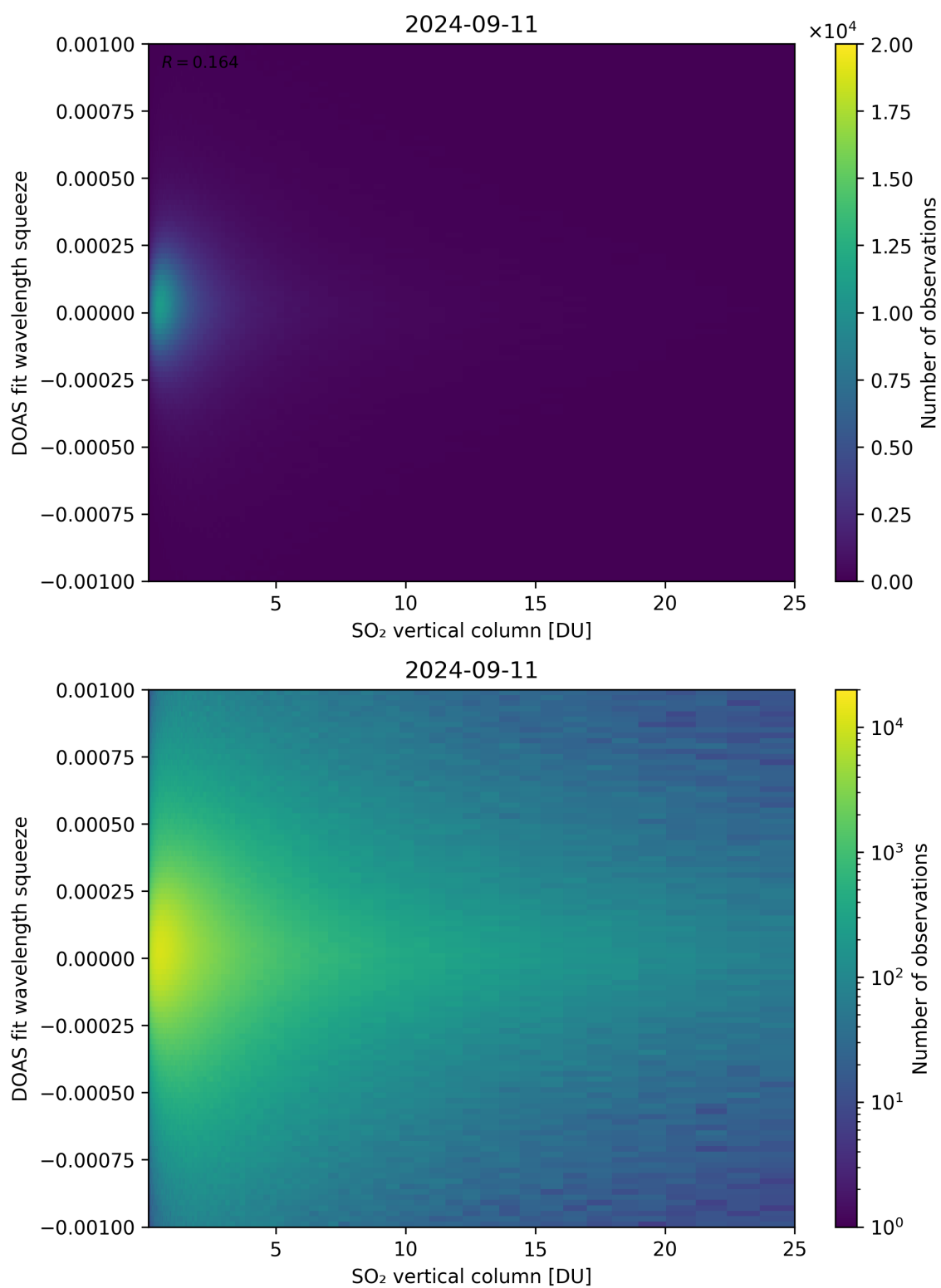
Figure 277: Scatter density plot of “SO 2 vertical column” against “DOAS fit wavelength squeeze” for 2024-09-10 to 2024-09-12.
