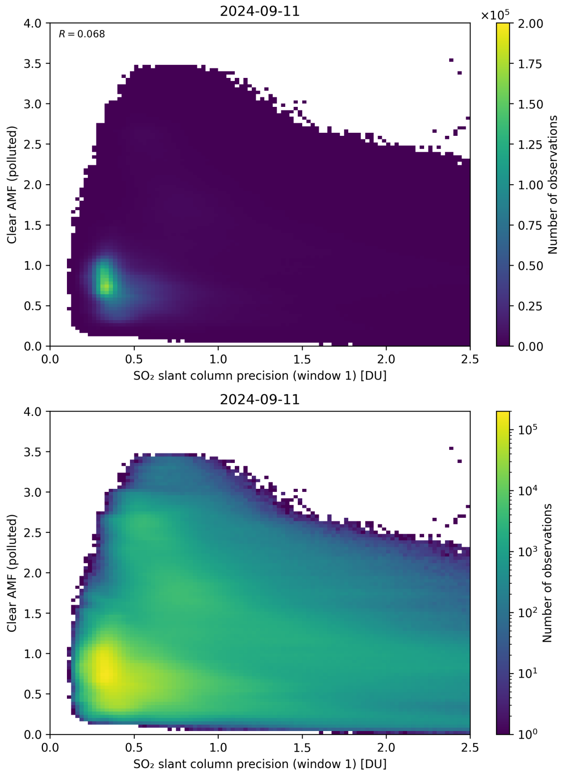
Figure 224: Scatter density plot of “SO 2 slant column precision (window 1)” against “Clear AMF (polluted)” for 2024-09-10 to 2024-09-12.
