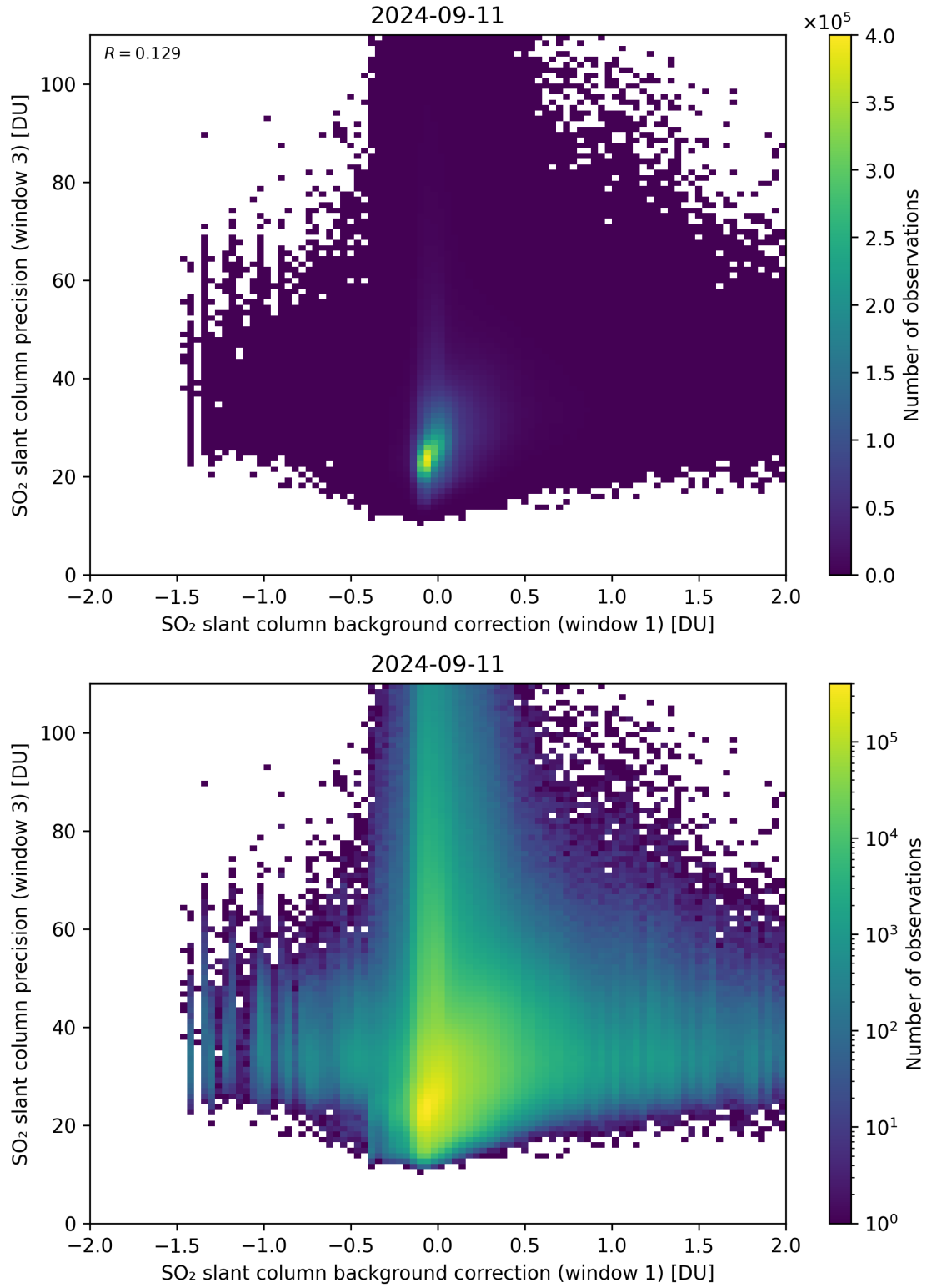
Figure 108: Scatter density plot of “SO 2 slant column background correction (window 1)” against “SO 2 slant column precision (window 3)” for 2024-09-10 to 2024-09-12.
