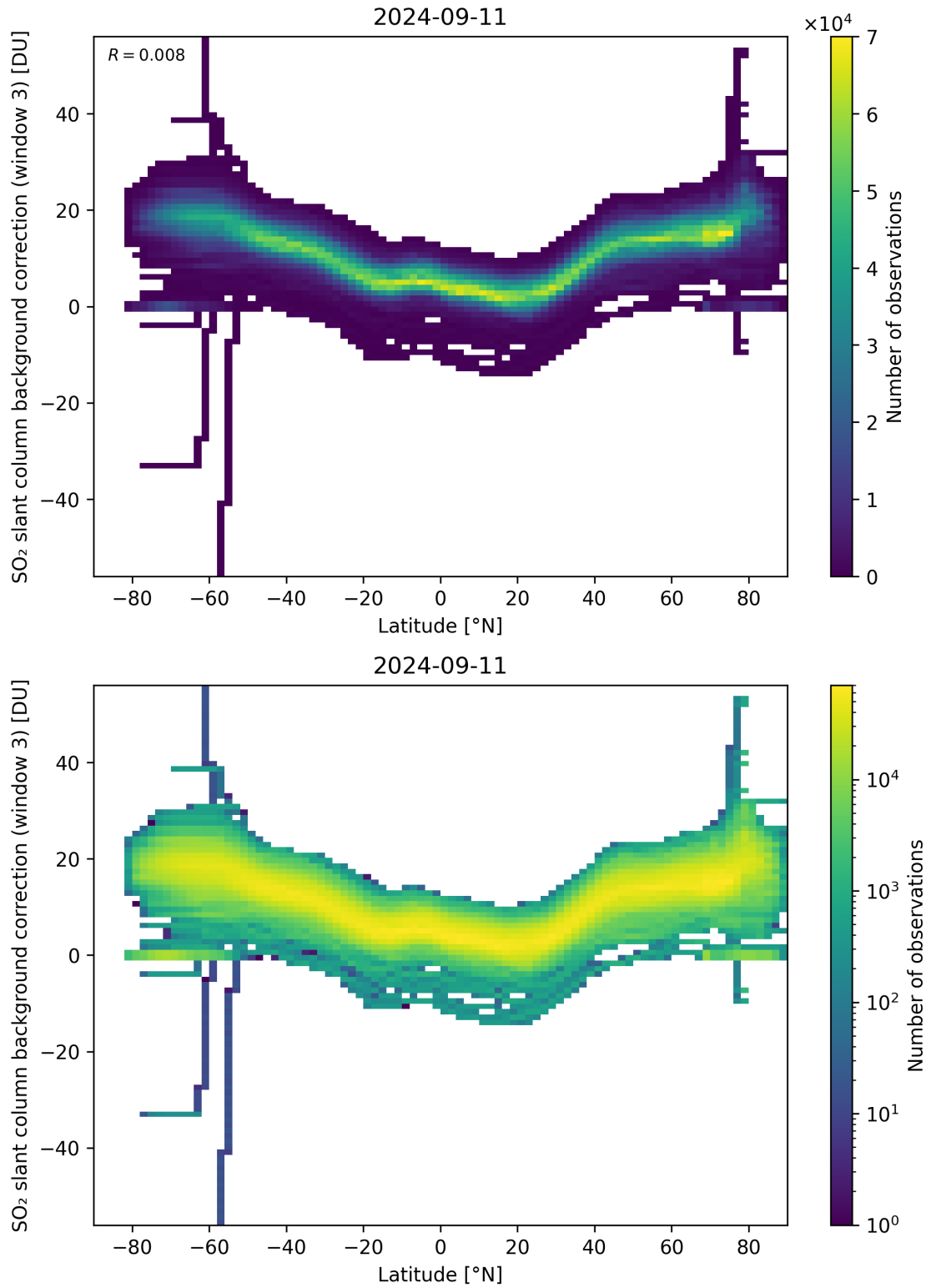
Figure 141: Scatter density plot of “Latitude” against “SO 2 slant column background correction (window 3)” for 2024-09-10 to 2024-09-12.
