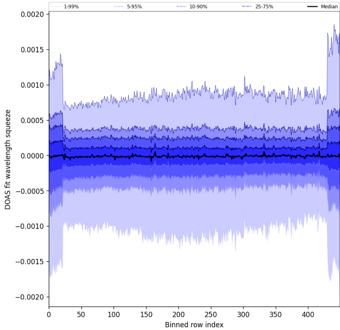
Figure 92: Along track statistics of “DOAS fit wavelength squeeze” for 2024-09-10 to 2024-09-12
