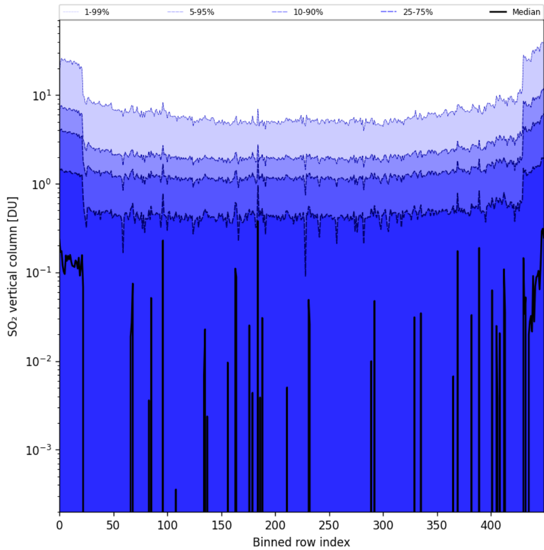
Figure 76: Along track statistics of “SO 2 vertical column” for 2024-09-10 to 2024-09-12
