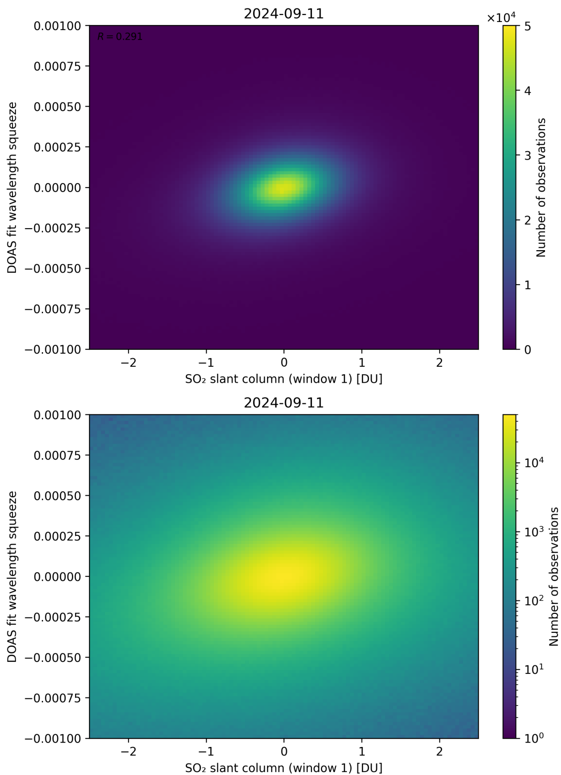
Figure 216: Scatter density plot of “SO 2 slant column (window 1)” against “DOAS fit wavelength squeeze” for 2024-09-10 to 2024-09-12.
