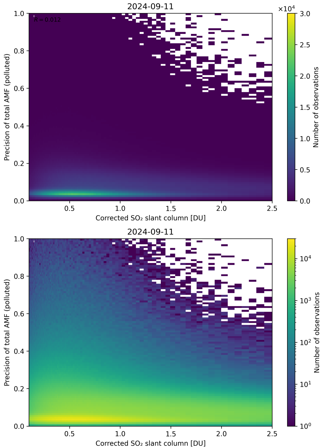
Figure 193: Scatter density plot of “Corrected SO 2 slant column” against “Precision of total AMF (polluted)” for 2024-09-10 to 2024-09-12.
