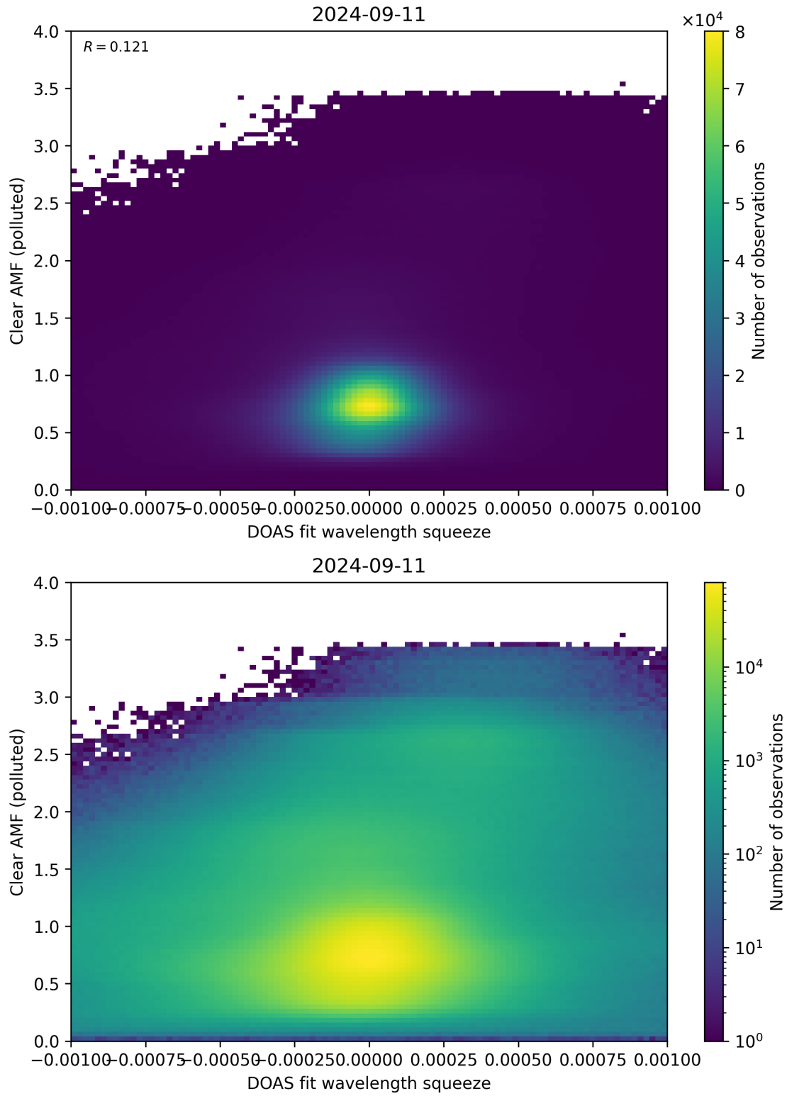
Figure 133: Scatter density plot of “DOAS fit wavelength squeeze” against “Clear AMF (polluted)” for 2024-09-10 to 2024-09-12.
