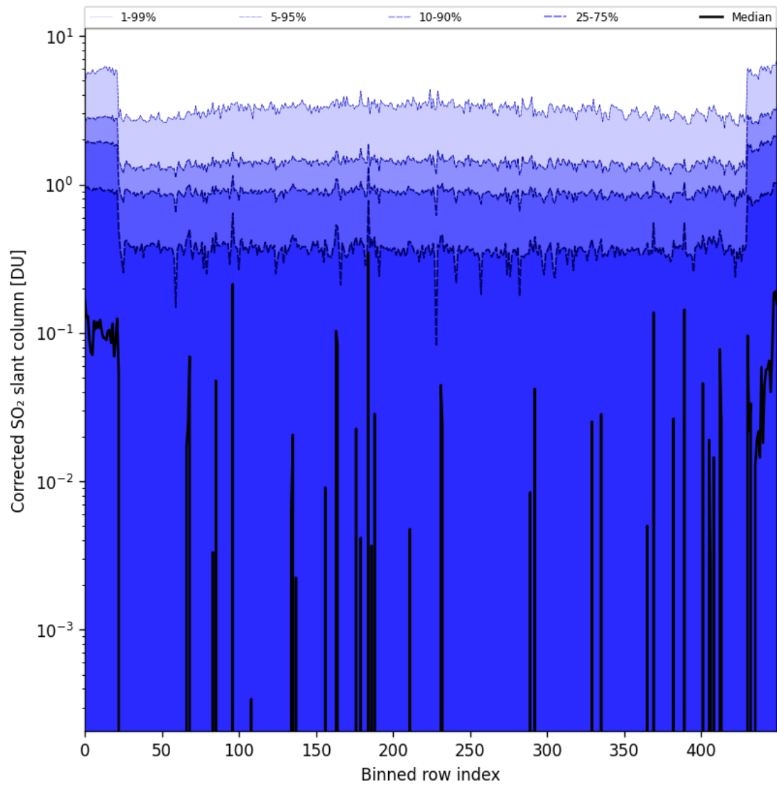
Figure 78: Along track statistics of “Corrected SO 2 slant column” for 2024-09-10 to 2024-09-12
