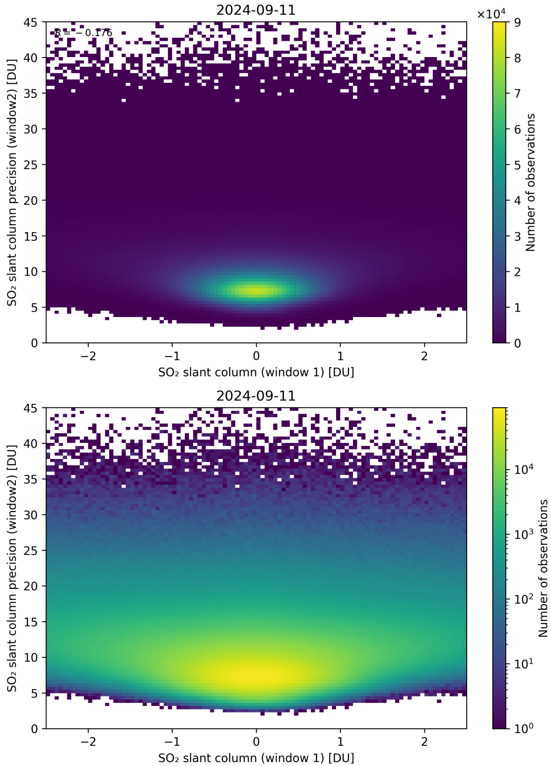
Figure 236: Scatter density plot of “SO 2 slant column (window 1)” against “SO 2 slant column precision (window2)” for 2024-09-10 to 2024-09-12.
