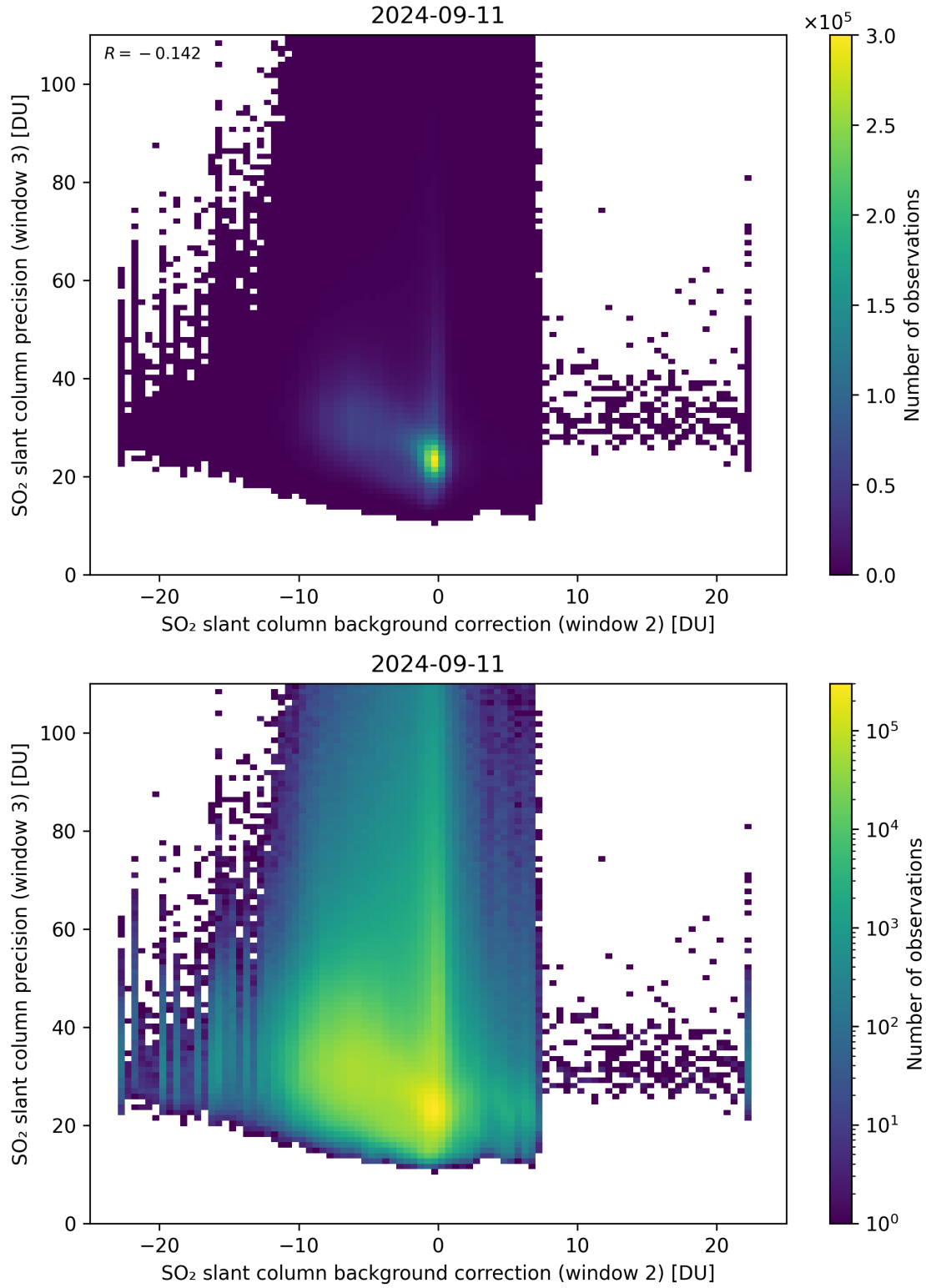
Figure 118: Scatter density plot of “SO 2 slant column background correction (window 2)” against “SO 2 slant column precision (window 3)” for 2024-09-10 to 2024-09-12.
