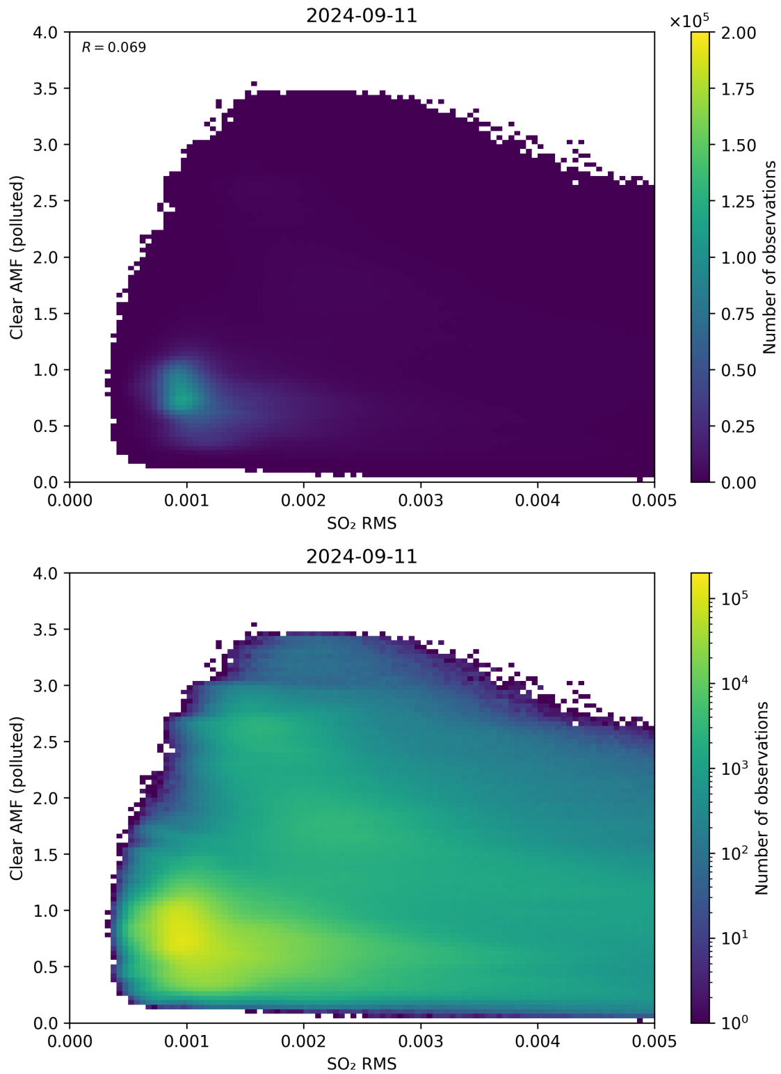
Figure 136: Scatter density plot of “SO 2 RMS” against “Clear AMF (polluted)” for 2024-09-10 to 2024-09-12.
