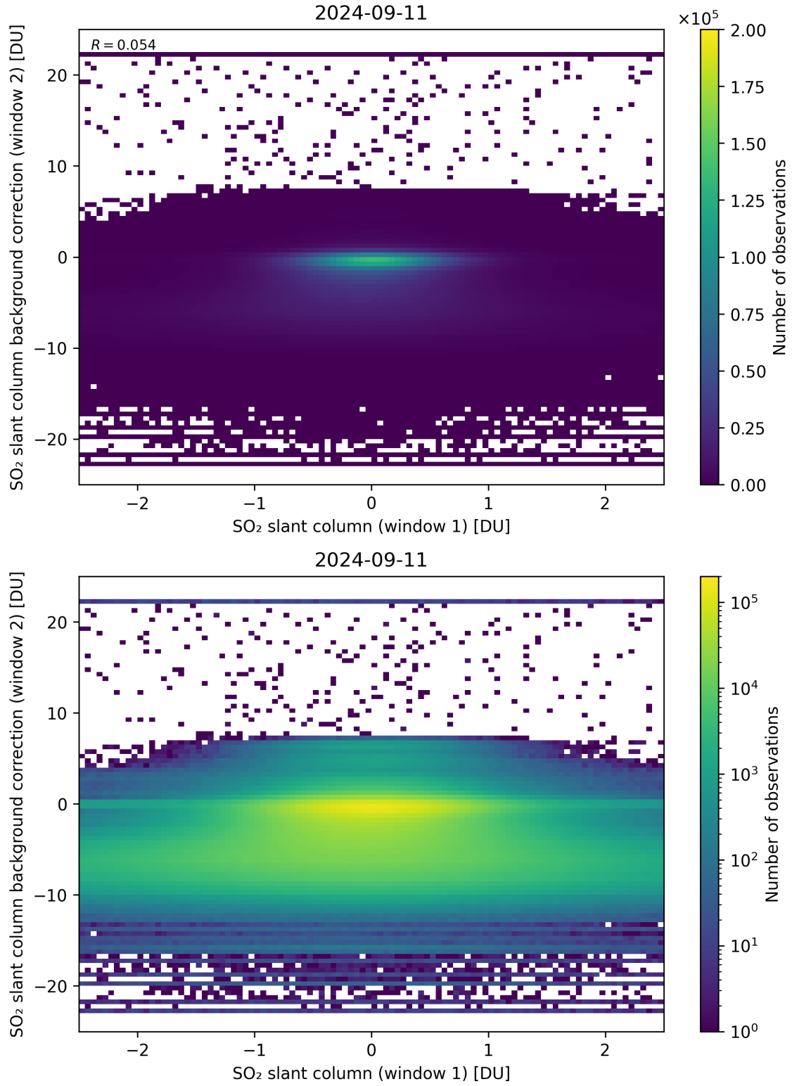
Figure 213: Scatter density plot of “SO 2 slant column (window 1)” against “SO 2 slant column background correction (window 2)” for 2024-09-10 to 2024-09-12.
