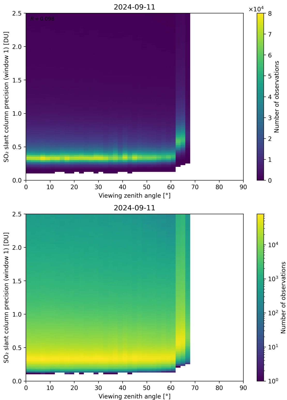
Figure 321: Scatter density plot of “Viewing zenith angle” against “SO 2 slant column precision (window 1)” for 2024-09-10 to 2024-09-12.
