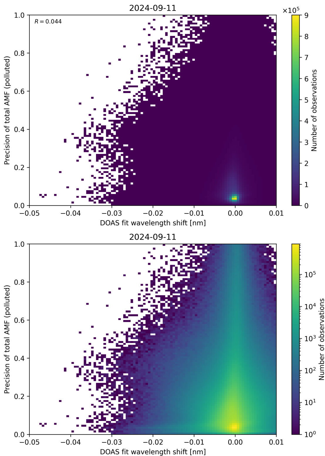
Figure 131: Scatter density plot of “DOAS fit wavelength shift” against “Precision of total AMF (polluted)” for 2024-09-10 to 2024-09-12.
