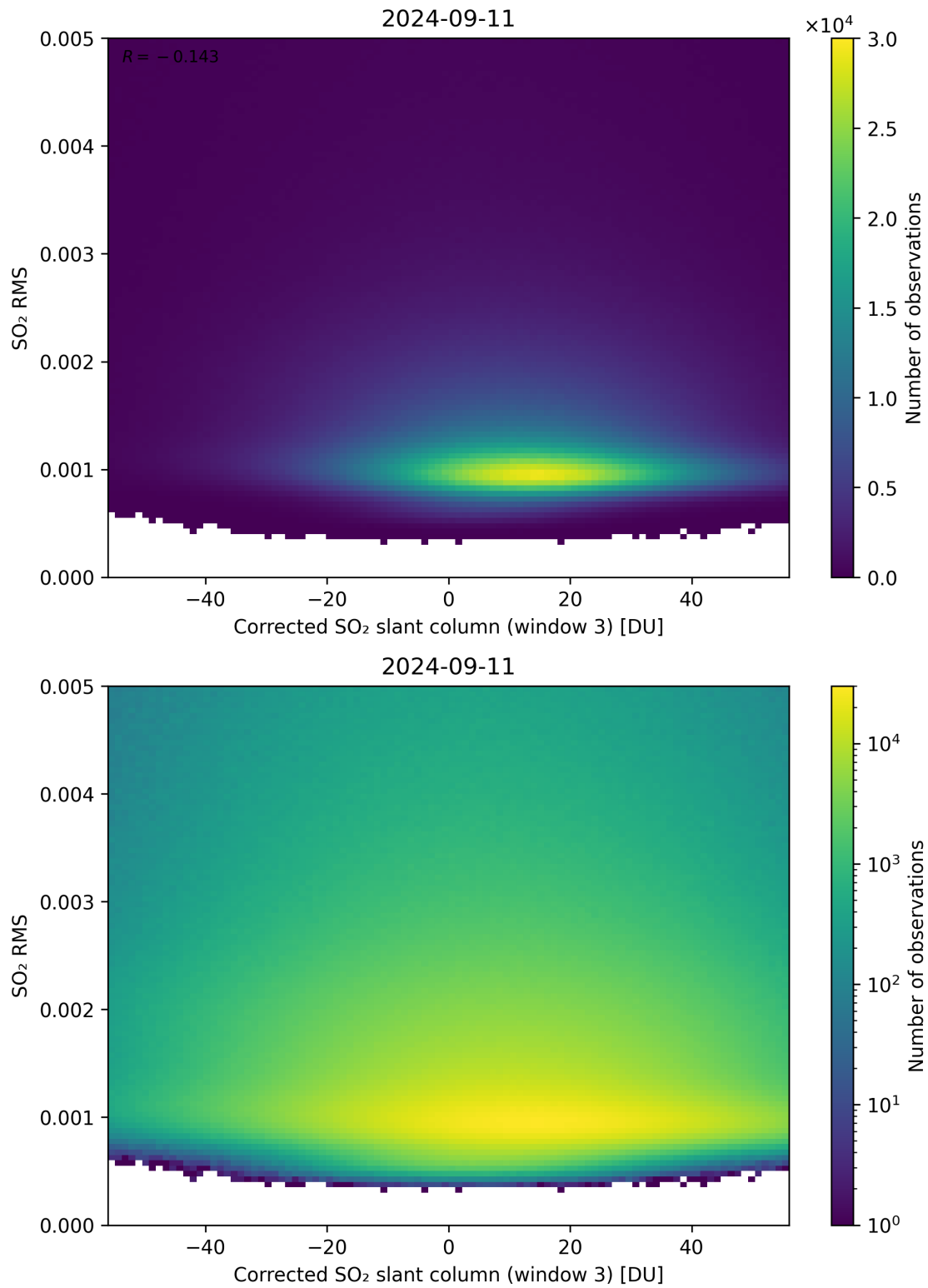
Figure 208: Scatter density plot of “Corrected SO 2 slant column (window 3)” against “SO 2 RMS” for 2024-09-10 to 2024-09-12.
