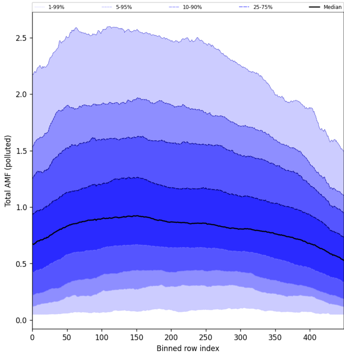
Figure 94: Along track statistics of “Total AMF (polluted)” for 2024-09-10 to 2024-09-12
