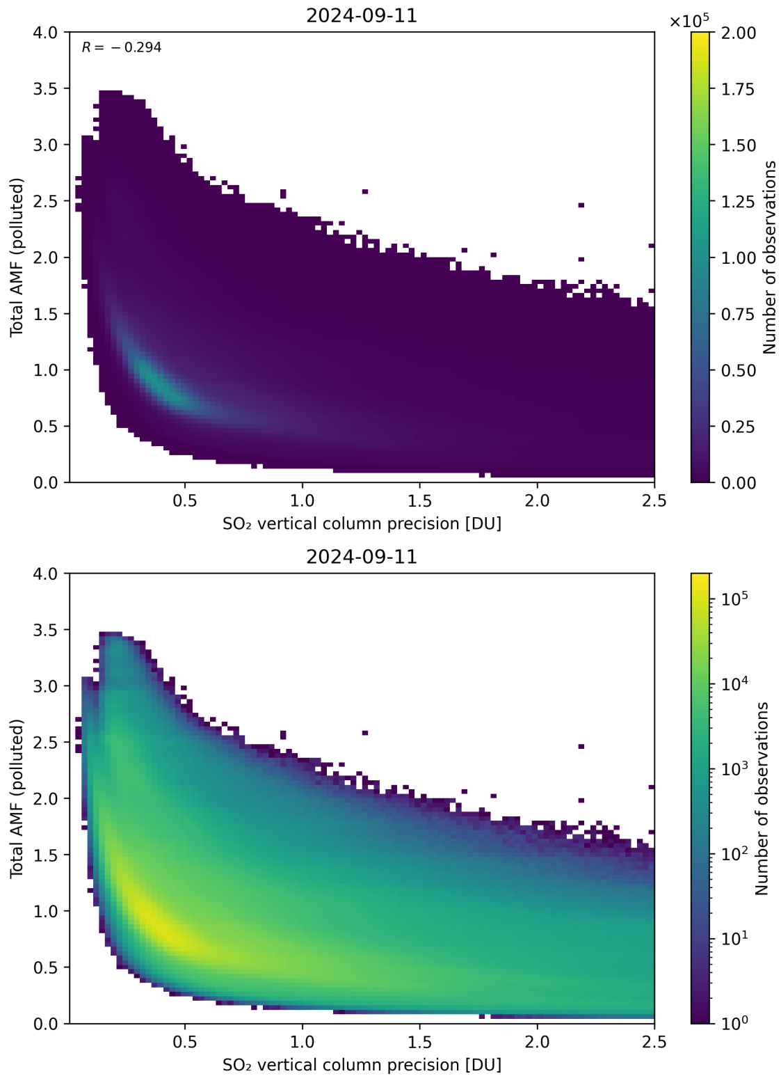
Figure 294: Scatter density plot of “SO 2 vertical column precision” against “Total AMF (polluted)” for 2024-09-10 to 2024-09-12.
