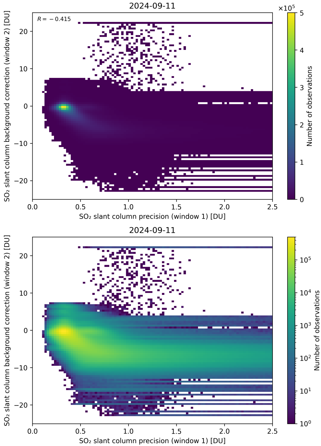
Figure 219: Scatter density plot of “SO 2 slant column precision (window 1)” against “SO 2 slant column background correction (window 2)” for 2024-09-10 to 2024-09-12.
