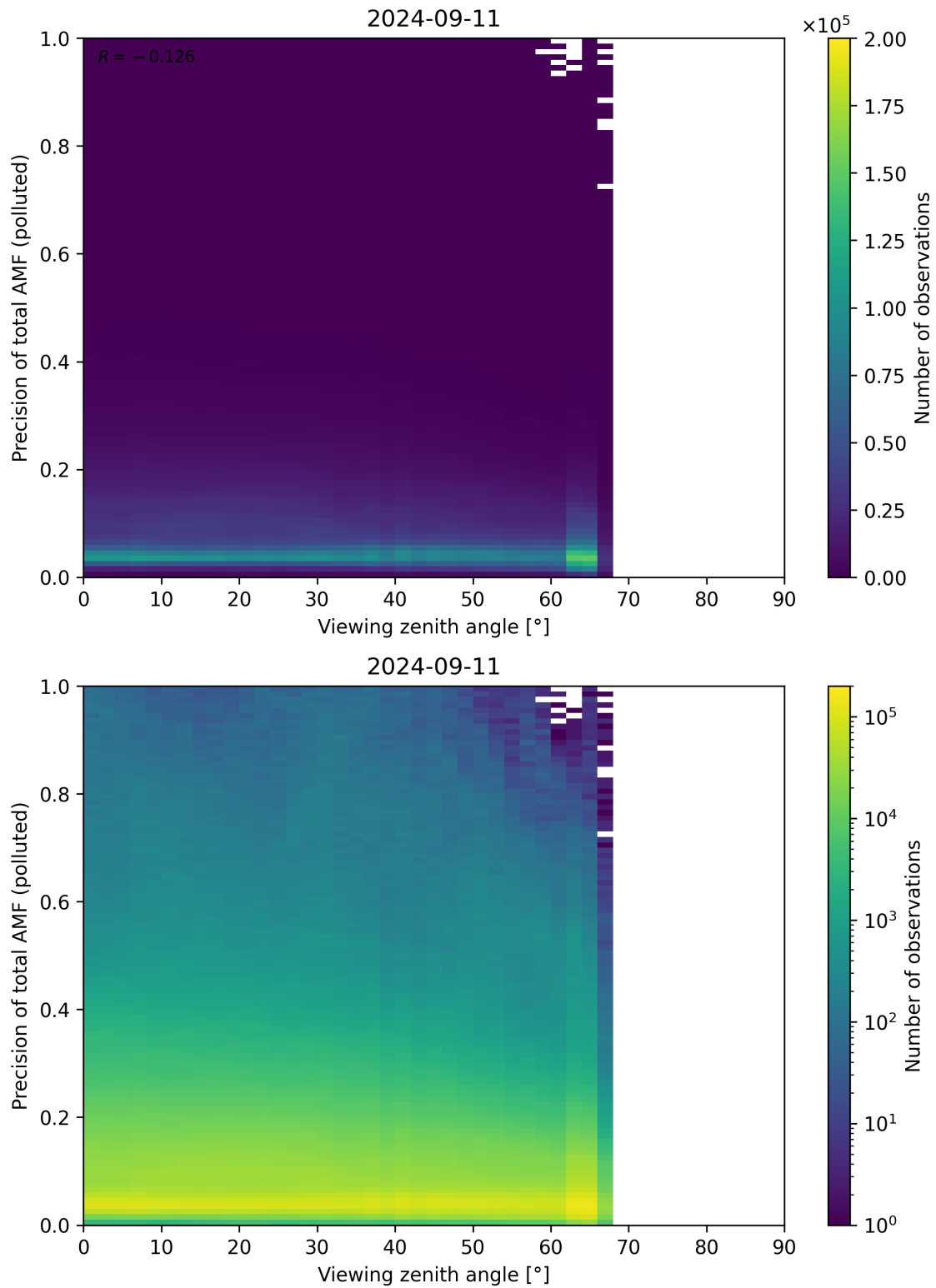
Figure 326: Scatter density plot of “Viewing zenith angle” against “Precision of total AMF (polluted)” for 2024-09-10 to 2024-09-12.
