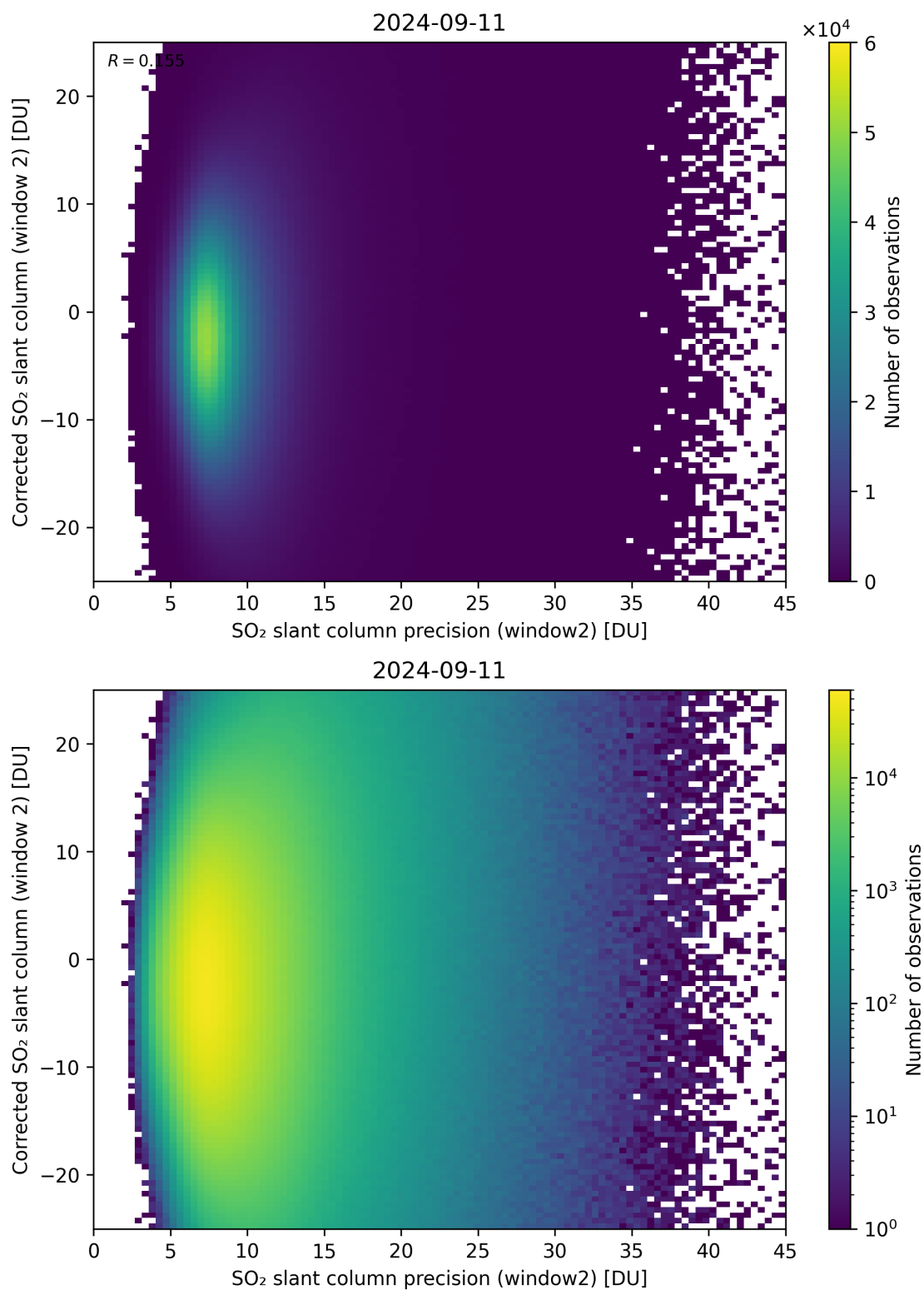
Figure 247: Scatter density plot of “SO 2 slant column precision (window2)” against “Corrected SO 2 slant column (window 2)” for 2024-09-10 to 2024-09-12.
