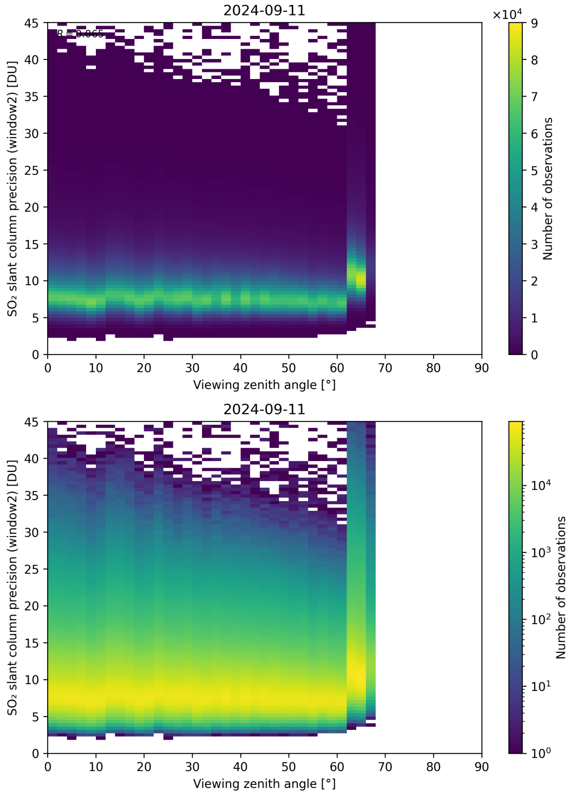
Figure 322: Scatter density plot of “Viewing zenith angle” against “SO 2 slant column precision (window2)” for 2024-09-10 to 2024-09-12.
