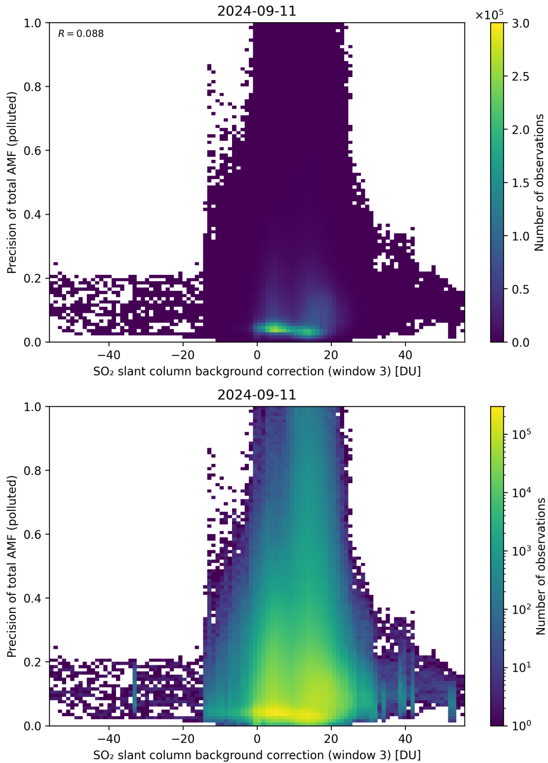
Figure 126: Scatter density plot of “SO 2 slant column background correction (window 3)” against “Precision of total AMF (polluted)” for 2024-09-10 to 2024-09-12.
