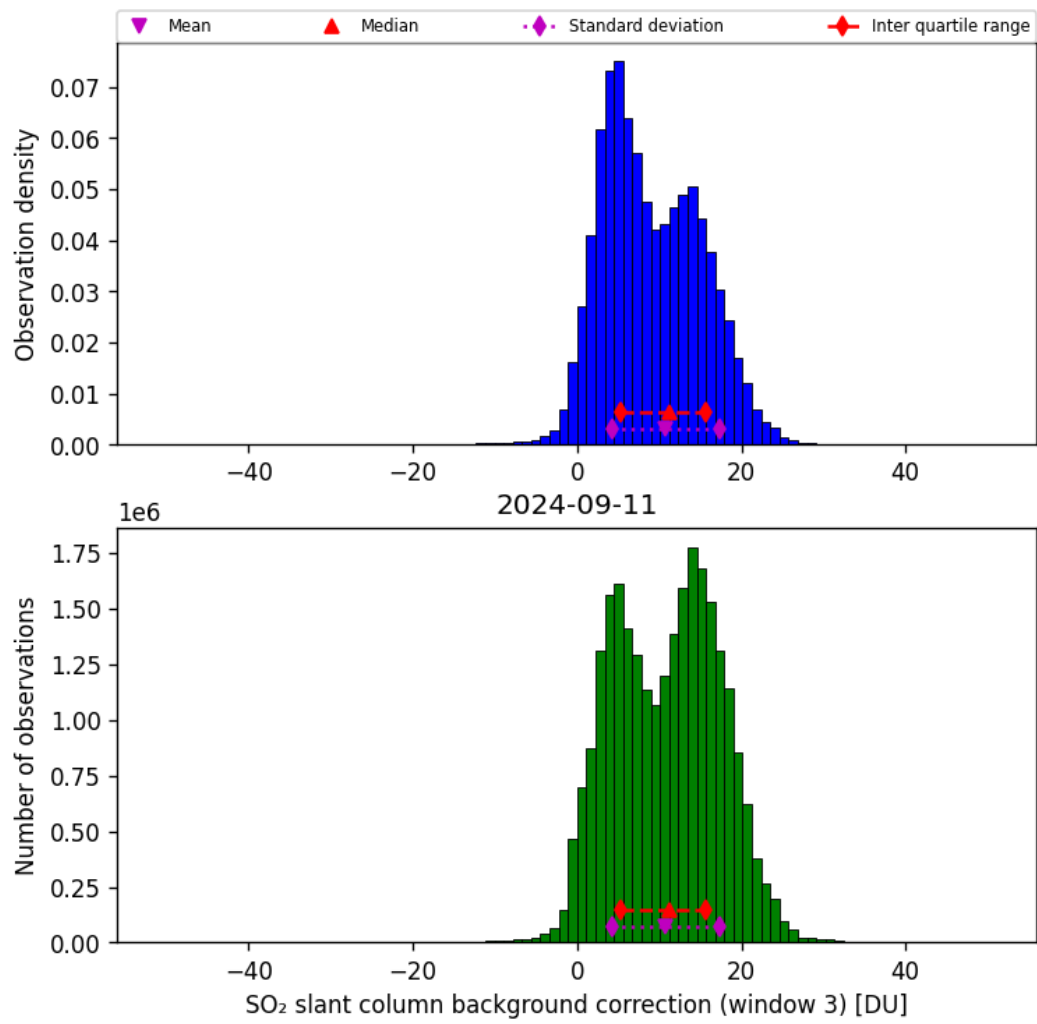
Figure 67: Histogram of “SO 2 slant column background correction (window 3)” for 2024-09-10 to 2024-09-12
