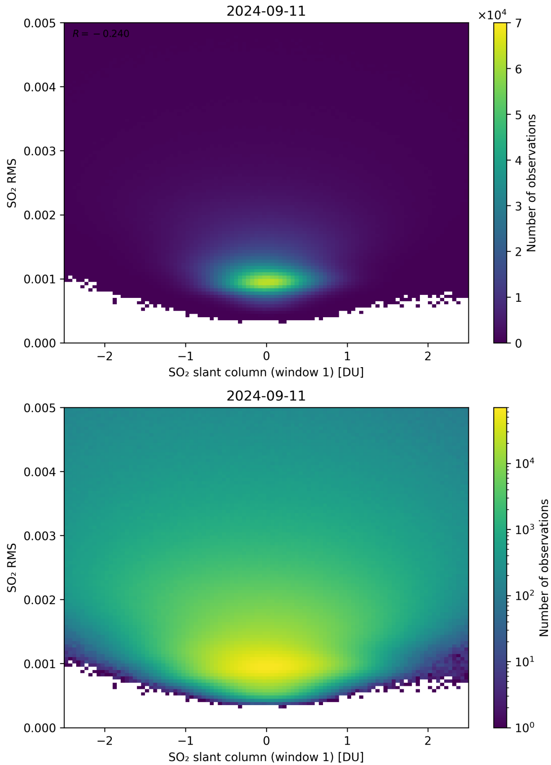
Figure 217: Scatter density plot of “SO 2 slant column (window 1)” against “SO 2 RMS” for 2024-09-10 to 2024-09-12.
