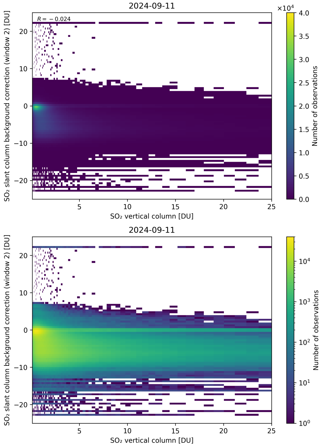
Figure 274: Scatter density plot of “SO 2 vertical column” against “SO 2 slant column background correction (window 2)” for 2024-09-10 to 2024-09-12.
