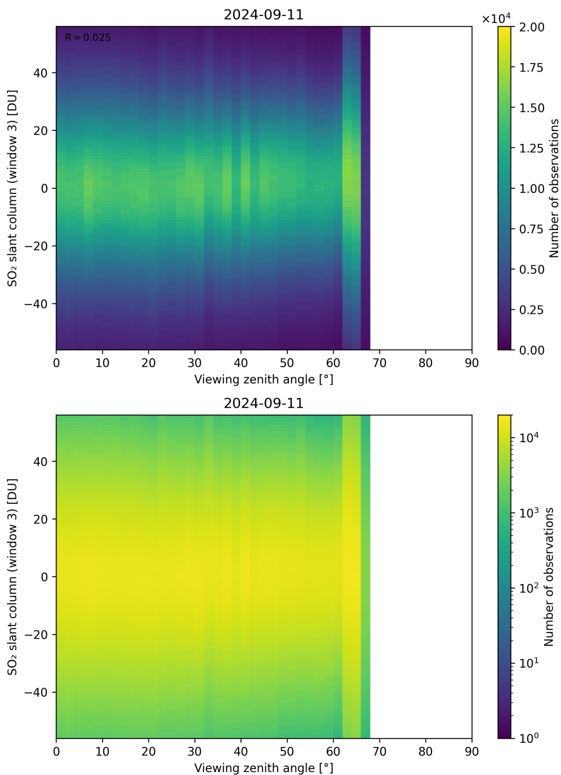
Figure 323: Scatter density plot of “Viewing zenith angle” against “SO 2 slant column (window 3)” for 2024-09-10 to 2024-09-12.
