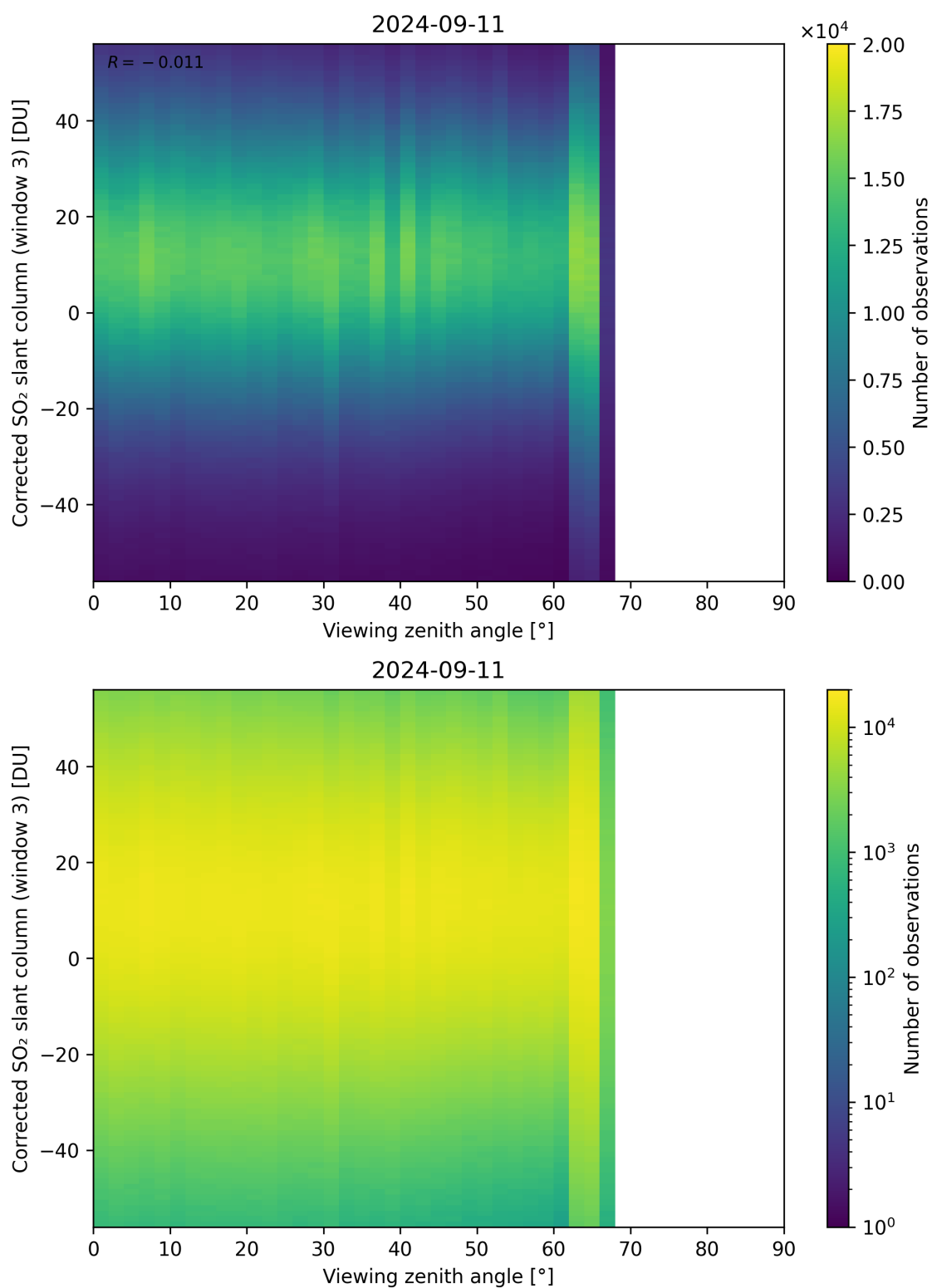
Figure 319: Scatter density plot of “Viewing zenith angle” against “Corrected SO 2 slant column (window 3)” for 2024-09-10 to 2024-09-12.
