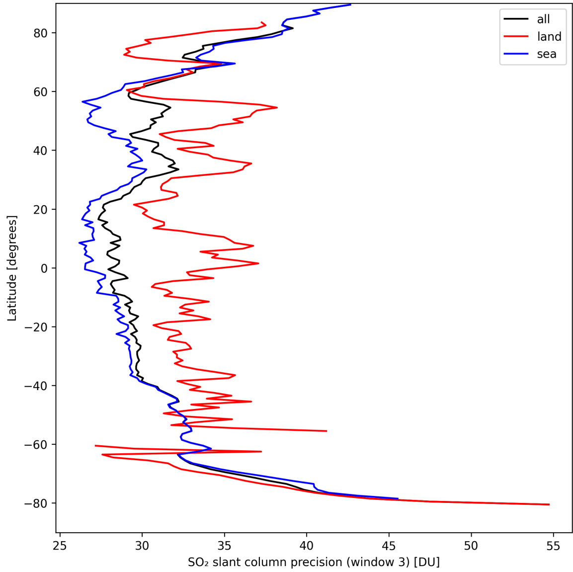
Figure 42: Zonal average of “SO 2 slant column precision (window 3)” for 2024-09-10 to 2024-09-12.
