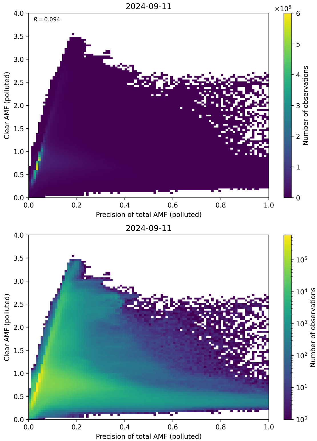
Figure 270: Scatter density plot of “Precision of total AMF (polluted)” against “Clear AMF (polluted)” for 2024-09-10 to 2024-09-12.
