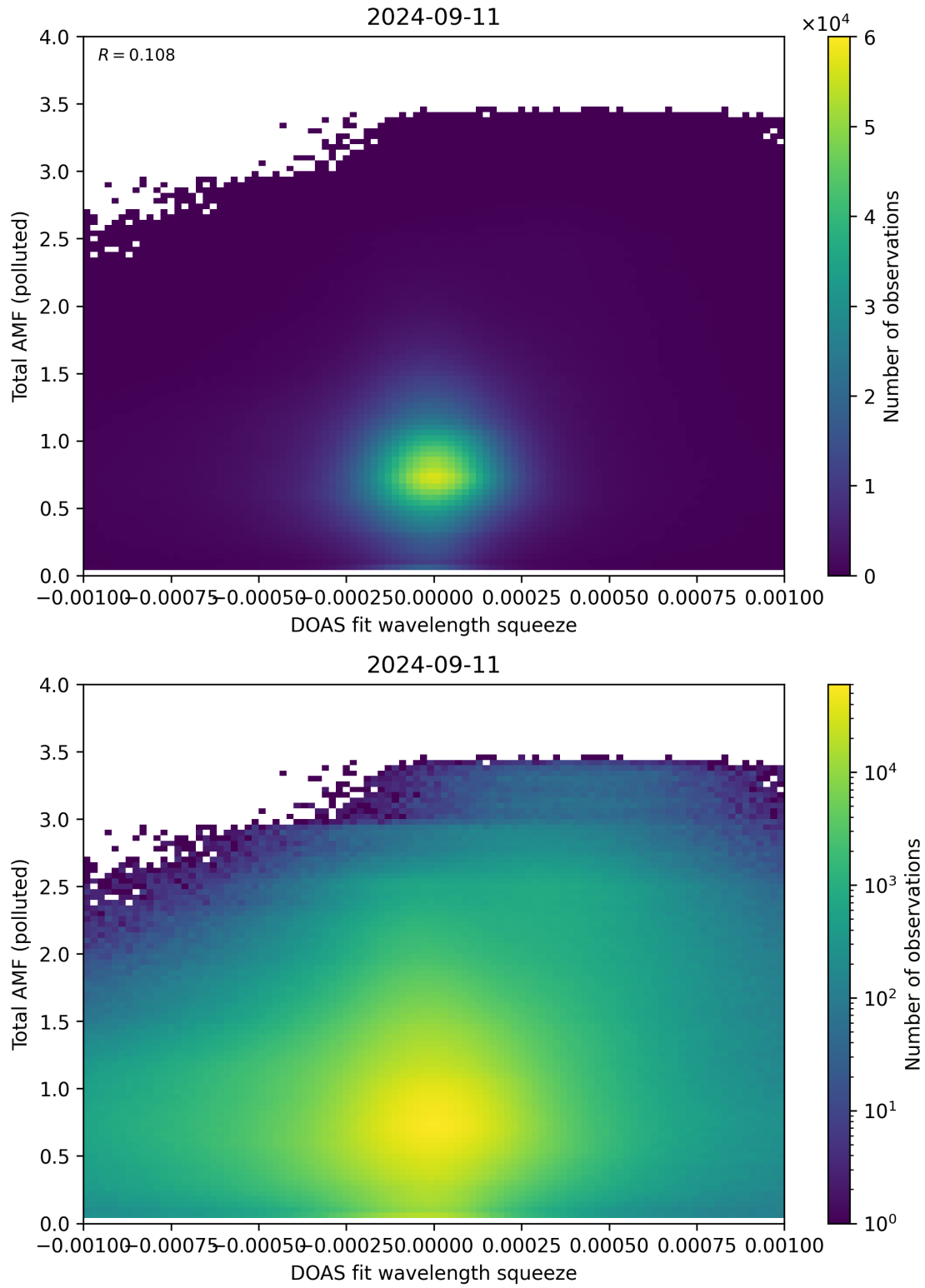
Figure 134: Scatter density plot of “DOAS fit wavelength squeeze” against “Total AMF (polluted)” for 2024-09-10 to 2024-09-12.
