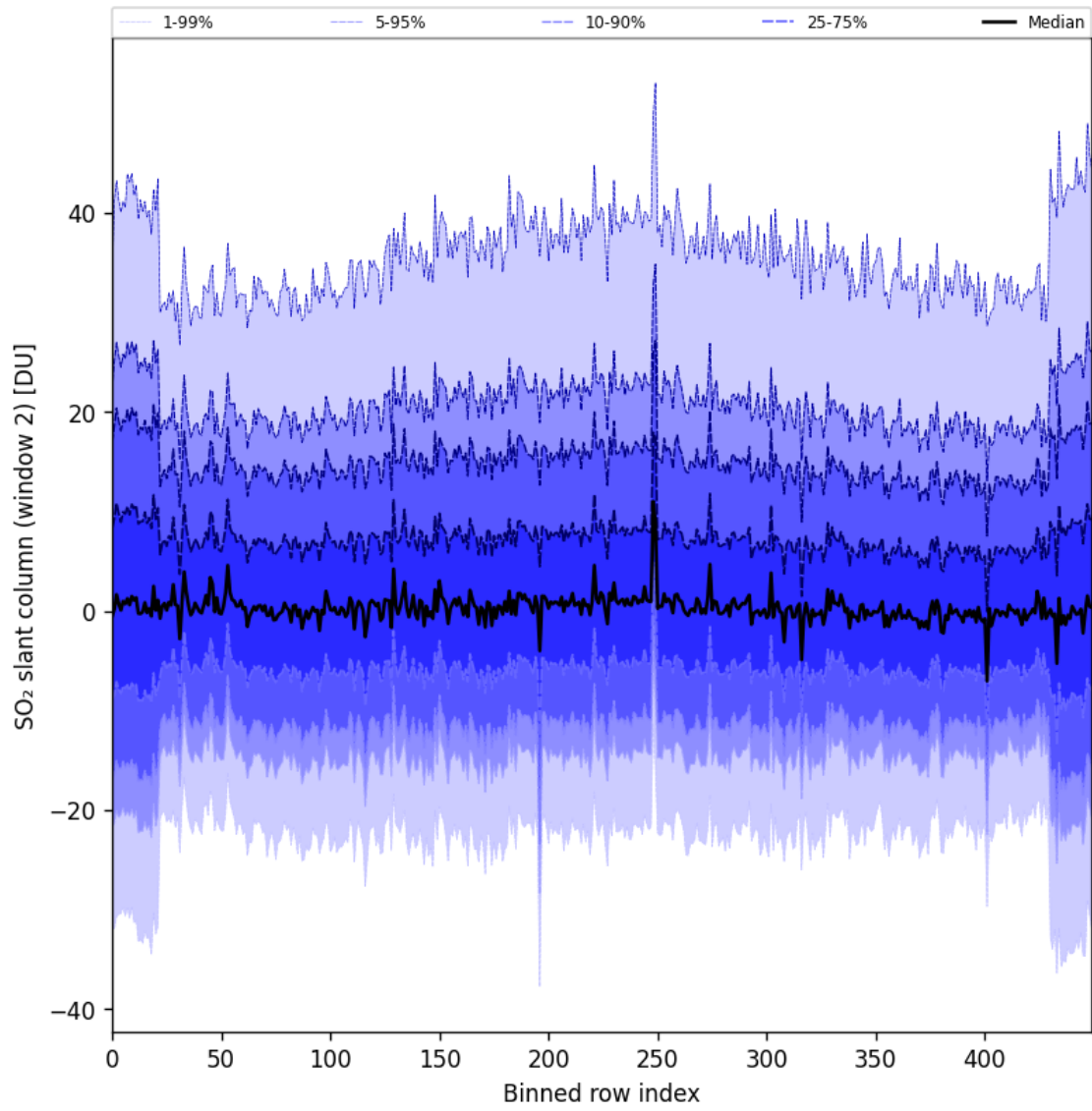
Figure 83: Along track statistics of “SO 2 slant column (window 2)” for 2024-09-10 to 2024-09-12
