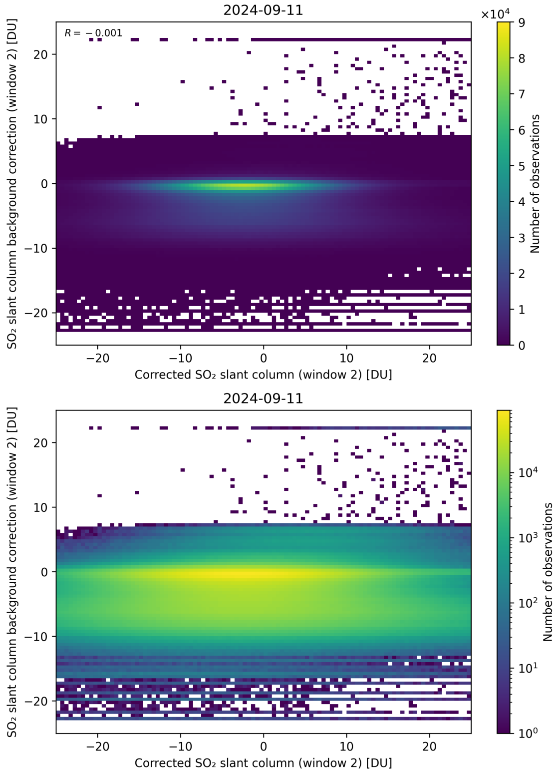
Figure 194: Scatter density plot of “Corrected SO 2 slant column (window 2)” against “SO 2 slant column background correction (window 2)” for 2024-09-10 to 2024-09-12.
