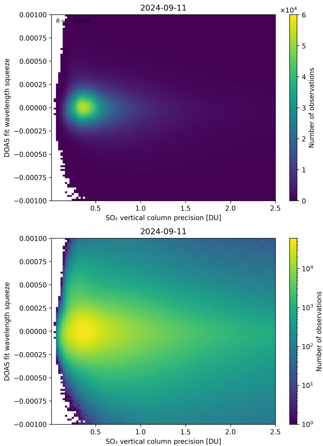
Figure 283: Scatter density plot of “SO 2 vertical column precision” against “DOAS fit wavelength squeeze” for 2024-09-10 to 2024-09-12.
