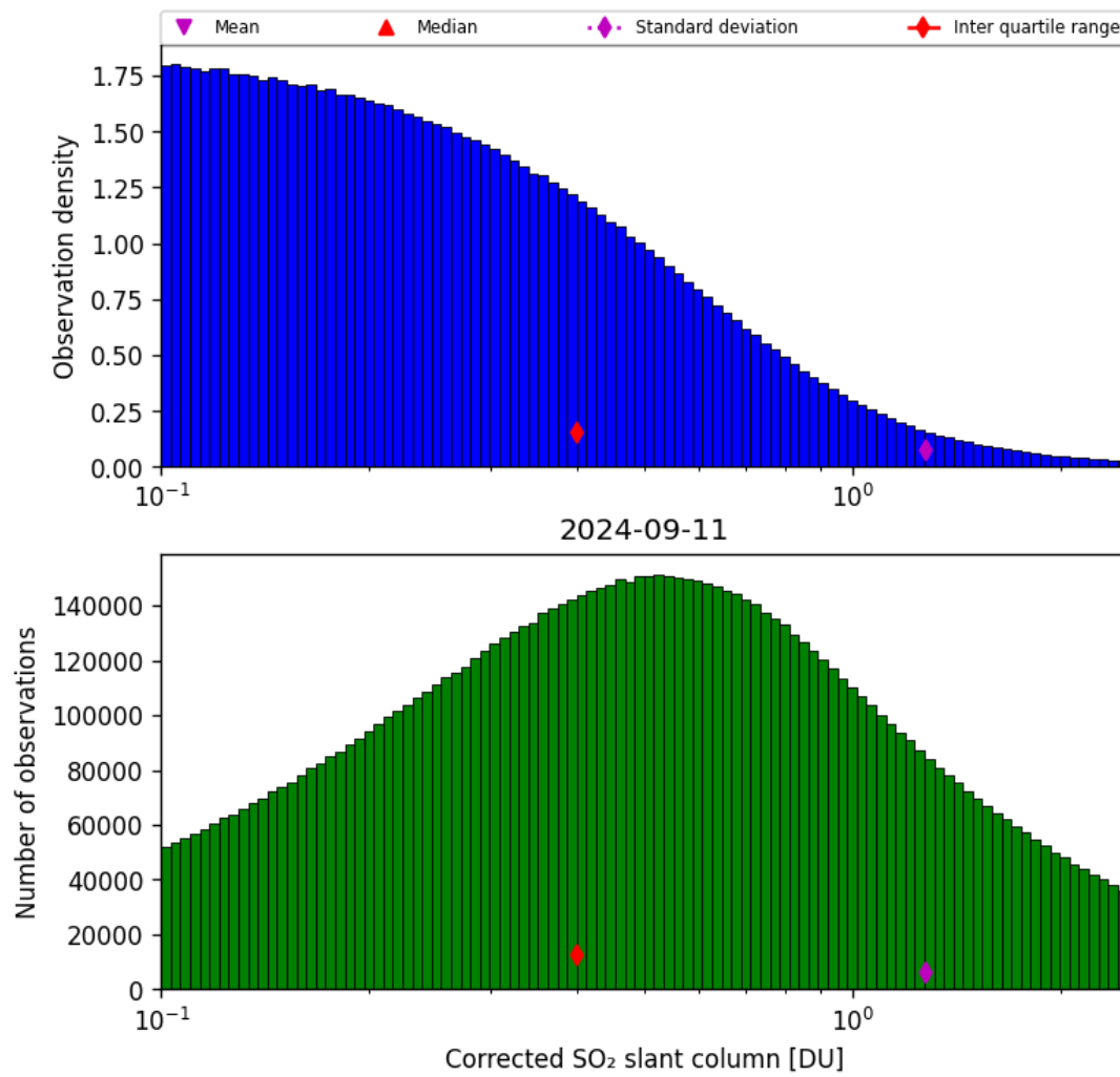
Figure 55: Histogram of “Corrected SO 2 slant column” for 2024-09-10 to 2024-09-12
