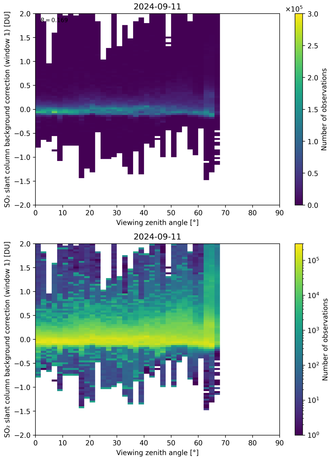
Figure 308: Scatter density plot of “Viewing zenith angle” against “SO 2 slant column background correction (window 1)” for 2024-09-10 to 2024-09-12.
