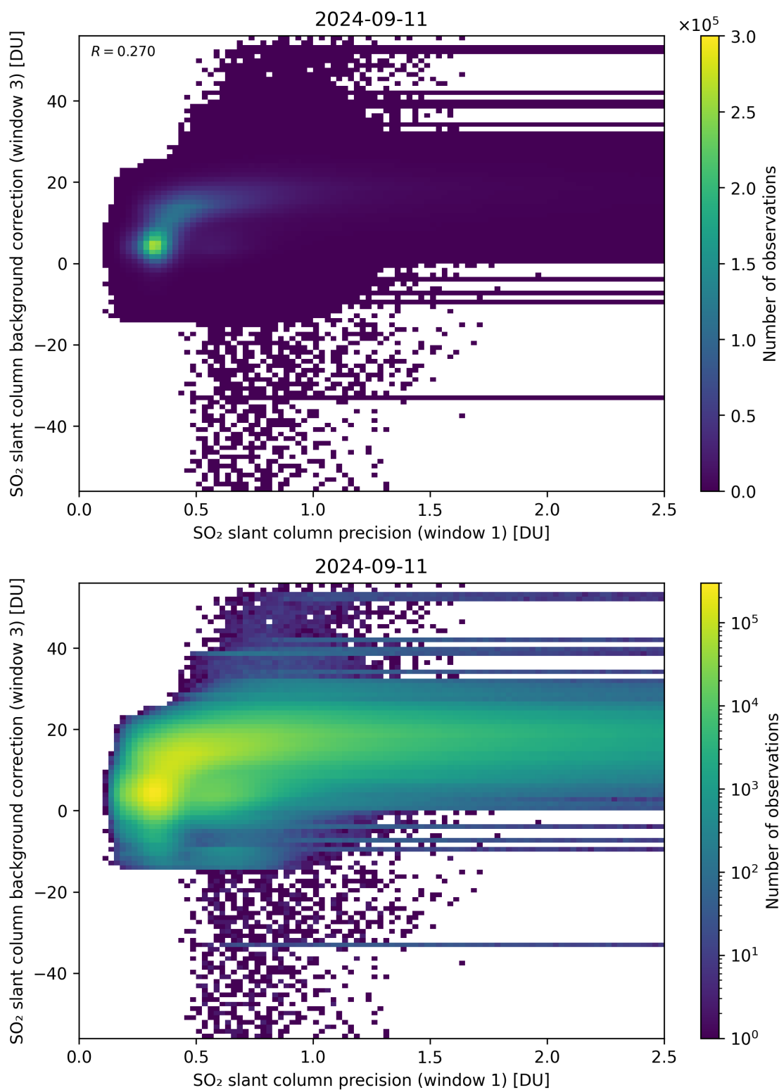
Figure 220: Scatter density plot of “SO 2 slant column precision (window 1)” against “SO 2 slant column background correction (window 3)” for 2024-09-10 to 2024-09-12.
