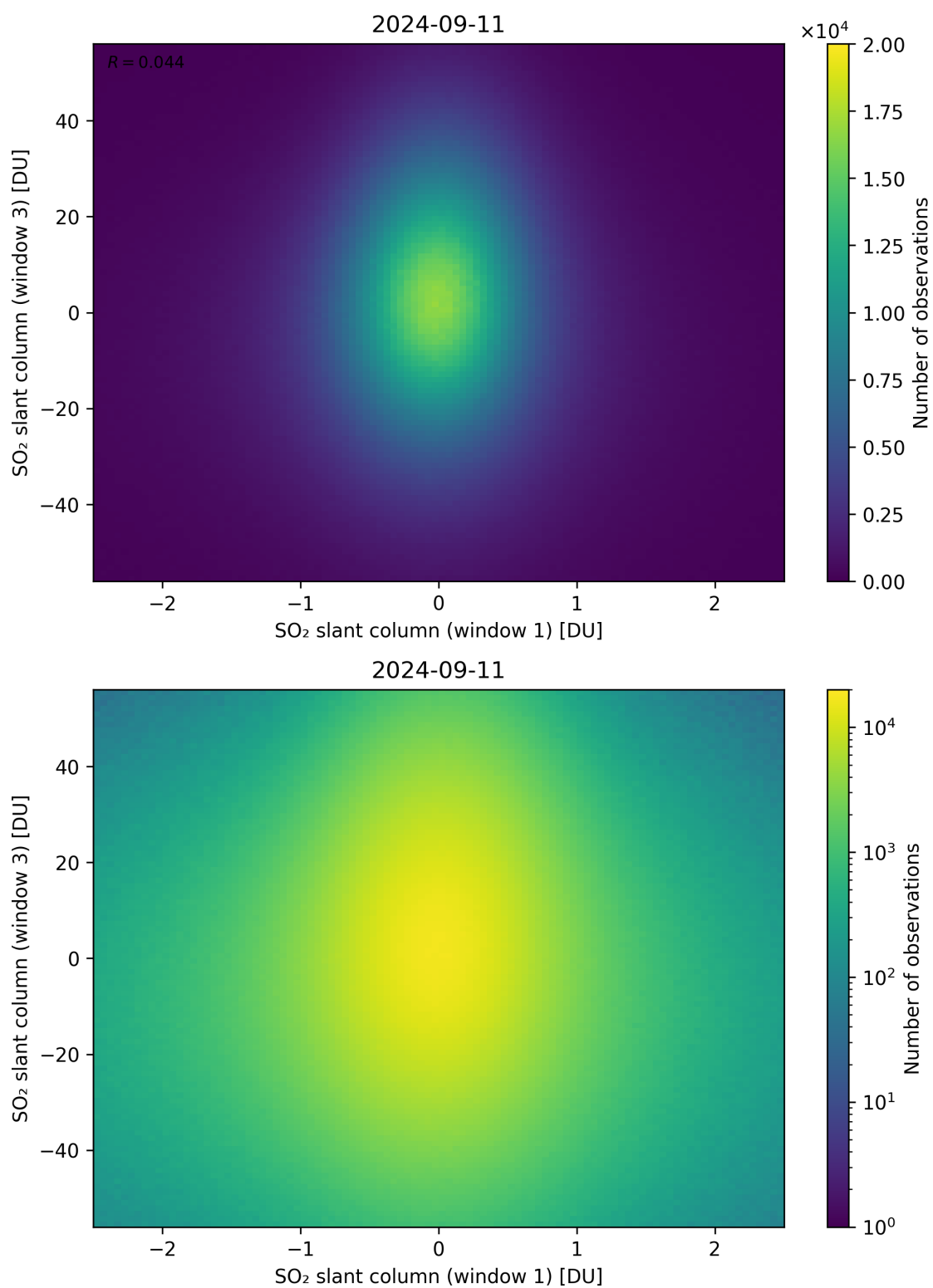
Figure 237: Scatter density plot of “SO 2 slant column (window 1)” against “SO 2 slant column (window 3)” for 2024-09-10 to 2024-09-12.
