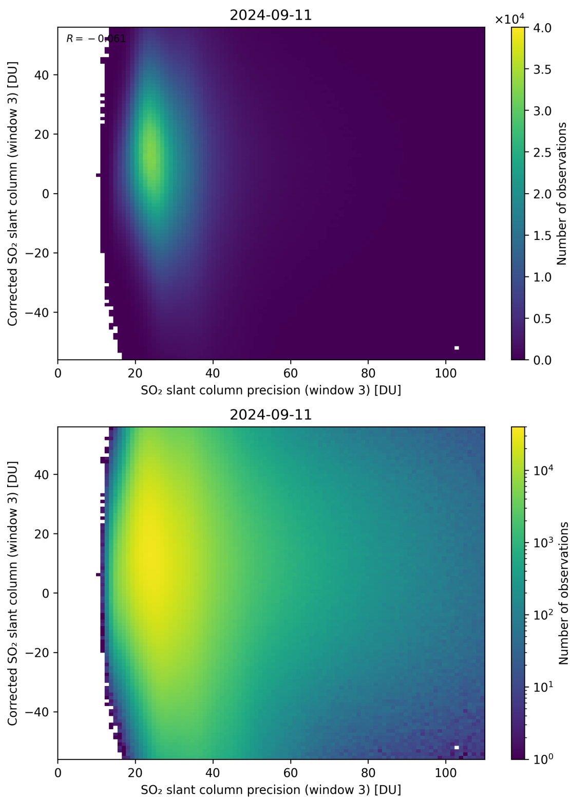
Figure 262: Scatter density plot of “SO 2 slant column precision (window 3)” against “Corrected SO 2 slant column (window 3)” for 2024-09-10 to 2024-09-12.
