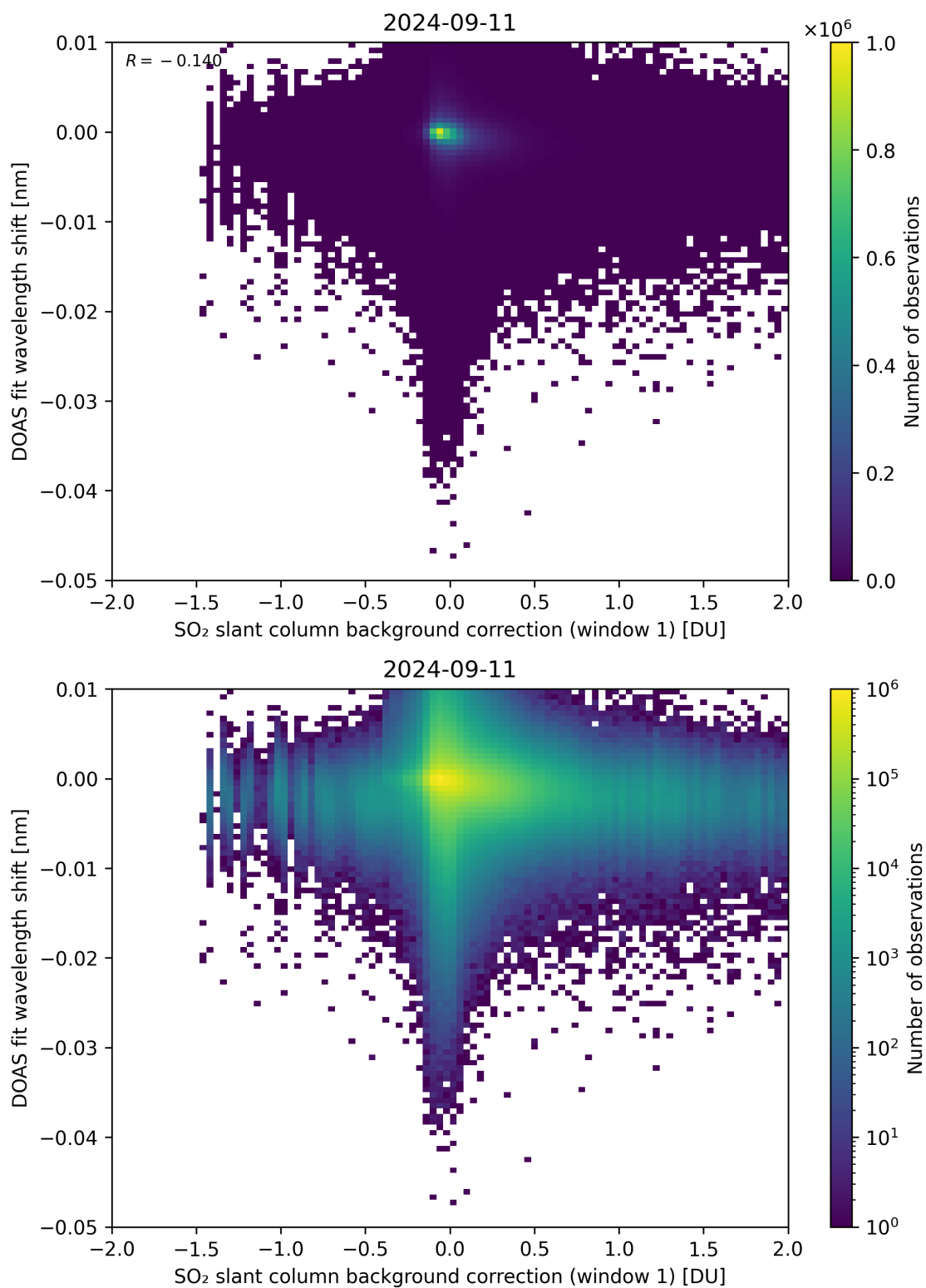
Figure 100: Scatter density plot of “SO 2 slant column background correction (window 1)” against “DOAS fit wavelength shift” for 2024-09-10 to 2024-09-12.
