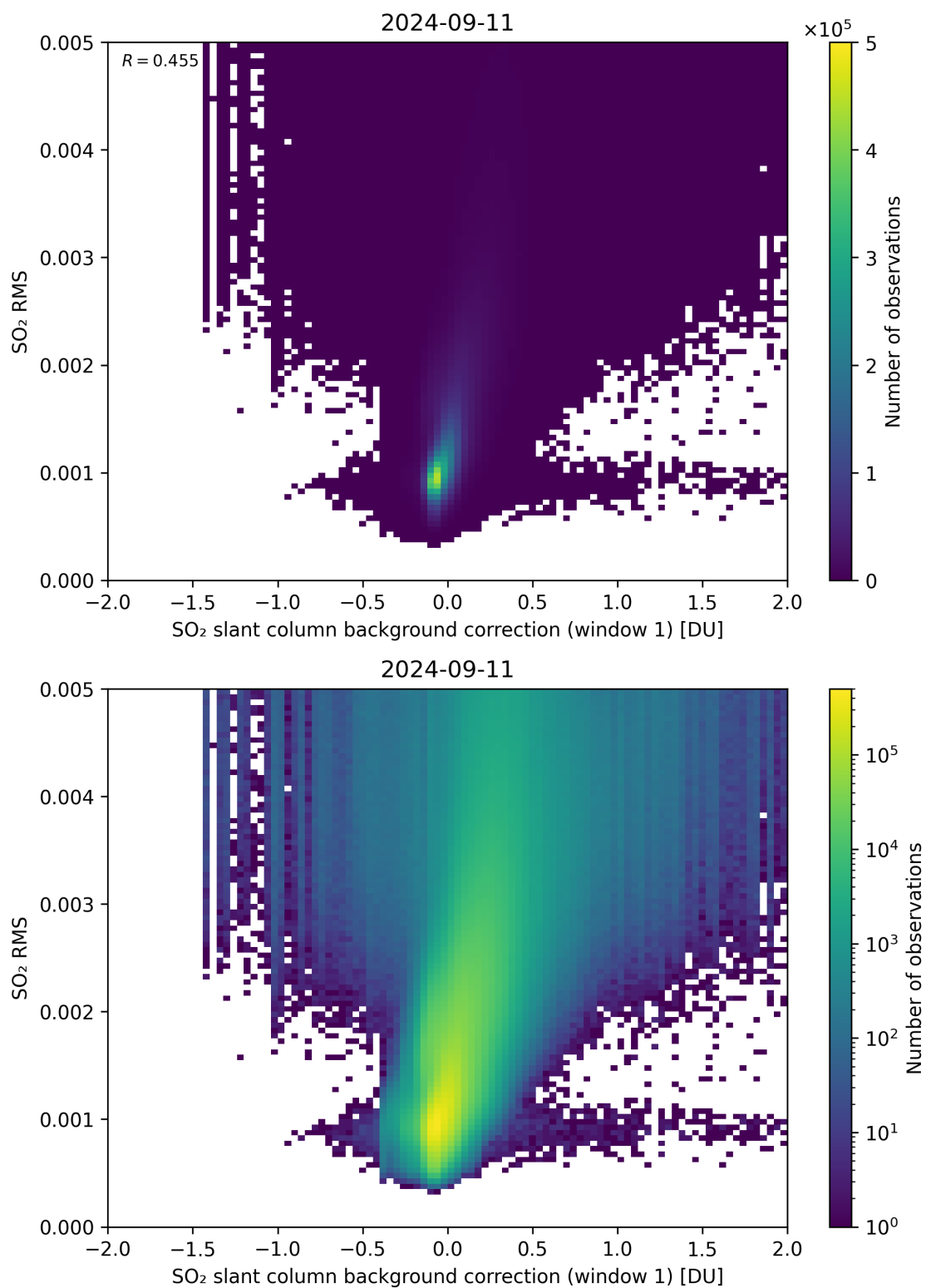
Figure 102: Scatter density plot of “SO 2 slant column background correction (window 1)” against “SO 2 RMS” for 2024-09-10 to 2024-09-12.
