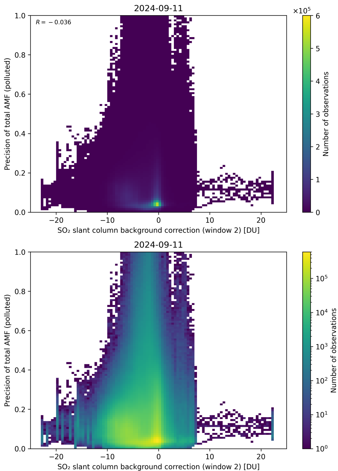
Figure 120: Scatter density plot of “SO 2 slant column background correction (window 2)” against “Precision of total AMF (polluted)” for 2024-09-10 to 2024-09-12.
