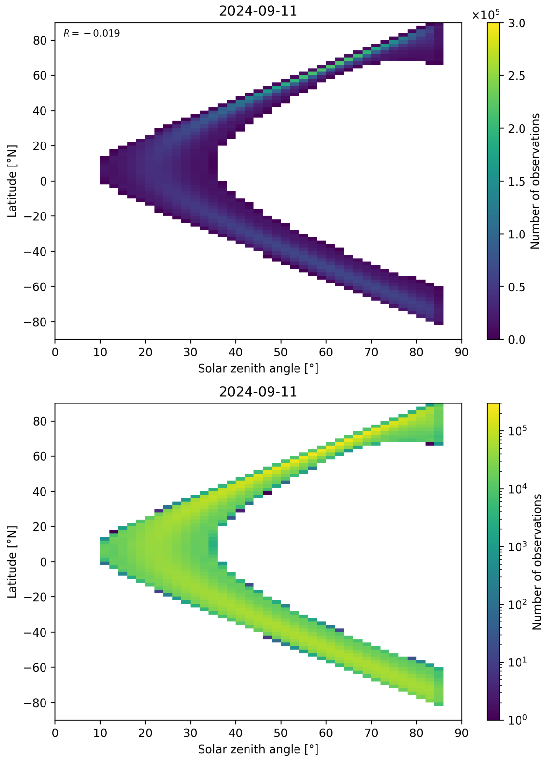
Figure 164: Scatter density plot of “Solar zenith angle” against “Latitude” for 2024-09-10 to 2024-09-12.
