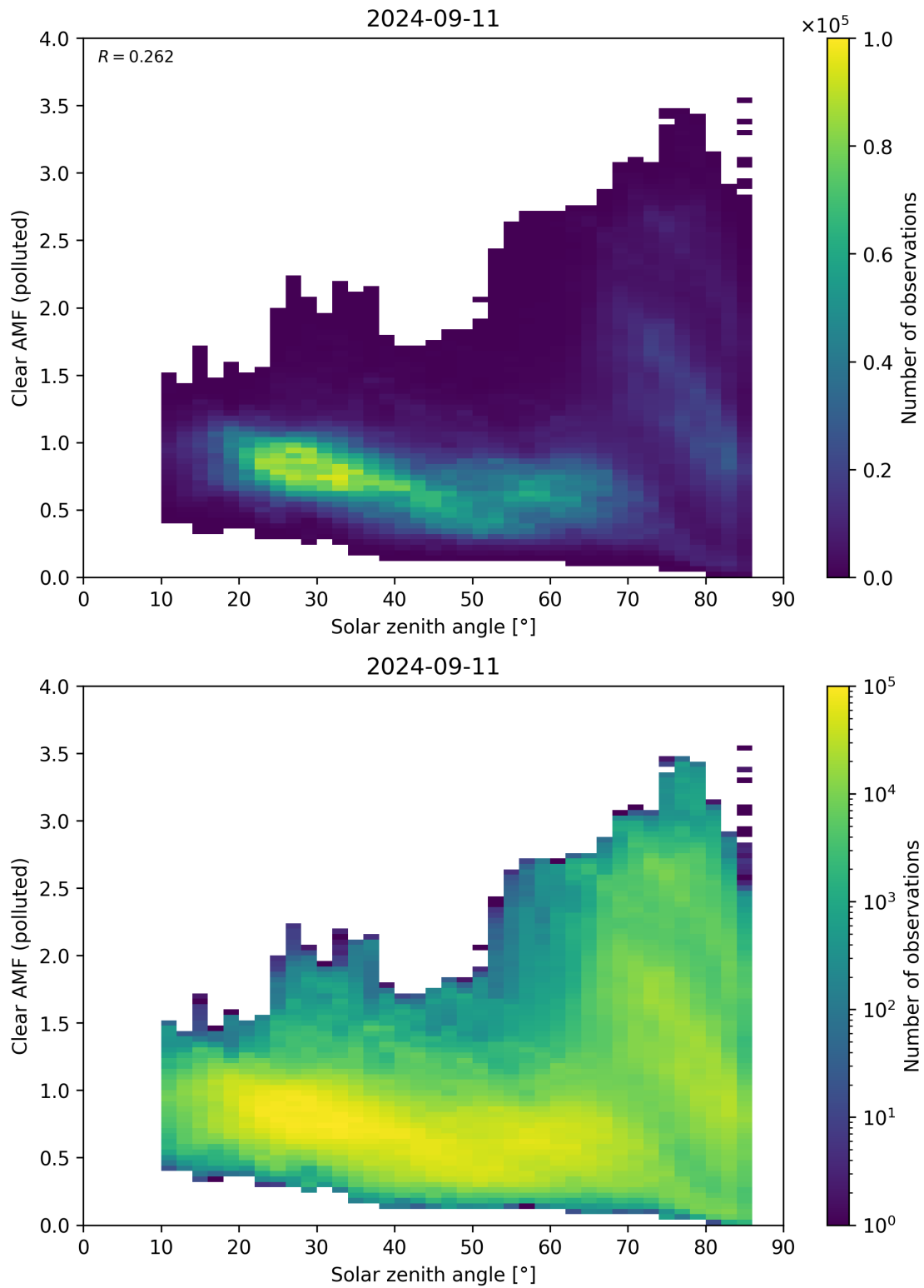
Figure 165: Scatter density plot of “Solar zenith angle” against “Clear AMF (polluted)” for 2024-09-10 to 2024-09-12.
