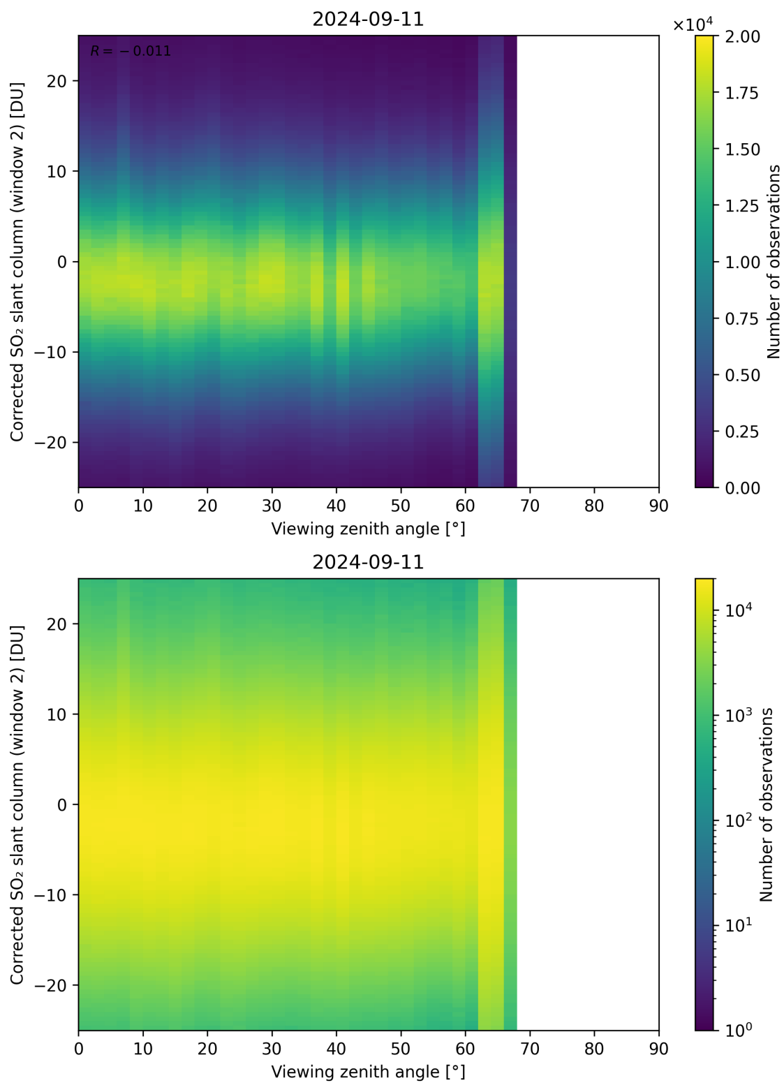
Figure 318: Scatter density plot of “Viewing zenith angle” against “Corrected SO 2 slant column (window 2)” for 2024-09-10 to 2024-09-12.
