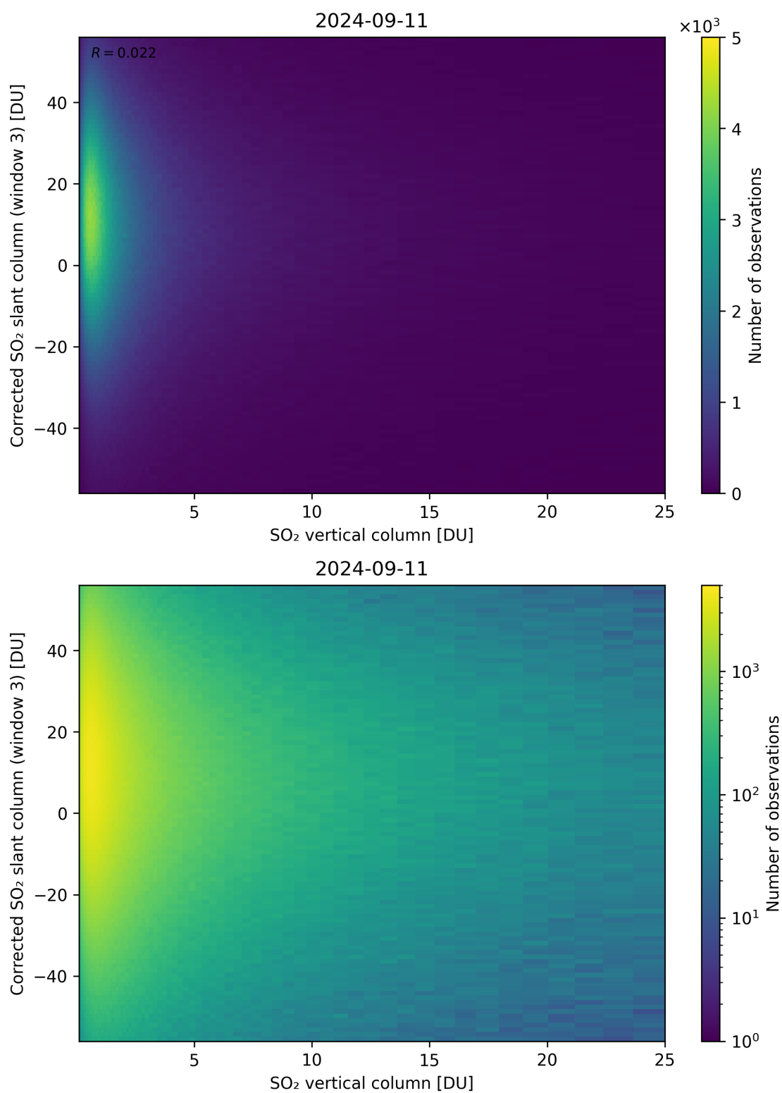
Figure 299: Scatter density plot of “SO 2 vertical column” against “Corrected SO 2 slant column (window 3)” for 2024-09-10 to 2024-09-12.
