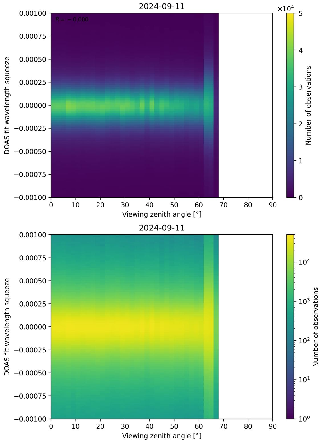
Figure 312: Scatter density plot of “Viewing zenith angle” against “DOAS fit wavelength squeeze” for 2024-09-10 to 2024-09-12.
