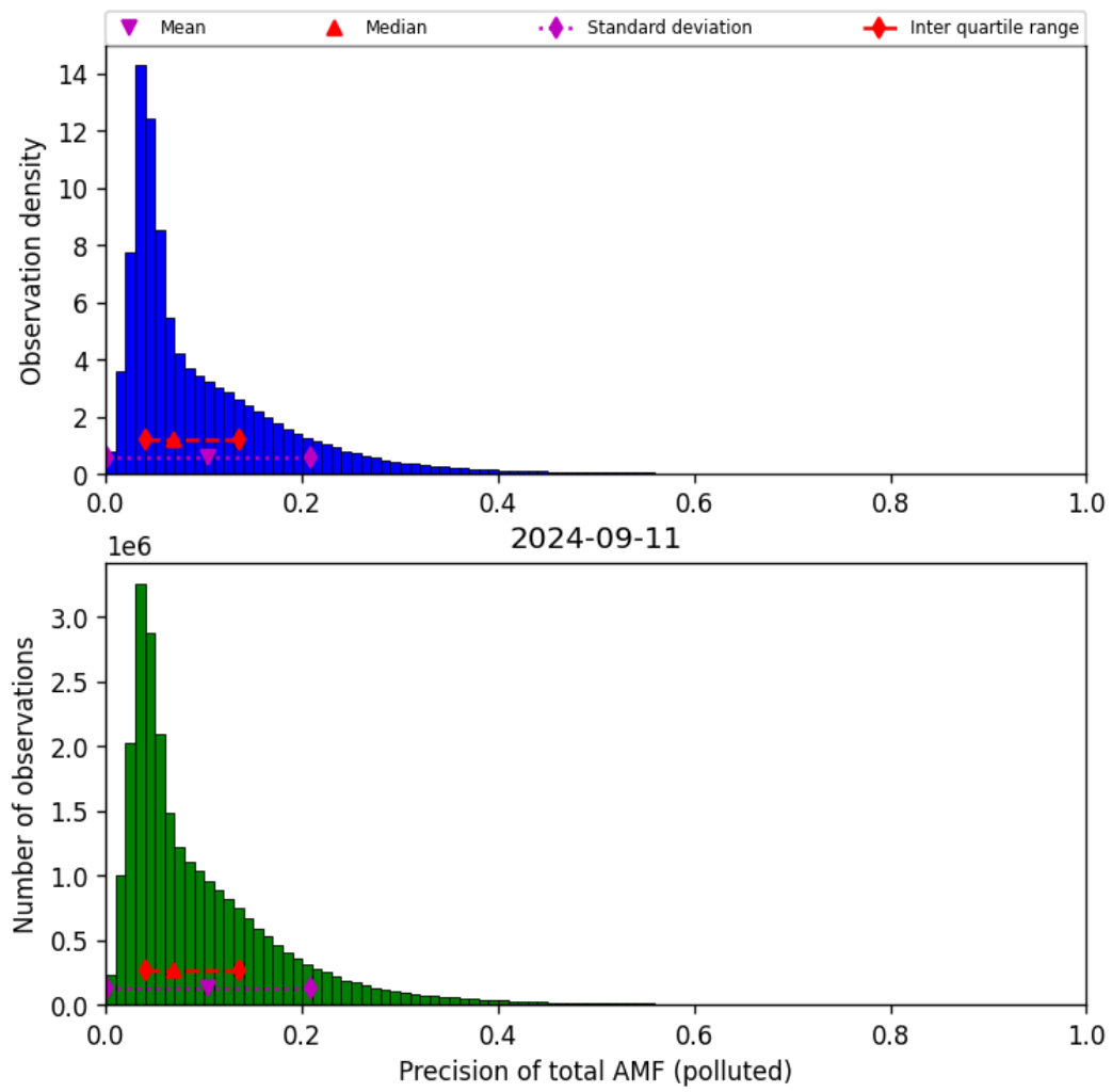
Figure 72: Histogram of “Precision of total AMF (polluted)” for 2024-09-10 to 2024-09-12
