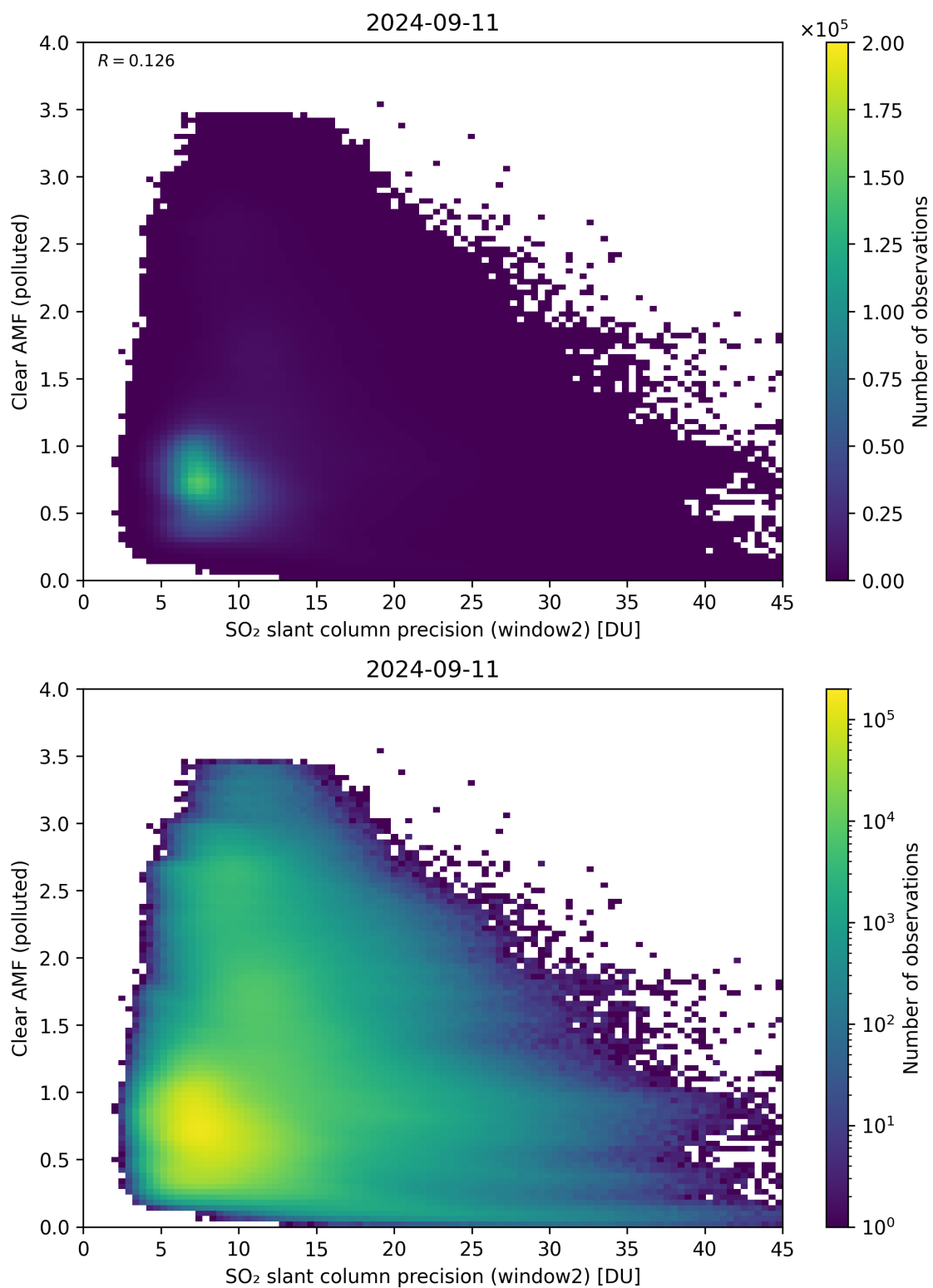
Figure 246: Scatter density plot of “SO 2 slant column precision (window2)” against “Clear AMF (polluted)” for 2024-09-10 to 2024-09-12.
