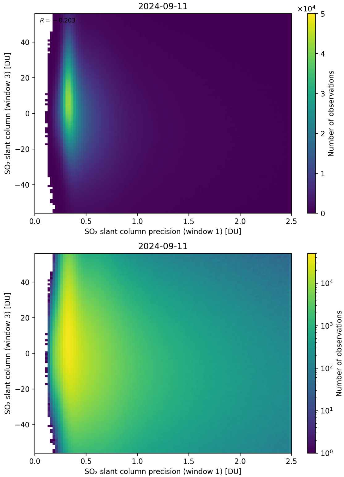
Figure 228: Scatter density plot of “SO 2 slant column precision (window 1)” against “SO 2 slant column (window 3)” for 2024-09-10 to 2024-09-12.
