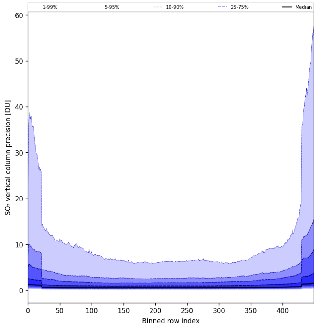
Figure 77: Along track statistics of “SO 2 vertical column precision” for 2024-09-10 to 2024-09-12
