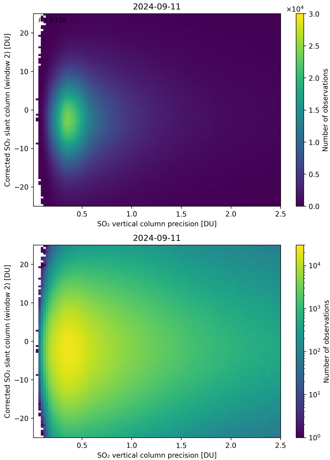
Figure 287: Scatter density plot of “SO 2 vertical column precision” against “Corrected SO 2 slant column (window 2)” for 2024-09-10 to 2024-09-12.
