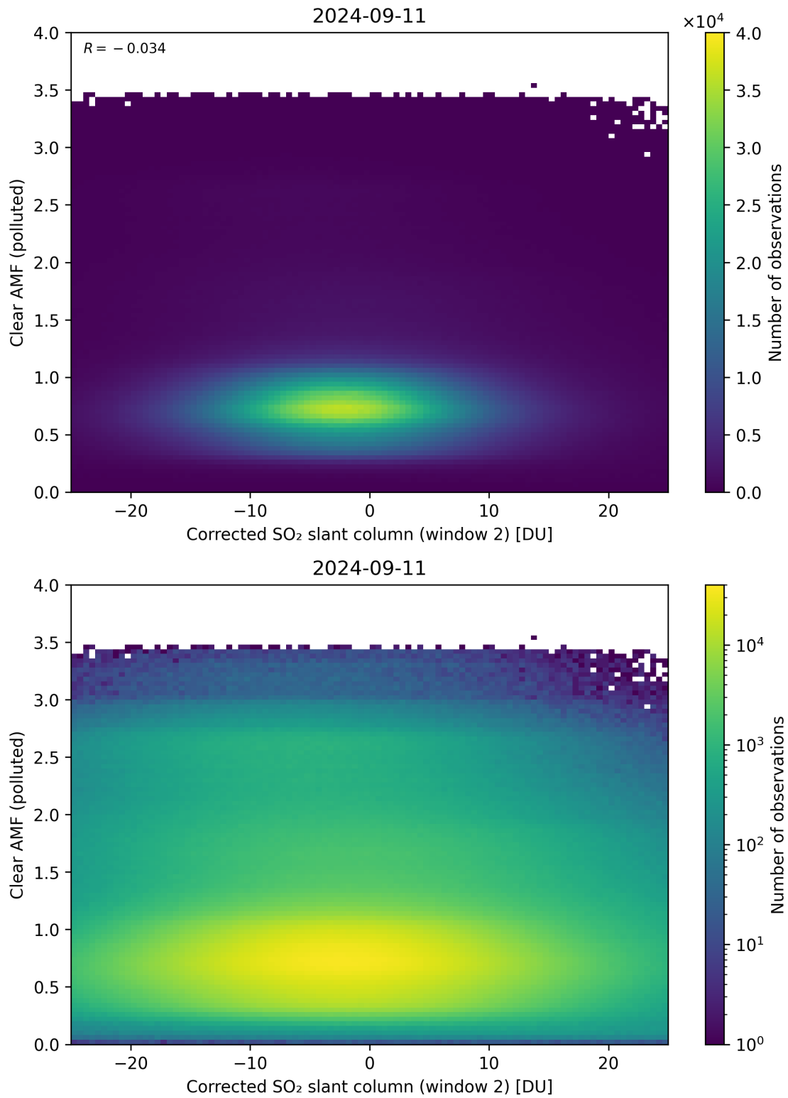
Figure 199: Scatter density plot of “Corrected SO 2 slant column (window 2)” against “Clear AMF (polluted)” for 2024-09-10 to 2024-09-12.
