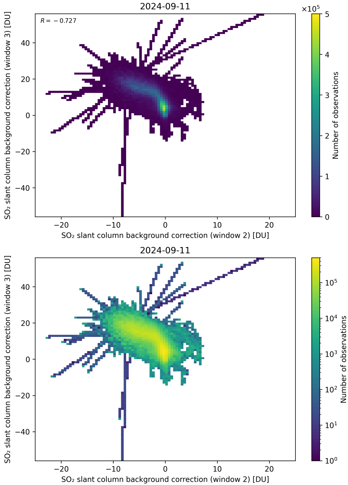
Figure 111: Scatter density plot of “SO 2 slant column background correction (window 2)” against “SO 2 slant column background correction (window 3)” for 2024-09-10 to 2024-09-12.
