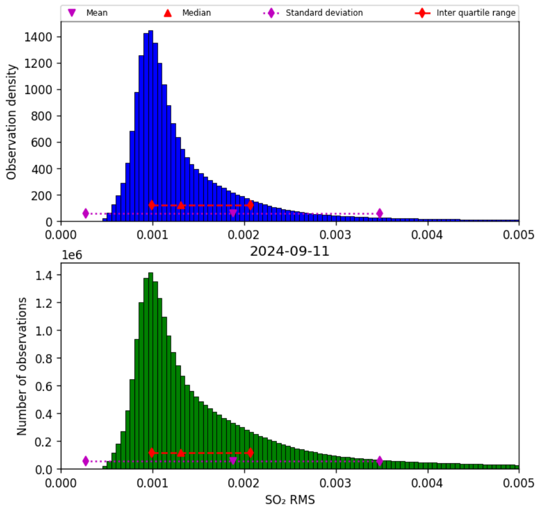
Figure 70: Histogram of “SO 2 RMS” for 2024-09-10 to 2024-09-12
