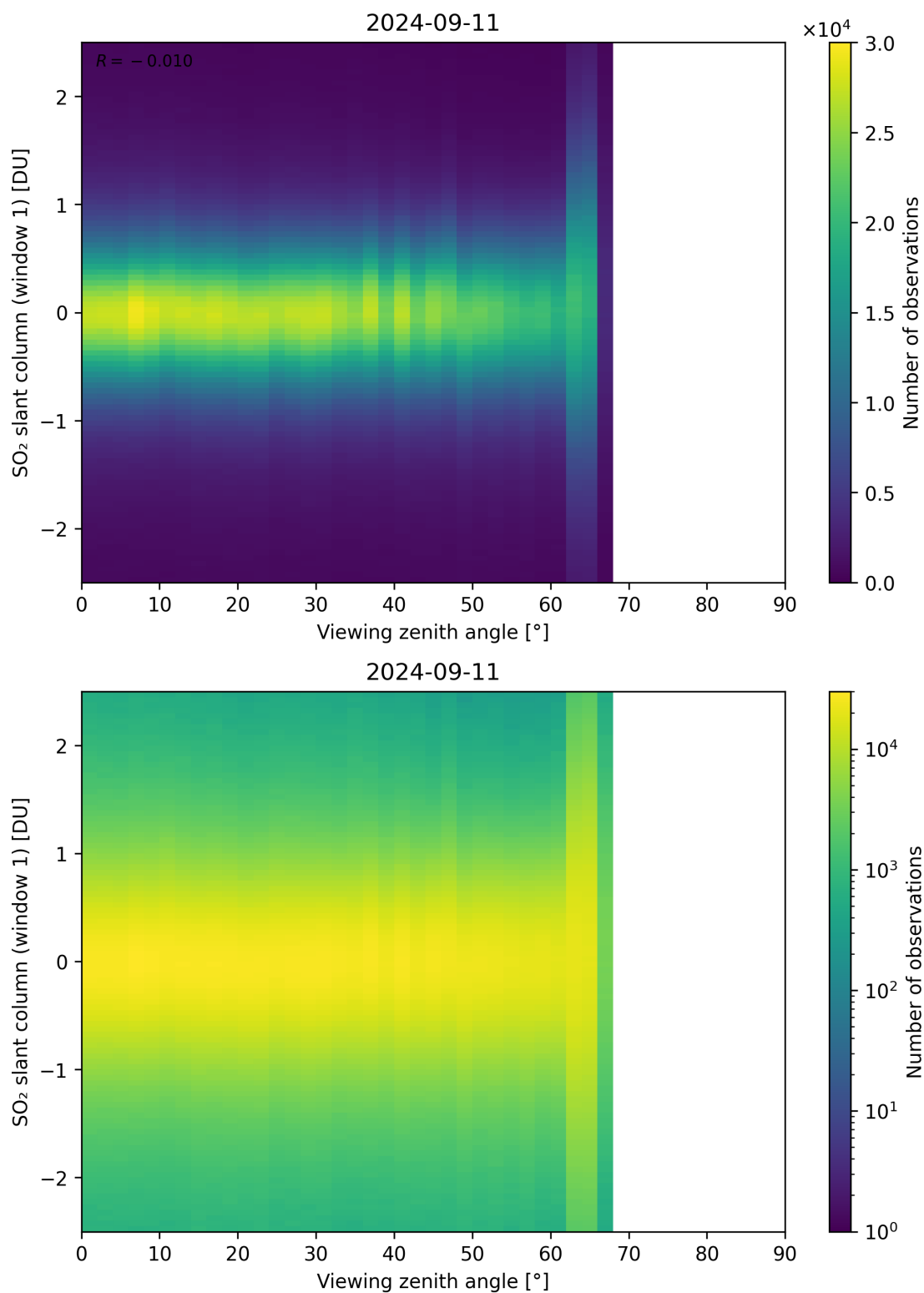
Figure 320: Scatter density plot of “Viewing zenith angle” against “SO 2 slant column (window 1)” for 2024-09-10 to 2024-09-12.
