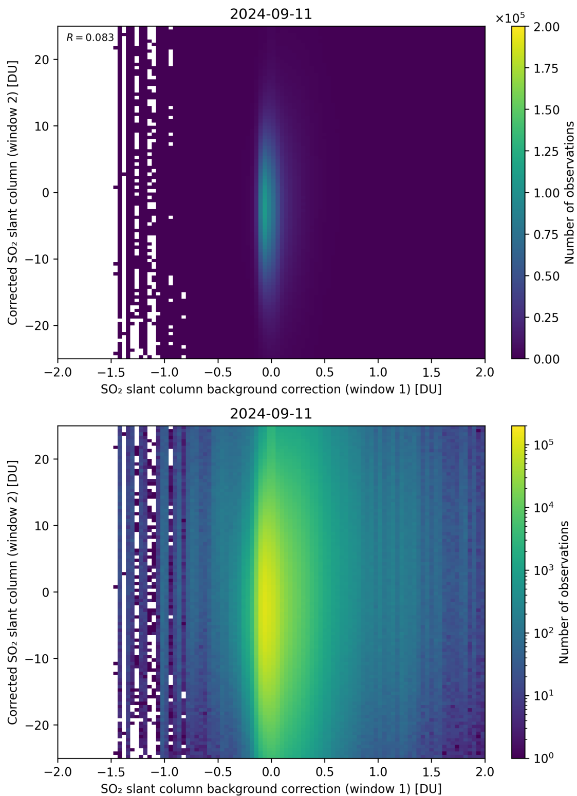
Figure 104: Scatter density plot of “SO 2 slant column background correction (window 1)” against “Corrected SO 2 slant column (window 2)” for 2024-09-10 to 2024-09-12.
