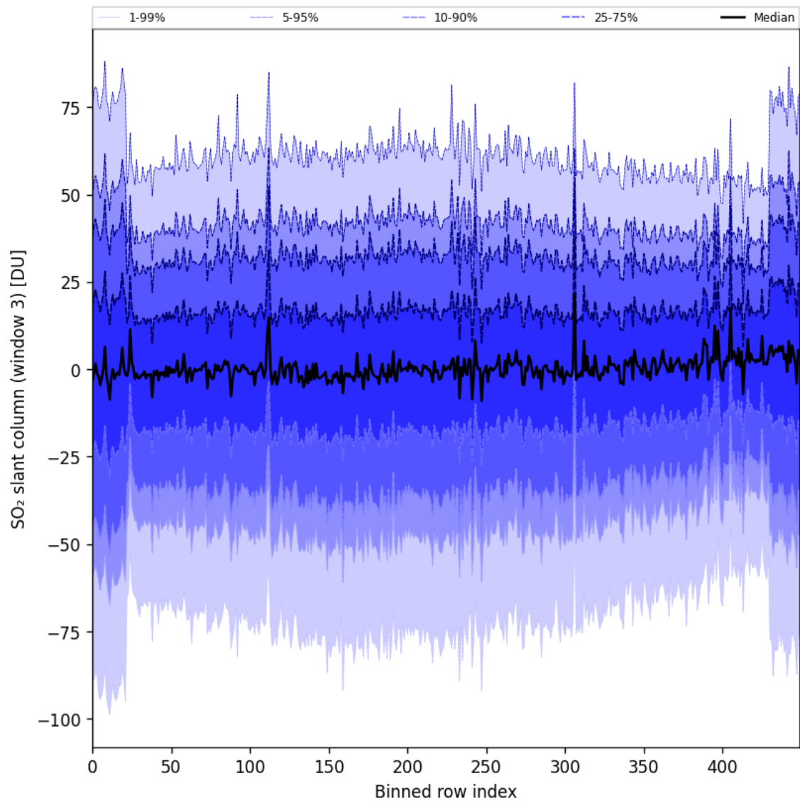
Figure 87: Along track statistics of “SO 2 slant column (window 3)” for 2024-09-10 to 2024-09-12
