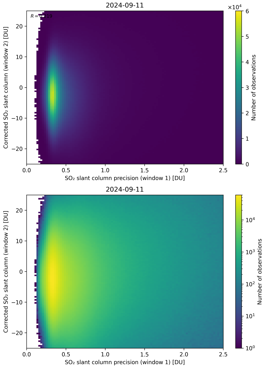
Figure 225: Scatter density plot of “SO 2 slant column precision (window 1)” against “Corrected SO 2 slant column (window 2)” for 2024-09-10 to 2024-09-12.
