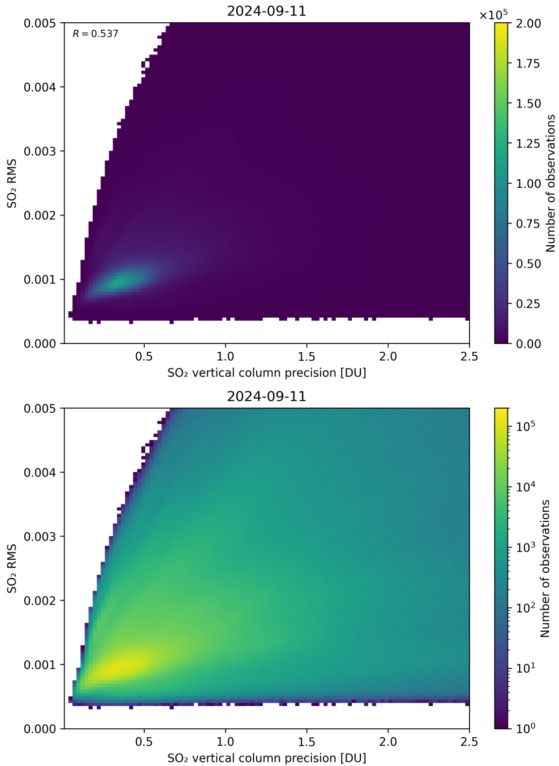
Figure 284: Scatter density plot of “SO 2 vertical column precision” against “SO 2 RMS” for 2024-09-10 to 2024-09-12.
