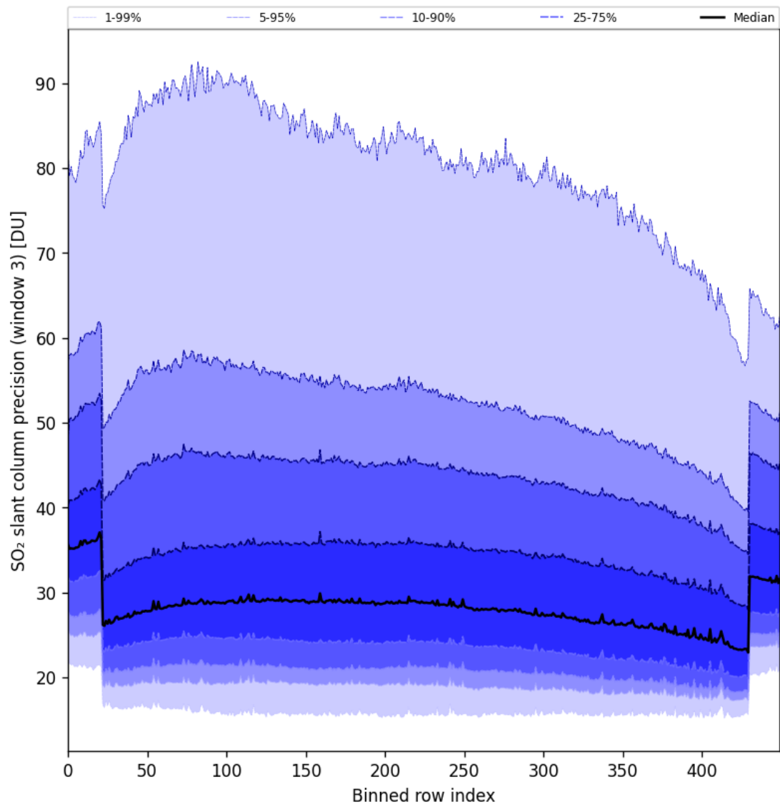
Figure 88: Along track statistics of “SO 2 slant column precision (window 3)” for 2024-09-10 to 2024-09-12
