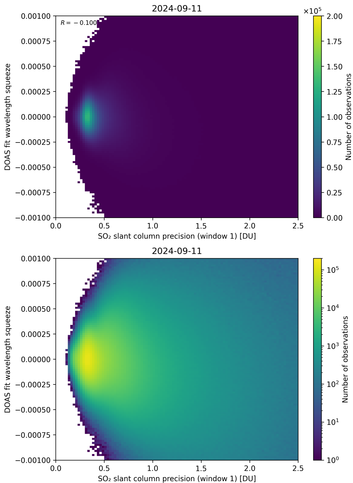
Figure 222: Scatter density plot of “SO 2 slant column precision (window 1)” against “DOAS fit wavelength squeeze” for 2024-09-10 to 2024-09-12.
