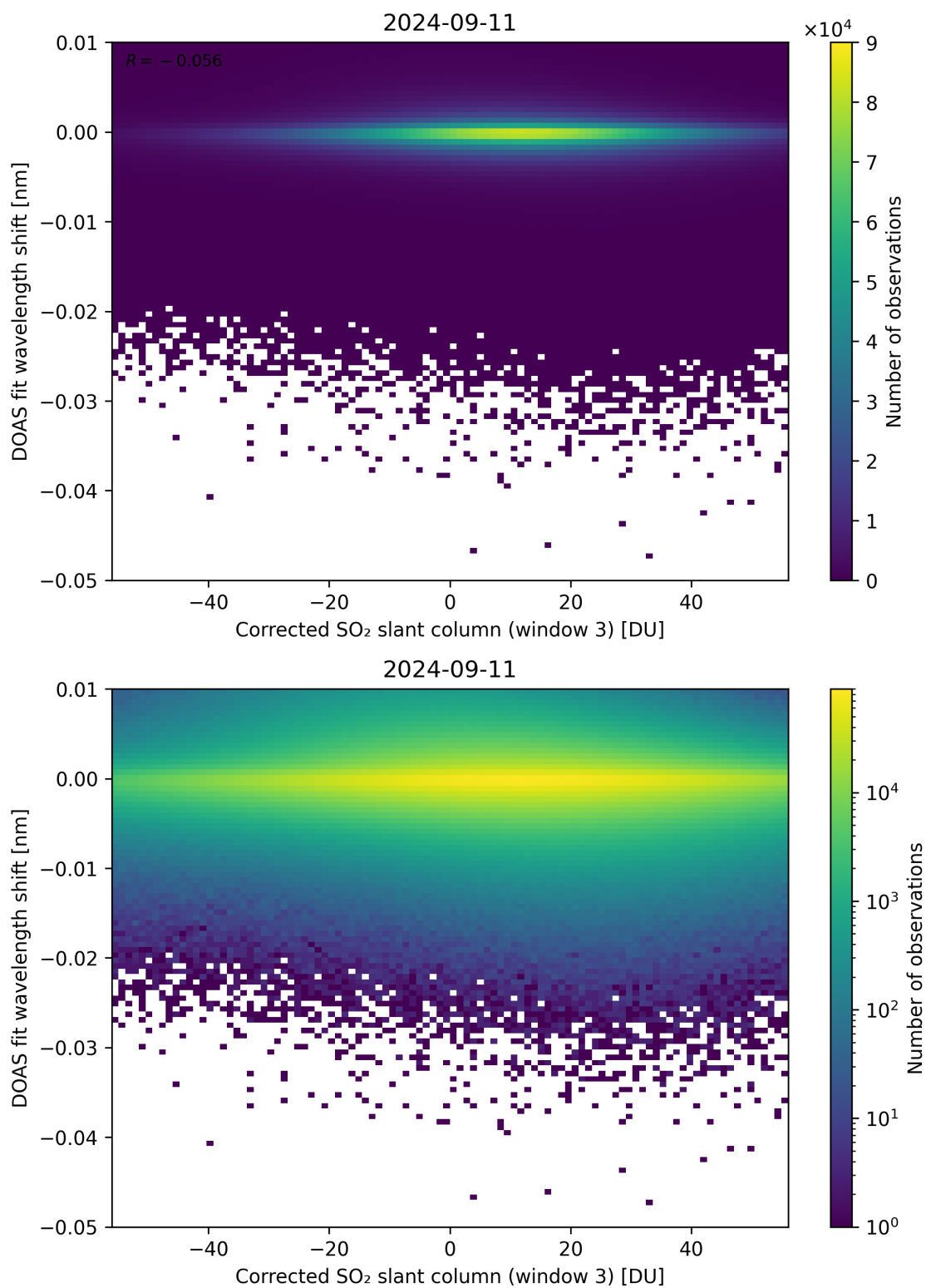
Figure 206: Scatter density plot of “Corrected SO 2 slant column (window 3)” against “DOAS fit wavelength shift” for 2024-09-10 to 2024-09-12.
