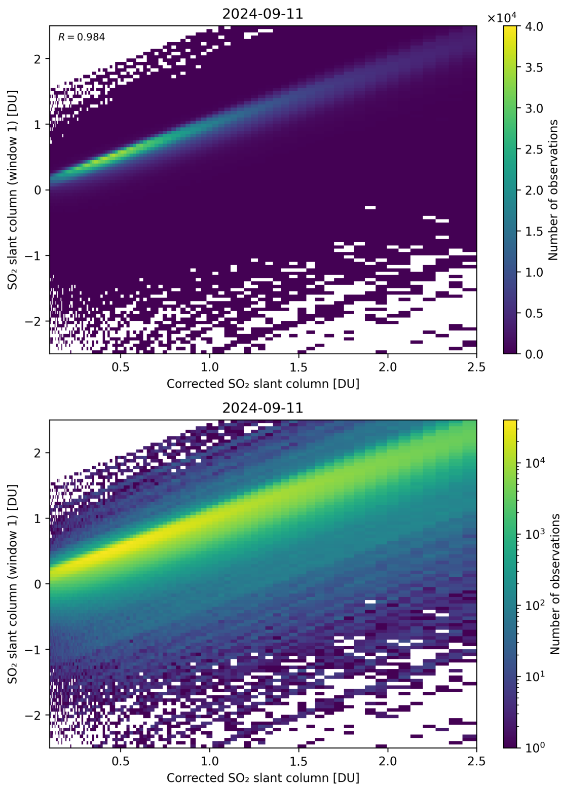
Figure 187: Scatter density plot of “Corrected SO 2 slant column” against “SO 2 slant column (window 1)” for 2024-09-10 to 2024-09-12.
