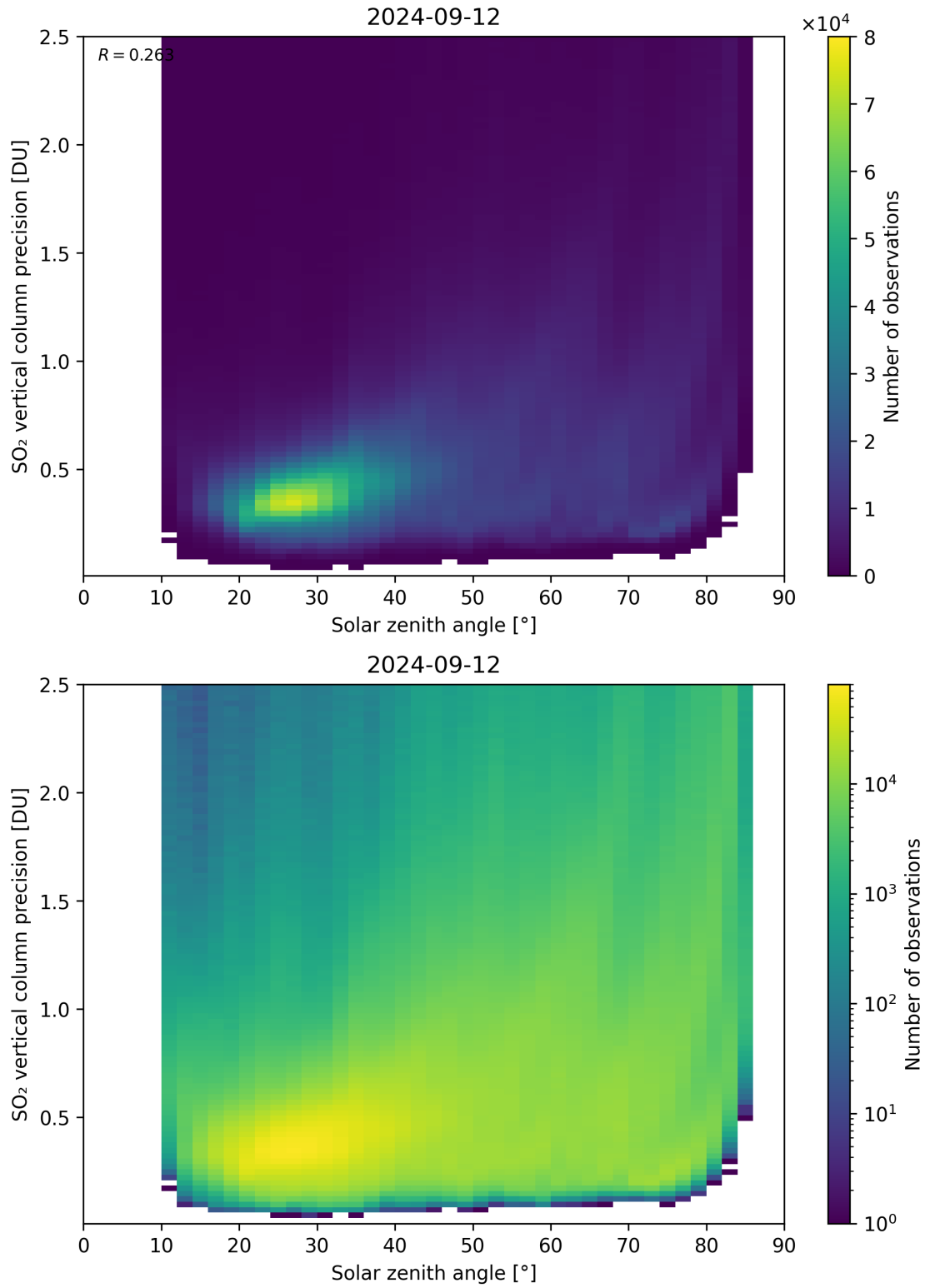
Figure 177: Scatter density plot of “Solar zenith angle” against “SO 2 vertical column precision” for 2024-09-12 to 2024-09-13.
