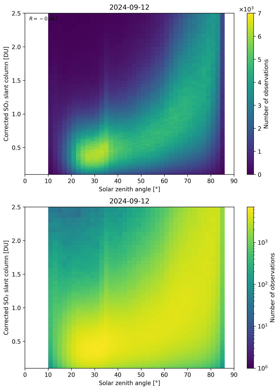
Figure 166: Scatter density plot of “Solar zenith angle” against “Corrected SO 2 slant column” for 2024-09-12 to 2024-09-13.
