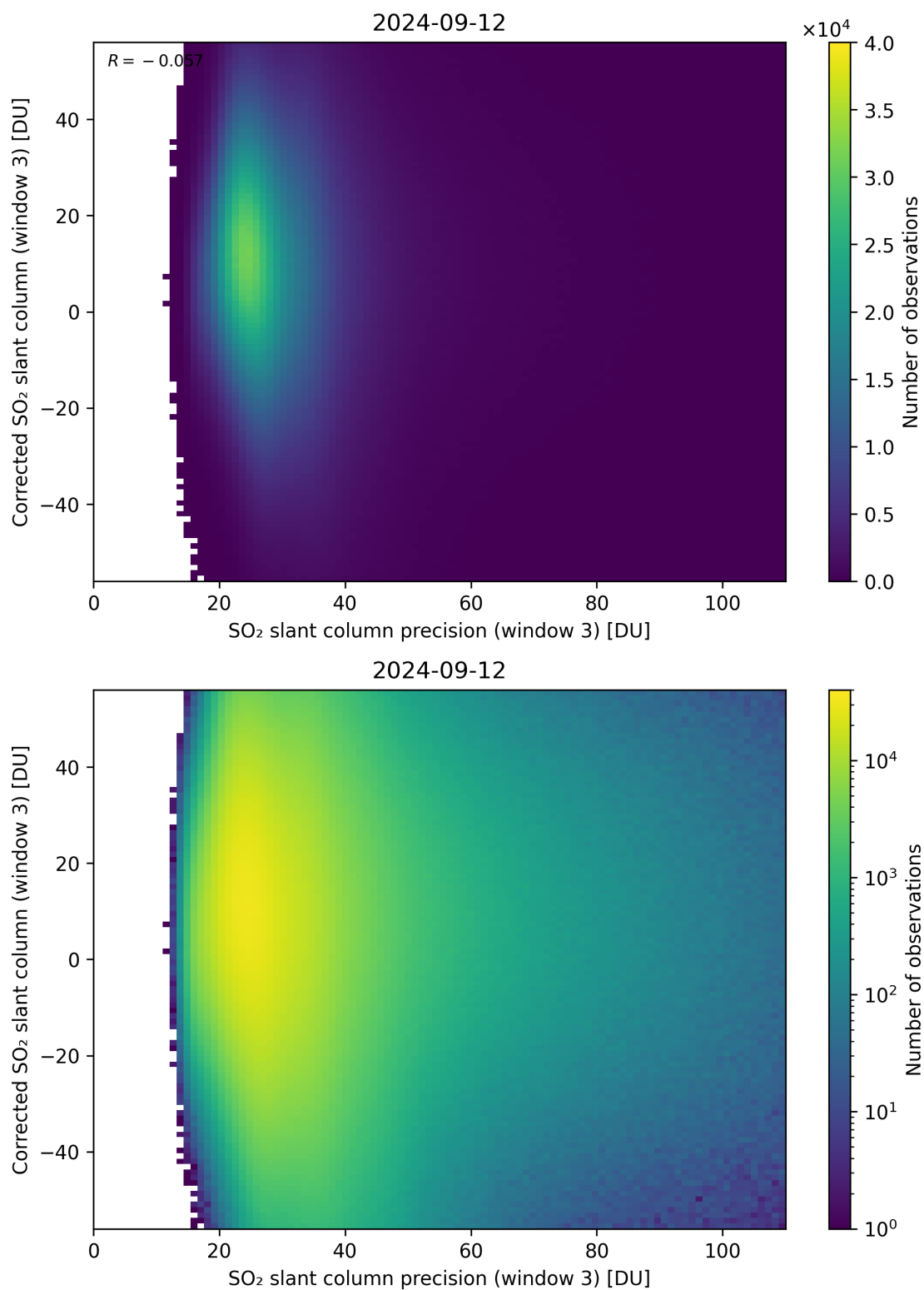
Figure 262: Scatter density plot of “SO 2 slant column precision (window 3)” against “Corrected SO 2 slant column (window 3)” for 2024-09-12 to 2024-09-13.
