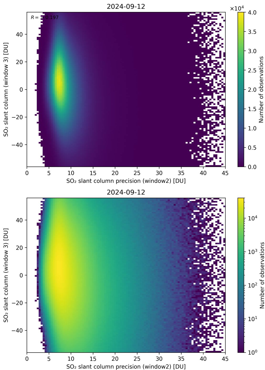
Figure 249: Scatter density plot of “SO 2 slant column precision (window2)” against “SO 2 slant column (window 3)” for 2024-09-12 to 2024-09-13.
