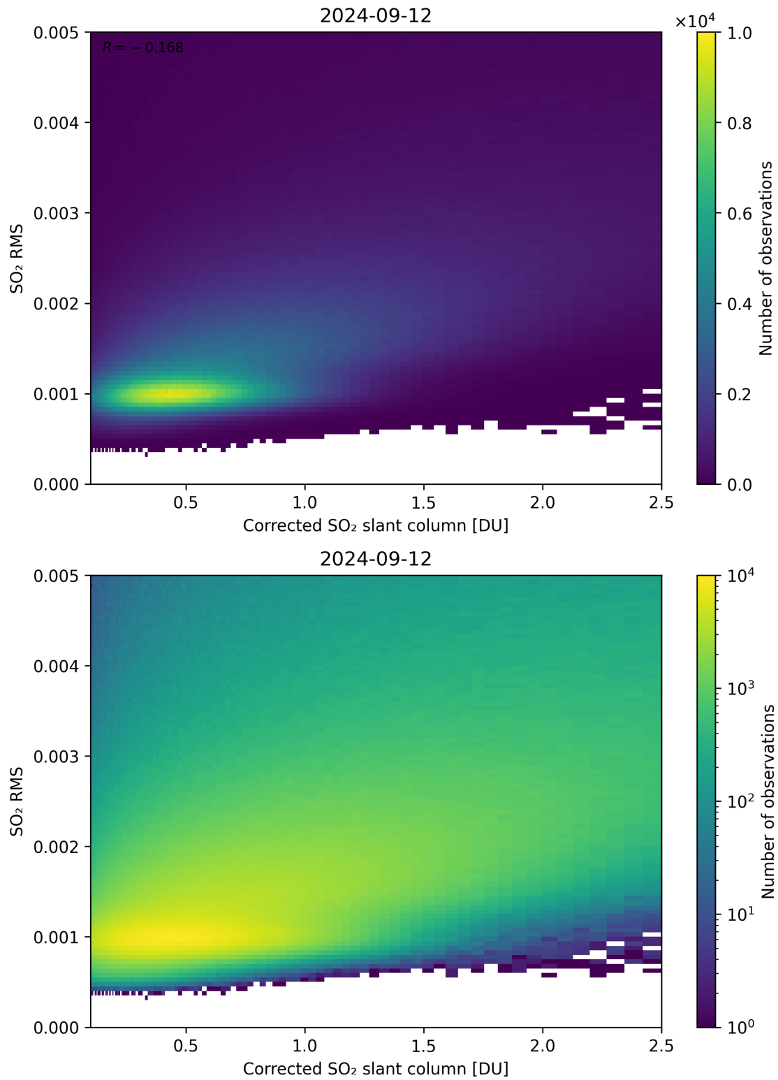
Figure 183: Scatter density plot of “Corrected SO 2 slant column” against “SO 2 RMS” for 2024-09-12 to 2024-09-13.
