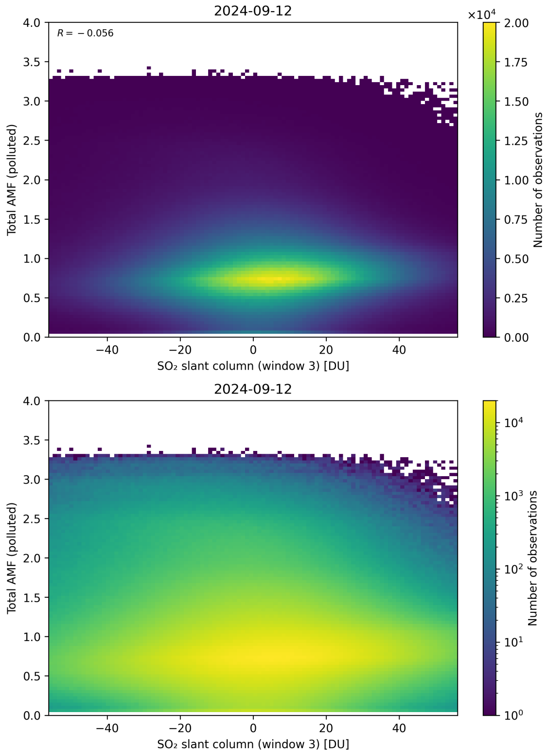
Figure 268: Scatter density plot of “SO 2 slant column (window 3)” against “Total AMF (polluted)” for 2024-09-12 to 2024-09-13.
