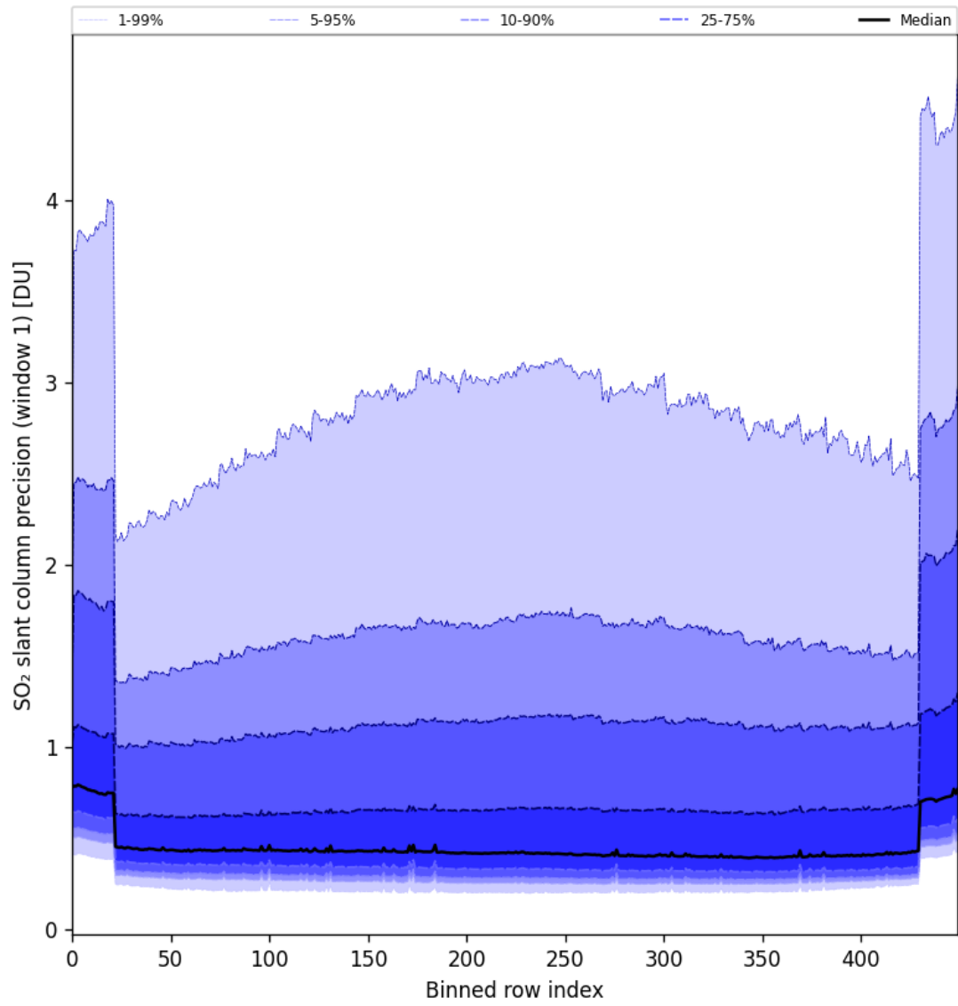
Figure 80: Along track statistics of “SO 2 slant column precision (window 1)” for 2024-09-12 to 2024-09-13
