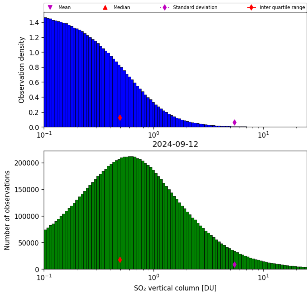
Figure 53: Histogram of “SO 2 vertical column” for 2024-09-12 to 2024-09-13
