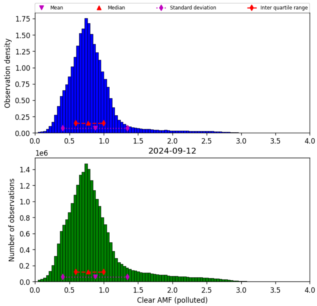
Figure 73: Histogram of “Clear AMF (polluted)” for 2024-09-12 to 2024-09-13
