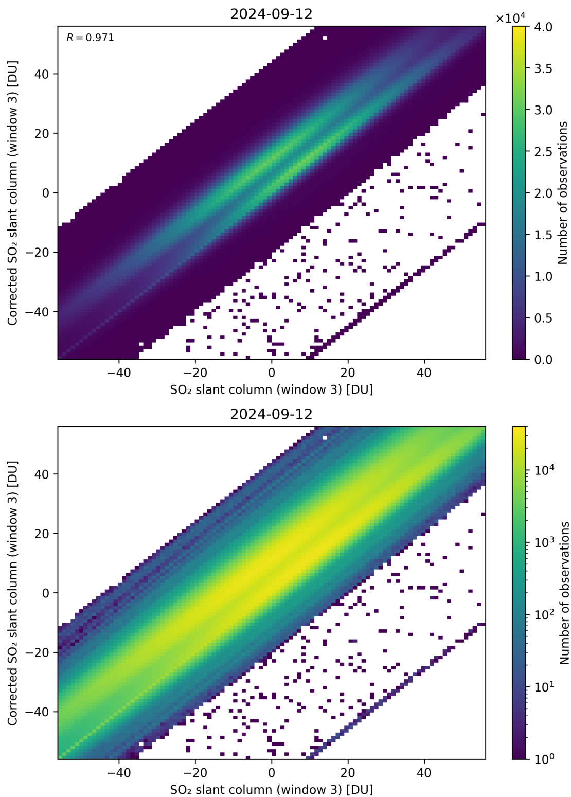
Figure 266: Scatter density plot of “SO 2 slant column (window 3)” against “Corrected SO 2 slant column (window 3)” for 2024-09-12 to 2024-09-13.
