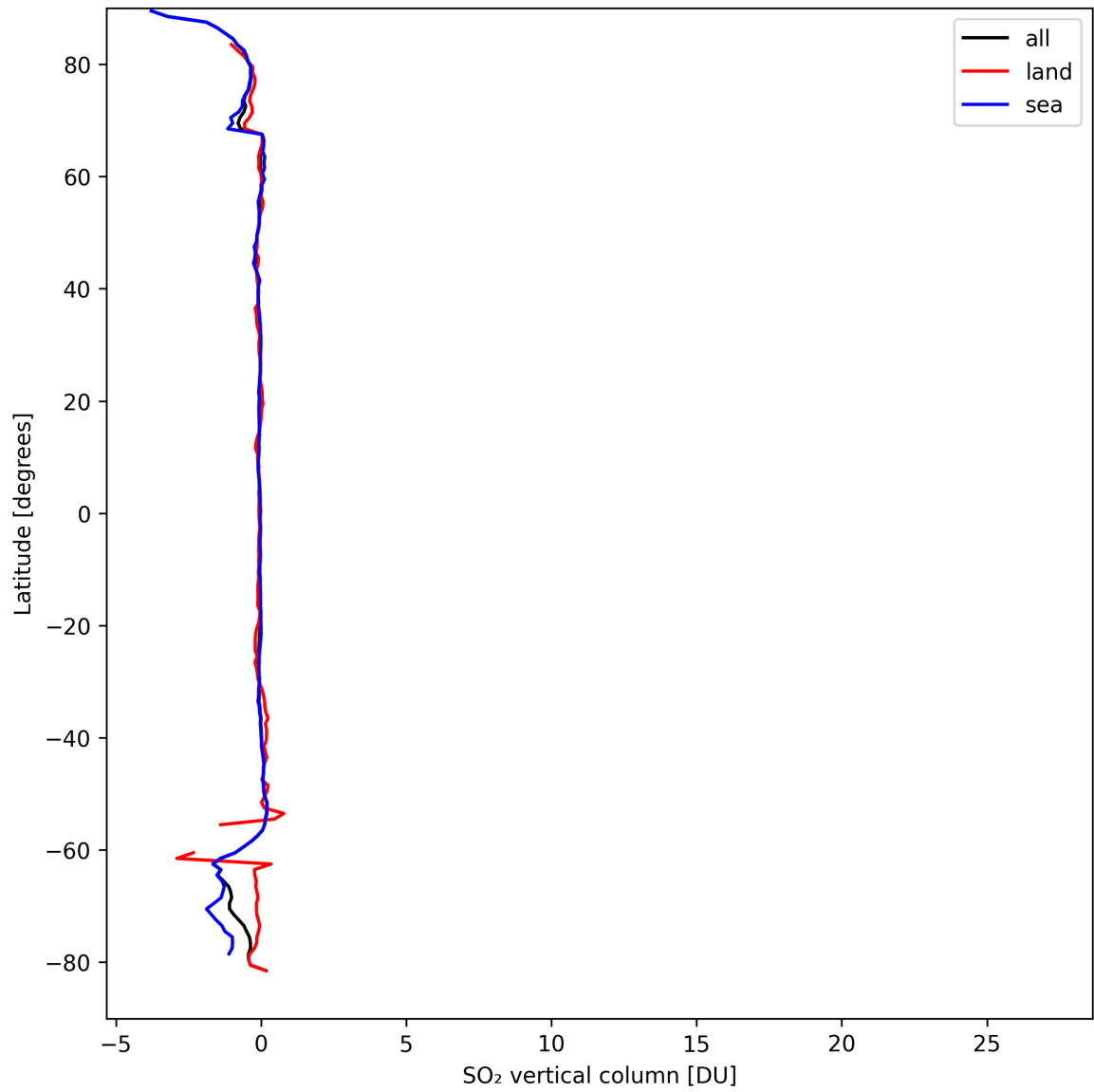
Figure 30: Zonal average of “SO 2 vertical column” for 2024-09-12 to 2024-09-13.
