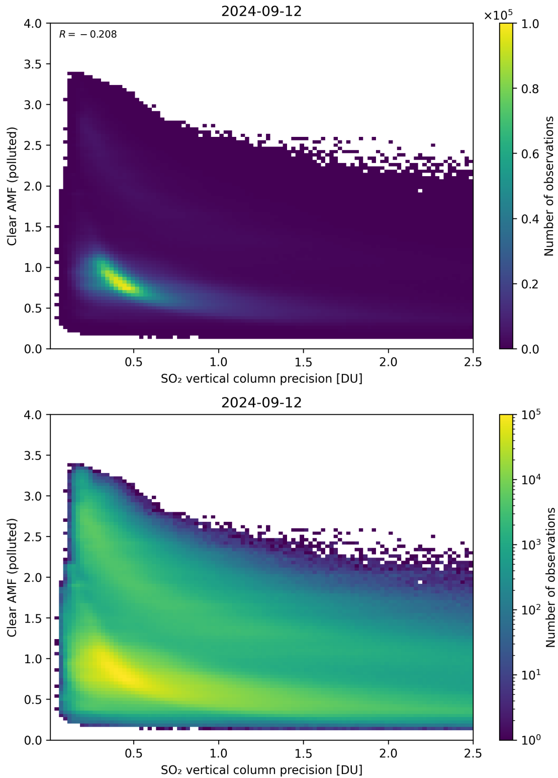
Figure 285: Scatter density plot of “SO 2 vertical column precision” against “Clear AMF (polluted)” for 2024-09-12 to 2024-09-13.
