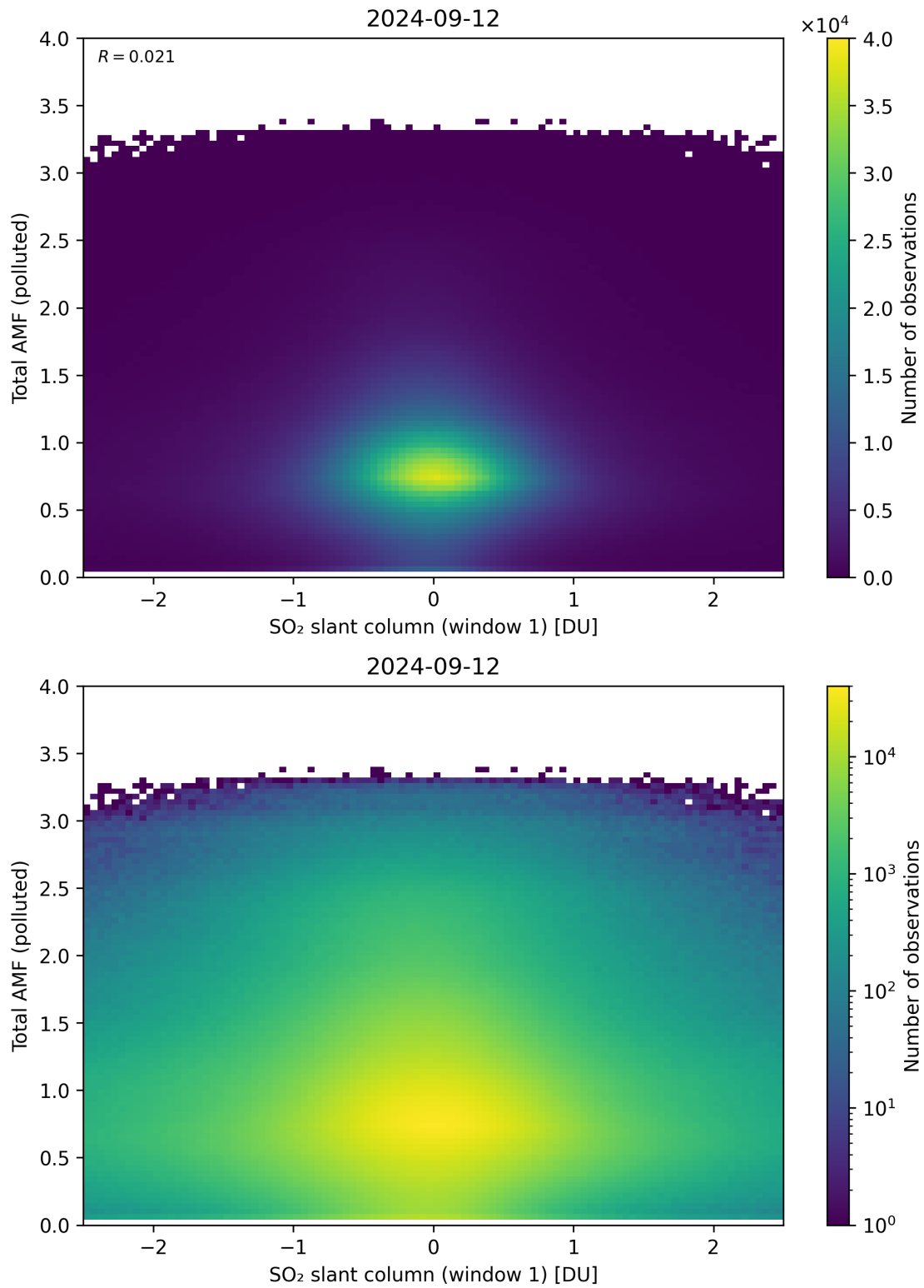
Figure 239: Scatter density plot of “SO 2 slant column (window 1)” against “Total AMF (polluted)” for 2024-09-12 to 2024-09-13.
