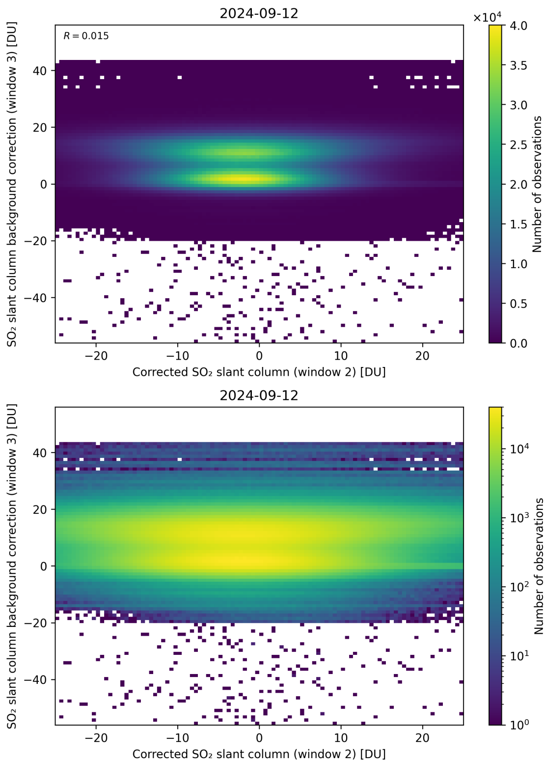
Figure 195: Scatter density plot of “Corrected SO 2 slant column (window 2)” against “SO 2 slant column background correction (window 3)” for 2024-09-12 to 2024-09-13.
