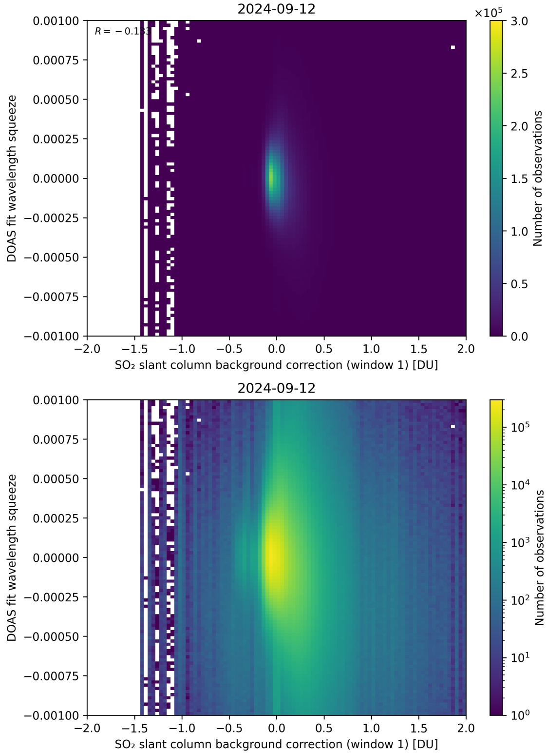
Figure 101: Scatter density plot of “SO 2 slant column background correction (window 1)” against “DOAS fit wavelength squeeze” for 2024-09-12 to 2024-09-13.
