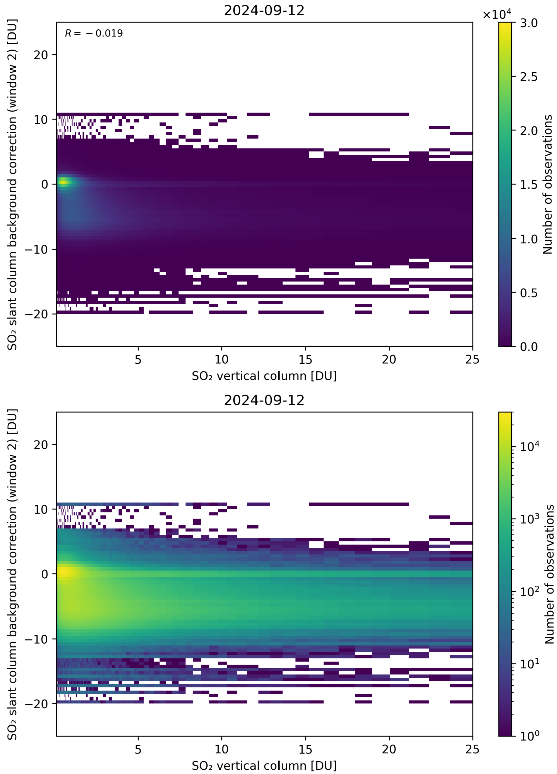
Figure 274: Scatter density plot of “SO 2 vertical column” against “SO 2 slant column background correction (window 2)” for 2024-09-12 to 2024-09-13.
