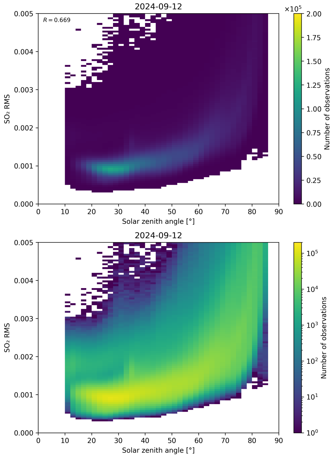
Figure 163: Scatter density plot of “Solar zenith angle” against “SO 2 RMS” for 2024-09-12 to 2024-09-13.
