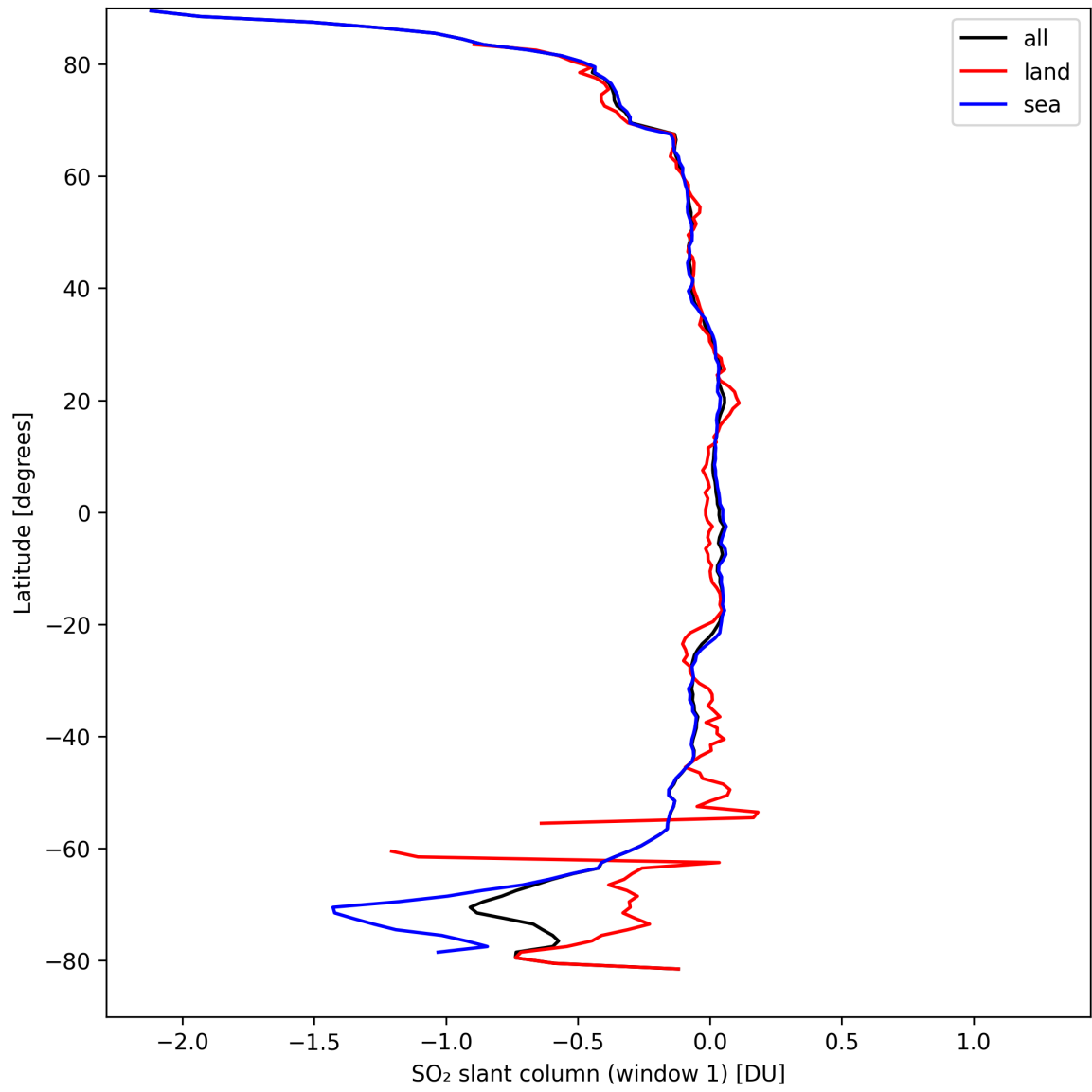
Figure 33: Zonal average of “SO 2 slant column (window 1)” for 2024-09-12 to 2024-09-13.
