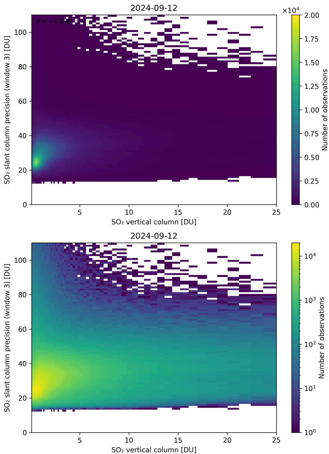
Figure 304: Scatter density plot of “SO 2 vertical column” against “SO 2 slant column precision (window 3)” for 2024-09-12 to 2024-09-13.
