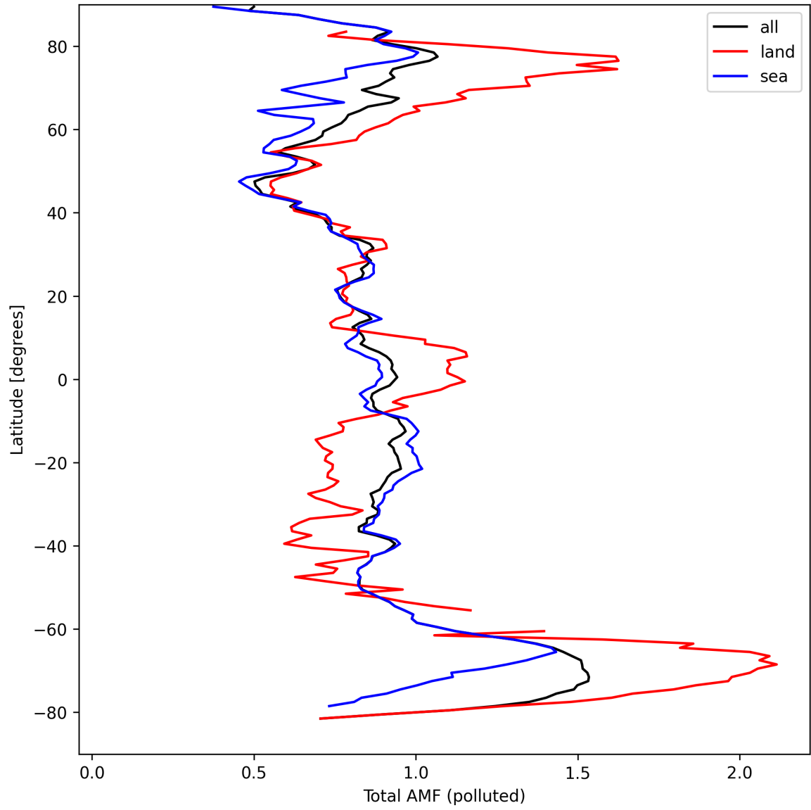
Figure 48: Zonal average of “Total AMF (polluted)” for 2024-09-12 to 2024-09-13.
