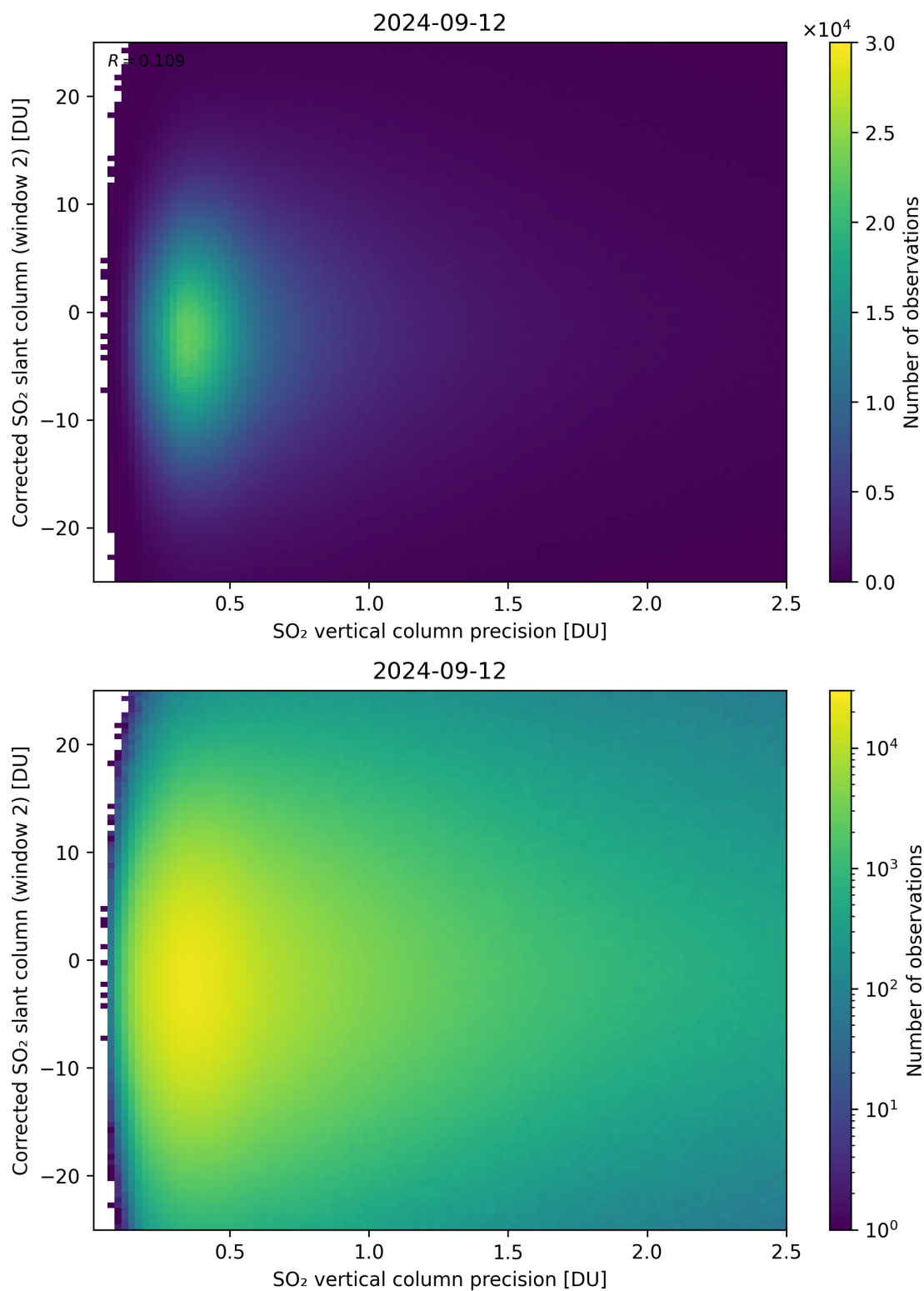
Figure 287: Scatter density plot of “SO 2 vertical column precision” against “Corrected SO 2 slant column (window 2)” for 2024-09-12 to 2024-09-13.
