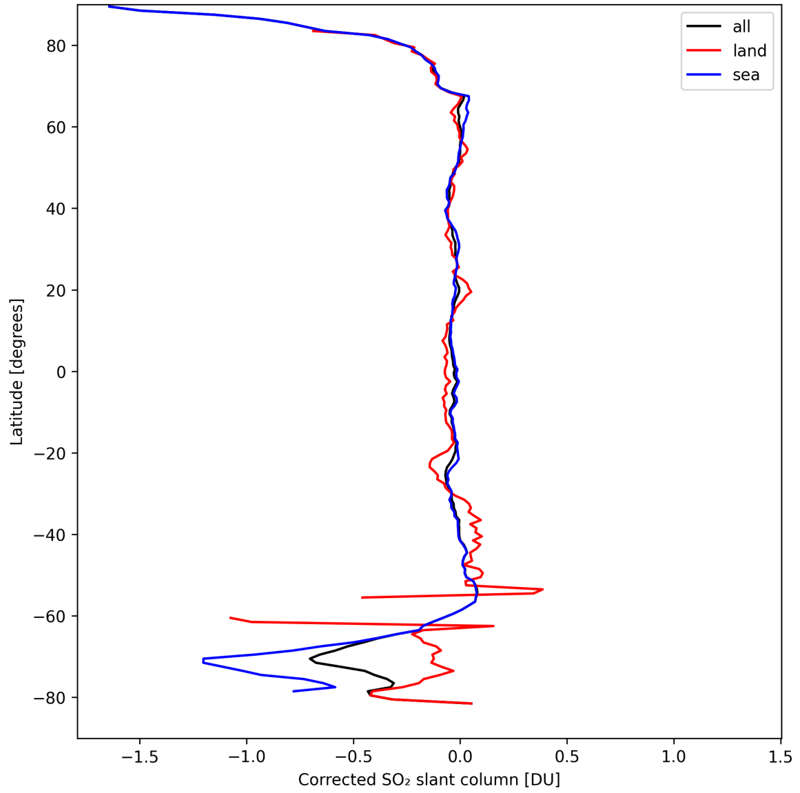
Figure 32: Zonal average of “Corrected SO 2 slant column” for 2024-09-12 to 2024-09-13.
