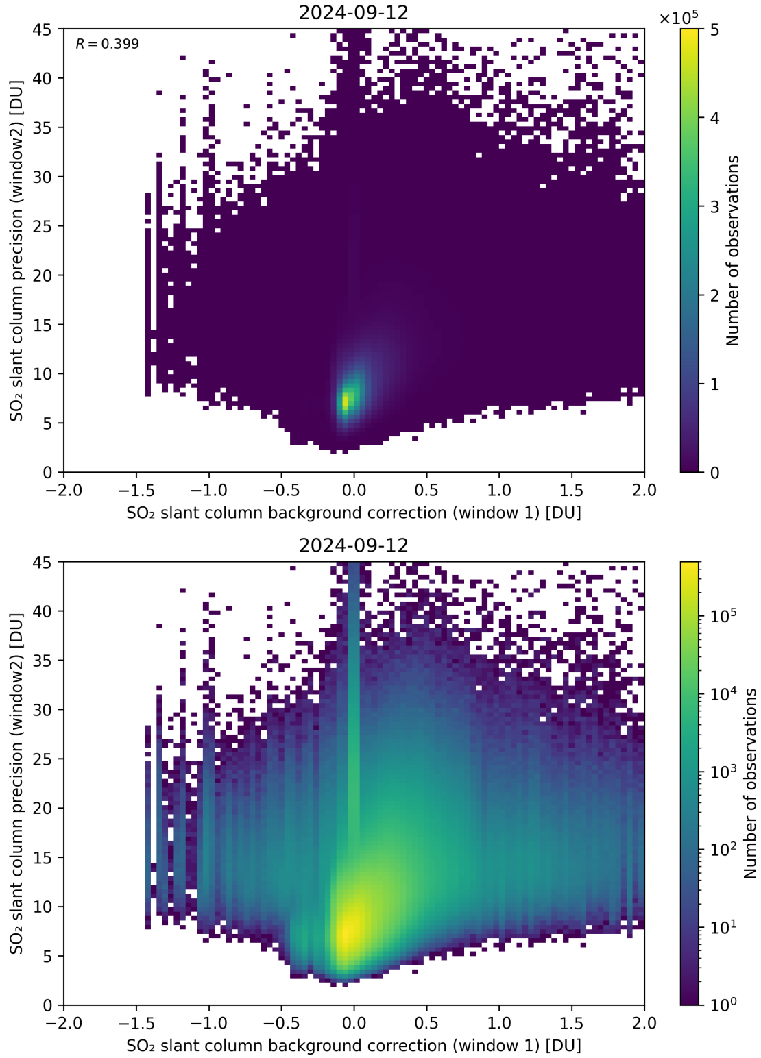
Figure 106: Scatter density plot of “SO 2 slant column background correction (window 1)” against “SO 2 slant column precision (window2)” for 2024-09-12 to 2024-09-13.
