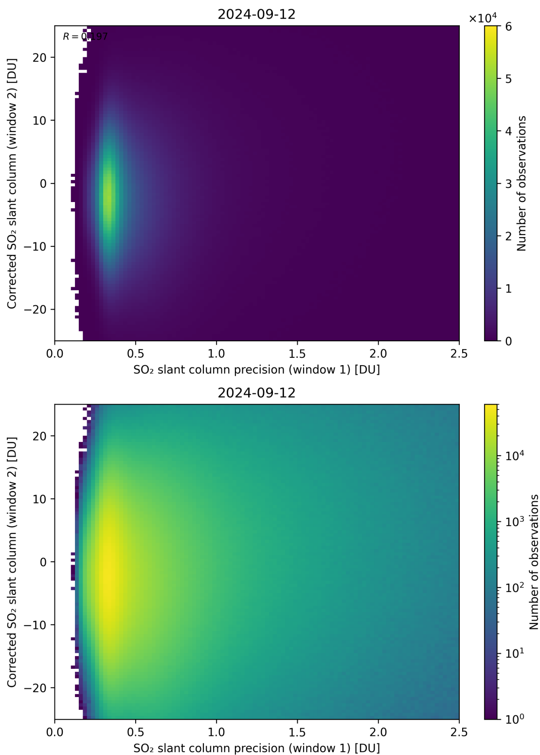
Figure 225: Scatter density plot of “SO 2 slant column precision (window 1)” against “Corrected SO 2 slant column (window 2)” for 2024-09-12 to 2024-09-13.
