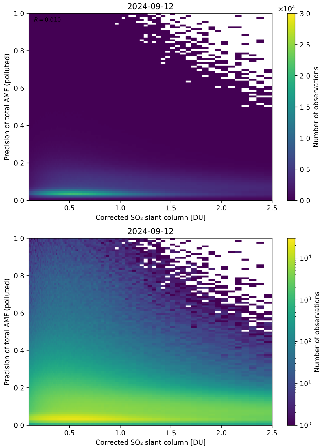
Figure 193: Scatter density plot of “Corrected SO 2 slant column” against “Precision of total AMF (polluted)” for 2024-09-12 to 2024-09-13.
