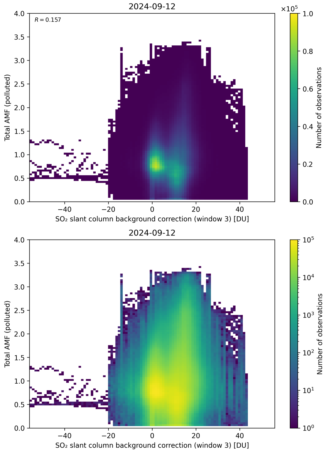
Figure 125: Scatter density plot of “SO 2 slant column background correction (window 3)” against “Total AMF (polluted)” for 2024-09-12 to 2024-09-13.
