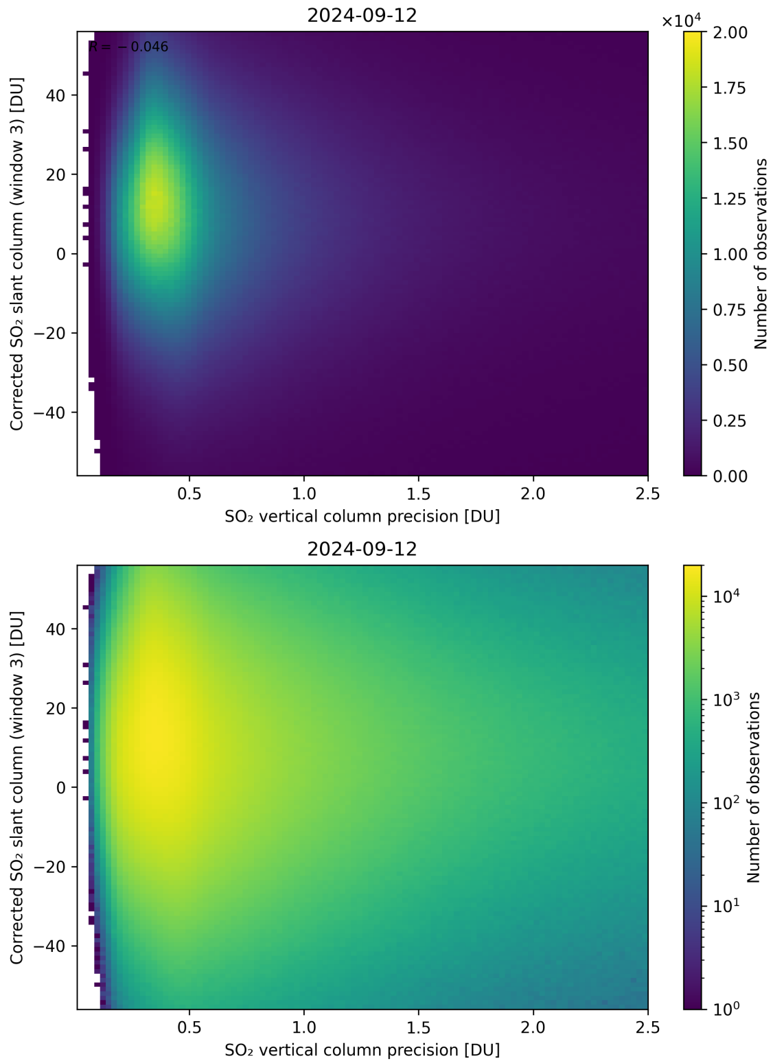
Figure 288: Scatter density plot of “SO 2 vertical column precision” against “Corrected SO 2 slant column (window 3)” for 2024-09-12 to 2024-09-13.
