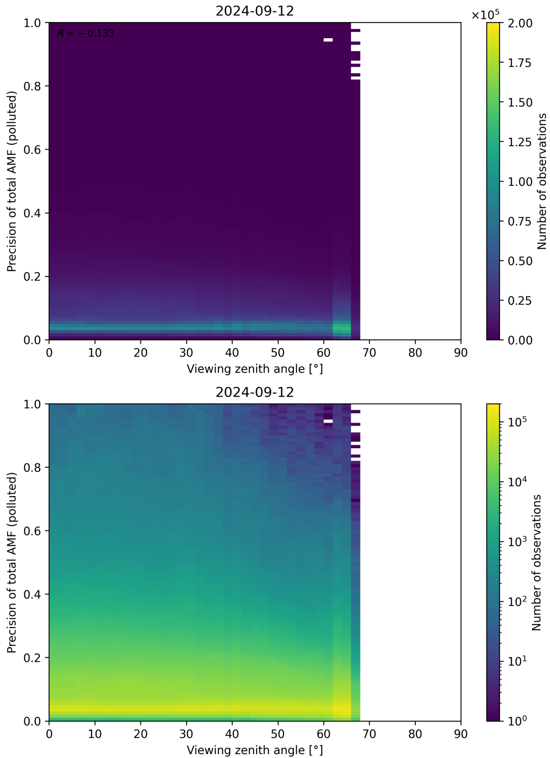
Figure 326: Scatter density plot of “Viewing zenith angle” against “Precision of total AMF (polluted)” for 2024-09-12 to 2024-09-13.
