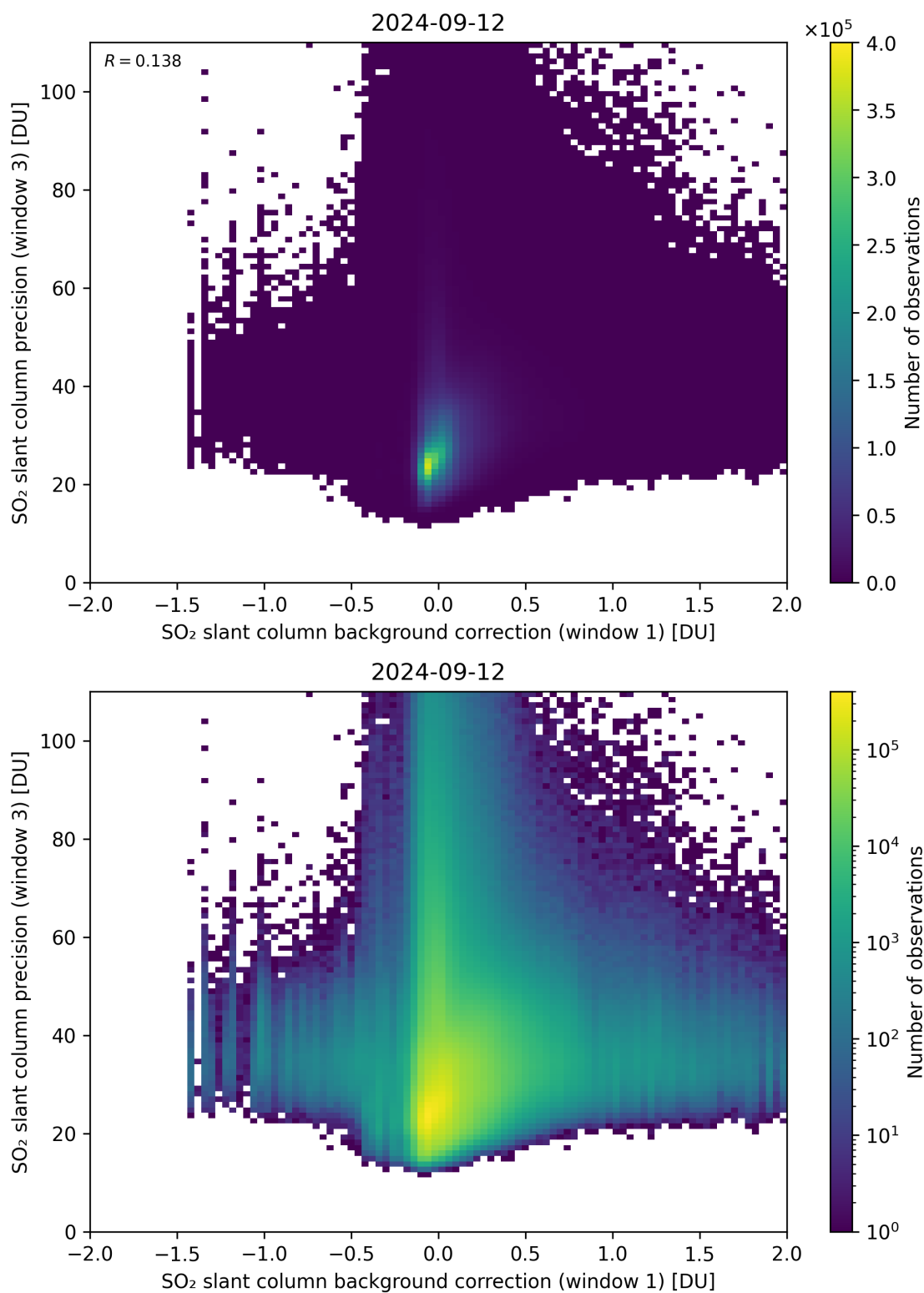
Figure 108: Scatter density plot of “SO 2 slant column background correction (window 1)” against “SO 2 slant column precision (window 3)” for 2024-09-12 to 2024-09-13.
