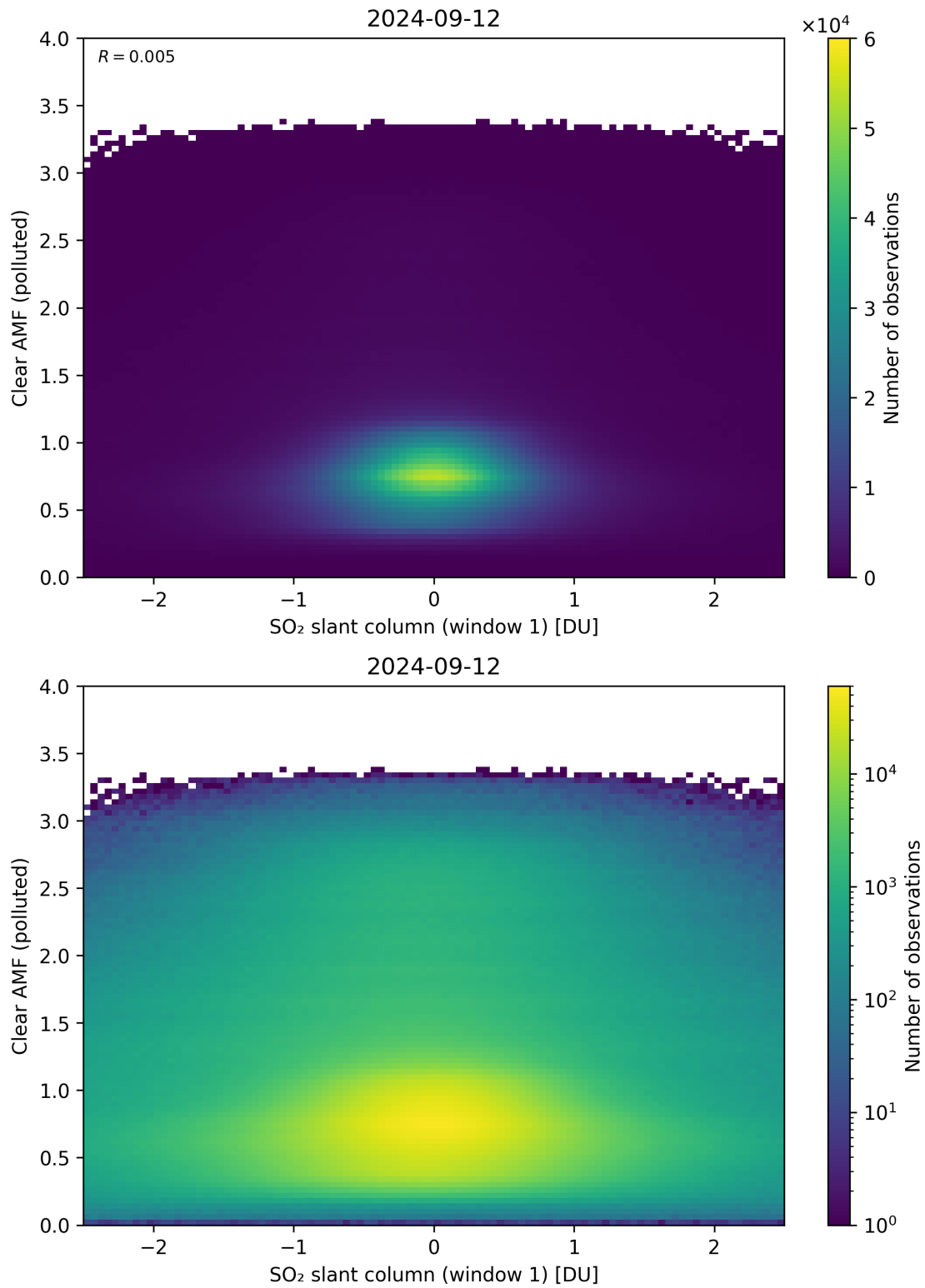
Figure 232: Scatter density plot of “SO 2 slant column (window 1)” against “Clear AMF (polluted)” for 2024-09-12 to 2024-09-13.
