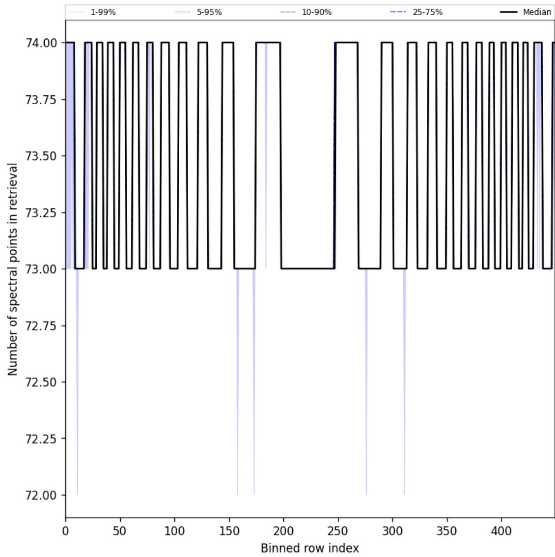
Figure 97: Along track statistics of “Number of spectral points in retrieval” for 2024-09-12 to 2024-09-13
