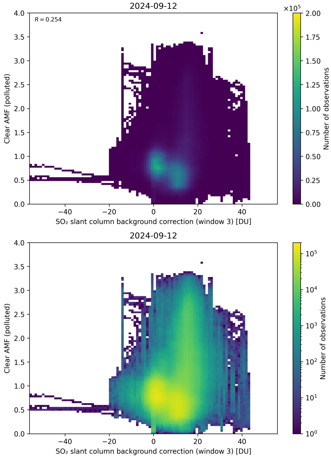
Figure 124: Scatter density plot of “SO 2 slant column background correction (window 3)” against “Clear AMF (polluted)” for 2024-09-12 to 2024-09-13.
