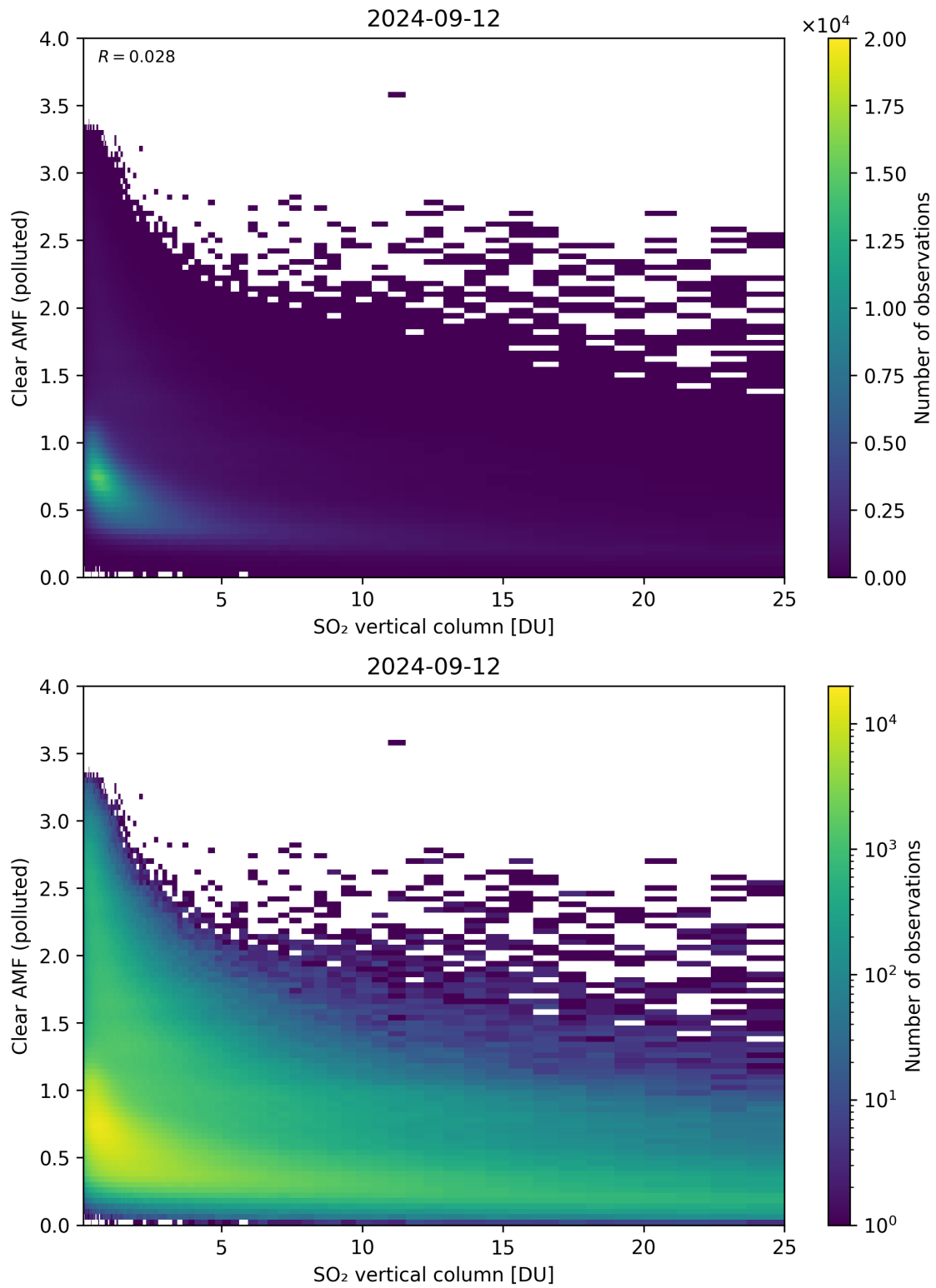
Figure 296: Scatter density plot of “SO 2 vertical column” against “Clear AMF (polluted)” for 2024-09-12 to 2024-09-13.
