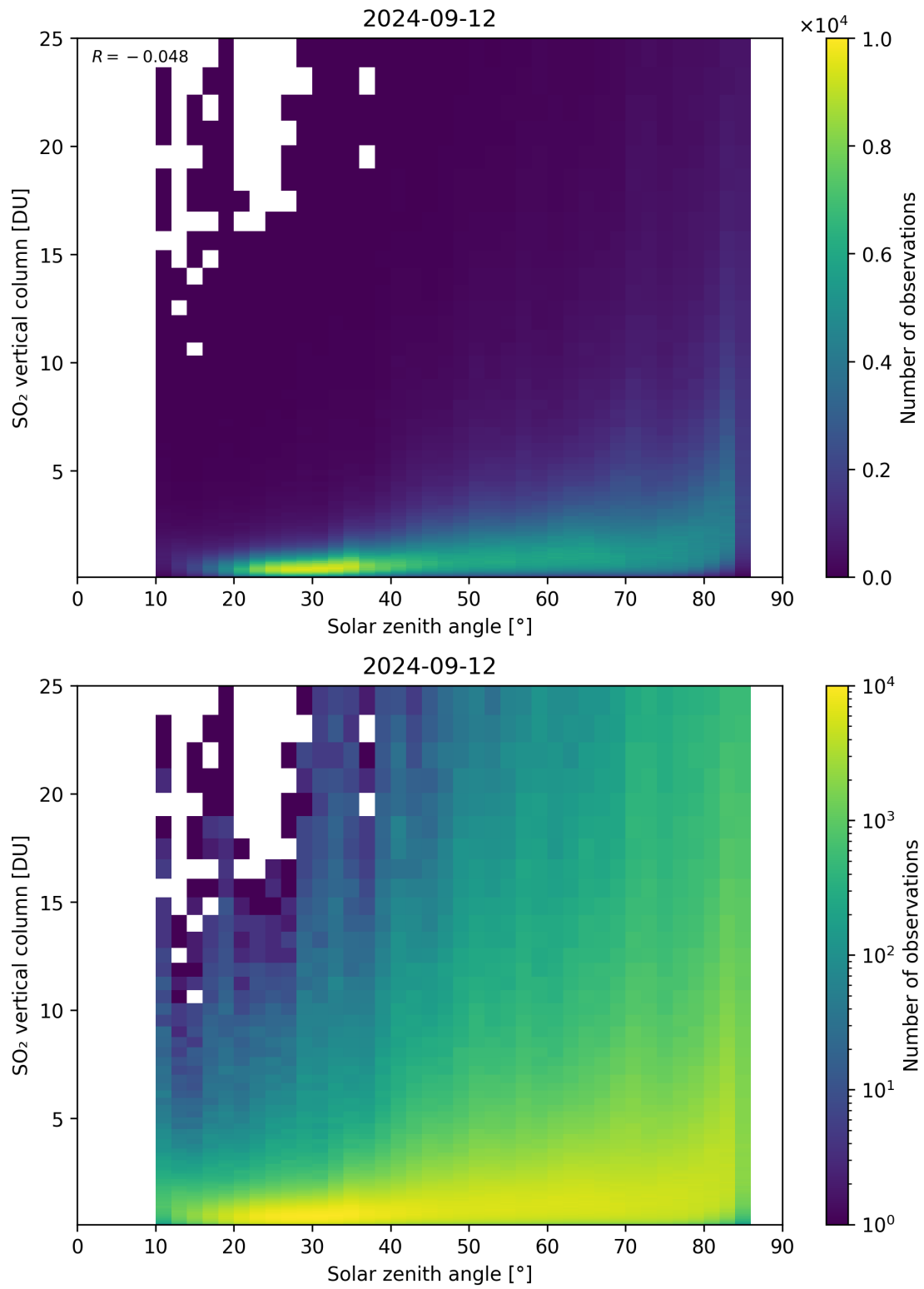
Figure 176: Scatter density plot of “Solar zenith angle” against “SO 2 vertical column” for 2024-09-12 to 2024-09-13.
