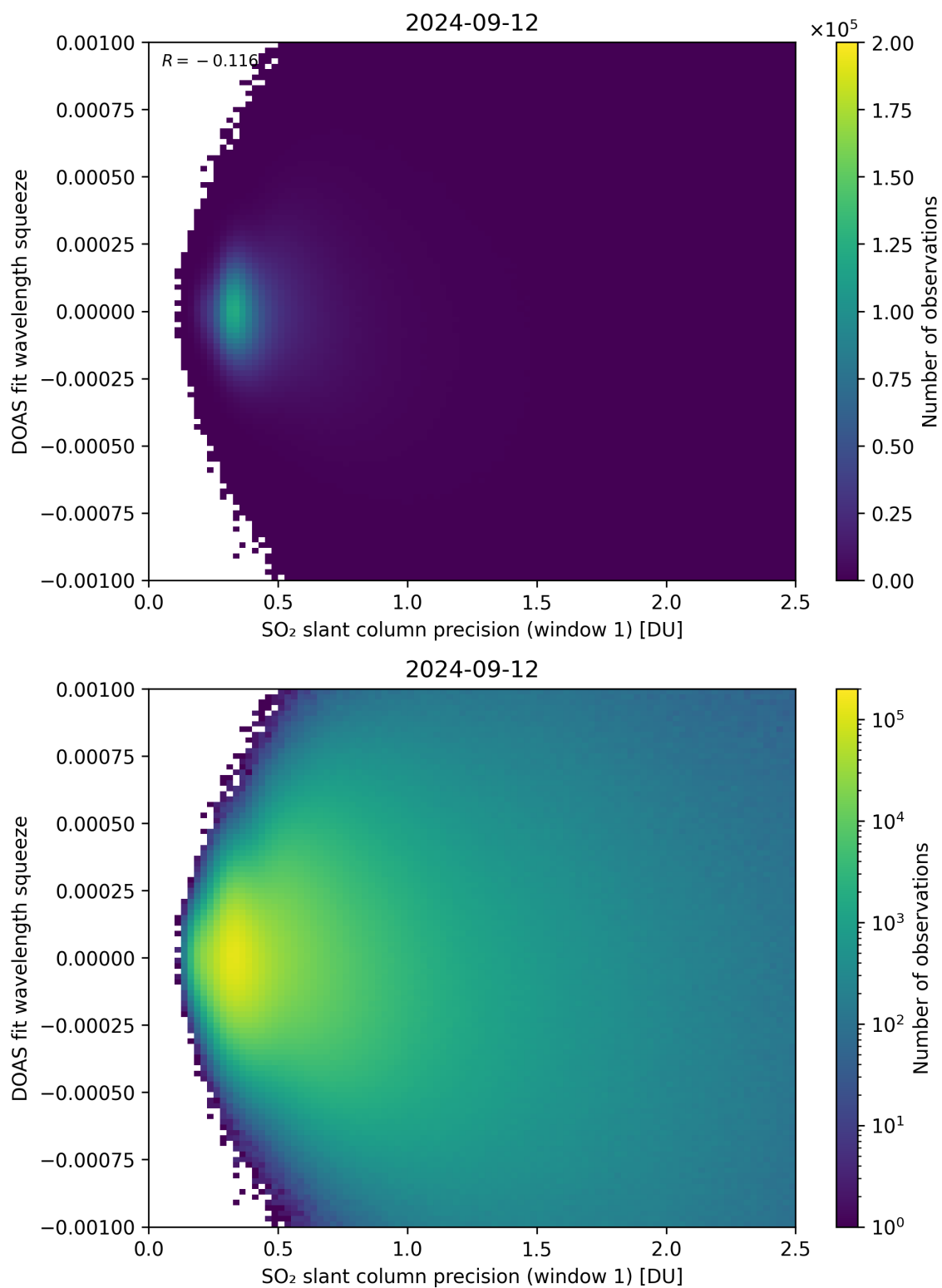
Figure 222: Scatter density plot of “SO 2 slant column precision (window 1)” against “DOAS fit wavelength squeeze” for 2024-09-12 to 2024-09-13.
