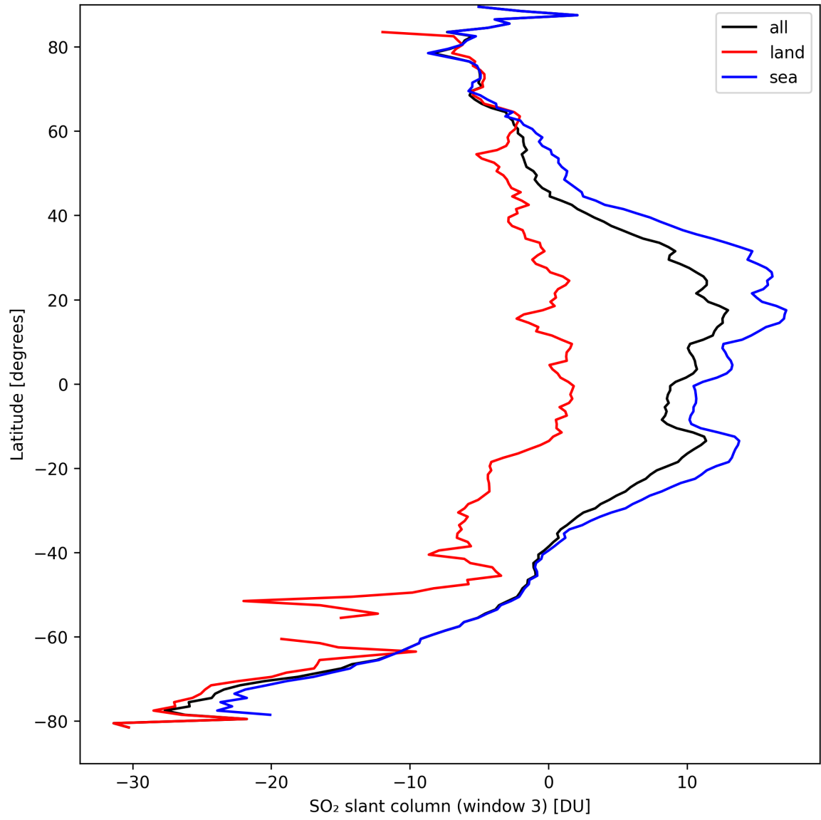
Figure 41: Zonal average of “SO 2 slant column (window 3)” for 2024-09-12 to 2024-09-13.
