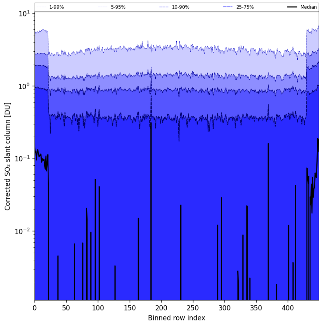
Figure 78: Along track statistics of “Corrected SO 2 slant column” for 2024-09-12 to 2024-09-13
