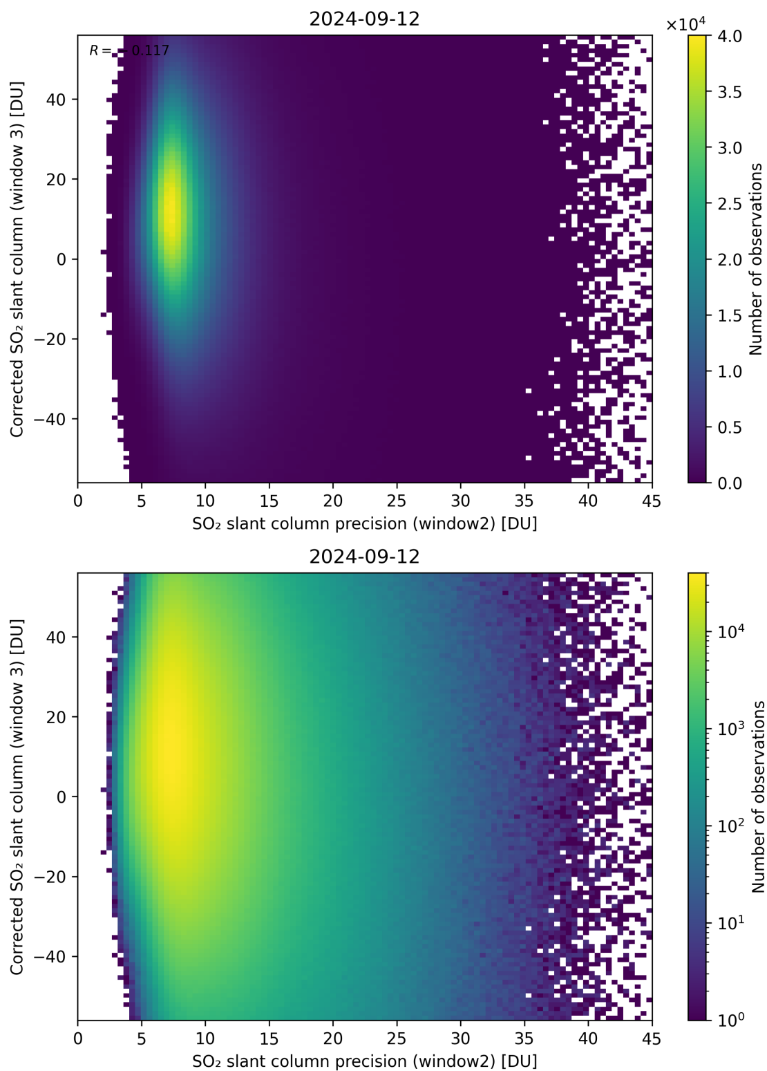
Figure 248: Scatter density plot of “SO 2 slant column precision (window2)” against “Corrected SO 2 slant column (window 3)” for 2024-09-12 to 2024-09-13.
