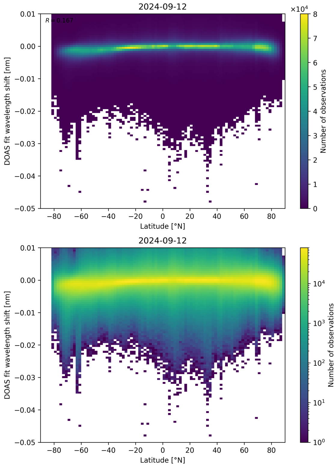
Figure 142: Scatter density plot of “Latitude” against “DOAS fit wavelength shift” for 2024-09-12 to 2024-09-13.
