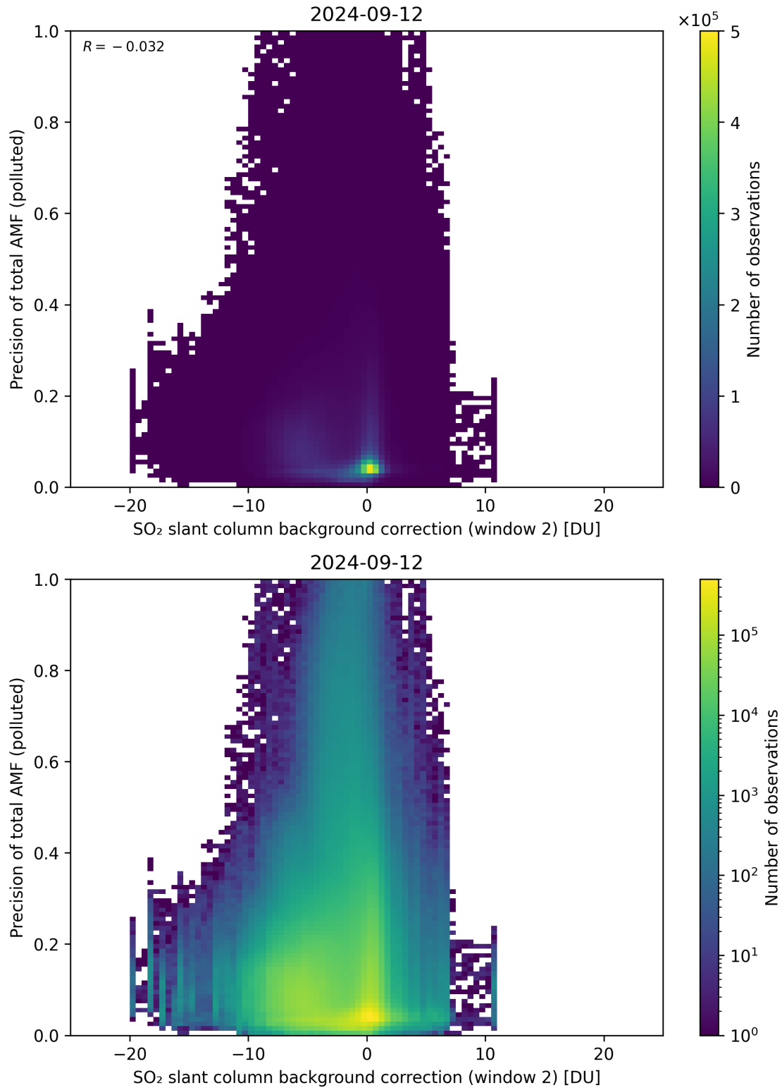
Figure 120: Scatter density plot of “SO 2 slant column background correction (window 2)” against “Precision of total AMF (polluted)” for 2024-09-12 to 2024-09-13.
