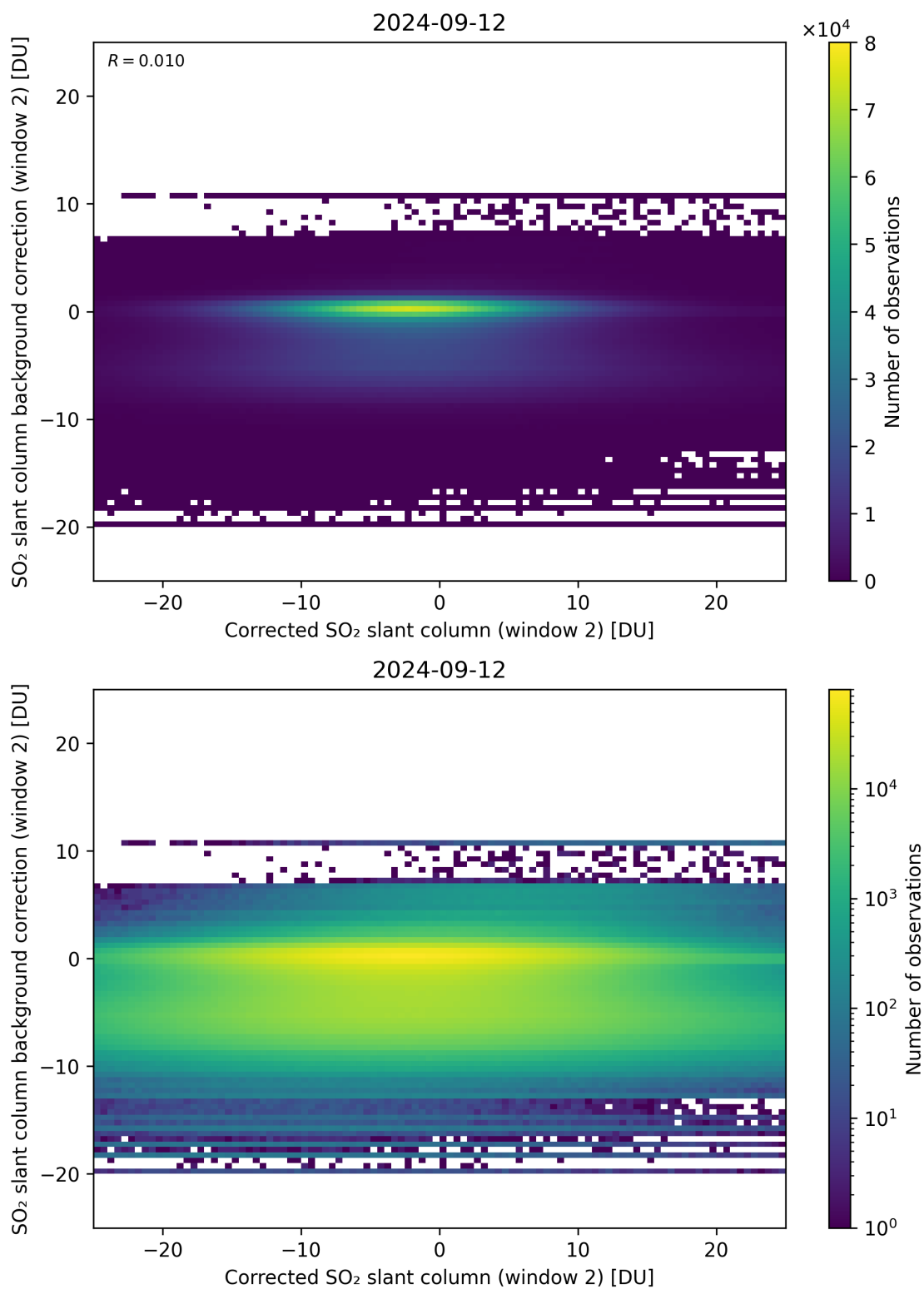
Figure 194: Scatter density plot of “Corrected SO 2 slant column (window 2)” against “SO 2 slant column background correction (window 2)” for 2024-09-12 to 2024-09-13.
