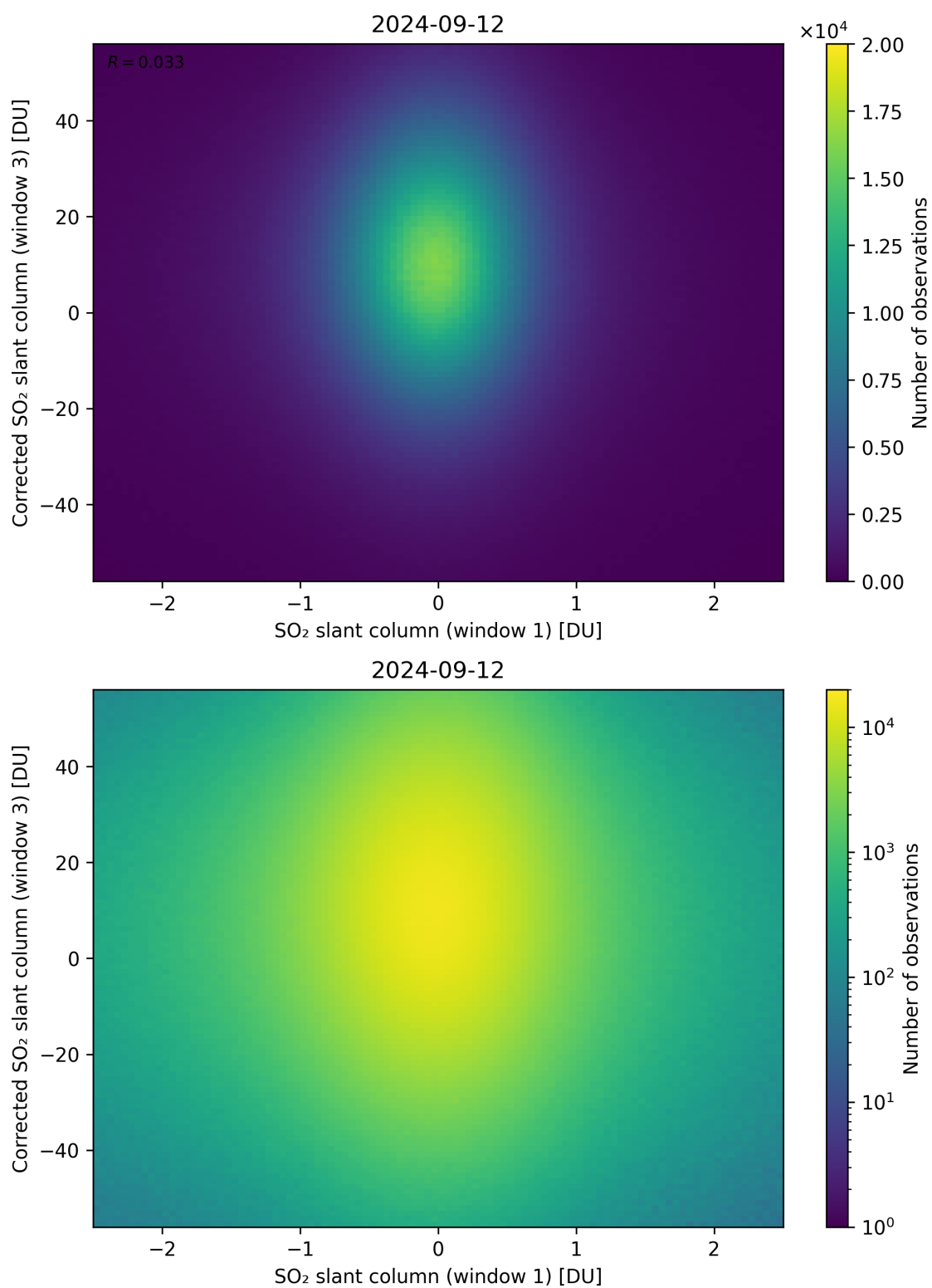
Figure 234: Scatter density plot of “SO 2 slant column (window 1)” against “Corrected SO 2 slant column (window 3)” for 2024-09-12 to 2024-09-13.
