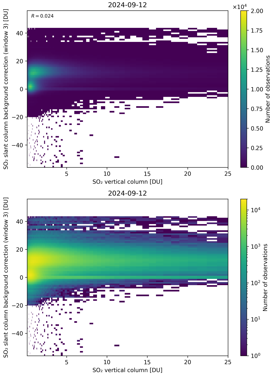
Figure 275: Scatter density plot of “SO 2 vertical column” against “SO 2 slant column background correction (window 3)” for 2024-09-12 to 2024-09-13.
