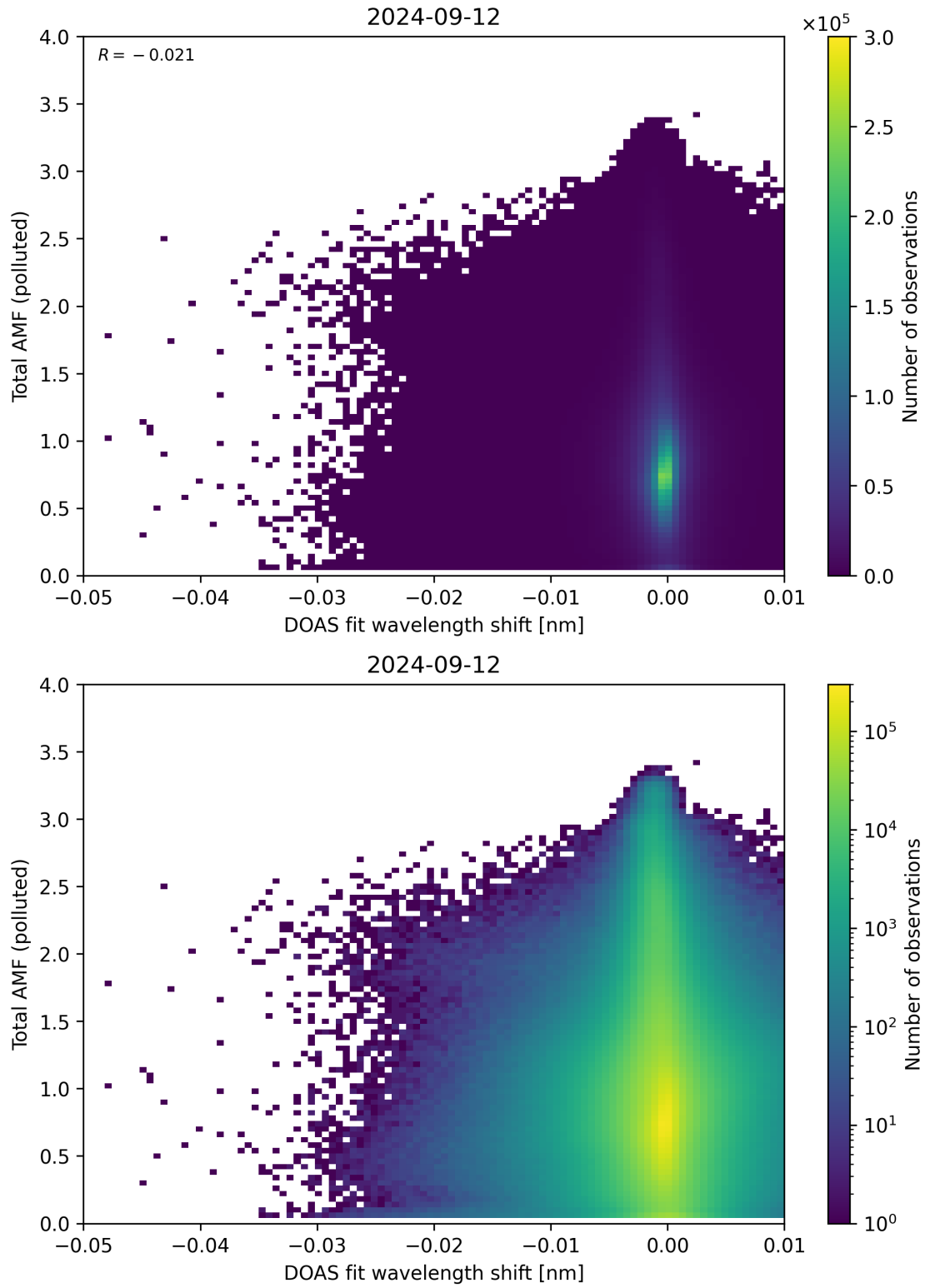
Figure 130: Scatter density plot of “DOAS fit wavelength shift” against “Total AMF (polluted)” for 2024-09-12 to 2024-09-13.
