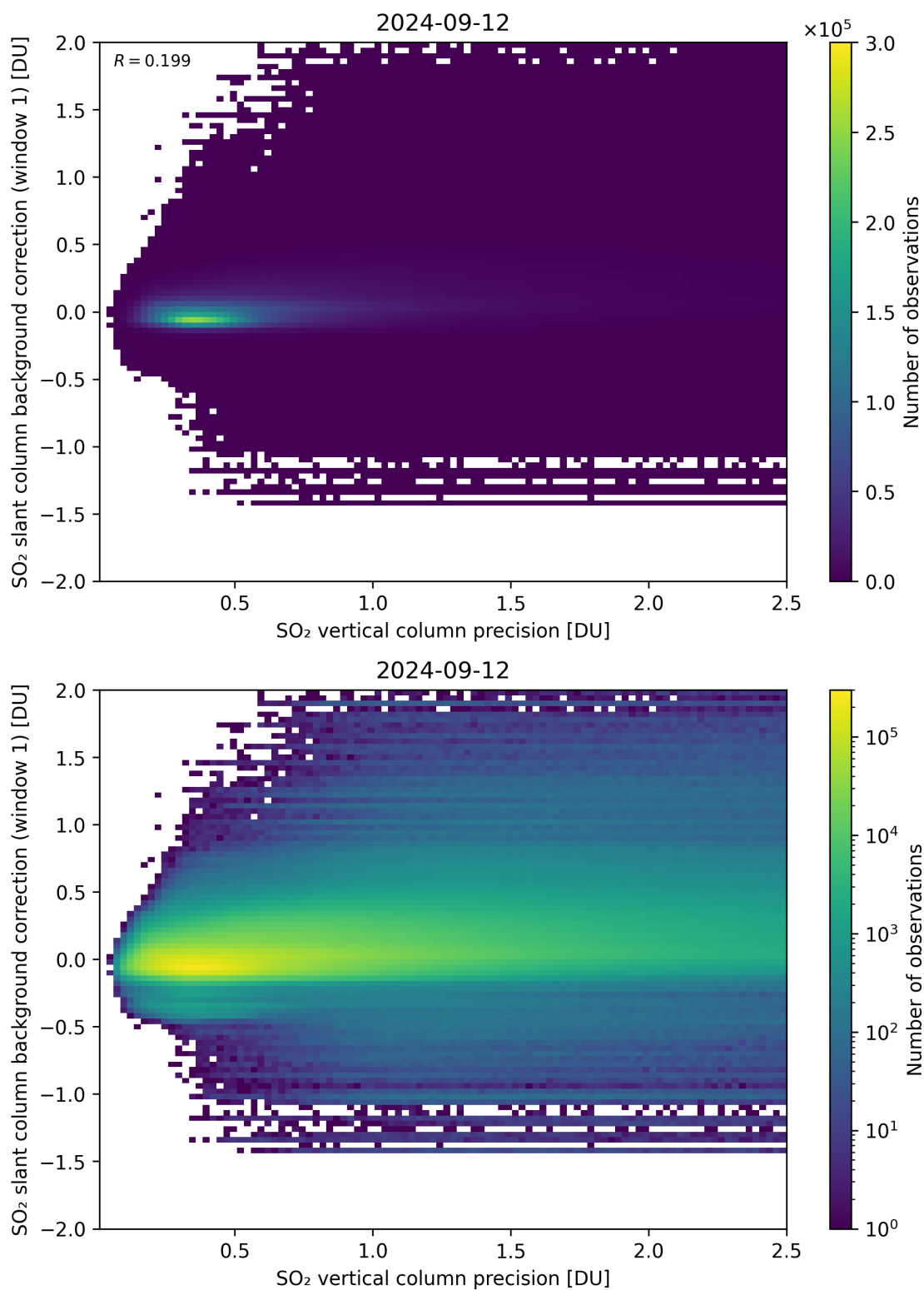
Figure 279: Scatter density plot of “SO 2 vertical column precision” against “SO 2 slant column background correction (window 1)” for 2024-09-12 to 2024-09-13.
