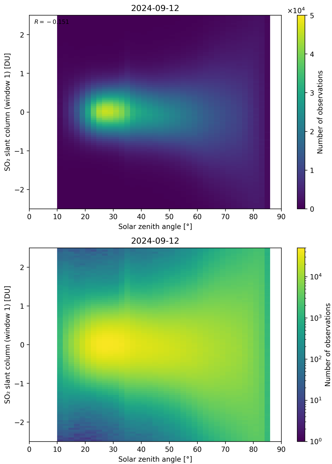
Figure 169: Scatter density plot of “Solar zenith angle” against “SO 2 slant column (window 1)” for 2024-09-12 to 2024-09-13.
