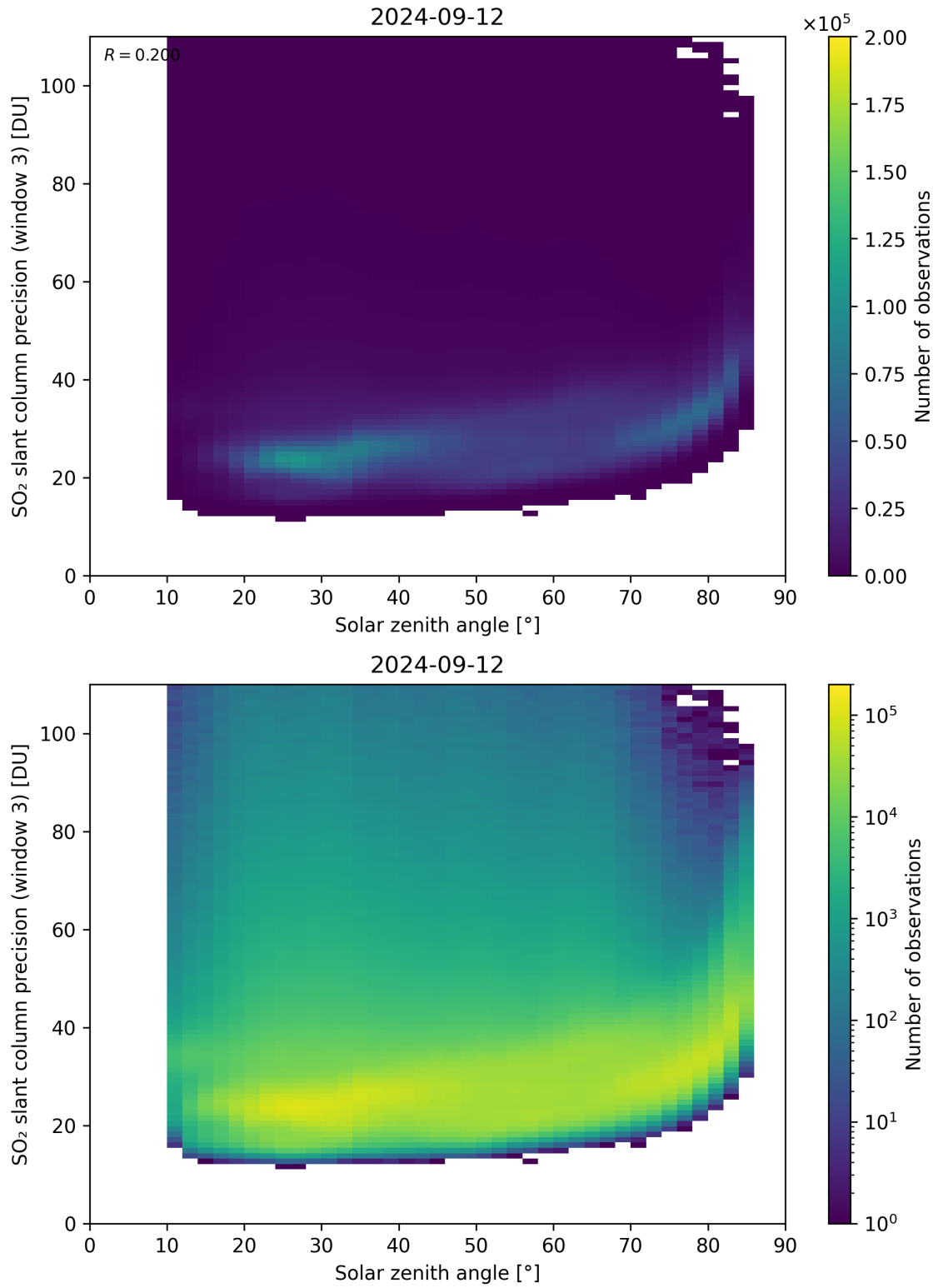
Figure 173: Scatter density plot of “Solar zenith angle” against “SO 2 slant column precision (window 3)” for 2024-09-12 to 2024-09-13.
