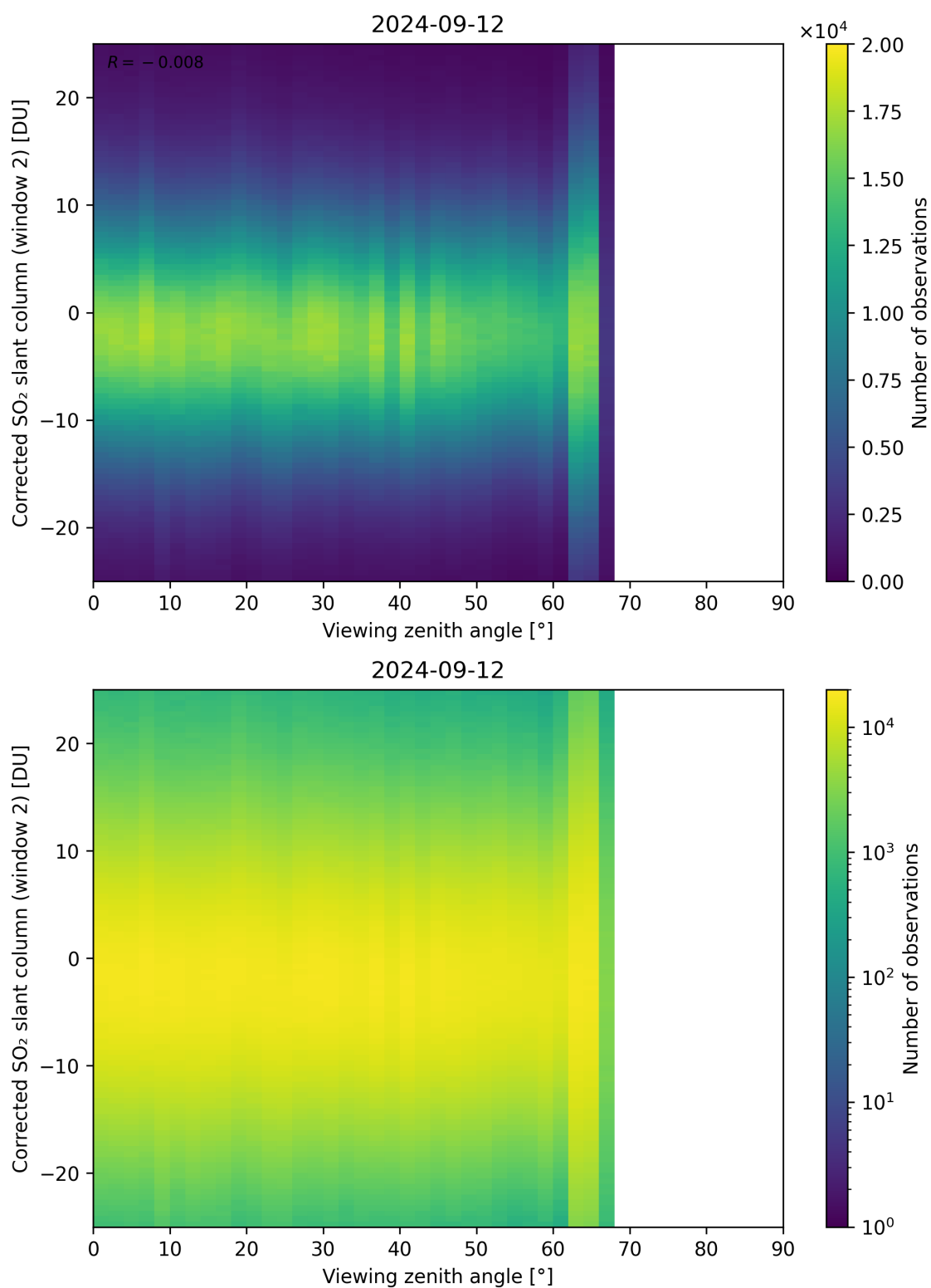
Figure 318: Scatter density plot of “Viewing zenith angle” against “Corrected SO 2 slant column (window 2)” for 2024-09-12 to 2024-09-13.
