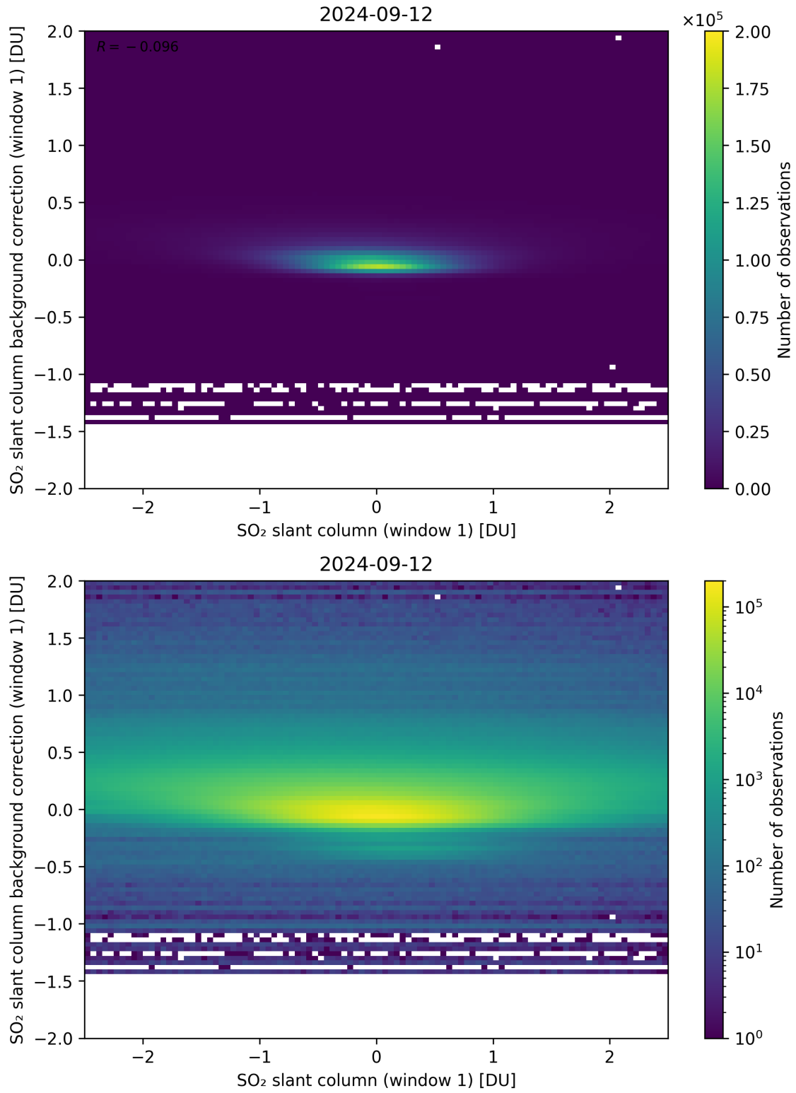
Figure 212: Scatter density plot of “SO 2 slant column (window 1)” against “SO 2 slant column background correction (window 1)” for 2024-09-12 to 2024-09-13.
