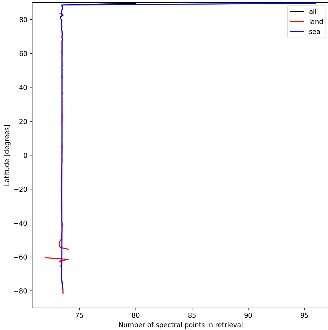
Figure 51: Zonal average of “Number of spectral points in retrieval” for 2024-09-12 to 2024-09-13.
