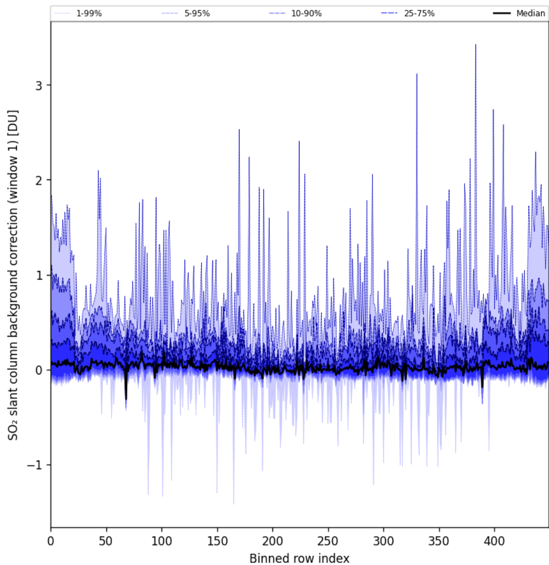
Figure 82: Along track statistics of “SO 2 slant column background correction (window 1)” for 2024-09-12 to 2024-09-13
