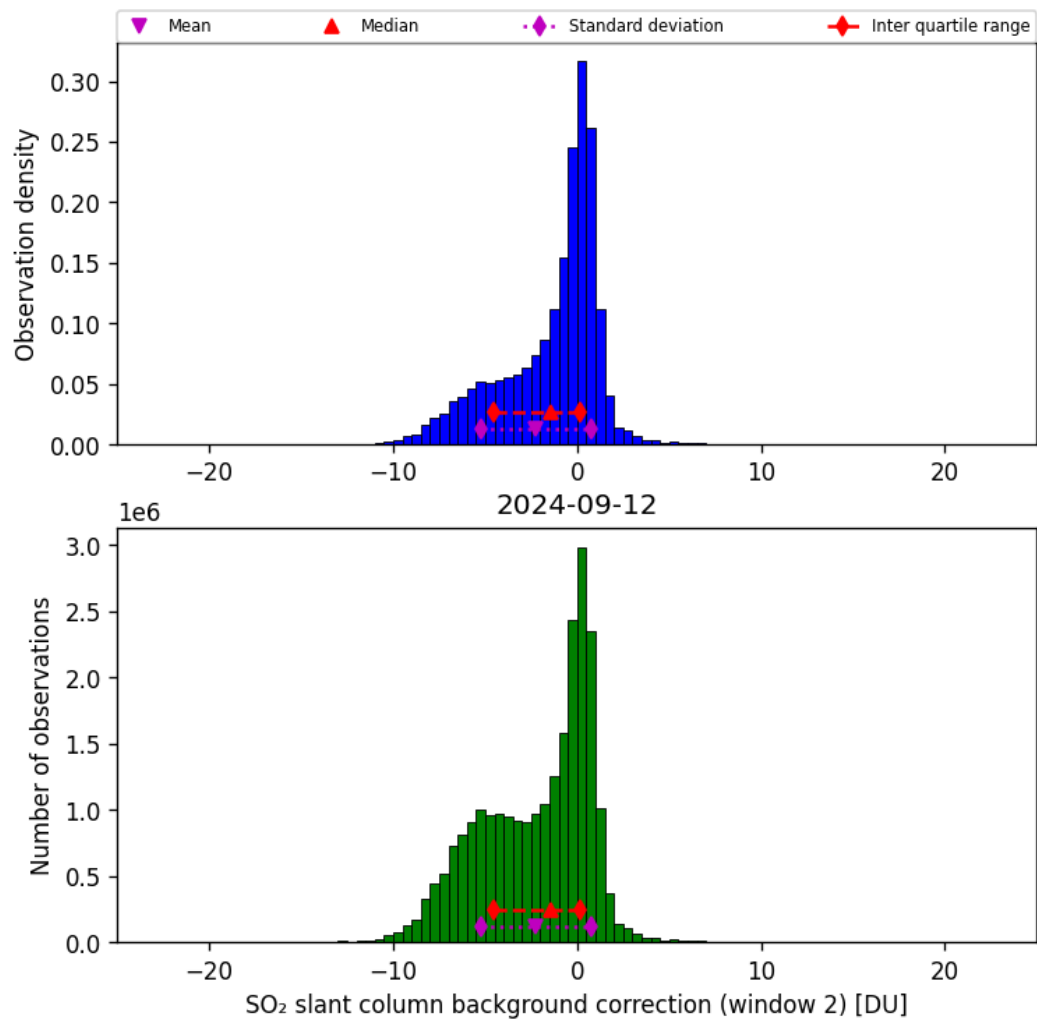
Figure 63: Histogram of “SO 2 slant column background correction (window 2)” for 2024-09-12 to 2024-09-13
