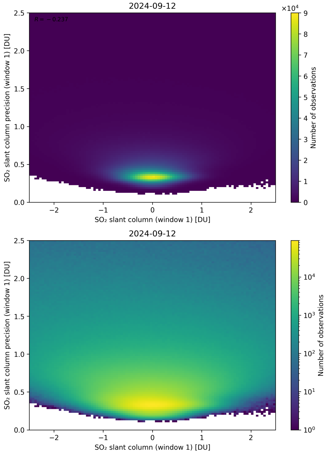
Figure 235: Scatter density plot of “SO 2 slant column (window 1)” against “SO 2 slant column precision (window 1)” for 2024-09-12 to 2024-09-13.
