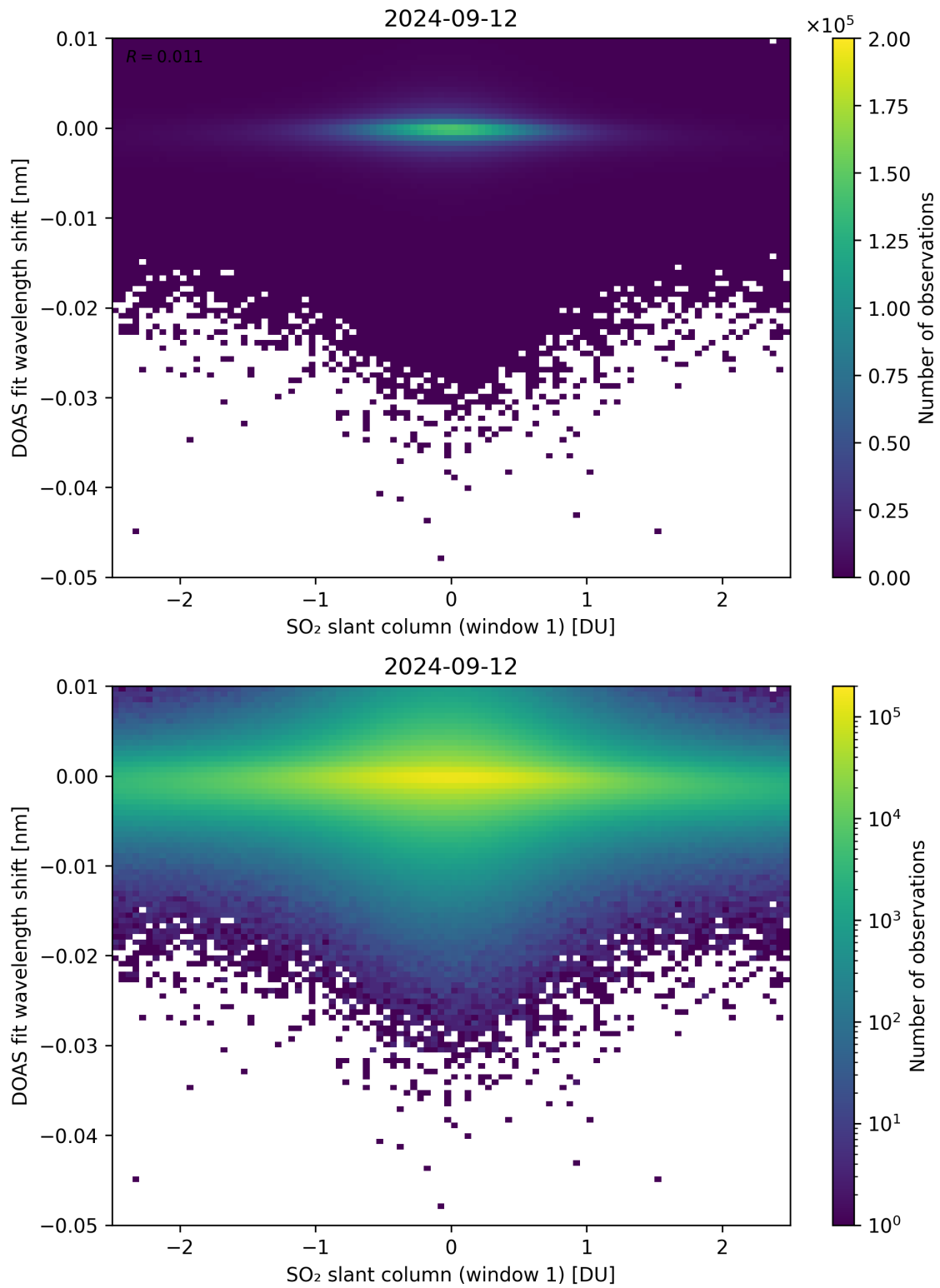
Figure 215: Scatter density plot of “SO 2 slant column (window 1)” against “DOAS fit wavelength shift” for 2024-09-12 to 2024-09-13.
