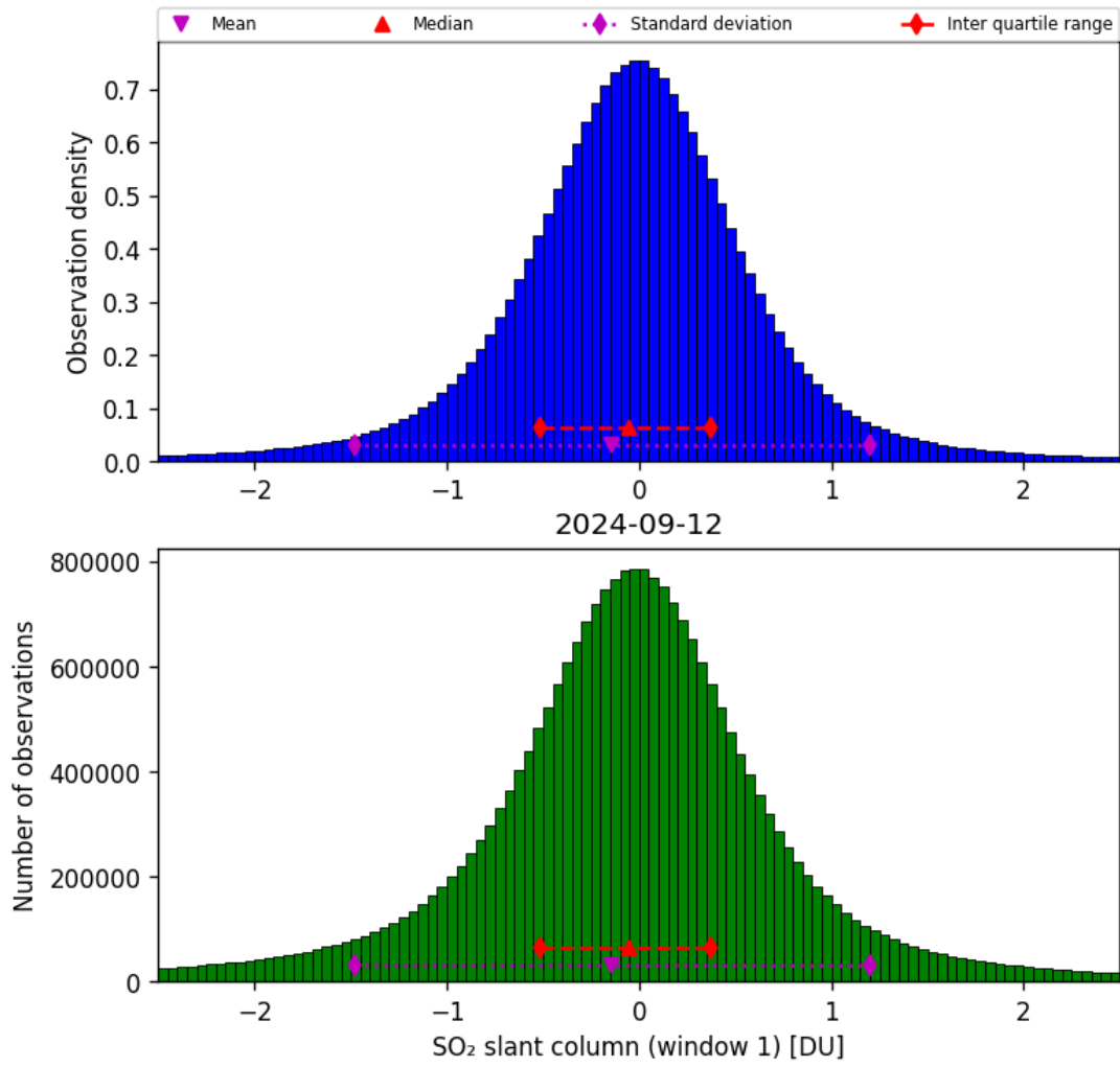
Figure 56: Histogram of “SO 2 slant column (window 1)” for 2024-09-12 to 2024-09-13
