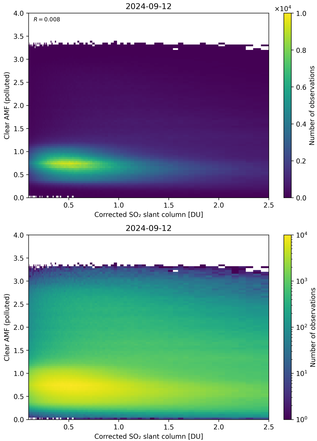
Figure 184: Scatter density plot of “Corrected SO 2 slant column” against “Clear AMF (polluted)” for 2024-09-12 to 2024-09-13.
