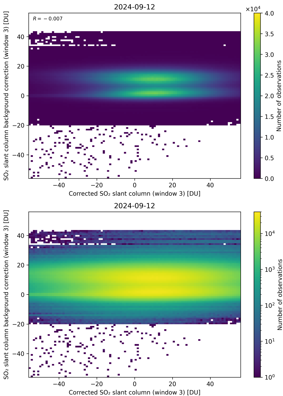
Figure 205: Scatter density plot of “Corrected SO 2 slant column (window 3)” against “SO 2 slant column background correction (window 3)” for 2024-09-12 to 2024-09-13.
