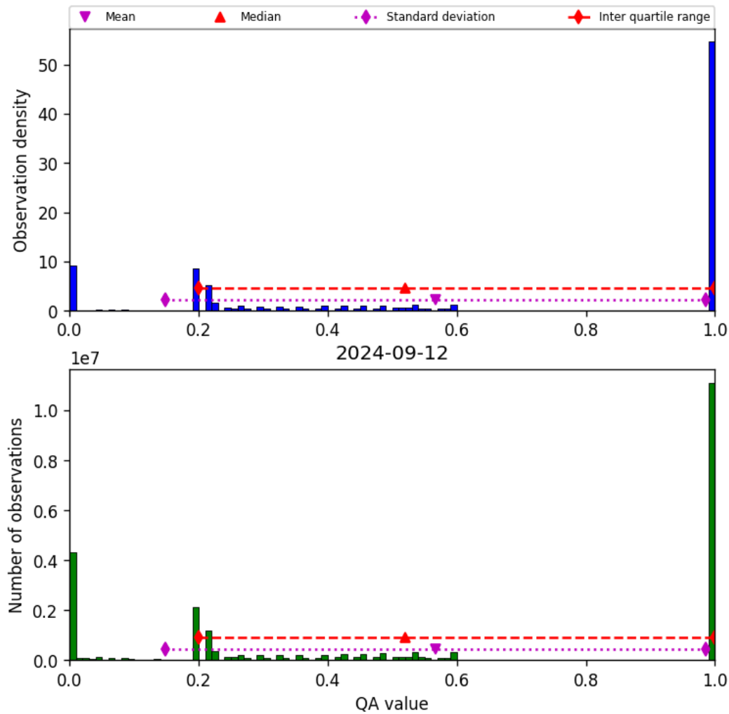
Figure 52: Histogram of “QA value” for 2024-09-12 to 2024-09-13
