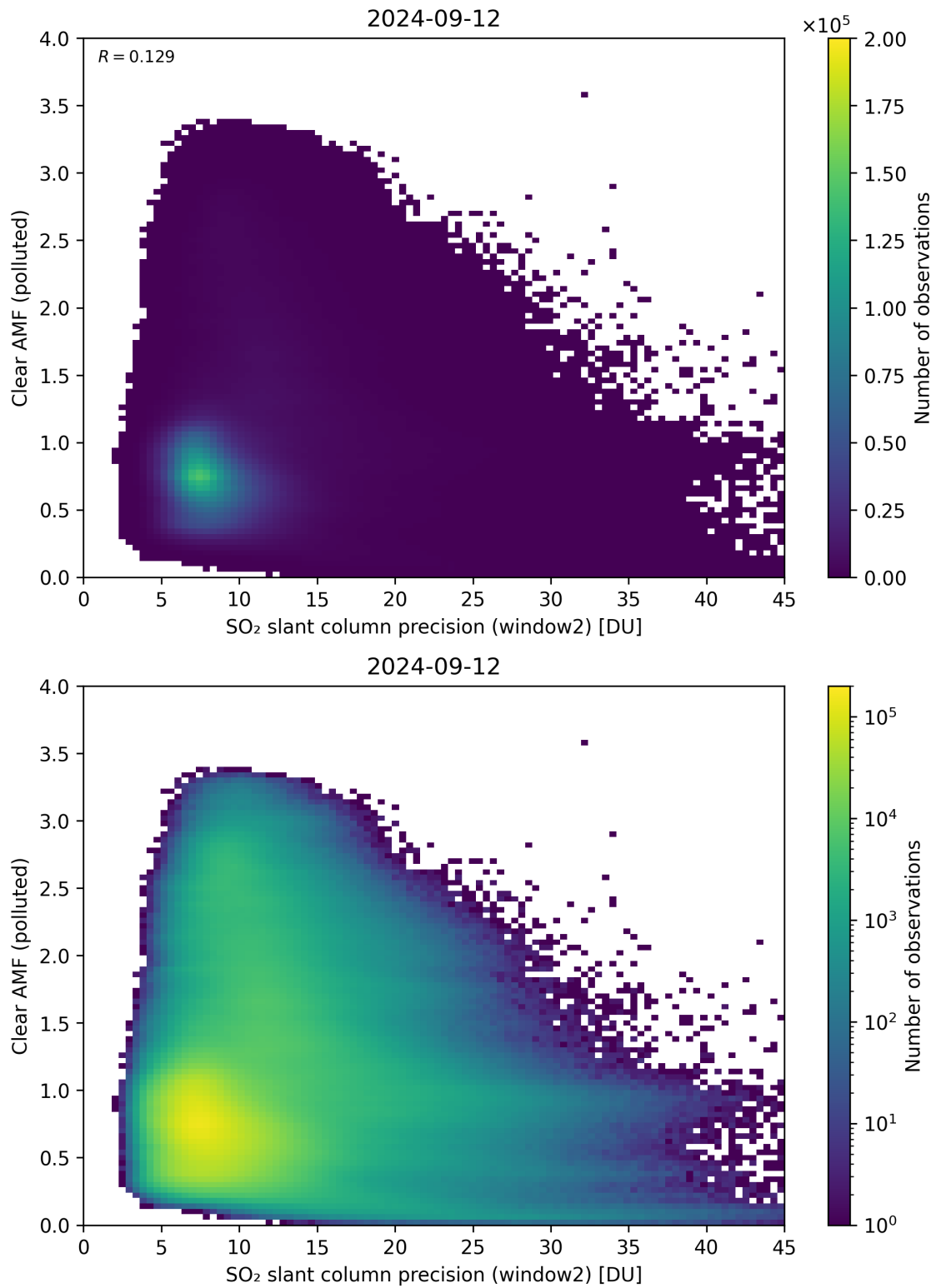
Figure 246: Scatter density plot of “SO 2 slant column precision (window2)” against “Clear AMF (polluted)” for 2024-09-12 to 2024-09-13.
