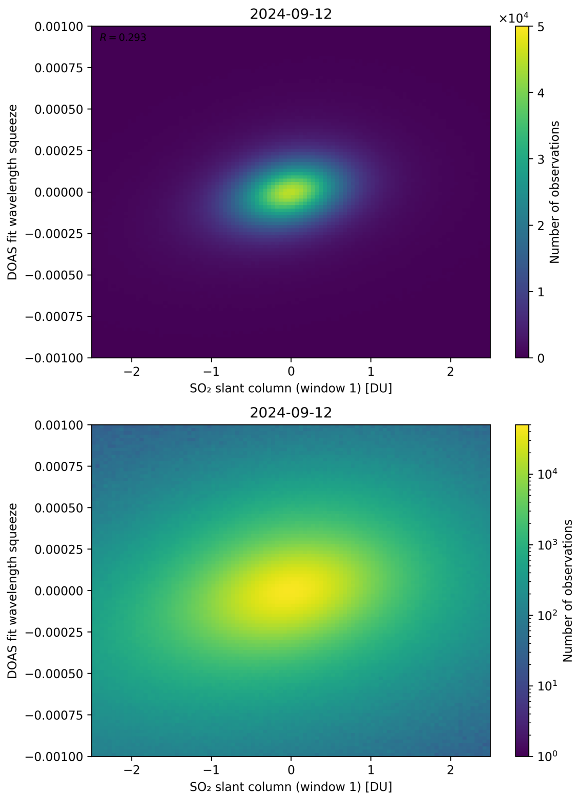
Figure 216: Scatter density plot of “SO 2 slant column (window 1)” against “DOAS fit wavelength squeeze” for 2024-09-12 to 2024-09-13.
