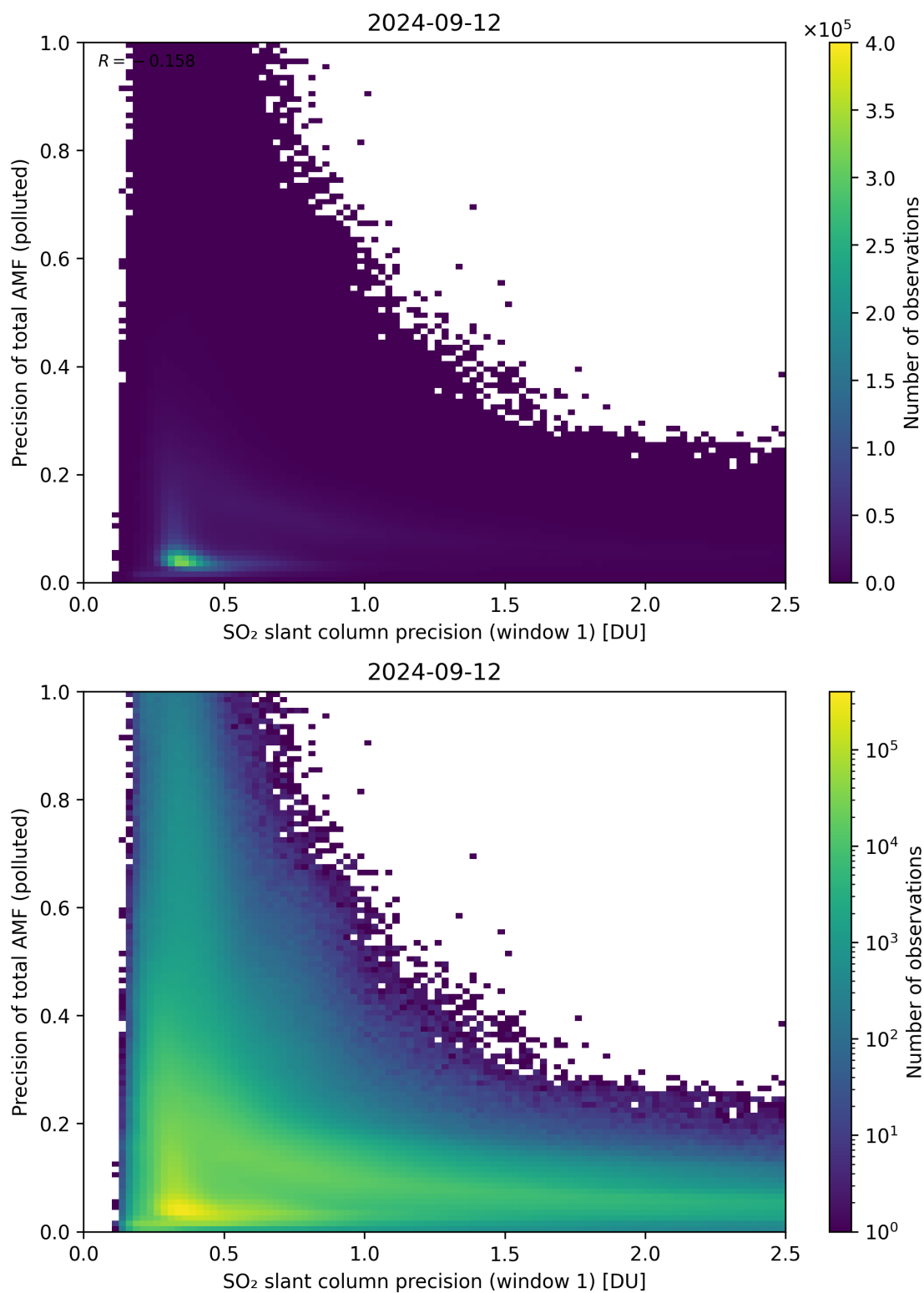
Figure 231: Scatter density plot of “SO 2 slant column precision (window 1)” against “Precision of total AMF (polluted)” for 2024-09-12 to 2024-09-13.
