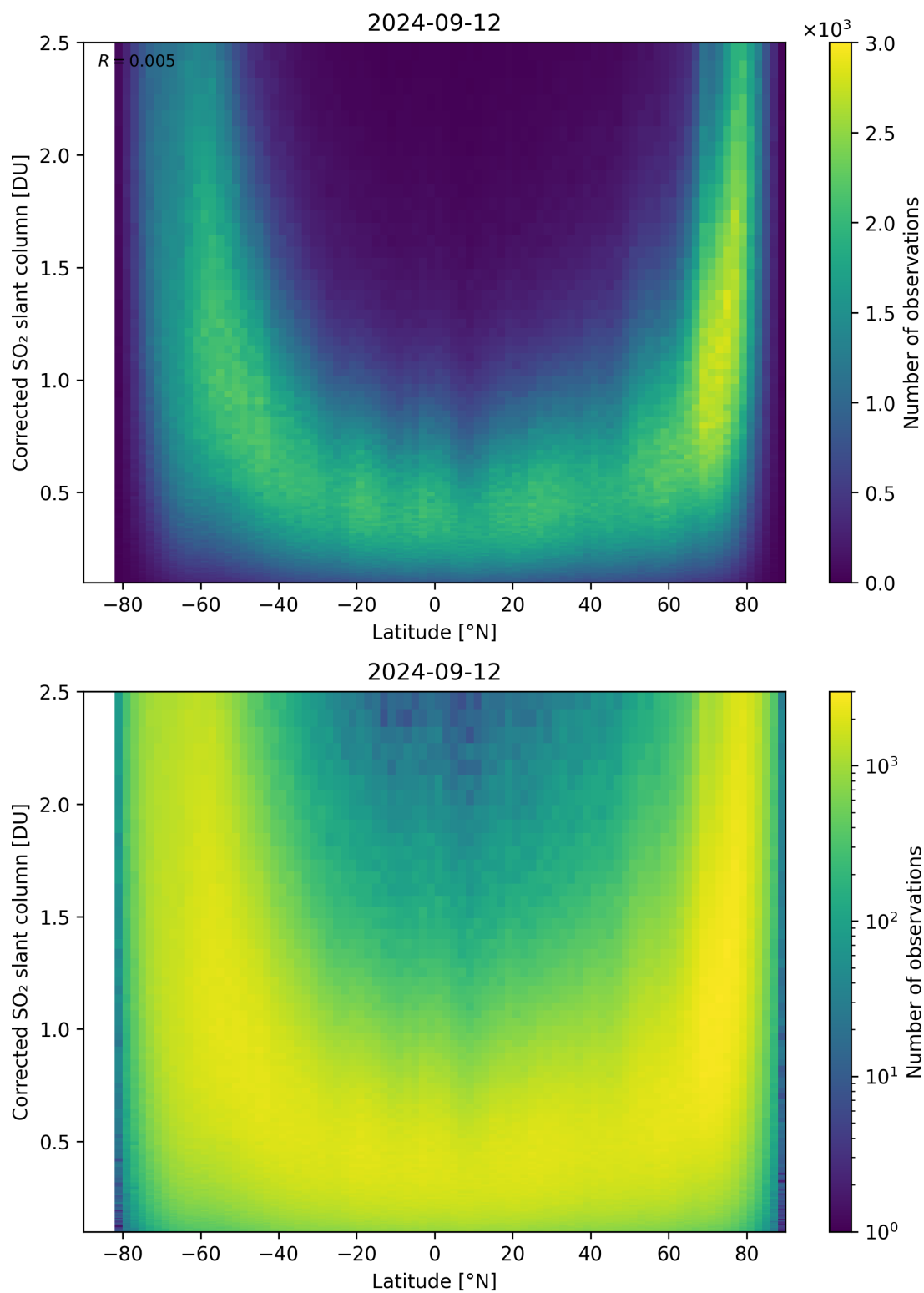
Figure 146: Scatter density plot of “Latitude” against “Corrected SO 2 slant column” for 2024-09-12 to 2024-09-13.
