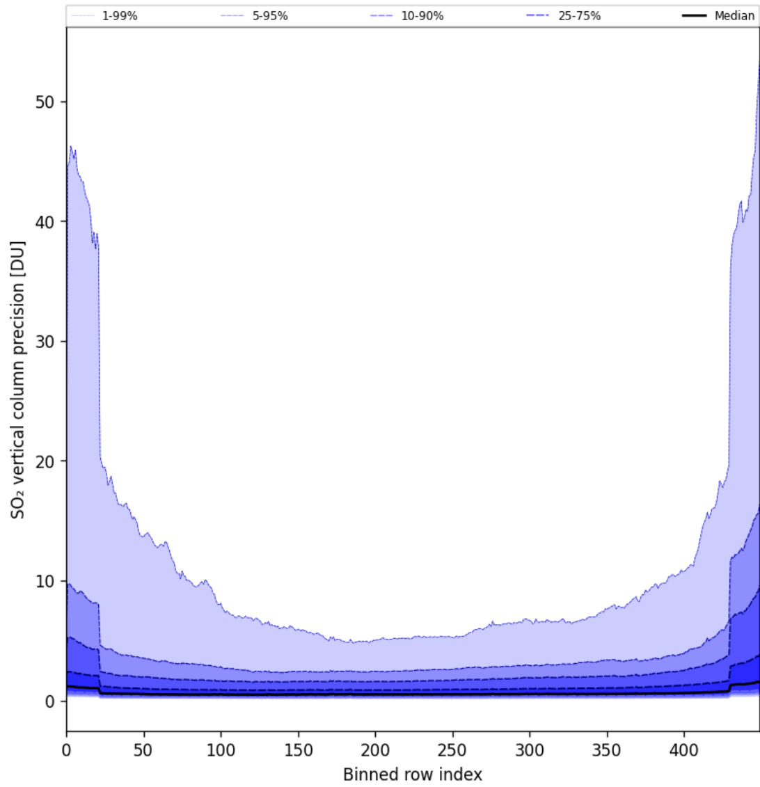
Figure 77: Along track statistics of “SO 2 vertical column precision” for 2024-09-12 to 2024-09-13
