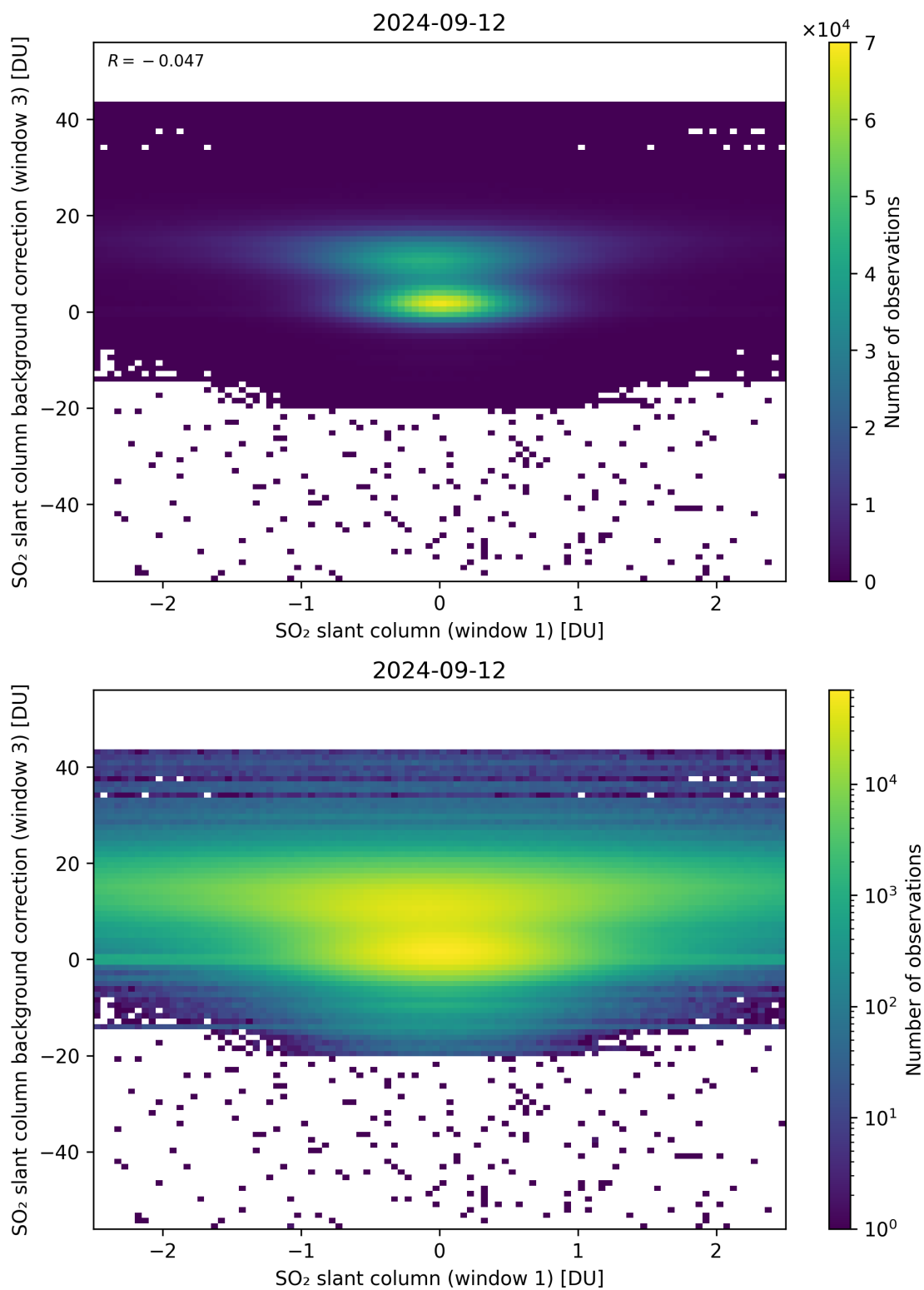
Figure 214: Scatter density plot of “SO 2 slant column (window 1)” against “SO 2 slant column background correction (window 3)” for 2024-09-12 to 2024-09-13.
