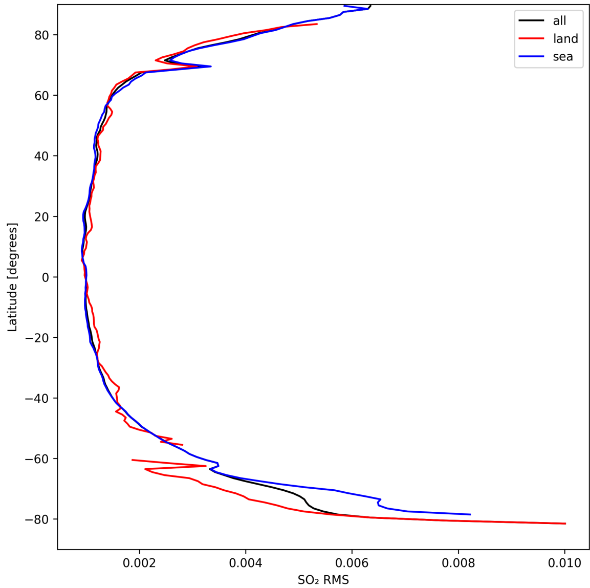
Figure 47: Zonal average of “SO 2 RMS” for 2024-09-12 to 2024-09-13.
