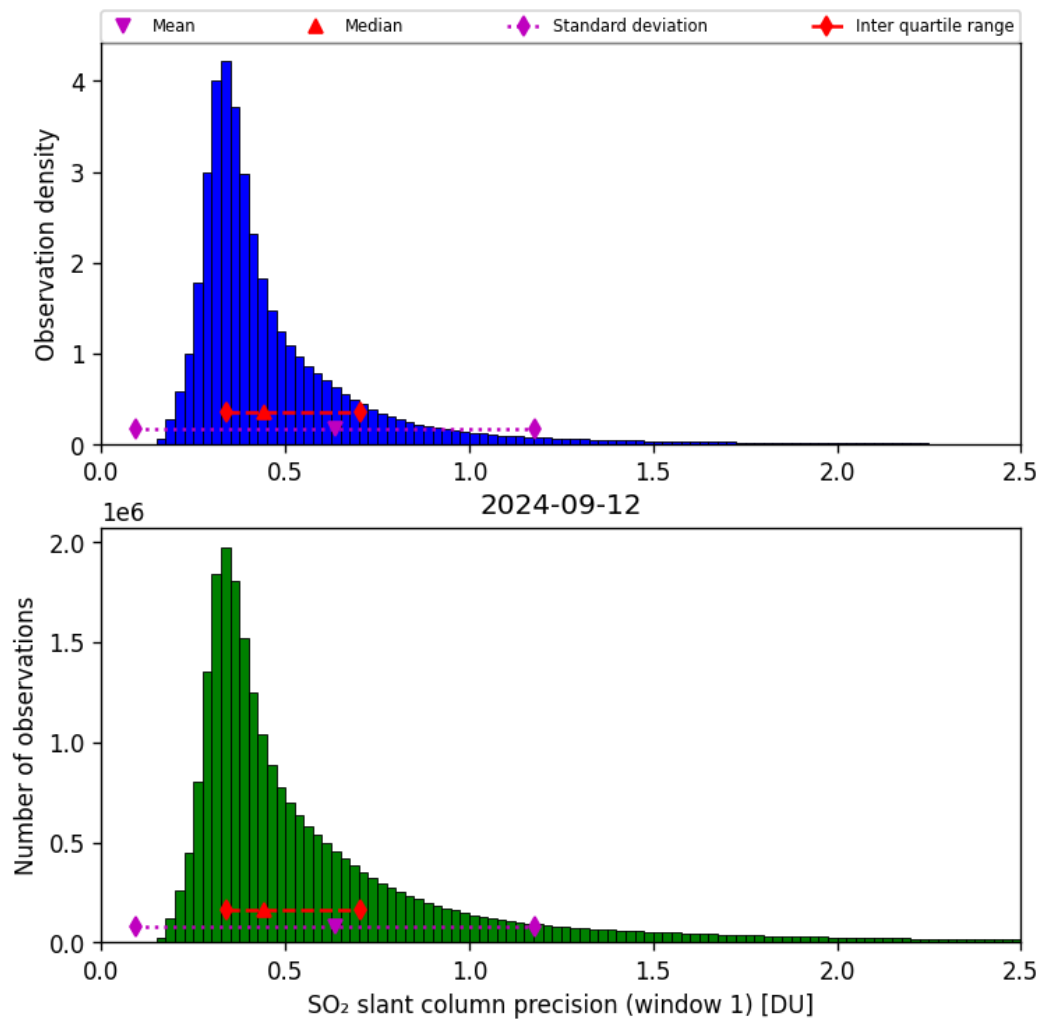
Figure 57: Histogram of “SO 2 slant column precision (window 1)” for 2024-09-12 to 2024-09-13
