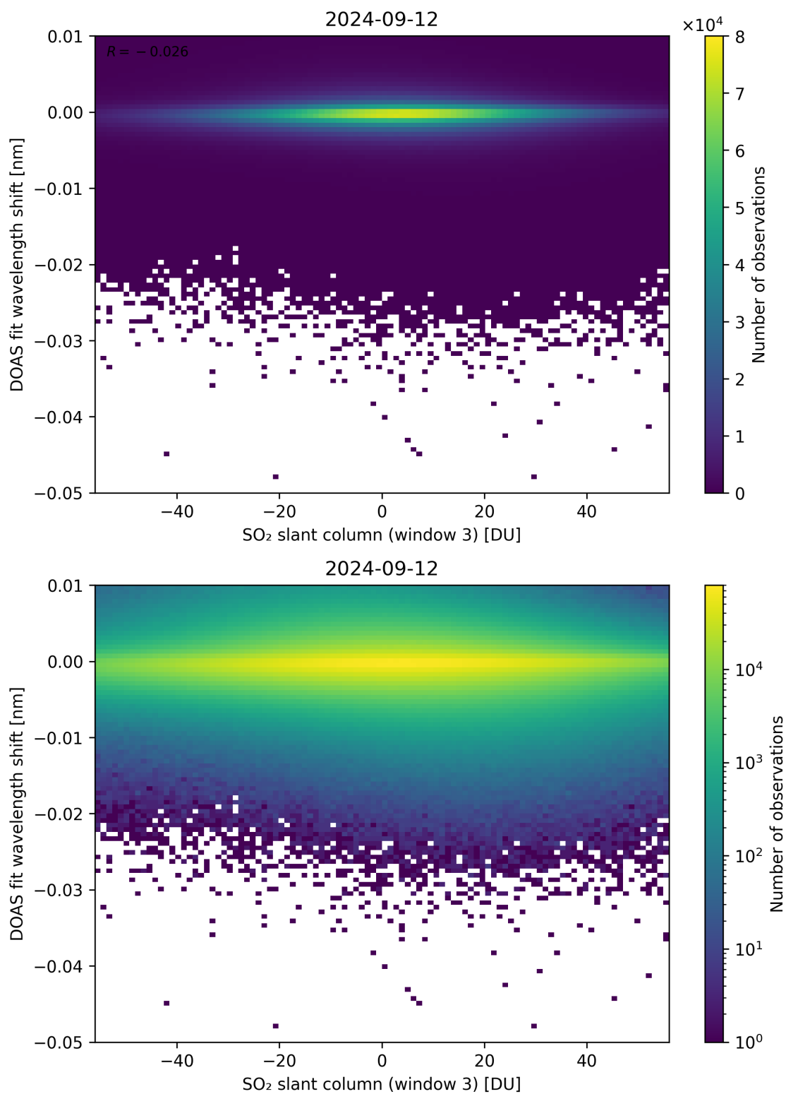
Figure 254: Scatter density plot of “SO 2 slant column (window 3)” against “DOAS fit wavelength shift” for 2024-09-12 to 2024-09-13.
