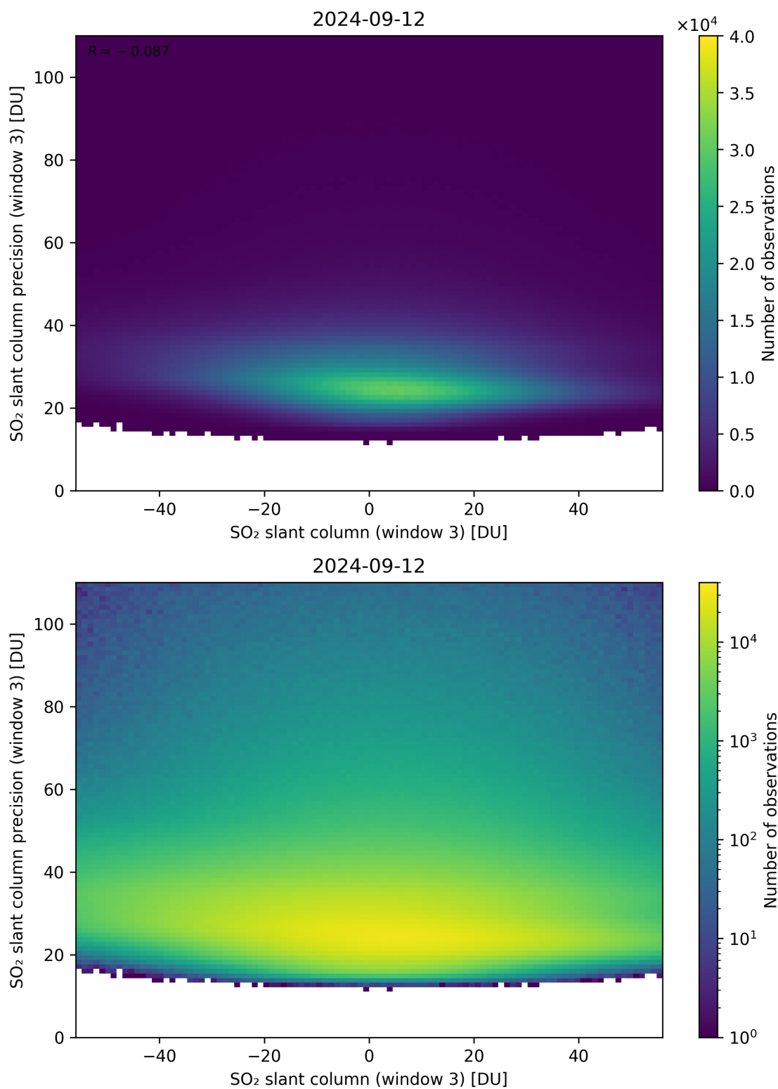
Figure 267: Scatter density plot of “SO 2 slant column (window 3)” against “SO 2 slant column precision (window 3)” for 2024-09-12 to 2024-09-13.
