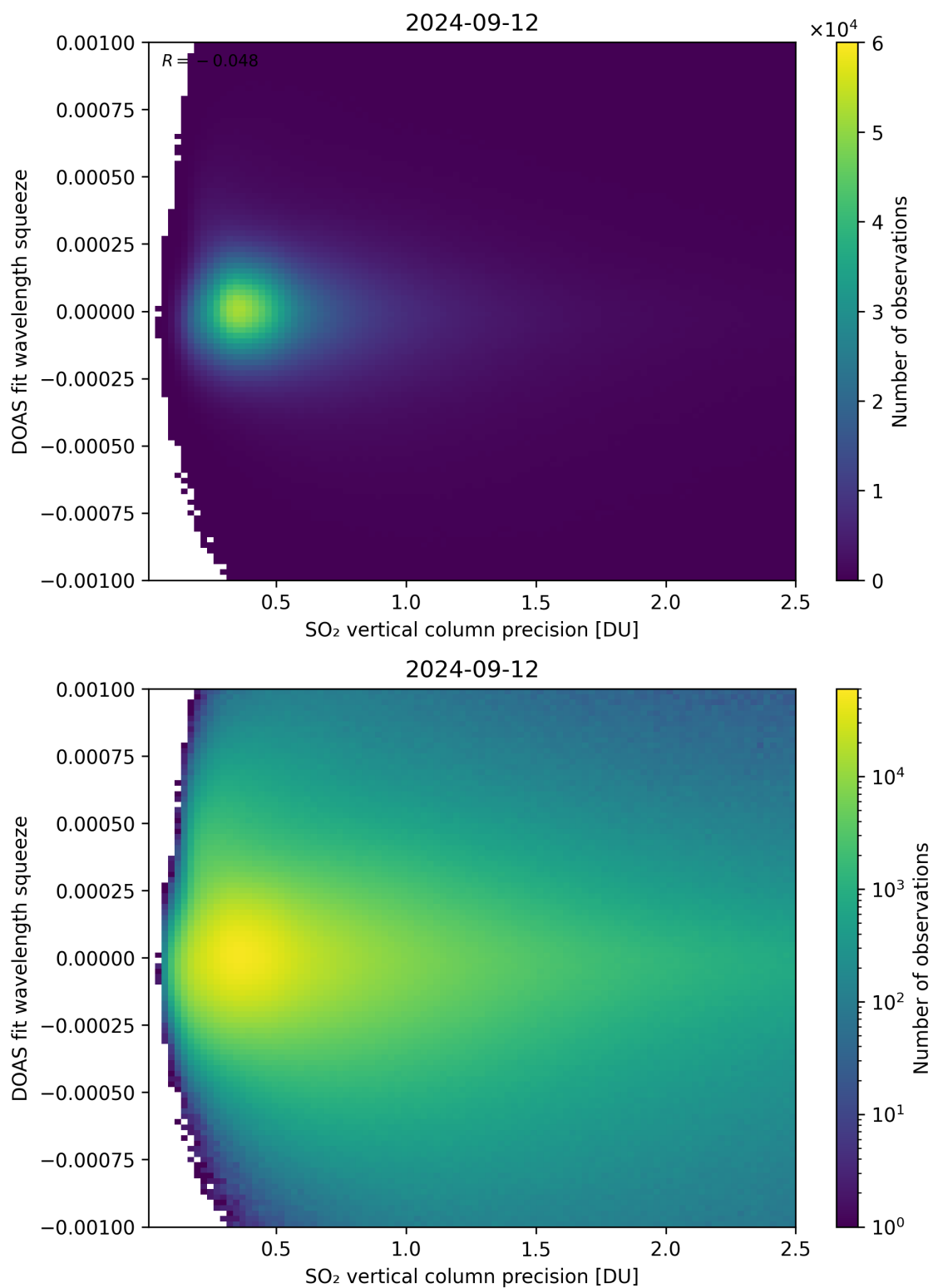
Figure 283: Scatter density plot of “SO 2 vertical column precision” against “DOAS fit wavelength squeeze” for 2024-09-12 to 2024-09-13.
