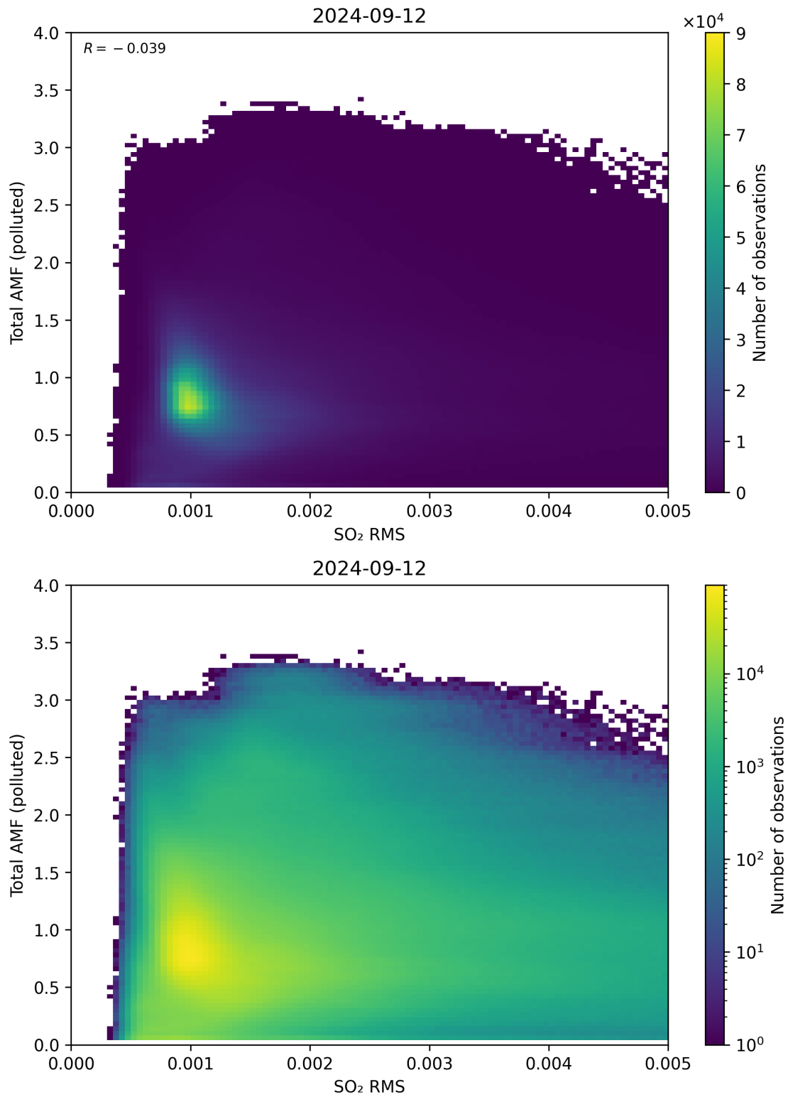
Figure 137: Scatter density plot of “SO 2 RMS” against “Total AMF (polluted)” for 2024-09-12 to 2024-09-13.
