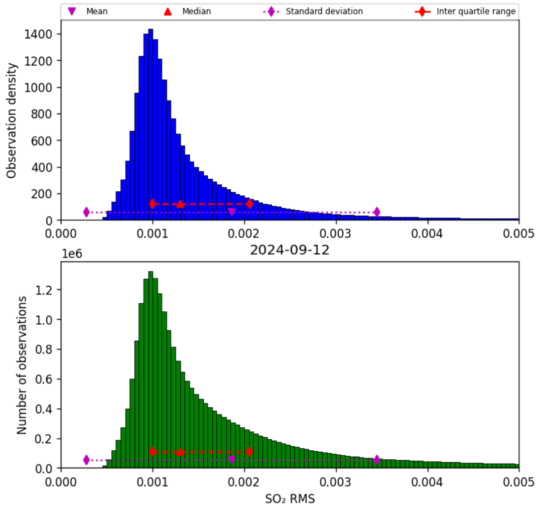
Figure 70: Histogram of “SO 2 RMS” for 2024-09-12 to 2024-09-13
