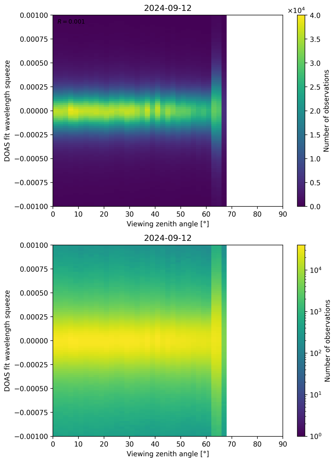
Figure 312: Scatter density plot of “Viewing zenith angle” against “DOAS fit wavelength squeeze” for 2024-09-12 to 2024-09-13.
