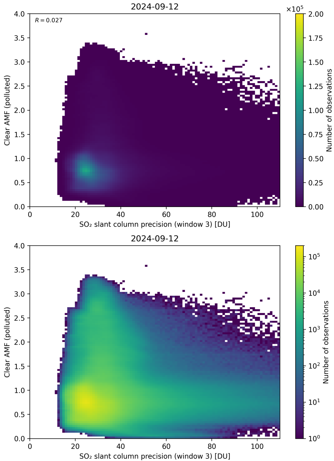
Figure 261: Scatter density plot of “SO 2 slant column precision (window 3)” against “Clear AMF (polluted)” for 2024-09-12 to 2024-09-13.
