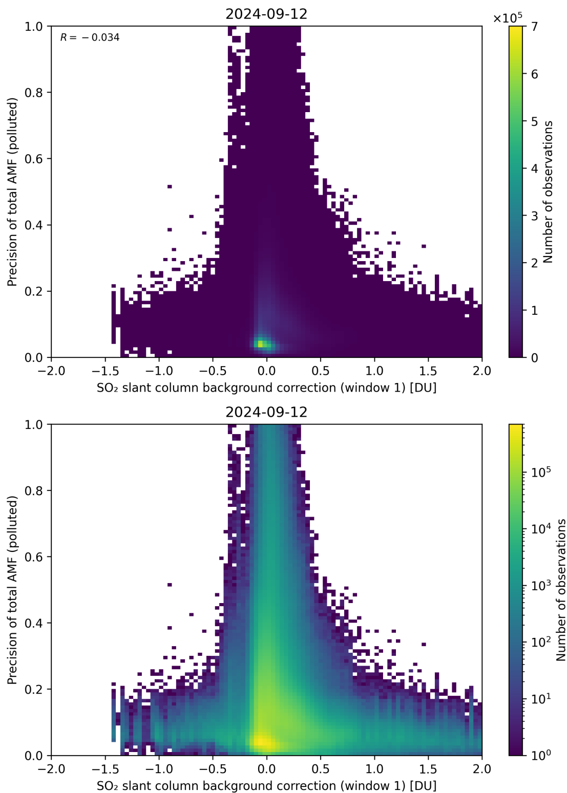
Figure 110: Scatter density plot of “SO 2 slant column background correction (window 1)” against “Precision of total AMF (polluted)” for 2024-09-12 to 2024-09-13.
