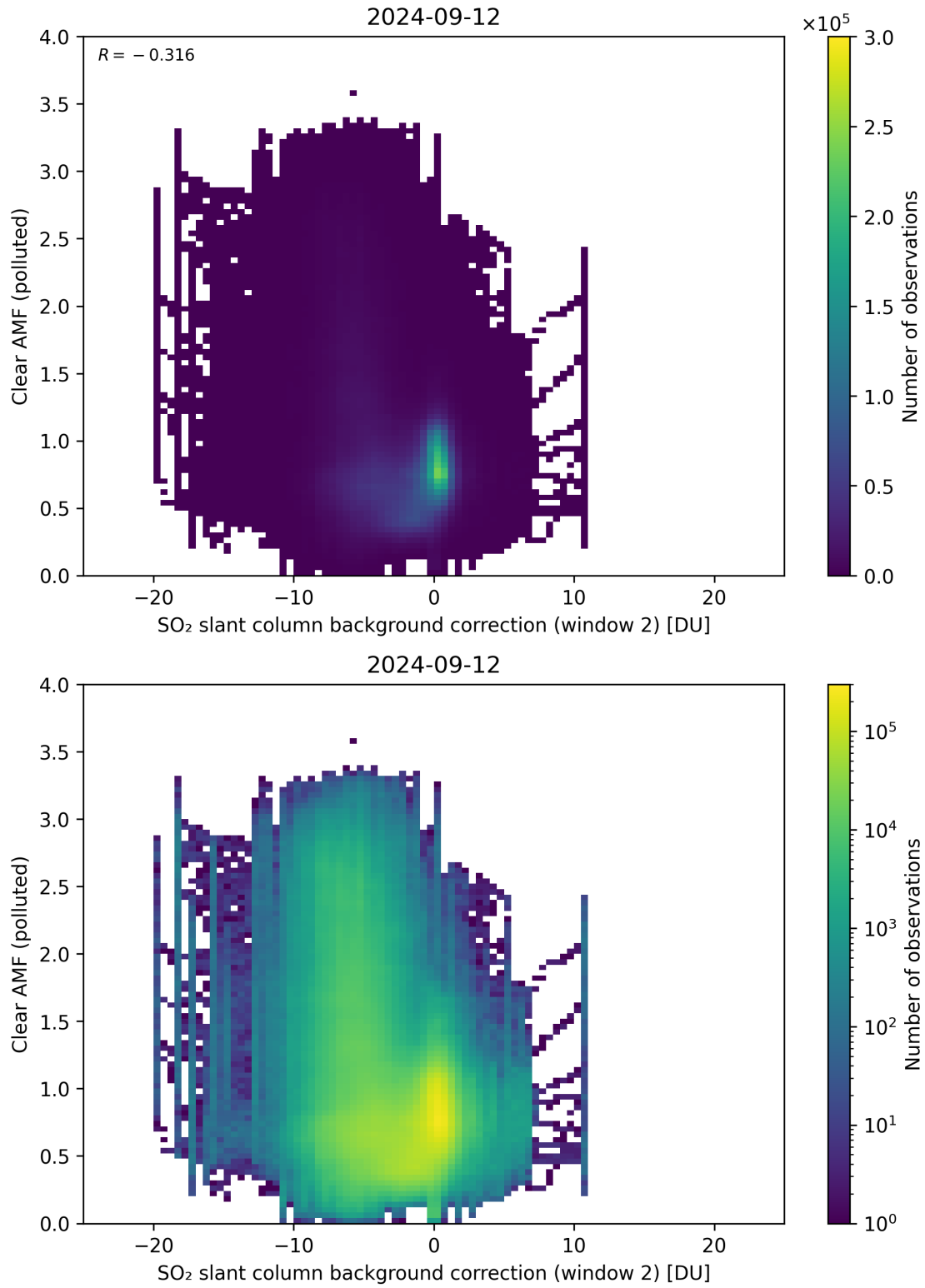
Figure 115: Scatter density plot of “SO 2 slant column background correction (window 2)” against “Clear AMF (polluted)” for 2024-09-12 to 2024-09-13.
