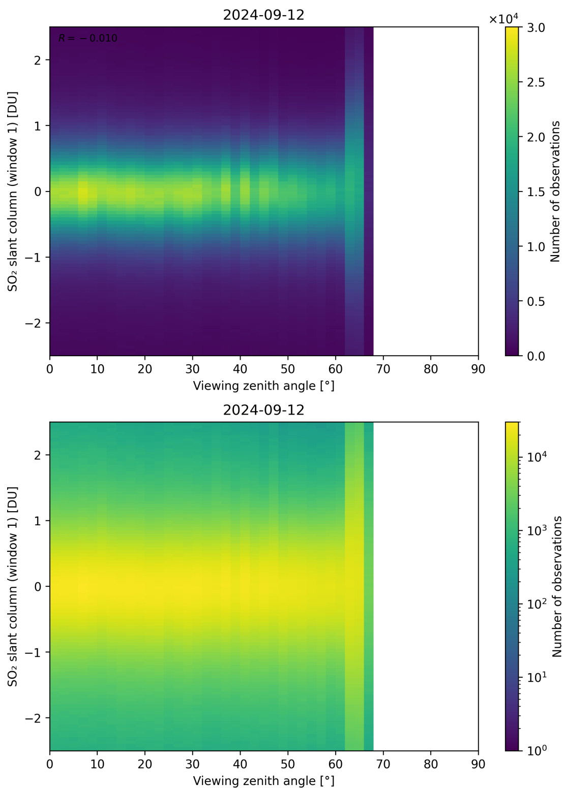
Figure 320: Scatter density plot of “Viewing zenith angle” against “SO 2 slant column (window 1)” for 2024-09-12 to 2024-09-13.
