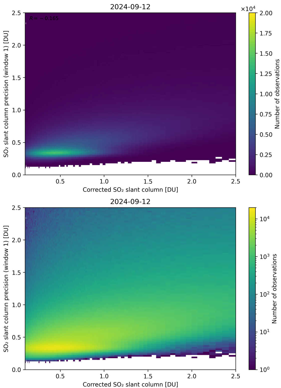
Figure 188: Scatter density plot of “Corrected SO 2 slant column” against “SO 2 slant column precision (window 1)” for 2024-09-12 to 2024-09-13.
