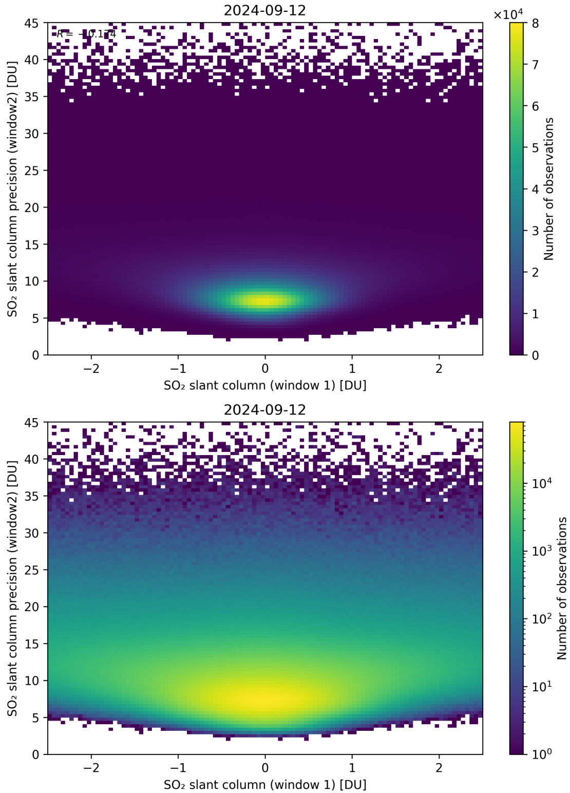
Figure 236: Scatter density plot of “SO 2 slant column (window 1)” against “SO 2 slant column precision (window2)” for 2024-09-12 to 2024-09-13.
