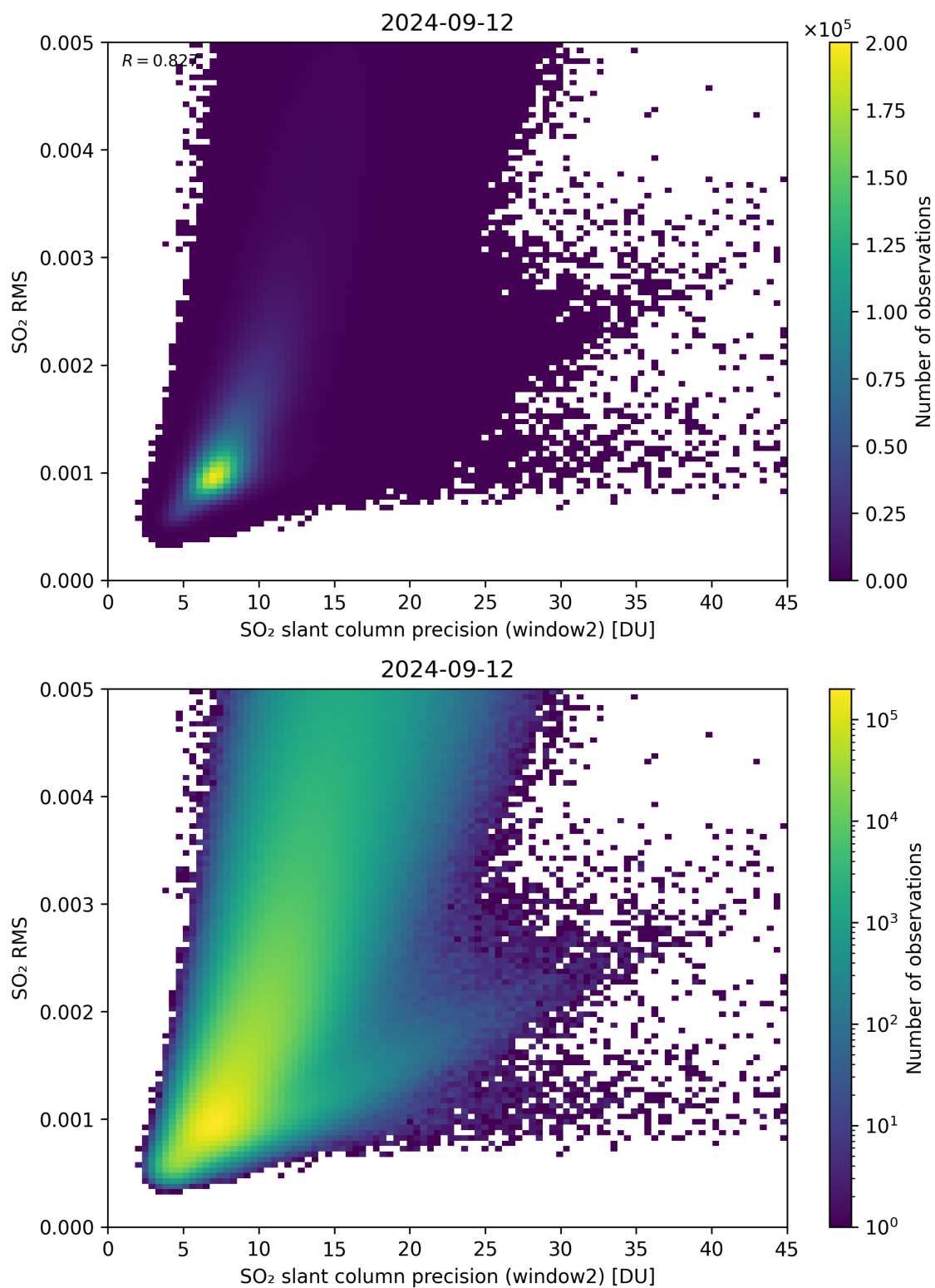
Figure 245: Scatter density plot of “SO 2 slant column precision (window2)” against “SO 2 RMS” for 2024-09-12 to 2024-09-13.
