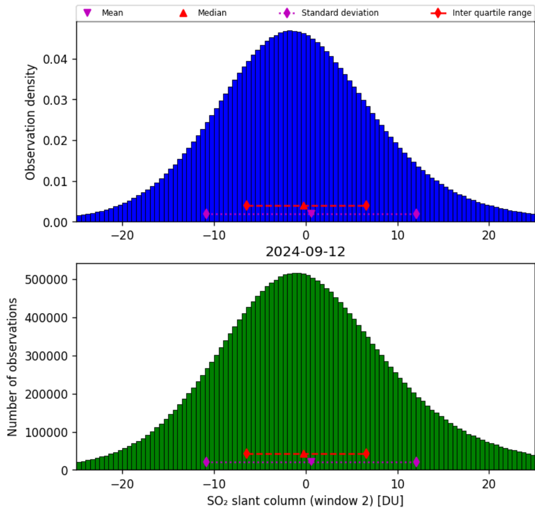
Figure 60: Histogram of “SO 2 slant column (window 2)” for 2024-09-12 to 2024-09-13
