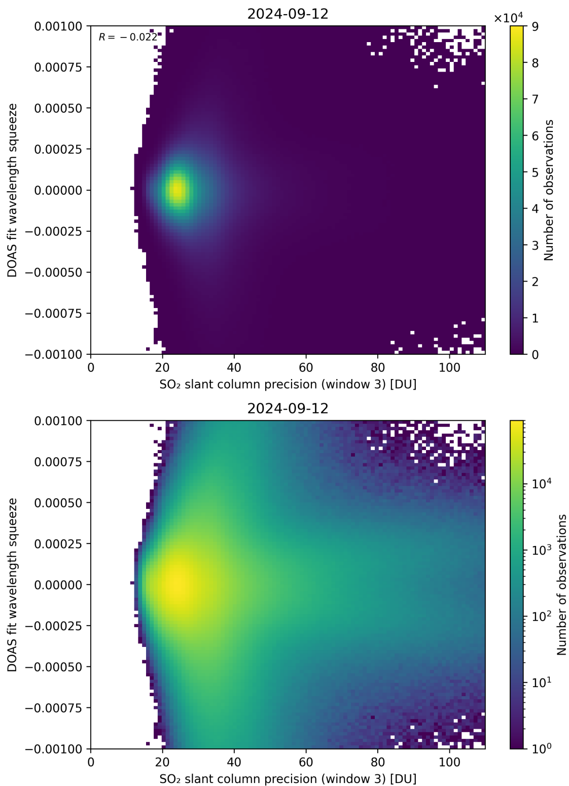
Figure 259: Scatter density plot of “SO 2 slant column precision (window 3)” against “DOAS fit wavelength squeeze” for 2024-09-12 to 2024-09-13.
