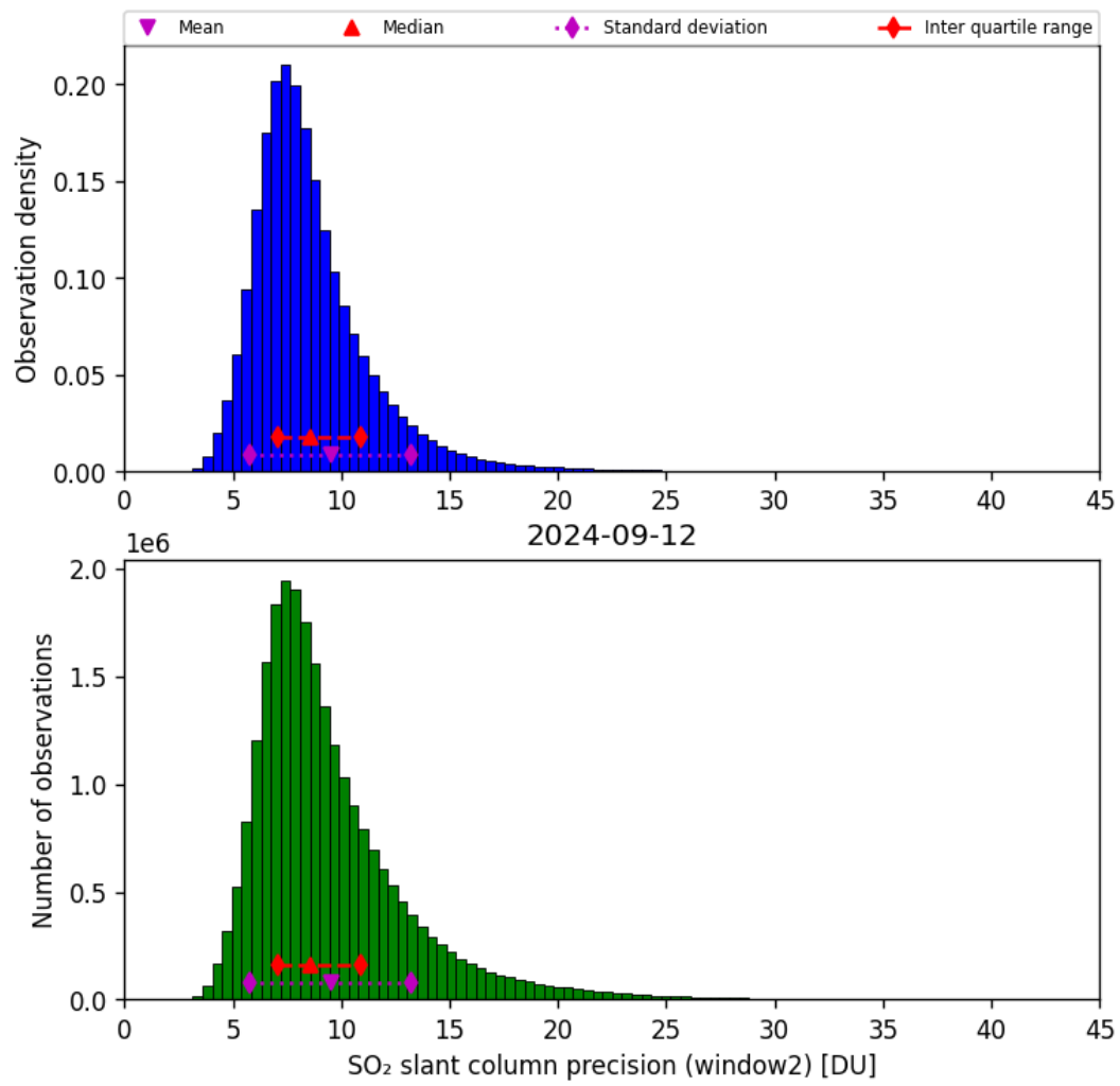
Figure 61: Histogram of “SO 2 slant column precision (window2)” for 2024-09-12 to 2024-09-13
