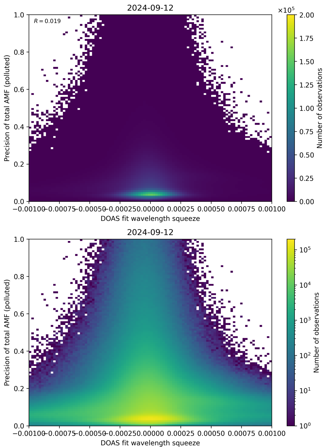
Figure 135: Scatter density plot of “DOAS fit wavelength squeeze” against “Precision of total AMF (polluted)” for 2024-09-12 to 2024-09-13.
