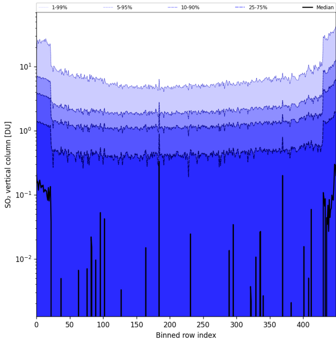
Figure 76: Along track statistics of “SO 2 vertical column” for 2024-09-12 to 2024-09-13
