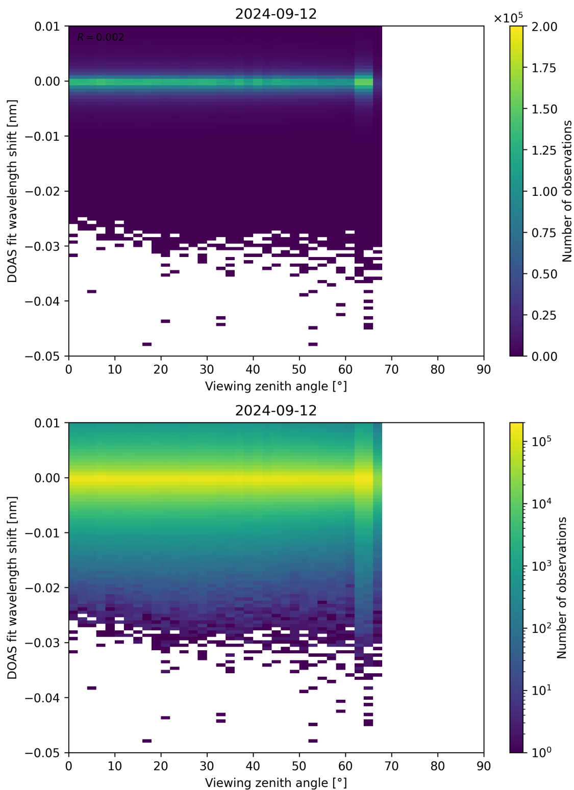
Figure 311: Scatter density plot of “Viewing zenith angle” against “DOAS fit wavelength shift” for 2024-09-12 to 2024-09-13.
