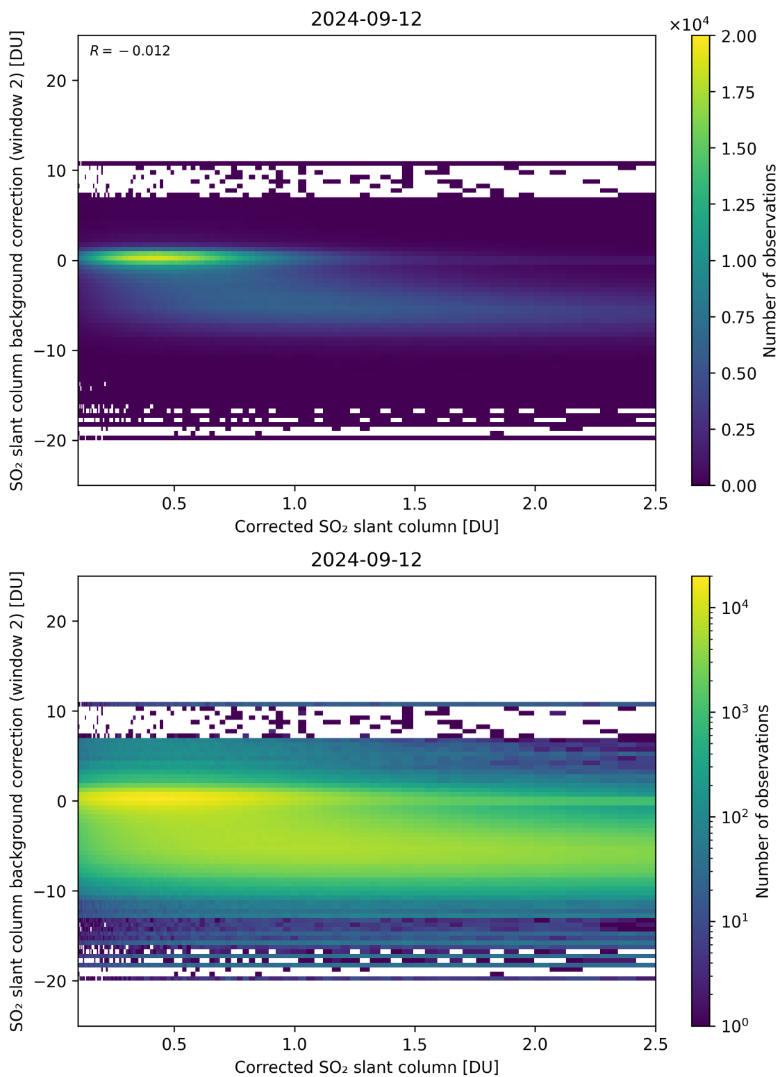
Figure 179: Scatter density plot of “Corrected SO 2 slant column” against “SO 2 slant column background correction (window 2)” for 2024-09-12 to 2024-09-13.
