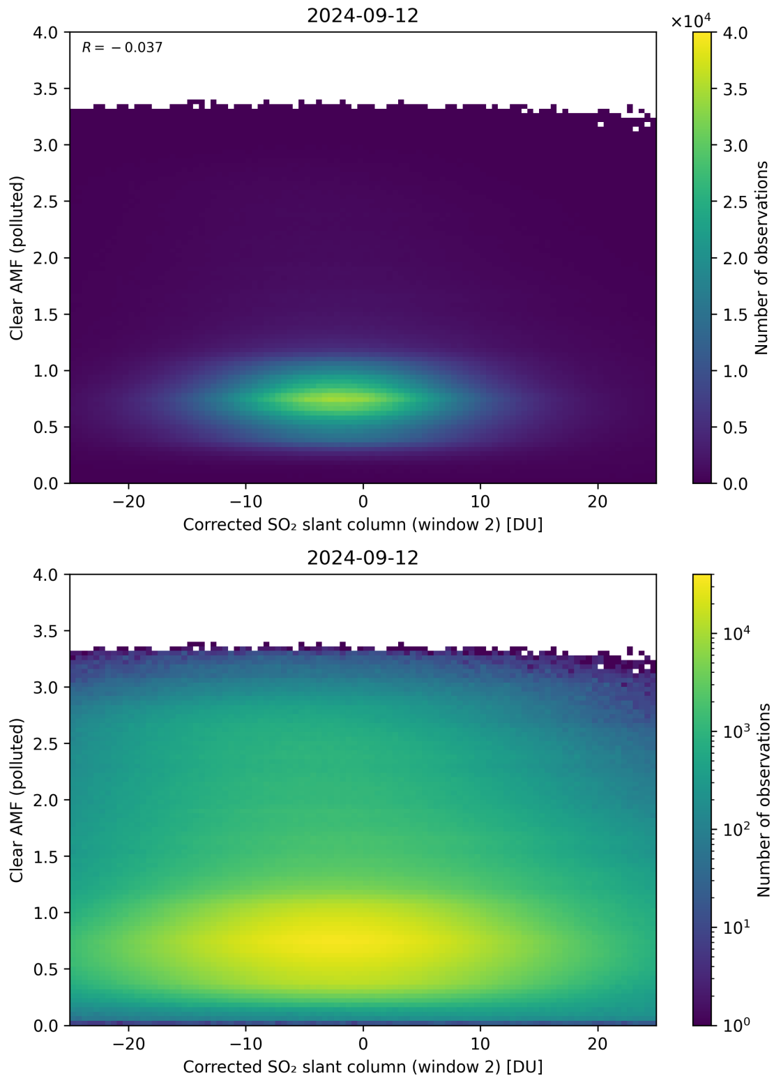
Figure 199: Scatter density plot of “Corrected SO 2 slant column (window 2)” against “Clear AMF (polluted)” for 2024-09-12 to 2024-09-13.
