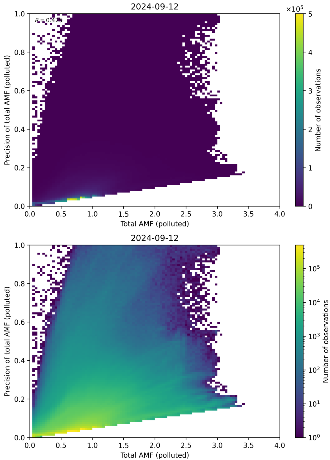
Figure 272: Scatter density plot of “Total AMF (polluted)” against “Precision of total AMF (polluted)” for 2024-09-12 to 2024-09-13.
