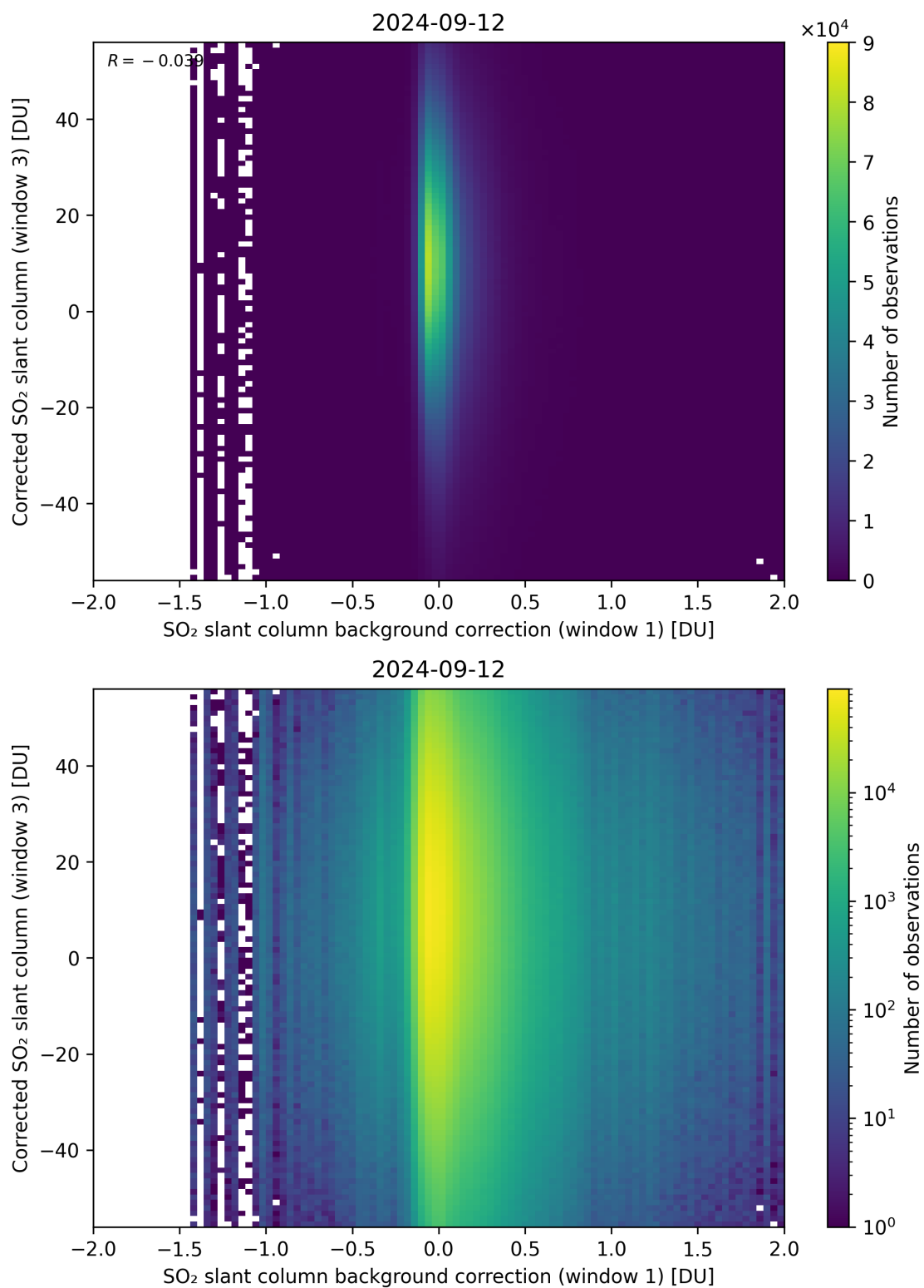
Figure 105: Scatter density plot of “SO 2 slant column background correction (window 1)” against “Corrected SO 2 slant column (window 3)” for 2024-09-12 to 2024-09-13.
