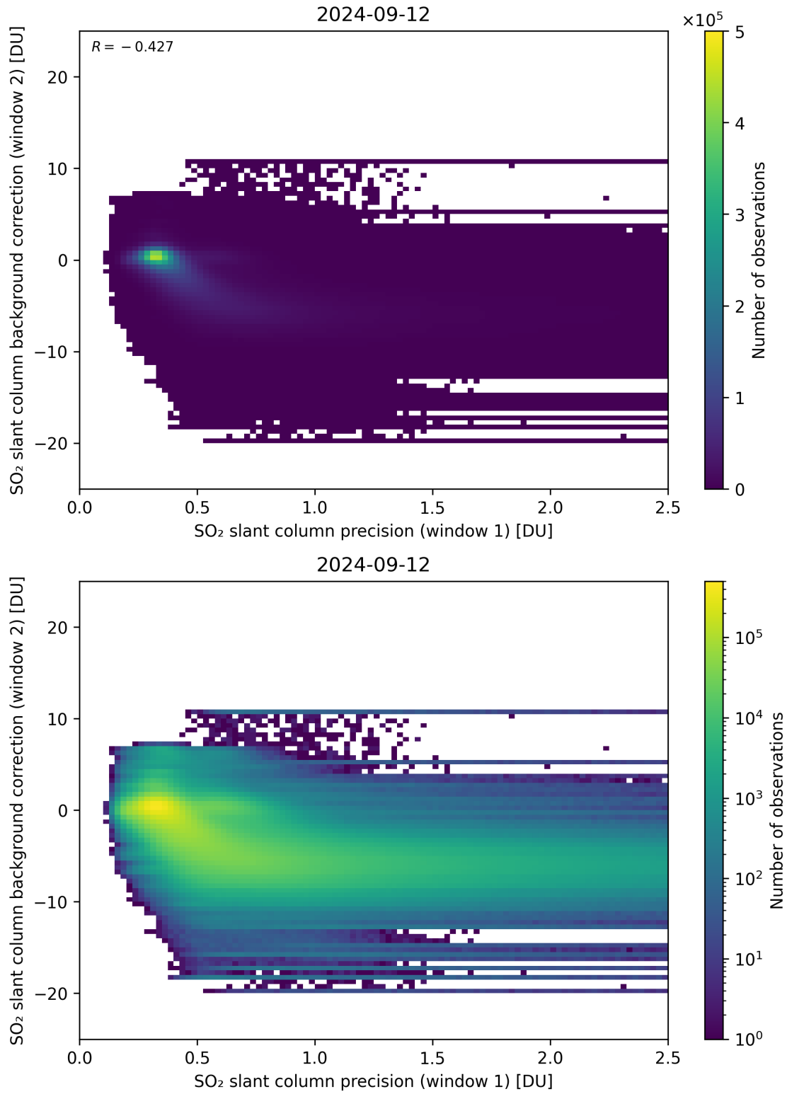
Figure 219: Scatter density plot of “SO 2 slant column precision (window 1)” against “SO 2 slant column background correction (window 2)” for 2024-09-12 to 2024-09-13.
