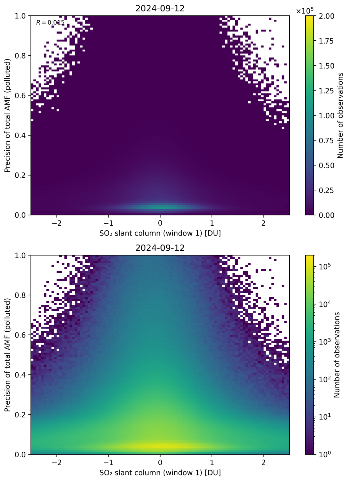
Figure 240: Scatter density plot of “SO 2 slant column (window 1)” against “Precision of total AMF (polluted)” for 2024-09-12 to 2024-09-13.
