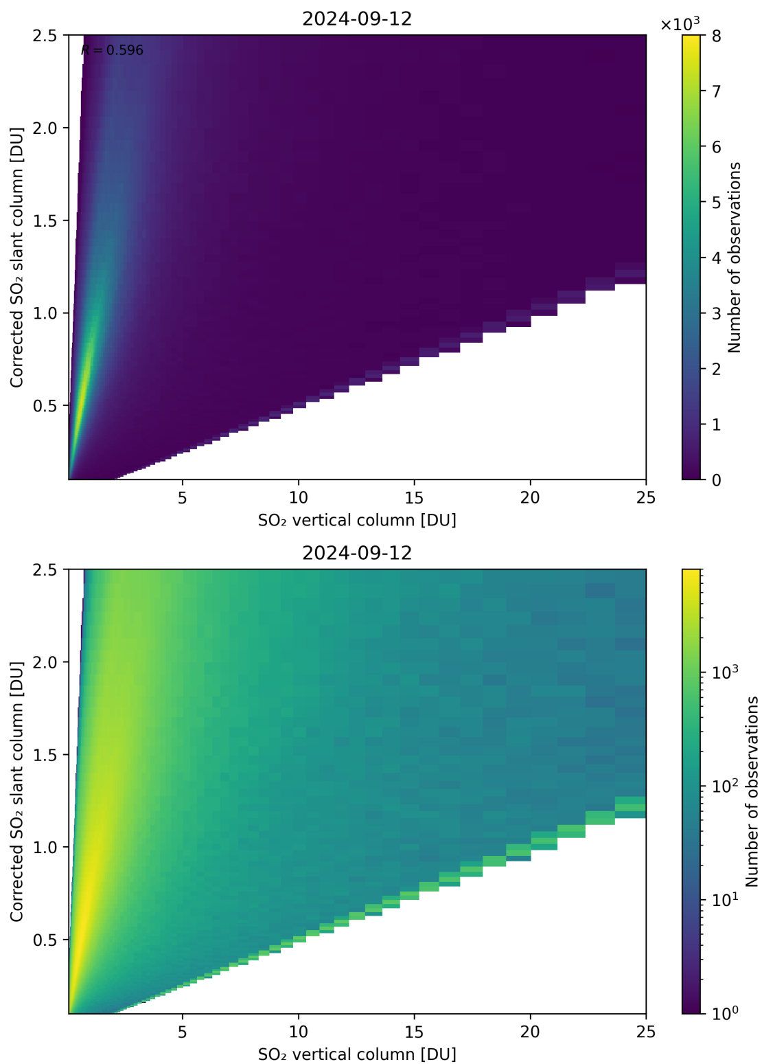
Figure 297: Scatter density plot of “SO 2 vertical column” against “Corrected SO 2 slant column” for 2024-09-12 to 2024-09-13.
