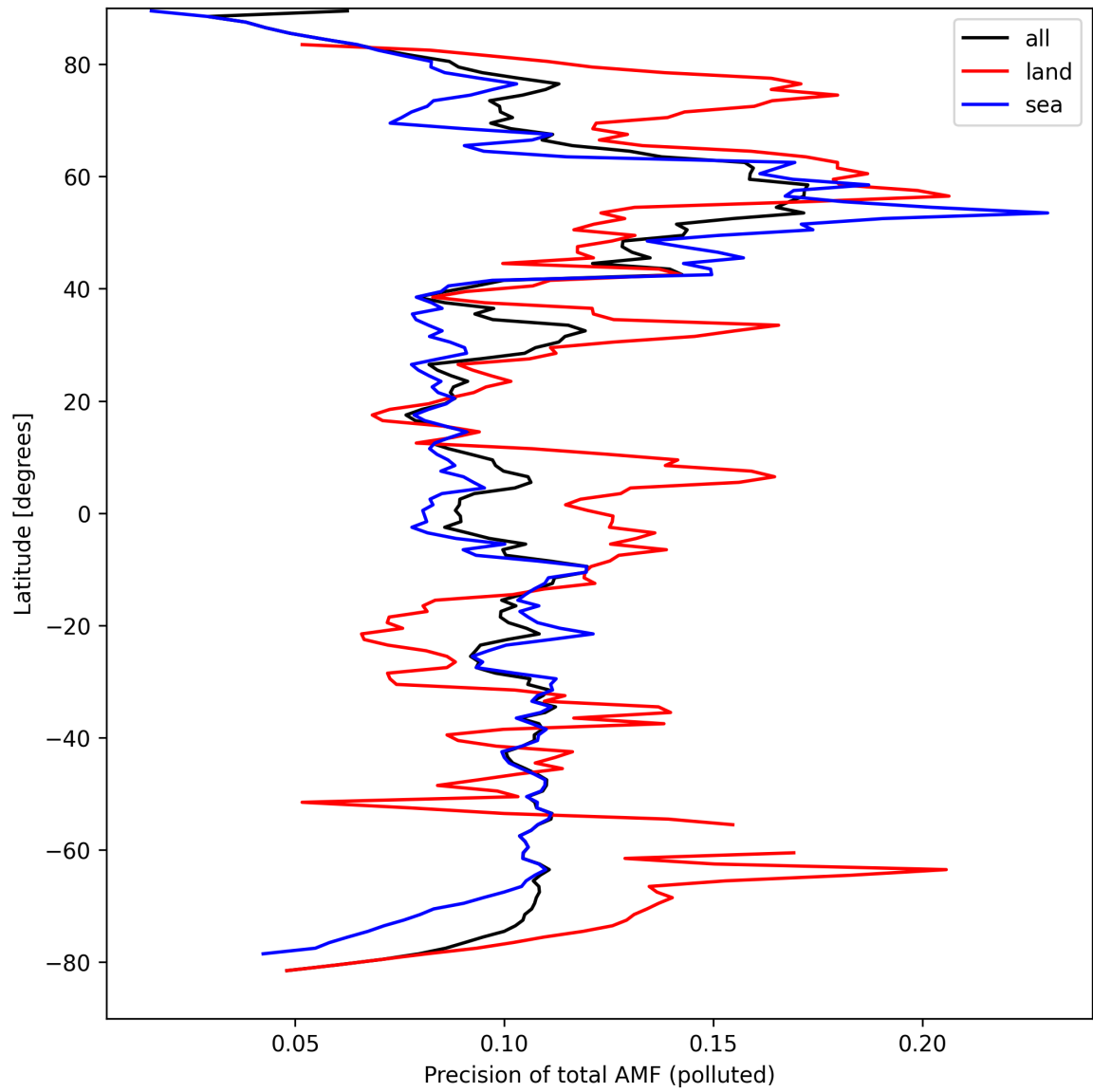
Figure 49: Zonal average of “Precision of total AMF (polluted)” for 2024-09-12 to 2024-09-13.
