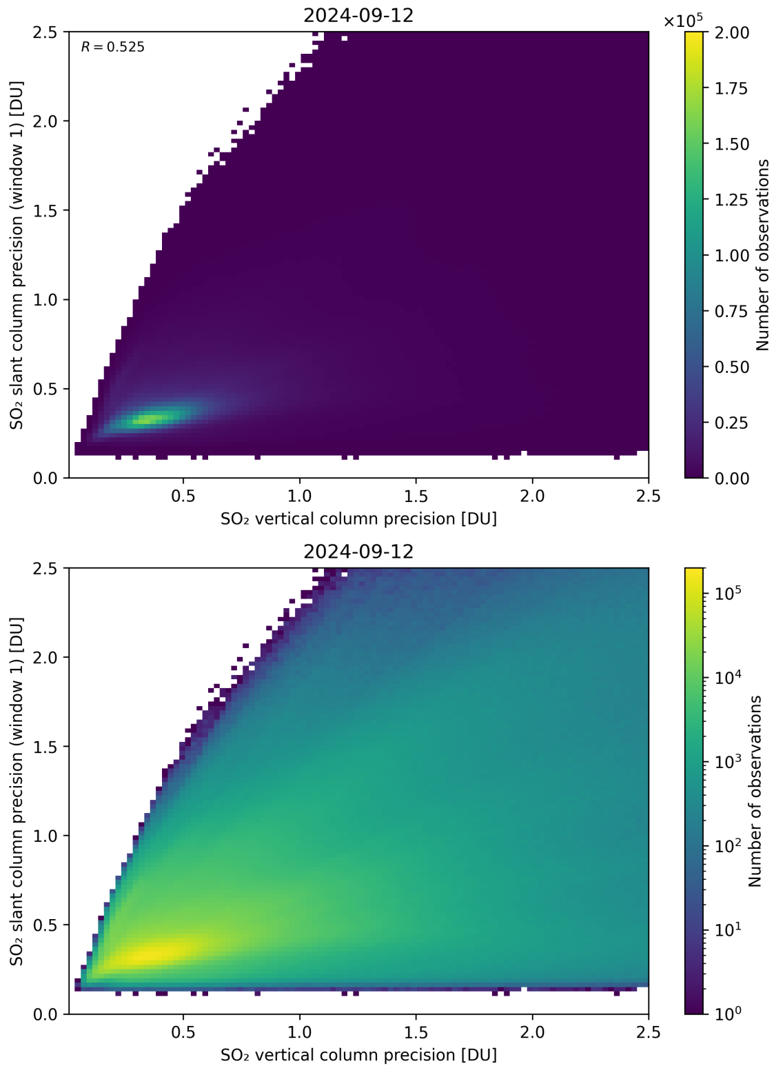
Figure 290: Scatter density plot of “SO 2 vertical column precision” against “SO 2 slant column precision (window 1)” for 2024-09-12 to 2024-09-13.
