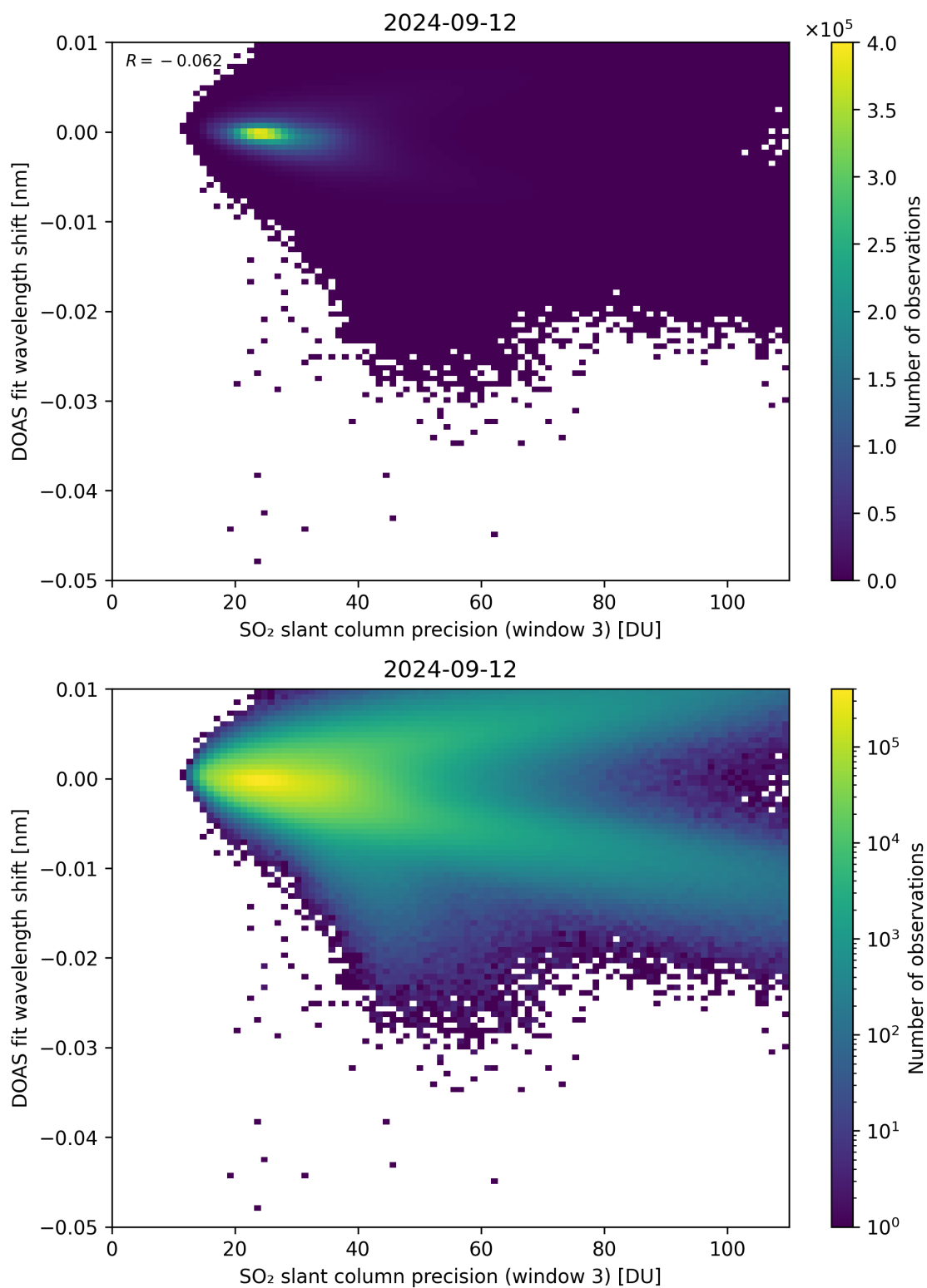
Figure 258: Scatter density plot of “SO 2 slant column precision (window 3)” against “DOAS fit wavelength shift” for 2024-09-12 to 2024-09-13.
