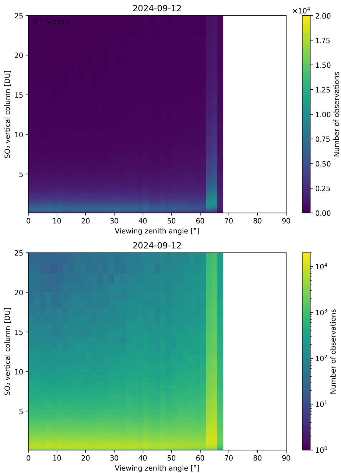
Figure 327: Scatter density plot of “Viewing zenith angle” against “SO 2 vertical column” for 2024-09-12 to 2024-09-13.
