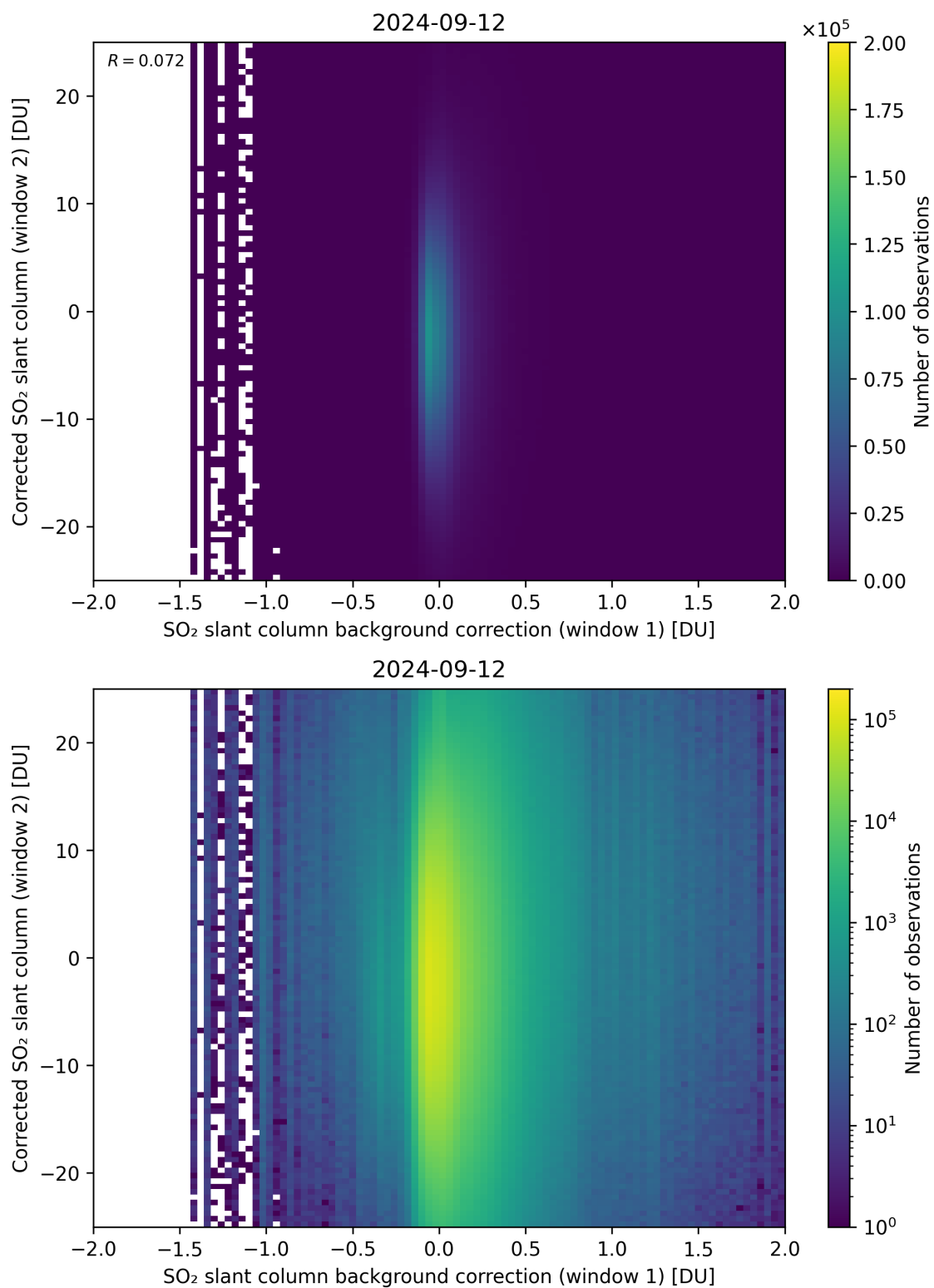
Figure 104: Scatter density plot of “SO 2 slant column background correction (window 1)” against “Corrected SO 2 slant column (window 2)” for 2024-09-12 to 2024-09-13.
