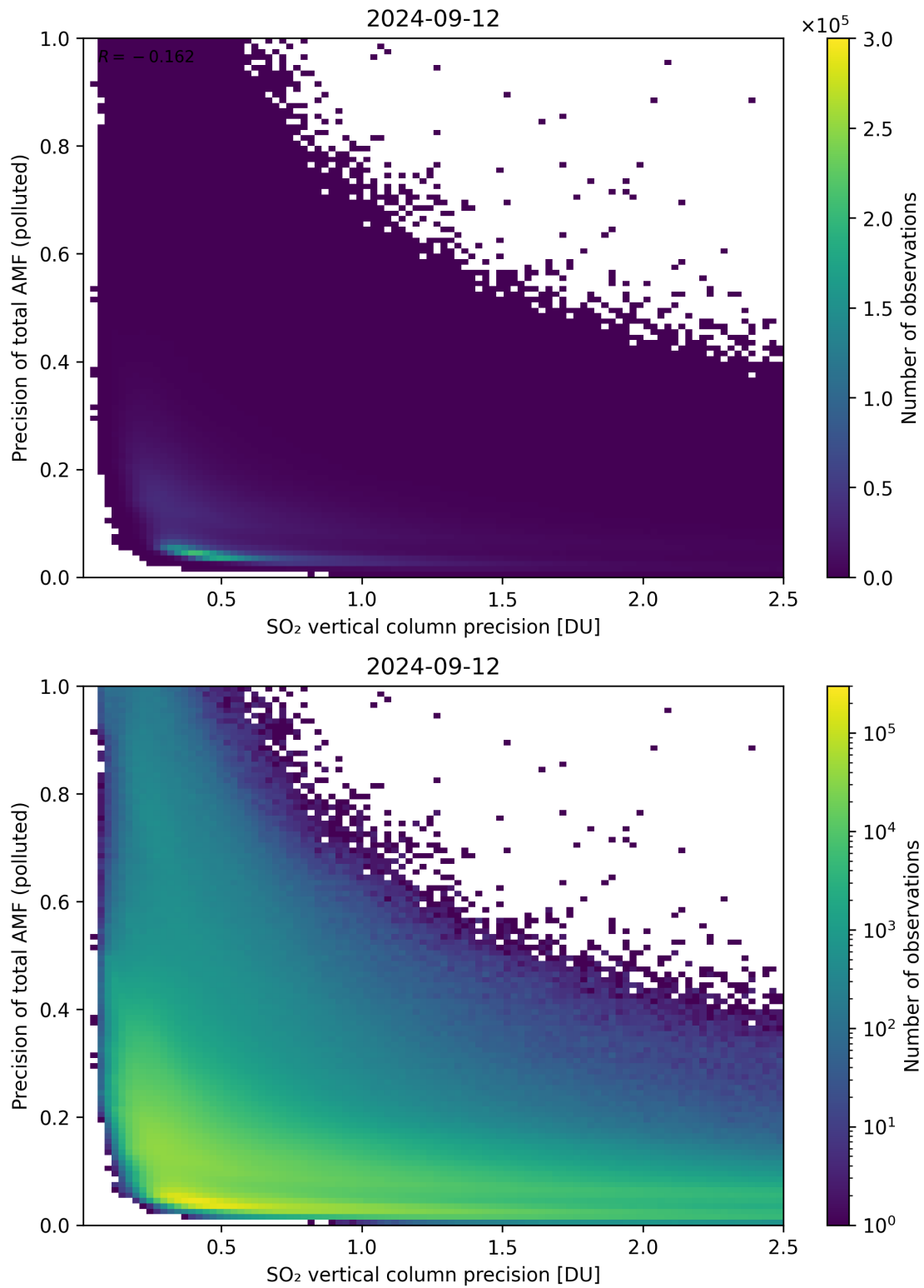
Figure 295: Scatter density plot of “SO 2 vertical column precision” against “Precision of total AMF (polluted)” for 2024-09-12 to 2024-09-13.
