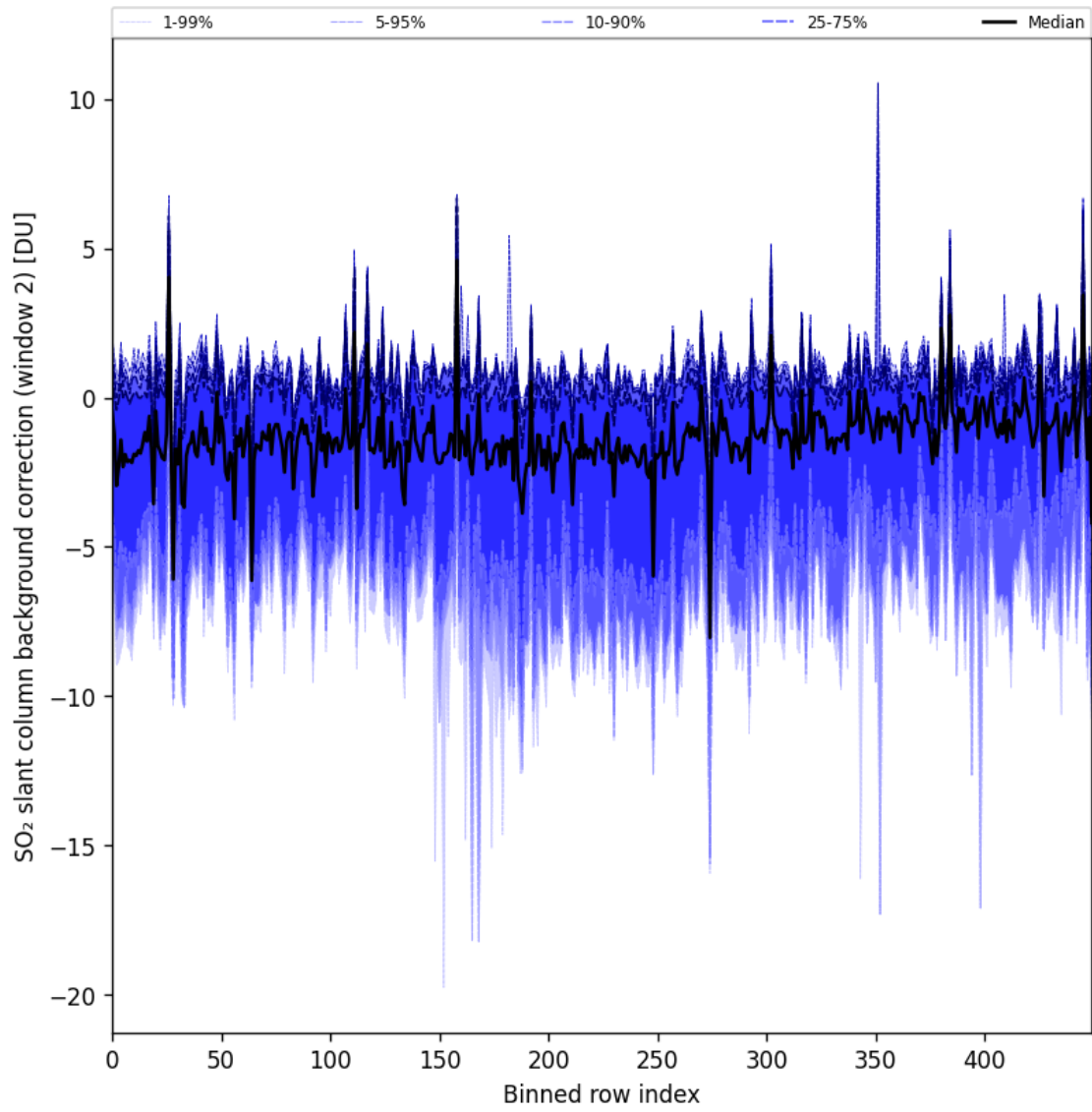
Figure 86: Along track statistics of “SO 2 slant column background correction (window 2)” for 2024-09-12 to 2024-09-13
