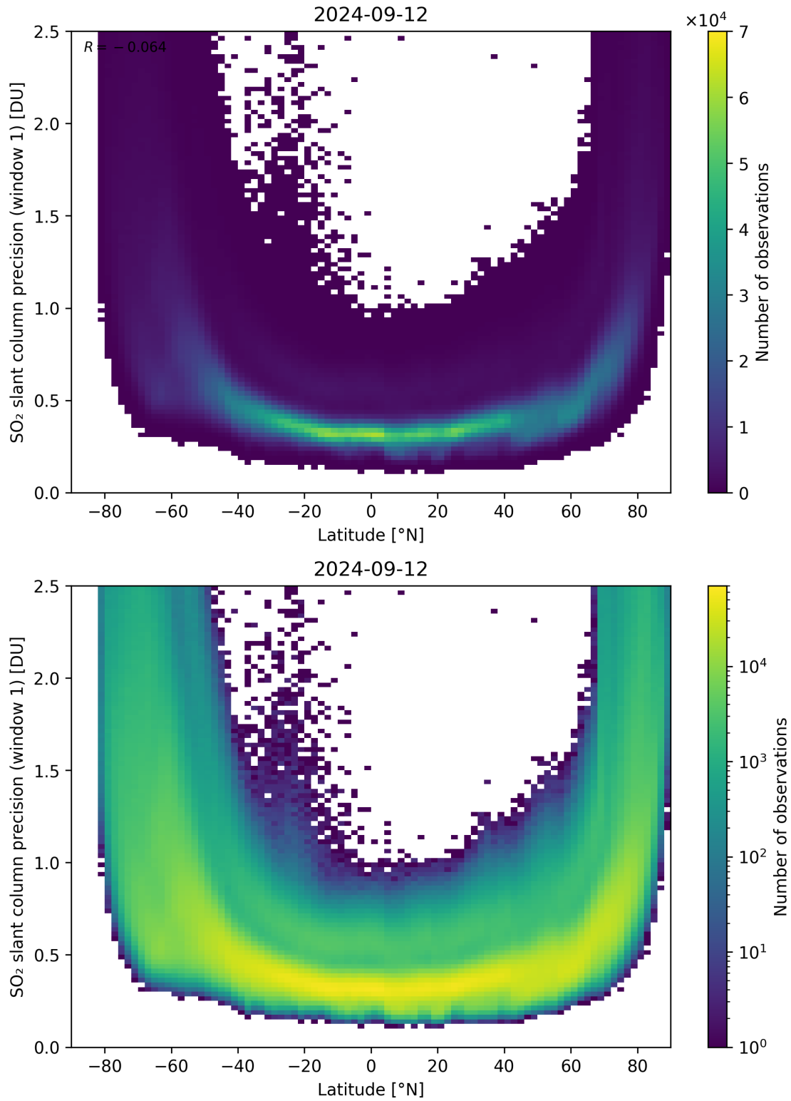
Figure 150: Scatter density plot of “Latitude” against “SO 2 slant column precision (window 1)” for 2024-09-12 to 2024-09-13.
