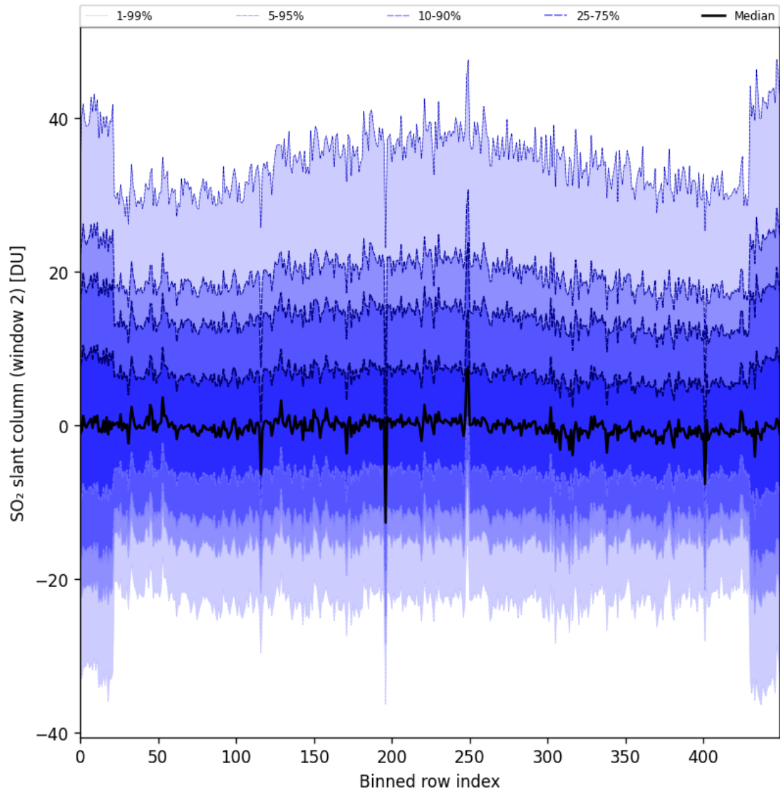
Figure 83: Along track statistics of “SO 2 slant column (window 2)” for 2024-09-12 to 2024-09-13
