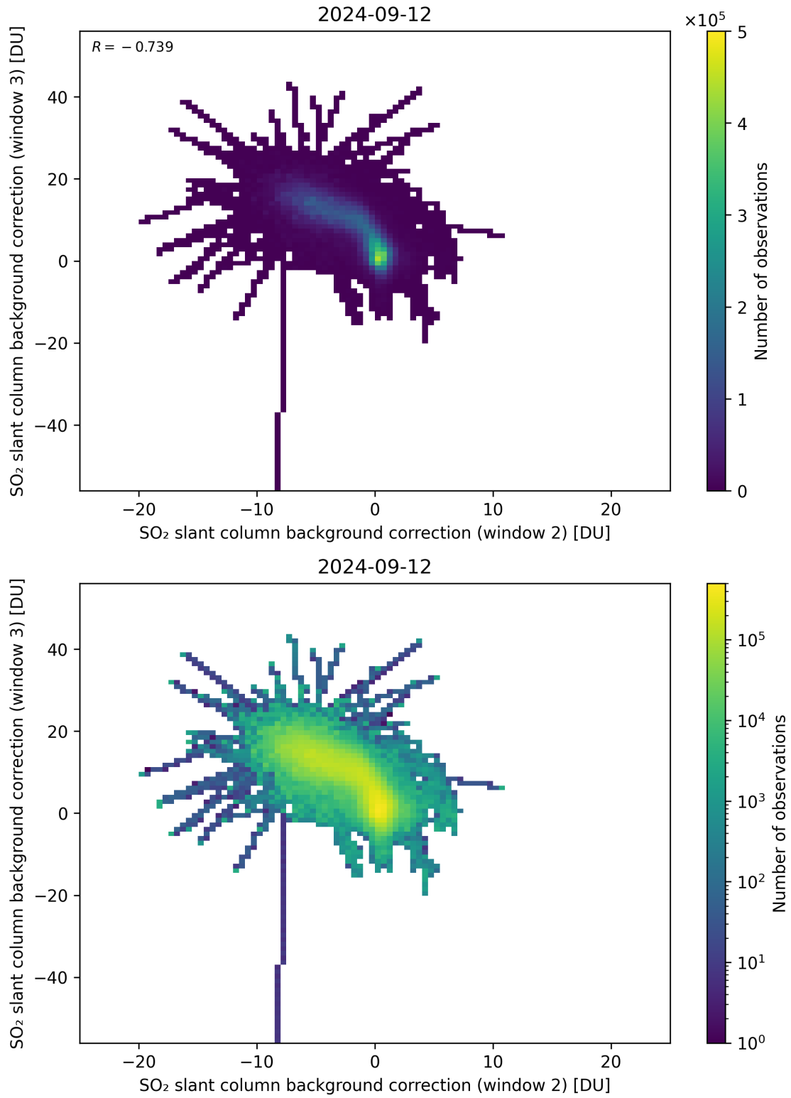
Figure 111: Scatter density plot of “SO 2 slant column background correction (window 2)” against “SO 2 slant column background correction (window 3)” for 2024-09-12 to 2024-09-13.
