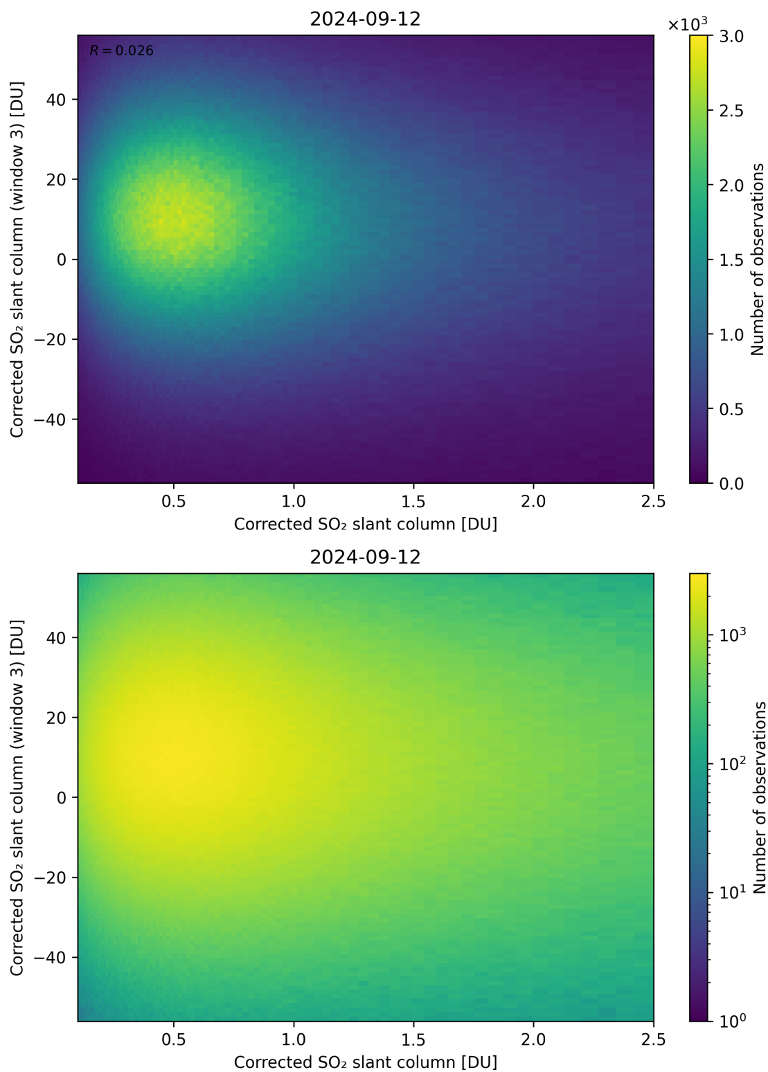
Figure 186: Scatter density plot of “Corrected SO 2 slant column” against “Corrected SO 2 slant column (window 3)” for 2024-09-12 to 2024-09-13.
