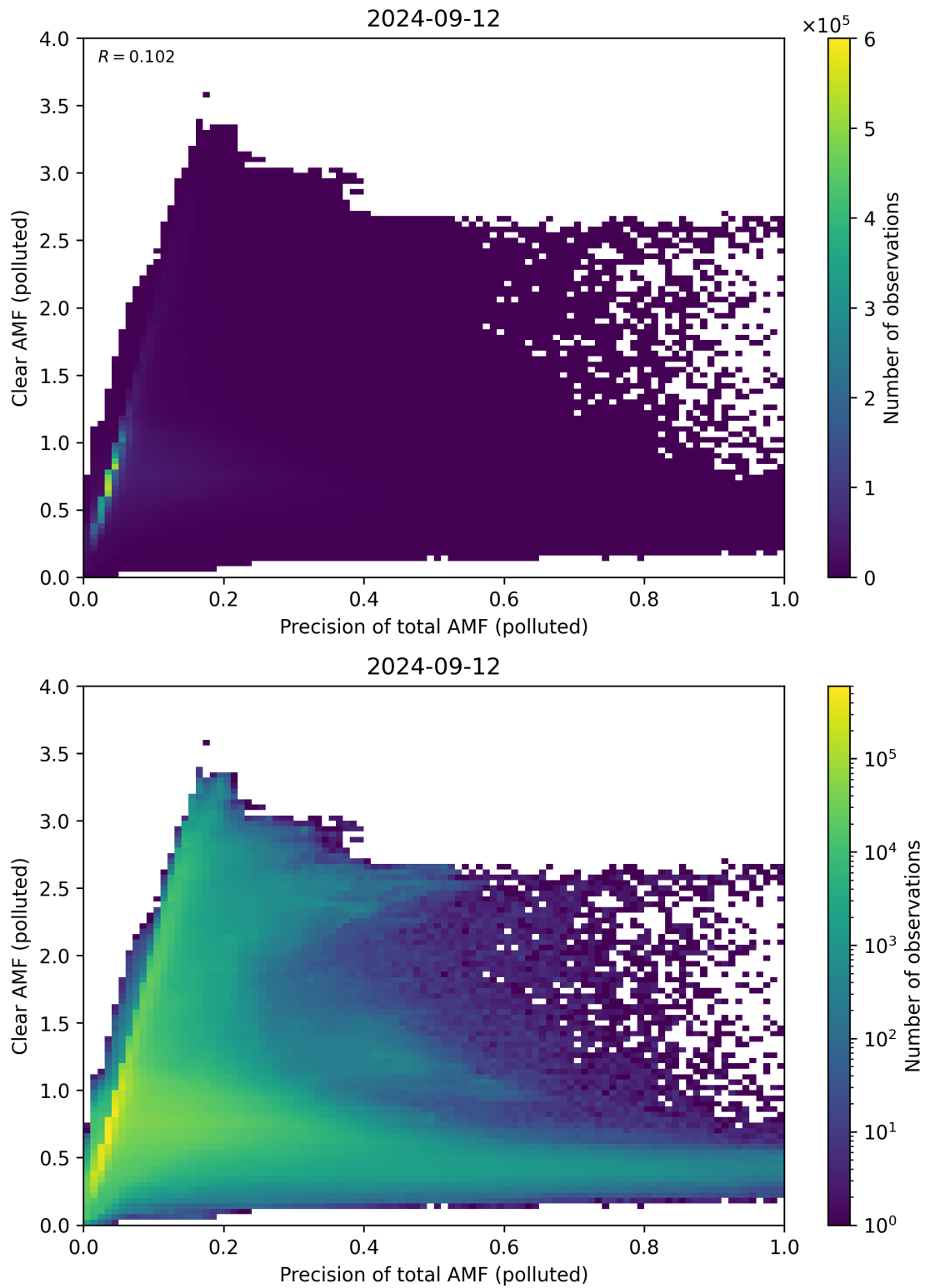
Figure 270: Scatter density plot of “Precision of total AMF (polluted)” against “Clear AMF (polluted)” for 2024-09-12 to 2024-09-13.
