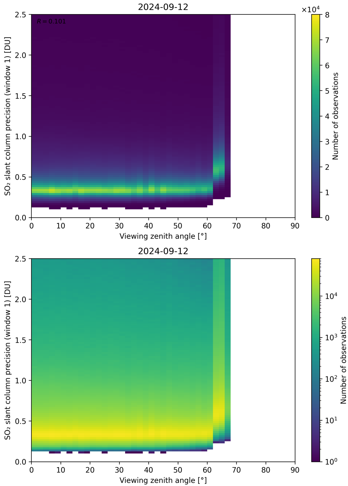
Figure 321: Scatter density plot of “Viewing zenith angle” against “SO 2 slant column precision (window 1)” for 2024-09-12 to 2024-09-13.
