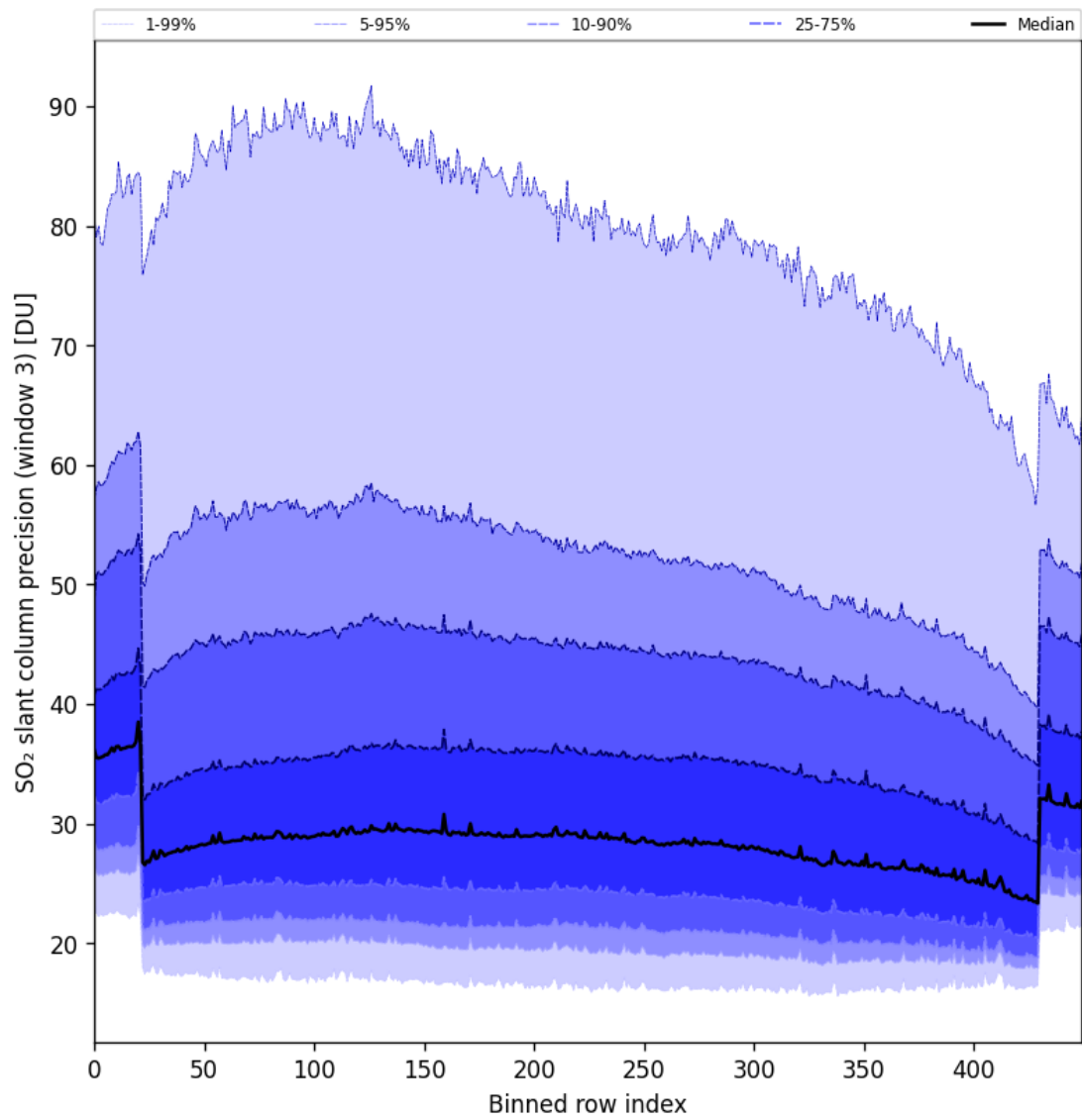
Figure 88: Along track statistics of “SO 2 slant column precision (window 3)” for 2024-09-12 to 2024-09-13
