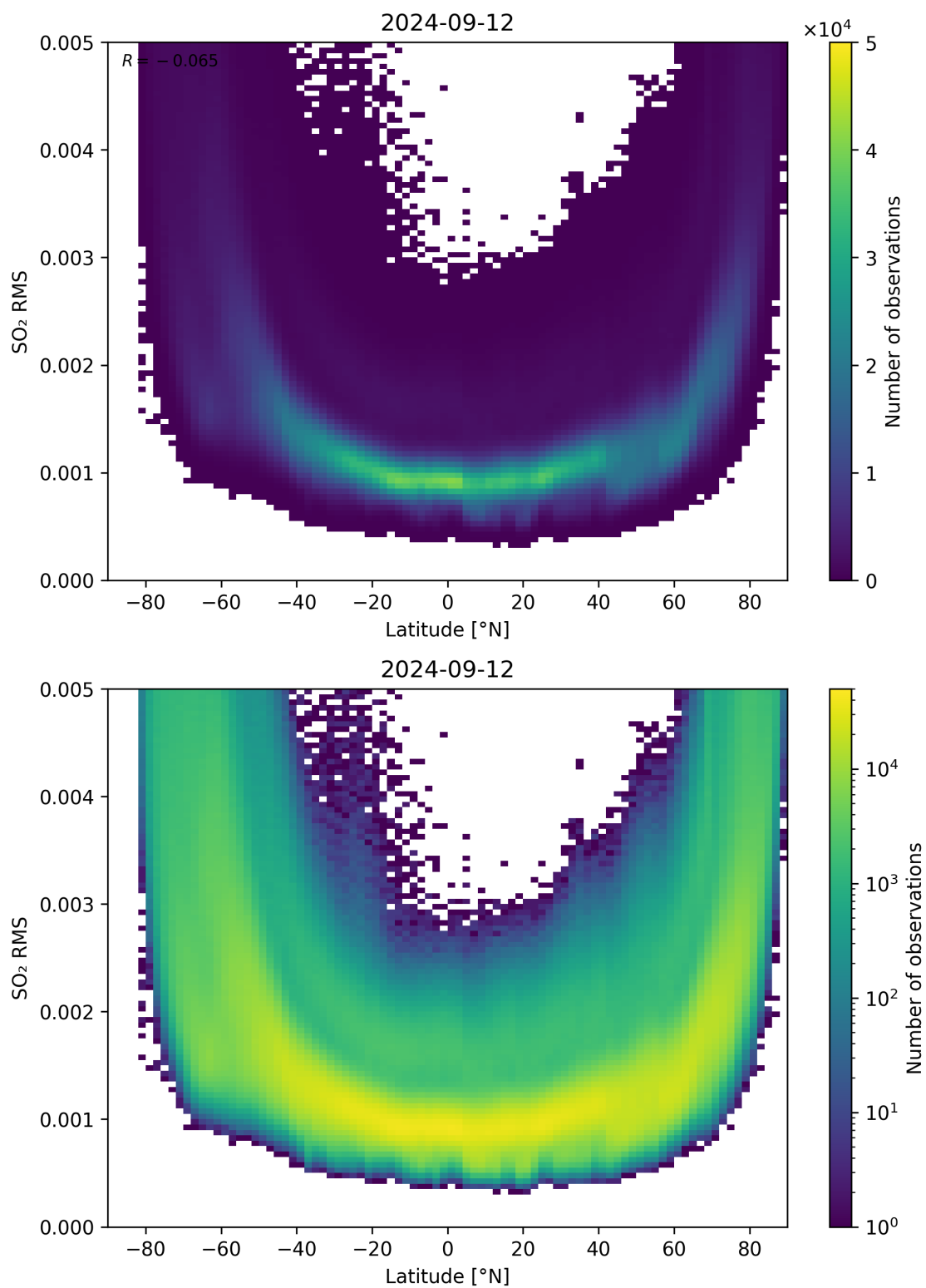
Figure 144: Scatter density plot of “Latitude” against “SO 2 RMS” for 2024-09-12 to 2024-09-13.
