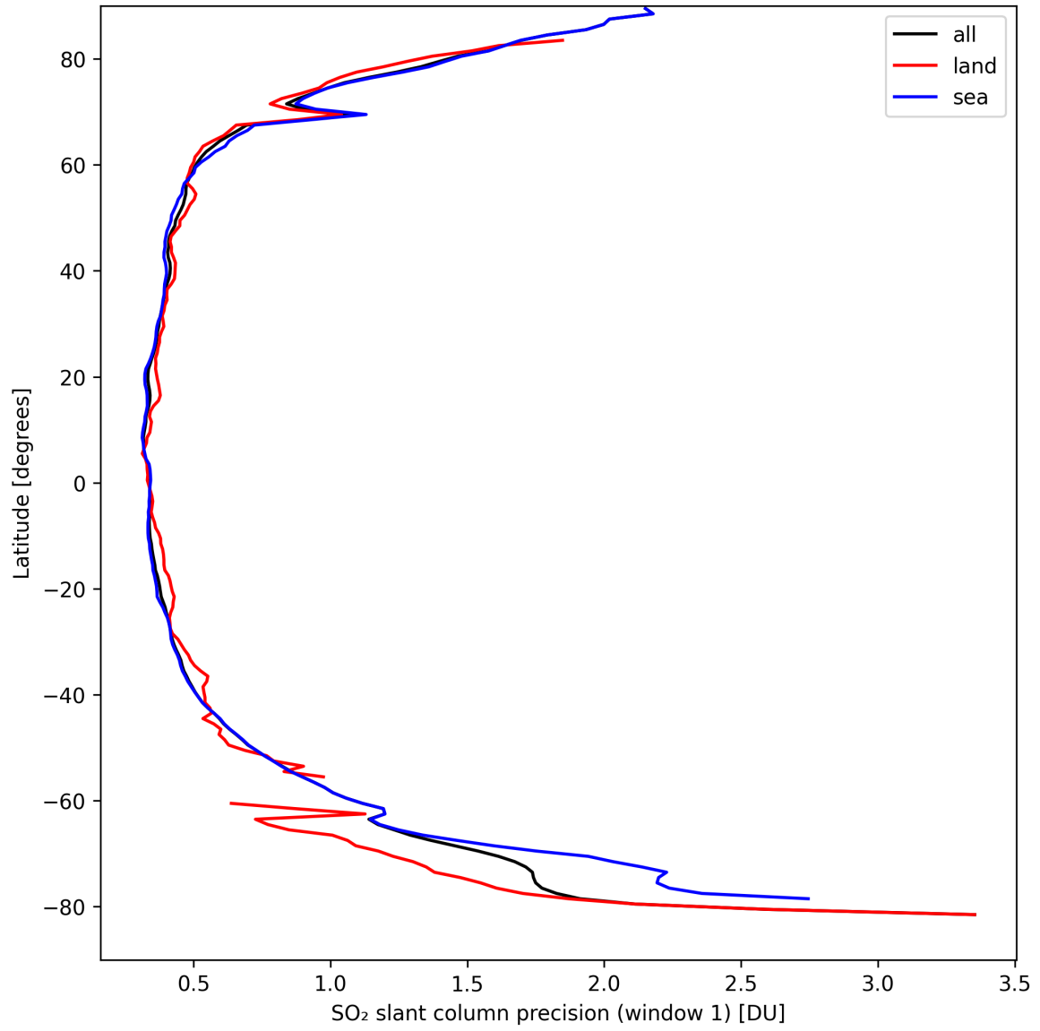
Figure 34: Zonal average of “SO 2 slant column precision (window 1)” for 2024-09-12 to 2024-09-13.
