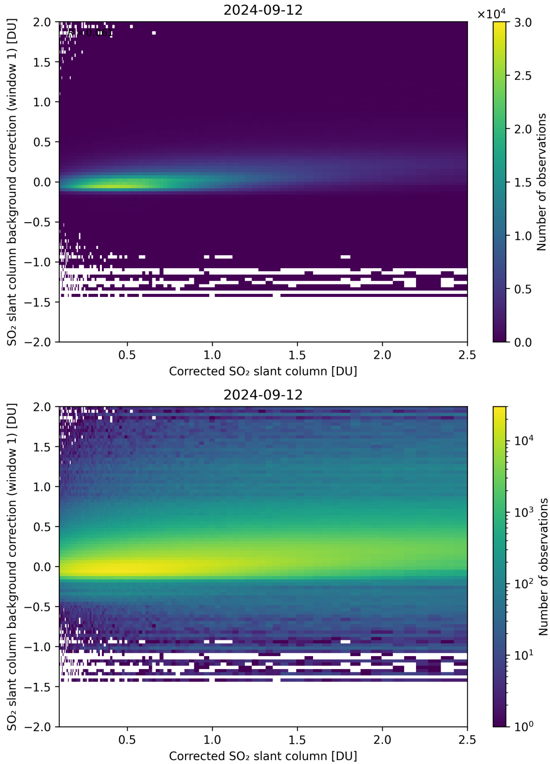
Figure 178: Scatter density plot of “Corrected SO 2 slant column” against “SO 2 slant column background correction (window 1)” for 2024-09-12 to 2024-09-13.
