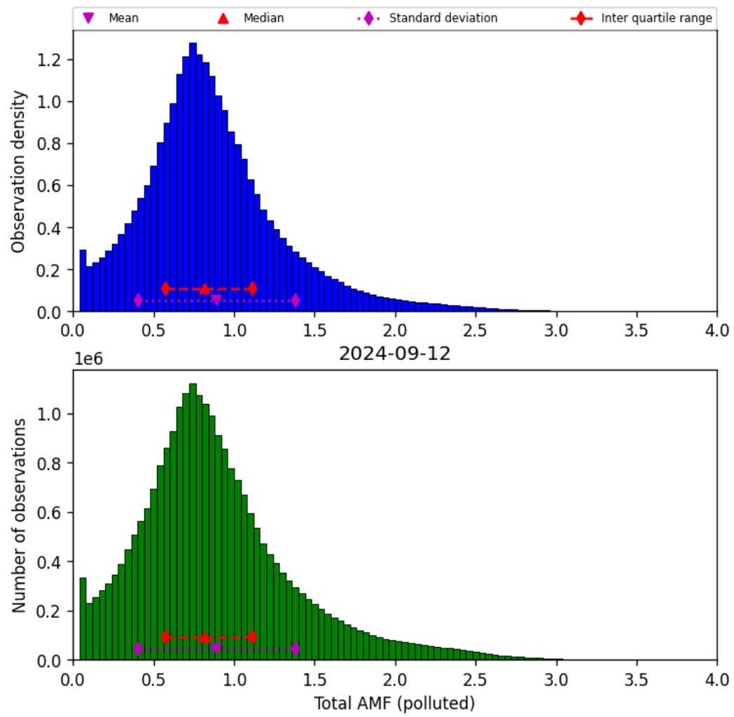
Figure 71: Histogram of “Total AMF (polluted)” for 2024-09-12 to 2024-09-13
