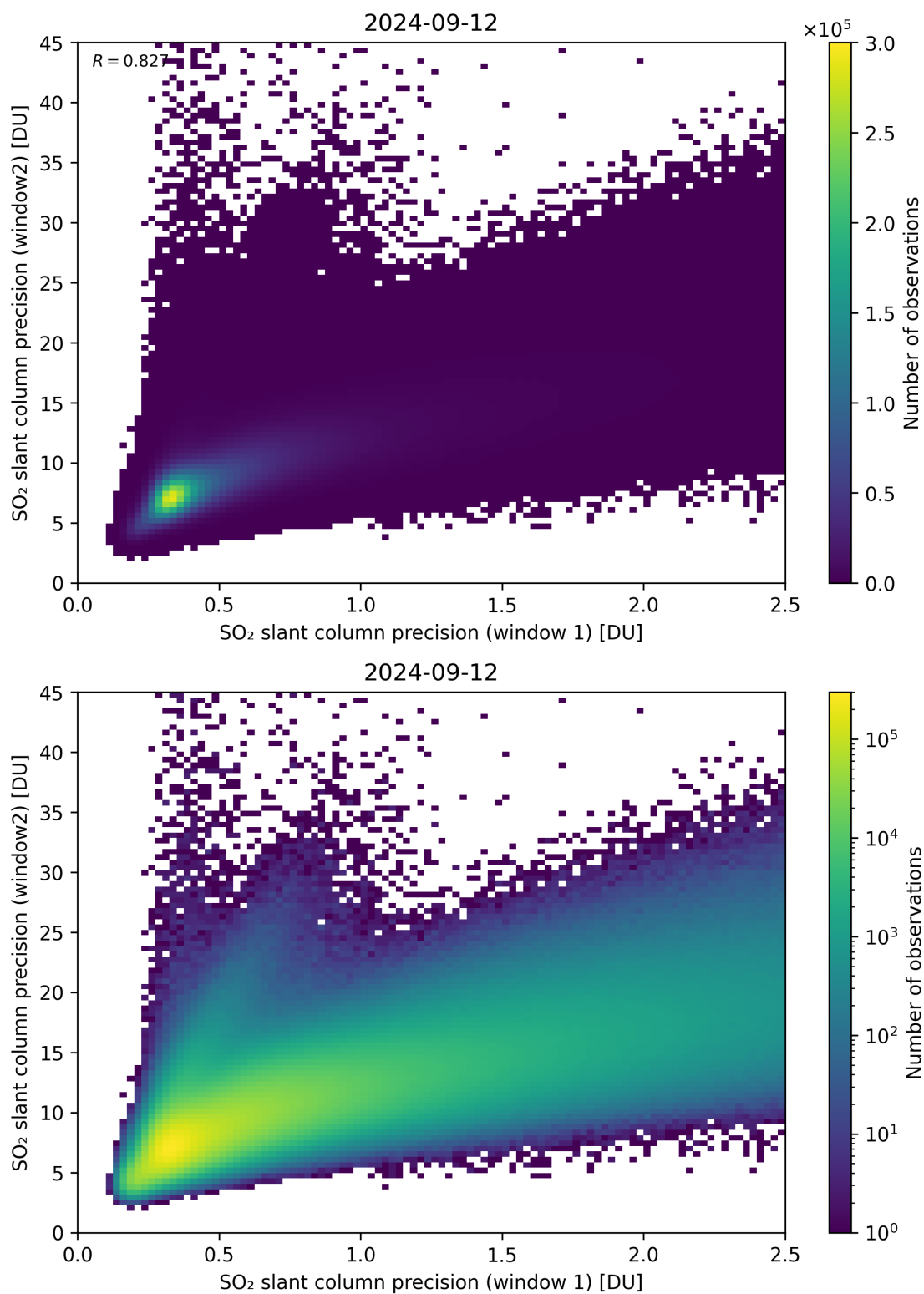
Figure 227: Scatter density plot of “SO 2 slant column precision (window 1)” against “SO 2 slant column precision (window2)” for 2024-09-12 to 2024-09-13.
