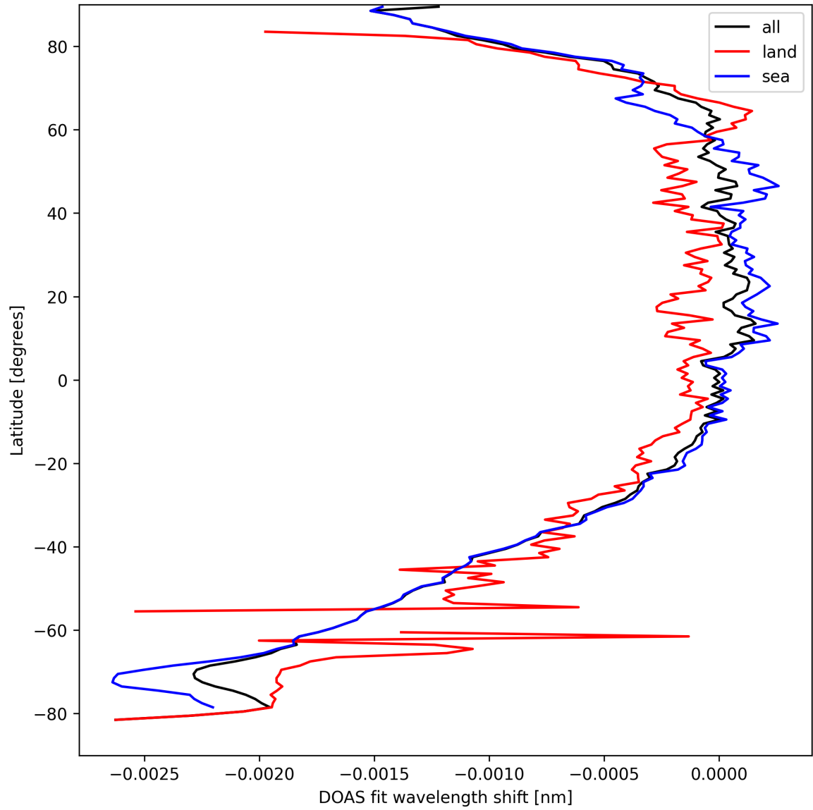
Figure 45: Zonal average of “DOAS fit wavelength shift” for 2024-09-12 to 2024-09-13.
