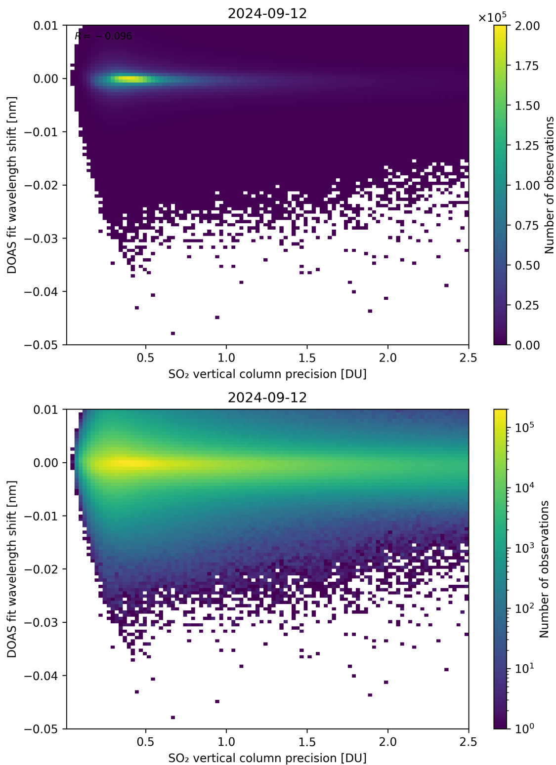
Figure 282: Scatter density plot of “SO 2 vertical column precision” against “DOAS fit wavelength shift” for 2024-09-12 to 2024-09-13.
