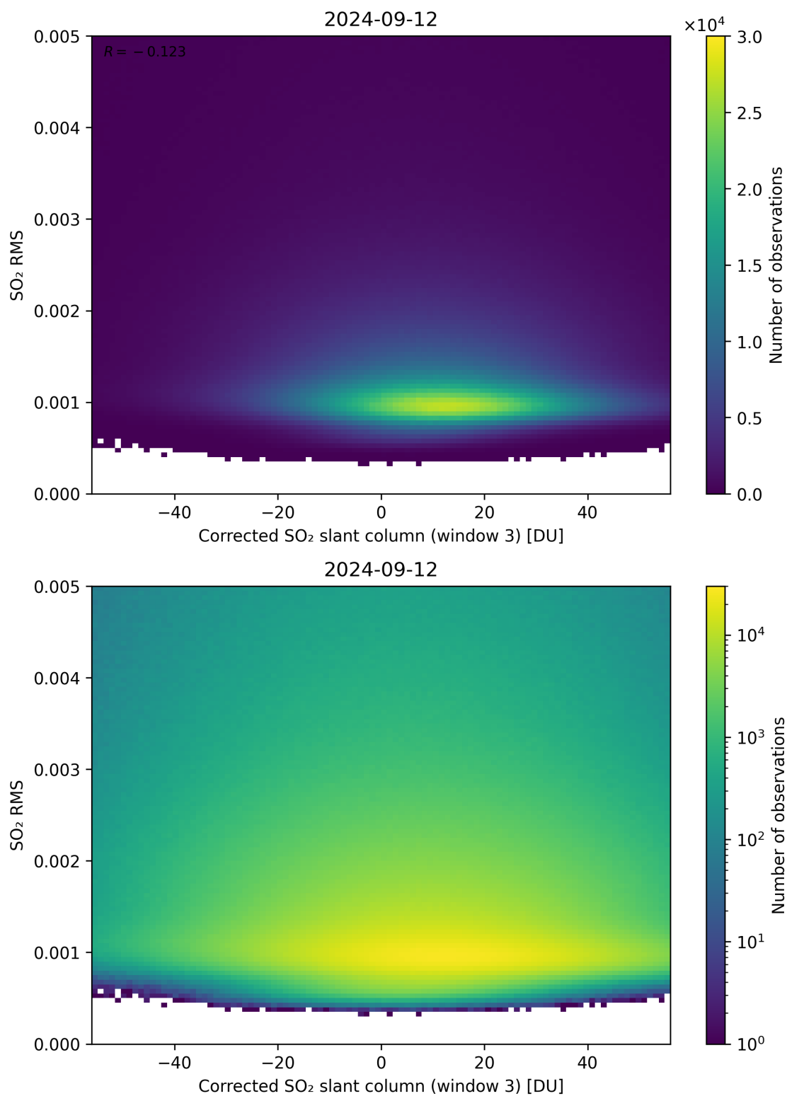
Figure 208: Scatter density plot of “Corrected SO 2 slant column (window 3)” against “SO 2 RMS” for 2024-09-12 to 2024-09-13.
