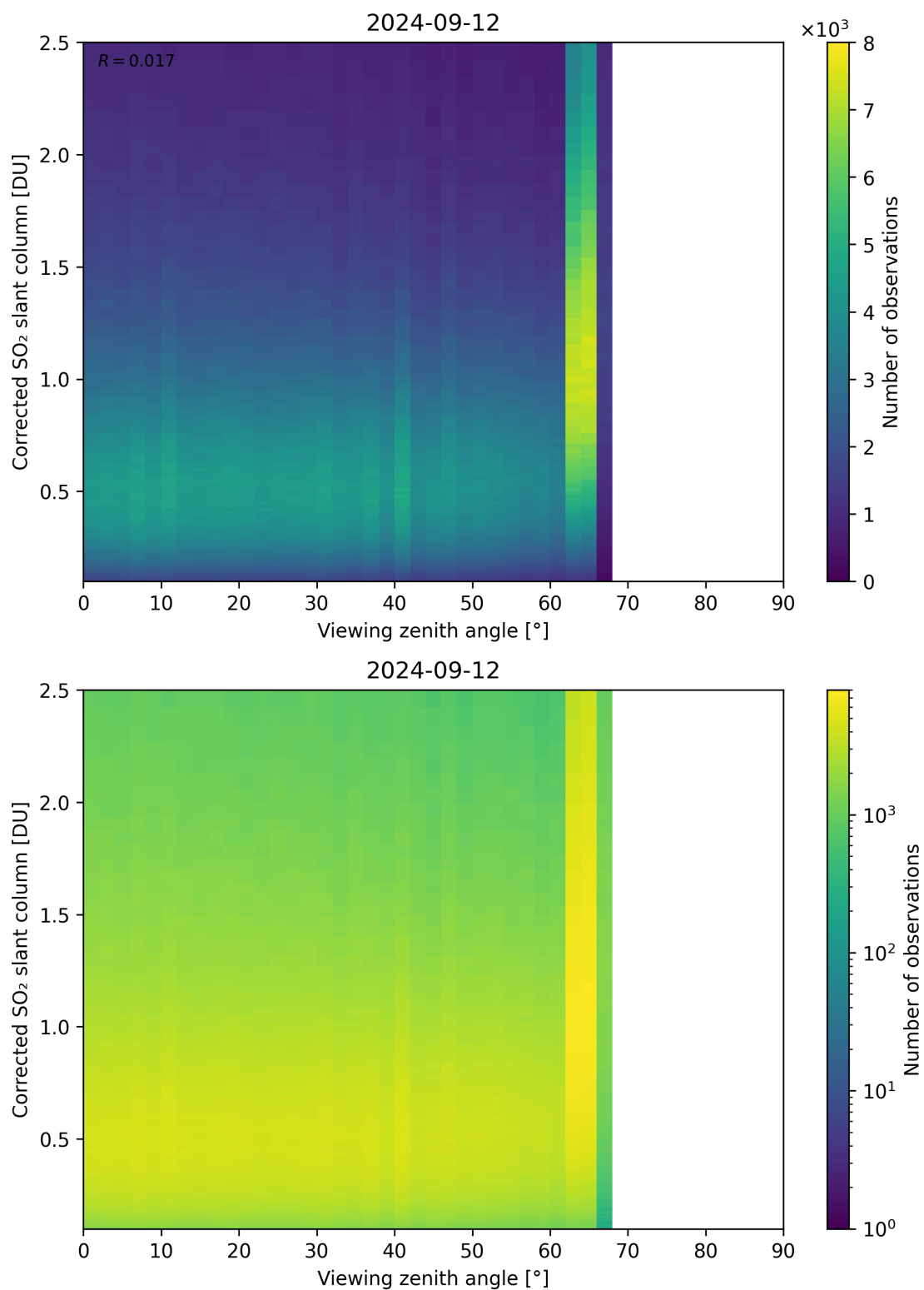
Figure 317: Scatter density plot of “Viewing zenith angle” against “Corrected SO 2 slant column” for 2024-09-12 to 2024-09-13.
