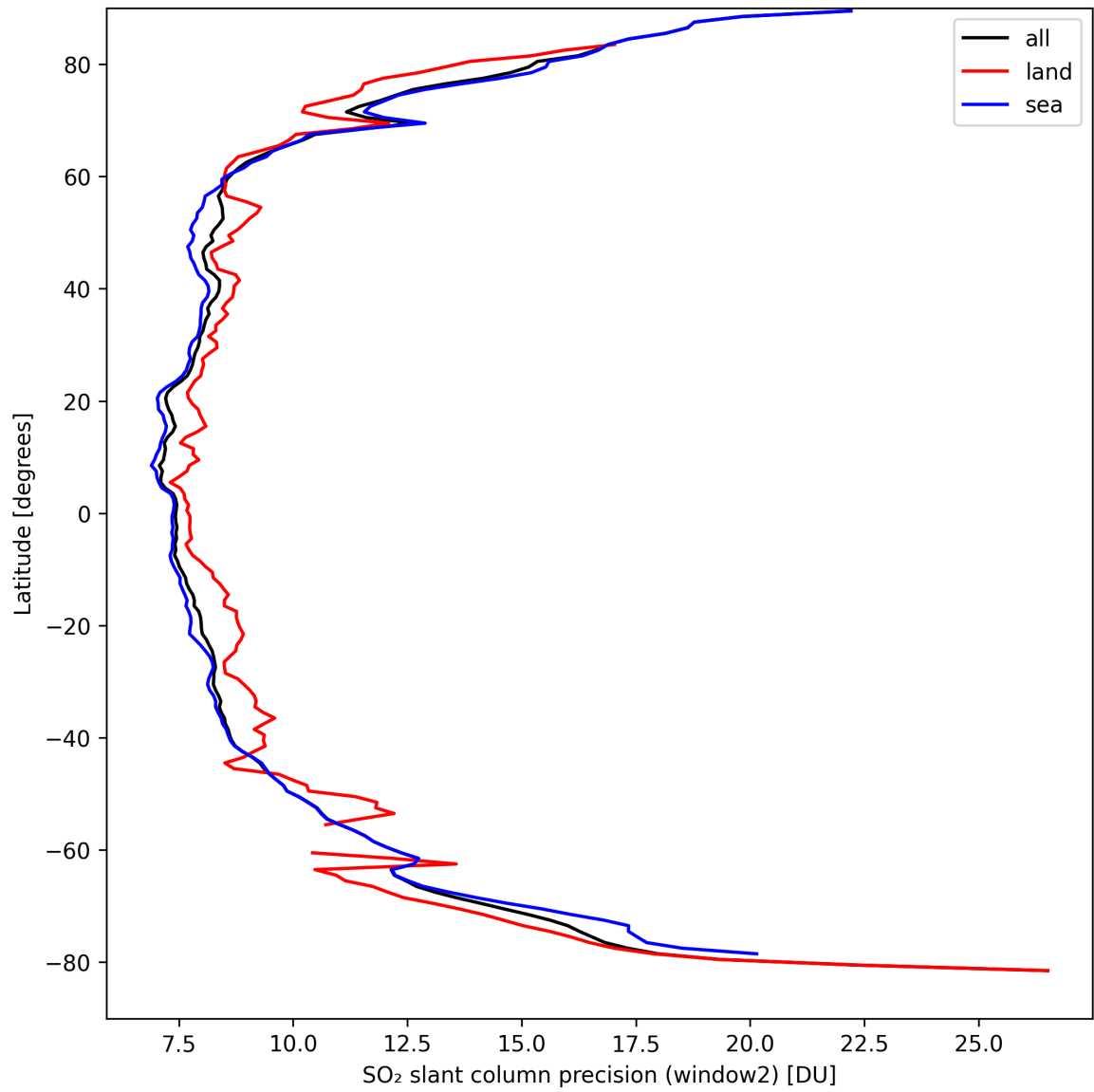
Figure 38: Zonal average of “SO 2 slant column precision (window2)” for 2024-09-12 to 2024-09-13.
