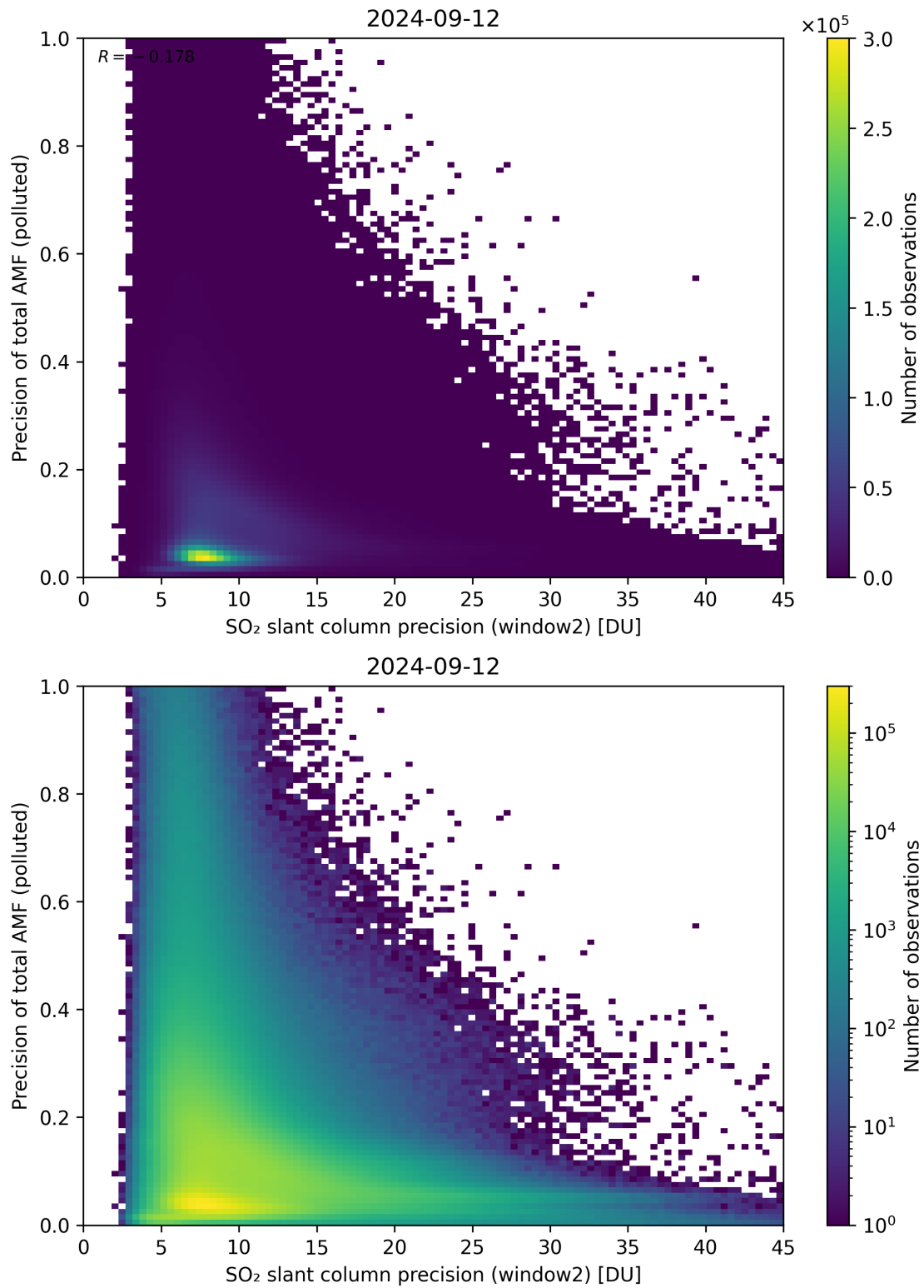
Figure 252: Scatter density plot of “SO 2 slant column precision (window2)” against “Precision of total AMF (polluted)” for 2024-09-12 to 2024-09-13.
