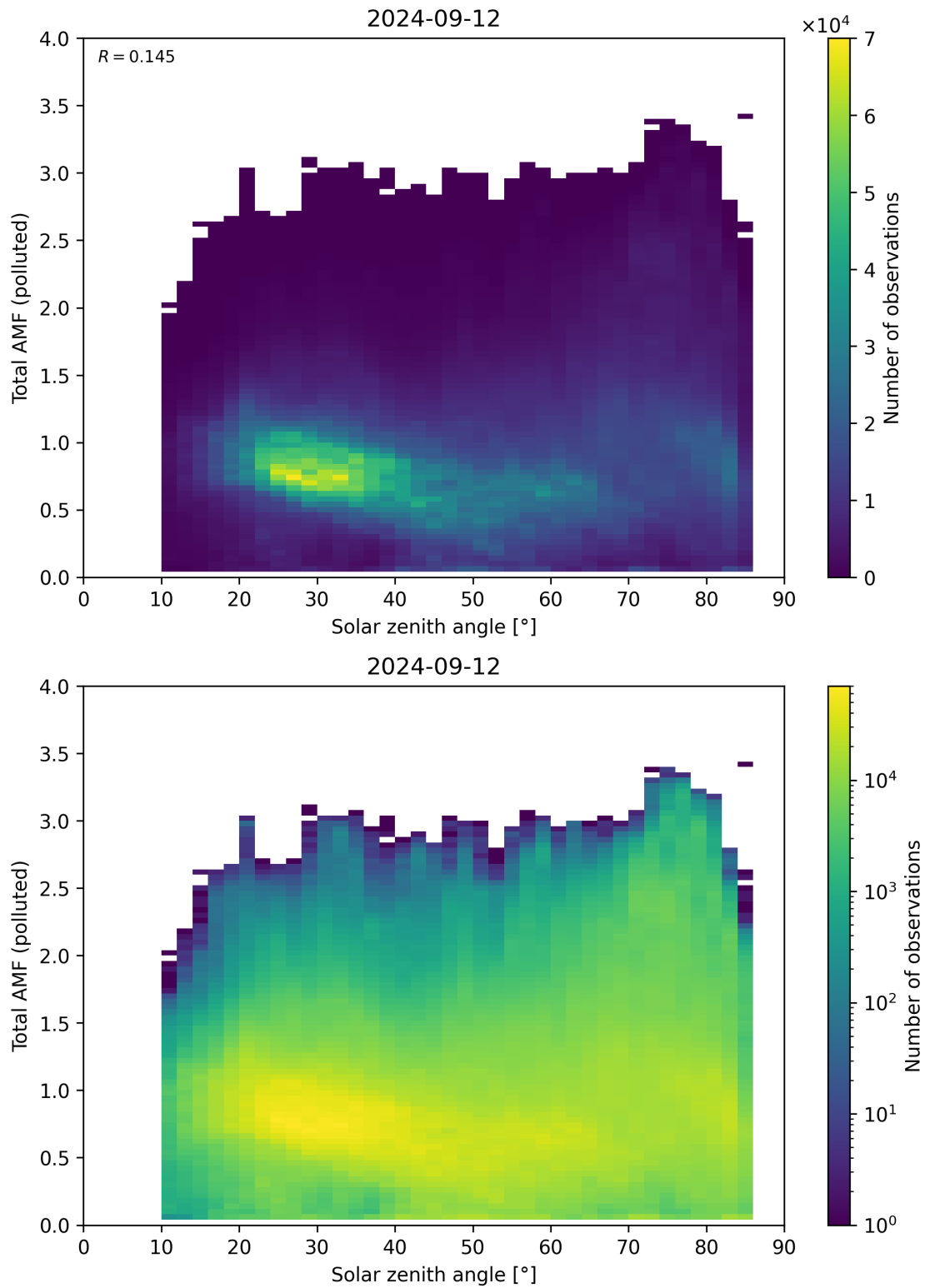
Figure 174: Scatter density plot of “Solar zenith angle” against “Total AMF (polluted)” for 2024-09-12 to 2024-09-13.
