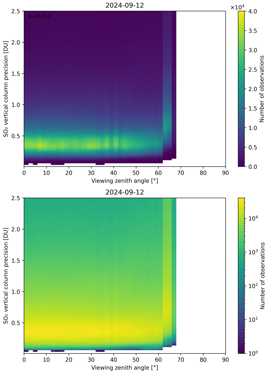
Figure 328: Scatter density plot of “Viewing zenith angle” against “SO 2 vertical column precision” for 2024-09-12 to 2024-09-13.
