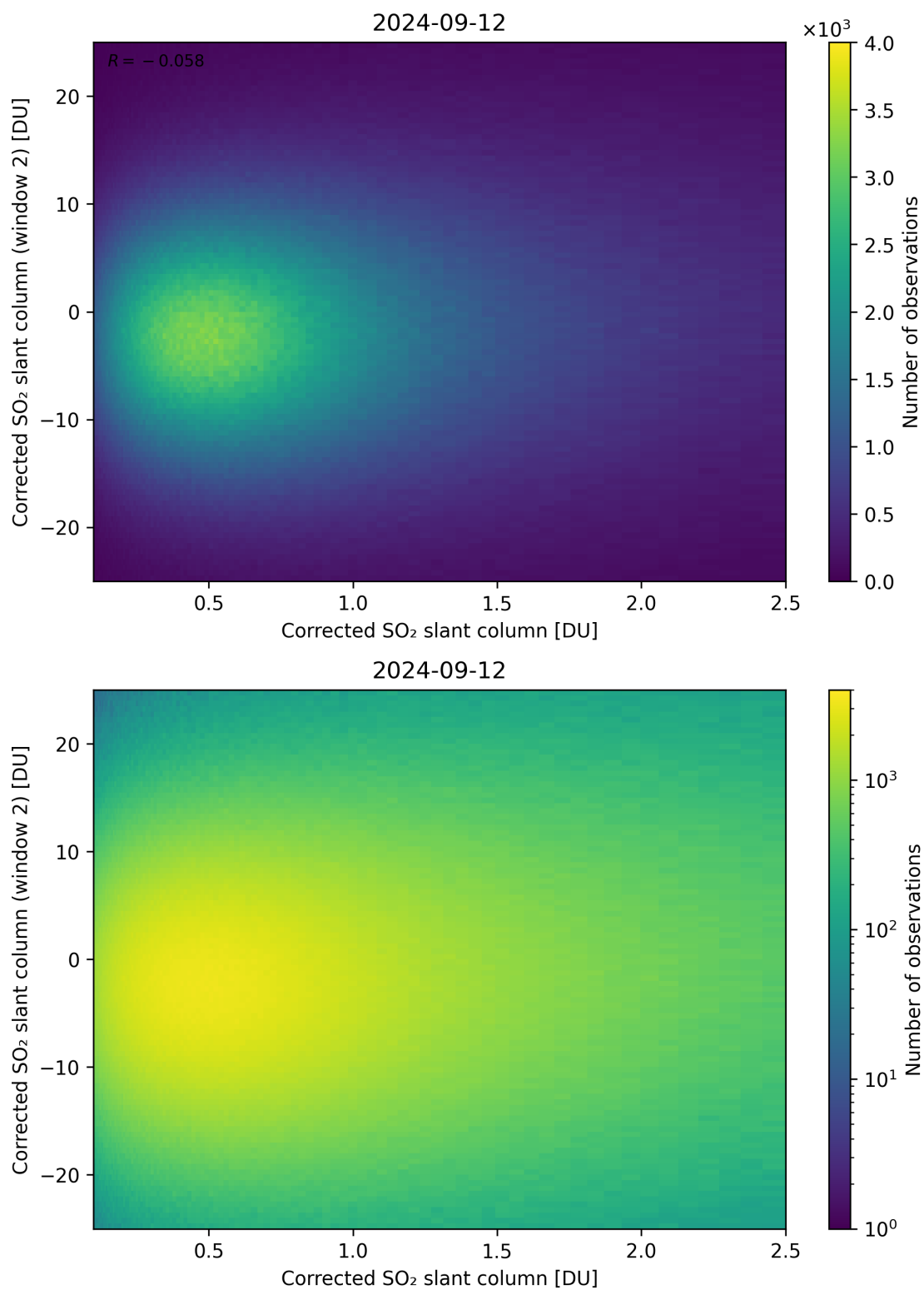
Figure 185: Scatter density plot of “Corrected SO 2 slant column” against “Corrected SO 2 slant column (window 2)” for 2024-09-12 to 2024-09-13.
