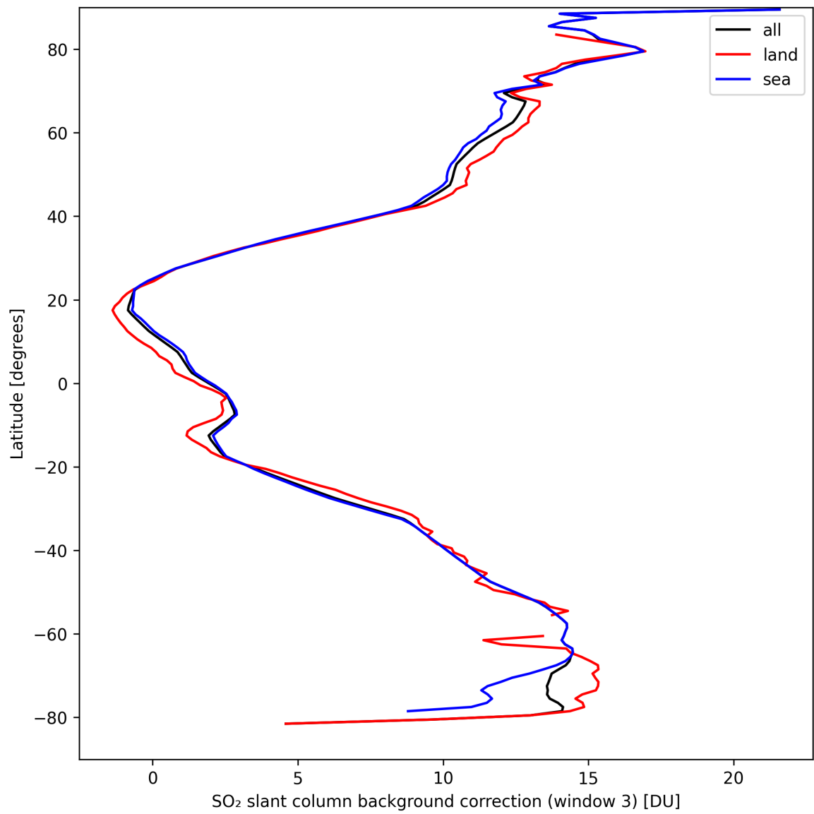
Figure 44: Zonal average of “SO 2 slant column background correction (window 3)” for 2024-09-12 to 2024-09-13.
