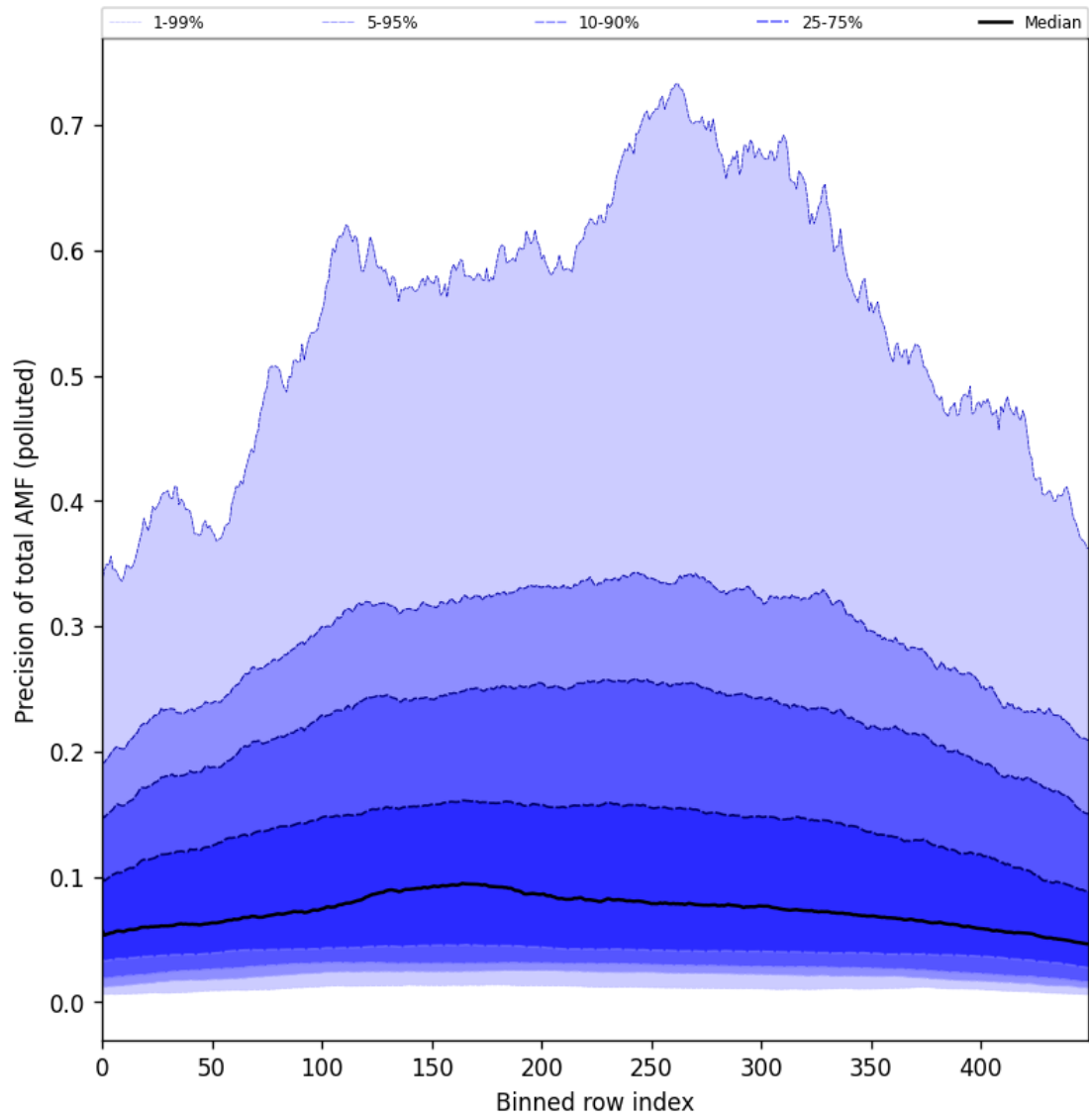
Figure 95: Along track statistics of “Precision of total AMF (polluted)” for 2024-09-12 to 2024-09-13
