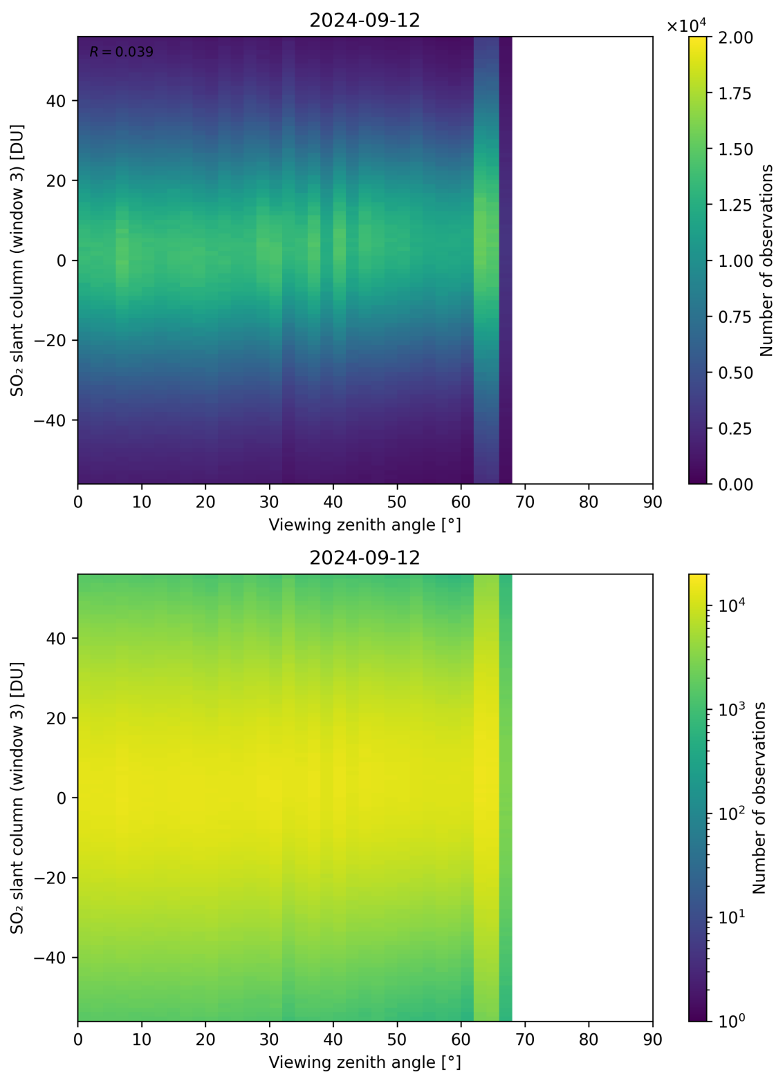
Figure 323: Scatter density plot of “Viewing zenith angle” against “SO 2 slant column (window 3)” for 2024-09-12 to 2024-09-13.
