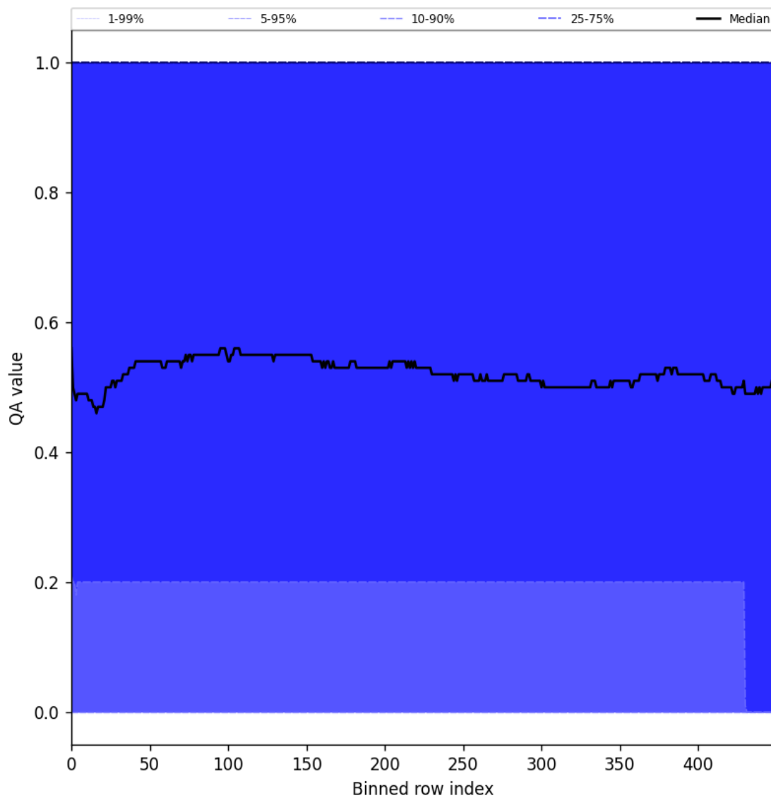
Figure 75: Along track statistics of “QA value” for 2024-09-12 to 2024-09-13
