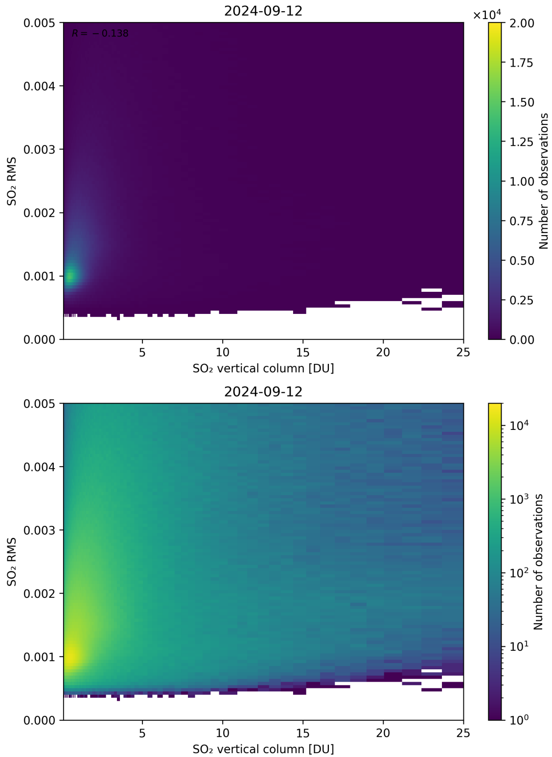
Figure 278: Scatter density plot of “SO 2 vertical column” against “SO 2 RMS” for 2024-09-12 to 2024-09-13.
