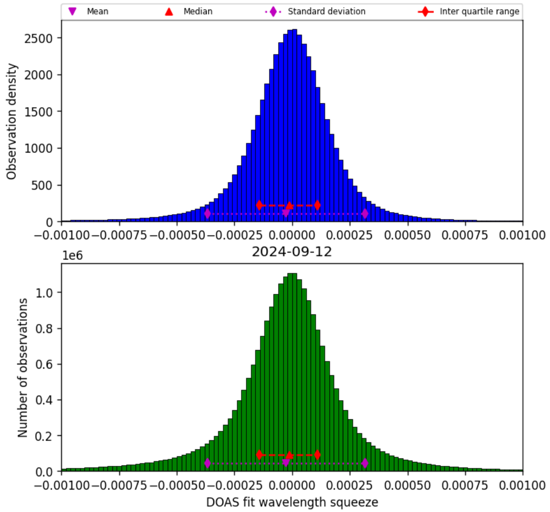
Figure 69: Histogram of “DOAS fit wavelength squeeze” for 2024-09-12 to 2024-09-13
