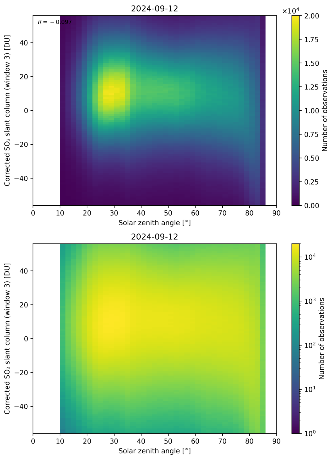
Figure 168: Scatter density plot of “Solar zenith angle” against “Corrected SO 2 slant column (window 3)” for 2024-09-12 to 2024-09-13.
