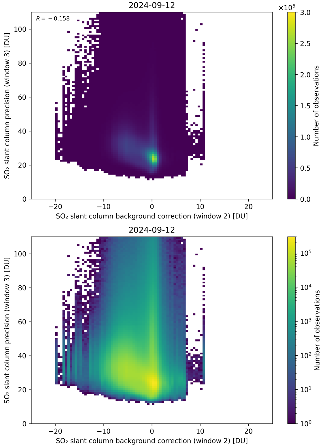
Figure 118: Scatter density plot of “SO 2 slant column background correction (window 2)” against “SO 2 slant column precision (window 3)” for 2024-09-12 to 2024-09-13.
