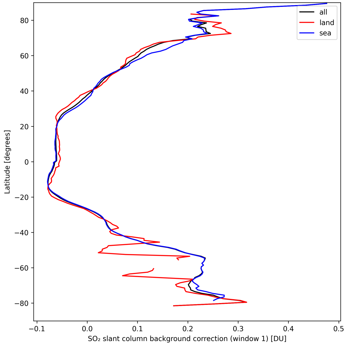
Figure 36: Zonal average of “SO 2 slant column background correction (window 1)” for 2024-09-12 to 2024-09-13.
