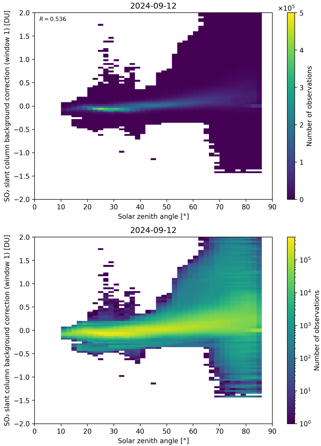
Figure 158: Scatter density plot of “Solar zenith angle” against “SO 2 slant column background correction (window 1)” for 2024-09-12 to 2024-09-13.
