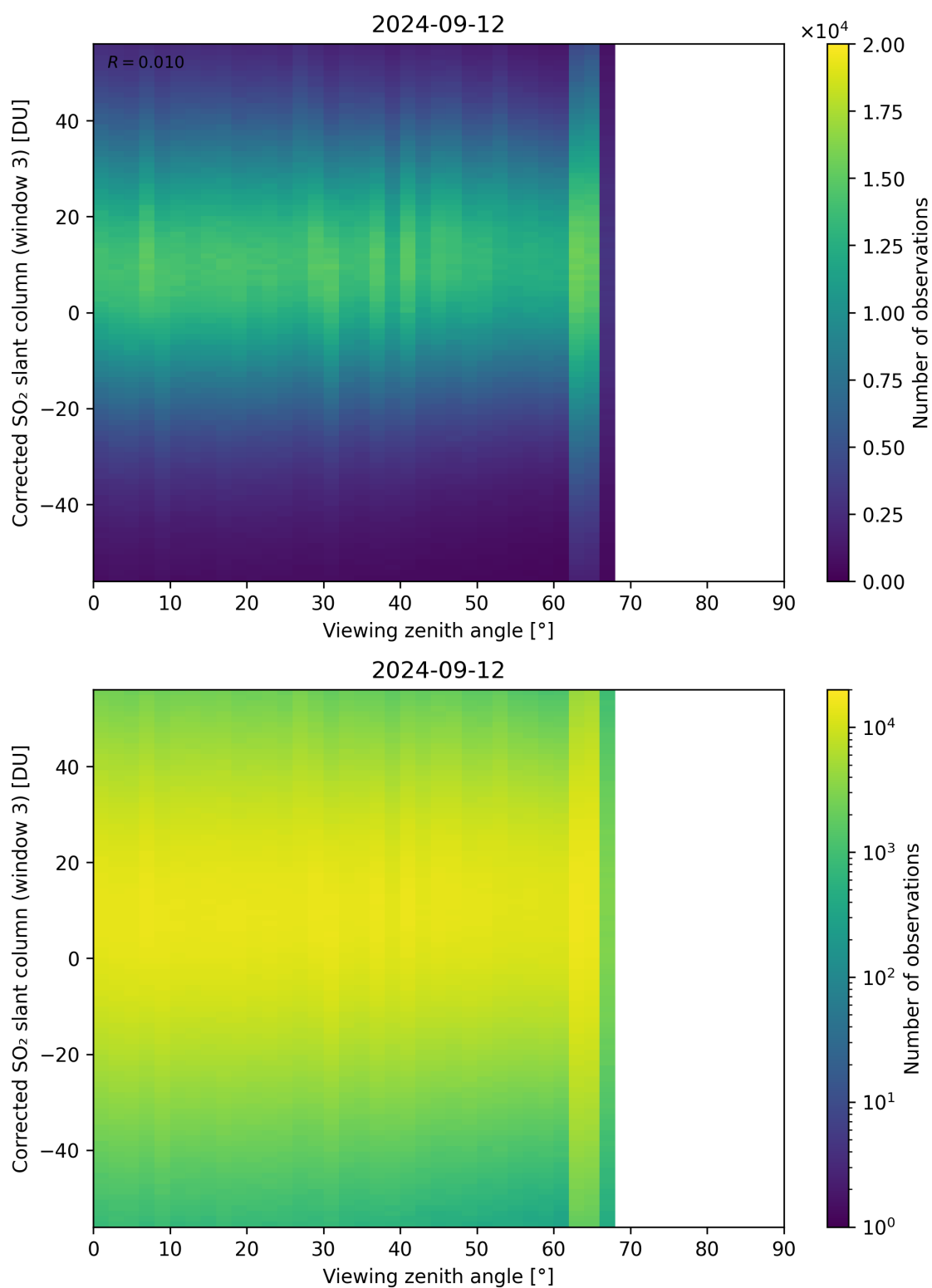
Figure 319: Scatter density plot of “Viewing zenith angle” against “Corrected SO 2 slant column (window 3)” for 2024-09-12 to 2024-09-13.
