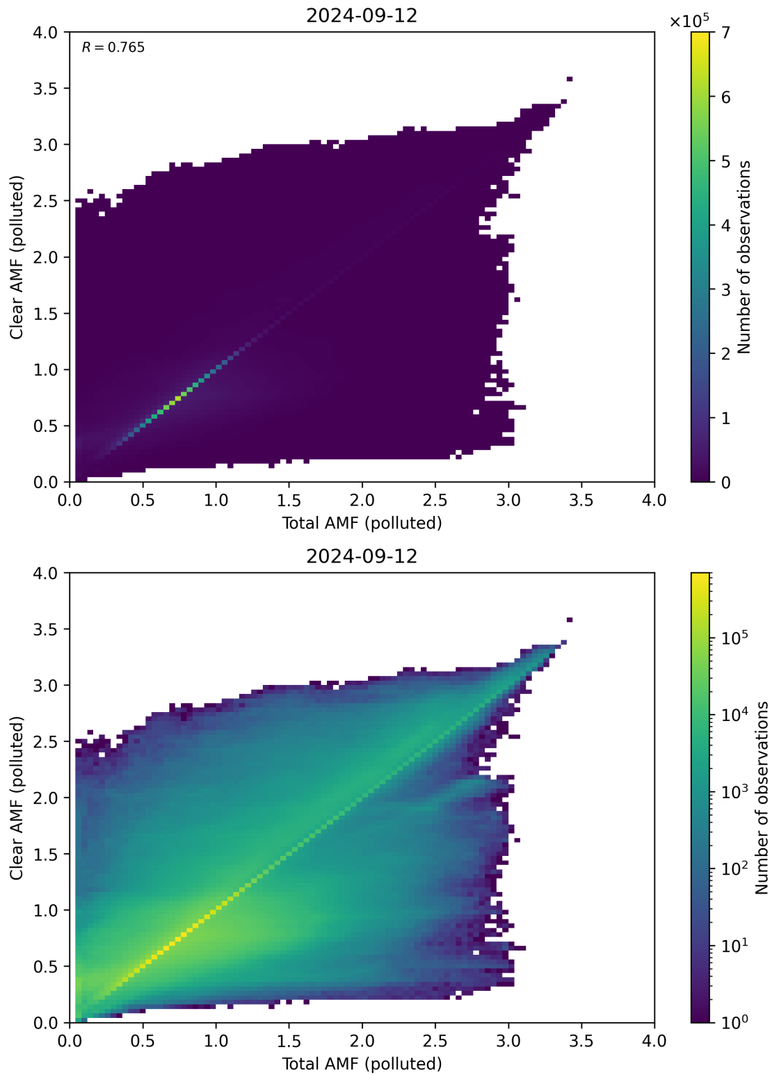
Figure 271: Scatter density plot of “Total AMF (polluted)” against “Clear AMF (polluted)” for 2024-09-12 to 2024-09-13.
