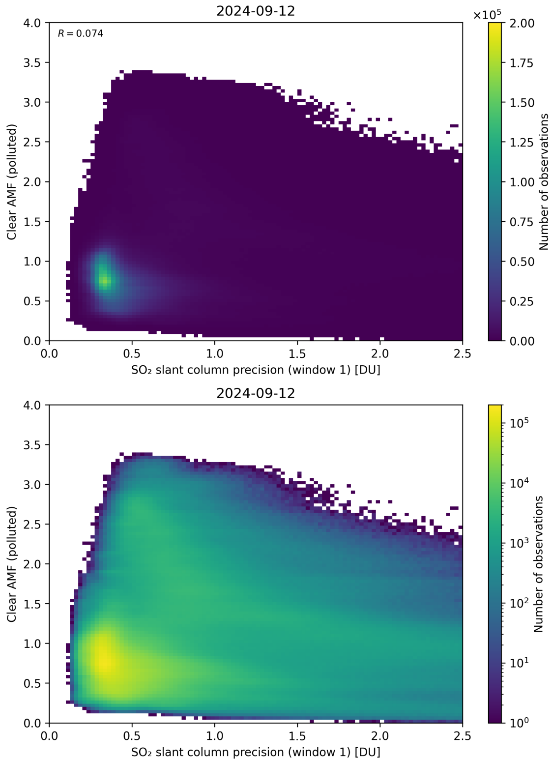
Figure 224: Scatter density plot of “SO 2 slant column precision (window 1)” against “Clear AMF (polluted)” for 2024-09-12 to 2024-09-13.
