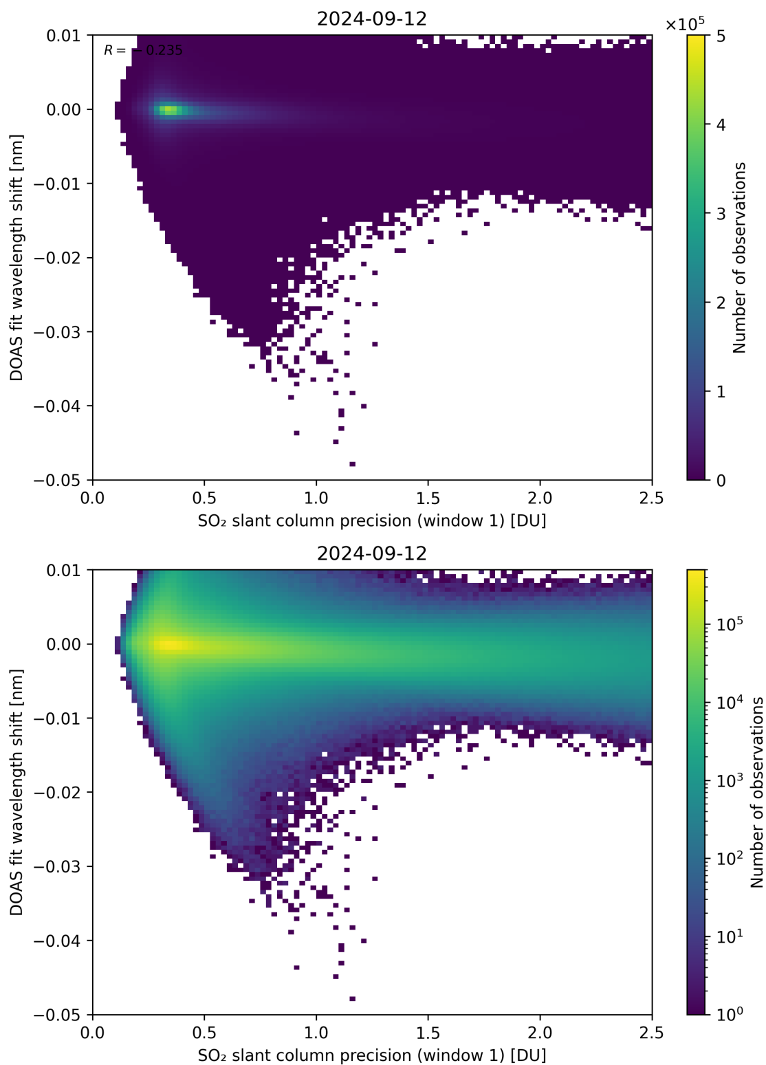
Figure 221: Scatter density plot of “SO 2 slant column precision (window 1)” against “DOAS fit wavelength shift” for 2024-09-12 to 2024-09-13.
