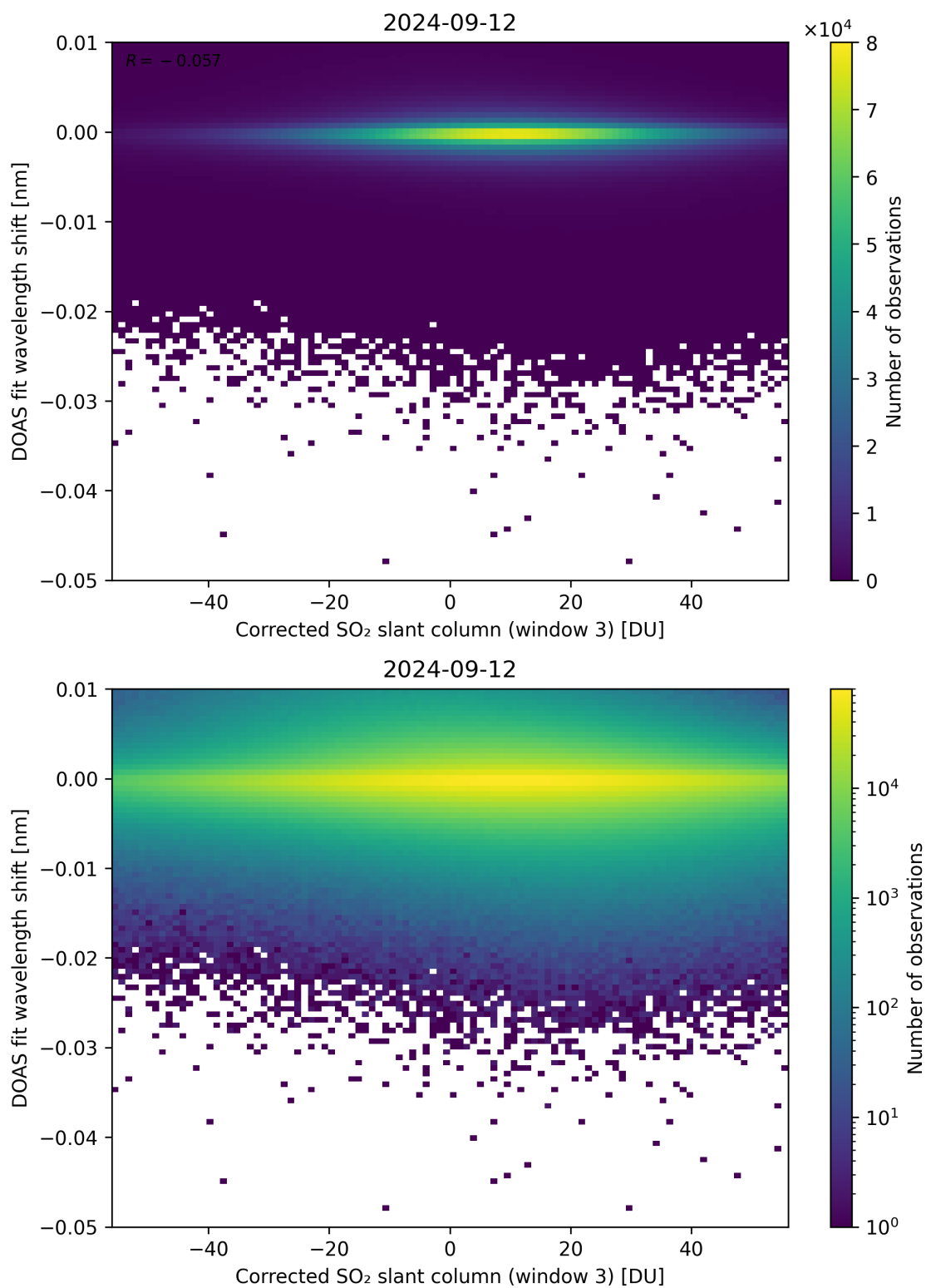
Figure 206: Scatter density plot of “Corrected SO 2 slant column (window 3)” against “DOAS fit wavelength shift” for 2024-09-12 to 2024-09-13.
