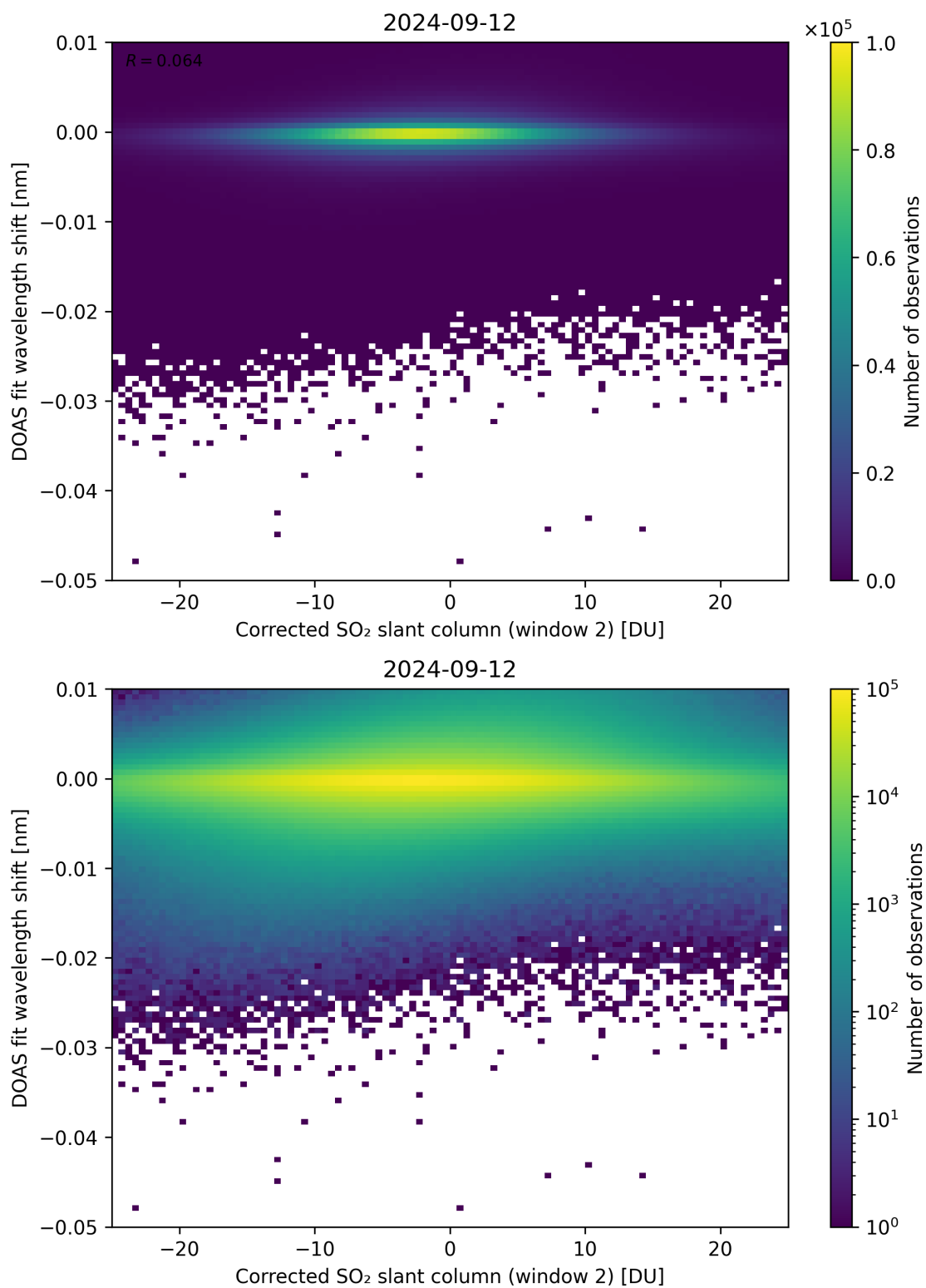
Figure 196: Scatter density plot of “Corrected SO 2 slant column (window 2)” against “DOAS fit wavelength shift” for 2024-09-12 to 2024-09-13.
