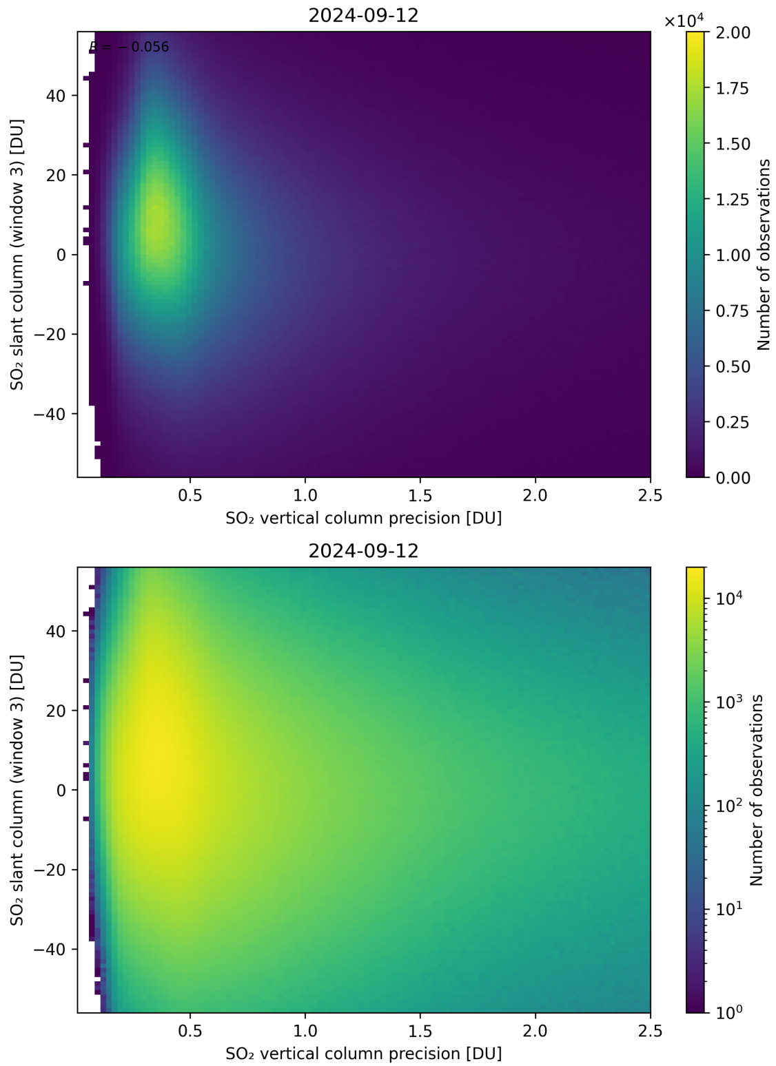
Figure 292: Scatter density plot of “SO 2 vertical column precision” against “SO 2 slant column (window 3)” for 2024-09-12 to 2024-09-13.
