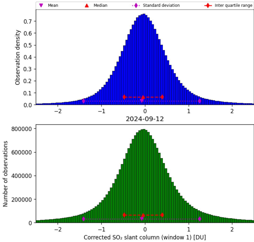
Figure 58: Histogram of “Corrected SO 2 slant column (window 1)” for 2024-09-12 to 2024-09-13
