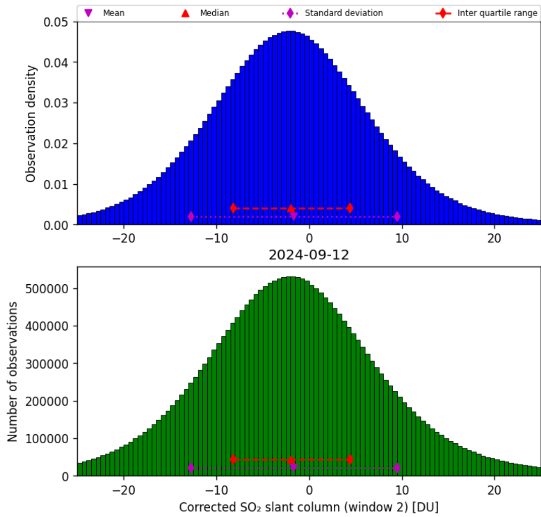
Figure 62: Histogram of “Corrected SO 2 slant column (window 2)” for 2024-09-12 to 2024-09-13
