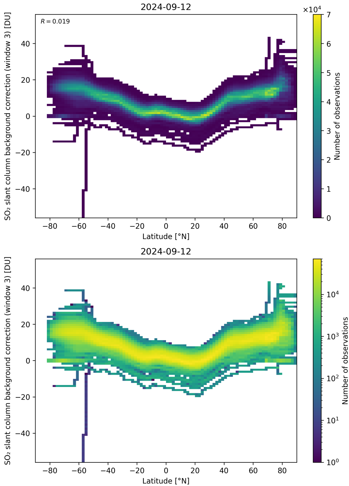
Figure 141: Scatter density plot of “Latitude” against “SO 2 slant column background correction (window 3)” for 2024-09-12 to 2024-09-13.
