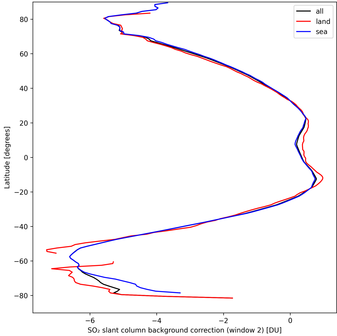
Figure 40: Zonal average of “SO 2 slant column background correction (window 2)” for 2024-09-12 to 2024-09-13.
