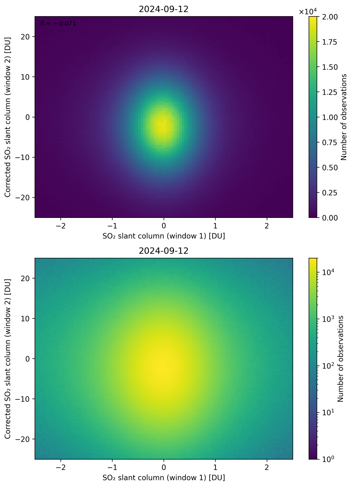
Figure 233: Scatter density plot of “SO 2 slant column (window 1)” against “Corrected SO 2 slant column (window 2)” for 2024-09-12 to 2024-09-13.
