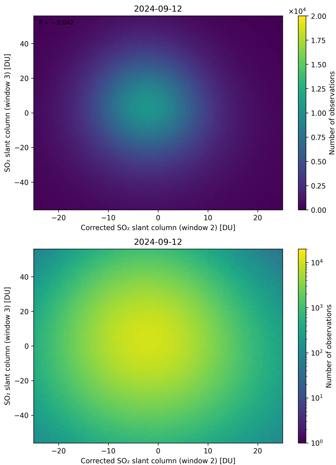
Figure 201: Scatter density plot of “Corrected SO 2 slant column (window 2)” against “SO 2 slant column (window 3)” for 2024-09-12 to 2024-09-13.
