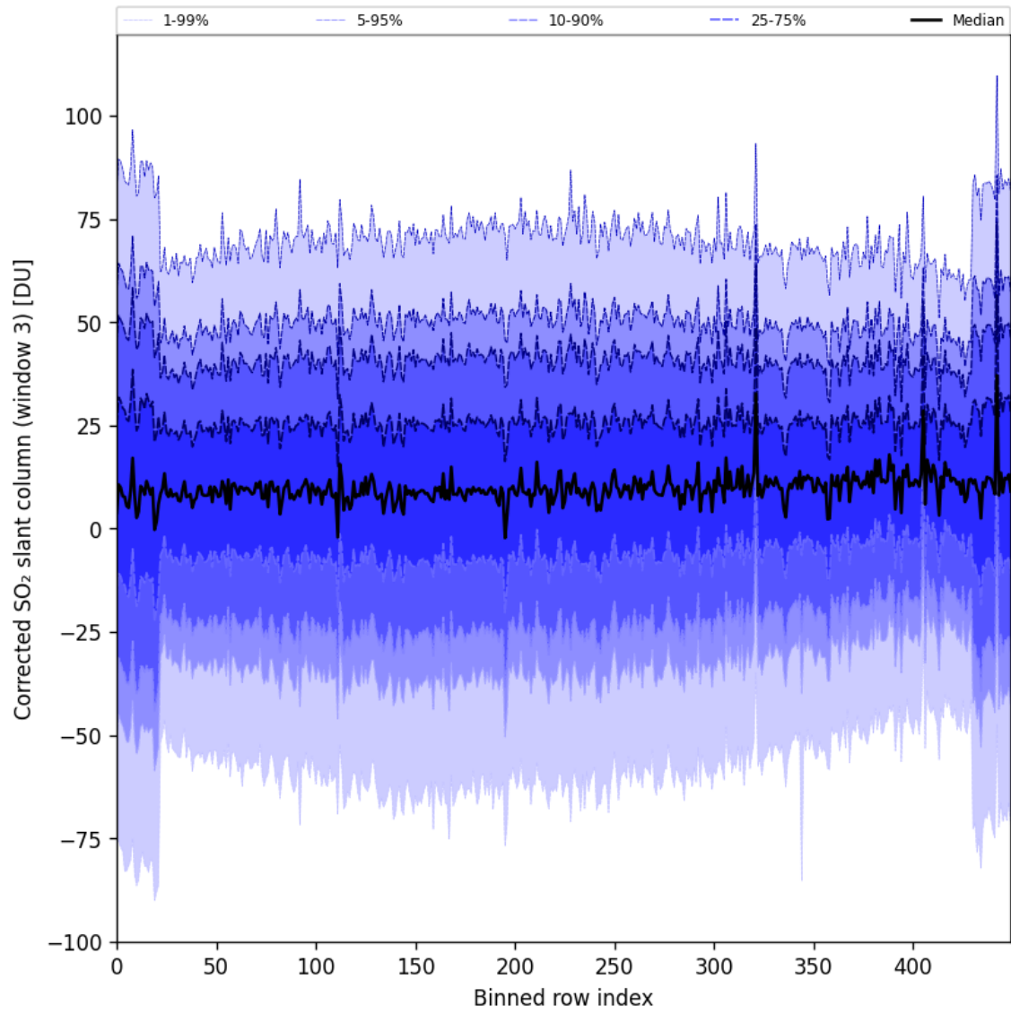
Figure 89: Along track statistics of “Corrected SO 2 slant column (window 3)” for 2024-09-12 to 2024-09-13
