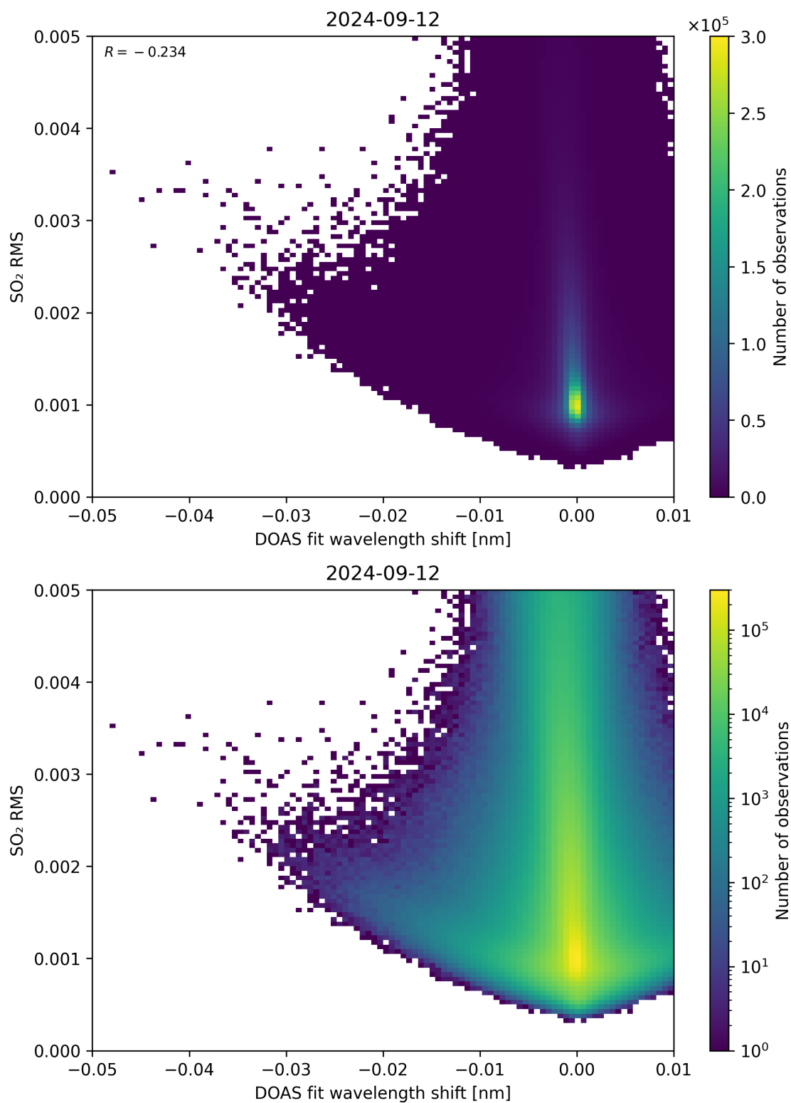
Figure 128: Scatter density plot of “DOAS fit wavelength shift” against “SO 2 RMS” for 2024-09-12 to 2024-09-13.
