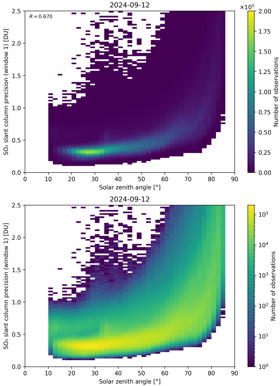
Figure 170: Scatter density plot of “Solar zenith angle” against “SO 2 slant column precision (window 1)” for 2024-09-12 to 2024-09-13.
