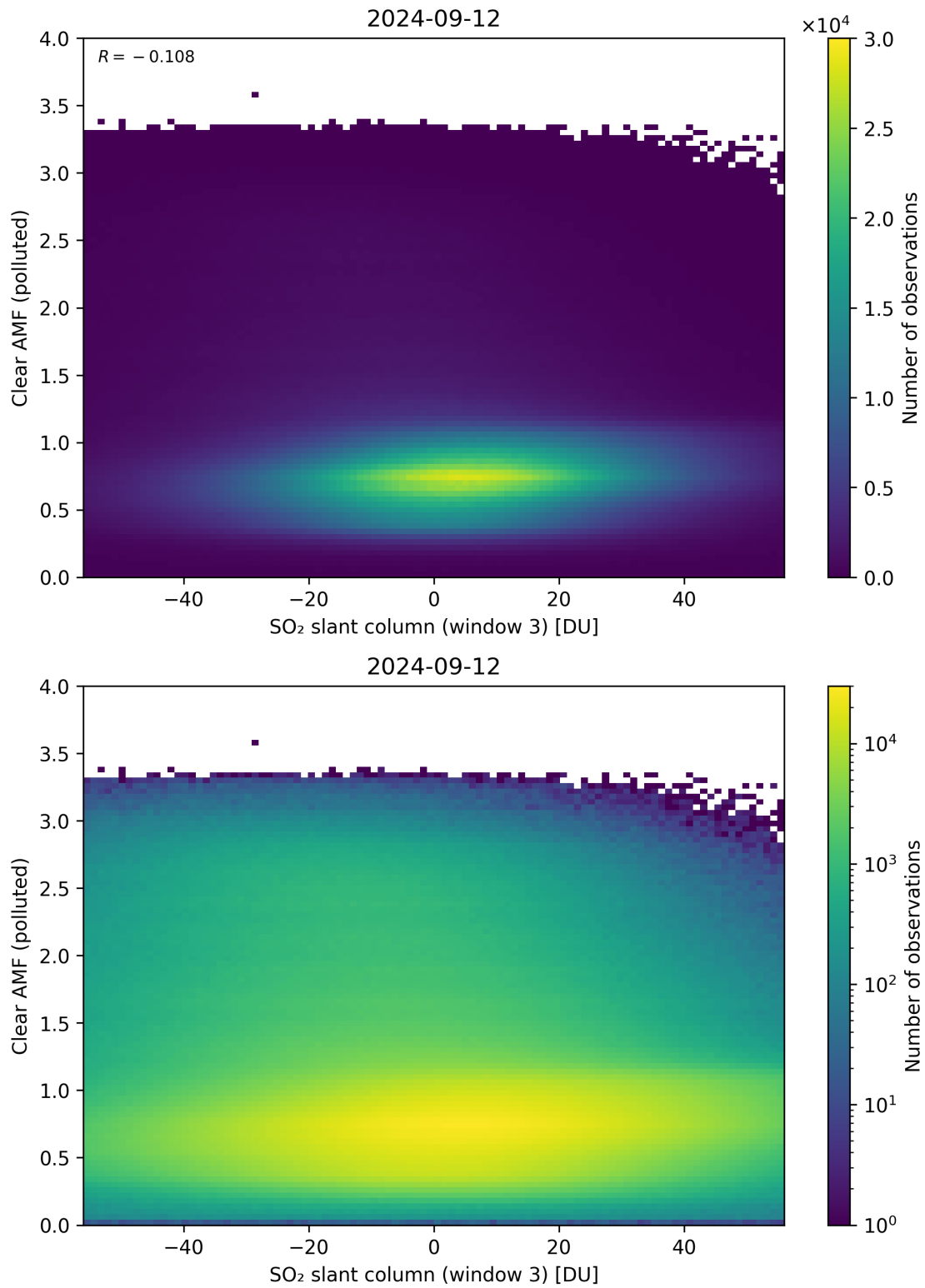
Figure 265: Scatter density plot of “SO 2 slant column (window 3)” against “Clear AMF (polluted)” for 2024-09-12 to 2024-09-13.
