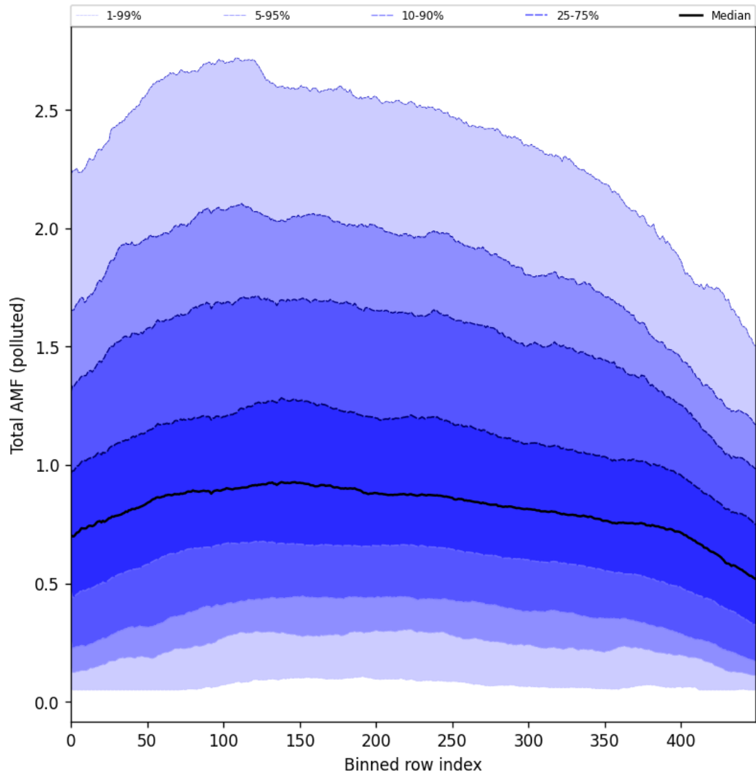
Figure 94: Along track statistics of “Total AMF (polluted)” for 2024-09-12 to 2024-09-13
