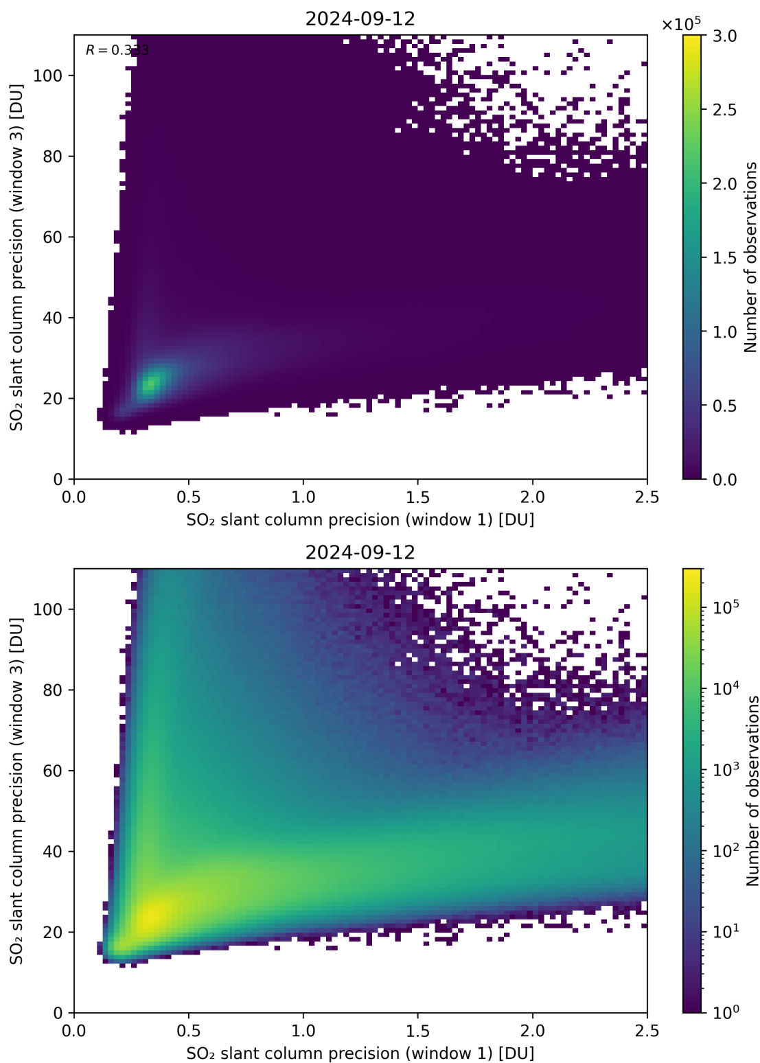
Figure 229: Scatter density plot of “SO 2 slant column precision (window 1)” against “SO 2 slant column precision (window 3)” for 2024-09-12 to 2024-09-13.
