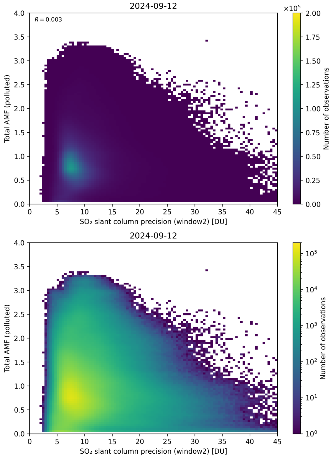
Figure 251: Scatter density plot of “SO 2 slant column precision (window2)” against “Total AMF (polluted)” for 2024-09-12 to 2024-09-13.
