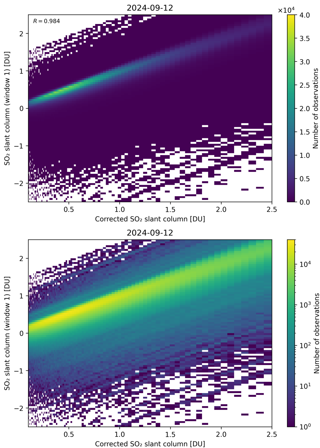
Figure 187: Scatter density plot of “Corrected SO 2 slant column” against “SO 2 slant column (window 1)” for 2024-09-12 to 2024-09-13.
