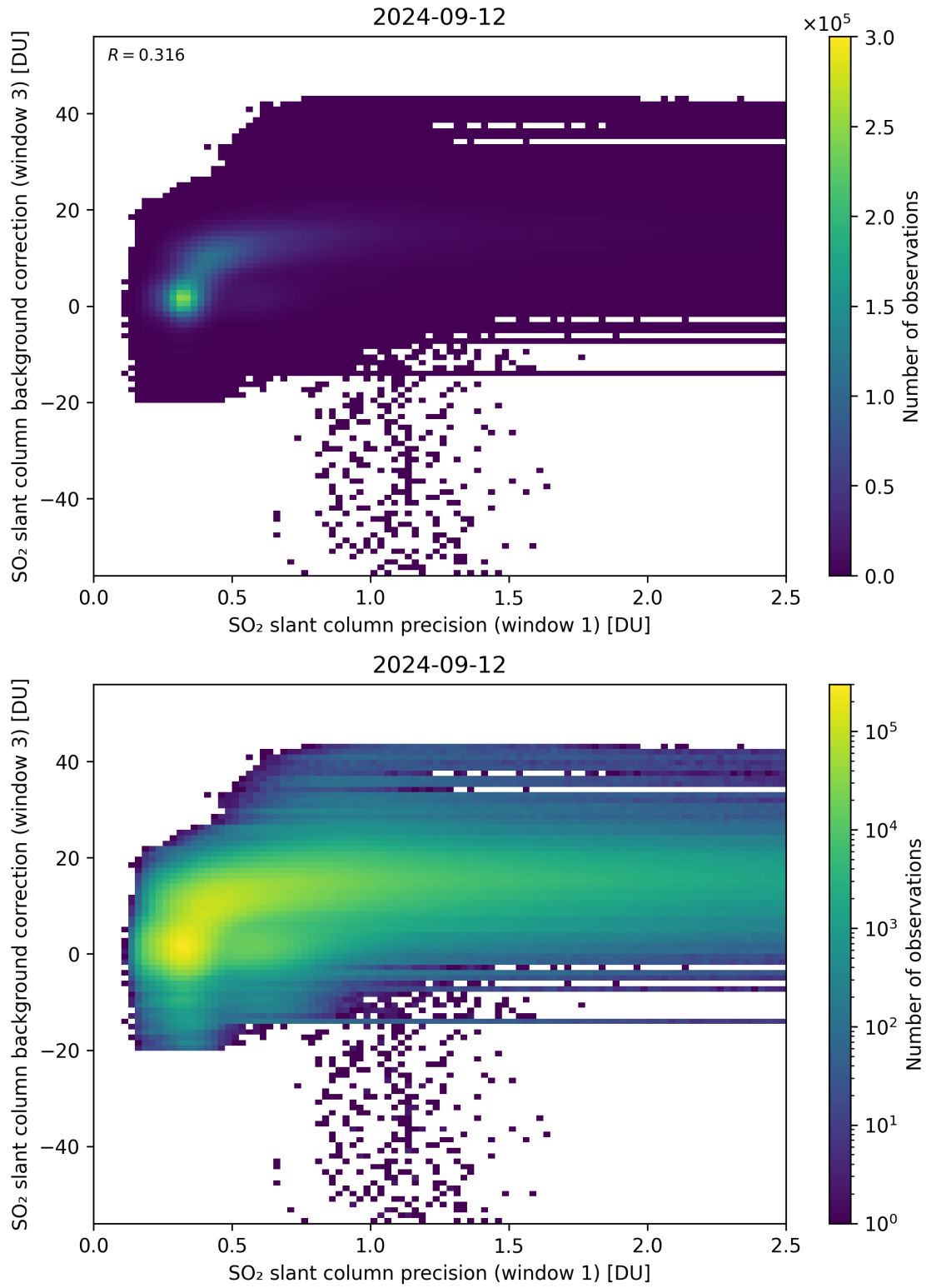
Figure 220: Scatter density plot of “SO 2 slant column precision (window 1)” against “SO 2 slant column background correction (window 3)” for 2024-09-12 to 2024-09-13.
