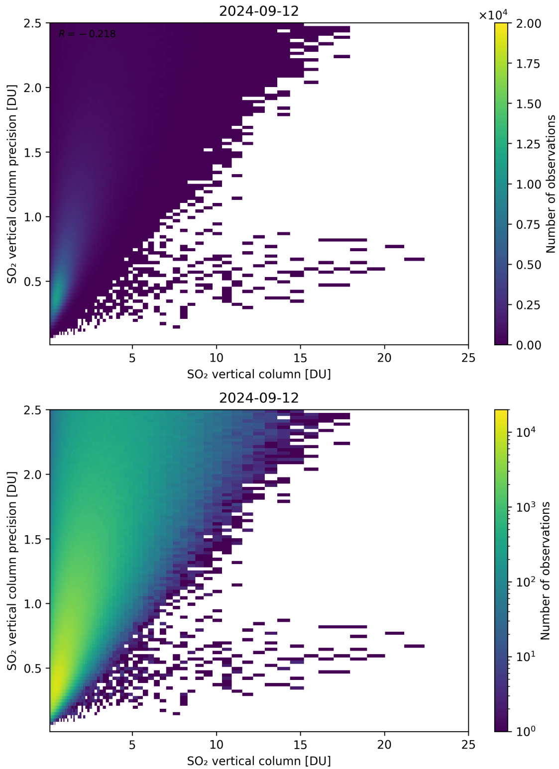
Figure 307: Scatter density plot of “SO 2 vertical column” against “SO 2 vertical column precision” for 2024-09-12 to 2024-09-13.
