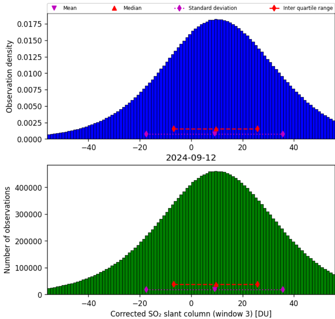
Figure 66: Histogram of “Corrected SO 2 slant column (window 3)” for 2024-09-12 to 2024-09-13
