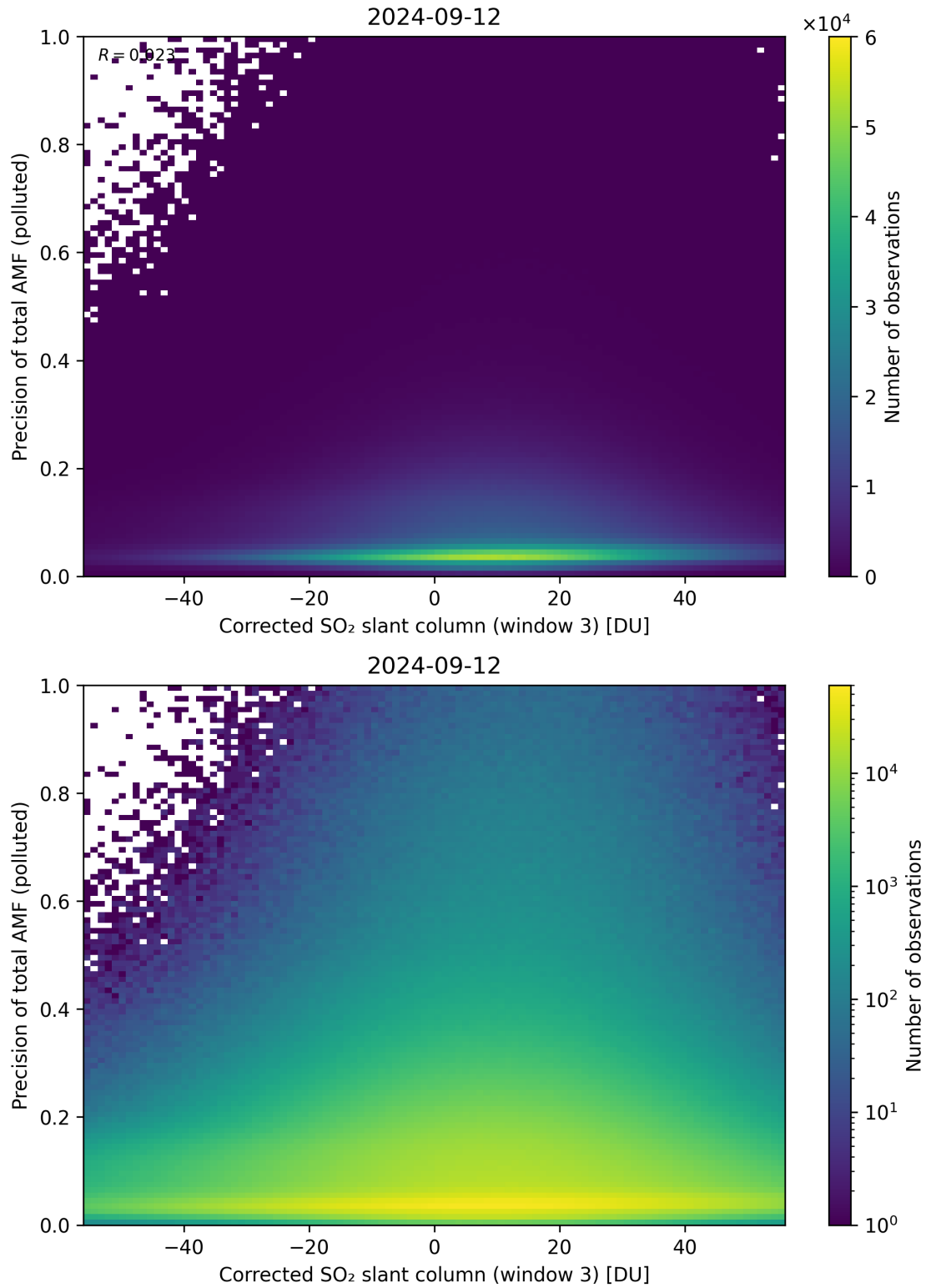
Figure 211: Scatter density plot of “Corrected SO 2 slant column (window 3)” against “Precision of total AMF (polluted)” for 2024-09-12 to 2024-09-13.
