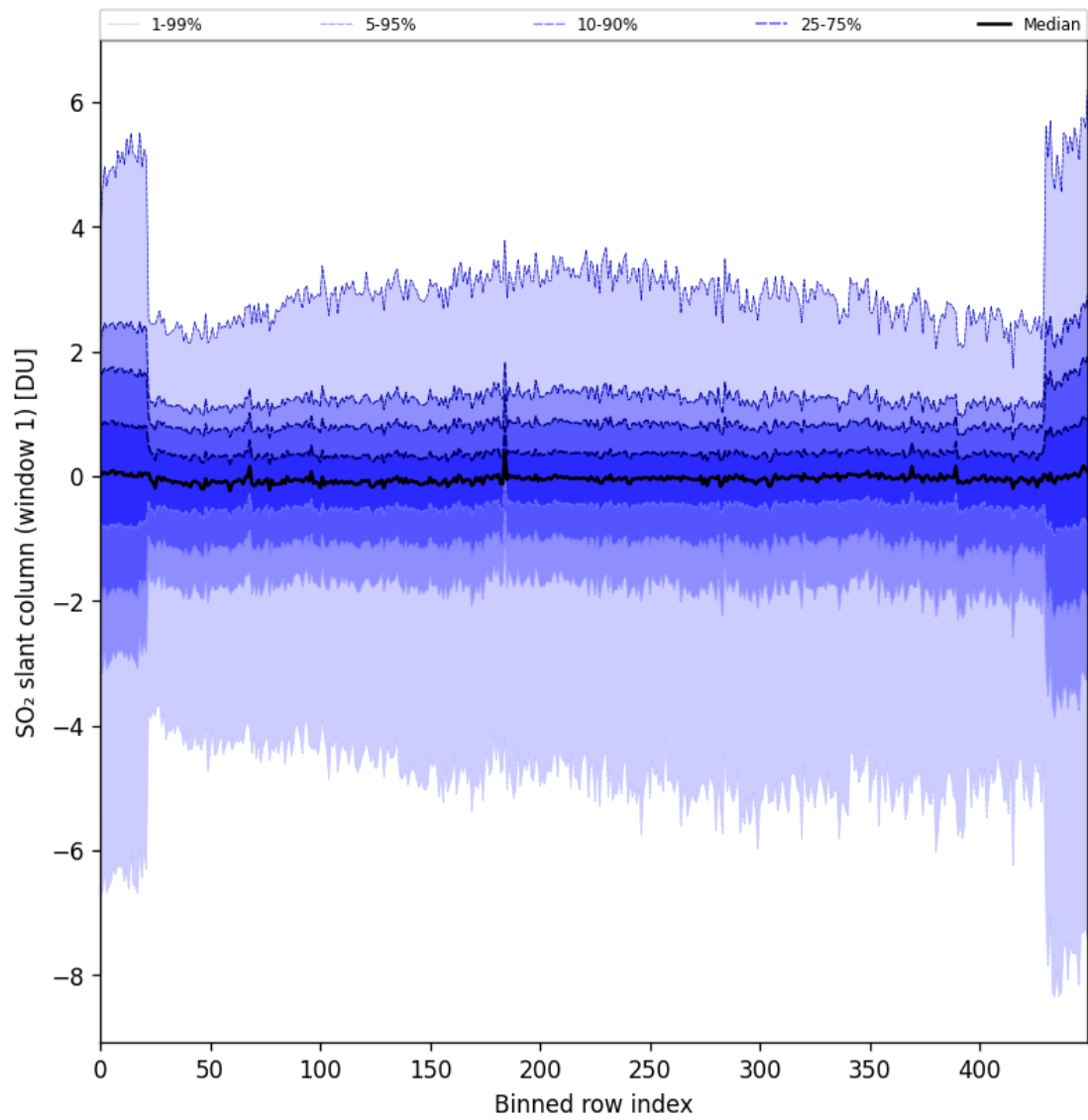
Figure 79: Along track statistics of “SO 2 slant column (window 1)” for 2024-09-12 to 2024-09-13
