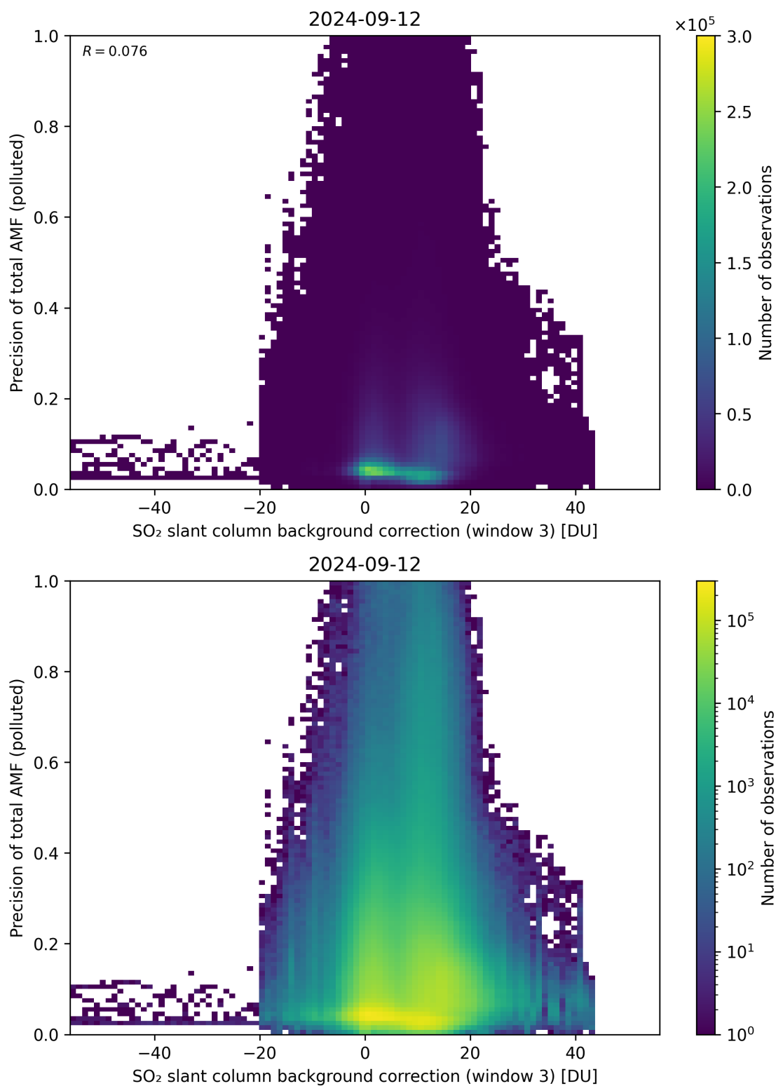
Figure 126: Scatter density plot of “SO 2 slant column background correction (window 3)” against “Precision of total AMF (polluted)” for 2024-09-12 to 2024-09-13.
