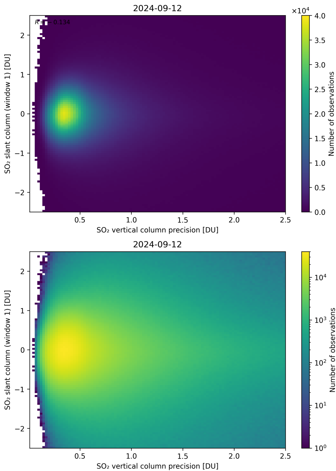
Figure 289: Scatter density plot of “SO 2 vertical column precision” against “SO 2 slant column (window 1)” for 2024-09-12 to 2024-09-13.
