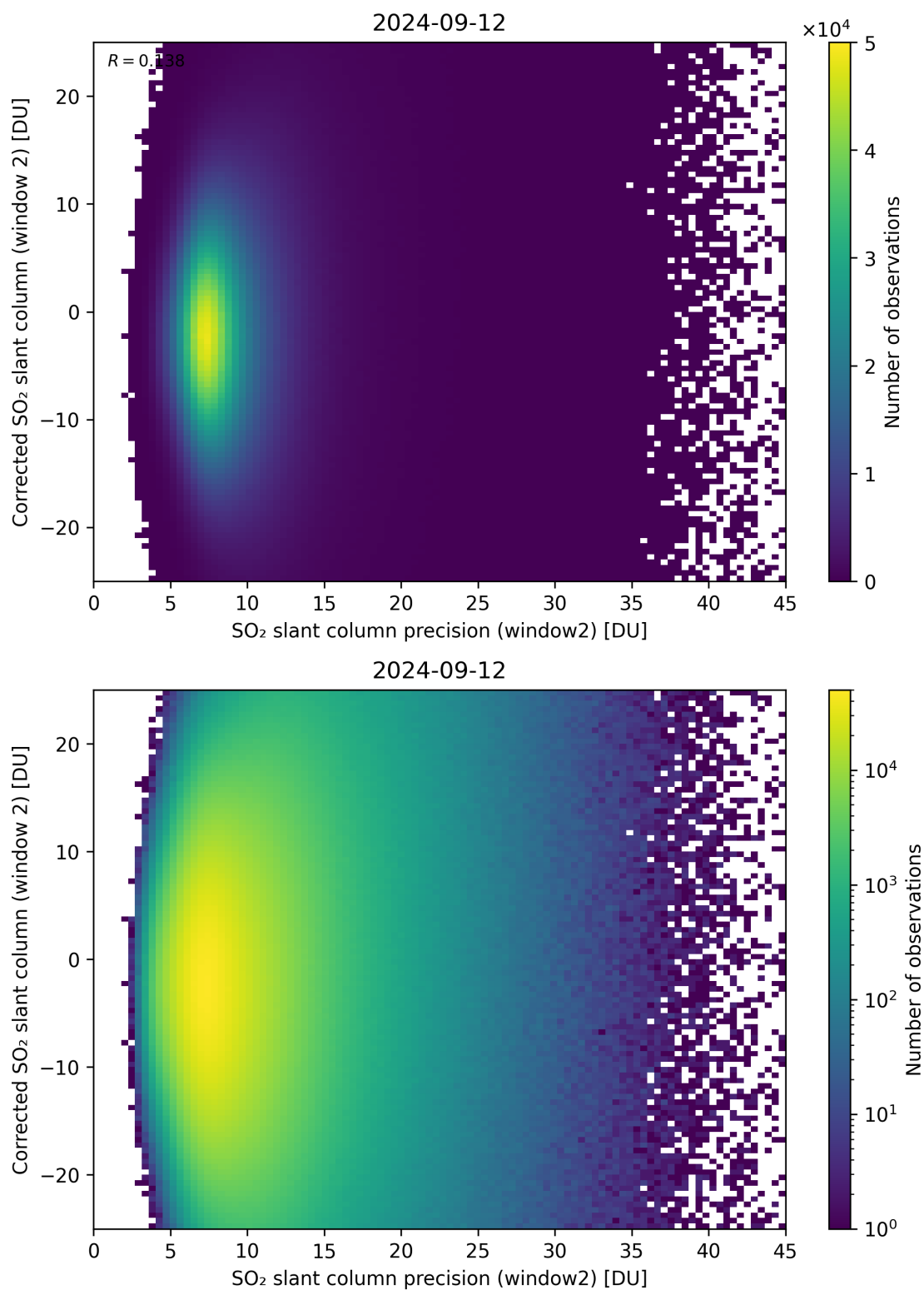
Figure 247: Scatter density plot of “SO 2 slant column precision (window2)” against “Corrected SO 2 slant column (window 2)” for 2024-09-12 to 2024-09-13.
