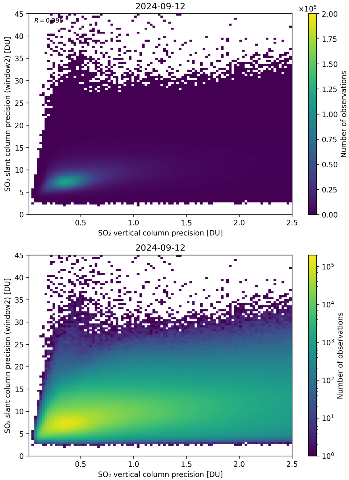
Figure 291: Scatter density plot of “SO 2 vertical column precision” against “SO 2 slant column precision (window2)” for 2024-09-12 to 2024-09-13.
