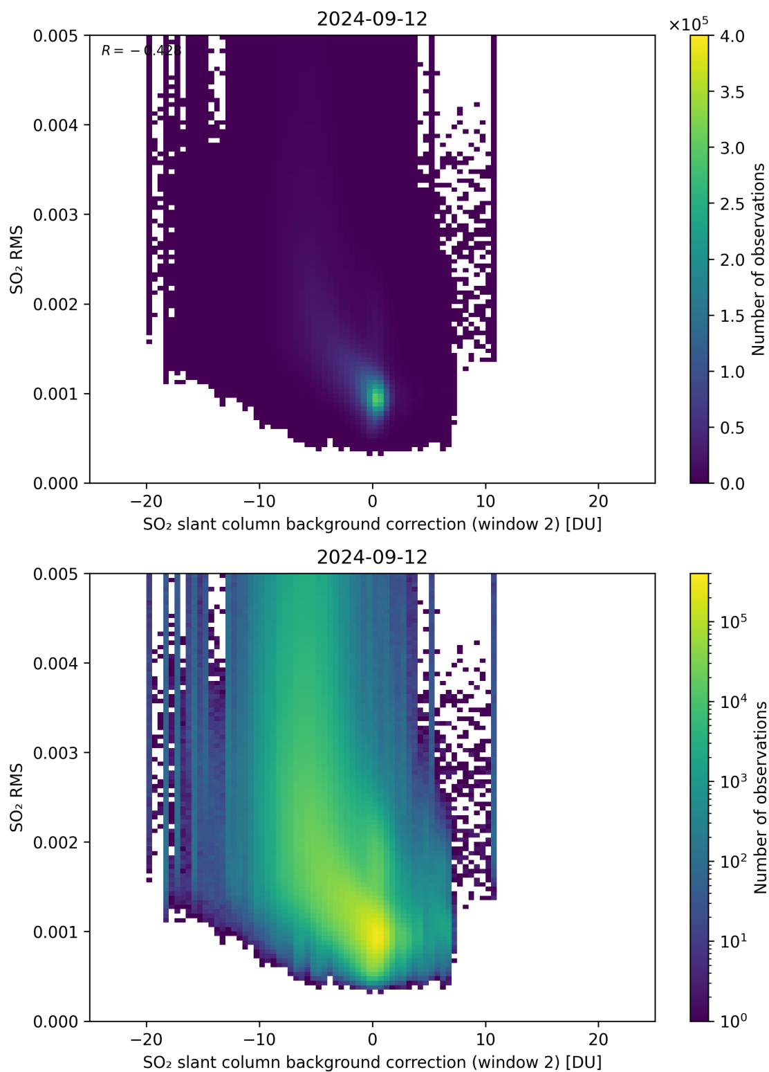
Figure 114: Scatter density plot of “SO 2 slant column background correction (window 2)” against “SO 2 RMS” for 2024-09-12 to 2024-09-13.
