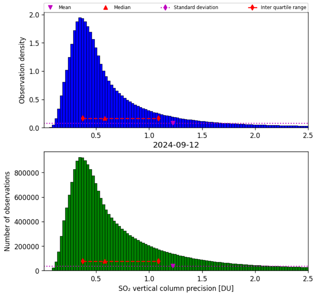
Figure 54: Histogram of “SO 2 vertical column precision” for 2024-09-12 to 2024-09-13
