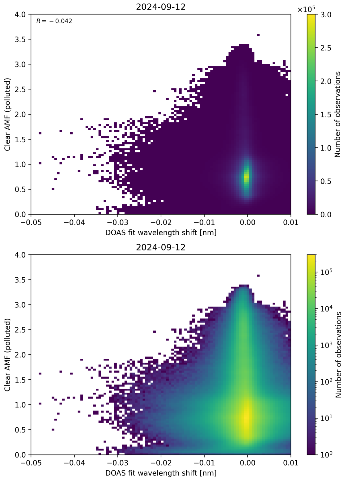
Figure 129: Scatter density plot of “DOAS fit wavelength shift” against “Clear AMF (polluted)” for 2024-09-12 to 2024-09-13.
