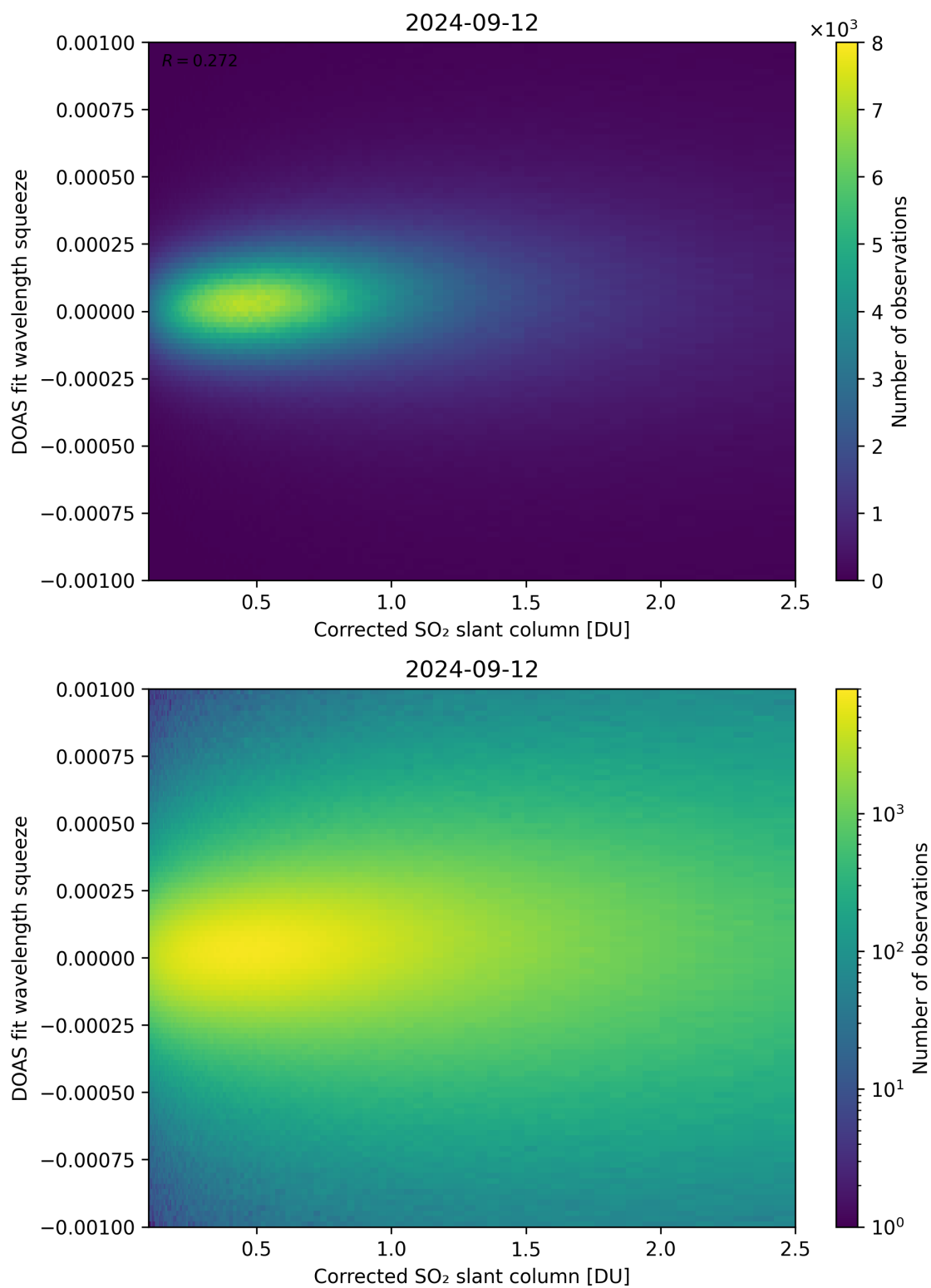
Figure 182: Scatter density plot of “Corrected SO 2 slant column” against “DOAS fit wavelength squeeze” for 2024-09-12 to 2024-09-13.
