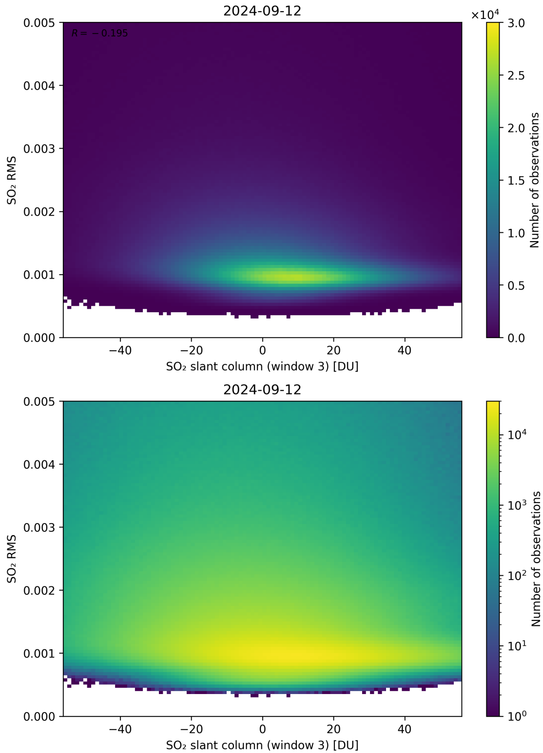
Figure 256: Scatter density plot of “SO 2 slant column (window 3)” against “SO 2 RMS” for 2024-09-12 to 2024-09-13.
