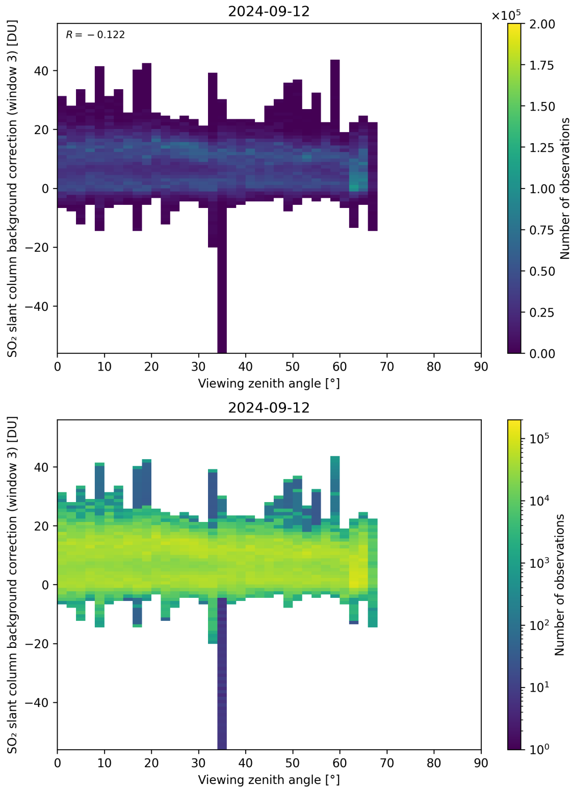
Figure 310: Scatter density plot of “Viewing zenith angle” against “SO 2 slant column background correction (window 3)” for 2024-09-12 to 2024-09-13.
