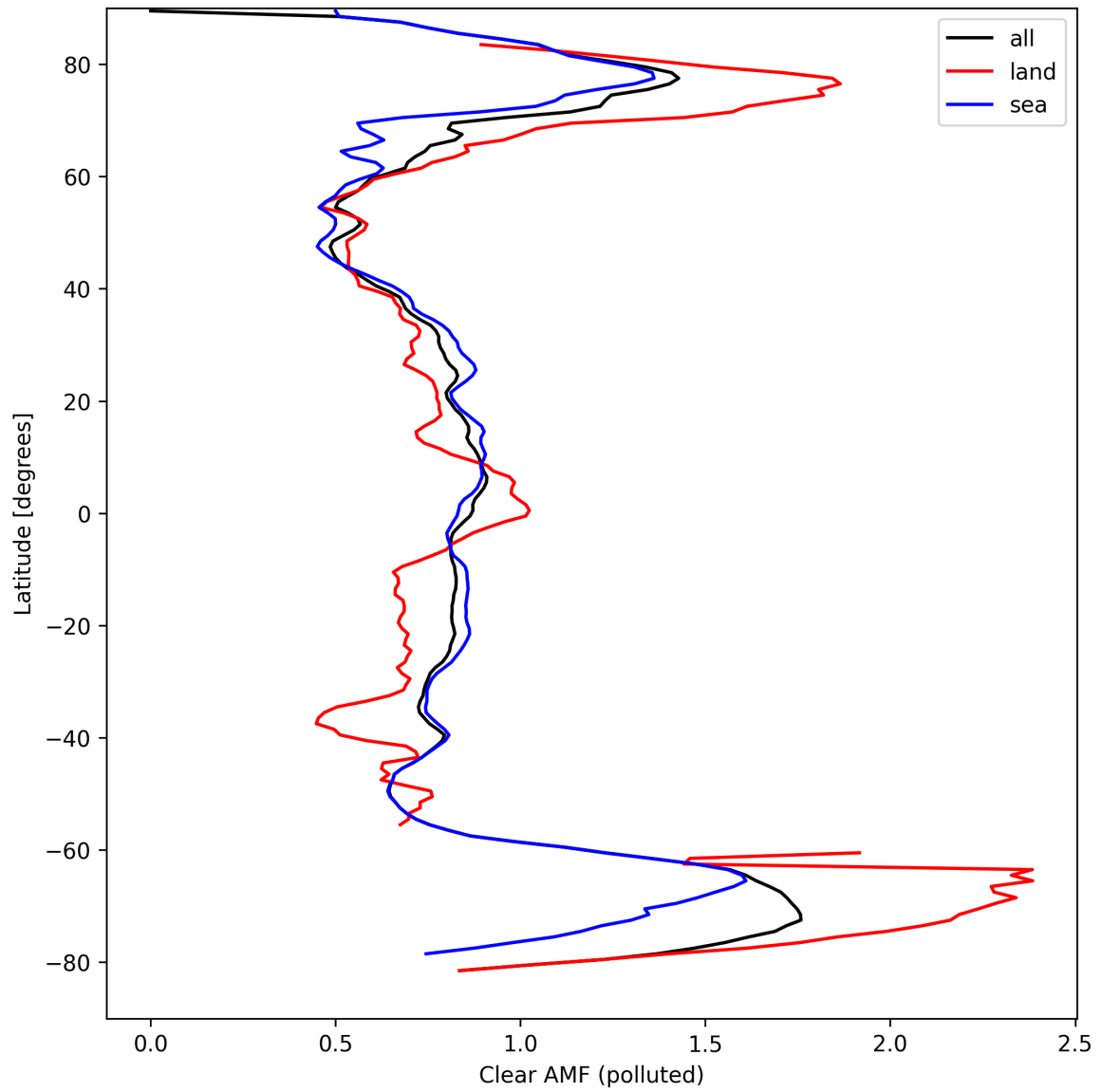
Figure 50: Zonal average of “Clear AMF (polluted)” for 2024-09-12 to 2024-09-13.
