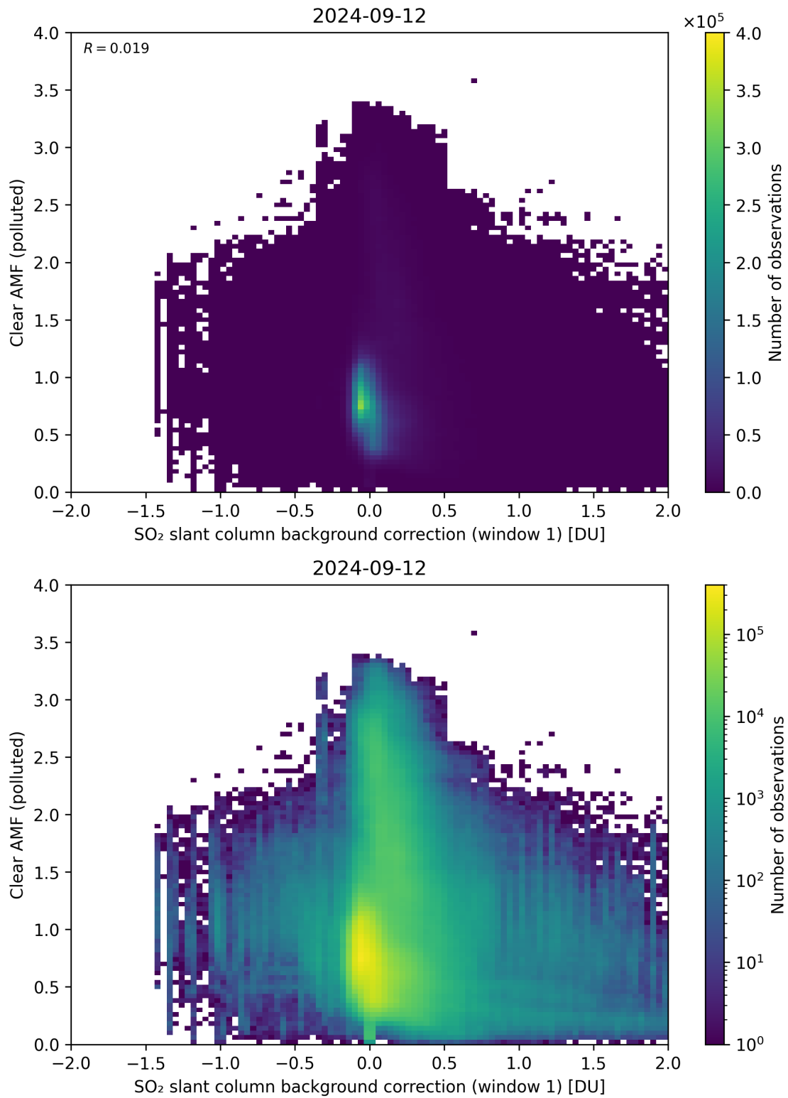
Figure 103: Scatter density plot of “SO 2 slant column background correction (window 1)” against “Clear AMF (polluted)” for 2024-09-12 to 2024-09-13.
