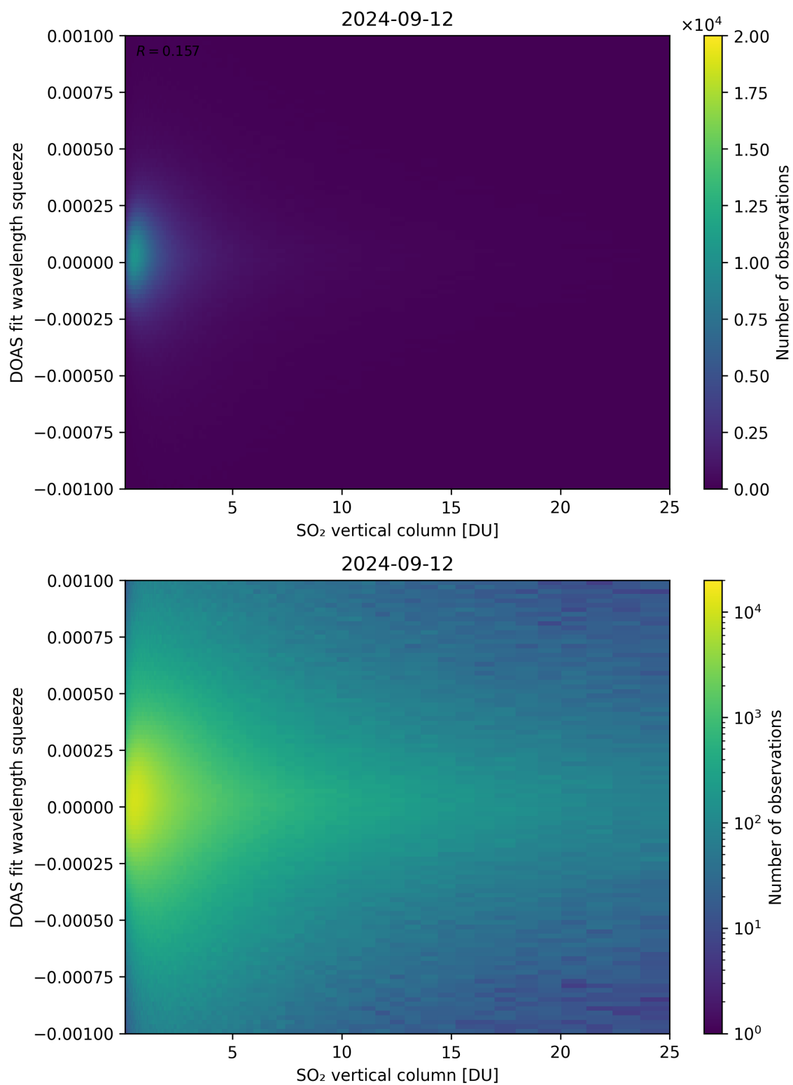
Figure 277: Scatter density plot of “SO 2 vertical column” against “DOAS fit wavelength squeeze” for 2024-09-12 to 2024-09-13.
