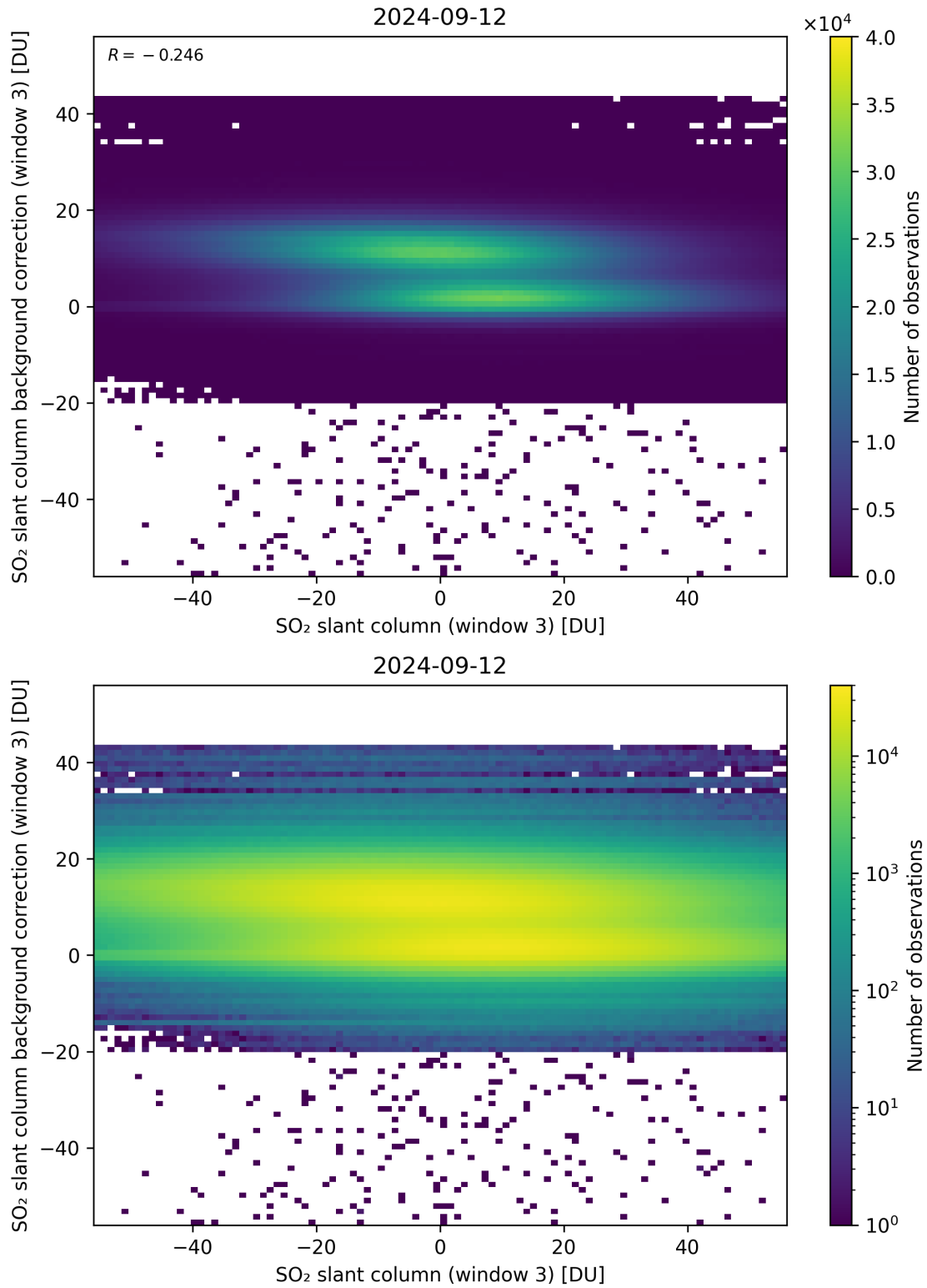
Figure 253: Scatter density plot of “SO 2 slant column (window 3)” against “SO 2 slant column background correction (window 3)” for 2024-09-12 to 2024-09-13.
