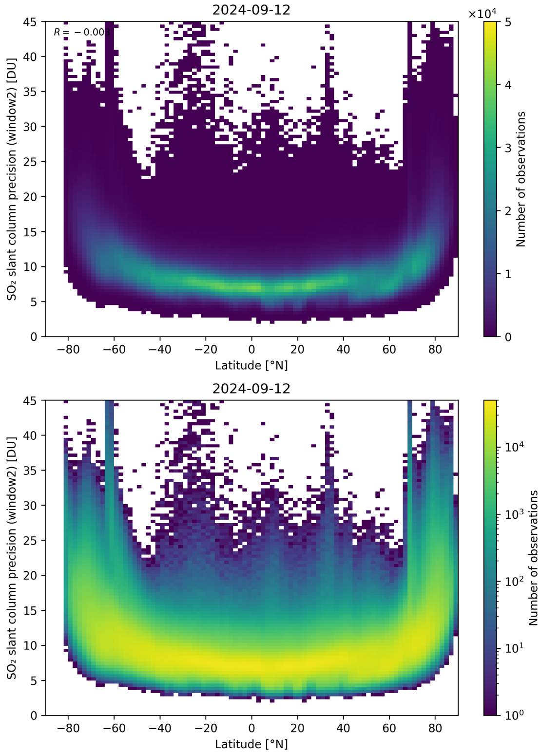
Figure 151: Scatter density plot of “Latitude” against “SO 2 slant column precision (window2)” for 2024-09-12 to 2024-09-13.
