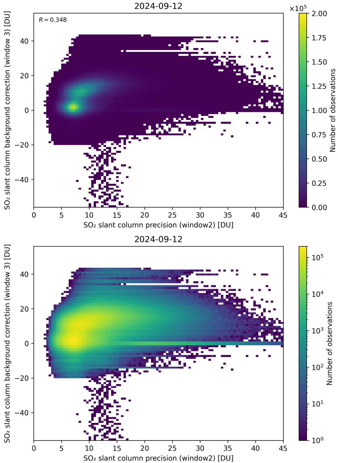
Figure 242: Scatter density plot of “SO 2 slant column precision (window2)” against “SO 2 slant column background correction (window 3)” for 2024-09-12 to 2024-09-13.
