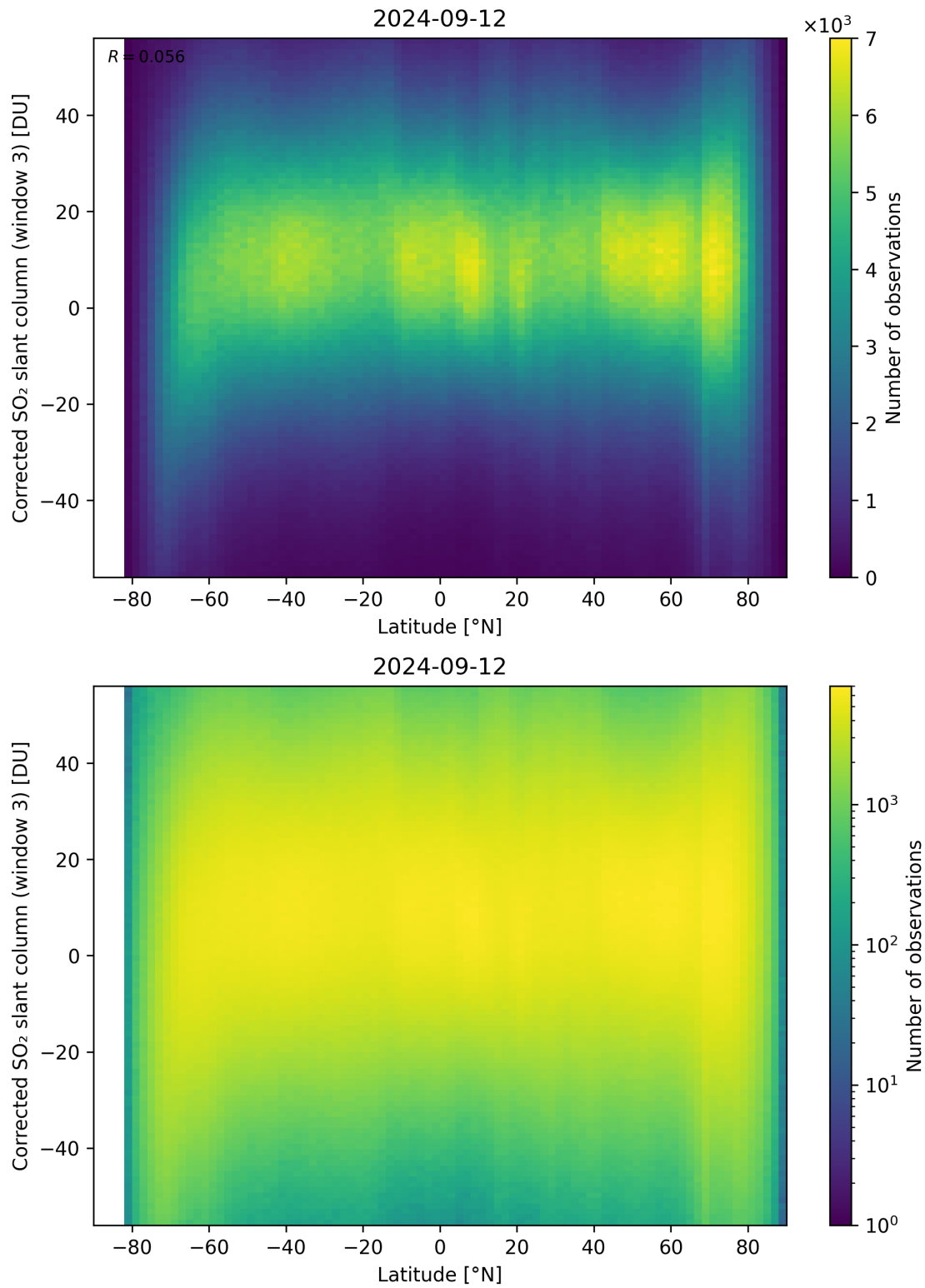
Figure 148: Scatter density plot of “Latitude” against “Corrected SO 2 slant column (window 3)” for 2024-09-12 to 2024-09-13.
