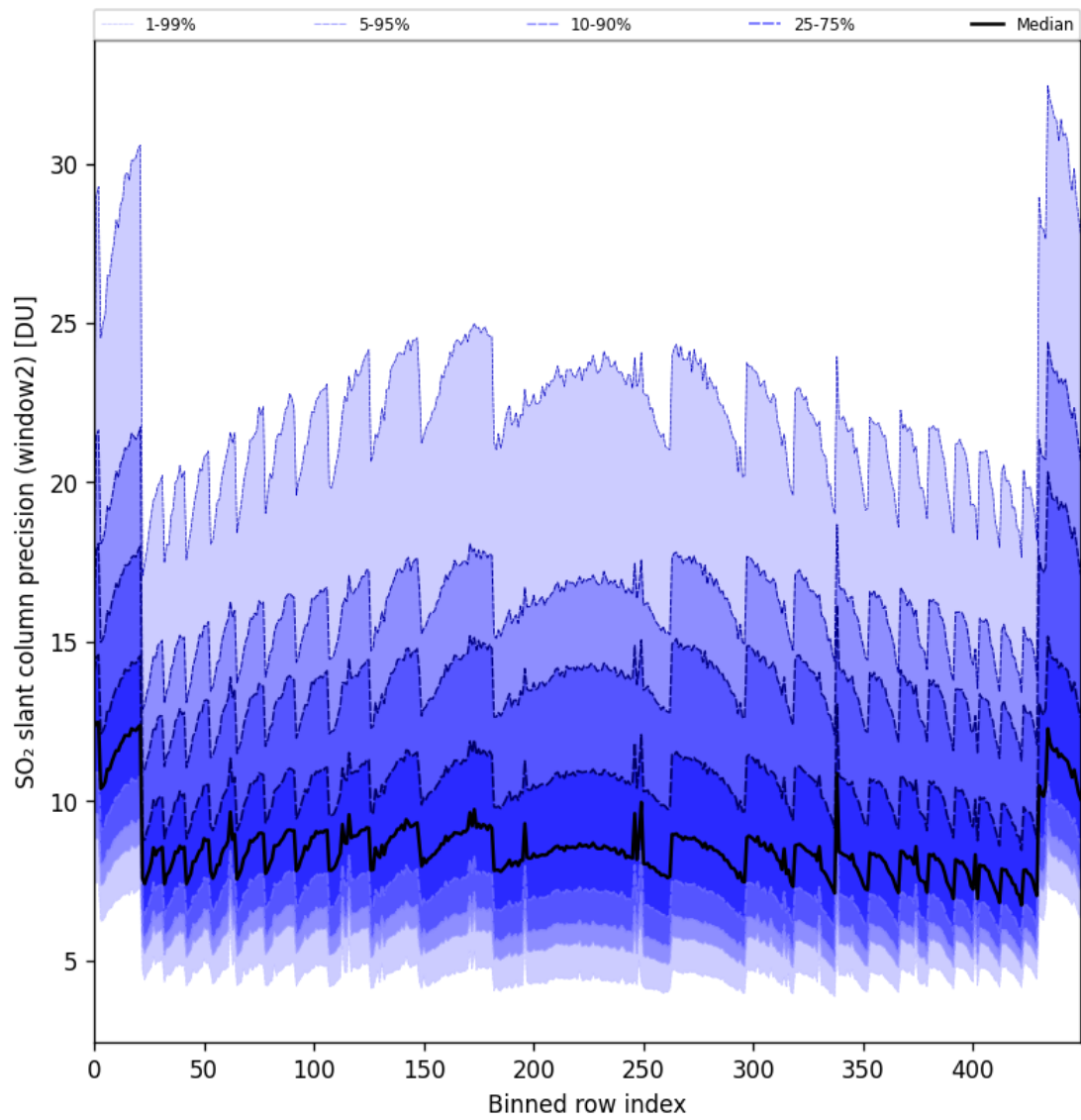
Figure 84: Along track statistics of “SO 2 slant column precision (window2)” for 2024-09-12 to 2024-09-13
