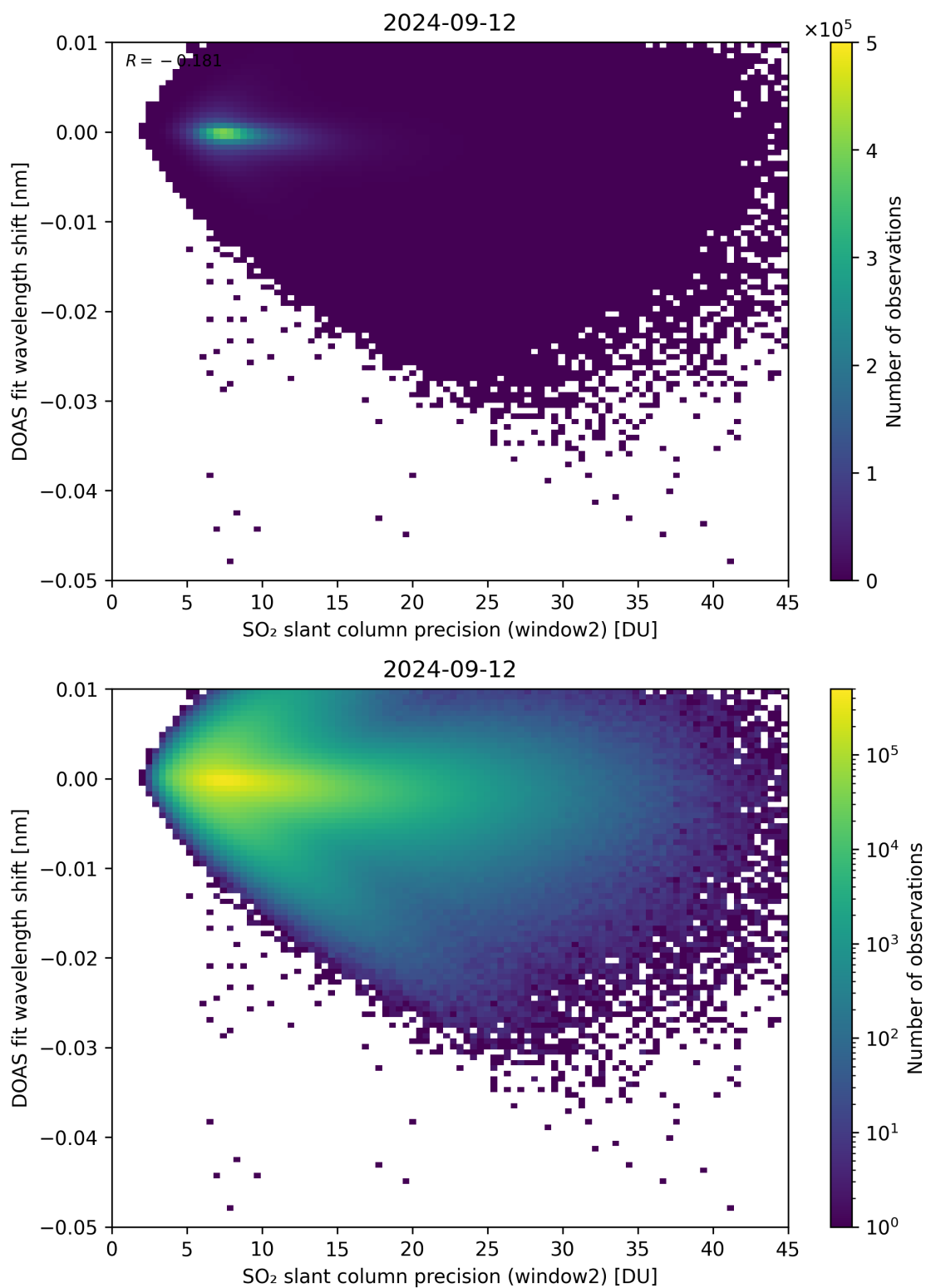
Figure 243: Scatter density plot of “SO 2 slant column precision (window2)” against “DOAS fit wavelength shift” for 2024-09-12 to 2024-09-13.
