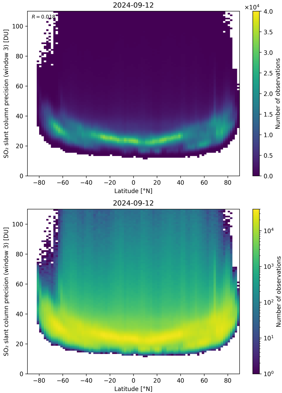
Figure 153: Scatter density plot of “Latitude” against “SO 2 slant column precision (window 3)” for 2024-09-12 to 2024-09-13.
