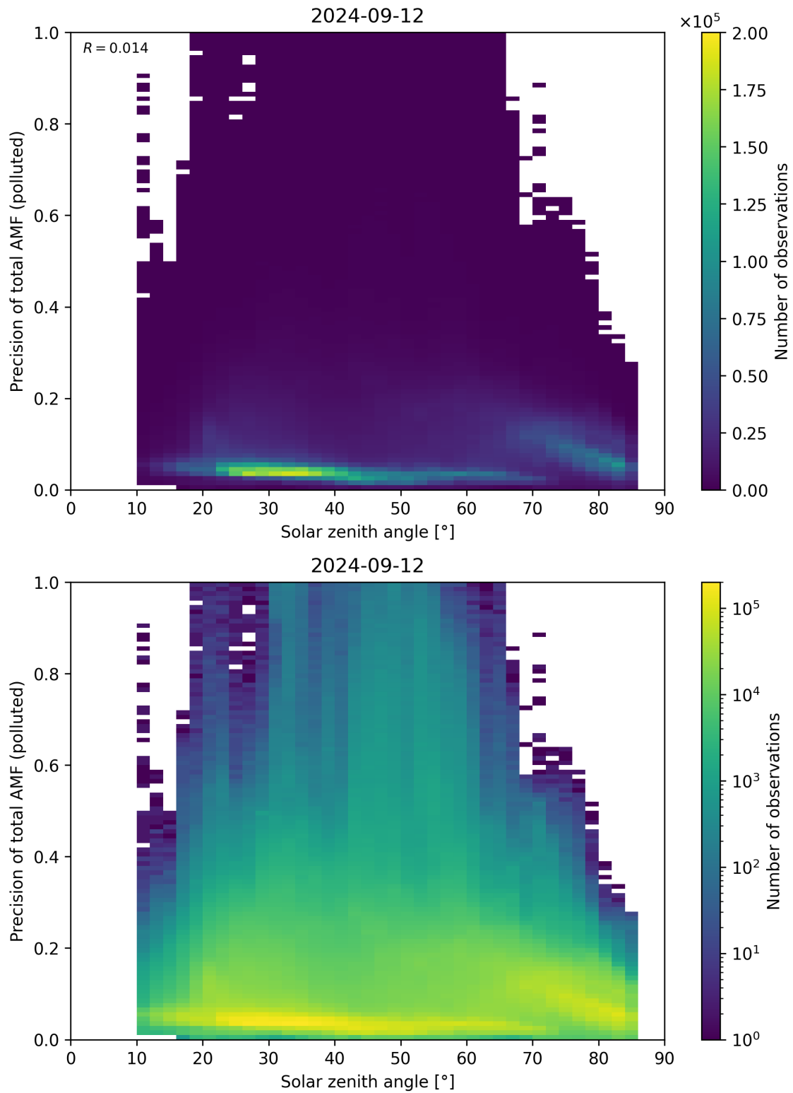
Figure 175: Scatter density plot of “Solar zenith angle” against “Precision of total AMF (polluted)” for 2024-09-12 to 2024-09-13.
