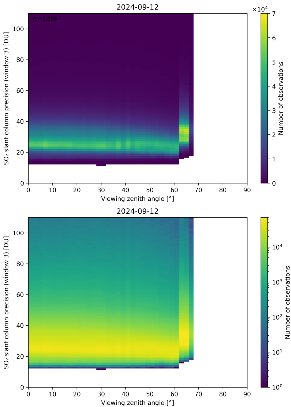
Figure 324: Scatter density plot of “Viewing zenith angle” against “SO 2 slant column precision (window 3)” for 2024-09-12 to 2024-09-13.
