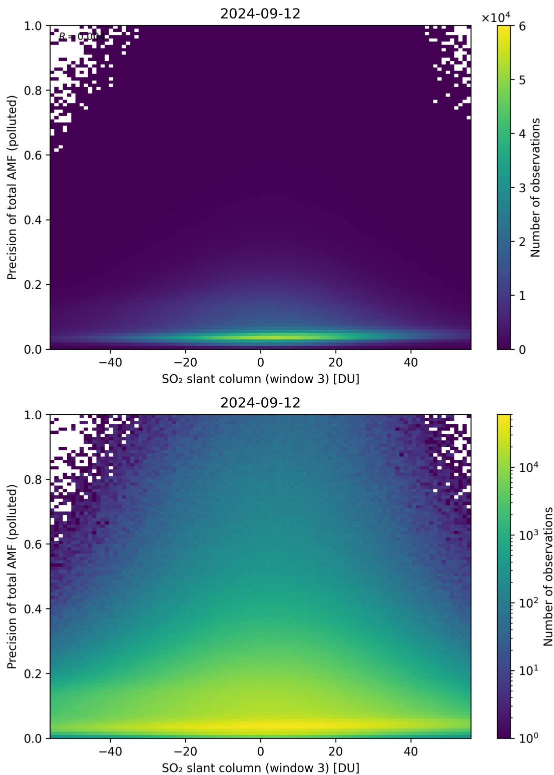
Figure 269: Scatter density plot of “SO 2 slant column (window 3)” against “Precision of total AMF (polluted)” for 2024-09-12 to 2024-09-13.
