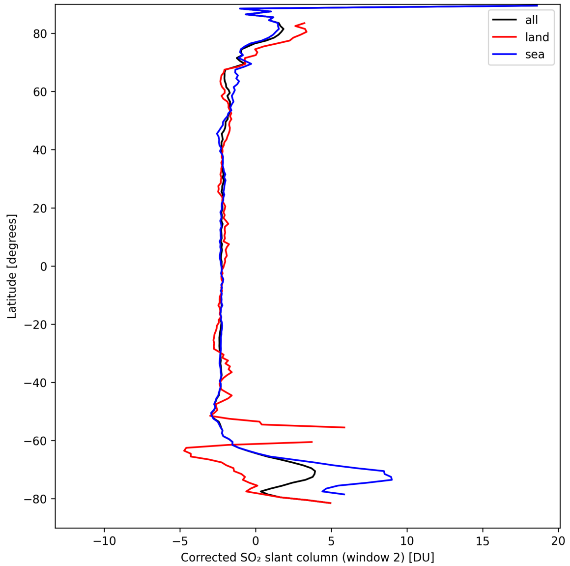
Figure 39: Zonal average of “Corrected SO 2 slant column (window 2)” for 2024-09-12 to 2024-09-13.
