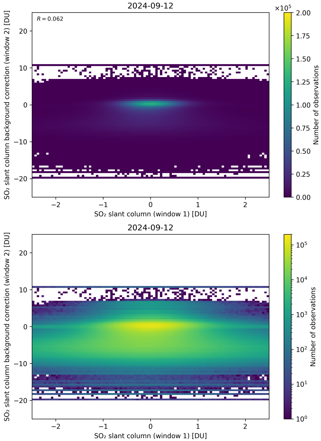
Figure 213: Scatter density plot of “SO 2 slant column (window 1)” against “SO 2 slant column background correction (window 2)” for 2024-09-12 to 2024-09-13.
