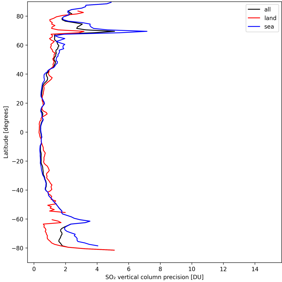
Figure 31: Zonal average of “SO 2 vertical column precision” for 2024-09-12 to 2024-09-13.
