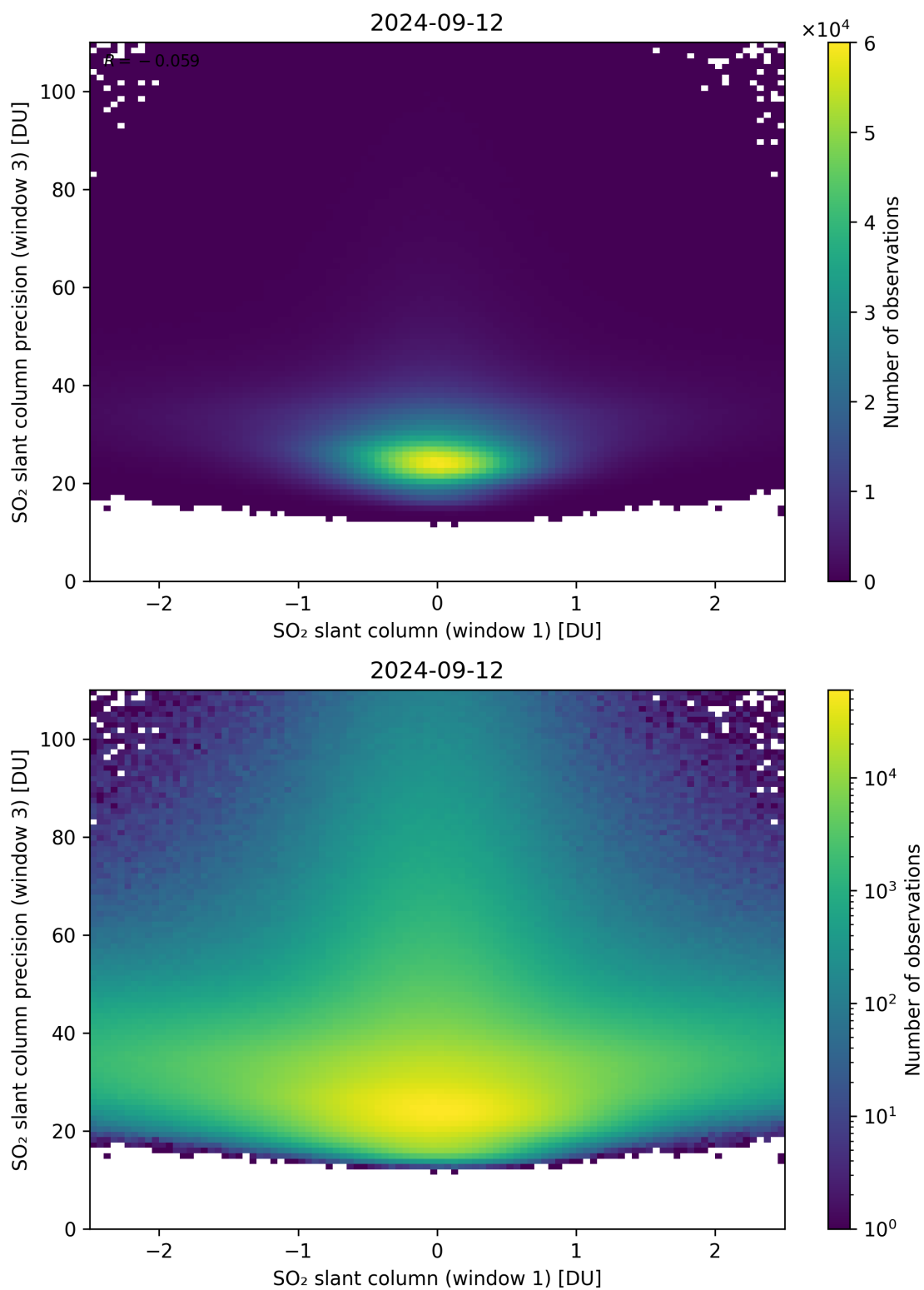
Figure 238: Scatter density plot of “SO 2 slant column (window 1)” against “SO 2 slant column precision (window 3)” for 2024-09-12 to 2024-09-13.
