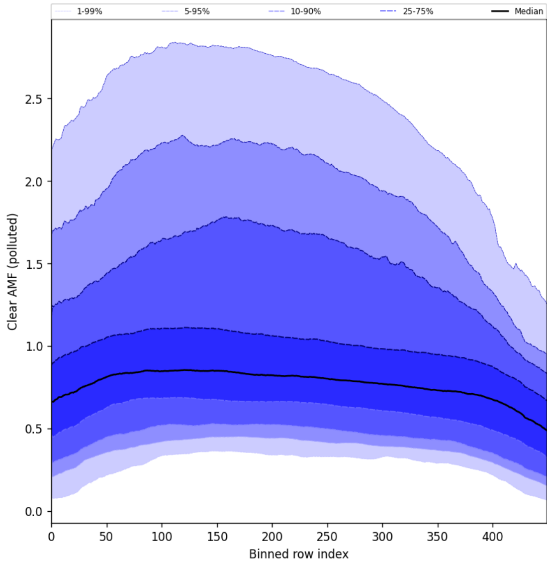
Figure 96: Along track statistics of “Clear AMF (polluted)” for 2024-09-12 to 2024-09-13
