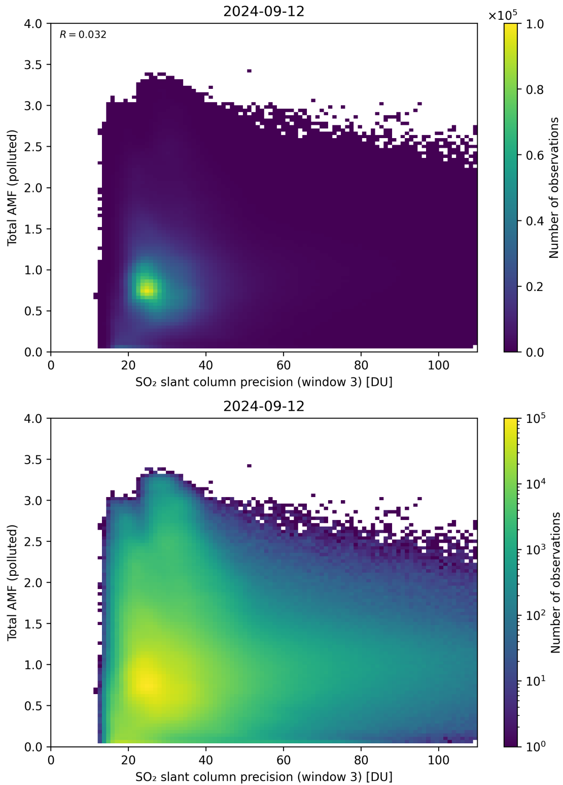
Figure 263: Scatter density plot of “SO 2 slant column precision (window 3)” against “Total AMF (polluted)” for 2024-09-12 to 2024-09-13.
