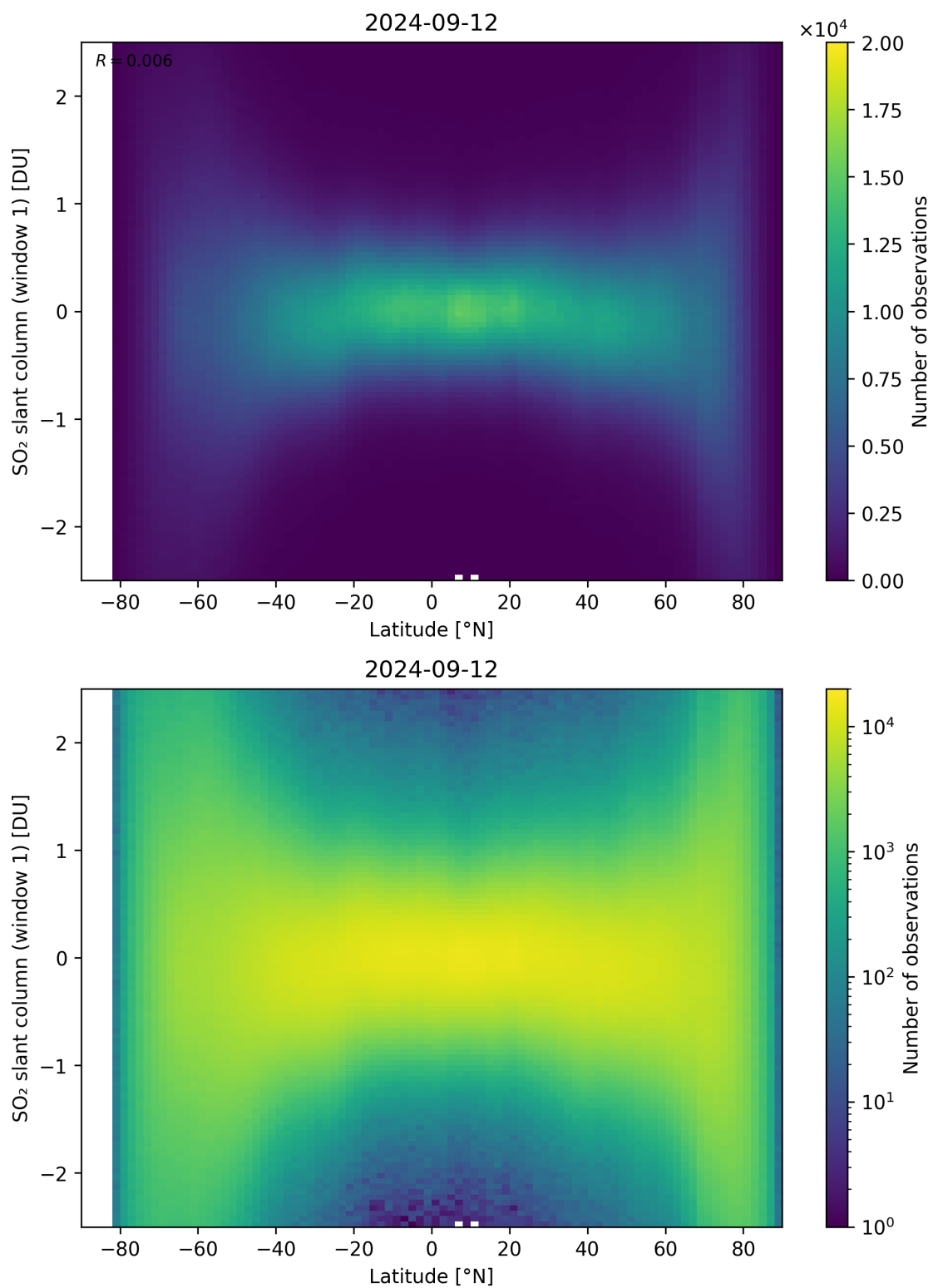
Figure 149: Scatter density plot of “Latitude” against “SO 2 slant column (window 1)” for 2024-09-12 to 2024-09-13.
