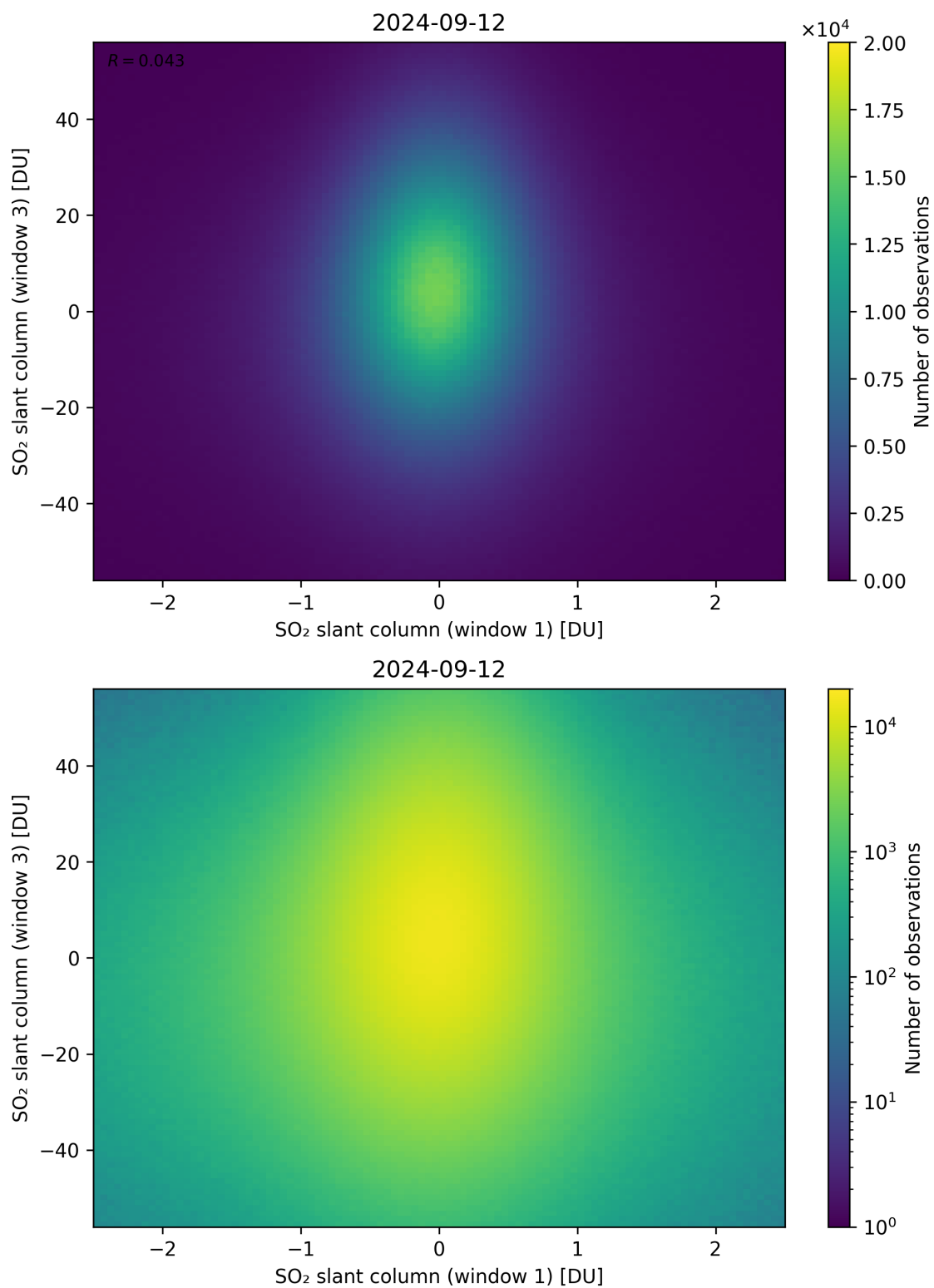
Figure 237: Scatter density plot of “SO 2 slant column (window 1)” against “SO 2 slant column (window 3)” for 2024-09-12 to 2024-09-13.
