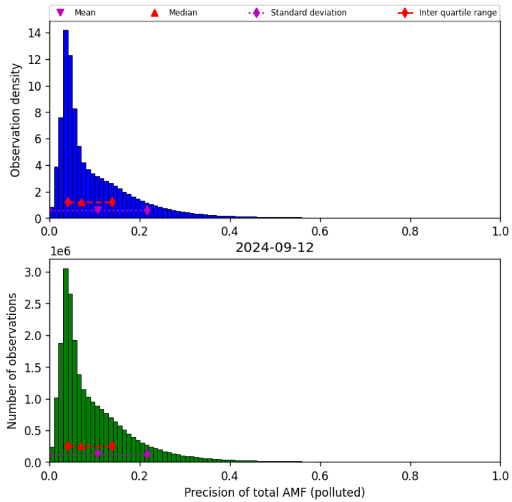
Figure 72: Histogram of “Precision of total AMF (polluted)” for 2024-09-12 to 2024-09-13
