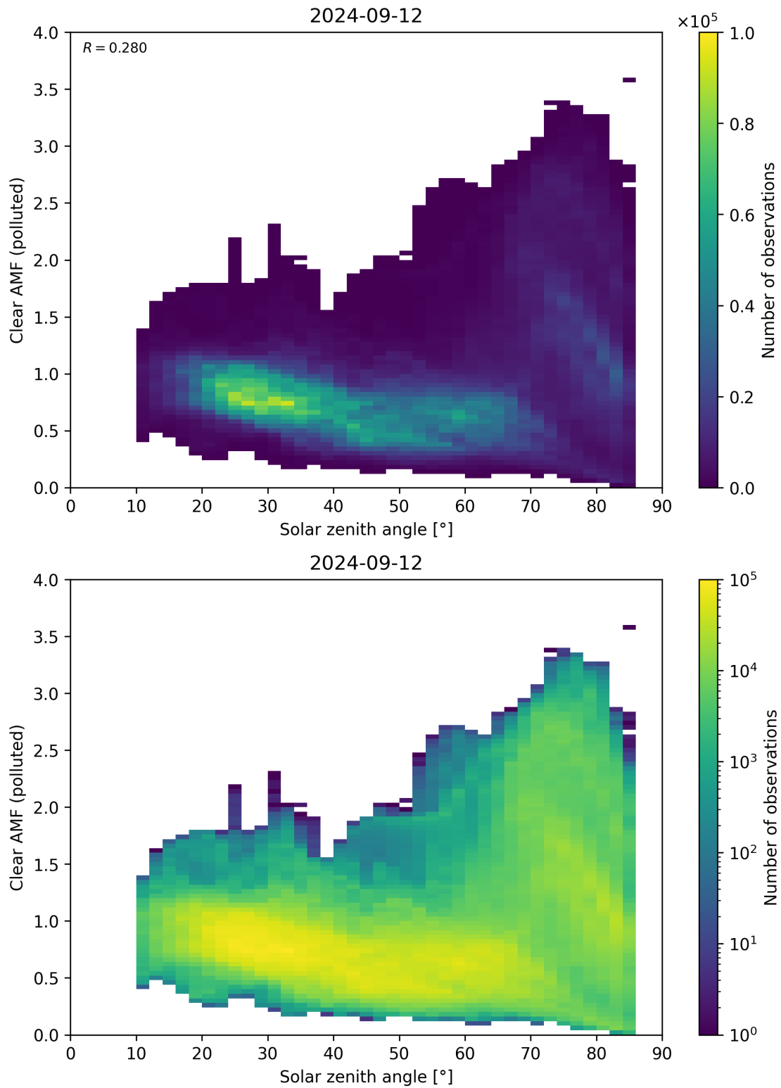
Figure 165: Scatter density plot of “Solar zenith angle” against “Clear AMF (polluted)” for 2024-09-12 to 2024-09-13.
