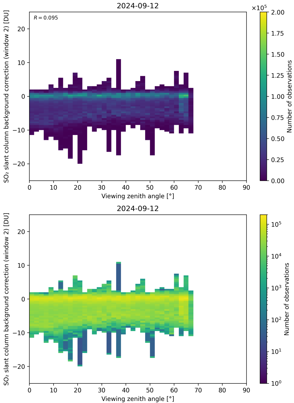
Figure 309: Scatter density plot of “Viewing zenith angle” against “SO 2 slant column background correction (window 2)” for 2024-09-12 to 2024-09-13.
