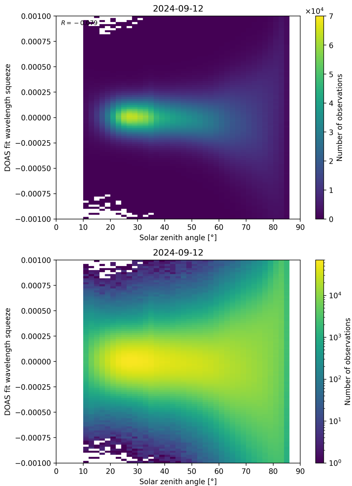
Figure 162: Scatter density plot of “Solar zenith angle” against “DOAS fit wavelength squeeze” for 2024-09-12 to 2024-09-13.
