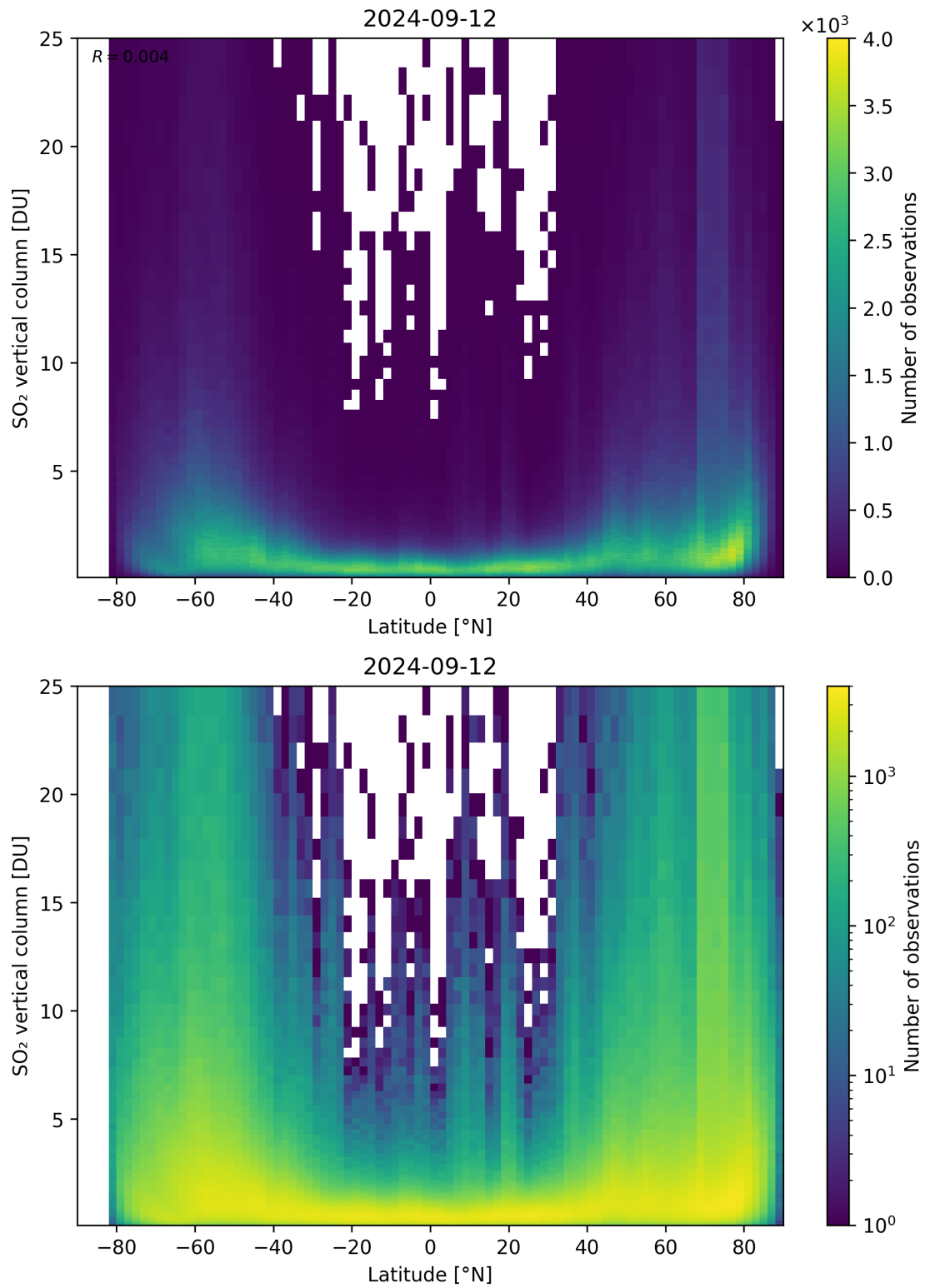
Figure 156: Scatter density plot of “Latitude” against “SO 2 vertical column” for 2024-09-12 to 2024-09-13.
