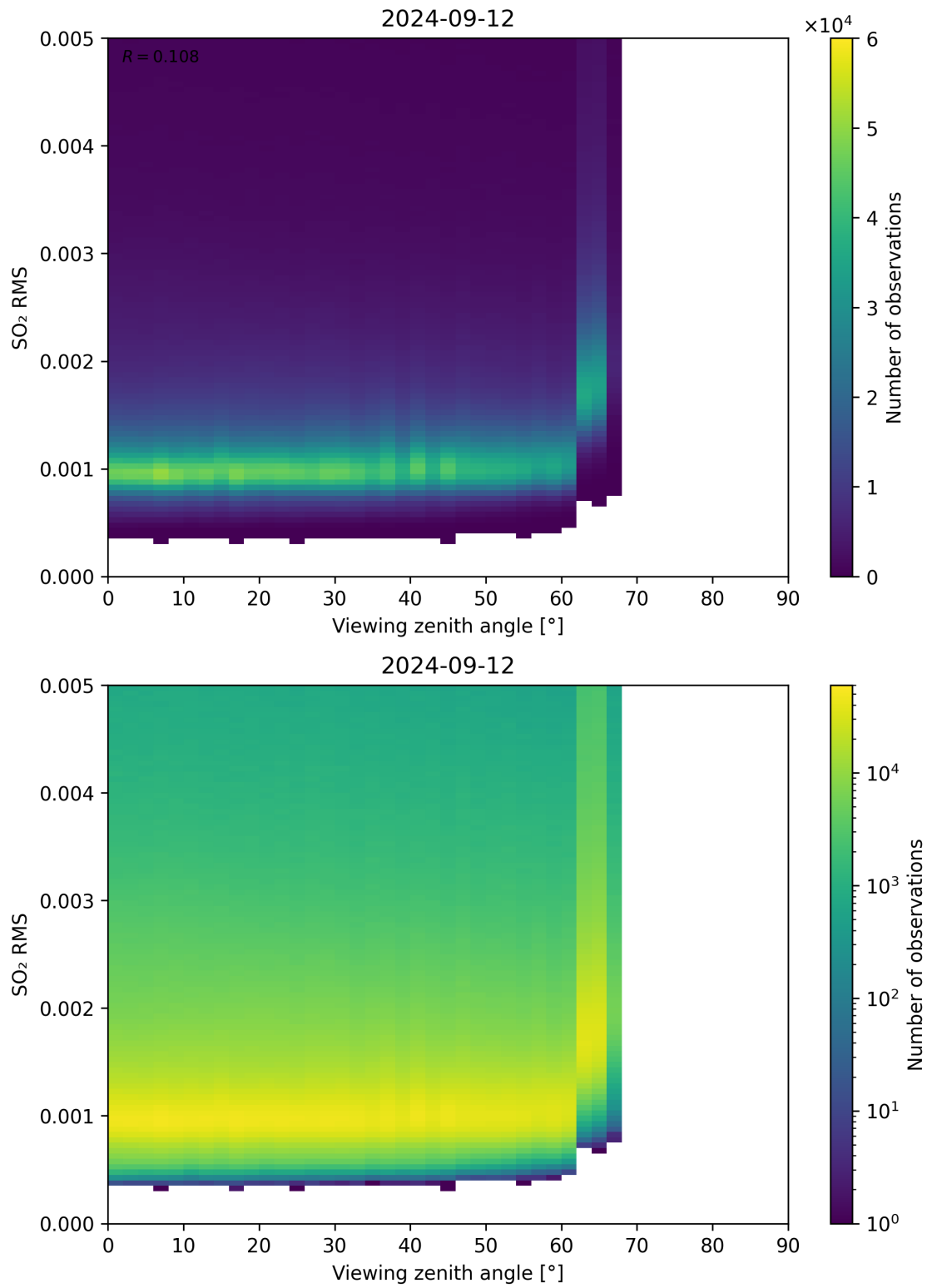
Figure 313: Scatter density plot of “Viewing zenith angle” against “SO 2 RMS” for 2024-09-12 to 2024-09-13.
