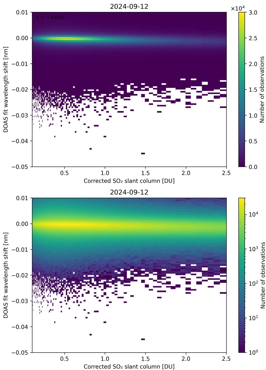
Figure 181: Scatter density plot of “Corrected SO 2 slant column” against “DOAS fit wavelength shift” for 2024-09-12 to 2024-09-13.
