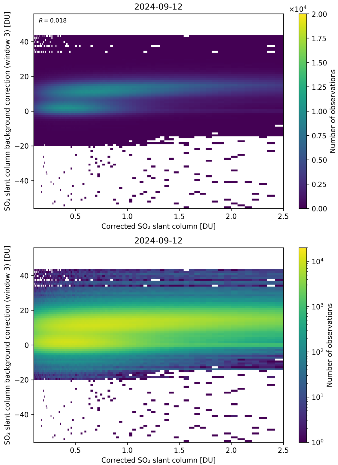
Figure 180: Scatter density plot of “Corrected SO 2 slant column” against “SO 2 slant column background correction (window 3)” for 2024-09-12 to 2024-09-13.
