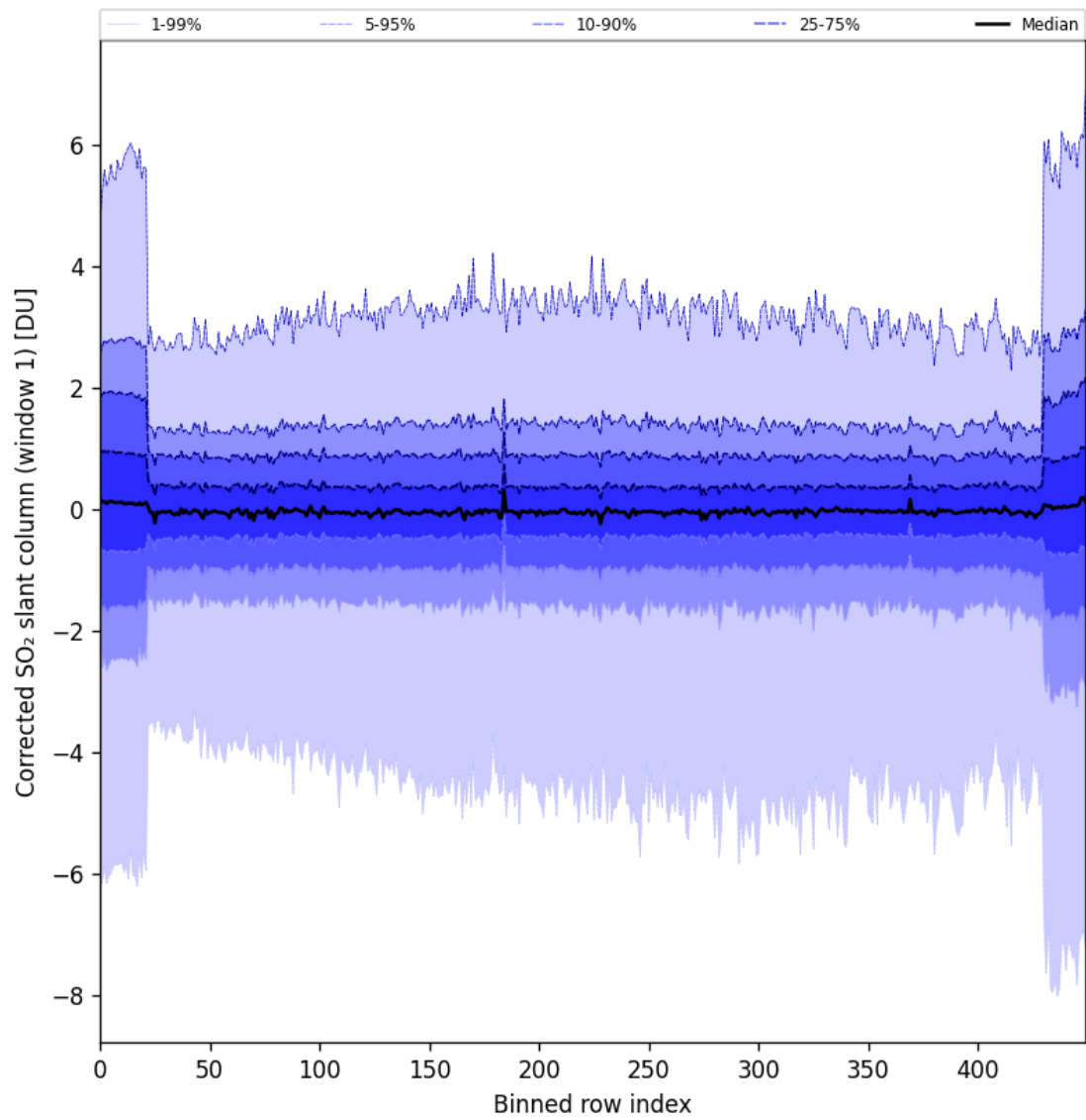
Figure 81: Along track statistics of “Corrected SO 2 slant column (window 1)” for 2024-09-12 to 2024-09-13
