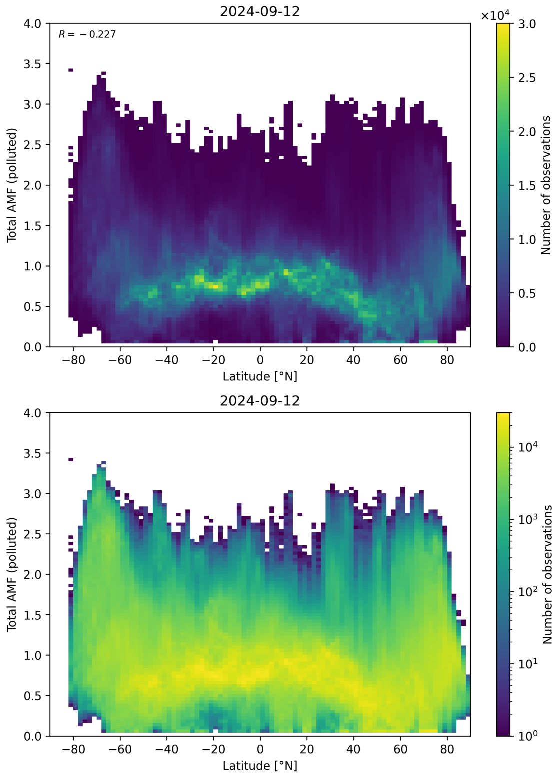
Figure 154: Scatter density plot of “Latitude” against “Total AMF (polluted)” for 2024-09-12 to 2024-09-13.
