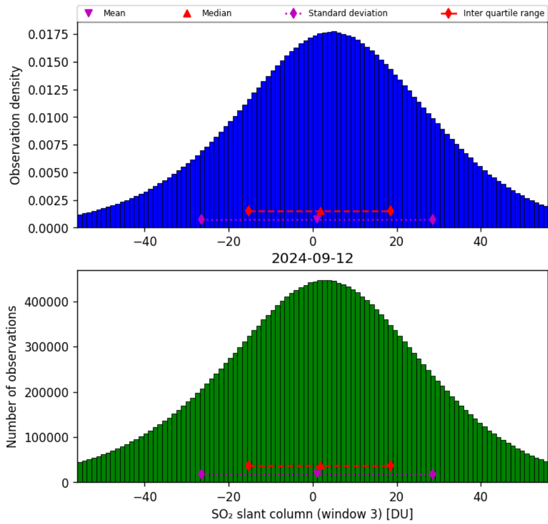
Figure 64: Histogram of “SO 2 slant column (window 3)” for 2024-09-12 to 2024-09-13
