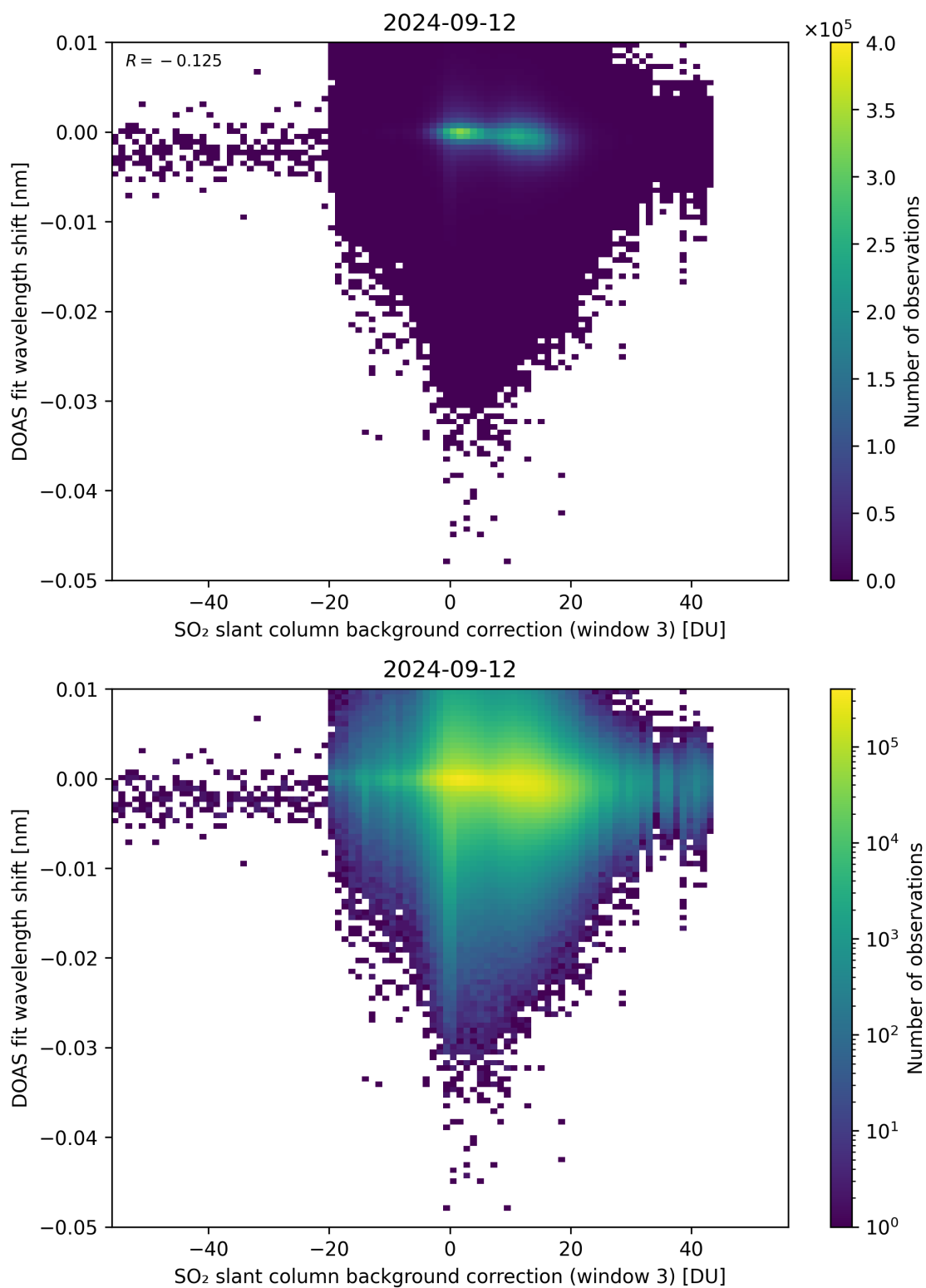
Figure 121: Scatter density plot of “SO 2 slant column background correction (window 3)” against “DOAS fit wavelength shift” for 2024-09-12 to 2024-09-13.
