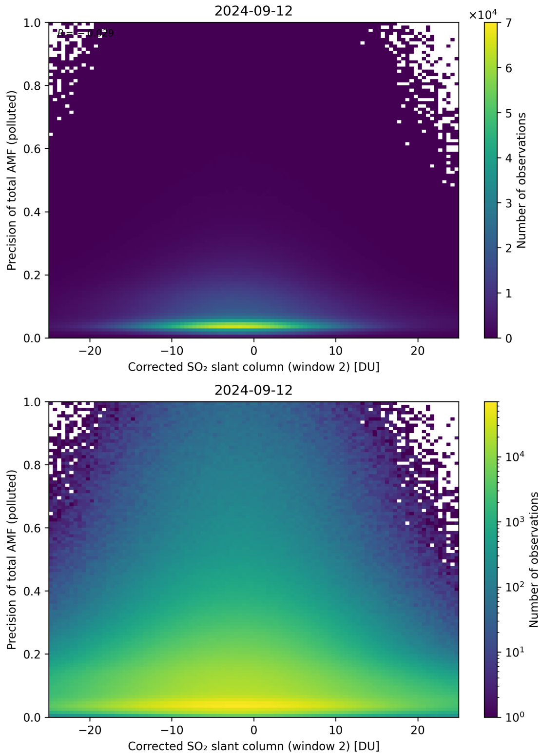
Figure 204: Scatter density plot of “Corrected SO 2 slant column (window 2)” against “Precision of total AMF (polluted)” for 2024-09-12 to 2024-09-13.
