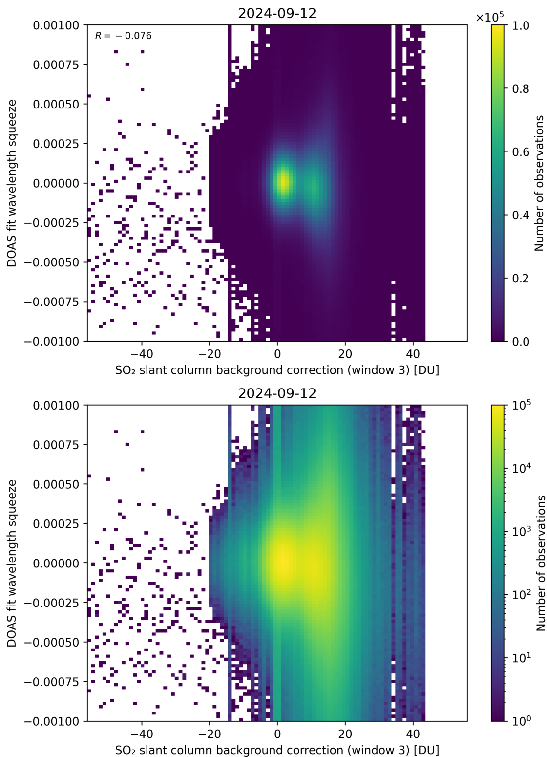
Figure 122: Scatter density plot of “SO 2 slant column background correction (window 3)” against “DOAS fit wavelength squeeze” for 2024-09-12 to 2024-09-13.
