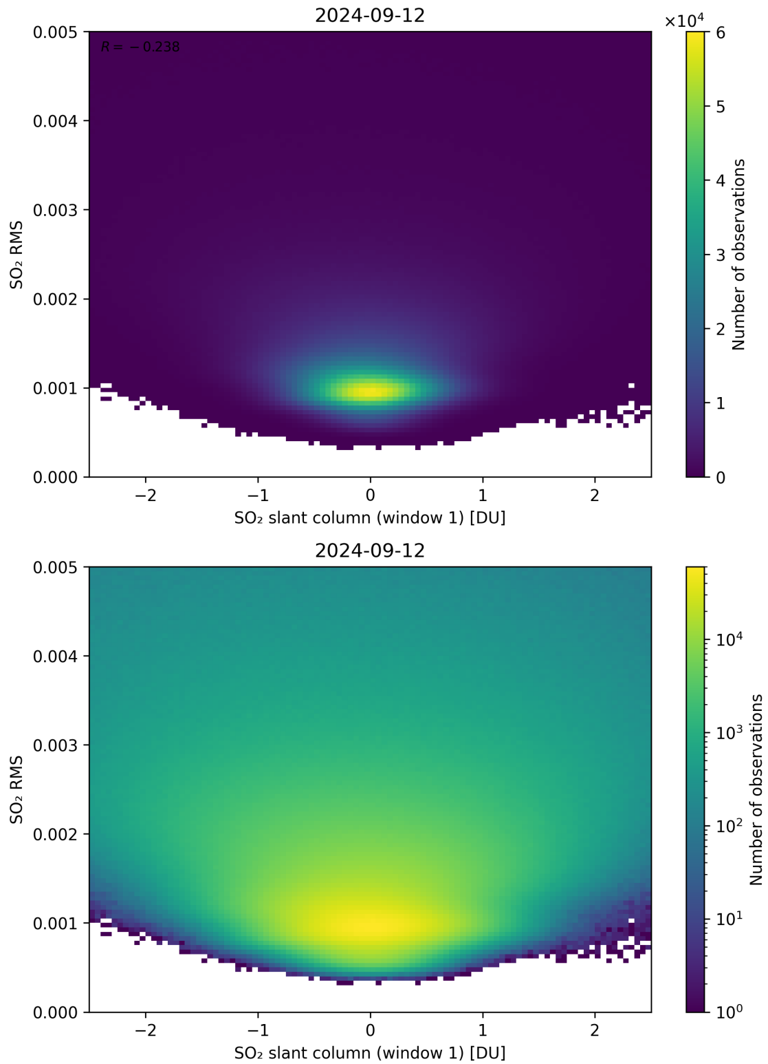
Figure 217: Scatter density plot of “SO 2 slant column (window 1)” against “SO 2 RMS” for 2024-09-12 to 2024-09-13.
