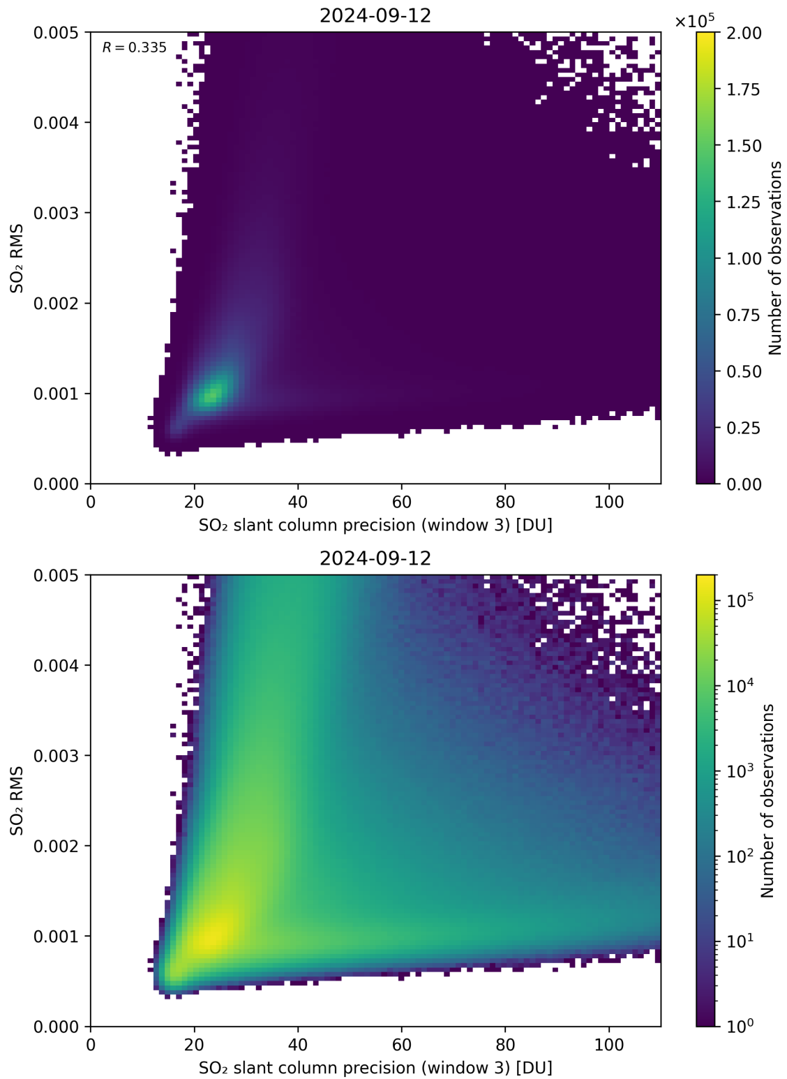
Figure 260: Scatter density plot of “SO 2 slant column precision (window 3)” against “SO 2 RMS” for 2024-09-12 to 2024-09-13.
