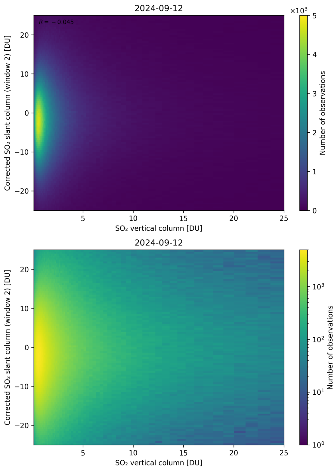
Figure 298: Scatter density plot of “SO 2 vertical column” against “Corrected SO 2 slant column (window 2)” for 2024-09-12 to 2024-09-13.
