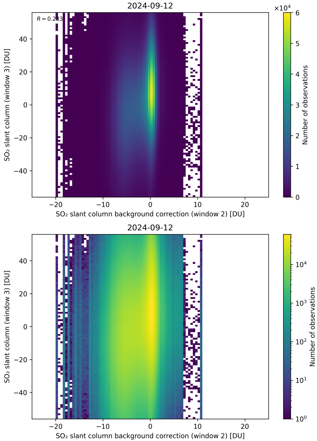
Figure 117: Scatter density plot of “SO 2 slant column background correction (window 2)” against “SO 2 slant column (window 3)” for 2024-09-12 to 2024-09-13.
