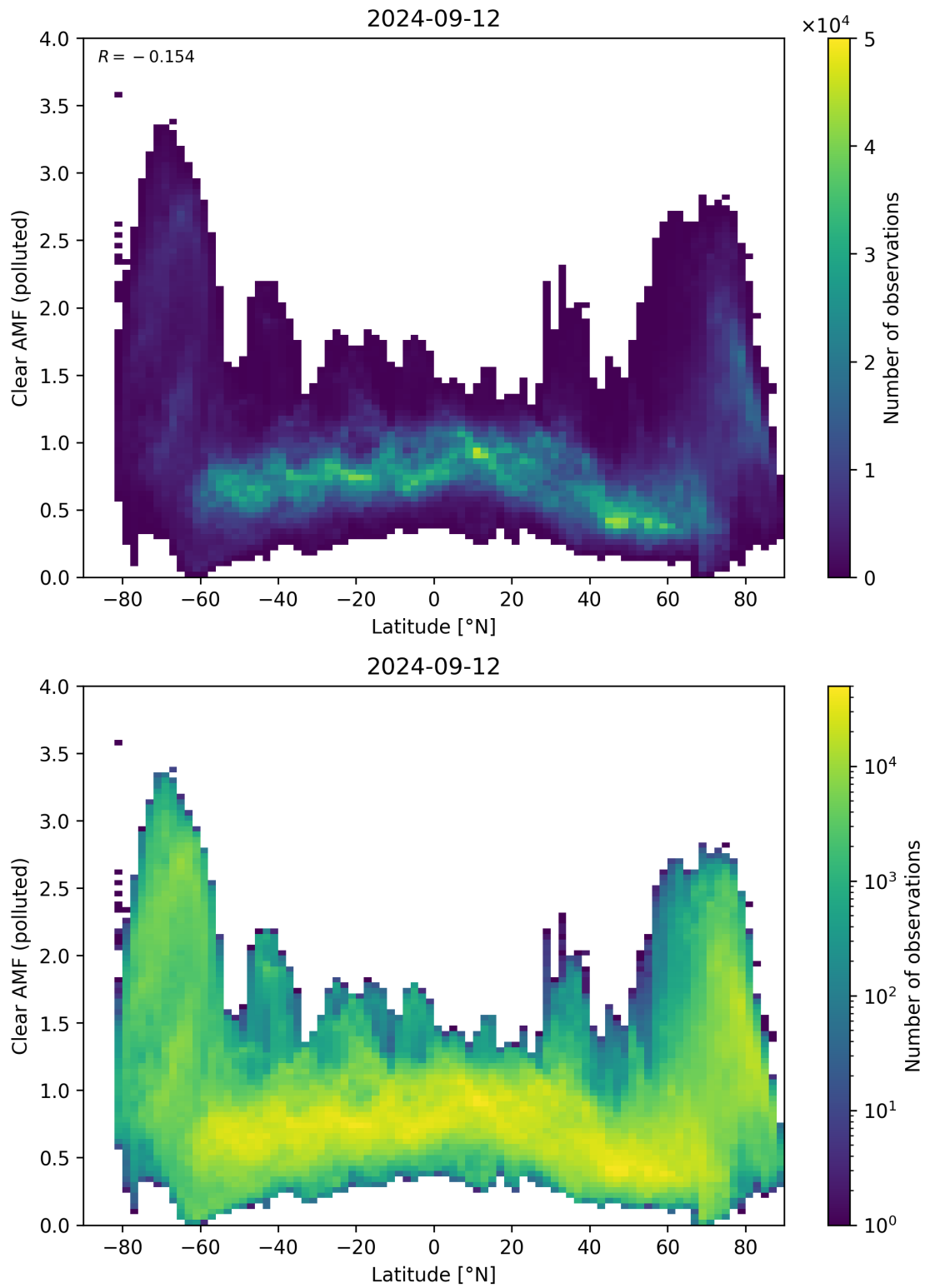
Figure 145: Scatter density plot of “Latitude” against “Clear AMF (polluted)” for 2024-09-12 to 2024-09-13.
