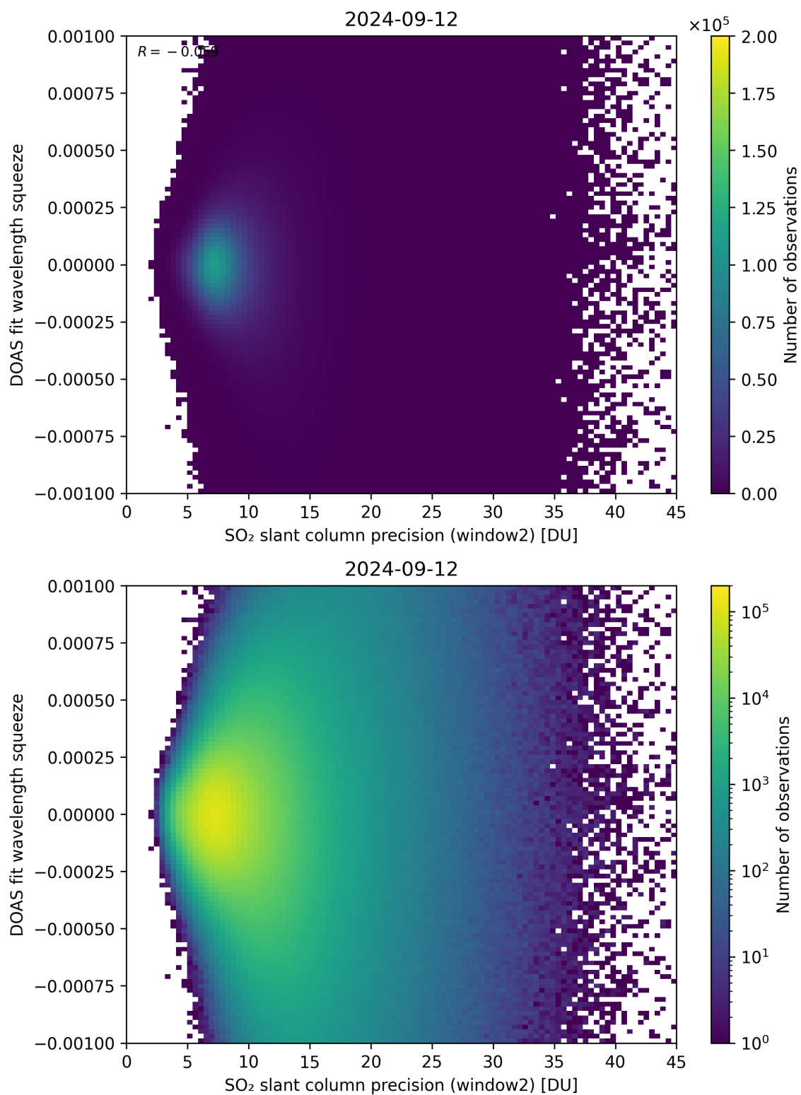
Figure 244: Scatter density plot of “SO 2 slant column precision (window2)” against “DOAS fit wavelength squeeze” for 2024-09-12 to 2024-09-13.
