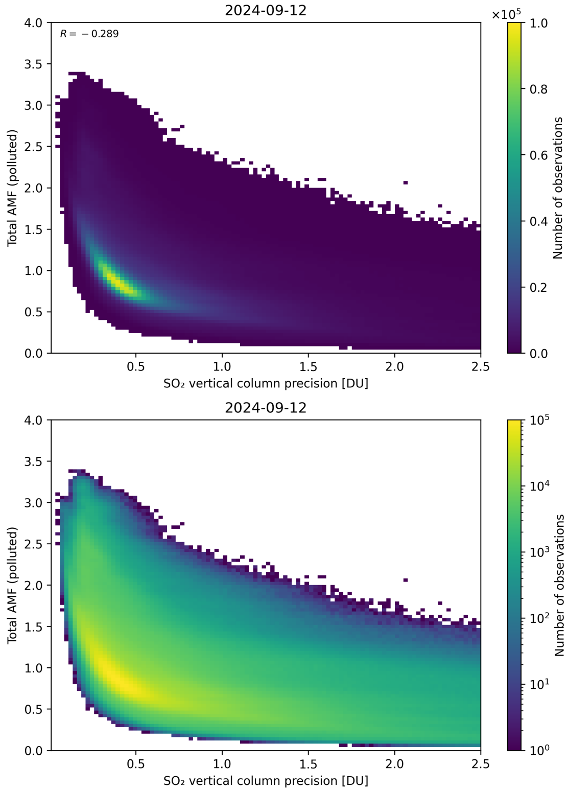
Figure 294: Scatter density plot of “SO 2 vertical column precision” against “Total AMF (polluted)” for 2024-09-12 to 2024-09-13.
