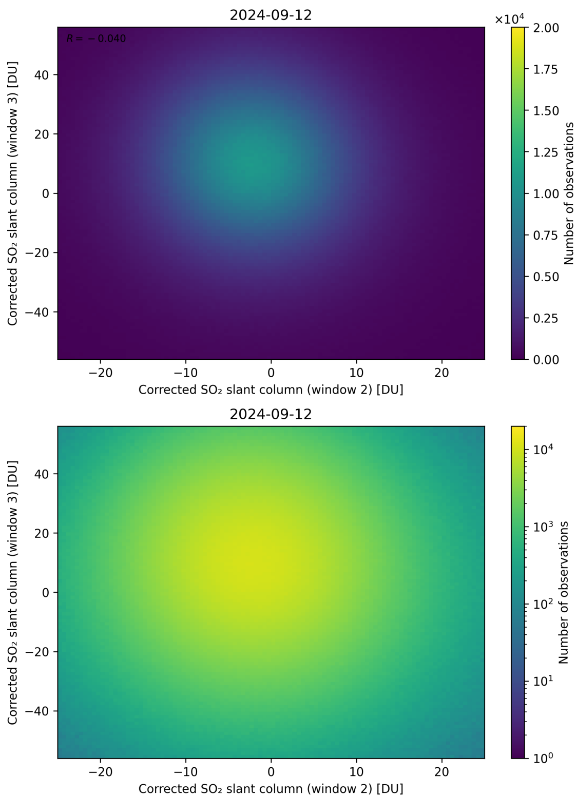
Figure 200: Scatter density plot of “Corrected SO 2 slant column (window 2)” against “Corrected SO 2 slant column (window 3)” for 2024-09-12 to 2024-09-13.
