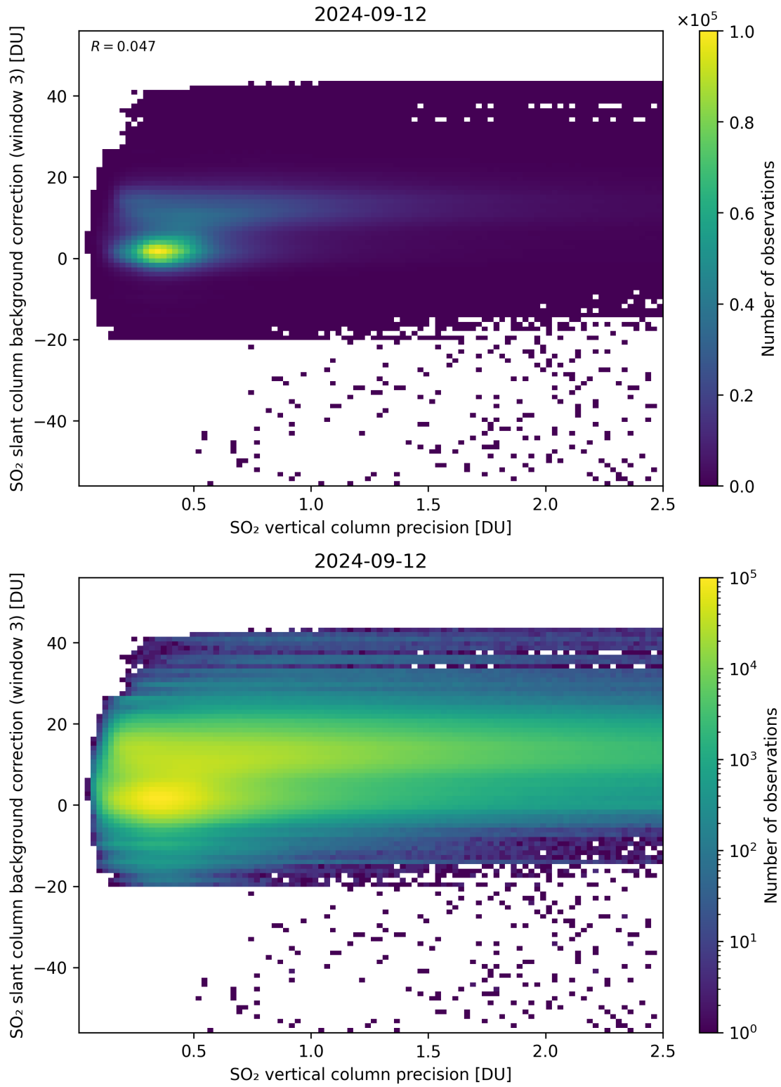
Figure 281: Scatter density plot of “SO 2 vertical column precision” against “SO 2 slant column background correction (window 3)” for 2024-09-12 to 2024-09-13.
