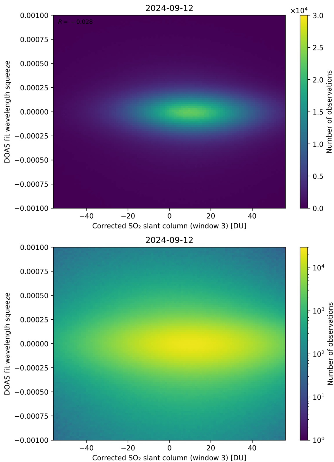
Figure 207: Scatter density plot of “Corrected SO 2 slant column (window 3)” against “DOAS fit wavelength squeeze” for 2024-09-12 to 2024-09-13.
