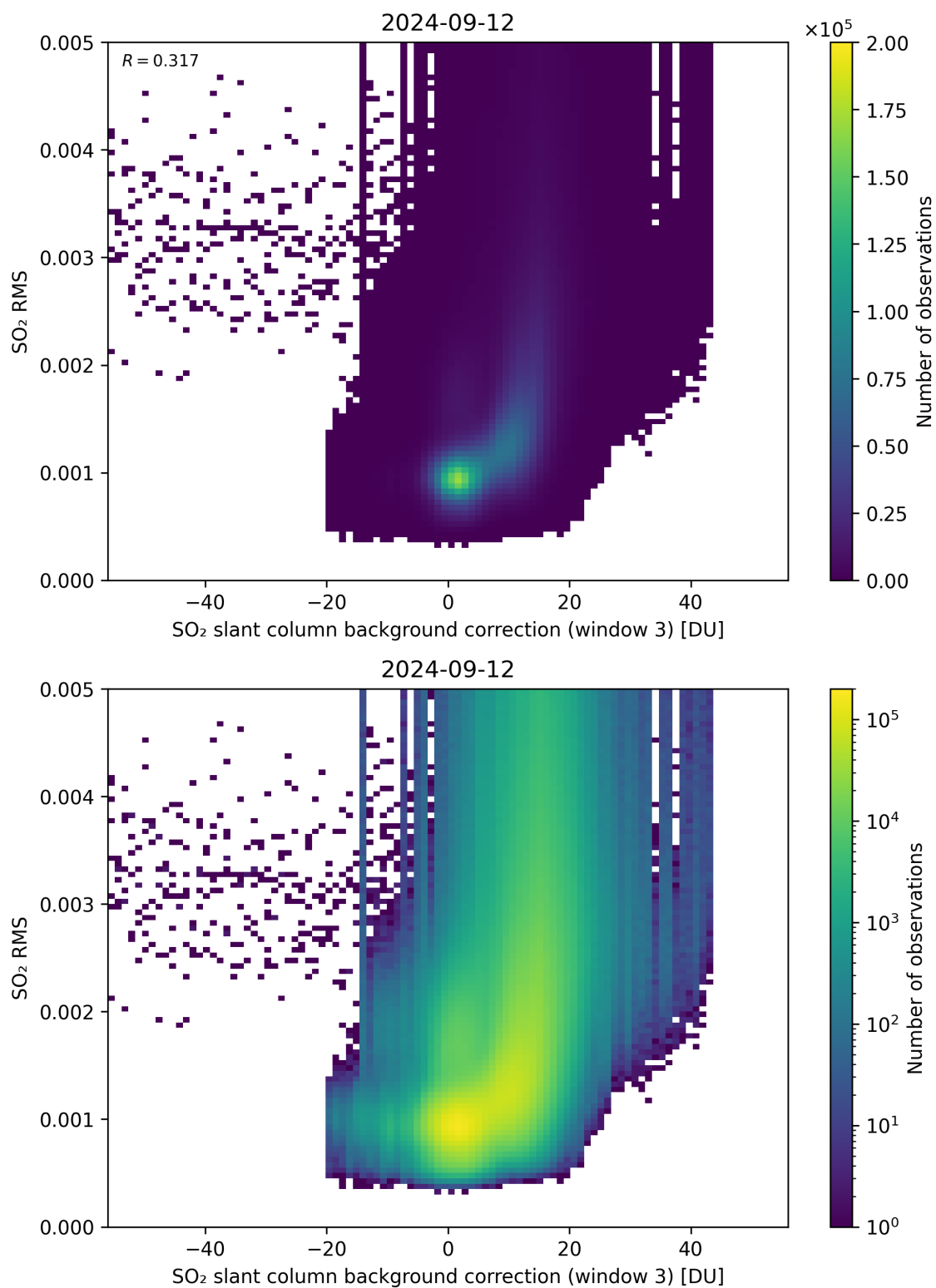
Figure 123: Scatter density plot of “SO 2 slant column background correction (window 3)” against “SO 2 RMS” for 2024-09-12 to 2024-09-13.
