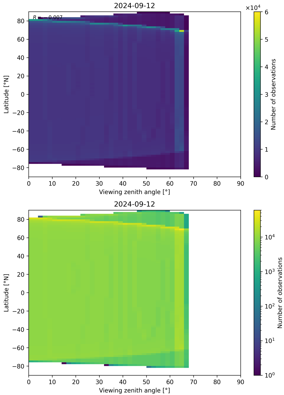
Figure 314: Scatter density plot of “Viewing zenith angle” against “Latitude” for 2024-09-12 to 2024-09-13.
