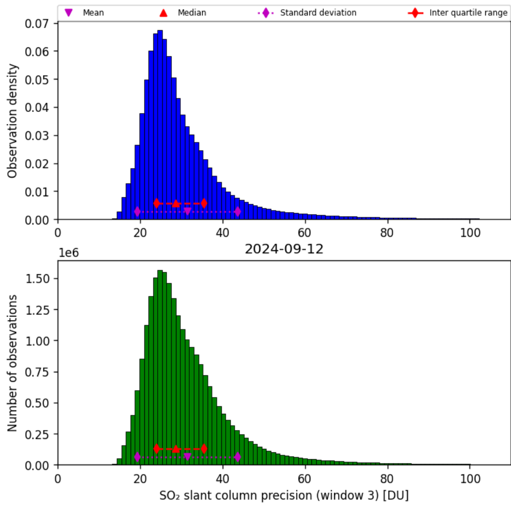
Figure 65: Histogram of “SO 2 slant column precision (window 3)” for 2024-09-12 to 2024-09-13
