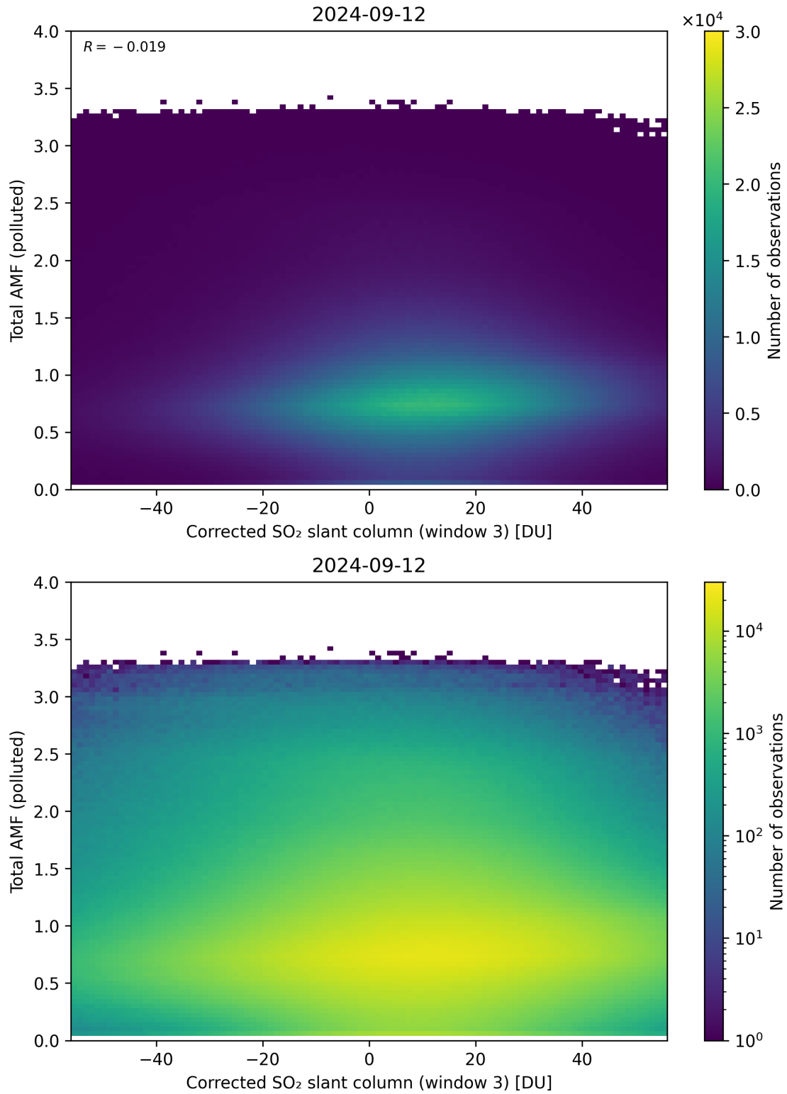
Figure 210: Scatter density plot of “Corrected SO 2 slant column (window 3)” against “Total AMF (polluted)” for 2024-09-12 to 2024-09-13.
