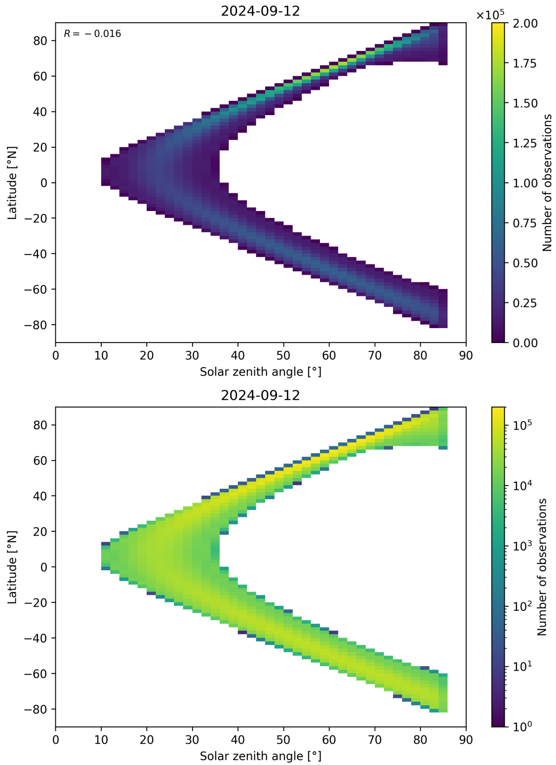
Figure 164: Scatter density plot of “Solar zenith angle” against “Latitude” for 2024-09-12 to 2024-09-13.
