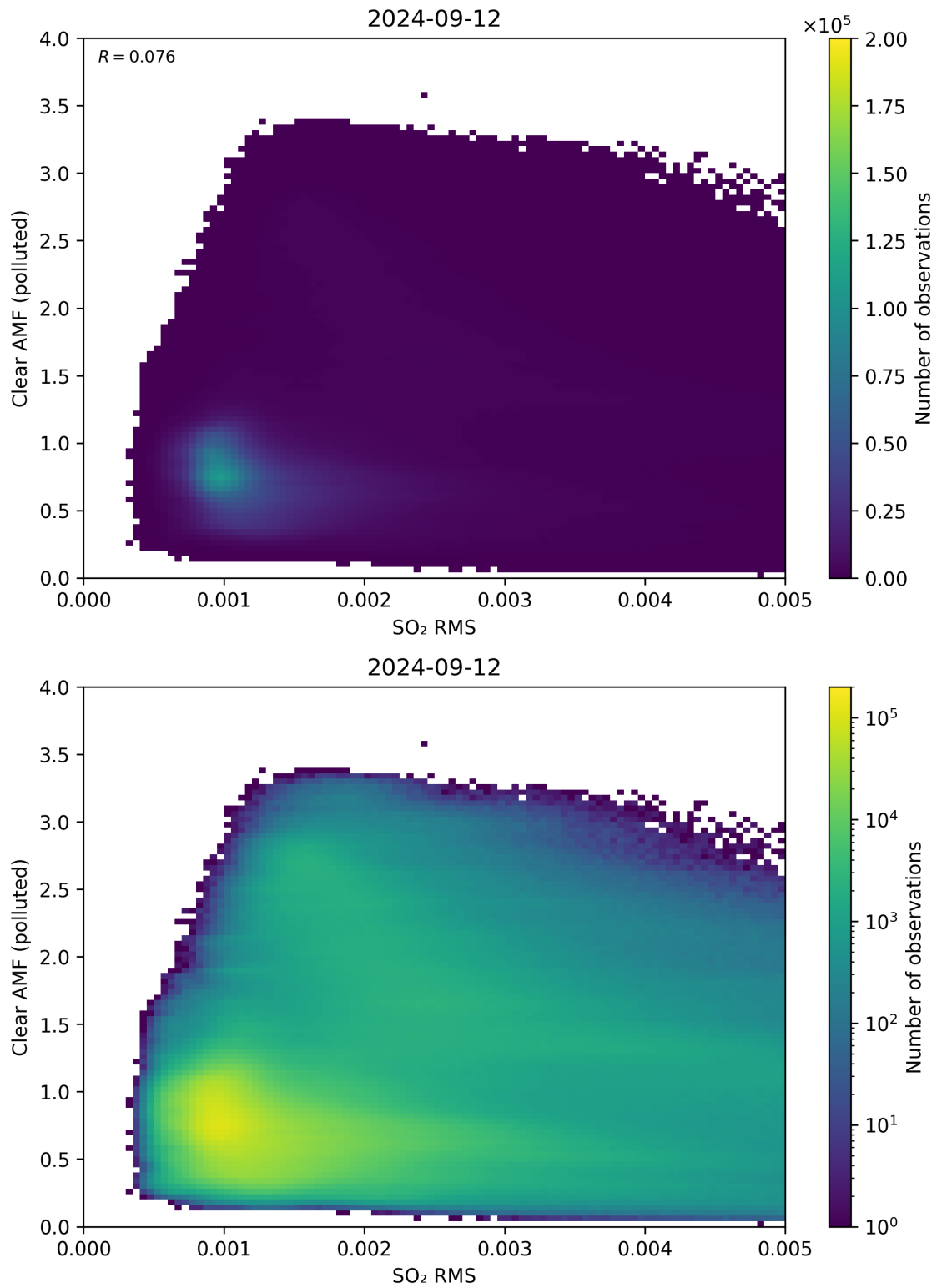
Figure 136: Scatter density plot of “SO 2 RMS” against “Clear AMF (polluted)” for 2024-09-12 to 2024-09-13.
