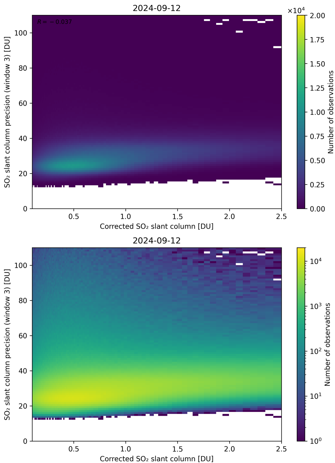
Figure 191: Scatter density plot of “Corrected SO 2 slant column” against “SO 2 slant column precision (window 3)” for 2024-09-12 to 2024-09-13.
