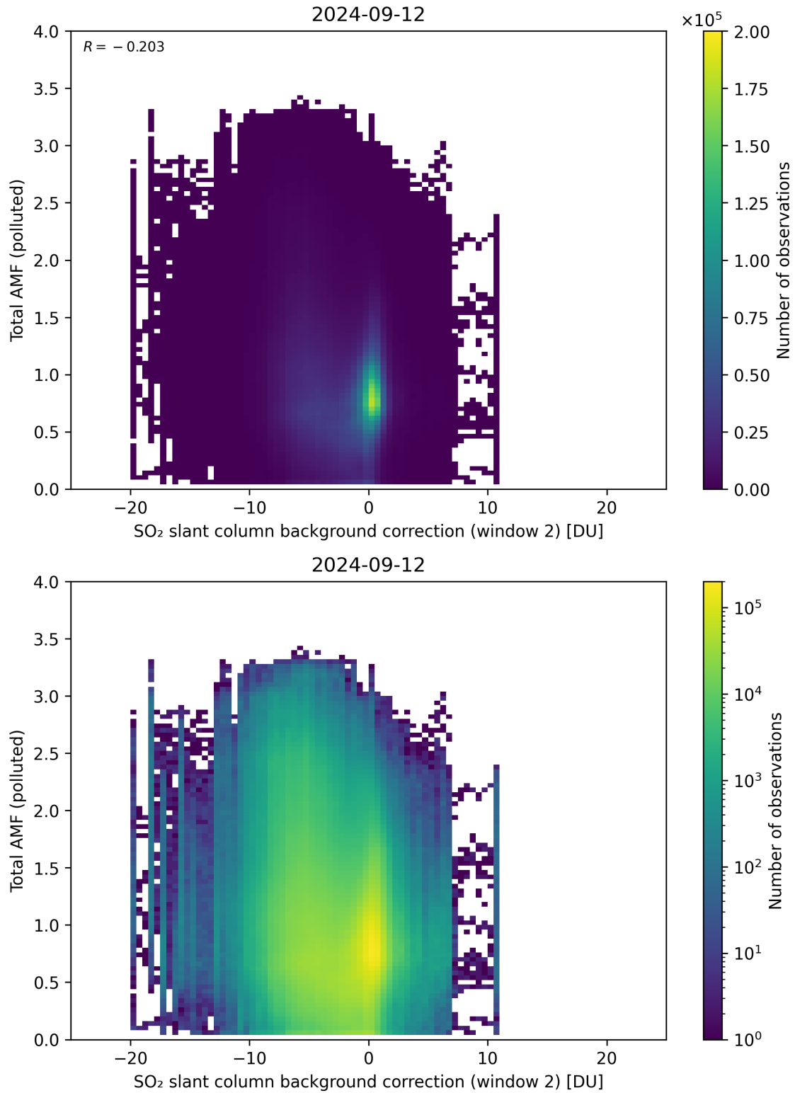
Figure 119: Scatter density plot of “SO 2 slant column background correction (window 2)” against “Total AMF (polluted)” for 2024-09-12 to 2024-09-13.
