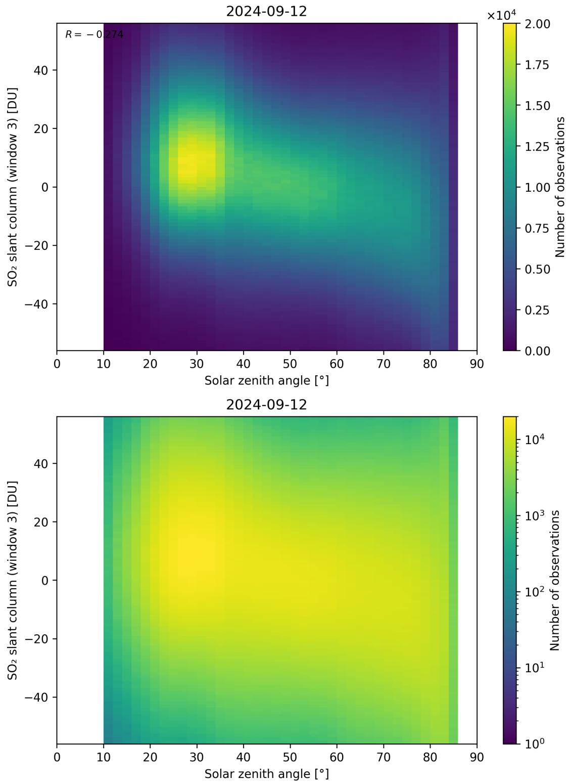
Figure 172: Scatter density plot of “Solar zenith angle” against “SO 2 slant column (window 3)” for 2024-09-12 to 2024-09-13.
