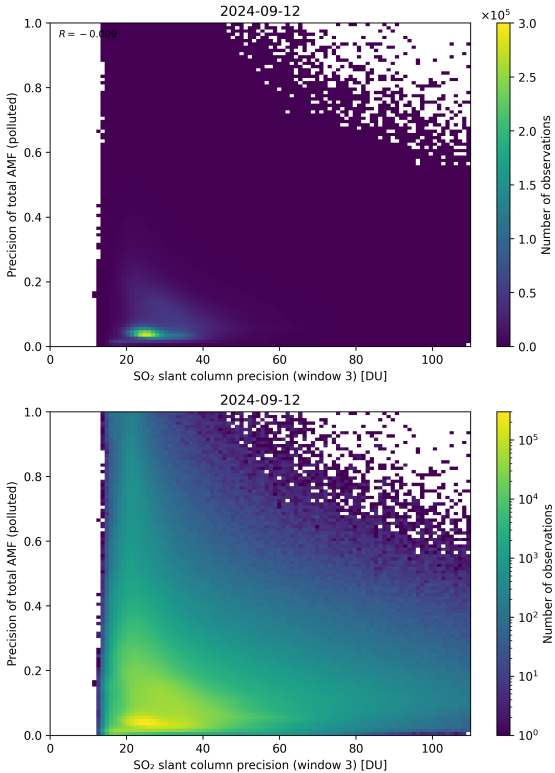
Figure 264: Scatter density plot of “SO 2 slant column precision (window 3)” against “Precision of total AMF (polluted)” for 2024-09-12 to 2024-09-13.
