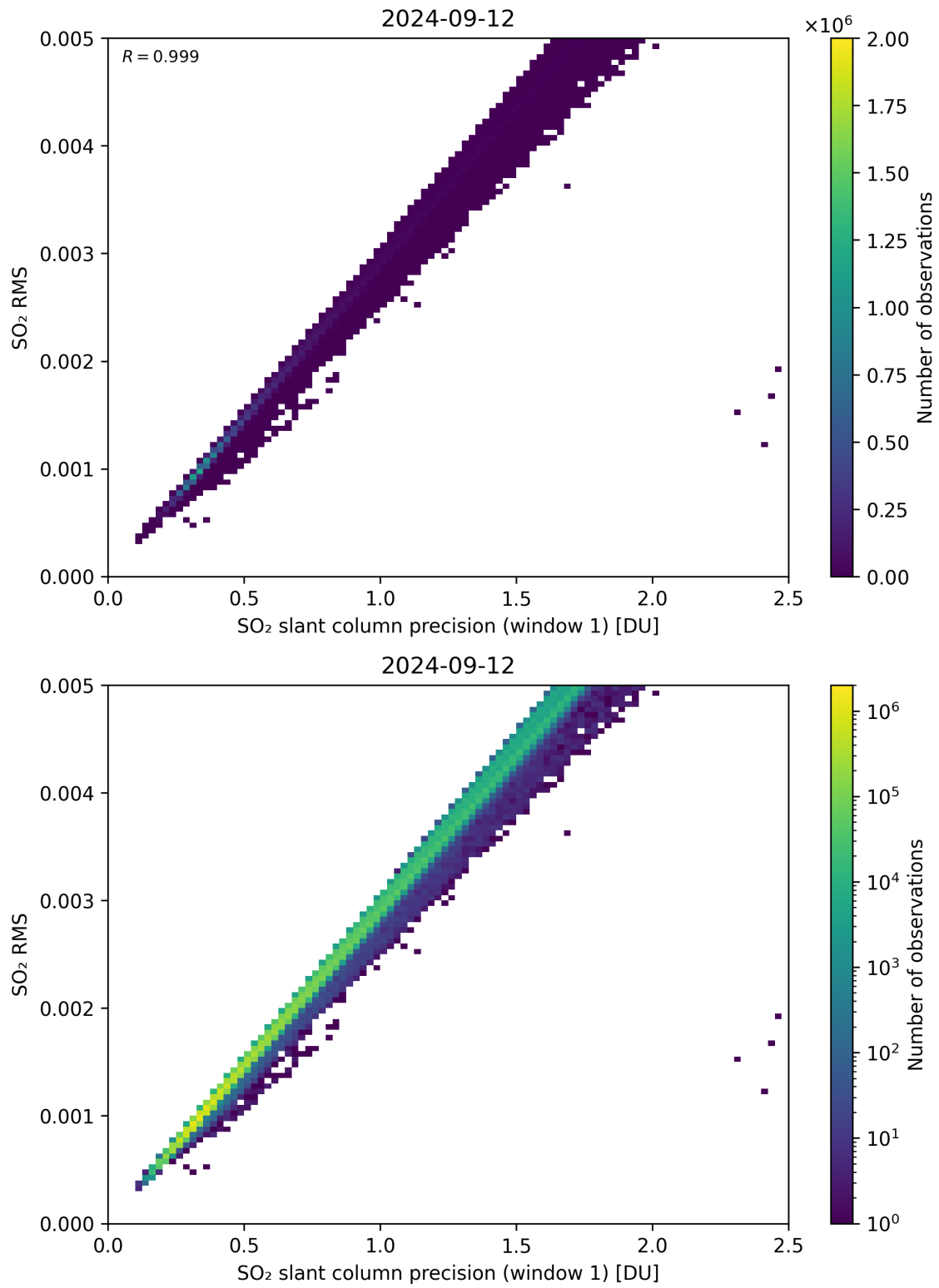
Figure 223: Scatter density plot of “SO 2 slant column precision (window 1)” against “SO 2 RMS” for 2024-09-12 to 2024-09-13.
