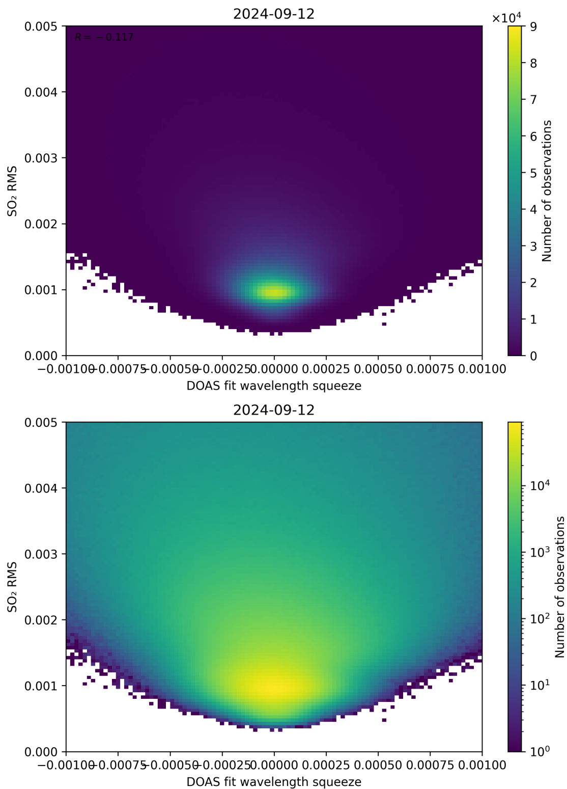
Figure 132: Scatter density plot of “DOAS fit wavelength squeeze” against “SO 2 RMS” for 2024-09-12 to 2024-09-13.
