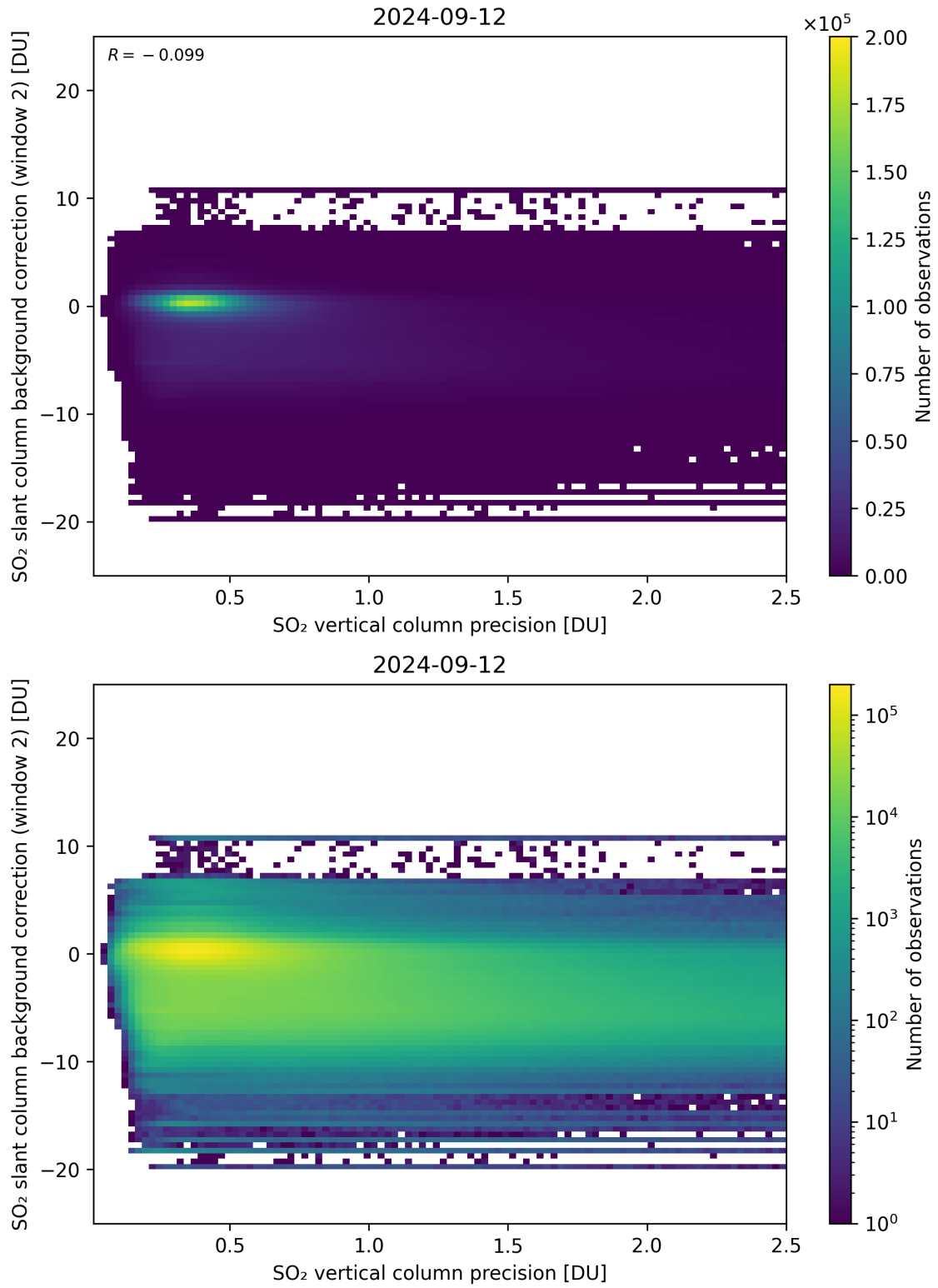
Figure 280: Scatter density plot of “SO 2 vertical column precision” against “SO 2 slant column background correction (window 2)” for 2024-09-12 to 2024-09-13.
