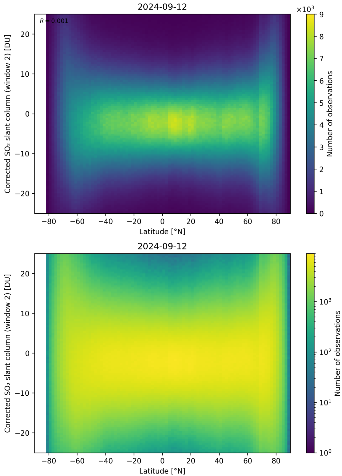
Figure 147: Scatter density plot of “Latitude” against “Corrected SO 2 slant column (window 2)” for 2024-09-12 to 2024-09-13.
