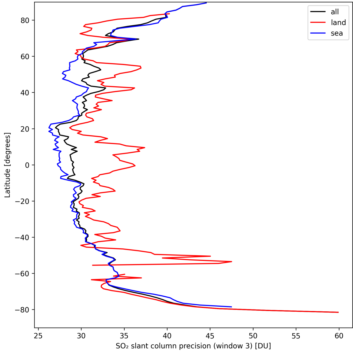
Figure 42: Zonal average of “SO 2 slant column precision (window 3)” for 2024-09-12 to 2024-09-13.
