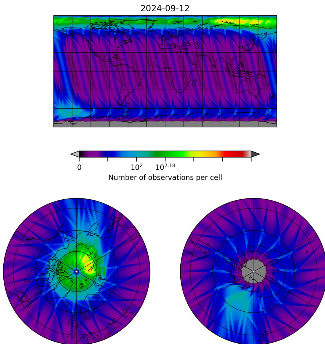
Figure 28: Map of the number of observations for 2024-09-12 to 2024-09-13
