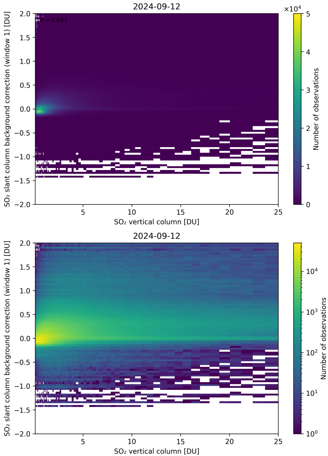
Figure 273: Scatter density plot of “SO 2 vertical column” against “SO 2 slant column background correction (window 1)” for 2024-09-12 to 2024-09-13.
