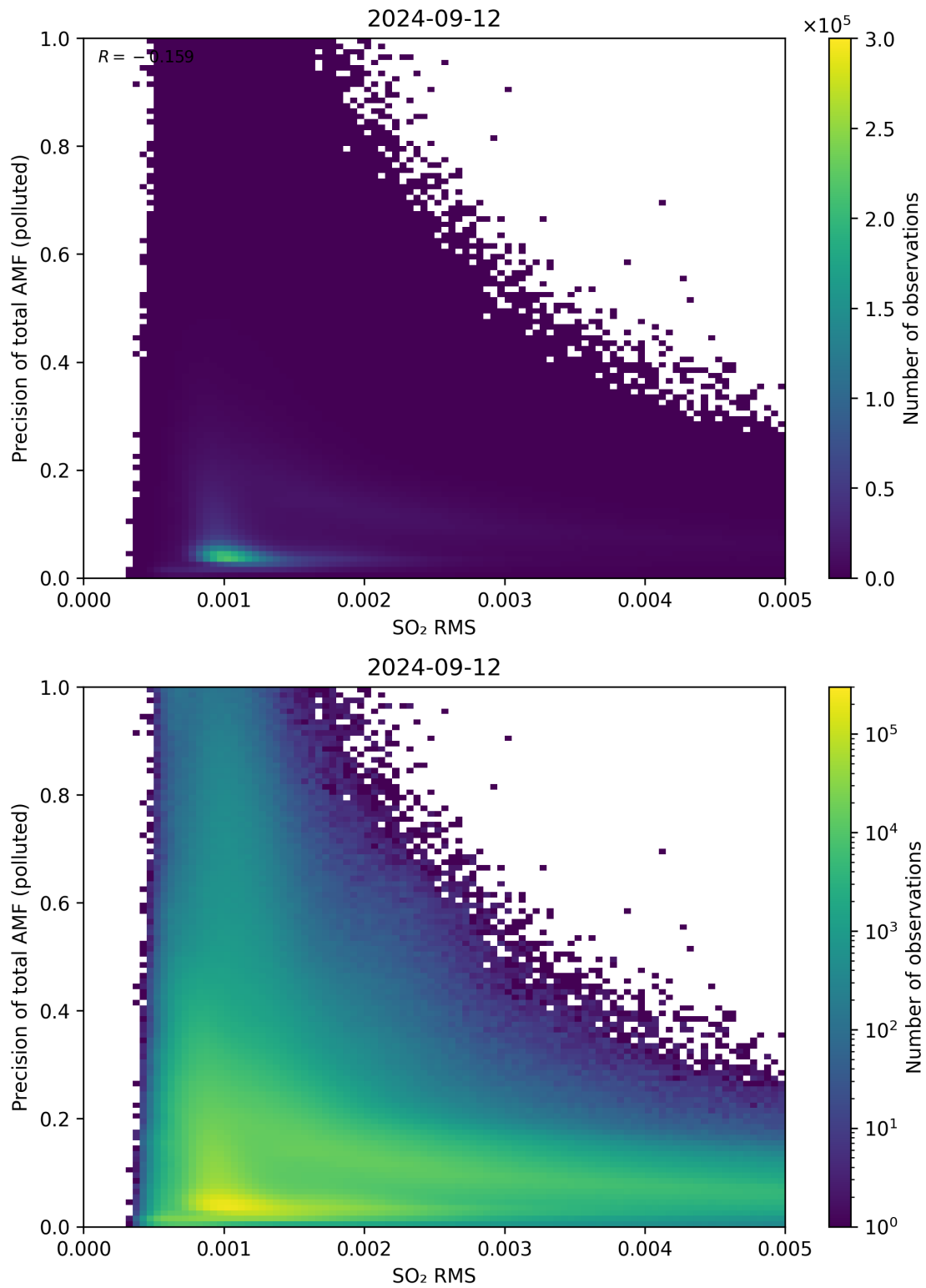
Figure 138: Scatter density plot of “SO 2 RMS” against “Precision of total AMF (polluted)” for 2024-09-12 to 2024-09-13.
