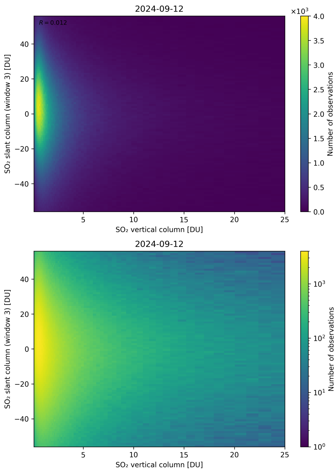
Figure 303: Scatter density plot of “SO 2 vertical column” against “SO 2 slant column (window 3)” for 2024-09-12 to 2024-09-13.
