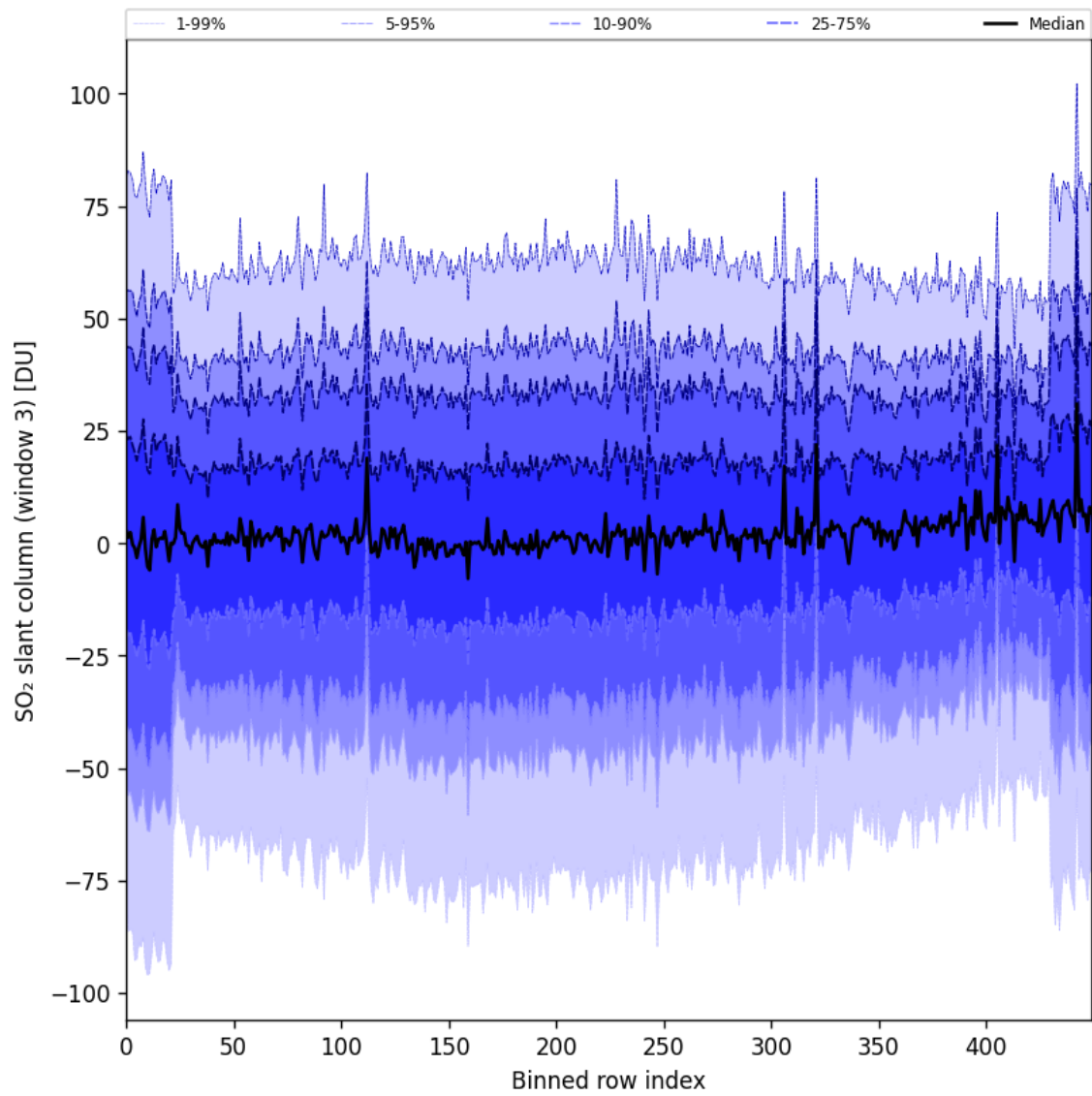
Figure 87: Along track statistics of “SO 2 slant column (window 3)” for 2024-09-12 to 2024-09-13
