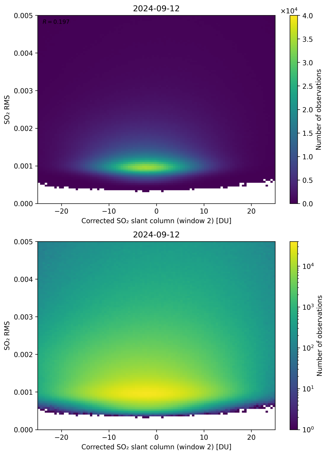
Figure 198: Scatter density plot of “Corrected SO 2 slant column (window 2)” against “SO 2 RMS” for 2024-09-12 to 2024-09-13.
