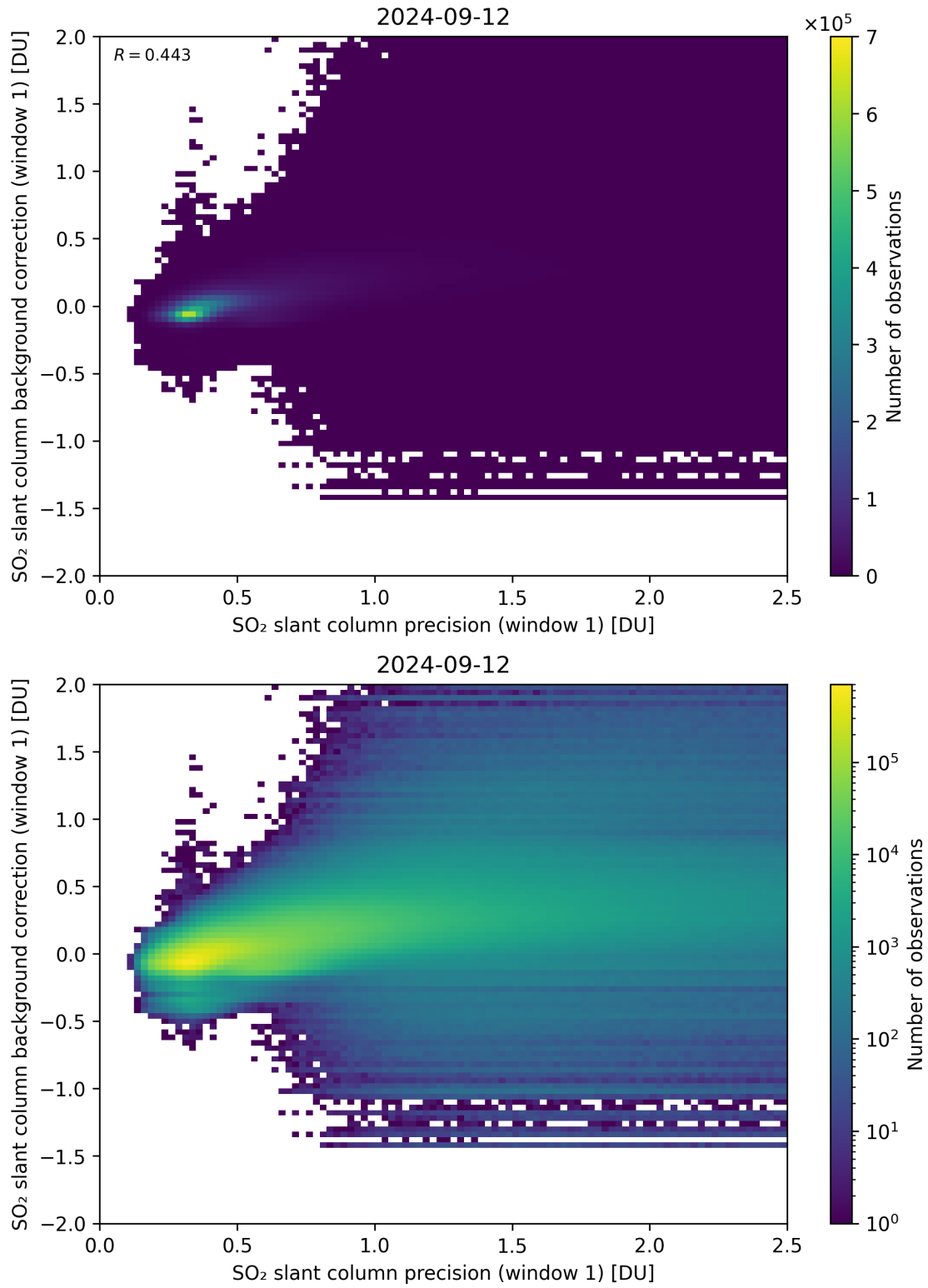
Figure 218: Scatter density plot of “SO 2 slant column precision (window 1)” against “SO 2 slant column background correction (window 1)” for 2024-09-12 to 2024-09-13.
