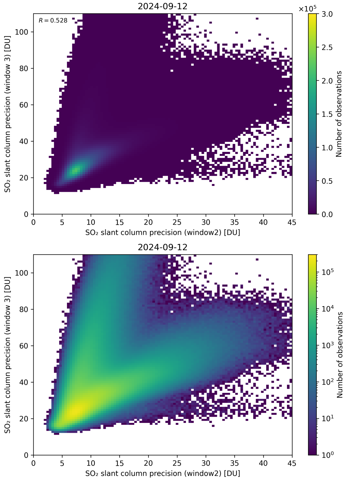
Figure 250: Scatter density plot of “SO 2 slant column precision (window2)” against “SO 2 slant column precision (window 3)” for 2024-09-12 to 2024-09-13.
