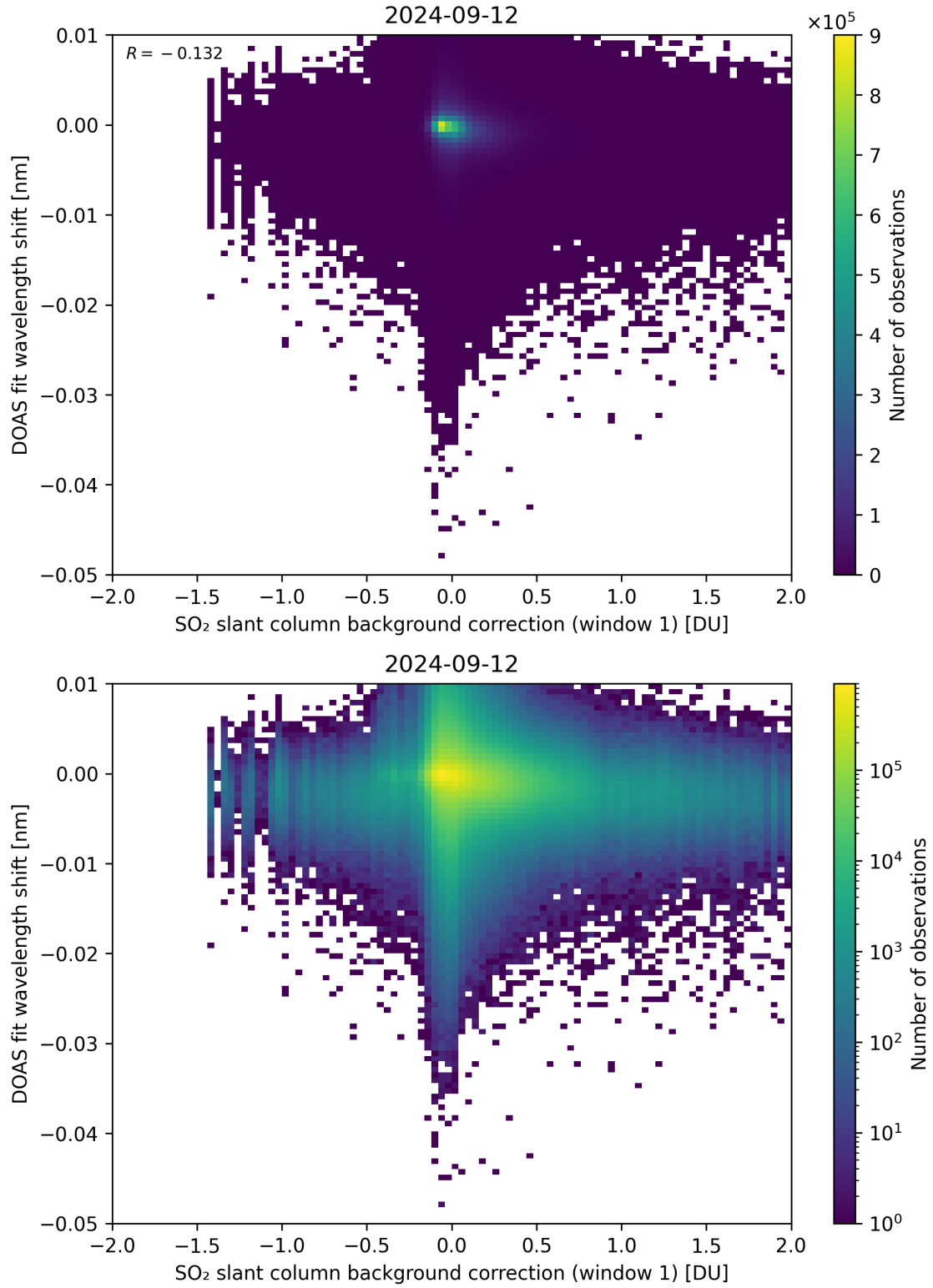
Figure 100: Scatter density plot of “SO 2 slant column background correction (window 1)” against “DOAS fit wavelength shift” for 2024-09-12 to 2024-09-13.
