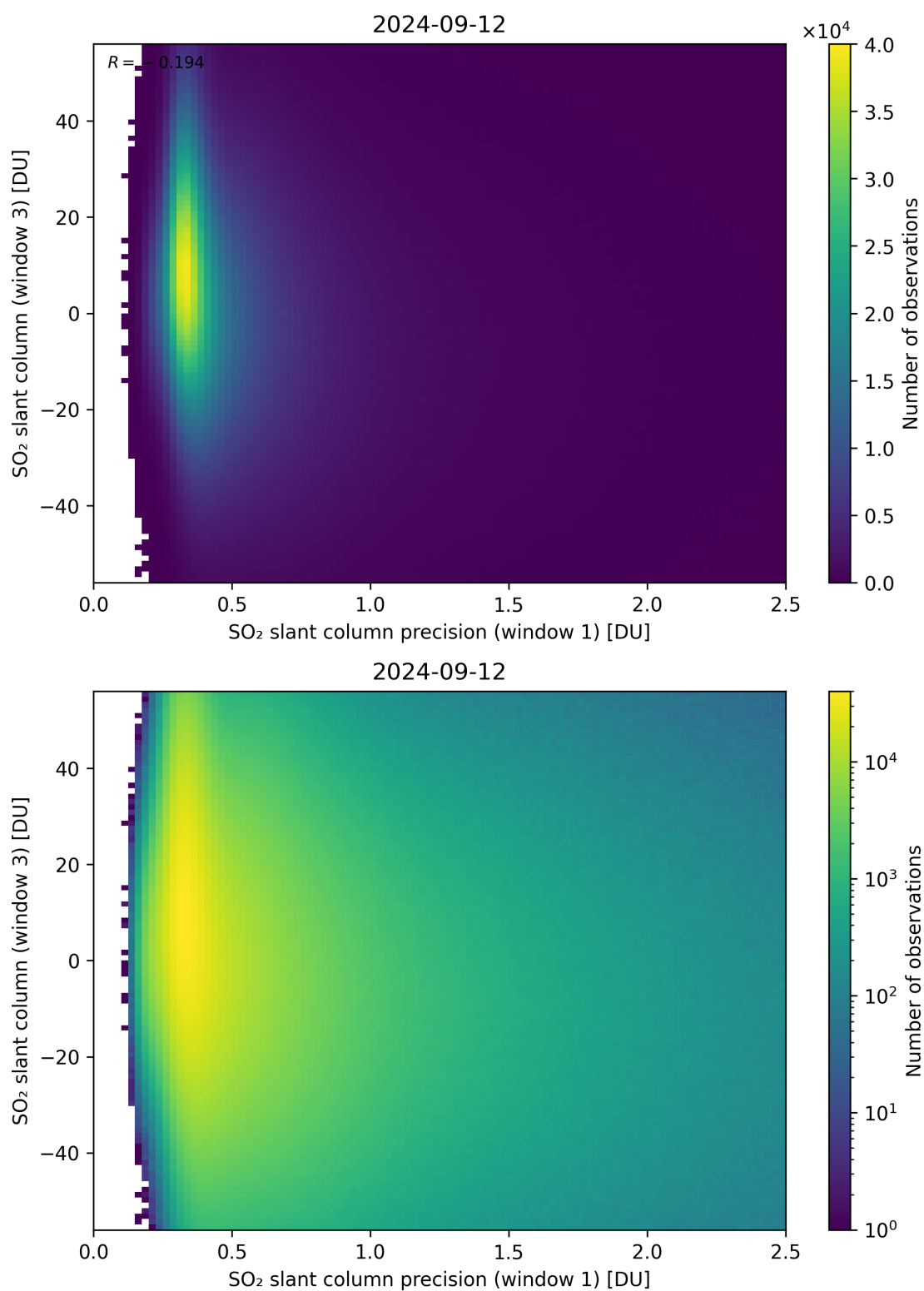
Figure 228: Scatter density plot of “SO 2 slant column precision (window 1)” against “SO 2 slant column (window 3)” for 2024-09-12 to 2024-09-13.
