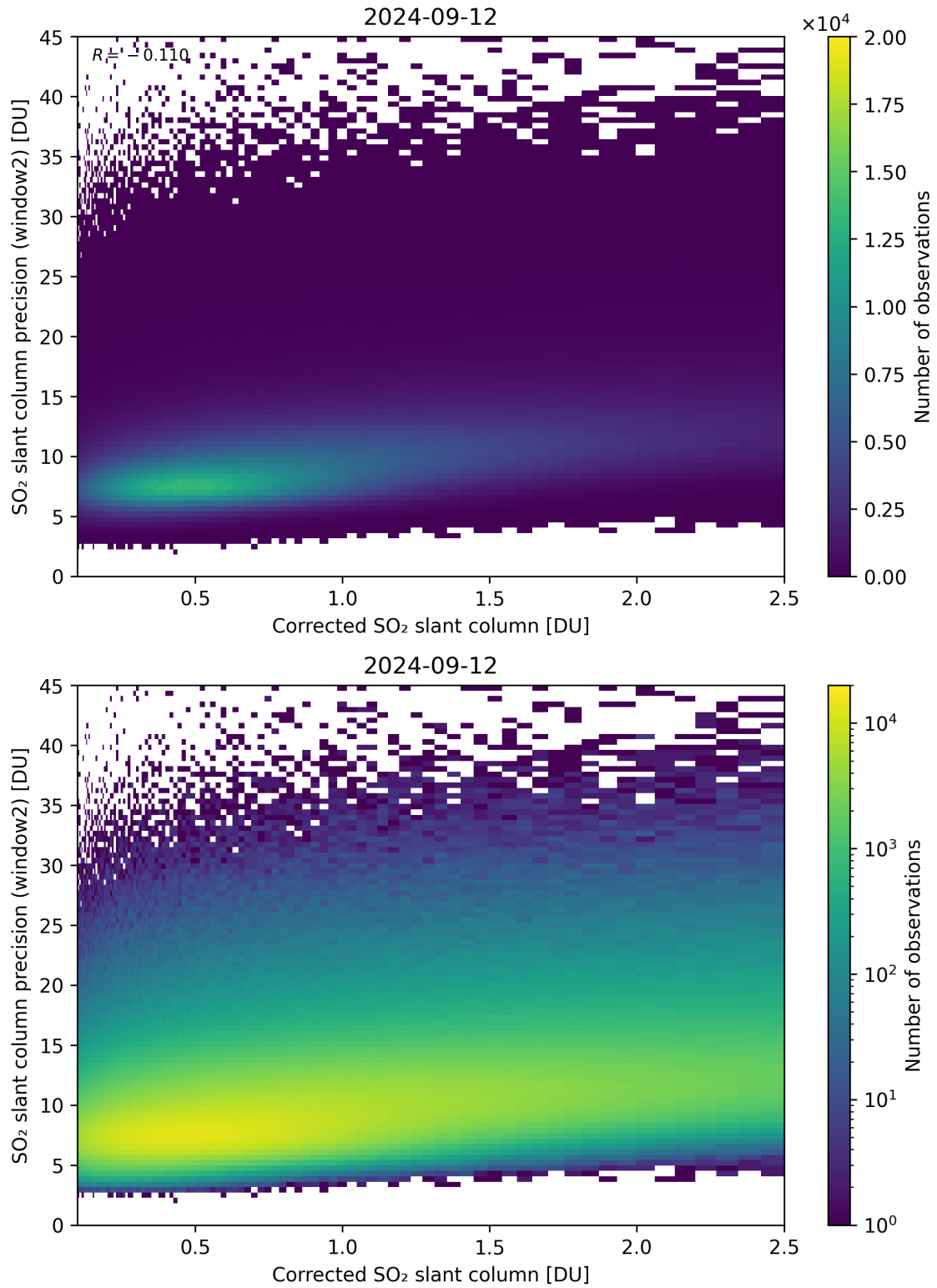
Figure 189: Scatter density plot of “Corrected SO 2 slant column” against “SO 2 slant column precision (window2)” for 2024-09-12 to 2024-09-13.
