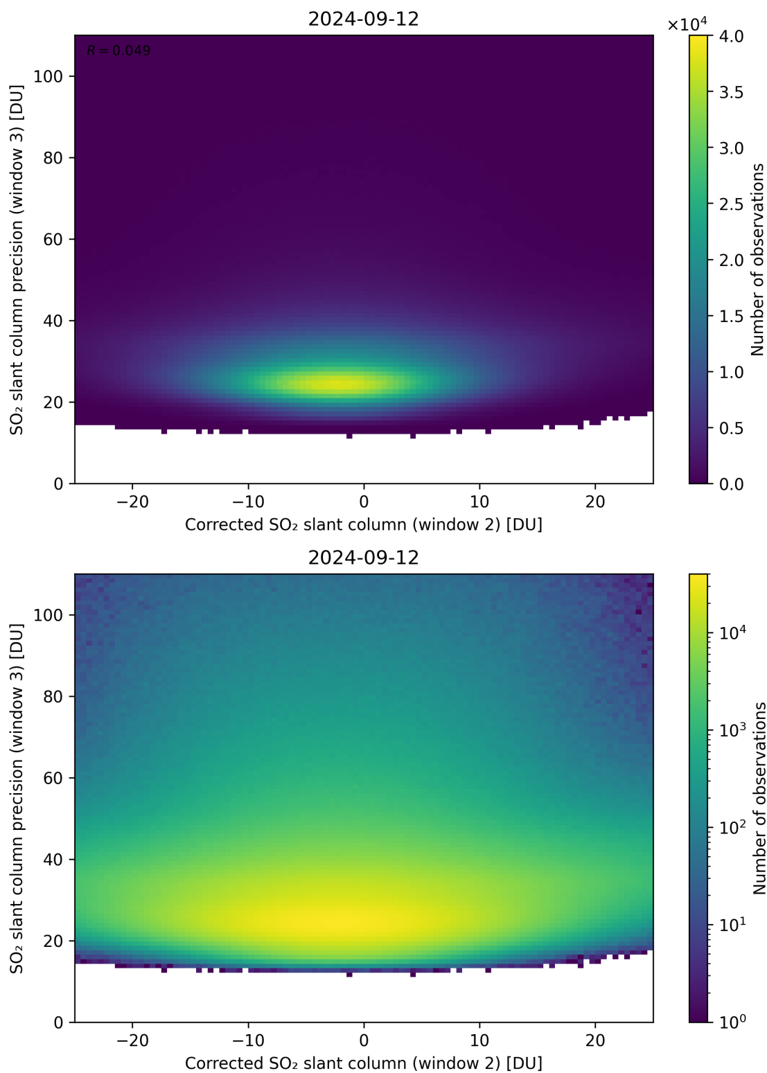
Figure 202: Scatter density plot of “Corrected SO 2 slant column (window 2)” against “SO 2 slant column precision (window 3)” for 2024-09-12 to 2024-09-13.
