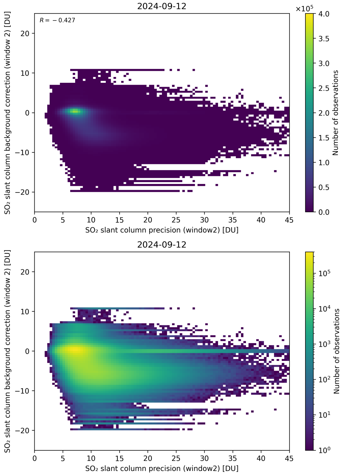
Figure 241: Scatter density plot of “SO 2 slant column precision (window2)” against “SO 2 slant column background correction (window 2)” for 2024-09-12 to 2024-09-13.
