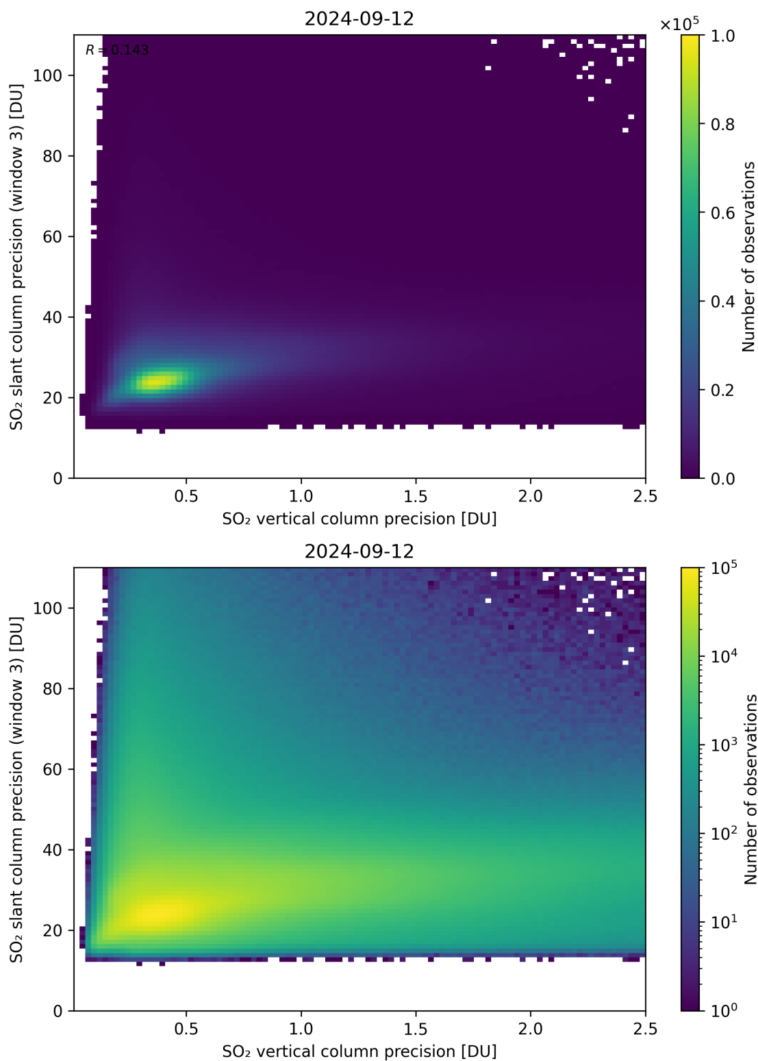
Figure 293: Scatter density plot of “SO 2 vertical column precision” against “SO 2 slant column precision (window 3)” for 2024-09-12 to 2024-09-13.
