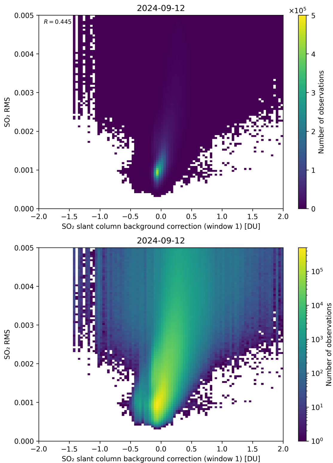
Figure 102: Scatter density plot of “SO 2 slant column background correction (window 1)” against “SO 2 RMS” for 2024-09-12 to 2024-09-13.
