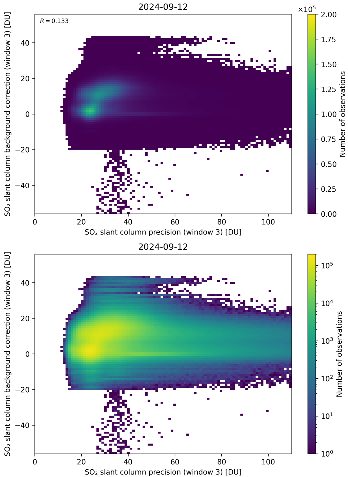
Figure 257: Scatter density plot of “SO 2 slant column precision (window 3)” against “SO 2 slant column background correction (window 3)” for 2024-09-12 to 2024-09-13.
