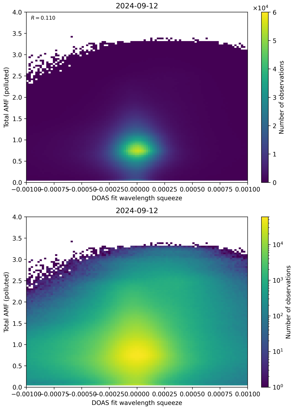
Figure 134: Scatter density plot of “DOAS fit wavelength squeeze” against “Total AMF (polluted)” for 2024-09-12 to 2024-09-13.
