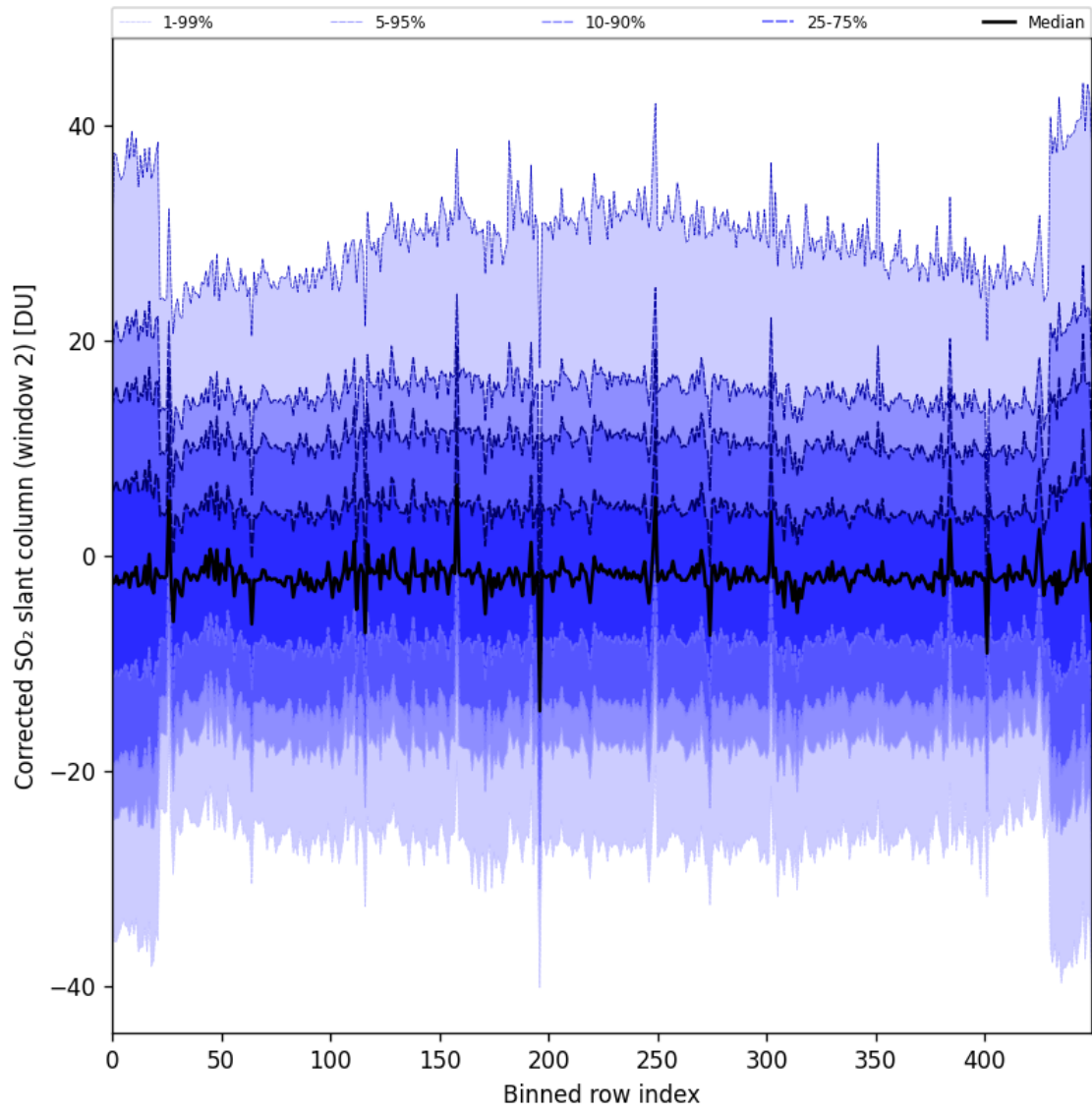
Figure 85: Along track statistics of “Corrected SO 2 slant column (window 2)” for 2024-09-12 to 2024-09-13
