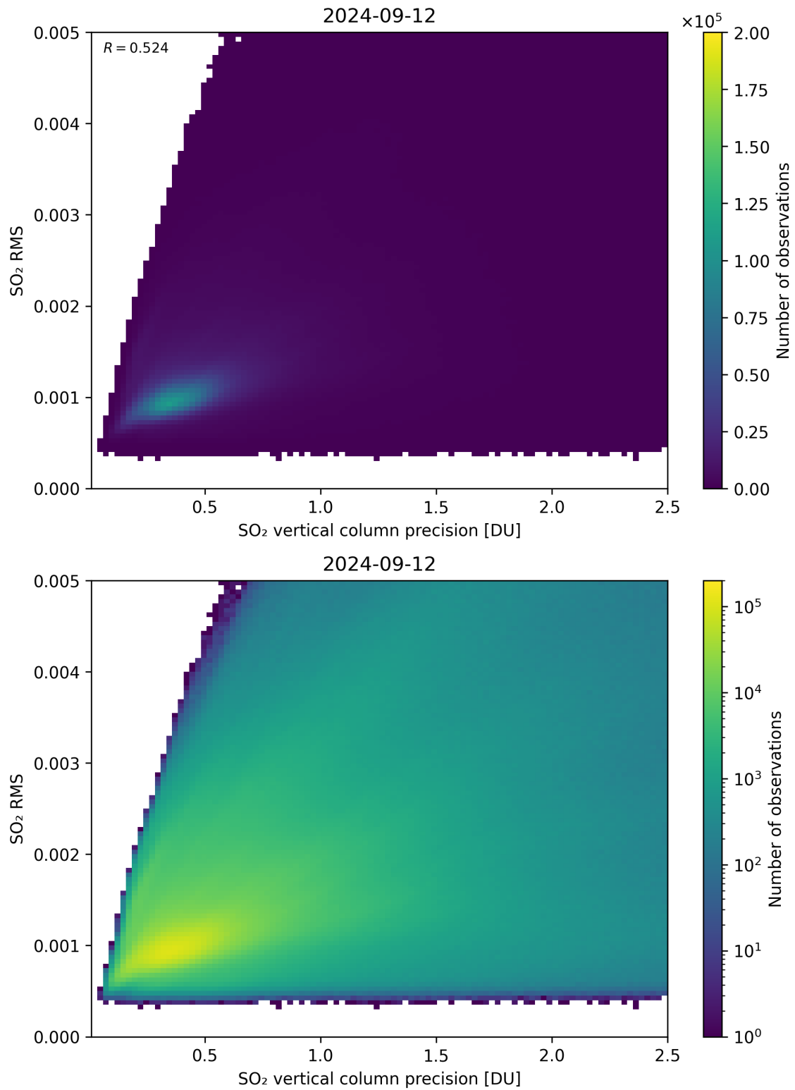
Figure 284: Scatter density plot of “SO 2 vertical column precision” against “SO 2 RMS” for 2024-09-12 to 2024-09-13.
