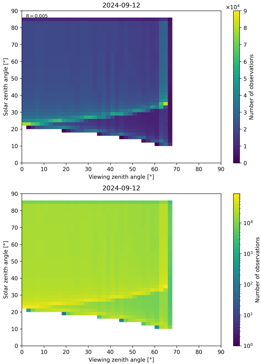
Figure 315: Scatter density plot of “Viewing zenith angle” against “Solar zenith angle” for 2024-09-12 to 2024-09-13.
