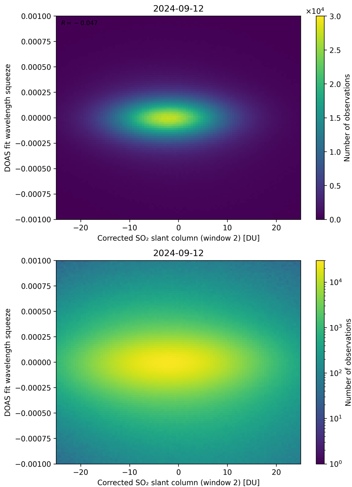
Figure 197: Scatter density plot of “Corrected SO 2 slant column (window 2)” against “DOAS fit wavelength squeeze” for 2024-09-12 to 2024-09-13.
