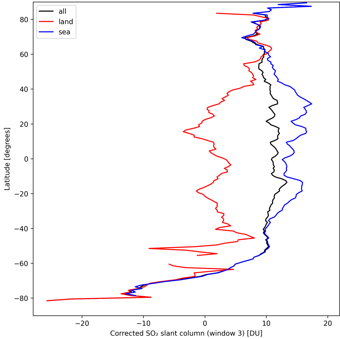
Figure 43: Zonal average of “Corrected SO 2 slant column (window 3)” for 2024-09-12 to 2024-09-13.
