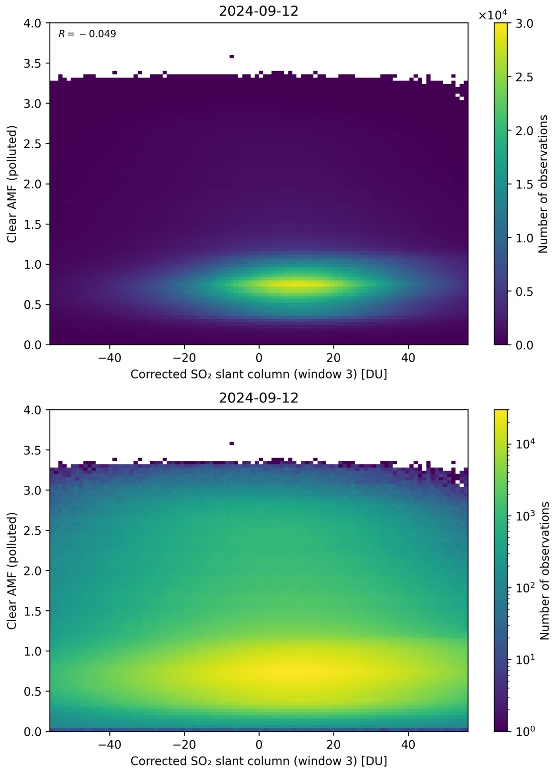
Figure 209: Scatter density plot of “Corrected SO 2 slant column (window 3)” against “Clear AMF (polluted)” for 2024-09-12 to 2024-09-13.
