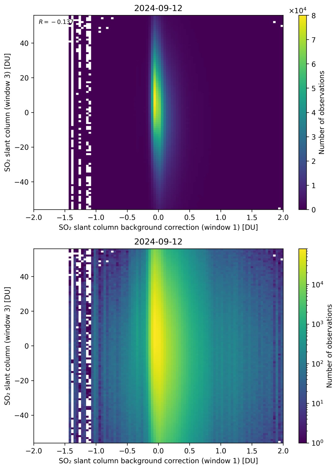
Figure 107: Scatter density plot of “SO 2 slant column background correction (window 1)” against “SO 2 slant column (window 3)” for 2024-09-12 to 2024-09-13.
