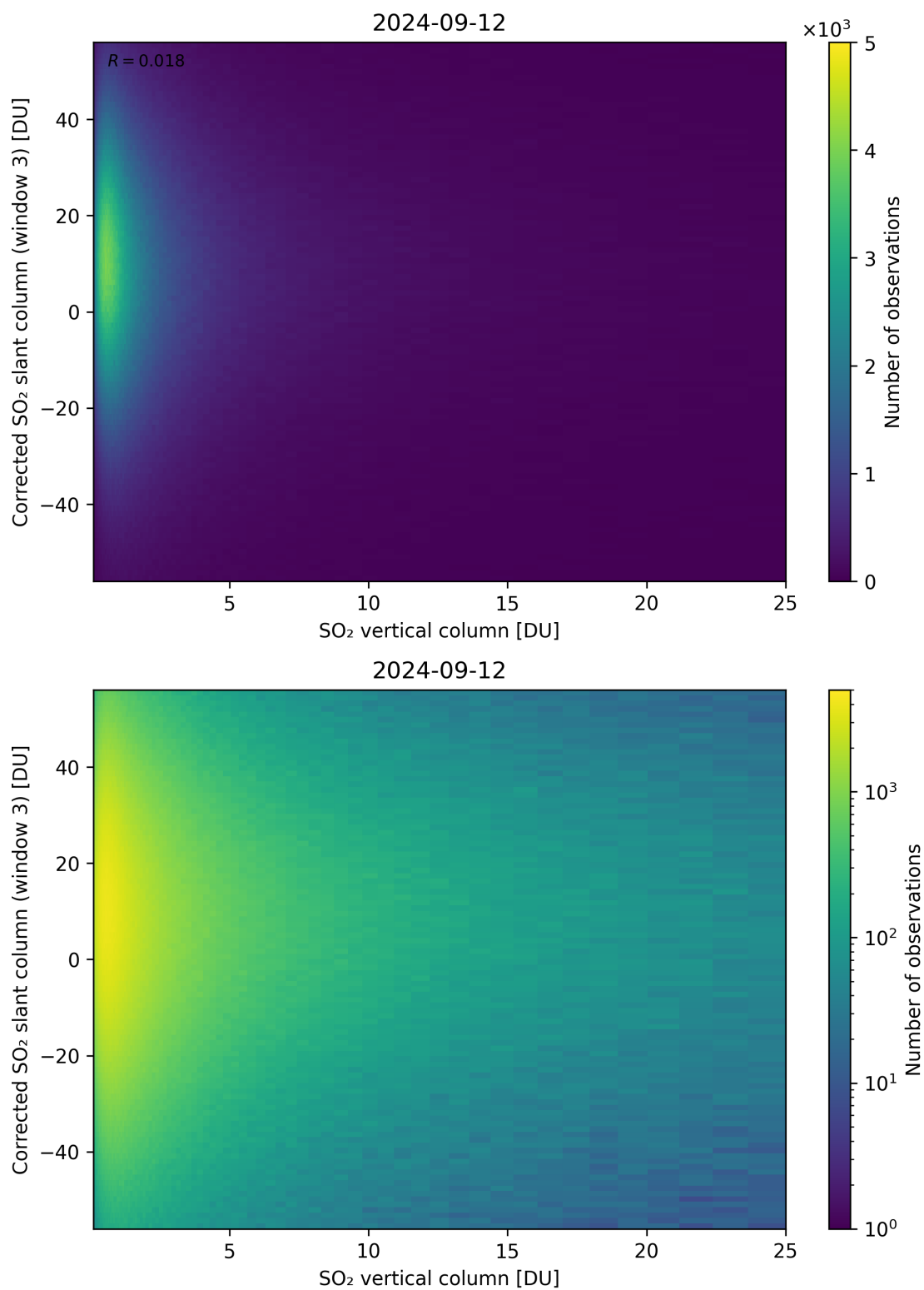
Figure 299: Scatter density plot of “SO 2 vertical column” against “Corrected SO 2 slant column (window 3)” for 2024-09-12 to 2024-09-13.
