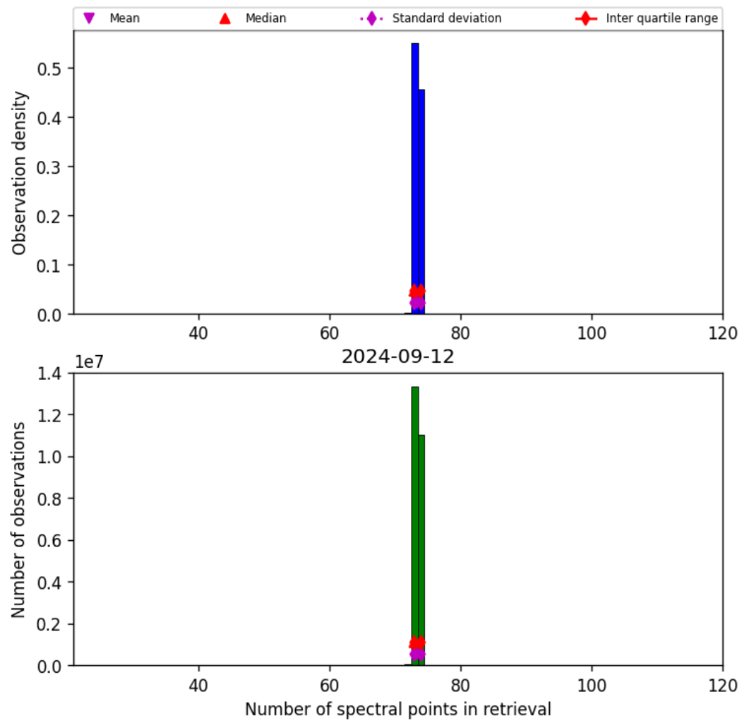
Figure 74: Histogram of “Number of spectral points in retrieval” for 2024-09-12 to 2024-09-13
