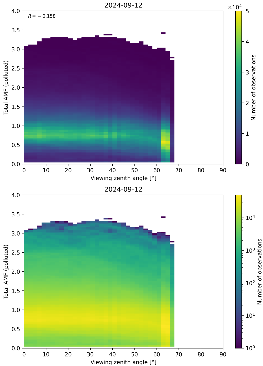
Figure 325: Scatter density plot of “Viewing zenith angle” against “Total AMF (polluted)” for 2024-09-12 to 2024-09-13.
