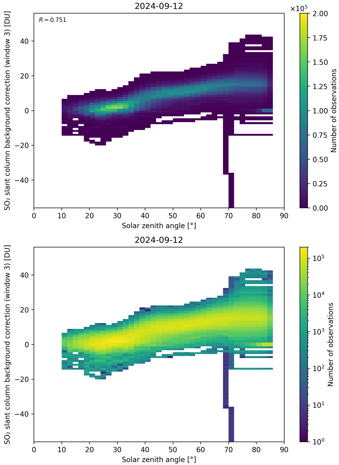
Figure 160: Scatter density plot of “Solar zenith angle” against “SO 2 slant column background correction (window 3)” for 2024-09-12 to 2024-09-13.
