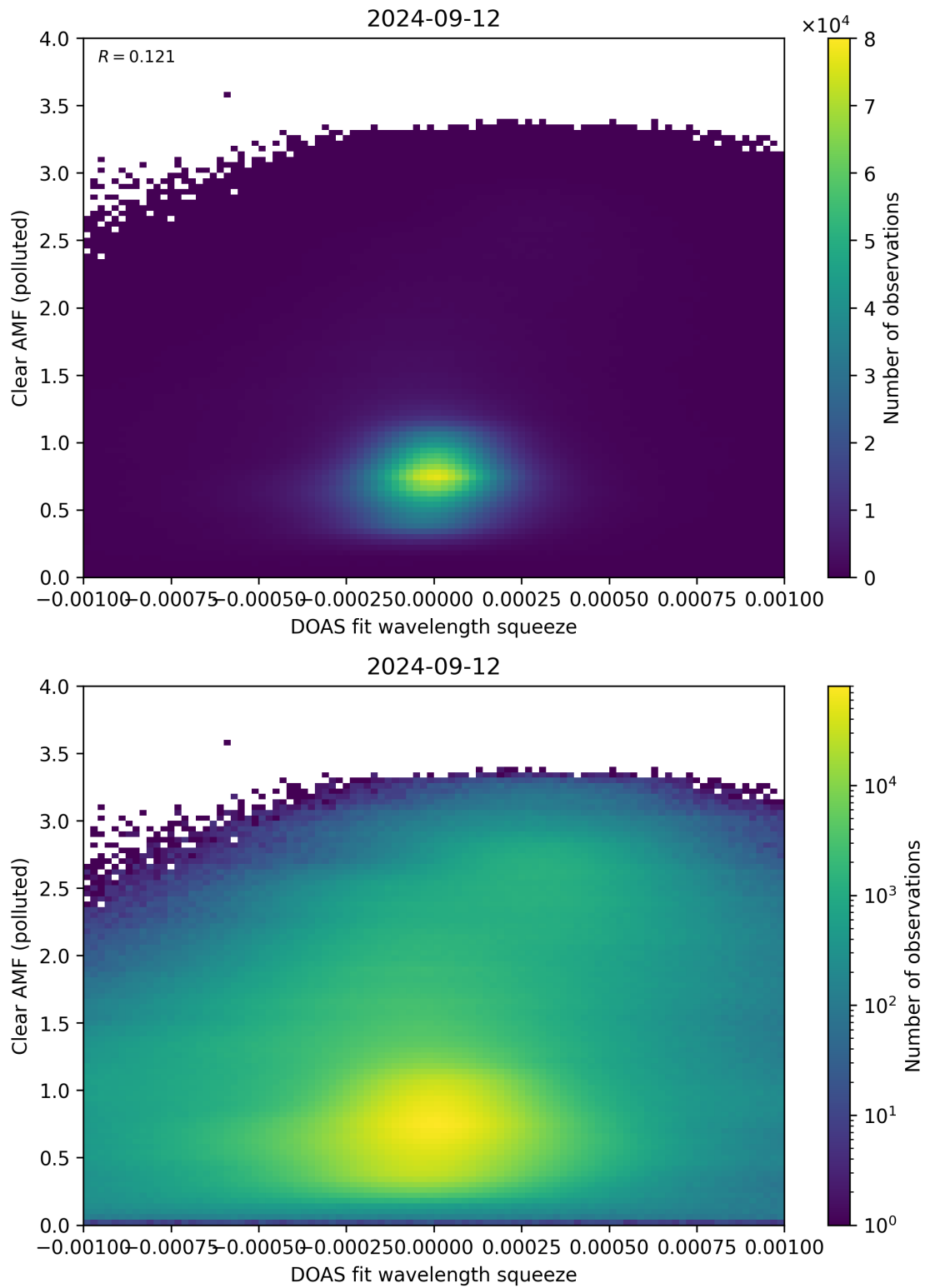
Figure 133: Scatter density plot of “DOAS fit wavelength squeeze” against “Clear AMF (polluted)” for 2024-09-12 to 2024-09-13.
