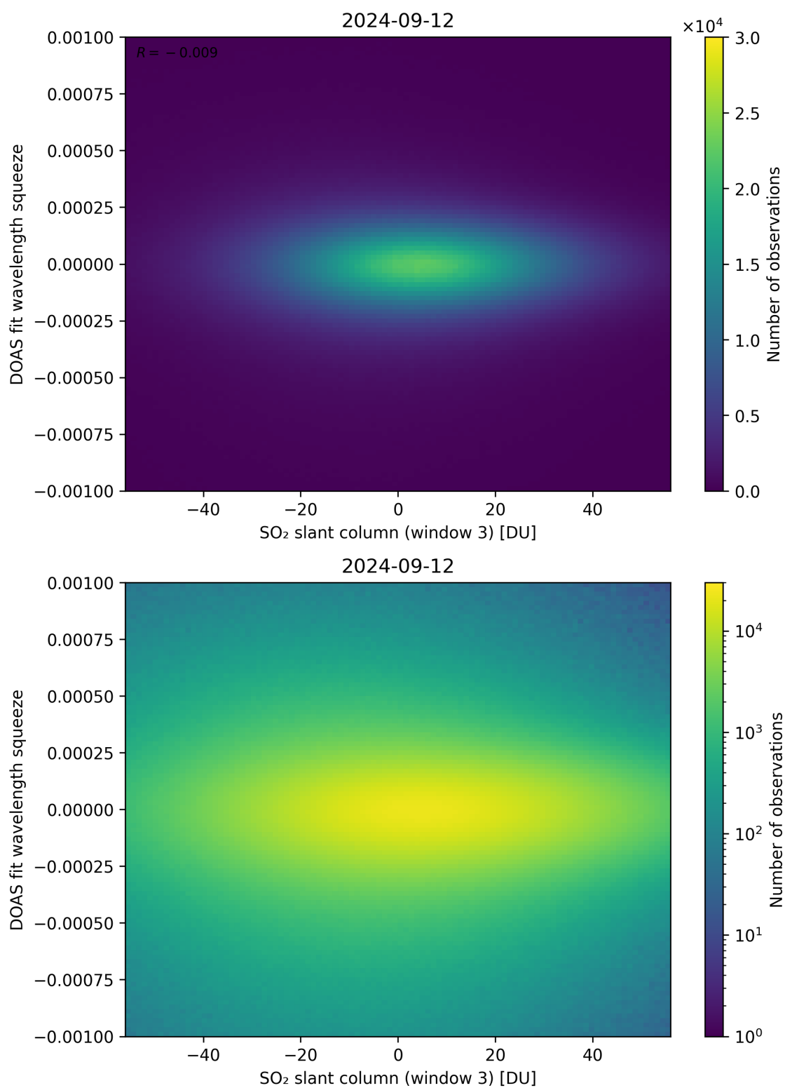
Figure 255: Scatter density plot of “SO 2 slant column (window 3)” against “DOAS fit wavelength squeeze” for 2024-09-12 to 2024-09-13.
