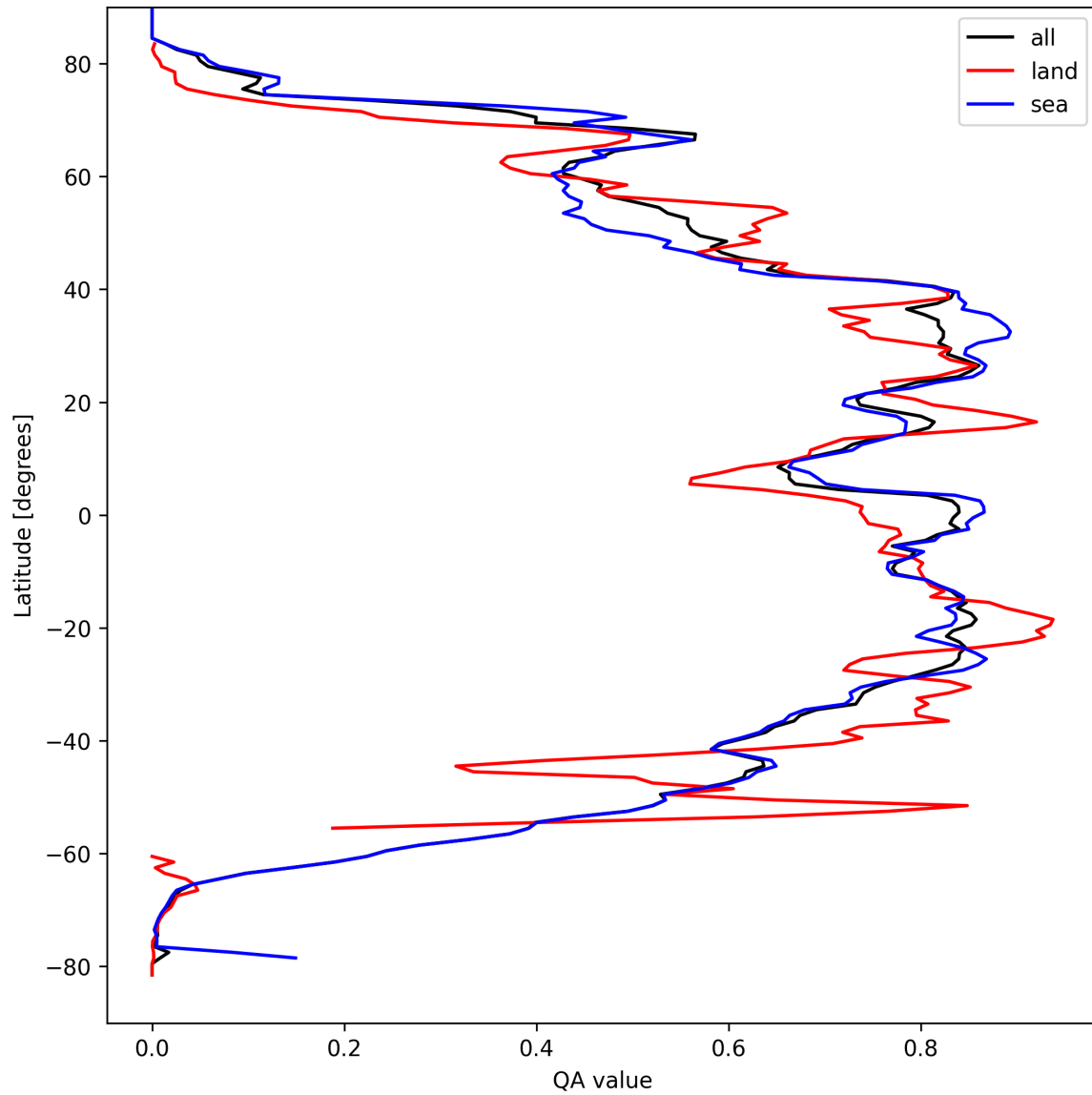
Figure 29: Zonal average of “QA value” for 2024-09-12 to 2024-09-13.
