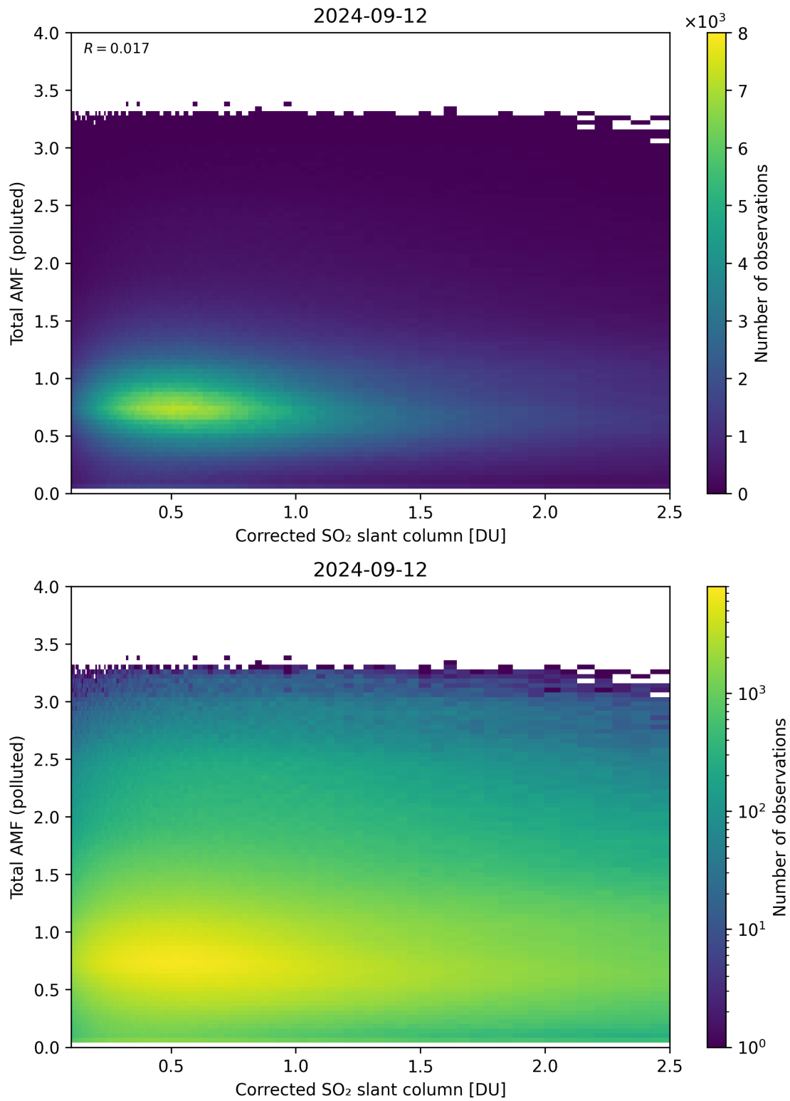
Figure 192: Scatter density plot of “Corrected SO 2 slant column” against “Total AMF (polluted)” for 2024-09-12 to 2024-09-13.
