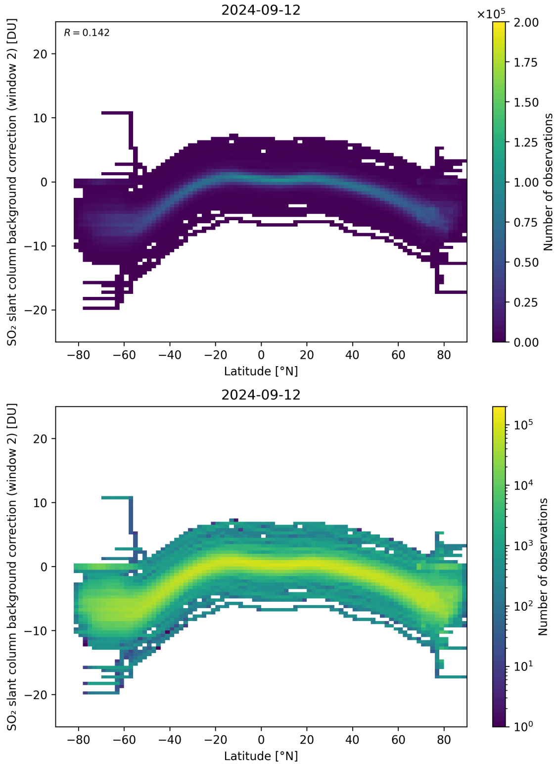
Figure 140: Scatter density plot of “Latitude” against “SO 2 slant column background correction (window 2)” for 2024-09-12 to 2024-09-13.
