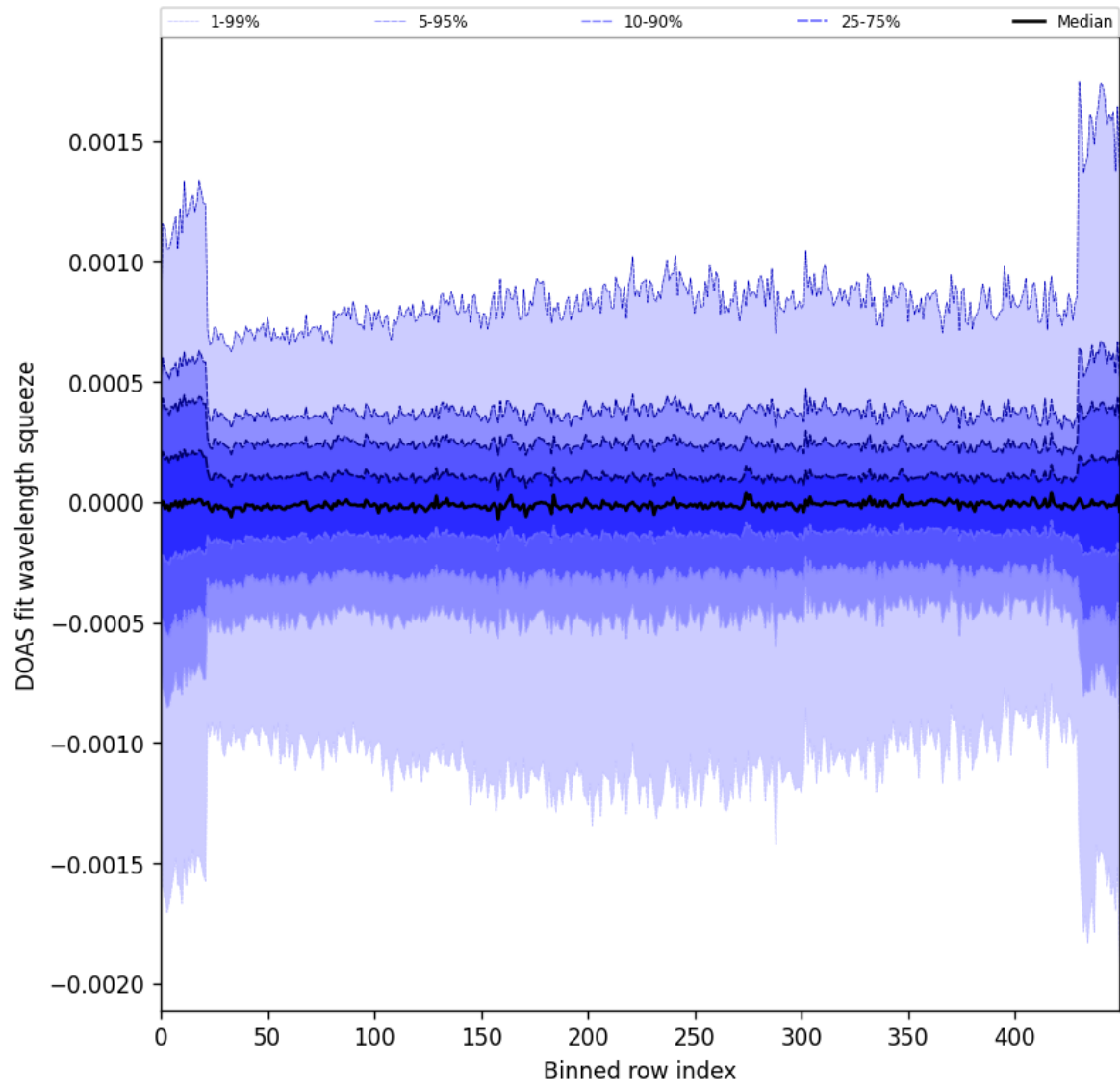
Figure 92: Along track statistics of “DOAS fit wavelength squeeze” for 2024-09-12 to 2024-09-13
