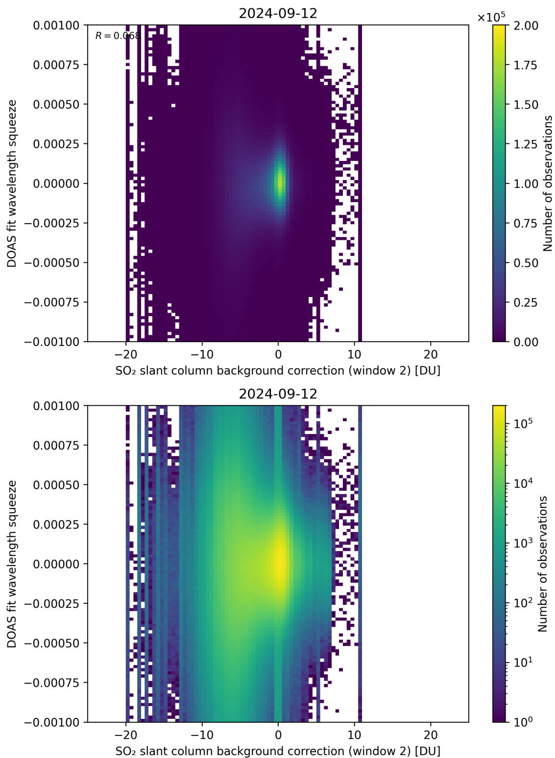
Figure 113: Scatter density plot of “SO 2 slant column background correction (window 2)” against “DOAS fit wavelength squeeze” for 2024-09-12 to 2024-09-13.
