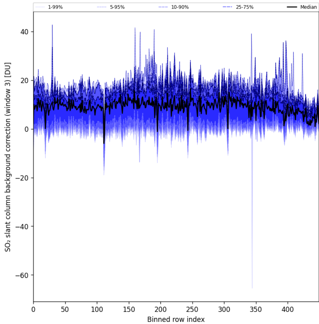
Figure 90: Along track statistics of “SO 2 slant column background correction (window 3)” for 2024-09-12 to 2024-09-13
