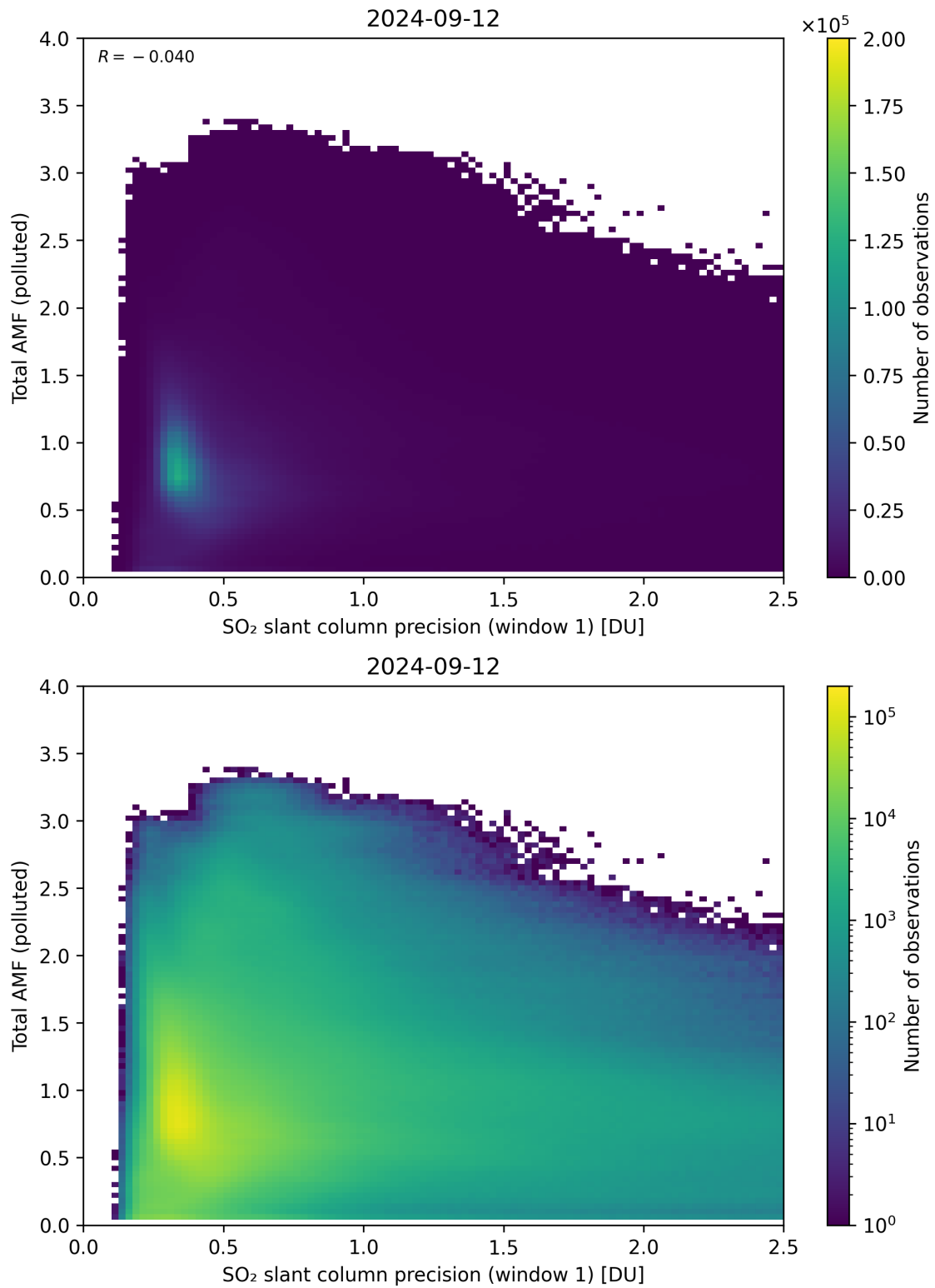
Figure 230: Scatter density plot of “SO 2 slant column precision (window 1)” against “Total AMF (polluted)” for 2024-09-12 to 2024-09-13.
