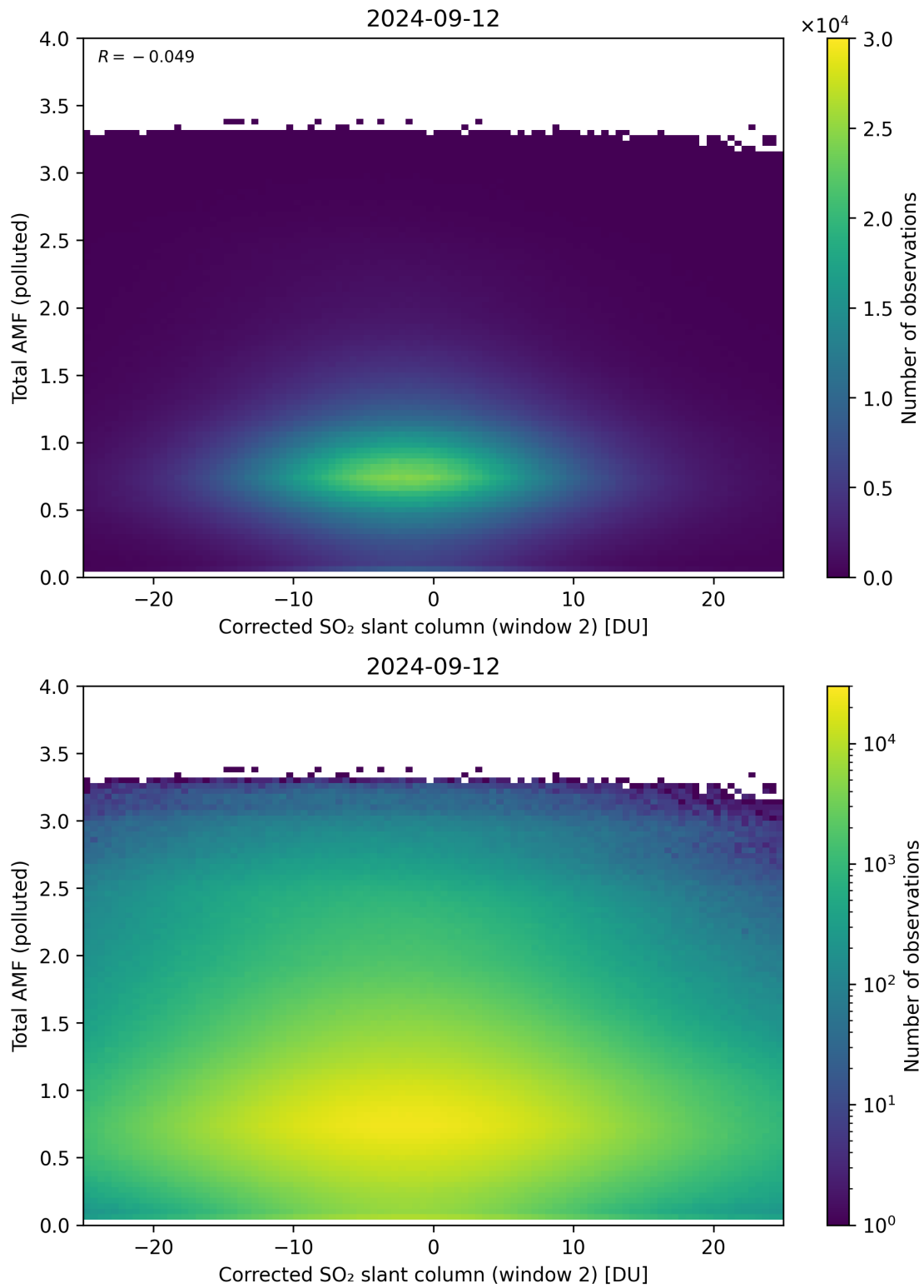
Figure 203: Scatter density plot of “Corrected SO 2 slant column (window 2)” against “Total AMF (polluted)” for 2024-09-12 to 2024-09-13.
