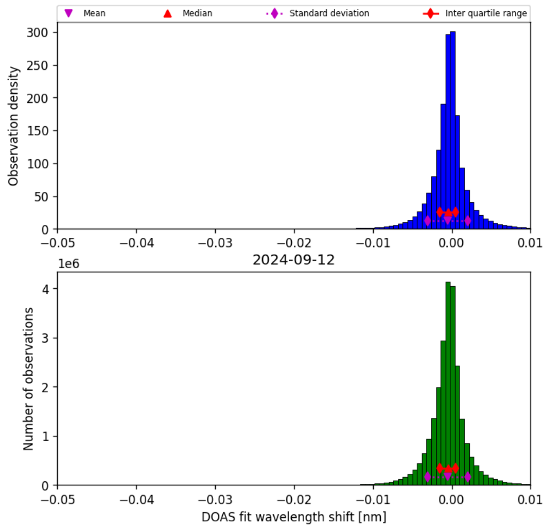
Figure 68: Histogram of “DOAS fit wavelength shift” for 2024-09-12 to 2024-09-13
