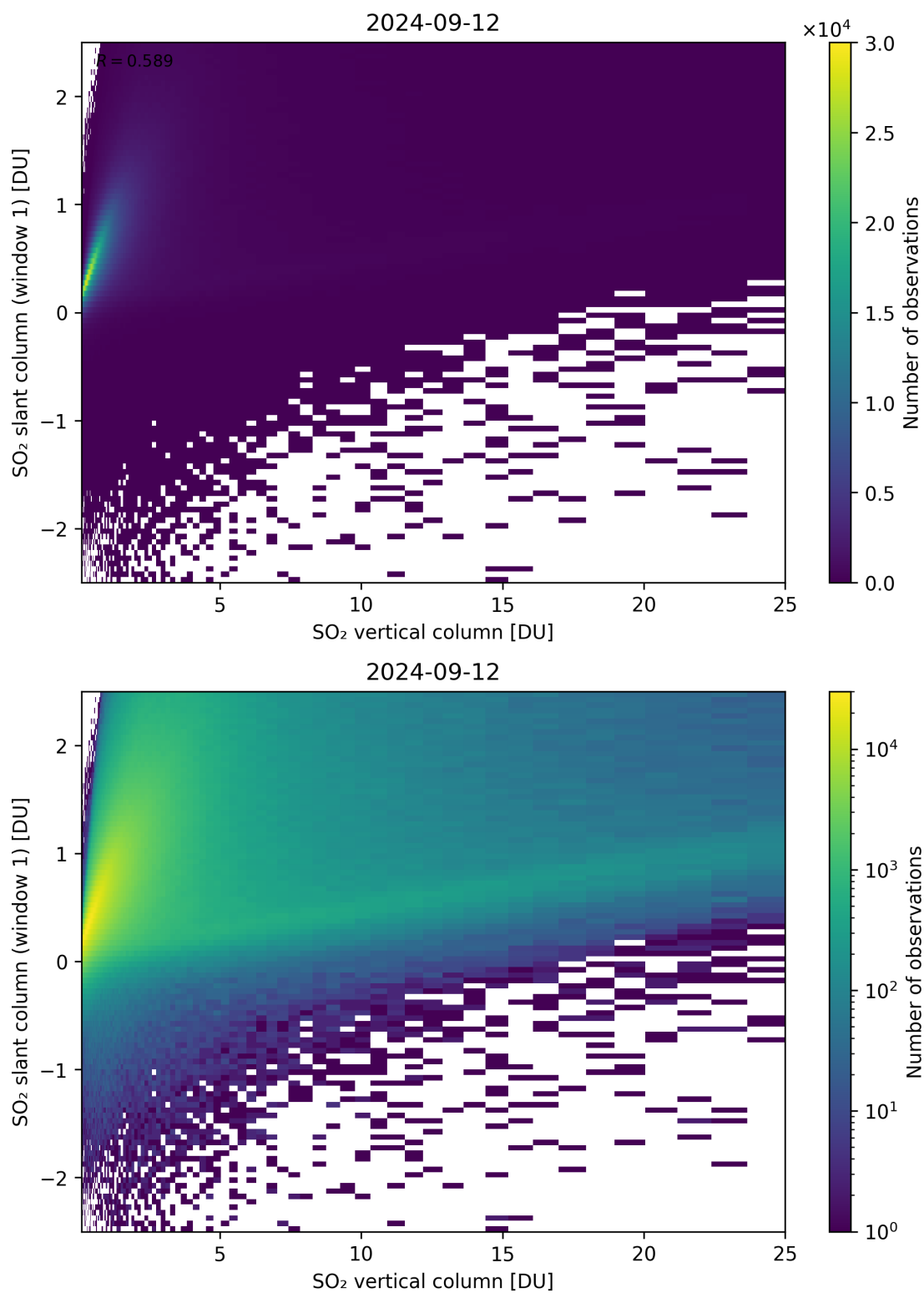
Figure 300: Scatter density plot of “SO 2 vertical column” against “SO 2 slant column (window 1)” for 2024-09-12 to 2024-09-13.
