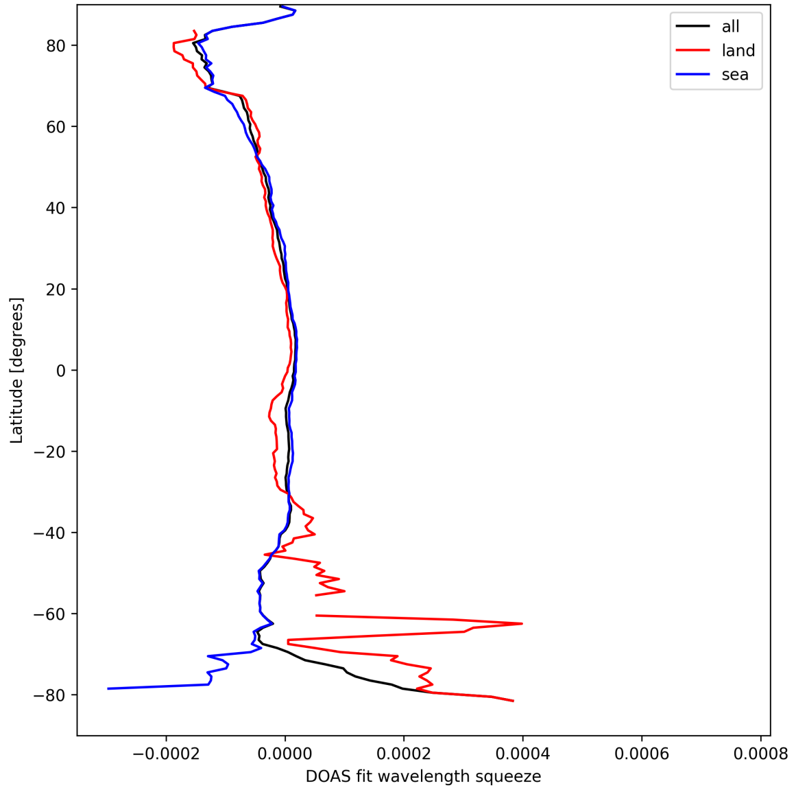
Figure 46: Zonal average of “DOAS fit wavelength squeeze” for 2024-09-12 to 2024-09-13.
