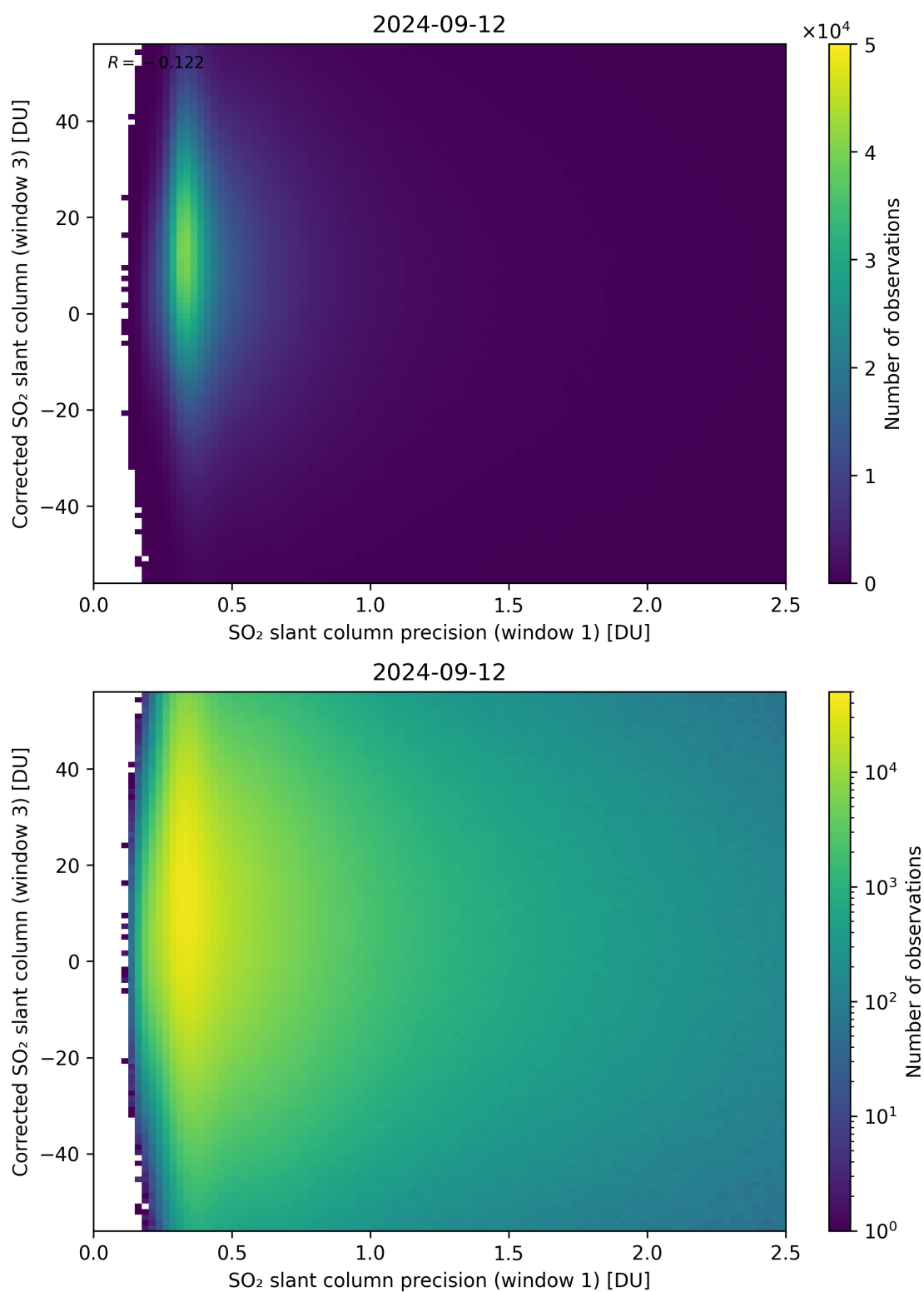
Figure 226: Scatter density plot of “SO 2 slant column precision (window 1)” against “Corrected SO 2 slant column (window 3)” for 2024-09-12 to 2024-09-13.
