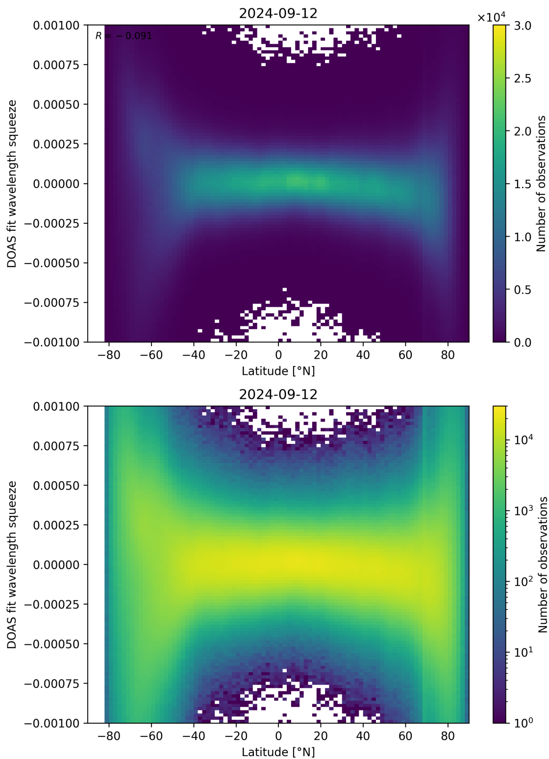
Figure 143: Scatter density plot of “Latitude” against “DOAS fit wavelength squeeze” for 2024-09-12 to 2024-09-13.
