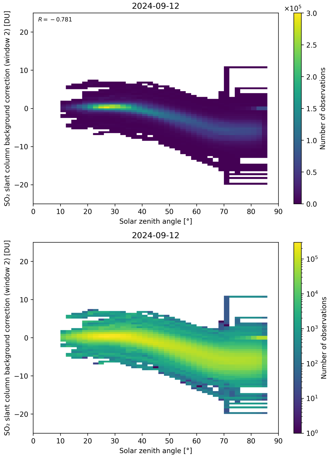
Figure 159: Scatter density plot of “Solar zenith angle” against “SO 2 slant column background correction (window 2)” for 2024-09-12 to 2024-09-13.
