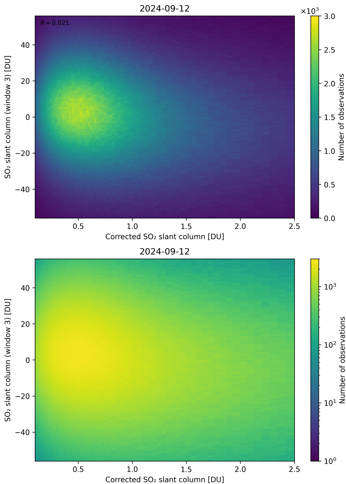
Figure 190: Scatter density plot of “Corrected SO 2 slant column” against “SO 2 slant column (window 3)” for 2024-09-12 to 2024-09-13.
