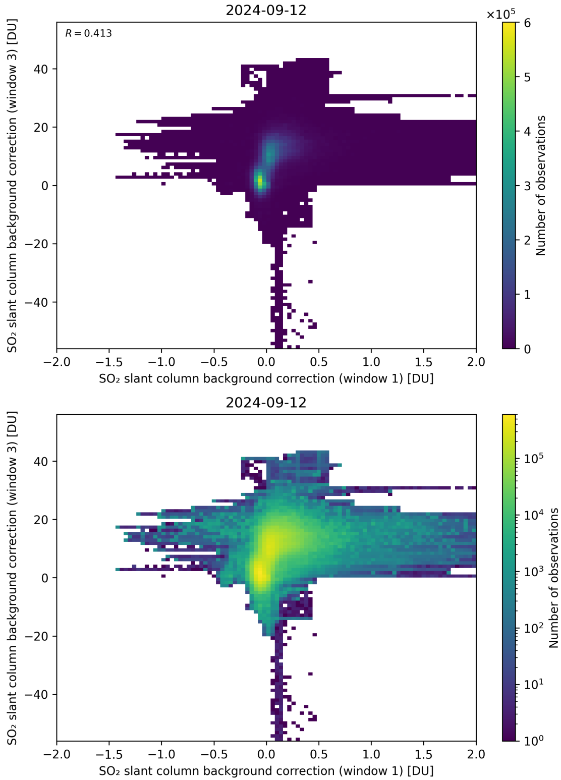
Figure 99: Scatter density plot of “SO 2 slant column background correction (window 1)” against “SO 2 slant column background correction (window 3)” for 2024-09-12 to 2024-09-13.
