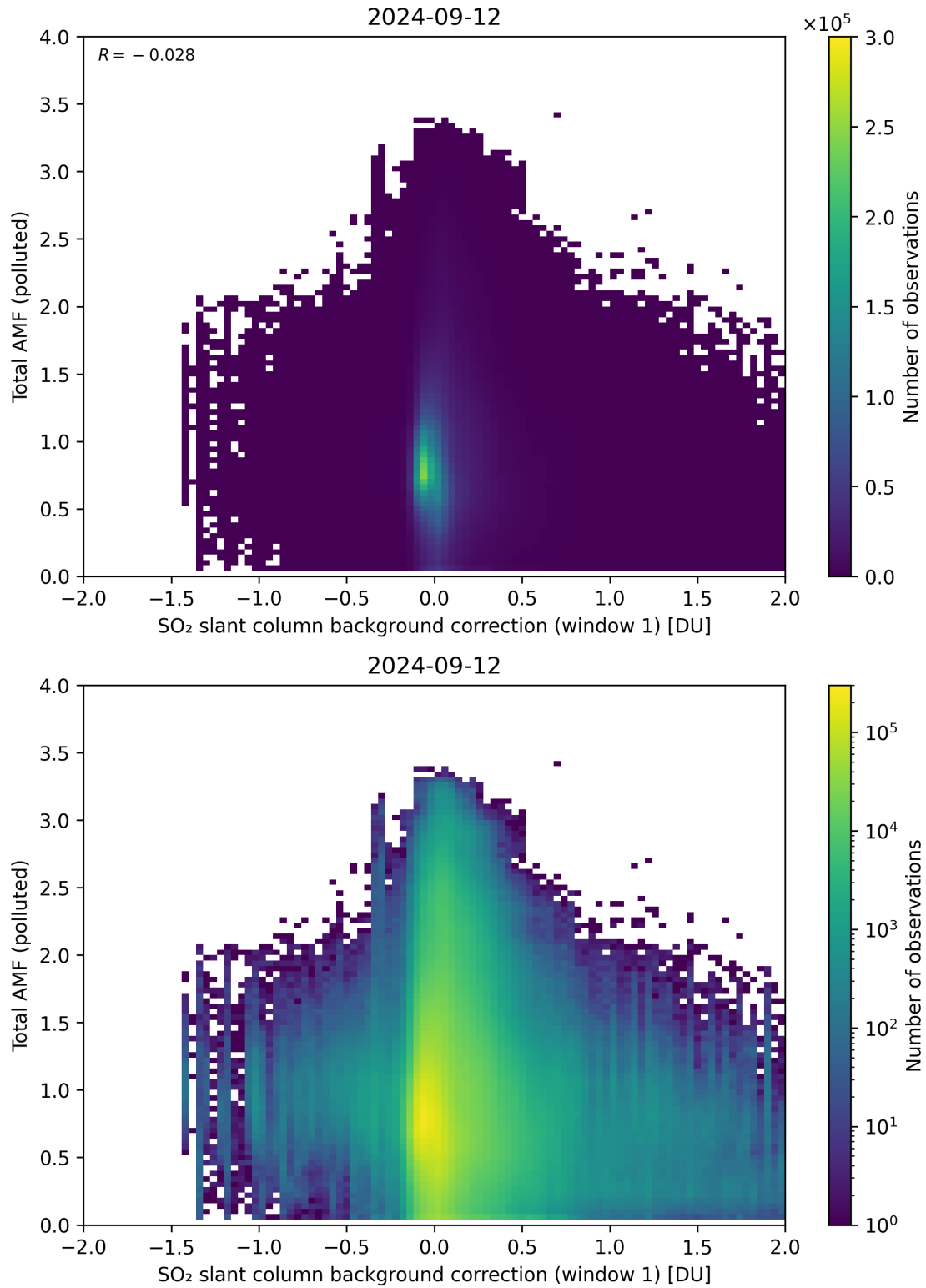
Figure 109: Scatter density plot of “SO 2 slant column background correction (window 1)” against “Total AMF (polluted)” for 2024-09-12 to 2024-09-13.
