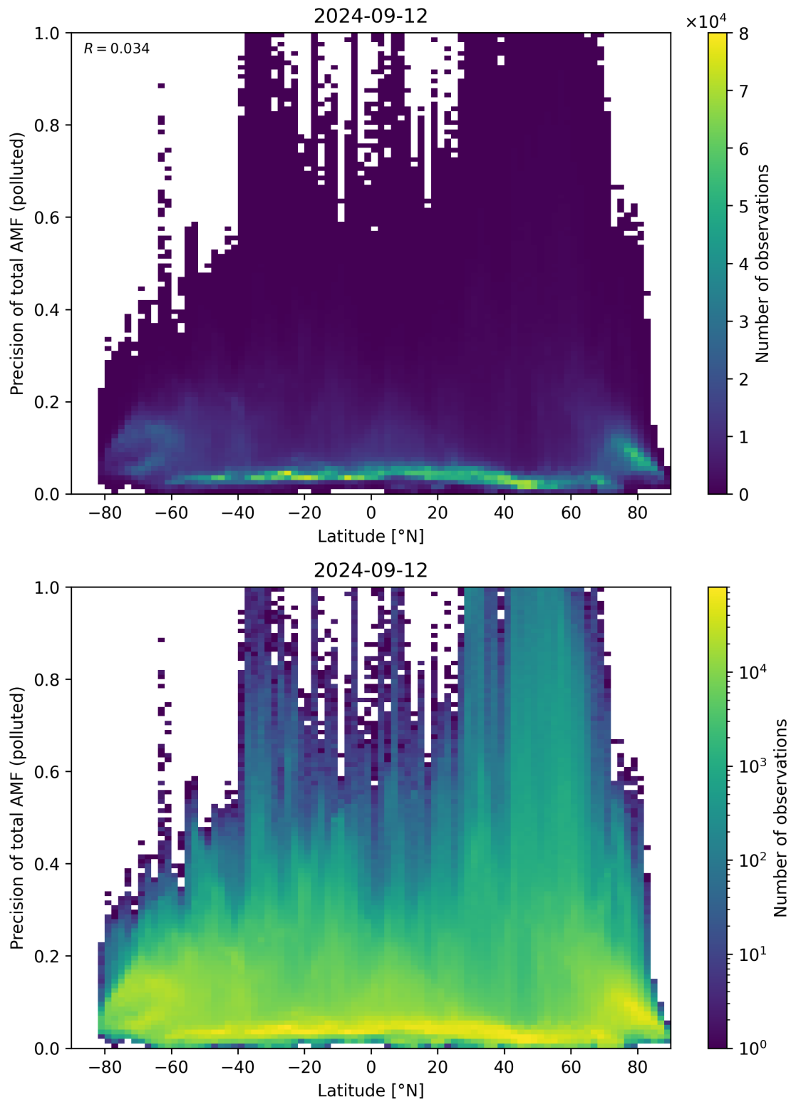
Figure 155: Scatter density plot of “Latitude” against “Precision of total AMF (polluted)” for 2024-09-12 to 2024-09-13.
