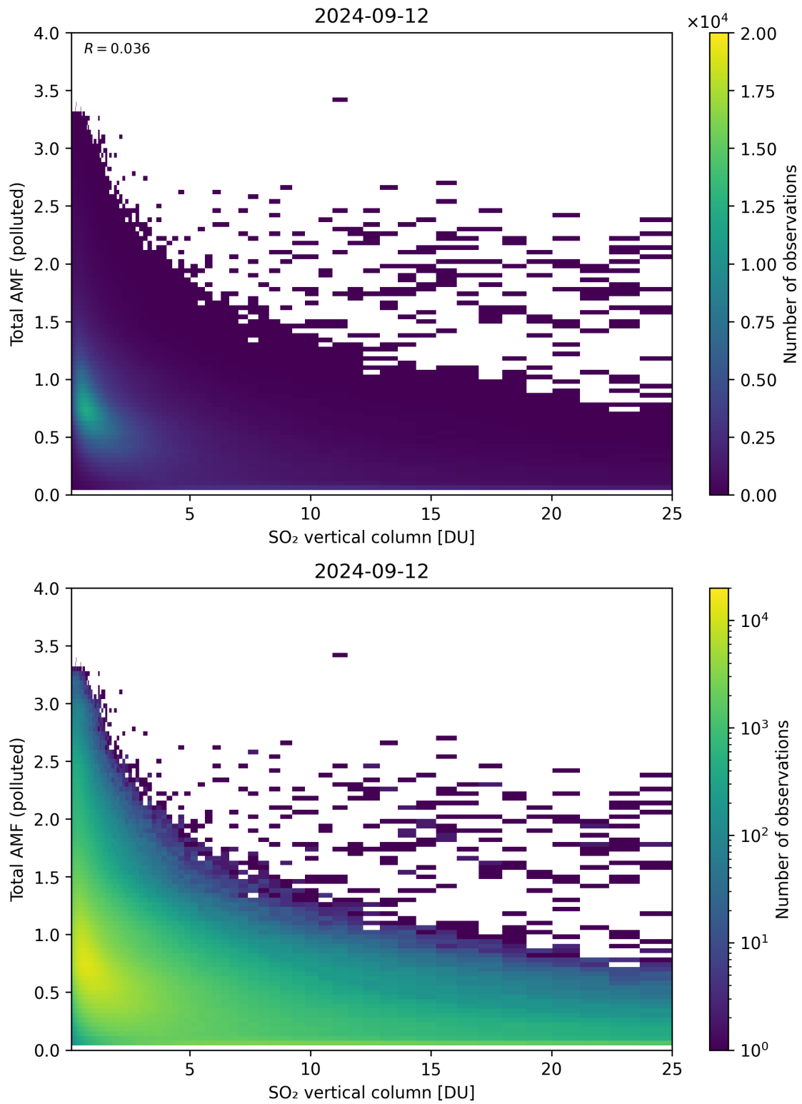
Figure 305: Scatter density plot of “SO 2 vertical column” against “Total AMF (polluted)” for 2024-09-12 to 2024-09-13.
