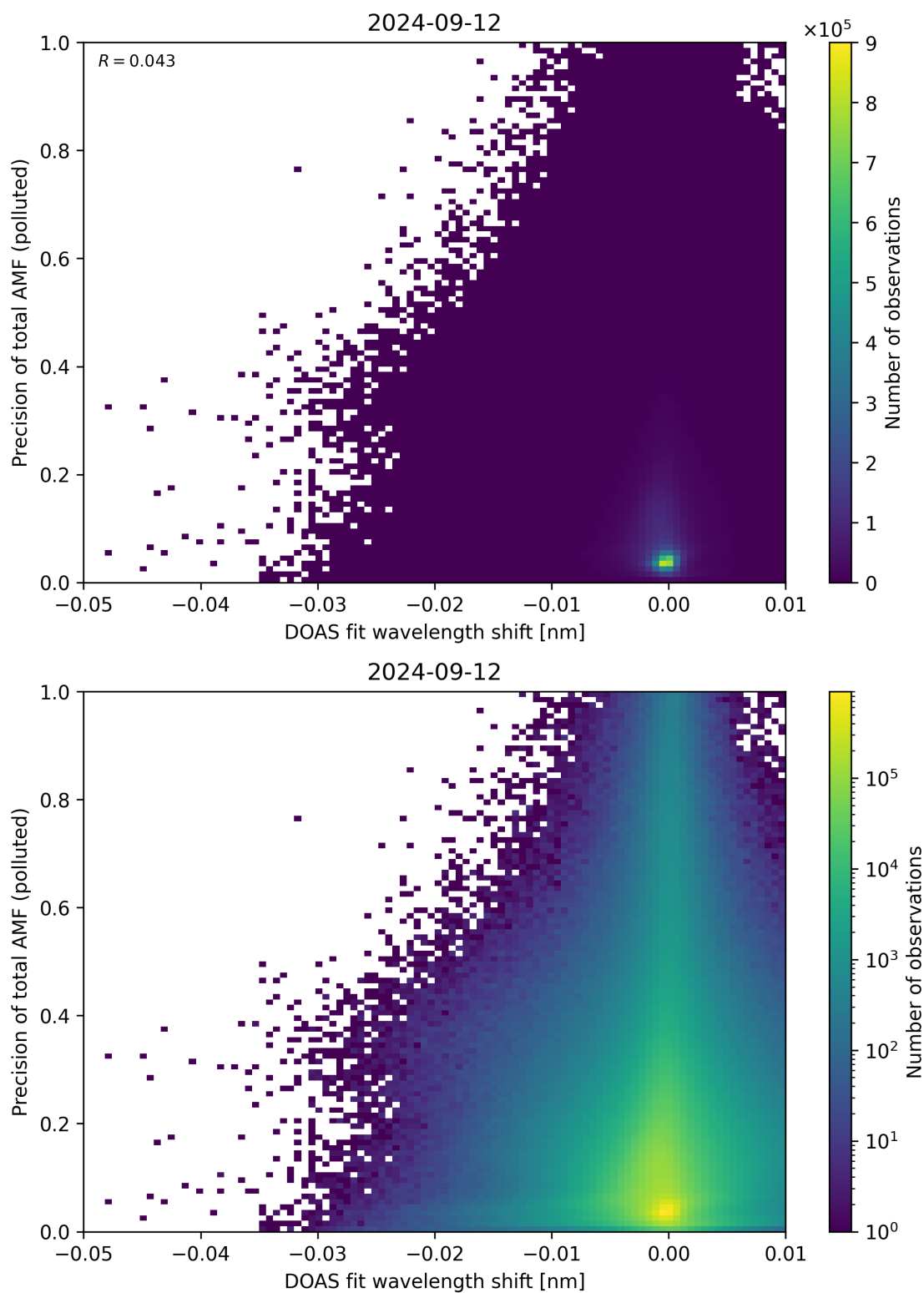
Figure 131: Scatter density plot of “DOAS fit wavelength shift” against “Precision of total AMF (polluted)” for 2024-09-12 to 2024-09-13.
