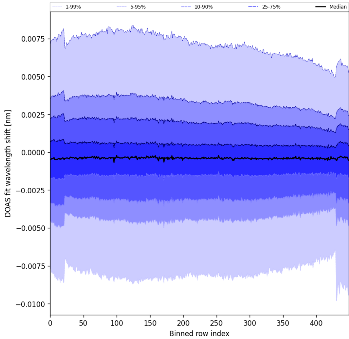
Figure 91: Along track statistics of “DOAS fit wavelength shift” for 2024-09-12 to 2024-09-13
