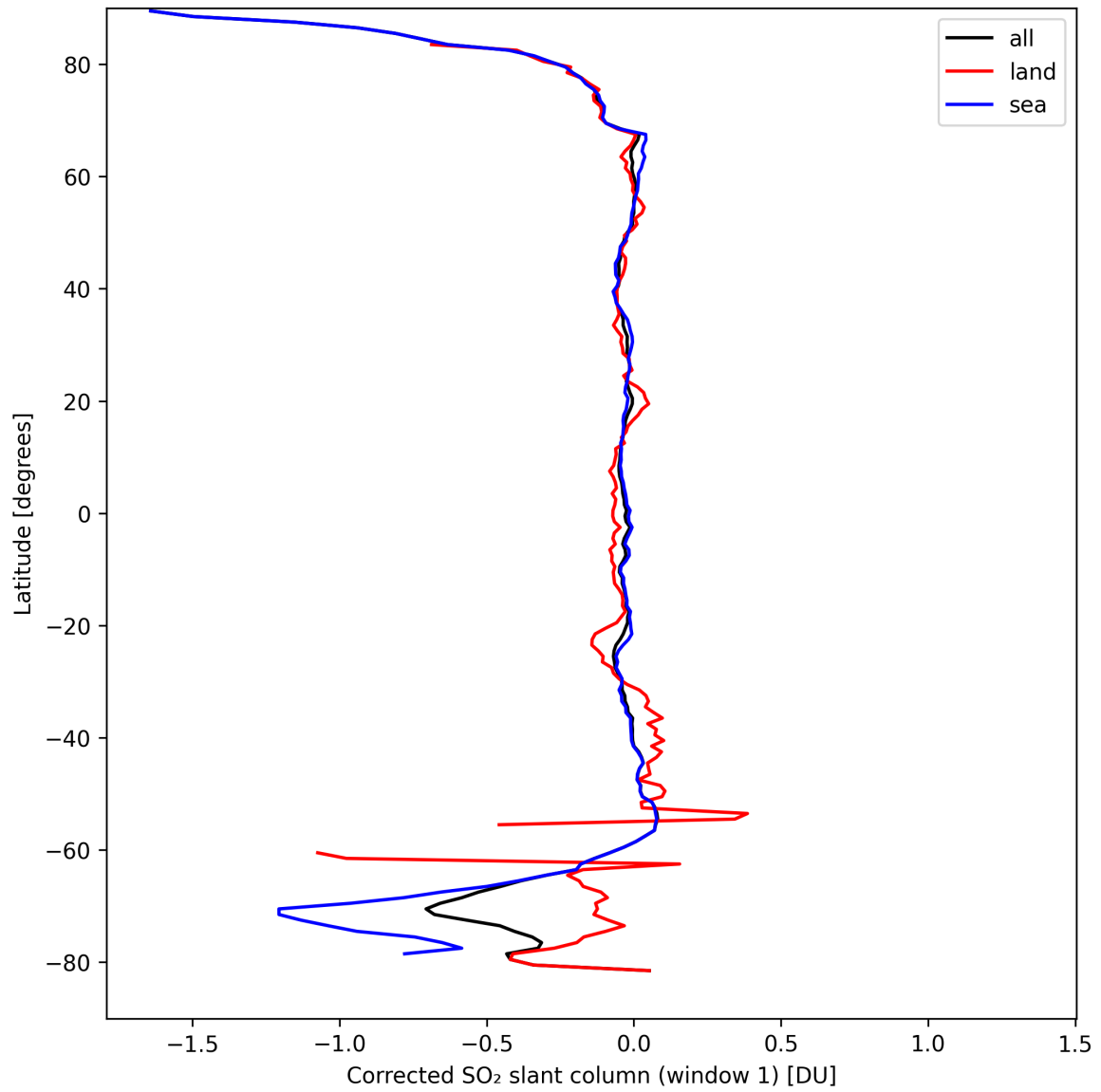
Figure 35: Zonal average of “Corrected SO 2 slant column (window 1)” for 2024-09-12 to 2024-09-13.
