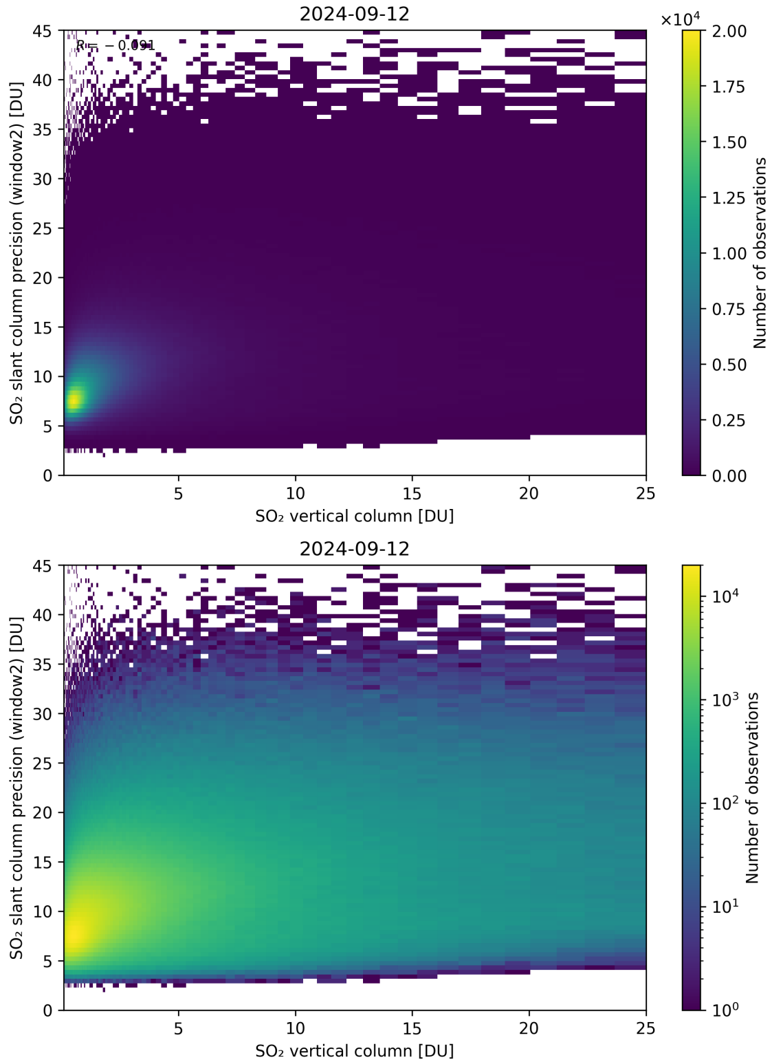
Figure 302: Scatter density plot of “SO 2 vertical column” against “SO 2 slant column precision (window2)” for 2024-09-12 to 2024-09-13.
