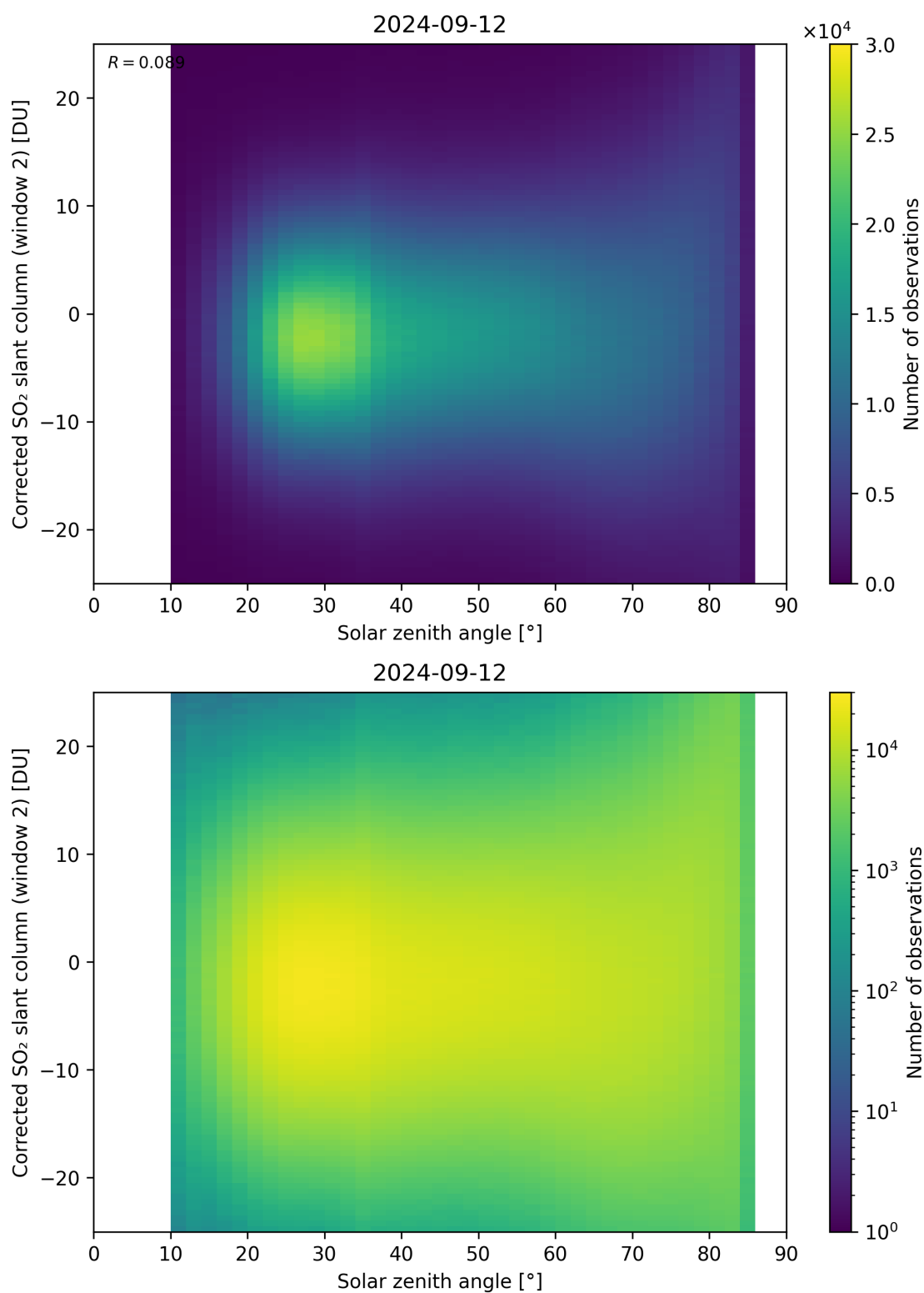
Figure 167: Scatter density plot of “Solar zenith angle” against “Corrected SO 2 slant column (window 2)” for 2024-09-12 to 2024-09-13.
