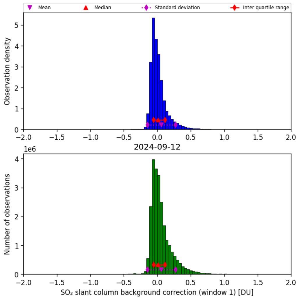
Figure 59: Histogram of “SO 2 slant column background correction (window 1)” for 2024-09-12 to 2024-09-13
