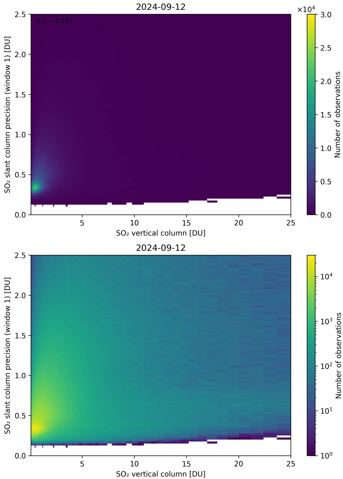
Figure 301: Scatter density plot of “SO 2 vertical column” against “SO 2 slant column precision (window 1)” for 2024-09-12 to 2024-09-13.
