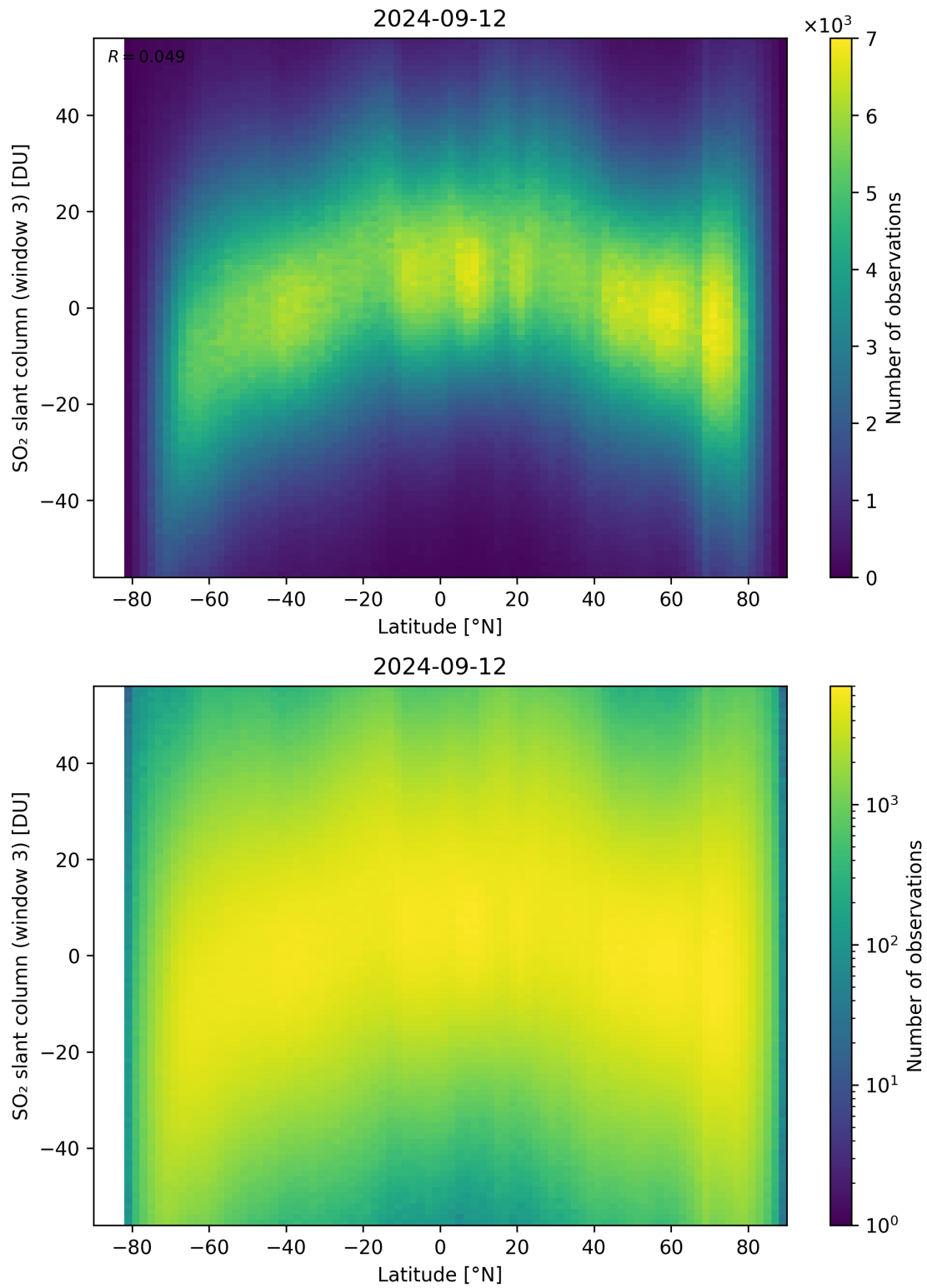
Figure 152: Scatter density plot of “Latitude” against “SO 2 slant column (window 3)” for 2024-09-12 to 2024-09-13.
