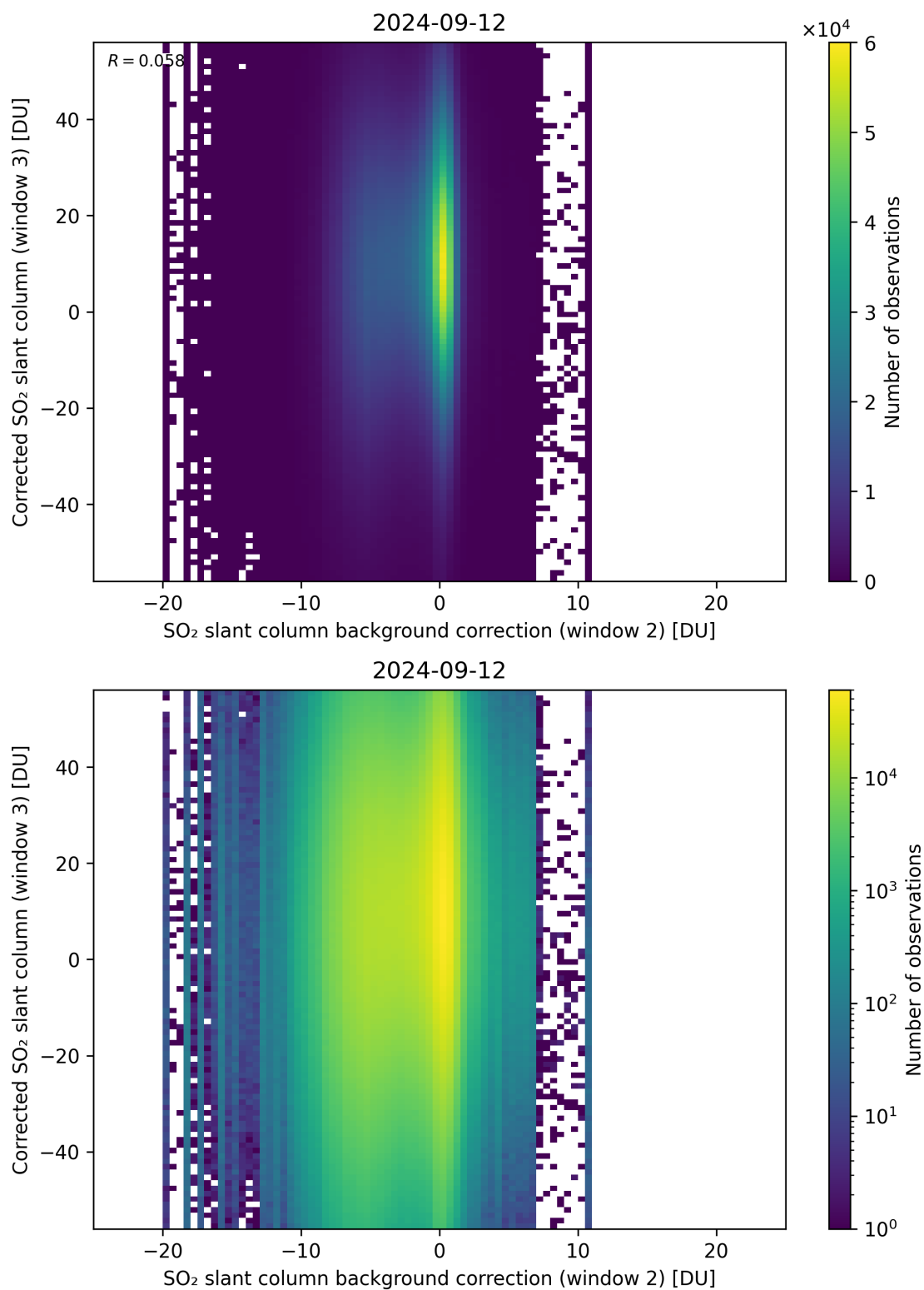
Figure 116: Scatter density plot of “SO 2 slant column background correction (window 2)” against “Corrected SO 2 slant column (window 3)” for 2024-09-12 to 2024-09-13.
