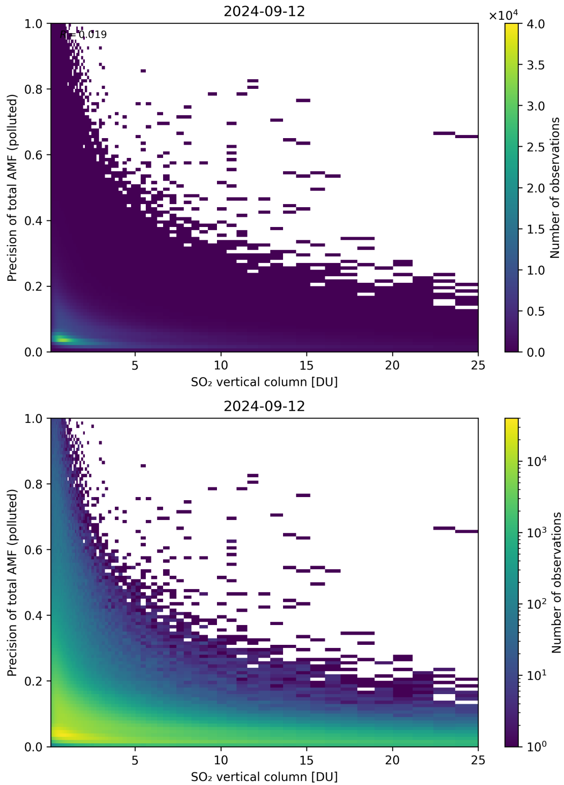
Figure 306: Scatter density plot of “SO 2 vertical column” against “Precision of total AMF (polluted)” for 2024-09-12 to 2024-09-13.
