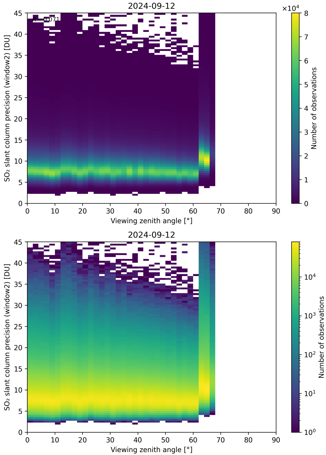
Figure 322: Scatter density plot of “Viewing zenith angle” against “SO 2 slant column precision (window2)” for 2024-09-12 to 2024-09-13.
