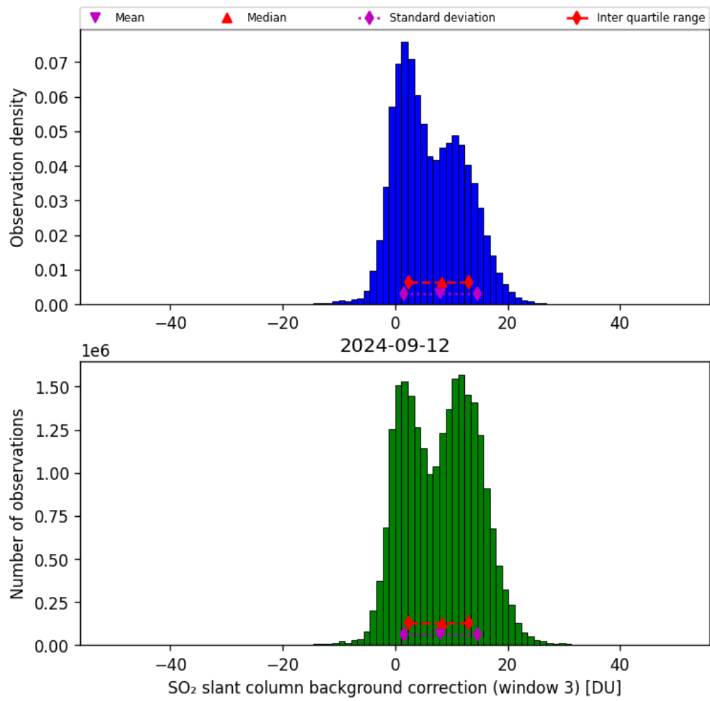
Figure 67: Histogram of “SO 2 slant column background correction (window 3)” for 2024-09-12 to 2024-09-13
