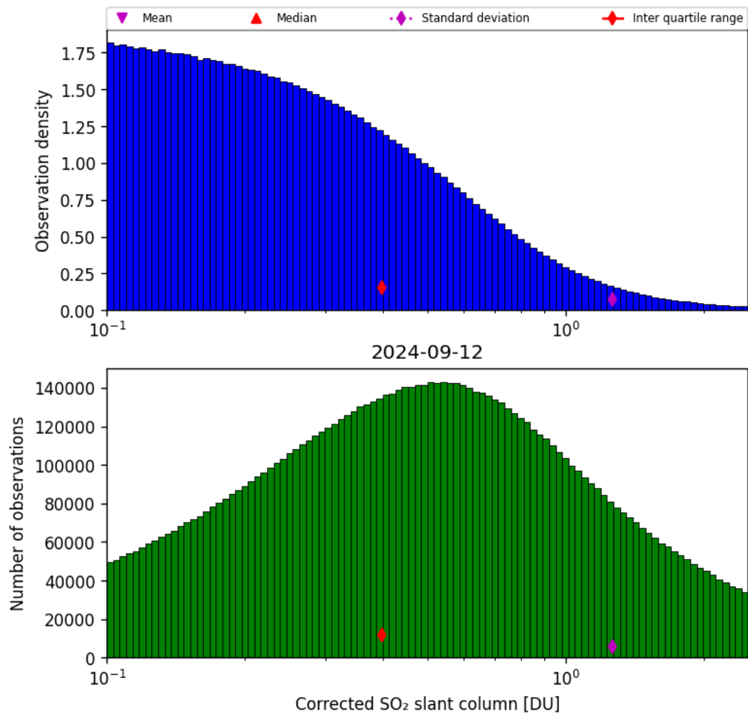
Figure 55: Histogram of “Corrected SO 2 slant column” for 2024-09-12 to 2024-09-13
