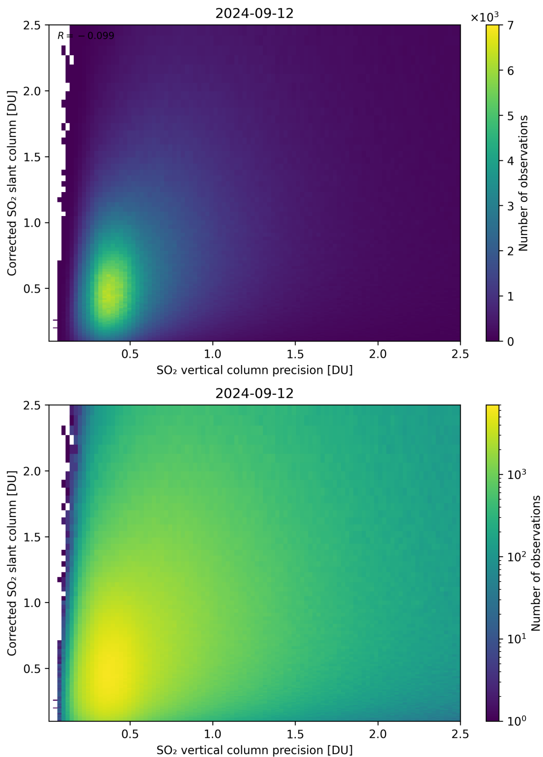
Figure 286: Scatter density plot of “SO 2 vertical column precision” against “Corrected SO 2 slant column” for 2024-09-12 to 2024-09-13.
