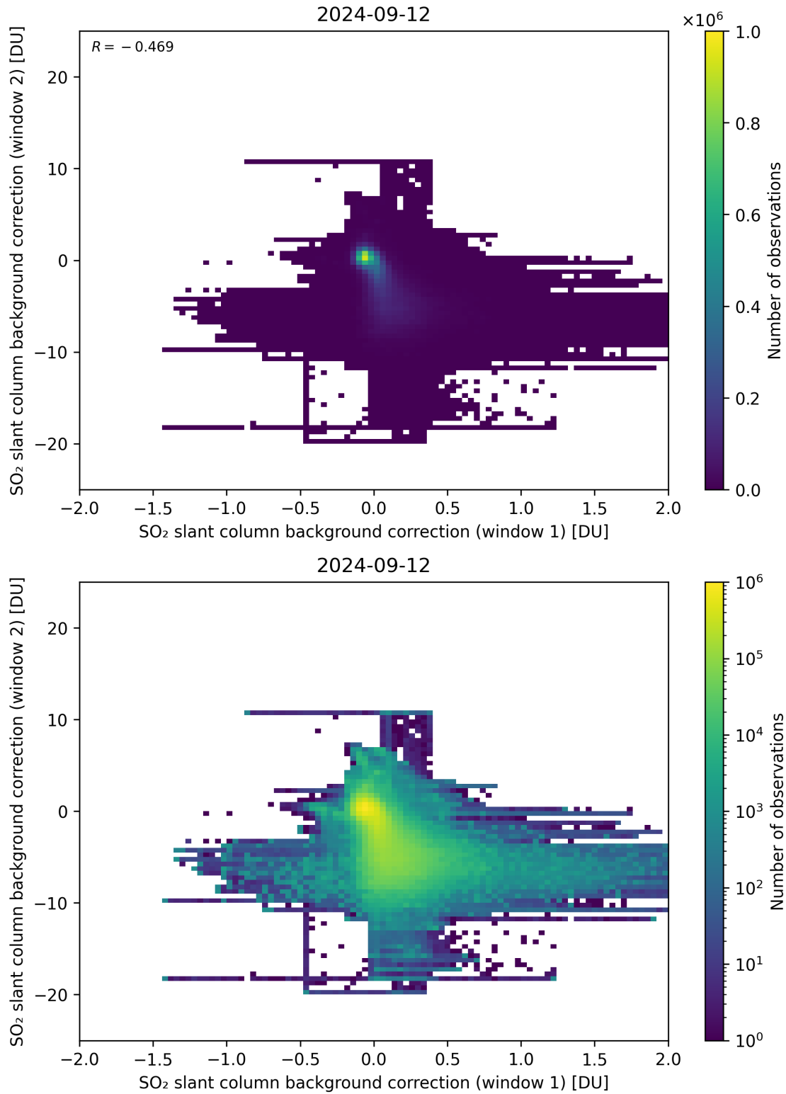
Figure 98: Scatter density plot of “SO 2 slant column background correction (window 1)” against “SO 2 slant column background correction (window 2)” for 2024-09-12 to 2024-09-13.
