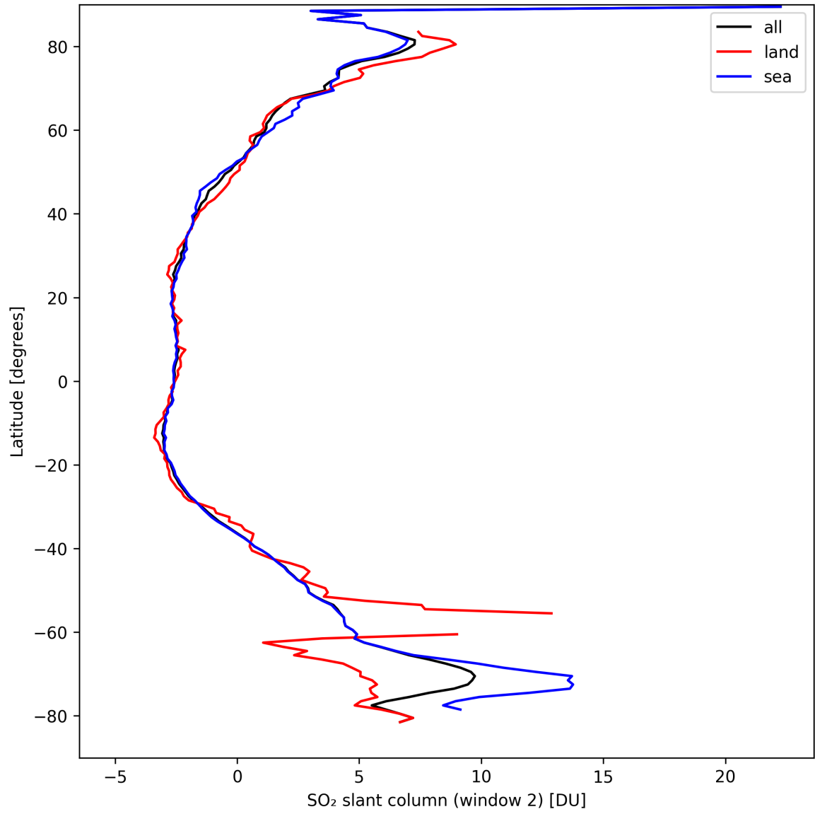
Figure 37: Zonal average of “SO 2 slant column (window 2)” for 2024-09-12 to 2024-09-13.
