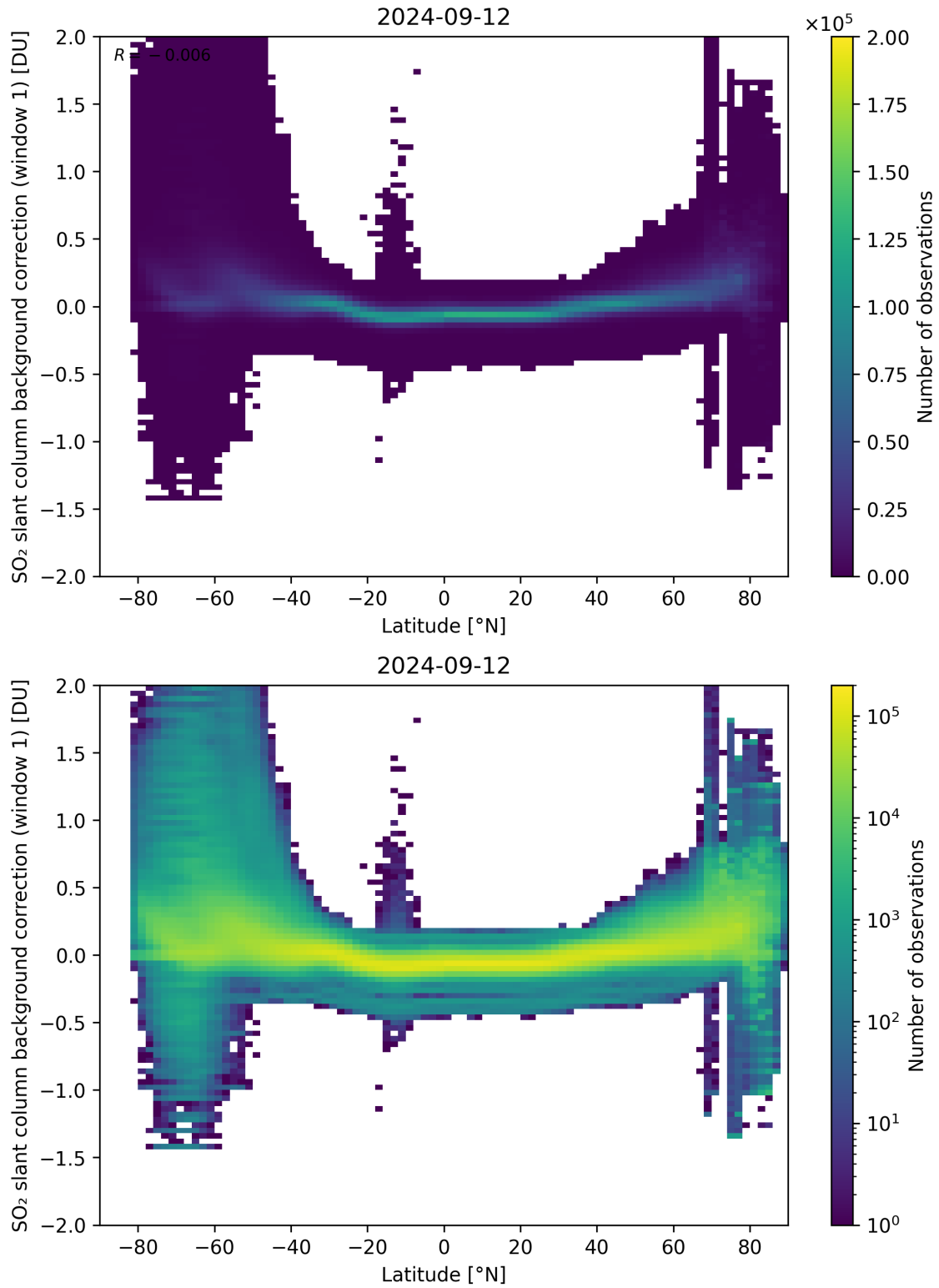
Figure 139: Scatter density plot of “Latitude” against “SO 2 slant column background correction (window 1)” for 2024-09-12 to 2024-09-13.
