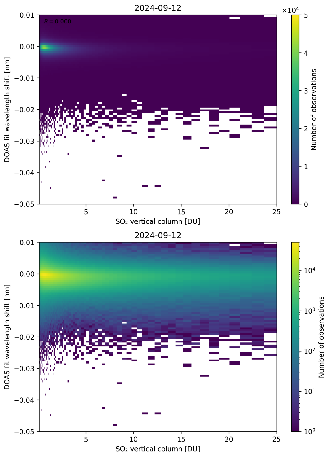
Figure 276: Scatter density plot of “SO 2 vertical column” against “DOAS fit wavelength shift” for 2024-09-12 to 2024-09-13.
