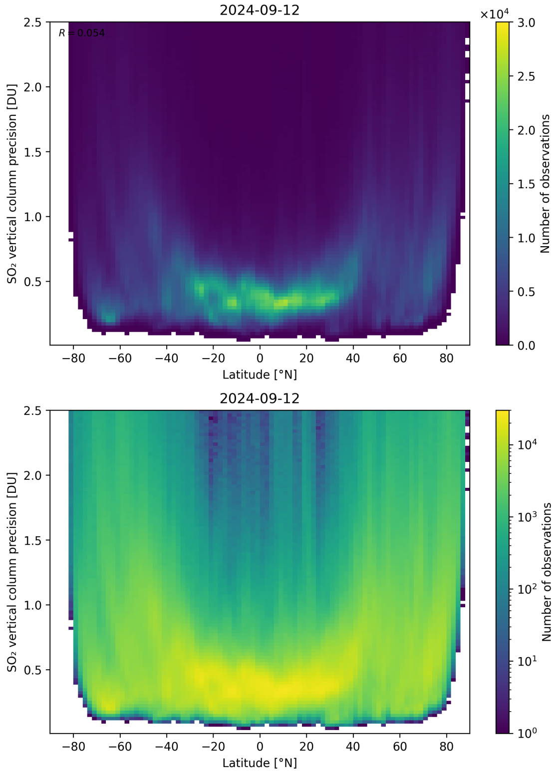
Figure 157: Scatter density plot of “Latitude” against “SO 2 vertical column precision” for 2024-09-12 to 2024-09-13.
