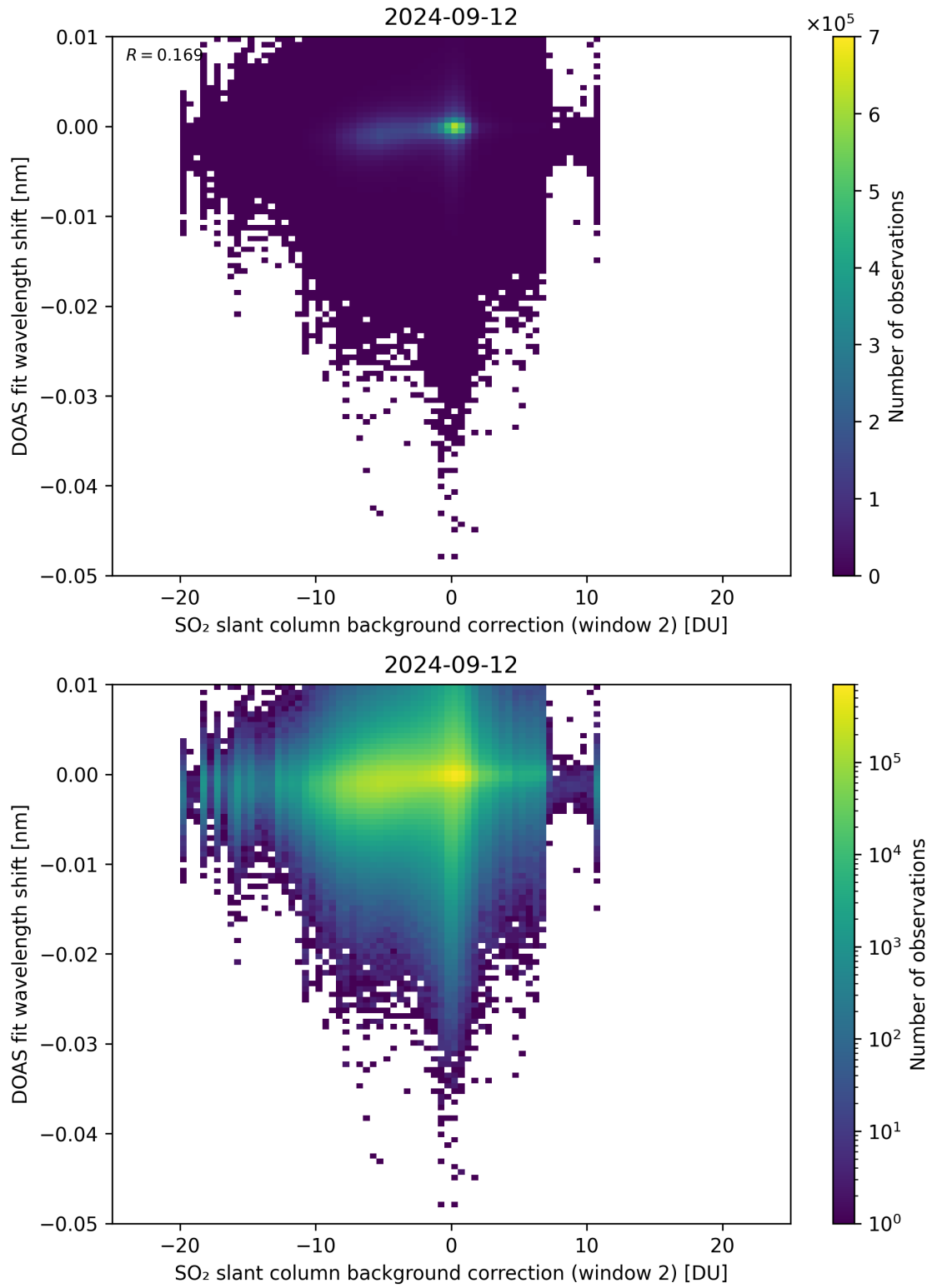
Figure 112: Scatter density plot of “SO 2 slant column background correction (window 2)” against “DOAS fit wavelength shift” for 2024-09-12 to 2024-09-13.
