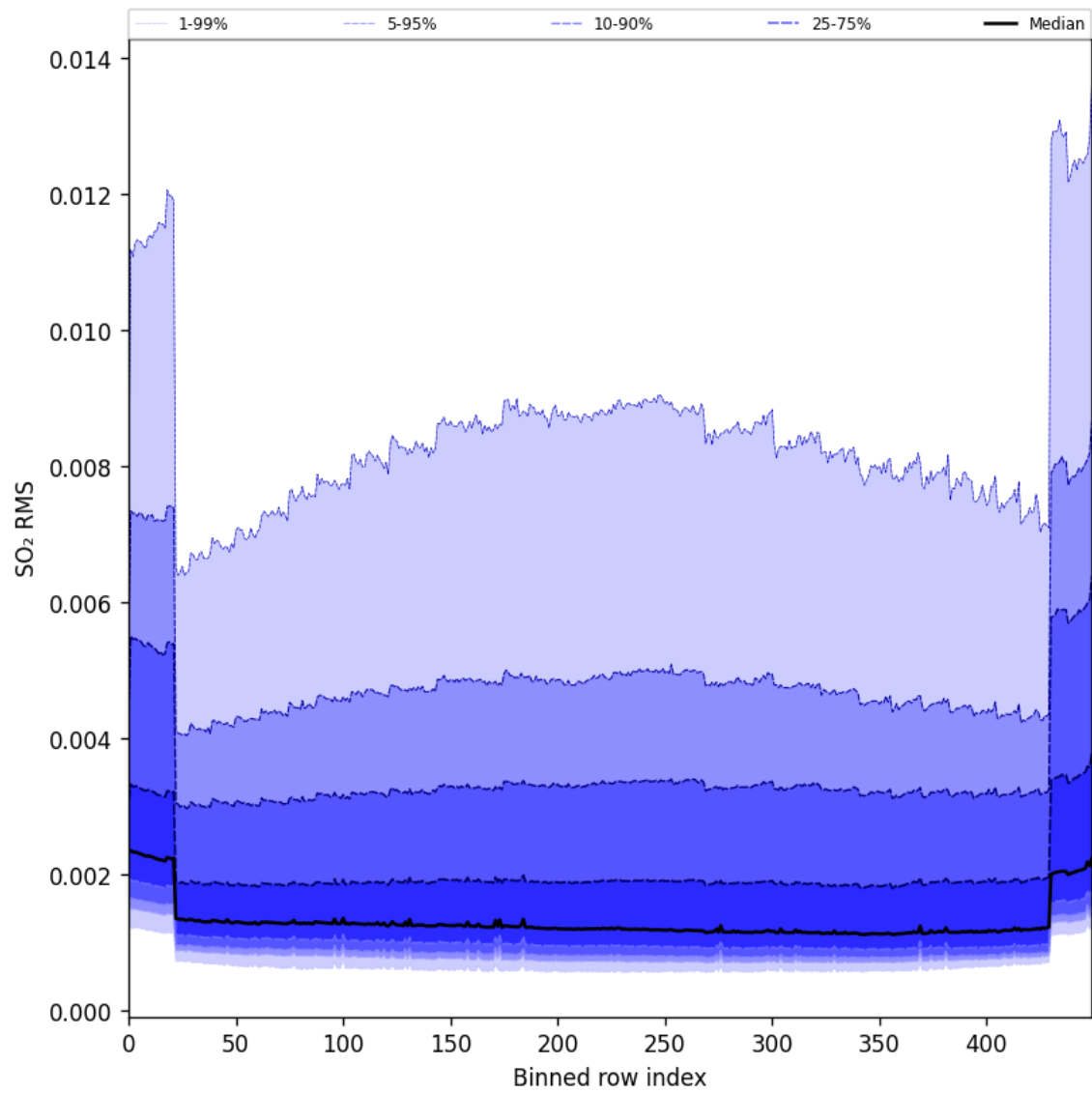
Figure 93: Along track statistics of “SO 2 RMS” for 2024-09-12 to 2024-09-13
