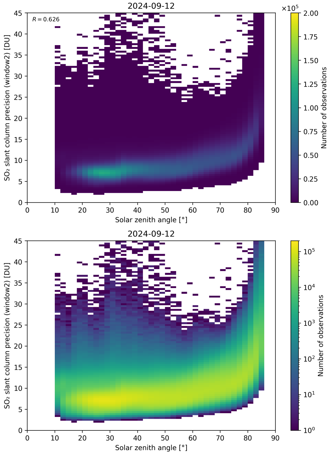
Figure 171: Scatter density plot of “Solar zenith angle” against “SO 2 slant column precision (window2)” for 2024-09-12 to 2024-09-13.
