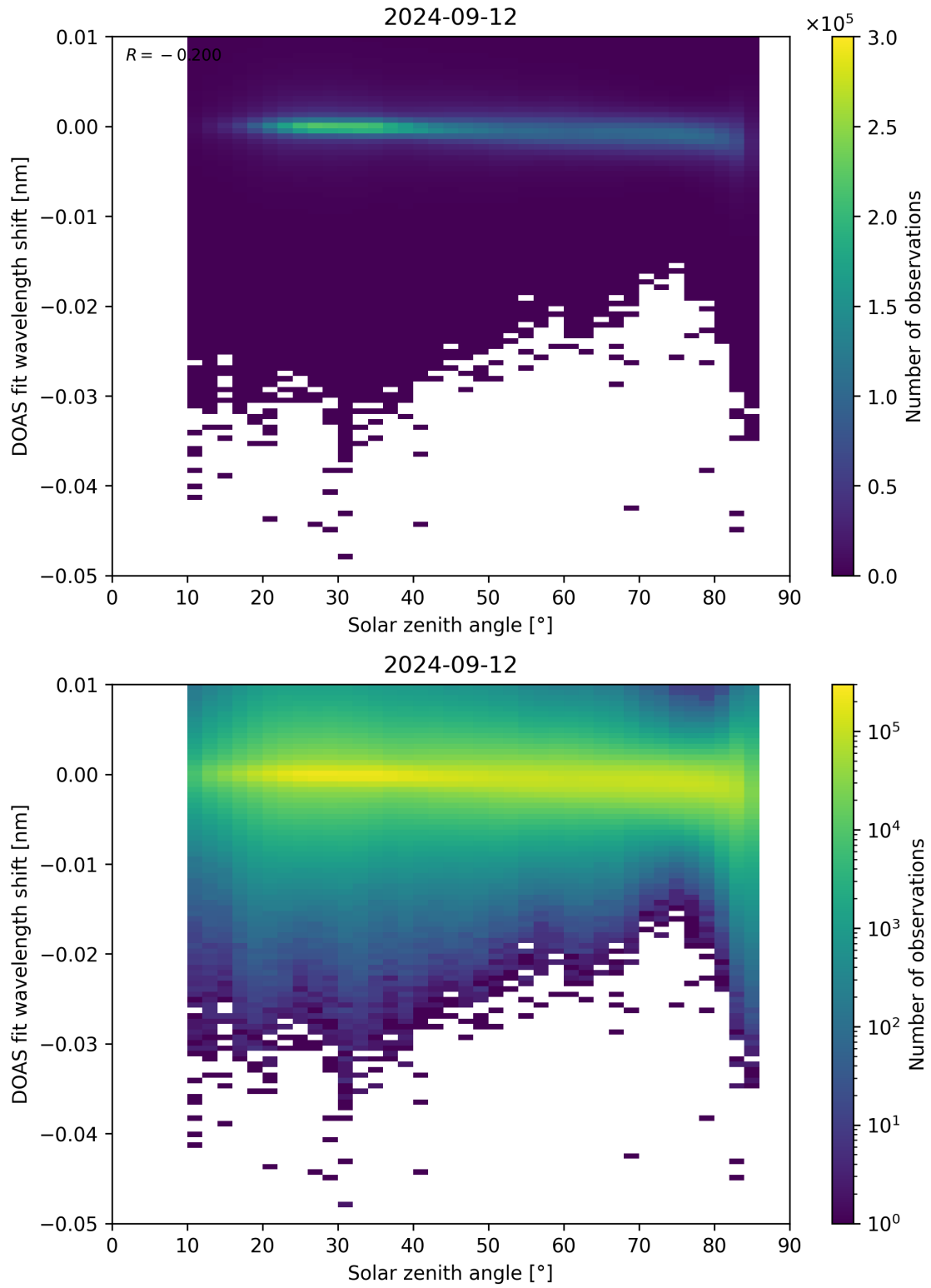
Figure 161: Scatter density plot of “Solar zenith angle” against “DOAS fit wavelength shift” for 2024-09-12 to 2024-09-13.
