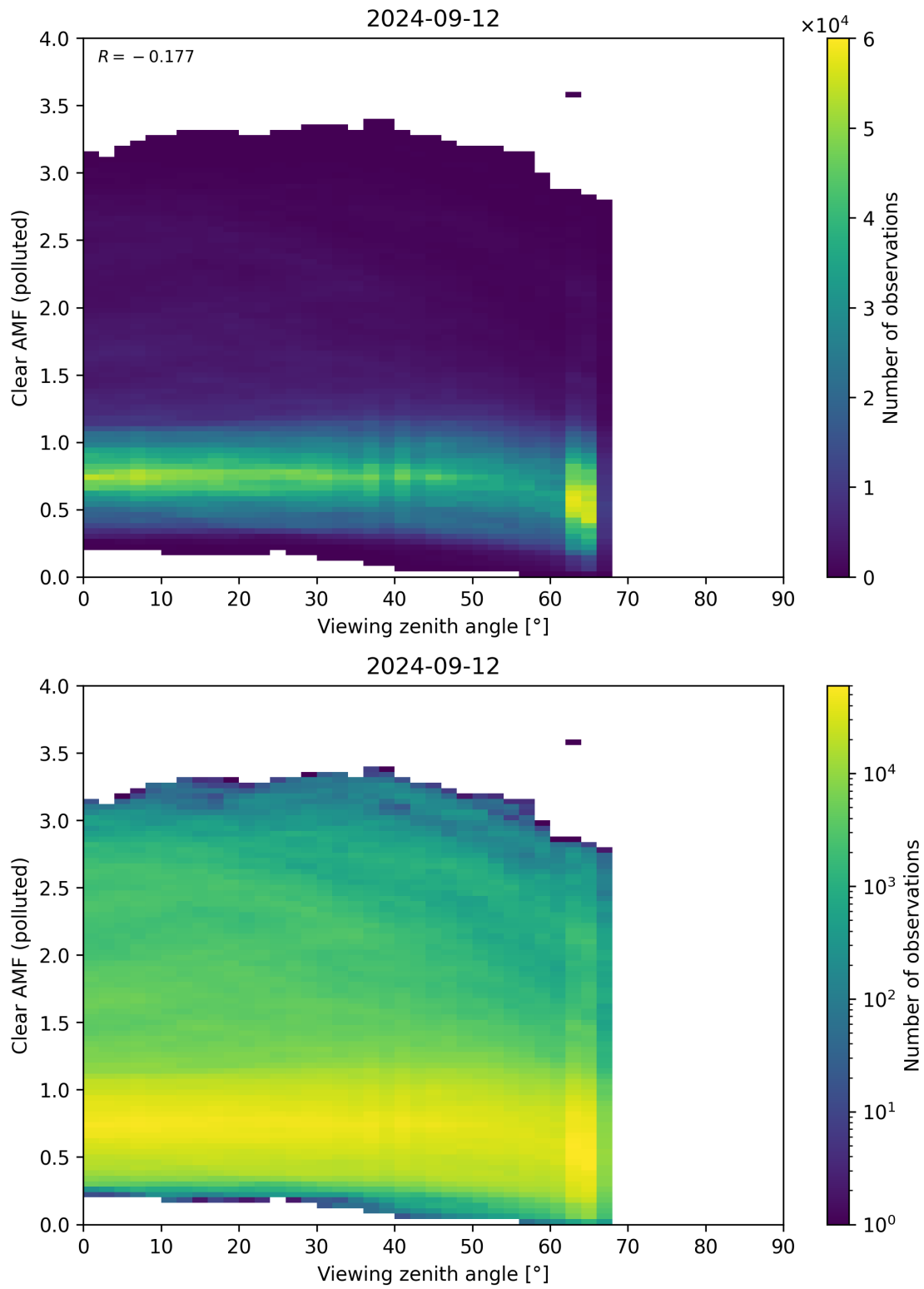
Figure 316: Scatter density plot of “Viewing zenith angle” against “Clear AMF (polluted)” for 2024-09-12 to 2024-09-13.
