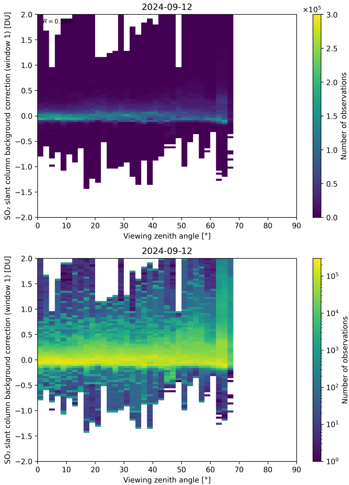
Figure 308: Scatter density plot of “Viewing zenith angle” against “SO 2 slant column background correction (window 1)” for 2024-09-12 to 2024-09-13.
