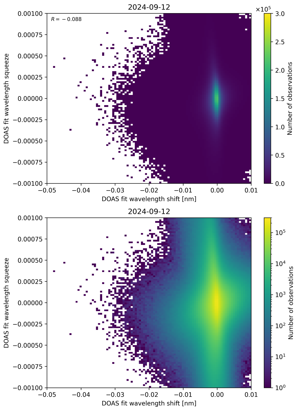
Figure 127: Scatter density plot of “DOAS fit wavelength shift” against “DOAS fit wavelength squeeze” for 2024-09-12 to 2024-09-13.
