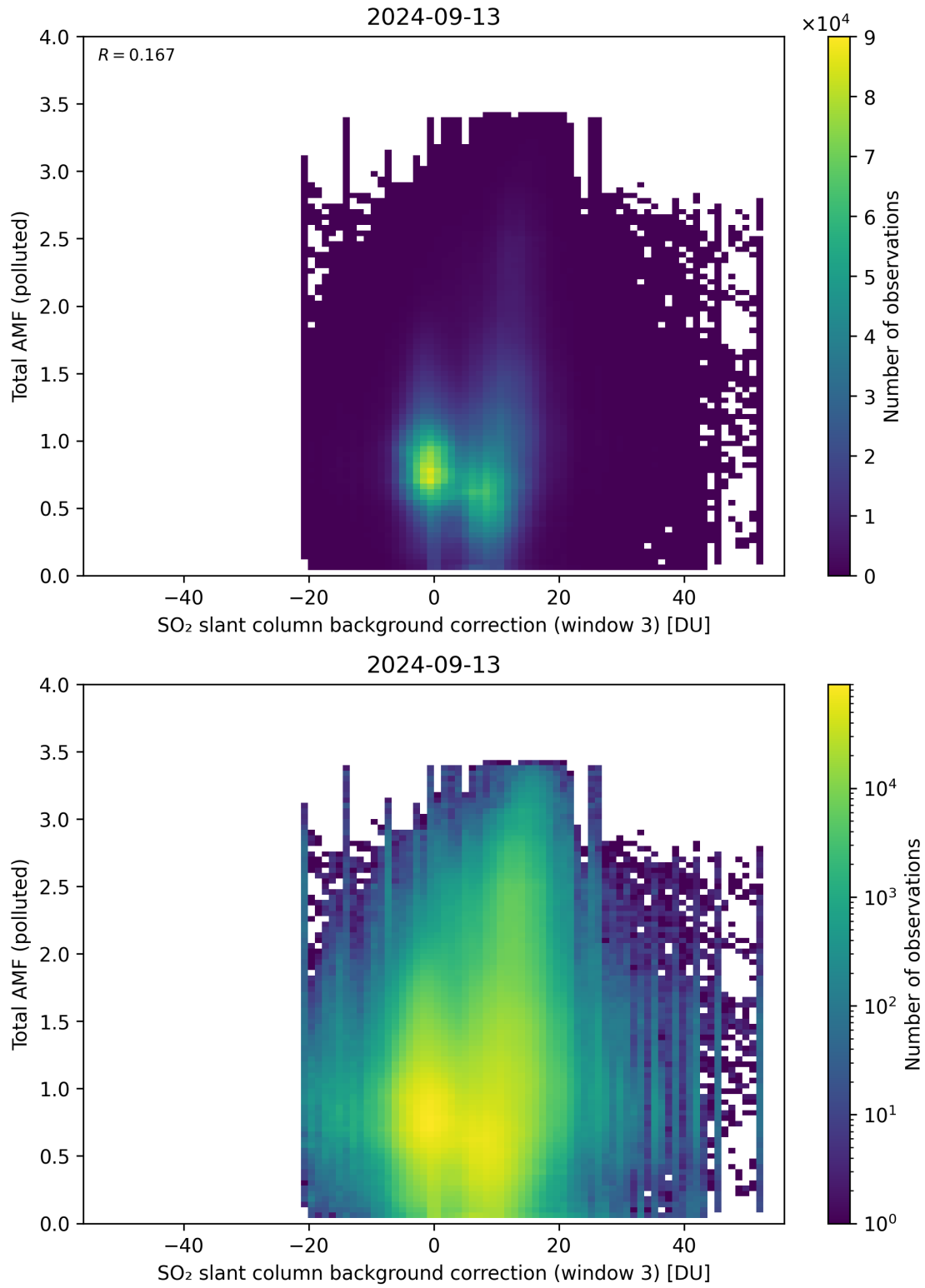
Figure 125: Scatter density plot of “SO 2 slant column background correction (window 3)” against “Total AMF (polluted)” for 2024-09-12 to 2024-09-14.
