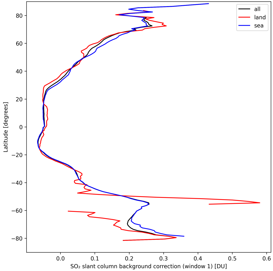
Figure 36: Zonal average of “SO 2 slant column background correction (window 1)” for 2024-09-12 to 2024-09-14.
