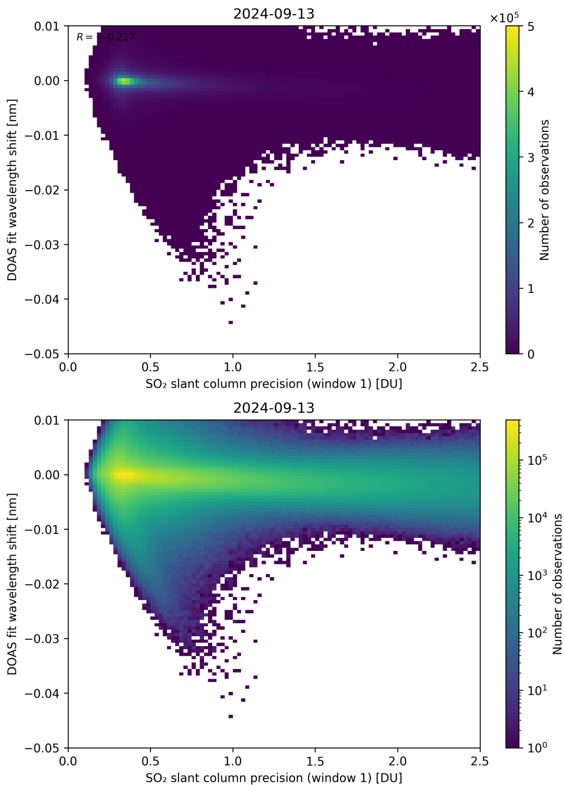
Figure 221: Scatter density plot of “SO 2 slant column precision (window 1)” against “DOAS fit wavelength shift” for 2024-09-12 to 2024-09-14.
