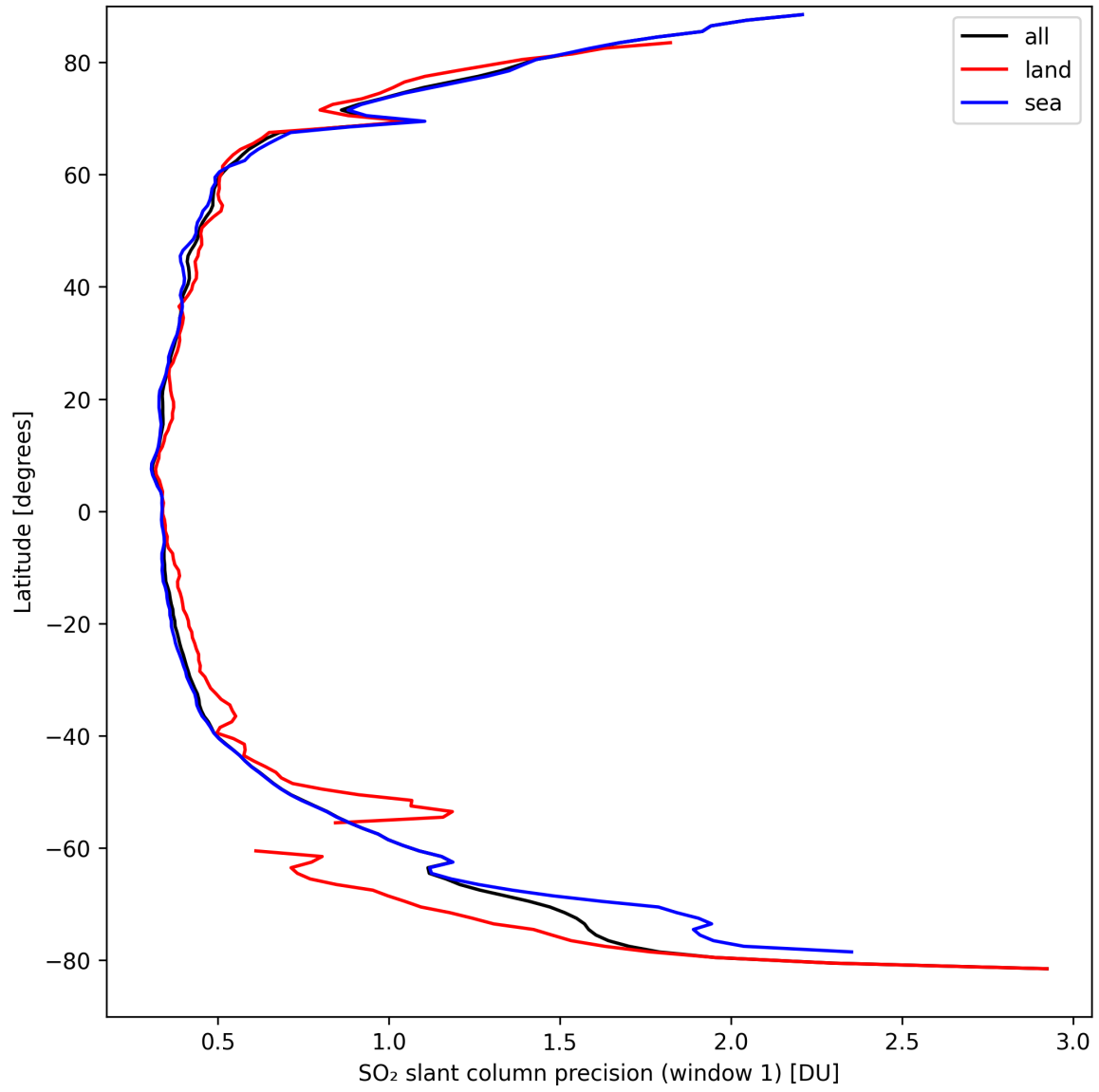
Figure 34: Zonal average of “SO 2 slant column precision (window 1)” for 2024-09-12 to 2024-09-14.
