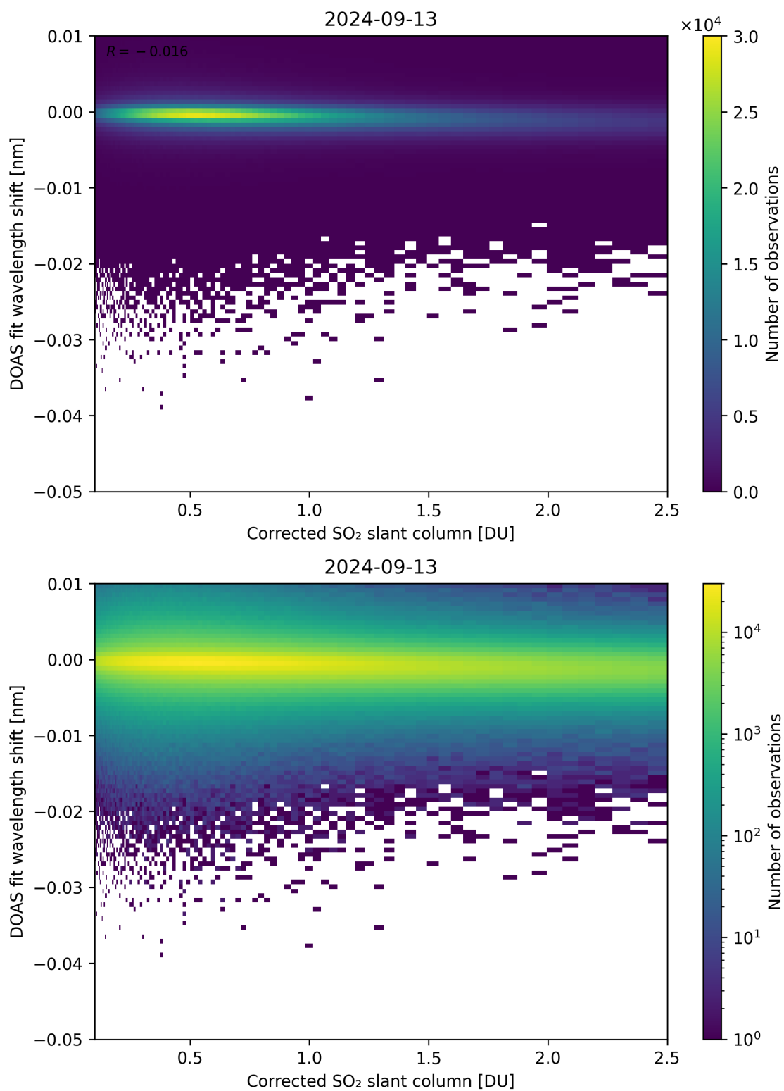
Figure 181: Scatter density plot of “Corrected SO 2 slant column” against “DOAS fit wavelength shift” for 2024-09-12 to 2024-09-14.
