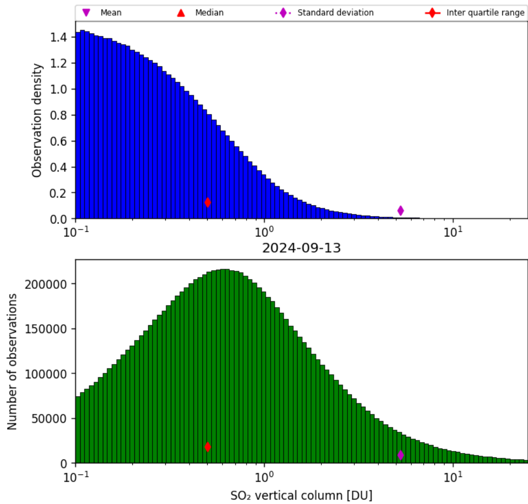
Figure 53: Histogram of “SO 2 vertical column” for 2024-09-12 to 2024-09-14
