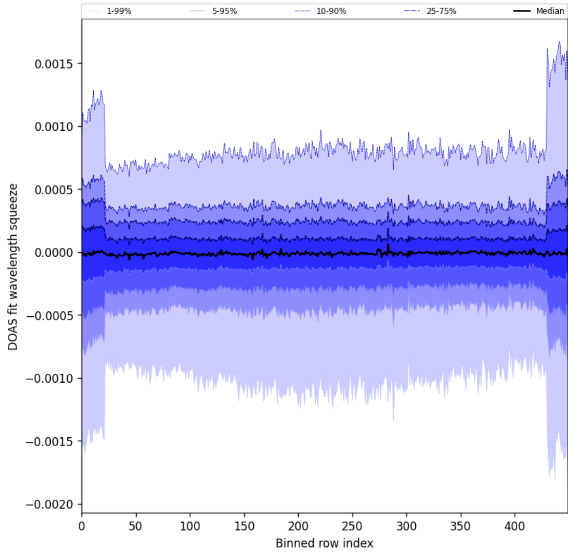
Figure 92: Along track statistics of “DOAS fit wavelength squeeze” for 2024-09-12 to 2024-09-14
