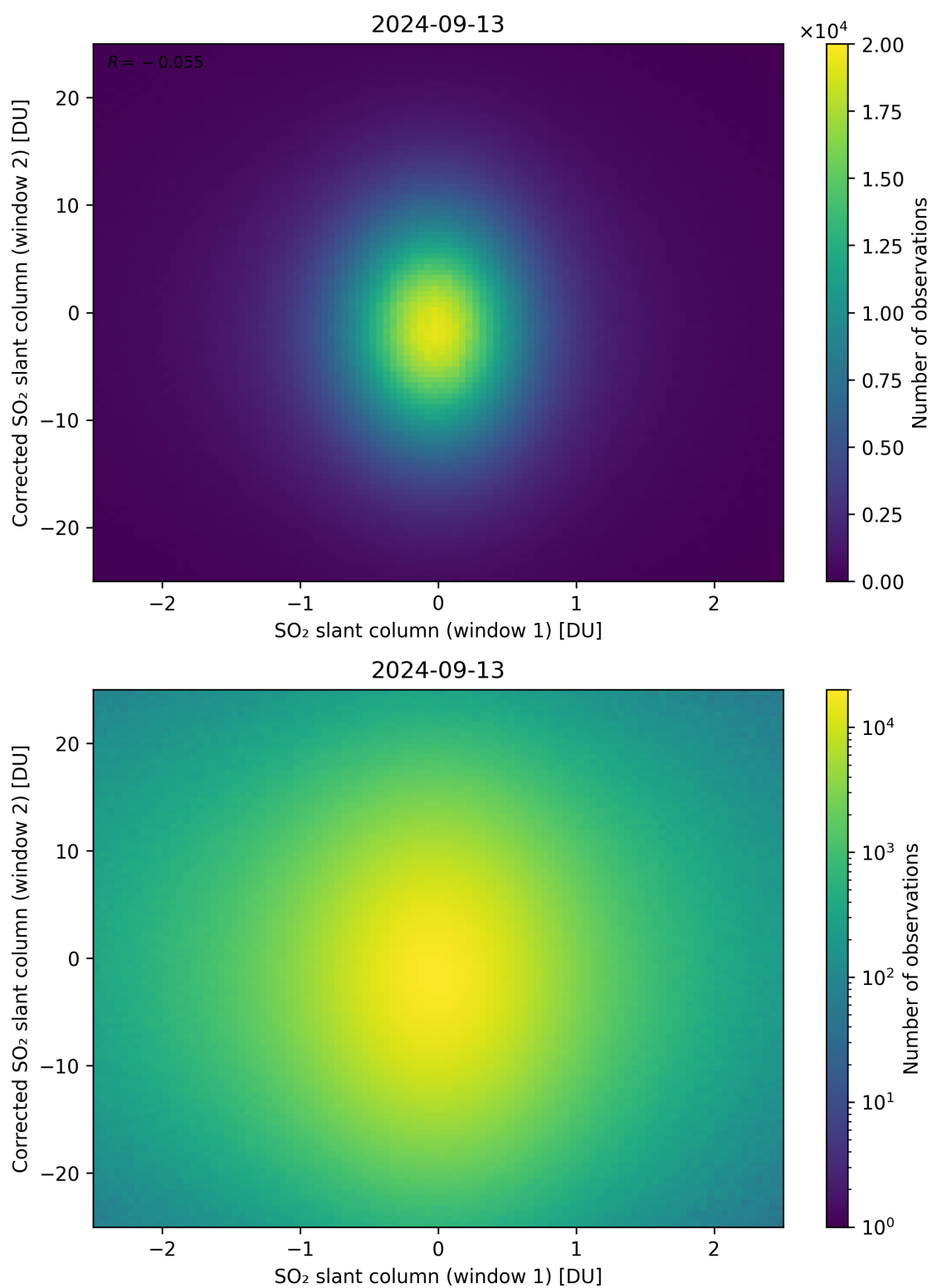
Figure 233: Scatter density plot of “SO 2 slant column (window 1)” against “Corrected SO 2 slant column (window 2)” for 2024-09-12 to 2024-09-14.
