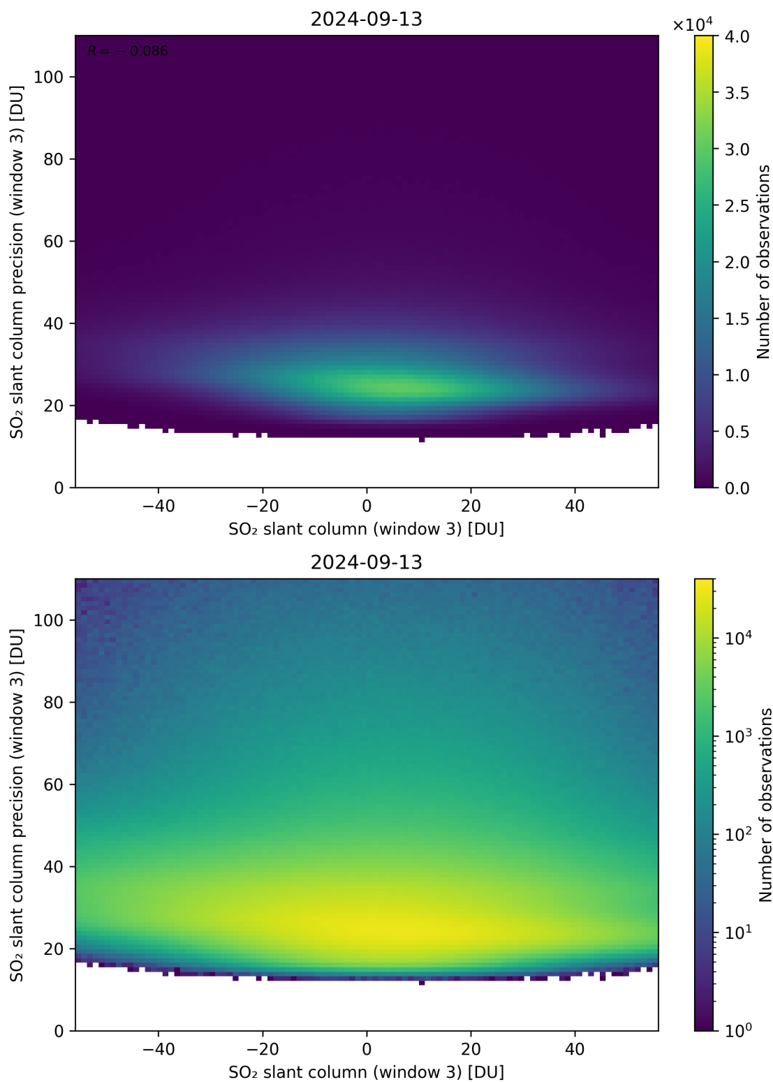
Figure 267: Scatter density plot of “SO 2 slant column (window 3)” against “SO 2 slant column precision (window 3)” for 2024-09-12 to 2024-09-14.
