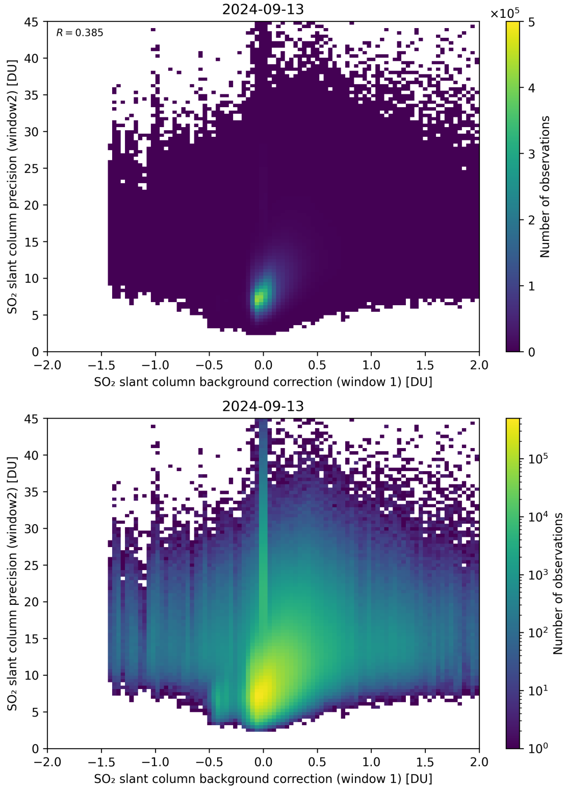
Figure 106: Scatter density plot of “SO 2 slant column background correction (window 1)” against “SO 2 slant column precision (window2)” for 2024-09-12 to 2024-09-14.
