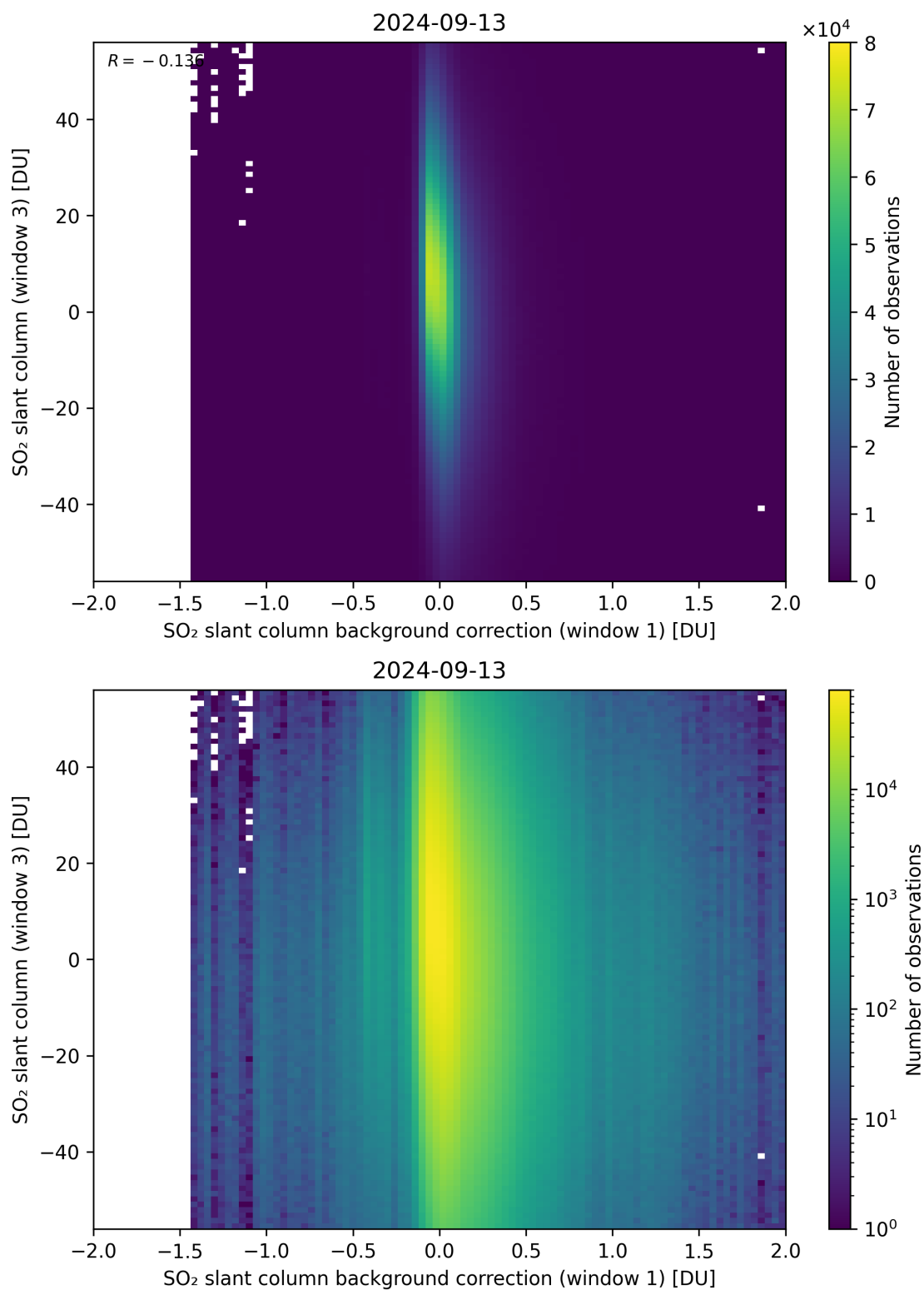
Figure 107: Scatter density plot of “SO 2 slant column background correction (window 1)” against “SO 2 slant column (window 3)” for 2024-09-12 to 2024-09-14.
