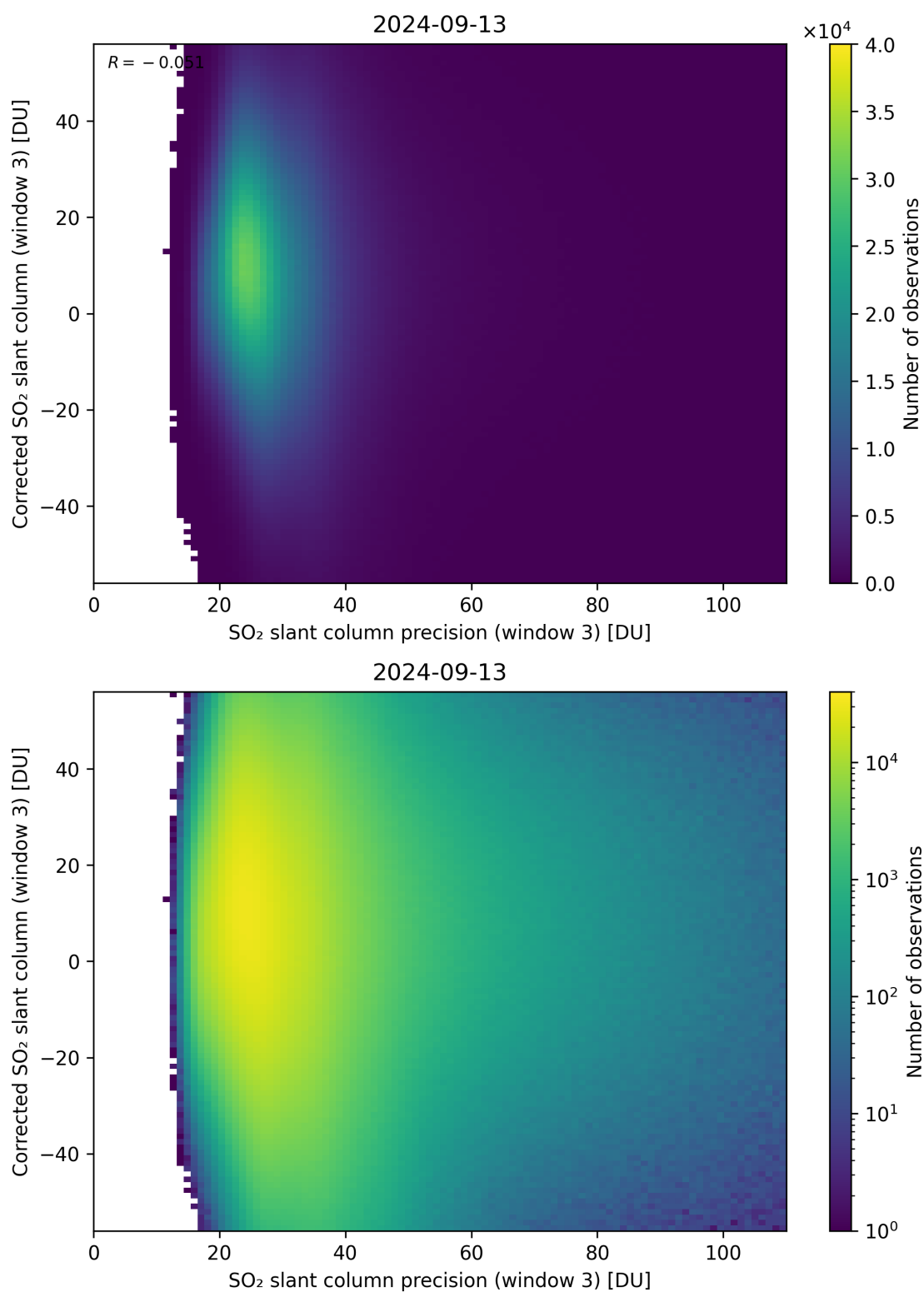
Figure 262: Scatter density plot of “SO 2 slant column precision (window 3)” against “Corrected SO 2 slant column (window 3)” for 2024-09-12 to 2024-09-14.
