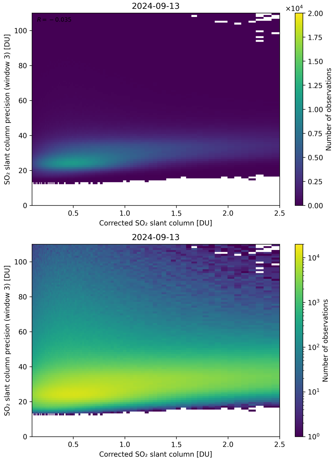
Figure 191: Scatter density plot of “Corrected SO 2 slant column” against “SO 2 slant column precision (window 3)” for 2024-09-12 to 2024-09-14.
