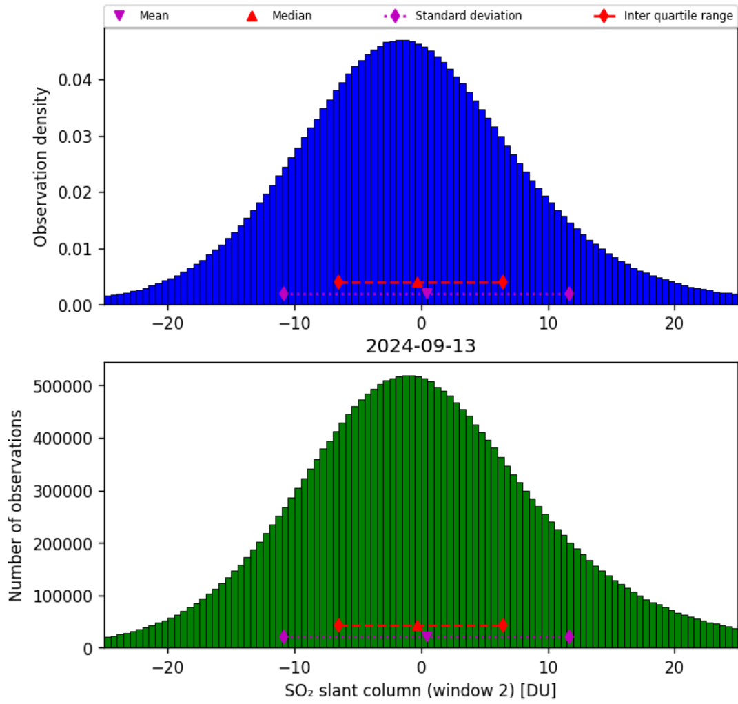
Figure 60: Histogram of “SO 2 slant column (window 2)” for 2024-09-12 to 2024-09-14
