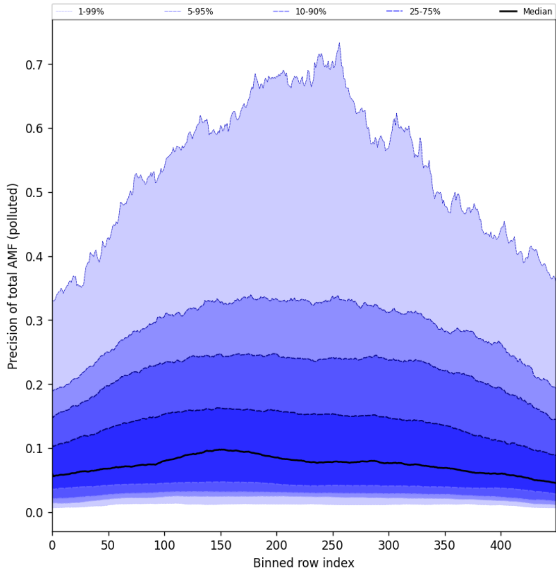
Figure 95: Along track statistics of “Precision of total AMF (polluted)” for 2024-09-12 to 2024-09-14
