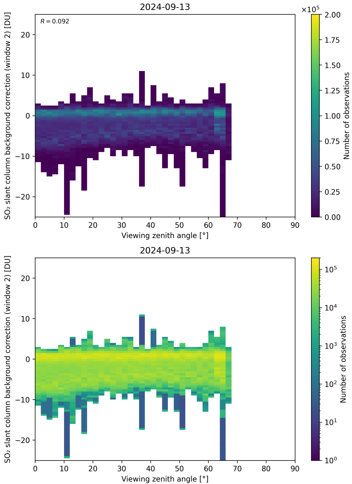
Figure 309: Scatter density plot of “Viewing zenith angle” against “SO 2 slant column background correction (window 2)” for 2024-09-12 to 2024-09-14.
