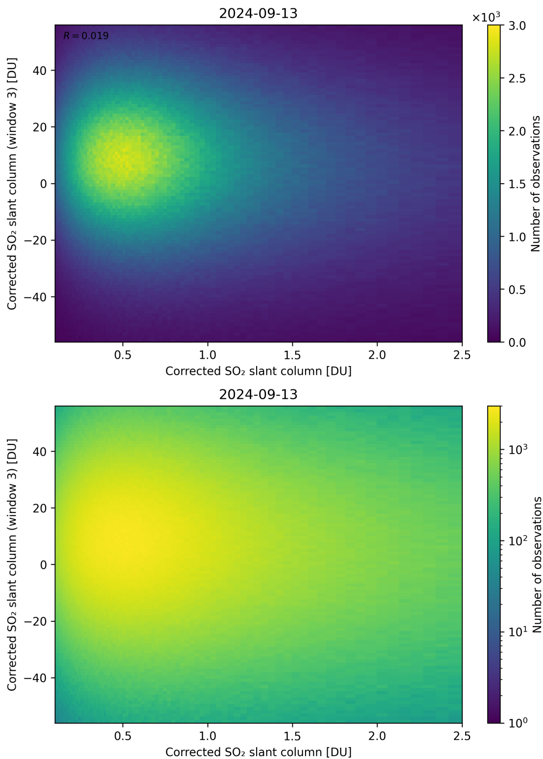
Figure 186: Scatter density plot of “Corrected SO 2 slant column” against “Corrected SO 2 slant column (window 3)” for 2024-09-12 to 2024-09-14.
