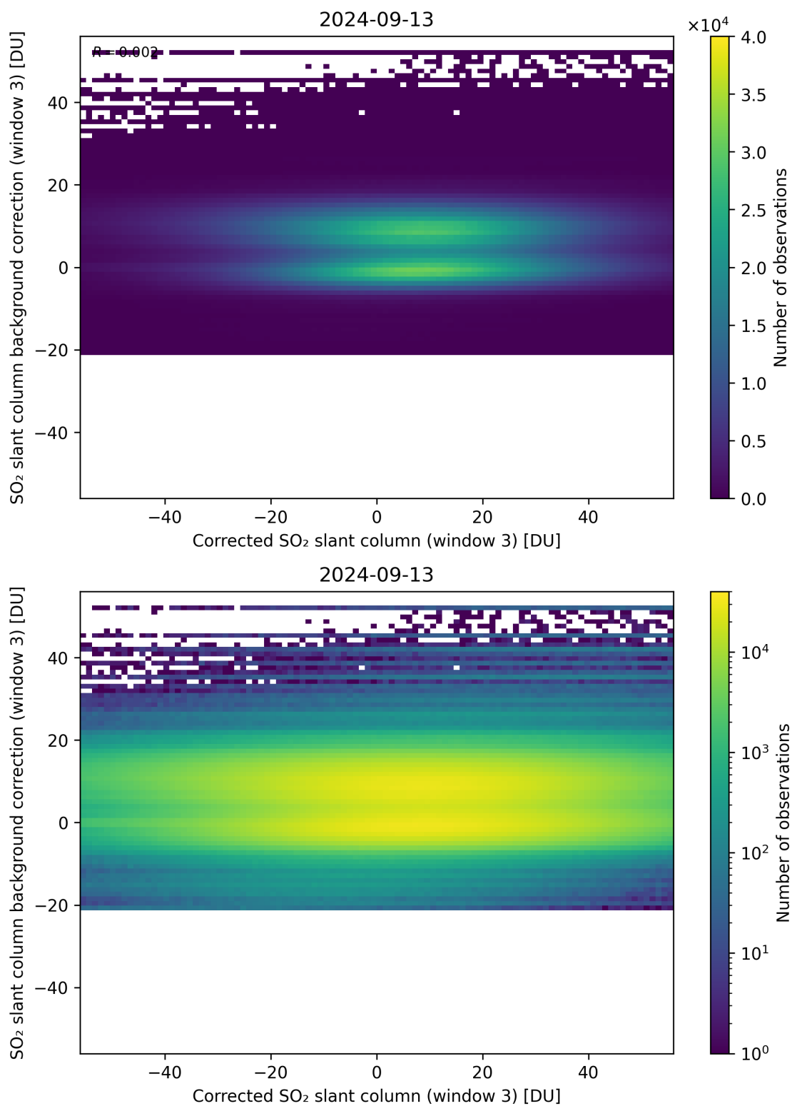
Figure 205: Scatter density plot of “Corrected SO 2 slant column (window 3)” against “SO 2 slant column background correction (window 3)” for 2024-09-12 to 2024-09-14.
