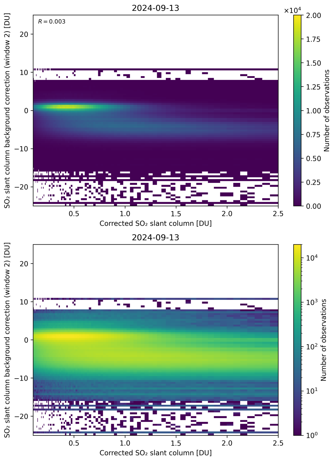
Figure 179: Scatter density plot of “Corrected SO 2 slant column” against “SO 2 slant column background correction (window 2)” for 2024-09-12 to 2024-09-14.
