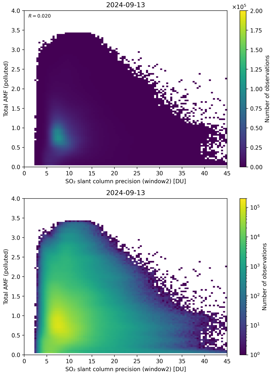
Figure 251: Scatter density plot of “SO 2 slant column precision (window2)” against “Total AMF (polluted)” for 2024-09-12 to 2024-09-14.
