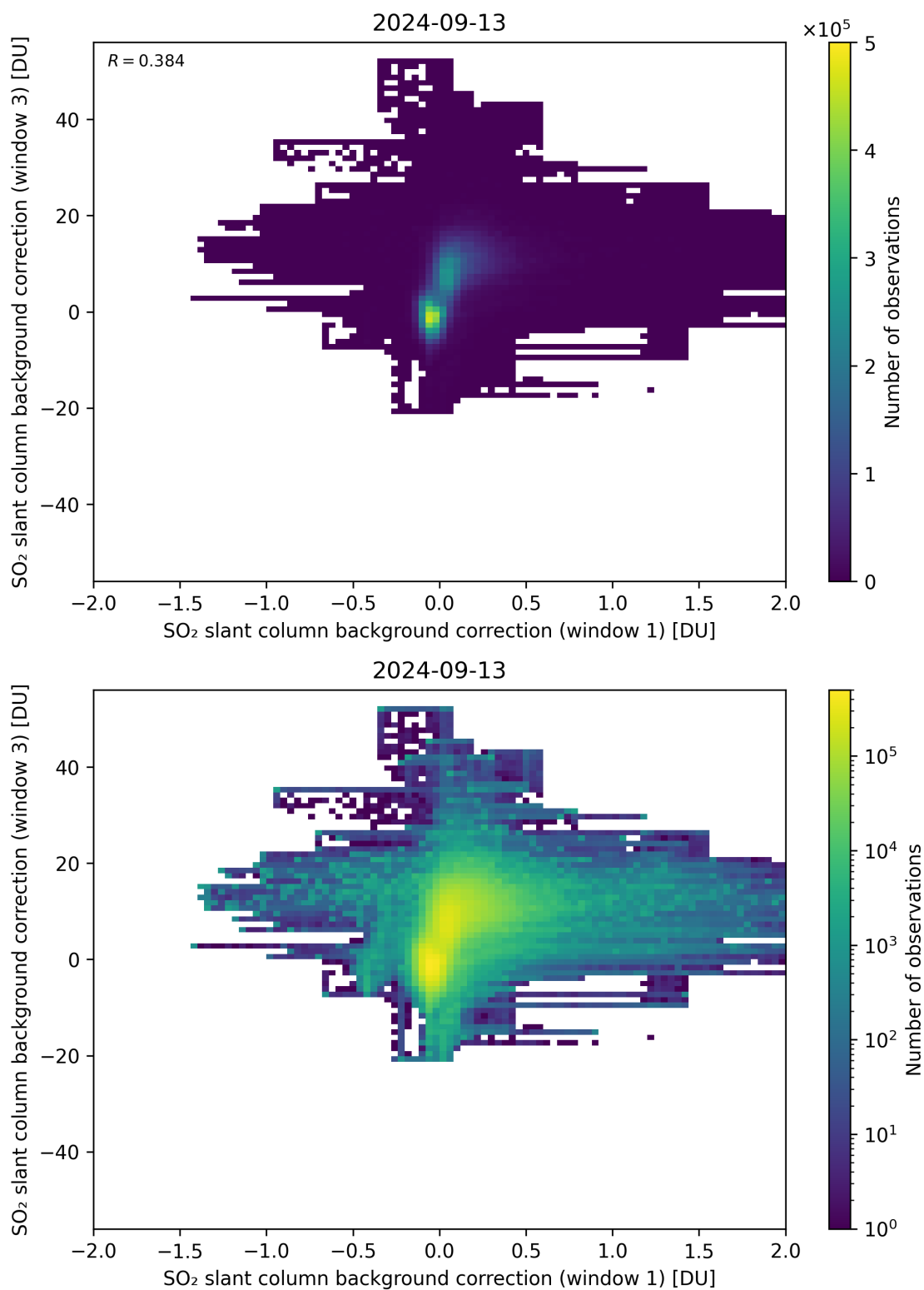
Figure 99: Scatter density plot of “SO 2 slant column background correction (window 1)” against “SO 2 slant column background correction (window 3)” for 2024-09-12 to 2024-09-14.
