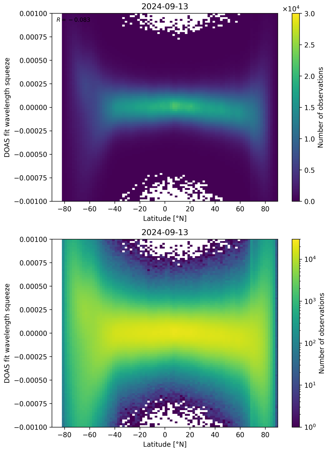
Figure 143: Scatter density plot of “Latitude” against “DOAS fit wavelength squeeze” for 2024-09-12 to 2024-09-14.
