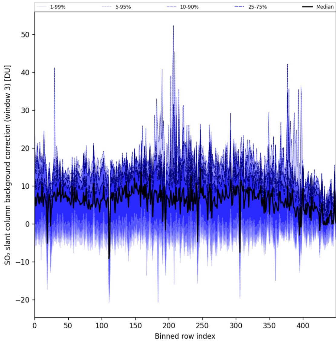
Figure 90: Along track statistics of "SO 2 slant column background correction (window 3)" for 2024-09-12 to 2024-09-14
