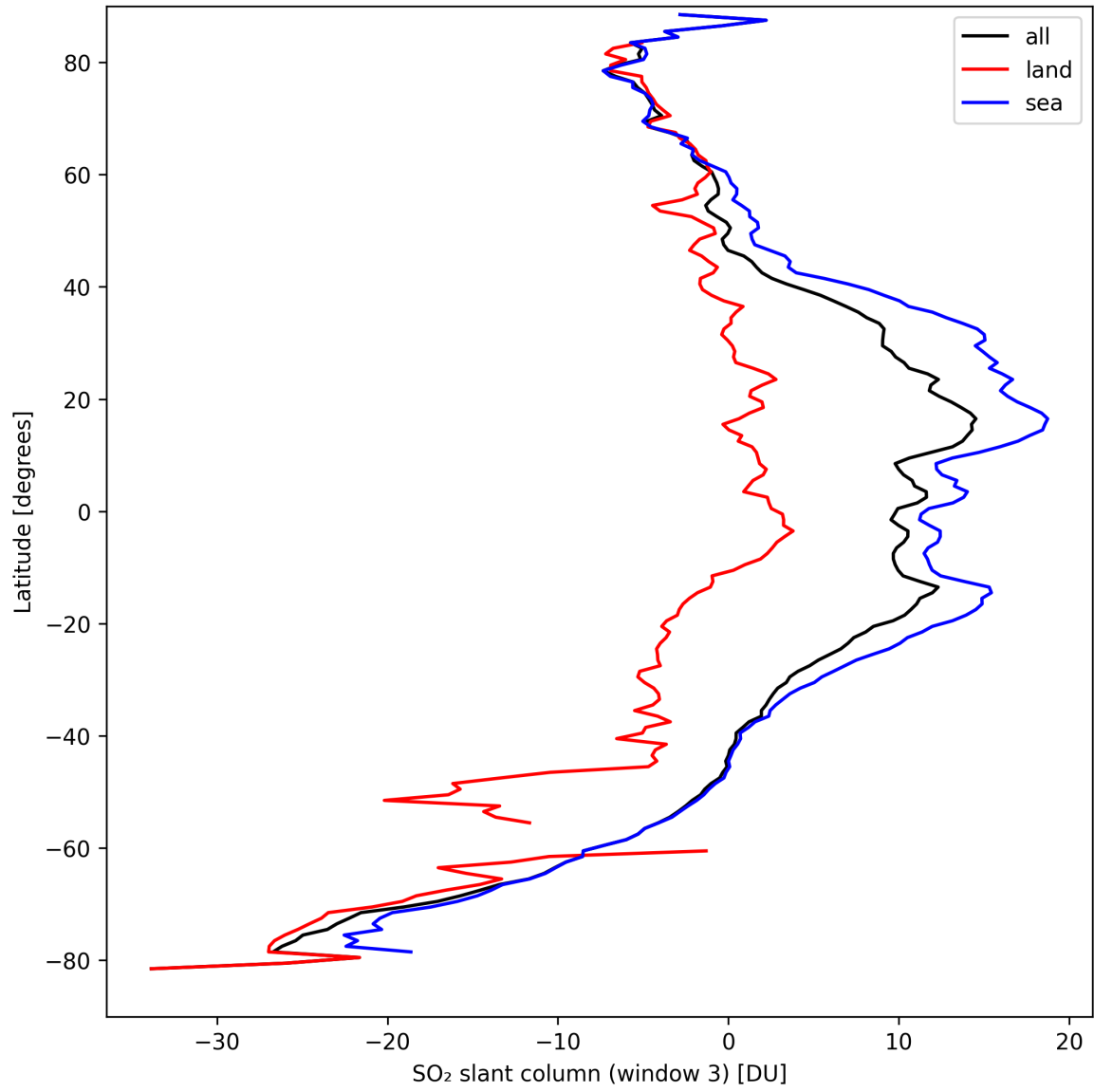
Figure 41: Zonal average of “SO 2 slant column (window 3)” for 2024-09-12 to 2024-09-14.
