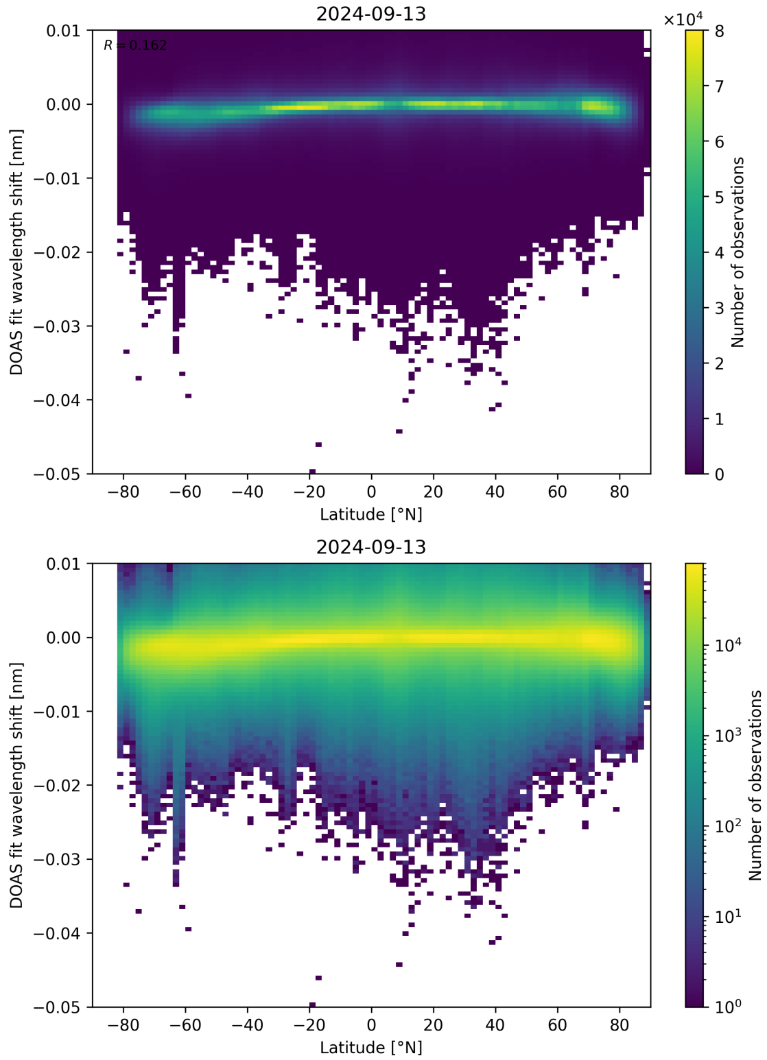
Figure 142: Scatter density plot of “Latitude” against “DOAS fit wavelength shift” for 2024-09-12 to 2024-09-14.
