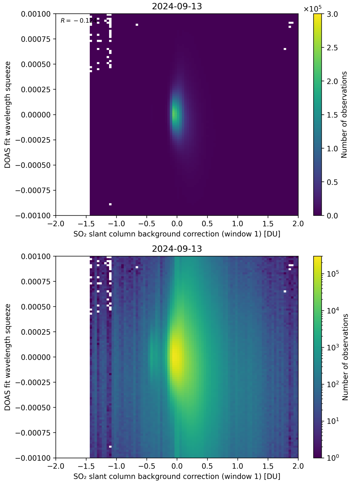
Figure 101: Scatter density plot of “SO 2 slant column background correction (window 1)” against “DOAS fit wavelength squeeze” for 2024-09-12 to 2024-09-14.
