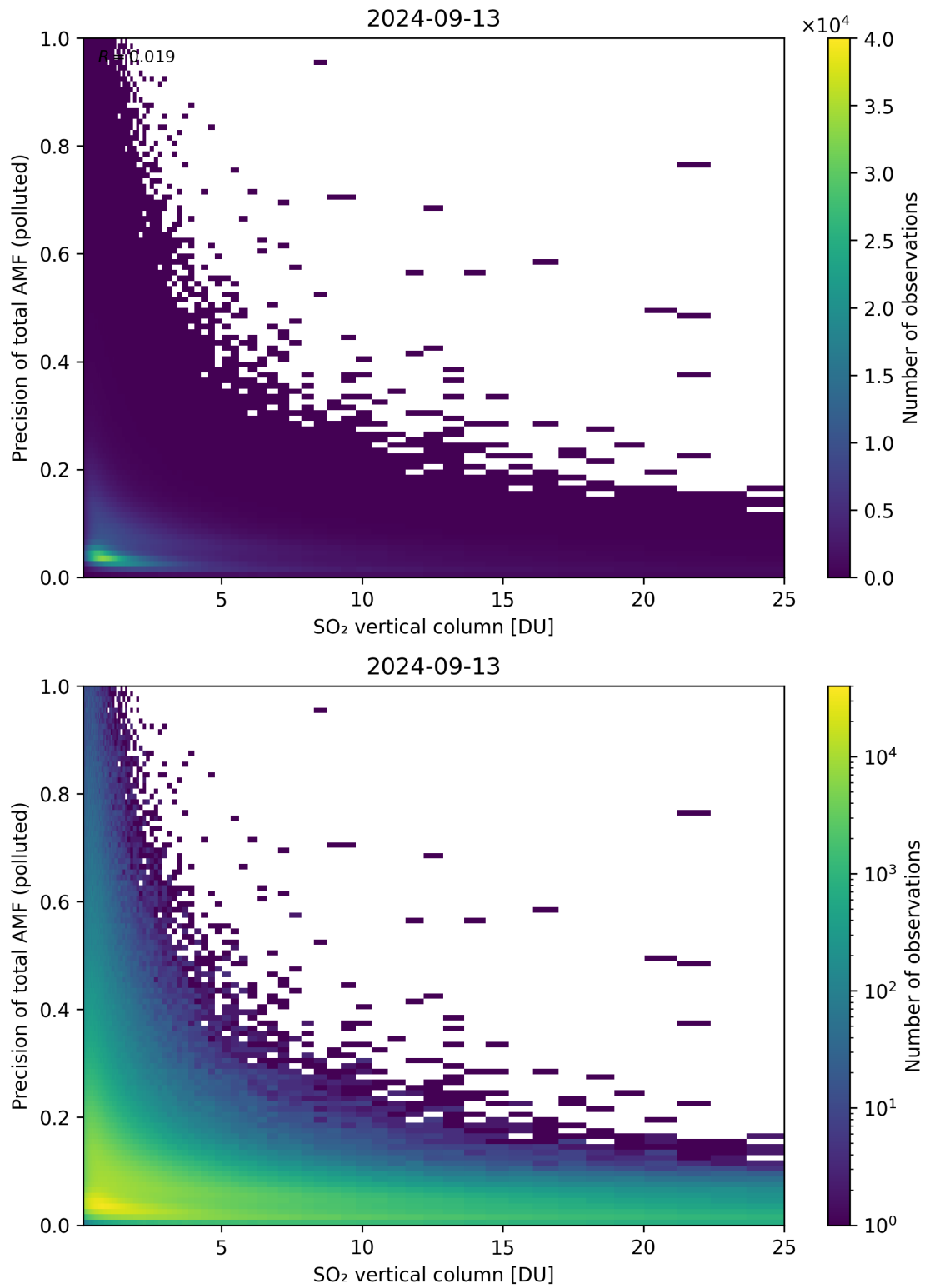
Figure 306: Scatter density plot of “SO 2 vertical column” against “Precision of total AMF (polluted)” for 2024-09-12 to 2024-09-14.
