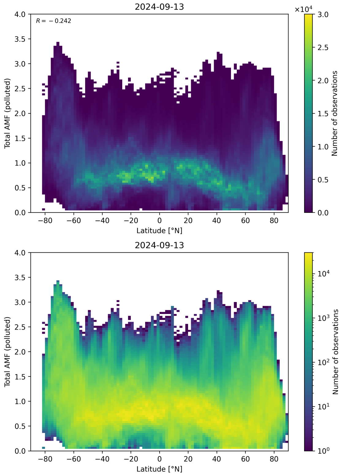
Figure 154: Scatter density plot of “Latitude” against “Total AMF (polluted)” for 2024-09-12 to 2024-09-14.
