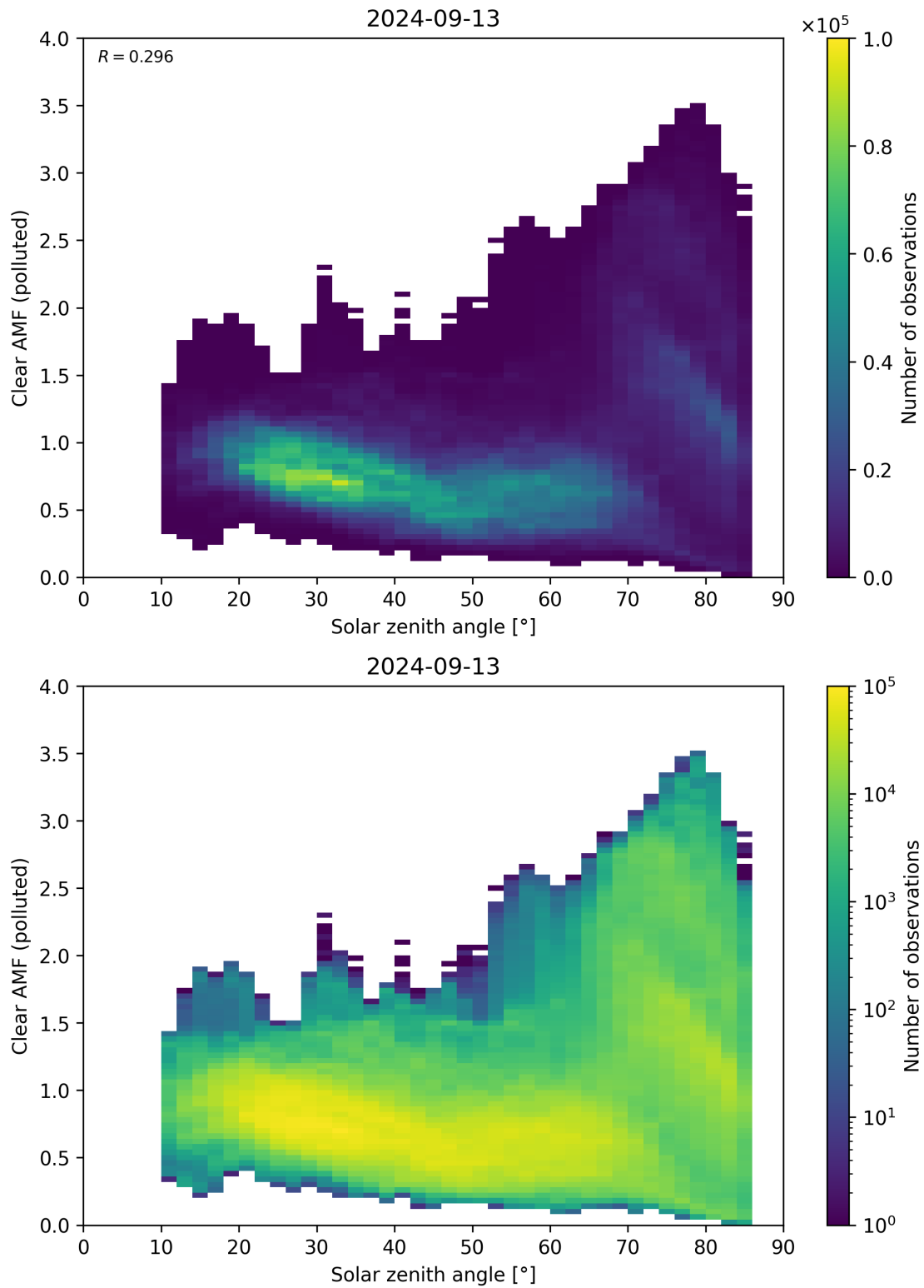
Figure 165: Scatter density plot of “Solar zenith angle” against “Clear AMF (polluted)” for 2024-09-12 to 2024-09-14.
