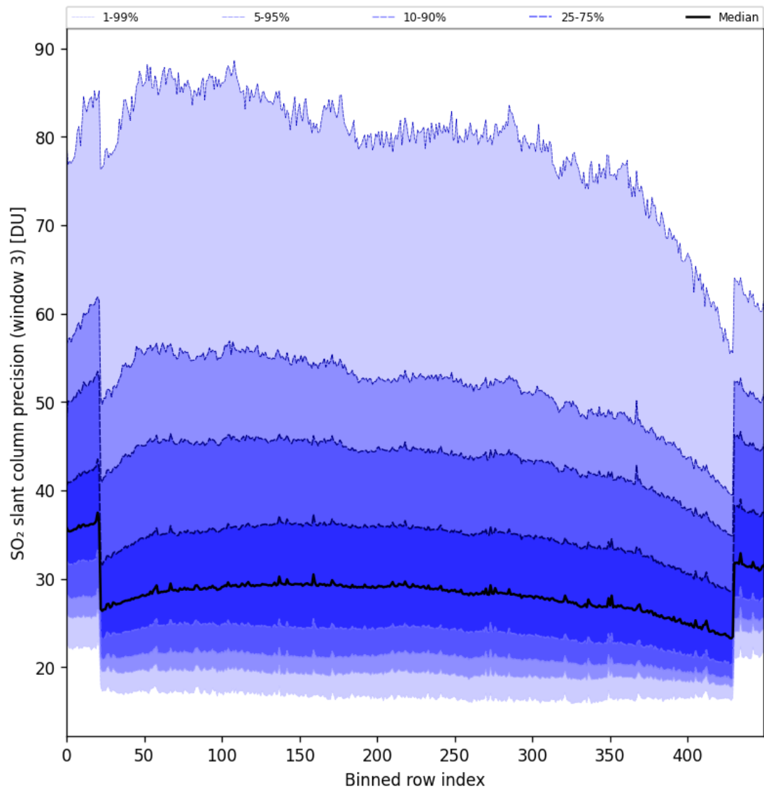
Figure 88: Along track statistics of “SO 2 slant column precision (window 3)” for 2024-09-12 to 2024-09-14
