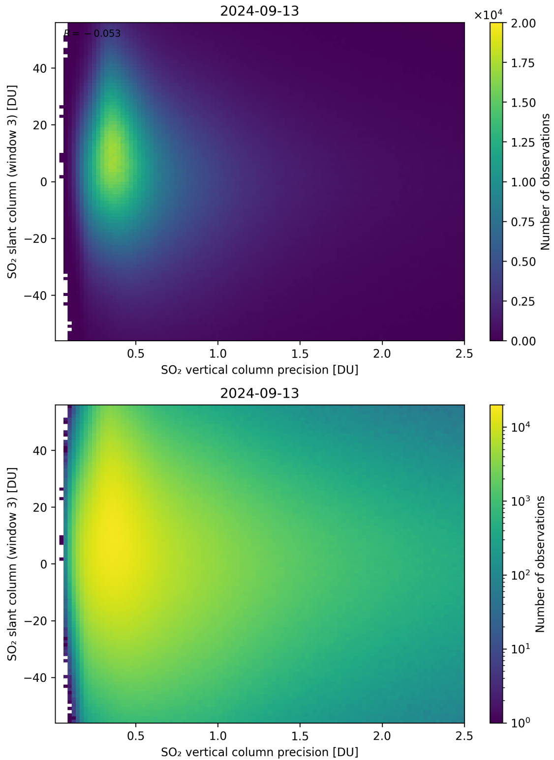
Figure 292: Scatter density plot of “SO 2 vertical column precision” against “SO 2 slant column (window 3)” for 2024-09-12 to 2024-09-14.
