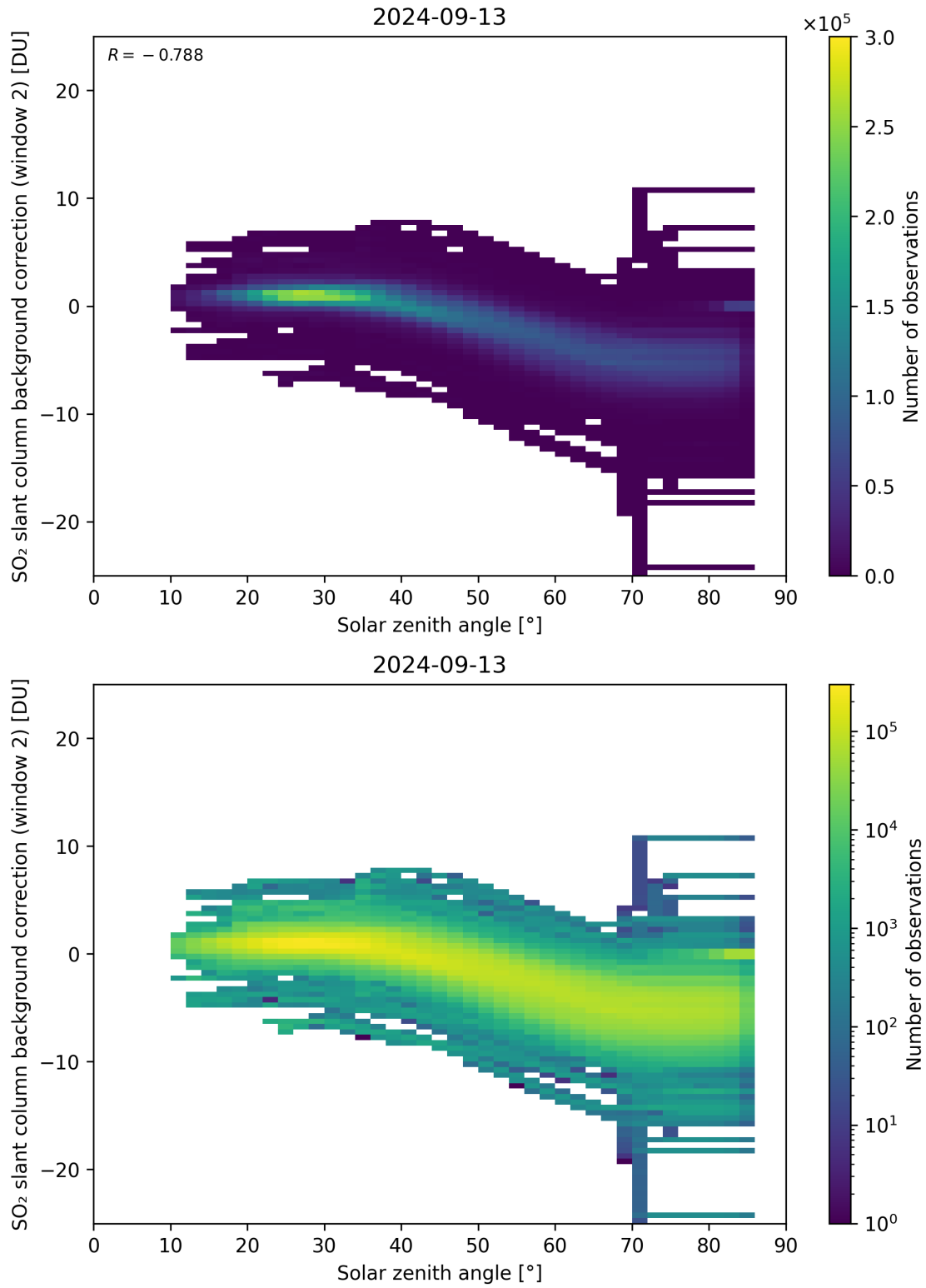
Figure 159: Scatter density plot of “Solar zenith angle” against “SO 2 slant column background correction (window 2)” for 2024-09-12 to 2024-09-14.
