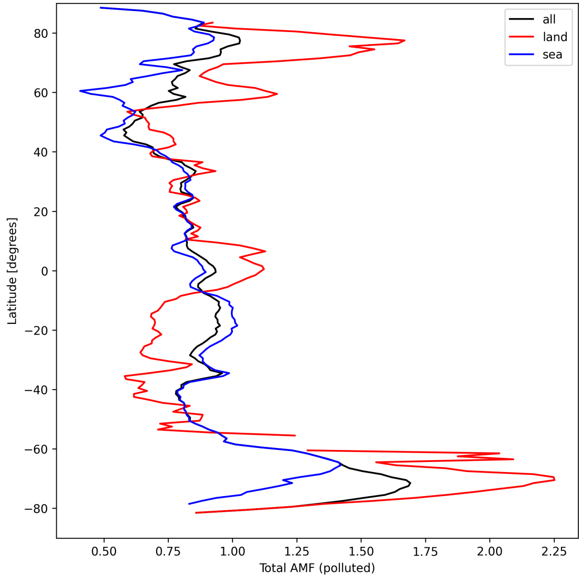
Figure 48: Zonal average of “Total AMF (polluted)” for 2024-09-12 to 2024-09-14.
