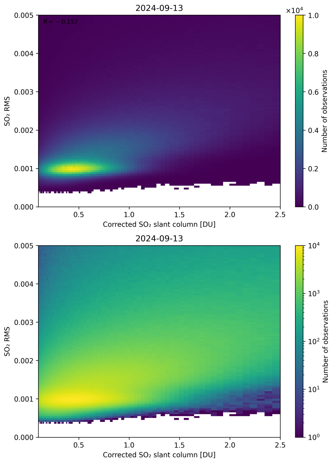
Figure 183: Scatter density plot of “Corrected SO 2 slant column” against “SO 2 RMS” for 2024-09-12 to 2024-09-14.
