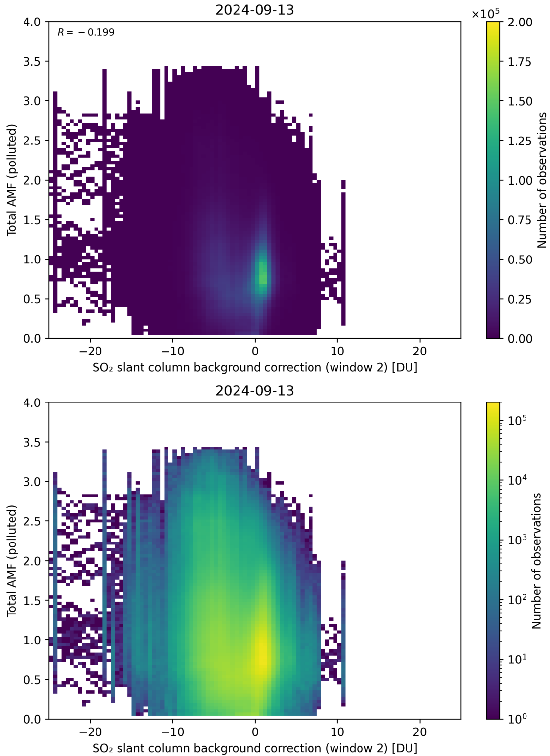
Figure 119: Scatter density plot of “SO 2 slant column background correction (window 2)” against “Total AMF (polluted)” for 2024-09-12 to 2024-09-14.
