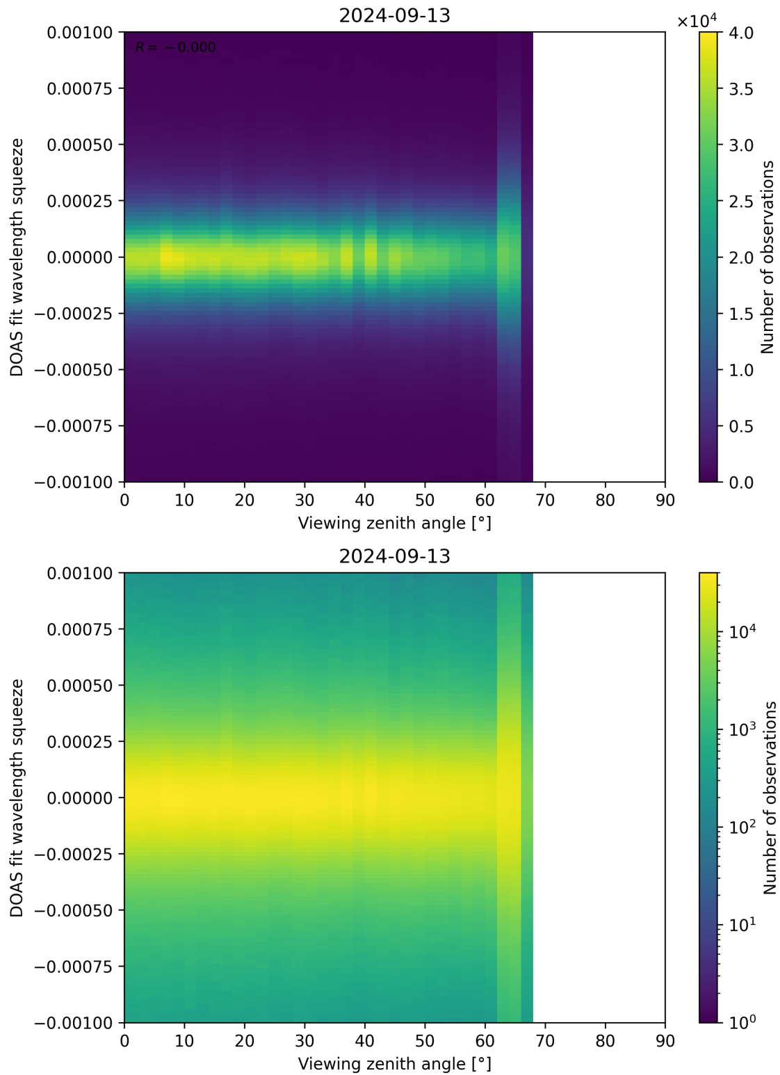
Figure 312: Scatter density plot of “Viewing zenith angle” against “DOAS fit wavelength squeeze” for 2024-09-12 to 2024-09-14.
