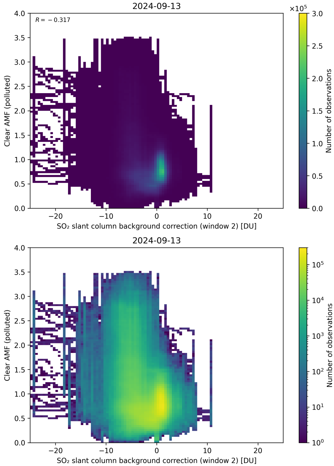
Figure 115: Scatter density plot of “SO 2 slant column background correction (window 2)” against “Clear AMF (polluted)” for 2024-09-12 to 2024-09-14.
