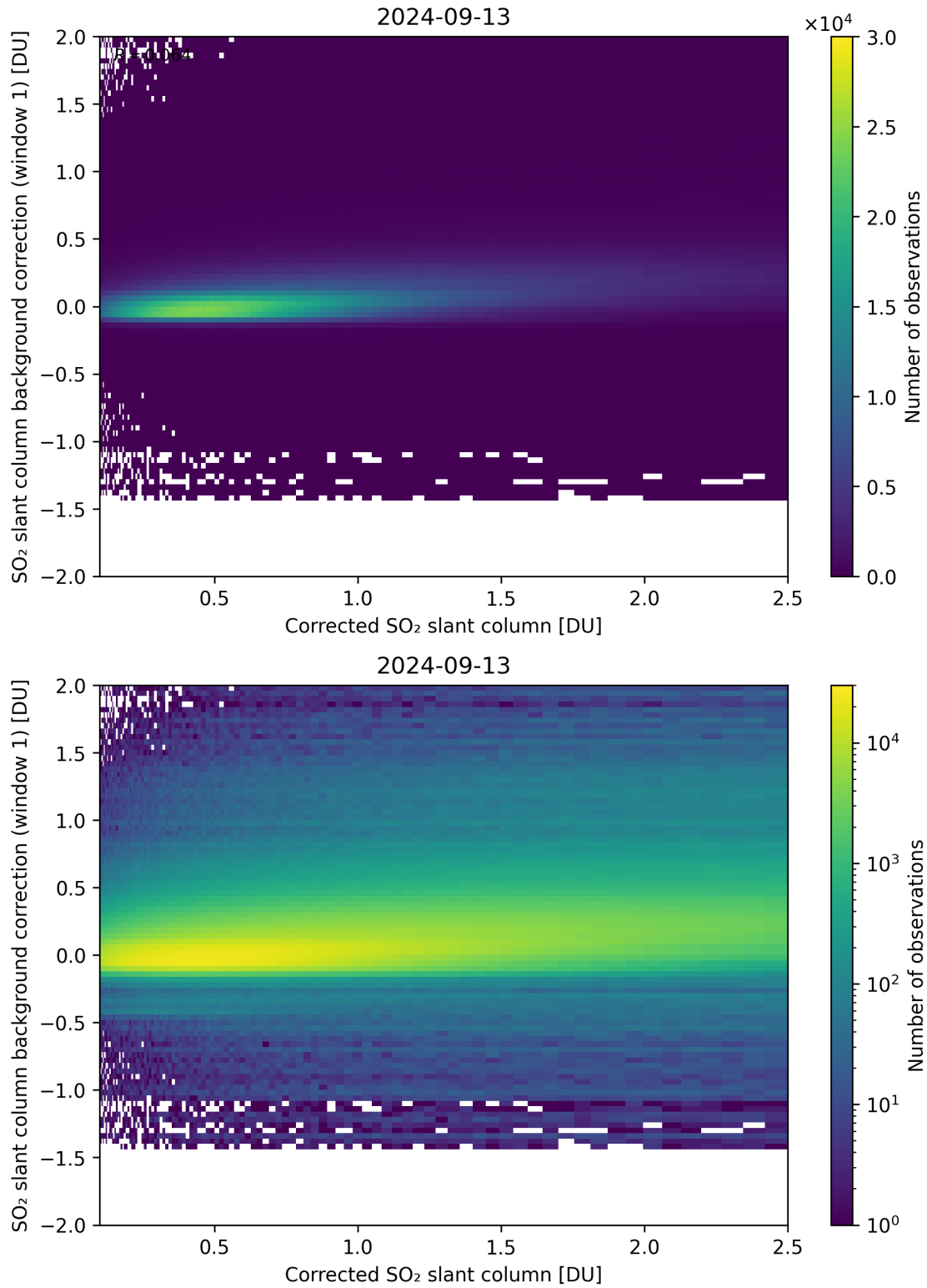
Figure 178: Scatter density plot of “Corrected SO 2 slant column” against “SO 2 slant column background correction (window 1)” for 2024-09-12 to 2024-09-14.
