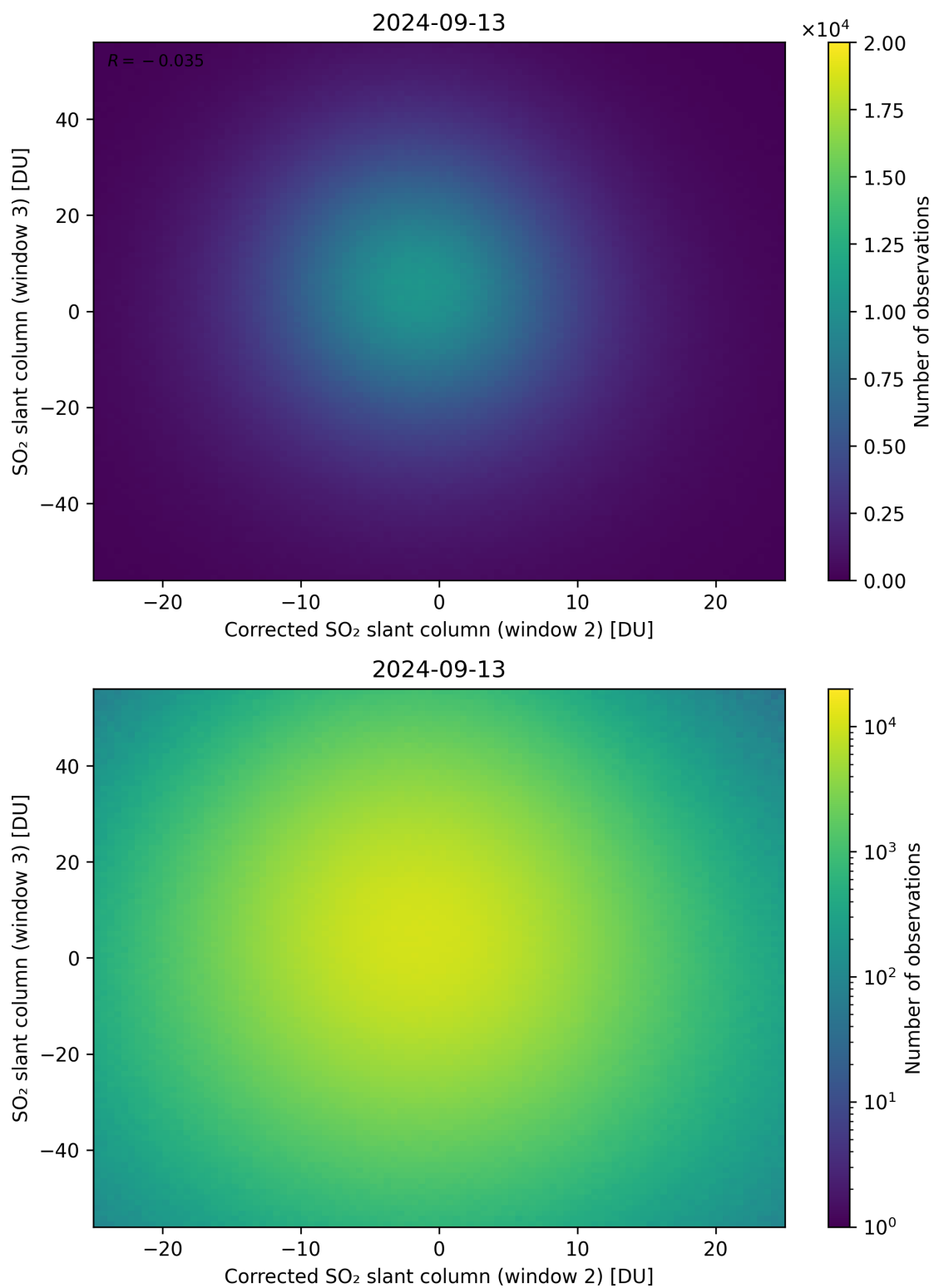
Figure 201: Scatter density plot of “Corrected SO 2 slant column (window 2)” against “SO 2 slant column (window 3)” for 2024-09-12 to 2024-09-14.
