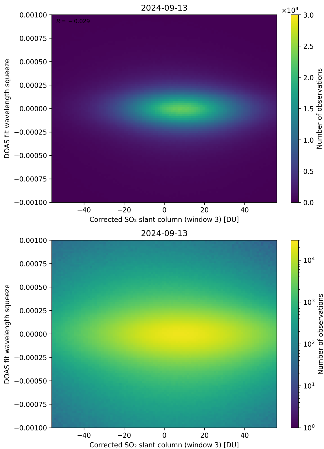
Figure 207: Scatter density plot of “Corrected SO 2 slant column (window 3)” against “DOAS fit wavelength squeeze” for 2024-09-12 to 2024-09-14.
