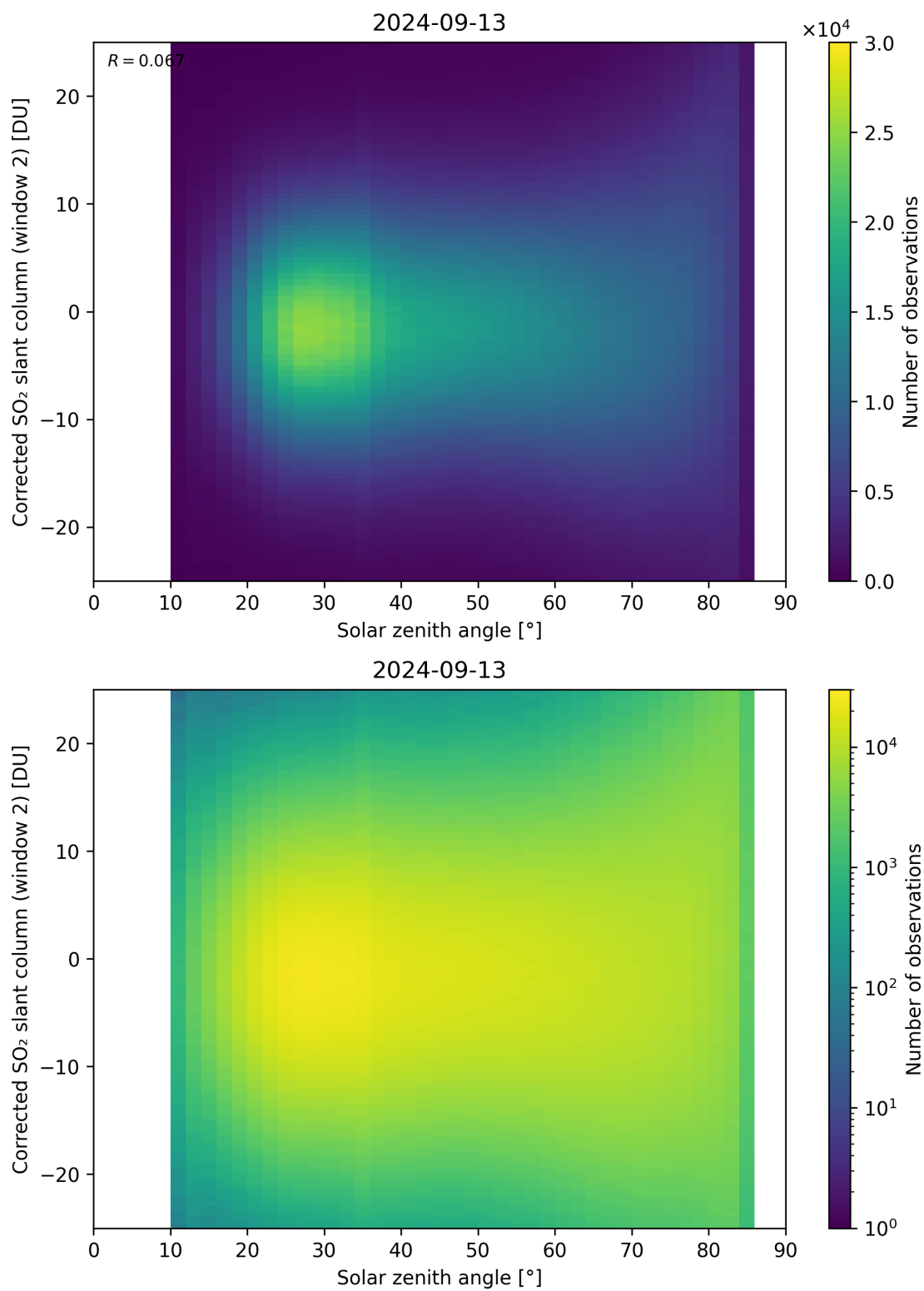
Figure 167: Scatter density plot of “Solar zenith angle” against “Corrected SO 2 slant column (window 2)” for 2024-09-12 to 2024-09-14.
