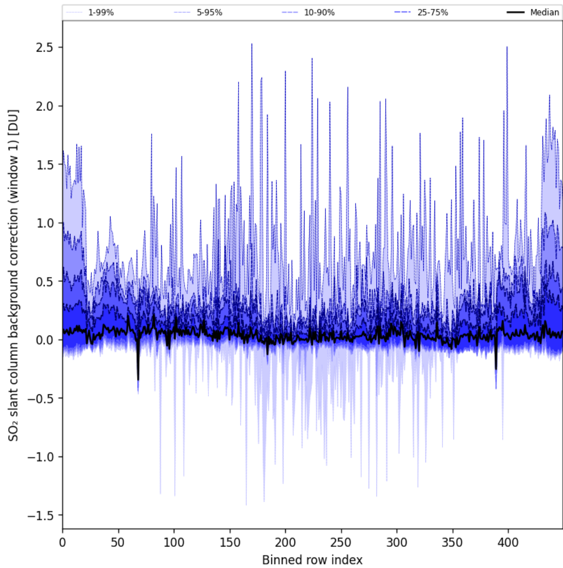
Figure 82: Along track statistics of “SO 2 slant column background correction (window 1)” for 2024-09-12 to 2024-09-14
