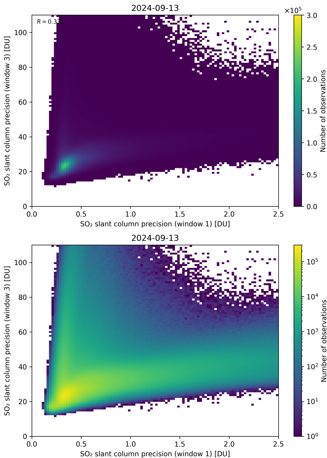
Figure 229: Scatter density plot of “SO 2 slant column precision (window 1)” against “SO 2 slant column precision (window 3)” for 2024-09-12 to 2024-09-14.
