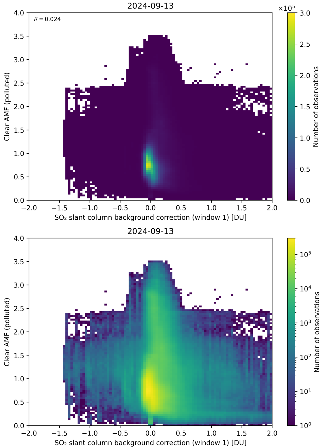
Figure 103: Scatter density plot of “SO 2 slant column background correction (window 1)” against “Clear AMF (polluted)” for 2024-09-12 to 2024-09-14.
