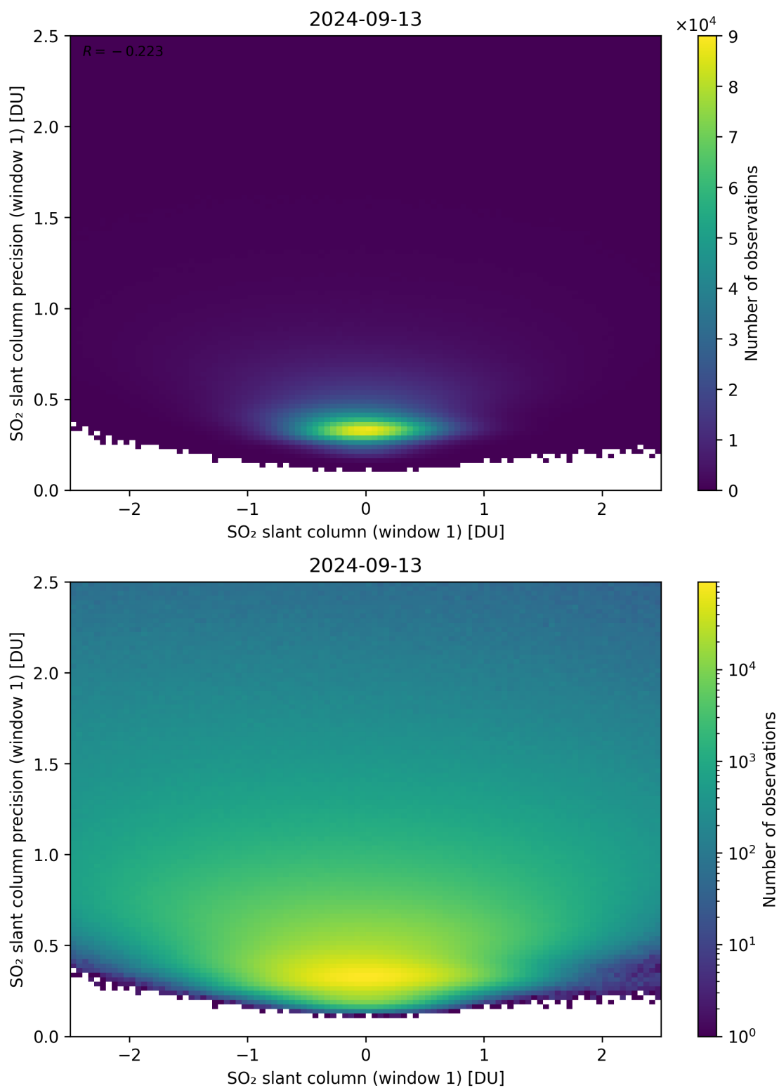
Figure 235: Scatter density plot of “SO 2 slant column (window 1)” against “SO 2 slant column precision (window 1)” for 2024-09-12 to 2024-09-14.
