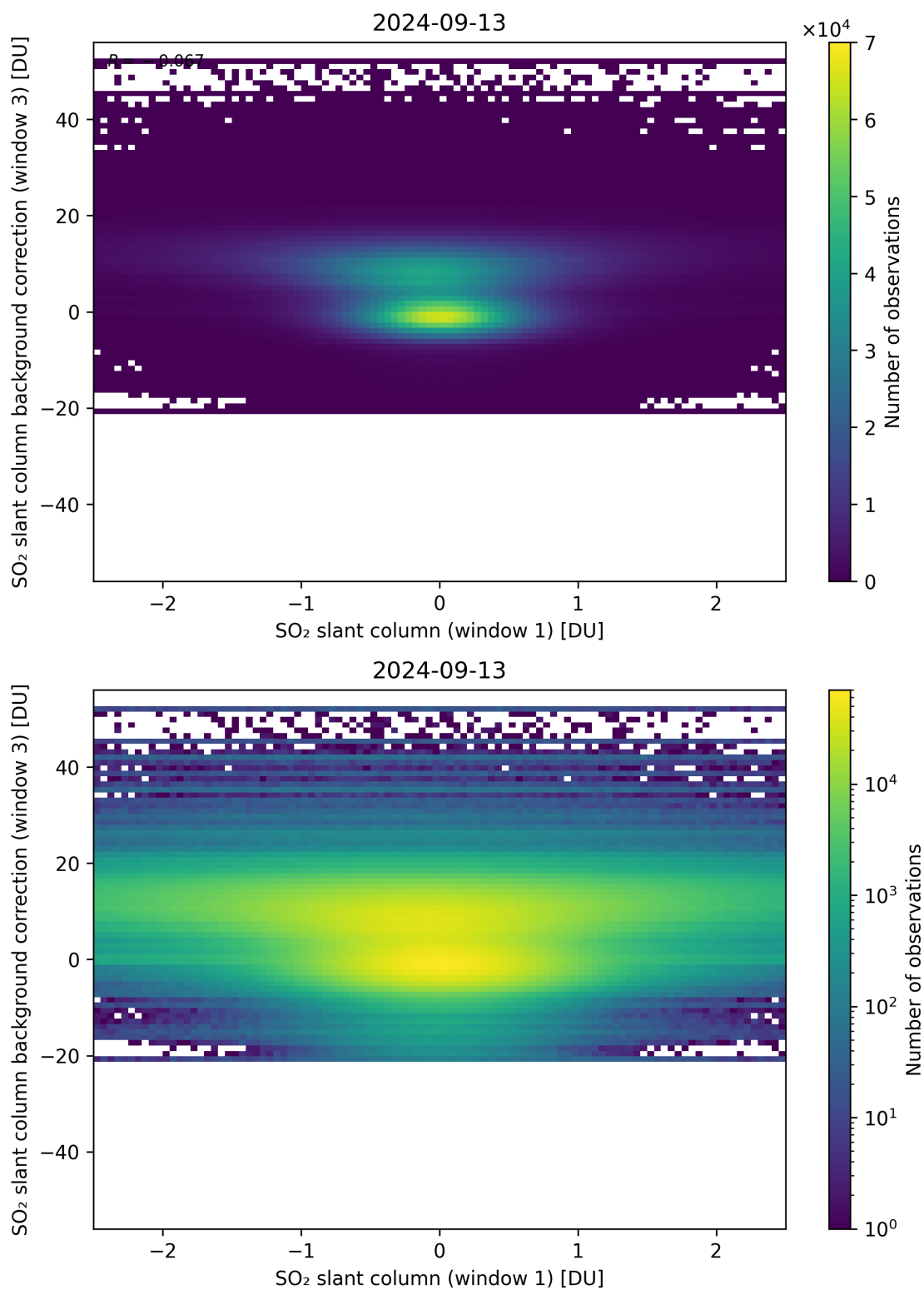
Figure 214: Scatter density plot of “SO 2 slant column (window 1)” against “SO 2 slant column background correction (window 3)” for 2024-09-12 to 2024-09-14.
