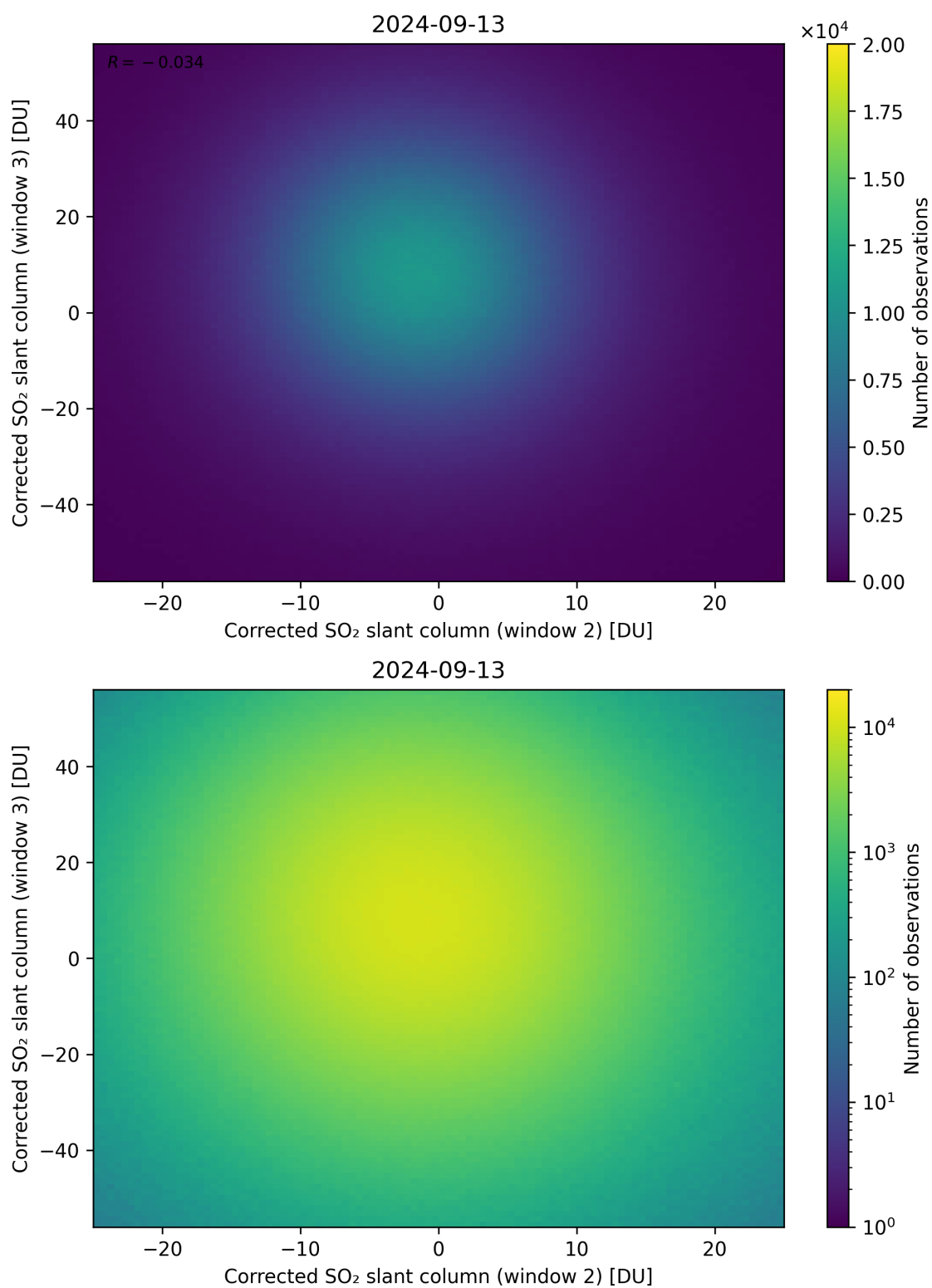
Figure 200: Scatter density plot of “Corrected SO 2 slant column (window 2)” against “Corrected SO 2 slant column (window 3)” for 2024-09-12 to 2024-09-14.
