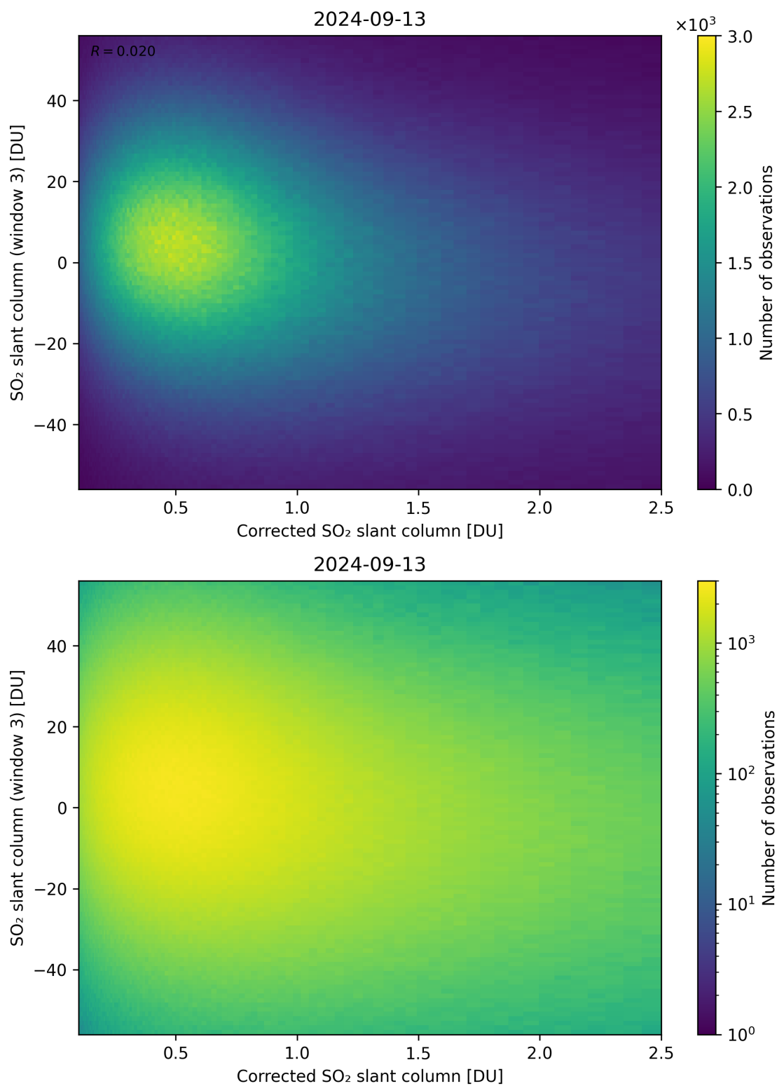
Figure 190: Scatter density plot of “Corrected SO 2 slant column” against “SO 2 slant column (window 3)” for 2024-09-12 to 2024-09-14.
