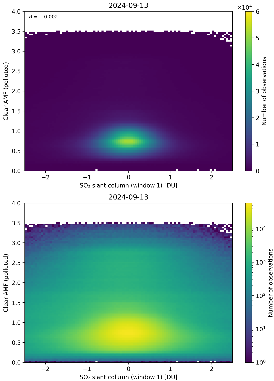
Figure 232: Scatter density plot of “SO 2 slant column (window 1)” against “Clear AMF (polluted)” for 2024-09-12 to 2024-09-14.
