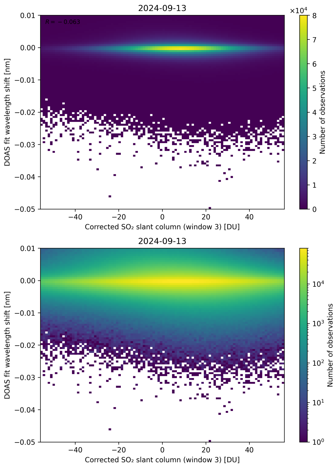
Figure 206: Scatter density plot of “Corrected SO 2 slant column (window 3)” against “DOAS fit wavelength shift” for 2024-09-12 to 2024-09-14.
