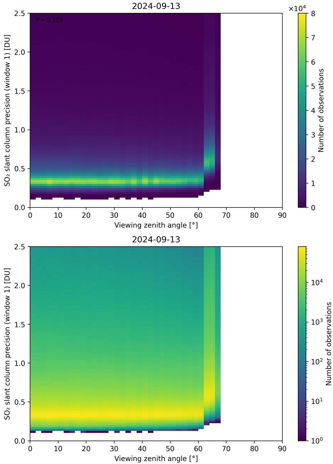
Figure 321: Scatter density plot of “Viewing zenith angle” against “SO 2 slant column precision (window 1)” for 2024-09-12 to 2024-09-14.
