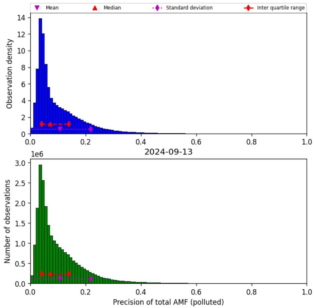
Figure 72: Histogram of “Precision of total AMF (polluted)” for 2024-09-12 to 2024-09-14
