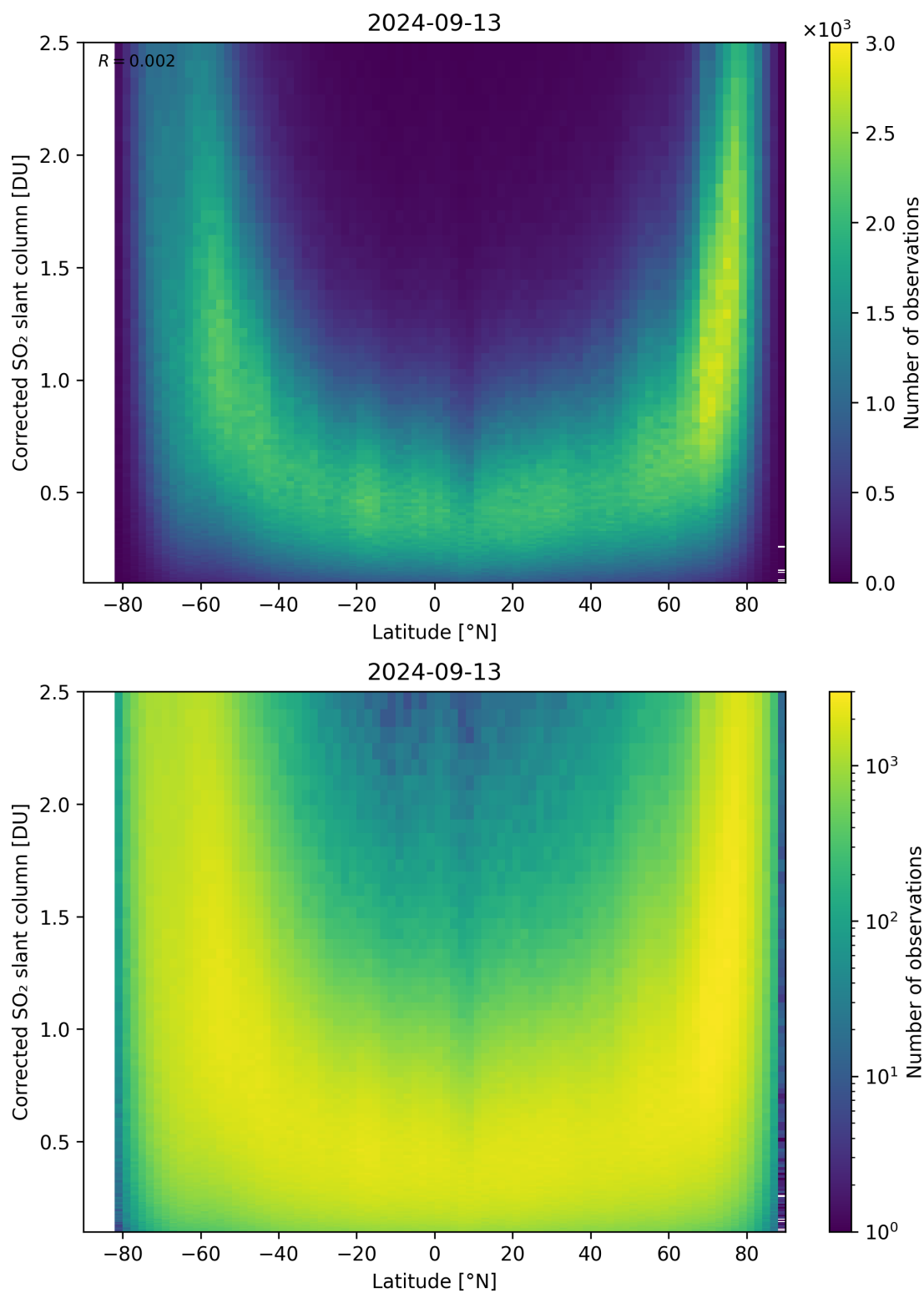
Figure 146: Scatter density plot of “Latitude” against “Corrected SO 2 slant column” for 2024-09-12 to 2024-09-14.
