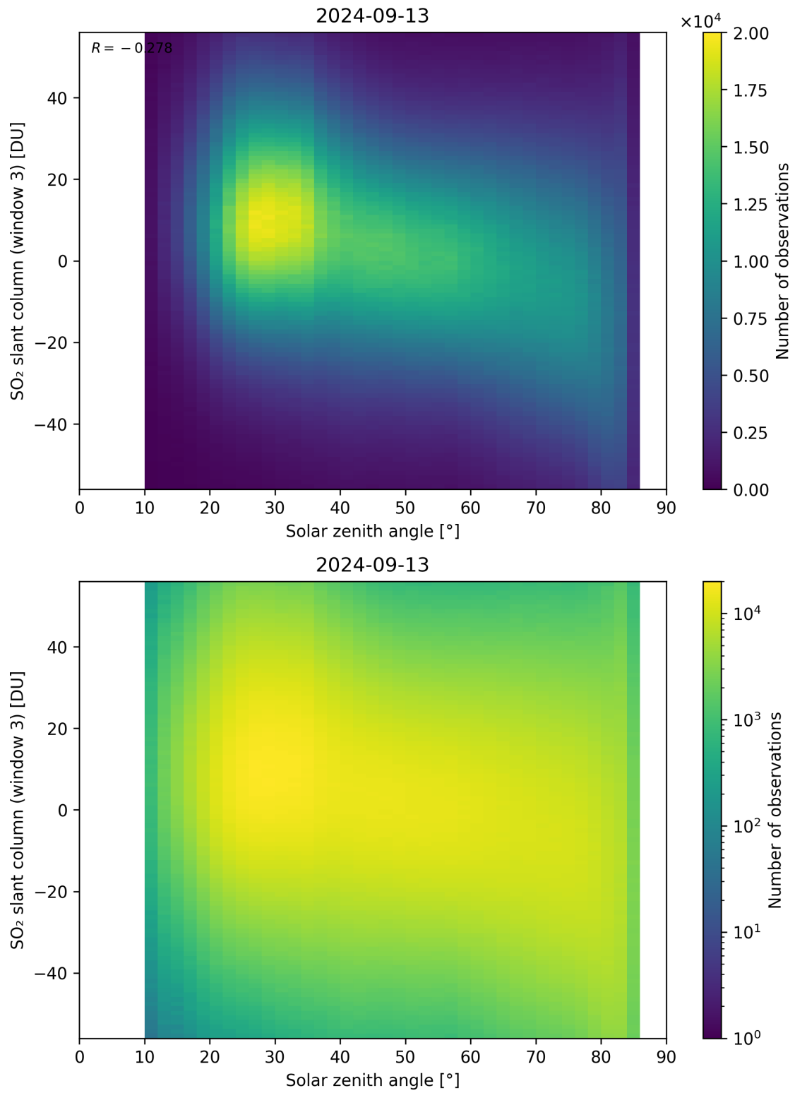
Figure 172: Scatter density plot of “Solar zenith angle” against “SO 2 slant column (window 3)” for 2024-09-12 to 2024-09-14.
