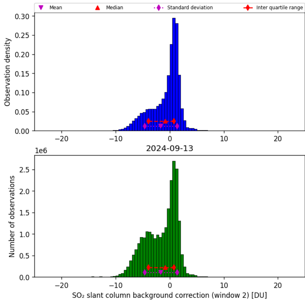
Figure 63: Histogram of “SO 2 slant column background correction (window 2)” for 2024-09-12 to 2024-09-14
