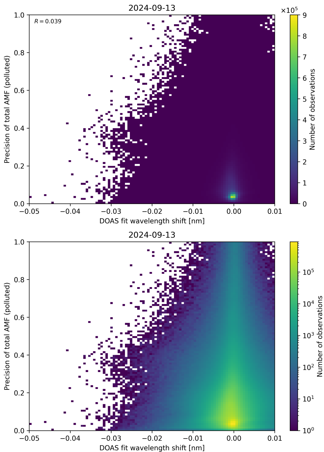
Figure 131: Scatter density plot of “DOAS fit wavelength shift” against “Precision of total AMF (polluted)” for 2024-09-12 to 2024-09-14.
