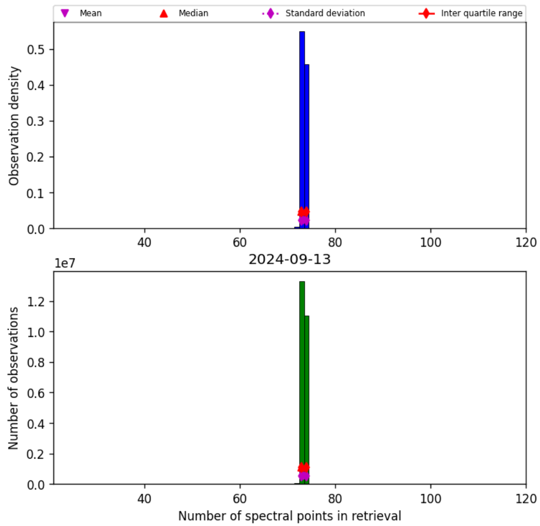
Figure 74: Histogram of “Number of spectral points in retrieval” for 2024-09-12 to 2024-09-14
