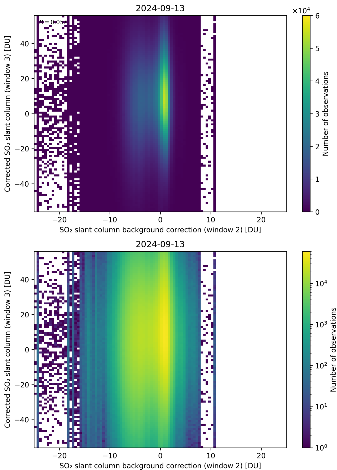
Figure 116: Scatter density plot of “SO 2 slant column background correction (window 2)” against “Corrected SO 2 slant column (window 3)” for 2024-09-12 to 2024-09-14.
