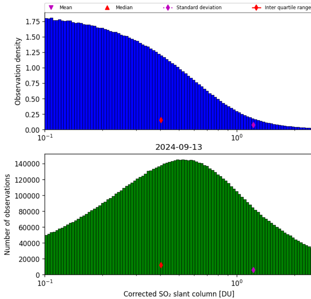
Figure 55: Histogram of “Corrected SO 2 slant column” for 2024-09-12 to 2024-09-14
