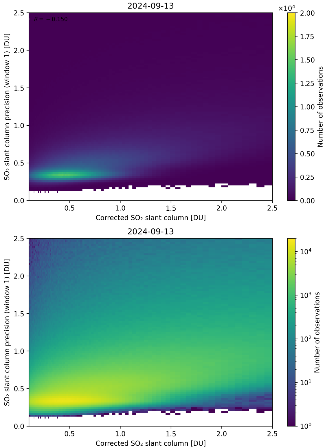
Figure 188: Scatter density plot of “Corrected SO 2 slant column” against “SO 2 slant column precision (window 1)” for 2024-09-12 to 2024-09-14.
