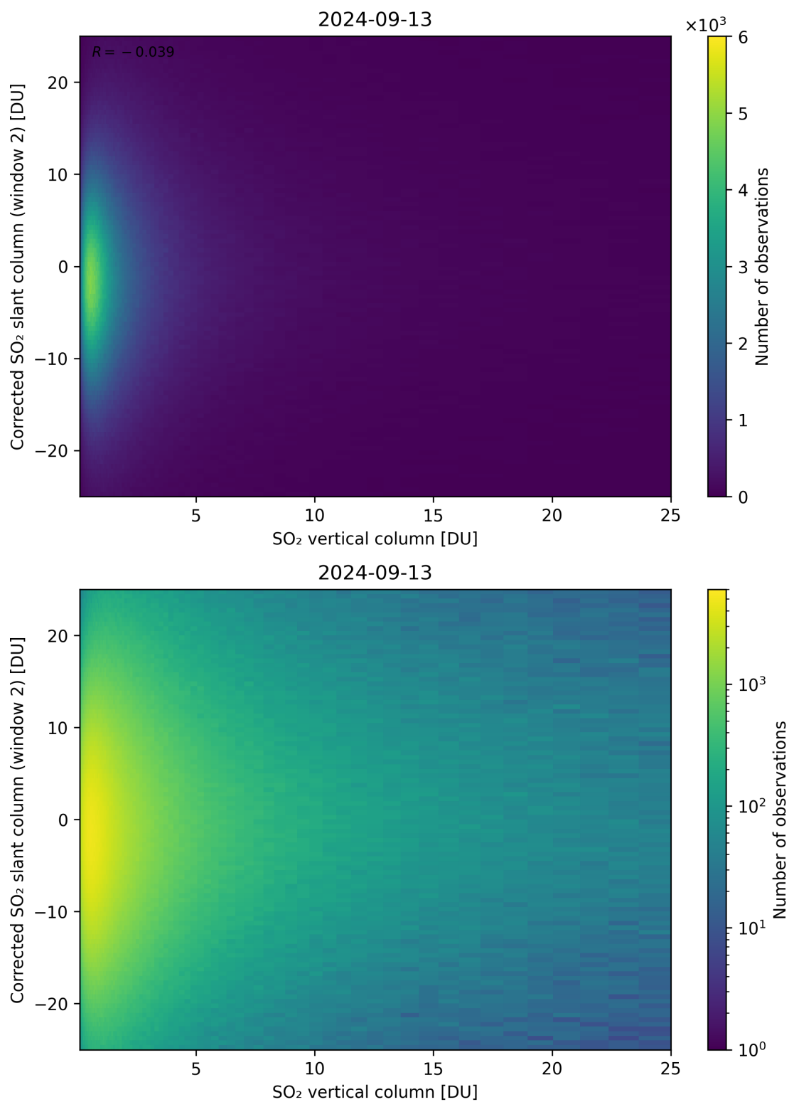
Figure 298: Scatter density plot of “SO 2 vertical column” against “Corrected SO 2 slant column (window 2)” for 2024-09-12 to 2024-09-14.
