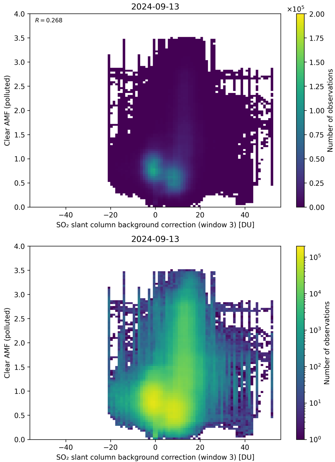
Figure 124: Scatter density plot of “SO 2 slant column background correction (window 3)” against “Clear AMF (polluted)” for 2024-09-12 to 2024-09-14.
