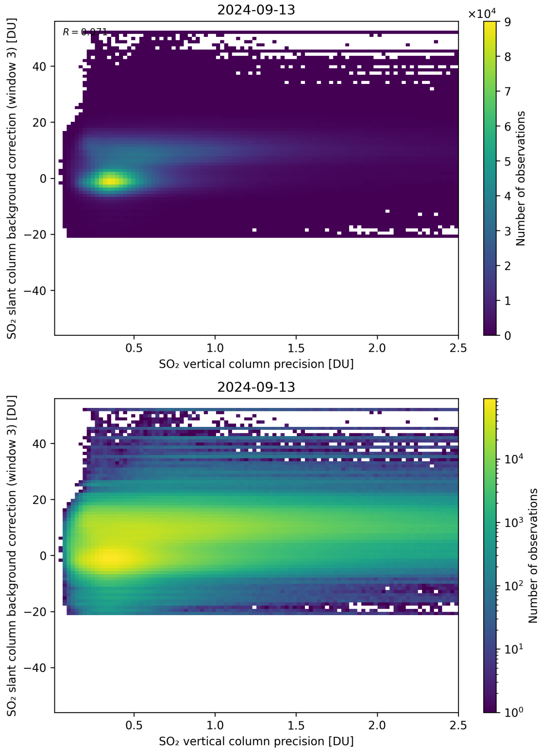
Figure 281: Scatter density plot of “SO 2 vertical column precision” against “SO 2 slant column background correction (window 3)” for 2024-09-12 to 2024-09-14.
