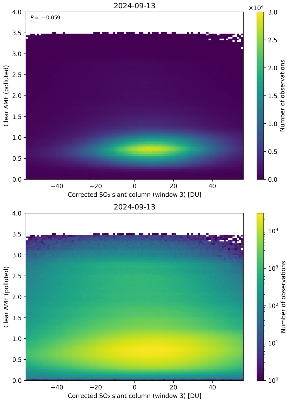
Figure 209: Scatter density plot of “Corrected SO 2 slant column (window 3)” against “Clear AMF (polluted)” for 2024-09-12 to 2024-09-14.
