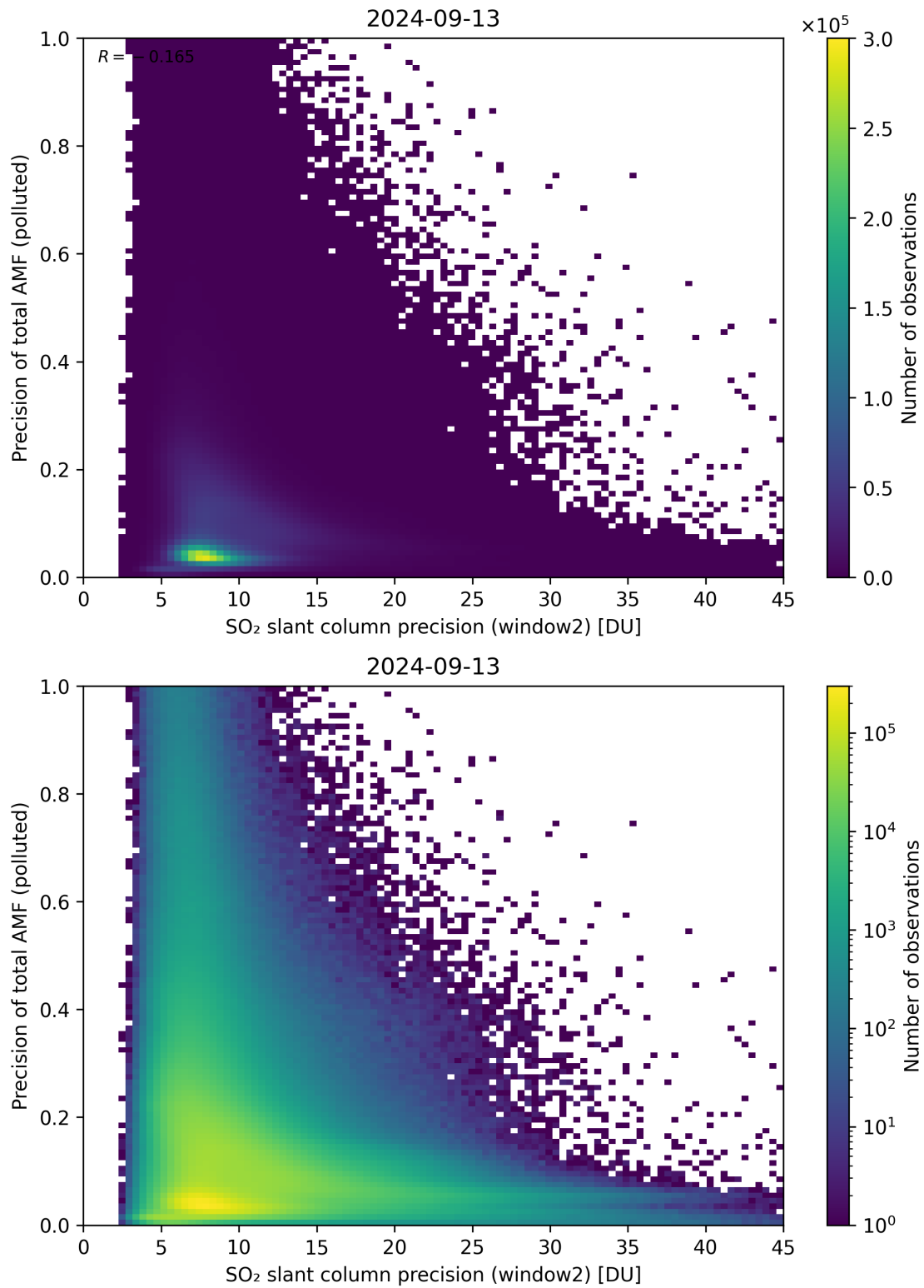
Figure 252: Scatter density plot of “SO 2 slant column precision (window2)” against “Precision of total AMF (polluted)” for 2024-09-12 to 2024-09-14.
