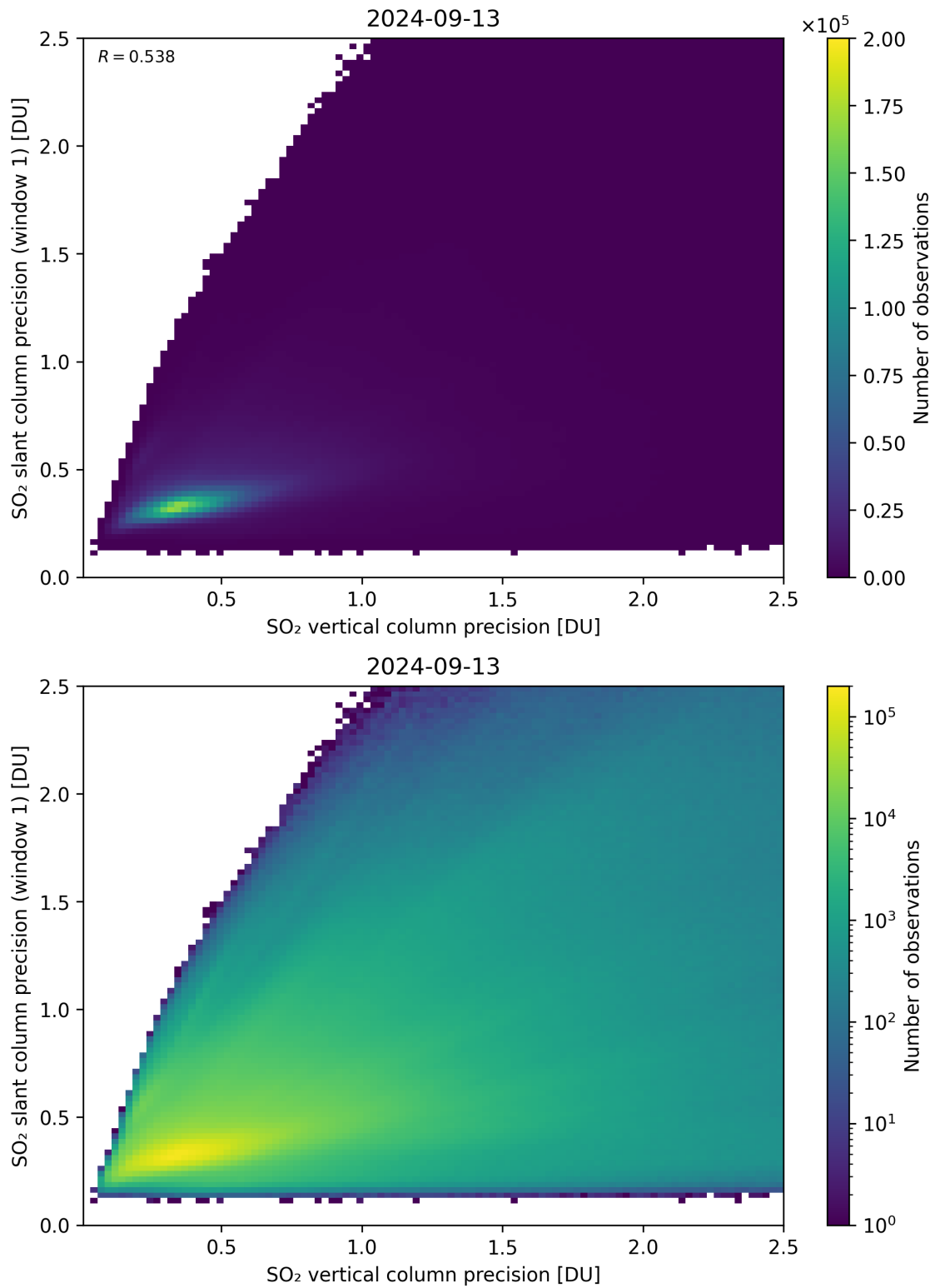
Figure 290: Scatter density plot of “SO 2 vertical column precision” against “SO 2 slant column precision (window 1)” for 2024-09-12 to 2024-09-14.
