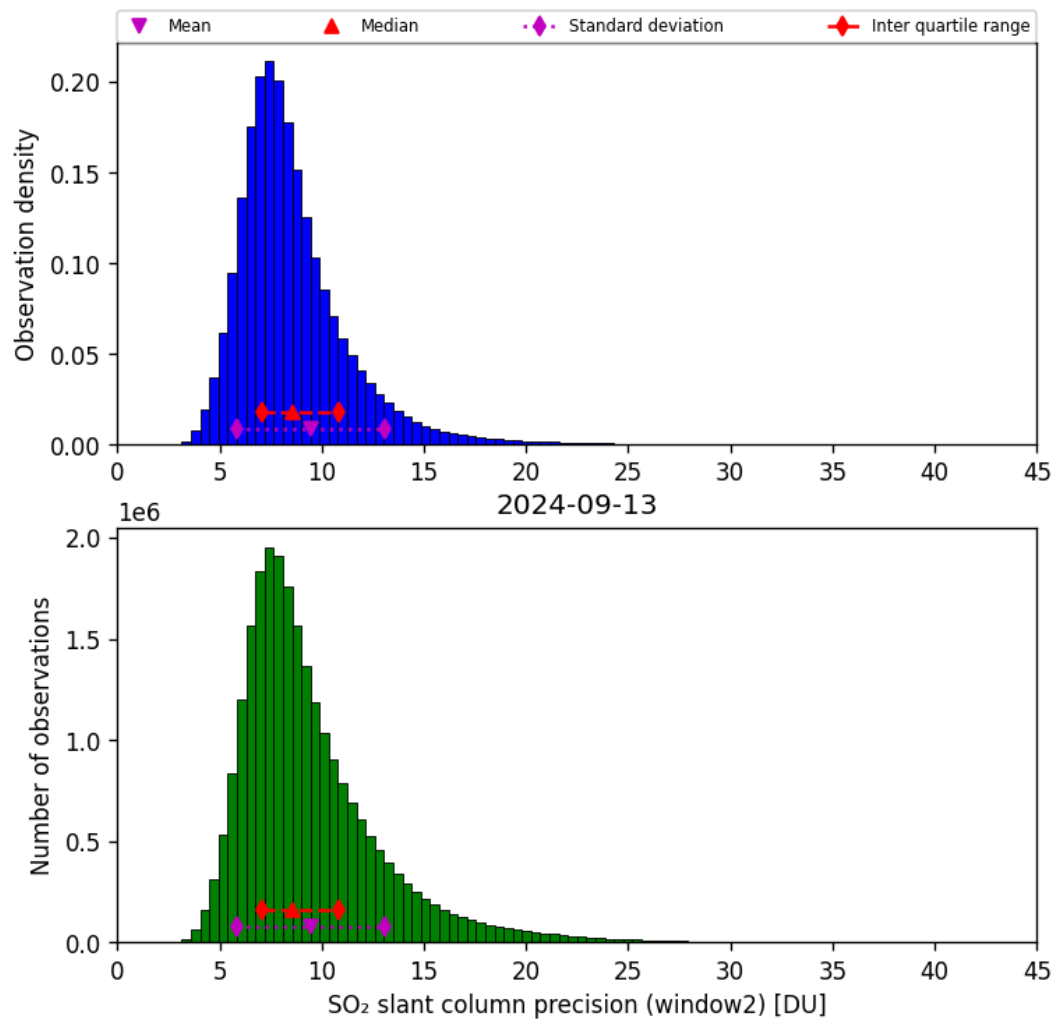
Figure 61: Histogram of “SO 2 slant column precision (window2)” for 2024-09-12 to 2024-09-14
