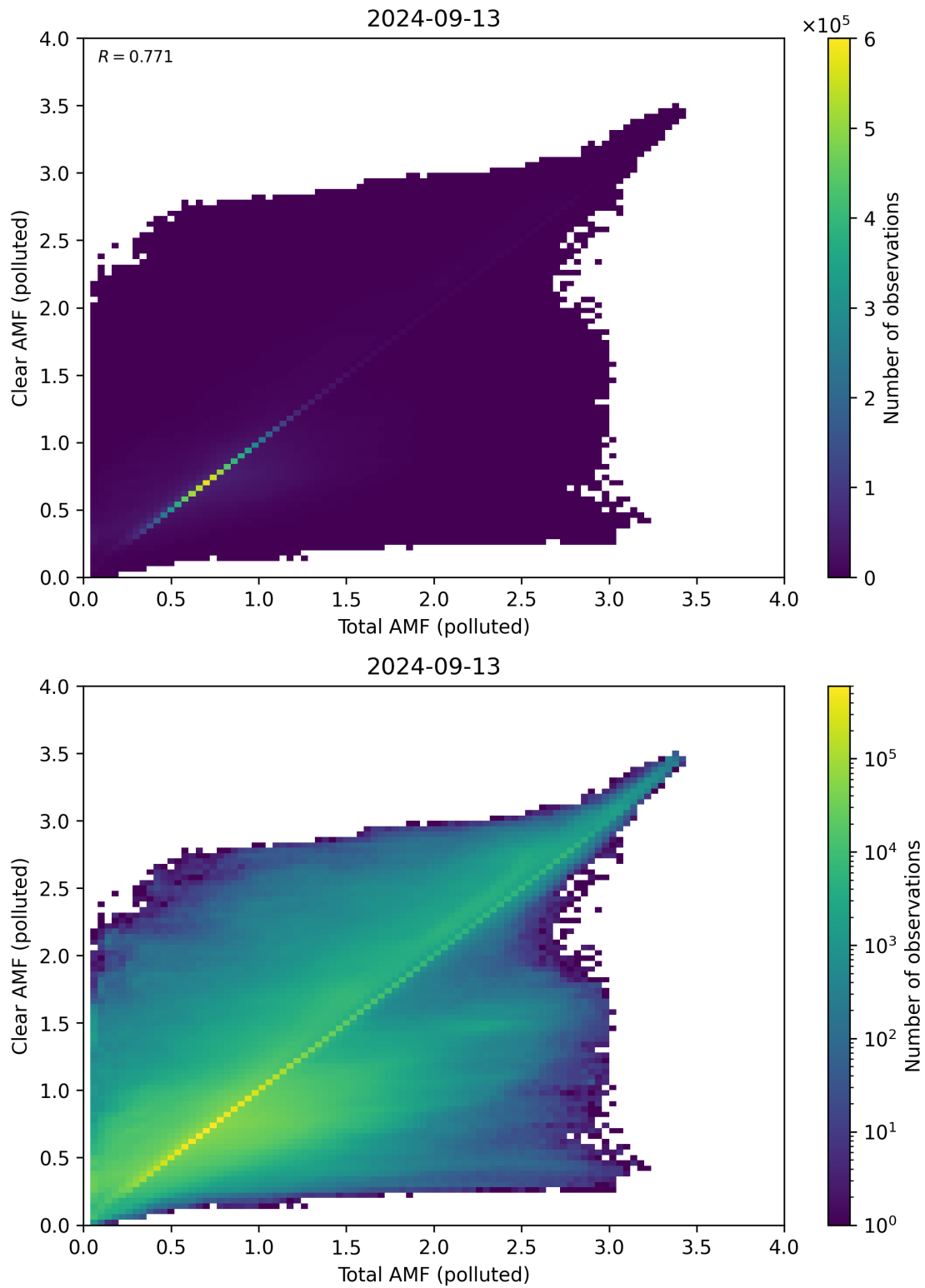
Figure 271: Scatter density plot of “Total AMF (polluted)” against “Clear AMF (polluted)” for 2024-09-12 to 2024-09-14.
