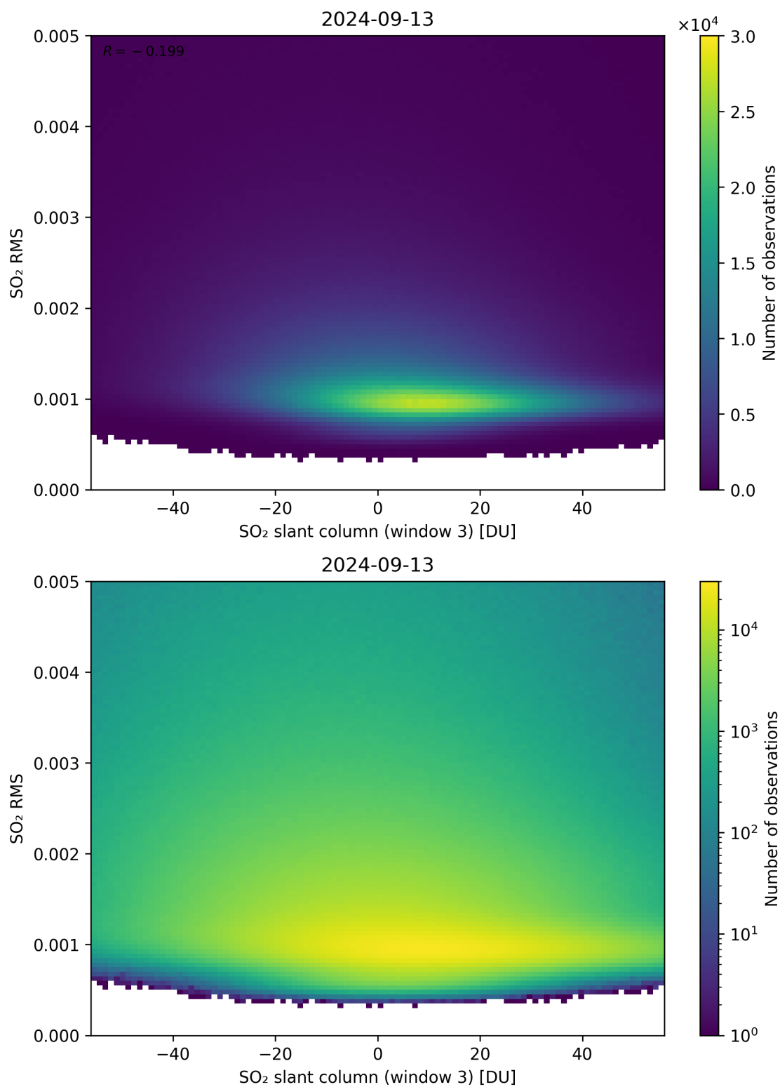
Figure 256: Scatter density plot of “SO 2 slant column (window 3)” against “SO 2 RMS” for 2024-09-12 to 2024-09-14.
