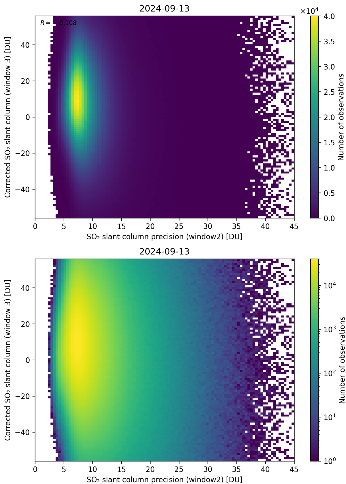
Figure 248: Scatter density plot of “SO 2 slant column precision (window2)” against “Corrected SO 2 slant column (window 3)” for 2024-09-12 to 2024-09-14.
