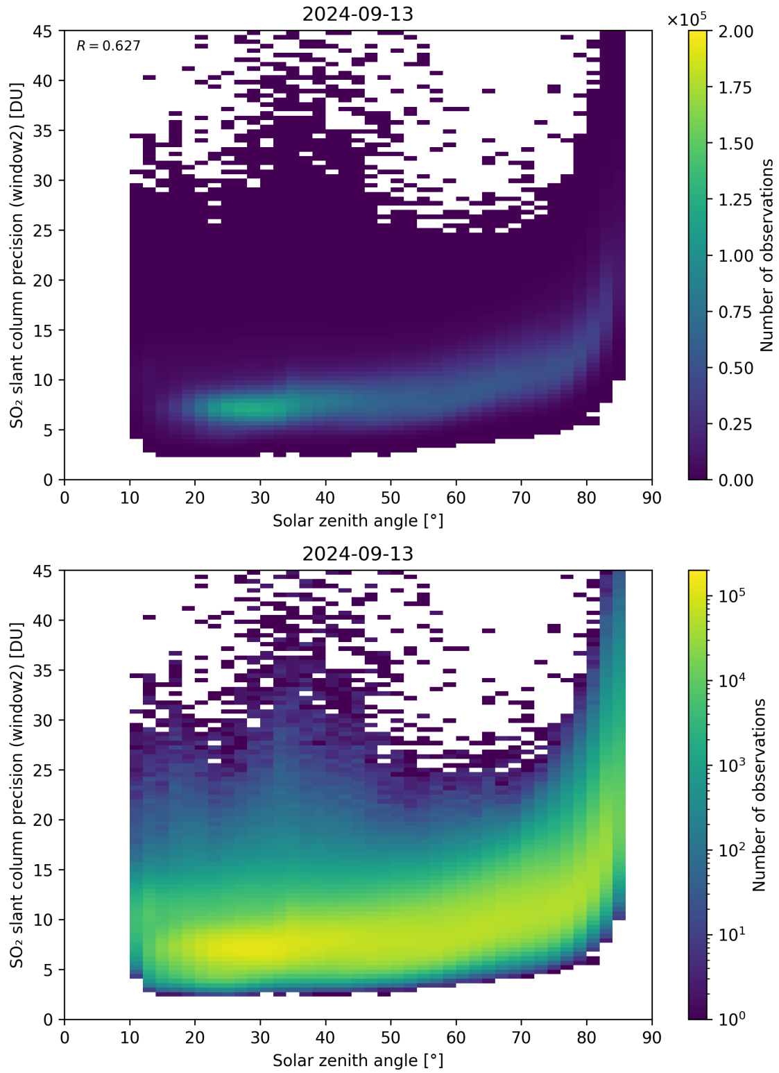
Figure 171: Scatter density plot of “Solar zenith angle” against “SO 2 slant column precision (window2)” for 2024-09-12 to 2024-09-14.
