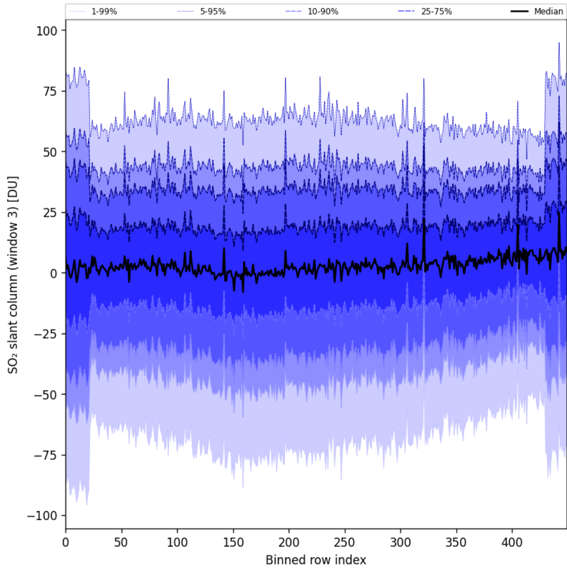
Figure 87: Along track statistics of “SO 2 slant column (window 3)” for 2024-09-12 to 2024-09-14
