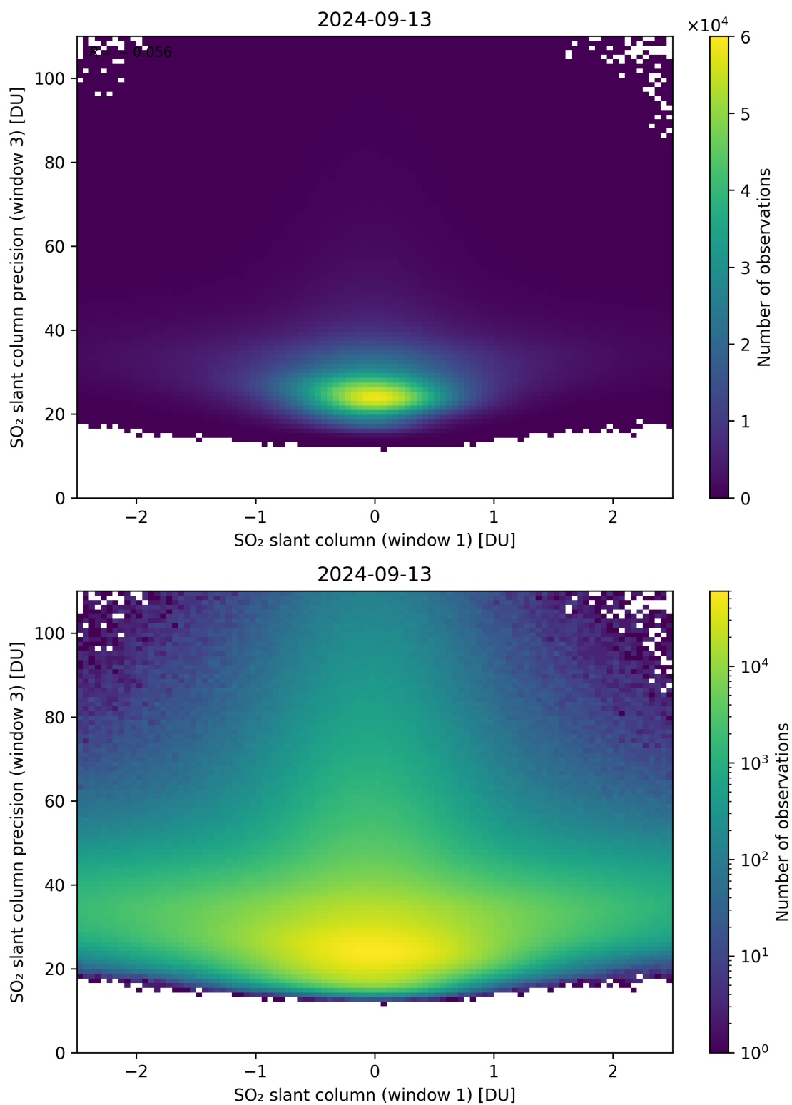
Figure 238: Scatter density plot of “SO 2 slant column (window 1)” against “SO 2 slant column precision (window 3)” for 2024-09-12 to 2024-09-14.
