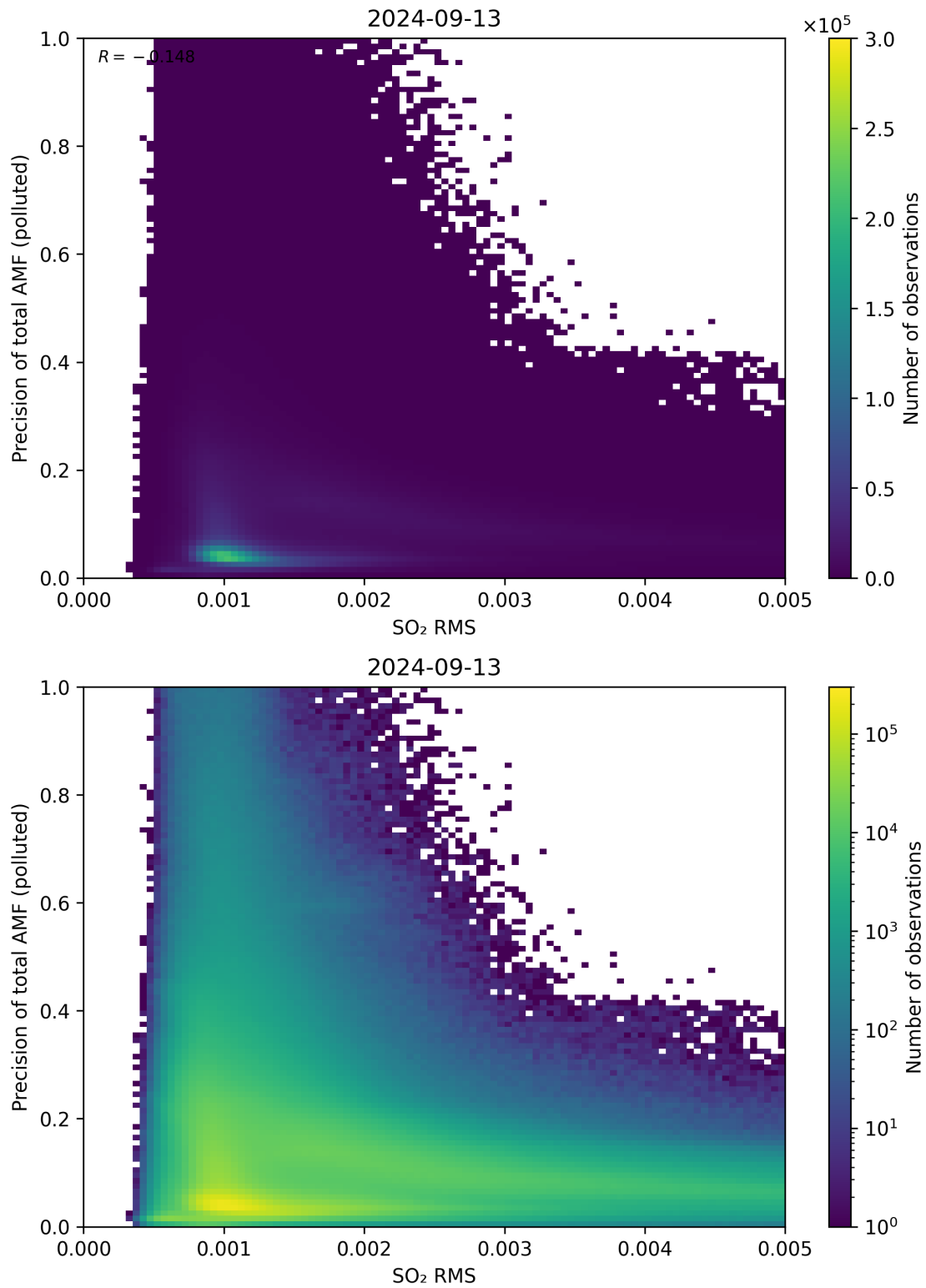
Figure 138: Scatter density plot of “SO 2 RMS” against “Precision of total AMF (polluted)” for 2024-09-12 to 2024-09-14.
