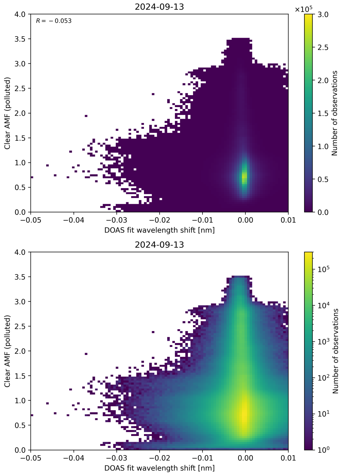
Figure 129: Scatter density plot of “DOAS fit wavelength shift” against “Clear AMF (polluted)” for 2024-09-12 to 2024-09-14.
