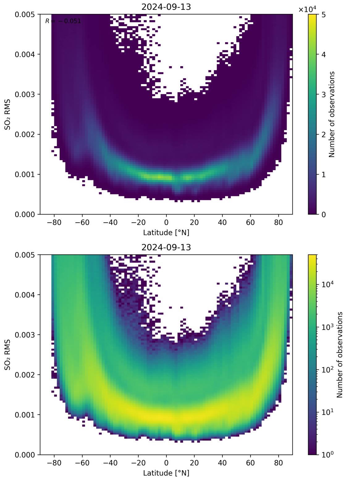
Figure 144: Scatter density plot of “Latitude” against “SO 2 RMS” for 2024-09-12 to 2024-09-14.
