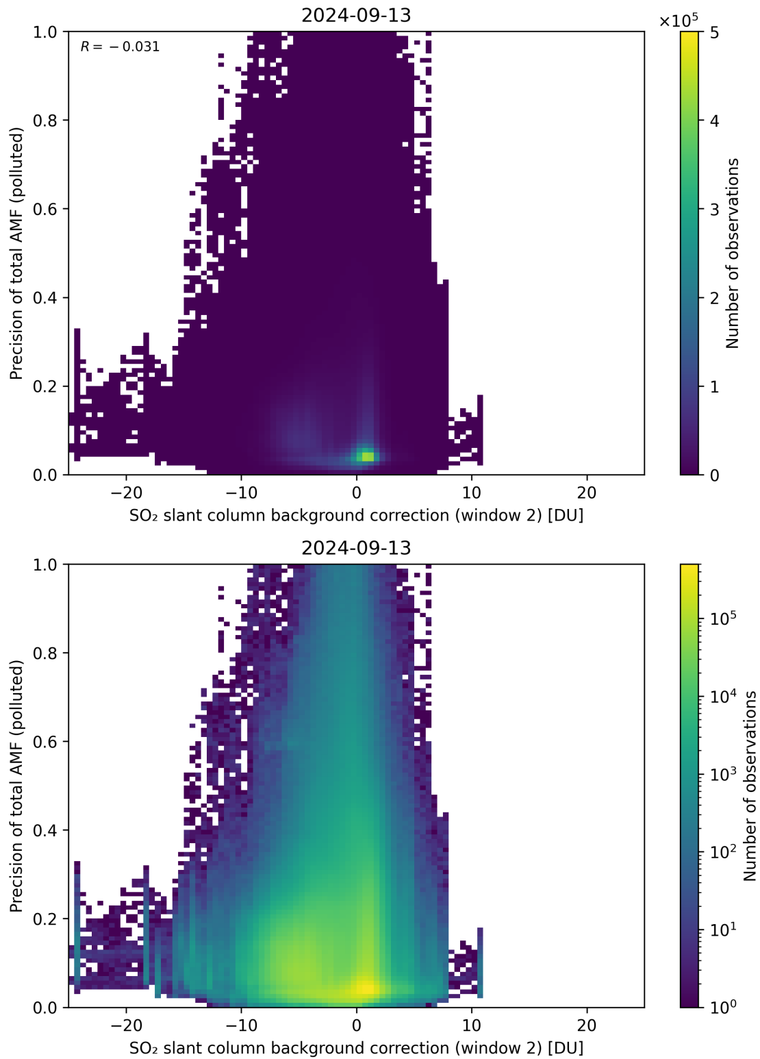
Figure 120: Scatter density plot of “SO 2 slant column background correction (window 2)” against “Precision of total AMF (polluted)” for 2024-09-12 to 2024-09-14.
