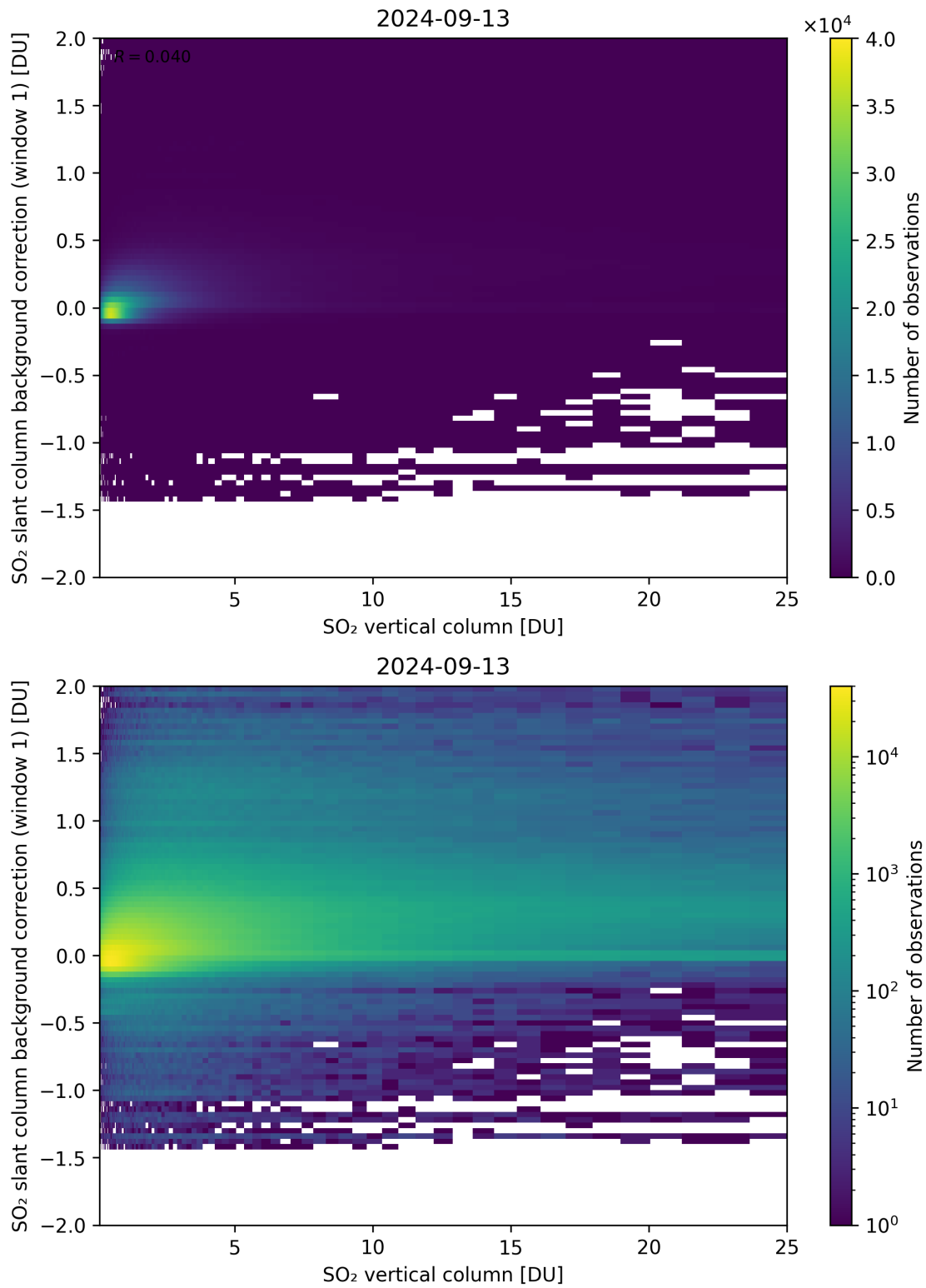
Figure 273: Scatter density plot of “SO 2 vertical column” against “SO 2 slant column background correction (window 1)” for 2024-09-12 to 2024-09-14.
