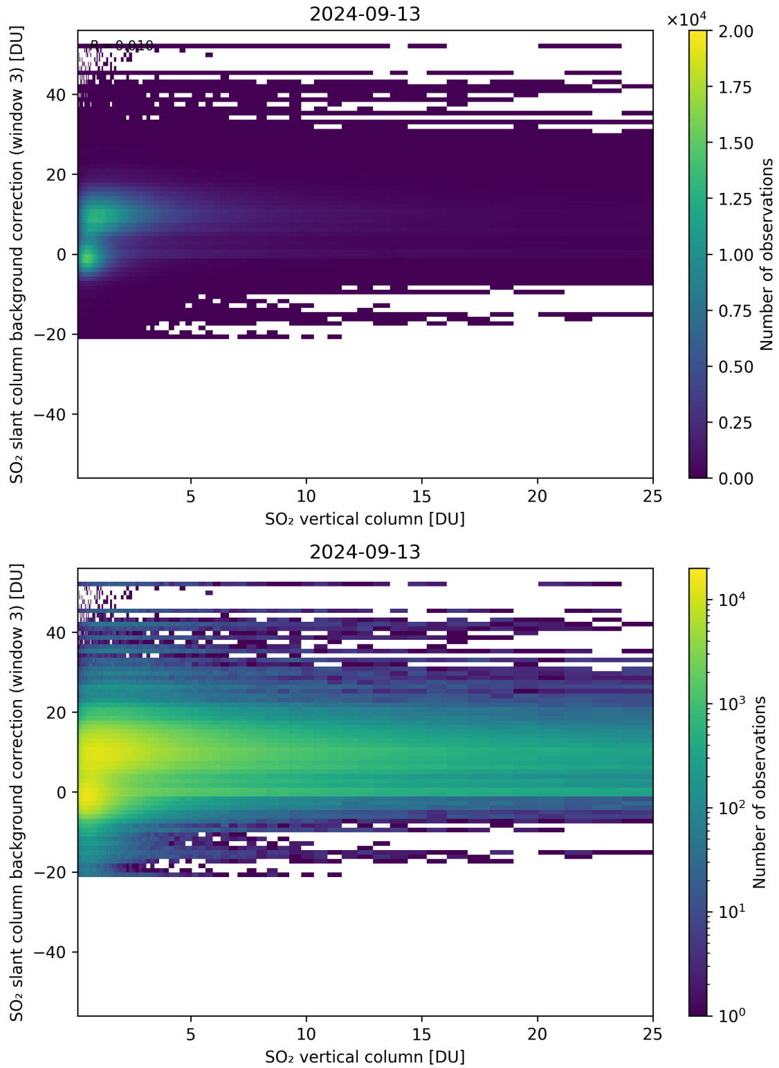
Figure 275: Scatter density plot of “SO 2 vertical column” against “SO 2 slant column background correction (window 3)” for 2024-09-12 to 2024-09-14.
