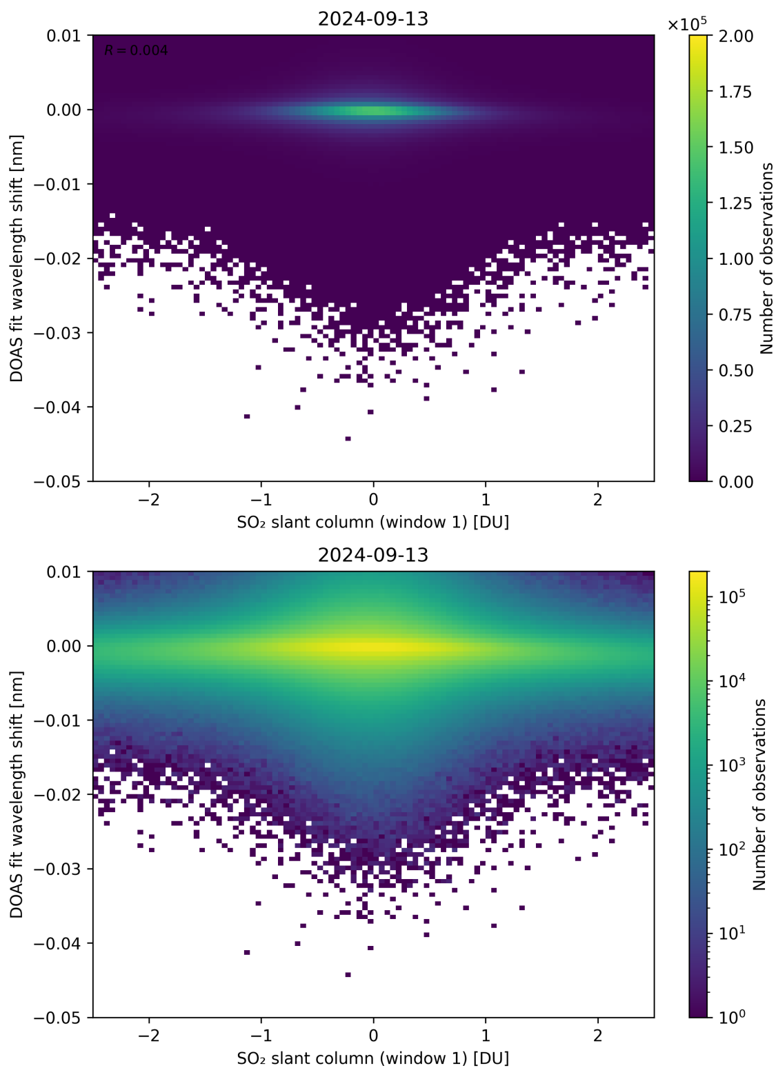
Figure 215: Scatter density plot of “SO 2 slant column (window 1)” against “DOAS fit wavelength shift” for 2024-09-12 to 2024-09-14.
