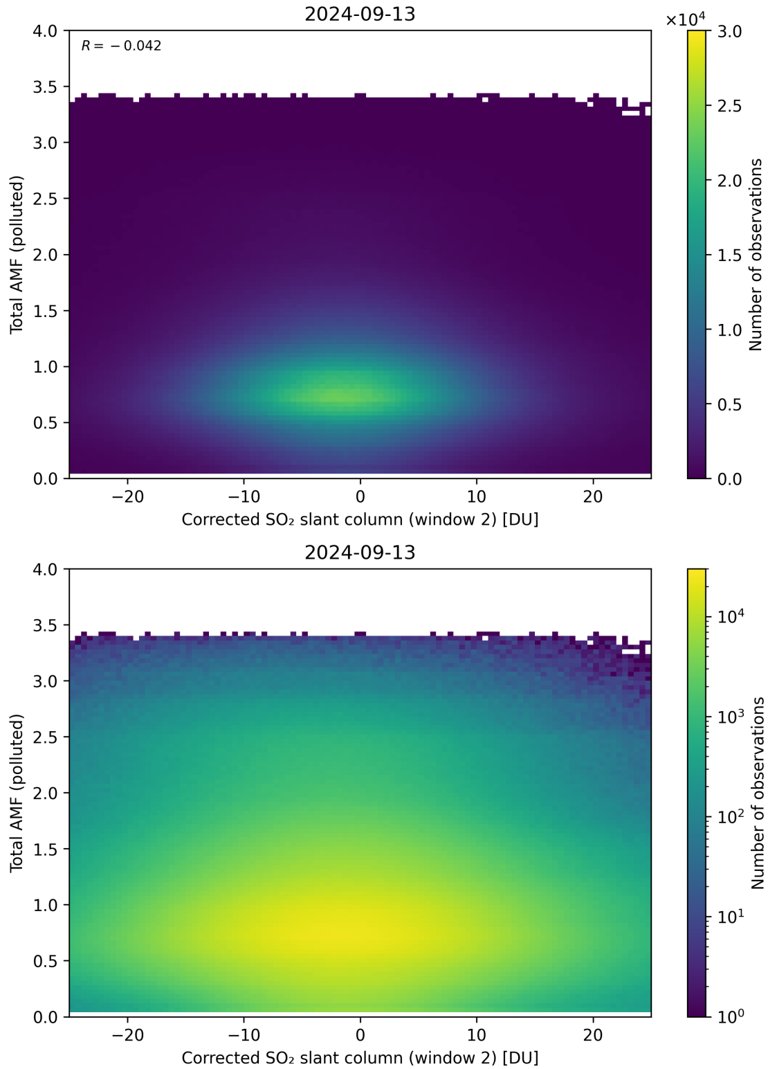
Figure 203: Scatter density plot of “Corrected SO 2 slant column (window 2)” against “Total AMF (polluted)” for 2024-09-12 to 2024-09-14.
