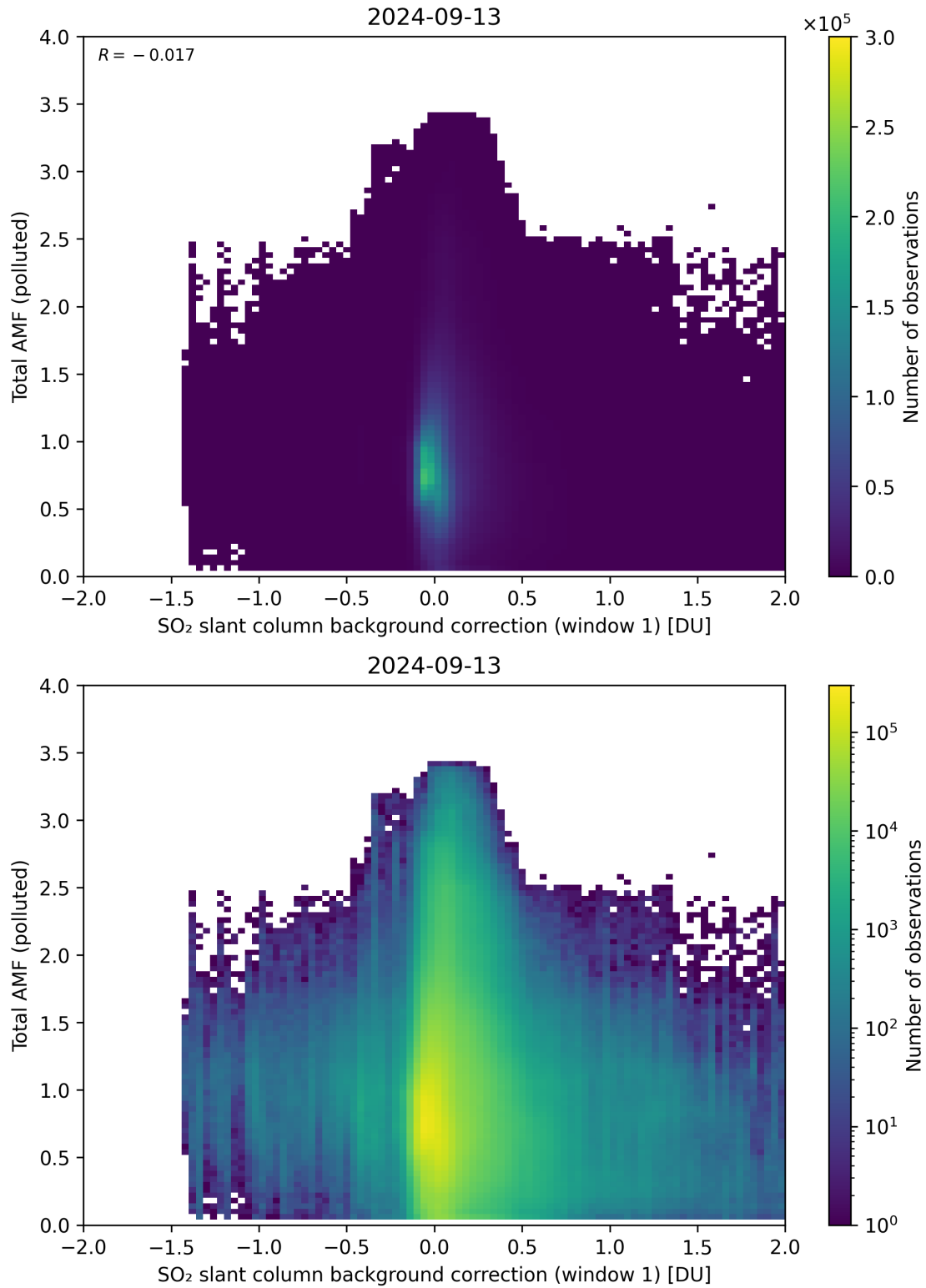
Figure 109: Scatter density plot of “SO 2 slant column background correction (window 1)” against “Total AMF (polluted)” for 2024-09-12 to 2024-09-14.
