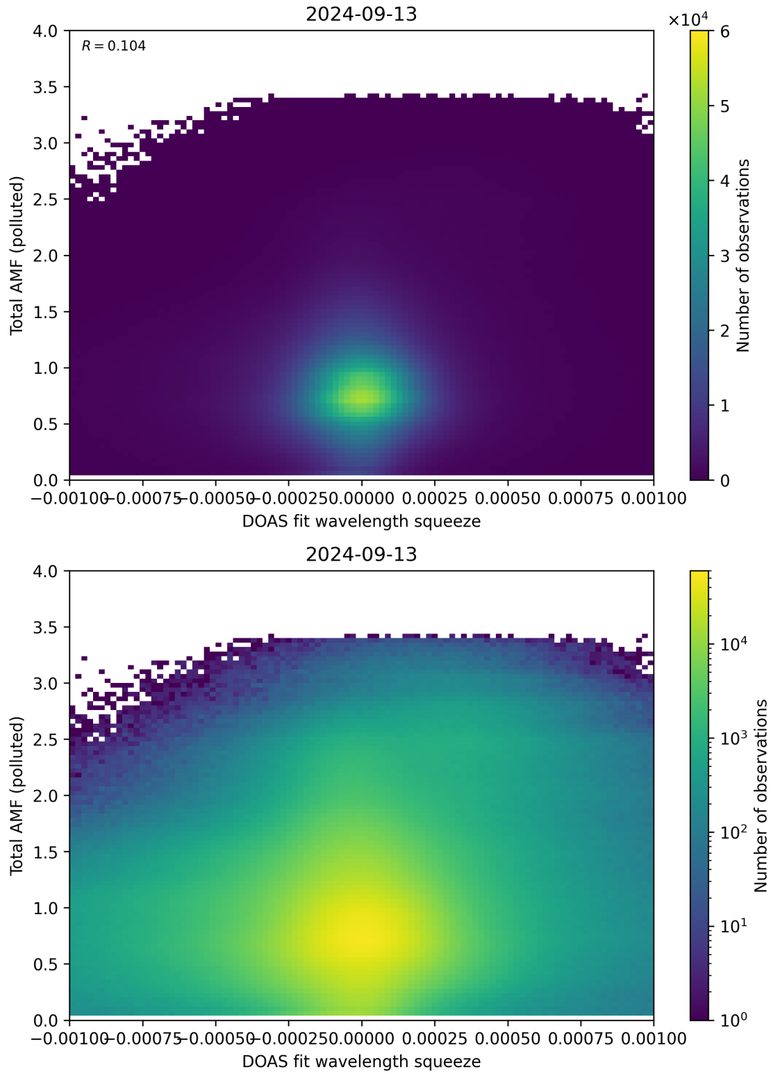
Figure 134: Scatter density plot of “DOAS fit wavelength squeeze” against “Total AMF (polluted)” for 2024-09-12 to 2024-09-14.
