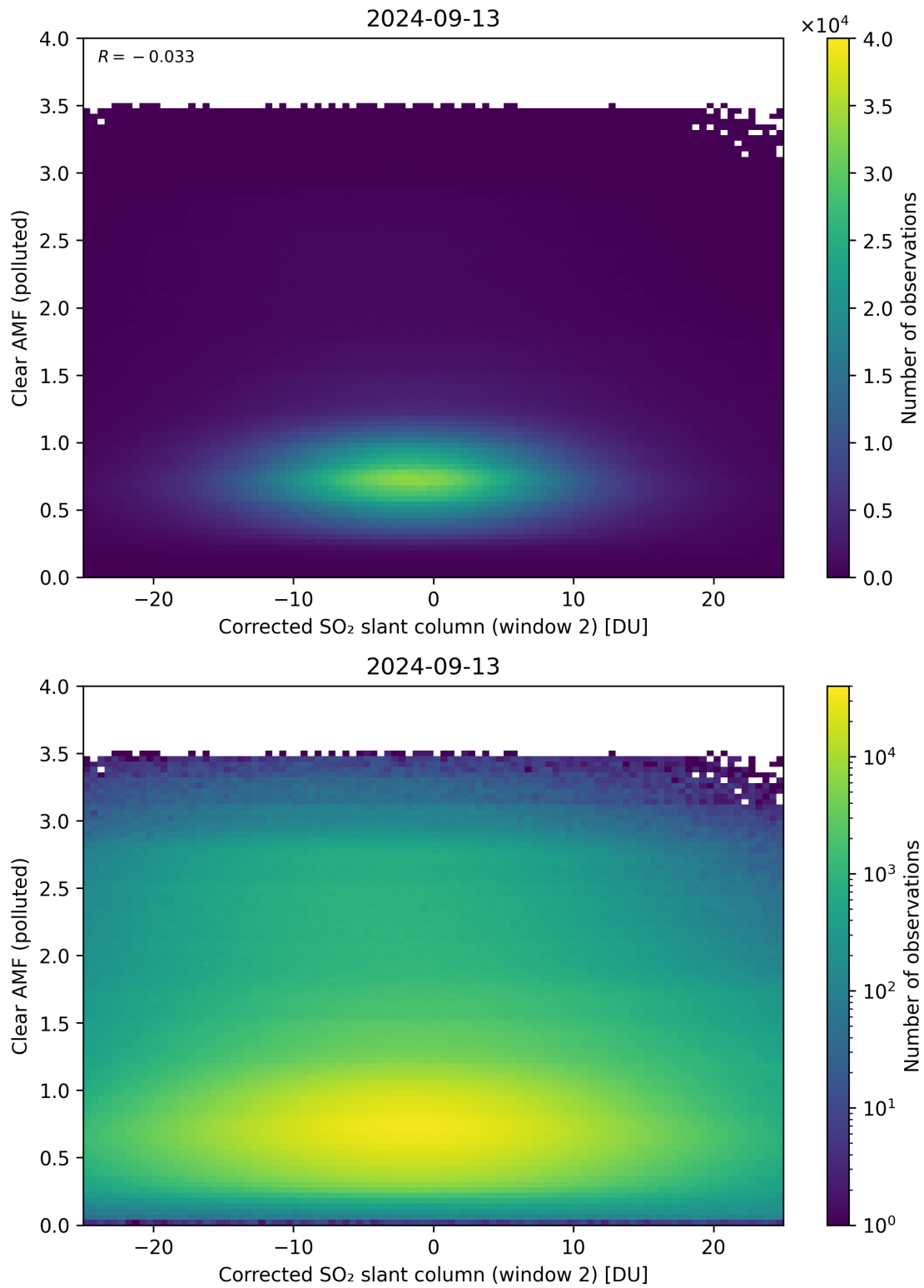
Figure 199: Scatter density plot of “Corrected SO 2 slant column (window 2)” against “Clear AMF (polluted)” for 2024-09-12 to 2024-09-14.
