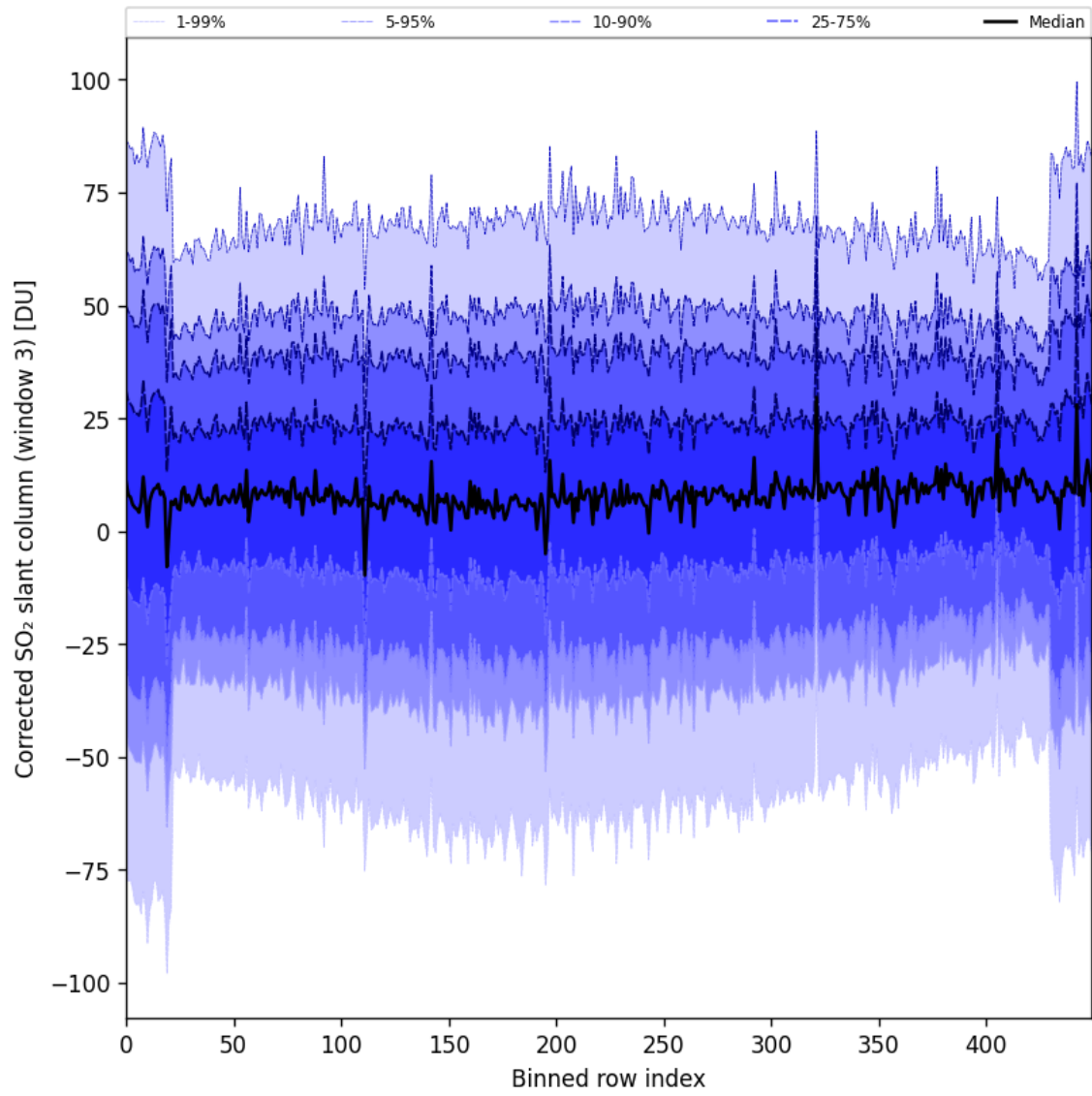
Figure 89: Along track statistics of “Corrected SO 2 slant column (window 3)” for 2024-09-12 to 2024-09-14
