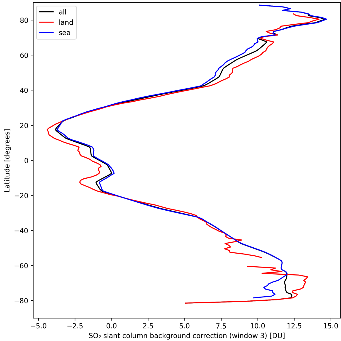
Figure 44: Zonal average of “SO 2 slant column background correction (window 3)” for 2024-09-12 to 2024-09-14.
