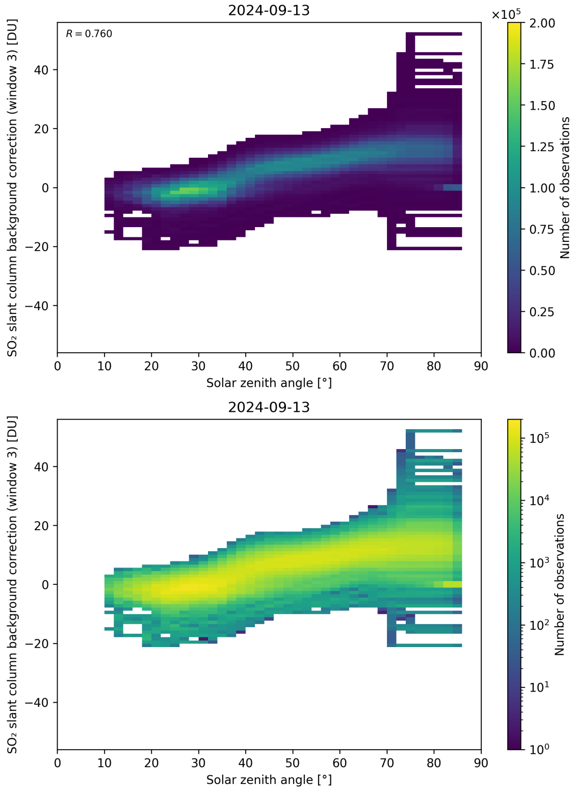
Figure 160: Scatter density plot of “Solar zenith angle” against “SO 2 slant column background correction (window 3)” for 2024-09-12 to 2024-09-14.
