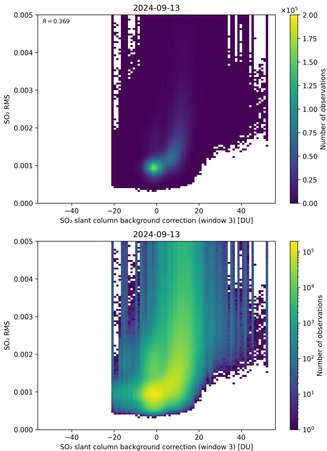
Figure 123: Scatter density plot of “SO 2 slant column background correction (window 3)” against “SO 2 RMS” for 2024-09-12 to 2024-09-14.
