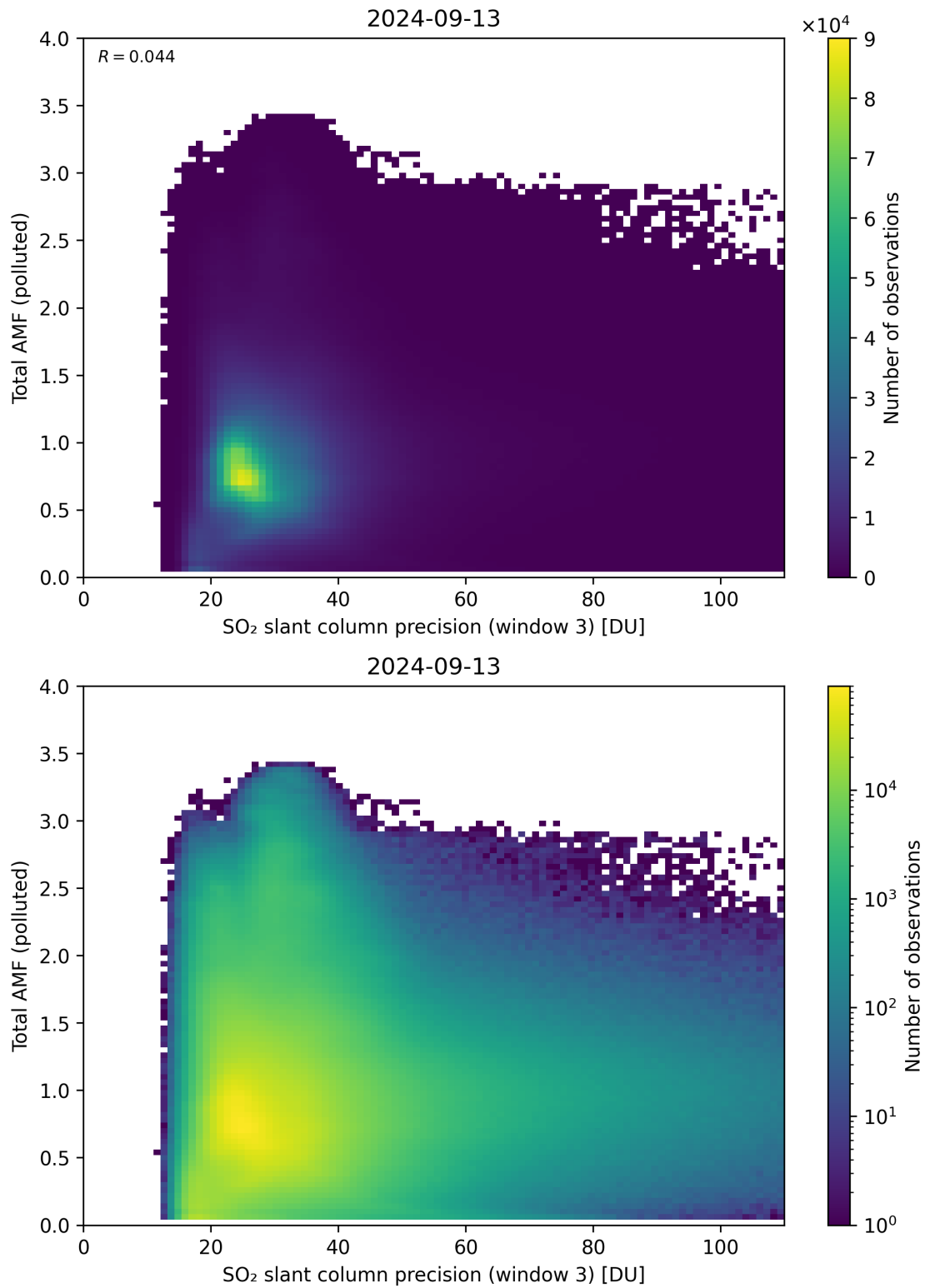
Figure 263: Scatter density plot of “SO 2 slant column precision (window 3)” against “Total AMF (polluted)” for 2024-09-12 to 2024-09-14.
