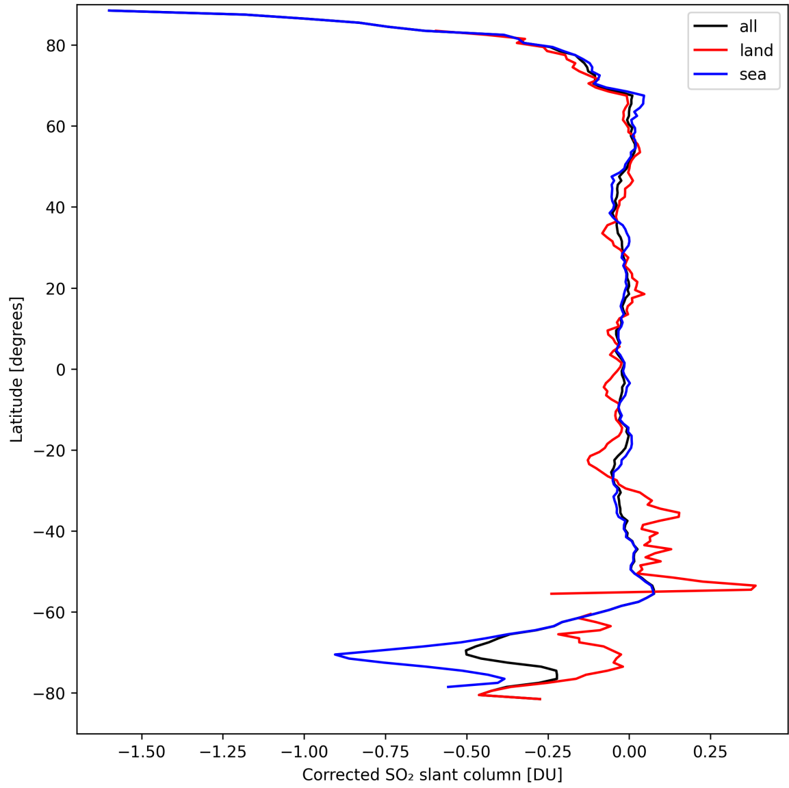
Figure 32: Zonal average of “Corrected SO 2 slant column” for 2024-09-12 to 2024-09-14.
