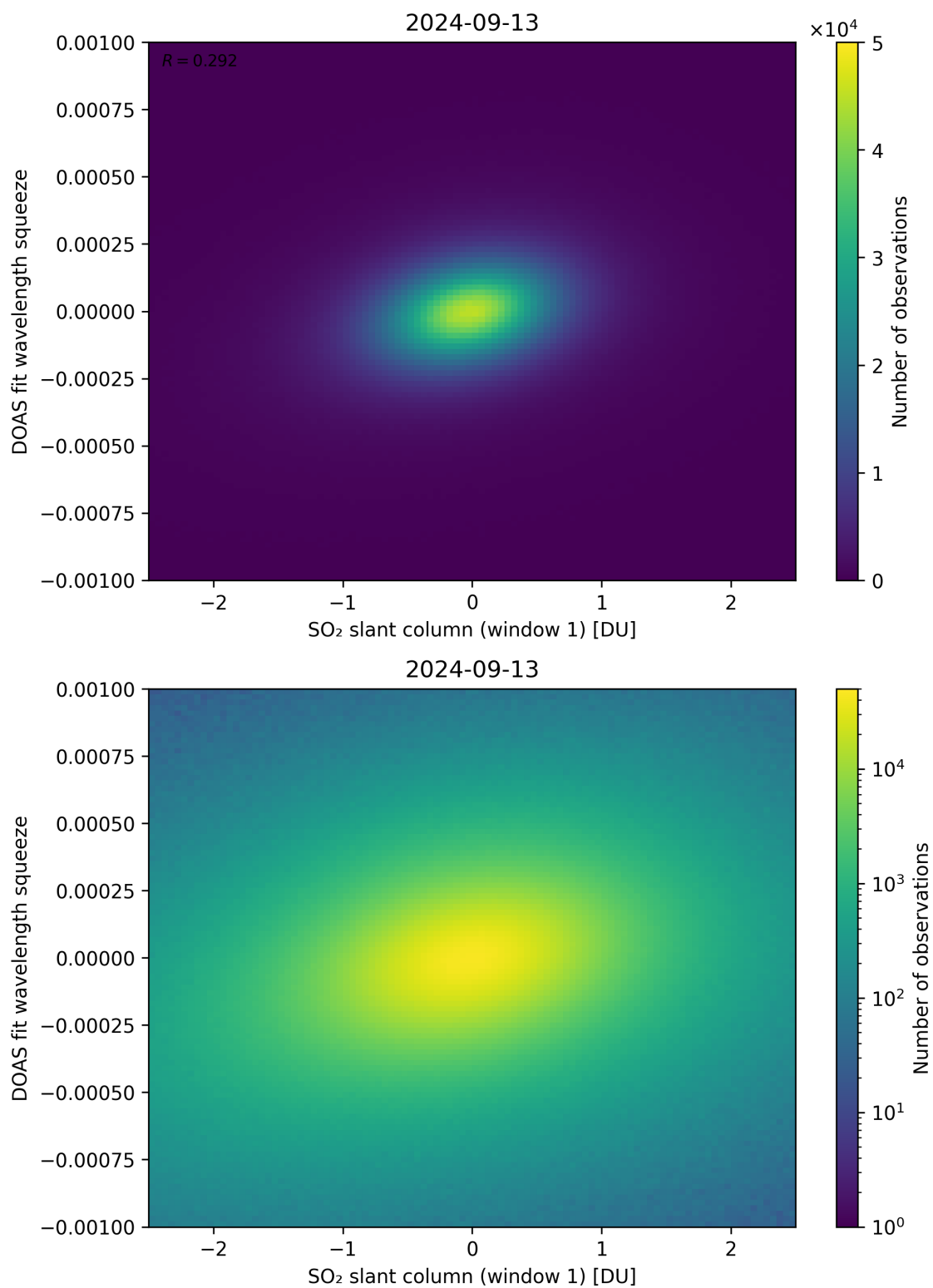
Figure 216: Scatter density plot of “SO 2 slant column (window 1)” against “DOAS fit wavelength squeeze” for 2024-09-12 to 2024-09-14.
