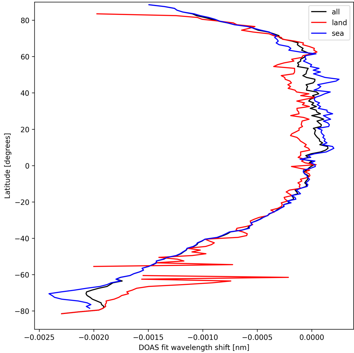
Figure 45: Zonal average of “DOAS fit wavelength shift” for 2024-09-12 to 2024-09-14.
