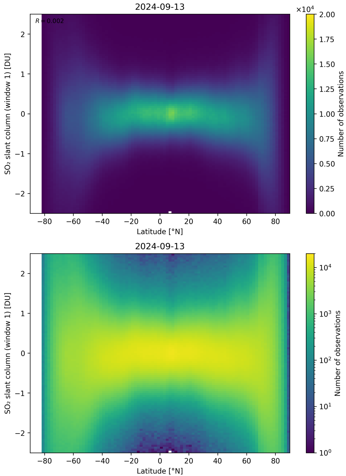
Figure 149: Scatter density plot of “Latitude” against “SO 2 slant column (window 1)” for 2024-09-12 to 2024-09-14.
