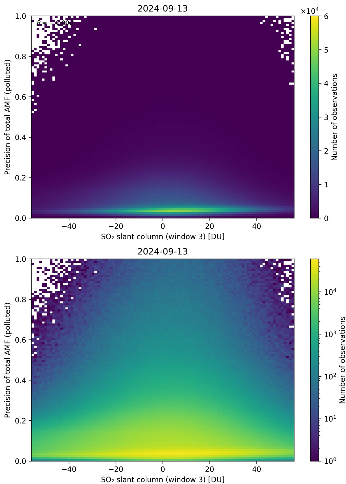
Figure 269: Scatter density plot of “SO 2 slant column (window 3)” against “Precision of total AMF (polluted)” for 2024-09-12 to 2024-09-14.
