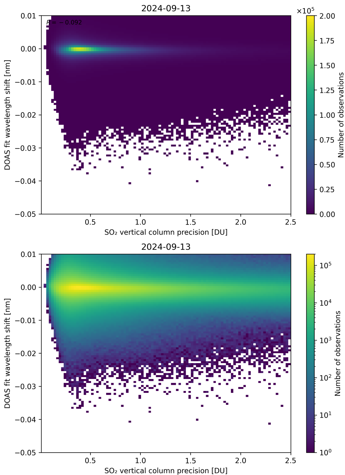
Figure 282: Scatter density plot of “SO 2 vertical column precision” against “DOAS fit wavelength shift” for 2024-09-12 to 2024-09-14.
