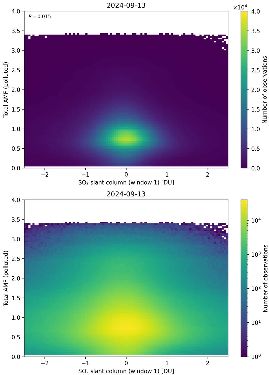
Figure 239: Scatter density plot of “SO 2 slant column (window 1)” against “Total AMF (polluted)” for 2024-09-12 to 2024-09-14.
