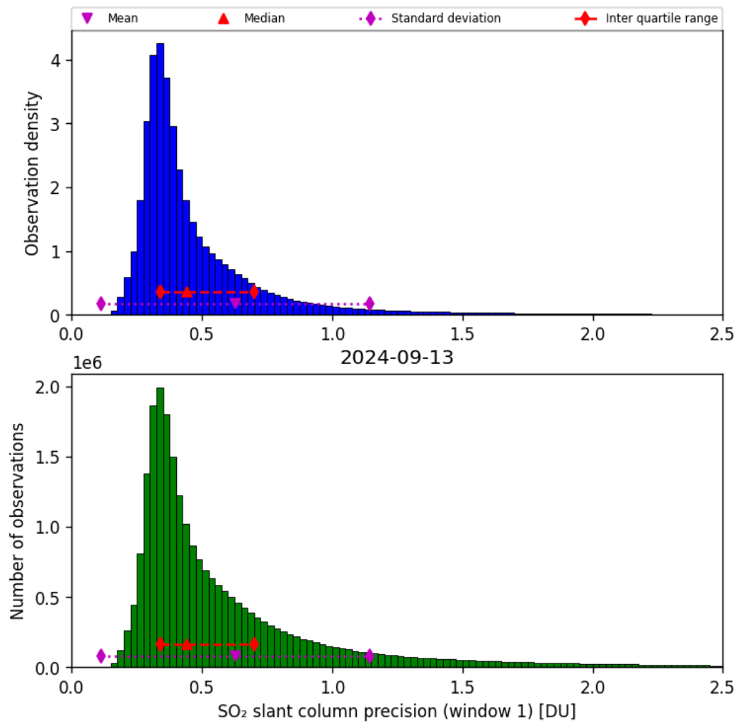
Figure 57: Histogram of “SO 2 slant column precision (window 1)” for 2024-09-12 to 2024-09-14
