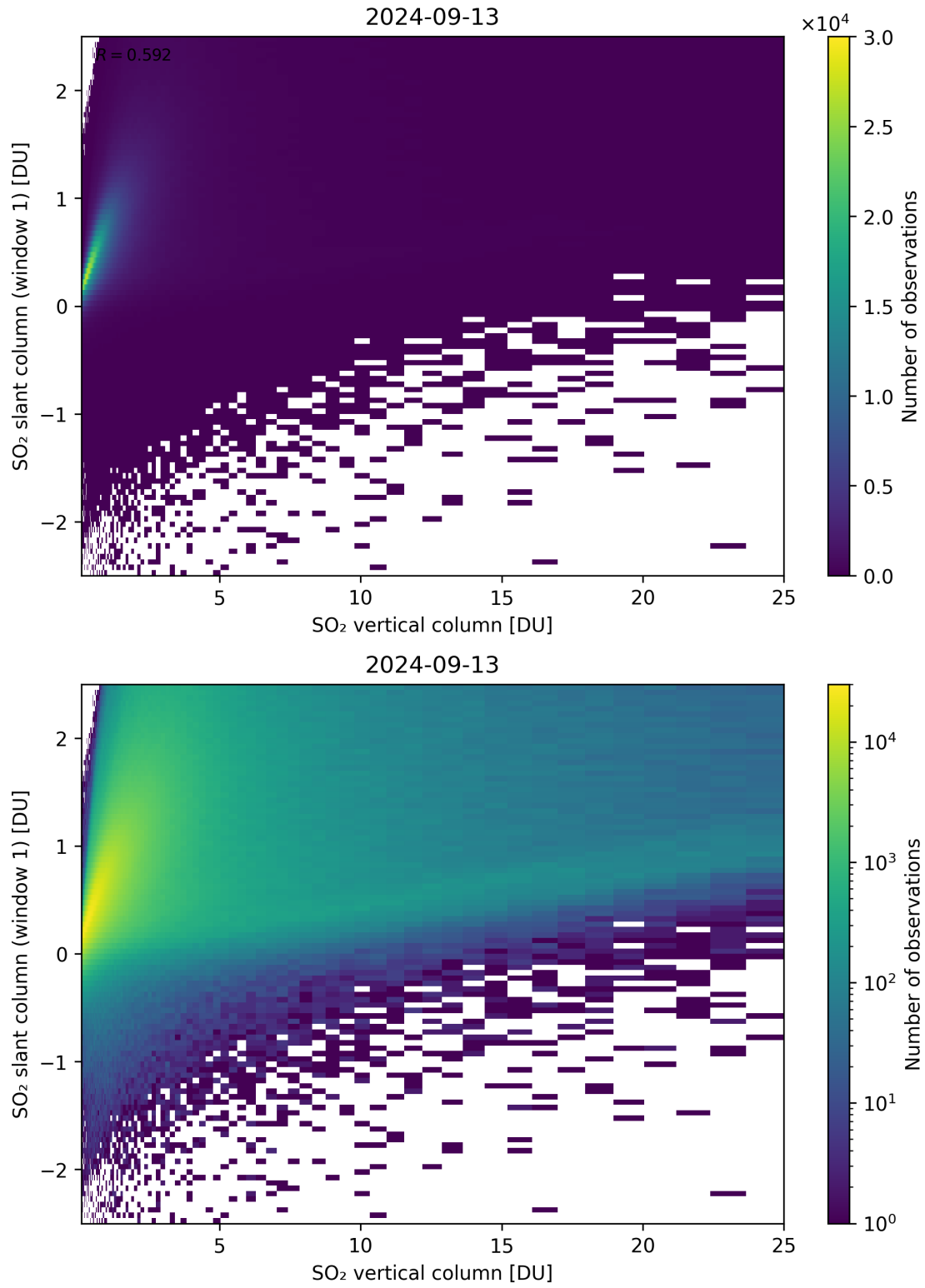
Figure 300: Scatter density plot of “SO 2 vertical column” against “SO 2 slant column (window 1)” for 2024-09-12 to 2024-09-14.
