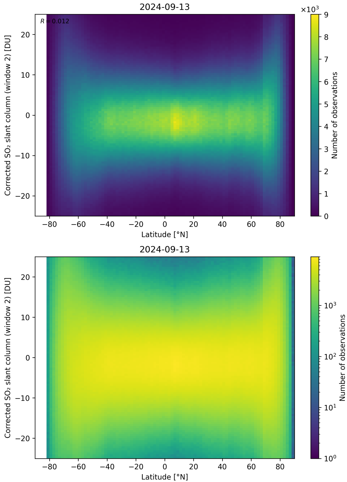
Figure 147: Scatter density plot of “Latitude” against “Corrected SO 2 slant column (window 2)” for 2024-09-12 to 2024-09-14.
