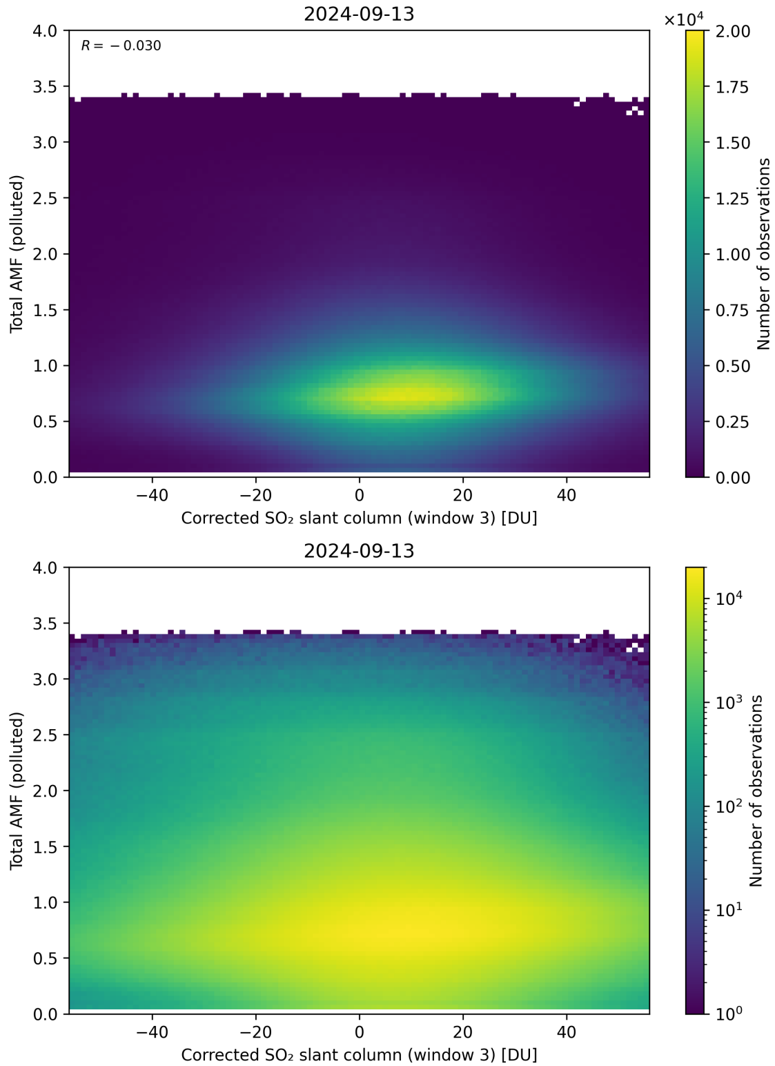
Figure 210: Scatter density plot of “Corrected SO 2 slant column (window 3)” against “Total AMF (polluted)” for 2024-09-12 to 2024-09-14.
