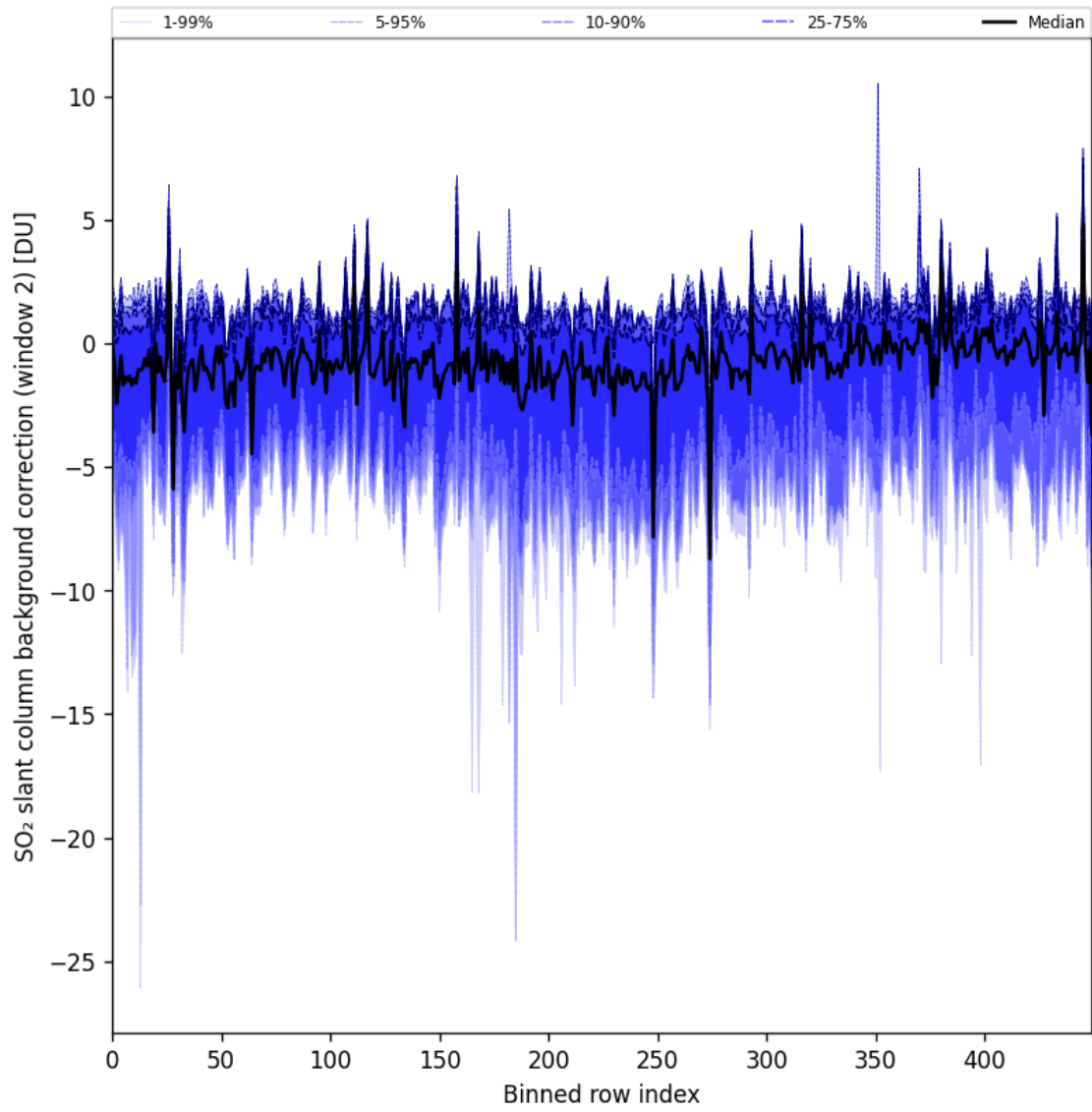
Figure 86: Along track statistics of “SO 2 slant column background correction (window 2)” for 2024-09-12 to 2024-09-14
