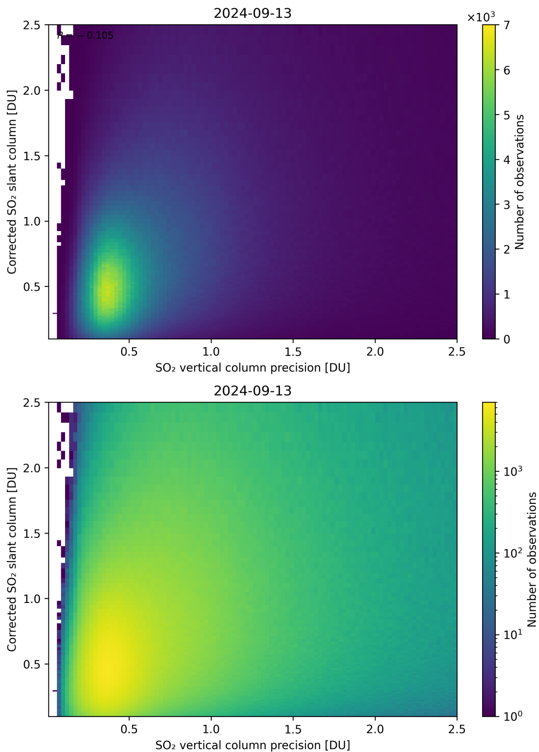
Figure 286: Scatter density plot of “SO 2 vertical column precision” against “Corrected SO 2 slant column” for 2024-09-12 to 2024-09-14.
