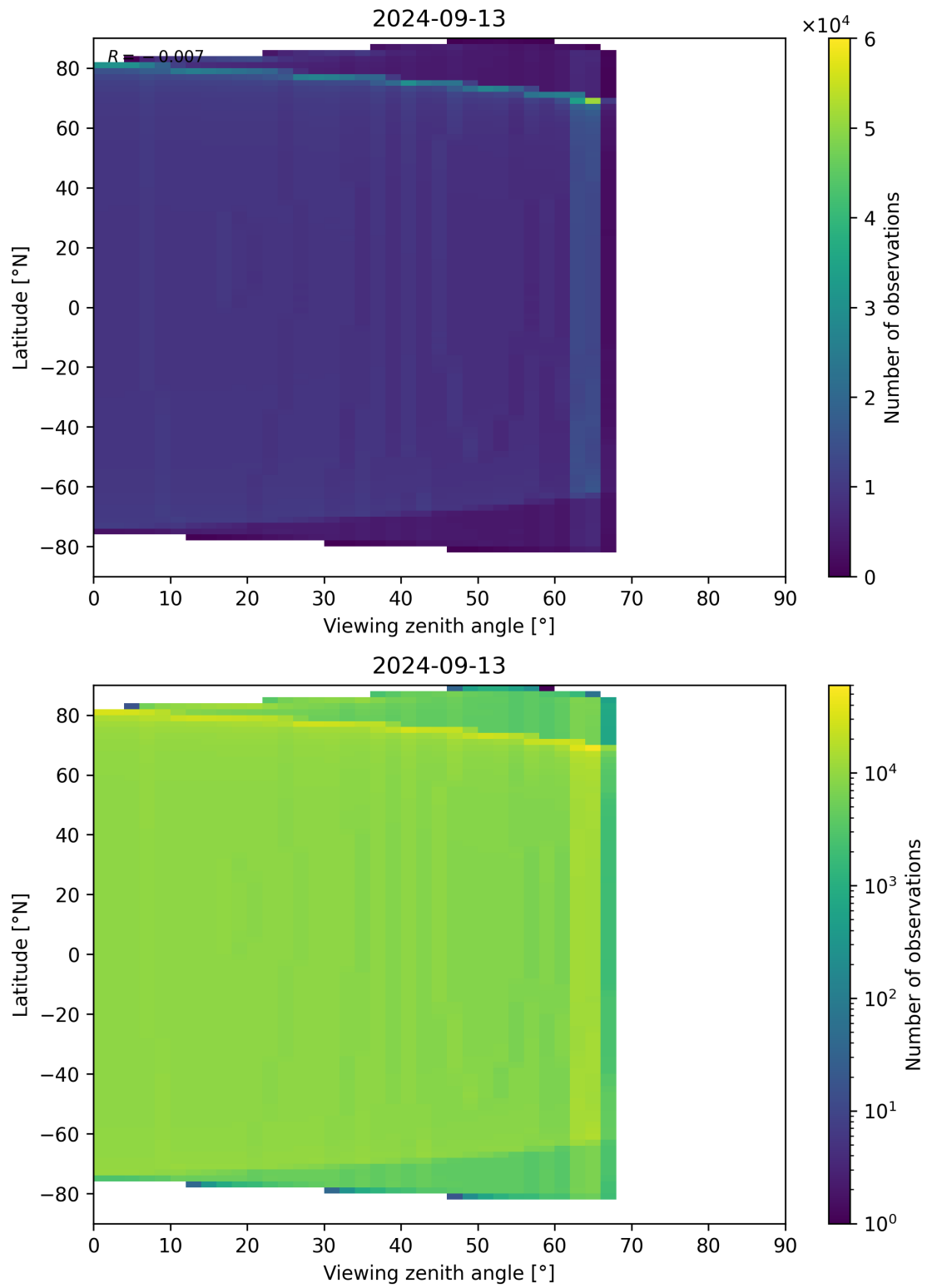
Figure 314: Scatter density plot of “Viewing zenith angle” against “Latitude” for 2024-09-12 to 2024-09-14.
