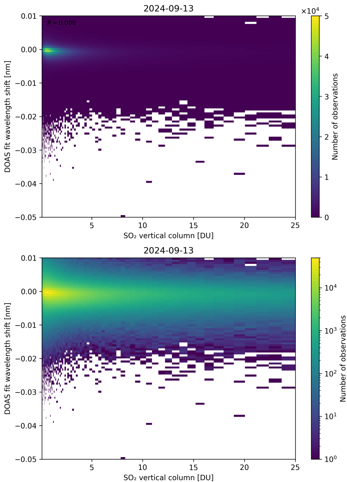
Figure 276: Scatter density plot of “SO 2 vertical column” against “DOAS fit wavelength shift” for 2024-09-12 to 2024-09-14.
