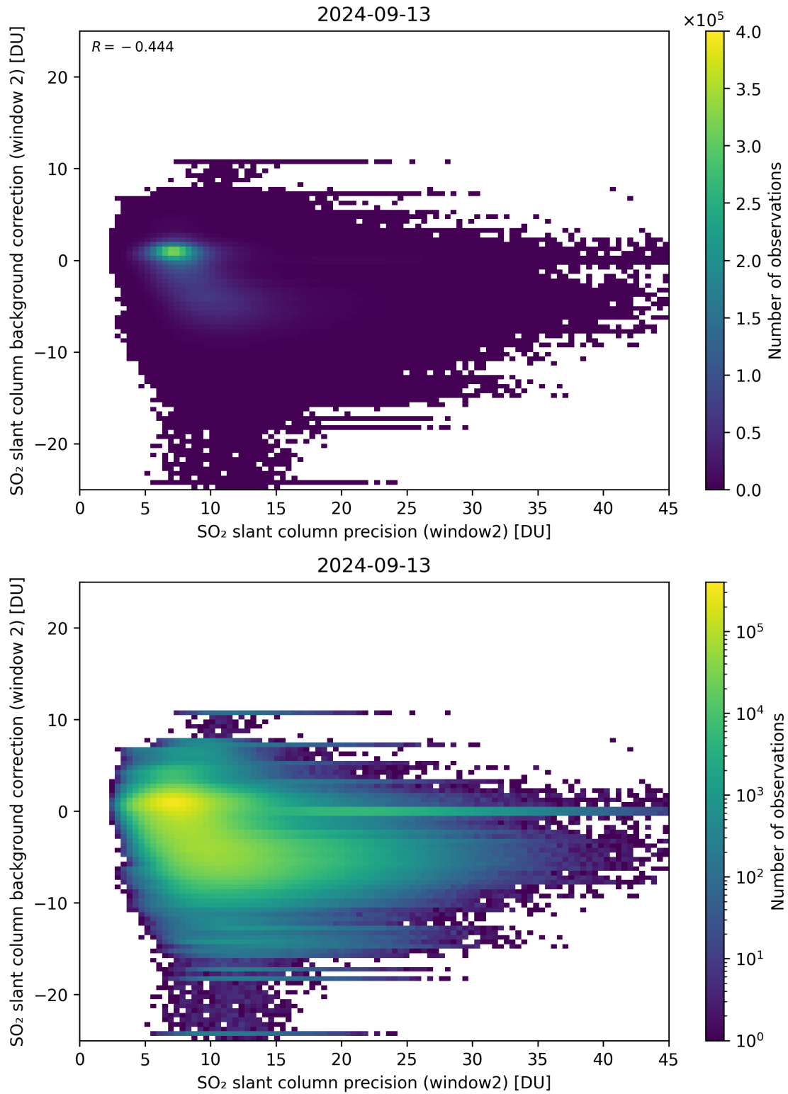
Figure 241: Scatter density plot of “SO 2 slant column precision (window2)” against “SO 2 slant column background correction (window 2)” for 2024-09-12 to 2024-09-14.
