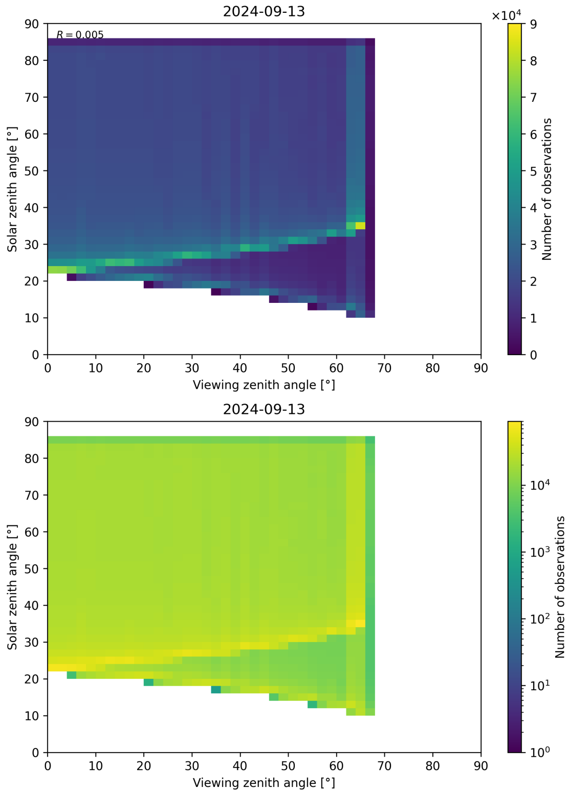
Figure 315: Scatter density plot of “Viewing zenith angle” against “Solar zenith angle” for 2024-09-12 to 2024-09-14.
