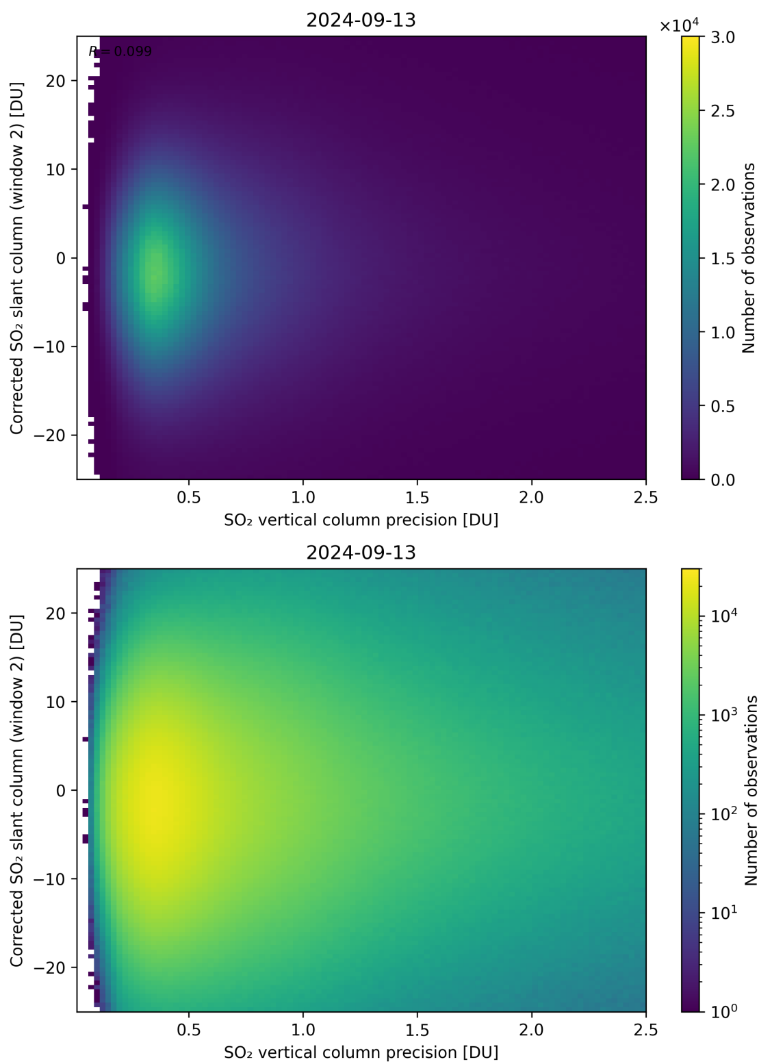
Figure 287: Scatter density plot of “SO 2 vertical column precision” against “Corrected SO 2 slant column (window 2)” for 2024-09-12 to 2024-09-14.
