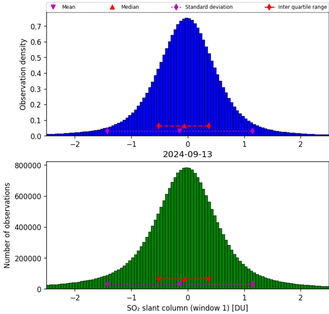
Figure 56: Histogram of “SO 2 slant column (window 1)” for 2024-09-12 to 2024-09-14
