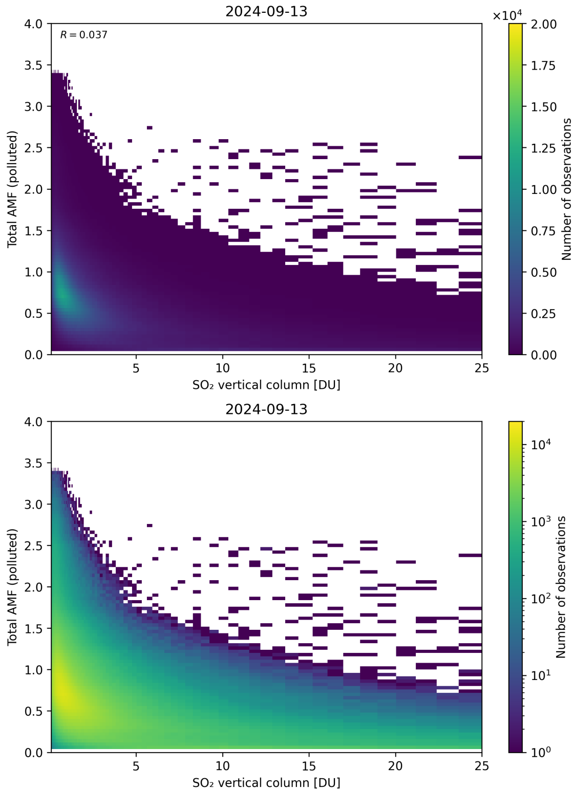
Figure 305: Scatter density plot of “SO 2 vertical column” against “Total AMF (polluted)” for 2024-09-12 to 2024-09-14.
