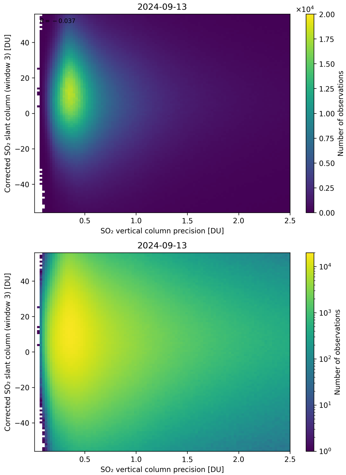
Figure 288: Scatter density plot of “SO 2 vertical column precision” against “Corrected SO 2 slant column (window 3)” for 2024-09-12 to 2024-09-14.
