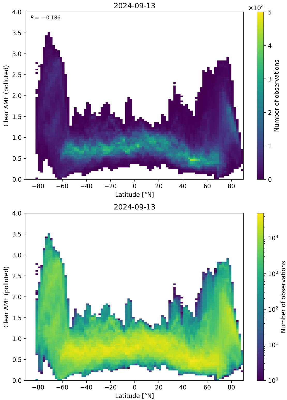
Figure 145: Scatter density plot of “Latitude” against “Clear AMF (polluted)” for 2024-09-12 to 2024-09-14.
