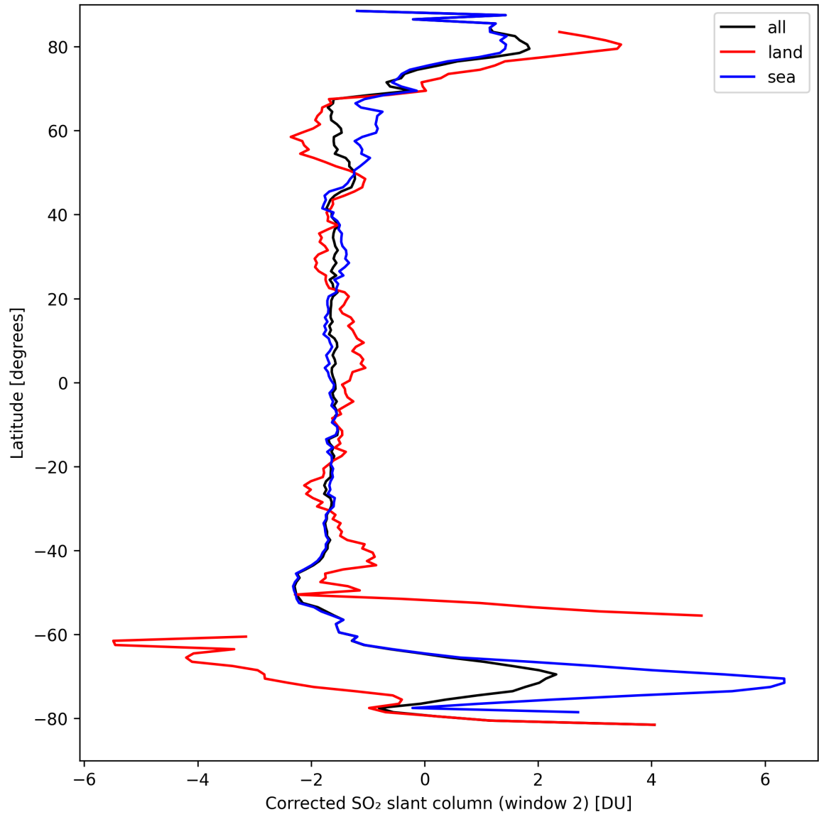
Figure 39: Zonal average of “Corrected SO 2 slant column (window 2)” for 2024-09-12 to 2024-09-14.
