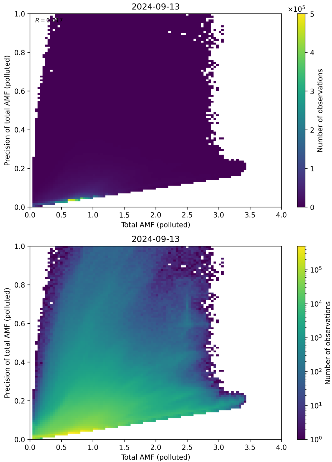
Figure 272: Scatter density plot of “Total AMF (polluted)” against “Precision of total AMF (polluted)” for 2024-09-12 to 2024-09-14.
