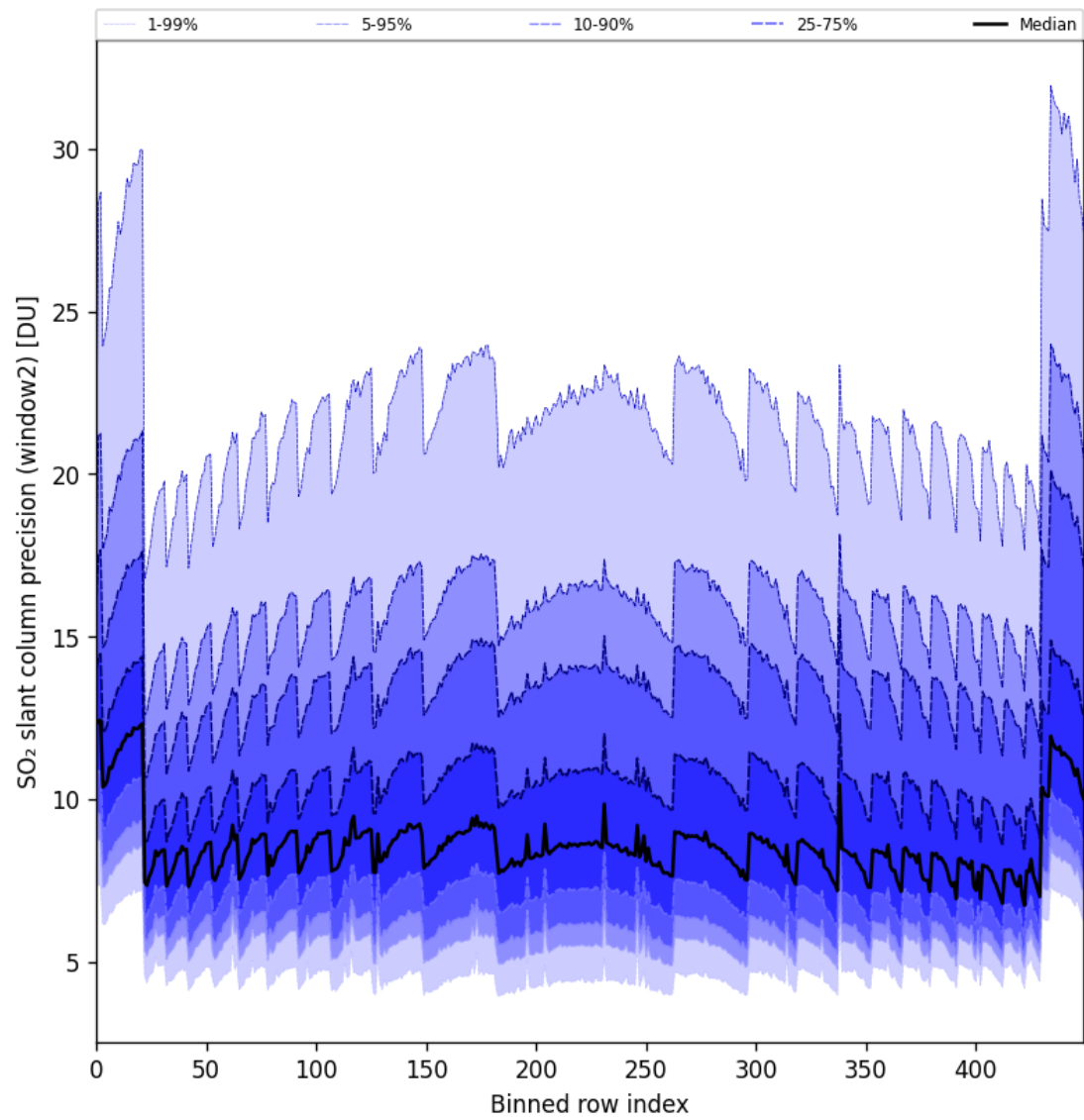
Figure 84: Along track statistics of “SO 2 slant column precision (window2)” for 2024-09-12 to 2024-09-14
