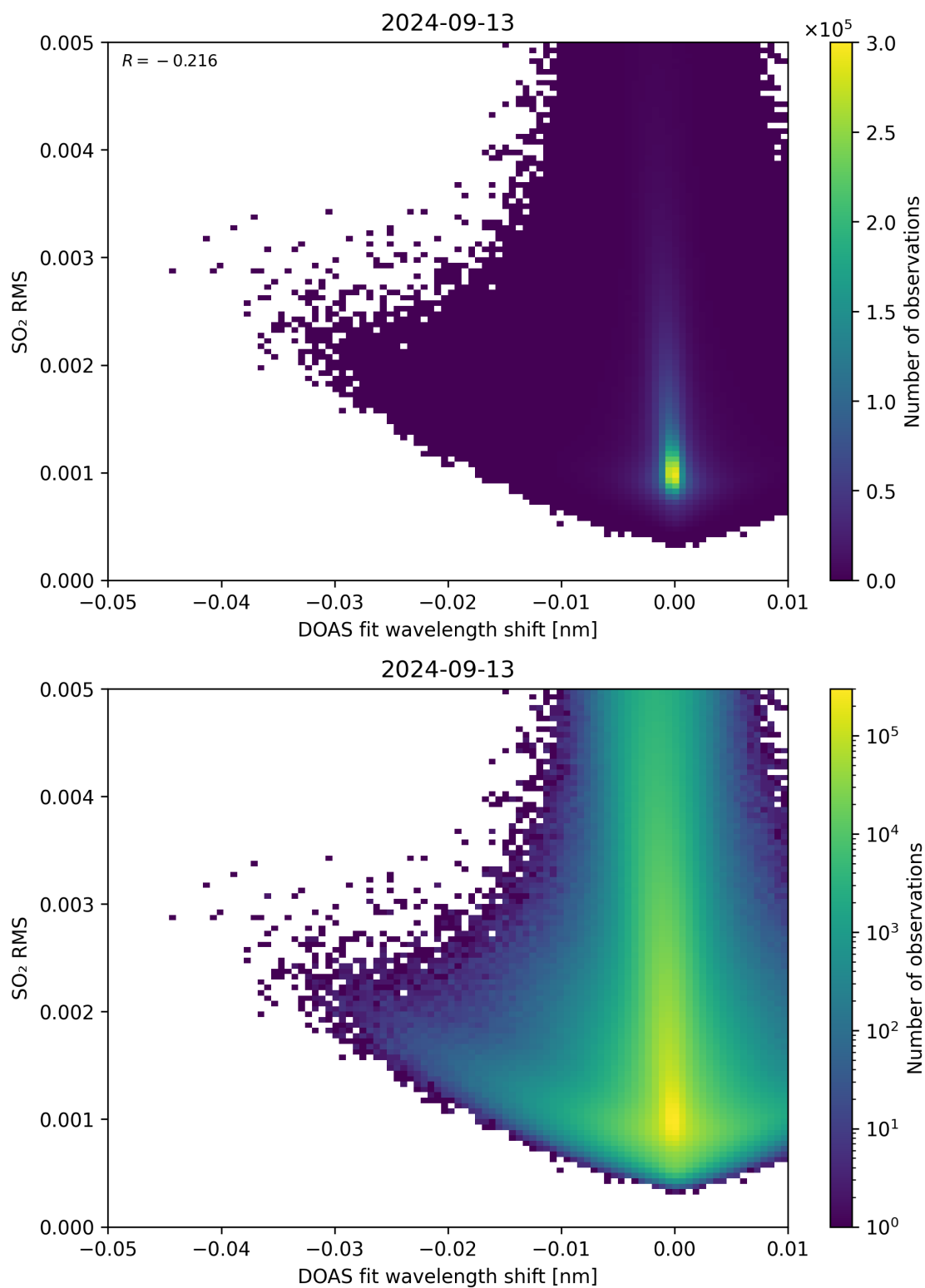
Figure 128: Scatter density plot of “DOAS fit wavelength shift” against “SO 2 RMS” for 2024-09-12 to 2024-09-14.
