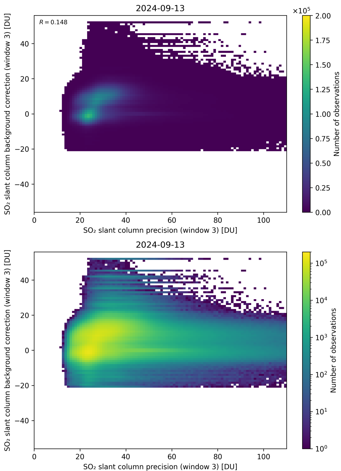
Figure 257: Scatter density plot of “SO 2 slant column precision (window 3)” against “SO 2 slant column background correction (window 3)” for 2024-09-12 to 2024-09-14.
