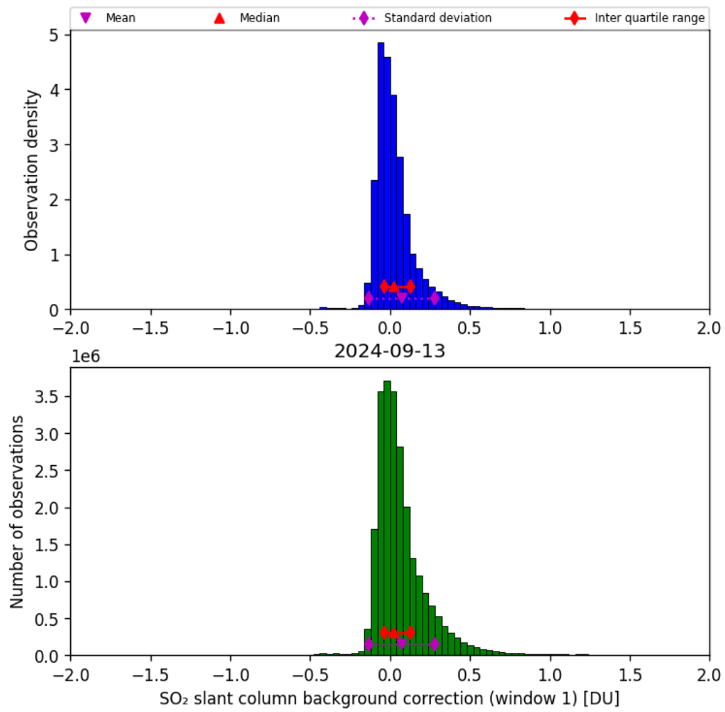
Figure 59: Histogram of “SO 2 slant column background correction (window 1)” for 2024-09-12 to 2024-09-14
