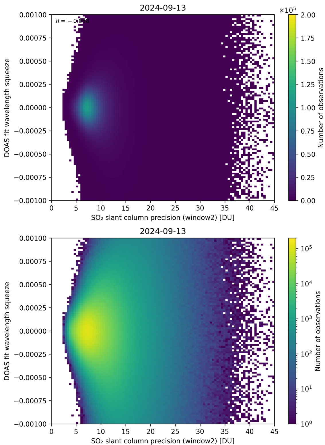
Figure 244: Scatter density plot of “SO 2 slant column precision (window2)” against “DOAS fit wavelength squeeze” for 2024-09-12 to 2024-09-14.
