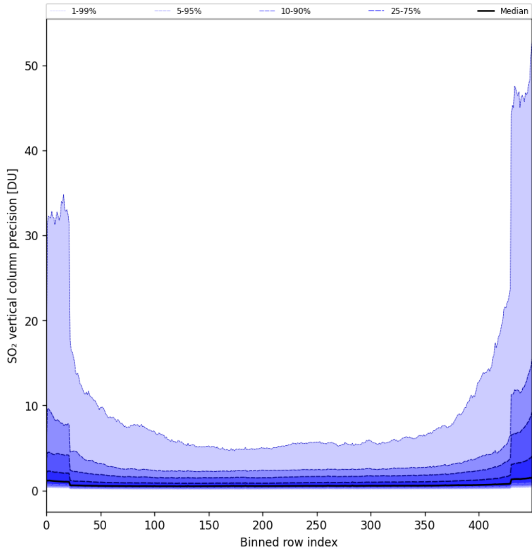
Figure 77: Along track statistics of “SO 2 vertical column precision” for 2024-09-12 to 2024-09-14
