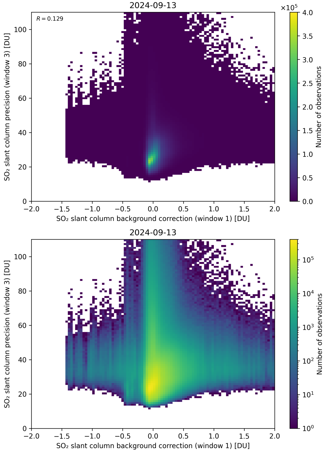
Figure 108: Scatter density plot of “SO 2 slant column background correction (window 1)” against “SO 2 slant column precision (window 3)” for 2024-09-12 to 2024-09-14.
