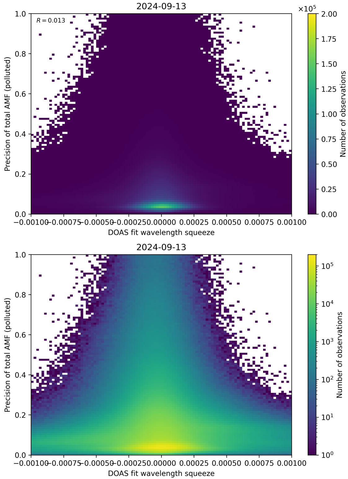
Figure 135: Scatter density plot of “DOAS fit wavelength squeeze” against “Precision of total AMF (polluted)” for 2024-09-12 to 2024-09-14.
