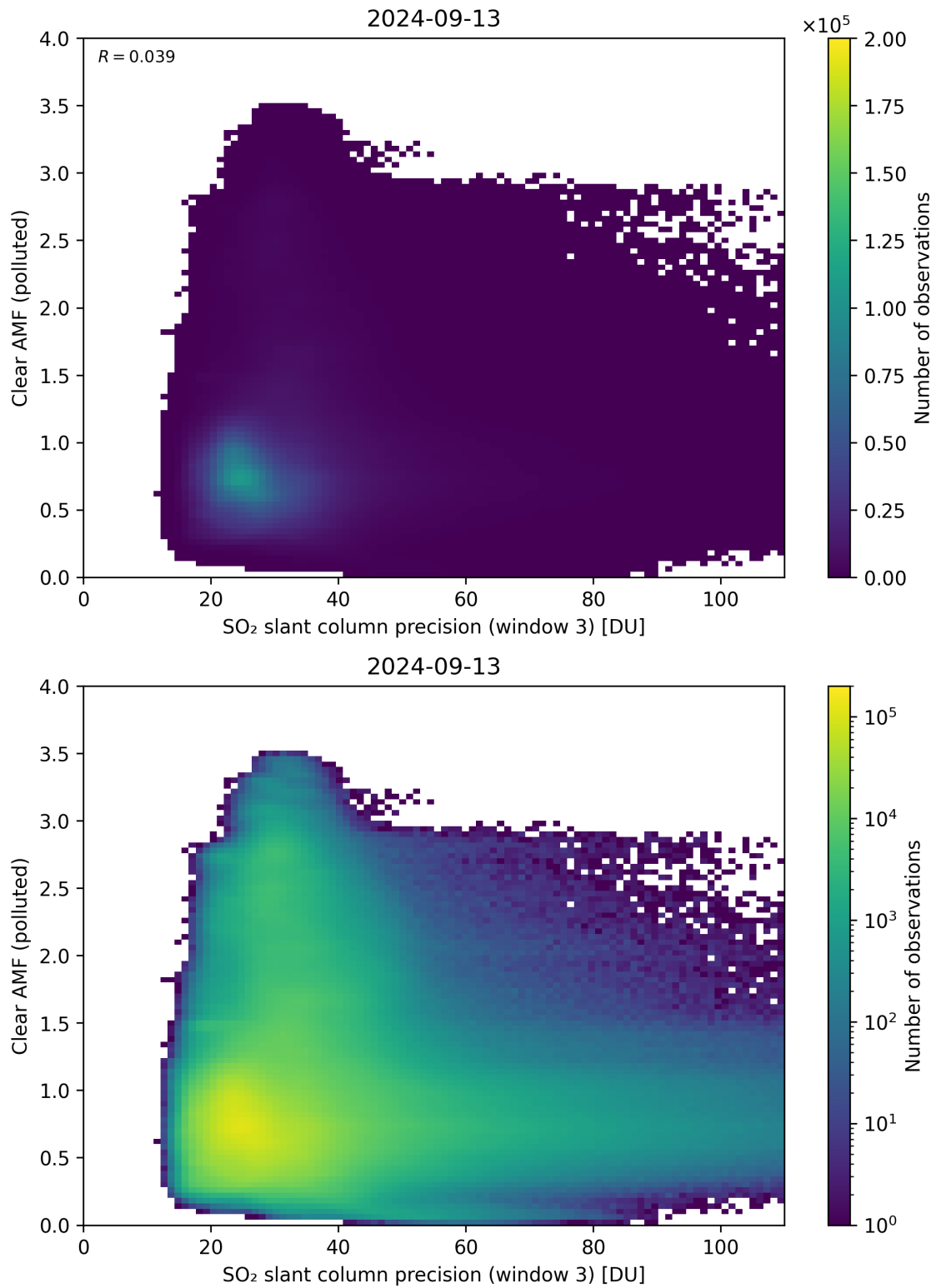
Figure 261: Scatter density plot of “SO 2 slant column precision (window 3)” against “Clear AMF (polluted)” for 2024-09-12 to 2024-09-14.
