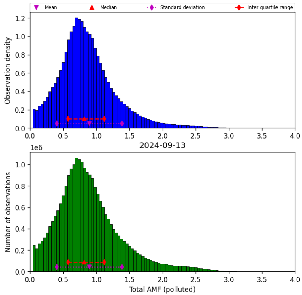
Figure 71: Histogram of “Total AMF (polluted)” for 2024-09-12 to 2024-09-14
