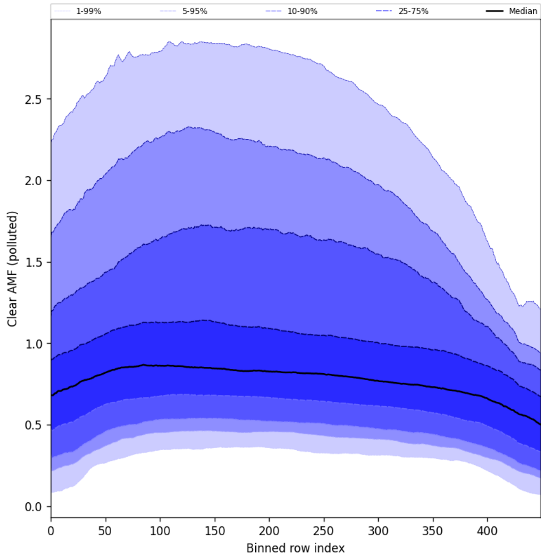
Figure 96: Along track statistics of “Clear AMF (polluted)” for 2024-09-12 to 2024-09-14
