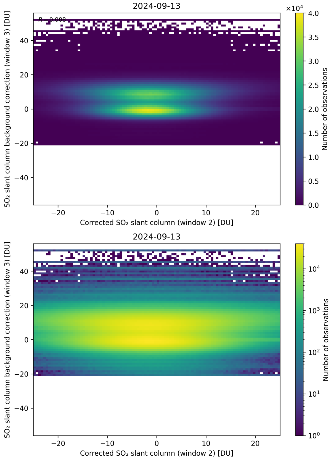
Figure 195: Scatter density plot of “Corrected SO 2 slant column (window 2)” against “SO 2 slant column background correction (window 3)” for 2024-09-12 to 2024-09-14.
