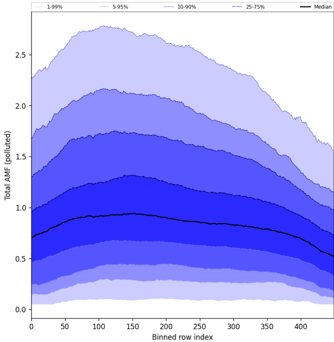
Figure 94: Along track statistics of “Total AMF (polluted)” for 2024-09-12 to 2024-09-14
