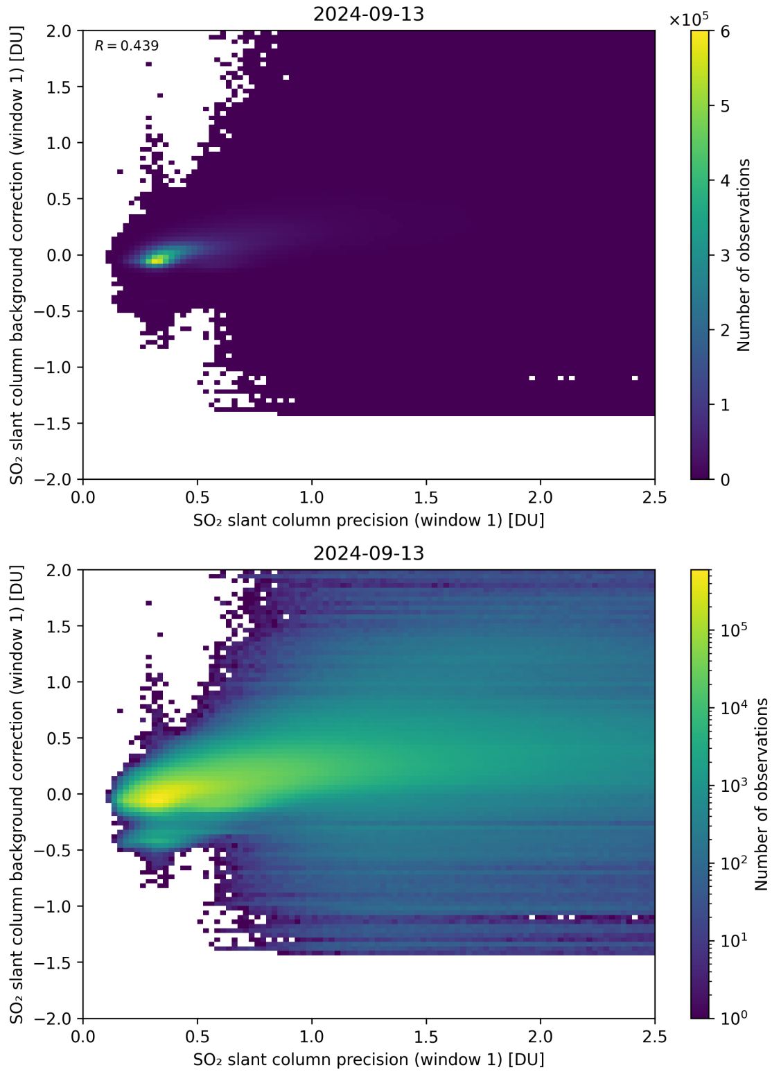
Figure 218: Scatter density plot of “SO 2 slant column precision (window 1)” against “SO 2 slant column background correction (window 1)” for 2024-09-12 to 2024-09-14.
