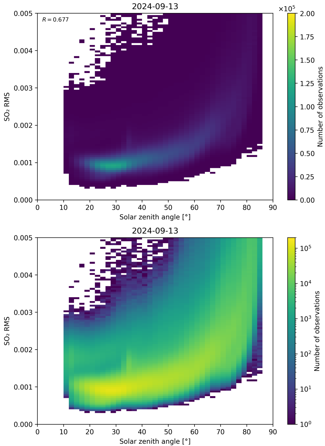
Figure 163: Scatter density plot of “Solar zenith angle” against “SO 2 RMS” for 2024-09-12 to 2024-09-14.
