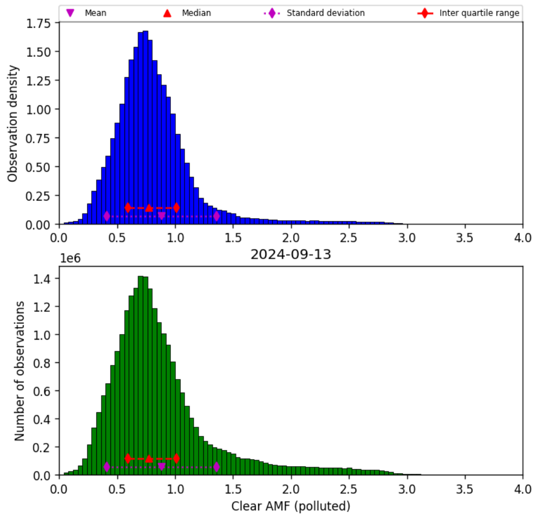
Figure 73: Histogram of “Clear AMF (polluted)” for 2024-09-12 to 2024-09-14
