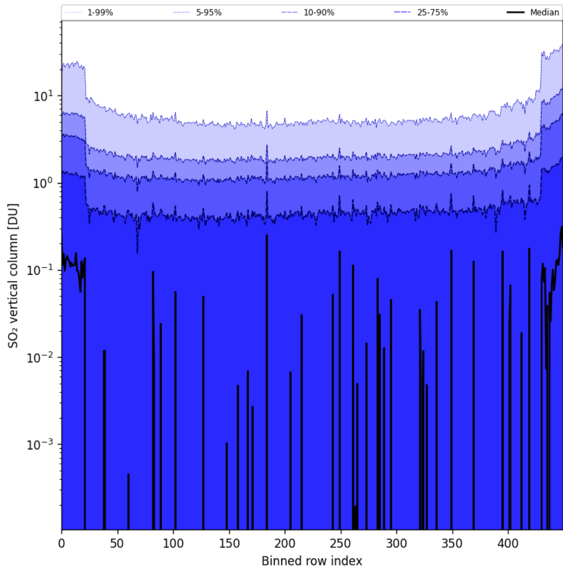
Figure 76: Along track statistics of “SO 2 vertical column” for 2024-09-12 to 2024-09-14
