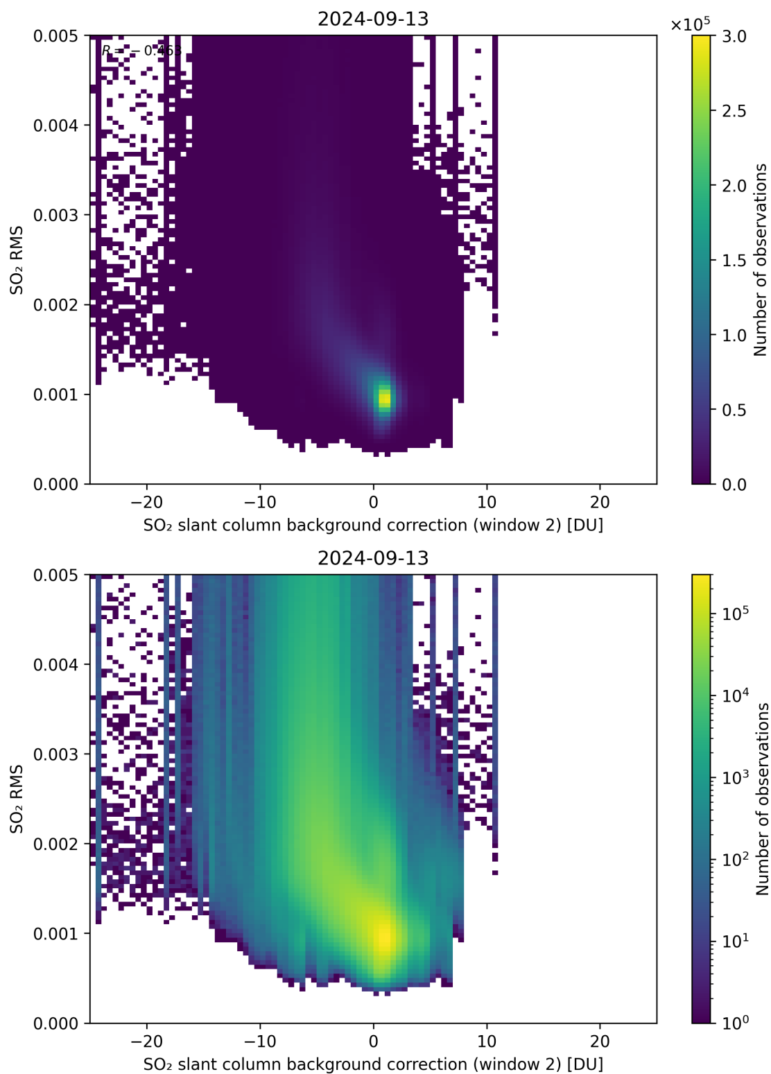
Figure 114: Scatter density plot of “SO 2 slant column background correction (window 2)” against “SO 2 RMS” for 2024-09-12 to 2024-09-14.
