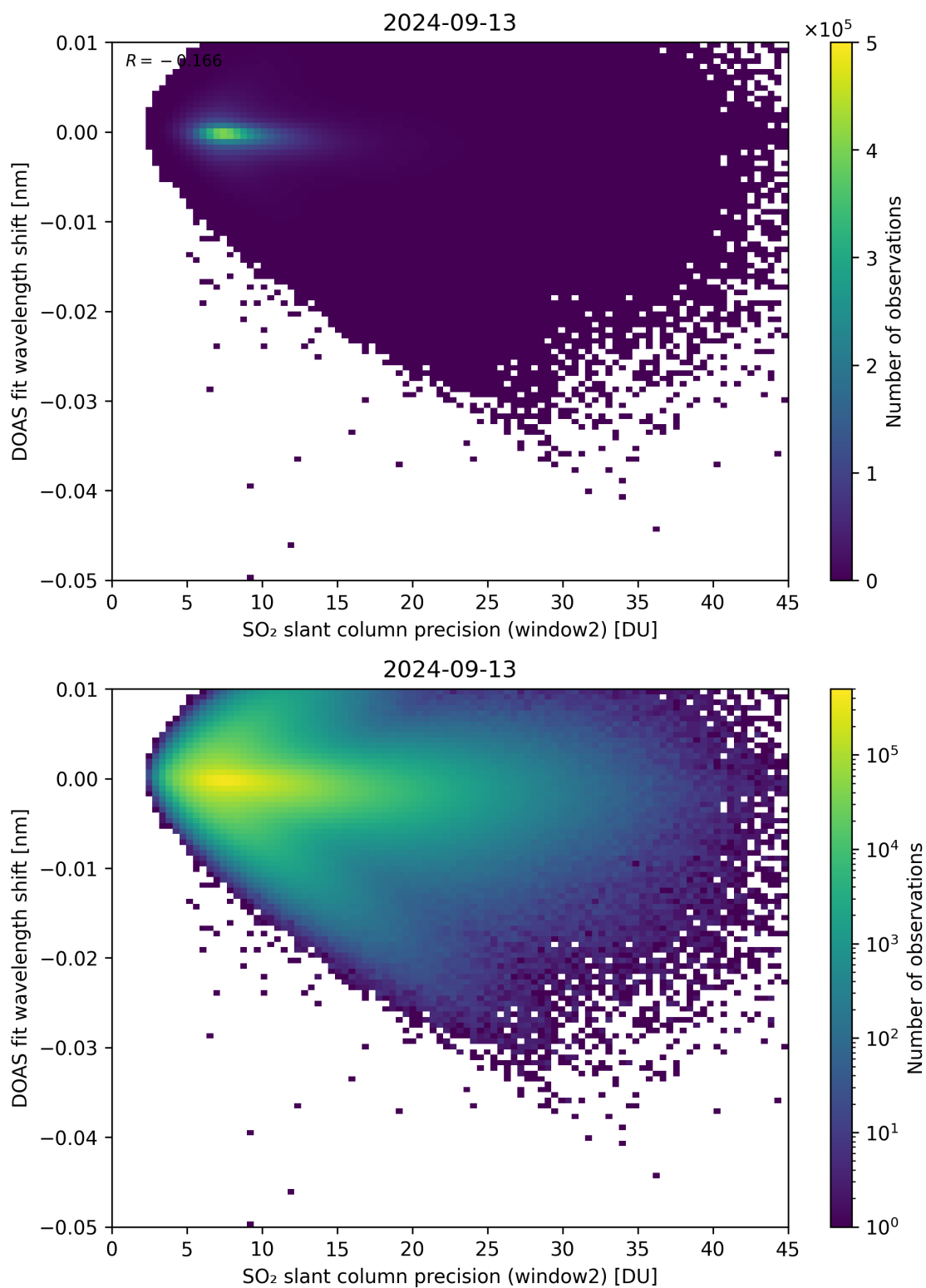
Figure 243: Scatter density plot of “SO 2 slant column precision (window2)” against “DOAS fit wavelength shift” for 2024-09-12 to 2024-09-14.
