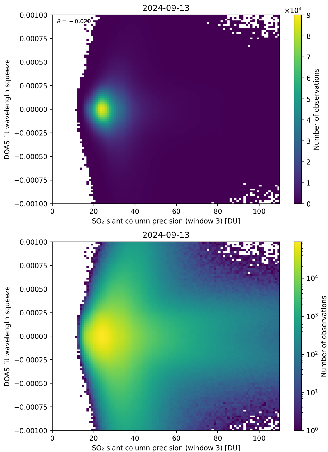
Figure 259: Scatter density plot of “SO 2 slant column precision (window 3)” against “DOAS fit wavelength squeeze” for 2024-09-12 to 2024-09-14.
