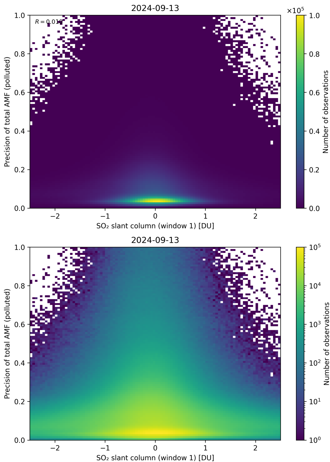
Figure 240: Scatter density plot of “SO 2 slant column (window 1)” against “Precision of total AMF (polluted)” for 2024-09-12 to 2024-09-14.
