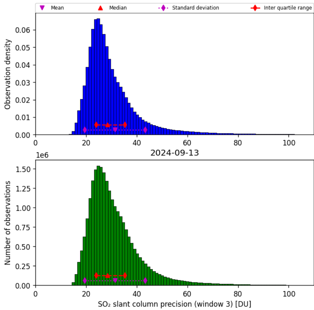
Figure 65: Histogram of “SO 2 slant column precision (window 3)” for 2024-09-12 to 2024-09-14
