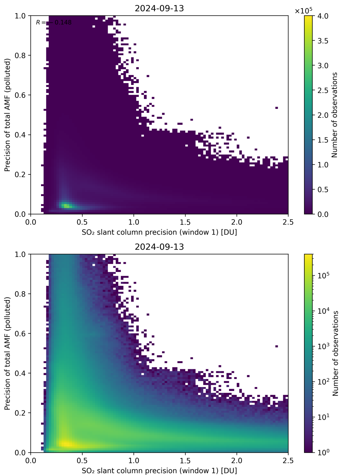
Figure 231: Scatter density plot of “SO 2 slant column precision (window 1)” against “Precision of total AMF (polluted)” for 2024-09-12 to 2024-09-14.
