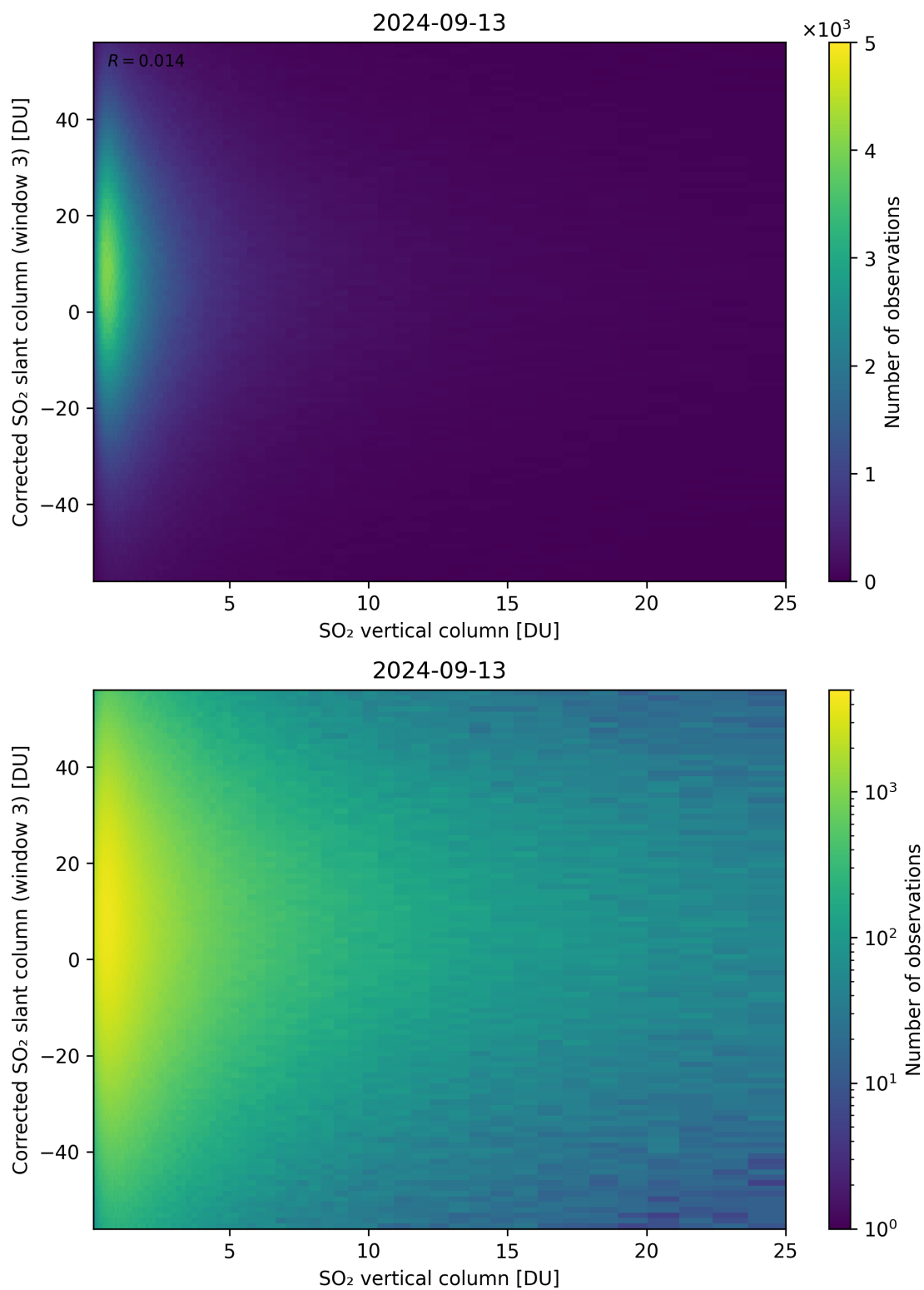
Figure 299: Scatter density plot of “SO 2 vertical column” against “Corrected SO 2 slant column (window 3)” for 2024-09-12 to 2024-09-14.
