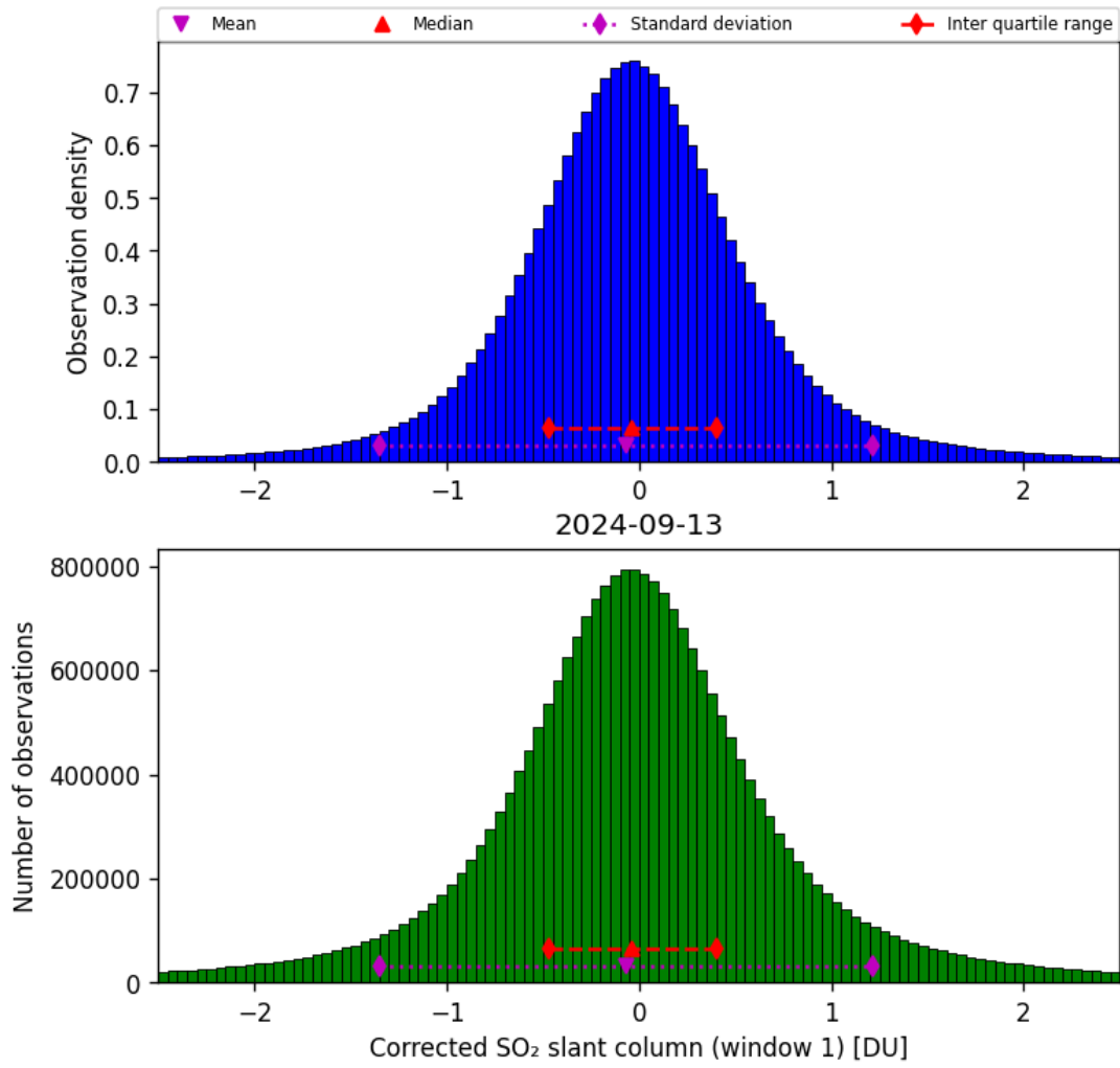
Figure 58: Histogram of “Corrected SO 2 slant column (window 1)” for 2024-09-12 to 2024-09-14
