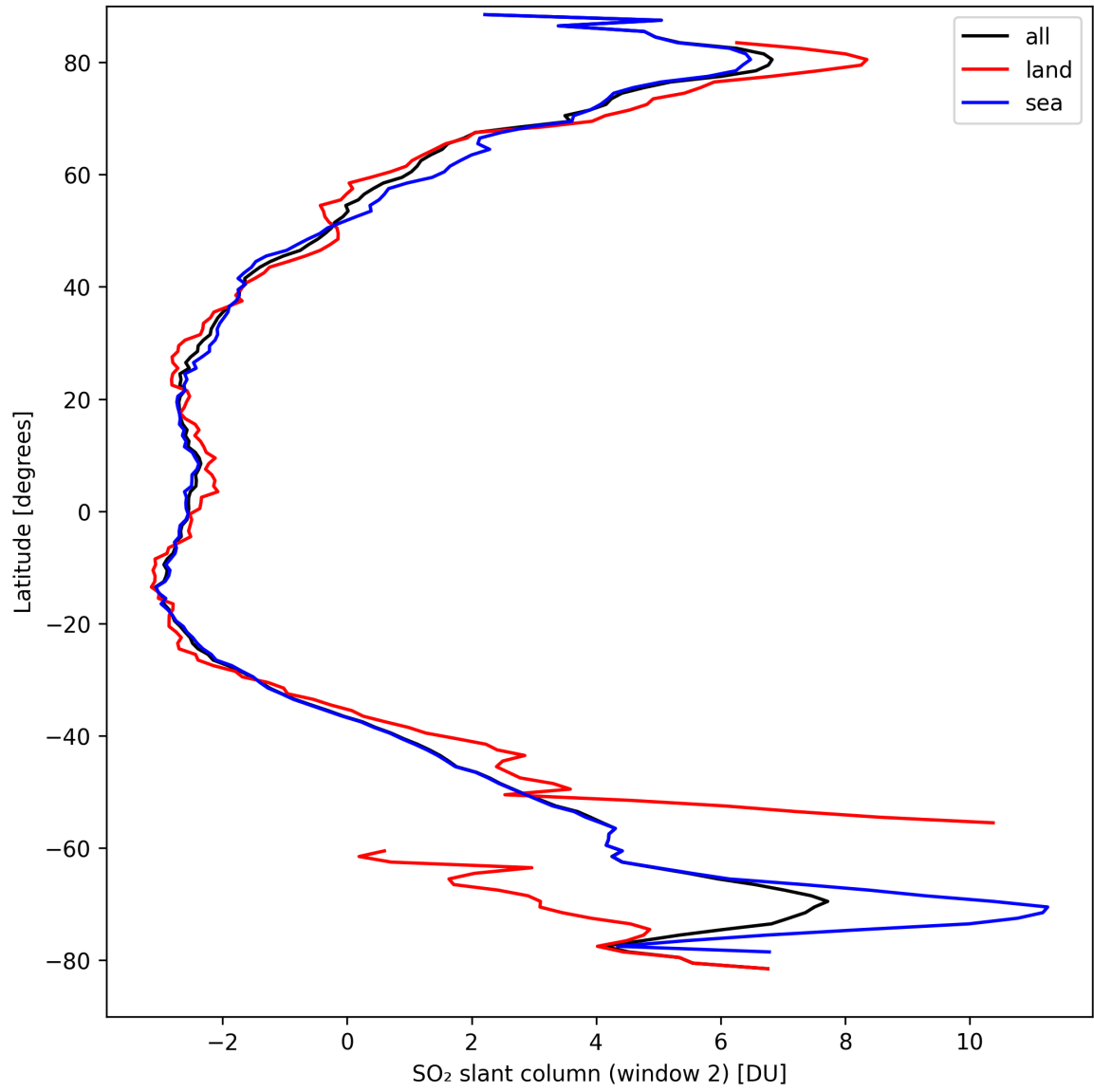
Figure 37: Zonal average of “SO 2 slant column (window 2)” for 2024-09-12 to 2024-09-14.
