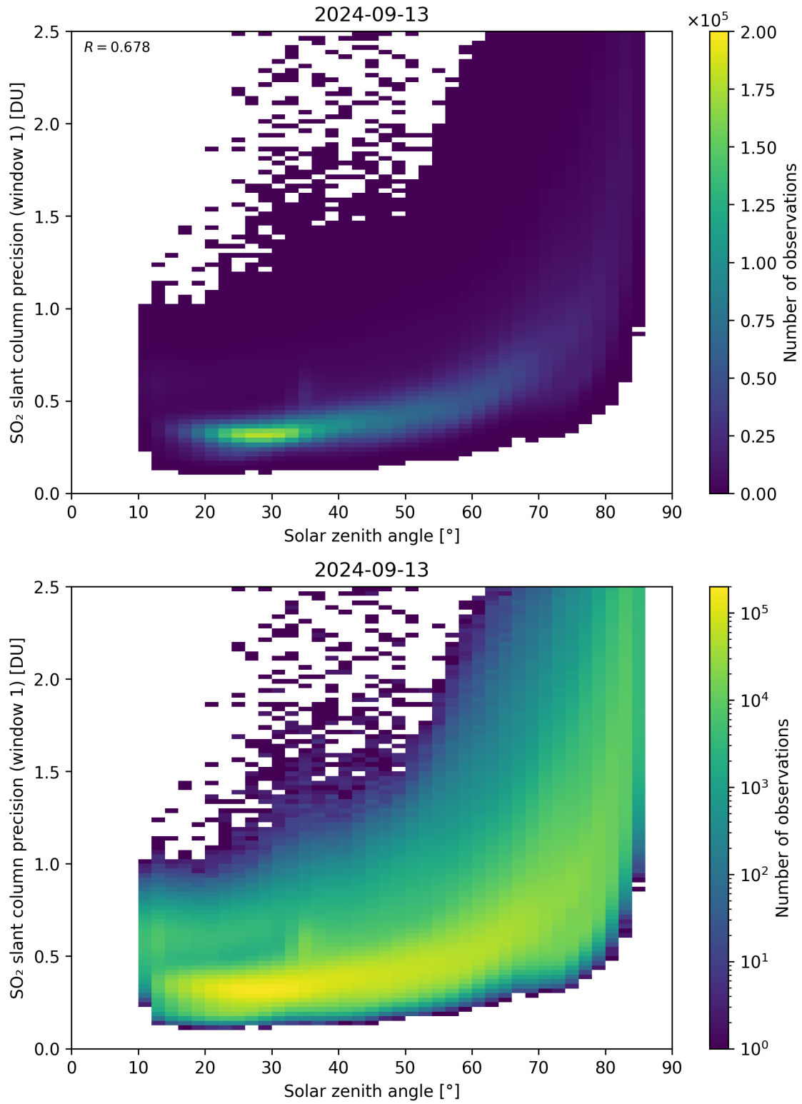
Figure 170: Scatter density plot of “Solar zenith angle” against “SO 2 slant column precision (window 1)” for 2024-09-12 to 2024-09-14.
