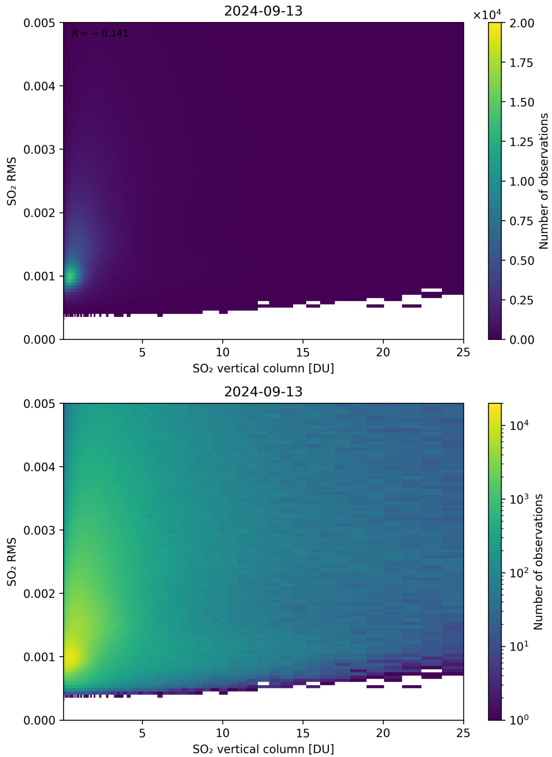
Figure 278: Scatter density plot of “SO 2 vertical column” against “SO 2 RMS” for 2024-09-12 to 2024-09-14.
