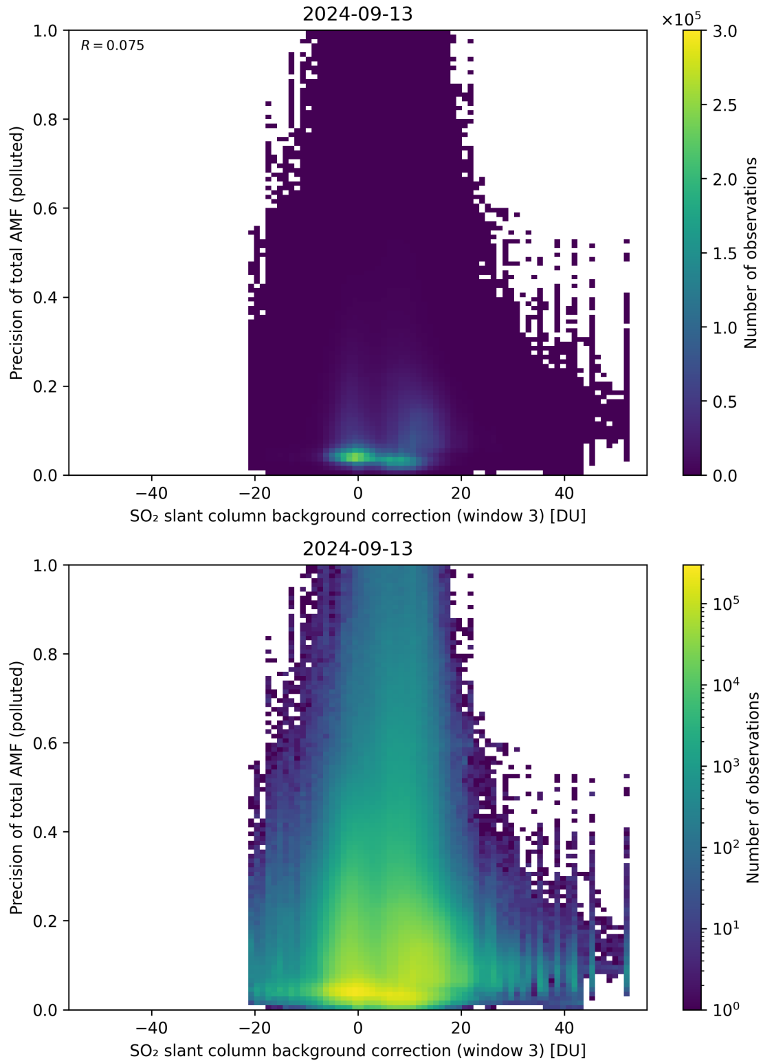
Figure 126: Scatter density plot of “SO 2 slant column background correction (window 3)” against “Precision of total AMF (polluted)” for 2024-09-12 to 2024-09-14.
