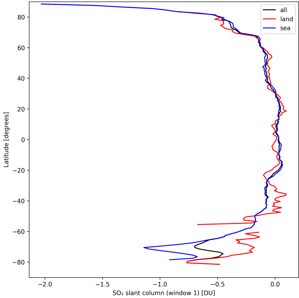
Figure 33: Zonal average of “SO 2 slant column (window 1)” for 2024-09-12 to 2024-09-14.
