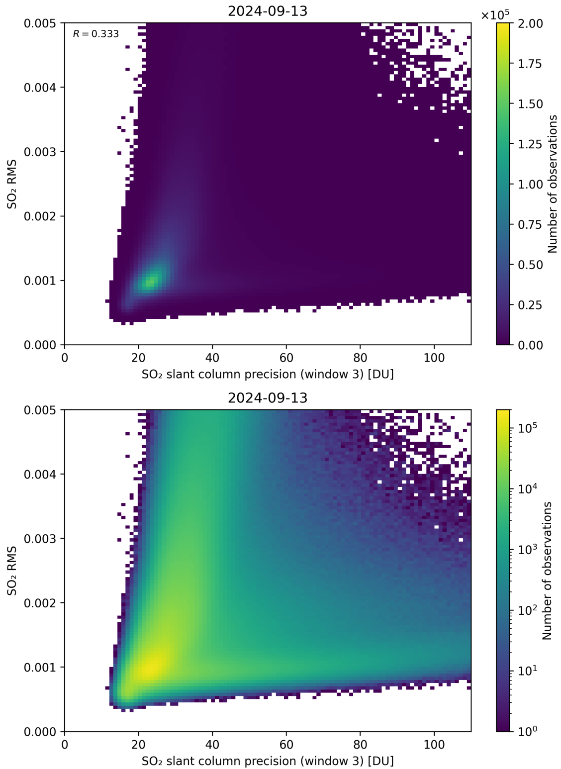
Figure 260: Scatter density plot of “SO 2 slant column precision (window 3)” against “SO 2 RMS” for 2024-09-12 to 2024-09-14.
