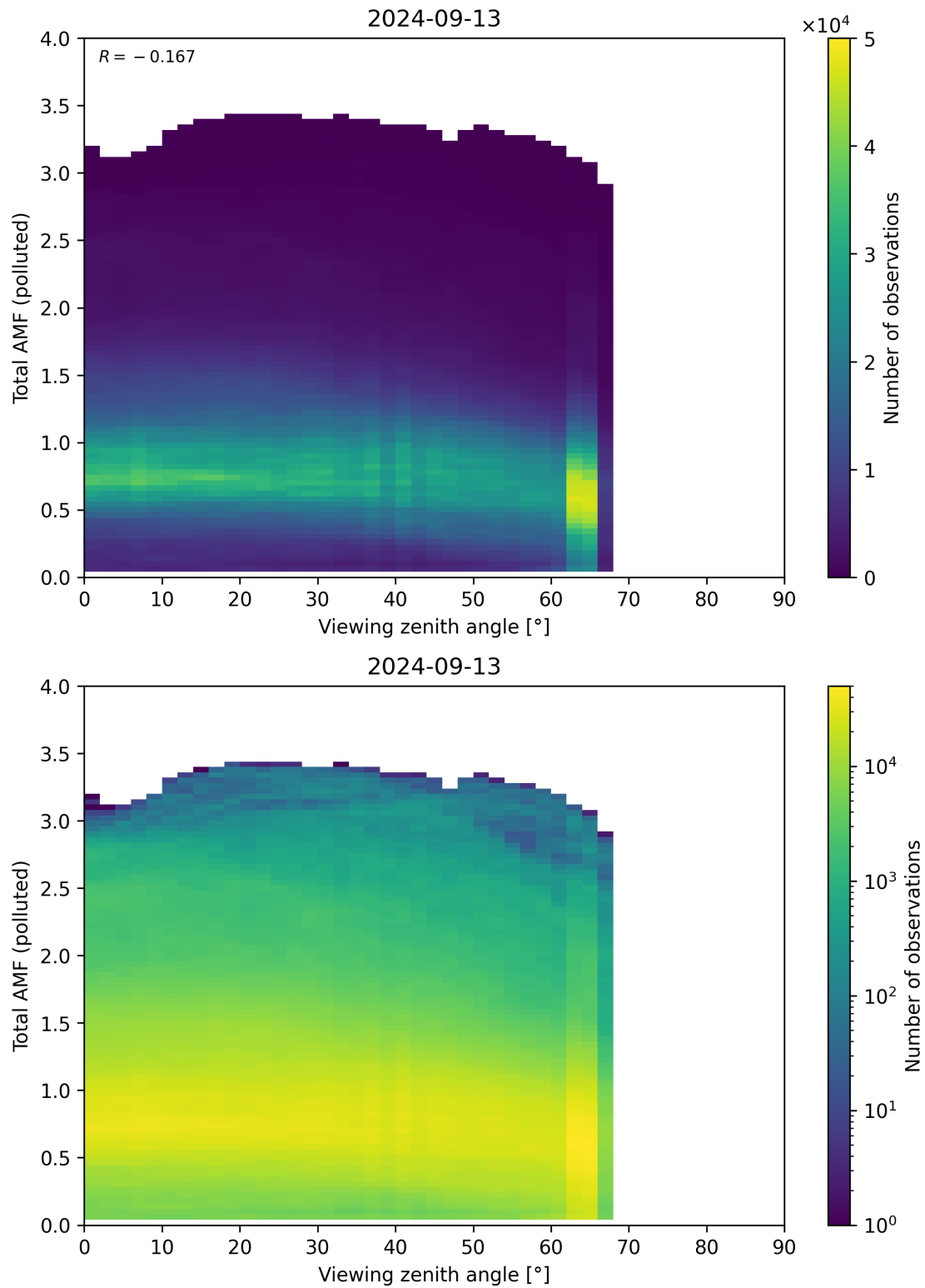
Figure 325: Scatter density plot of “Viewing zenith angle” against “Total AMF (polluted)” for 2024-09-12 to 2024-09-14.
