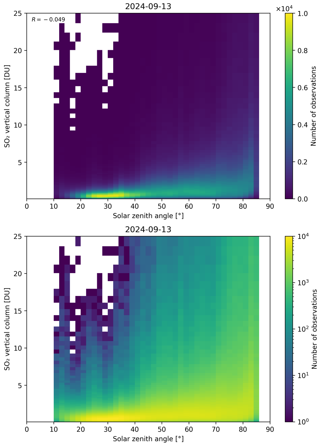
Figure 176: Scatter density plot of “Solar zenith angle” against “SO 2 vertical column” for 2024-09-12 to 2024-09-14.
