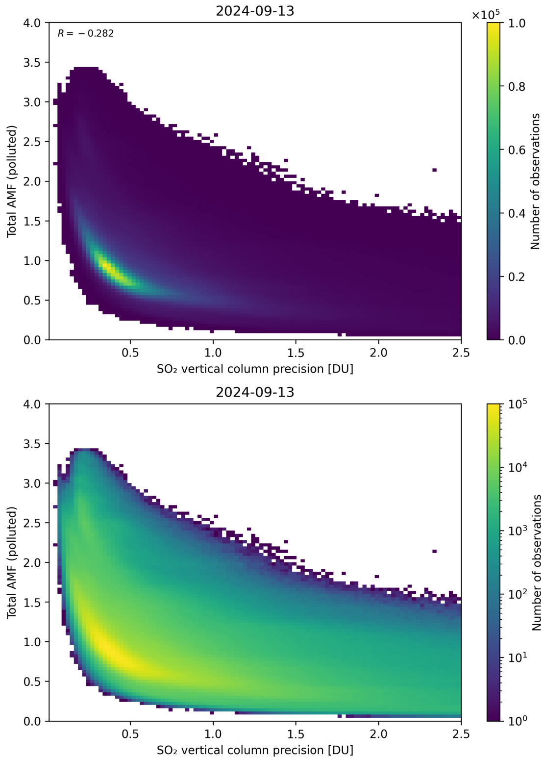
Figure 294: Scatter density plot of “SO 2 vertical column precision” against “Total AMF (polluted)” for 2024-09-12 to 2024-09-14.
