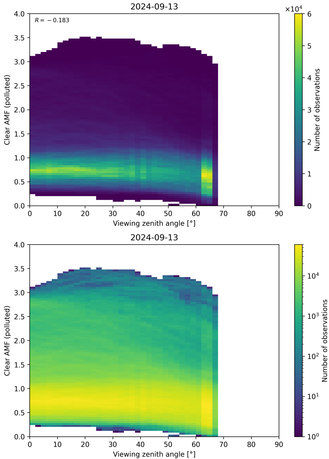
Figure 316: Scatter density plot of “Viewing zenith angle” against “Clear AMF (polluted)” for 2024-09-12 to 2024-09-14.
