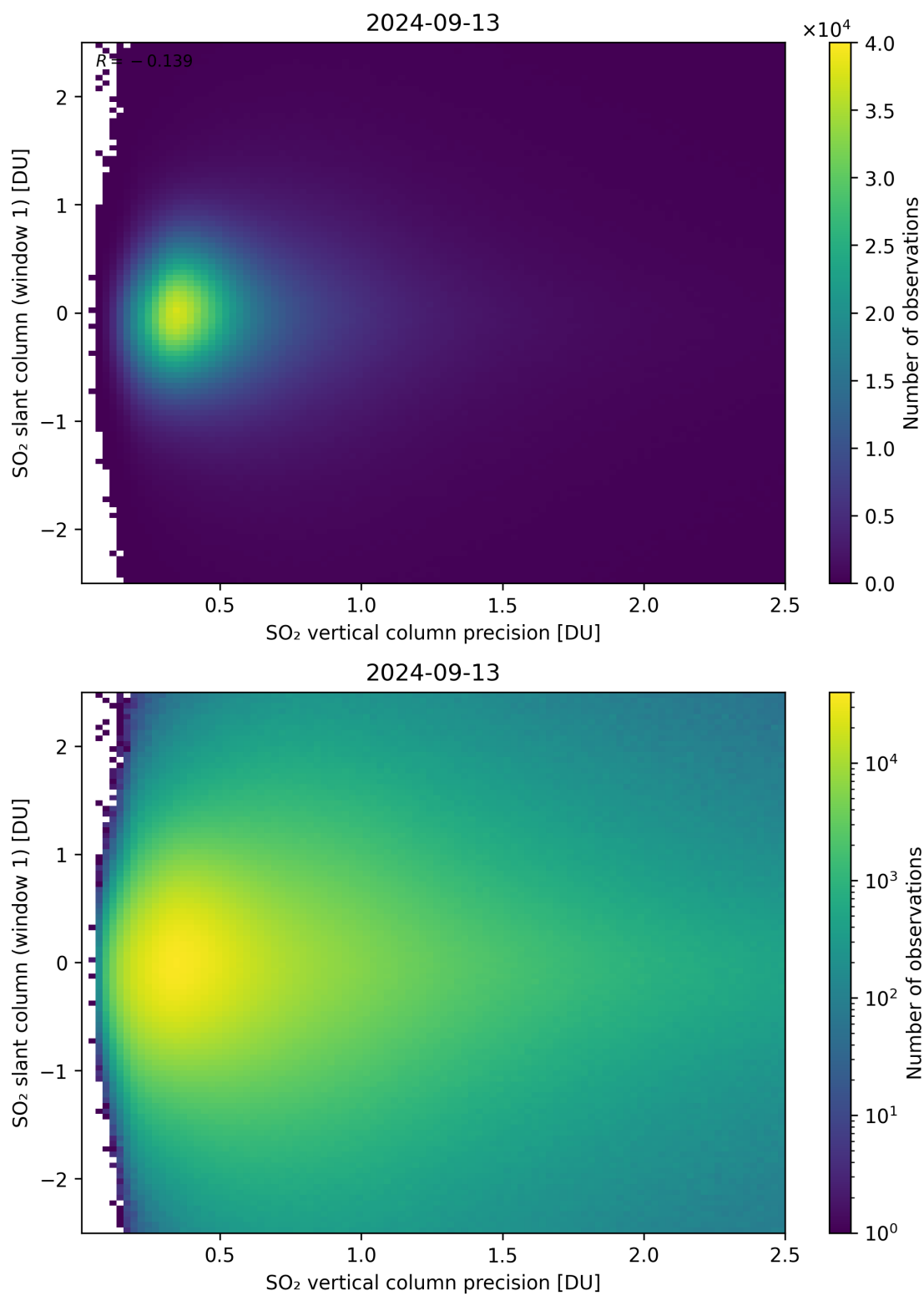
Figure 289: Scatter density plot of “SO 2 vertical column precision” against “SO 2 slant column (window 1)” for 2024-09-12 to 2024-09-14.
