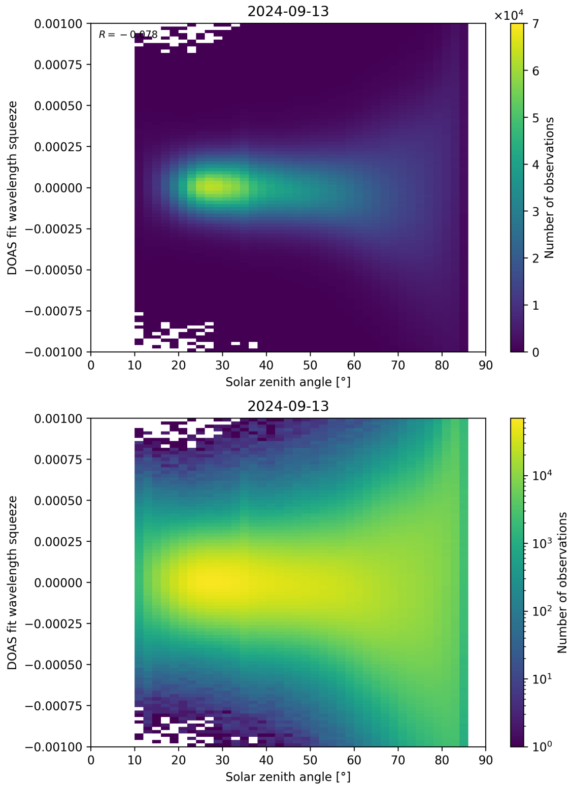
Figure 162: Scatter density plot of “Solar zenith angle” against “DOAS fit wavelength squeeze” for 2024-09-12 to 2024-09-14.
