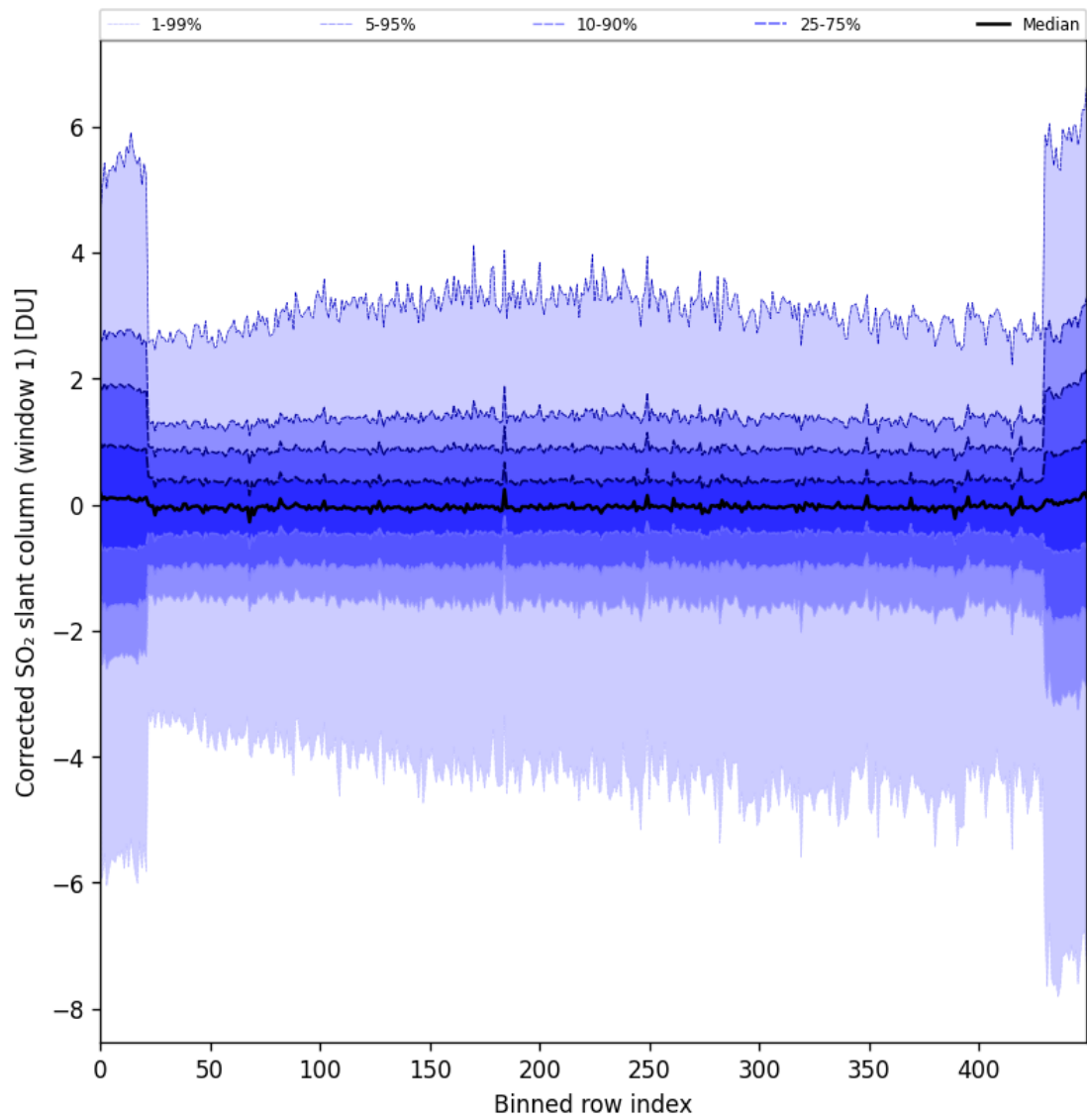
Figure 81: Along track statistics of “Corrected SO 2 slant column (window 1)” for 2024-09-12 to 2024-09-14
