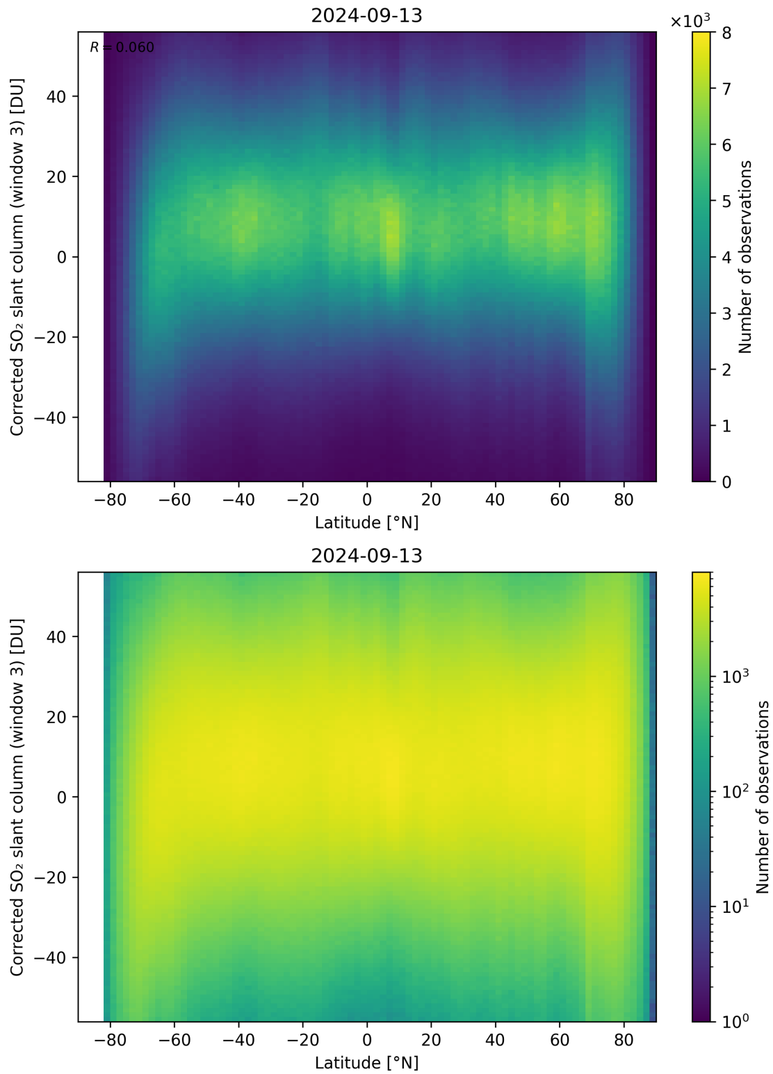
Figure 148: Scatter density plot of “Latitude” against “Corrected SO 2 slant column (window 3)” for 2024-09-12 to 2024-09-14.
