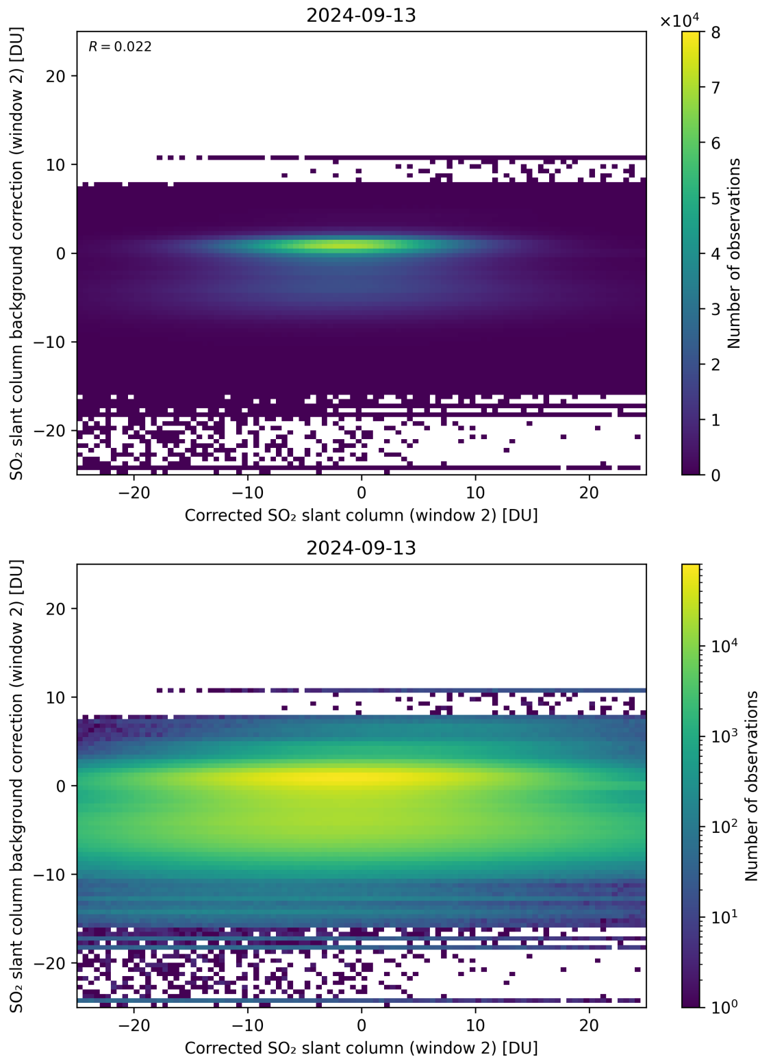
Figure 194: Scatter density plot of “Corrected SO 2 slant column (window 2)” against “SO 2 slant column background correction (window 2)” for 2024-09-12 to 2024-09-14.
