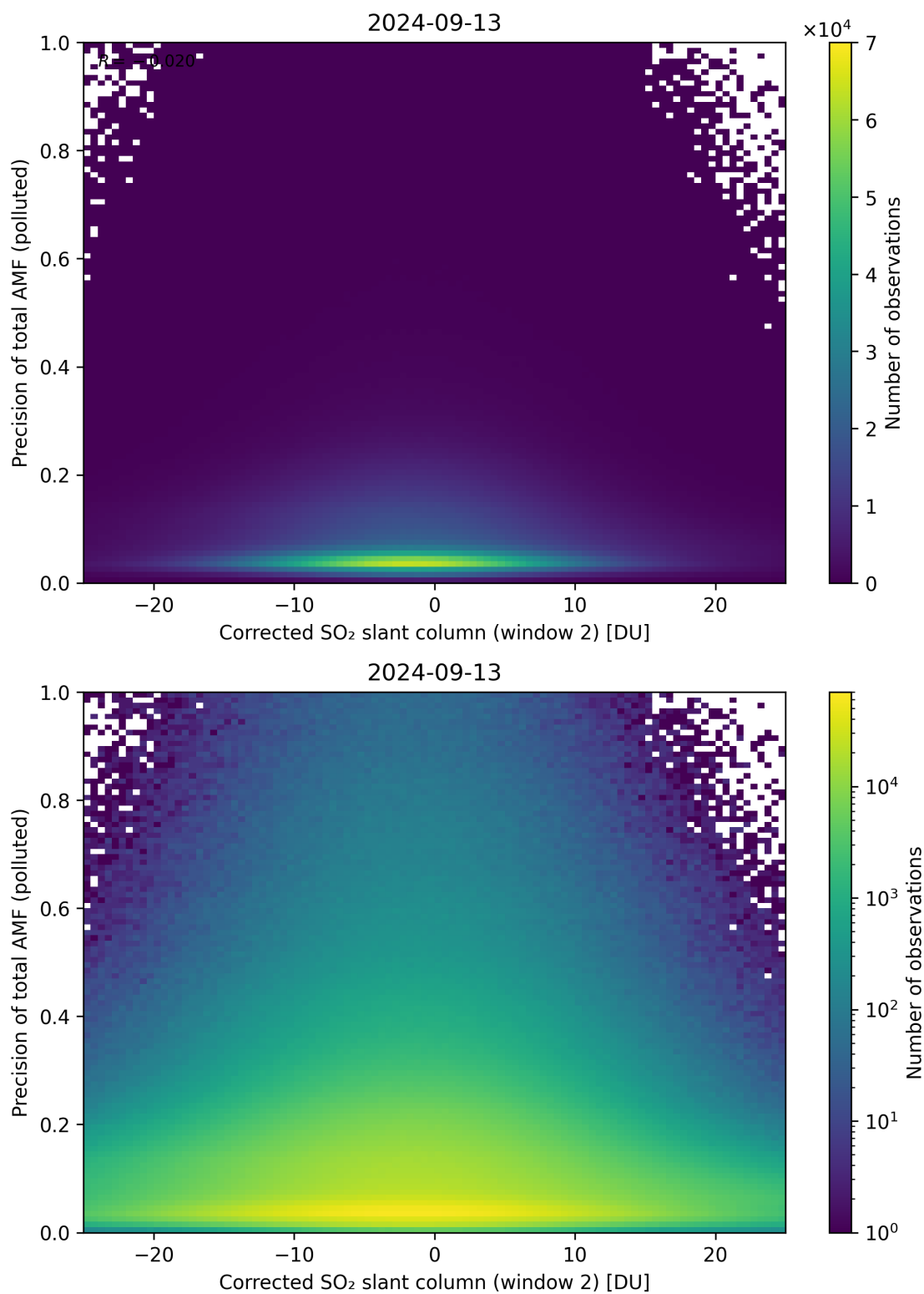
Figure 204: Scatter density plot of “Corrected SO 2 slant column (window 2)” against “Precision of total AMF (polluted)” for 2024-09-12 to 2024-09-14.
