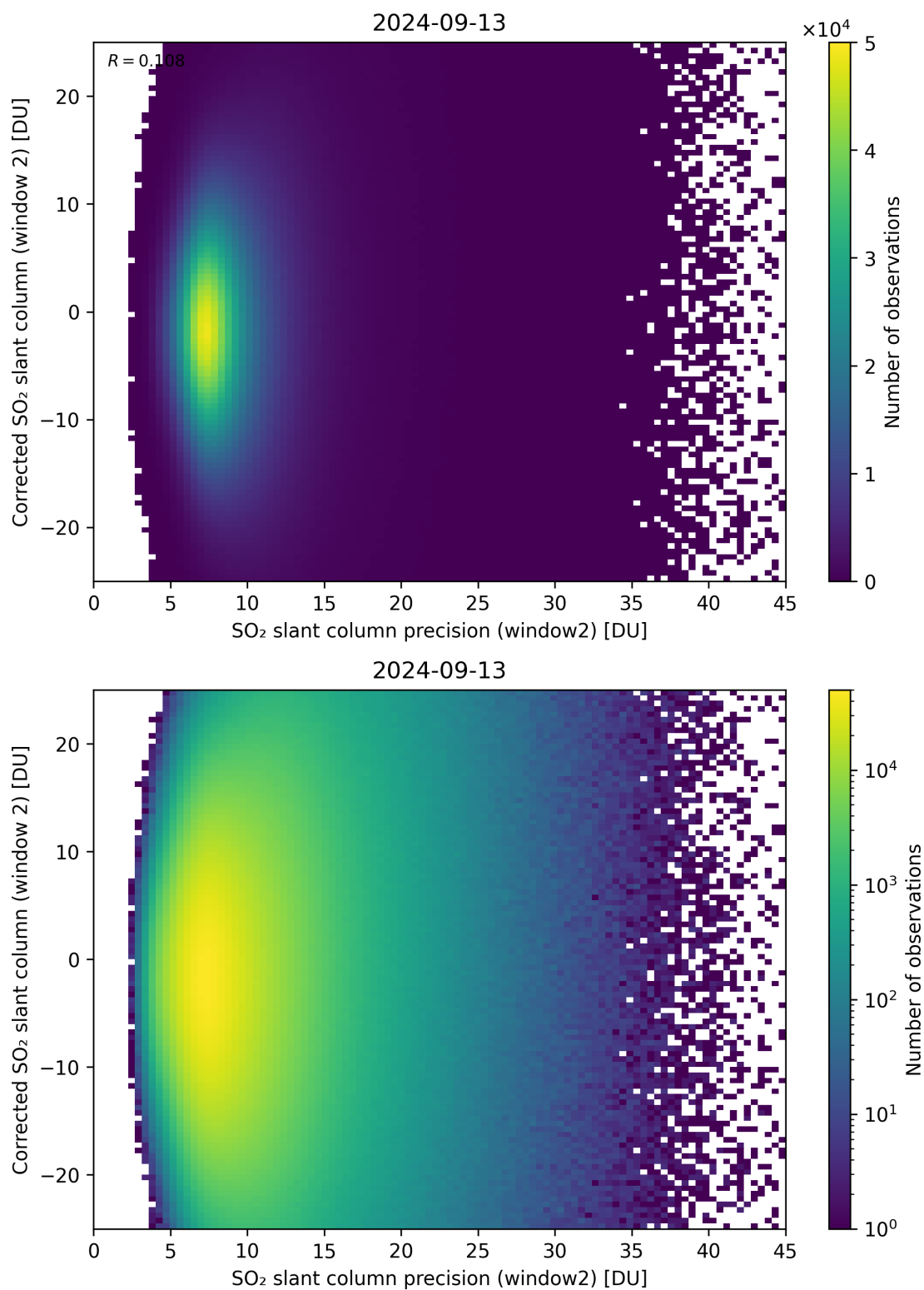
Figure 247: Scatter density plot of “SO 2 slant column precision (window2)” against “Corrected SO 2 slant column (window 2)” for 2024-09-12 to 2024-09-14.
