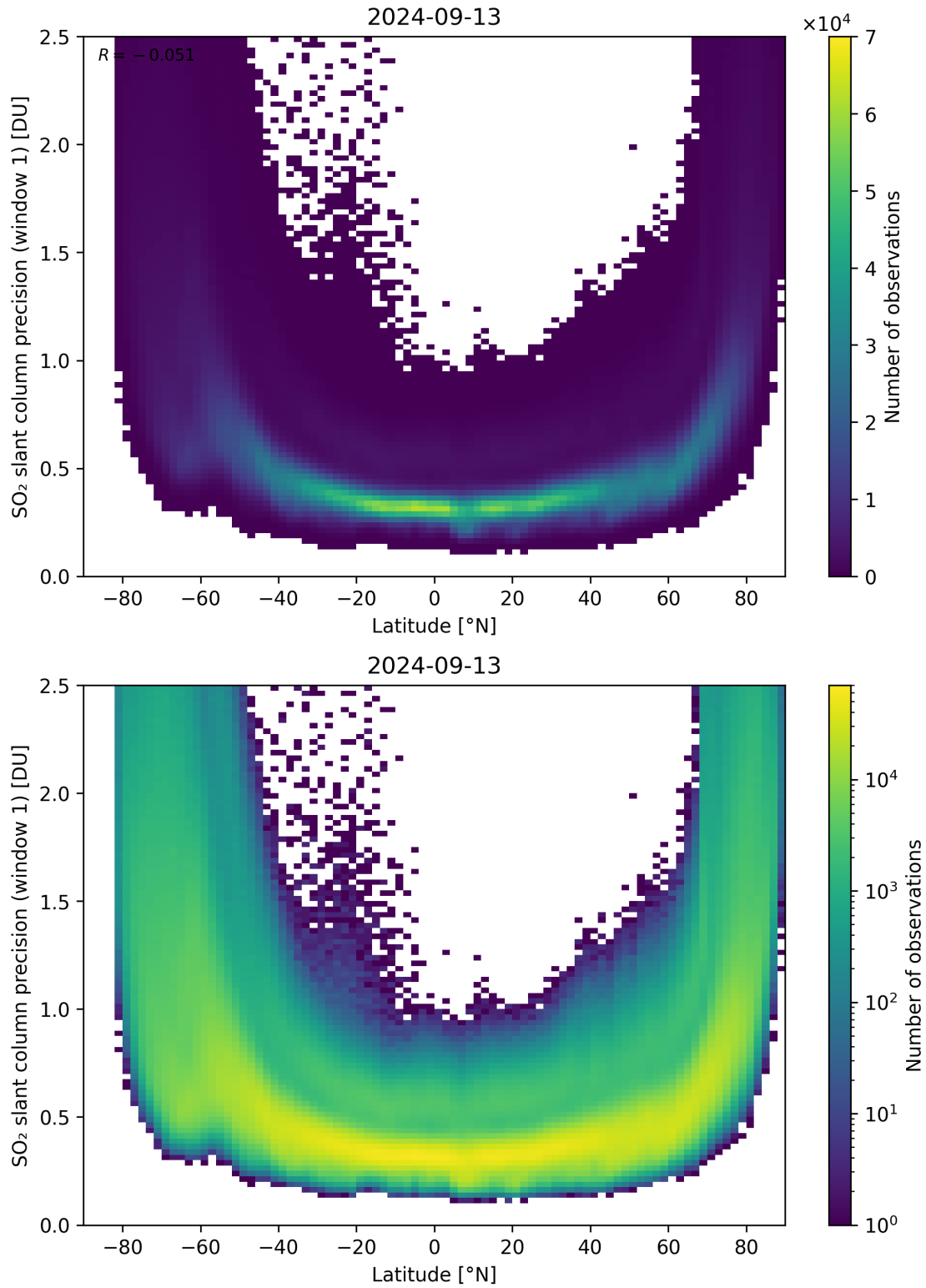
Figure 150: Scatter density plot of “Latitude” against “SO 2 slant column precision (window 1)” for 2024-09-12 to 2024-09-14.
