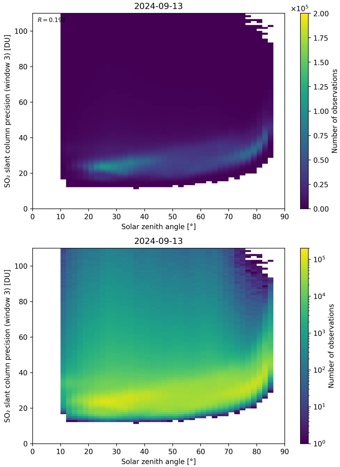
Figure 173: Scatter density plot of “Solar zenith angle” against “SO 2 slant column precision (window 3)” for 2024-09-12 to 2024-09-14.
