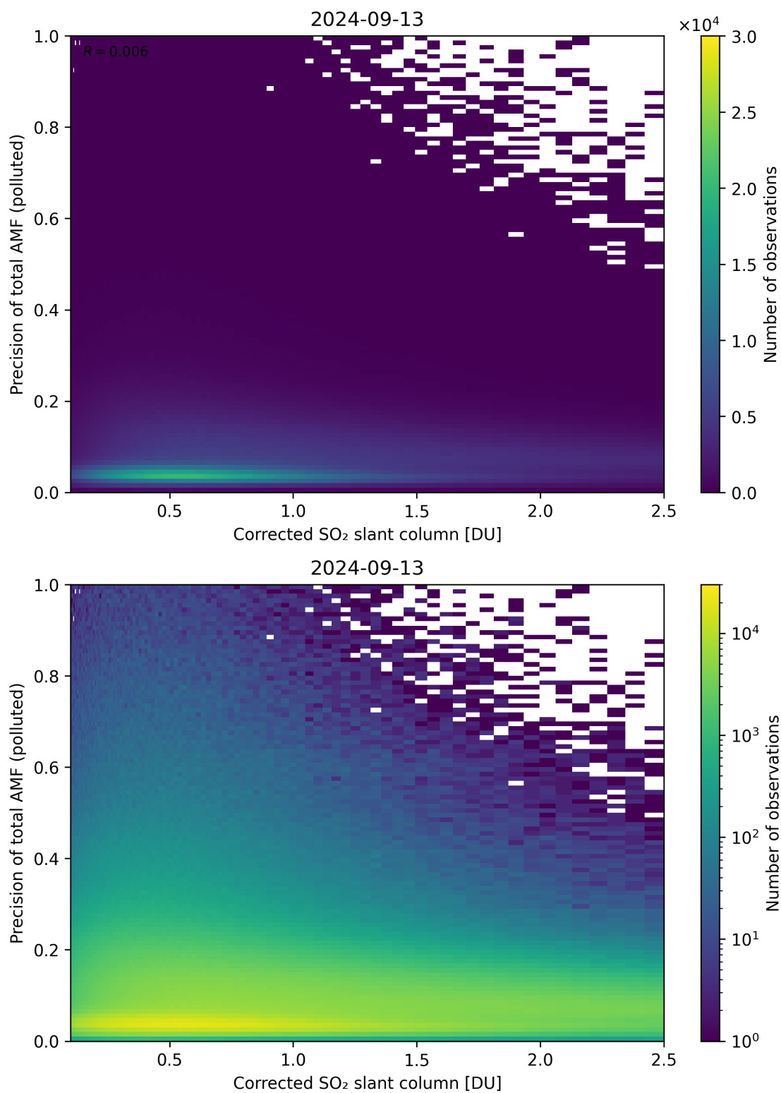
Figure 193: Scatter density plot of “Corrected SO 2 slant column” against “Precision of total AMF (polluted)” for 2024-09-12 to 2024-09-14.
