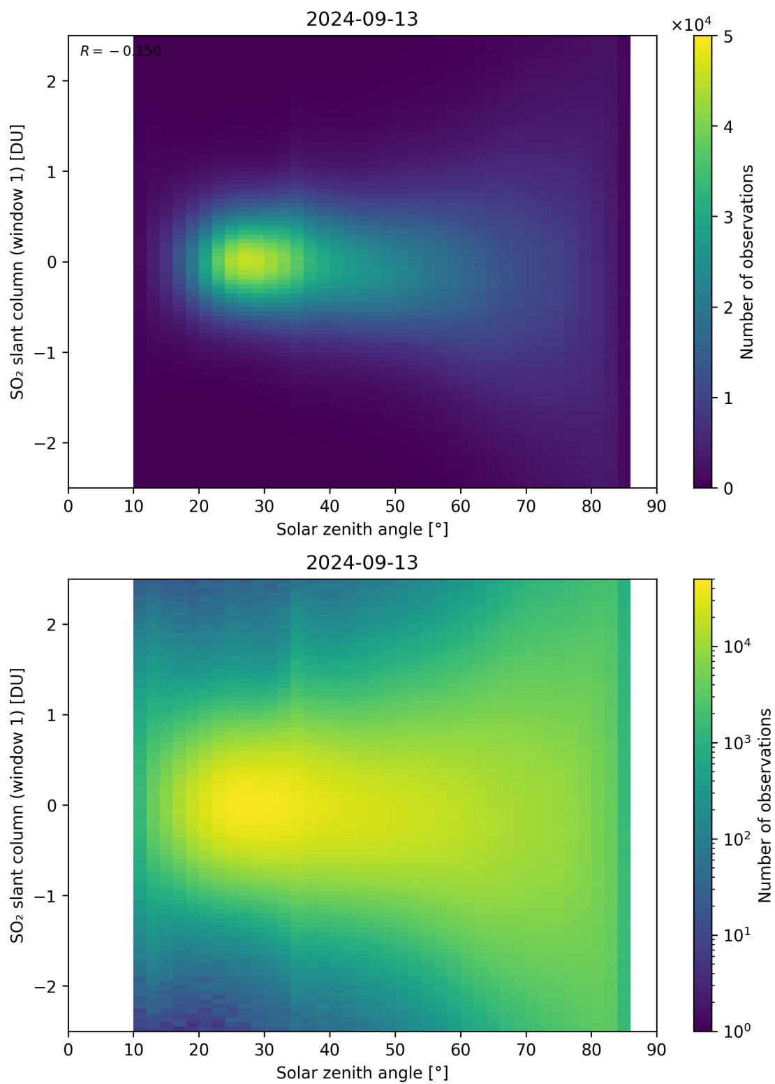
Figure 169: Scatter density plot of “Solar zenith angle” against “SO 2 slant column (window 1)” for 2024-09-12 to 2024-09-14.
