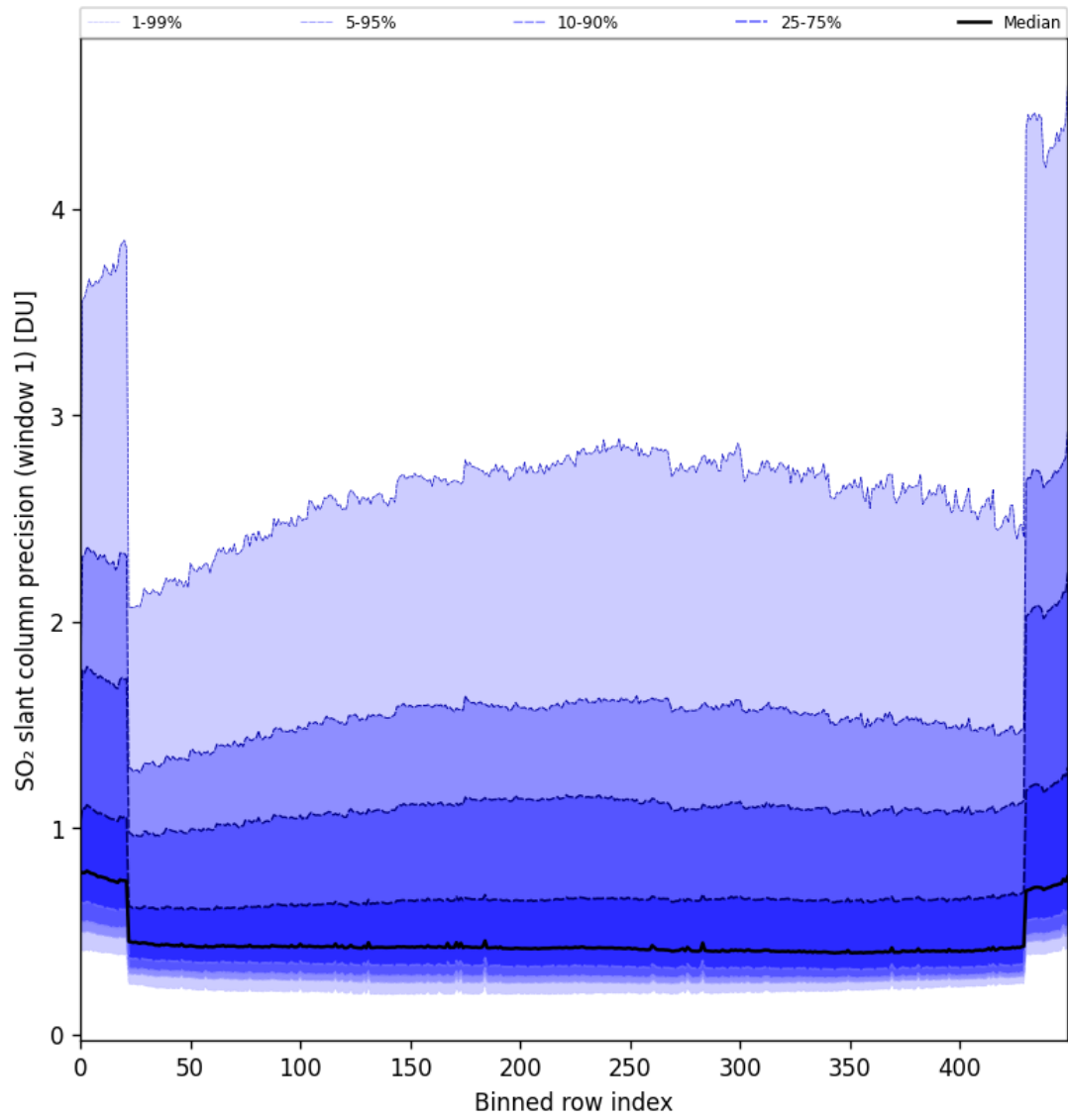
Figure 80: Along track statistics of “SO 2 slant column precision (window 1)” for 2024-09-12 to 2024-09-14
