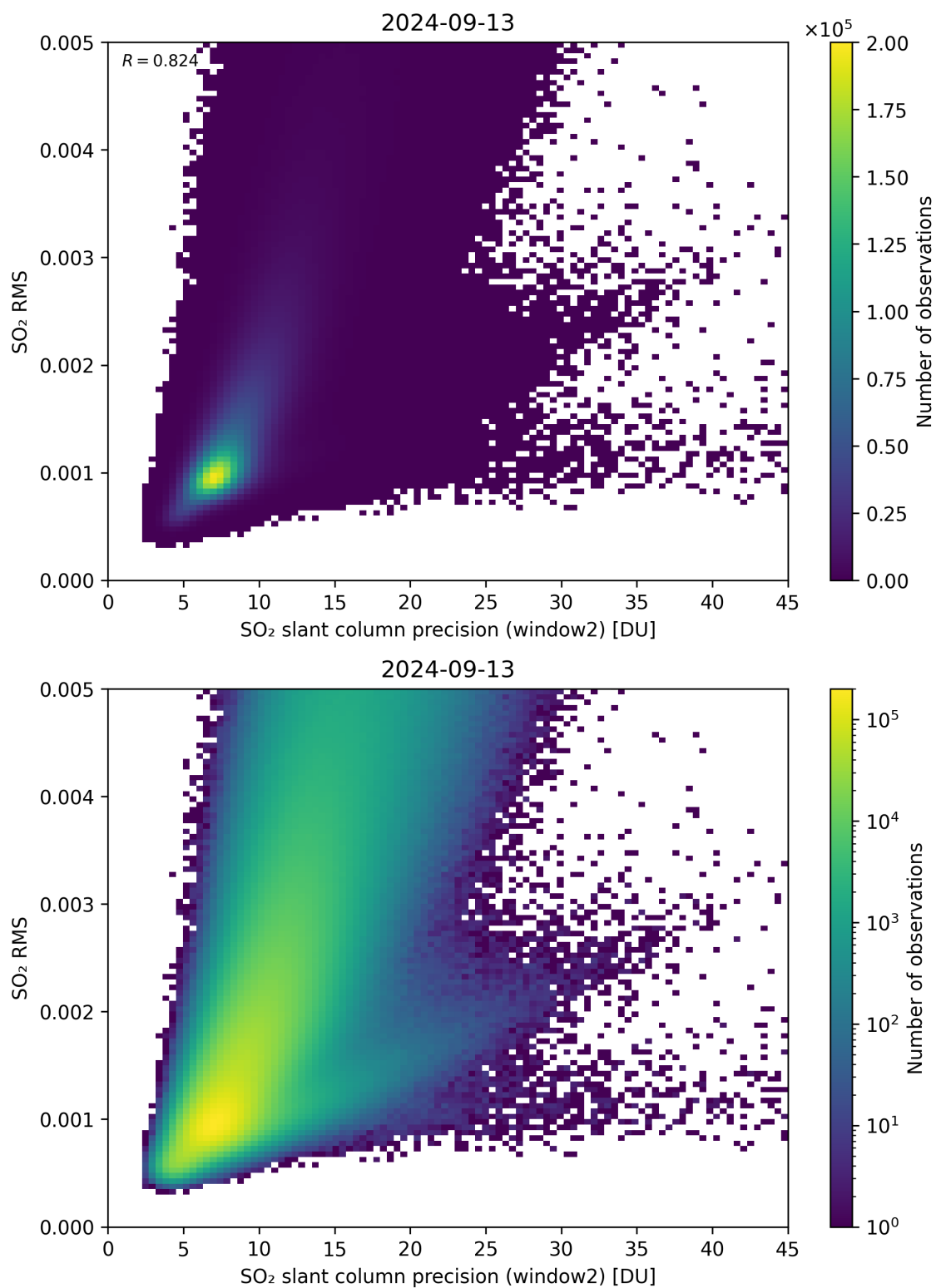
Figure 245: Scatter density plot of “SO 2 slant column precision (window2)” against “SO 2 RMS” for 2024-09-12 to 2024-09-14.
