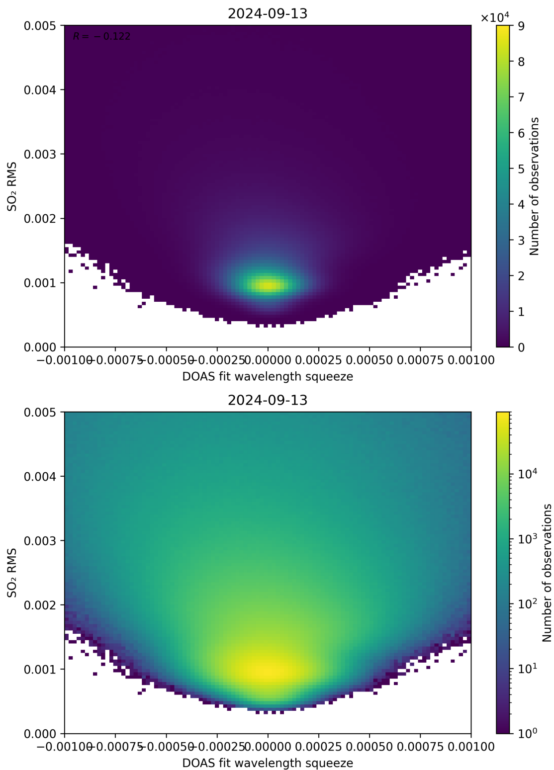
Figure 132: Scatter density plot of “DOAS fit wavelength squeeze” against “SO 2 RMS” for 2024-09-12 to 2024-09-14.
