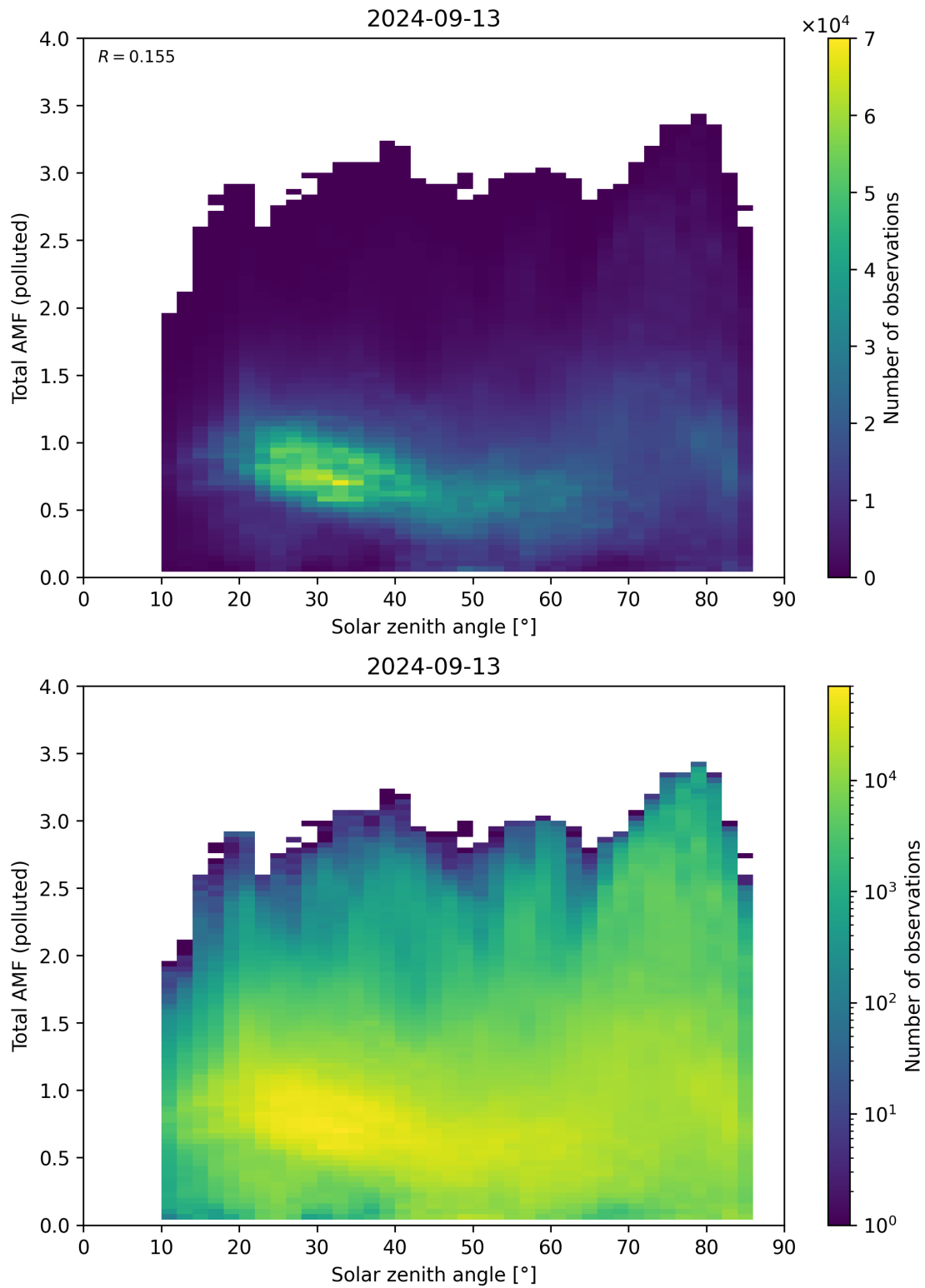
Figure 174: Scatter density plot of “Solar zenith angle” against “Total AMF (polluted)” for 2024-09-12 to 2024-09-14.
