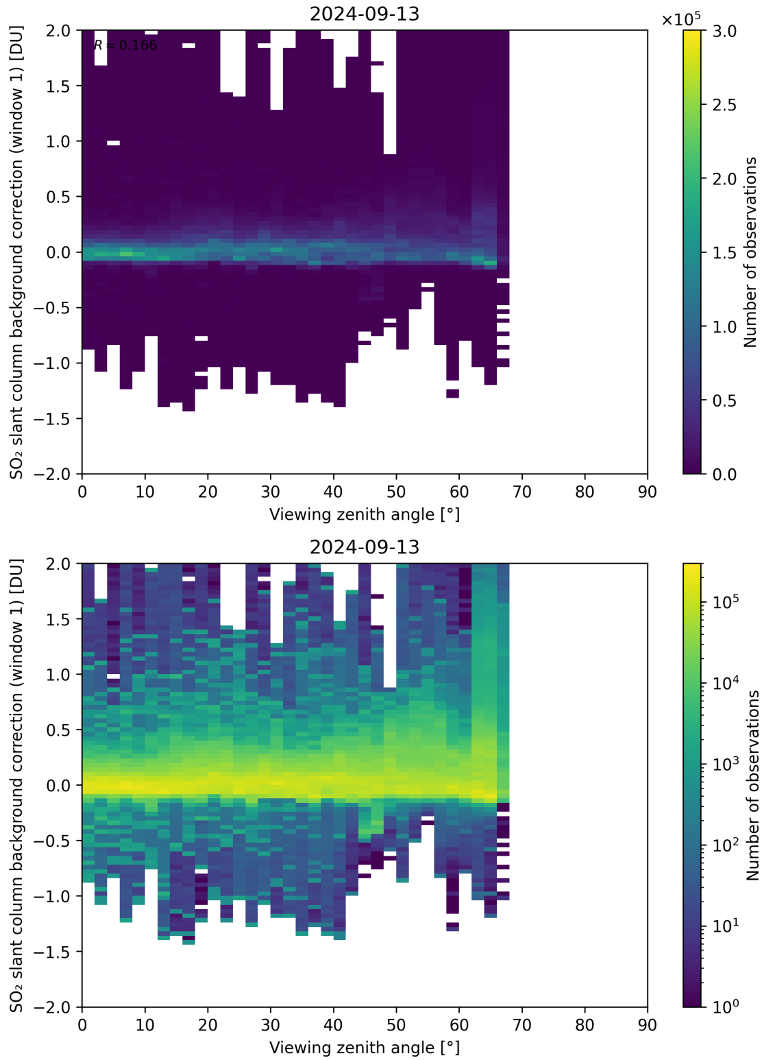
Figure 308: Scatter density plot of “Viewing zenith angle” against “SO 2 slant column background correction (window 1)” for 2024-09-12 to 2024-09-14.
