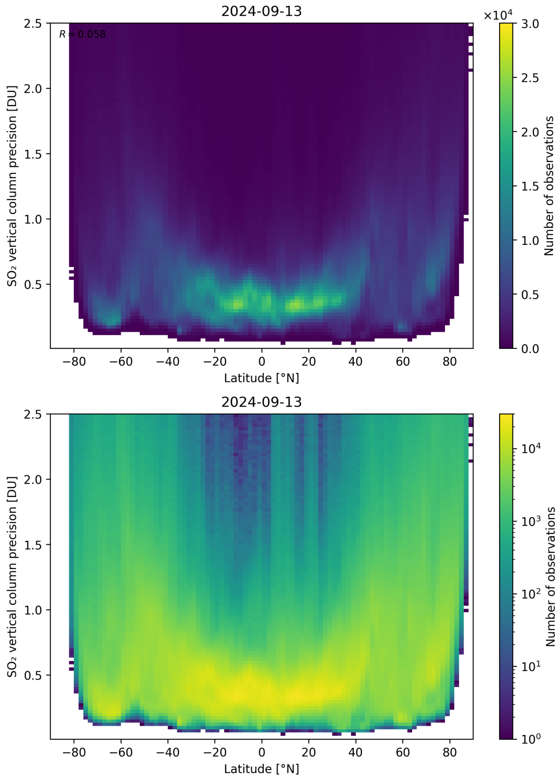
Figure 157: Scatter density plot of “Latitude” against “SO 2 vertical column precision” for 2024-09-12 to 2024-09-14.
