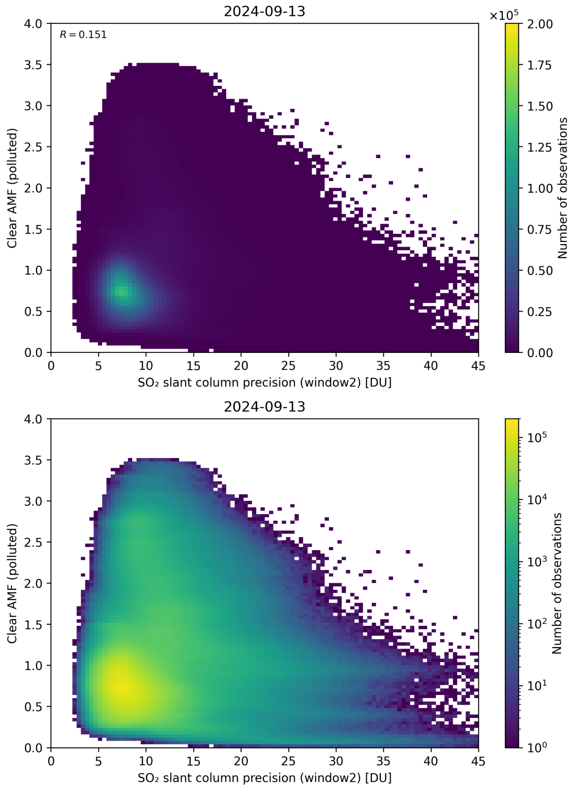
Figure 246: Scatter density plot of “SO 2 slant column precision (window2)” against “Clear AMF (polluted)” for 2024-09-12 to 2024-09-14.
