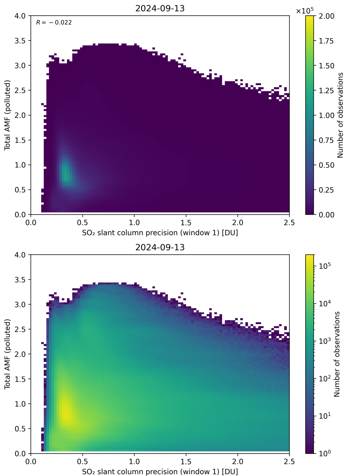
Figure 230: Scatter density plot of “SO 2 slant column precision (window 1)” against “Total AMF (polluted)” for 2024-09-12 to 2024-09-14.
