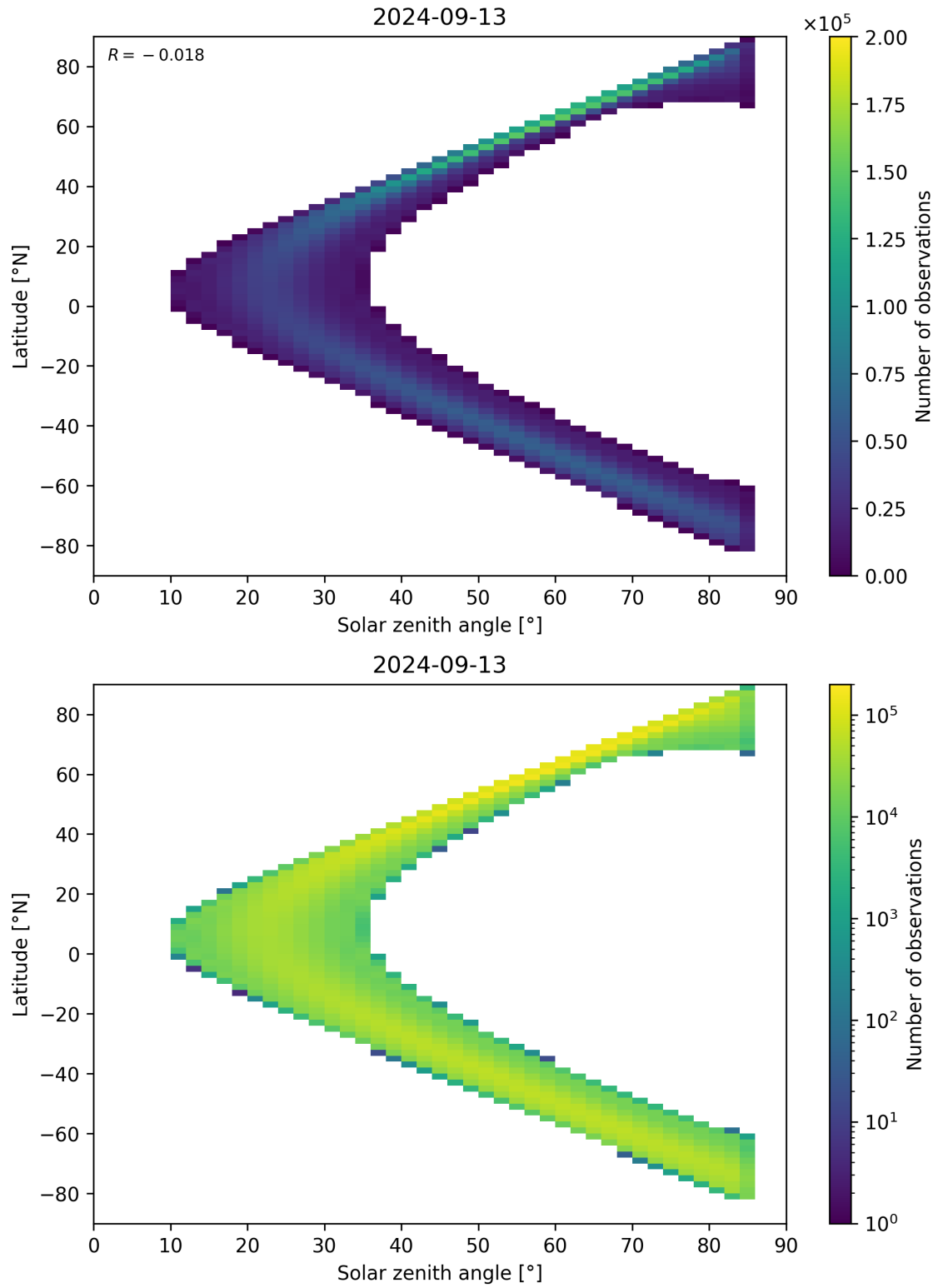
Figure 164: Scatter density plot of “Solar zenith angle” against “Latitude” for 2024-09-12 to 2024-09-14.
