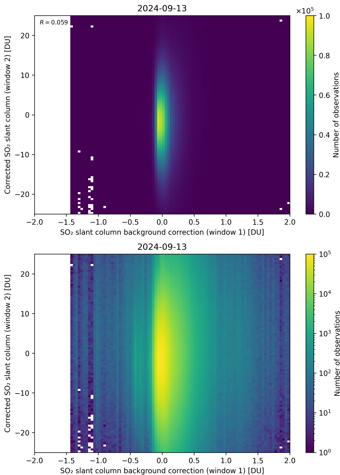
Figure 104: Scatter density plot of “SO 2 slant column background correction (window 1)” against “Corrected SO 2 slant column (window 2)” for 2024-09-12 to 2024-09-14.
