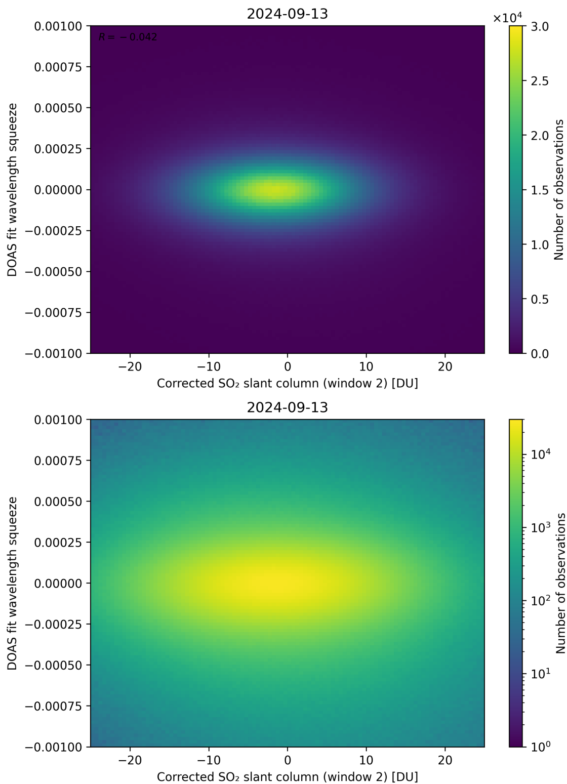
Figure 197: Scatter density plot of “Corrected SO 2 slant column (window 2)” against “DOAS fit wavelength squeeze” for 2024-09-12 to 2024-09-14.
