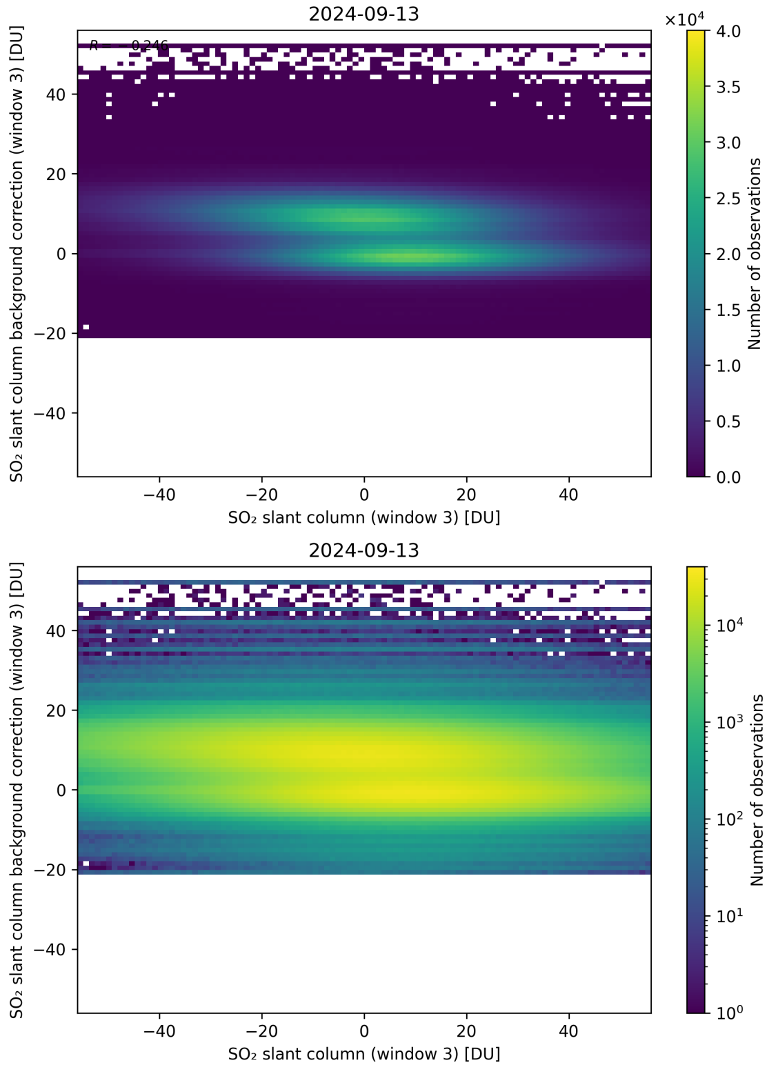
Figure 253: Scatter density plot of “SO 2 slant column (window 3)” against “SO 2 slant column background correction (window 3)” for 2024-09-12 to 2024-09-14.
