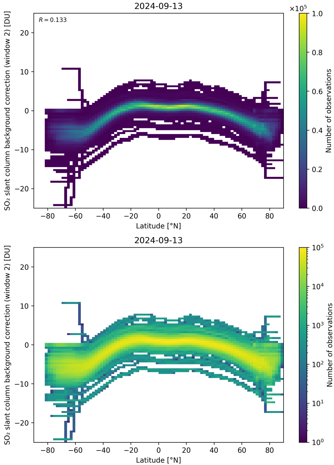
Figure 140: Scatter density plot of “Latitude” against “SO 2 slant column background correction (window 2)” for 2024-09-12 to 2024-09-14.
