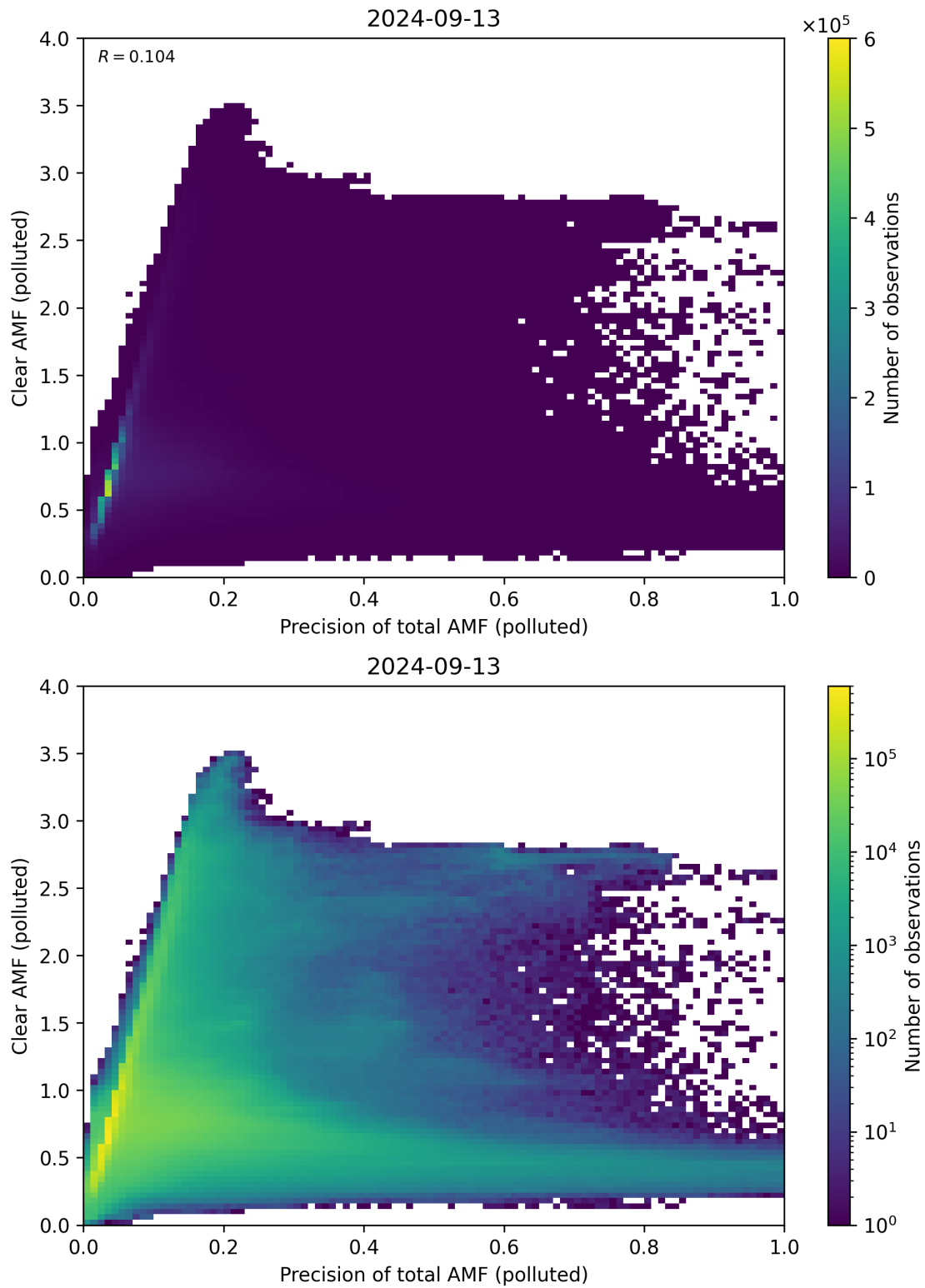
Figure 270: Scatter density plot of “Precision of total AMF (polluted)” against “Clear AMF (polluted)” for 2024-09-12 to 2024-09-14.
