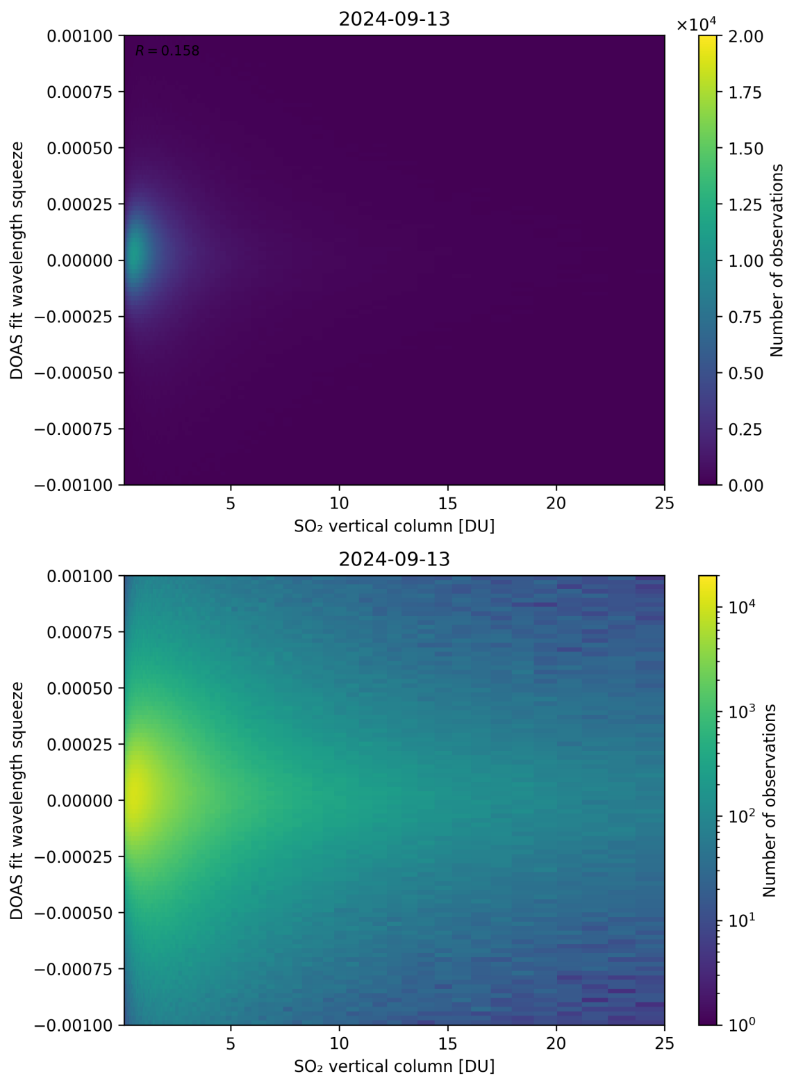
Figure 277: Scatter density plot of “SO 2 vertical column” against “DOAS fit wavelength squeeze” for 2024-09-12 to 2024-09-14.
