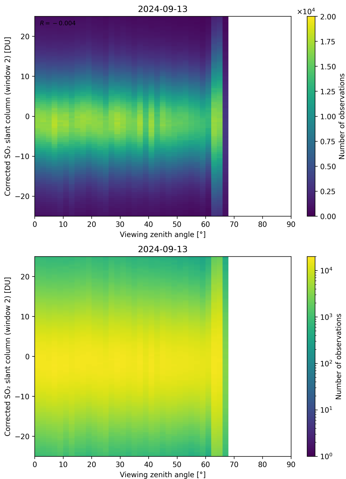
Figure 318: Scatter density plot of “Viewing zenith angle” against “Corrected SO 2 slant column (window 2)” for 2024-09-12 to 2024-09-14.
