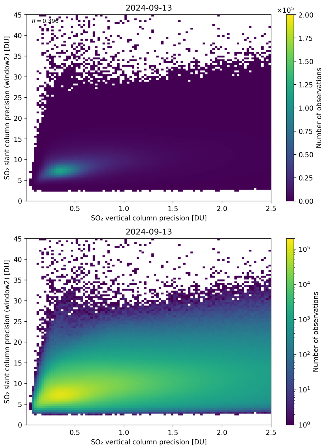
Figure 291: Scatter density plot of “SO 2 vertical column precision” against “SO 2 slant column precision (window2)” for 2024-09-12 to 2024-09-14.
