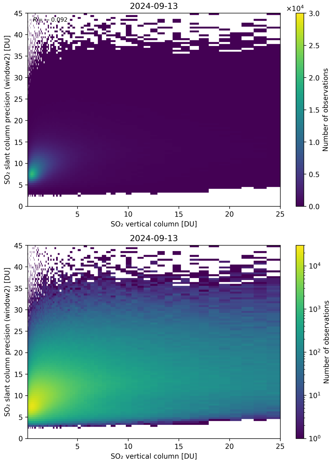
Figure 302: Scatter density plot of “SO 2 vertical column” against “SO 2 slant column precision (window2)” for 2024-09-12 to 2024-09-14.
