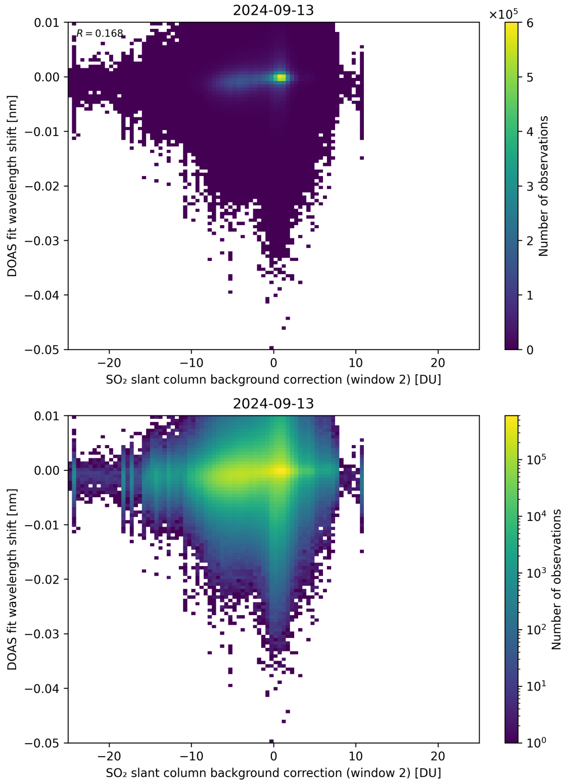
Figure 112: Scatter density plot of “SO 2 slant column background correction (window 2)” against “DOAS fit wavelength shift” for 2024-09-12 to 2024-09-14.
