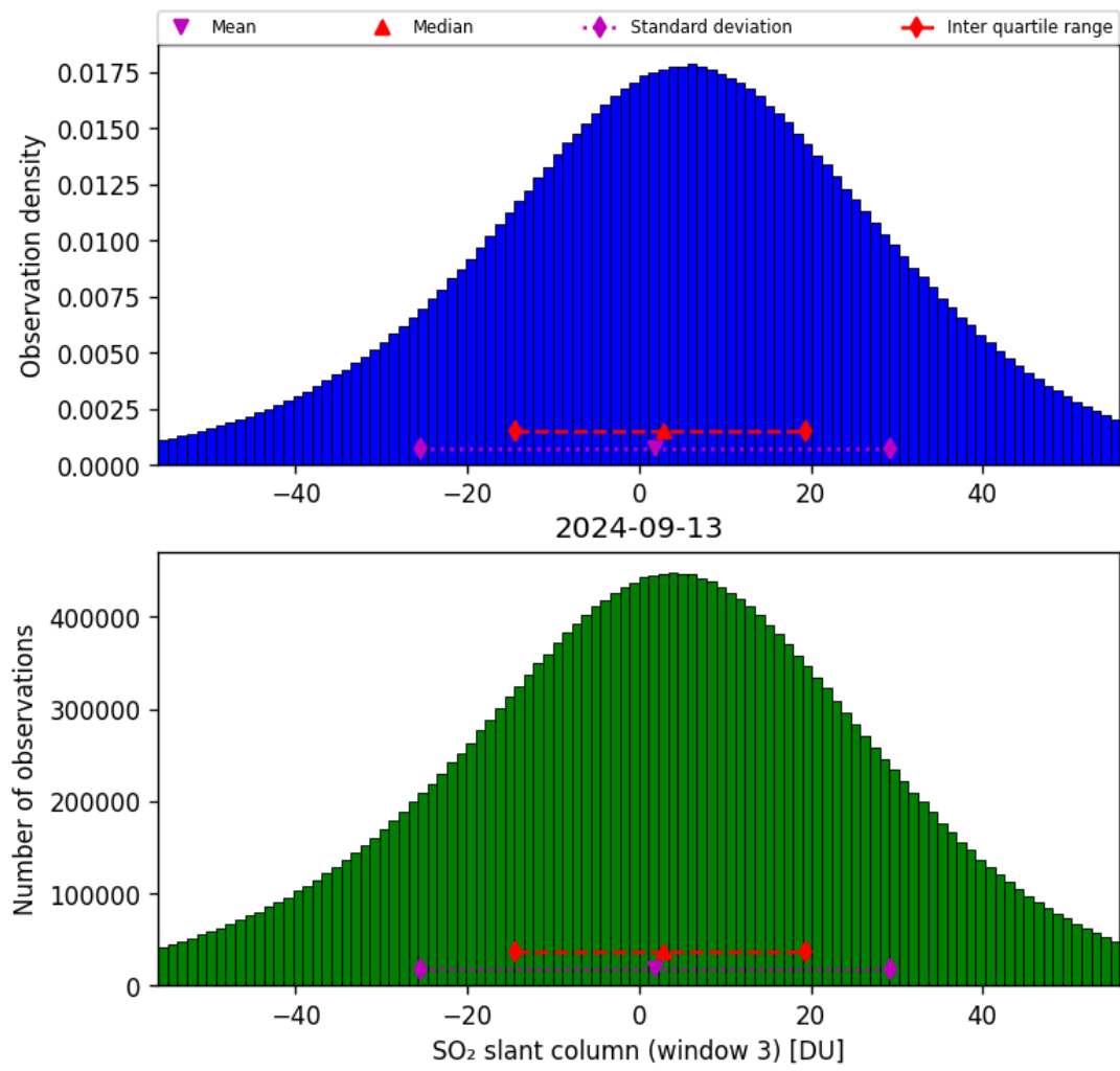
Figure 64: Histogram of “SO 2 slant column (window 3)” for 2024-09-12 to 2024-09-14
