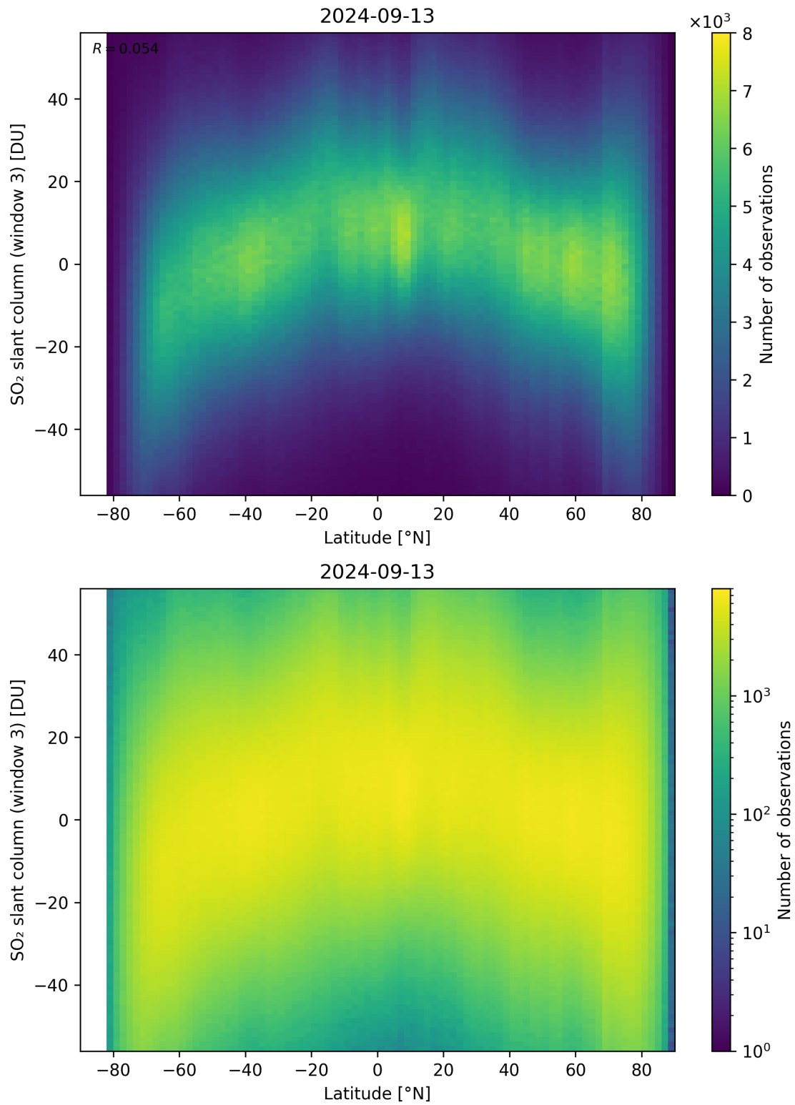
Figure 152: Scatter density plot of “Latitude” against “SO 2 slant column (window 3)” for 2024-09-12 to 2024-09-14.
