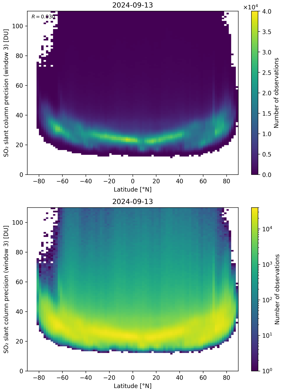
Figure 153: Scatter density plot of “Latitude” against “SO 2 slant column precision (window 3)” for 2024-09-12 to 2024-09-14.
