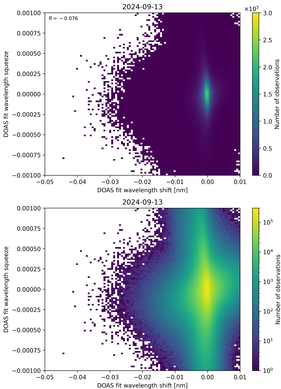
Figure 127: Scatter density plot of “DOAS fit wavelength shift” against “DOAS fit wavelength squeeze” for 2024-09-12 to 2024-09-14.
