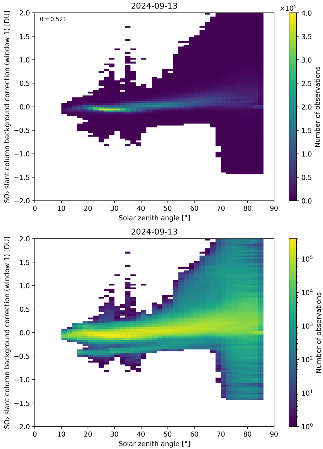
Figure 158: Scatter density plot of “Solar zenith angle” against “SO 2 slant column background correction (window 1)” for 2024-09-12 to 2024-09-14.
