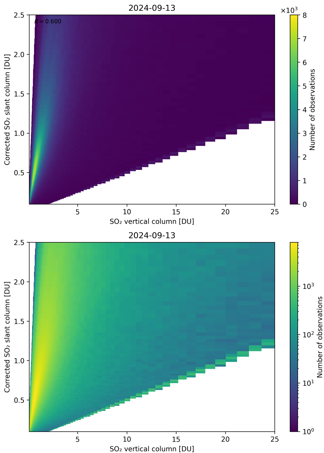
Figure 297: Scatter density plot of “SO 2 vertical column” against “Corrected SO 2 slant column” for 2024-09-12 to 2024-09-14.
