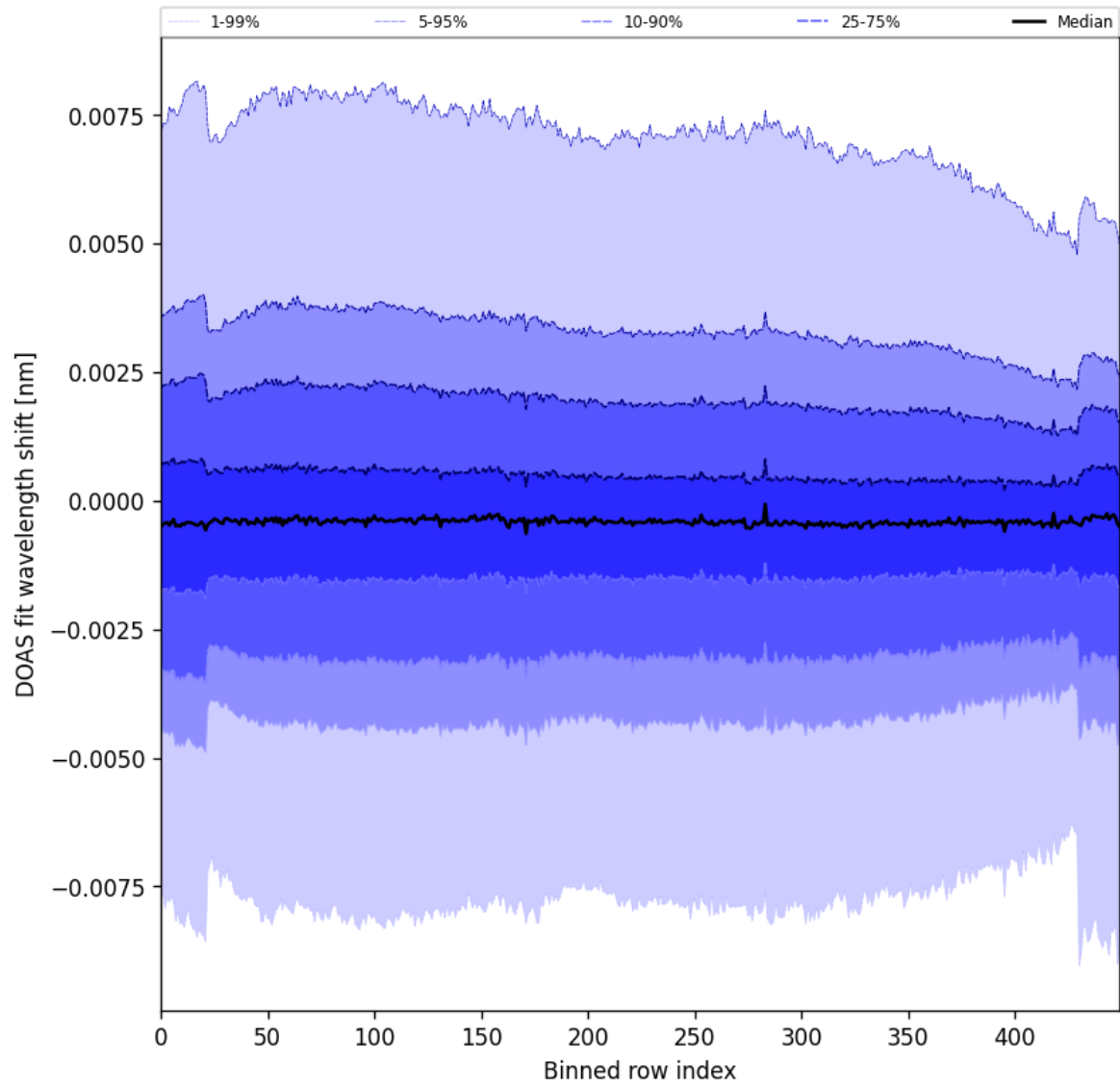
Figure 91: Along track statistics of “DOAS fit wavelength shift” for 2024-09-12 to 2024-09-14
