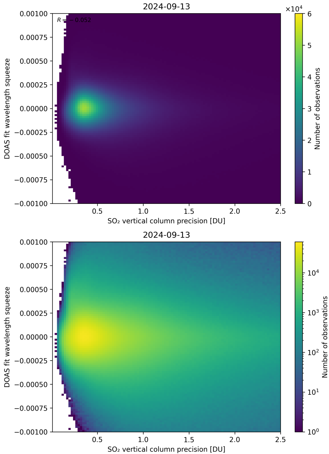
Figure 283: Scatter density plot of “SO 2 vertical column precision” against “DOAS fit wavelength squeeze” for 2024-09-12 to 2024-09-14.
