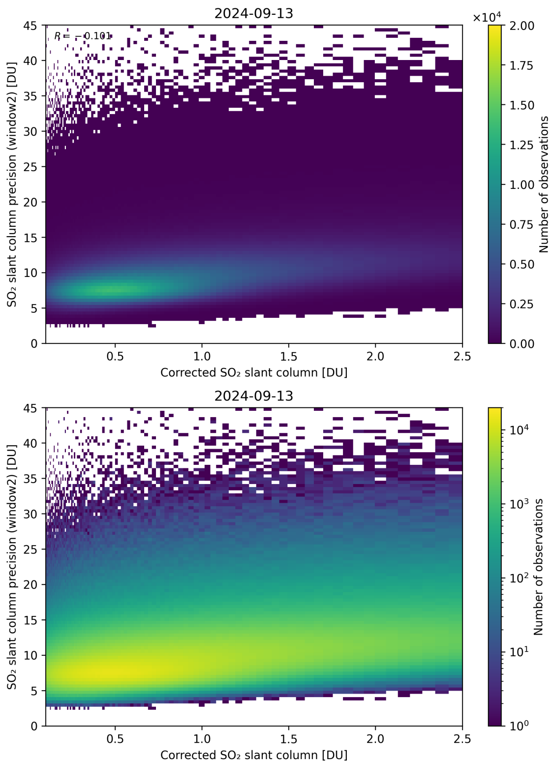
Figure 189: Scatter density plot of “Corrected SO 2 slant column” against “SO 2 slant column precision (window2)” for 2024-09-12 to 2024-09-14.
