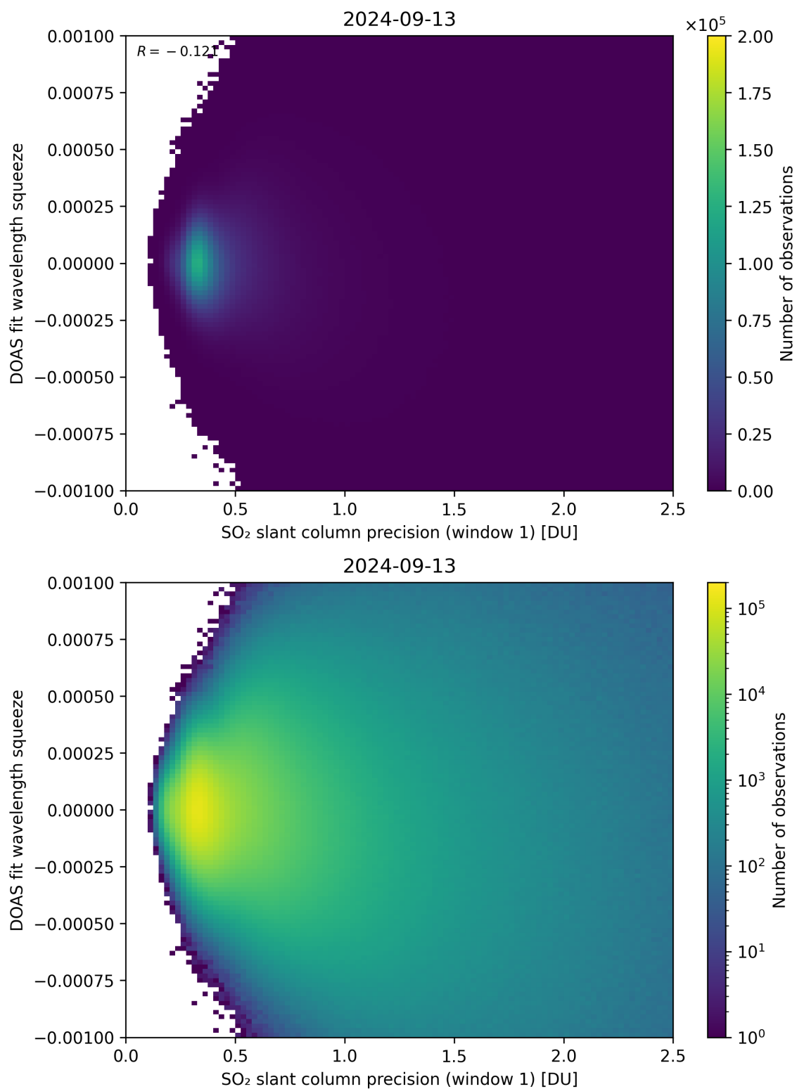
Figure 222: Scatter density plot of “SO 2 slant column precision (window 1)” against “DOAS fit wavelength squeeze” for 2024-09-12 to 2024-09-14.
