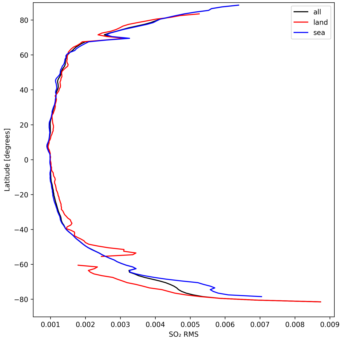
Figure 47: Zonal average of “ \text{SO}_2 RMS” for 2024-09-12 to 2024-09-14.
