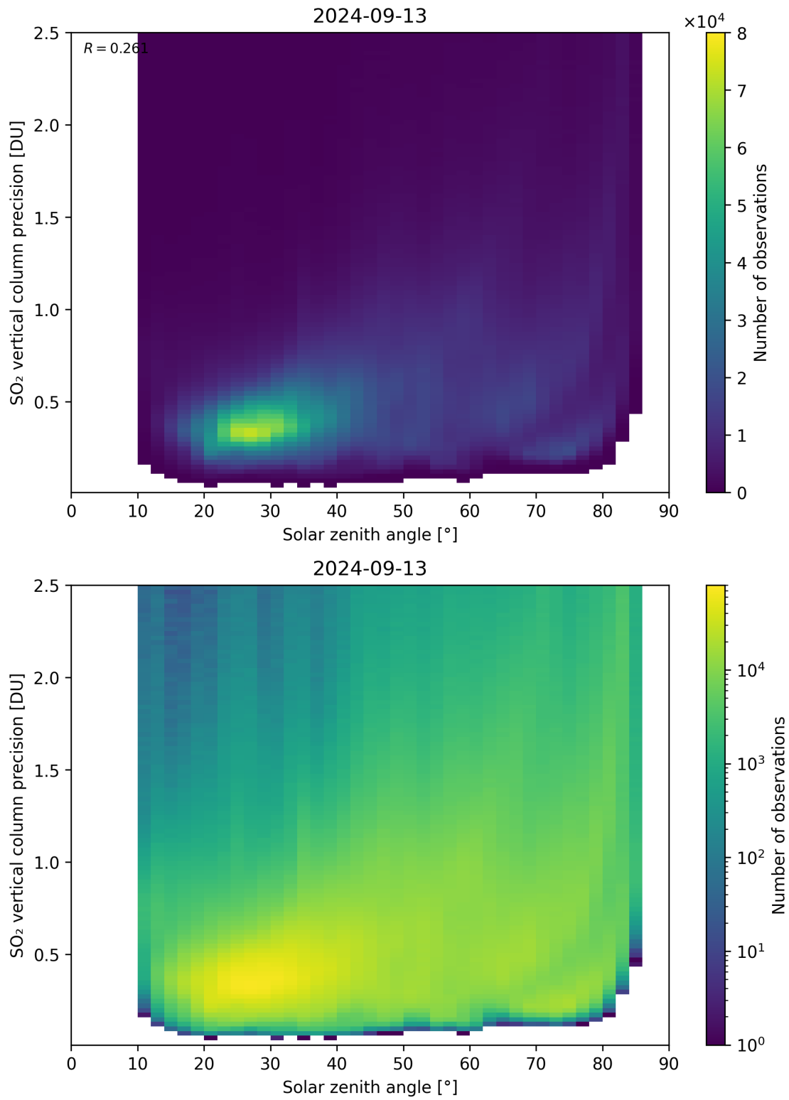
Figure 177: Scatter density plot of “Solar zenith angle” against “SO 2 vertical column precision” for 2024-09-12 to 2024-09-14.
