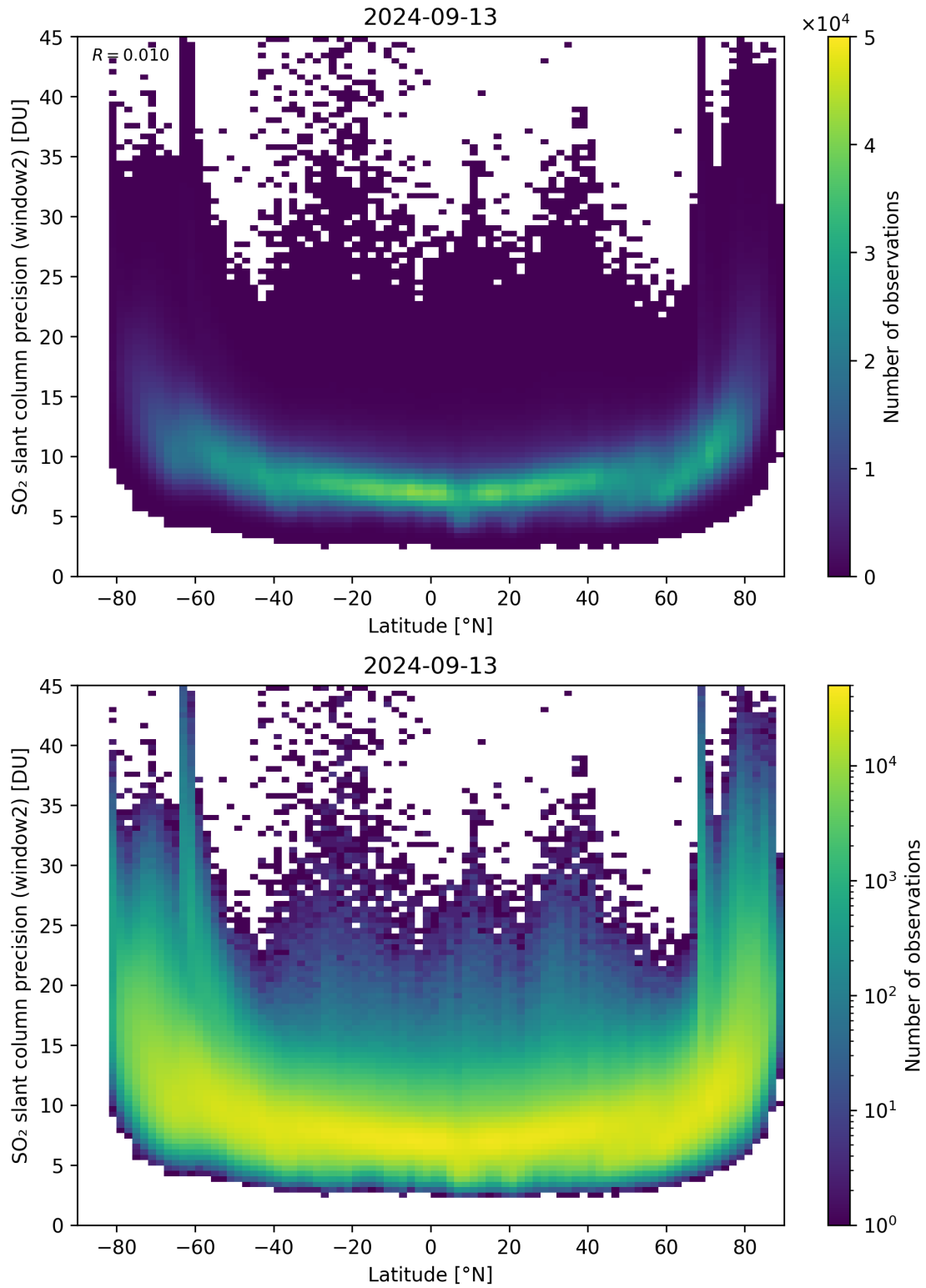
Figure 151: Scatter density plot of “Latitude” against “SO 2 slant column precision (window2)” for 2024-09-12 to 2024-09-14.
