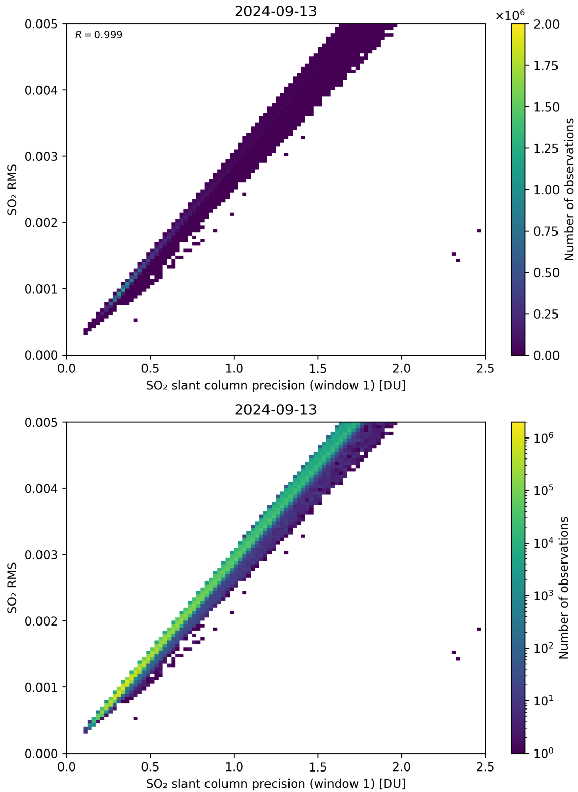
Figure 223: Scatter density plot of “SO 2 slant column precision (window 1)” against “SO 2 RMS” for 2024-09-12 to 2024-09-14.
