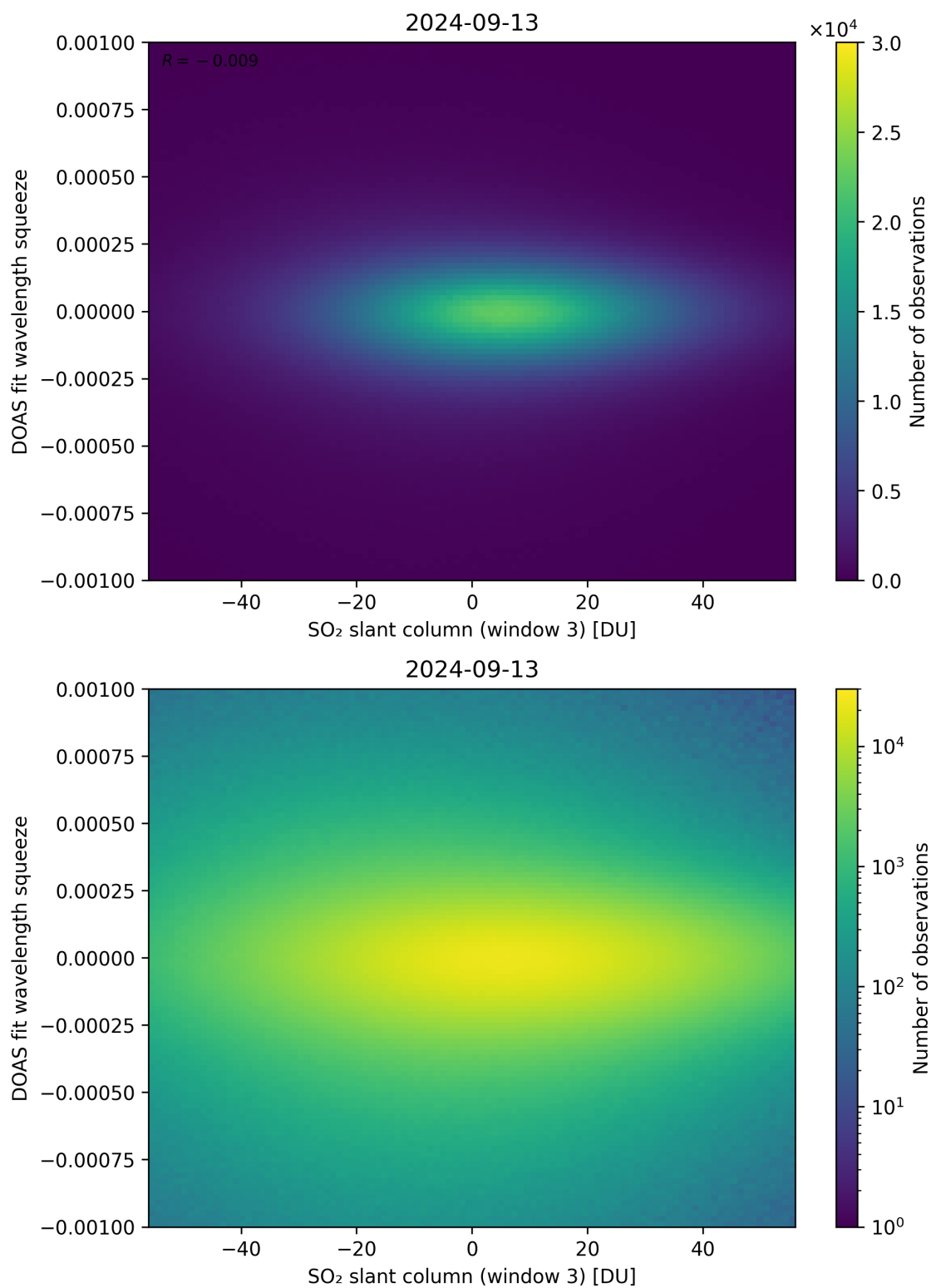
Figure 255: Scatter density plot of “SO 2 slant column (window 3)” against “DOAS fit wavelength squeeze” for 2024-09-12 to 2024-09-14.
