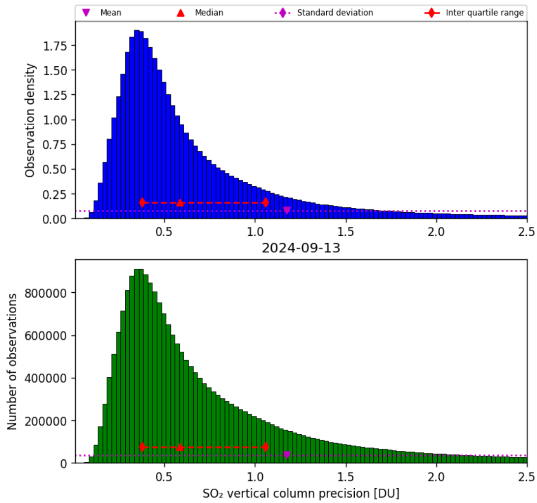
Figure 54: Histogram of “SO 2 vertical column precision” for 2024-09-12 to 2024-09-14
