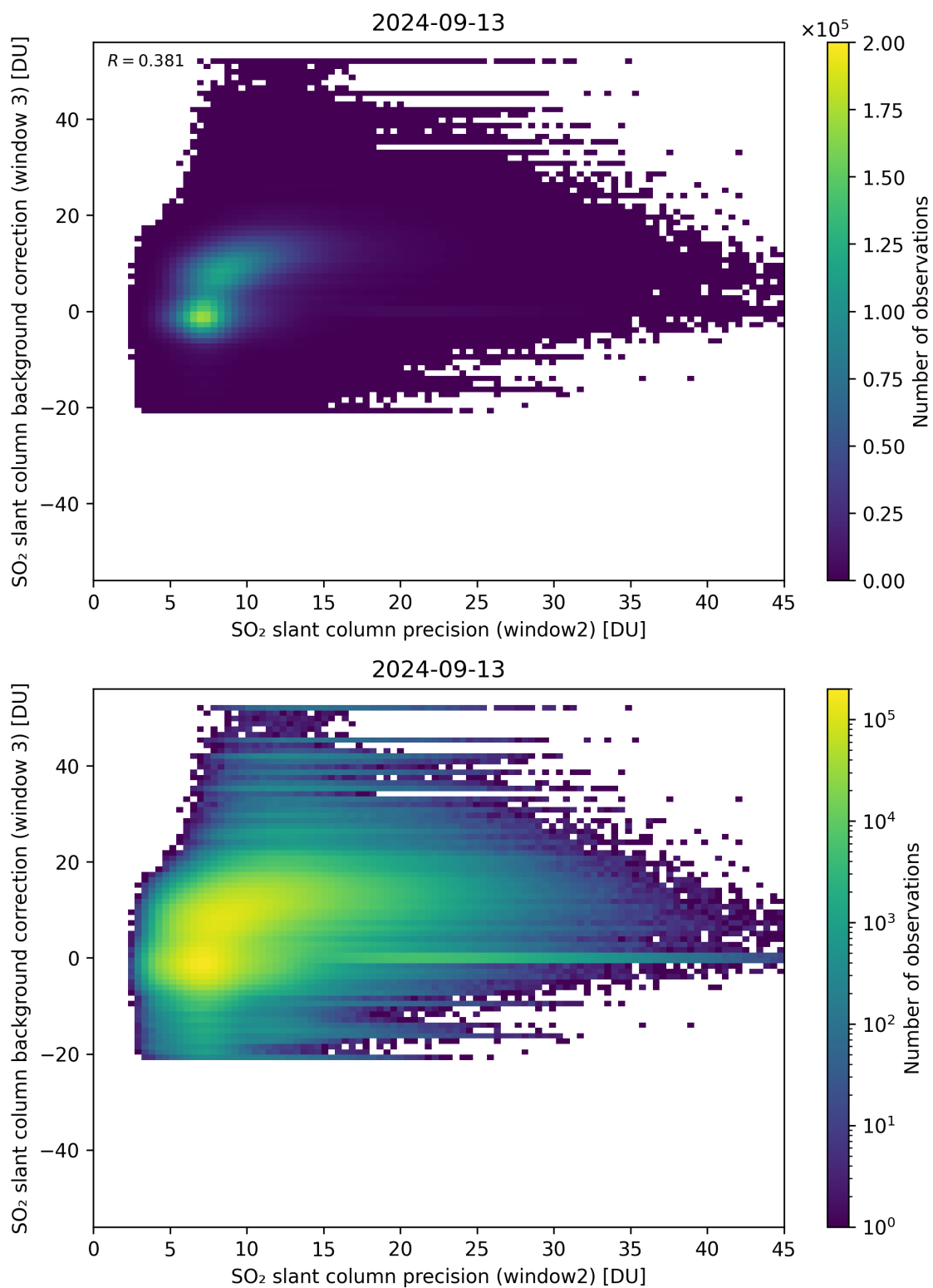
Figure 242: Scatter density plot of “SO 2 slant column precision (window2)” against “SO 2 slant column background correction (window 3)” for 2024-09-12 to 2024-09-14.
