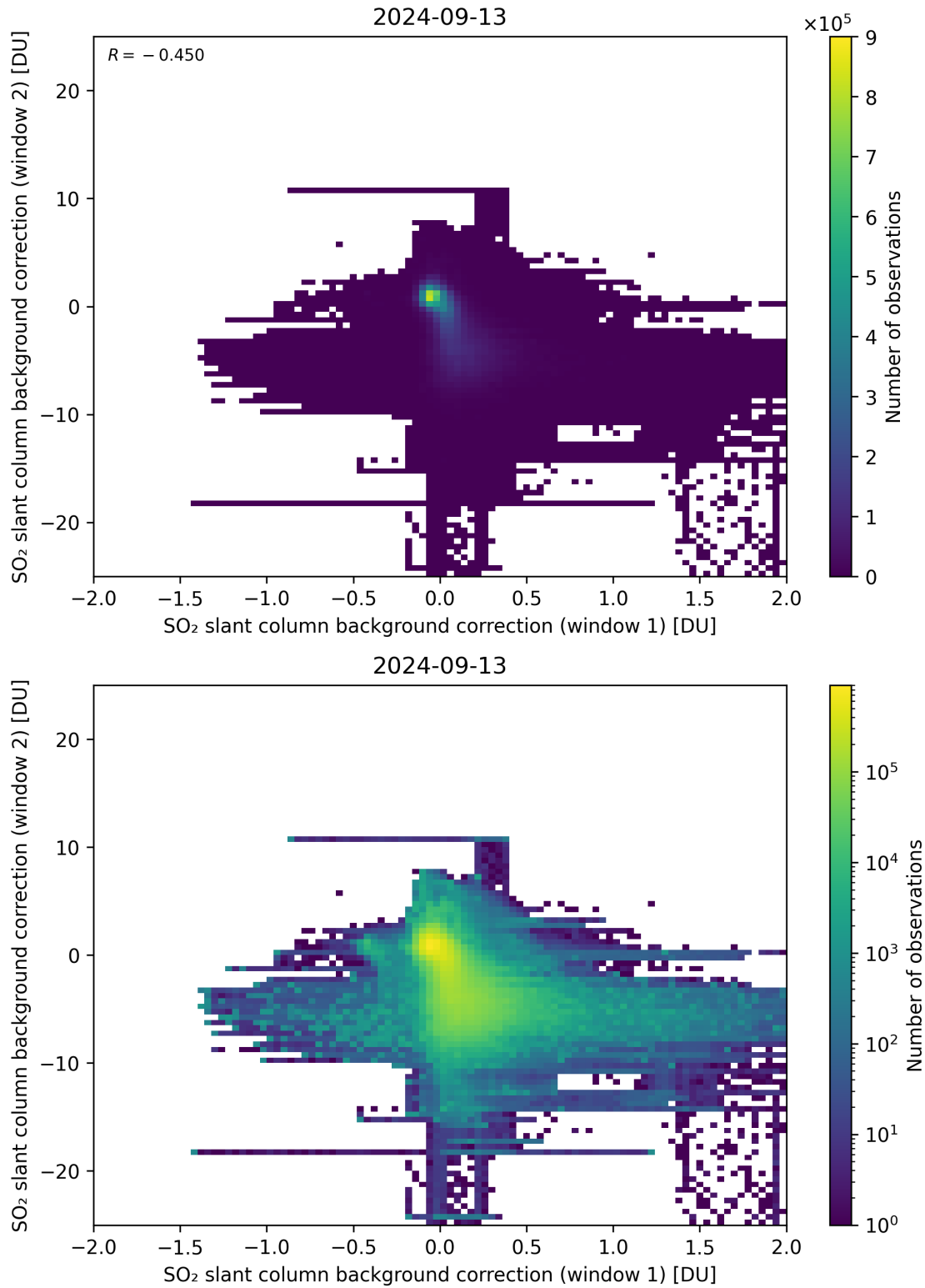
Figure 98: Scatter density plot of “SO 2 slant column background correction (window 1)” against “SO 2 slant column background correction (window 2)” for 2024-09-12 to 2024-09-14.
