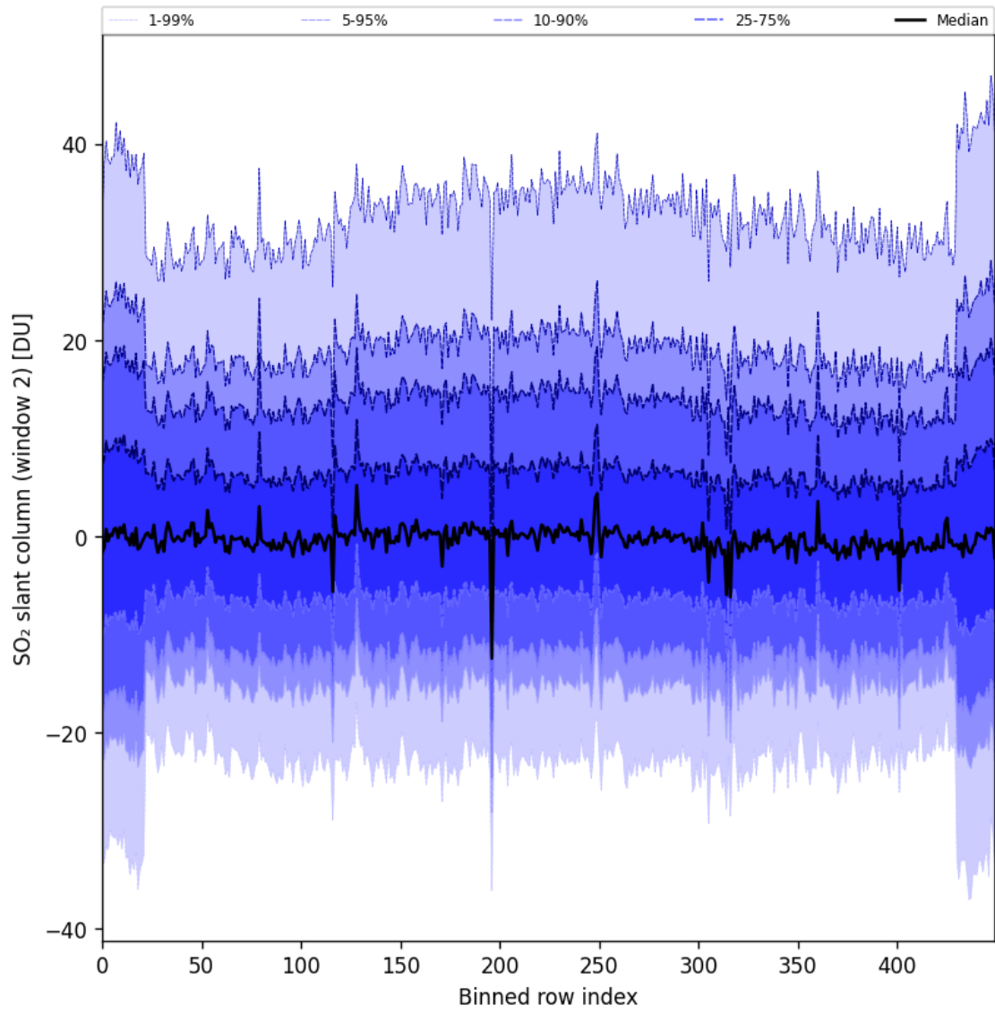
Figure 83: Along track statistics of “SO 2 slant column (window 2)” for 2024-09-12 to 2024-09-14
