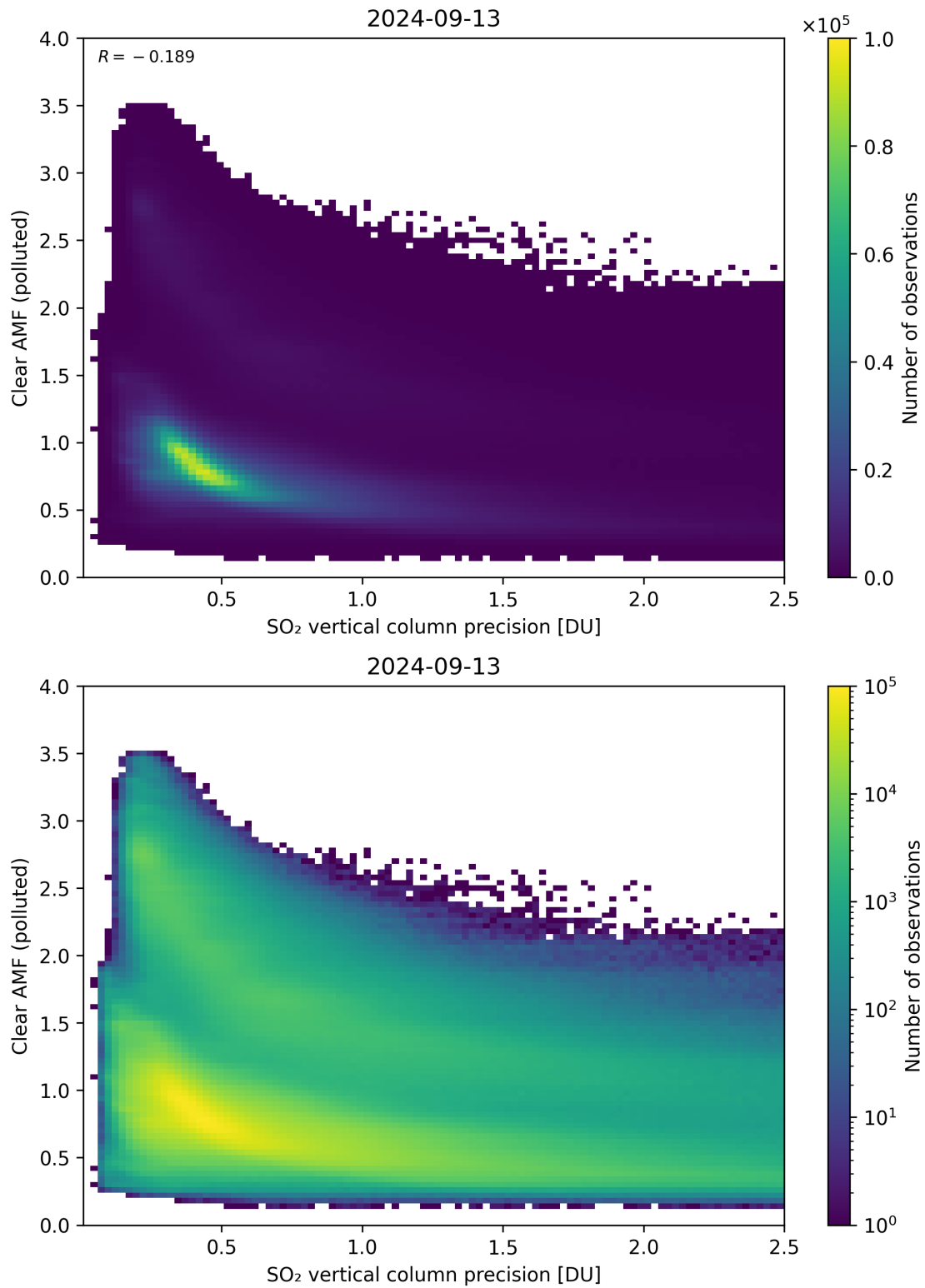
Figure 285: Scatter density plot of “SO 2 vertical column precision” against “Clear AMF (polluted)” for 2024-09-12 to 2024-09-14.
