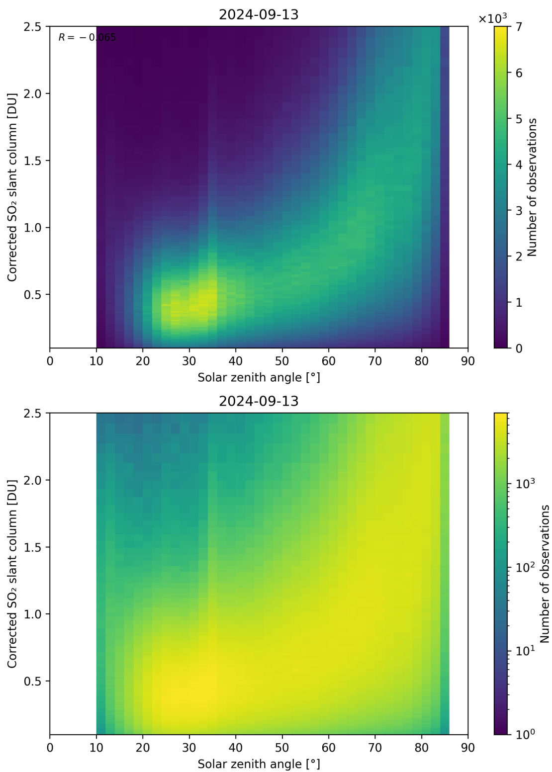
Figure 166: Scatter density plot of “Solar zenith angle” against “Corrected SO 2 slant column” for 2024-09-12 to 2024-09-14.
