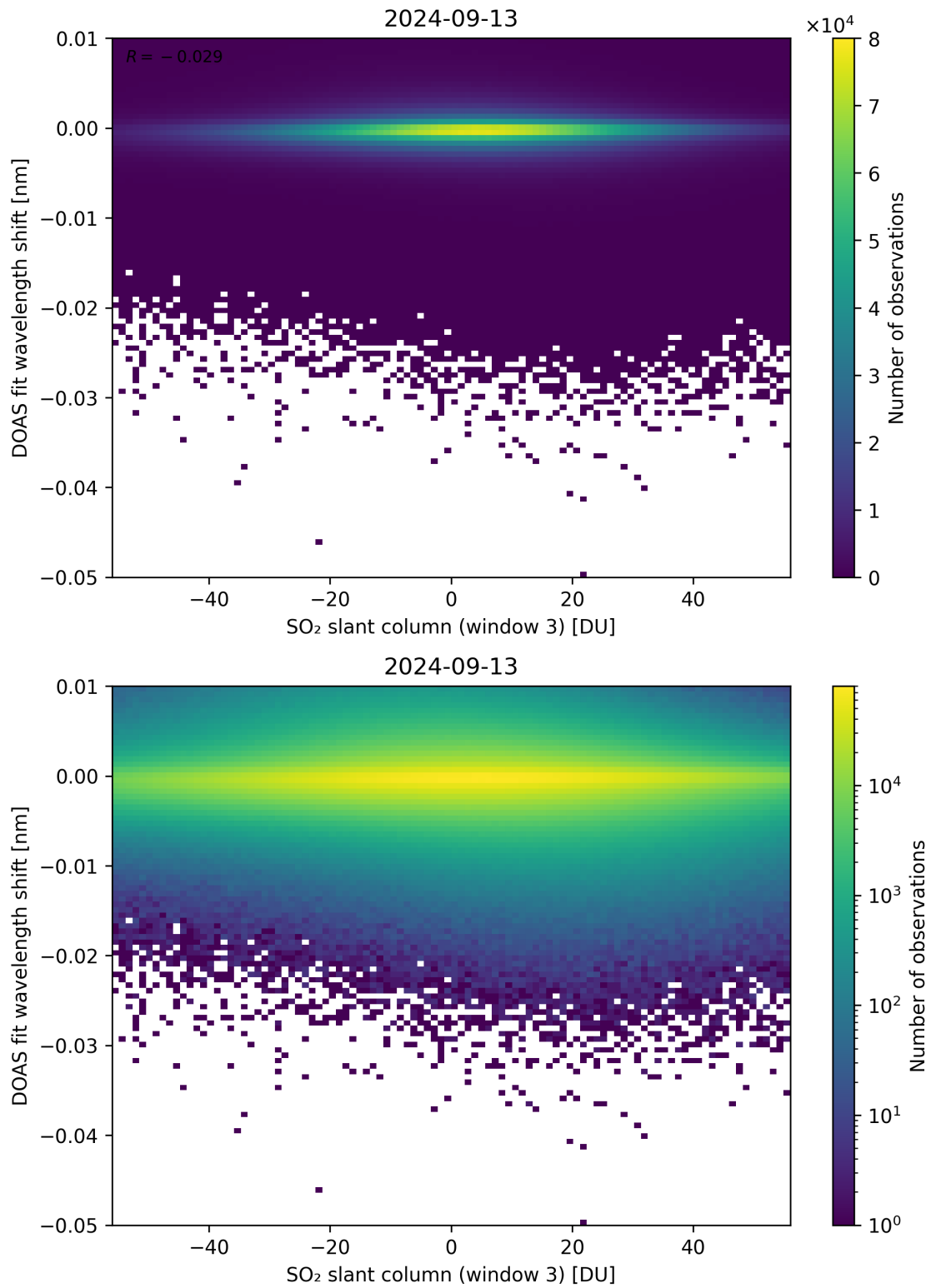
Figure 254: Scatter density plot of “SO 2 slant column (window 3)” against “DOAS fit wavelength shift” for 2024-09-12 to 2024-09-14.
