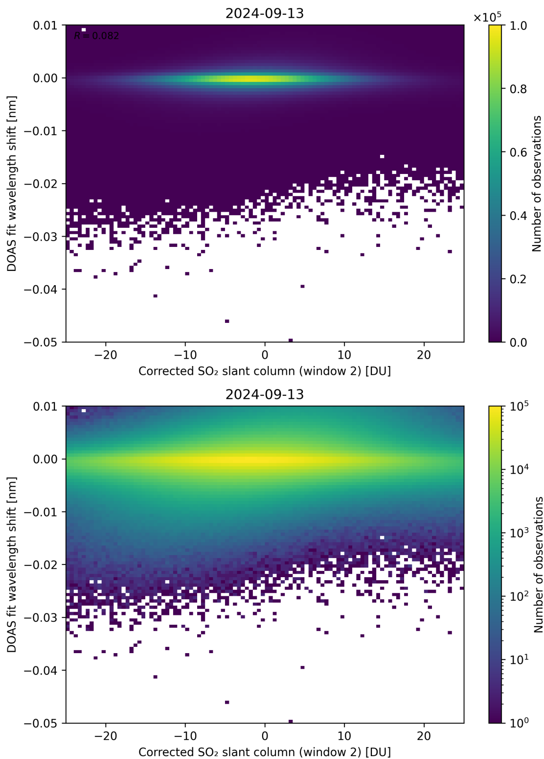
Figure 196: Scatter density plot of “Corrected SO 2 slant column (window 2)” against “DOAS fit wavelength shift” for 2024-09-12 to 2024-09-14.
