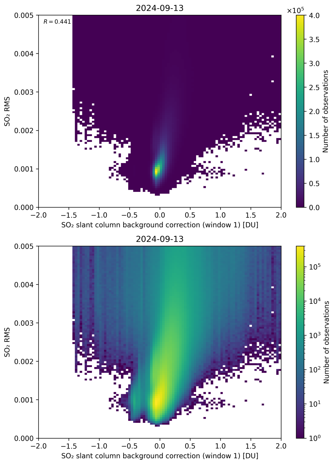
Figure 102: Scatter density plot of “SO 2 slant column background correction (window 1)” against “SO 2 RMS” for 2024-09-12 to 2024-09-14.
