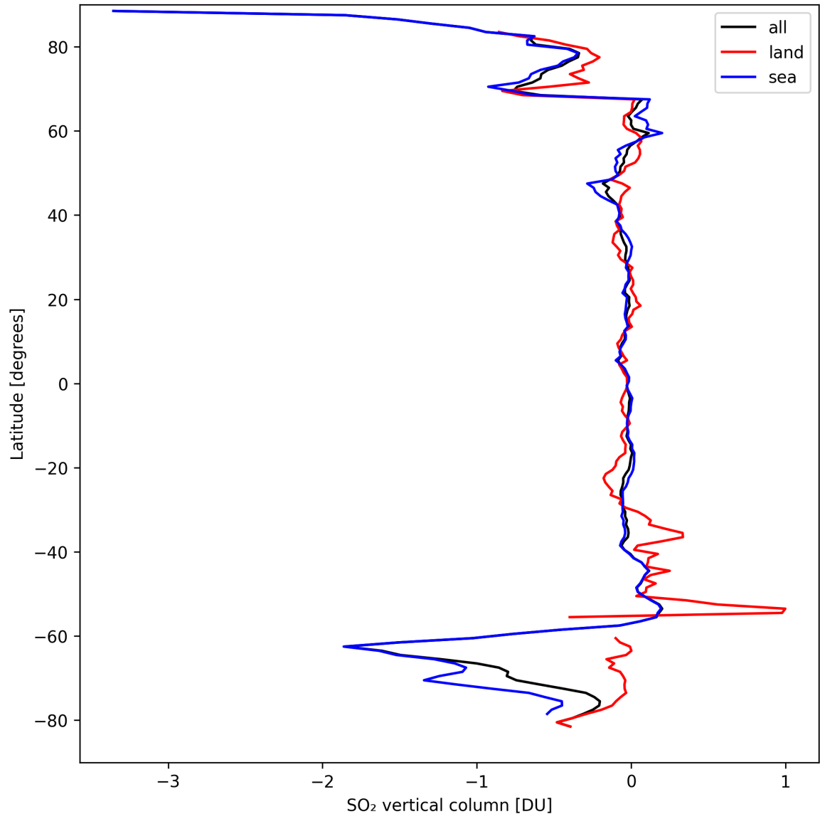
Figure 30: Zonal average of “SO 2 vertical column” for 2024-09-12 to 2024-09-14.
