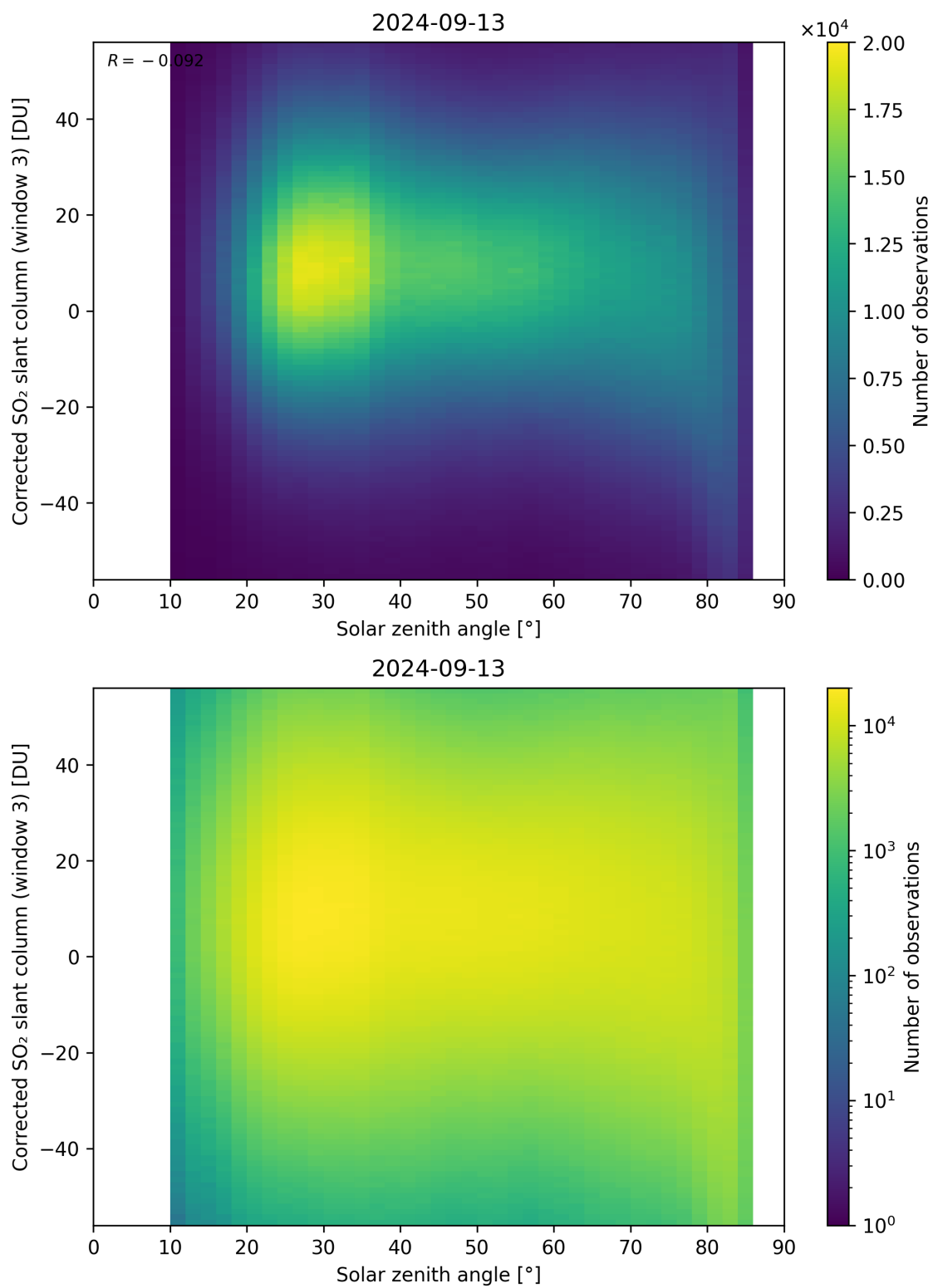
Figure 168: Scatter density plot of “Solar zenith angle” against “Corrected SO 2 slant column (window 3)” for 2024-09-12 to 2024-09-14.
