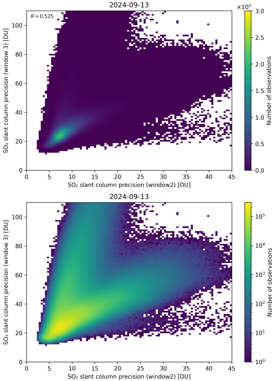
Figure 250: Scatter density plot of “SO 2 slant column precision (window2)” against “SO 2 slant column precision (window 3)” for 2024-09-12 to 2024-09-14.
