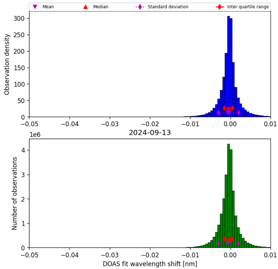
Figure 68: Histogram of “DOAS fit wavelength shift” for 2024-09-12 to 2024-09-14
