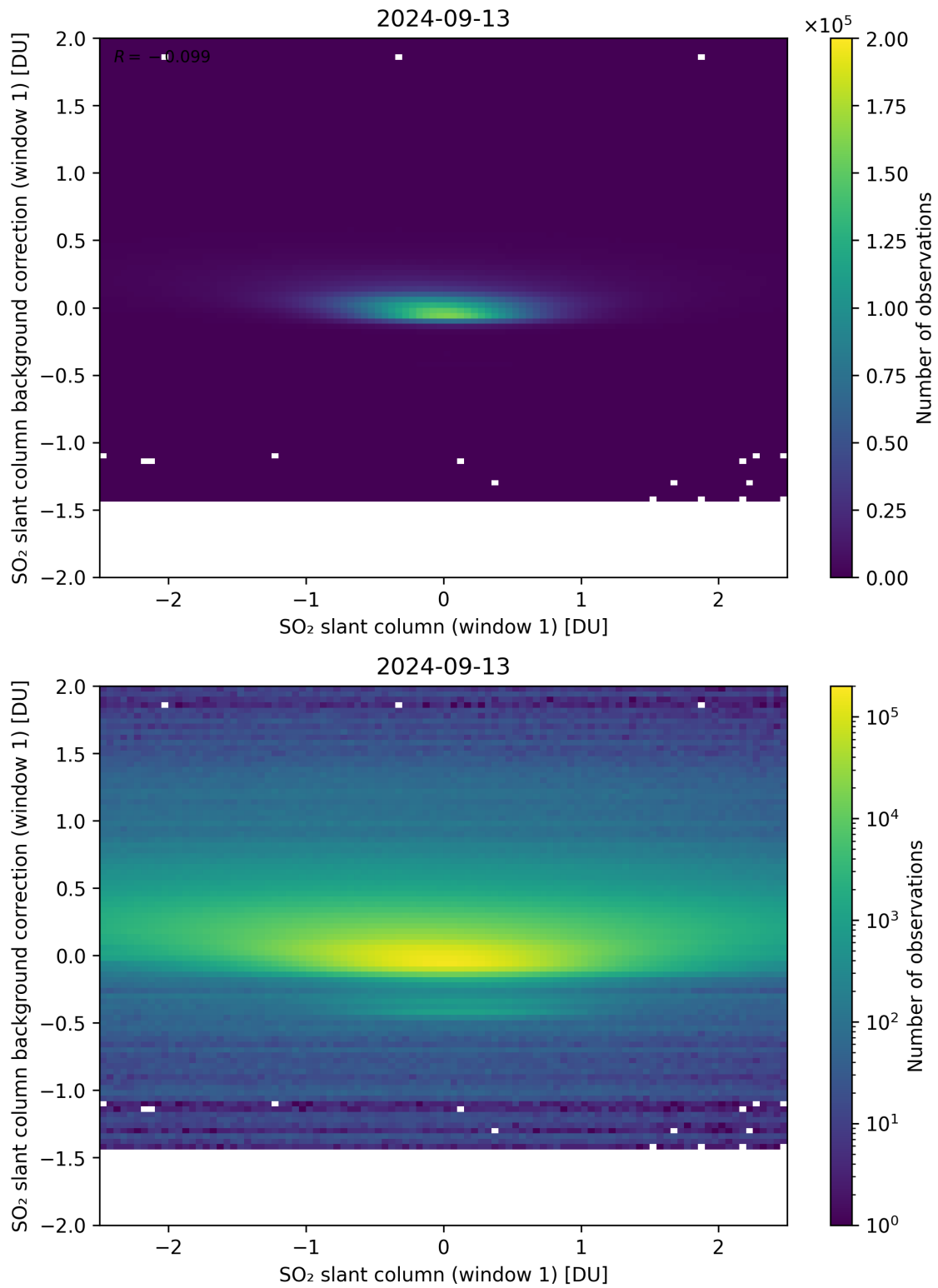
Figure 212: Scatter density plot of “SO 2 slant column (window 1)” against “SO 2 slant column background correction (window 1)” for 2024-09-12 to 2024-09-14.
