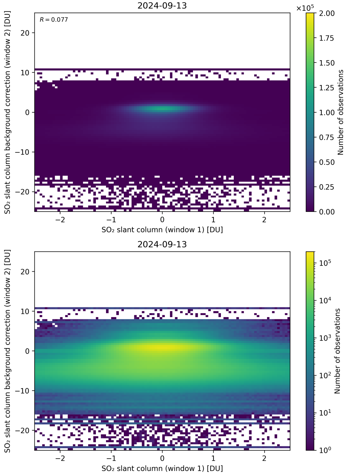
Figure 213: Scatter density plot of “SO 2 slant column (window 1)” against “SO 2 slant column background correction (window 2)” for 2024-09-12 to 2024-09-14.
