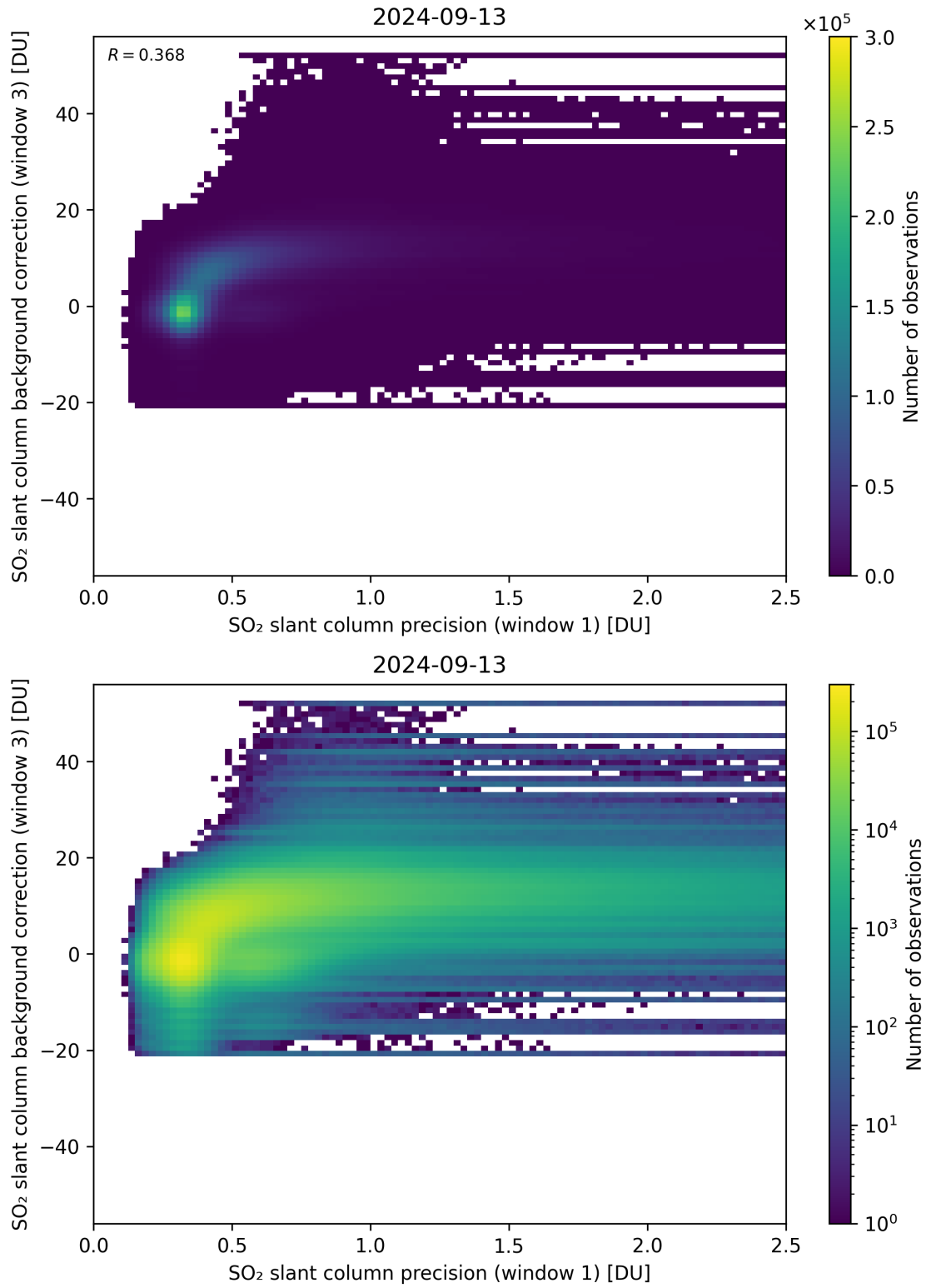
Figure 220: Scatter density plot of “SO 2 slant column precision (window 1)” against “SO 2 slant column background correction (window 3)” for 2024-09-12 to 2024-09-14.
