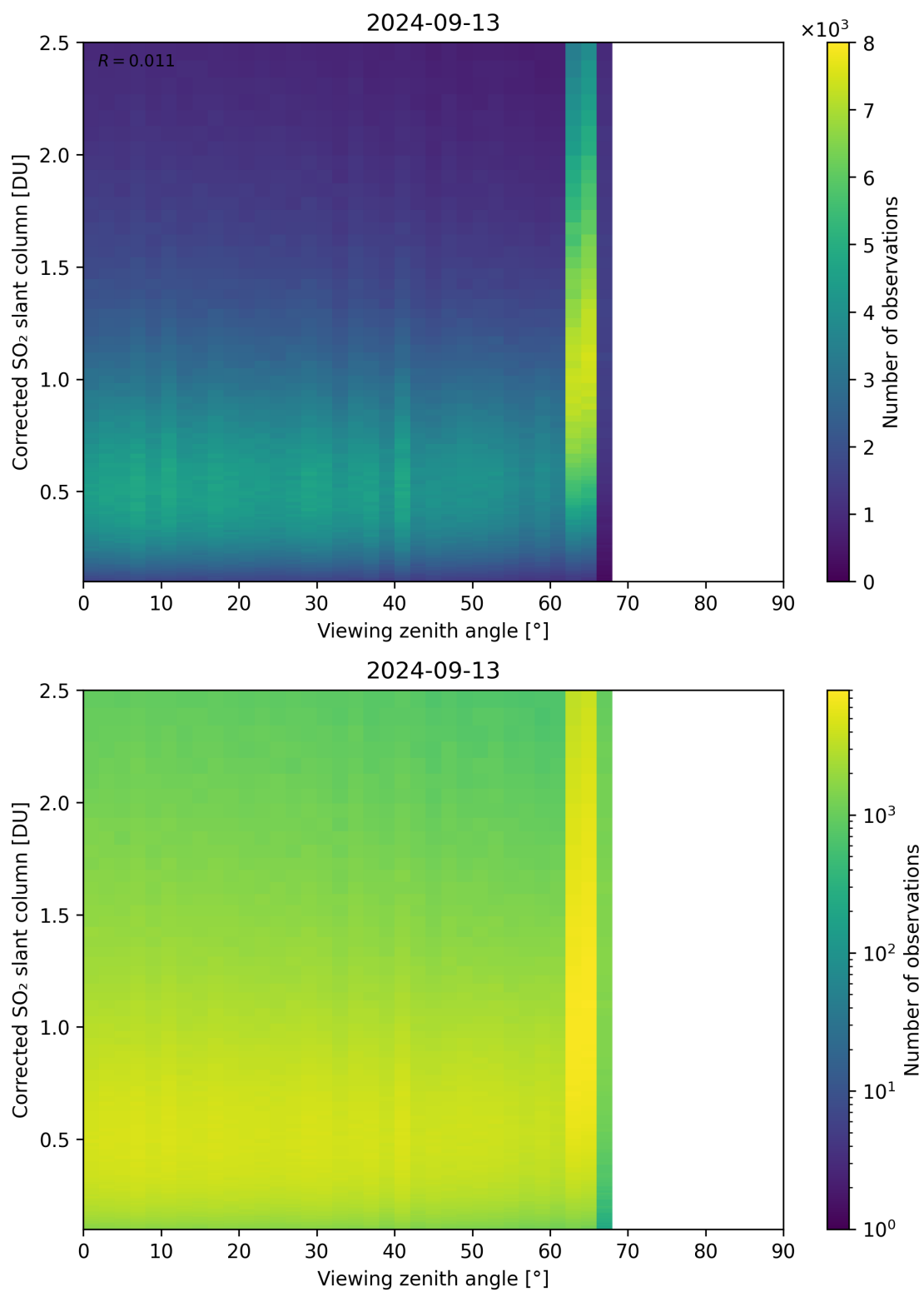
Figure 317: Scatter density plot of “Viewing zenith angle” against “Corrected SO 2 slant column” for 2024-09-12 to 2024-09-14.
