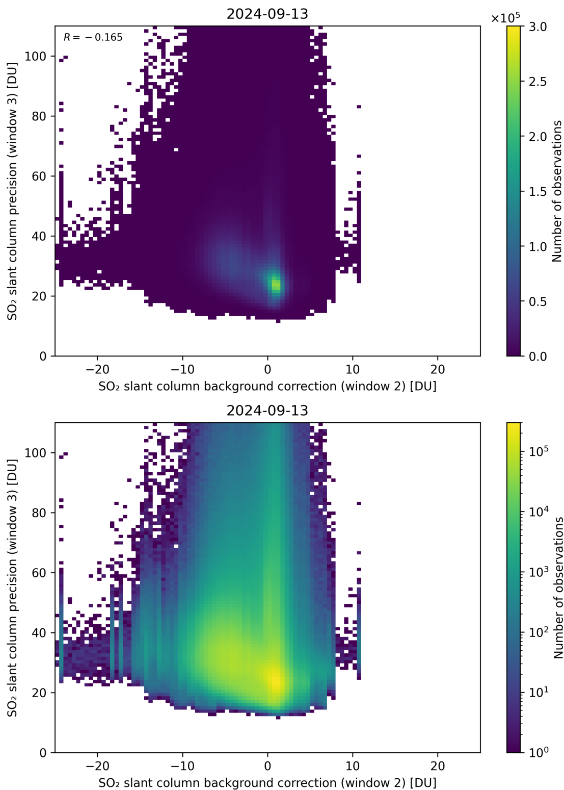
Figure 118: Scatter density plot of “SO 2 slant column background correction (window 2)” against “SO 2 slant column precision (window 3)” for 2024-09-12 to 2024-09-14.
