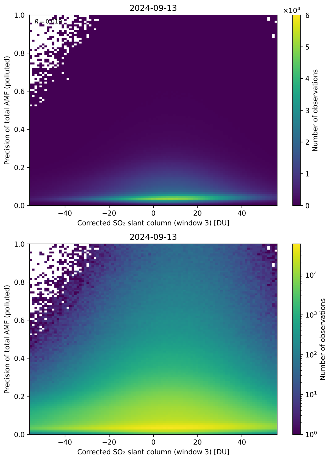
Figure 211: Scatter density plot of “Corrected SO 2 slant column (window 3)” against “Precision of total AMF (polluted)” for 2024-09-12 to 2024-09-14.
