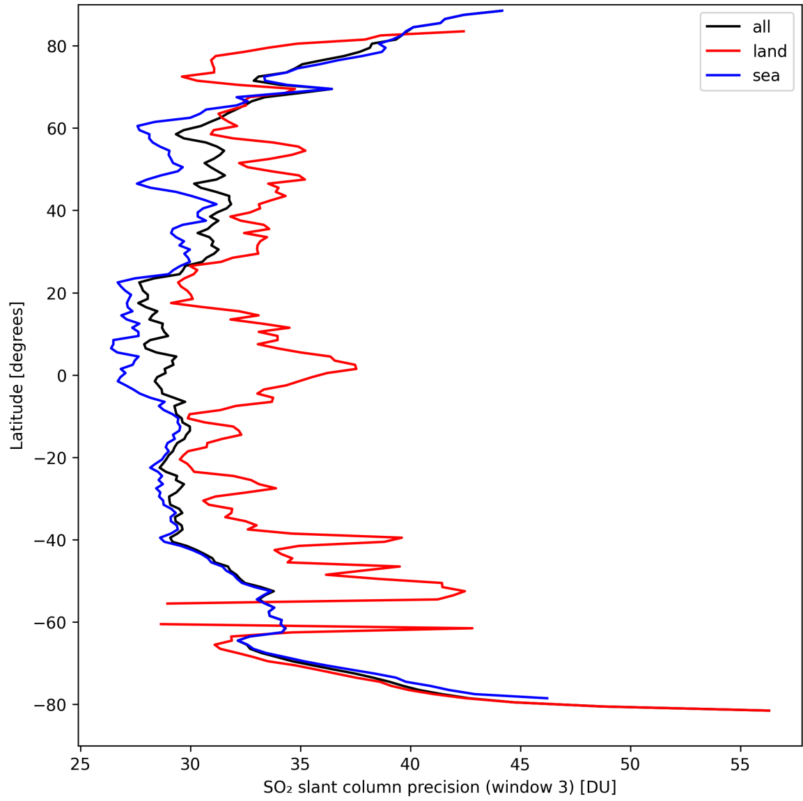
Figure 42: Zonal average of “SO 2 slant column precision (window 3)” for 2024-09-12 to 2024-09-14.
