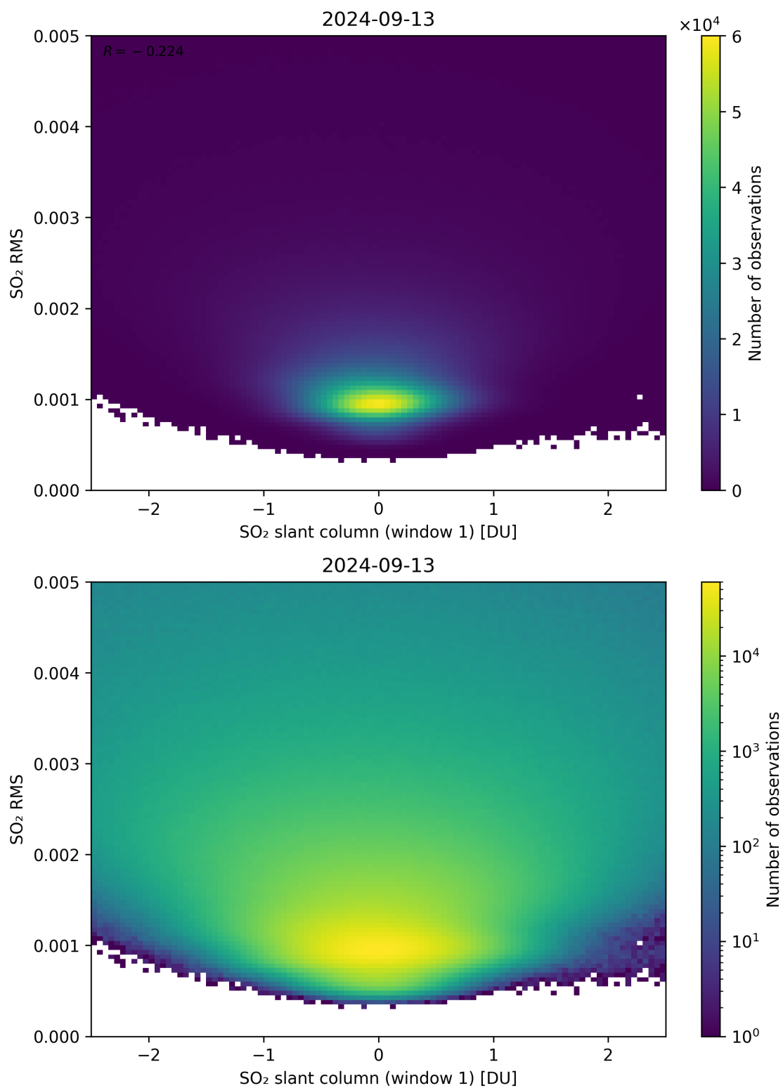
Figure 217: Scatter density plot of “SO 2 slant column (window 1)” against “SO 2 RMS” for 2024-09-12 to 2024-09-14.
