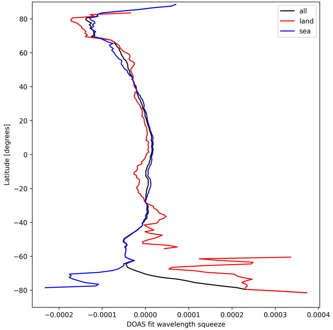
Figure 46: Zonal average of “DOAS fit wavelength squeeze” for 2024-09-12 to 2024-09-14.
