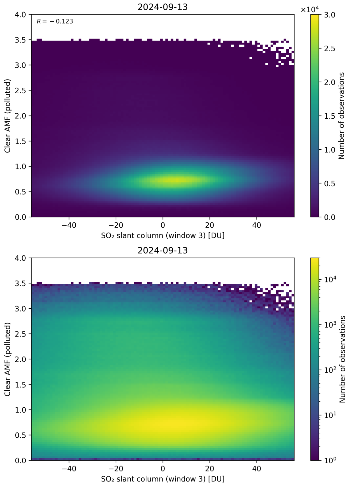
Figure 265: Scatter density plot of “SO 2 slant column (window 3)” against “Clear AMF (polluted)” for 2024-09-12 to 2024-09-14.
