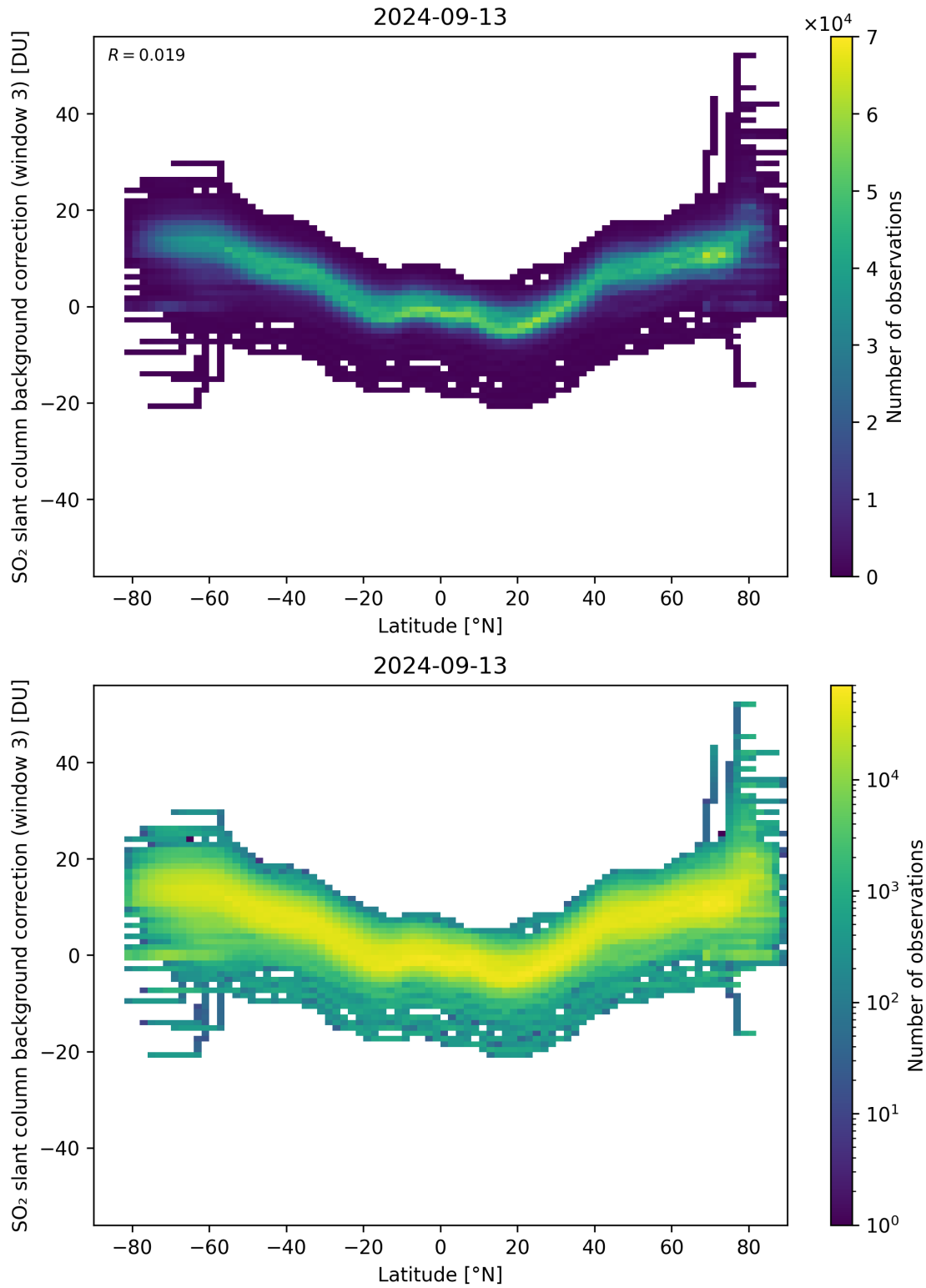
Figure 141: Scatter density plot of “Latitude” against “SO 2 slant column background correction (window 3)” for 2024-09-12 to 2024-09-14.
