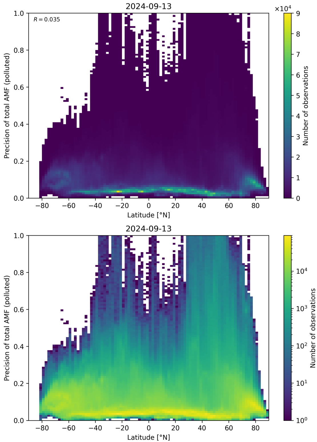
Figure 155: Scatter density plot of “Latitude” against “Precision of total AMF (polluted)” for 2024-09-12 to 2024-09-14.
