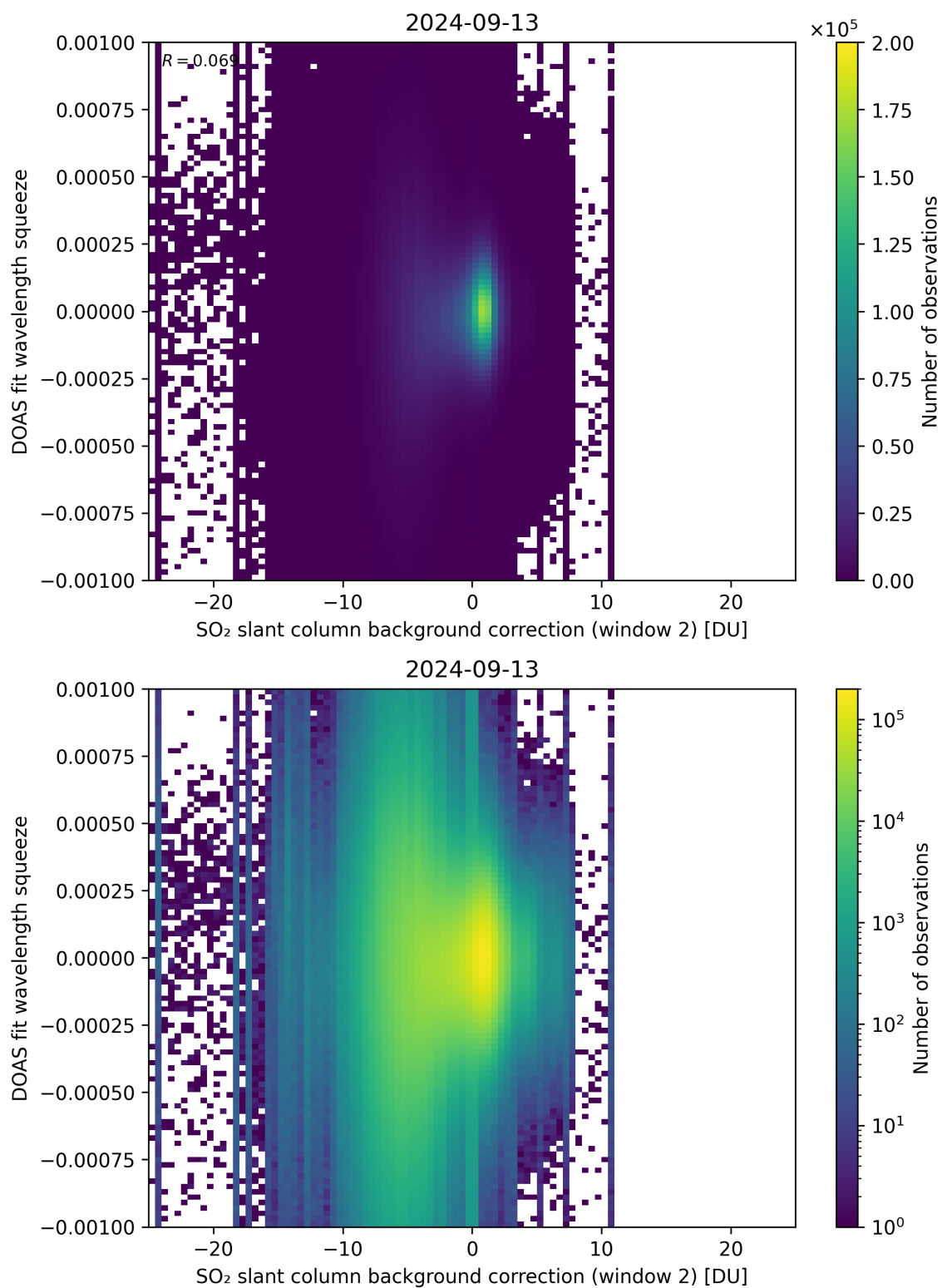
Figure 113: Scatter density plot of “SO 2 slant column background correction (window 2)” against “DOAS fit wavelength squeeze” for 2024-09-12 to 2024-09-14.
