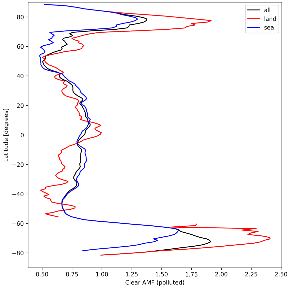
Figure 50: Zonal average of “Clear AMF (polluted)” for 2024-09-12 to 2024-09-14.
