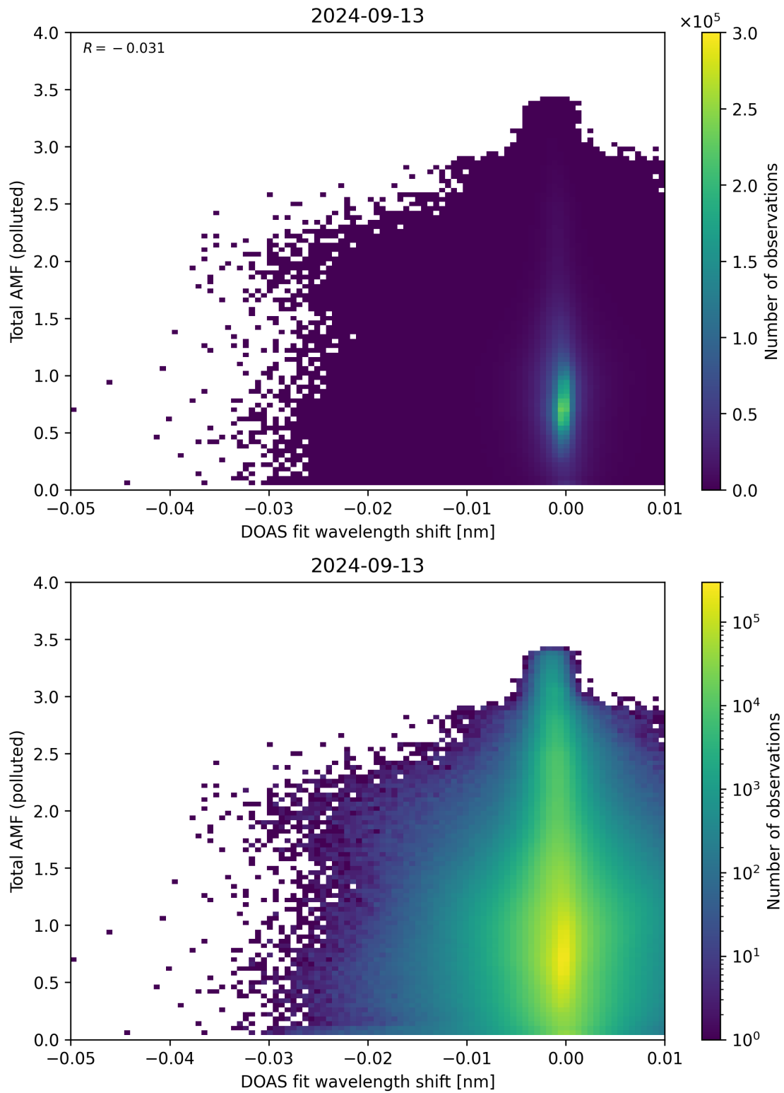
Figure 130: Scatter density plot of “DOAS fit wavelength shift” against “Total AMF (polluted)” for 2024-09-12 to 2024-09-14.
