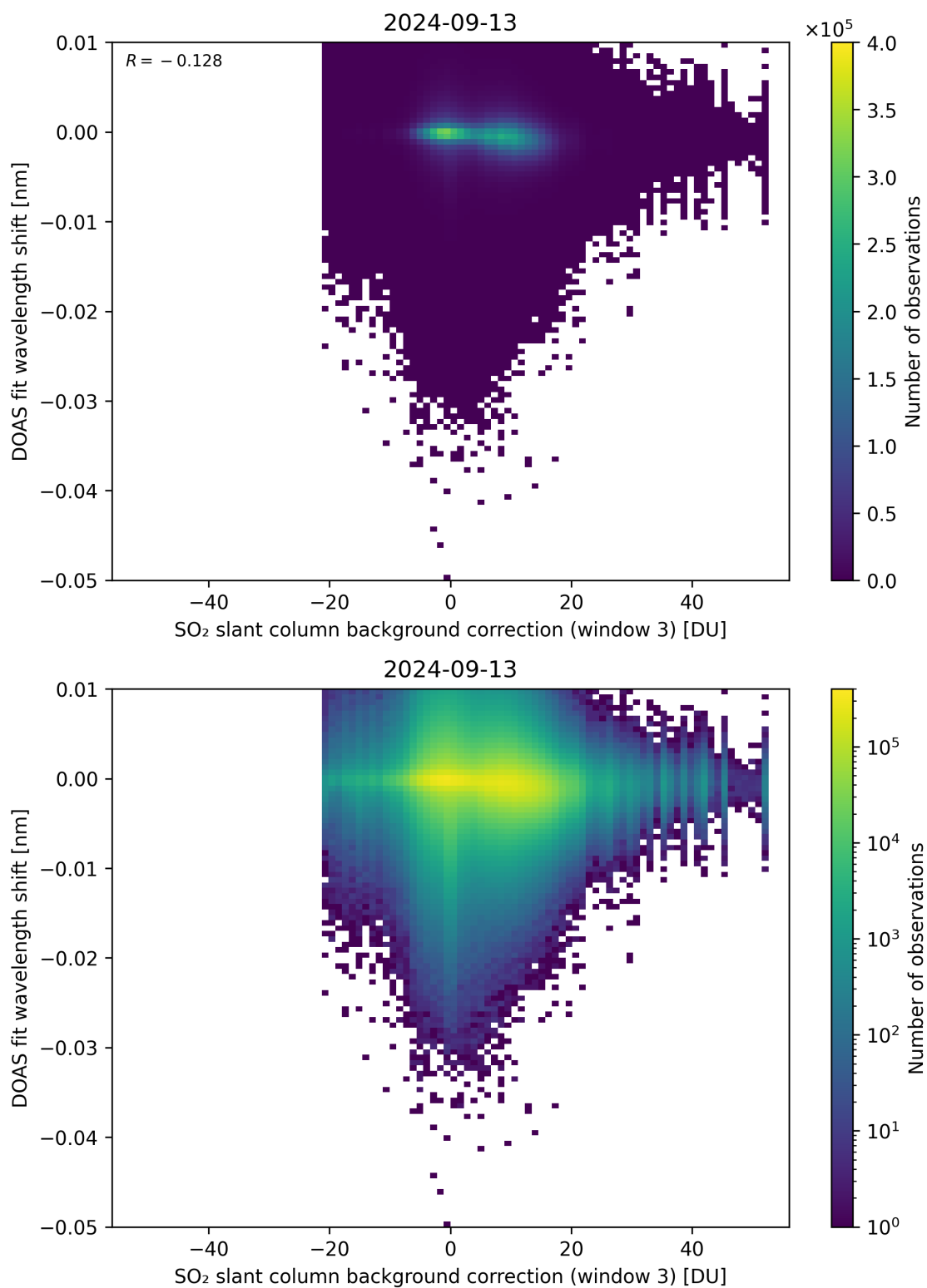
Figure 121: Scatter density plot of “SO 2 slant column background correction (window 3)” against “DOAS fit wavelength shift” for 2024-09-12 to 2024-09-14.
