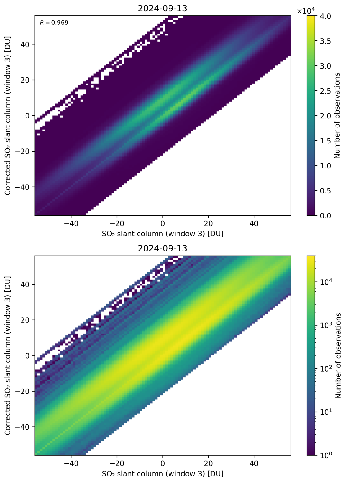
Figure 266: Scatter density plot of “SO 2 slant column (window 3)” against “Corrected SO 2 slant column (window 3)” for 2024-09-12 to 2024-09-14.
