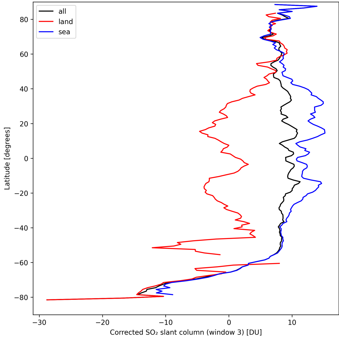
Figure 43: Zonal average of “Corrected SO 2 slant column (window 3)” for 2024-09-12 to 2024-09-14.
