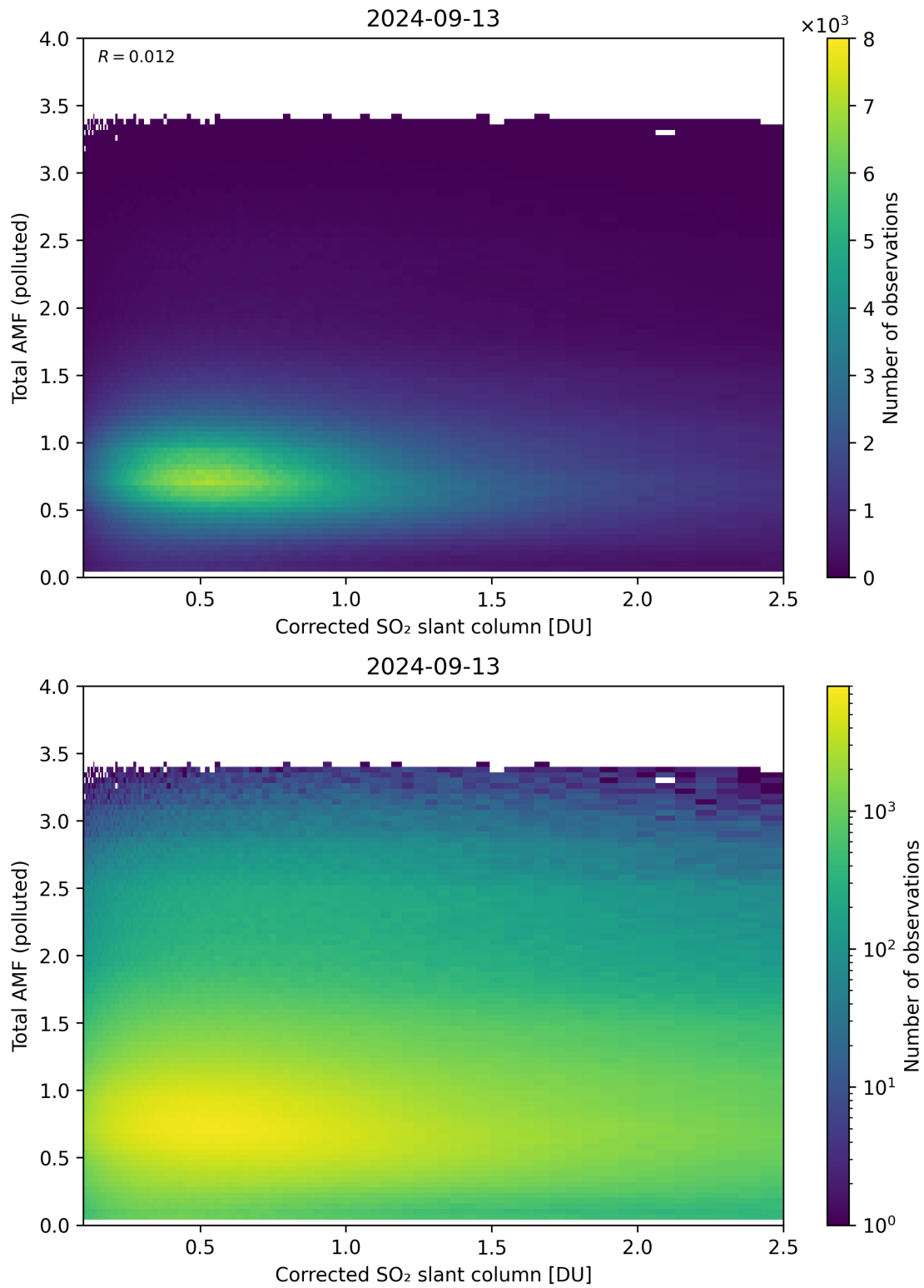
Figure 192: Scatter density plot of “Corrected SO 2 slant column” against “Total AMF (polluted)” for 2024-09-12 to 2024-09-14.
