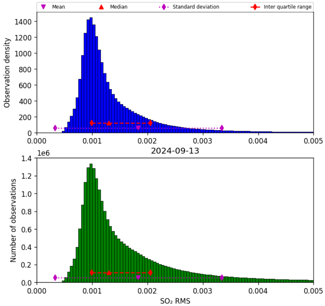
Figure 70: Histogram of “SO 2 RMS” for 2024-09-12 to 2024-09-14
