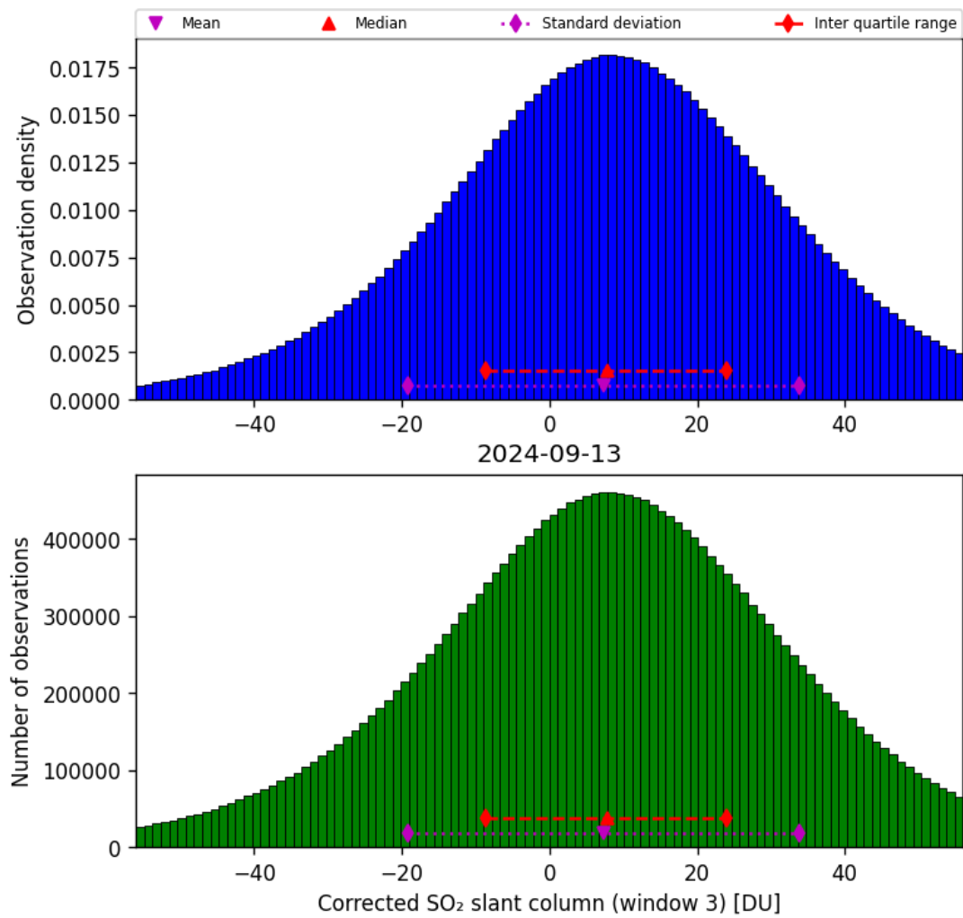
Figure 66: Histogram of “Corrected SO 2 slant column (window 3)” for 2024-09-12 to 2024-09-14
