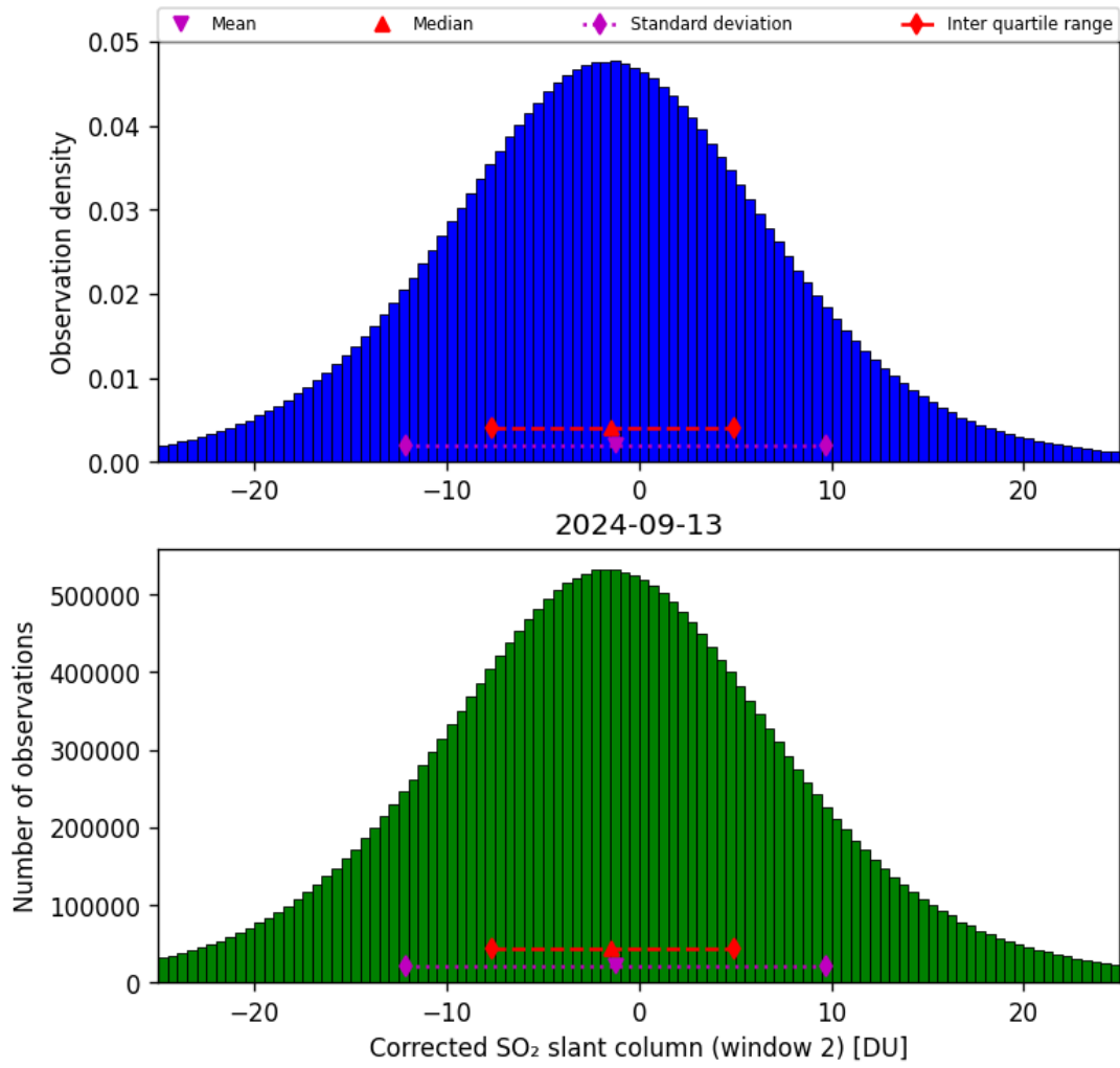
Figure 62: Histogram of “Corrected SO 2 slant column (window 2)” for 2024-09-12 to 2024-09-14
