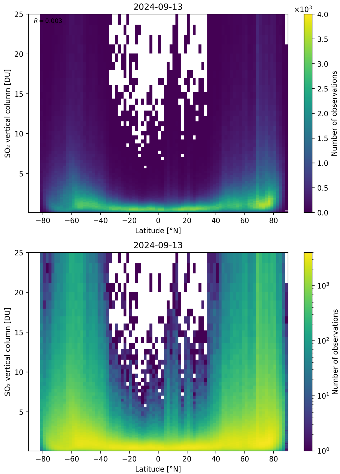
Figure 156: Scatter density plot of “Latitude” against “SO 2 vertical column” for 2024-09-12 to 2024-09-14.
