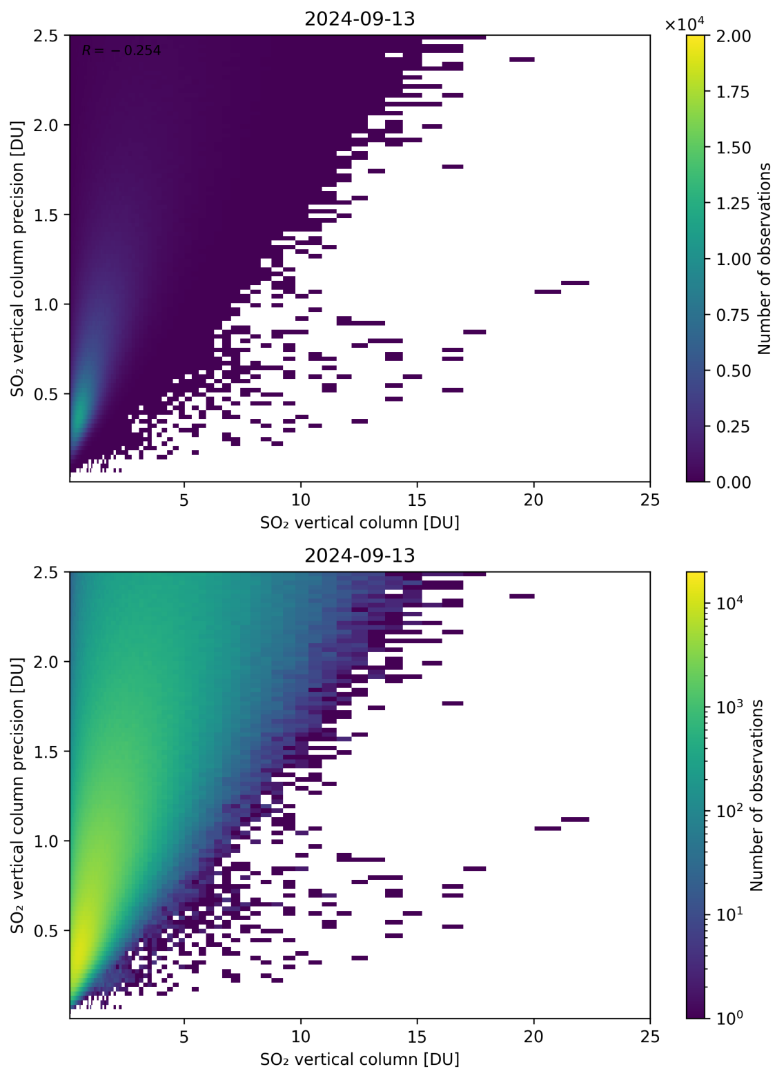
Figure 307: Scatter density plot of “SO 2 vertical column” against “SO 2 vertical column precision” for 2024-09-12 to 2024-09-14.
