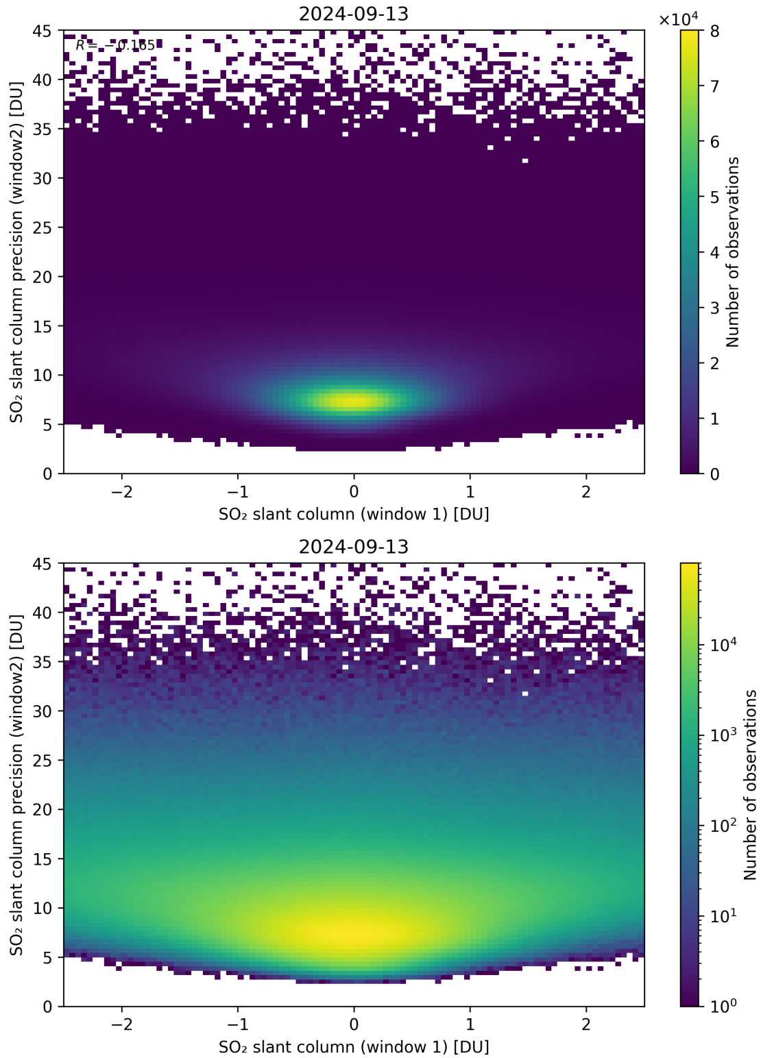
Figure 236: Scatter density plot of “SO 2 slant column (window 1)” against “SO 2 slant column precision (window2)” for 2024-09-12 to 2024-09-14.
