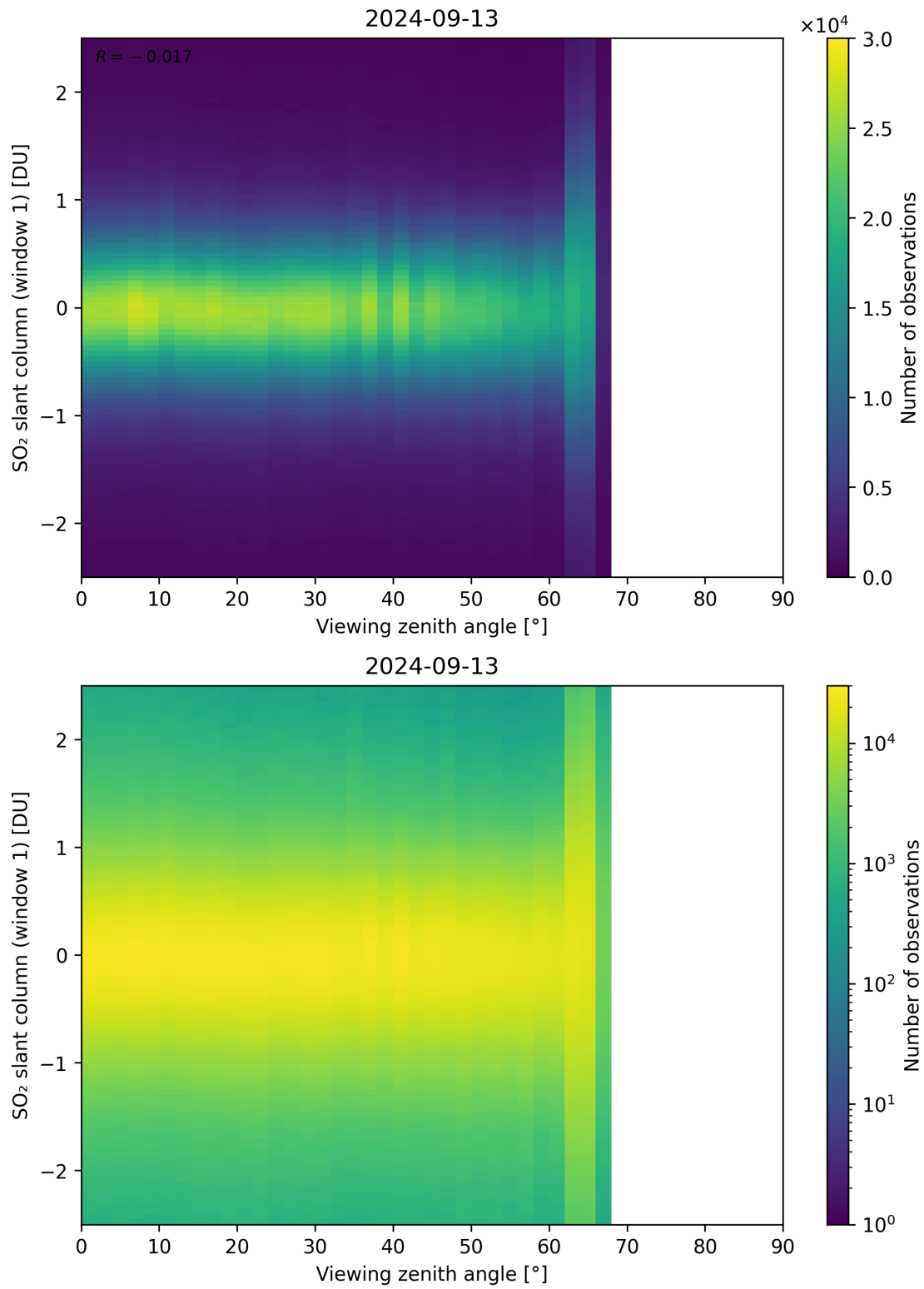
Figure 320: Scatter density plot of “Viewing zenith angle” against “SO 2 slant column (window 1)” for 2024-09-12 to 2024-09-14.
