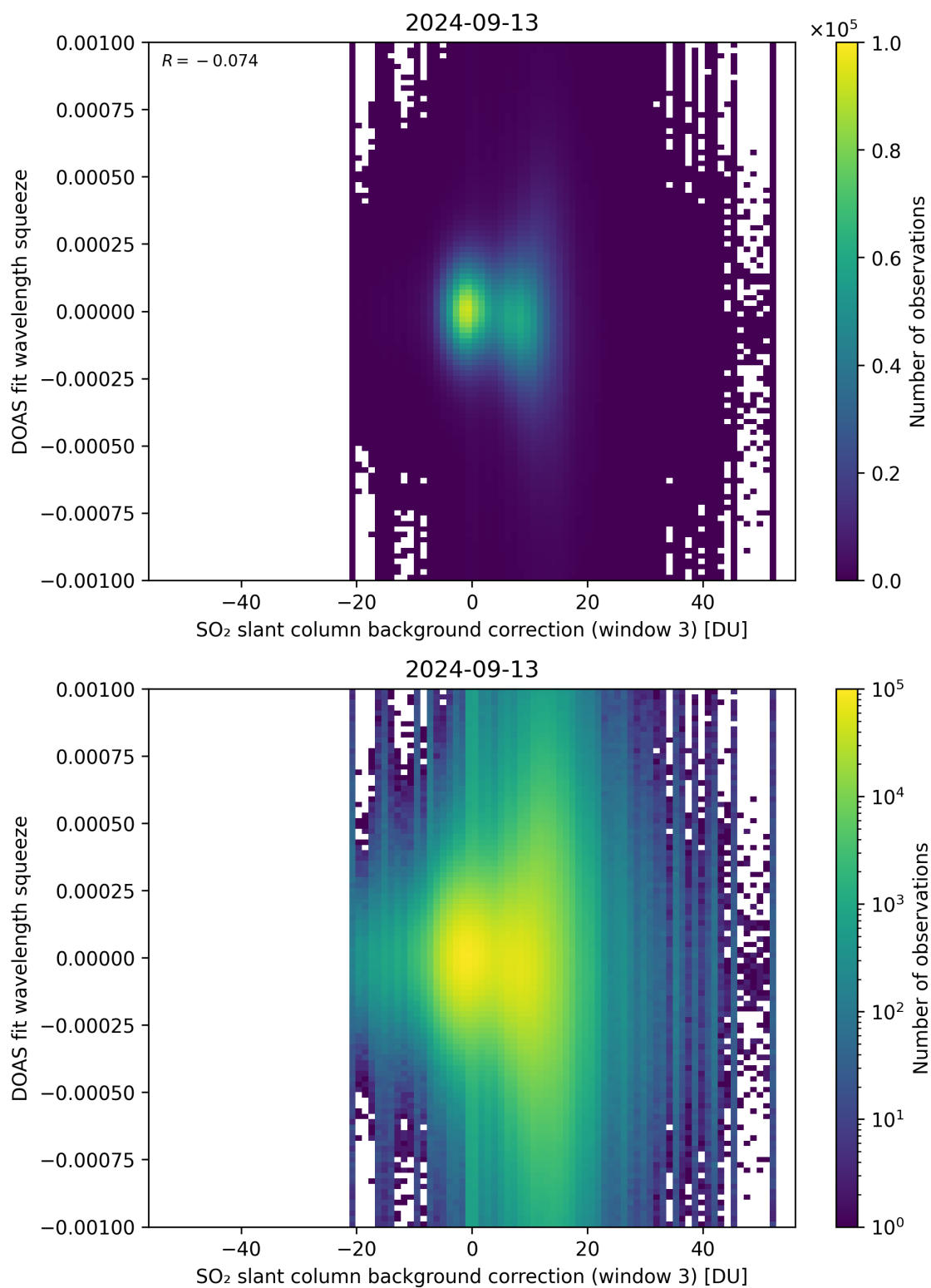
Figure 122: Scatter density plot of “SO 2 slant column background correction (window 3)” against “DOAS fit wavelength squeeze” for 2024-09-12 to 2024-09-14.
