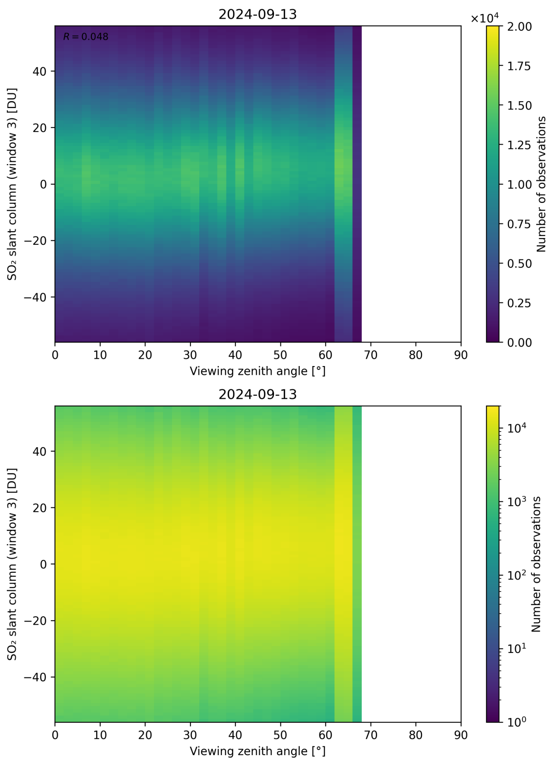
Figure 323: Scatter density plot of “Viewing zenith angle” against “SO 2 slant column (window 3)” for 2024-09-12 to 2024-09-14.
