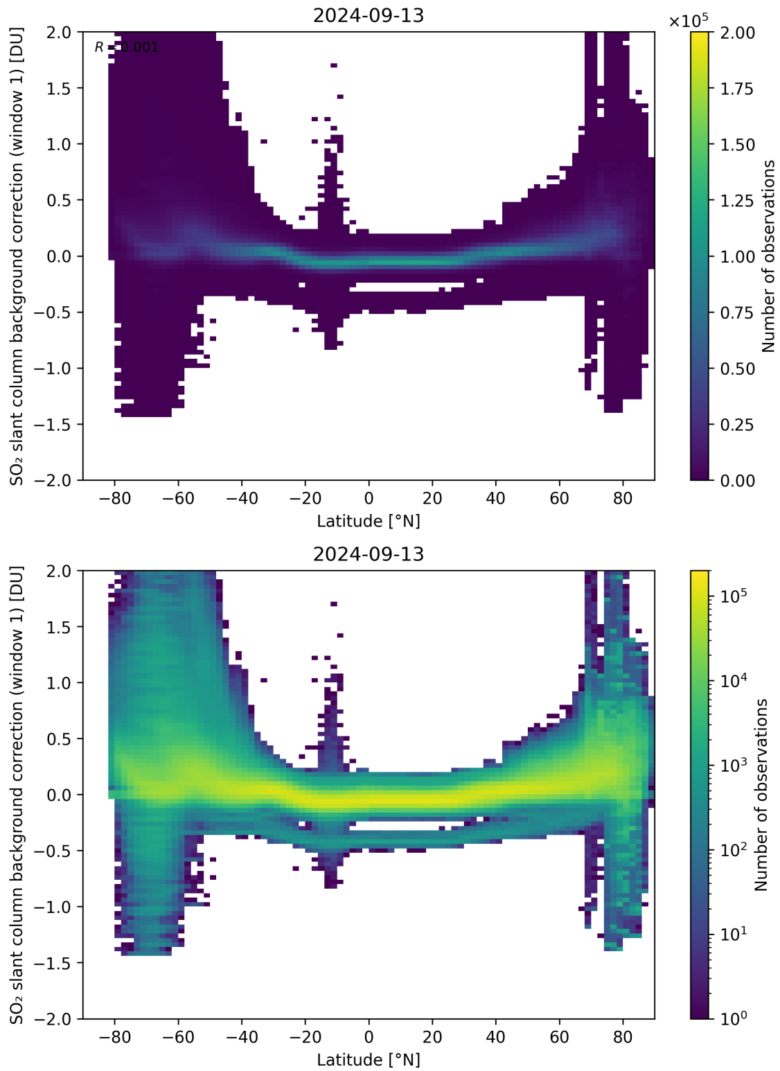
Figure 139: Scatter density plot of “Latitude” against “SO 2 slant column background correction (window 1)” for 2024-09-12 to 2024-09-14.
