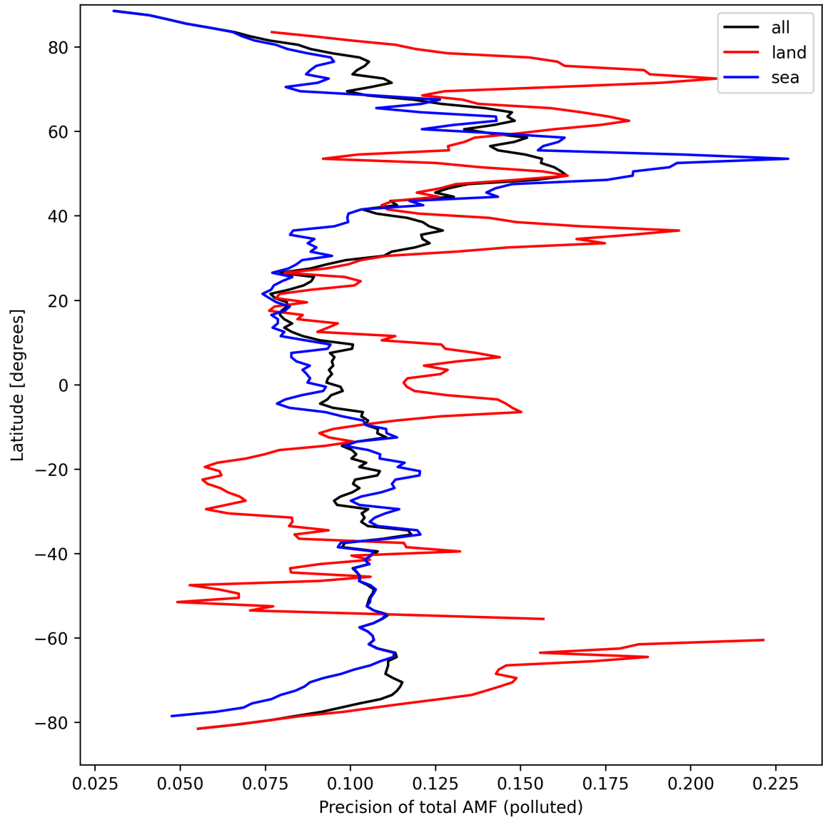
Figure 49: Zonal average of “Precision of total AMF (polluted)” for 2024-09-12 to 2024-09-14.
