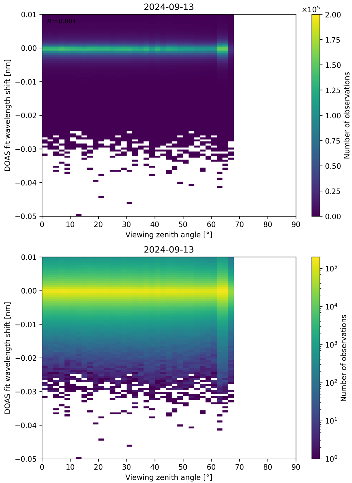
Figure 311: Scatter density plot of “Viewing zenith angle” against “DOAS fit wavelength shift” for 2024-09-12 to 2024-09-14.
