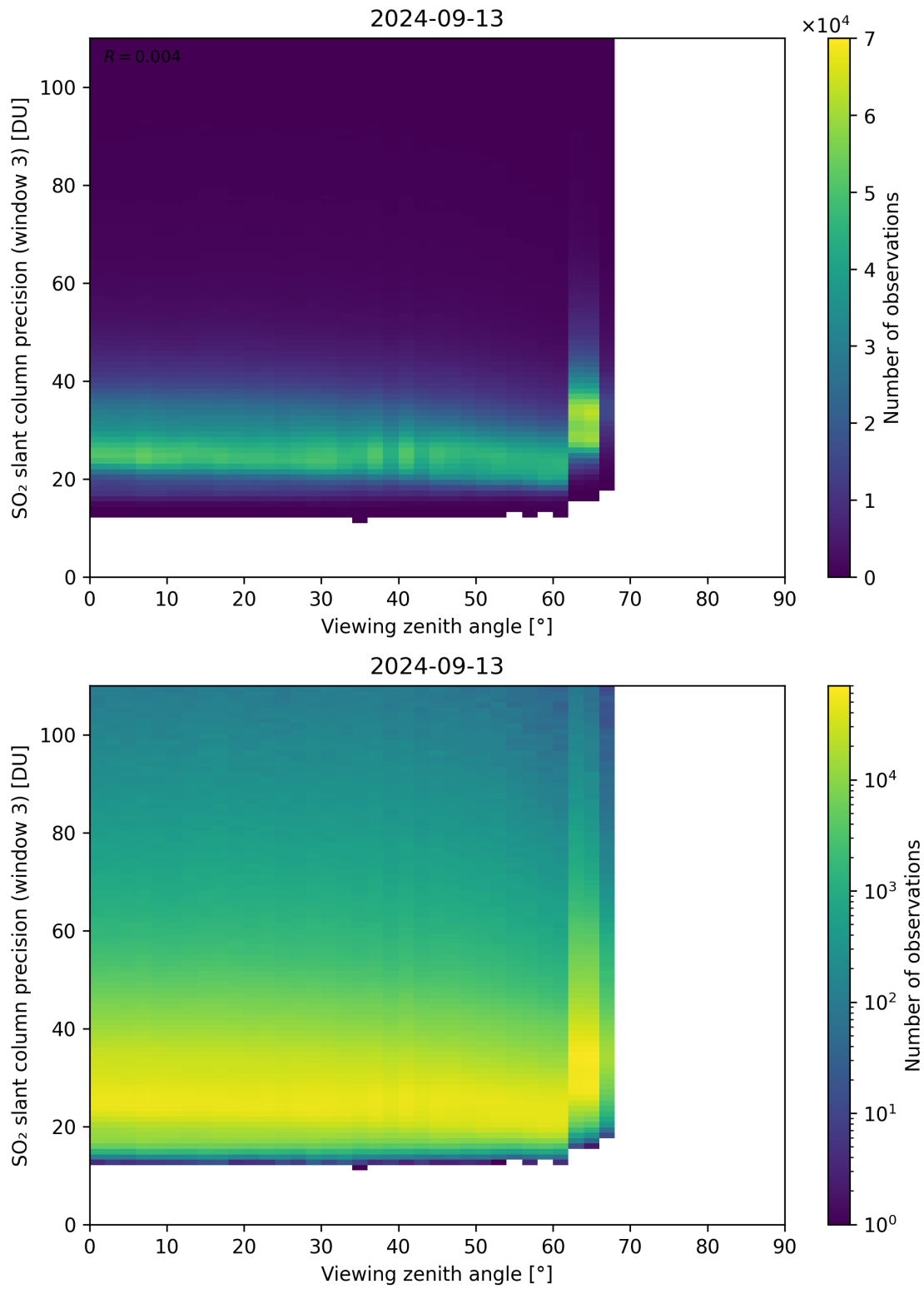
Figure 324: Scatter density plot of “Viewing zenith angle” against “SO 2 slant column precision (window 3)” for 2024-09-12 to 2024-09-14.
