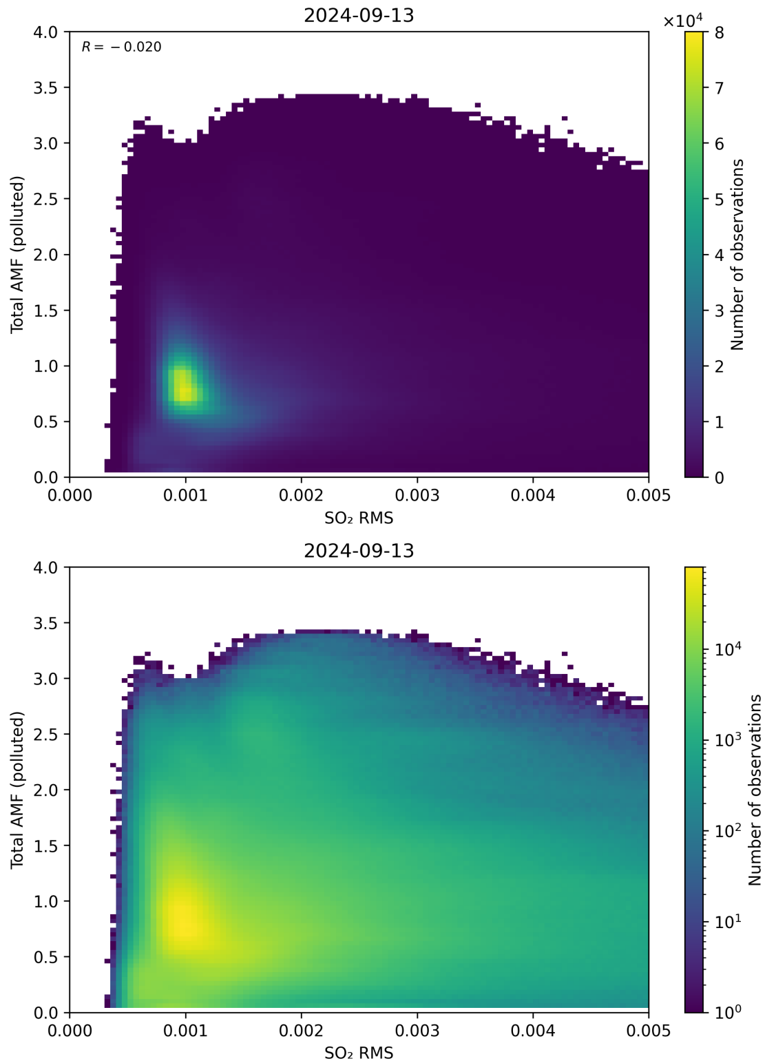
Figure 137: Scatter density plot of “SO 2 RMS” against “Total AMF (polluted)” for 2024-09-12 to 2024-09-14.
