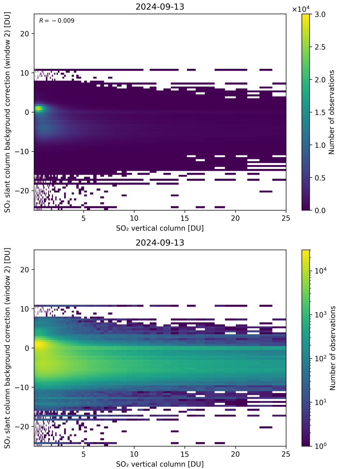
Figure 274: Scatter density plot of “SO 2 vertical column” against “SO 2 slant column background correction (window 2)” for 2024-09-12 to 2024-09-14.
