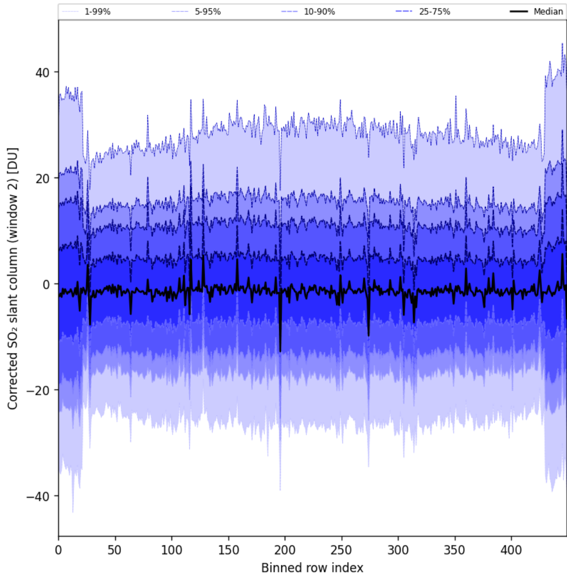
Figure 85: Along track statistics of “Corrected SO 2 slant column (window 2)” for 2024-09-12 to 2024-09-14
