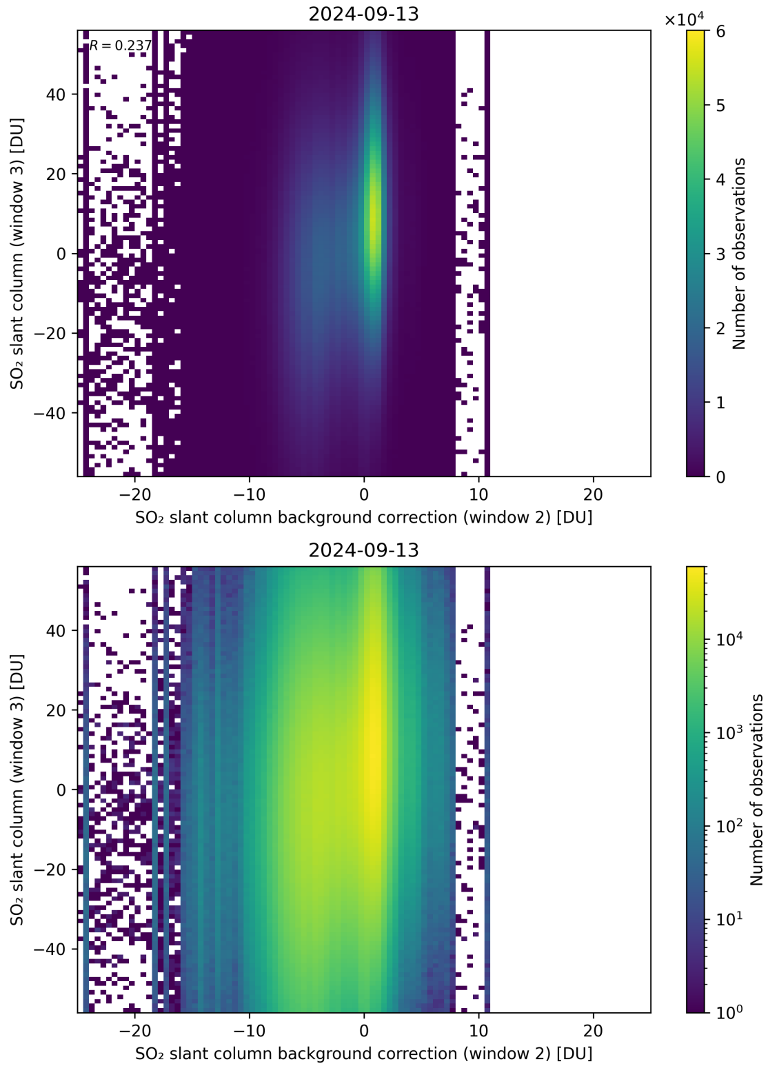
Figure 117: Scatter density plot of “SO 2 slant column background correction (window 2)” against “SO 2 slant column (window 3)” for 2024-09-12 to 2024-09-14.
