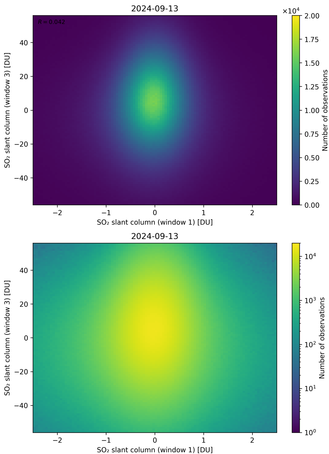
Figure 237: Scatter density plot of “SO 2 slant column (window 1)” against “SO 2 slant column (window 3)” for 2024-09-12 to 2024-09-14.
