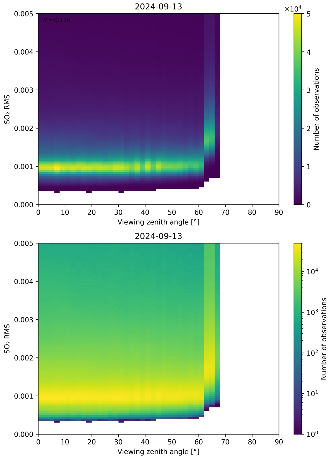
Figure 313: Scatter density plot of “Viewing zenith angle” against “SO 2 RMS” for 2024-09-12 to 2024-09-14.
