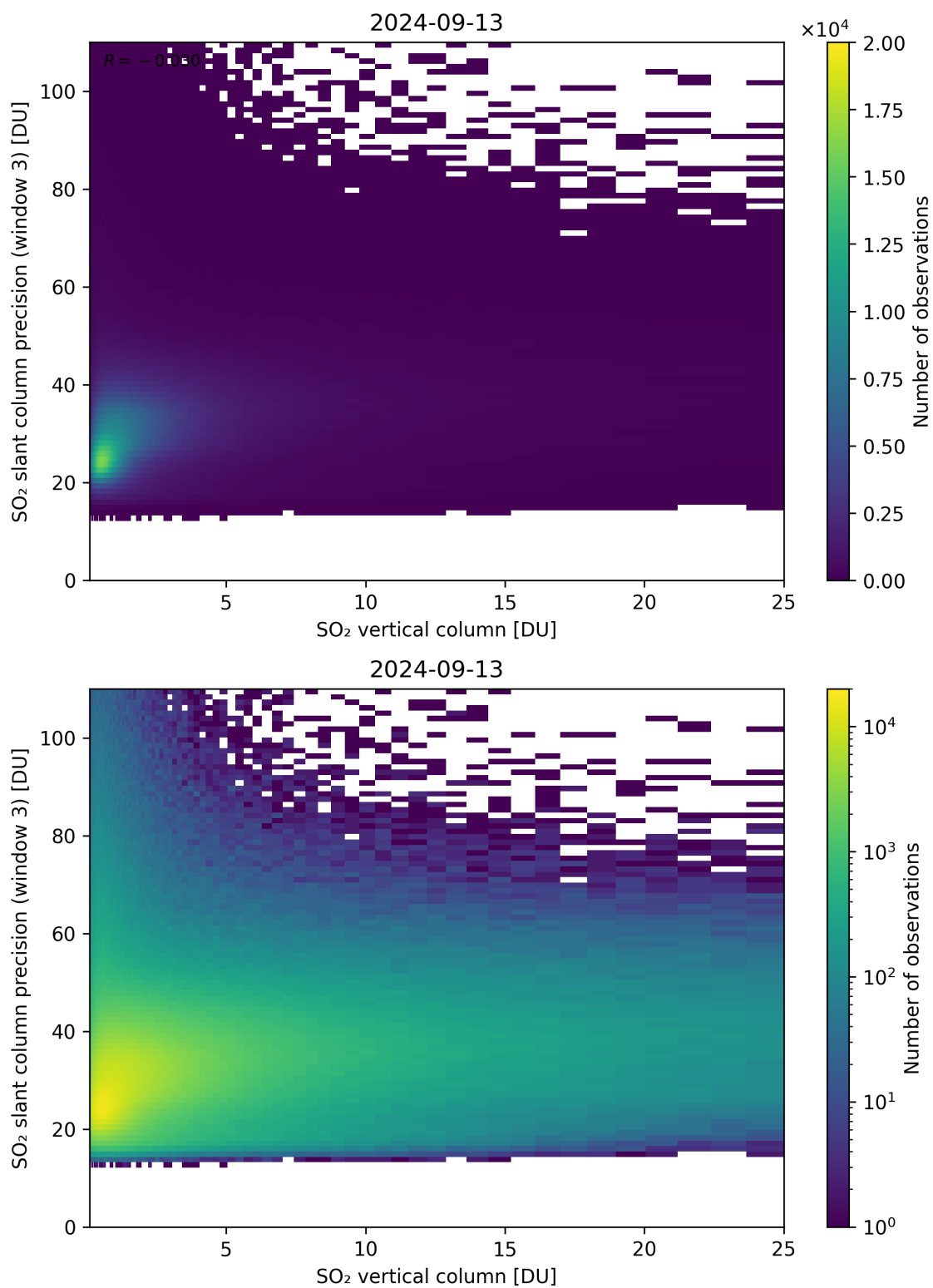
Figure 304: Scatter density plot of “SO 2 vertical column” against “SO 2 slant column precision (window 3)” for 2024-09-12 to 2024-09-14.
