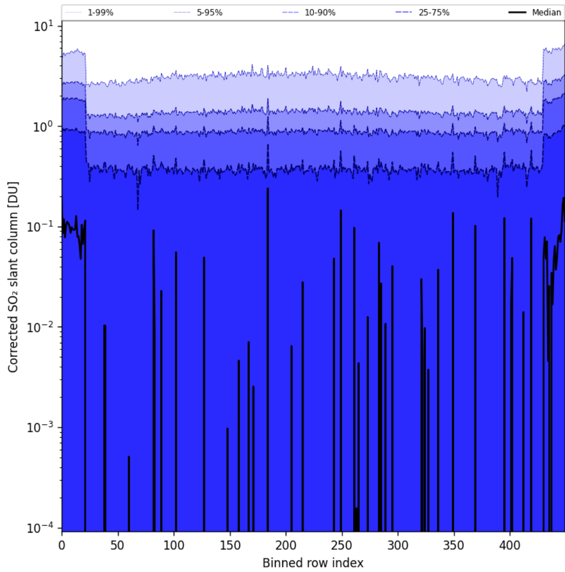
Figure 78: Along track statistics of “Corrected SO 2 slant column” for 2024-09-12 to 2024-09-14
