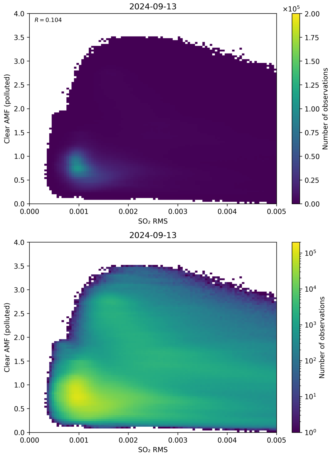
Figure 136: Scatter density plot of “SO 2 RMS” against “Clear AMF (polluted)” for 2024-09-12 to 2024-09-14.
