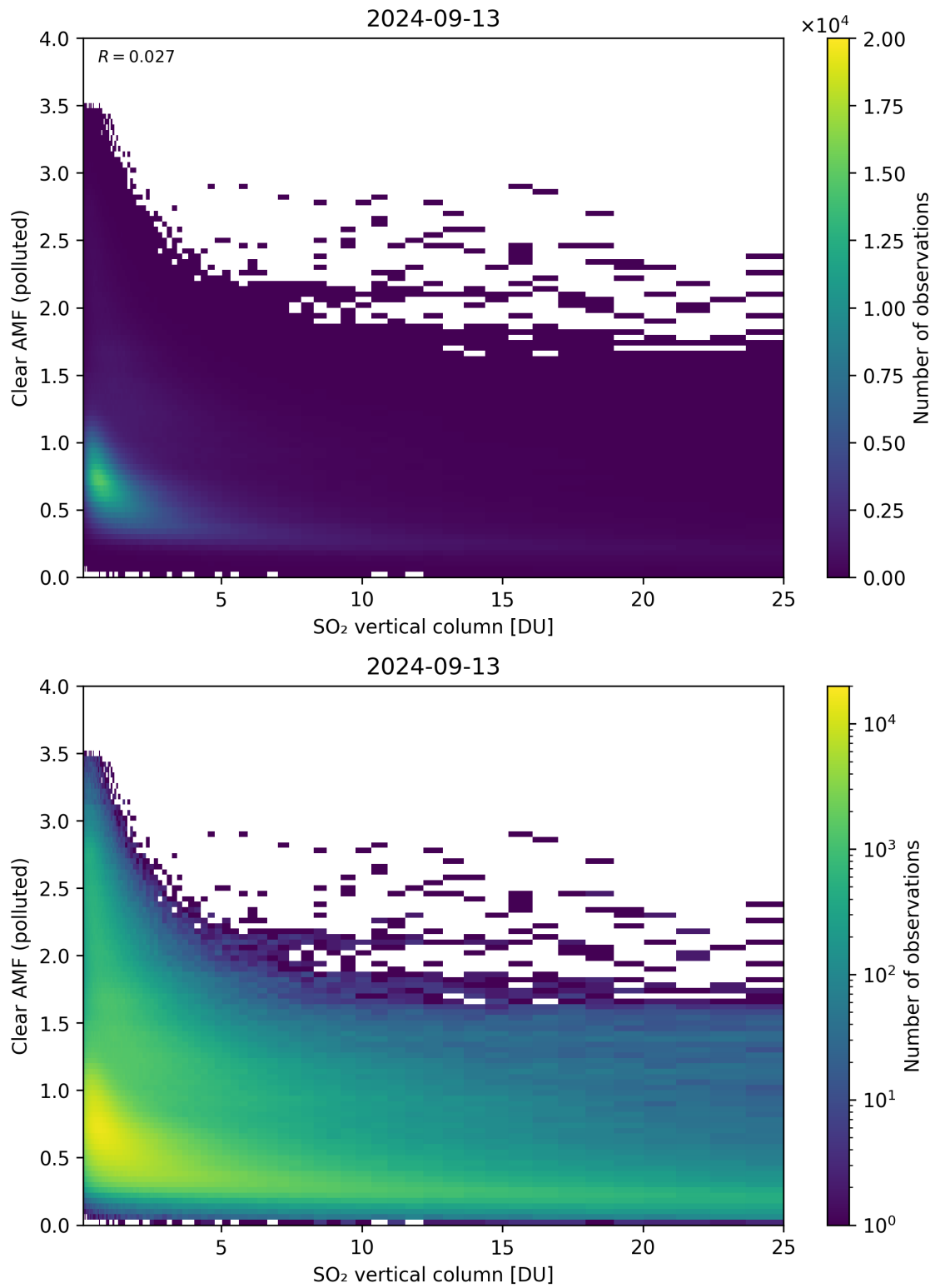
Figure 296: Scatter density plot of “SO 2 vertical column” against “Clear AMF (polluted)” for 2024-09-12 to 2024-09-14.
