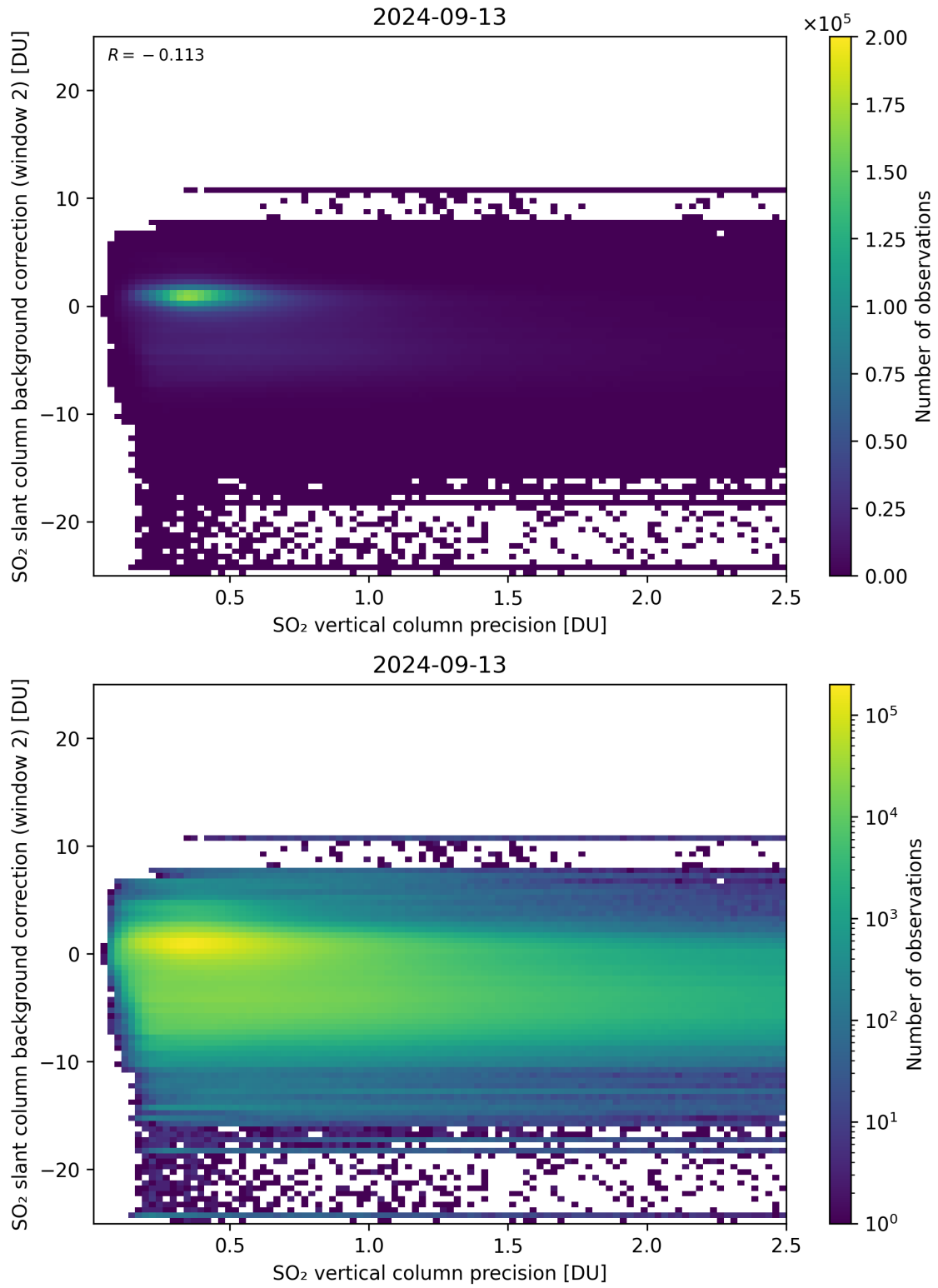
Figure 280: Scatter density plot of “SO 2 vertical column precision” against “SO 2 slant column background correction (window 2)” for 2024-09-12 to 2024-09-14.
