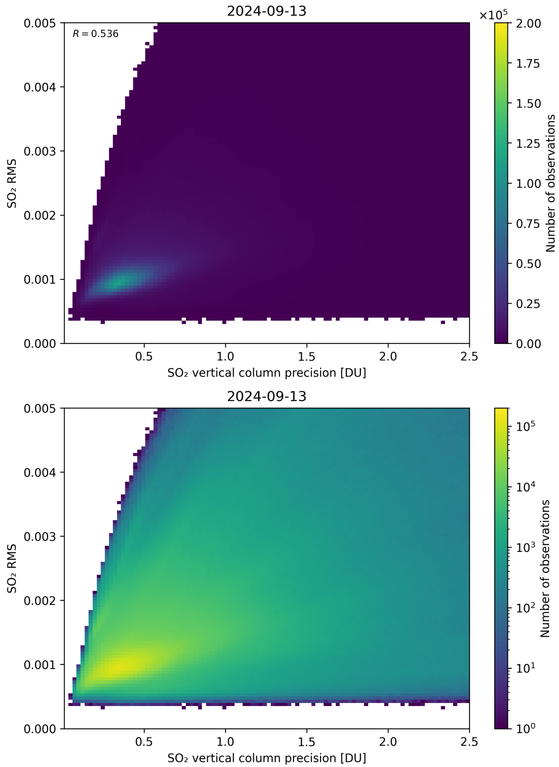
Figure 284: Scatter density plot of “SO 2 vertical column precision” against “SO 2 RMS” for 2024-09-12 to 2024-09-14.
