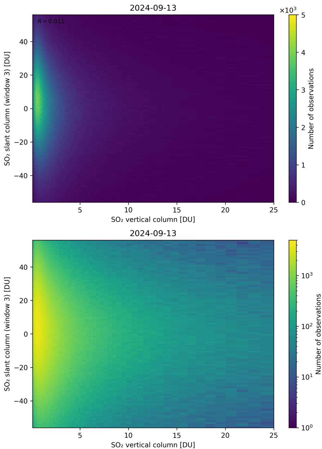
Figure 303: Scatter density plot of “SO 2 vertical column” against “SO 2 slant column (window 3)” for 2024-09-12 to 2024-09-14.
