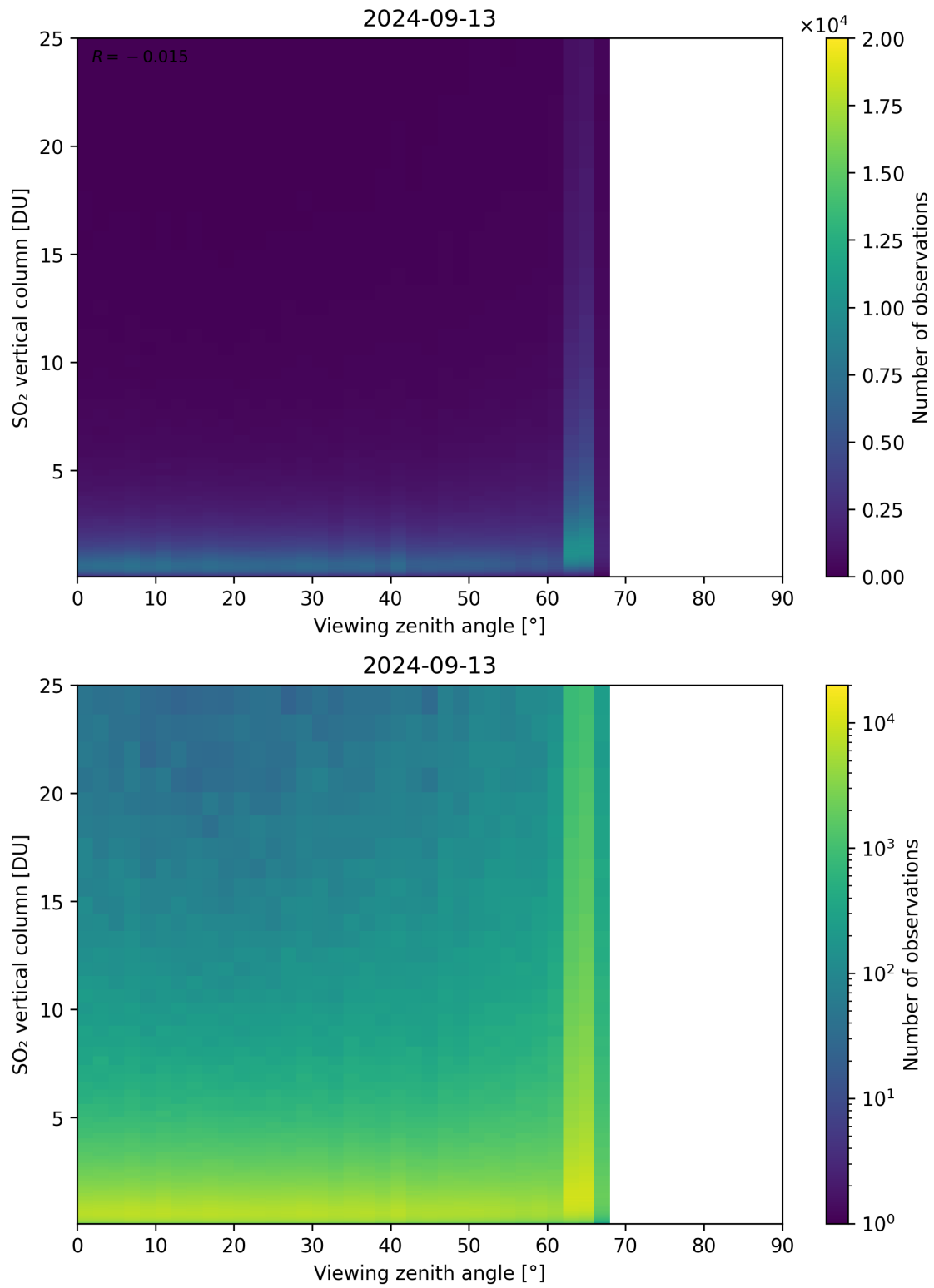
Figure 327: Scatter density plot of “Viewing zenith angle” against “SO 2 vertical column” for 2024-09-12 to 2024-09-14.
