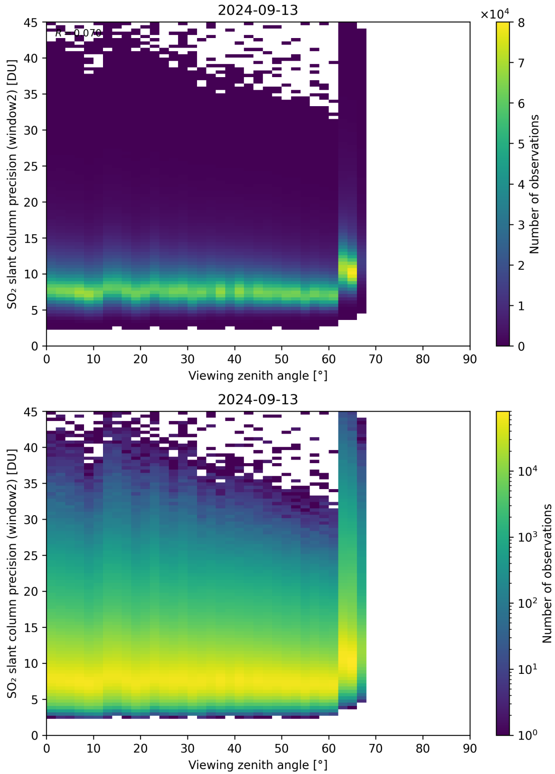
Figure 322: Scatter density plot of “Viewing zenith angle” against “SO 2 slant column precision (window2)” for 2024-09-12 to 2024-09-14.
