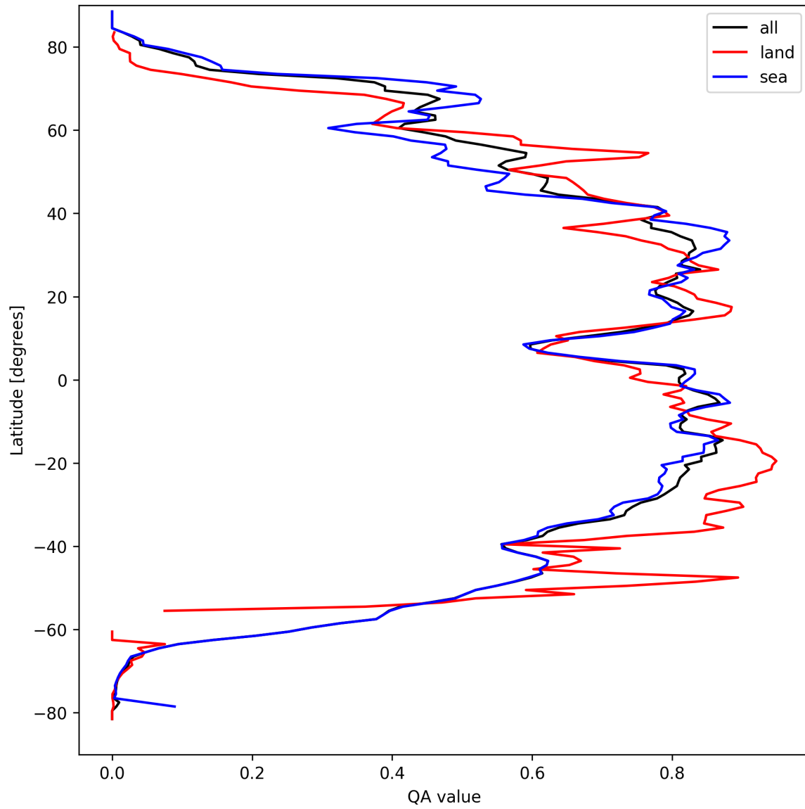
Figure 29: Zonal average of “QA value” for 2024-09-12 to 2024-09-14.
