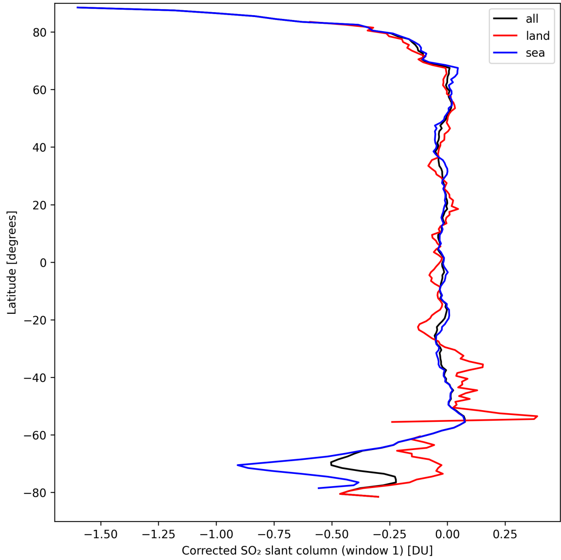
Figure 35: Zonal average of “Corrected SO 2 slant column (window 1)” for 2024-09-12 to 2024-09-14.
