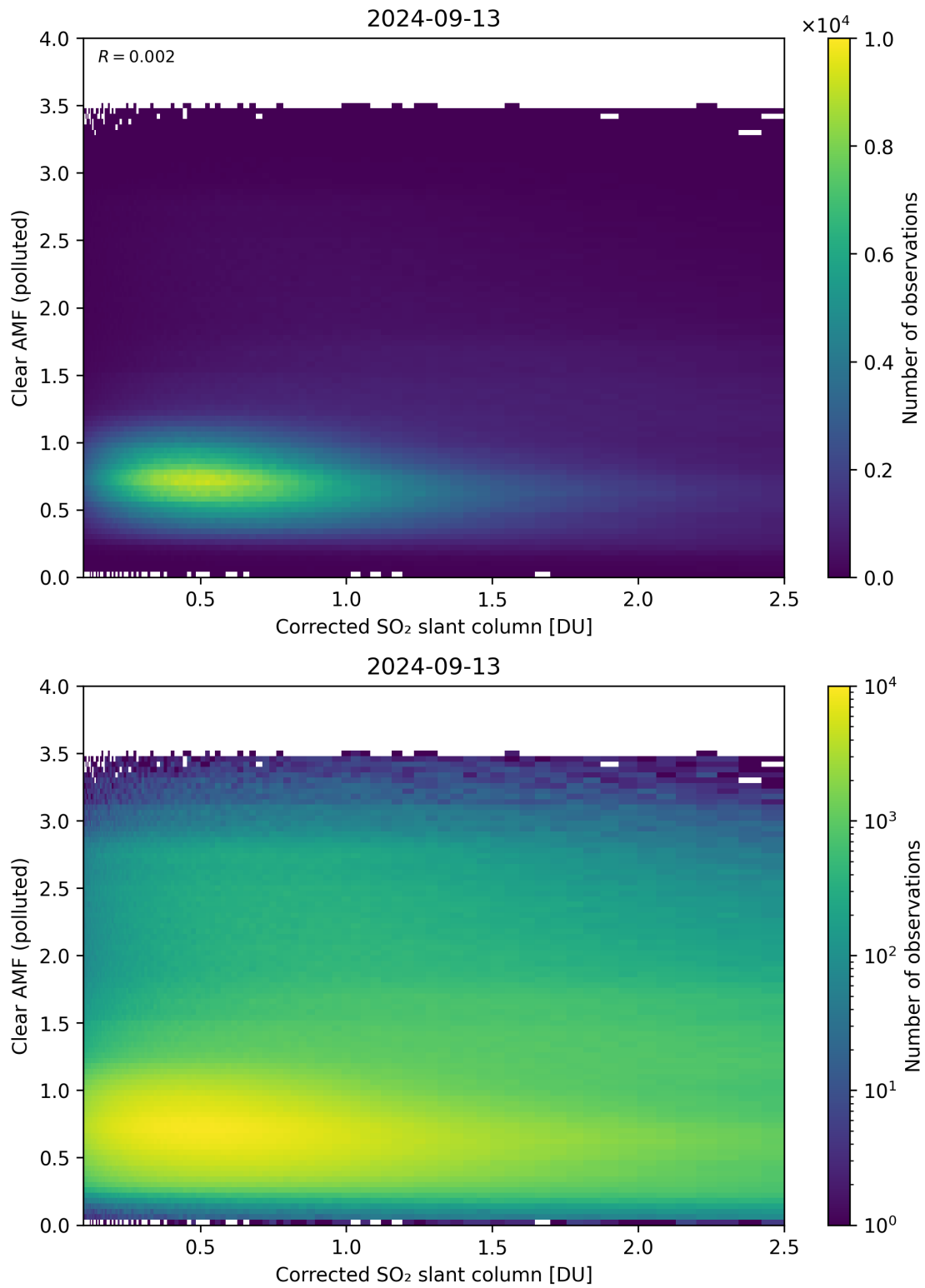
Figure 184: Scatter density plot of “Corrected SO 2 slant column” against “Clear AMF (polluted)” for 2024-09-12 to 2024-09-14.
