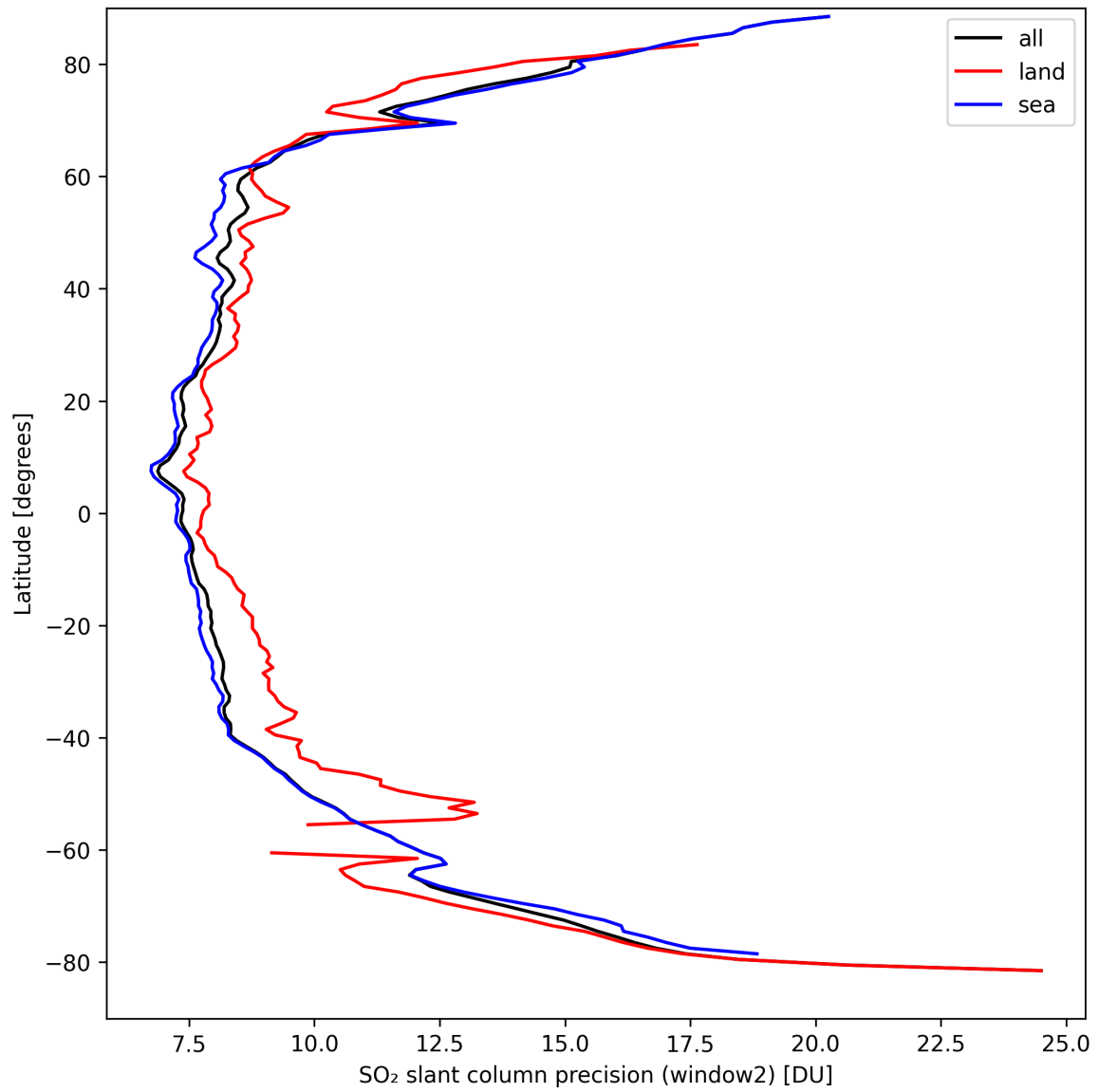
Figure 38: Zonal average of “SO 2 slant column precision (window2)” for 2024-09-12 to 2024-09-14.
