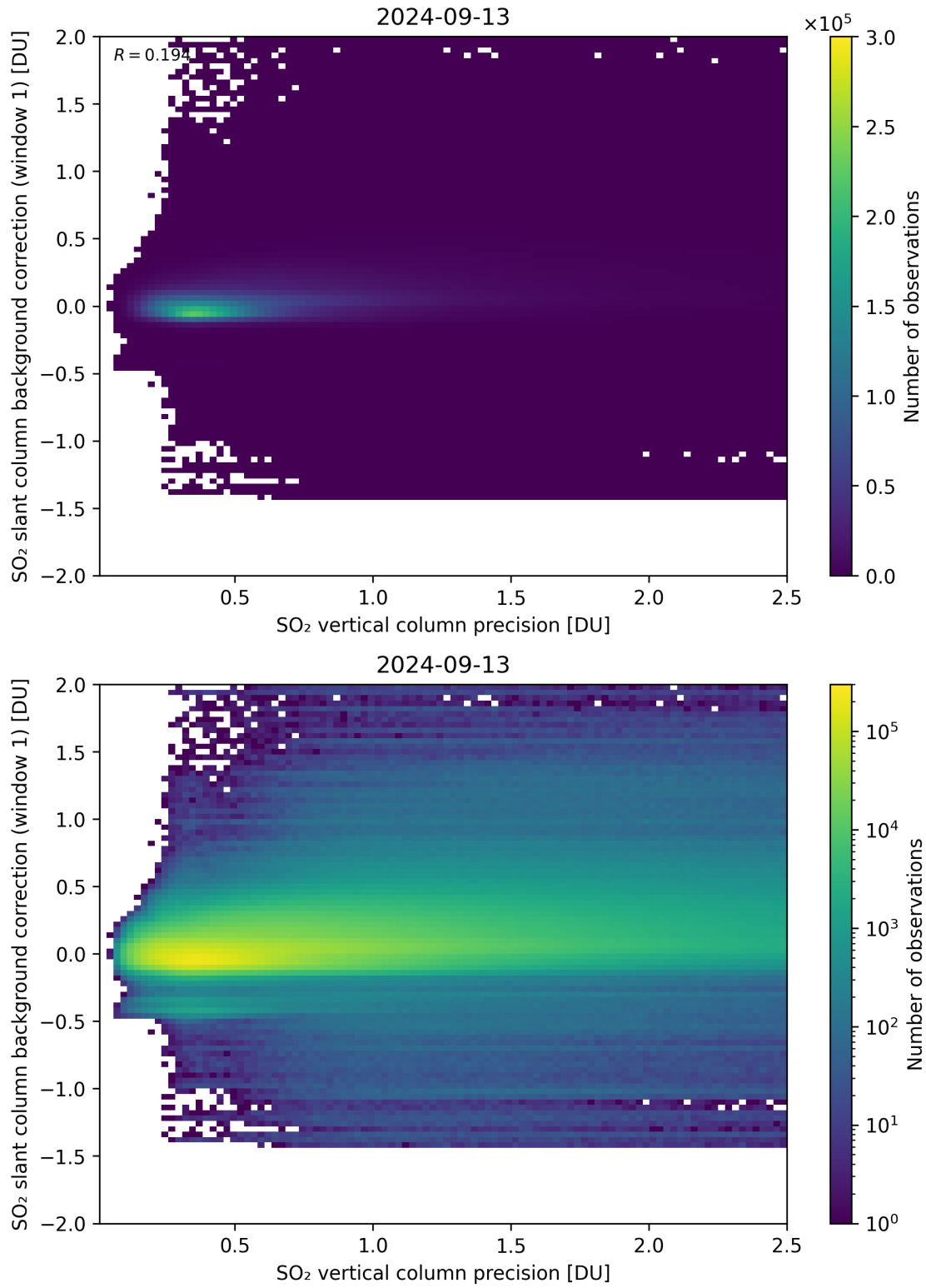
Figure 279: Scatter density plot of “SO 2 vertical column precision” against “SO 2 slant column background correction (window 1)” for 2024-09-12 to 2024-09-14.
