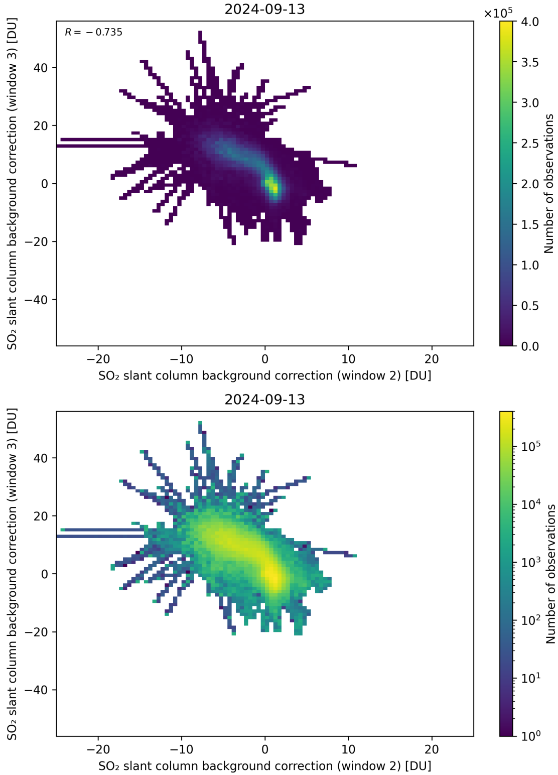
Figure 111: Scatter density plot of “SO 2 slant column background correction (window 2)” against “SO 2 slant column background correction (window 3)” for 2024-09-12 to 2024-09-14.
