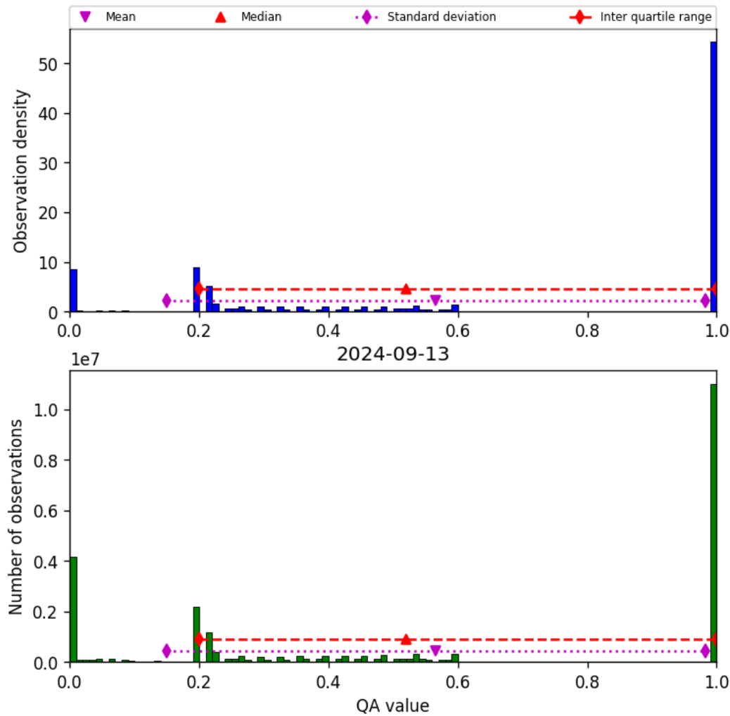
Figure 52: Histogram of “QA value” for 2024-09-12 to 2024-09-14
