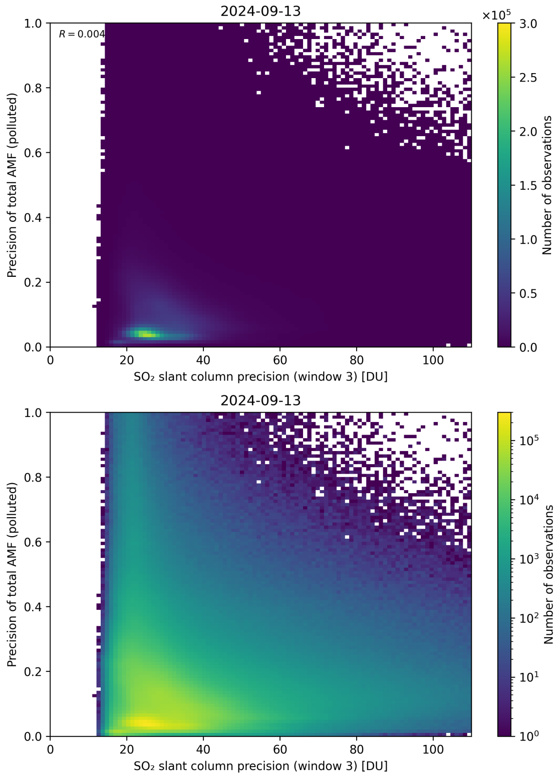
Figure 264: Scatter density plot of “SO 2 slant column precision (window 3)” against “Precision of total AMF (polluted)” for 2024-09-12 to 2024-09-14.
