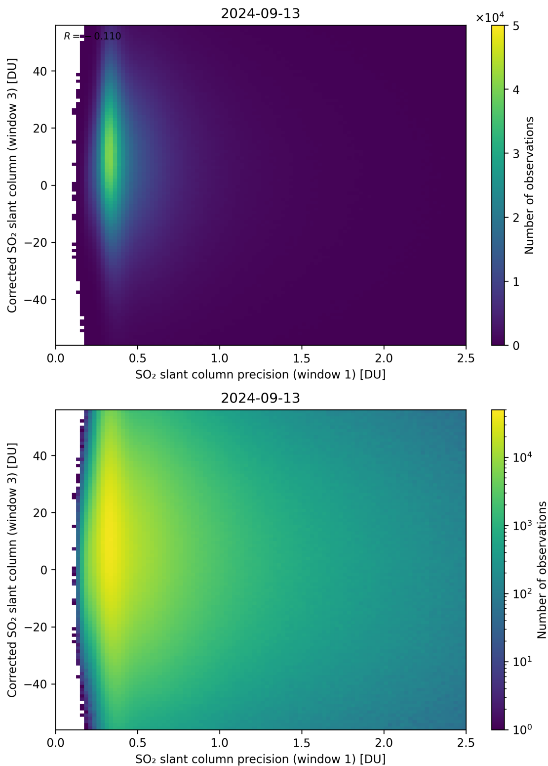
Figure 226: Scatter density plot of “SO 2 slant column precision (window 1)” against “Corrected SO 2 slant column (window 3)” for 2024-09-12 to 2024-09-14.
