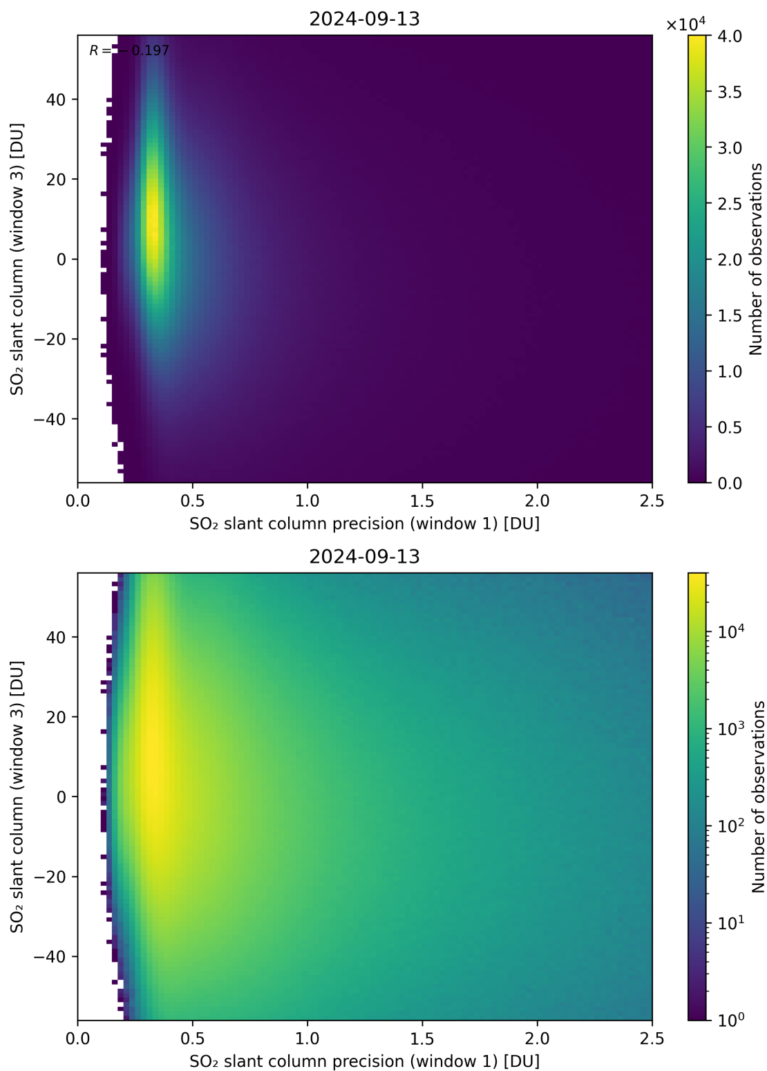
Figure 228: Scatter density plot of “SO 2 slant column precision (window 1)” against “SO 2 slant column (window 3)” for 2024-09-12 to 2024-09-14.
