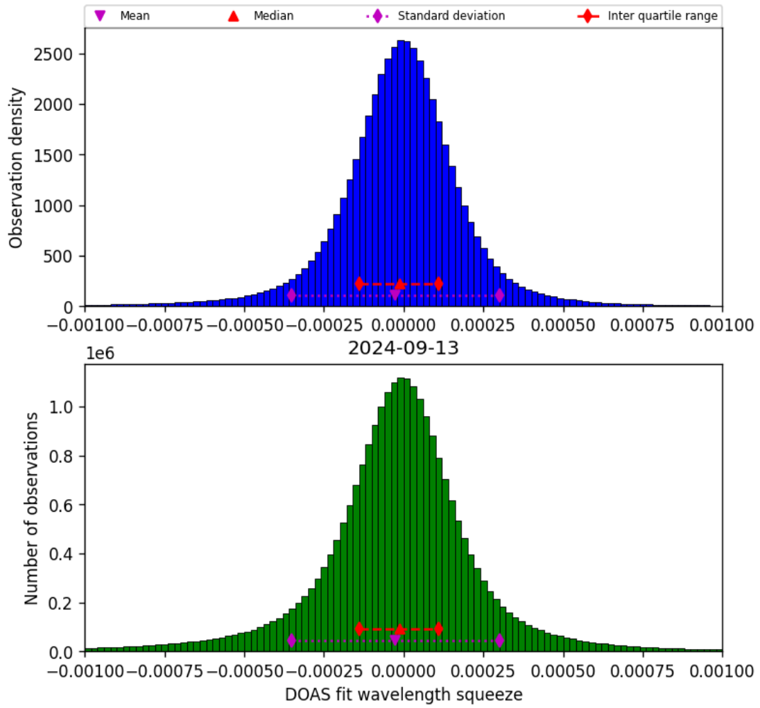
Figure 69: Histogram of “DOAS fit wavelength squeeze” for 2024-09-12 to 2024-09-14
