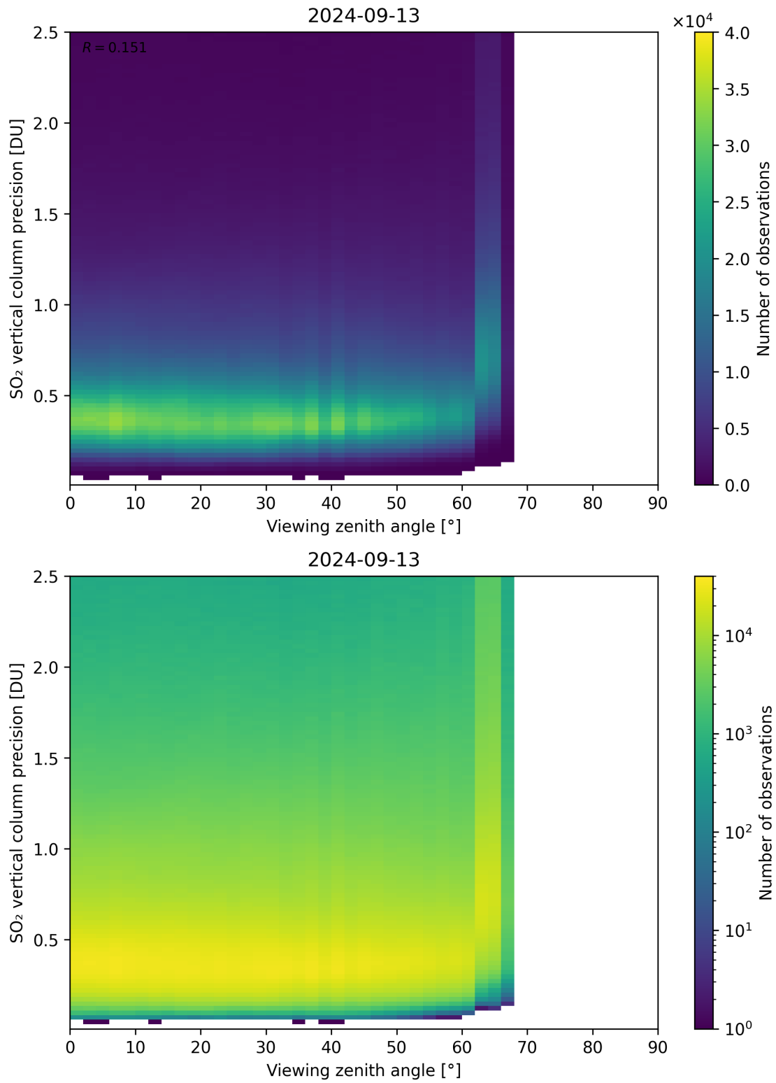
Figure 328: Scatter density plot of “Viewing zenith angle” against “SO 2 vertical column precision” for 2024-09-12 to 2024-09-14.
