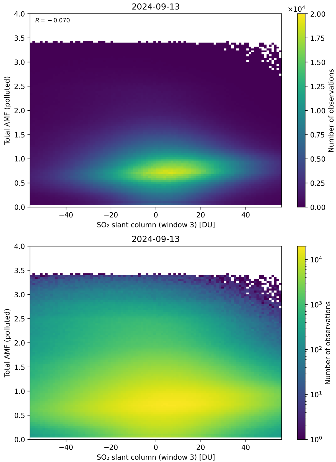
Figure 268: Scatter density plot of “SO 2 slant column (window 3)” against “Total AMF (polluted)” for 2024-09-12 to 2024-09-14.
