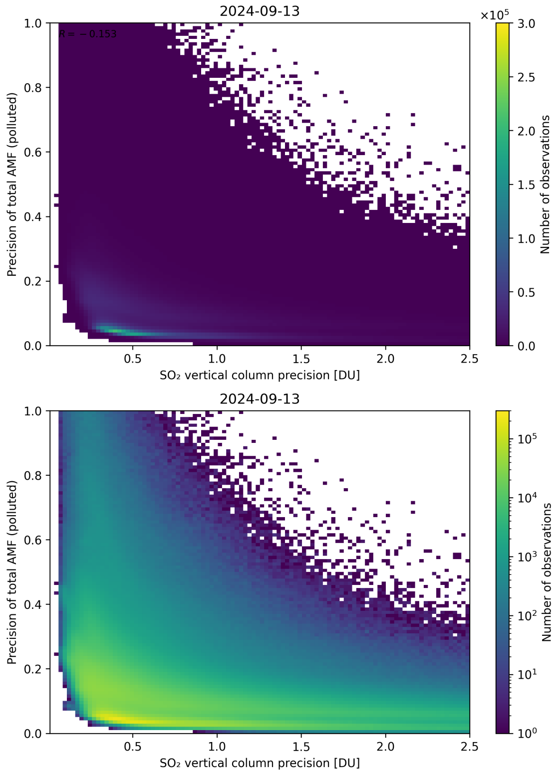
Figure 295: Scatter density plot of “SO 2 vertical column precision” against “Precision of total AMF (polluted)” for 2024-09-12 to 2024-09-14.
