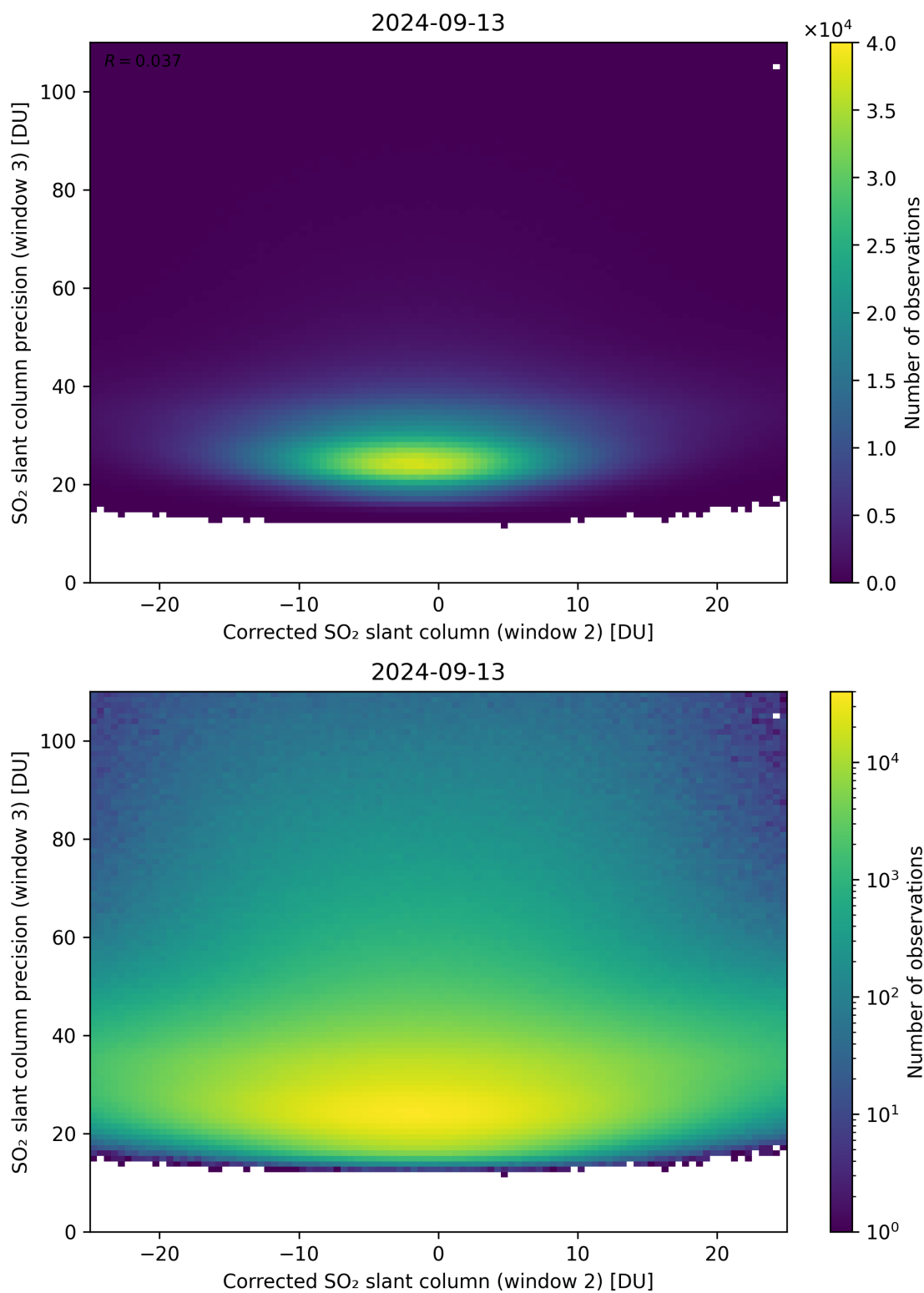
Figure 202: Scatter density plot of “Corrected SO 2 slant column (window 2)” against “SO 2 slant column precision (window 3)” for 2024-09-12 to 2024-09-14.
