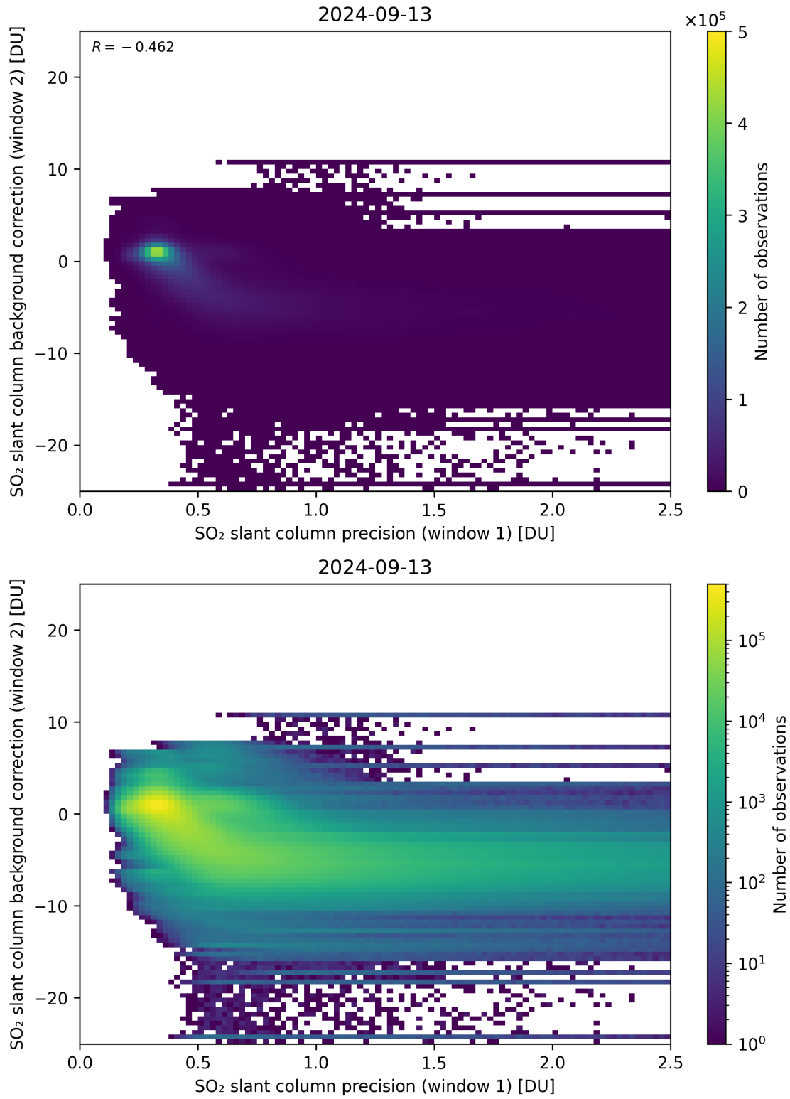
Figure 219: Scatter density plot of “SO 2 slant column precision (window 1)” against “SO 2 slant column background correction (window 2)” for 2024-09-12 to 2024-09-14.
