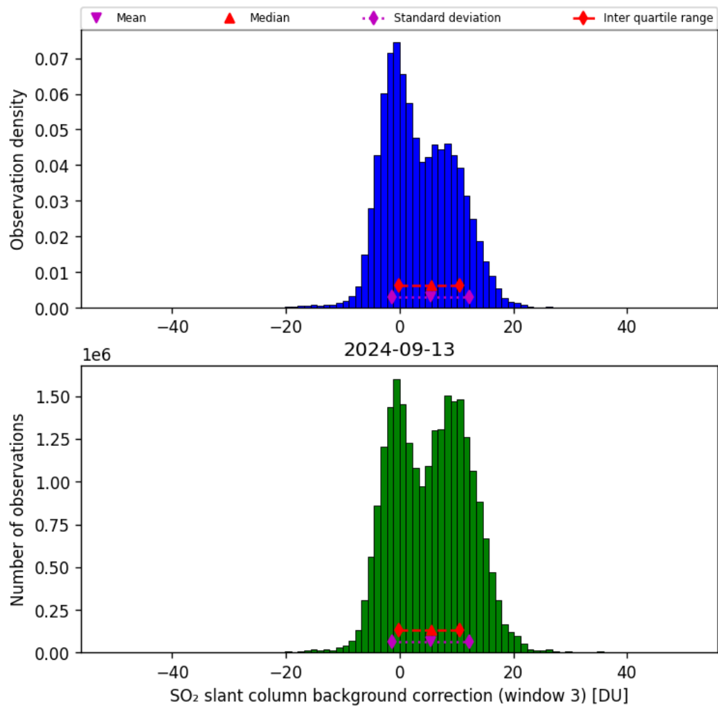
Figure 67: Histogram of “SO 2 slant column background correction (window 3)” for 2024-09-12 to 2024-09-14
