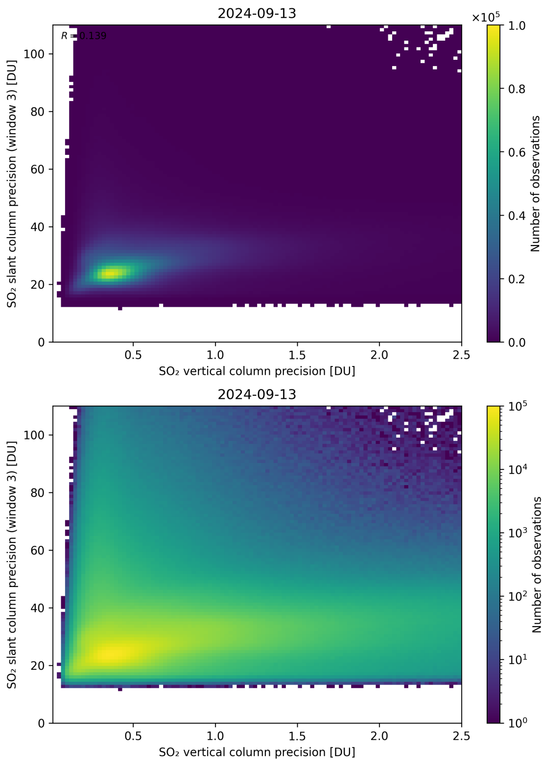
Figure 293: Scatter density plot of “SO 2 vertical column precision” against “SO 2 slant column precision (window 3)” for 2024-09-12 to 2024-09-14.
