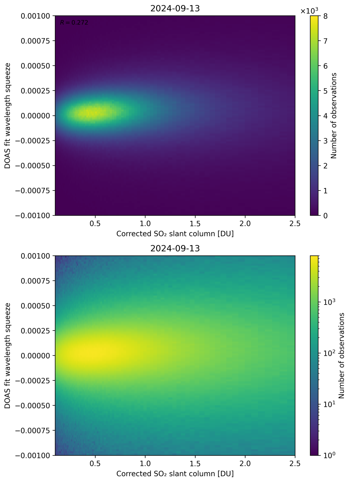
Figure 182: Scatter density plot of “Corrected SO 2 slant column” against “DOAS fit wavelength squeeze” for 2024-09-12 to 2024-09-14.
