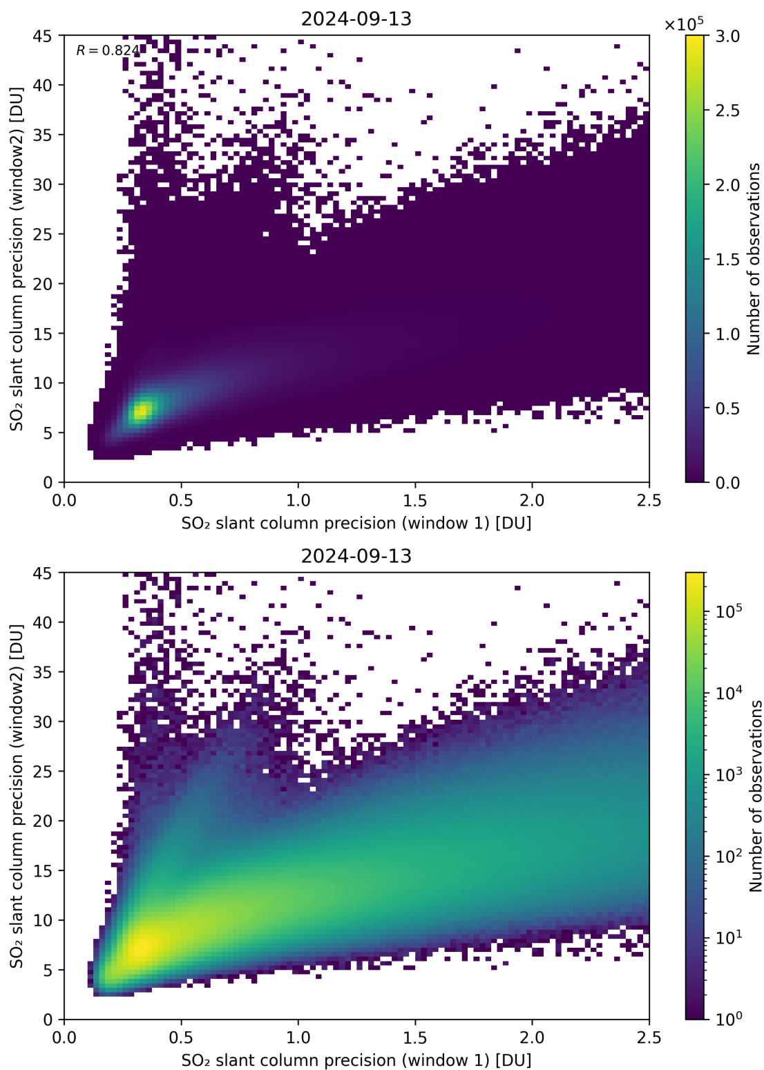
Figure 227: Scatter density plot of “SO 2 slant column precision (window 1)” against “SO 2 slant column precision (window2)” for 2024-09-12 to 2024-09-14.
