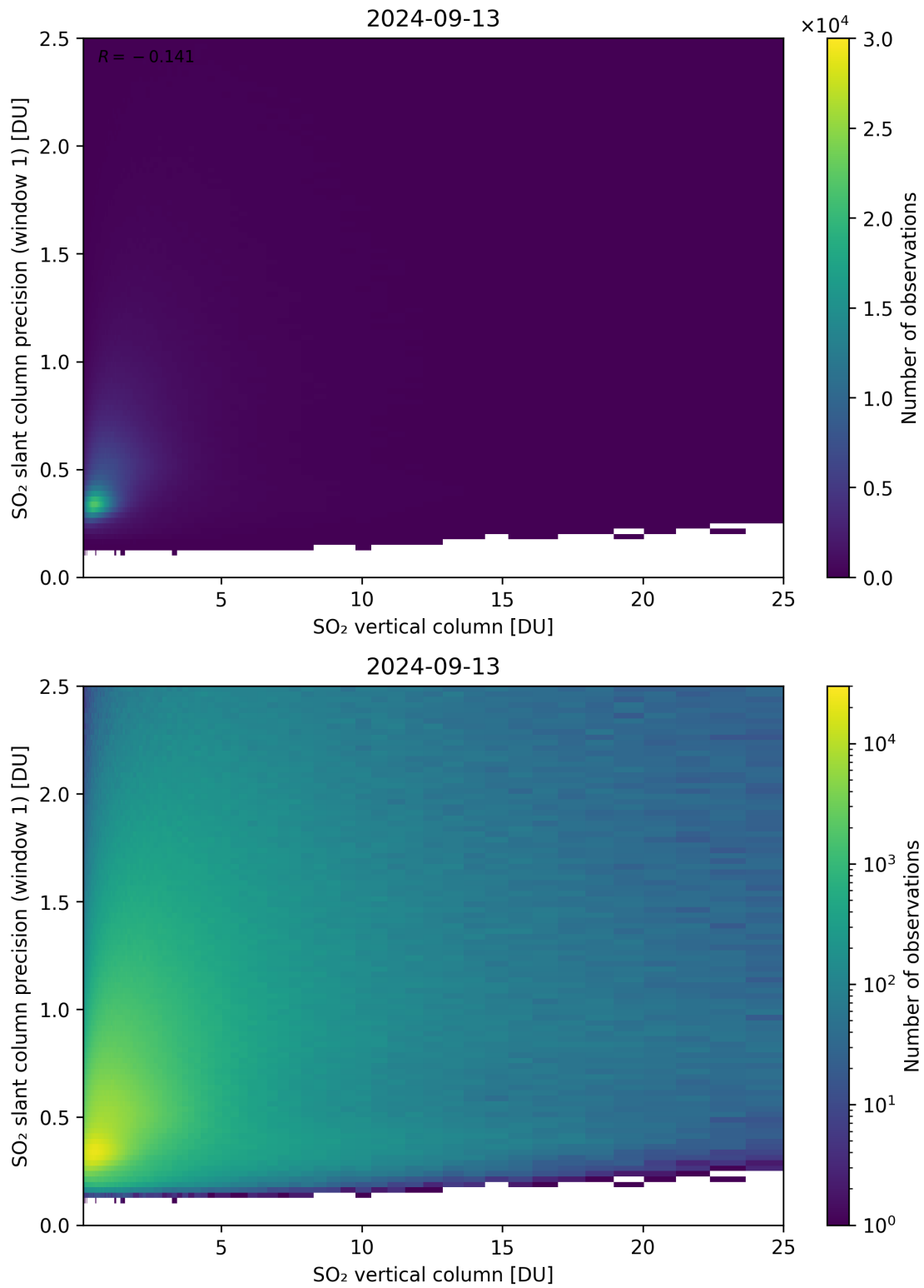
Figure 301: Scatter density plot of “SO 2 vertical column” against “SO 2 slant column precision (window 1)” for 2024-09-12 to 2024-09-14.
