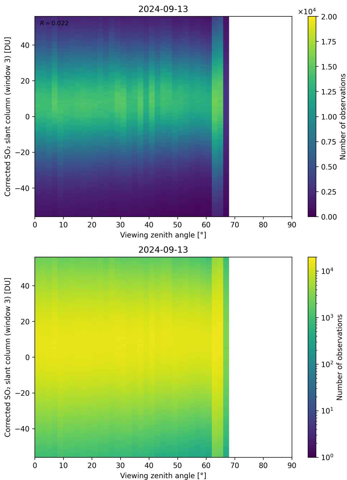
Figure 319: Scatter density plot of “Viewing zenith angle” against “Corrected SO 2 slant column (window 3)” for 2024-09-12 to 2024-09-14.
