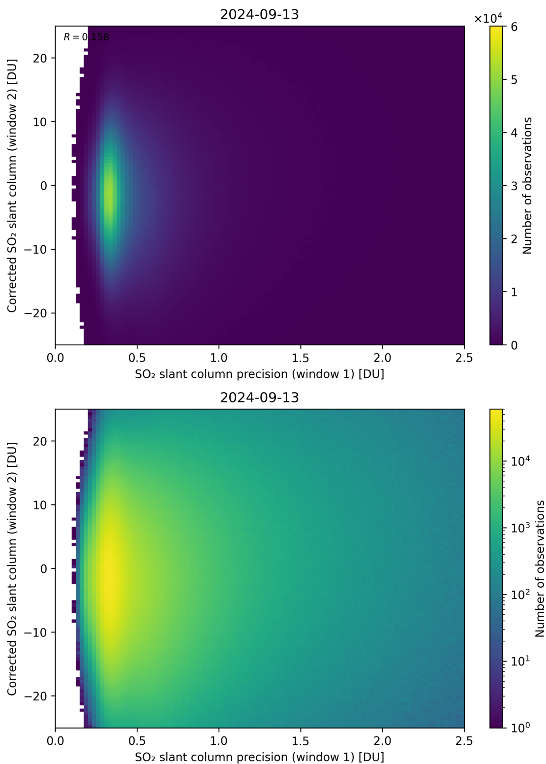
Figure 225: Scatter density plot of “SO 2 slant column precision (window 1)” against “Corrected SO 2 slant column (window 2)” for 2024-09-12 to 2024-09-14.
