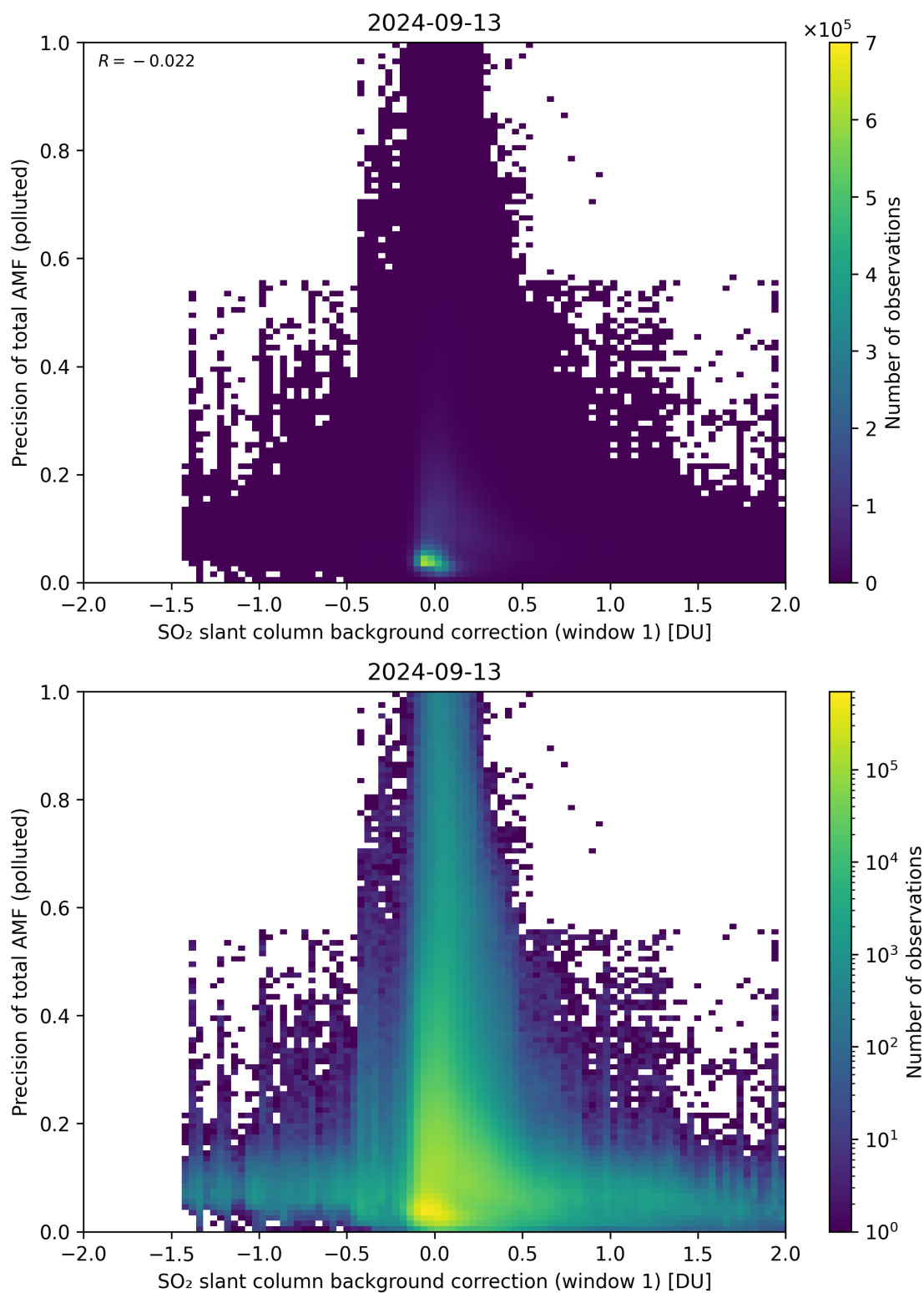
Figure 110: Scatter density plot of “SO 2 slant column background correction (window 1)” against “Precision of total AMF (polluted)” for 2024-09-12 to 2024-09-14.
