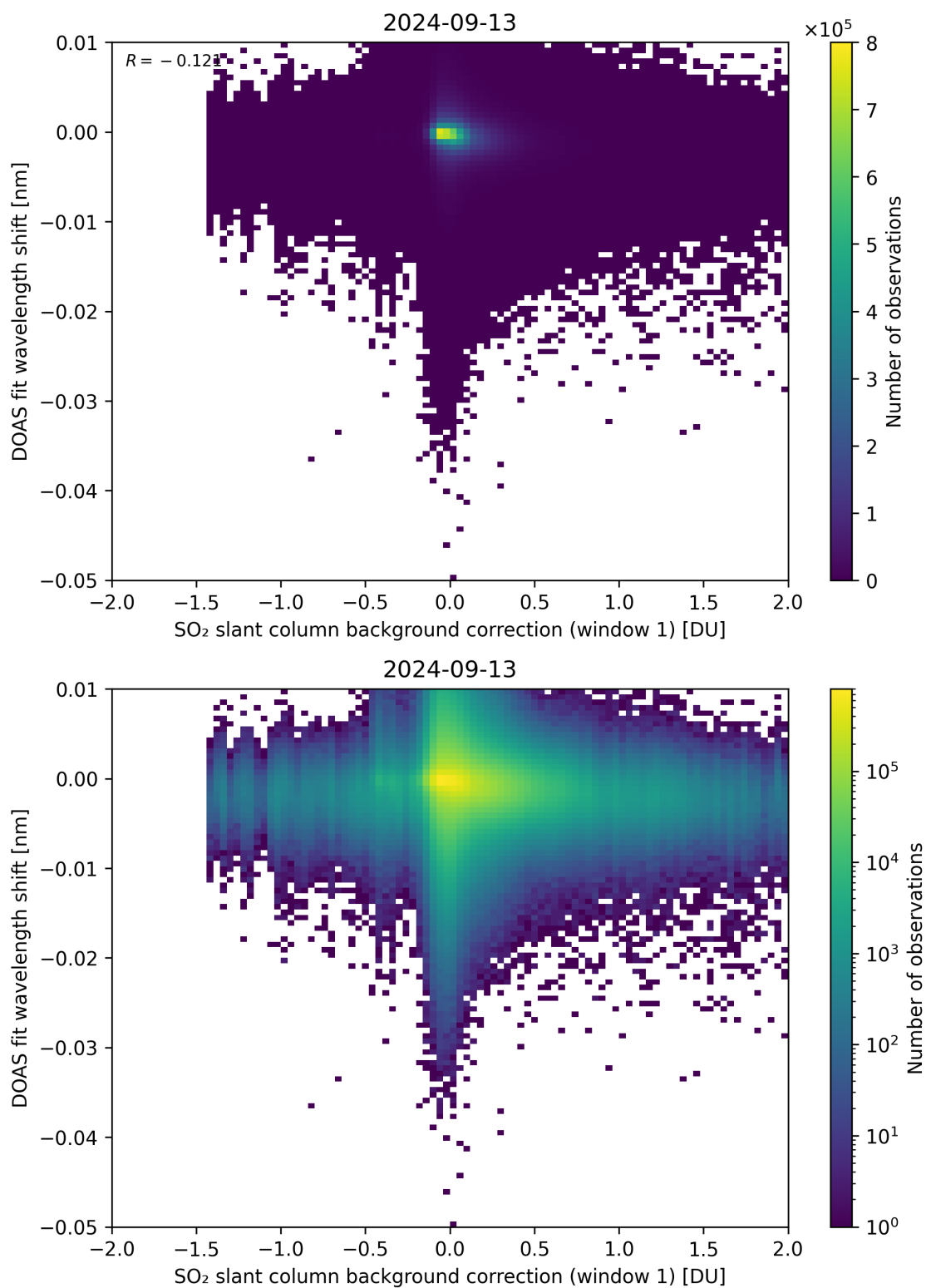
Figure 100: Scatter density plot of “SO 2 slant column background correction (window 1)” against “DOAS fit wavelength shift” for 2024-09-12 to 2024-09-14.
