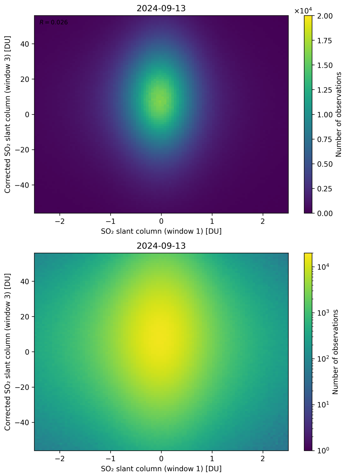
Figure 234: Scatter density plot of “SO 2 slant column (window 1)” against “Corrected SO 2 slant column (window 3)” for 2024-09-12 to 2024-09-14.
