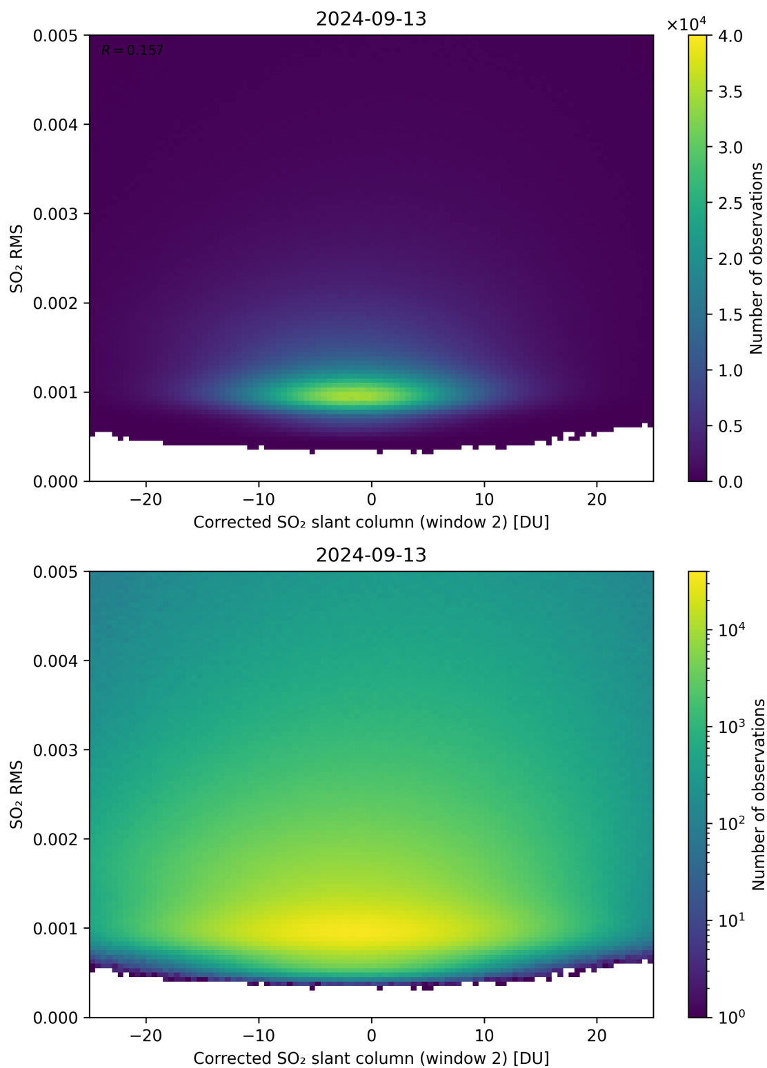
Figure 198: Scatter density plot of “Corrected SO 2 slant column (window 2)” against “SO 2 RMS” for 2024-09-12 to 2024-09-14.
