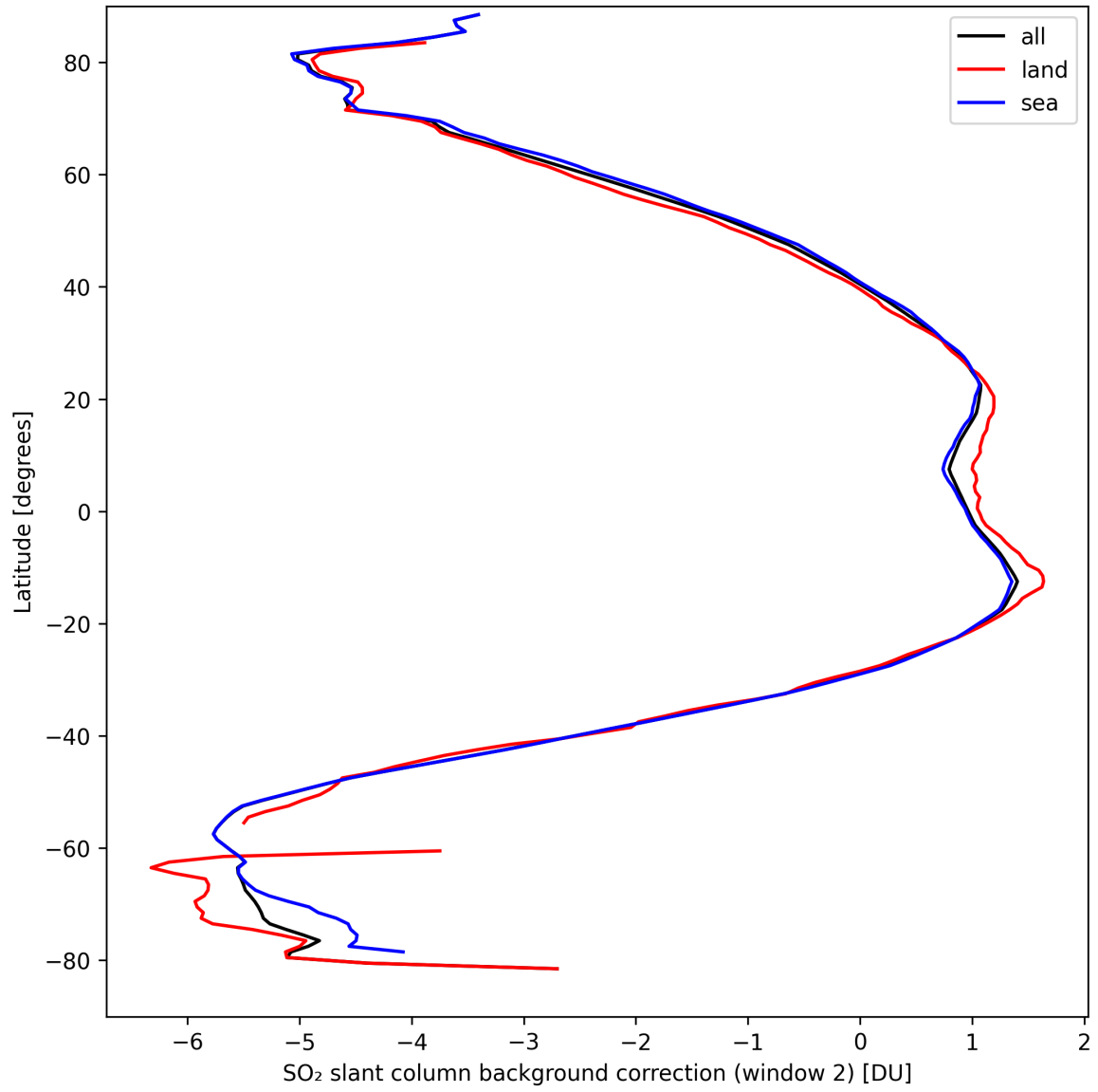
Figure 40: Zonal average of "SO 2 slant column background correction (window 2)" for 2024-09-12 to 2024-09-14.
