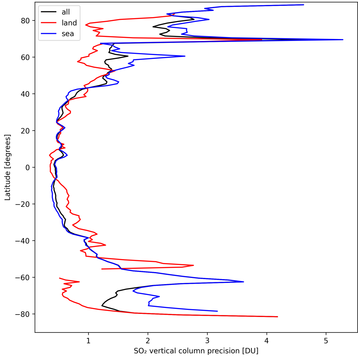
Figure 31: Zonal average of “SO 2 vertical column precision” for 2024-09-12 to 2024-09-14.
