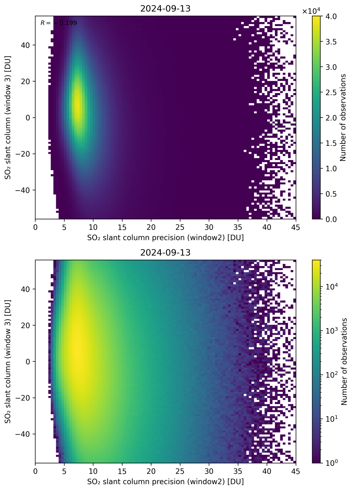
Figure 249: Scatter density plot of “SO 2 slant column precision (window2)” against “SO 2 slant column (window 3)” for 2024-09-12 to 2024-09-14.
