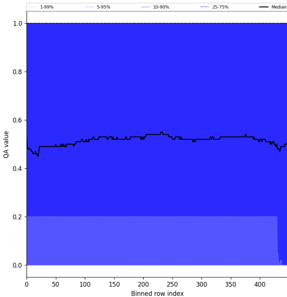
Figure 75: Along track statistics of “QA value” for 2024-09-12 to 2024-09-14
