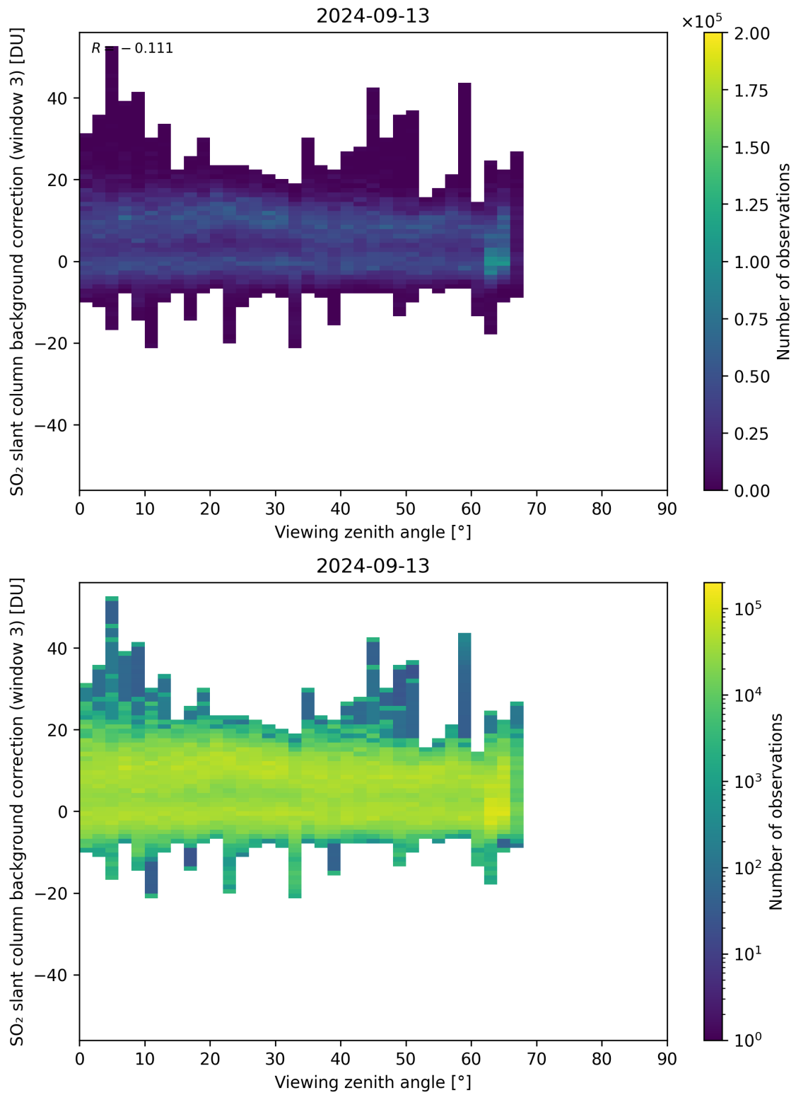
Figure 310: Scatter density plot of “Viewing zenith angle” against “SO 2 slant column background correction (window 3)” for 2024-09-12 to 2024-09-14.
