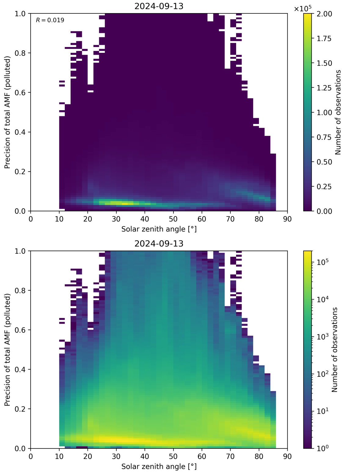
Figure 175: Scatter density plot of “Solar zenith angle” against “Precision of total AMF (polluted)” for 2024-09-12 to 2024-09-14.
