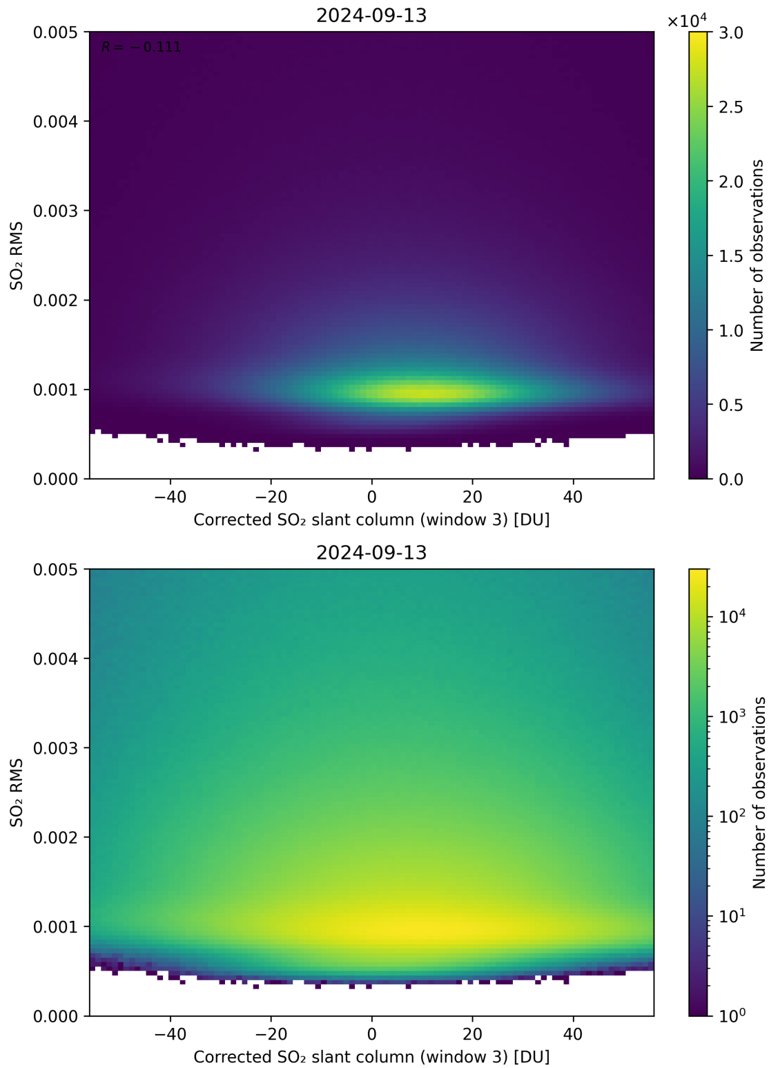
Figure 208: Scatter density plot of “Corrected SO 2 slant column (window 3)” against “SO 2 RMS” for 2024-09-12 to 2024-09-14.
