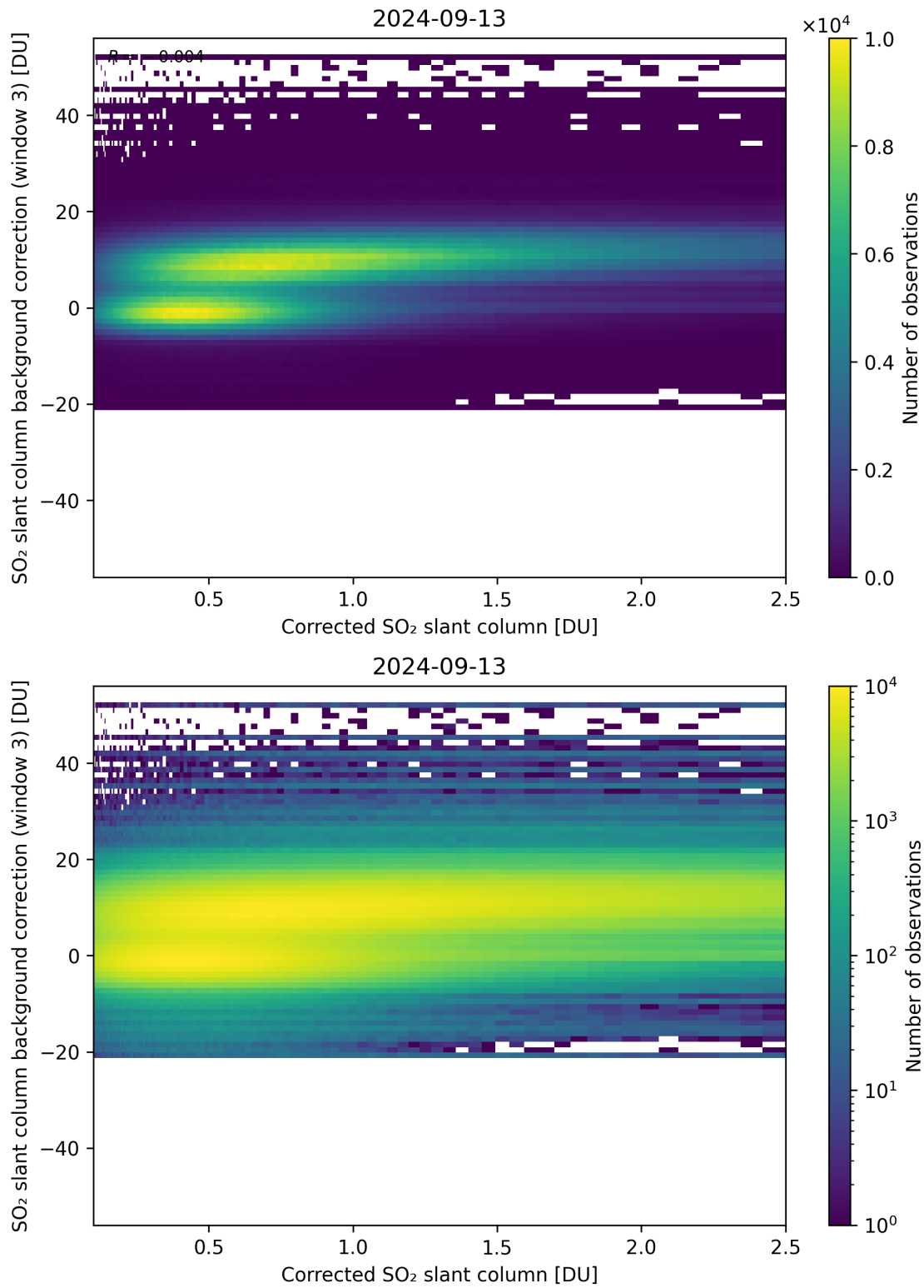
Figure 180: Scatter density plot of “Corrected SO 2 slant column” against “SO 2 slant column background correction (window 3)” for 2024-09-12 to 2024-09-14.
