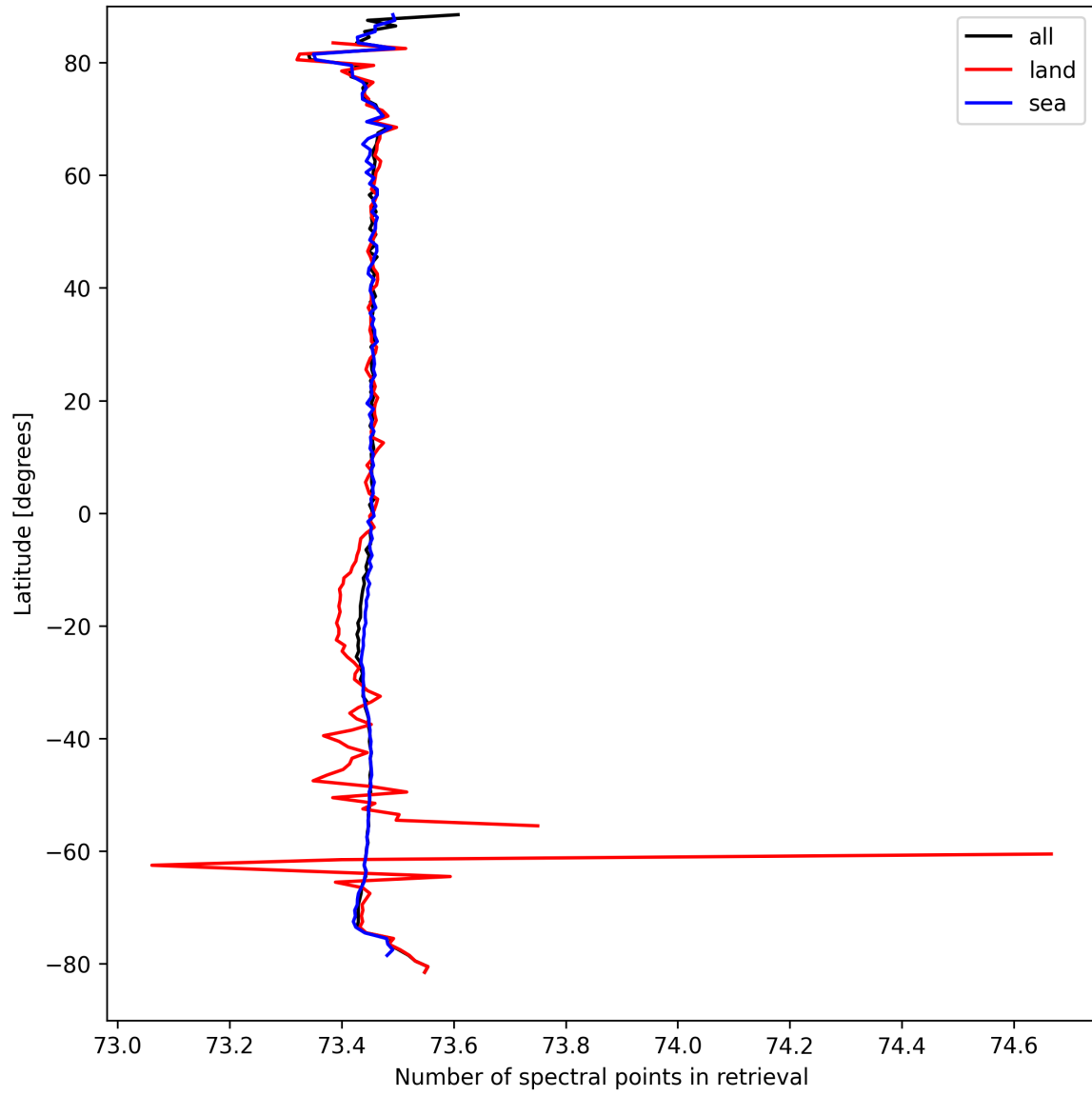
Figure 51: Zonal average of “Number of spectral points in retrieval” for 2024-09-12 to 2024-09-14.
