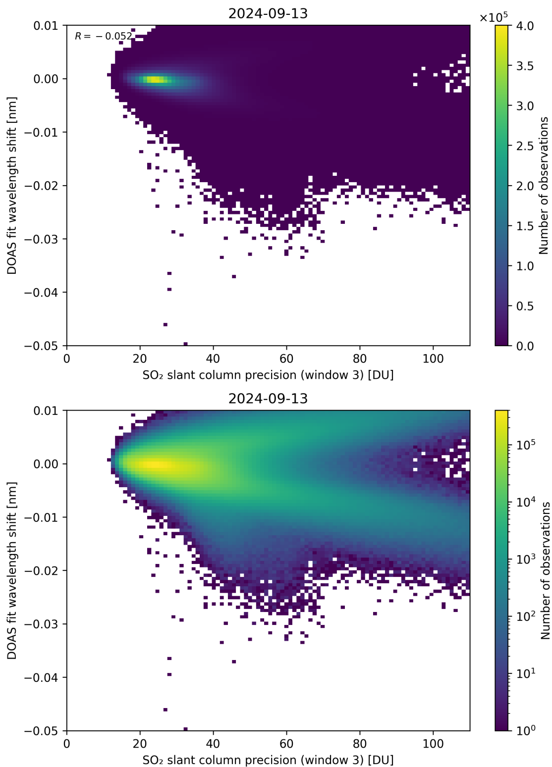
Figure 258: Scatter density plot of “SO 2 slant column precision (window 3)” against “DOAS fit wavelength shift” for 2024-09-12 to 2024-09-14.
