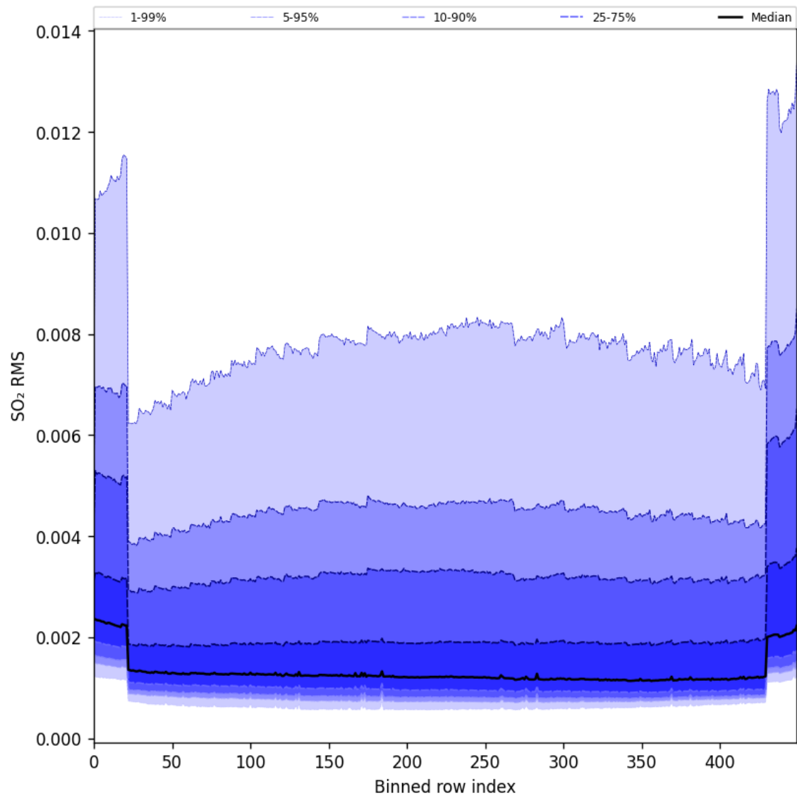
Figure 93: Along track statistics of “SO 2 RMS” for 2024-09-12 to 2024-09-14
