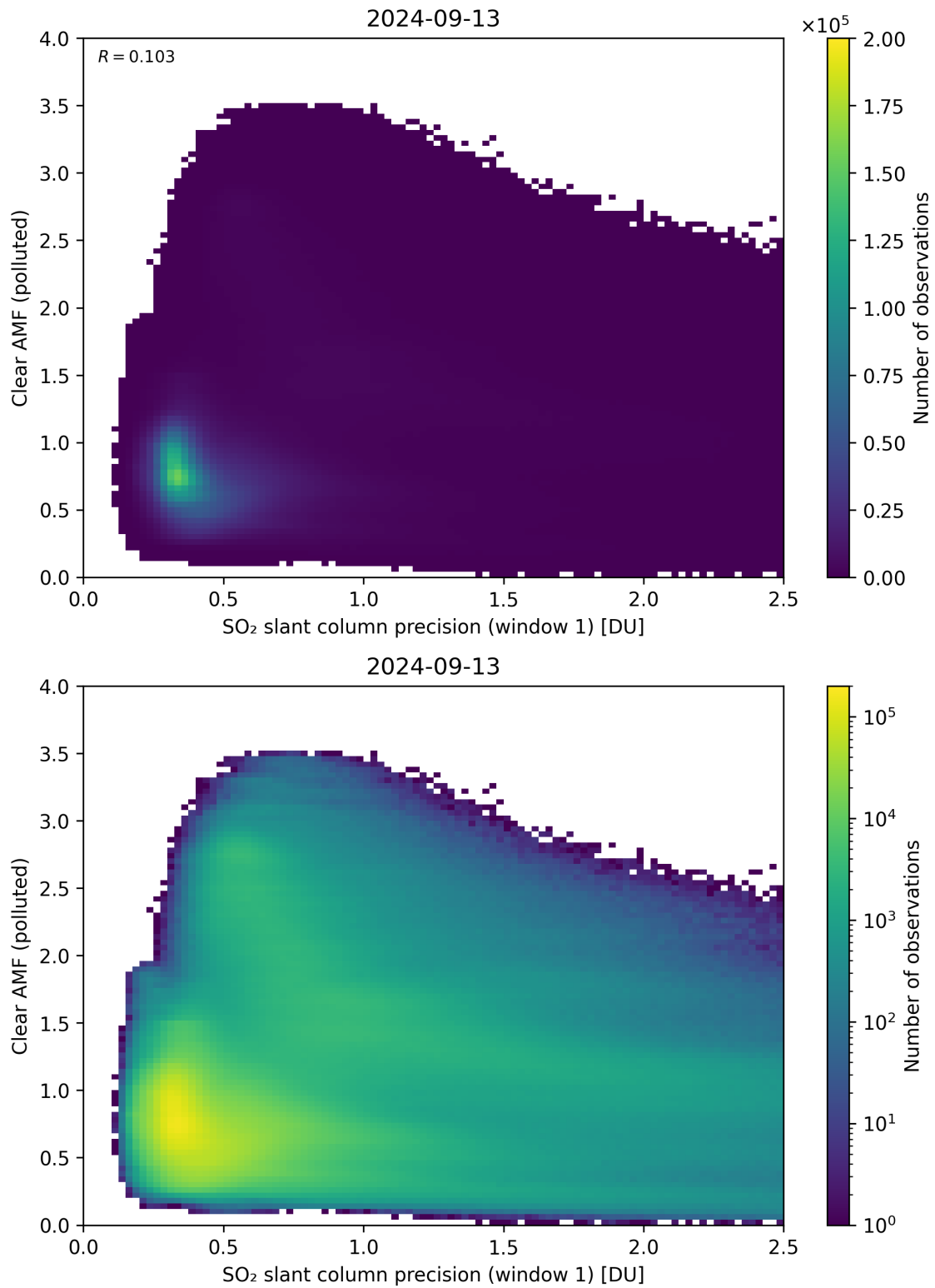
Figure 224: Scatter density plot of “SO 2 slant column precision (window 1)” against “Clear AMF (polluted)” for 2024-09-12 to 2024-09-14.
