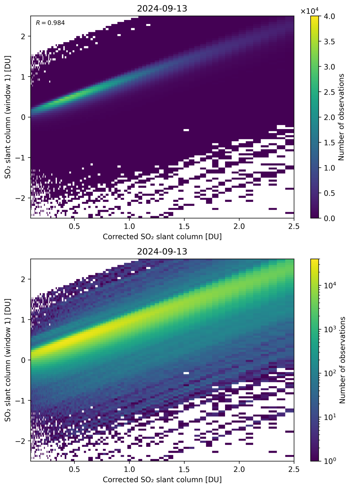
Figure 187: Scatter density plot of “Corrected SO 2 slant column” against “SO 2 slant column (window 1)” for 2024-09-12 to 2024-09-14.
