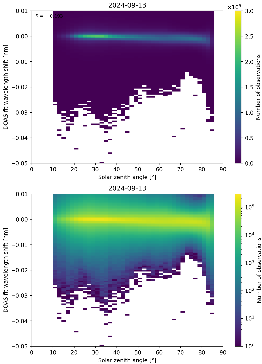
Figure 161: Scatter density plot of “Solar zenith angle” against “DOAS fit wavelength shift” for 2024-09-12 to 2024-09-14.
