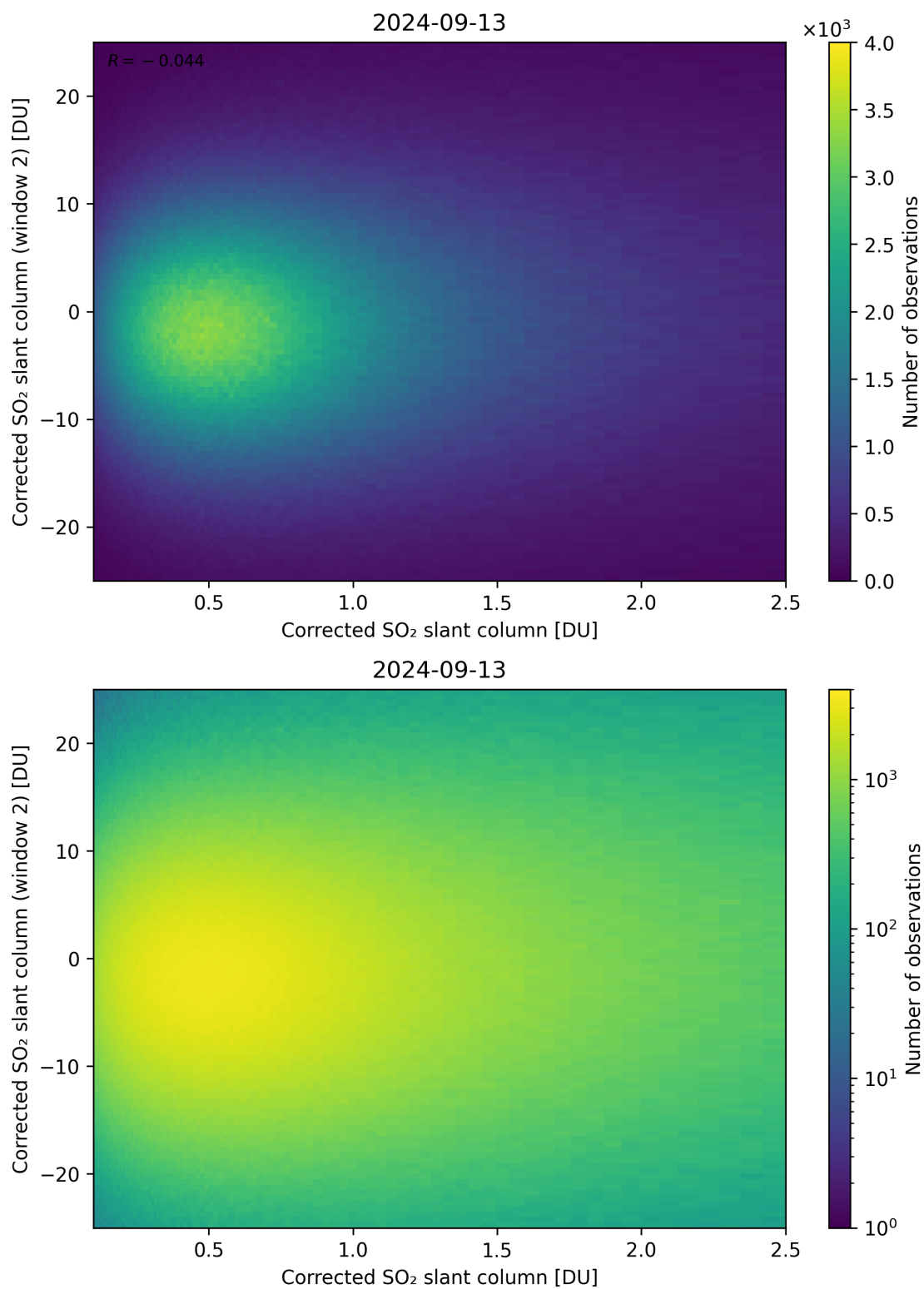
Figure 185: Scatter density plot of “Corrected SO 2 slant column” against “Corrected SO 2 slant column (window 2)” for 2024-09-12 to 2024-09-14.
