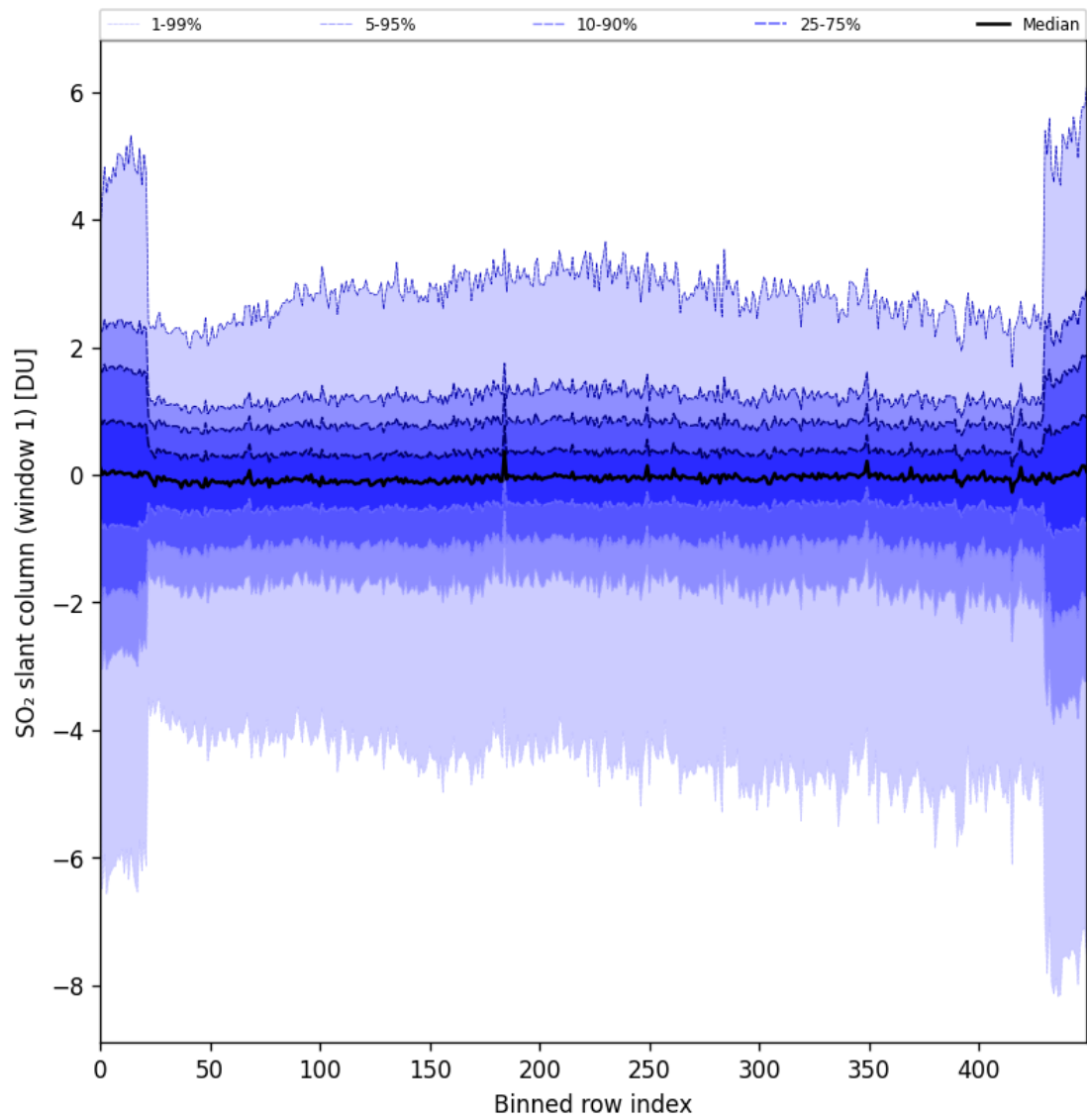
Figure 79: Along track statistics of “SO 2 slant column (window 1)” for 2024-09-12 to 2024-09-14
