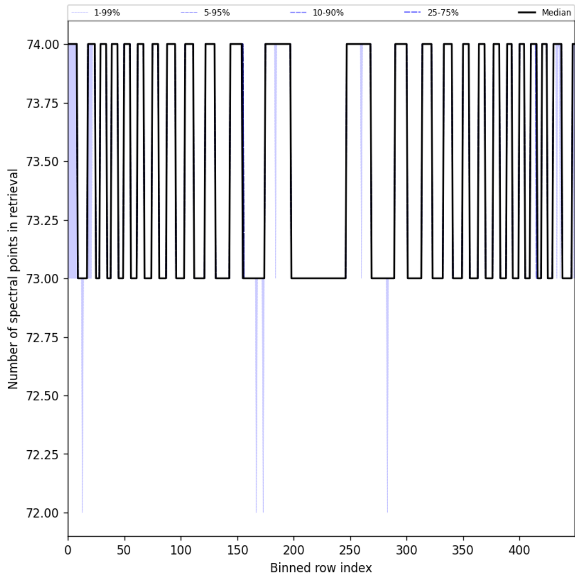
Figure 97: Along track statistics of “Number of spectral points in retrieval” for 2024-09-12 to 2024-09-14
