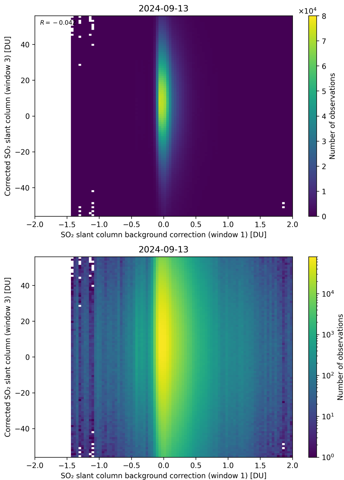
Figure 105: Scatter density plot of “SO 2 slant column background correction (window 1)” against “Corrected SO 2 slant column (window 3)” for 2024-09-12 to 2024-09-14.
