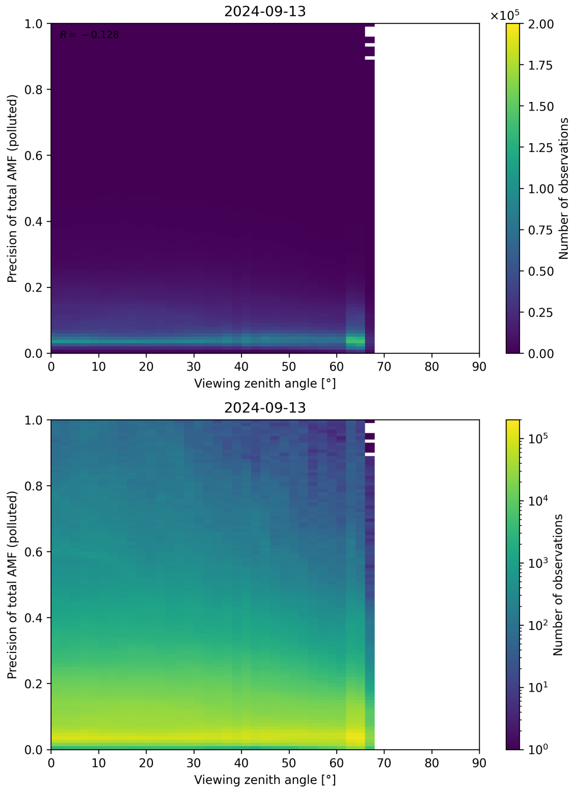
Figure 326: Scatter density plot of “Viewing zenith angle” against “Precision of total AMF (polluted)” for 2024-09-12 to 2024-09-14.
