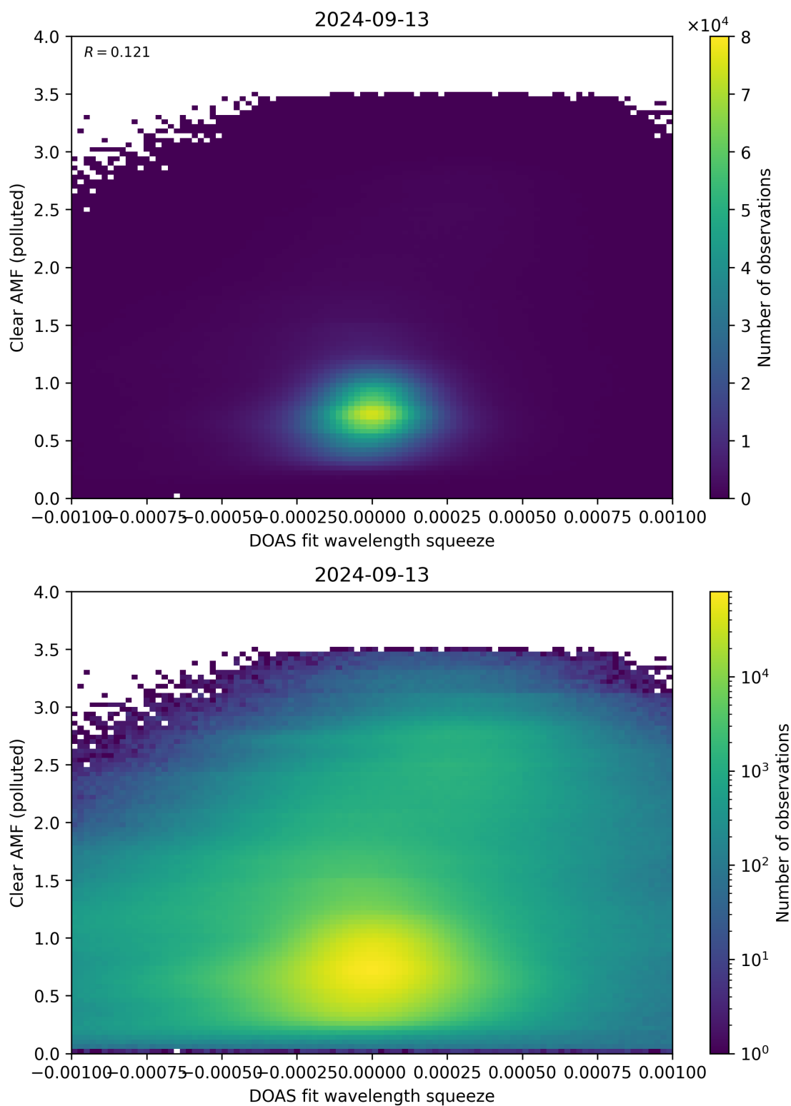
Figure 133: Scatter density plot of “DOAS fit wavelength squeeze” against “Clear AMF (polluted)” for 2024-09-12 to 2024-09-14.
