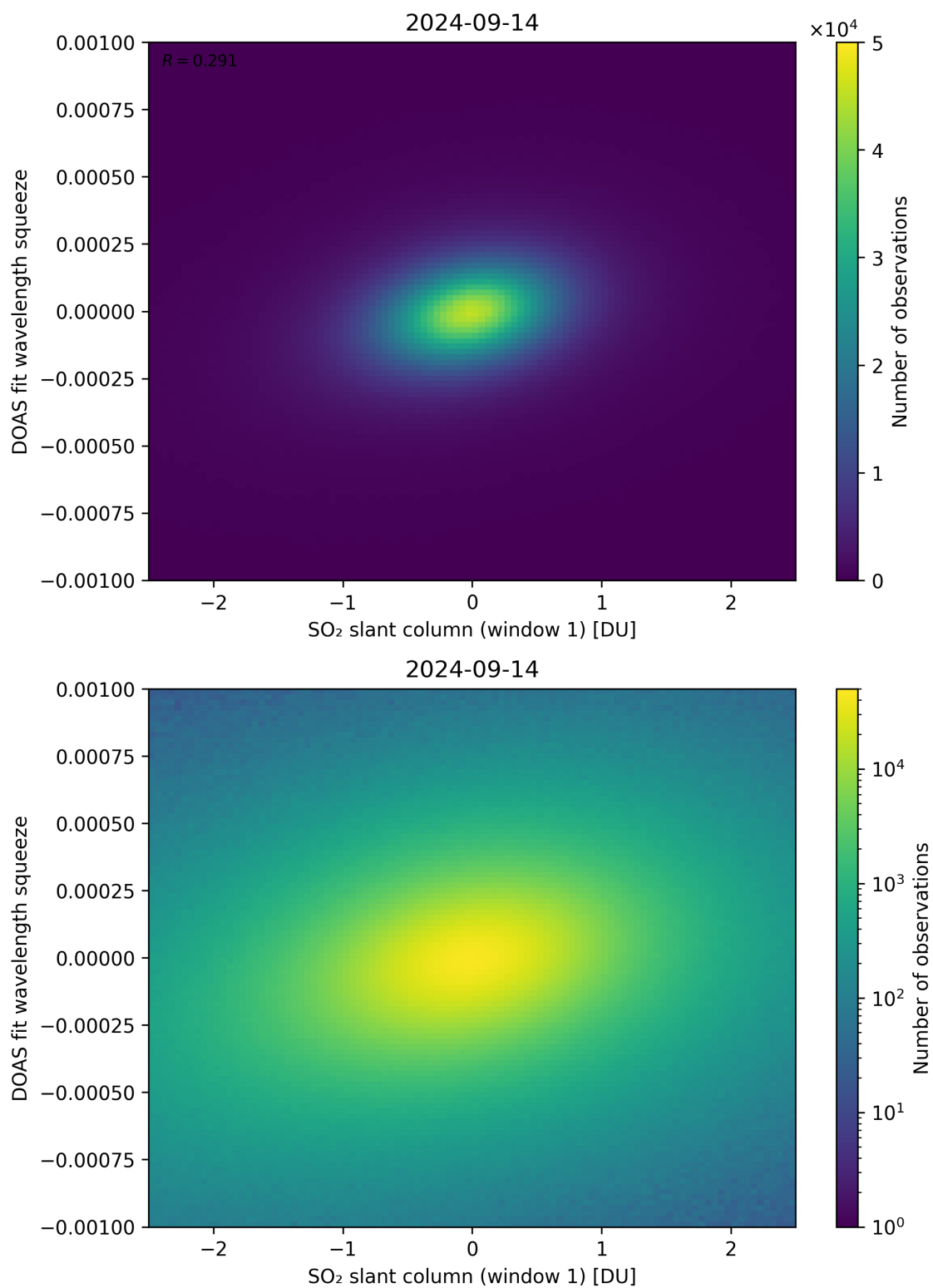
Figure 216: Scatter density plot of “SO 2 slant column (window 1)” against “DOAS fit wavelength squeeze” for 2024-09-13 to 2024-09-15.
