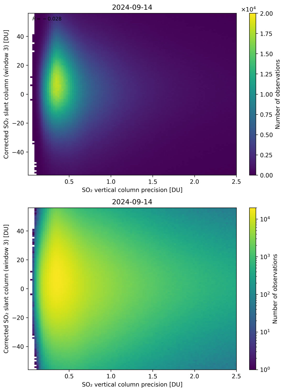
Figure 288: Scatter density plot of “SO 2 vertical column precision” against “Corrected SO 2 slant column (window 3)” for 2024-09-13 to 2024-09-15.
