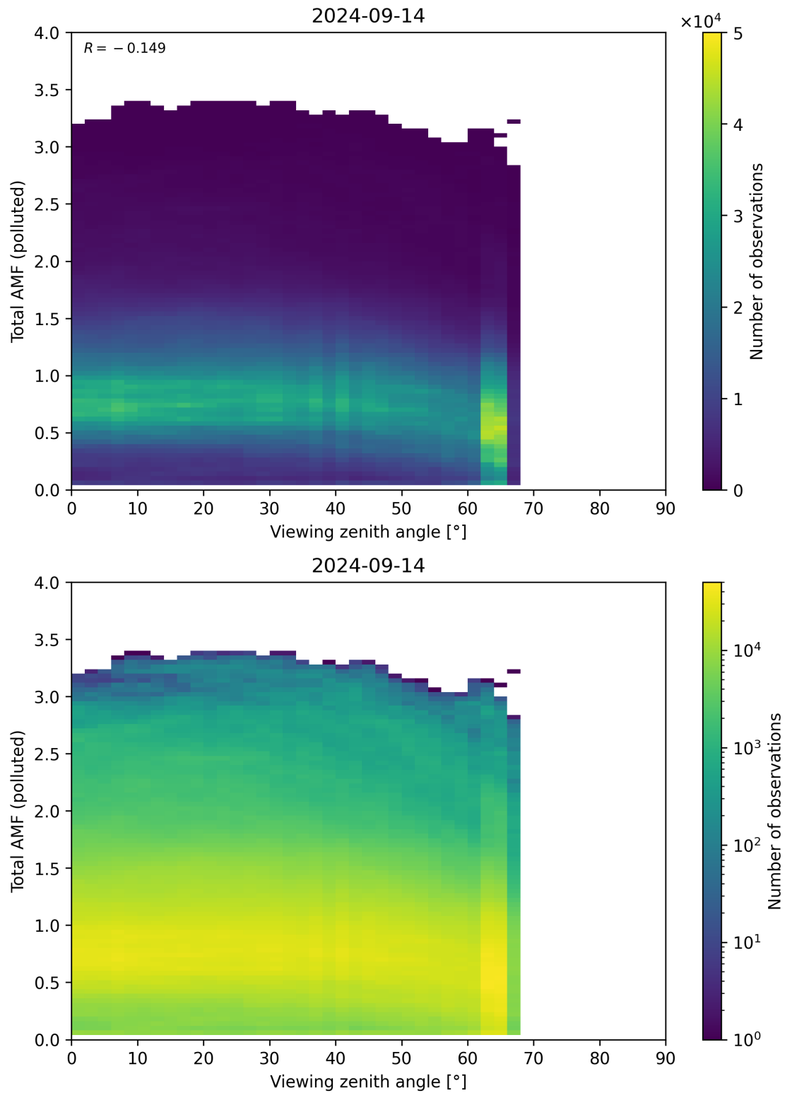
Figure 325: Scatter density plot of “Viewing zenith angle” against “Total AMF (polluted)” for 2024-09-13 to 2024-09-15.
