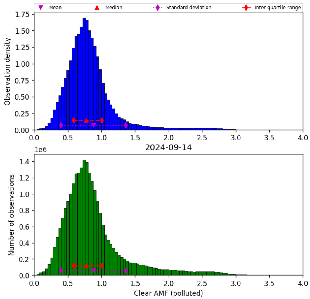
Figure 73: Histogram of “Clear AMF (polluted)” for 2024-09-13 to 2024-09-15
