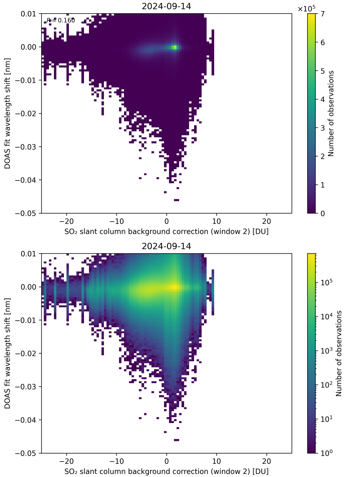
Figure 112: Scatter density plot of “SO 2 slant column background correction (window 2)” against “DOAS fit wavelength shift” for 2024-09-13 to 2024-09-15.
