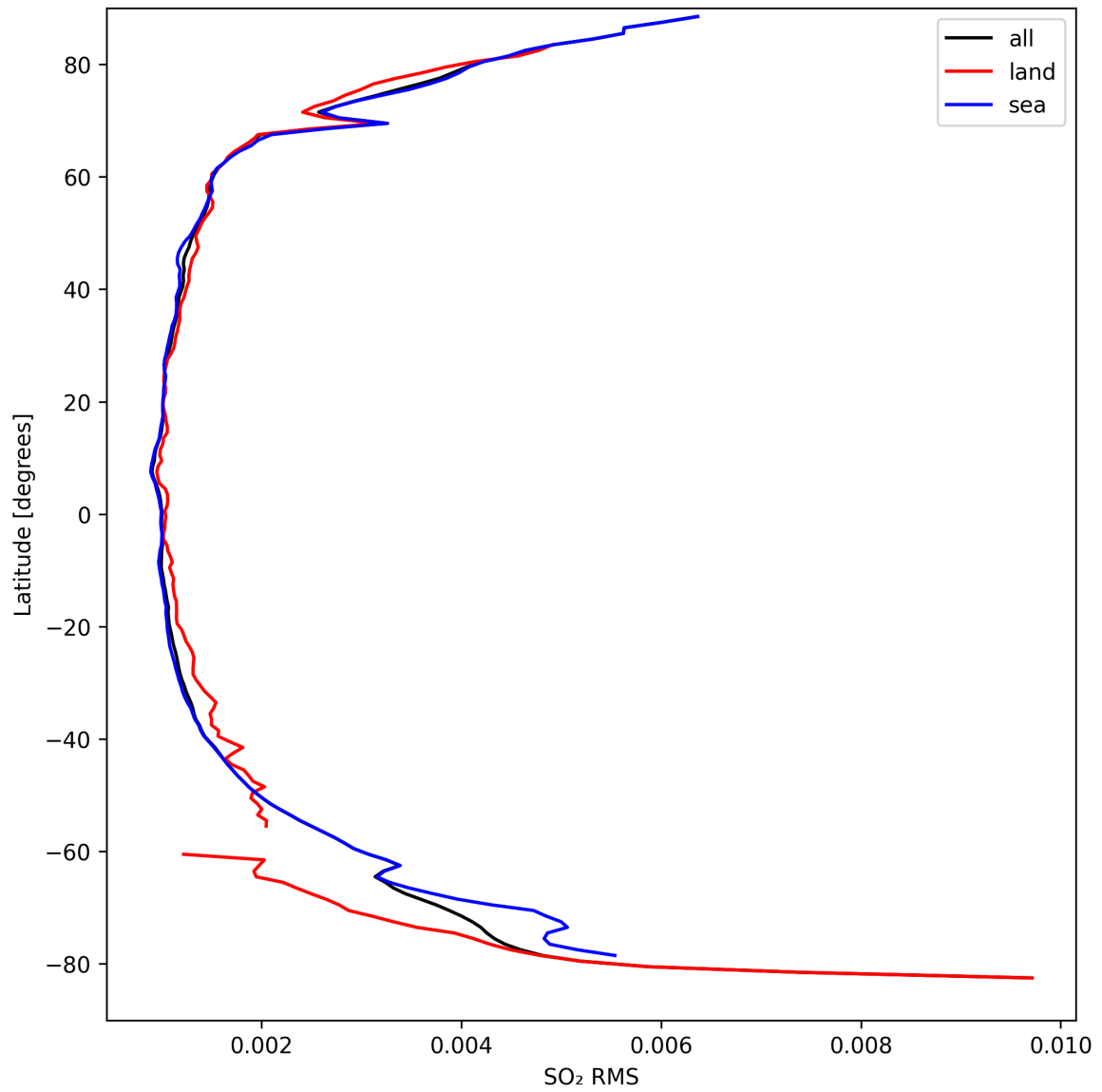
Figure 47: Zonal average of “SO 2 RMS” for 2024-09-13 to 2024-09-15.
