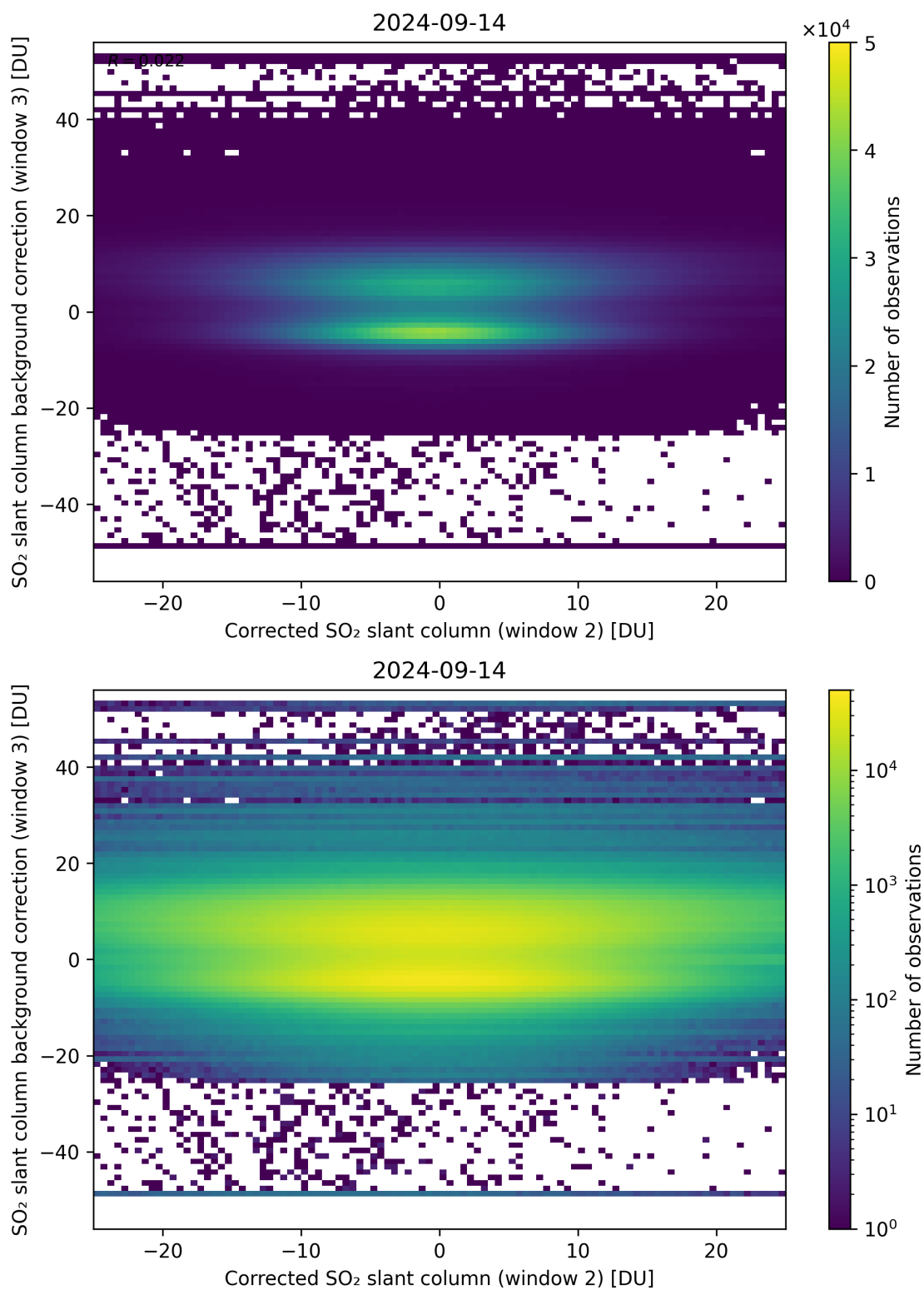
Figure 195: Scatter density plot of “Corrected SO 2 slant column (window 2)” against “SO 2 slant column background correction (window 3)” for 2024-09-13 to 2024-09-15.
