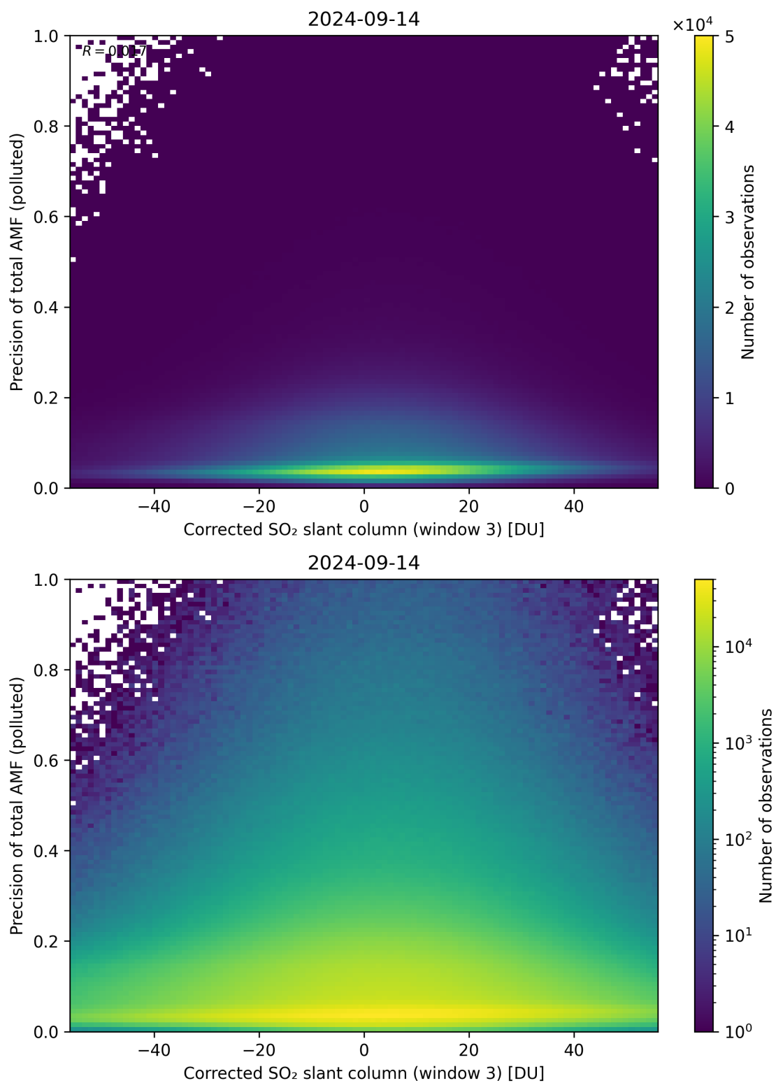
Figure 211: Scatter density plot of “Corrected SO 2 slant column (window 3)” against “Precision of total AMF (polluted)” for 2024-09-13 to 2024-09-15.
