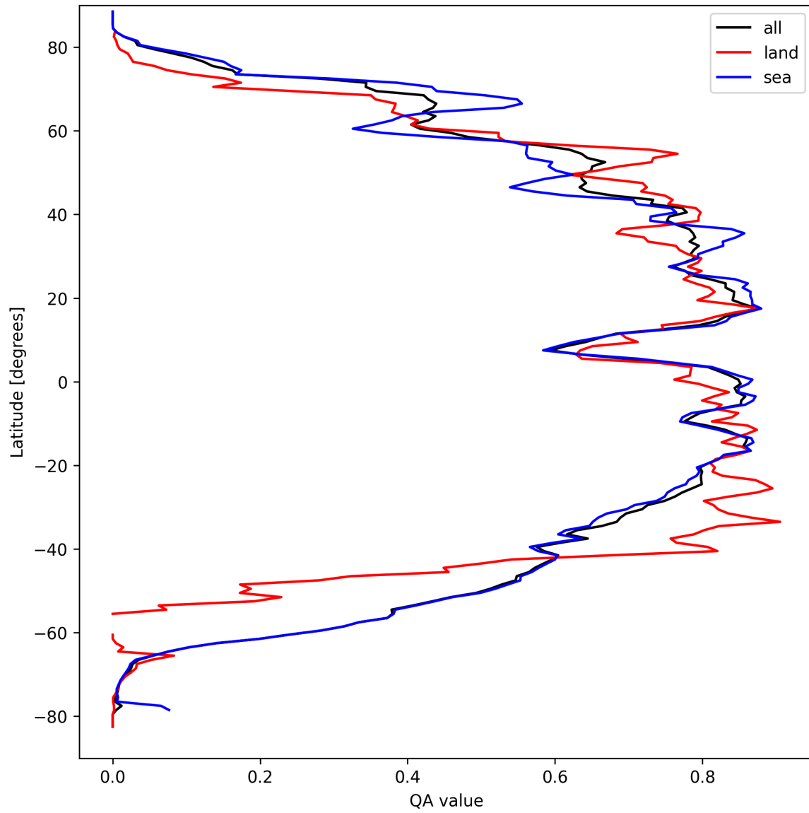
Figure 29: Zonal average of “QA value” for 2024-09-13 to 2024-09-15.
