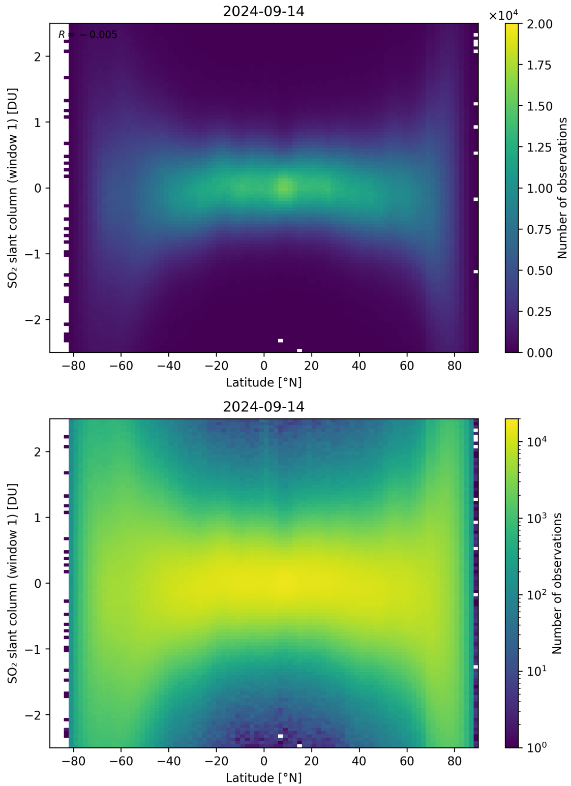
Figure 149: Scatter density plot of “Latitude” against “SO 2 slant column (window 1)” for 2024-09-13 to 2024-09-15.
