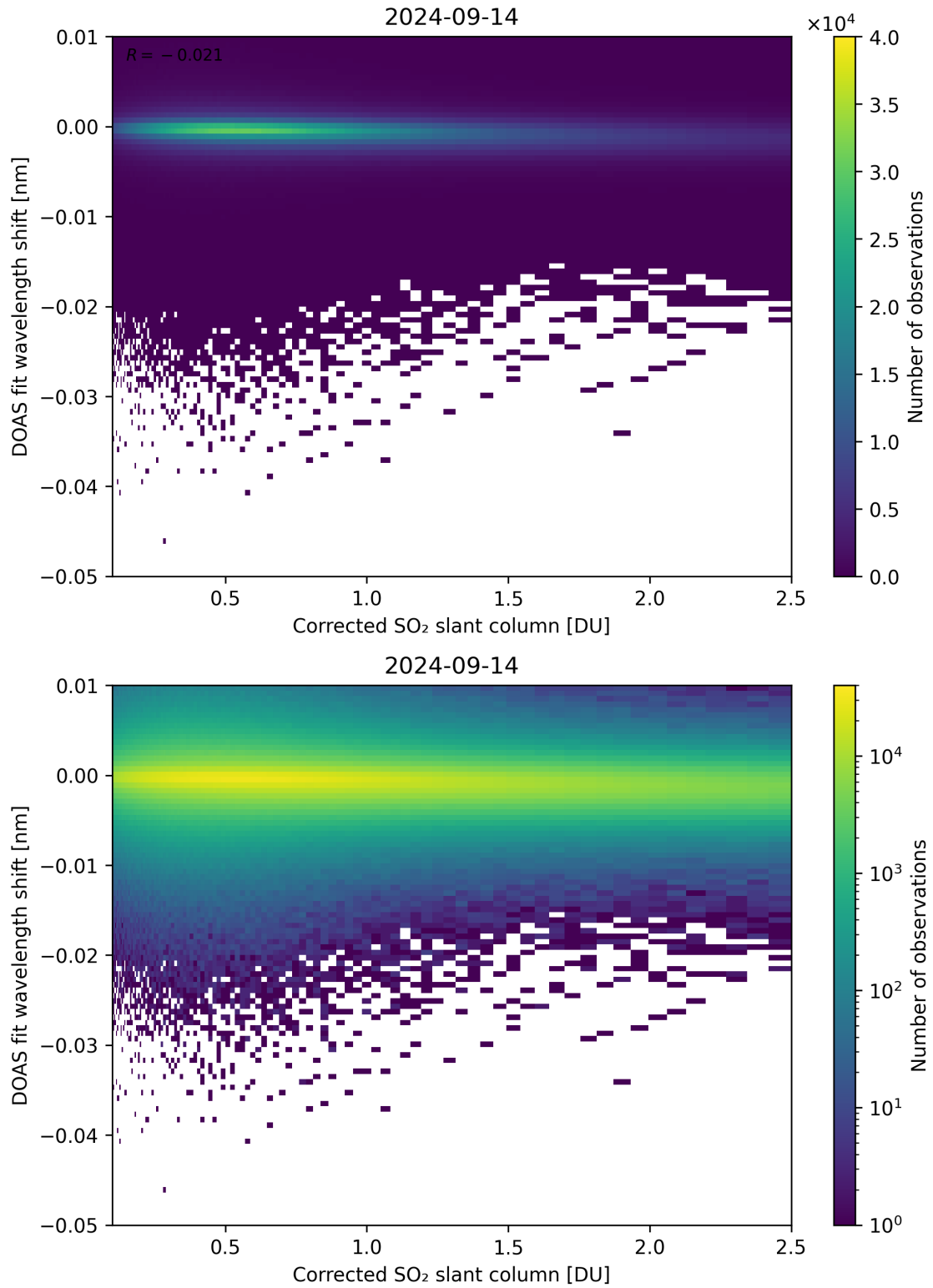
Figure 181: Scatter density plot of “Corrected SO 2 slant column” against “DOAS fit wavelength shift” for 2024-09-13 to 2024-09-15.
