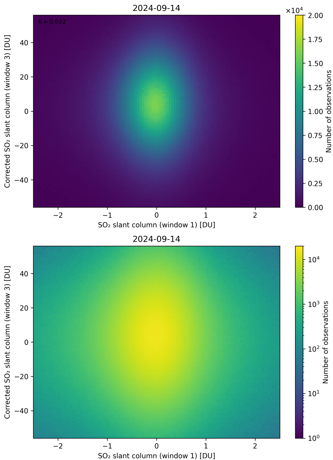
Figure 234: Scatter density plot of “SO 2 slant column (window 1)” against “Corrected SO 2 slant column (window 3)” for 2024-09-13 to 2024-09-15.
