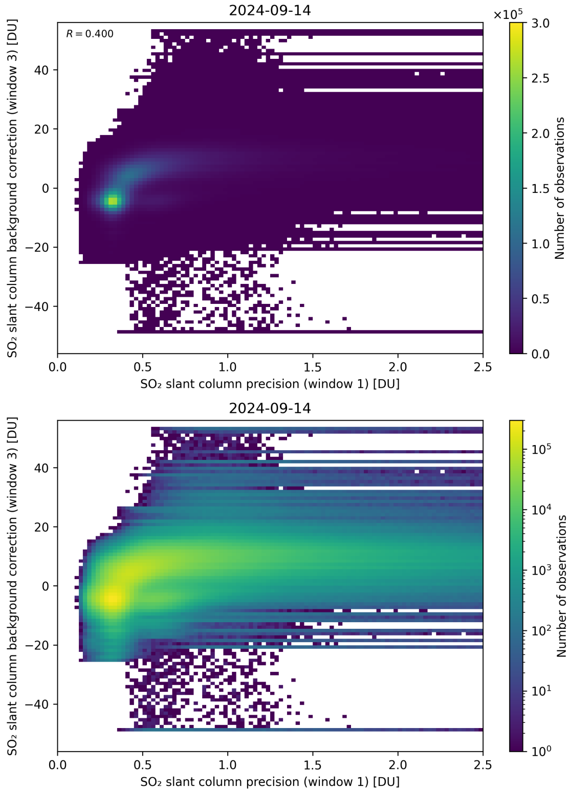
Figure 220: Scatter density plot of “SO 2 slant column precision (window 1)” against “SO 2 slant column background correction (window 3)” for 2024-09-13 to 2024-09-15.
