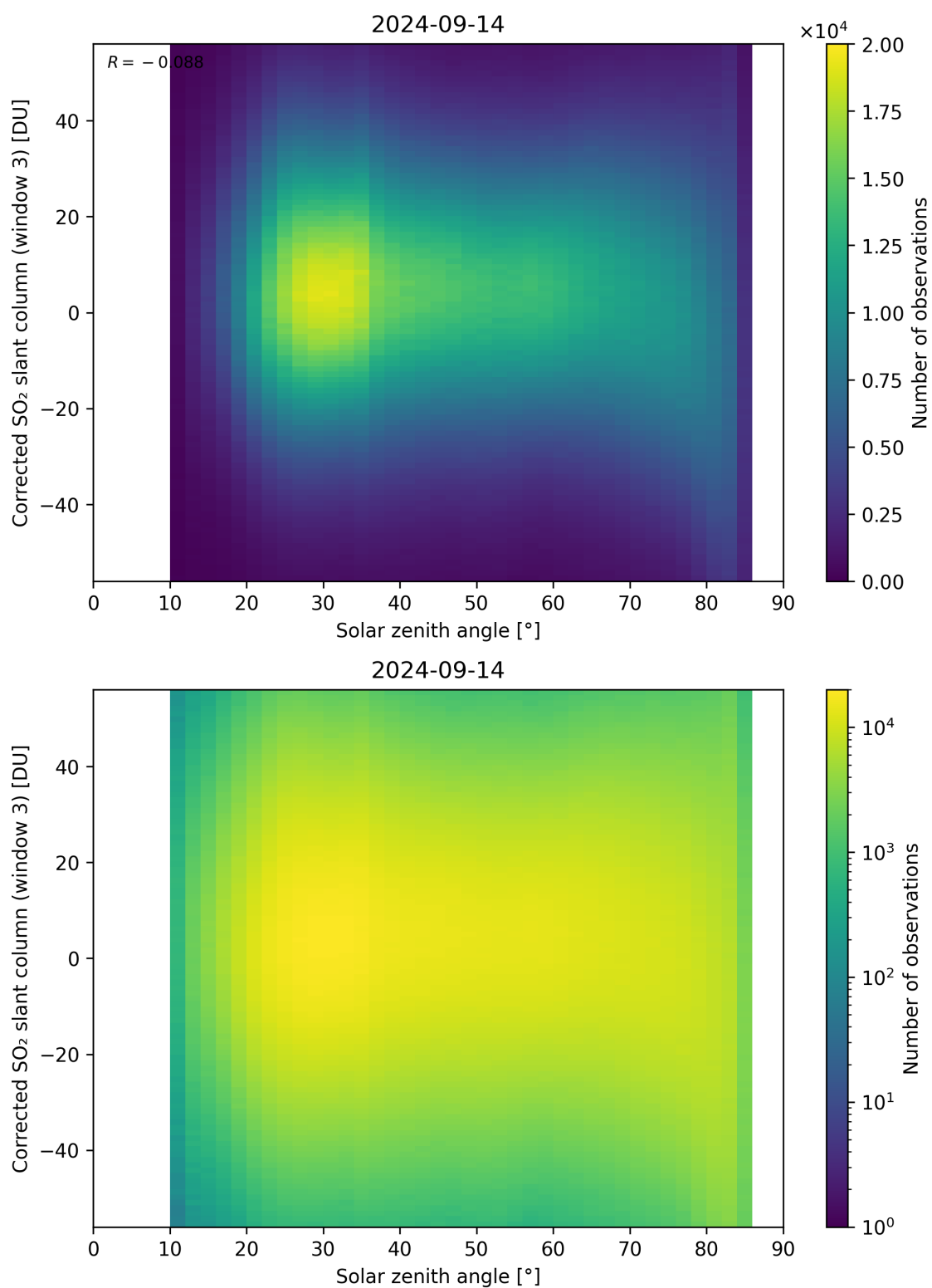
Figure 168: Scatter density plot of “Solar zenith angle” against “Corrected SO 2 slant column (window 3)” for 2024-09-13 to 2024-09-15.
