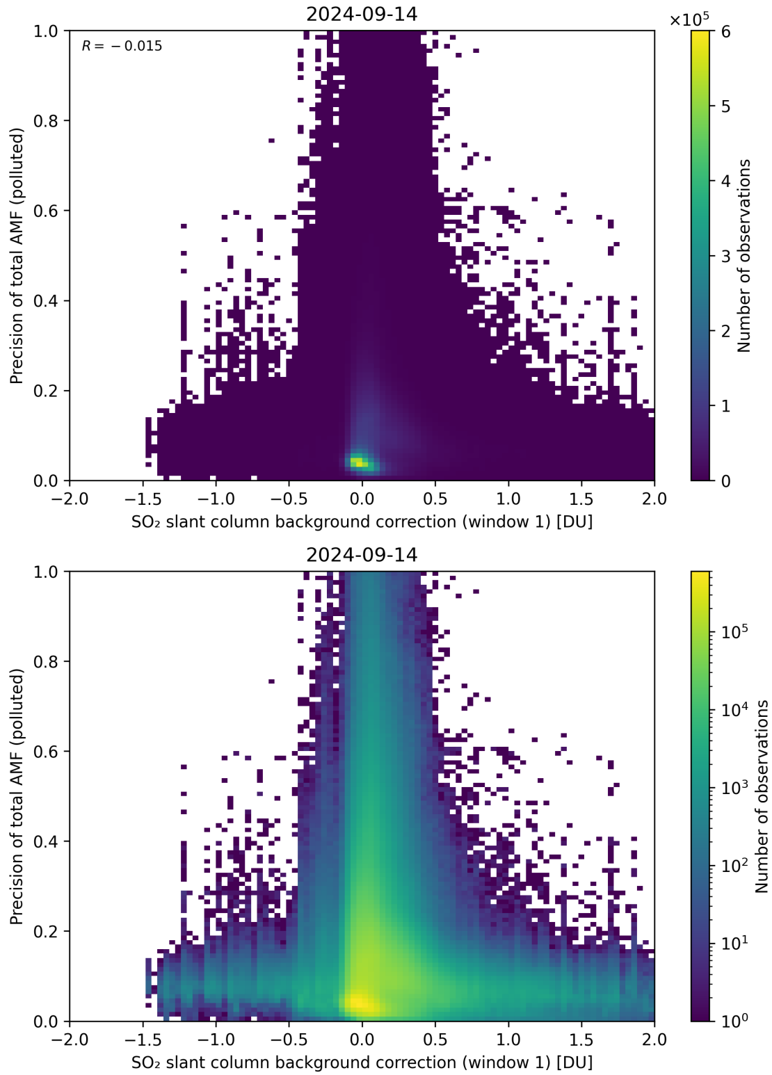
Figure 110: Scatter density plot of “SO 2 slant column background correction (window 1)” against “Precision of total AMF (polluted)” for 2024-09-13 to 2024-09-15.
