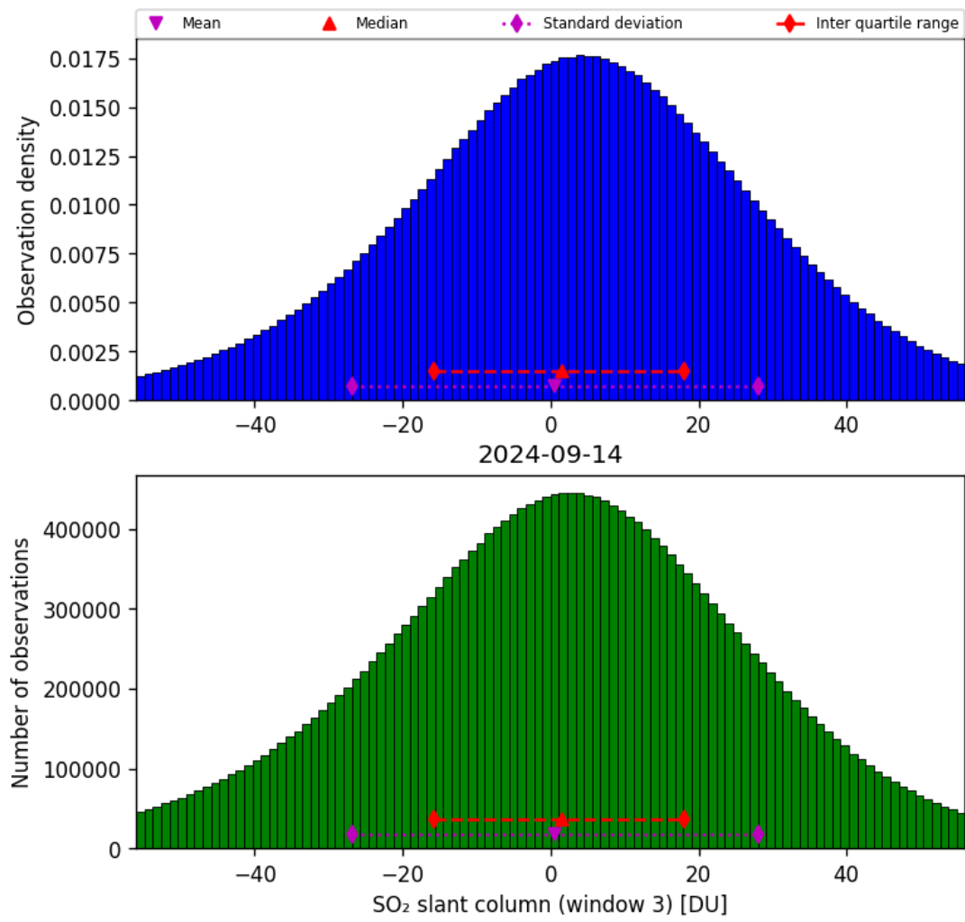
Figure 64: Histogram of “SO 2 slant column (window 3)” for 2024-09-13 to 2024-09-15
