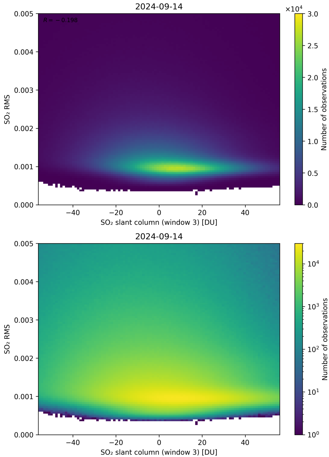
Figure 256: Scatter density plot of “SO 2 slant column (window 3)” against “SO 2 RMS” for 2024-09-13 to 2024-09-15.
