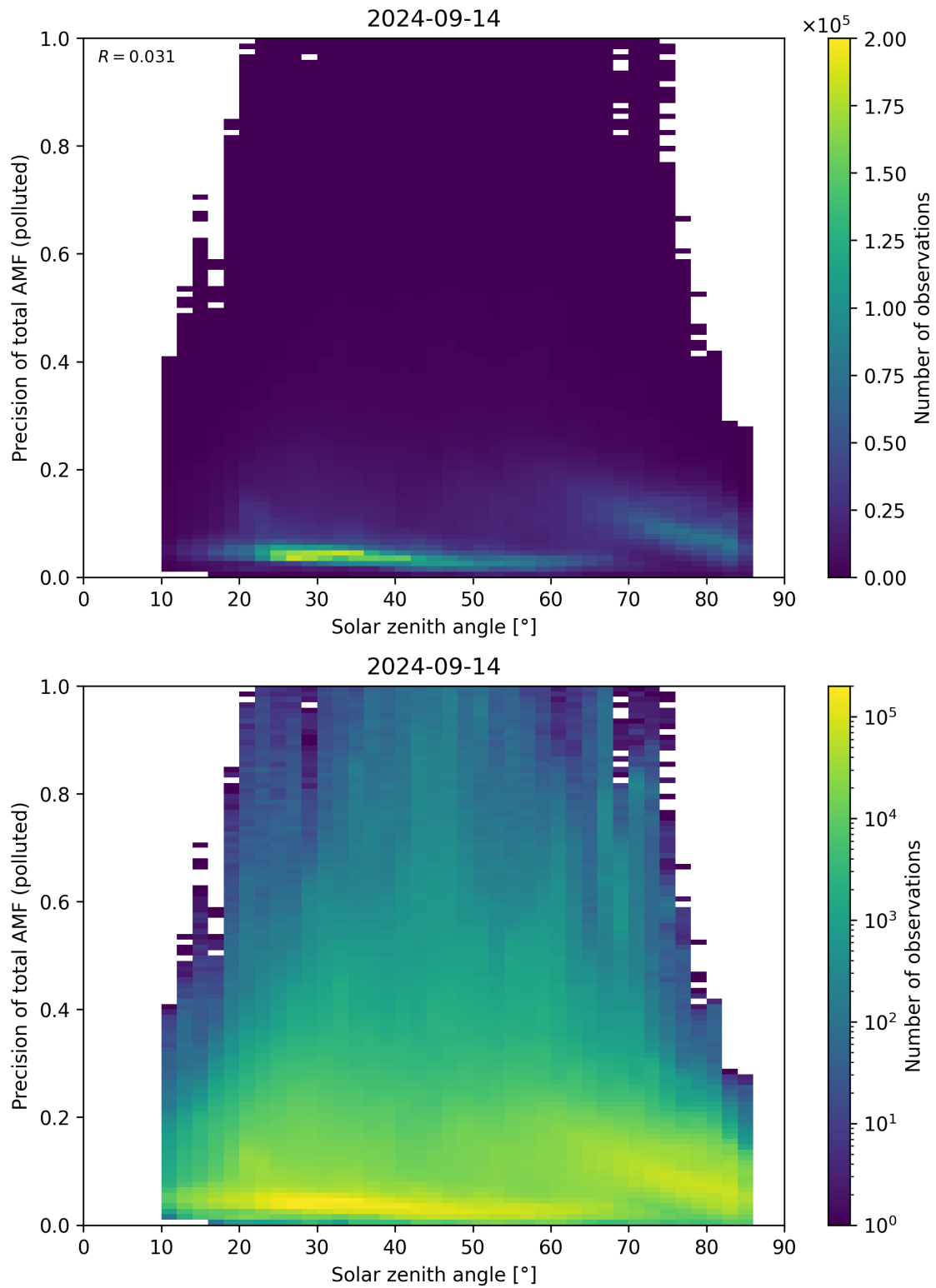
Figure 175: Scatter density plot of “Solar zenith angle” against “Precision of total AMF (polluted)” for 2024-09-13 to 2024-09-15.
