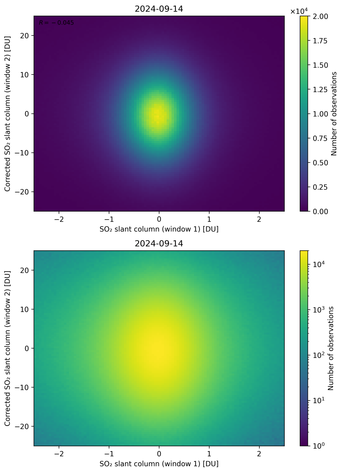
Figure 233: Scatter density plot of “SO 2 slant column (window 1)” against “Corrected SO 2 slant column (window 2)” for 2024-09-13 to 2024-09-15.
