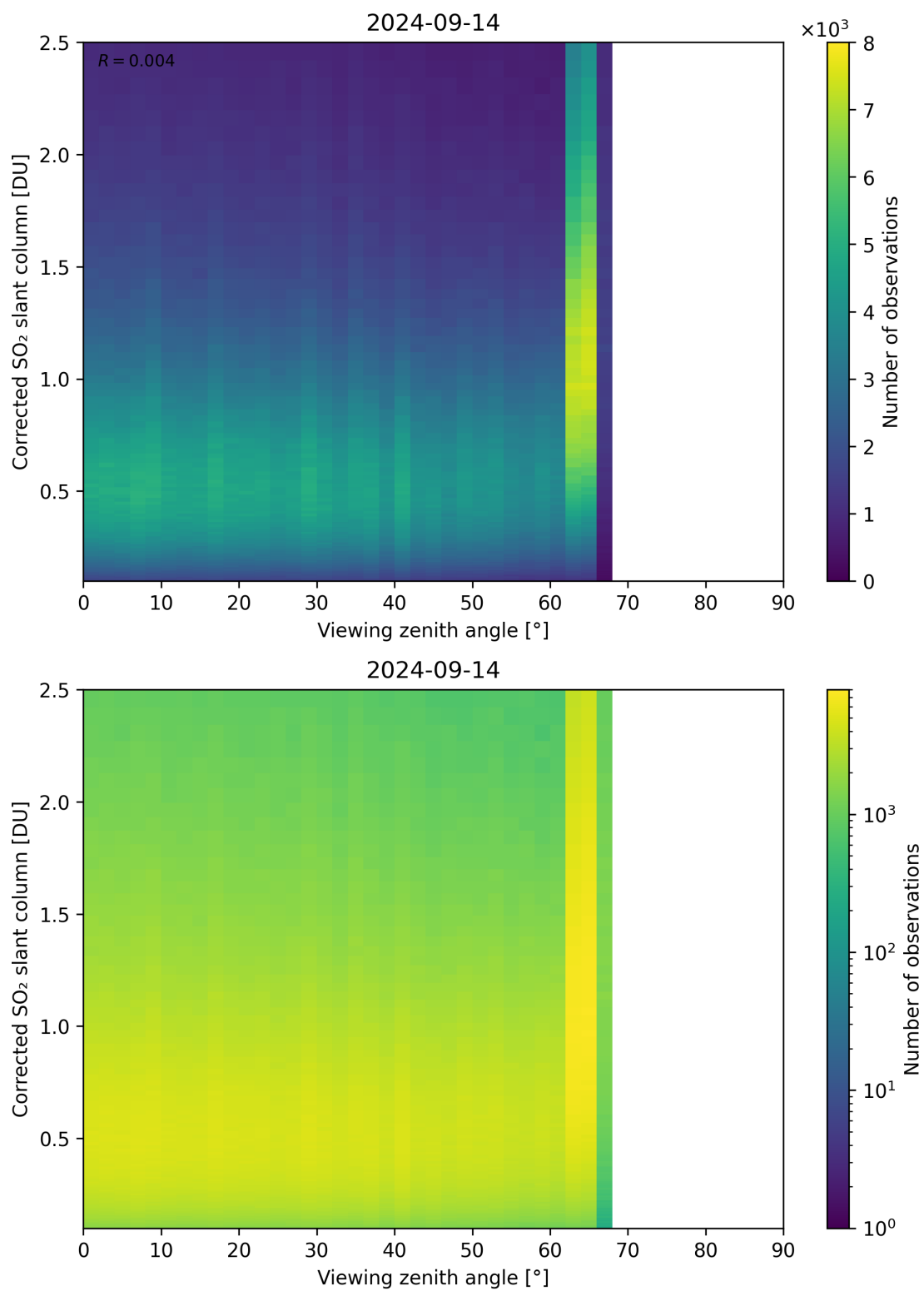
Figure 317: Scatter density plot of “Viewing zenith angle” against “Corrected SO 2 slant column” for 2024-09-13 to 2024-09-15.
