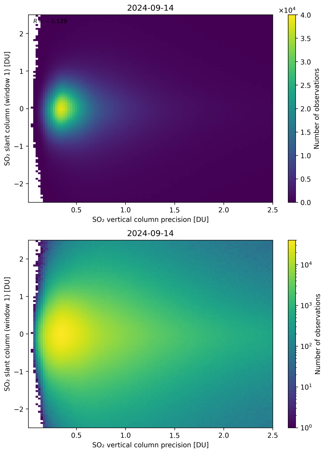
Figure 289: Scatter density plot of “SO 2 vertical column precision” against “SO 2 slant column (window 1)” for 2024-09-13 to 2024-09-15.
