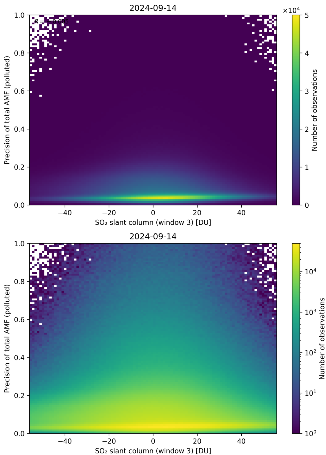
Figure 269: Scatter density plot of “SO 2 slant column (window 3)” against “Precision of total AMF (polluted)” for 2024-09-13 to 2024-09-15.
