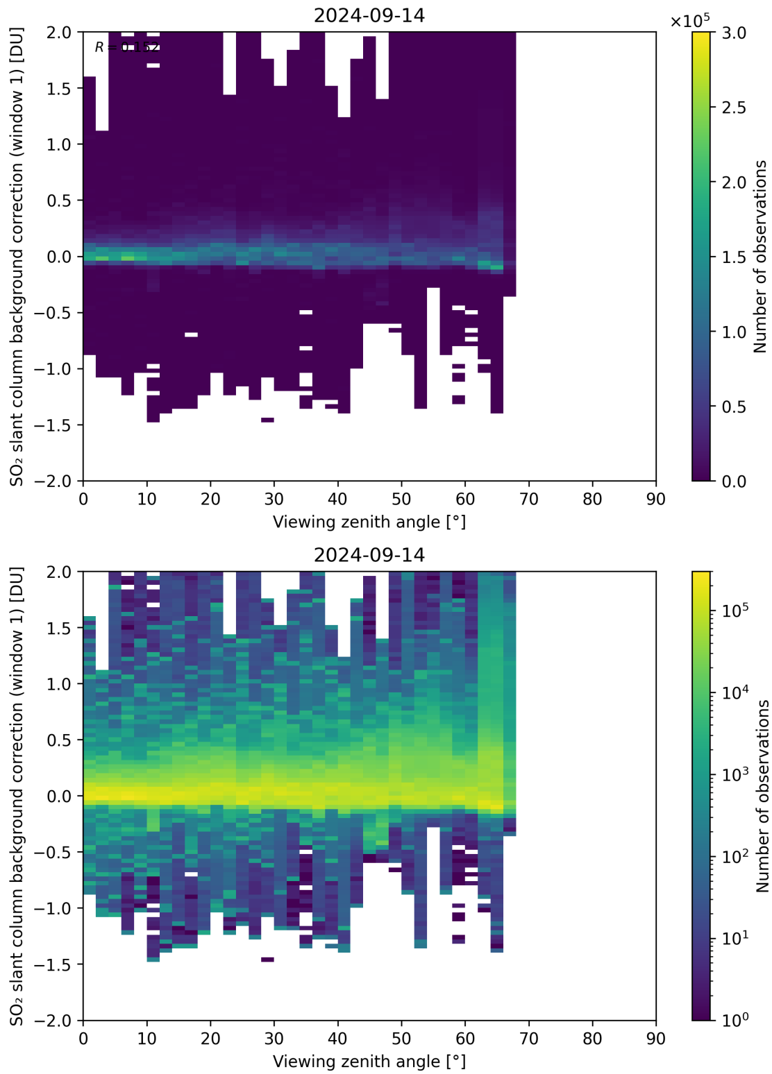
Figure 308: Scatter density plot of “Viewing zenith angle” against “SO 2 slant column background correction (window 1)” for 2024-09-13 to 2024-09-15.
