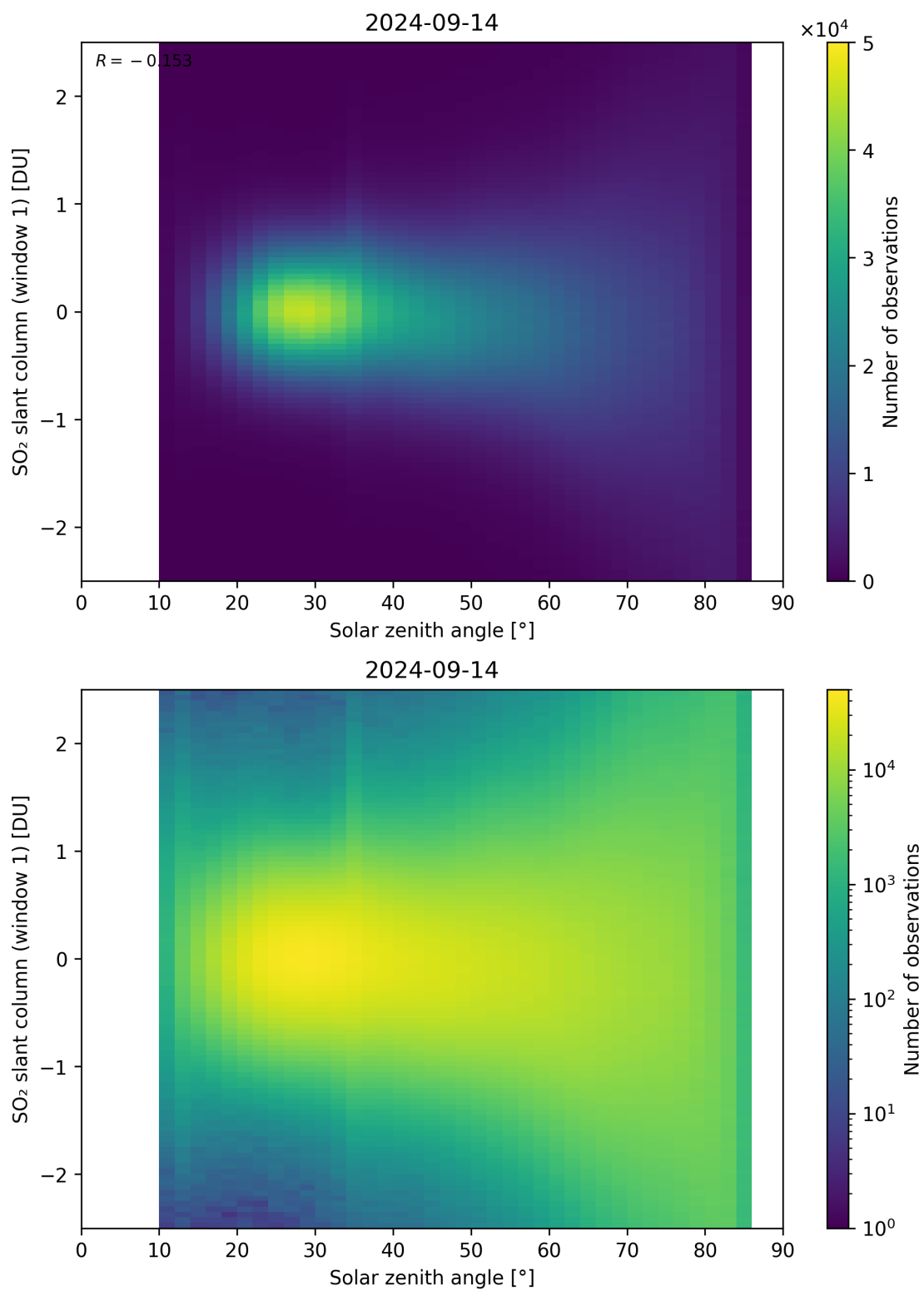
Figure 169: Scatter density plot of “Solar zenith angle” against “SO 2 slant column (window 1)” for 2024-09-13 to 2024-09-15.
