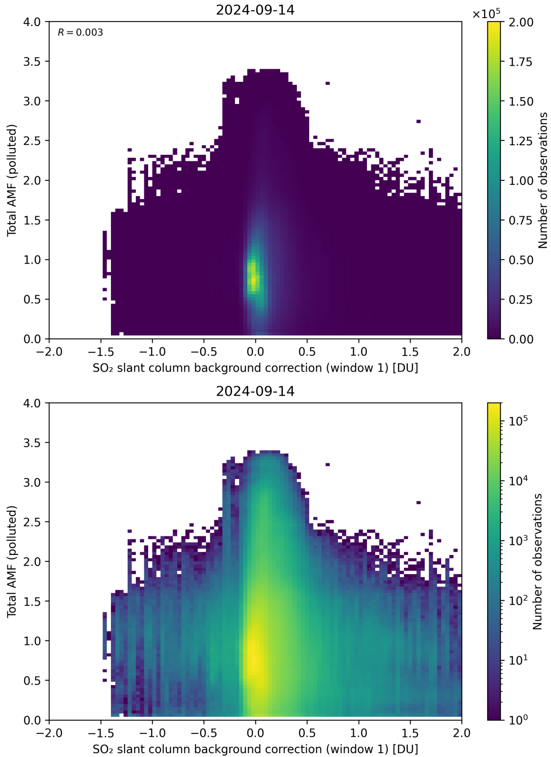
Figure 109: Scatter density plot of “SO 2 slant column background correction (window 1)” against “Total AMF (polluted)” for 2024-09-13 to 2024-09-15.
