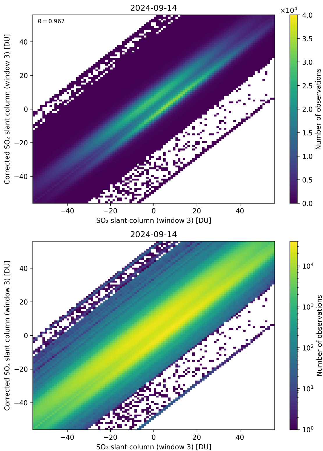
Figure 266: Scatter density plot of “SO 2 slant column (window 3)” against “Corrected SO 2 slant column (window 3)” for 2024-09-13 to 2024-09-15.
