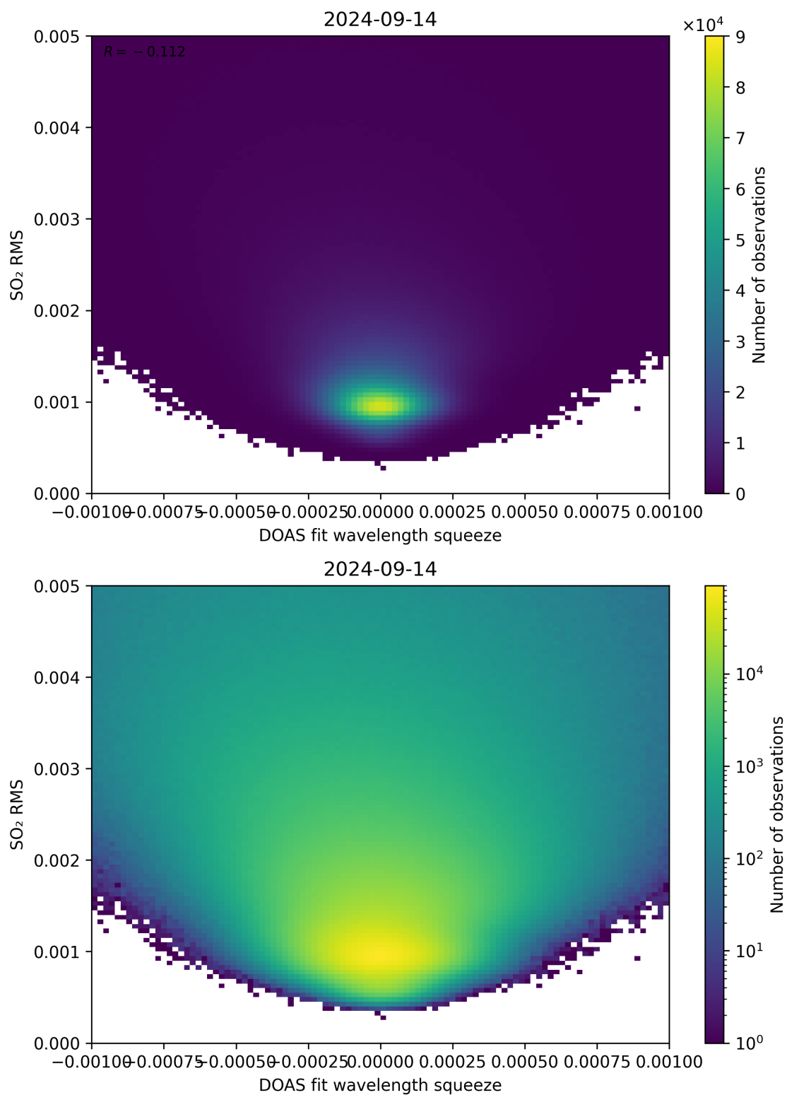
Figure 132: Scatter density plot of “DOAS fit wavelength squeeze” against “SO 2 RMS” for 2024-09-13 to 2024-09-15.
