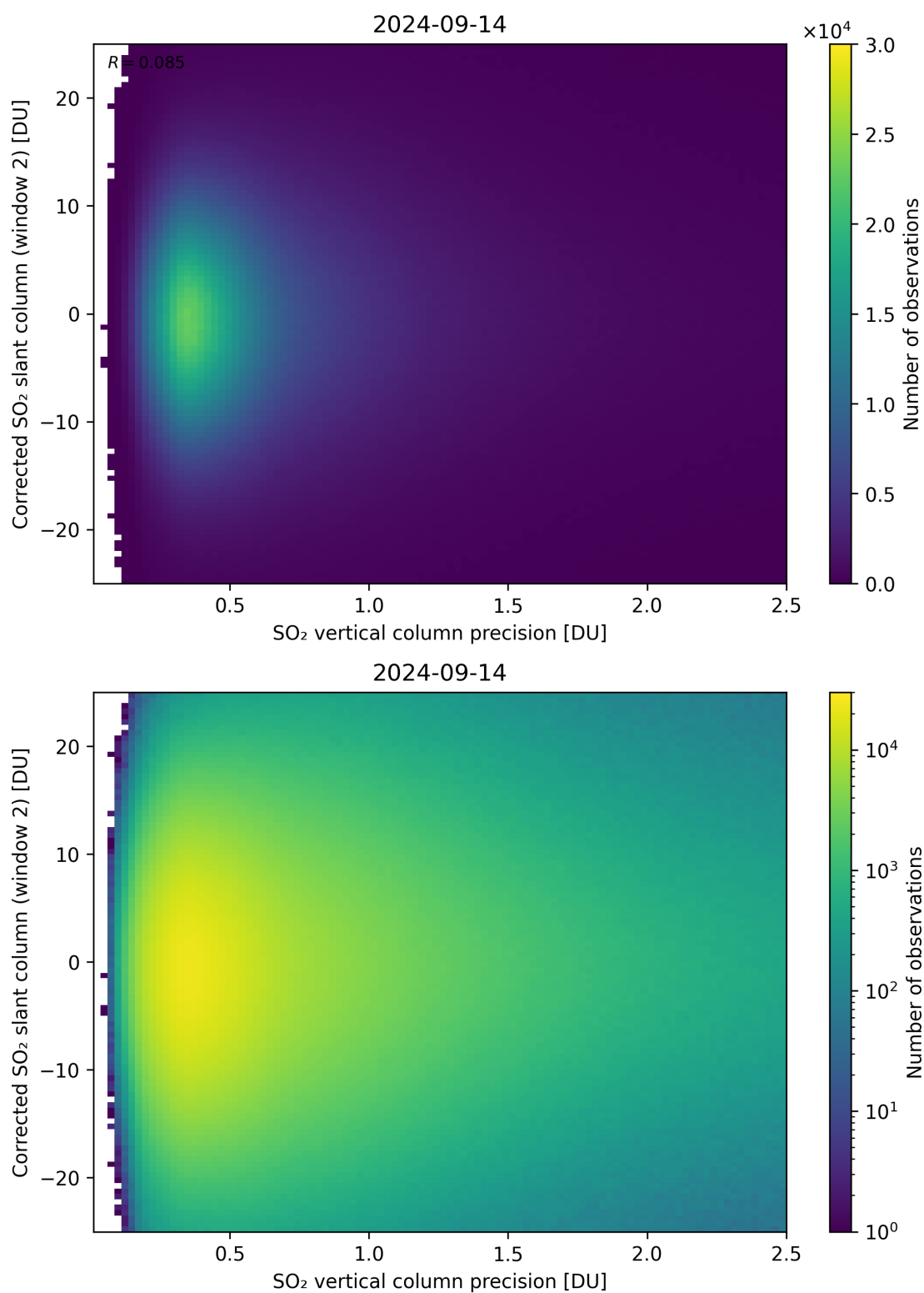
Figure 287: Scatter density plot of “SO 2 vertical column precision” against “Corrected SO 2 slant column (window 2)” for 2024-09-13 to 2024-09-15.
