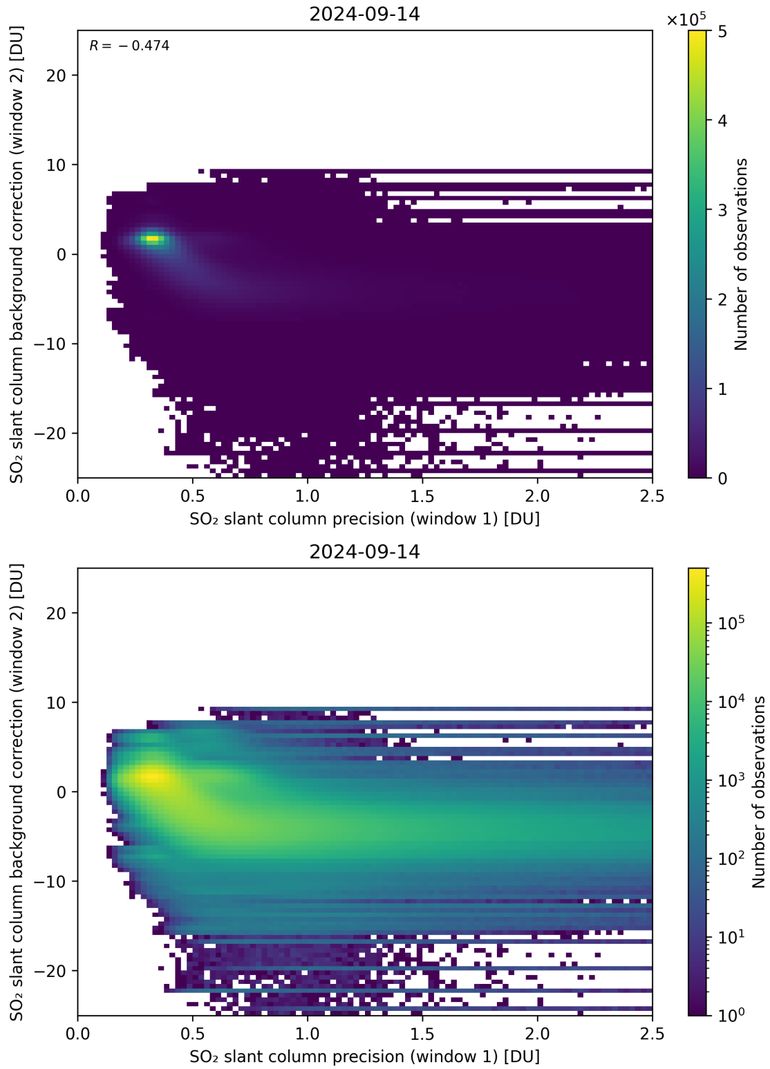
Figure 219: Scatter density plot of “SO 2 slant column precision (window 1)” against “SO 2 slant column background correction (window 2)” for 2024-09-13 to 2024-09-15.
