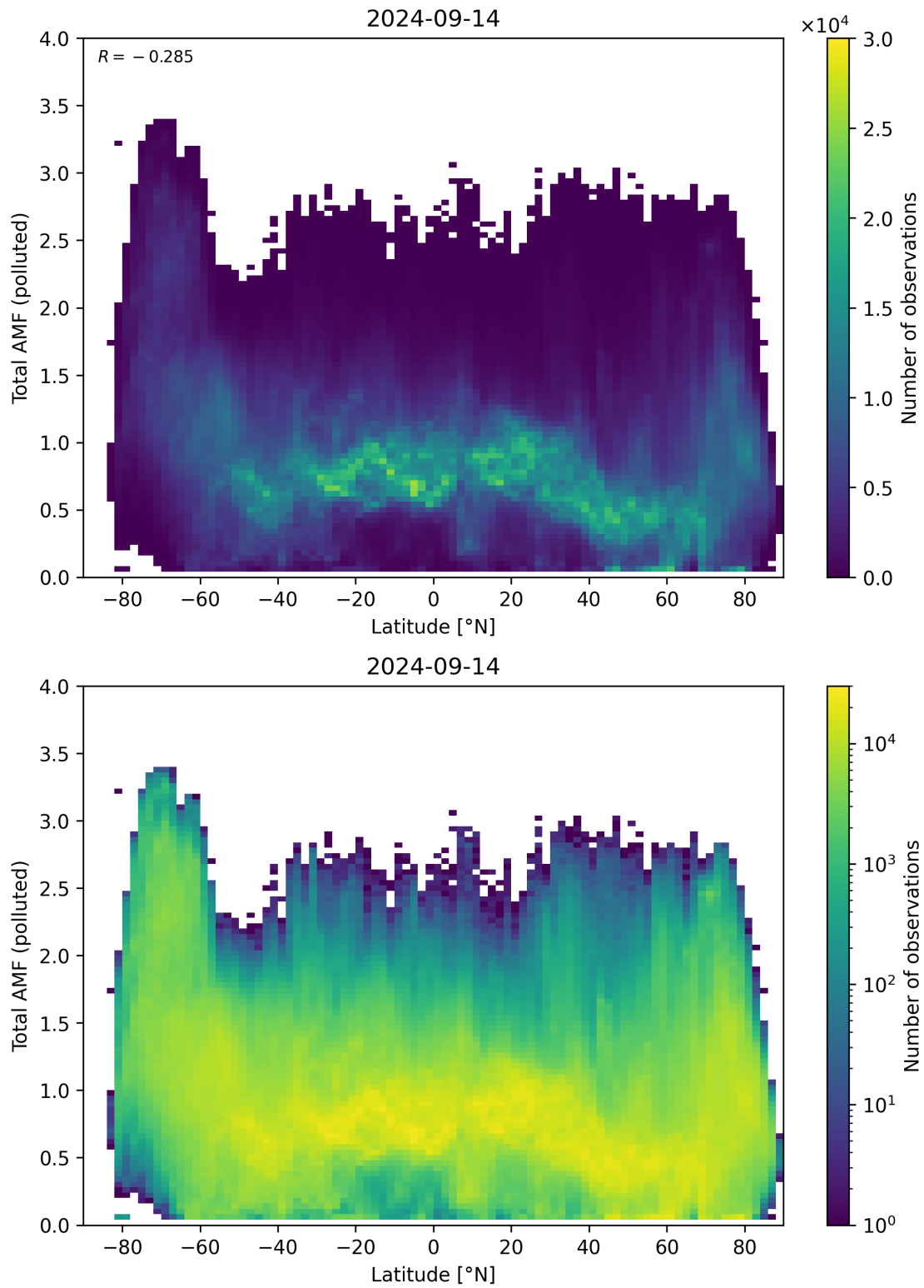
Figure 154: Scatter density plot of “Latitude” against “Total AMF (polluted)” for 2024-09-13 to 2024-09-15.
