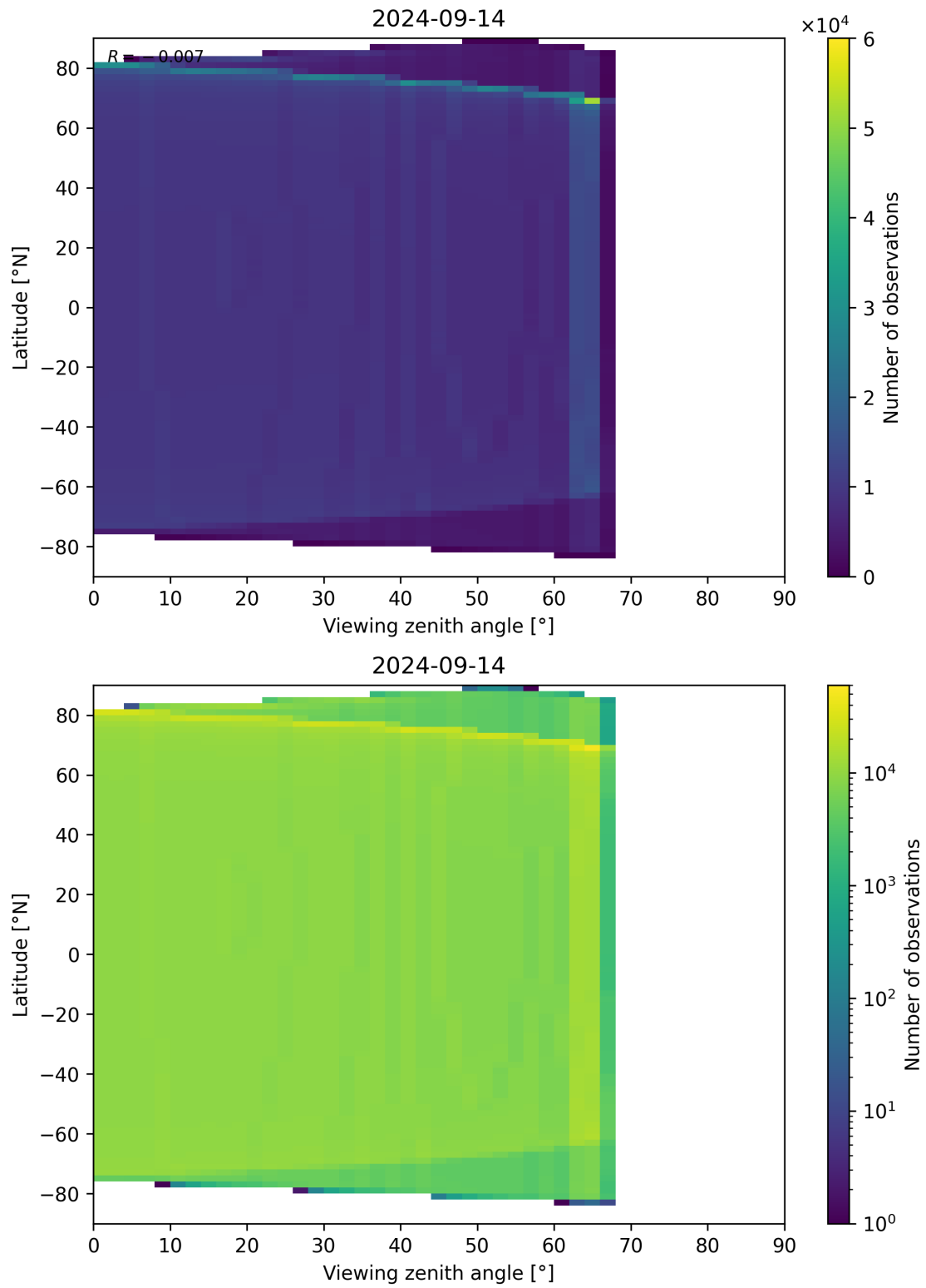
Figure 314: Scatter density plot of “Viewing zenith angle” against “Latitude” for 2024-09-13 to 2024-09-15.
