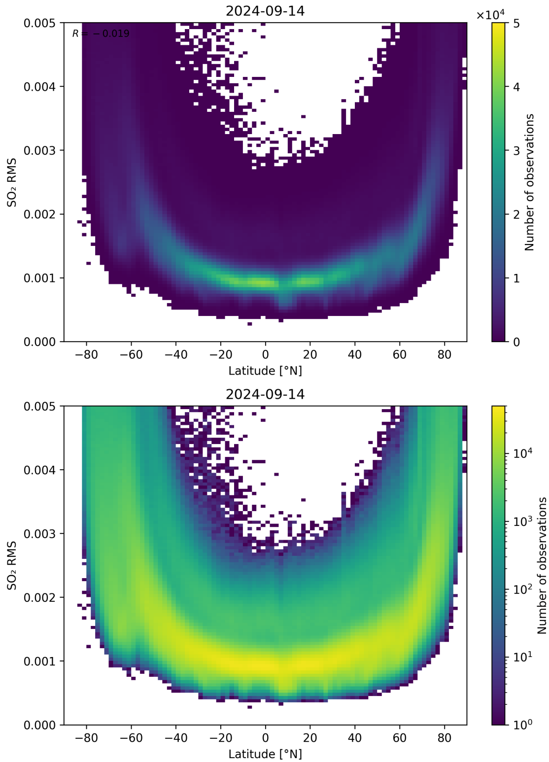
Figure 144: Scatter density plot of “Latitude” against “SO 2 RMS” for 2024-09-13 to 2024-09-15.
