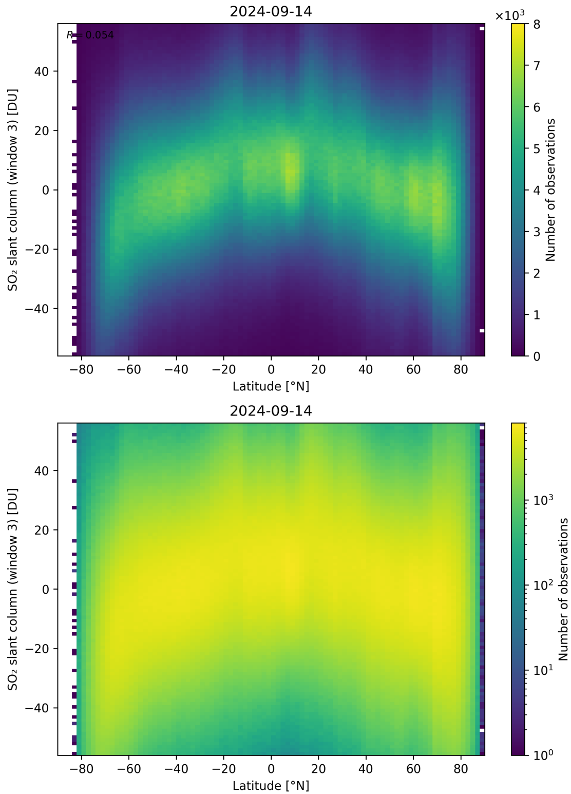
Figure 152: Scatter density plot of “Latitude” against “SO 2 slant column (window 3)” for 2024-09-13 to 2024-09-15.
