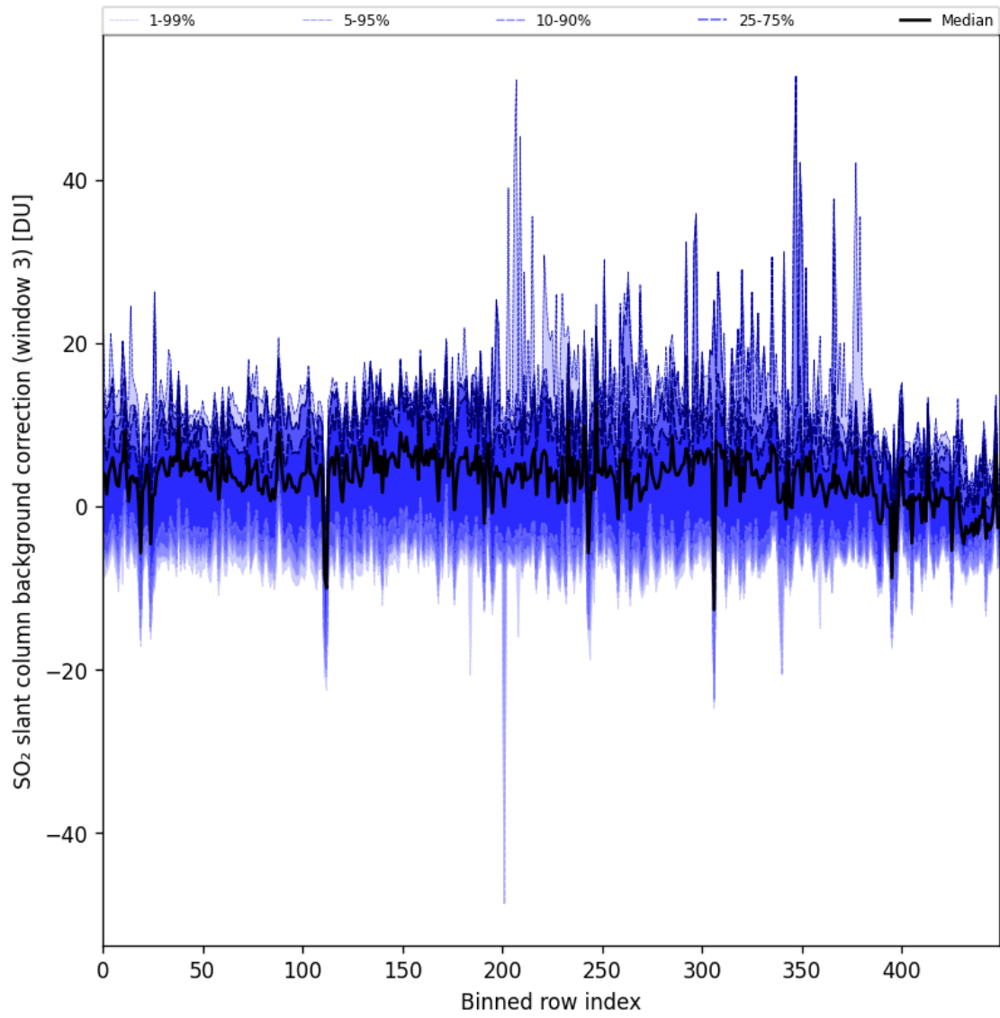
Figure 90: Along track statistics of “SO 2 slant column background correction (window 3)” for 2024-09-13 to 2024-09-15
