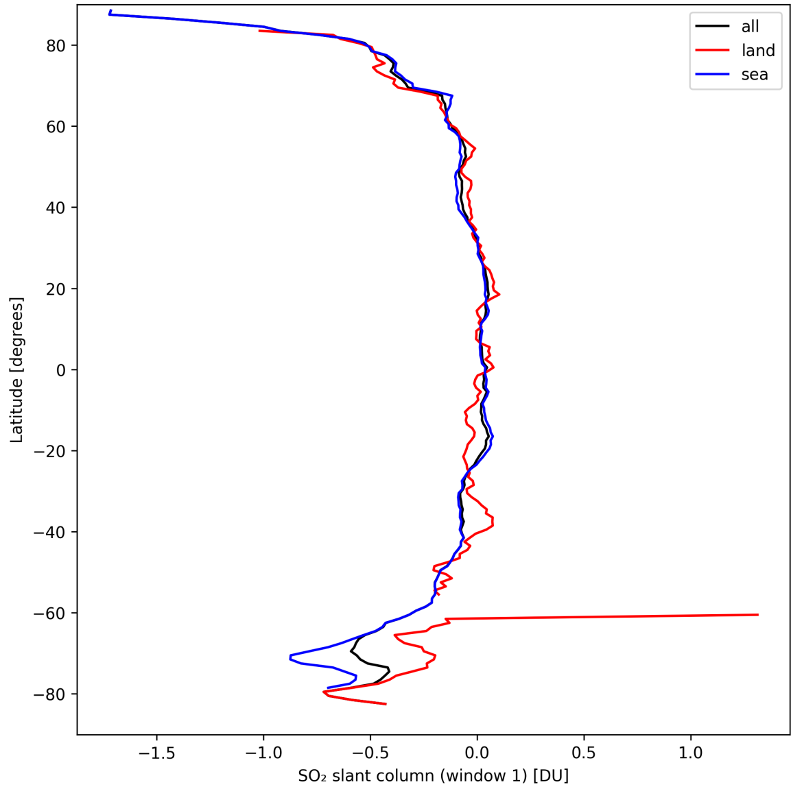
Figure 33: Zonal average of “SO 2 slant column (window 1)” for 2024-09-13 to 2024-09-15.
