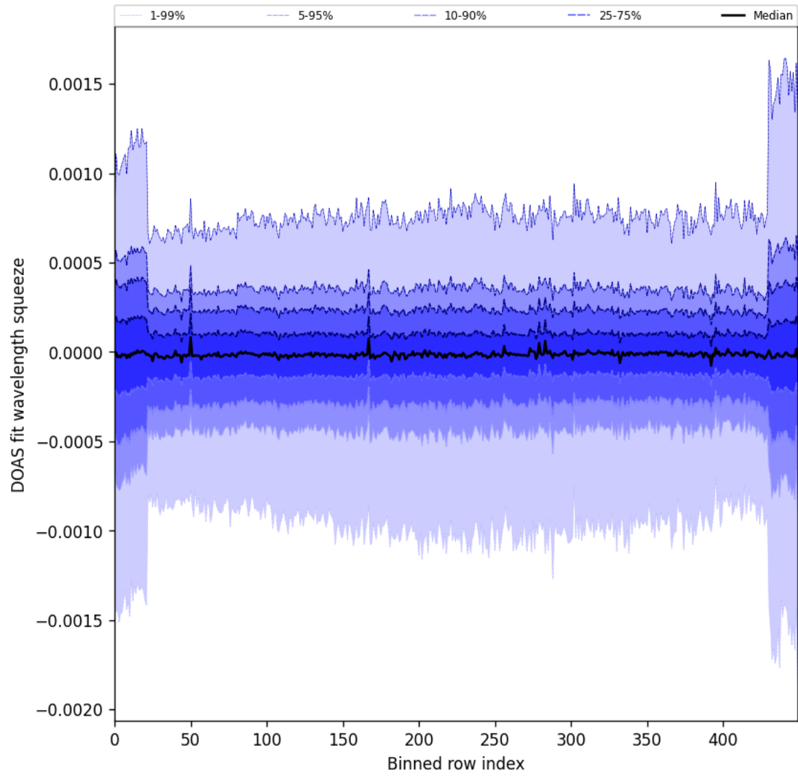
Figure 92: Along track statistics of “DOAS fit wavelength squeeze” for 2024-09-13 to 2024-09-15
