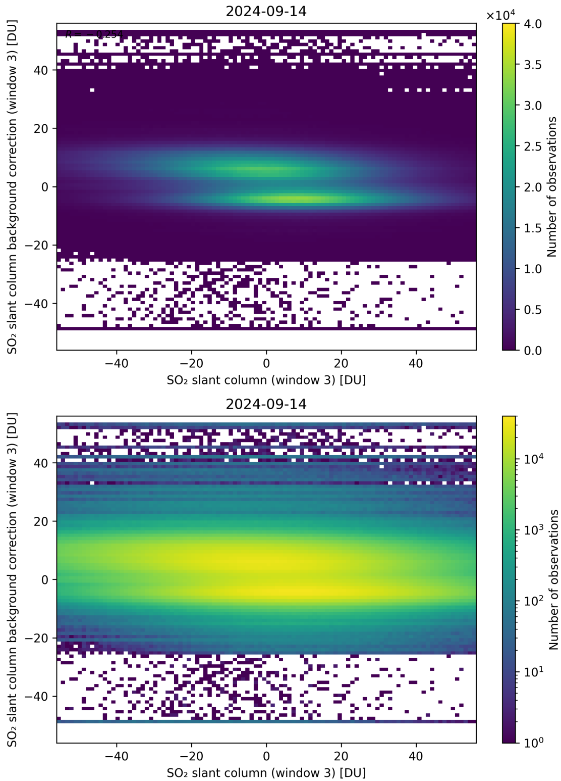
Figure 253: Scatter density plot of “SO 2 slant column (window 3)” against “SO 2 slant column background correction (window 3)” for 2024-09-13 to 2024-09-15.
