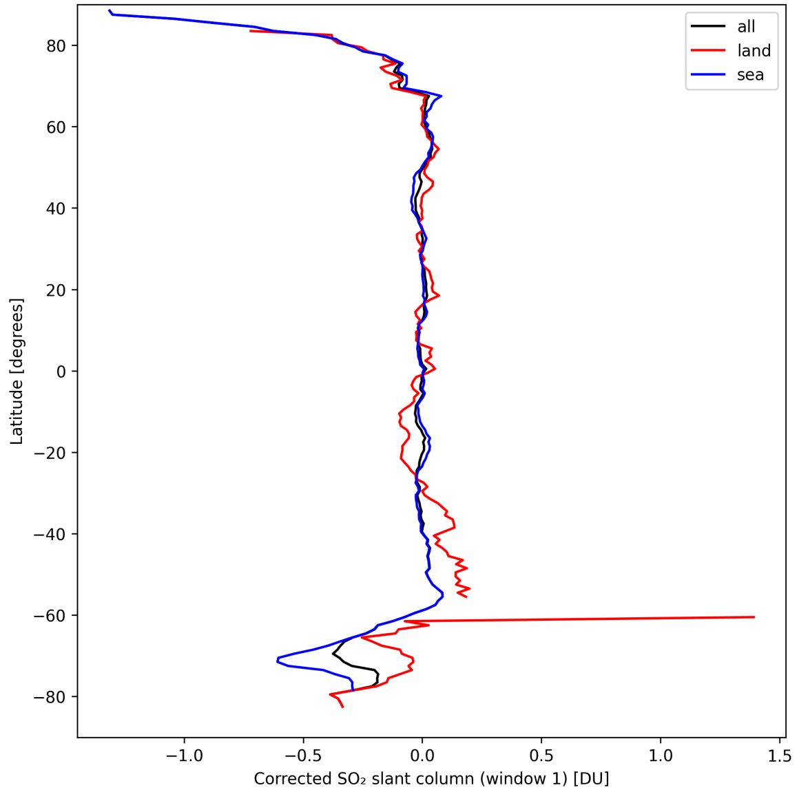
Figure 35: Zonal average of “Corrected SO 2 slant column (window 1)” for 2024-09-13 to 2024-09-15.
