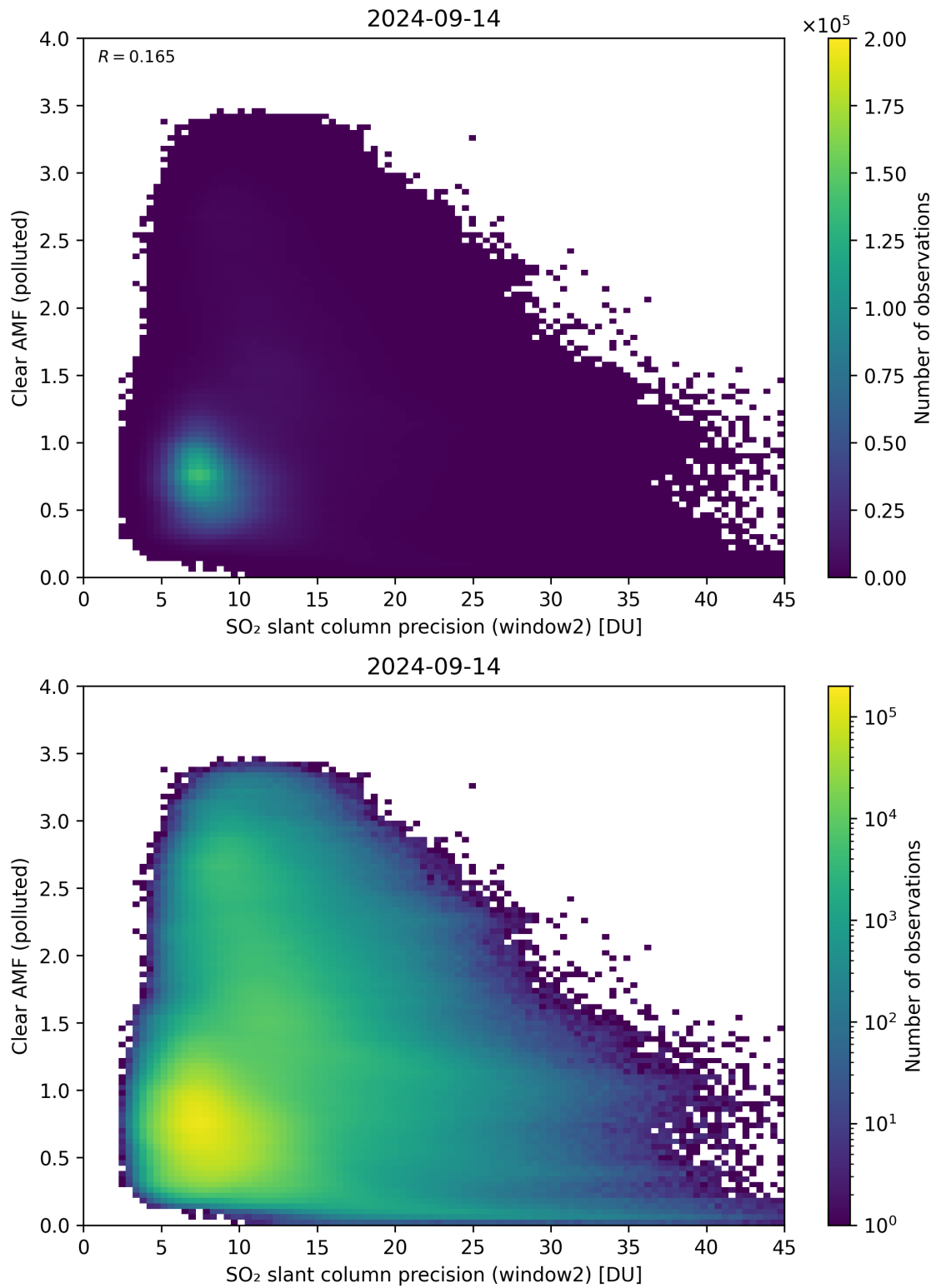
Figure 246: Scatter density plot of “SO 2 slant column precision (window2)” against “Clear AMF (polluted)” for 2024-09-13 to 2024-09-15.
