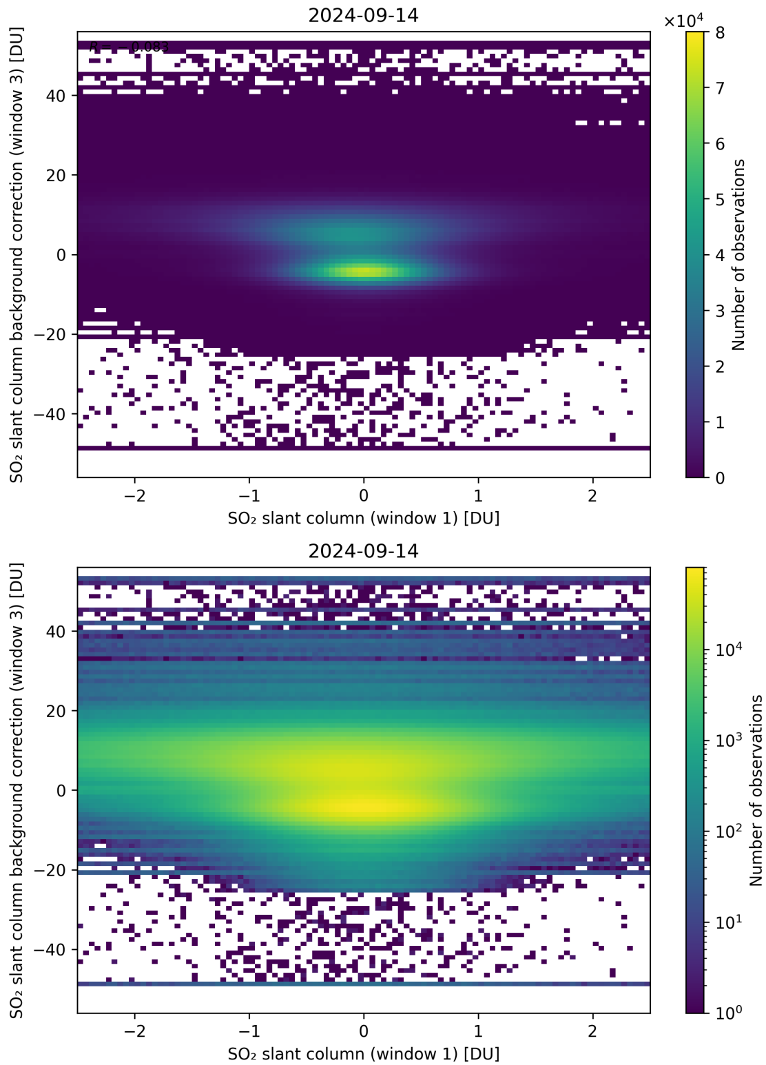
Figure 214: Scatter density plot of “SO 2 slant column (window 1)” against “SO 2 slant column background correction (window 3)” for 2024-09-13 to 2024-09-15.
