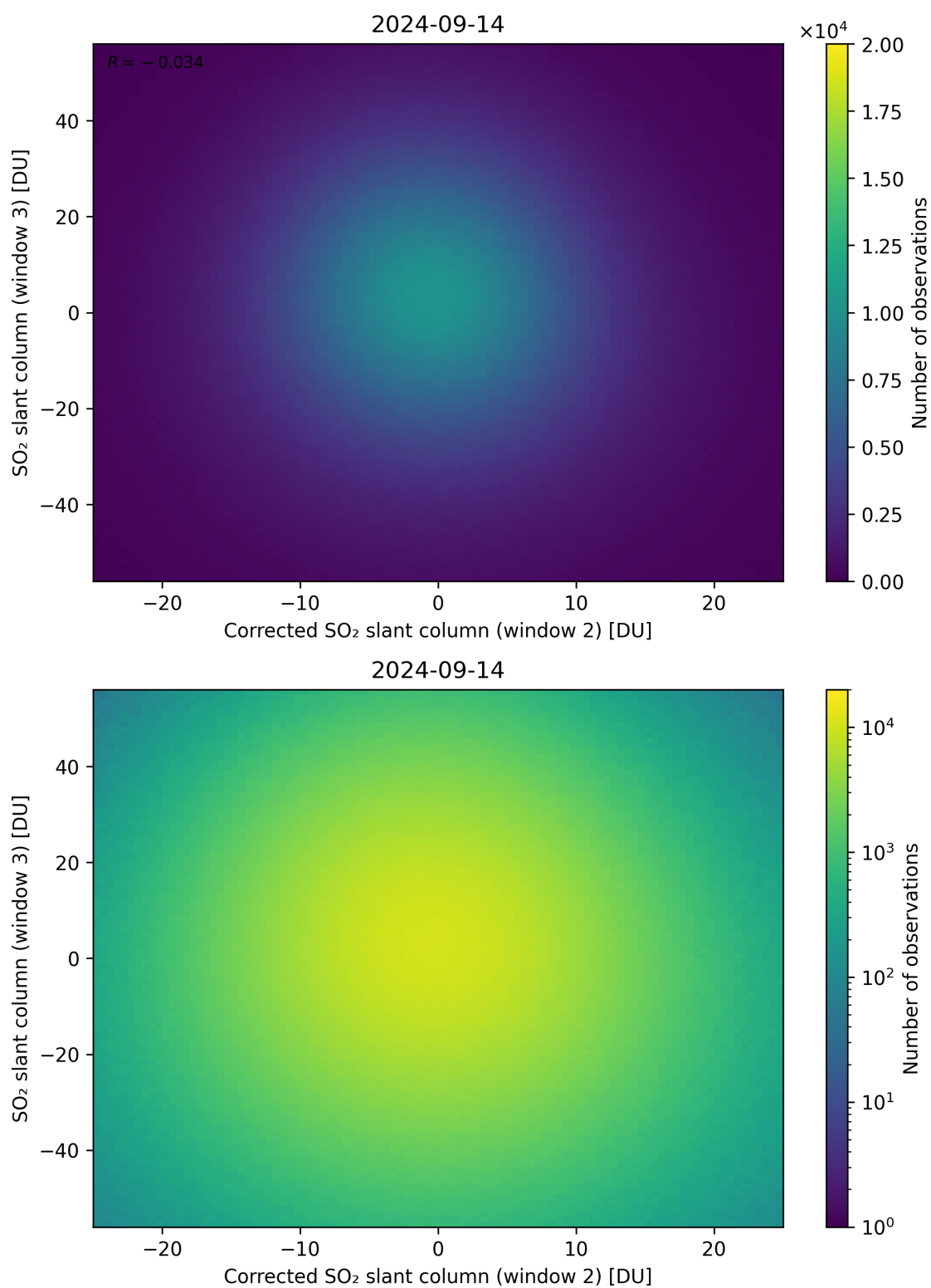
Figure 201: Scatter density plot of “Corrected SO 2 slant column (window 2)” against “SO 2 slant column (window 3)” for 2024-09-13 to 2024-09-15.
