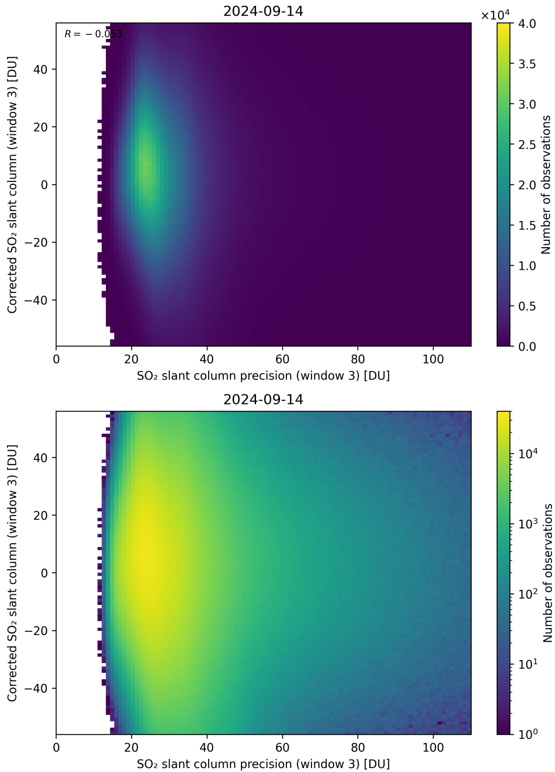
Figure 262: Scatter density plot of “SO 2 slant column precision (window 3)” against “Corrected SO 2 slant column (window 3)” for 2024-09-13 to 2024-09-15.
