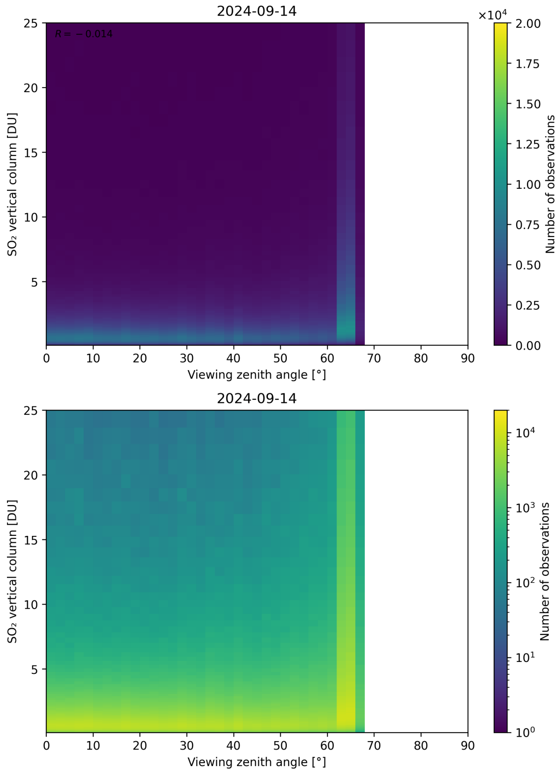
Figure 327: Scatter density plot of “Viewing zenith angle” against “SO 2 vertical column” for 2024-09-13 to 2024-09-15.
