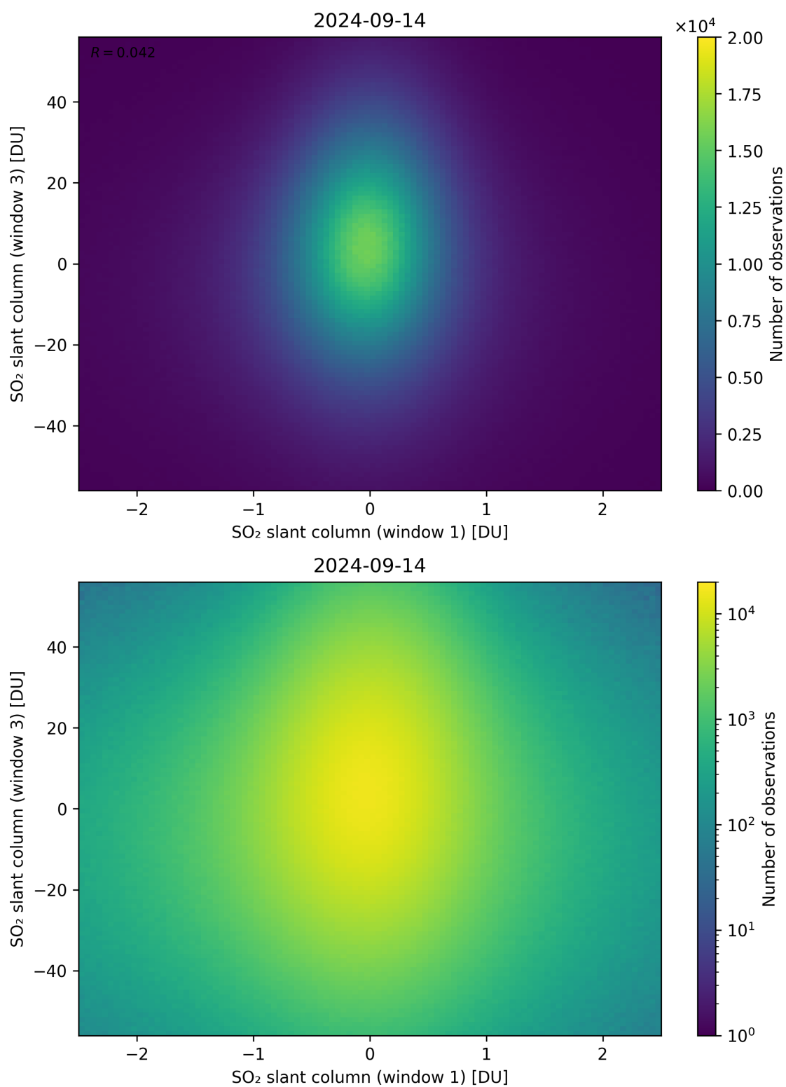
Figure 237: Scatter density plot of “SO 2 slant column (window 1)” against “SO 2 slant column (window 3)” for 2024-09-13 to 2024-09-15.
