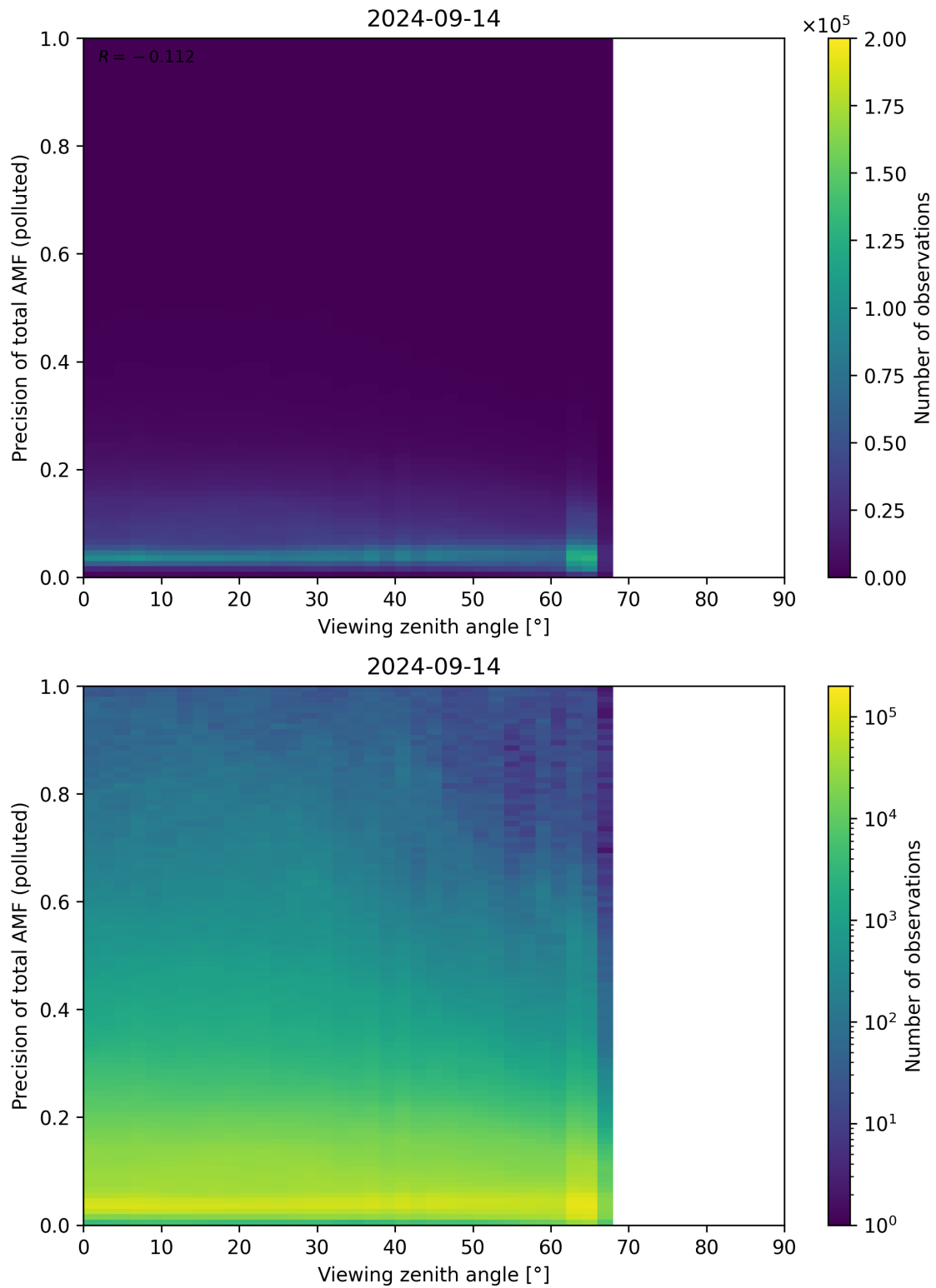
Figure 326: Scatter density plot of “Viewing zenith angle” against “Precision of total AMF (polluted)” for 2024-09-13 to 2024-09-15.
