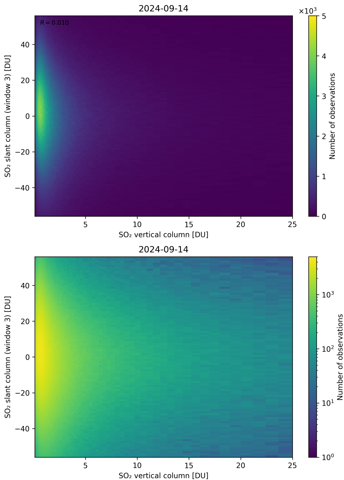
Figure 303: Scatter density plot of “SO 2 vertical column” against “SO 2 slant column (window 3)” for 2024-09-13 to 2024-09-15.
