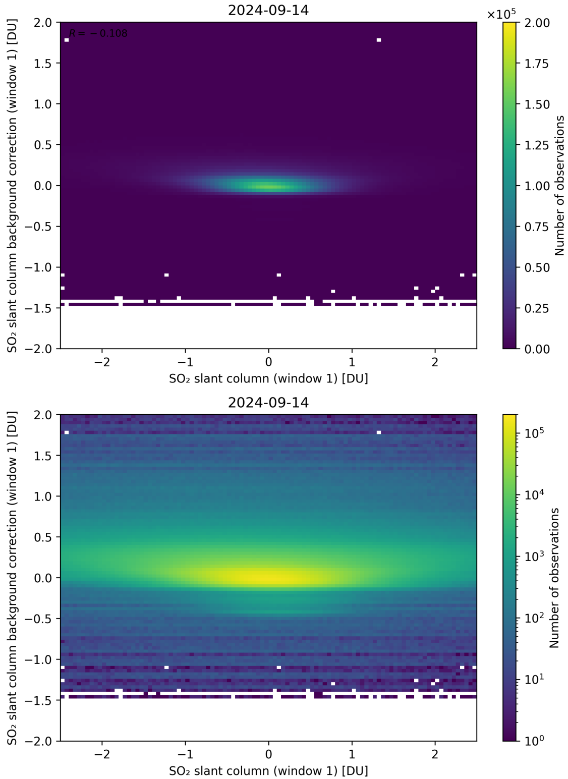
Figure 212: Scatter density plot of “SO 2 slant column (window 1)” against “SO 2 slant column background correction (window 1)” for 2024-09-13 to 2024-09-15.
