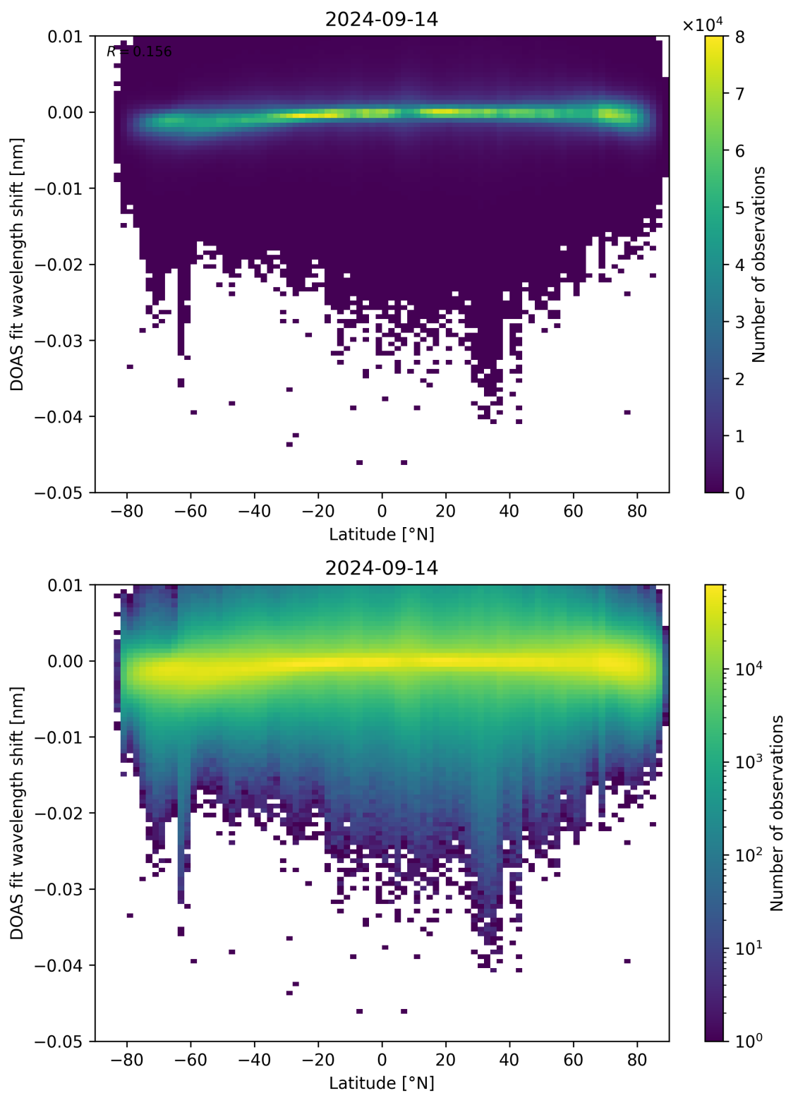
Figure 142: Scatter density plot of “Latitude” against “DOAS fit wavelength shift” for 2024-09-13 to 2024-09-15.
