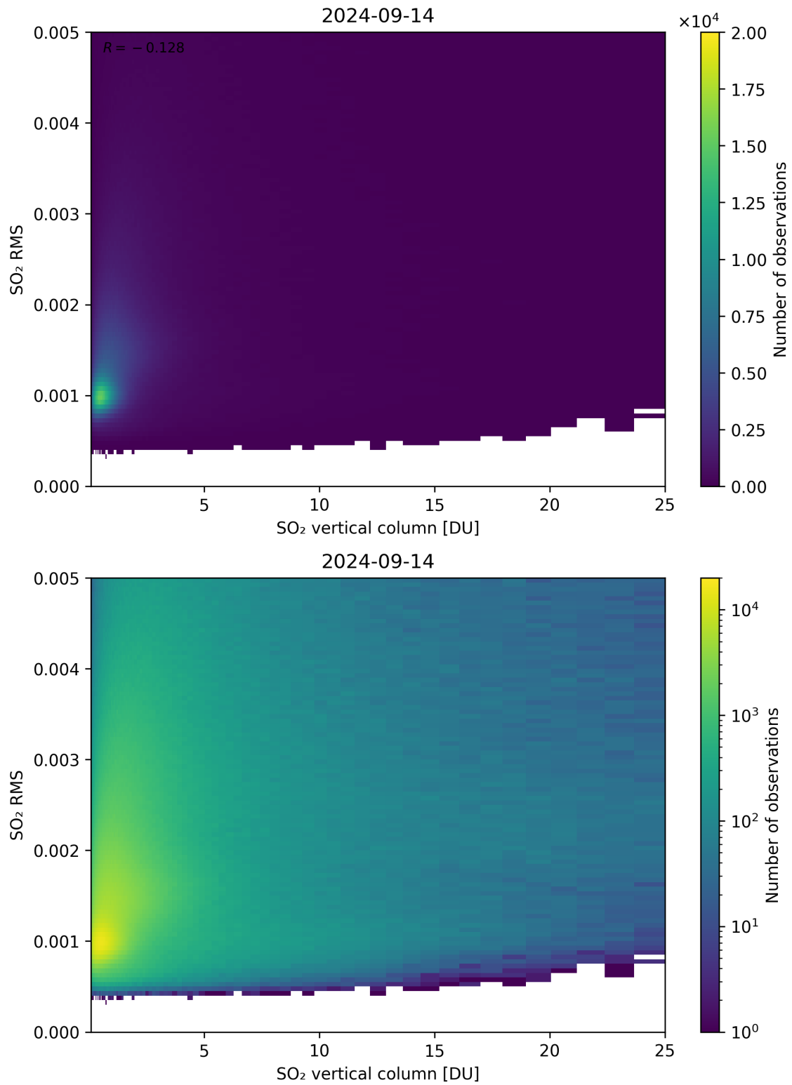
Figure 278: Scatter density plot of “SO 2 vertical column” against “SO 2 RMS” for 2024-09-13 to 2024-09-15.
