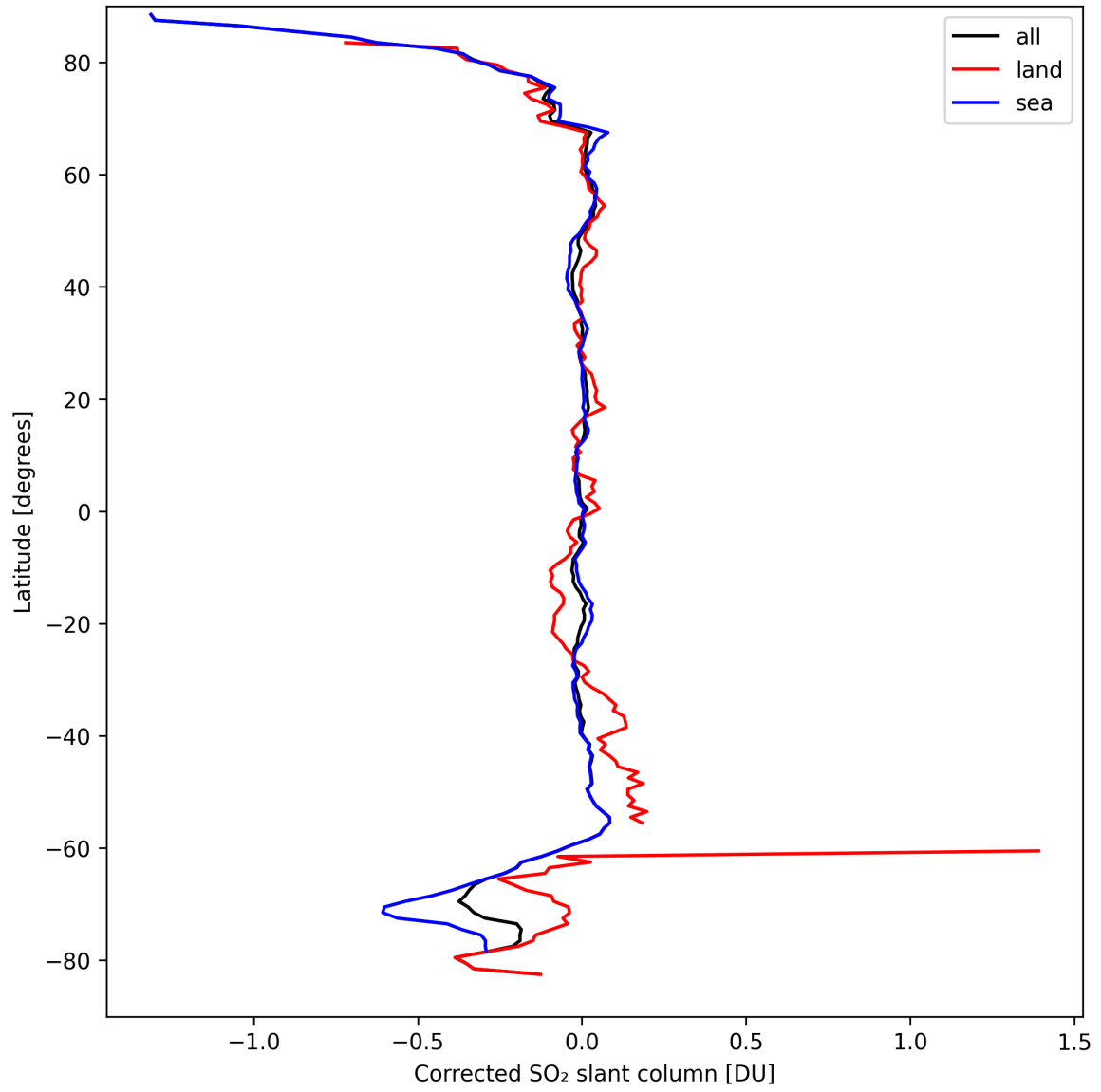
Figure 32: Zonal average of “Corrected SO 2 slant column” for 2024-09-13 to 2024-09-15.
