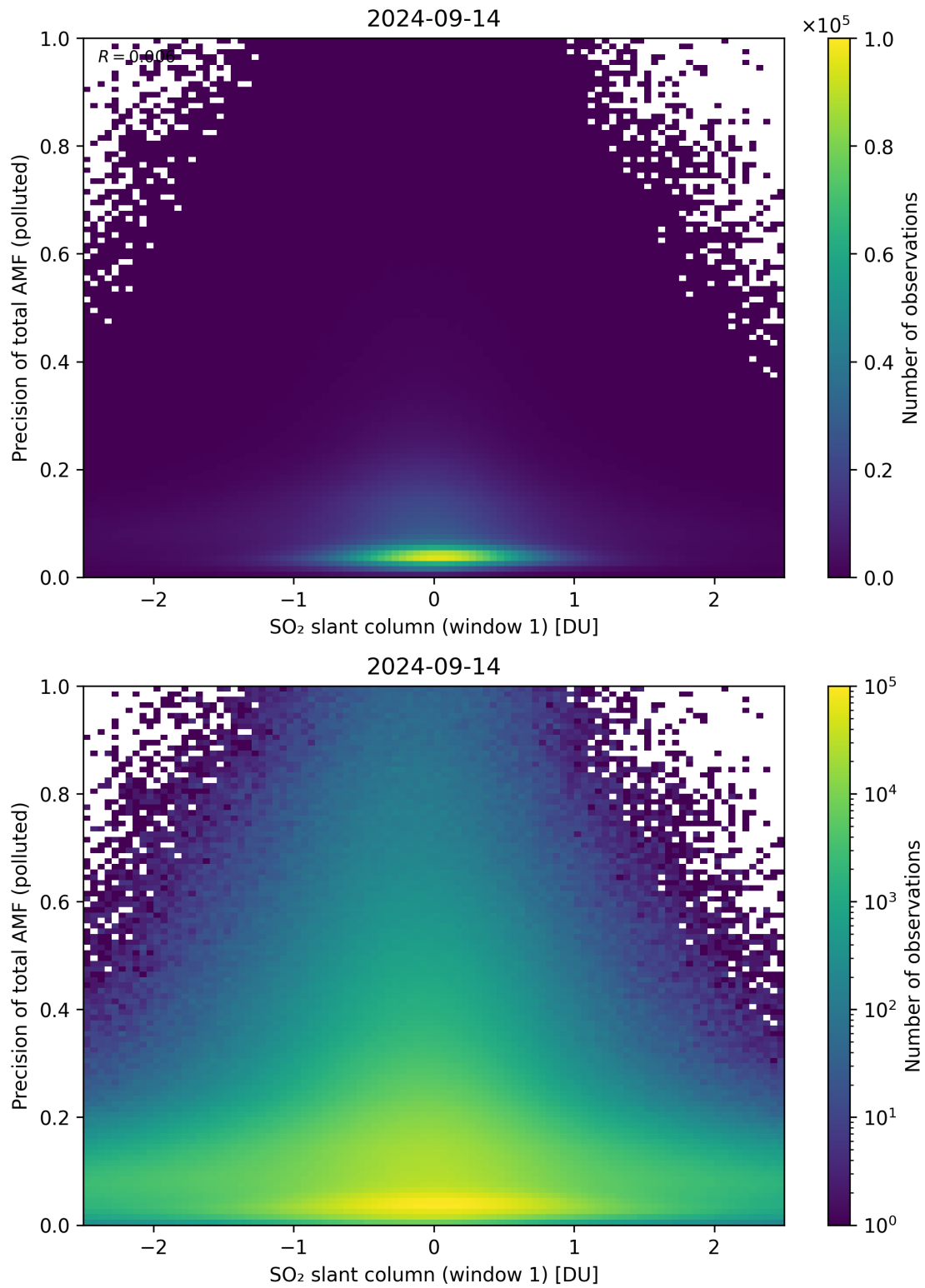
Figure 240: Scatter density plot of “SO 2 slant column (window 1)” against “Precision of total AMF (polluted)” for 2024-09-13 to 2024-09-15.
