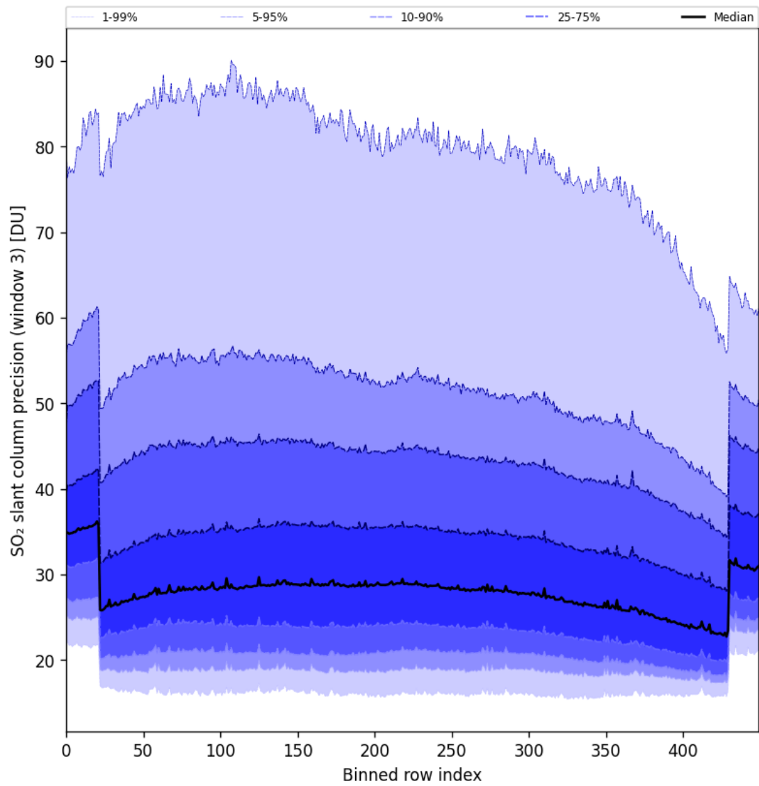
Figure 88: Along track statistics of “SO 2 slant column precision (window 3)” for 2024-09-13 to 2024-09-15
