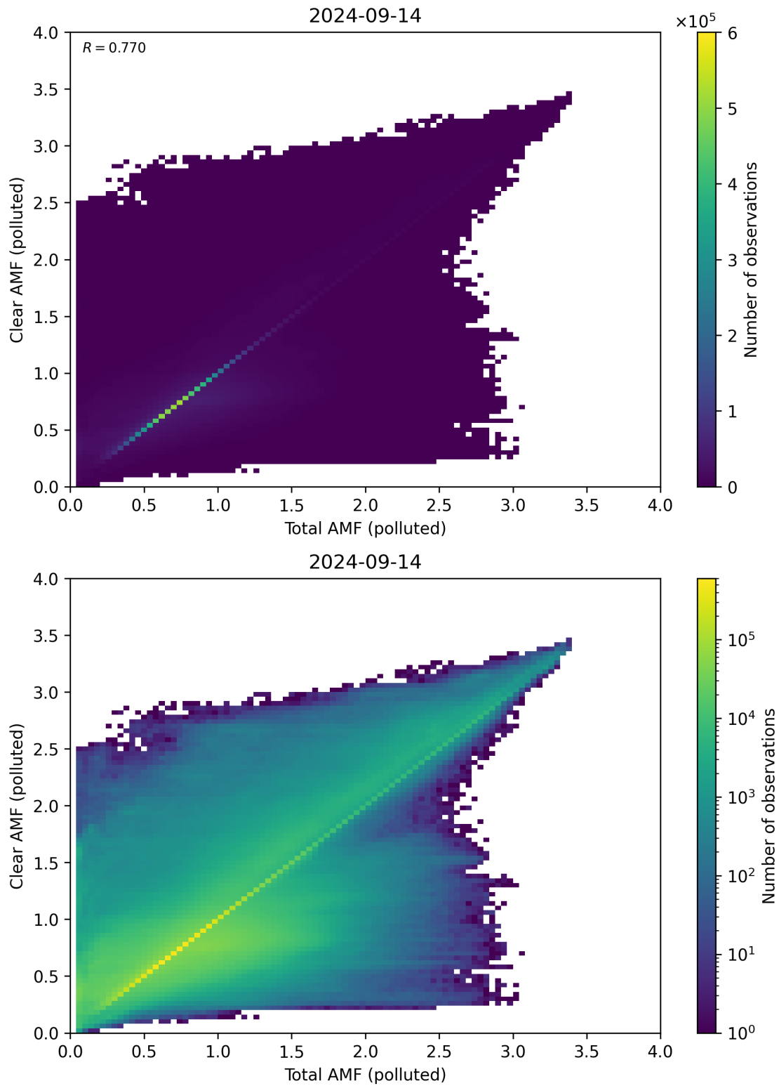
Figure 271: Scatter density plot of “Total AMF (polluted)” against “Clear AMF (polluted)” for 2024-09-13 to 2024-09-15.
