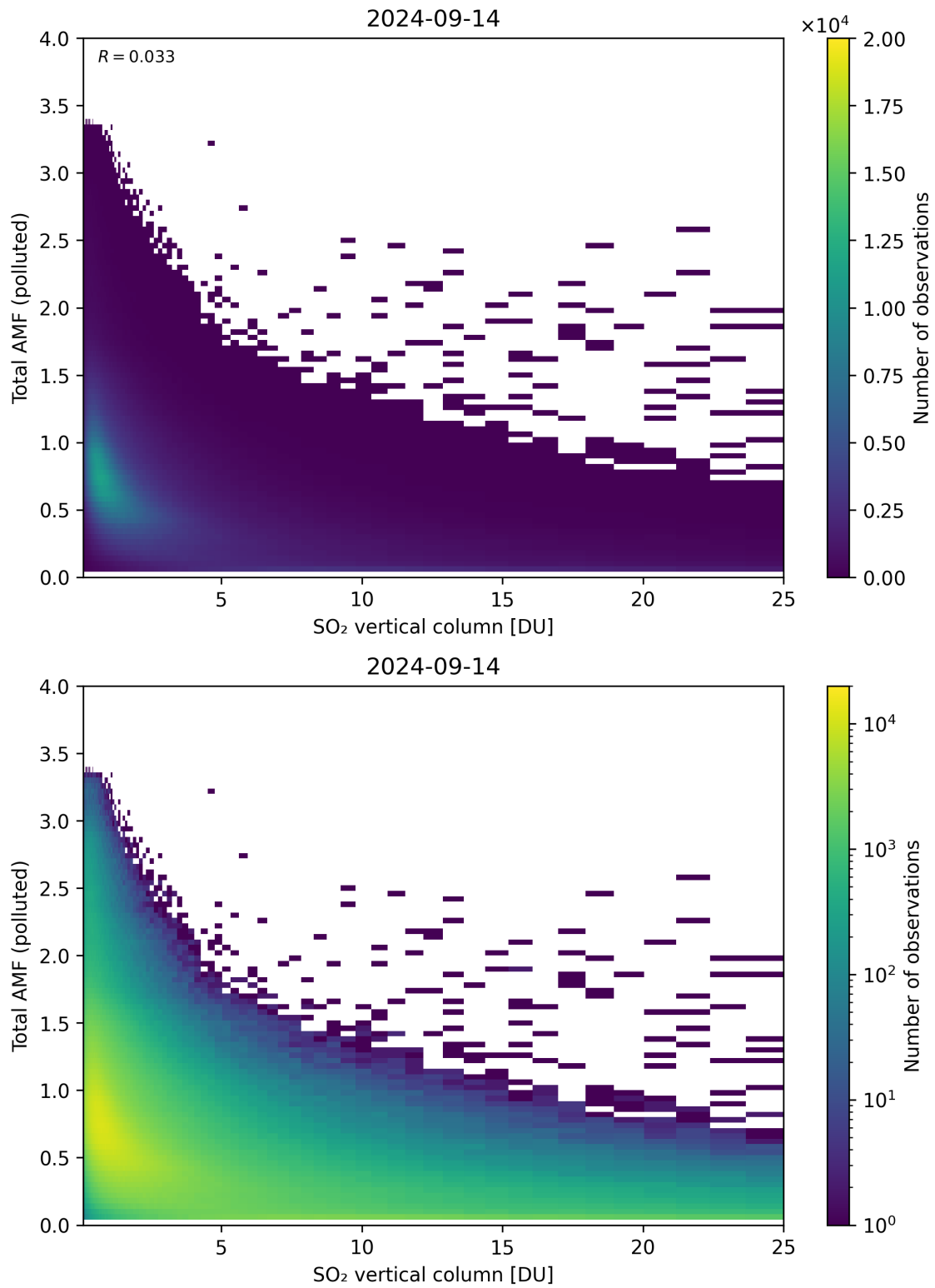
Figure 305: Scatter density plot of “SO 2 vertical column” against “Total AMF (polluted)” for 2024-09-13 to 2024-09-15.
