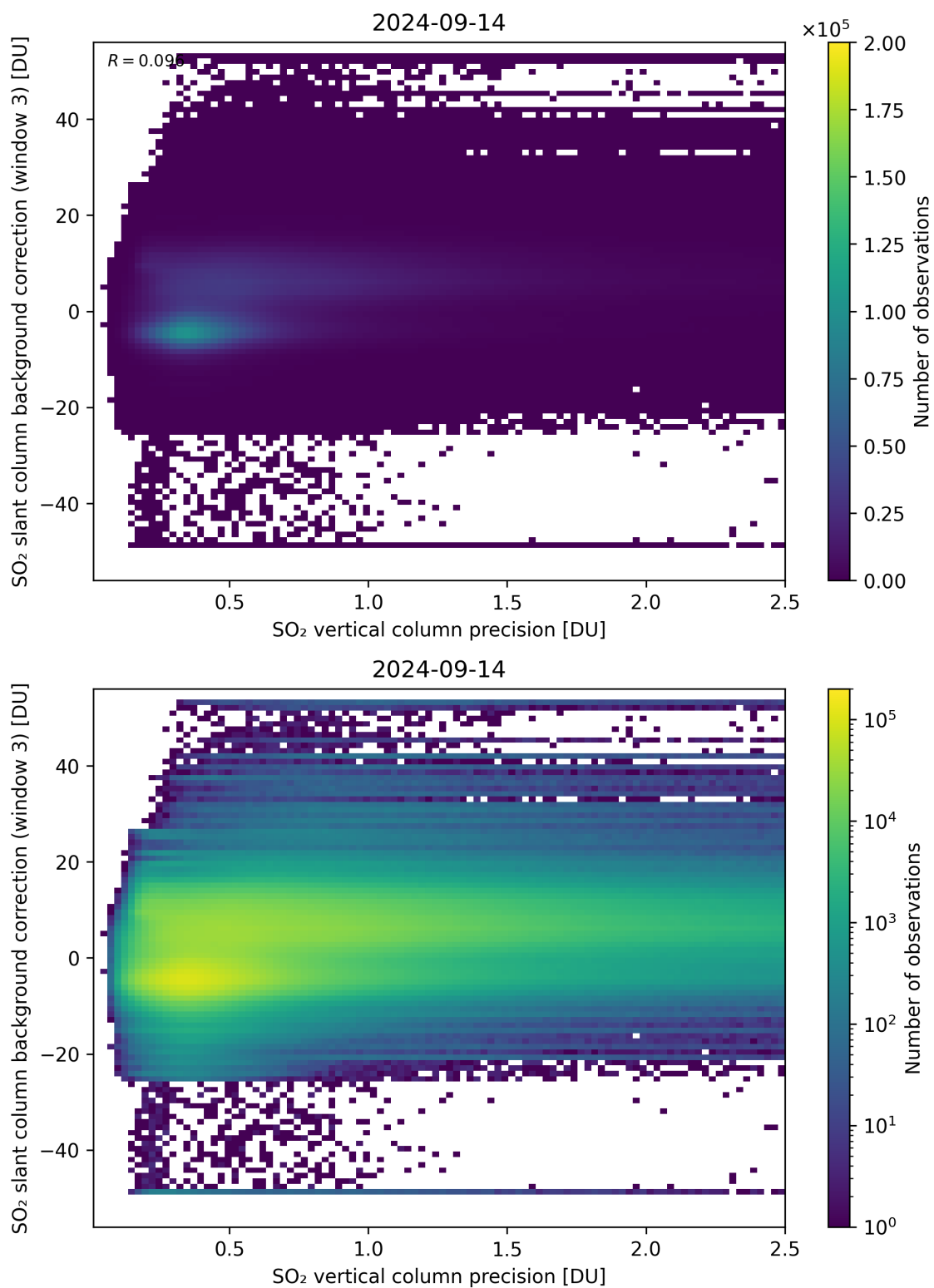
Figure 281: Scatter density plot of “SO 2 vertical column precision” against “SO 2 slant column background correction (window 3)” for 2024-09-13 to 2024-09-15.
