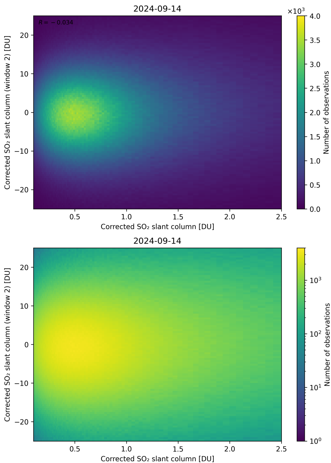
Figure 185: Scatter density plot of “Corrected SO 2 slant column” against “Corrected SO 2 slant column (window 2)” for 2024-09-13 to 2024-09-15.
