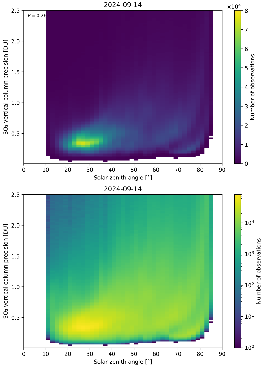
Figure 177: Scatter density plot of “Solar zenith angle” against “SO 2 vertical column precision” for 2024-09-13 to 2024-09-15.
