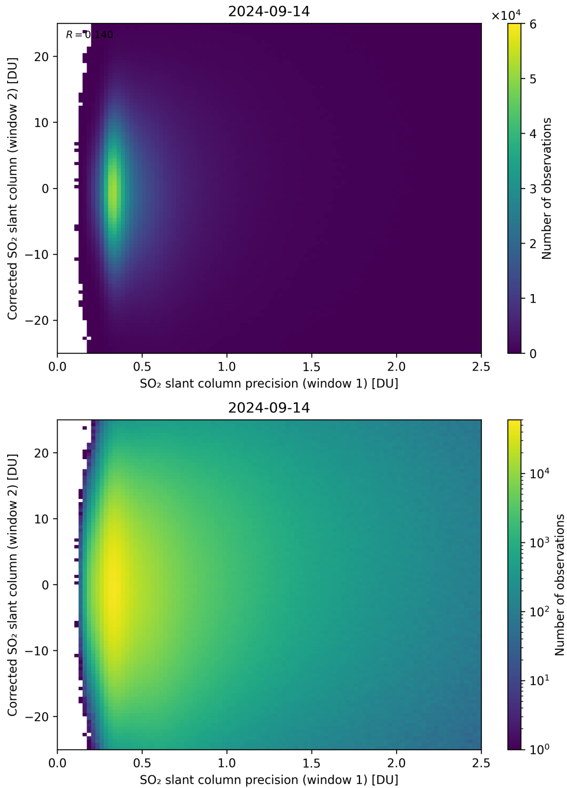
Figure 225: Scatter density plot of “SO 2 slant column precision (window 1)” against “Corrected SO 2 slant column (window 2)” for 2024-09-13 to 2024-09-15.
