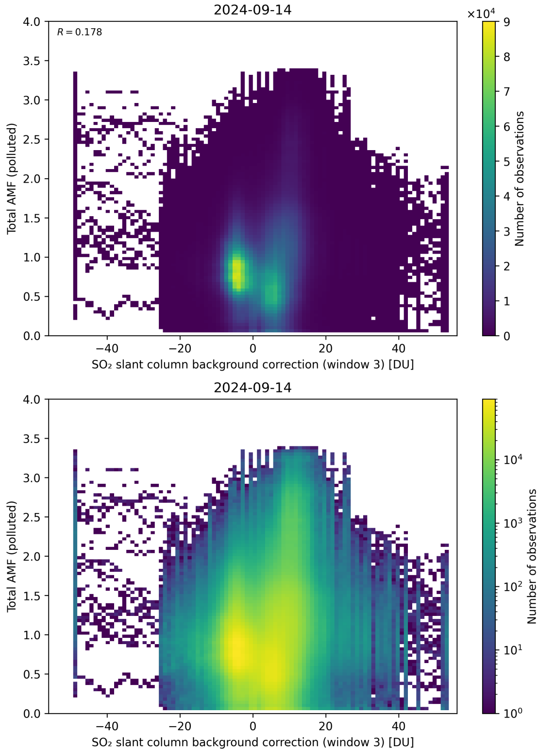
Figure 125: Scatter density plot of “SO 2 slant column background correction (window 3)” against “Total AMF (polluted)” for 2024-09-13 to 2024-09-15.
