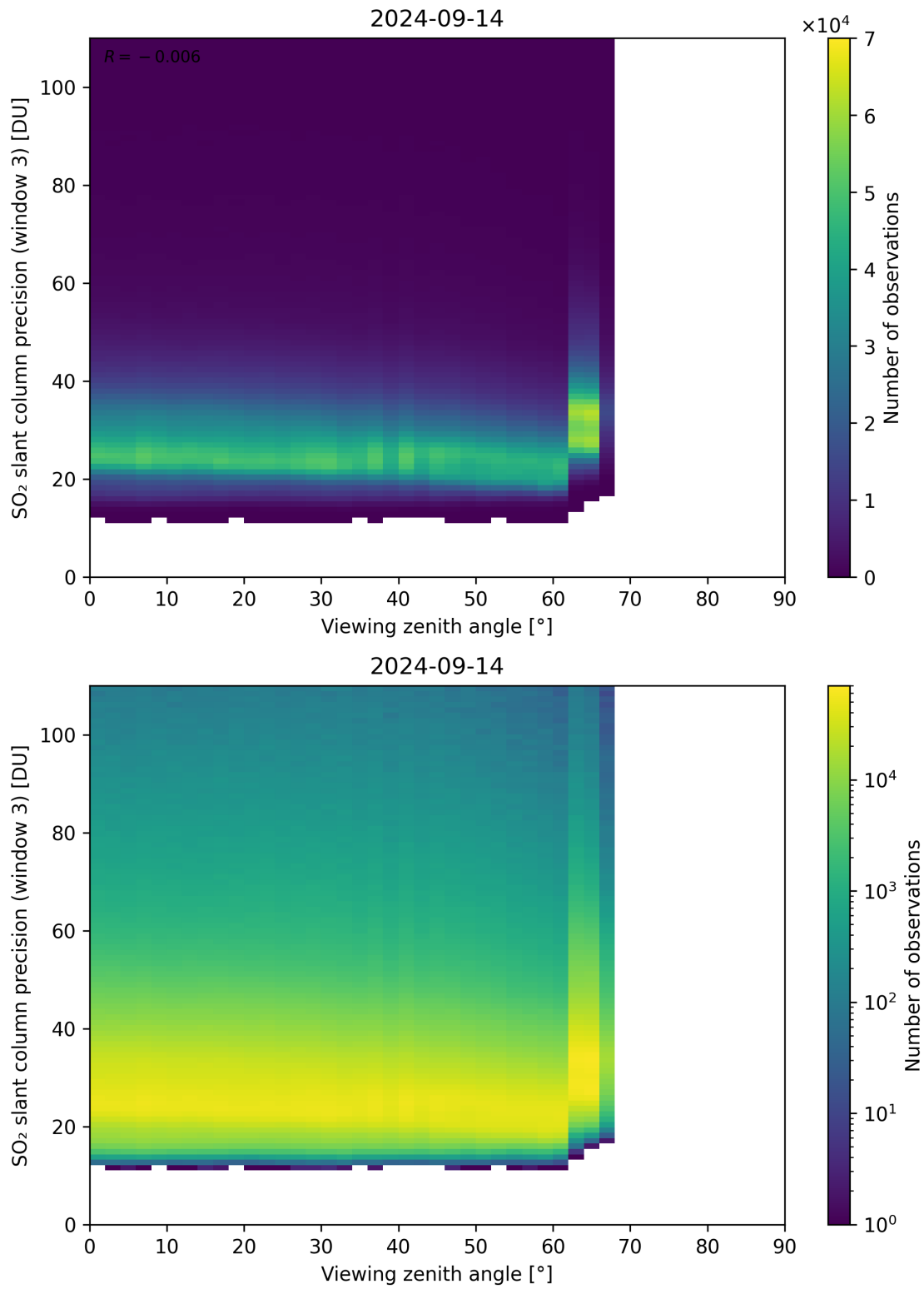
Figure 324: Scatter density plot of “Viewing zenith angle” against “SO 2 slant column precision (window 3)” for 2024-09-13 to 2024-09-15.
