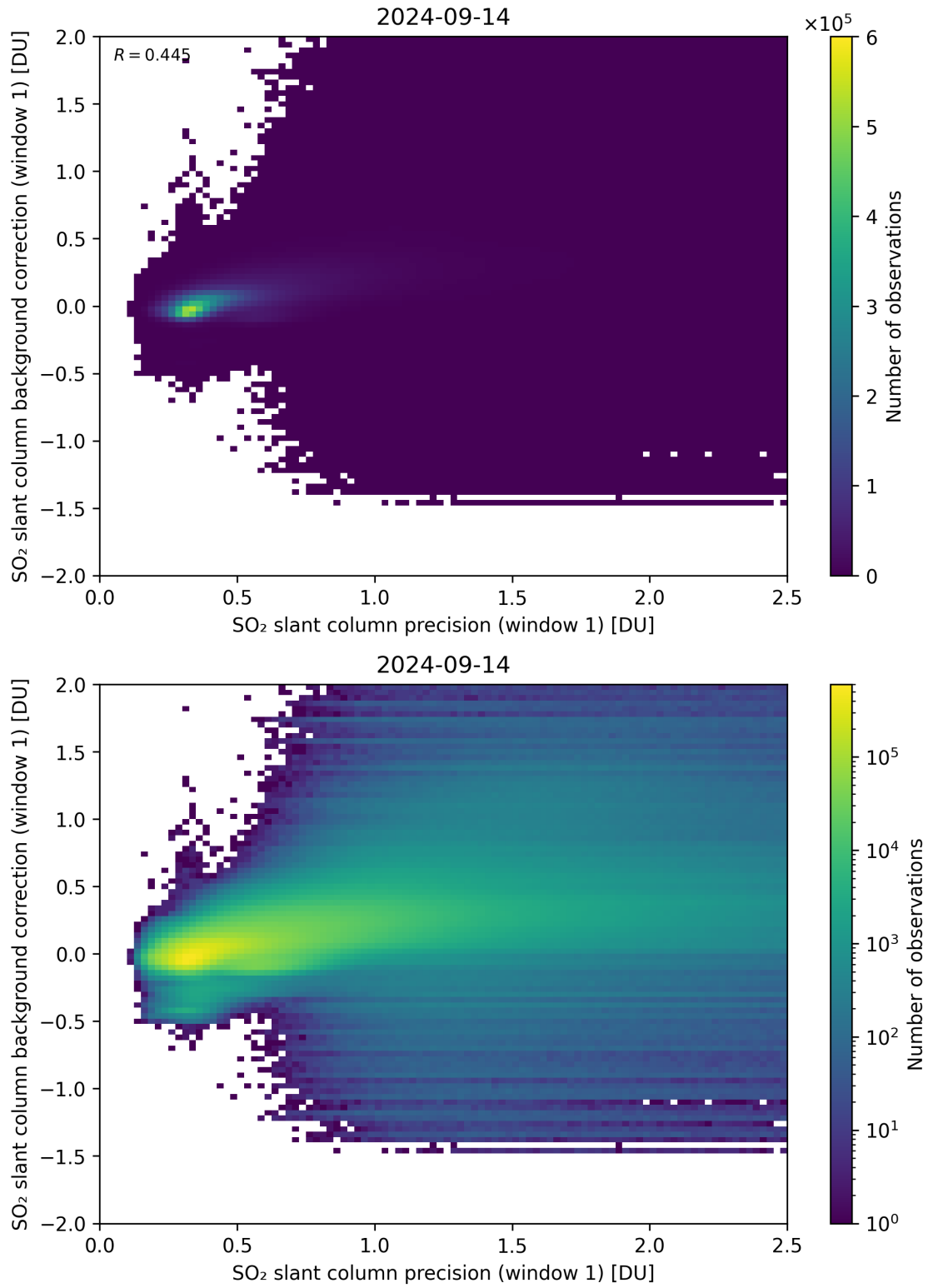
Figure 218: Scatter density plot of “SO 2 slant column precision (window 1)” against “SO 2 slant column background correction (window 1)” for 2024-09-13 to 2024-09-15.
