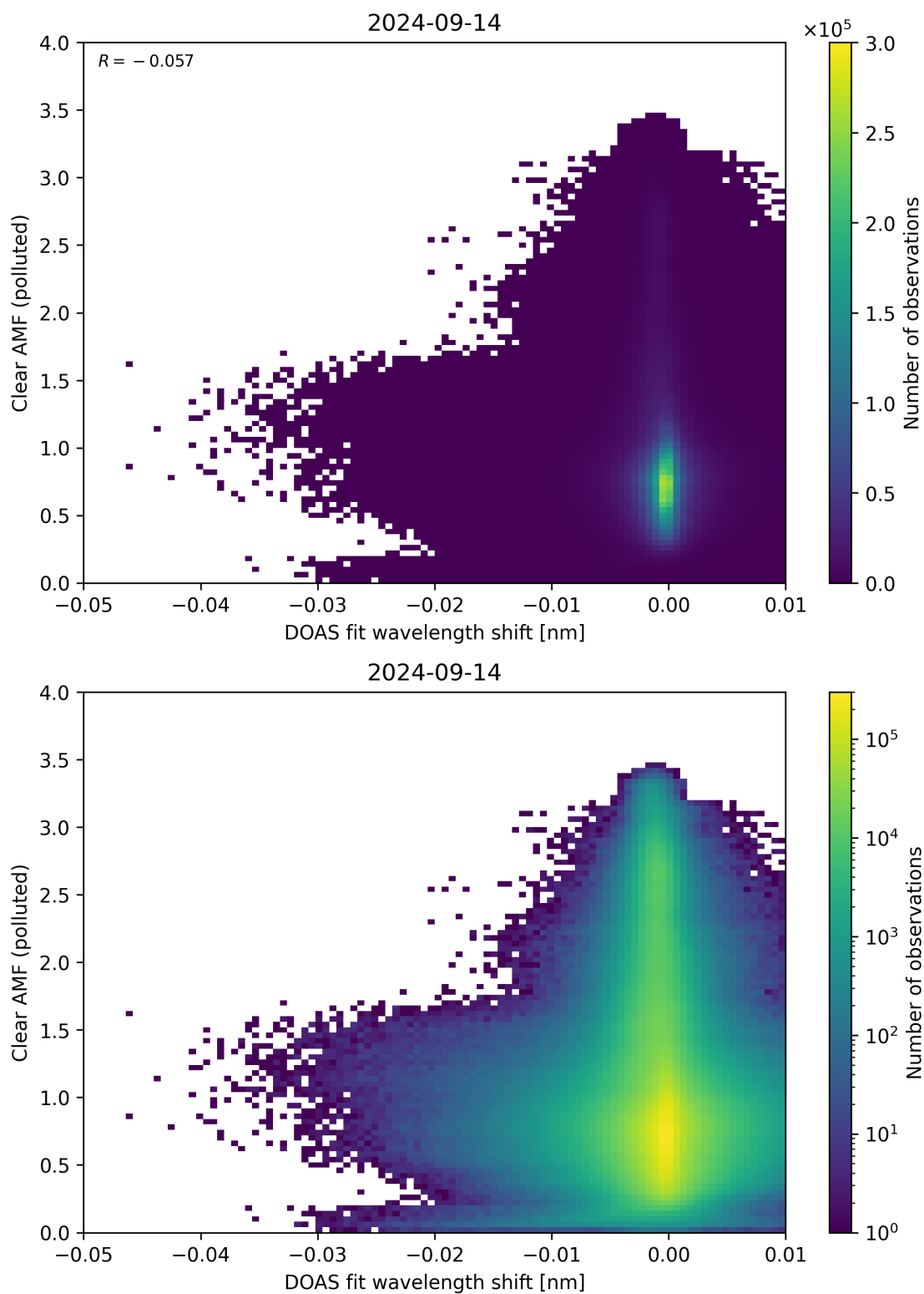
Figure 129: Scatter density plot of “DOAS fit wavelength shift” against “Clear AMF (polluted)” for 2024-09-13 to 2024-09-15.
