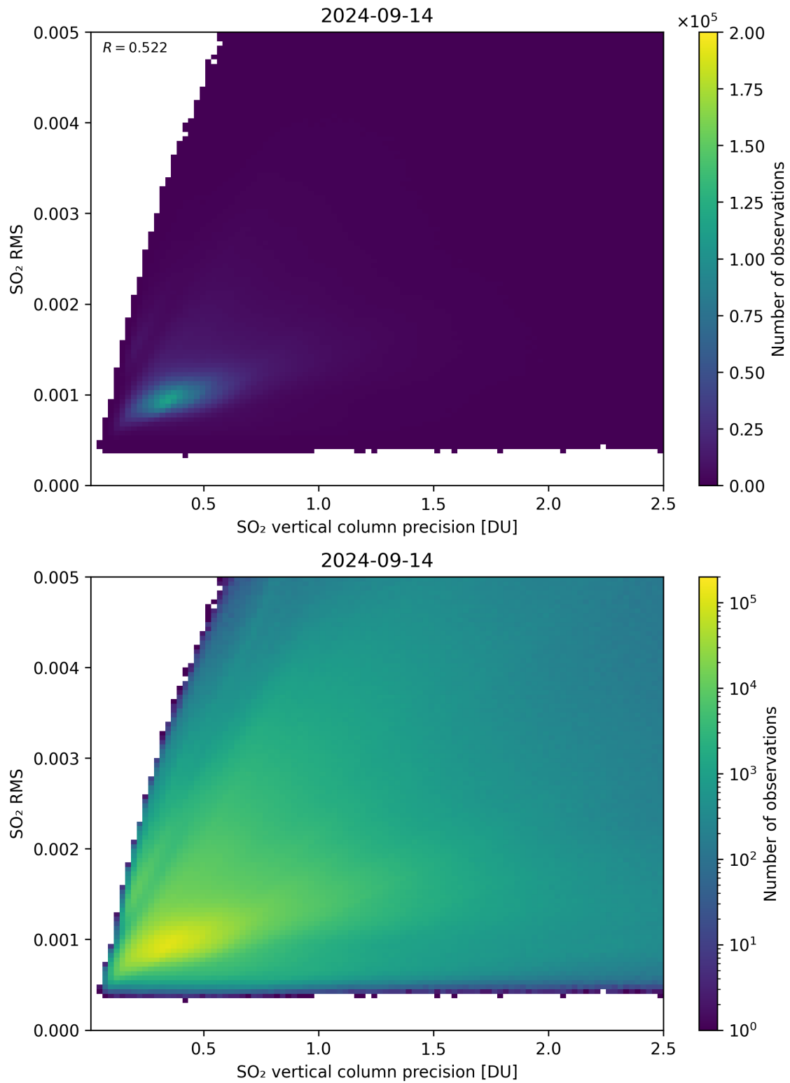
Figure 284: Scatter density plot of “SO 2 vertical column precision” against “SO 2 RMS” for 2024-09-13 to 2024-09-15.
