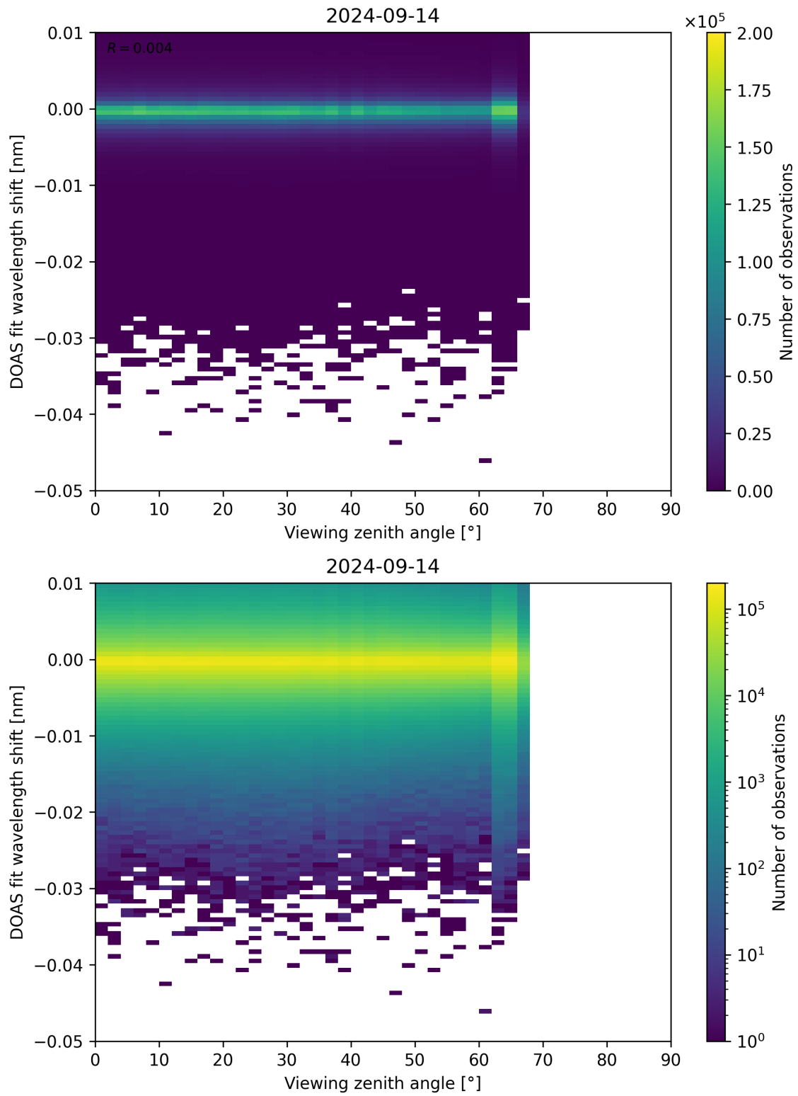
Figure 311: Scatter density plot of “Viewing zenith angle” against “DOAS fit wavelength shift” for 2024-09-13 to 2024-09-15.
