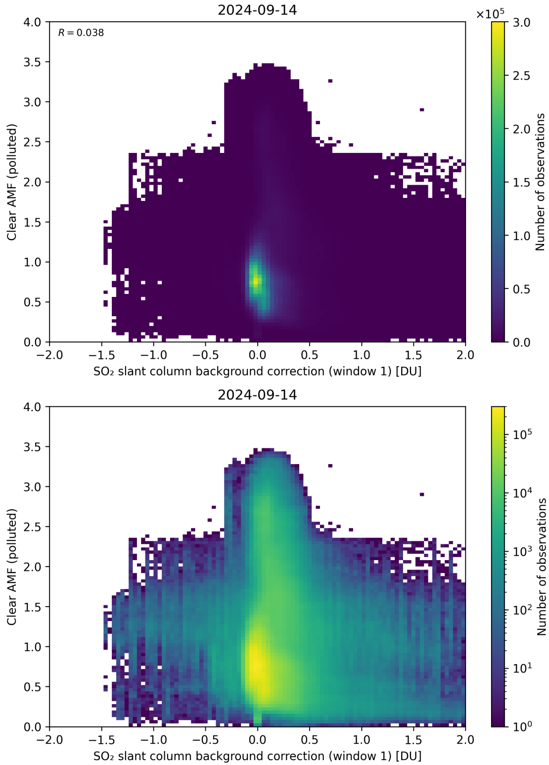
Figure 103: Scatter density plot of “SO 2 slant column background correction (window 1)” against “Clear AMF (polluted)” for 2024-09-13 to 2024-09-15.
