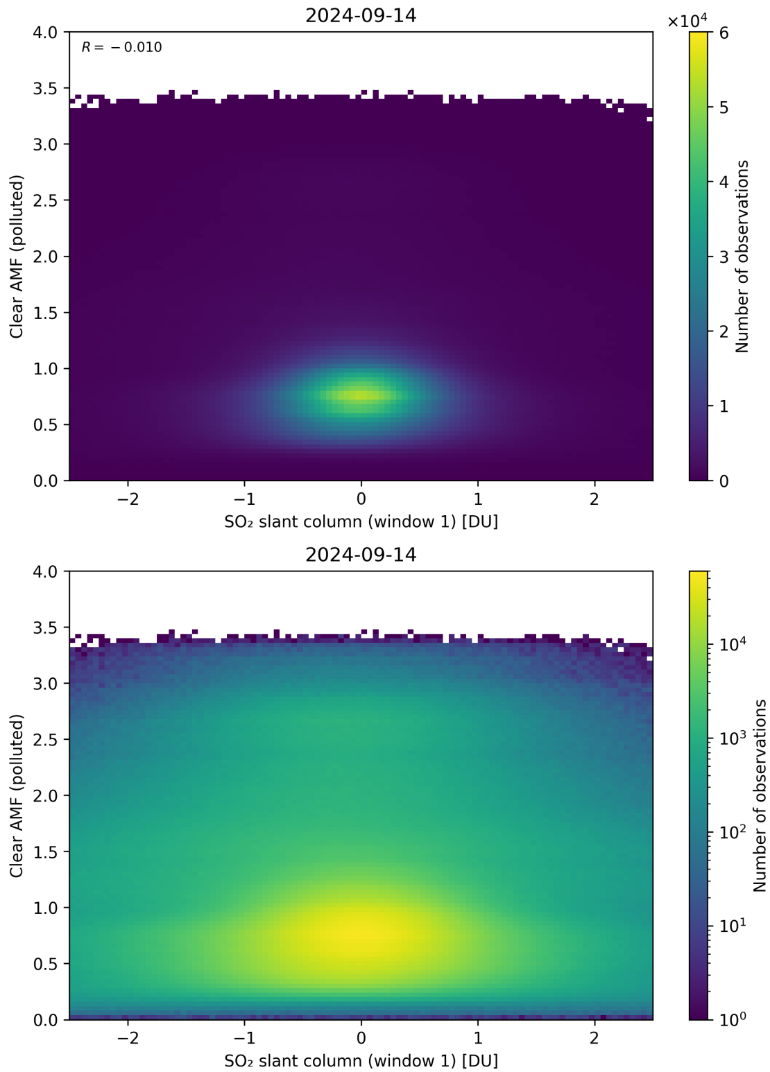
Figure 232: Scatter density plot of “SO 2 slant column (window 1)” against “Clear AMF (polluted)” for 2024-09-13 to 2024-09-15.
