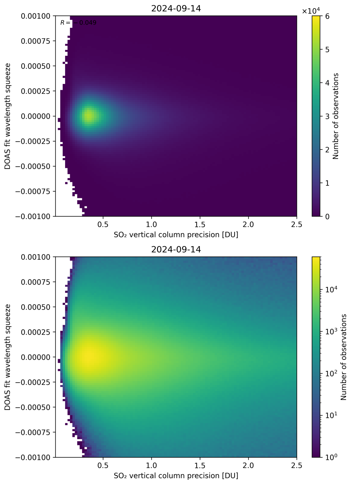
Figure 283: Scatter density plot of “SO 2 vertical column precision” against “DOAS fit wavelength squeeze” for 2024-09-13 to 2024-09-15.
