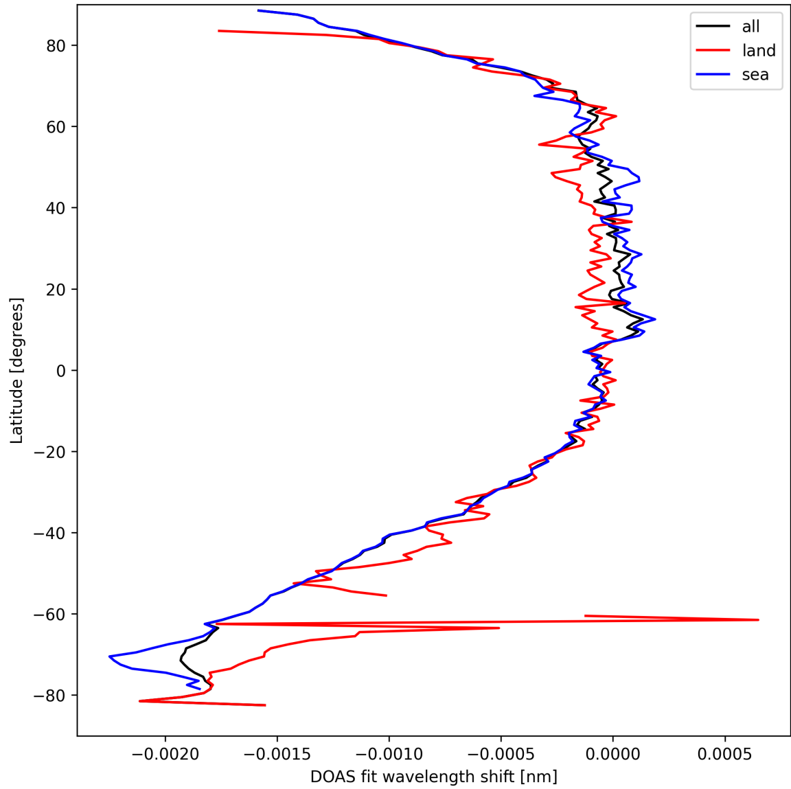
Figure 45: Zonal average of "DOAS fit wavelength shift" for 2024-09-13 to 2024-09-15.
