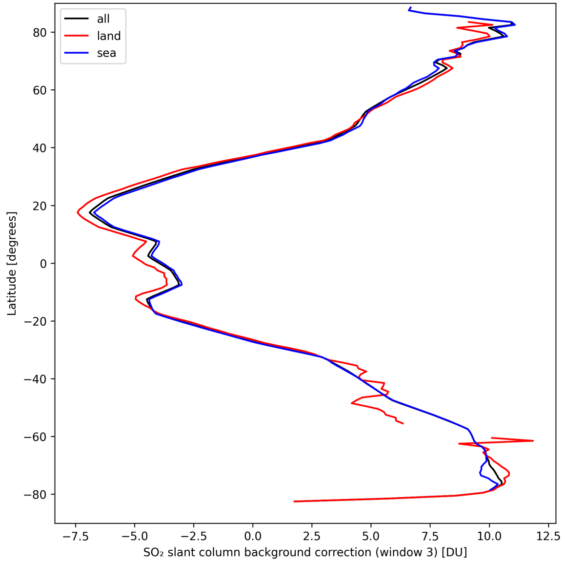
Figure 44: Zonal average of "SO 2 slant column background correction (window 3)" for 2024-09-13 to 2024-09-15.
