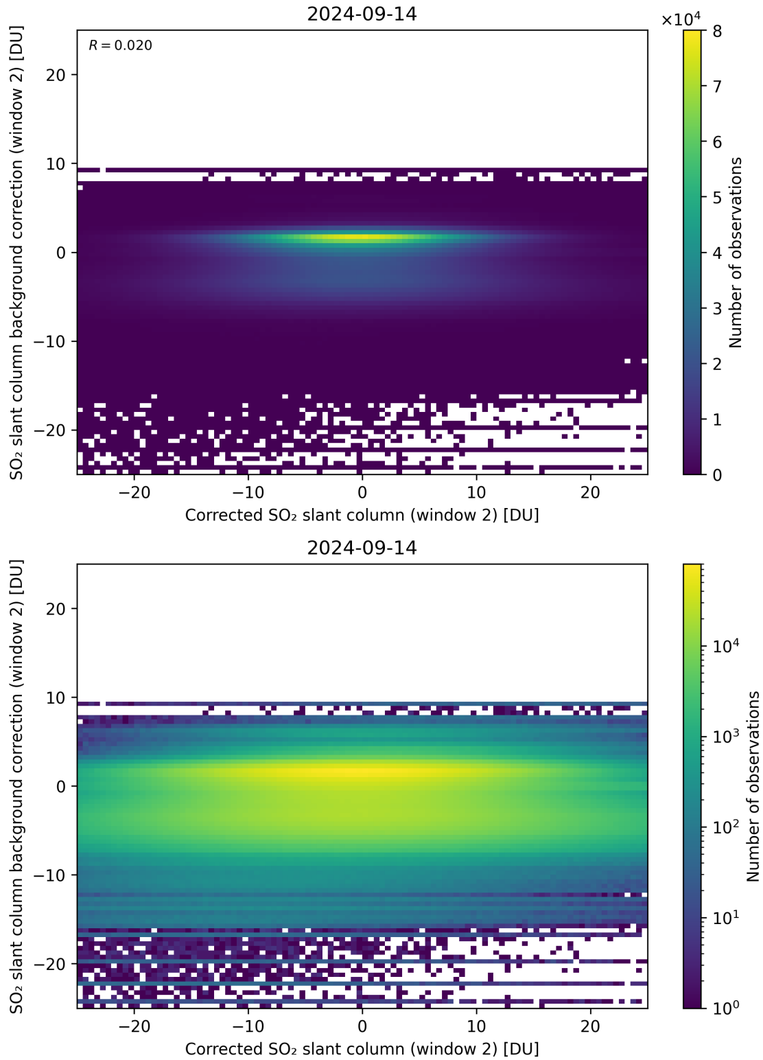
Figure 194: Scatter density plot of “Corrected SO 2 slant column (window 2)” against “SO 2 slant column background correction (window 2)” for 2024-09-13 to 2024-09-15.
