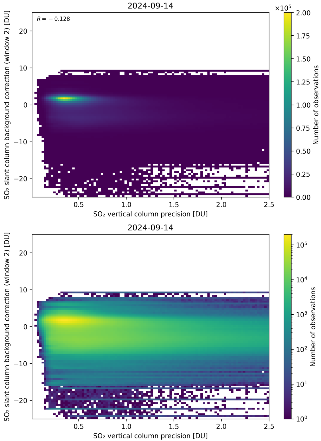
Figure 280: Scatter density plot of “SO 2 vertical column precision” against “SO 2 slant column background correction (window 2)” for 2024-09-13 to 2024-09-15.
