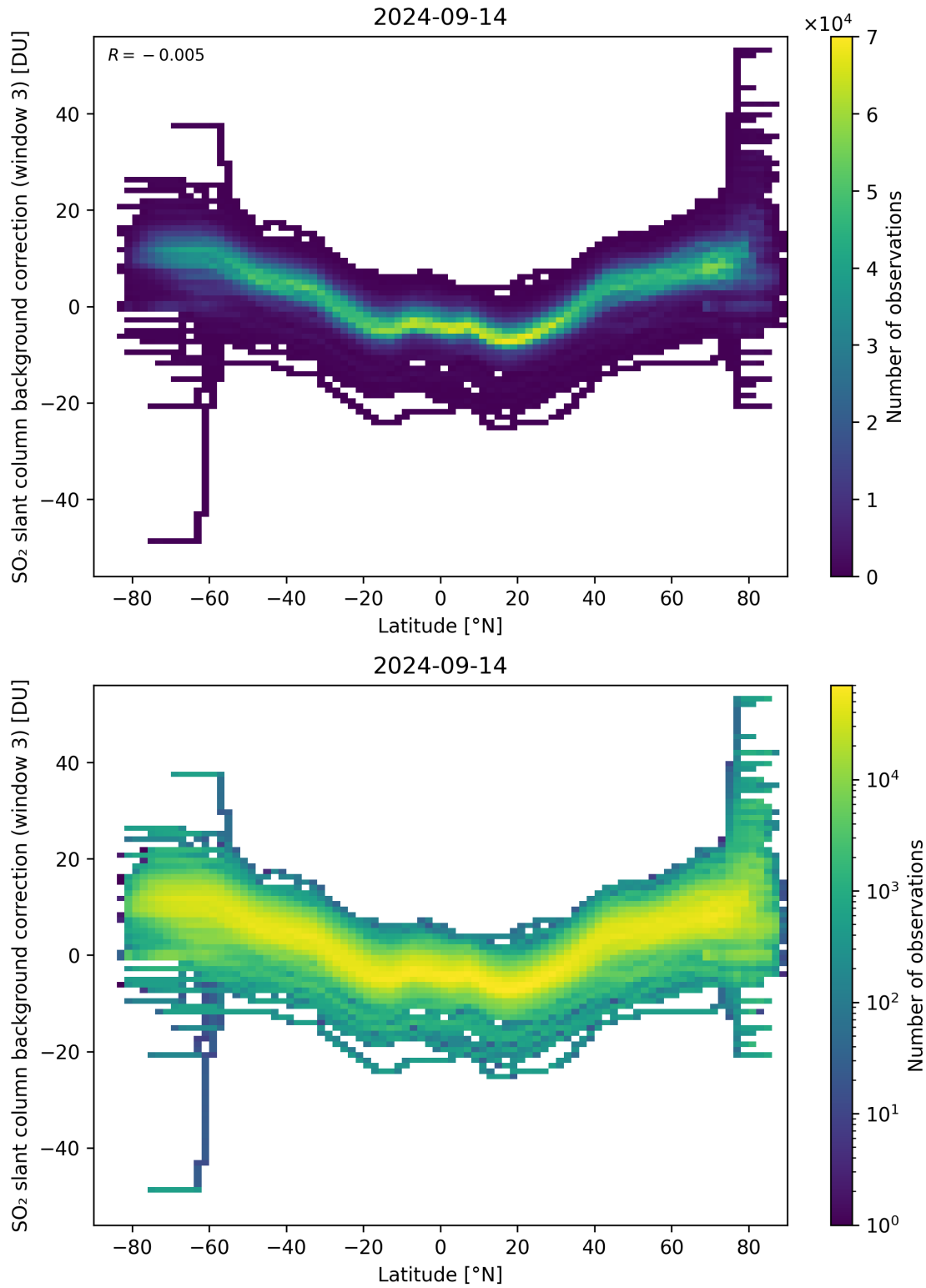
Figure 141: Scatter density plot of “Latitude” against “SO 2 slant column background correction (window 3)” for 2024-09-13 to 2024-09-15.
