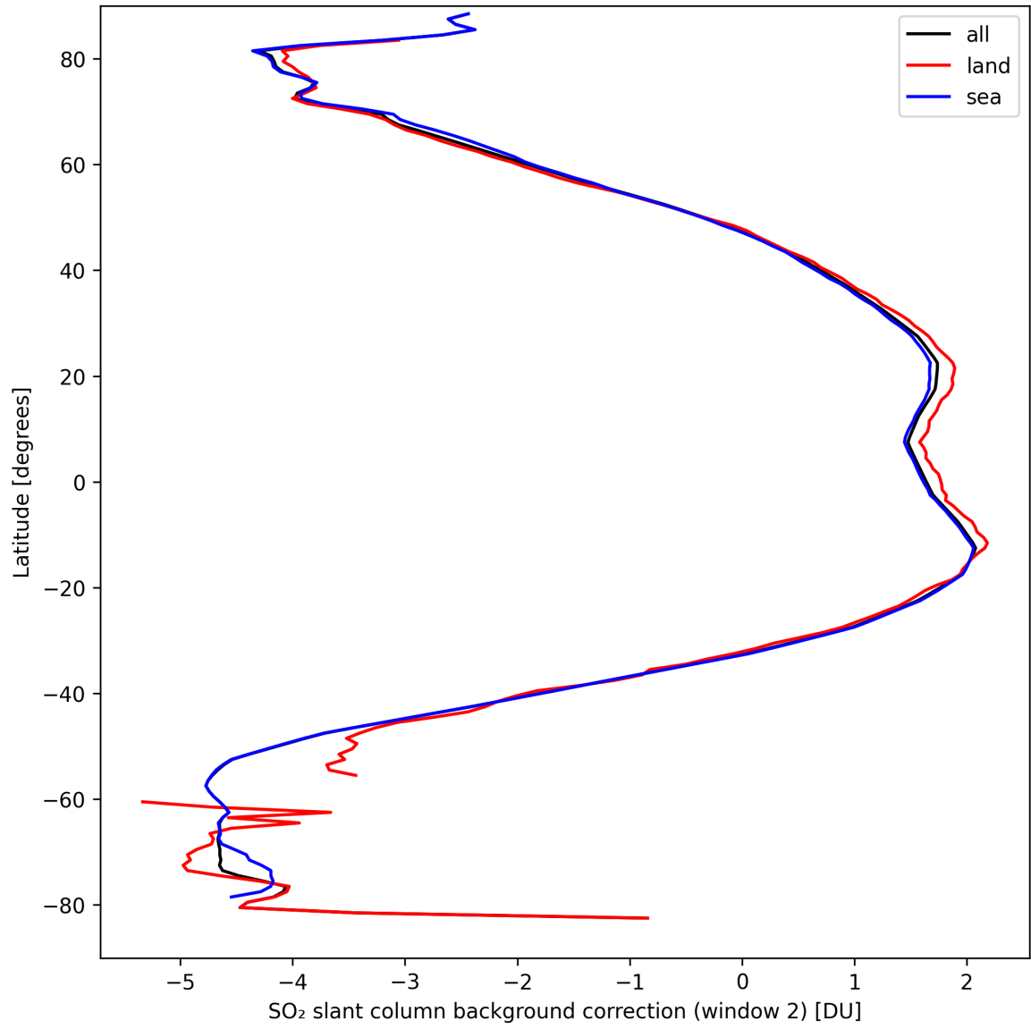
Figure 40: Zonal average of “SO 2 slant column background correction (window 2)” for 2024-09-13 to 2024-09-15.
