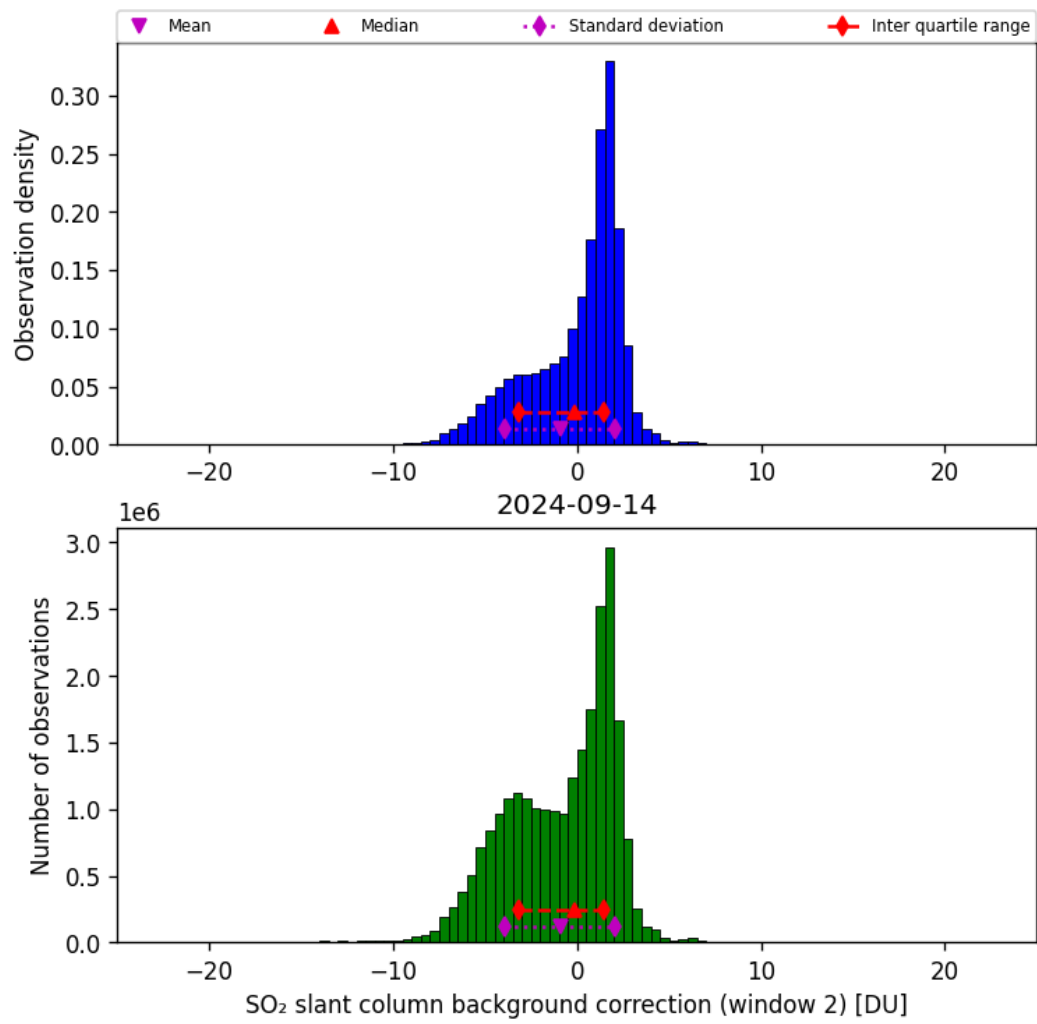
Figure 63: Histogram of “SO 2 slant column background correction (window 2)” for 2024-09-13 to 2024-09-15
