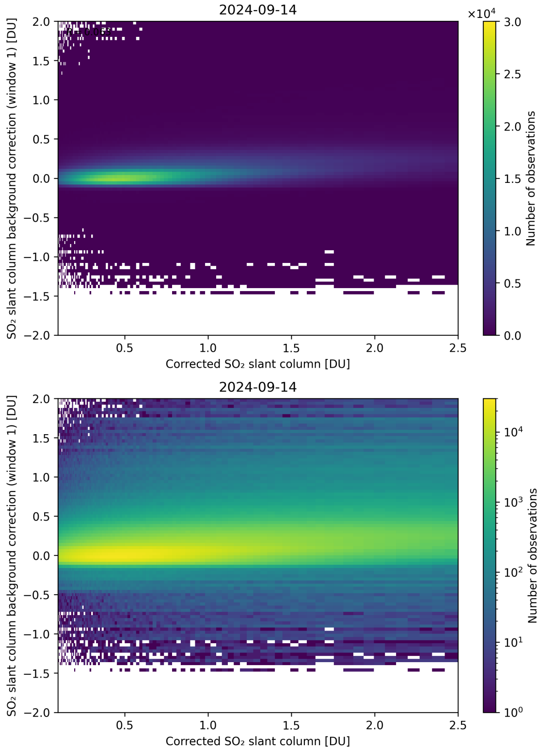
Figure 178: Scatter density plot of “Corrected SO 2 slant column” against “SO 2 slant column background correction (window 1)” for 2024-09-13 to 2024-09-15.
