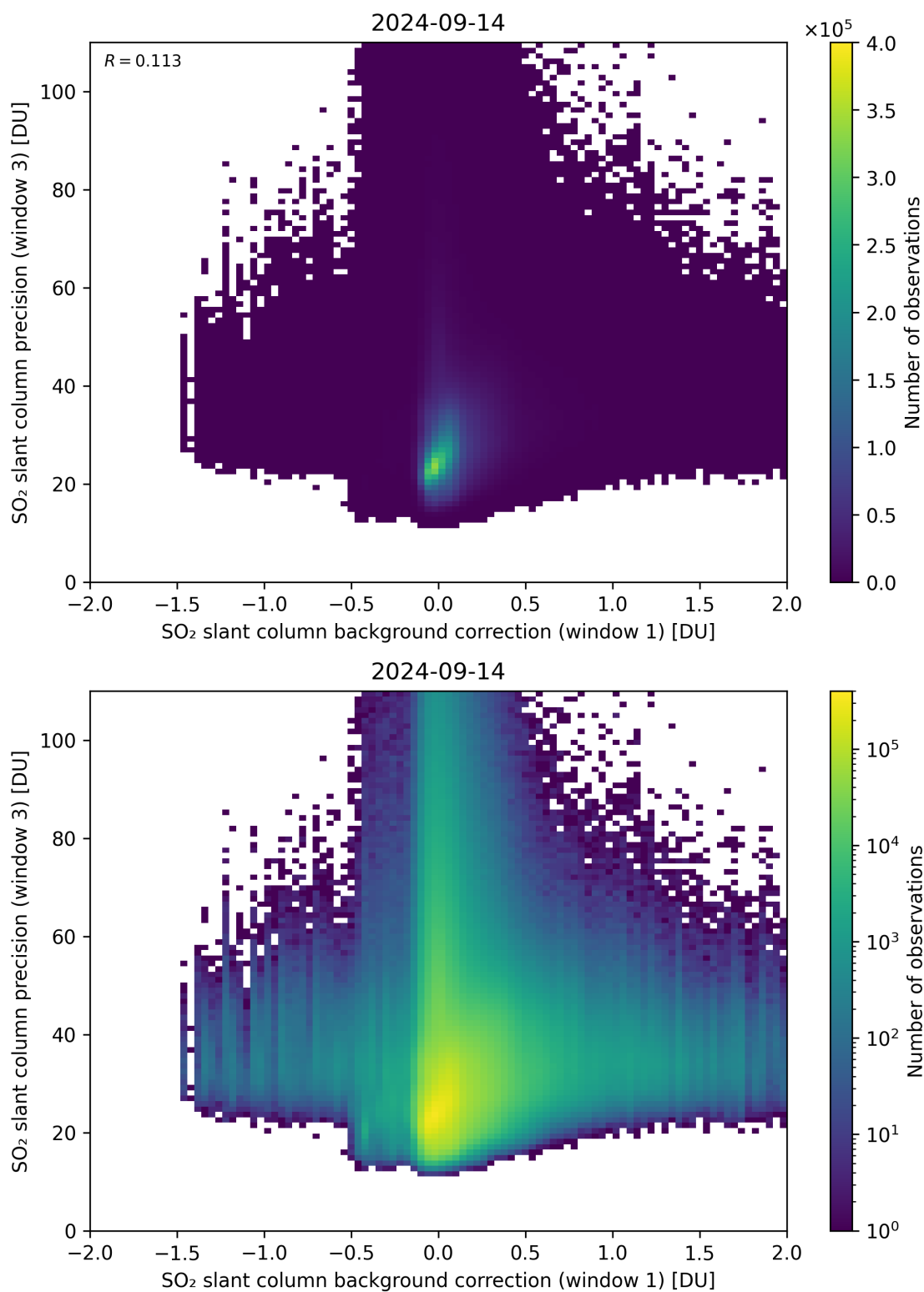
Figure 108: Scatter density plot of “SO 2 slant column background correction (window 1)” against “SO 2 slant column precision (window 3)” for 2024-09-13 to 2024-09-15.
