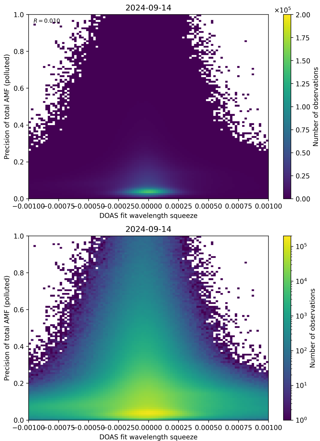
Figure 135: Scatter density plot of “DOAS fit wavelength squeeze” against “Precision of total AMF (polluted)” for 2024-09-13 to 2024-09-15.
