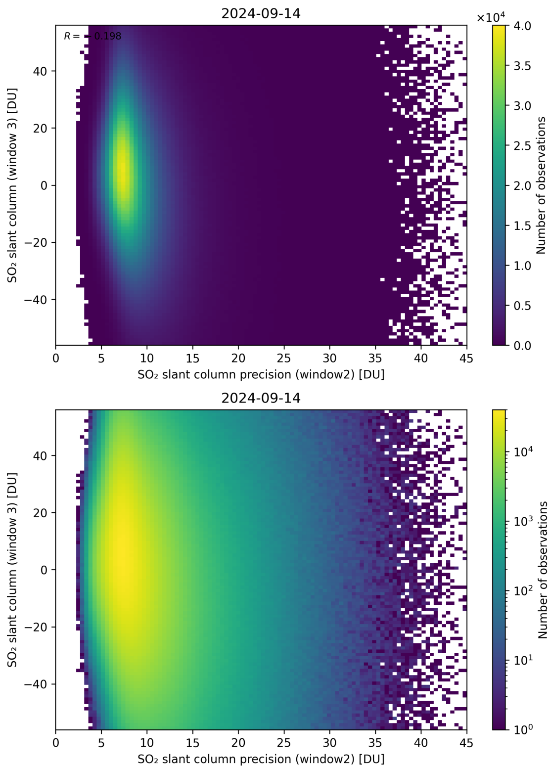
Figure 249: Scatter density plot of “SO 2 slant column precision (window2)” against “SO 2 slant column (window 3)” for 2024-09-13 to 2024-09-15.
