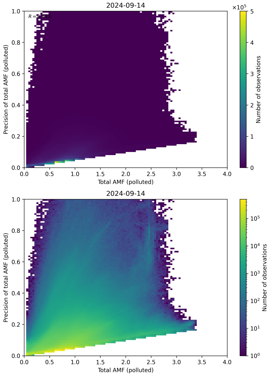
Figure 272: Scatter density plot of “Total AMF (polluted)” against “Precision of total AMF (polluted)” for 2024-09-13 to 2024-09-15.
