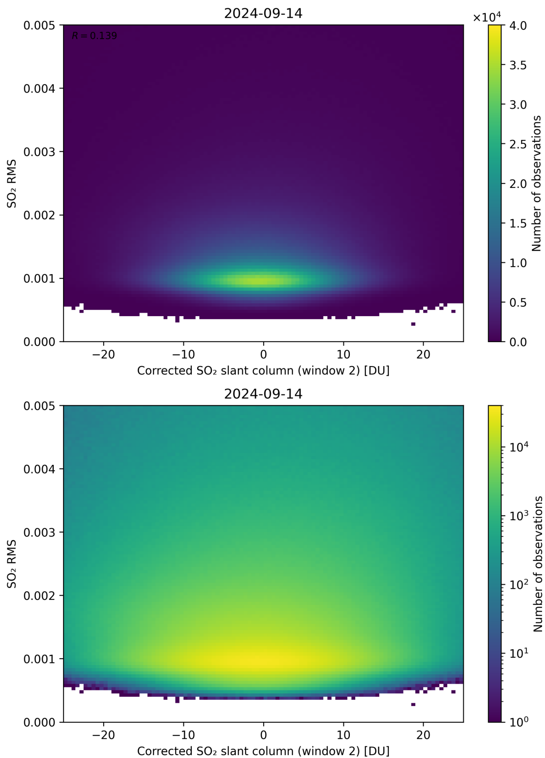
Figure 198: Scatter density plot of “Corrected SO 2 slant column (window 2)” against “SO 2 RMS” for 2024-09-13 to 2024-09-15.
