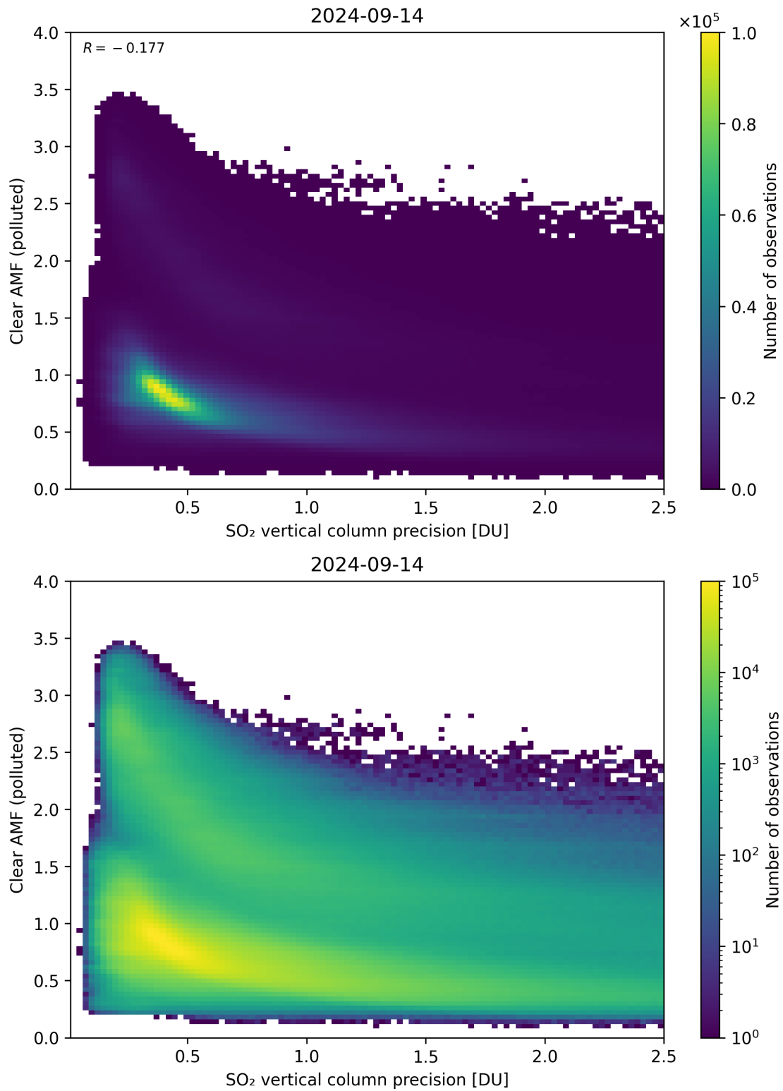
Figure 285: Scatter density plot of “SO 2 vertical column precision” against “Clear AMF (polluted)” for 2024-09-13 to 2024-09-15.
