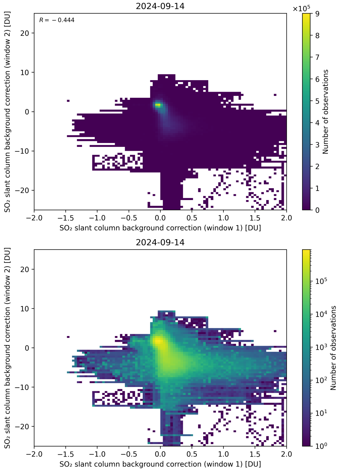
Figure 98: Scatter density plot of “SO 2 slant column background correction (window 1)” against “SO 2 slant column background correction (window 2)” for 2024-09-13 to 2024-09-15.
