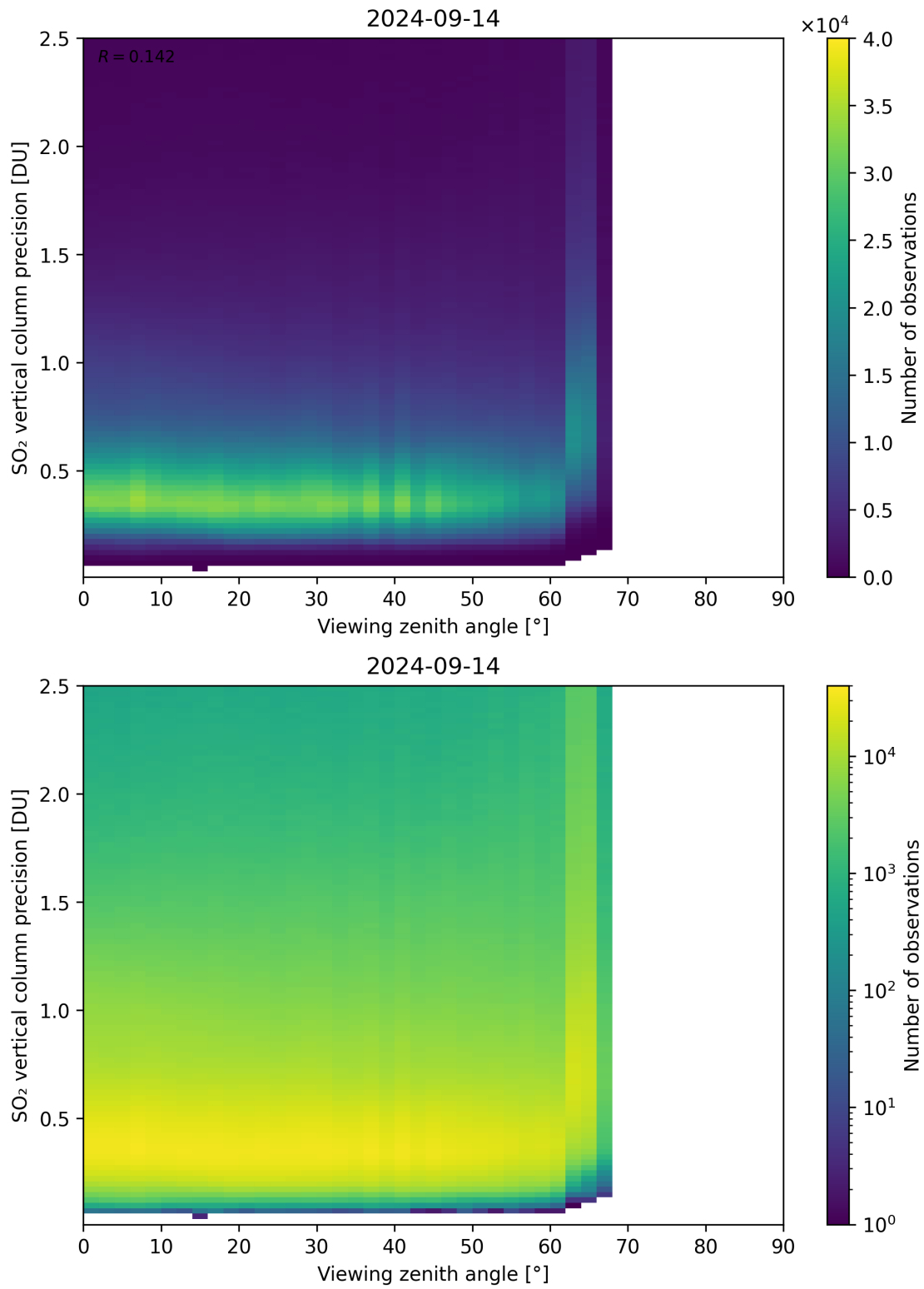
Figure 328: Scatter density plot of “Viewing zenith angle” against “SO 2 vertical column precision” for 2024-09-13 to 2024-09-15.
