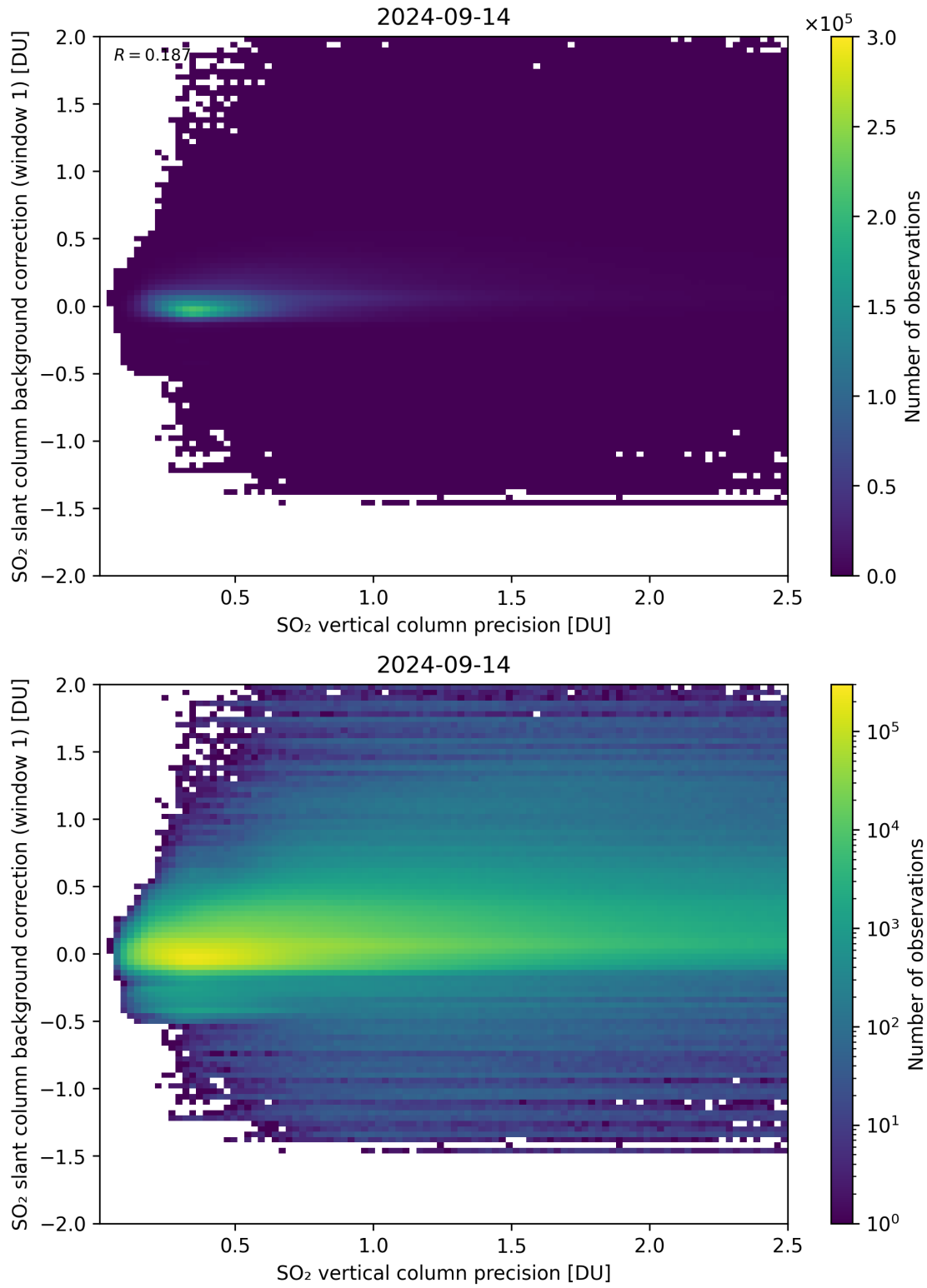
Figure 279: Scatter density plot of “SO 2 vertical column precision” against “SO 2 slant column background correction (window 1)” for 2024-09-13 to 2024-09-15.
