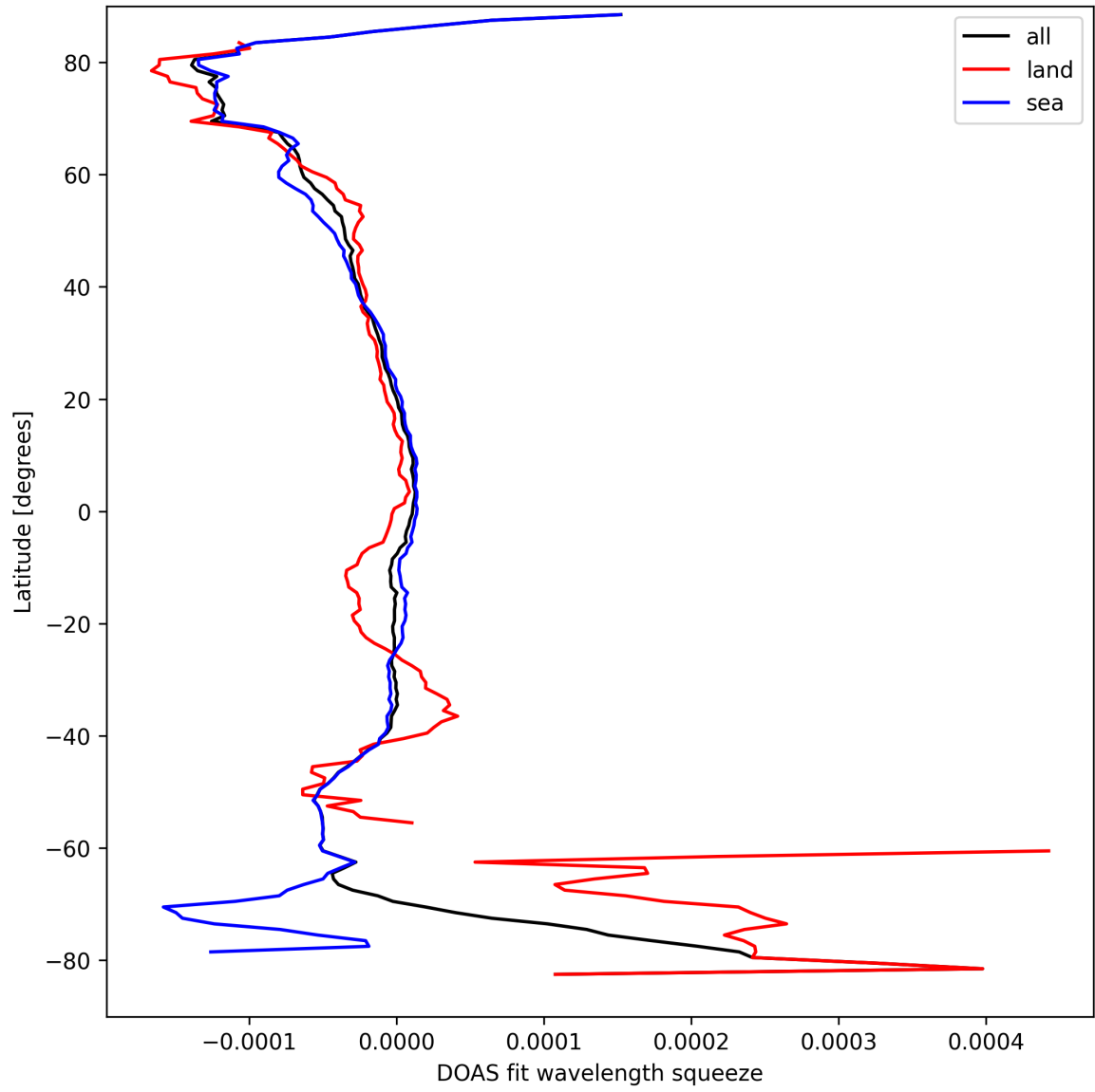
Figure 46: Zonal average of "DOAS fit wavelength squeeze" for 2024-09-13 to 2024-09-15.
