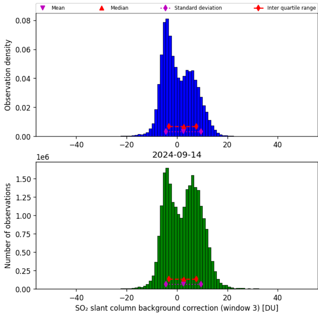
Figure 67: Histogram of “SO 2 slant column background correction (window 3)” for 2024-09-13 to 2024-09-15
