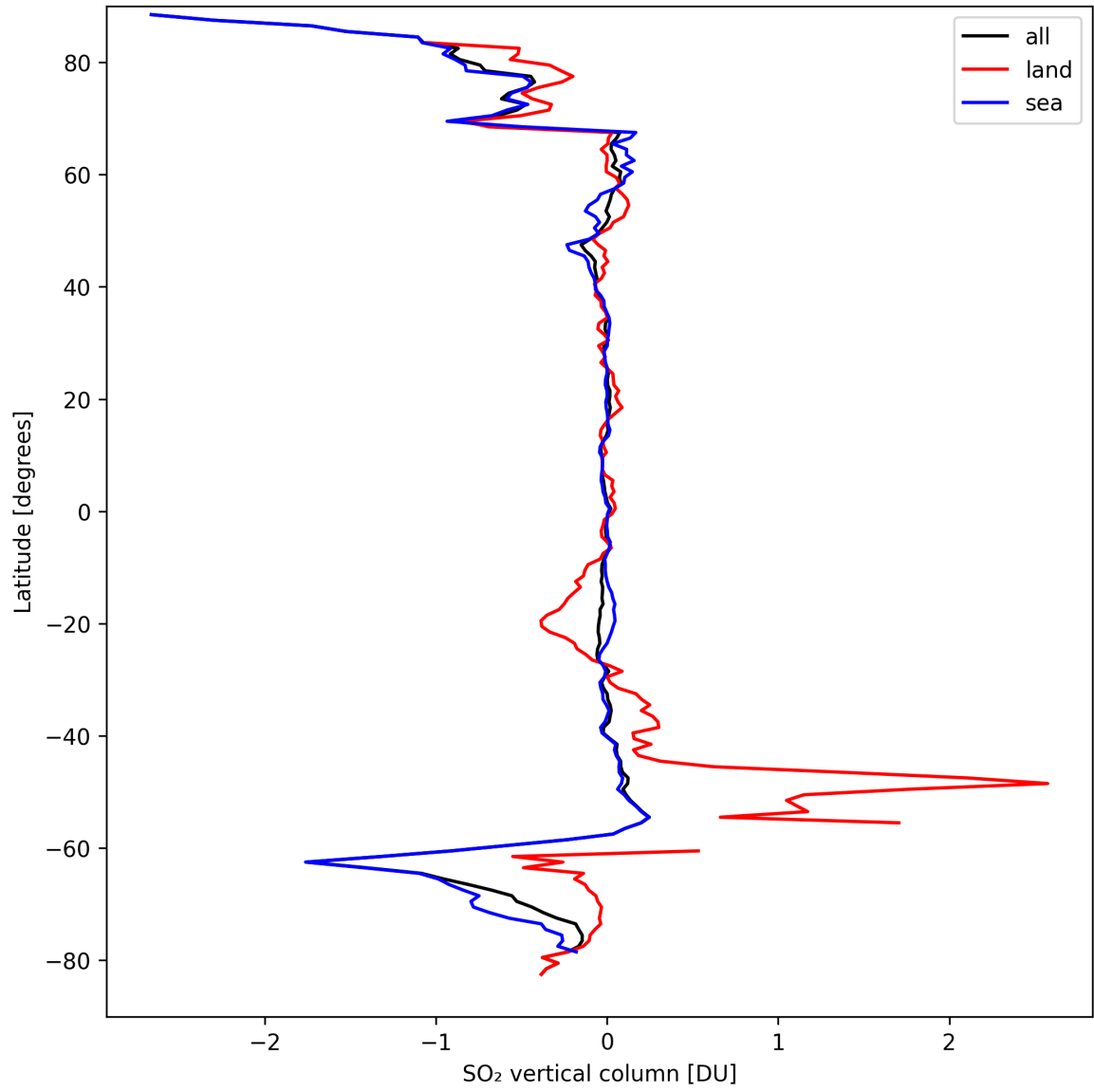
Figure 30: Zonal average of “SO 2 vertical column” for 2024-09-13 to 2024-09-15.
