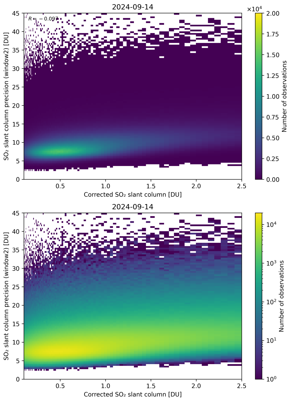
Figure 189: Scatter density plot of “Corrected SO 2 slant column” against “SO 2 slant column precision (window2)” for 2024-09-13 to 2024-09-15.
