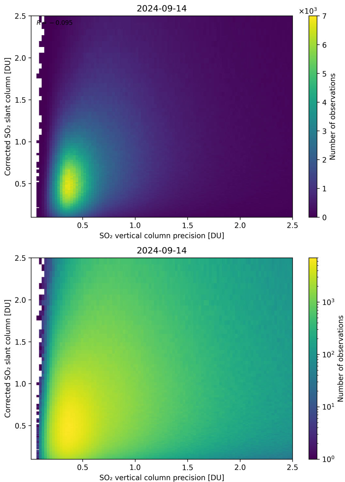
Figure 286: Scatter density plot of “SO 2 vertical column precision” against “Corrected SO 2 slant column” for 2024-09-13 to 2024-09-15.
