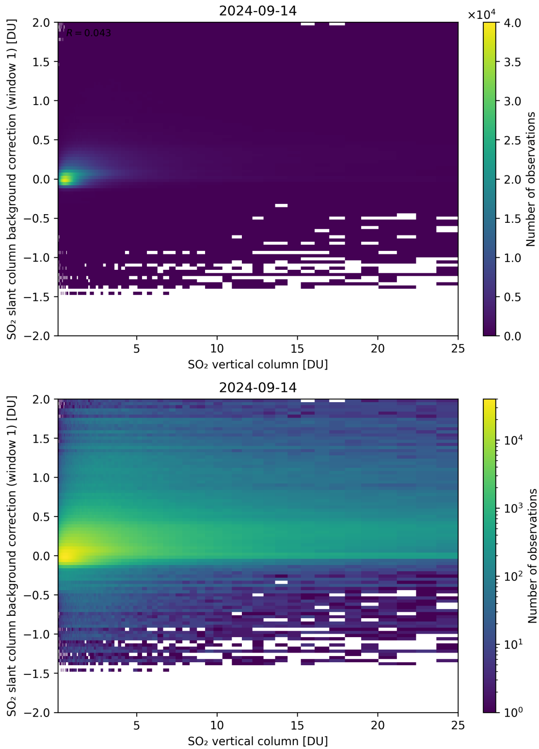
Figure 273: Scatter density plot of “SO 2 vertical column” against “SO 2 slant column background correction (window 1)” for 2024-09-13 to 2024-09-15.
