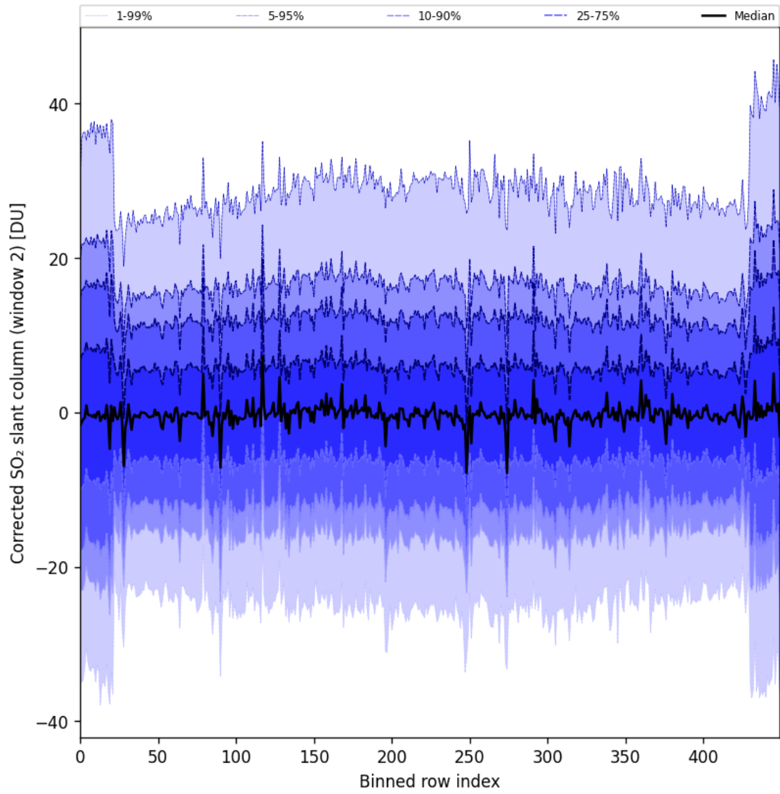
Figure 85: Along track statistics of “Corrected SO 2 slant column (window 2)” for 2024-09-13 to 2024-09-15
