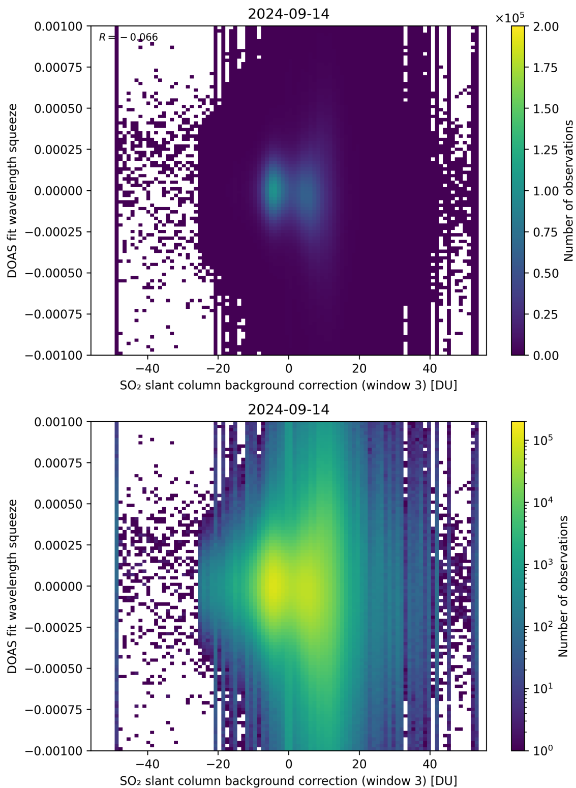
Figure 122: Scatter density plot of “SO 2 slant column background correction (window 3)” against “DOAS fit wavelength squeeze” for 2024-09-13 to 2024-09-15.
