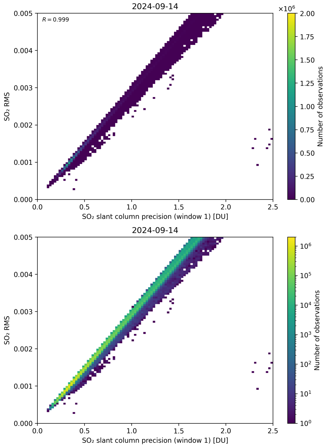
Figure 223: Scatter density plot of “SO 2 slant column precision (window 1)” against “SO 2 RMS” for 2024-09-13 to 2024-09-15.
