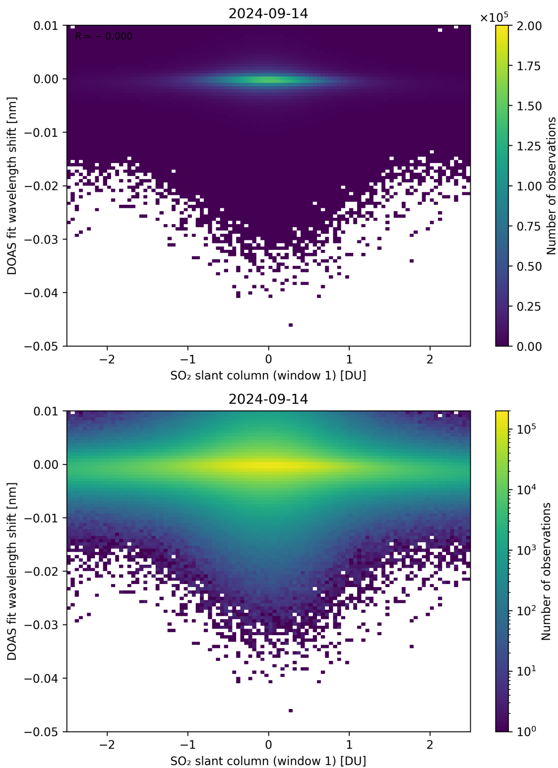
Figure 215: Scatter density plot of “SO 2 slant column (window 1)” against “DOAS fit wavelength shift” for 2024-09-13 to 2024-09-15.
