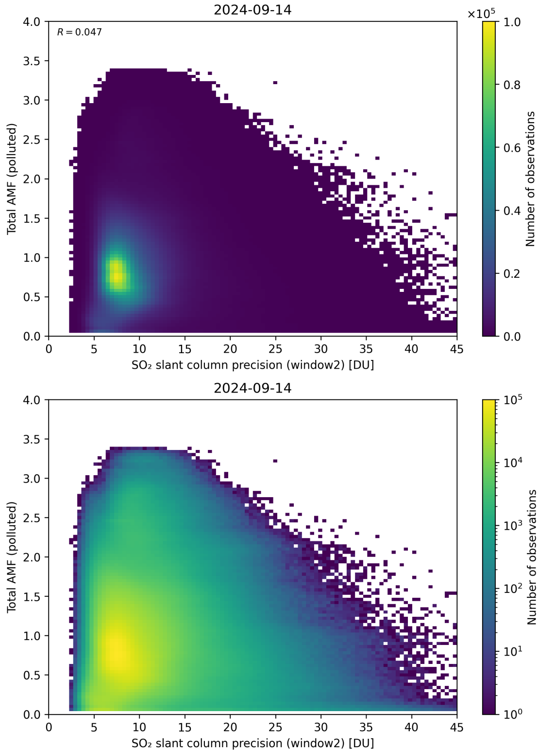
Figure 251: Scatter density plot of “SO 2 slant column precision (window2)” against “Total AMF (polluted)” for 2024-09-13 to 2024-09-15.
