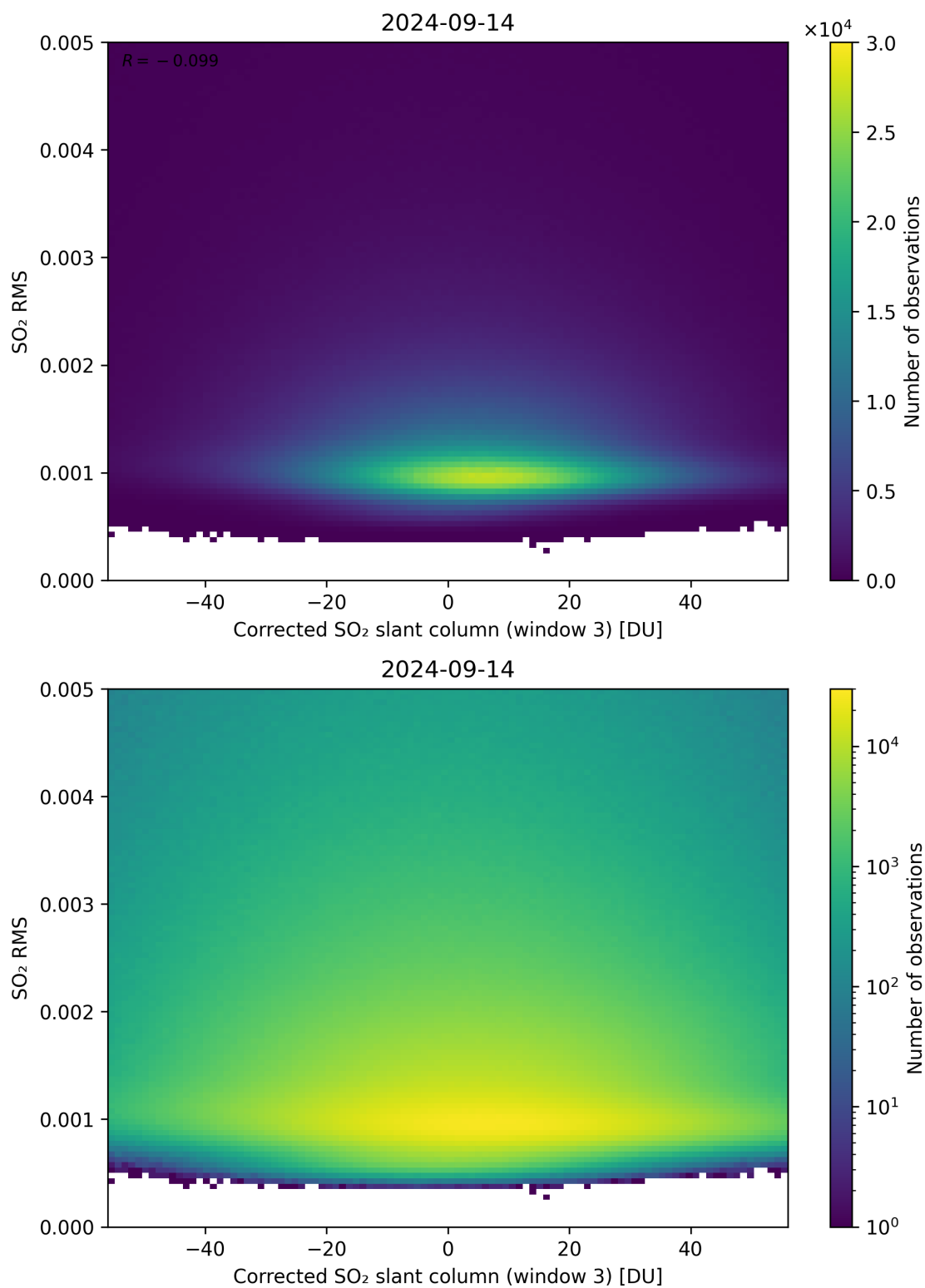
Figure 208: Scatter density plot of “Corrected SO 2 slant column (window 3)” against “SO 2 RMS” for 2024-09-13 to 2024-09-15.
