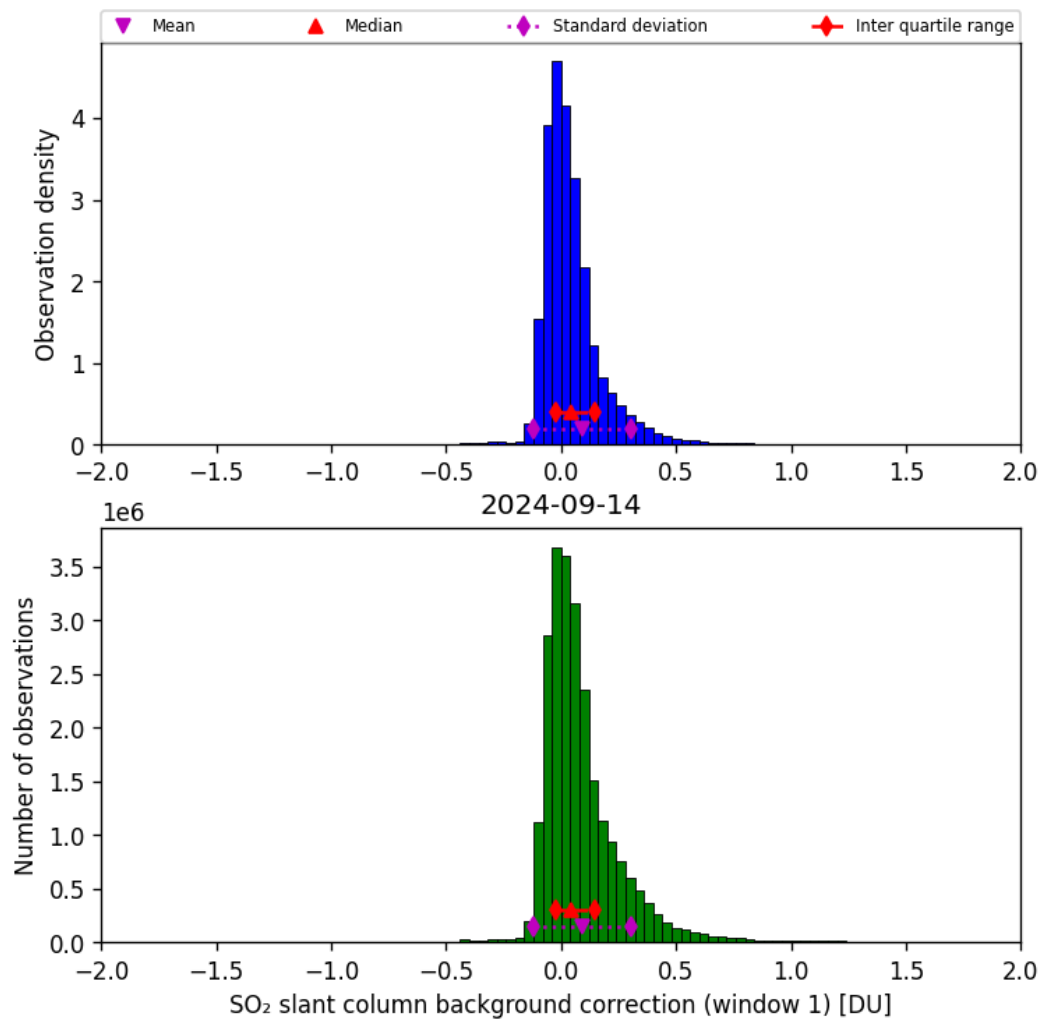
Figure 59: Histogram of “SO 2 slant column background correction (window 1)” for 2024-09-13 to 2024-09-15
