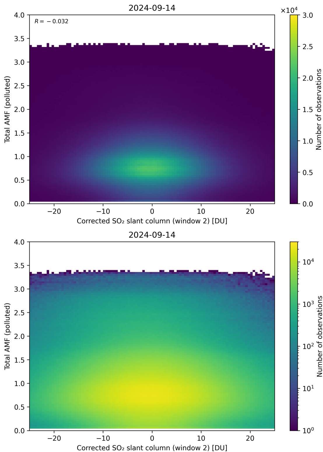
Figure 203: Scatter density plot of “Corrected SO 2 slant column (window 2)” against “Total AMF (polluted)” for 2024-09-13 to 2024-09-15.
