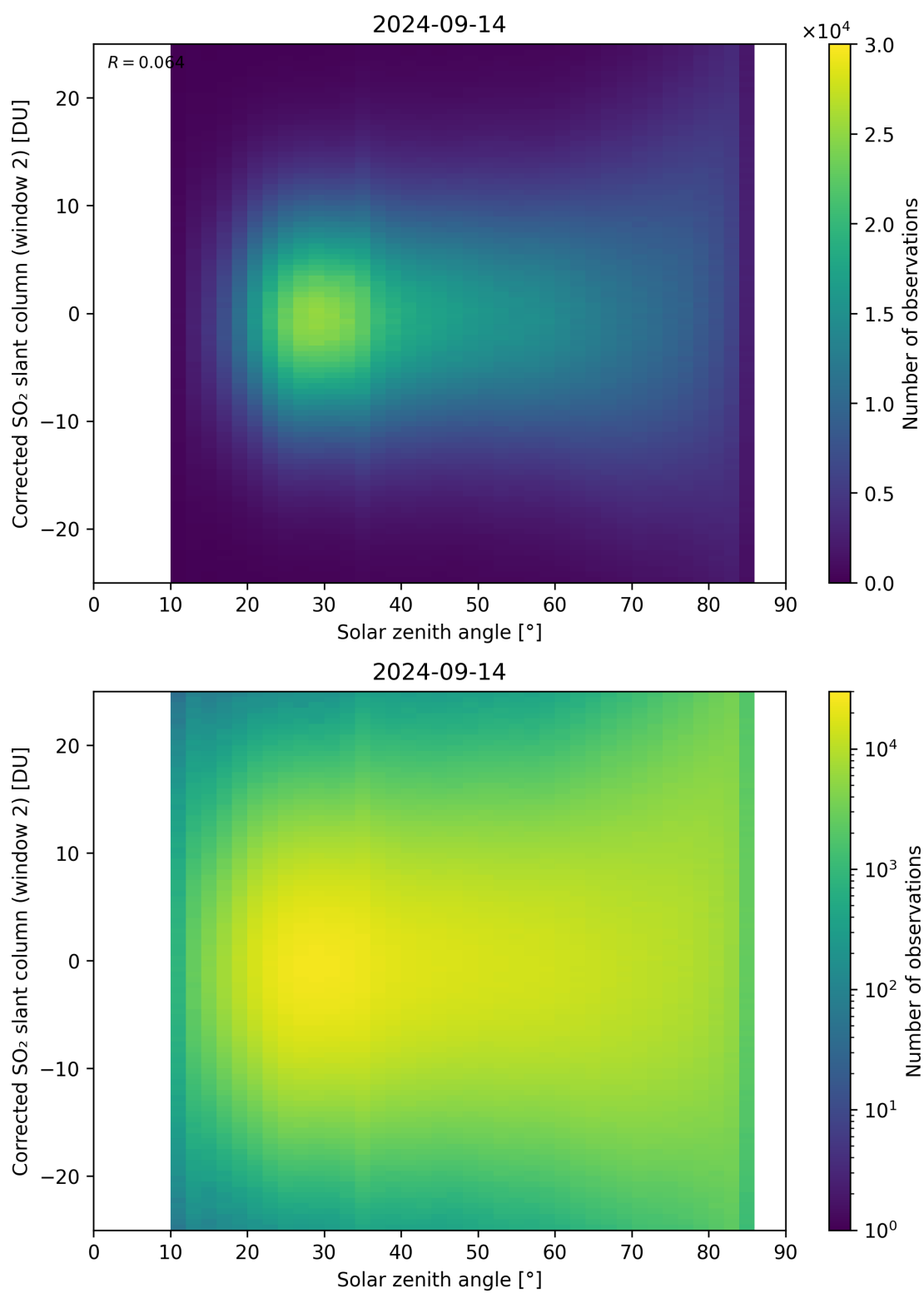
Figure 167: Scatter density plot of “Solar zenith angle” against “Corrected SO 2 slant column (window 2)” for 2024-09-13 to 2024-09-15.
