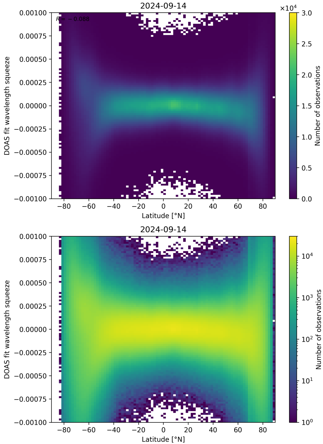
Figure 143: Scatter density plot of “Latitude” against “DOAS fit wavelength squeeze” for 2024-09-13 to 2024-09-15.
