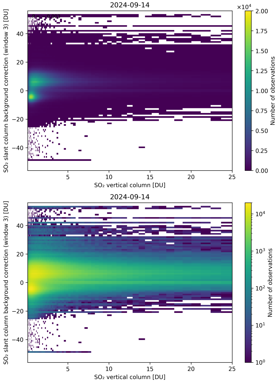
Figure 275: Scatter density plot of “SO 2 vertical column” against “SO 2 slant column background correction (window 3)” for 2024-09-13 to 2024-09-15.
