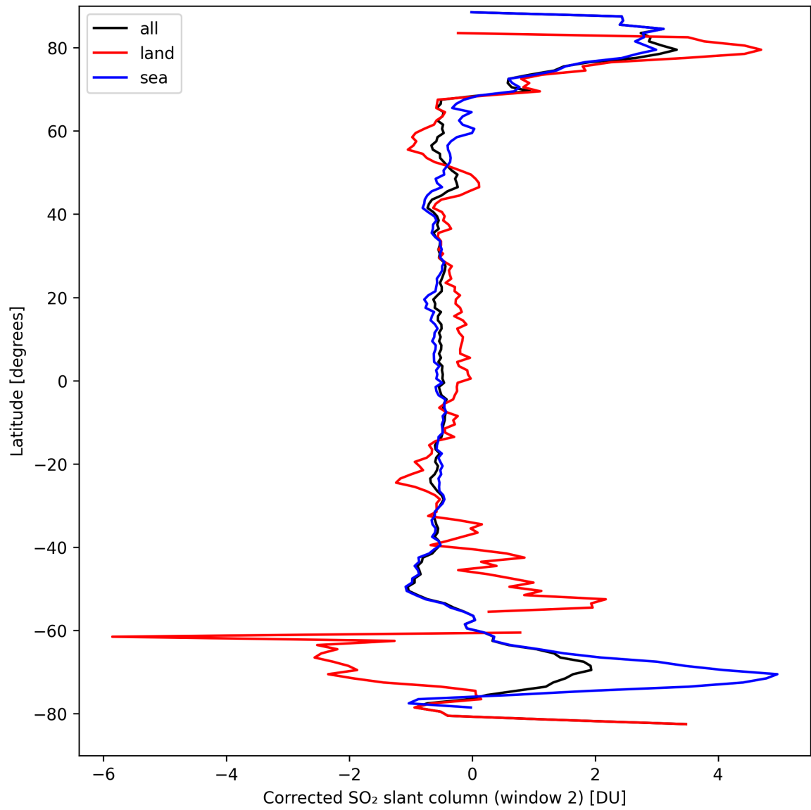
Figure 39: Zonal average of “Corrected SO 2 slant column (window 2)” for 2024-09-13 to 2024-09-15.
