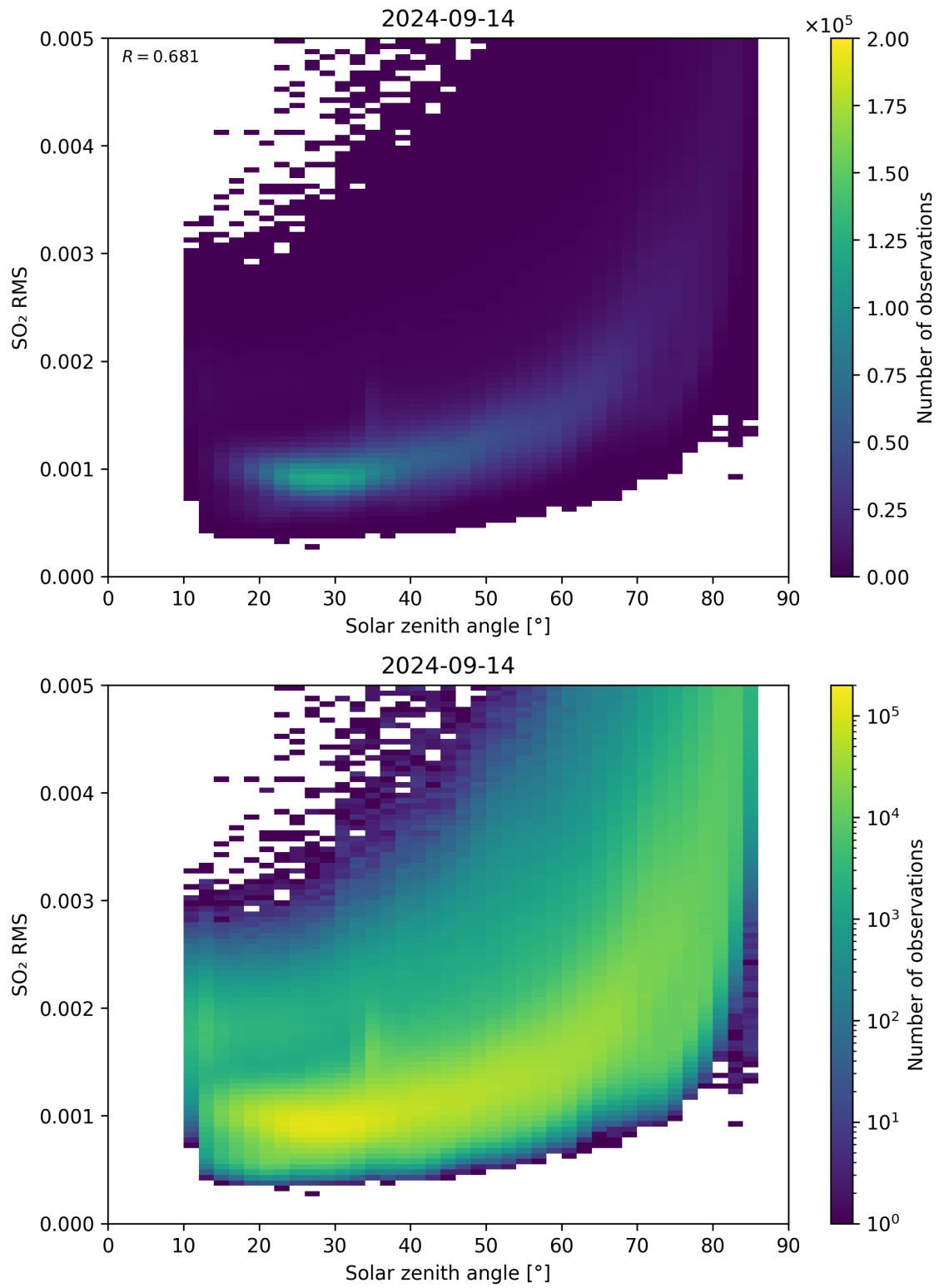
Figure 163: Scatter density plot of “Solar zenith angle” against “SO 2 RMS” for 2024-09-13 to 2024-09-15.
