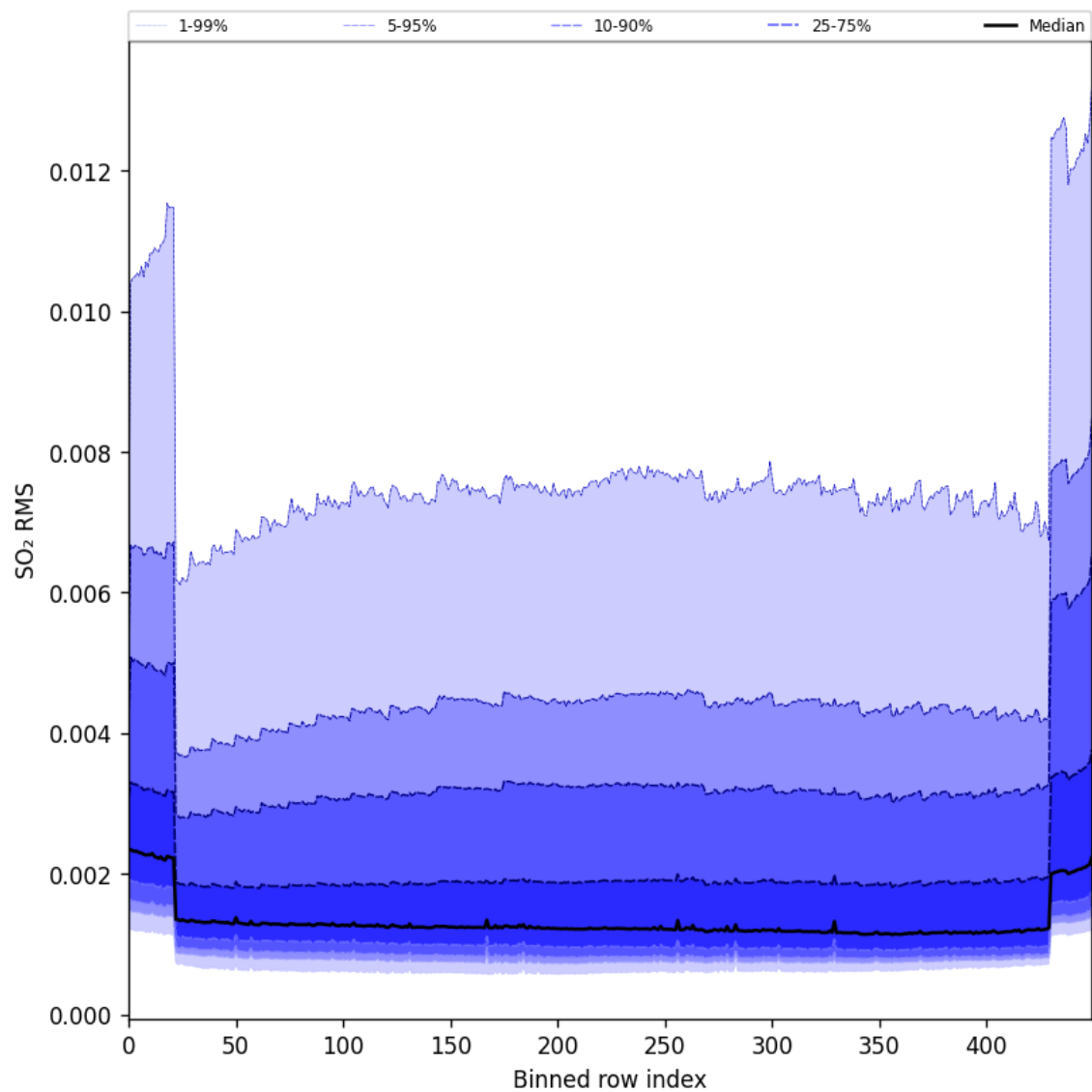
Figure 93: Along track statistics of “SO 2 RMS” for 2024-09-13 to 2024-09-15
