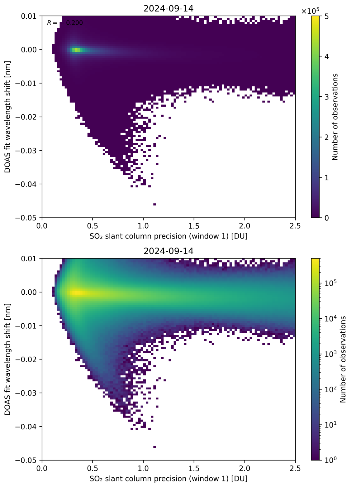
Figure 221: Scatter density plot of “SO 2 slant column precision (window 1)” against “DOAS fit wavelength shift” for 2024-09-13 to 2024-09-15.
