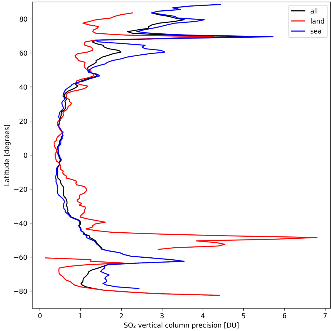
Figure 31: Zonal average of “SO 2 vertical column precision” for 2024-09-13 to 2024-09-15.
