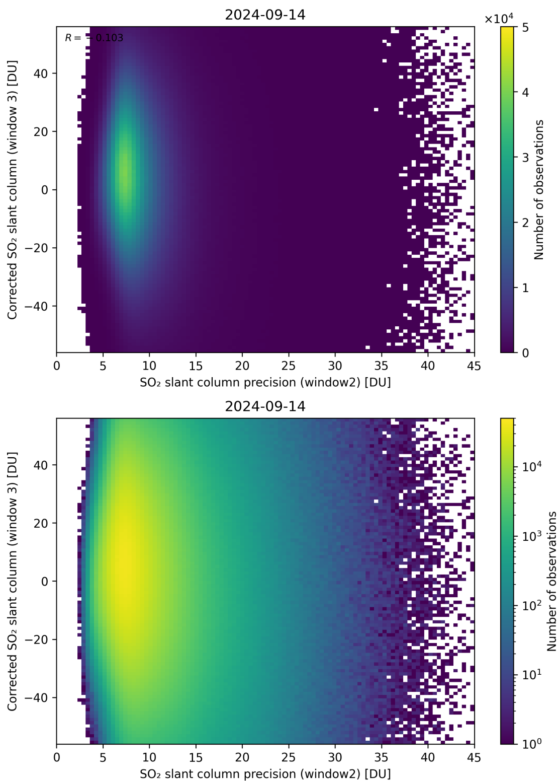
Figure 248: Scatter density plot of “SO 2 slant column precision (window2)” against “Corrected SO 2 slant column (window 3)” for 2024-09-13 to 2024-09-15.
