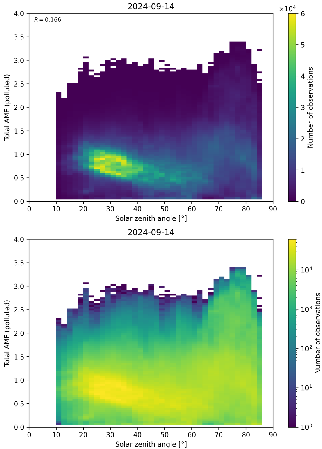
Figure 174: Scatter density plot of “Solar zenith angle” against “Total AMF (polluted)” for 2024-09-13 to 2024-09-15.
