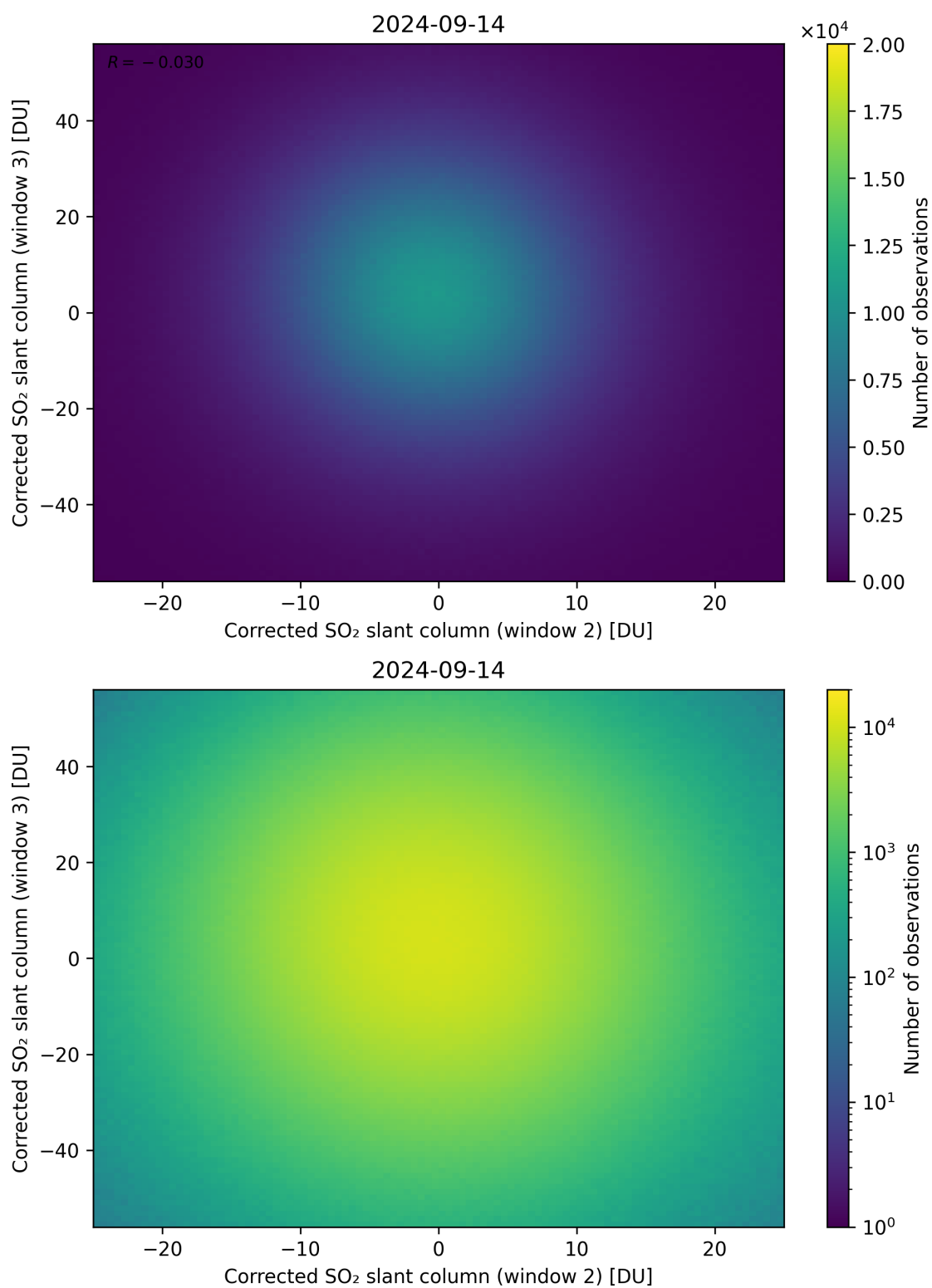
Figure 200: Scatter density plot of “Corrected SO 2 slant column (window 2)” against “Corrected SO 2 slant column (window 3)” for 2024-09-13 to 2024-09-15.
