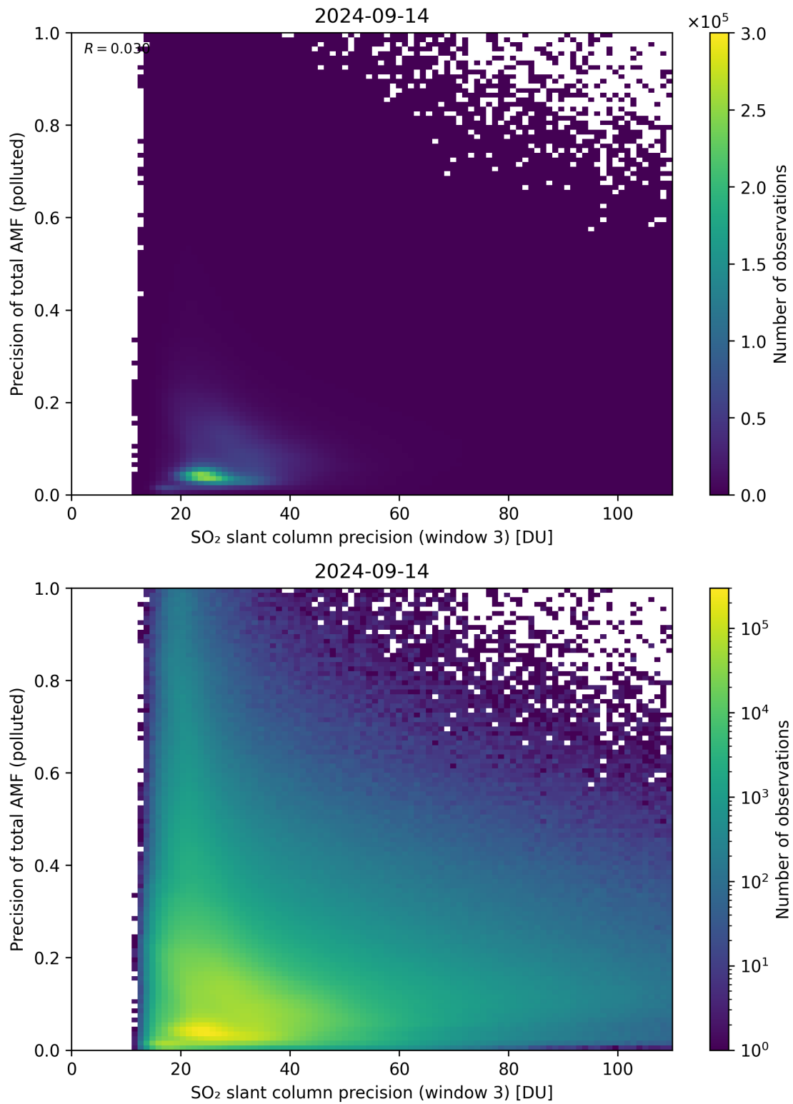
Figure 264: Scatter density plot of “SO 2 slant column precision (window 3)” against “Precision of total AMF (polluted)” for 2024-09-13 to 2024-09-15.
