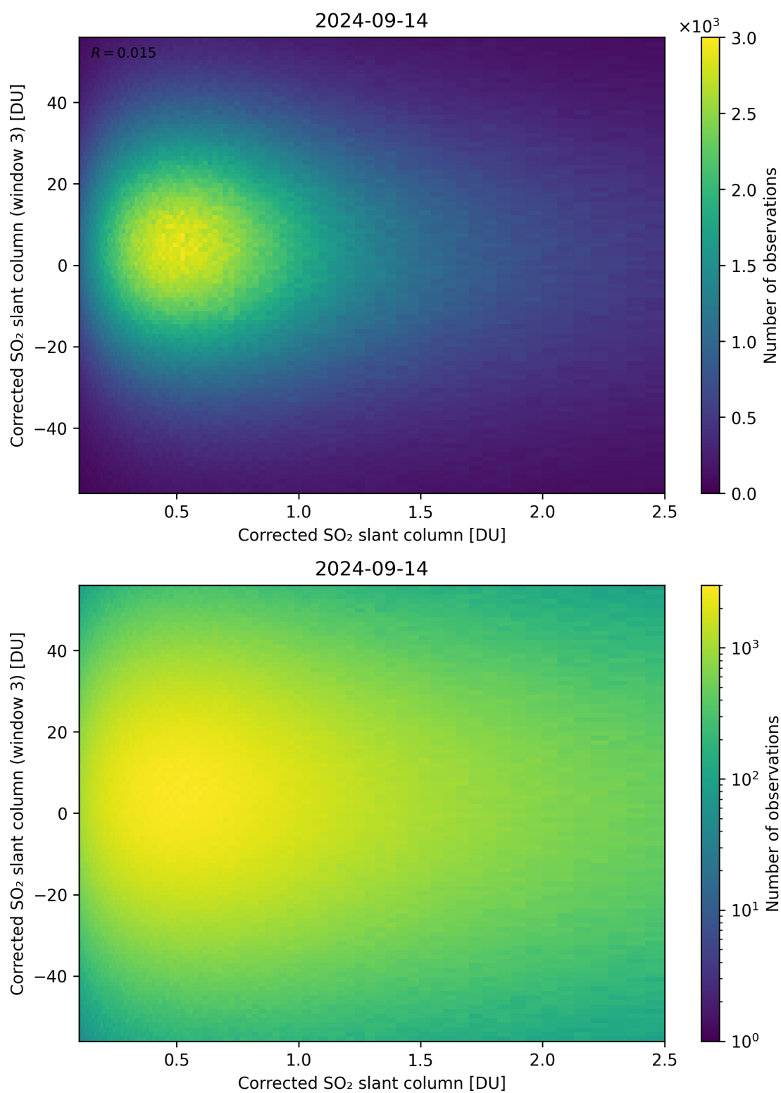
Figure 186: Scatter density plot of “Corrected SO 2 slant column” against “Corrected SO 2 slant column (window 3)” for 2024-09-13 to 2024-09-15.
