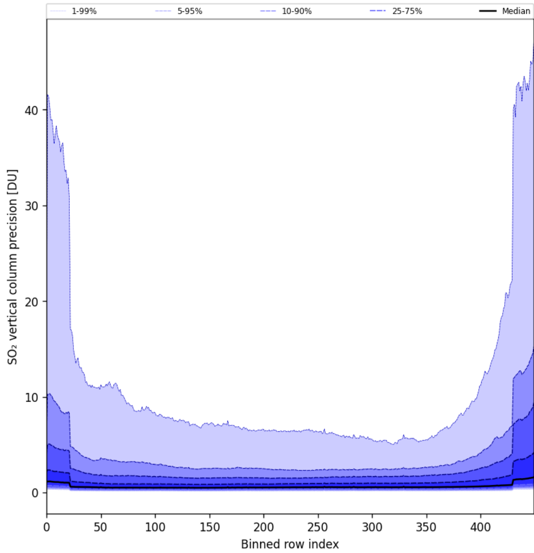
Figure 77: Along track statistics of “SO 2 vertical column precision” for 2024-09-13 to 2024-09-15
