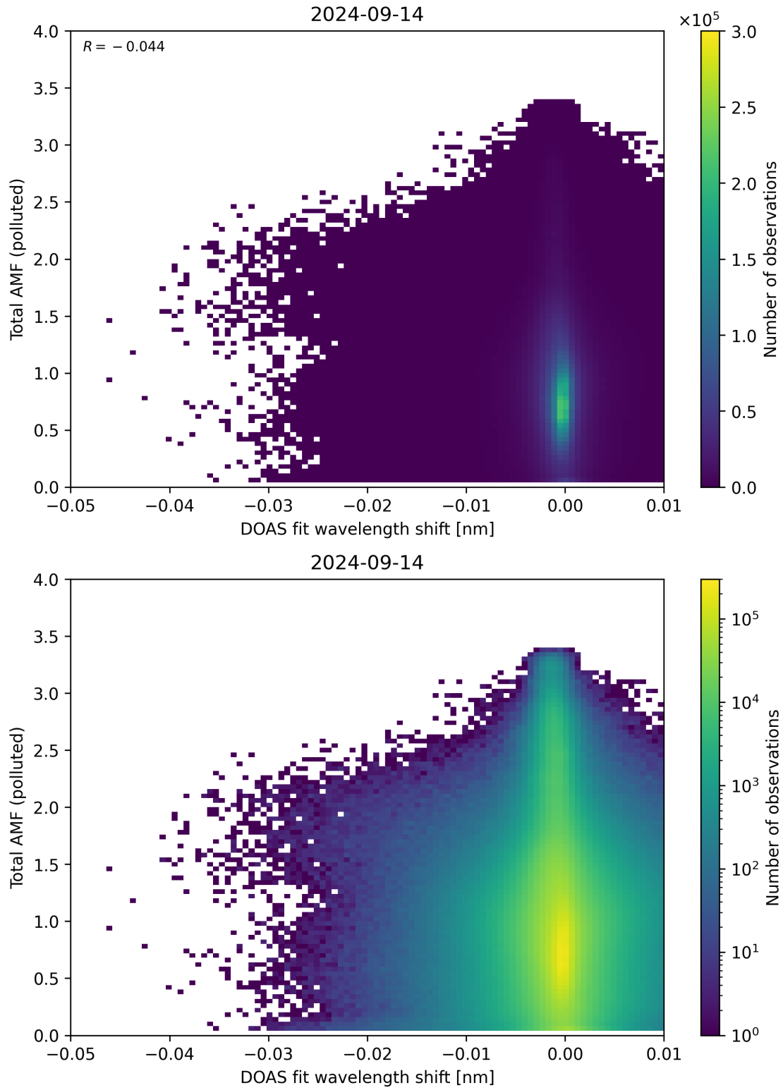
Figure 130: Scatter density plot of “DOAS fit wavelength shift” against “Total AMF (polluted)” for 2024-09-13 to 2024-09-15.
