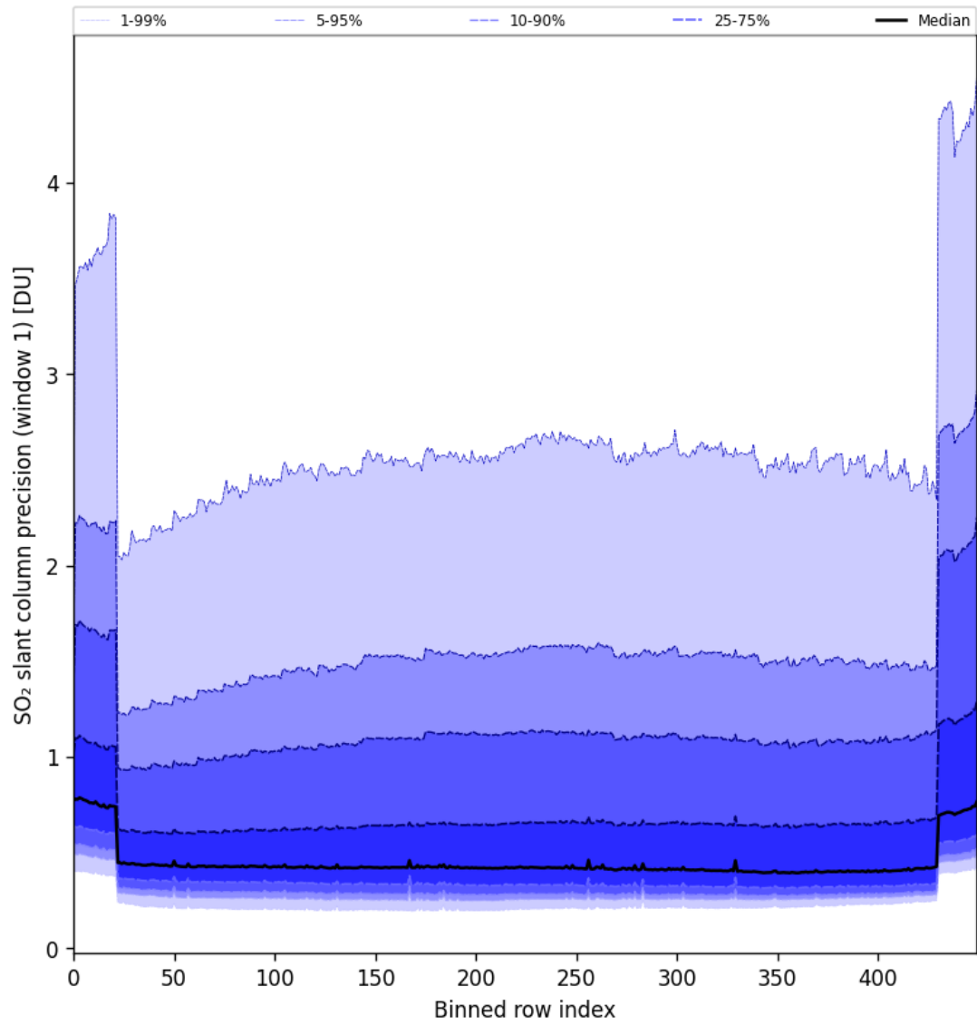
Figure 80: Along track statistics of “SO 2 slant column precision (window 1)” for 2024-09-13 to 2024-09-15
