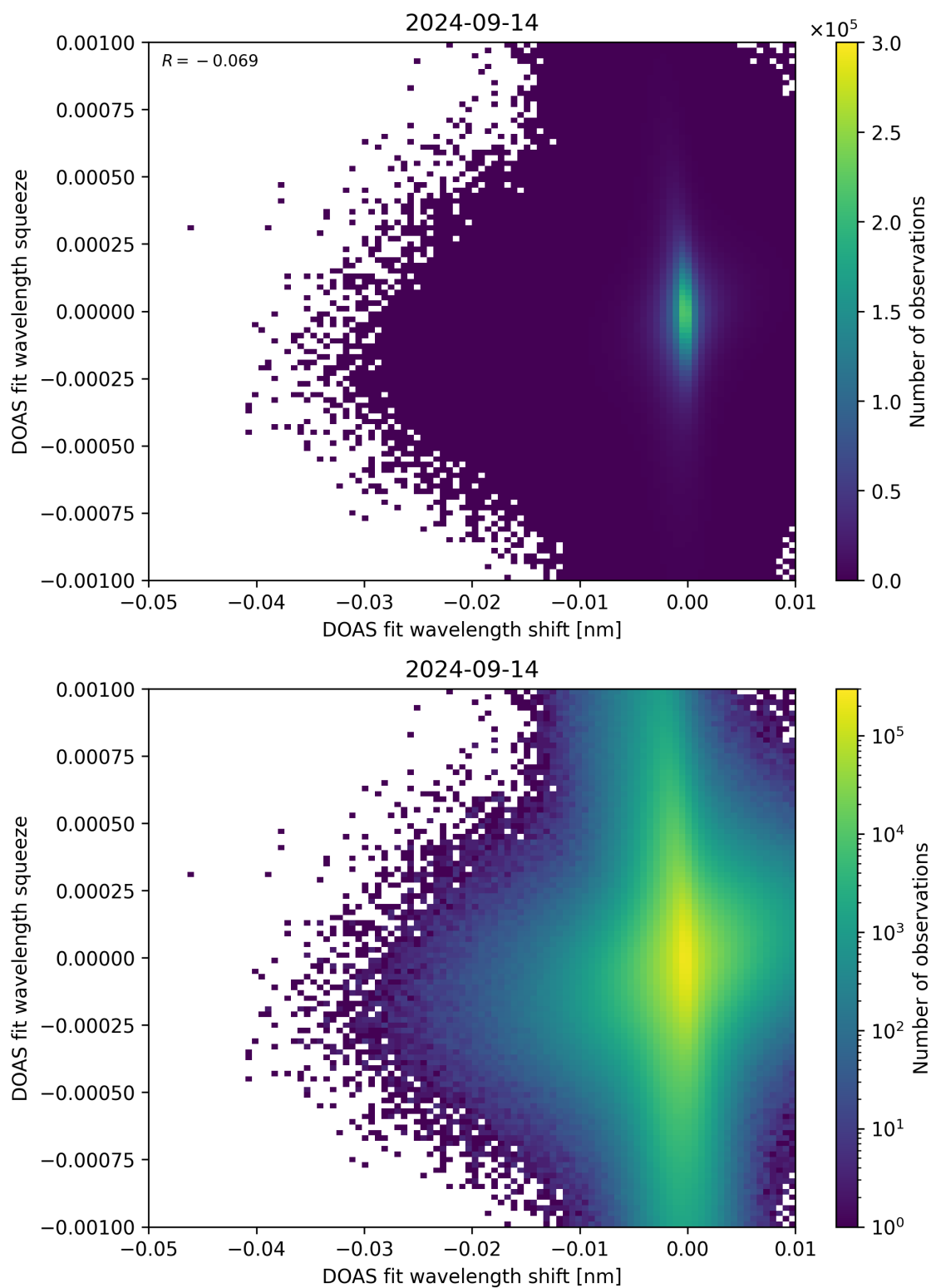
Figure 127: Scatter density plot of “DOAS fit wavelength shift” against “DOAS fit wavelength squeeze” for 2024-09-13 to 2024-09-15.
