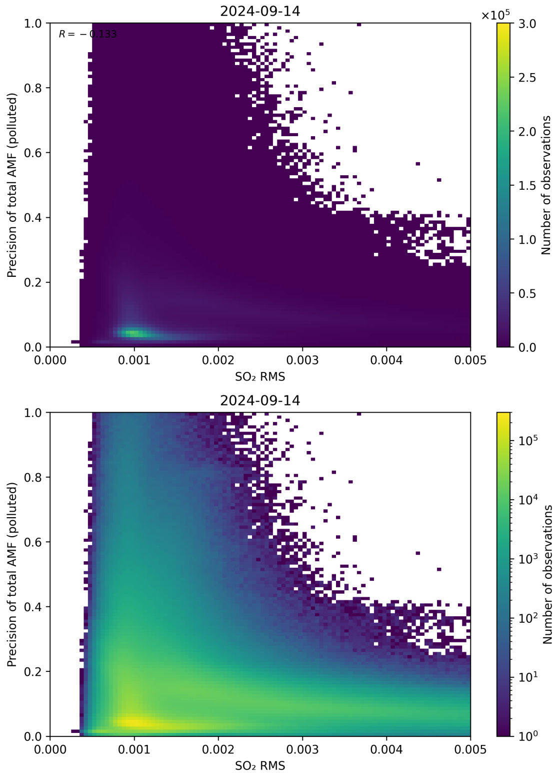
Figure 138: Scatter density plot of “SO 2 RMS” against “Precision of total AMF (polluted)” for 2024-09-13 to 2024-09-15.
