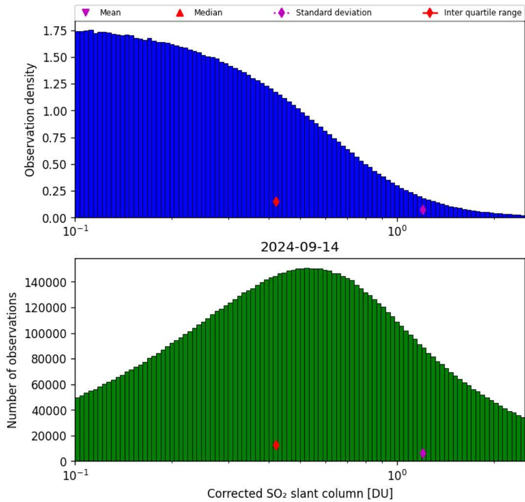
Figure 55: Histogram of “Corrected SO 2 slant column” for 2024-09-13 to 2024-09-15
