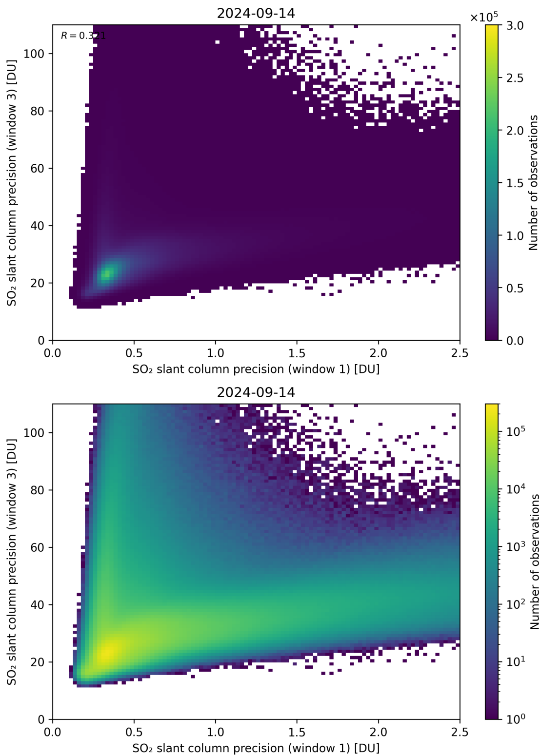
Figure 229: Scatter density plot of “SO 2 slant column precision (window 1)” against “SO 2 slant column precision (window 3)” for 2024-09-13 to 2024-09-15.
