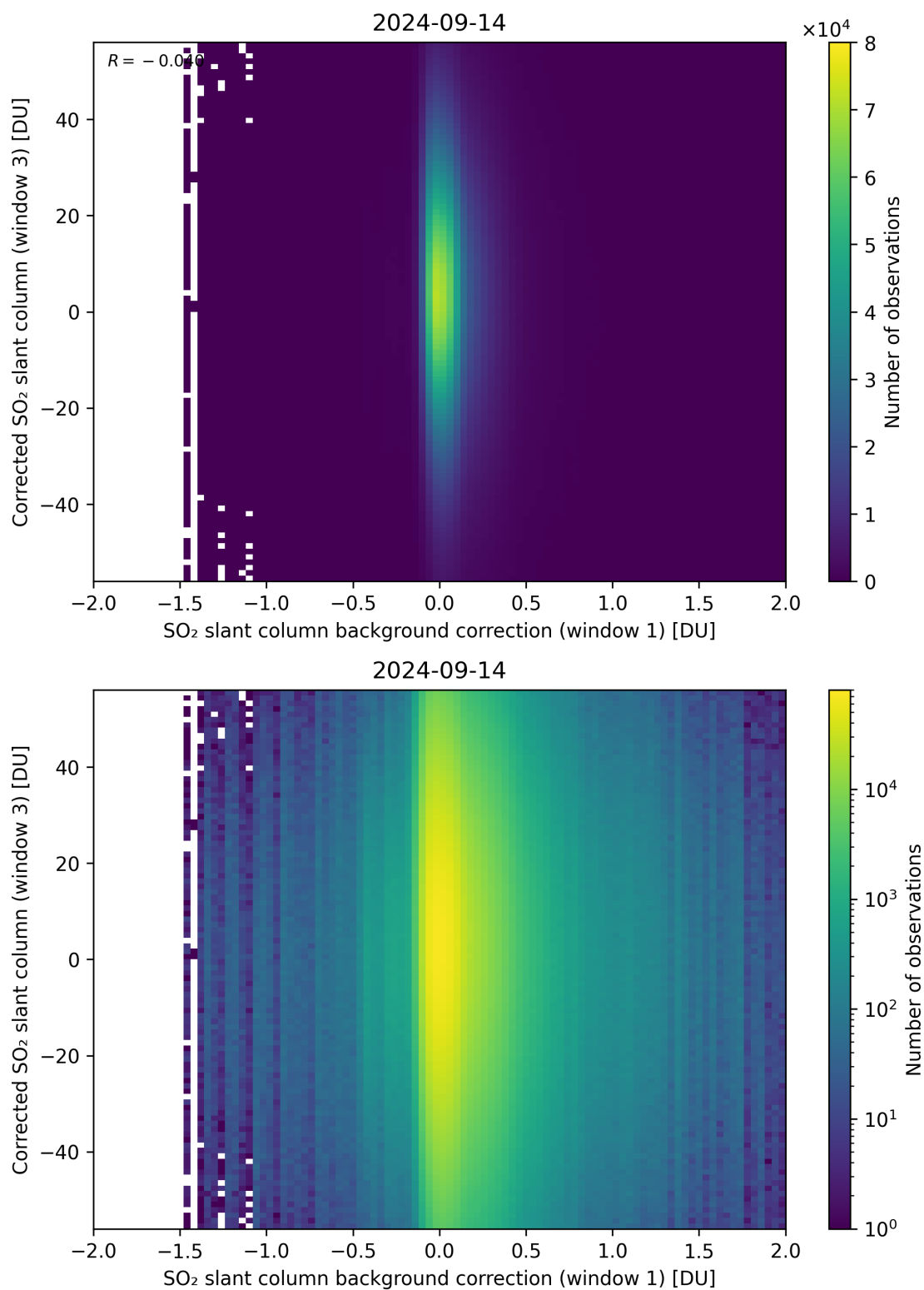
Figure 105: Scatter density plot of “SO 2 slant column background correction (window 1)” against “Corrected SO 2 slant column (window 3)” for 2024-09-13 to 2024-09-15.
