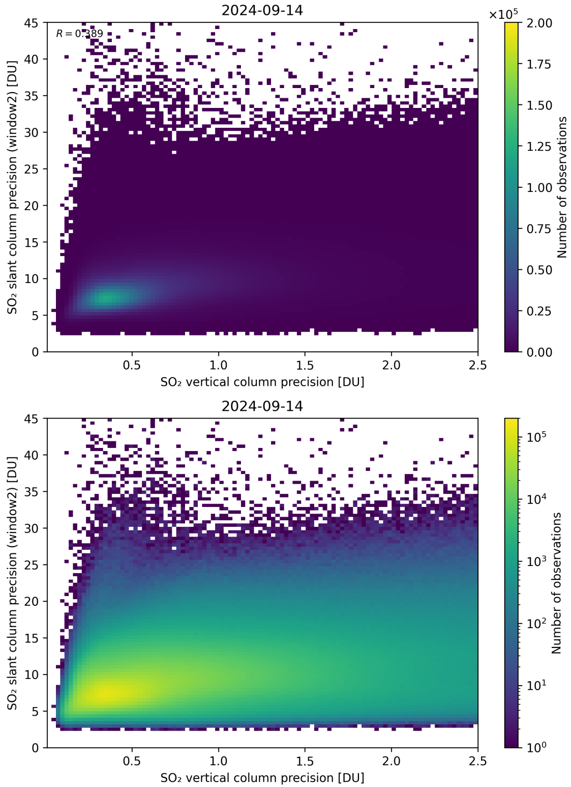
Figure 291: Scatter density plot of “SO 2 vertical column precision” against “SO 2 slant column precision (window2)” for 2024-09-13 to 2024-09-15.
