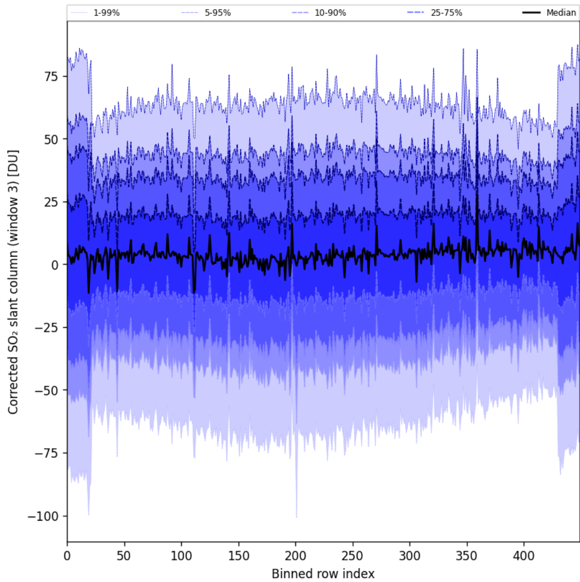
Figure 89: Along track statistics of “Corrected SO 2 slant column (window 3)” for 2024-09-13 to 2024-09-15
