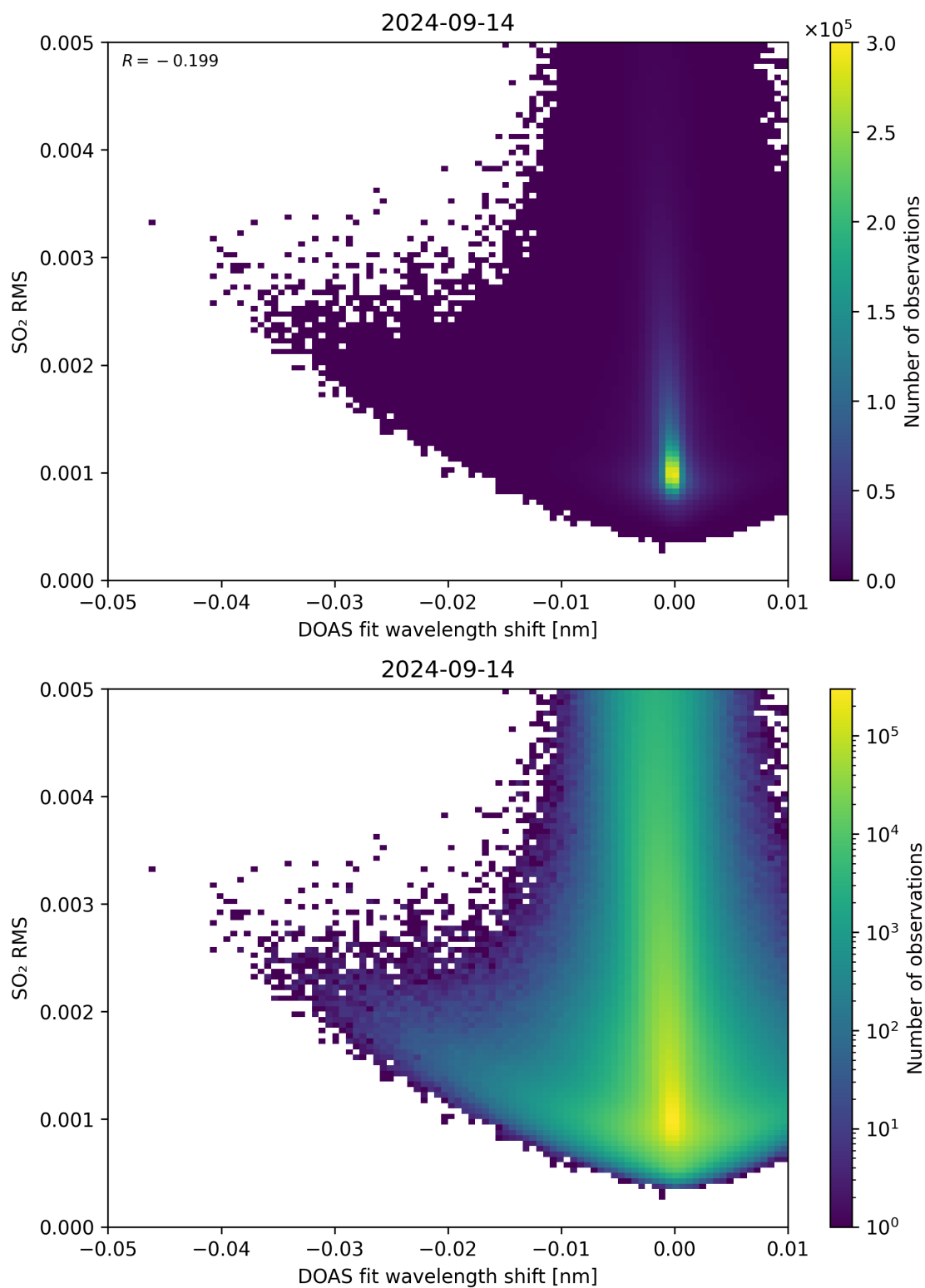
Figure 128: Scatter density plot of “DOAS fit wavelength shift” against “SO 2 RMS” for 2024-09-13 to 2024-09-15.
