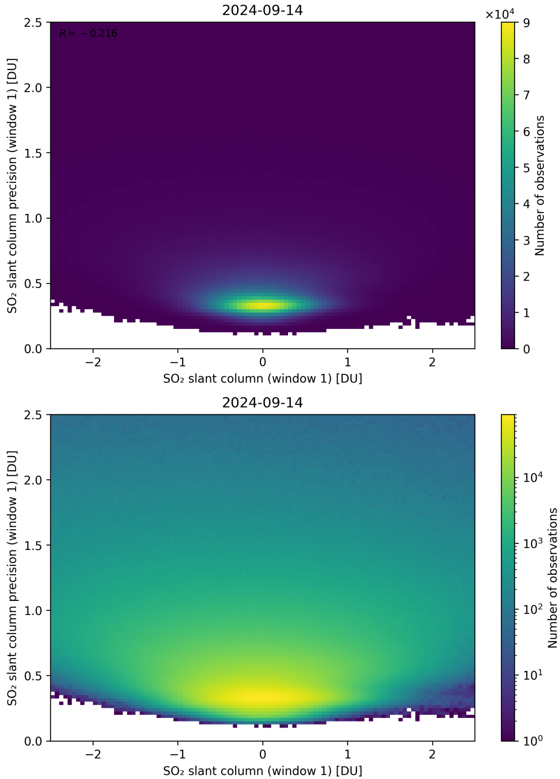
Figure 235: Scatter density plot of “SO 2 slant column (window 1)” against “SO 2 slant column precision (window 1)” for 2024-09-13 to 2024-09-15.
