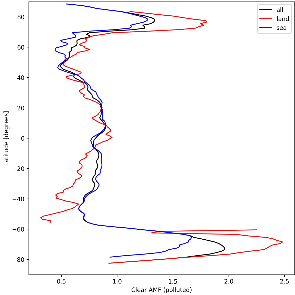
Figure 50: Zonal average of “Clear AMF (polluted)” for 2024-09-13 to 2024-09-15.
