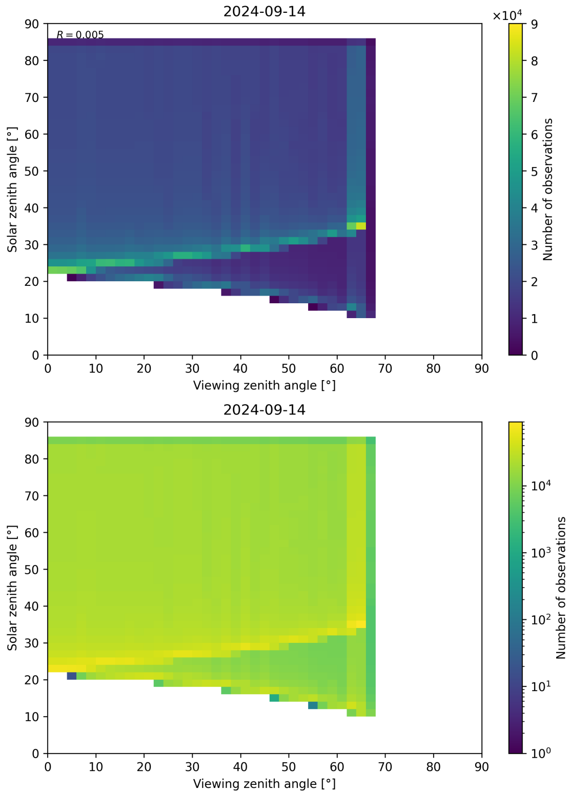
Figure 315: Scatter density plot of “Viewing zenith angle” against “Solar zenith angle” for 2024-09-13 to 2024-09-15.
