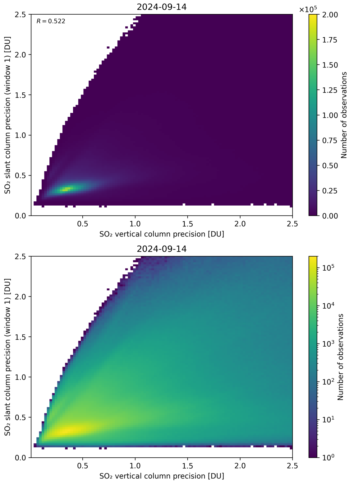
Figure 290: Scatter density plot of “SO 2 vertical column precision” against “SO 2 slant column precision (window 1)” for 2024-09-13 to 2024-09-15.
