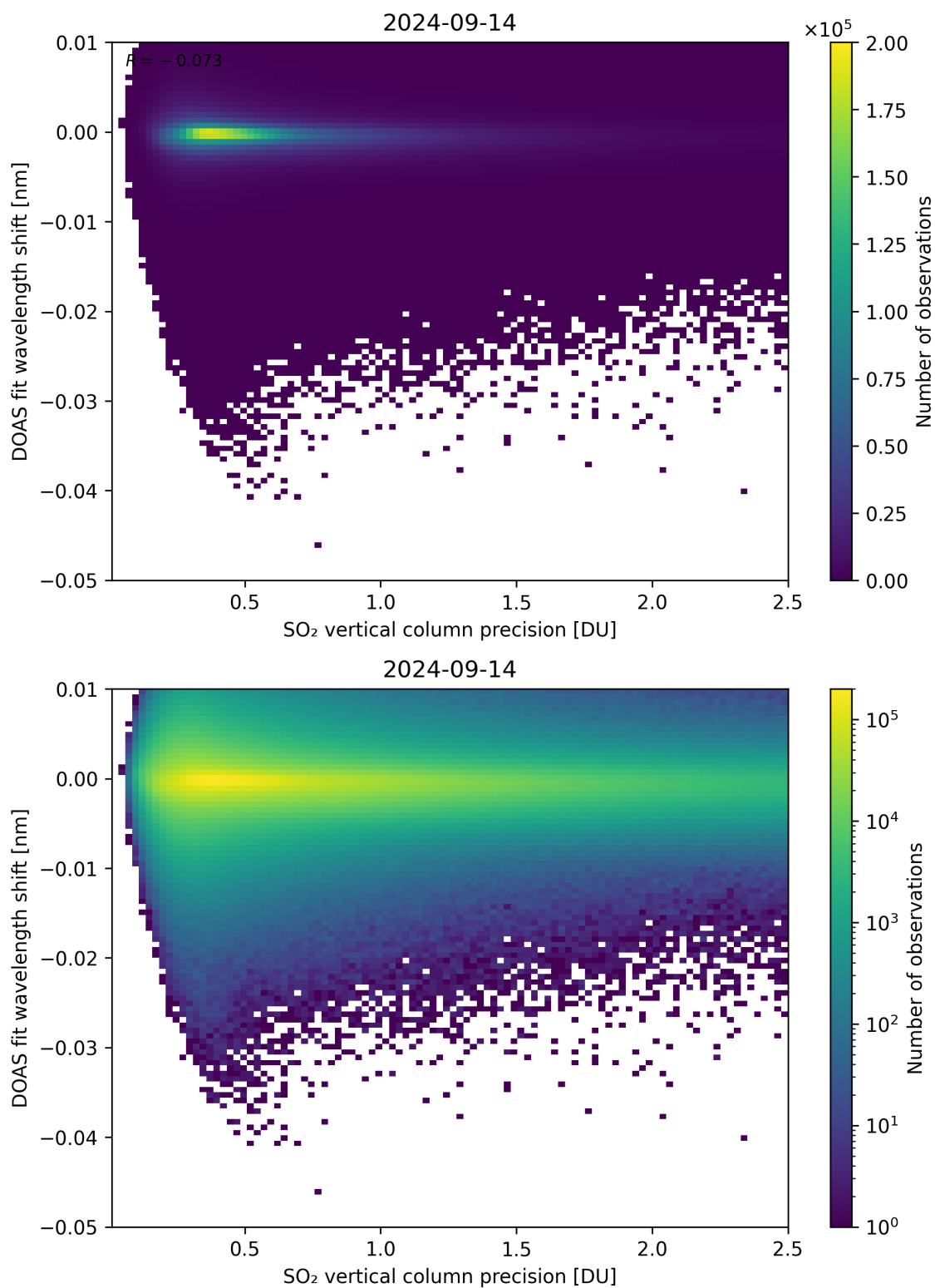
Figure 282: Scatter density plot of “SO 2 vertical column precision” against “DOAS fit wavelength shift” for 2024-09-13 to 2024-09-15.
