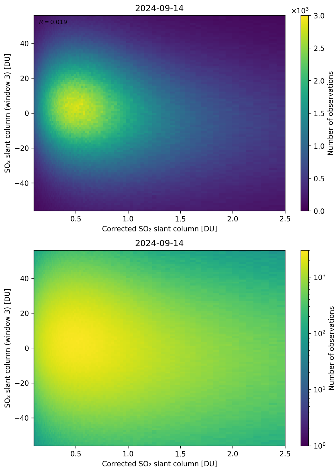
Figure 190: Scatter density plot of “Corrected SO 2 slant column” against “SO 2 slant column (window 3)” for 2024-09-13 to 2024-09-15.
