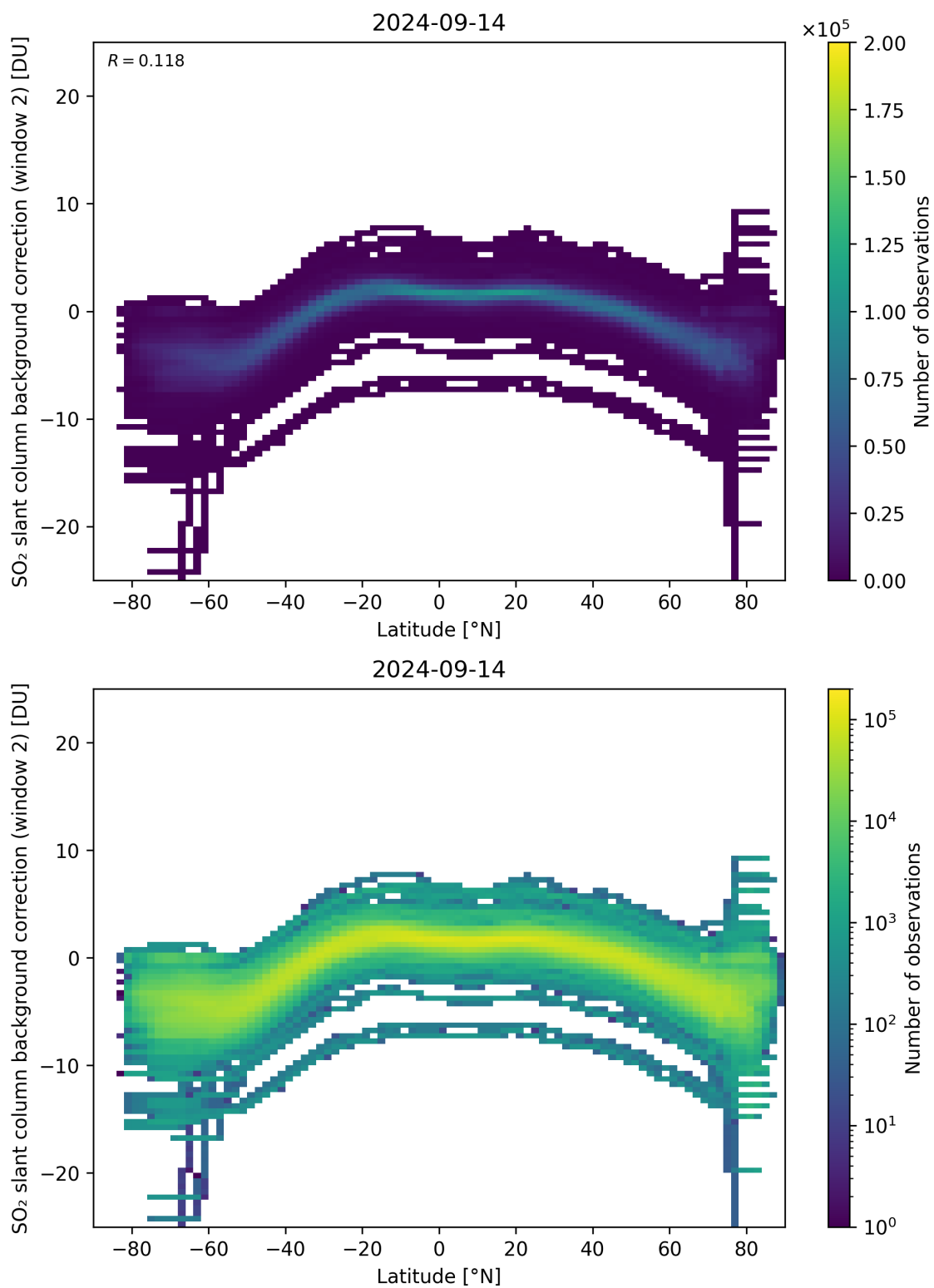
Figure 140: Scatter density plot of “Latitude” against “SO 2 slant column background correction (window 2)” for 2024-09-13 to 2024-09-15.
