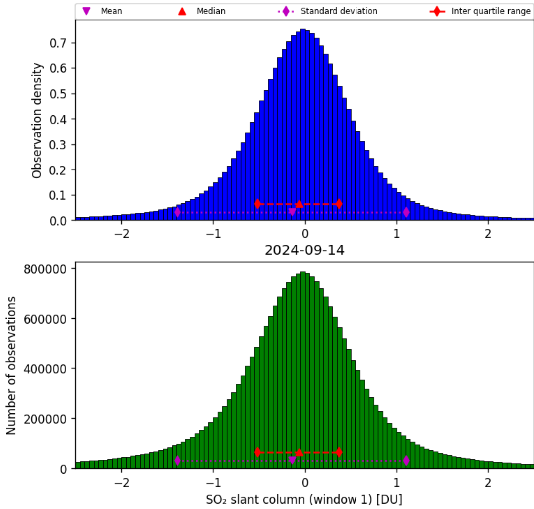
Figure 56: Histogram of “SO 2 slant column (window 1)” for 2024-09-13 to 2024-09-15
