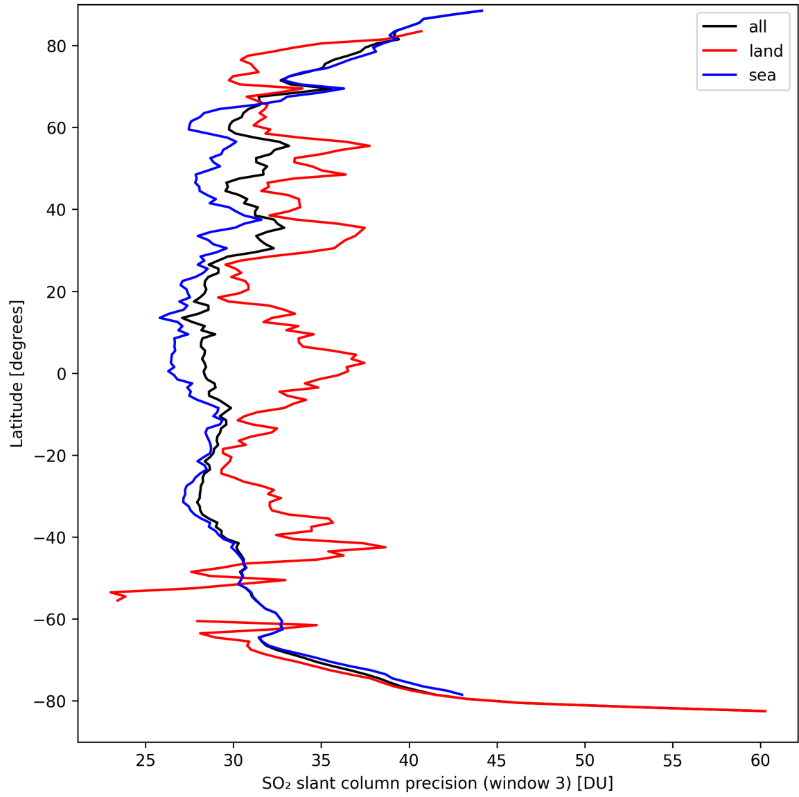
Figure 42: Zonal average of “SO 2 slant column precision (window 3)” for 2024-09-13 to 2024-09-15.
