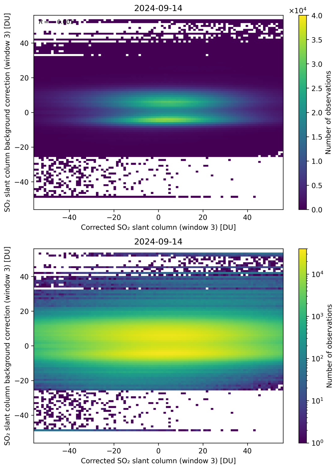
Figure 205: Scatter density plot of “Corrected SO 2 slant column (window 3)” against “SO 2 slant column background correction (window 3)” for 2024-09-13 to 2024-09-15.
