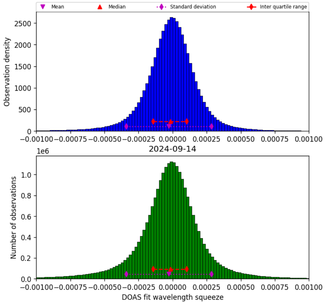
Figure 69: Histogram of “DOAS fit wavelength squeeze” for 2024-09-13 to 2024-09-15
