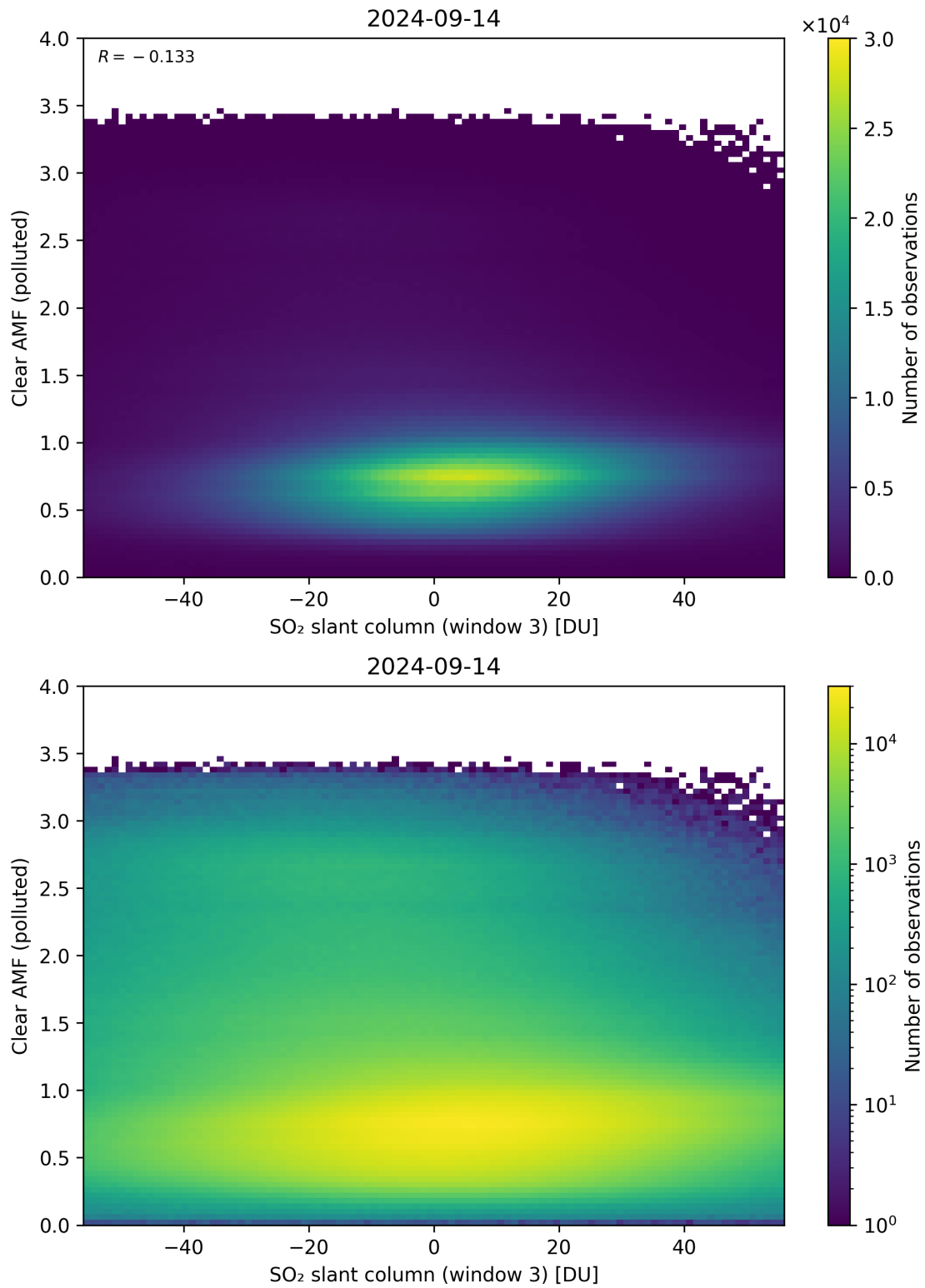
Figure 265: Scatter density plot of “SO 2 slant column (window 3)” against “Clear AMF (polluted)” for 2024-09-13 to 2024-09-15.
