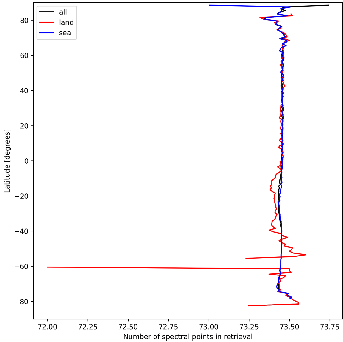
Figure 51: Zonal average of “Number of spectral points in retrieval” for 2024-09-13 to 2024-09-15.
