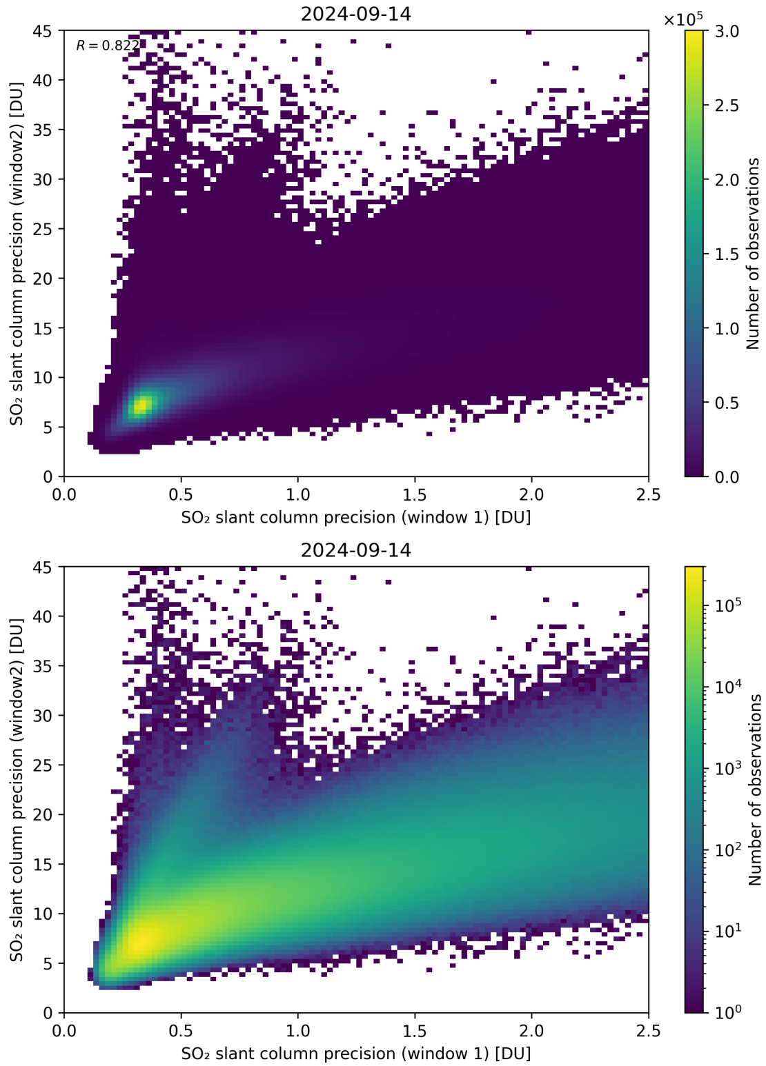
Figure 227: Scatter density plot of “SO 2 slant column precision (window 1)” against “SO 2 slant column precision (window 2)” for 2024-09-13 to 2024-09-15.
