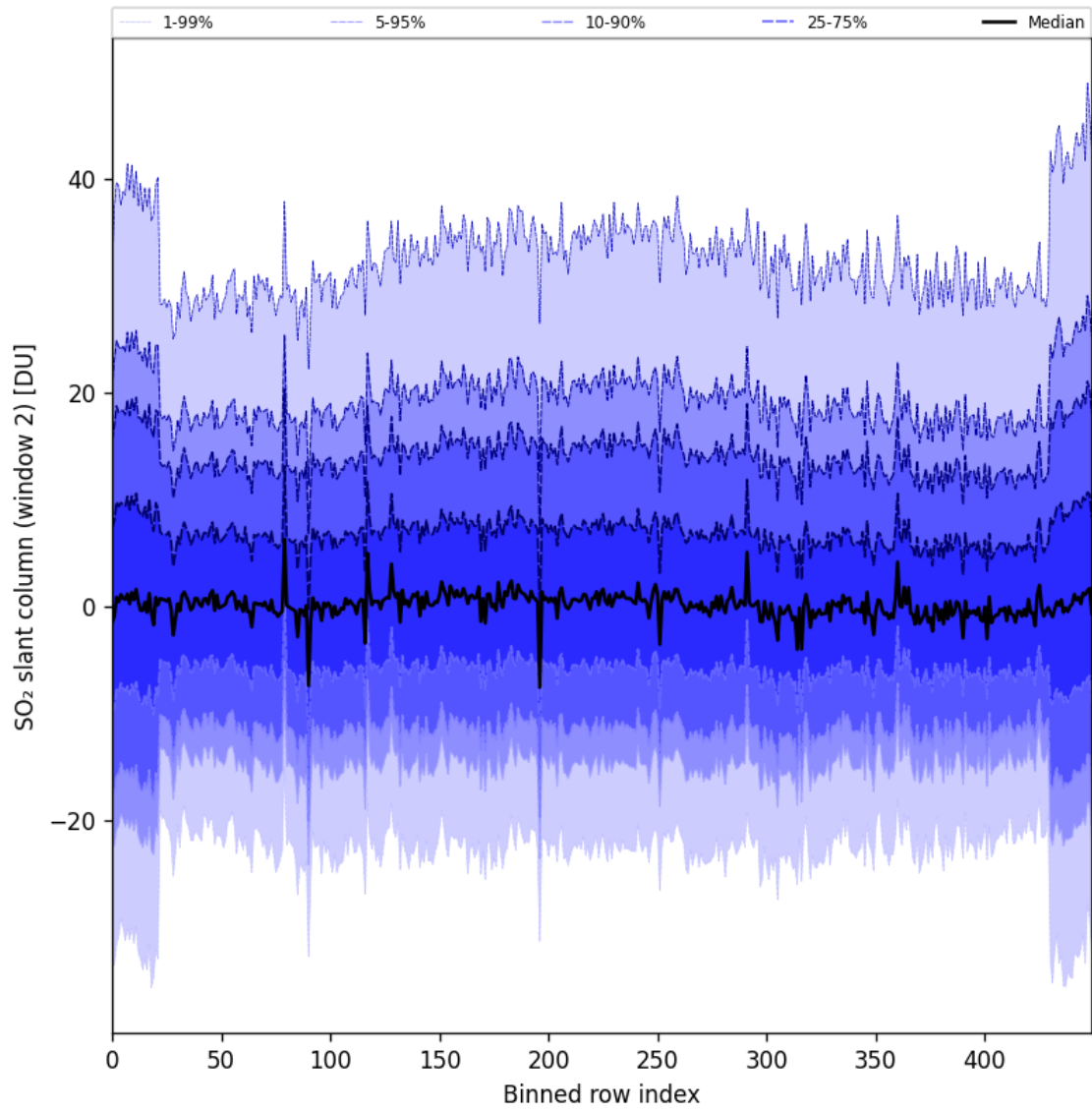
Figure 83: Along track statistics of “SO 2 slant column (window 2)” for 2024-09-13 to 2024-09-15
