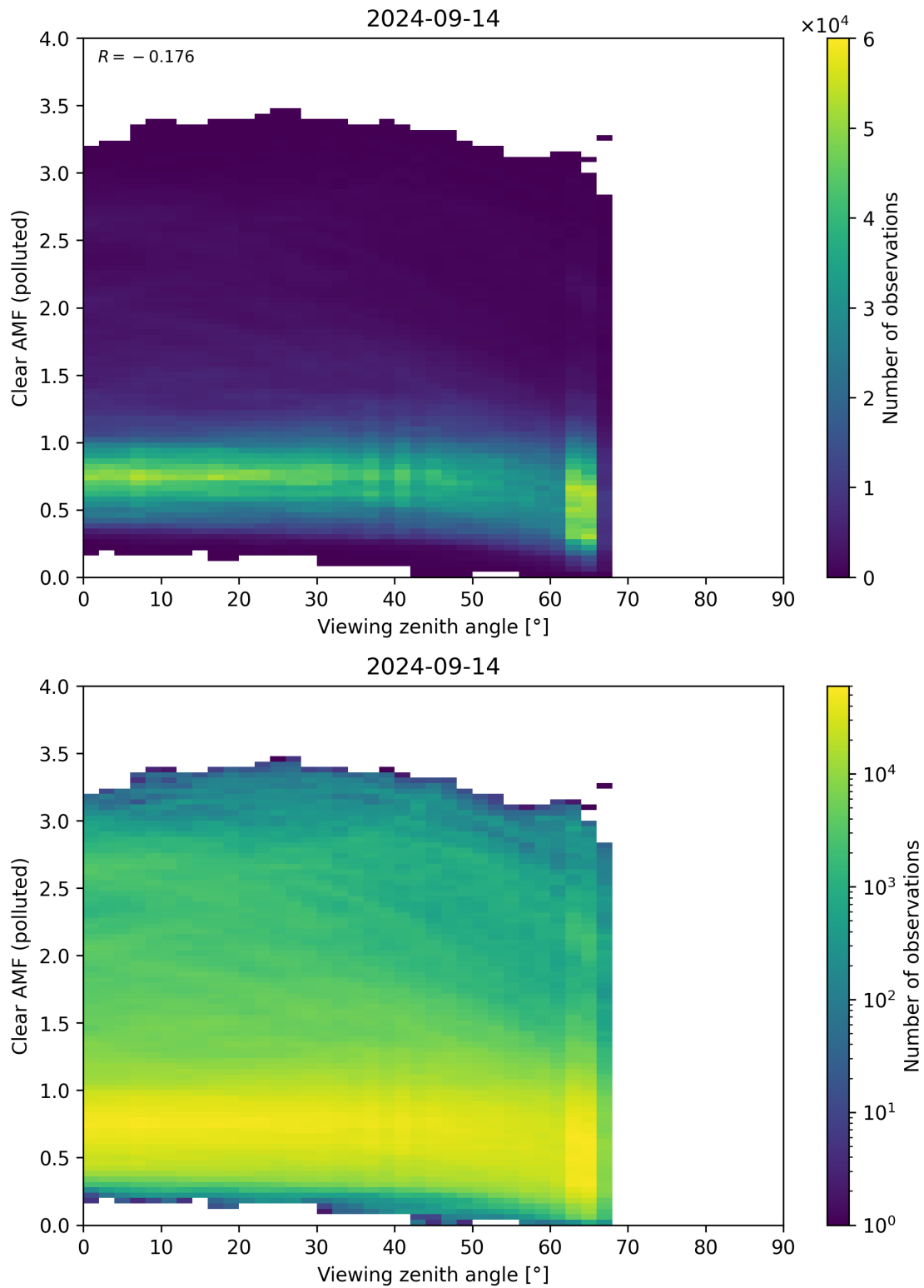
Figure 316: Scatter density plot of “Viewing zenith angle” against “Clear AMF (polluted)” for 2024-09-13 to 2024-09-15.
