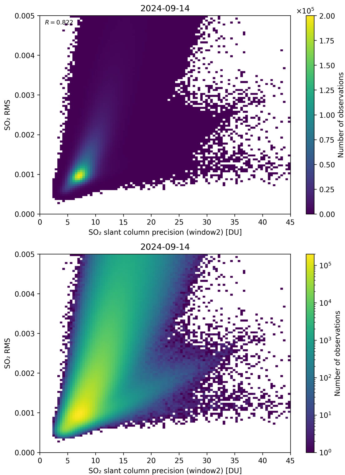
Figure 245: Scatter density plot of “SO 2 slant column precision (window2)” against “SO 2 RMS” for 2024-09-13 to 2024-09-15.
