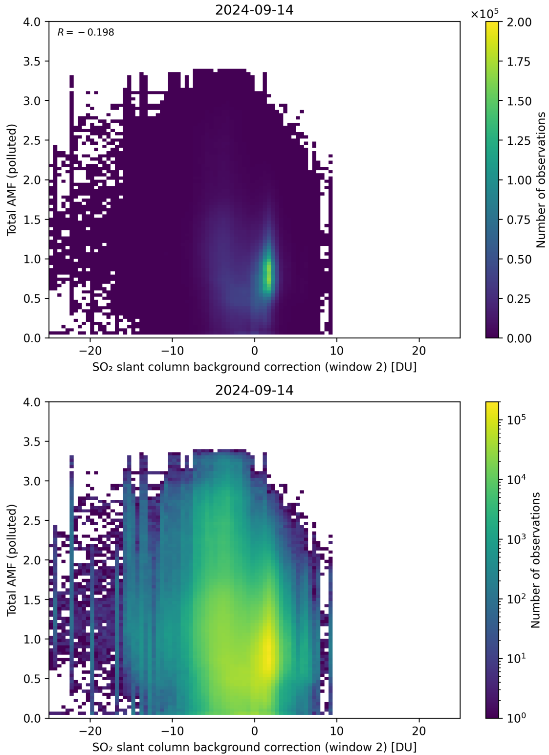
Figure 119: Scatter density plot of “SO 2 slant column background correction (window 2)” against “Total AMF (polluted)” for 2024-09-13 to 2024-09-15.
