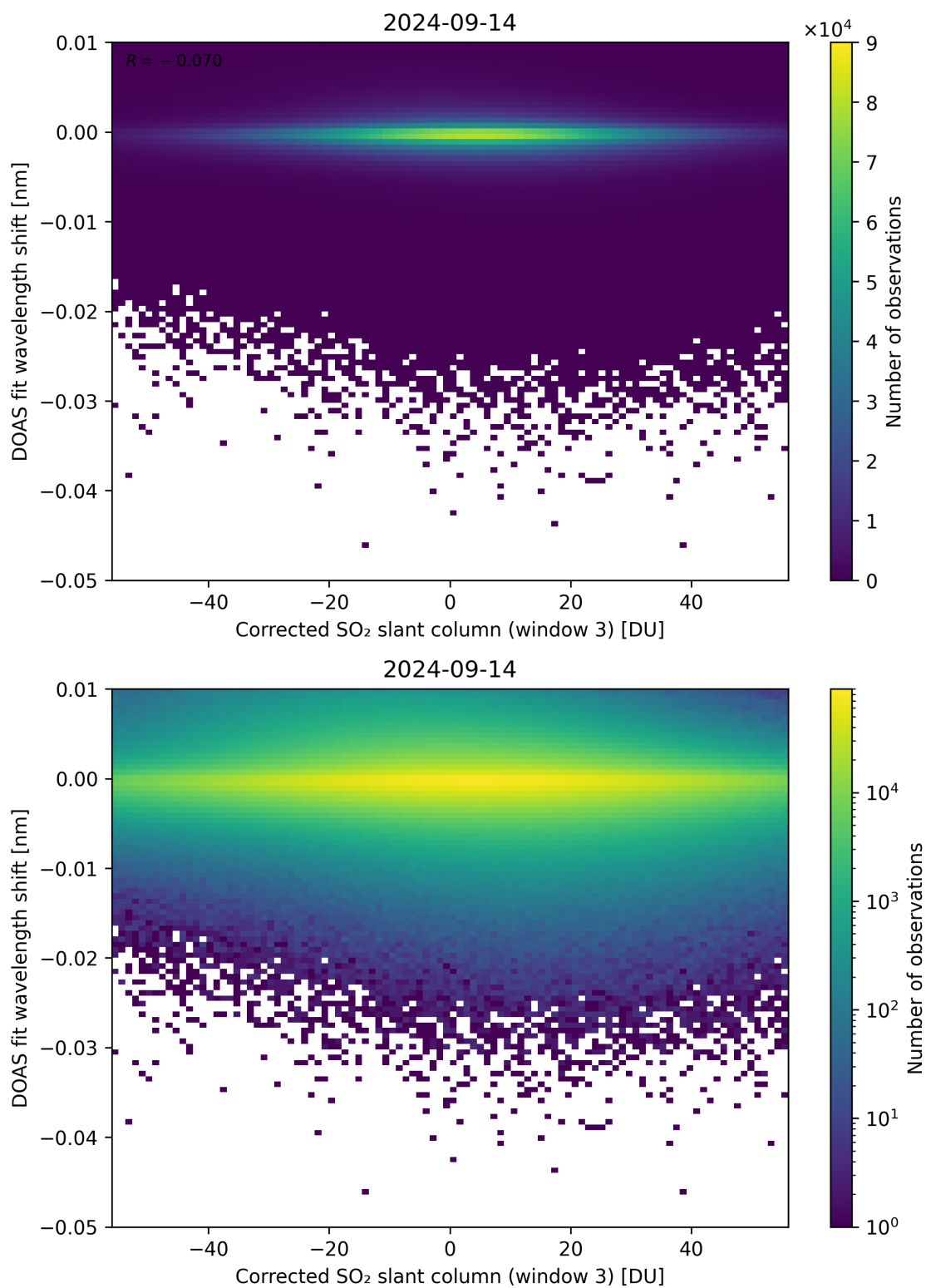
Figure 206: Scatter density plot of “Corrected SO 2 slant column (window 3)” against “DOAS fit wavelength shift” for 2024-09-13 to 2024-09-15.
