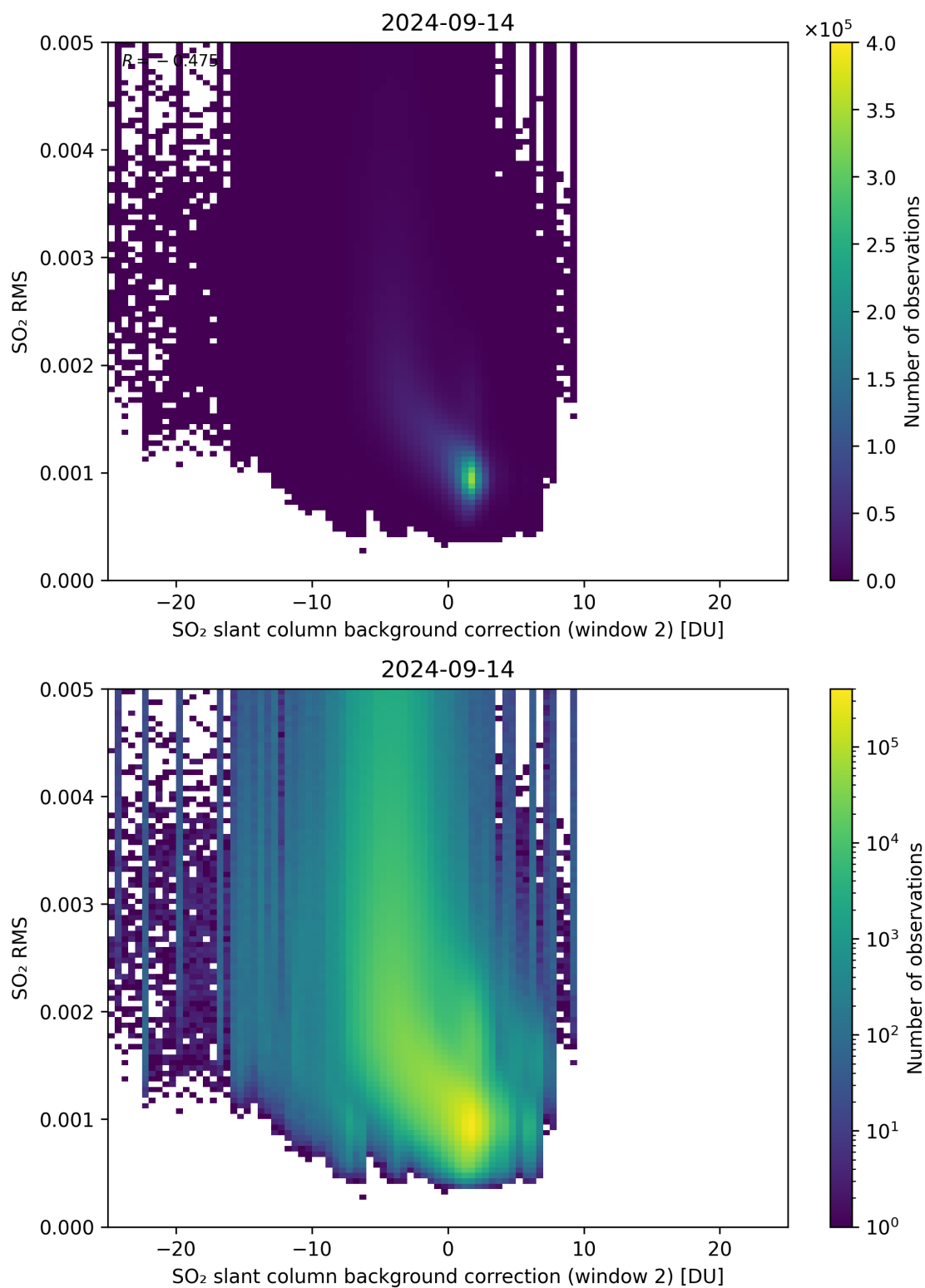
Figure 114: Scatter density plot of “SO 2 slant column background correction (window 2)” against “SO 2 RMS” for 2024-09-13 to 2024-09-15.
