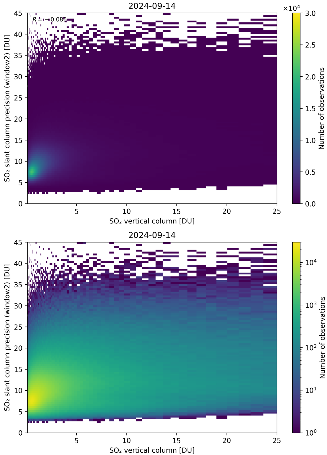
Figure 302: Scatter density plot of “SO 2 vertical column” against “SO 2 slant column precision (window2)” for 2024-09-13 to 2024-09-15.
