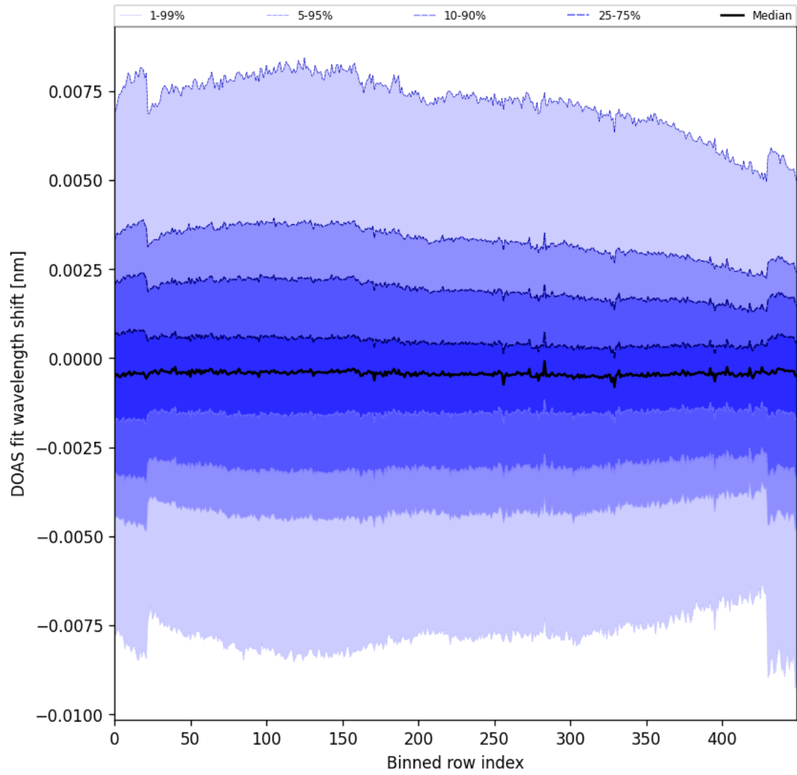
Figure 91: Along track statistics of “DOAS fit wavelength shift” for 2024-09-13 to 2024-09-15
