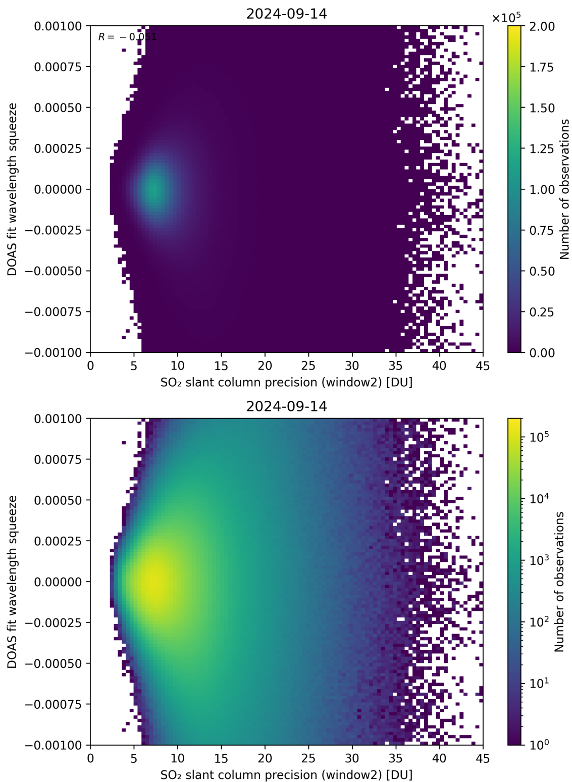
Figure 244: Scatter density plot of “SO 2 slant column precision (window2)” against “DOAS fit wavelength squeeze” for 2024-09-13 to 2024-09-15.
