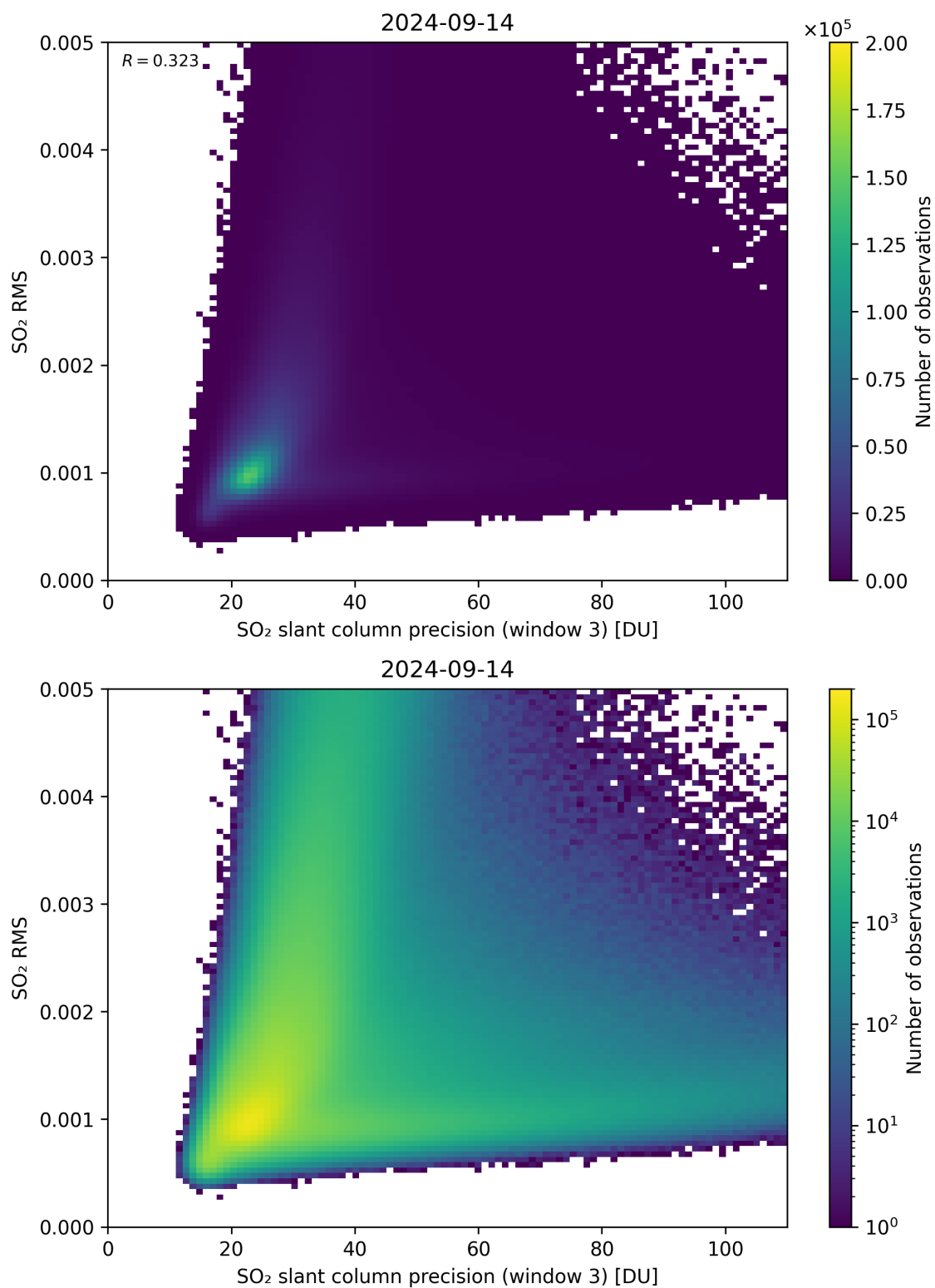
Figure 260: Scatter density plot of “SO 2 slant column precision (window 3)” against “SO 2 RMS” for 2024-09-13 to 2024-09-15.
