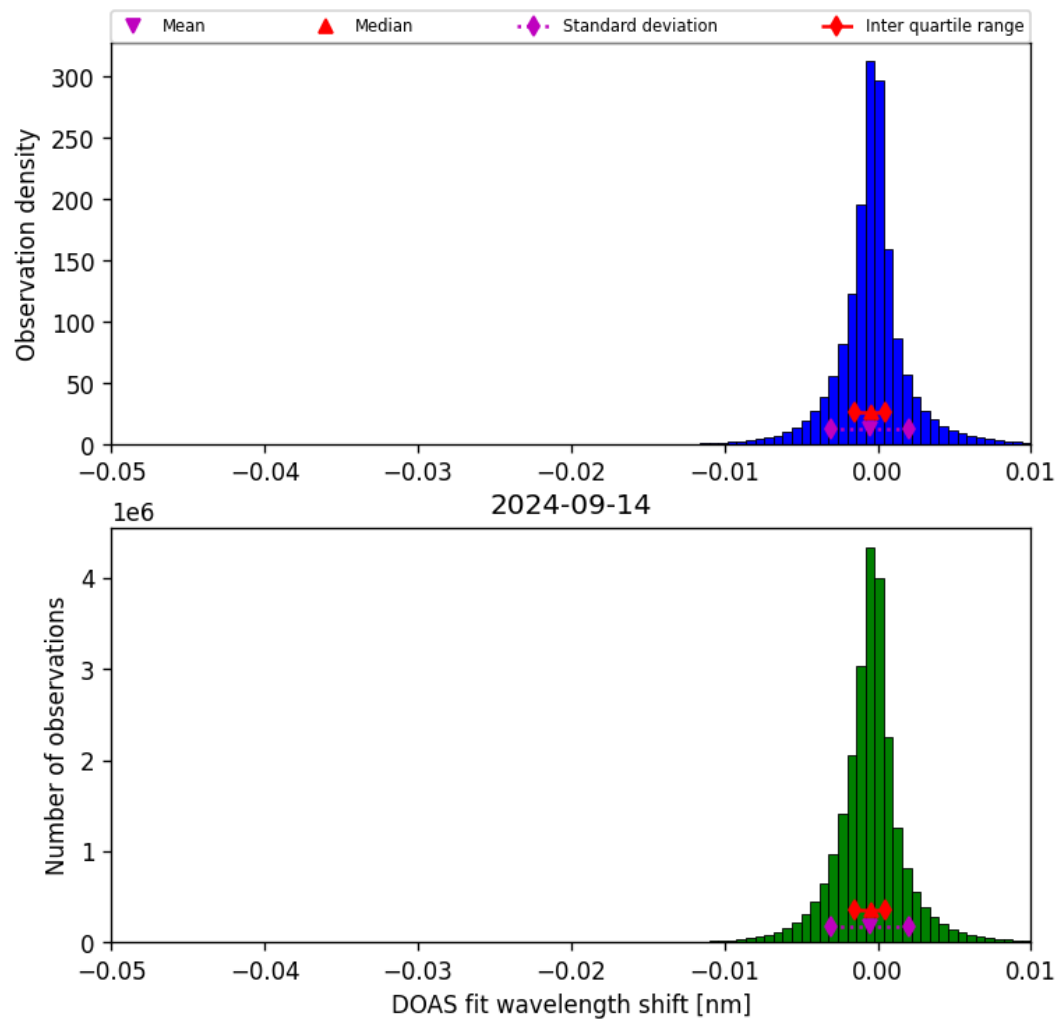
Figure 68: Histogram of “DOAS fit wavelength shift” for 2024-09-13 to 2024-09-15
