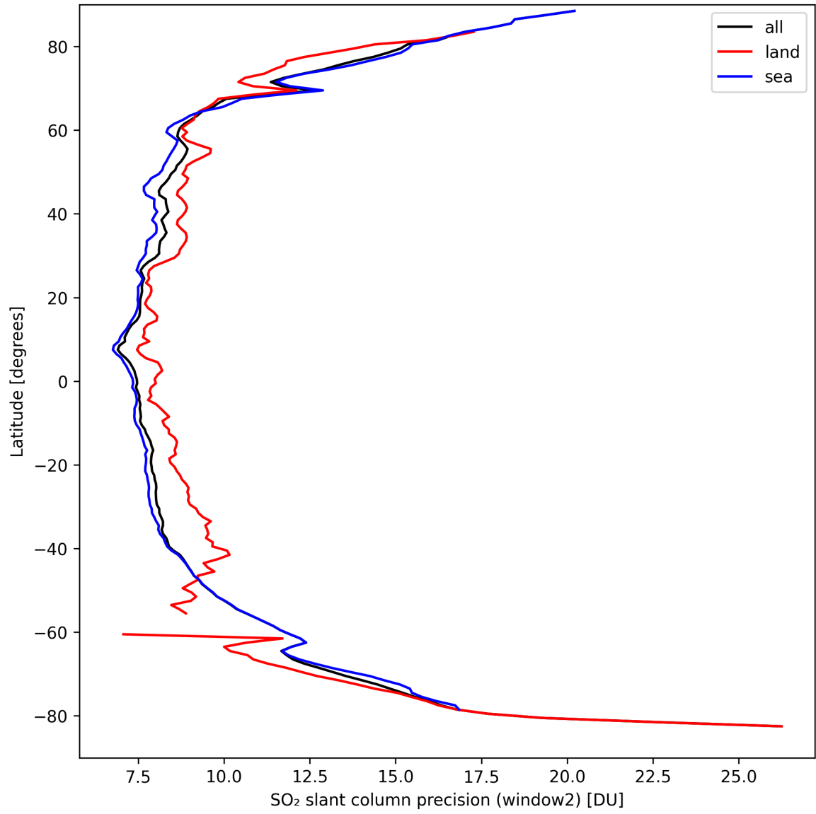
Figure 38: Zonal average of “SO 2 slant column precision (window2)” for 2024-09-13 to 2024-09-15.
