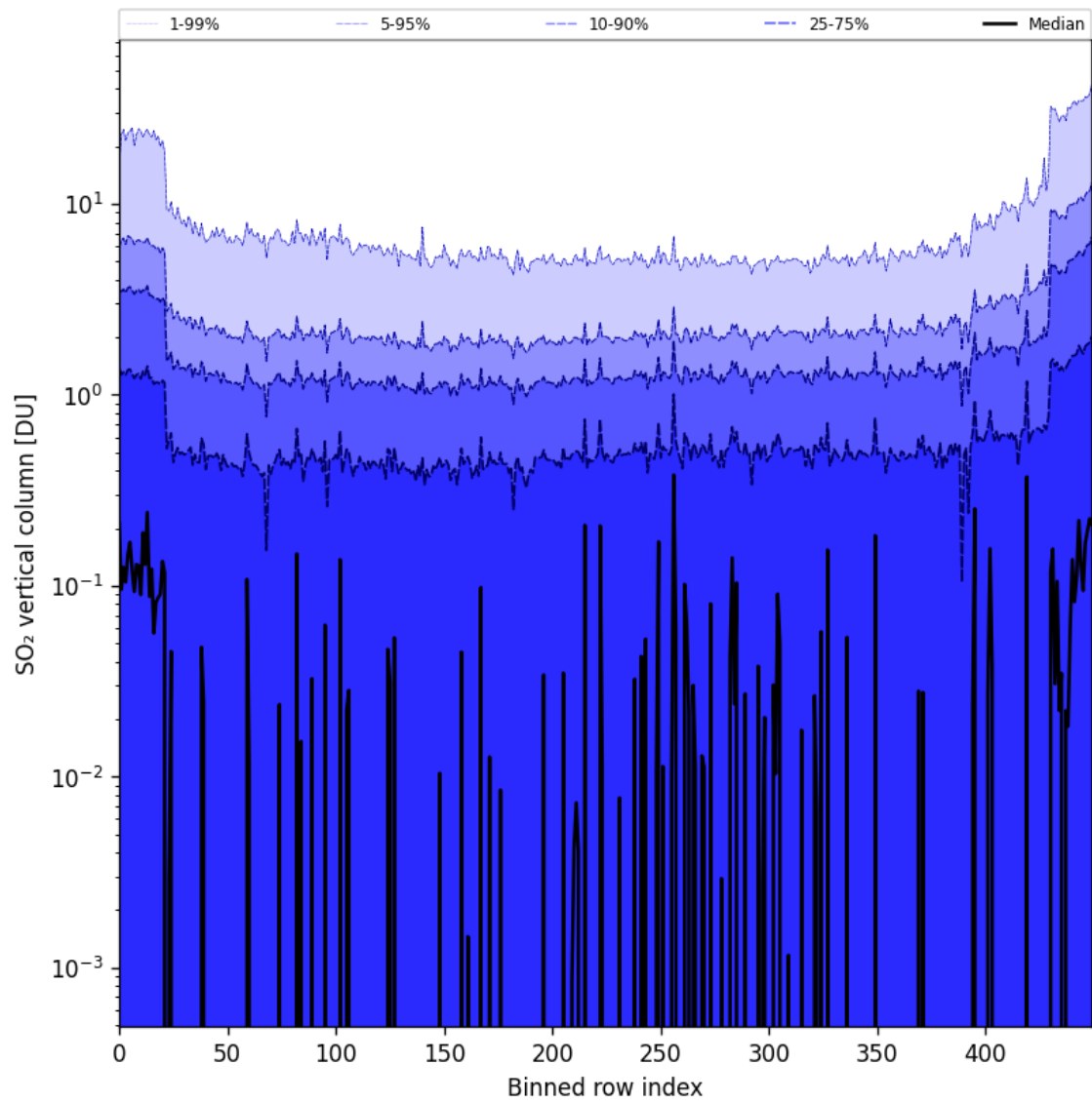
Figure 76: Along track statistics of “SO 2 vertical column” for 2024-09-13 to 2024-09-15
