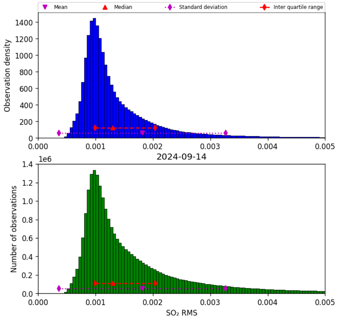
Figure 70: Histogram of “SO 2 RMS” for 2024-09-13 to 2024-09-15
