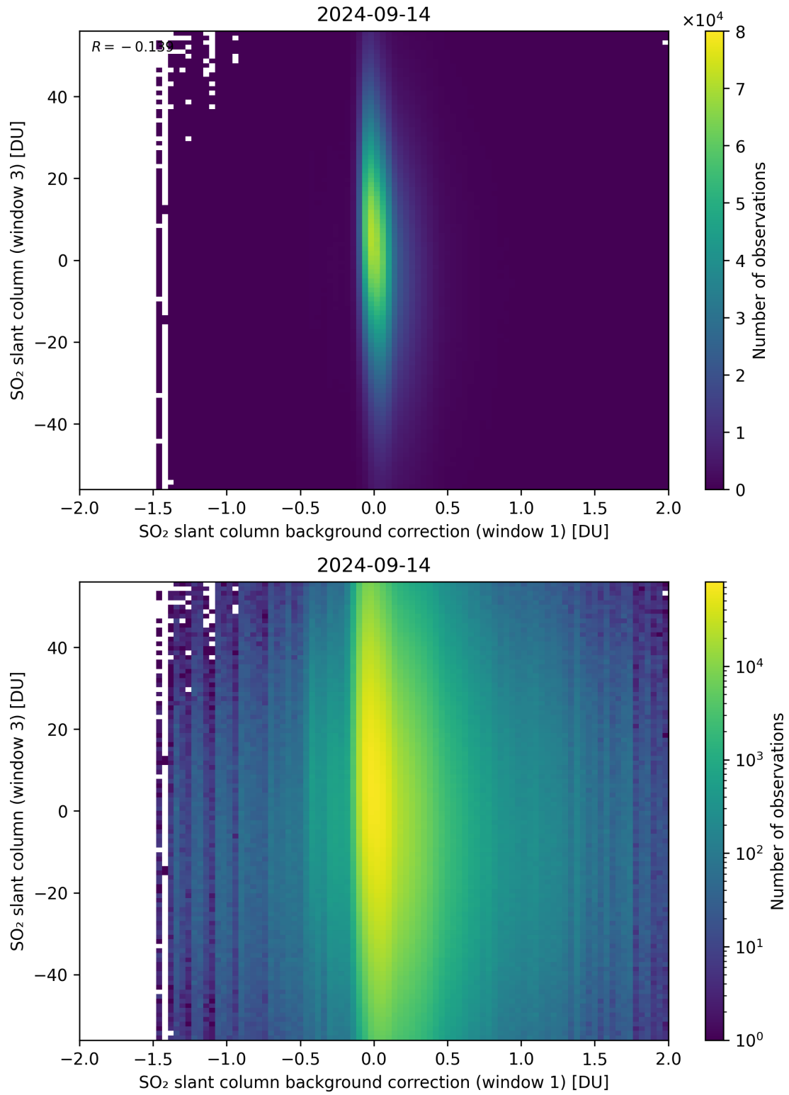
Figure 107: Scatter density plot of “SO 2 slant column background correction (window 1)” against “SO 2 slant column (window 3)” for 2024-09-13 to 2024-09-15.
