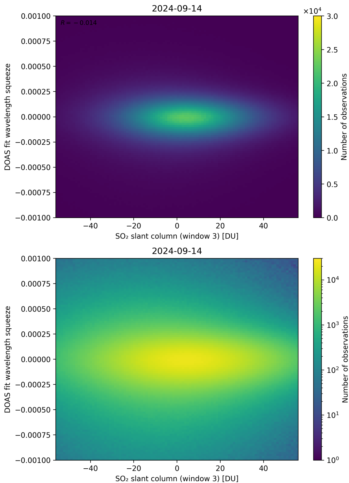
Figure 255: Scatter density plot of “SO 2 slant column (window 3)” against “DOAS fit wavelength squeeze” for 2024-09-13 to 2024-09-15.
