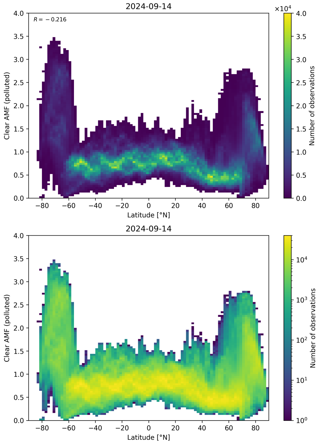
Figure 145: Scatter density plot of “Latitude” against “Clear AMF (polluted)” for 2024-09-13 to 2024-09-15.
