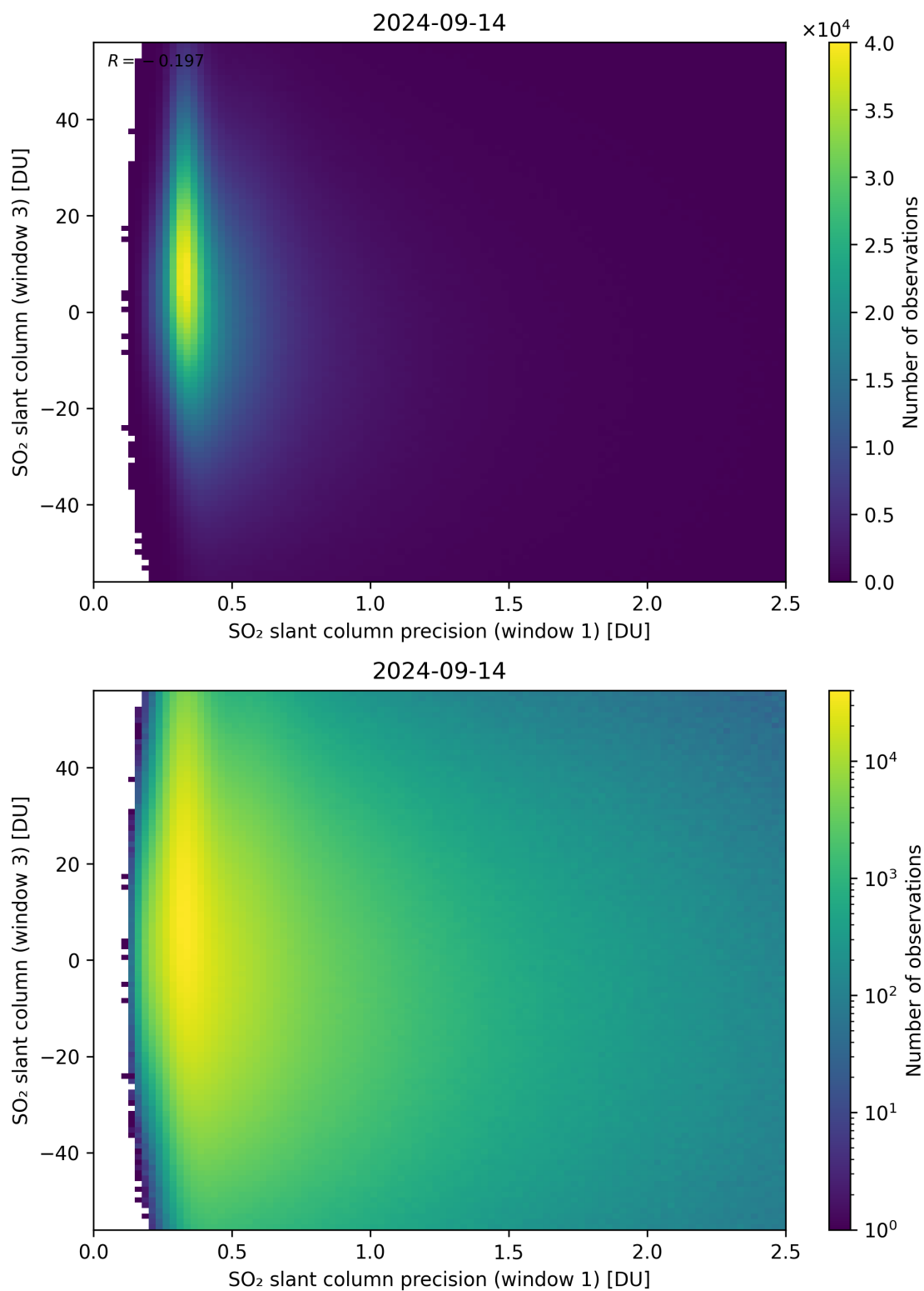
Figure 228: Scatter density plot of “SO 2 slant column precision (window 1)” against “SO 2 slant column (window 3)” for 2024-09-13 to 2024-09-15.
