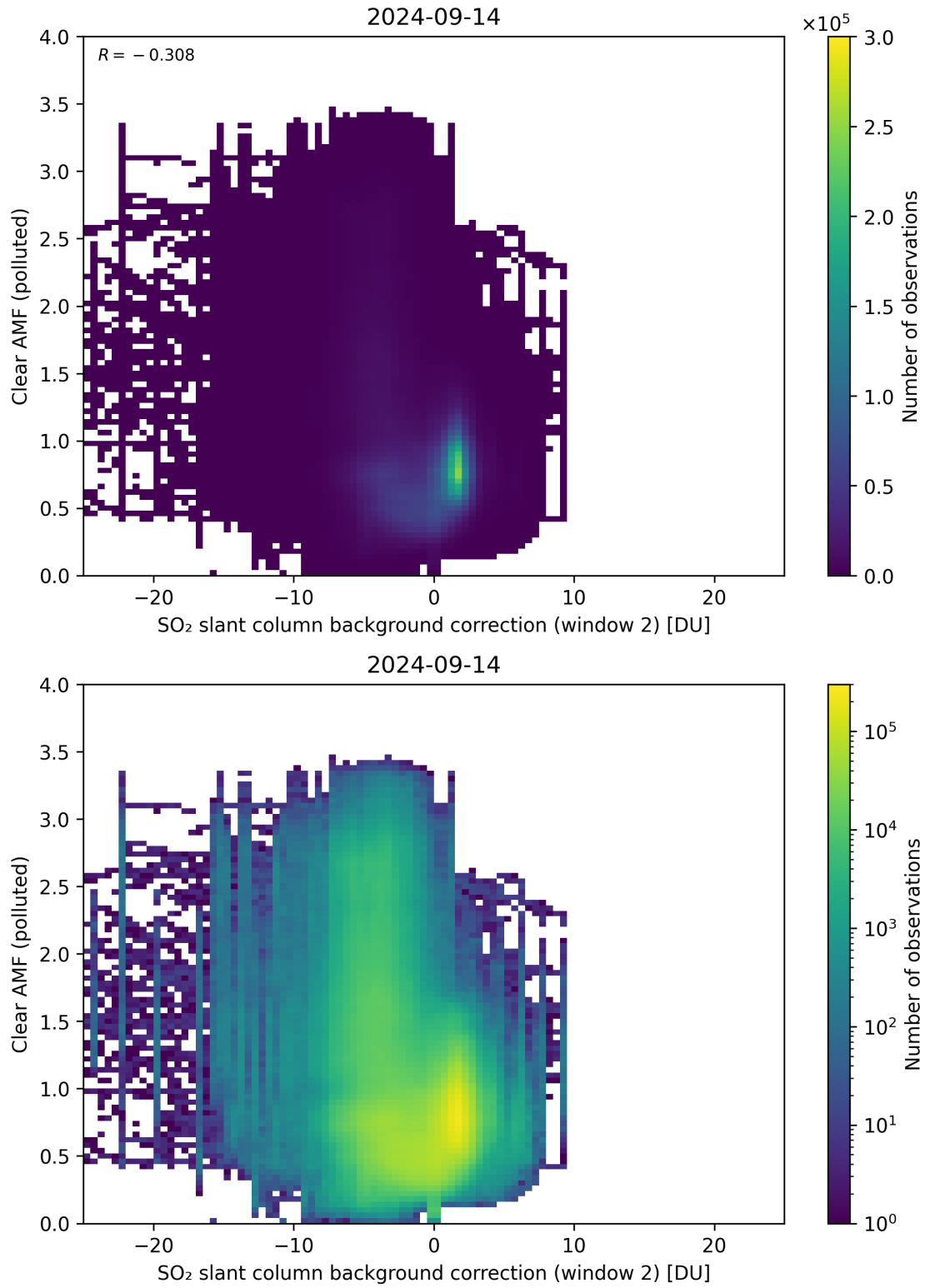
Figure 115: Scatter density plot of “SO 2 slant column background correction (window 2)” against “Clear AMF (polluted)” for 2024-09-13 to 2024-09-15.
