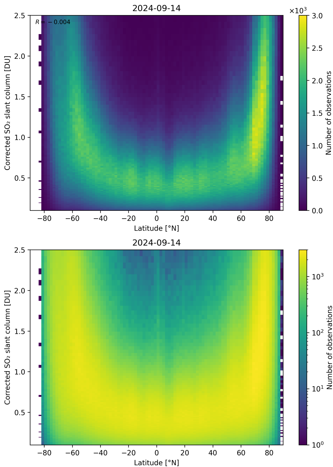
Figure 146: Scatter density plot of “Latitude” against “Corrected SO 2 slant column” for 2024-09-13 to 2024-09-15.
