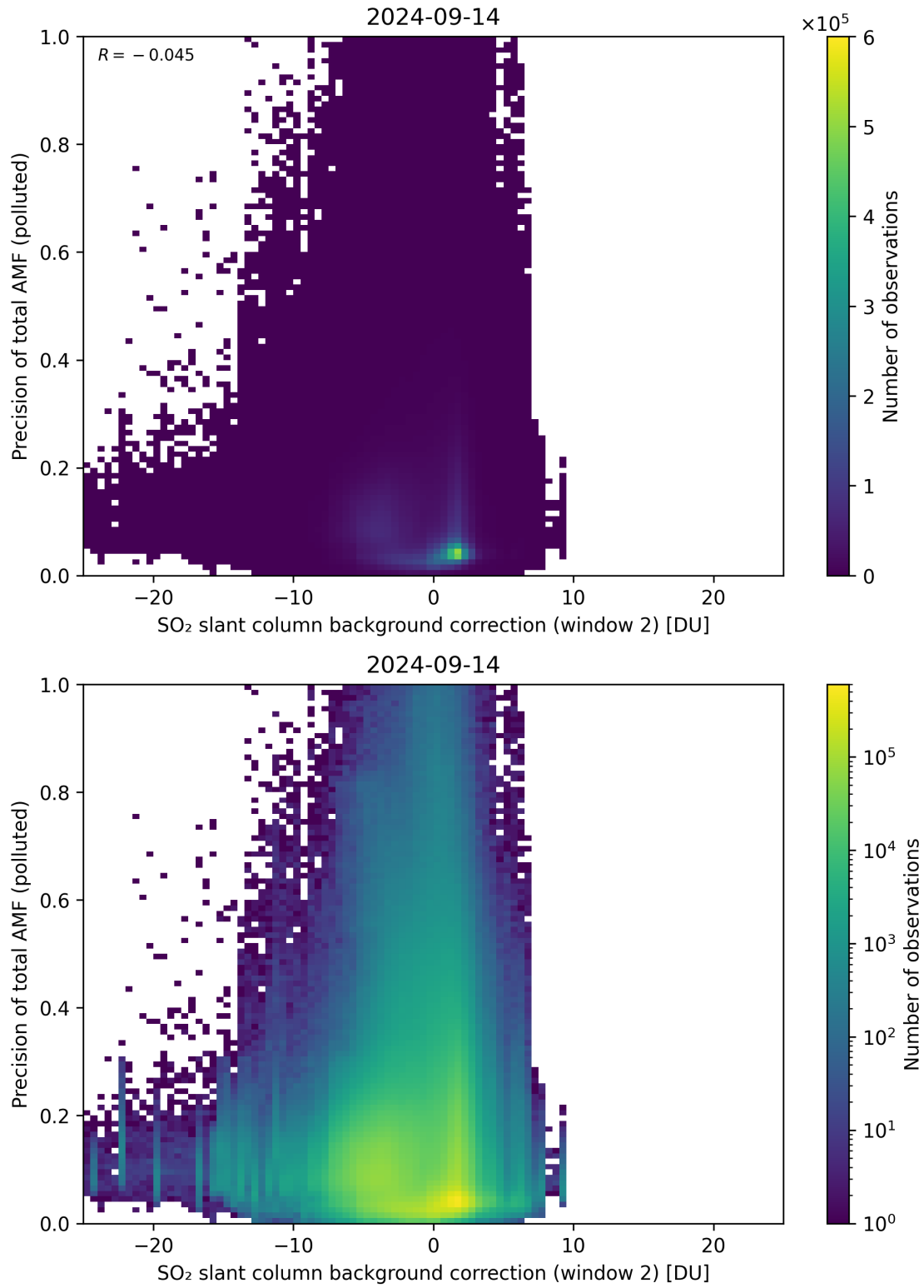
Figure 120: Scatter density plot of “SO 2 slant column background correction (window 2)” against “Precision of total AMF (polluted)” for 2024-09-13 to 2024-09-15.
