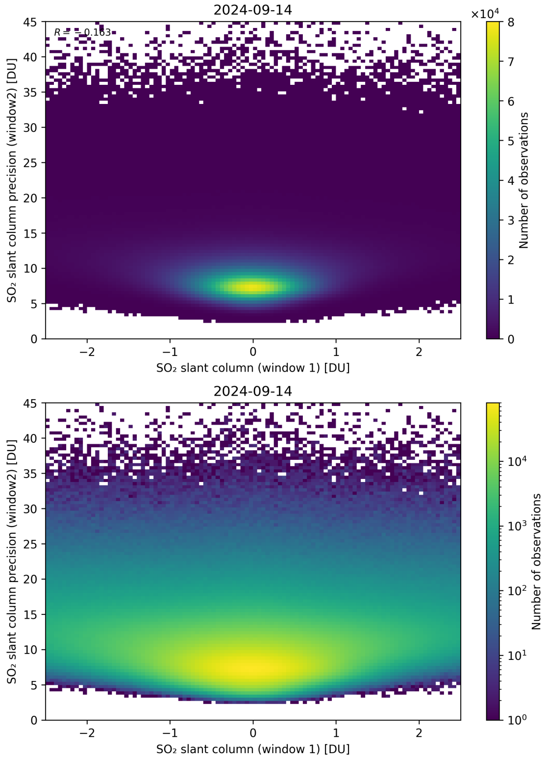
Figure 236: Scatter density plot of “SO 2 slant column (window 1)” against “SO 2 slant column precision (window2)” for 2024-09-13 to 2024-09-15.
