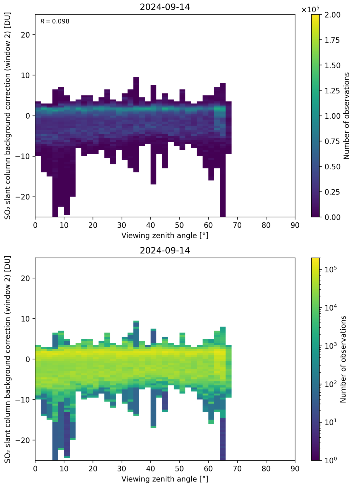
Figure 309: Scatter density plot of “Viewing zenith angle” against “SO 2 slant column background correction (window 2)” for 2024-09-13 to 2024-09-15.
