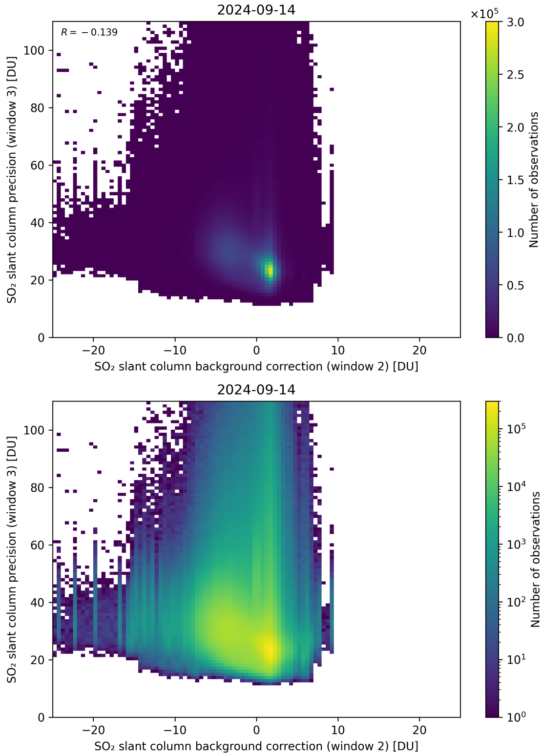
Figure 118: Scatter density plot of “SO 2 slant column background correction (window 2)” against “SO 2 slant column precision (window 3)” for 2024-09-13 to 2024-09-15.
