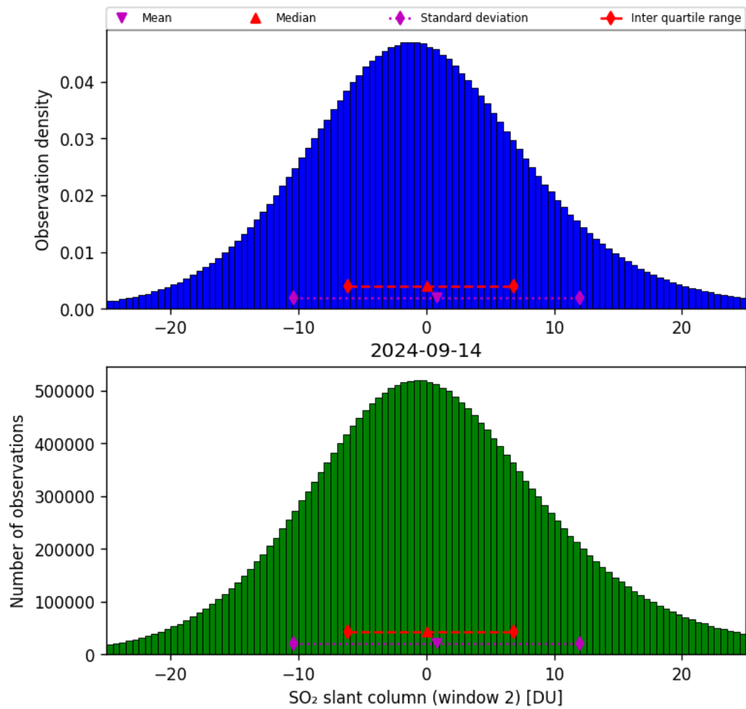
Figure 60: Histogram of “SO 2 slant column (window 2)” for 2024-09-13 to 2024-09-15
