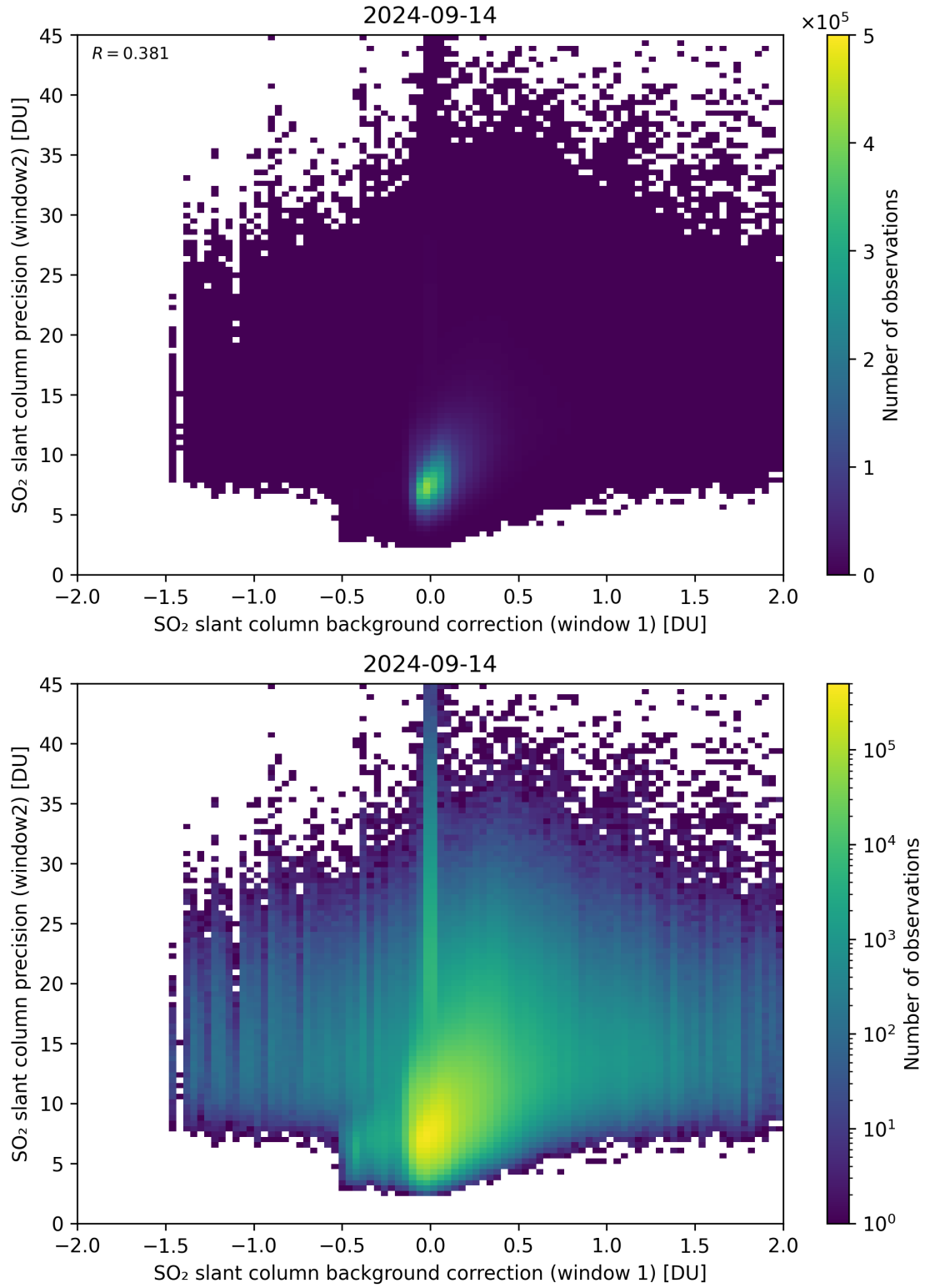
Figure 106: Scatter density plot of “SO 2 slant column background correction (window 1)” against “SO 2 slant column precision (window2)” for 2024-09-13 to 2024-09-15.
