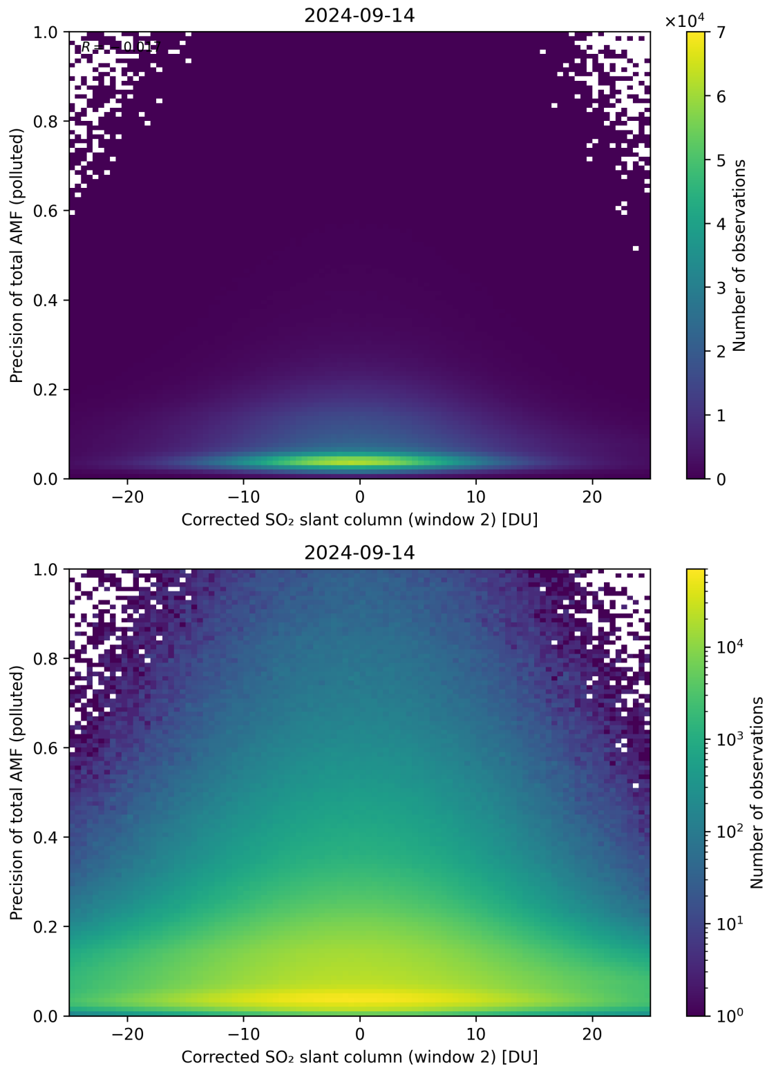
Figure 204: Scatter density plot of “Corrected SO 2 slant column (window 2)” against “Precision of total AMF (polluted)” for 2024-09-13 to 2024-09-15.
