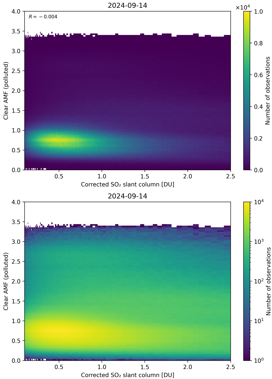
Figure 184: Scatter density plot of “Corrected SO 2 slant column” against “Clear AMF (polluted)” for 2024-09-13 to 2024-09-15.
