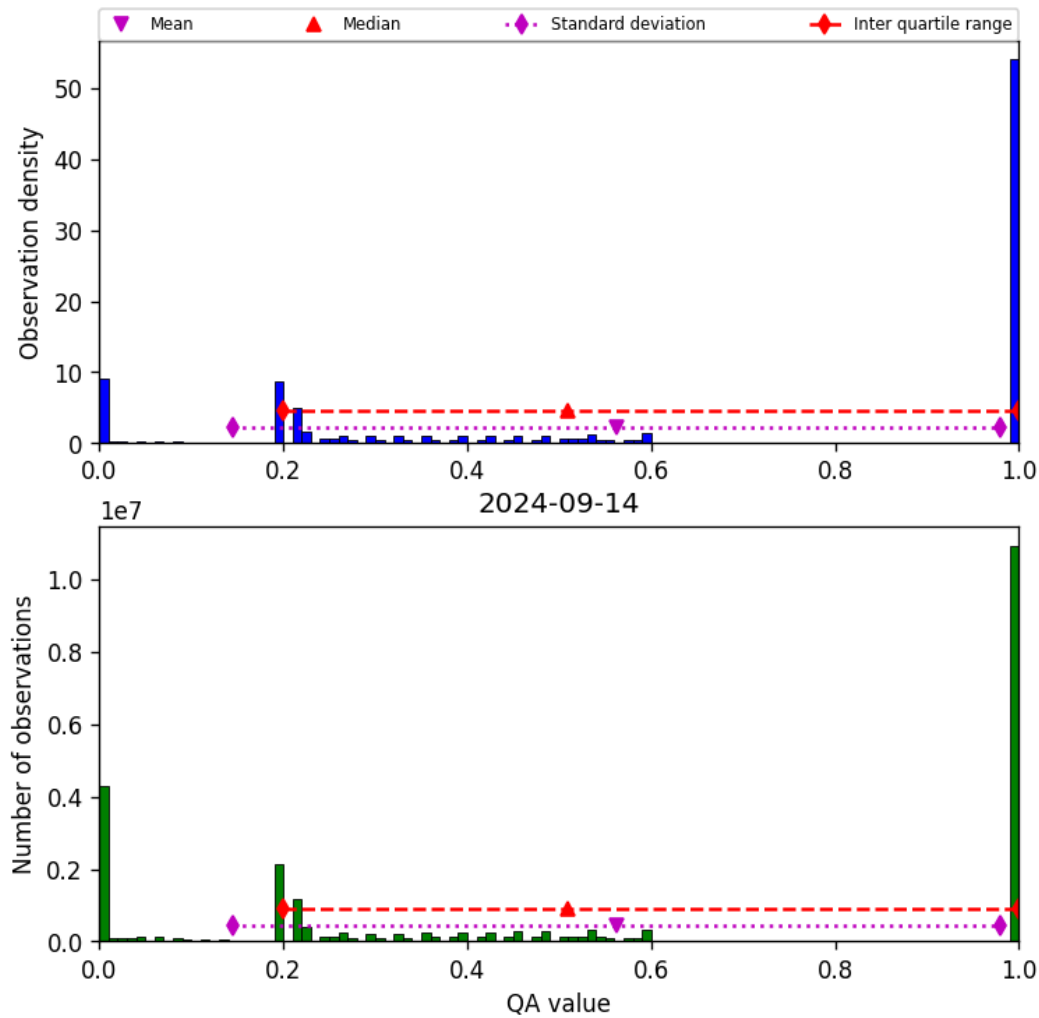
Figure 52: Histogram of “QA value” for 2024-09-13 to 2024-09-15
