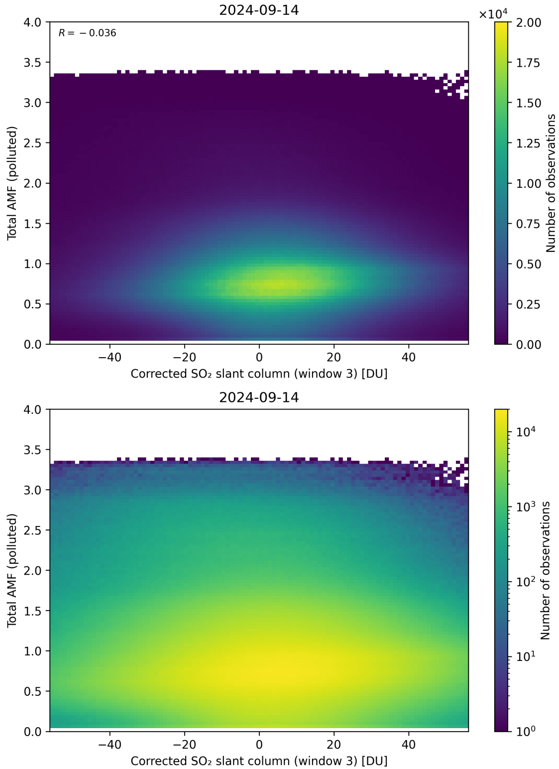
Figure 210: Scatter density plot of “Corrected SO 2 slant column (window 3)” against “Total AMF (polluted)” for 2024-09-13 to 2024-09-15.
