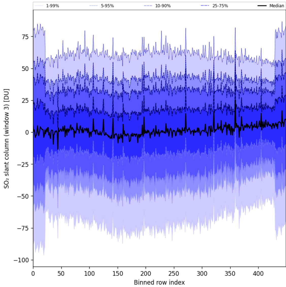
Figure 87: Along track statistics of “SO 2 slant column (window 3)” for 2024-09-13 to 2024-09-15
