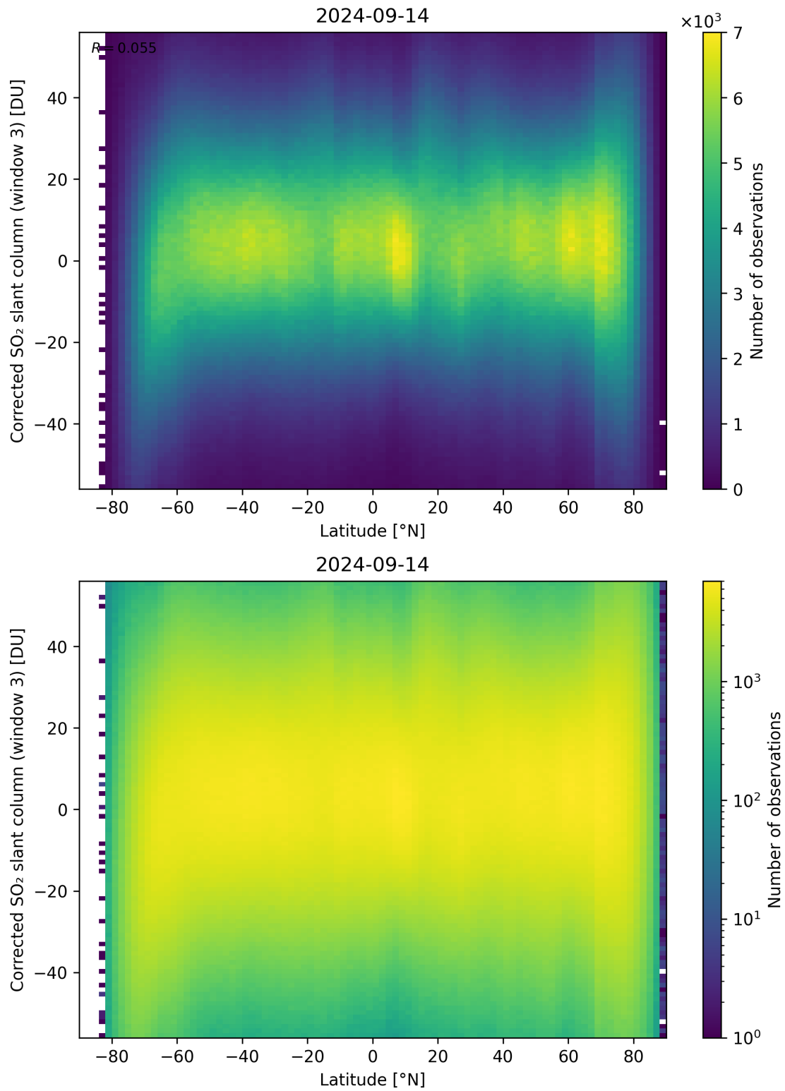
Figure 148: Scatter density plot of “Latitude” against “Corrected SO 2 slant column (window 3)” for 2024-09-13 to 2024-09-15.
