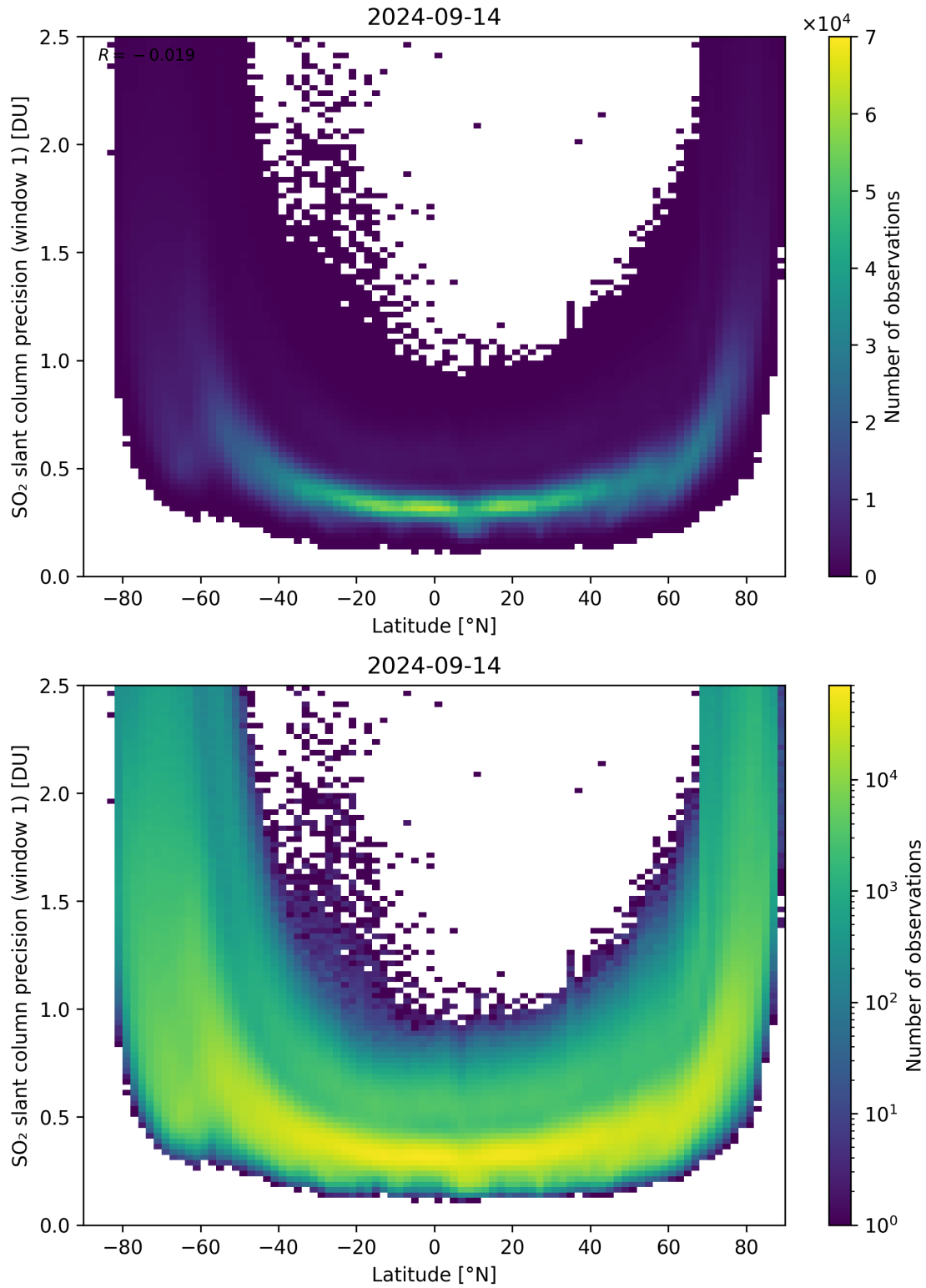
Figure 150: Scatter density plot of “Latitude” against “SO 2 slant column precision (window 1)” for 2024-09-13 to 2024-09-15.
