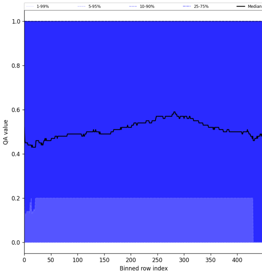
Figure 75: Along track statistics of “QA value” for 2024-09-13 to 2024-09-15
