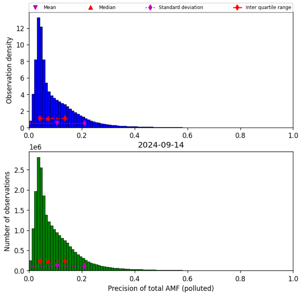
Figure 72: Histogram of “Precision of total AMF (polluted)” for 2024-09-13 to 2024-09-15
