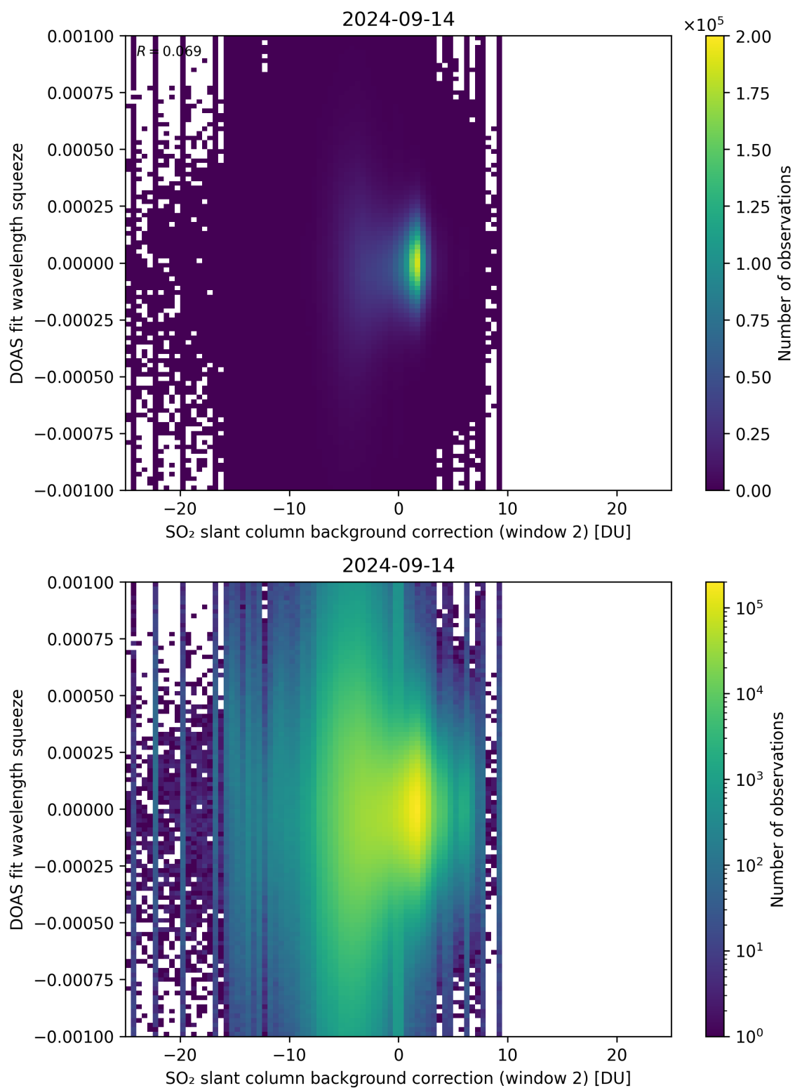
Figure 113: Scatter density plot of “SO 2 slant column background correction (window 2)” against “DOAS fit wavelength squeeze” for 2024-09-13 to 2024-09-15.
