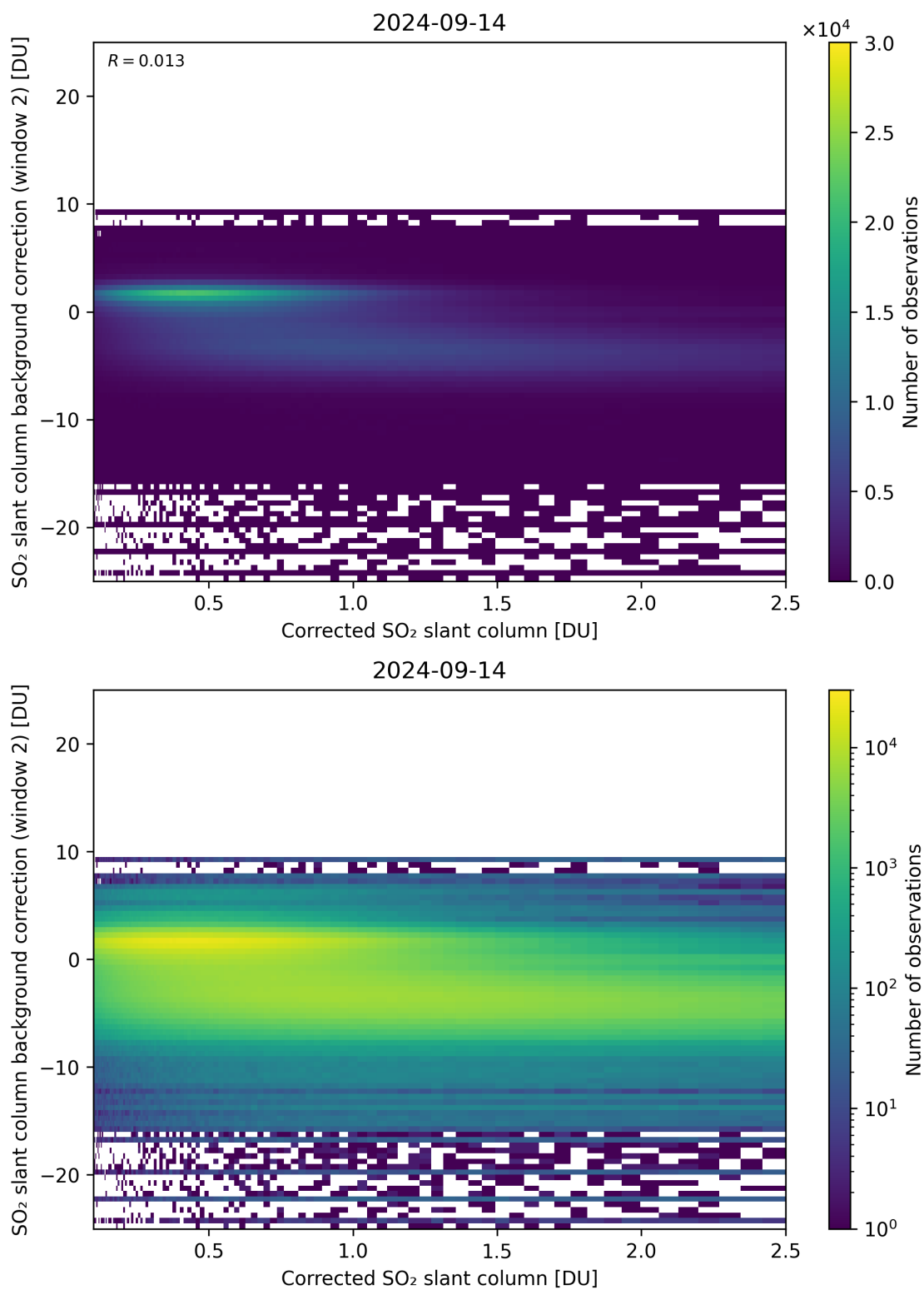
Figure 179: Scatter density plot of “Corrected SO 2 slant column” against “SO 2 slant column background correction (window 2)” for 2024-09-13 to 2024-09-15.
