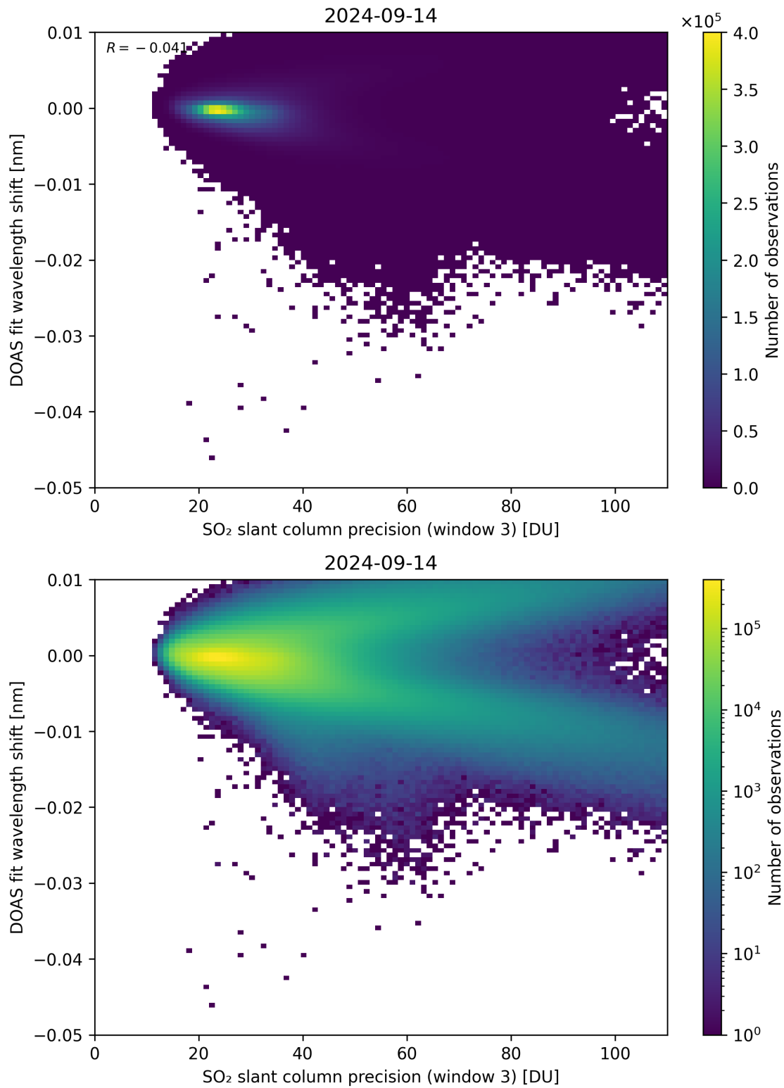
Figure 258: Scatter density plot of “SO 2 slant column precision (window 3)” against “DOAS fit wavelength shift” for 2024-09-13 to 2024-09-15.
