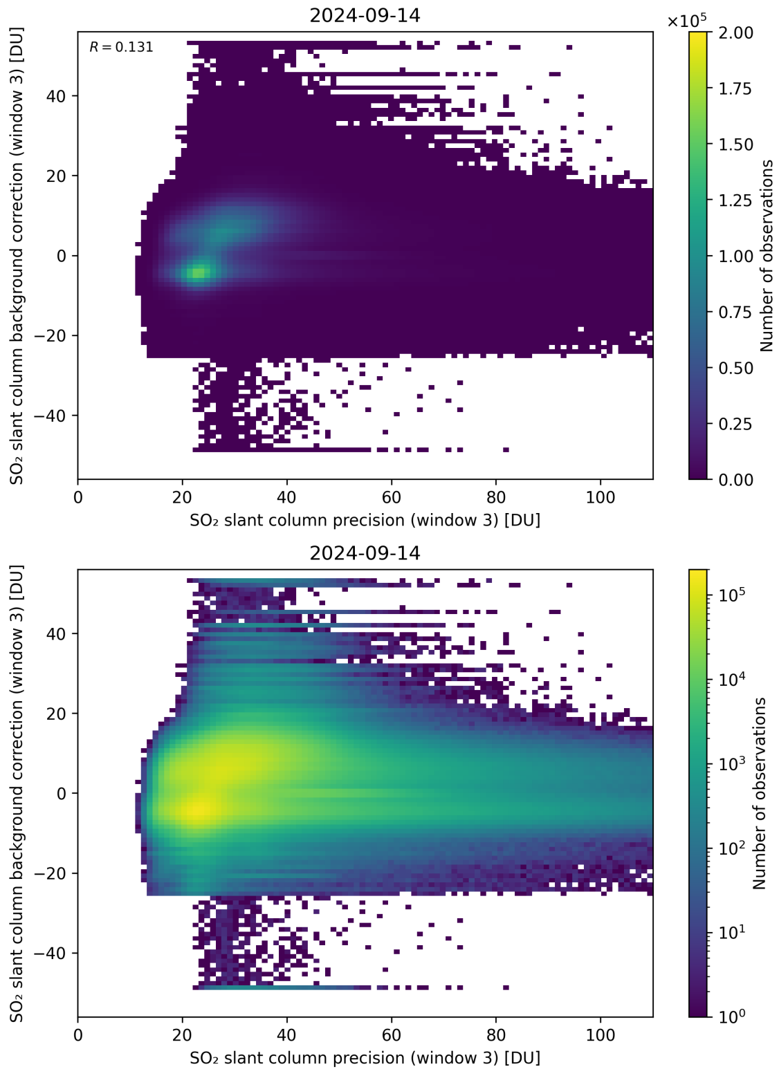
Figure 257: Scatter density plot of “SO 2 slant column precision (window 3)” against “SO 2 slant column background correction (window 3)” for 2024-09-13 to 2024-09-15.
