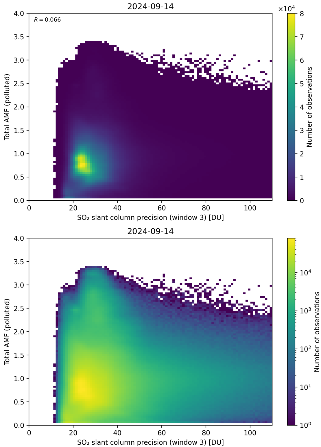
Figure 263: Scatter density plot of “SO 2 slant column precision (window 3)” against “Total AMF (polluted)” for 2024-09-13 to 2024-09-15.
