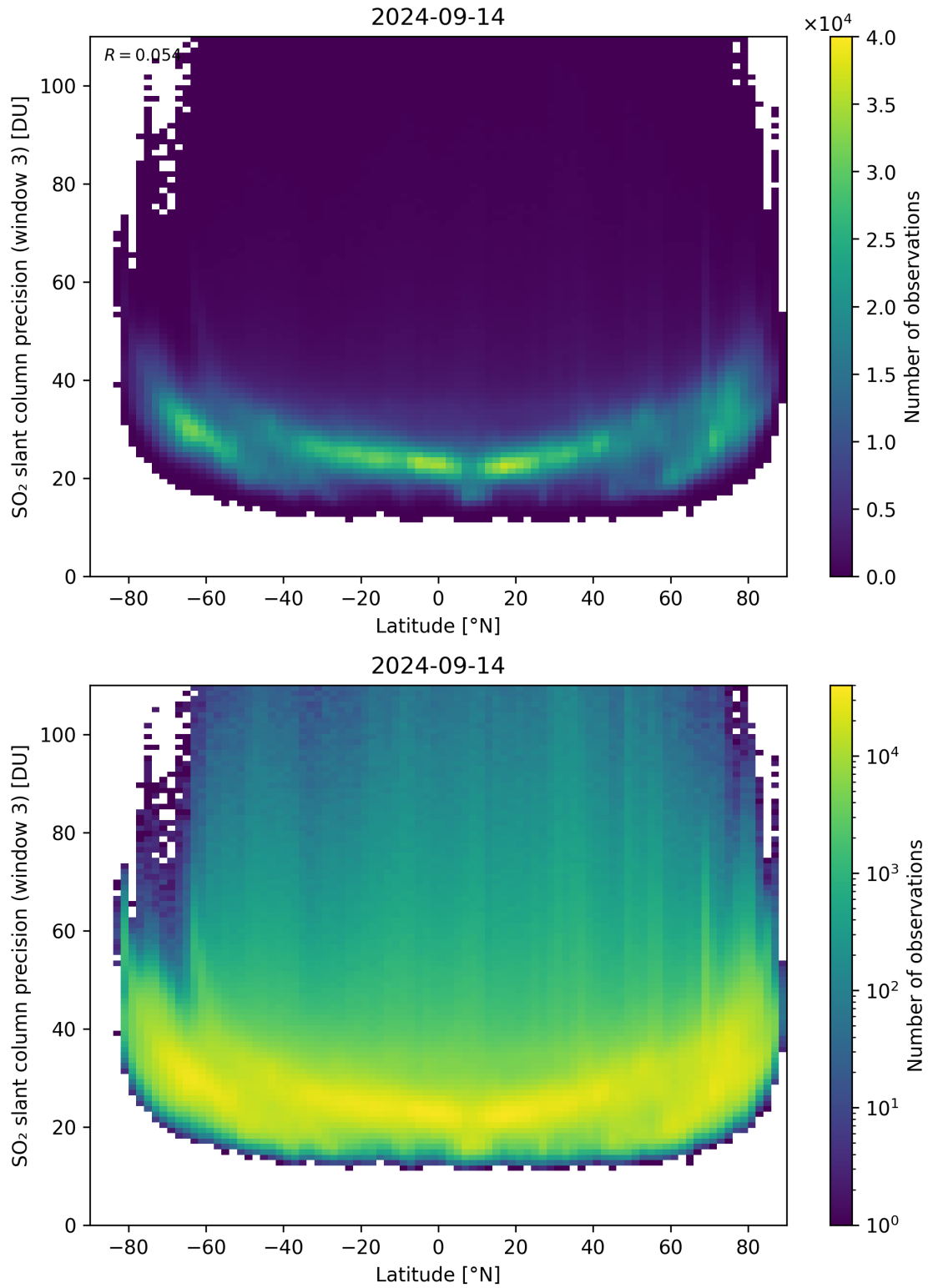
Figure 153: Scatter density plot of “Latitude” against “SO 2 slant column precision (window 3)” for 2024-09-13 to 2024-09-15.
