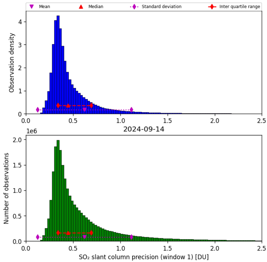
Figure 57: Histogram of “SO 2 slant column precision (window 1)” for 2024-09-13 to 2024-09-15
