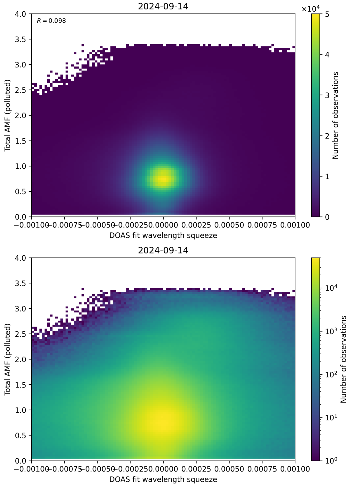
Figure 134: Scatter density plot of “DOAS fit wavelength squeeze” against “Total AMF (polluted)” for 2024-09-13 to 2024-09-15.
