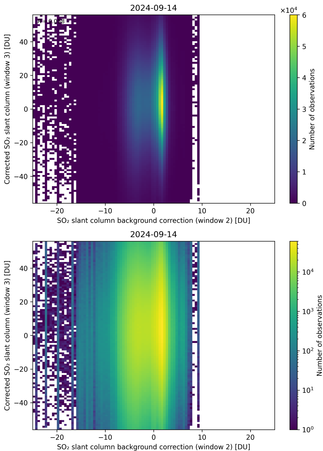
Figure 116: Scatter density plot of “SO 2 slant column background correction (window 2)” against “Corrected SO 2 slant column (window 3)” for 2024-09-13 to 2024-09-15.
