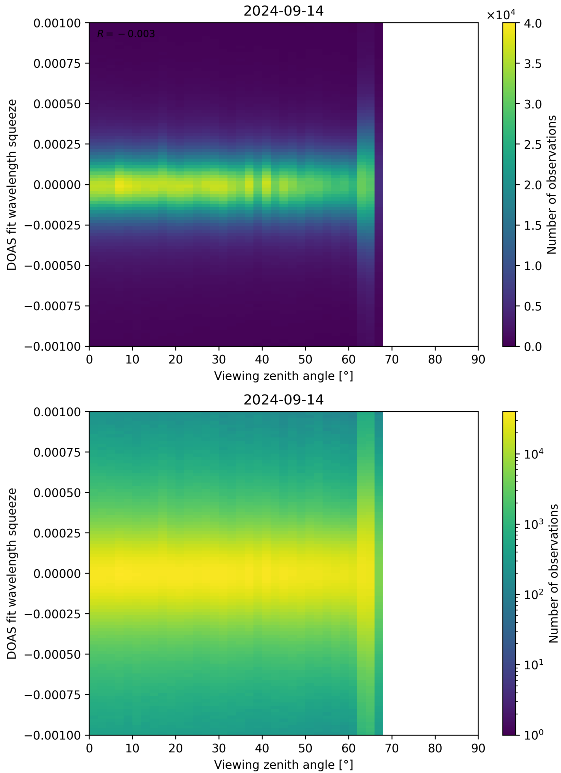
Figure 312: Scatter density plot of “Viewing zenith angle” against “DOAS fit wavelength squeeze” for 2024-09-13 to 2024-09-15.
