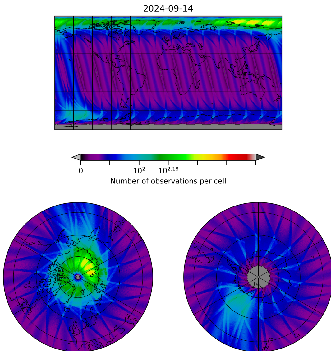
Figure 28: Map of the number of observations for 2024-09-13 to 2024-09-15
