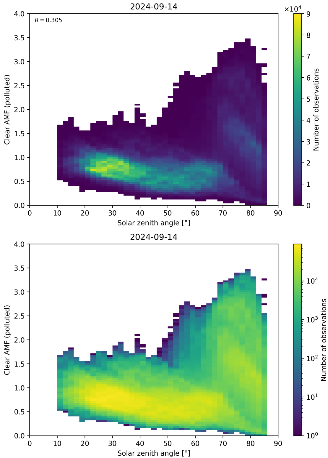
Figure 165: Scatter density plot of “Solar zenith angle” against “Clear AMF (polluted)” for 2024-09-13 to 2024-09-15.
