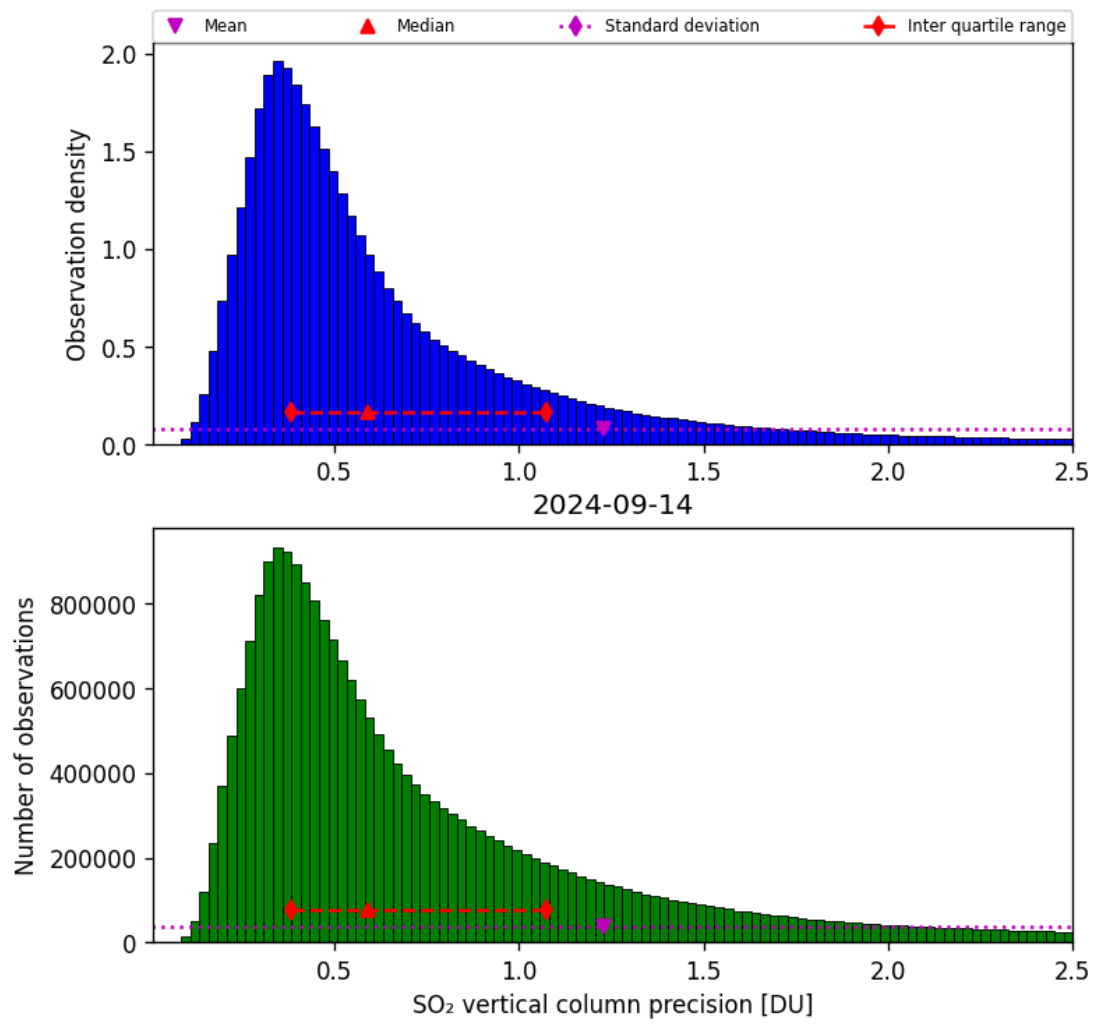
Figure 54: Histogram of “SO 2 vertical column precision” for 2024-09-13 to 2024-09-15
