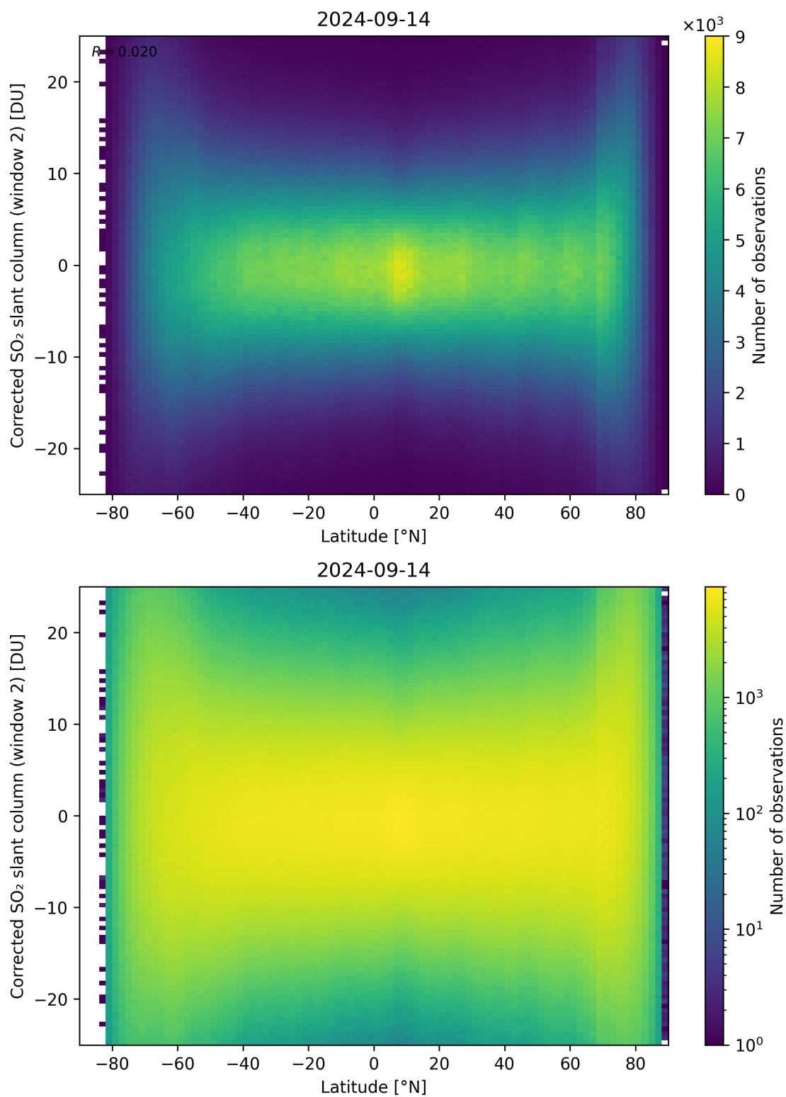
Figure 147: Scatter density plot of “Latitude” against “Corrected SO 2 slant column (window 2)” for 2024-09-13 to 2024-09-15.
