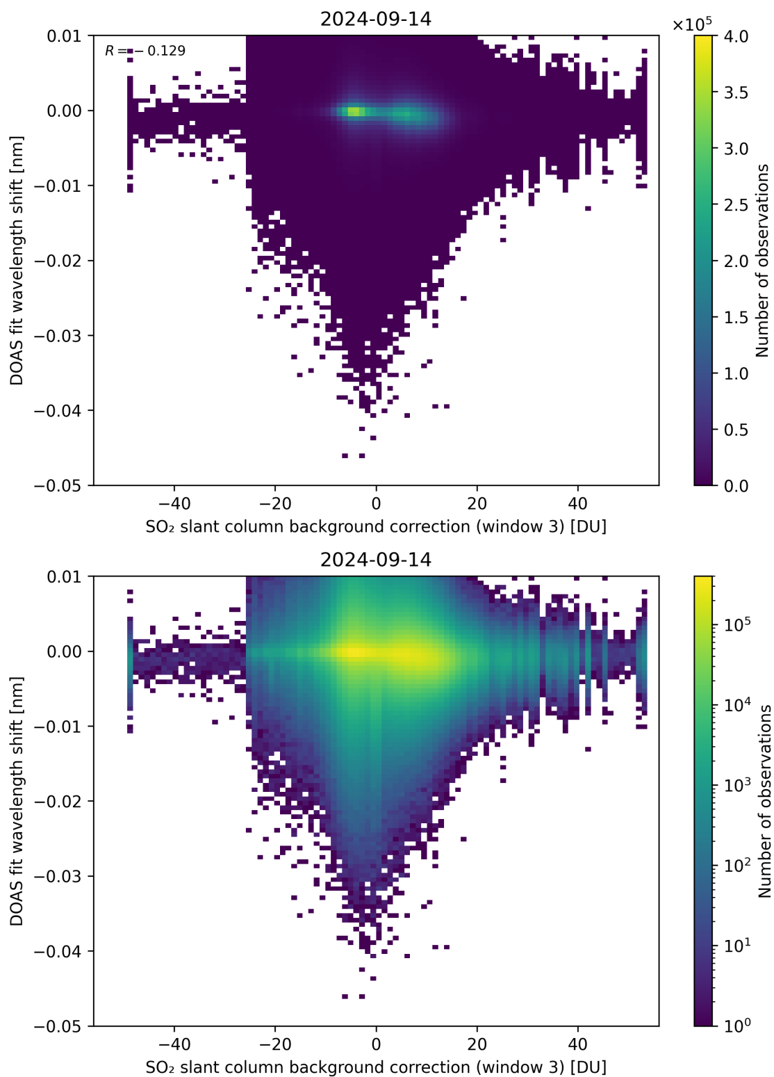
Figure 121: Scatter density plot of “SO 2 slant column background correction (window 3)” against “DOAS fit wavelength shift” for 2024-09-13 to 2024-09-15.
