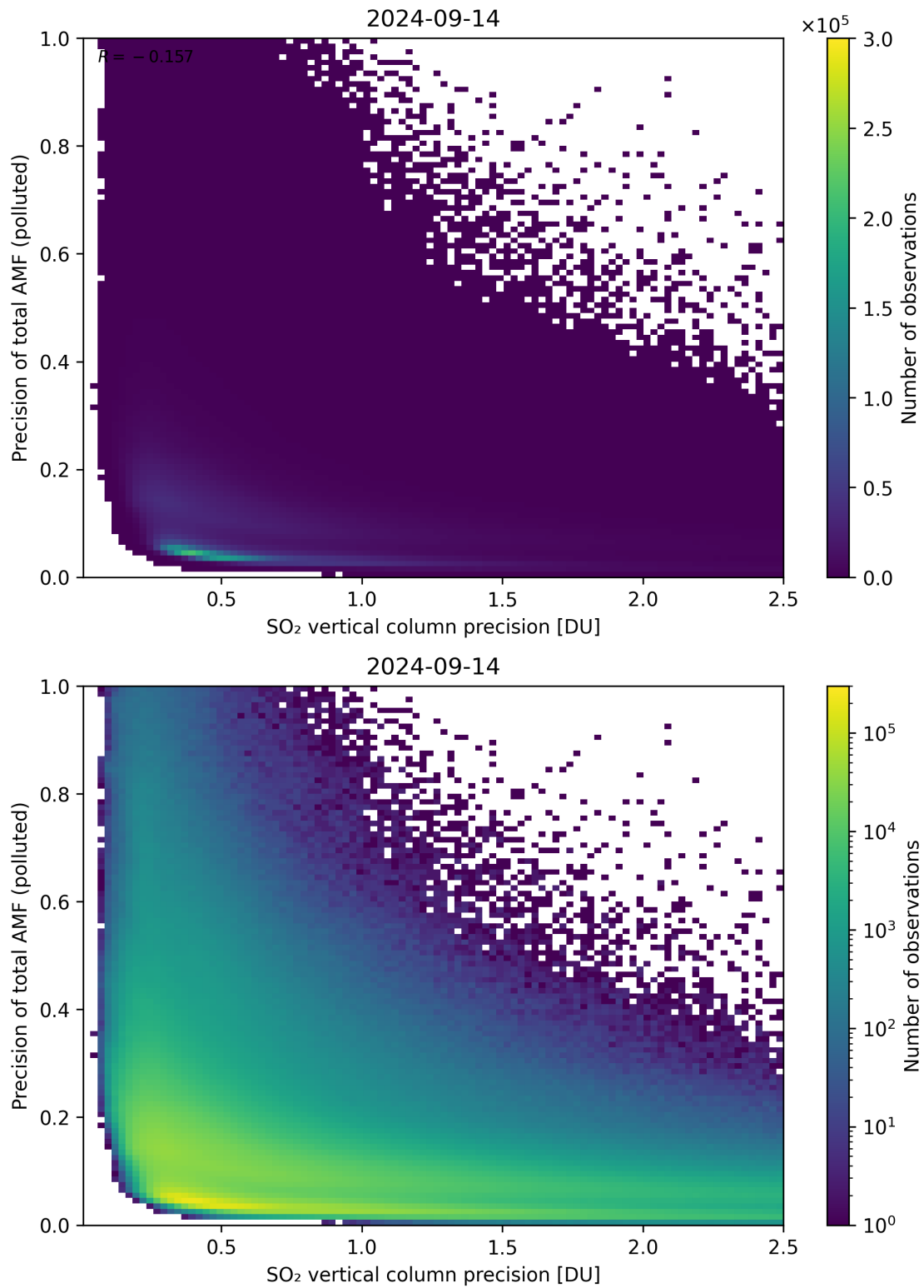
Figure 295: Scatter density plot of “SO 2 vertical column precision” against “Precision of total AMF (polluted)” for 2024-09-13 to 2024-09-15.
