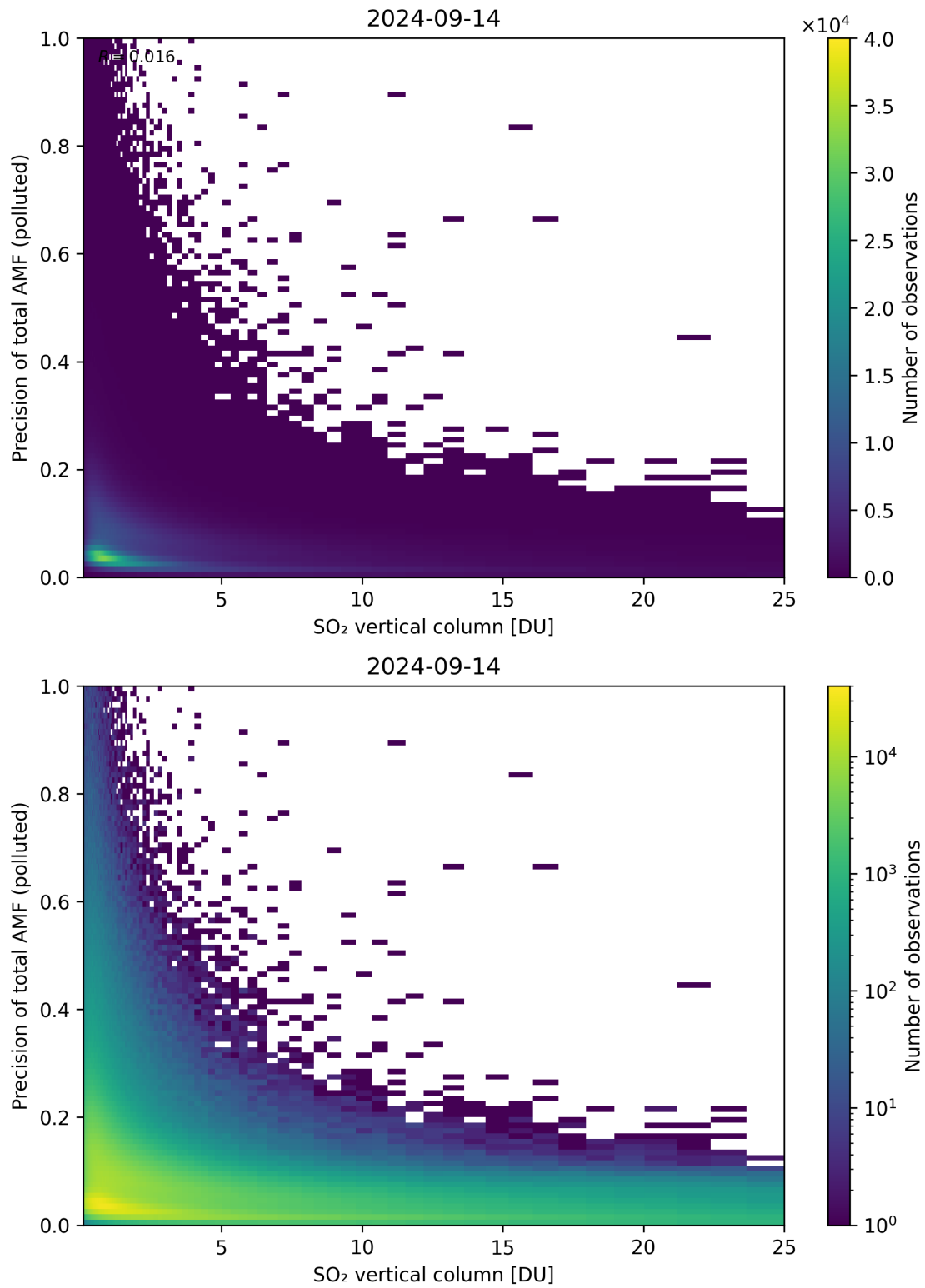
Figure 306: Scatter density plot of “SO 2 vertical column” against “Precision of total AMF (polluted)” for 2024-09-13 to 2024-09-15.
