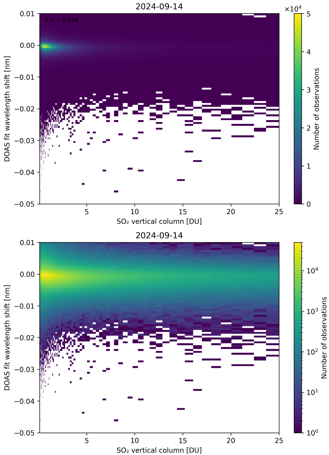
Figure 276: Scatter density plot of “SO 2 vertical column” against “DOAS fit wavelength shift” for 2024-09-13 to 2024-09-15.
