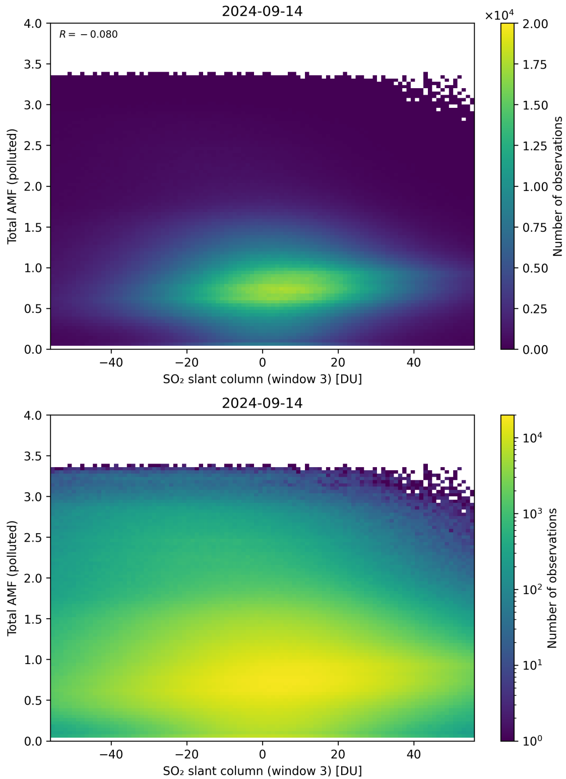
Figure 268: Scatter density plot of “SO 2 slant column (window 3)” against “Total AMF (polluted)” for 2024-09-13 to 2024-09-15.
