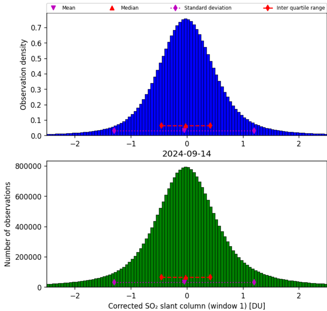
Figure 58: Histogram of “Corrected SO 2 slant column (window 1)” for 2024-09-13 to 2024-09-15
