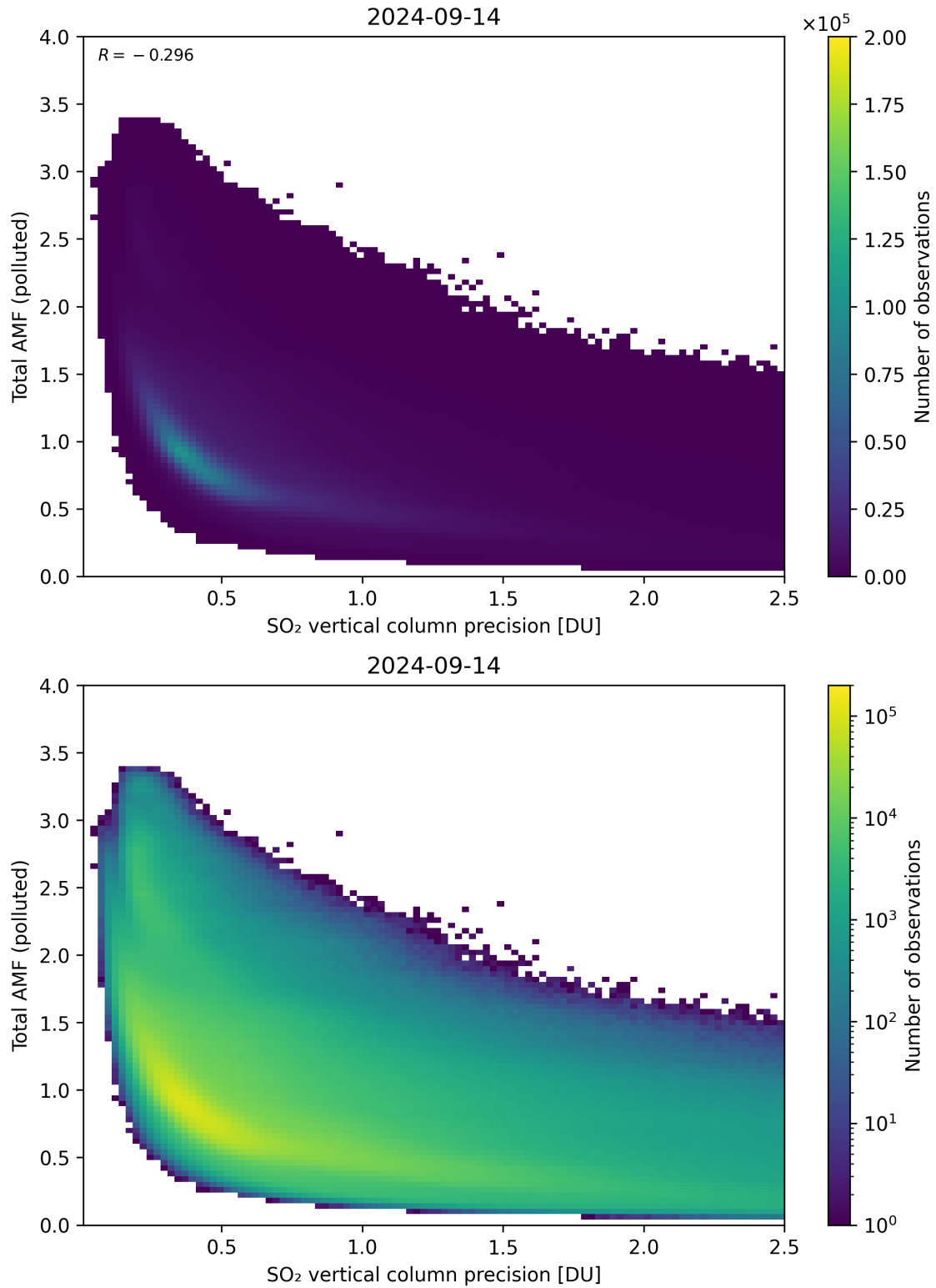
Figure 294: Scatter density plot of “SO 2 vertical column precision” against “Total AMF (polluted)” for 2024-09-13 to 2024-09-15.
