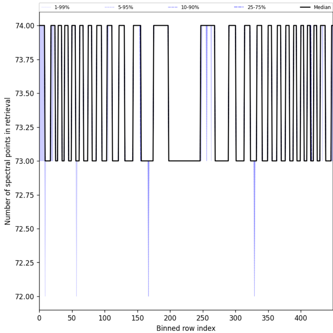
Figure 97: Along track statistics of “Number of spectral points in retrieval” for 2024-09-13 to 2024-09-15
