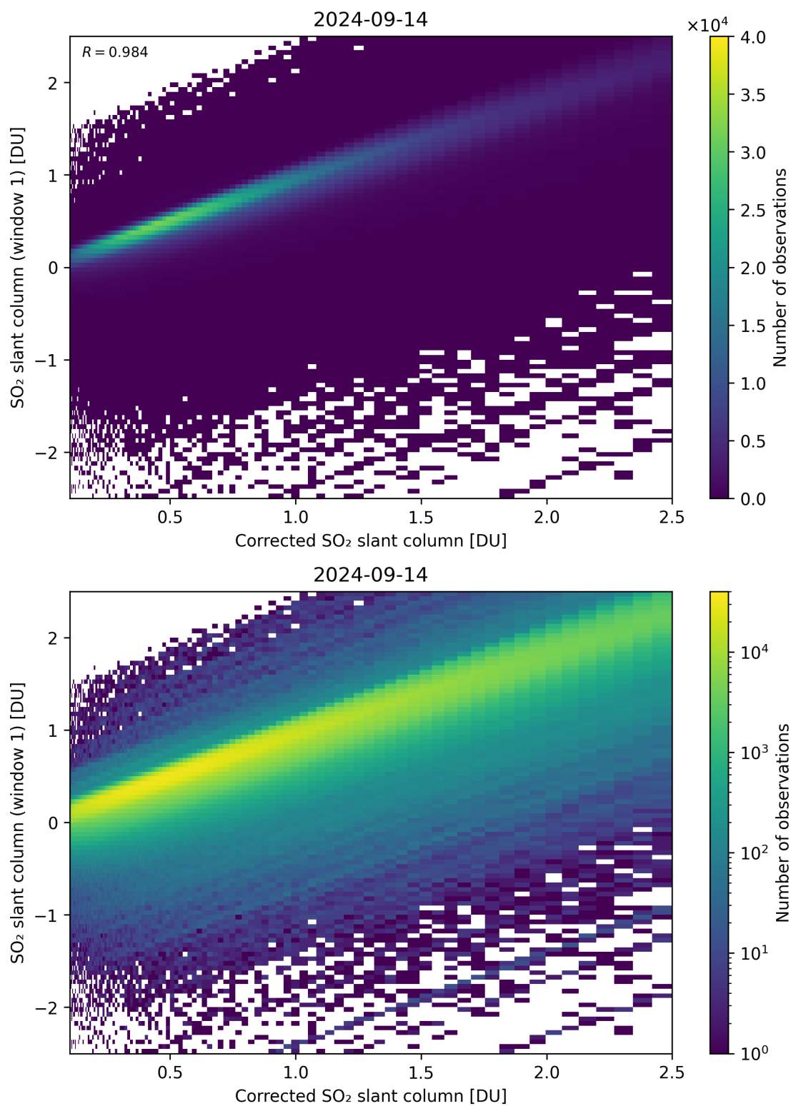
Figure 187: Scatter density plot of “Corrected SO 2 slant column” against “SO 2 slant column (window 1)” for 2024-09-13 to 2024-09-15.
