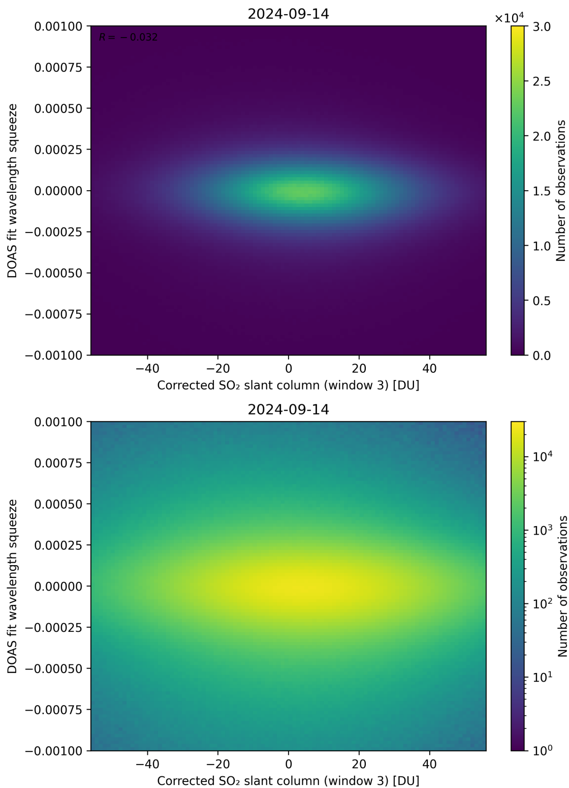
Figure 207: Scatter density plot of “Corrected SO 2 slant column (window 3)” against “DOAS fit wavelength squeeze” for 2024-09-13 to 2024-09-15.
