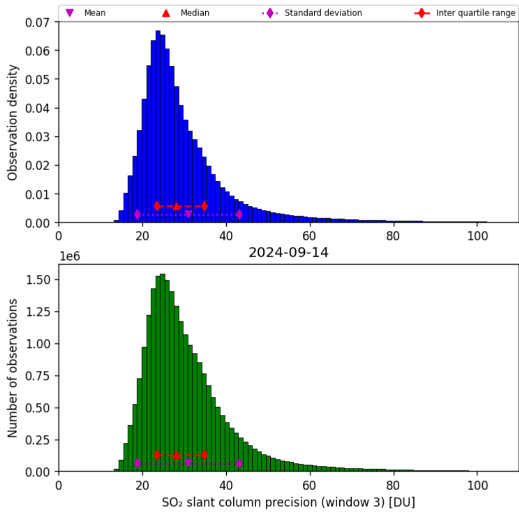
Figure 65: Histogram of “SO 2 slant column precision (window 3)” for 2024-09-13 to 2024-09-15
