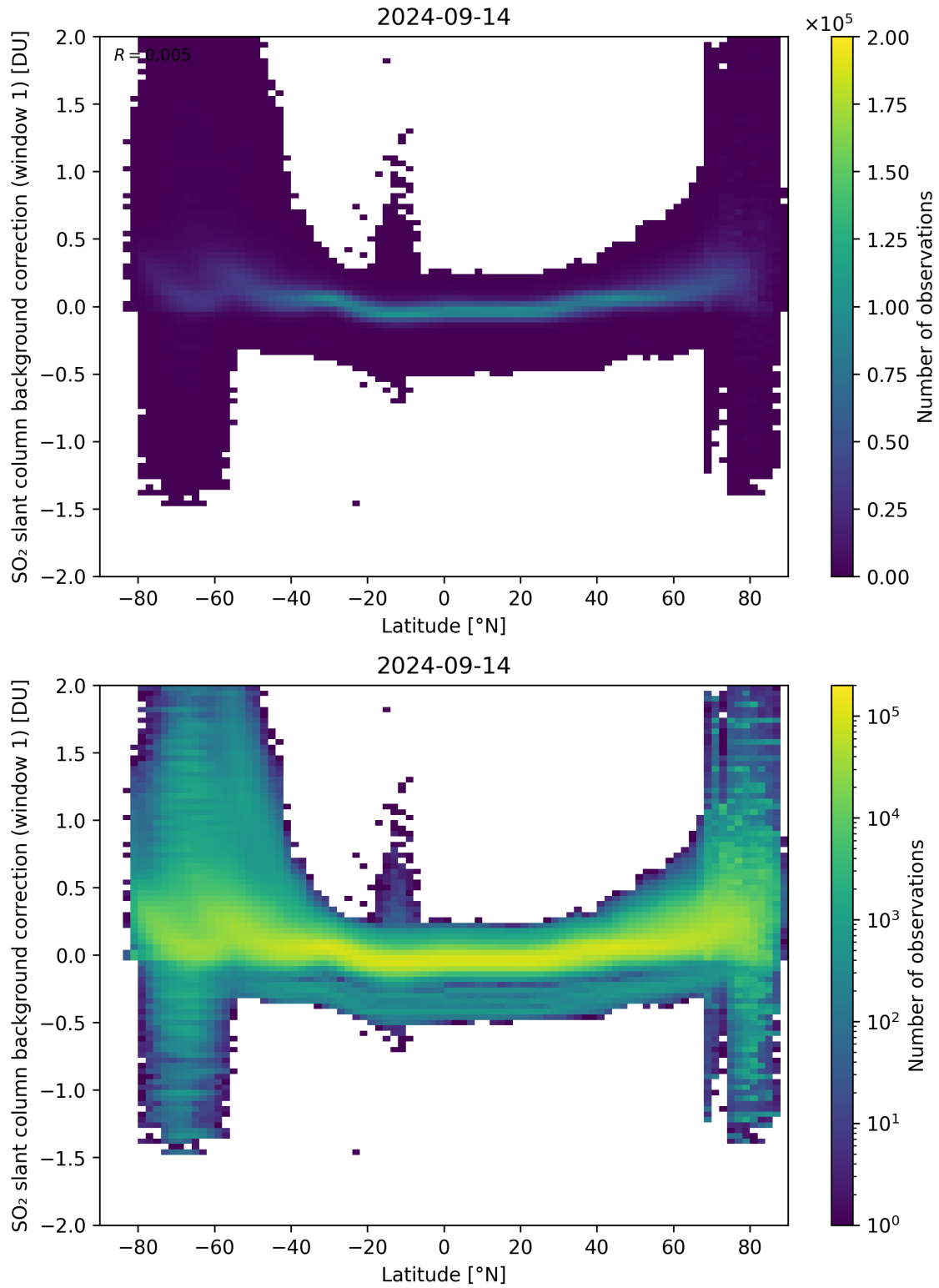
Figure 139: Scatter density plot of “Latitude” against “SO 2 slant column background correction (window 1)” for 2024-09-13 to 2024-09-15.
