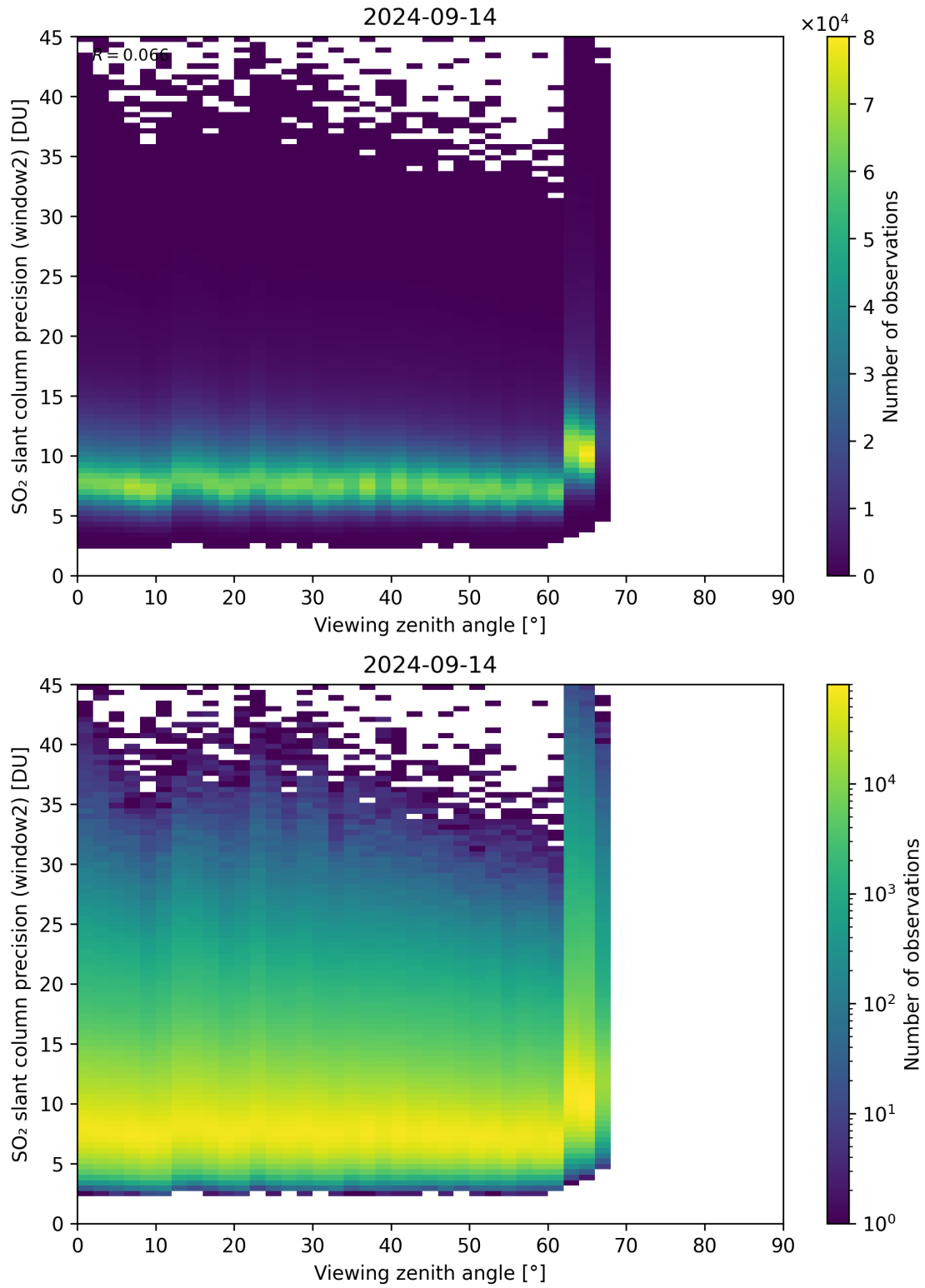
Figure 322: Scatter density plot of “Viewing zenith angle” against “SO 2 slant column precision (window2)” for 2024-09-13 to 2024-09-15.
