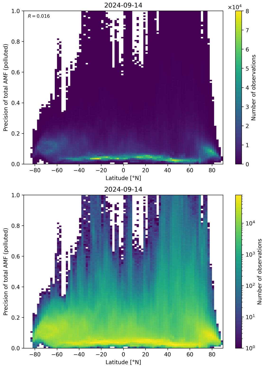
Figure 155: Scatter density plot of “Latitude” against “Precision of total AMF (polluted)” for 2024-09-13 to 2024-09-15.
