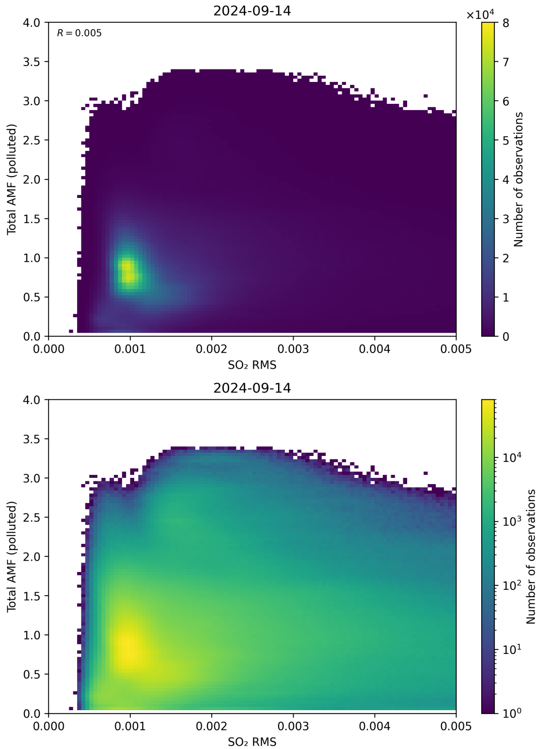
Figure 137: Scatter density plot of “SO 2 RMS” against “Total AMF (polluted)” for 2024-09-13 to 2024-09-15.
