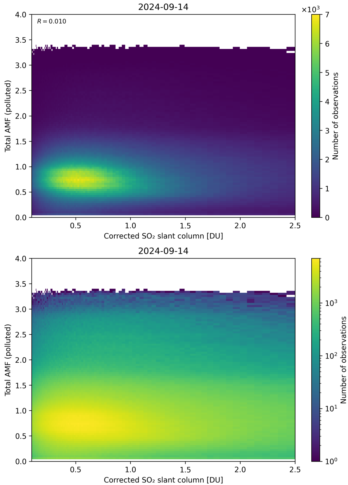
Figure 192: Scatter density plot of “Corrected SO 2 slant column” against “Total AMF (polluted)” for 2024-09-13 to 2024-09-15.
