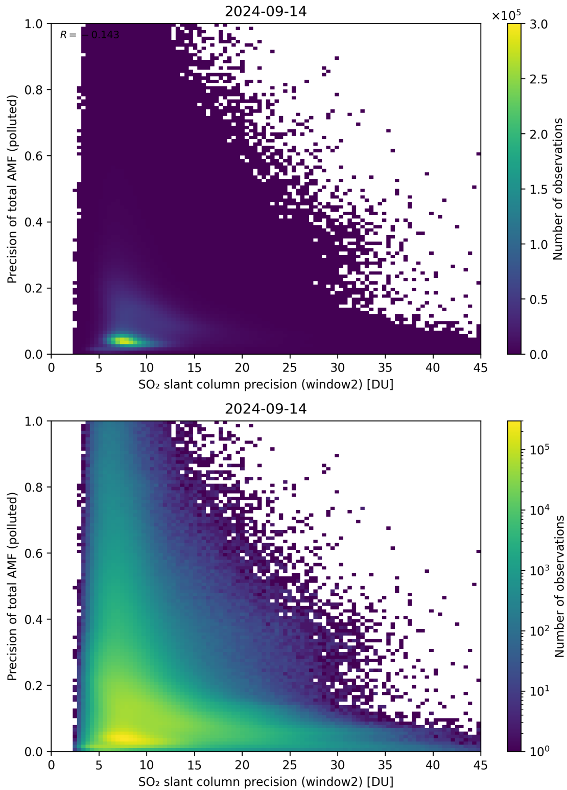
Figure 252: Scatter density plot of “SO 2 slant column precision (window2)” against “Precision of total AMF (polluted)” for 2024-09-13 to 2024-09-15.
