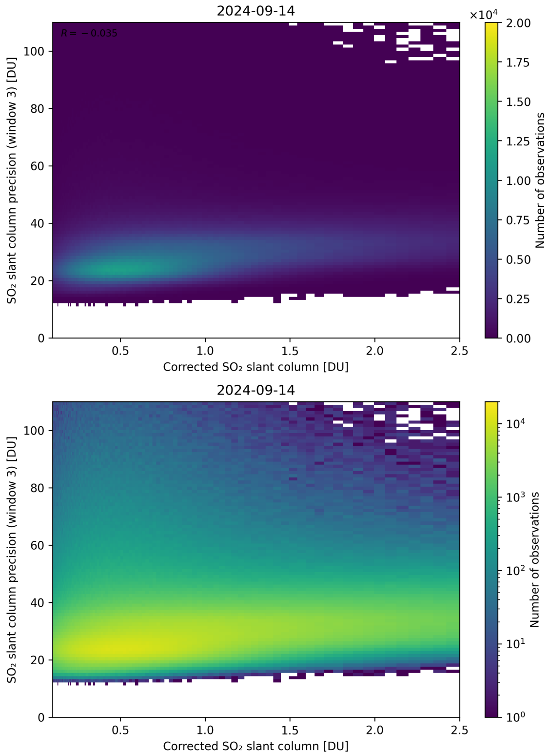
Figure 191: Scatter density plot of “Corrected SO 2 slant column” against “SO 2 slant column precision (window 3)” for 2024-09-13 to 2024-09-15.
