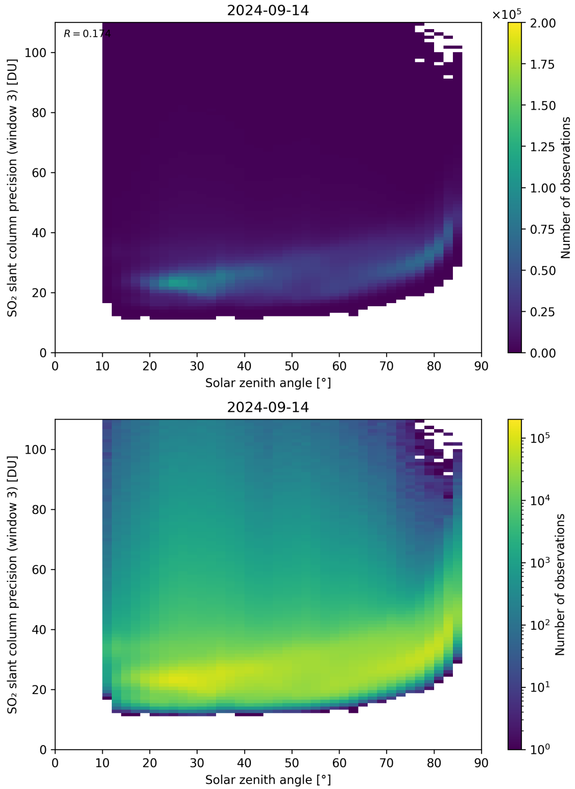
Figure 173: Scatter density plot of “Solar zenith angle” against “SO 2 slant column precision (window 3)” for 2024-09-13 to 2024-09-15.
