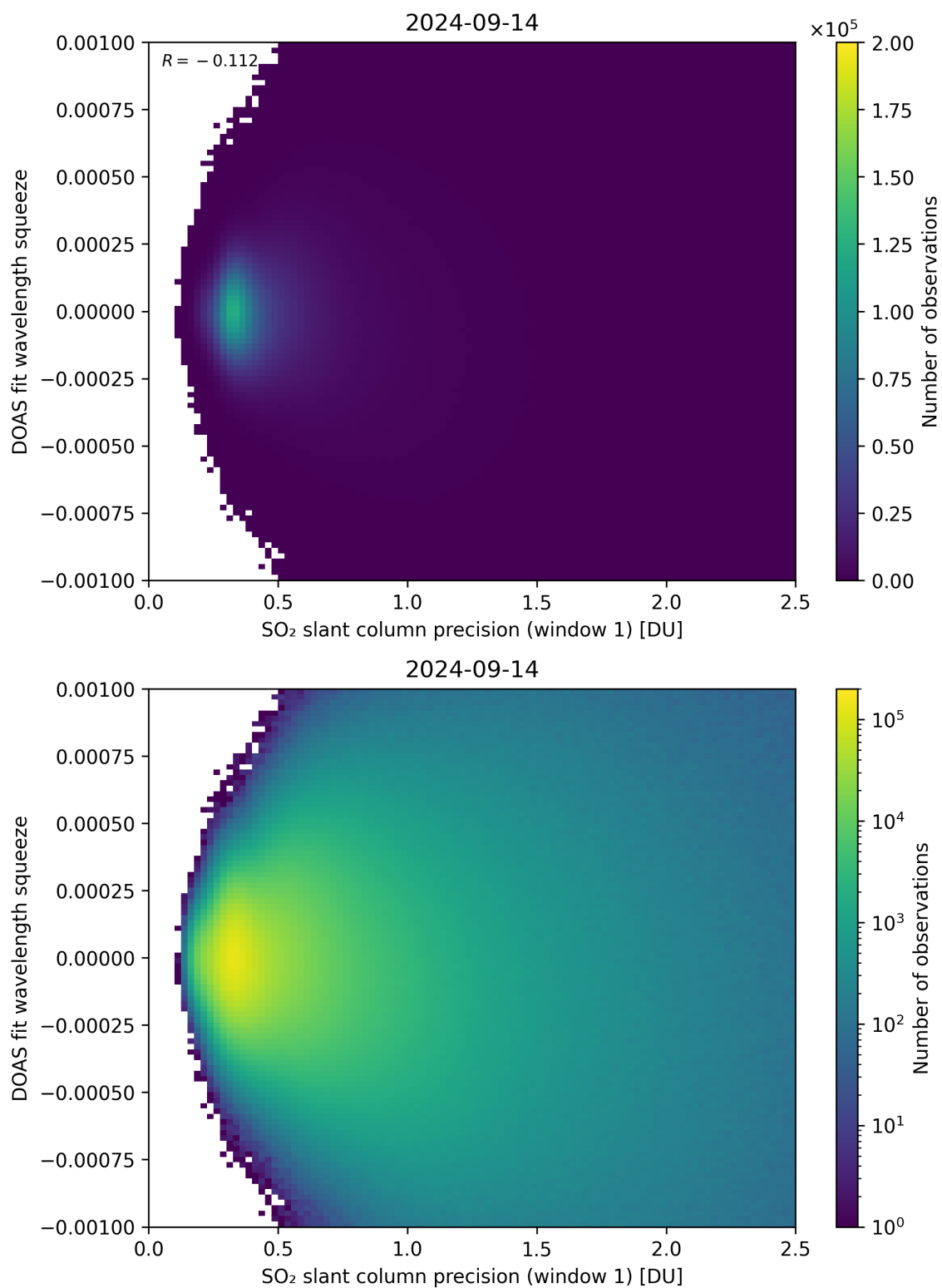
Figure 222: Scatter density plot of “SO 2 slant column precision (window 1)” against “DOAS fit wavelength squeeze” for 2024-09-13 to 2024-09-15.
