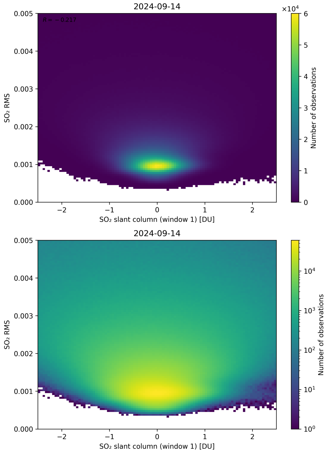
Figure 217: Scatter density plot of “SO 2 slant column (window 1)” against “SO 2 RMS” for 2024-09-13 to 2024-09-15.
