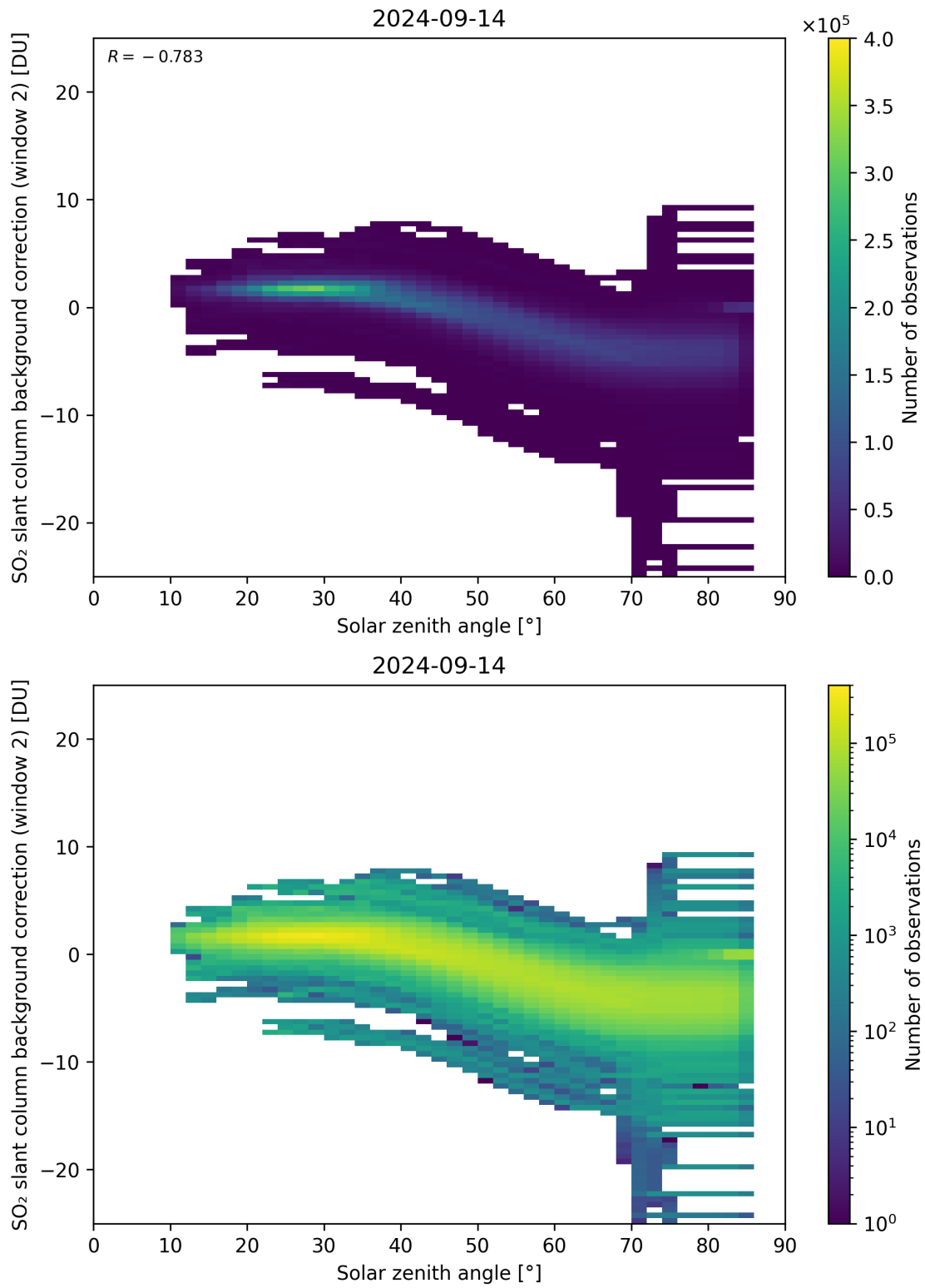
Figure 159: Scatter density plot of “Solar zenith angle” against “SO 2 slant column background correction (window 2)” for 2024-09-13 to 2024-09-15.
