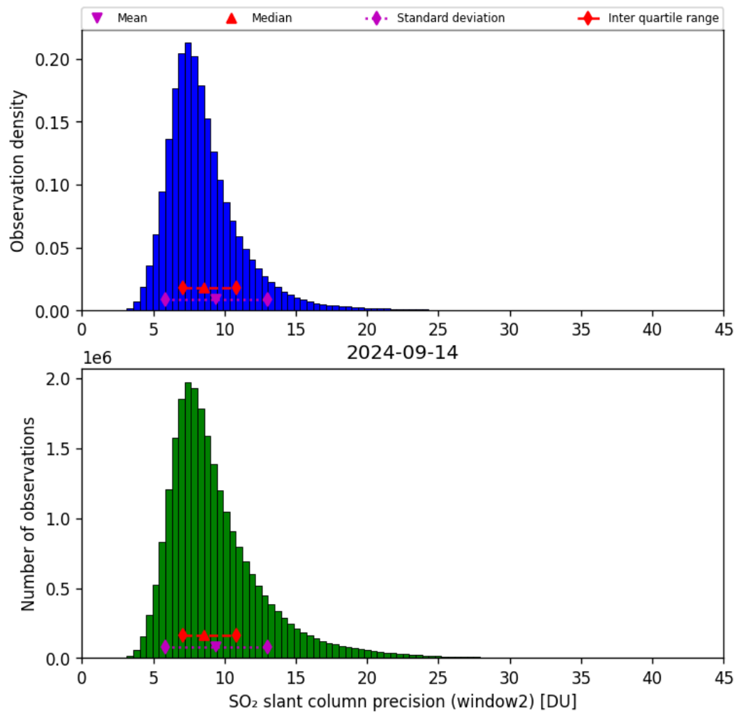
Figure 61: Histogram of “SO 2 slant column precision (window2)” for 2024-09-13 to 2024-09-15
