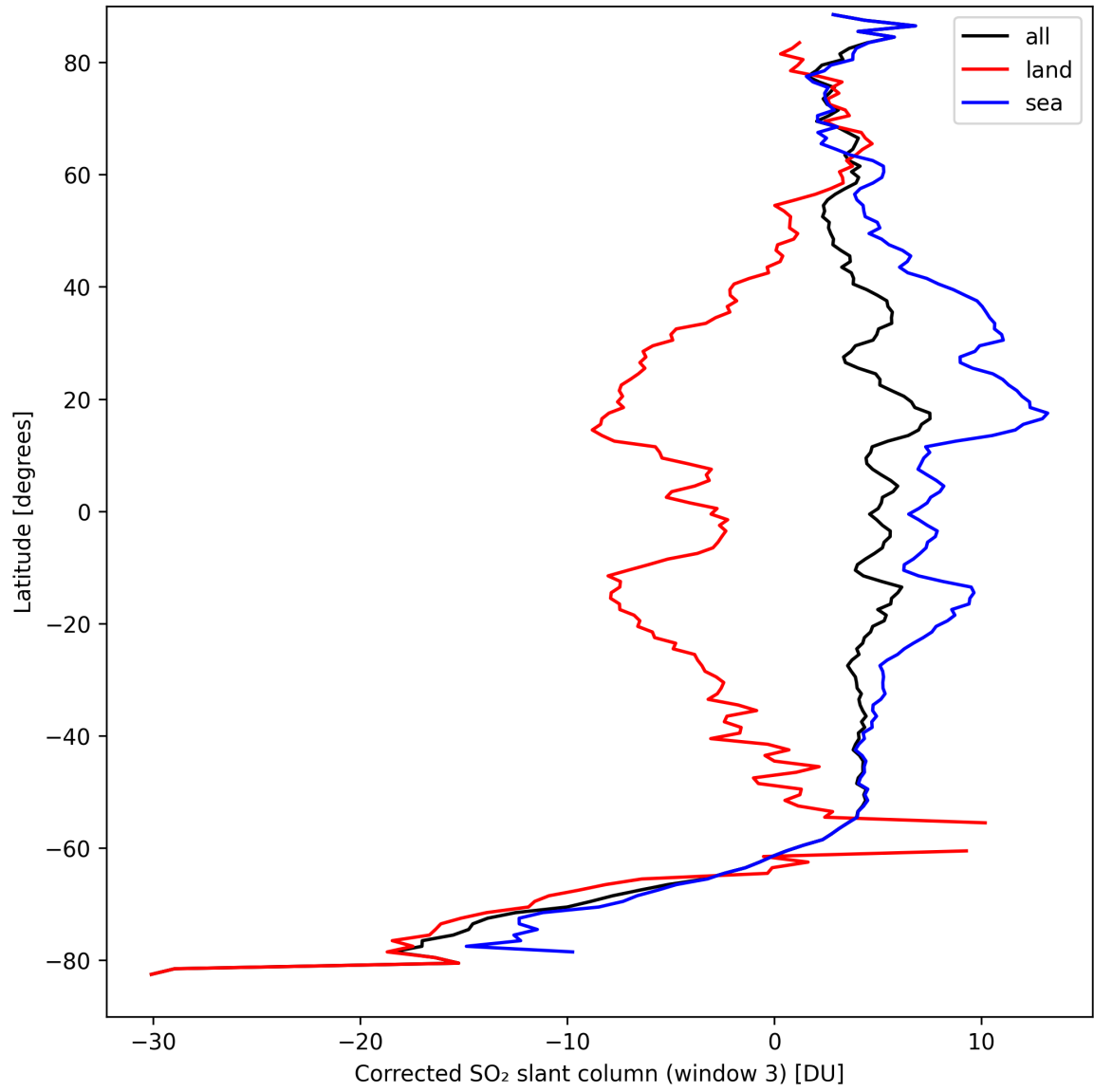
Figure 43: Zonal average of “Corrected SO 2 slant column (window 3)” for 2024-09-13 to 2024-09-15.
