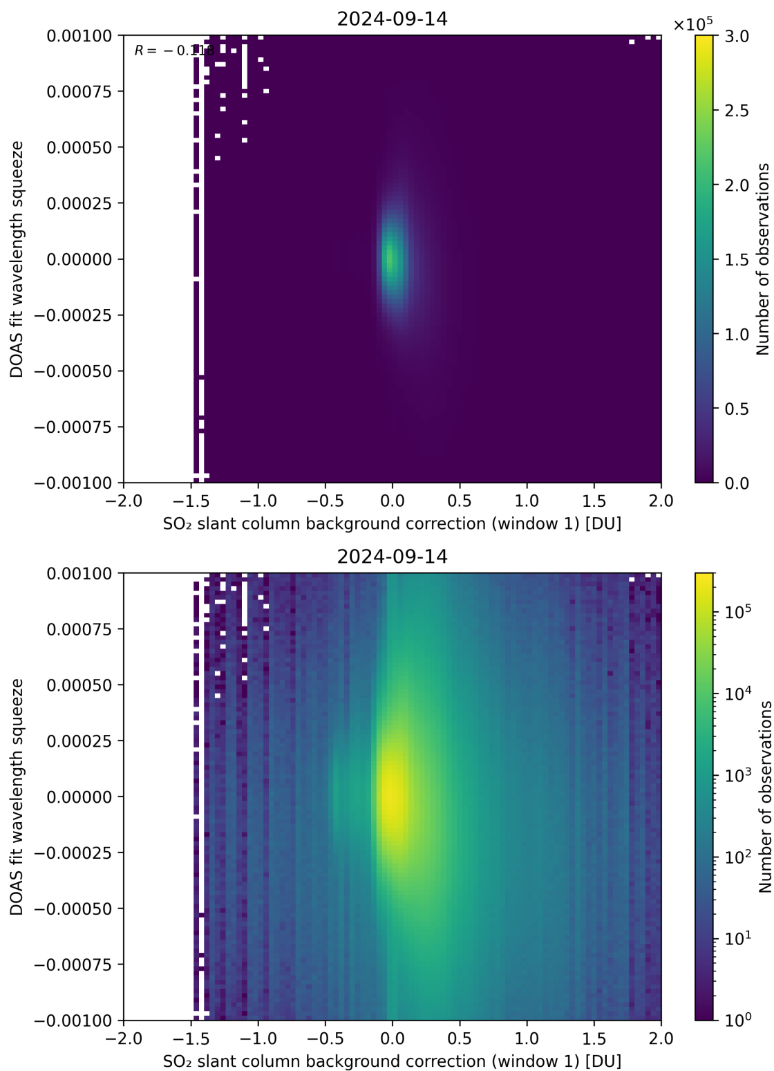
Figure 101: Scatter density plot of “SO 2 slant column background correction (window 1)” against “DOAS fit wavelength squeeze” for 2024-09-13 to 2024-09-15.
