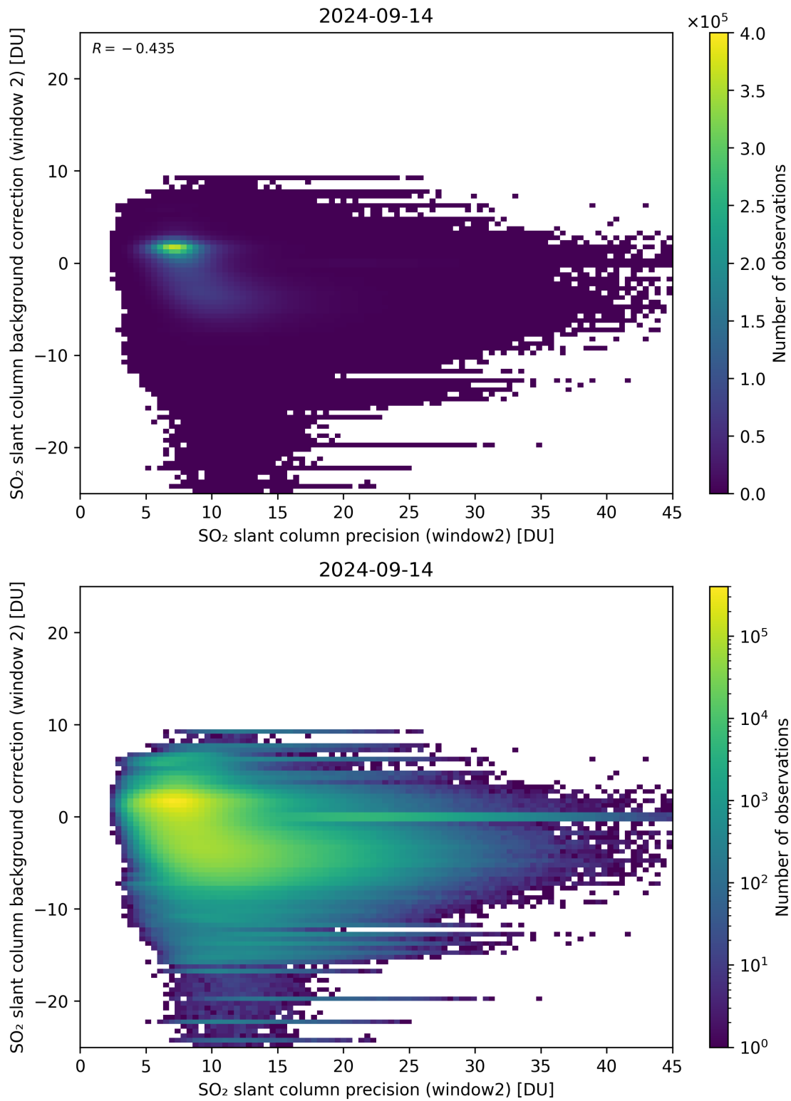
Figure 241: Scatter density plot of “SO 2 slant column precision (window2)” against “SO 2 slant column background correction (window 2)” for 2024-09-13 to 2024-09-15.
