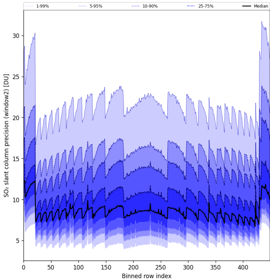
Figure 84: Along track statistics of “SO 2 slant column precision (window2)” for 2024-09-13 to 2024-09-15
