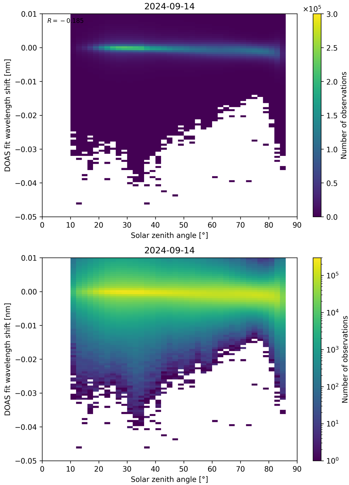
Figure 161: Scatter density plot of “Solar zenith angle” against “DOAS fit wavelength shift” for 2024-09-13 to 2024-09-15.
