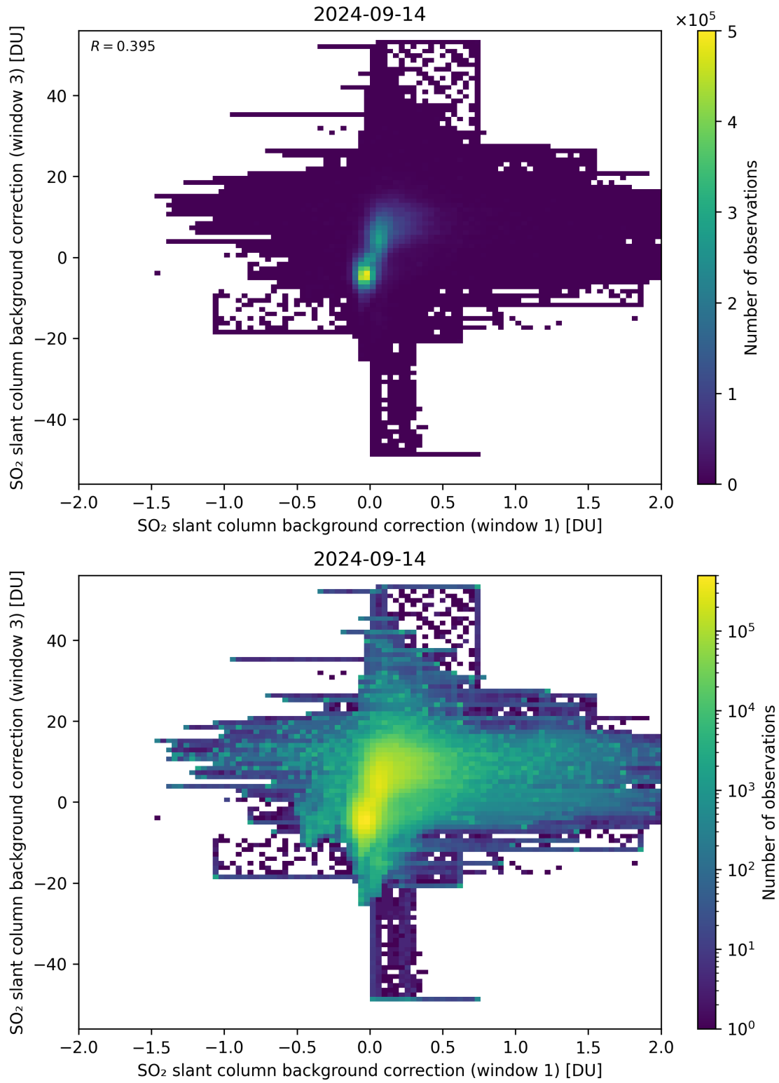
Figure 99: Scatter density plot of “SO 2 slant column background correction (window 1)” against “SO 2 slant column background correction (window 3)” for 2024-09-13 to 2024-09-15.
