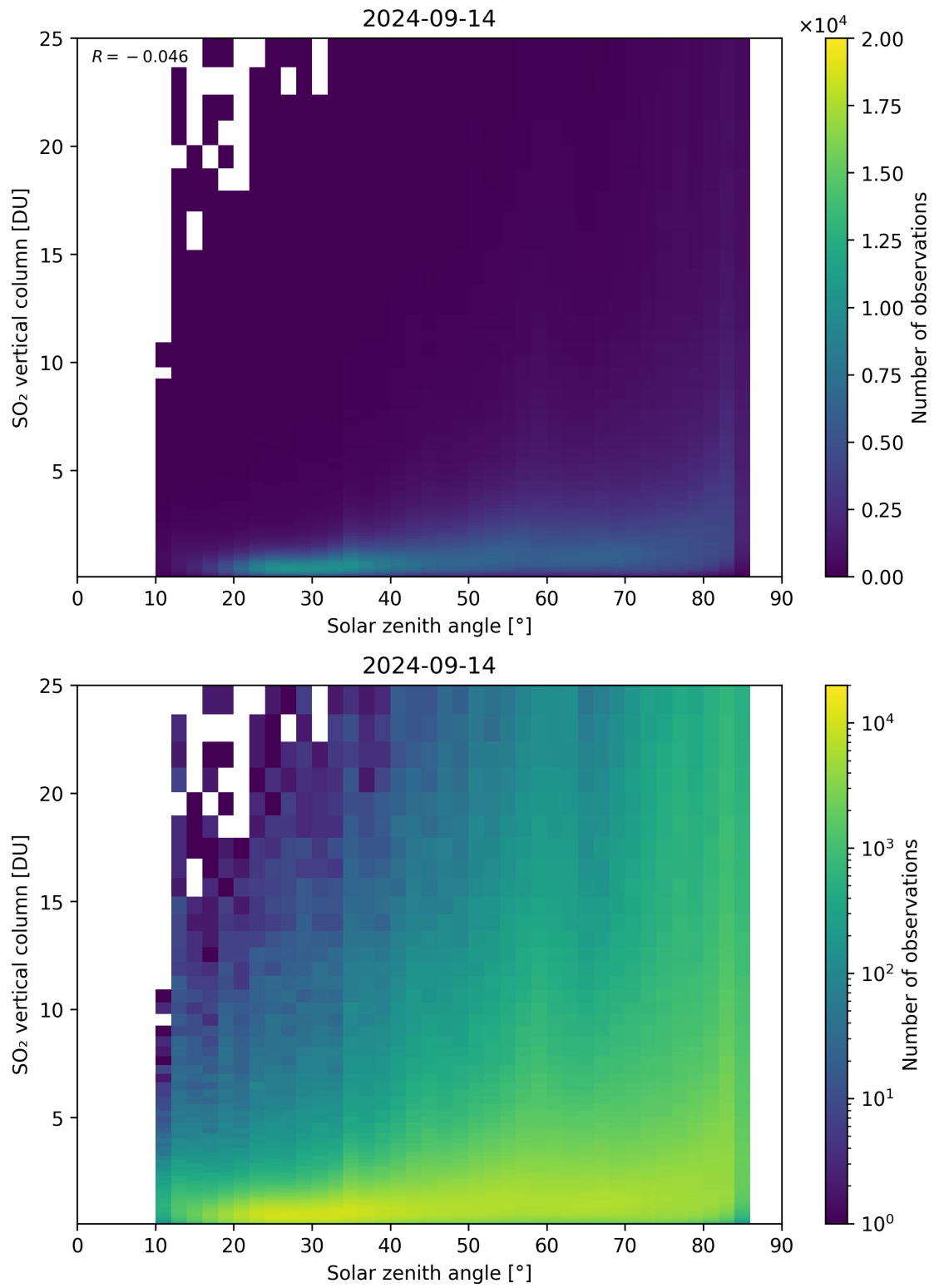
Figure 176: Scatter density plot of “Solar zenith angle” against “SO 2 vertical column” for 2024-09-13 to 2024-09-15.
