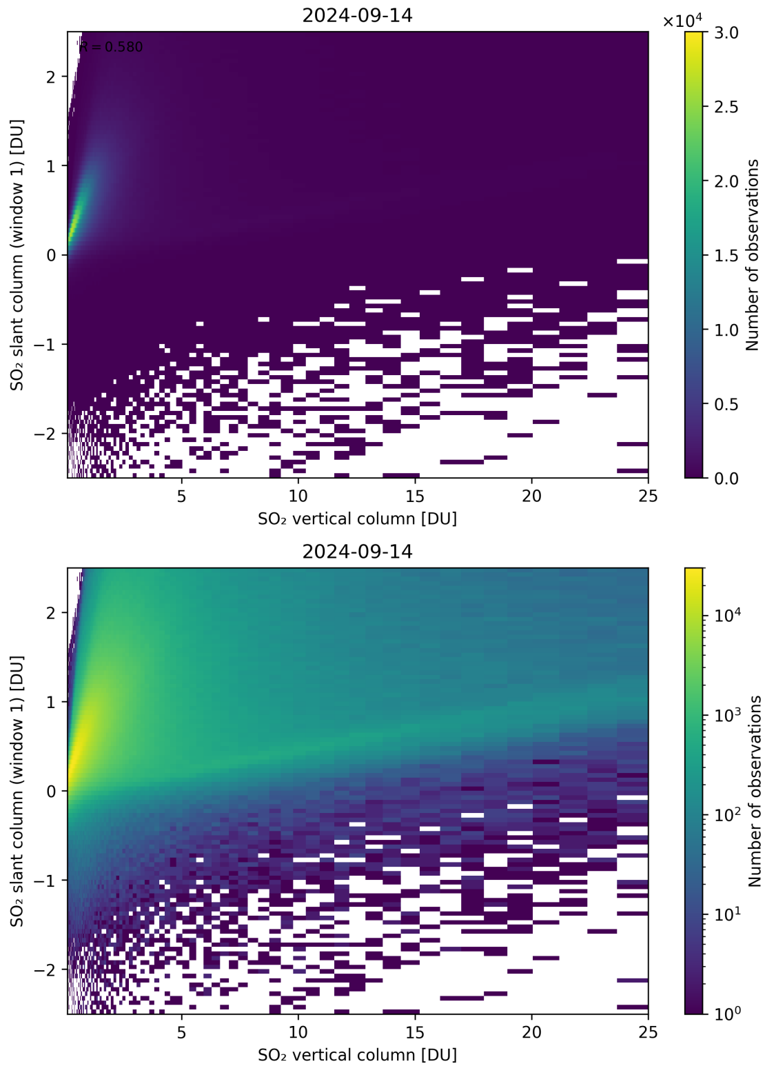
Figure 300: Scatter density plot of “SO 2 vertical column” against “SO 2 slant column (window 1)” for 2024-09-13 to 2024-09-15.
