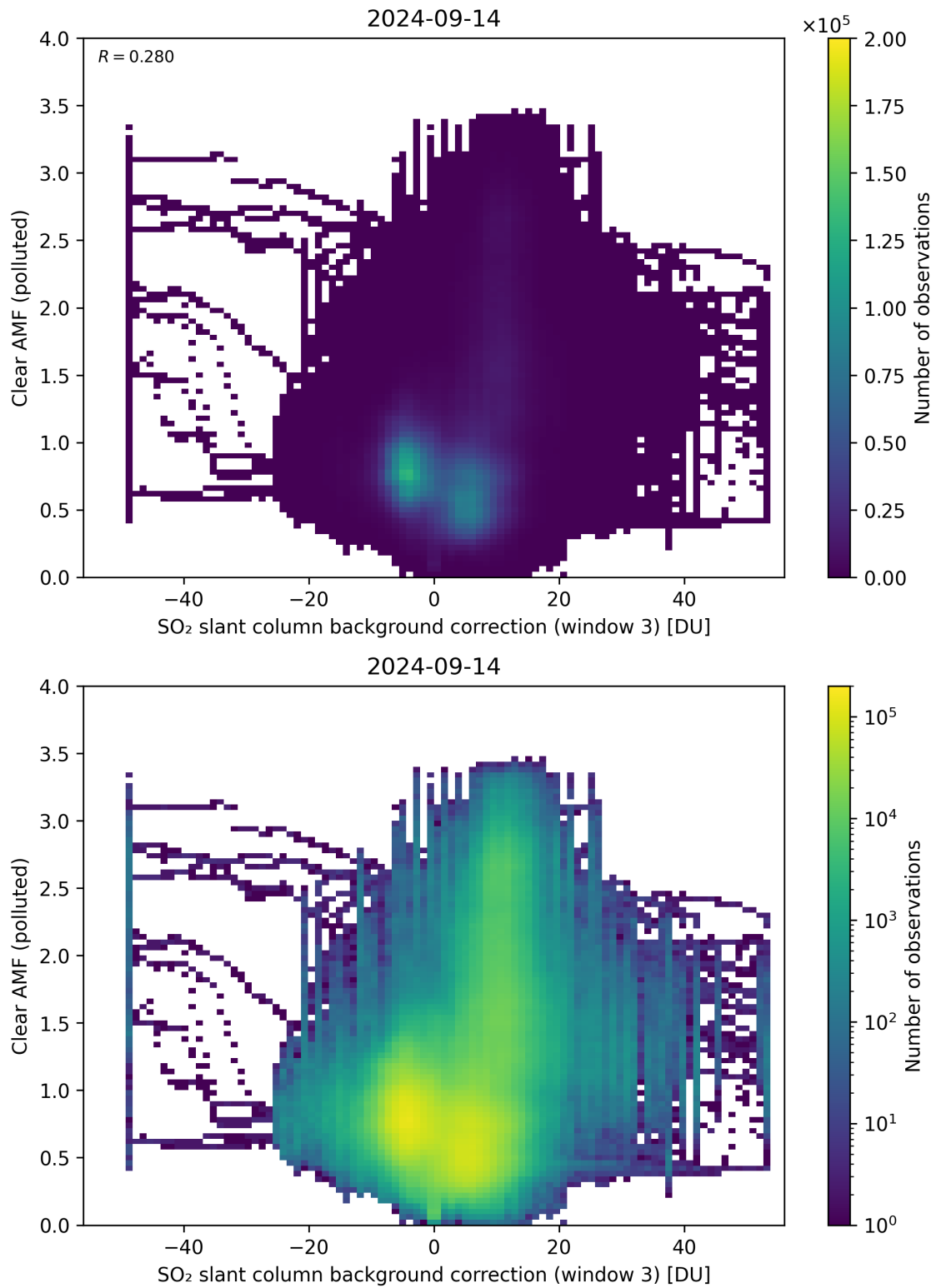
Figure 124: Scatter density plot of “SO 2 slant column background correction (window 3)” against “Clear AMF (polluted)” for 2024-09-13 to 2024-09-15.
