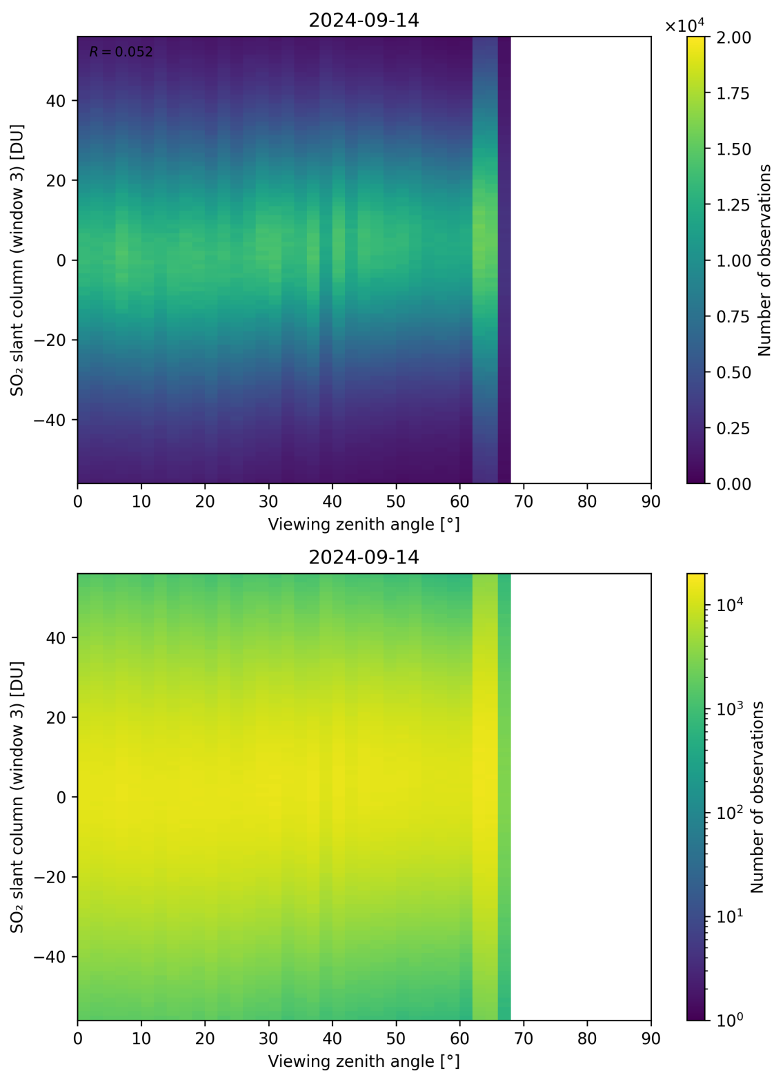
Figure 323: Scatter density plot of “Viewing zenith angle” against “SO 2 slant column (window 3)” for 2024-09-13 to 2024-09-15.
