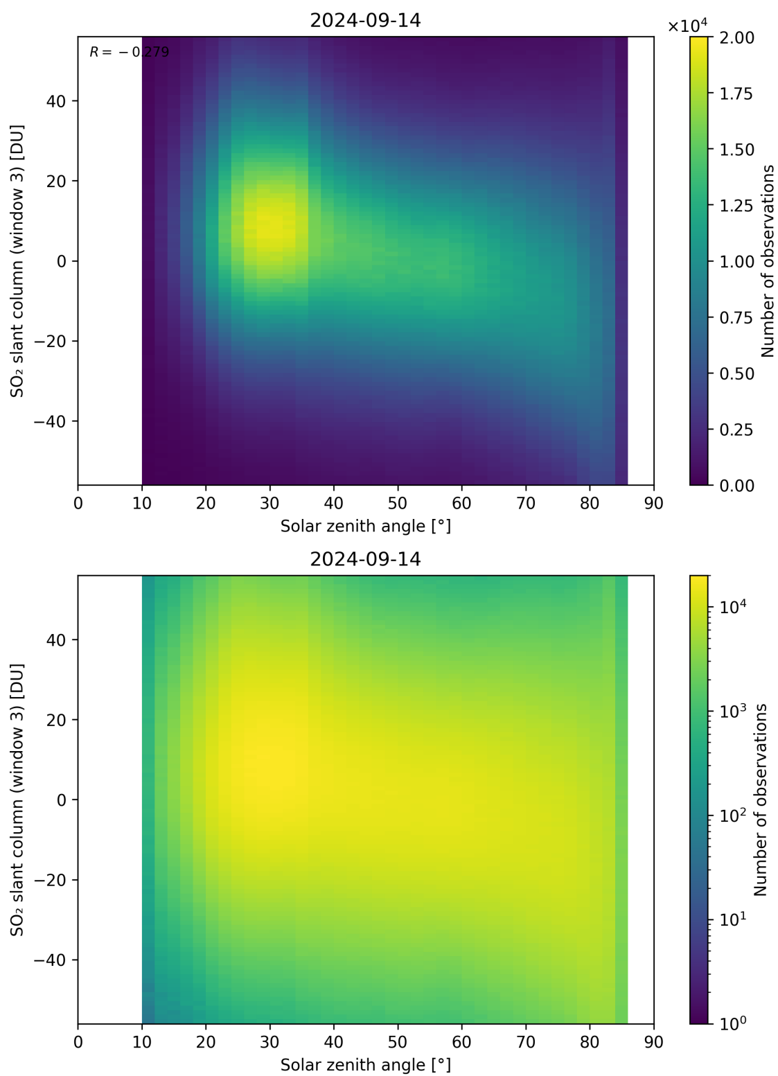
Figure 172: Scatter density plot of “Solar zenith angle” against “SO 2 slant column (window 3)” for 2024-09-13 to 2024-09-15.
