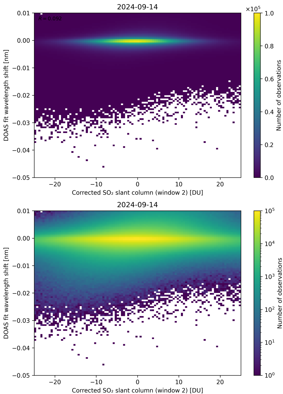
Figure 196: Scatter density plot of “Corrected SO 2 slant column (window 2)” against “DOAS fit wavelength shift” for 2024-09-13 to 2024-09-15.
