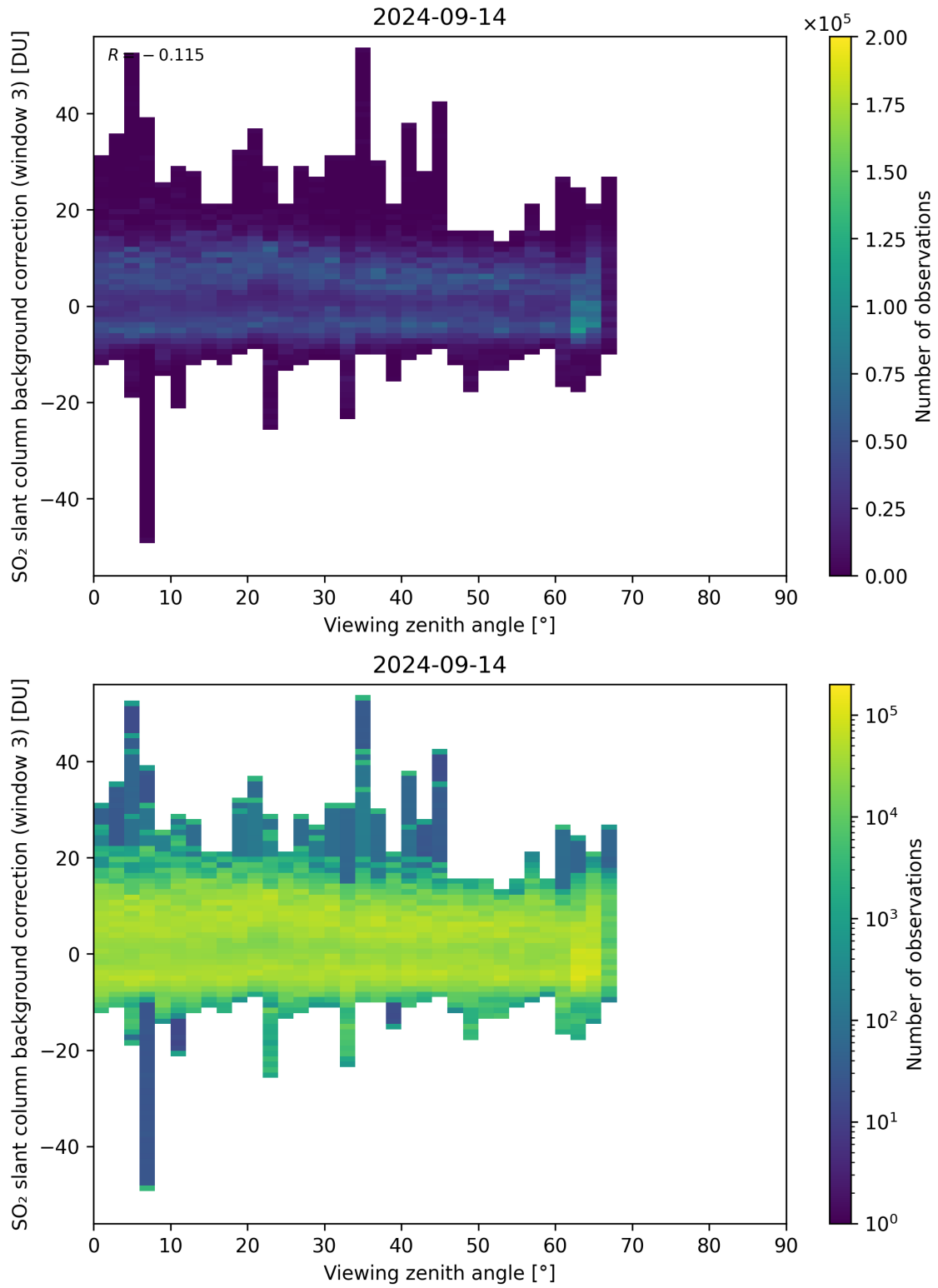
Figure 310: Scatter density plot of “Viewing zenith angle” against “SO 2 slant column background correction (window 3)” for 2024-09-13 to 2024-09-15.
