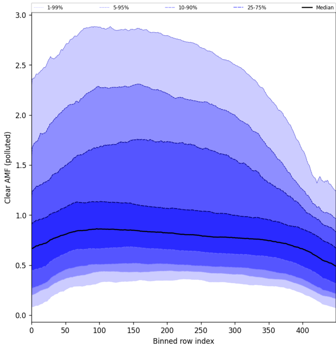
Figure 96: Along track statistics of “Clear AMF (polluted)” for 2024-09-13 to 2024-09-15
