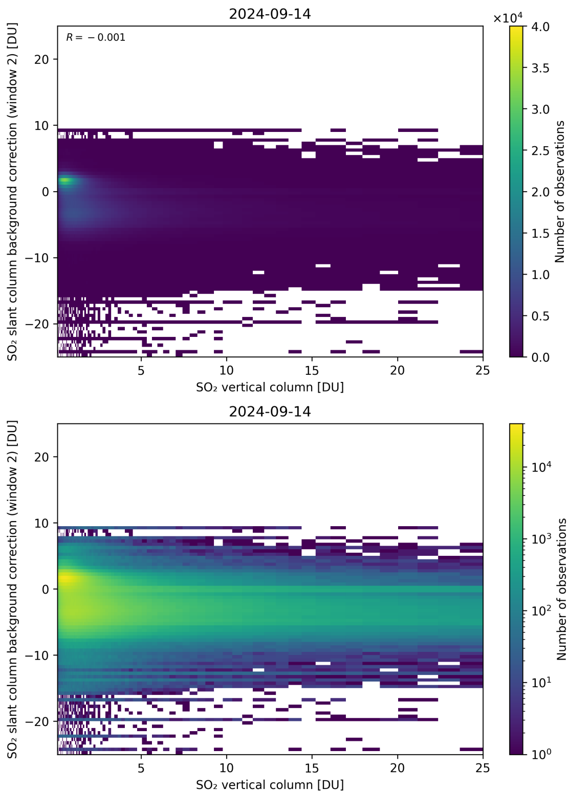
Figure 274: Scatter density plot of “SO 2 vertical column” against “SO 2 slant column background correction (window 2)” for 2024-09-13 to 2024-09-15.
