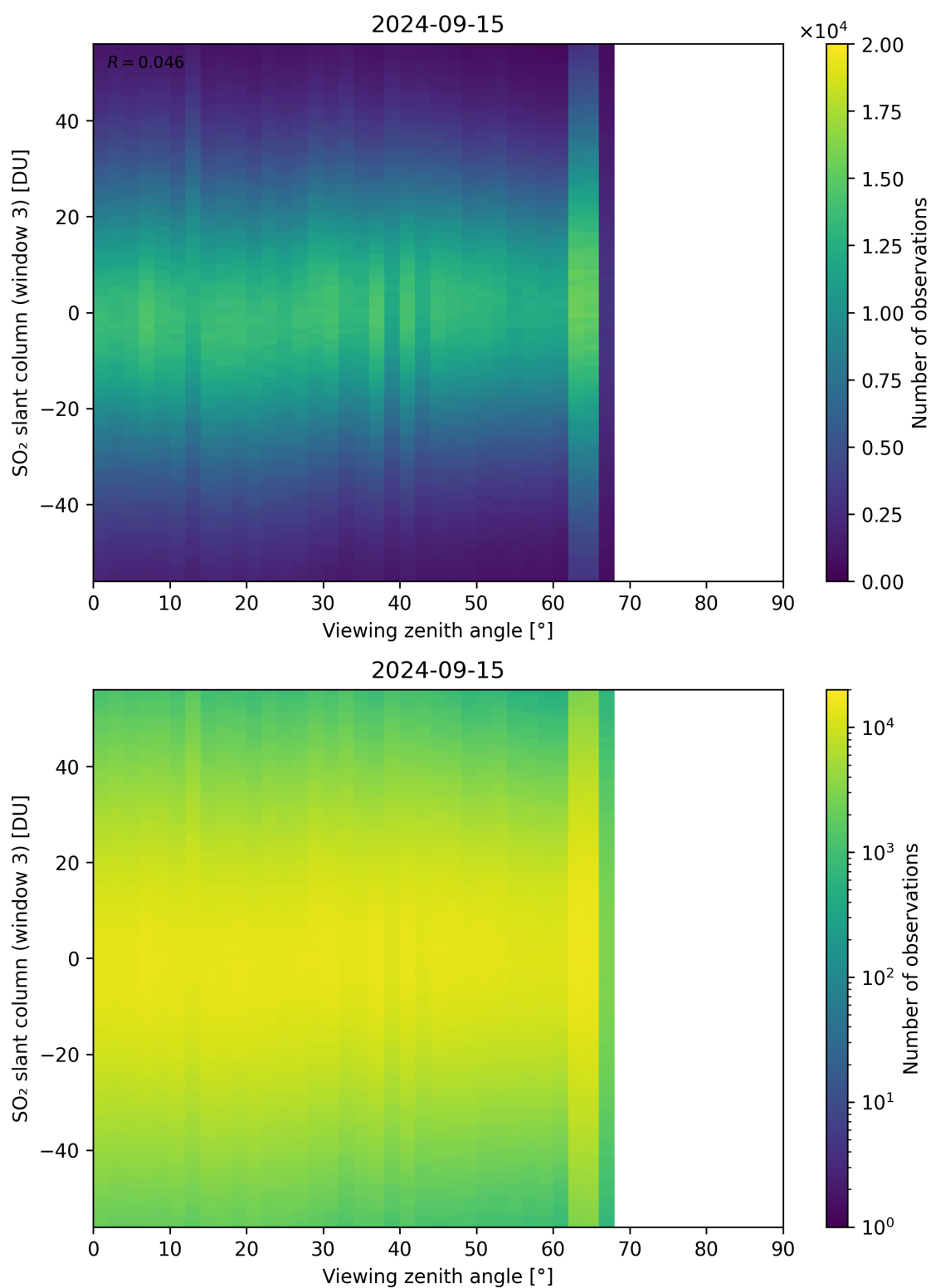
Figure 323: Scatter density plot of “Viewing zenith angle” against “SO 2 slant column (window 3)” for 2024-09-14 to 2024-09-16.
