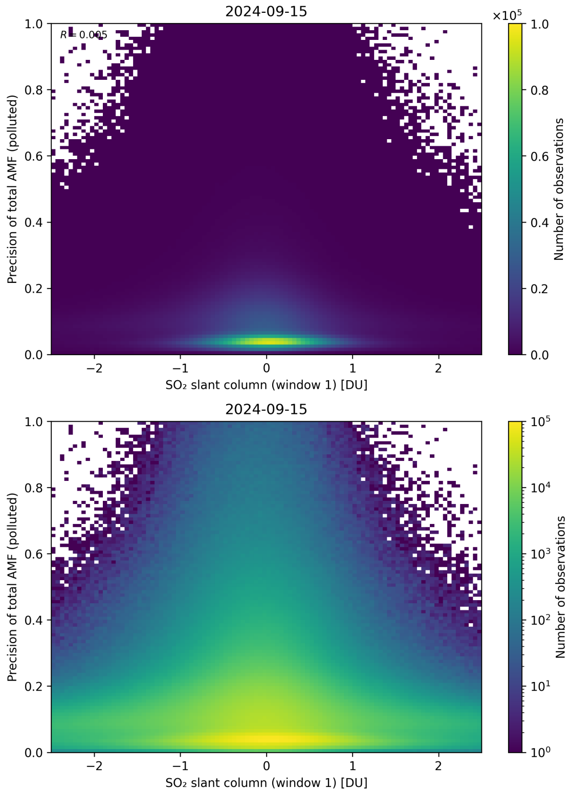
Figure 240: Scatter density plot of “SO 2 slant column (window 1)” against “Precision of total AMF (polluted)” for 2024-09-14 to 2024-09-16.
