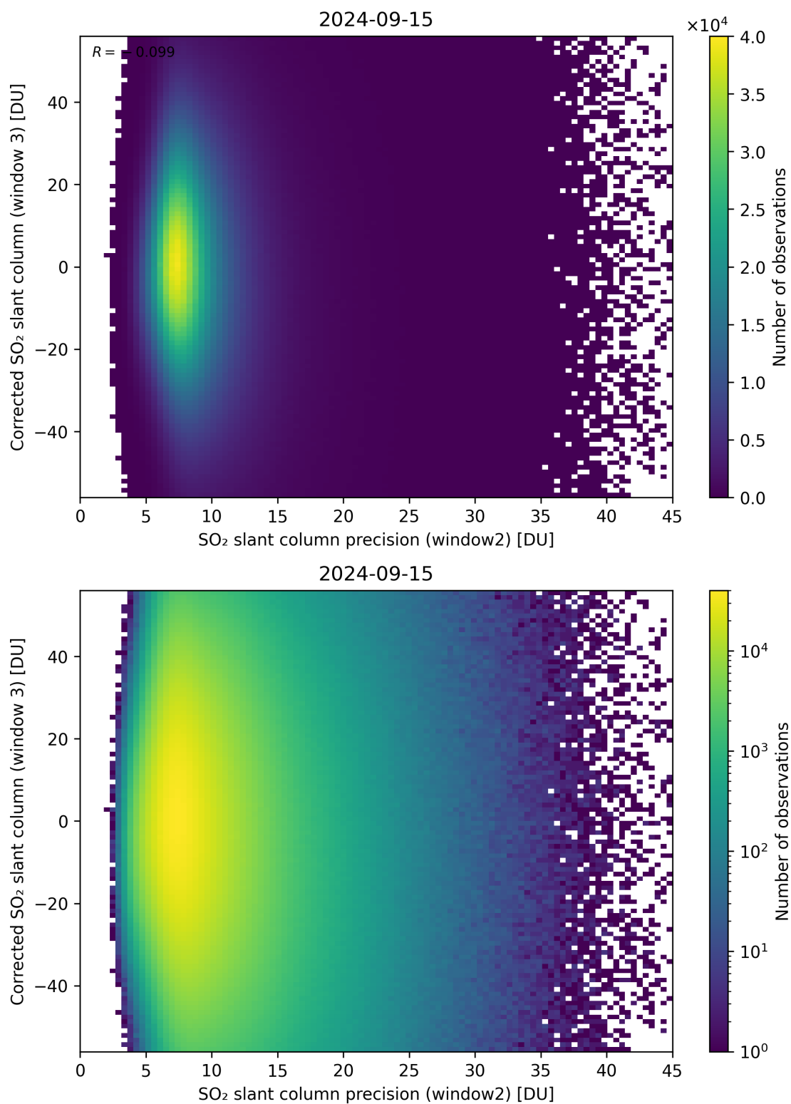
Figure 248: Scatter density plot of “SO 2 slant column precision (window2)” against “Corrected SO 2 slant column (window 3)” for 2024-09-14 to 2024-09-16.
