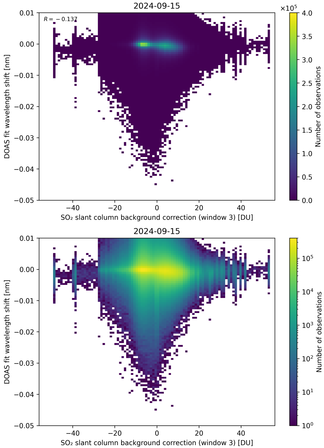
Figure 121: Scatter density plot of “SO 2 slant column background correction (window 3)” against “DOAS fit wavelength shift” for 2024-09-14 to 2024-09-16.
