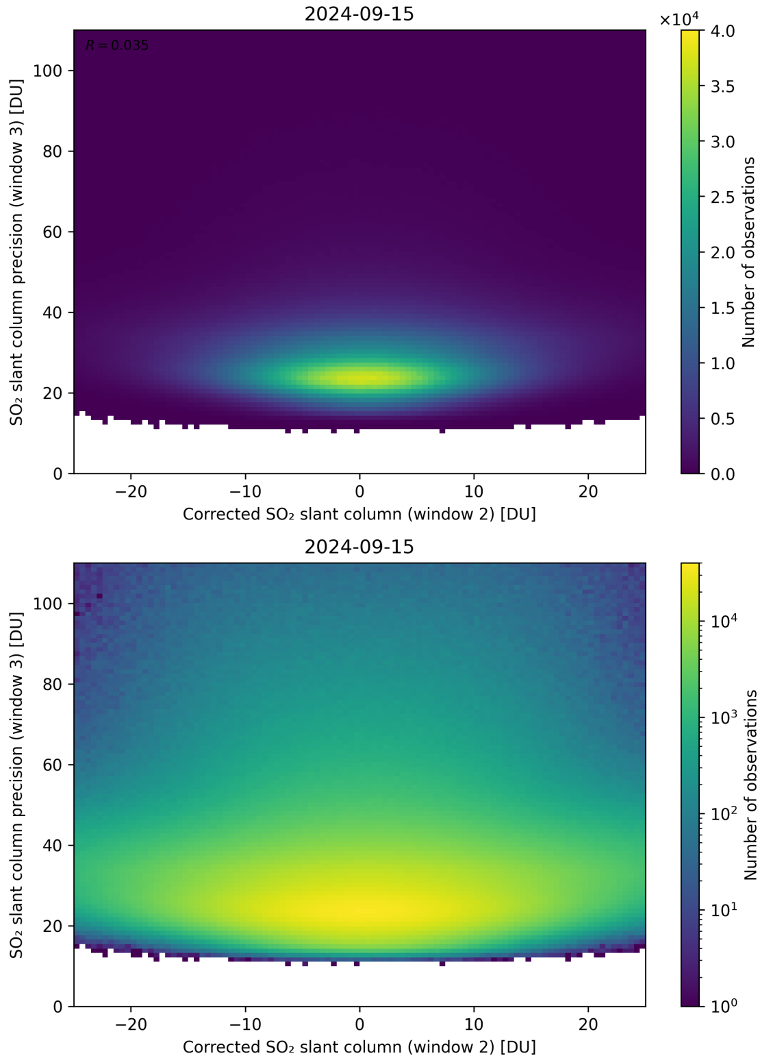
Figure 202: Scatter density plot of “Corrected SO 2 slant column (window 2)” against “SO 2 slant column precision (window 3)” for 2024-09-14 to 2024-09-16.
