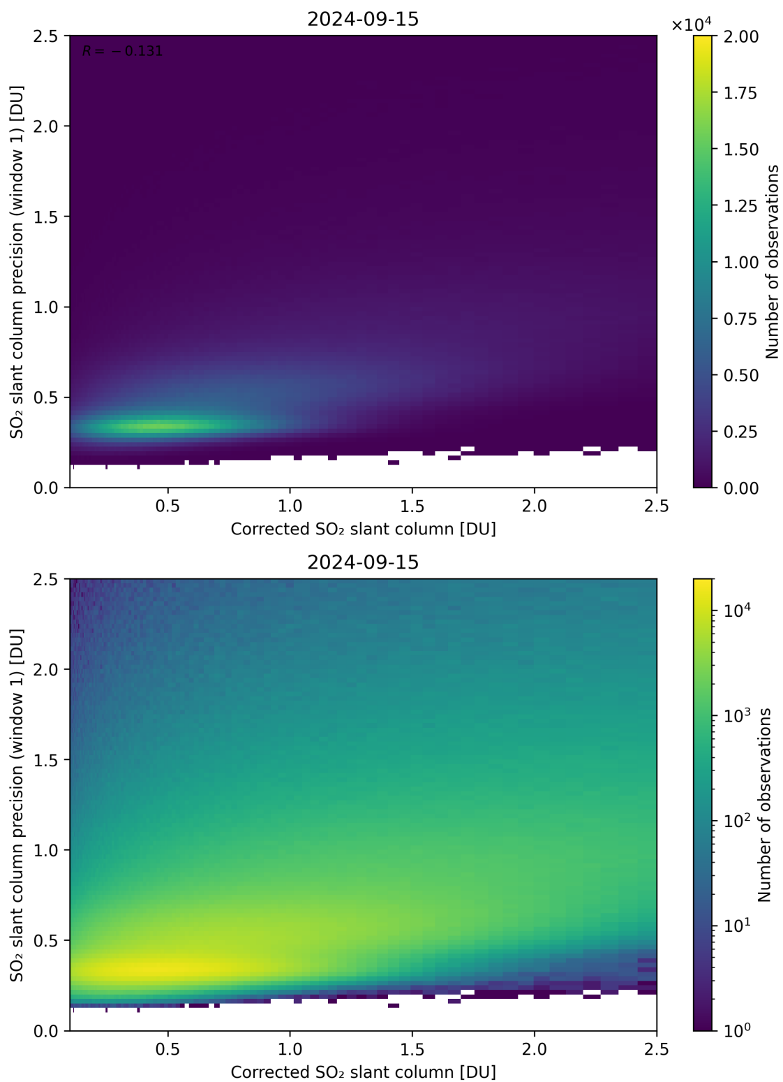
Figure 188: Scatter density plot of “Corrected SO 2 slant column” against “SO 2 slant column precision (window 1)” for 2024-09-14 to 2024-09-16.
