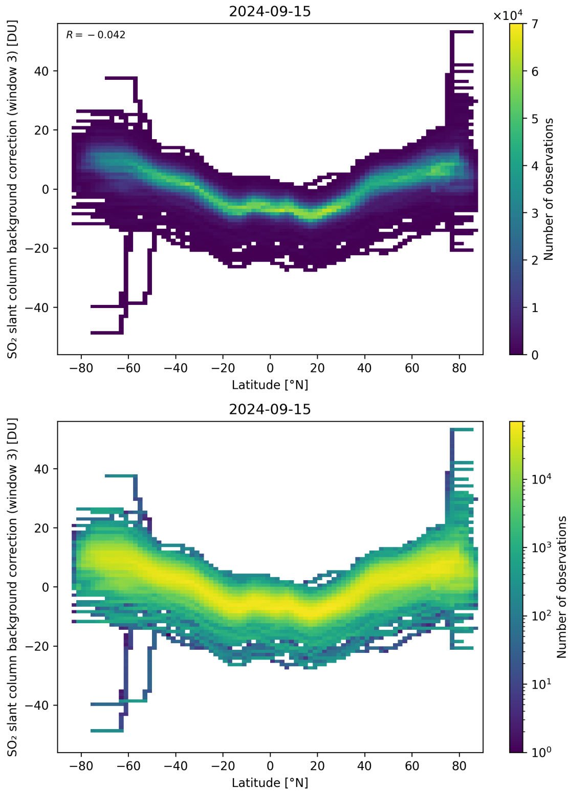
Figure 141: Scatter density plot of “Latitude” against “SO 2 slant column background correction (window 3)” for 2024-09-14 to 2024-09-16.
