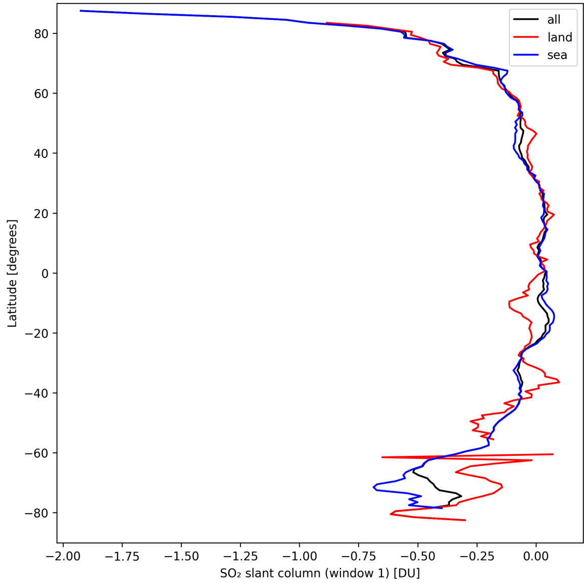
Figure 33: Zonal average of “SO 2 slant column (window 1)” for 2024-09-14 to 2024-09-16.
