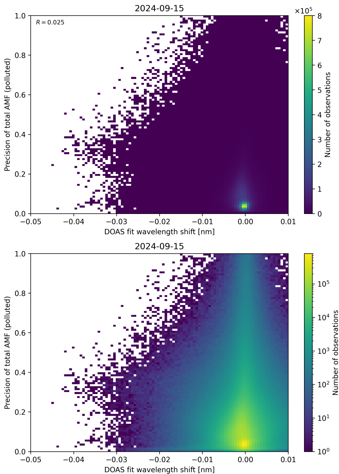
Figure 131: Scatter density plot of “DOAS fit wavelength shift” against “Precision of total AMF (polluted)” for 2024-09-14 to 2024-09-16.
