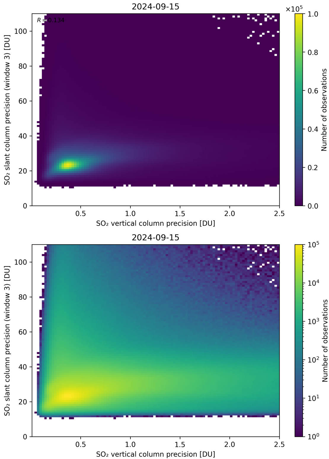
Figure 293: Scatter density plot of “SO 2 vertical column precision” against “SO 2 slant column precision (window 3)” for 2024-09-14 to 2024-09-16.
