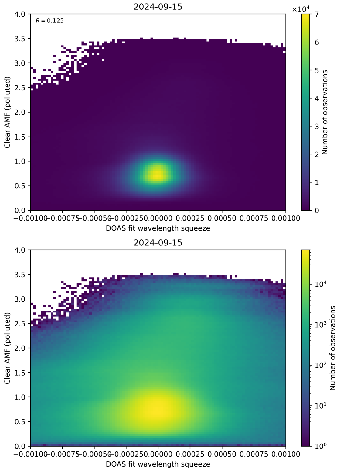
Figure 133: Scatter density plot of “DOAS fit wavelength squeeze” against “Clear AMF (polluted)” for 2024-09-14 to 2024-09-16.
