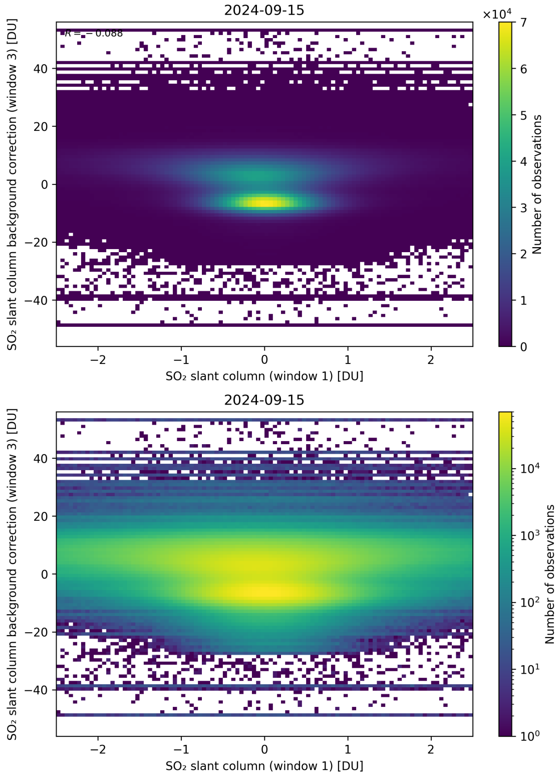
Figure 214: Scatter density plot of “SO 2 slant column (window 1)” against “SO 2 slant column background correction (window 3)” for 2024-09-14 to 2024-09-16.
