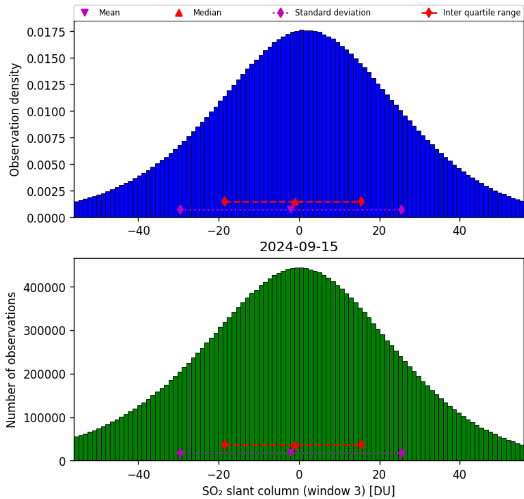
Figure 64: Histogram of “SO 2 slant column (window 3)” for 2024-09-14 to 2024-09-16
