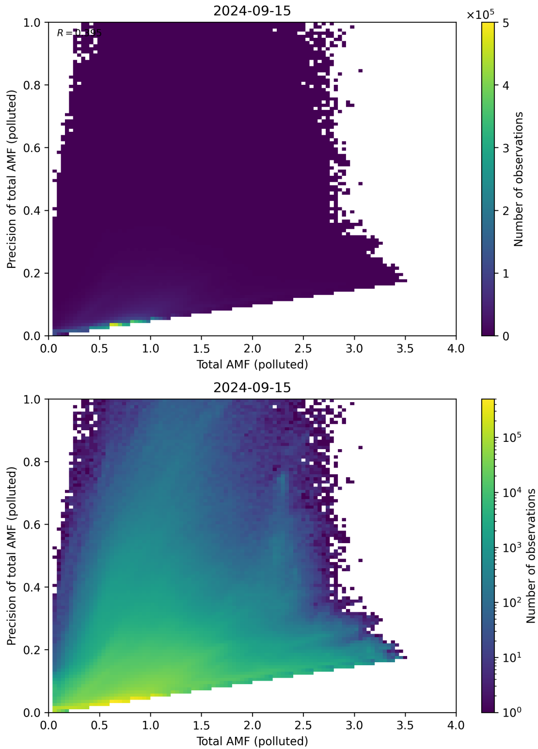
Figure 272: Scatter density plot of “Total AMF (polluted)” against “Precision of total AMF (polluted)” for 2024-09-14 to 2024-09-16.
