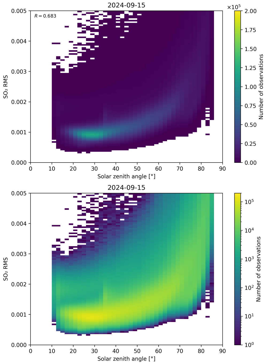
Figure 163: Scatter density plot of “Solar zenith angle” against “SO 2 RMS” for 2024-09-14 to 2024-09-16.
