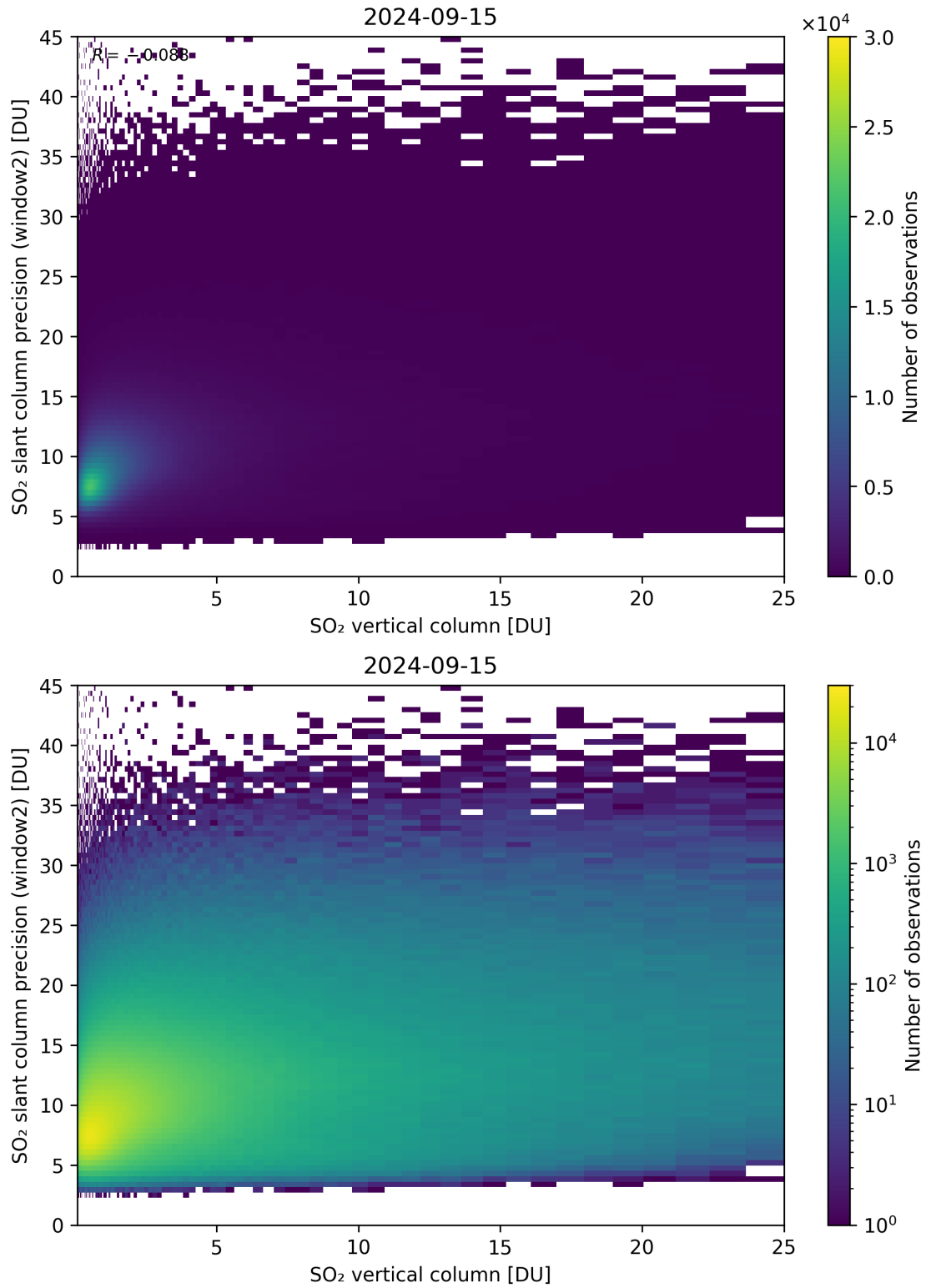
Figure 302: Scatter density plot of “SO 2 vertical column” against “SO 2 slant column precision (window2)” for 2024-09-14 to 2024-09-16.
