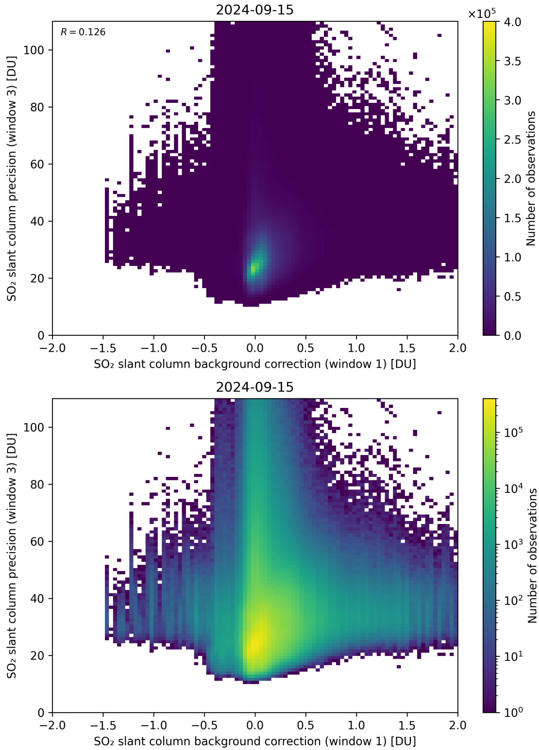
Figure 108: Scatter density plot of “SO 2 slant column background correction (window 1)” against “SO 2 slant column precision (window 3)” for 2024-09-14 to 2024-09-16.
