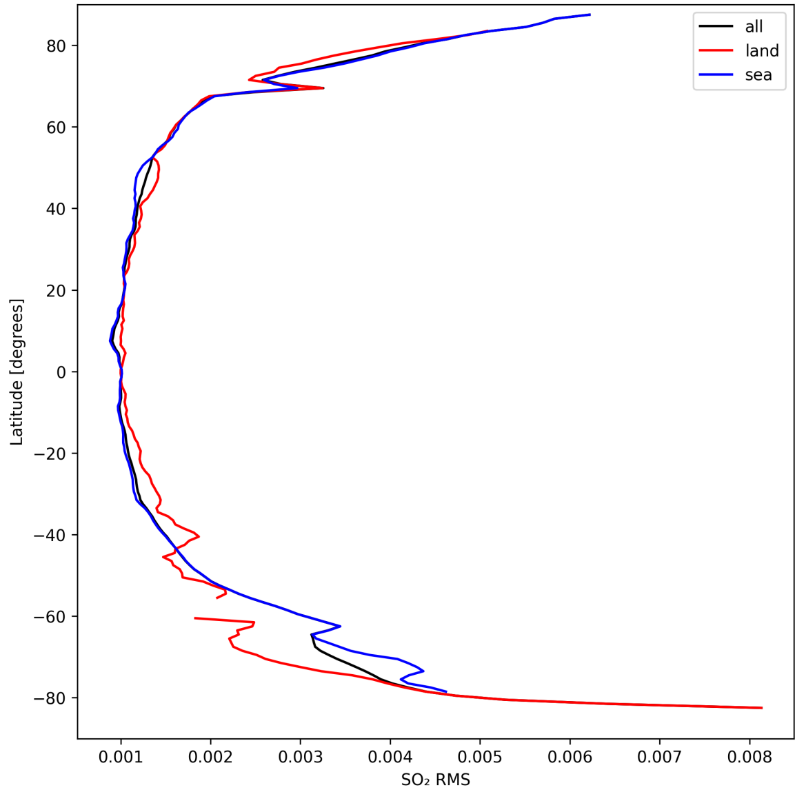
Figure 47: Zonal average of “SO 2 RMS” for 2024-09-14 to 2024-09-16.
