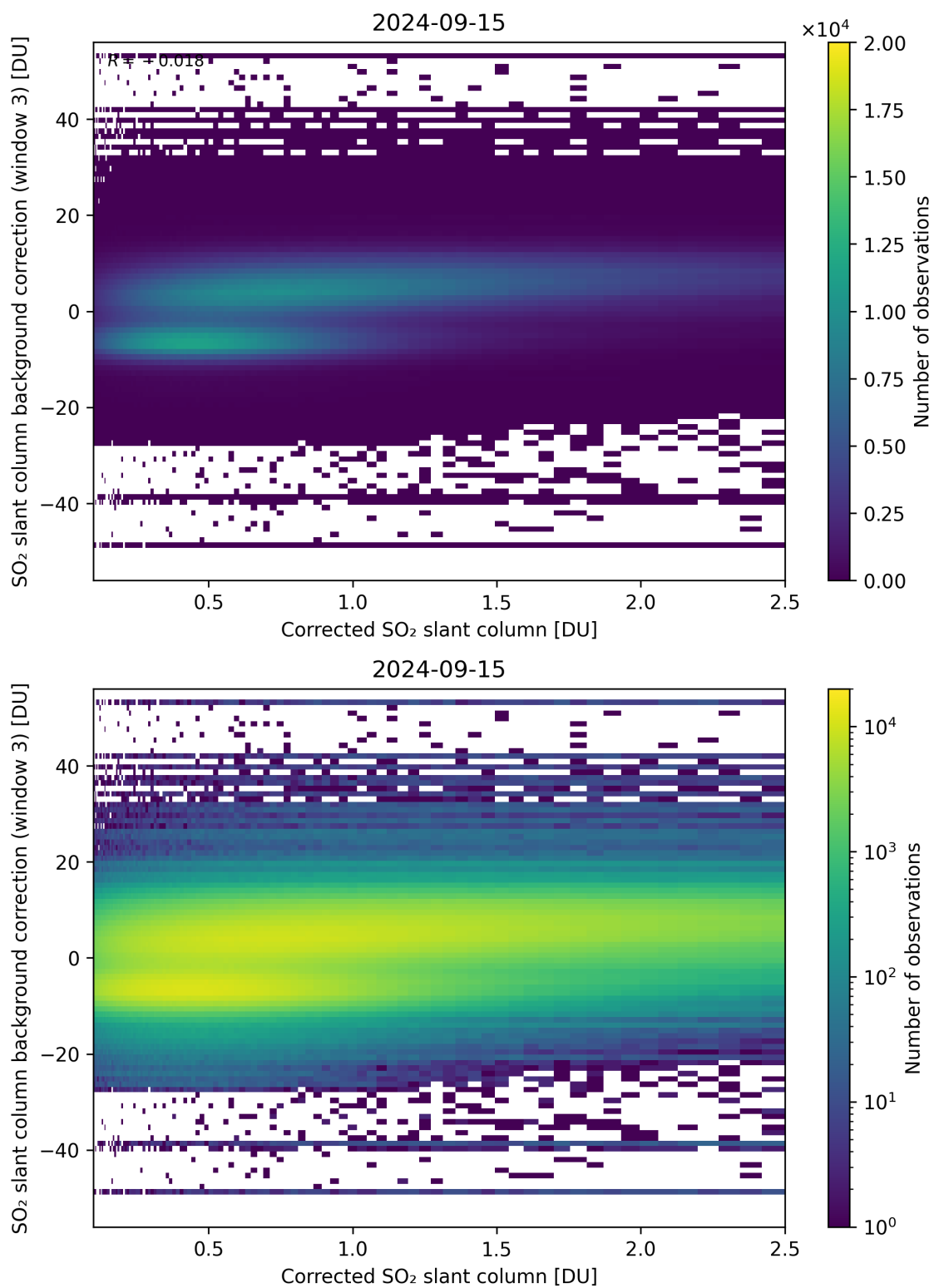
Figure 180: Scatter density plot of “Corrected SO 2 slant column” against “SO 2 slant column background correction (window 3)” for 2024-09-14 to 2024-09-16.
