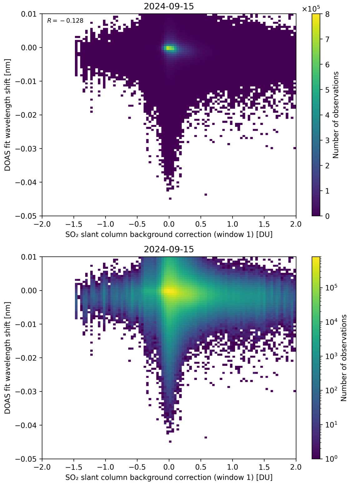
Figure 100: Scatter density plot of “SO 2 slant column background correction (window 1)” against “DOAS fit wavelength shift” for 2024-09-14 to 2024-09-16.
