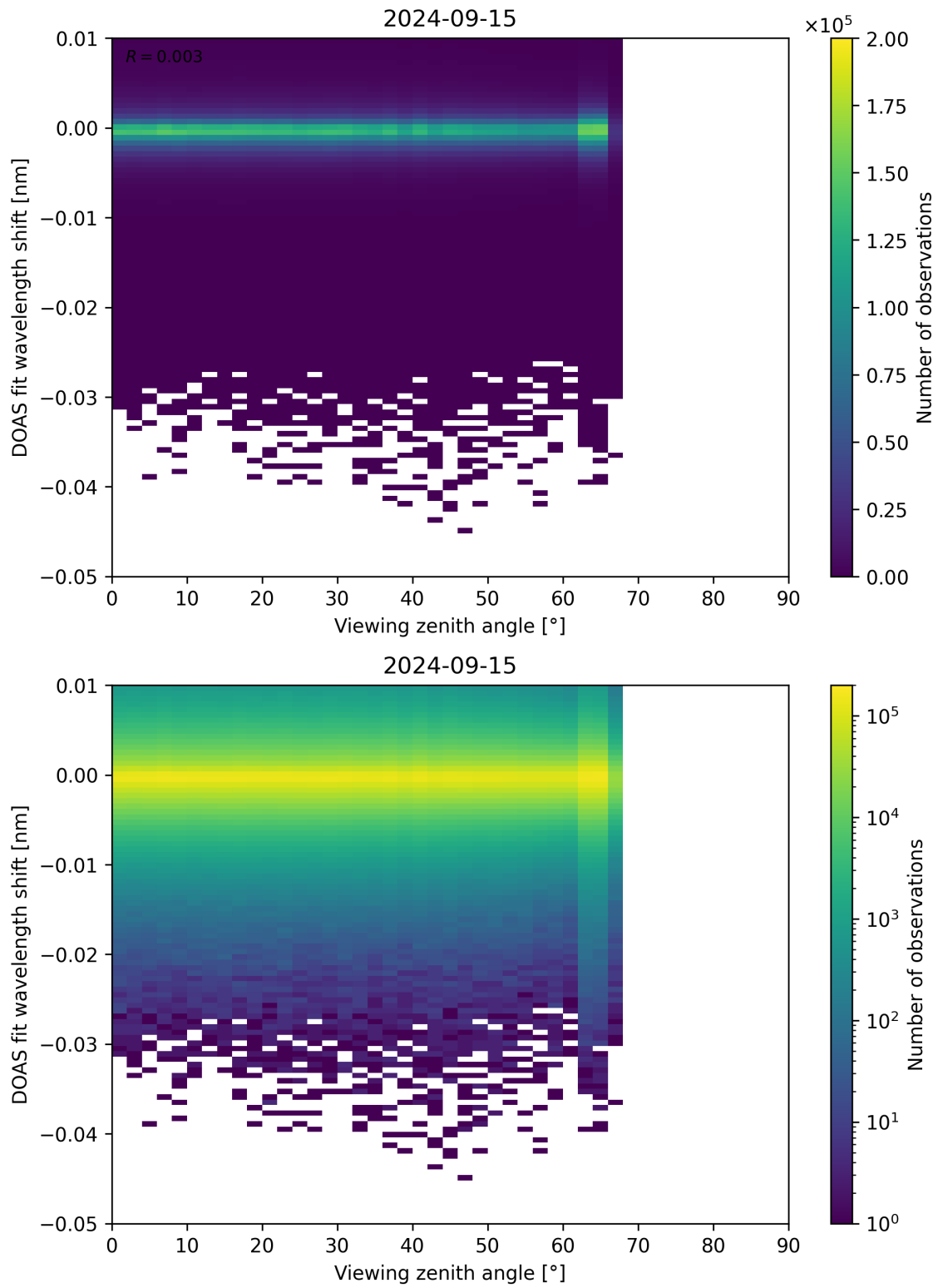
Figure 311: Scatter density plot of “Viewing zenith angle” against “DOAS fit wavelength shift” for 2024-09-14 to 2024-09-16.
