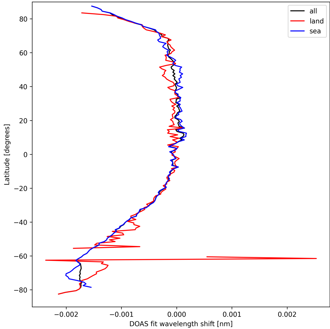
Figure 45: Zonal average of “DOAS fit wavelength shift” for 2024-09-14 to 2024-09-16.
