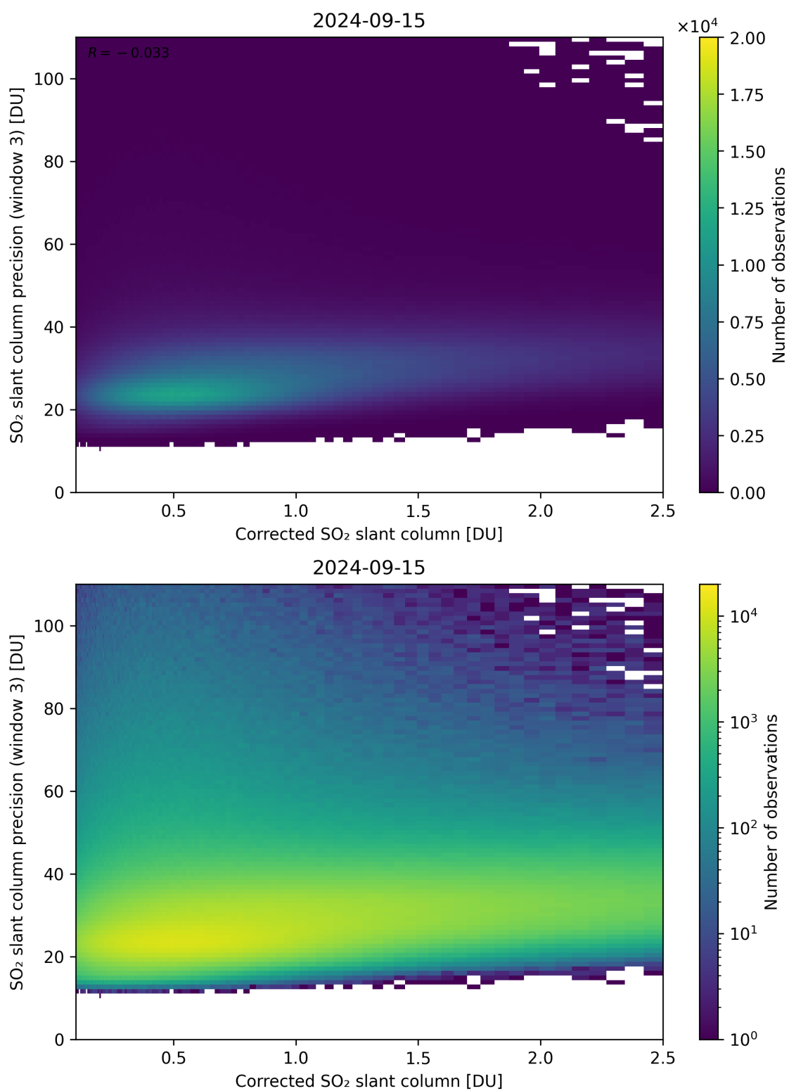
Figure 191: Scatter density plot of “Corrected SO 2 slant column” against “SO 2 slant column precision (window 3)” for 2024-09-14 to 2024-09-16.
