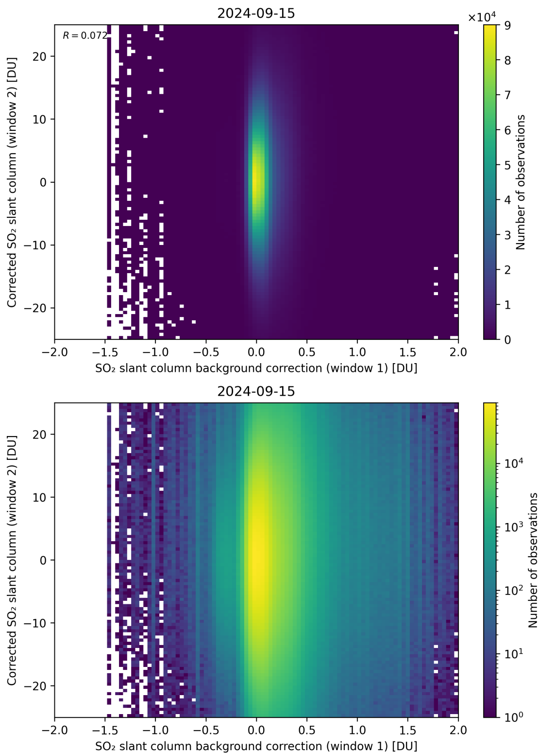
Figure 104: Scatter density plot of “SO 2 slant column background correction (window 1)” against “Corrected SO 2 slant column (window 2)” for 2024-09-14 to 2024-09-16.
