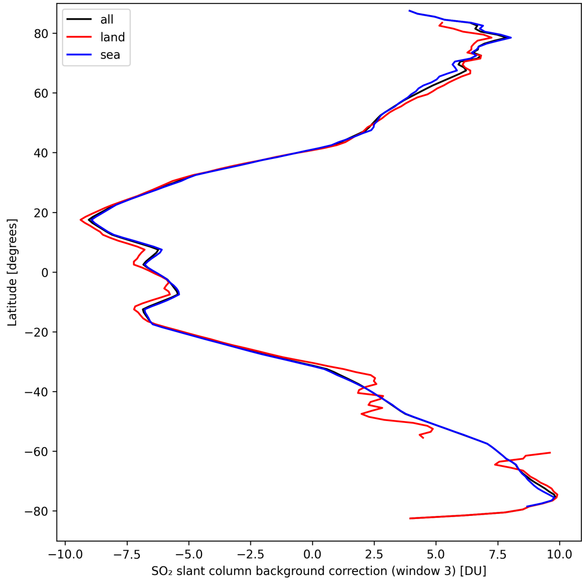
Figure 44: Zonal average of “SO 2 slant column background correction (window 3)” for 2024-09-14 to 2024-09-16.
