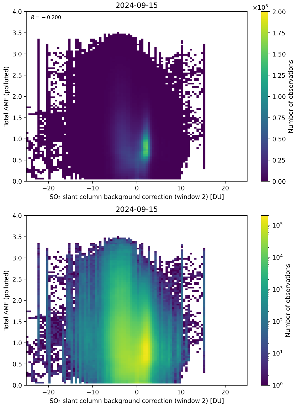
Figure 119: Scatter density plot of “SO 2 slant column background correction (window 2)” against “Total AMF (polluted)” for 2024-09-14 to 2024-09-16.
