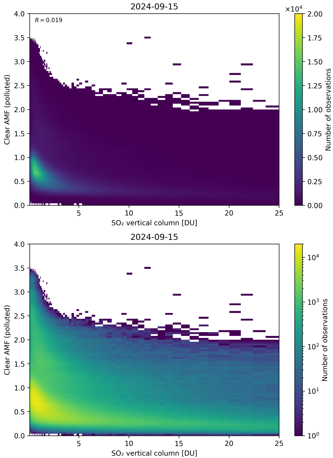
Figure 296: Scatter density plot of “SO 2 vertical column” against “Clear AMF (polluted)” for 2024-09-14 to 2024-09-16.
