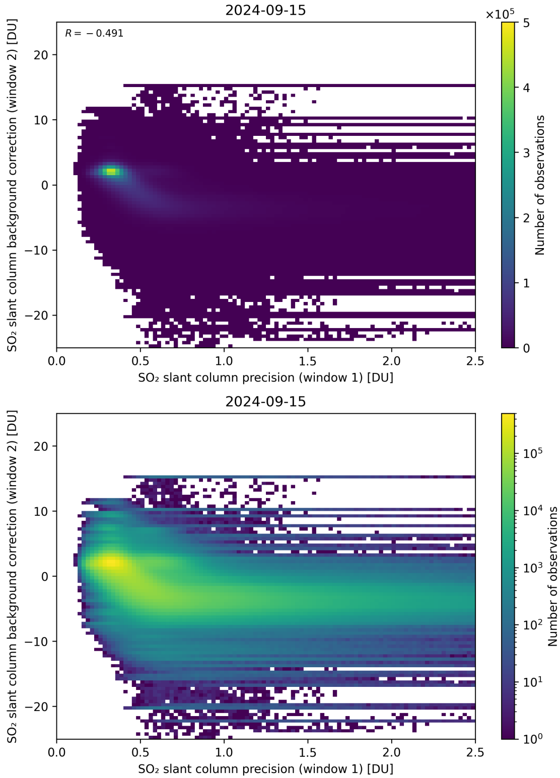
Figure 219: Scatter density plot of “SO 2 slant column precision (window 1)” against “SO 2 slant column background correction (window 2)” for 2024-09-14 to 2024-09-16.
