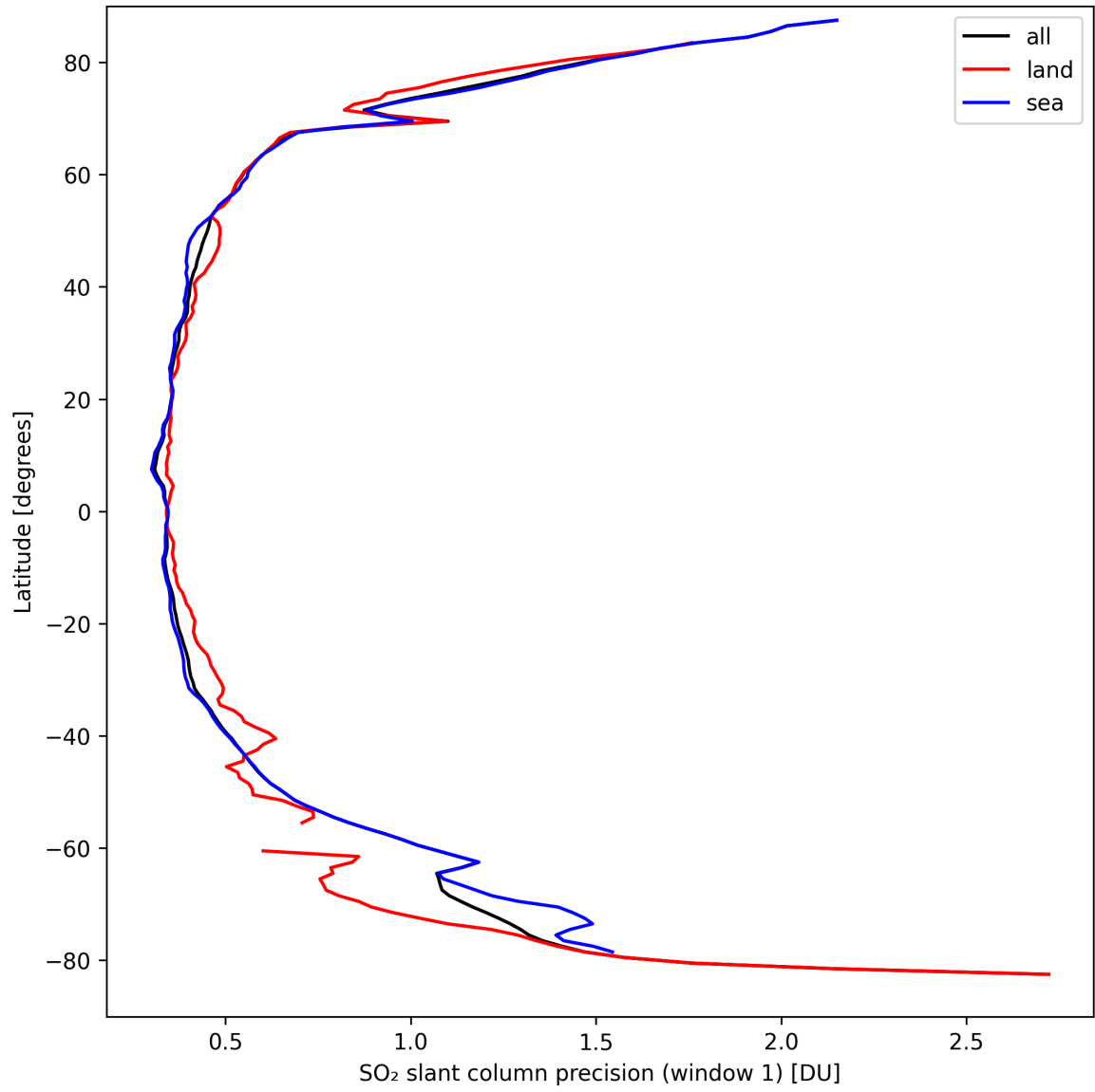
Figure 34: Zonal average of “SO 2 slant column precision (window 1)” for 2024-09-14 to 2024-09-16.
