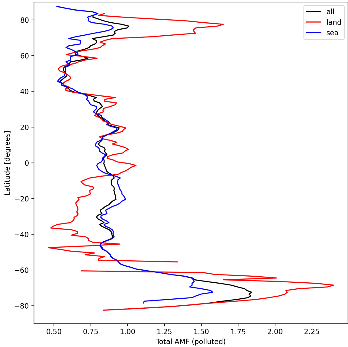
Figure 48: Zonal average of “Total AMF (polluted)” for 2024-09-14 to 2024-09-16.
