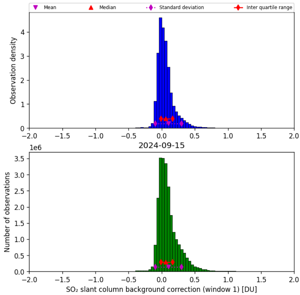
Figure 59: Histogram of “SO 2 slant column background correction (window 1)” for 2024-09-14 to 2024-09-16
