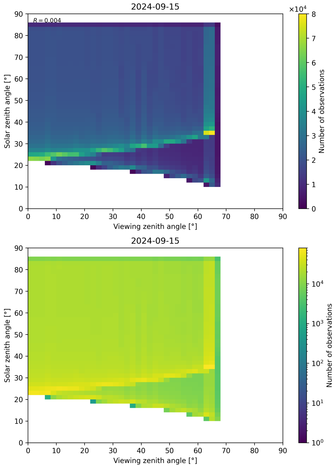
Figure 315: Scatter density plot of “Viewing zenith angle” against “Solar zenith angle” for 2024-09-14 to 2024-09-16.
