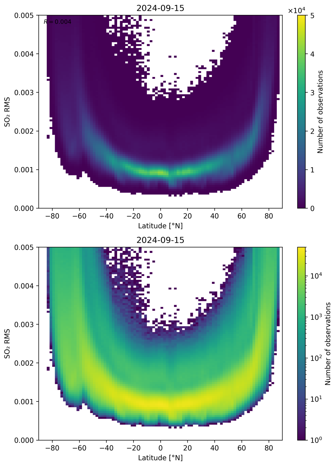
Figure 144: Scatter density plot of “Latitude” against “SO 2 RMS” for 2024-09-14 to 2024-09-16.
