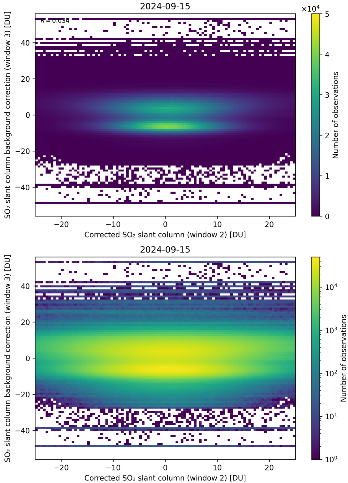
Figure 195: Scatter density plot of “Corrected SO 2 slant column (window 2)” against “SO 2 slant column background correction (window 3)” for 2024-09-14 to 2024-09-16.
