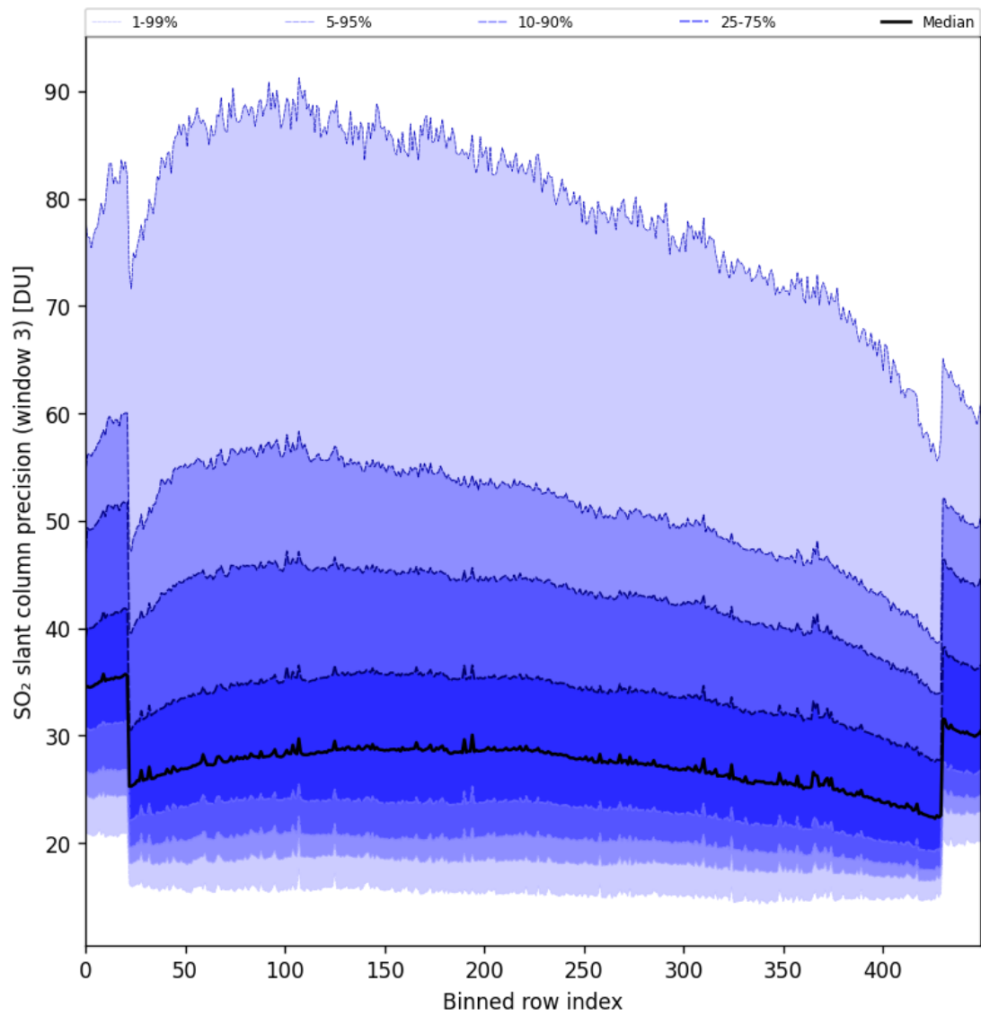
Figure 88: Along track statistics of “SO 2 slant column precision (window 3)” for 2024-09-14 to 2024-09-16
