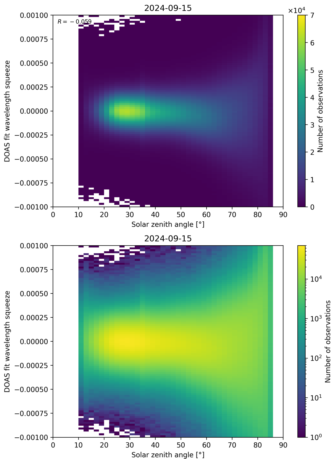
Figure 162: Scatter density plot of “Solar zenith angle” against “DOAS fit wavelength squeeze” for 2024-09-14 to 2024-09-16.
