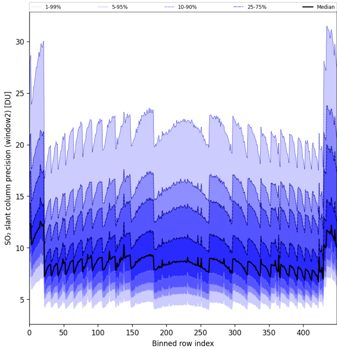
Figure 84: Along track statistics of “SO 2 slant column precision (window2)” for 2024-09-14 to 2024-09-16
