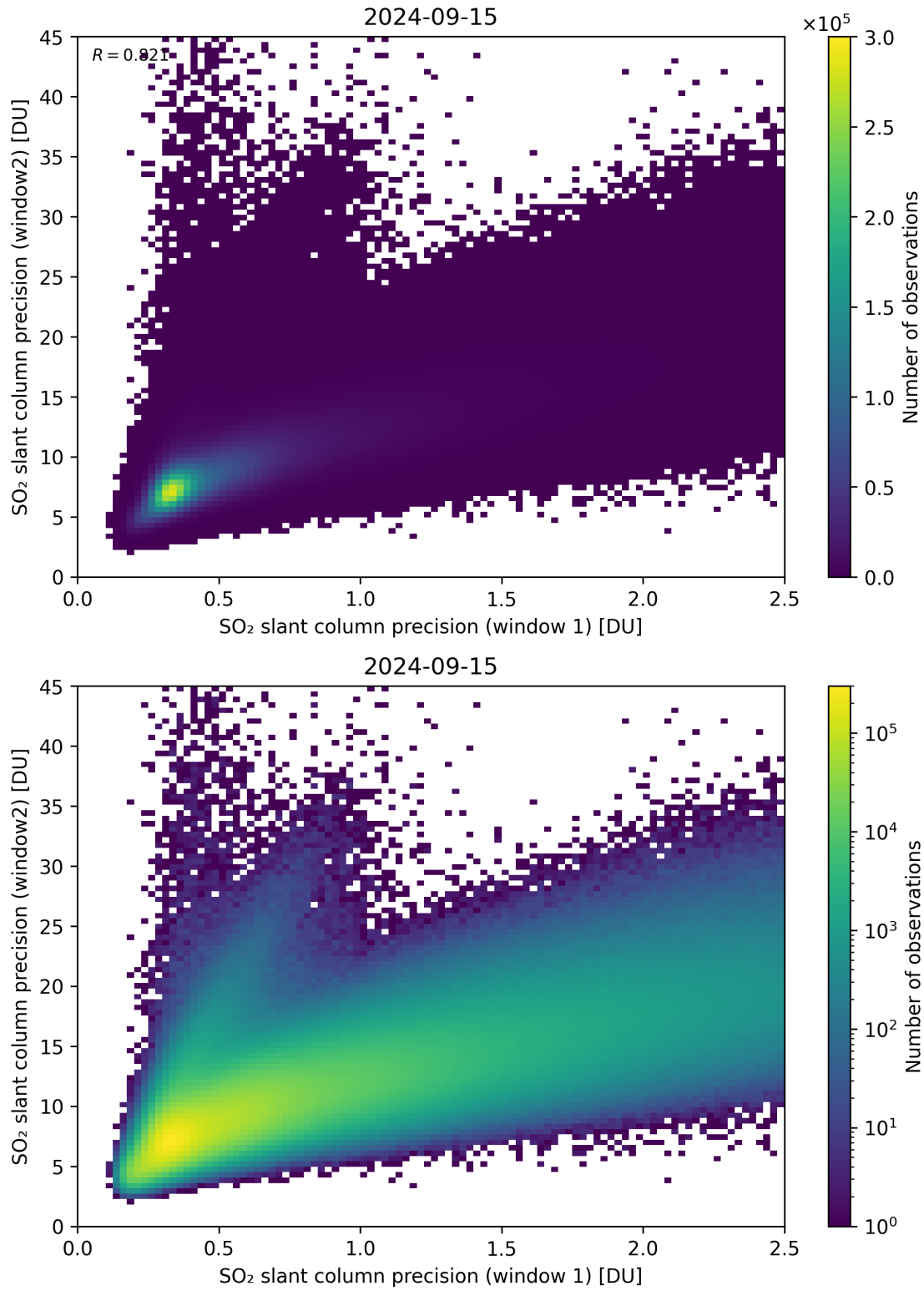
Figure 227: Scatter density plot of “SO 2 slant column precision (window 1)” against “SO 2 slant column precision (window2)” for 2024-09-14 to 2024-09-16.
