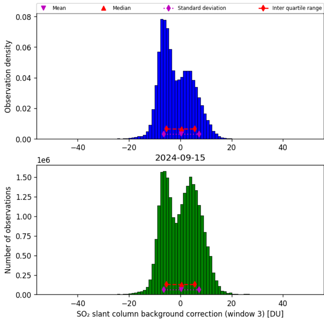
Figure 67: Histogram of “SO 2 slant column background correction (window 3)” for 2024-09-14 to 2024-09-16
