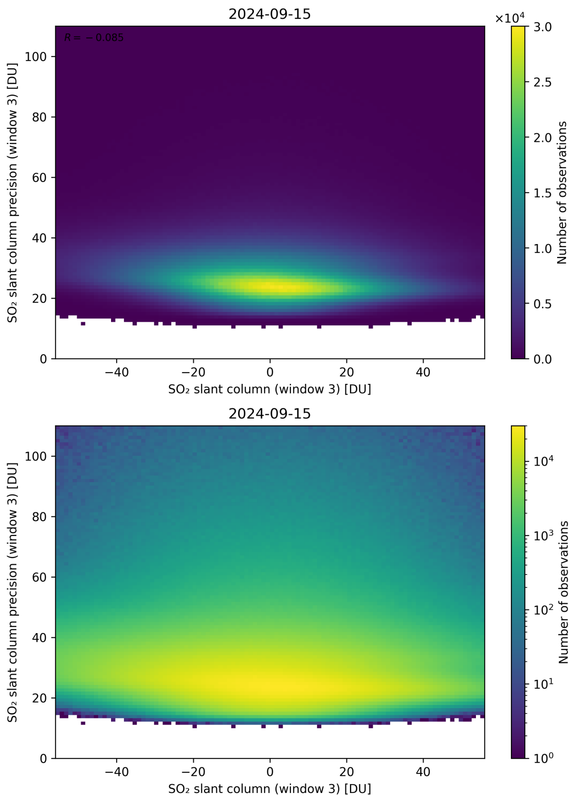
Figure 267: Scatter density plot of “SO 2 slant column (window 3)” against “SO 2 slant column precision (window 3)” for 2024-09-14 to 2024-09-16.
