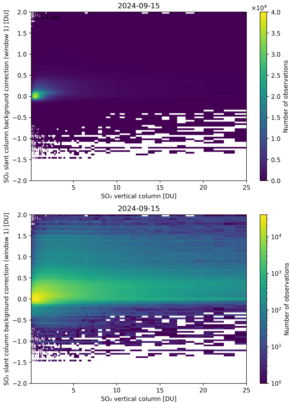
Figure 273: Scatter density plot of “SO 2 vertical column” against “SO 2 slant column background correction (window 1)” for 2024-09-14 to 2024-09-16.
