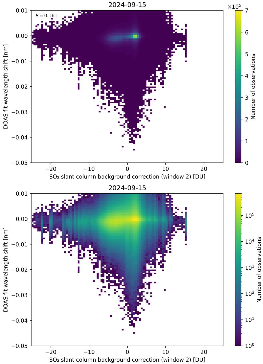
Figure 112: Scatter density plot of “SO 2 slant column background correction (window 2)” against “DOAS fit wavelength shift” for 2024-09-14 to 2024-09-16.
