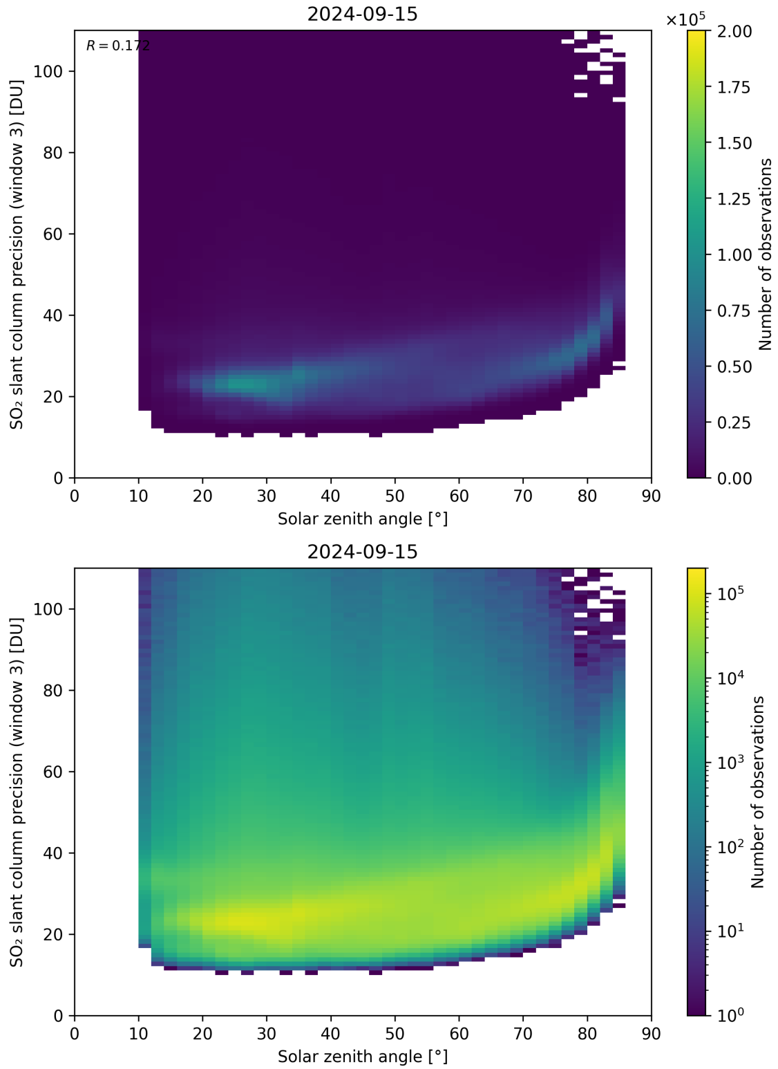
Figure 173: Scatter density plot of “Solar zenith angle” against “SO 2 slant column precision (window 3)” for 2024-09-14 to 2024-09-16.
