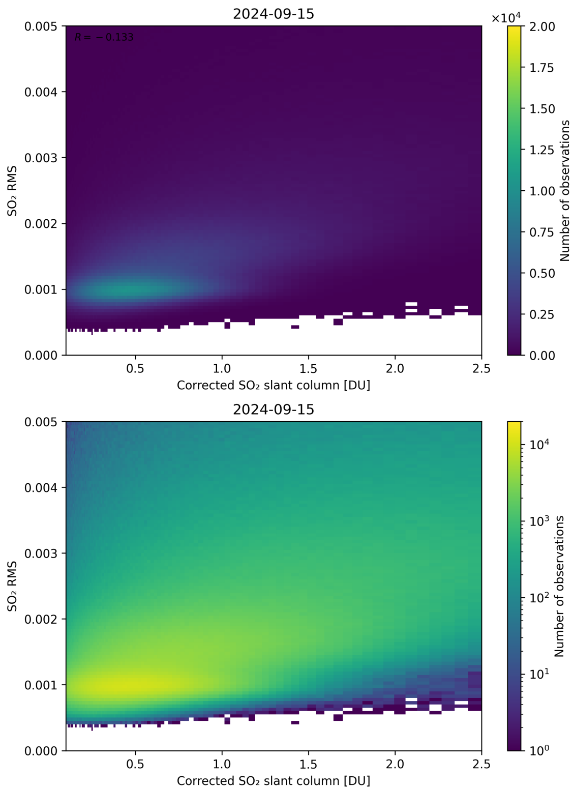
Figure 183: Scatter density plot of “Corrected SO 2 slant column” against “SO 2 RMS” for 2024-09-14 to 2024-09-16.
