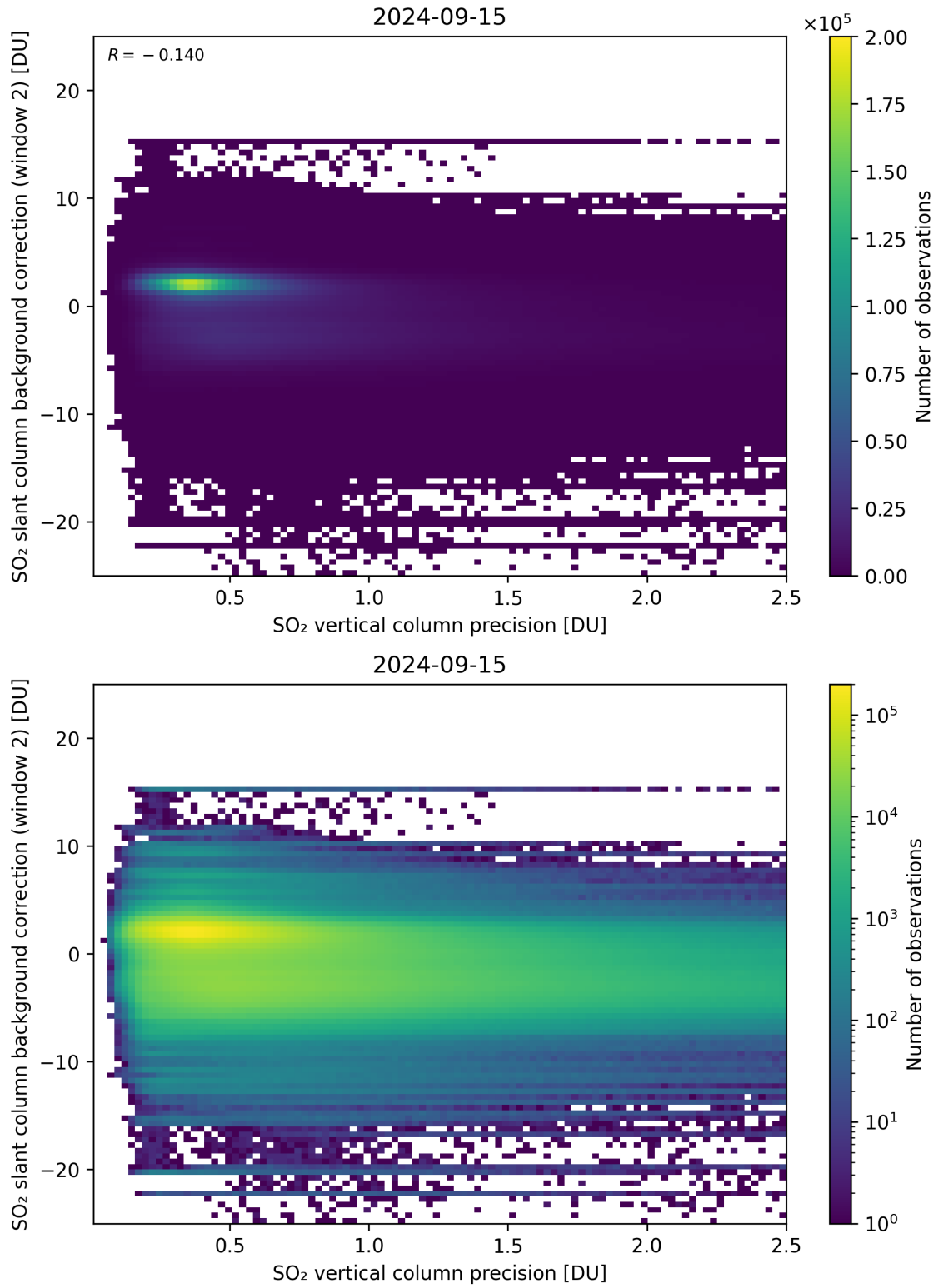
Figure 280: Scatter density plot of “SO 2 vertical column precision” against “SO 2 slant column background correction (window 2)” for 2024-09-14 to 2024-09-16.
