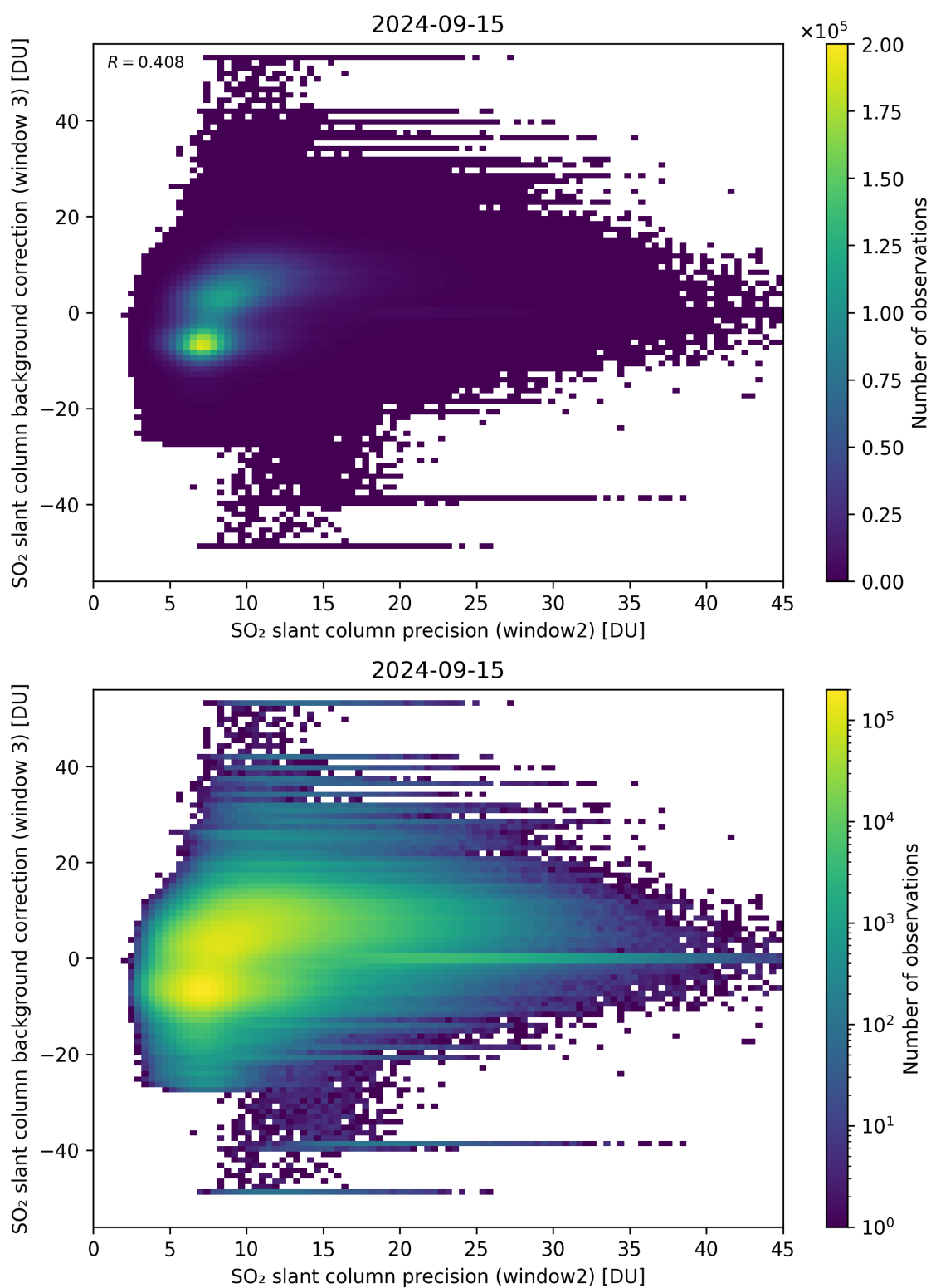
Figure 242: Scatter density plot of “SO 2 slant column precision (window2)” against “SO 2 slant column background correction (window 3)” for 2024-09-14 to 2024-09-16.
