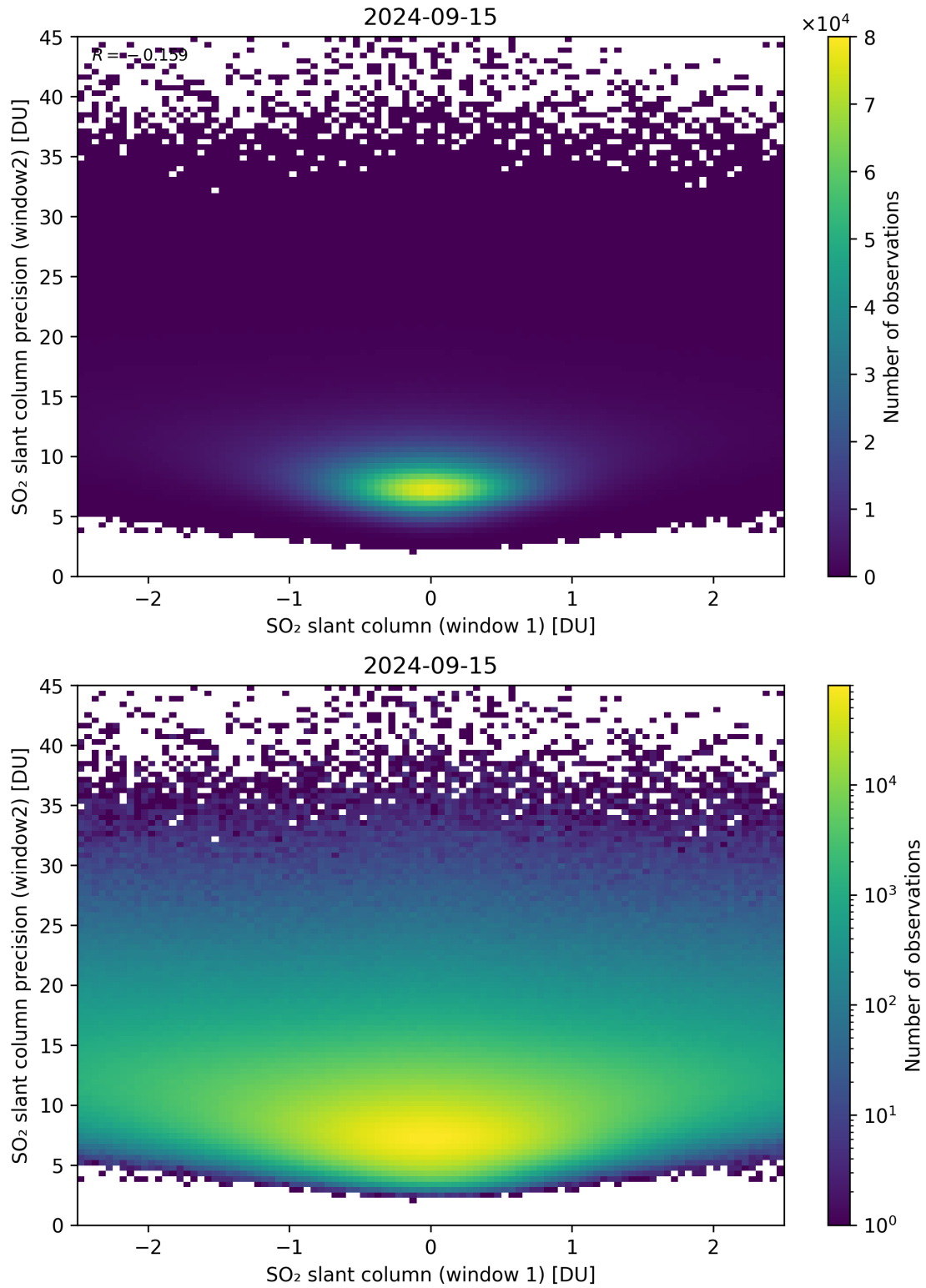
Figure 236: Scatter density plot of “SO 2 slant column (window 1)” against “SO 2 slant column precision (window2)” for 2024-09-14 to 2024-09-16.
