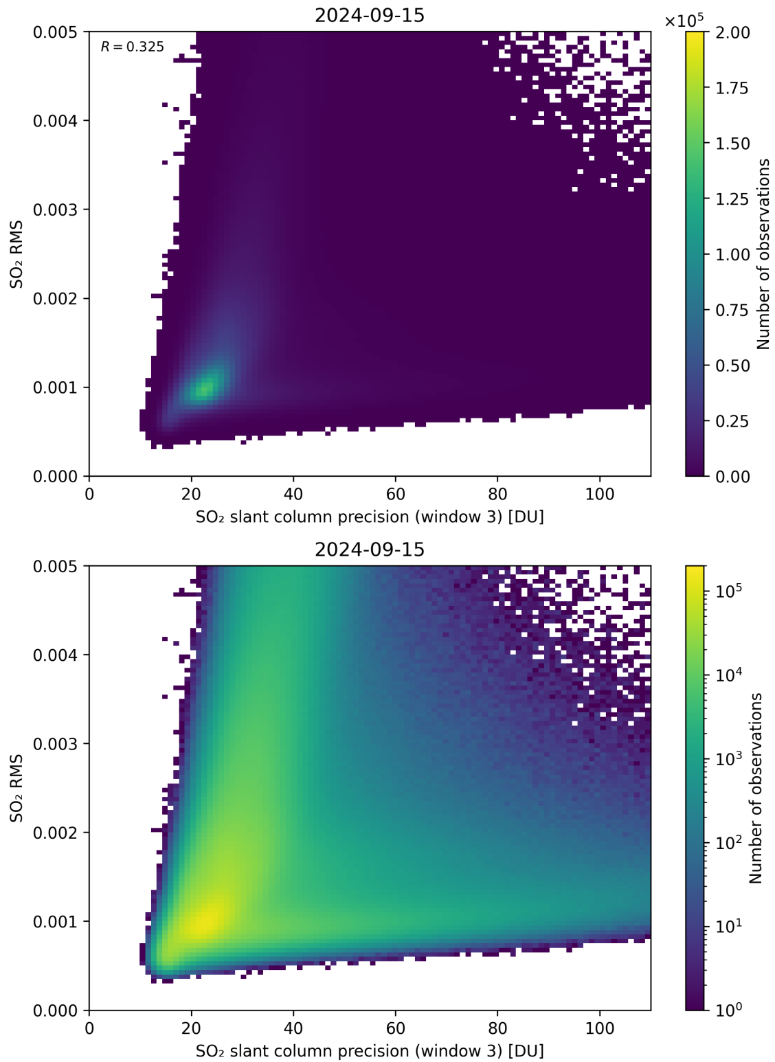
Figure 260: Scatter density plot of “SO 2 slant column precision (window 3)” against “SO 2 RMS” for 2024-09-14 to 2024-09-16.
