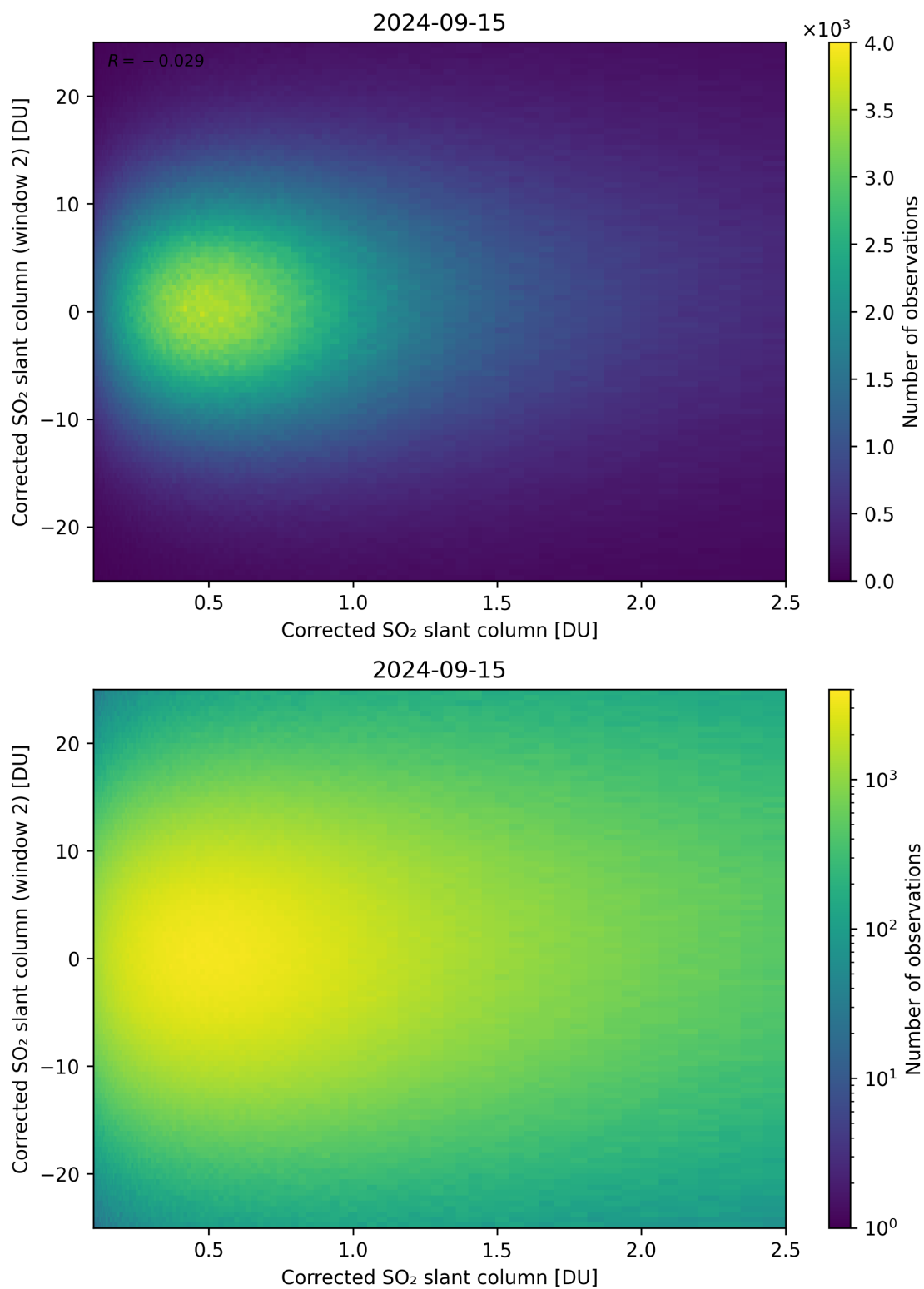
Figure 185: Scatter density plot of “Corrected SO 2 slant column” against “Corrected SO 2 slant column (window 2)” for 2024-09-14 to 2024-09-16.
