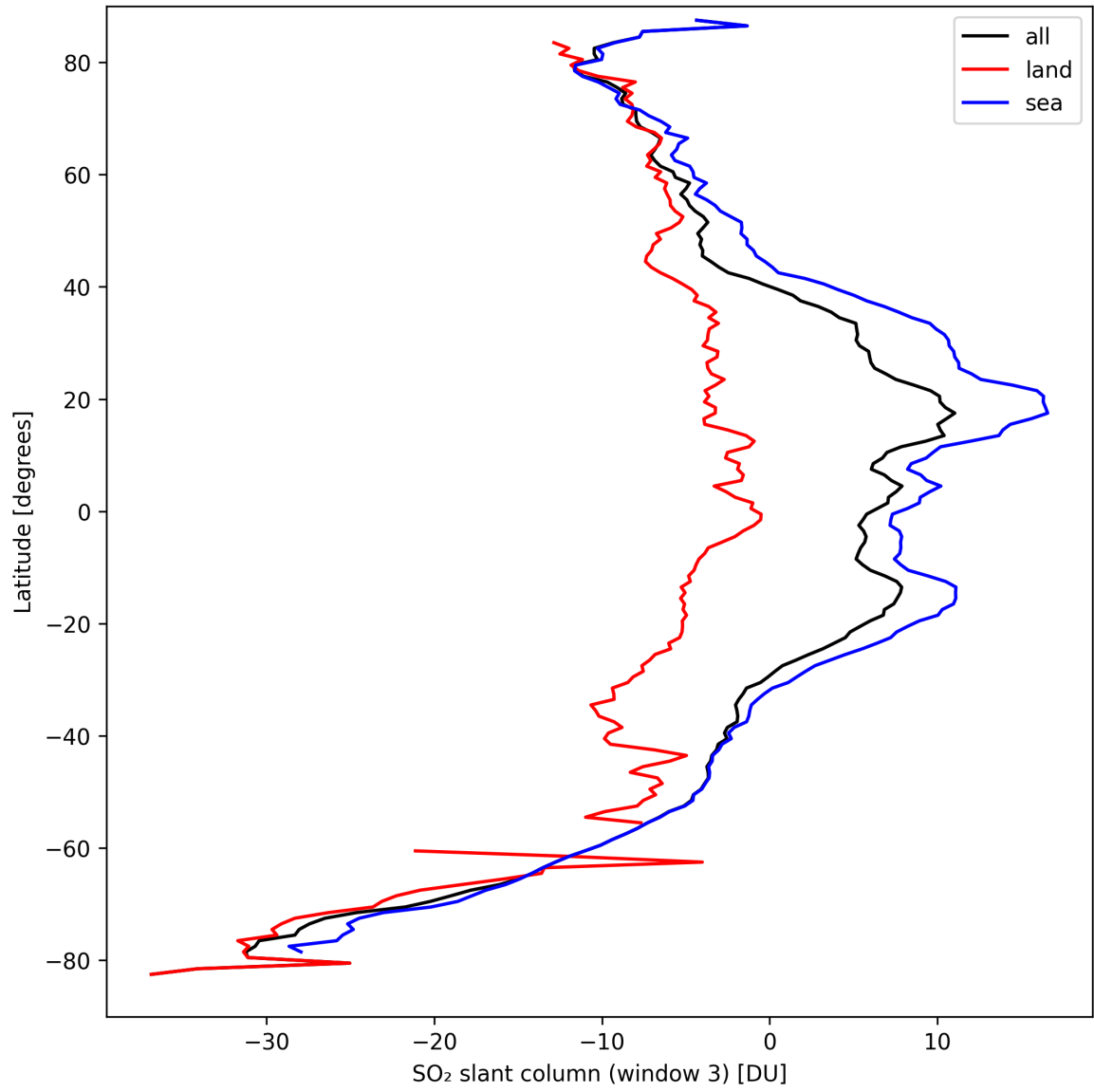
Figure 41: Zonal average of “SO 2 slant column (window 3)” for 2024-09-14 to 2024-09-16.
