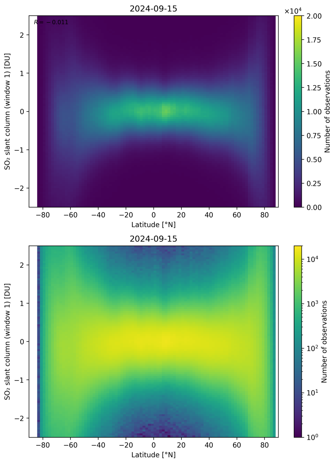
Figure 149: Scatter density plot of “Latitude” against “SO 2 slant column (window 1)” for 2024-09-14 to 2024-09-16.
