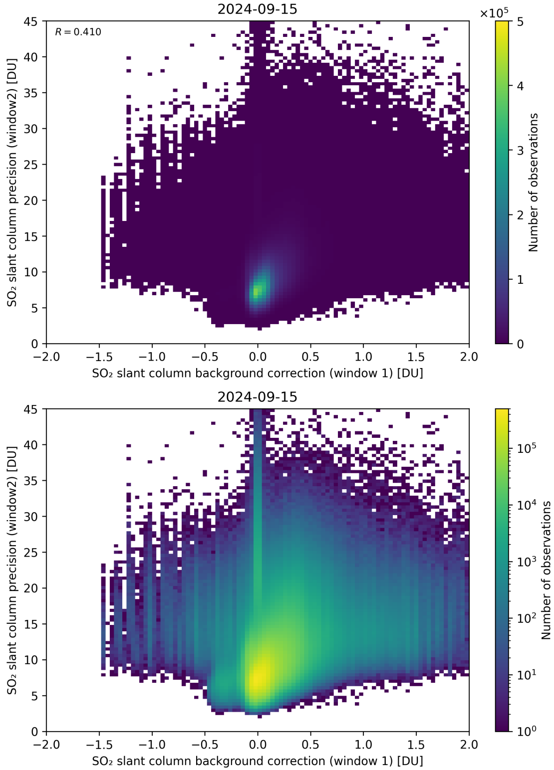
Figure 106: Scatter density plot of “SO 2 slant column background correction (window 1)” against “SO 2 slant column precision (window2)” for 2024-09-14 to 2024-09-16.
