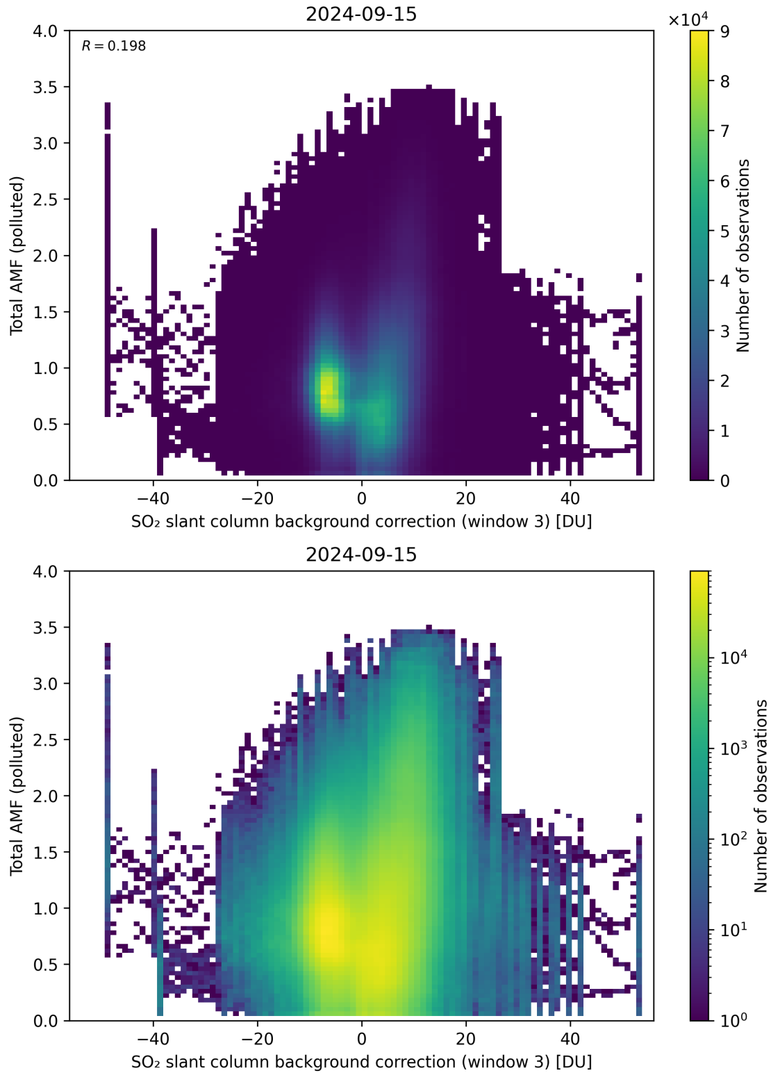
Figure 125: Scatter density plot of “SO 2 slant column background correction (window 3)” against “Total AMF (polluted)” for 2024-09-14 to 2024-09-16.
