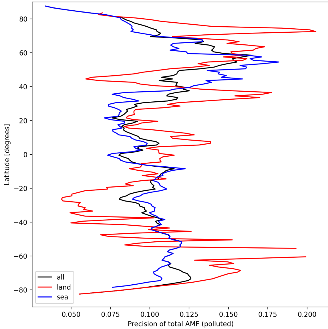
Figure 49: Zonal average of “Precision of total AMF (polluted)” for 2024-09-14 to 2024-09-16.
