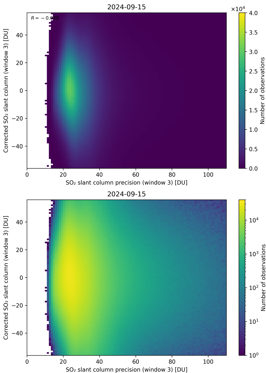
Figure 262: Scatter density plot of “SO 2 slant column precision (window 3)” against “Corrected SO 2 slant column (window 3)” for 2024-09-14 to 2024-09-16.
