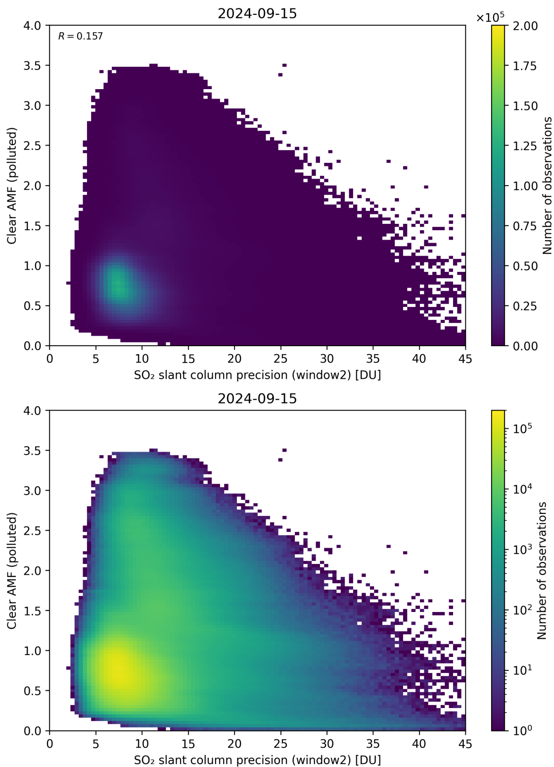
Figure 246: Scatter density plot of “SO 2 slant column precision (window2)” against “Clear AMF (polluted)” for 2024-09-14 to 2024-09-16.
