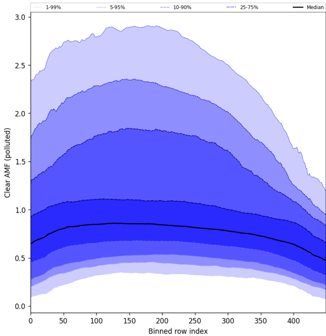
Figure 96: Along track statistics of “Clear AMF (polluted)” for 2024-09-14 to 2024-09-16
