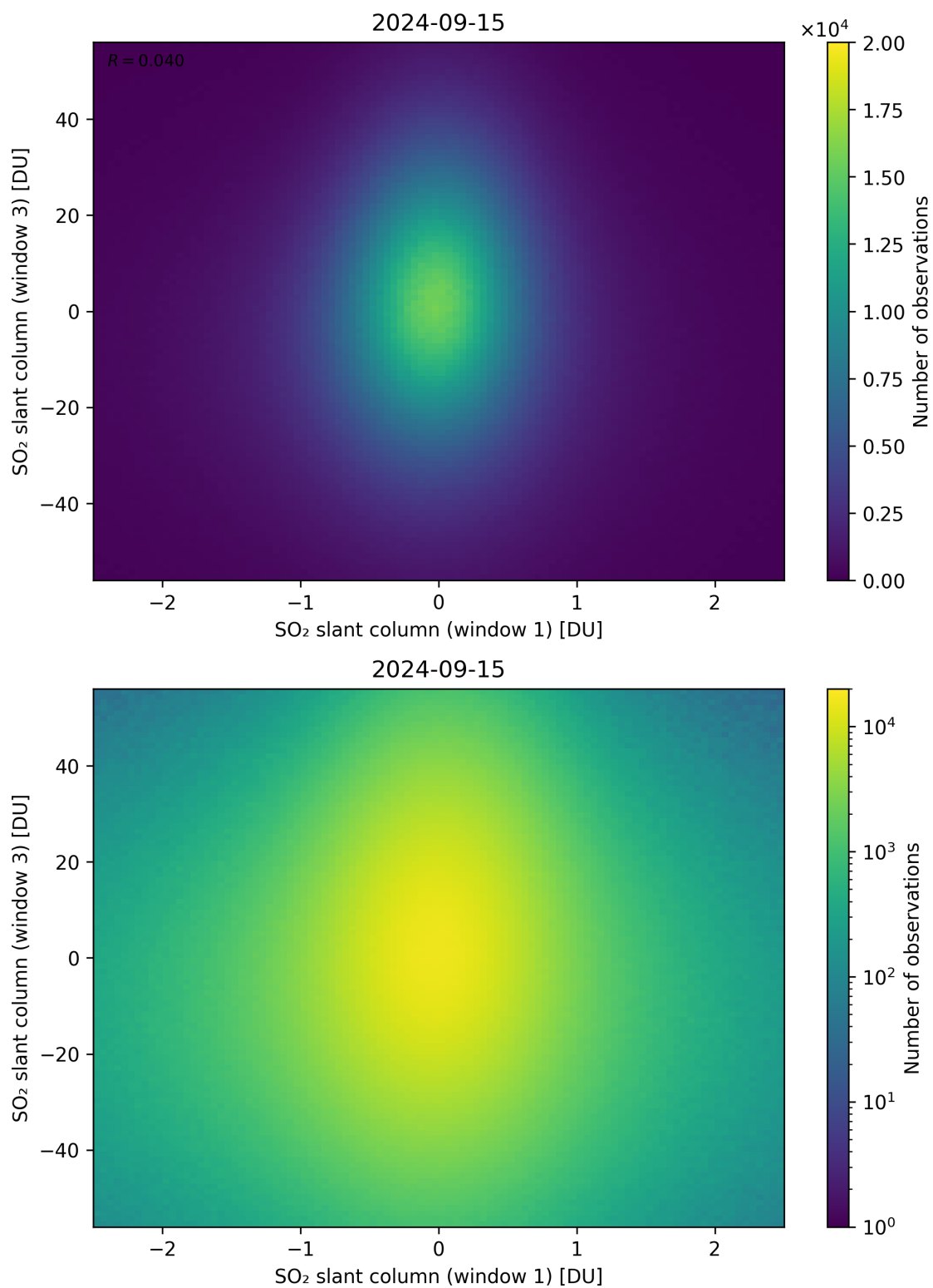
Figure 237: Scatter density plot of “SO 2 slant column (window 1)” against “SO 2 slant column (window 3)” for 2024-09-14 to 2024-09-16.
