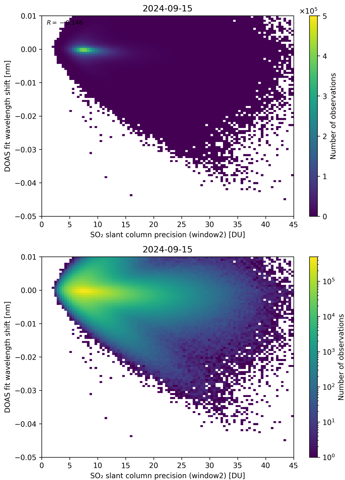
Figure 243: Scatter density plot of “SO 2 slant column precision (window2)” against “DOAS fit wavelength shift” for 2024-09-14 to 2024-09-16.
