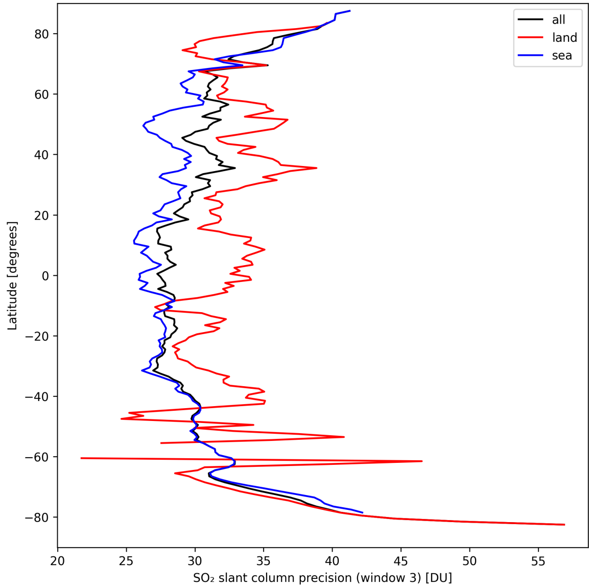
Figure 42: Zonal average of “SO 2 slant column precision (window 3)” for 2024-09-14 to 2024-09-16.
