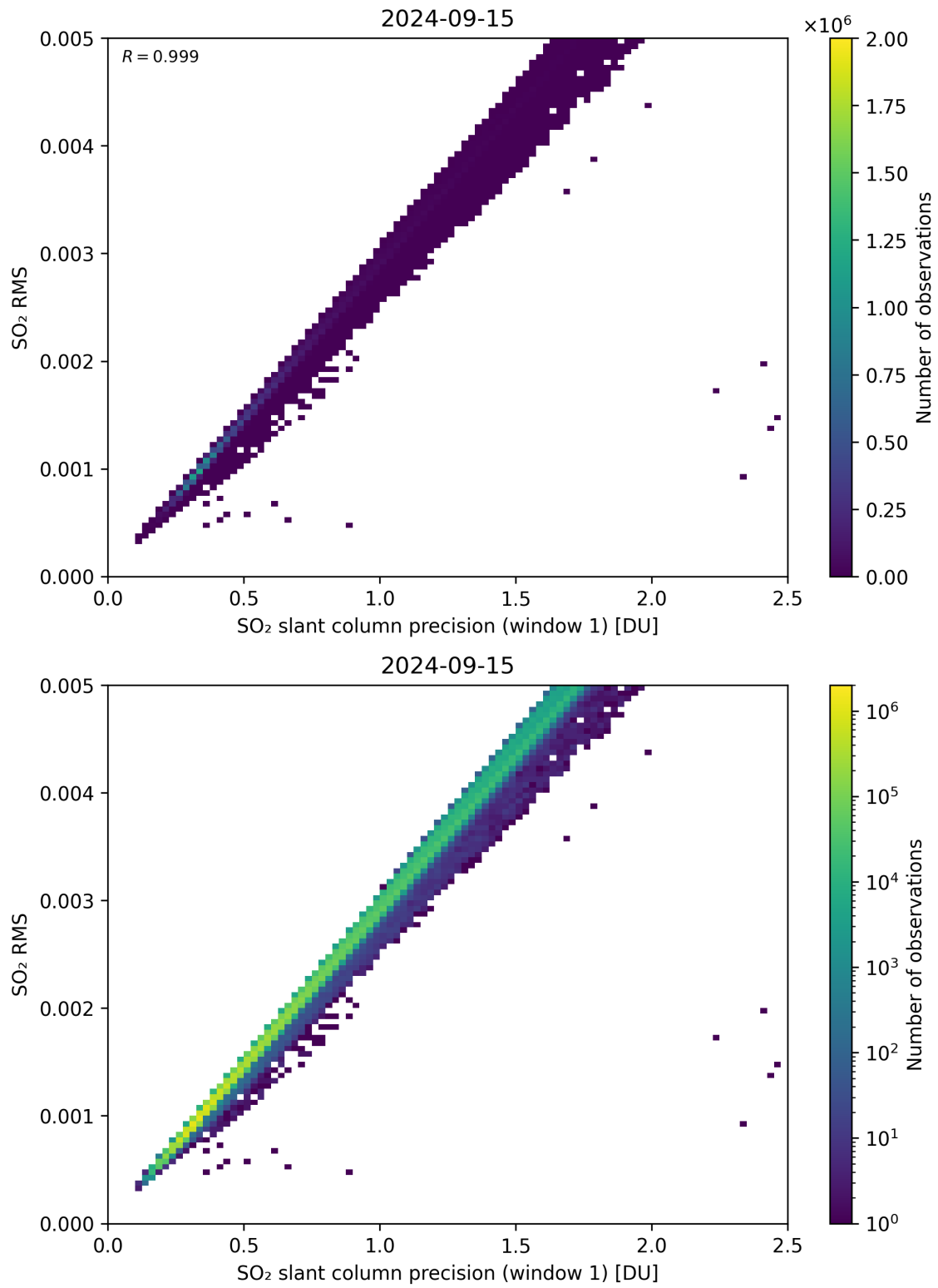
Figure 223: Scatter density plot of “SO 2 slant column precision (window 1)” against “SO 2 RMS” for 2024-09-14 to 2024-09-16.
