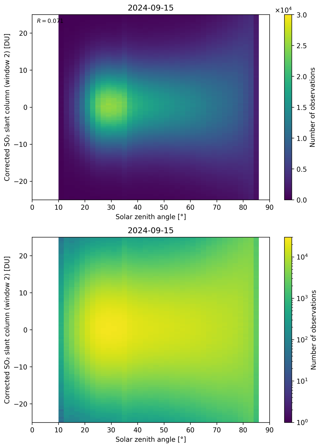
Figure 167: Scatter density plot of “Solar zenith angle” against “Corrected SO 2 slant column (window 2)” for 2024-09-14 to 2024-09-16.
