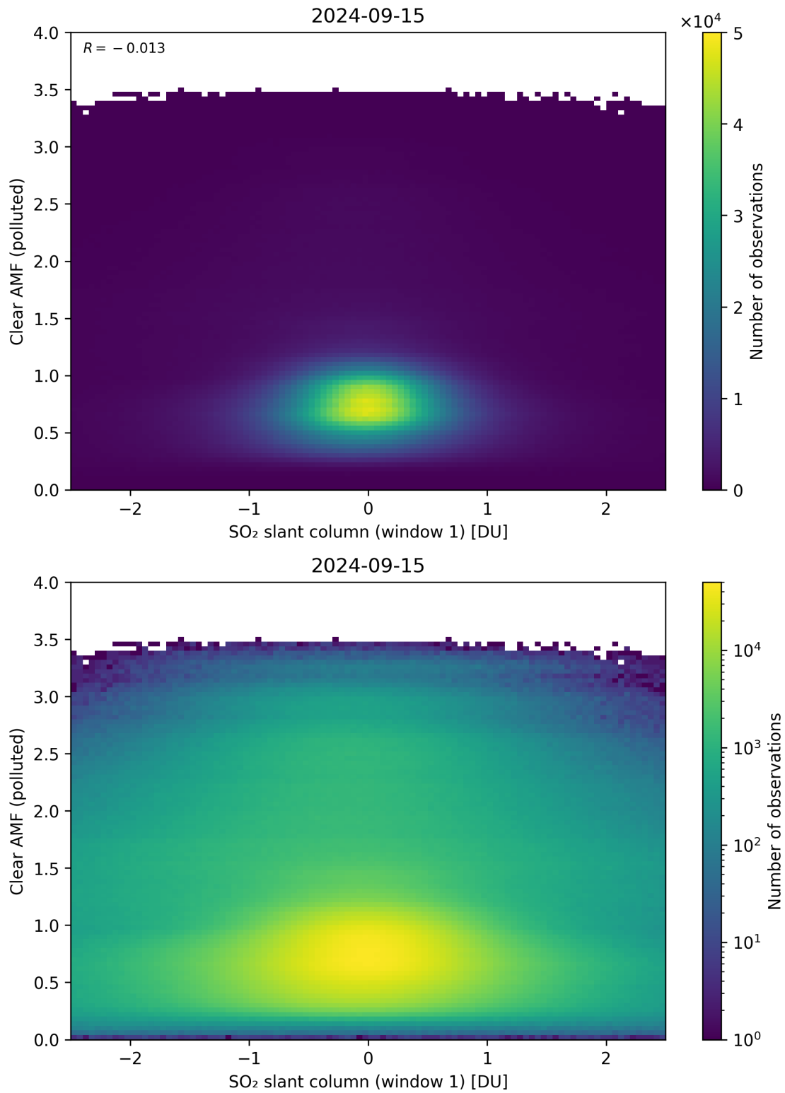
Figure 232: Scatter density plot of “SO 2 slant column (window 1)” against “Clear AMF (polluted)” for 2024-09-14 to 2024-09-16.
