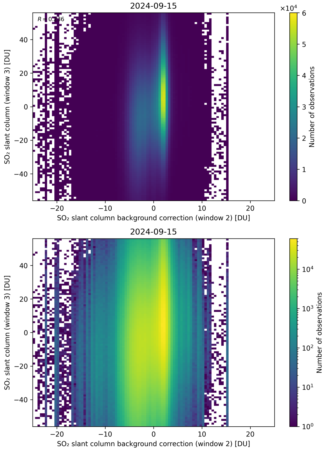
Figure 117: Scatter density plot of “SO 2 slant column background correction (window 2)” against “SO 2 slant column (window 3)” for 2024-09-14 to 2024-09-16.
