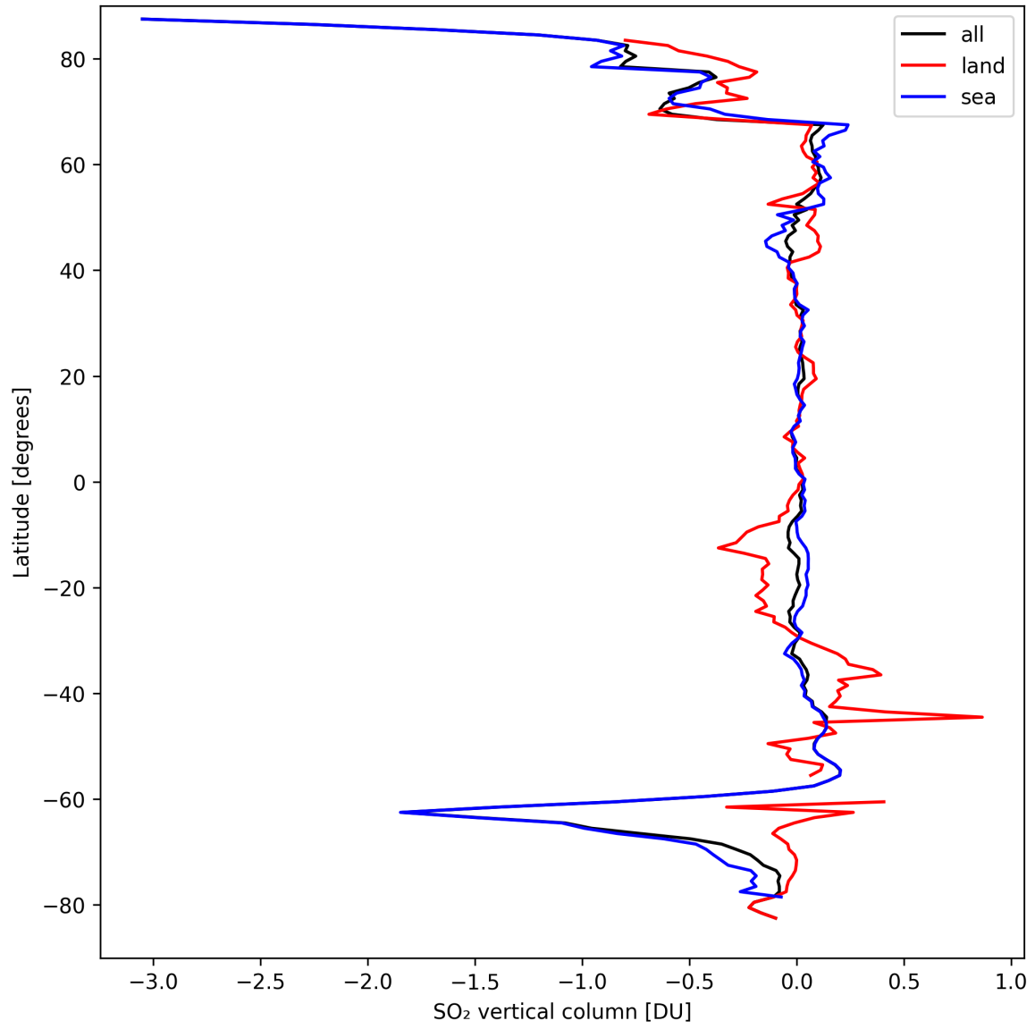
Figure 30: Zonal average of “SO 2 vertical column” for 2024-09-14 to 2024-09-16.
