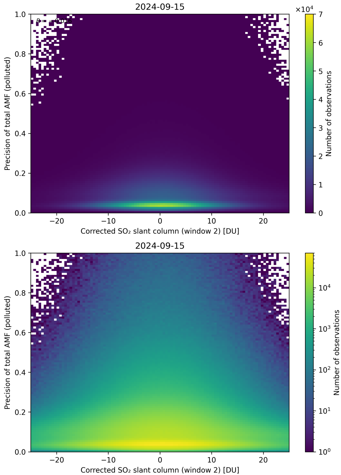
Figure 204: Scatter density plot of “Corrected SO 2 slant column (window 2)” against “Precision of total AMF (polluted)” for 2024-09-14 to 2024-09-16.
