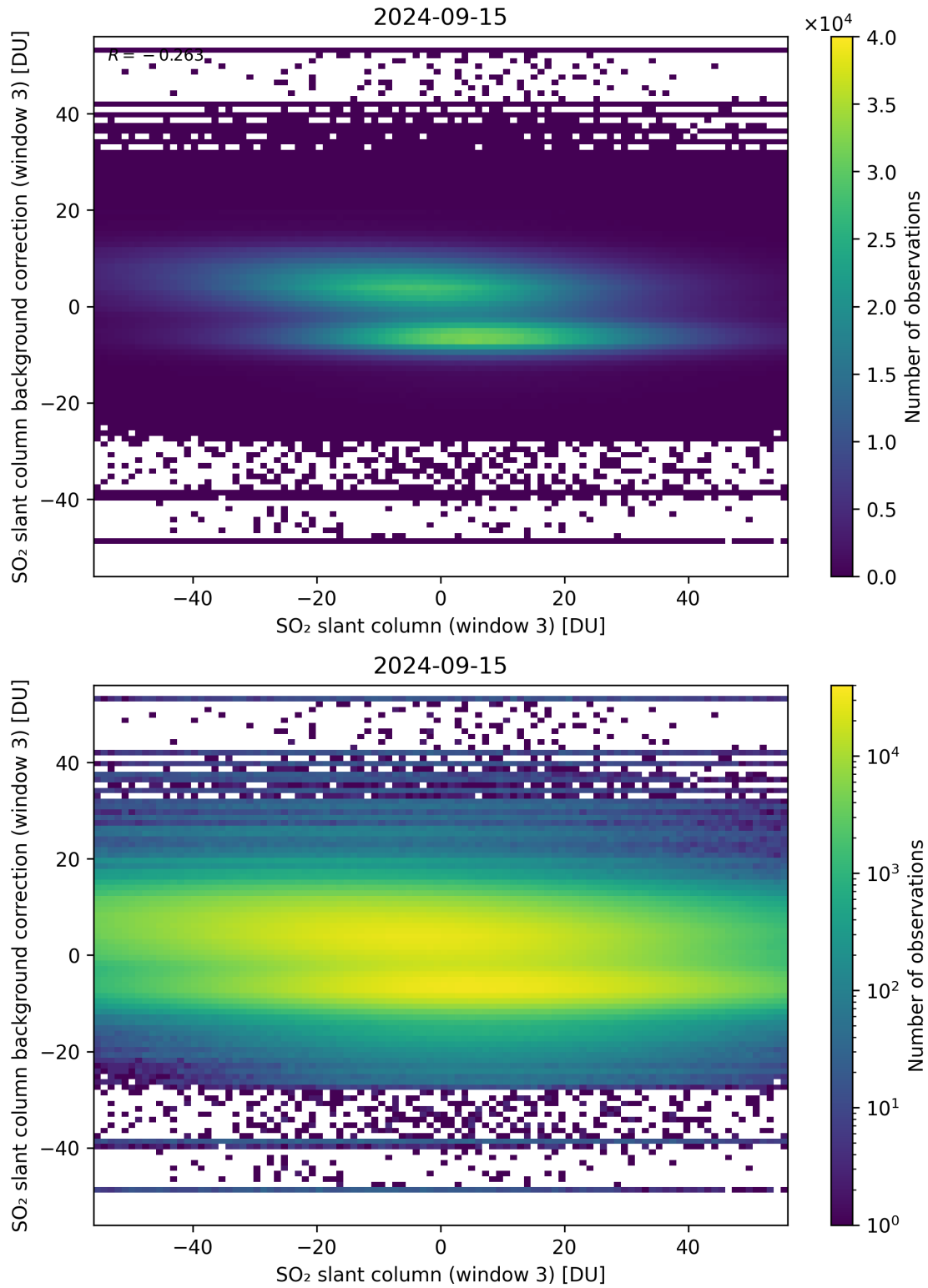
Figure 253: Scatter density plot of “SO 2 slant column (window 3)” against “SO 2 slant column background correction (window 3)” for 2024-09-14 to 2024-09-16.
