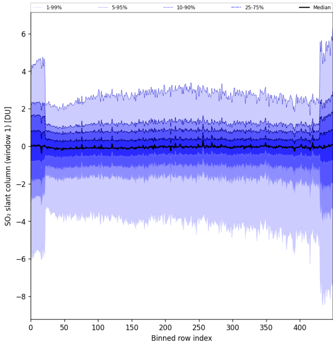
Figure 79: Along track statistics of “SO 2 slant column (window 1)” for 2024-09-14 to 2024-09-16
