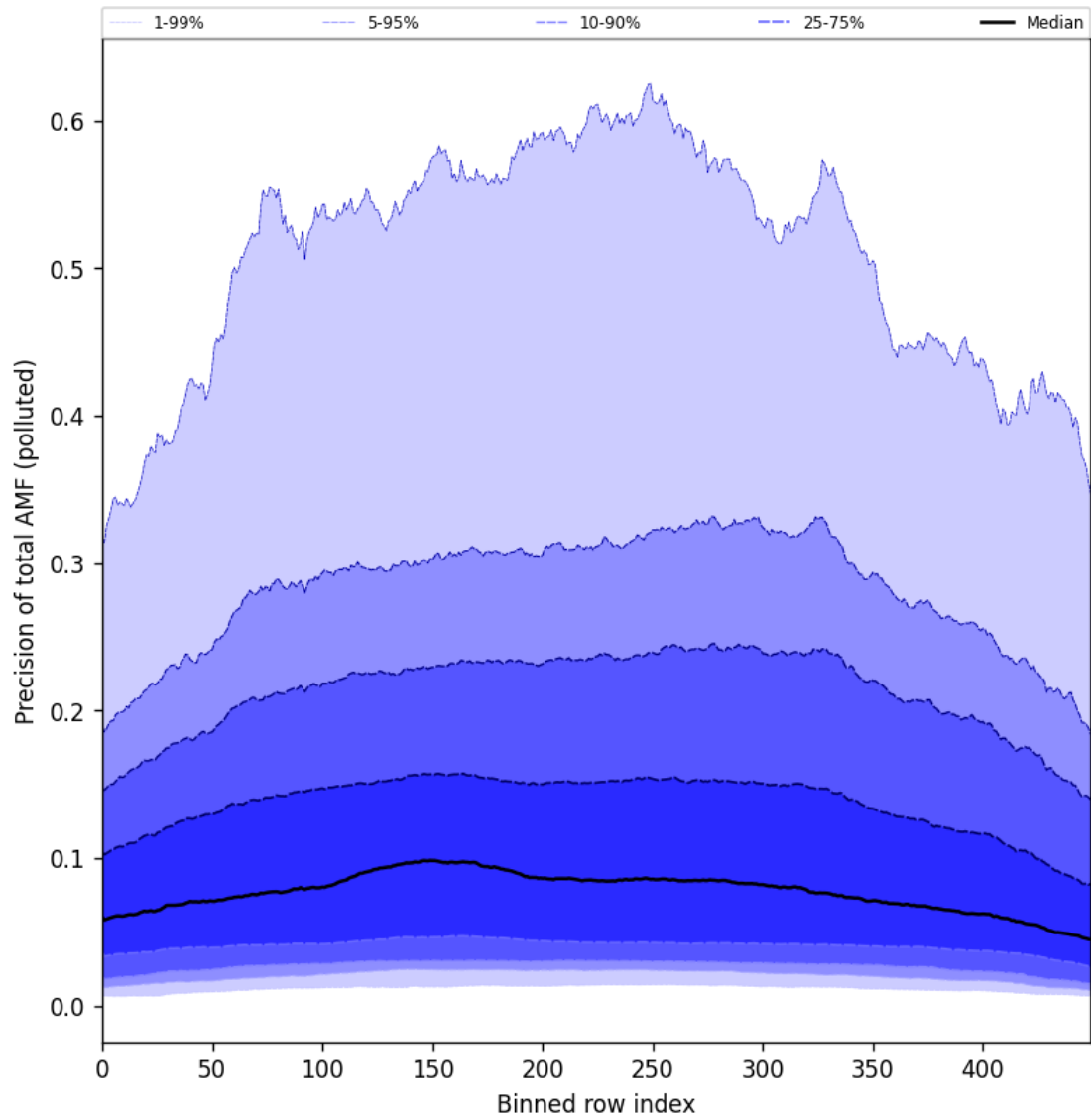
Figure 95: Along track statistics of “Precision of total AMF (polluted)” for 2024-09-14 to 2024-09-16
