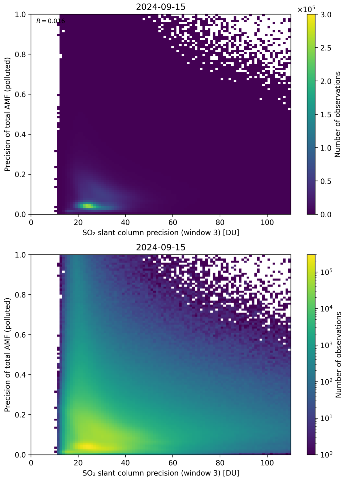
Figure 264: Scatter density plot of “SO 2 slant column precision (window 3)” against “Precision of total AMF (polluted)” for 2024-09-14 to 2024-09-16.
