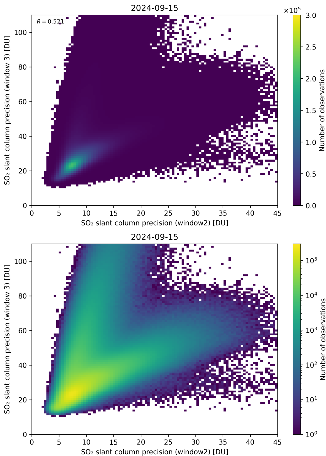
Figure 250: Scatter density plot of “SO 2 slant column precision (window2)” against “SO 2 slant column precision (window 3)” for 2024-09-14 to 2024-09-16.
