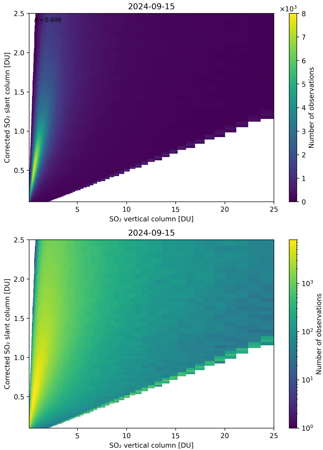
Figure 297: Scatter density plot of “SO 2 vertical column” against “Corrected SO 2 slant column” for 2024-09-14 to 2024-09-16.
