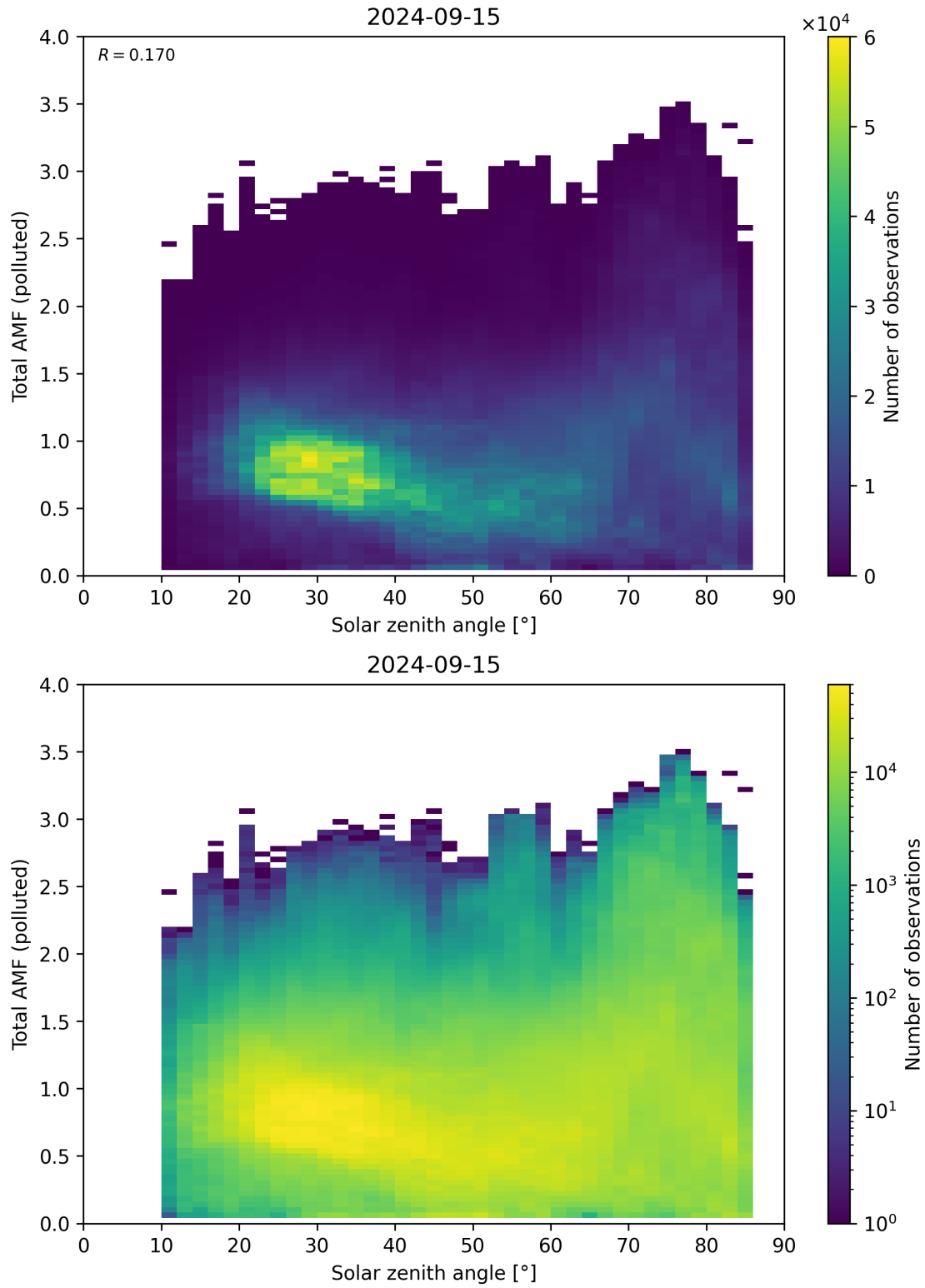
Figure 174: Scatter density plot of “Solar zenith angle” against “Total AMF (polluted)” for 2024-09-14 to 2024-09-16.
