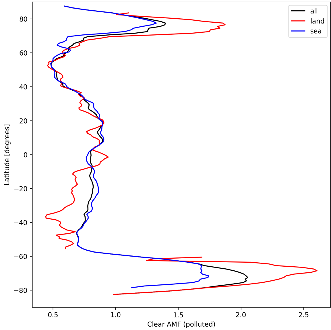
Figure 50: Zonal average of “Clear AMF (polluted)” for 2024-09-14 to 2024-09-16.
