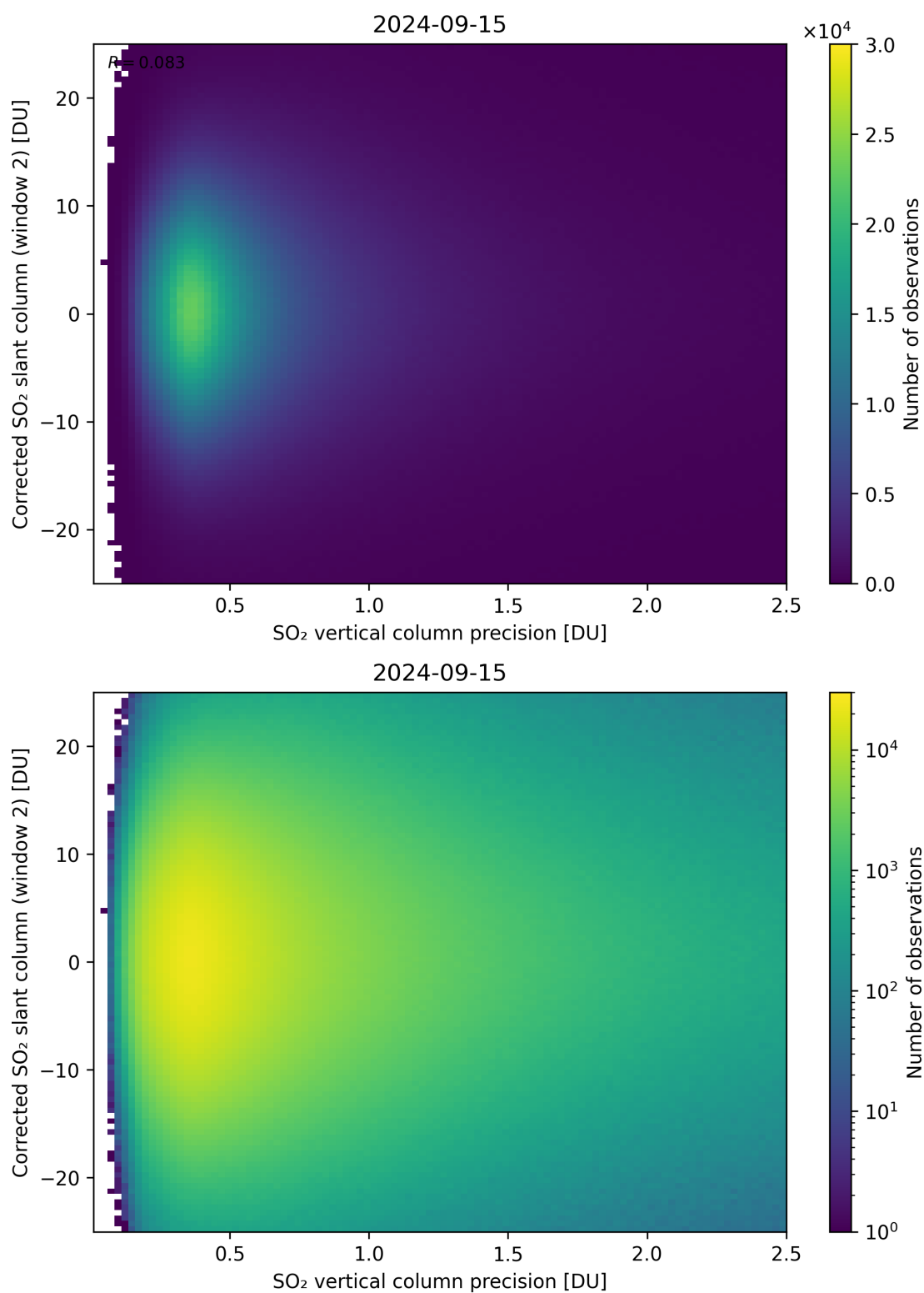
Figure 287: Scatter density plot of “SO 2 vertical column precision” against “Corrected SO 2 slant column (window 2)” for 2024-09-14 to 2024-09-16.
