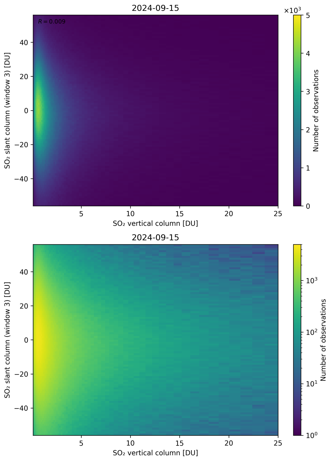
Figure 303: Scatter density plot of “SO 2 vertical column” against “SO 2 slant column (window 3)” for 2024-09-14 to 2024-09-16.
