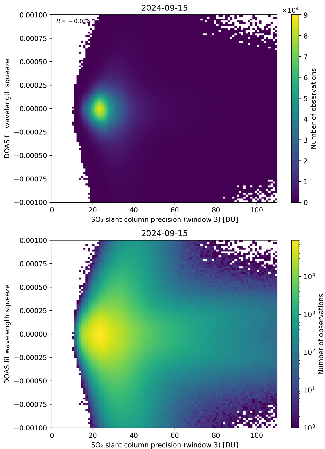
Figure 259: Scatter density plot of “SO 2 slant column precision (window 3)” against “DOAS fit wavelength squeeze” for 2024-09-14 to 2024-09-16.
