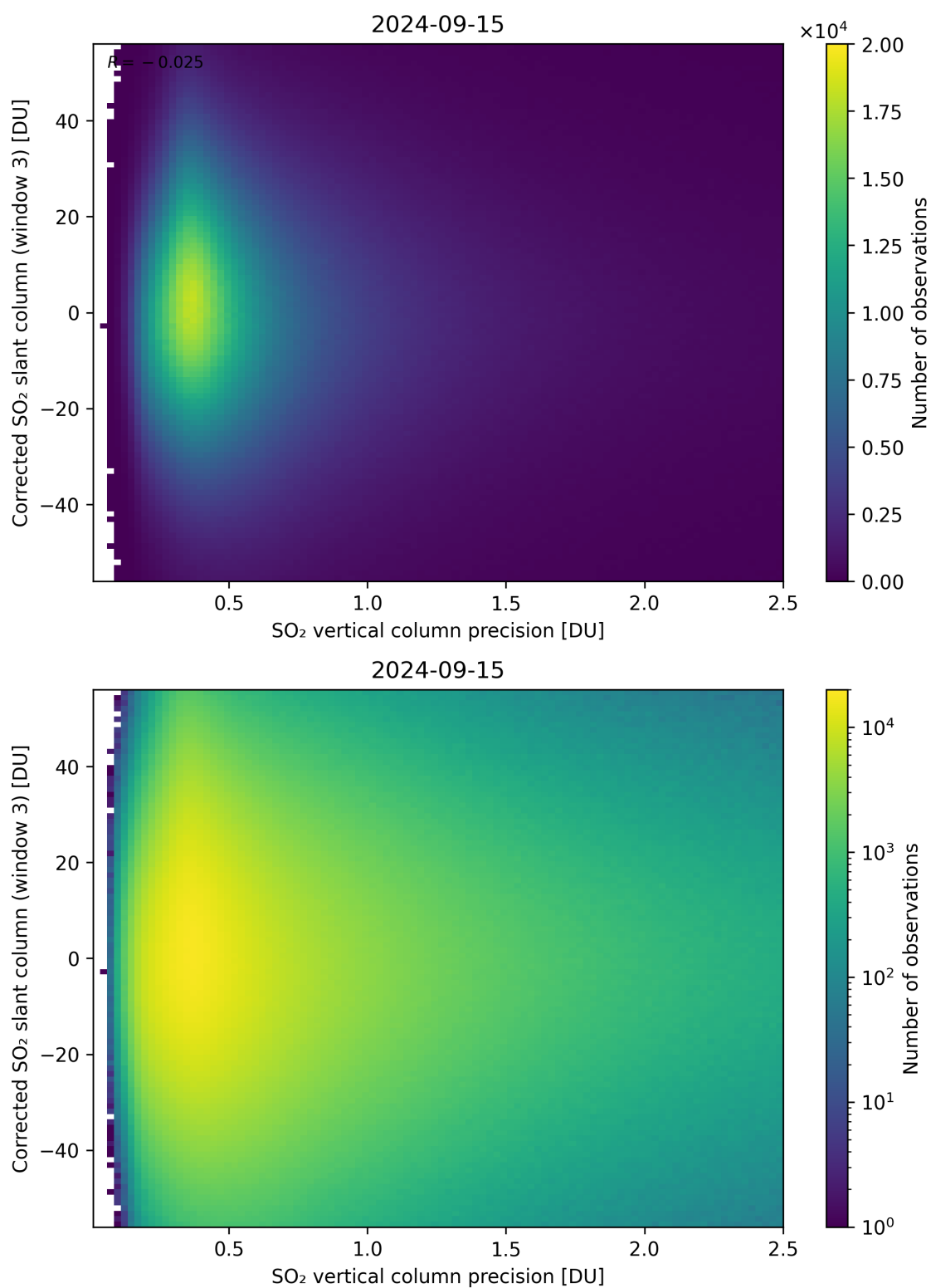
Figure 288: Scatter density plot of “SO 2 vertical column precision” against “Corrected SO 2 slant column (window 3)” for 2024-09-14 to 2024-09-16.
