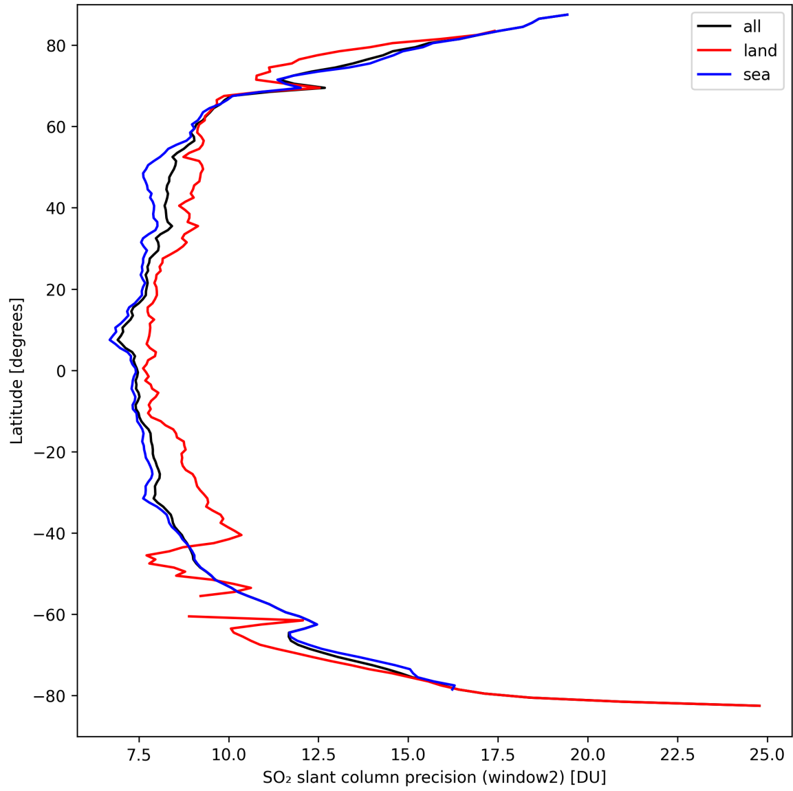
Figure 38: Zonal average of “SO 2 slant column precision (window2)” for 2024-09-14 to 2024-09-16.
