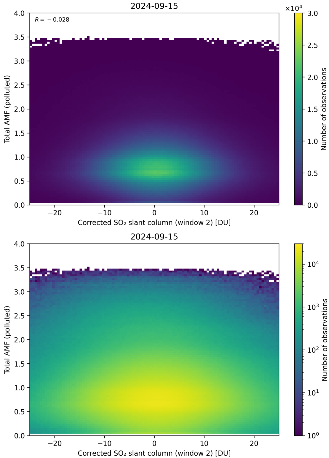
Figure 203: Scatter density plot of “Corrected SO 2 slant column (window 2)” against “Total AMF (polluted)” for 2024-09-14 to 2024-09-16.
