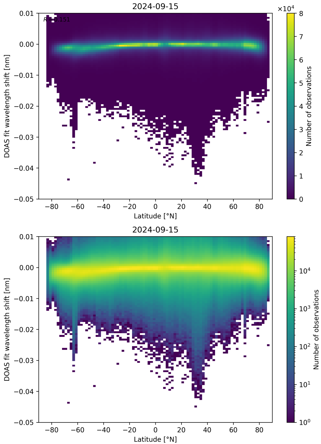
Figure 142: Scatter density plot of “Latitude” against “DOAS fit wavelength shift” for 2024-09-14 to 2024-09-16.
