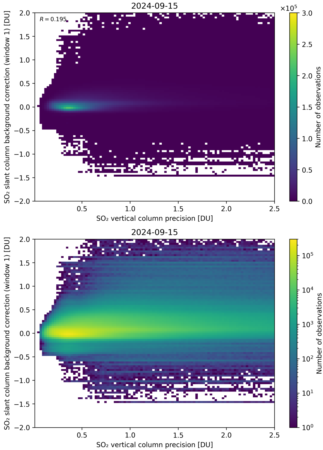
Figure 279: Scatter density plot of “SO 2 vertical column precision” against “SO 2 slant column background correction (window 1)” for 2024-09-14 to 2024-09-16.
