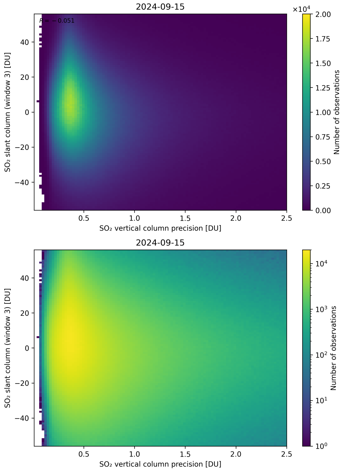
Figure 292: Scatter density plot of “SO 2 vertical column precision” against “SO 2 slant column (window 3)” for 2024-09-14 to 2024-09-16.
