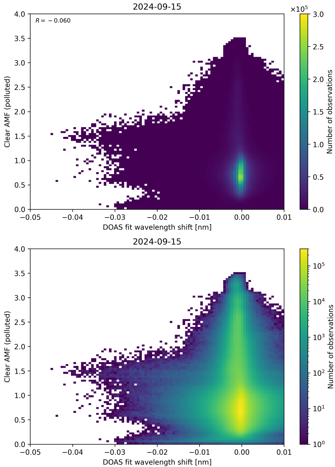
Figure 129: Scatter density plot of “DOAS fit wavelength shift” against “Clear AMF (polluted)” for 2024-09-14 to 2024-09-16.
