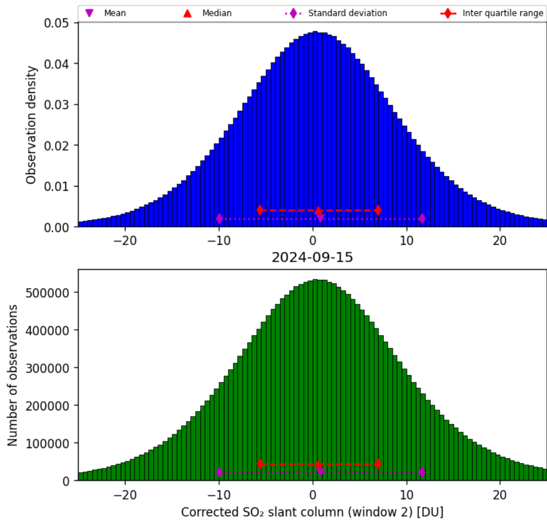
Figure 62: Histogram of “Corrected SO 2 slant column (window 2)” for 2024-09-14 to 2024-09-16
