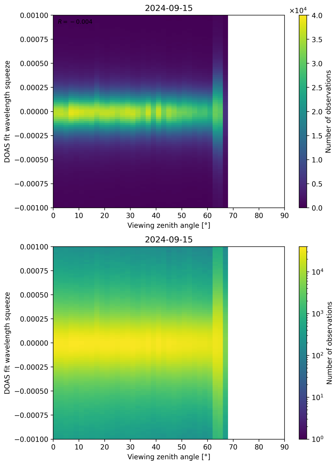
Figure 312: Scatter density plot of “Viewing zenith angle” against “DOAS fit wavelength squeeze” for 2024-09-14 to 2024-09-16.
