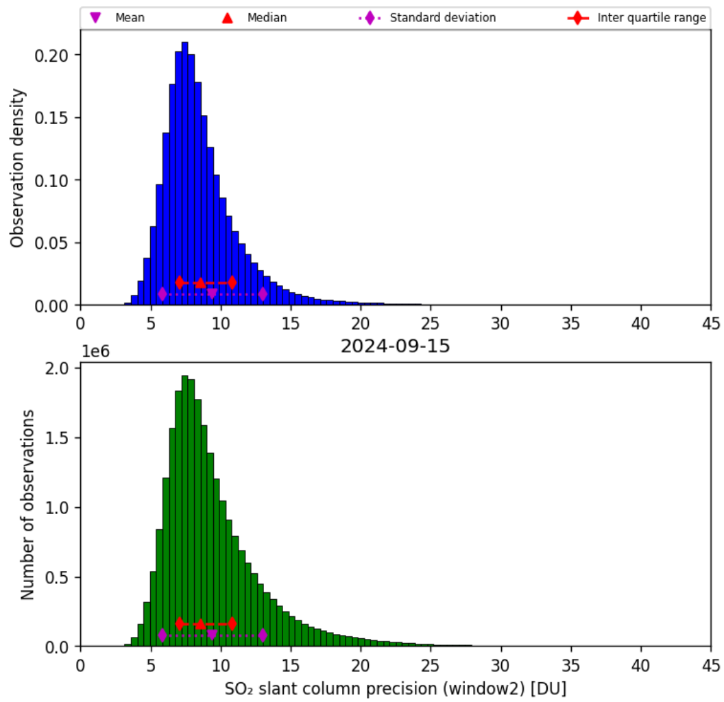
Figure 61: Histogram of “SO 2 slant column precision (window2)” for 2024-09-14 to 2024-09-16
