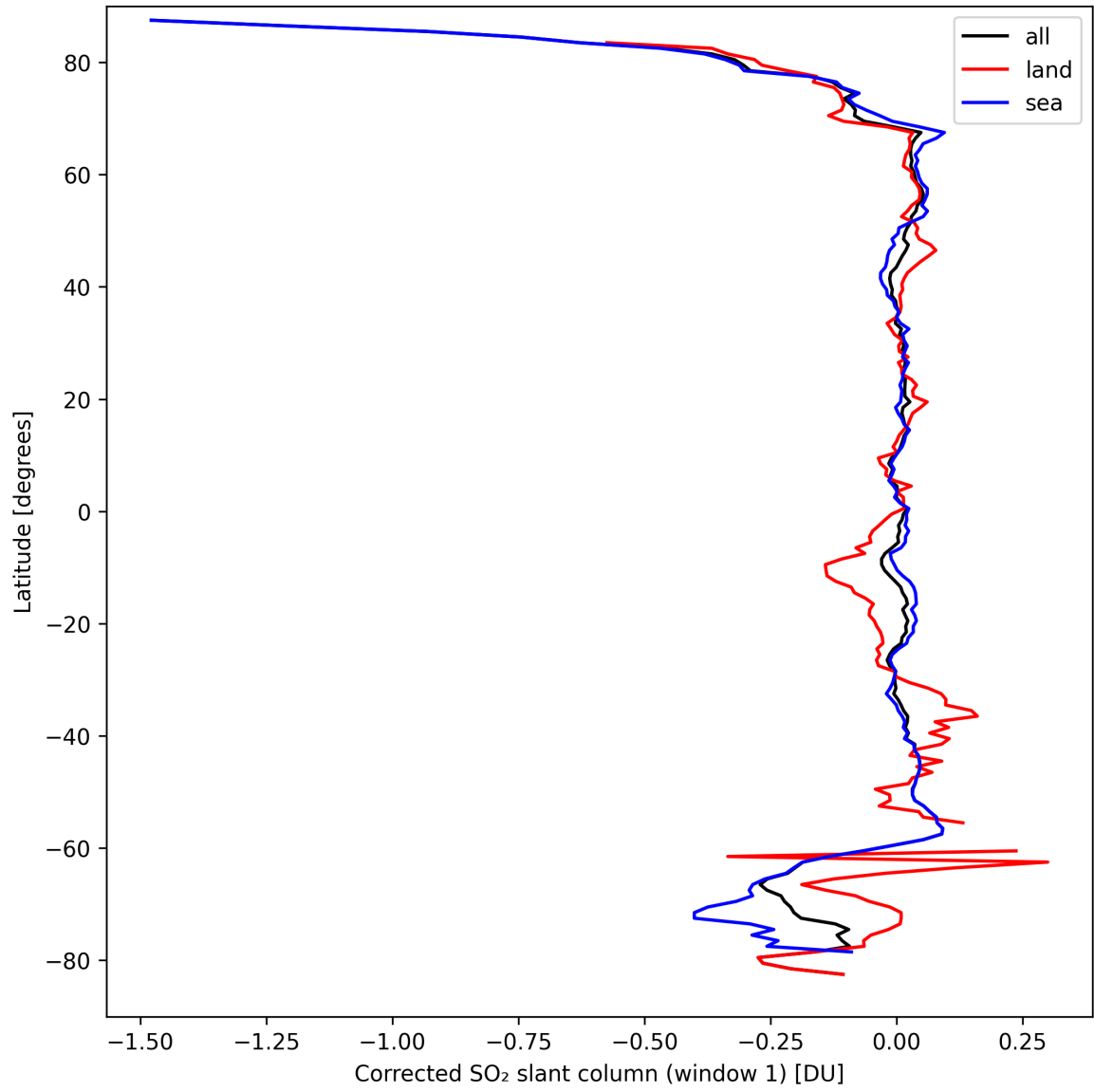
Figure 35: Zonal average of “Corrected SO 2 slant column (window 1)” for 2024-09-14 to 2024-09-16.
