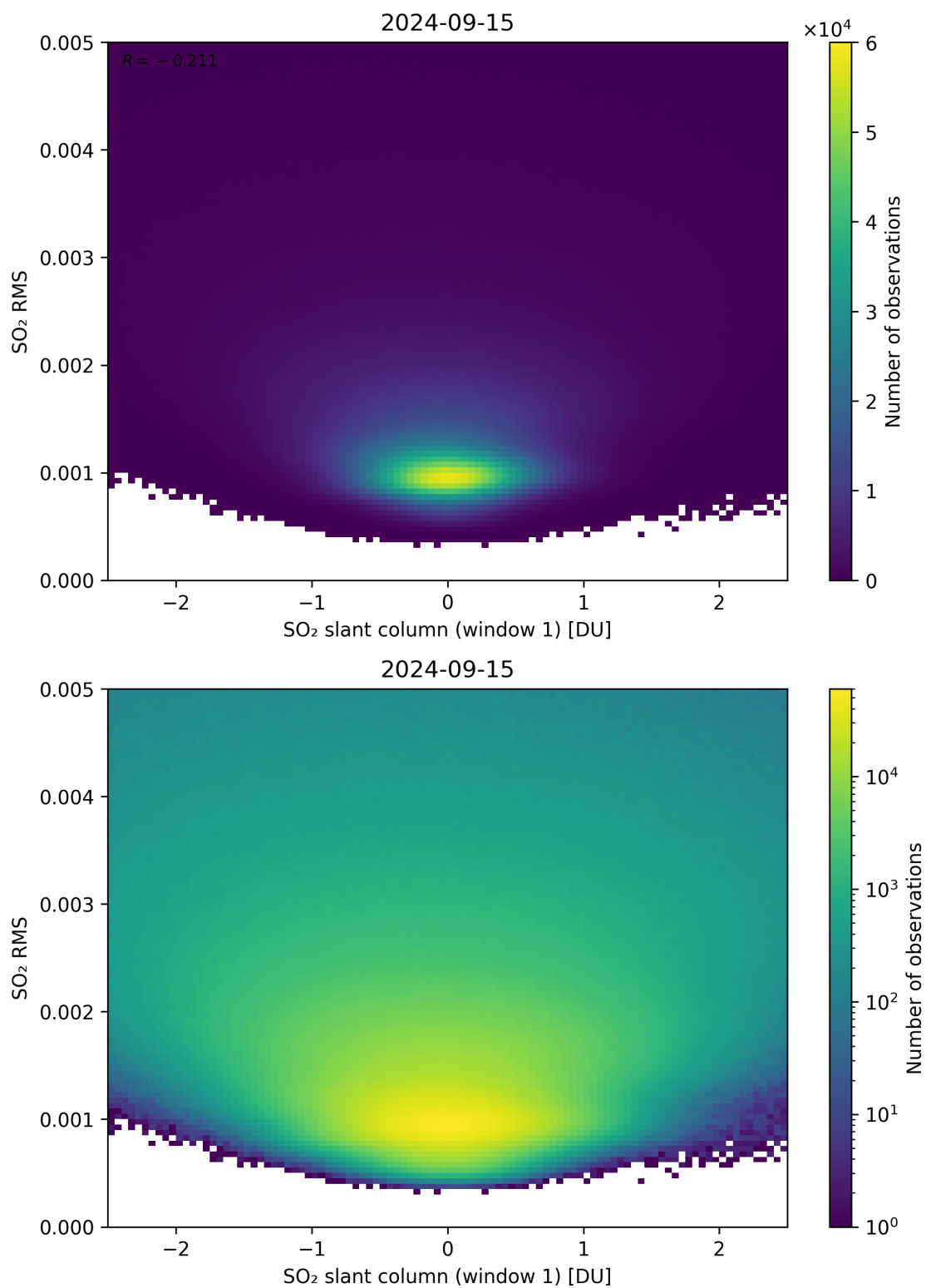
Figure 217: Scatter density plot of “SO 2 slant column (window 1)” against “SO 2 RMS” for 2024-09-14 to 2024-09-16.
