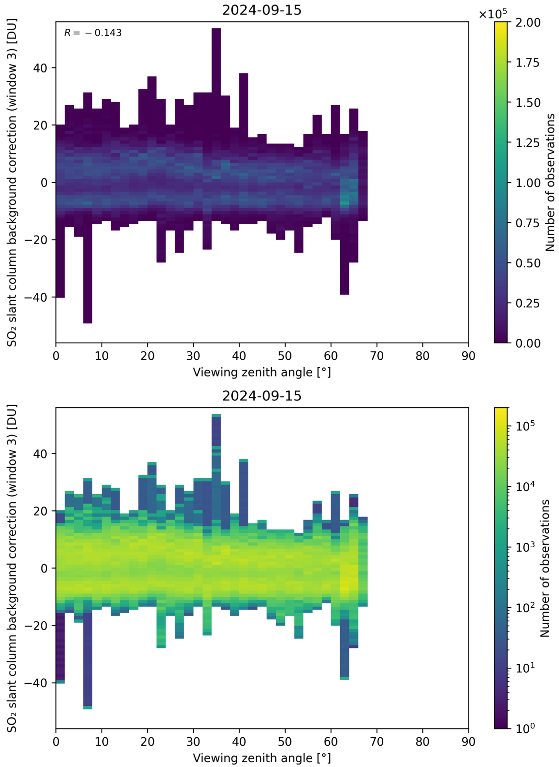
Figure 310: Scatter density plot of “Viewing zenith angle” against “SO 2 slant column background correction (window 3)” for 2024-09-14 to 2024-09-16.
