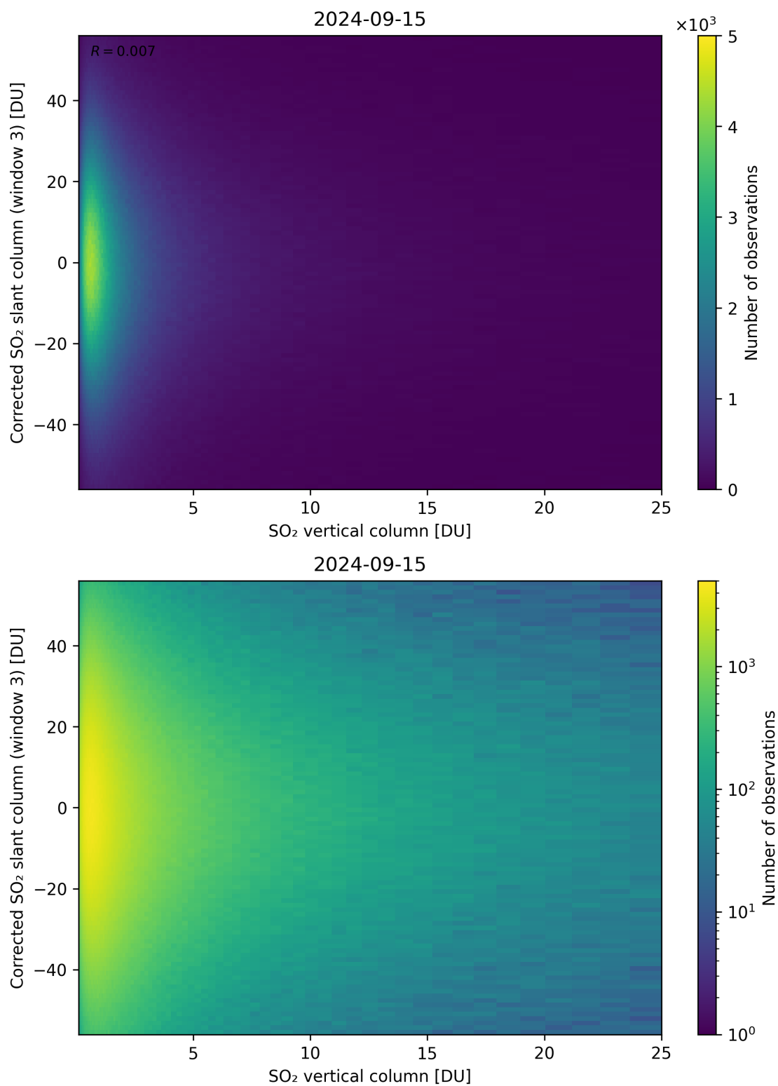
Figure 299: Scatter density plot of “SO 2 vertical column” against “Corrected SO 2 slant column (window 3)” for 2024-09-14 to 2024-09-16.
