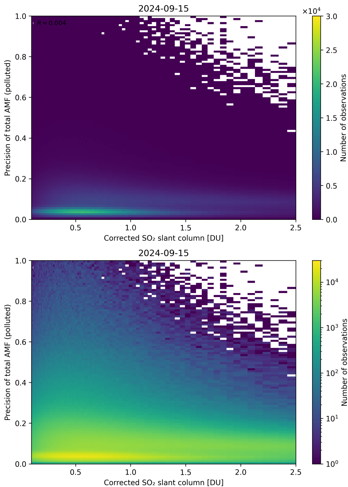
Figure 193: Scatter density plot of “Corrected SO 2 slant column” against “Precision of total AMF (polluted)” for 2024-09-14 to 2024-09-16.
