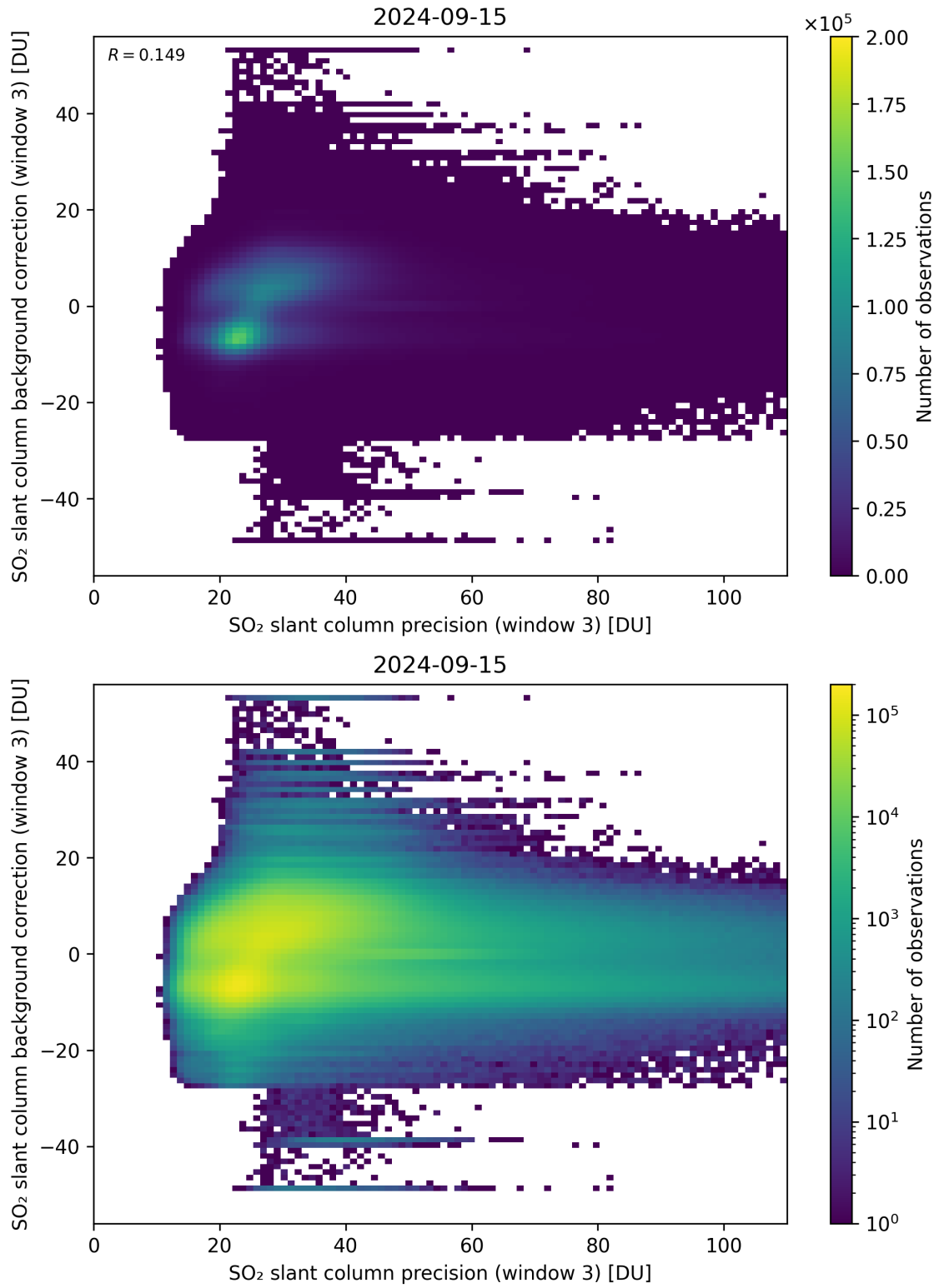
Figure 257: Scatter density plot of “SO 2 slant column precision (window 3)” against “SO 2 slant column background correction (window 3)” for 2024-09-14 to 2024-09-16.
