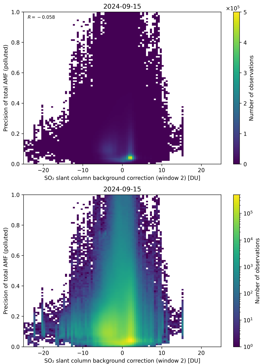
Figure 120: Scatter density plot of “SO 2 slant column background correction (window 2)” against “Precision of total AMF (polluted)” for 2024-09-14 to 2024-09-16.
