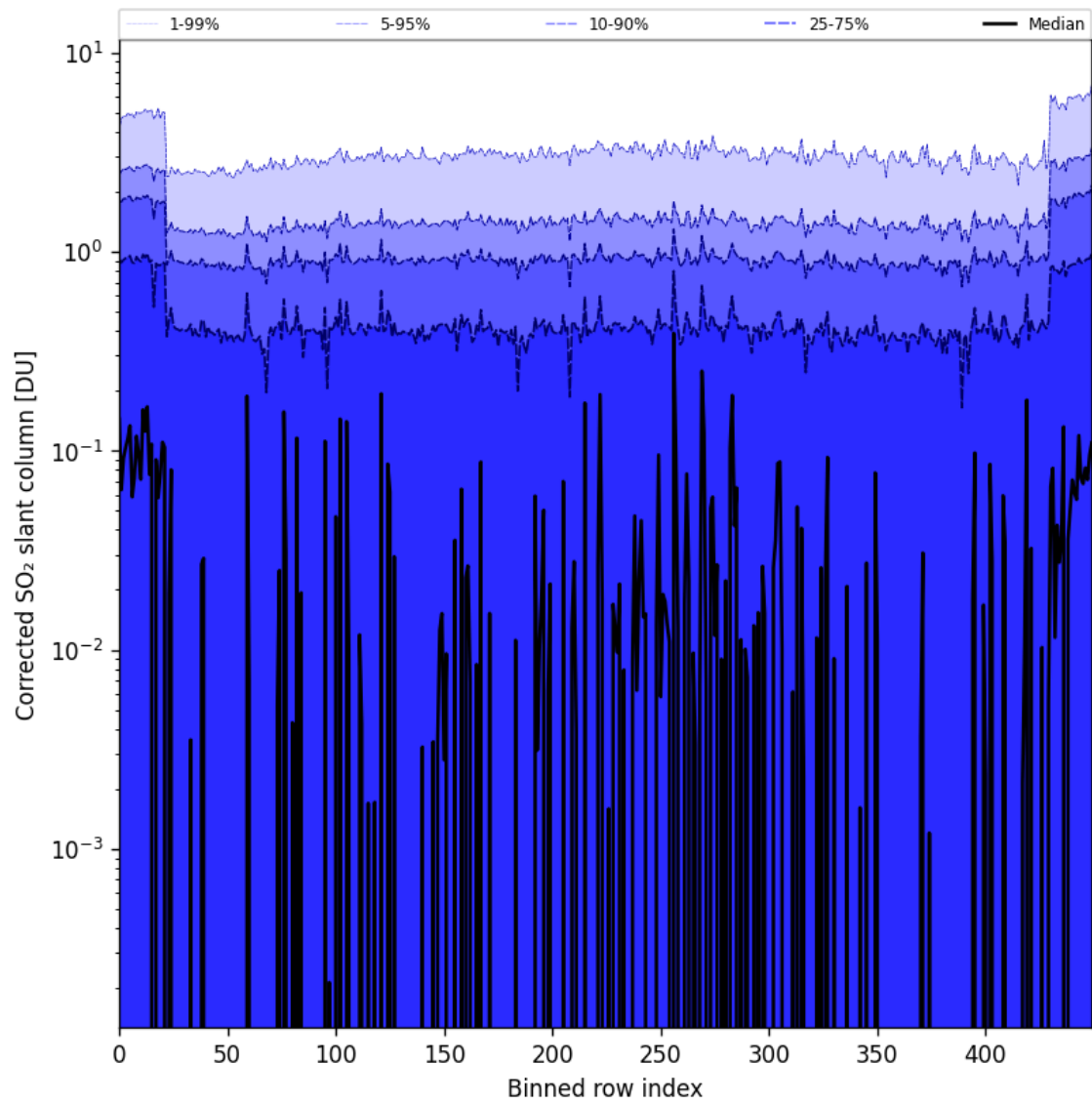
Figure 78: Along track statistics of "Corrected SO 2 slant column" for 2024-09-14 to 2024-09-16
