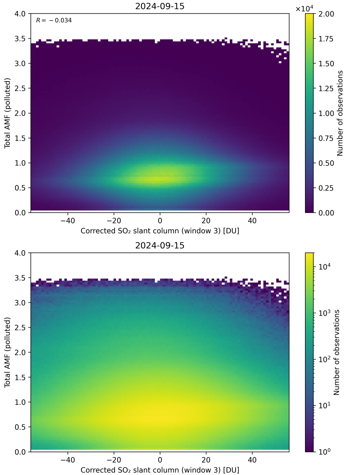
Figure 210: Scatter density plot of “Corrected SO 2 slant column (window 3)” against “Total AMF (polluted)” for 2024-09-14 to 2024-09-16.
