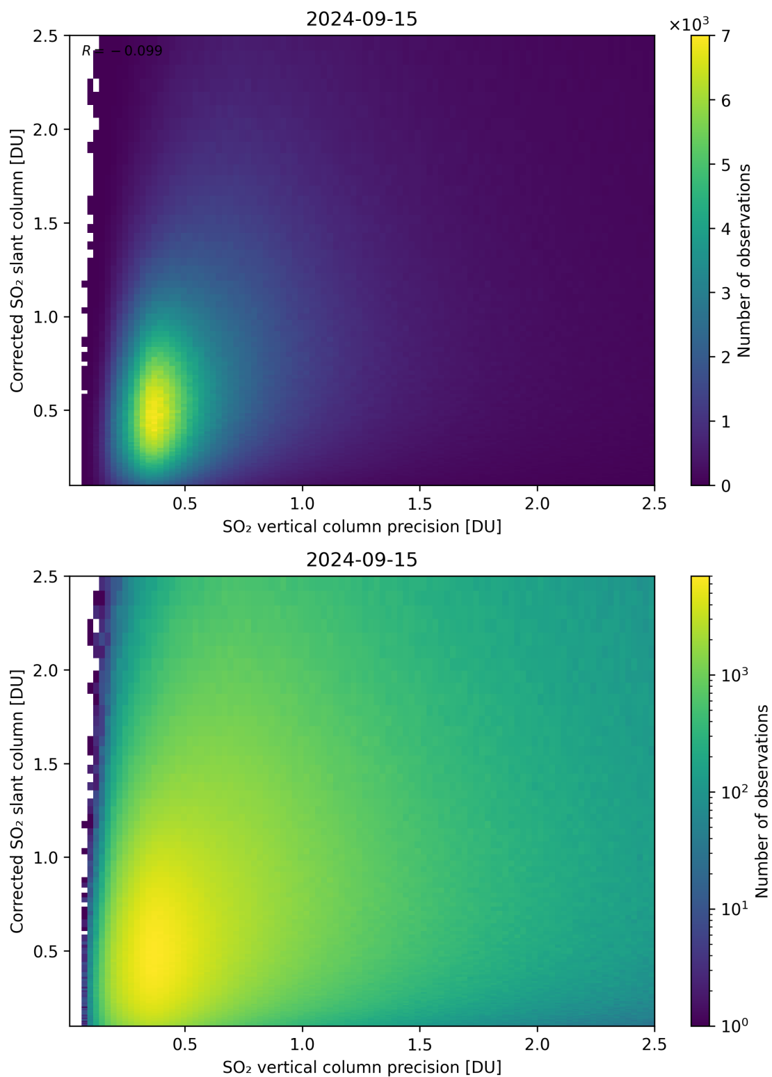
Figure 286: Scatter density plot of “SO 2 vertical column precision” against “Corrected SO 2 slant column” for 2024-09-14 to 2024-09-16.
