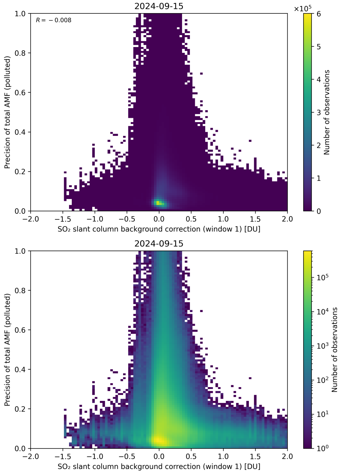
Figure 110: Scatter density plot of “SO 2 slant column background correction (window 1)” against “Precision of total AMF (polluted)” for 2024-09-14 to 2024-09-16.
