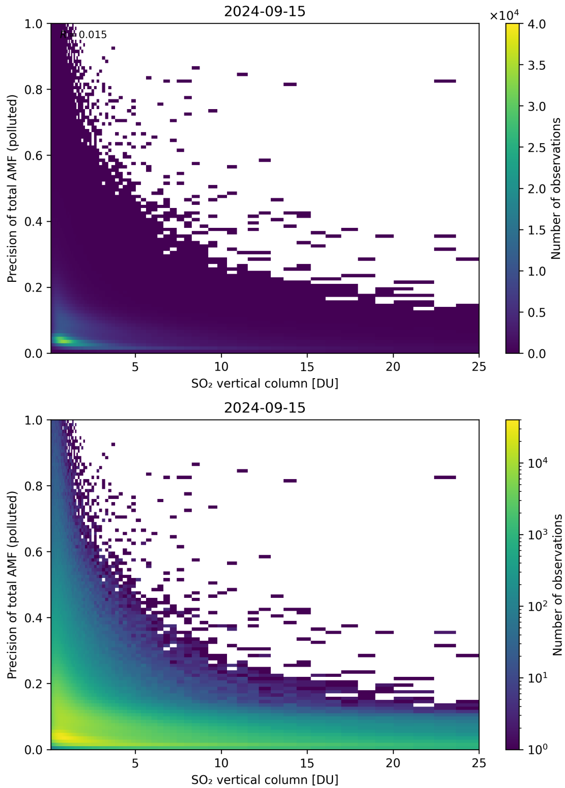
Figure 306: Scatter density plot of “SO 2 vertical column” against “Precision of total AMF (polluted)” for 2024-09-14 to 2024-09-16.
