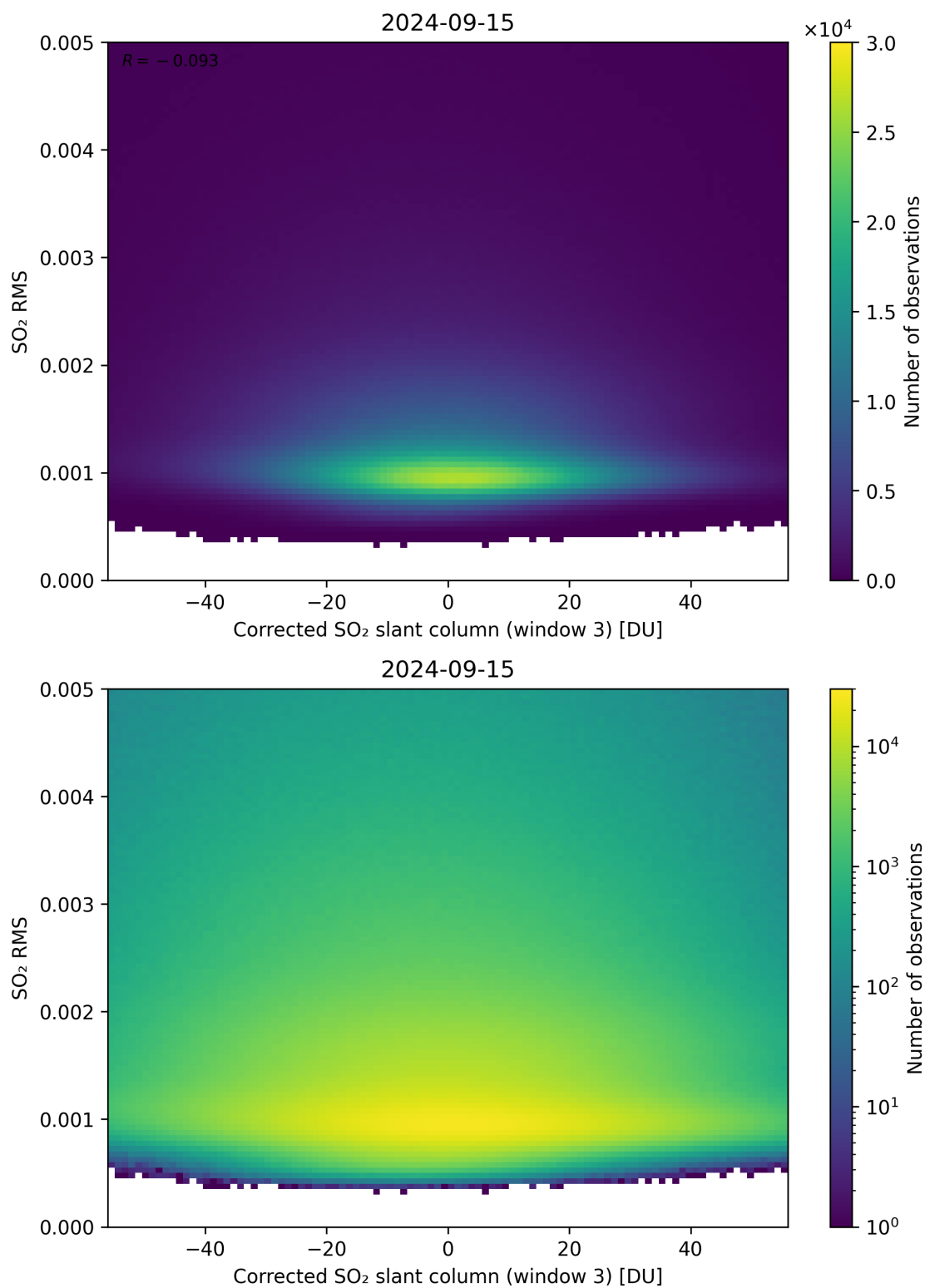
Figure 208: Scatter density plot of “Corrected SO 2 slant column (window 3)” against “SO 2 RMS” for 2024-09-14 to 2024-09-16.
