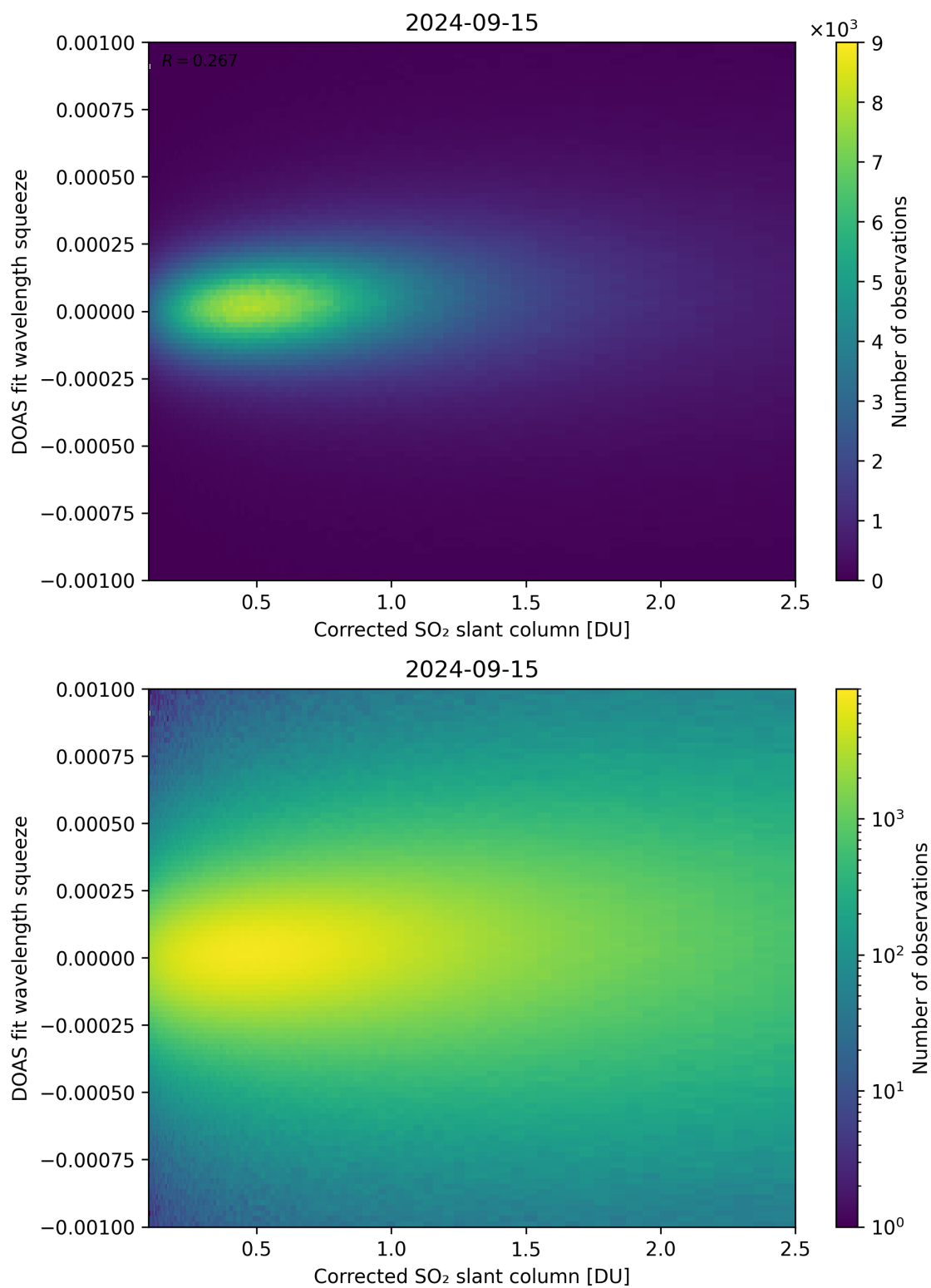
Figure 182: Scatter density plot of “Corrected SO 2 slant column” against “DOAS fit wavelength squeeze” for 2024-09-14 to 2024-09-16.
