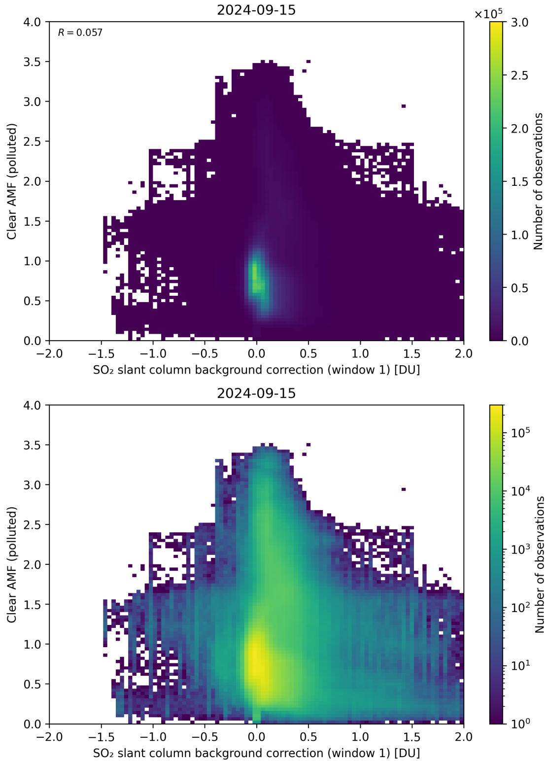
Figure 103: Scatter density plot of “SO 2 slant column background correction (window 1)” against “Clear AMF (polluted)” for 2024-09-14 to 2024-09-16.
