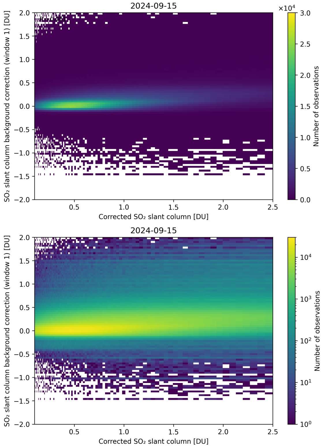
Figure 178: Scatter density plot of “Corrected SO 2 slant column” against “SO 2 slant column background correction (window 1)” for 2024-09-14 to 2024-09-16.
