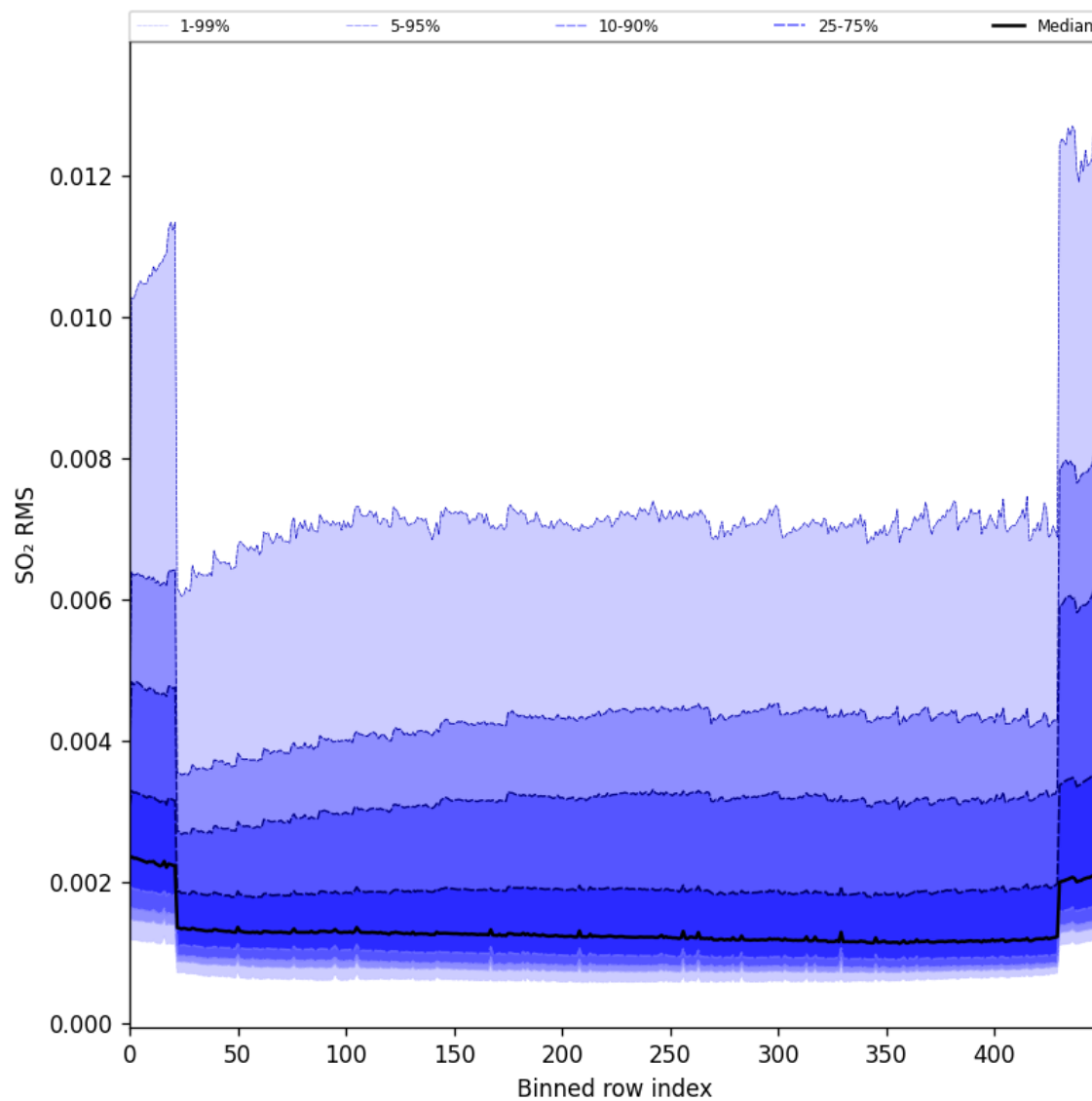
Figure 93: Along track statistics of “SO 2 RMS” for 2024-09-14 to 2024-09-16
