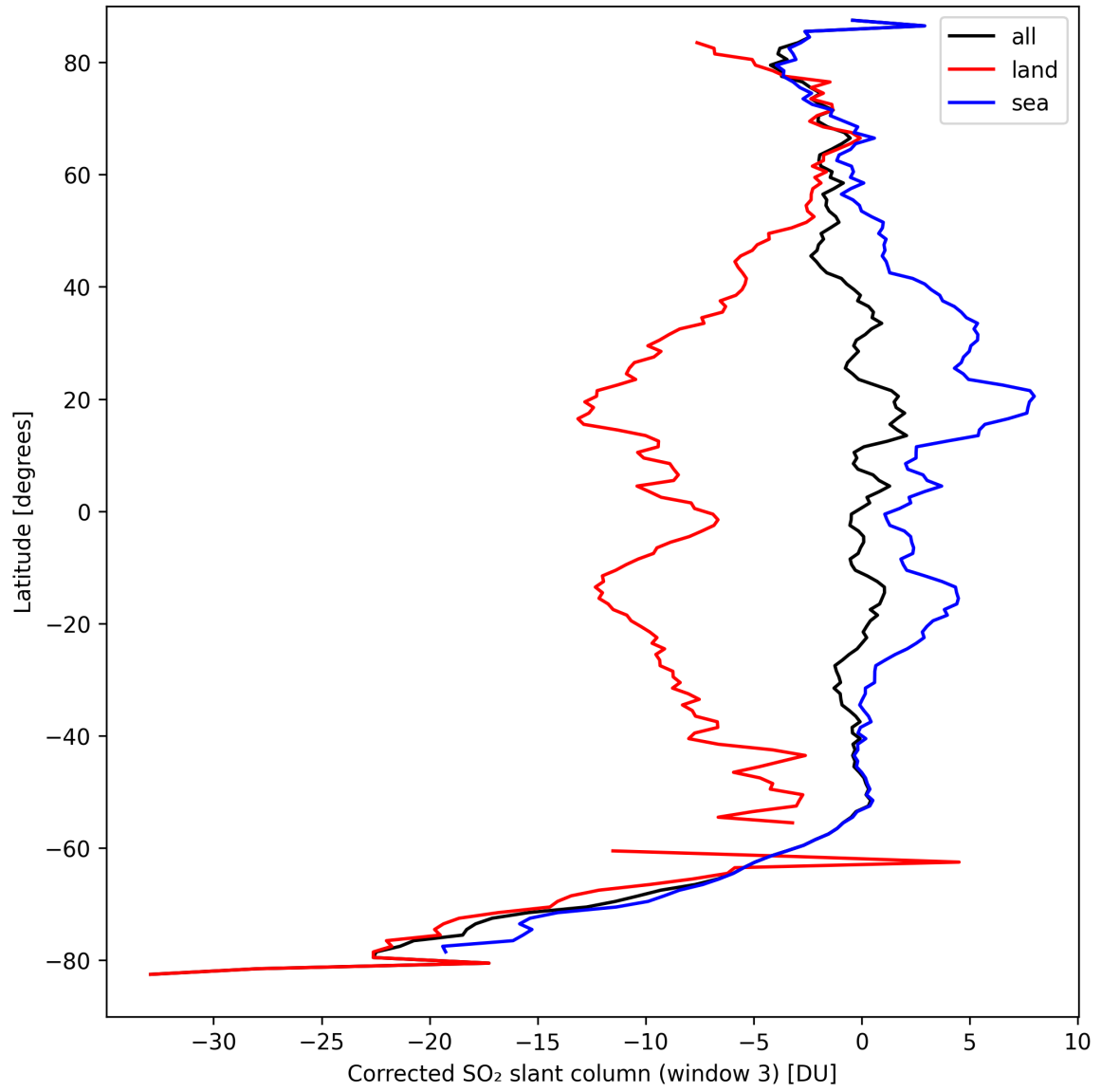
Figure 43: Zonal average of “Corrected SO 2 slant column (window 3)” for 2024-09-14 to 2024-09-16.
