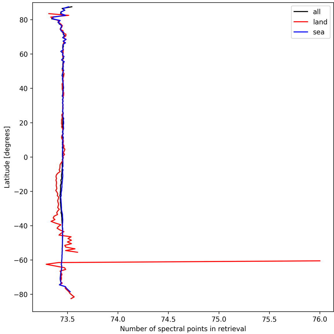
Figure 51: Zonal average of “Number of spectral points in retrieval” for 2024-09-14 to 2024-09-16.
