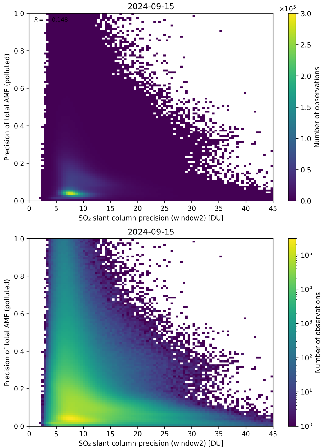
Figure 252: Scatter density plot of “SO 2 slant column precision (window2)” against “Precision of total AMF (polluted)” for 2024-09-14 to 2024-09-16.
