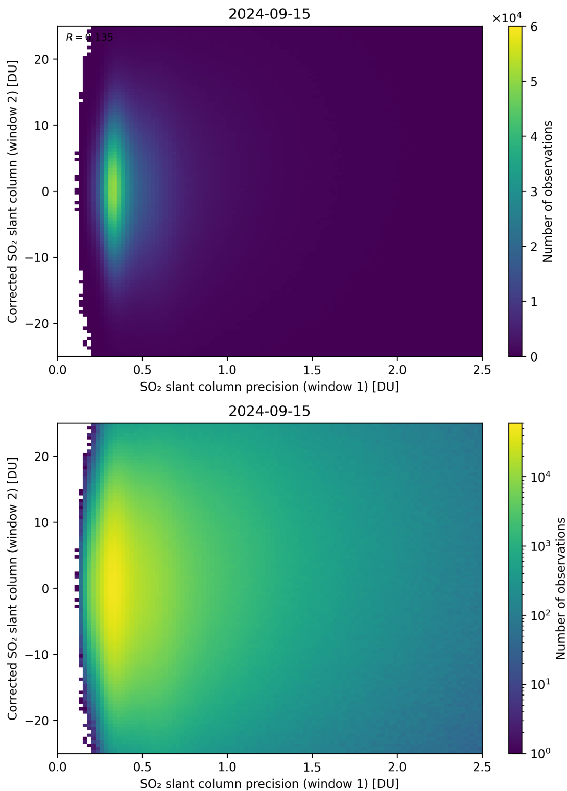
Figure 225: Scatter density plot of “SO 2 slant column precision (window 1)” against “Corrected SO 2 slant column (window 2)” for 2024-09-14 to 2024-09-16.
