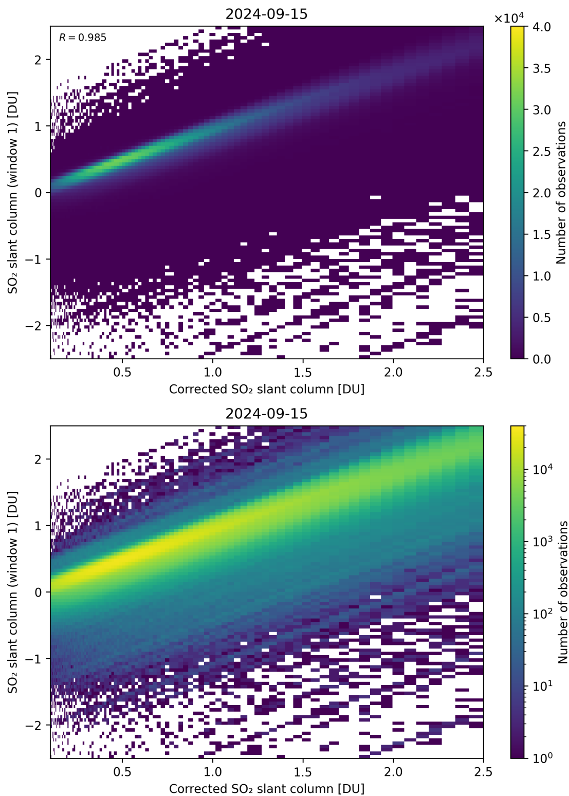
Figure 187: Scatter density plot of “Corrected SO 2 slant column” against “SO 2 slant column (window 1)” for 2024-09-14 to 2024-09-16.
