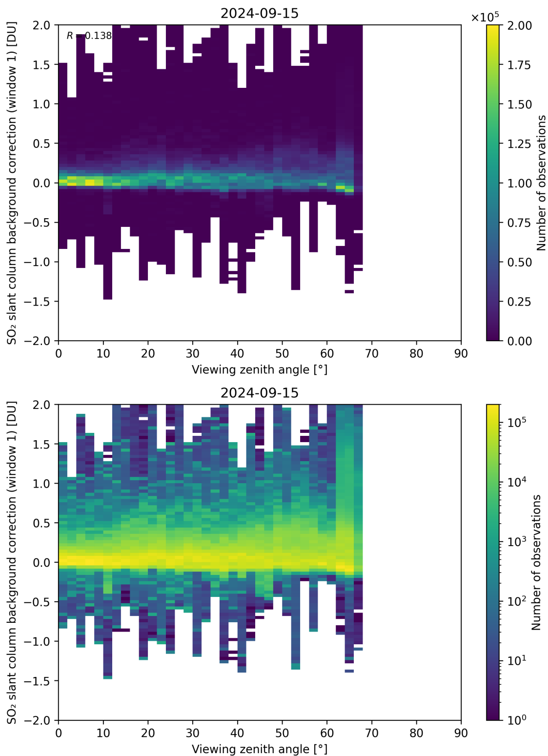
Figure 308: Scatter density plot of “Viewing zenith angle” against “SO 2 slant column background correction (window 1)” for 2024-09-14 to 2024-09-16.
