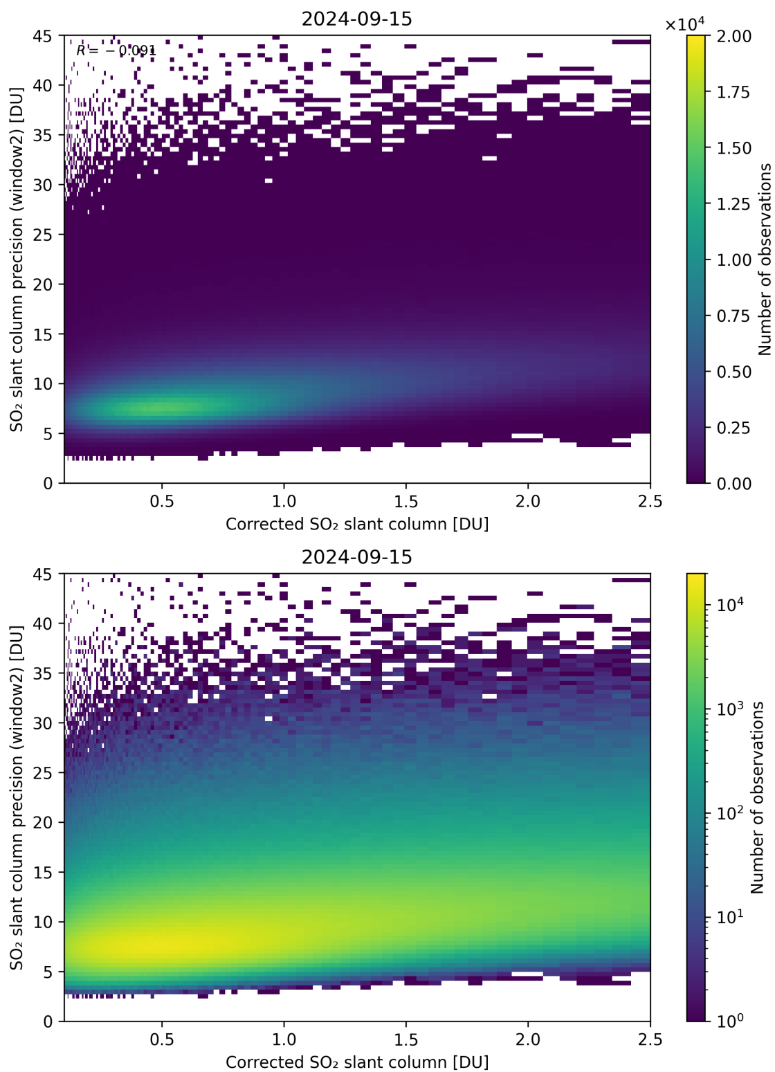
Figure 189: Scatter density plot of “Corrected SO 2 slant column” against “SO 2 slant column precision (window2)” for 2024-09-14 to 2024-09-16.
