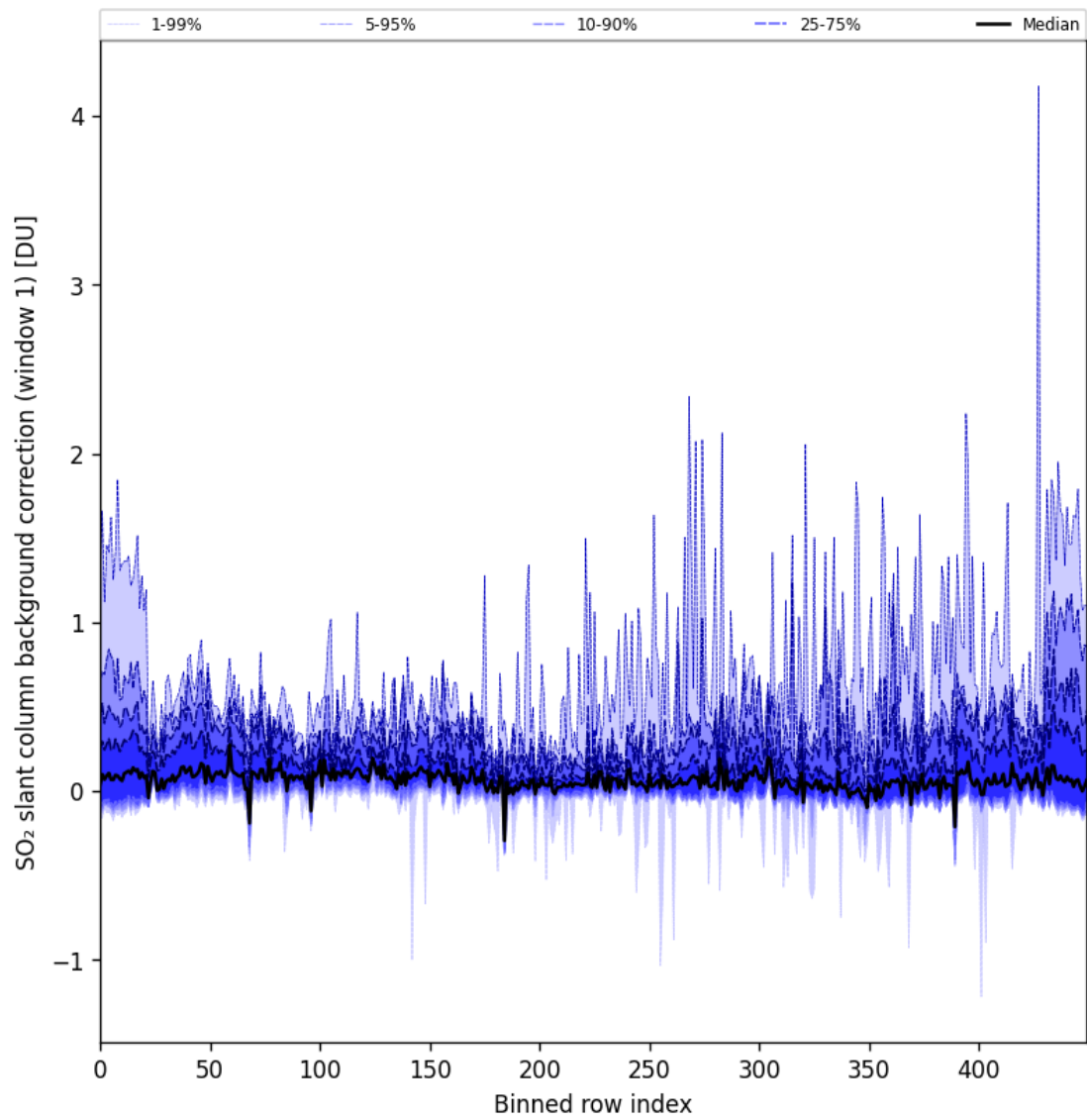
Figure 82: Along track statistics of “SO 2 slant column background correction (window 1)” for 2024-09-14 to 2024-09-16
