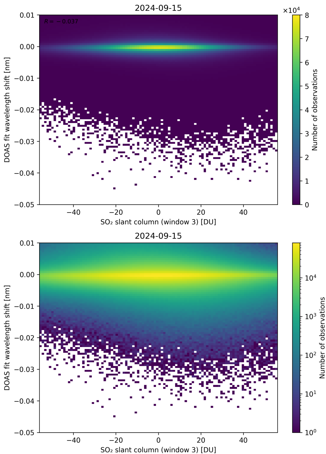
Figure 254: Scatter density plot of “SO 2 slant column (window 3)” against “DOAS fit wavelength shift” for 2024-09-14 to 2024-09-16.
