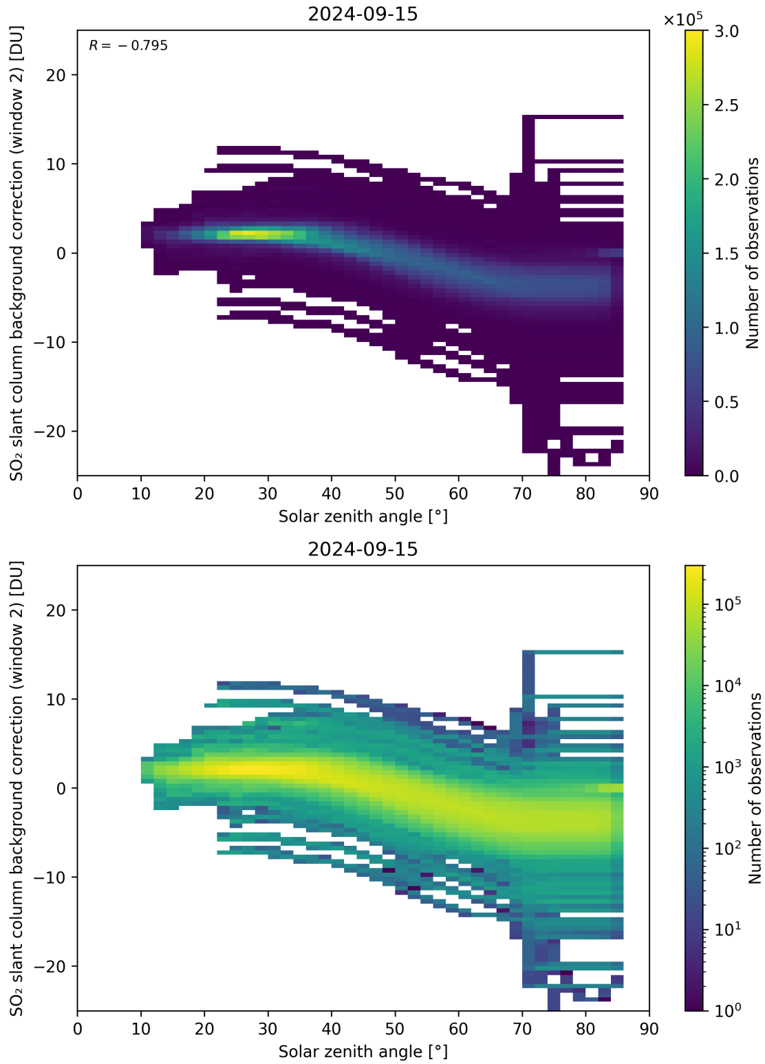
Figure 159: Scatter density plot of “Solar zenith angle” against “SO 2 slant column background correction (window 2)” for 2024-09-14 to 2024-09-16.
