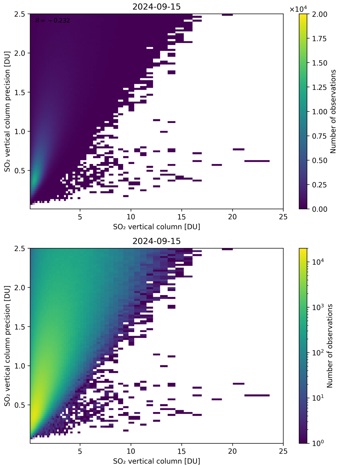
Figure 307: Scatter density plot of “SO 2 vertical column” against “SO 2 vertical column precision” for 2024-09-14 to 2024-09-16.
