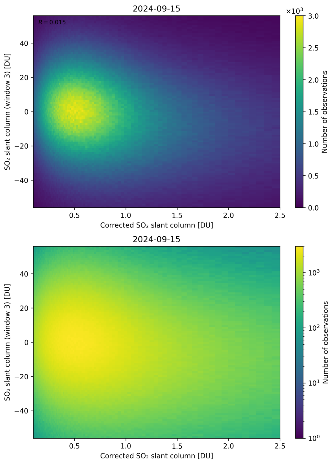
Figure 190: Scatter density plot of “Corrected SO 2 slant column” against “SO 2 slant column (window 3)” for 2024-09-14 to 2024-09-16.
