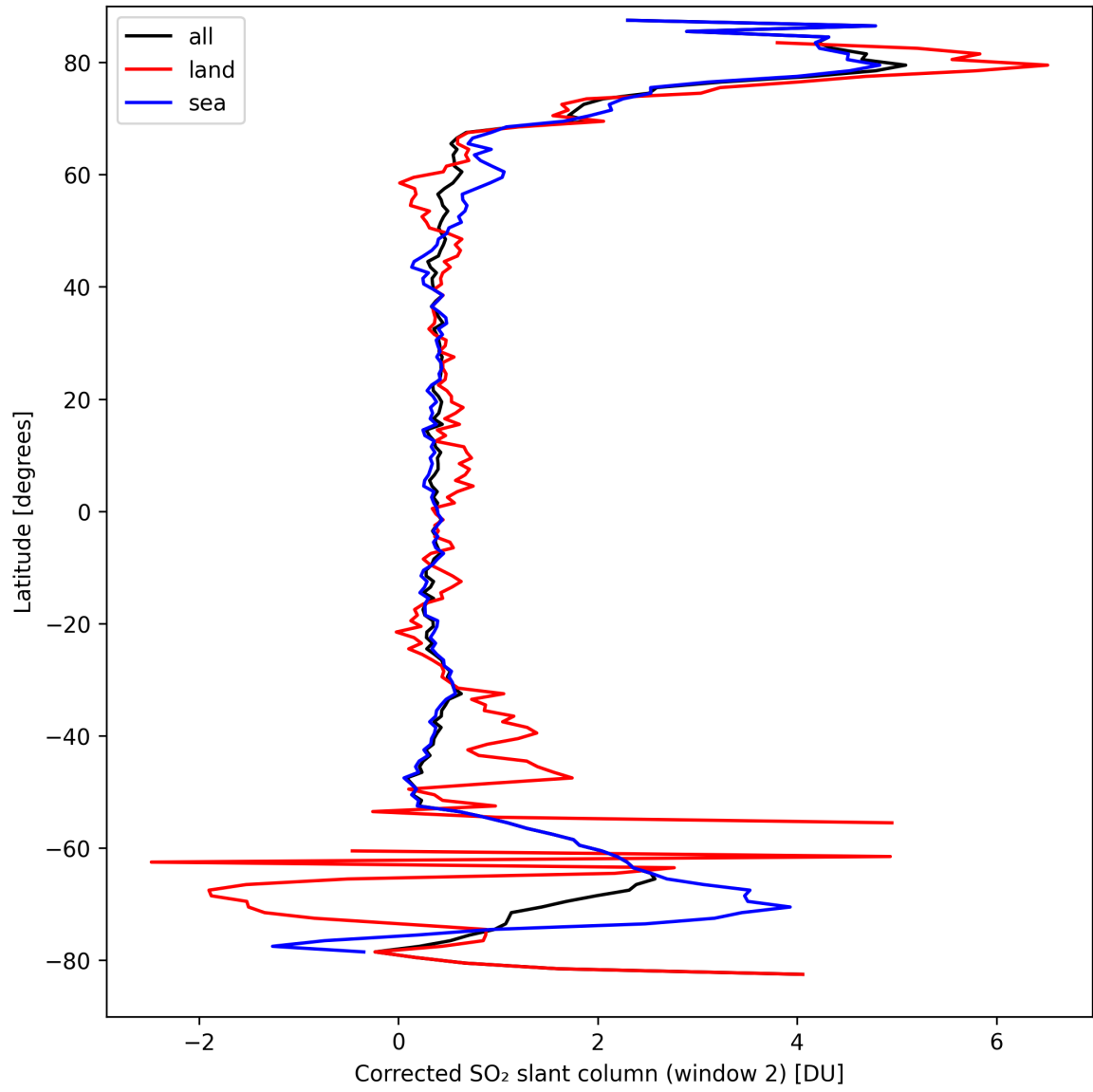
Figure 39: Zonal average of “Corrected SO 2 slant column (window 2)” for 2024-09-14 to 2024-09-16.
