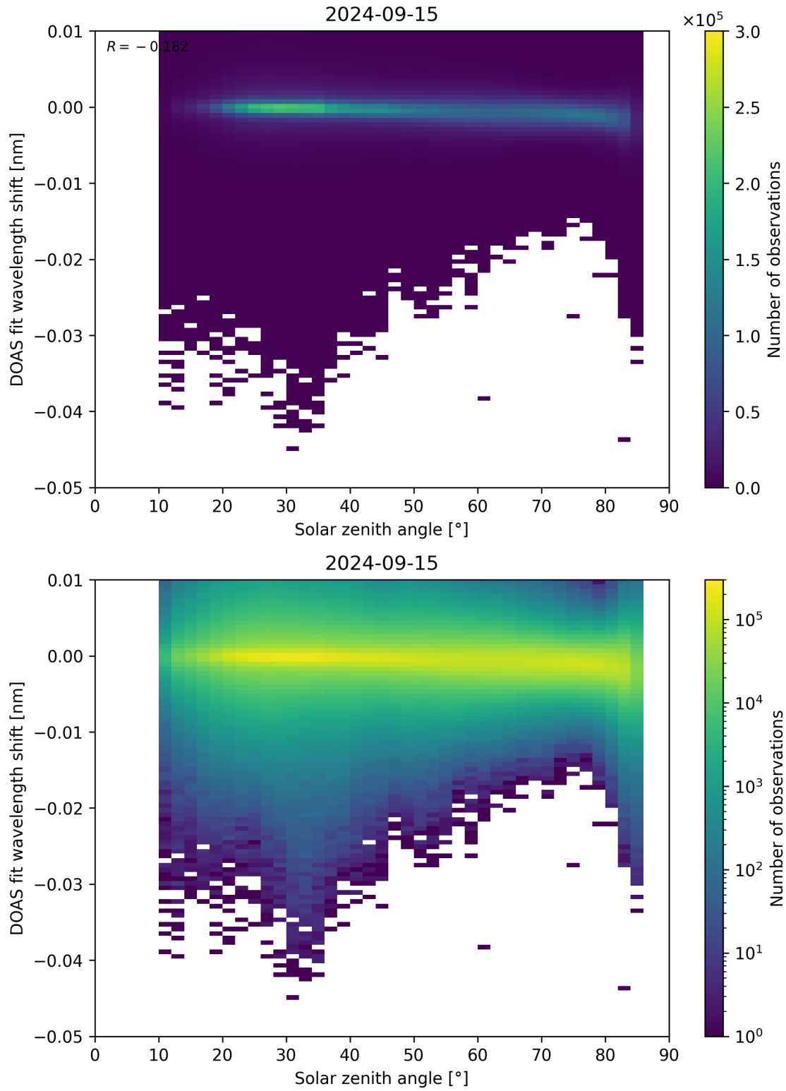
Figure 161: Scatter density plot of “Solar zenith angle” against “DOAS fit wavelength shift” for 2024-09-14 to 2024-09-16.
