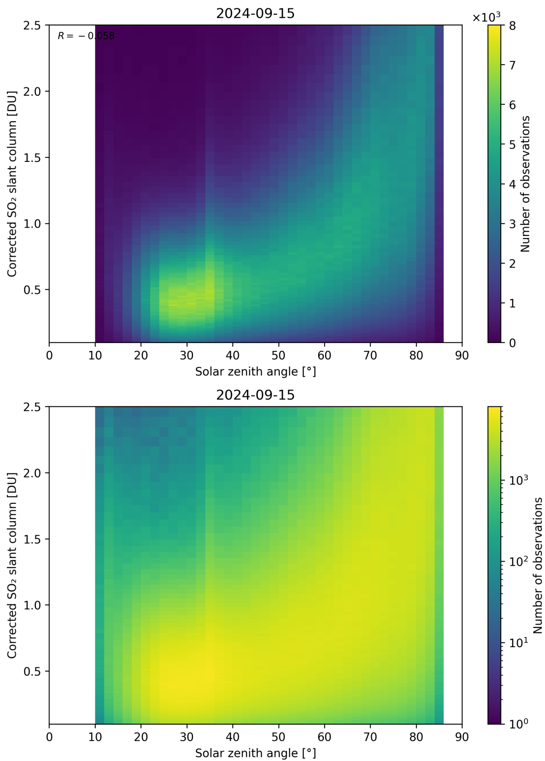
Figure 166: Scatter density plot of “Solar zenith angle” against “Corrected SO 2 slant column” for 2024-09-14 to 2024-09-16.
