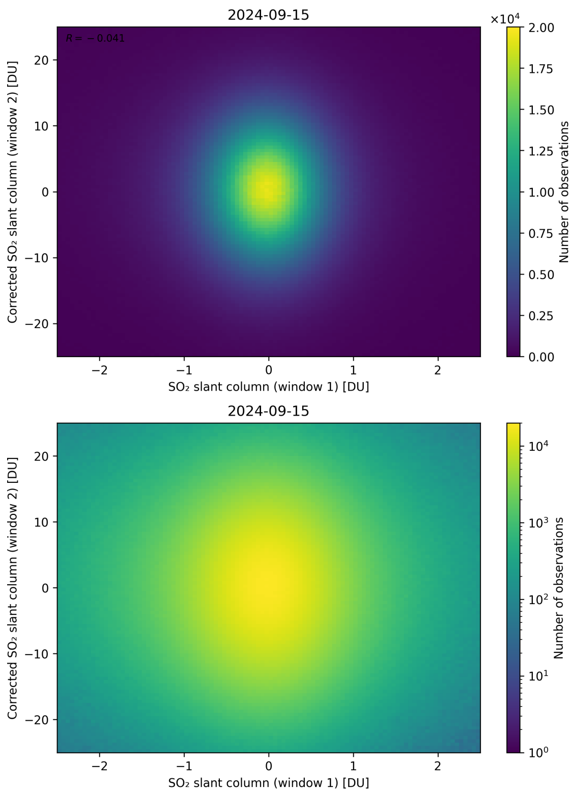
Figure 233: Scatter density plot of “SO 2 slant column (window 1)” against “Corrected SO 2 slant column (window 2)” for 2024-09-14 to 2024-09-16.
