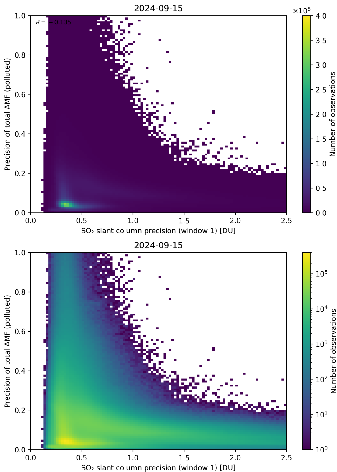
Figure 231: Scatter density plot of “SO 2 slant column precision (window 1)” against “Precision of total AMF (polluted)” for 2024-09-14 to 2024-09-16.
