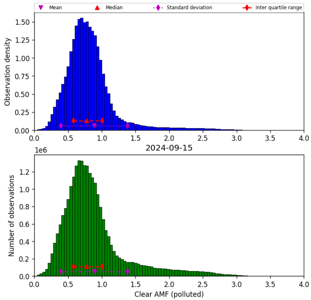
Figure 73: Histogram of “Clear AMF (polluted)” for 2024-09-14 to 2024-09-16
