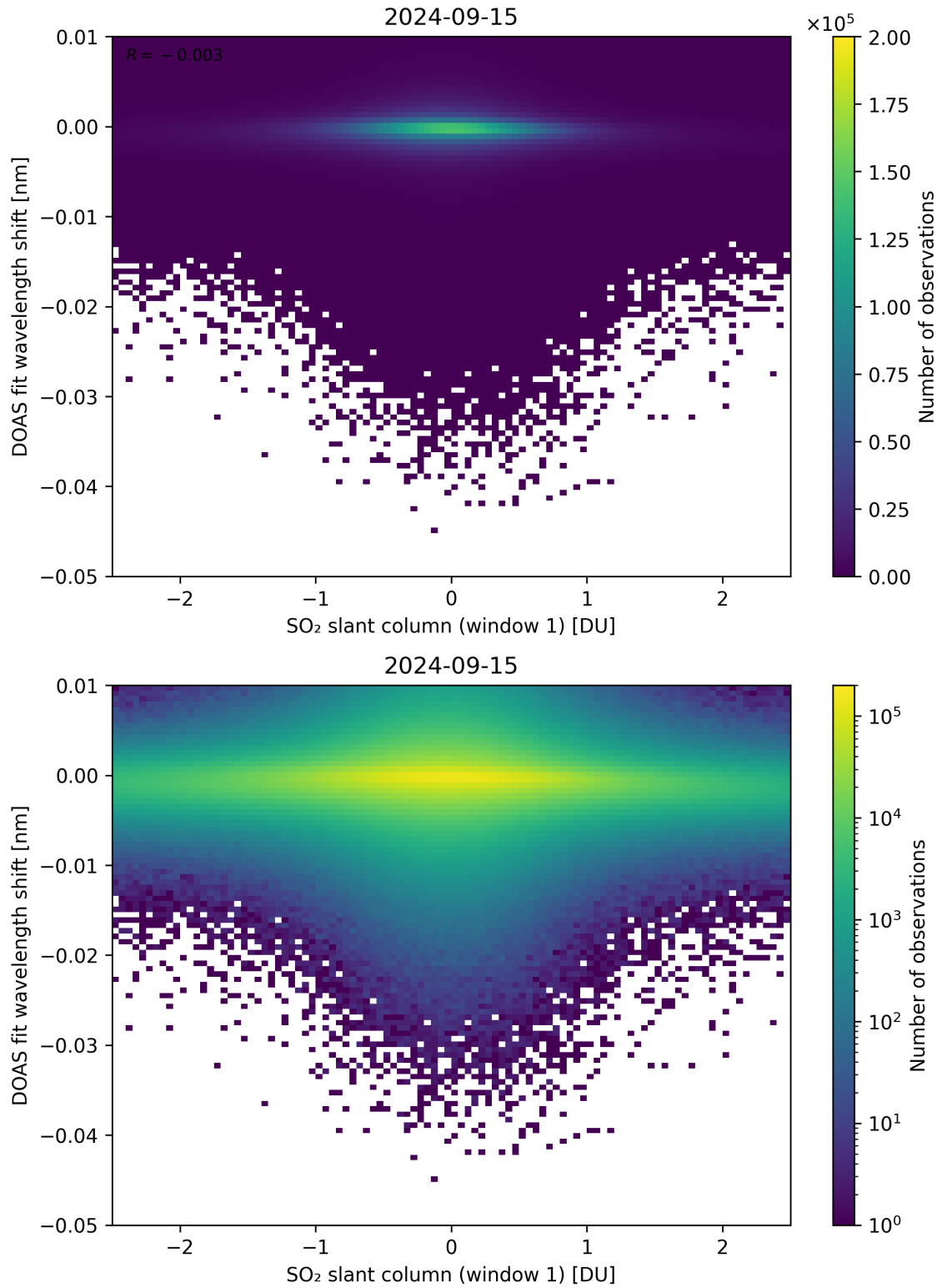
Figure 215: Scatter density plot of “SO 2 slant column (window 1)” against “DOAS fit wavelength shift” for 2024-09-14 to 2024-09-16.
