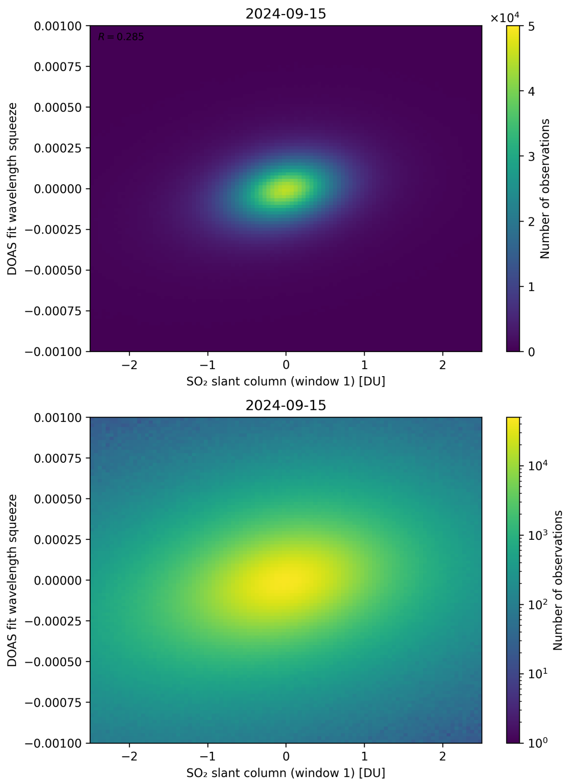
Figure 216: Scatter density plot of “SO 2 slant column (window 1)” against “DOAS fit wavelength squeeze” for 2024-09-14 to 2024-09-16.
