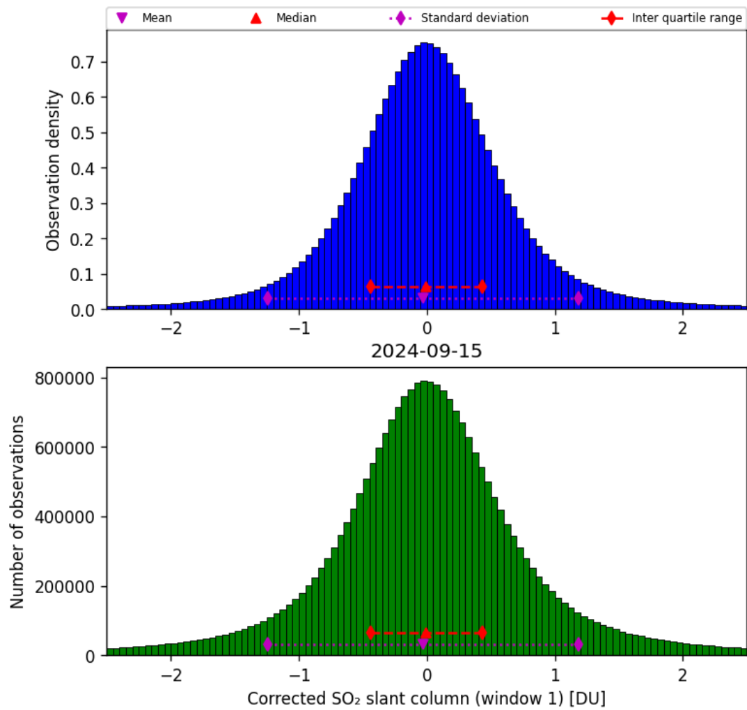
Figure 58: Histogram of “Corrected SO 2 slant column (window 1)” for 2024-09-14 to 2024-09-16
