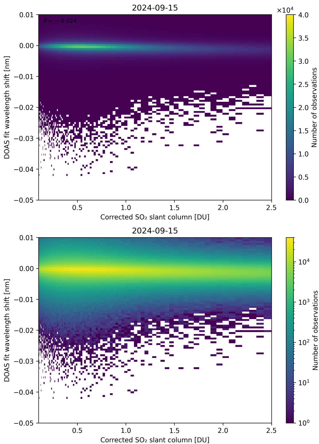
Figure 181: Scatter density plot of “Corrected SO 2 slant column” against “DOAS fit wavelength shift” for 2024-09-14 to 2024-09-16.
