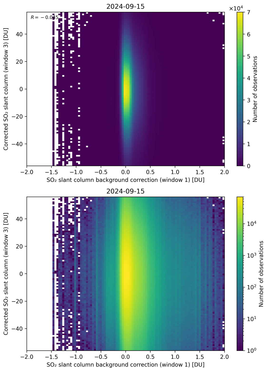
Figure 105: Scatter density plot of “SO 2 slant column background correction (window 1)” against “Corrected SO 2 slant column (window 3)” for 2024-09-14 to 2024-09-16.
