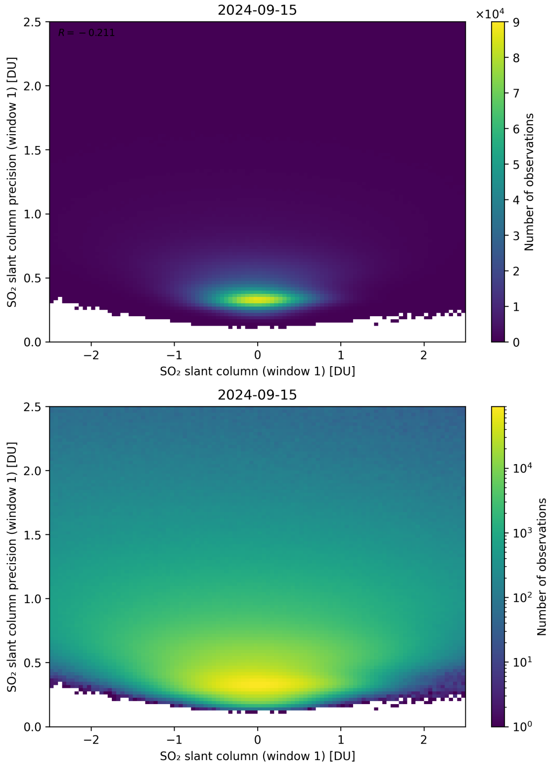
Figure 235: Scatter density plot of “SO 2 slant column (window 1)” against “SO 2 slant column precision (window 1)” for 2024-09-14 to 2024-09-16.
