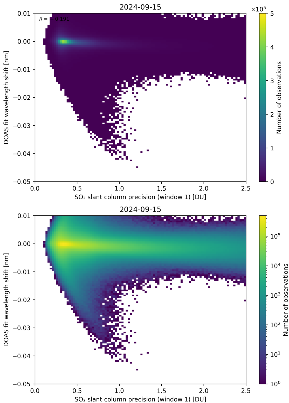
Figure 221: Scatter density plot of “SO 2 slant column precision (window 1)” against “DOAS fit wavelength shift” for 2024-09-14 to 2024-09-16.
