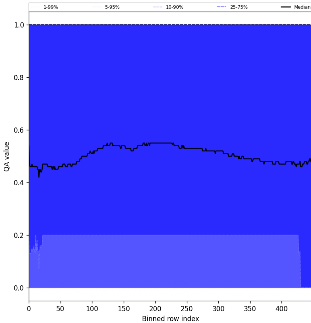
Figure 75: Along track statistics of “QA value” for 2024-09-14 to 2024-09-16
