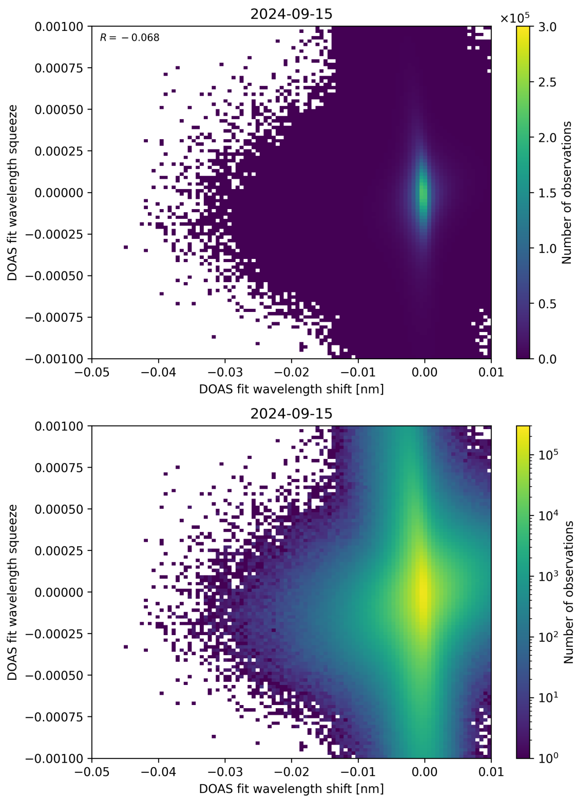
Figure 127: Scatter density plot of “DOAS fit wavelength shift” against “DOAS fit wavelength squeeze” for 2024-09-14 to 2024-09-16.
