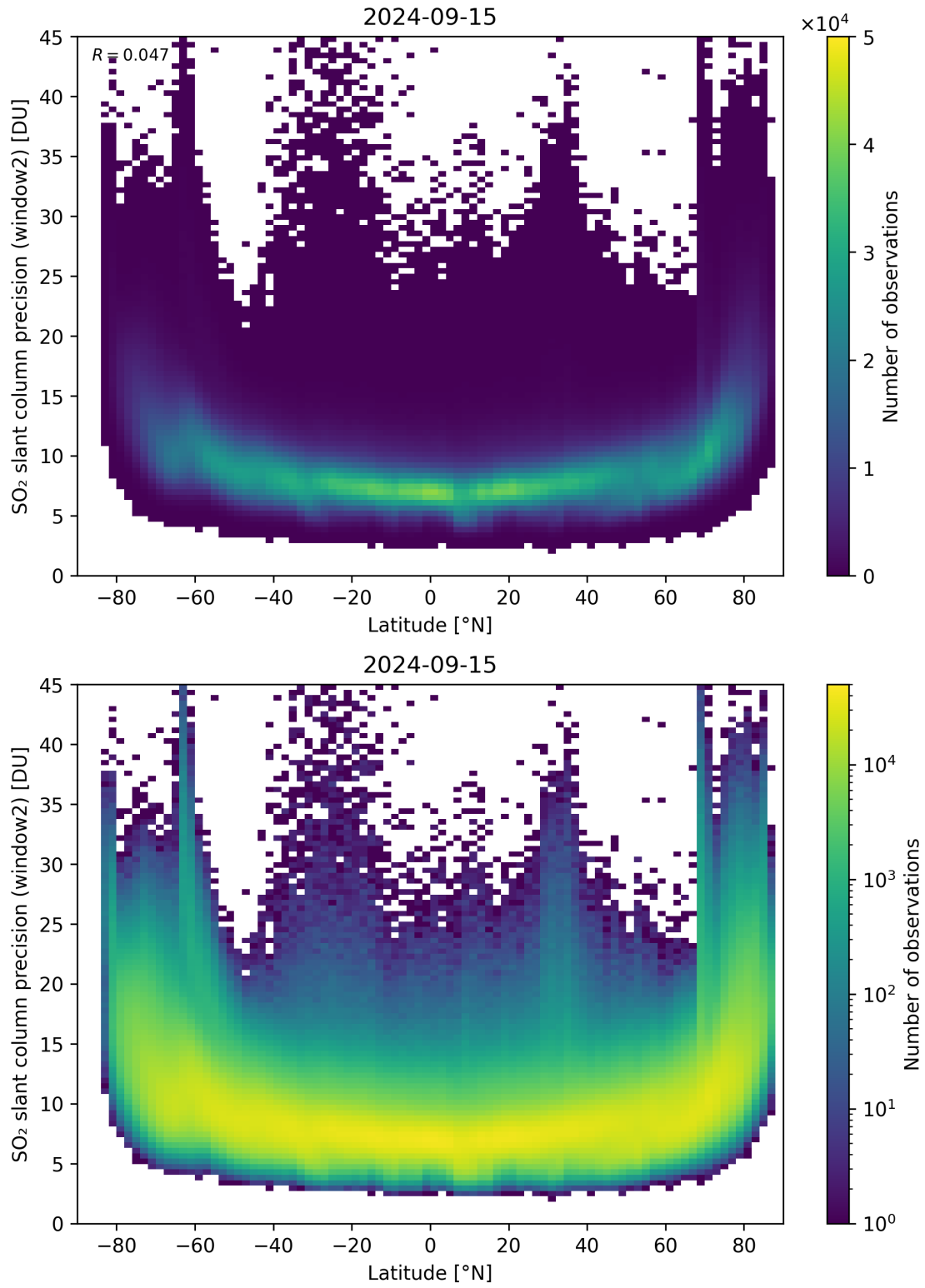
Figure 151: Scatter density plot of “Latitude” against “SO 2 slant column precision (window2)” for 2024-09-14 to 2024-09-16.
