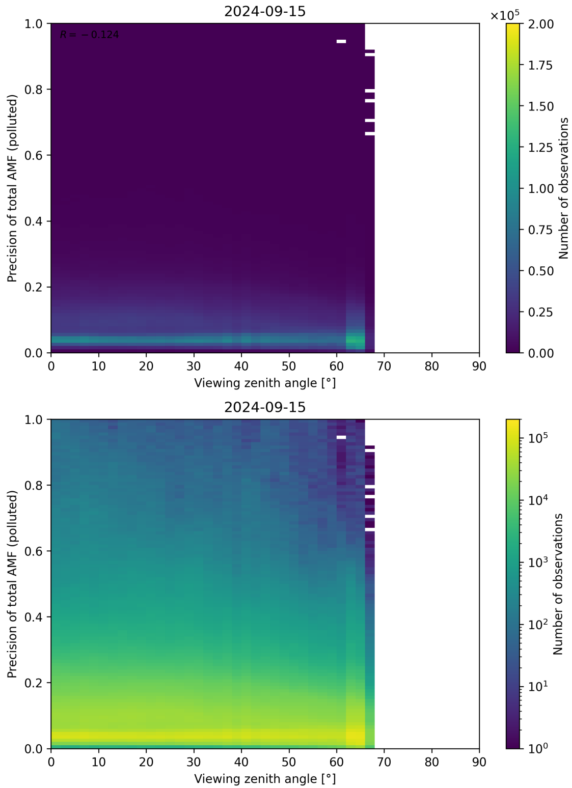
Figure 326: Scatter density plot of “Viewing zenith angle” against “Precision of total AMF (polluted)” for 2024-09-14 to 2024-09-16.
