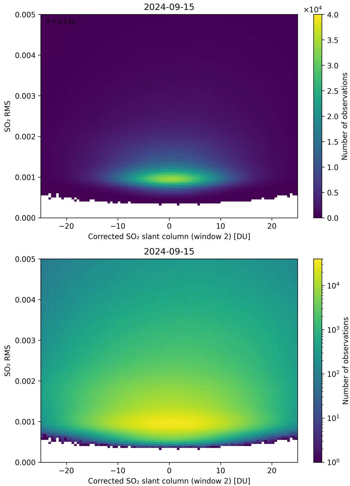
Figure 198: Scatter density plot of “Corrected SO 2 slant column (window 2)” against “SO 2 RMS” for 2024-09-14 to 2024-09-16.
