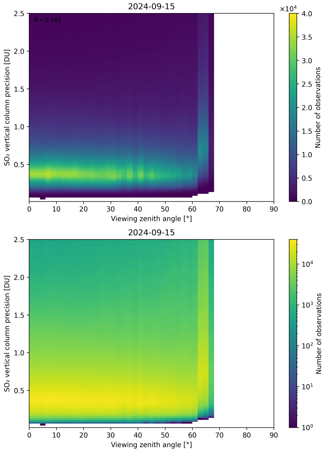
Figure 328: Scatter density plot of “Viewing zenith angle” against “SO 2 vertical column precision” for 2024-09-14 to 2024-09-16.
