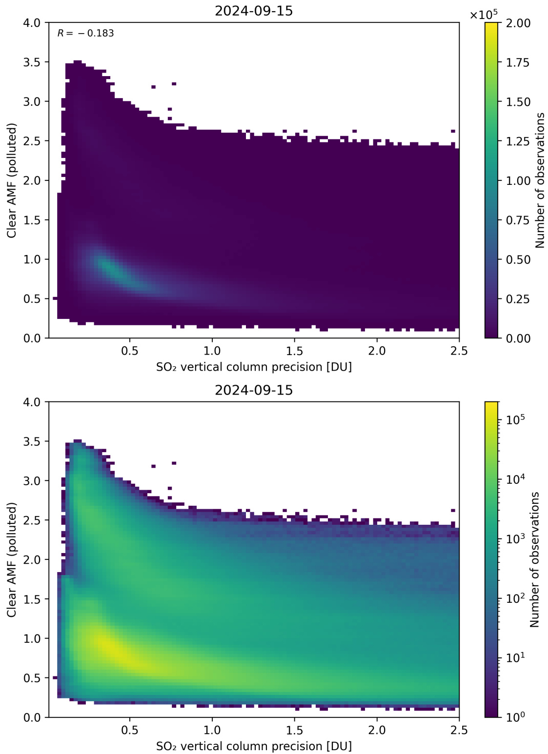
Figure 285: Scatter density plot of “SO 2 vertical column precision” against “Clear AMF (polluted)” for 2024-09-14 to 2024-09-16.
