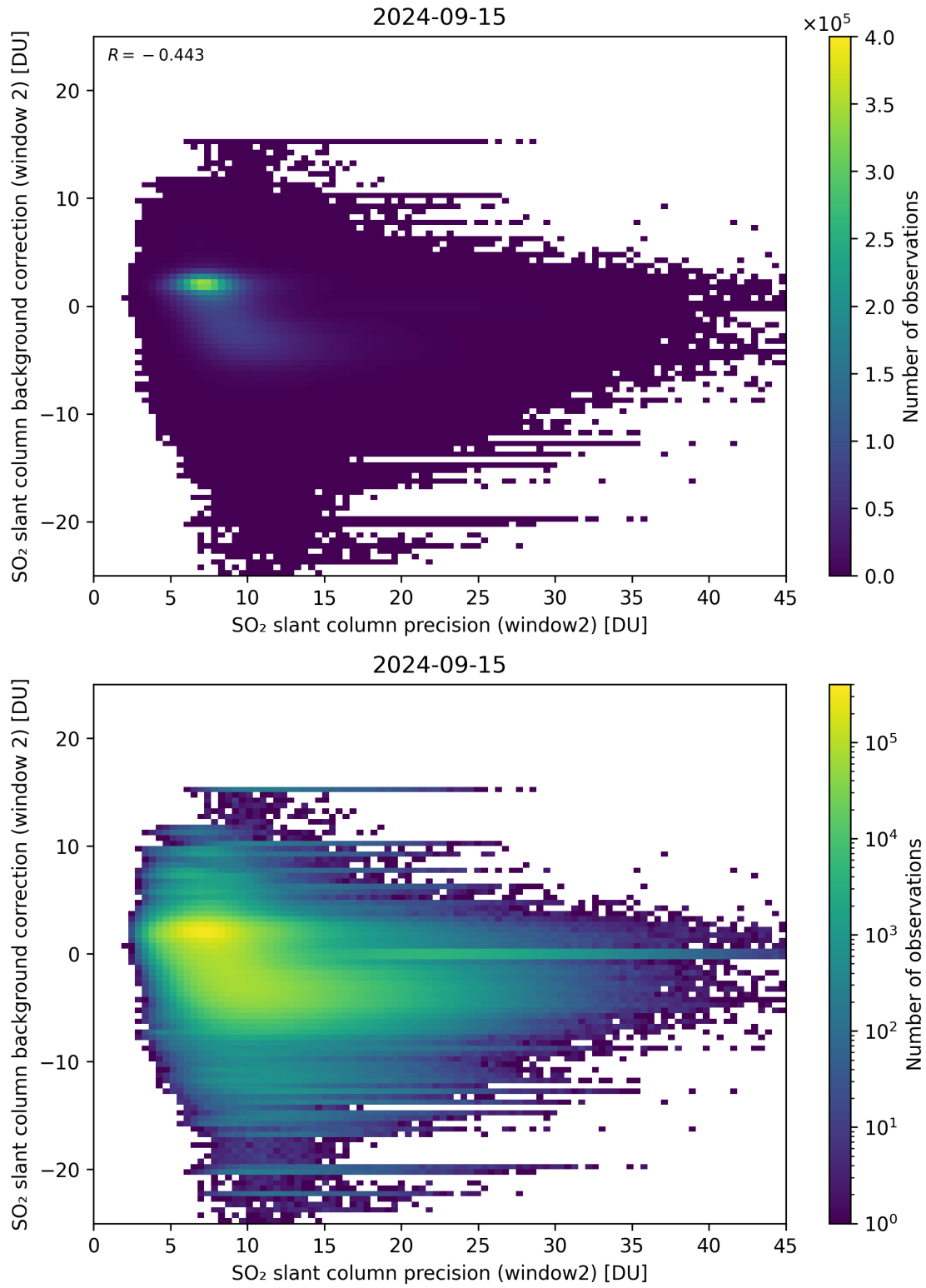
Figure 241: Scatter density plot of “SO 2 slant column precision (window2)” against “SO 2 slant column background correction (window 2)” for 2024-09-14 to 2024-09-16.
