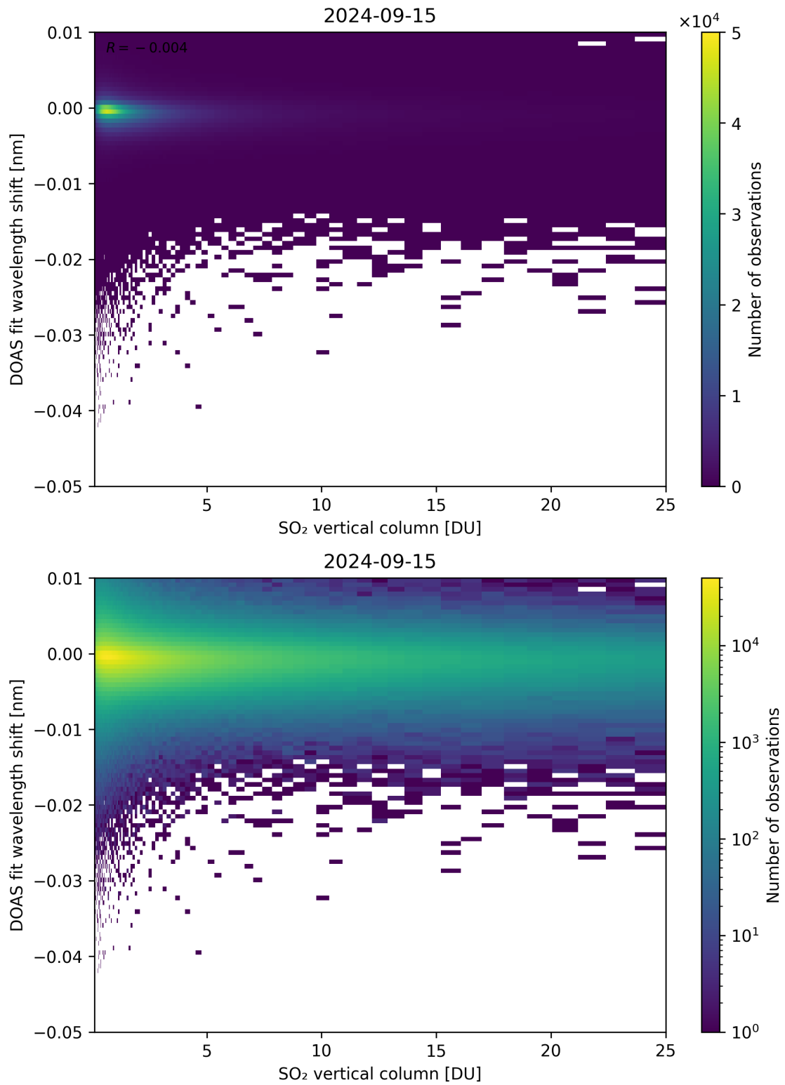
Figure 276: Scatter density plot of “SO 2 vertical column” against “DOAS fit wavelength shift” for 2024-09-14 to 2024-09-16.
