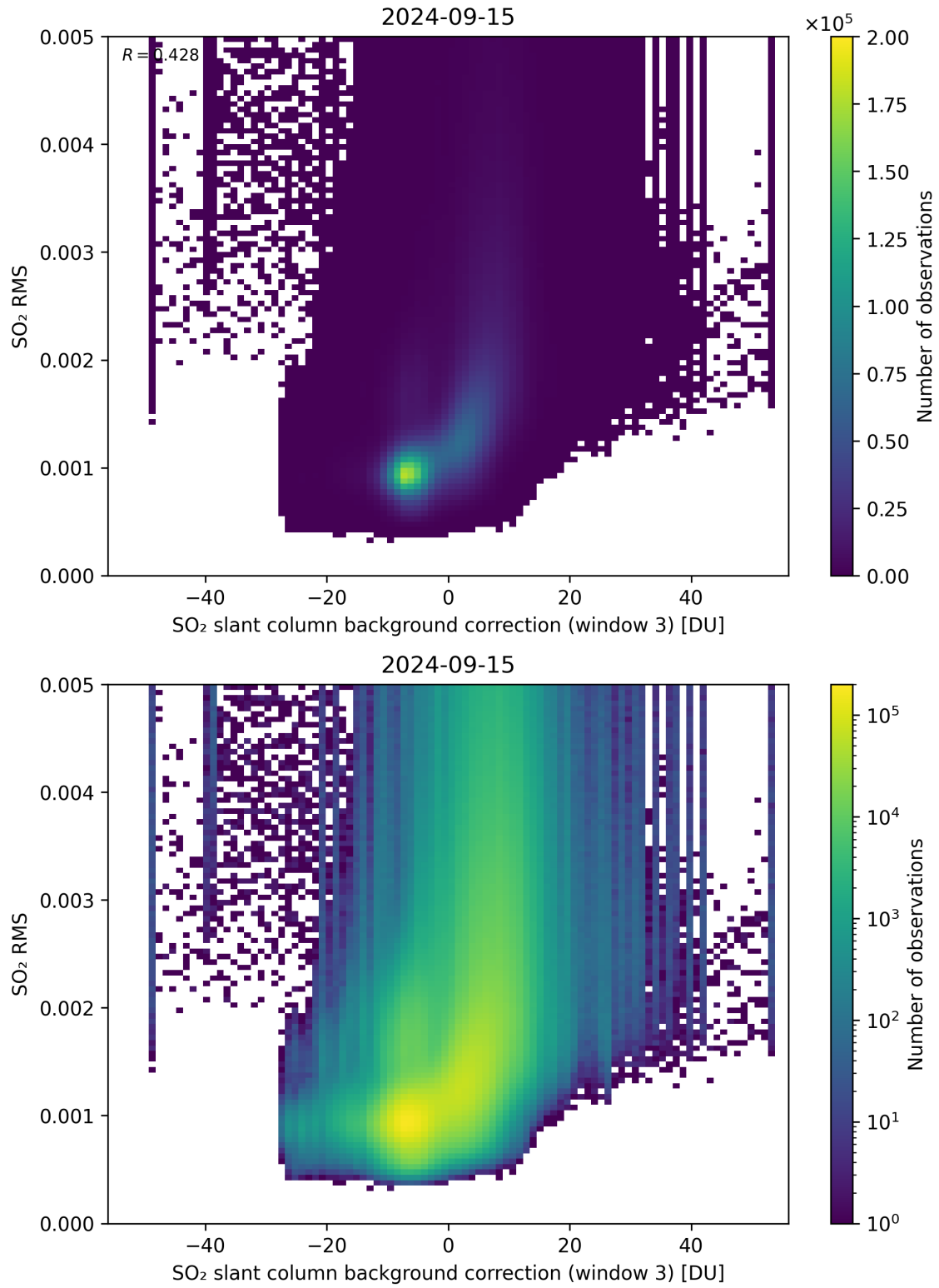
Figure 123: Scatter density plot of “SO 2 slant column background correction (window 3)” against “SO 2 RMS” for 2024-09-14 to 2024-09-16.
