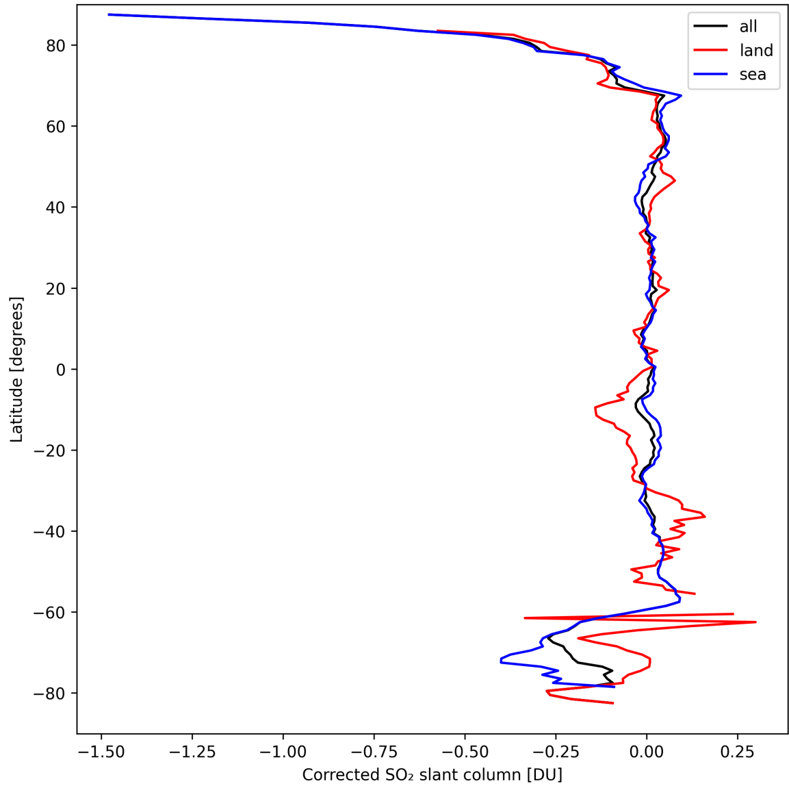
Figure 32: Zonal average of “Corrected SO 2 slant column” for 2024-09-14 to 2024-09-16.
