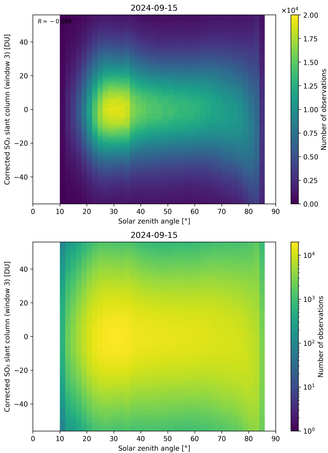
Figure 168: Scatter density plot of “Solar zenith angle” against “Corrected SO 2 slant column (window 3)” for 2024-09-14 to 2024-09-16.
