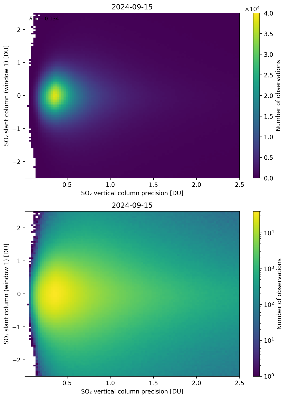
Figure 289: Scatter density plot of “SO 2 vertical column precision” against “SO 2 slant column (window 1)” for 2024-09-14 to 2024-09-16.
