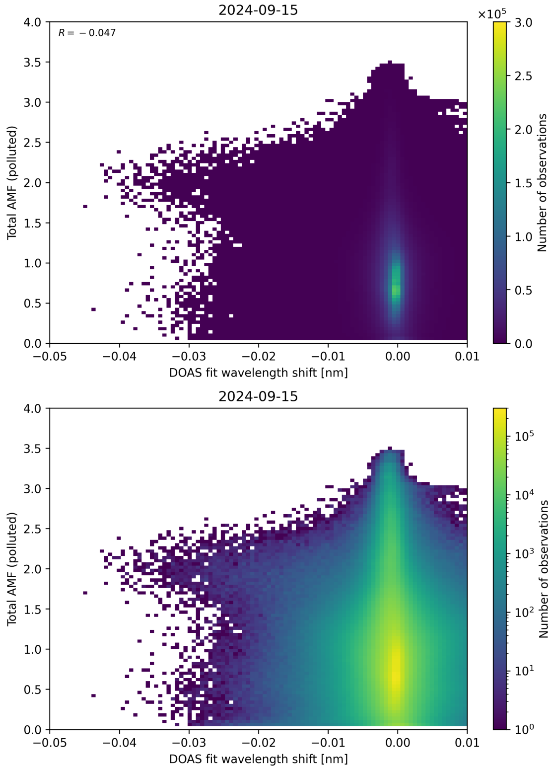
Figure 130: Scatter density plot of “DOAS fit wavelength shift” against “Total AMF (polluted)” for 2024-09-14 to 2024-09-16.
