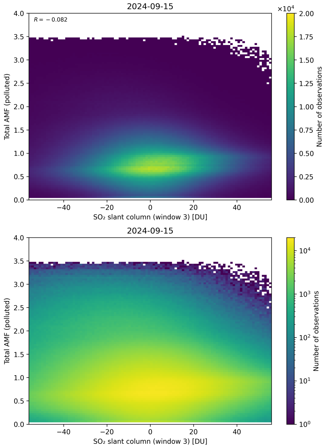
Figure 268: Scatter density plot of “SO 2 slant column (window 3)” against “Total AMF (polluted)” for 2024-09-14 to 2024-09-16.
