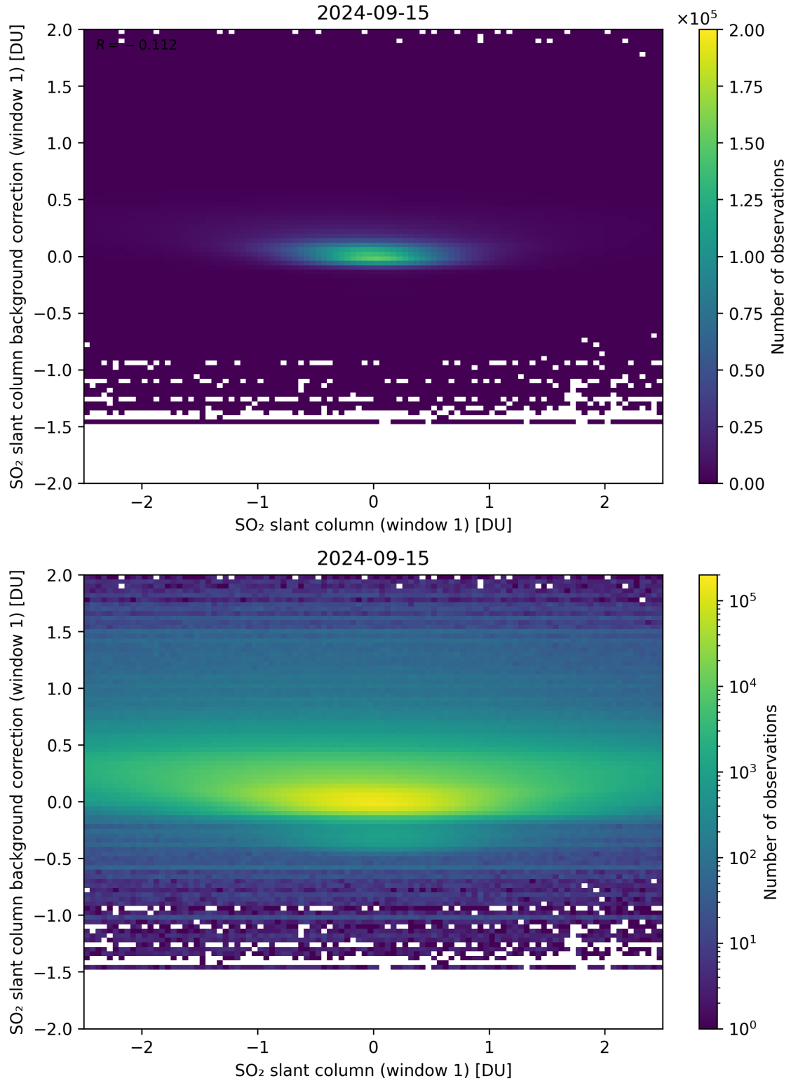
Figure 212: Scatter density plot of “SO 2 slant column (window 1)” against “SO 2 slant column background correction (window 1)” for 2024-09-14 to 2024-09-16.
