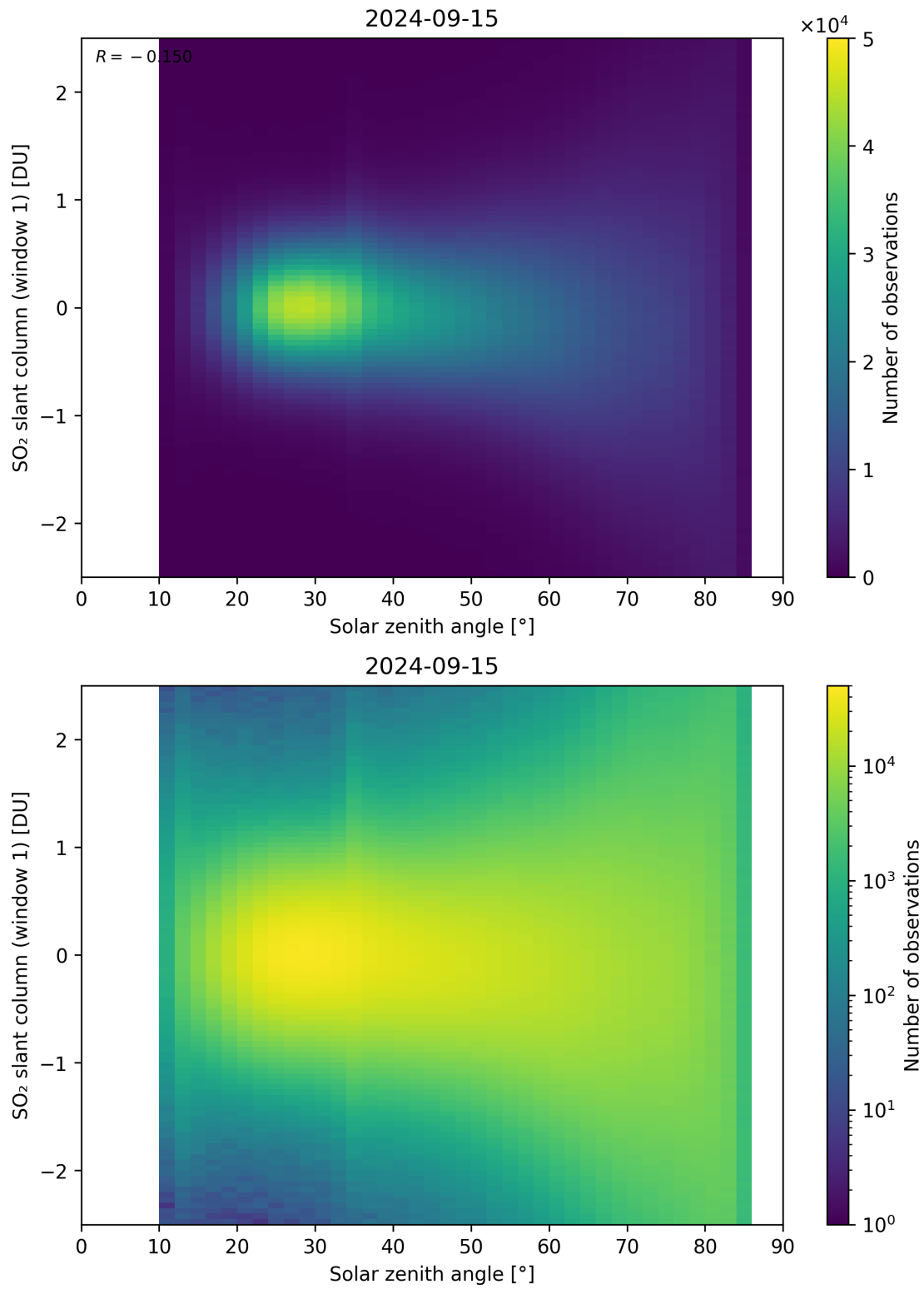
Figure 169: Scatter density plot of “Solar zenith angle” against “SO 2 slant column (window 1)” for 2024-09-14 to 2024-09-16.
