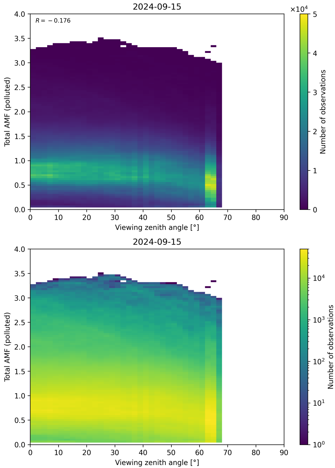
Figure 325: Scatter density plot of “Viewing zenith angle” against “Total AMF (polluted)” for 2024-09-14 to 2024-09-16.
