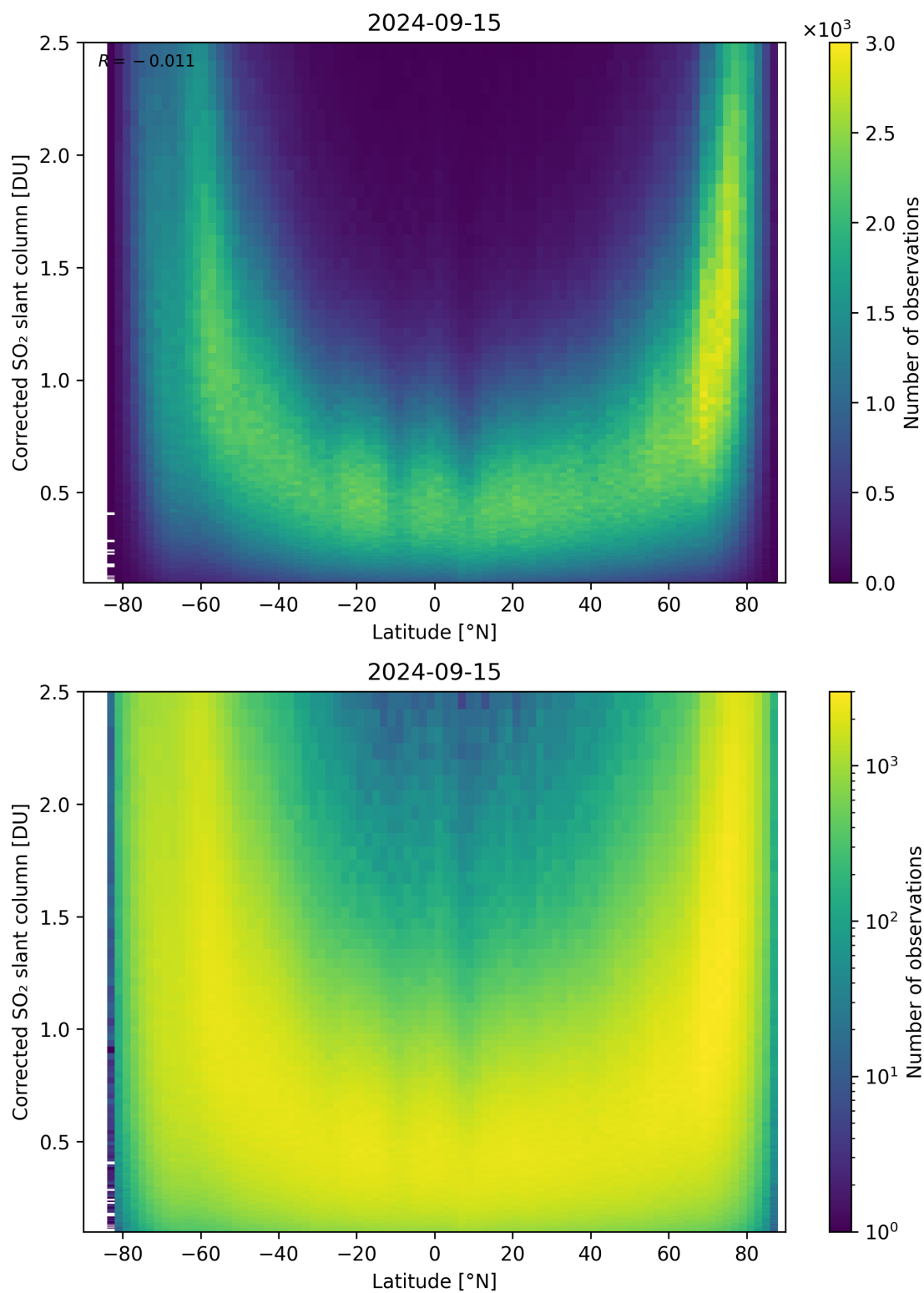
Figure 146: Scatter density plot of “Latitude” against “Corrected SO 2 slant column” for 2024-09-14 to 2024-09-16.
