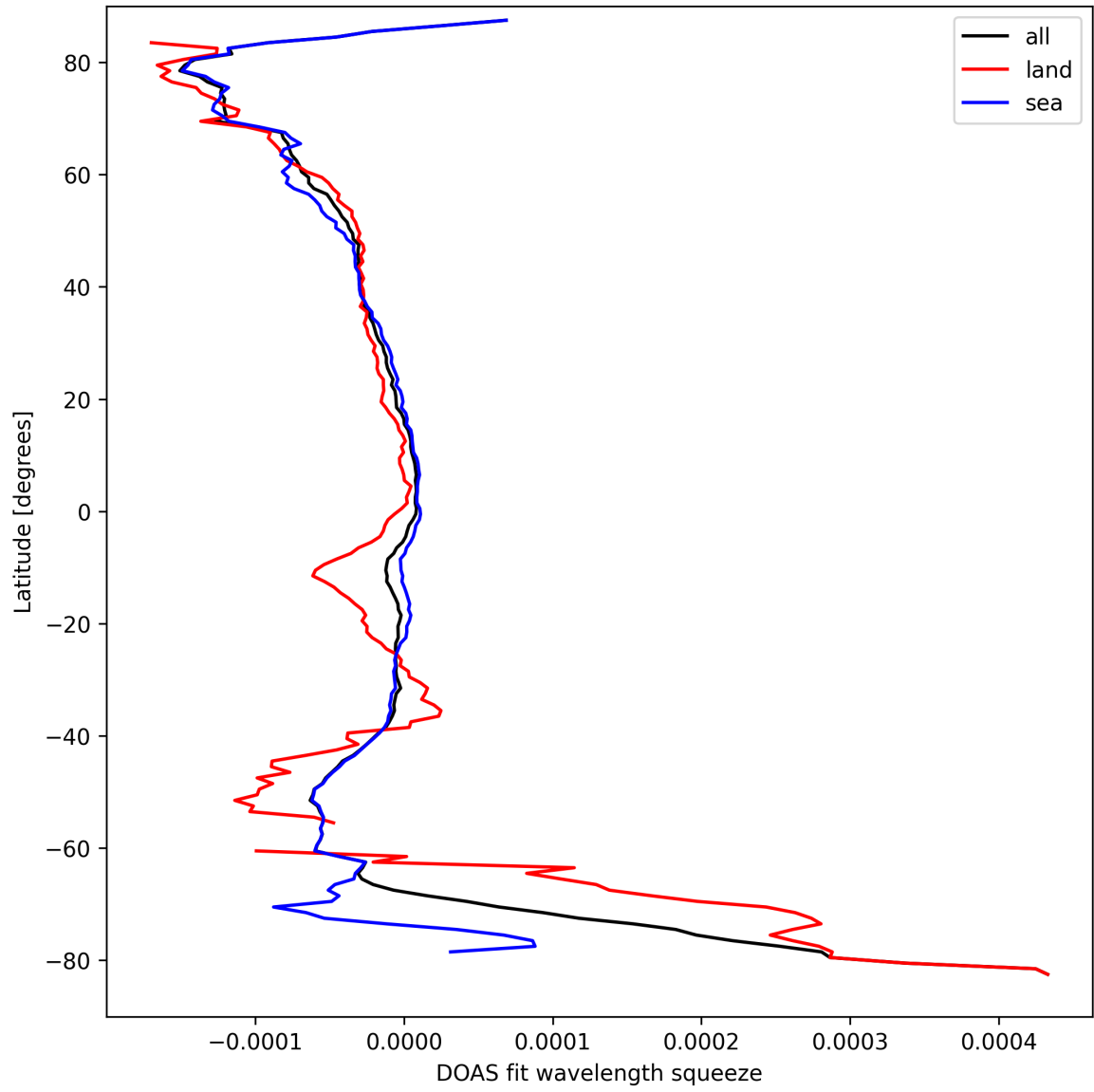
Figure 46: Zonal average of “DOAS fit wavelength squeeze” for 2024-09-14 to 2024-09-16.
