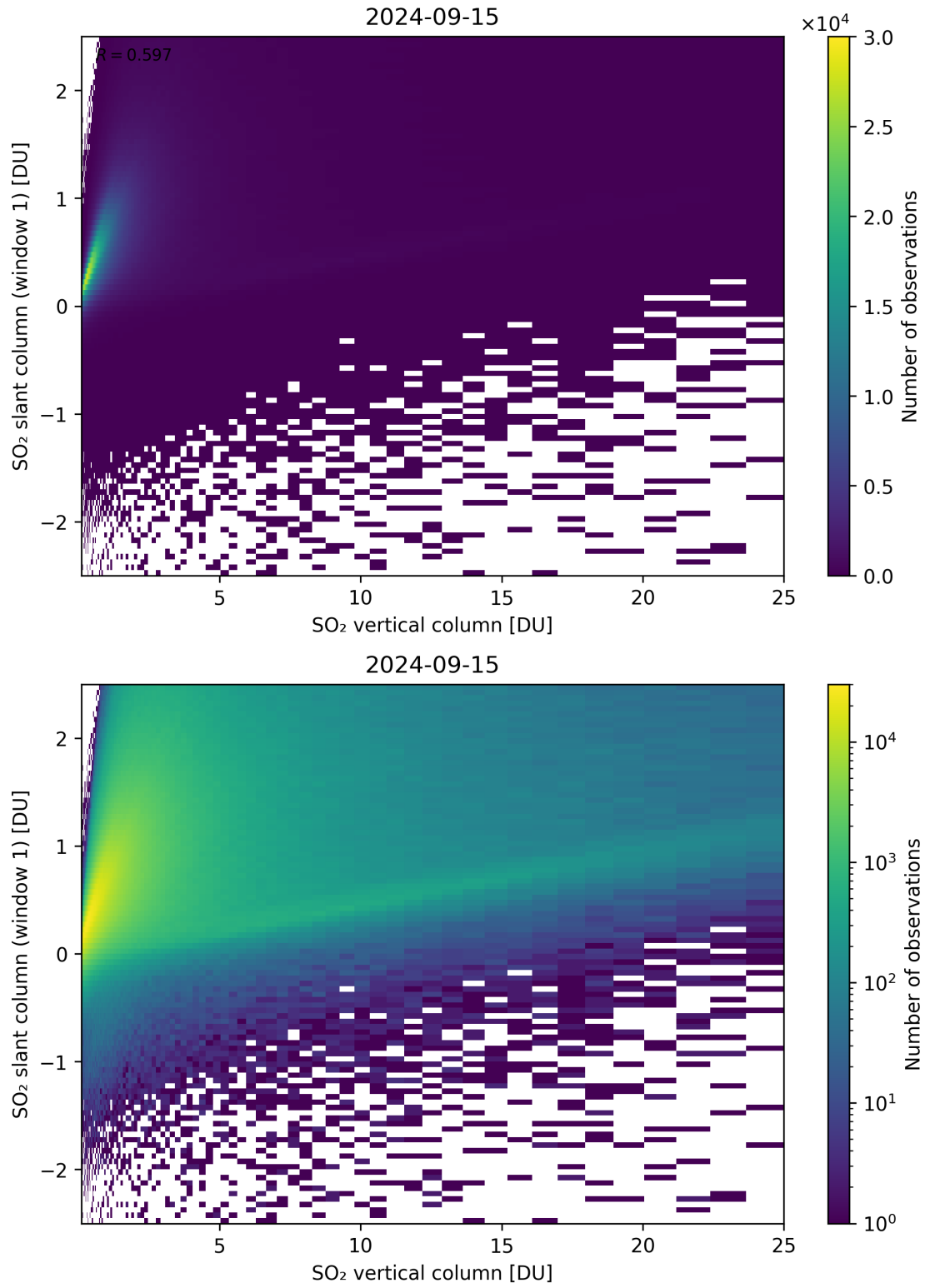
Figure 300: Scatter density plot of “SO 2 vertical column” against “SO 2 slant column (window 1)” for 2024-09-14 to 2024-09-16.
