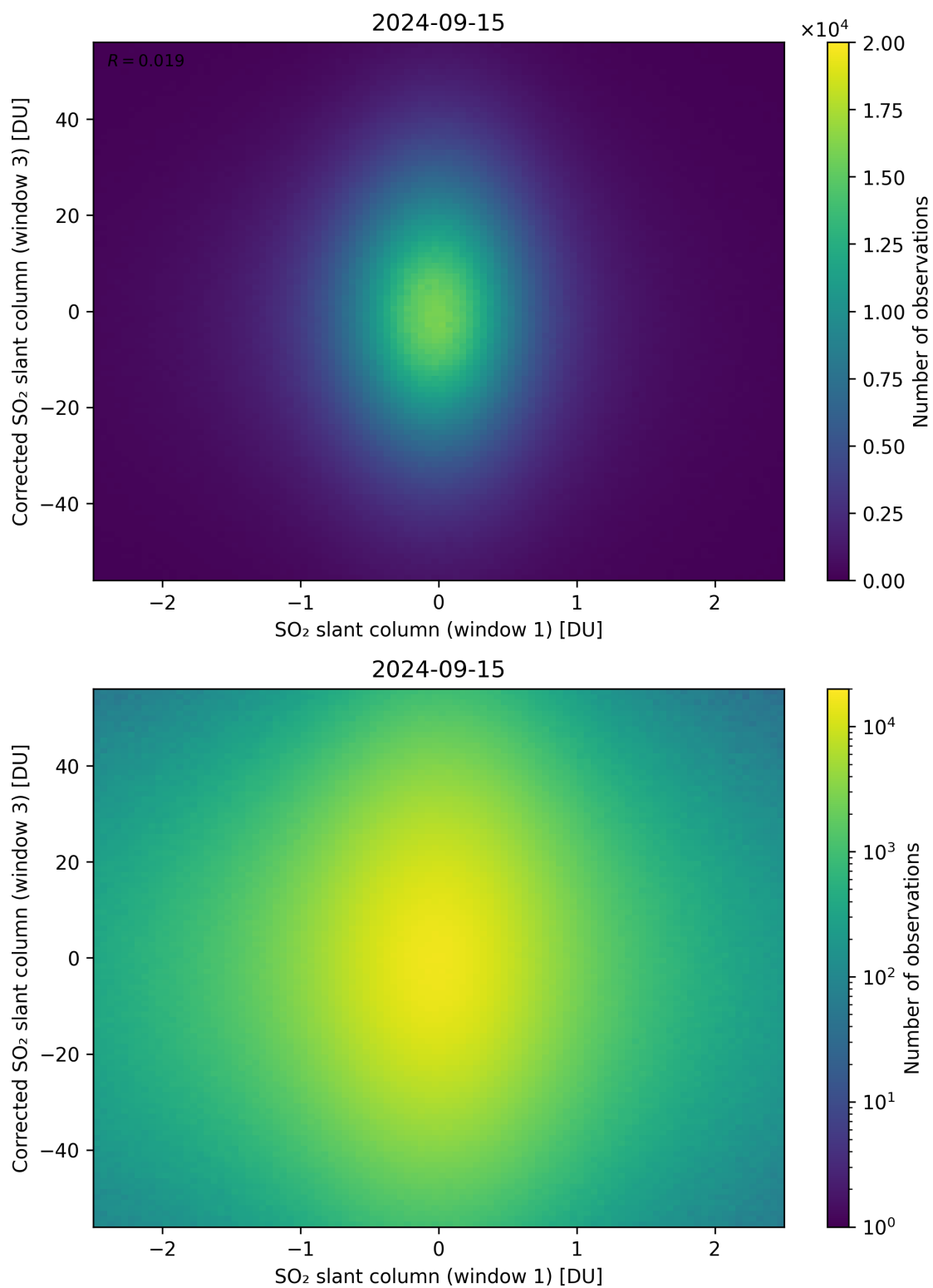
Figure 234: Scatter density plot of “SO 2 slant column (window 1)” against “Corrected SO 2 slant column (window 3)” for 2024-09-14 to 2024-09-16.
