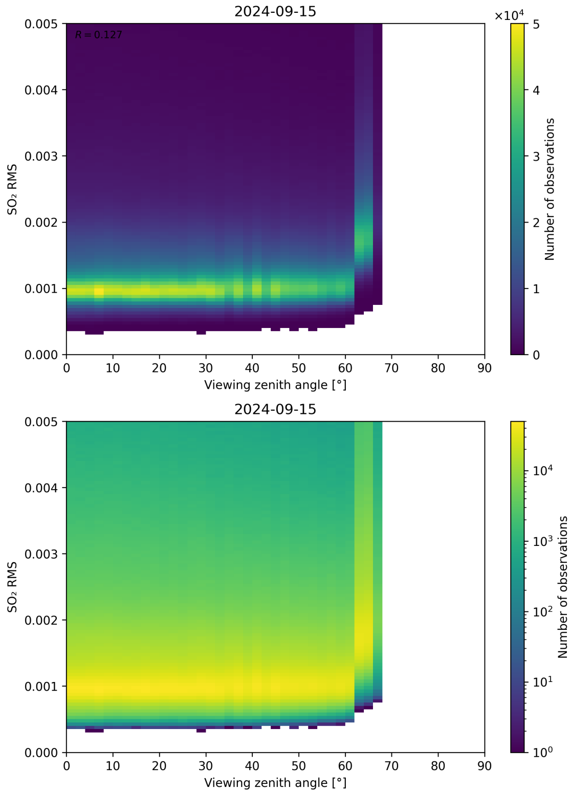
Figure 313: Scatter density plot of “Viewing zenith angle” against “SO 2 RMS” for 2024-09-14 to 2024-09-16.
