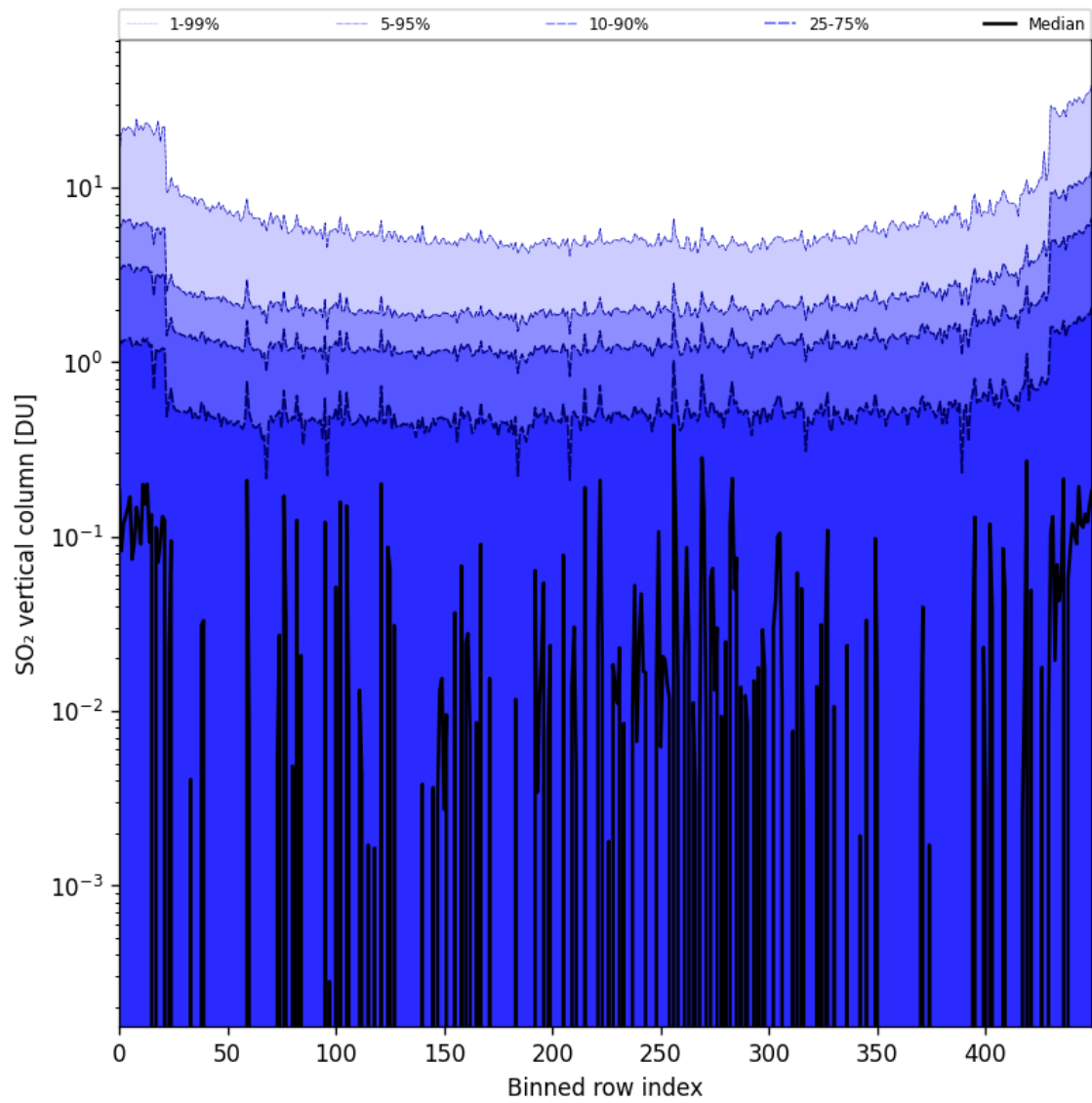
Figure 76: Along track statistics of “SO 2 vertical column” for 2024-09-14 to 2024-09-16
