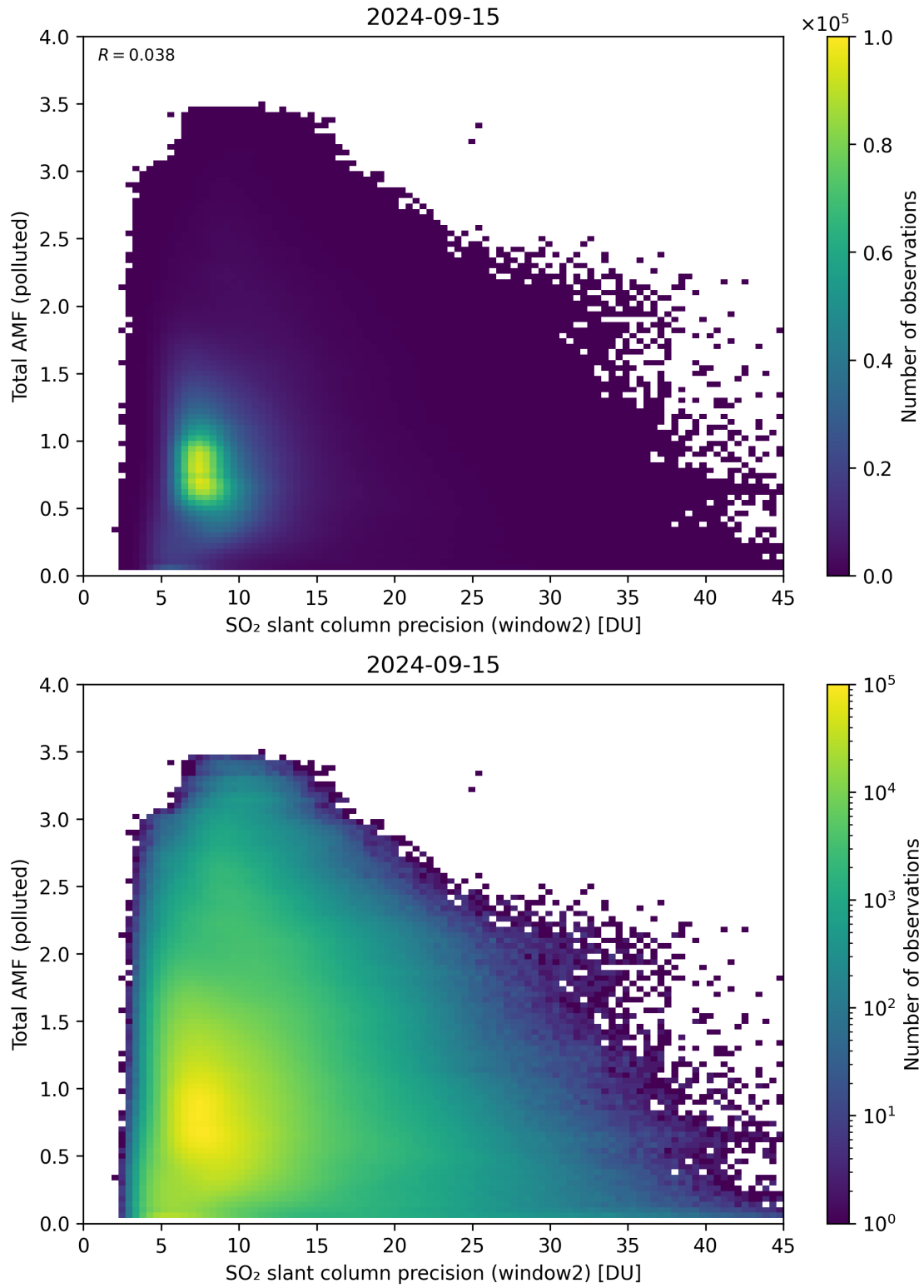
Figure 251: Scatter density plot of “SO 2 slant column precision (window2)” against “Total AMF (polluted)” for 2024-09-14 to 2024-09-16.
