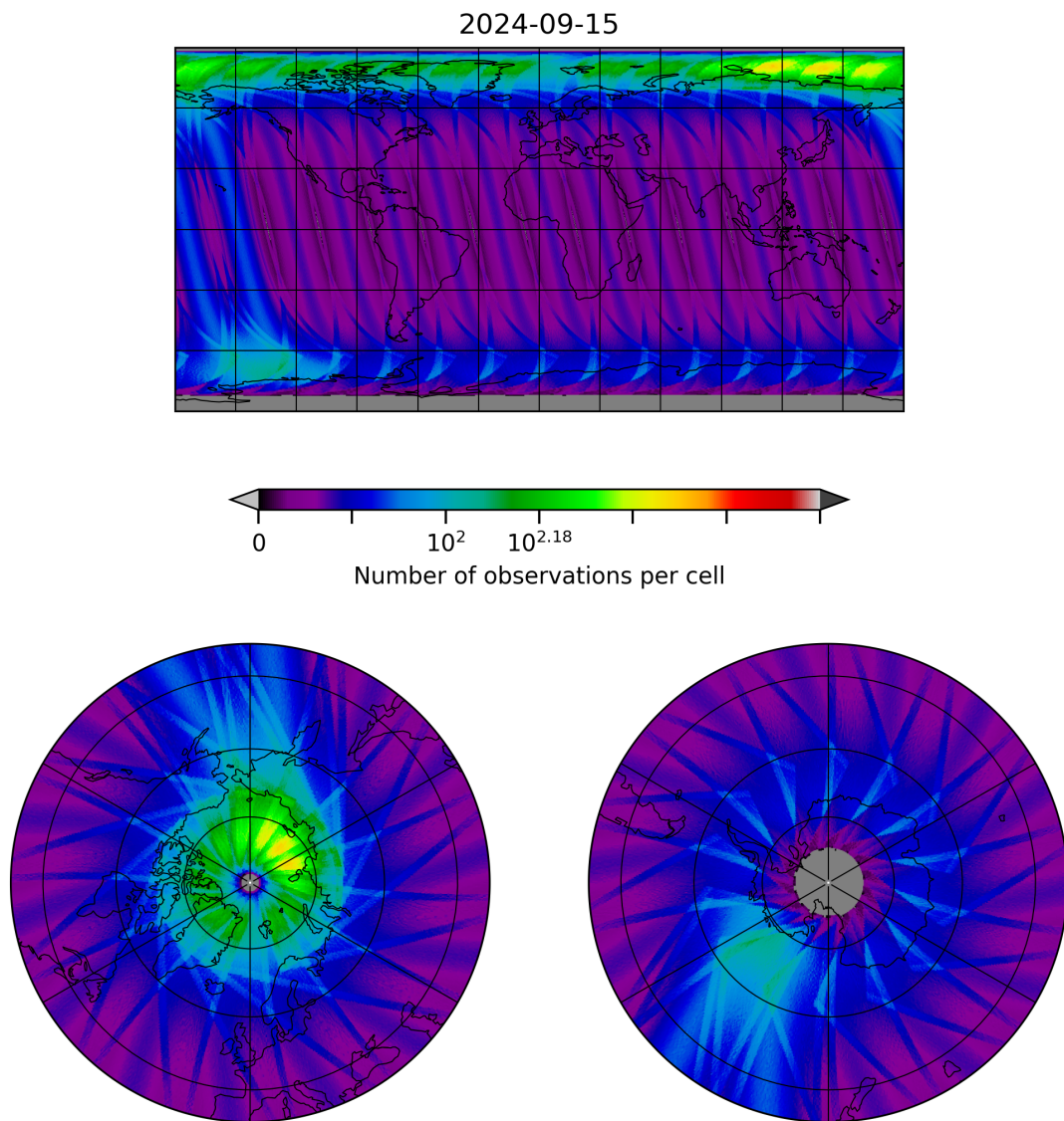
Figure 28: Map of the number of observations for 2024-09-14 to 2024-09-16
