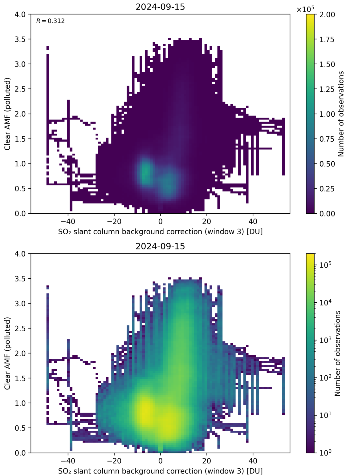
Figure 124: Scatter density plot of “SO 2 slant column background correction (window 3)” against “Clear AMF (polluted)” for 2024-09-14 to 2024-09-16.
