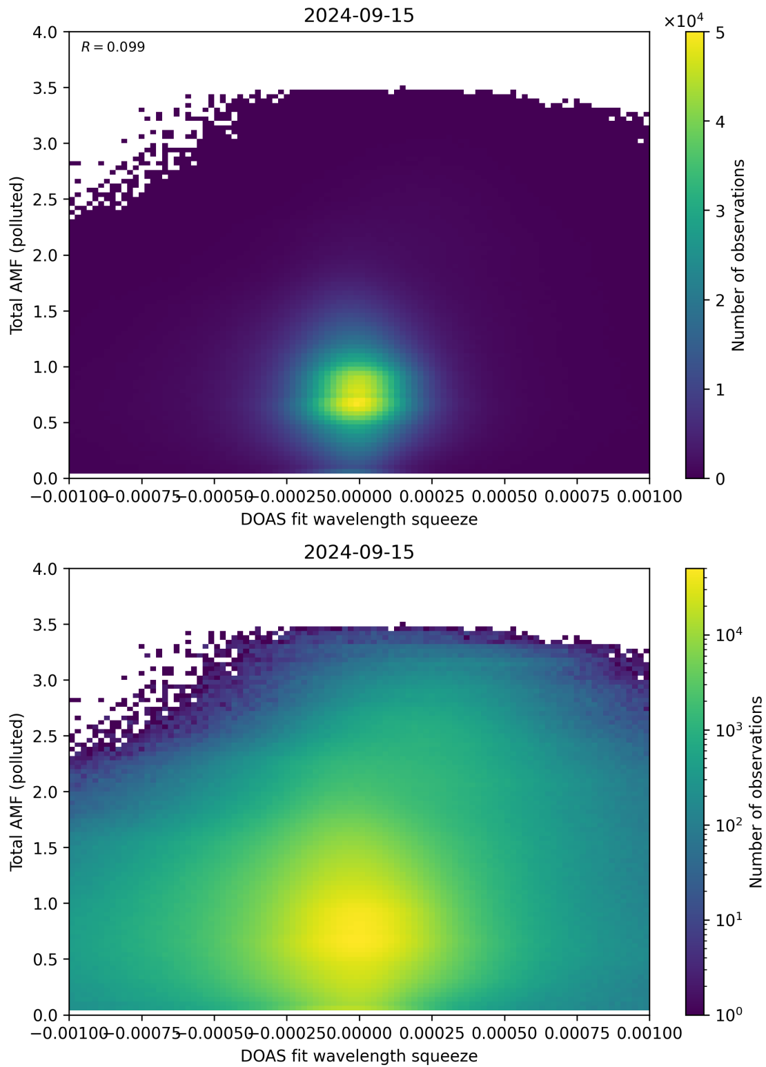
Figure 134: Scatter density plot of “DOAS fit wavelength squeeze” against “Total AMF (polluted)” for 2024-09-14 to 2024-09-16.
