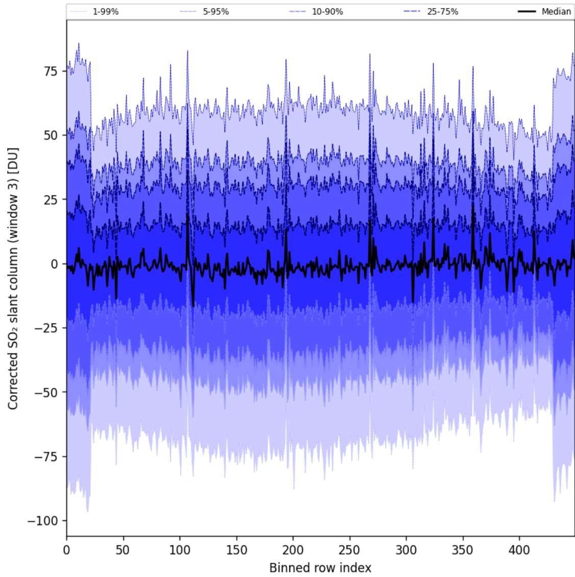
Figure 89: Along track statistics of “Corrected SO 2 slant column (window 3)” for 2024-09-14 to 2024-09-16
