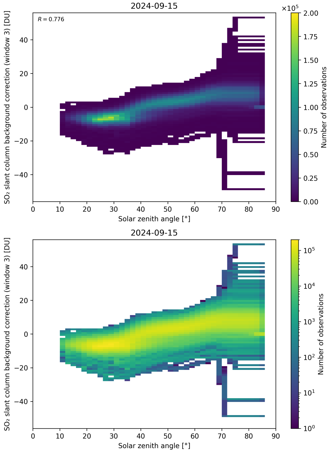
Figure 160: Scatter density plot of “Solar zenith angle” against “SO 2 slant column background correction (window 3)” for 2024-09-14 to 2024-09-16.
