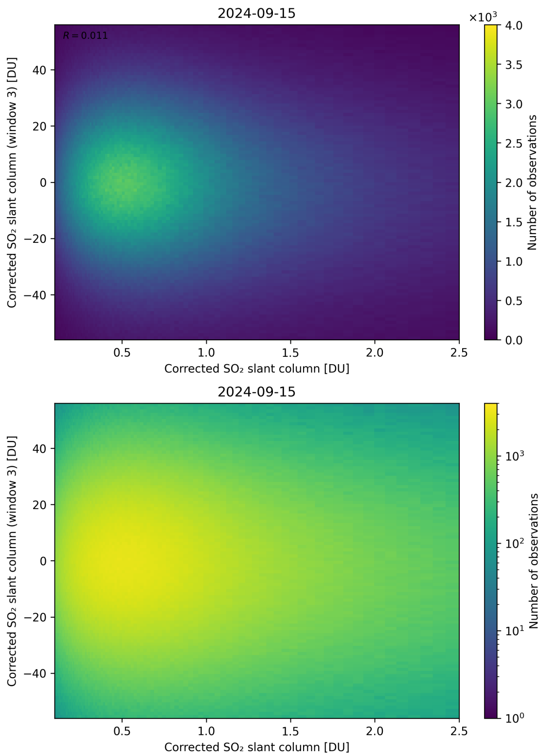
Figure 186: Scatter density plot of “Corrected SO 2 slant column” against “Corrected SO 2 slant column (window 3)” for 2024-09-14 to 2024-09-16.
