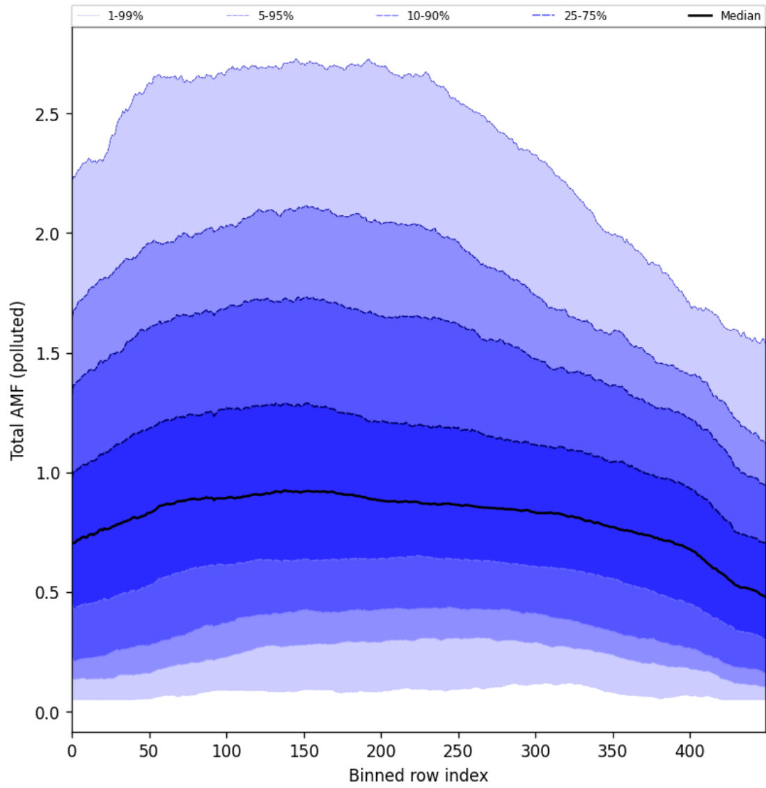
Figure 94: Along track statistics of “Total AMF (polluted)” for 2024-09-14 to 2024-09-16
