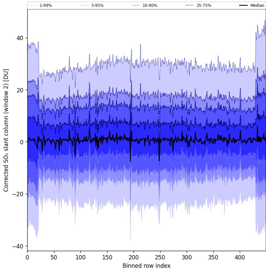
Figure 85: Along track statistics of “Corrected SO 2 slant column (window 2)” for 2024-09-14 to 2024-09-16
