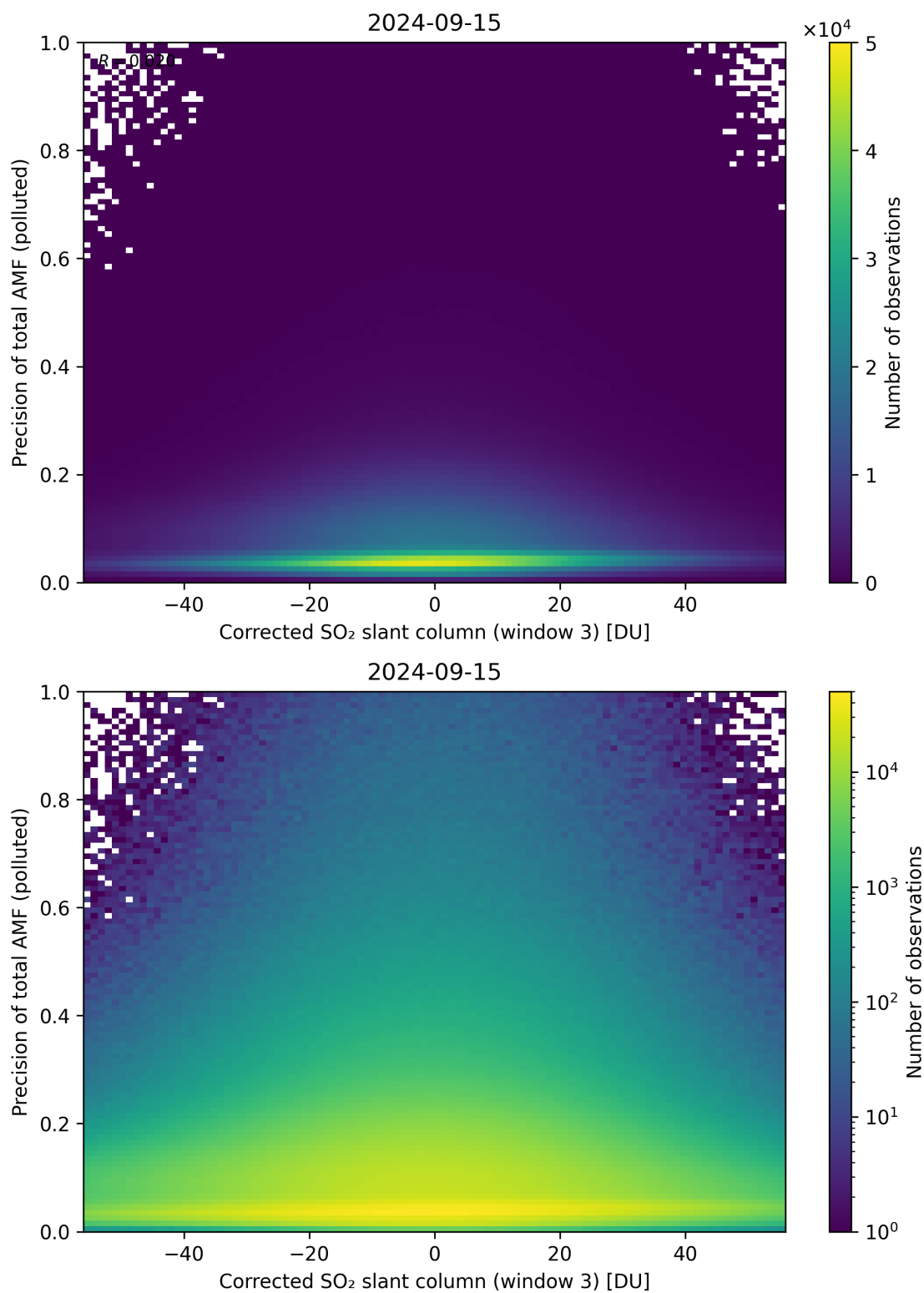
Figure 211: Scatter density plot of “Corrected SO 2 slant column (window 3)” against “Precision of total AMF (polluted)” for 2024-09-14 to 2024-09-16.
