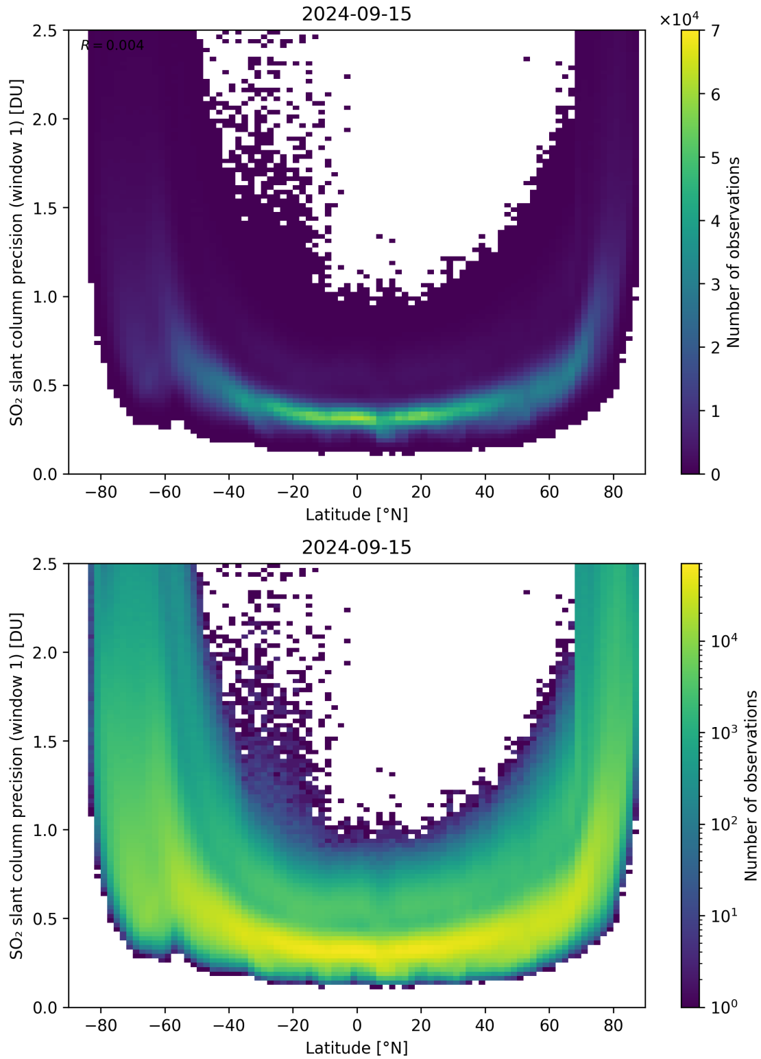
Figure 150: Scatter density plot of “Latitude” against “SO 2 slant column precision (window 1)” for 2024-09-14 to 2024-09-16.
