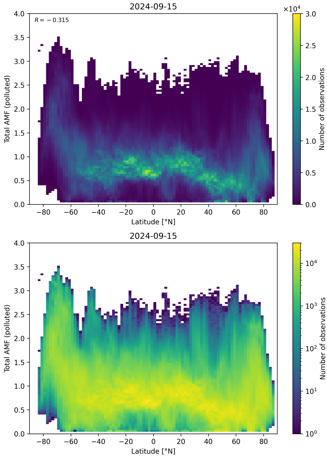
Figure 154: Scatter density plot of “Latitude” against “Total AMF (polluted)” for 2024-09-14 to 2024-09-16.
