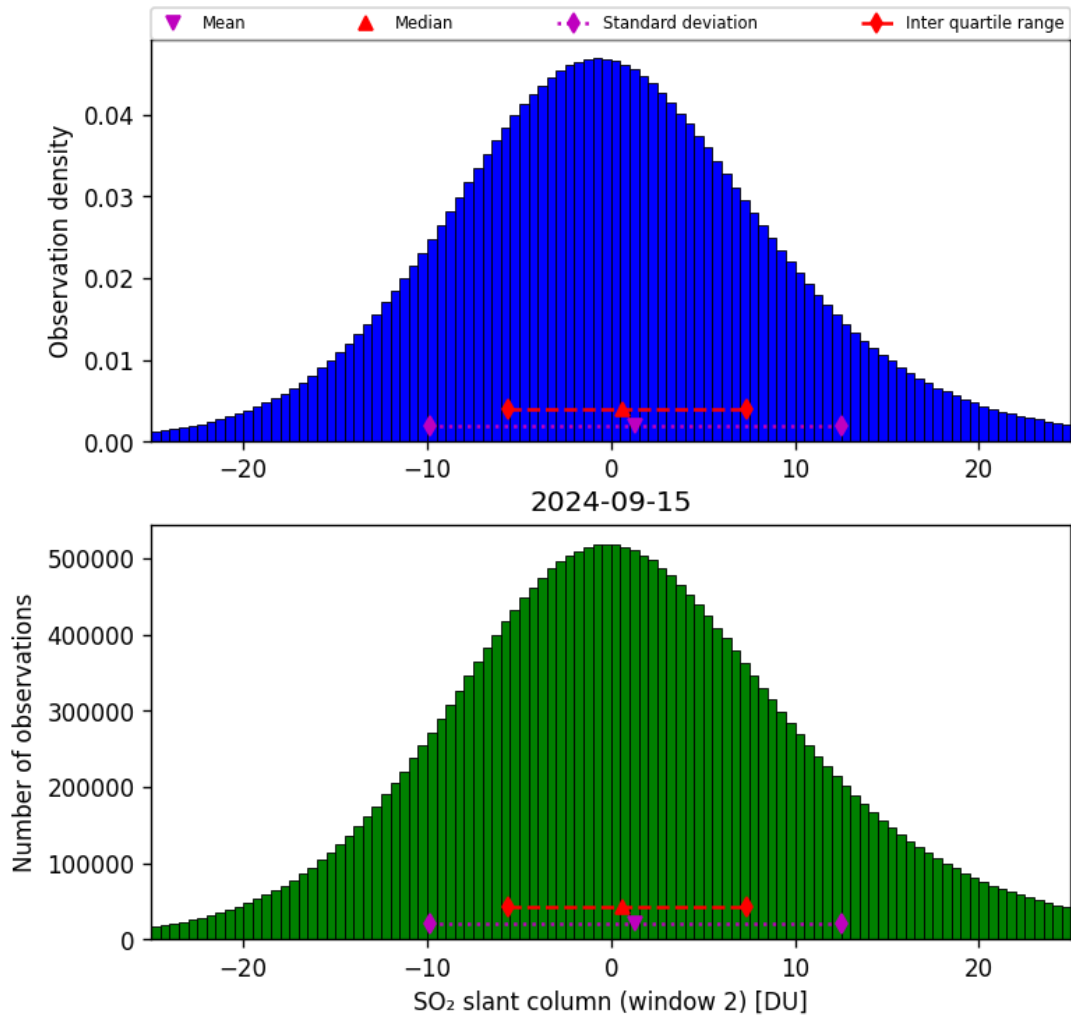
Figure 60: Histogram of “SO 2 slant column (window 2)” for 2024-09-14 to 2024-09-16
