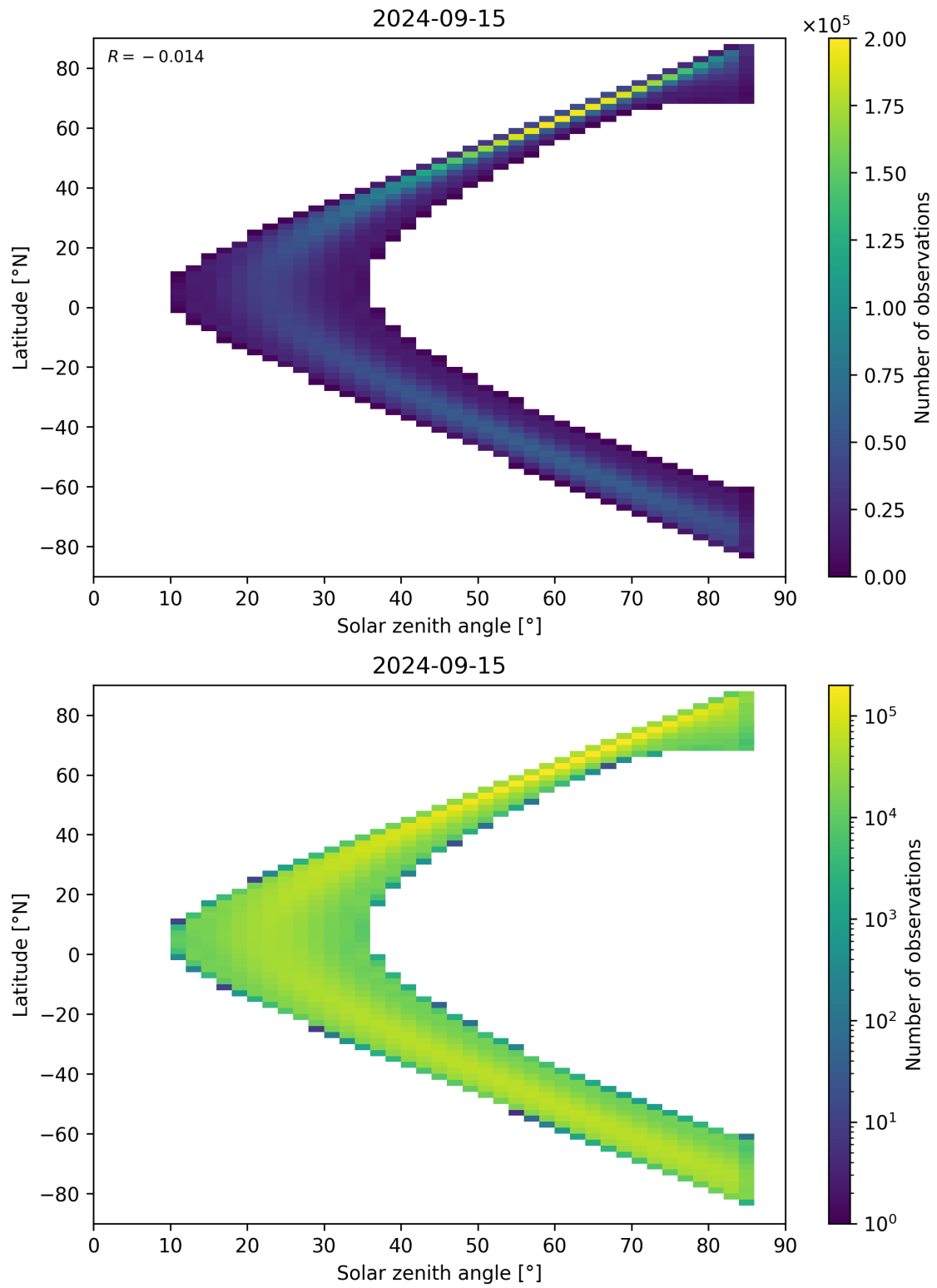
Figure 164: Scatter density plot of “Solar zenith angle” against “Latitude” for 2024-09-14 to 2024-09-16.
