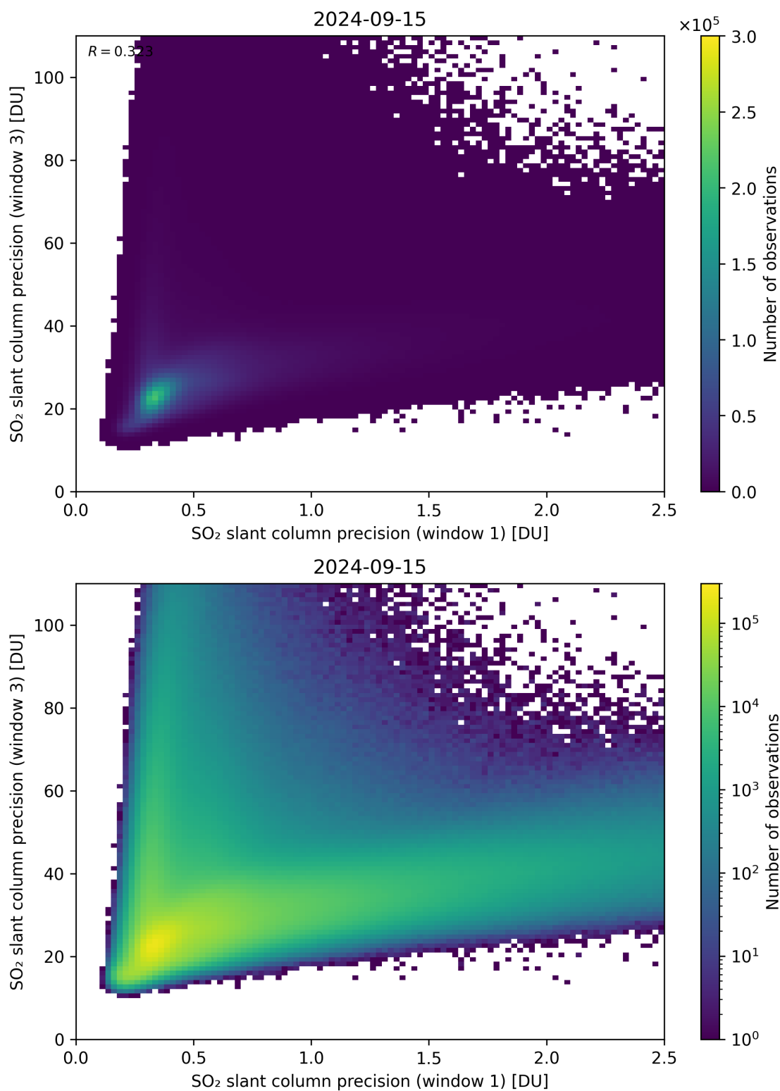
Figure 229: Scatter density plot of “SO 2 slant column precision (window 1)” against “SO 2 slant column precision (window 3)” for 2024-09-14 to 2024-09-16.
