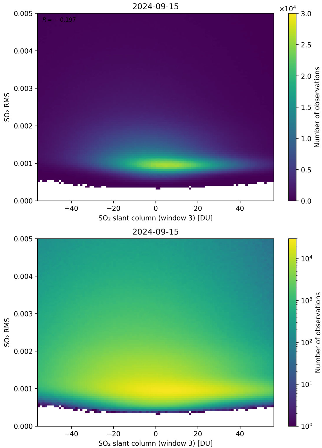
Figure 256: Scatter density plot of “SO 2 slant column (window 3)” against “SO 2 RMS” for 2024-09-14 to 2024-09-16.
