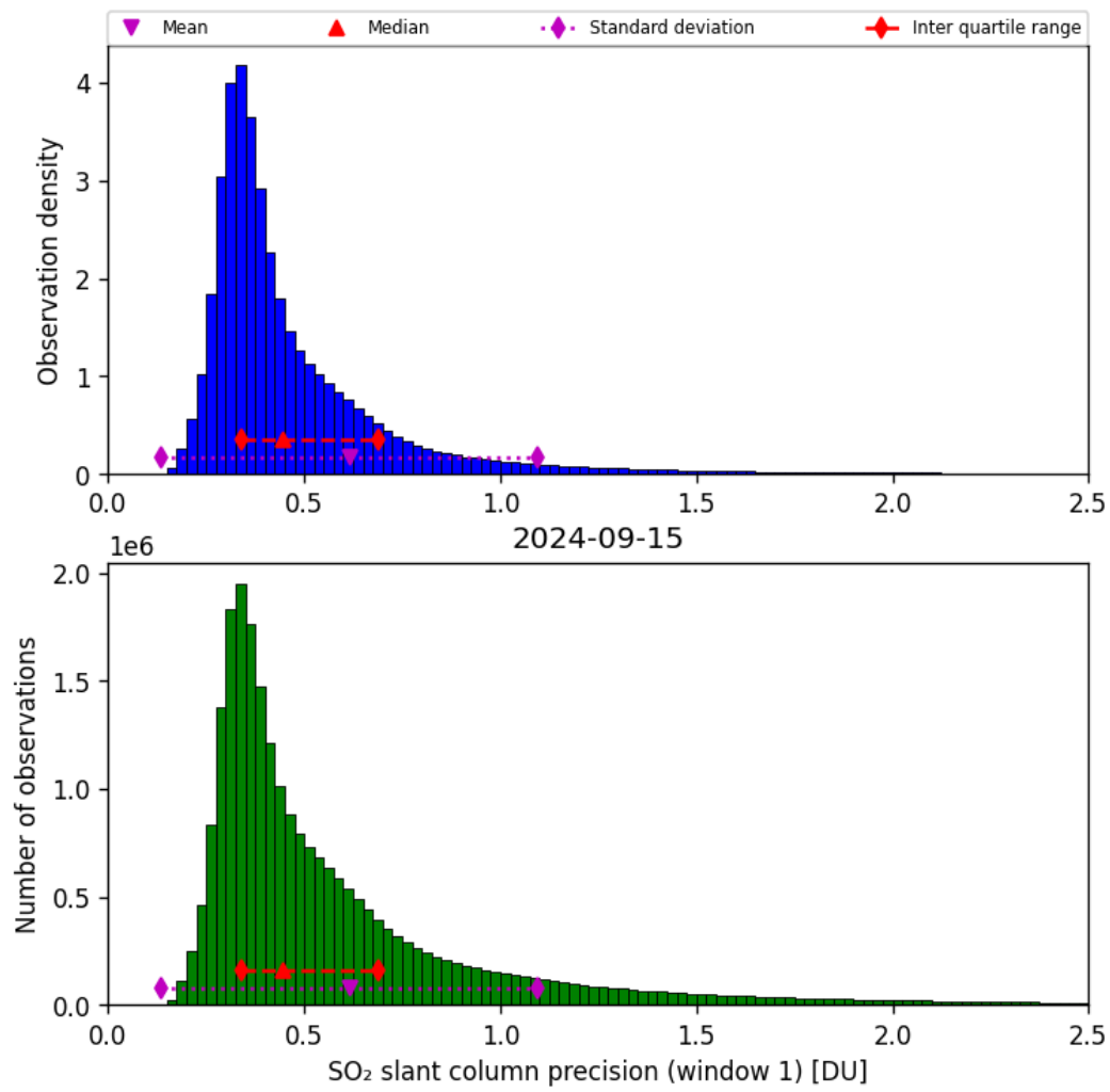
Figure 57: Histogram of “SO 2 slant column precision (window 1)” for 2024-09-14 to 2024-09-16
