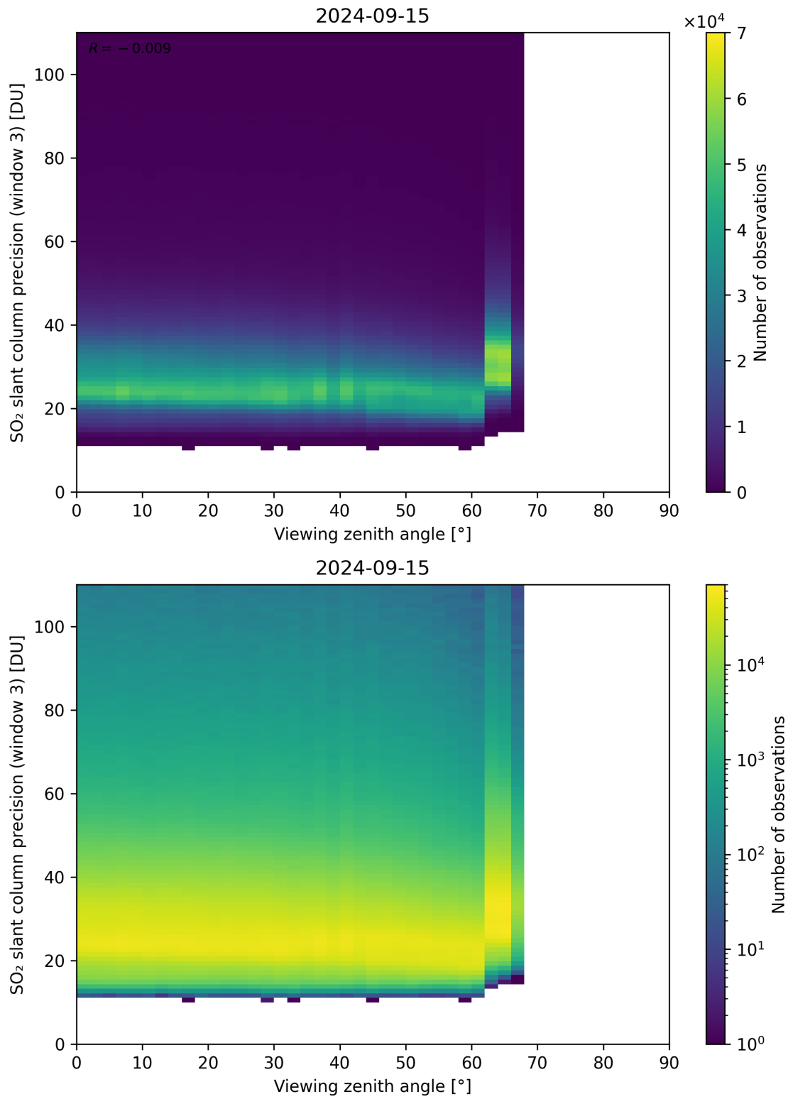
Figure 324: Scatter density plot of “Viewing zenith angle” against “SO 2 slant column precision (window 3)” for 2024-09-14 to 2024-09-16.
