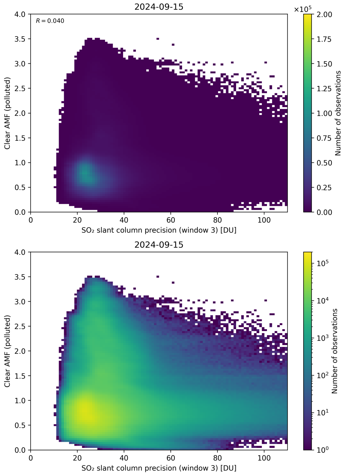
Figure 261: Scatter density plot of “SO 2 slant column precision (window 3)” against “Clear AMF (polluted)” for 2024-09-14 to 2024-09-16.
