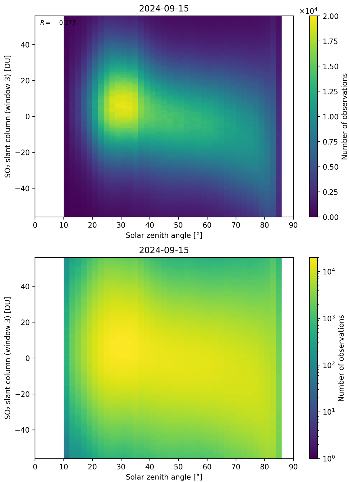
Figure 172: Scatter density plot of “Solar zenith angle” against “SO 2 slant column (window 3)” for 2024-09-14 to 2024-09-16.
