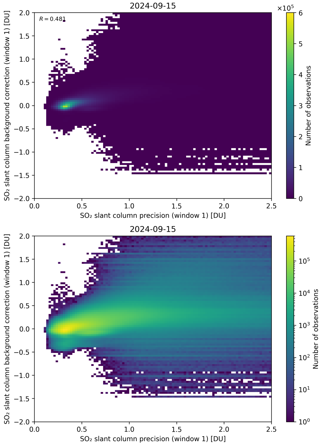
Figure 218: Scatter density plot of “SO 2 slant column precision (window 1)” against “SO 2 slant column background correction (window 1)” for 2024-09-14 to 2024-09-16.
