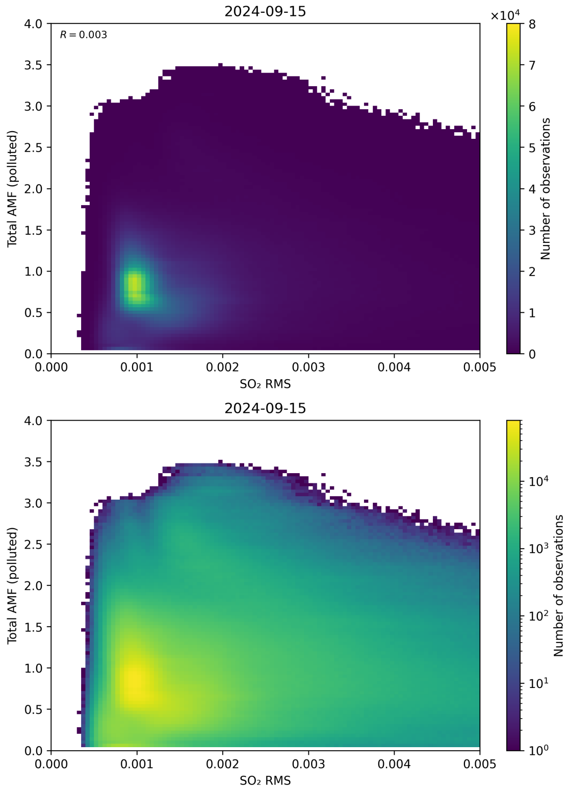
Figure 137: Scatter density plot of “SO 2 RMS” against “Total AMF (polluted)” for 2024-09-14 to 2024-09-16.
