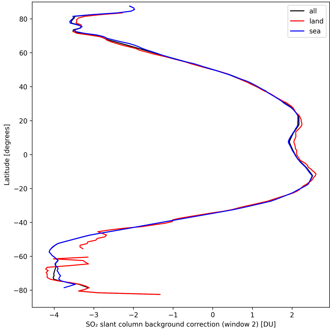
Figure 40: Zonal average of “SO 2 slant column background correction (window 2)” for 2024-09-14 to 2024-09-16.
