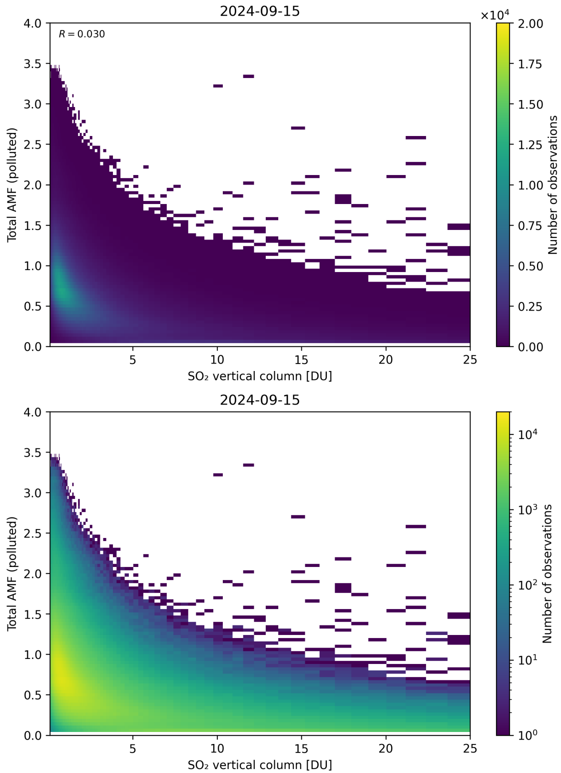
Figure 305: Scatter density plot of “SO 2 vertical column” against “Total AMF (polluted)” for 2024-09-14 to 2024-09-16.
