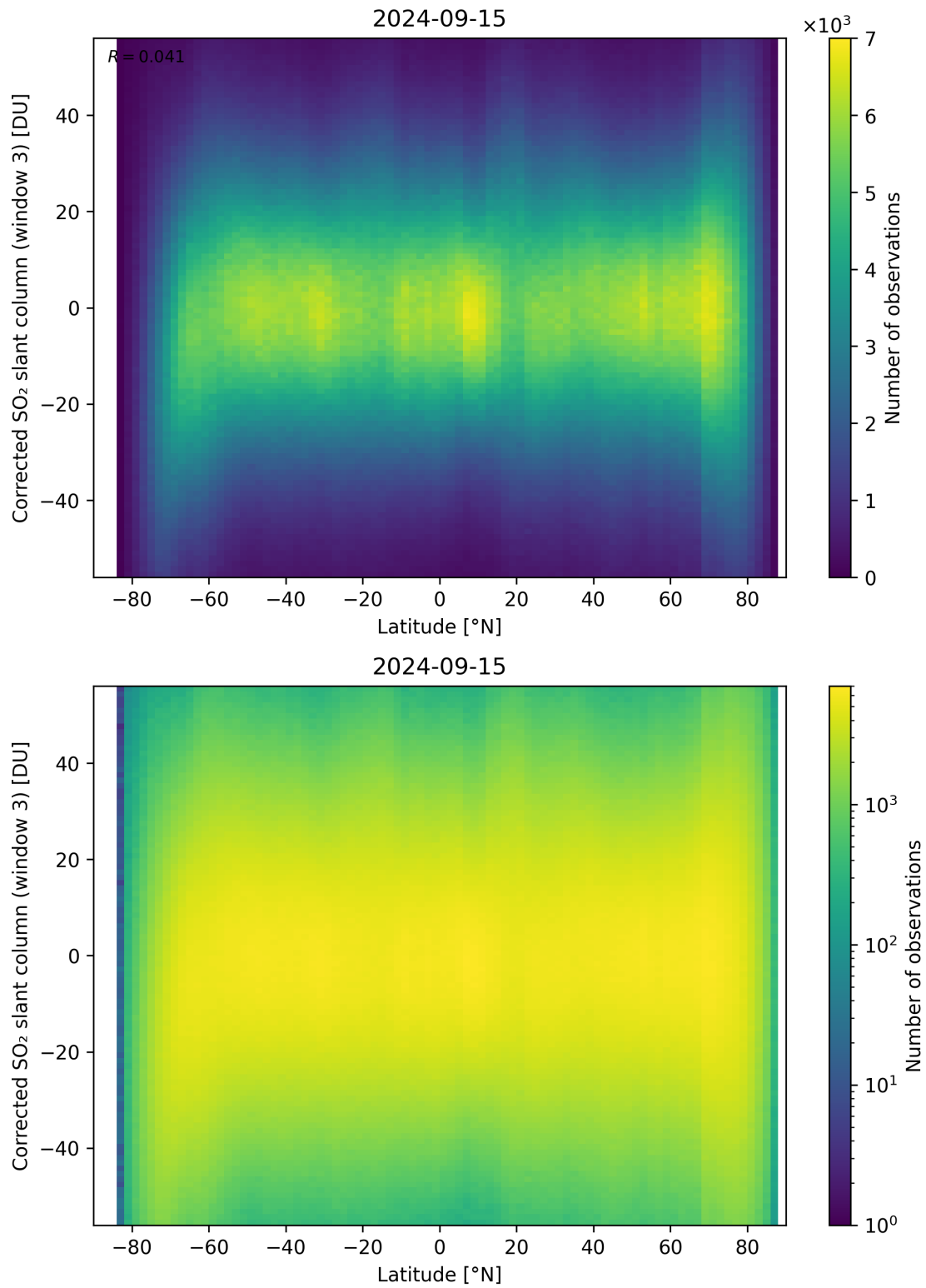
Figure 148: Scatter density plot of “Latitude” against “Corrected SO 2 slant column (window 3)” for 2024-09-14 to 2024-09-16.
