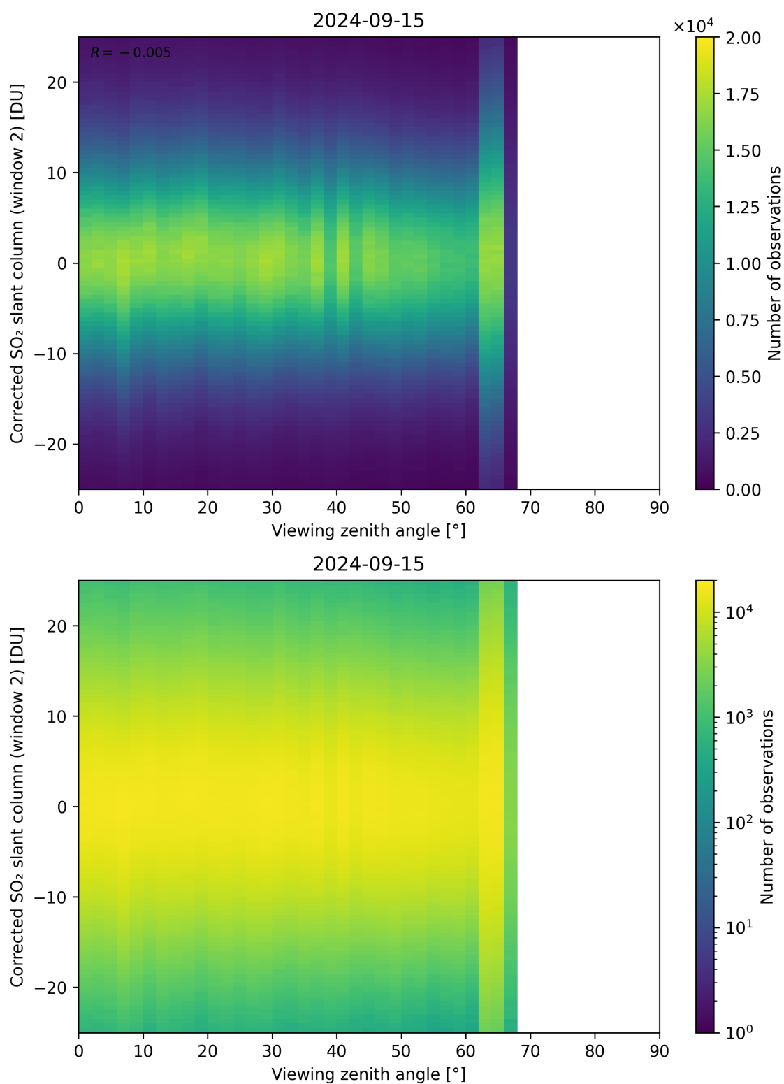
Figure 318: Scatter density plot of “Viewing zenith angle” against “Corrected SO 2 slant column (window 2)” for 2024-09-14 to 2024-09-16.
