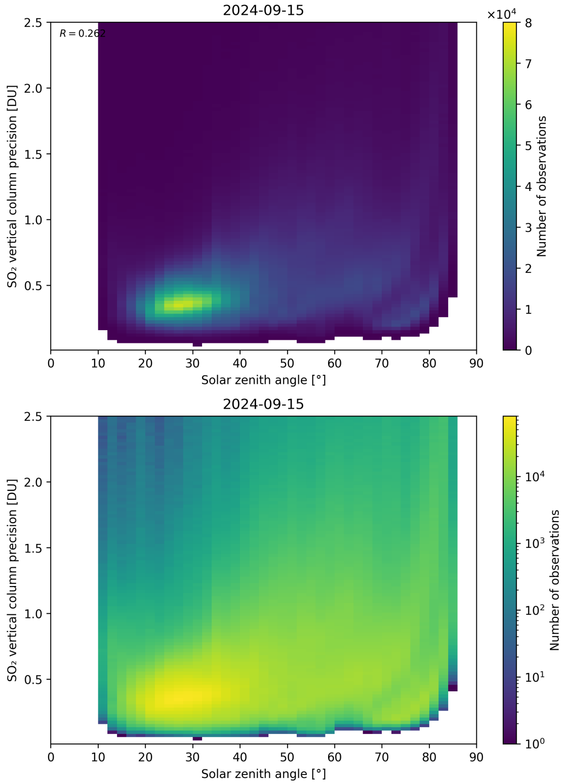
Figure 177: Scatter density plot of “Solar zenith angle” against “SO 2 vertical column precision” for 2024-09-14 to 2024-09-16.
