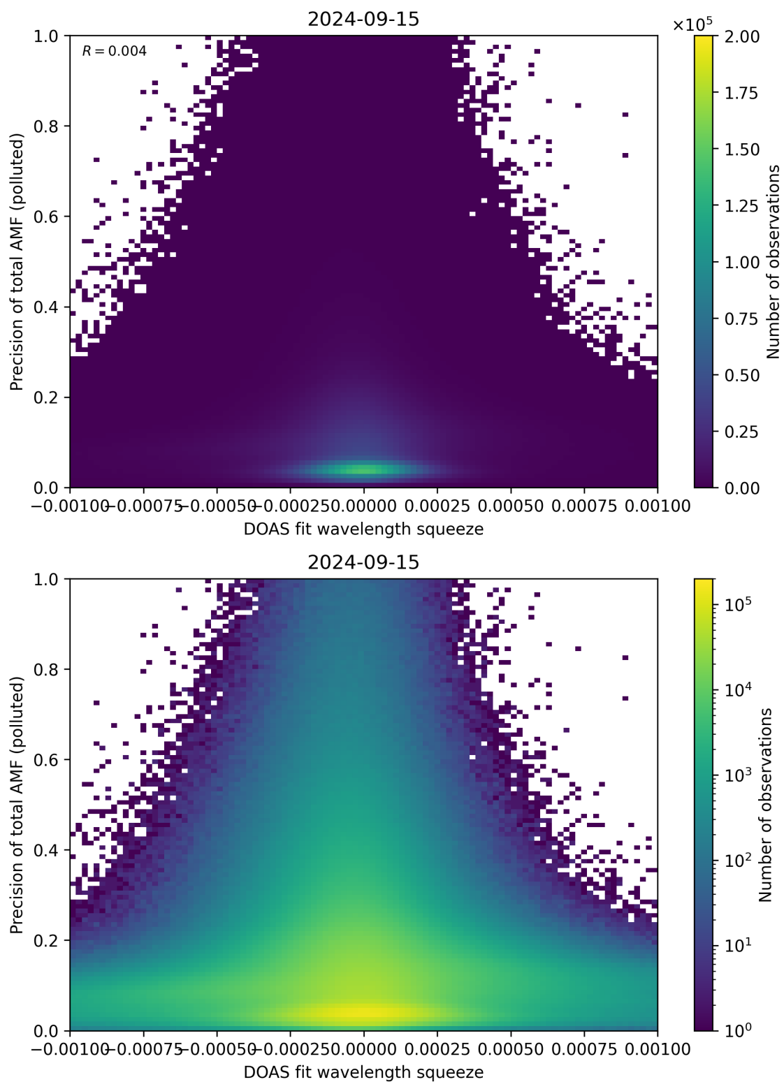
Figure 135: Scatter density plot of “DOAS fit wavelength squeeze” against “Precision of total AMF (polluted)” for 2024-09-14 to 2024-09-16.
