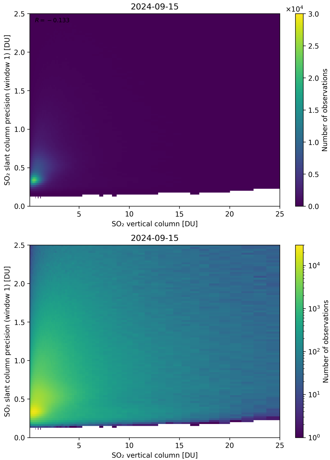
Figure 301: Scatter density plot of “SO 2 vertical column” against “SO 2 slant column precision (window 1)” for 2024-09-14 to 2024-09-16.
