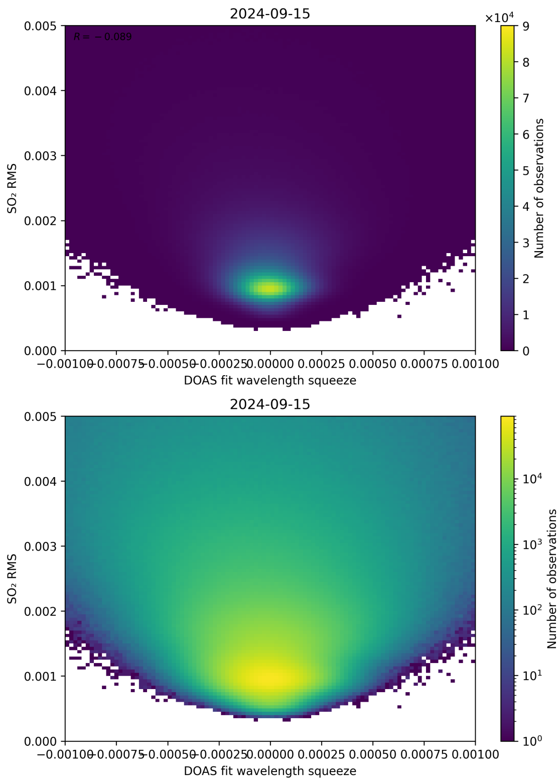
Figure 132: Scatter density plot of “DOAS fit wavelength squeeze” against “SO 2 RMS” for 2024-09-14 to 2024-09-16.
