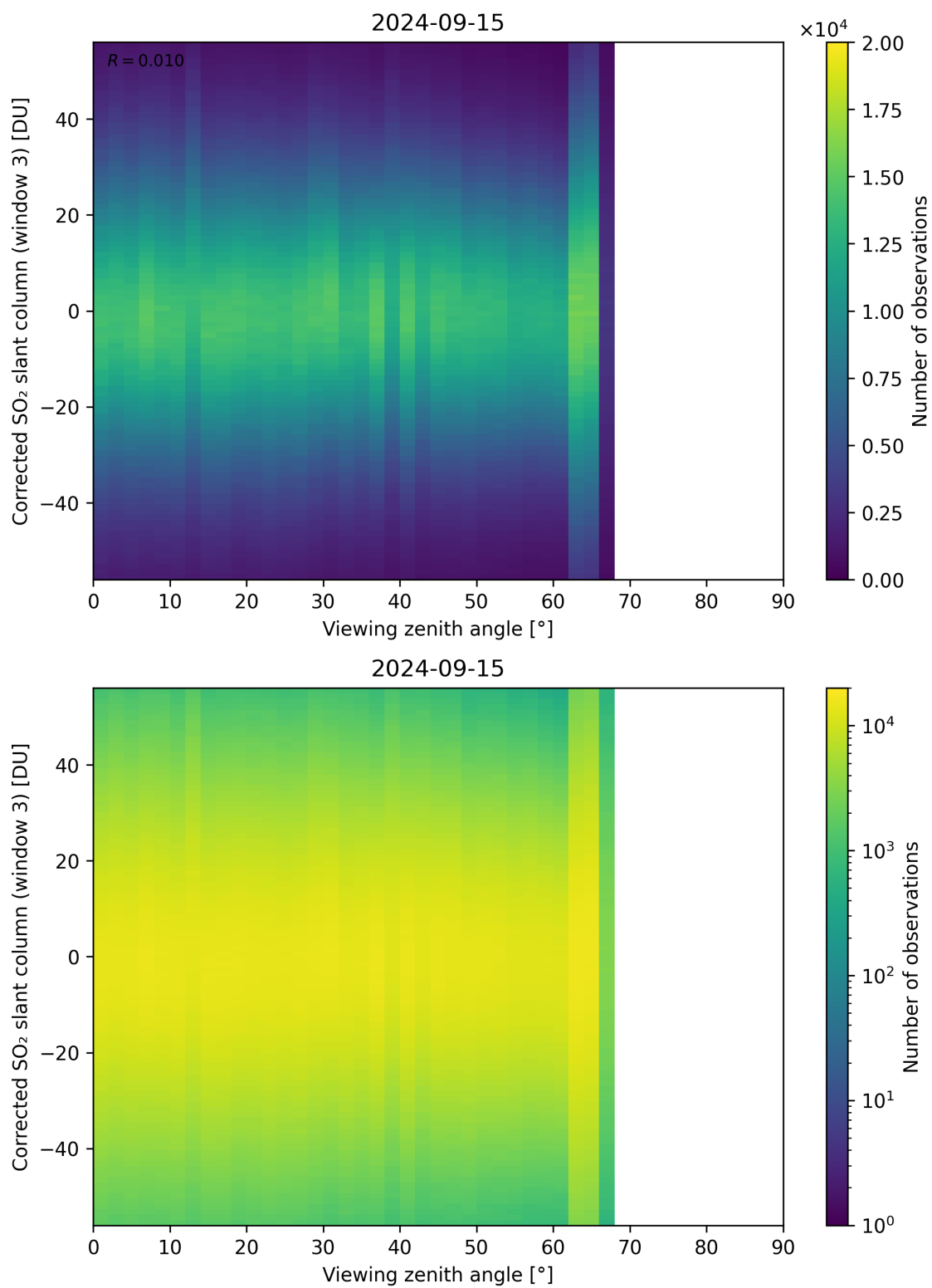
Figure 319: Scatter density plot of “Viewing zenith angle” against “Corrected SO 2 slant column (window 3)” for 2024-09-14 to 2024-09-16.
