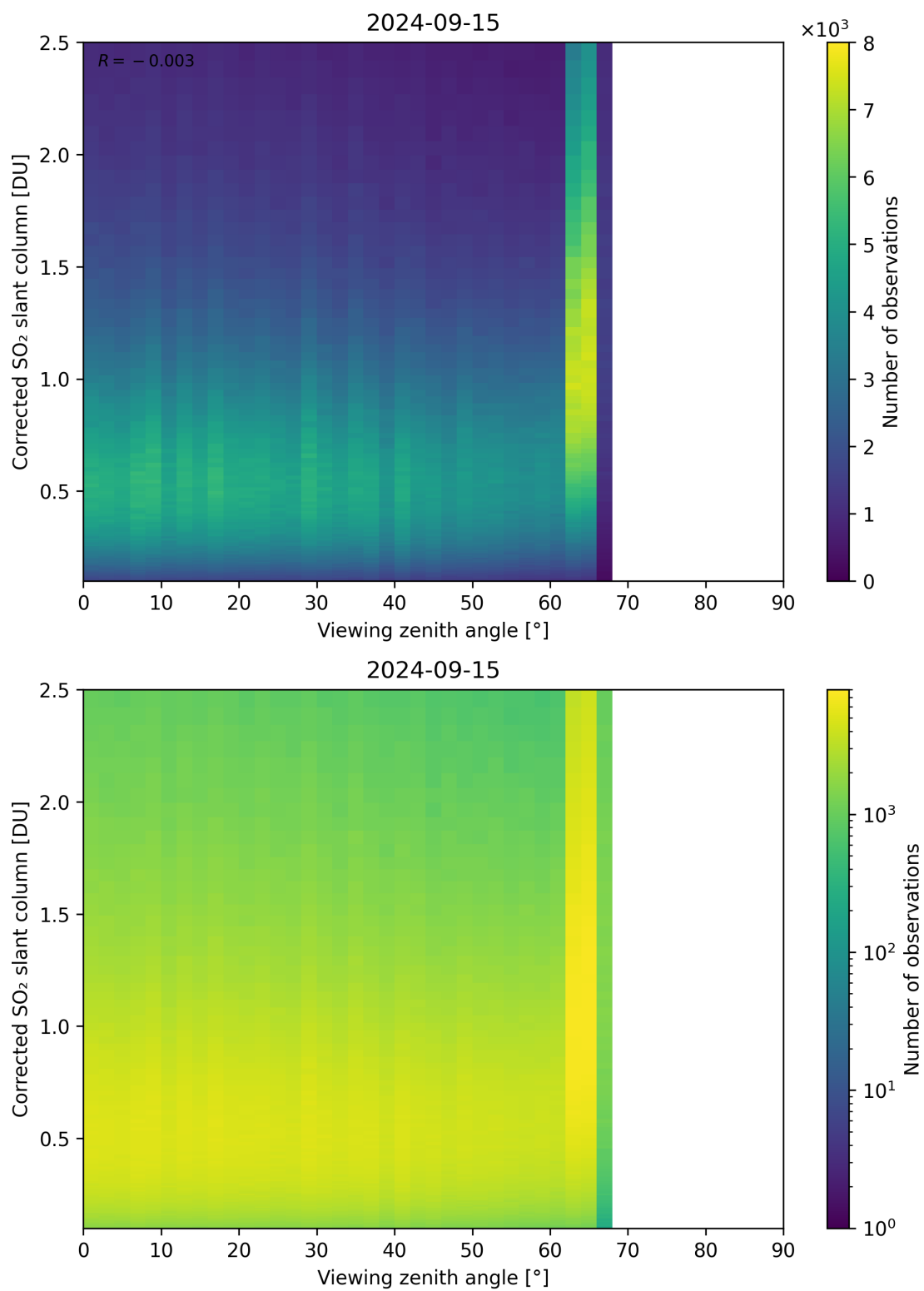
Figure 317: Scatter density plot of “Viewing zenith angle” against “Corrected SO 2 slant column” for 2024-09-14 to 2024-09-16.
