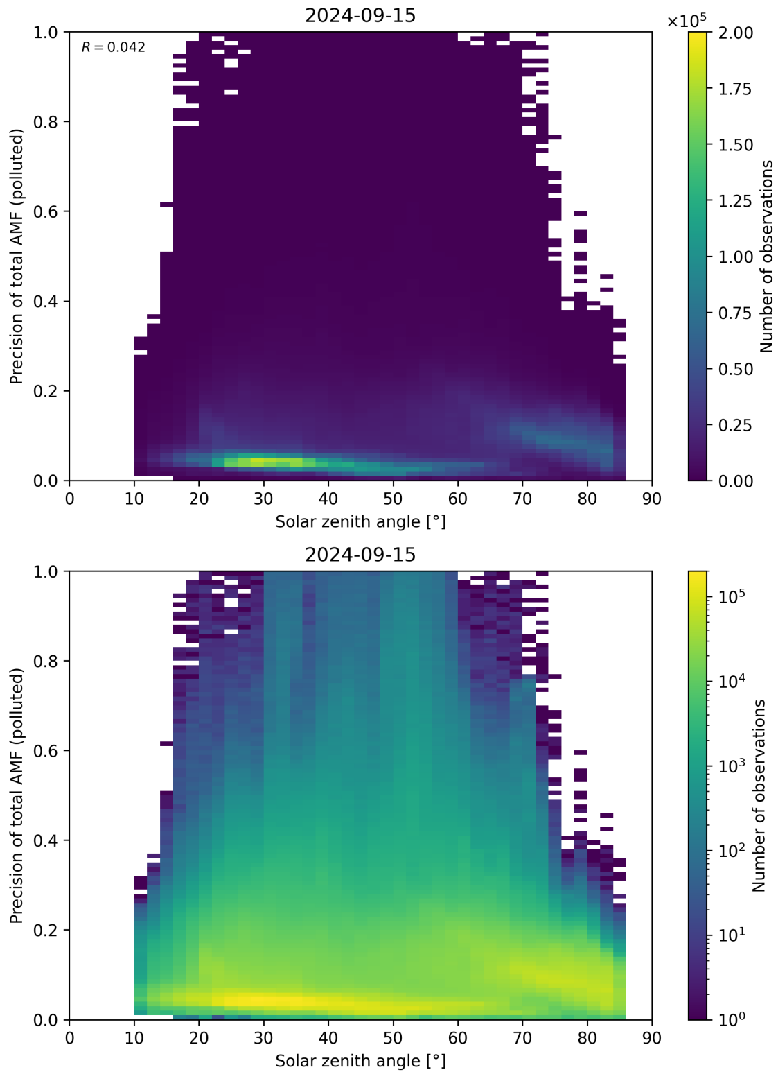
Figure 175: Scatter density plot of “Solar zenith angle” against “Precision of total AMF (polluted)” for 2024-09-14 to 2024-09-16.
