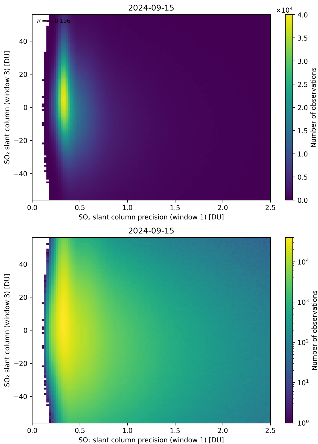
Figure 228: Scatter density plot of “SO 2 slant column precision (window 1)” against “SO 2 slant column (window 3)” for 2024-09-14 to 2024-09-16.
