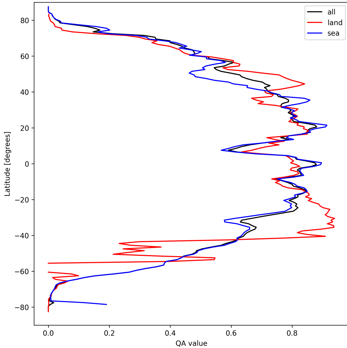
Figure 29: Zonal average of “QA value” for 2024-09-14 to 2024-09-16.
