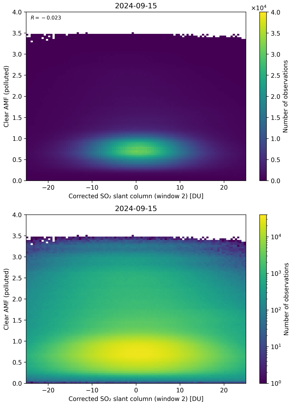
Figure 199: Scatter density plot of “Corrected SO 2 slant column (window 2)” against “Clear AMF (polluted)” for 2024-09-14 to 2024-09-16.
