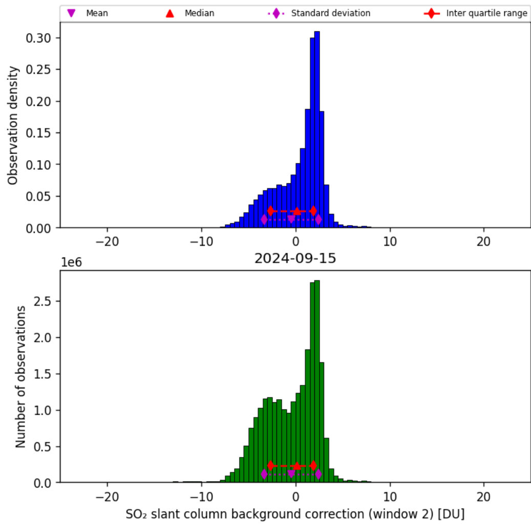
Figure 63: Histogram of “SO 2 slant column background correction (window 2)” for 2024-09-14 to 2024-09-16
