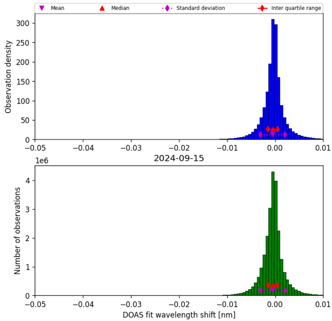
Figure 68: Histogram of “DOAS fit wavelength shift” for 2024-09-14 to 2024-09-16
