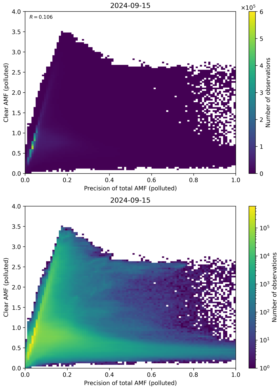
Figure 270: Scatter density plot of “Precision of total AMF (polluted)” against “Clear AMF (polluted)” for 2024-09-14 to 2024-09-16.
