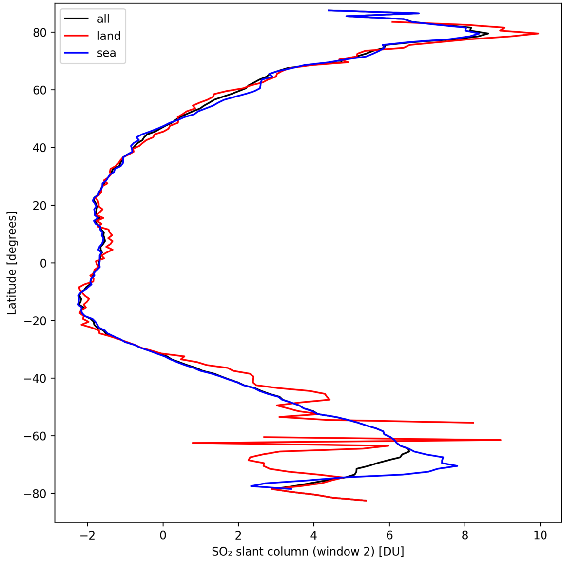
Figure 37: Zonal average of “SO 2 slant column (window 2)” for 2024-09-14 to 2024-09-16.
