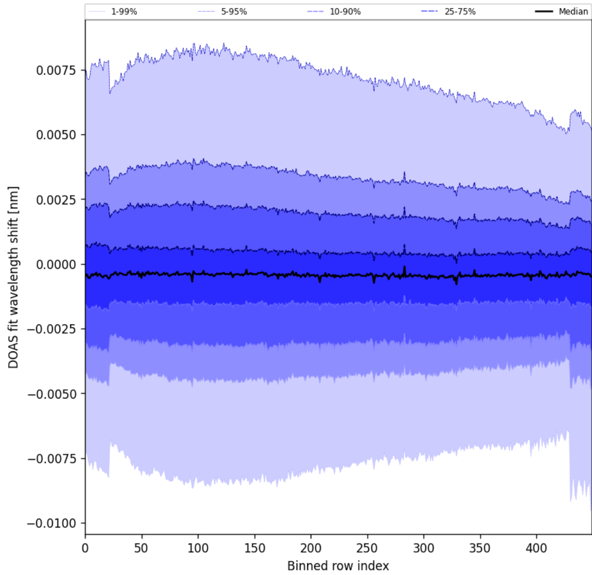
Figure 91: Along track statistics of “DOAS fit wavelength shift” for 2024-09-14 to 2024-09-16
