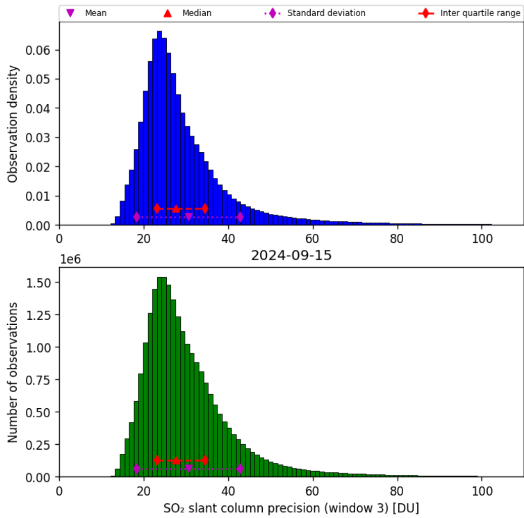
Figure 65: Histogram of “SO 2 slant column precision (window 3)” for 2024-09-14 to 2024-09-16
