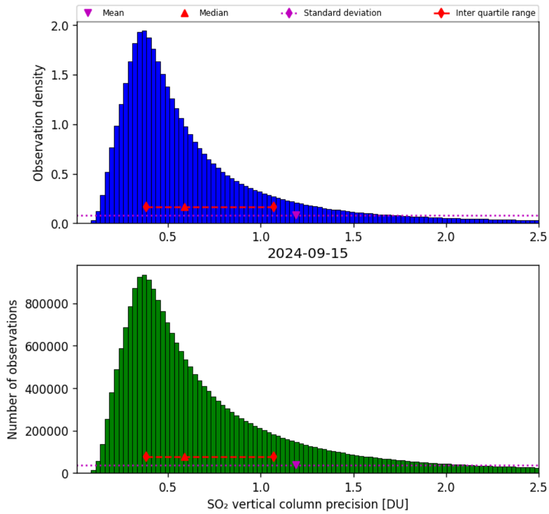
Figure 54: Histogram of “SO 2 vertical column precision” for 2024-09-14 to 2024-09-16
