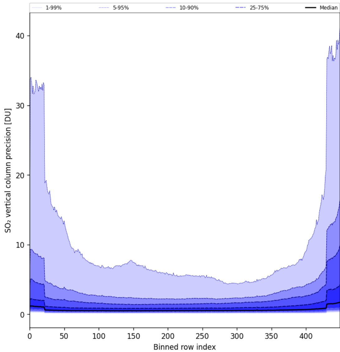
Figure 77: Along track statistics of “SO 2 vertical column precision” for 2024-09-14 to 2024-09-16
