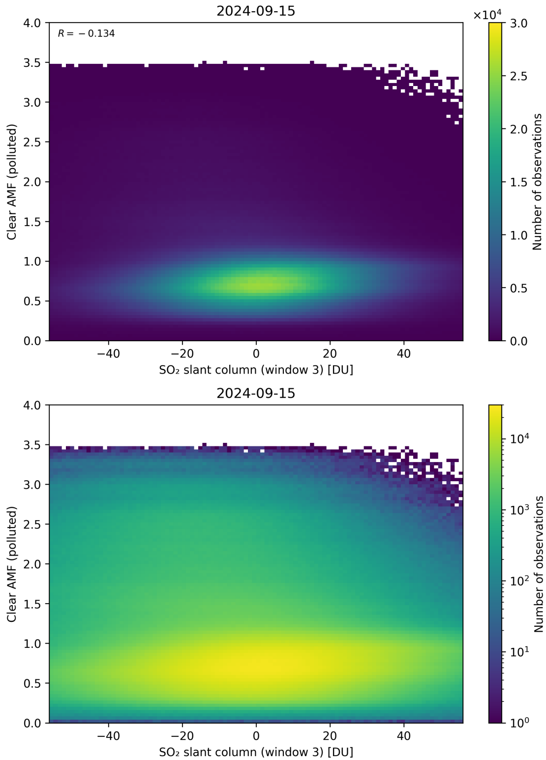
Figure 265: Scatter density plot of “SO 2 slant column (window 3)” against “Clear AMF (polluted)” for 2024-09-14 to 2024-09-16.
