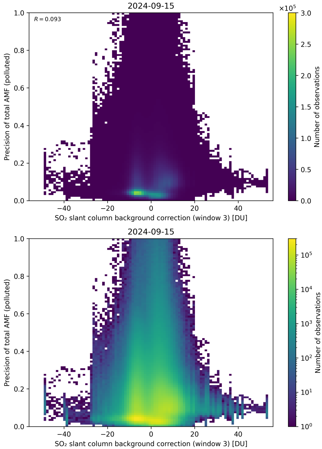
Figure 126: Scatter density plot of “SO 2 slant column background correction (window 3)” against “Precision of total AMF (polluted)” for 2024-09-14 to 2024-09-16.
