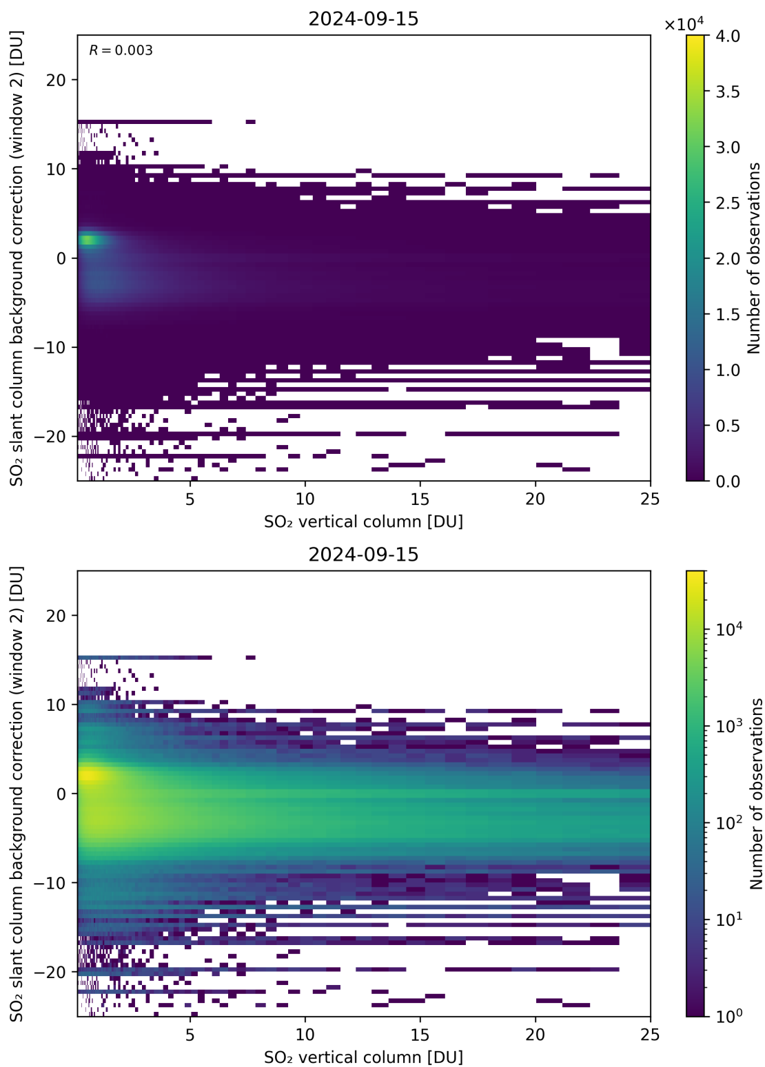
Figure 274: Scatter density plot of “SO 2 vertical column” against “SO 2 slant column background correction (window 2)” for 2024-09-14 to 2024-09-16.
