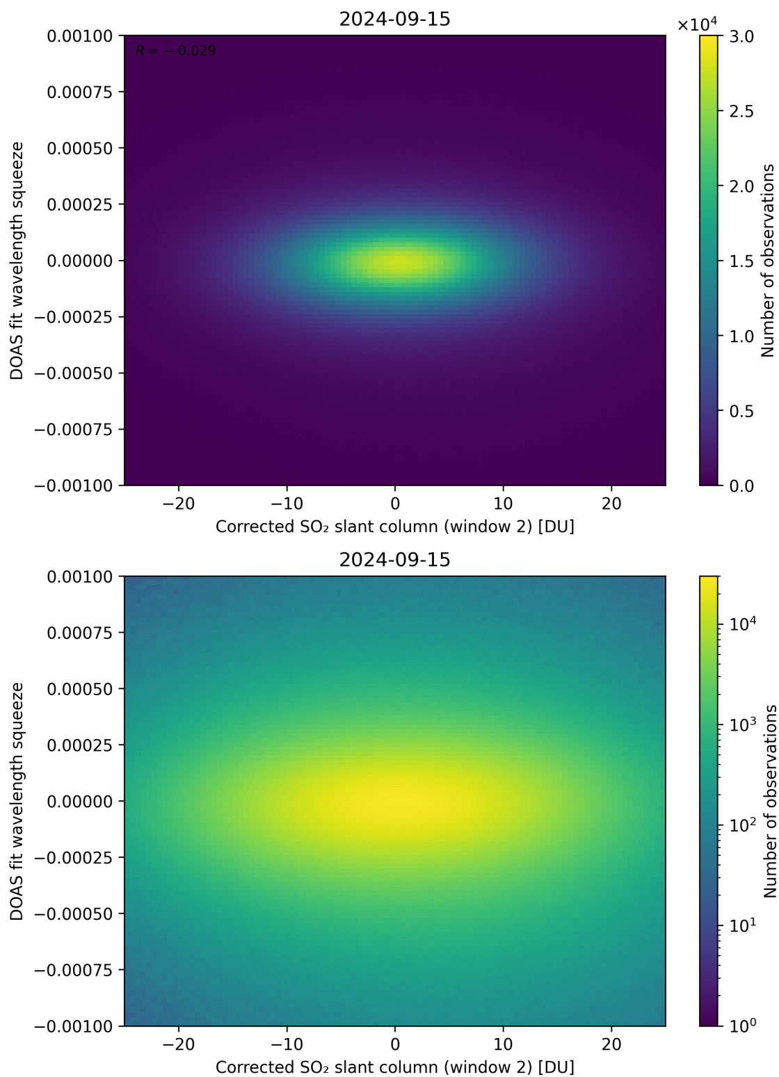
Figure 197: Scatter density plot of “Corrected SO 2 slant column (window 2)” against “DOAS fit wavelength squeeze” for 2024-09-14 to 2024-09-16.
