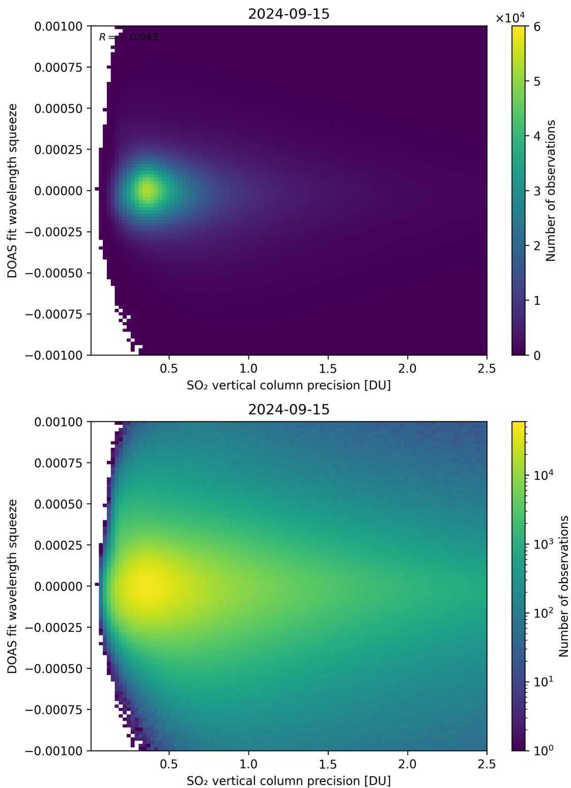
Figure 283: Scatter density plot of “SO 2 vertical column precision” against “DOAS fit wavelength squeeze” for 2024-09-14 to 2024-09-16.
