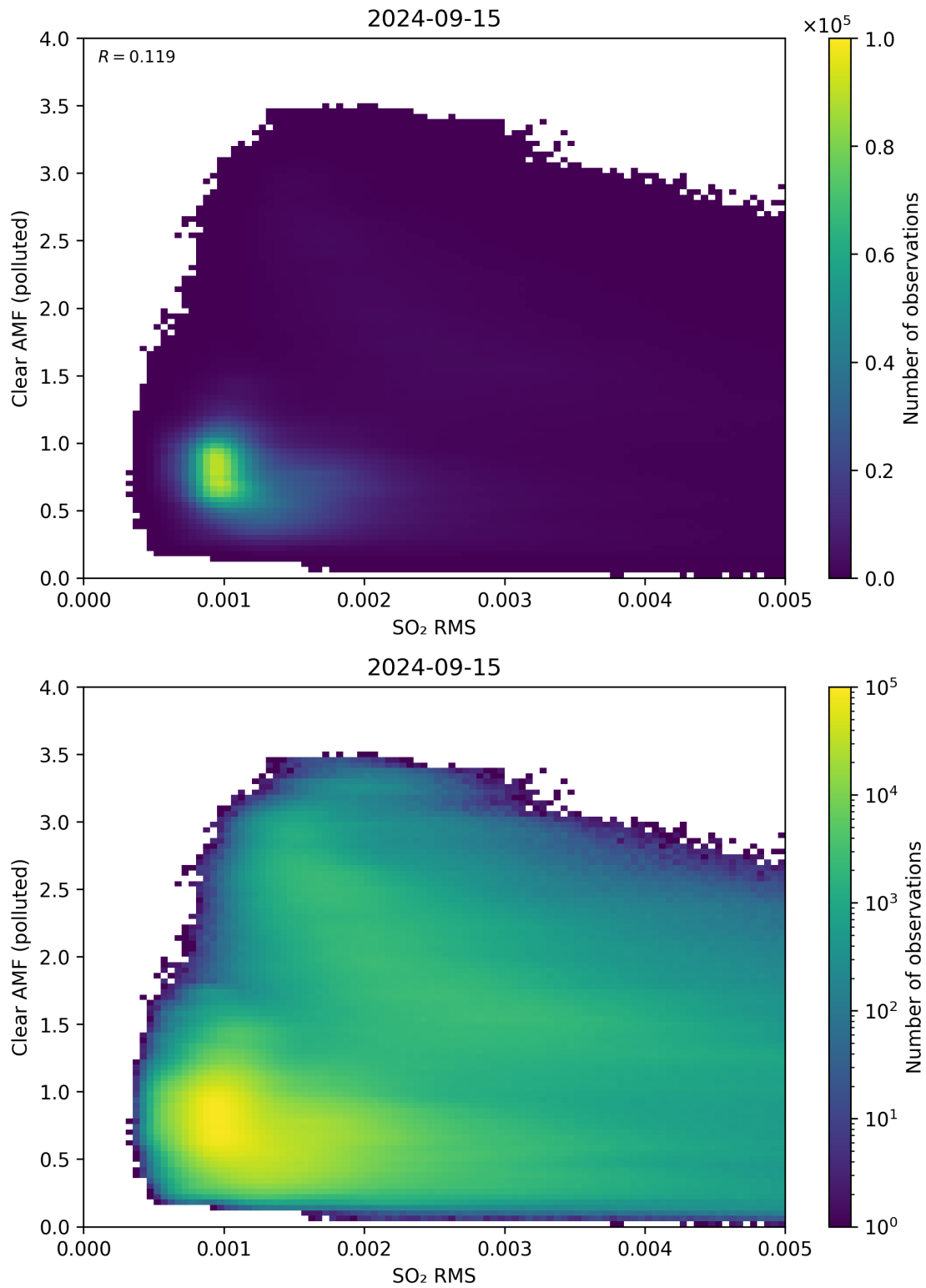
Figure 136: Scatter density plot of “SO 2 RMS” against “Clear AMF (polluted)” for 2024-09-14 to 2024-09-16.
