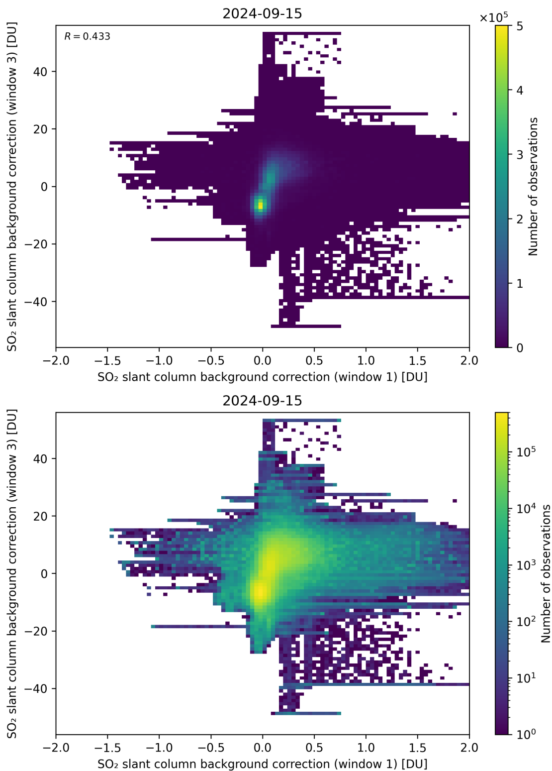
Figure 99: Scatter density plot of “SO 2 slant column background correction (window 1)” against “SO 2 slant column background correction (window 3)” for 2024-09-14 to 2024-09-16.
