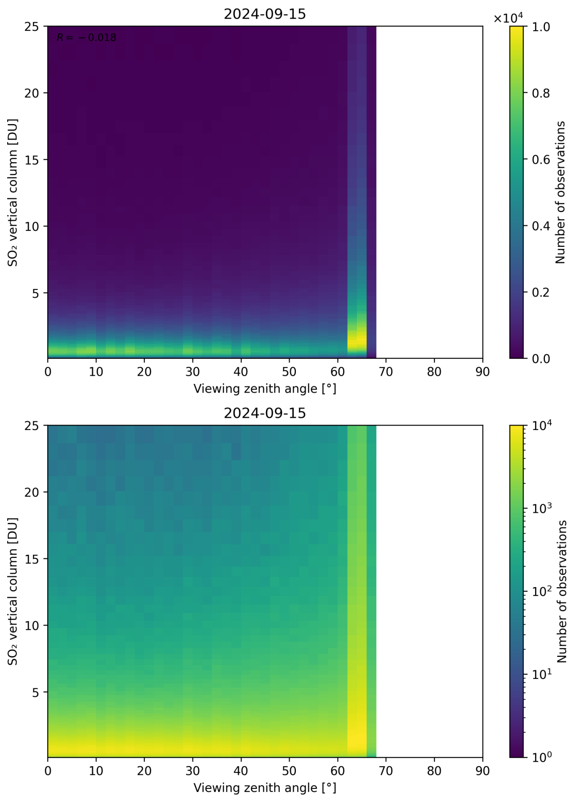
Figure 327: Scatter density plot of “Viewing zenith angle” against “SO 2 vertical column” for 2024-09-14 to 2024-09-16.
