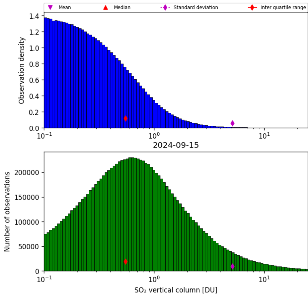
Figure 53: Histogram of “SO 2 vertical column” for 2024-09-14 to 2024-09-16
