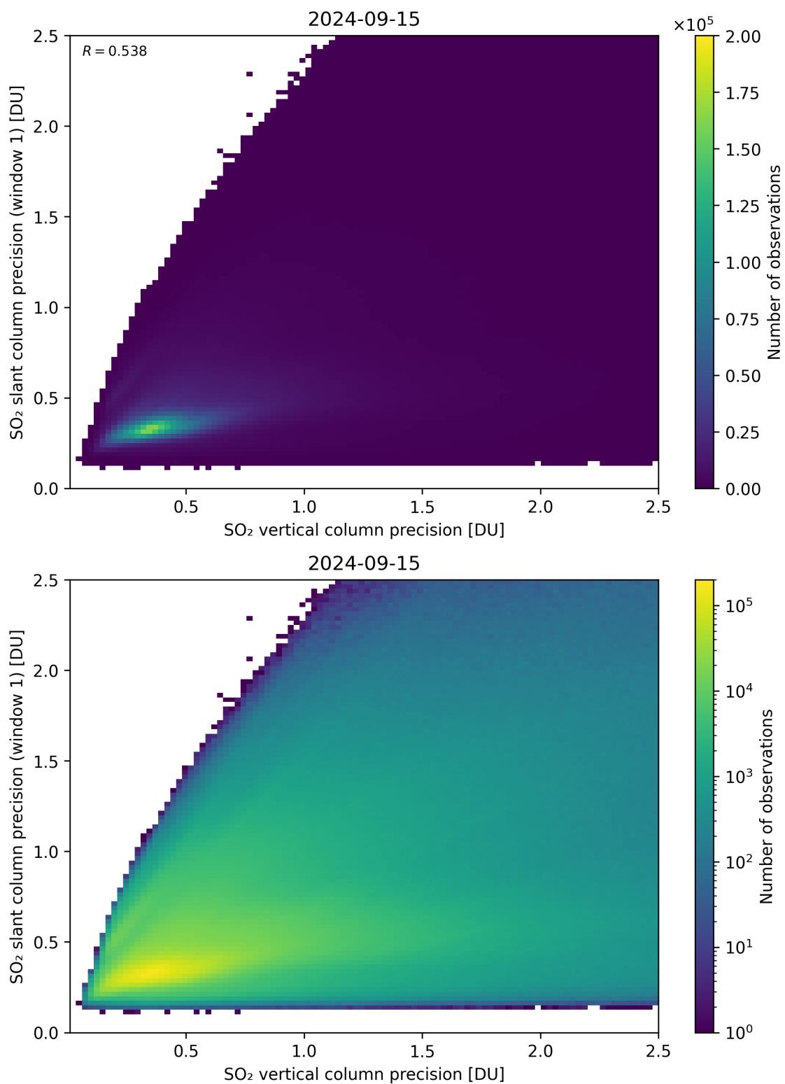
Figure 290: Scatter density plot of “SO 2 vertical column precision” against “SO 2 slant column precision (window 1)” for 2024-09-14 to 2024-09-16.
