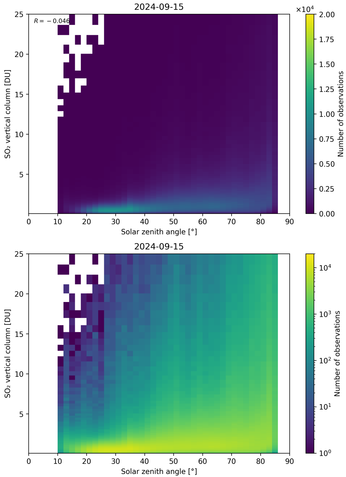
Figure 176: Scatter density plot of “Solar zenith angle” against “SO 2 vertical column” for 2024-09-14 to 2024-09-16.
