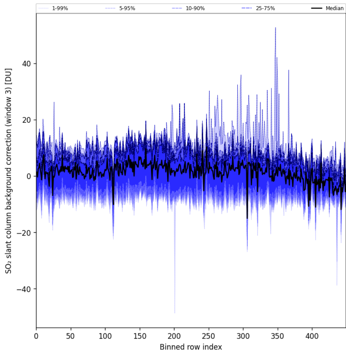
Figure 90: Along track statistics of “SO 2 slant column background correction (window 3)” for 2024-09-14 to 2024-09-16
