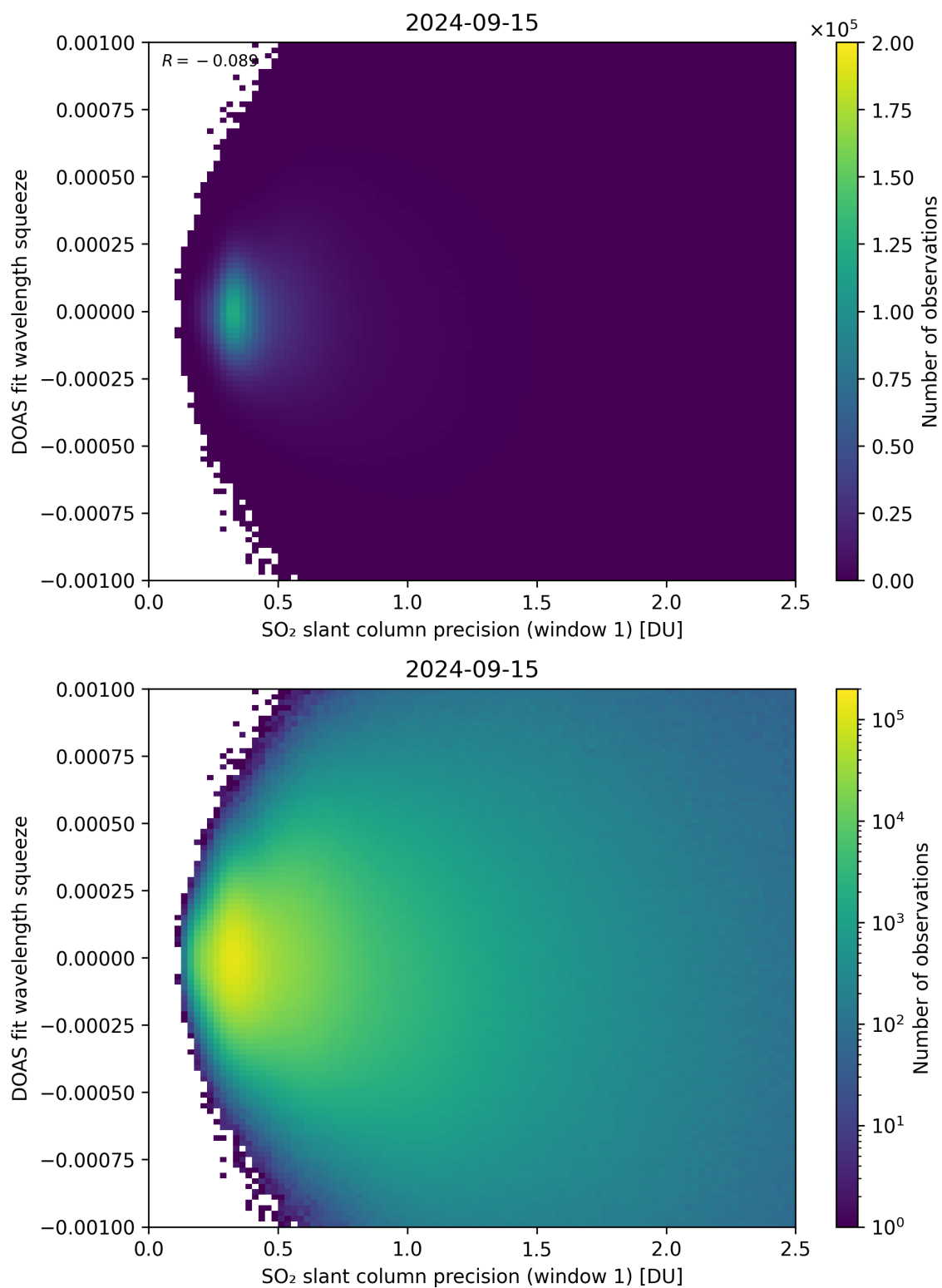
Figure 222: Scatter density plot of “SO 2 slant column precision (window 1)” against “DOAS fit wavelength squeeze” for 2024-09-14 to 2024-09-16.
