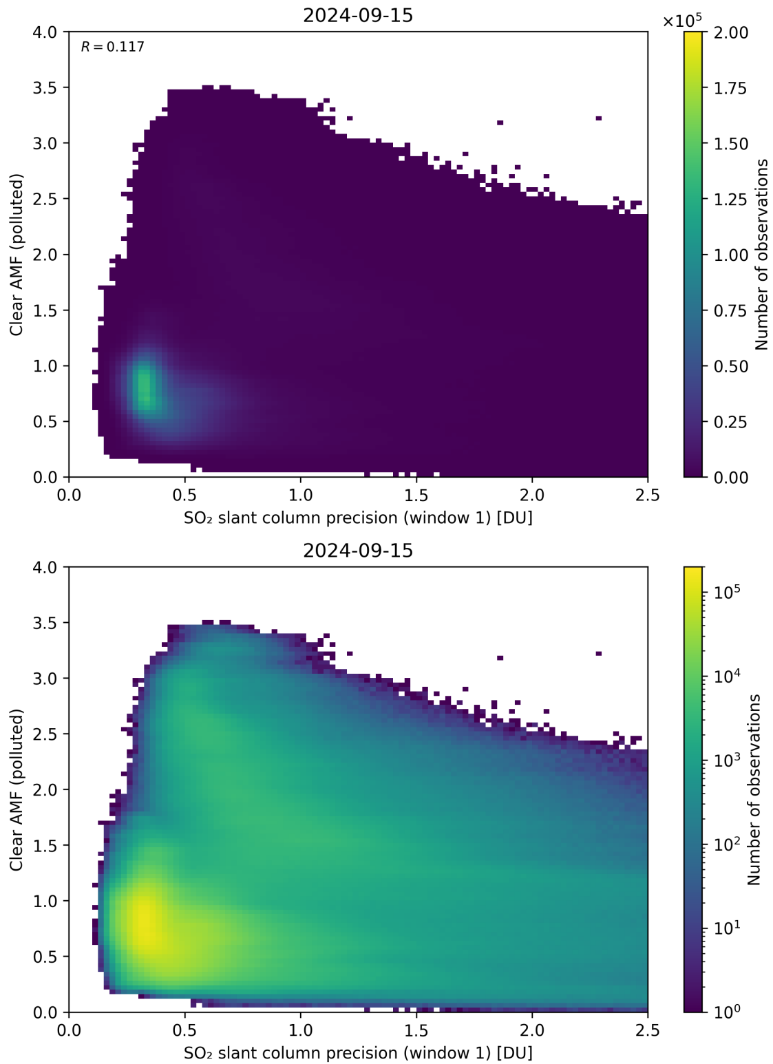
Figure 224: Scatter density plot of “SO 2 slant column precision (window 1)” against “Clear AMF (polluted)” for 2024-09-14 to 2024-09-16.
