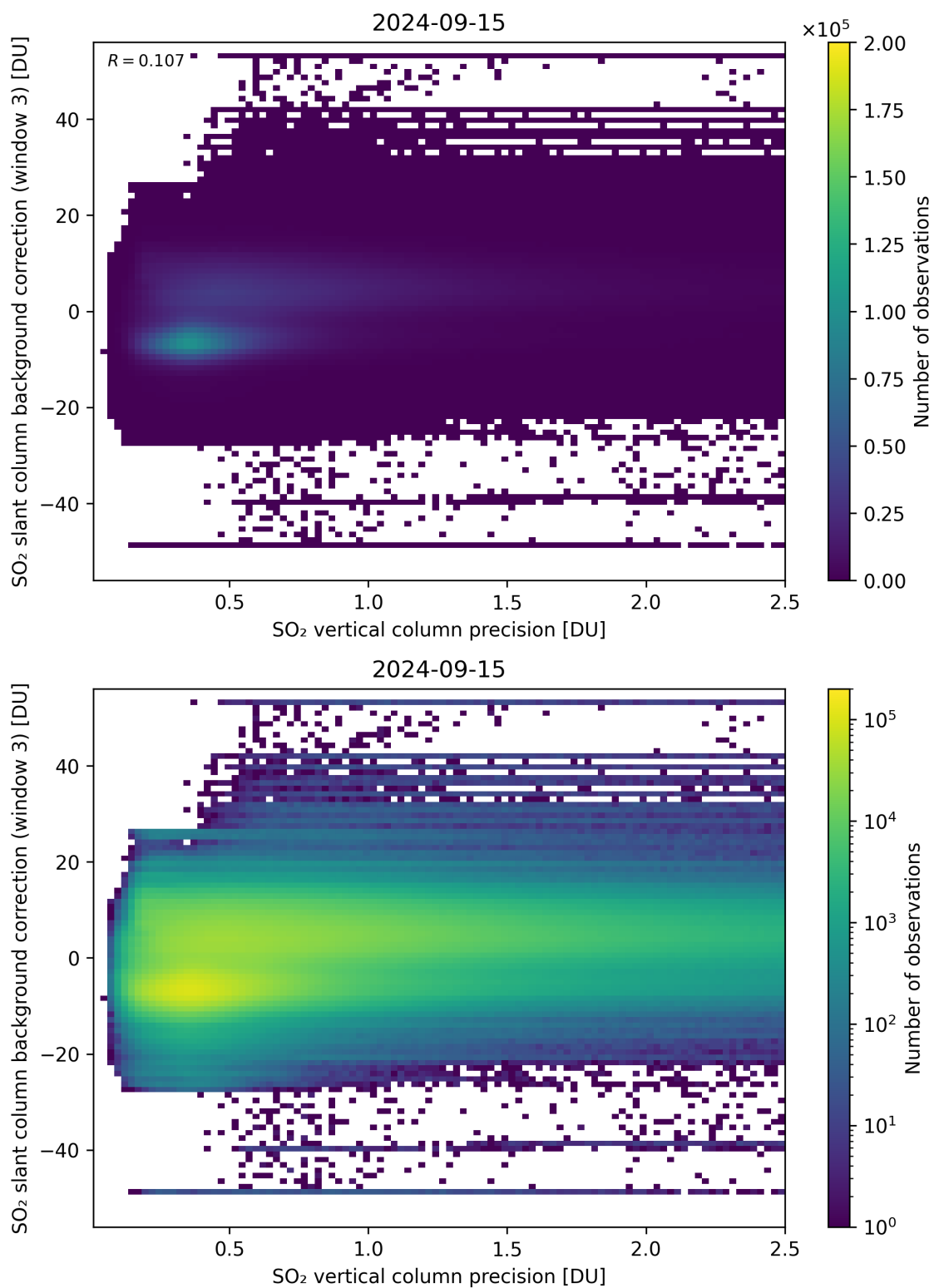
Figure 281: Scatter density plot of “SO 2 vertical column precision” against “SO 2 slant column background correction (window 3)” for 2024-09-14 to 2024-09-16.
