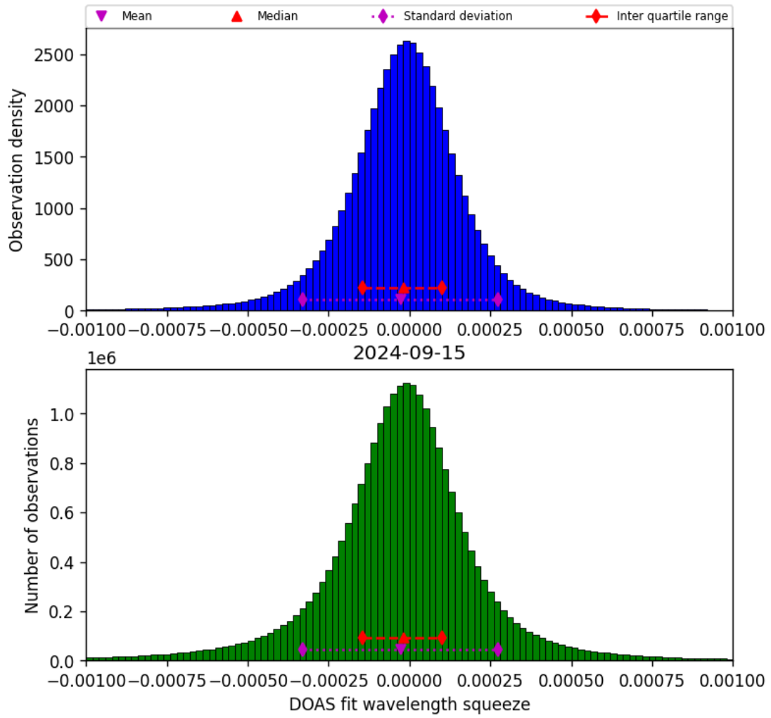
Figure 69: Histogram of “DOAS fit wavelength squeeze” for 2024-09-14 to 2024-09-16
