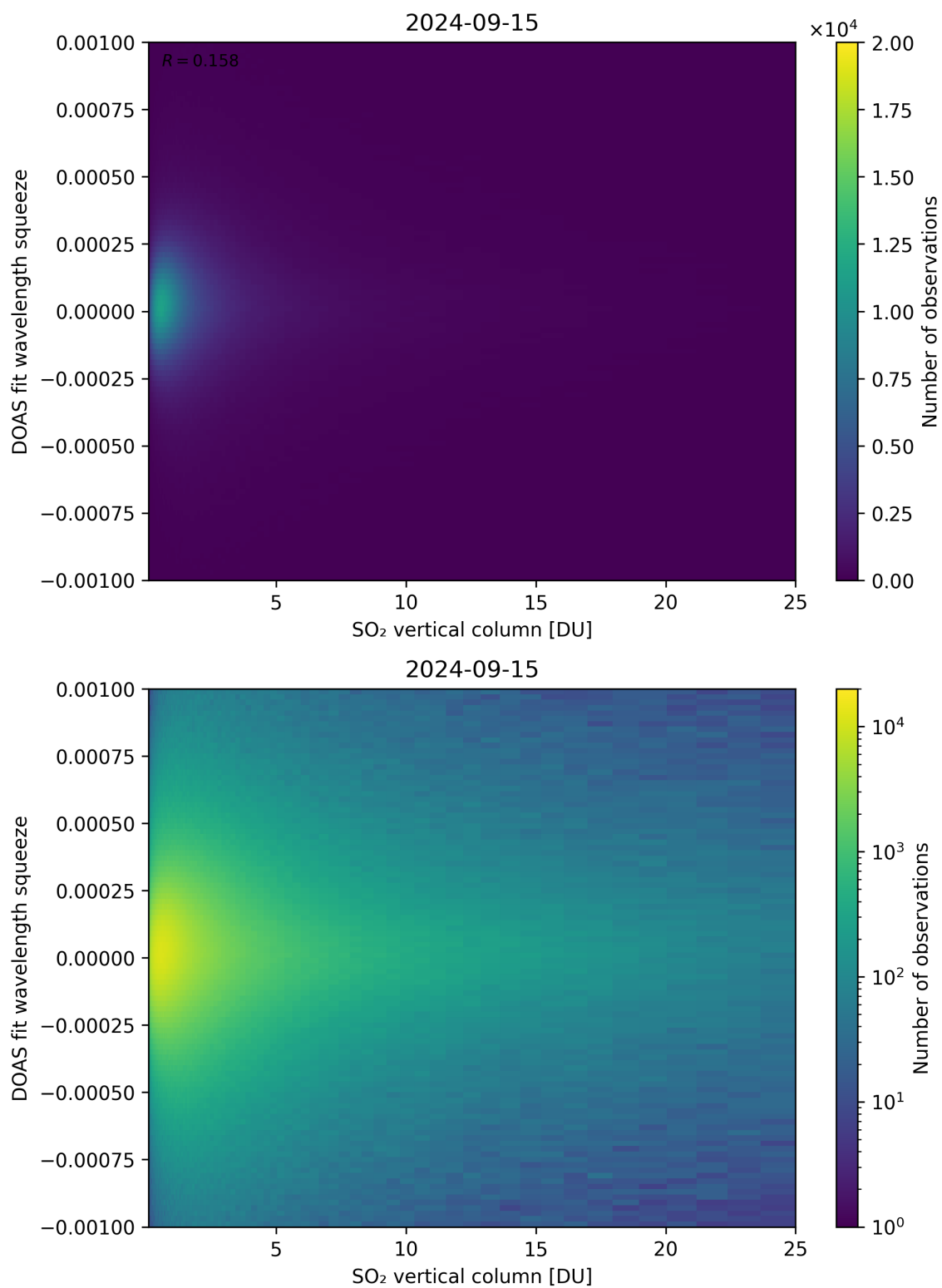
Figure 277: Scatter density plot of “SO 2 vertical column” against “DOAS fit wavelength squeeze” for 2024-09-14 to 2024-09-16.
