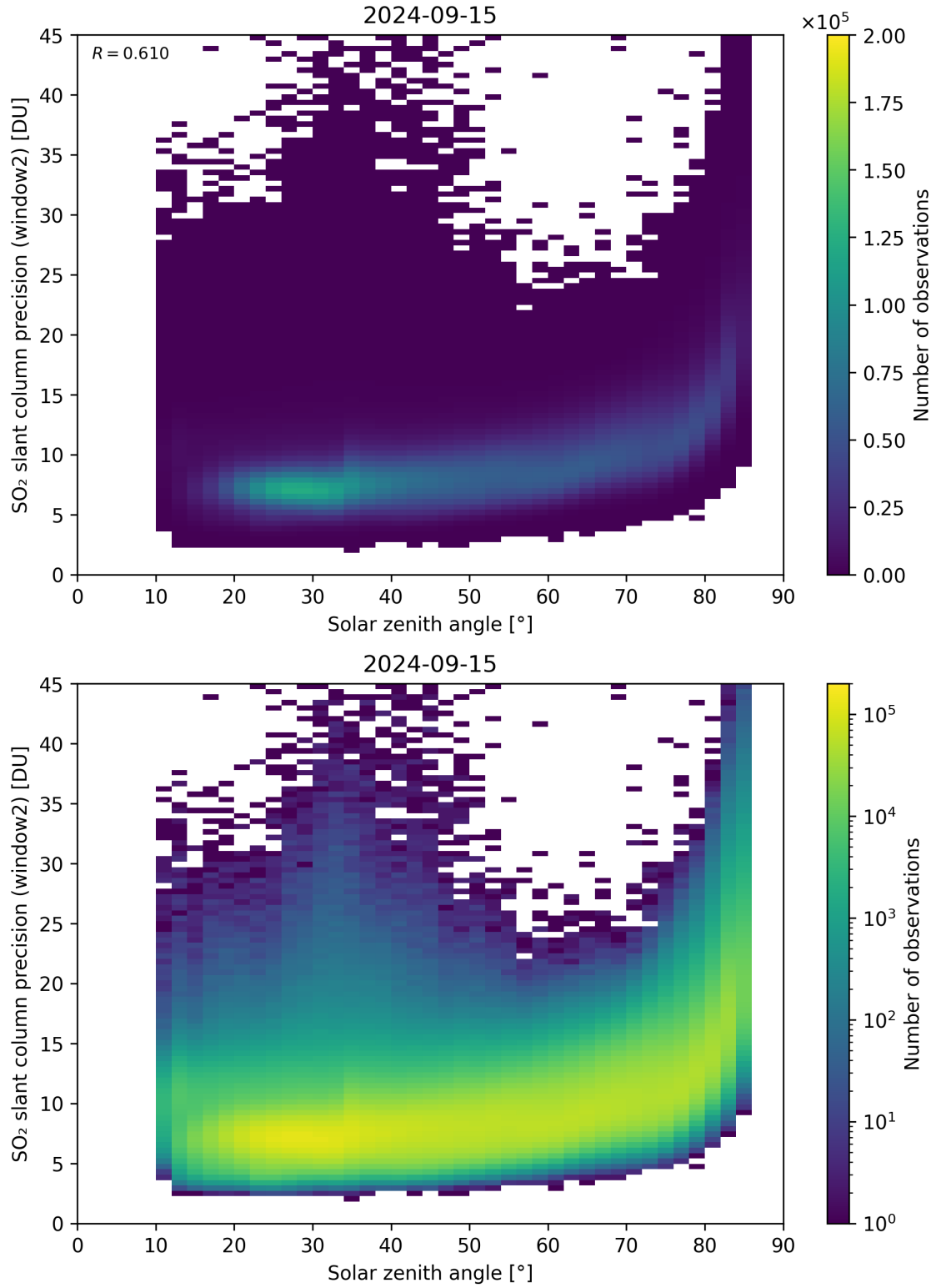
Figure 171: Scatter density plot of “Solar zenith angle” against “SO 2 slant column precision (window2)” for 2024-09-14 to 2024-09-16.
