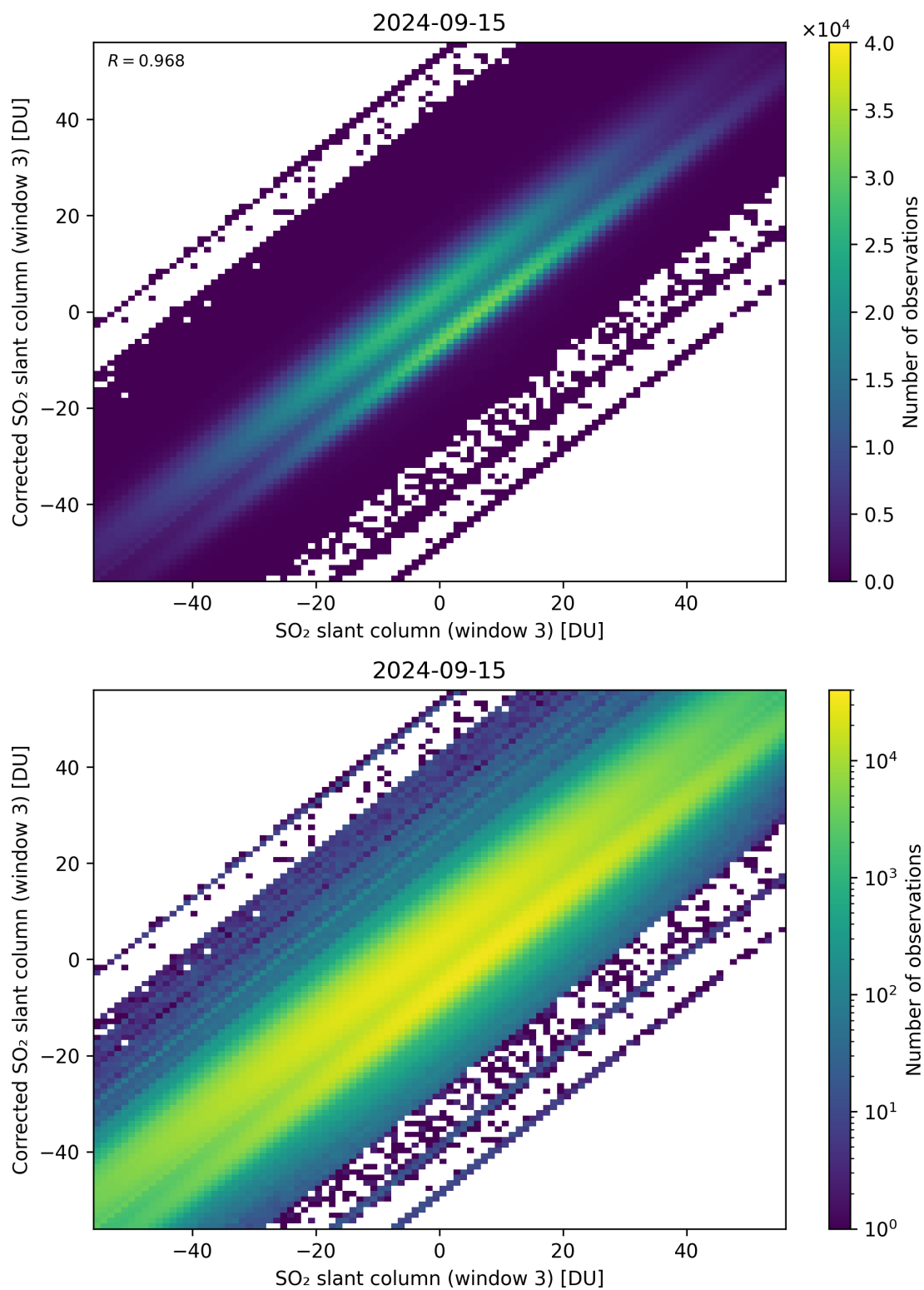
Figure 266: Scatter density plot of “SO 2 slant column (window 3)” against “Corrected SO 2 slant column (window 3)” for 2024-09-14 to 2024-09-16.
