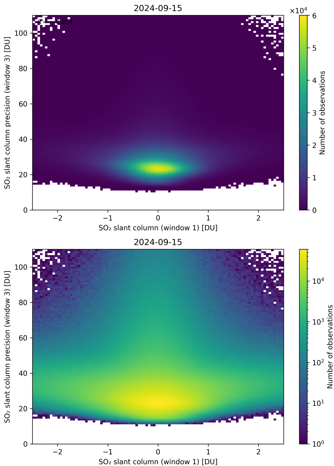
Figure 238: Scatter density plot of “SO 2 slant column (window 1)” against “SO 2 slant column precision (window 3)” for 2024-09-14 to 2024-09-16.
