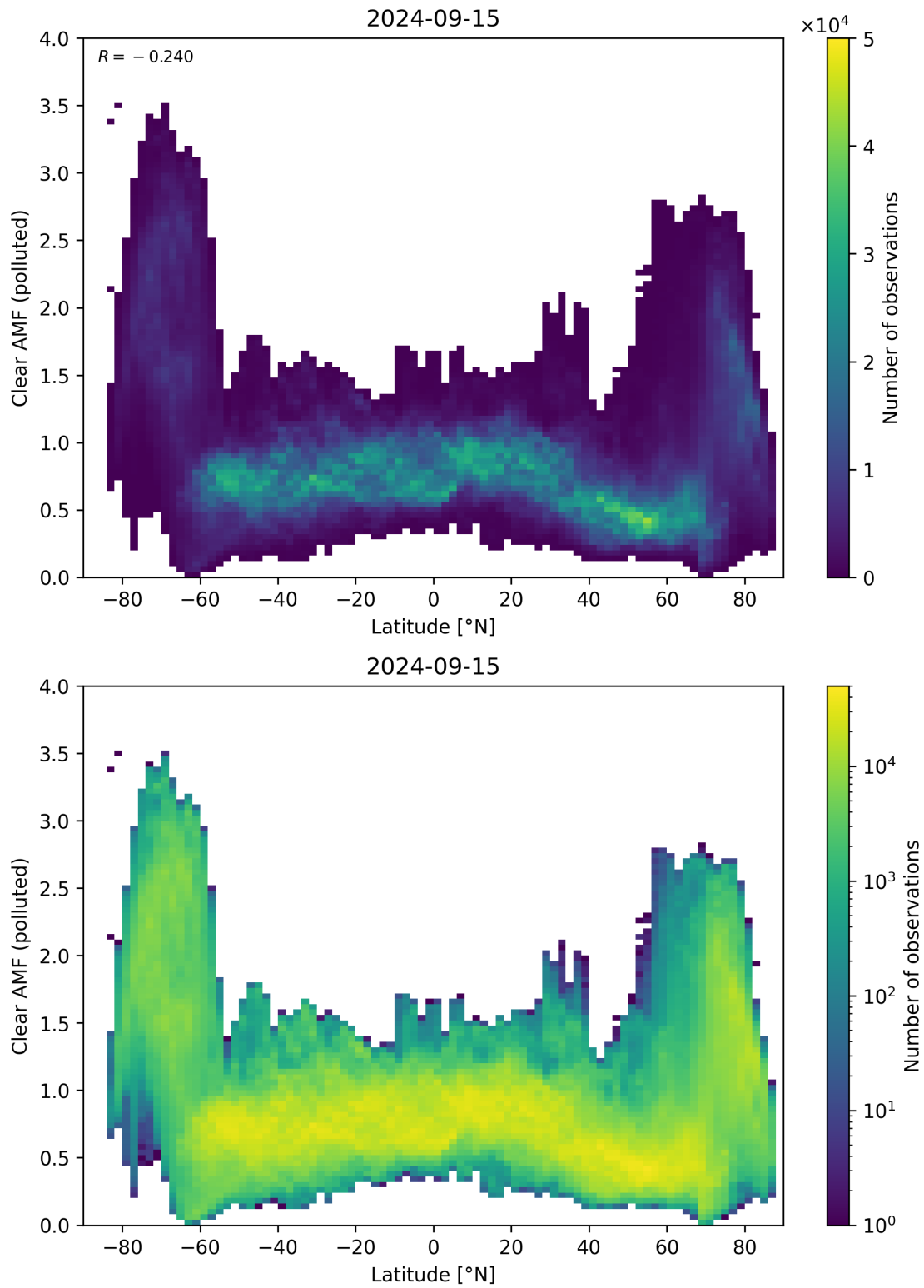
Figure 145: Scatter density plot of “Latitude” against “Clear AMF (polluted)” for 2024-09-14 to 2024-09-16.
