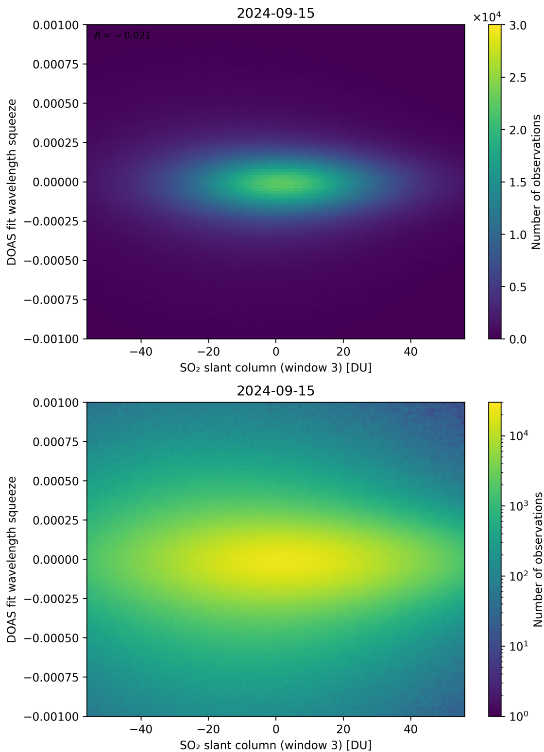
Figure 255: Scatter density plot of “SO 2 slant column (window 3)” against “DOAS fit wavelength squeeze” for 2024-09-14 to 2024-09-16.
