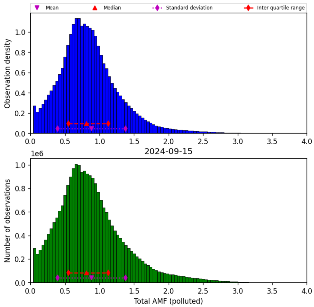
Figure 71: Histogram of “Total AMF (polluted)” for 2024-09-14 to 2024-09-16
