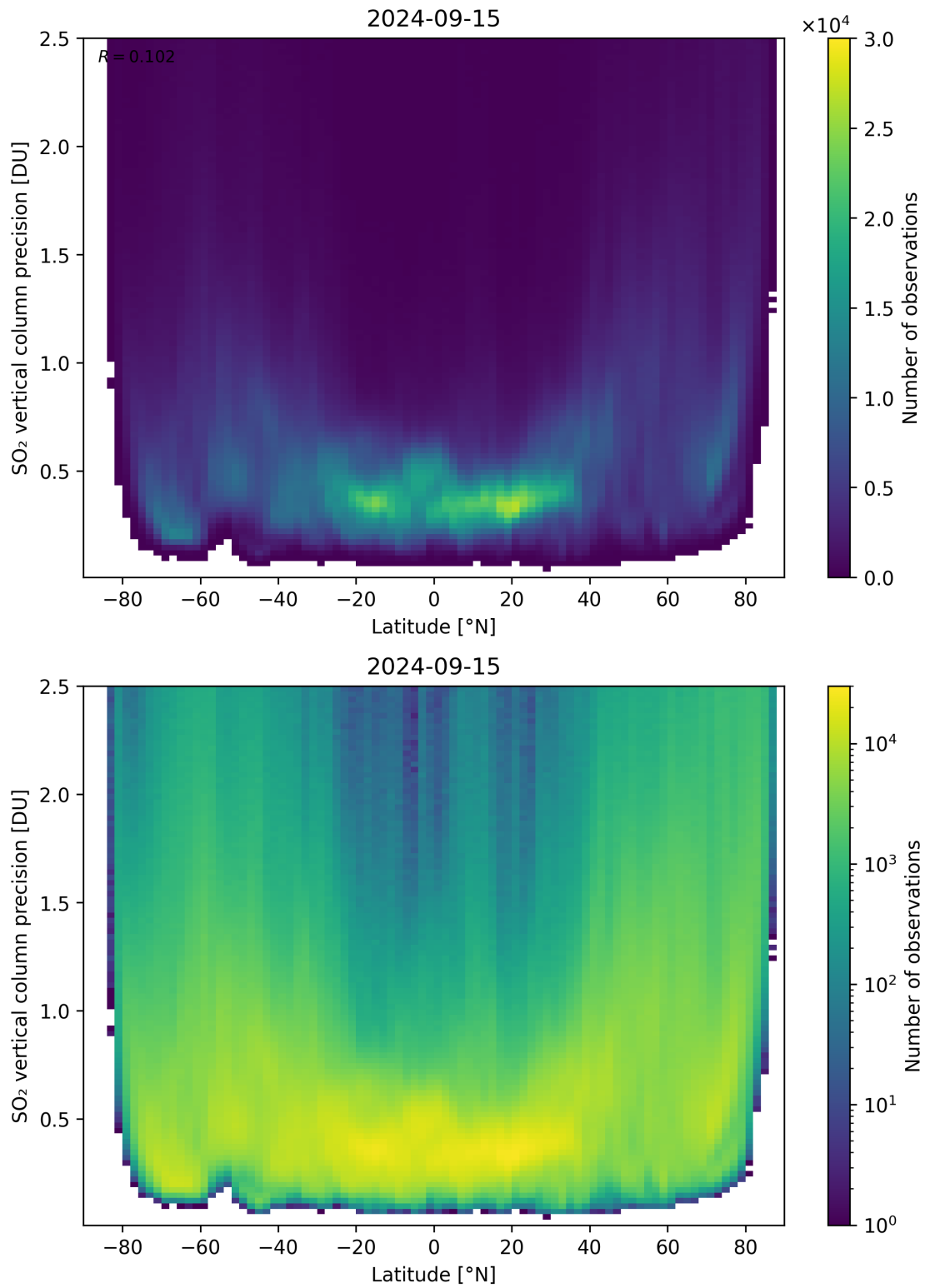
Figure 157: Scatter density plot of “Latitude” against “SO 2 vertical column precision” for 2024-09-14 to 2024-09-16.
