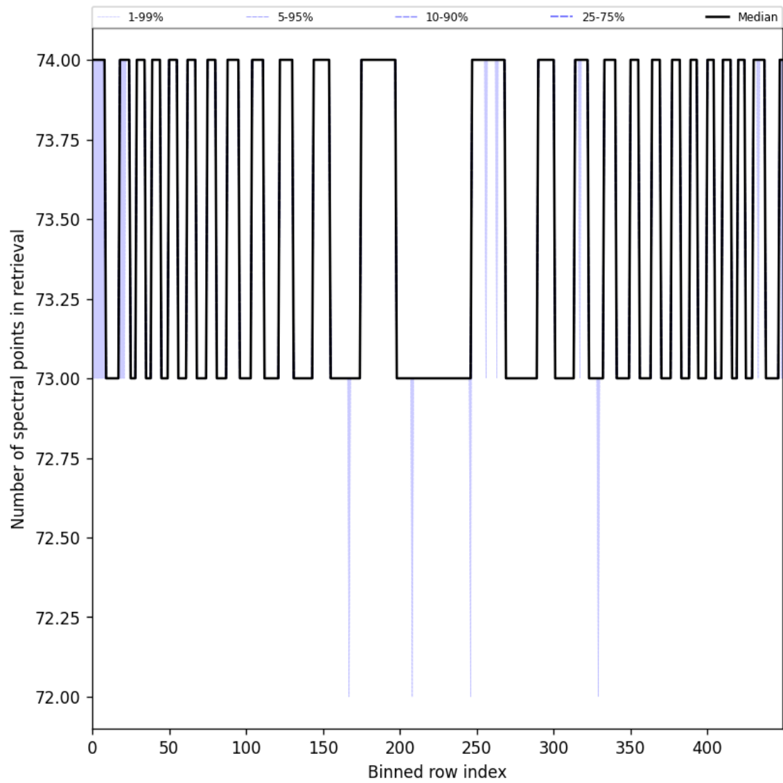
Figure 97: Along track statistics of “Number of spectral points in retrieval” for 2024-09-14 to 2024-09-16
