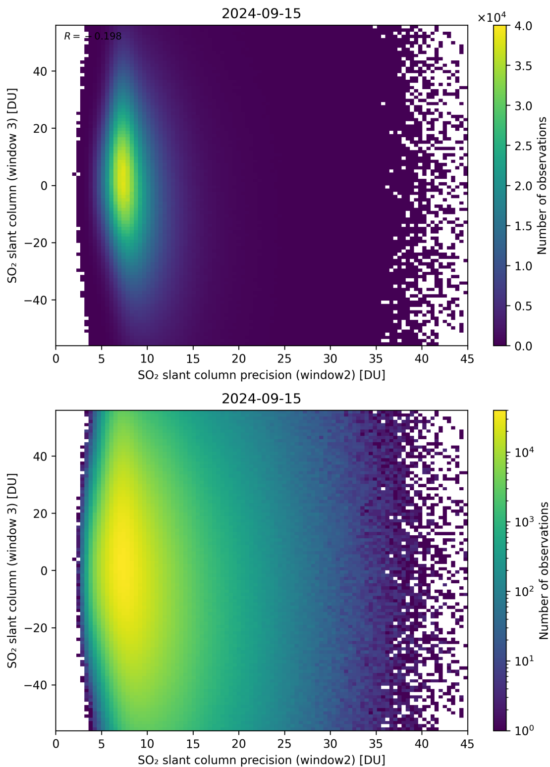
Figure 249: Scatter density plot of “SO 2 slant column precision (window2)” against “SO 2 slant column (window 3)” for 2024-09-14 to 2024-09-16.
