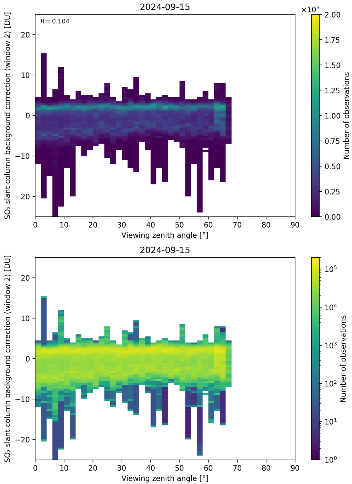
Figure 309: Scatter density plot of “Viewing zenith angle” against “SO 2 slant column background correction (window 2)” for 2024-09-14 to 2024-09-16.
