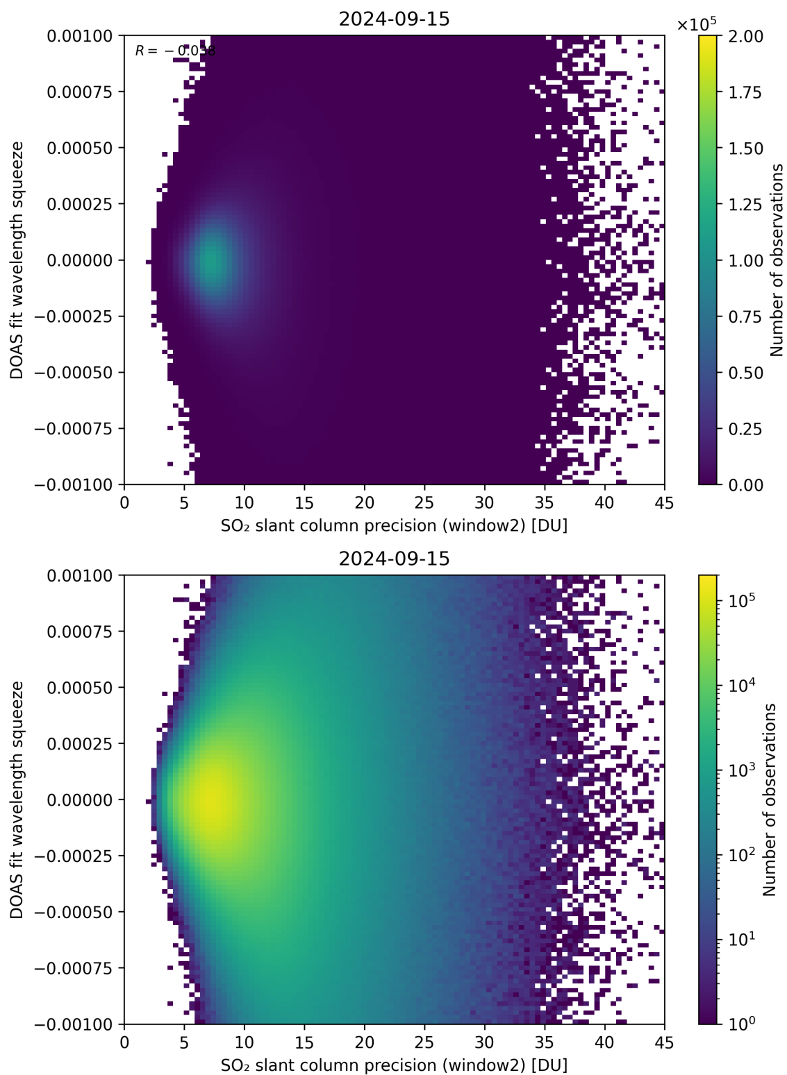
Figure 244: Scatter density plot of “SO 2 slant column precision (window2)” against “DOAS fit wavelength squeeze” for 2024-09-14 to 2024-09-16.
