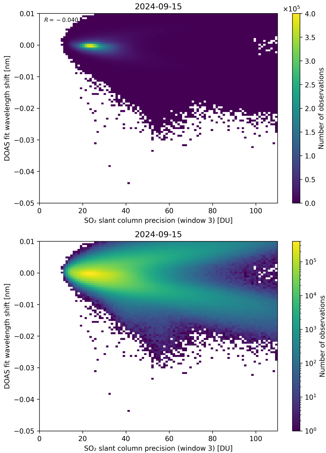
Figure 258: Scatter density plot of “SO 2 slant column precision (window 3)” against “DOAS fit wavelength shift” for 2024-09-14 to 2024-09-16.
