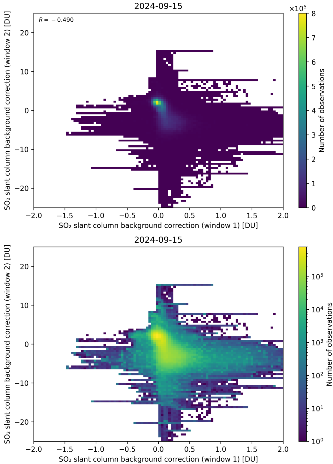
Figure 98: Scatter density plot of “SO 2 slant column background correction (window 1)” against “SO 2 slant column background correction (window 2)” for 2024-09-14 to 2024-09-16.
