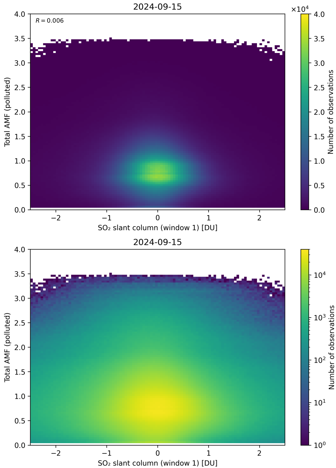
Figure 239: Scatter density plot of “SO 2 slant column (window 1)” against “Total AMF (polluted)” for 2024-09-14 to 2024-09-16.
