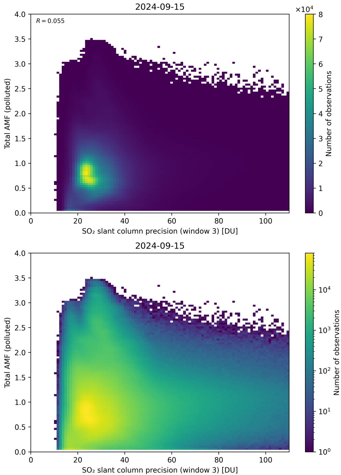
Figure 263: Scatter density plot of “SO 2 slant column precision (window 3)” against “Total AMF (polluted)” for 2024-09-14 to 2024-09-16.
