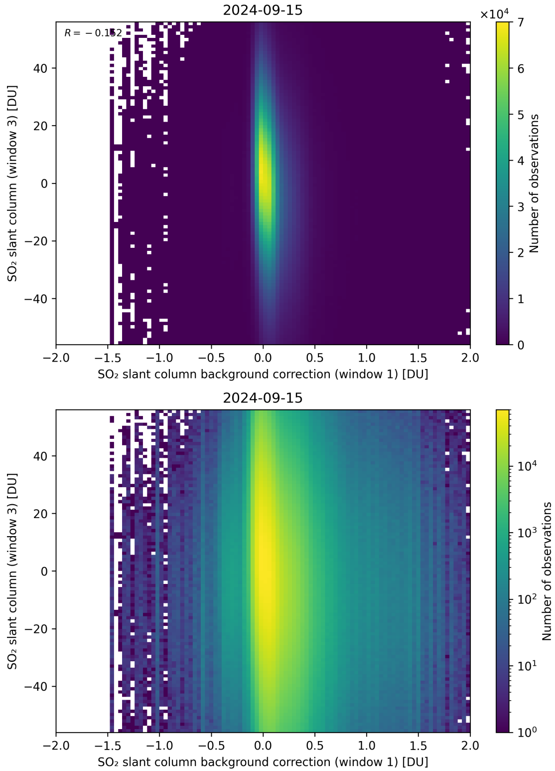
Figure 107: Scatter density plot of “SO 2 slant column background correction (window 1)” against “SO 2 slant column (window 3)” for 2024-09-14 to 2024-09-16.
