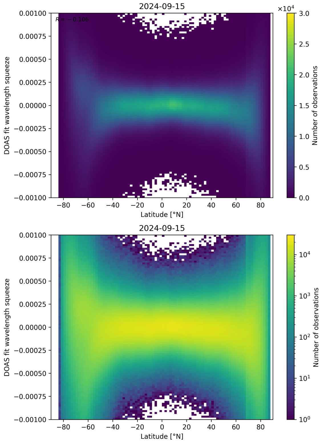
Figure 143: Scatter density plot of “Latitude” against “DOAS fit wavelength squeeze” for 2024-09-14 to 2024-09-16.
