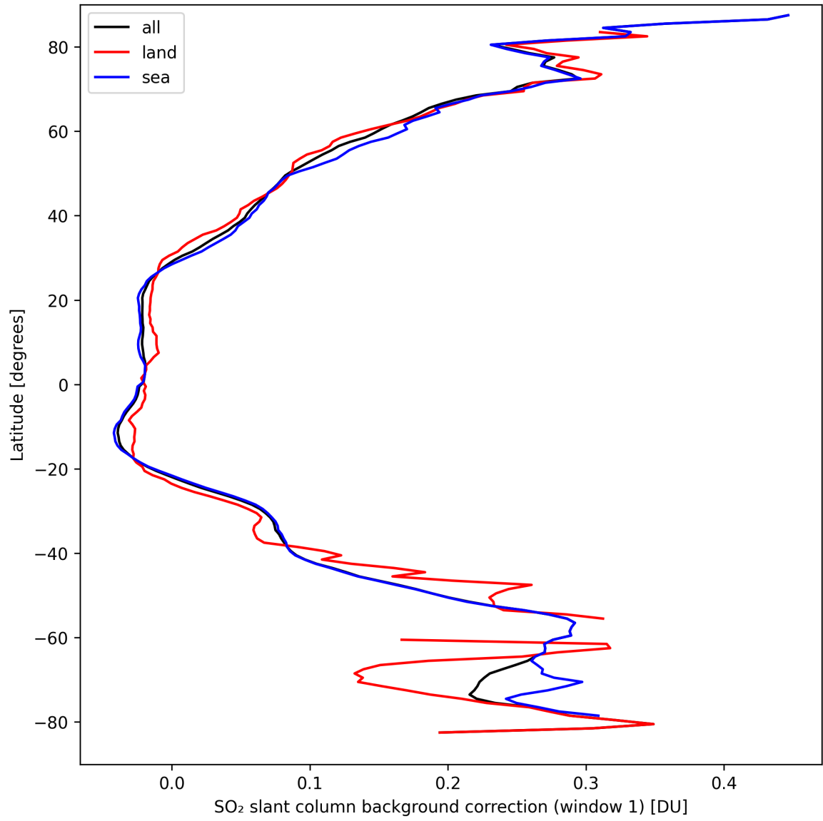
Figure 36: Zonal average of “SO 2 slant column background correction (window 1)” for 2024-09-14 to 2024-09-16.
