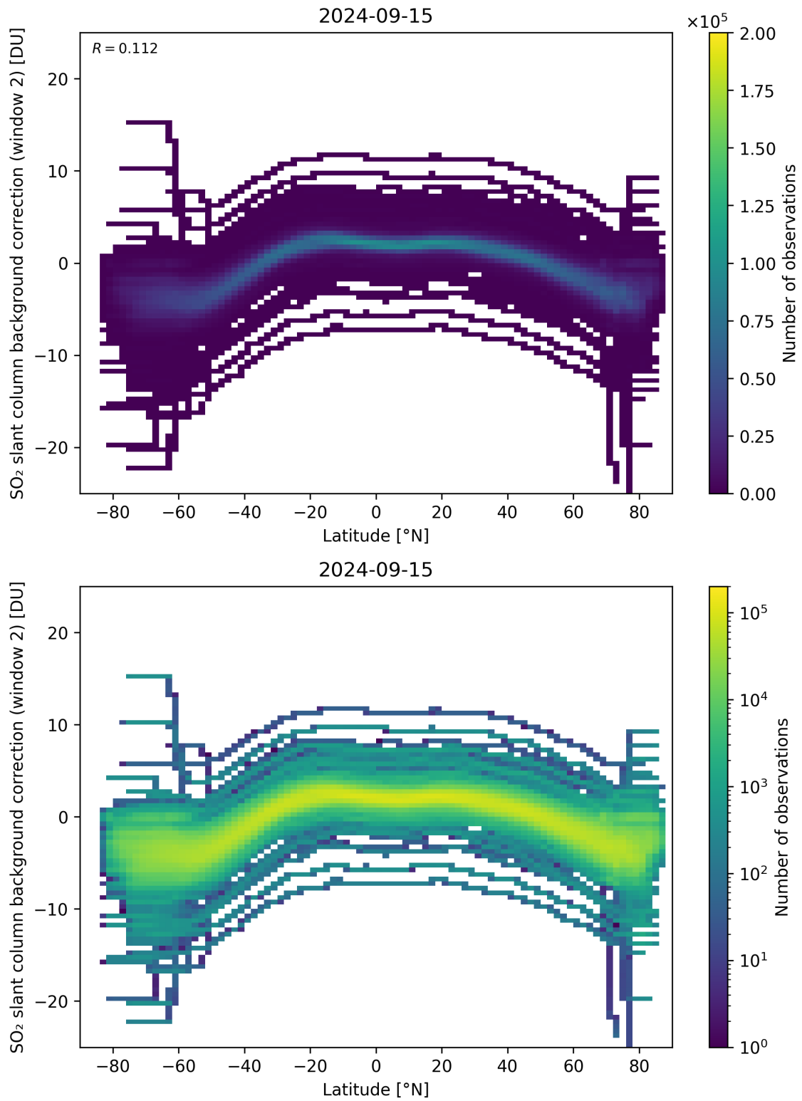
Figure 140: Scatter density plot of “Latitude” against “SO 2 slant column background correction (window 2)” for 2024-09-14 to 2024-09-16.
