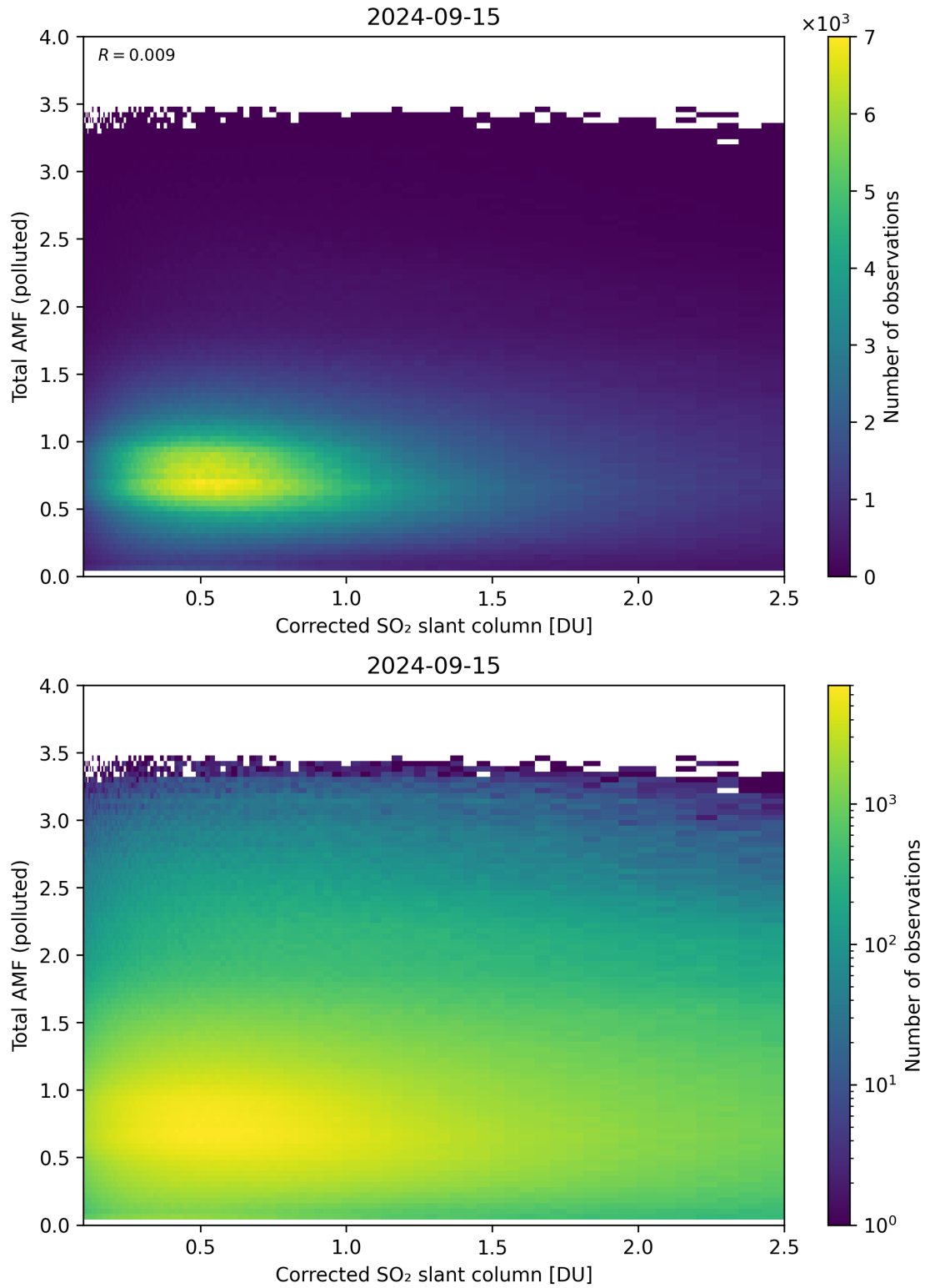
Figure 192: Scatter density plot of “Corrected SO 2 slant column” against “Total AMF (polluted)” for 2024-09-14 to 2024-09-16.
