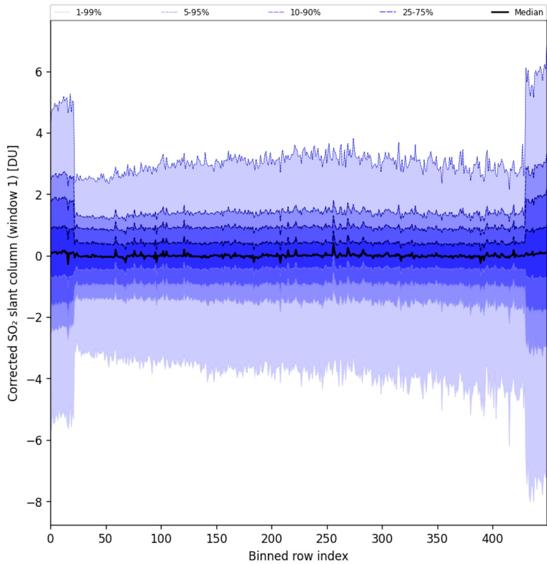
Figure 81: Along track statistics of “Corrected SO 2 slant column (window 1)” for 2024-09-14 to 2024-09-16
