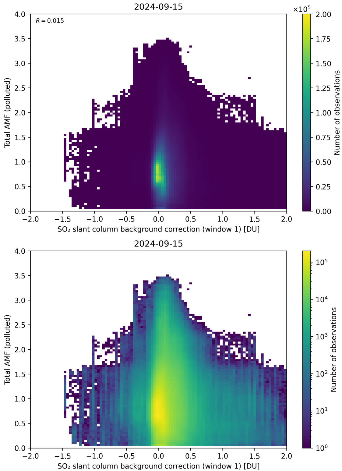
Figure 109: Scatter density plot of “SO 2 slant column background correction (window 1)” against “Total AMF (polluted)” for 2024-09-14 to 2024-09-16.
