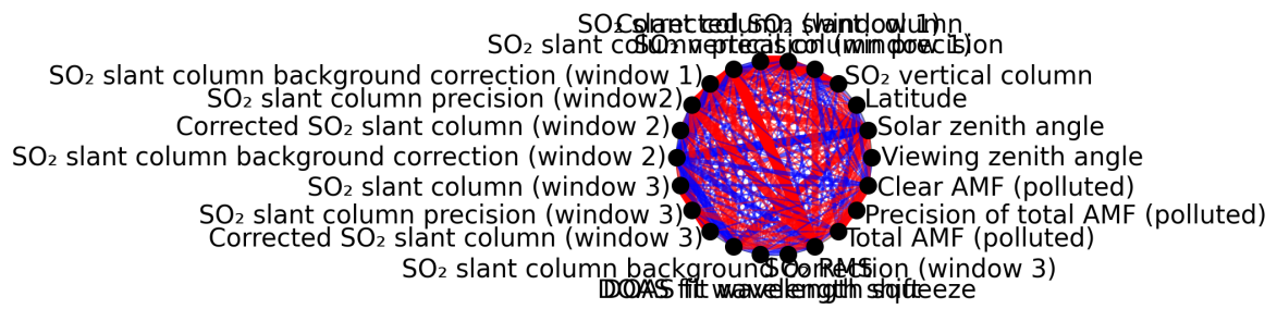
Figure 1: Map of correlation graph for 2024-09-14 to 2024-09-16.
