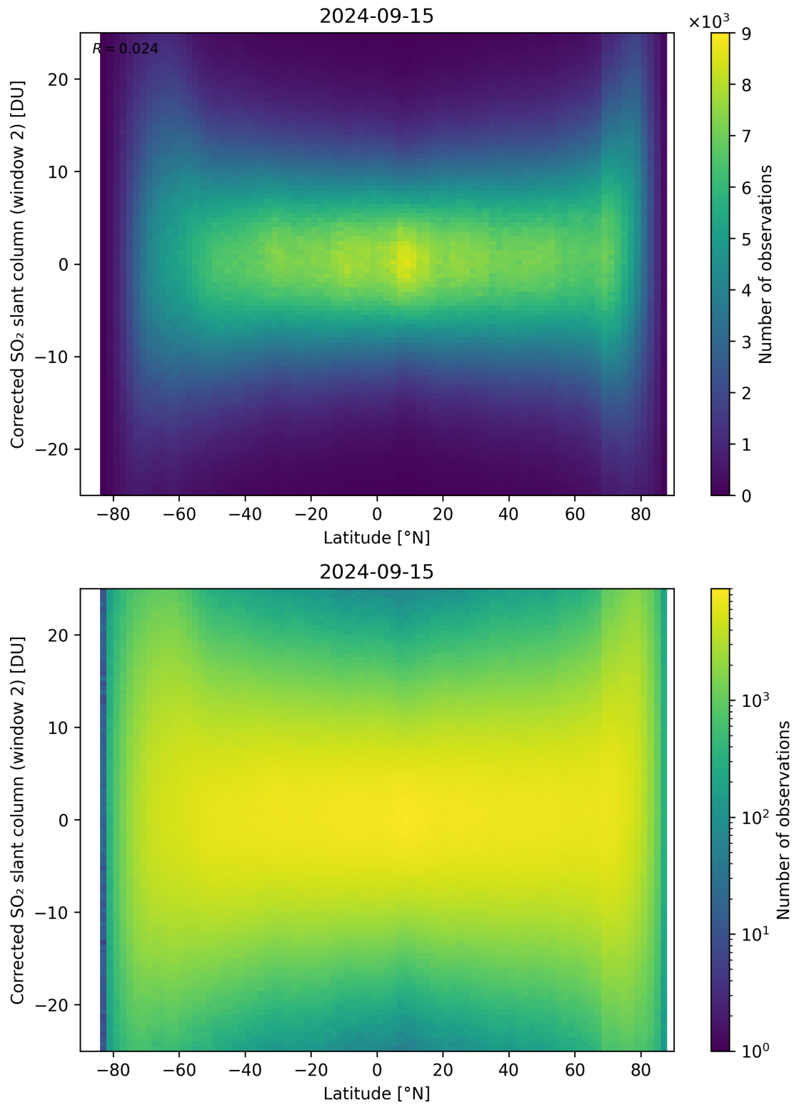
Figure 147: Scatter density plot of “Latitude” against “Corrected SO 2 slant column (window 2)” for 2024-09-14 to 2024-09-16.
