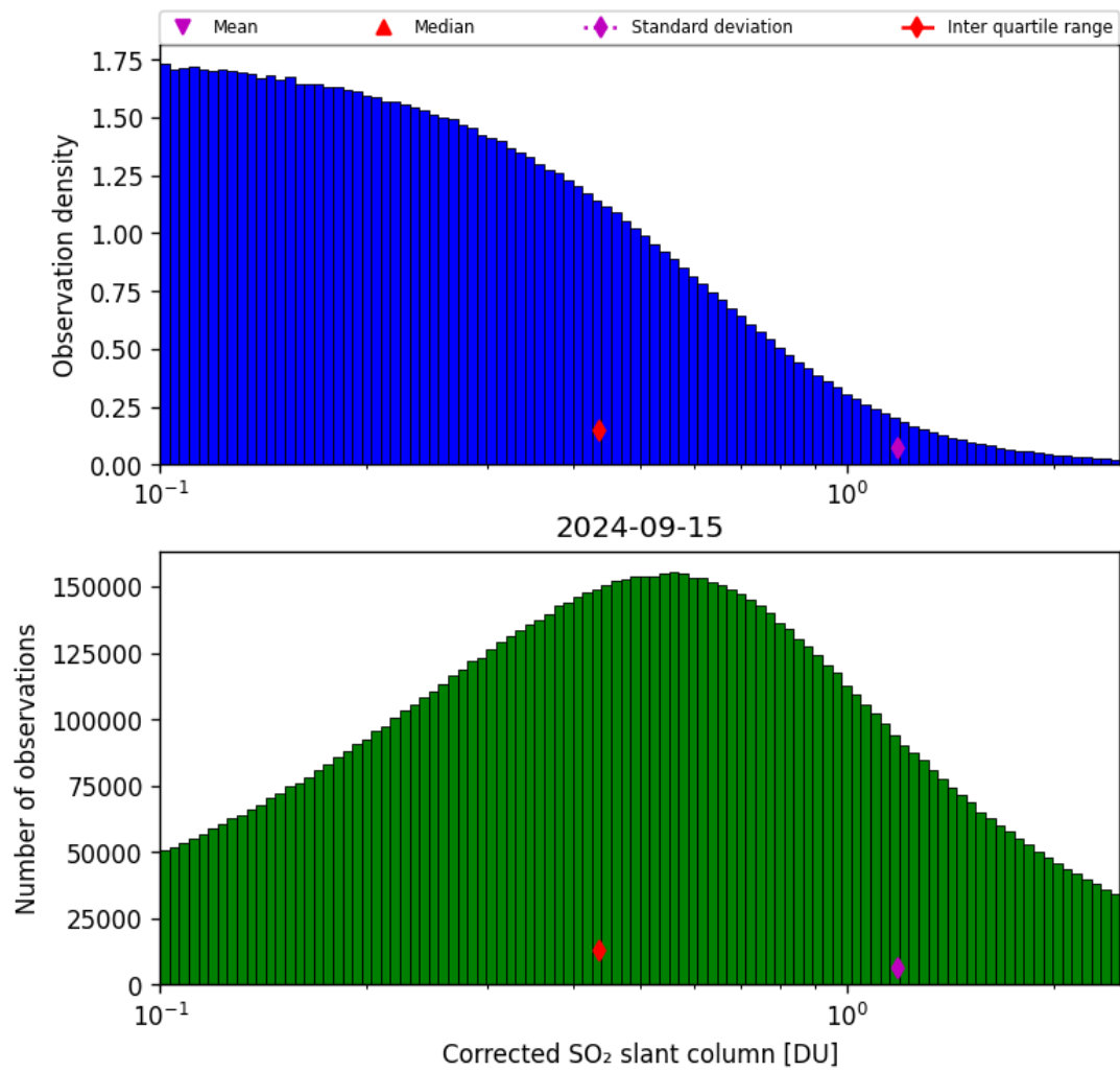
Figure 55: Histogram of “Corrected SO 2 slant column” for 2024-09-14 to 2024-09-16
