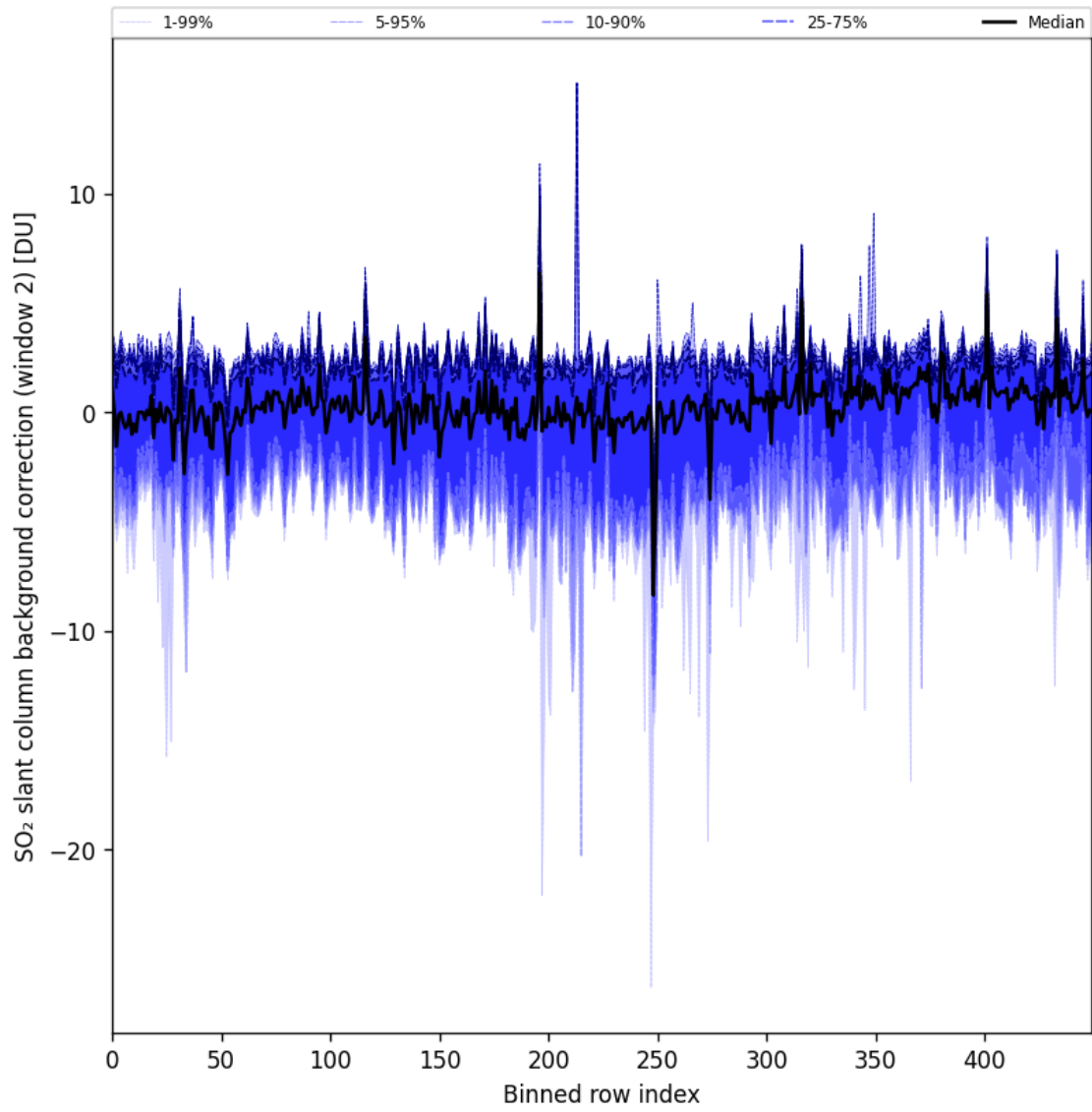
Figure 86: Along track statistics of “SO 2 slant column background correction (window 2)” for 2024-09-14 to 2024-09-16
