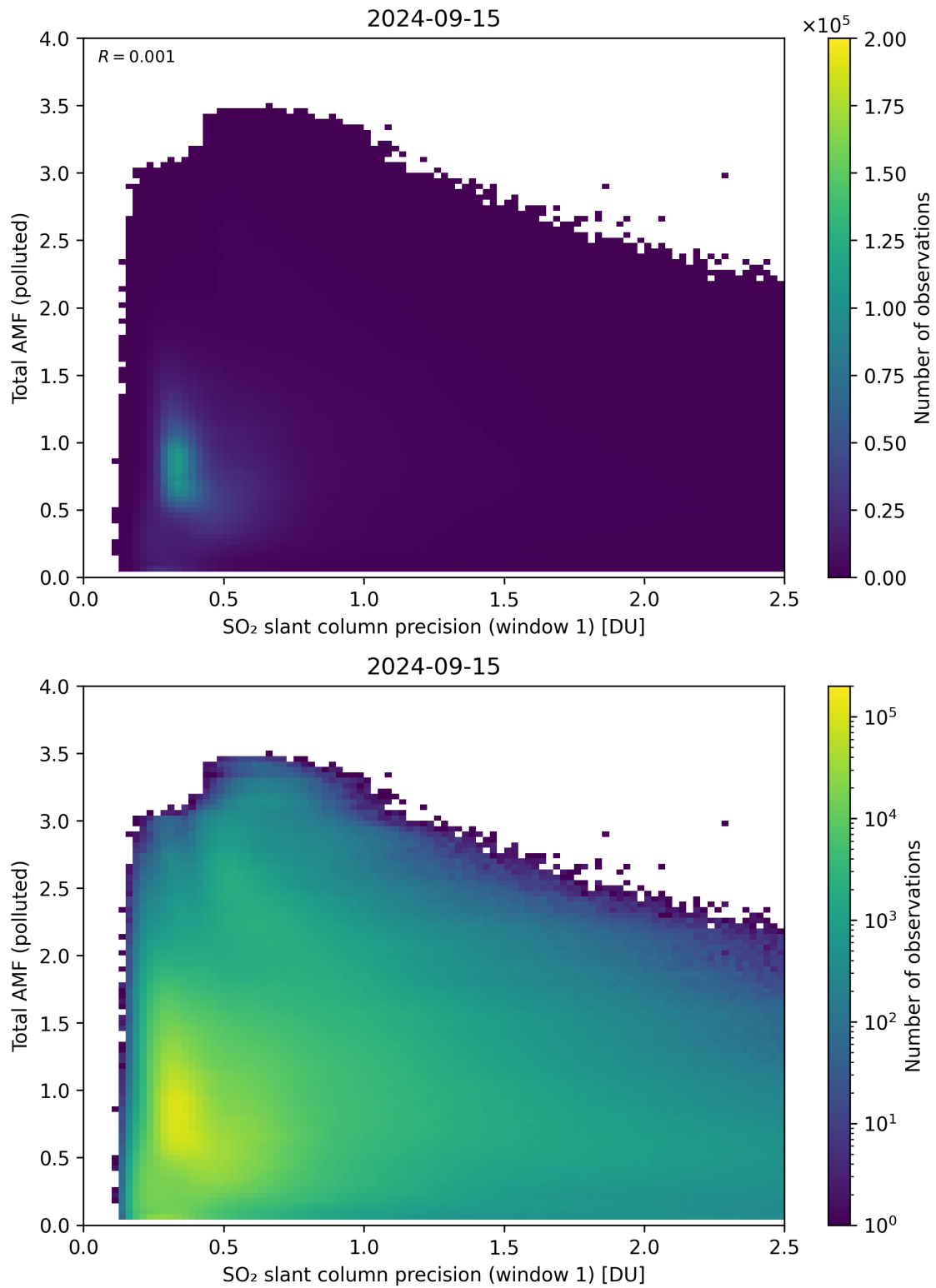
Figure 230: Scatter density plot of “SO 2 slant column precision (window 1)” against “Total AMF (polluted)” for 2024-09-14 to 2024-09-16.
