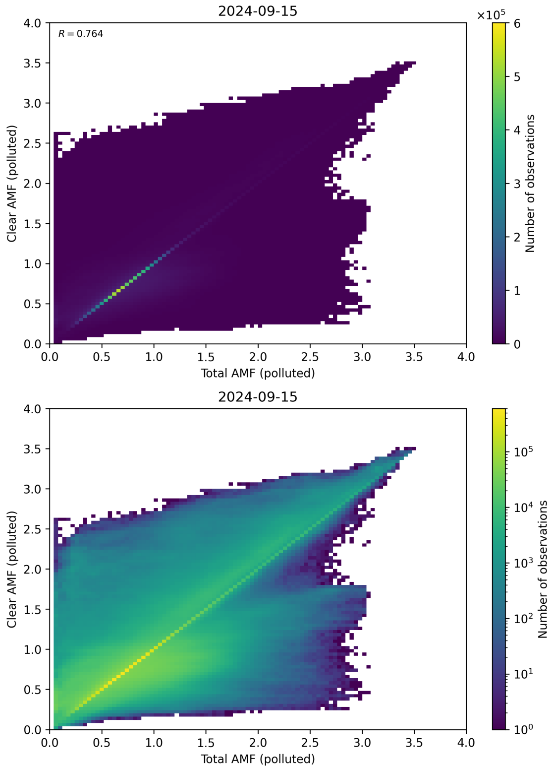
Figure 271: Scatter density plot of “Total AMF (polluted)” against “Clear AMF (polluted)” for 2024-09-14 to 2024-09-16.
