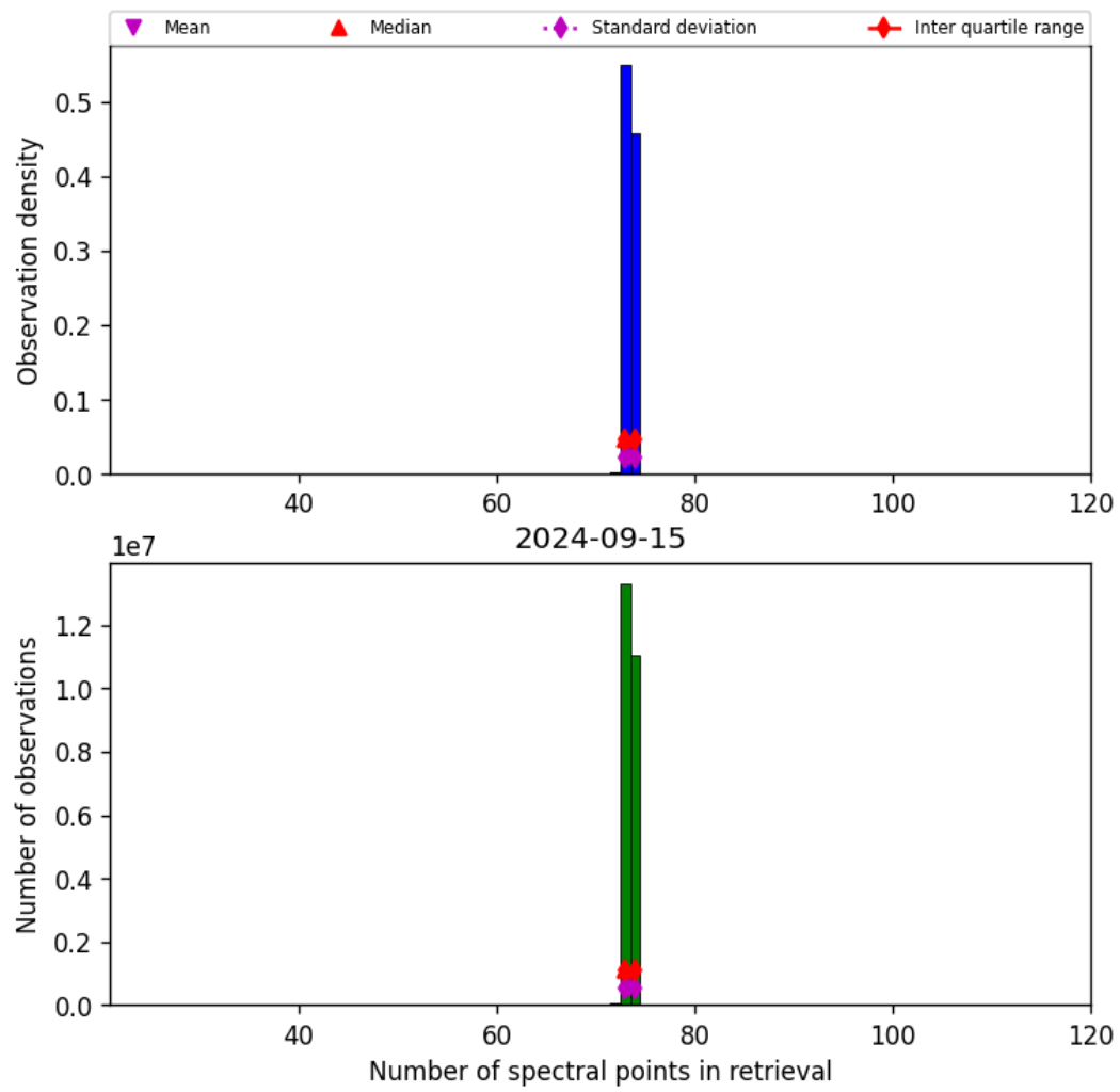
Figure 74: Histogram of “Number of spectral points in retrieval” for 2024-09-14 to 2024-09-16
