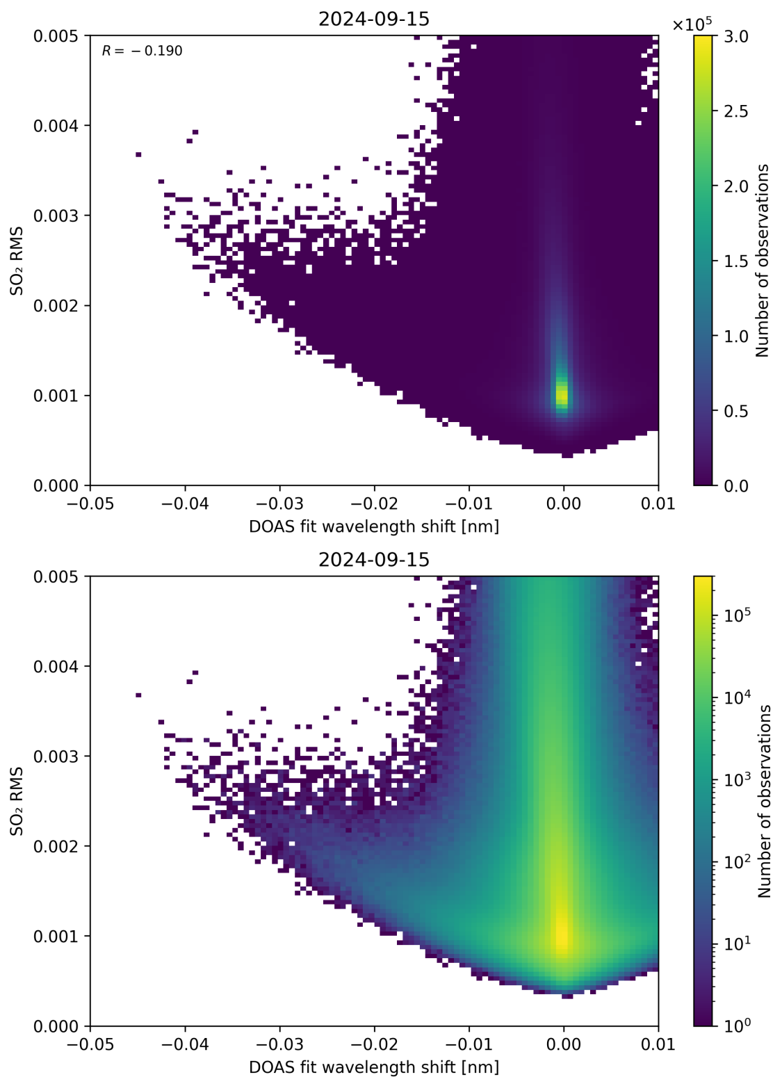
Figure 128: Scatter density plot of “DOAS fit wavelength shift” against “SO 2 RMS” for 2024-09-14 to 2024-09-16.
