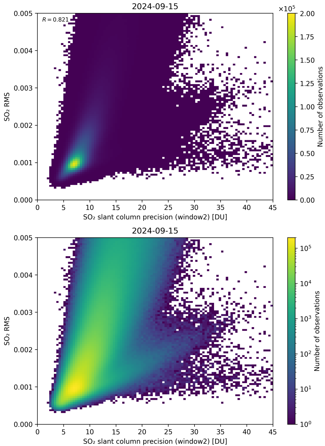
Figure 245: Scatter density plot of “SO 2 slant column precision (window2)” against “SO 2 RMS” for 2024-09-14 to 2024-09-16.
