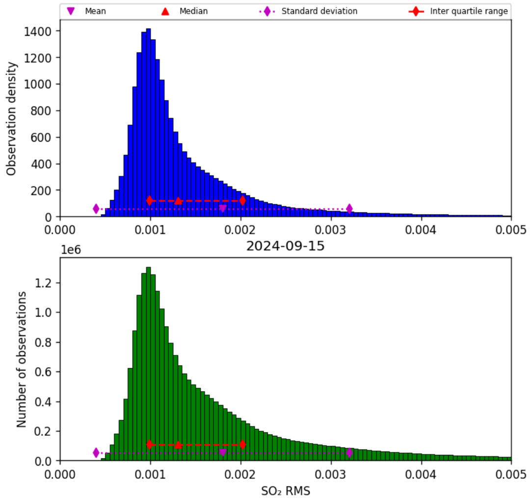
Figure 70: Histogram of “SO 2 RMS” for 2024-09-14 to 2024-09-16
