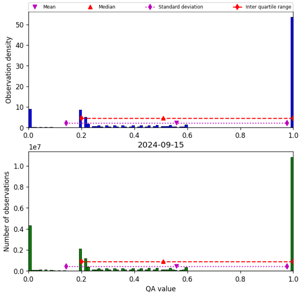
Figure 52: Histogram of “QA value” for 2024-09-14 to 2024-09-16
