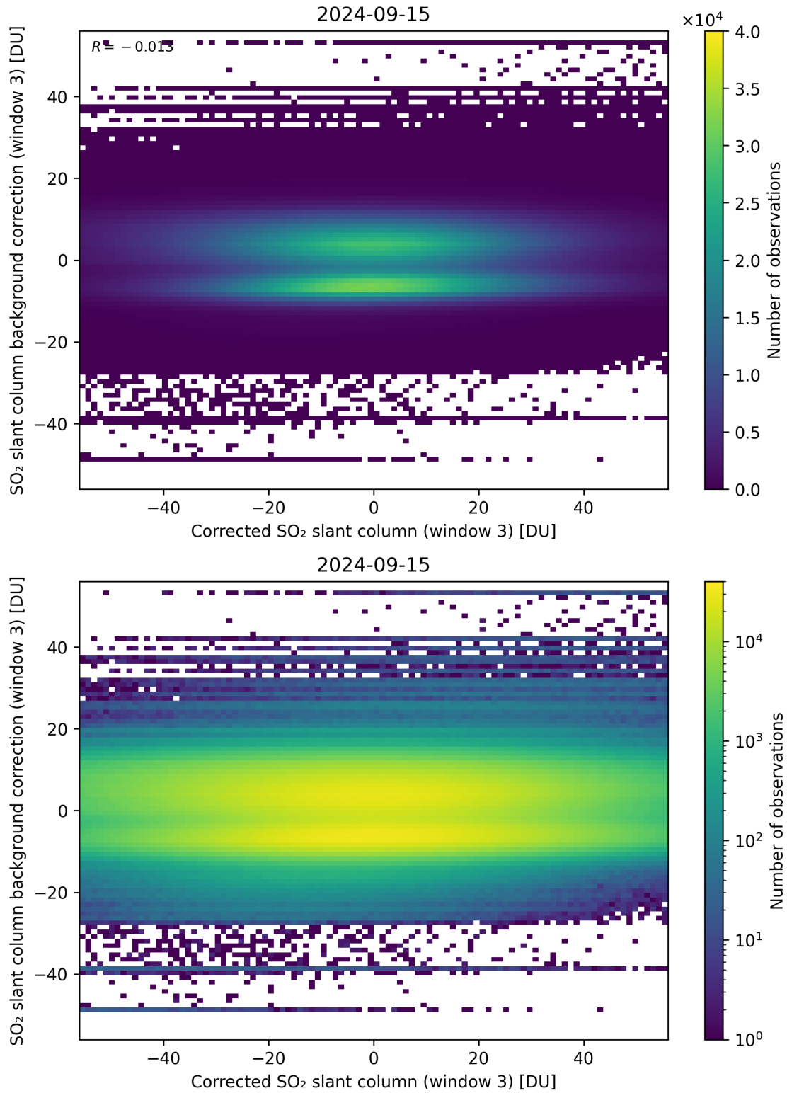
Figure 205: Scatter density plot of “Corrected SO 2 slant column (window 3)” against “SO 2 slant column background correction (window 3)” for 2024-09-14 to 2024-09-16.
