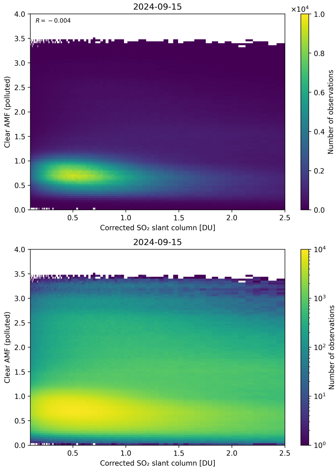
Figure 184: Scatter density plot of “Corrected SO 2 slant column” against “Clear AMF (polluted)” for 2024-09-14 to 2024-09-16.
