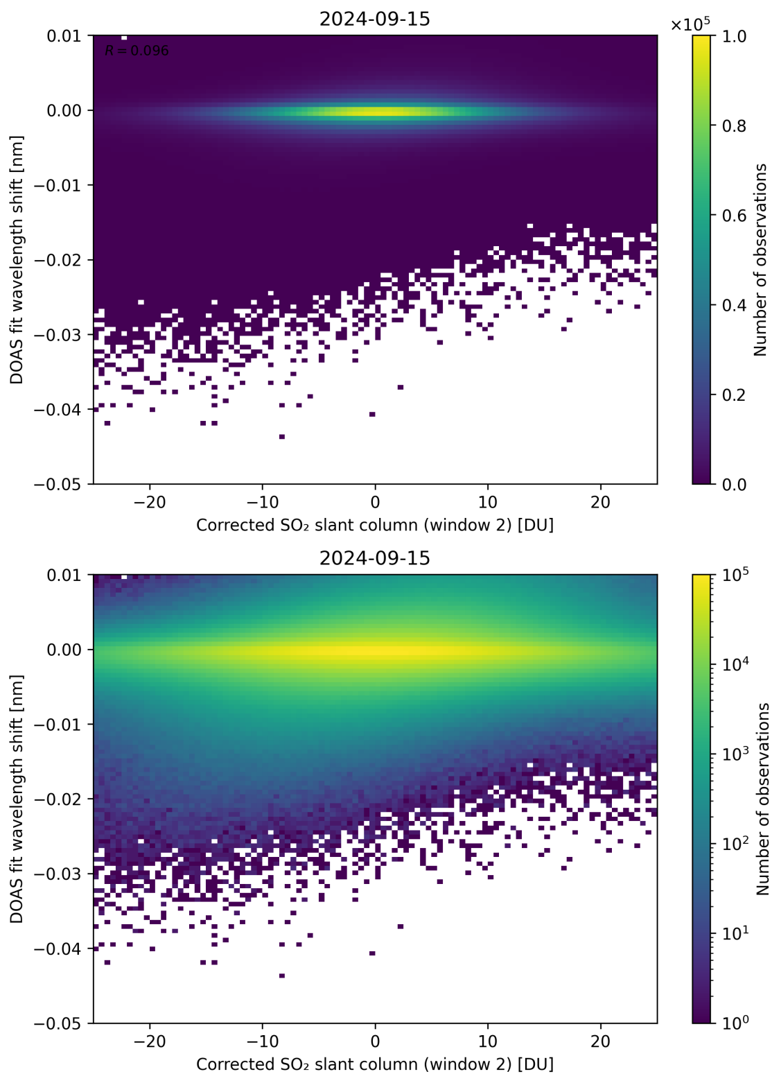
Figure 196: Scatter density plot of “Corrected SO 2 slant column (window 2)” against “DOAS fit wavelength shift” for 2024-09-14 to 2024-09-16.
