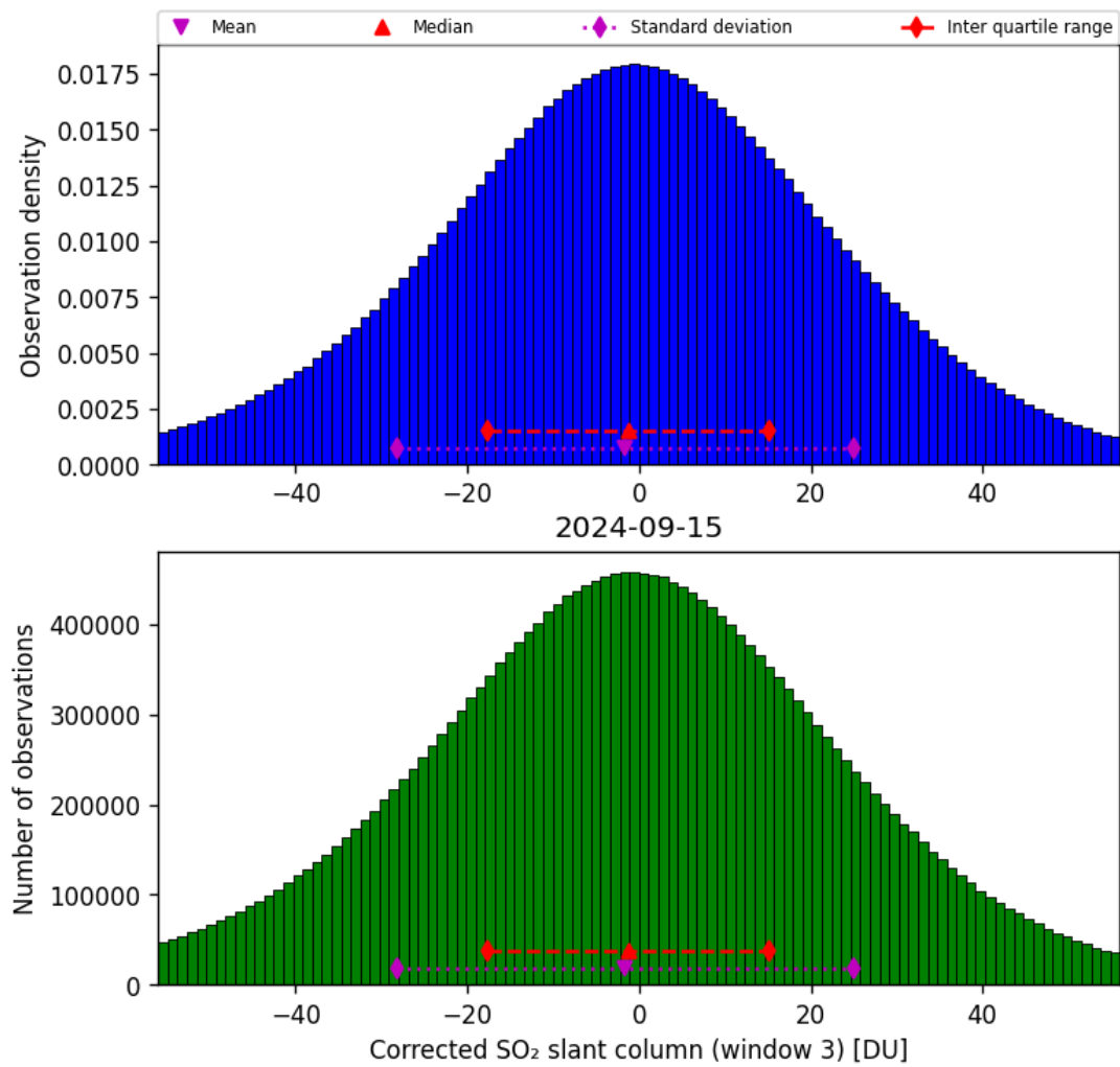
Figure 66: Histogram of “Corrected SO 2 slant column (window 3)” for 2024-09-14 to 2024-09-16
