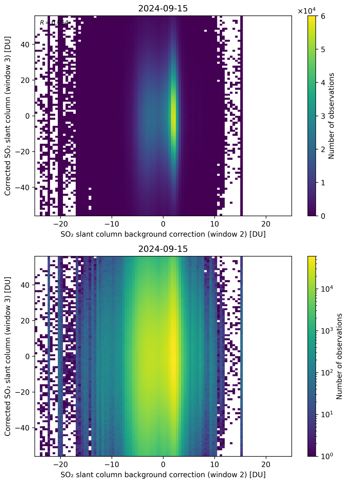
Figure 116: Scatter density plot of “SO 2 slant column background correction (window 2)” against “Corrected SO 2 slant column (window 3)” for 2024-09-14 to 2024-09-16.
