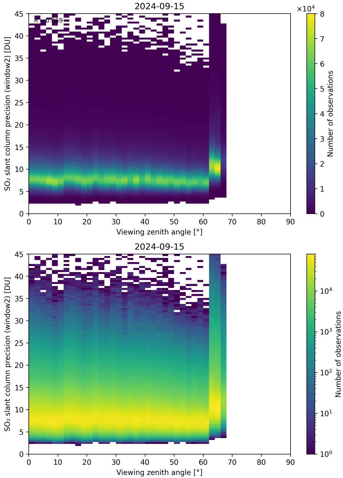
Figure 322: Scatter density plot of “Viewing zenith angle” against “SO 2 slant column precision (window2)” for 2024-09-14 to 2024-09-16.
