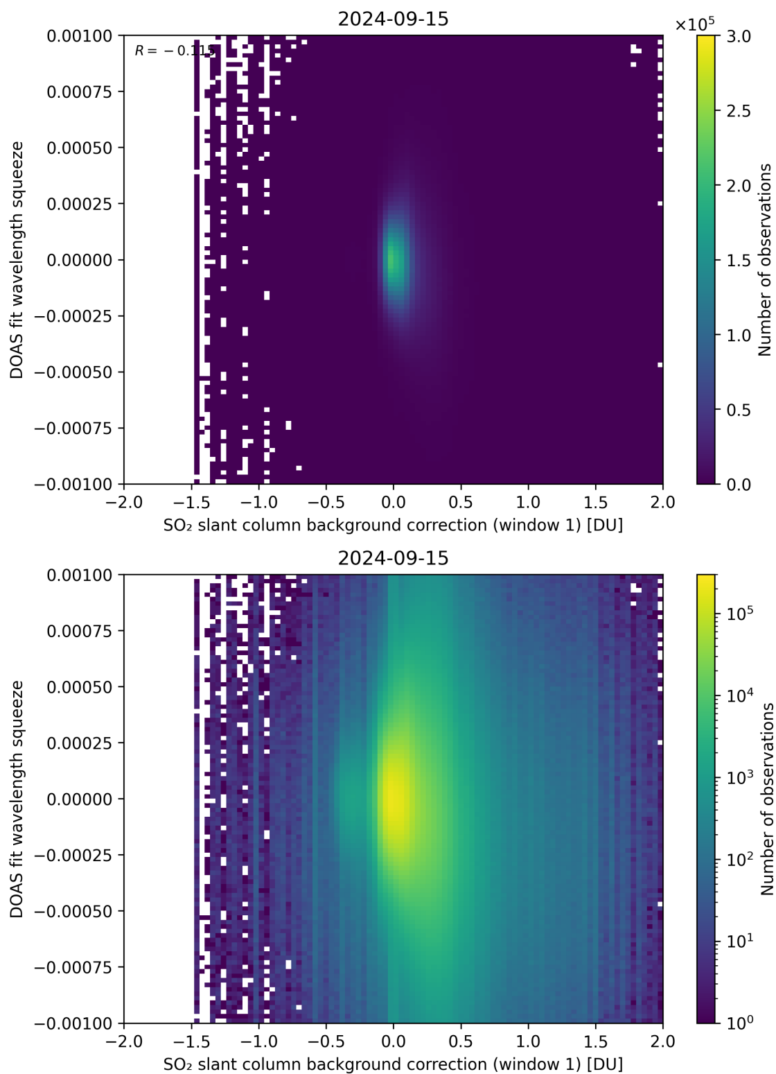
Figure 101: Scatter density plot of “SO 2 slant column background correction (window 1)” against “DOAS fit wavelength squeeze” for 2024-09-14 to 2024-09-16.
