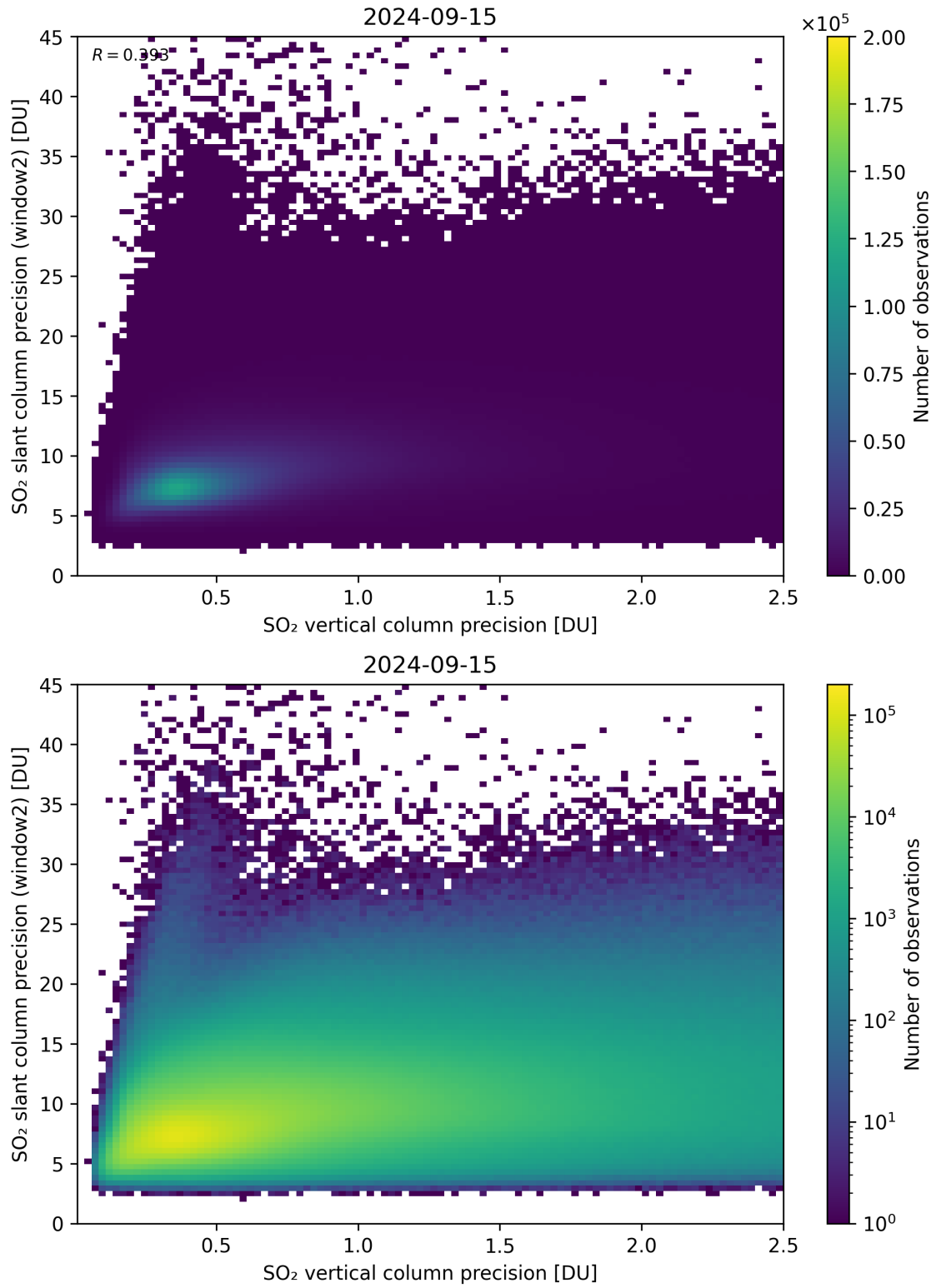
Figure 291: Scatter density plot of “SO 2 vertical column precision” against “SO 2 slant column precision (window2)” for 2024-09-14 to 2024-09-16.
