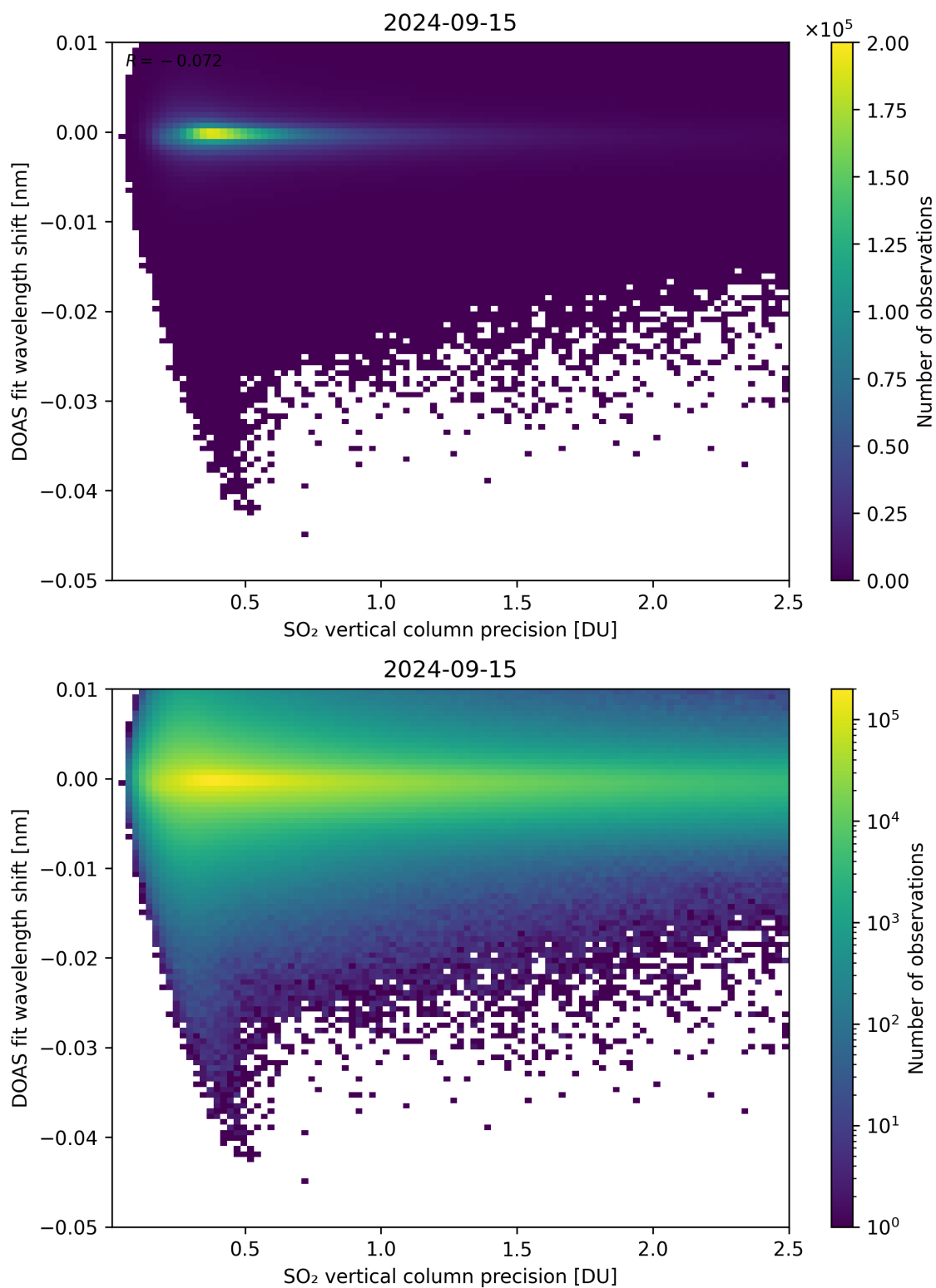
Figure 282: Scatter density plot of “SO 2 vertical column precision” against “DOAS fit wavelength shift” for 2024-09-14 to 2024-09-16.
