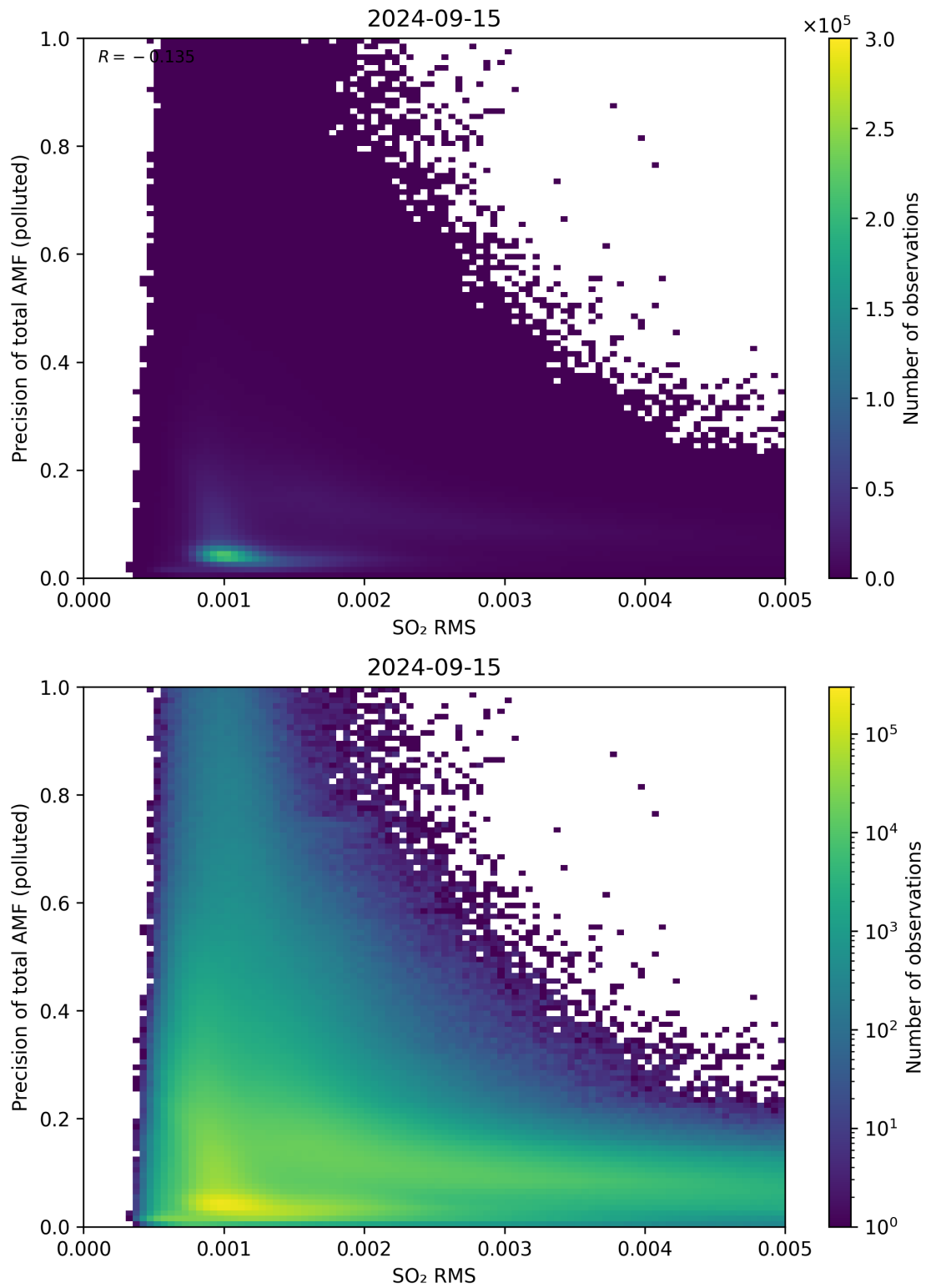
Figure 138: Scatter density plot of “SO 2 RMS” against “Precision of total AMF (polluted)” for 2024-09-14 to 2024-09-16.
