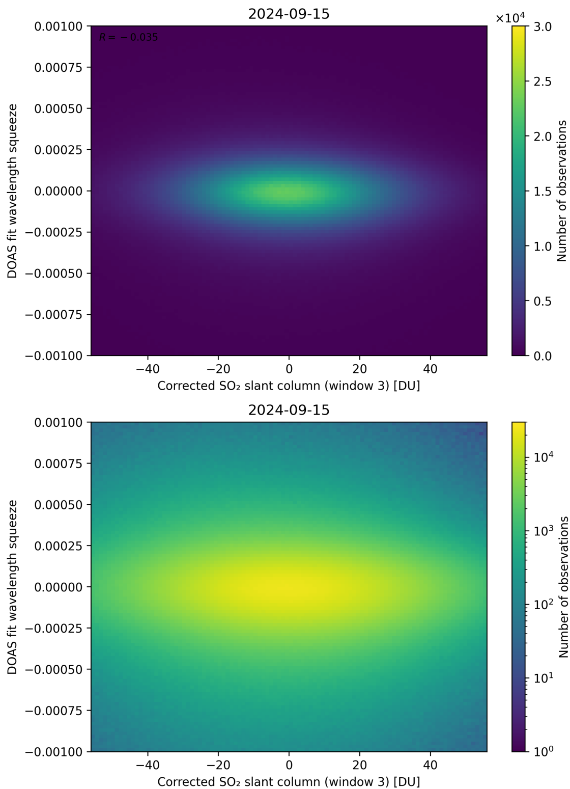
Figure 207: Scatter density plot of “Corrected SO 2 slant column (window 3)” against “DOAS fit wavelength squeeze” for 2024-09-14 to 2024-09-16.
