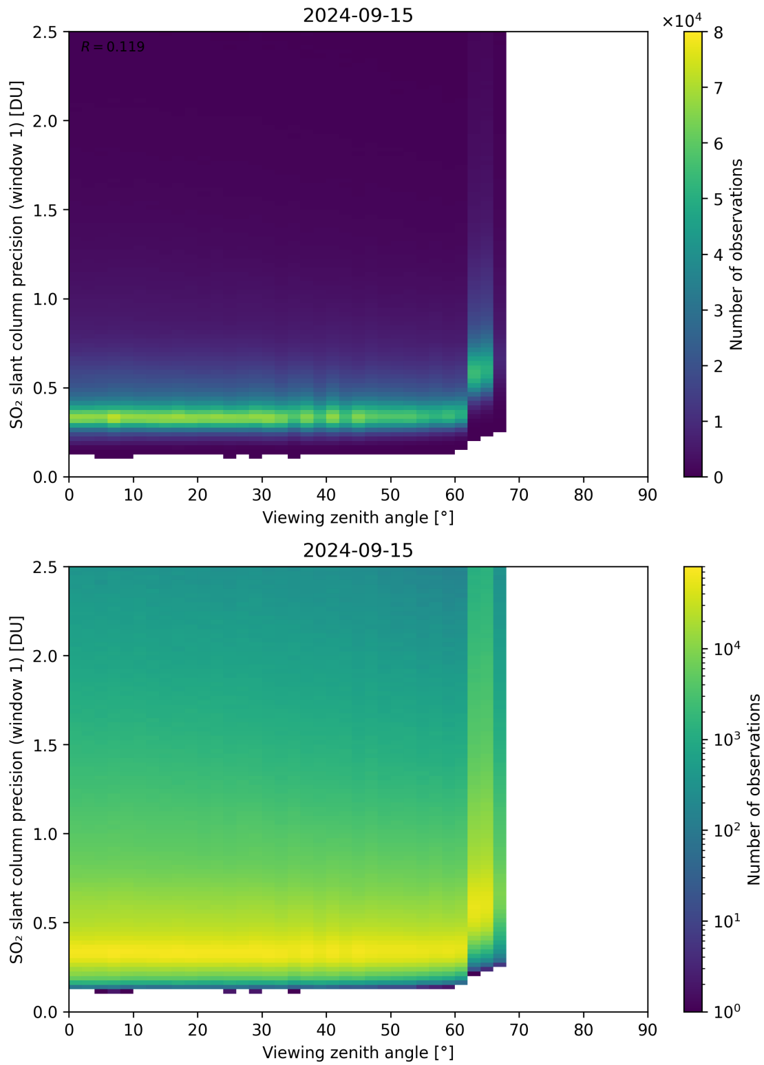
Figure 321: Scatter density plot of “Viewing zenith angle” against “SO 2 slant column precision (window 1)” for 2024-09-14 to 2024-09-16.
