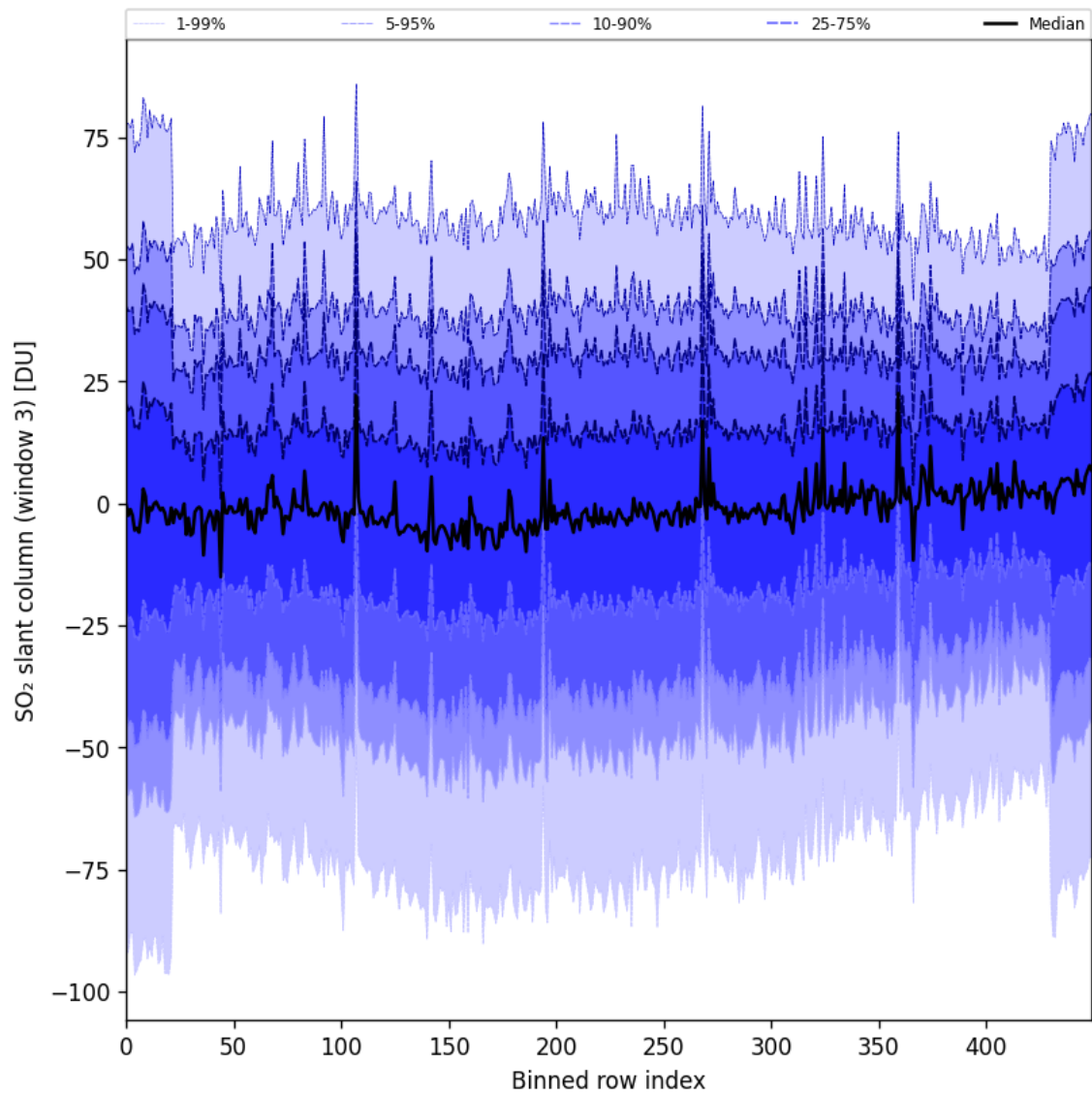
Figure 87: Along track statistics of “SO 2 slant column (window 3)” for 2024-09-14 to 2024-09-16
