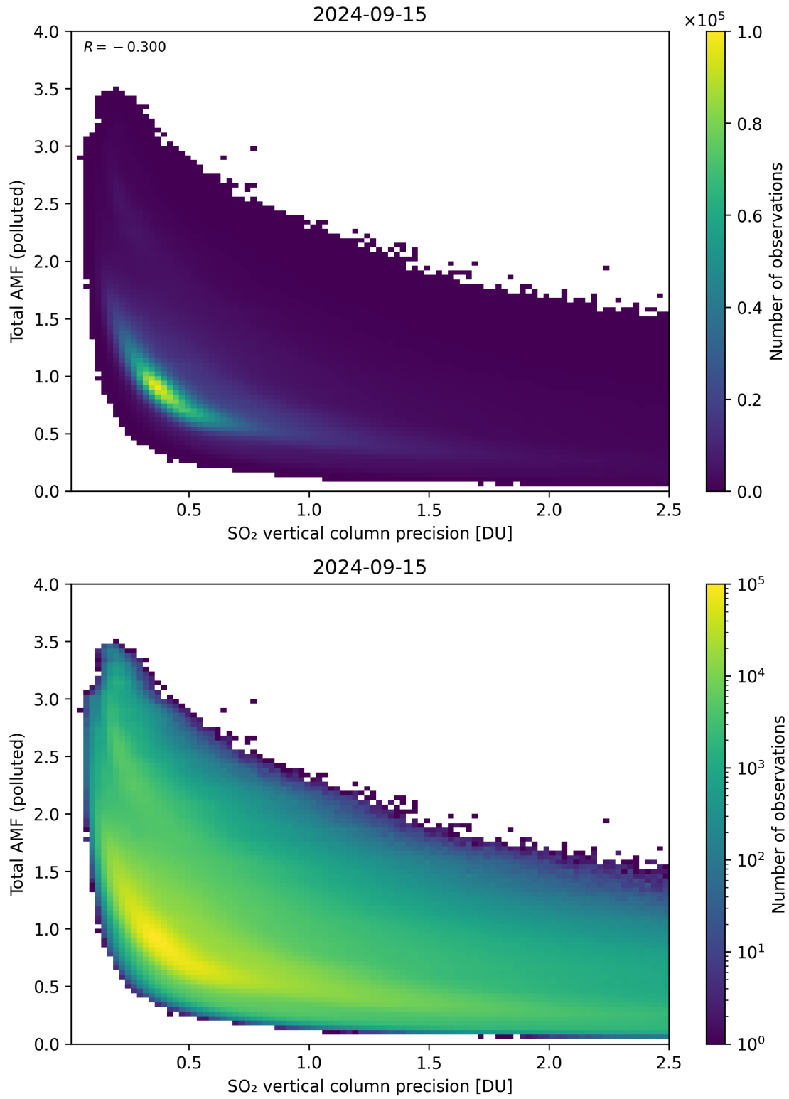
Figure 294: Scatter density plot of “SO 2 vertical column precision” against “Total AMF (polluted)” for 2024-09-14 to 2024-09-16.
