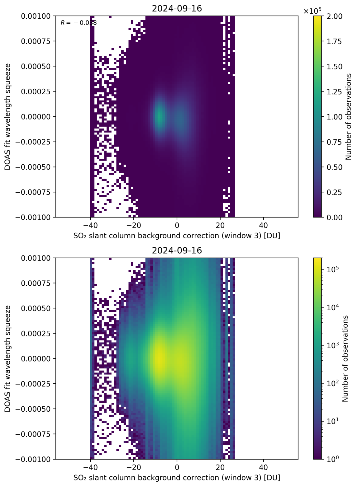
Figure 122: Scatter density plot of “SO 2 slant column background correction (window 3)” against “DOAS fit wavelength squeeze” for 2024-09-15 to 2024-09-17.
