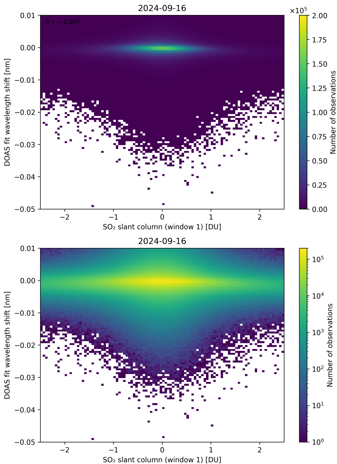
Figure 215: Scatter density plot of “SO 2 slant column (window 1)” against “DOAS fit wavelength shift” for 2024-09-15 to 2024-09-17.
