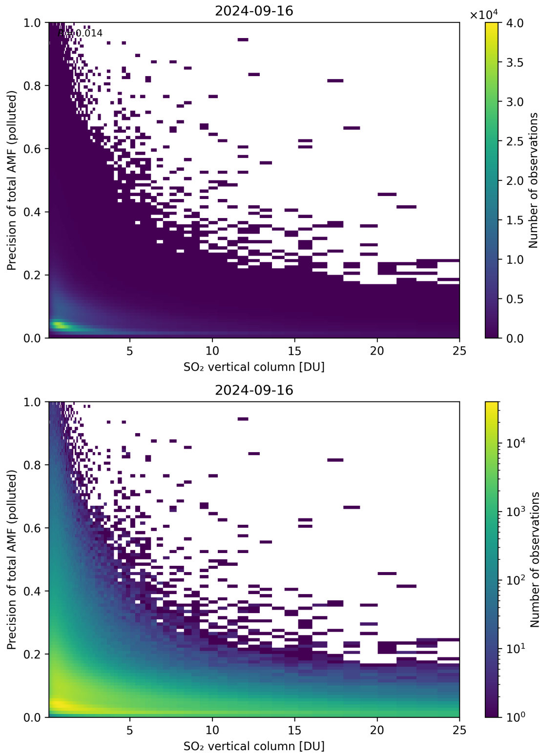
Figure 306: Scatter density plot of “SO 2 vertical column” against “Precision of total AMF (polluted)” for 2024-09-15 to 2024-09-17.
