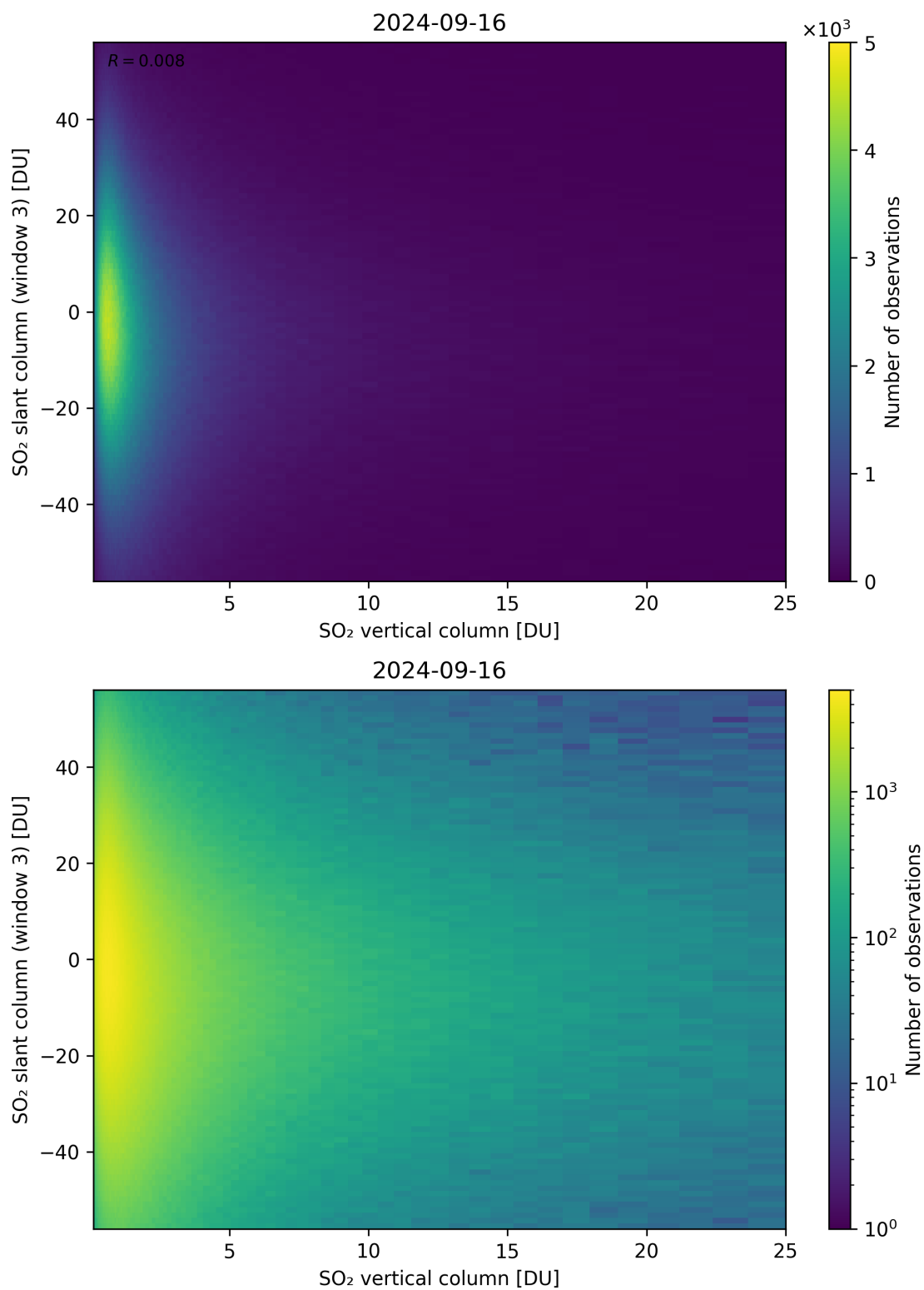
Figure 303: Scatter density plot of “SO 2 vertical column” against “SO 2 slant column (window 3)” for 2024-09-15 to 2024-09-17.
