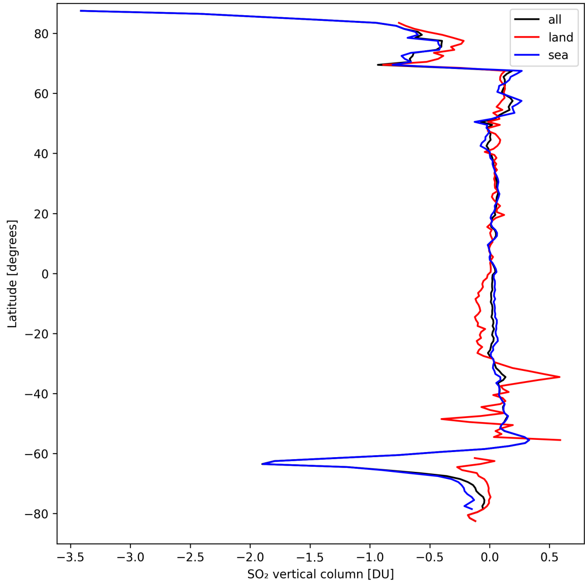
Figure 30: Zonal average of “SO 2 vertical column” for 2024-09-15 to 2024-09-17.
