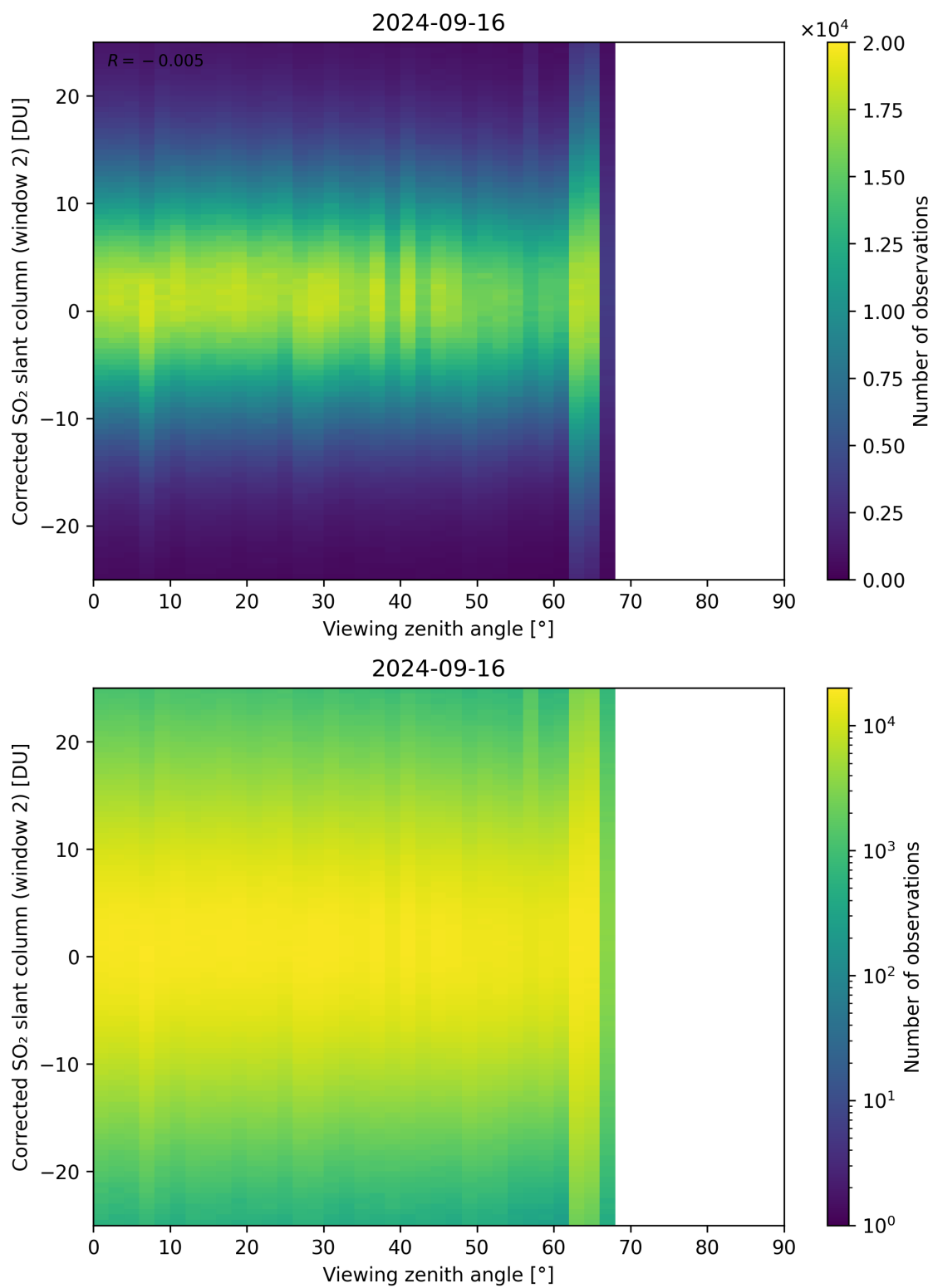
Figure 318: Scatter density plot of “Viewing zenith angle” against “Corrected SO 2 slant column (window 2)” for 2024-09-15 to 2024-09-17.
