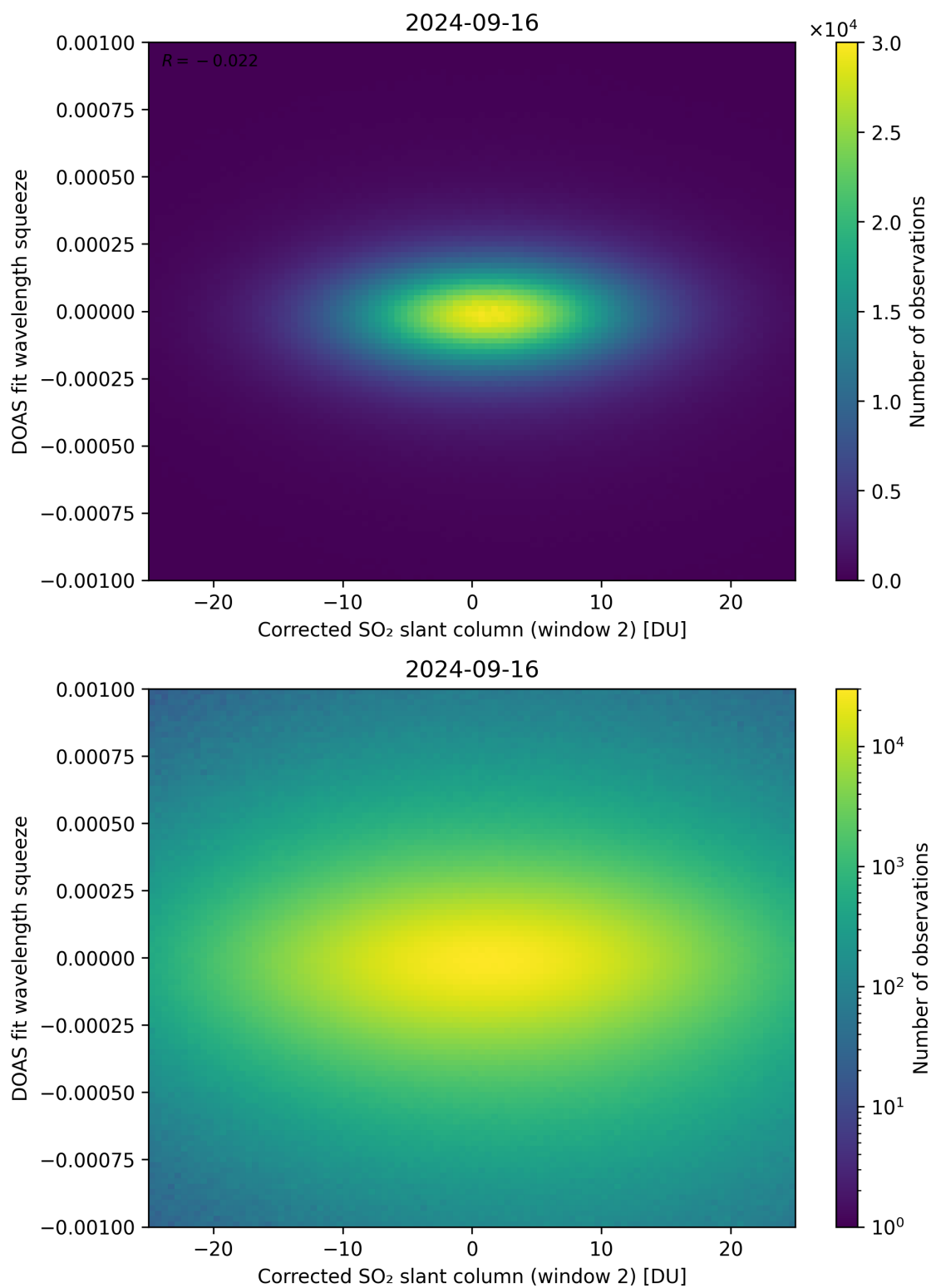
Figure 197: Scatter density plot of “Corrected SO 2 slant column (window 2)” against “DOAS fit wavelength squeeze” for 2024-09-15 to 2024-09-17.
