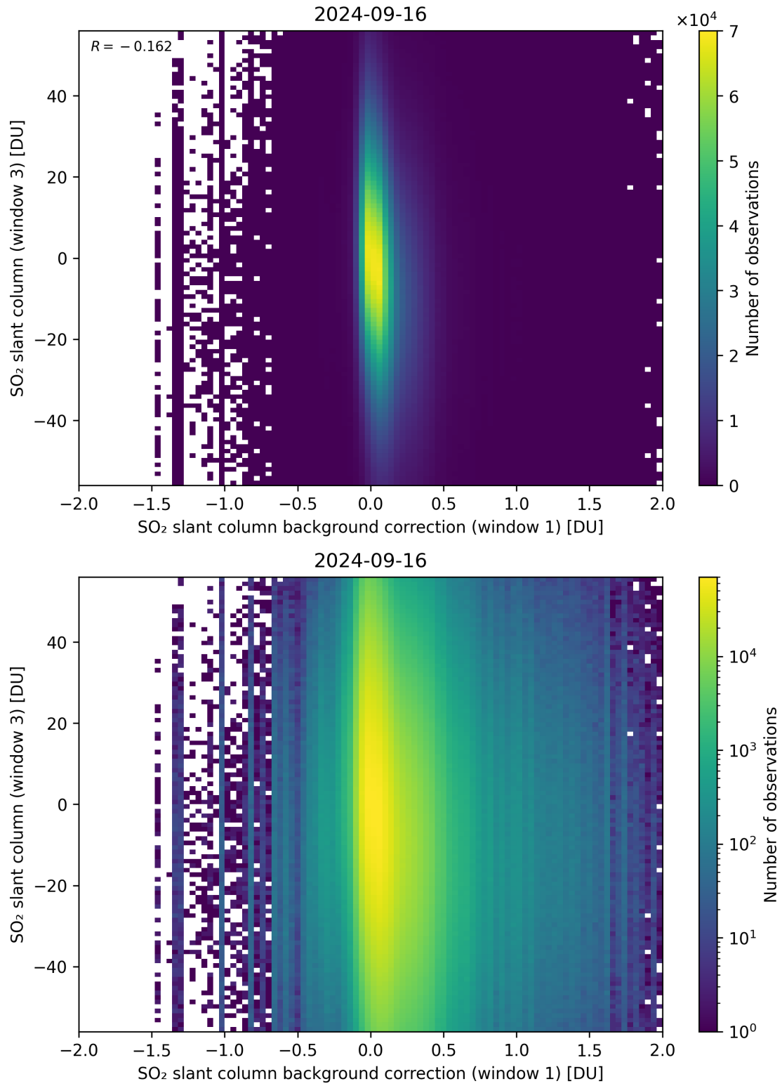
Figure 107: Scatter density plot of “SO 2 slant column background correction (window 1)” against “SO 2 slant column (window 3)” for 2024-09-15 to 2024-09-17.
