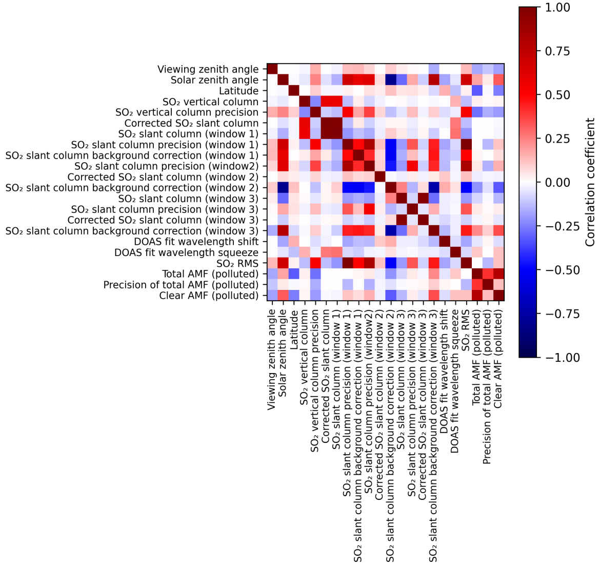
Figure 2: Map of correlation matrix for 2024-09-15 to 2024-09-17.
