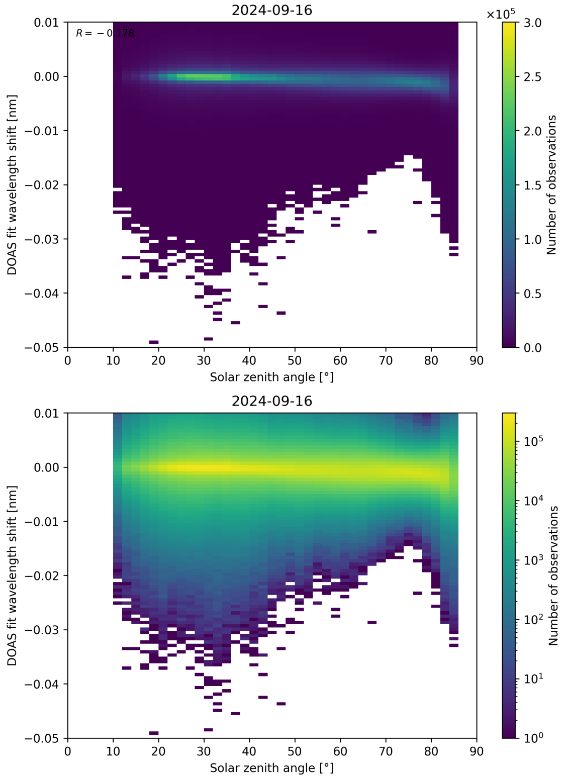
Figure 161: Scatter density plot of “Solar zenith angle” against “DOAS fit wavelength shift” for 2024-09-15 to 2024-09-17.
