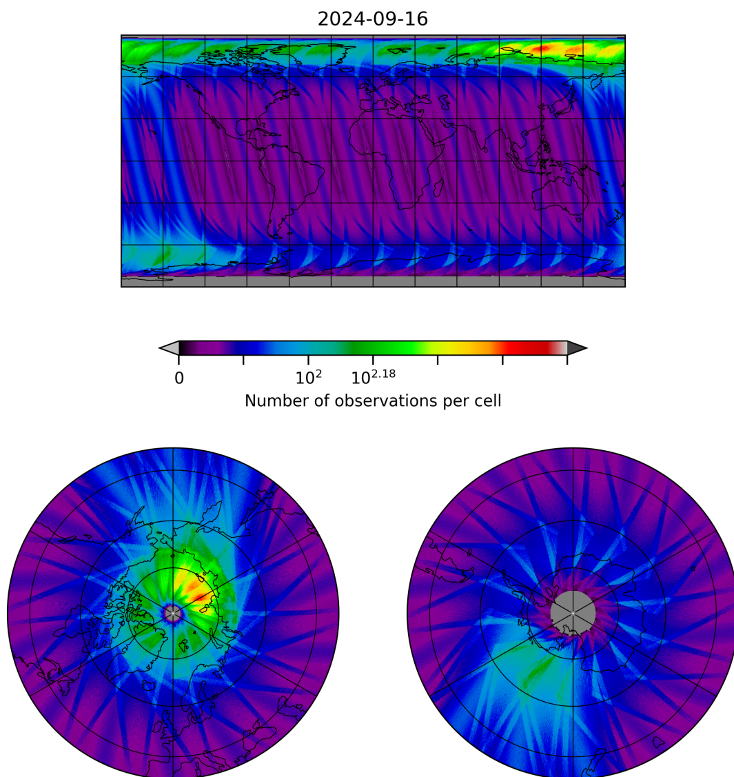
Figure 28: Map of the number of observations for 2024-09-15 to 2024-09-17
