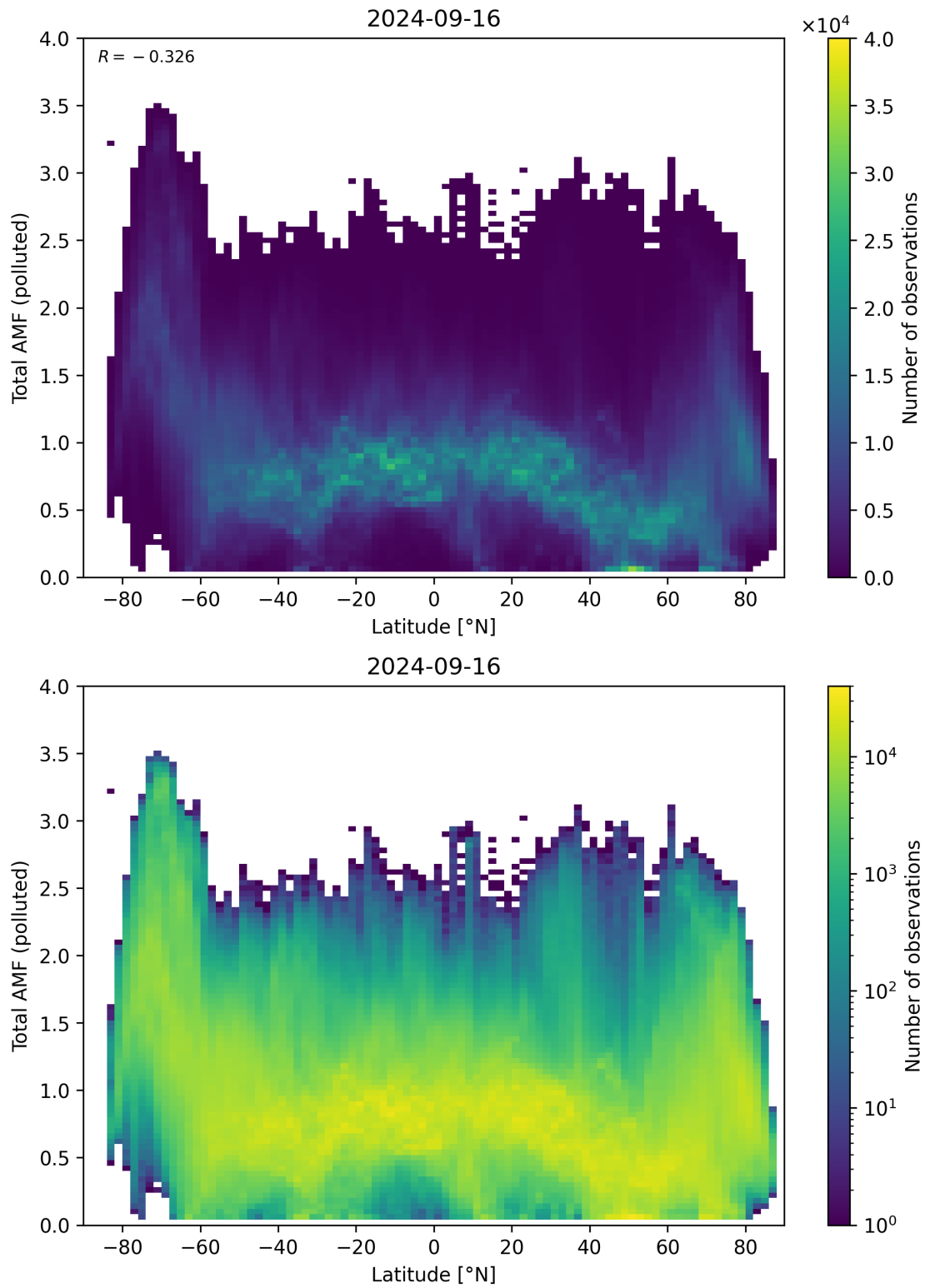
Figure 154: Scatter density plot of “Latitude” against “Total AMF (polluted)” for 2024-09-15 to 2024-09-17.
