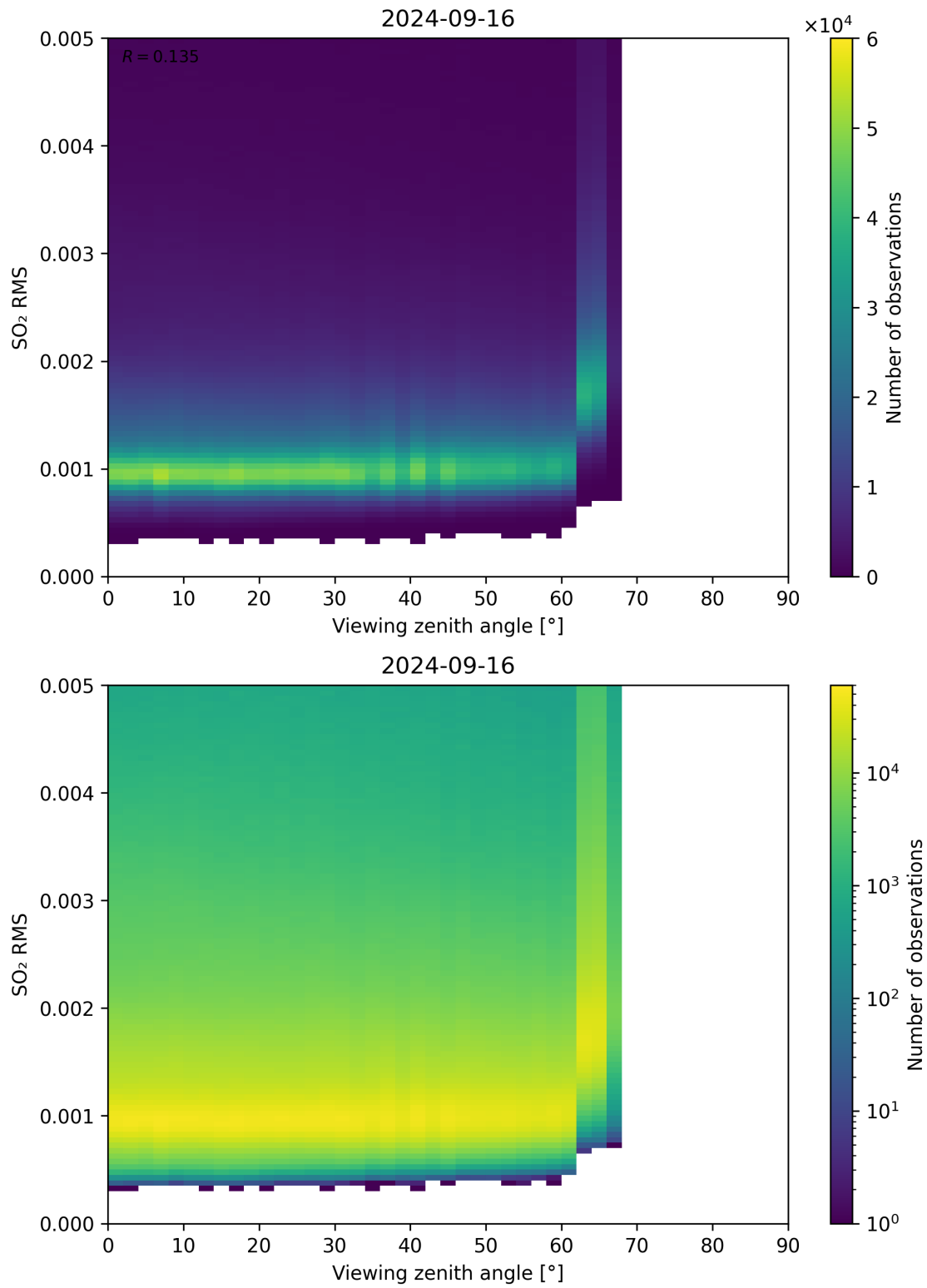
Figure 313: Scatter density plot of “Viewing zenith angle” against “SO 2 RMS” for 2024-09-15 to 2024-09-17.
