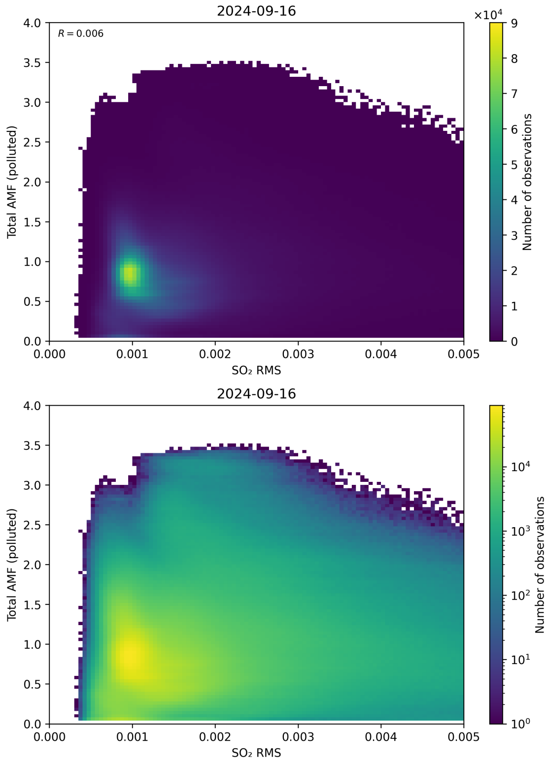
Figure 137: Scatter density plot of “SO 2 RMS” against “Total AMF (polluted)” for 2024-09-15 to 2024-09-17.
