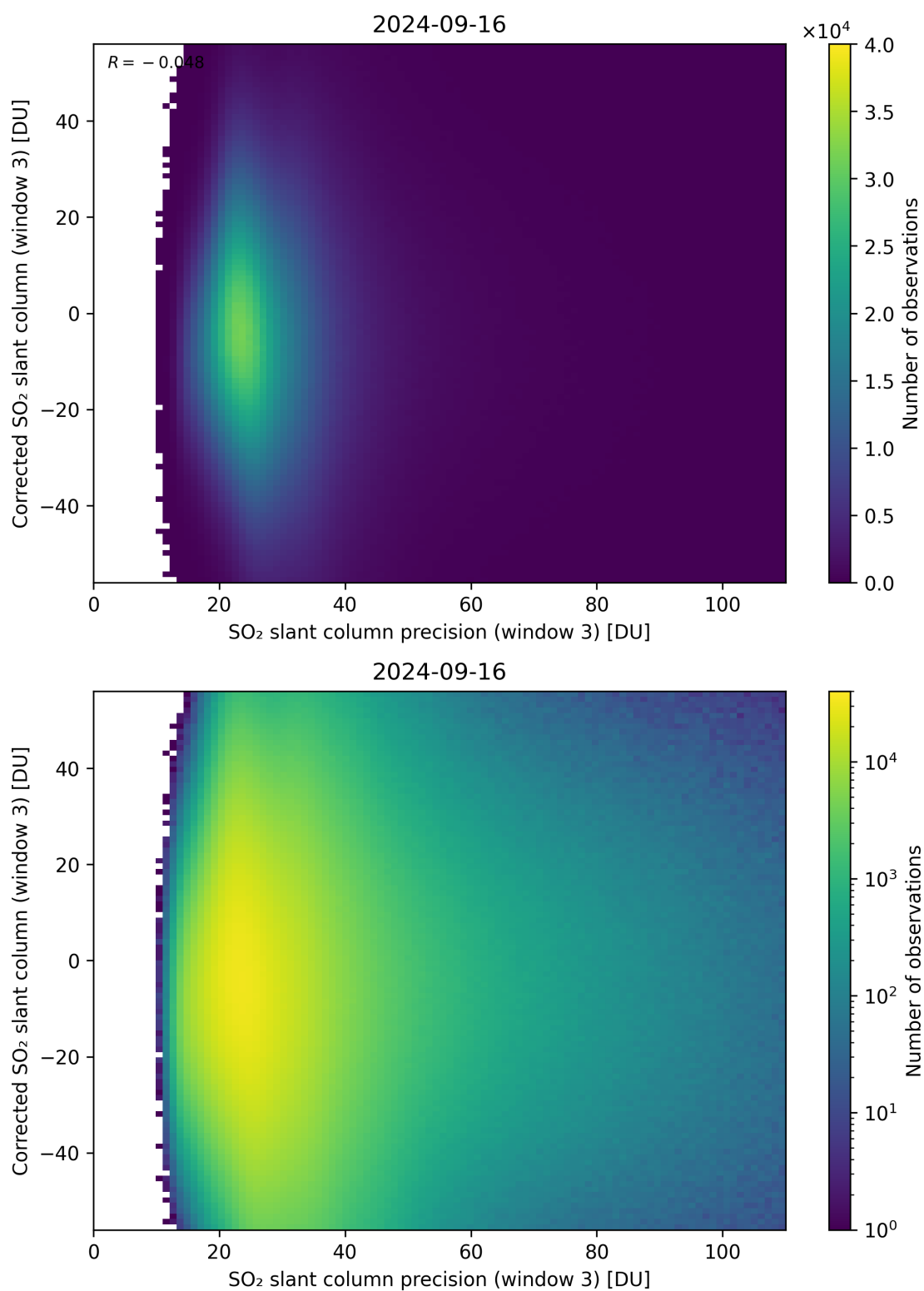
Figure 262: Scatter density plot of “SO 2 slant column precision (window 3)” against “Corrected SO 2 slant column (window 3)” for 2024-09-15 to 2024-09-17.
