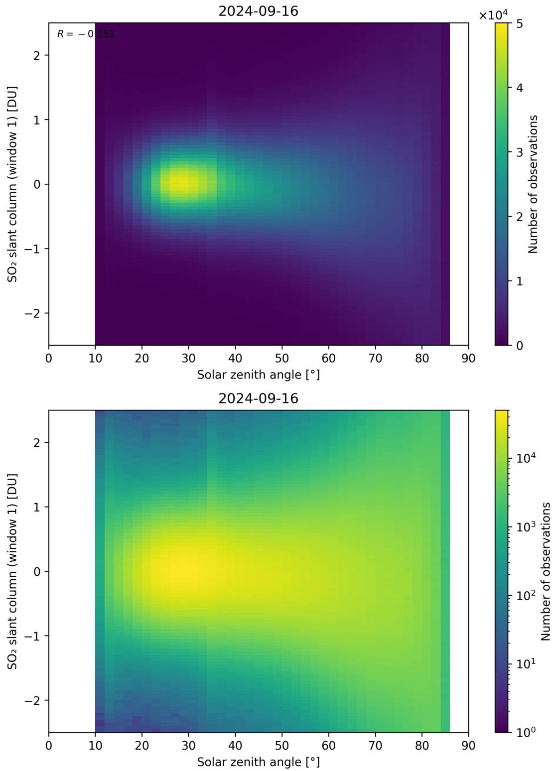
Figure 169: Scatter density plot of “Solar zenith angle” against “SO 2 slant column (window 1)” for 2024-09-15 to 2024-09-17.
