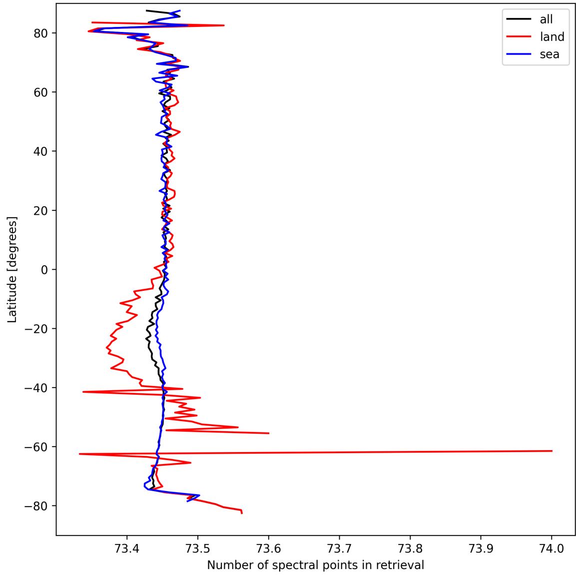
Figure 51: Zonal average of “Number of spectral points in retrieval” for 2024-09-15 to 2024-09-17.
