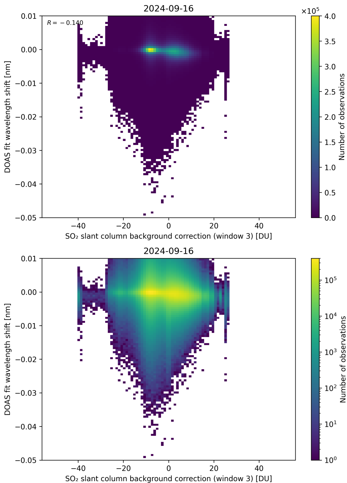
Figure 121: Scatter density plot of “SO 2 slant column background correction (window 3)” against “DOAS fit wavelength shift” for 2024-09-15 to 2024-09-17.
