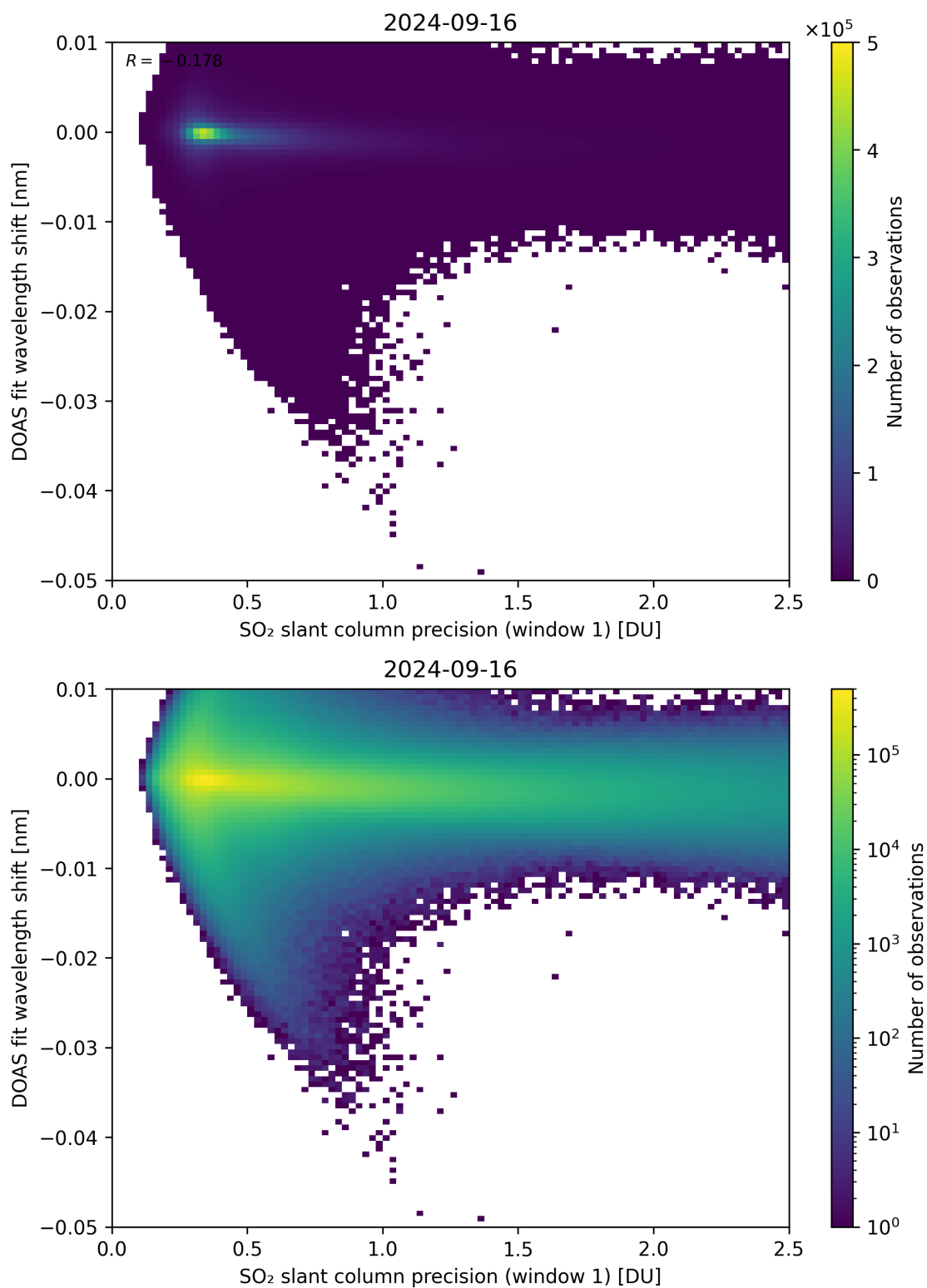
Figure 221: Scatter density plot of “SO 2 slant column precision (window 1)” against “DOAS fit wavelength shift” for 2024-09-15 to 2024-09-17.
