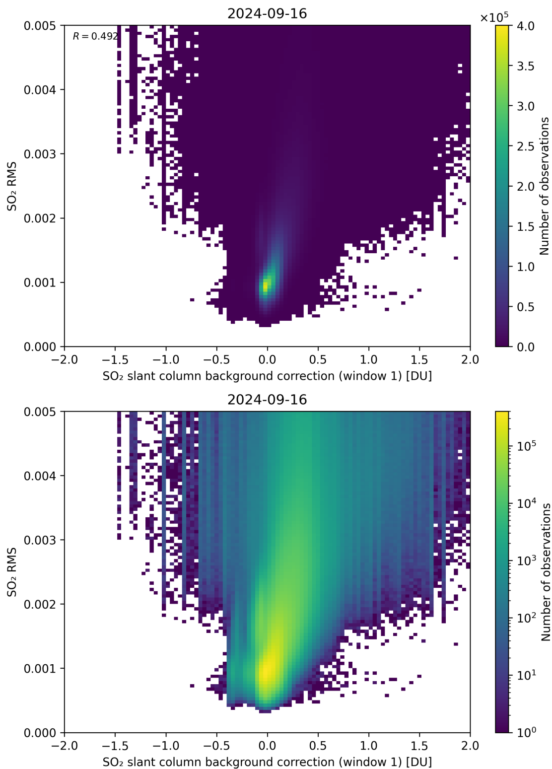
Figure 102: Scatter density plot of “SO 2 slant column background correction (window 1)” against “SO 2 RMS” for 2024-09-15 to 2024-09-17.
