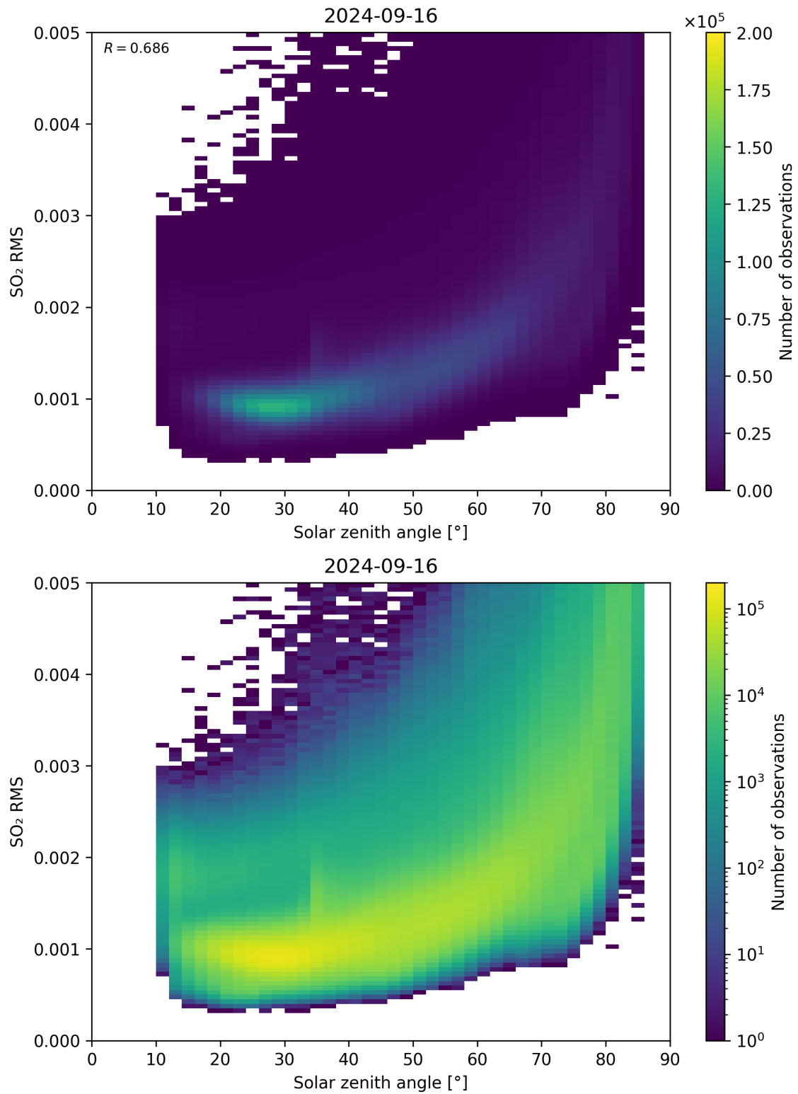
Figure 163: Scatter density plot of “Solar zenith angle” against “SO 2 RMS” for 2024-09-15 to 2024-09-17.
