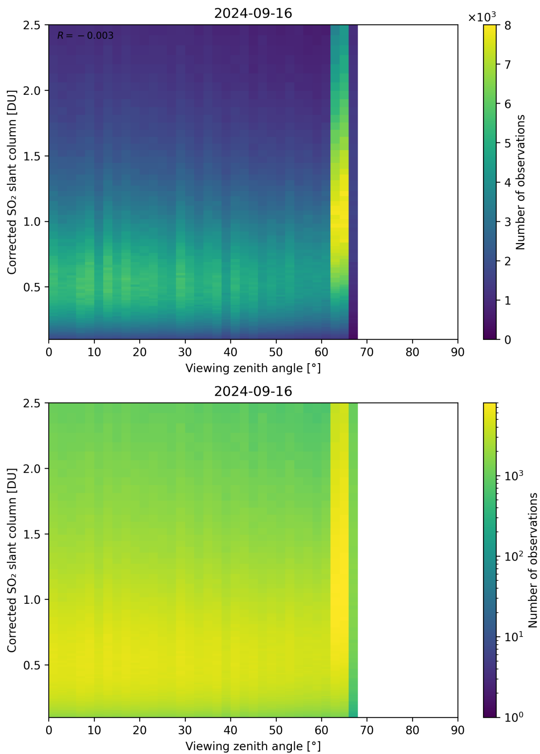
Figure 317: Scatter density plot of “Viewing zenith angle” against “Corrected SO 2 slant column” for 2024-09-15 to 2024-09-17.
