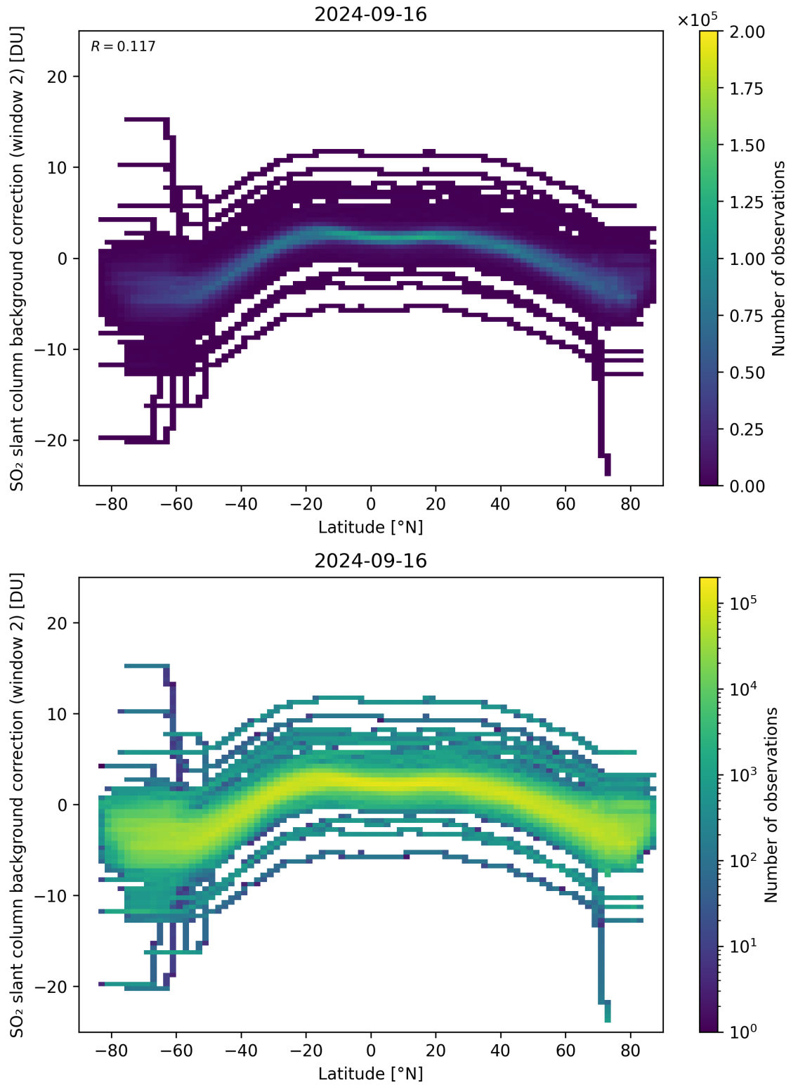
Figure 140: Scatter density plot of “Latitude” against “SO 2 slant column background correction (window 2)” for 2024-09-15 to 2024-09-17.
