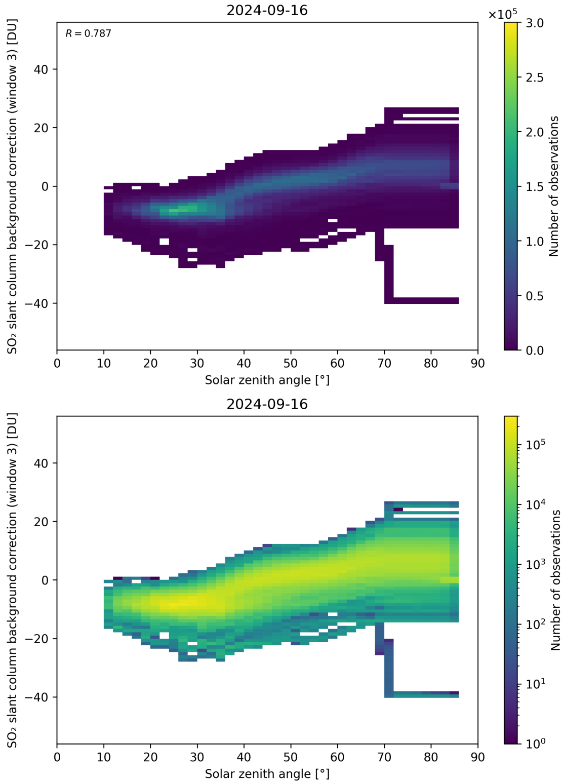
Figure 160: Scatter density plot of “Solar zenith angle” against “SO 2 slant column background correction (window 3)” for 2024-09-15 to 2024-09-17.
