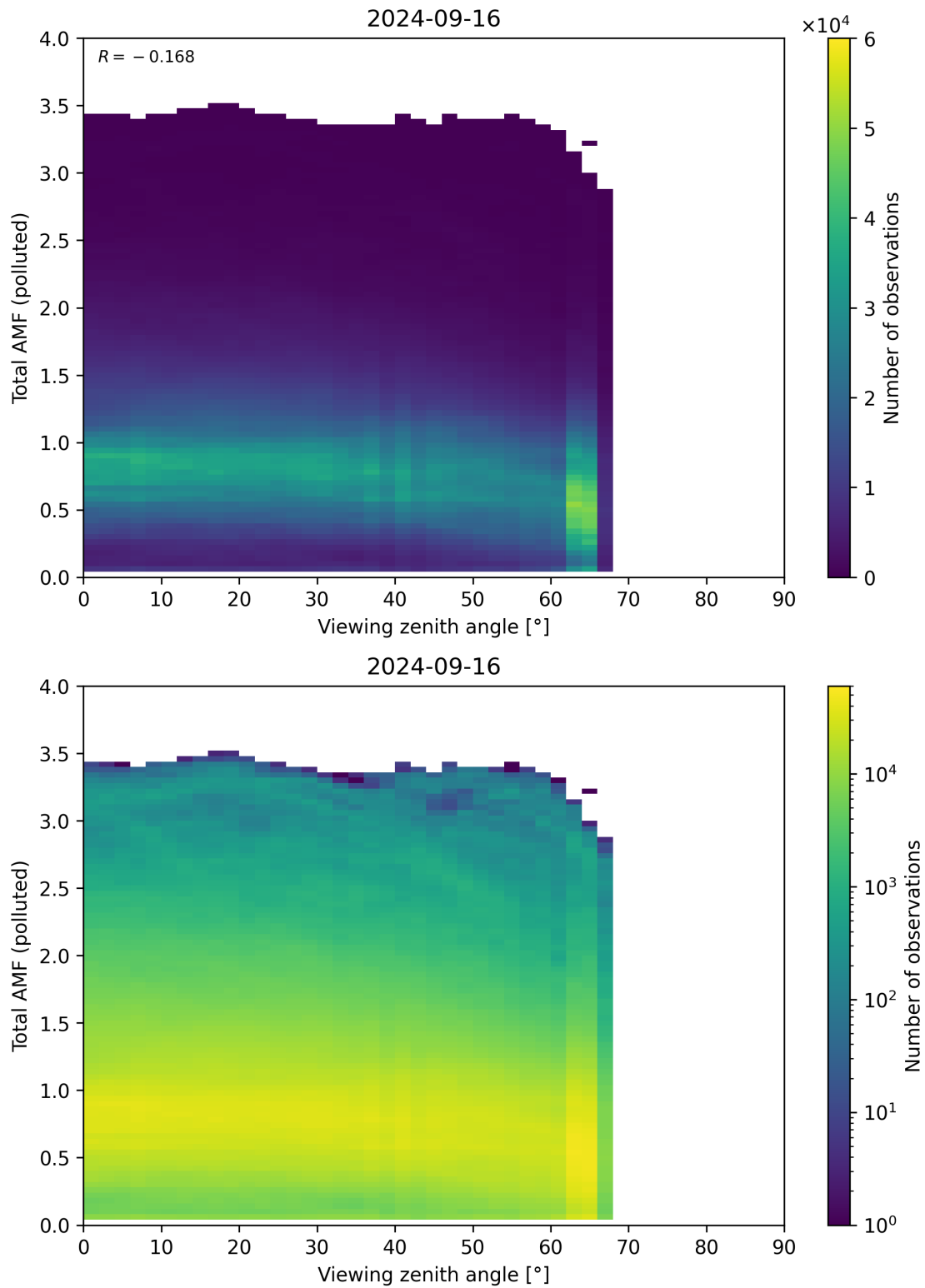
Figure 325: Scatter density plot of “Viewing zenith angle” against “Total AMF (polluted)” for 2024-09-15 to 2024-09-17.
