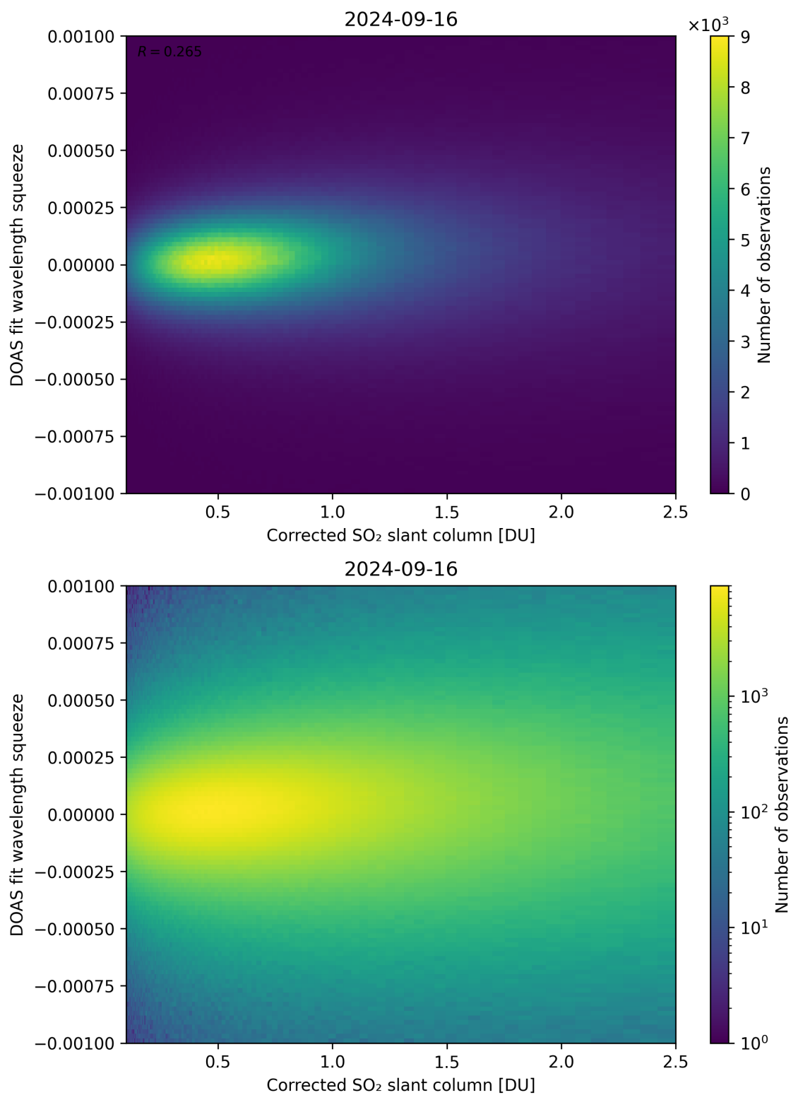
Figure 182: Scatter density plot of “Corrected SO 2 slant column” against “DOAS fit wavelength squeeze” for 2024-09-15 to 2024-09-17.
