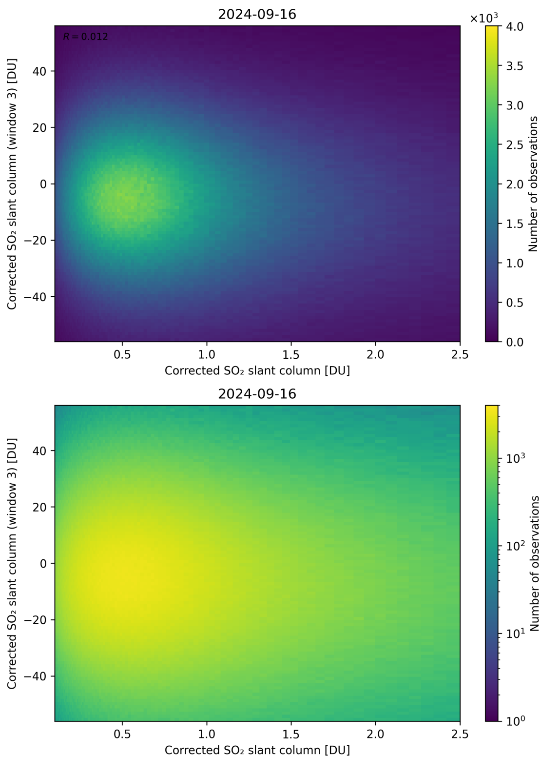
Figure 186: Scatter density plot of “Corrected SO 2 slant column” against “Corrected SO 2 slant column (window 3)” for 2024-09-15 to 2024-09-17.
