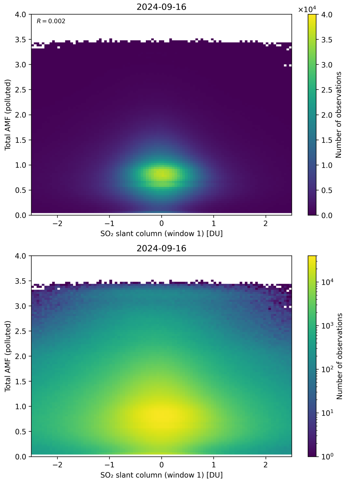
Figure 239: Scatter density plot of “SO 2 slant column (window 1)” against “Total AMF (polluted)” for 2024-09-15 to 2024-09-17.
