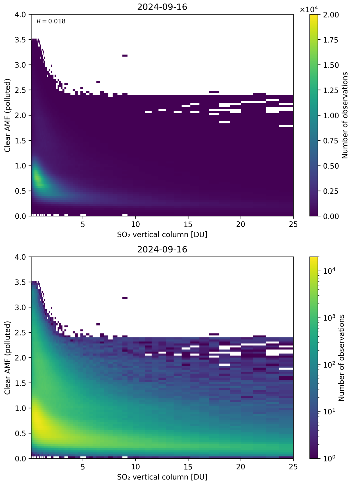
Figure 296: Scatter density plot of “SO 2 vertical column” against “Clear AMF (polluted)” for 2024-09-15 to 2024-09-17.
