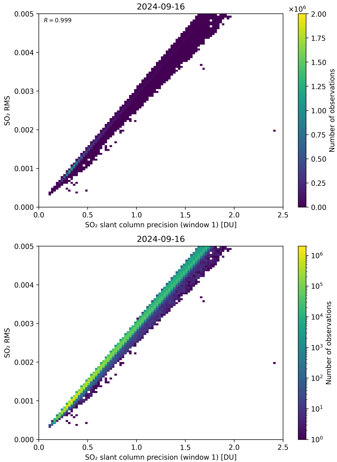
Figure 223: Scatter density plot of “SO 2 slant column precision (window 1)” against “SO 2 RMS” for 2024-09-15 to 2024-09-17.
