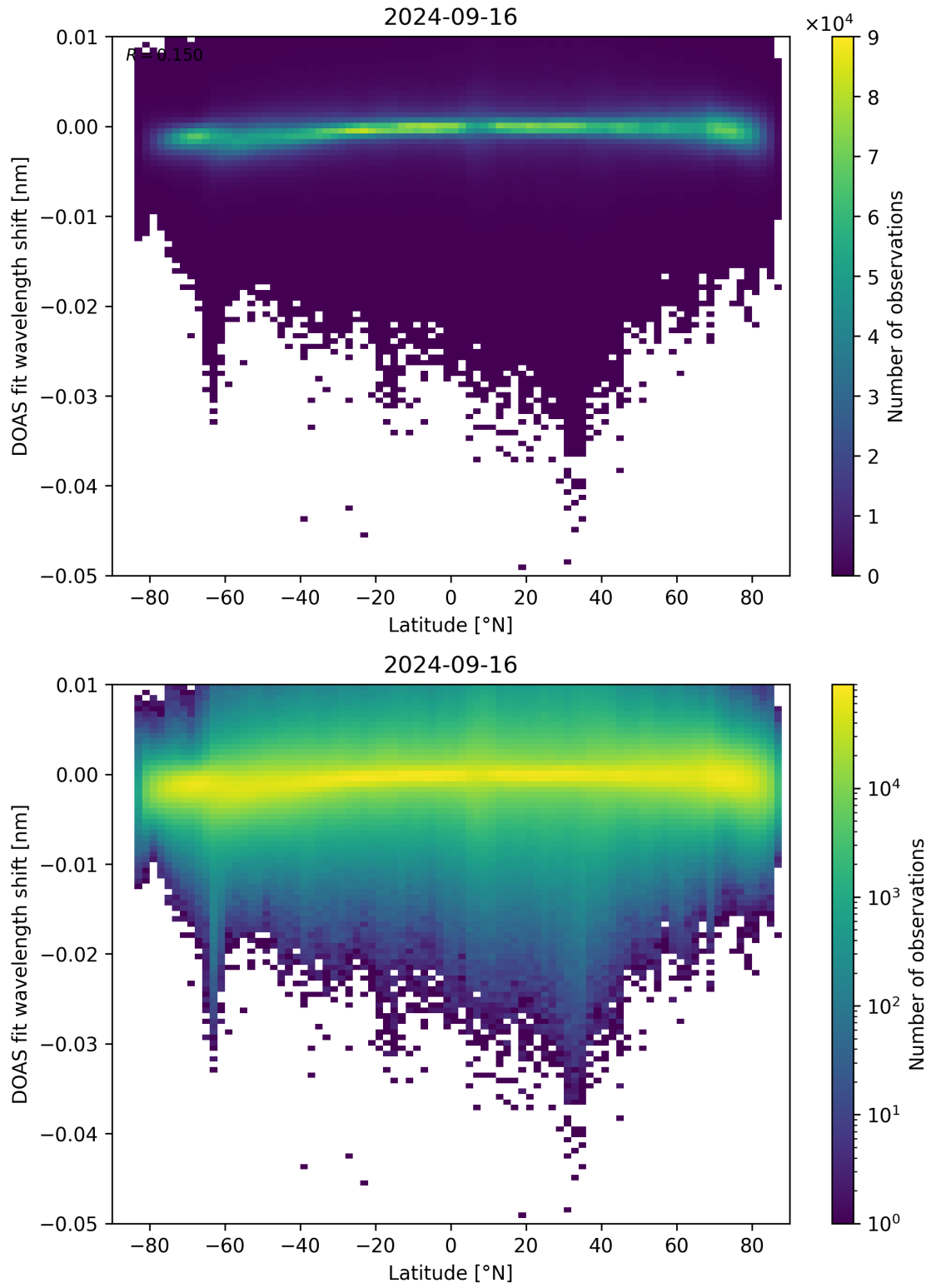
Figure 142: Scatter density plot of “Latitude” against “DOAS fit wavelength shift” for 2024-09-15 to 2024-09-17.
