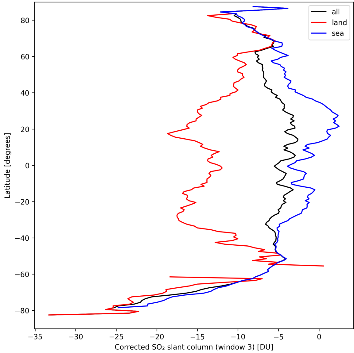
Figure 43: Zonal average of “Corrected SO 2 slant column (window 3)” for 2024-09-15 to 2024-09-17.
