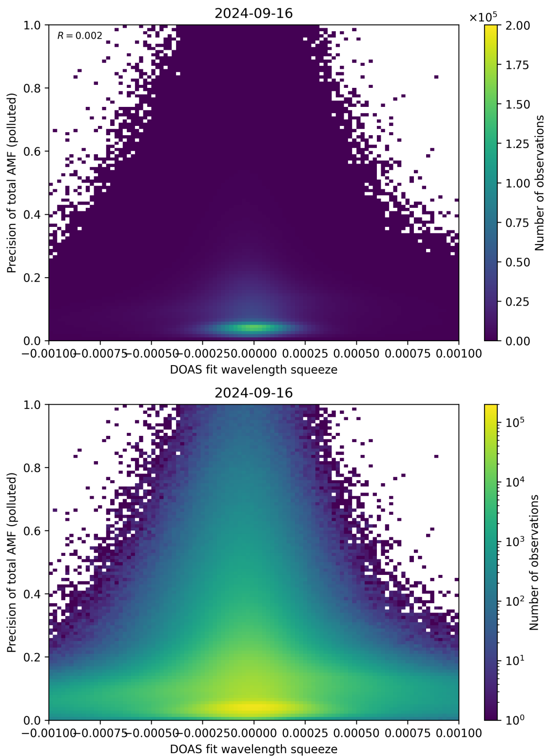
Figure 135: Scatter density plot of “DOAS fit wavelength squeeze” against “Precision of total AMF (polluted)” for 2024-09-15 to 2024-09-17.
