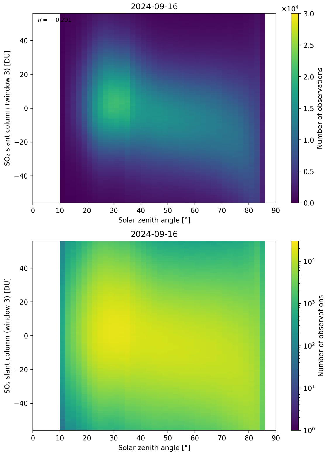
Figure 172: Scatter density plot of “Solar zenith angle” against “SO 2 slant column (window 3)” for 2024-09-15 to 2024-09-17.
