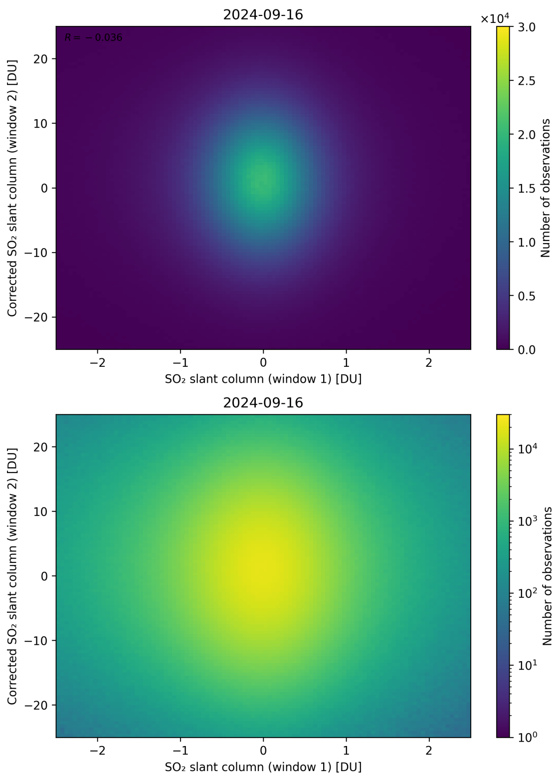
Figure 233: Scatter density plot of “SO 2 slant column (window 1)” against “Corrected SO 2 slant column (window 2)” for 2024-09-15 to 2024-09-17.
