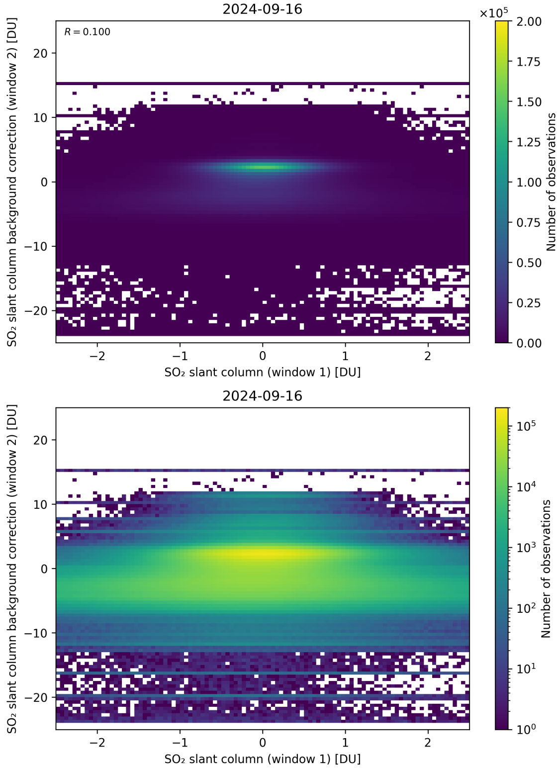
Figure 213: Scatter density plot of “SO 2 slant column (window 1)” against “SO 2 slant column background correction (window 2)” for 2024-09-15 to 2024-09-17.
