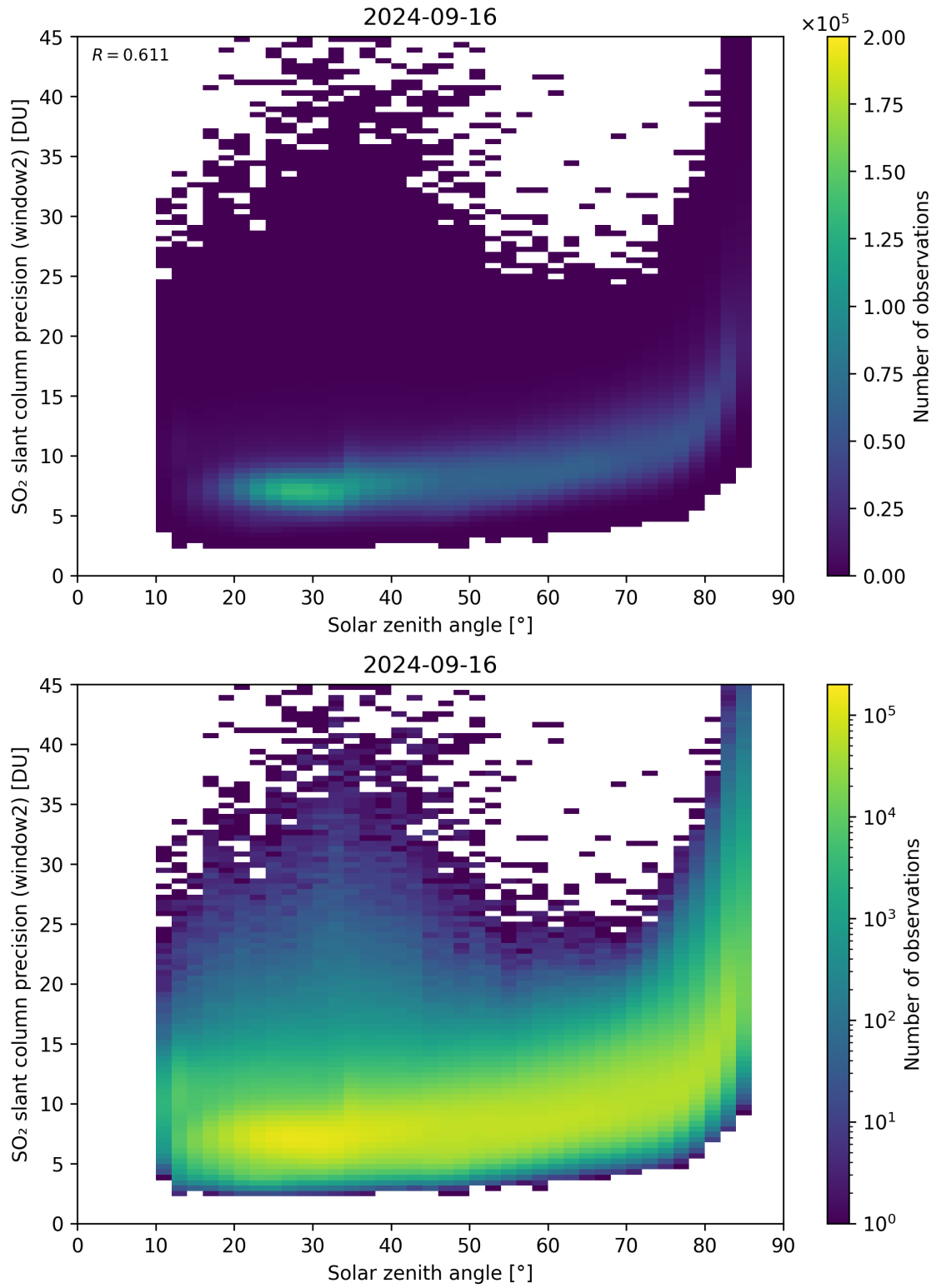
Figure 171: Scatter density plot of “Solar zenith angle” against “SO 2 slant column precision (window2)” for 2024-09-15 to 2024-09-17.
