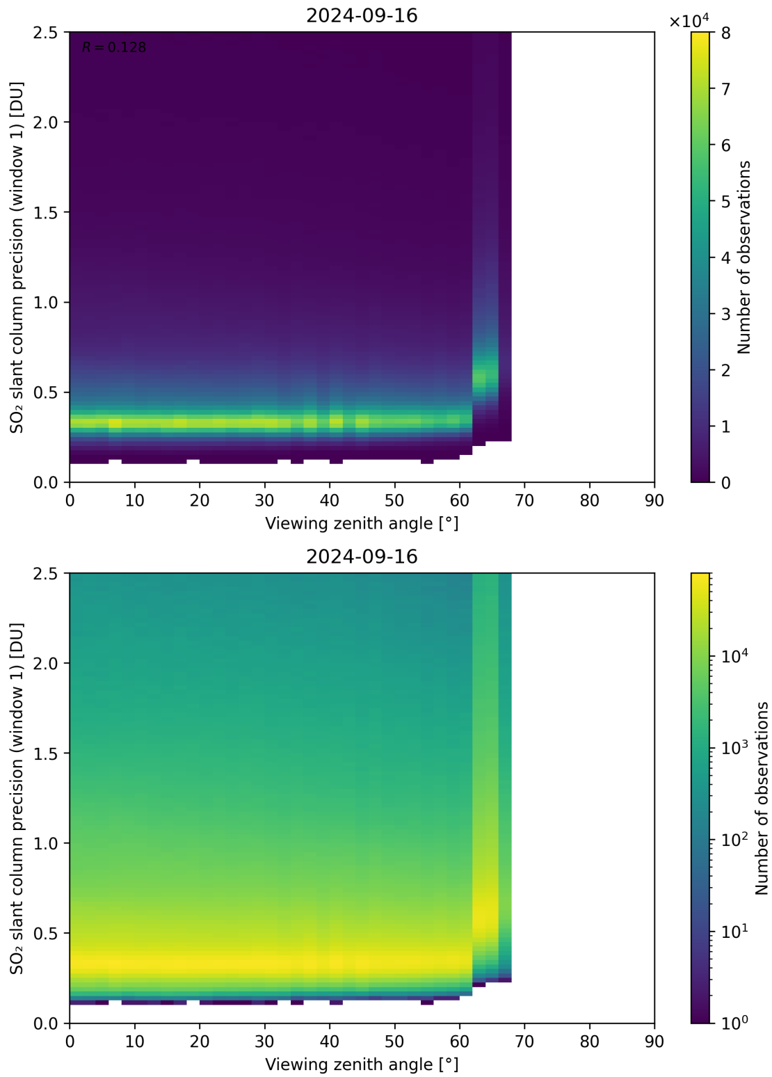
Figure 321: Scatter density plot of “Viewing zenith angle” against “SO 2 slant column precision (window 1)” for 2024-09-15 to 2024-09-17.
