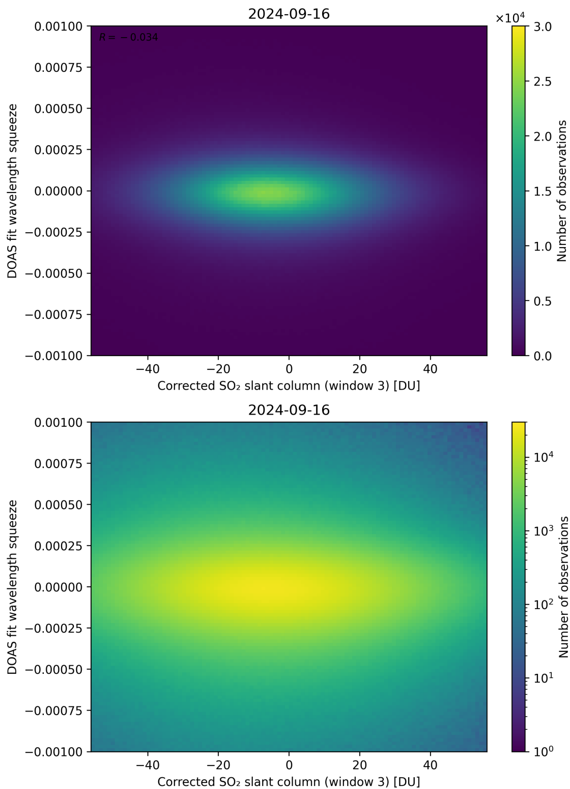
Figure 207: Scatter density plot of “Corrected SO 2 slant column (window 3)” against “DOAS fit wavelength squeeze” for 2024-09-15 to 2024-09-17.
