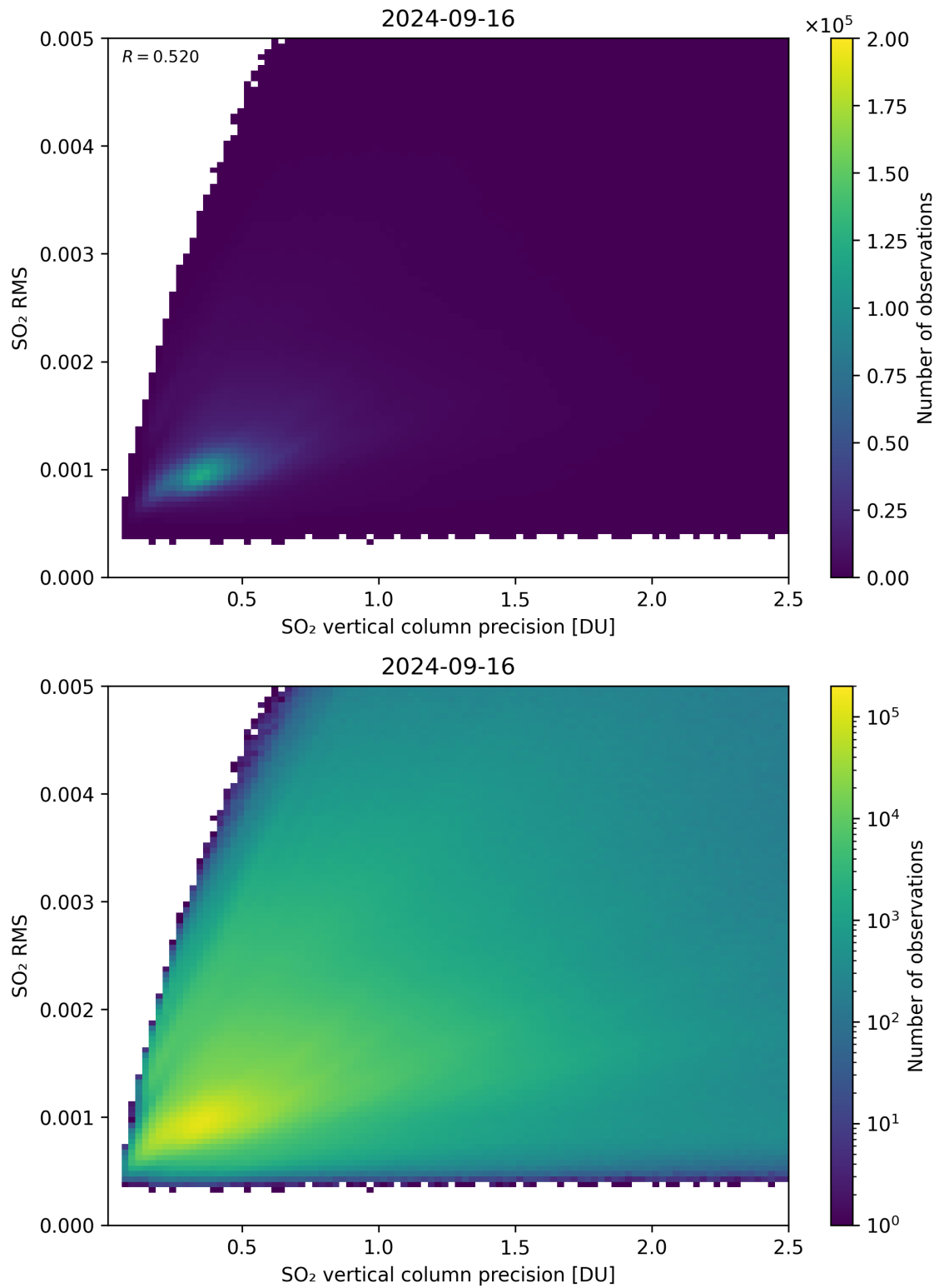
Figure 284: Scatter density plot of “SO 2 vertical column precision” against “SO 2 RMS” for 2024-09-15 to 2024-09-17.
