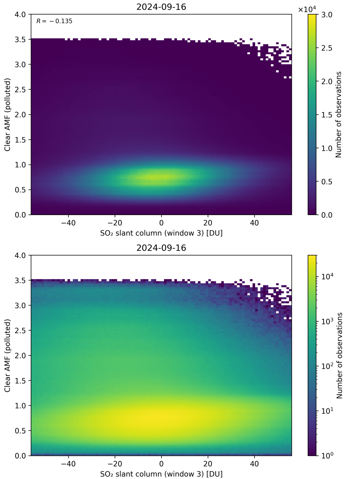
Figure 265: Scatter density plot of “SO 2 slant column (window 3)” against “Clear AMF (polluted)” for 2024-09-15 to 2024-09-17.
