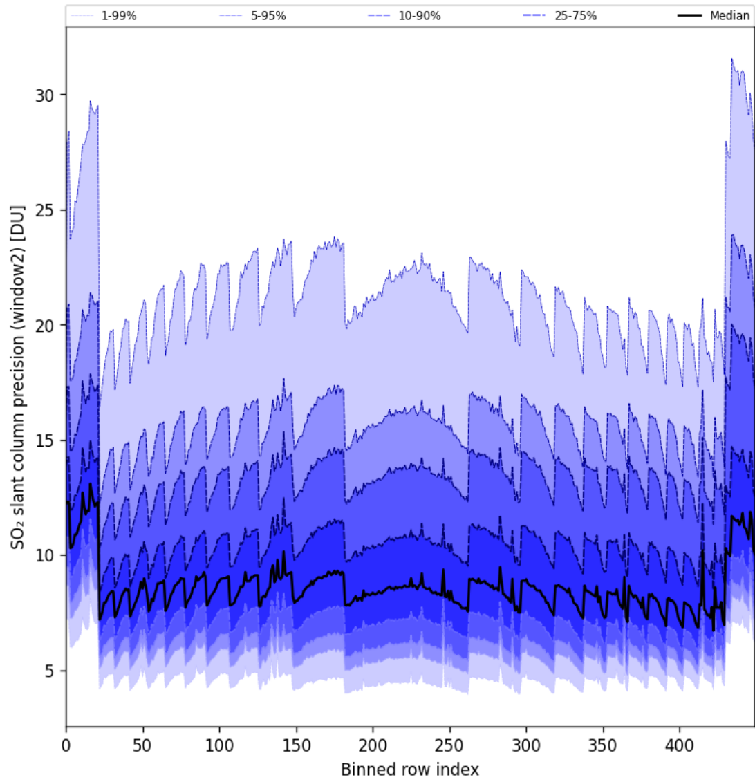
Figure 84: Along track statistics of “SO 2 slant column precision (window2)” for 2024-09-15 to 2024-09-17
