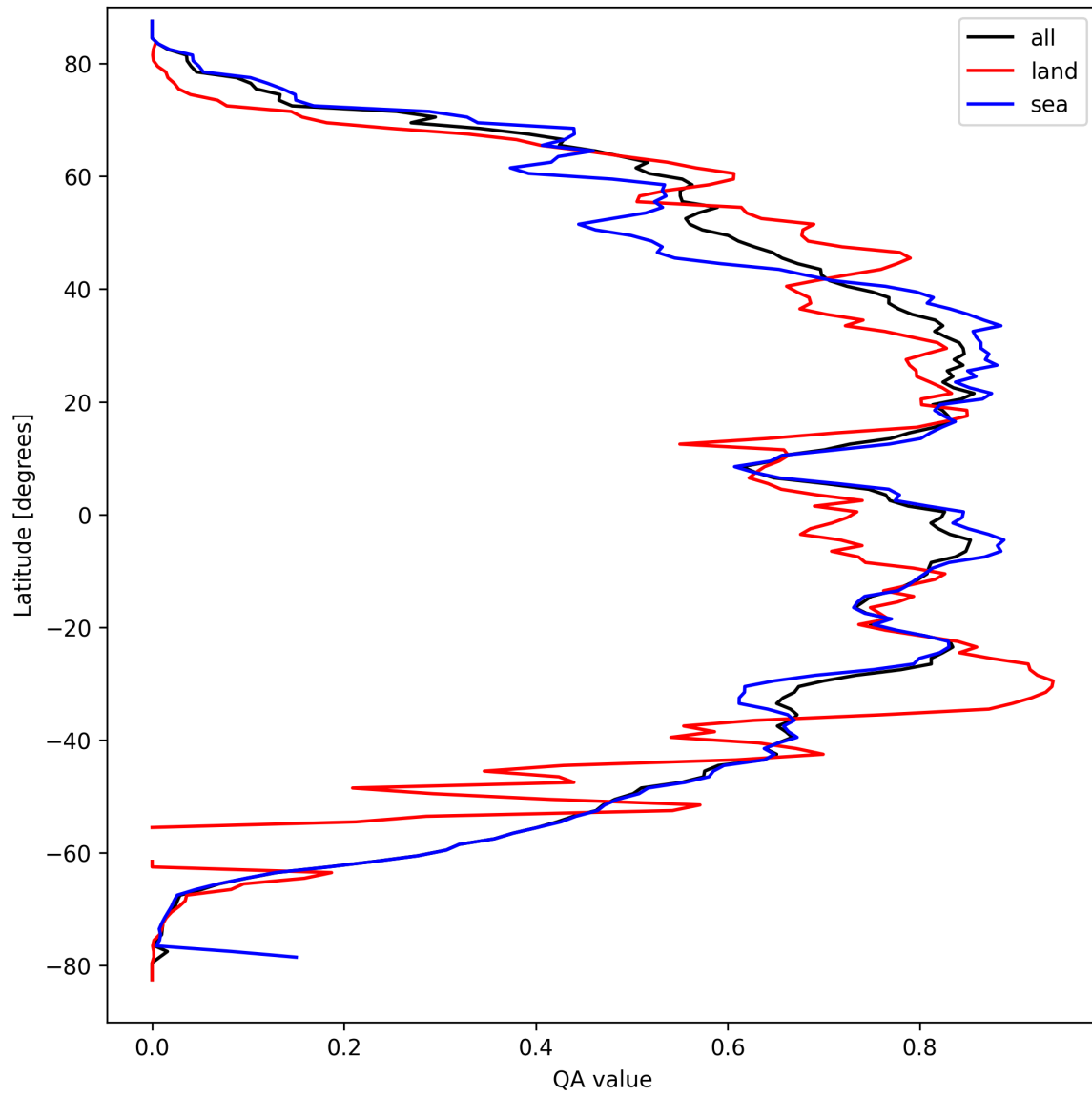
Figure 29: Zonal average of “QA value” for 2024-09-15 to 2024-09-17.
