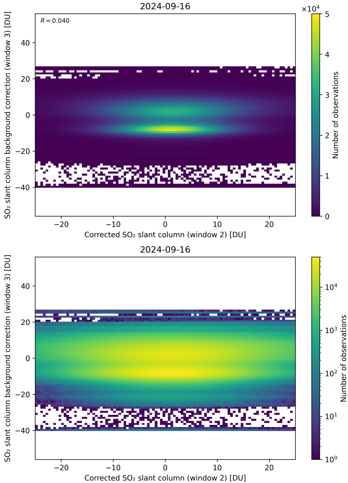
Figure 195: Scatter density plot of “Corrected SO 2 slant column (window 2)” against “SO 2 slant column background correction (window 3)” for 2024-09-15 to 2024-09-17.
