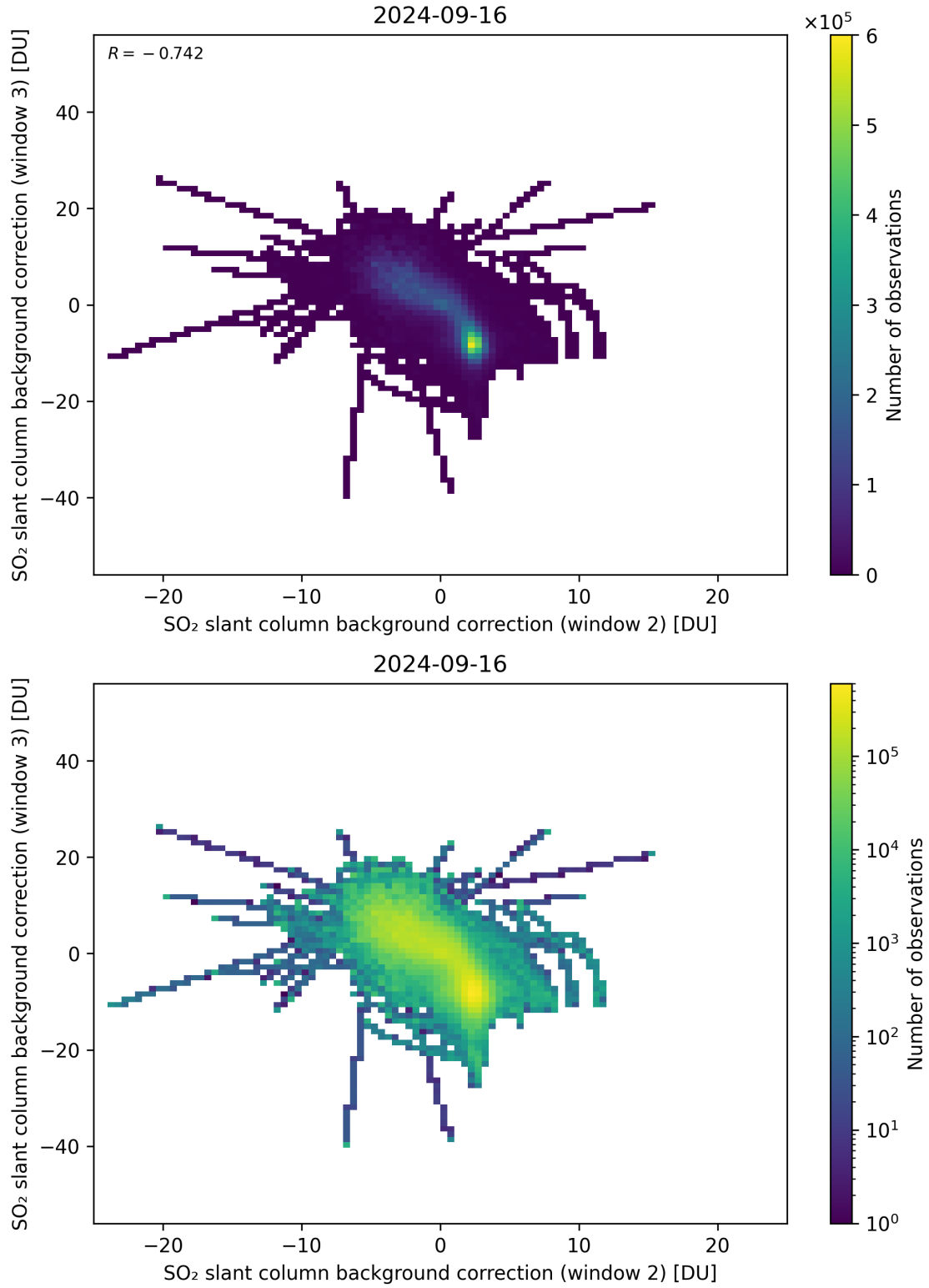
Figure 111: Scatter density plot of “SO 2 slant column background correction (window 2)” against “SO 2 slant column background correction (window 3)” for 2024-09-15 to 2024-09-17.
