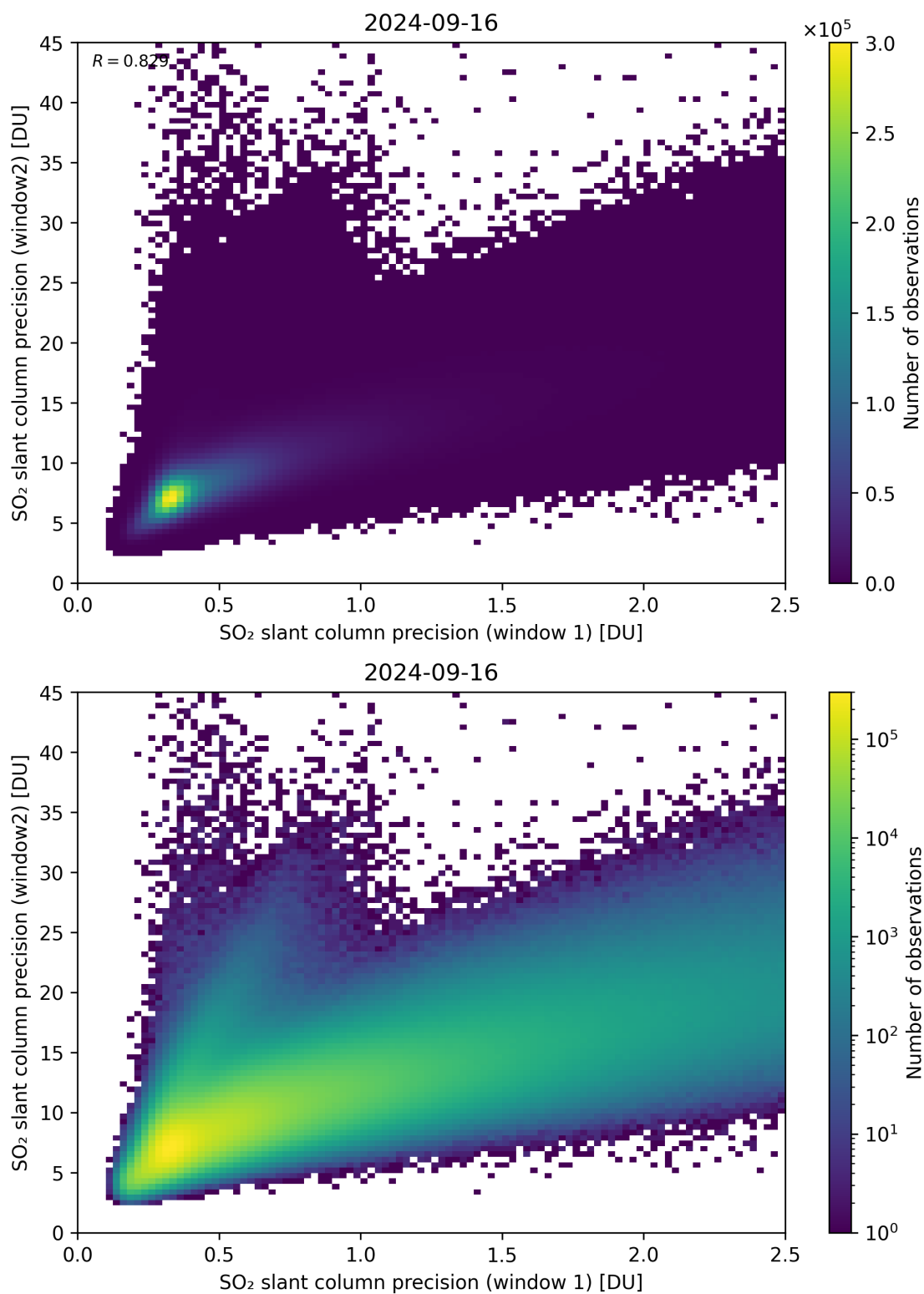
Figure 227: Scatter density plot of “SO 2 slant column precision (window 1)” against “SO 2 slant column precision (window2)” for 2024-09-15 to 2024-09-17.
