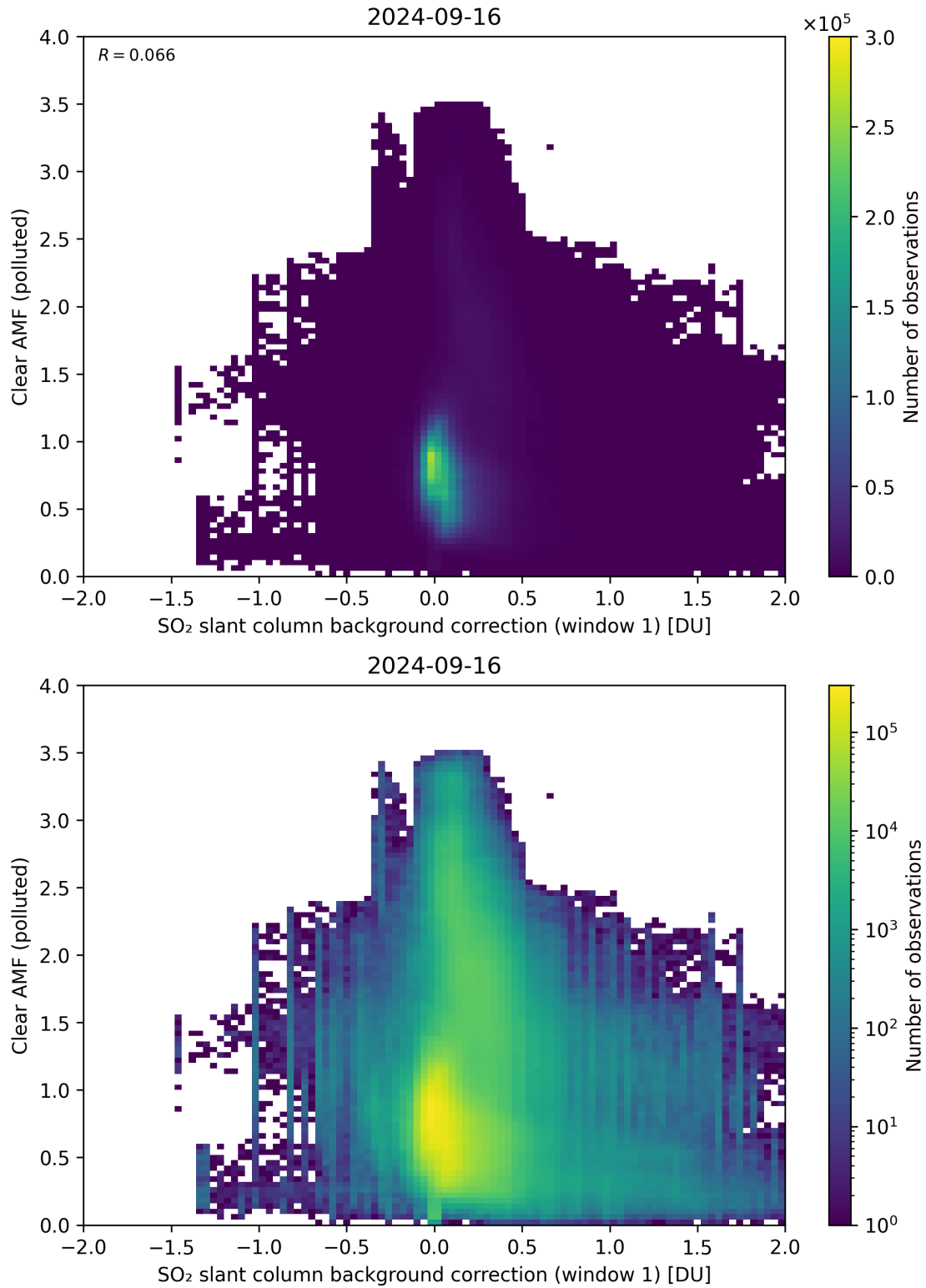
Figure 103: Scatter density plot of “SO 2 slant column background correction (window 1)” against “Clear AMF (polluted)” for 2024-09-15 to 2024-09-17.
