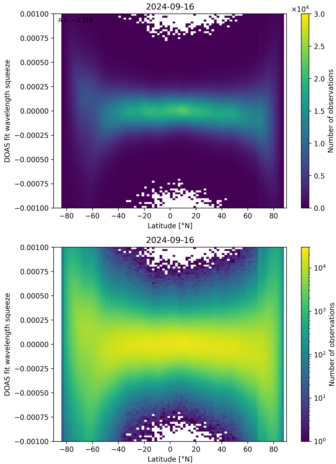
Figure 143: Scatter density plot of “Latitude” against “DOAS fit wavelength squeeze” for 2024-09-15 to 2024-09-17.
