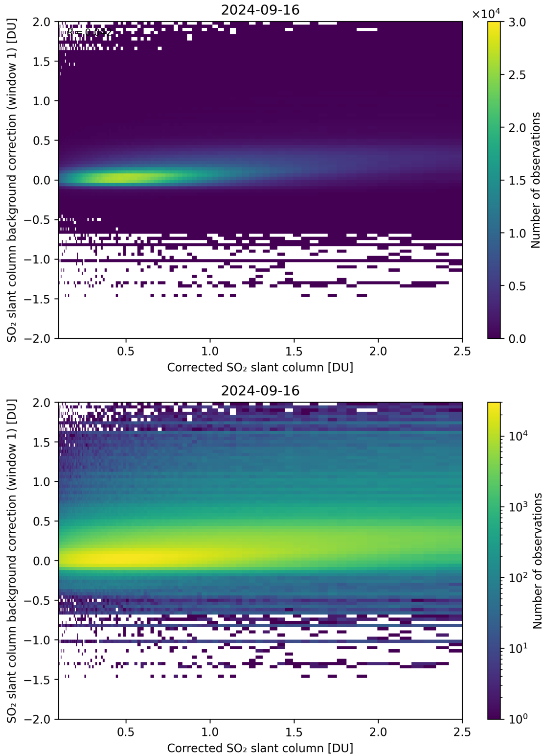
Figure 178: Scatter density plot of “Corrected SO 2 slant column” against “SO 2 slant column background correction (window 1)” for 2024-09-15 to 2024-09-17.
