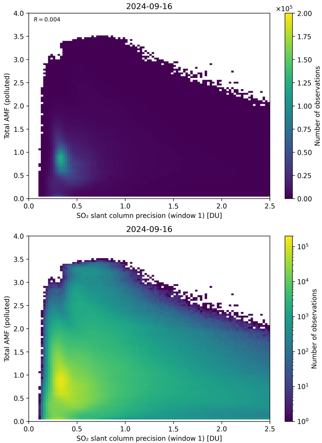
Figure 230: Scatter density plot of “SO 2 slant column precision (window 1)” against “Total AMF (polluted)” for 2024-09-15 to 2024-09-17.
