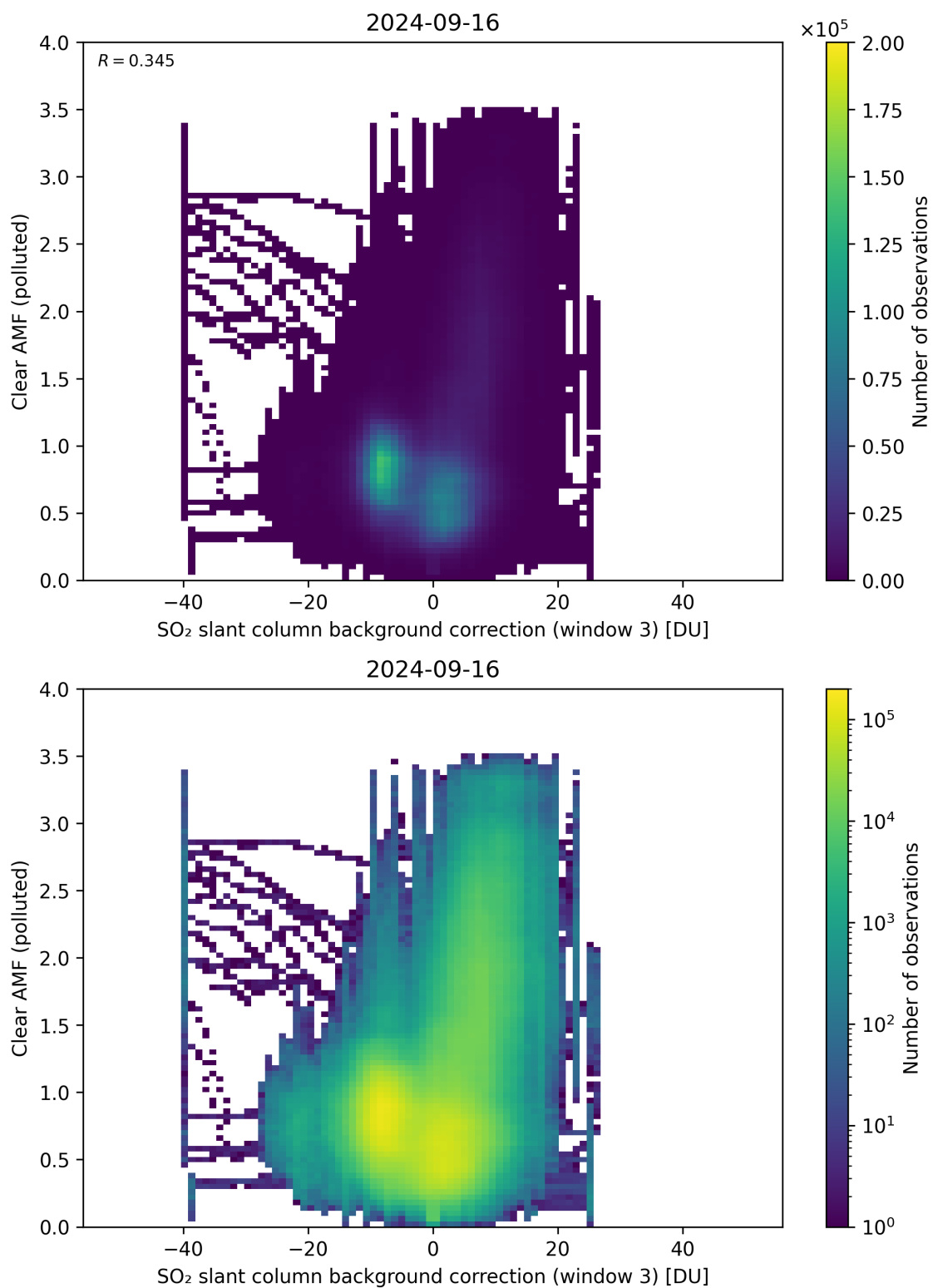
Figure 124: Scatter density plot of “SO 2 slant column background correction (window 3)” against “Clear AMF (polluted)” for 2024-09-15 to 2024-09-17.
