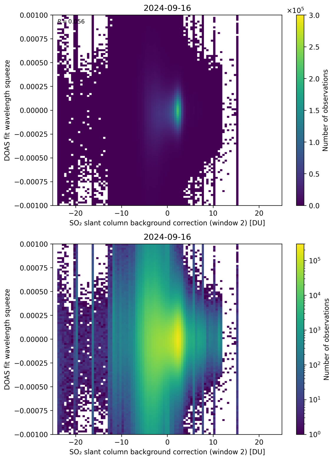
Figure 113: Scatter density plot of “SO 2 slant column background correction (window 2)” against “DOAS fit wavelength squeeze” for 2024-09-15 to 2024-09-17.
