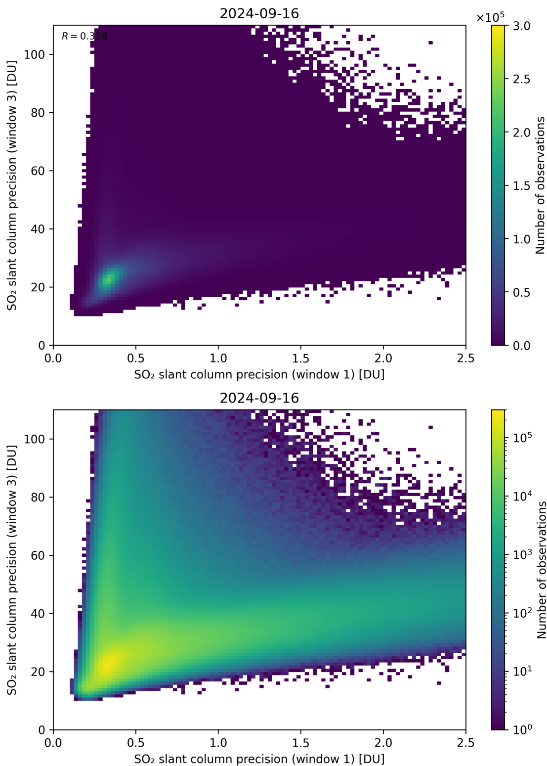
Figure 229: Scatter density plot of “SO 2 slant column precision (window 1)” against “SO 2 slant column precision (window 3)” for 2024-09-15 to 2024-09-17.
