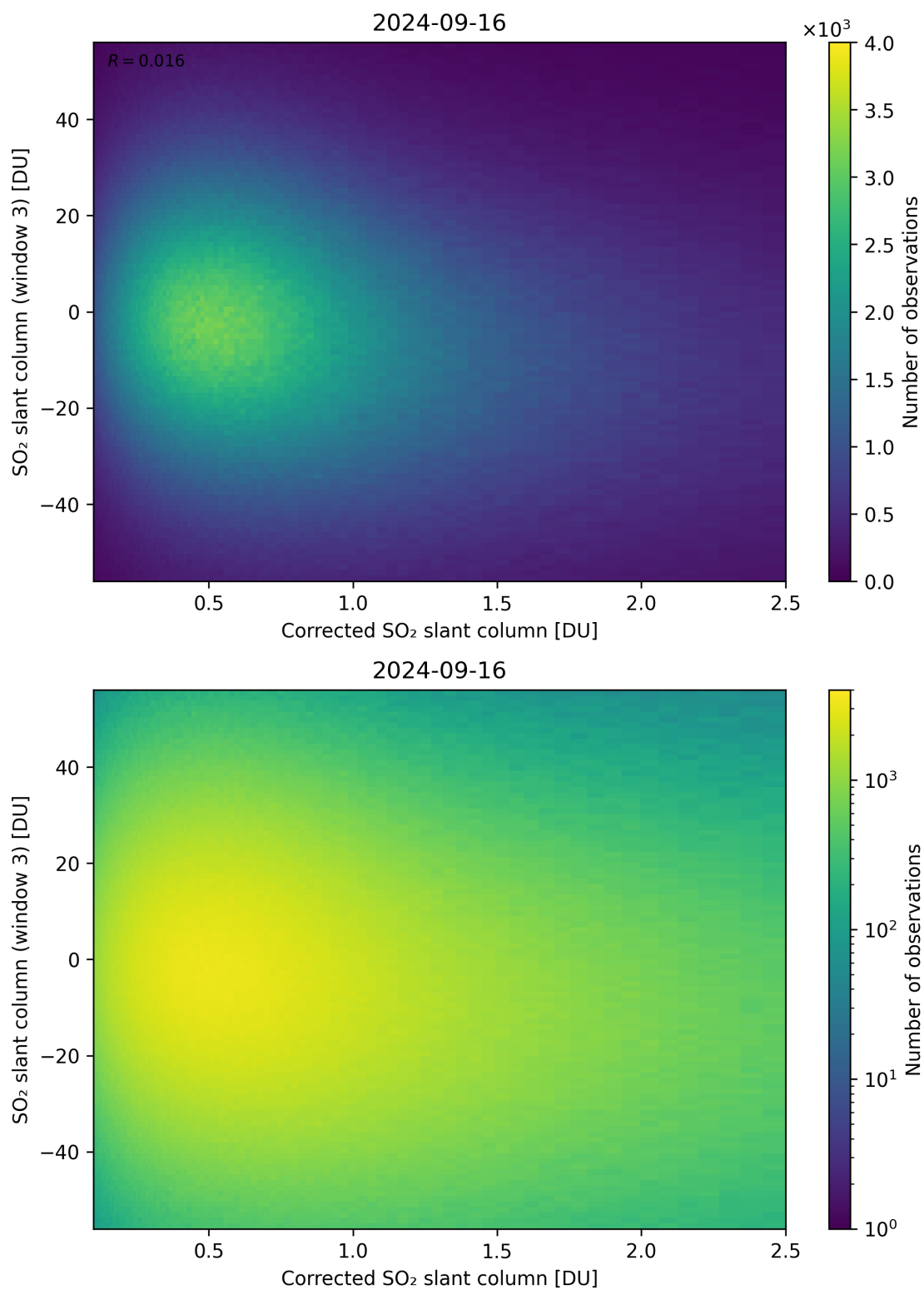
Figure 190: Scatter density plot of “Corrected SO 2 slant column” against “SO 2 slant column (window 3)” for 2024-09-15 to 2024-09-17.
