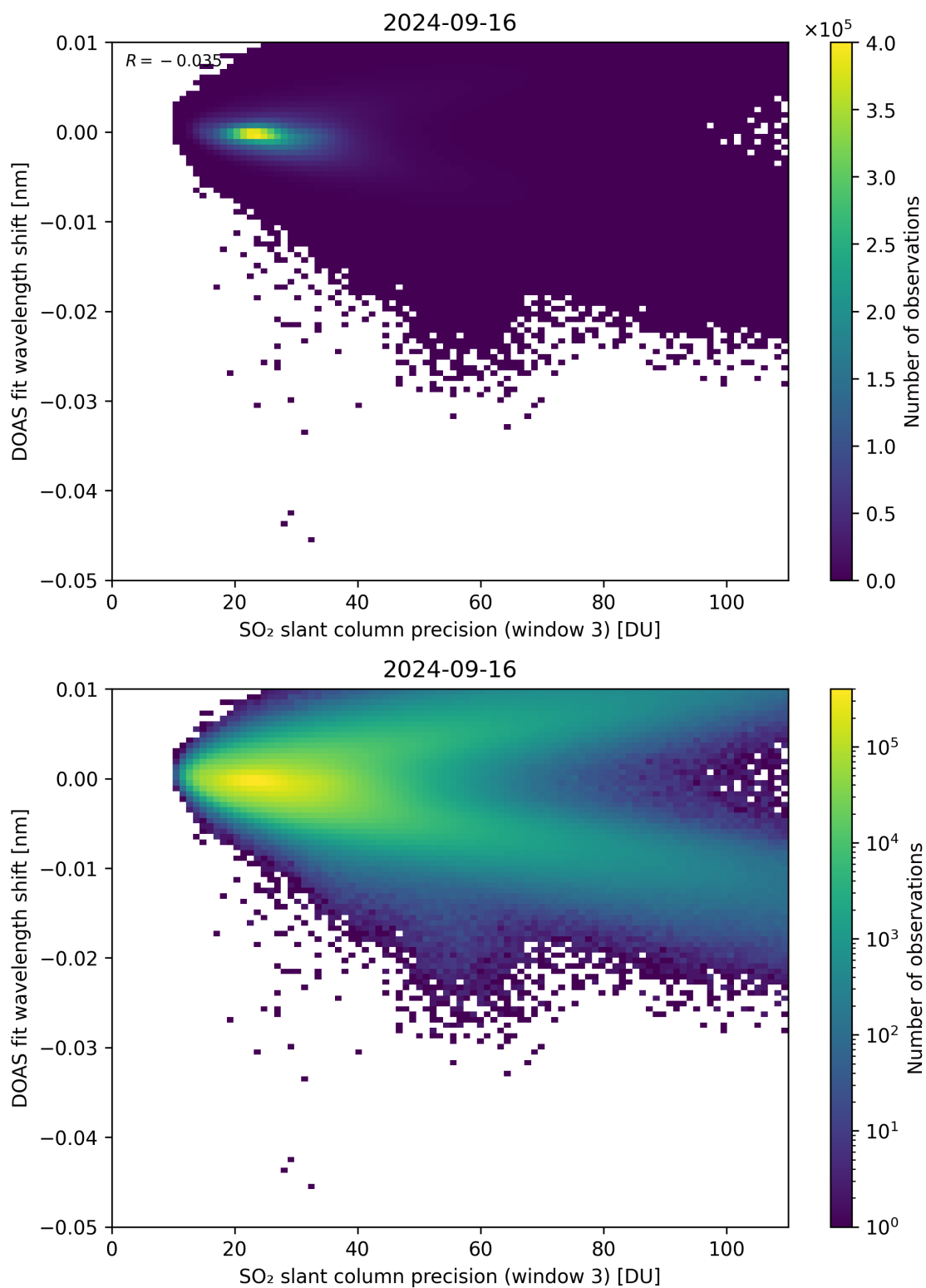
Figure 258: Scatter density plot of “SO 2 slant column precision (window 3)” against “DOAS fit wavelength shift” for 2024-09-15 to 2024-09-17.
