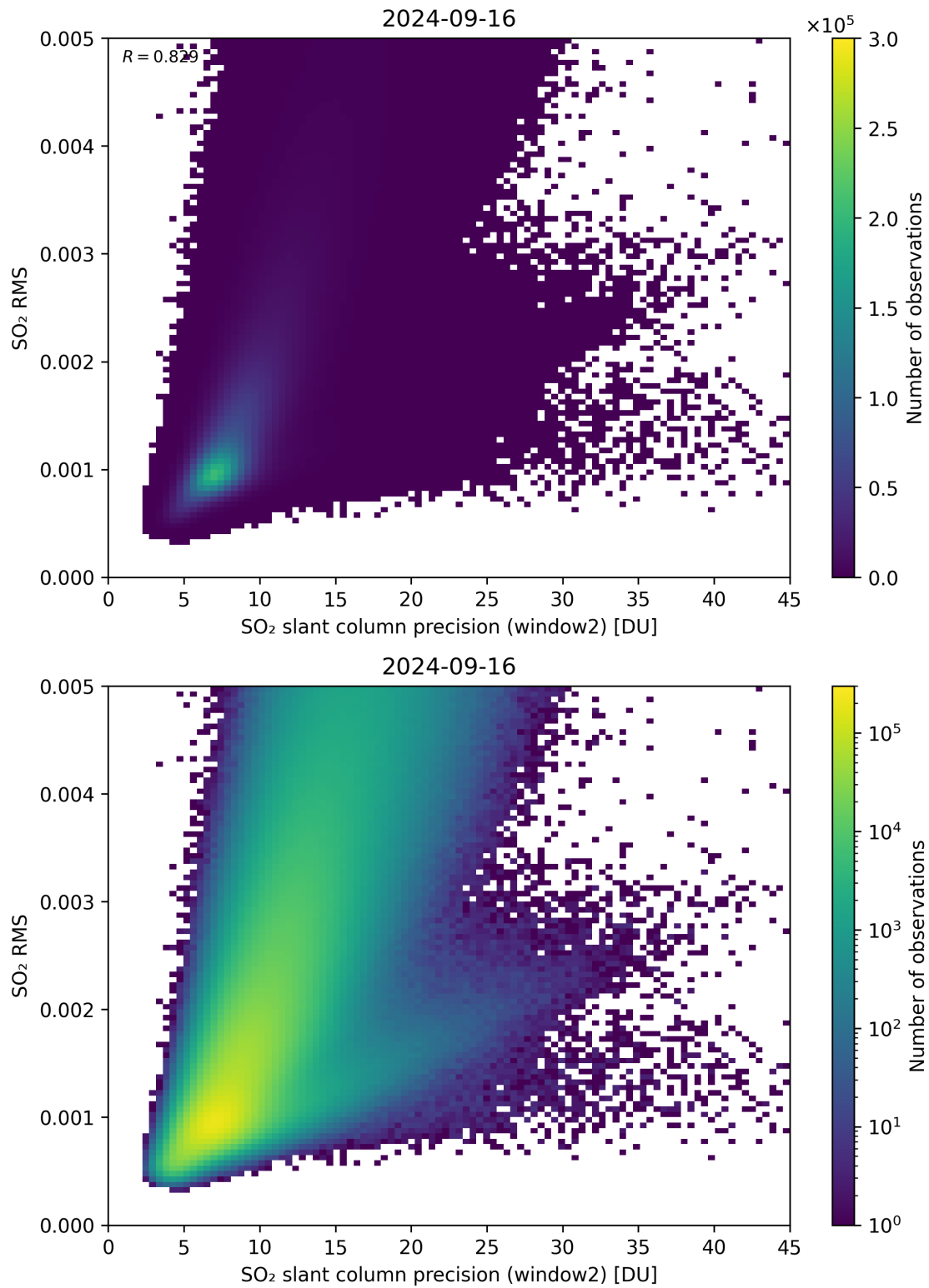
Figure 245: Scatter density plot of “SO 2 slant column precision (window2)” against “SO 2 RMS” for 2024-09-15 to 2024-09-17.
