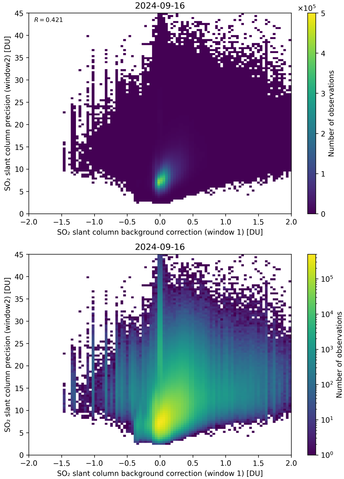
Figure 106: Scatter density plot of “SO 2 slant column background correction (window 1)” against “SO 2 slant column precision (window2)” for 2024-09-15 to 2024-09-17.
