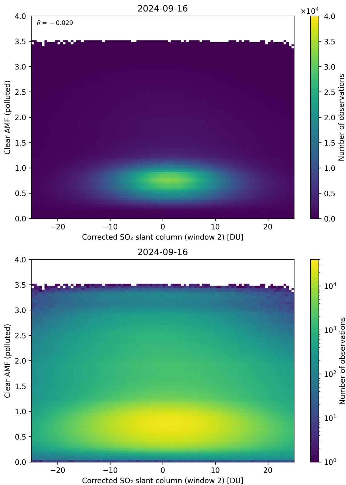
Figure 199: Scatter density plot of “Corrected SO 2 slant column (window 2)” against “Clear AMF (polluted)” for 2024-09-15 to 2024-09-17.
