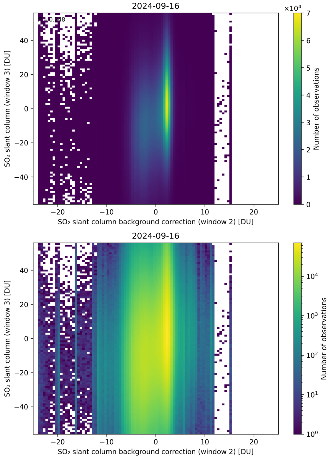
Figure 117: Scatter density plot of “SO 2 slant column background correction (window 2)” against “SO 2 slant column (window 3)” for 2024-09-15 to 2024-09-17.
