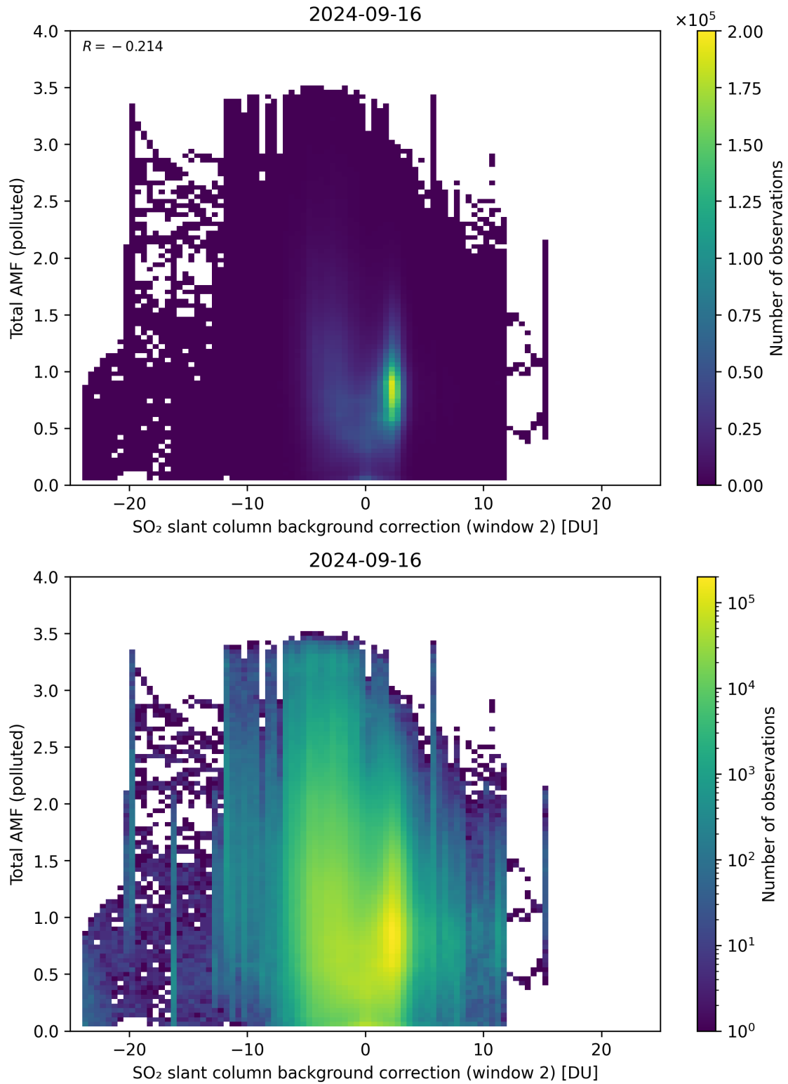
Figure 119: Scatter density plot of “SO 2 slant column background correction (window 2)” against “Total AMF (polluted)” for 2024-09-15 to 2024-09-17.
