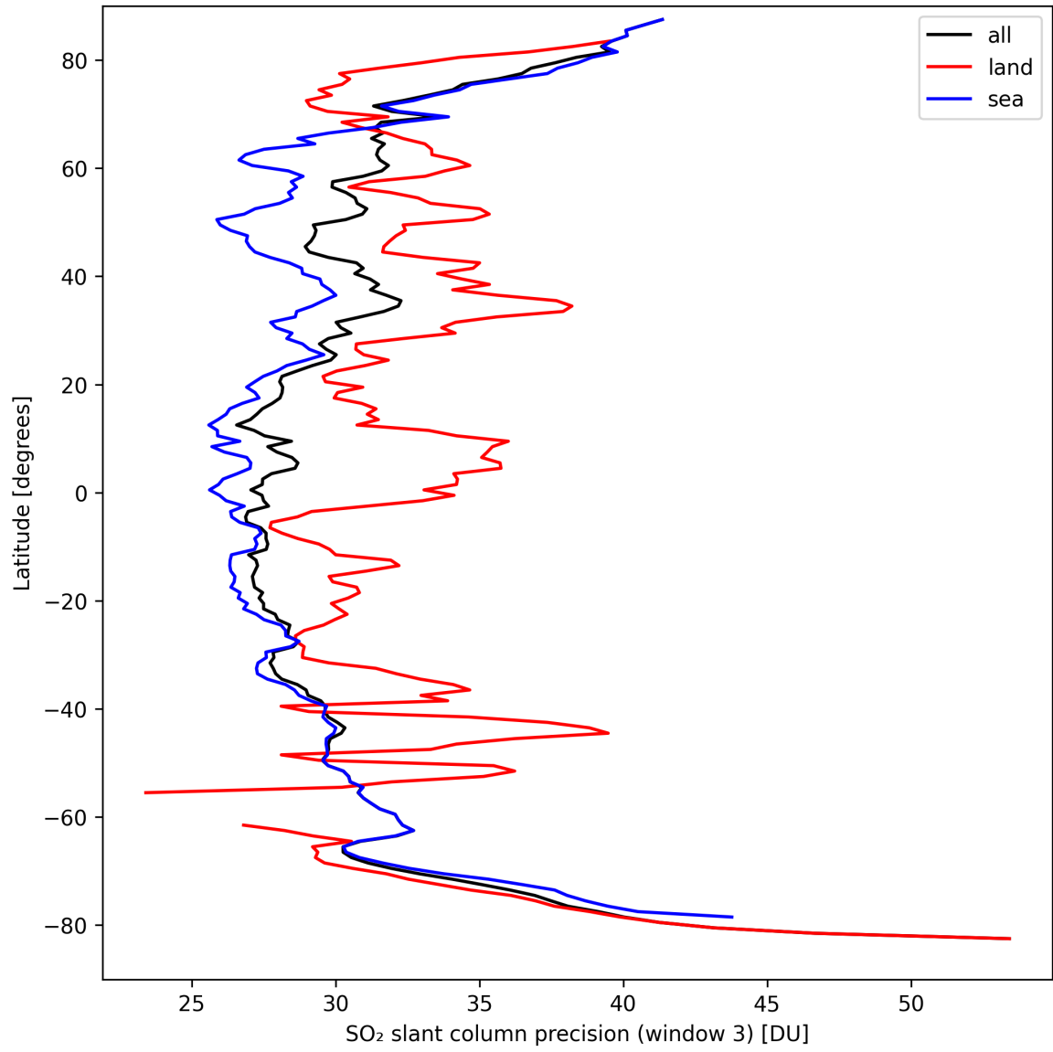
Figure 42: Zonal average of “SO 2 slant column precision (window 3)” for 2024-09-15 to 2024-09-17.
