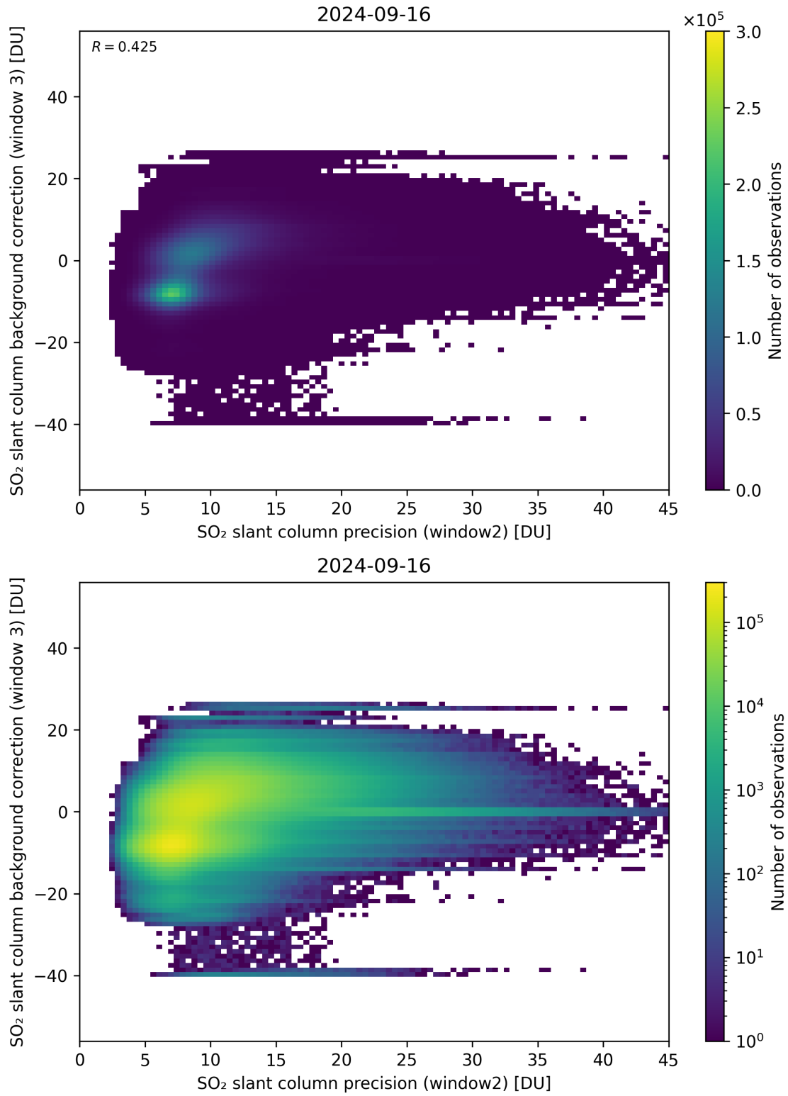
Figure 242: Scatter density plot of “SO 2 slant column precision (window2)” against “SO 2 slant column background correction (window 3)” for 2024-09-15 to 2024-09-17.
