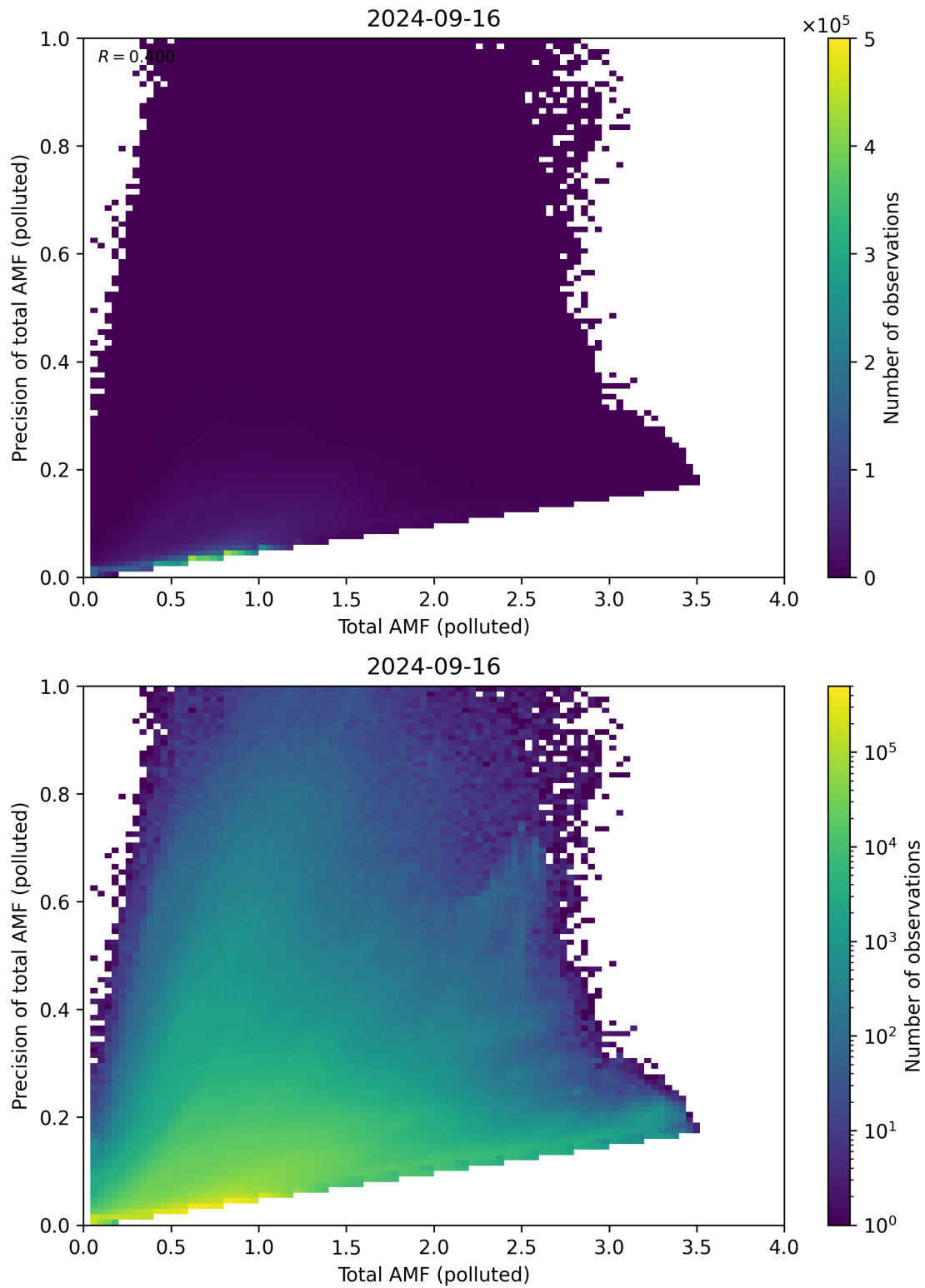
Figure 272: Scatter density plot of “Total AMF (polluted)” against “Precision of total AMF (polluted)” for 2024-09-15 to 2024-09-17.
