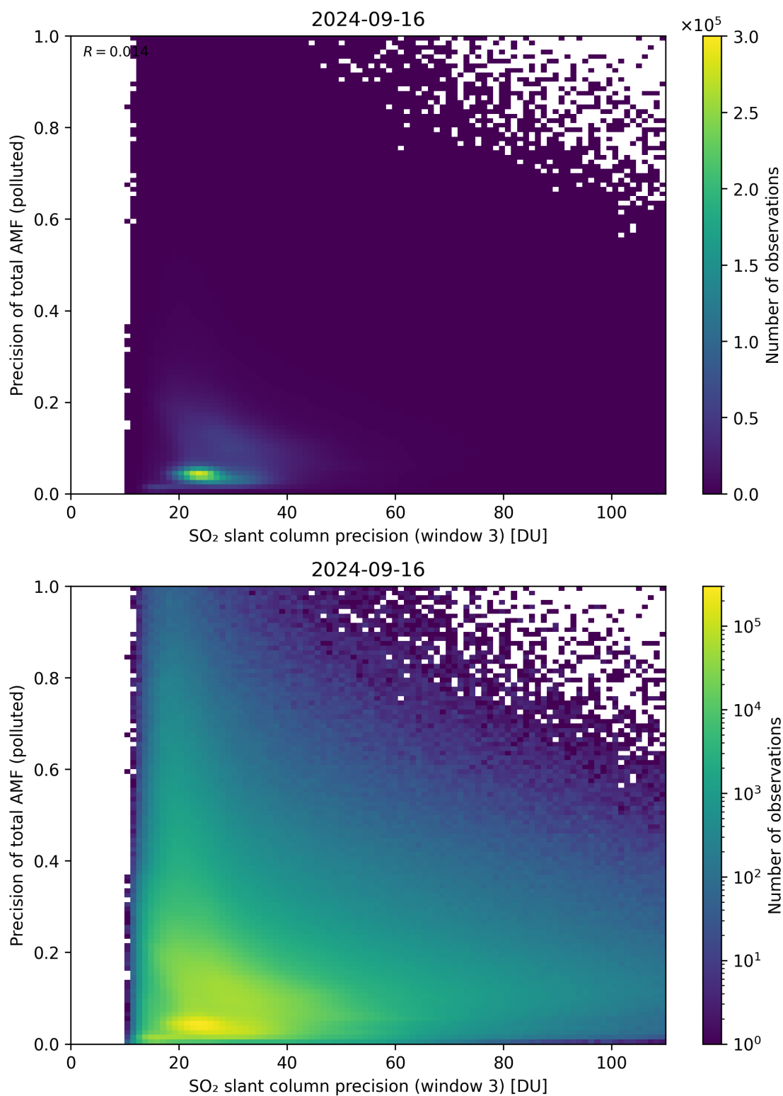
Figure 264: Scatter density plot of “SO 2 slant column precision (window 3)” against “Precision of total AMF (polluted)” for 2024-09-15 to 2024-09-17.
