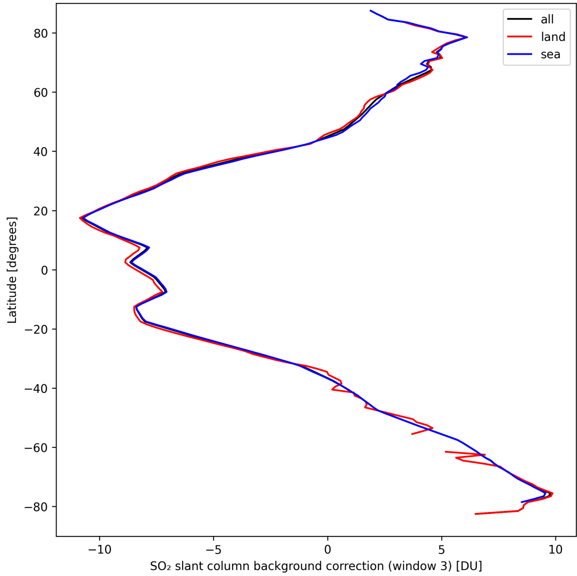
Figure 44: Zonal average of “SO 2 slant column background correction (window 3)” for 2024-09-15 to 2024-09-17.
