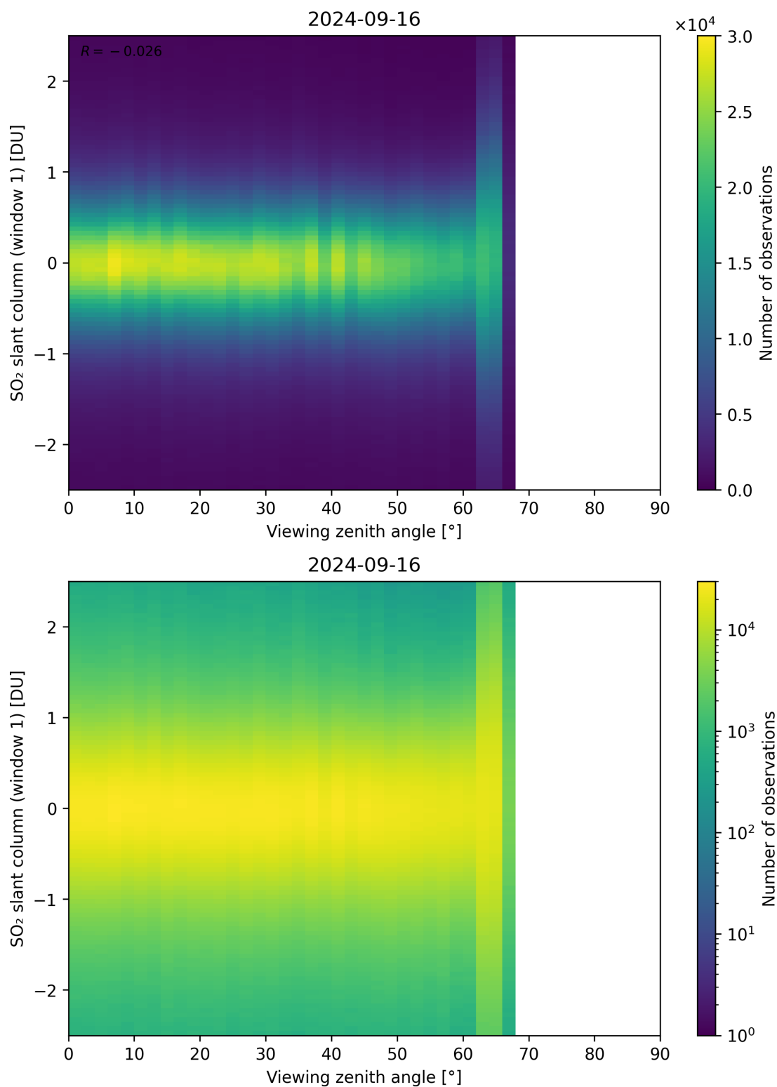
Figure 320: Scatter density plot of “Viewing zenith angle” against “SO 2 slant column (window 1)” for 2024-09-15 to 2024-09-17.
