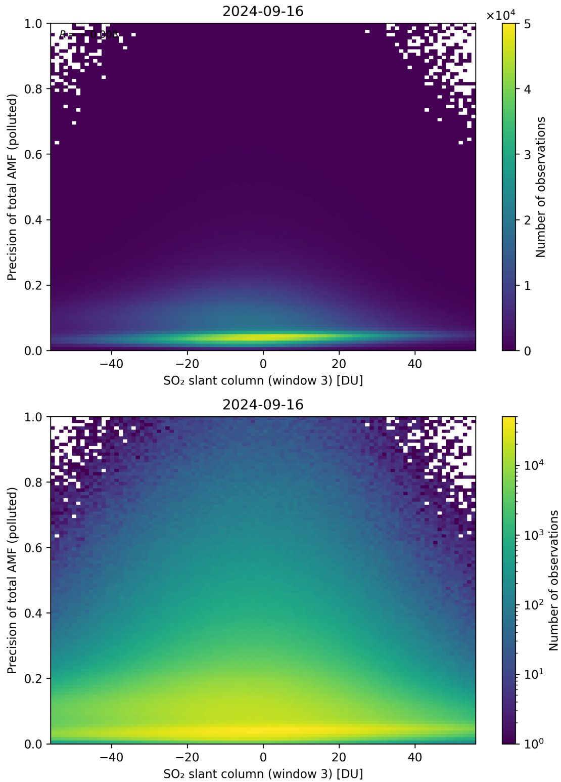
Figure 269: Scatter density plot of “SO 2 slant column (window 3)” against “Precision of total AMF (polluted)” for 2024-09-15 to 2024-09-17.
