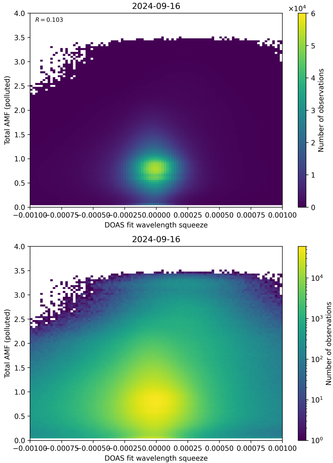
Figure 134: Scatter density plot of “DOAS fit wavelength squeeze” against “Total AMF (polluted)” for 2024-09-15 to 2024-09-17.
