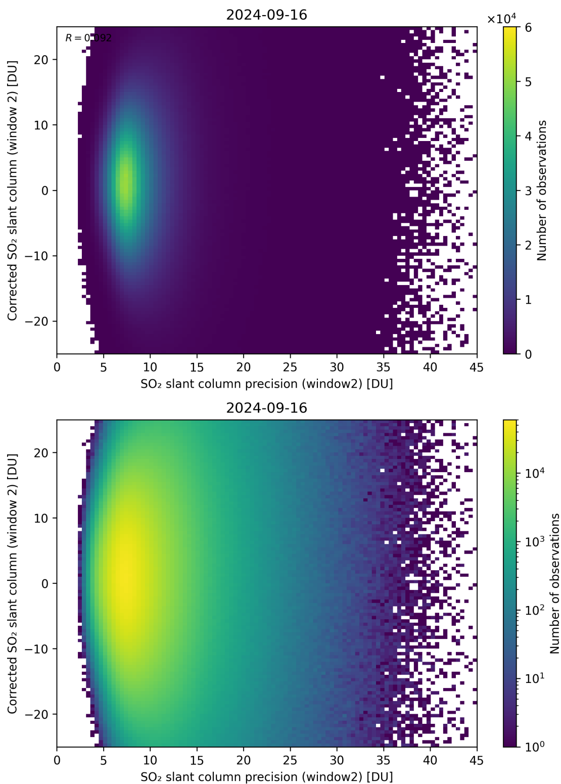
Figure 247: Scatter density plot of “SO 2 slant column precision (window2)” against “Corrected SO 2 slant column (window 2)” for 2024-09-15 to 2024-09-17.
