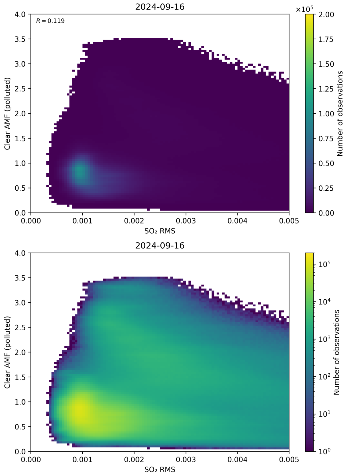
Figure 136: Scatter density plot of “SO 2 RMS” against “Clear AMF (polluted)” for 2024-09-15 to 2024-09-17.
