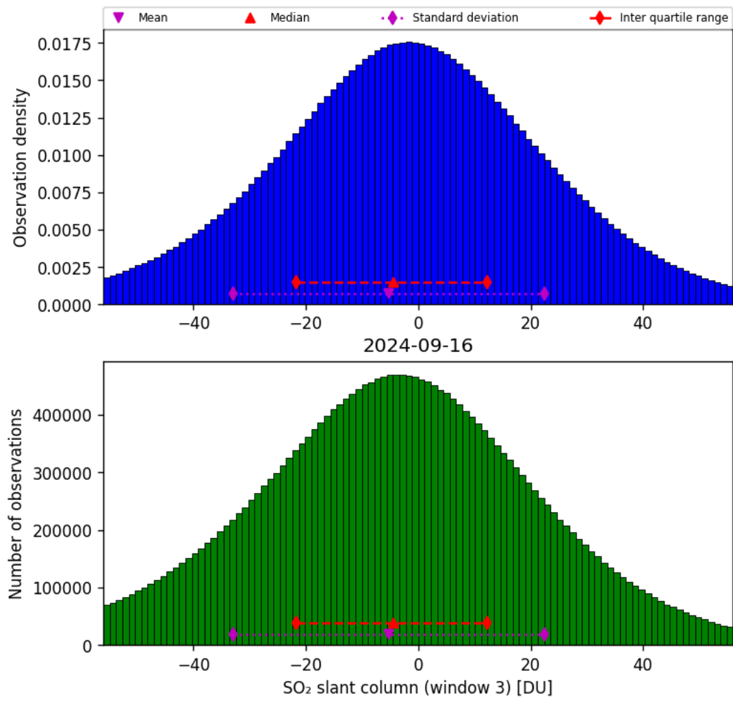
Figure 64: Histogram of “SO 2 slant column (window 3)” for 2024-09-15 to 2024-09-17
