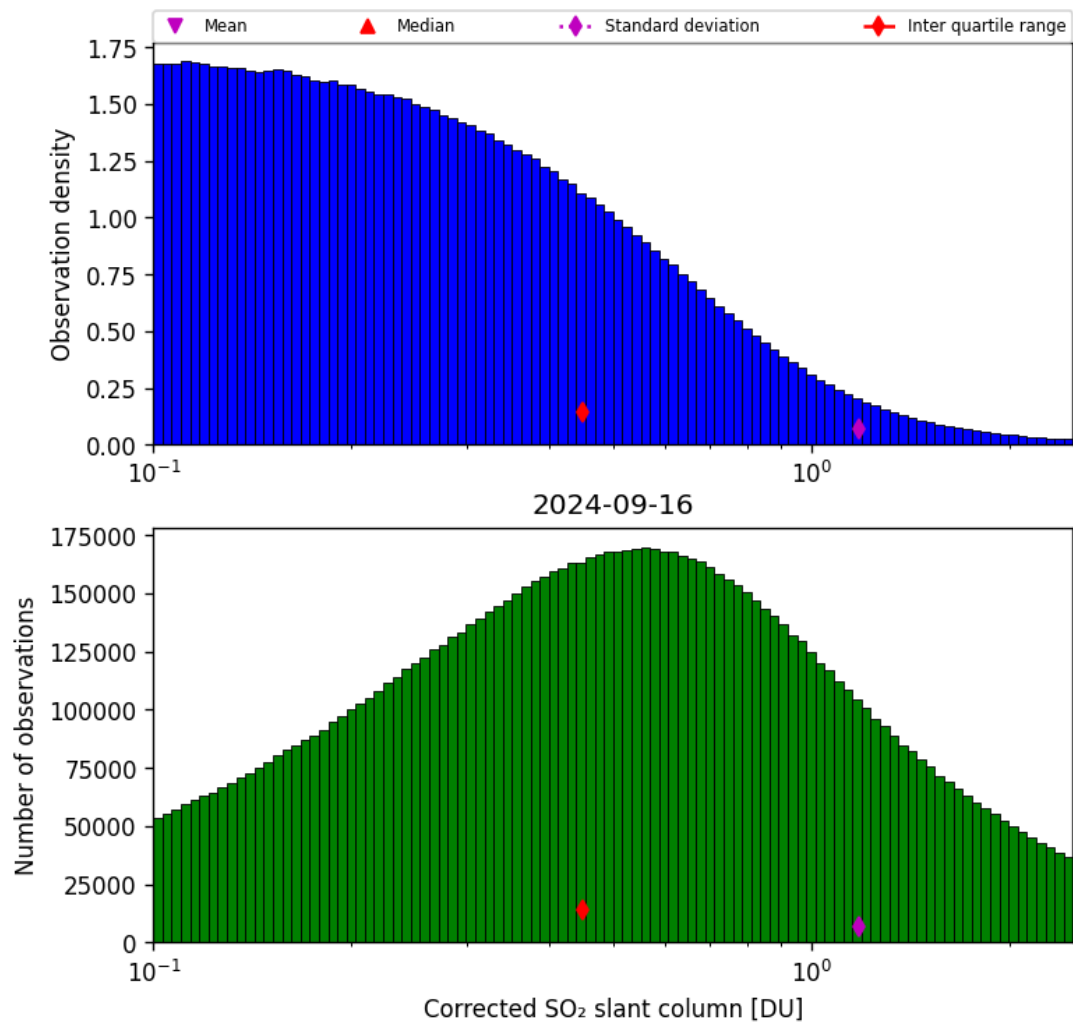
Figure 55: Histogram of “Corrected SO 2 slant column” for 2024-09-15 to 2024-09-17
