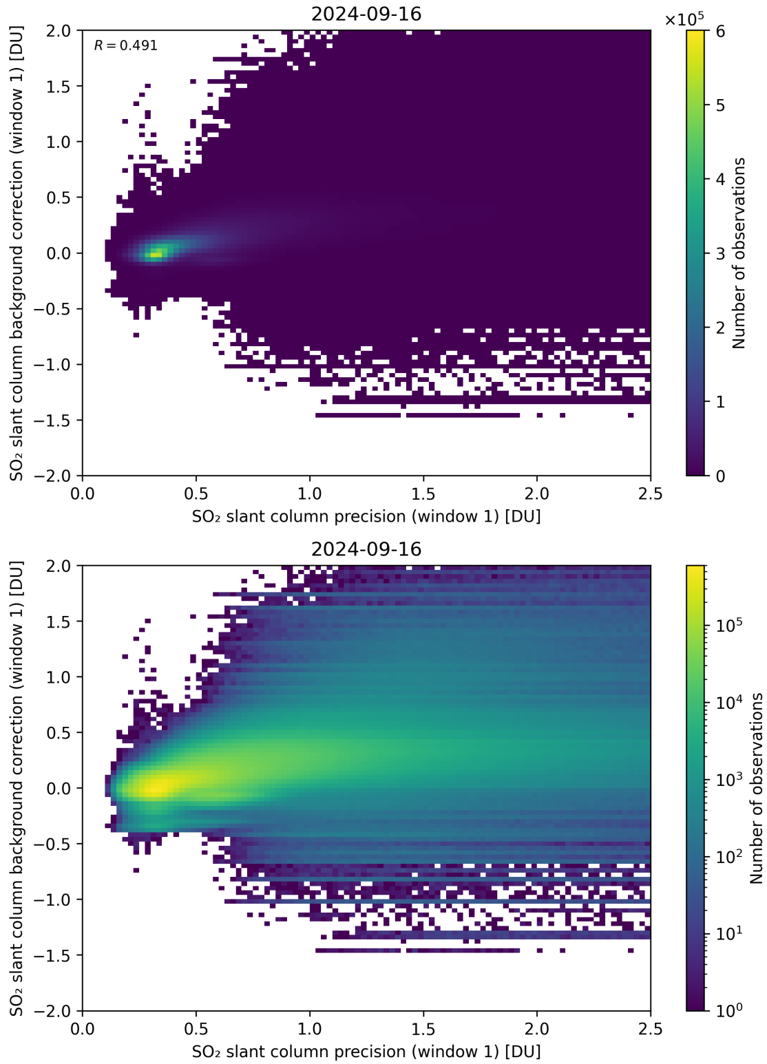
Figure 218: Scatter density plot of “SO 2 slant column precision (window 1)” against “SO 2 slant column background correction (window 1)” for 2024-09-15 to 2024-09-17.
