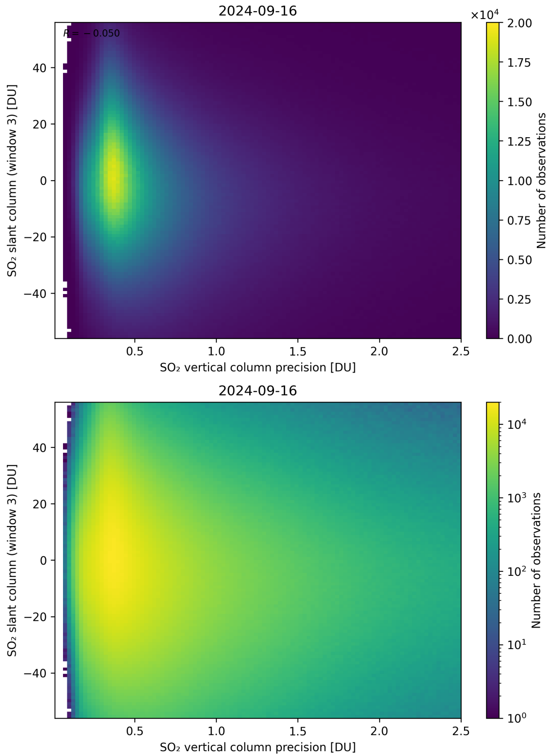
Figure 292: Scatter density plot of “SO 2 vertical column precision” against “SO 2 slant column (window 3)” for 2024-09-15 to 2024-09-17.
