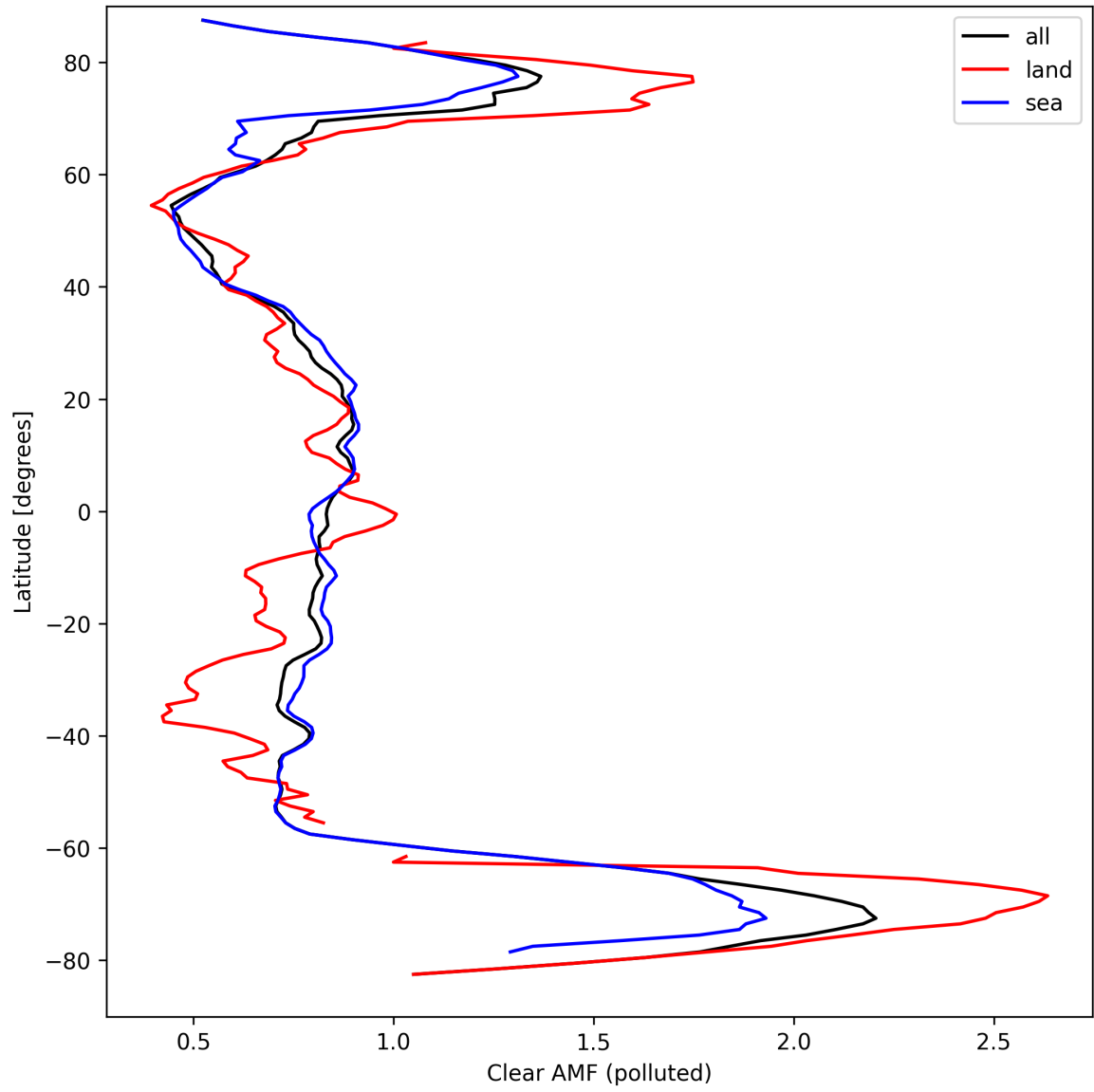
Figure 50: Zonal average of “Clear AMF (polluted)” for 2024-09-15 to 2024-09-17.
