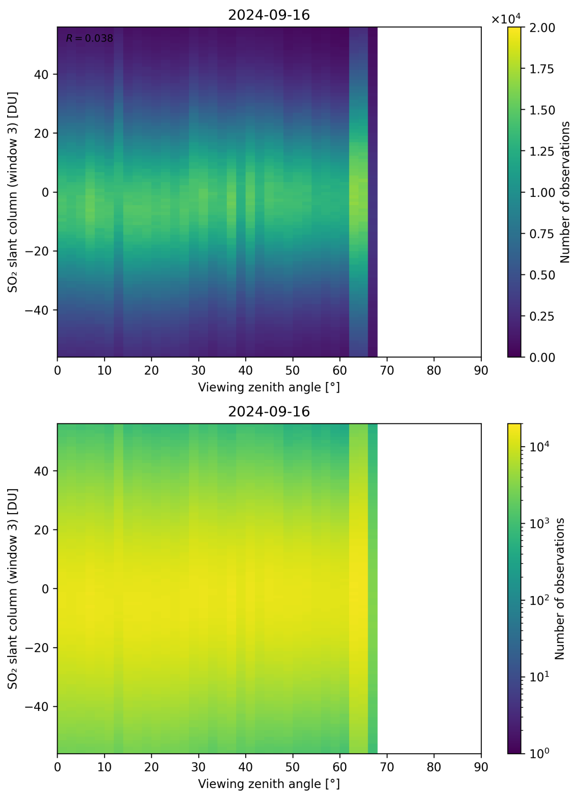
Figure 323: Scatter density plot of “Viewing zenith angle” against “SO 2 slant column (window 3)” for 2024-09-15 to 2024-09-17.
