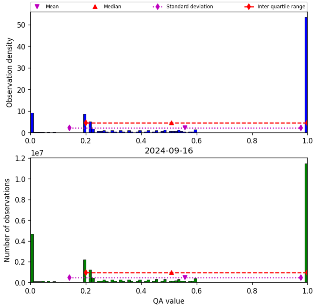
Figure 52: Histogram of “QA value” for 2024-09-15 to 2024-09-17
