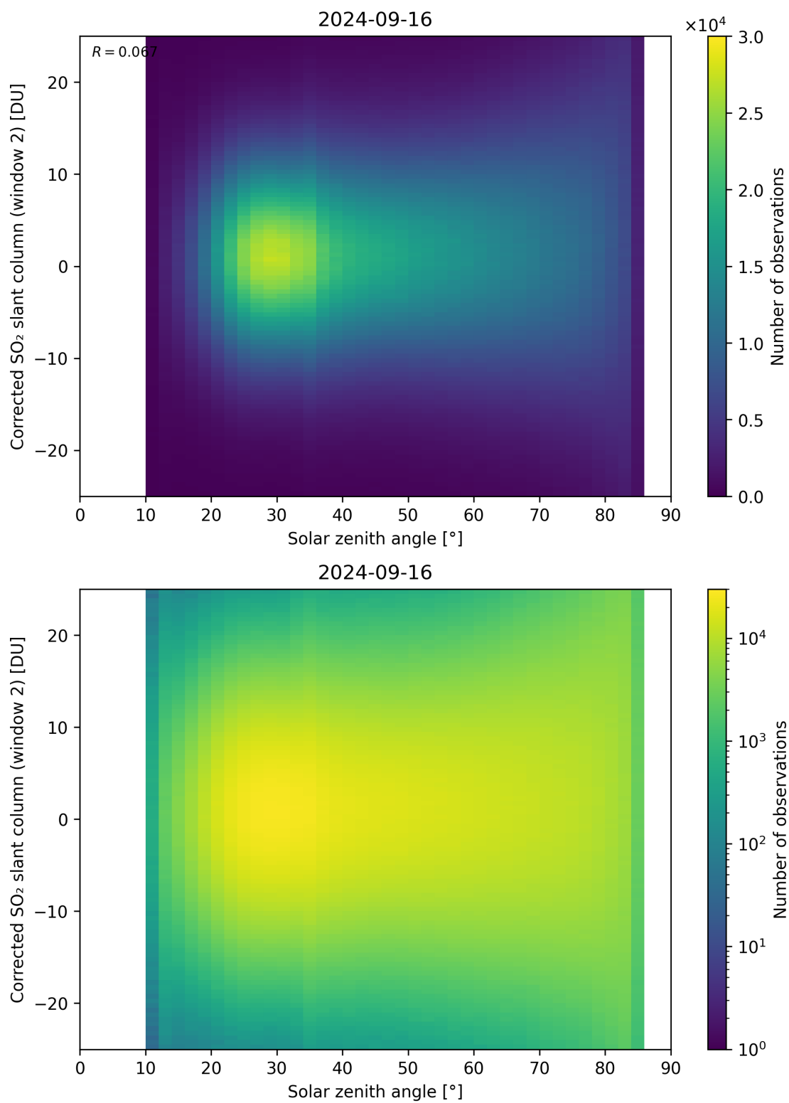
Figure 167: Scatter density plot of “Solar zenith angle” against “Corrected SO 2 slant column (window 2)” for 2024-09-15 to 2024-09-17.
