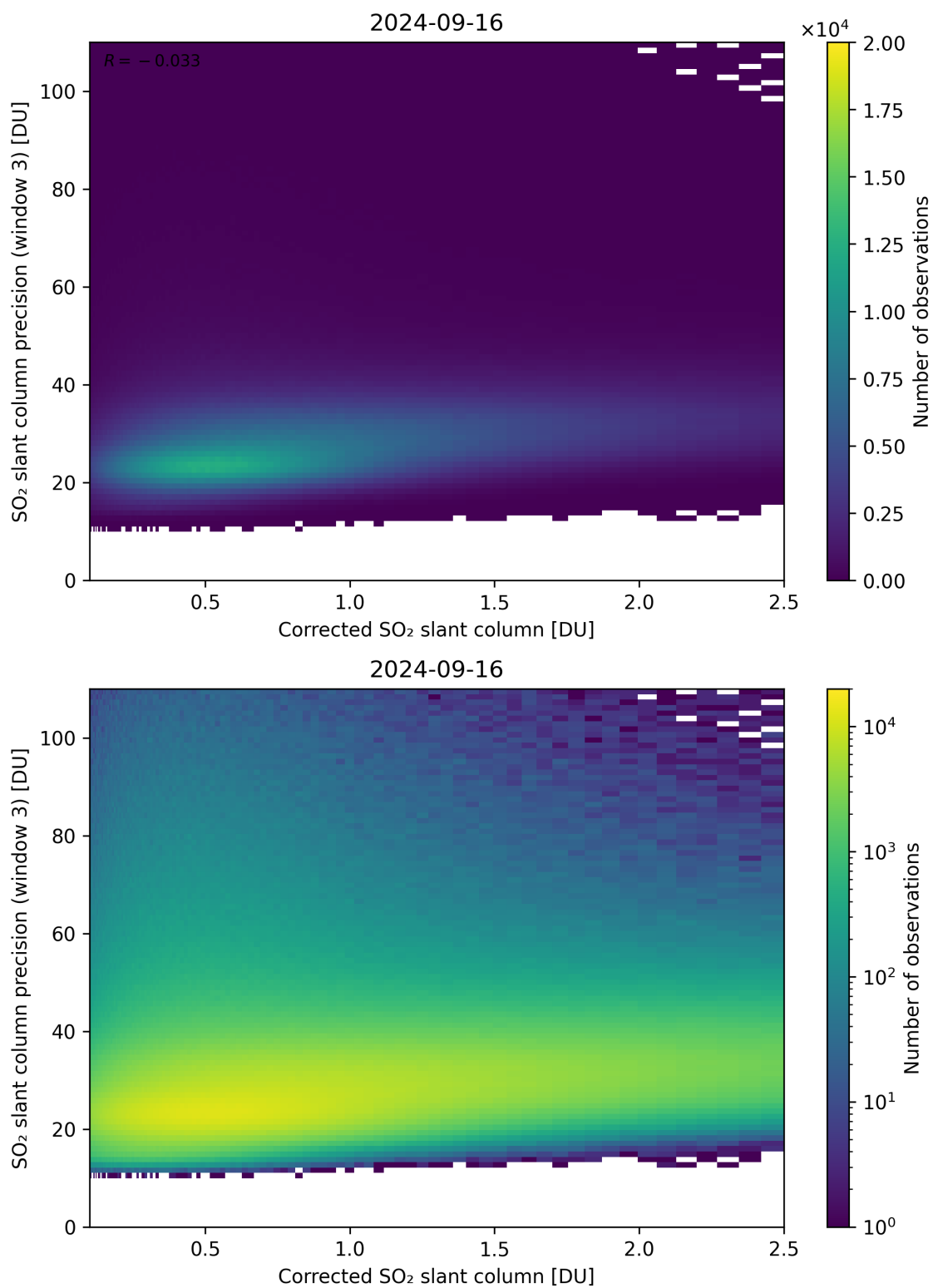
Figure 191: Scatter density plot of “Corrected SO 2 slant column” against “SO 2 slant column precision (window 3)” for 2024-09-15 to 2024-09-17.
