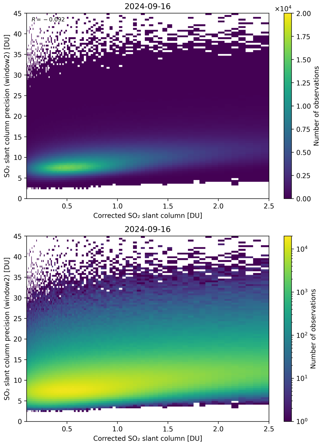
Figure 189: Scatter density plot of “Corrected SO 2 slant column” against “SO 2 slant column precision (window2)” for 2024-09-15 to 2024-09-17.
