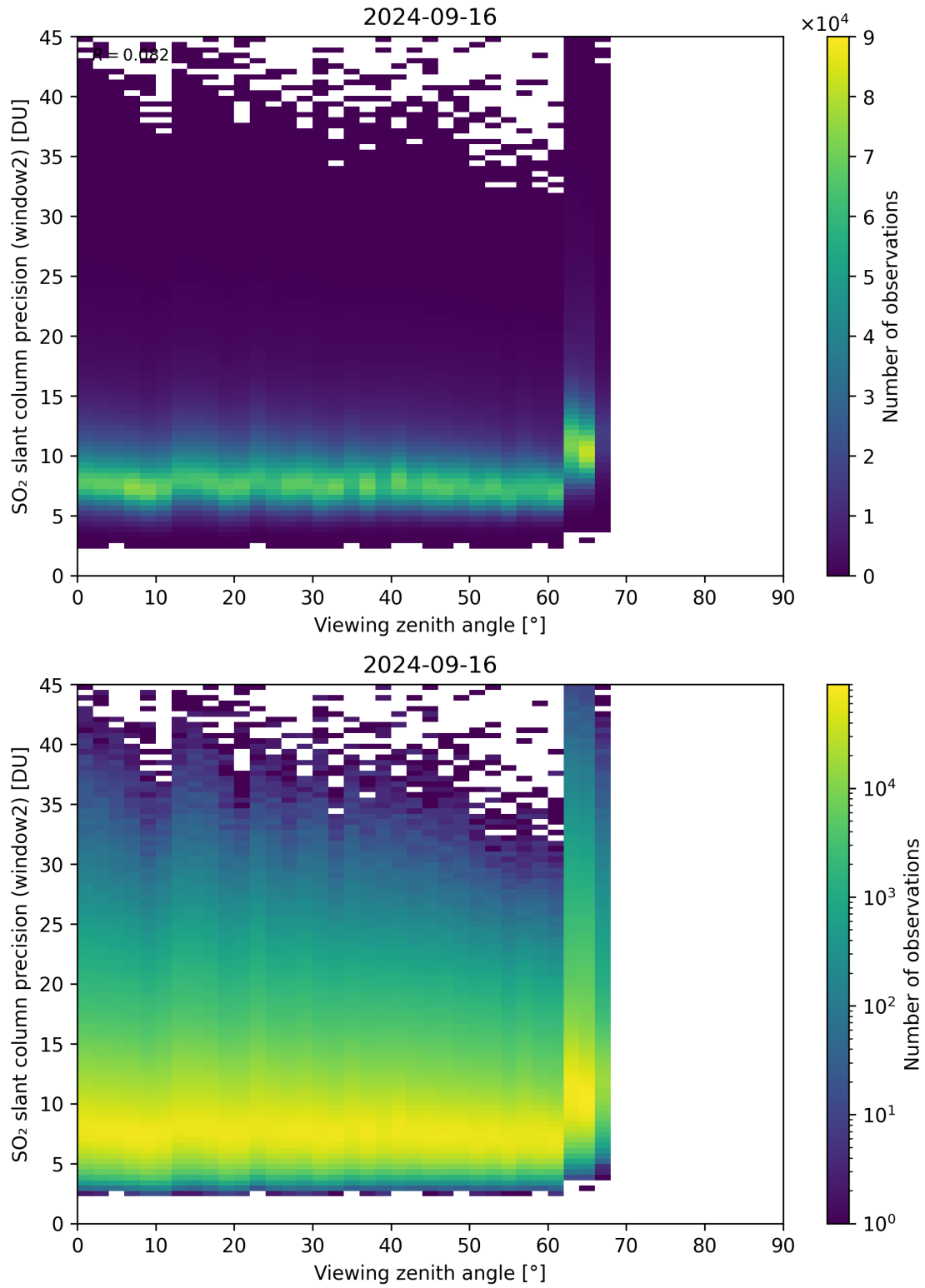
Figure 322: Scatter density plot of “Viewing zenith angle” against “SO 2 slant column precision (window2)” for 2024-09-15 to 2024-09-17.
