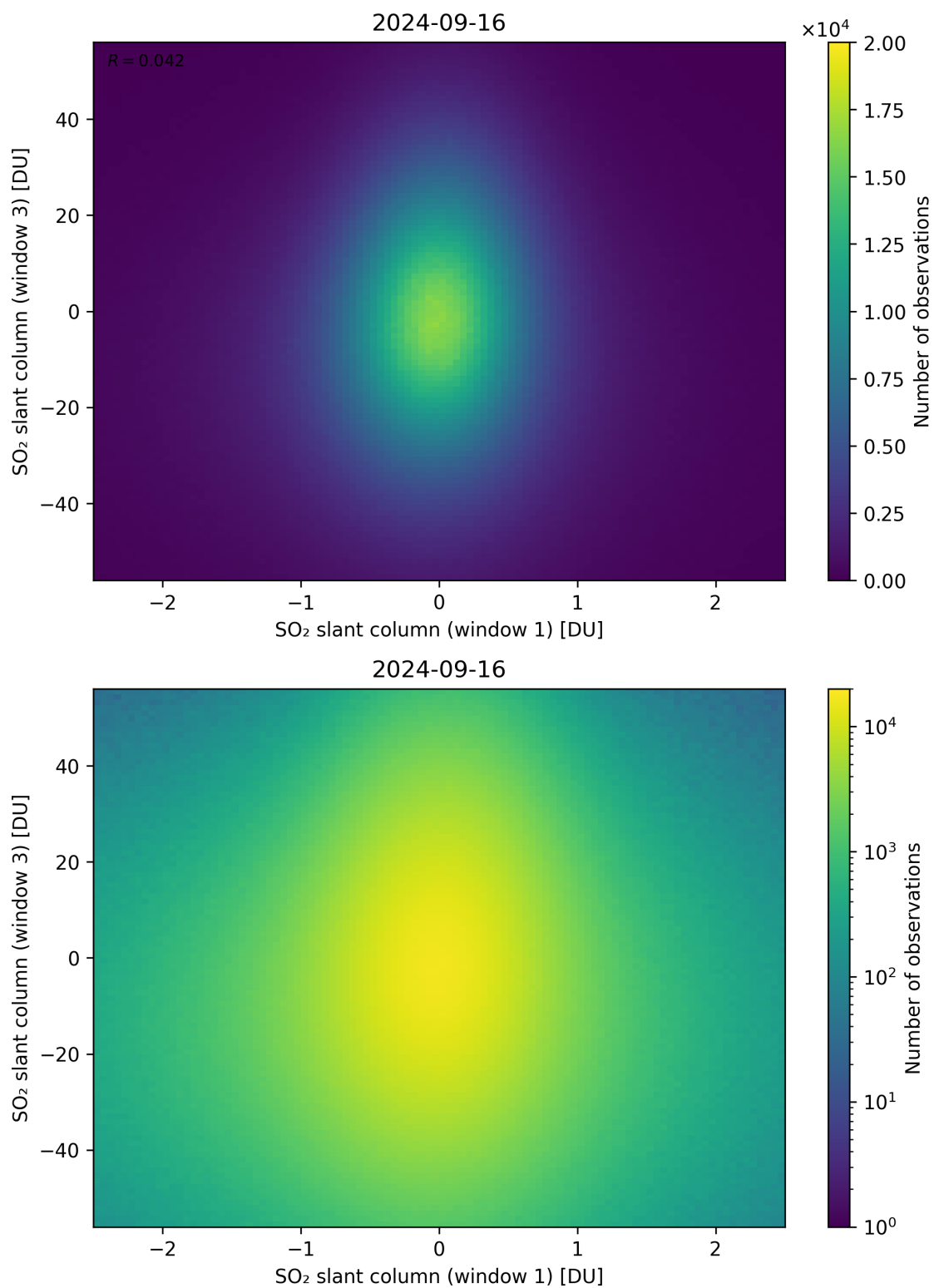
Figure 237: Scatter density plot of “SO 2 slant column (window 1)” against “SO 2 slant column (window 3)” for 2024-09-15 to 2024-09-17.
