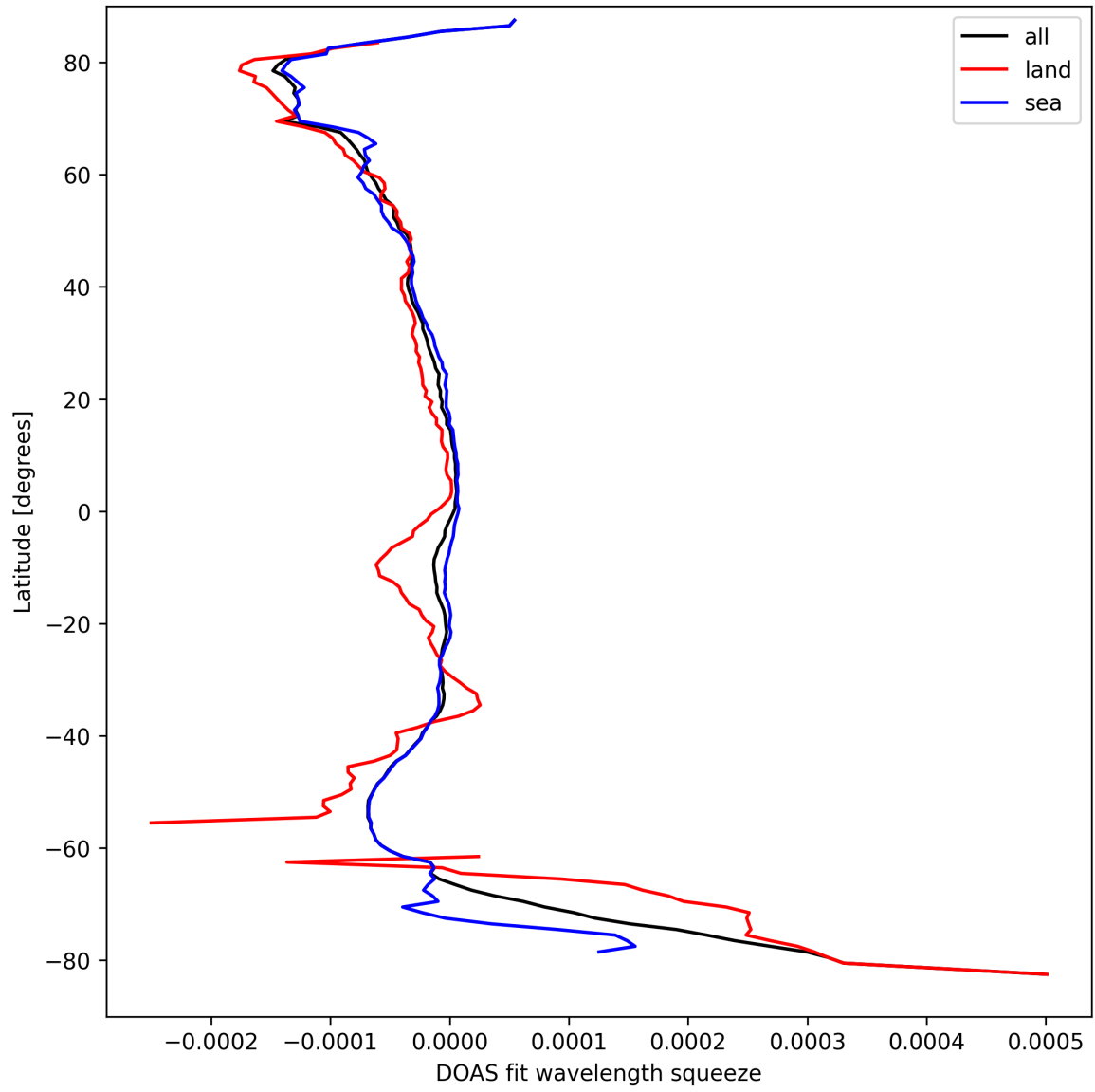
Figure 46: Zonal average of "DOAS fit wavelength squeeze" for 2024-09-15 to 2024-09-17.
