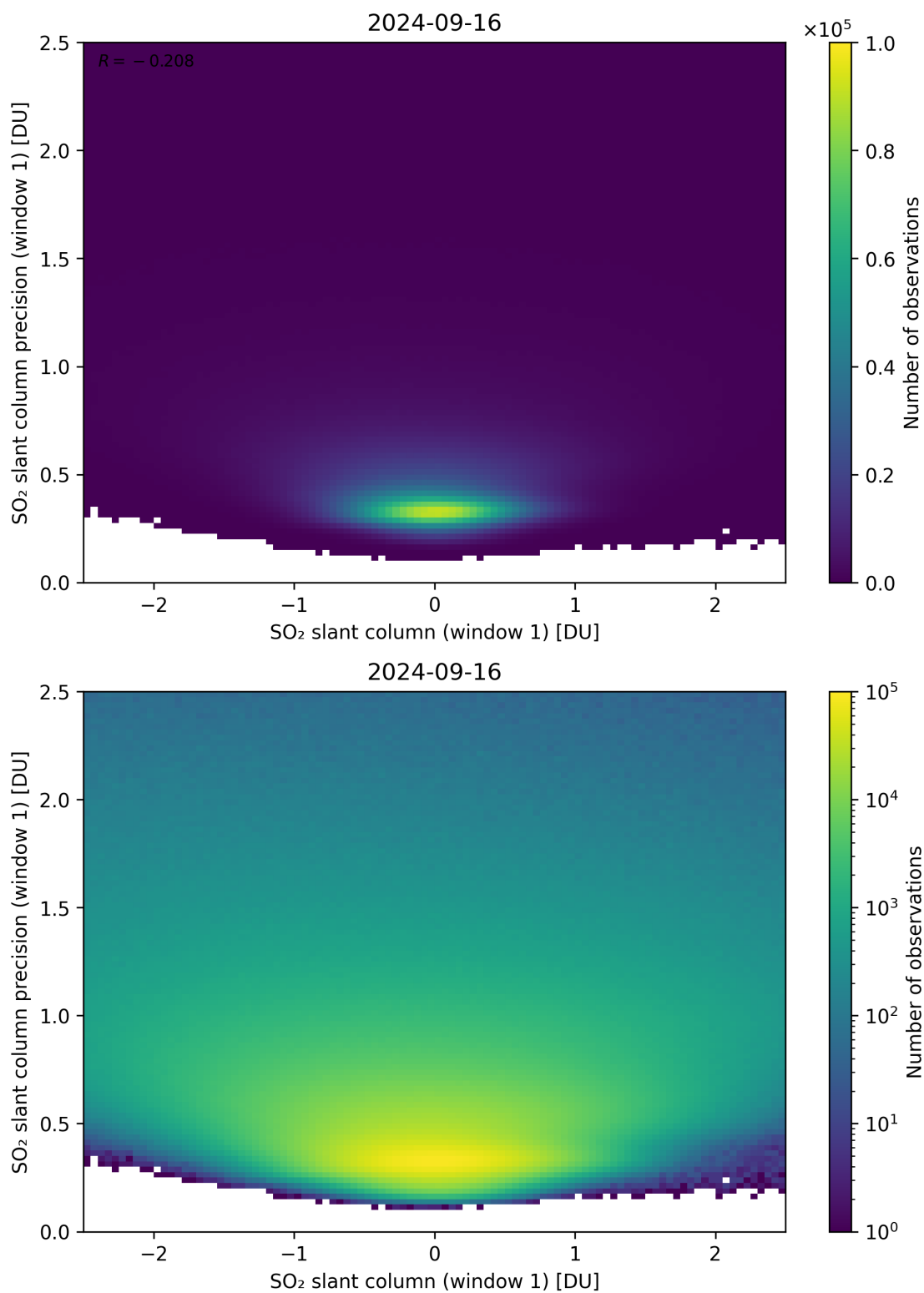
Figure 235: Scatter density plot of “SO 2 slant column (window 1)” against “SO 2 slant column precision (window 1)” for 2024-09-15 to 2024-09-17.
