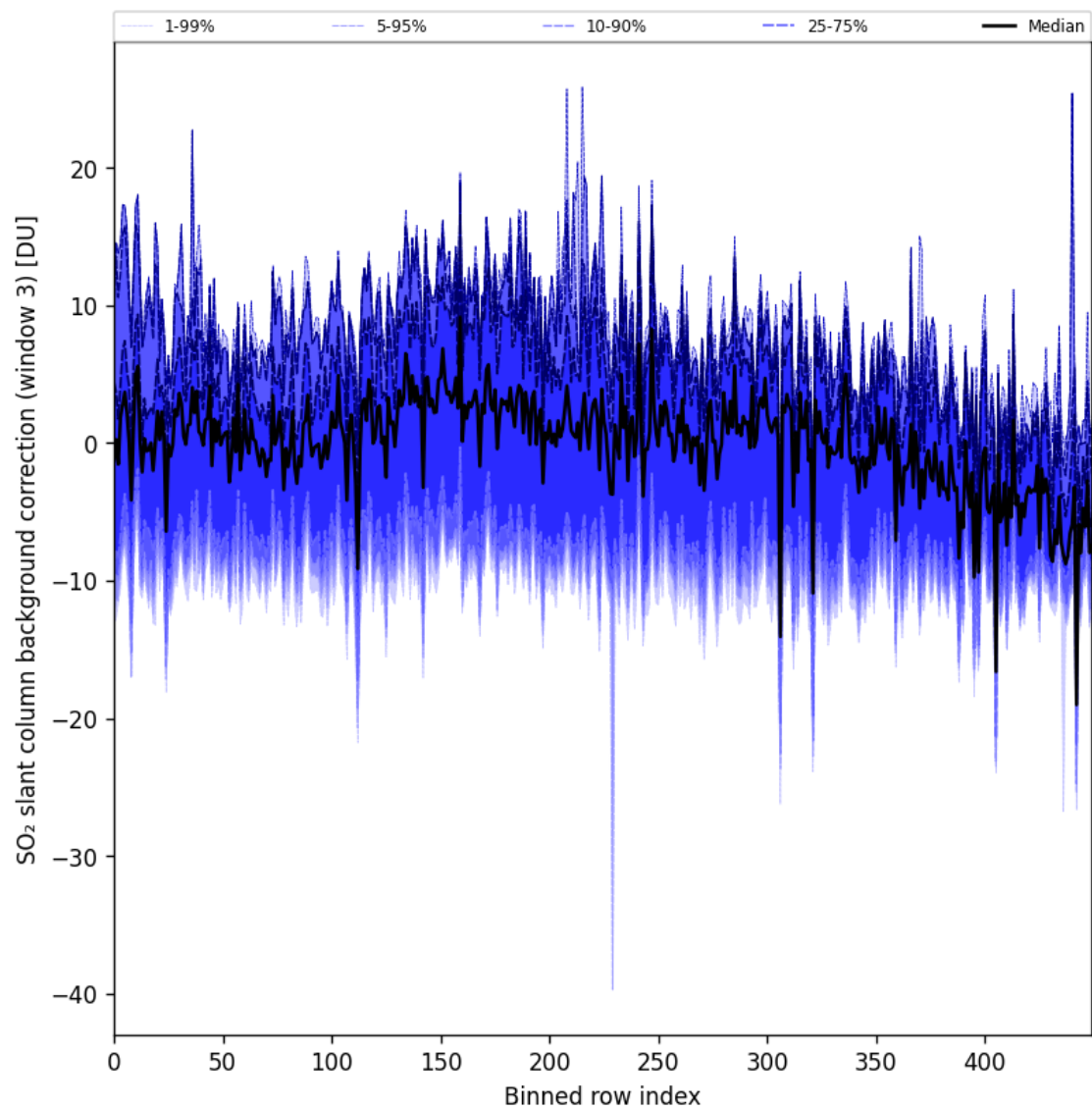
Figure 90: Along track statistics of “SO 2 slant column background correction (window 3)” for 2024-09-15 to 2024-09-17
