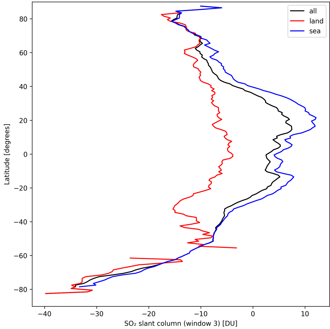
Figure 41: Zonal average of “SO 2 slant column (window 3)” for 2024-09-15 to 2024-09-17.
