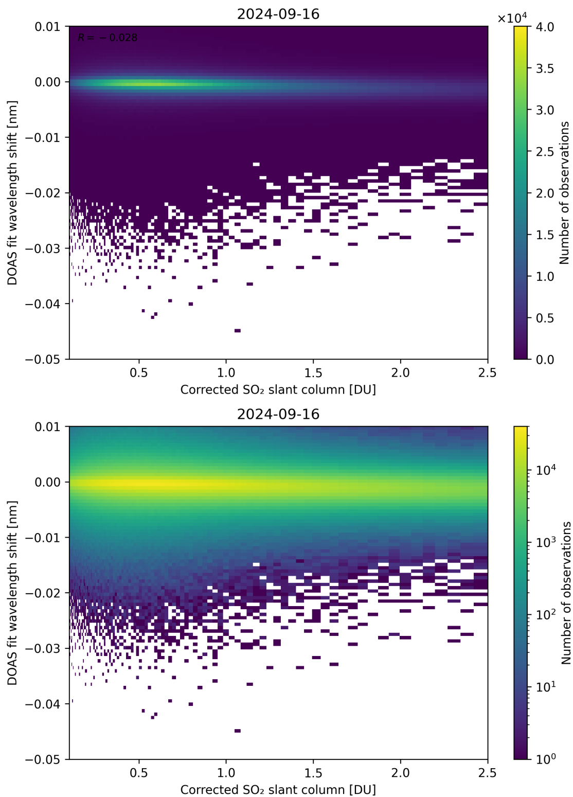
Figure 181: Scatter density plot of “Corrected SO 2 slant column” against “DOAS fit wavelength shift” for 2024-09-15 to 2024-09-17.
