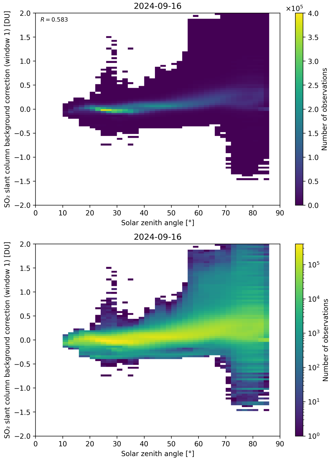
Figure 158: Scatter density plot of “Solar zenith angle” against “SO 2 slant column background correction (window 1)” for 2024-09-15 to 2024-09-17.
