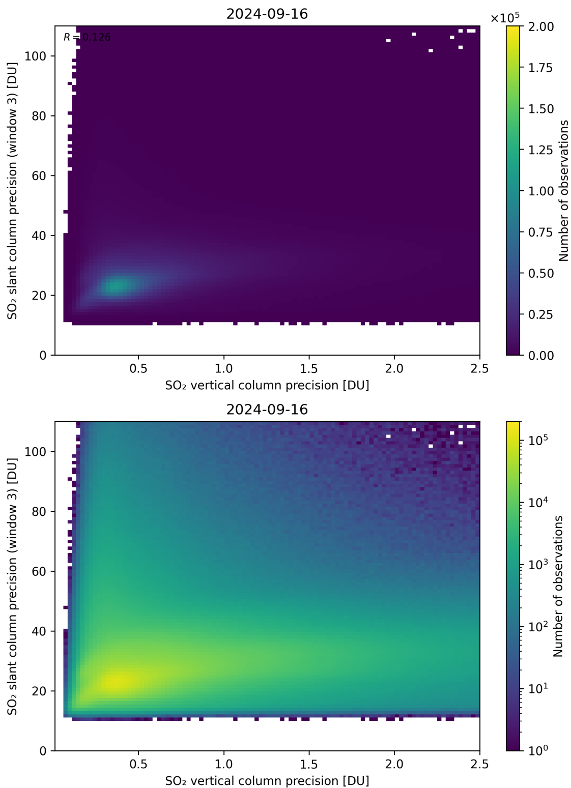
Figure 293: Scatter density plot of “SO 2 vertical column precision” against “SO 2 slant column precision (window 3)” for 2024-09-15 to 2024-09-17.
