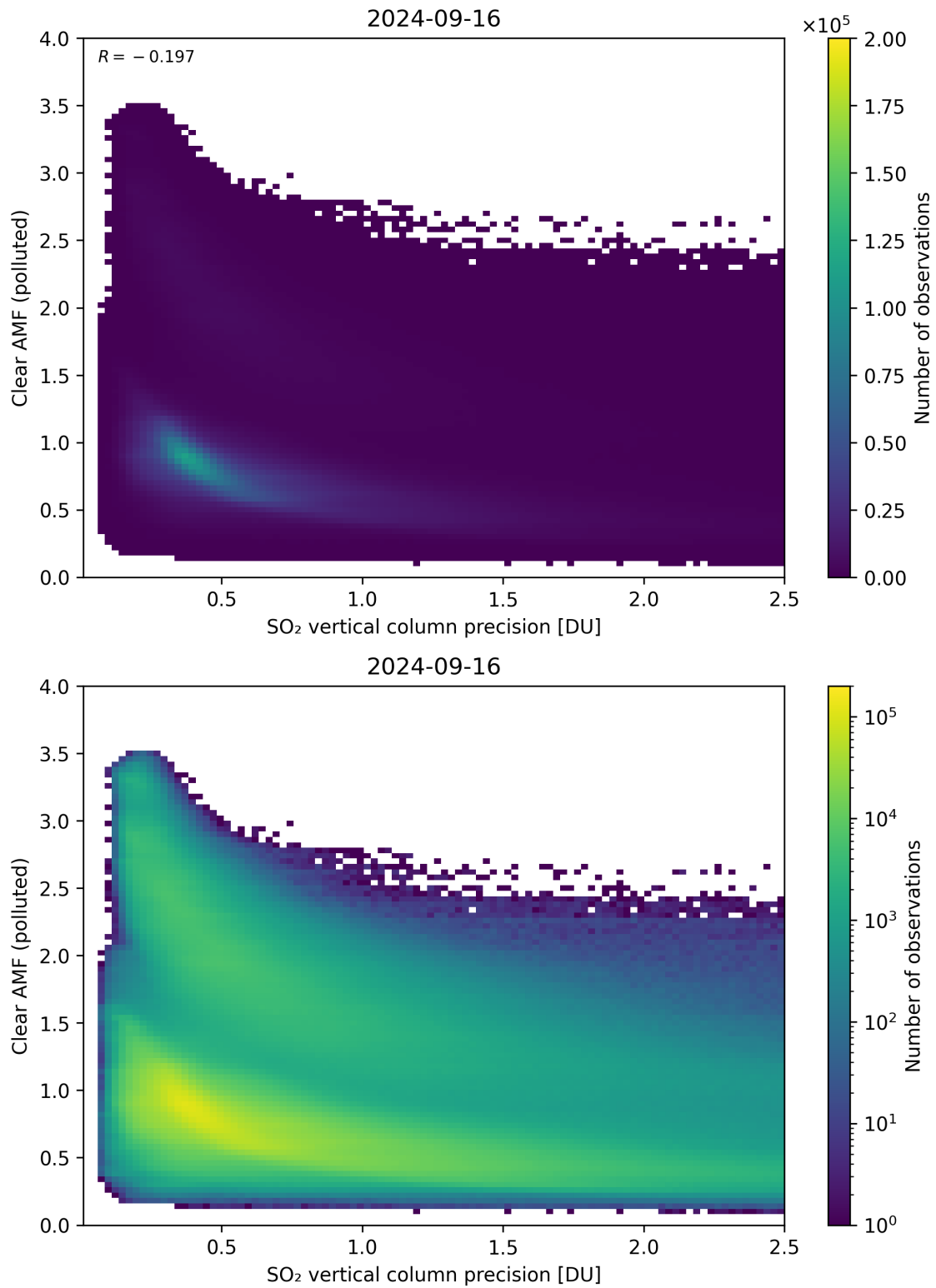
Figure 285: Scatter density plot of “SO 2 vertical column precision” against “Clear AMF (polluted)” for 2024-09-15 to 2024-09-17.
