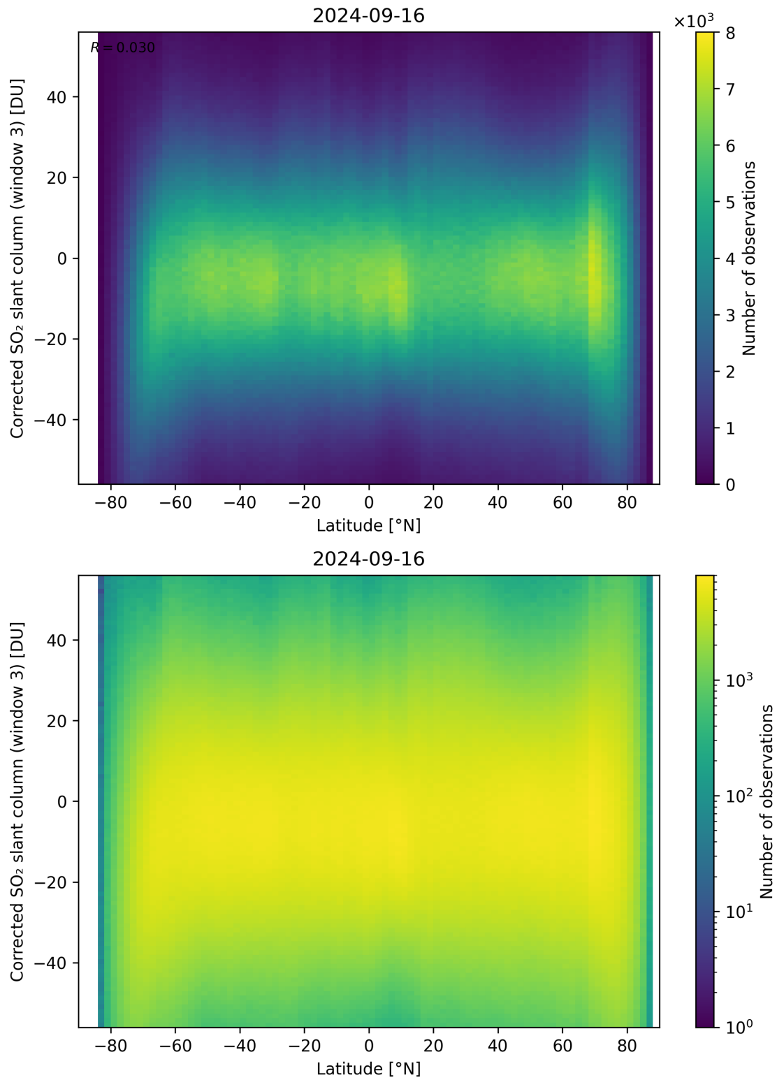
Figure 148: Scatter density plot of “Latitude” against “Corrected SO 2 slant column (window 3)” for 2024-09-15 to 2024-09-17.
