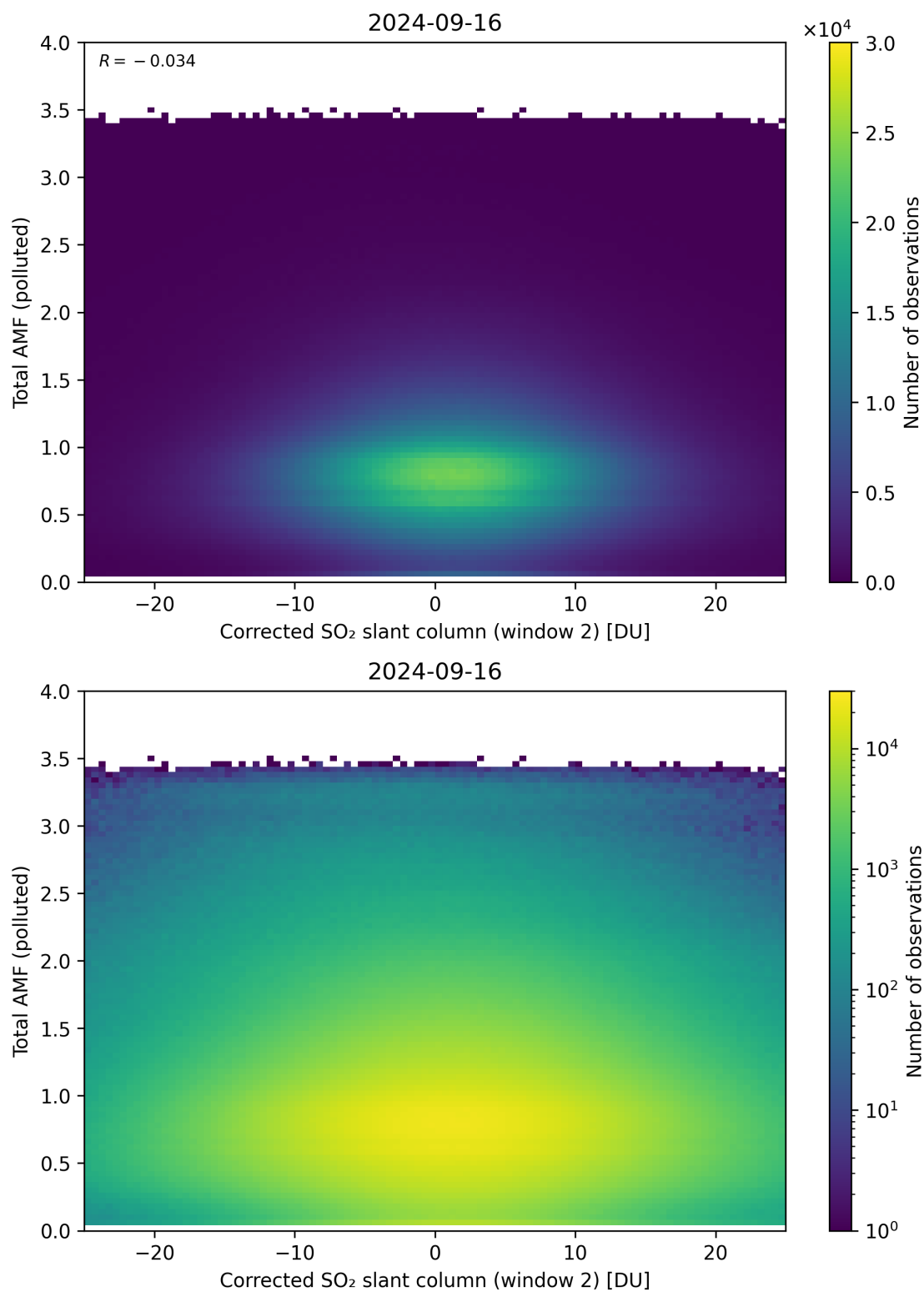
Figure 203: Scatter density plot of “Corrected SO 2 slant column (window 2)” against “Total AMF (polluted)” for 2024-09-15 to 2024-09-17.
