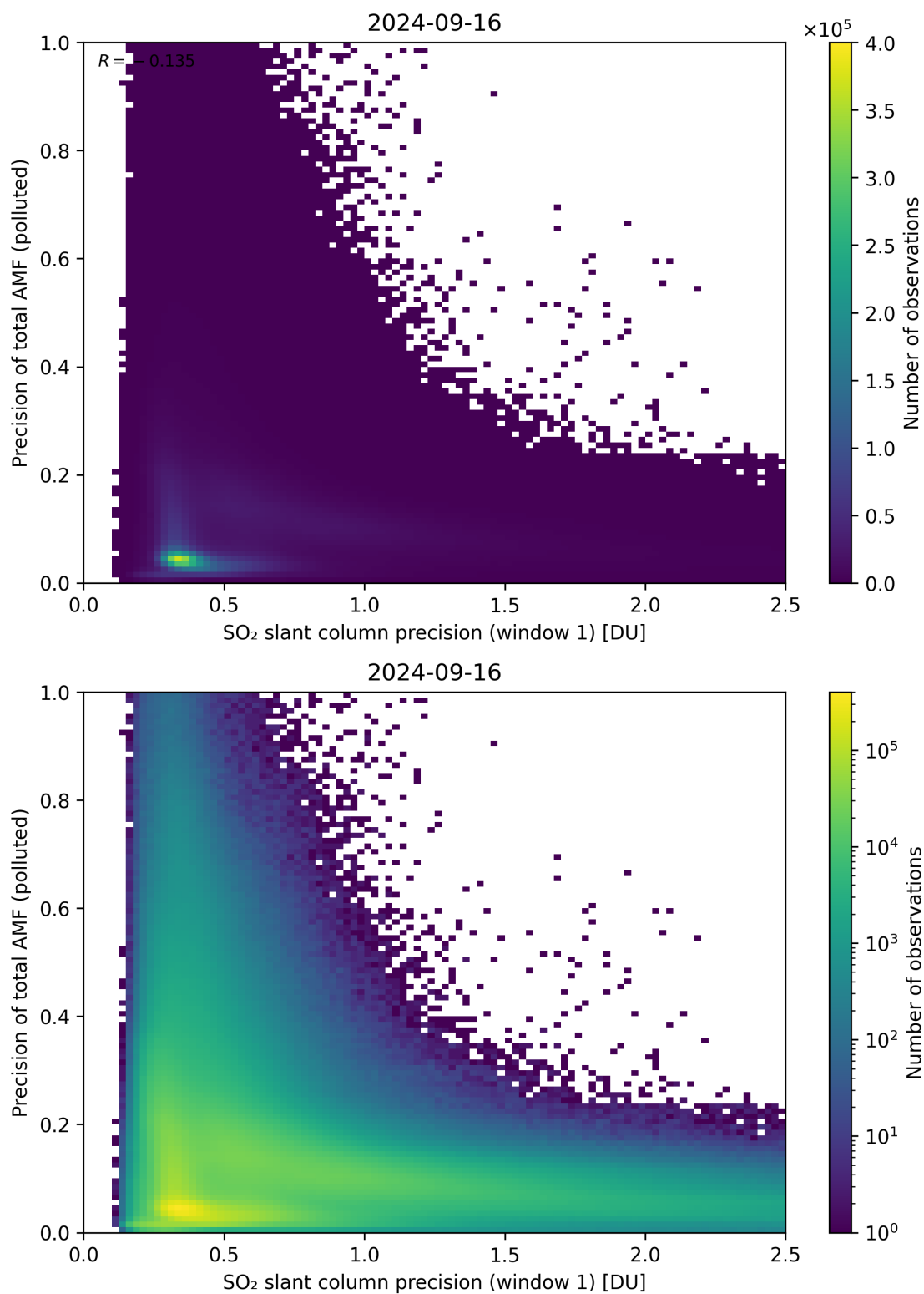
Figure 231: Scatter density plot of “SO 2 slant column precision (window 1)” against “Precision of total AMF (polluted)” for 2024-09-15 to 2024-09-17.
