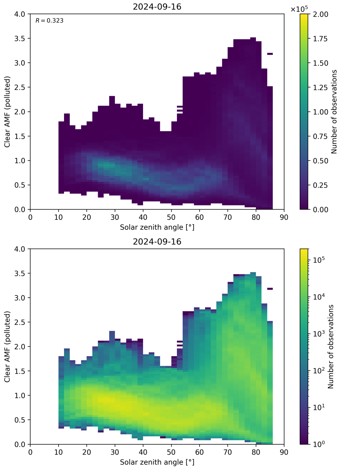
Figure 165: Scatter density plot of “Solar zenith angle” against “Clear AMF (polluted)” for 2024-09-15 to 2024-09-17.
