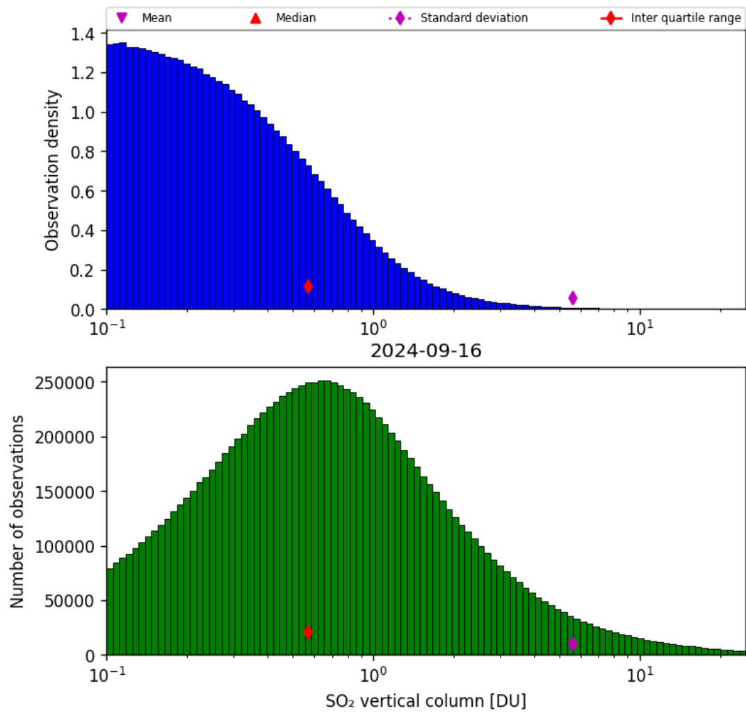
Figure 53: Histogram of “SO 2 vertical column” for 2024-09-15 to 2024-09-17
