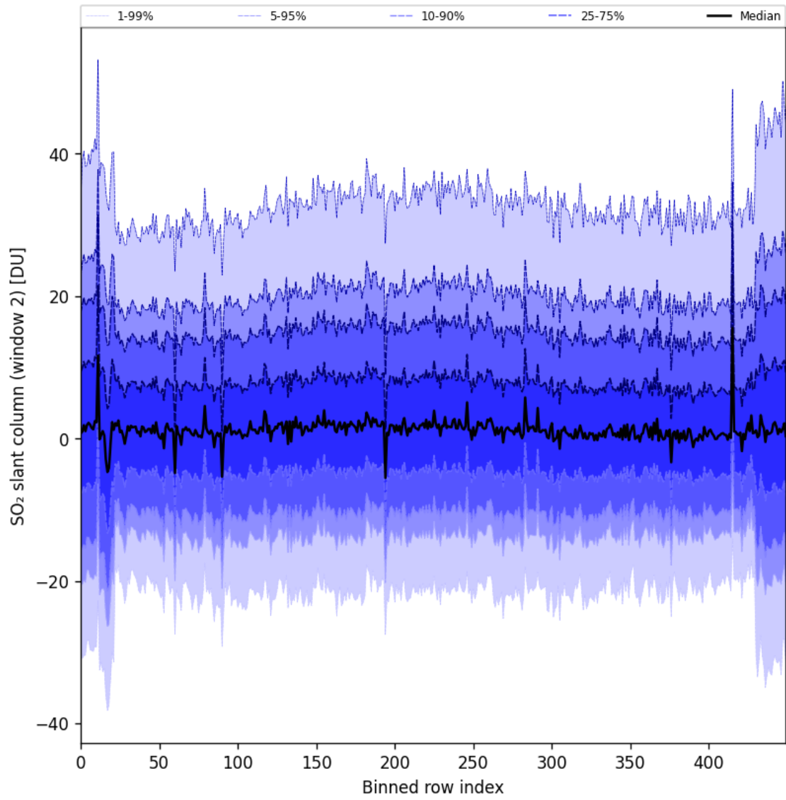
Figure 83: Along track statistics of “SO 2 slant column (window 2)” for 2024-09-15 to 2024-09-17
