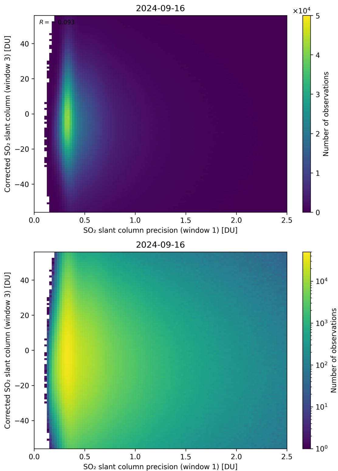
Figure 226: Scatter density plot of “SO 2 slant column precision (window 1)” against “Corrected SO 2 slant column (window 3)” for 2024-09-15 to 2024-09-17.
