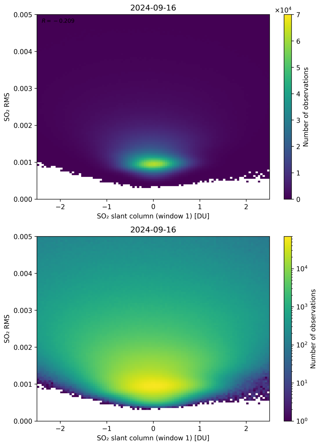
Figure 217: Scatter density plot of “SO 2 slant column (window 1)” against “SO 2 RMS” for 2024-09-15 to 2024-09-17.
