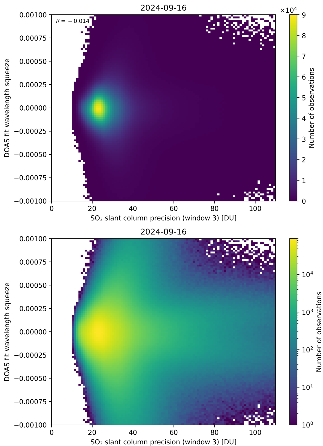
Figure 259: Scatter density plot of “SO 2 slant column precision (window 3)” against “DOAS fit wavelength squeeze” for 2024-09-15 to 2024-09-17.
