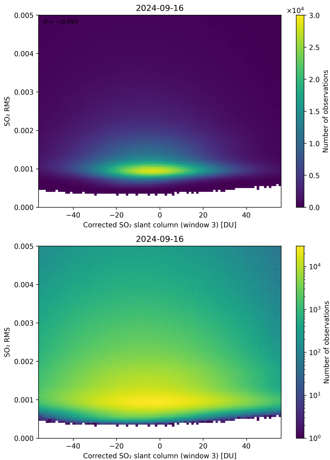
Figure 208: Scatter density plot of “Corrected SO 2 slant column (window 3)” against “SO 2 RMS” for 2024-09-15 to 2024-09-17.
