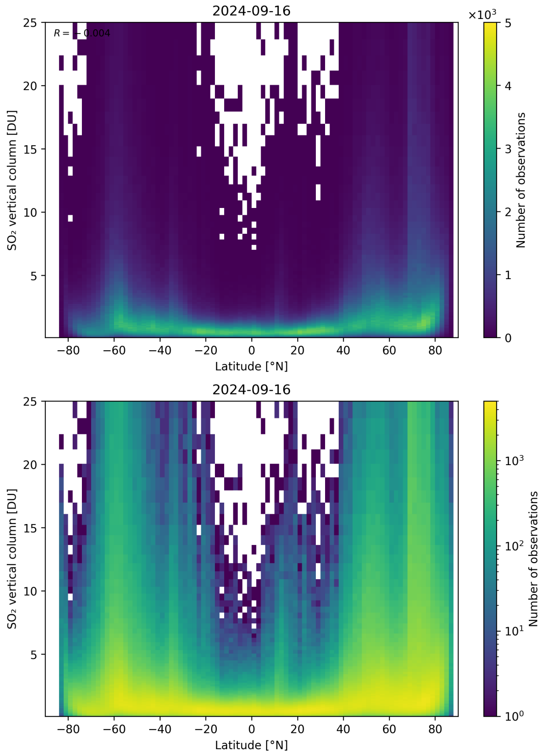
Figure 156: Scatter density plot of “Latitude” against “SO 2 vertical column” for 2024-09-15 to 2024-09-17.
