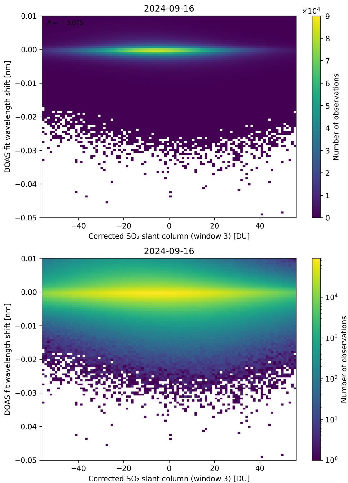
Figure 206: Scatter density plot of “Corrected SO 2 slant column (window 3)” against “DOAS fit wavelength shift” for 2024-09-15 to 2024-09-17.
