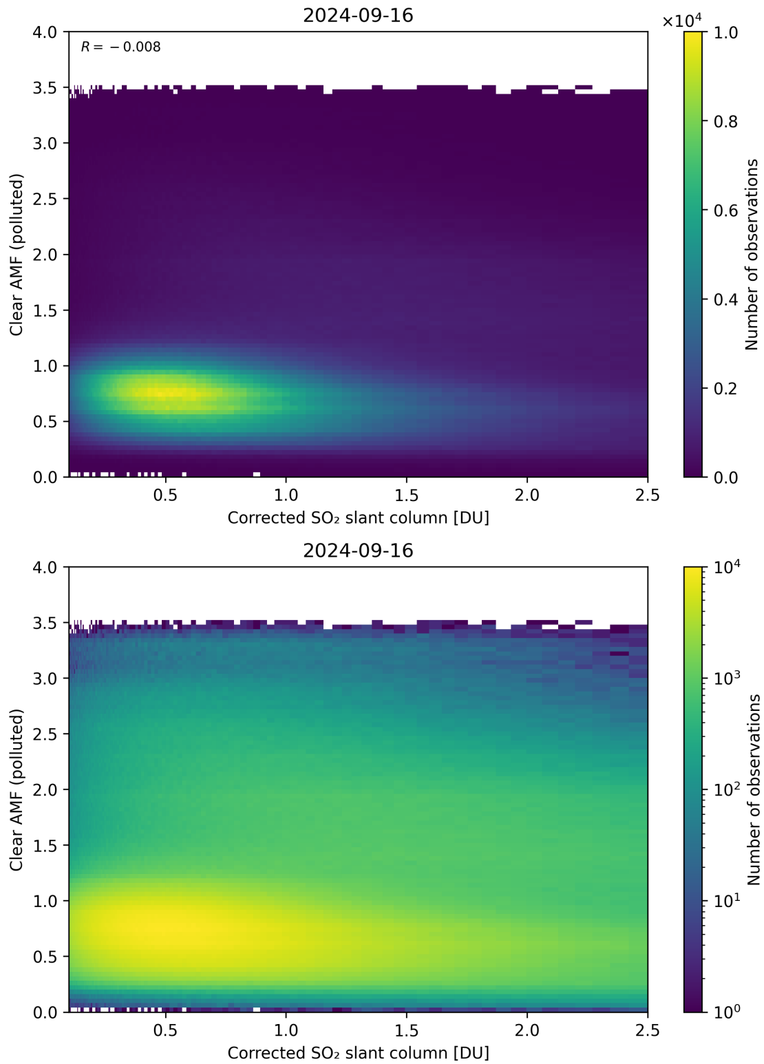
Figure 184: Scatter density plot of “Corrected SO 2 slant column” against “Clear AMF (polluted)” for 2024-09-15 to 2024-09-17.
