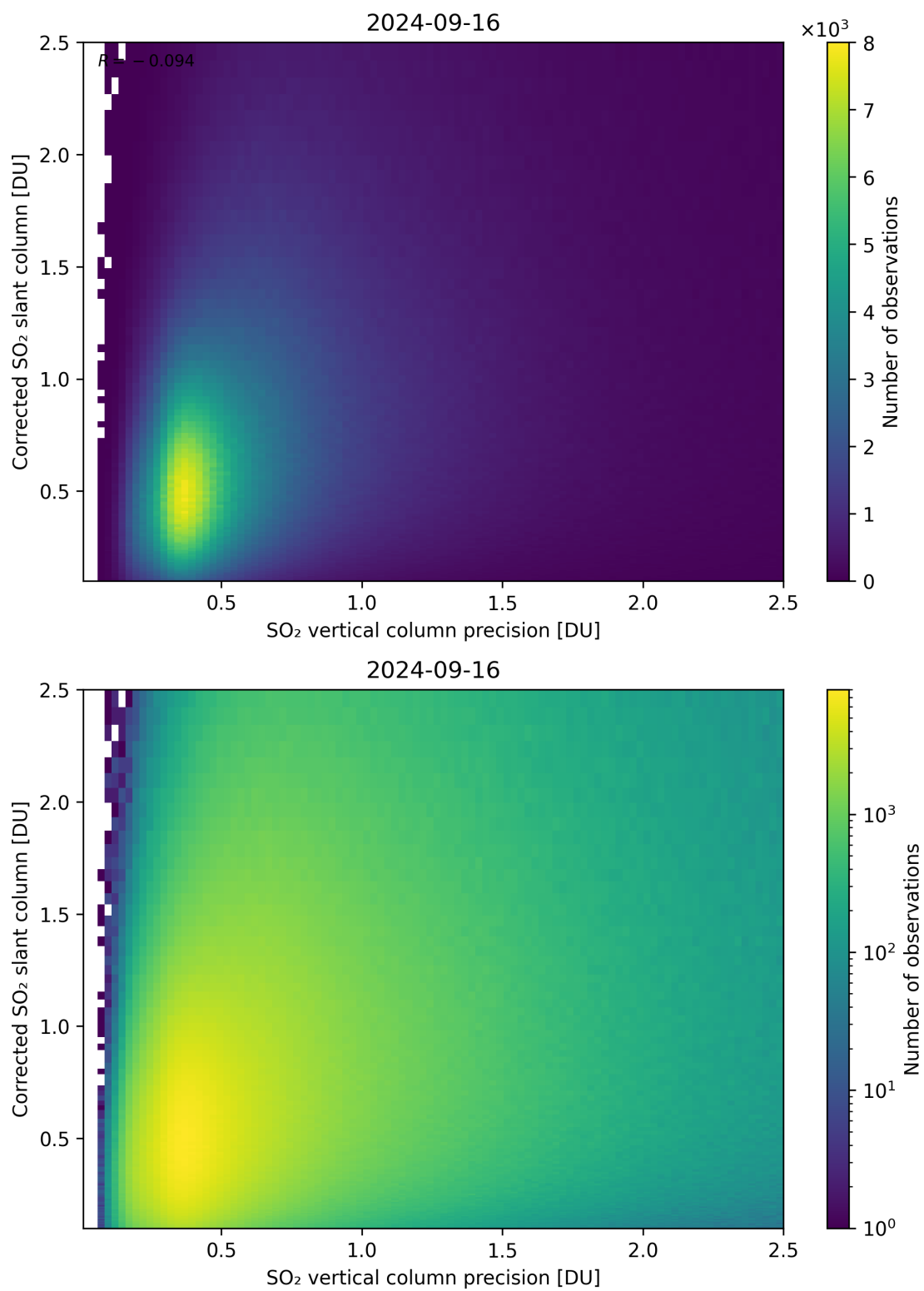
Figure 286: Scatter density plot of “SO 2 vertical column precision” against “Corrected SO 2 slant column” for 2024-09-15 to 2024-09-17.
