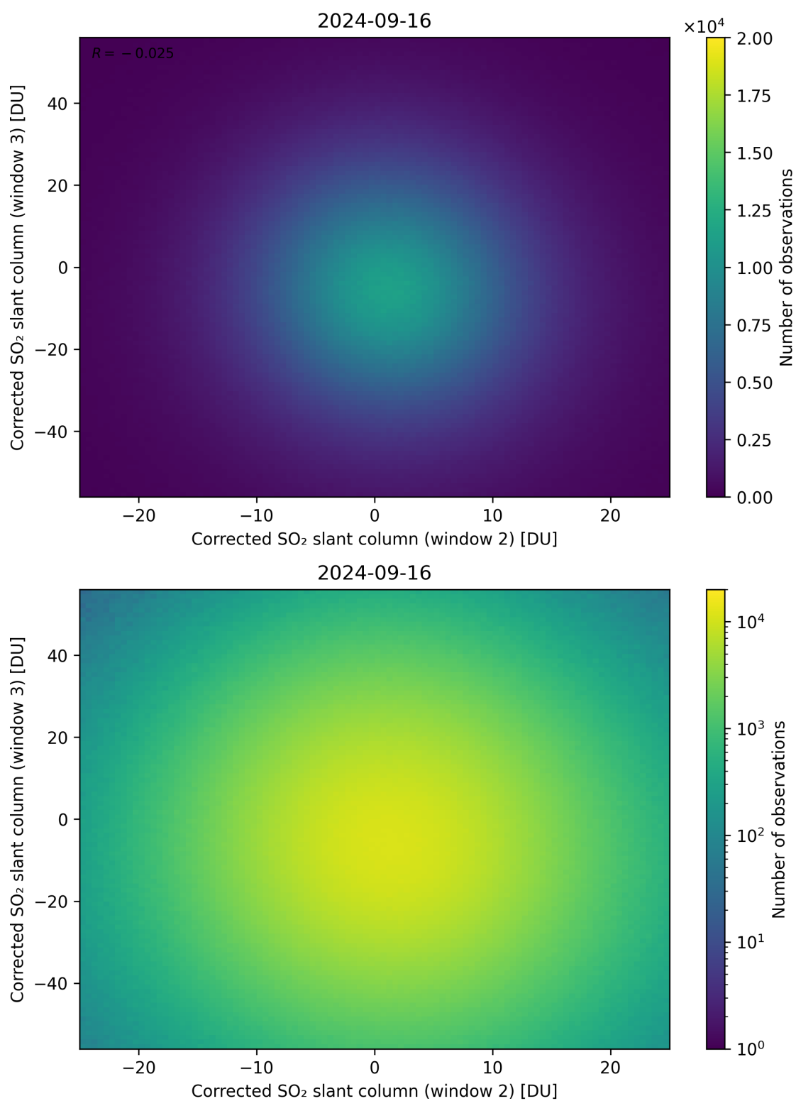
Figure 200: Scatter density plot of “Corrected SO 2 slant column (window 2)” against “Corrected SO 2 slant column (window 3)” for 2024-09-15 to 2024-09-17.
