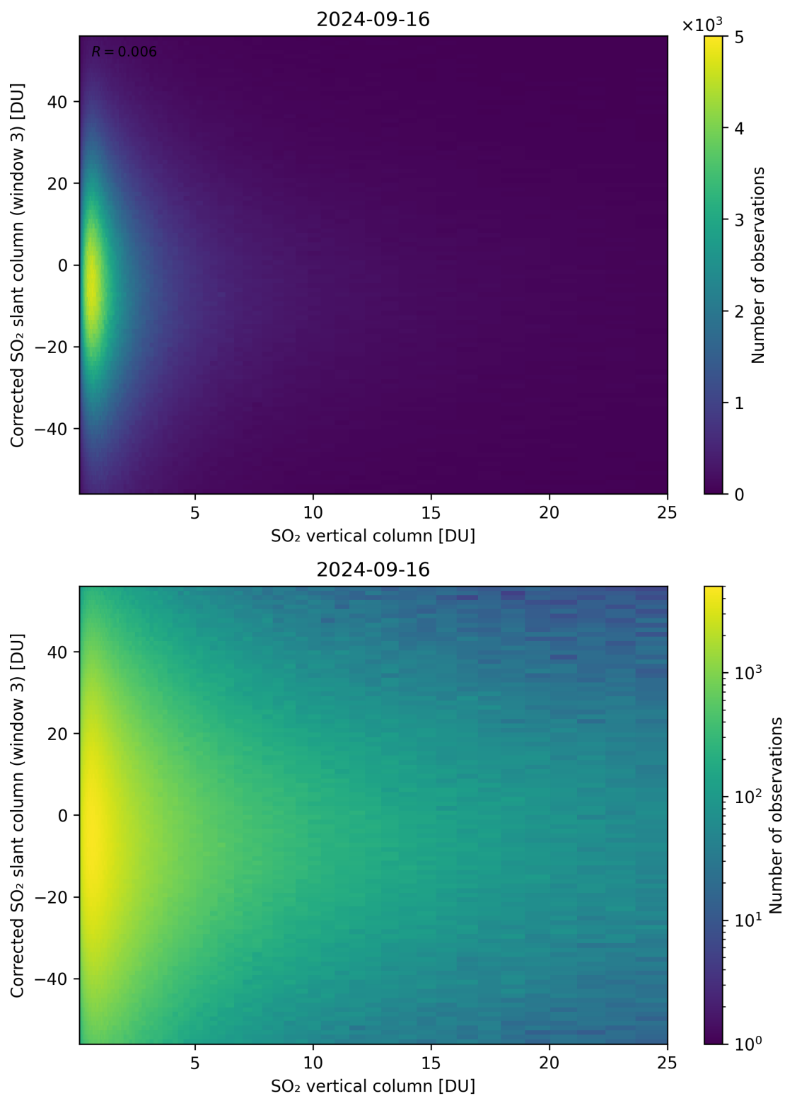
Figure 299: Scatter density plot of “SO 2 vertical column” against “Corrected SO 2 slant column (window 3)” for 2024-09-15 to 2024-09-17.
