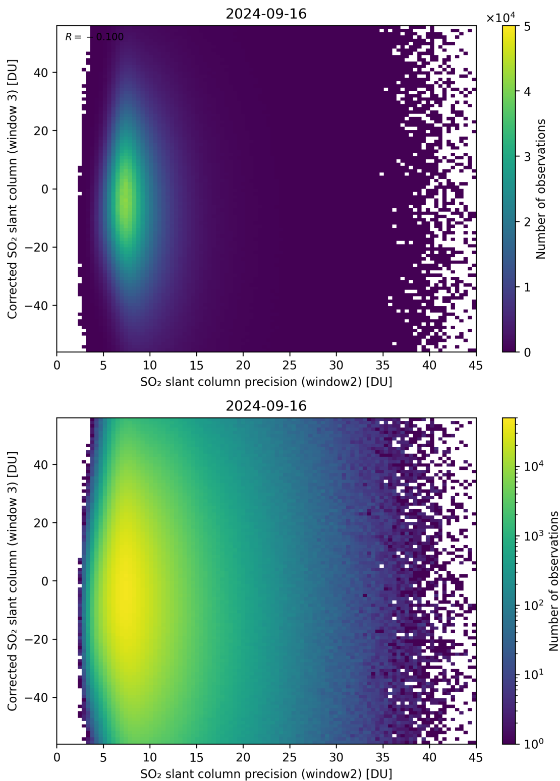
Figure 248: Scatter density plot of “SO 2 slant column precision (window2)” against “Corrected SO 2 slant column (window 3)” for 2024-09-15 to 2024-09-17.
