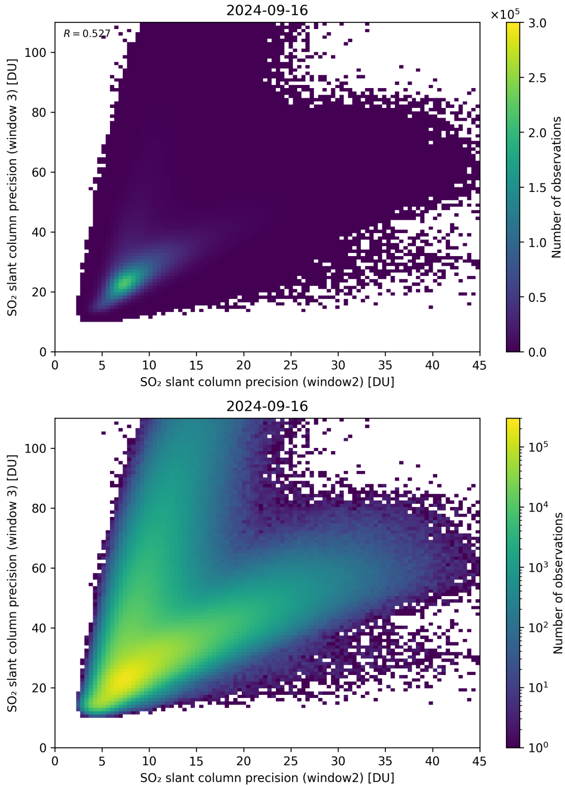
Figure 250: Scatter density plot of “SO 2 slant column precision (window2)” against “SO 2 slant column precision (window 3)” for 2024-09-15 to 2024-09-17.
