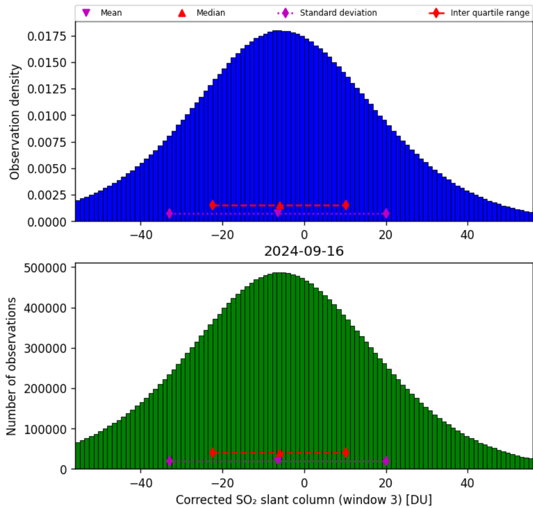
Figure 66: Histogram of “Corrected SO 2 slant column (window 3)” for 2024-09-15 to 2024-09-17
