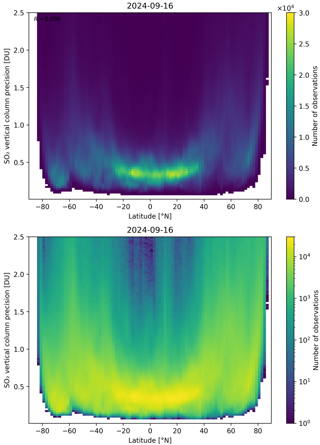
Figure 157: Scatter density plot of “Latitude” against “SO 2 vertical column precision” for 2024-09-15 to 2024-09-17.
