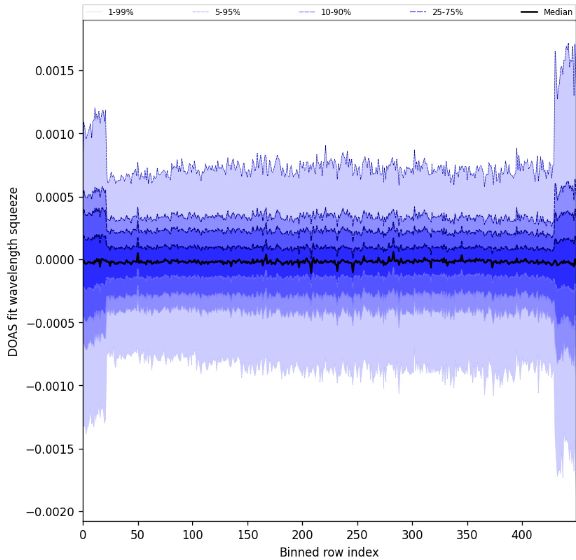
Figure 92: Along track statistics of “DOAS fit wavelength squeeze” for 2024-09-15 to 2024-09-17
