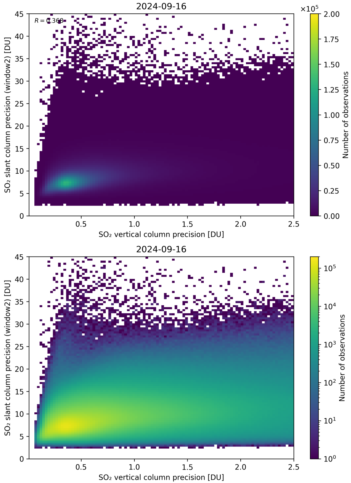
Figure 291: Scatter density plot of “SO 2 vertical column precision” against “SO 2 slant column precision (window2)” for 2024-09-15 to 2024-09-17.
