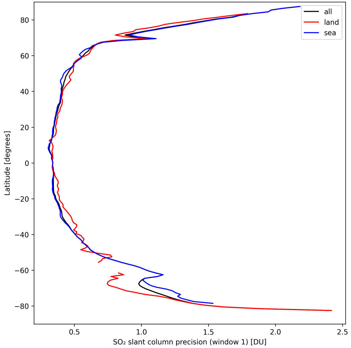
Figure 34: Zonal average of “SO 2 slant column precision (window 1)” for 2024-09-15 to 2024-09-17.
