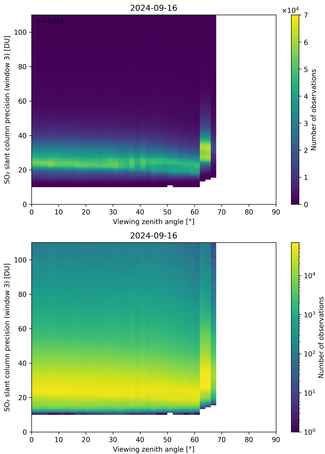
Figure 324: Scatter density plot of “Viewing zenith angle” against “SO 2 slant column precision (window 3)” for 2024-09-15 to 2024-09-17.
