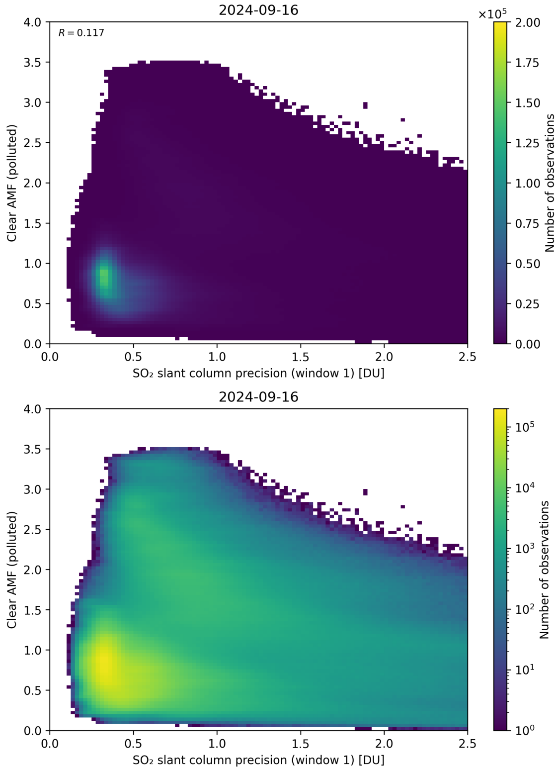
Figure 224: Scatter density plot of “SO 2 slant column precision (window 1)” against “Clear AMF (polluted)” for 2024-09-15 to 2024-09-17.
