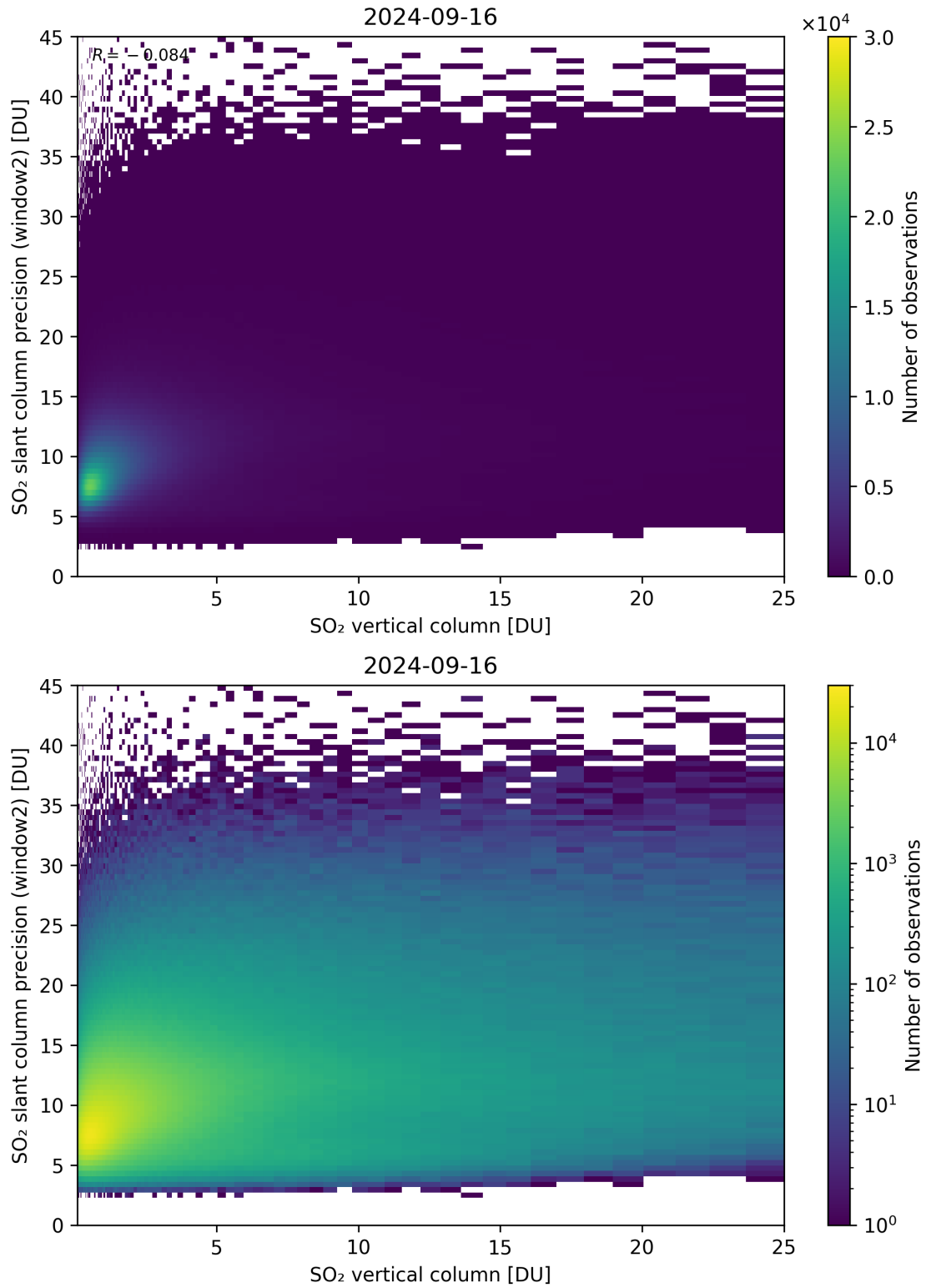
Figure 302: Scatter density plot of “SO 2 vertical column” against “SO 2 slant column precision (window2)” for 2024-09-15 to 2024-09-17.
