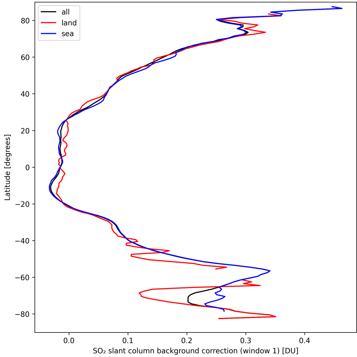
Figure 36: Zonal average of “SO 2 slant column background correction (window 1)” for 2024-09-15 to 2024-09-17.
