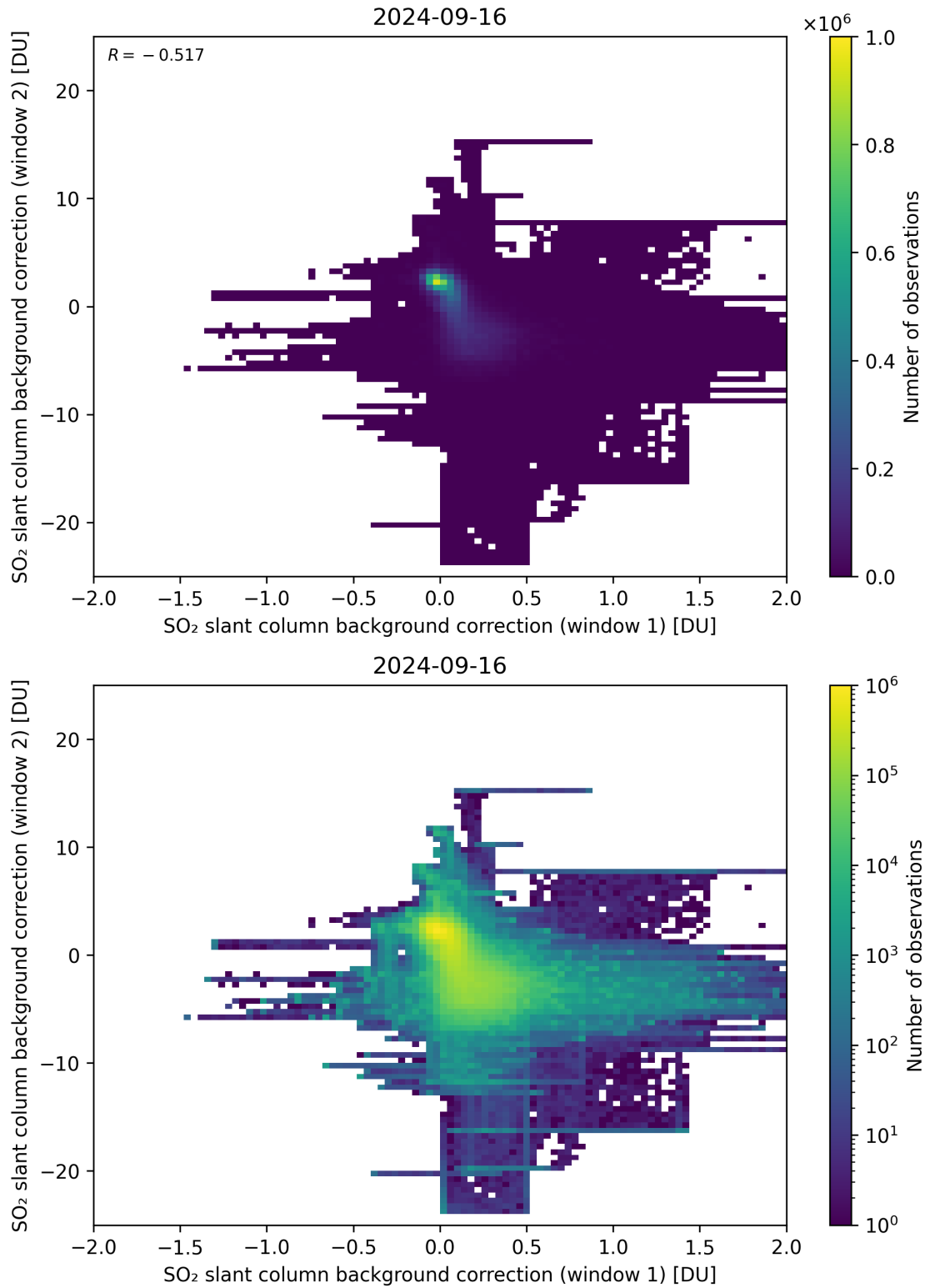
Figure 98: Scatter density plot of “SO 2 slant column background correction (window 1)” against “SO 2 slant column background correction (window 2)” for 2024-09-15 to 2024-09-17.
