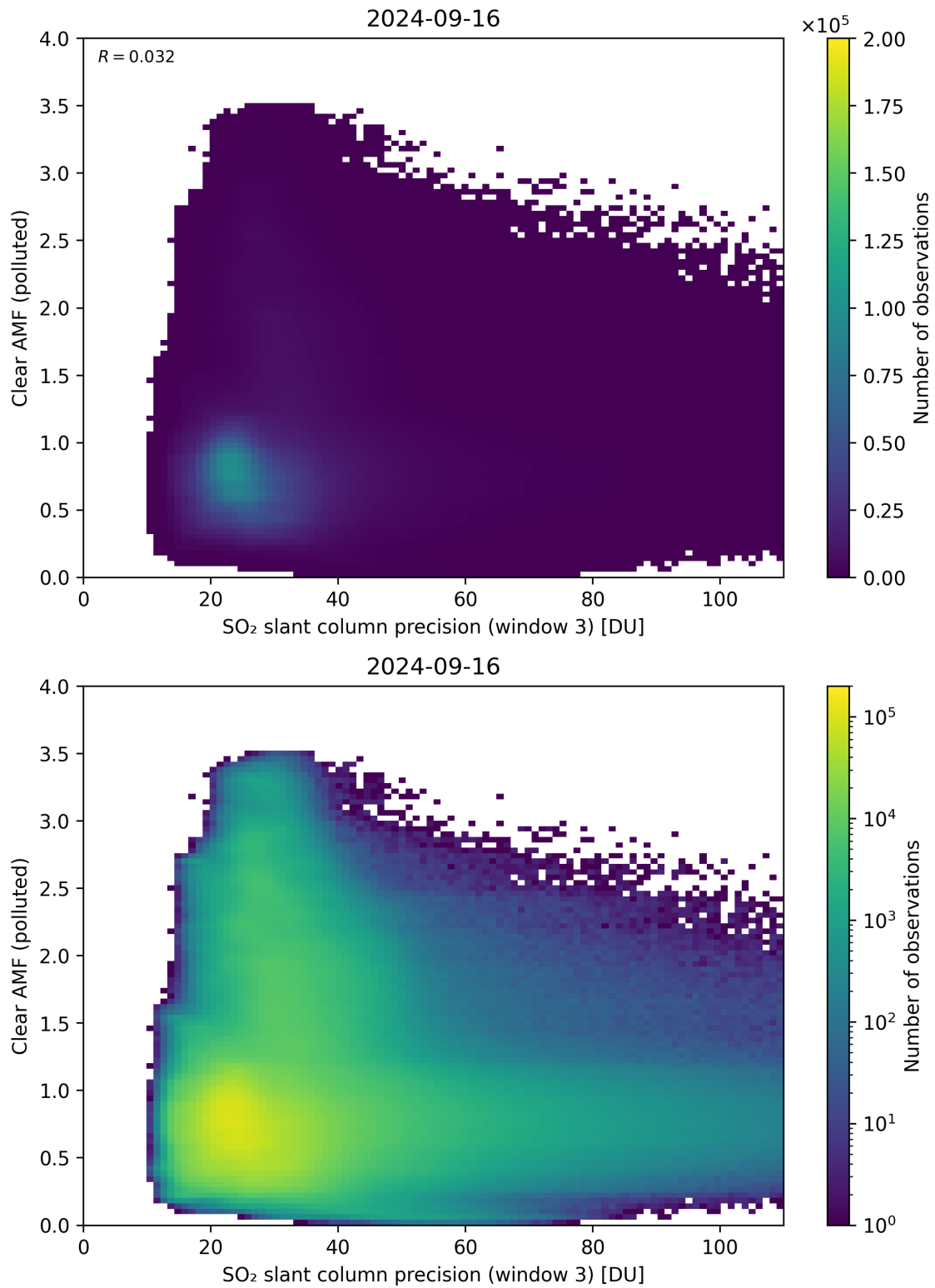
Figure 261: Scatter density plot of “SO 2 slant column precision (window 3)” against “Clear AMF (polluted)” for 2024-09-15 to 2024-09-17.
