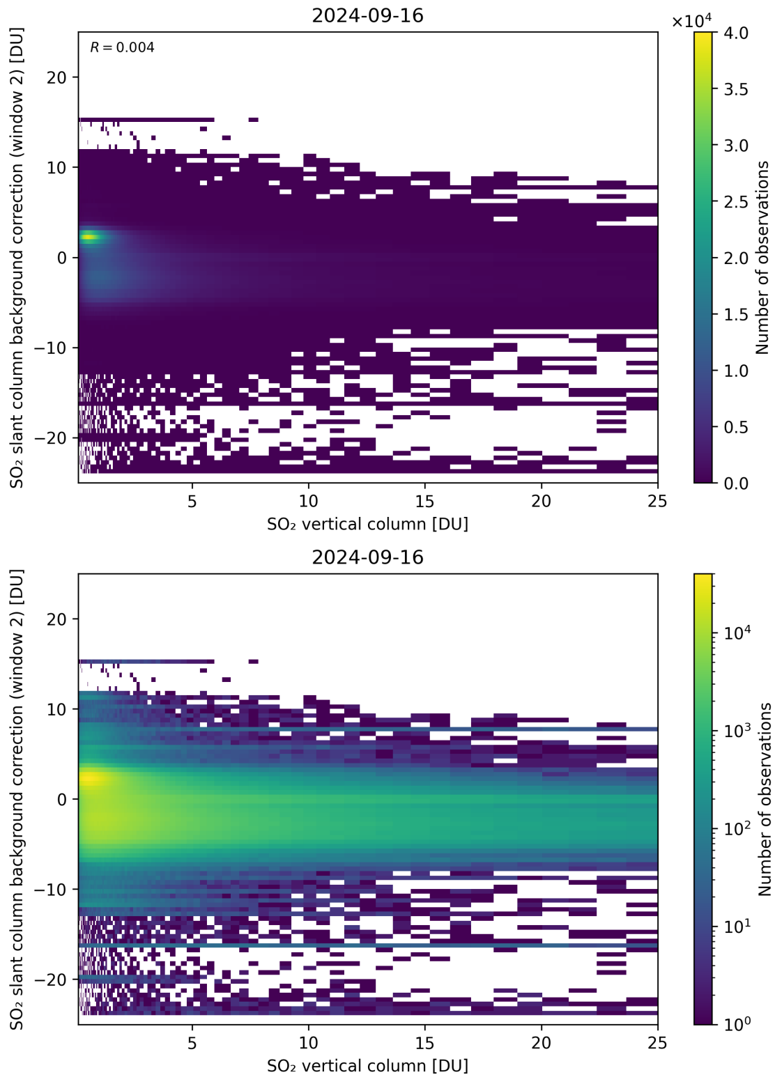
Figure 274: Scatter density plot of “SO 2 vertical column” against “SO 2 slant column background correction (window 2)” for 2024-09-15 to 2024-09-17.
