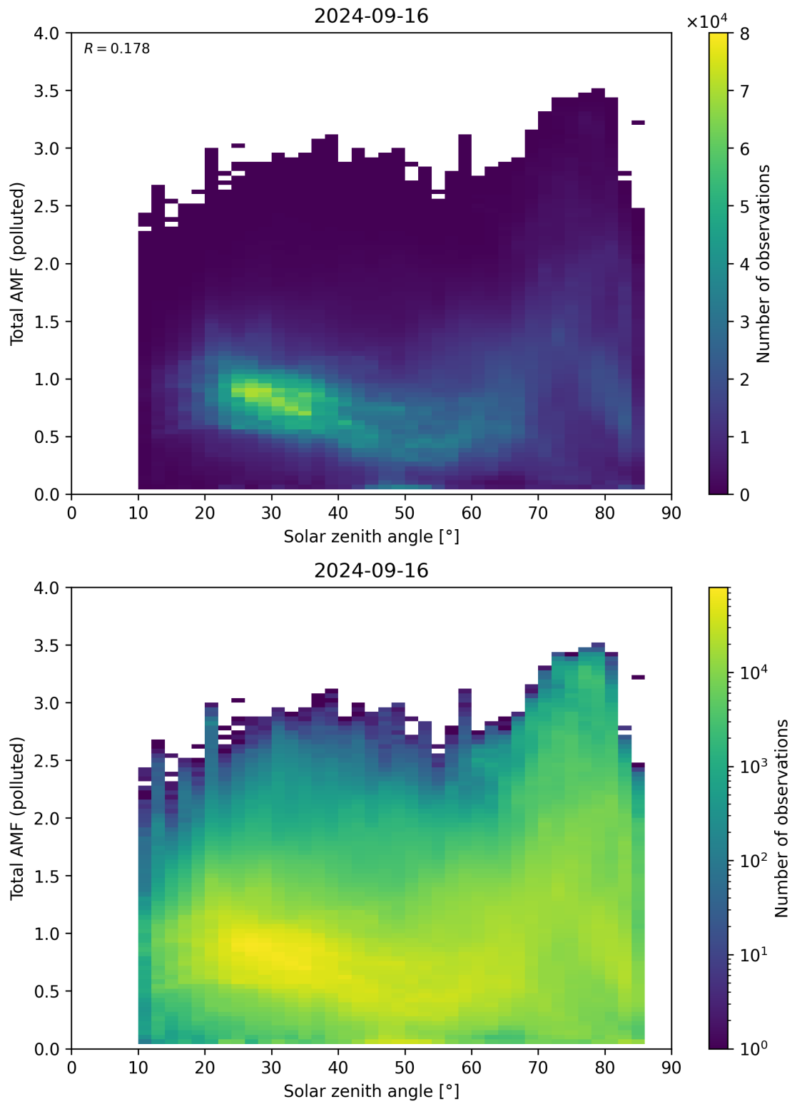
Figure 174: Scatter density plot of “Solar zenith angle” against “Total AMF (polluted)” for 2024-09-15 to 2024-09-17.
