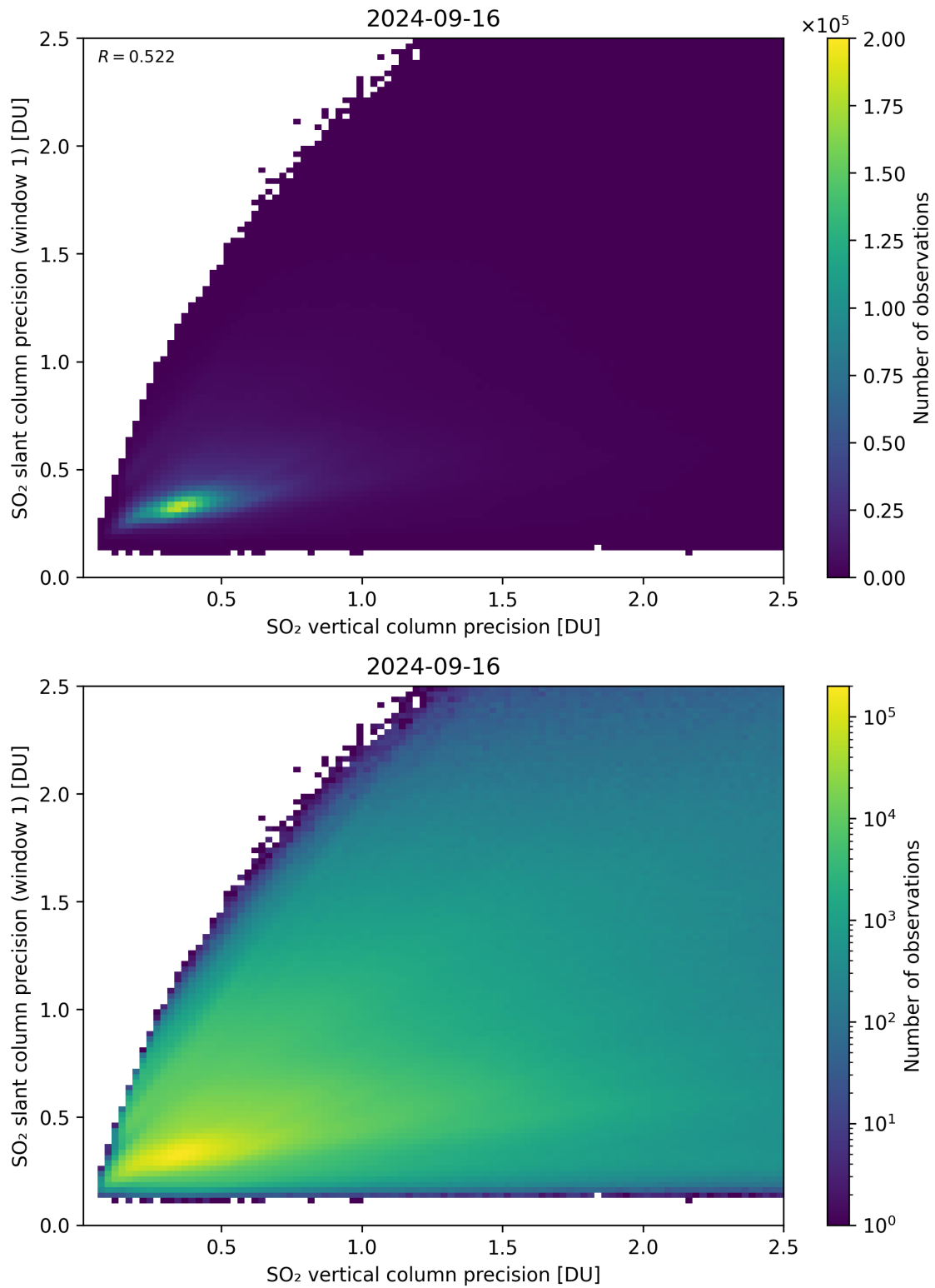
Figure 290: Scatter density plot of “SO 2 vertical column precision” against “SO 2 slant column precision (window 1)” for 2024-09-15 to 2024-09-17.
