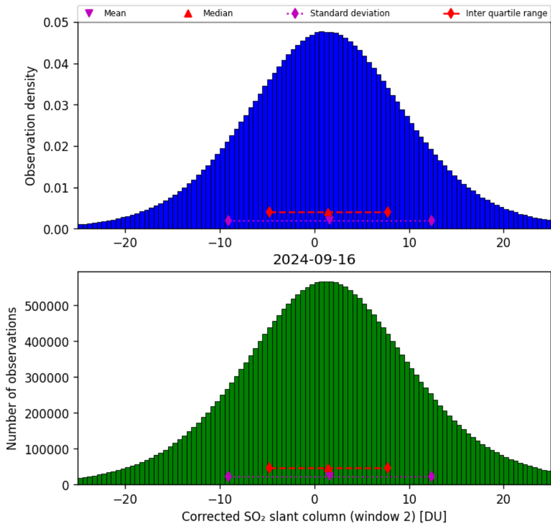
Figure 62: Histogram of “Corrected SO 2 slant column (window 2)” for 2024-09-15 to 2024-09-17
