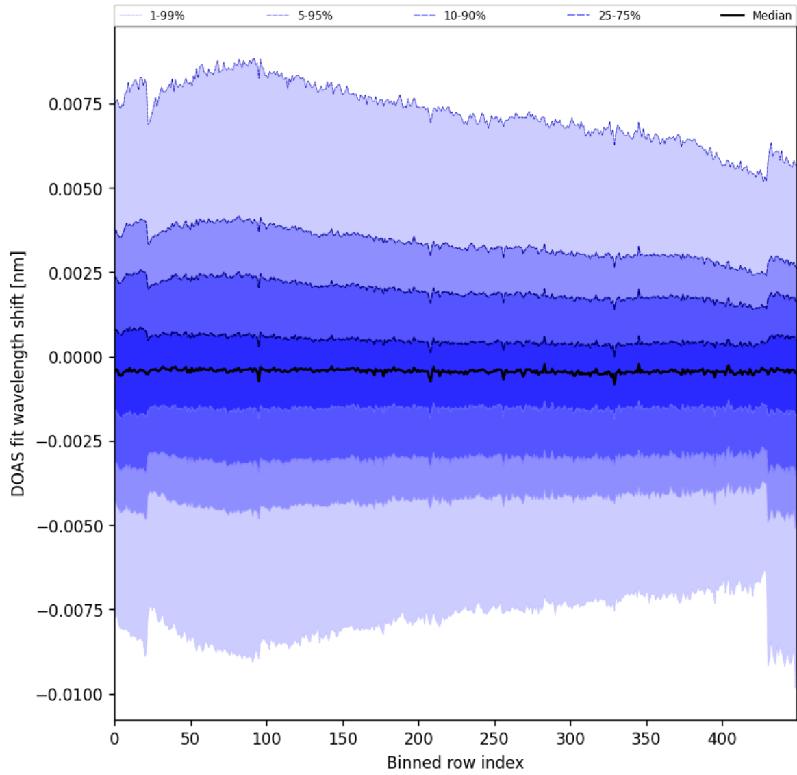
Figure 91: Along track statistics of “DOAS fit wavelength shift” for 2024-09-15 to 2024-09-17
