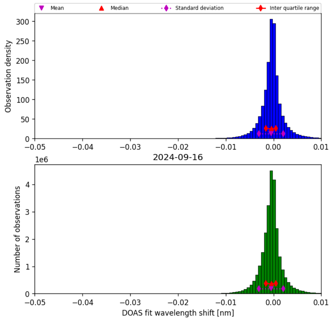
Figure 68: Histogram of “DOAS fit wavelength shift” for 2024-09-15 to 2024-09-17
