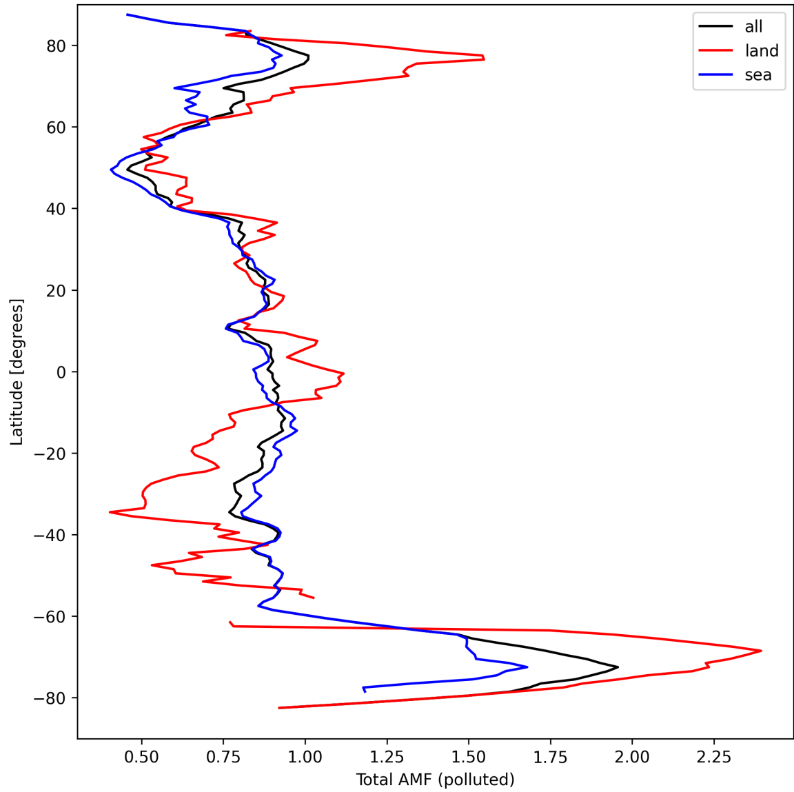
Figure 48: Zonal average of “Total AMF (polluted)” for 2024-09-15 to 2024-09-17.
