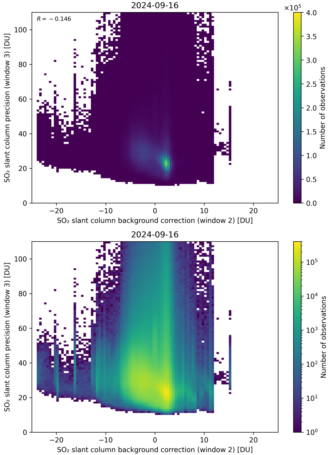
Figure 118: Scatter density plot of “SO 2 slant column background correction (window 2)” against “SO 2 slant column precision (window 3)” for 2024-09-15 to 2024-09-17.
