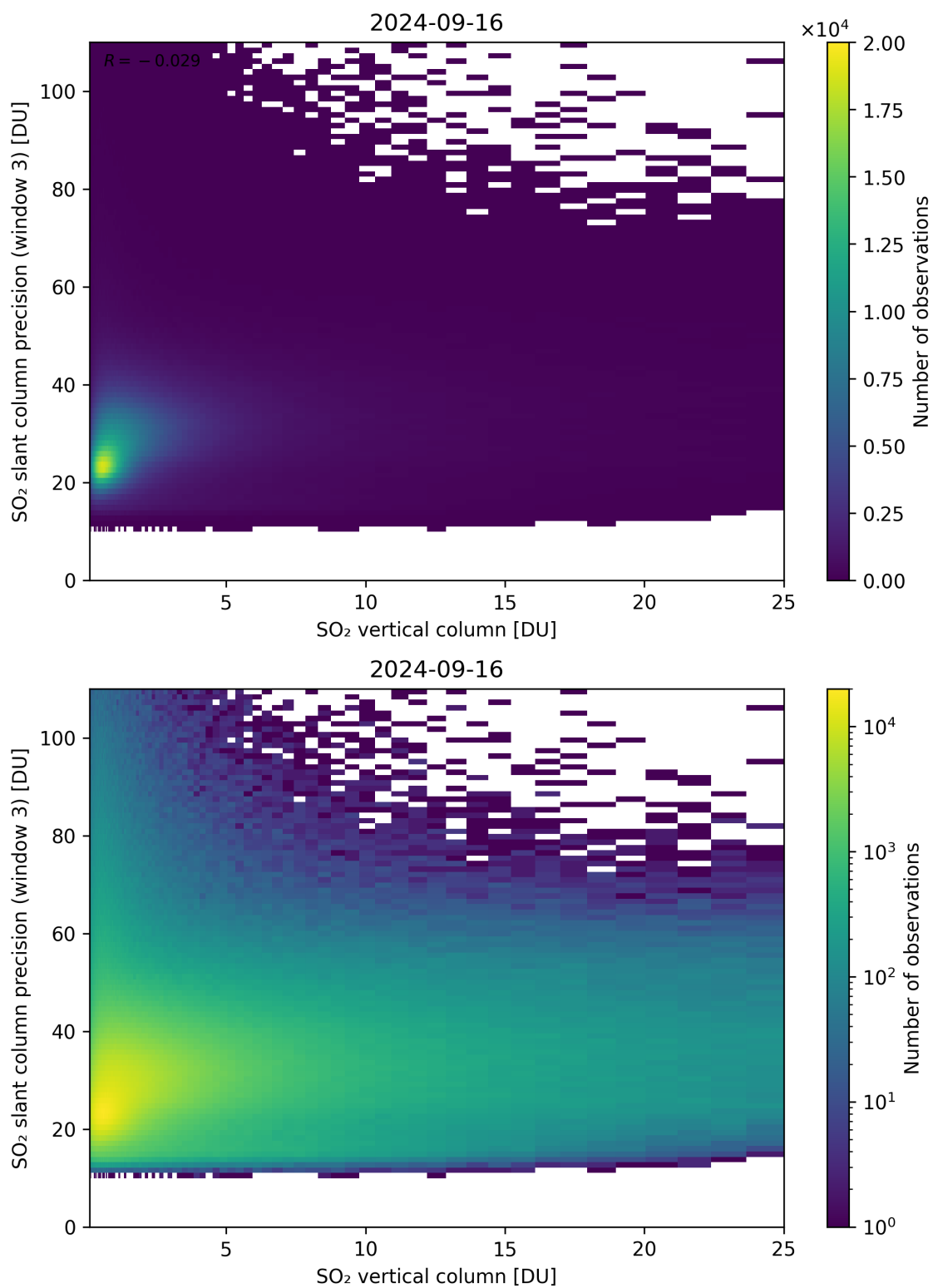
Figure 304: Scatter density plot of “SO 2 vertical column” against “SO 2 slant column precision (window 3)” for 2024-09-15 to 2024-09-17.
