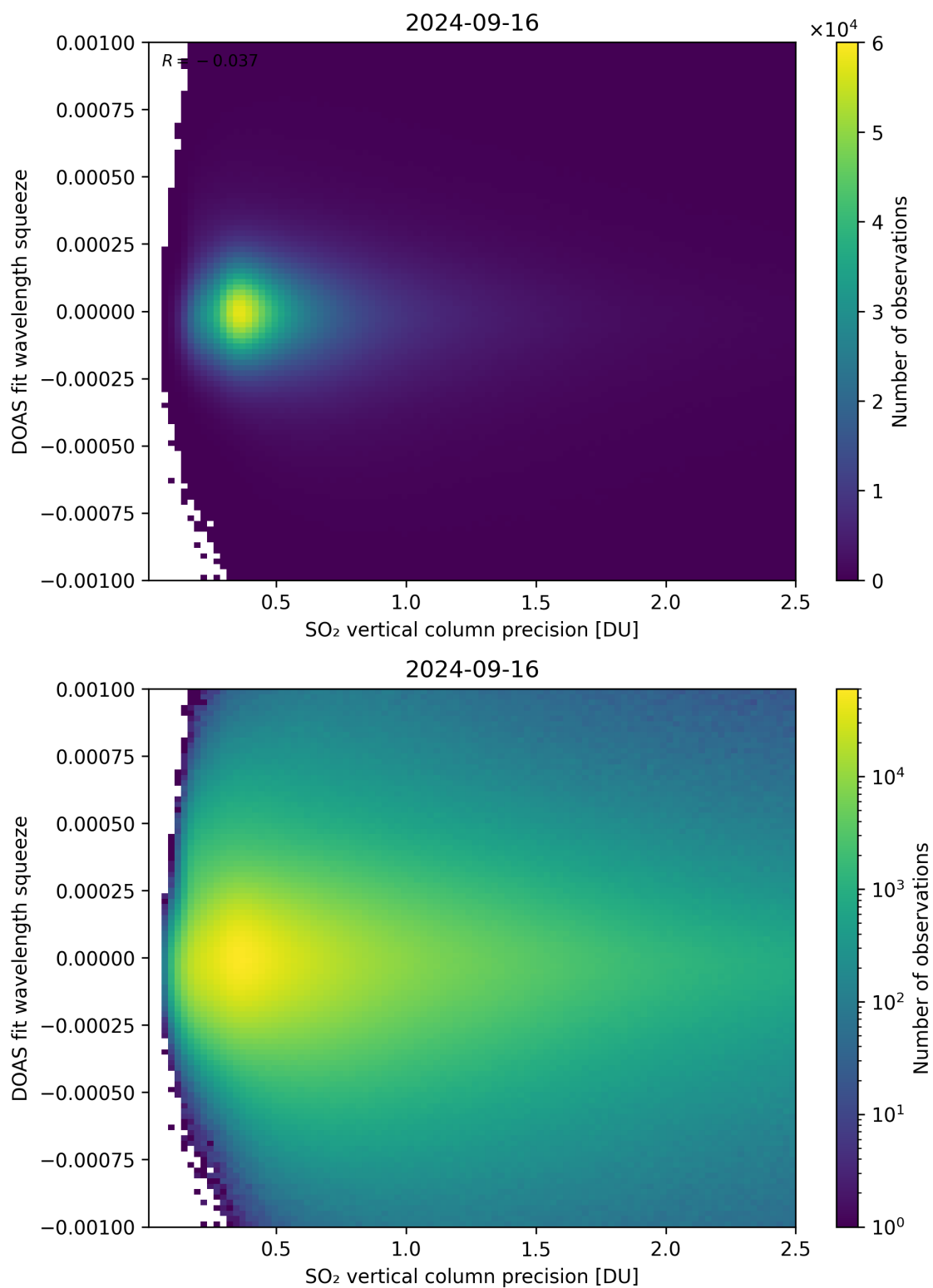
Figure 283: Scatter density plot of “SO 2 vertical column precision” against “DOAS fit wavelength squeeze” for 2024-09-15 to 2024-09-17.
