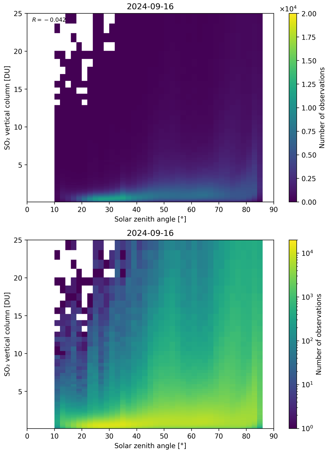
Figure 176: Scatter density plot of “Solar zenith angle” against “SO 2 vertical column” for 2024-09-15 to 2024-09-17.
