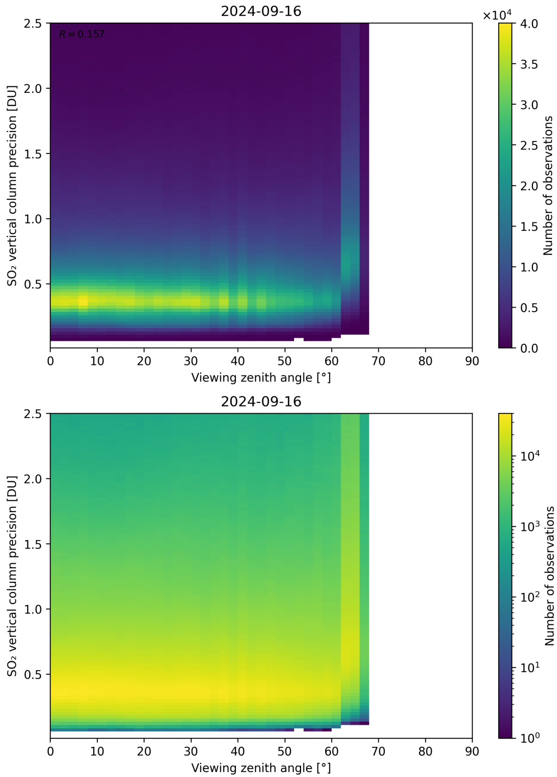
Figure 328: Scatter density plot of “Viewing zenith angle” against “SO 2 vertical column precision” for 2024-09-15 to 2024-09-17.
