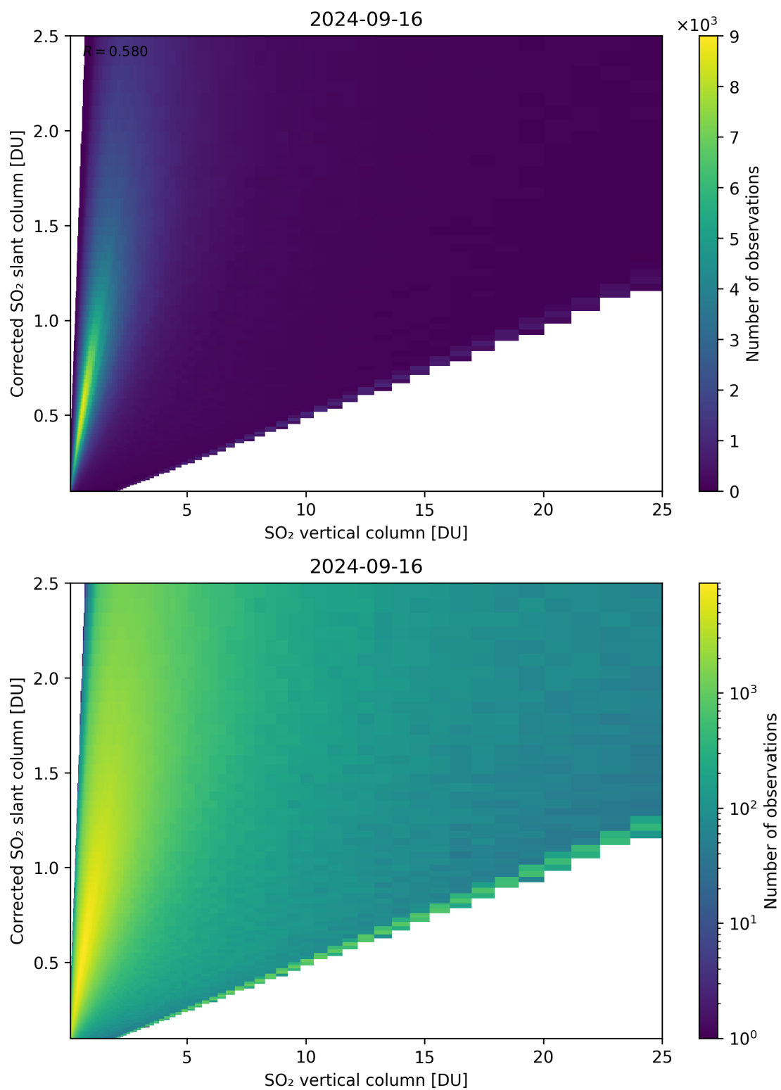
Figure 297: Scatter density plot of “SO 2 vertical column” against “Corrected SO 2 slant column” for 2024-09-15 to 2024-09-17.
