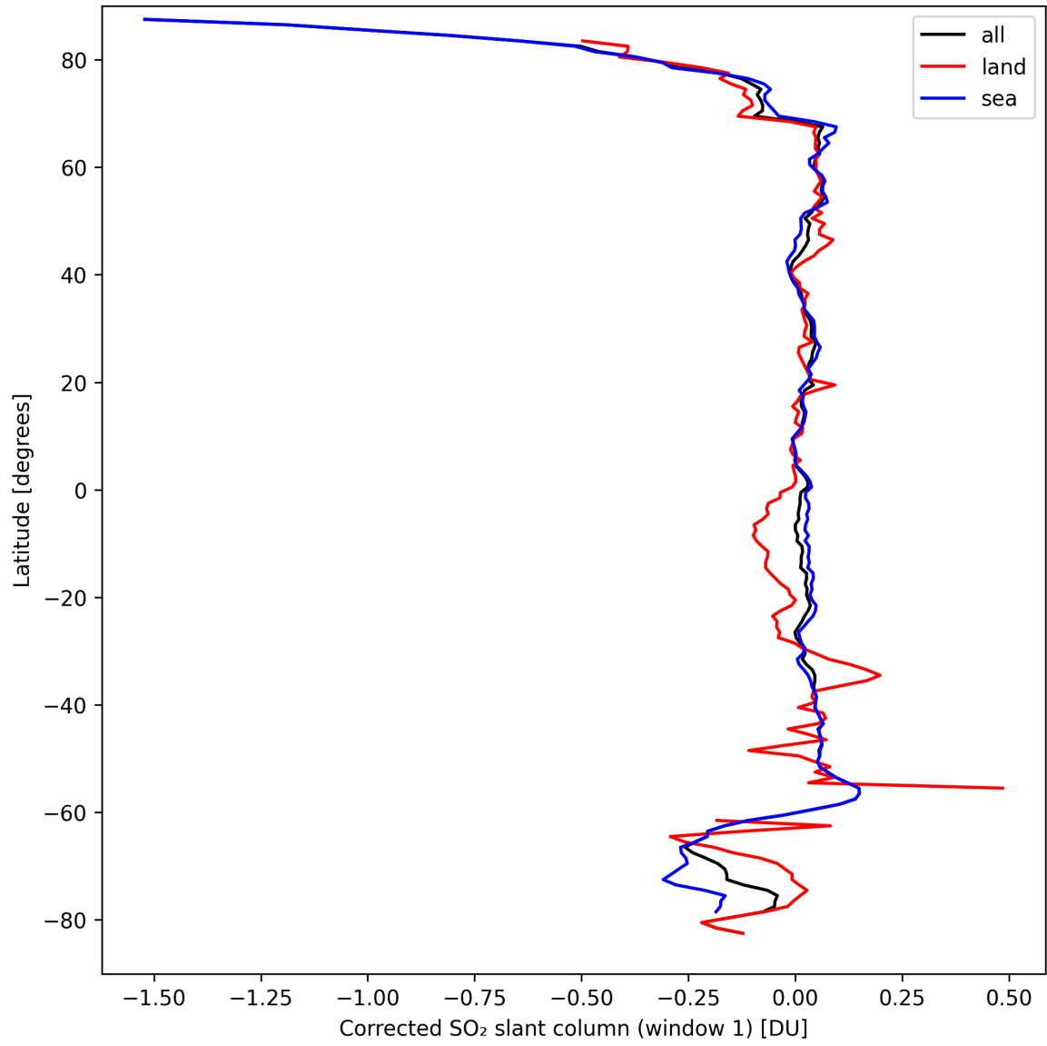
Figure 35: Zonal average of “Corrected SO 2 slant column (window 1)” for 2024-09-15 to 2024-09-17.
