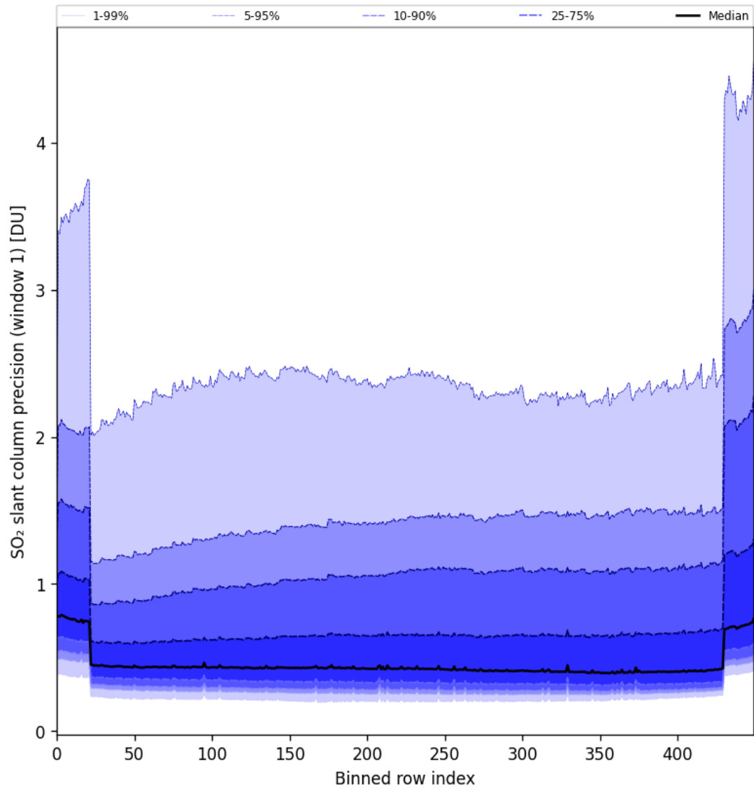
Figure 80: Along track statistics of “SO 2 slant column precision (window 1)” for 2024-09-15 to 2024-09-17
