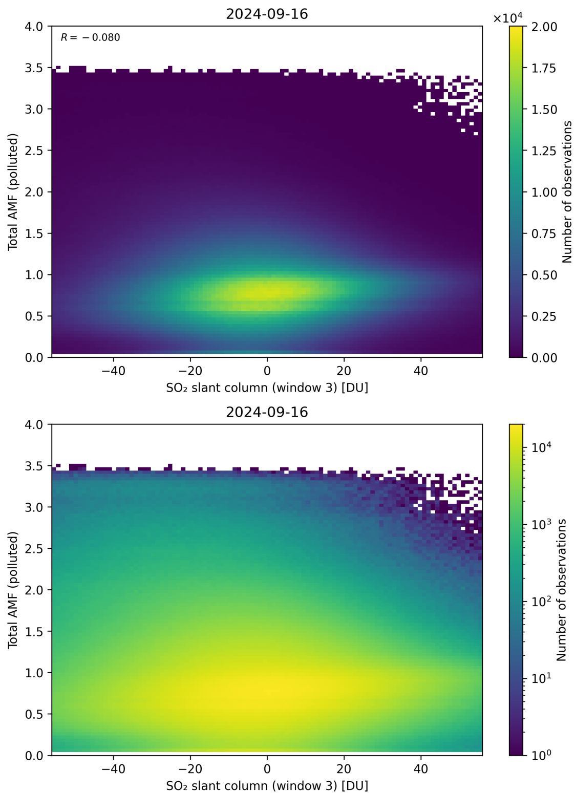
Figure 268: Scatter density plot of “SO 2 slant column (window 3)” against “Total AMF (polluted)” for 2024-09-15 to 2024-09-17.
