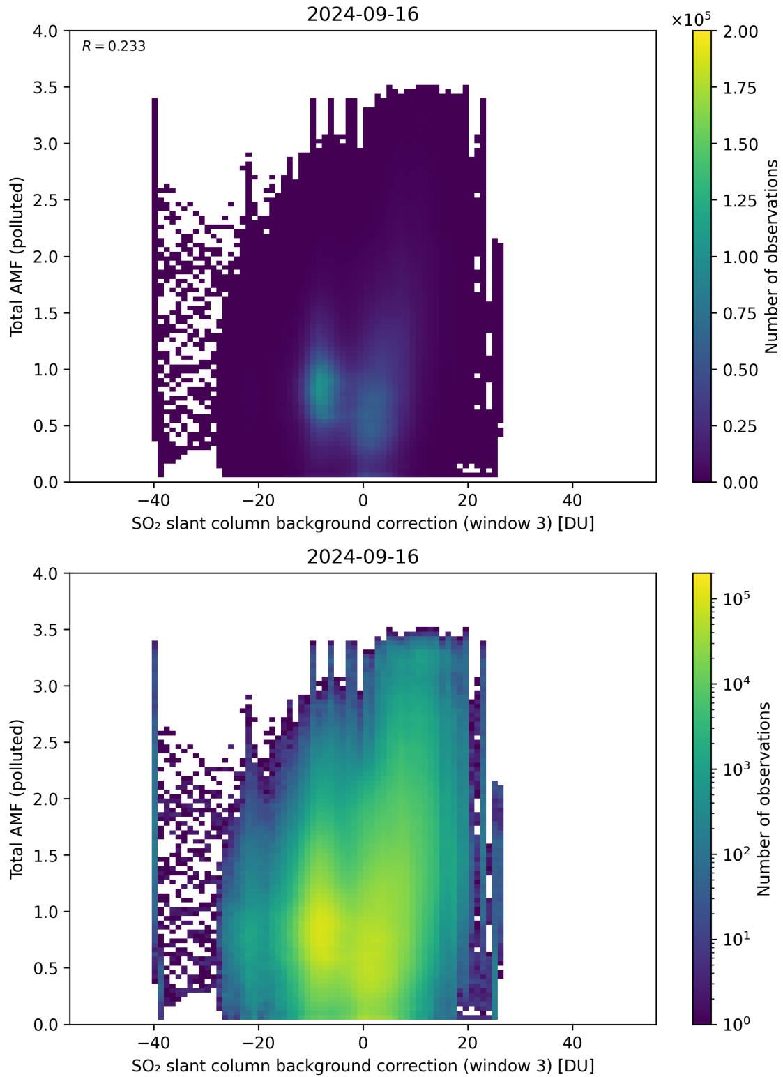
Figure 125: Scatter density plot of “SO 2 slant column background correction (window 3)” against “Total AMF (polluted)” for 2024-09-15 to 2024-09-17.
