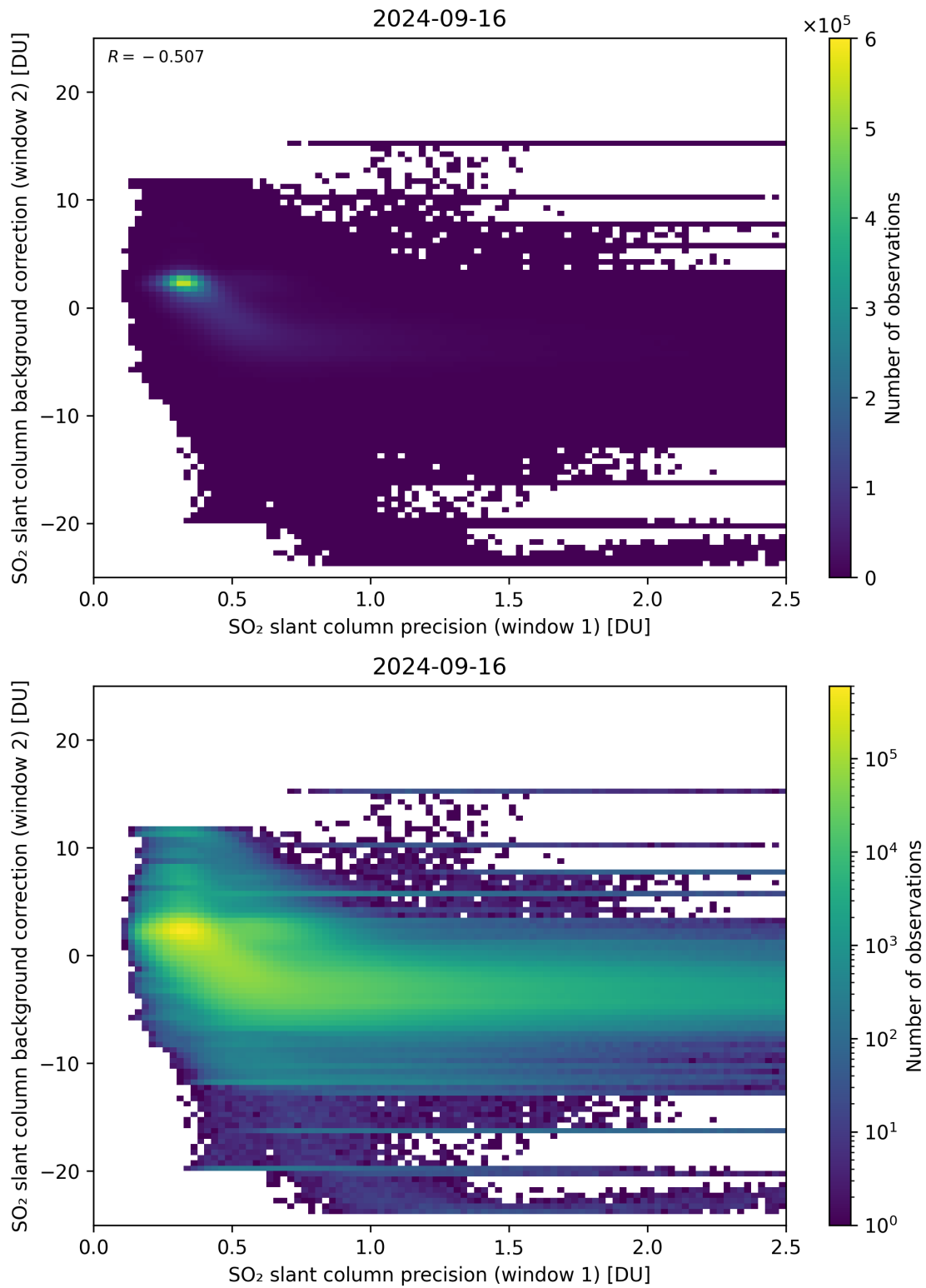
Figure 219: Scatter density plot of “SO 2 slant column precision (window 1)” against “SO 2 slant column background correction (window 2)” for 2024-09-15 to 2024-09-17.
