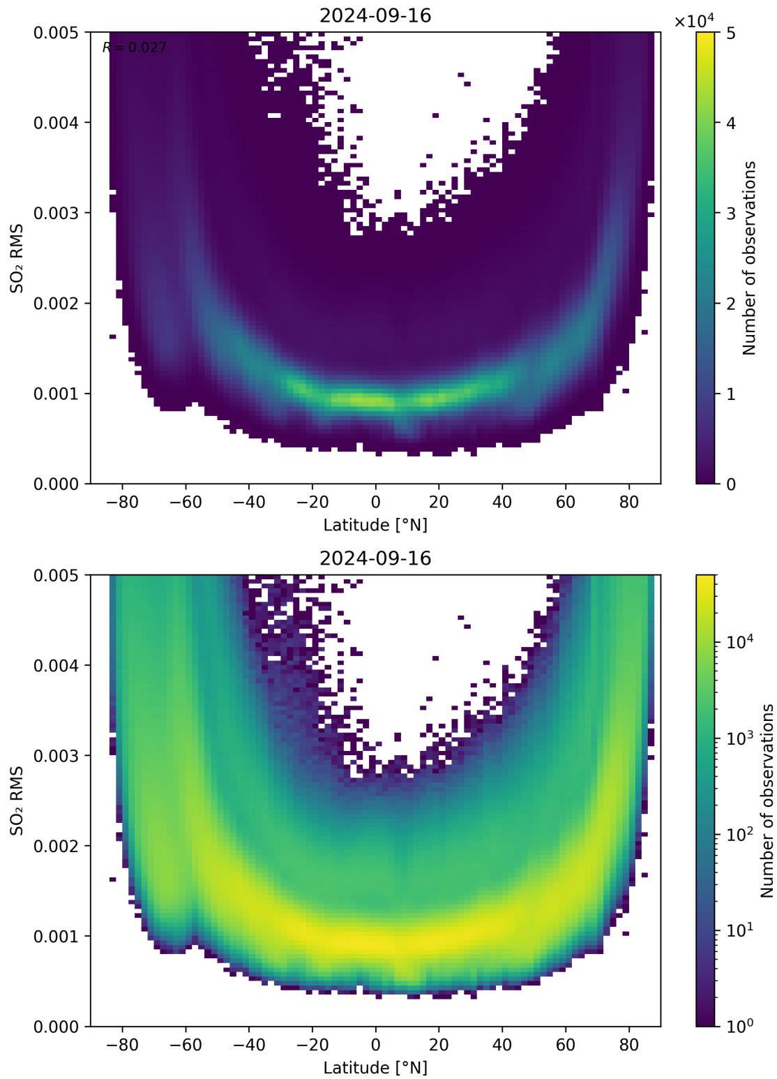
Figure 144: Scatter density plot of “Latitude” against “SO 2 RMS” for 2024-09-15 to 2024-09-17.
