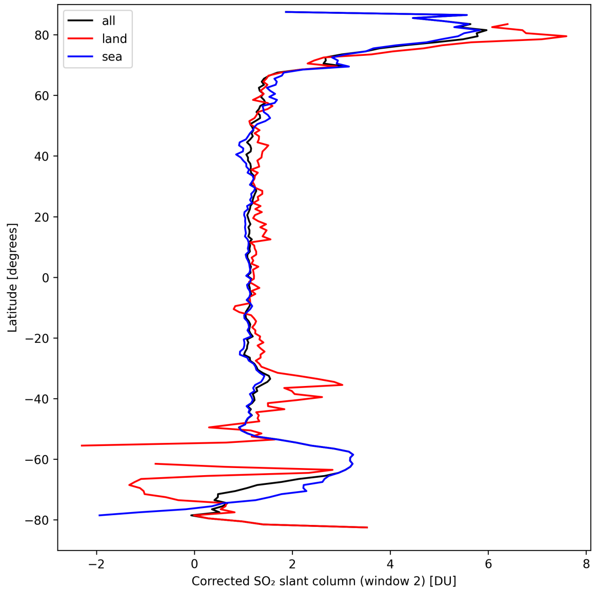
Figure 39: Zonal average of “Corrected SO 2 slant column (window 2)” for 2024-09-15 to 2024-09-17.
