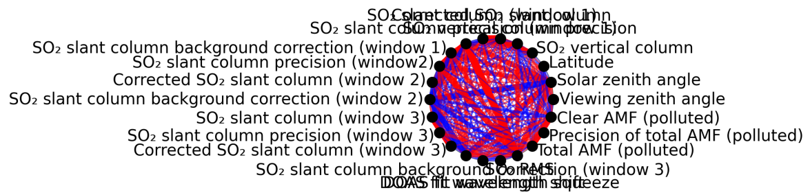
Figure 1: Map of correlation graph for 2024-09-15 to 2024-09-17.
