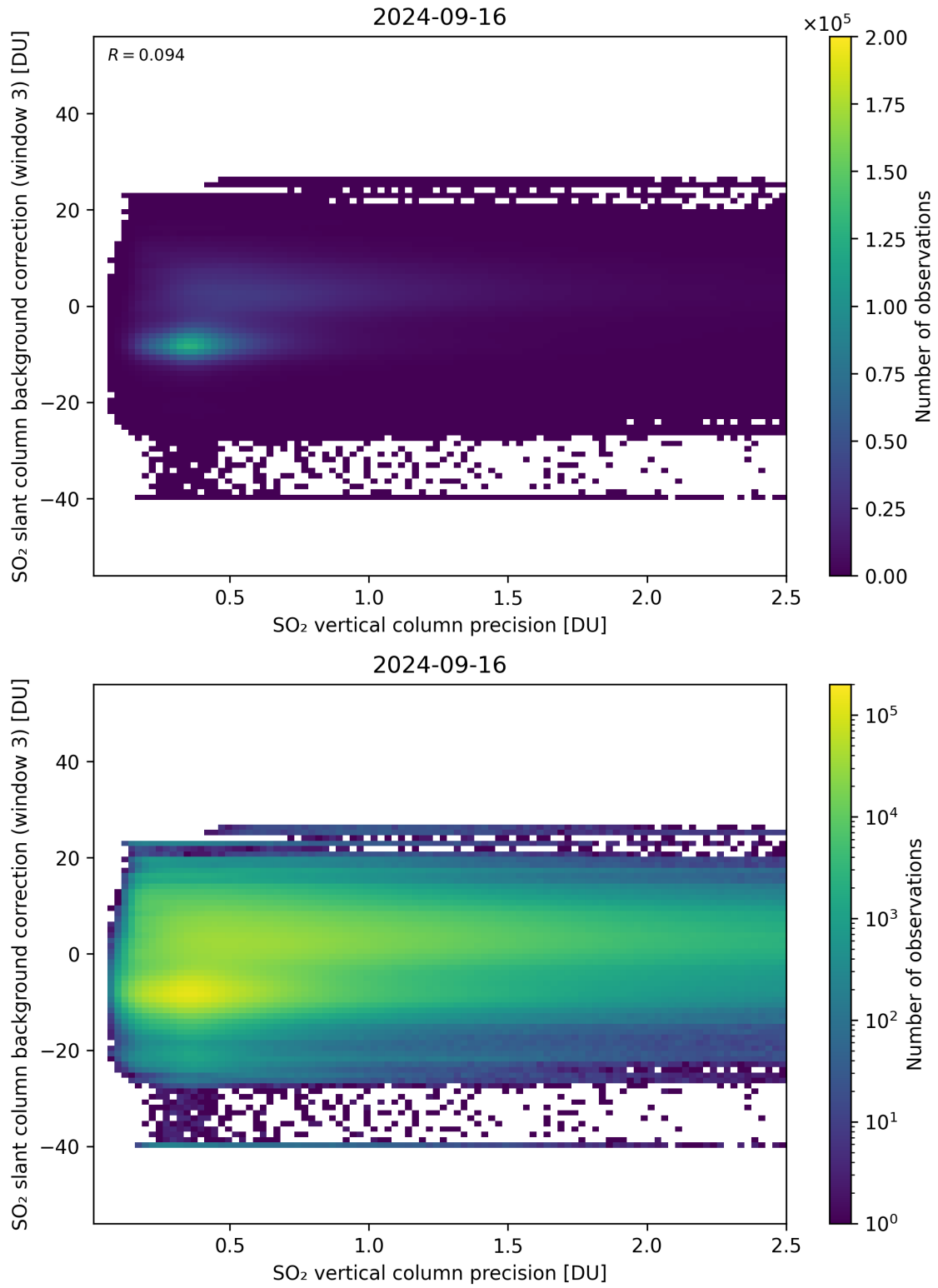
Figure 281: Scatter density plot of “SO 2 vertical column precision” against “SO 2 slant column background correction (window 3)” for 2024-09-15 to 2024-09-17.
