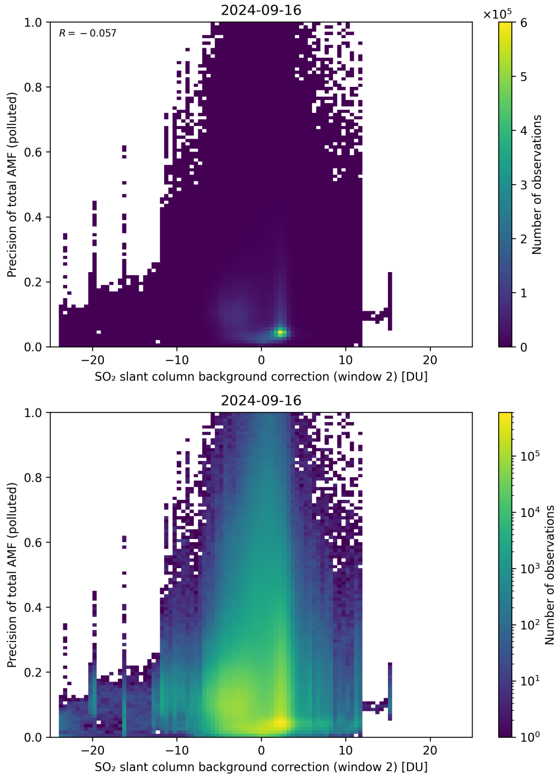
Figure 120: Scatter density plot of “SO 2 slant column background correction (window 2)” against “Precision of total AMF (polluted)” for 2024-09-15 to 2024-09-17.
