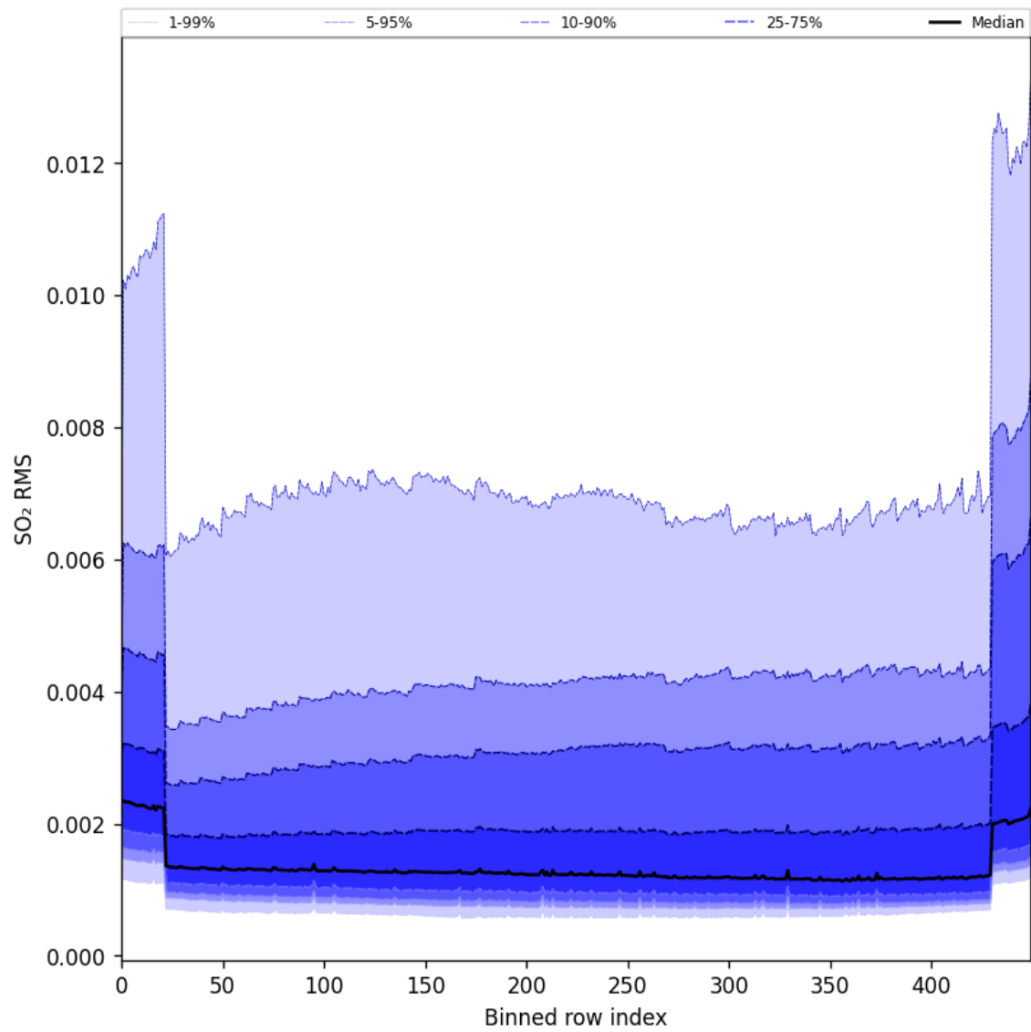
Figure 93: Along track statistics of “SO 2 RMS” for 2024-09-15 to 2024-09-17
