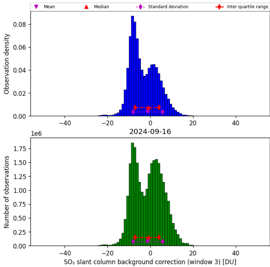
Figure 67: Histogram of “SO 2 slant column background correction (window 3)” for 2024-09-15 to 2024-09-17
