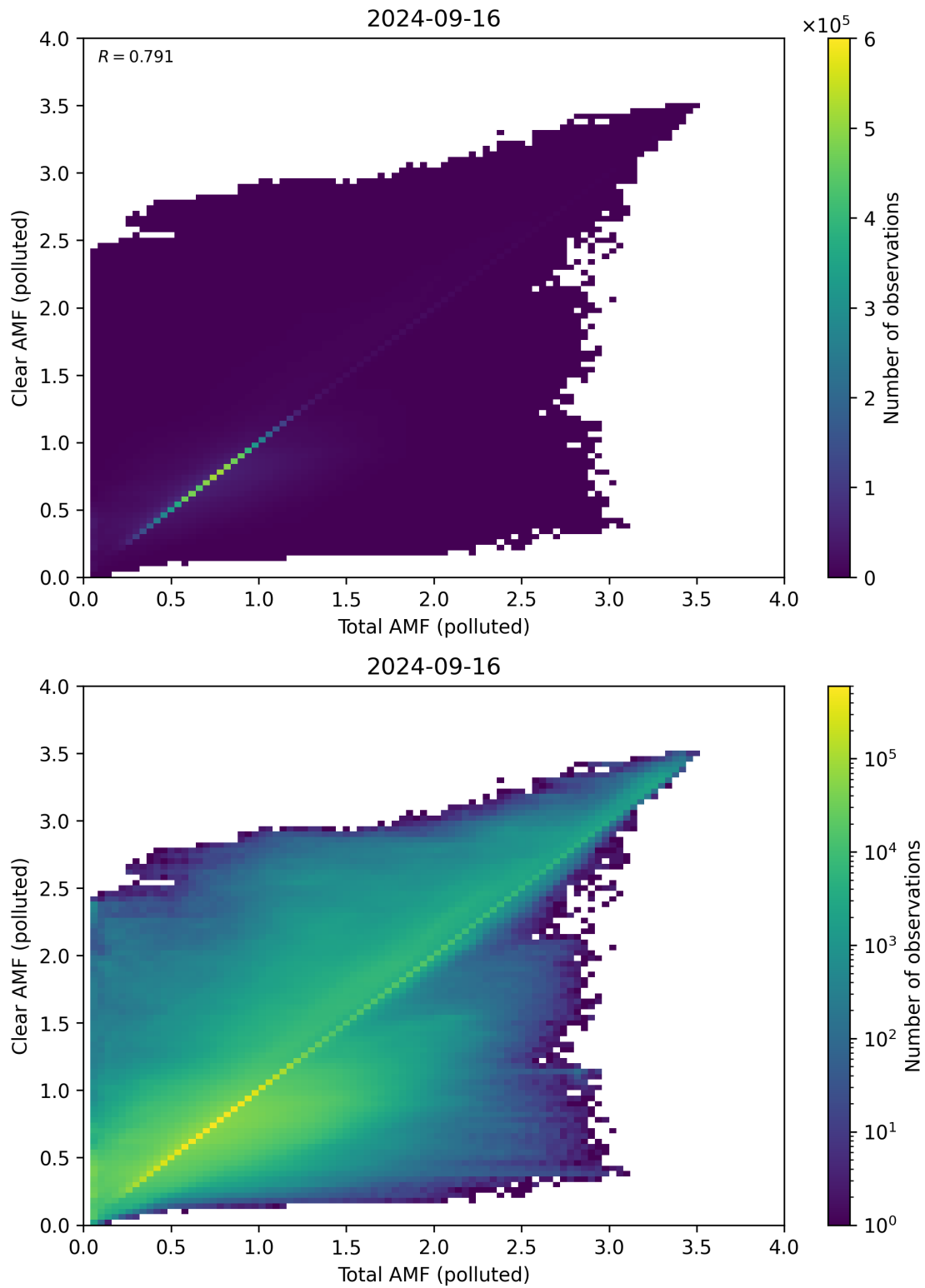
Figure 271: Scatter density plot of “Total AMF (polluted)” against “Clear AMF (polluted)” for 2024-09-15 to 2024-09-17.
