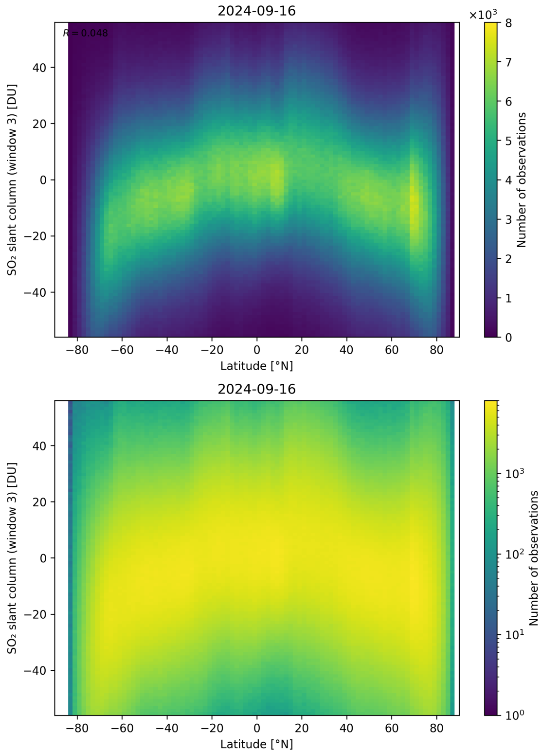
Figure 152: Scatter density plot of “Latitude” against “SO 2 slant column (window 3)” for 2024-09-15 to 2024-09-17.
