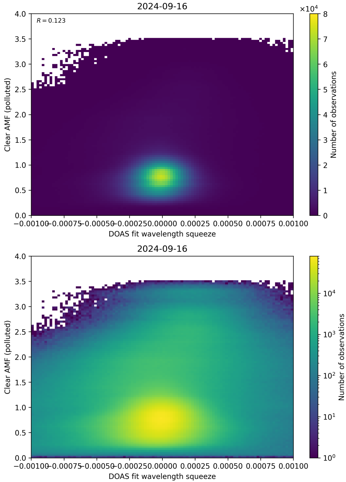
Figure 133: Scatter density plot of “DOAS fit wavelength squeeze” against “Clear AMF (polluted)” for 2024-09-15 to 2024-09-17.
