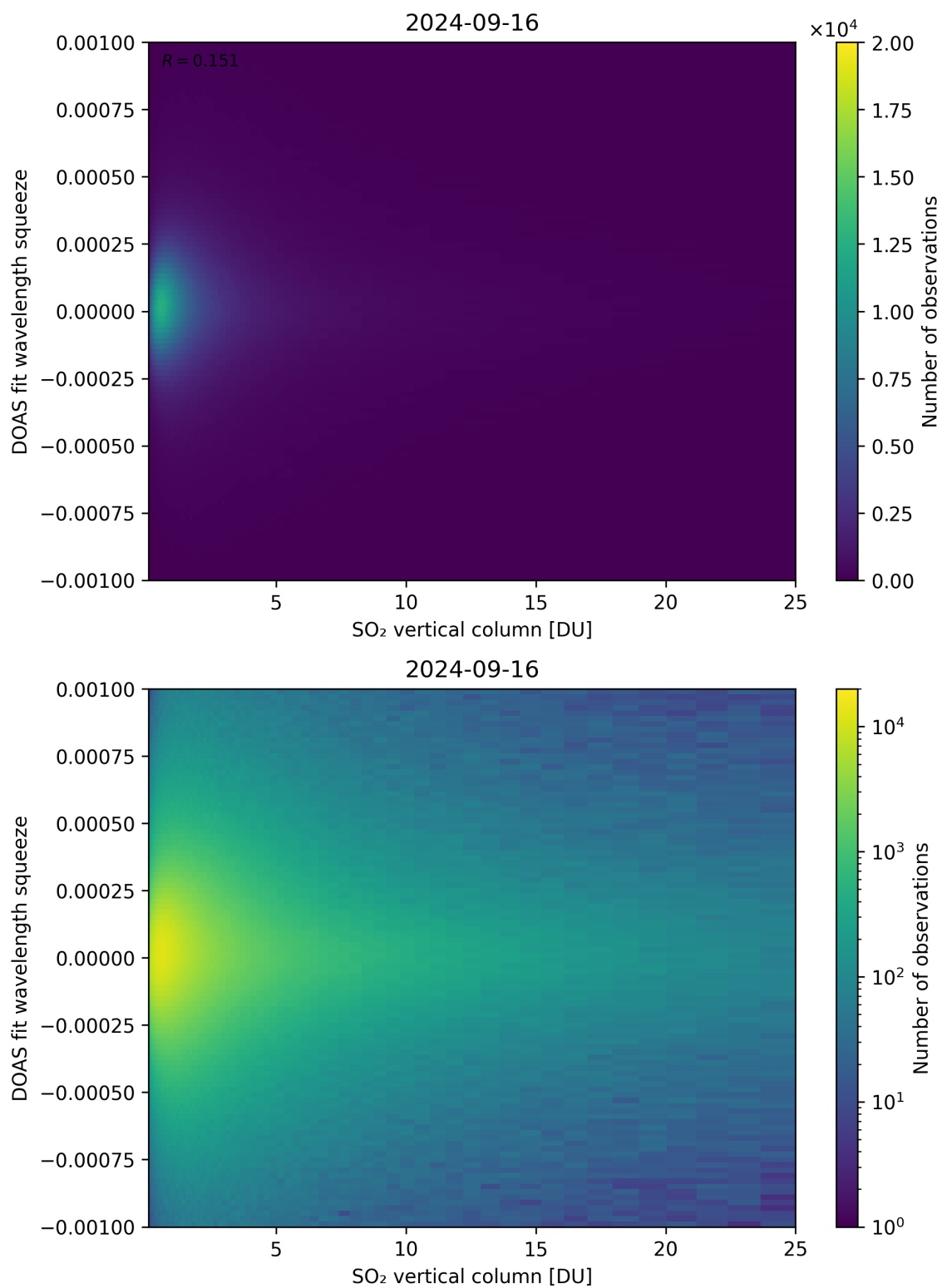
Figure 277: Scatter density plot of “SO 2 vertical column” against “DOAS fit wavelength squeeze” for 2024-09-15 to 2024-09-17.
