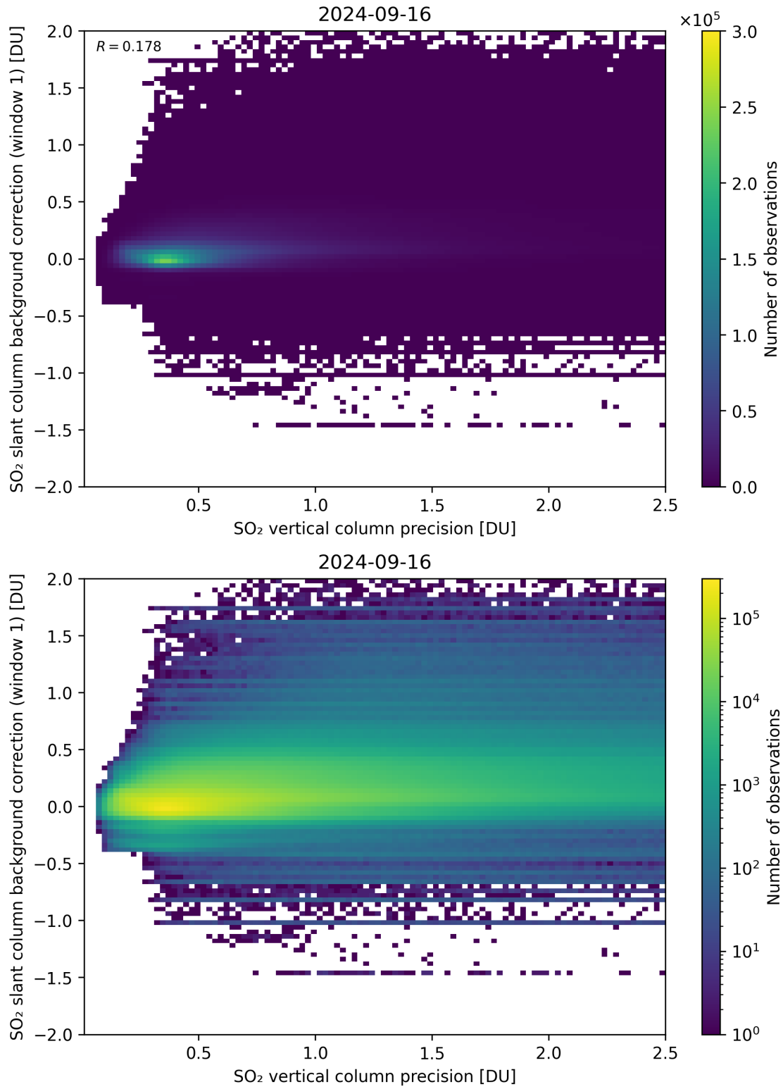
Figure 279: Scatter density plot of “SO 2 vertical column precision” against “SO 2 slant column background correction (window 1)” for 2024-09-15 to 2024-09-17.
