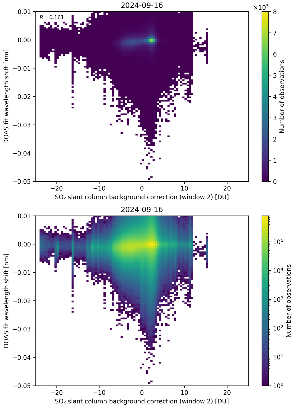
Figure 112: Scatter density plot of “SO 2 slant column background correction (window 2)” against “DOAS fit wavelength shift” for 2024-09-15 to 2024-09-17.
