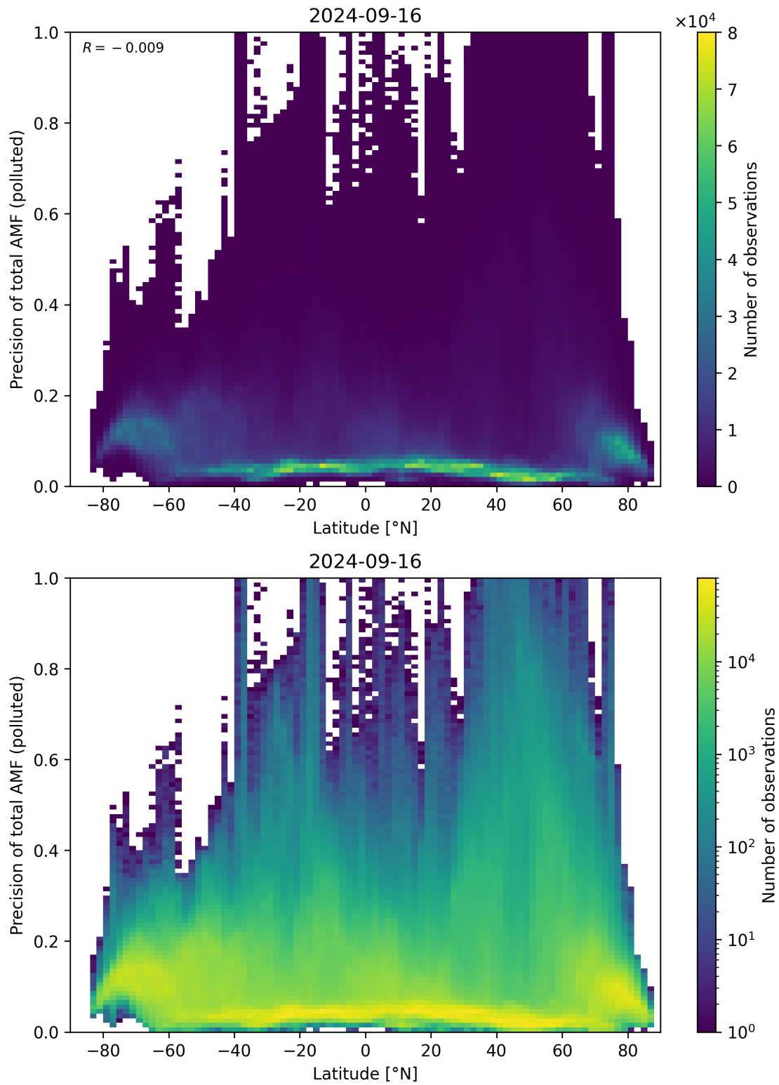
Figure 155: Scatter density plot of “Latitude” against “Precision of total AMF (polluted)” for 2024-09-15 to 2024-09-17.
