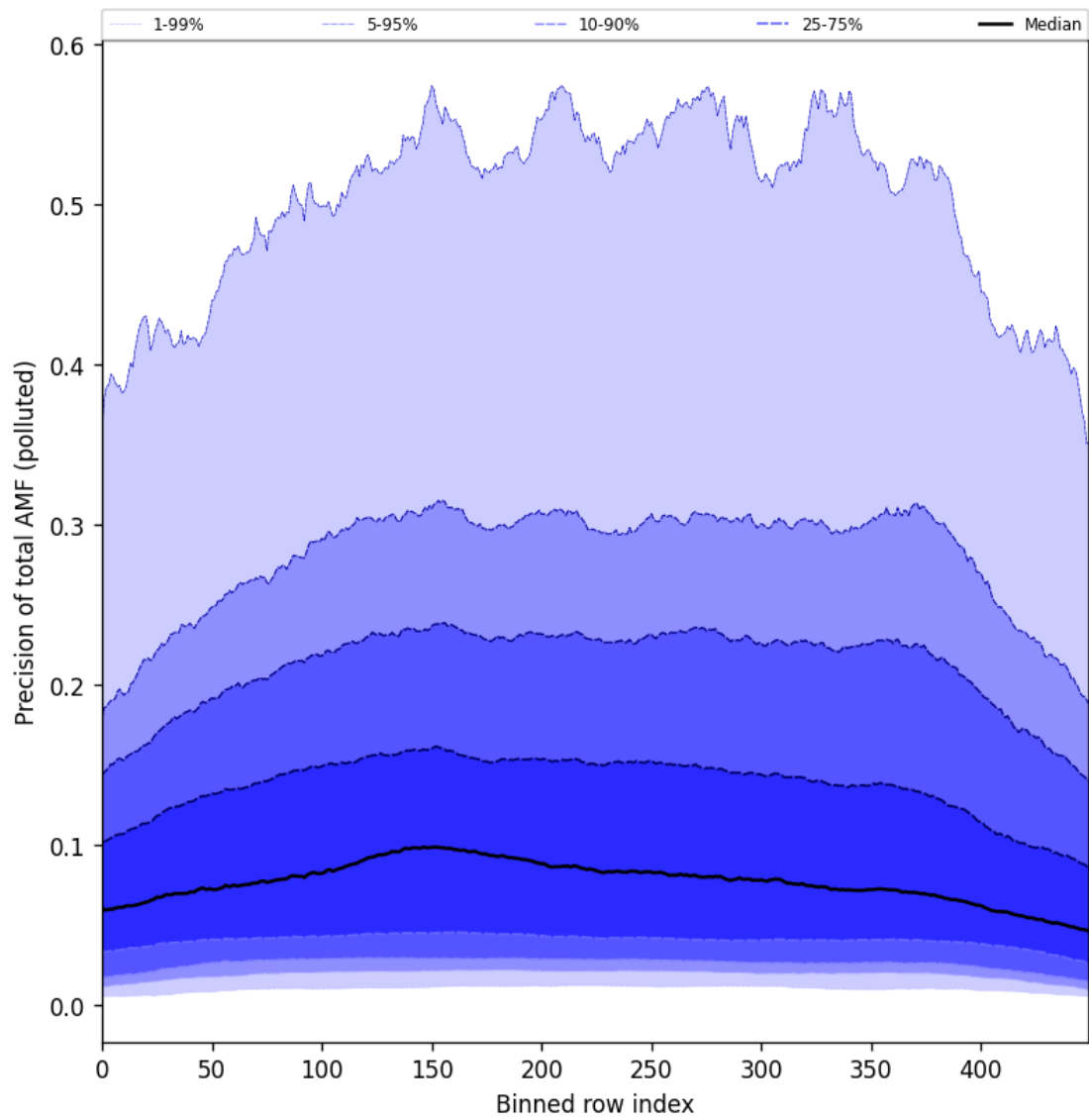
Figure 95: Along track statistics of “Precision of total AMF (polluted)” for 2024-09-15 to 2024-09-17
