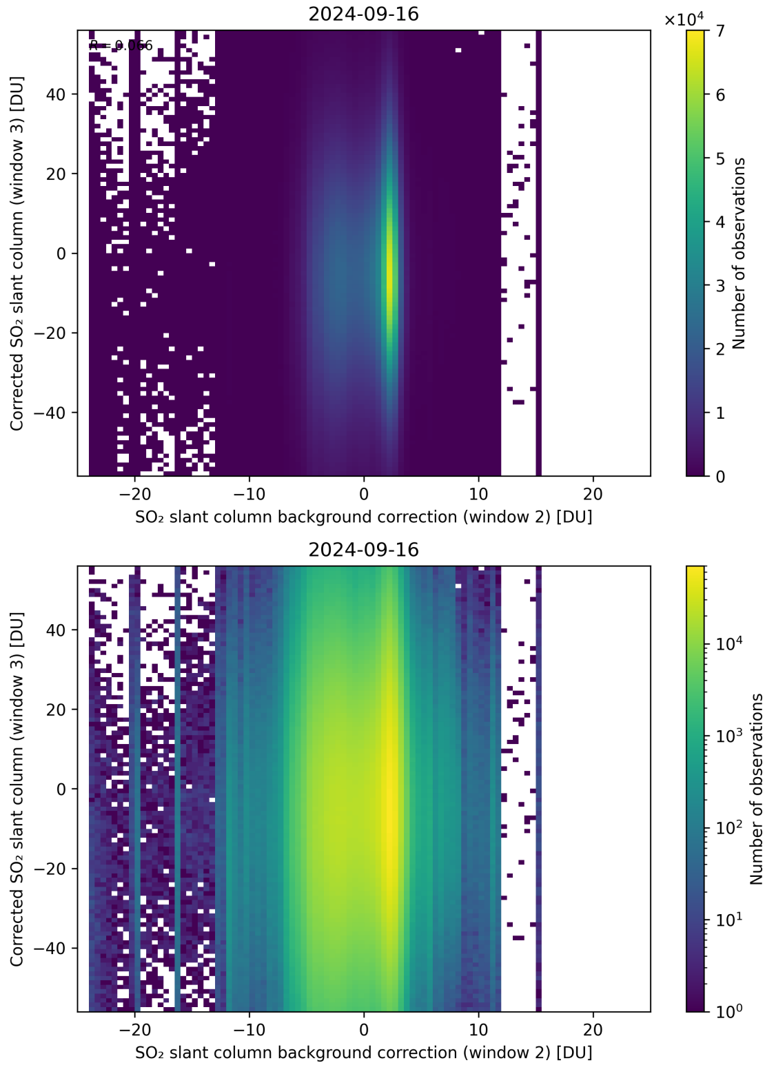
Figure 116: Scatter density plot of “SO 2 slant column background correction (window 2)” against “Corrected SO 2 slant column (window 3)” for 2024-09-15 to 2024-09-17.
