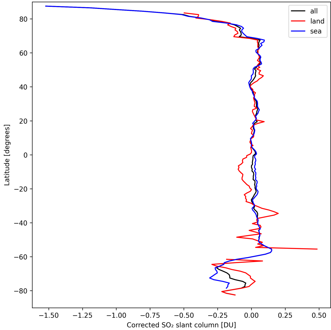
Figure 32: Zonal average of “Corrected SO 2 slant column” for 2024-09-15 to 2024-09-17.
