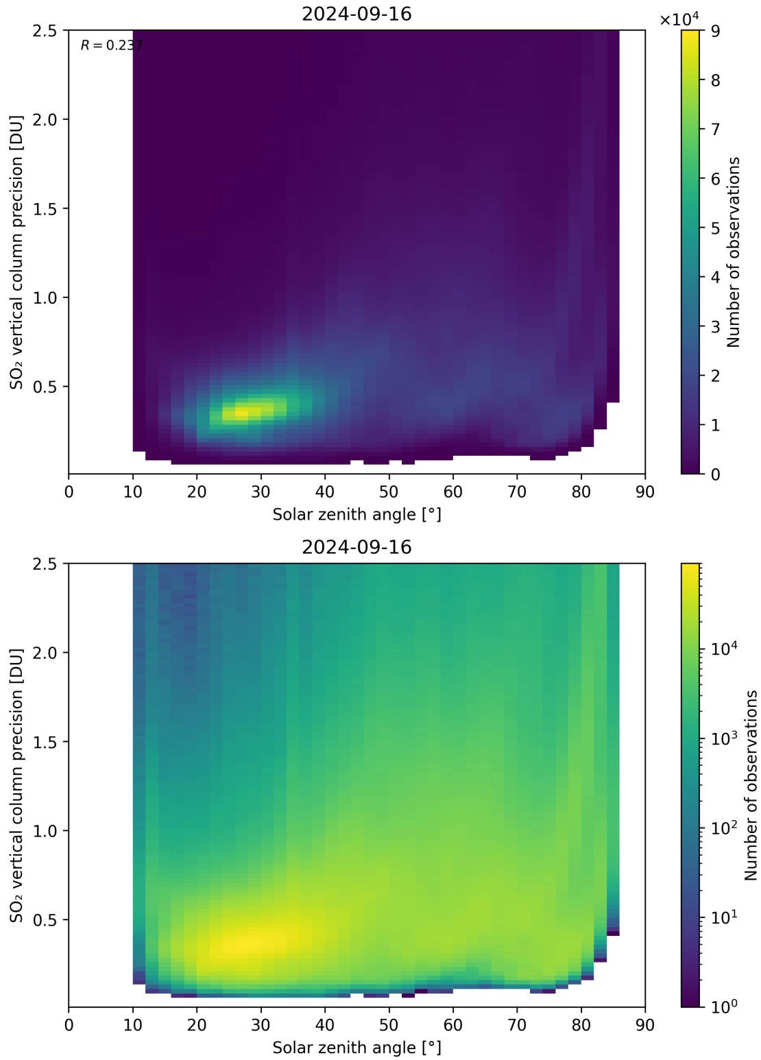
Figure 177: Scatter density plot of “Solar zenith angle” against “SO 2 vertical column precision” for 2024-09-15 to 2024-09-17.
