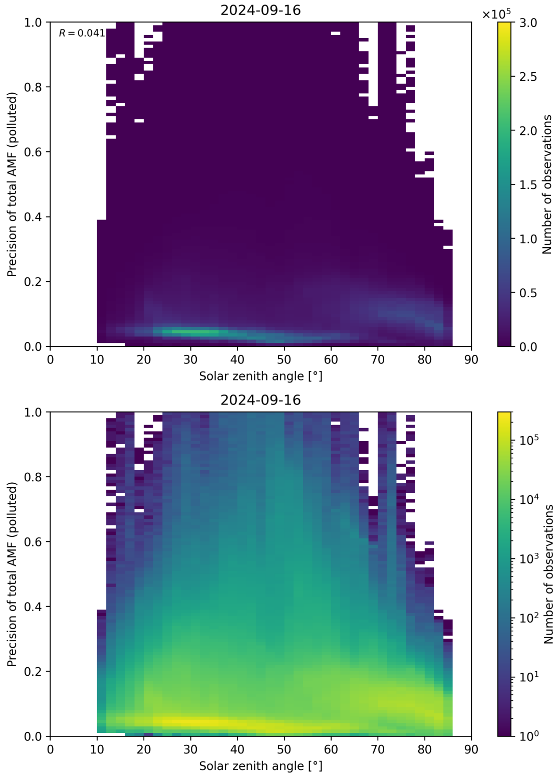
Figure 175: Scatter density plot of “Solar zenith angle” against “Precision of total AMF (polluted)” for 2024-09-15 to 2024-09-17.
