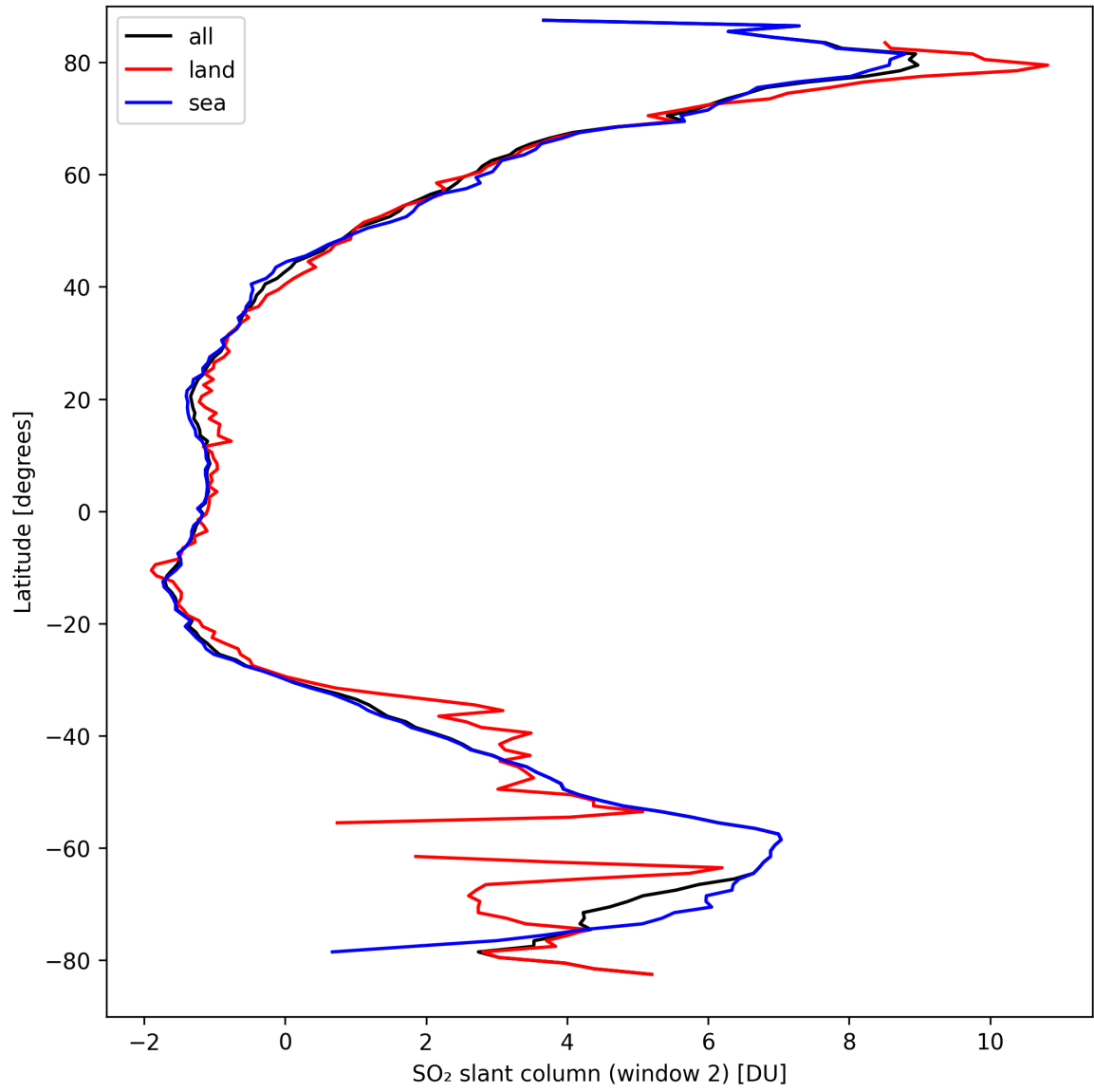
Figure 37: Zonal average of “SO 2 slant column (window 2)” for 2024-09-15 to 2024-09-17.
