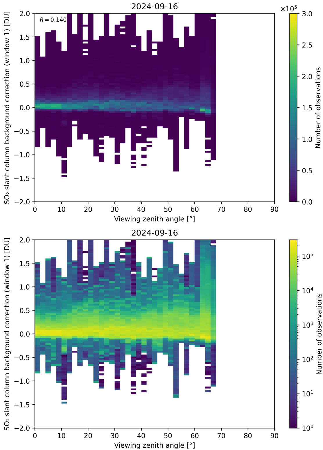
Figure 308: Scatter density plot of “Viewing zenith angle” against “SO 2 slant column background correction (window 1)” for 2024-09-15 to 2024-09-17.
