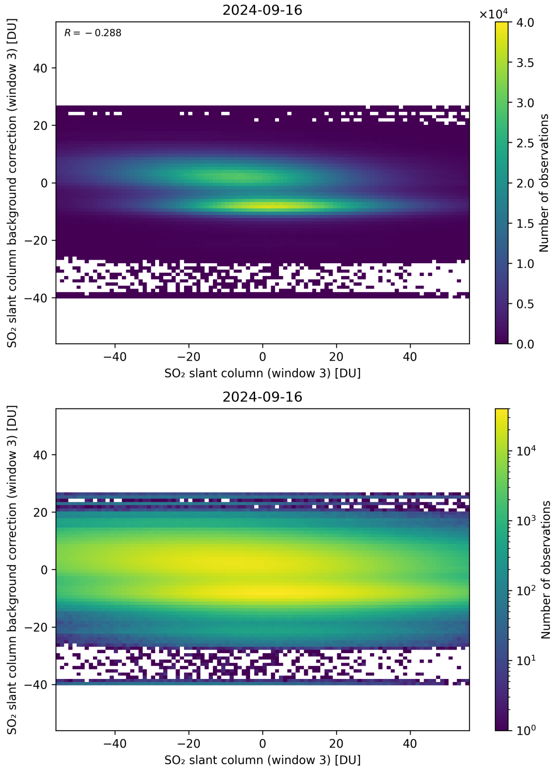
Figure 253: Scatter density plot of “SO 2 slant column (window 3)” against “SO 2 slant column background correction (window 3)” for 2024-09-15 to 2024-09-17.
