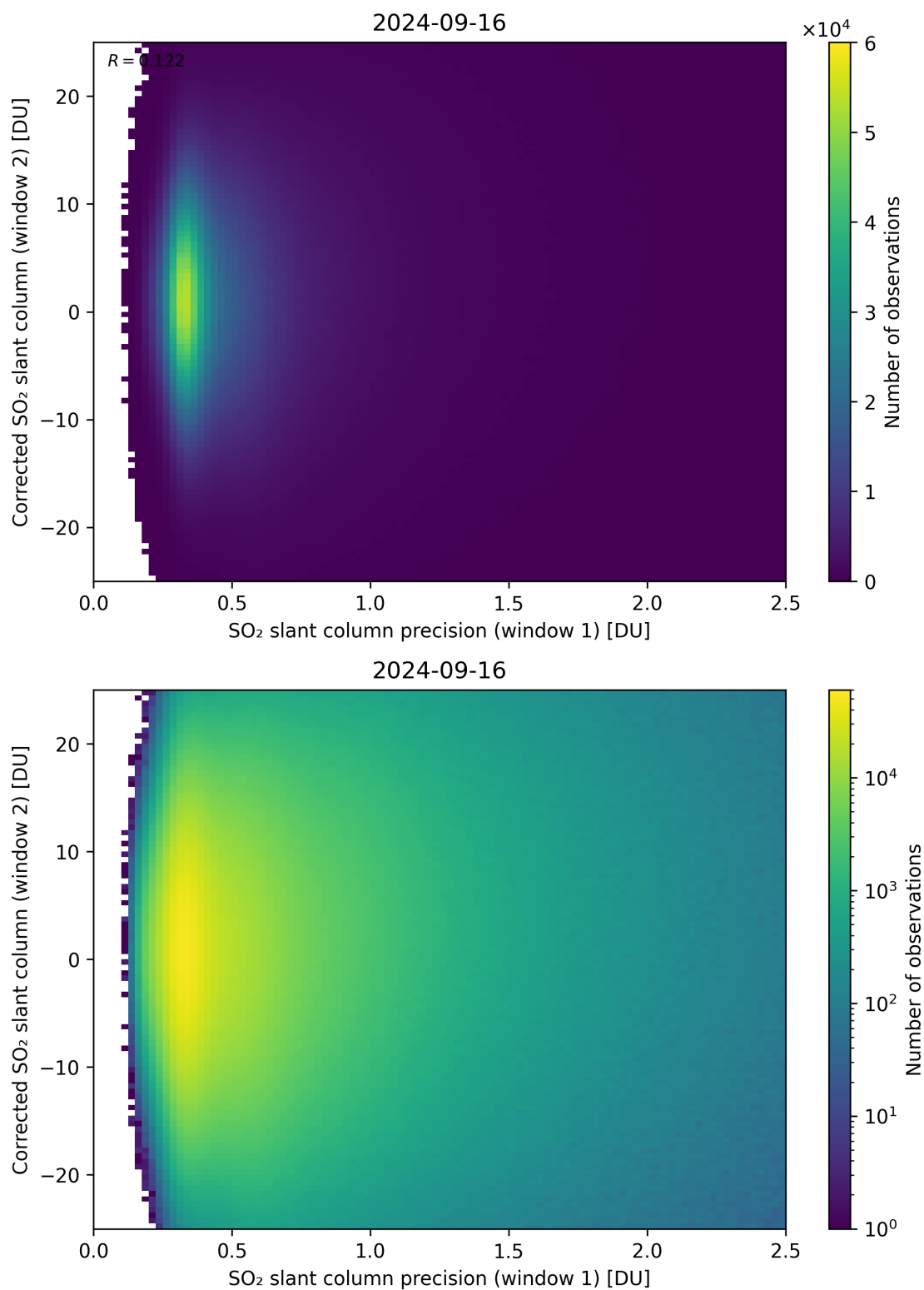
Figure 225: Scatter density plot of “SO 2 slant column precision (window 1)” against “Corrected SO 2 slant column (window 2)” for 2024-09-15 to 2024-09-17.
