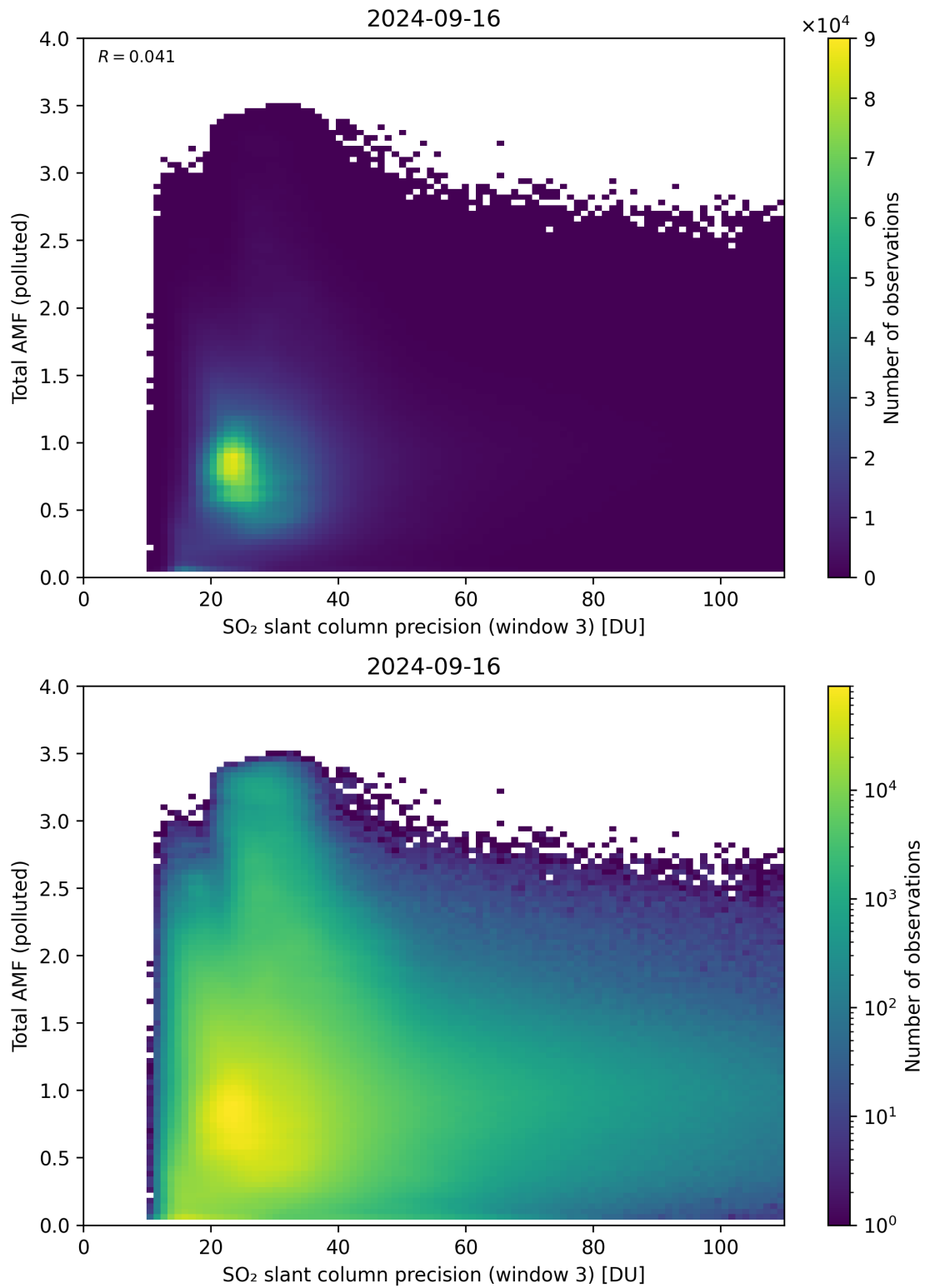
Figure 263: Scatter density plot of “SO 2 slant column precision (window 3)” against “Total AMF (polluted)” for 2024-09-15 to 2024-09-17.
