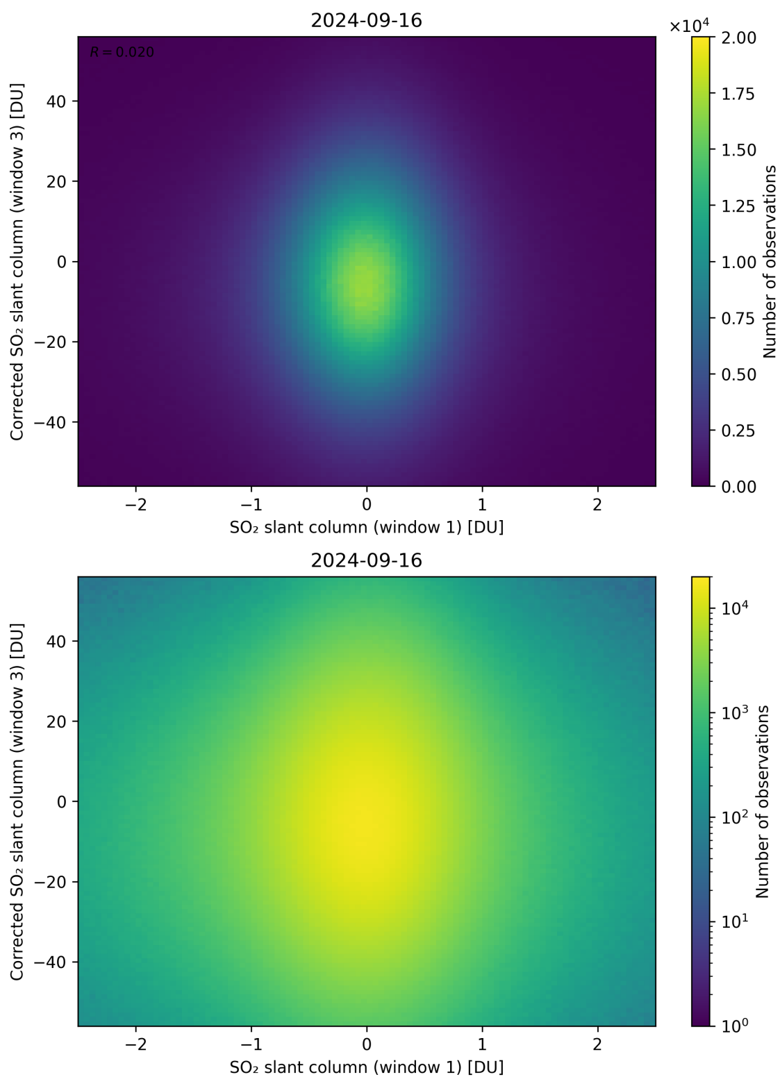
Figure 234: Scatter density plot of “SO 2 slant column (window 1)” against “Corrected SO 2 slant column (window 3)” for 2024-09-15 to 2024-09-17.
