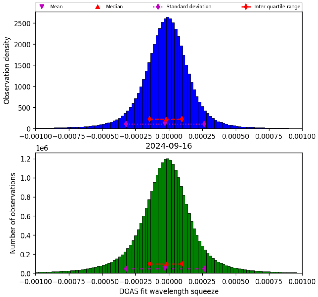
Figure 69: Histogram of “DOAS fit wavelength squeeze” for 2024-09-15 to 2024-09-17
