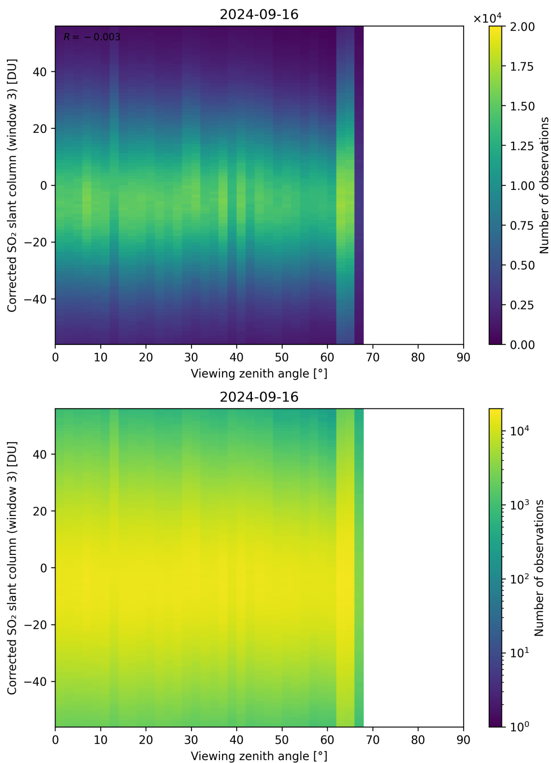
Figure 319: Scatter density plot of “Viewing zenith angle” against “Corrected SO 2 slant column (window 3)” for 2024-09-15 to 2024-09-17.
