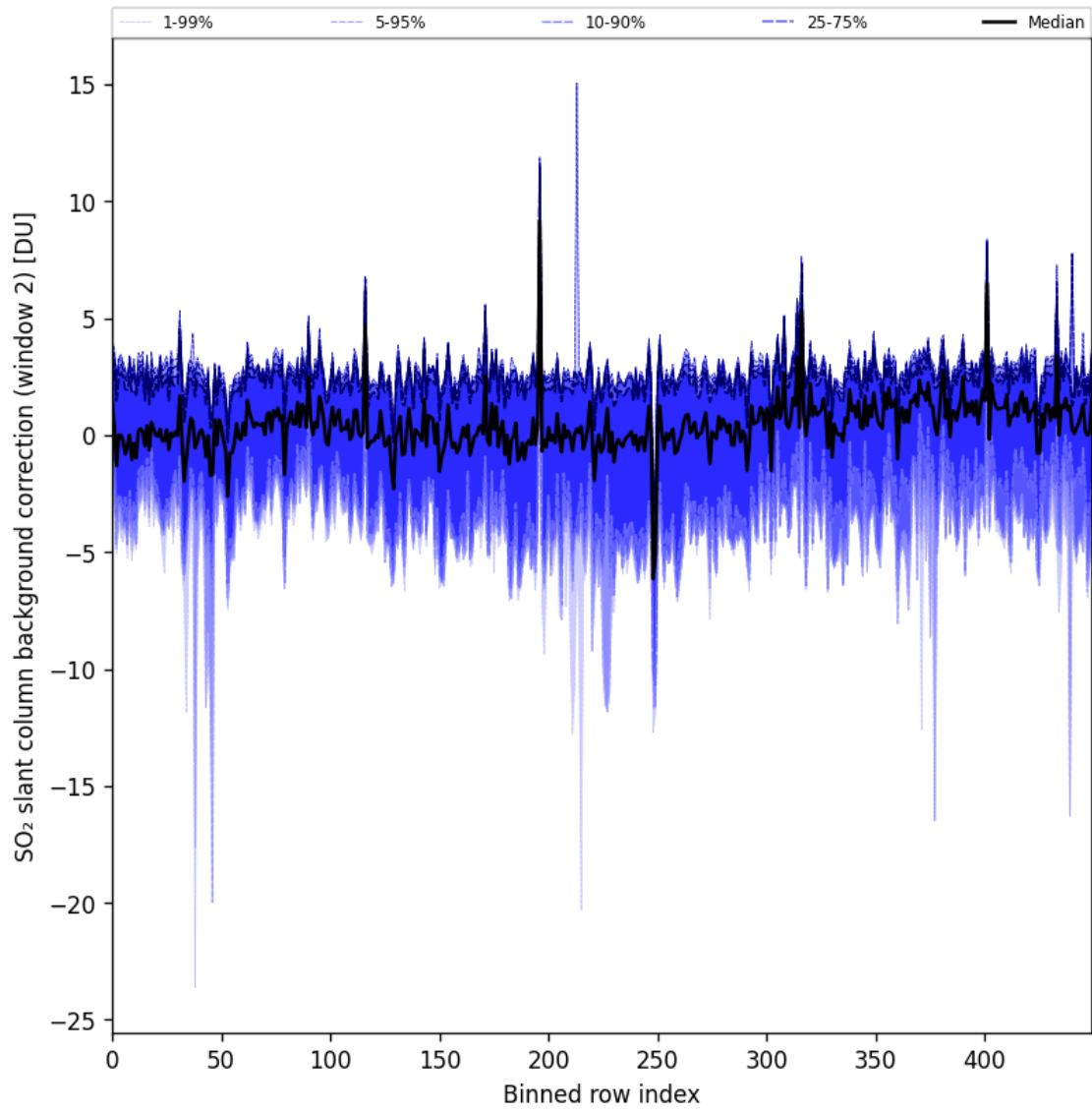
Figure 86: Along track statistics of “SO 2 slant column background correction (window 2)” for 2024-09-15 to 2024-09-17
