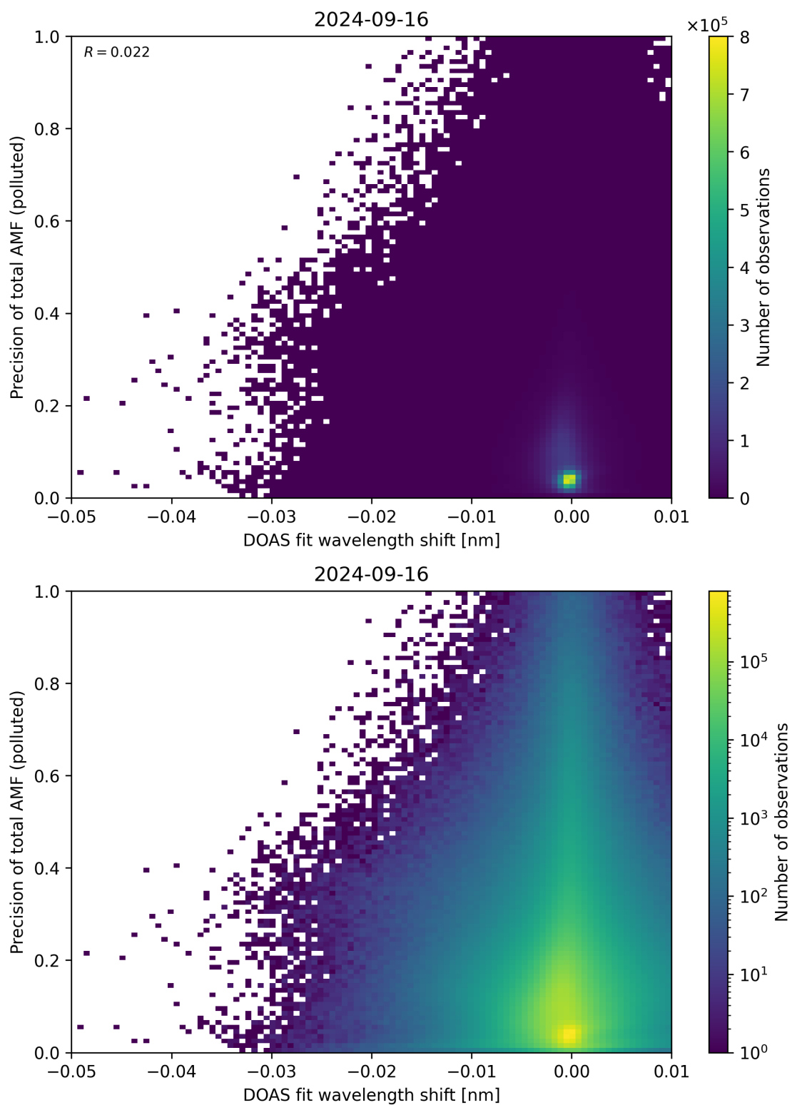
Figure 131: Scatter density plot of “DOAS fit wavelength shift” against “Precision of total AMF (polluted)” for 2024-09-15 to 2024-09-17.
