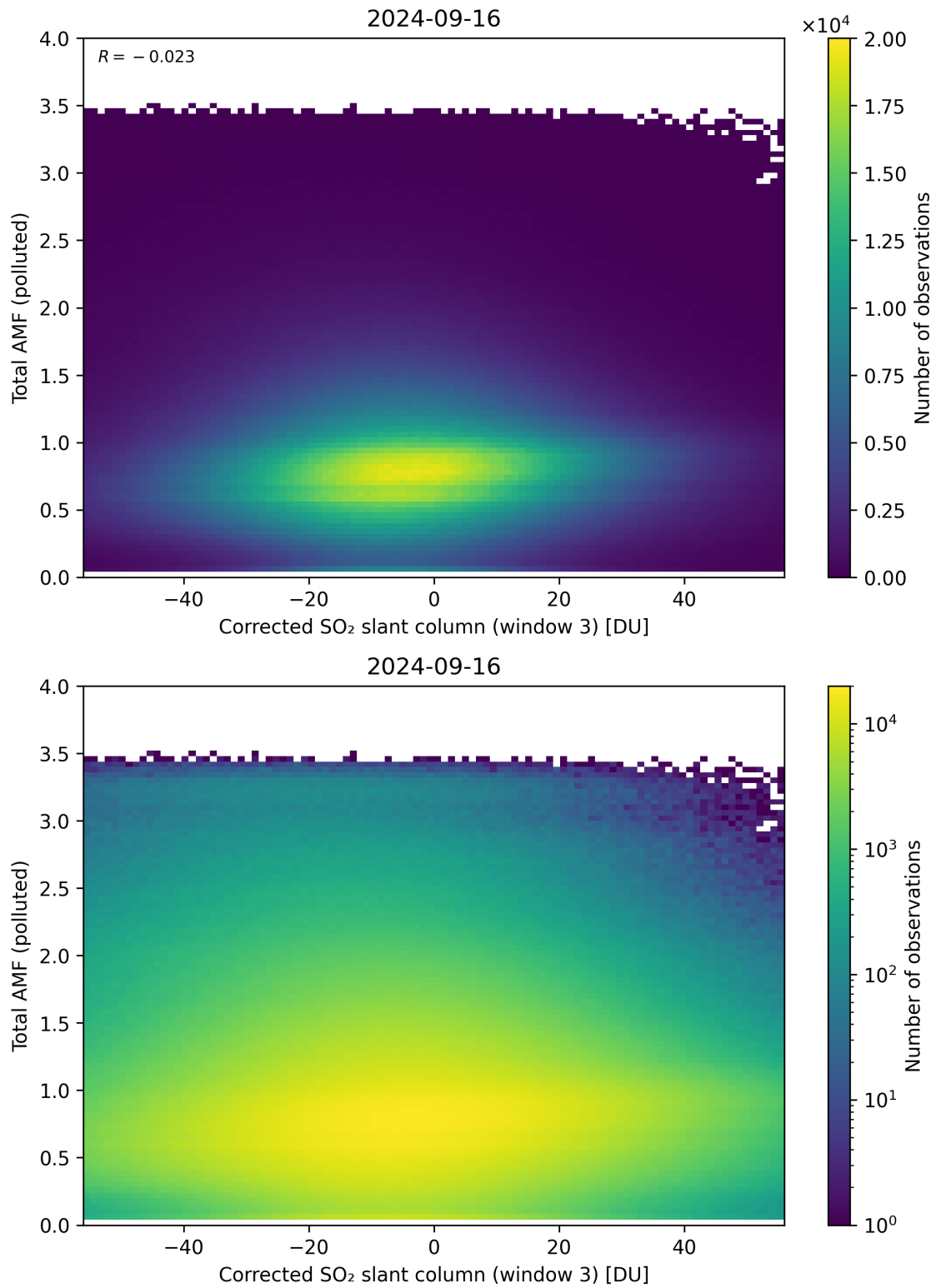
Figure 210: Scatter density plot of “Corrected SO 2 slant column (window 3)” against “Total AMF (polluted)” for 2024-09-15 to 2024-09-17.
