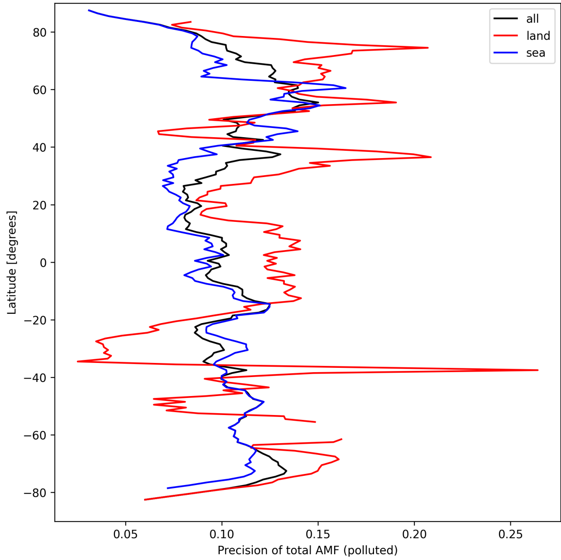
Figure 49: Zonal average of “Precision of total AMF (polluted)” for 2024-09-15 to 2024-09-17.
