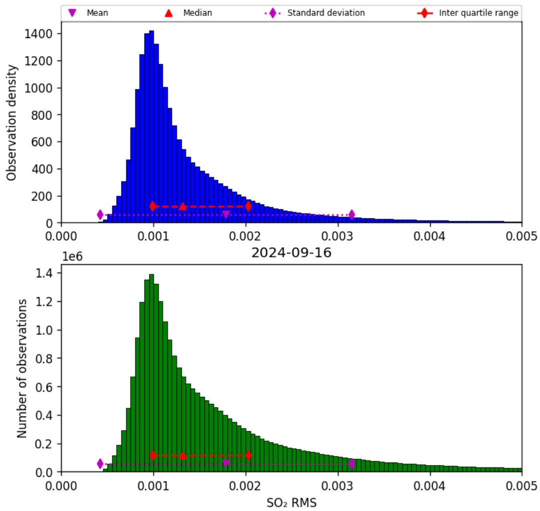
Figure 70: Histogram of “SO 2 RMS” for 2024-09-15 to 2024-09-17
