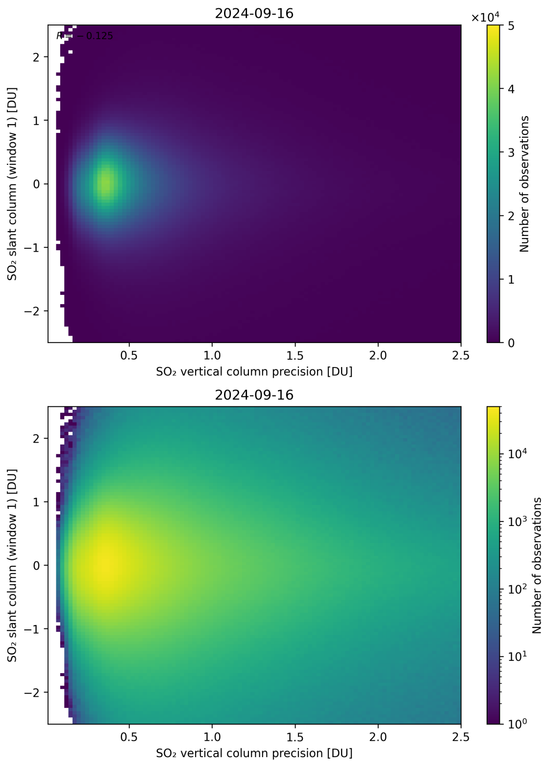
Figure 289: Scatter density plot of “SO 2 vertical column precision” against “SO 2 slant column (window 1)” for 2024-09-15 to 2024-09-17.
