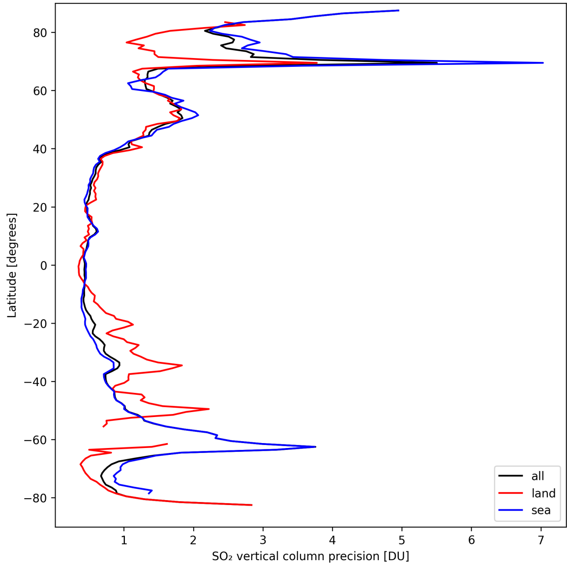
Figure 31: Zonal average of “SO 2 vertical column precision” for 2024-09-15 to 2024-09-17.
