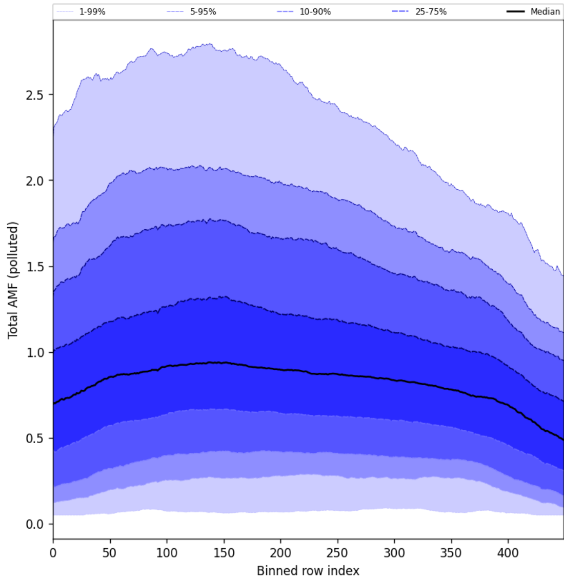
Figure 94: Along track statistics of “Total AMF (polluted)” for 2024-09-15 to 2024-09-17
