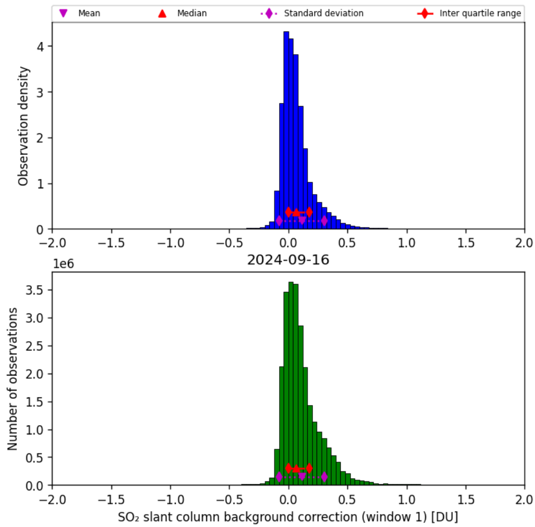
Figure 59: Histogram of “SO 2 slant column background correction (window 1)” for 2024-09-15 to 2024-09-17
