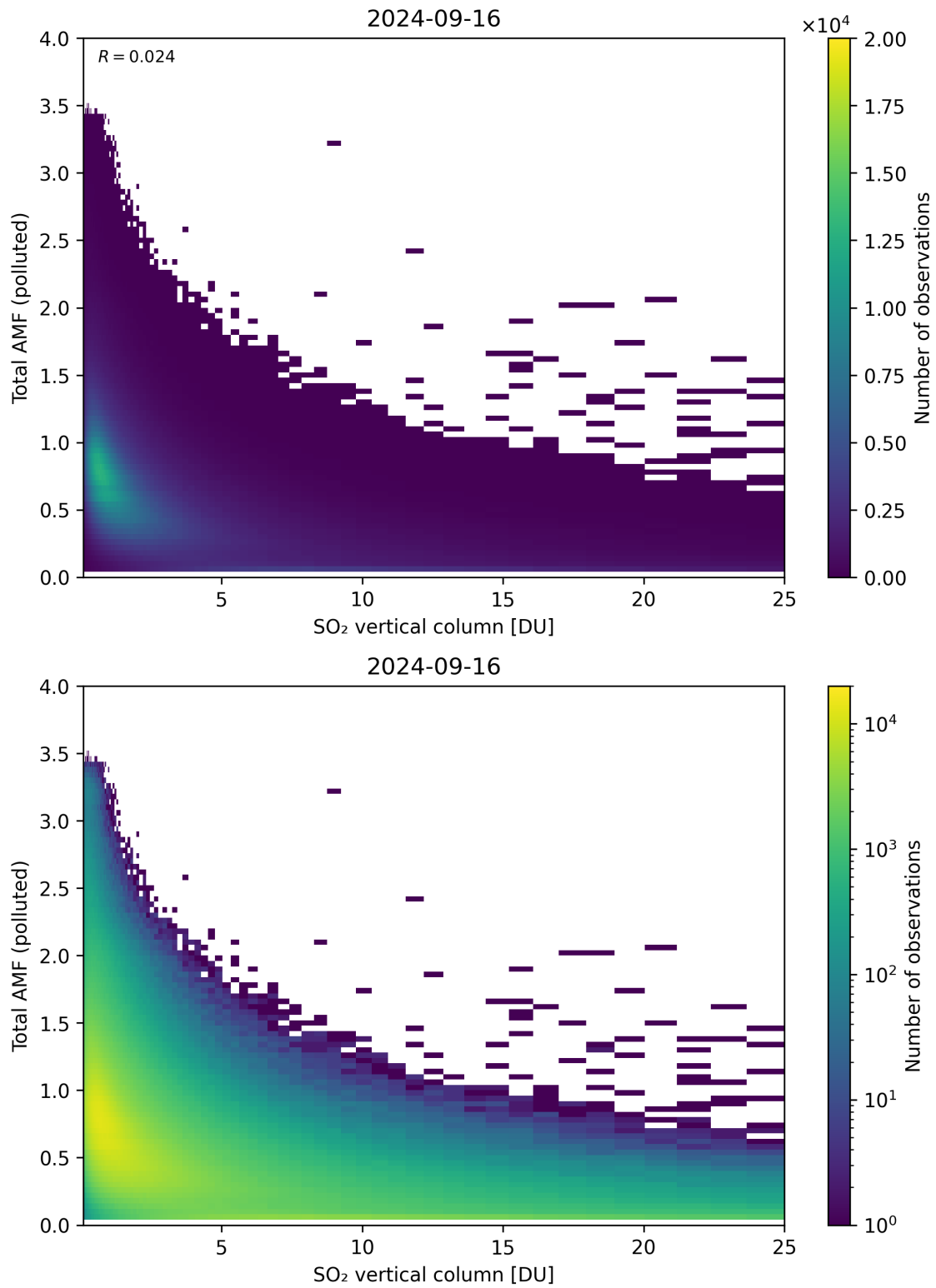
Figure 305: Scatter density plot of “SO 2 vertical column” against “Total AMF (polluted)” for 2024-09-15 to 2024-09-17.
