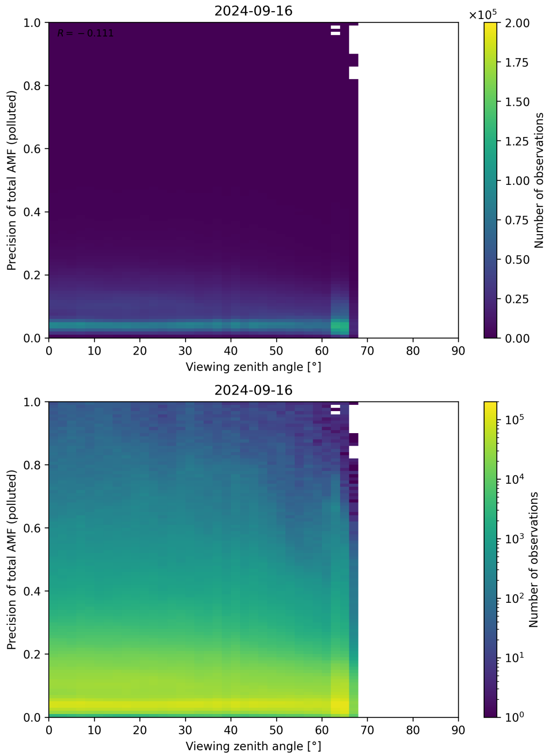
Figure 326: Scatter density plot of “Viewing zenith angle” against “Precision of total AMF (polluted)” for 2024-09-15 to 2024-09-17.
