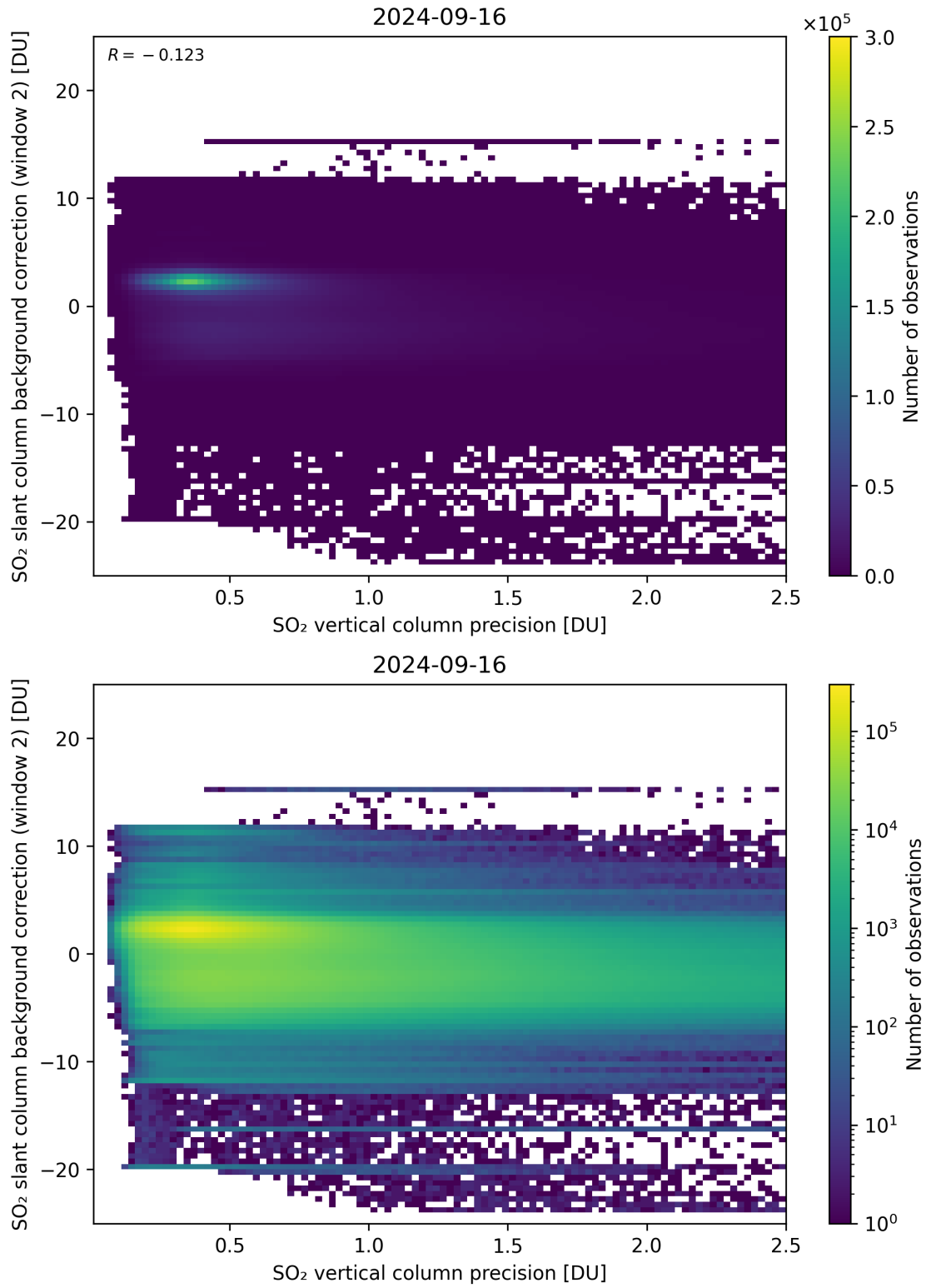
Figure 280: Scatter density plot of “SO 2 vertical column precision” against “SO 2 slant column background correction (window 2)” for 2024-09-15 to 2024-09-17.
