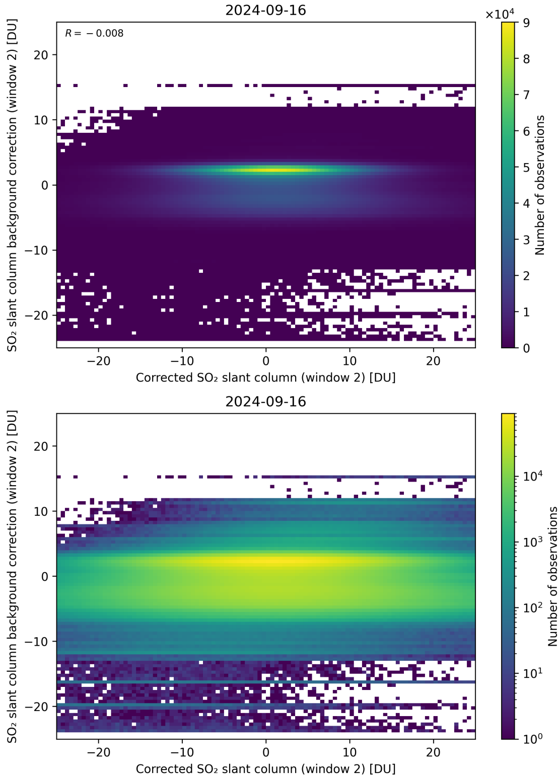
Figure 194: Scatter density plot of “Corrected SO 2 slant column (window 2)” against “SO 2 slant column background correction (window 2)” for 2024-09-15 to 2024-09-17.
