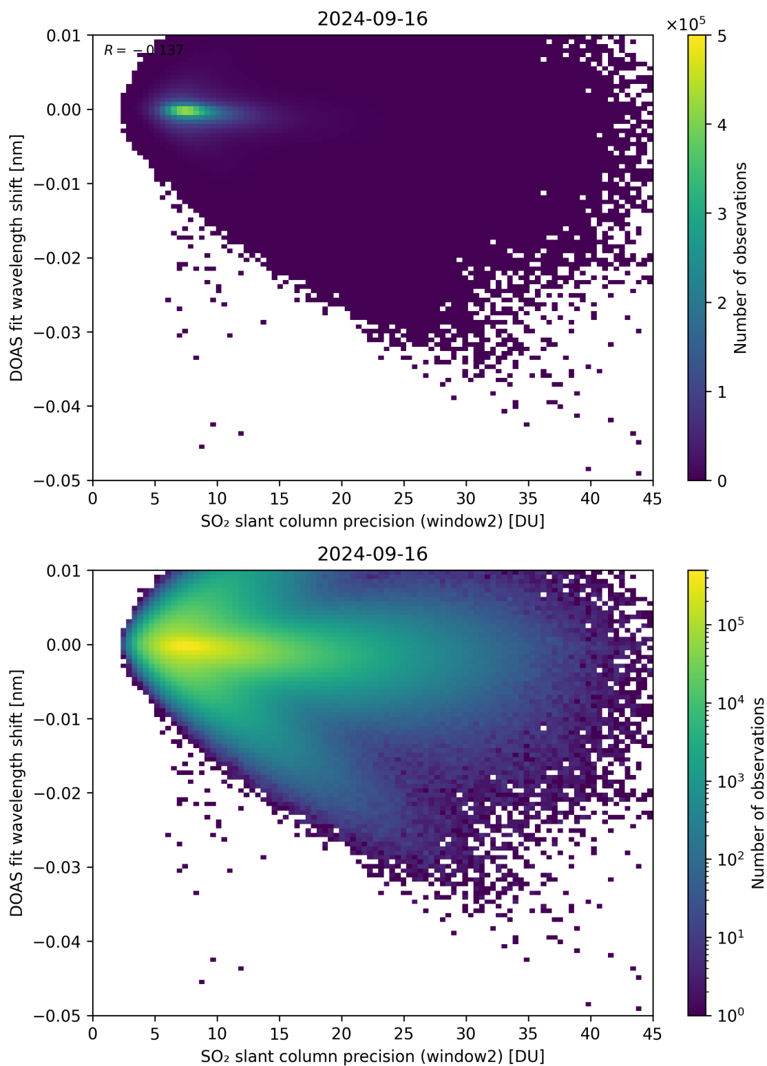
Figure 243: Scatter density plot of “SO 2 slant column precision (window2)” against “DOAS fit wavelength shift” for 2024-09-15 to 2024-09-17.
