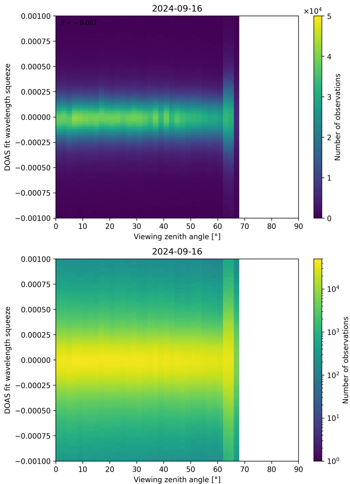
Figure 312: Scatter density plot of “Viewing zenith angle” against “DOAS fit wavelength squeeze” for 2024-09-15 to 2024-09-17.
