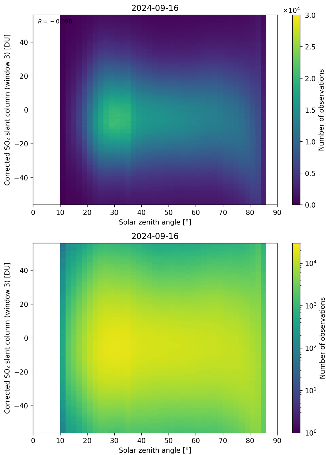
Figure 168: Scatter density plot of “Solar zenith angle” against “Corrected SO 2 slant column (window 3)” for 2024-09-15 to 2024-09-17.
