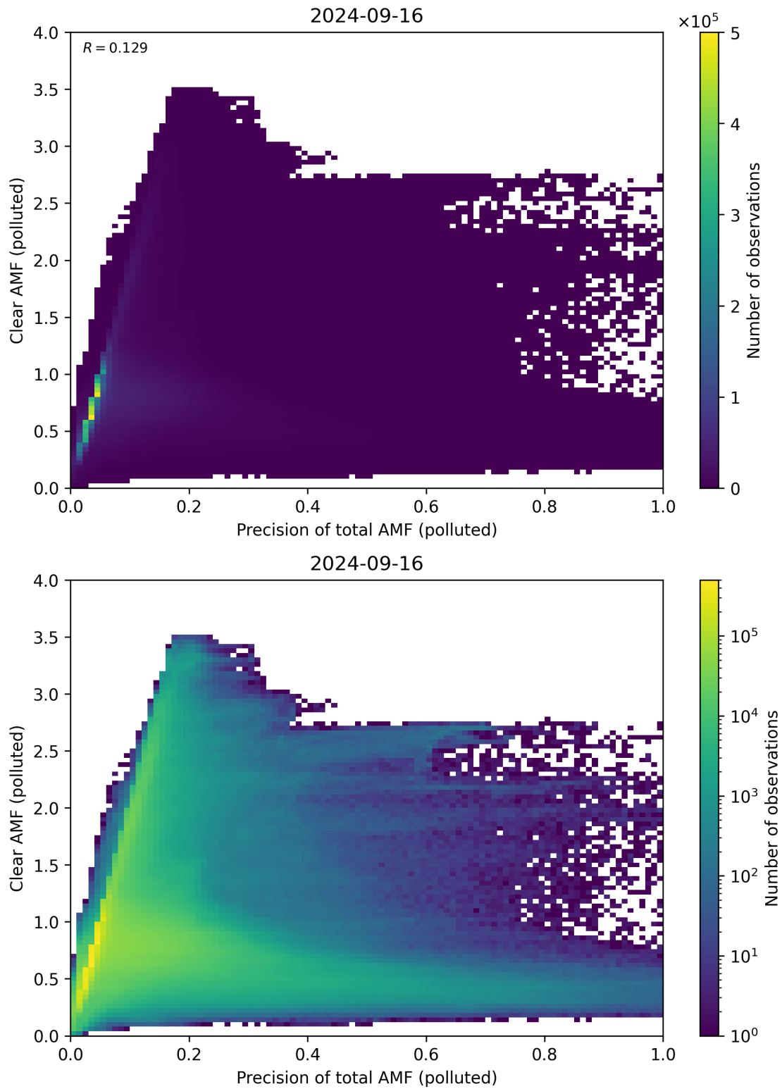
Figure 270: Scatter density plot of “Precision of total AMF (polluted)” against “Clear AMF (polluted)” for 2024-09-15 to 2024-09-17.
