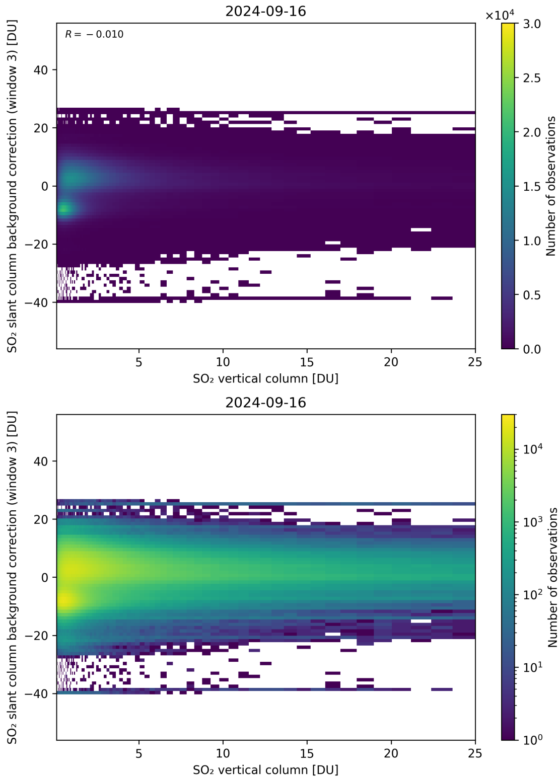
Figure 275: Scatter density plot of “SO 2 vertical column” against “SO 2 slant column background correction (window 3)” for 2024-09-15 to 2024-09-17.
