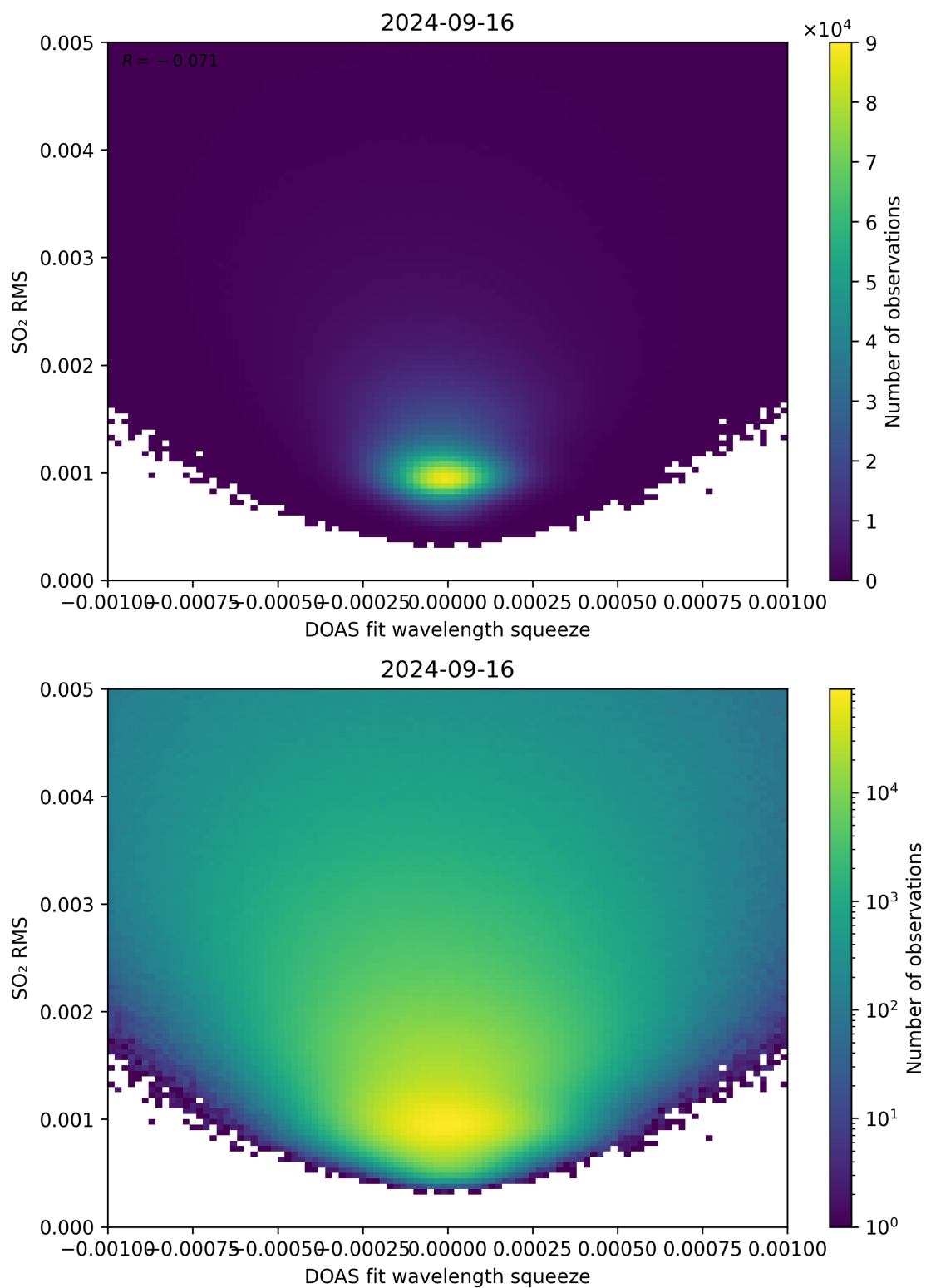
Figure 132: Scatter density plot of “DOAS fit wavelength squeeze” against “SO 2 RMS” for 2024-09-15 to 2024-09-17.
