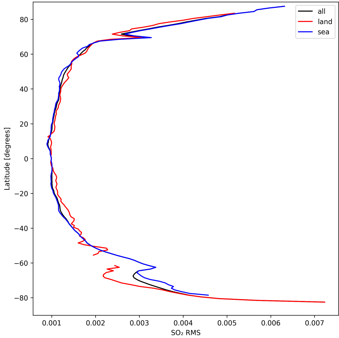
Figure 47: Zonal average of “SO 2 RMS” for 2024-09-15 to 2024-09-17.
