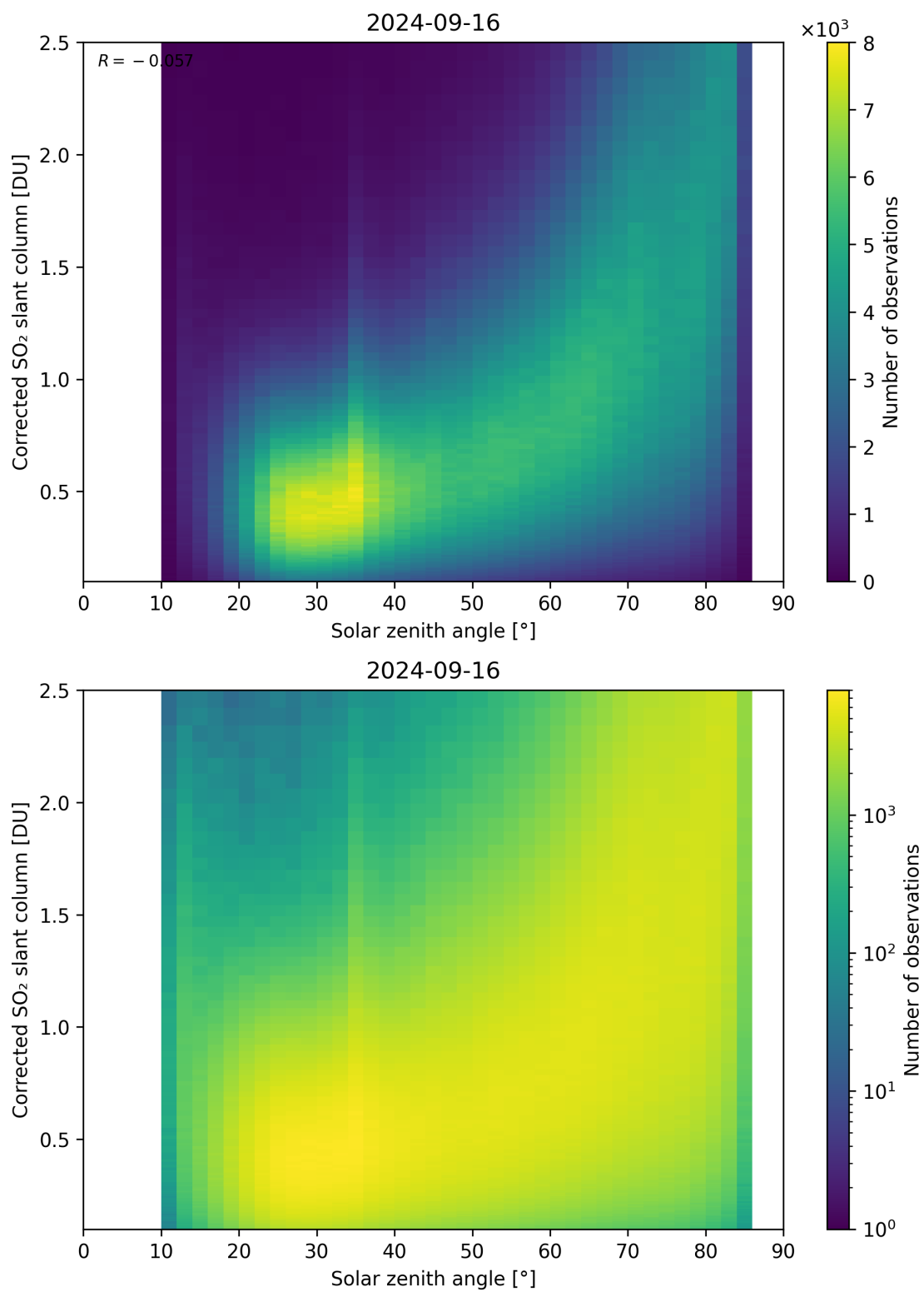
Figure 166: Scatter density plot of “Solar zenith angle” against “Corrected SO 2 slant column” for 2024-09-15 to 2024-09-17.
