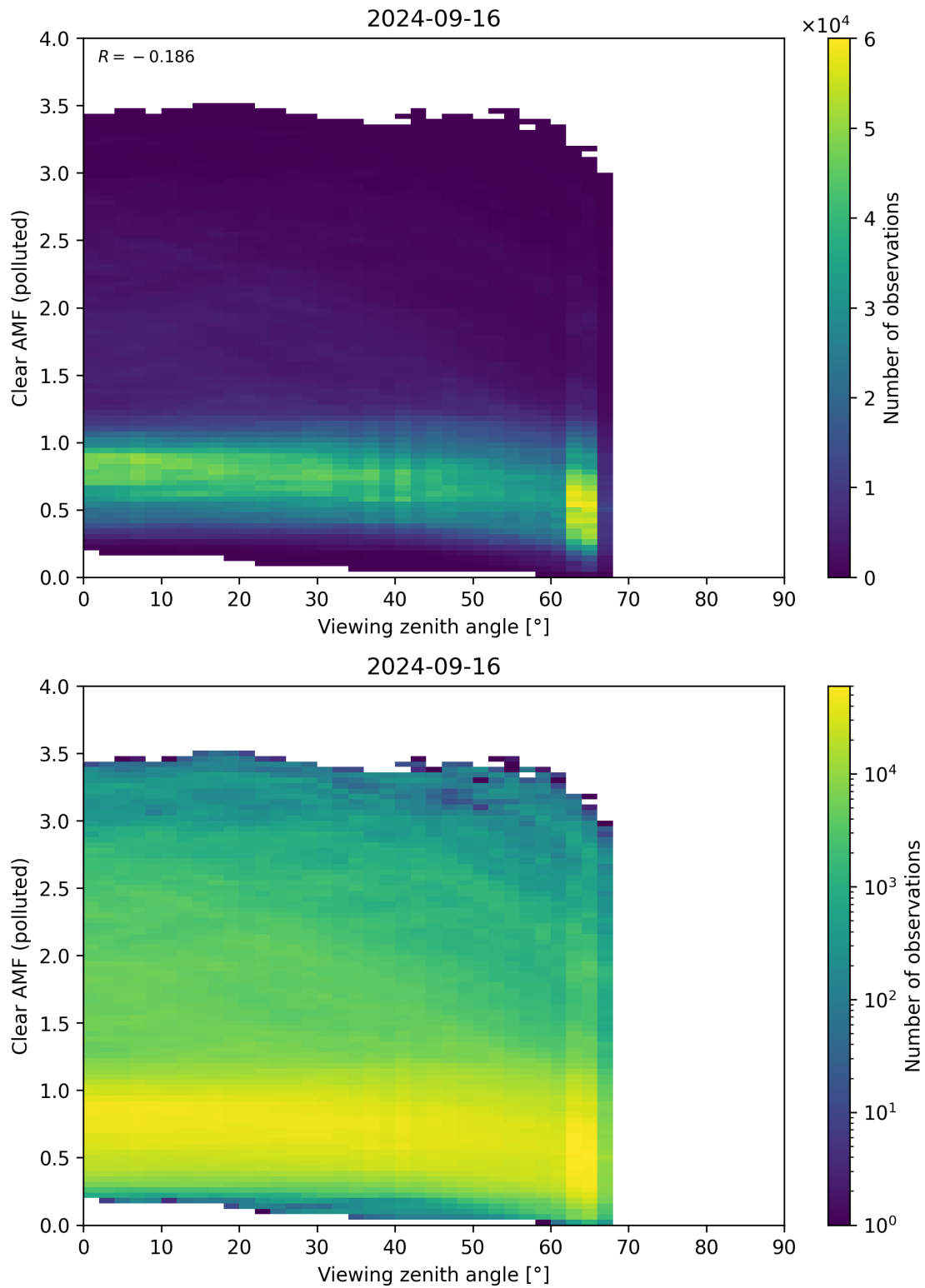
Figure 316: Scatter density plot of “Viewing zenith angle” against “Clear AMF (polluted)” for 2024-09-15 to 2024-09-17.
