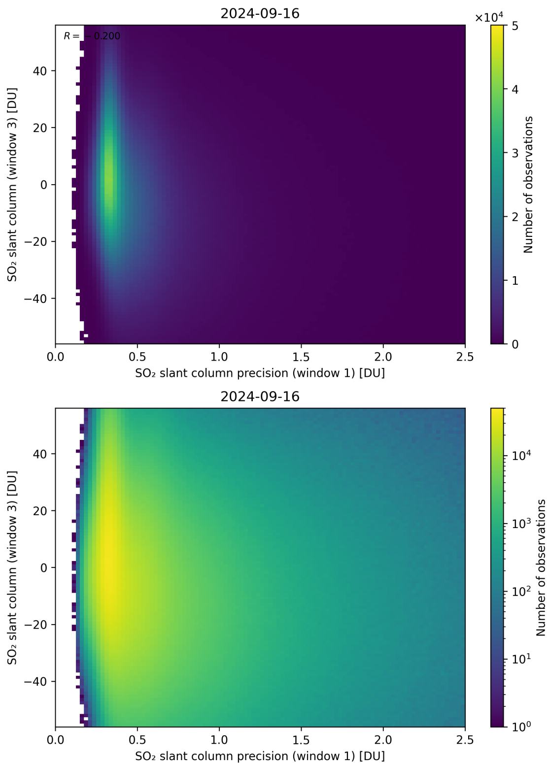
Figure 228: Scatter density plot of “SO 2 slant column precision (window 1)” against “SO 2 slant column (window 3)” for 2024-09-15 to 2024-09-17.
