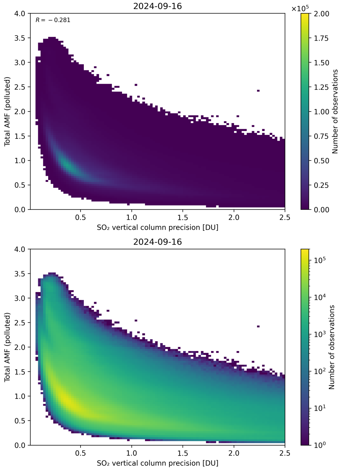
Figure 294: Scatter density plot of “SO 2 vertical column precision” against “Total AMF (polluted)” for 2024-09-15 to 2024-09-17.
