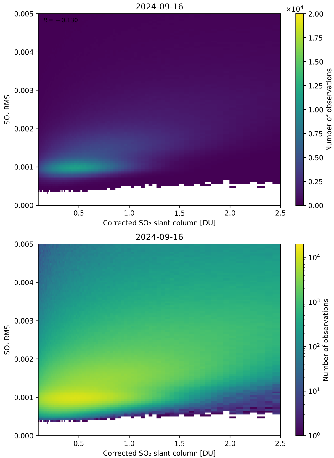
Figure 183: Scatter density plot of “Corrected SO 2 slant column” against “SO 2 RMS” for 2024-09-15 to 2024-09-17.
