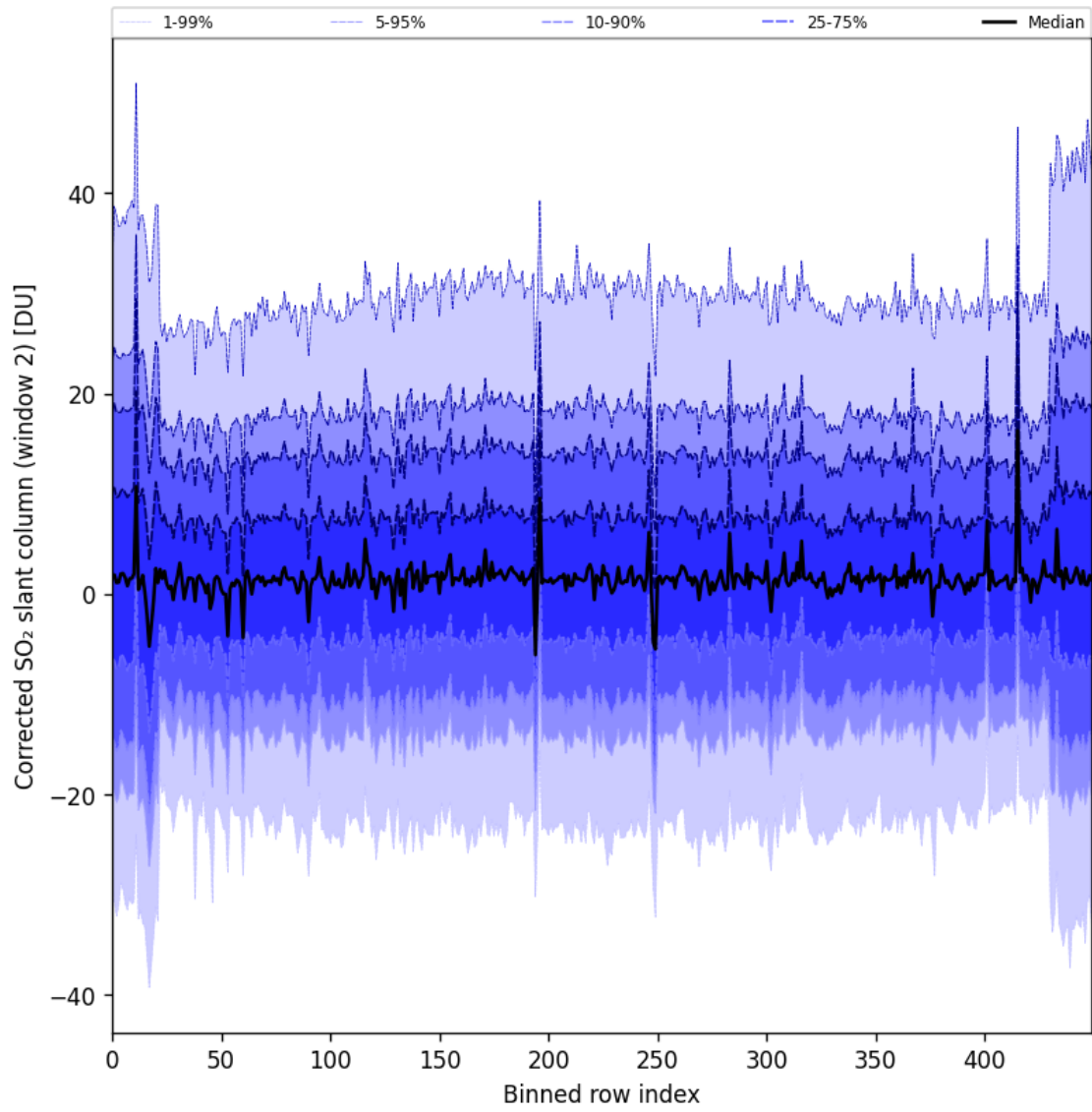
Figure 85: Along track statistics of “Corrected SO 2 slant column (window 2)” for 2024-09-15 to 2024-09-17
