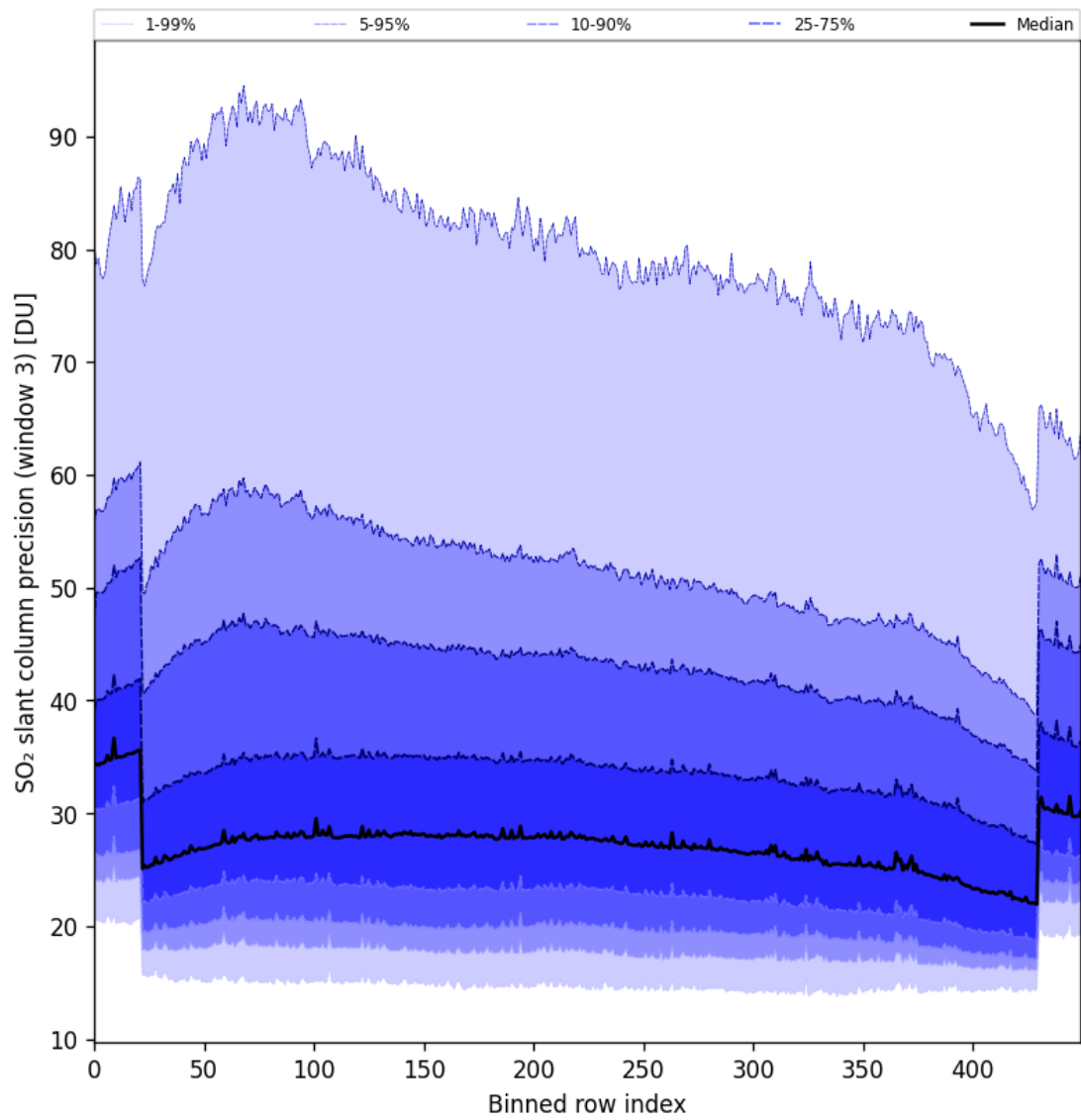
Figure 88: Along track statistics of “SO 2 slant column precision (window 3)” for 2024-09-15 to 2024-09-17
