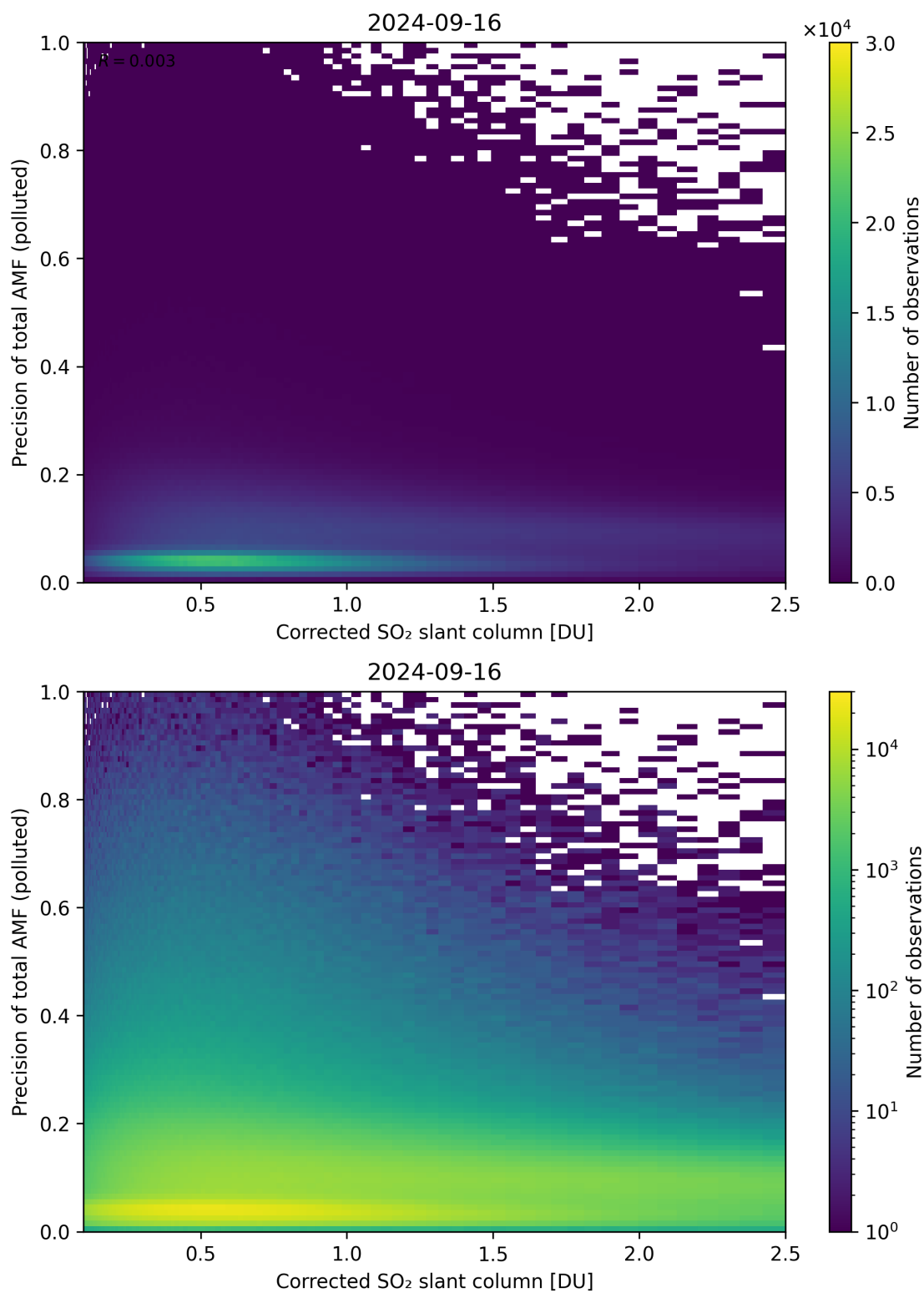
Figure 193: Scatter density plot of “Corrected SO 2 slant column” against “Precision of total AMF (polluted)” for 2024-09-15 to 2024-09-17.
