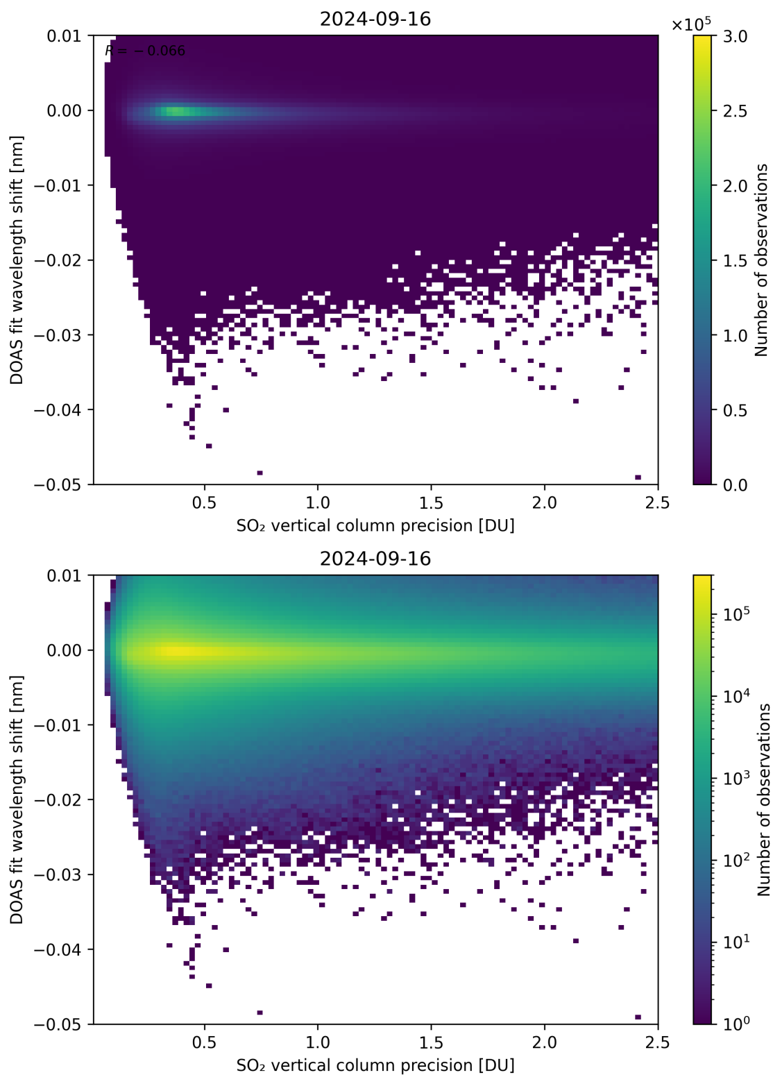
Figure 282: Scatter density plot of “SO 2 vertical column precision” against “DOAS fit wavelength shift” for 2024-09-15 to 2024-09-17.
