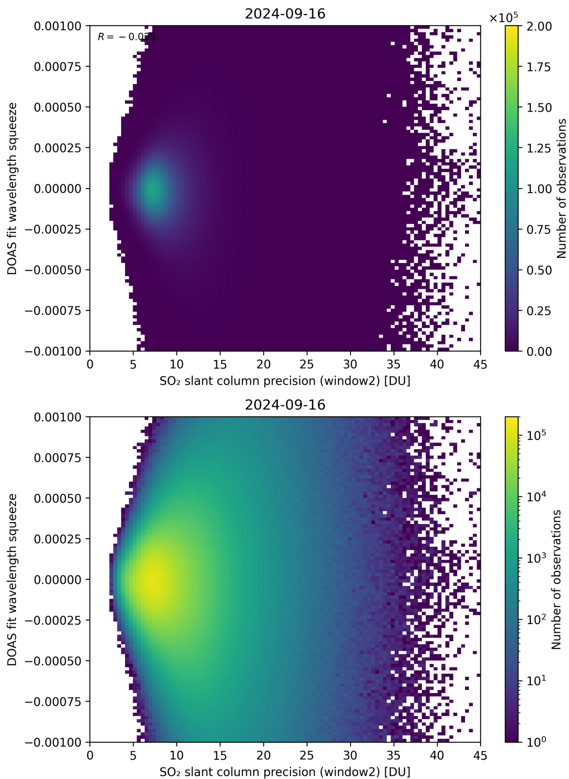
Figure 244: Scatter density plot of “SO 2 slant column precision (window2)” against “DOAS fit wavelength squeeze” for 2024-09-15 to 2024-09-17.
