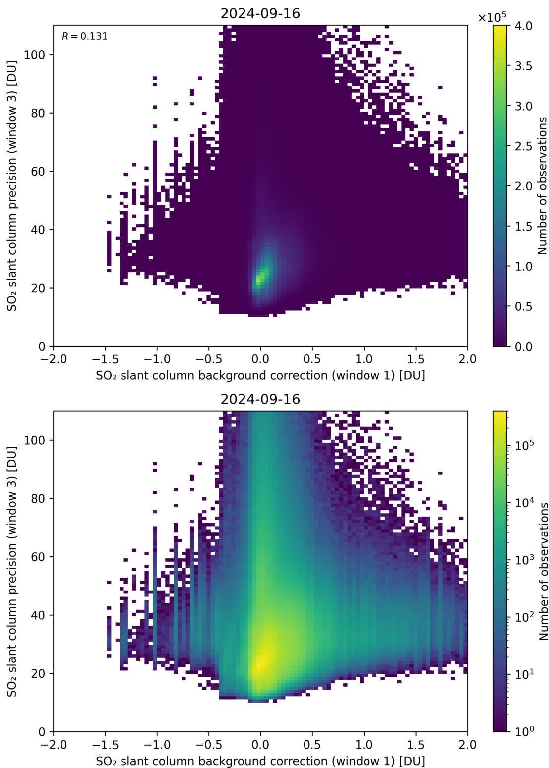
Figure 108: Scatter density plot of “SO 2 slant column background correction (window 1)” against “SO 2 slant column precision (window 3)” for 2024-09-15 to 2024-09-17.
