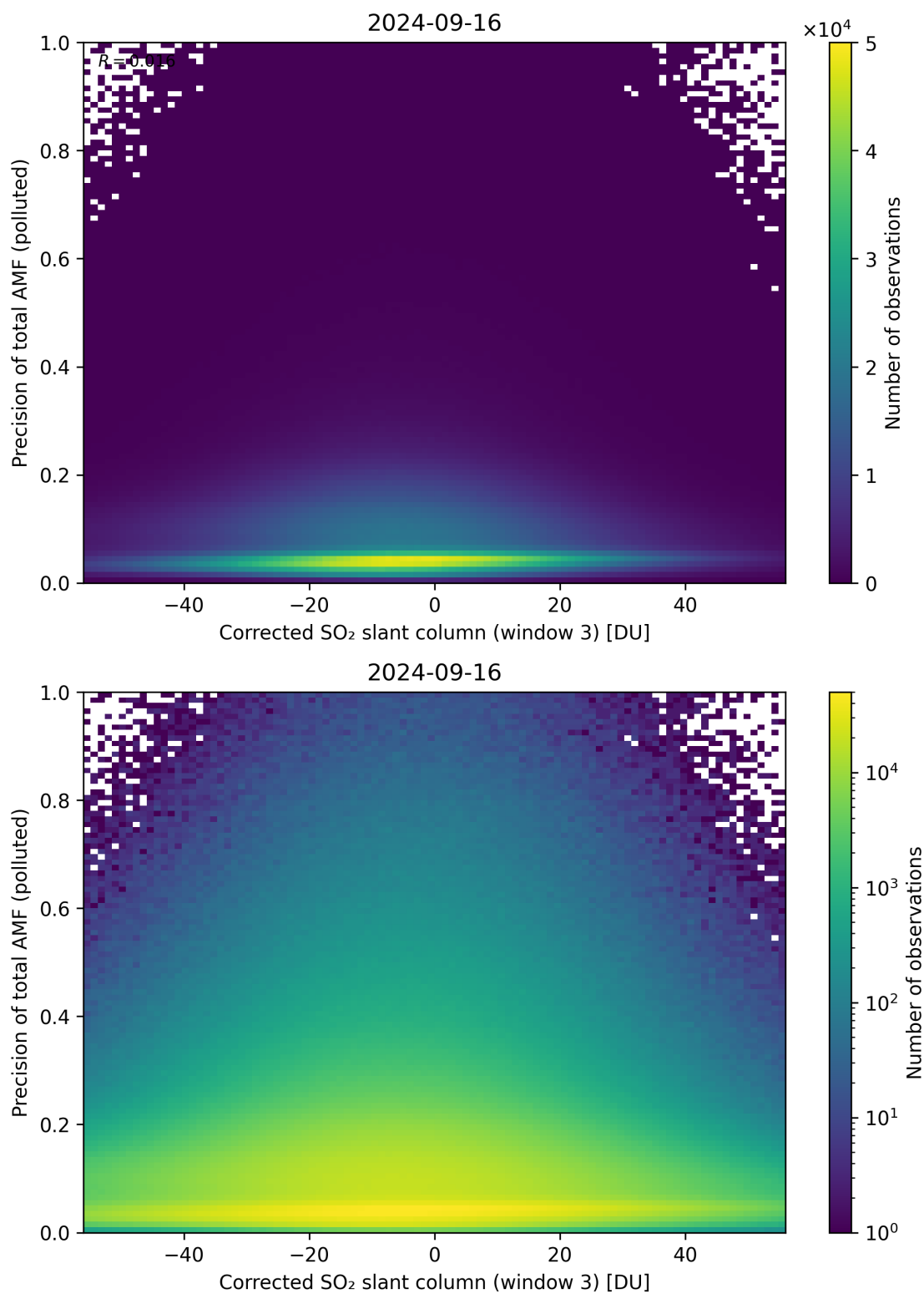
Figure 211: Scatter density plot of “Corrected SO 2 slant column (window 3)” against “Precision of total AMF (polluted)” for 2024-09-15 to 2024-09-17.
