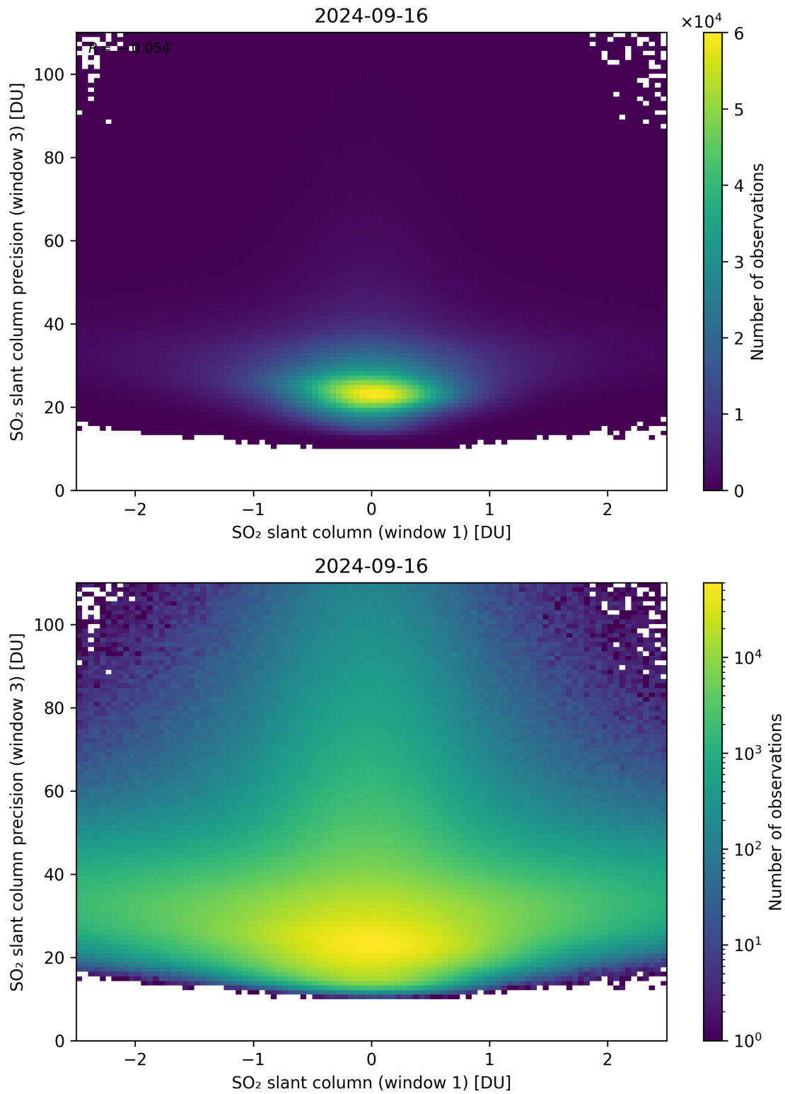
Figure 238: Scatter density plot of “SO 2 slant column (window 1)” against “SO 2 slant column precision (window 3)” for 2024-09-15 to 2024-09-17.
