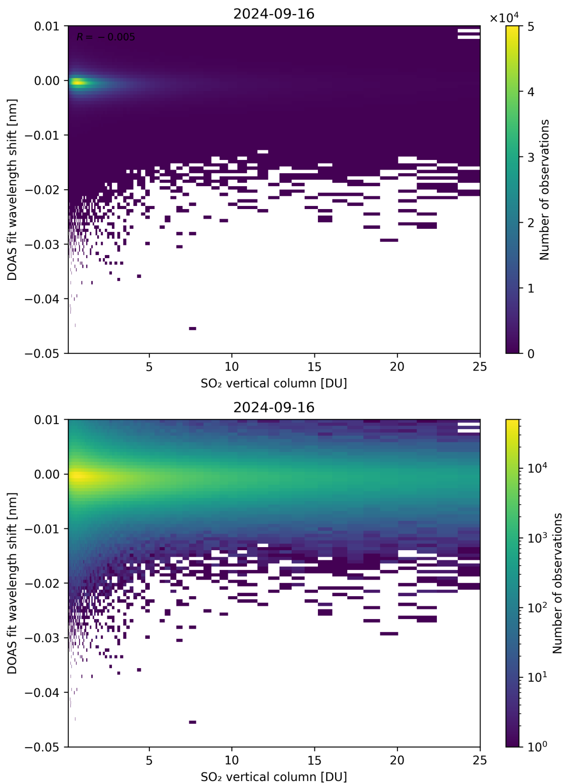
Figure 276: Scatter density plot of “SO 2 vertical column” against “DOAS fit wavelength shift” for 2024-09-15 to 2024-09-17.
