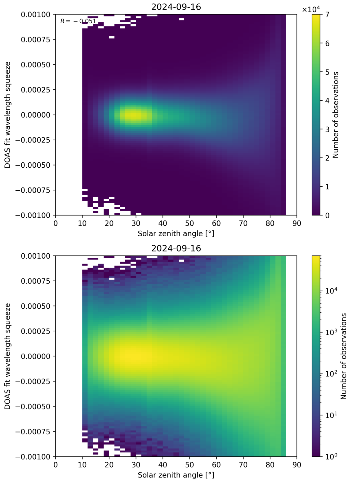
Figure 162: Scatter density plot of “Solar zenith angle” against “DOAS fit wavelength squeeze” for 2024-09-15 to 2024-09-17.
