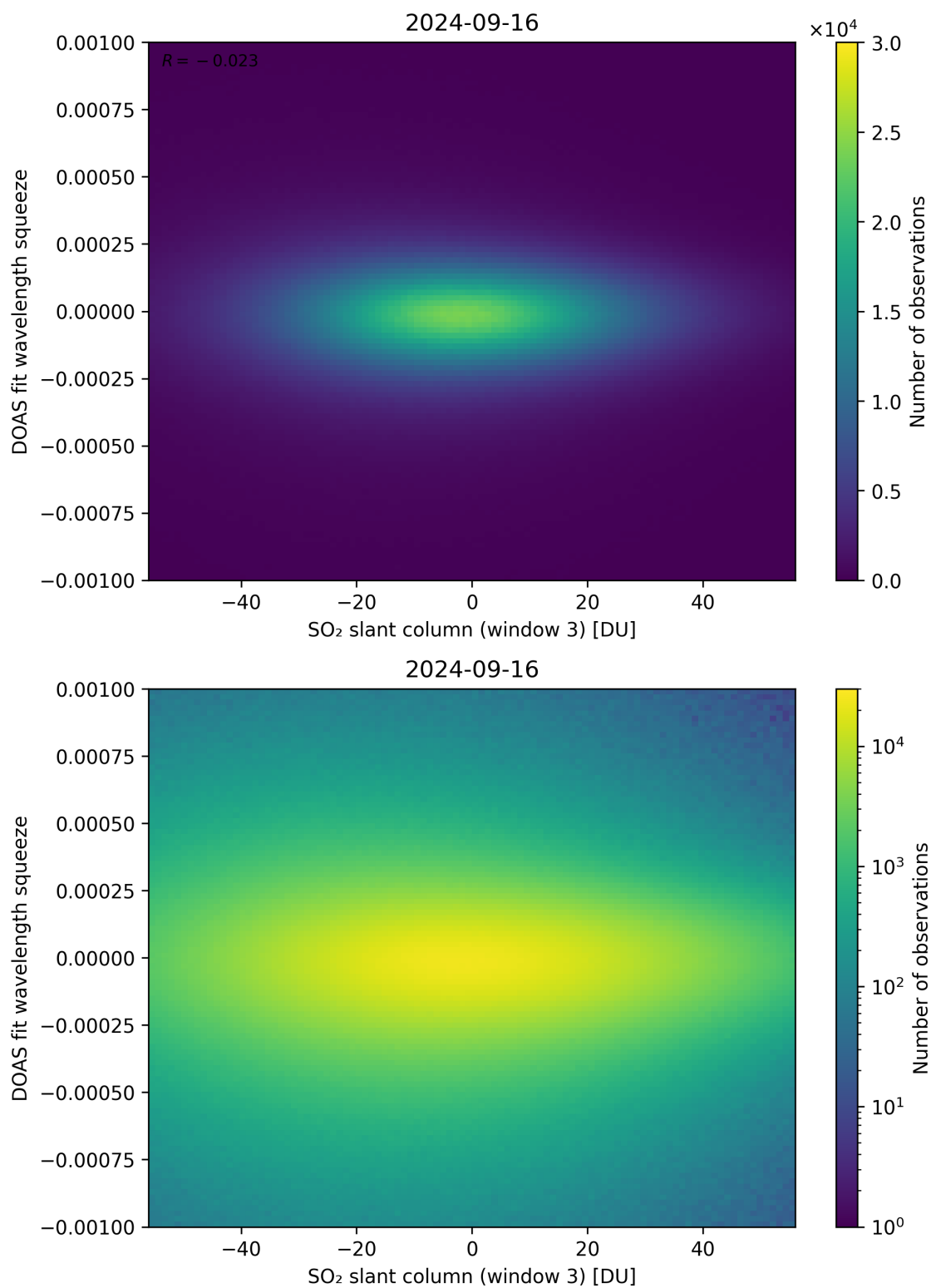
Figure 255: Scatter density plot of “SO 2 slant column (window 3)” against “DOAS fit wavelength squeeze” for 2024-09-15 to 2024-09-17.
