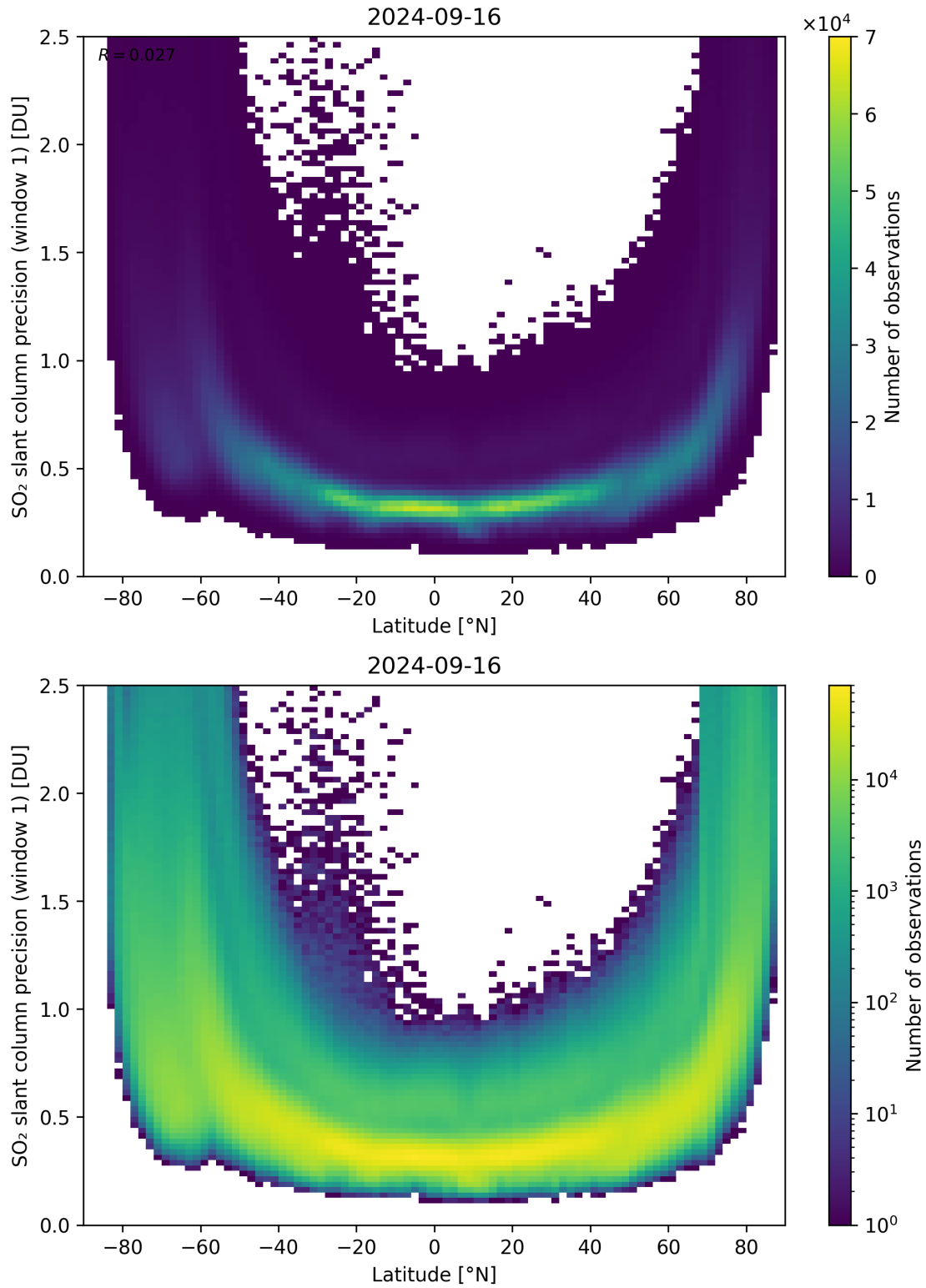
Figure 150: Scatter density plot of “Latitude” against “SO 2 slant column precision (window 1)” for 2024-09-15 to 2024-09-17.
