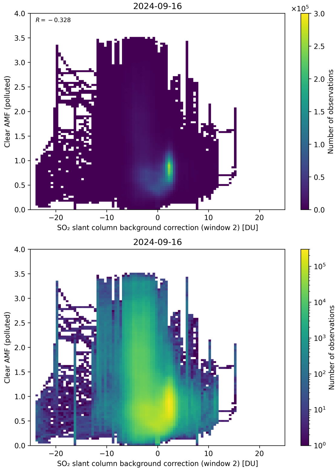
Figure 115: Scatter density plot of “SO 2 slant column background correction (window 2)” against “Clear AMF (polluted)” for 2024-09-15 to 2024-09-17.
