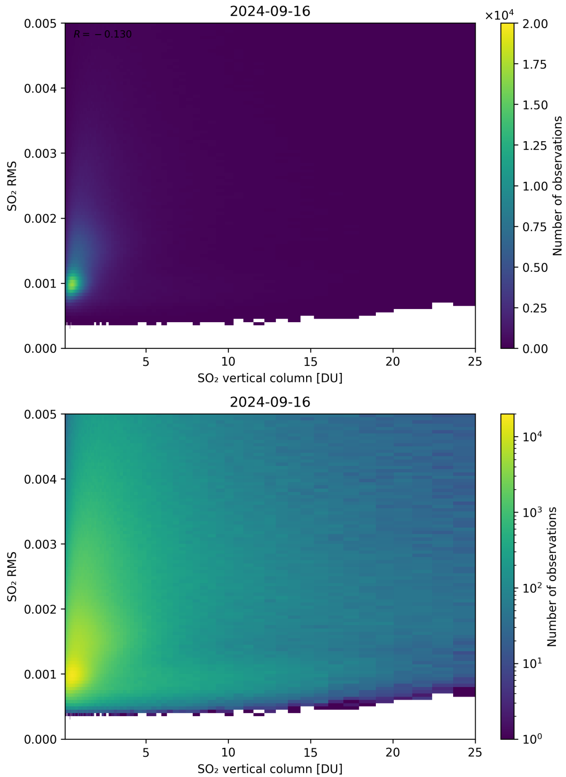
Figure 278: Scatter density plot of “SO 2 vertical column” against “SO 2 RMS” for 2024-09-15 to 2024-09-17.
