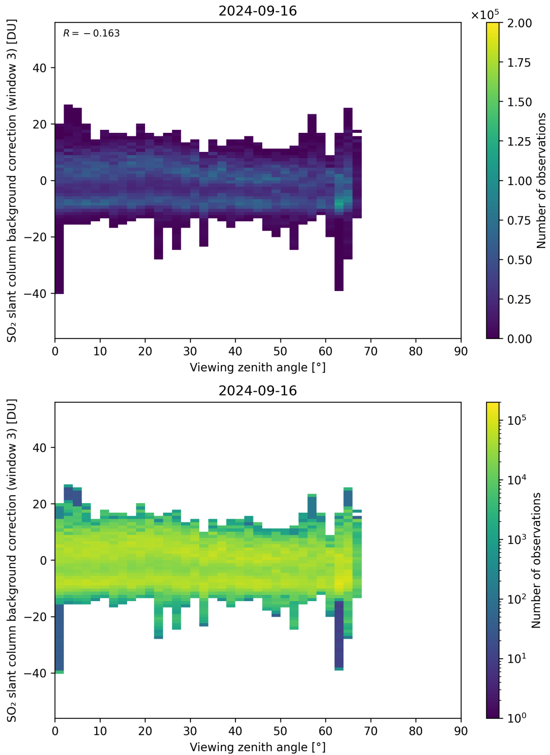
Figure 310: Scatter density plot of “Viewing zenith angle” against “SO 2 slant column background correction (window 3)” for 2024-09-15 to 2024-09-17.
