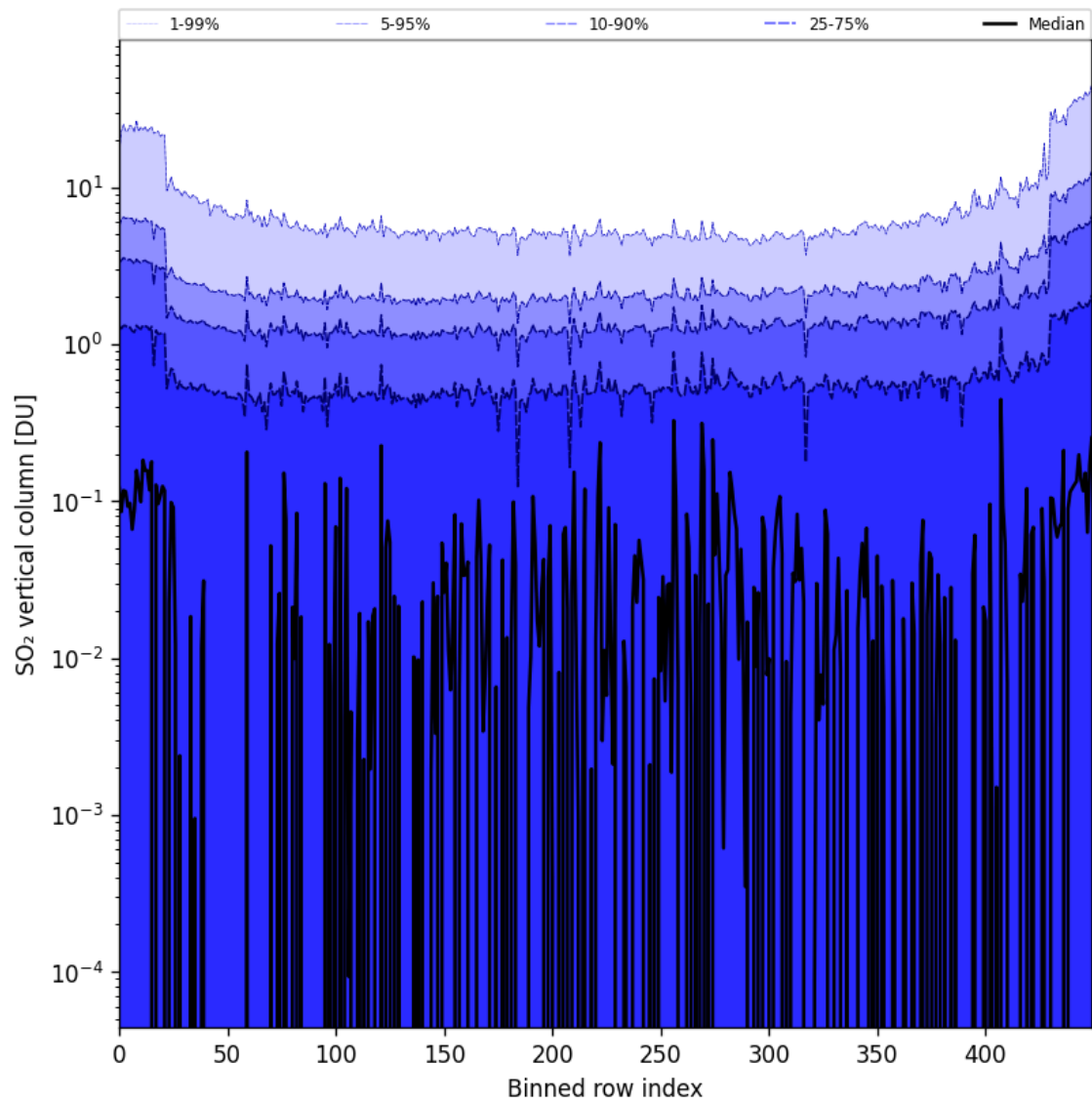
Figure 76: Along track statistics of “SO 2 vertical column” for 2024-09-15 to 2024-09-17
