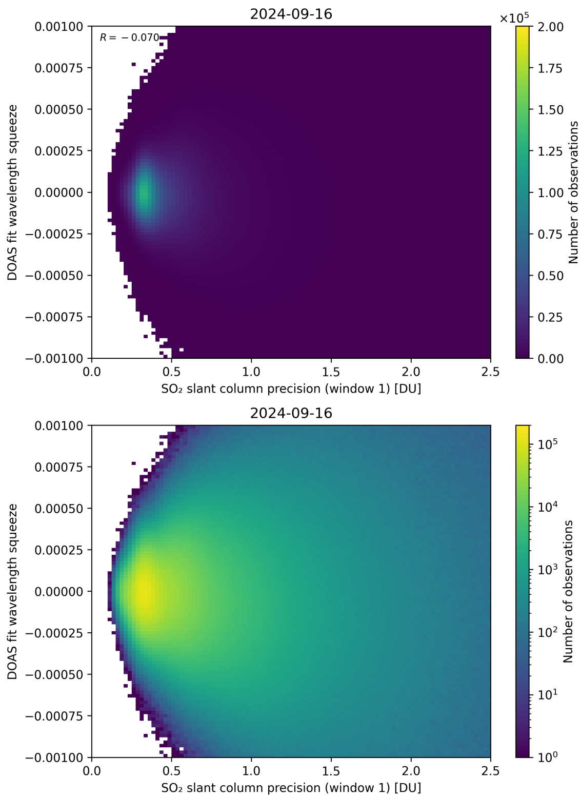
Figure 222: Scatter density plot of “SO 2 slant column precision (window 1)” against “DOAS fit wavelength squeeze” for 2024-09-15 to 2024-09-17.
