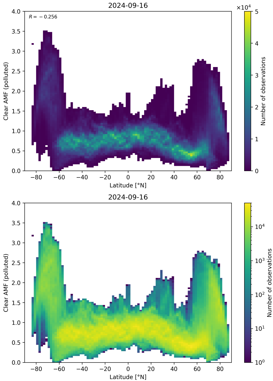
Figure 145: Scatter density plot of “Latitude” against “Clear AMF (polluted)” for 2024-09-15 to 2024-09-17.
