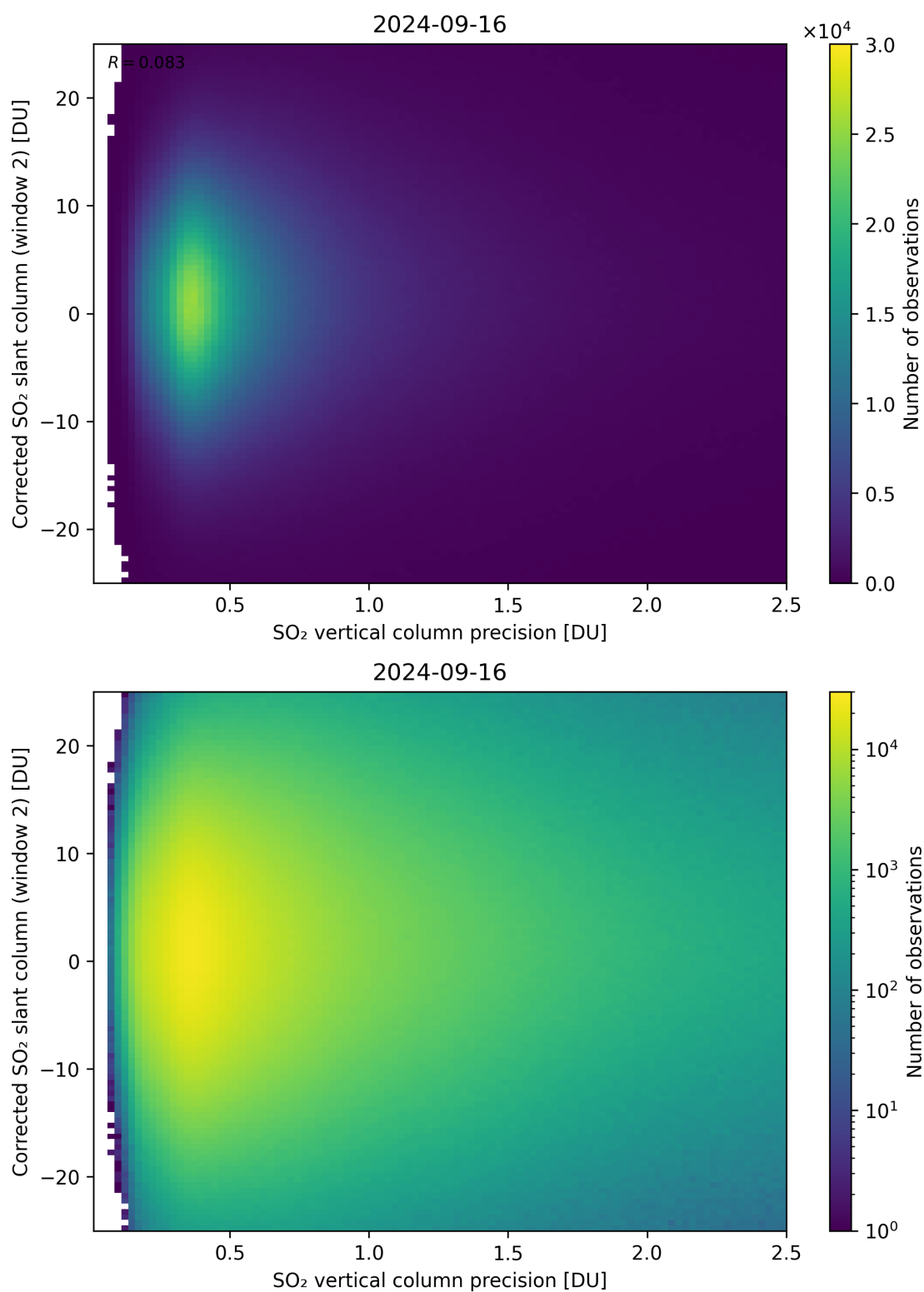
Figure 287: Scatter density plot of “SO 2 vertical column precision” against “Corrected SO 2 slant column (window 2)” for 2024-09-15 to 2024-09-17.
