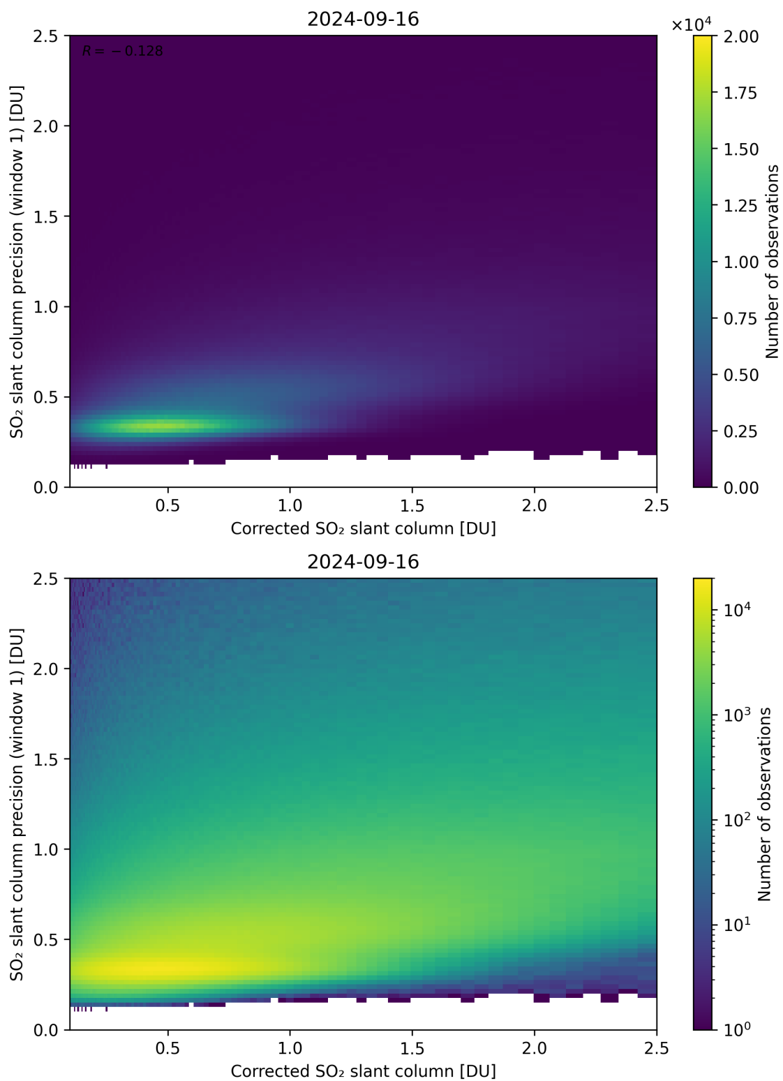
Figure 188: Scatter density plot of “Corrected SO 2 slant column” against “SO 2 slant column precision (window 1)” for 2024-09-15 to 2024-09-17.
