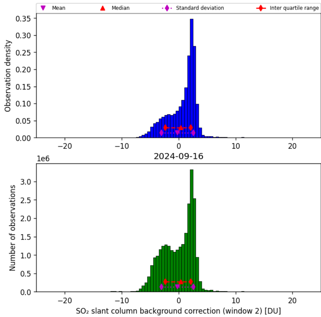
Figure 63: Histogram of “SO 2 slant column background correction (window 2)” for 2024-09-15 to 2024-09-17
