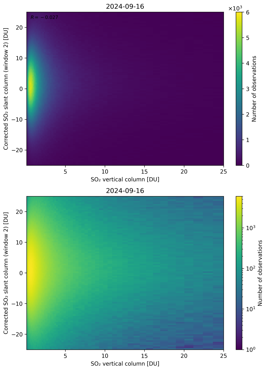
Figure 298: Scatter density plot of “SO 2 vertical column” against “Corrected SO 2 slant column (window 2)” for 2024-09-15 to 2024-09-17.
