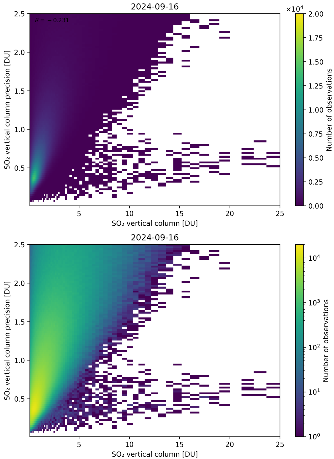
Figure 307: Scatter density plot of “SO 2 vertical column” against “SO 2 vertical column precision” for 2024-09-15 to 2024-09-17.
