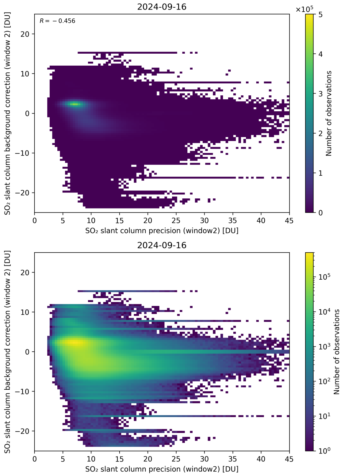
Figure 241: Scatter density plot of “SO 2 slant column precision (window2)” against “SO 2 slant column background correction (window 2)” for 2024-09-15 to 2024-09-17.
