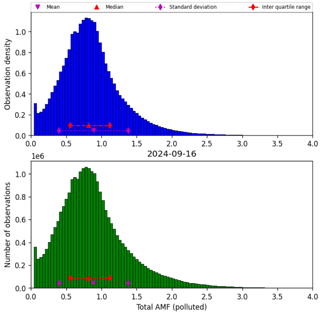
Figure 71: Histogram of “Total AMF (polluted)” for 2024-09-15 to 2024-09-17
