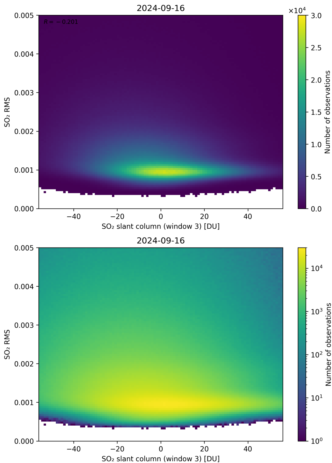
Figure 256: Scatter density plot of “SO 2 slant column (window 3)” against “SO 2 RMS” for 2024-09-15 to 2024-09-17.
