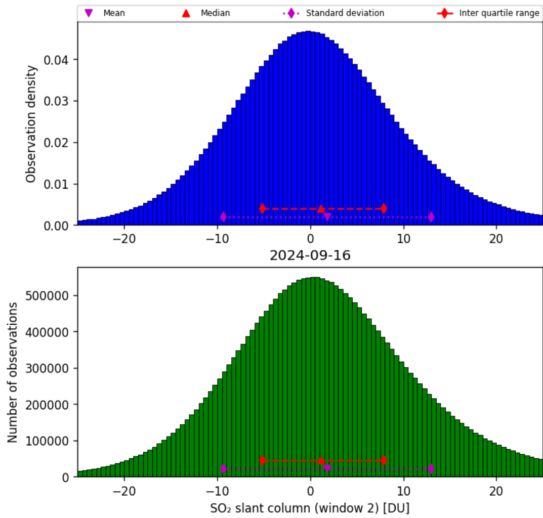
Figure 60: Histogram of “SO 2 slant column (window 2)” for 2024-09-15 to 2024-09-17
