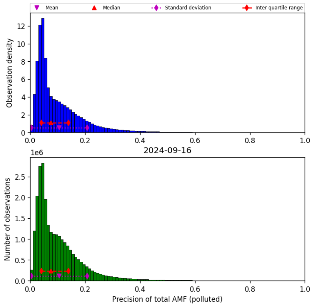
Figure 72: Histogram of “Precision of total AMF (polluted)” for 2024-09-15 to 2024-09-17
