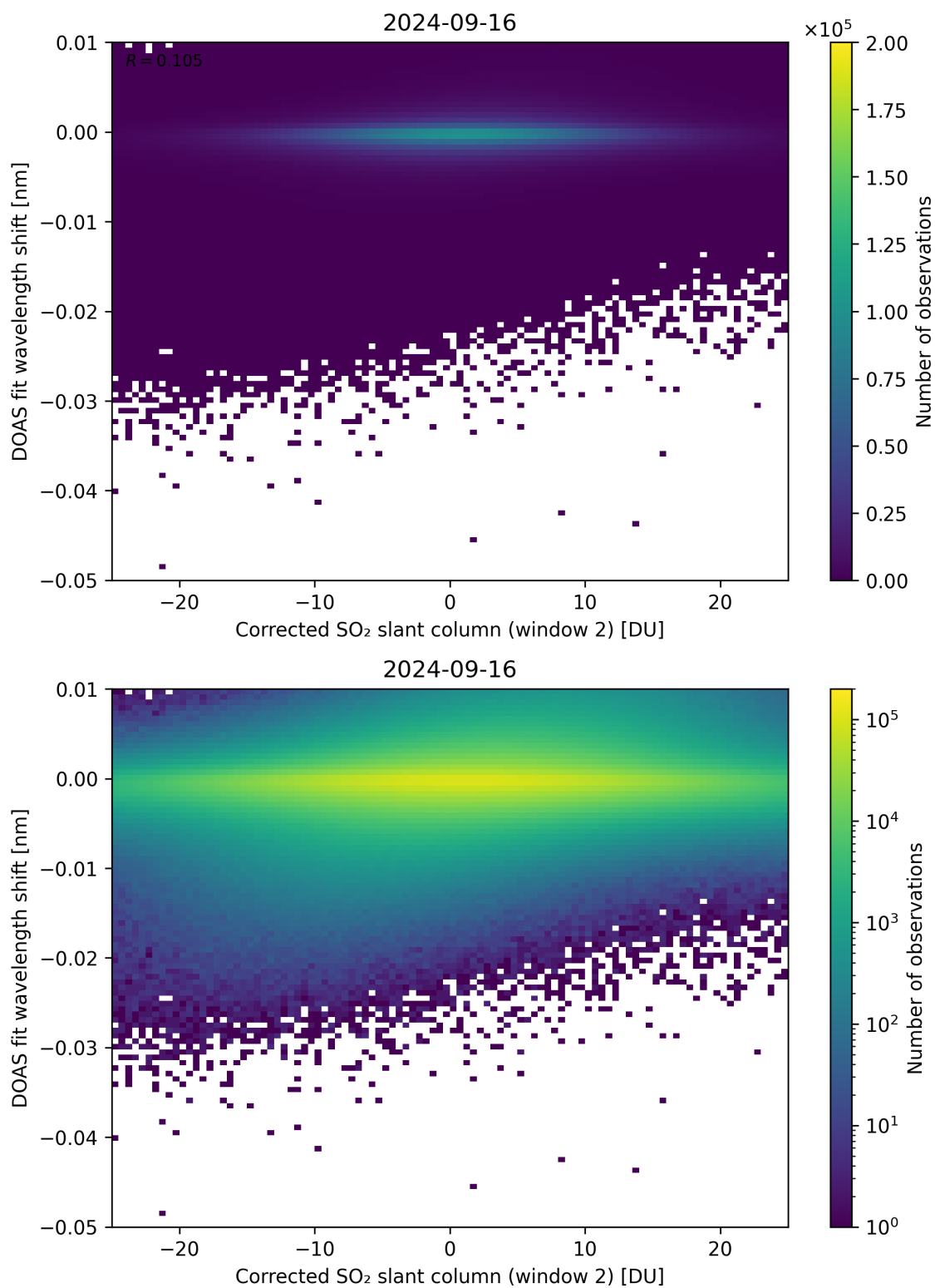
Figure 196: Scatter density plot of “Corrected SO 2 slant column (window 2)” against “DOAS fit wavelength shift” for 2024-09-15 to 2024-09-17.
