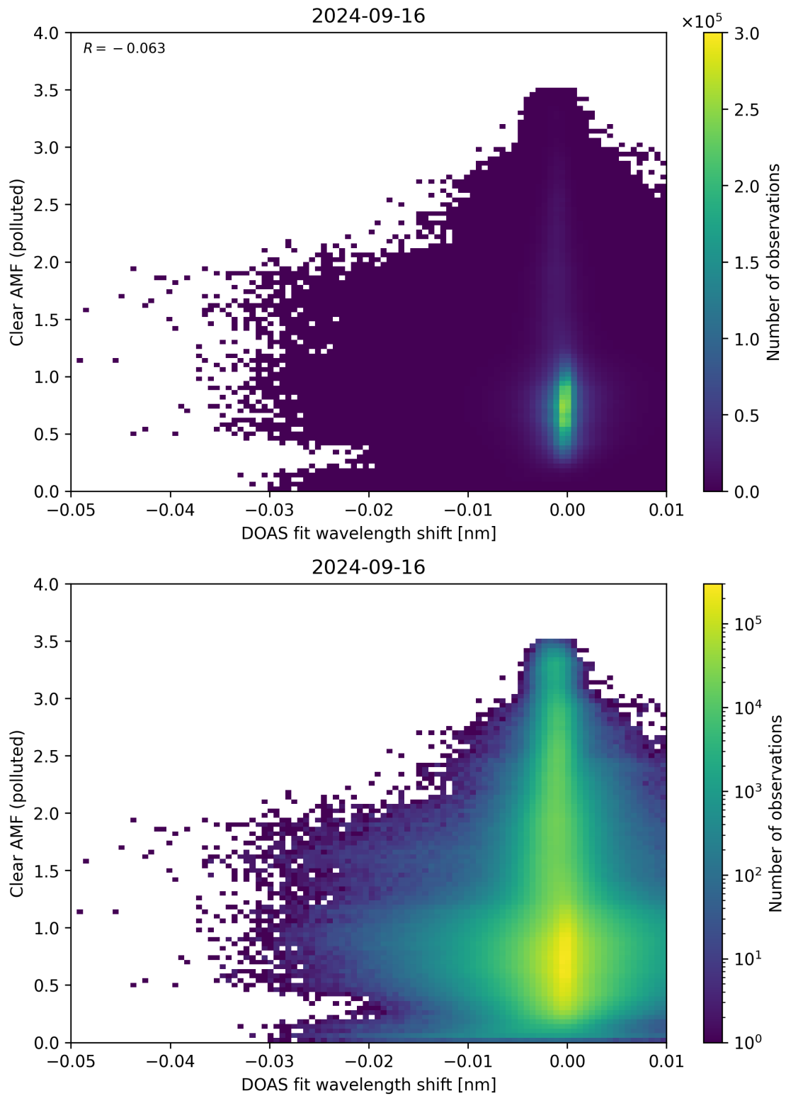
Figure 129: Scatter density plot of “DOAS fit wavelength shift” against “Clear AMF (polluted)” for 2024-09-15 to 2024-09-17.
