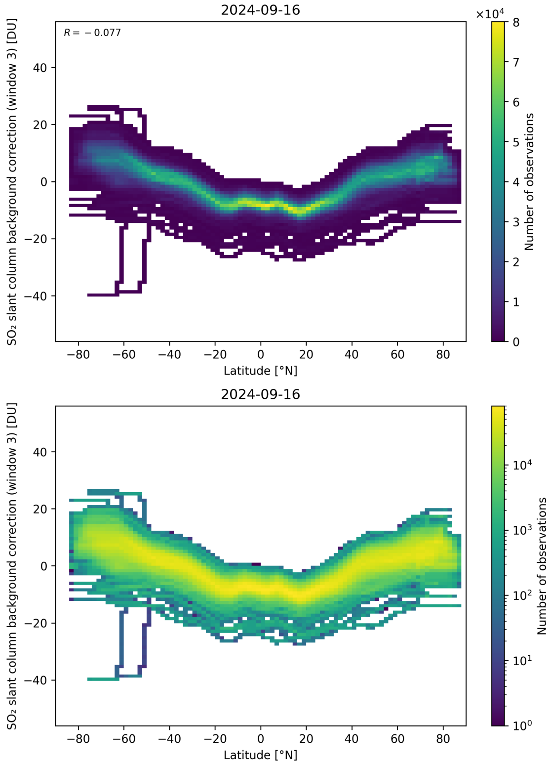
Figure 141: Scatter density plot of “Latitude” against “SO 2 slant column background correction (window 3)” for 2024-09-15 to 2024-09-17.
