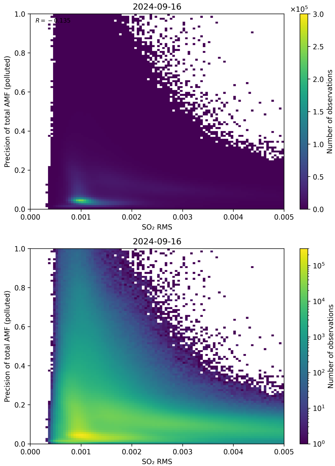
Figure 138: Scatter density plot of “SO 2 RMS” against “Precision of total AMF (polluted)” for 2024-09-15 to 2024-09-17.
