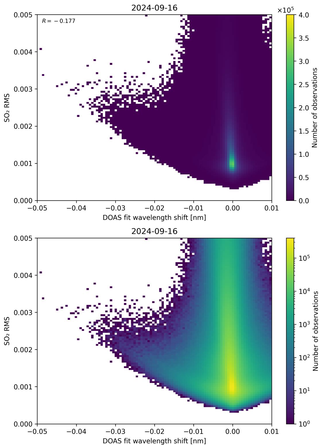
Figure 128: Scatter density plot of “DOAS fit wavelength shift” against “SO 2 RMS” for 2024-09-15 to 2024-09-17.
