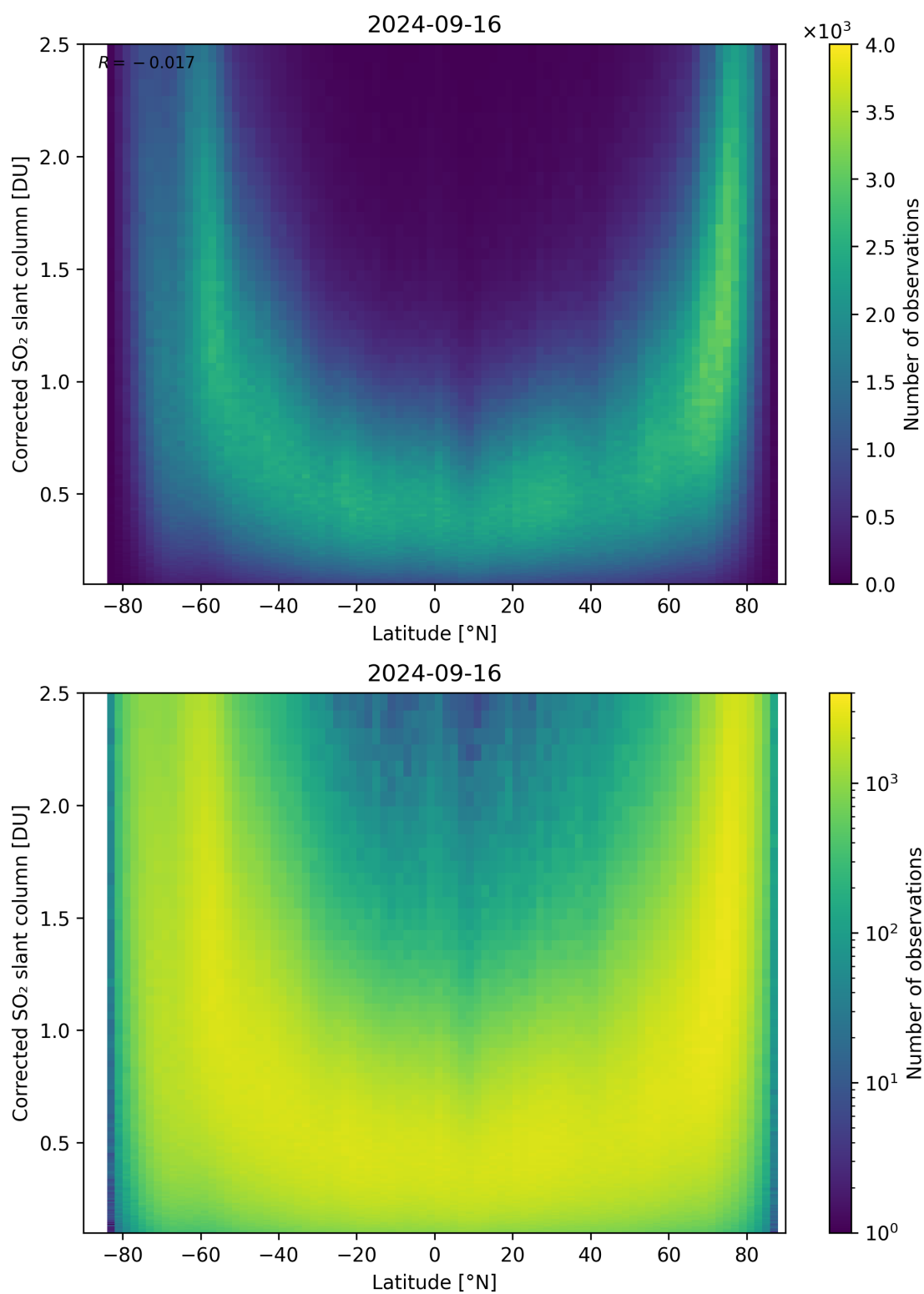
Figure 146: Scatter density plot of “Latitude” against “Corrected SO 2 slant column” for 2024-09-15 to 2024-09-17.
