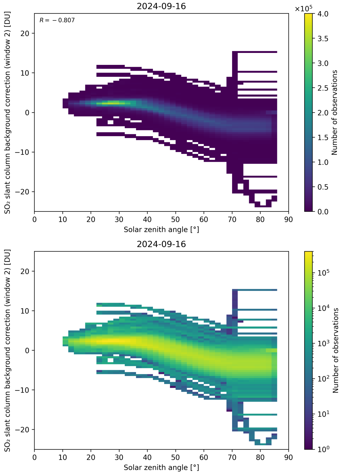
Figure 159: Scatter density plot of “Solar zenith angle” against “SO 2 slant column background correction (window 2)” for 2024-09-15 to 2024-09-17.
