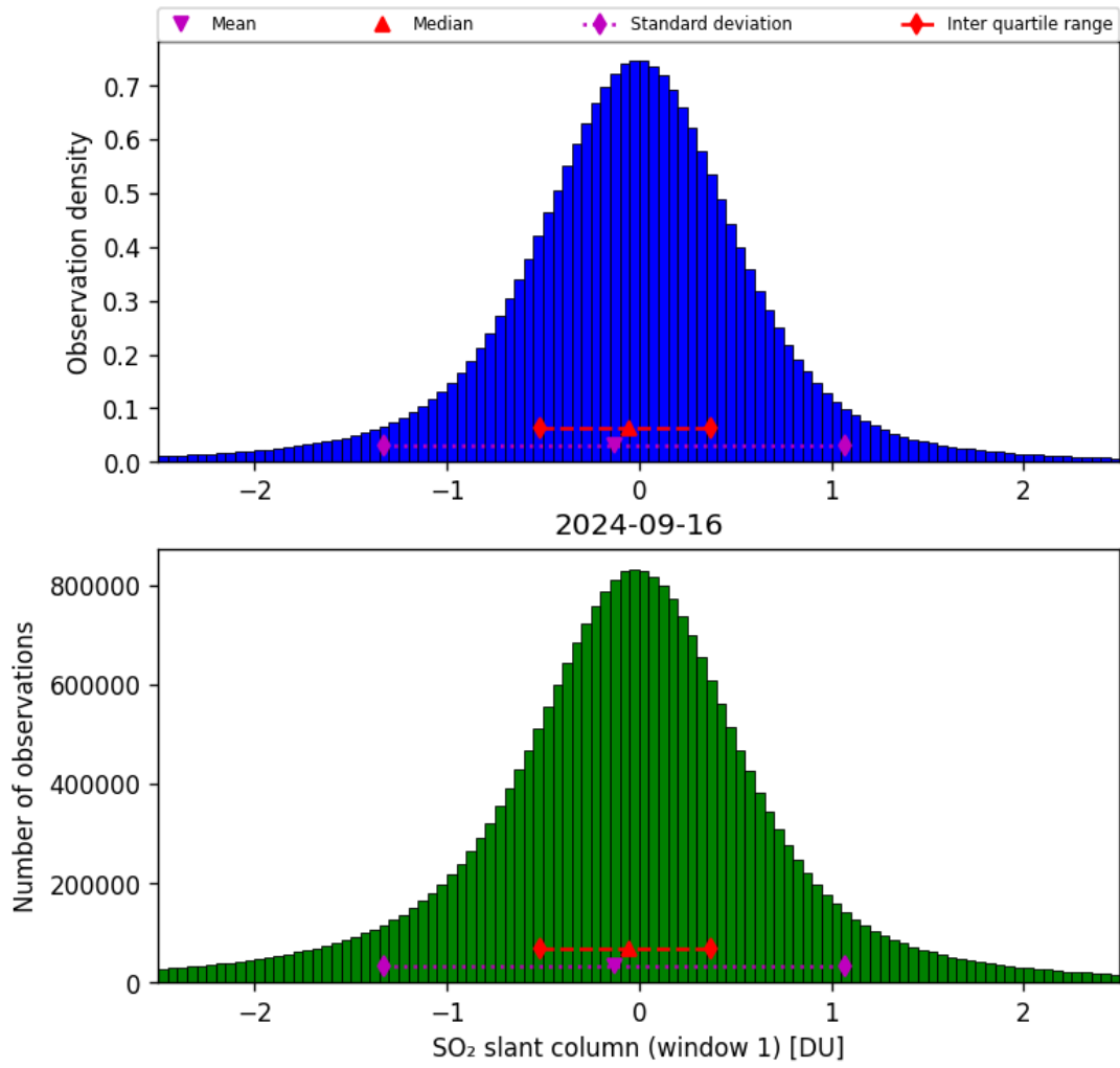
Figure 56: Histogram of “SO 2 slant column (window 1)” for 2024-09-15 to 2024-09-17
