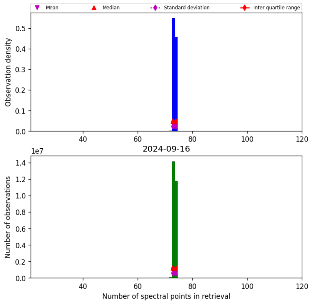
Figure 74: Histogram of “Number of spectral points in retrieval” for 2024-09-15 to 2024-09-17
