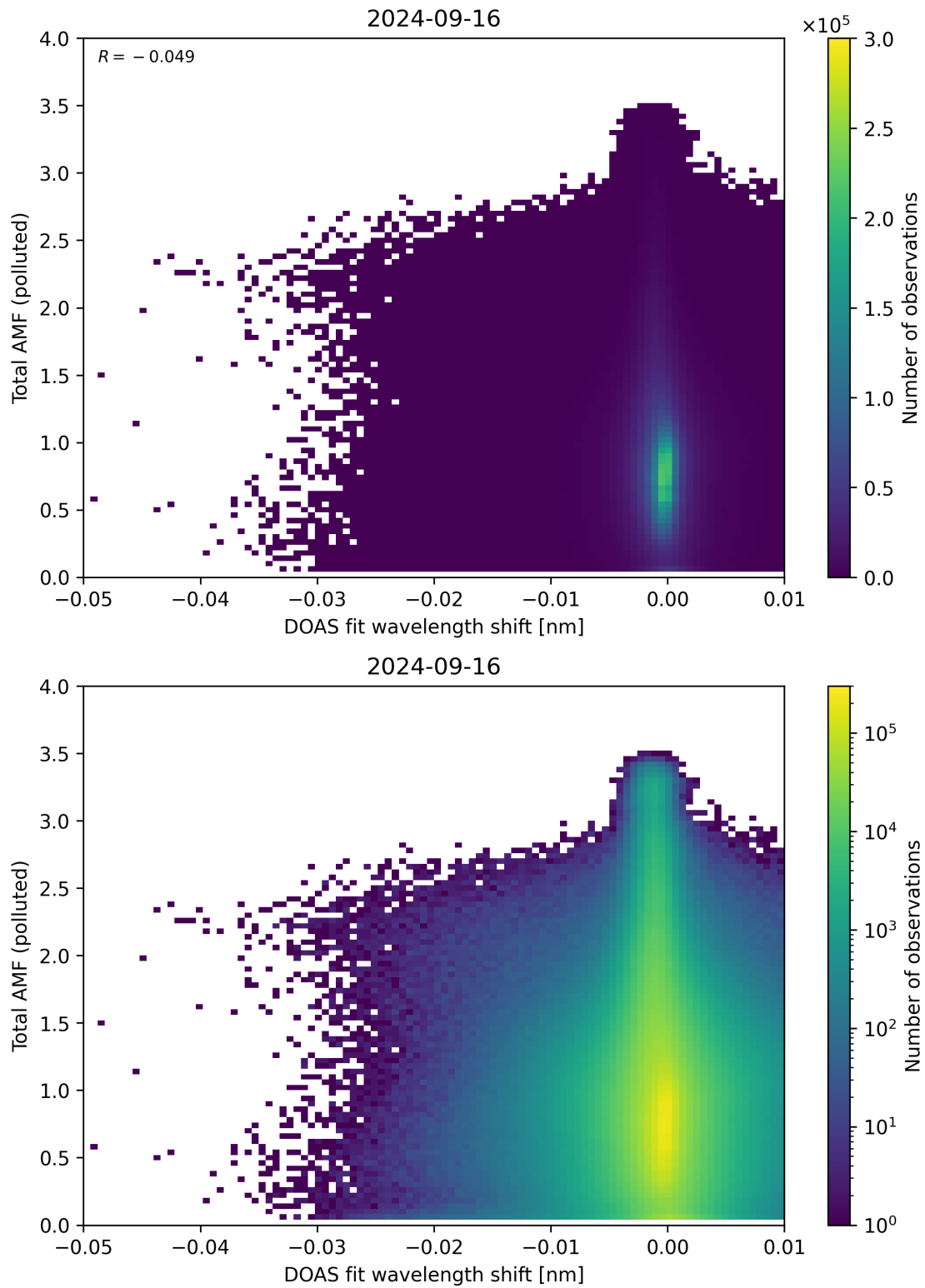
Figure 130: Scatter density plot of “DOAS fit wavelength shift” against “Total AMF (polluted)” for 2024-09-15 to 2024-09-17.
