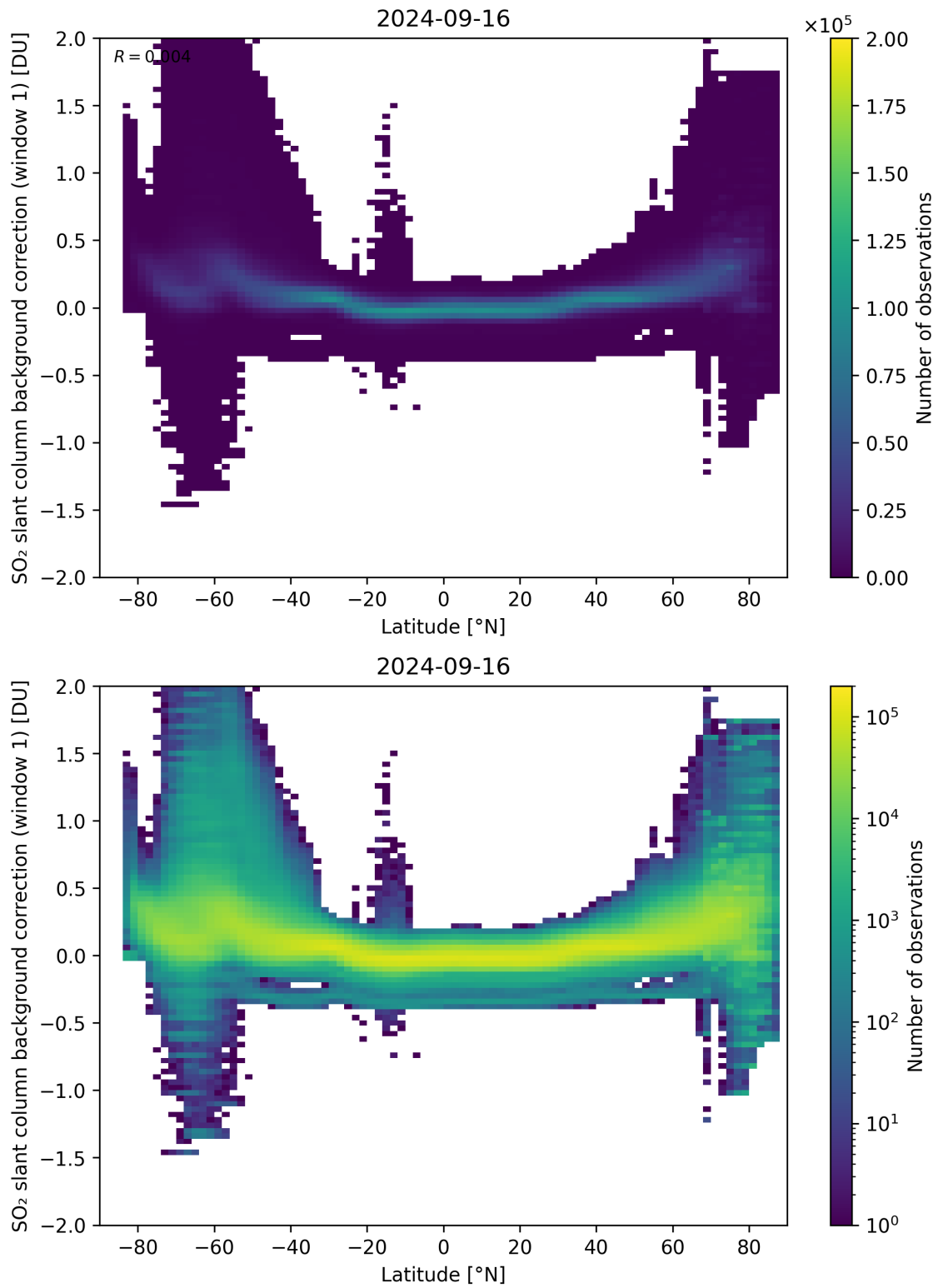
Figure 139: Scatter density plot of “Latitude” against “SO 2 slant column background correction (window 1)” for 2024-09-15 to 2024-09-17.
