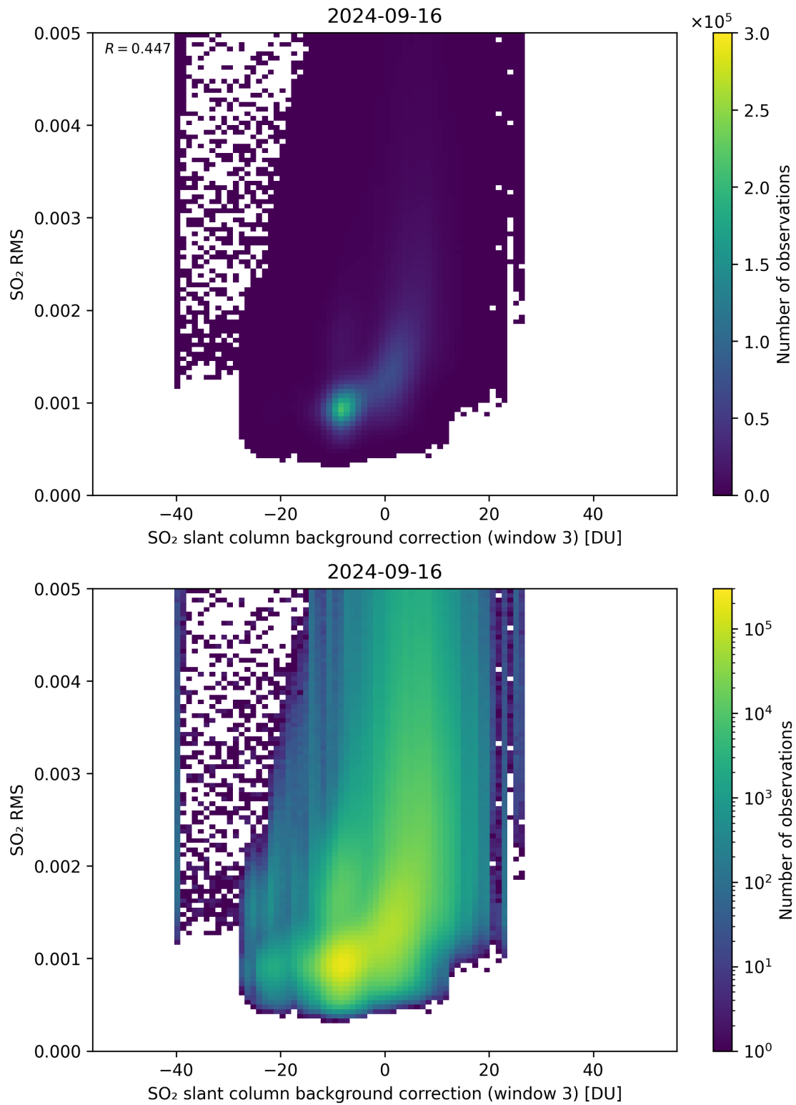
Figure 123: Scatter density plot of “SO 2 slant column background correction (window 3)” against “SO 2 RMS” for 2024-09-15 to 2024-09-17.
