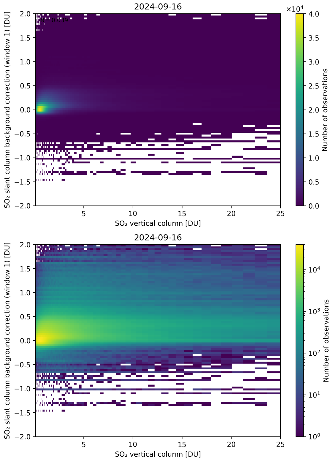
Figure 273: Scatter density plot of “SO 2 vertical column” against “SO 2 slant column background correction (window 1)” for 2024-09-15 to 2024-09-17.
