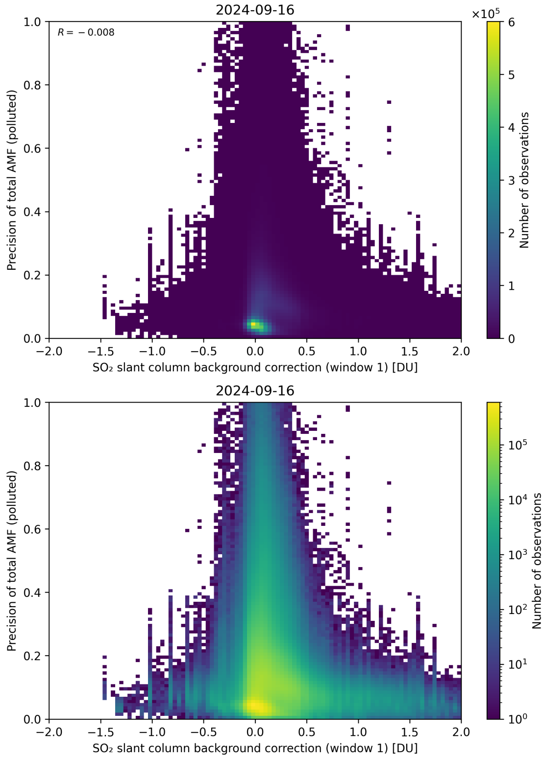
Figure 110: Scatter density plot of “SO 2 slant column background correction (window 1)” against “Precision of total AMF (polluted)” for 2024-09-15 to 2024-09-17.
