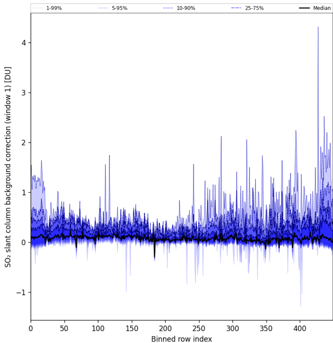
Figure 82: Along track statistics of “SO 2 slant column background correction (window 1)” for 2024-09-15 to 2024-09-17
