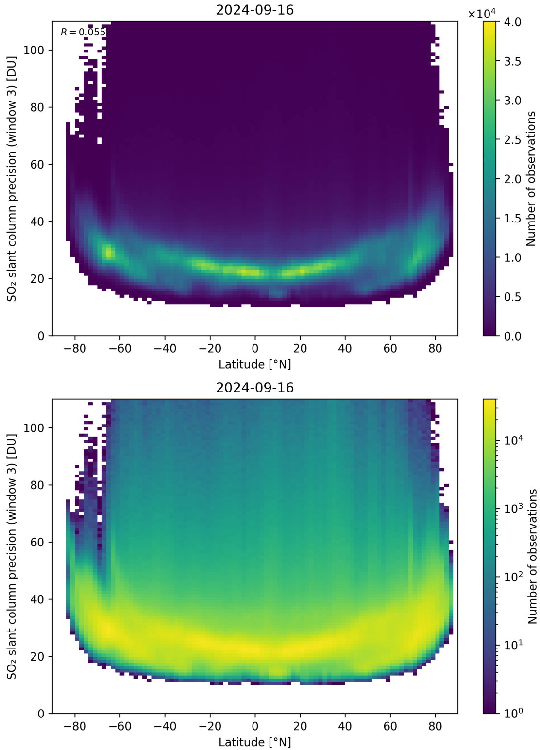
Figure 153: Scatter density plot of “Latitude” against “SO 2 slant column precision (window 3)” for 2024-09-15 to 2024-09-17.
