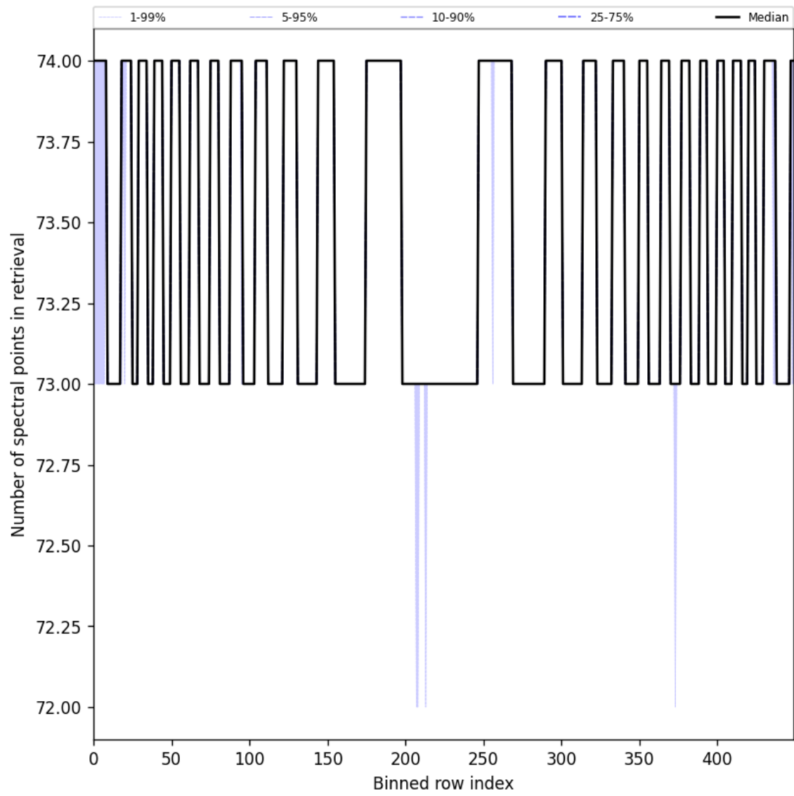
Figure 97: Along track statistics of “Number of spectral points in retrieval” for 2024-09-15 to 2024-09-17
