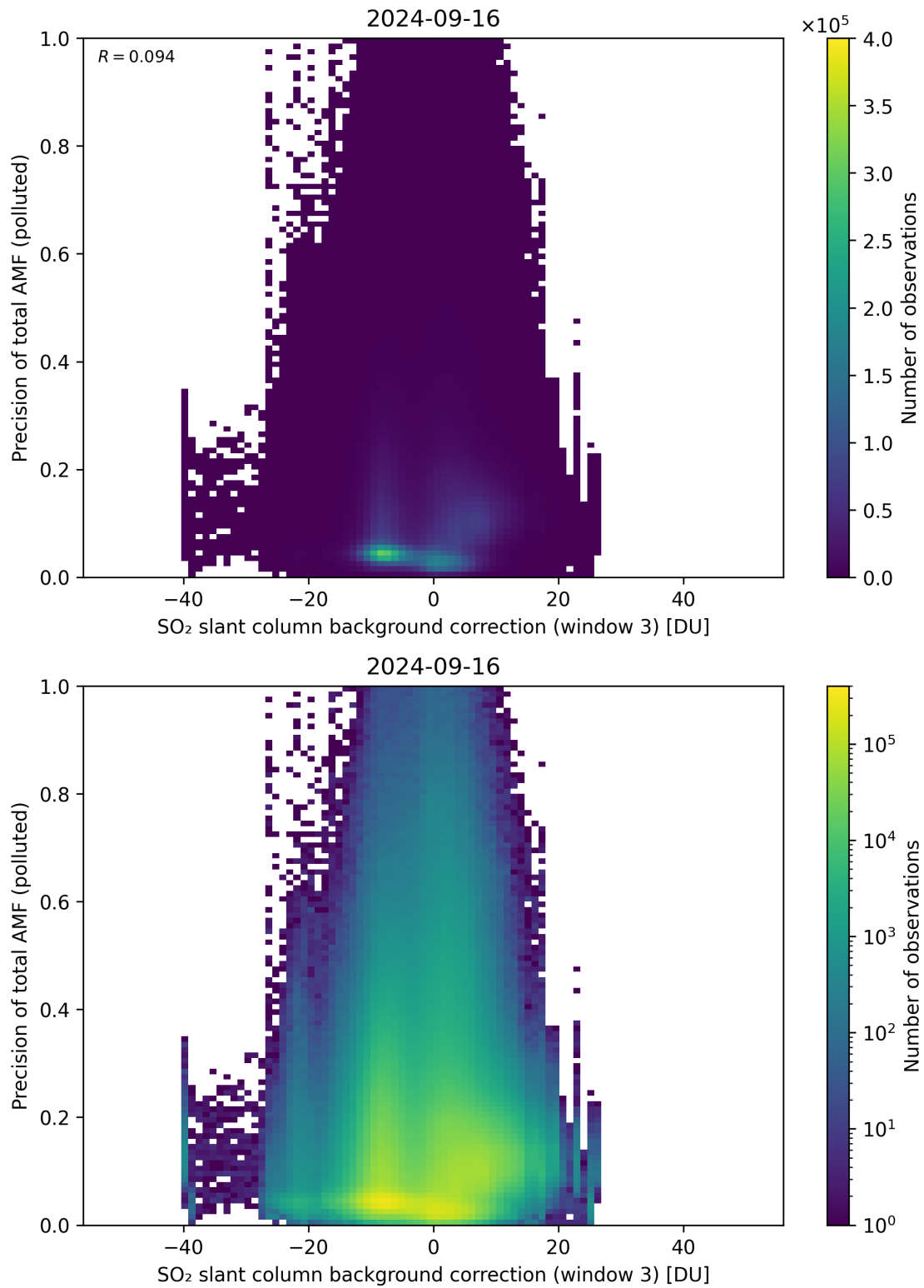
Figure 126: Scatter density plot of “SO 2 slant column background correction (window 3)” against “Precision of total AMF (polluted)” for 2024-09-15 to 2024-09-17.
