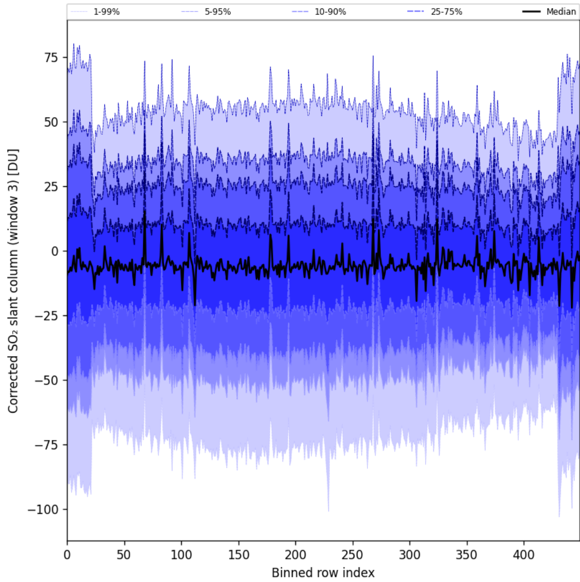
Figure 89: Along track statistics of “Corrected SO 2 slant column (window 3)” for 2024-09-15 to 2024-09-17
