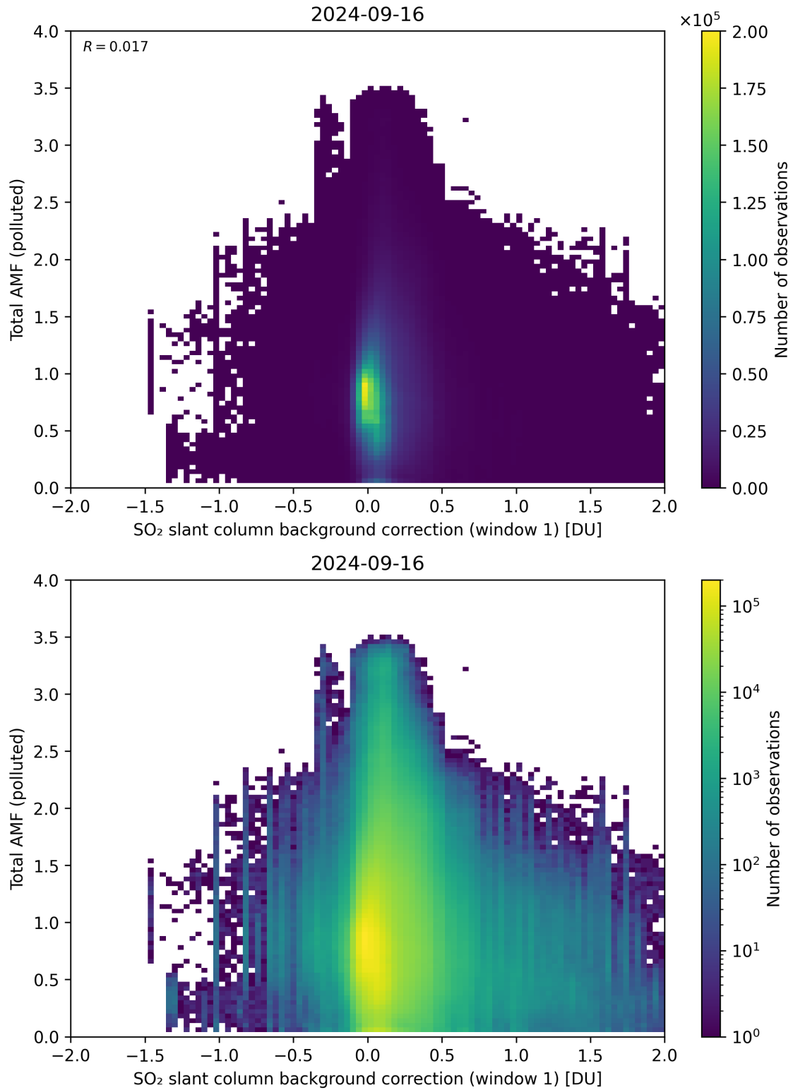
Figure 109: Scatter density plot of “SO 2 slant column background correction (window 1)” against “Total AMF (polluted)” for 2024-09-15 to 2024-09-17.
