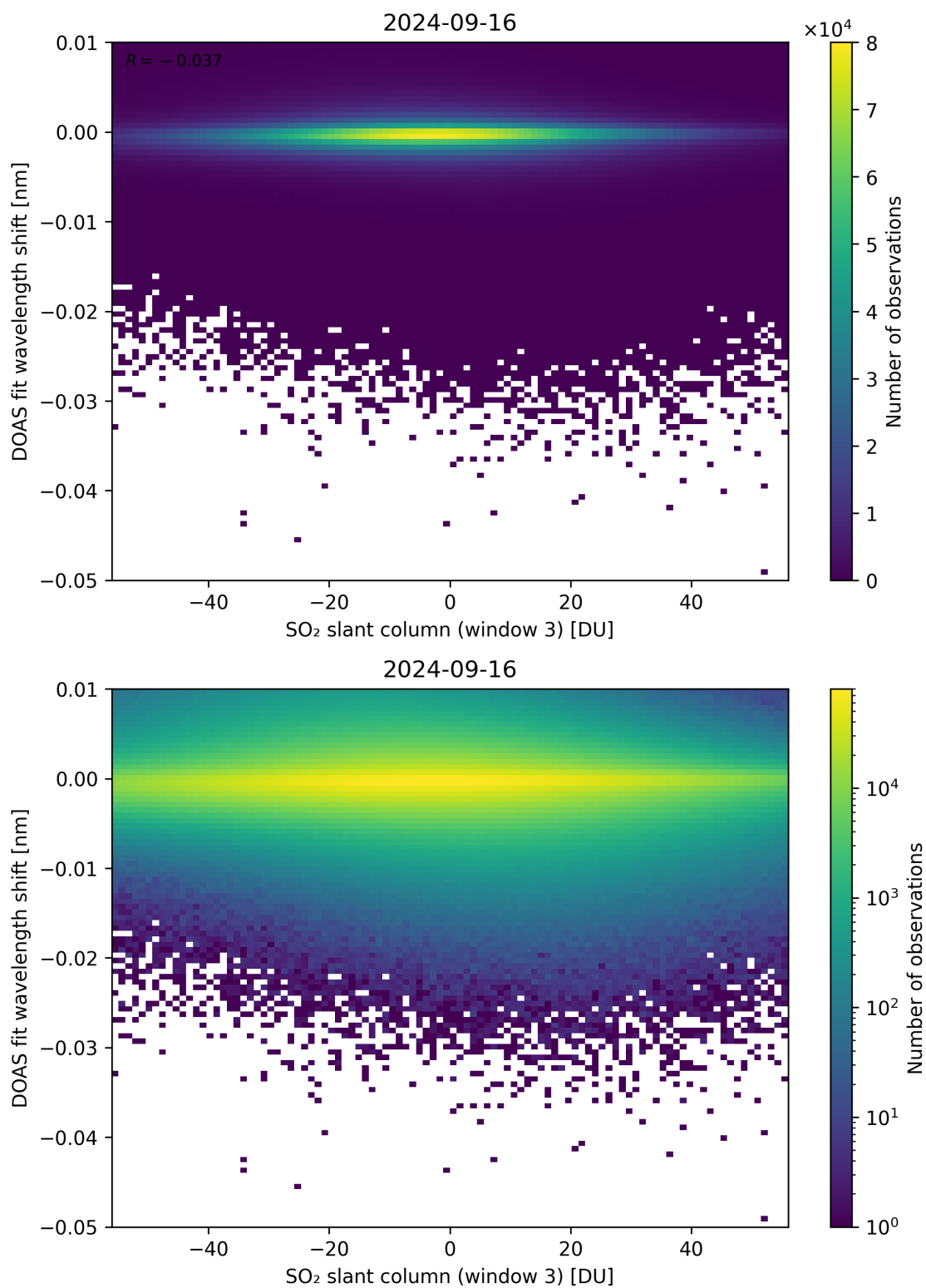
Figure 254: Scatter density plot of “SO 2 slant column (window 3)” against “DOAS fit wavelength shift” for 2024-09-15 to 2024-09-17.
