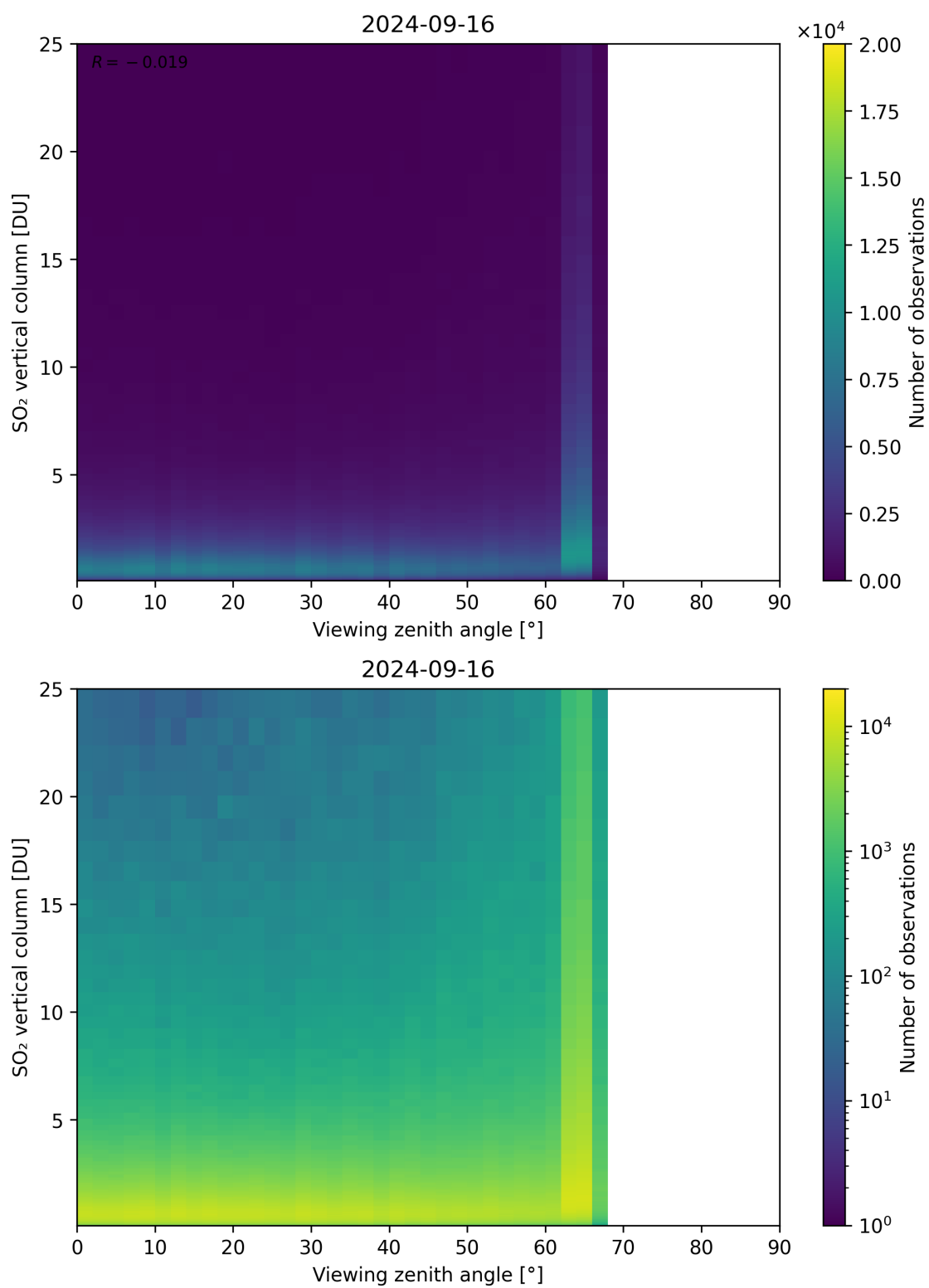
Figure 327: Scatter density plot of “Viewing zenith angle” against “SO 2 vertical column” for 2024-09-15 to 2024-09-17.
