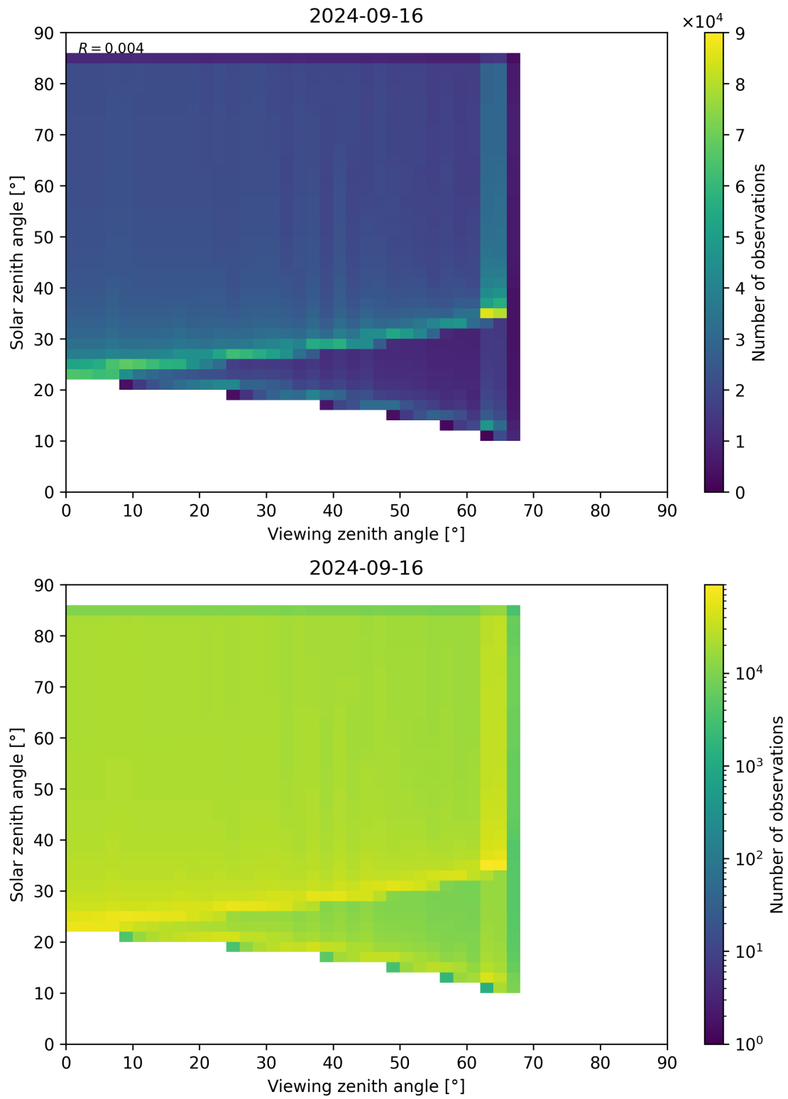
Figure 315: Scatter density plot of “Viewing zenith angle” against “Solar zenith angle” for 2024-09-15 to 2024-09-17.
