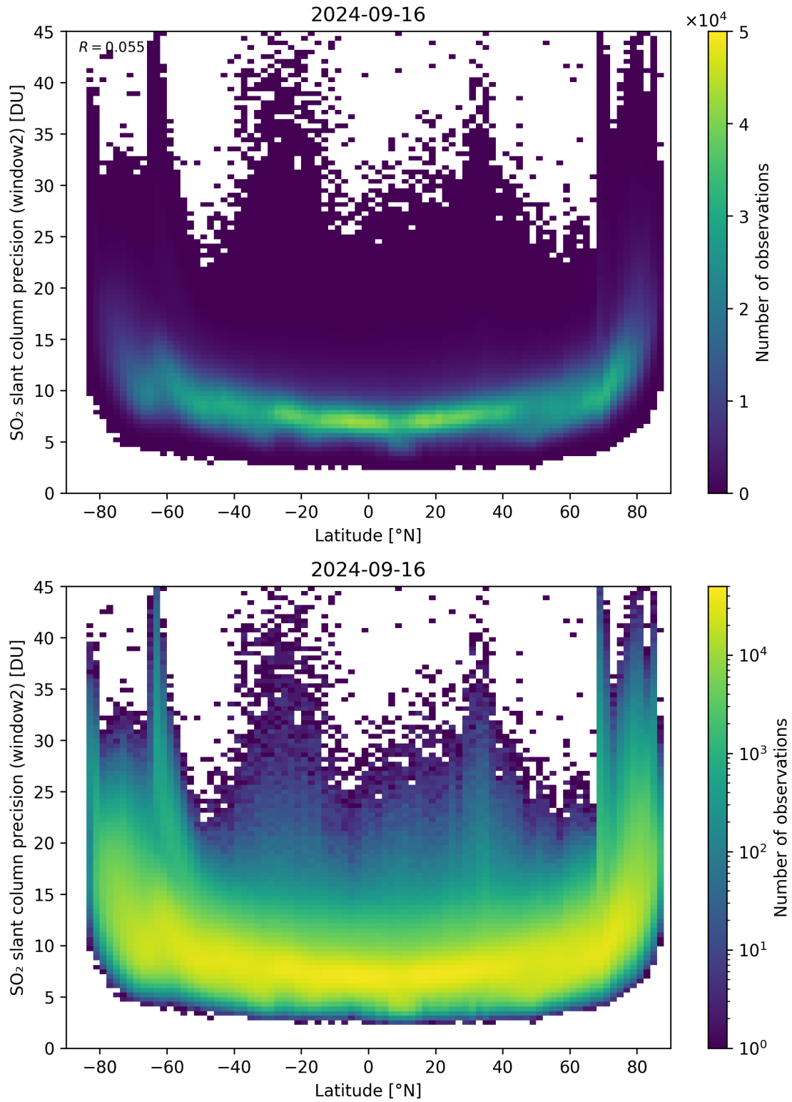
Figure 151: Scatter density plot of “Latitude” against “SO 2 slant column precision (window2)” for 2024-09-15 to 2024-09-17.
