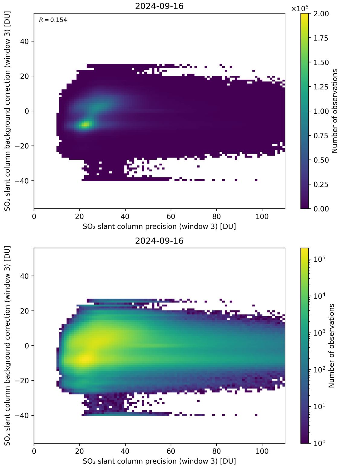
Figure 257: Scatter density plot of “SO 2 slant column precision (window 3)” against “SO 2 slant column background correction (window 3)” for 2024-09-15 to 2024-09-17.
