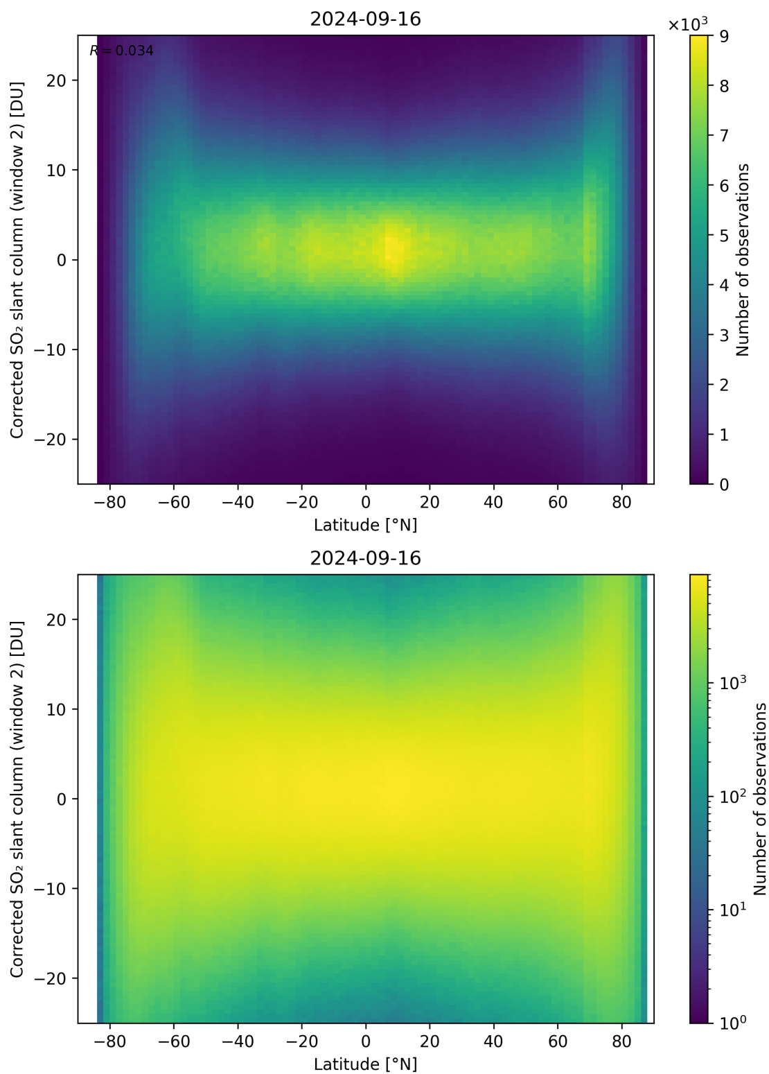
Figure 147: Scatter density plot of “Latitude” against “Corrected SO 2 slant column (window 2)” for 2024-09-15 to 2024-09-17.
