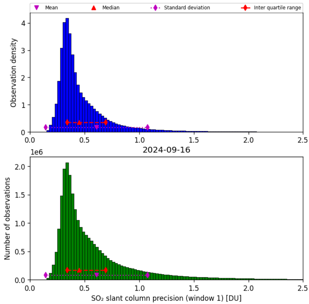
Figure 57: Histogram of “SO 2 slant column precision (window 1)” for 2024-09-15 to 2024-09-17
