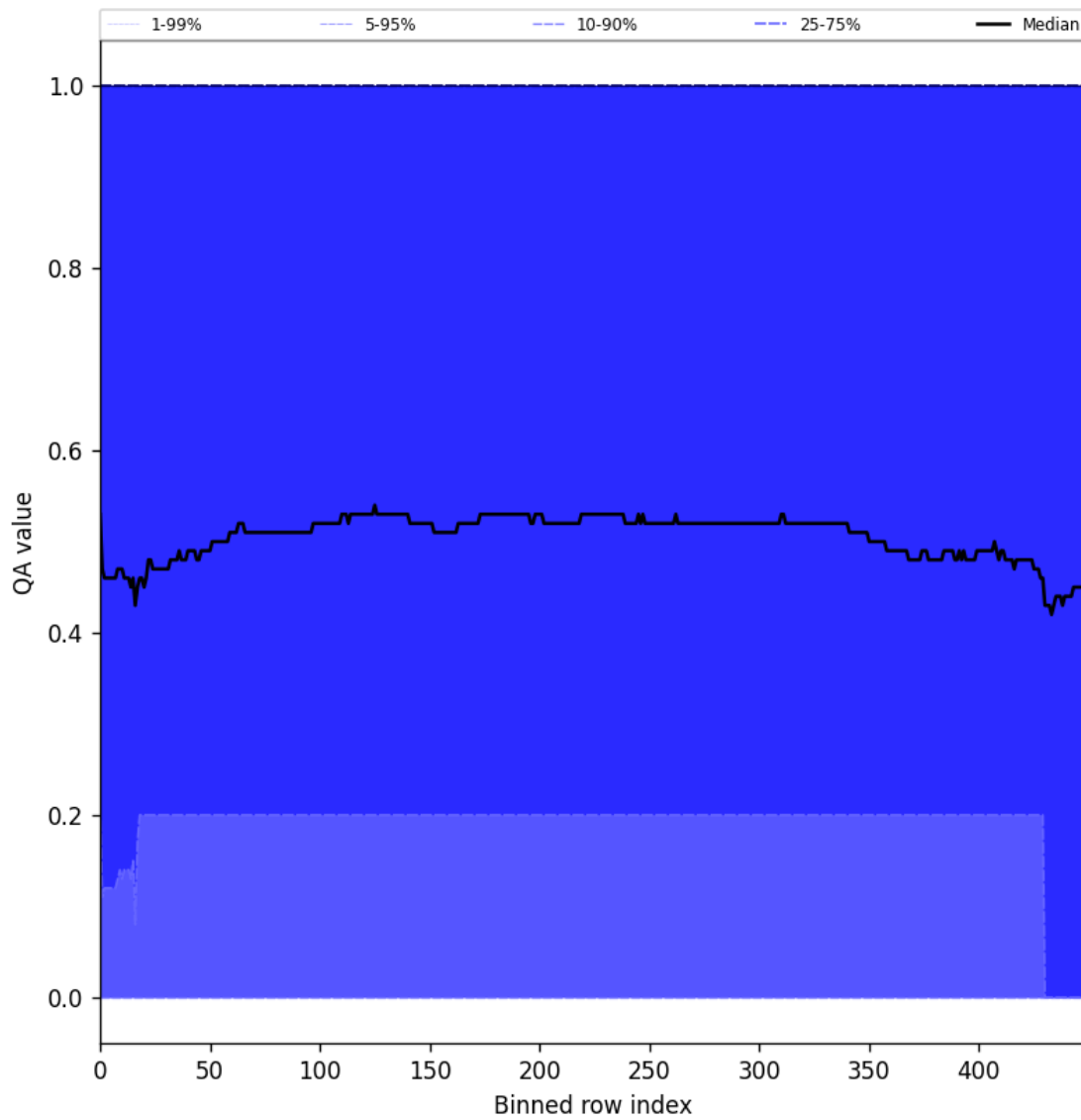
Figure 75: Along track statistics of “QA value” for 2024-09-15 to 2024-09-17
