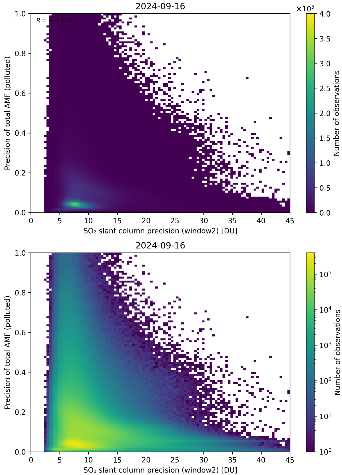
Figure 252: Scatter density plot of “SO 2 slant column precision (window2)” against “Precision of total AMF (polluted)” for 2024-09-15 to 2024-09-17.
