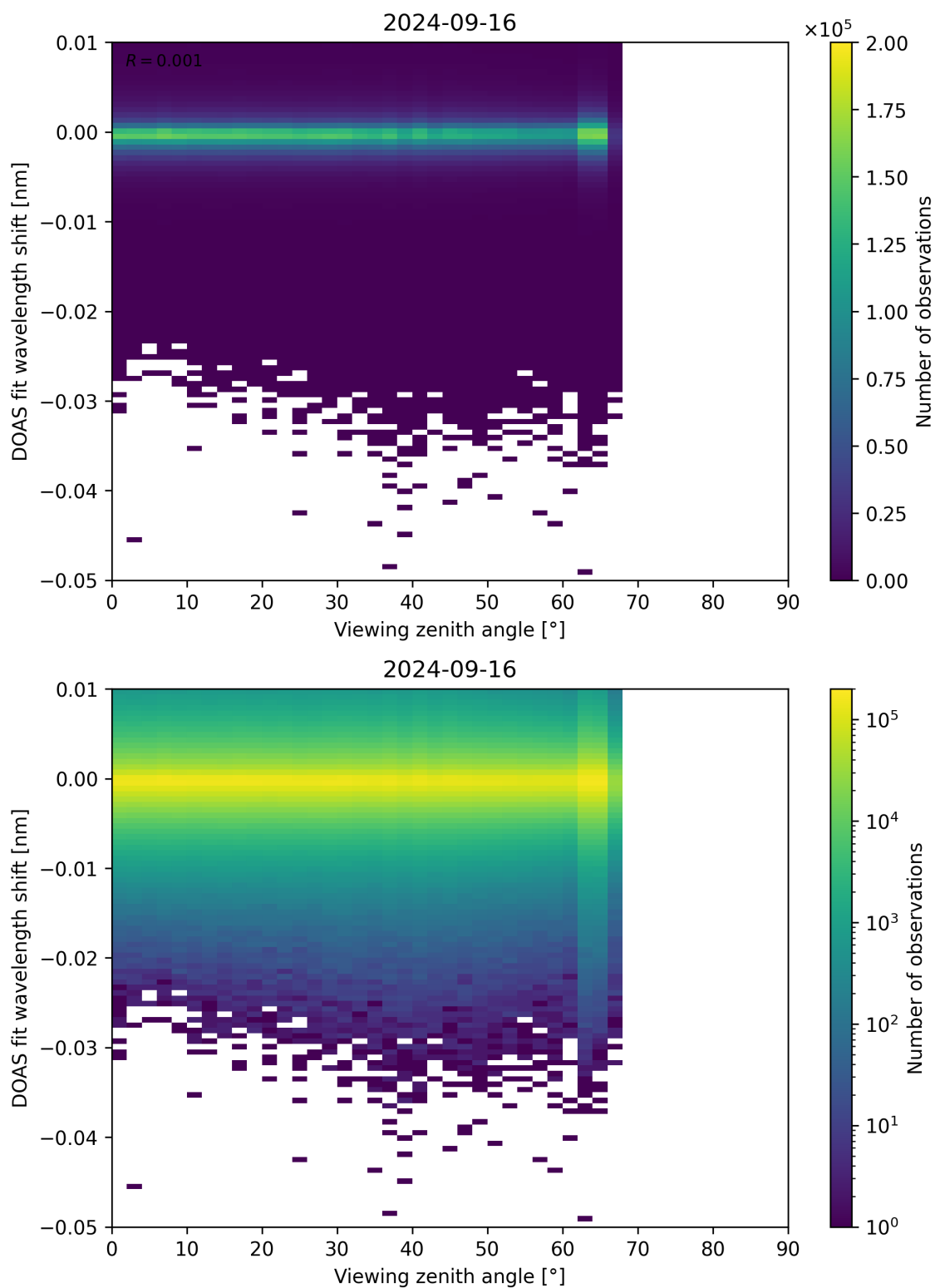
Figure 311: Scatter density plot of “Viewing zenith angle” against “DOAS fit wavelength shift” for 2024-09-15 to 2024-09-17.
