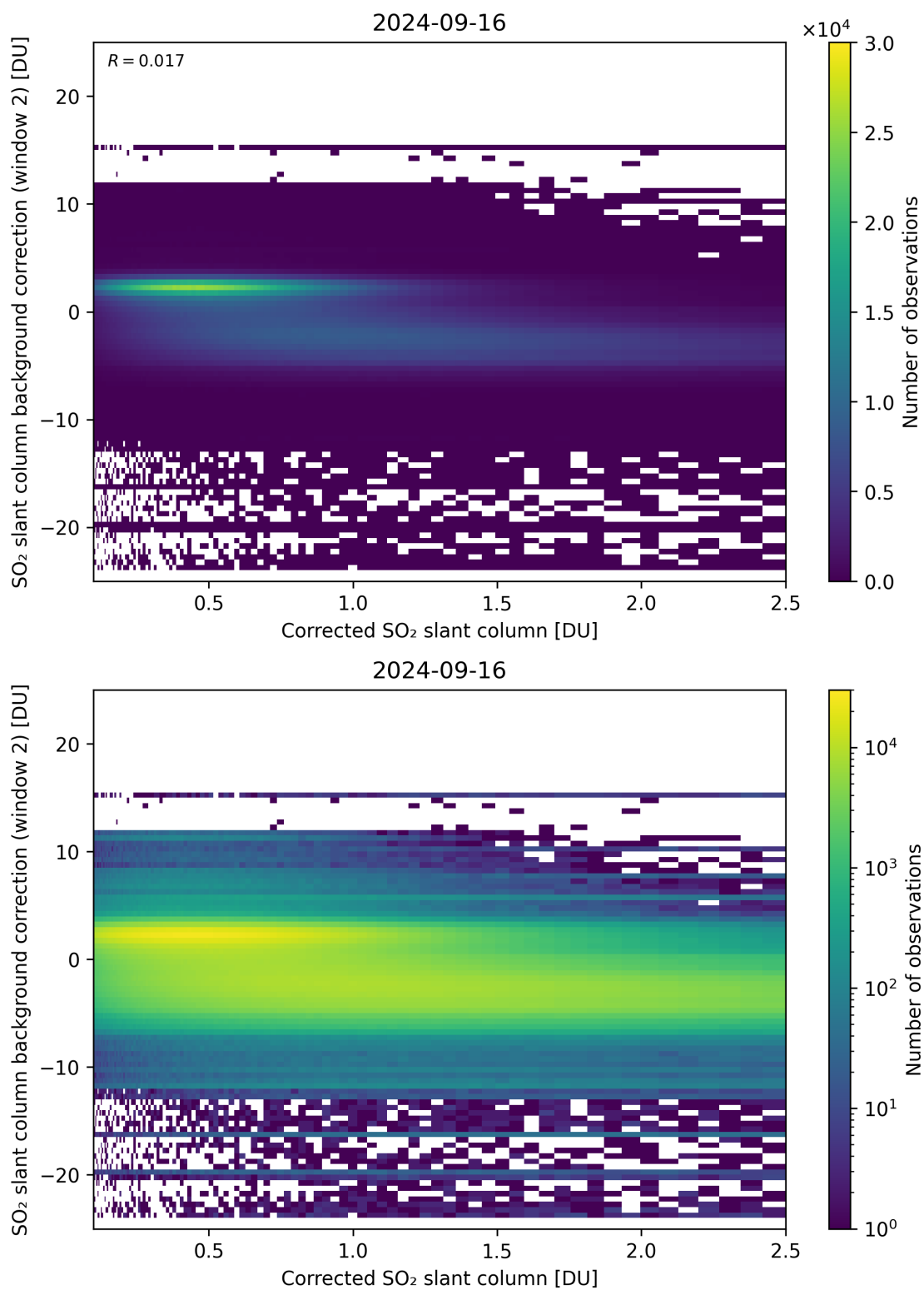
Figure 179: Scatter density plot of “Corrected SO 2 slant column” against “SO 2 slant column background correction (window 2)” for 2024-09-15 to 2024-09-17.
