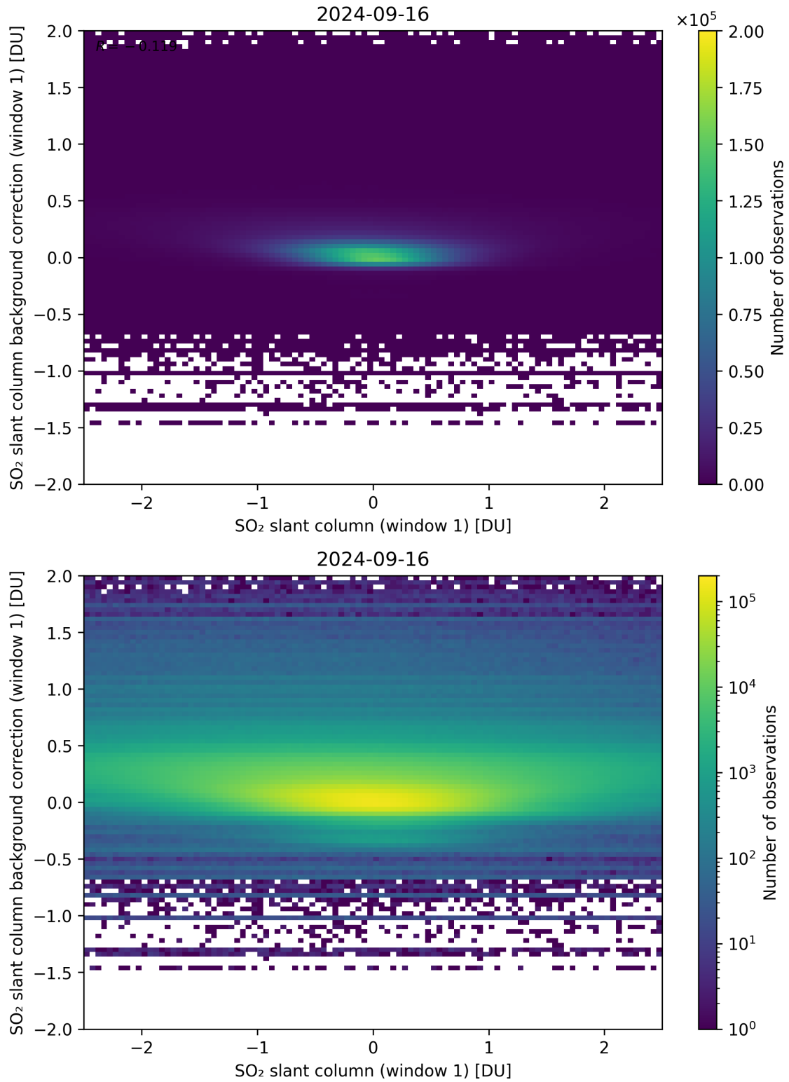
Figure 212: Scatter density plot of “SO 2 slant column (window 1)” against “SO 2 slant column background correction (window 1)” for 2024-09-15 to 2024-09-17.
