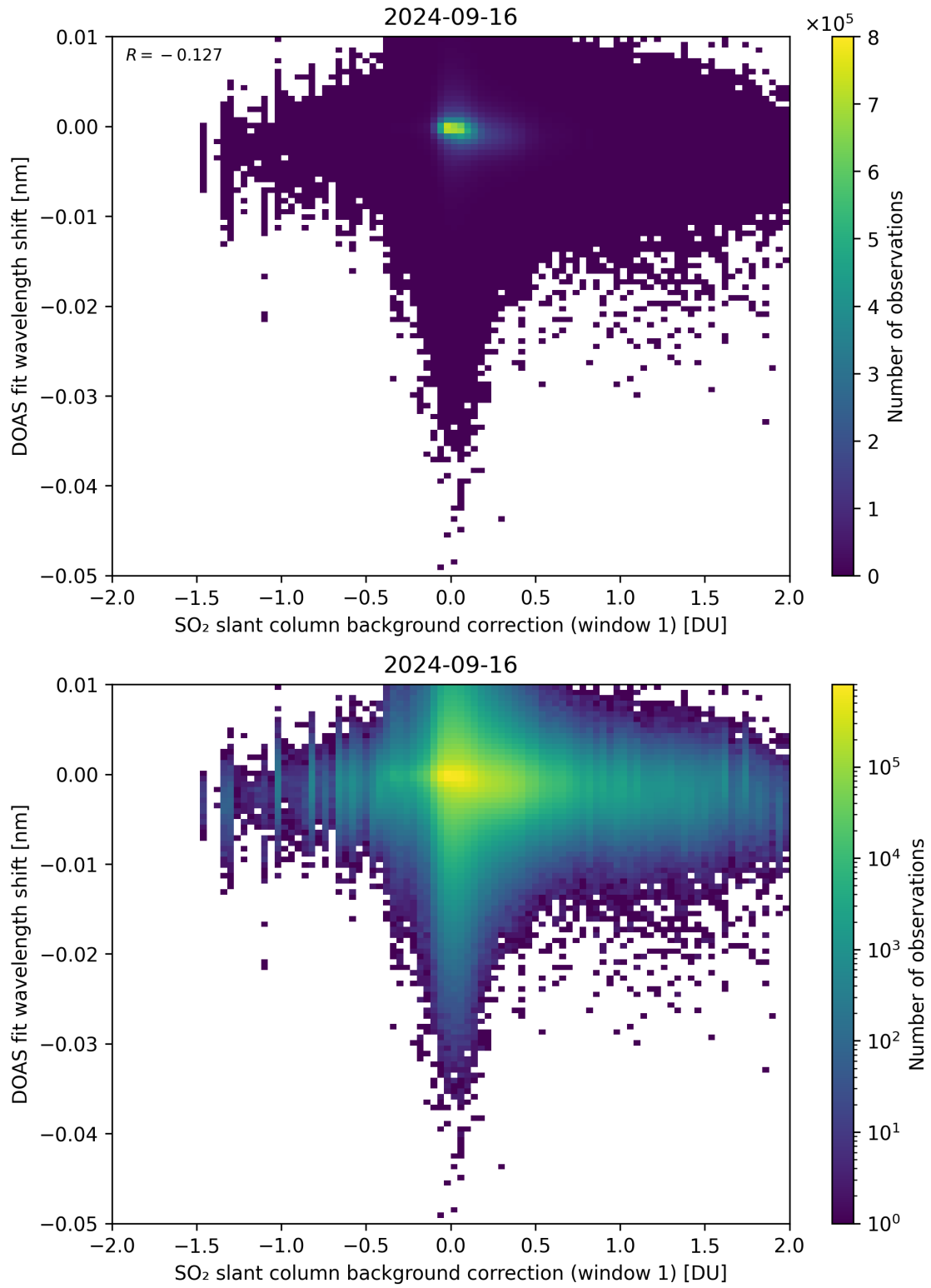
Figure 100: Scatter density plot of “SO 2 slant column background correction (window 1)” against “DOAS fit wavelength shift” for 2024-09-15 to 2024-09-17.
