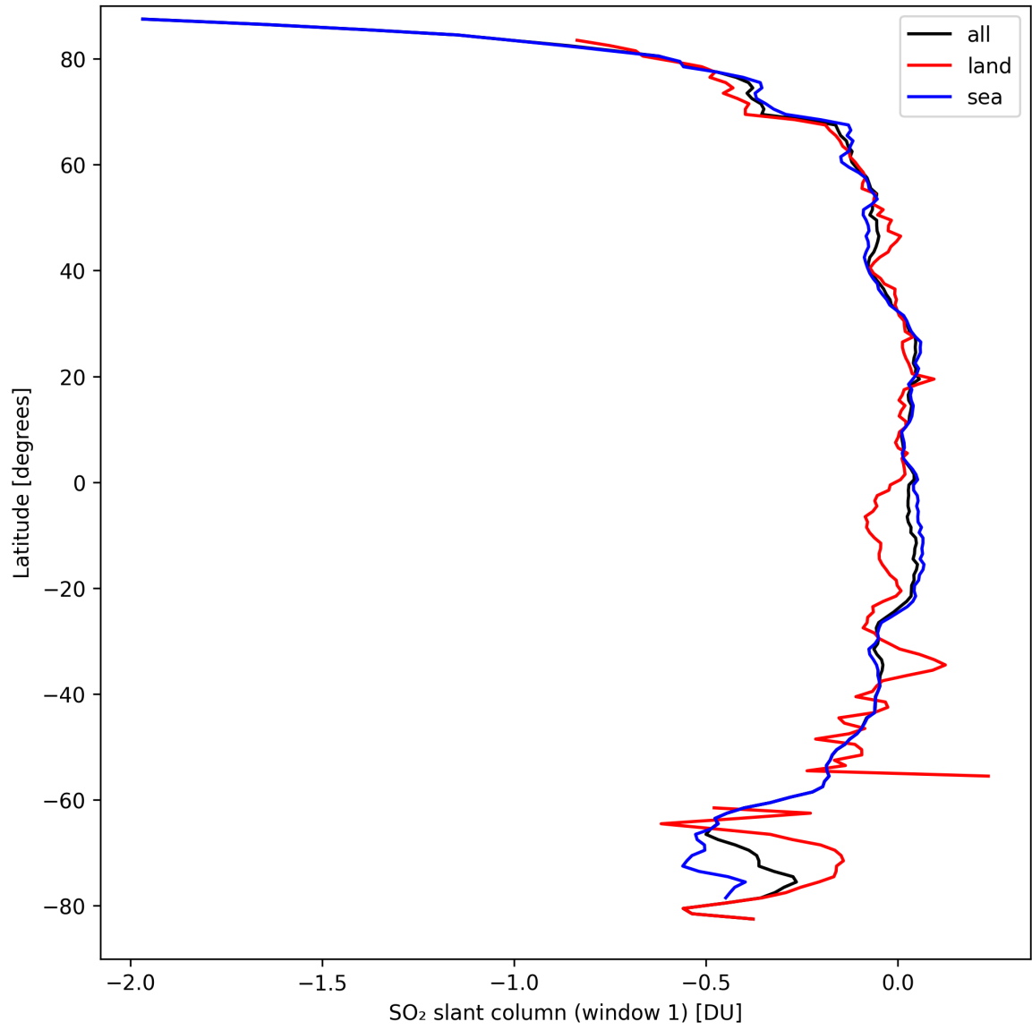
Figure 33: Zonal average of “SO 2 slant column (window 1)” for 2024-09-15 to 2024-09-17.
