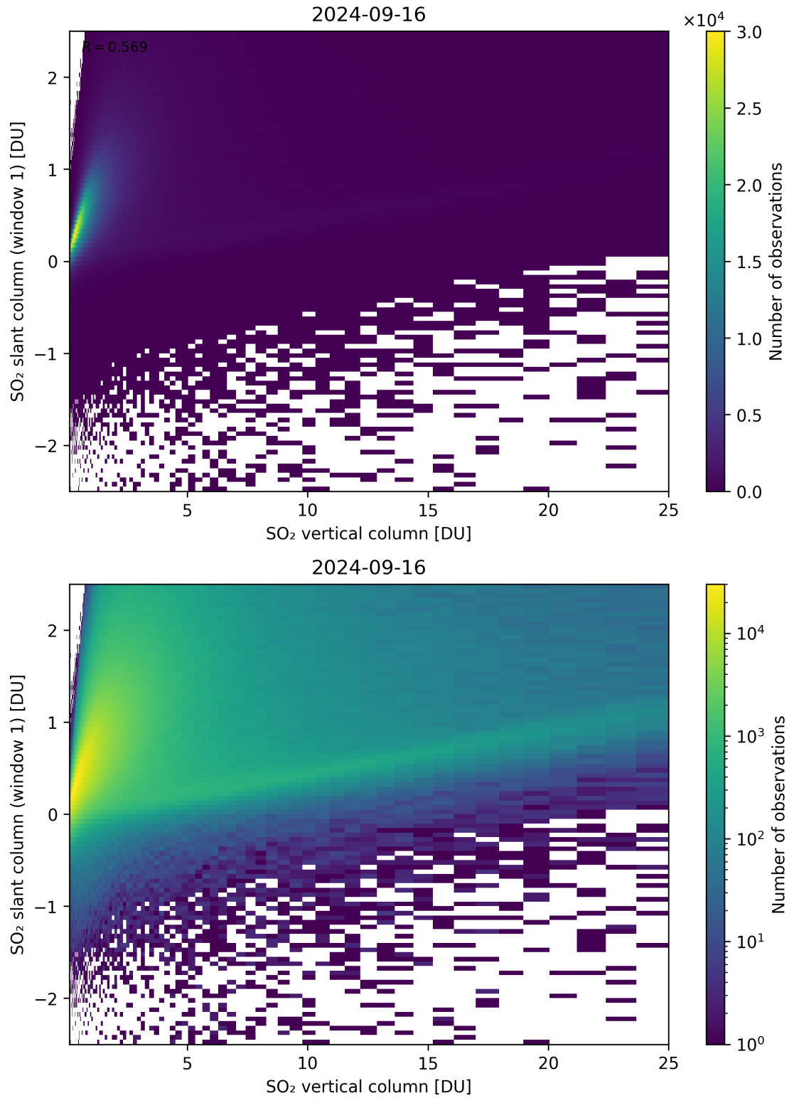
Figure 300: Scatter density plot of “SO 2 vertical column” against “SO 2 slant column (window 1)” for 2024-09-15 to 2024-09-17.
