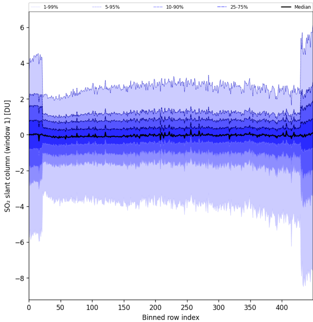
Figure 79: Along track statistics of “SO 2 slant column (window 1)” for 2024-09-15 to 2024-09-17
