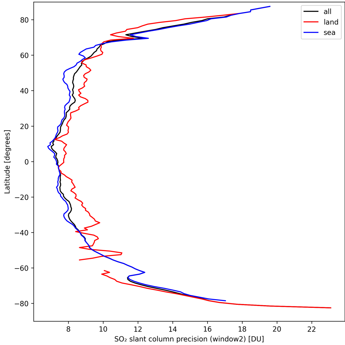
Figure 38: Zonal average of “SO 2 slant column precision (window2)” for 2024-09-15 to 2024-09-17.
