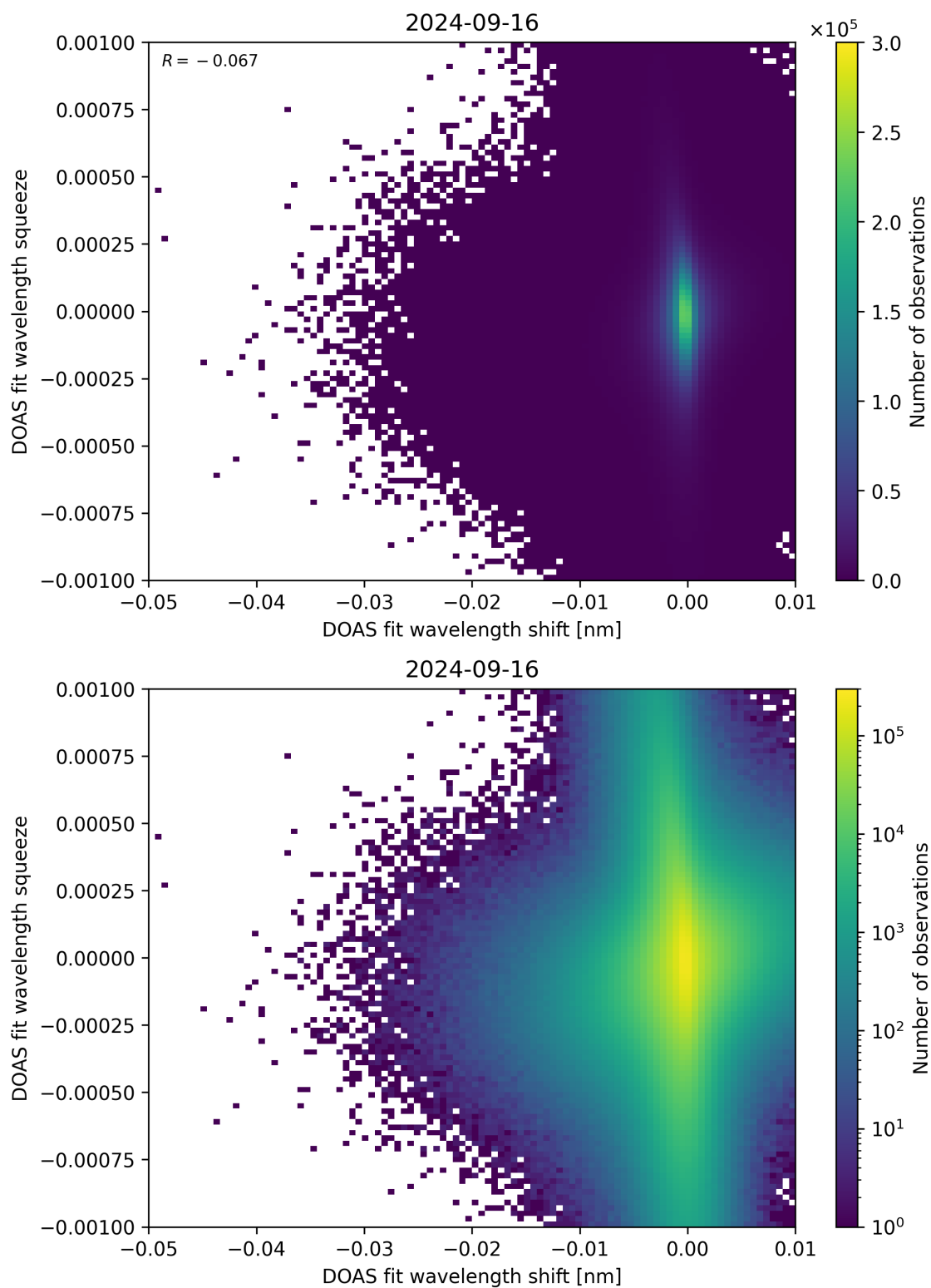
Figure 127: Scatter density plot of “DOAS fit wavelength shift” against “DOAS fit wavelength squeeze” for 2024-09-15 to 2024-09-17.
