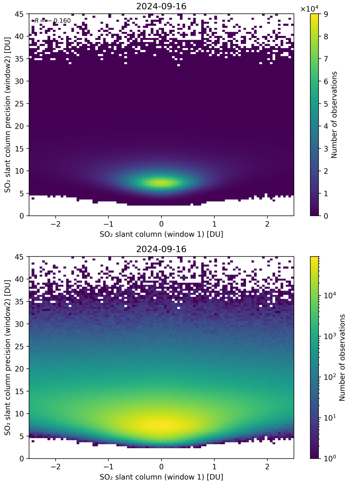
Figure 236: Scatter density plot of “SO 2 slant column (window 1)” against “SO 2 slant column precision (window2)” for 2024-09-15 to 2024-09-17.
