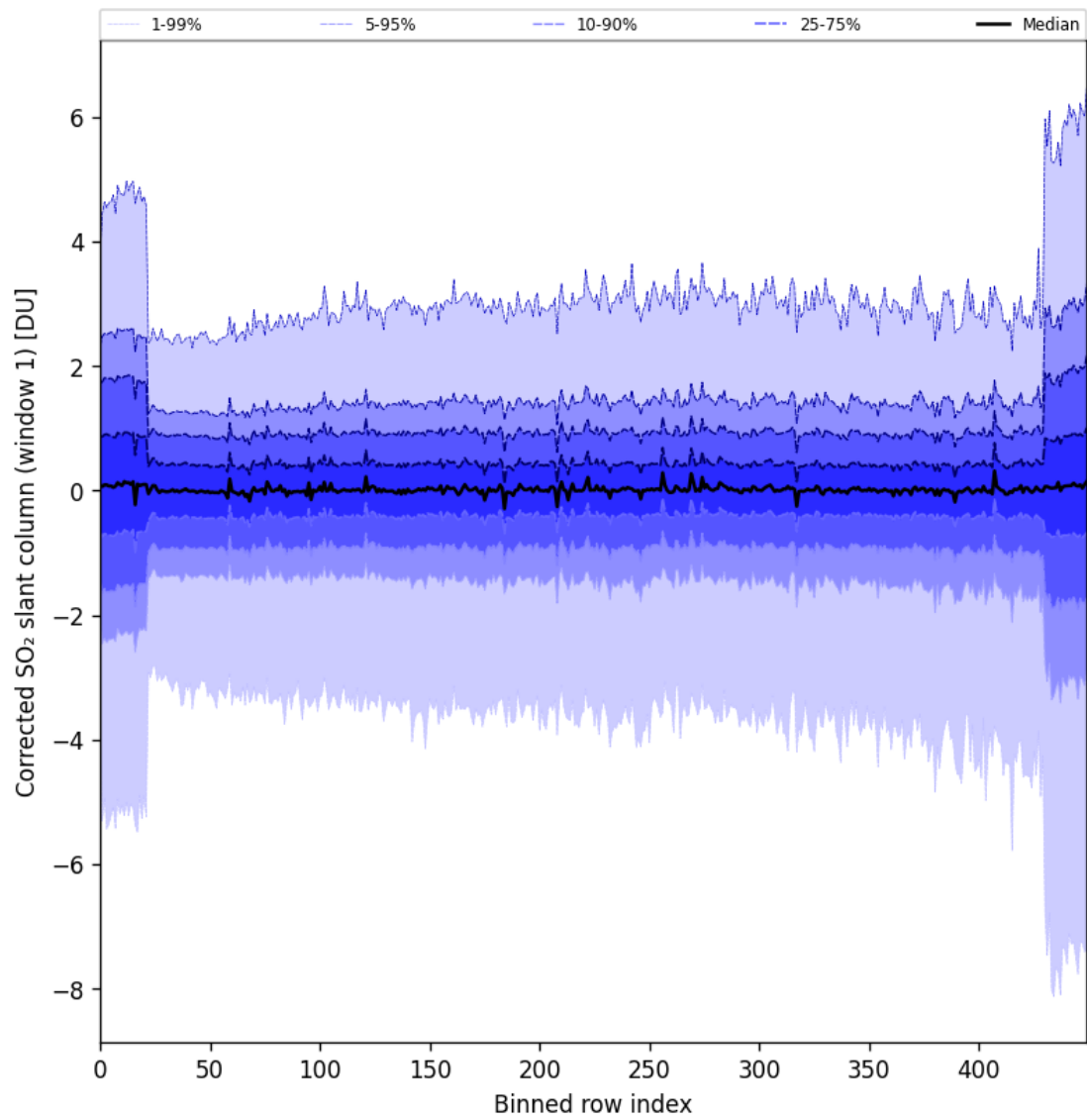
Figure 81: Along track statistics of “Corrected SO 2 slant column (window 1)” for 2024-09-15 to 2024-09-17
