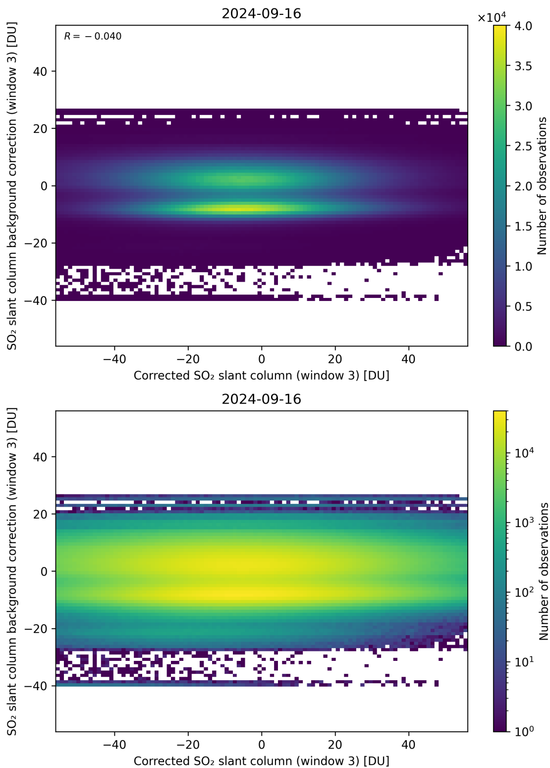
Figure 205: Scatter density plot of “Corrected SO 2 slant column (window 3)” against “SO 2 slant column background correction (window 3)” for 2024-09-15 to 2024-09-17.
