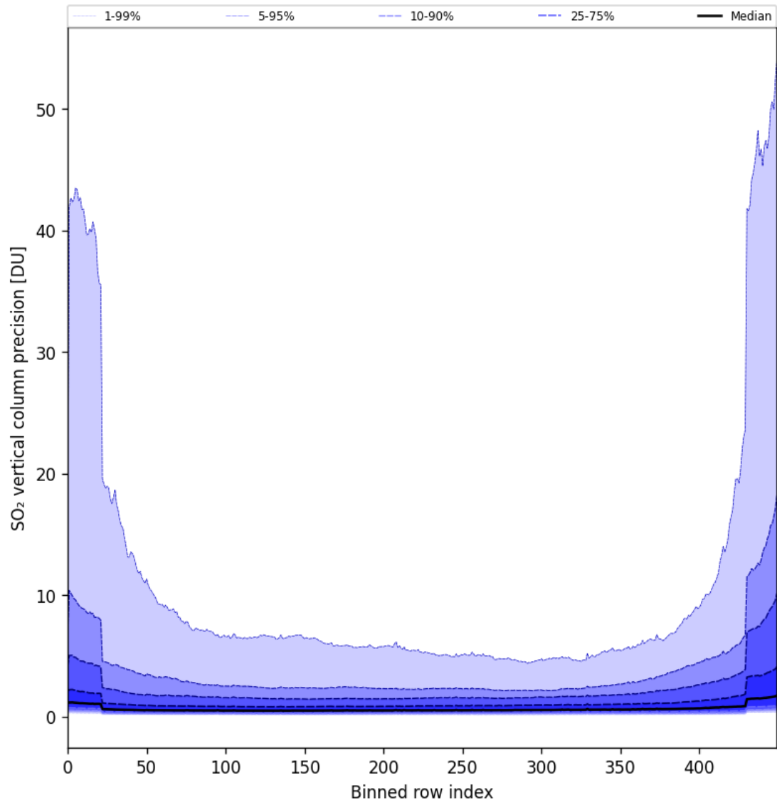
Figure 77: Along track statistics of “SO 2 vertical column precision” for 2024-09-15 to 2024-09-17
