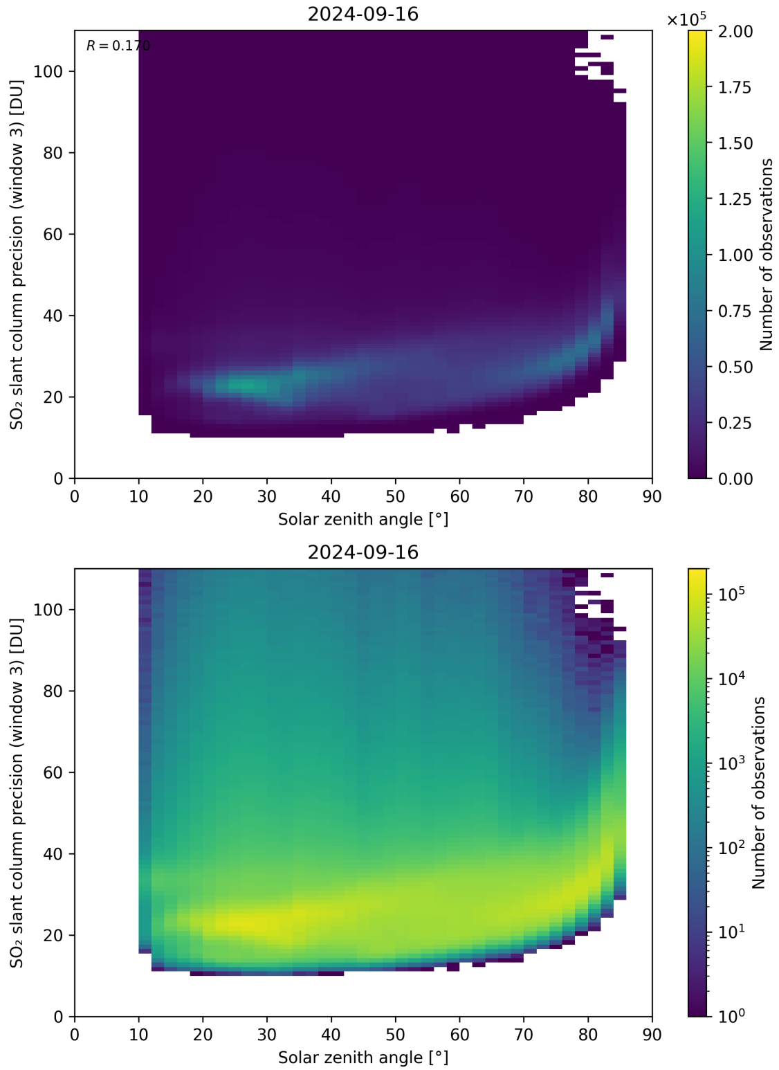
Figure 173: Scatter density plot of “Solar zenith angle” against “SO 2 slant column precision (window 3)” for 2024-09-15 to 2024-09-17.
