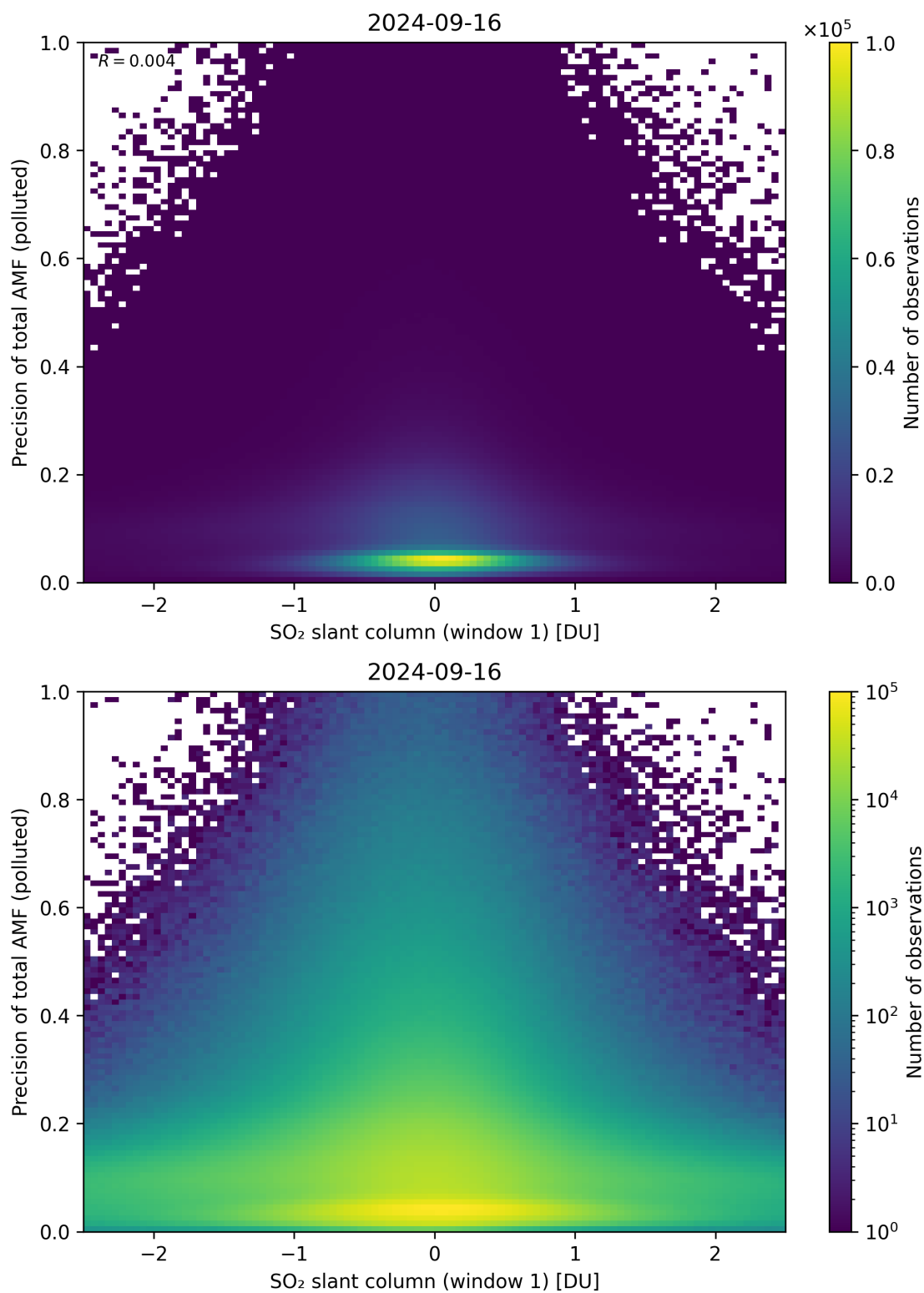
Figure 240: Scatter density plot of “SO 2 slant column (window 1)” against “Precision of total AMF (polluted)” for 2024-09-15 to 2024-09-17.
