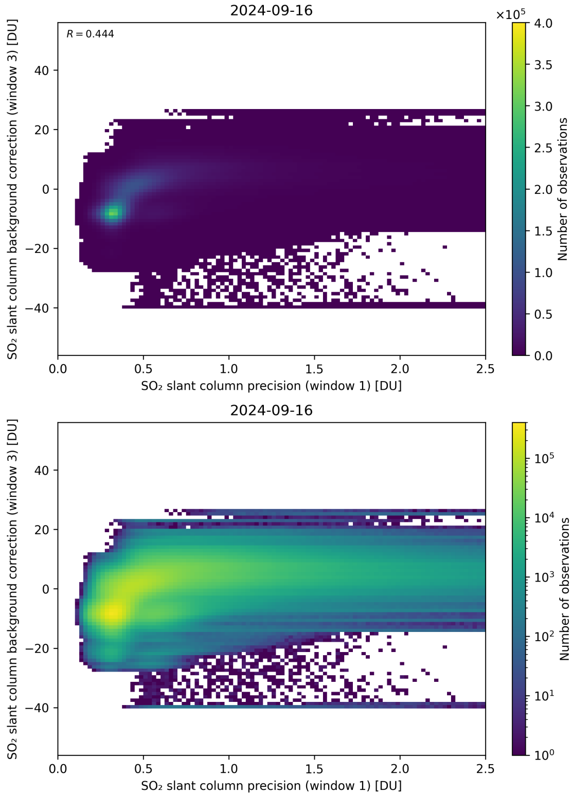
Figure 220: Scatter density plot of “SO 2 slant column precision (window 1)” against “SO 2 slant column background correction (window 3)” for 2024-09-15 to 2024-09-17.
