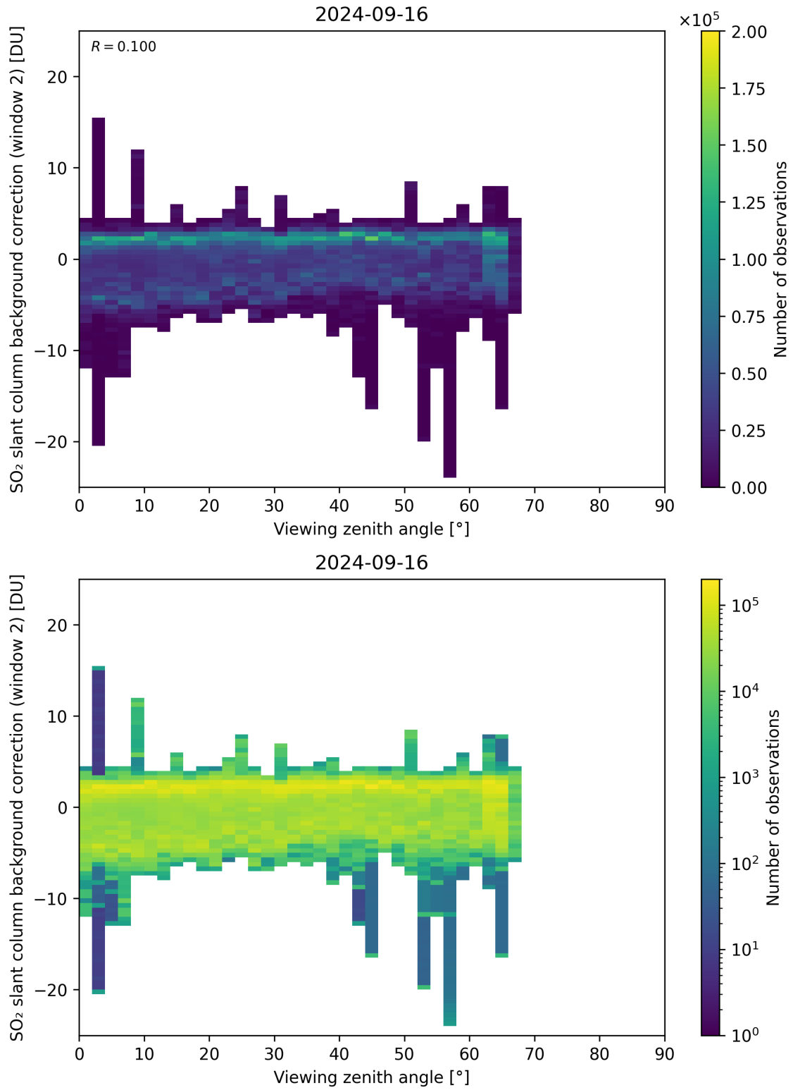
Figure 309: Scatter density plot of “Viewing zenith angle” against “SO 2 slant column background correction (window 2)” for 2024-09-15 to 2024-09-17.
