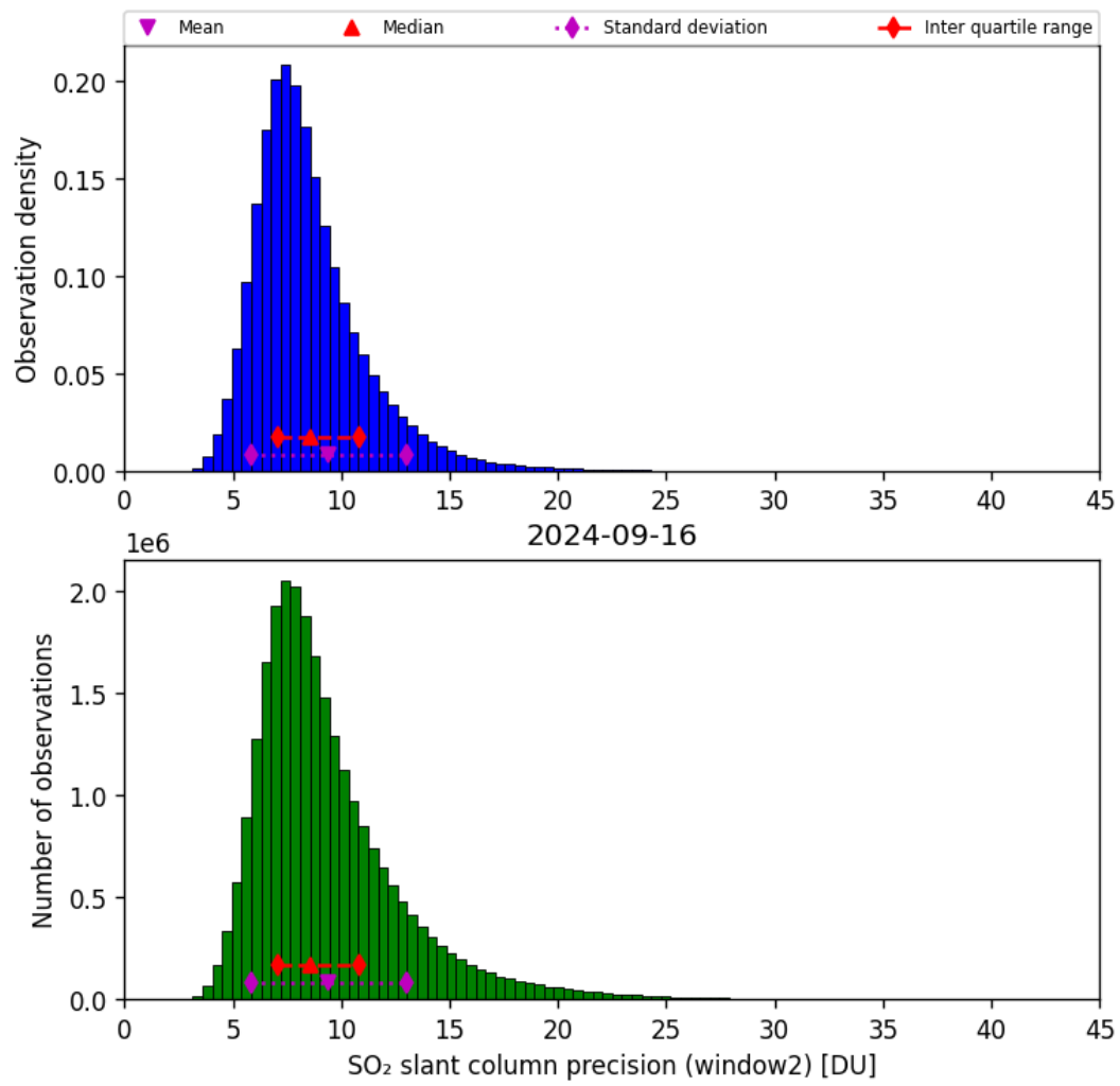
Figure 61: Histogram of “SO 2 slant column precision (window2)” for 2024-09-15 to 2024-09-17
