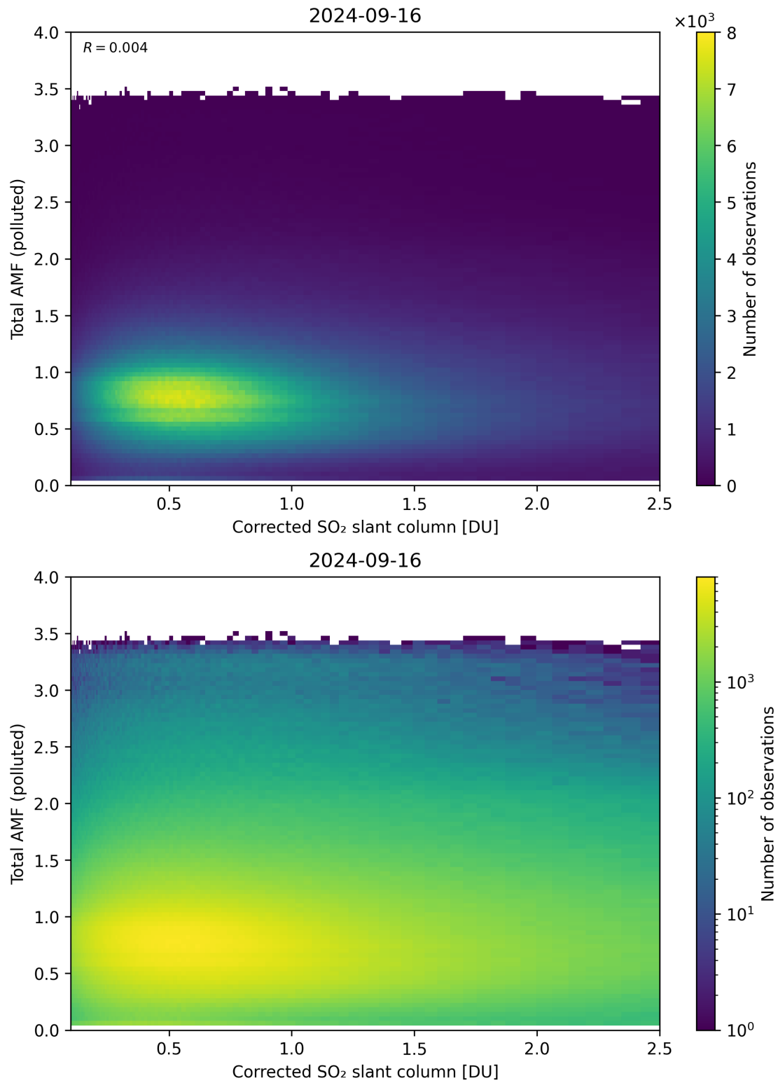
Figure 192: Scatter density plot of “Corrected SO 2 slant column” against “Total AMF (polluted)” for 2024-09-15 to 2024-09-17.
