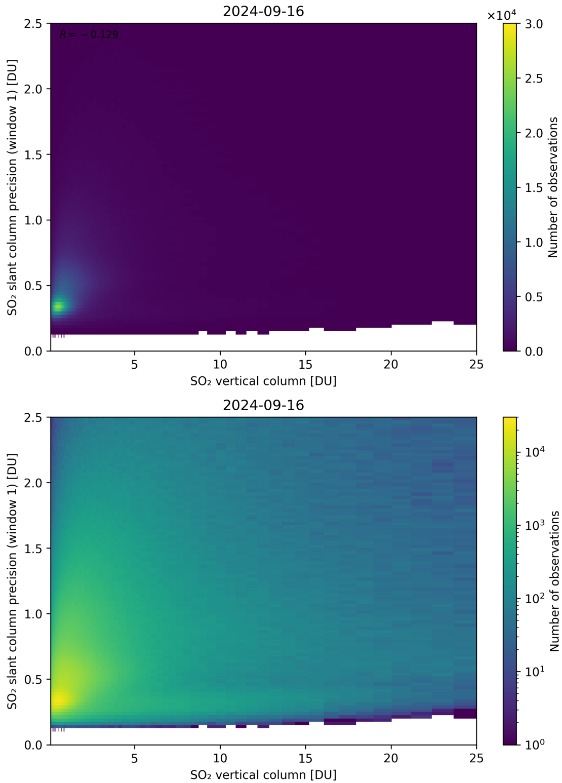
Figure 301: Scatter density plot of “SO 2 vertical column” against “SO 2 slant column precision (window 1)” for 2024-09-15 to 2024-09-17.
