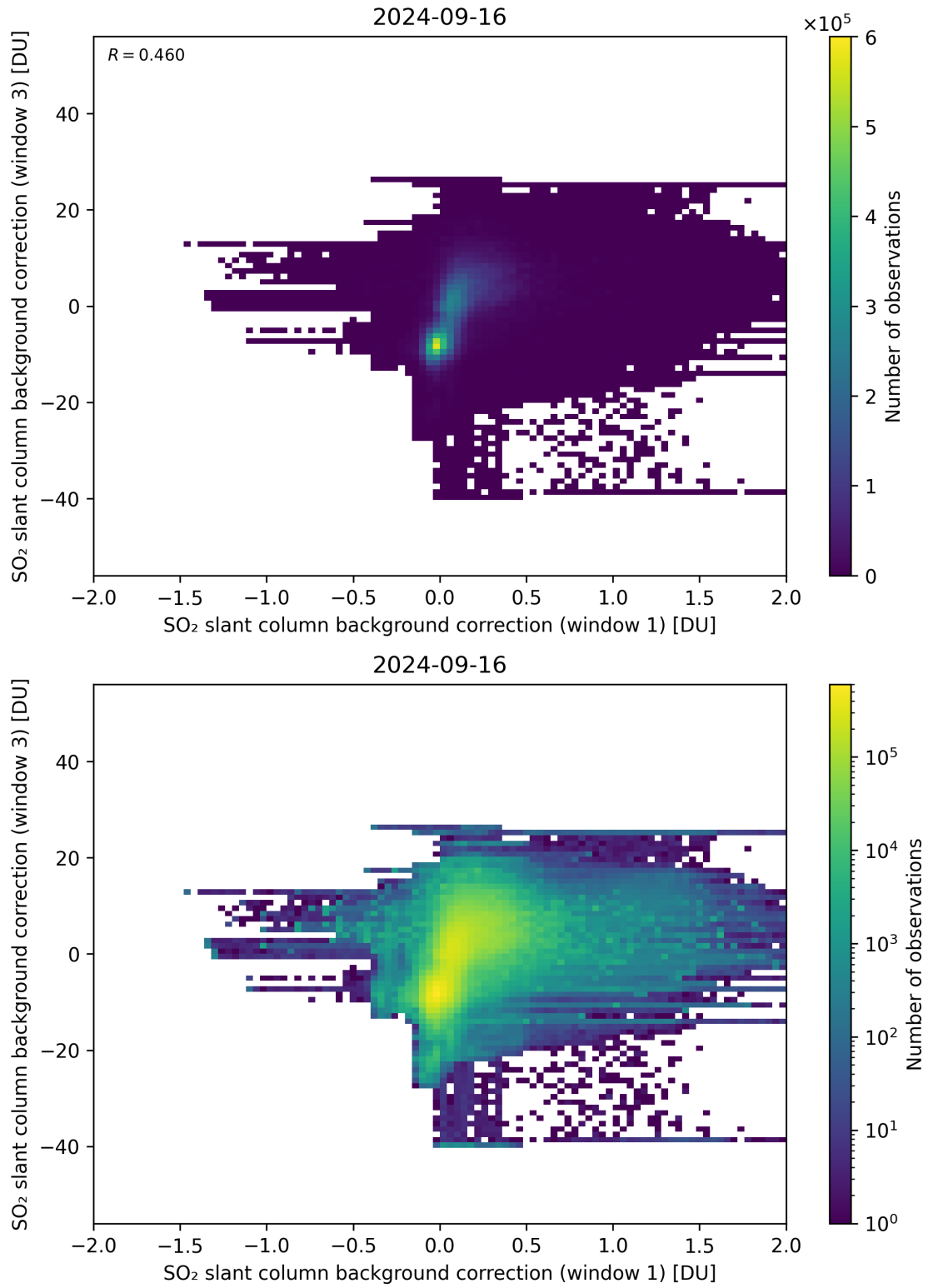
Figure 99: Scatter density plot of “SO 2 slant column background correction (window 1)” against “SO 2 slant column background correction (window 3)” for 2024-09-15 to 2024-09-17.
