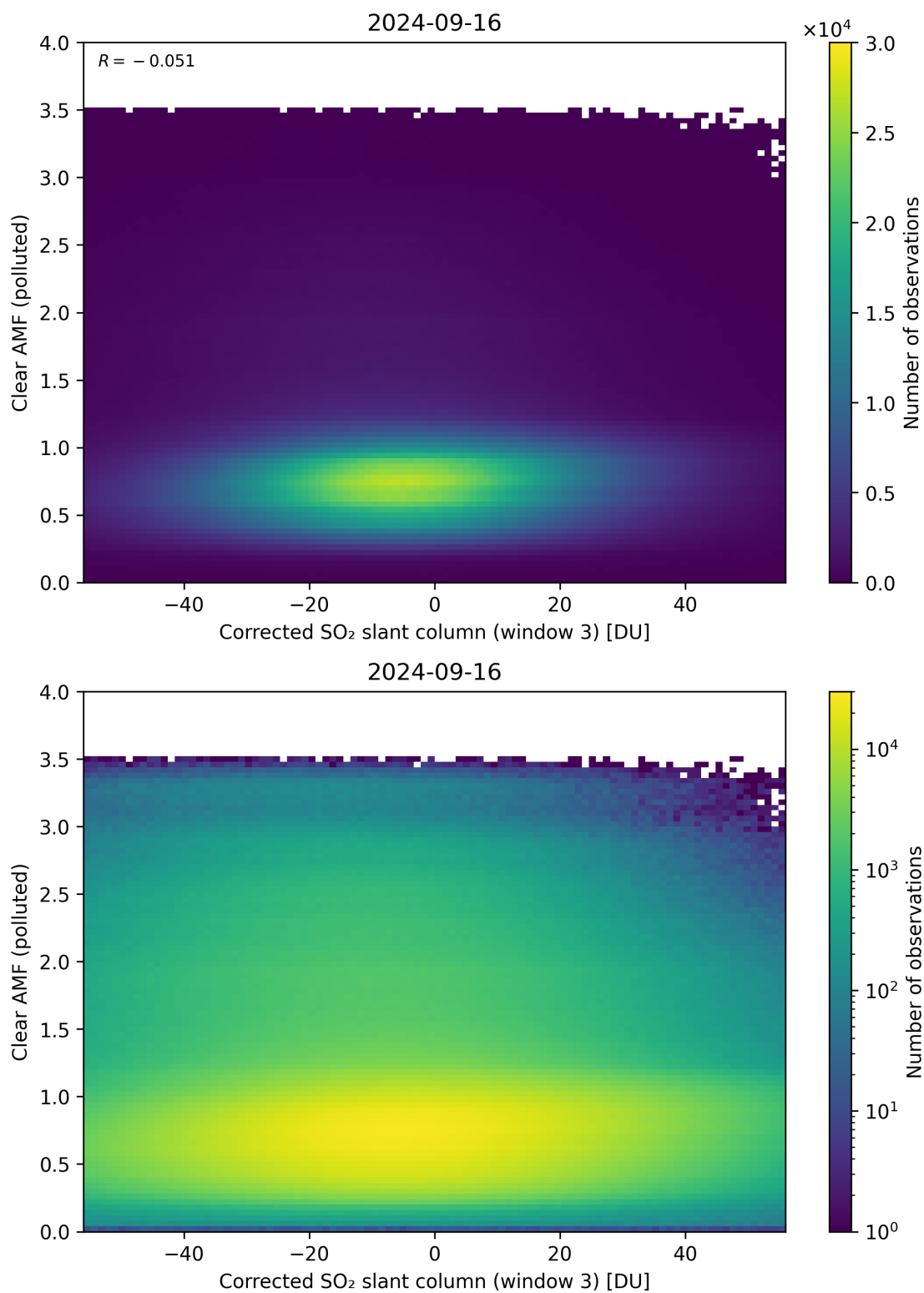
Figure 209: Scatter density plot of “Corrected SO 2 slant column (window 3)” against “Clear AMF (polluted)” for 2024-09-15 to 2024-09-17.
