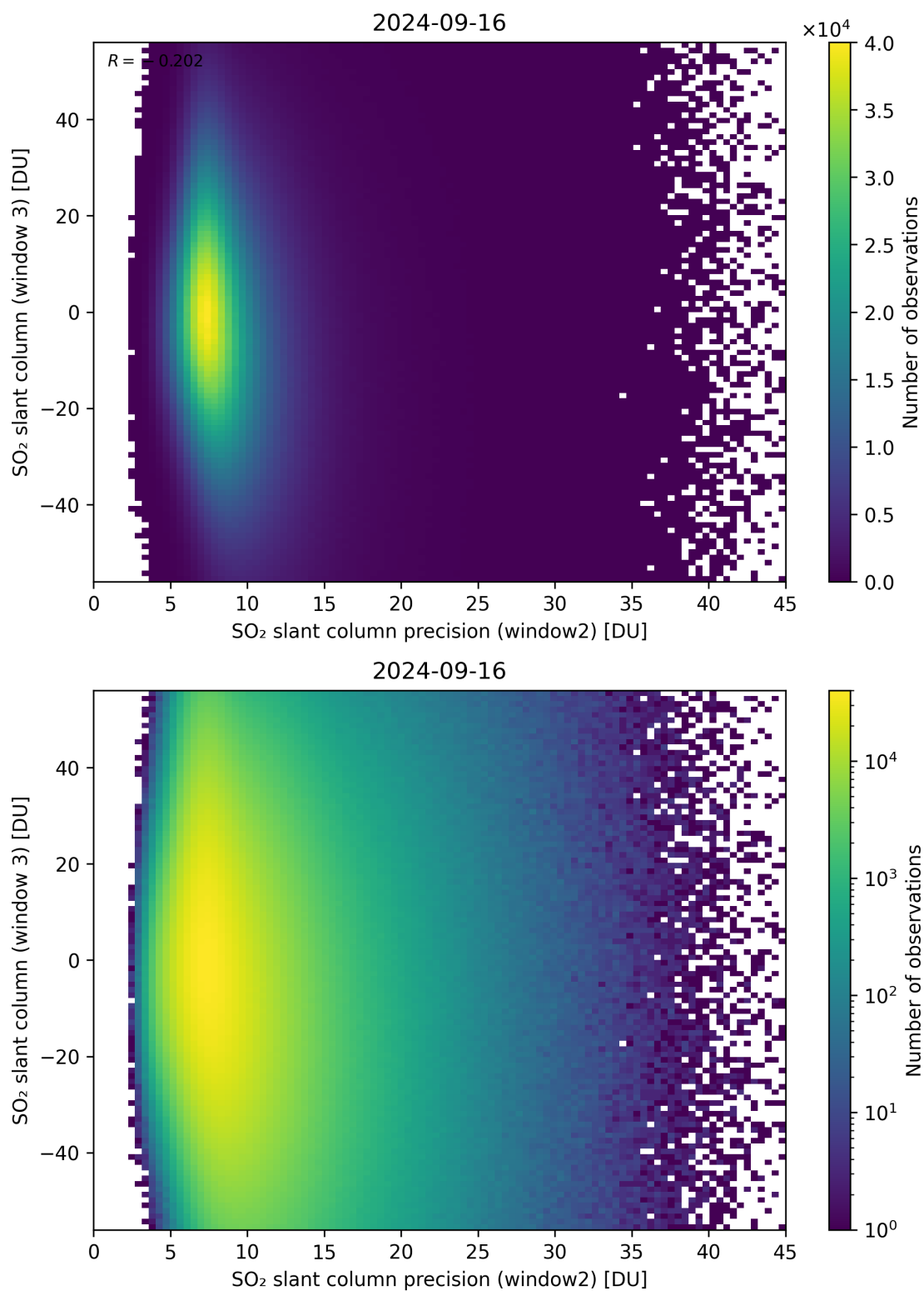
Figure 249: Scatter density plot of “SO 2 slant column precision (window2)” against “SO 2 slant column (window 3)” for 2024-09-15 to 2024-09-17.
