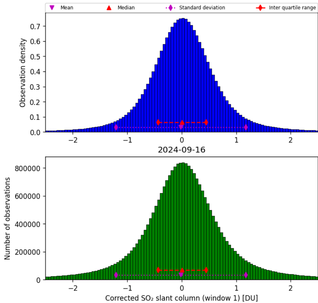
Figure 58: Histogram of “Corrected SO 2 slant column (window 1)” for 2024-09-15 to 2024-09-17
