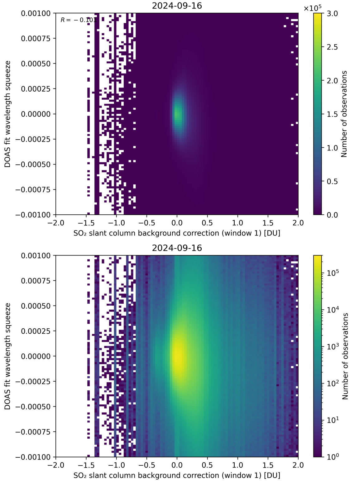
Figure 101: Scatter density plot of “SO 2 slant column background correction (window 1)” against “DOAS fit wavelength squeeze” for 2024-09-15 to 2024-09-17.
