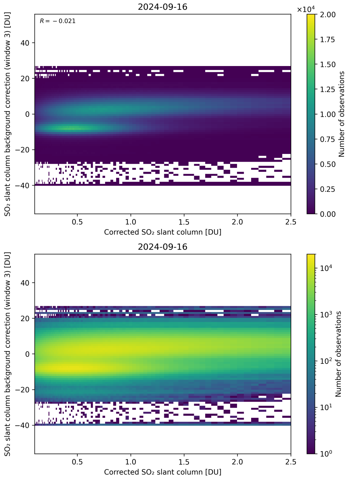
Figure 180: Scatter density plot of “Corrected SO 2 slant column” against “SO 2 slant column background correction (window 3)” for 2024-09-15 to 2024-09-17.
