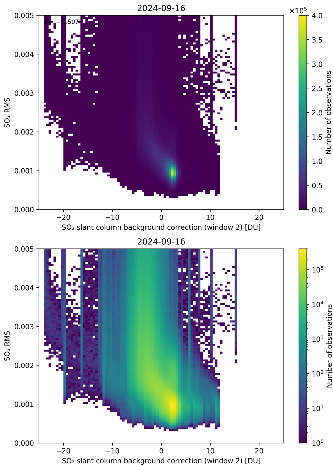
Figure 114: Scatter density plot of “SO 2 slant column background correction (window 2)” against “SO 2 RMS” for 2024-09-15 to 2024-09-17.
