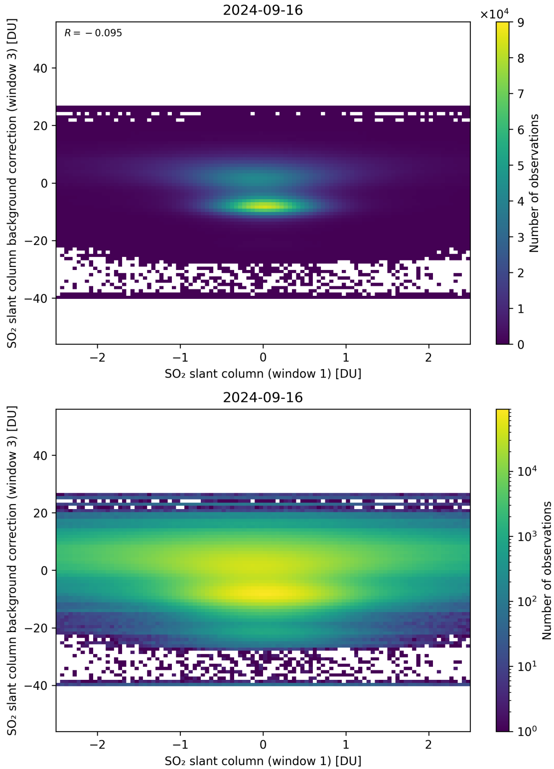
Figure 214: Scatter density plot of “SO 2 slant column (window 1)” against “SO 2 slant column background correction (window 3)” for 2024-09-15 to 2024-09-17.
