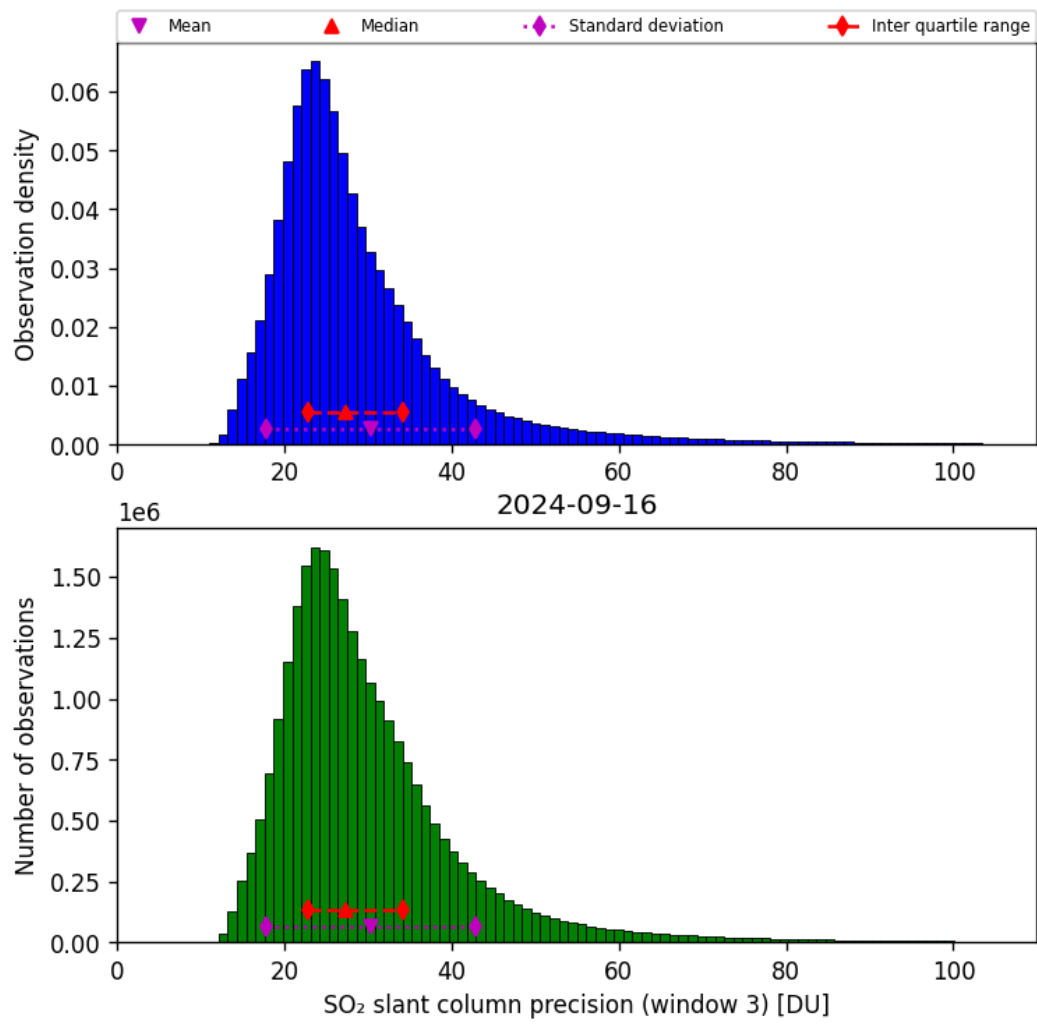
Figure 65: Histogram of “SO 2 slant column precision (window 3)” for 2024-09-15 to 2024-09-17
