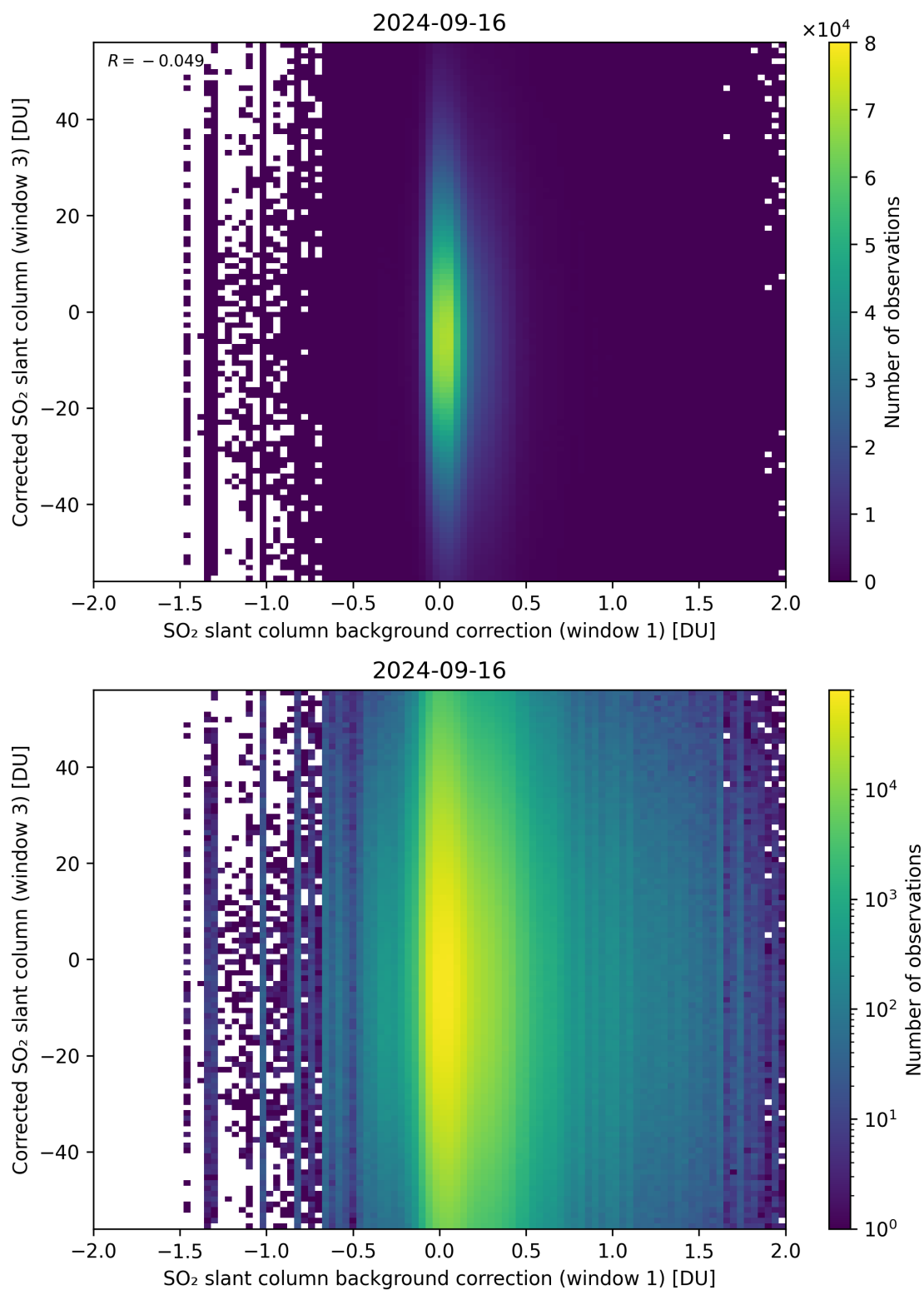
Figure 105: Scatter density plot of “SO 2 slant column background correction (window 1)” against “Corrected SO 2 slant column (window 3)” for 2024-09-15 to 2024-09-17.
