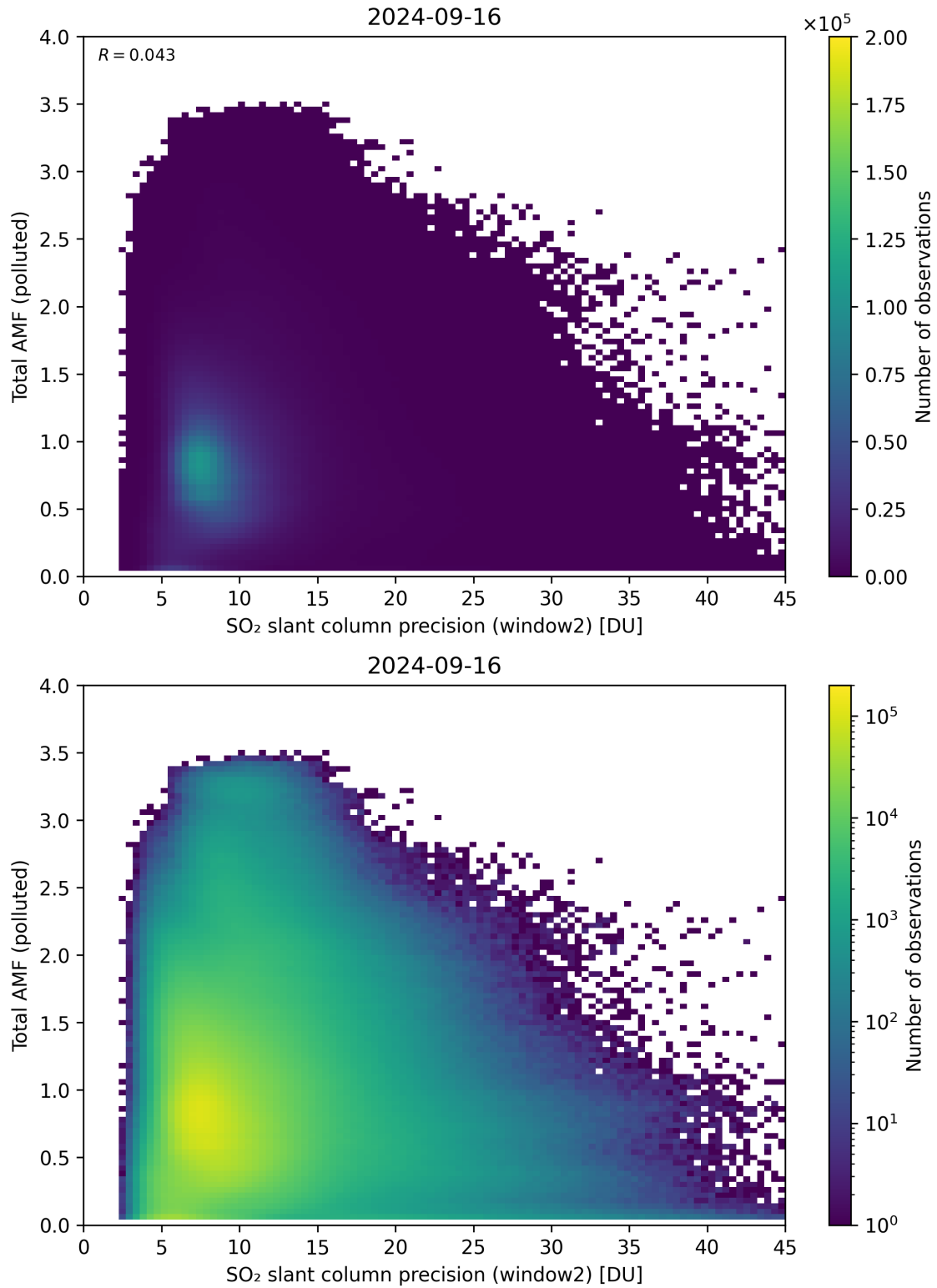
Figure 251: Scatter density plot of “SO 2 slant column precision (window2)” against “Total AMF (polluted)” for 2024-09-15 to 2024-09-17.
