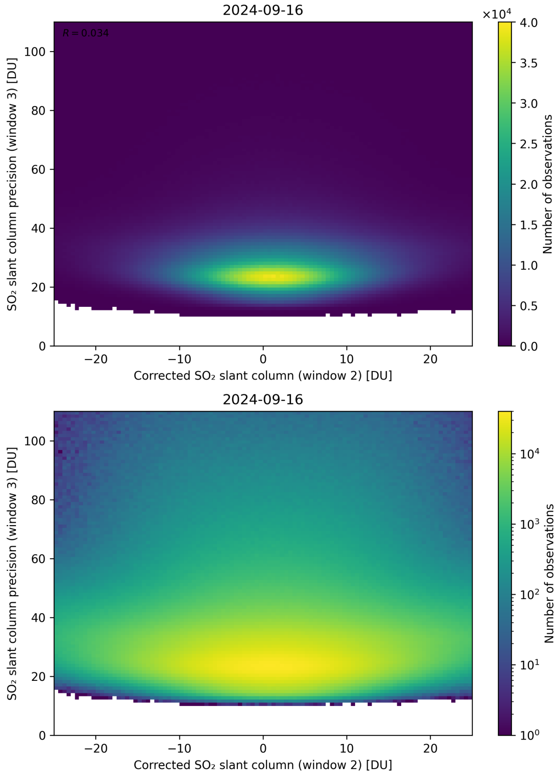
Figure 202: Scatter density plot of “Corrected SO 2 slant column (window 2)” against “SO 2 slant column precision (window 3)” for 2024-09-15 to 2024-09-17.
