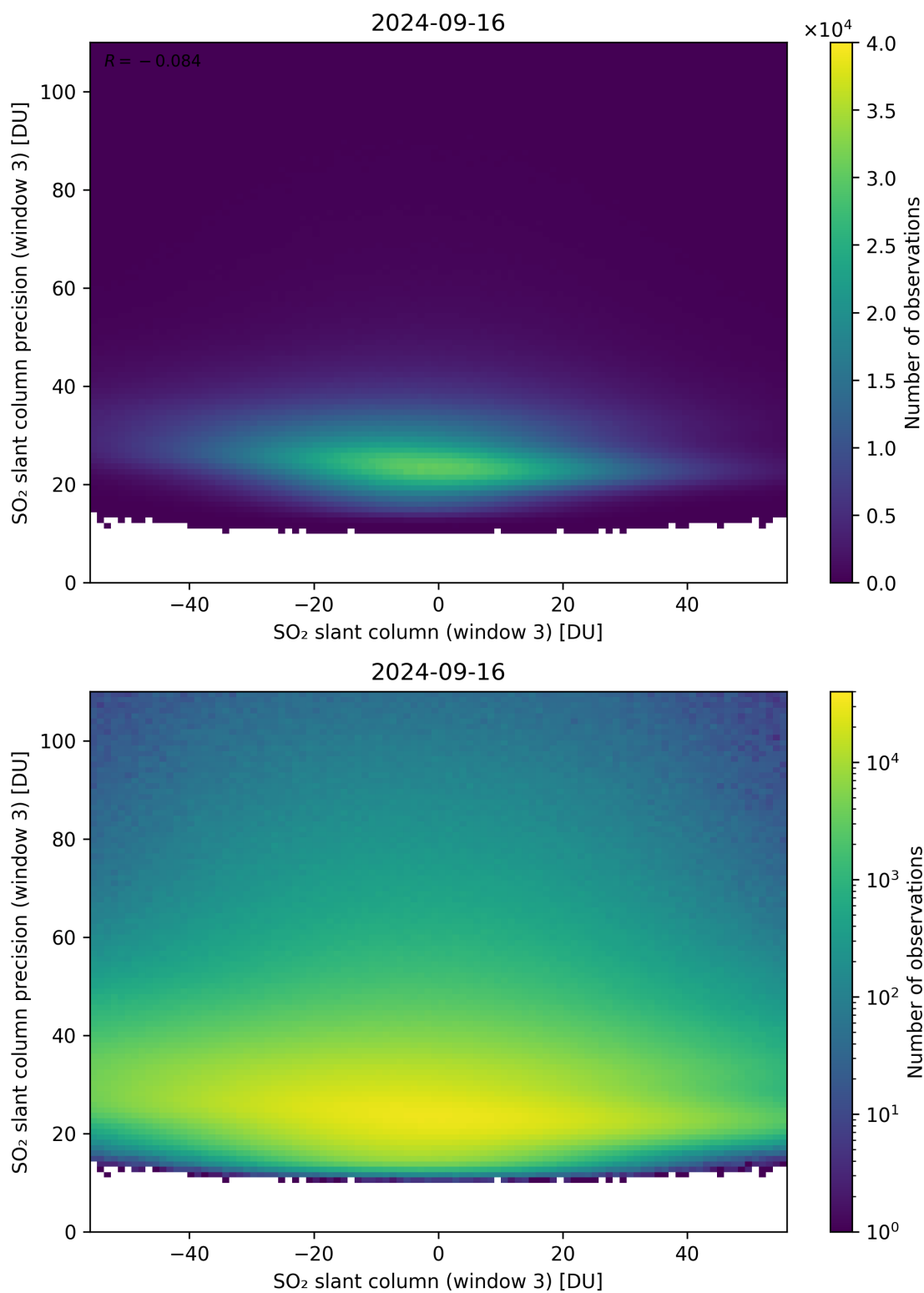
Figure 267: Scatter density plot of “SO 2 slant column (window 3)” against “SO 2 slant column precision (window 3)” for 2024-09-15 to 2024-09-17.
