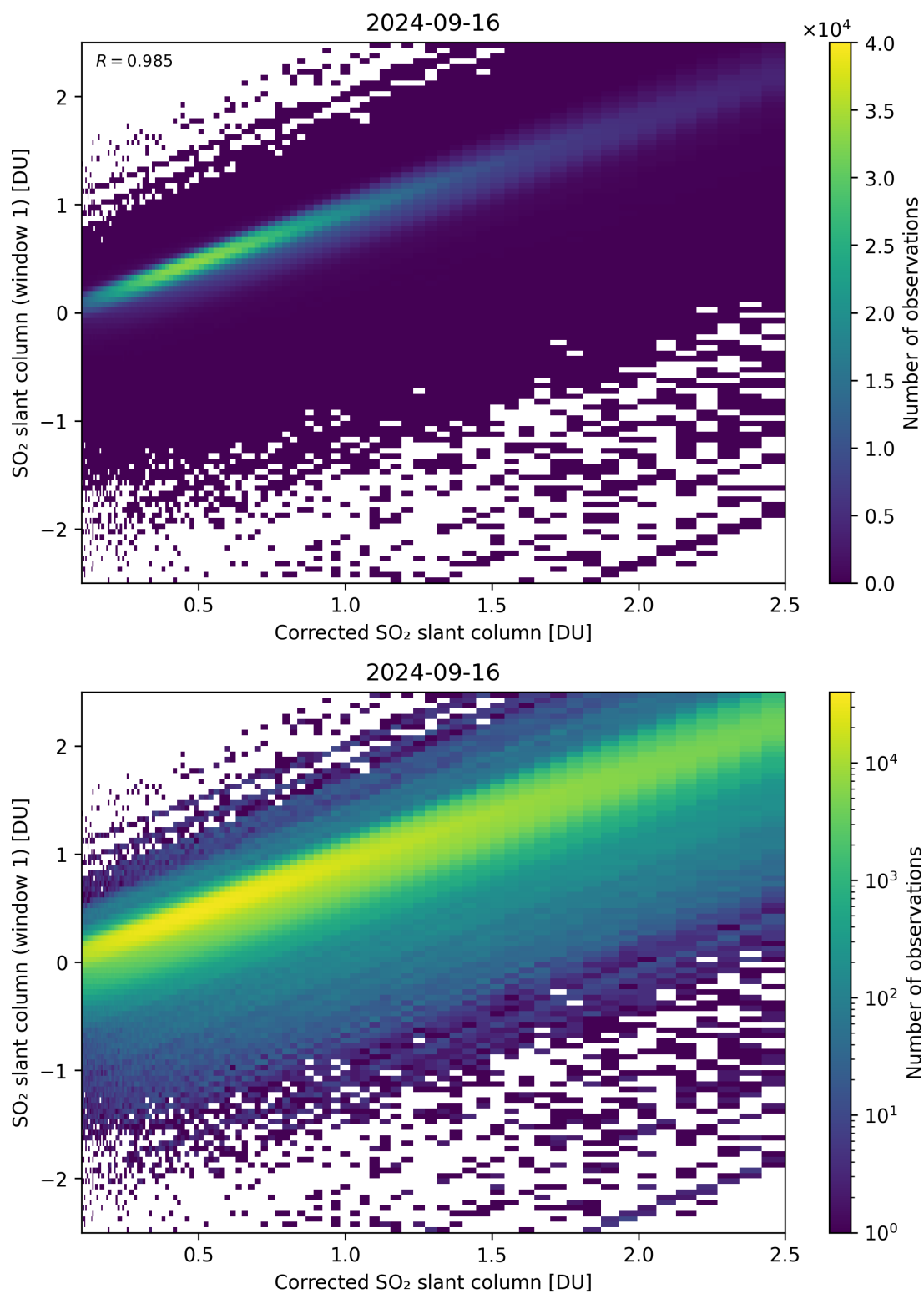
Figure 187: Scatter density plot of “Corrected SO 2 slant column” against “SO 2 slant column (window 1)” for 2024-09-15 to 2024-09-17.
