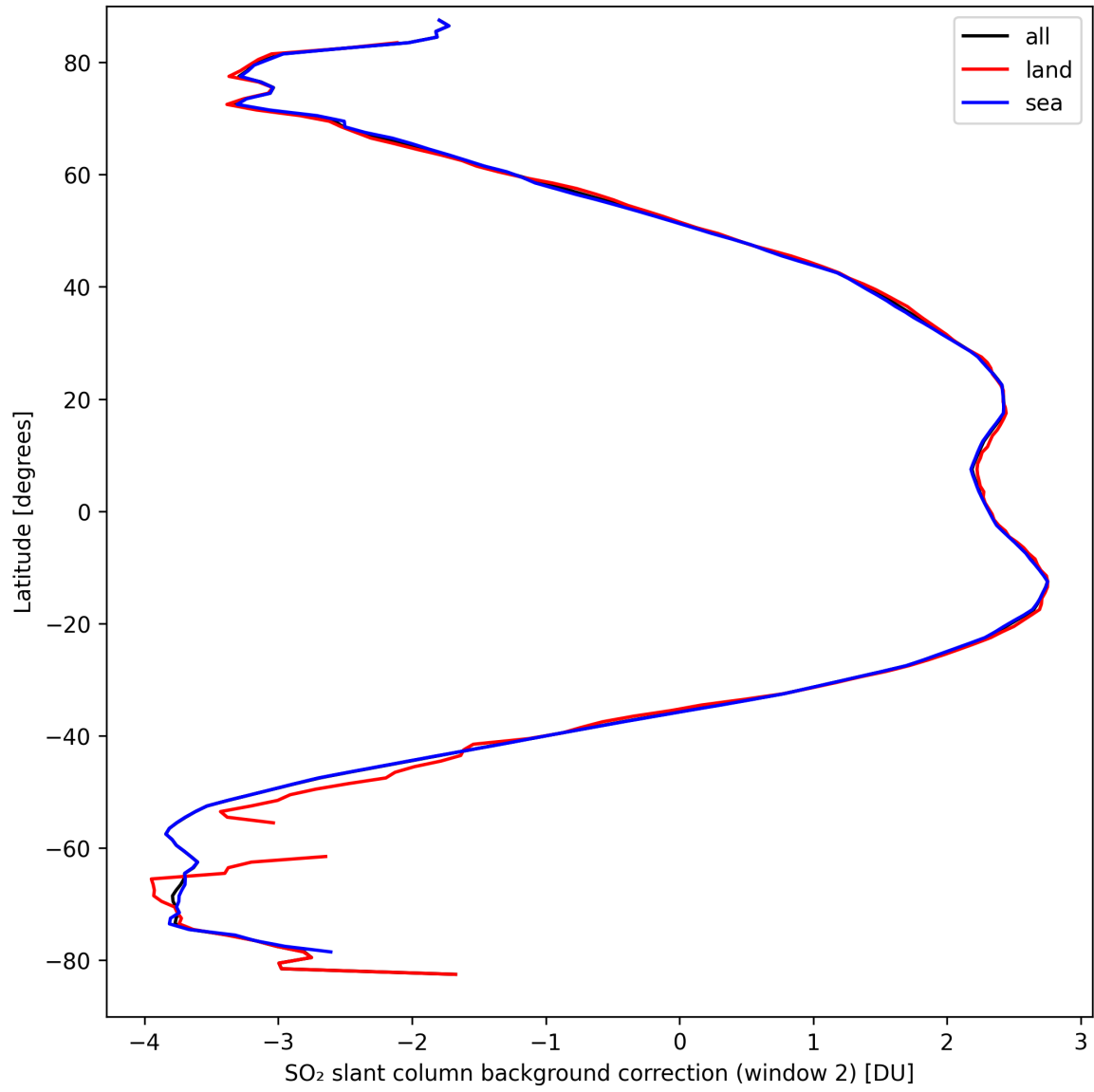
Figure 40: Zonal average of “SO 2 slant column background correction (window 2)” for 2024-09-15 to 2024-09-17.
