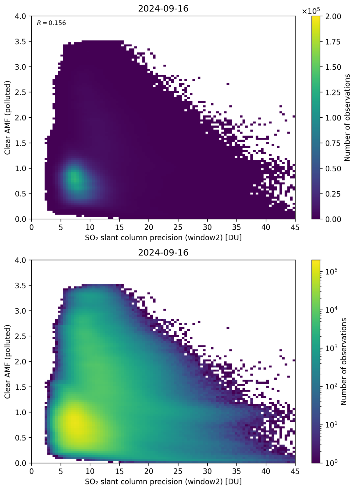
Figure 246: Scatter density plot of “SO 2 slant column precision (window2)” against “Clear AMF (polluted)” for 2024-09-15 to 2024-09-17.
