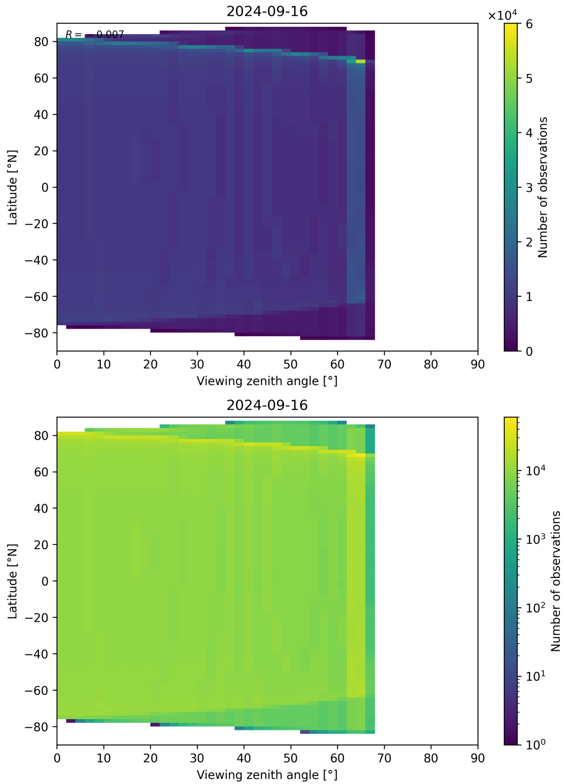
Figure 314: Scatter density plot of “Viewing zenith angle” against “Latitude” for 2024-09-15 to 2024-09-17.
