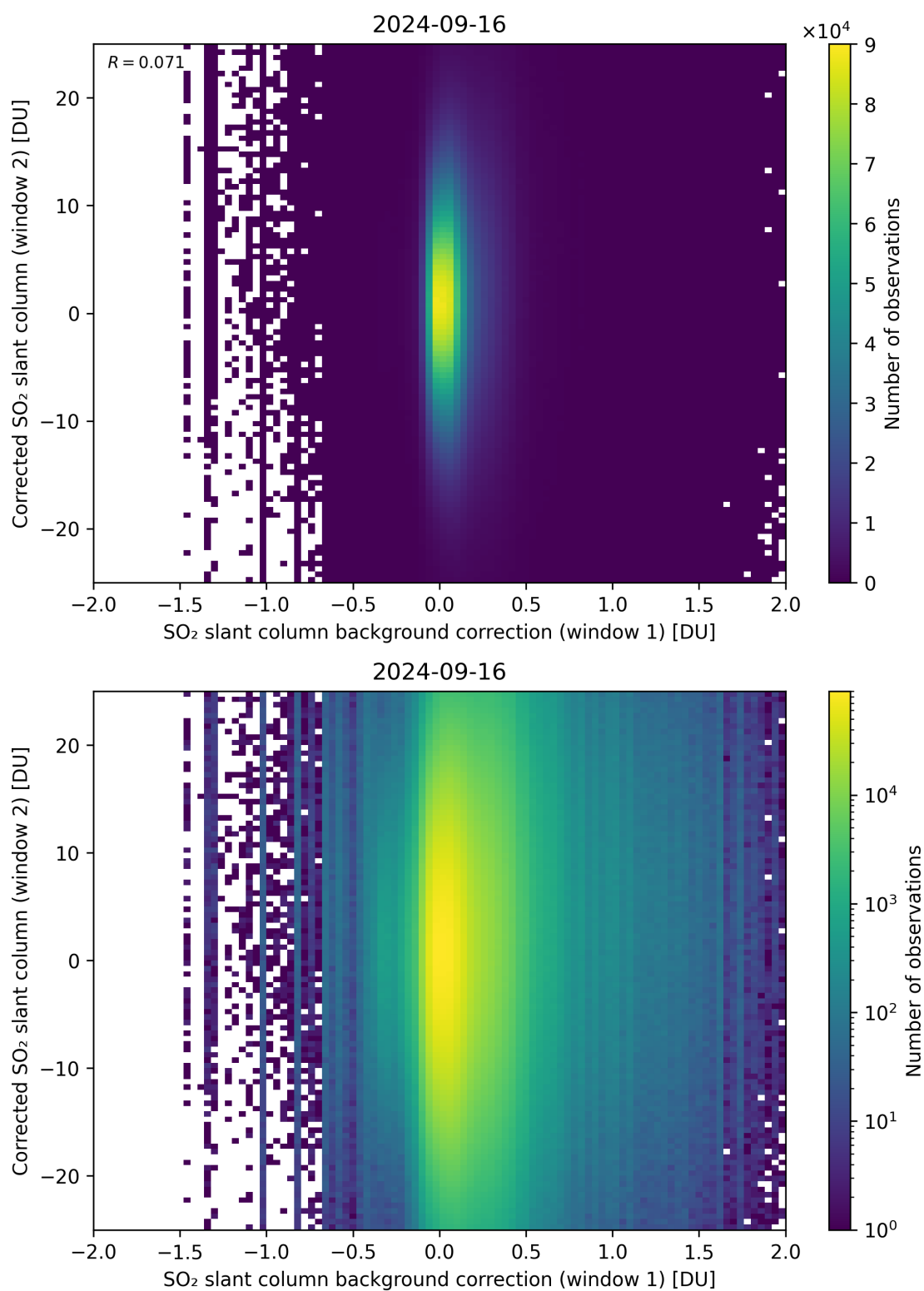
Figure 104: Scatter density plot of “SO 2 slant column background correction (window 1)” against “Corrected SO 2 slant column (window 2)” for 2024-09-15 to 2024-09-17.
