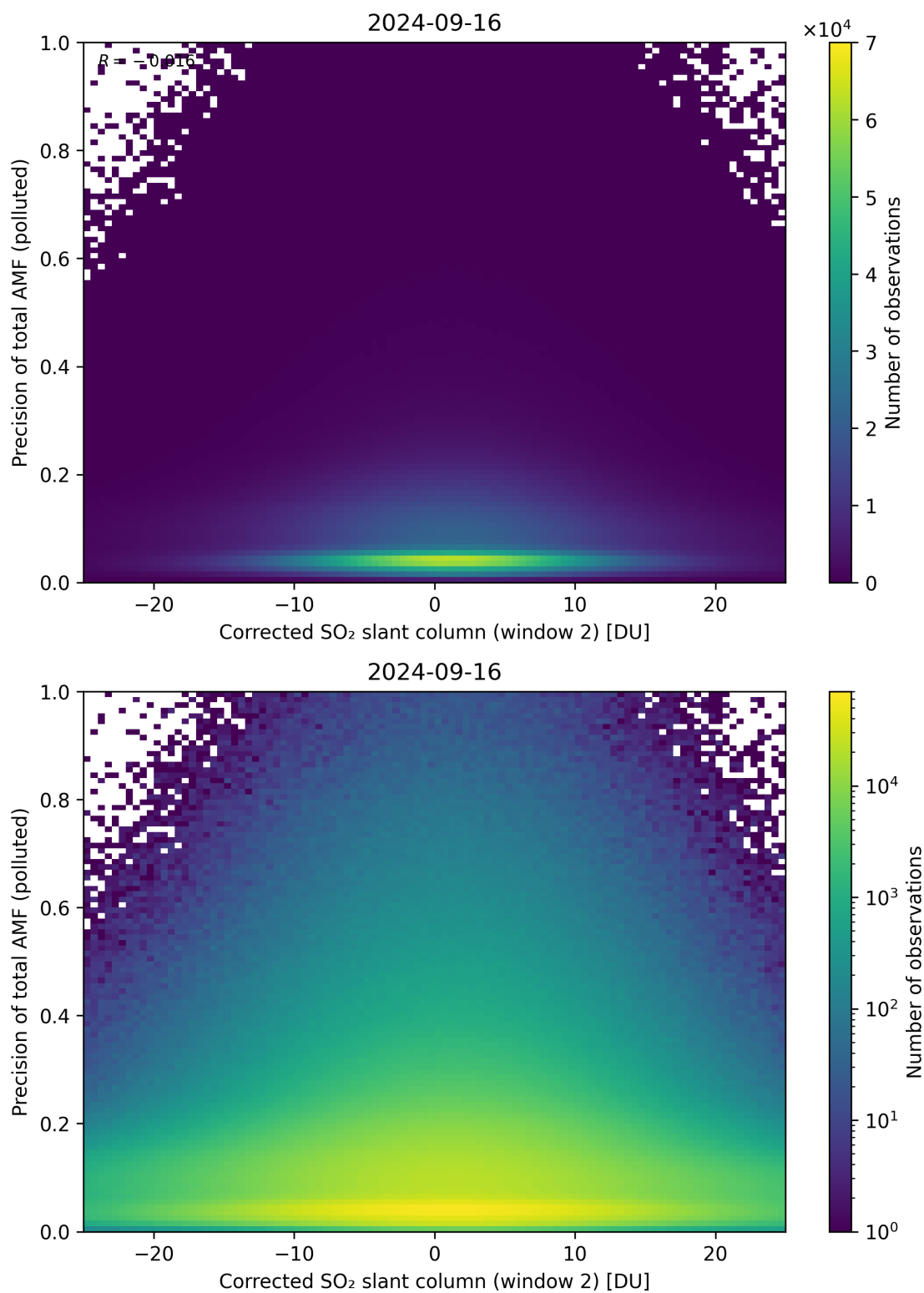
Figure 204: Scatter density plot of “Corrected SO 2 slant column (window 2)” against “Precision of total AMF (polluted)” for 2024-09-15 to 2024-09-17.
