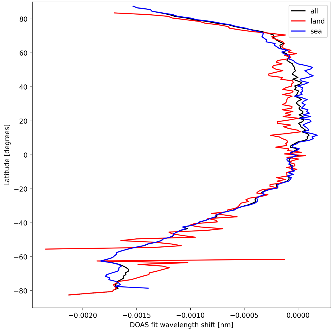
Figure 45: Zonal average of "DOAS fit wavelength shift" for 2024-09-15 to 2024-09-17.
