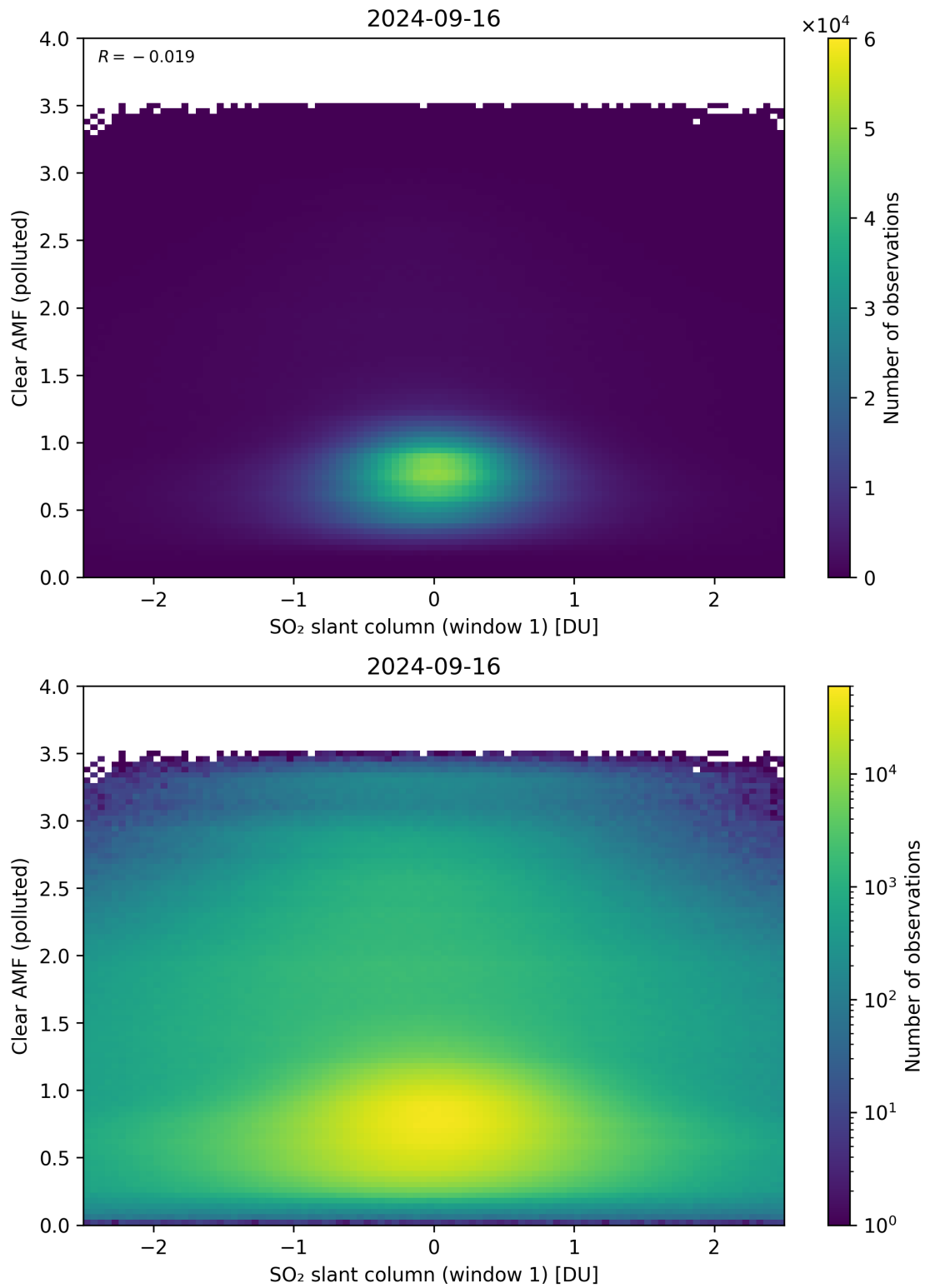
Figure 232: Scatter density plot of “SO 2 slant column (window 1)” against “Clear AMF (polluted)” for 2024-09-15 to 2024-09-17.
