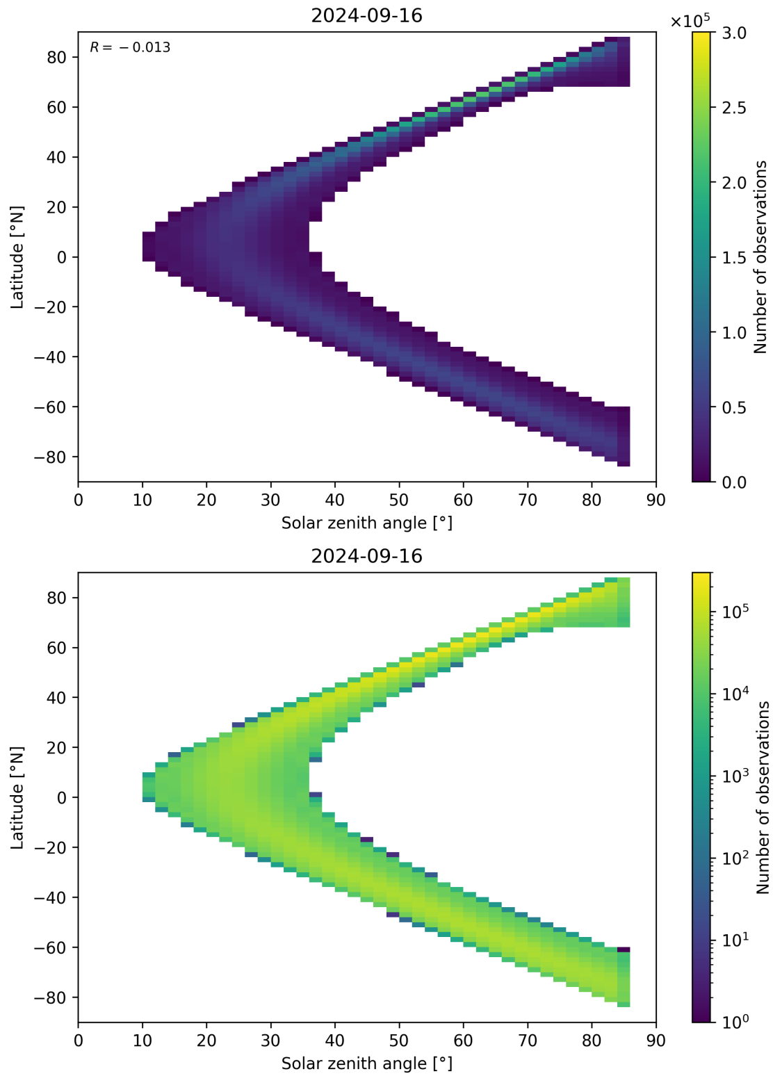
Figure 164: Scatter density plot of “Solar zenith angle” against “Latitude” for 2024-09-15 to 2024-09-17.
