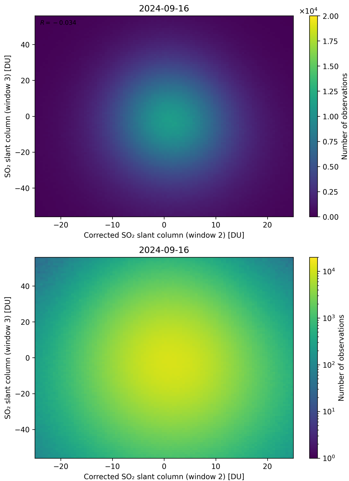
Figure 201: Scatter density plot of “Corrected SO 2 slant column (window 2)” against “SO 2 slant column (window 3)” for 2024-09-15 to 2024-09-17.
