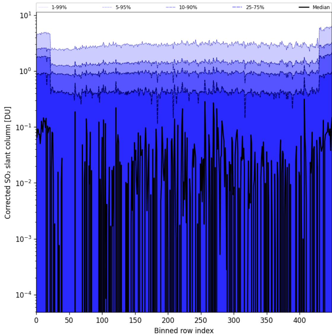
Figure 78: Along track statistics of “Corrected SO 2 slant column” for 2024-09-15 to 2024-09-17
