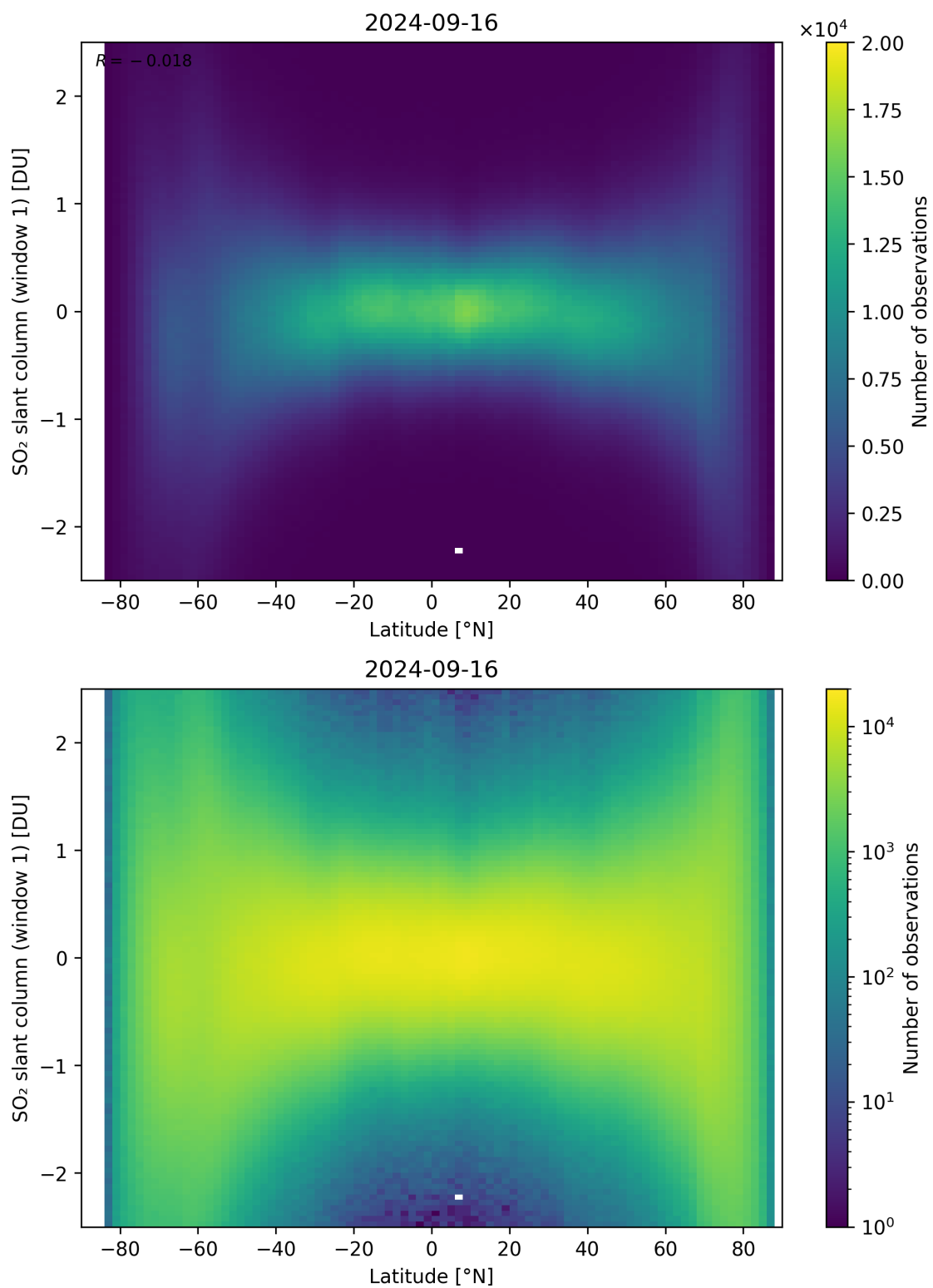
Figure 149: Scatter density plot of “Latitude” against “SO 2 slant column (window 1)” for 2024-09-15 to 2024-09-17.
