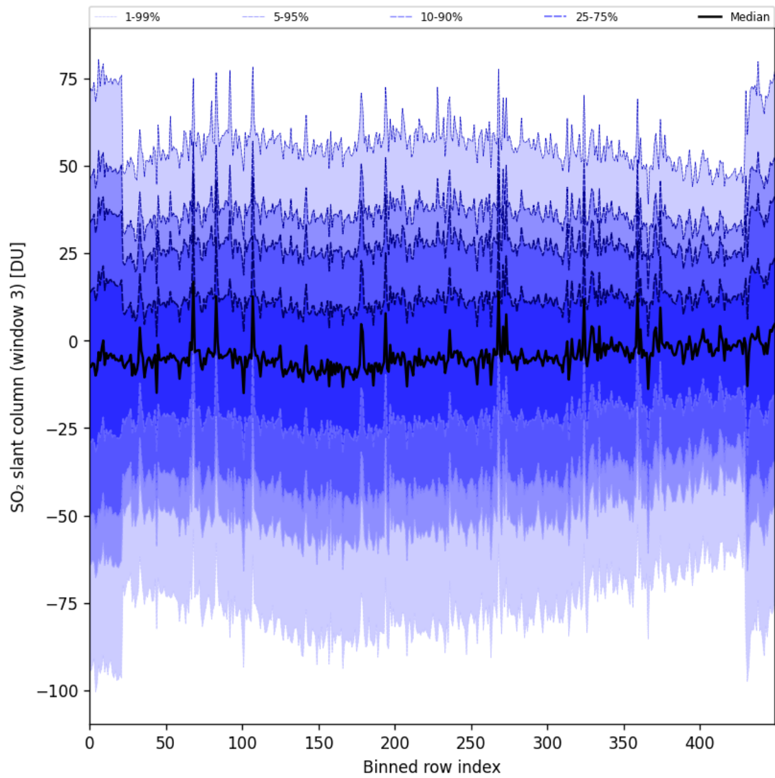
Figure 87: Along track statistics of “SO 2 slant column (window 3)” for 2024-09-15 to 2024-09-17
