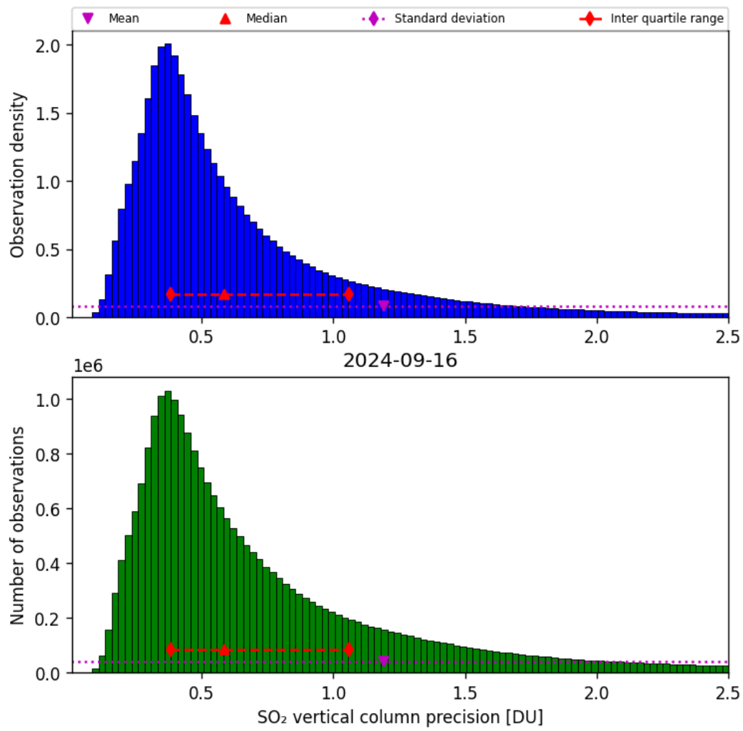
Figure 54: Histogram of “SO 2 vertical column precision” for 2024-09-15 to 2024-09-17
