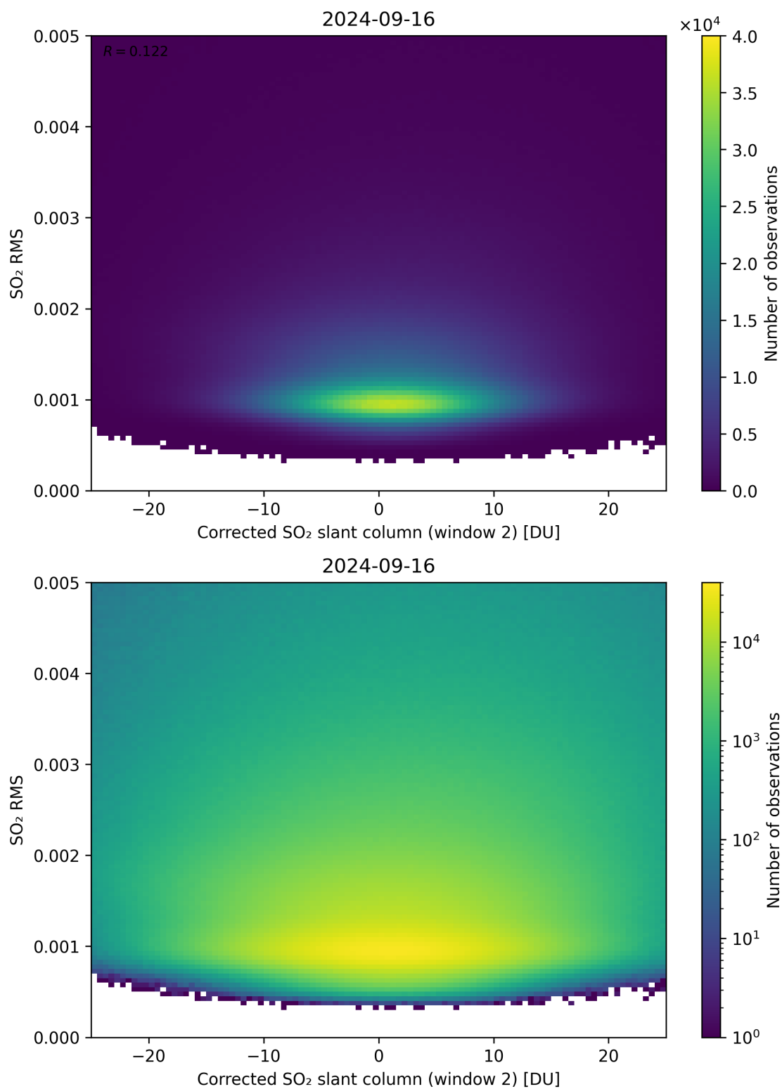
Figure 198: Scatter density plot of “Corrected SO 2 slant column (window 2)” against “SO 2 RMS” for 2024-09-15 to 2024-09-17.
