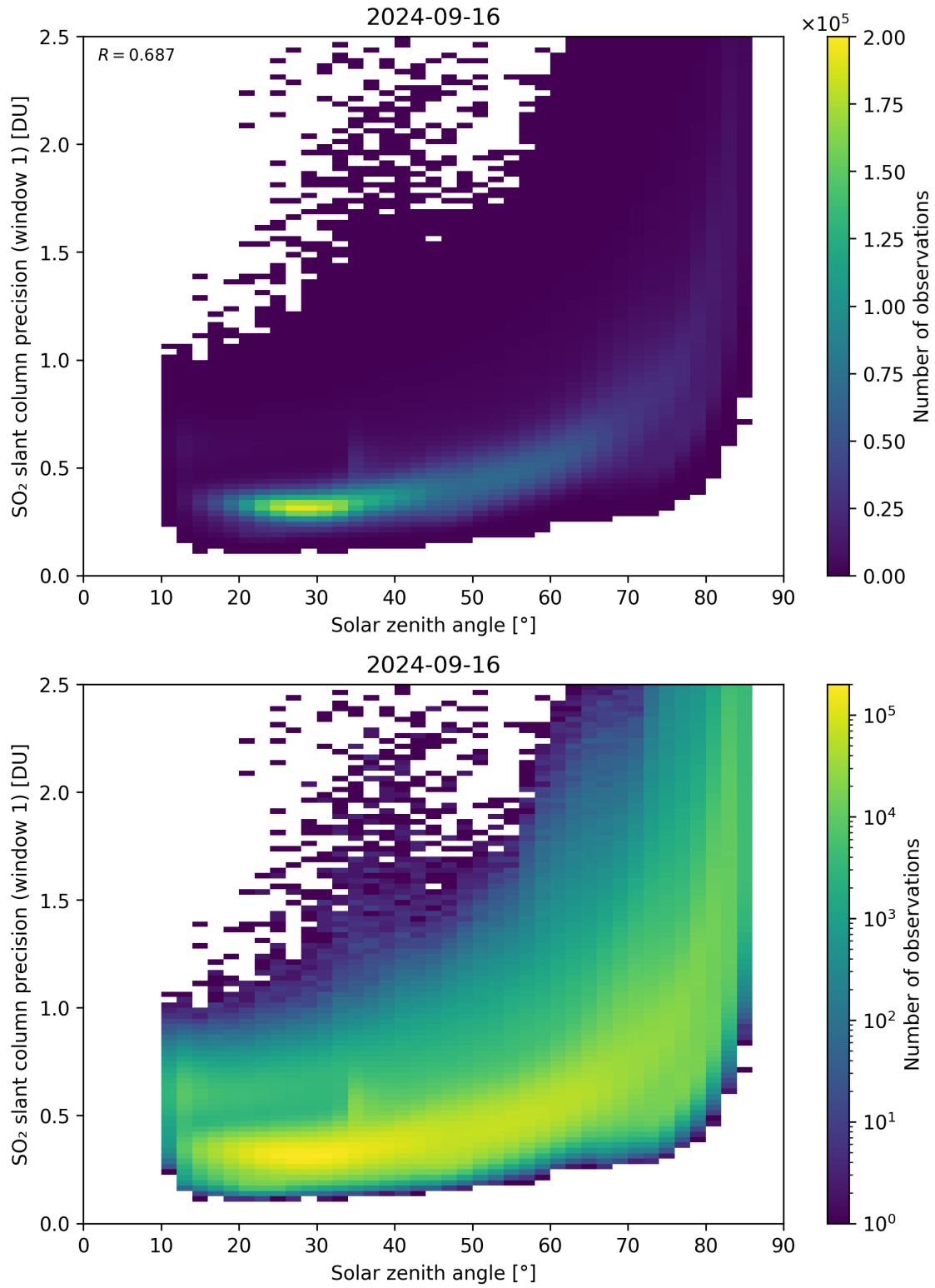
Figure 170: Scatter density plot of “Solar zenith angle” against “SO 2 slant column precision (window 1)” for 2024-09-15 to 2024-09-17.
