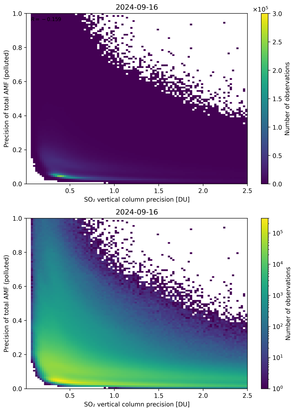
Figure 295: Scatter density plot of “SO 2 vertical column precision” against “Precision of total AMF (polluted)” for 2024-09-15 to 2024-09-17.
