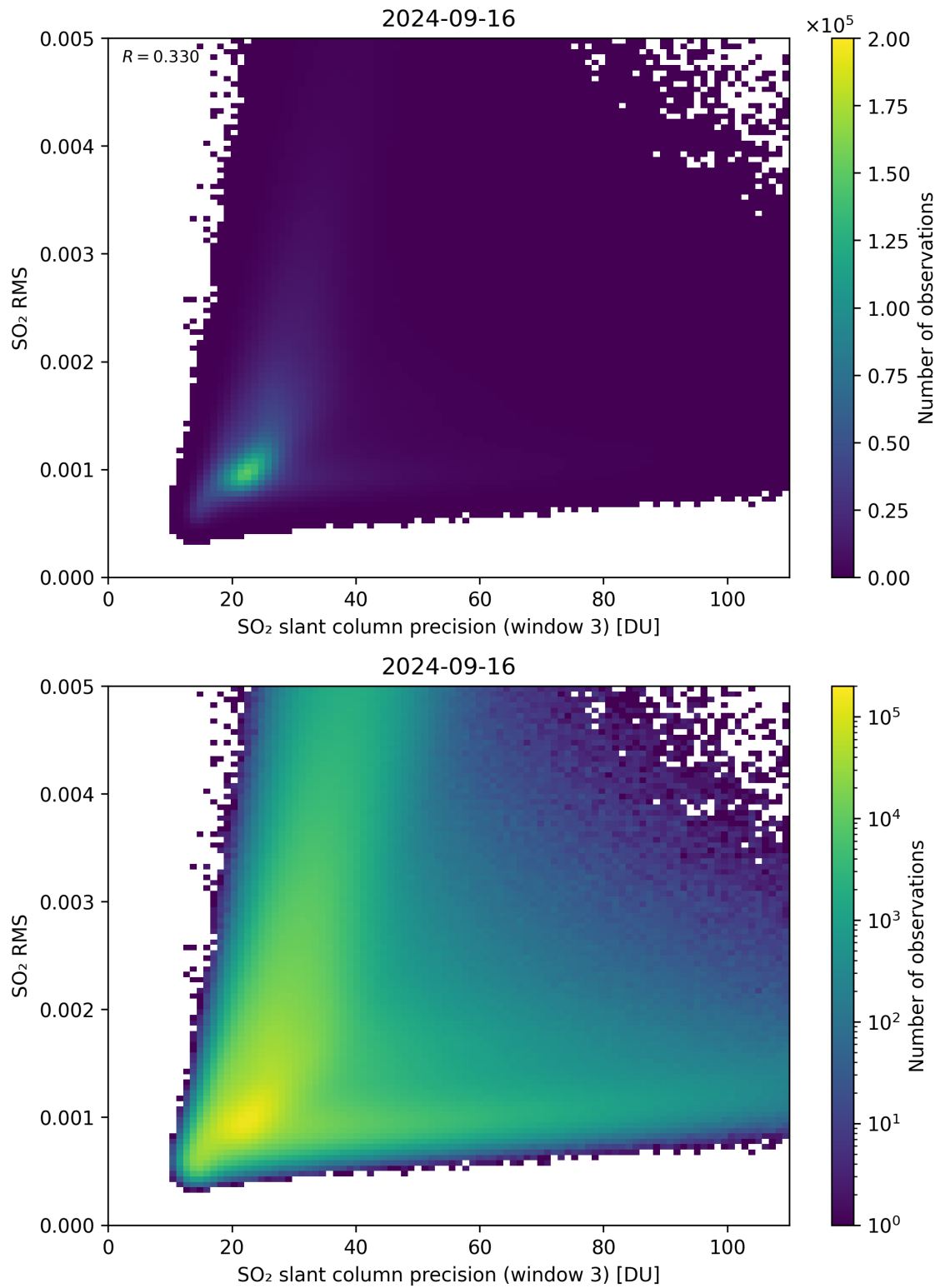
Figure 260: Scatter density plot of “SO 2 slant column precision (window 3)” against “SO 2 RMS” for 2024-09-15 to 2024-09-17.
