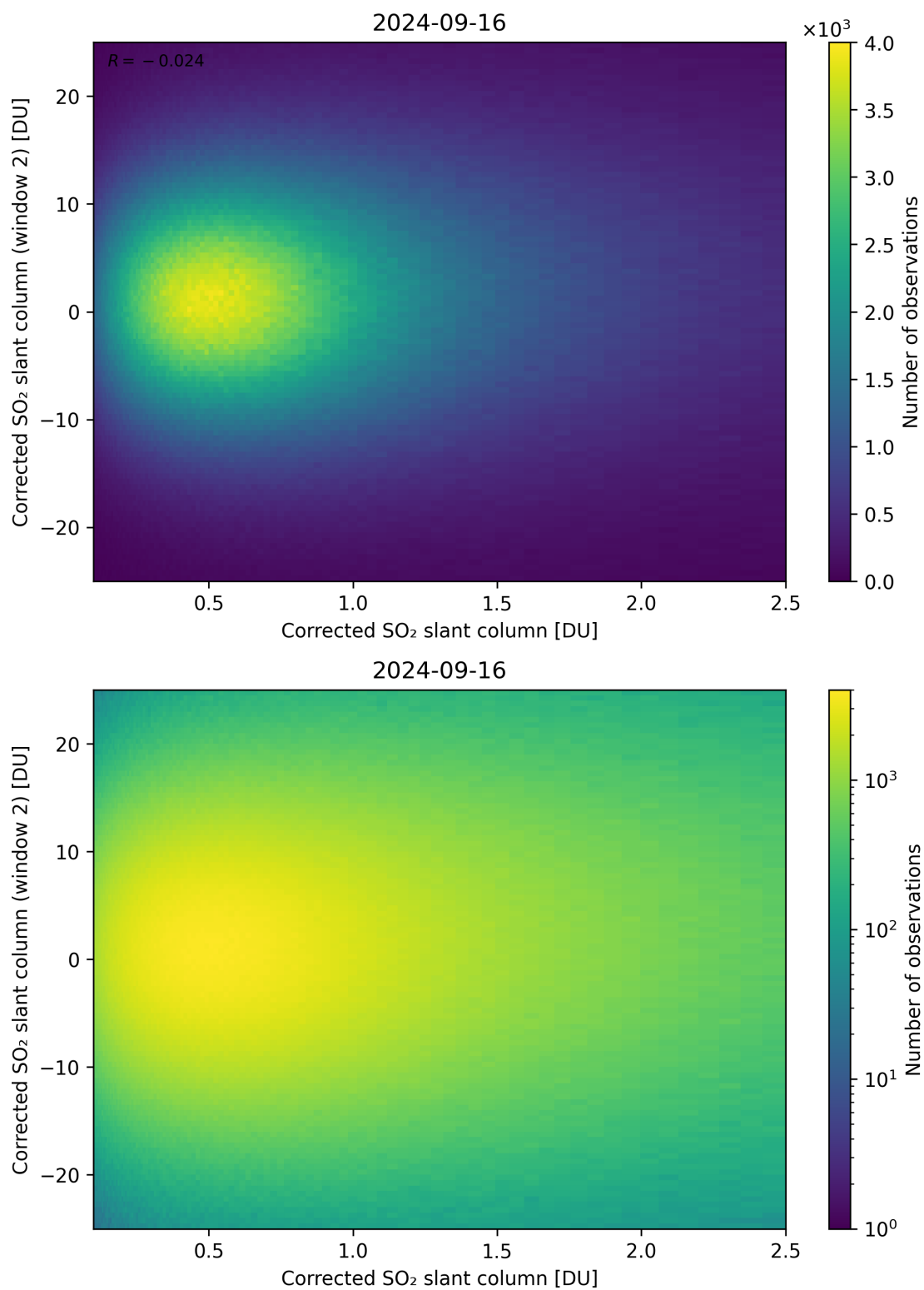
Figure 185: Scatter density plot of “Corrected SO 2 slant column” against “Corrected SO 2 slant column (window 2)” for 2024-09-15 to 2024-09-17.
