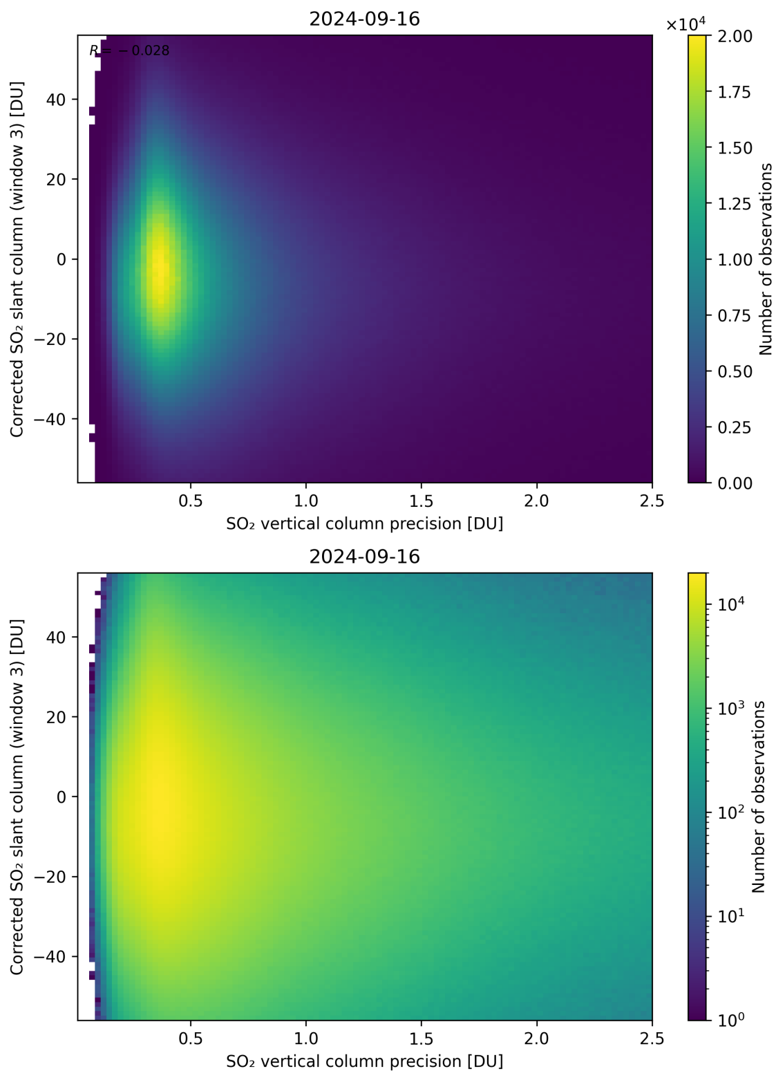
Figure 288: Scatter density plot of “SO 2 vertical column precision” against “Corrected SO 2 slant column (window 3)” for 2024-09-15 to 2024-09-17.
