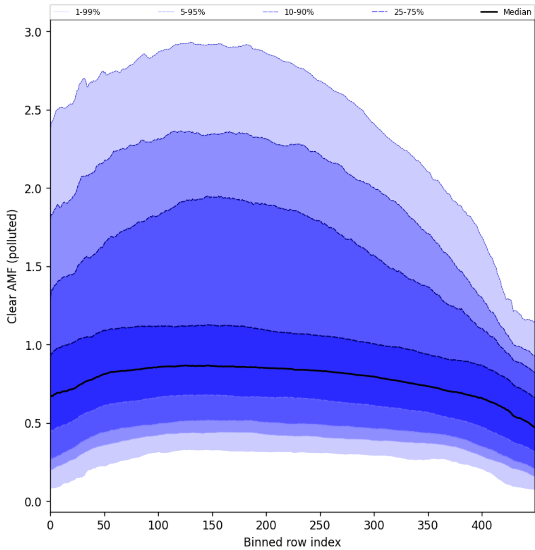
Figure 96: Along track statistics of “Clear AMF (polluted)” for 2024-09-15 to 2024-09-17
