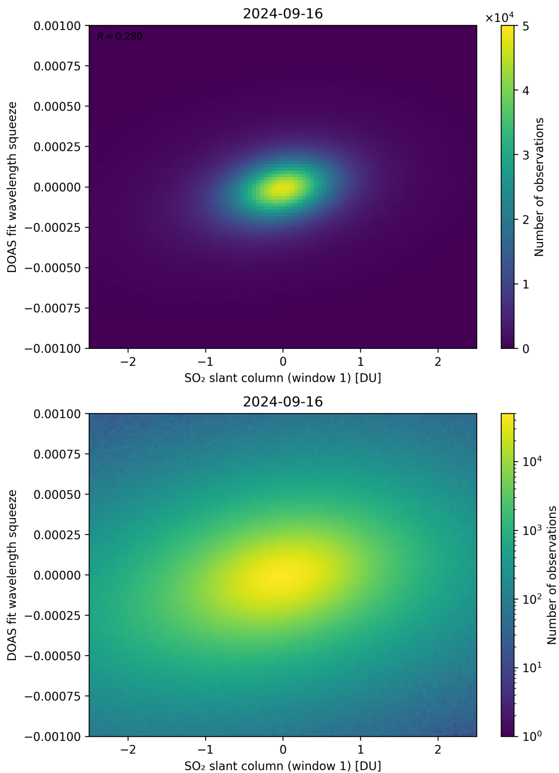
Figure 216: Scatter density plot of “SO 2 slant column (window 1)” against “DOAS fit wavelength squeeze” for 2024-09-15 to 2024-09-17.
