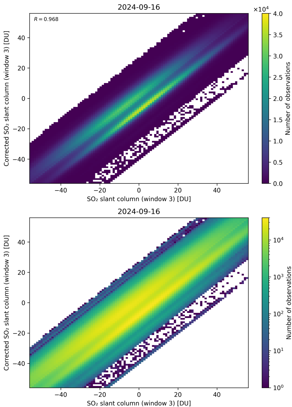
Figure 266: Scatter density plot of “SO 2 slant column (window 3)” against “Corrected SO 2 slant column (window 3)” for 2024-09-15 to 2024-09-17.
