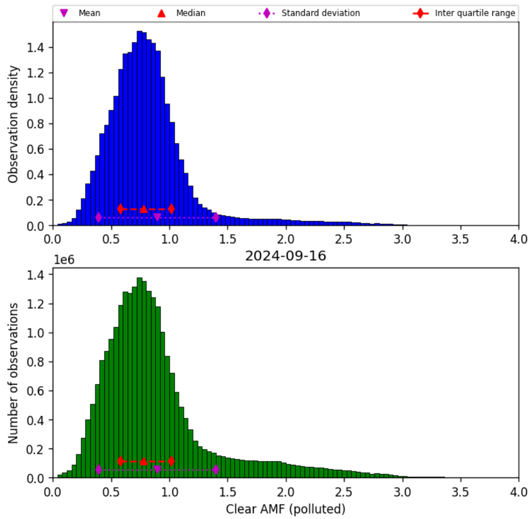
Figure 73: Histogram of “Clear AMF (polluted)” for 2024-09-15 to 2024-09-17
