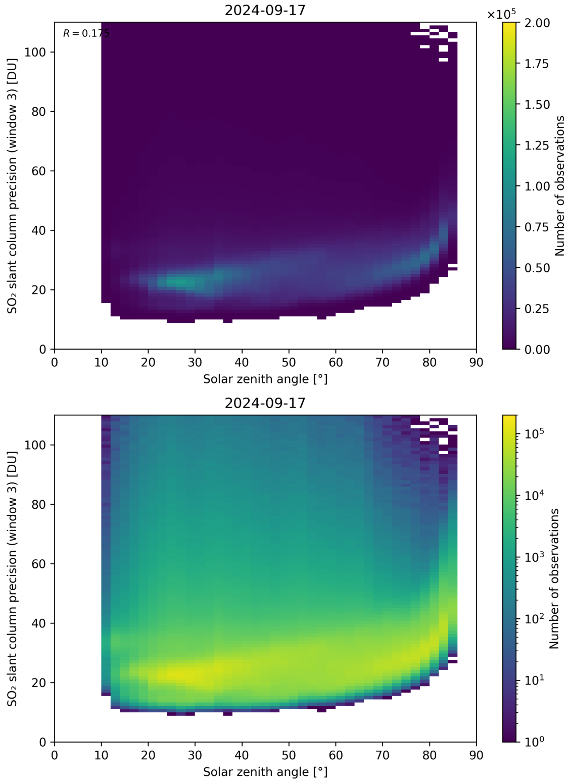
Figure 173: Scatter density plot of “Solar zenith angle” against “SO 2 slant column precision (window 3)” for 2024-09-17 to 2024-09-18.
