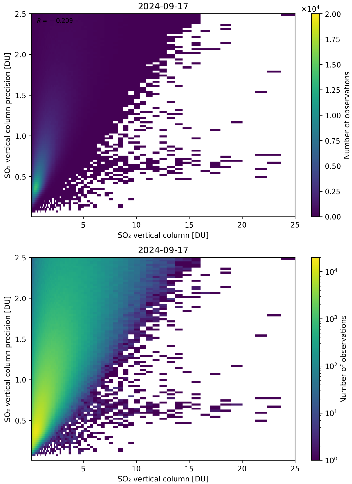
Figure 307: Scatter density plot of “SO 2 vertical column” against “SO 2 vertical column precision” for 2024-09-17 to 2024-09-18.
