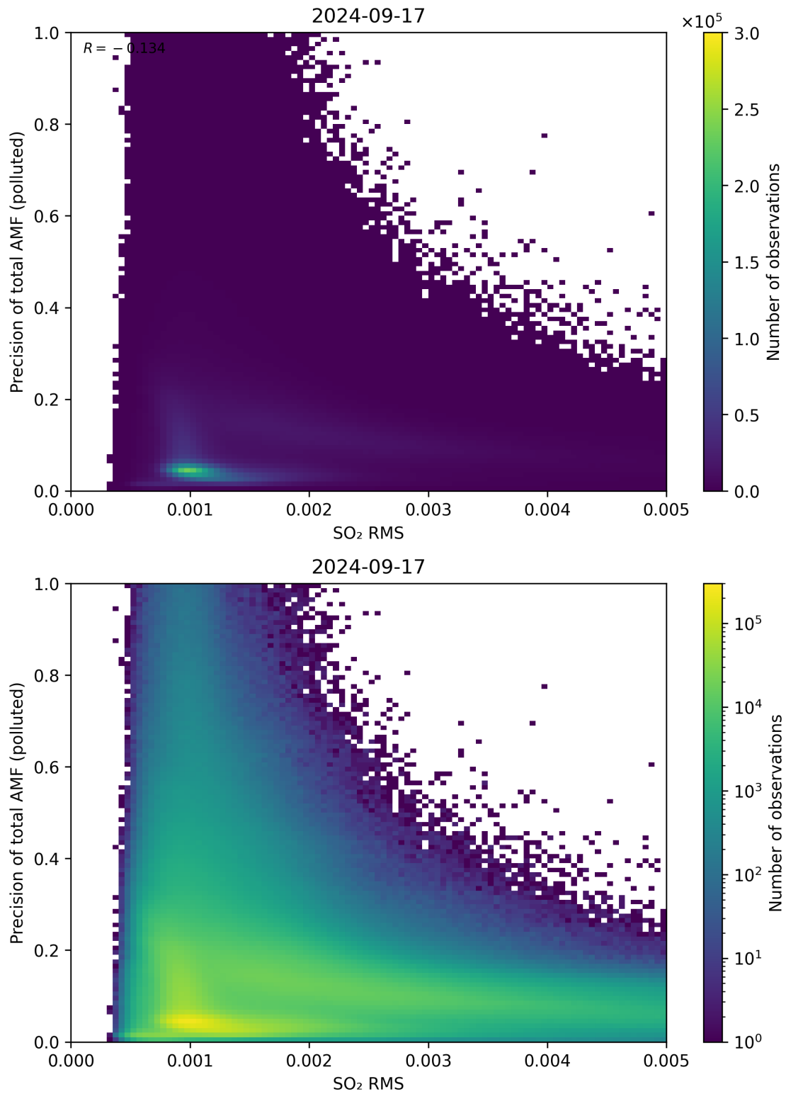
Figure 138: Scatter density plot of “SO 2 RMS” against “Precision of total AMF (polluted)” for 2024-09-17 to 2024-09-18.
