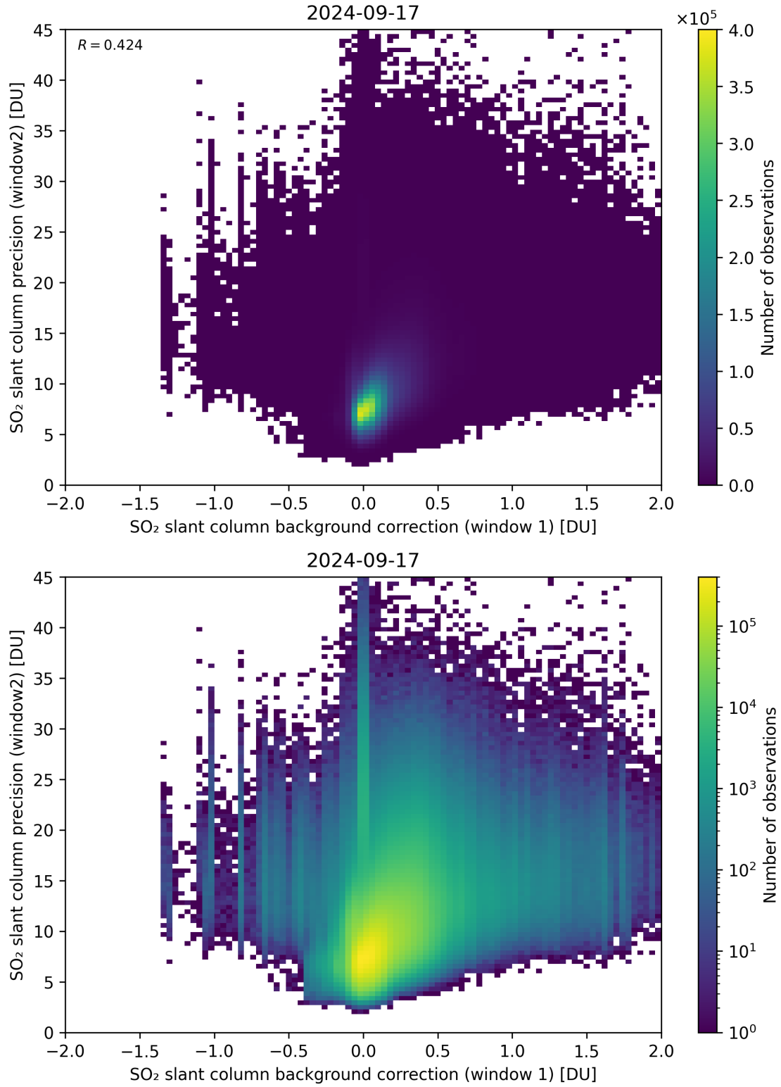
Figure 106: Scatter density plot of “SO 2 slant column background correction (window 1)” against “SO 2 slant column precision (window2)” for 2024-09-17 to 2024-09-18.
