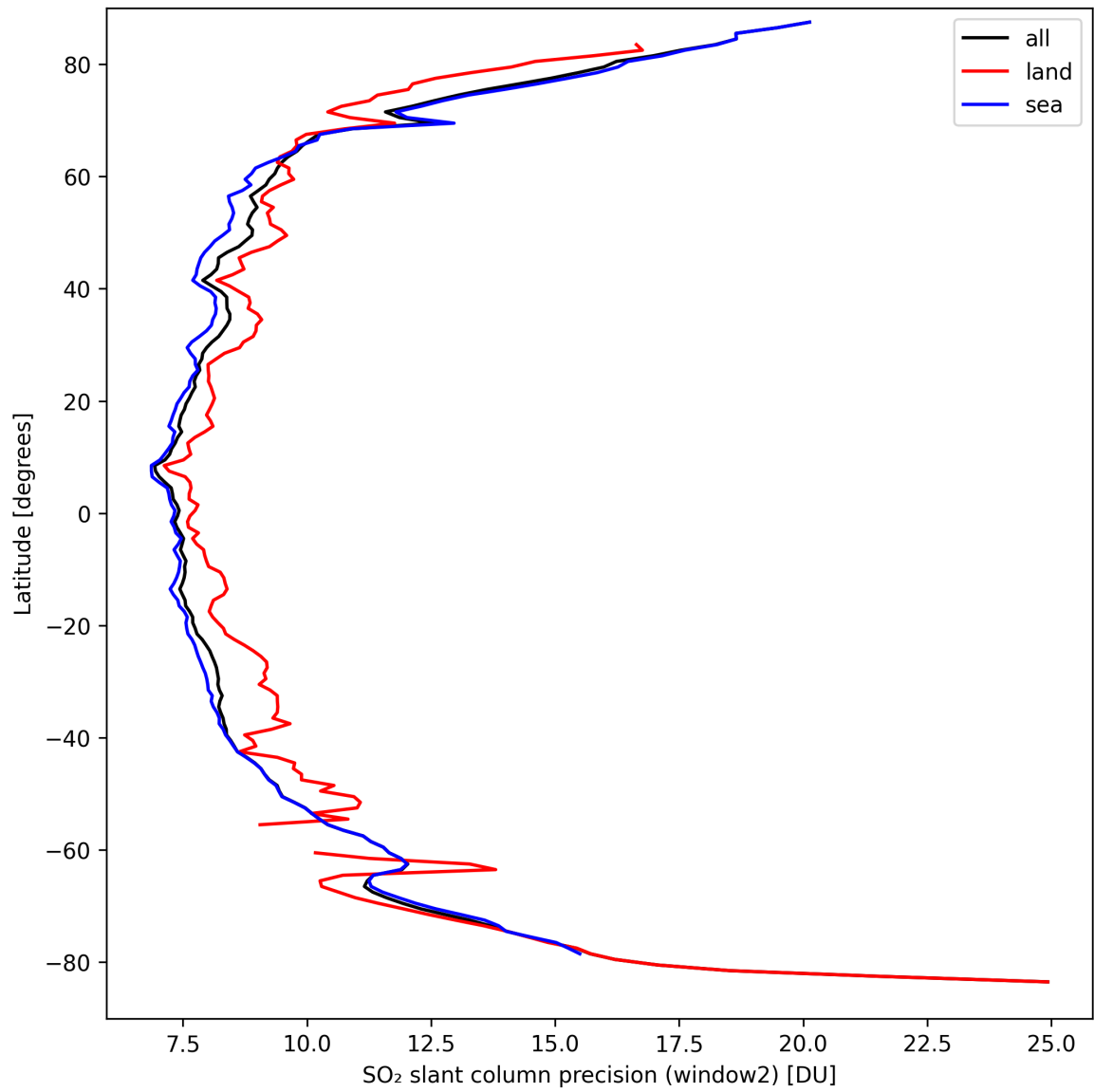
Figure 38: Zonal average of “SO 2 slant column precision (window2)” for 2024-09-17 to 2024-09-18.
