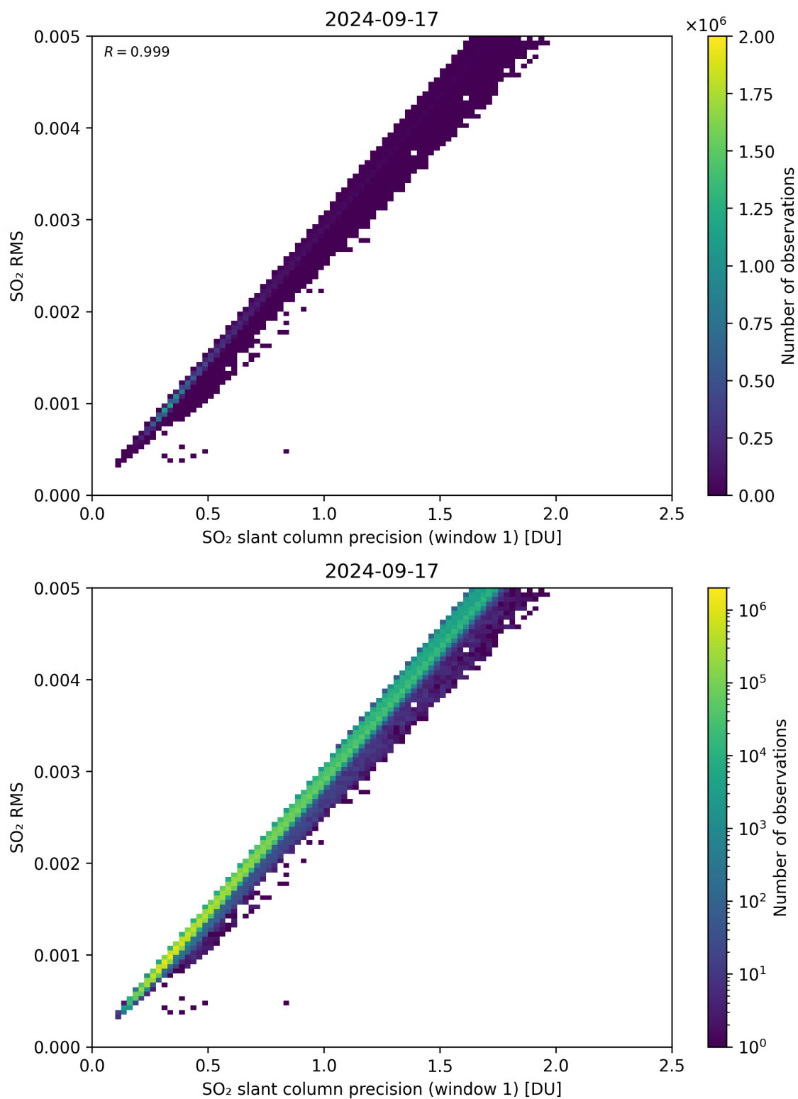
Figure 223: Scatter density plot of “SO 2 slant column precision (window 1)” against “SO 2 RMS” for 2024-09-17 to 2024-09-18.
