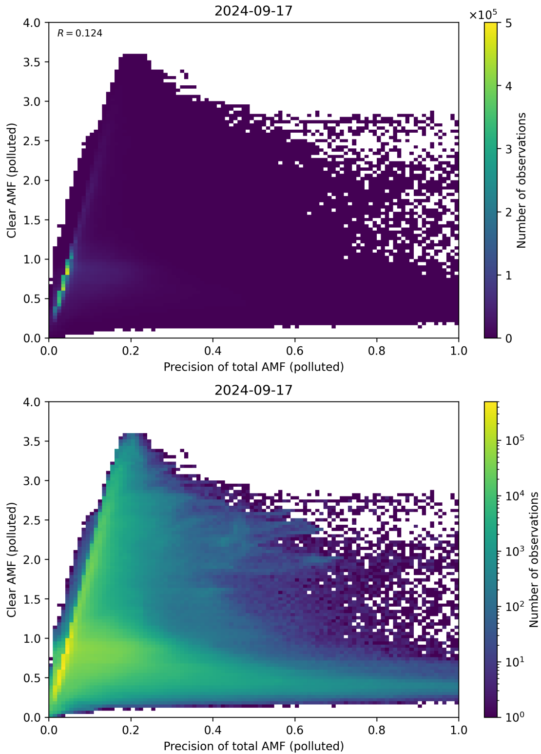
Figure 270: Scatter density plot of “Precision of total AMF (polluted)” against “Clear AMF (polluted)” for 2024-09-17 to 2024-09-18.
