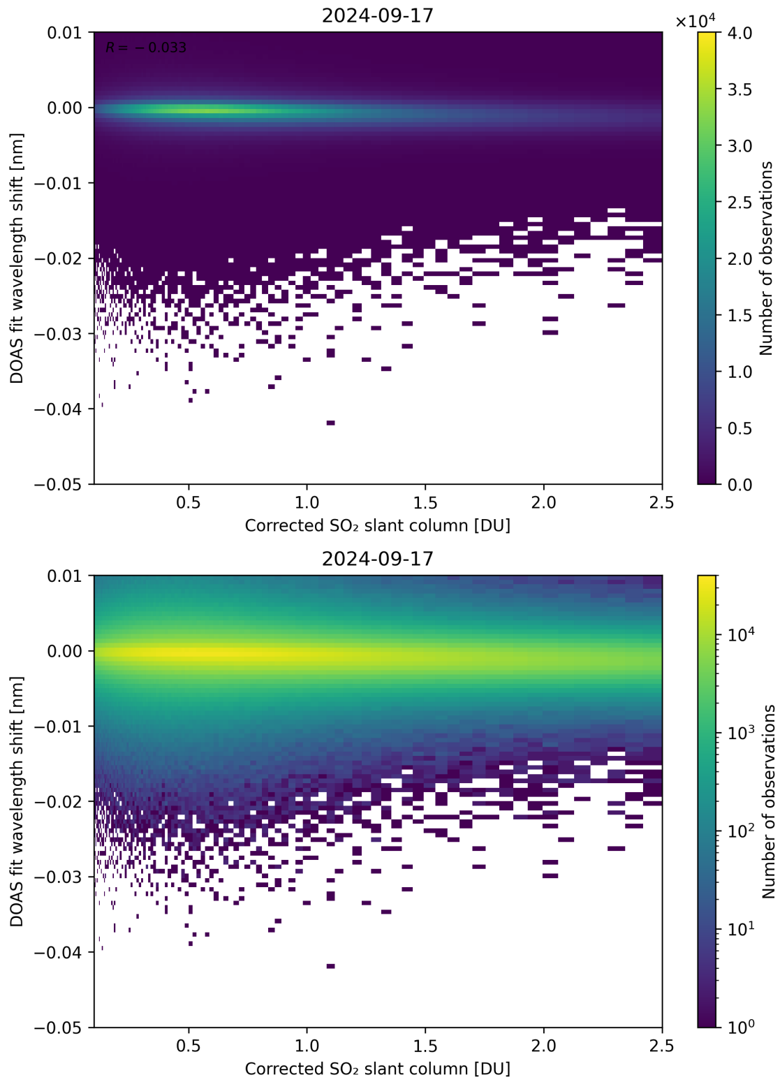
Figure 181: Scatter density plot of “Corrected SO 2 slant column” against “DOAS fit wavelength shift” for 2024-09-17 to 2024-09-18.
