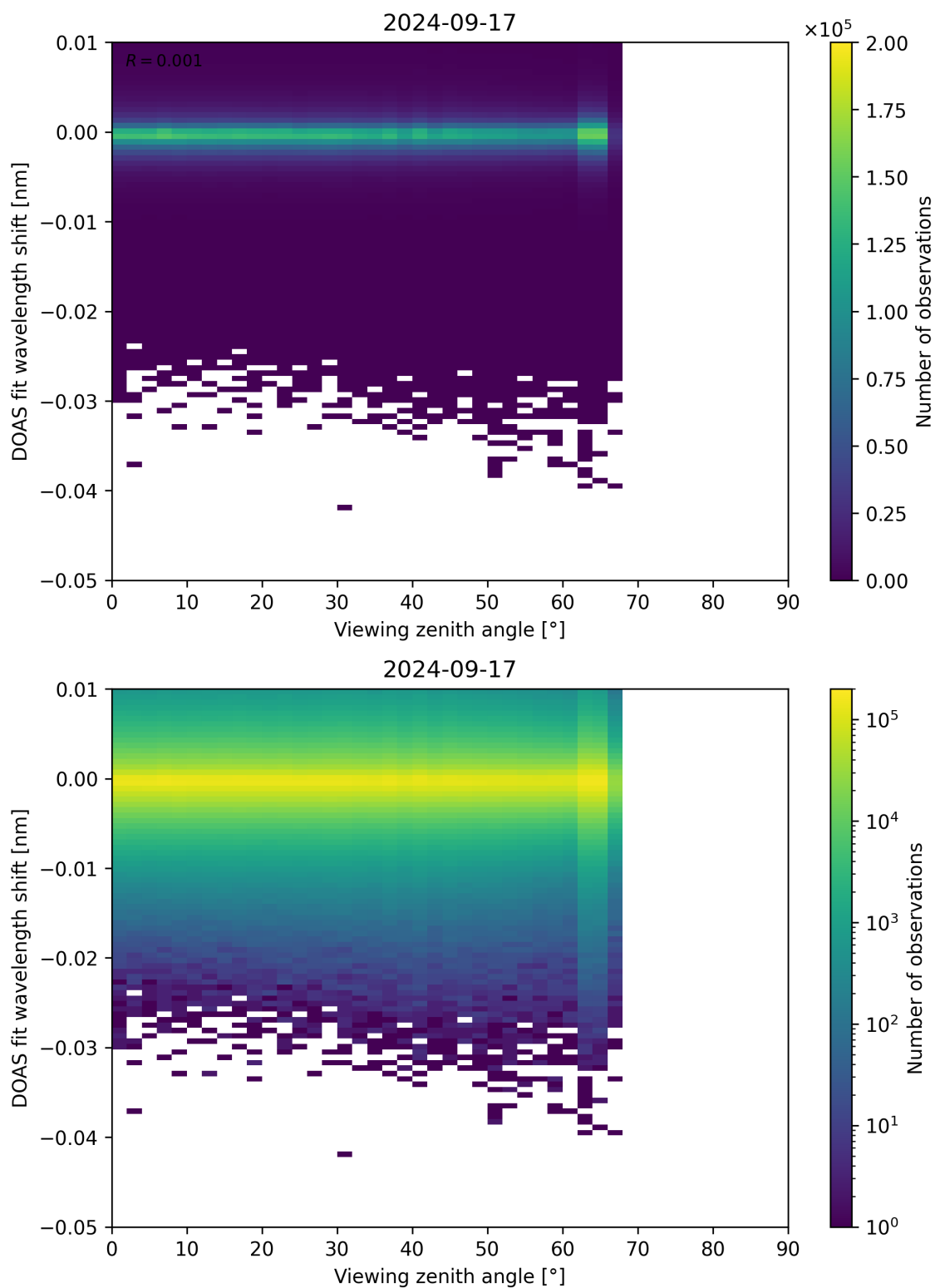
Figure 311: Scatter density plot of “Viewing zenith angle” against “DOAS fit wavelength shift” for 2024-09-17 to 2024-09-18.
