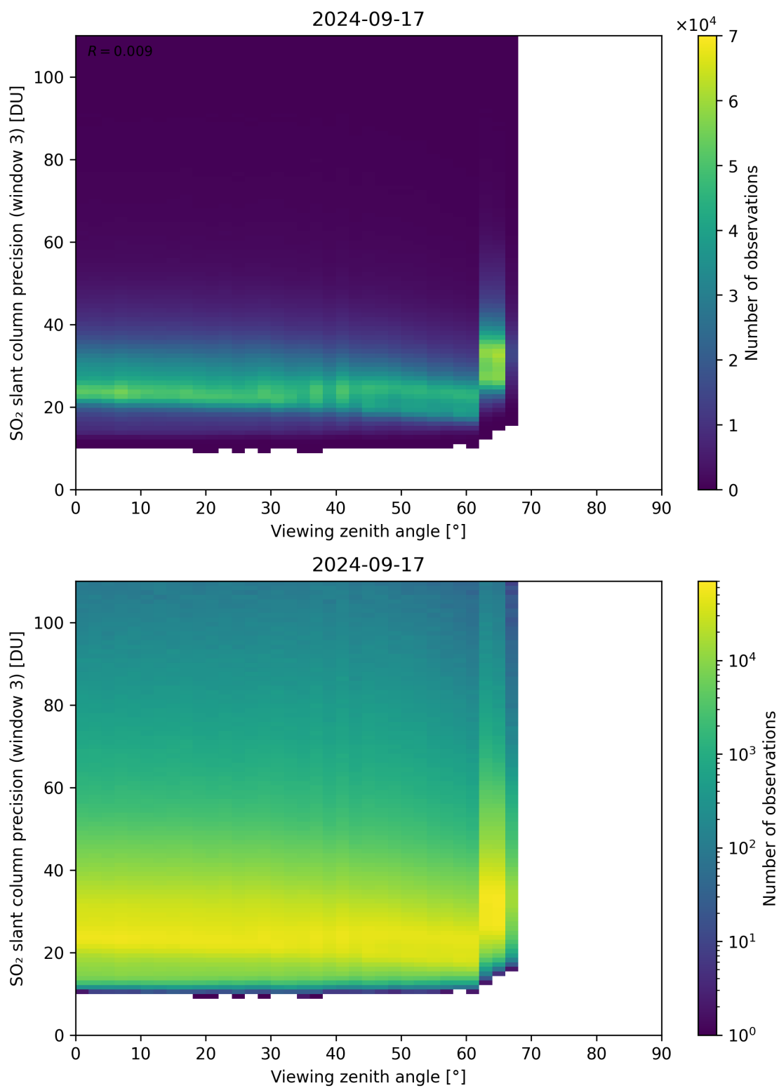
Figure 324: Scatter density plot of “Viewing zenith angle” against “SO 2 slant column precision (window 3)” for 2024-09-17 to 2024-09-18.
