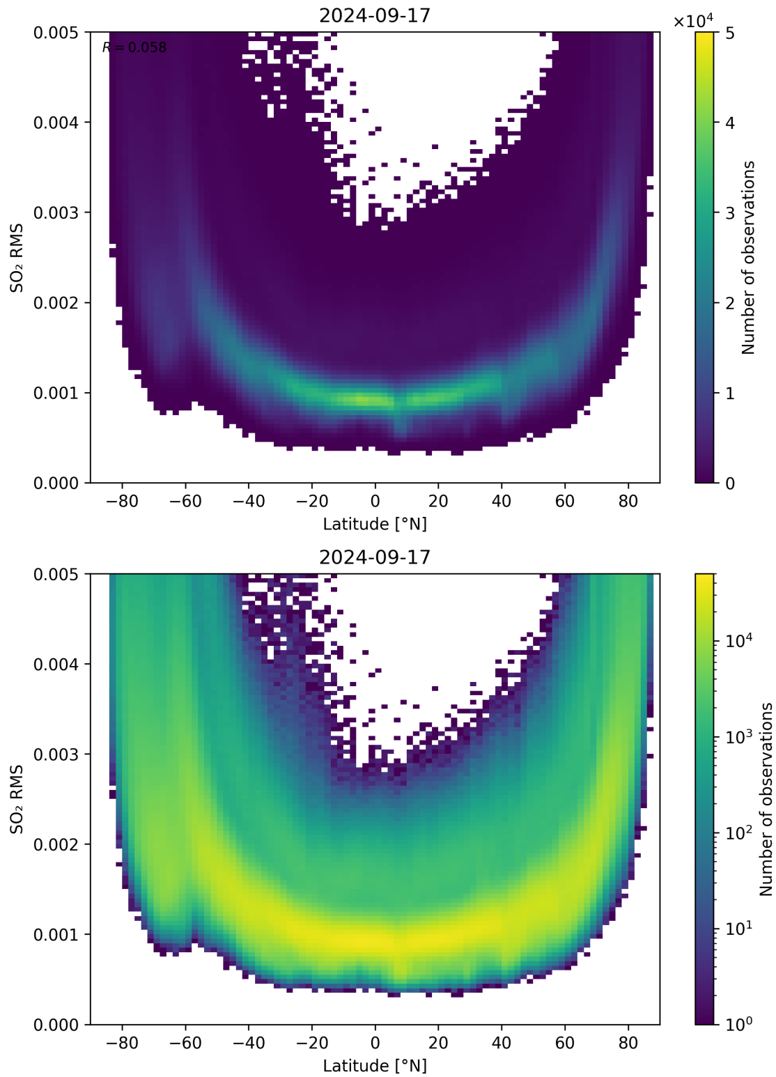
Figure 144: Scatter density plot of “Latitude” against “SO 2 RMS” for 2024-09-17 to 2024-09-18.
