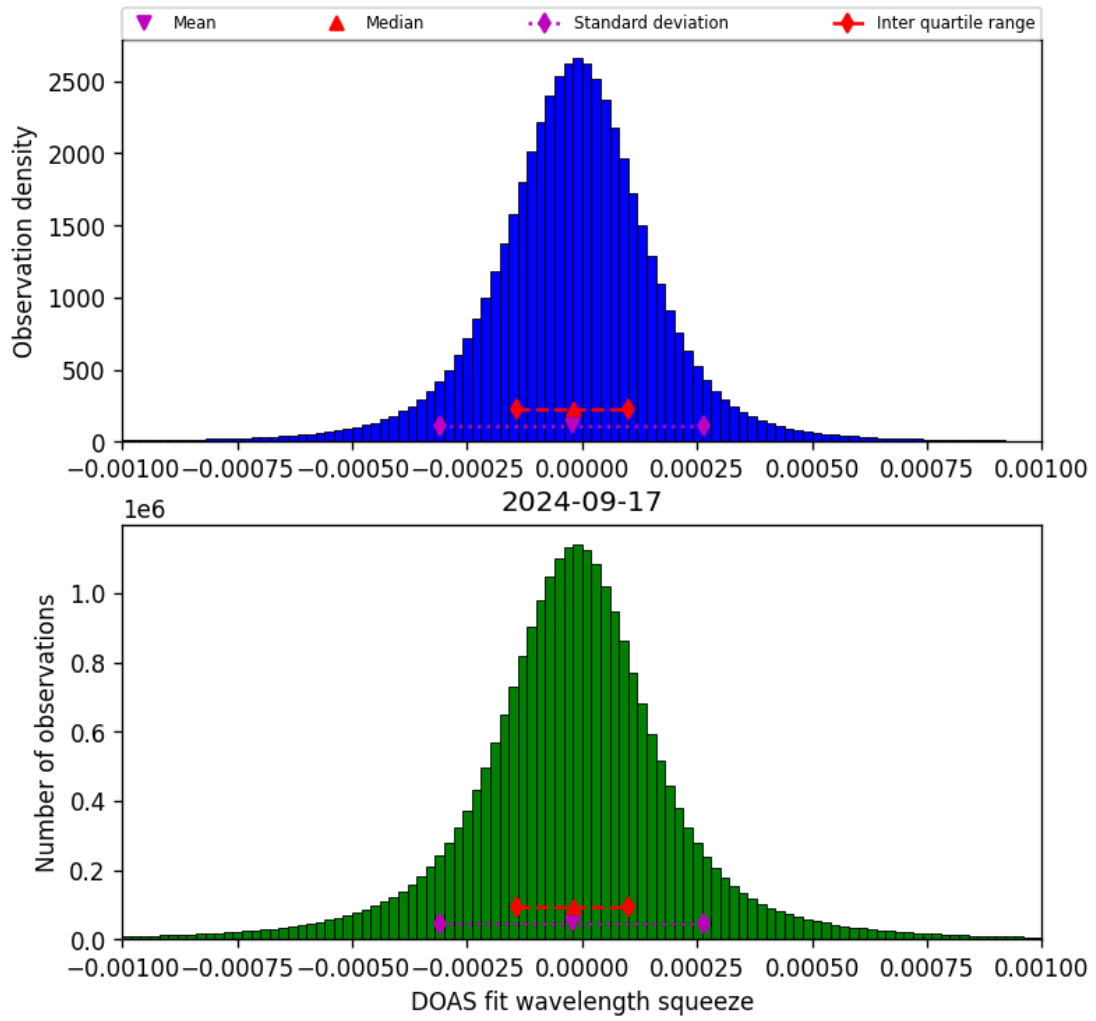
Figure 69: Histogram of “DOAS fit wavelength squeeze” for 2024-09-17 to 2024-09-18
