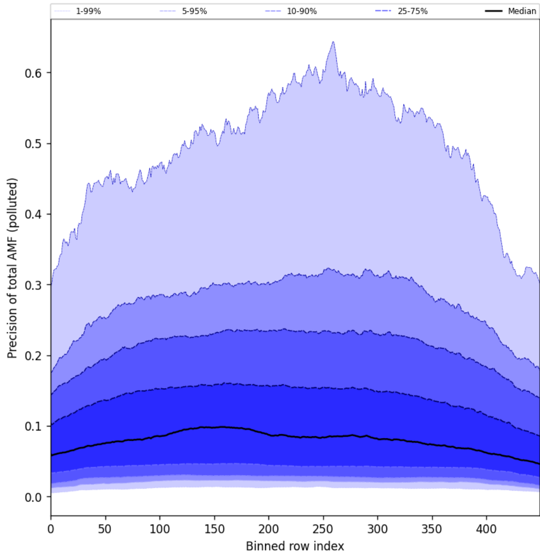
Figure 95: Along track statistics of “Precision of total AMF (polluted)” for 2024-09-17 to 2024-09-18
