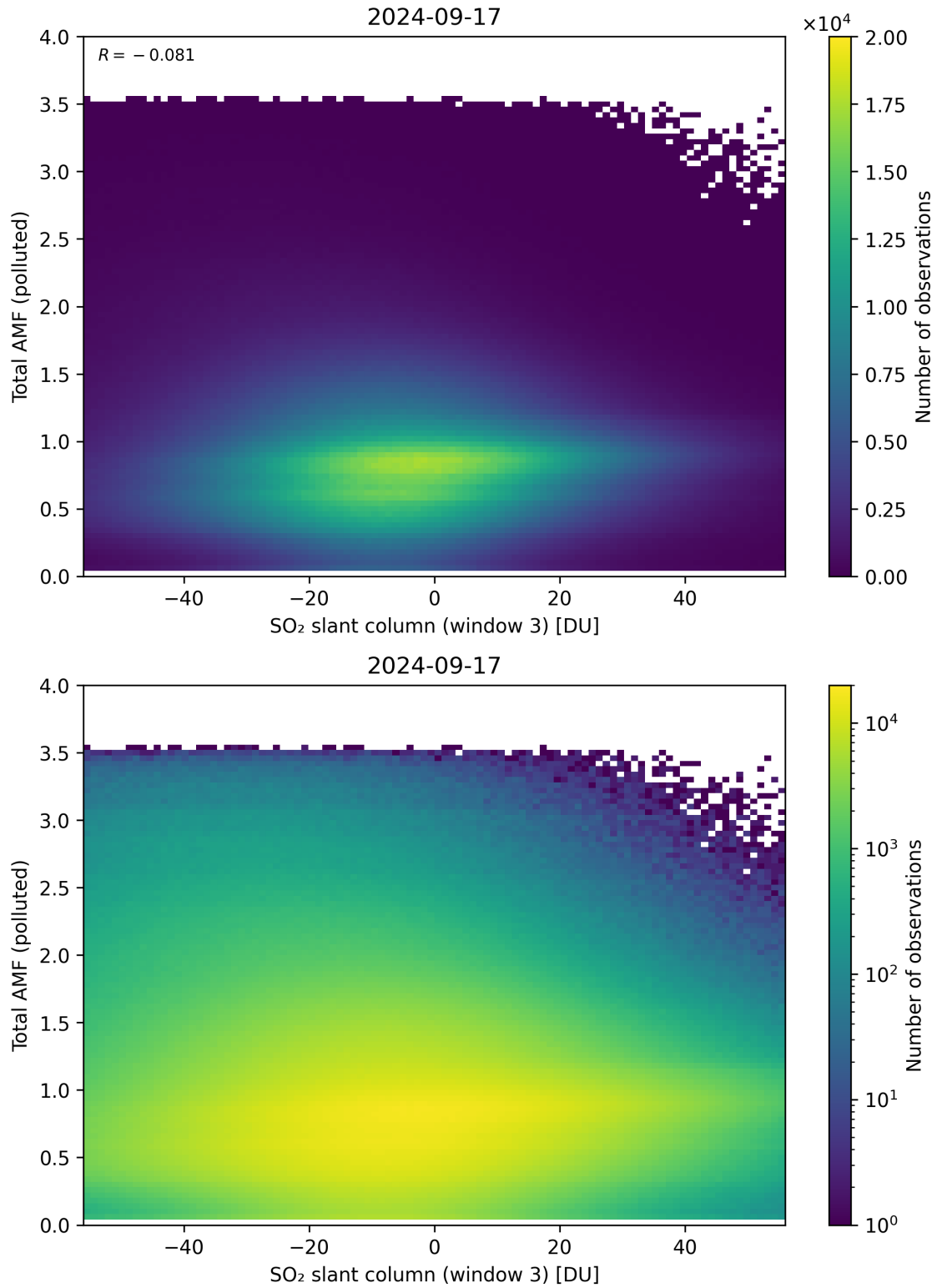
Figure 268: Scatter density plot of “SO 2 slant column (window 3)” against “Total AMF (polluted)” for 2024-09-17 to 2024-09-18.
