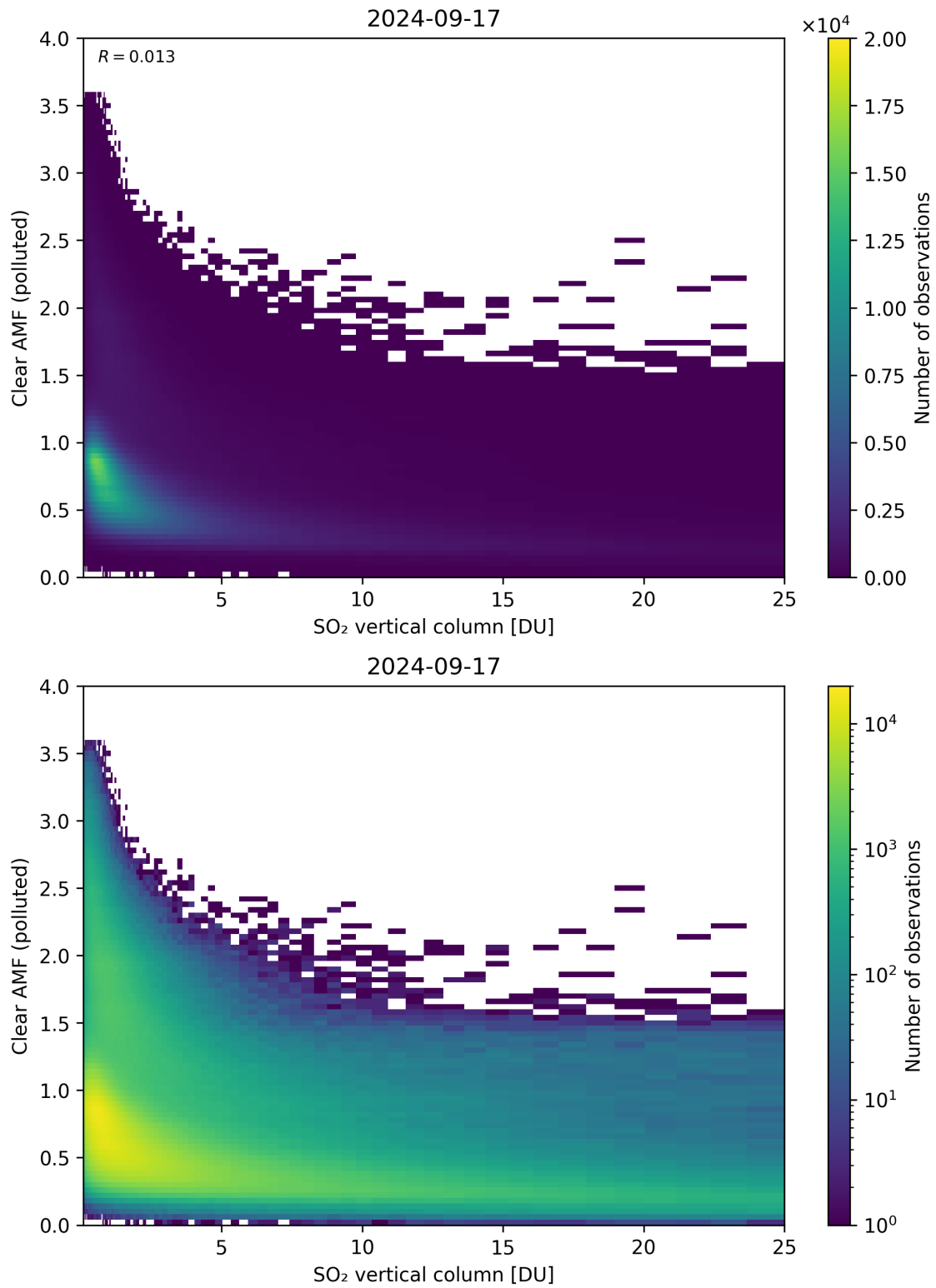
Figure 296: Scatter density plot of “SO 2 vertical column” against “Clear AMF (polluted)” for 2024-09-17 to 2024-09-18.
