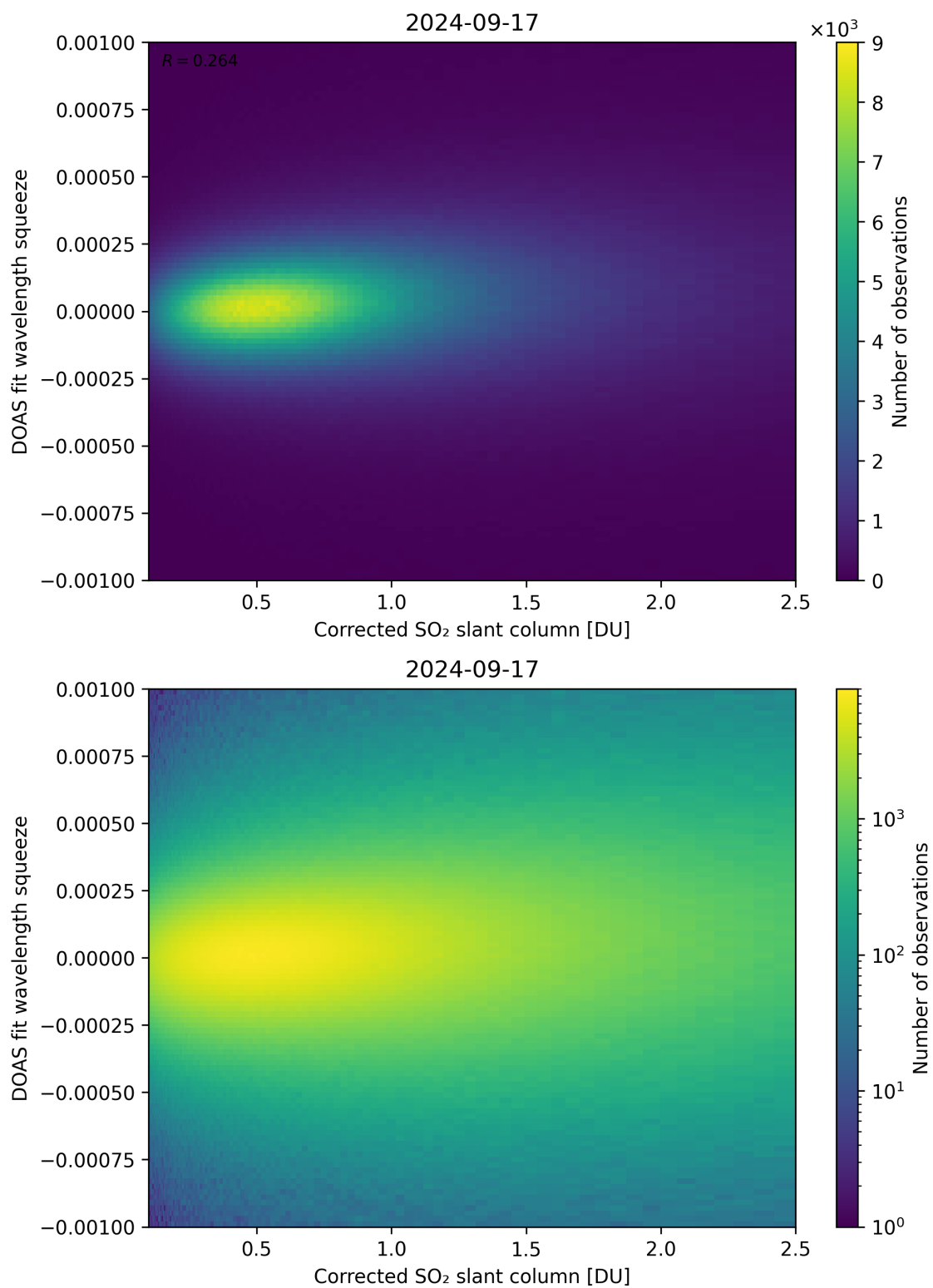
Figure 182: Scatter density plot of “Corrected SO 2 slant column” against “DOAS fit wavelength squeeze” for 2024-09-17 to 2024-09-18.
