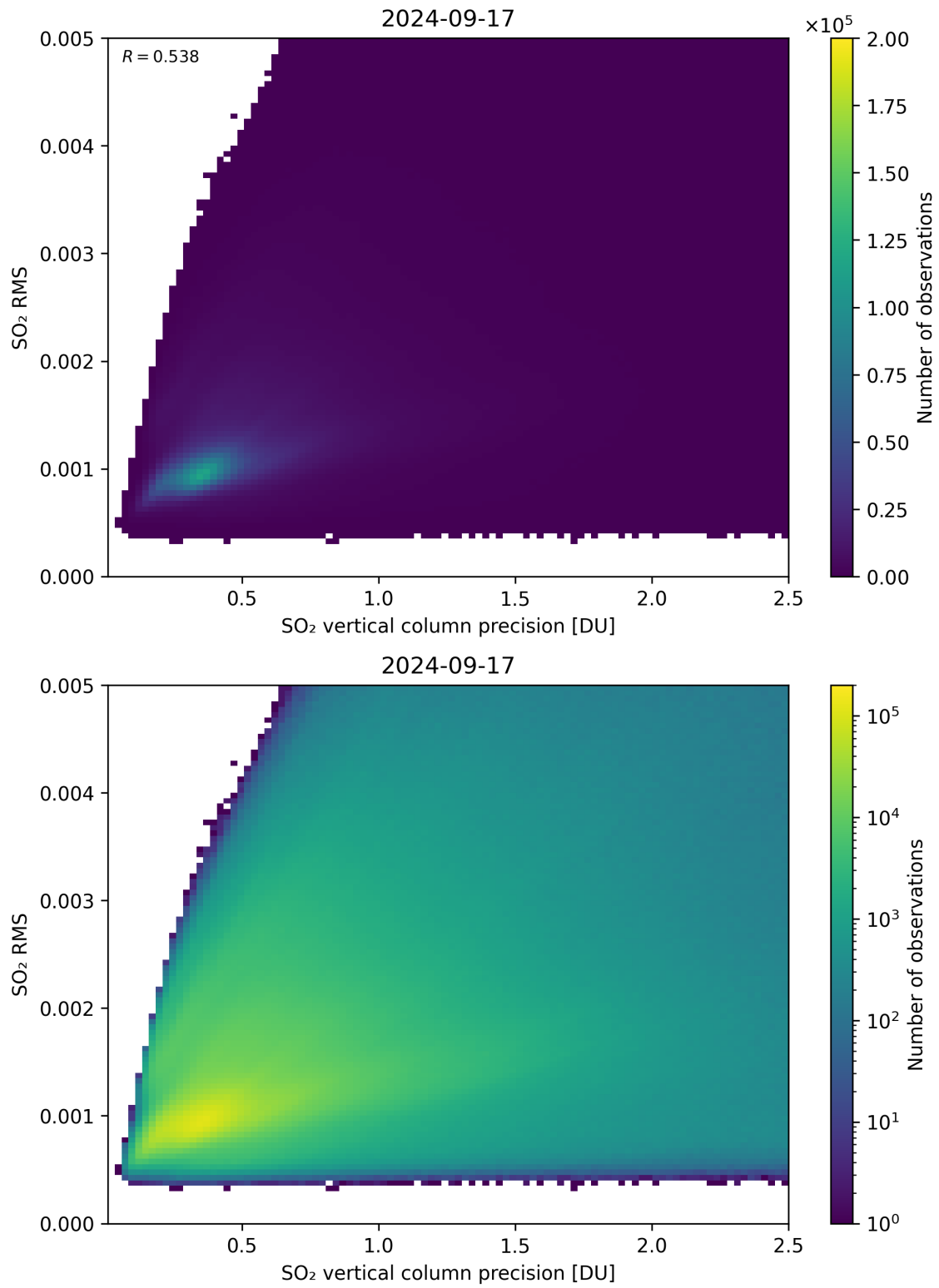
Figure 284: Scatter density plot of “SO 2 vertical column precision” against “SO 2 RMS” for 2024-09-17 to 2024-09-18.
