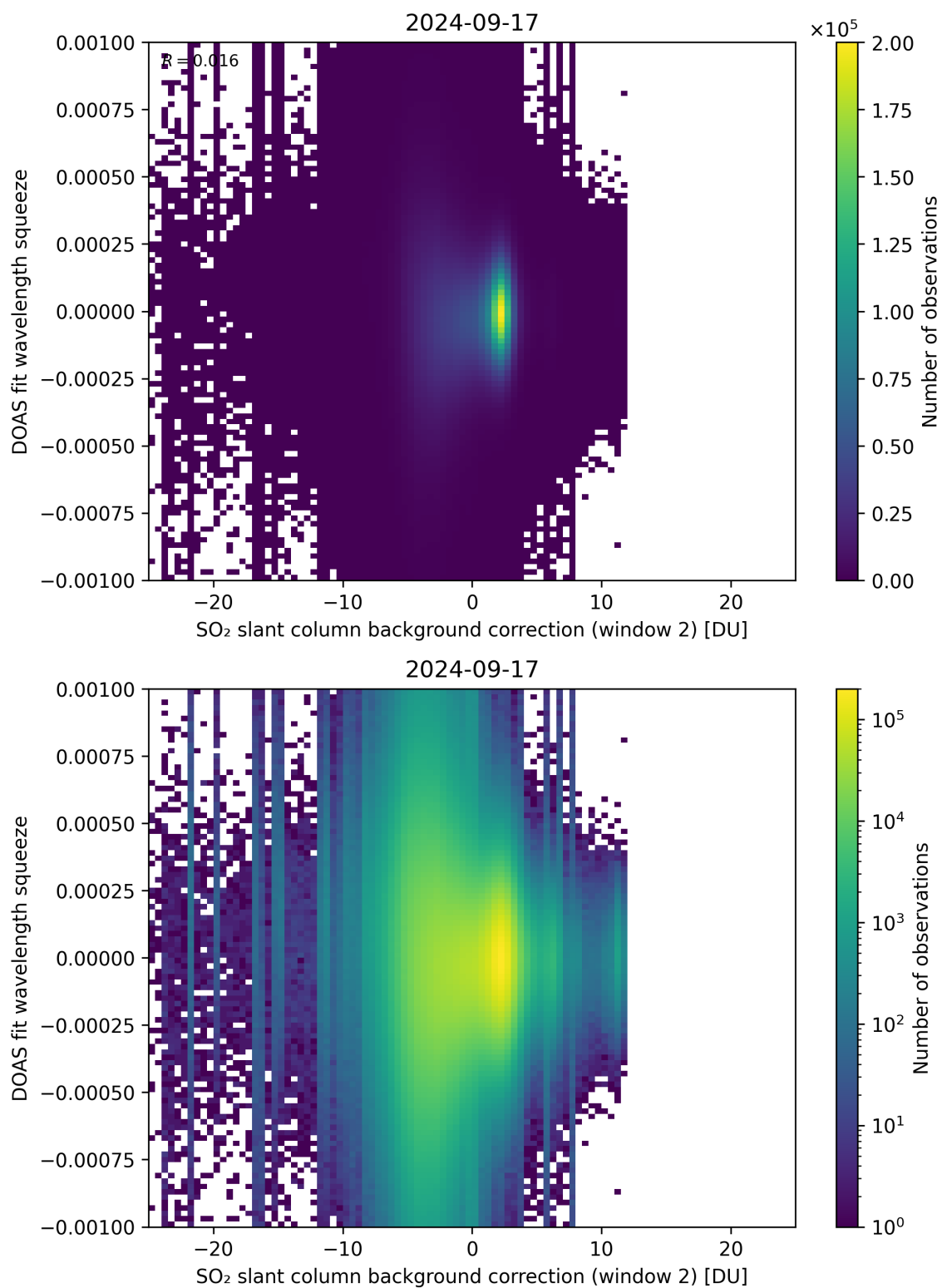
Figure 113: Scatter density plot of “SO 2 slant column background correction (window 2)” against “DOAS fit wavelength squeeze” for 2024-09-17 to 2024-09-18.
