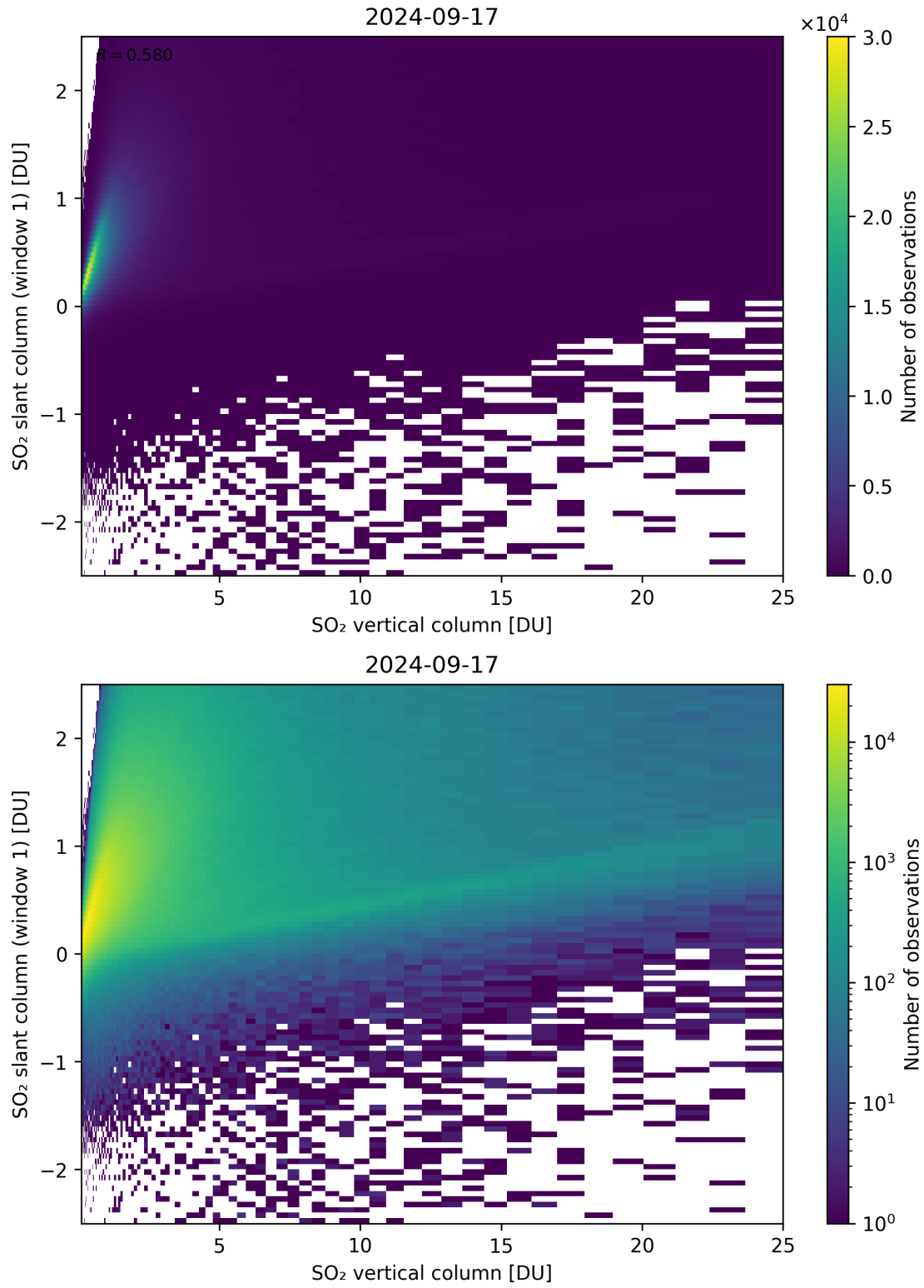
Figure 300: Scatter density plot of “SO 2 vertical column” against “SO 2 slant column (window 1)” for 2024-09-17 to 2024-09-18.
