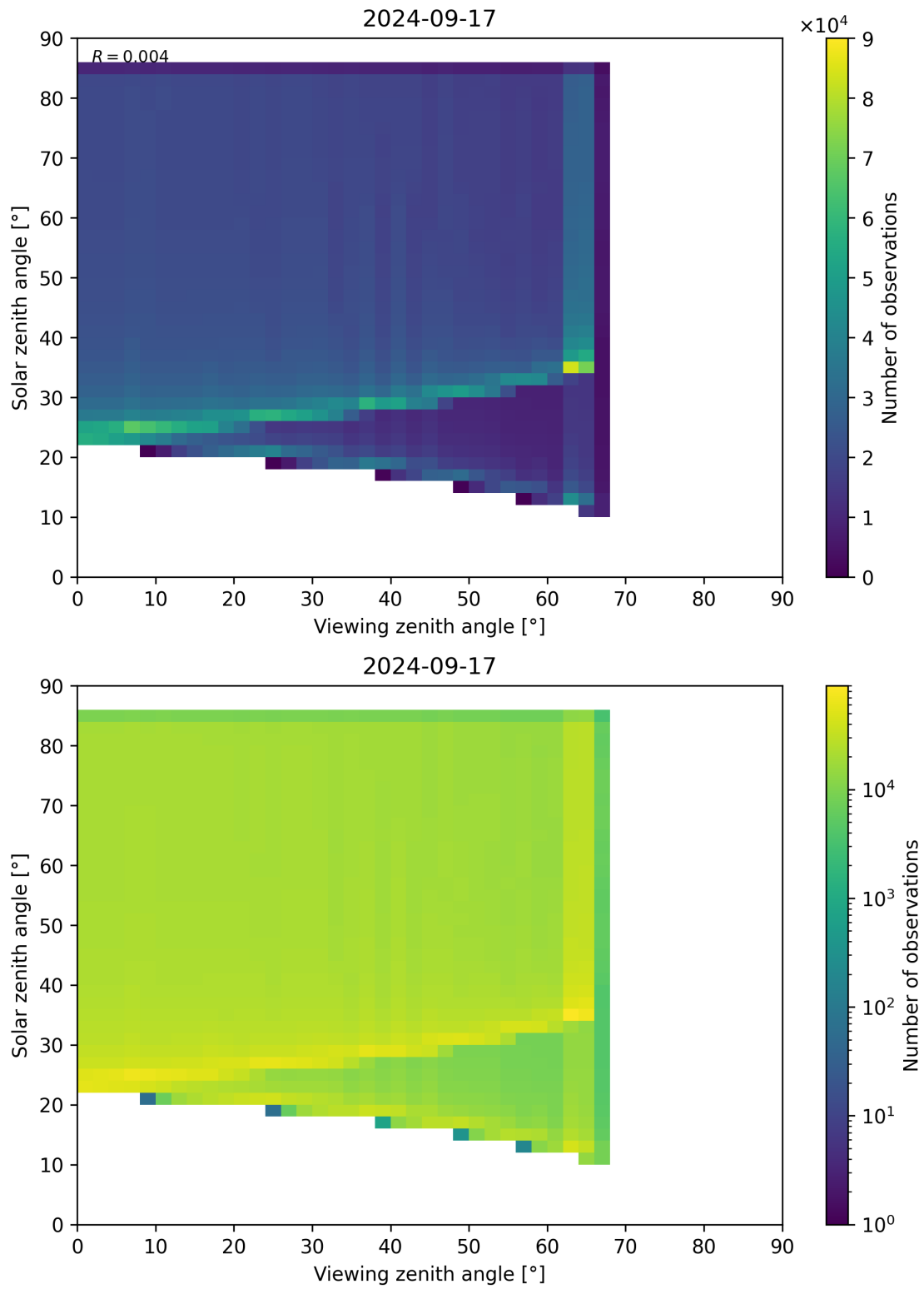
Figure 315: Scatter density plot of “Viewing zenith angle” against “Solar zenith angle” for 2024-09-17 to 2024-09-18.
