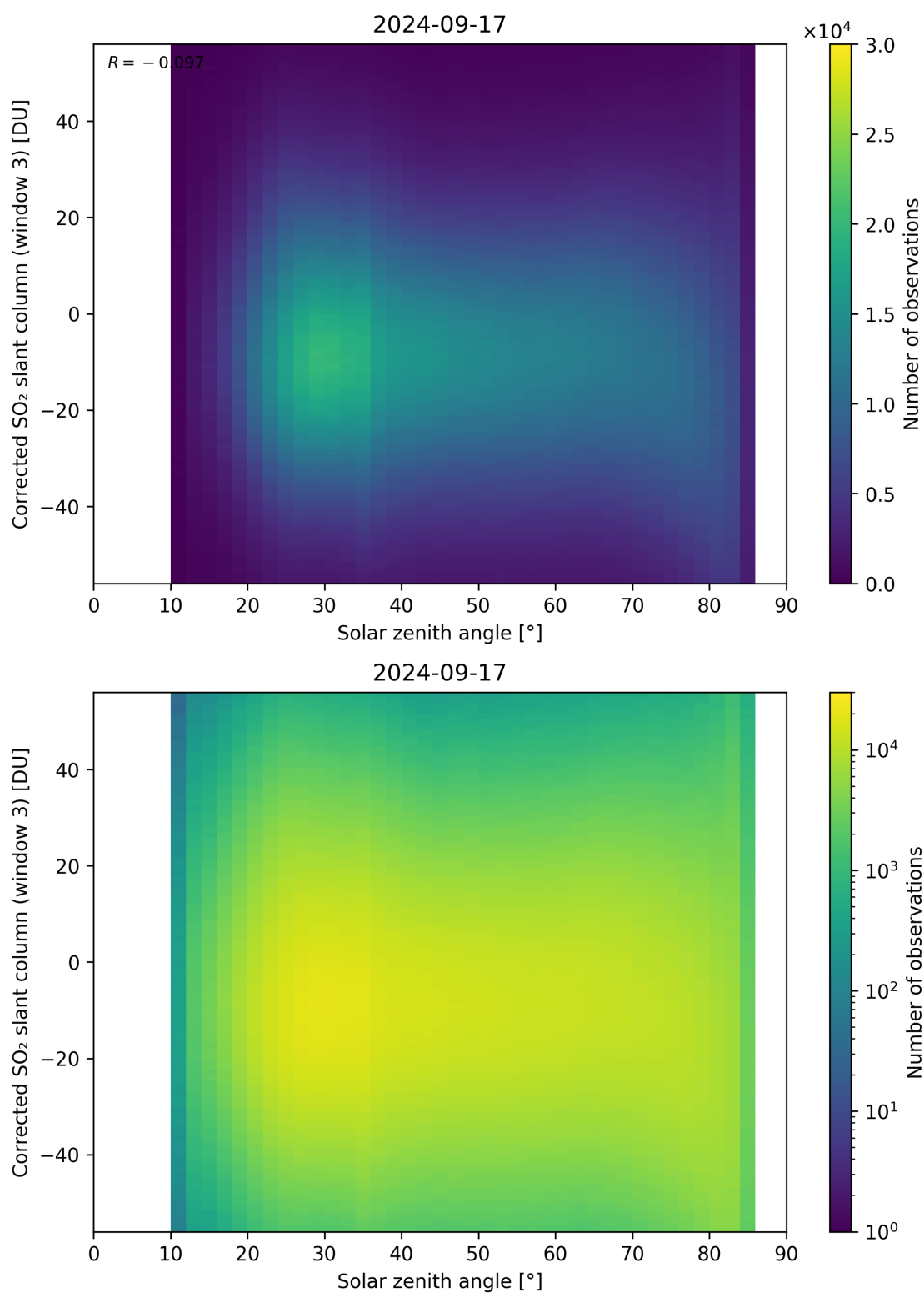
Figure 168: Scatter density plot of “Solar zenith angle” against “Corrected SO 2 slant column (window 3)” for 2024-09-17 to 2024-09-18.
