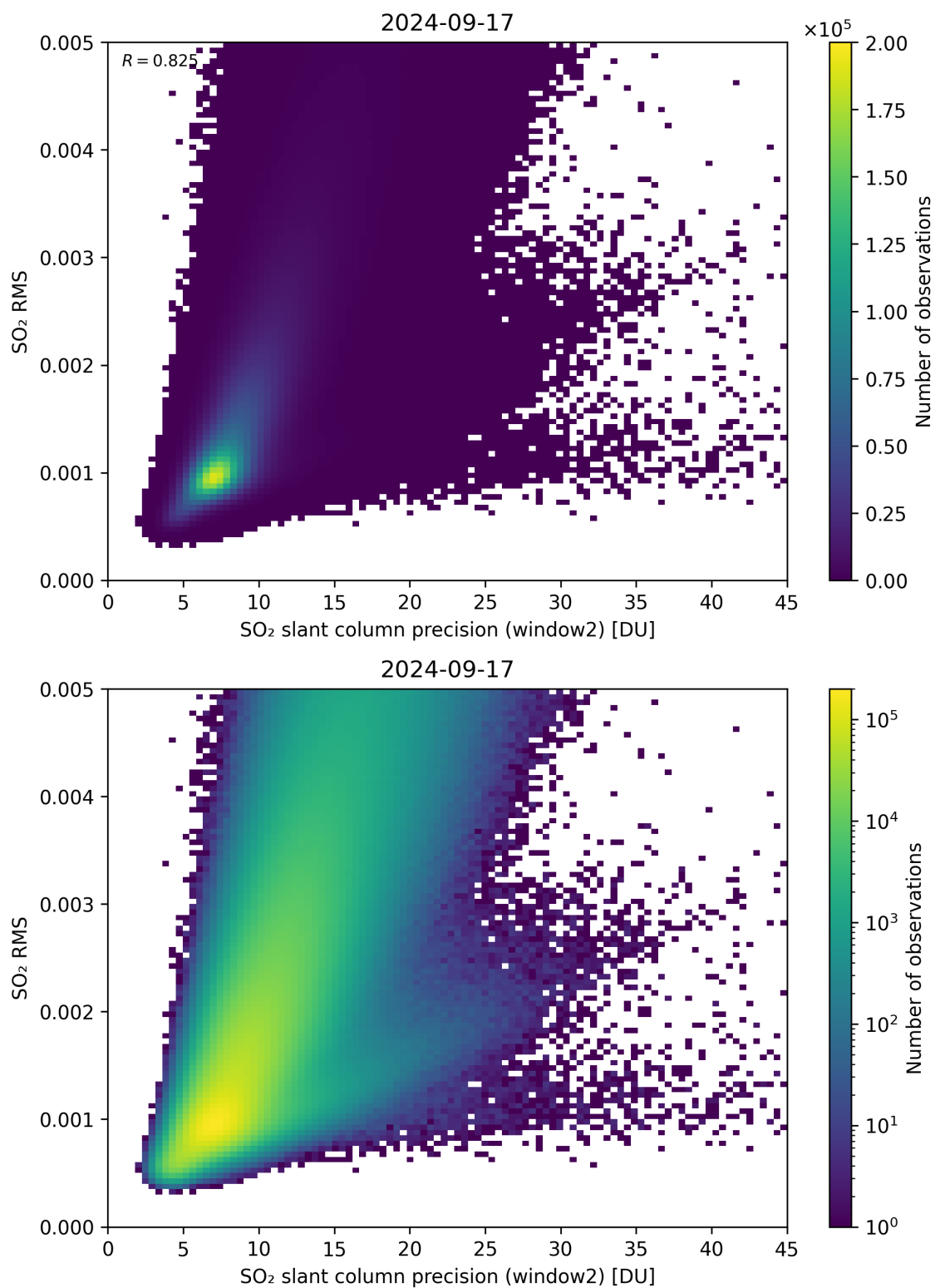
Figure 245: Scatter density plot of “SO 2 slant column precision (window2)” against “SO 2 RMS” for 2024-09-17 to 2024-09-18.
