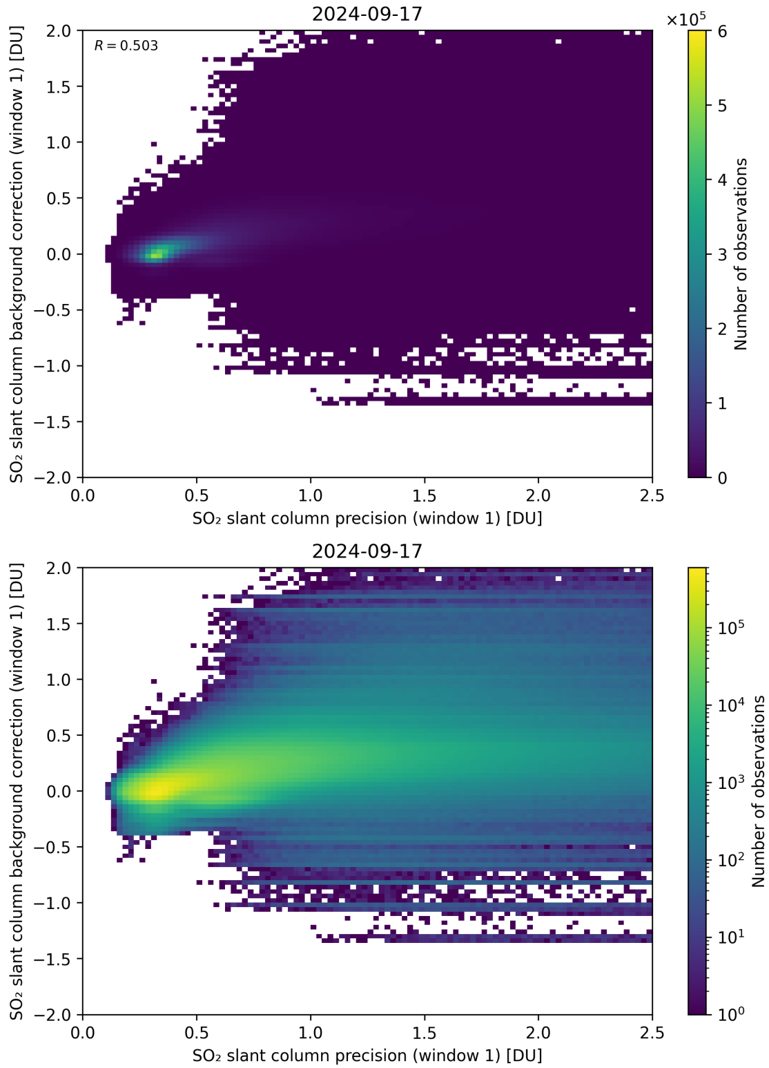
Figure 218: Scatter density plot of “SO 2 slant column precision (window 1)” against “SO 2 slant column background correction (window 1)” for 2024-09-17 to 2024-09-18.
