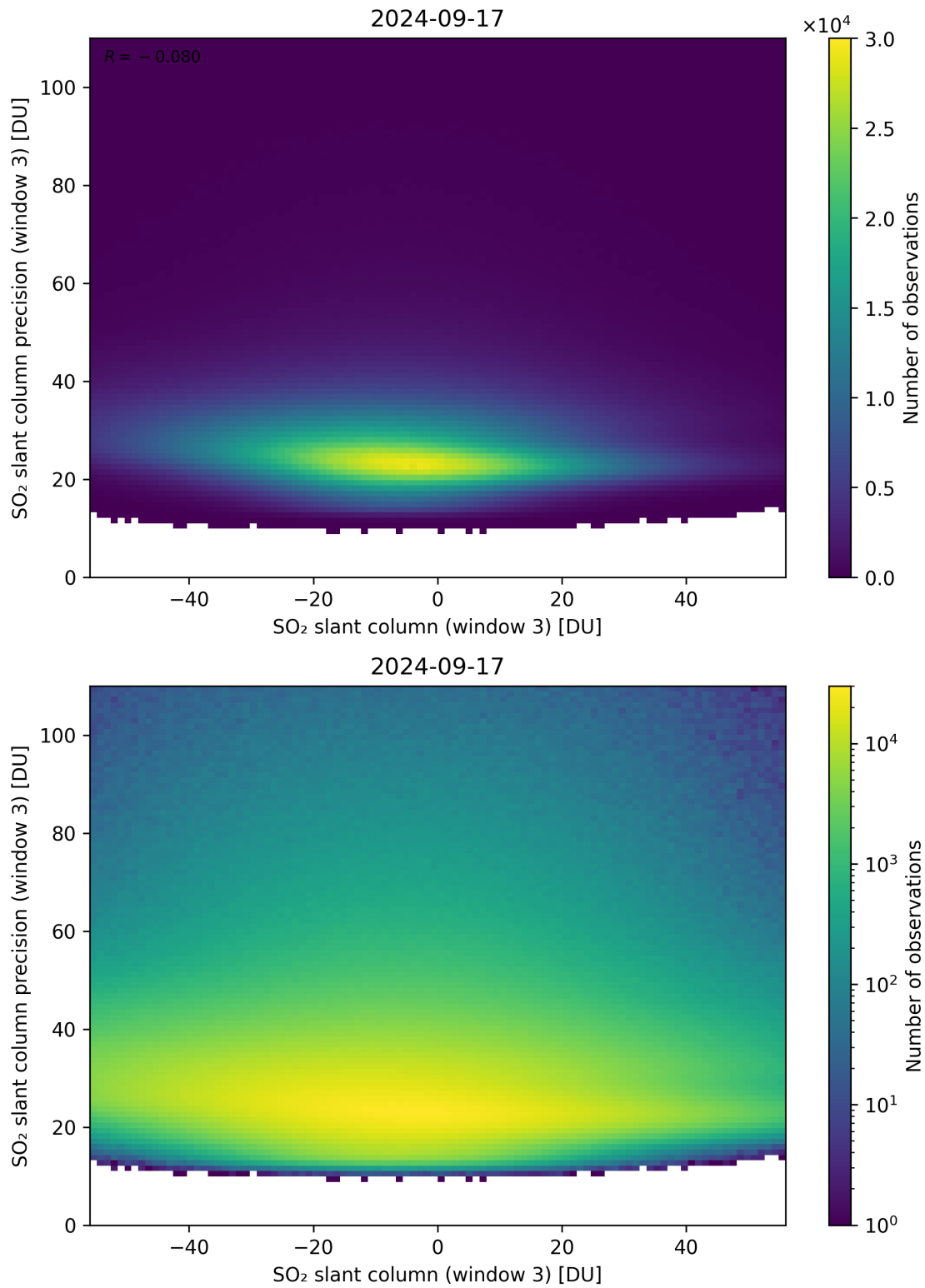
Figure 267: Scatter density plot of “SO 2 slant column (window 3)” against “SO 2 slant column precision (window 3)” for 2024-09-17 to 2024-09-18.
