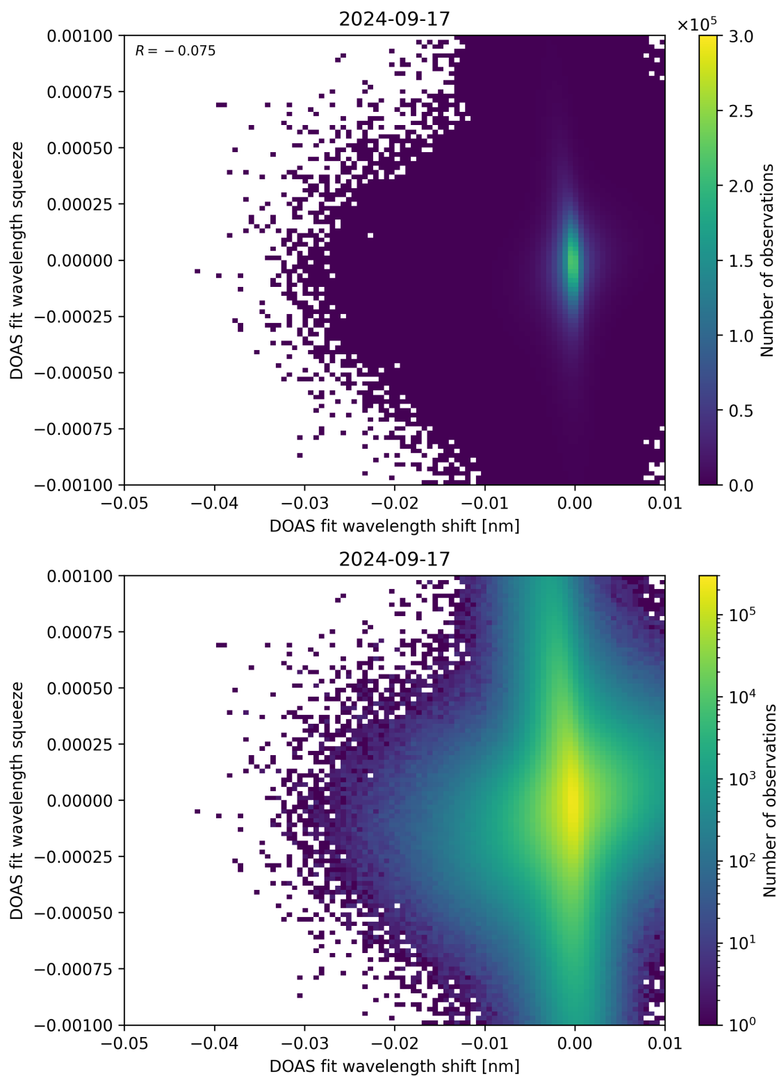
Figure 127: Scatter density plot of “DOAS fit wavelength shift” against “DOAS fit wavelength squeeze” for 2024-09-17 to 2024-09-18.
