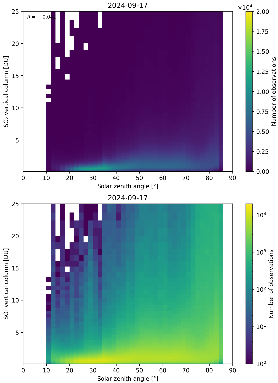
Figure 176: Scatter density plot of “Solar zenith angle” against “SO 2 vertical column” for 2024-09-17 to 2024-09-18.
