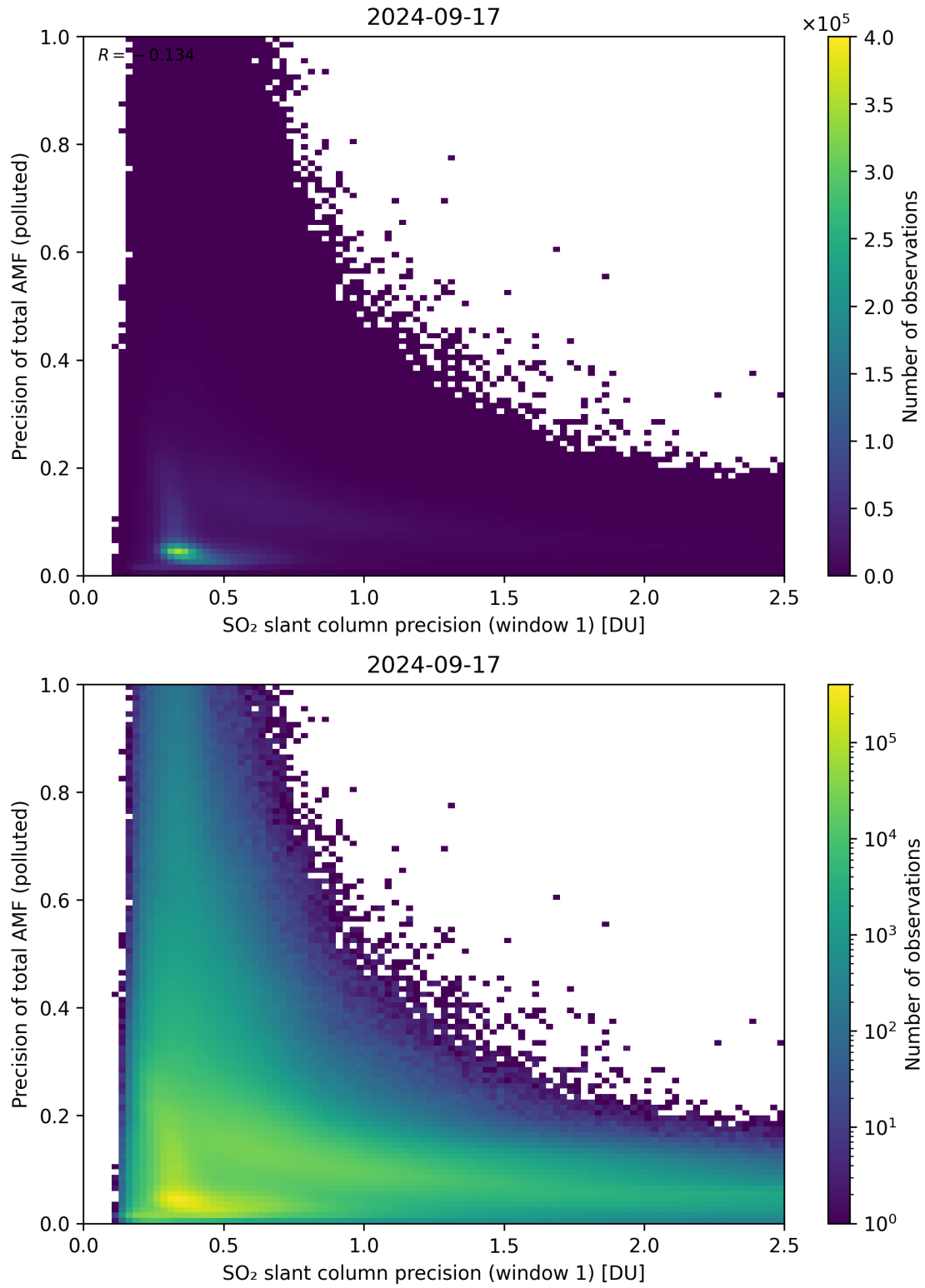
Figure 231: Scatter density plot of “SO 2 slant column precision (window 1)” against “Precision of total AMF (polluted)” for 2024-09-17 to 2024-09-18.
