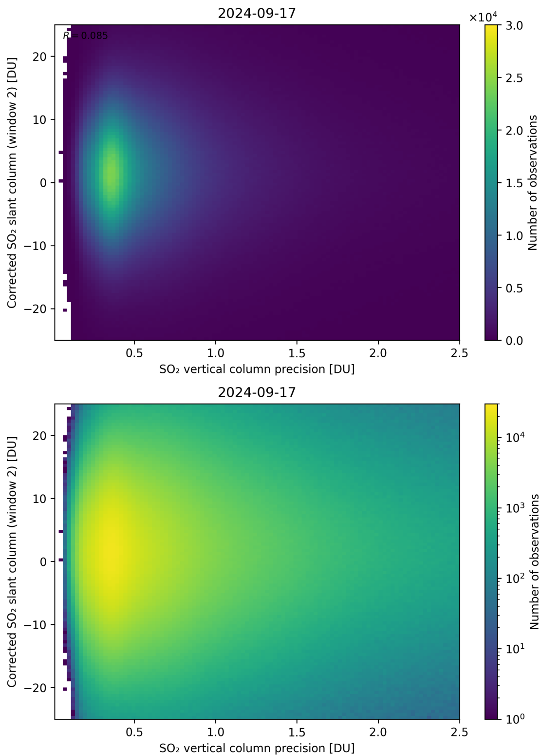
Figure 287: Scatter density plot of “SO 2 vertical column precision” against “Corrected SO 2 slant column (window 2)” for 2024-09-17 to 2024-09-18.
