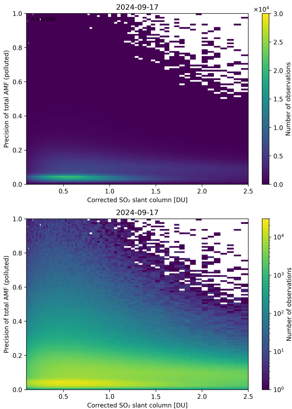
Figure 193: Scatter density plot of “Corrected SO 2 slant column” against “Precision of total AMF (polluted)” for 2024-09-17 to 2024-09-18.
