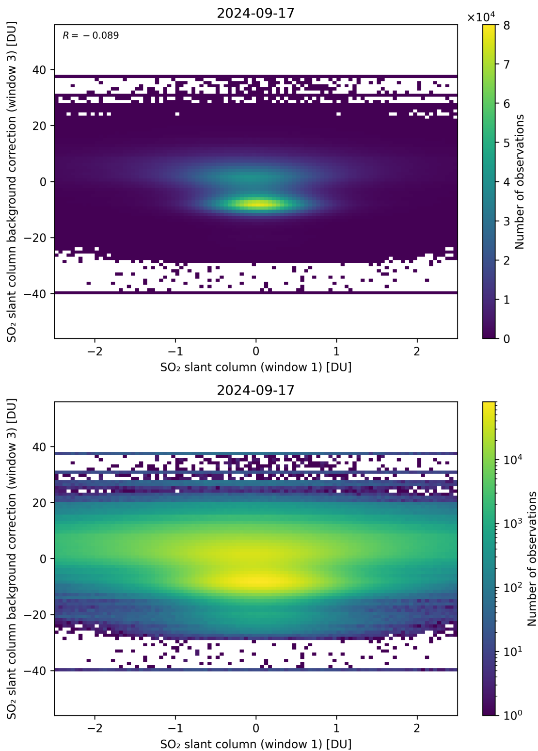
Figure 214: Scatter density plot of “SO 2 slant column (window 1)” against “SO 2 slant column background correction (window 3)” for 2024-09-17 to 2024-09-18.
