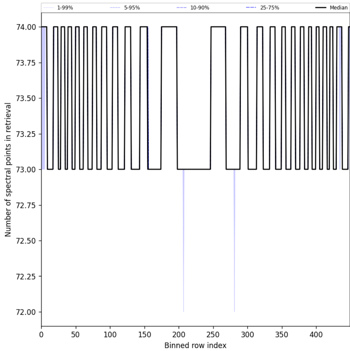
Figure 97: Along track statistics of “Number of spectral points in retrieval” for 2024-09-17 to 2024-09-18
