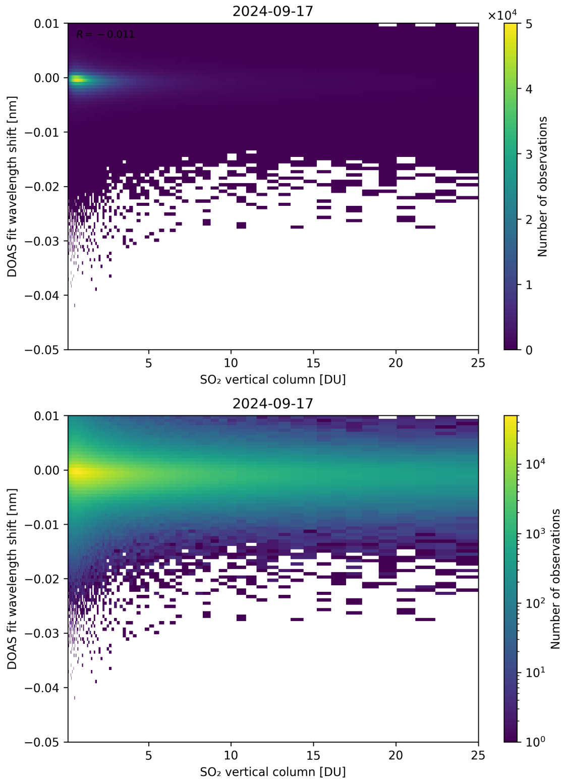
Figure 276: Scatter density plot of “SO 2 vertical column” against “DOAS fit wavelength shift” for 2024-09-17 to 2024-09-18.
