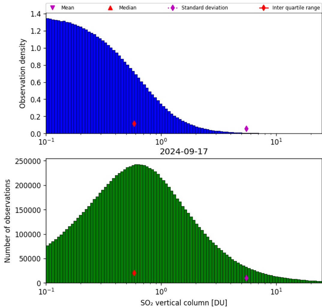
Figure 53: Histogram of “SO 2 vertical column” for 2024-09-17 to 2024-09-18
