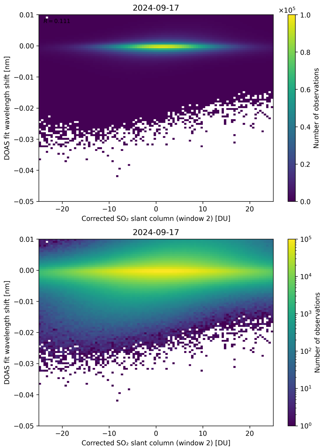
Figure 196: Scatter density plot of “Corrected SO 2 slant column (window 2)” against “DOAS fit wavelength shift” for 2024-09-17 to 2024-09-18.
