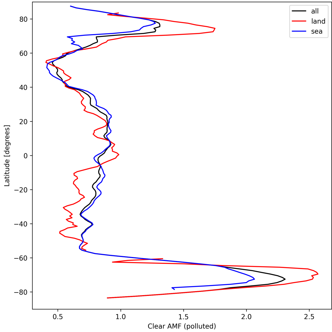
Figure 50: Zonal average of “Clear AMF (polluted)” for 2024-09-17 to 2024-09-18.
