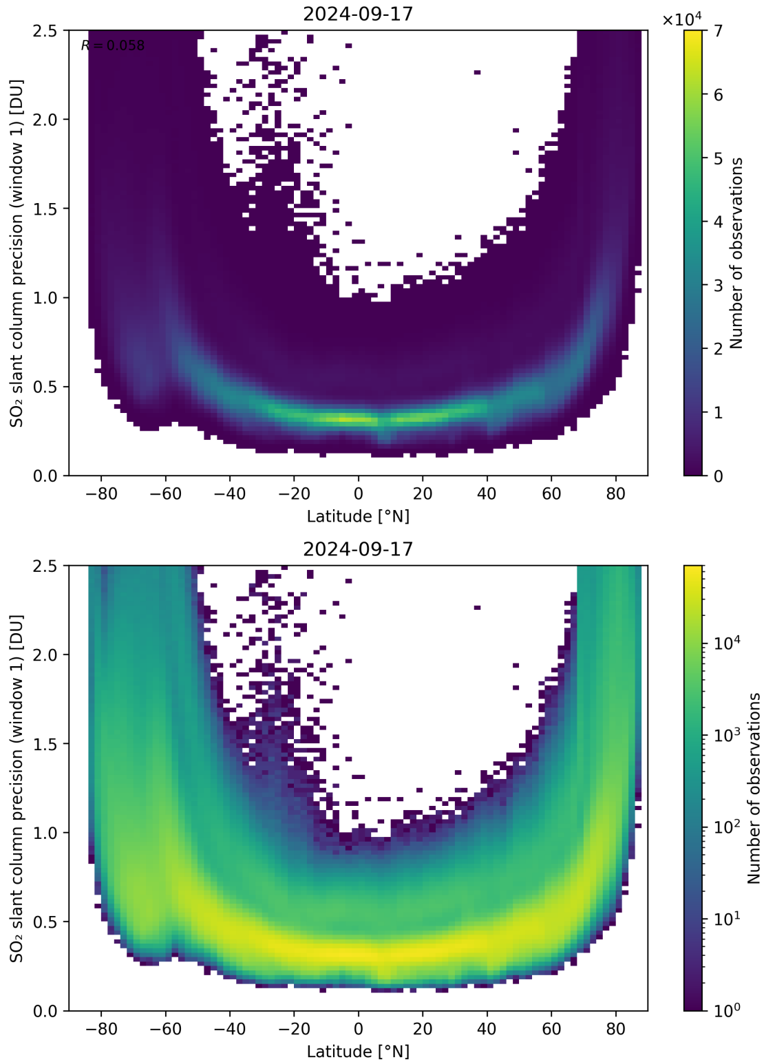
Figure 150: Scatter density plot of “Latitude” against “SO 2 slant column precision (window 1)” for 2024-09-17 to 2024-09-18.
