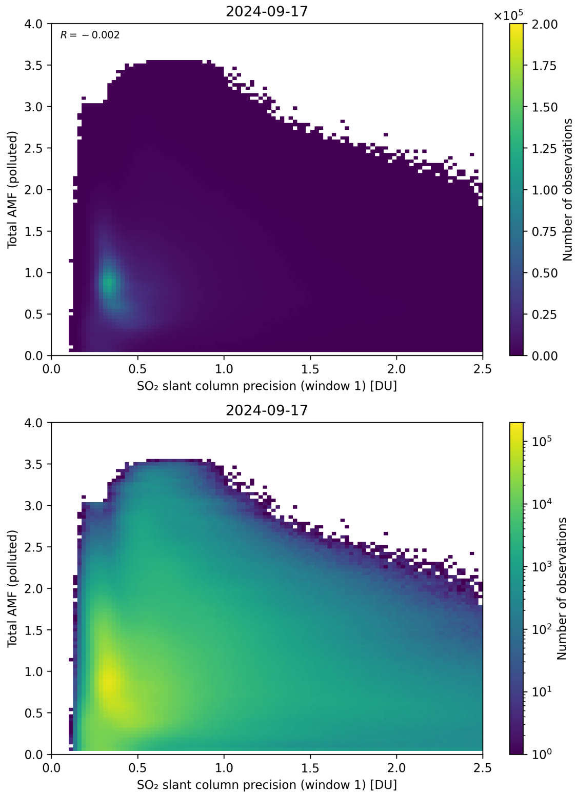
Figure 230: Scatter density plot of “SO 2 slant column precision (window 1)” against “Total AMF (polluted)” for 2024-09-17 to 2024-09-18.
