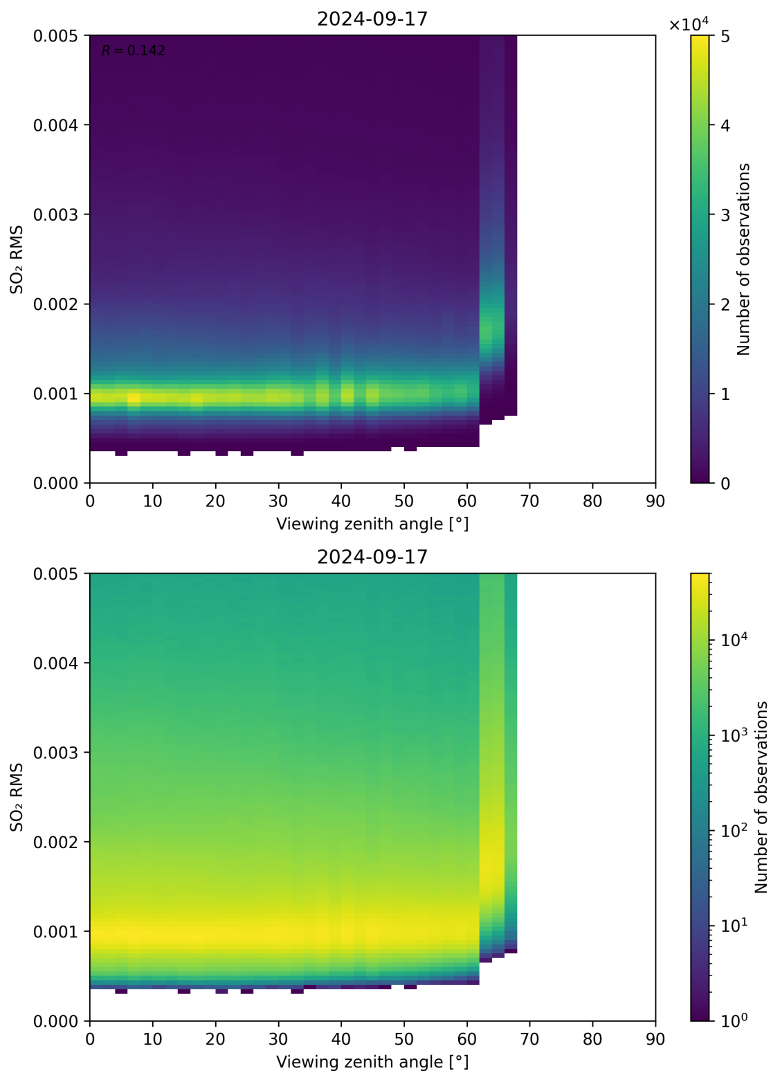
Figure 313: Scatter density plot of “Viewing zenith angle” against “SO 2 RMS” for 2024-09-17 to 2024-09-18.
