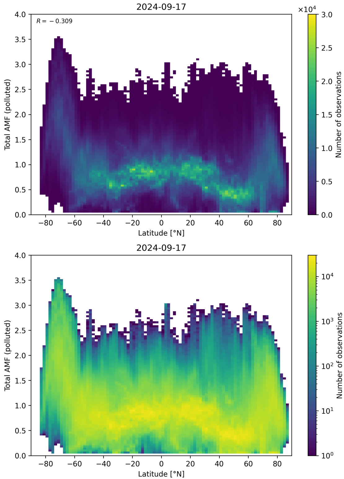
Figure 154: Scatter density plot of “Latitude” against “Total AMF (polluted)” for 2024-09-17 to 2024-09-18.
