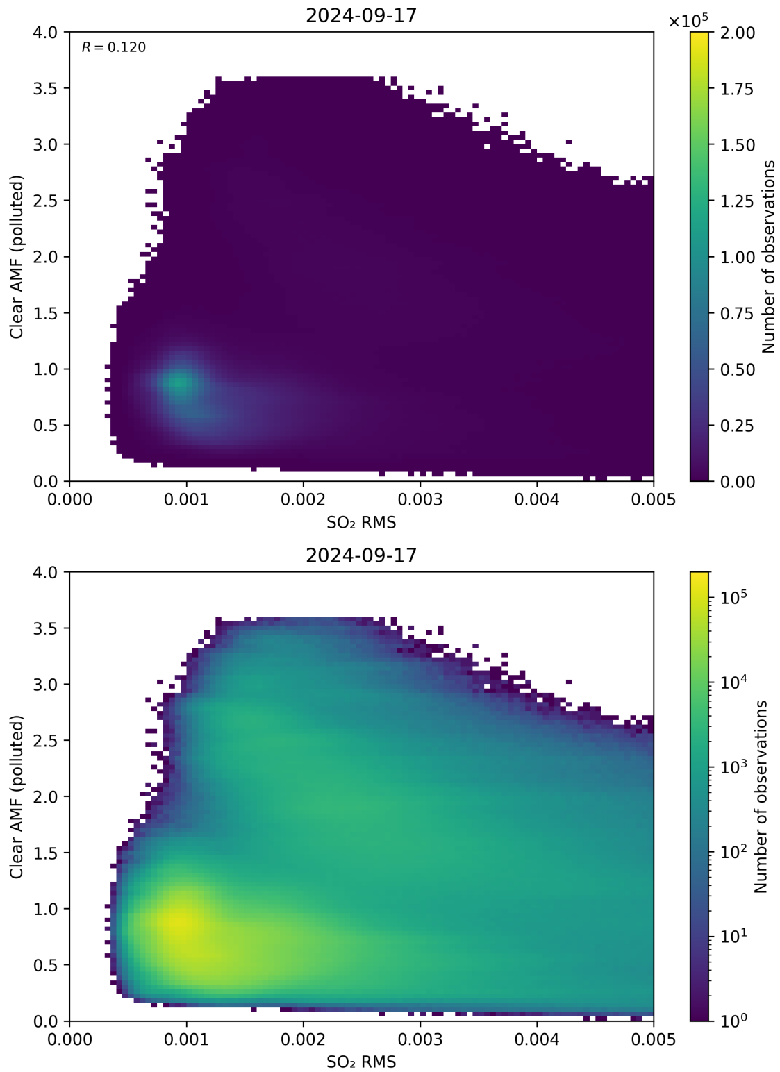
Figure 136: Scatter density plot of “SO 2 RMS” against “Clear AMF (polluted)” for 2024-09-17 to 2024-09-18.
