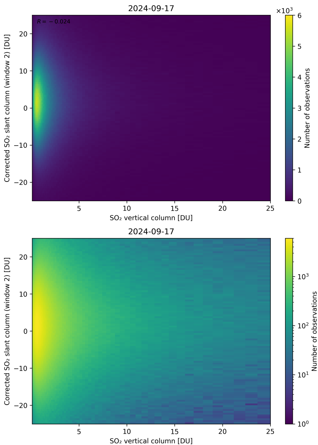
Figure 298: Scatter density plot of “SO 2 vertical column” against “Corrected SO 2 slant column (window 2)” for 2024-09-17 to 2024-09-18.
