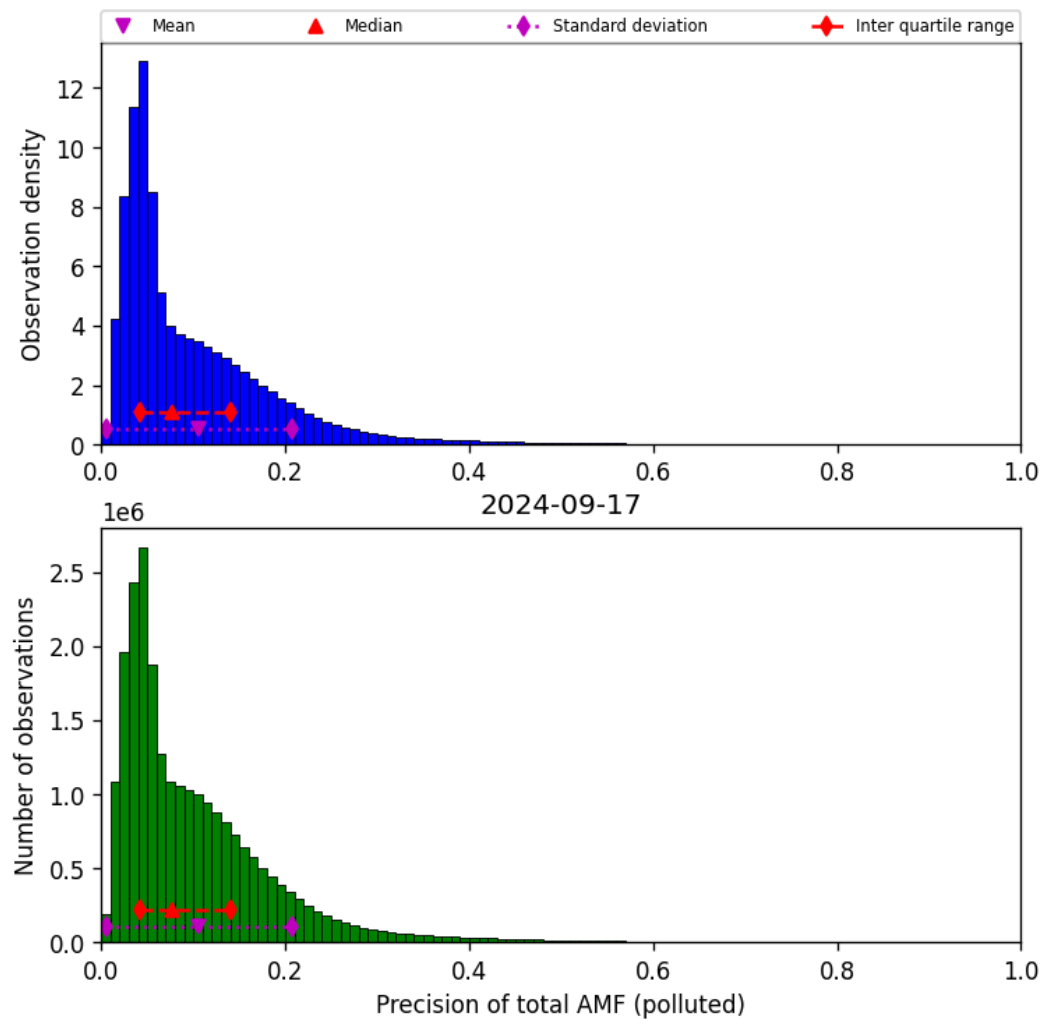
Figure 72: Histogram of “Precision of total AMF (polluted)” for 2024-09-17 to 2024-09-18
