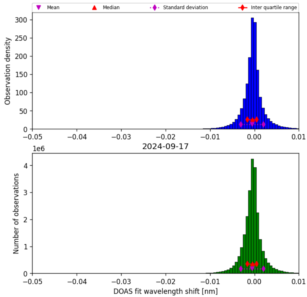
Figure 68: Histogram of “DOAS fit wavelength shift” for 2024-09-17 to 2024-09-18
