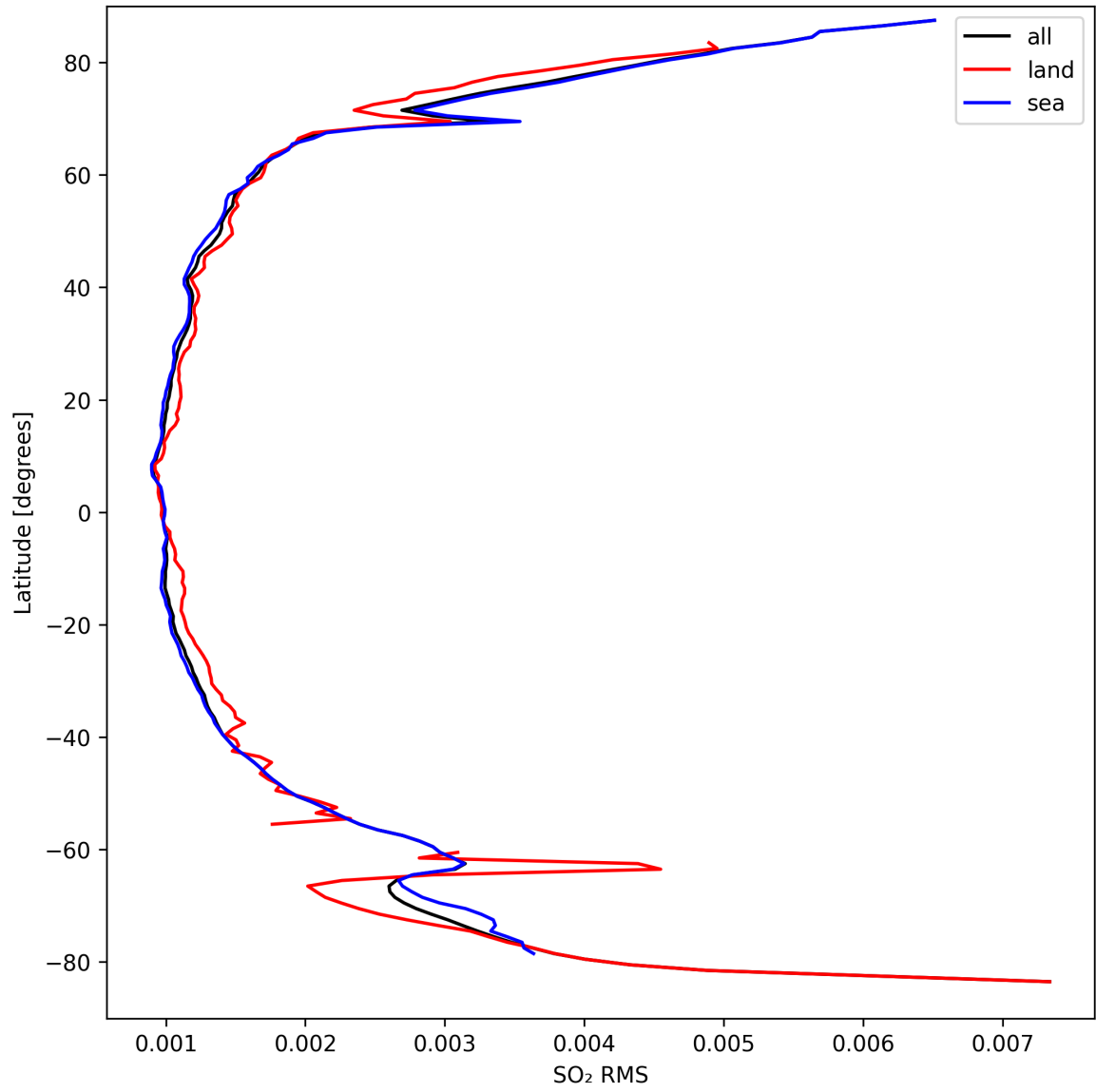
Figure 47: Zonal average of “SO 2 RMS” for 2024-09-17 to 2024-09-18.
