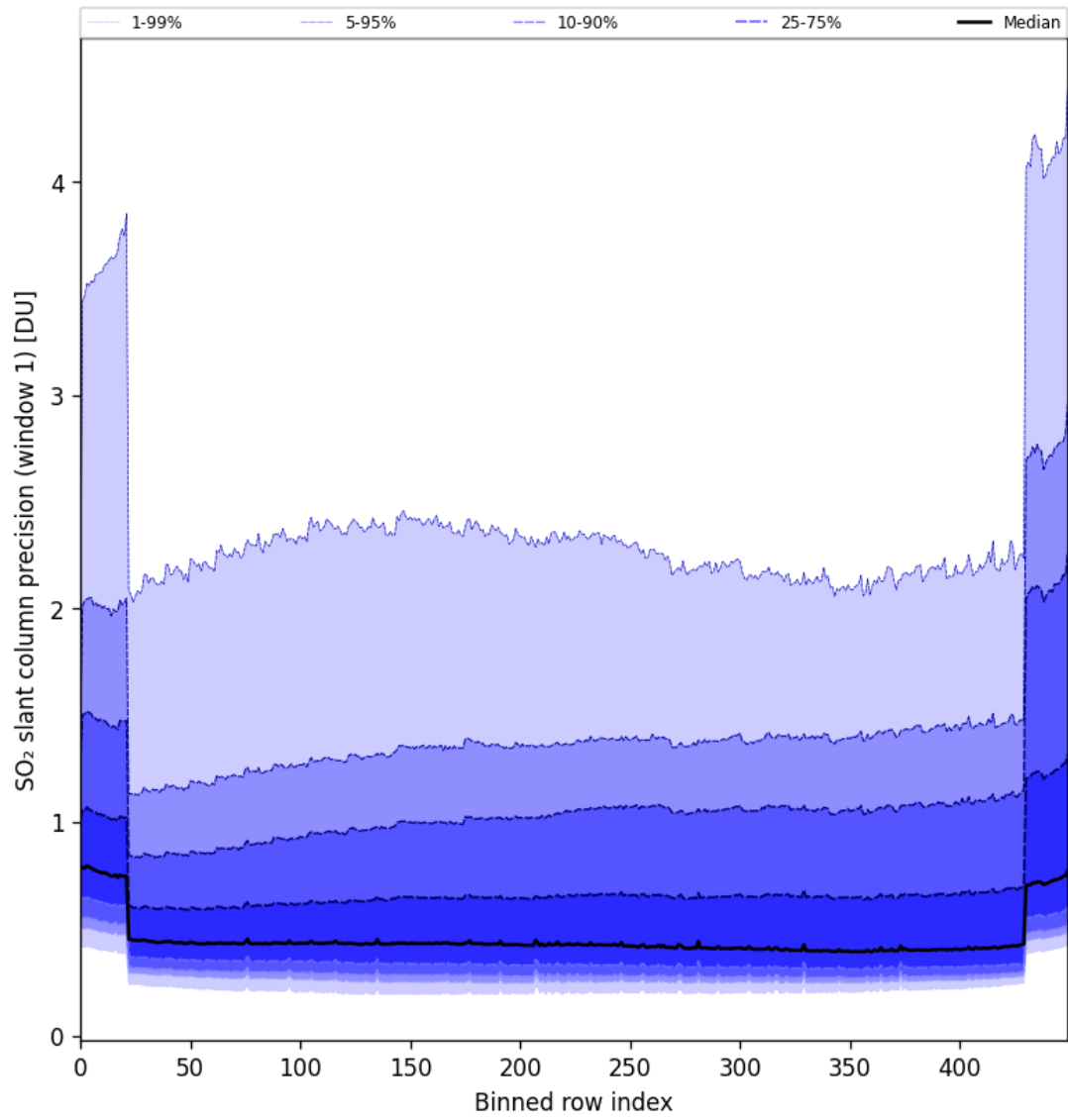
Figure 80: Along track statistics of “SO 2 slant column precision (window 1)” for 2024-09-17 to 2024-09-18
