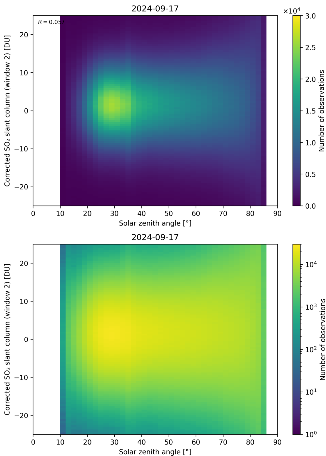
Figure 167: Scatter density plot of “Solar zenith angle” against “Corrected SO 2 slant column (window 2)” for 2024-09-17 to 2024-09-18.
