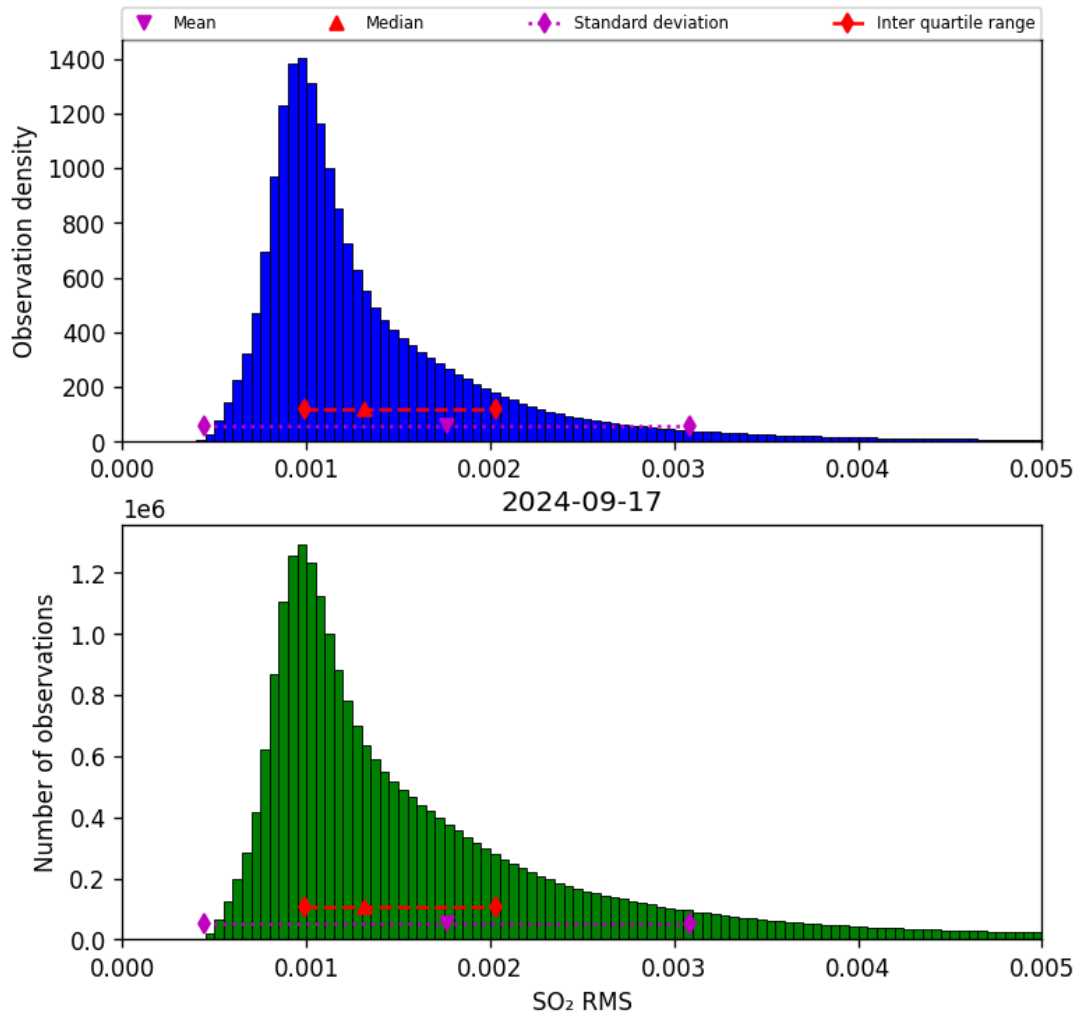
Figure 70: Histogram of “SO 2 RMS” for 2024-09-17 to 2024-09-18
