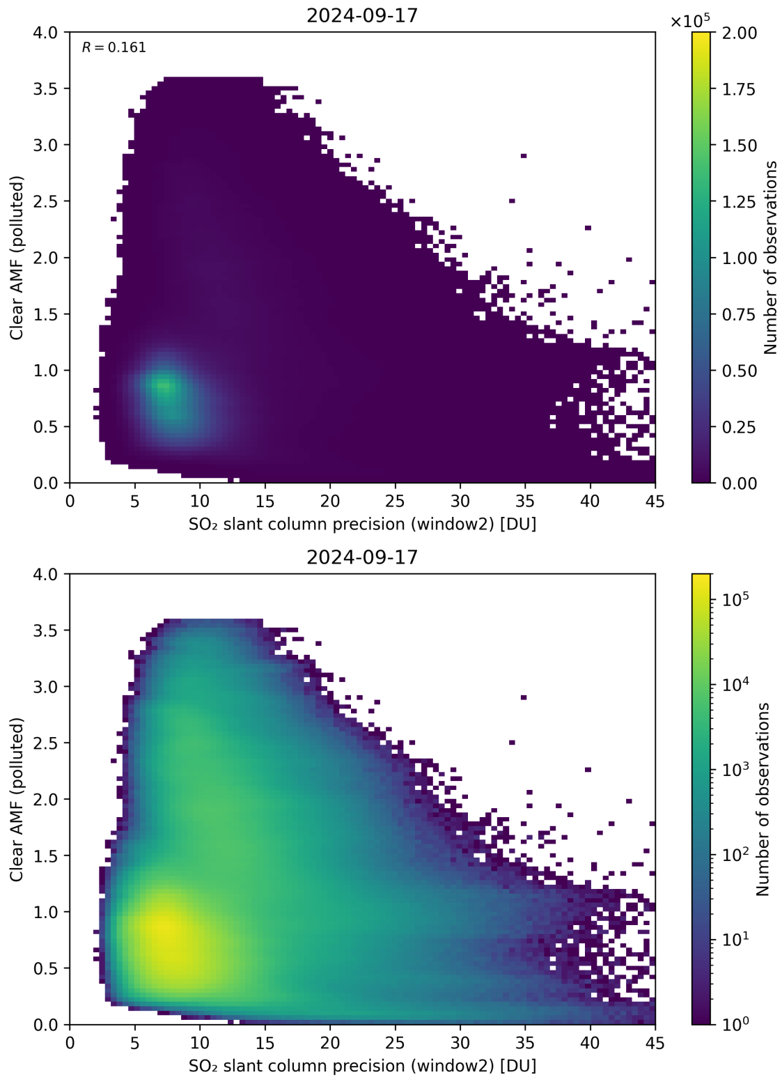
Figure 246: Scatter density plot of “SO 2 slant column precision (window2)” against “Clear AMF (polluted)” for 2024-09-17 to 2024-09-18.
