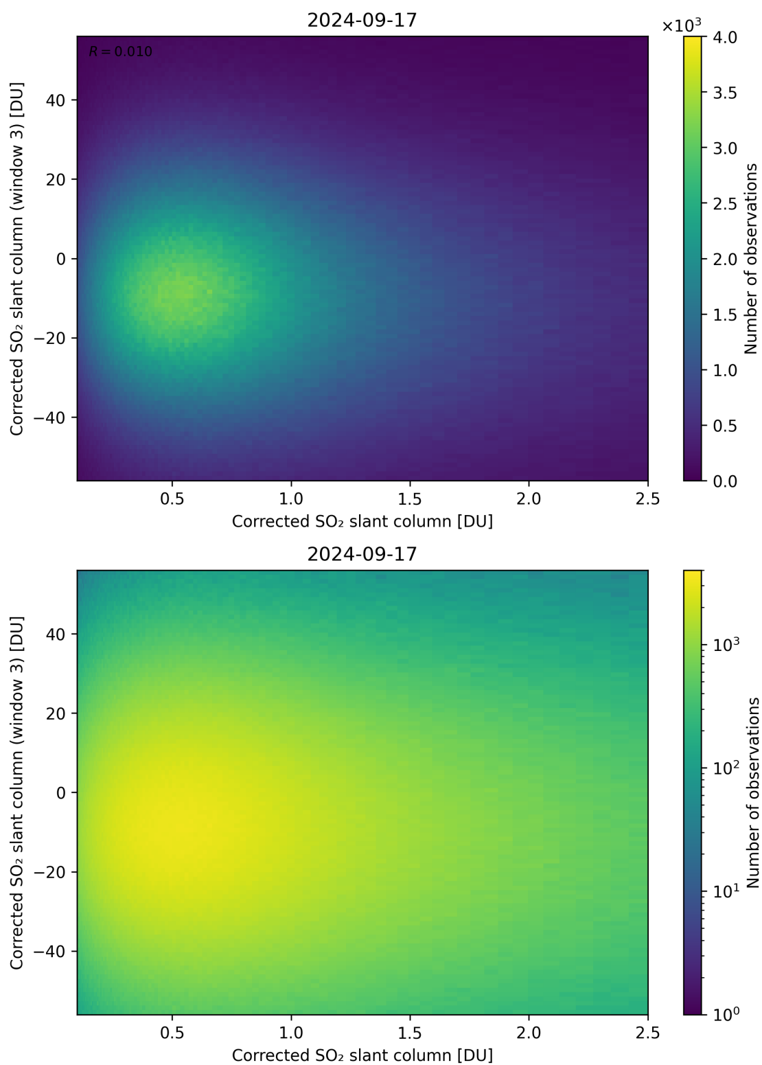
Figure 186: Scatter density plot of “Corrected SO 2 slant column” against “Corrected SO 2 slant column (window 3)” for 2024-09-17 to 2024-09-18.
