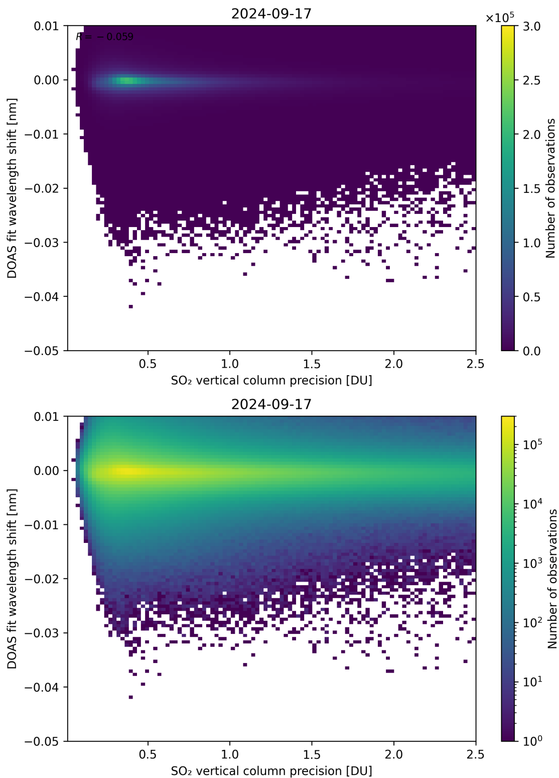
Figure 282: Scatter density plot of “SO 2 vertical column precision” against “DOAS fit wavelength shift” for 2024-09-17 to 2024-09-18.
