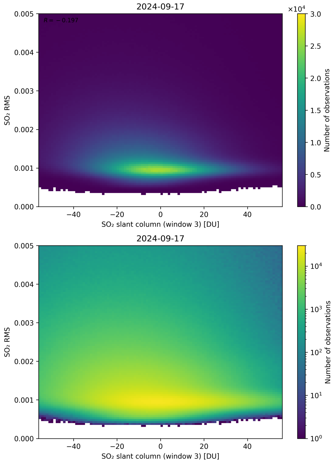
Figure 256: Scatter density plot of “SO 2 slant column (window 3)” against “SO 2 RMS” for 2024-09-17 to 2024-09-18.
