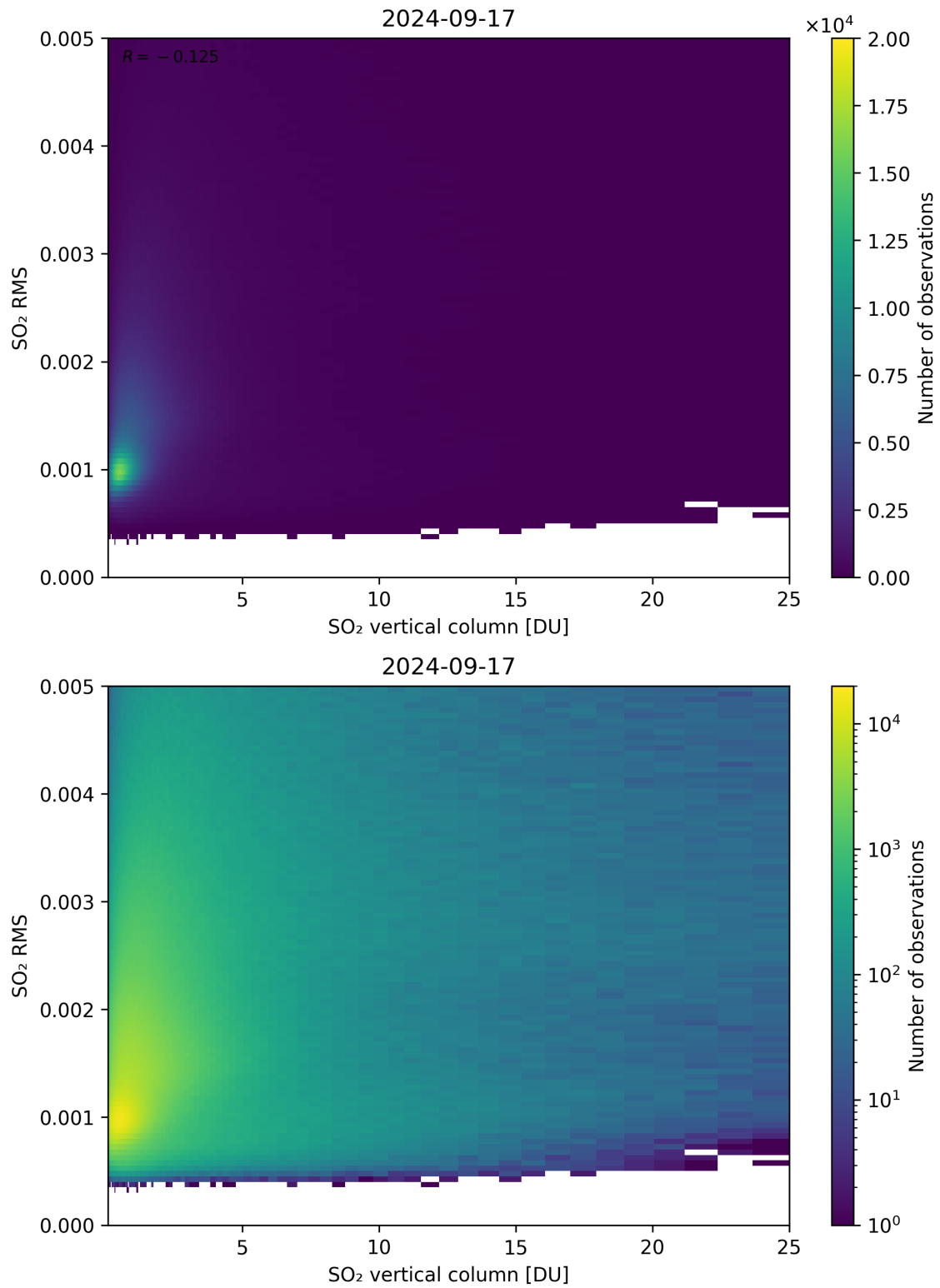
Figure 278: Scatter density plot of “SO 2 vertical column” against “SO 2 RMS” for 2024-09-17 to 2024-09-18.
