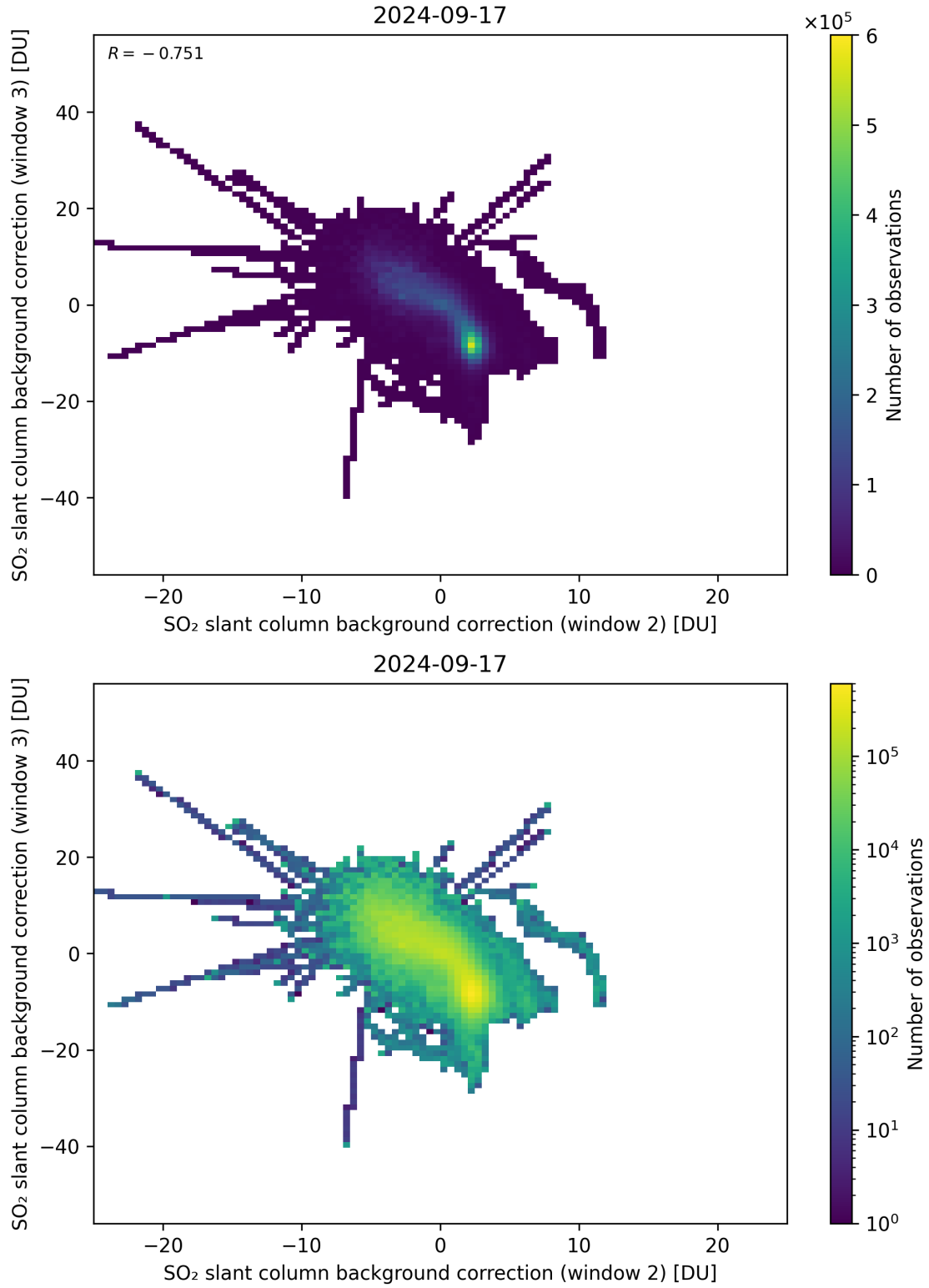
Figure 111: Scatter density plot of “SO 2 slant column background correction (window 2)” against “SO 2 slant column background correction (window 3)” for 2024-09-17 to 2024-09-18.
