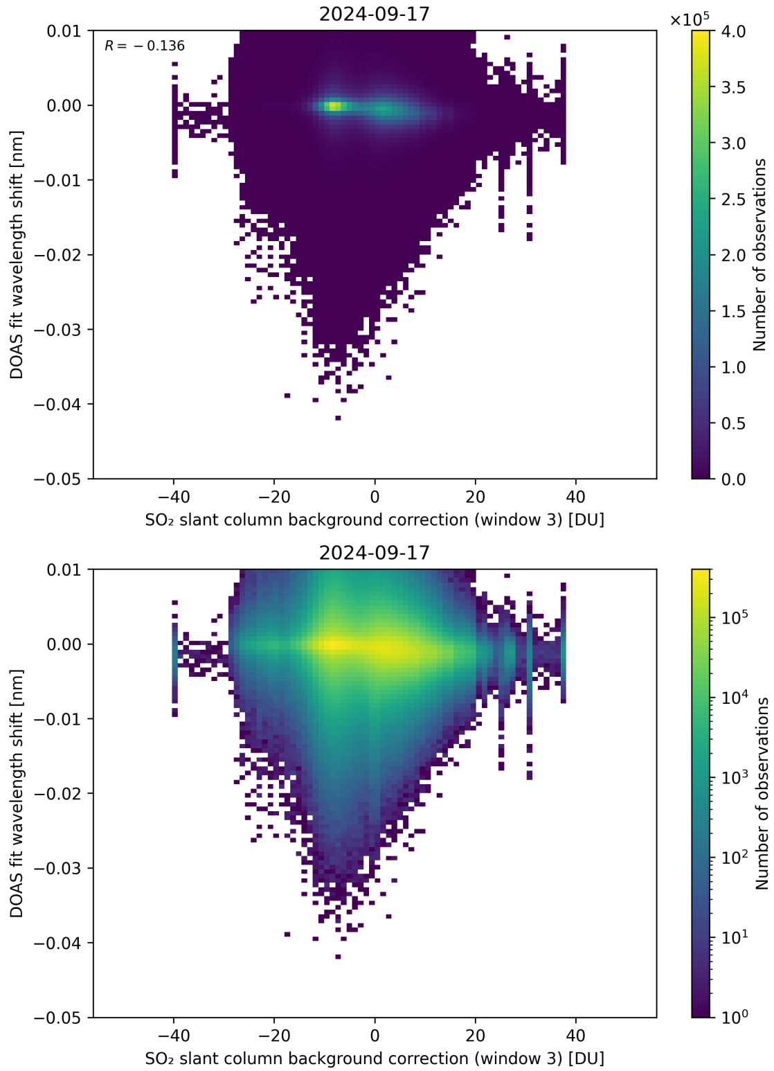
Figure 121: Scatter density plot of “SO 2 slant column background correction (window 3)” against “DOAS fit wavelength shift” for 2024-09-17 to 2024-09-18.
