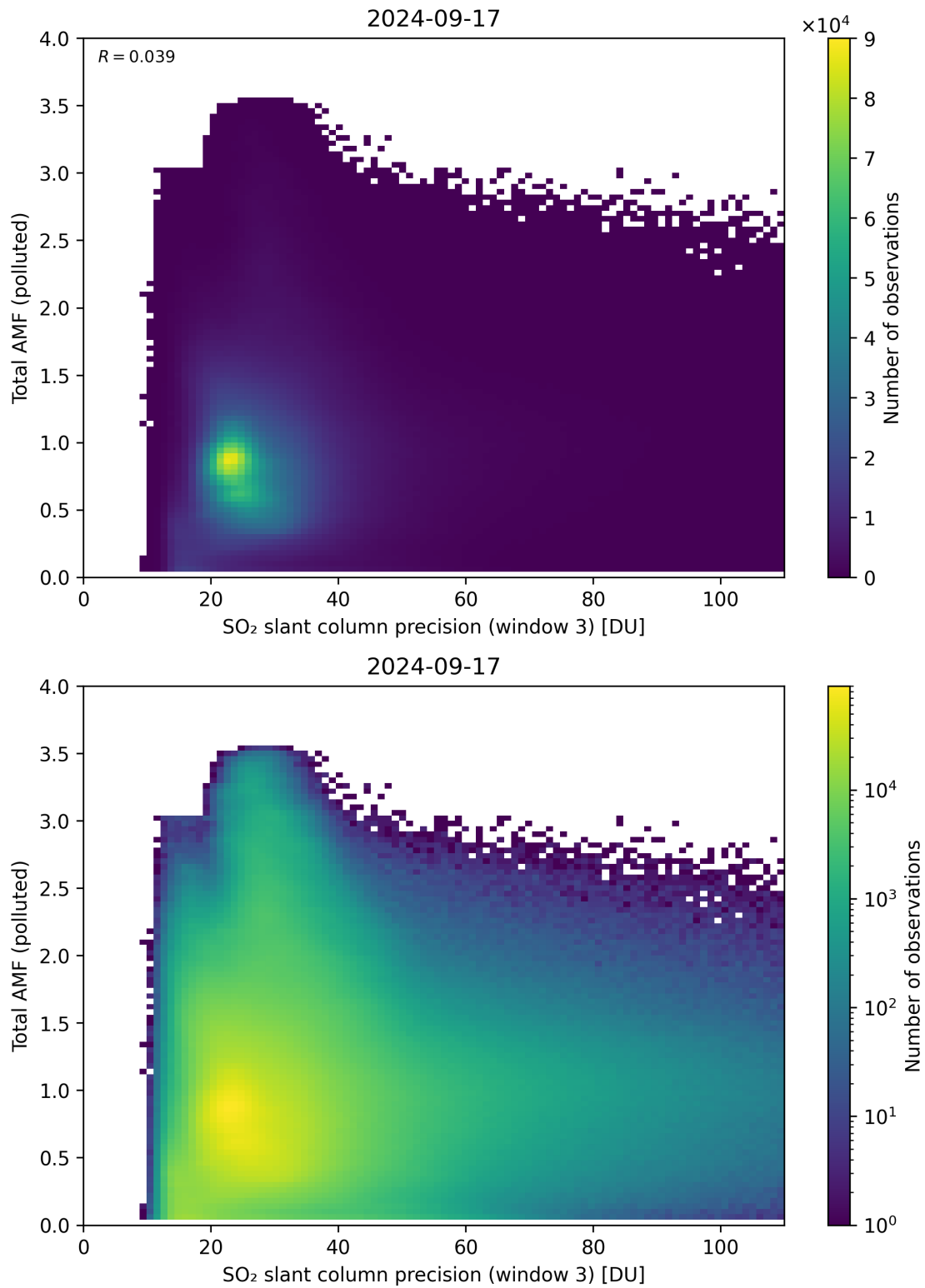
Figure 263: Scatter density plot of “SO 2 slant column precision (window 3)” against “Total AMF (polluted)” for 2024-09-17 to 2024-09-18.
