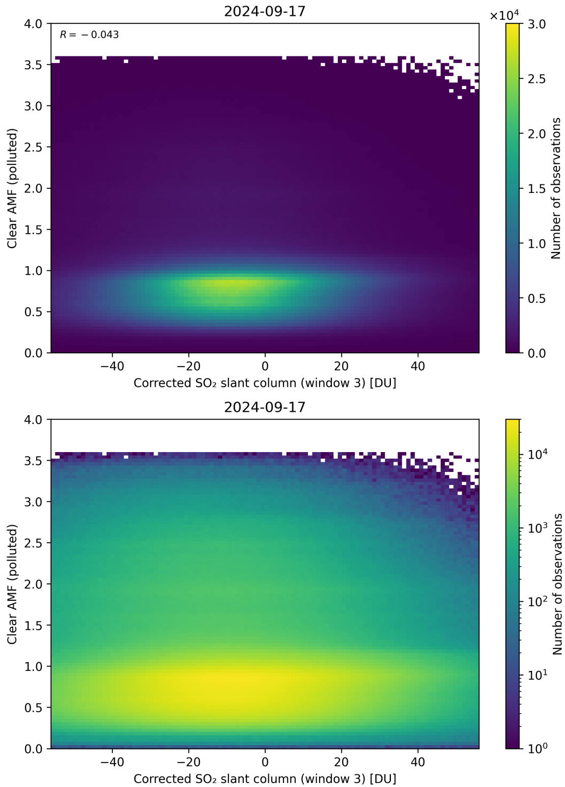
Figure 209: Scatter density plot of “Corrected SO 2 slant column (window 3)” against “Clear AMF (polluted)” for 2024-09-17 to 2024-09-18.
