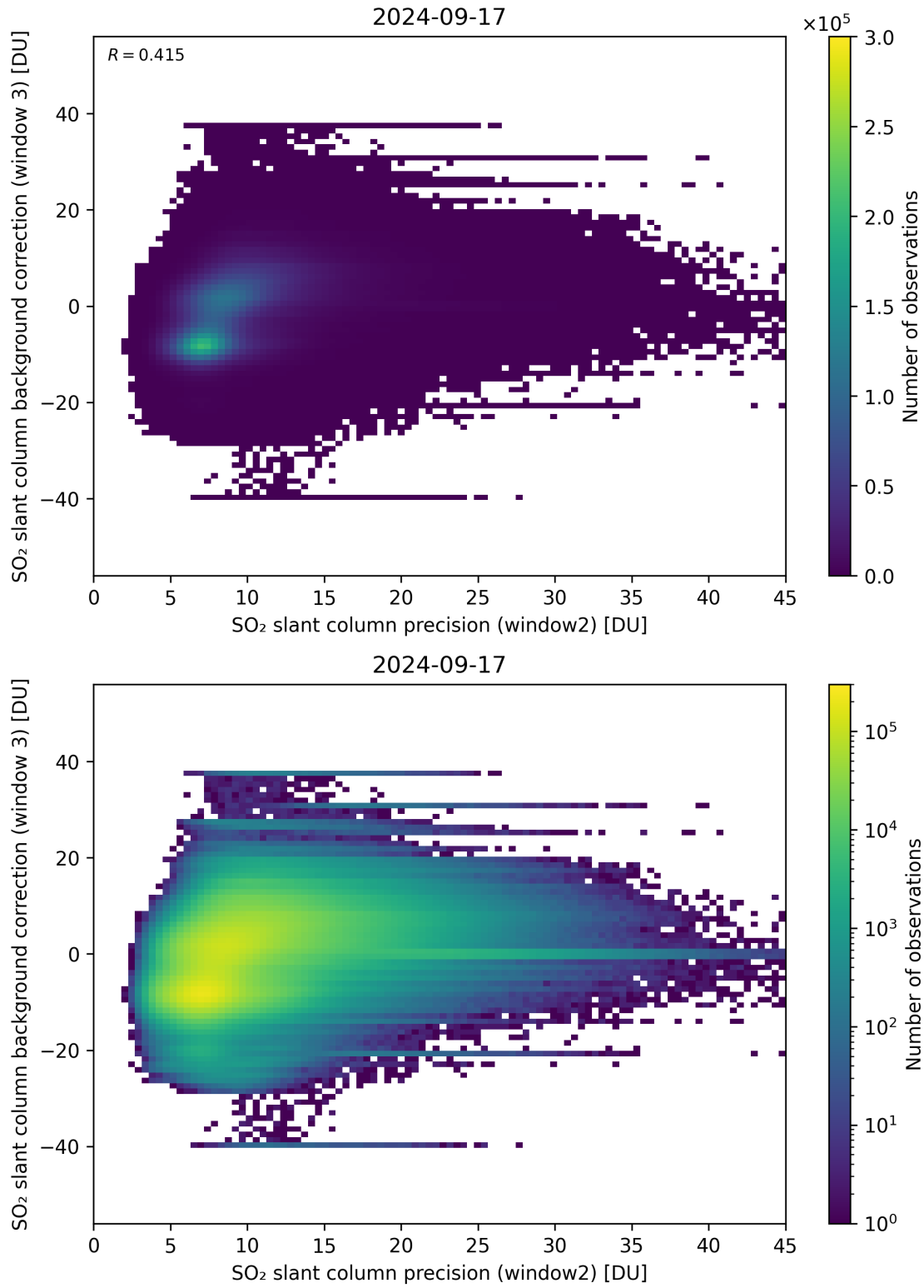
Figure 242: Scatter density plot of “SO 2 slant column precision (window2)” against “SO 2 slant column background correction (window 3)” for 2024-09-17 to 2024-09-18.
