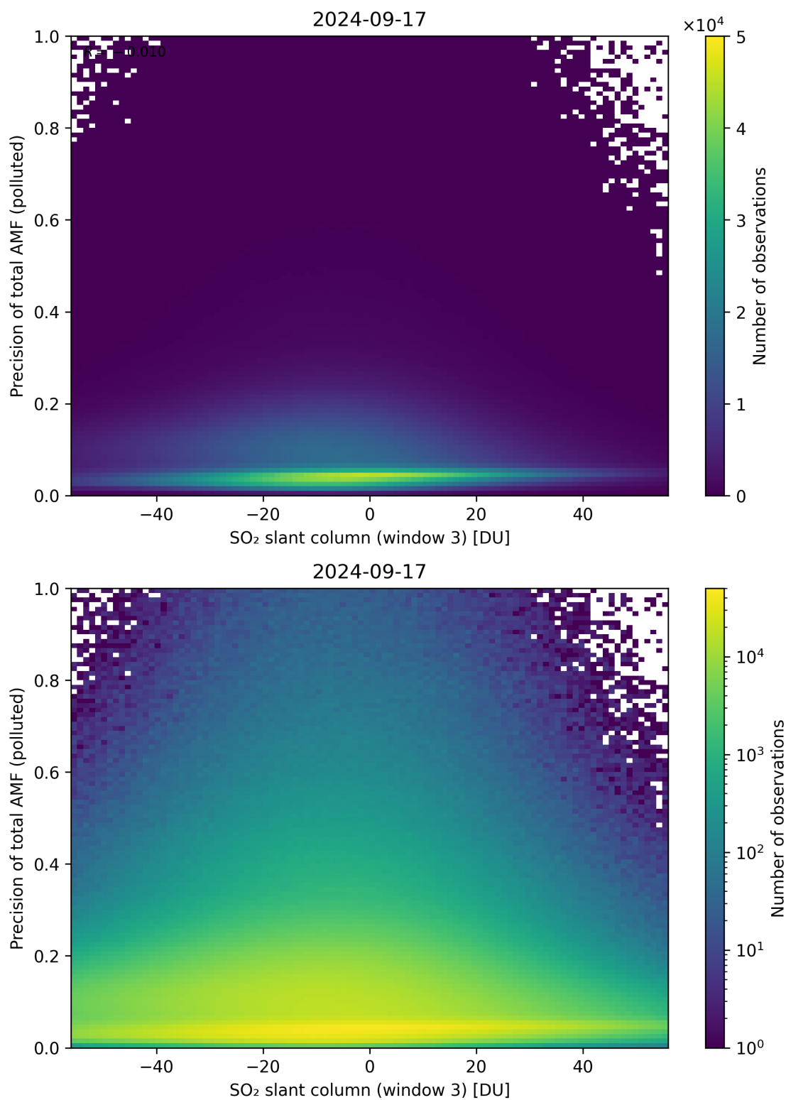
Figure 269: Scatter density plot of “SO 2 slant column (window 3)” against “Precision of total AMF (polluted)” for 2024-09-17 to 2024-09-18.
