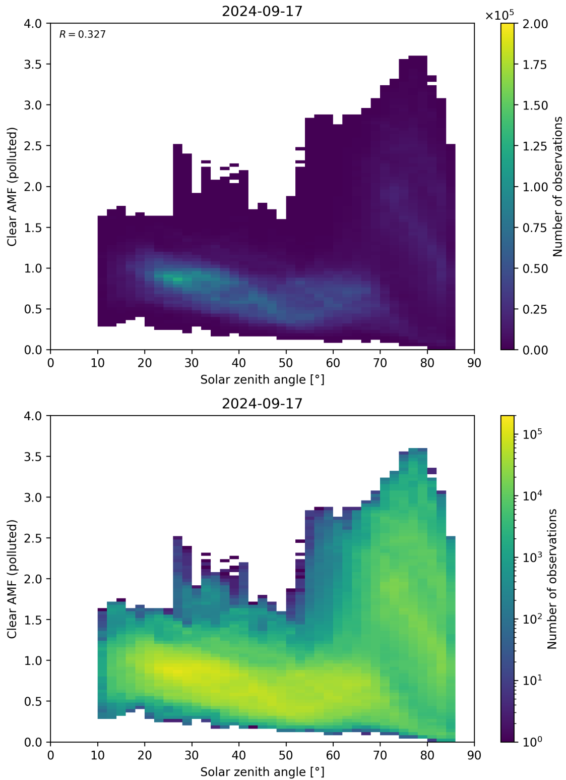
Figure 165: Scatter density plot of “Solar zenith angle” against “Clear AMF (polluted)” for 2024-09-17 to 2024-09-18.
