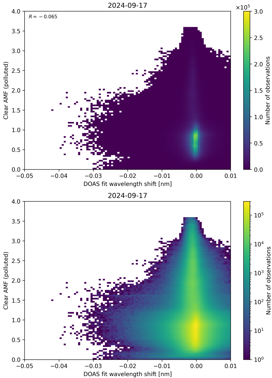
Figure 129: Scatter density plot of “DOAS fit wavelength shift” against “Clear AMF (polluted)” for 2024-09-17 to 2024-09-18.
