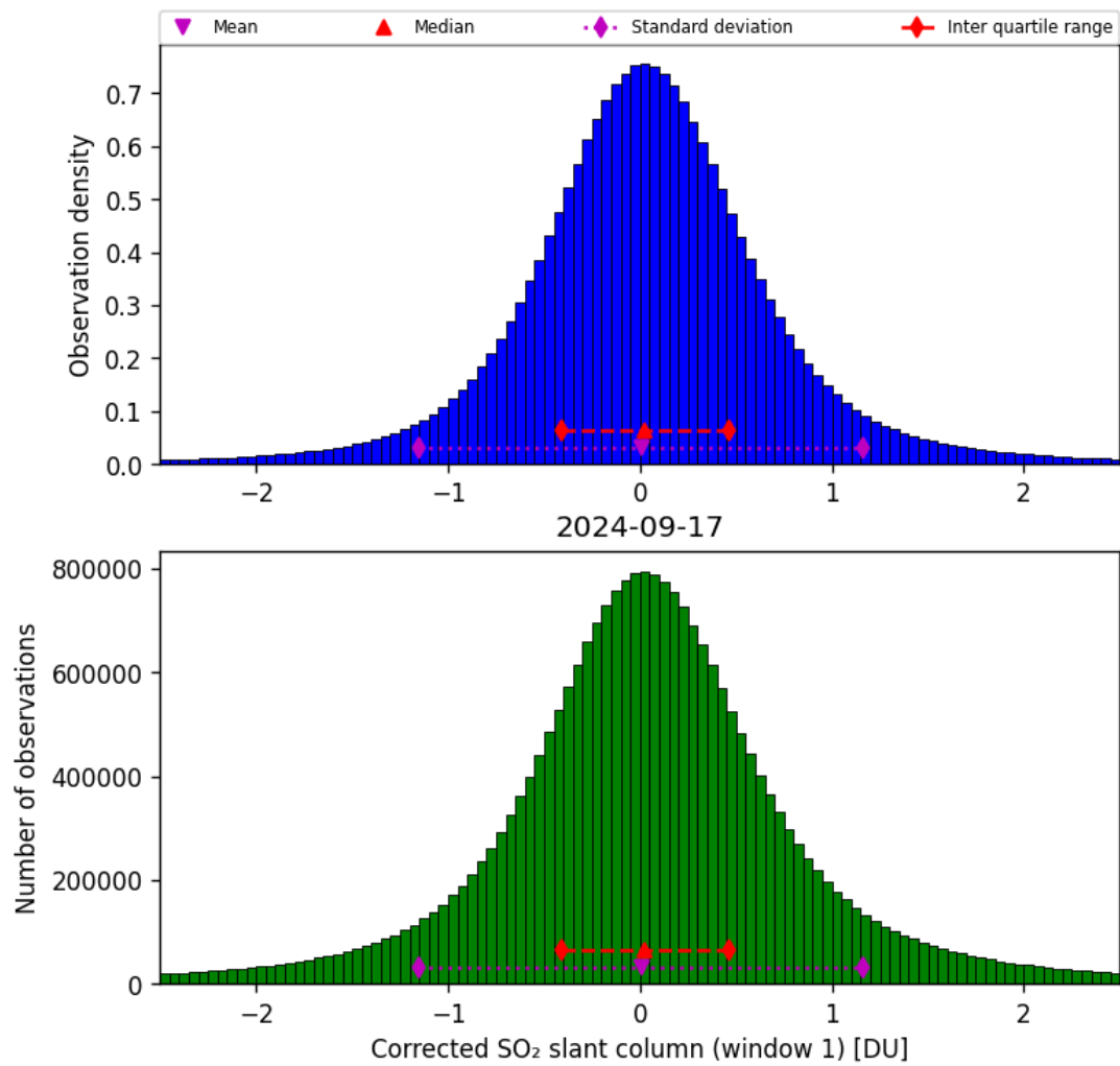
Figure 58: Histogram of “Corrected SO 2 slant column (window 1)” for 2024-09-17 to 2024-09-18
