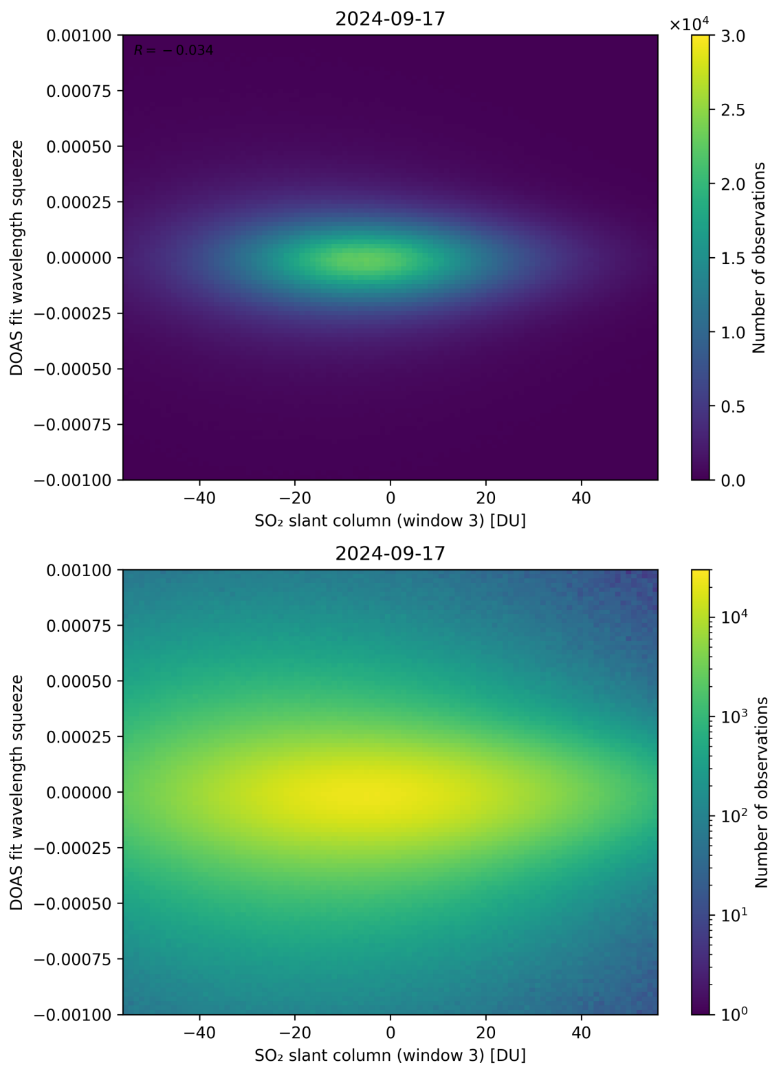
Figure 255: Scatter density plot of “SO 2 slant column (window 3)” against “DOAS fit wavelength squeeze” for 2024-09-17 to 2024-09-18.
