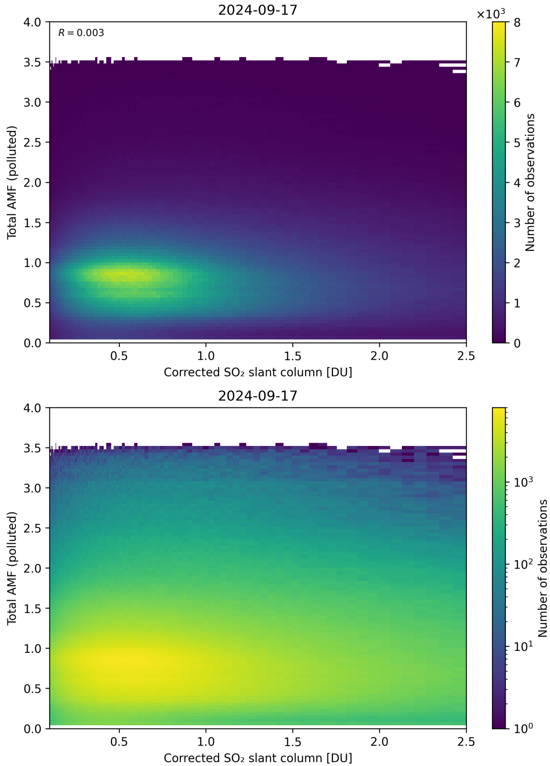
Figure 192: Scatter density plot of “Corrected SO 2 slant column” against “Total AMF (polluted)” for 2024-09-17 to 2024-09-18.
