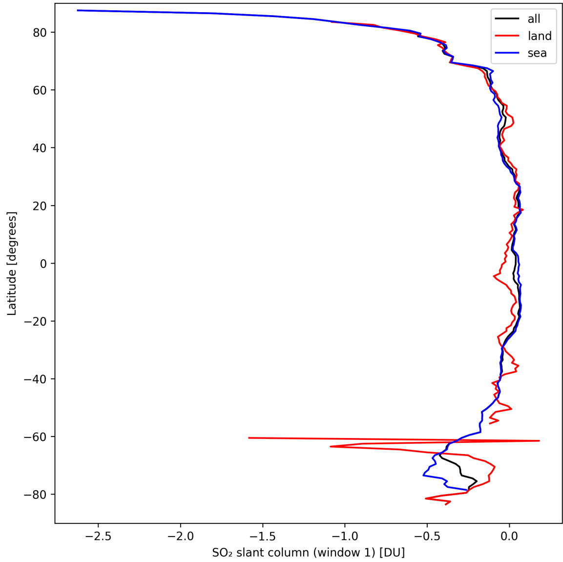
Figure 33: Zonal average of “SO 2 slant column (window 1)” for 2024-09-17 to 2024-09-18.
