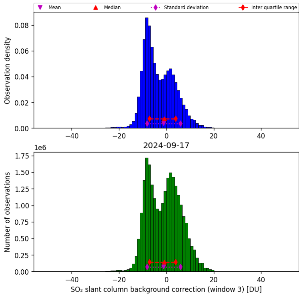
Figure 67: Histogram of “SO 2 slant column background correction (window 3)” for 2024-09-17 to 2024-09-18
