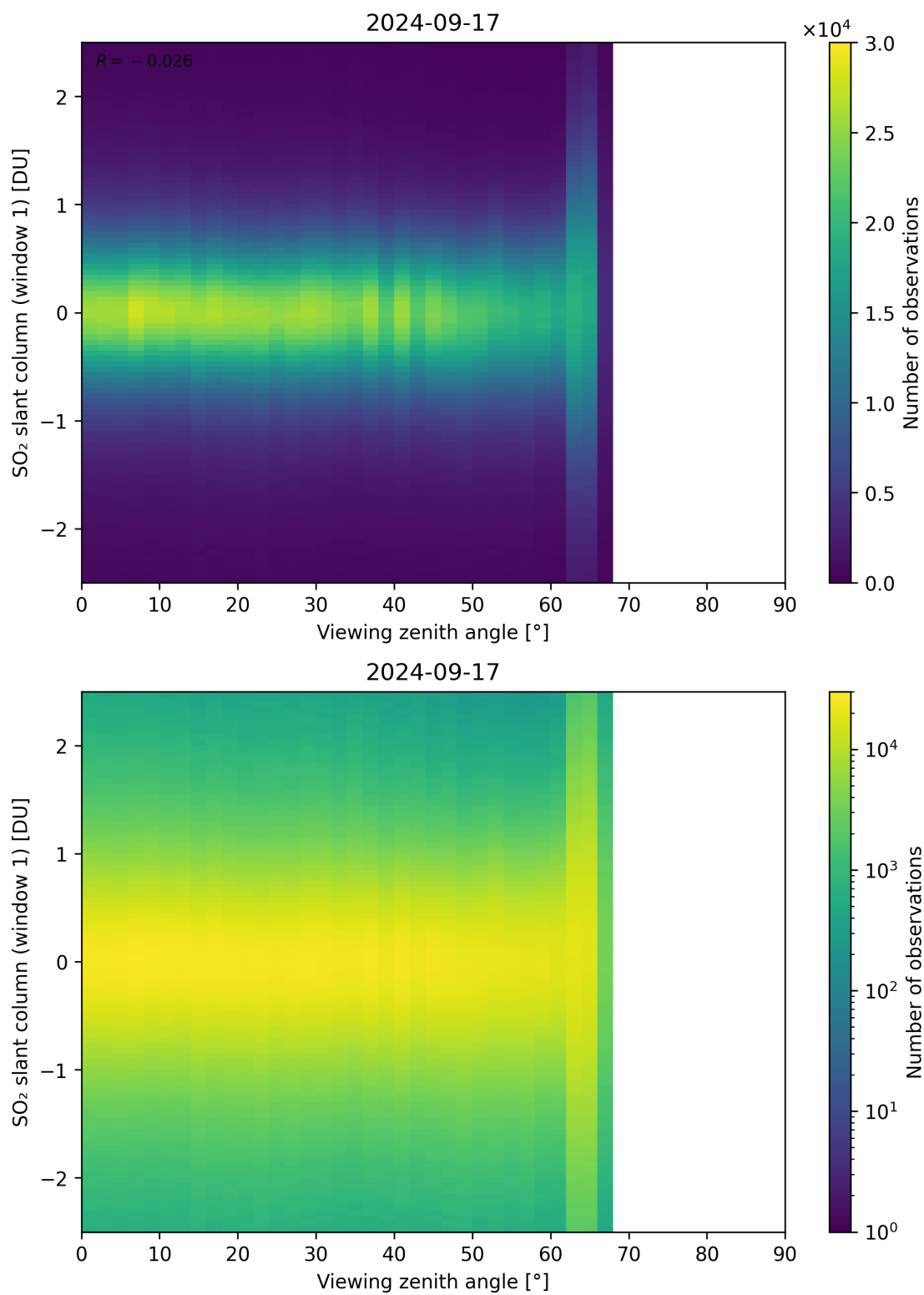
Figure 320: Scatter density plot of “Viewing zenith angle” against “SO 2 slant column (window 1)” for 2024-09-17 to 2024-09-18.
