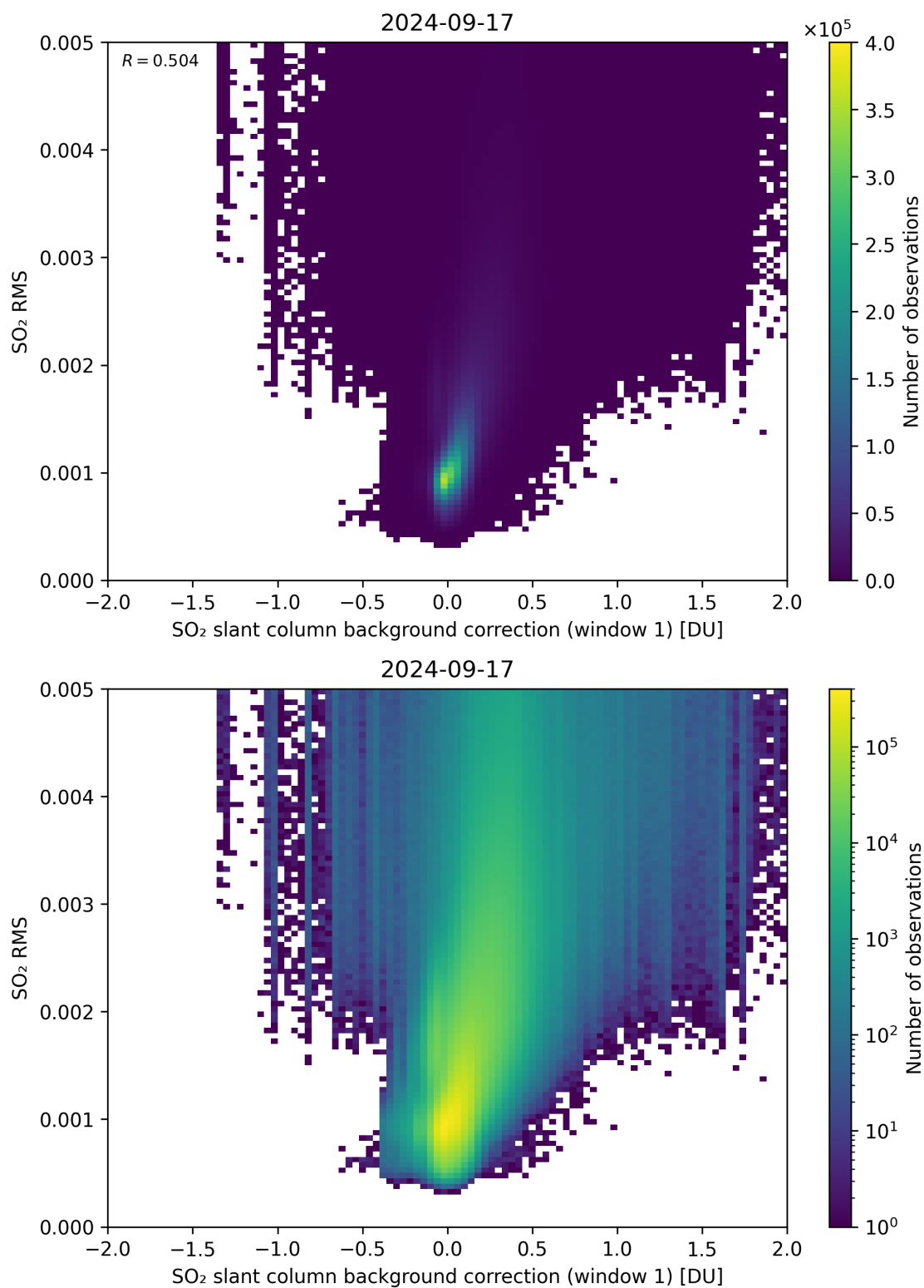
Figure 102: Scatter density plot of “SO 2 slant column background correction (window 1)” against “SO 2 RMS” for 2024-09-17 to 2024-09-18.
