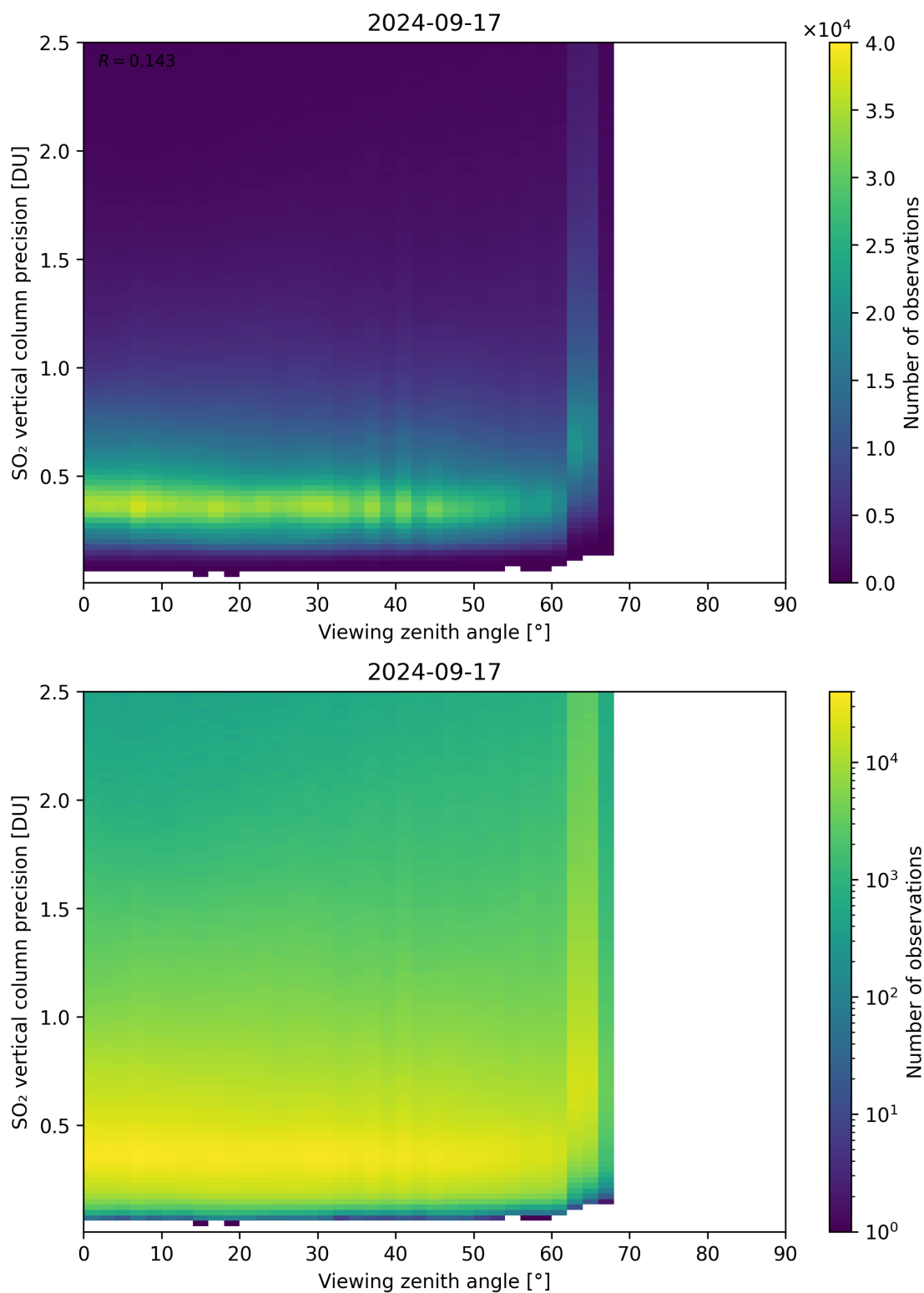
Figure 328: Scatter density plot of “Viewing zenith angle” against “SO 2 vertical column precision” for 2024-09-17 to 2024-09-18.
