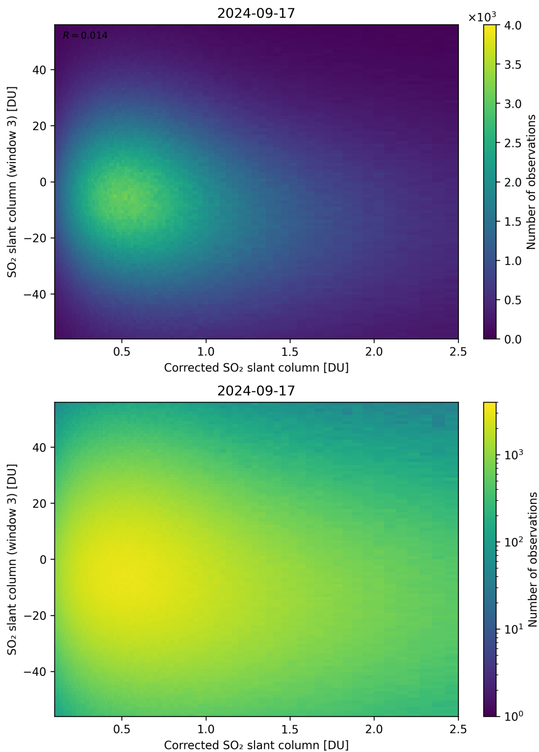
Figure 190: Scatter density plot of “Corrected SO 2 slant column” against “SO 2 slant column (window 3)” for 2024-09-17 to 2024-09-18.
