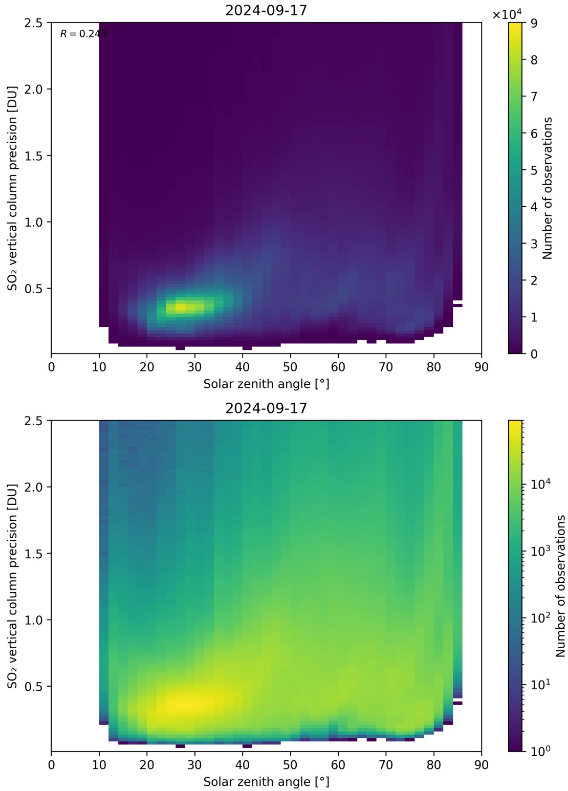
Figure 177: Scatter density plot of “Solar zenith angle” against “SO 2 vertical column precision” for 2024-09-17 to 2024-09-18.
