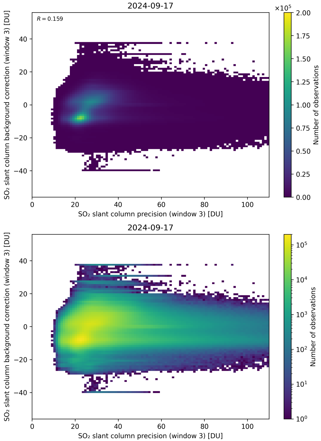
Figure 257: Scatter density plot of “SO 2 slant column precision (window 3)” against “SO 2 slant column background correction (window 3)” for 2024-09-17 to 2024-09-18.
