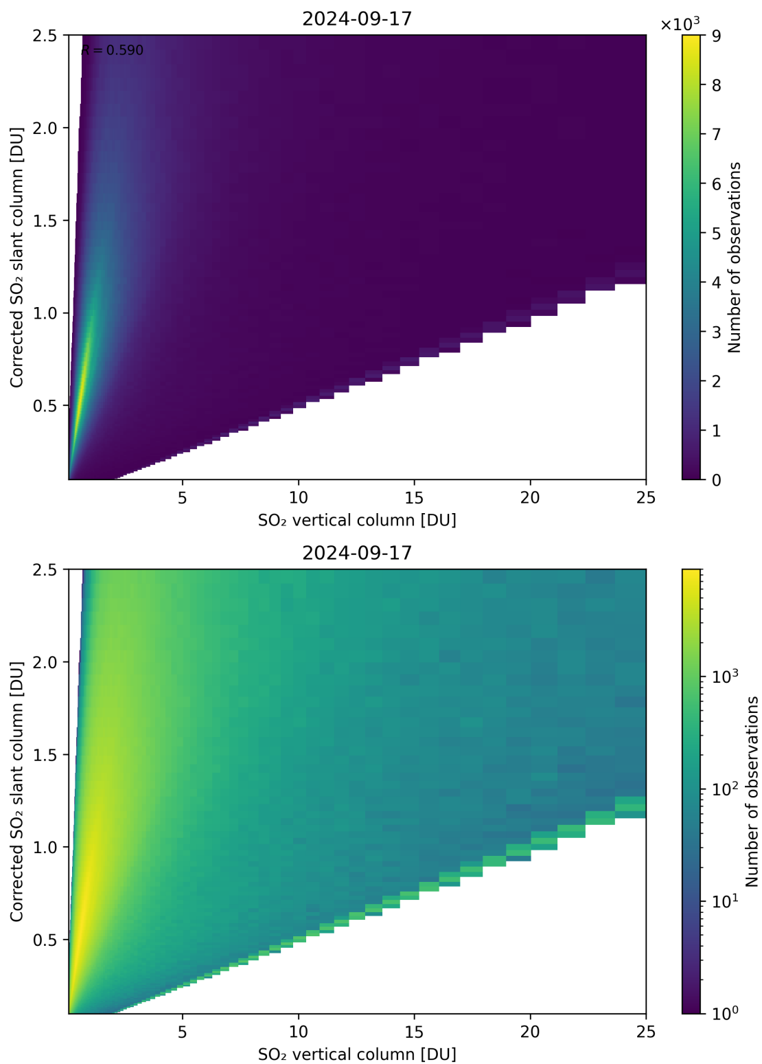
Figure 297: Scatter density plot of “SO 2 vertical column” against “Corrected SO 2 slant column” for 2024-09-17 to 2024-09-18.
