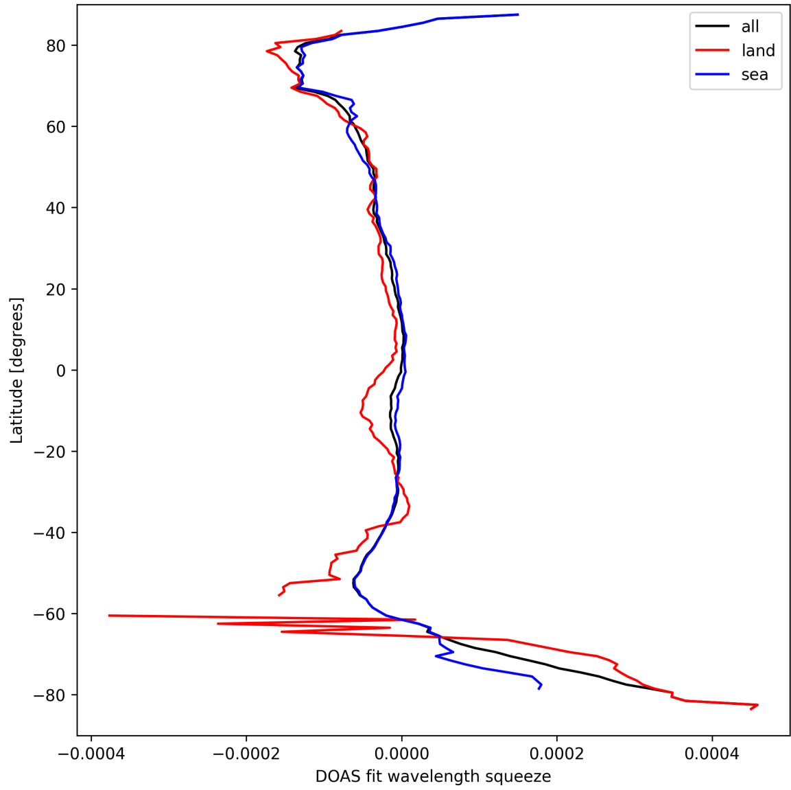
Figure 46: Zonal average of "DOAS fit wavelength squeeze" for 2024-09-17 to 2024-09-18.
