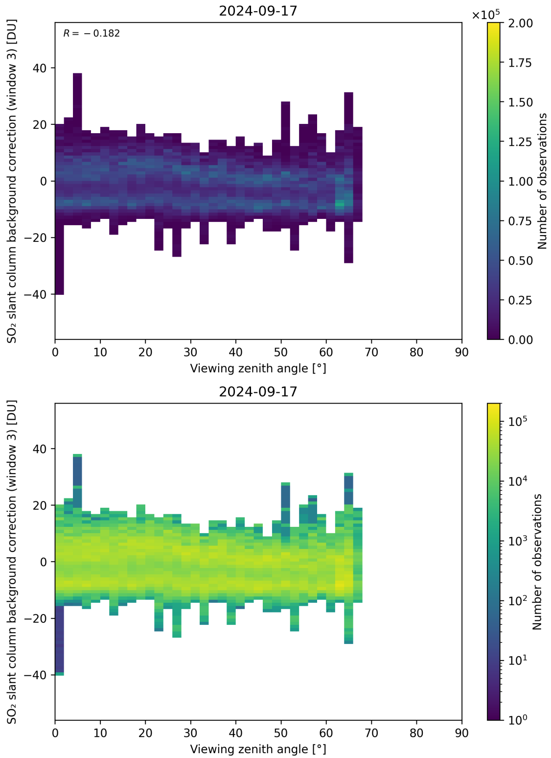
Figure 310: Scatter density plot of “Viewing zenith angle” against “SO 2 slant column background correction (window 3)” for 2024-09-17 to 2024-09-18.
