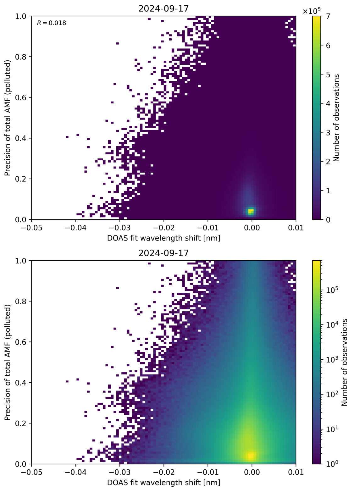
Figure 131: Scatter density plot of “DOAS fit wavelength shift” against “Precision of total AMF (polluted)” for 2024-09-17 to 2024-09-18.
