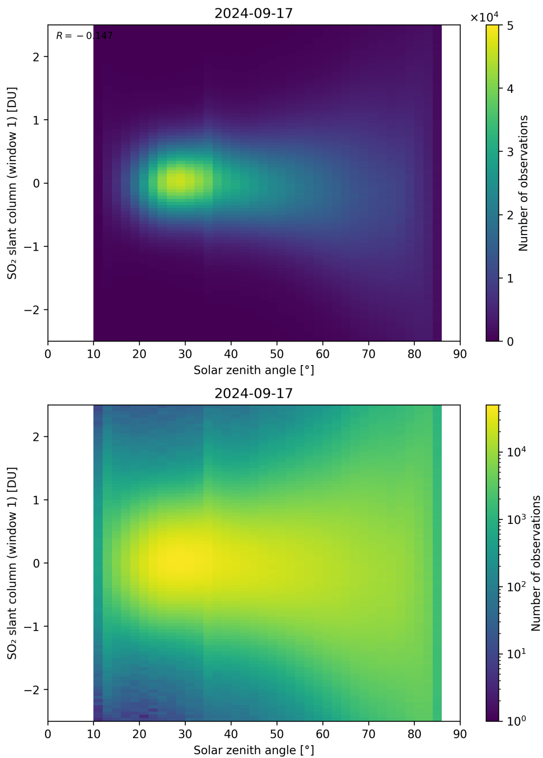
Figure 169: Scatter density plot of “Solar zenith angle” against “SO 2 slant column (window 1)” for 2024-09-17 to 2024-09-18.
