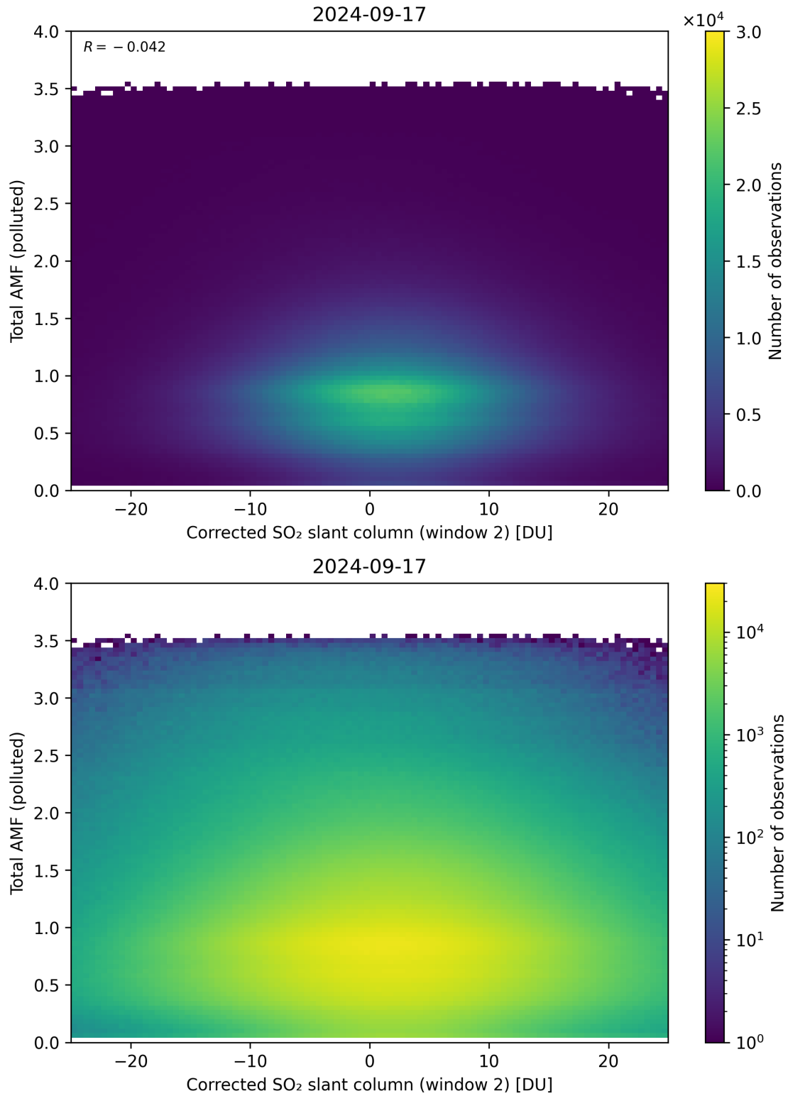
Figure 203: Scatter density plot of “Corrected SO 2 slant column (window 2)” against “Total AMF (polluted)” for 2024-09-17 to 2024-09-18.
