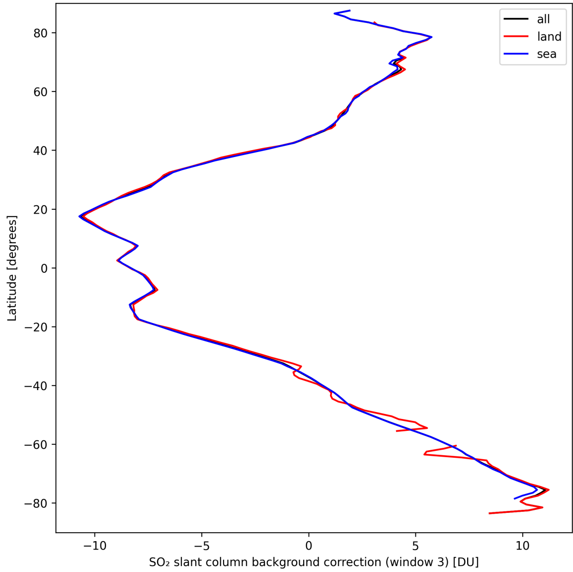
Figure 44: Zonal average of “SO 2 slant column background correction (window 3)” for 2024-09-17 to 2024-09-18.
