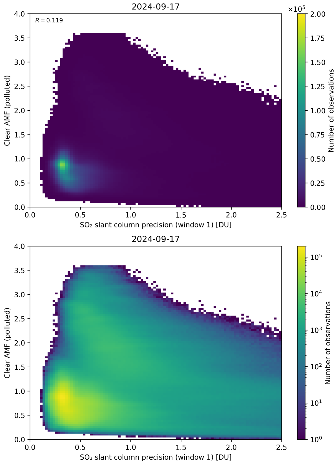
Figure 224: Scatter density plot of “SO 2 slant column precision (window 1)” against “Clear AMF (polluted)” for 2024-09-17 to 2024-09-18.
