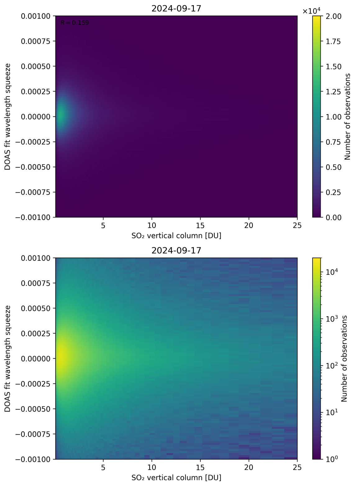
Figure 277: Scatter density plot of “SO 2 vertical column” against “DOAS fit wavelength squeeze” for 2024-09-17 to 2024-09-18.
