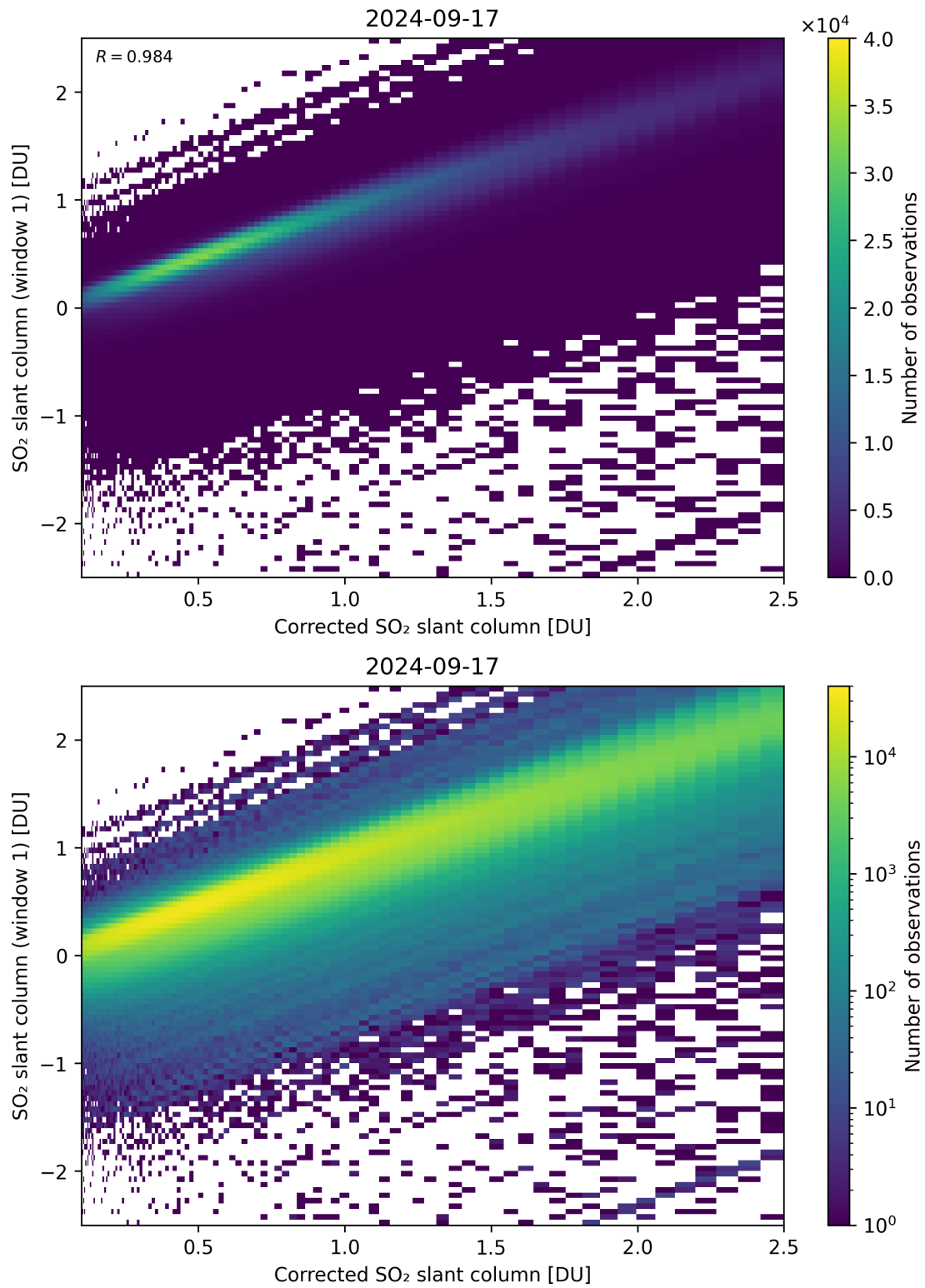
Figure 187: Scatter density plot of “Corrected SO 2 slant column” against “SO 2 slant column (window 1)” for 2024-09-17 to 2024-09-18.
