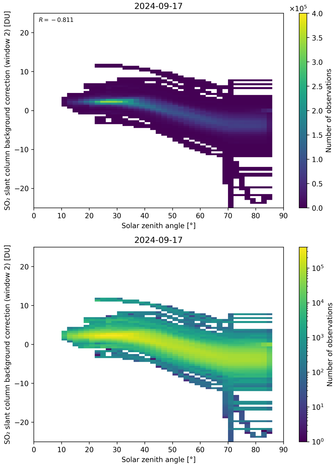
Figure 159: Scatter density plot of “Solar zenith angle” against “SO 2 slant column background correction (window 2)” for 2024-09-17 to 2024-09-18.
