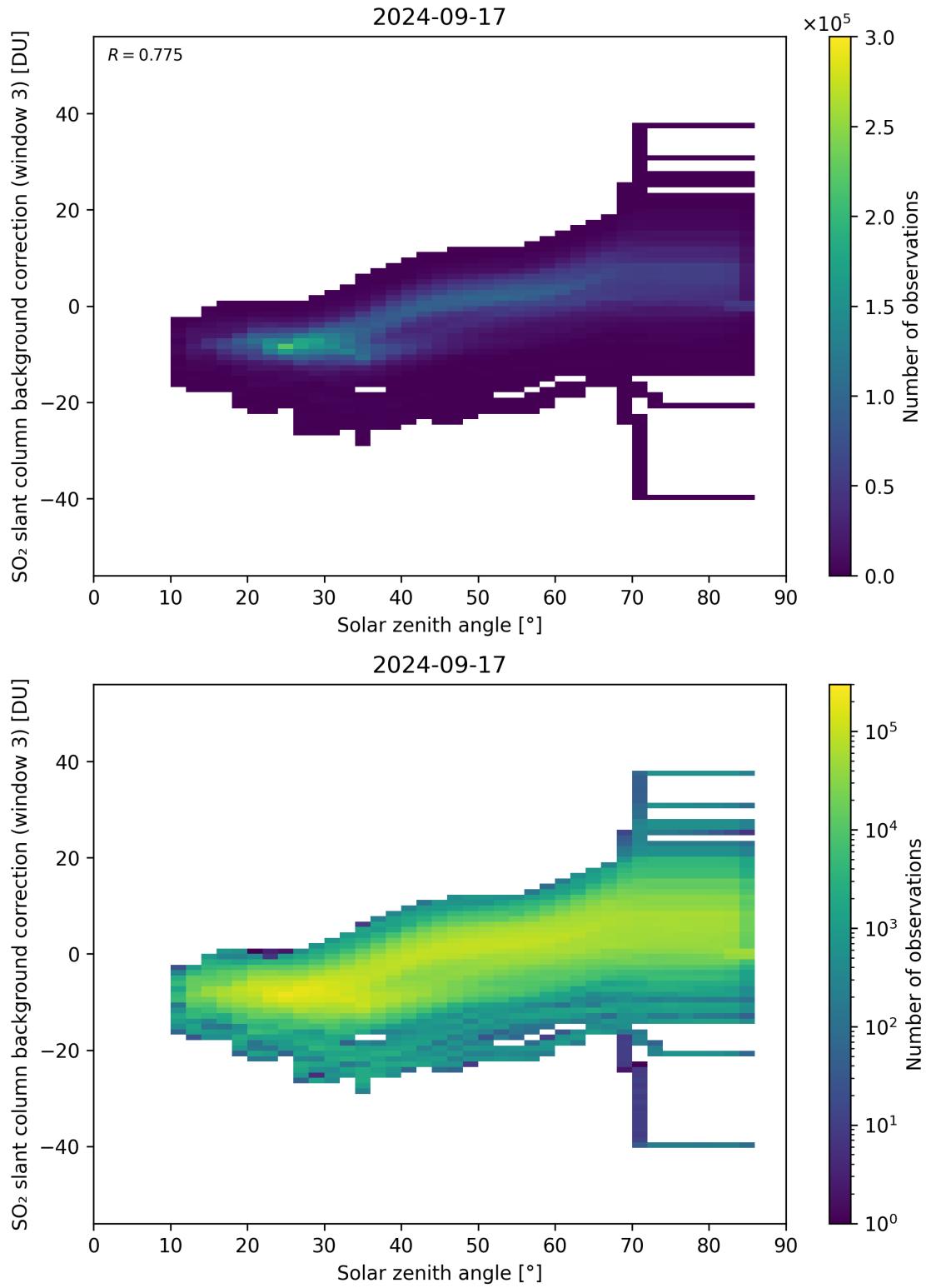
Figure 160: Scatter density plot of “Solar zenith angle” against “SO 2 slant column background correction (window 3)” for 2024-09-17 to 2024-09-18.
