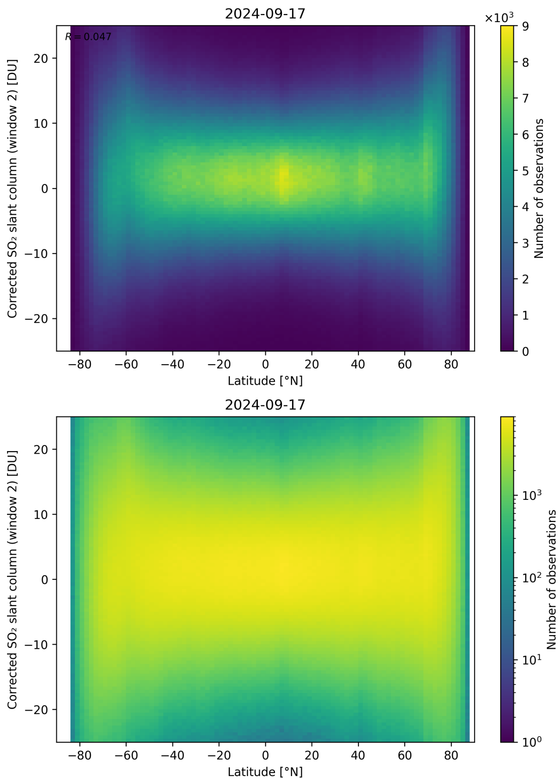
Figure 147: Scatter density plot of “Latitude” against “Corrected SO 2 slant column (window 2)” for 2024-09-17 to 2024-09-18.
