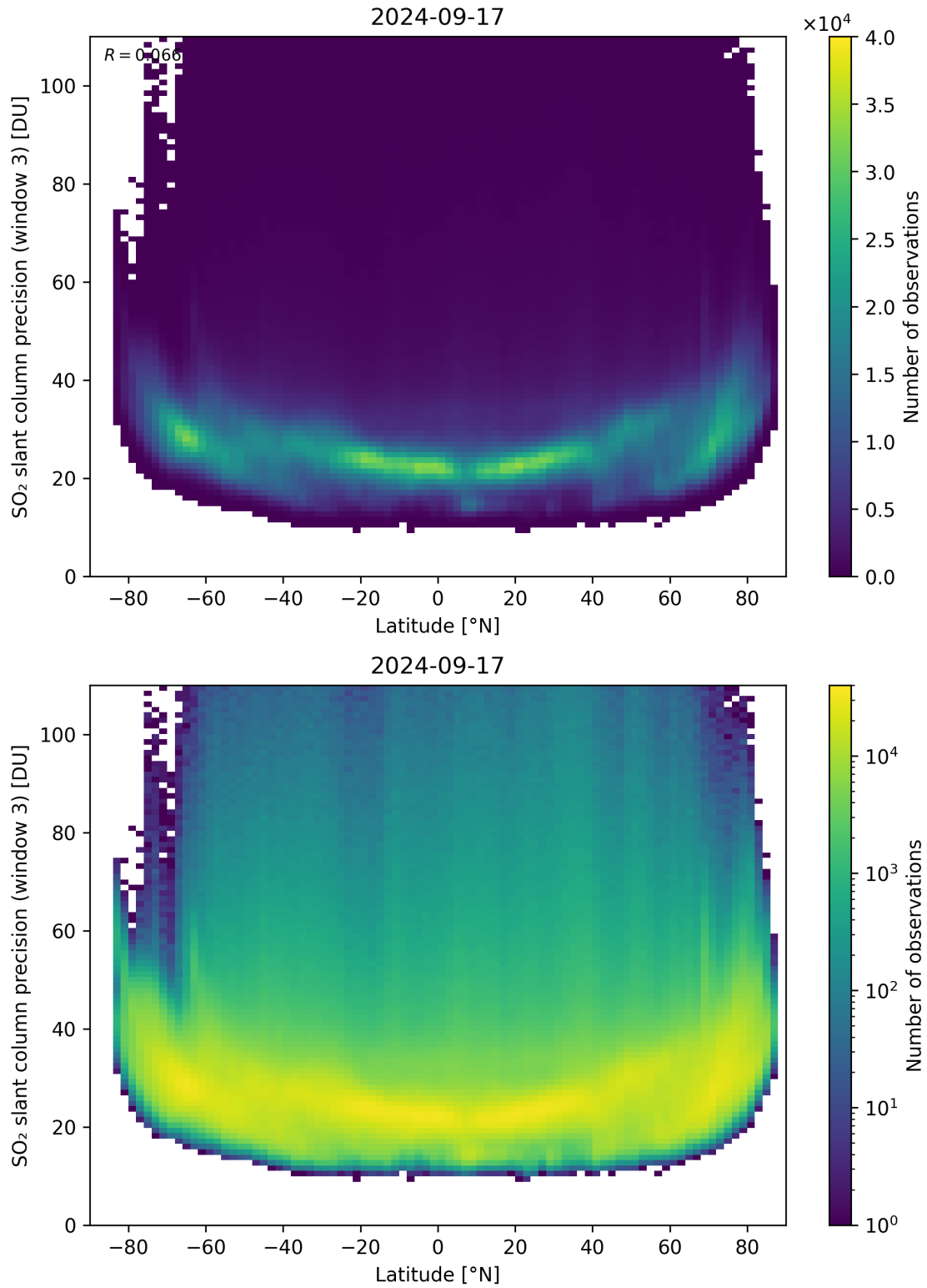
Figure 153: Scatter density plot of “Latitude” against “SO 2 slant column precision (window 3)” for 2024-09-17 to 2024-09-18.
