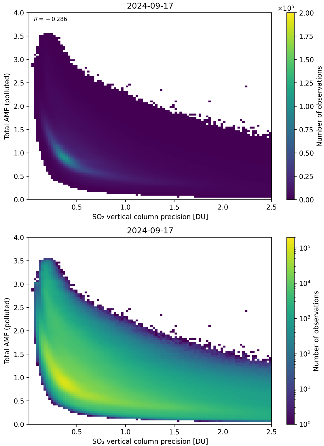
Figure 294: Scatter density plot of “SO 2 vertical column precision” against “Total AMF (polluted)” for 2024-09-17 to 2024-09-18.
