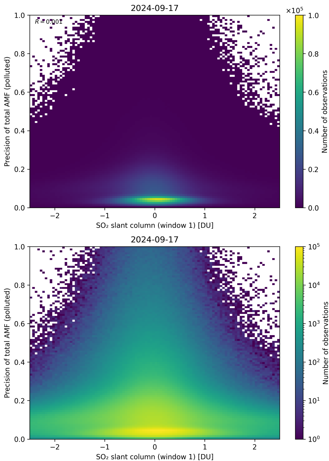
Figure 240: Scatter density plot of “SO 2 slant column (window 1)” against “Precision of total AMF (polluted)” for 2024-09-17 to 2024-09-18.
