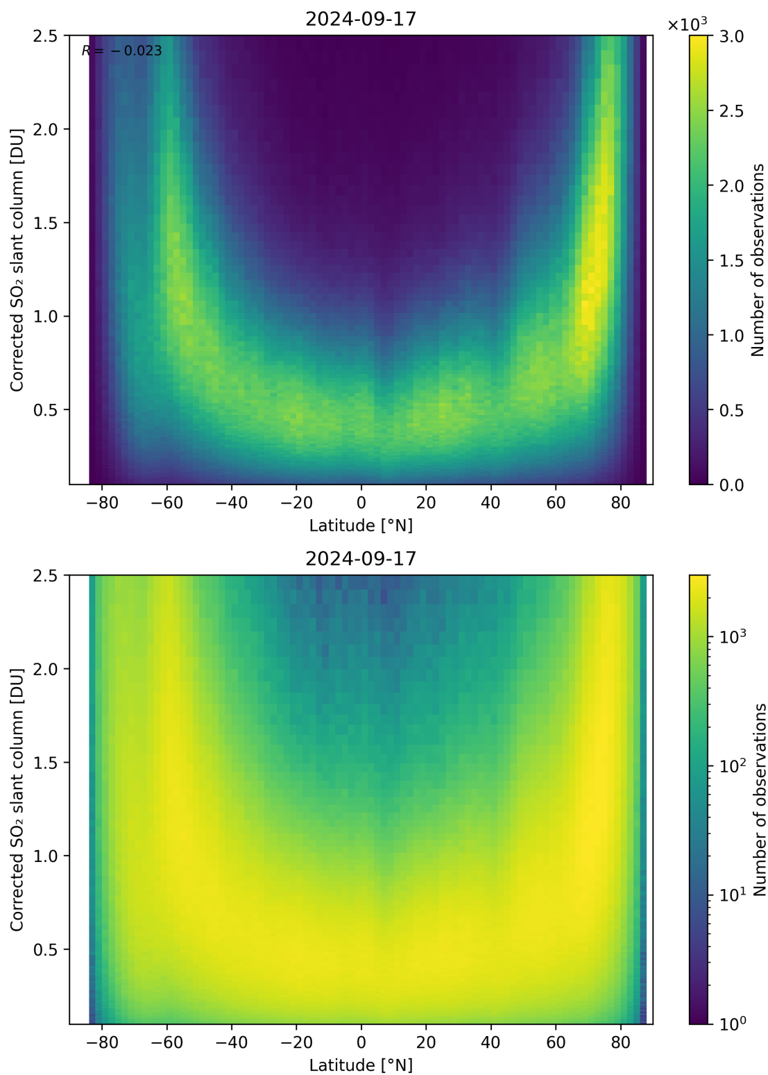
Figure 146: Scatter density plot of “Latitude” against “Corrected SO 2 slant column” for 2024-09-17 to 2024-09-18.
