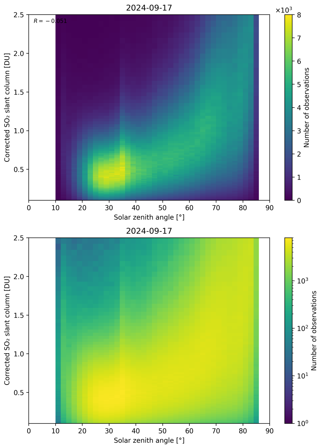
Figure 166: Scatter density plot of “Solar zenith angle” against “Corrected SO 2 slant column” for 2024-09-17 to 2024-09-18.
