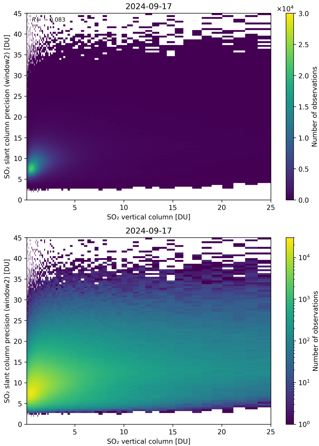
Figure 302: Scatter density plot of “SO 2 vertical column” against “SO 2 slant column precision (window2)” for 2024-09-17 to 2024-09-18.
