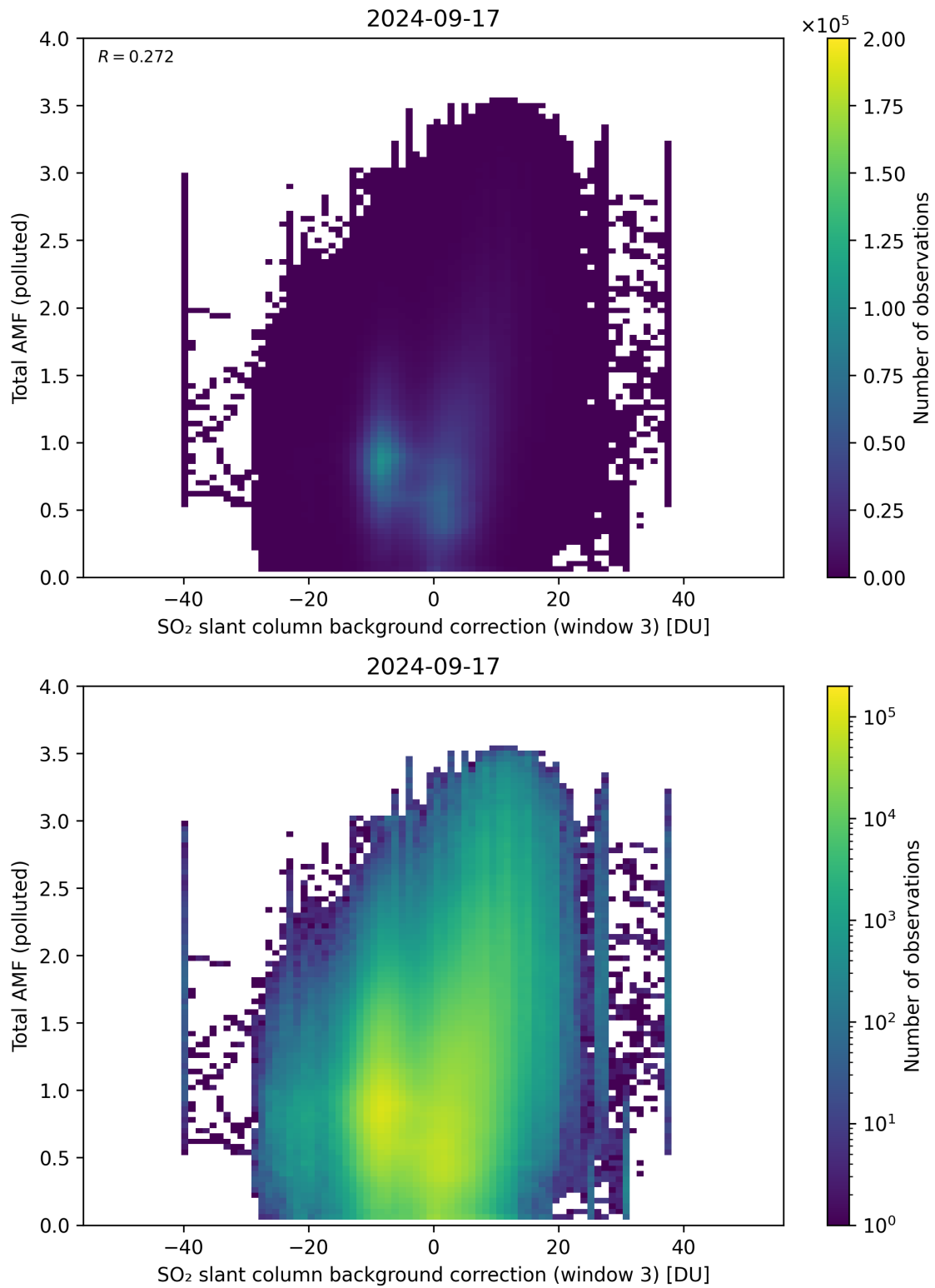
Figure 125: Scatter density plot of “SO 2 slant column background correction (window 3)” against “Total AMF (polluted)” for 2024-09-17 to 2024-09-18.
