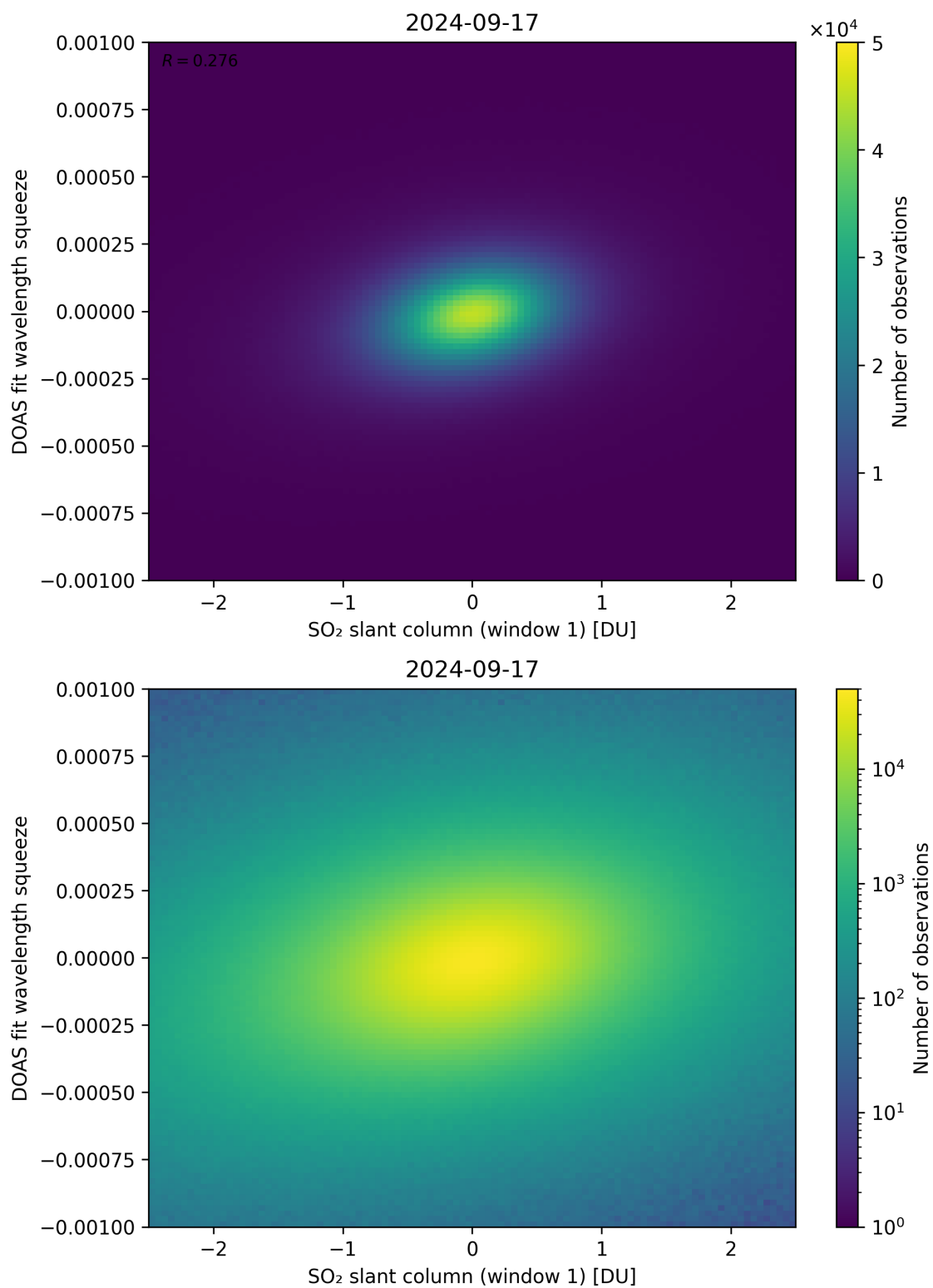
Figure 216: Scatter density plot of “SO 2 slant column (window 1)” against “DOAS fit wavelength squeeze” for 2024-09-17 to 2024-09-18.
