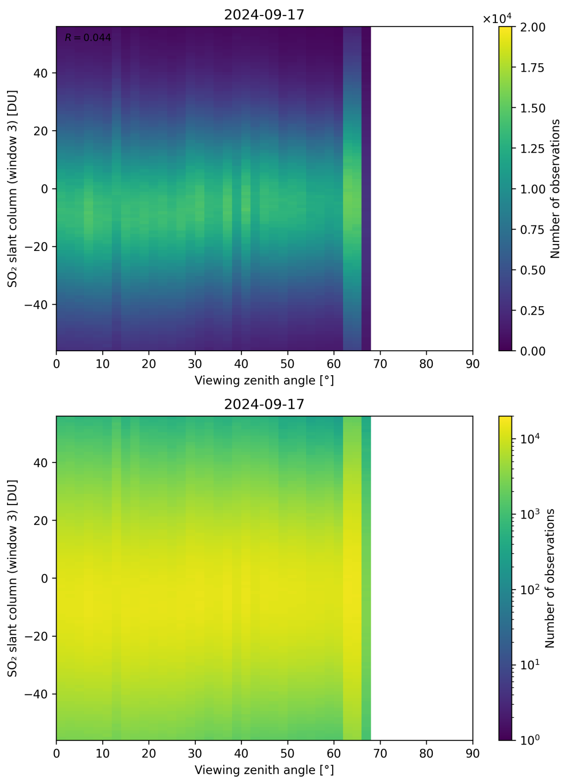
Figure 323: Scatter density plot of “Viewing zenith angle” against “SO 2 slant column (window 3)” for 2024-09-17 to 2024-09-18.
