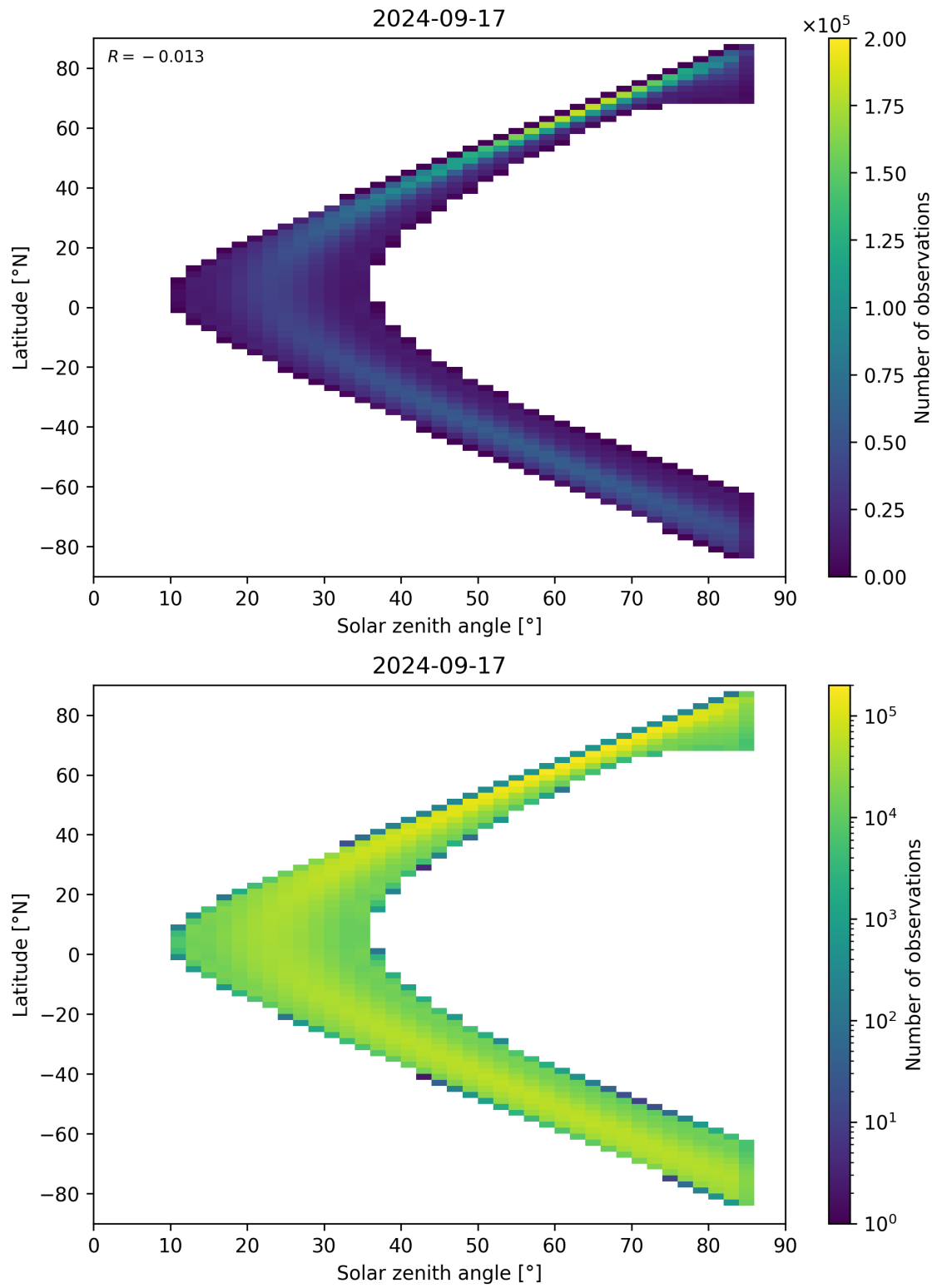
Figure 164: Scatter density plot of “Solar zenith angle” against “Latitude” for 2024-09-17 to 2024-09-18.
