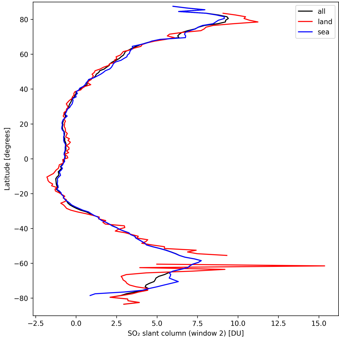
Figure 37: Zonal average of “SO 2 slant column (window 2)” for 2024-09-17 to 2024-09-18.
