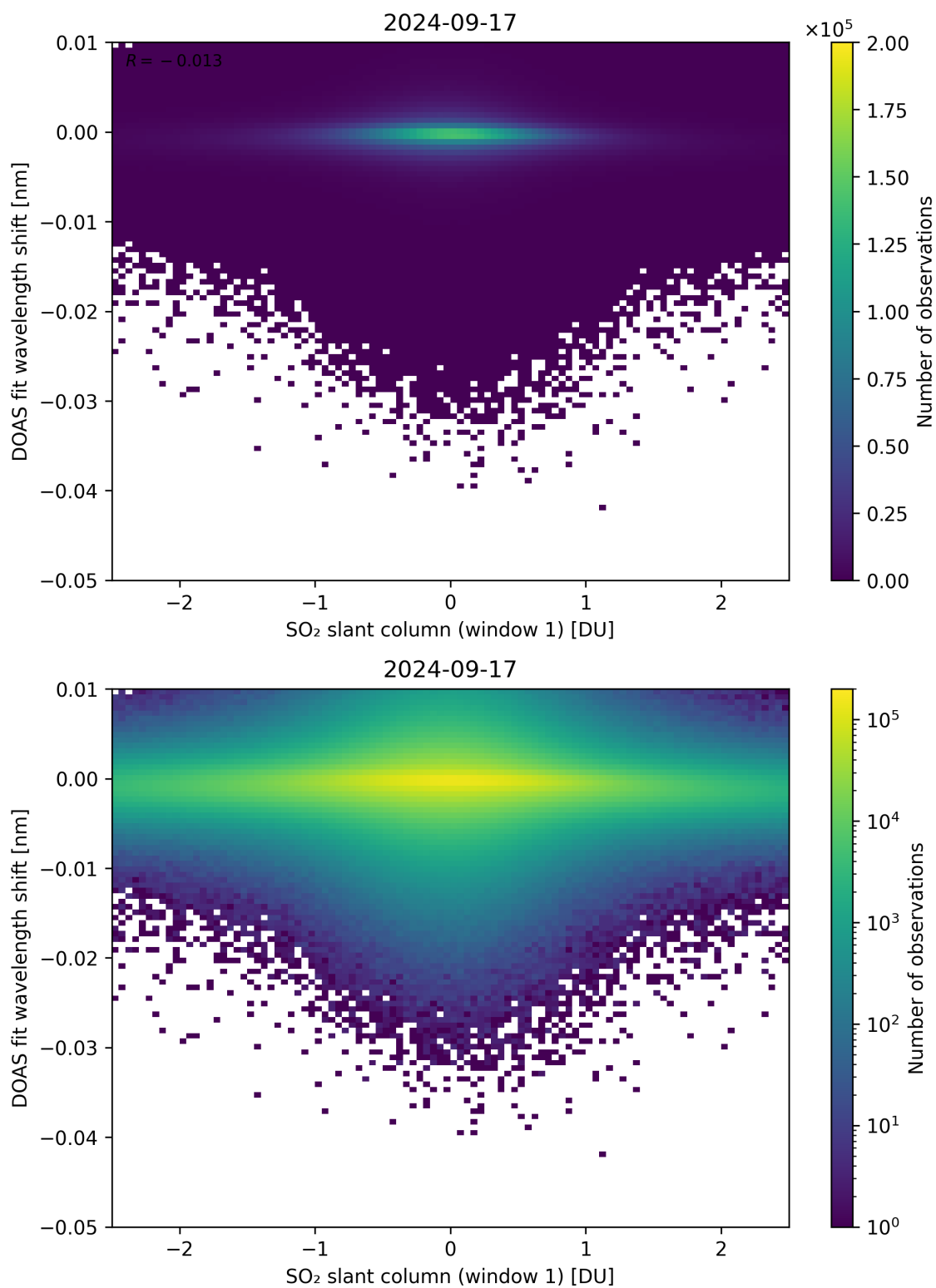
Figure 215: Scatter density plot of “SO 2 slant column (window 1)” against “DOAS fit wavelength shift” for 2024-09-17 to 2024-09-18.
