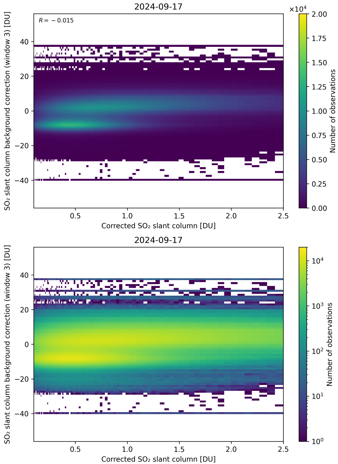
Figure 180: Scatter density plot of “Corrected SO 2 slant column” against “SO 2 slant column background correction (window 3)” for 2024-09-17 to 2024-09-18.
