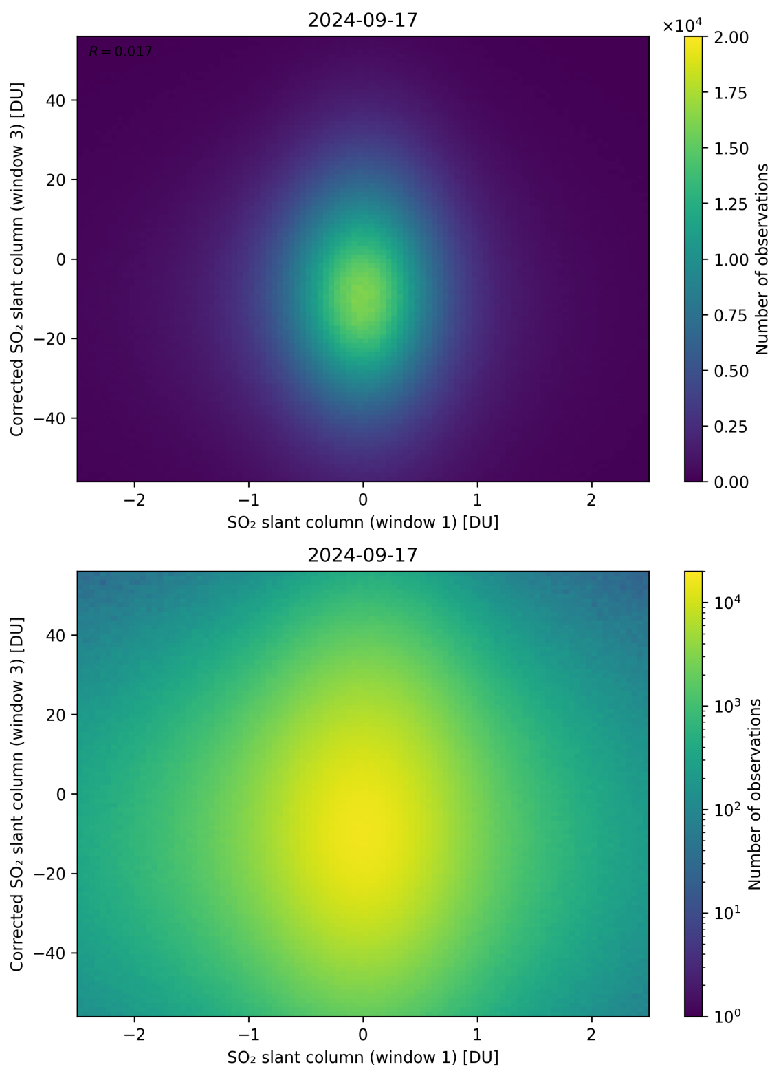
Figure 234: Scatter density plot of “SO 2 slant column (window 1)” against “Corrected SO 2 slant column (window 3)” for 2024-09-17 to 2024-09-18.
