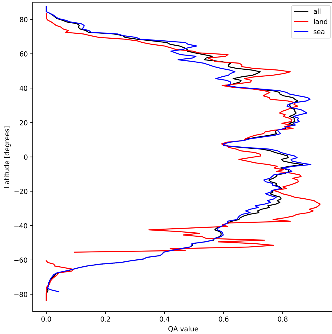
Figure 29: Zonal average of “QA value” for 2024-09-17 to 2024-09-18.
