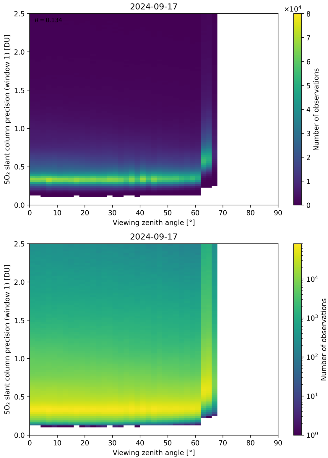
Figure 321: Scatter density plot of “Viewing zenith angle” against “SO 2 slant column precision (window 1)” for 2024-09-17 to 2024-09-18.
