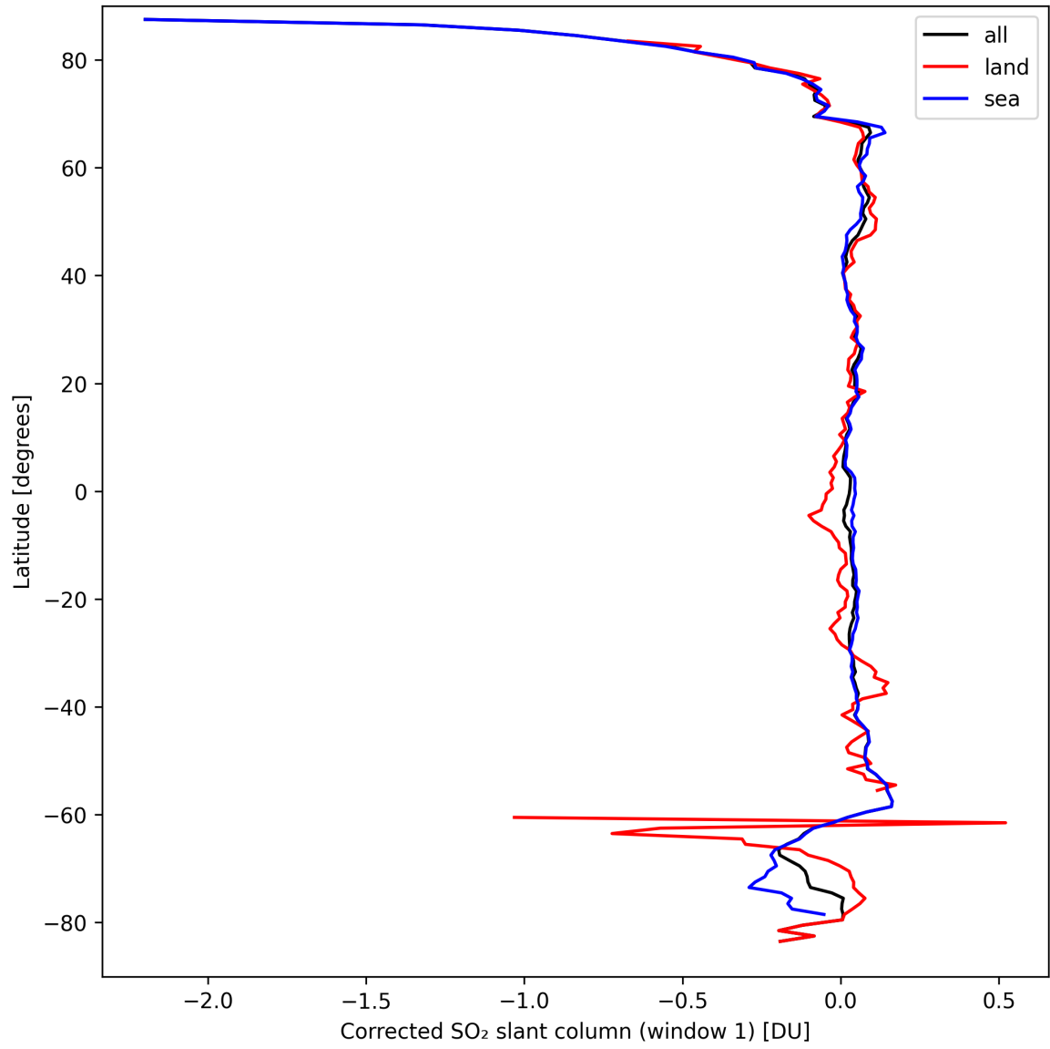
Figure 35: Zonal average of “Corrected SO 2 slant column (window 1)” for 2024-09-17 to 2024-09-18.
