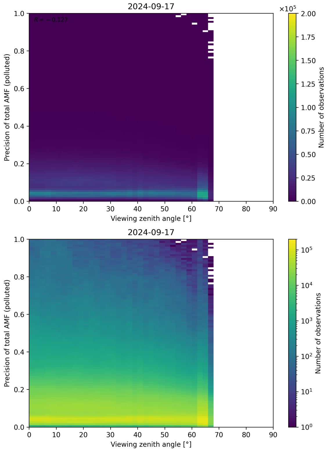
Figure 326: Scatter density plot of “Viewing zenith angle” against “Precision of total AMF (polluted)” for 2024-09-17 to 2024-09-18.
