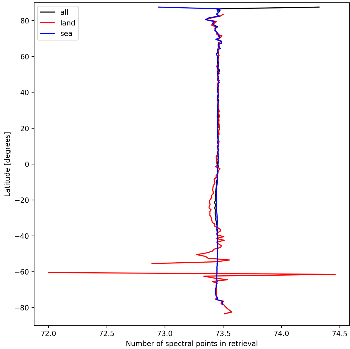
Figure 51: Zonal average of “Number of spectral points in retrieval” for 2024-09-17 to 2024-09-18.
