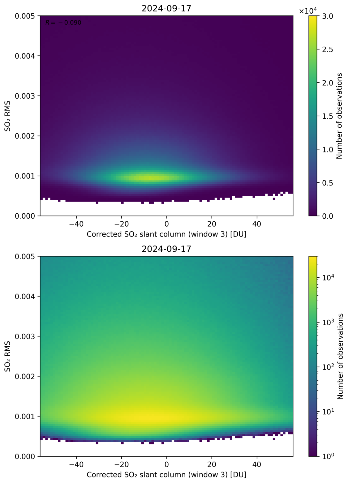
Figure 208: Scatter density plot of “Corrected SO 2 slant column (window 3)” against “SO 2 RMS” for 2024-09-17 to 2024-09-18.
