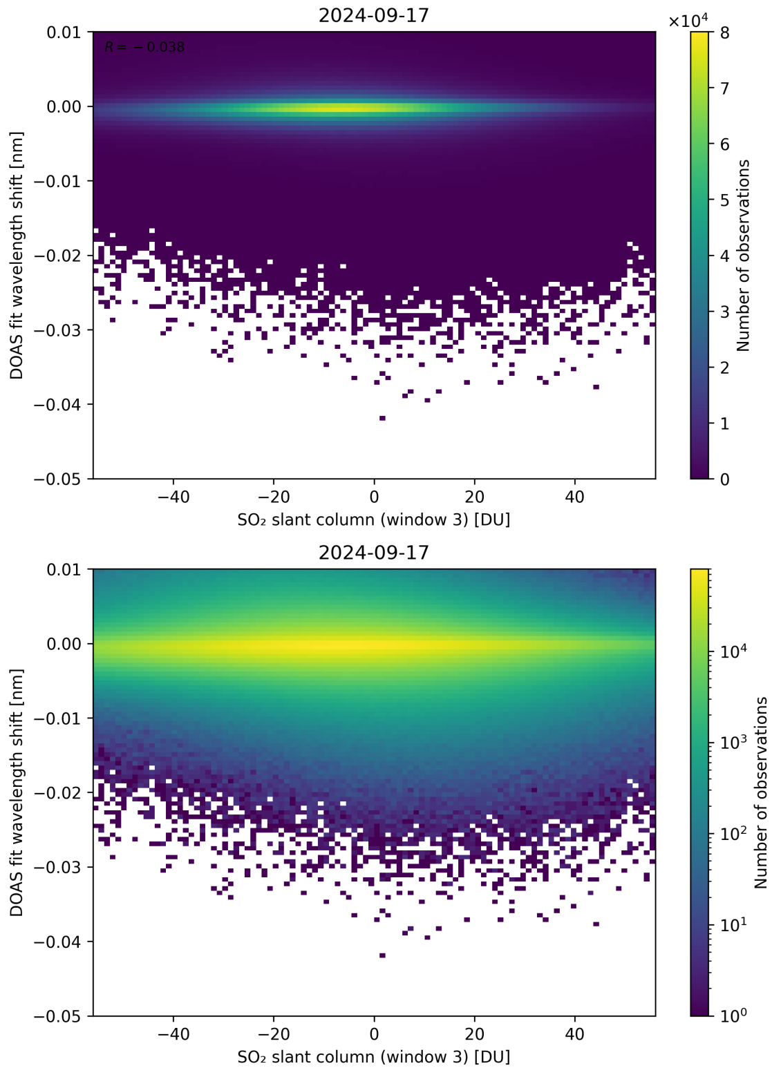
Figure 254: Scatter density plot of “SO 2 slant column (window 3)” against “DOAS fit wavelength shift” for 2024-09-17 to 2024-09-18.
