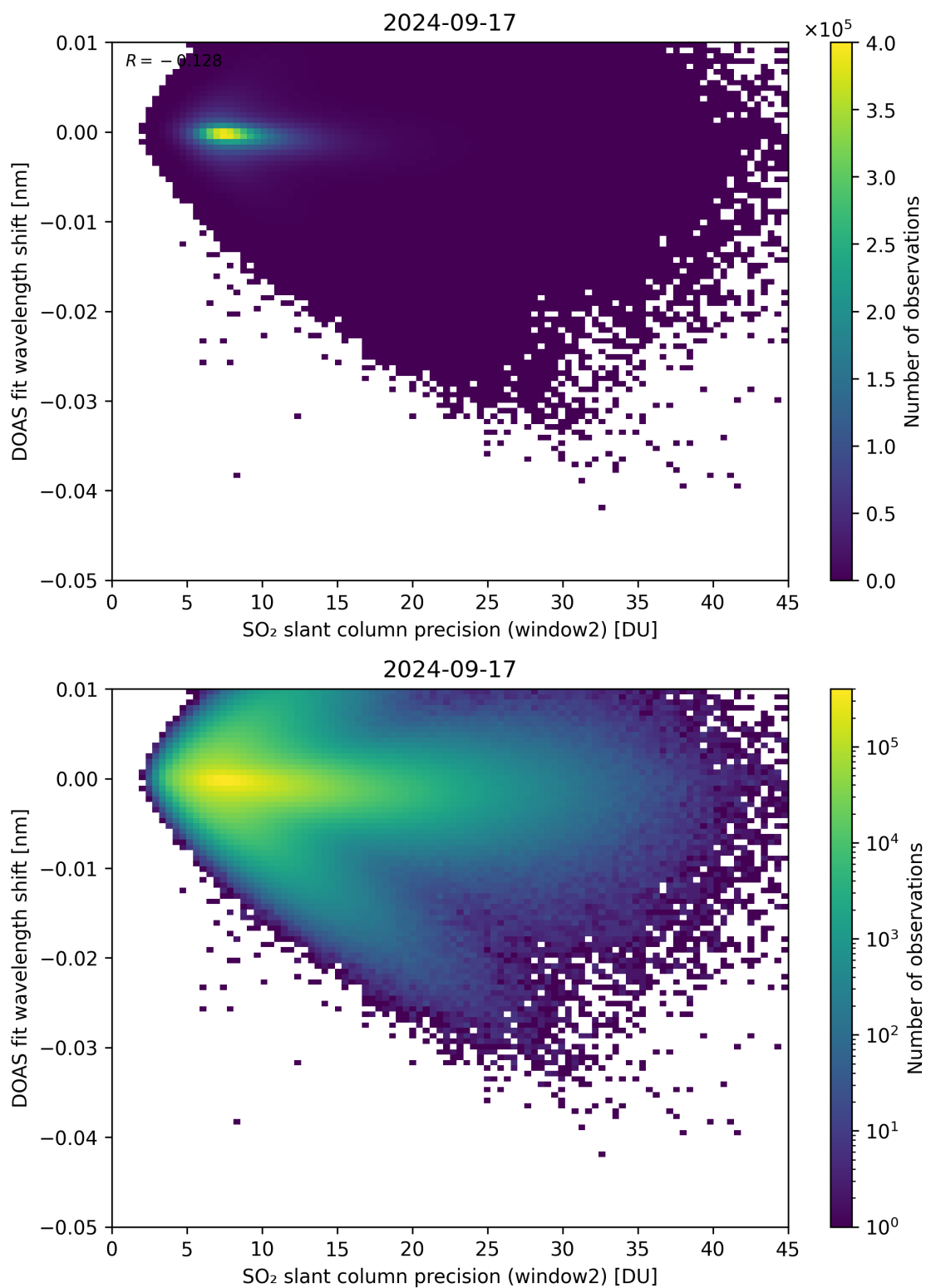
Figure 243: Scatter density plot of “SO 2 slant column precision (window2)” against “DOAS fit wavelength shift” for 2024-09-17 to 2024-09-18.
