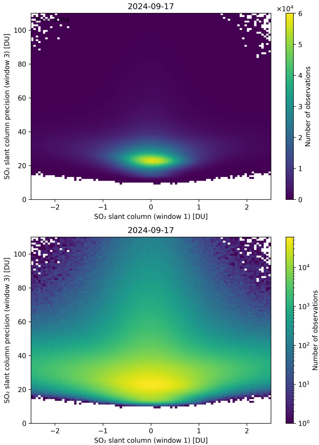
Figure 238: Scatter density plot of “SO 2 slant column (window 1)” against “SO 2 slant column precision (window 3)” for 2024-09-17 to 2024-09-18.
