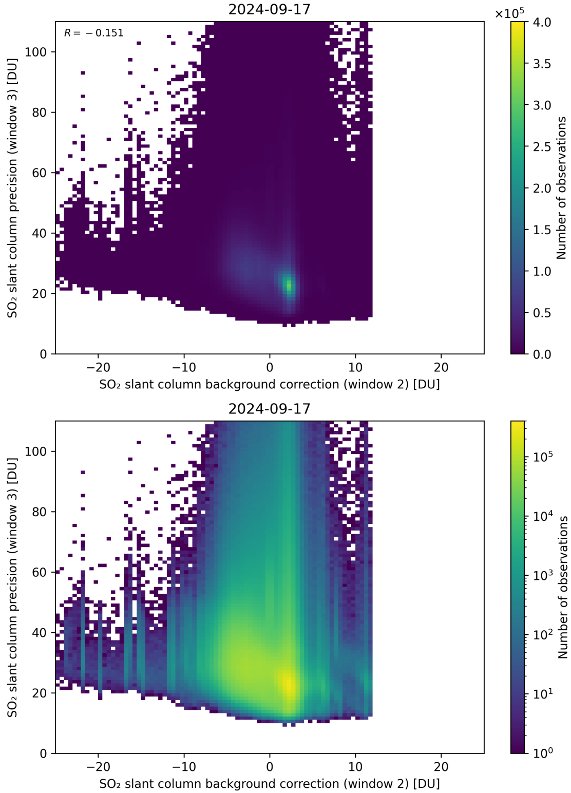
Figure 118: Scatter density plot of “SO 2 slant column background correction (window 2)” against “SO 2 slant column precision (window 3)” for 2024-09-17 to 2024-09-18.
