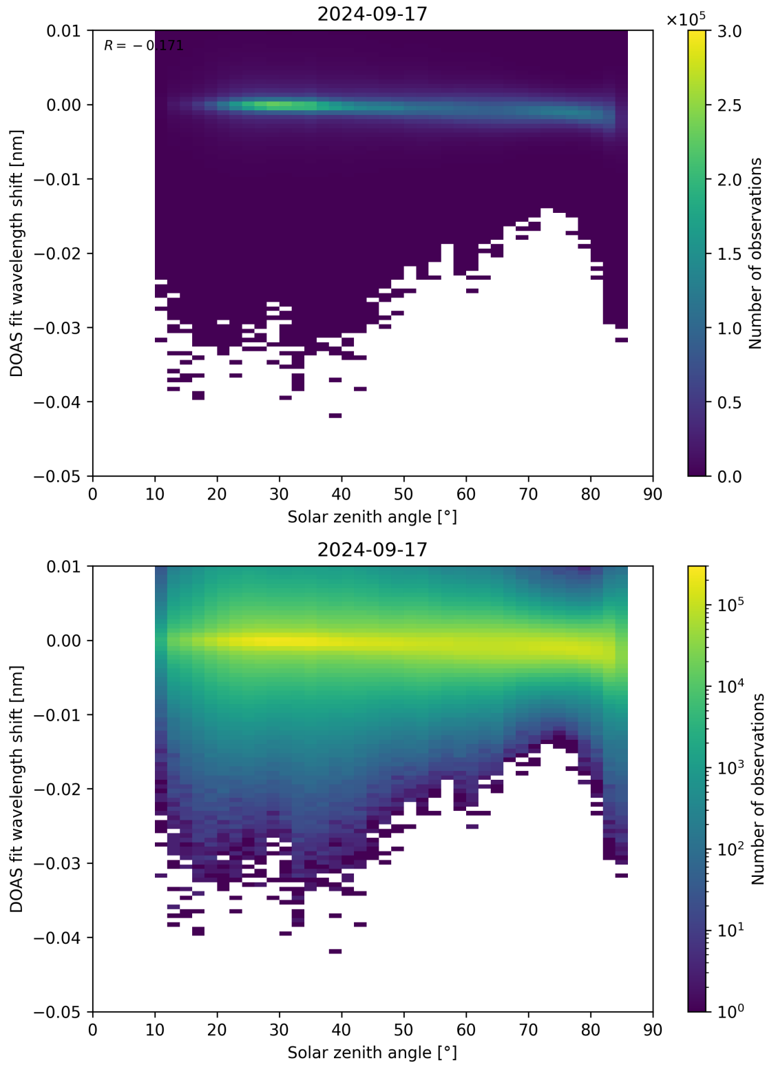
Figure 161: Scatter density plot of “Solar zenith angle” against “DOAS fit wavelength shift” for 2024-09-17 to 2024-09-18.
