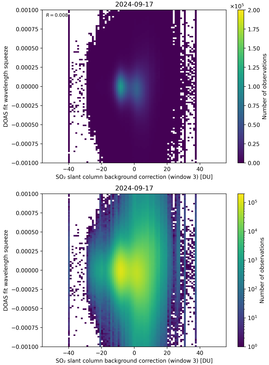
Figure 122: Scatter density plot of “SO 2 slant column background correction (window 3)” against “DOAS fit wavelength squeeze” for 2024-09-17 to 2024-09-18.
