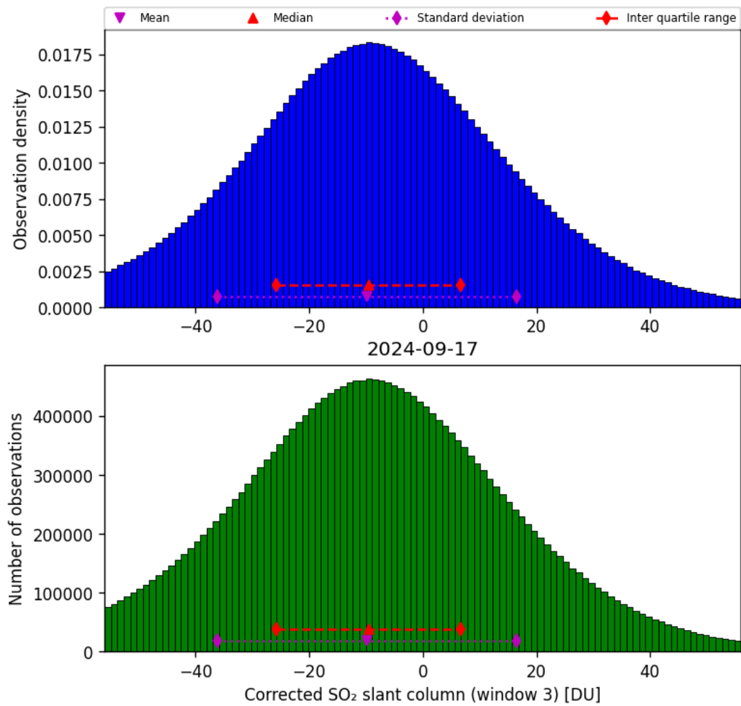
Figure 66: Histogram of “Corrected SO 2 slant column (window 3)” for 2024-09-17 to 2024-09-18
