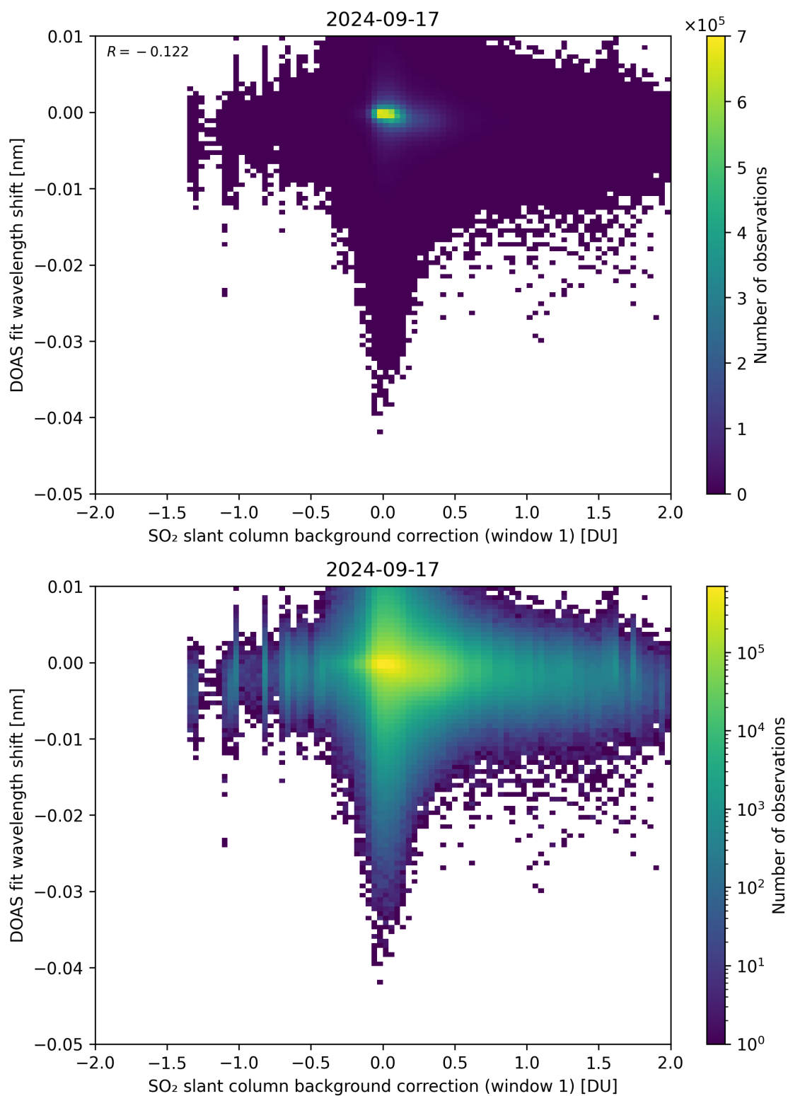
Figure 100: Scatter density plot of “SO 2 slant column background correction (window 1)” against “DOAS fit wavelength shift” for 2024-09-17 to 2024-09-18.
