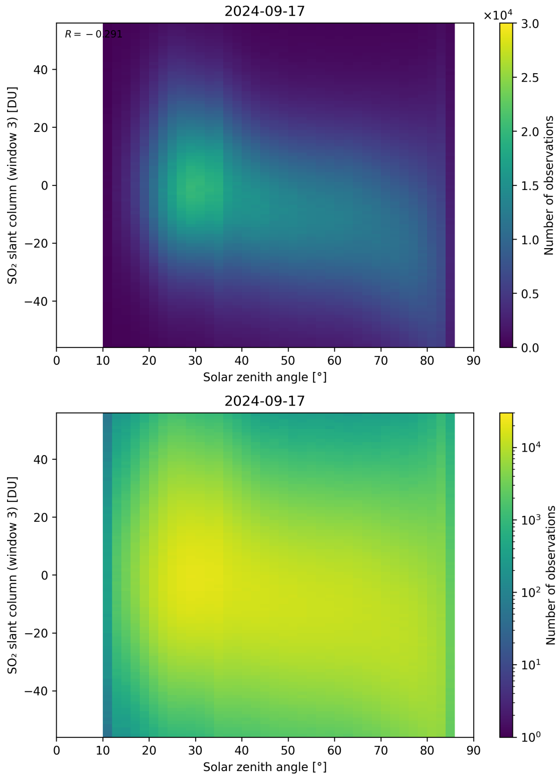
Figure 172: Scatter density plot of “Solar zenith angle” against “SO 2 slant column (window 3)” for 2024-09-17 to 2024-09-18.
