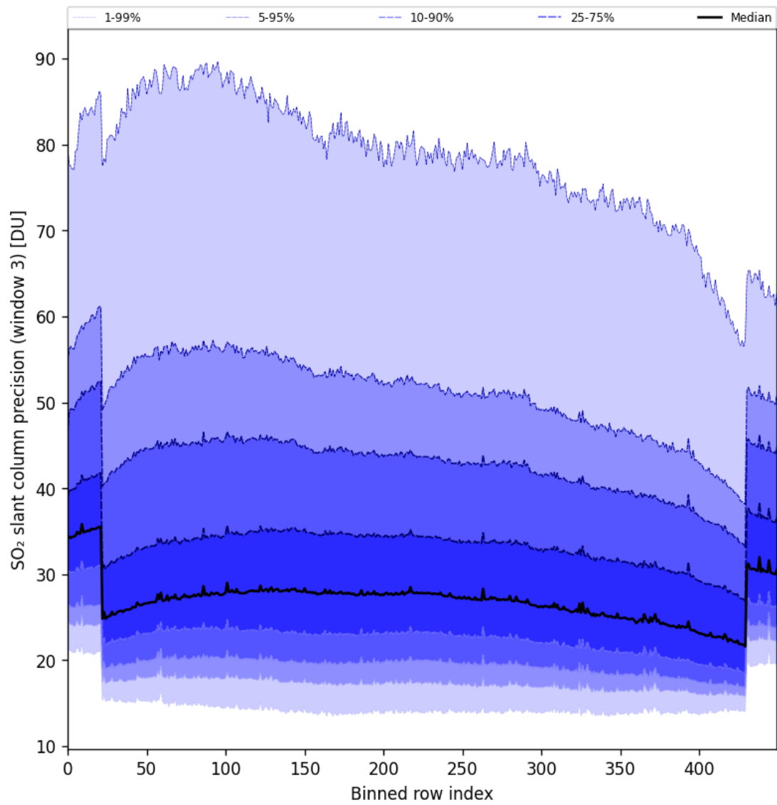
Figure 88: Along track statistics of “SO 2 slant column precision (window 3)” for 2024-09-17 to 2024-09-18
