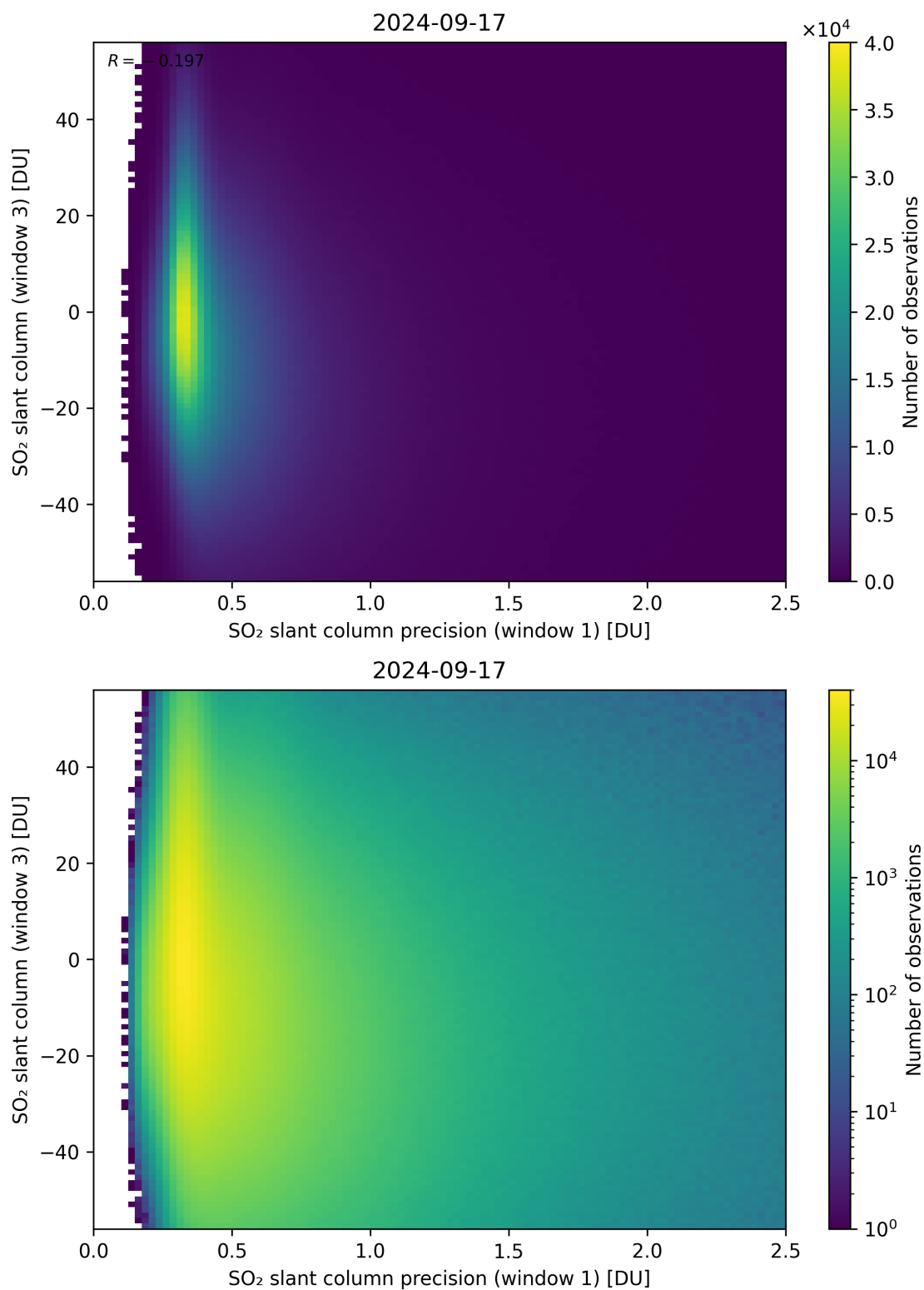
Figure 228: Scatter density plot of “SO 2 slant column precision (window 1)” against “SO 2 slant column (window 3)” for 2024-09-17 to 2024-09-18.
