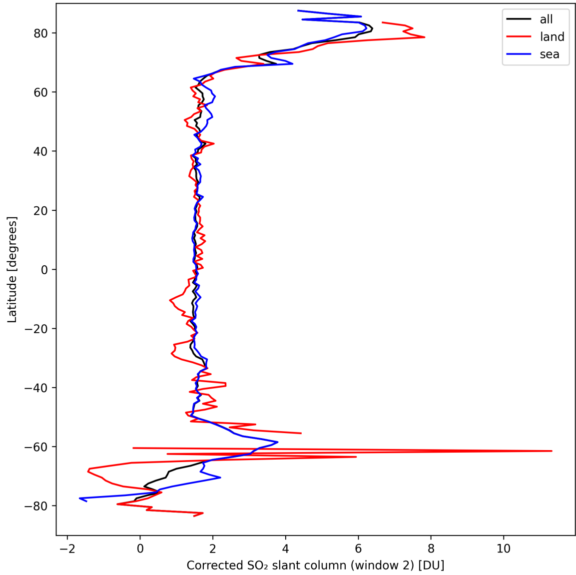
Figure 39: Zonal average of “Corrected SO 2 slant column (window 2)” for 2024-09-17 to 2024-09-18.
