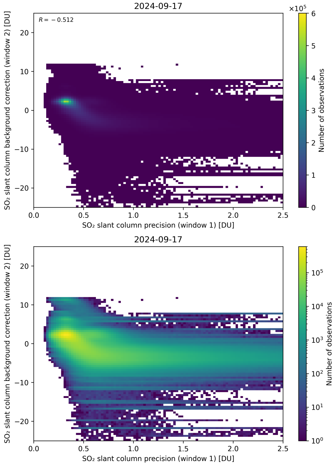
Figure 219: Scatter density plot of “SO 2 slant column precision (window 1)” against “SO 2 slant column background correction (window 2)” for 2024-09-17 to 2024-09-18.
