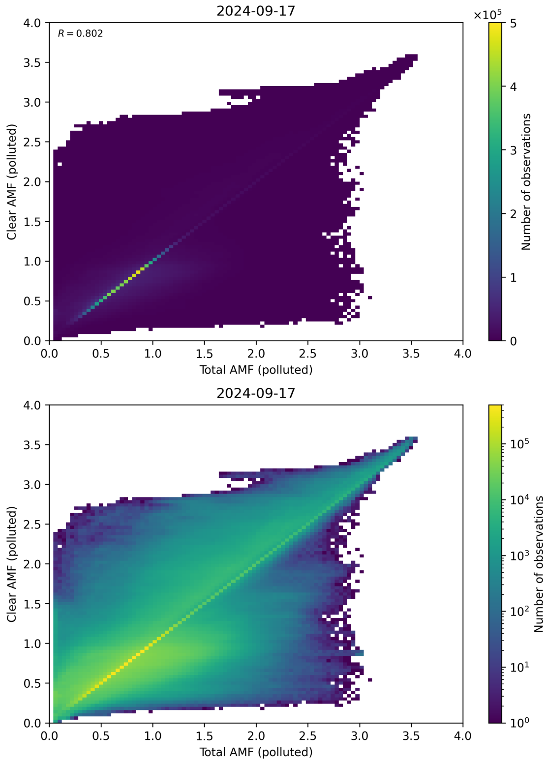
Figure 271: Scatter density plot of “Total AMF (polluted)” against “Clear AMF (polluted)” for 2024-09-17 to 2024-09-18.
