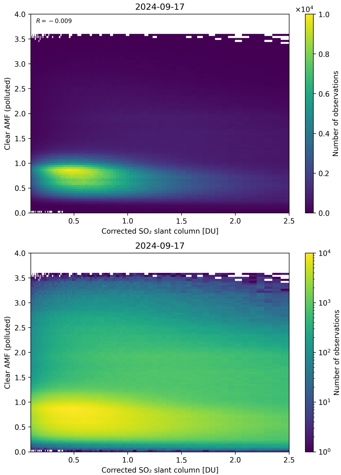
Figure 184: Scatter density plot of “Corrected SO 2 slant column” against “Clear AMF (polluted)” for 2024-09-17 to 2024-09-18.
