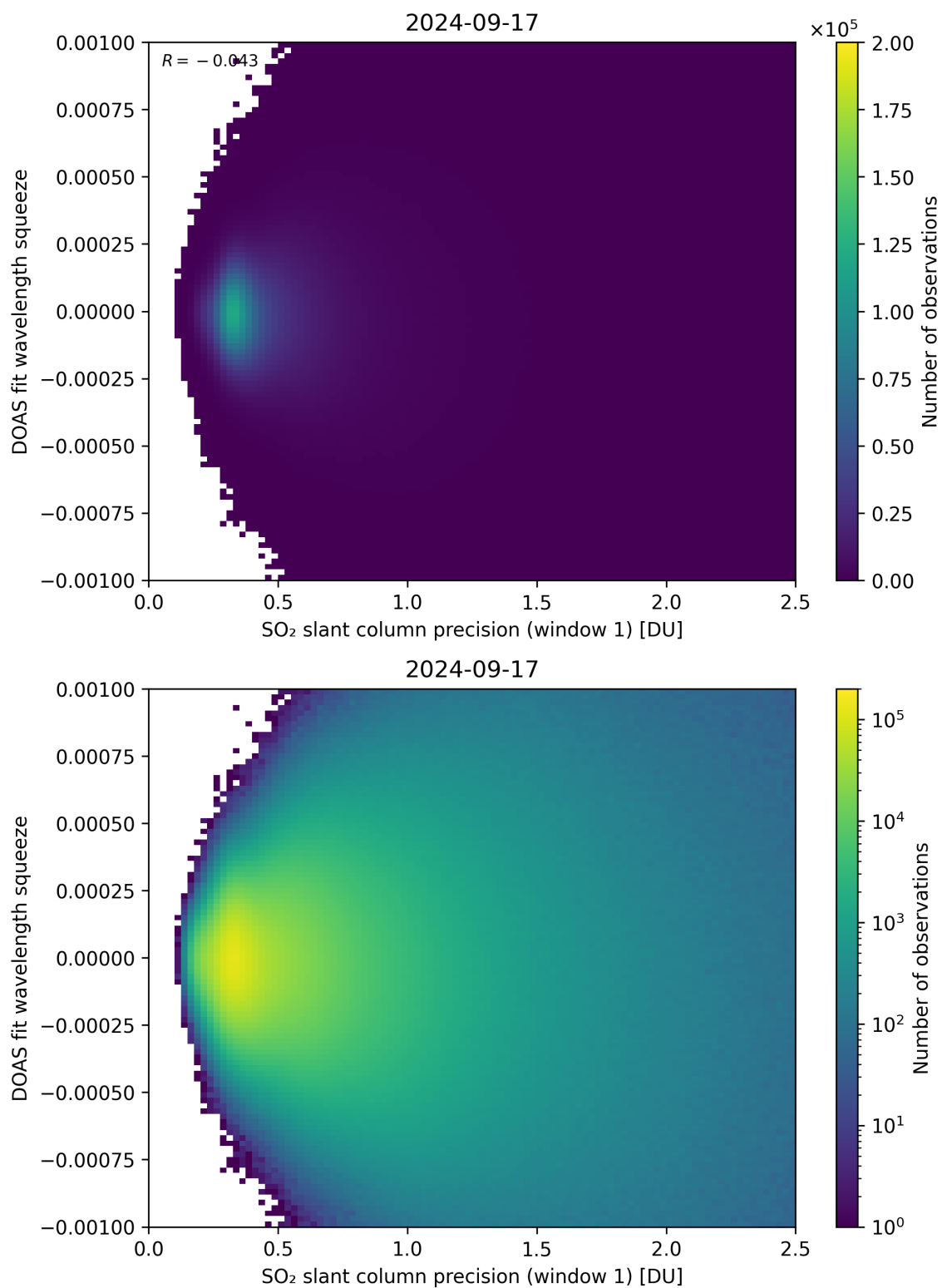
Figure 222: Scatter density plot of “SO 2 slant column precision (window 1)” against “DOAS fit wavelength squeeze” for 2024-09-17 to 2024-09-18.
