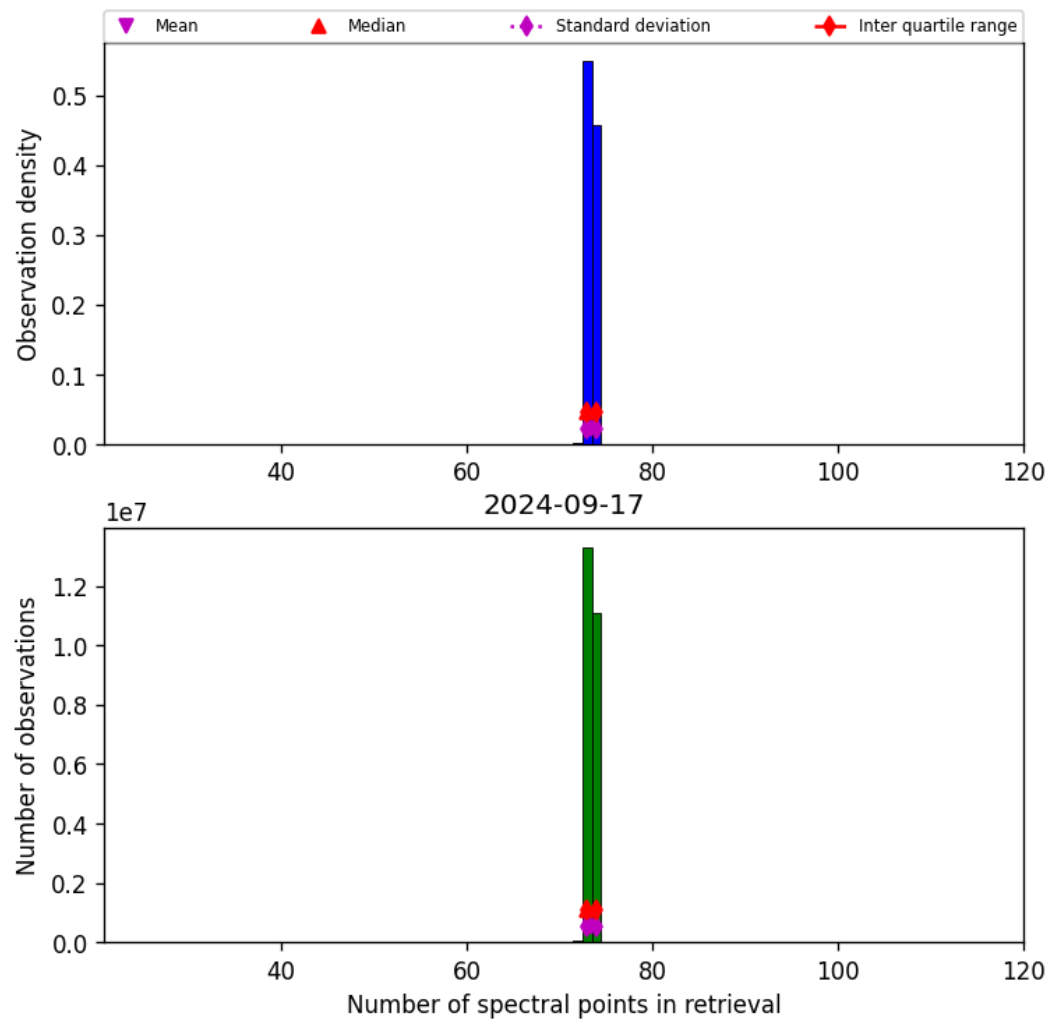
Figure 74: Histogram of “Number of spectral points in retrieval” for 2024-09-17 to 2024-09-18
