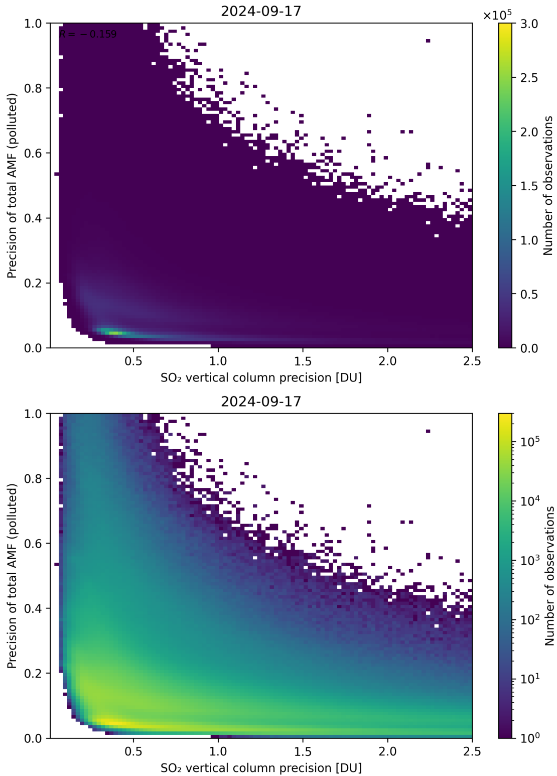
Figure 295: Scatter density plot of “SO 2 vertical column precision” against “Precision of total AMF (polluted)” for 2024-09-17 to 2024-09-18.
