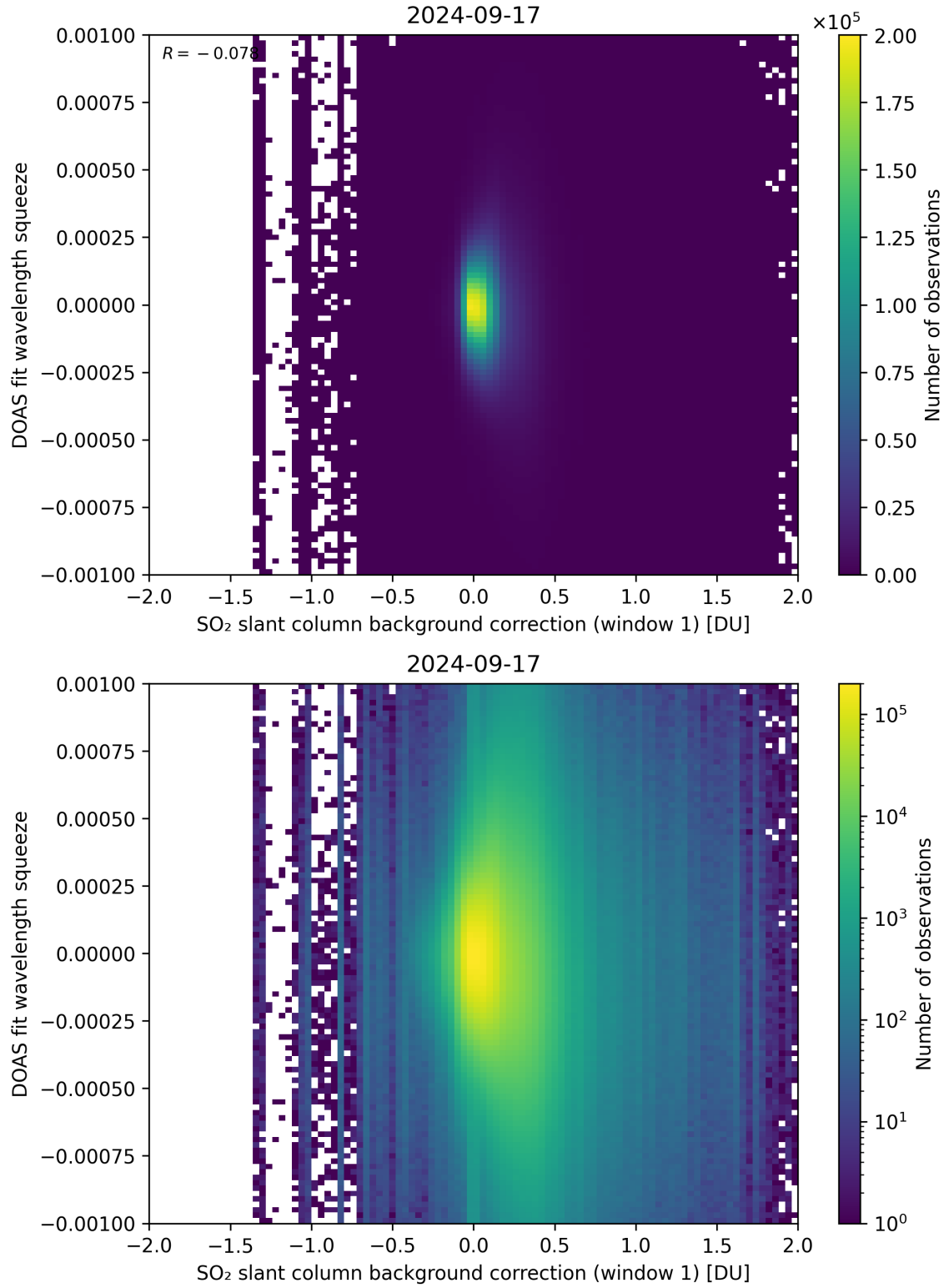
Figure 101: Scatter density plot of “SO 2 slant column background correction (window 1)” against “DOAS fit wavelength squeeze” for 2024-09-17 to 2024-09-18.
