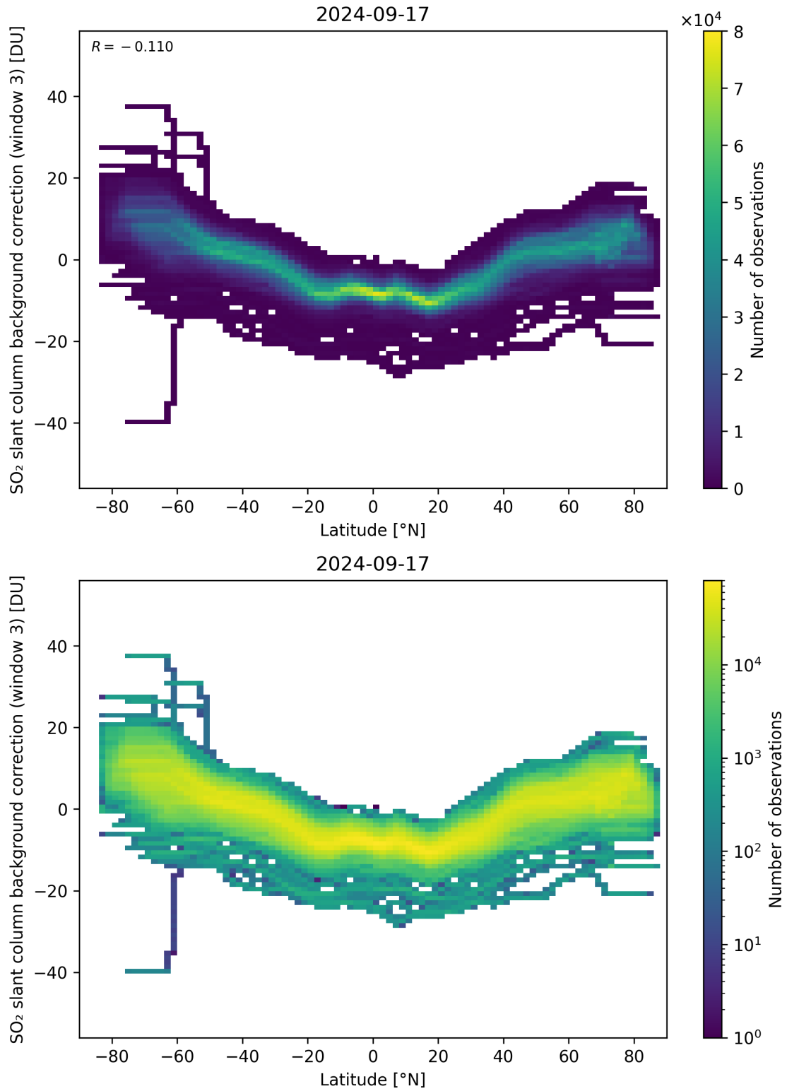
Figure 141: Scatter density plot of “Latitude” against “SO 2 slant column background correction (window 3)” for 2024-09-17 to 2024-09-18.
