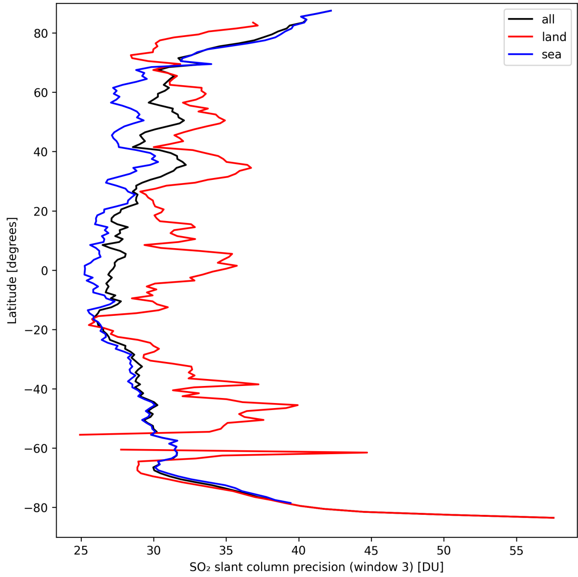
Figure 42: Zonal average of “SO 2 slant column precision (window 3)” for 2024-09-17 to 2024-09-18.
