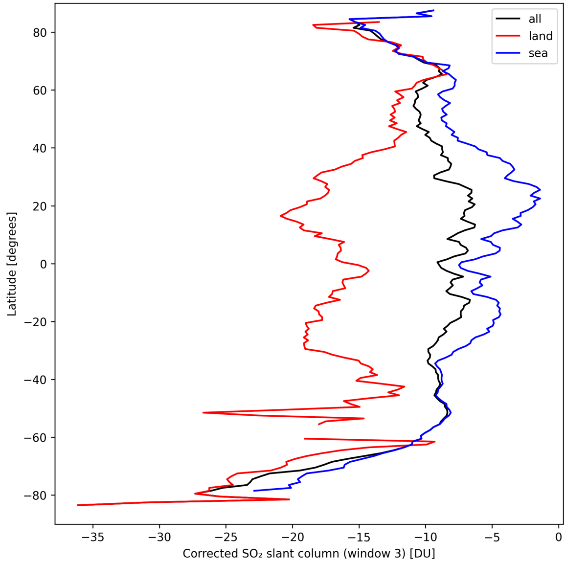
Figure 43: Zonal average of “Corrected SO 2 slant column (window 3)” for 2024-09-17 to 2024-09-18.
