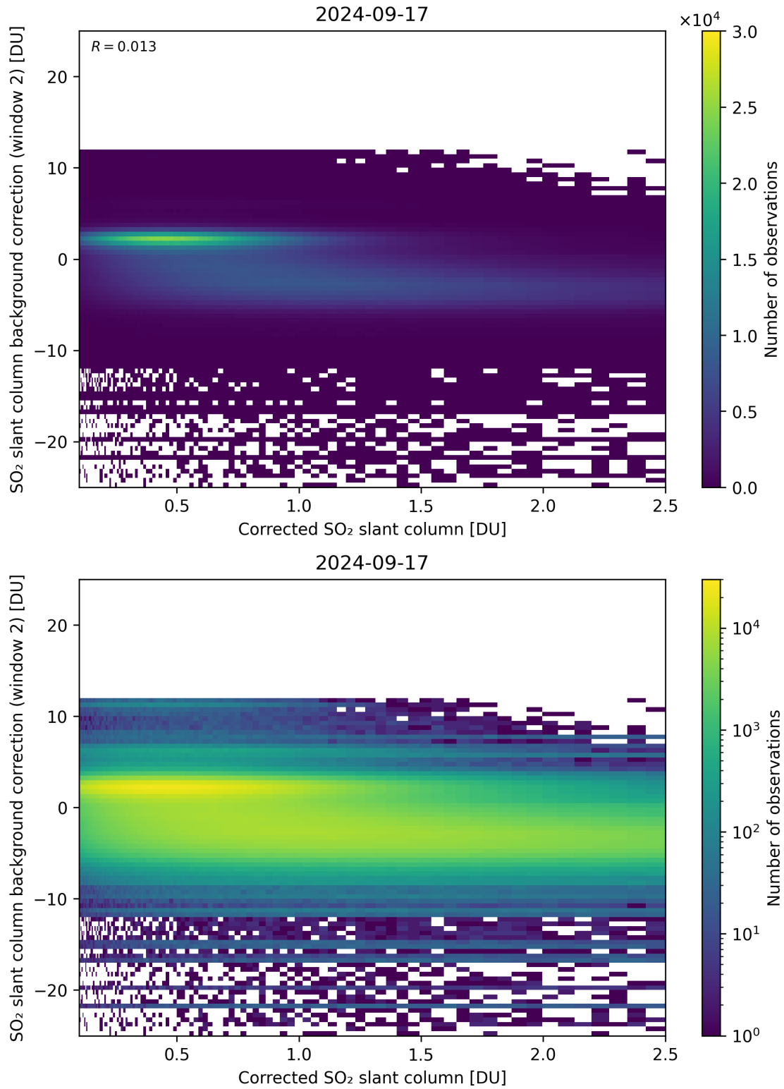
Figure 179: Scatter density plot of “Corrected SO 2 slant column” against “SO 2 slant column background correction (window 2)” for 2024-09-17 to 2024-09-18.
