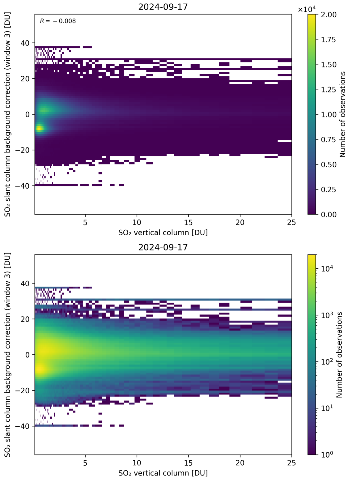
Figure 275: Scatter density plot of “SO 2 vertical column” against “SO 2 slant column background correction (window 3)” for 2024-09-17 to 2024-09-18.
