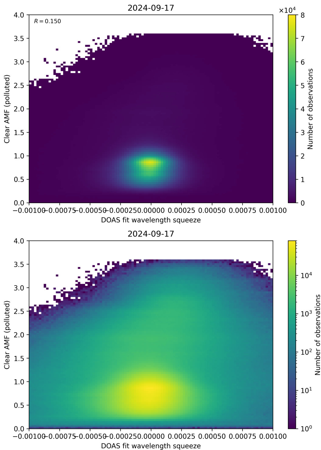
Figure 133: Scatter density plot of “DOAS fit wavelength squeeze” against “Clear AMF (polluted)” for 2024-09-17 to 2024-09-18.
