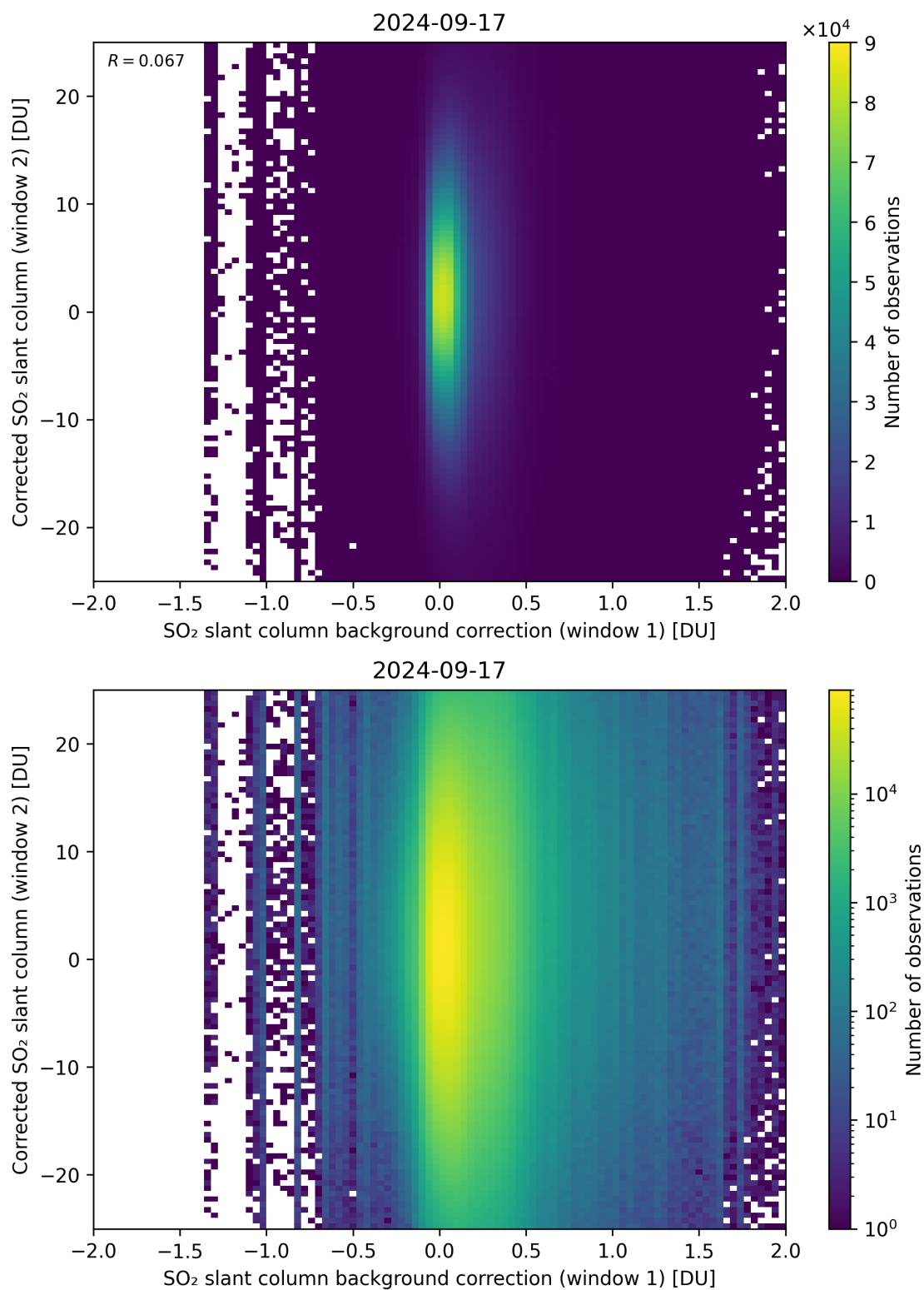
Figure 104: Scatter density plot of “SO 2 slant column background correction (window 1)” against “Corrected SO 2 slant column (window 2)” for 2024-09-17 to 2024-09-18.
