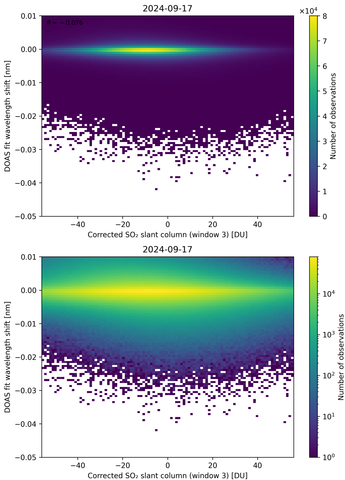
Figure 206: Scatter density plot of “Corrected SO 2 slant column (window 3)” against “DOAS fit wavelength shift” for 2024-09-17 to 2024-09-18.
