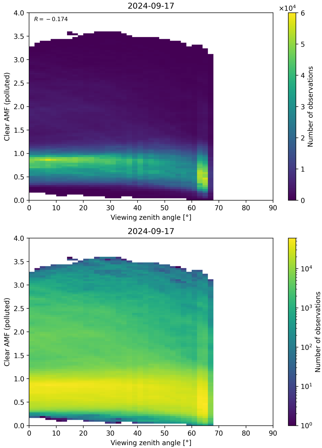
Figure 316: Scatter density plot of “Viewing zenith angle” against “Clear AMF (polluted)” for 2024-09-17 to 2024-09-18.
