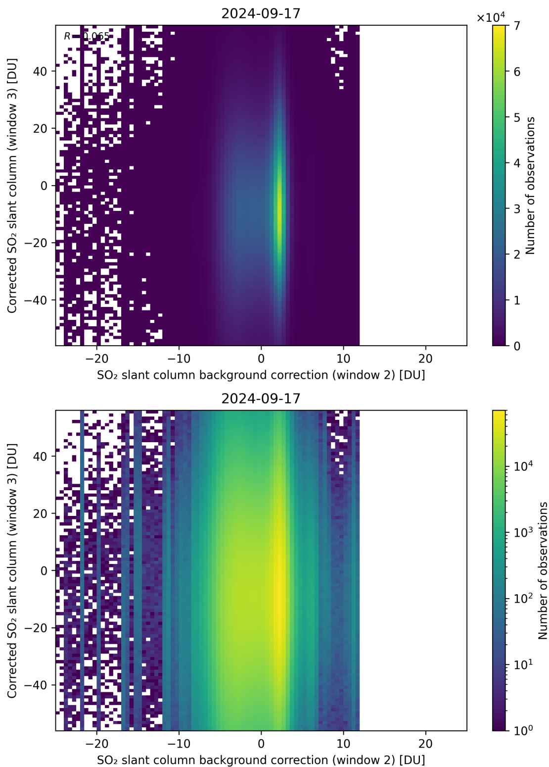
Figure 116: Scatter density plot of “SO 2 slant column background correction (window 2)” against “Corrected SO 2 slant column (window 3)” for 2024-09-17 to 2024-09-18.
