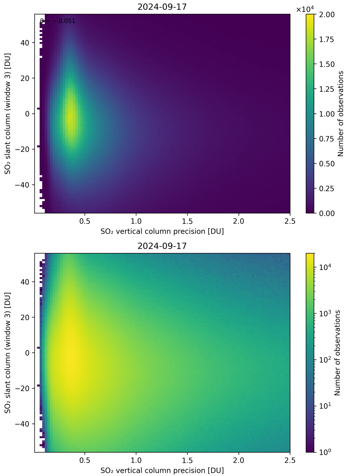
Figure 292: Scatter density plot of “SO 2 vertical column precision” against “SO 2 slant column (window 3)” for 2024-09-17 to 2024-09-18.
