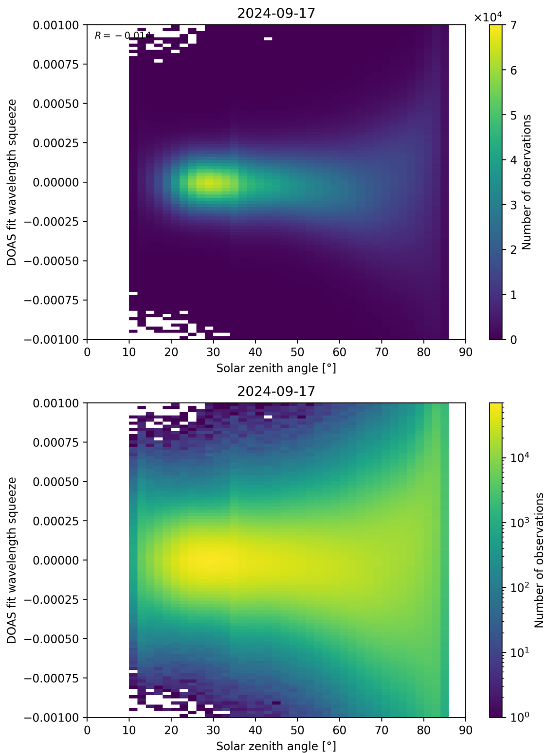
Figure 162: Scatter density plot of “Solar zenith angle” against “DOAS fit wavelength squeeze” for 2024-09-17 to 2024-09-18.
