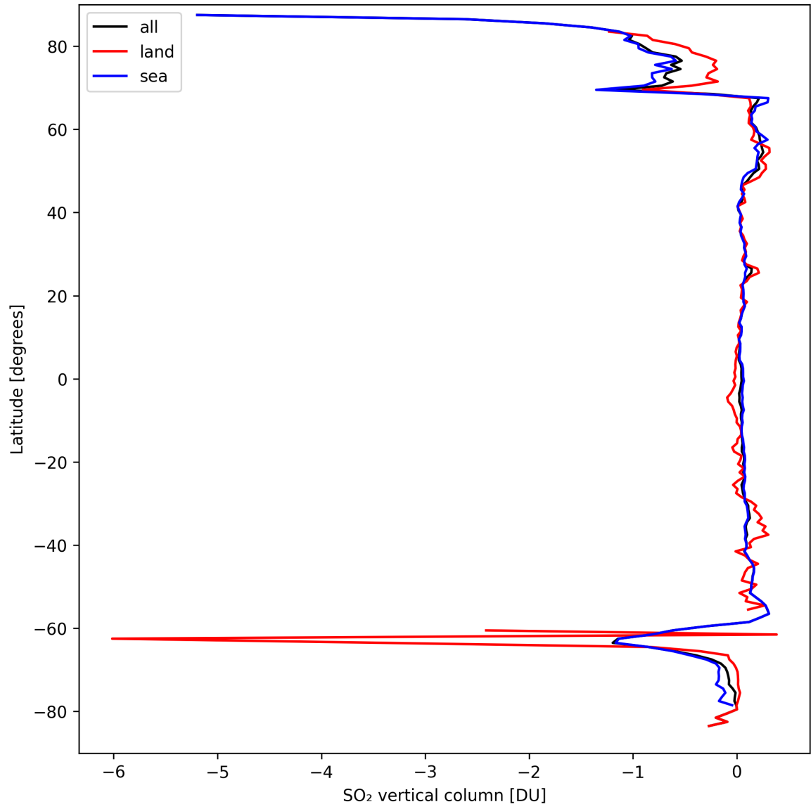
Figure 30: Zonal average of “SO 2 vertical column” for 2024-09-17 to 2024-09-18.
