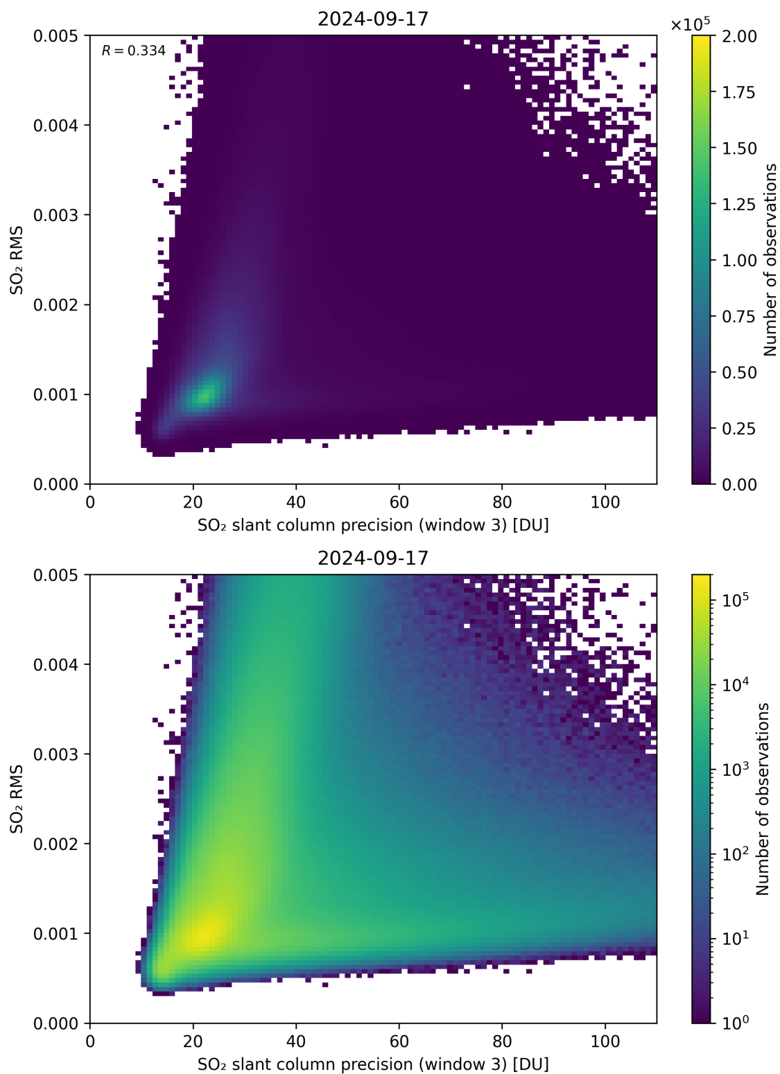
Figure 260: Scatter density plot of “SO 2 slant column precision (window 3)” against “SO 2 RMS” for 2024-09-17 to 2024-09-18.
