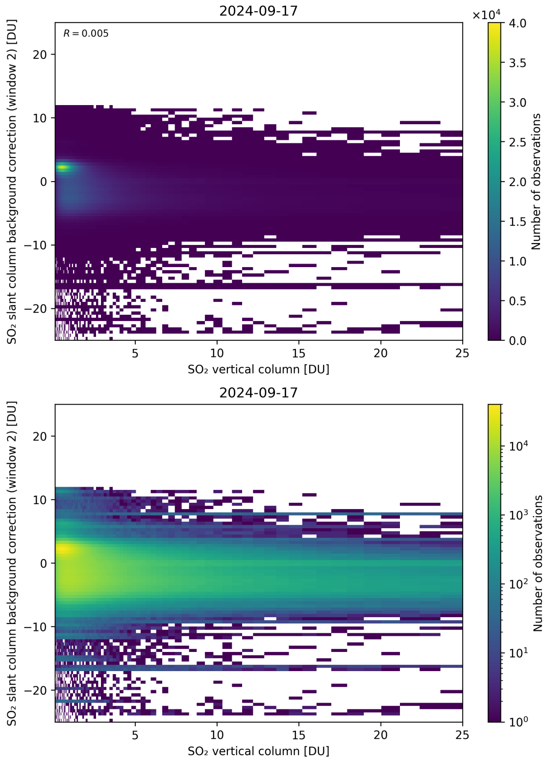
Figure 274: Scatter density plot of “SO 2 vertical column” against “SO 2 slant column background correction (window 2)” for 2024-09-17 to 2024-09-18.
