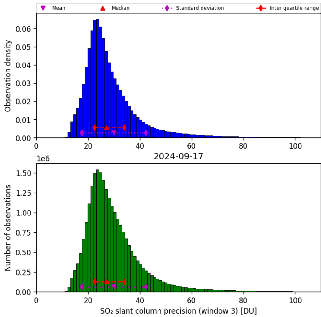
Figure 65: Histogram of “SO 2 slant column precision (window 3)” for 2024-09-17 to 2024-09-18
