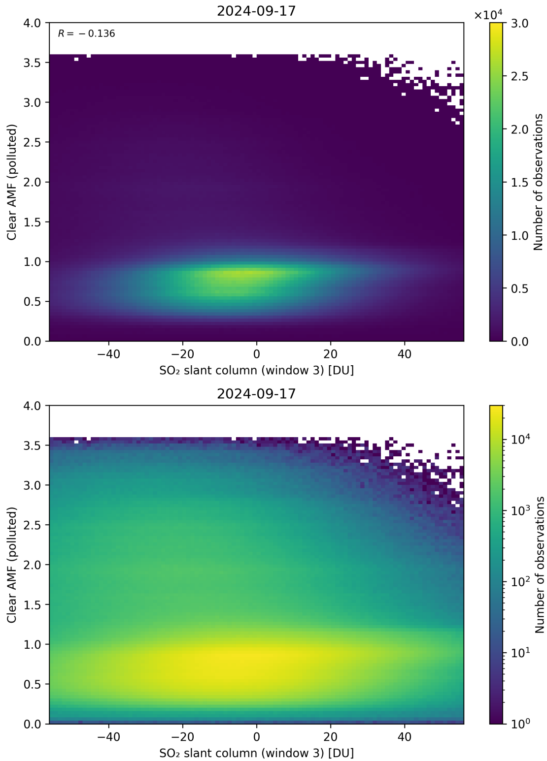
Figure 265: Scatter density plot of “SO 2 slant column (window 3)” against “Clear AMF (polluted)” for 2024-09-17 to 2024-09-18.
