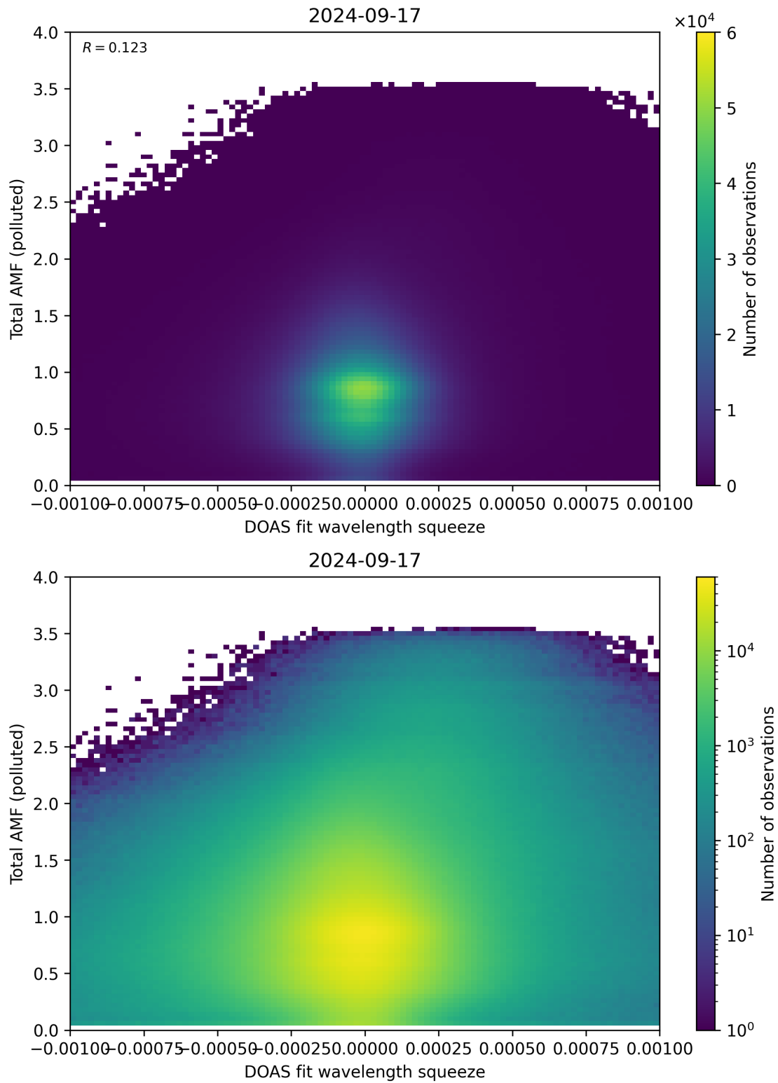
Figure 134: Scatter density plot of “DOAS fit wavelength squeeze” against “Total AMF (polluted)” for 2024-09-17 to 2024-09-18.
