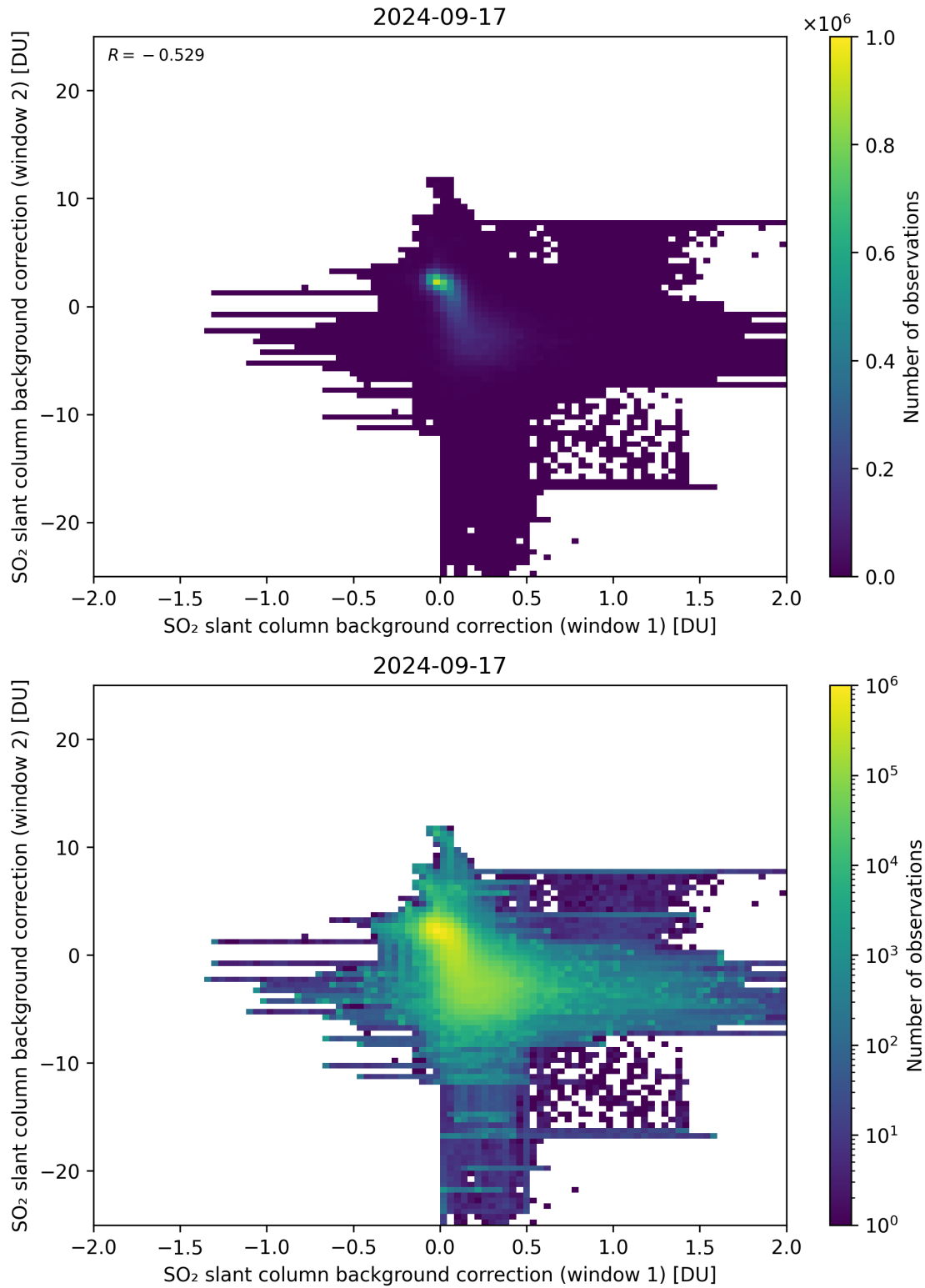
Figure 98: Scatter density plot of “SO 2 slant column background correction (window 1)” against “SO 2 slant column background correction (window 2)” for 2024-09-17 to 2024-09-18.
