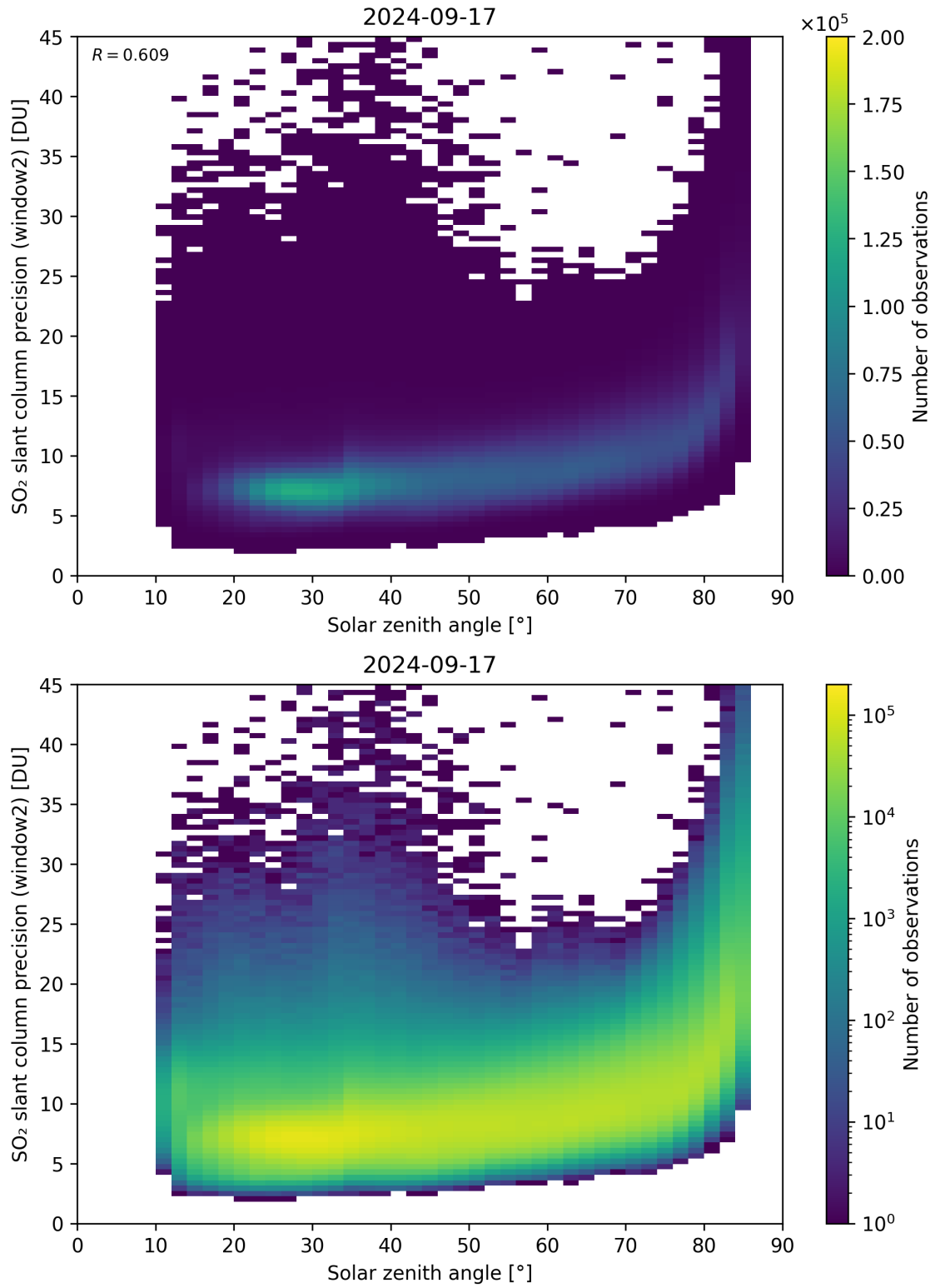
Figure 171: Scatter density plot of “Solar zenith angle” against “SO 2 slant column precision (window2)” for 2024-09-17 to 2024-09-18.
