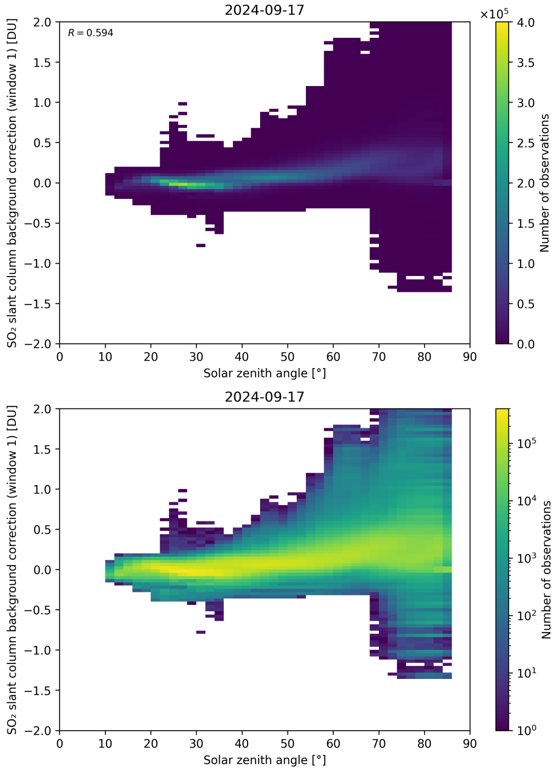
Figure 158: Scatter density plot of “Solar zenith angle” against “SO 2 slant column background correction (window 1)” for 2024-09-17 to 2024-09-18.
