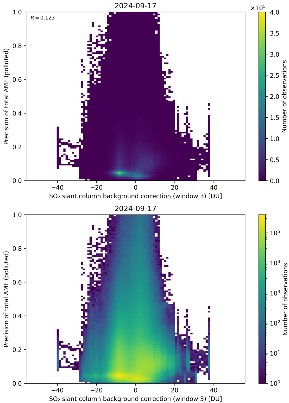
Figure 126: Scatter density plot of “SO 2 slant column background correction (window 3)” against “Precision of total AMF (polluted)” for 2024-09-17 to 2024-09-18.
