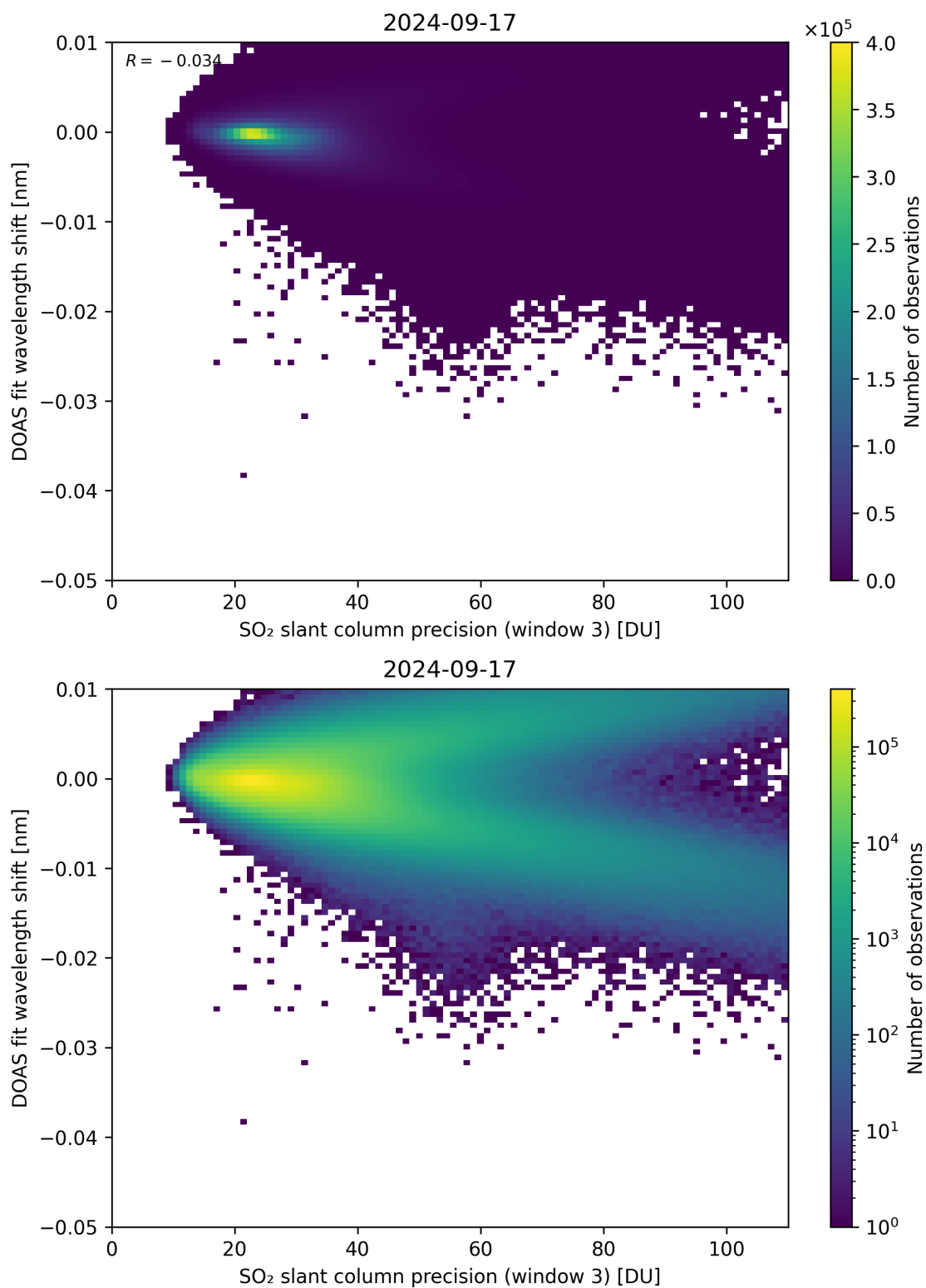
Figure 258: Scatter density plot of “SO 2 slant column precision (window 3)” against “DOAS fit wavelength shift” for 2024-09-17 to 2024-09-18.
