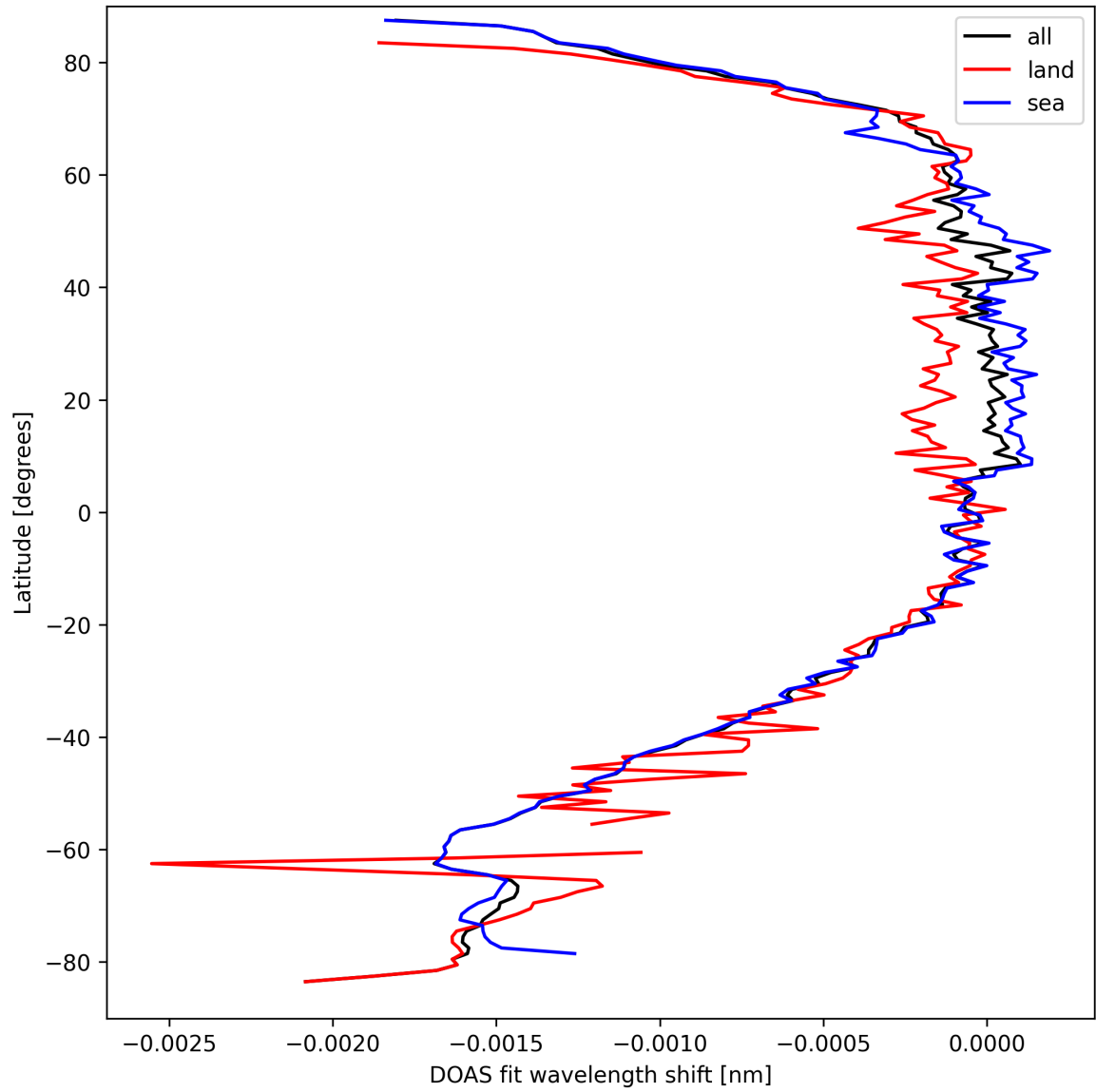
Figure 45: Zonal average of "DOAS fit wavelength shift" for 2024-09-17 to 2024-09-18.
