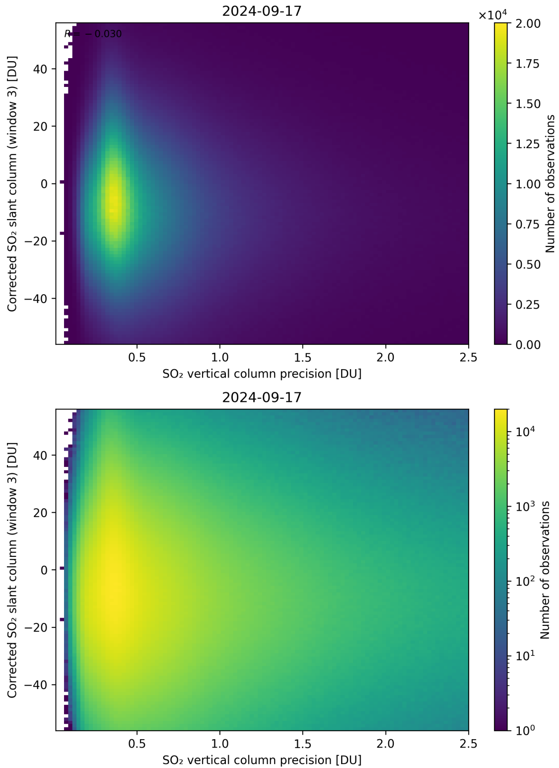
Figure 288: Scatter density plot of “SO 2 vertical column precision” against “Corrected SO 2 slant column (window 3)” for 2024-09-17 to 2024-09-18.
