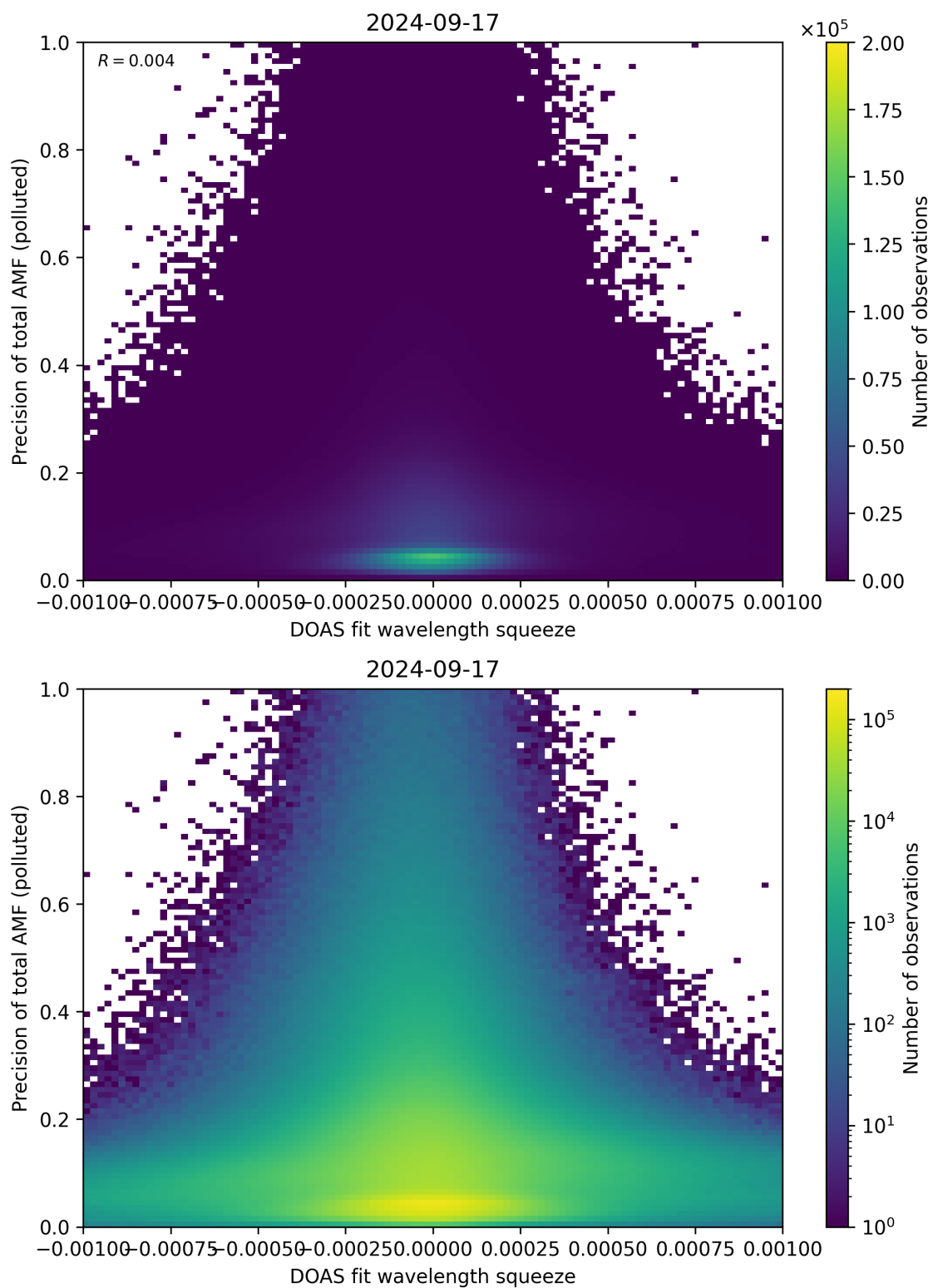
Figure 135: Scatter density plot of “DOAS fit wavelength squeeze” against “Precision of total AMF (polluted)” for 2024-09-17 to 2024-09-18.
