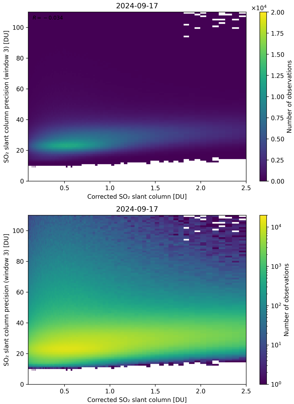
Figure 191: Scatter density plot of “Corrected SO 2 slant column” against “SO 2 slant column precision (window 3)” for 2024-09-17 to 2024-09-18.
