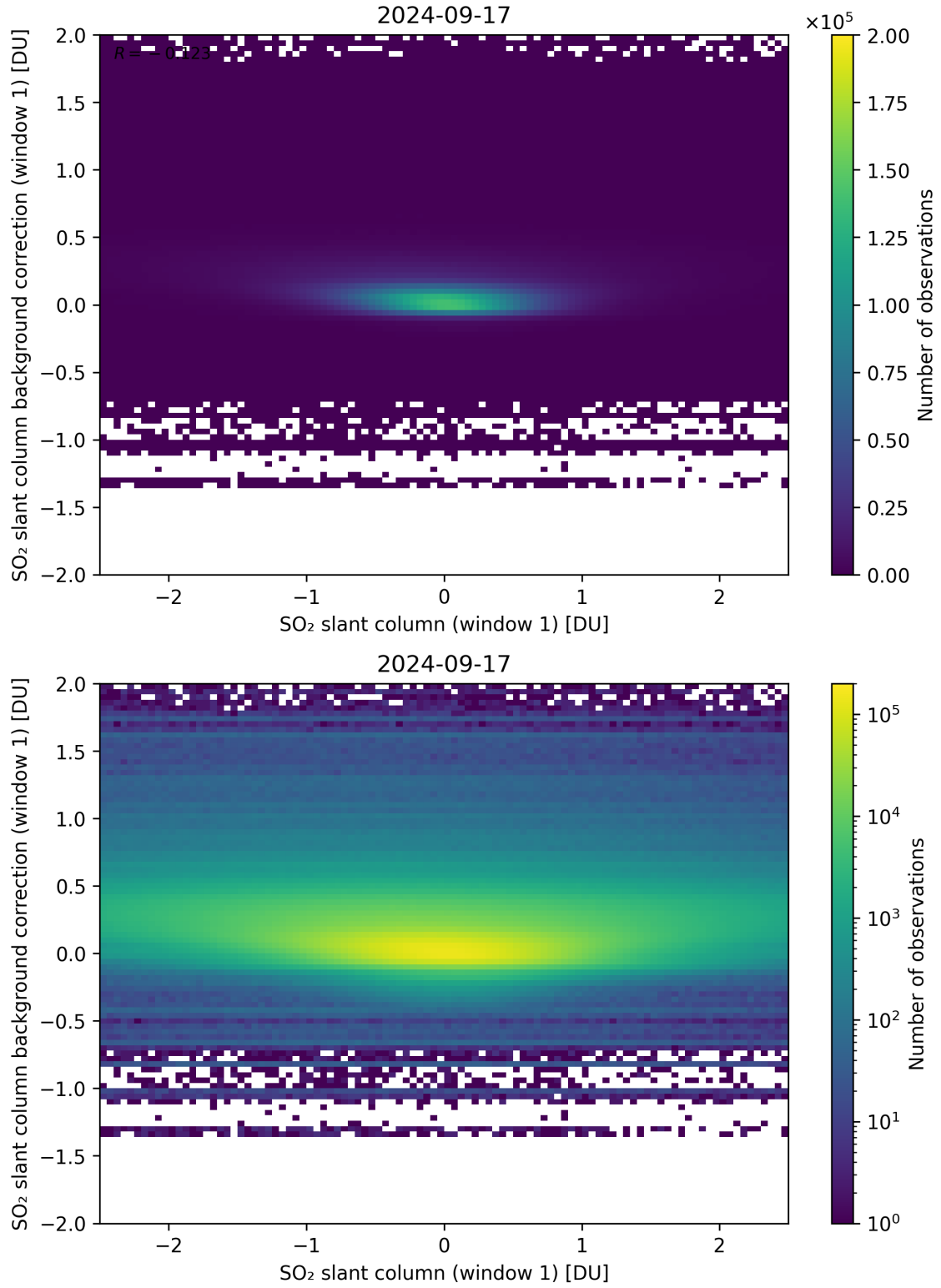
Figure 212: Scatter density plot of “SO 2 slant column (window 1)” against “SO 2 slant column background correction (window 1)” for 2024-09-17 to 2024-09-18.
