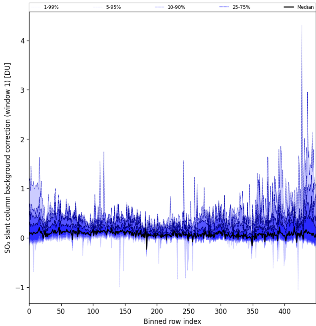
Figure 82: Along track statistics of “SO 2 slant column background correction (window 1)” for 2024-09-17 to 2024-09-18
