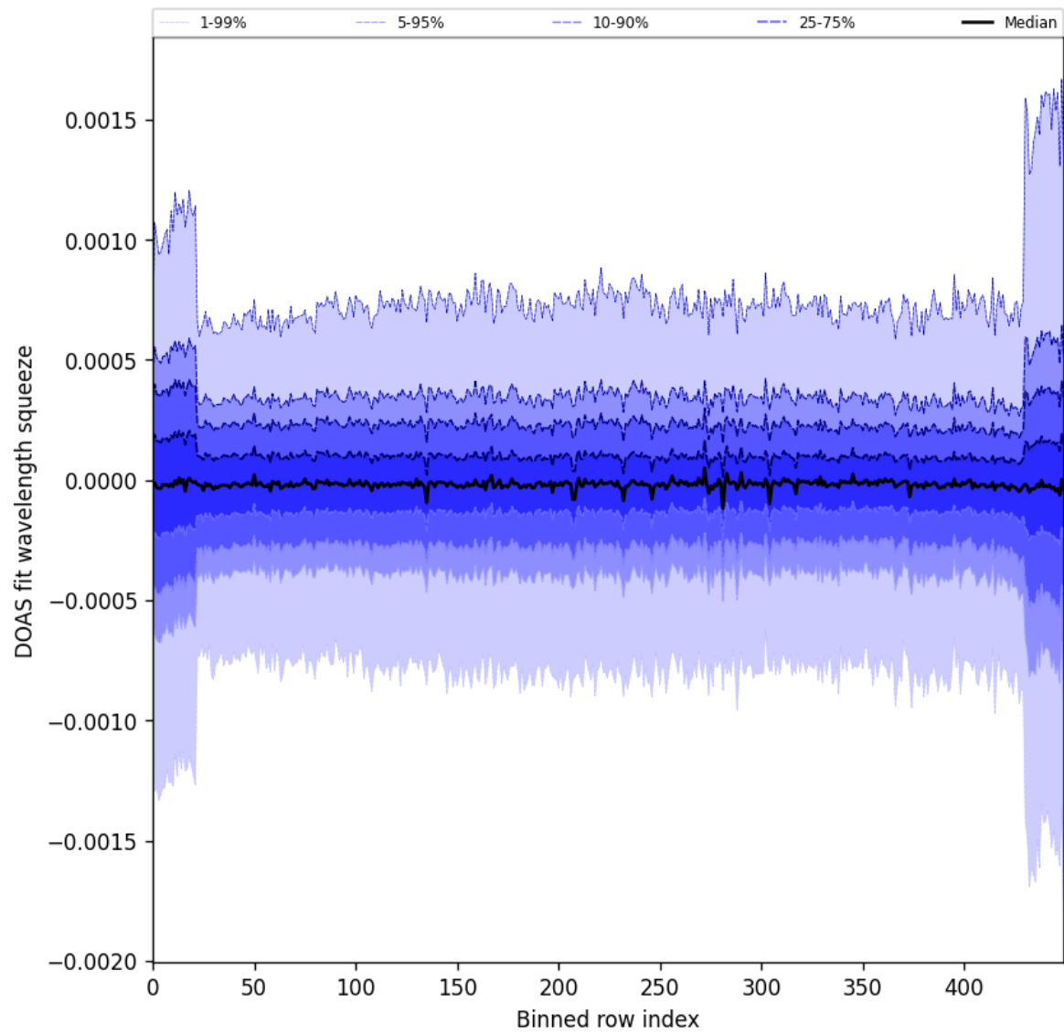
Figure 92: Along track statistics of “DOAS fit wavelength squeeze” for 2024-09-17 to 2024-09-18
