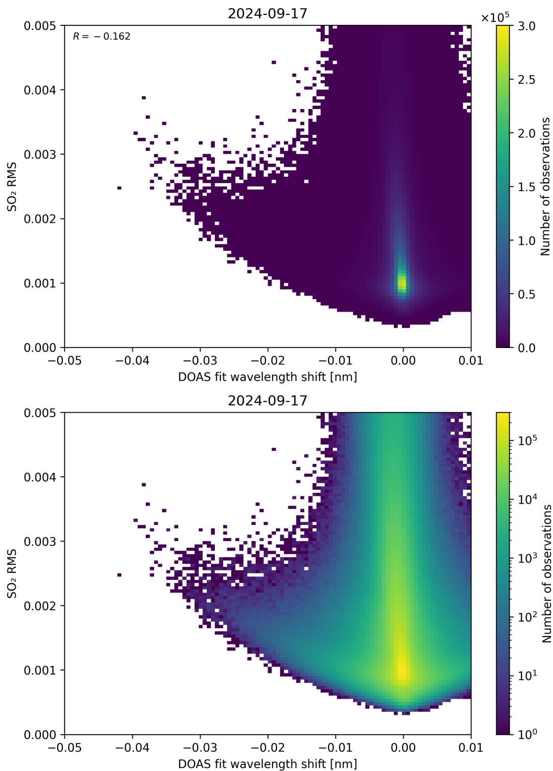
Figure 128: Scatter density plot of “DOAS fit wavelength shift” against “SO 2 RMS” for 2024-09-17 to 2024-09-18.
