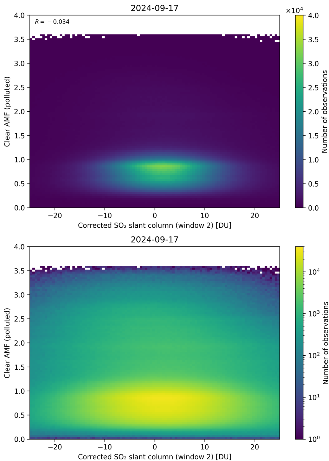
Figure 199: Scatter density plot of “Corrected SO 2 slant column (window 2)” against “Clear AMF (polluted)” for 2024-09-17 to 2024-09-18.
