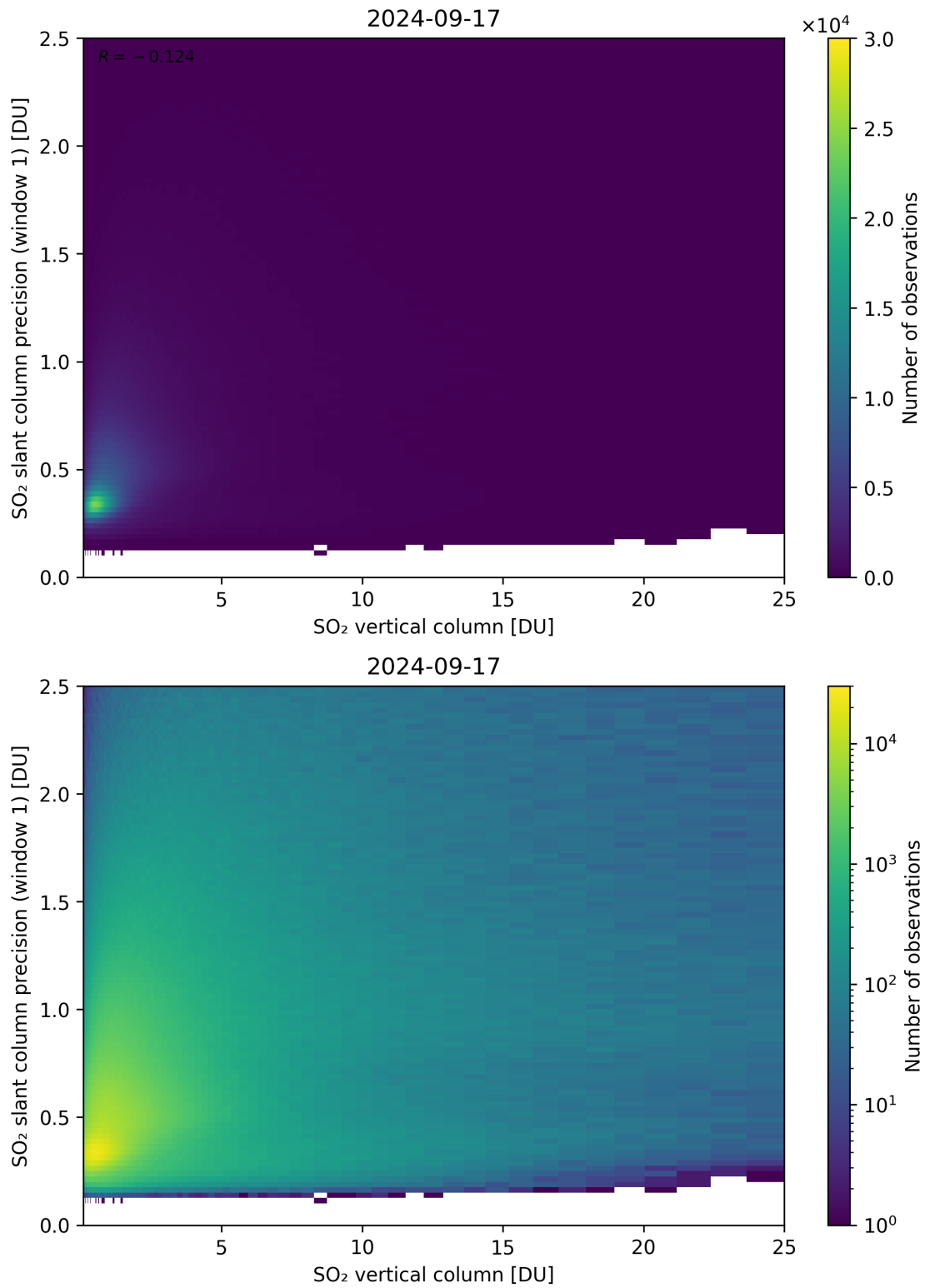
Figure 301: Scatter density plot of “SO 2 vertical column” against “SO 2 slant column precision (window 1)” for 2024-09-17 to 2024-09-18.
