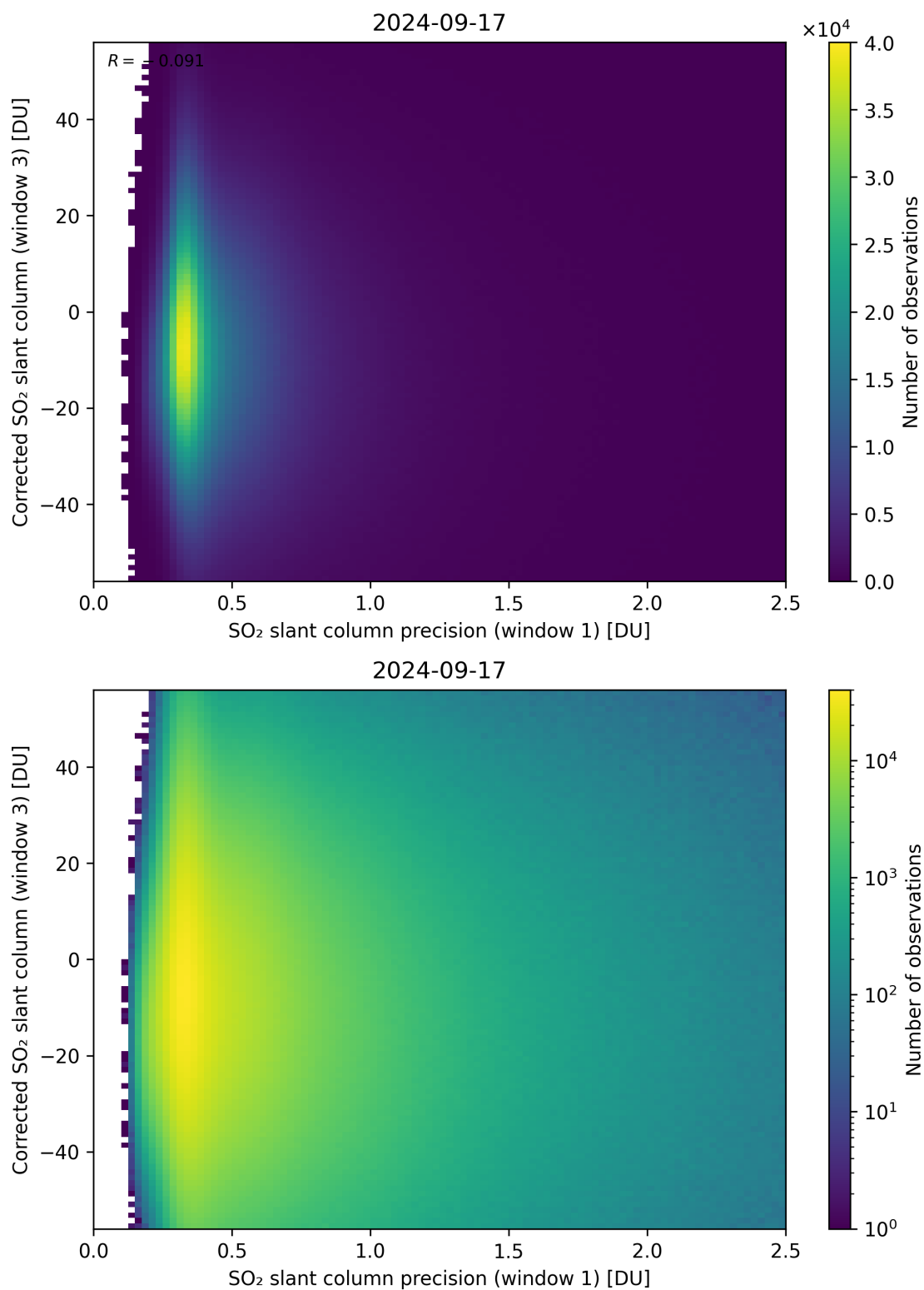
Figure 226: Scatter density plot of “SO 2 slant column precision (window 1)” against “Corrected SO 2 slant column (window 3)” for 2024-09-17 to 2024-09-18.
