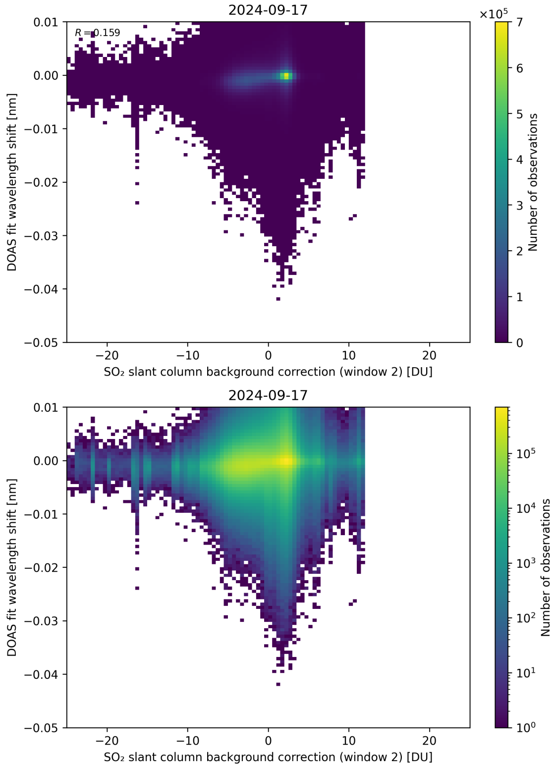
Figure 112: Scatter density plot of “SO 2 slant column background correction (window 2)” against “DOAS fit wavelength shift” for 2024-09-17 to 2024-09-18.
