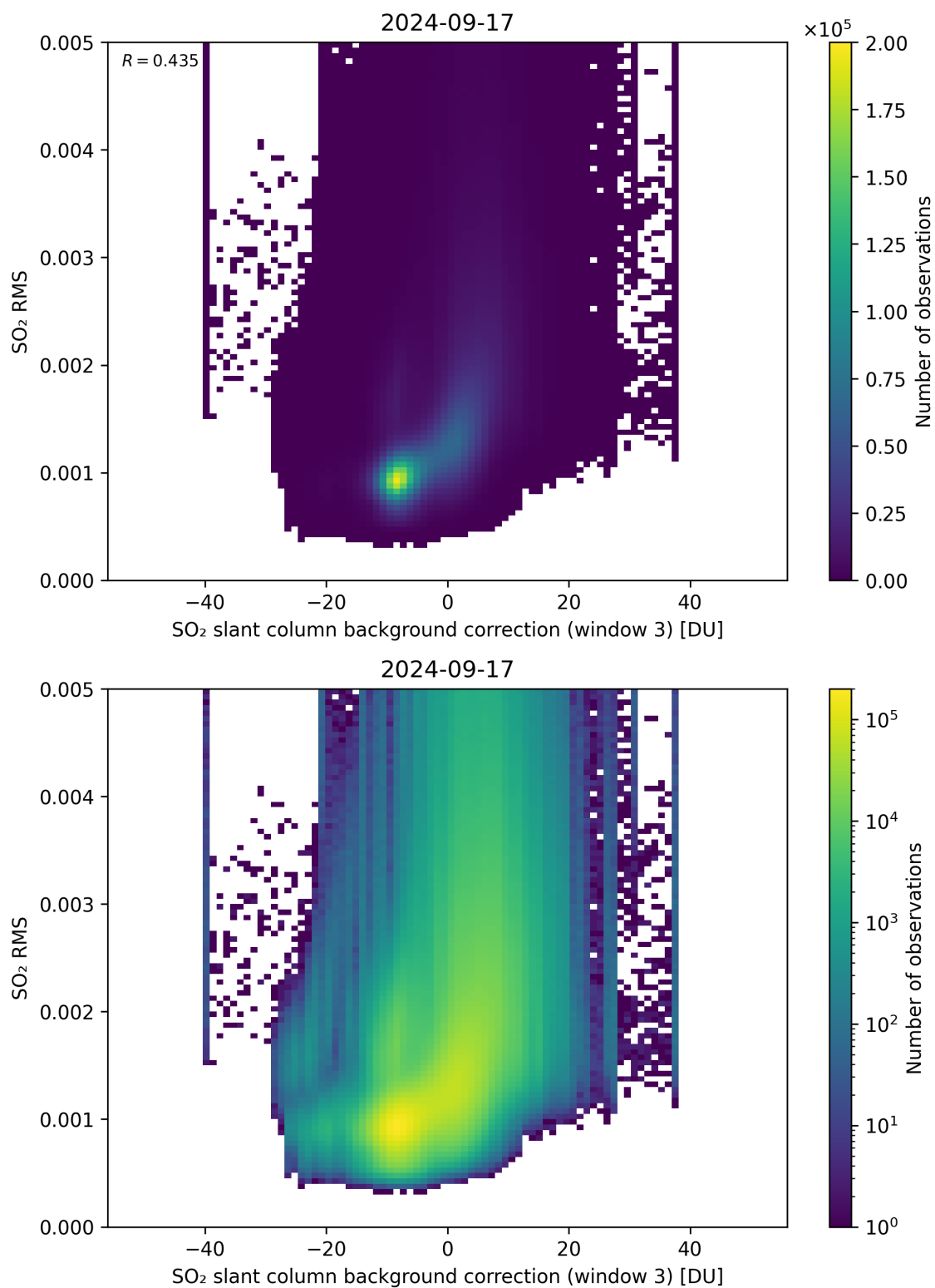
Figure 123: Scatter density plot of “SO 2 slant column background correction (window 3)” against “SO 2 RMS” for 2024-09-17 to 2024-09-18.
