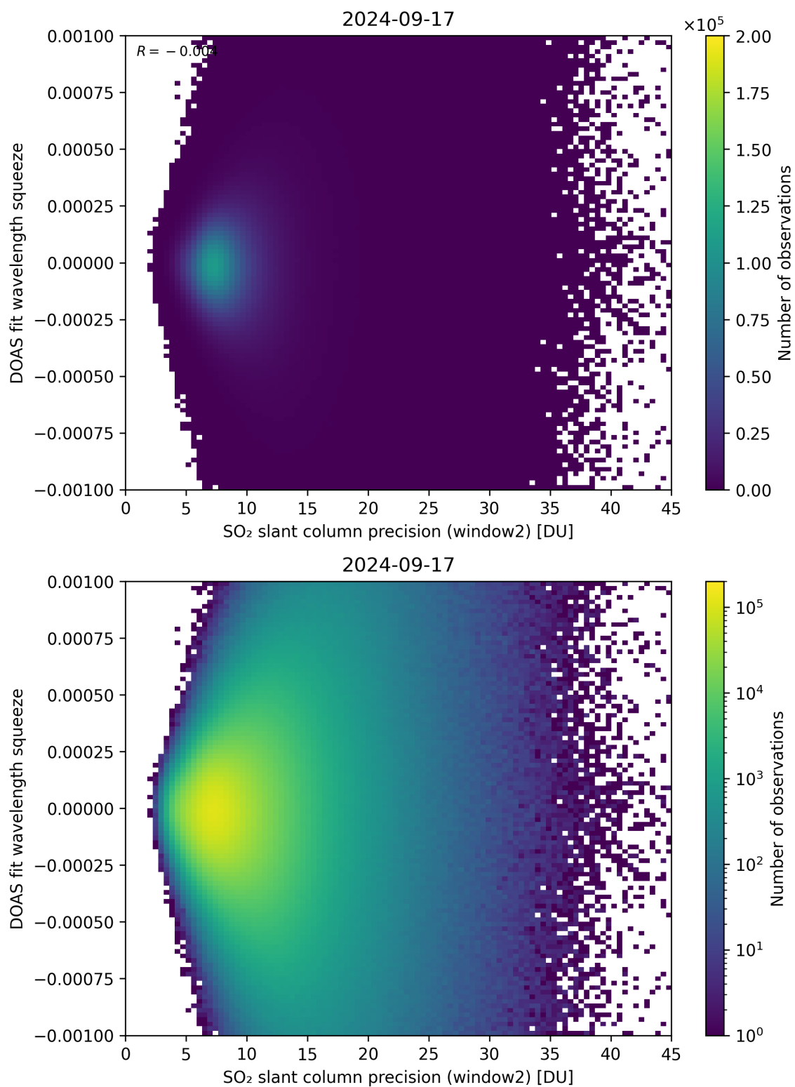
Figure 244: Scatter density plot of “SO 2 slant column precision (window2)” against “DOAS fit wavelength squeeze” for 2024-09-17 to 2024-09-18.
