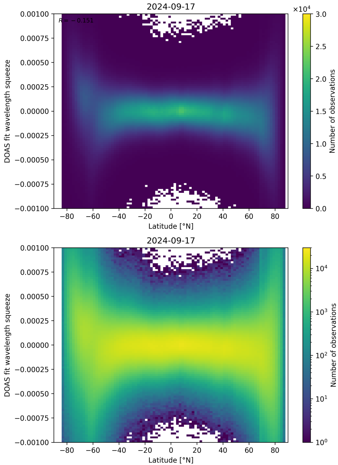
Figure 143: Scatter density plot of “Latitude” against “DOAS fit wavelength squeeze” for 2024-09-17 to 2024-09-18.
