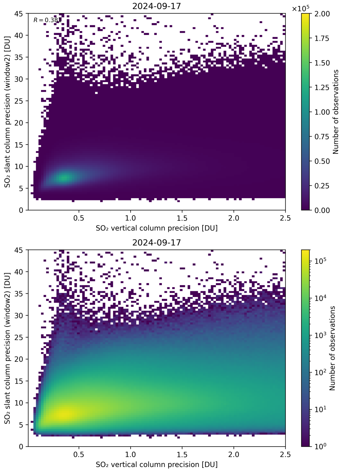
Figure 291: Scatter density plot of “SO 2 vertical column precision” against “SO 2 slant column precision (window2)” for 2024-09-17 to 2024-09-18.
