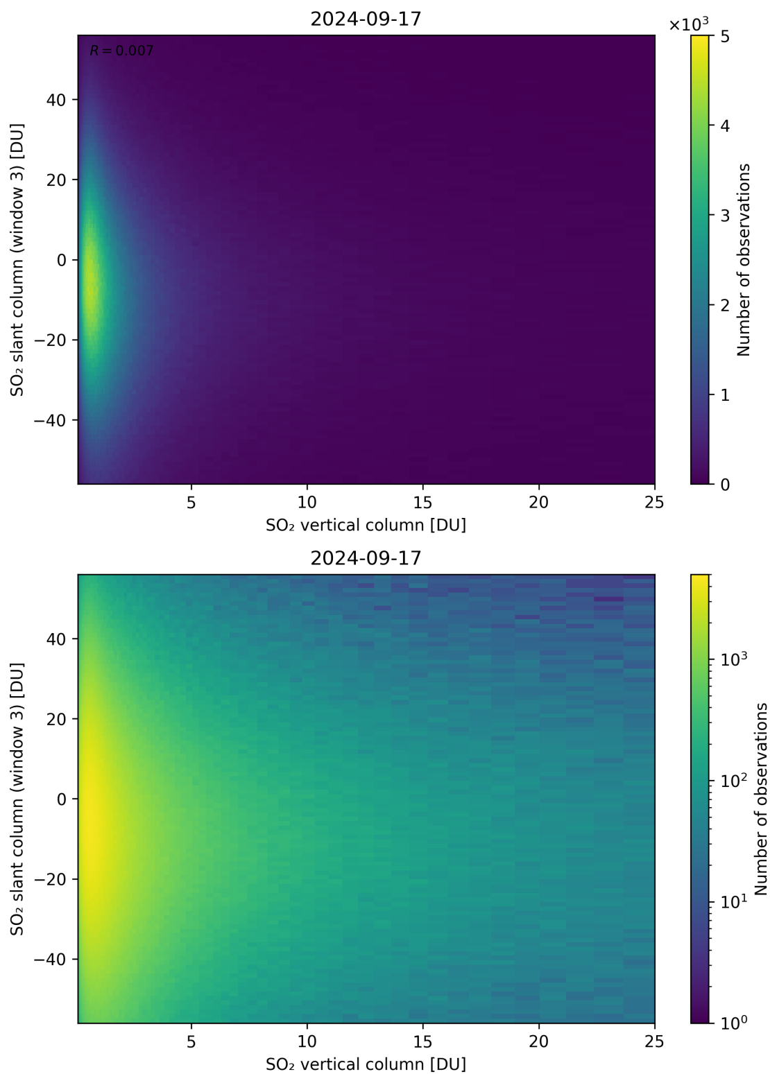
Figure 303: Scatter density plot of “SO 2 vertical column” against “SO 2 slant column (window 3)” for 2024-09-17 to 2024-09-18.
