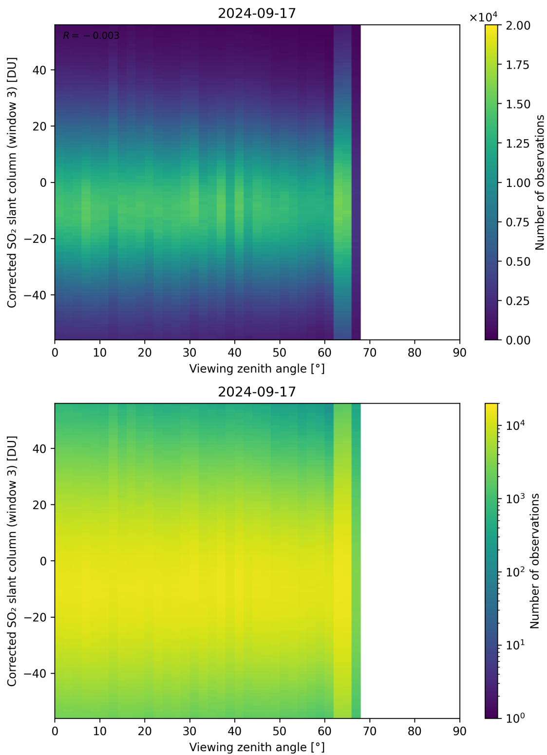
Figure 319: Scatter density plot of “Viewing zenith angle” against “Corrected SO 2 slant column (window 3)” for 2024-09-17 to 2024-09-18.
