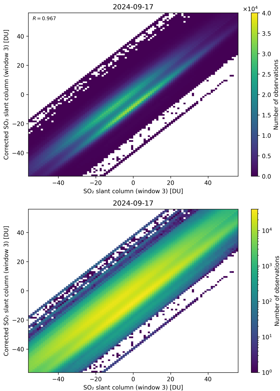
Figure 266: Scatter density plot of “SO 2 slant column (window 3)” against “Corrected SO 2 slant column (window 3)” for 2024-09-17 to 2024-09-18.
