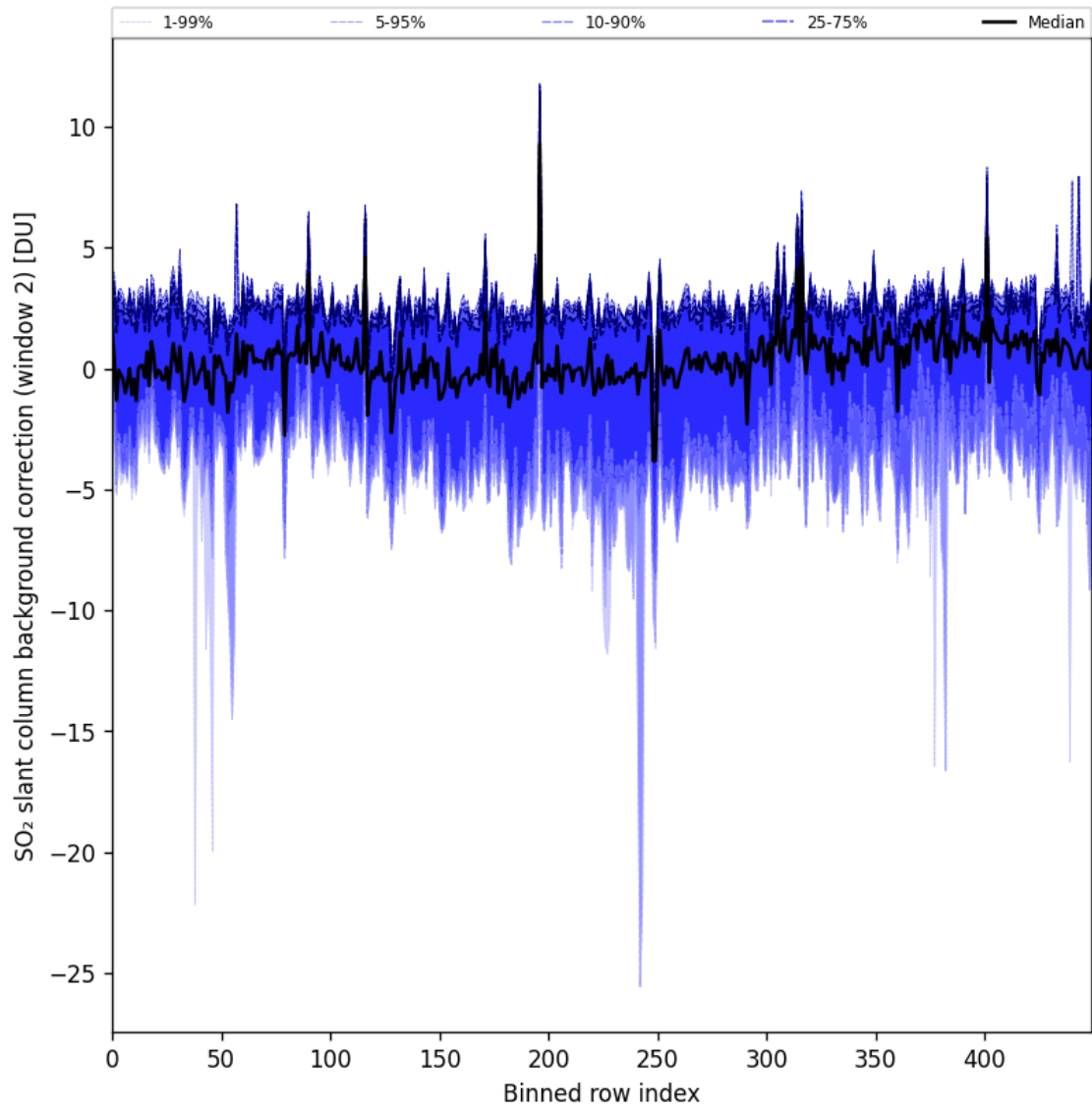
Figure 86: Along track statistics of “SO 2 slant column background correction (window 2)” for 2024-09-17 to 2024-09-18
