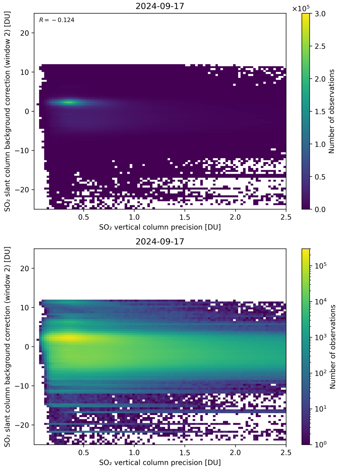
Figure 280: Scatter density plot of “SO 2 vertical column precision” against “SO 2 slant column background correction (window 2)” for 2024-09-17 to 2024-09-18.
