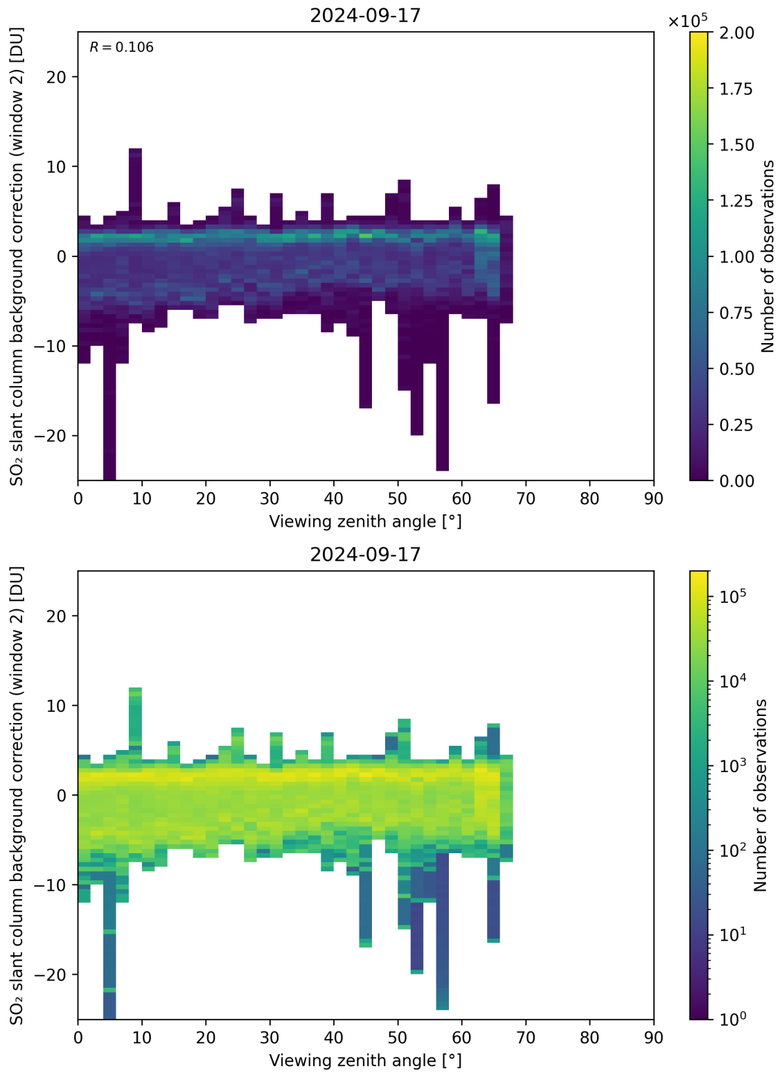
Figure 309: Scatter density plot of “Viewing zenith angle” against “SO 2 slant column background correction (window 2)” for 2024-09-17 to 2024-09-18.
