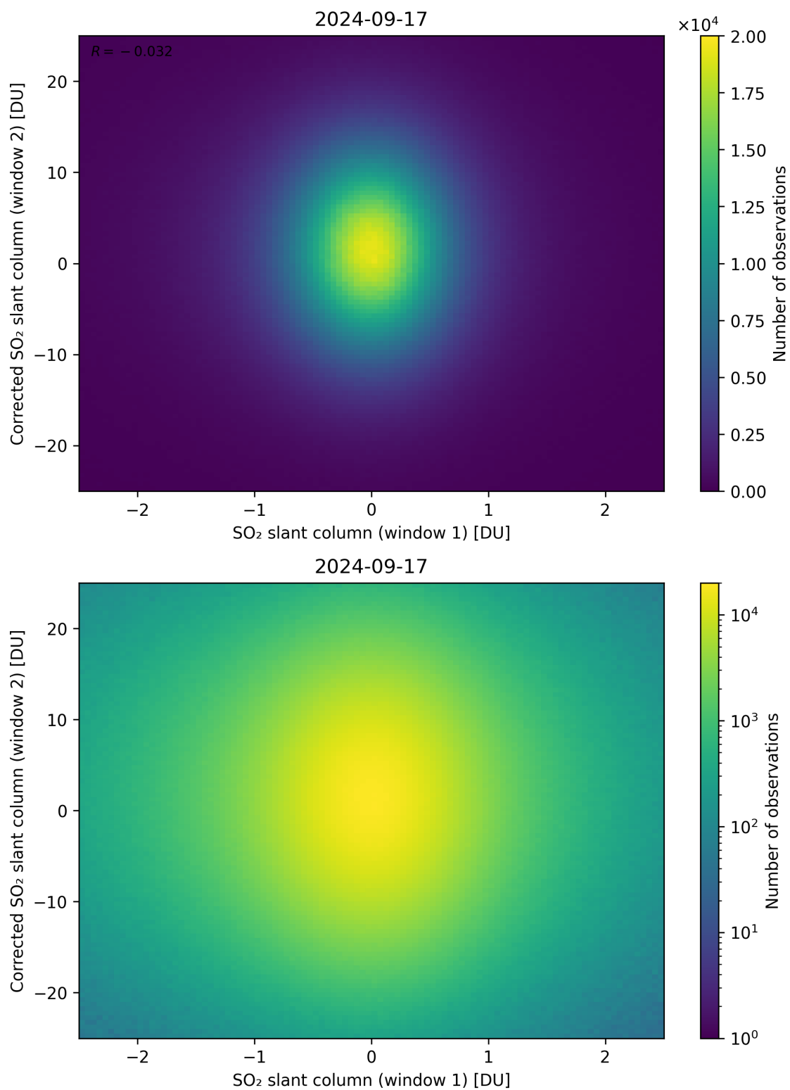
Figure 233: Scatter density plot of “SO 2 slant column (window 1)” against “Corrected SO 2 slant column (window 2)” for 2024-09-17 to 2024-09-18.
