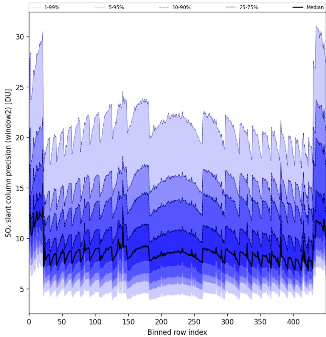
Figure 84: Along track statistics of “SO 2 slant column precision (window2)” for 2024-09-17 to 2024-09-18
