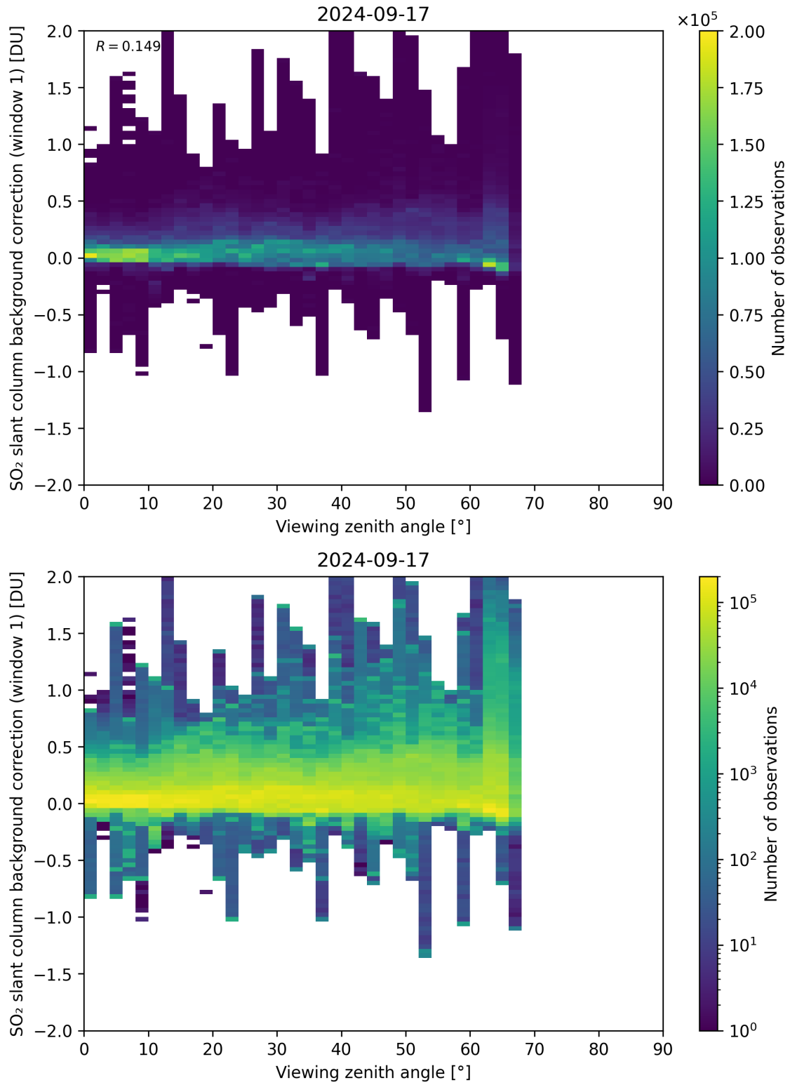
Figure 308: Scatter density plot of “Viewing zenith angle” against “SO 2 slant column background correction (window 1)” for 2024-09-17 to 2024-09-18.
