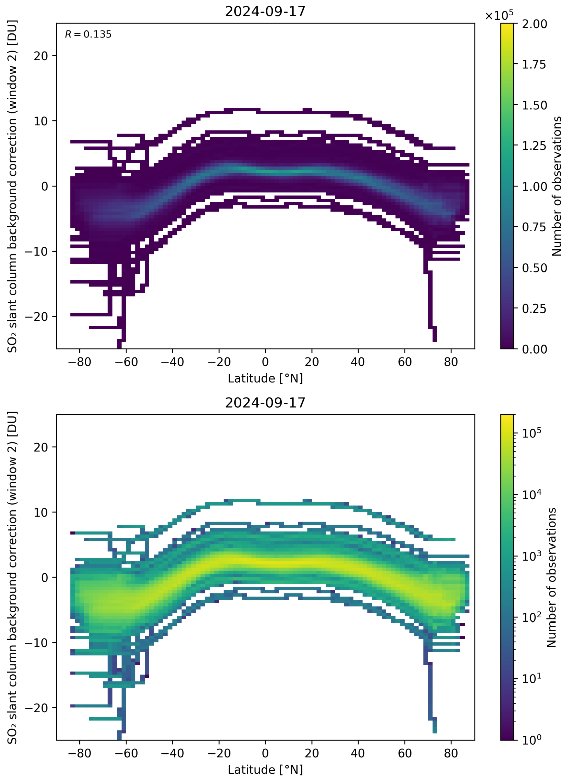
Figure 140: Scatter density plot of “Latitude” against “SO 2 slant column background correction (window 2)” for 2024-09-17 to 2024-09-18.
