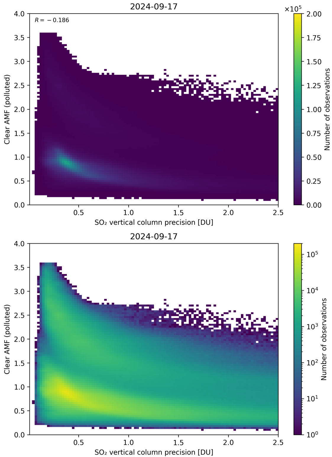
Figure 285: Scatter density plot of “SO 2 vertical column precision” against “Clear AMF (polluted)” for 2024-09-17 to 2024-09-18.
