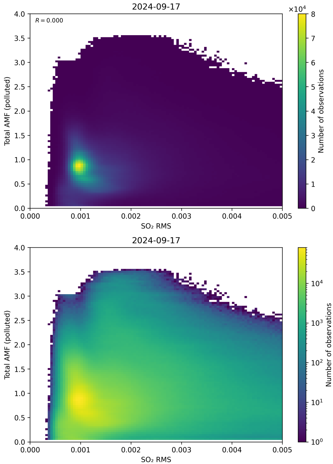
Figure 137: Scatter density plot of “SO 2 RMS” against “Total AMF (polluted)” for 2024-09-17 to 2024-09-18.
