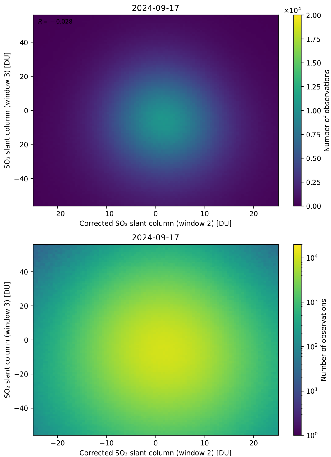
Figure 201: Scatter density plot of “Corrected SO 2 slant column (window 2)” against “SO 2 slant column (window 3)” for 2024-09-17 to 2024-09-18.
