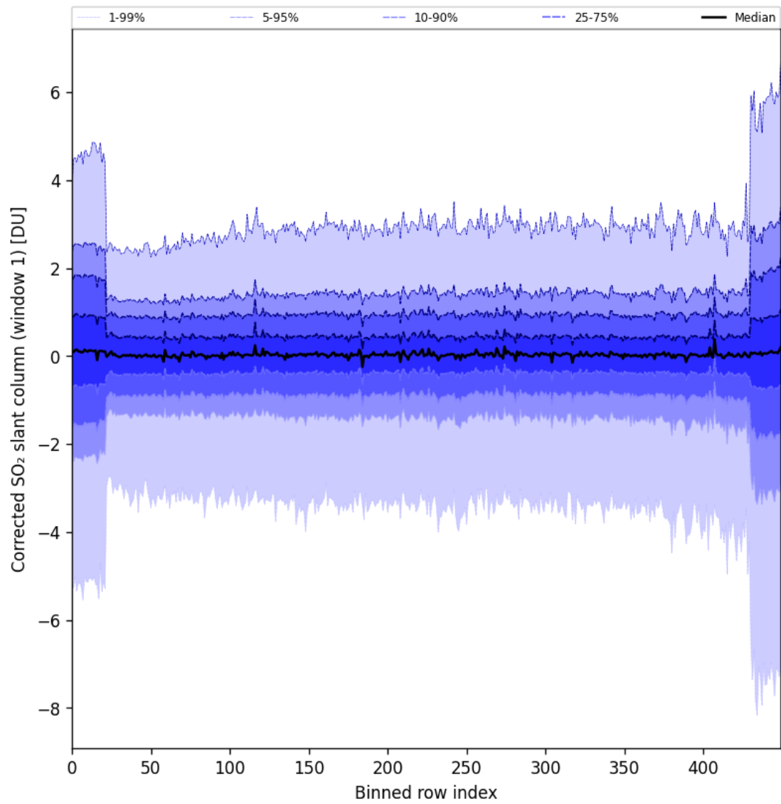
Figure 81: Along track statistics of “Corrected SO 2 slant column (window 1)” for 2024-09-17 to 2024-09-18
