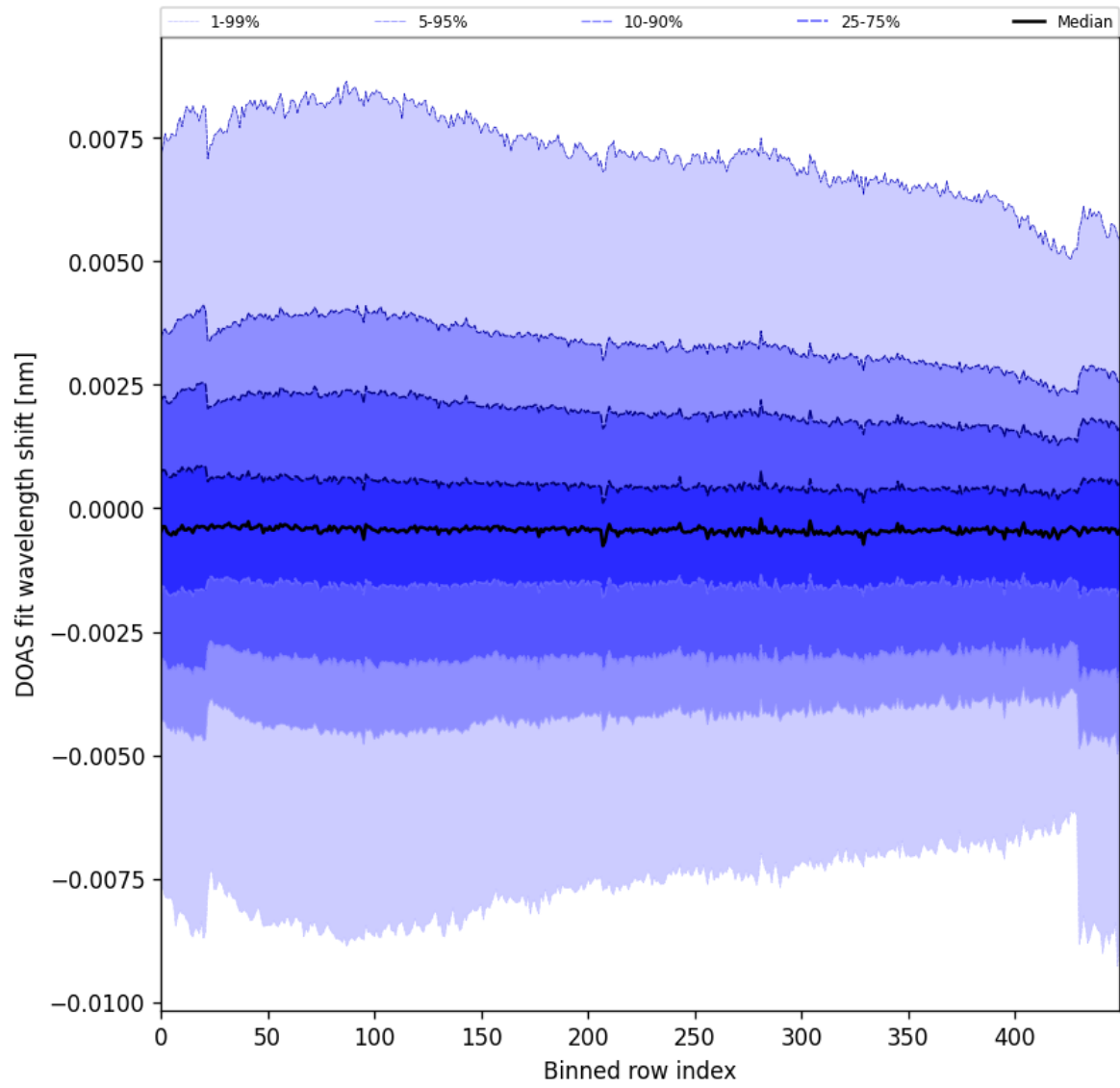
Figure 91: Along track statistics of “DOAS fit wavelength shift” for 2024-09-17 to 2024-09-18
