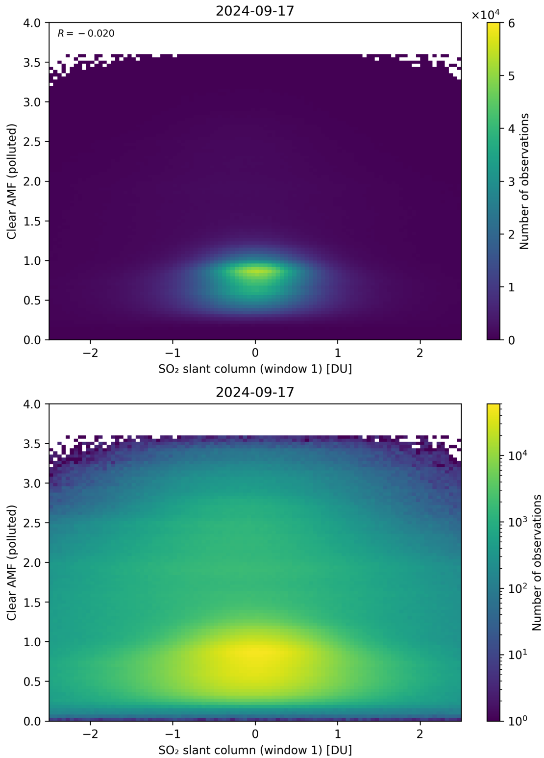
Figure 232: Scatter density plot of “SO 2 slant column (window 1)” against “Clear AMF (polluted)” for 2024-09-17 to 2024-09-18.
