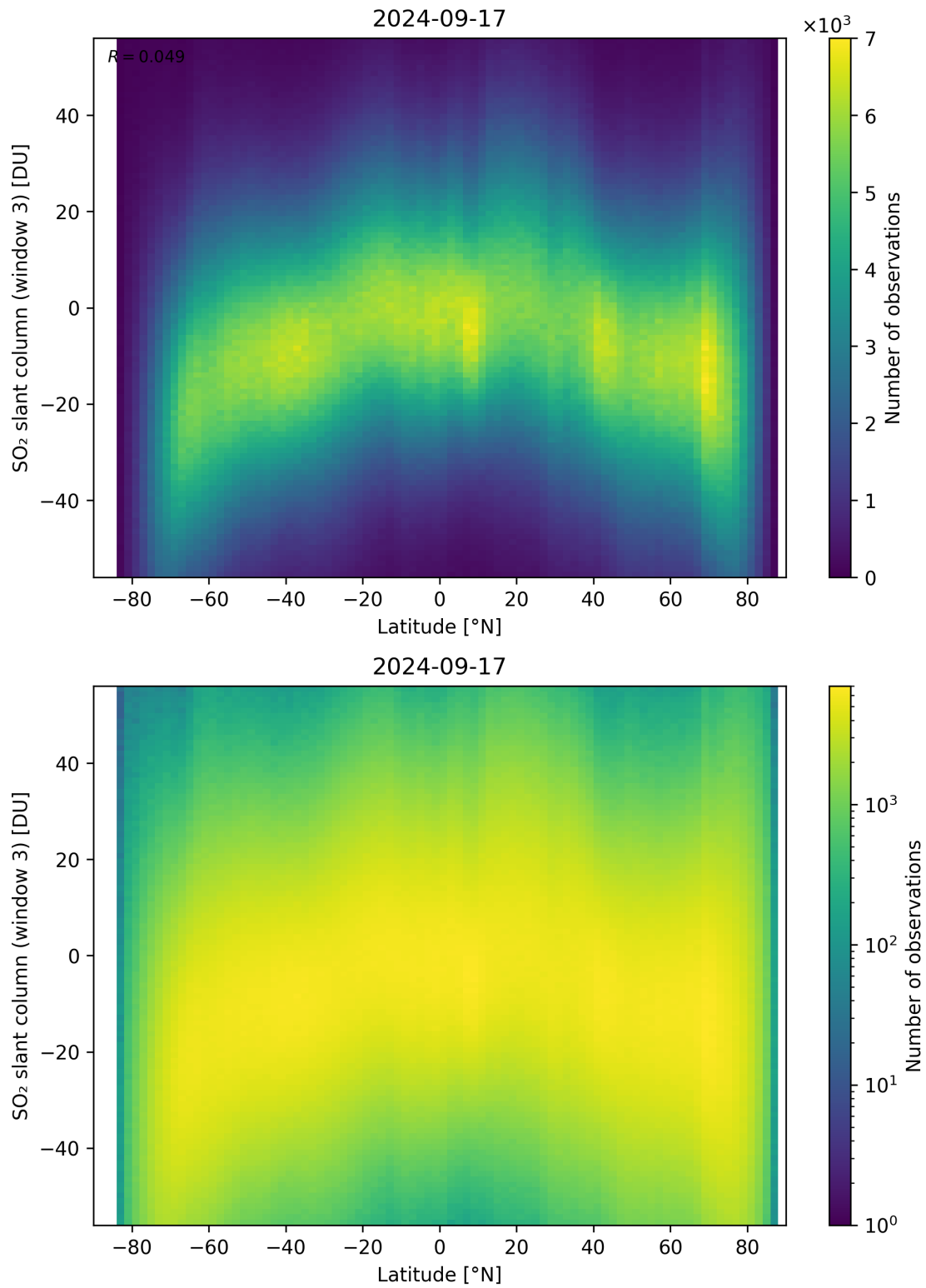
Figure 152: Scatter density plot of “Latitude” against “SO 2 slant column (window 3)” for 2024-09-17 to 2024-09-18.
