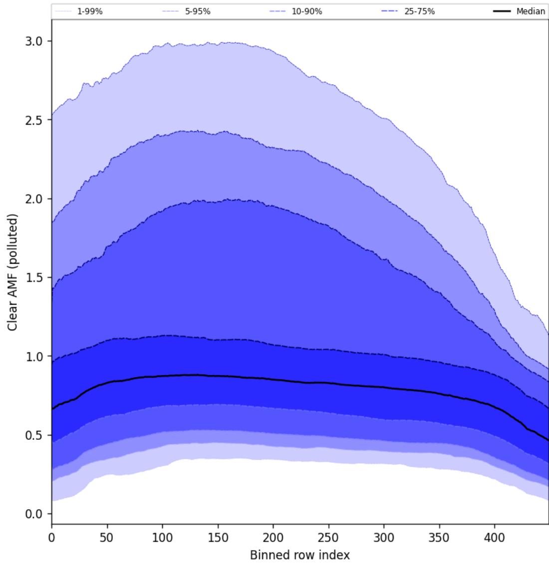
Figure 96: Along track statistics of “Clear AMF (polluted)” for 2024-09-17 to 2024-09-18
