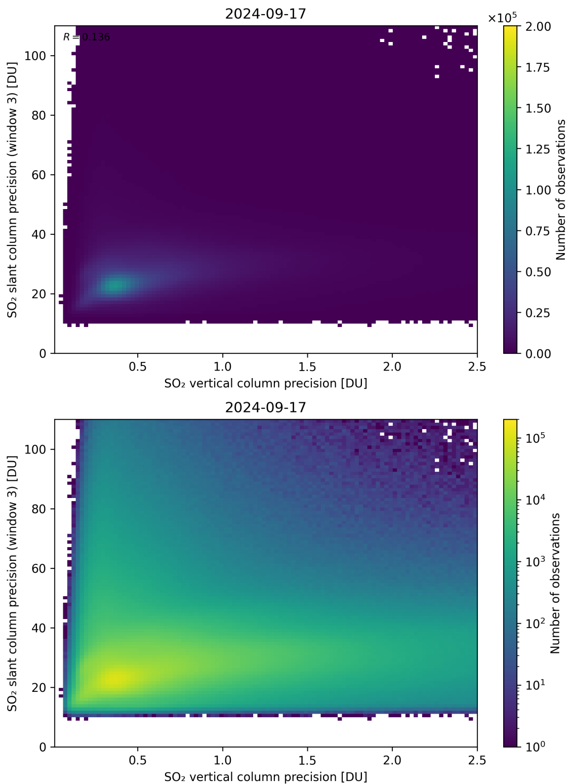
Figure 293: Scatter density plot of “SO 2 vertical column precision” against “SO 2 slant column precision (window 3)” for 2024-09-17 to 2024-09-18.
