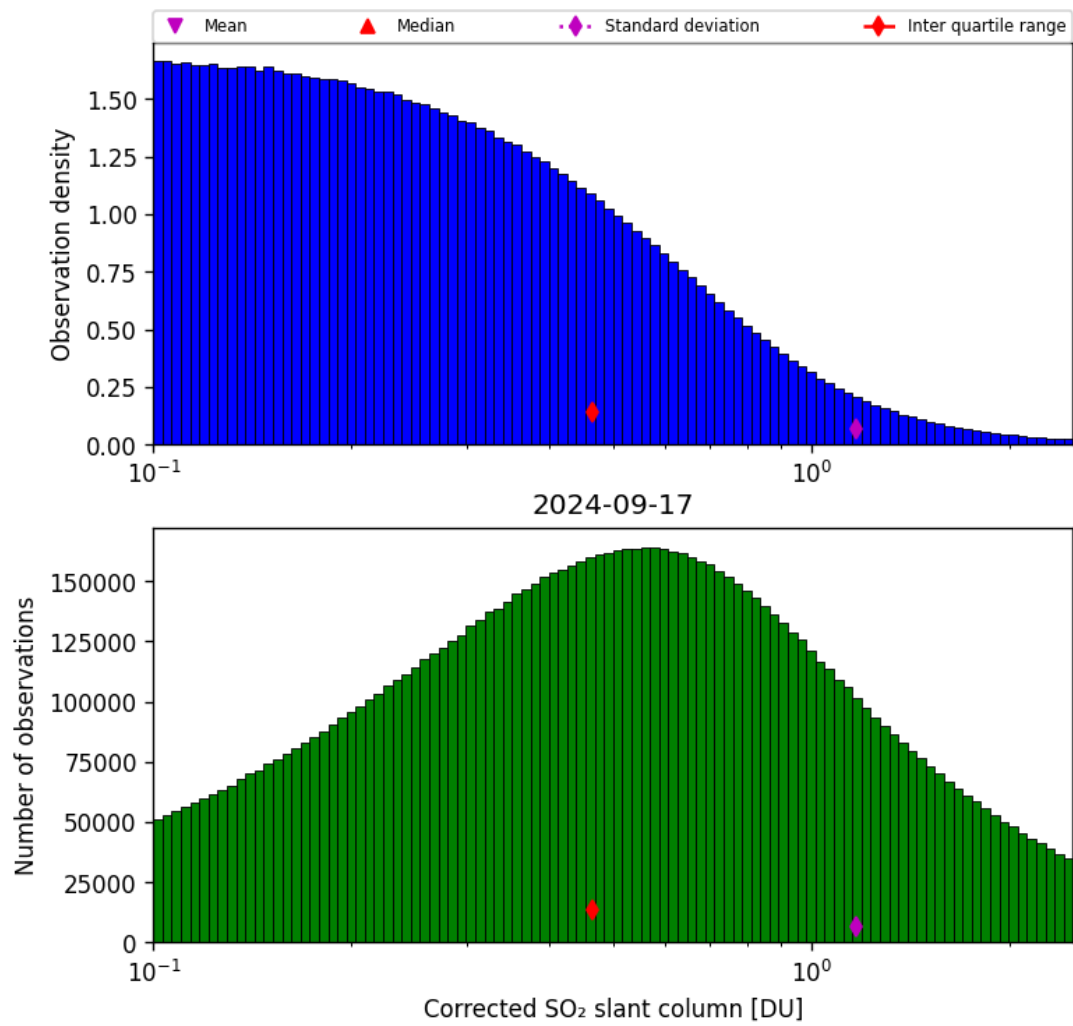
Figure 55: Histogram of “Corrected SO 2 slant column” for 2024-09-17 to 2024-09-18
