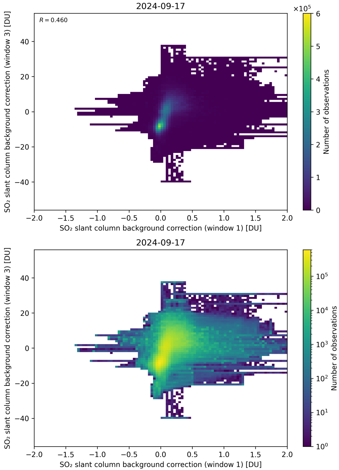
Figure 99: Scatter density plot of “SO 2 slant column background correction (window 1)” against “SO 2 slant column background correction (window 3)” for 2024-09-17 to 2024-09-18.
