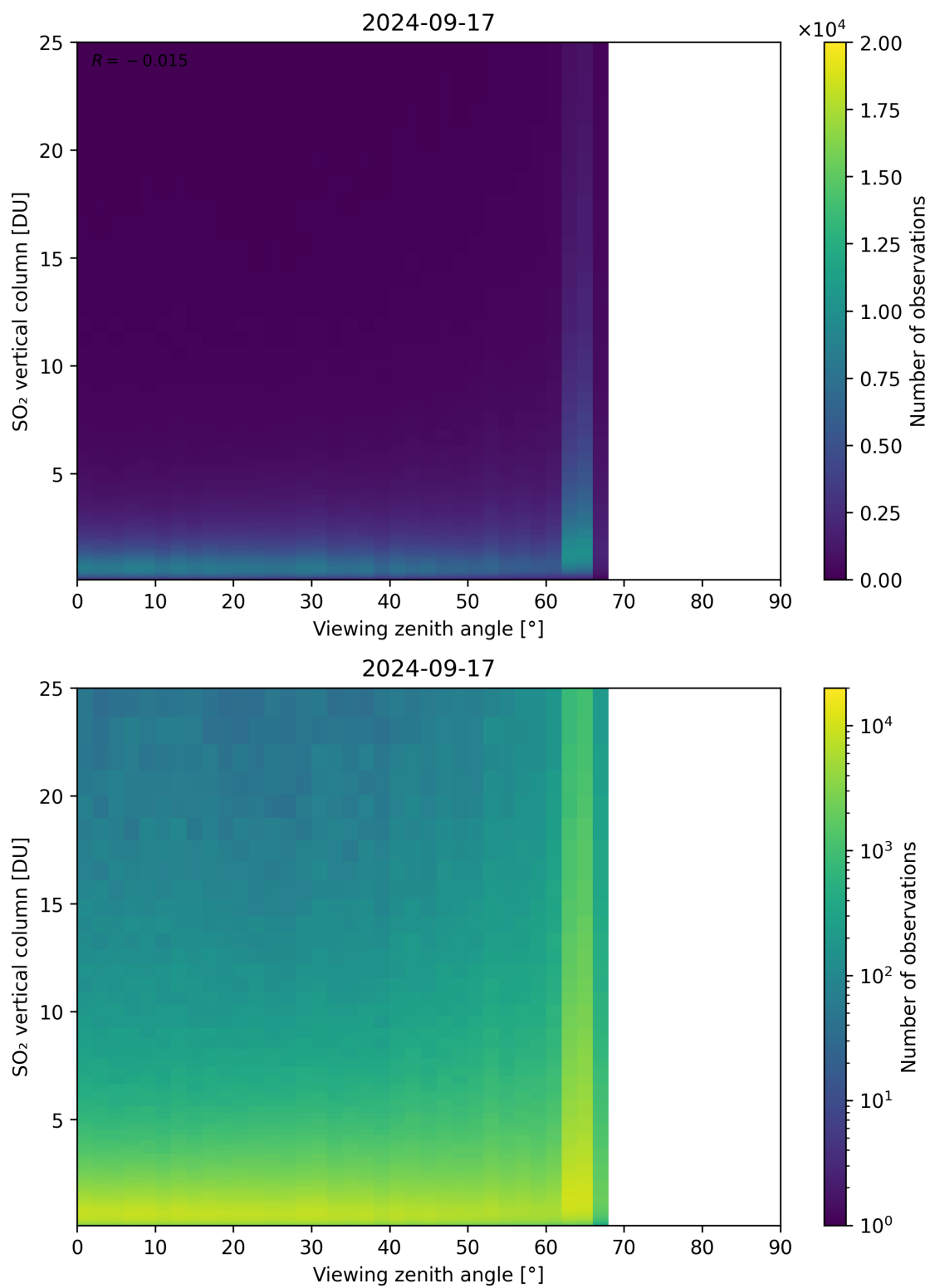
Figure 327: Scatter density plot of “Viewing zenith angle” against “SO 2 vertical column” for 2024-09-17 to 2024-09-18.
