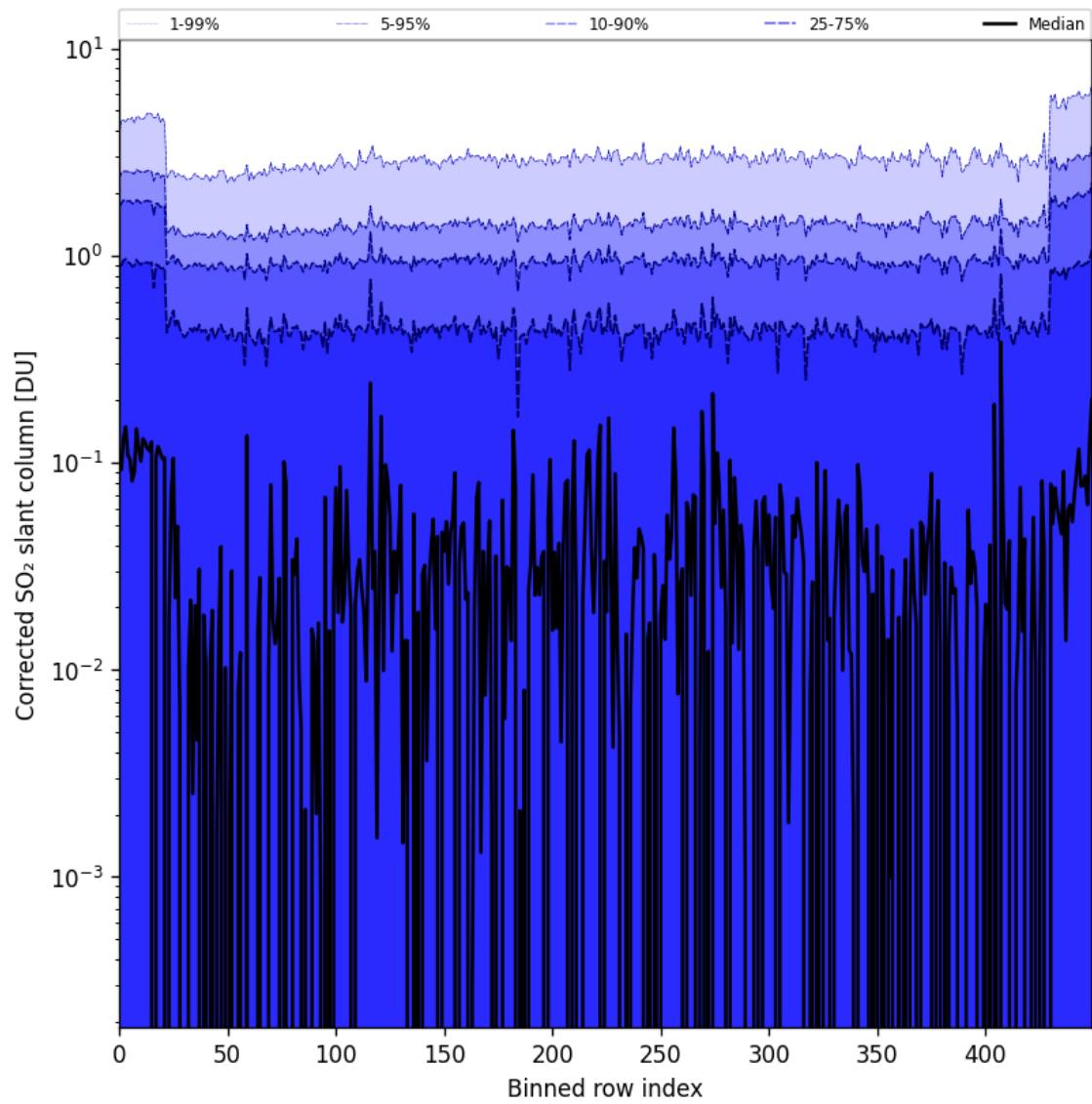
Figure 78: Along track statistics of “Corrected SO 2 slant column” for 2024-09-17 to 2024-09-18
