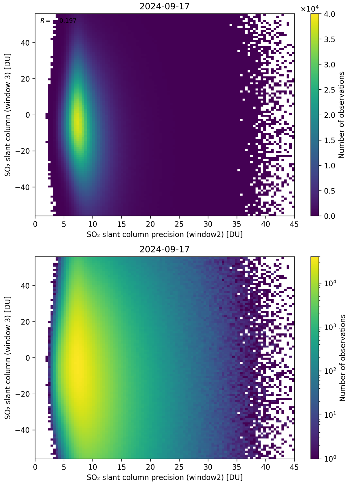
Figure 249: Scatter density plot of “SO 2 slant column precision (window2)” against “SO 2 slant column (window 3)” for 2024-09-17 to 2024-09-18.
