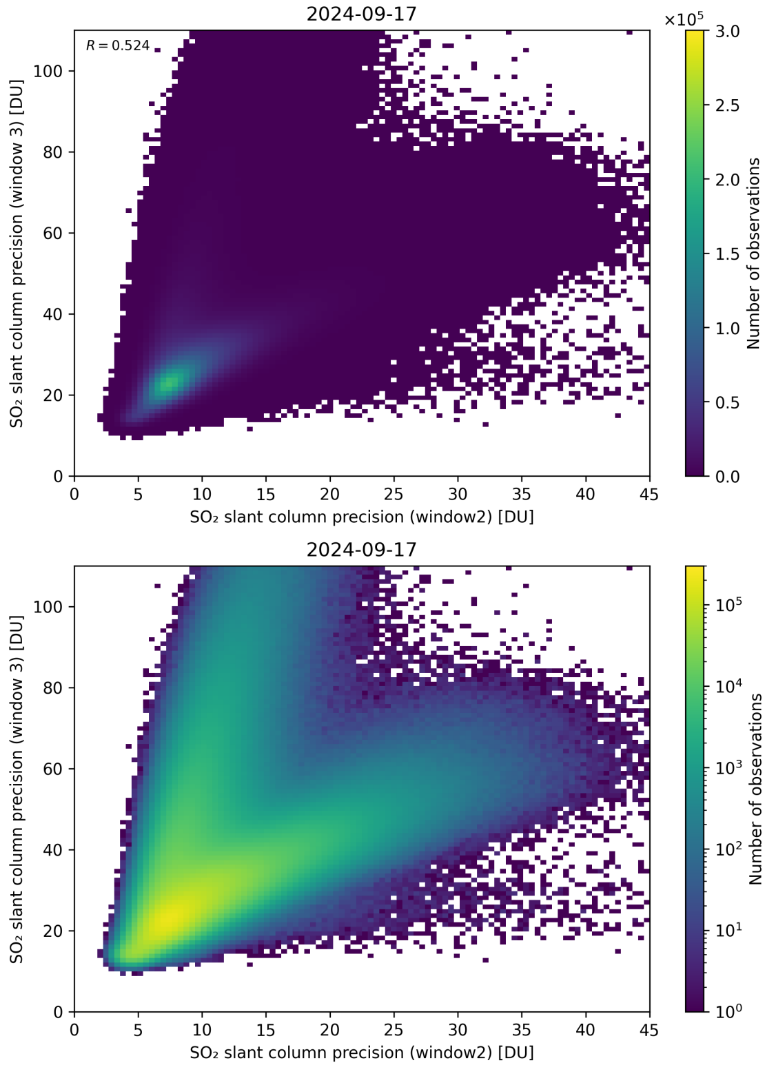
Figure 250: Scatter density plot of “SO 2 slant column precision (window2)” against “SO 2 slant column precision (window 3)” for 2024-09-17 to 2024-09-18.
