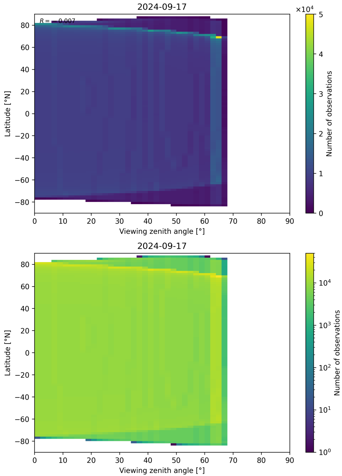
Figure 314: Scatter density plot of “Viewing zenith angle” against “Latitude” for 2024-09-17 to 2024-09-18.
