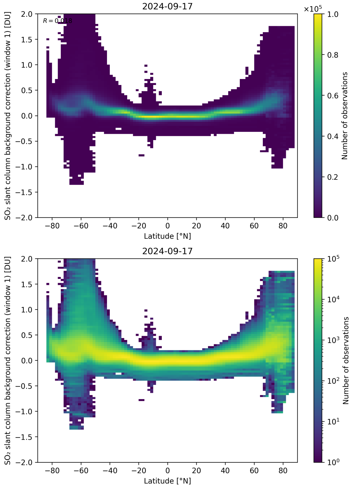
Figure 139: Scatter density plot of “Latitude” against “SO 2 slant column background correction (window 1)” for 2024-09-17 to 2024-09-18.
