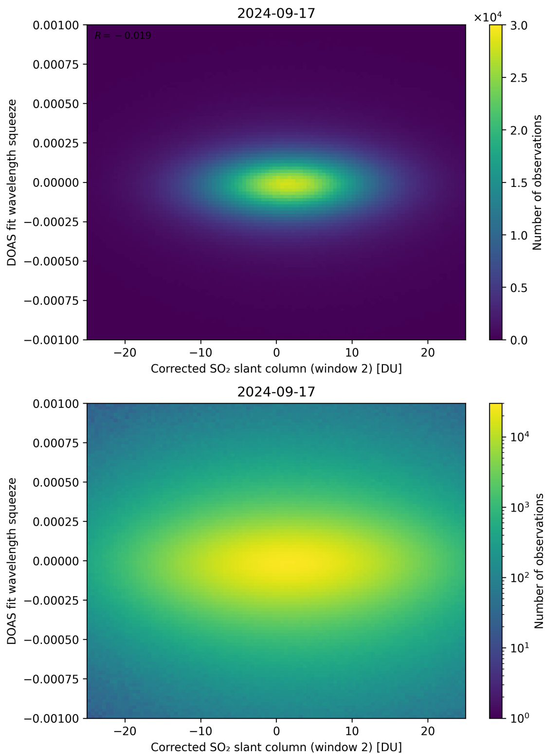
Figure 197: Scatter density plot of “Corrected SO 2 slant column (window 2)” against “DOAS fit wavelength squeeze” for 2024-09-17 to 2024-09-18.
