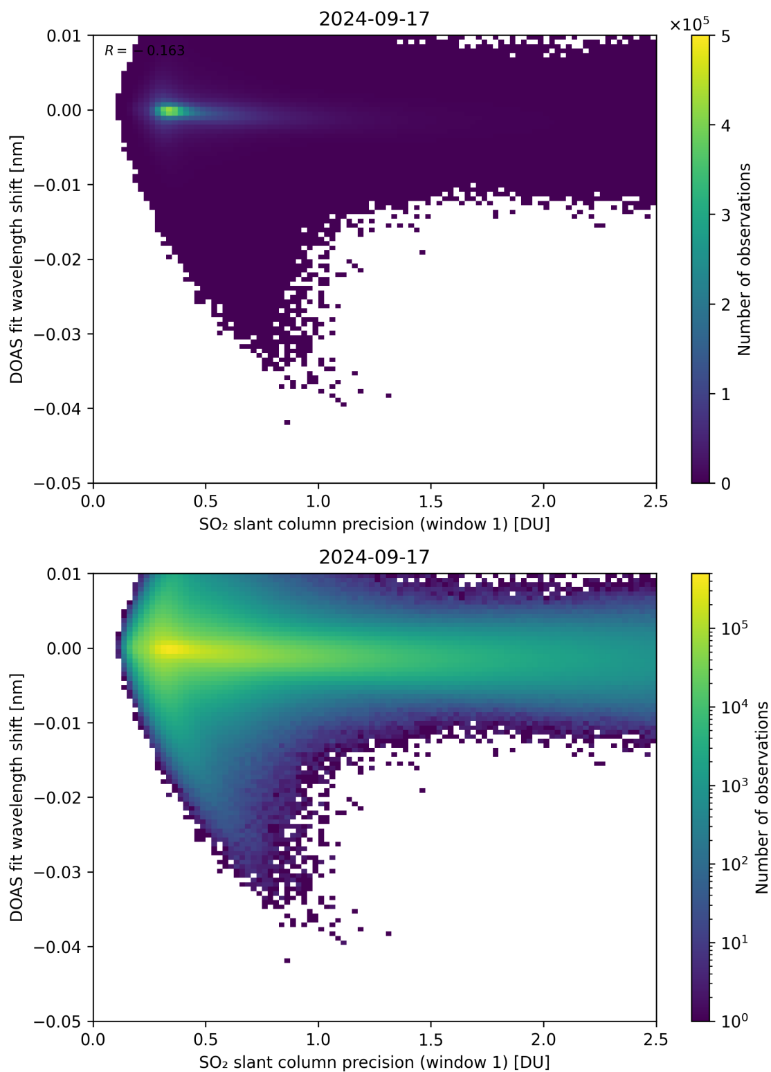
Figure 221: Scatter density plot of “SO 2 slant column precision (window 1)” against “DOAS fit wavelength shift” for 2024-09-17 to 2024-09-18.
