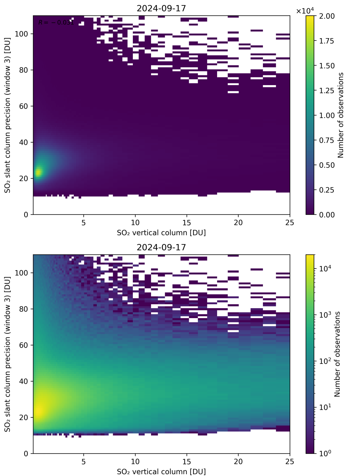
Figure 304: Scatter density plot of “SO 2 vertical column” against “SO 2 slant column precision (window 3)” for 2024-09-17 to 2024-09-18.
