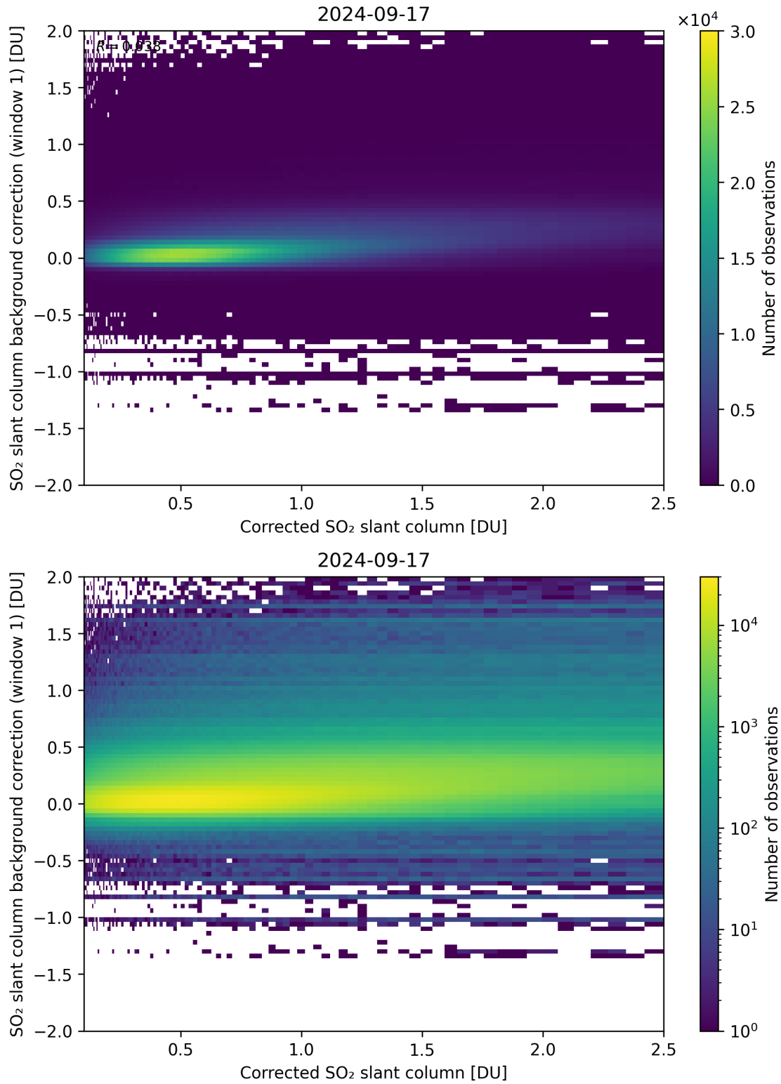
Figure 178: Scatter density plot of “Corrected SO 2 slant column” against “SO 2 slant column background correction (window 1)” for 2024-09-17 to 2024-09-18.
