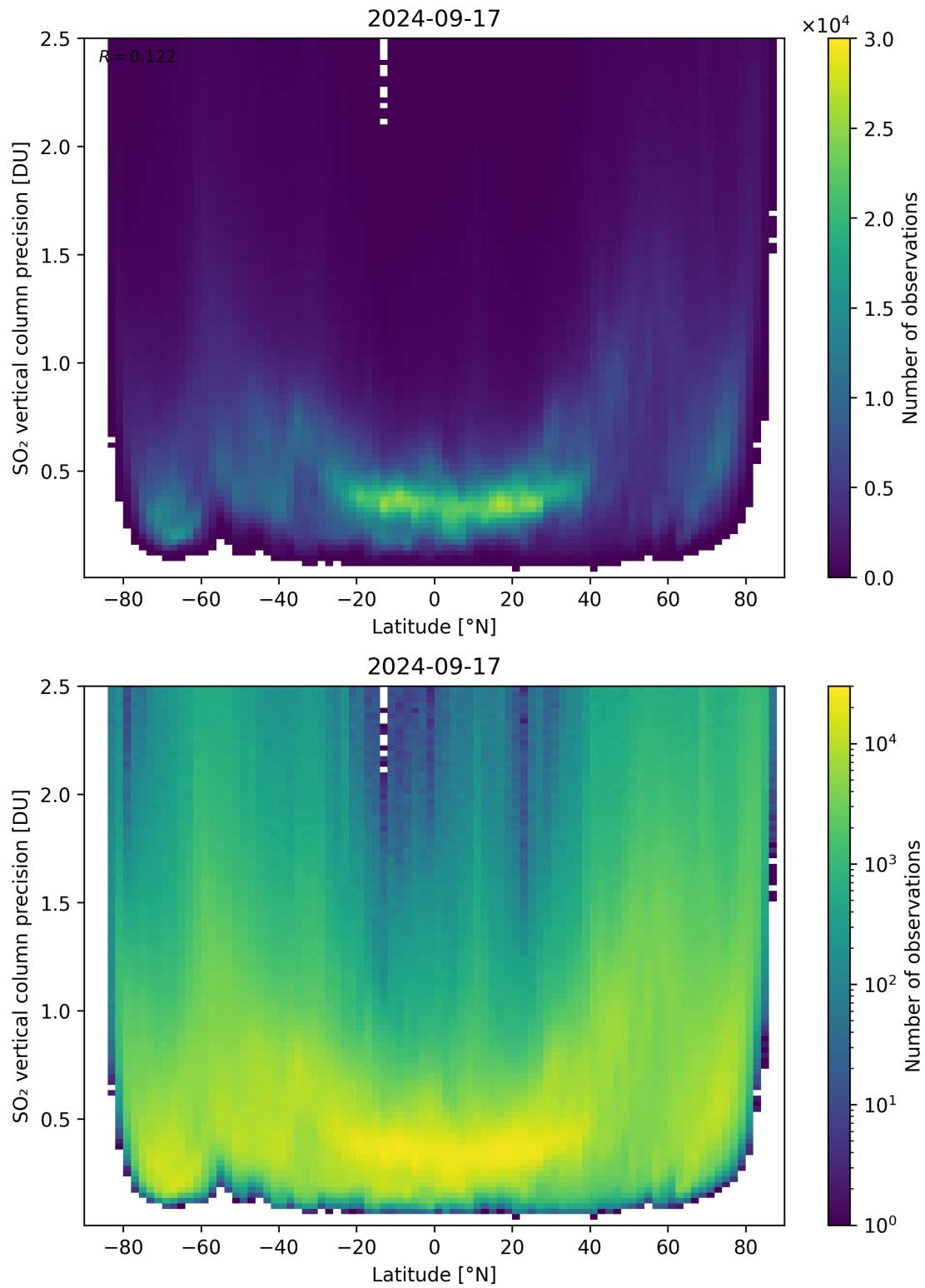
Figure 157: Scatter density plot of “Latitude” against “SO 2 vertical column precision” for 2024-09-17 to 2024-09-18.
