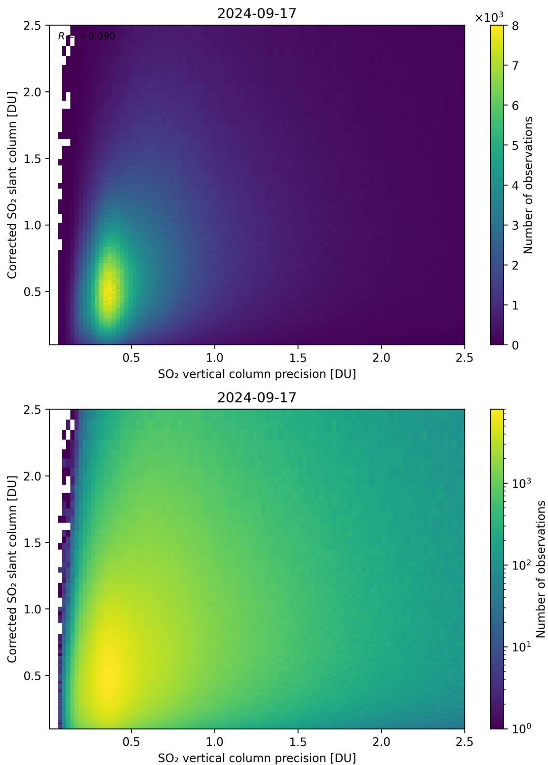
Figure 286: Scatter density plot of “SO 2 vertical column precision” against “Corrected SO 2 slant column” for 2024-09-17 to 2024-09-18.
