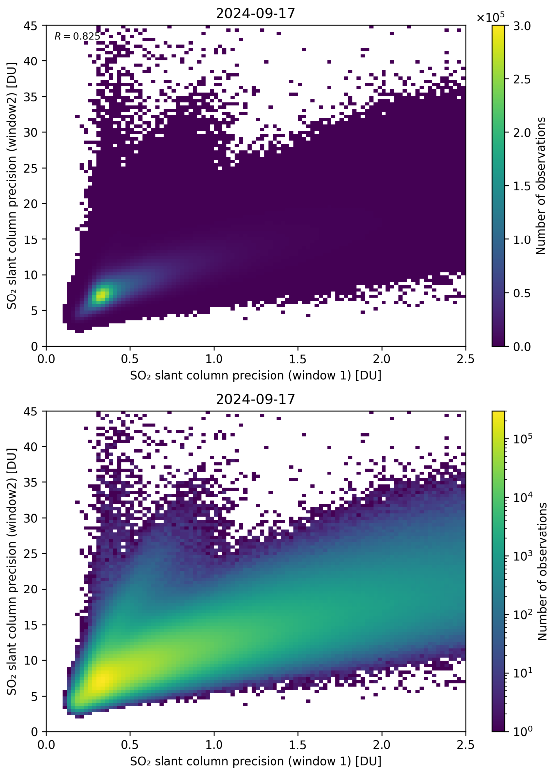
Figure 227: Scatter density plot of “SO 2 slant column precision (window 1)” against “SO 2 slant column precision (window2)” for 2024-09-17 to 2024-09-18.
