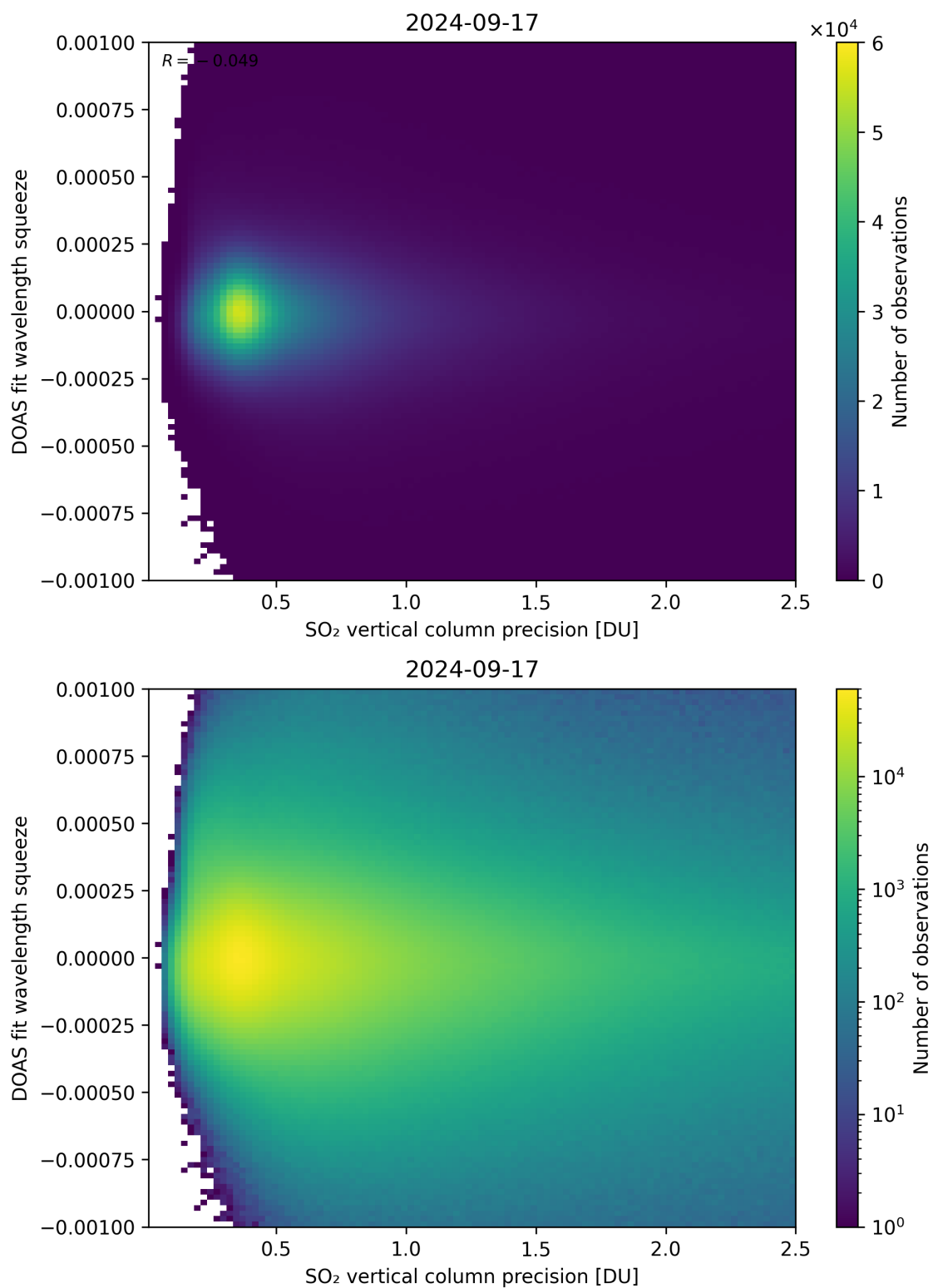
Figure 283: Scatter density plot of “SO 2 vertical column precision” against “DOAS fit wavelength squeeze” for 2024-09-17 to 2024-09-18.
