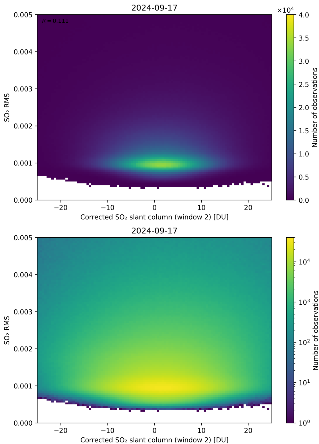
Figure 198: Scatter density plot of “Corrected SO 2 slant column (window 2)” against “SO 2 RMS” for 2024-09-17 to 2024-09-18.
