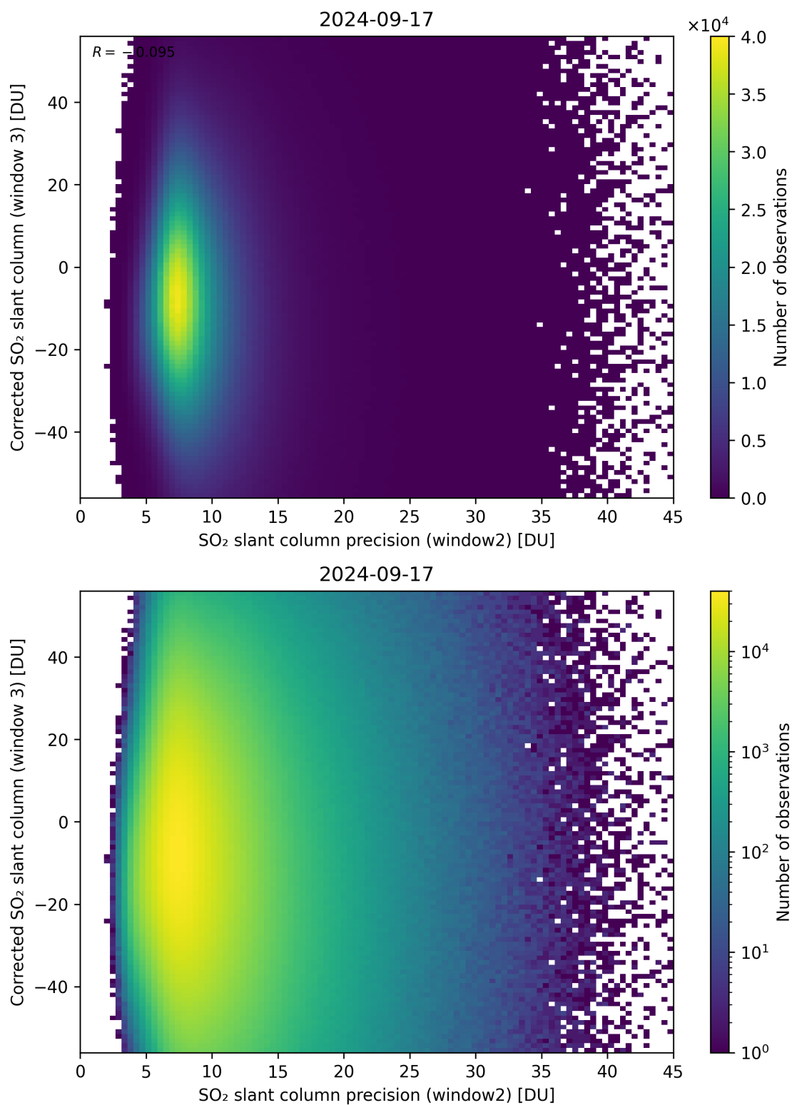
Figure 248: Scatter density plot of “SO 2 slant column precision (window2)” against “Corrected SO 2 slant column (window 3)” for 2024-09-17 to 2024-09-18.
