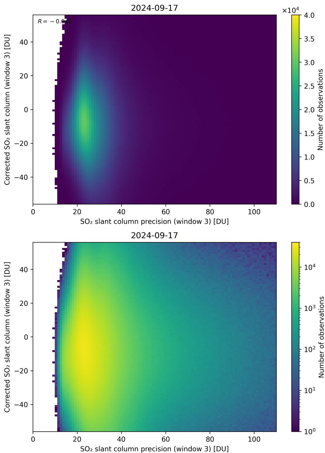
Figure 262: Scatter density plot of “SO 2 slant column precision (window 3)” against “Corrected SO 2 slant column (window 3)” for 2024-09-17 to 2024-09-18.
