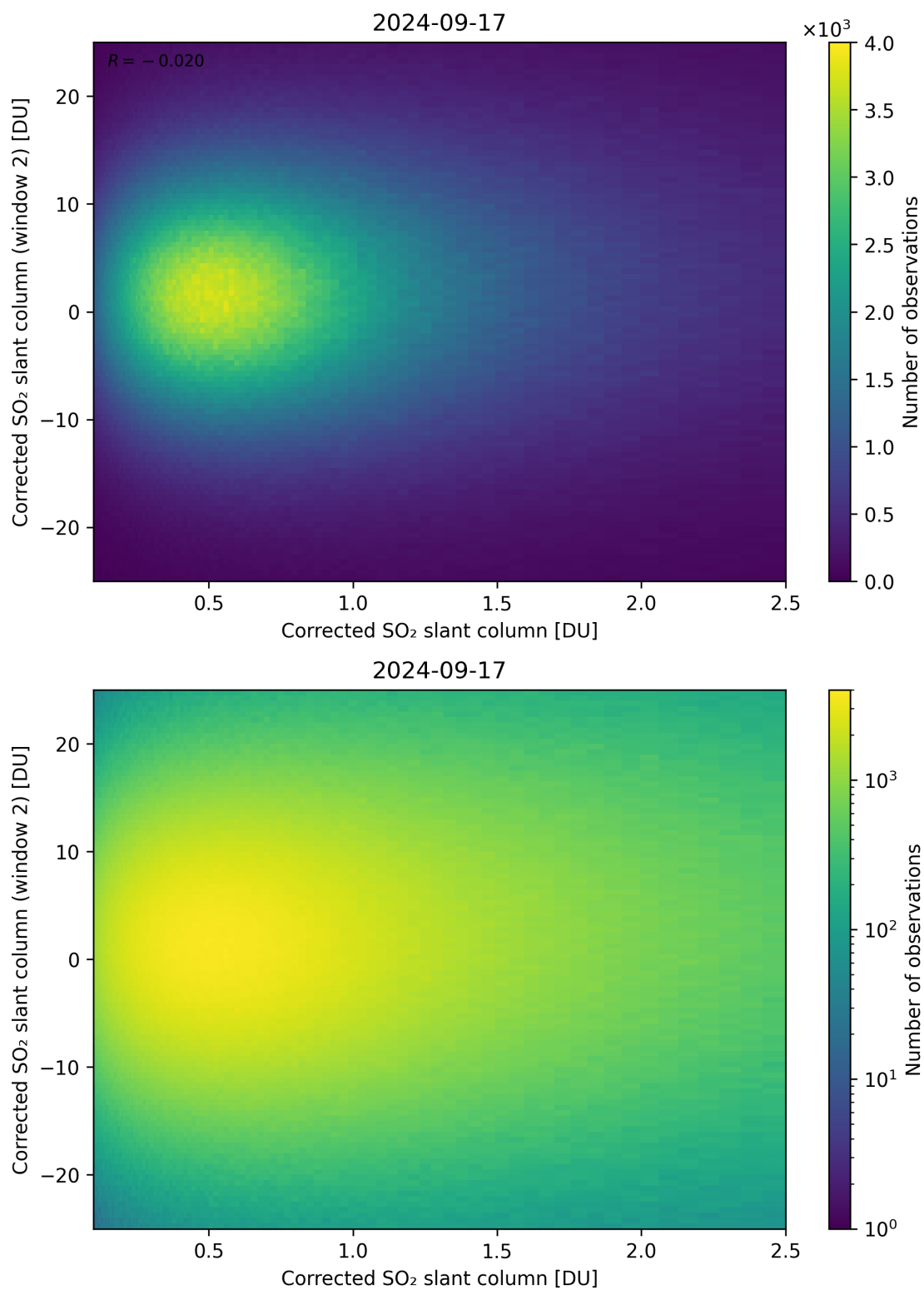
Figure 185: Scatter density plot of “Corrected SO 2 slant column” against “Corrected SO 2 slant column (window 2)” for 2024-09-17 to 2024-09-18.
