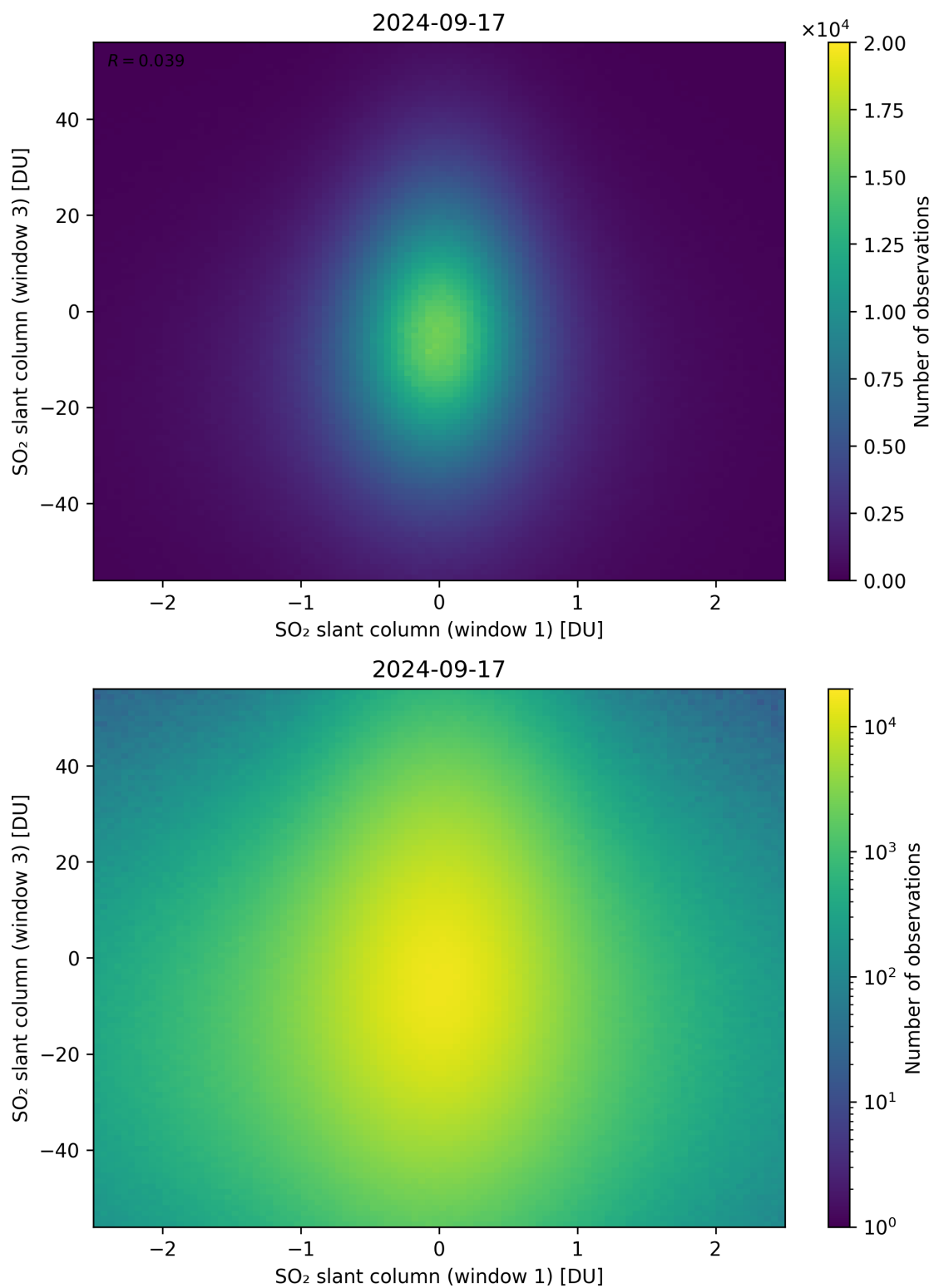
Figure 237: Scatter density plot of “SO 2 slant column (window 1)” against “SO 2 slant column (window 3)” for 2024-09-17 to 2024-09-18.
