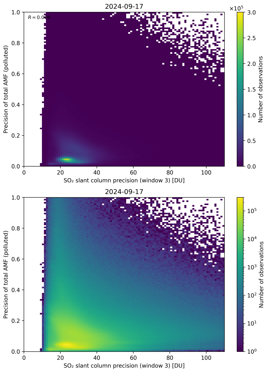
Figure 264: Scatter density plot of “SO 2 slant column precision (window 3)” against “Precision of total AMF (polluted)” for 2024-09-17 to 2024-09-18.
