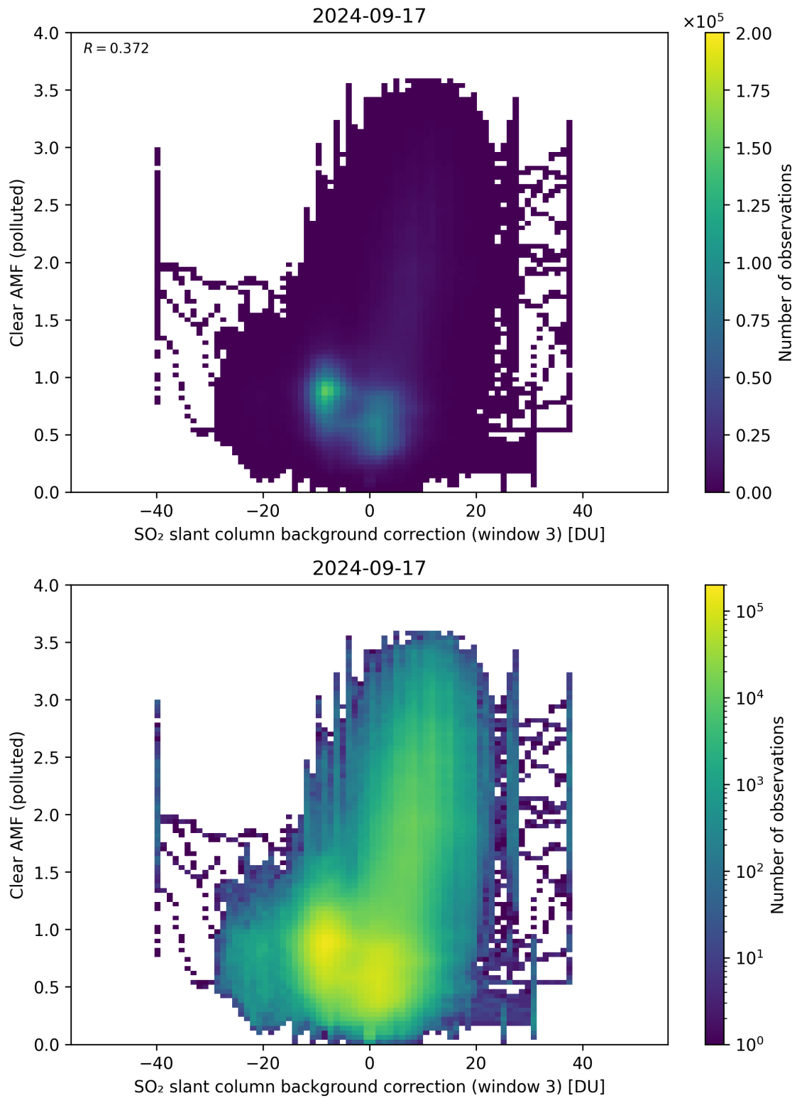
Figure 124: Scatter density plot of “SO 2 slant column background correction (window 3)” against “Clear AMF (polluted)” for 2024-09-17 to 2024-09-18.
