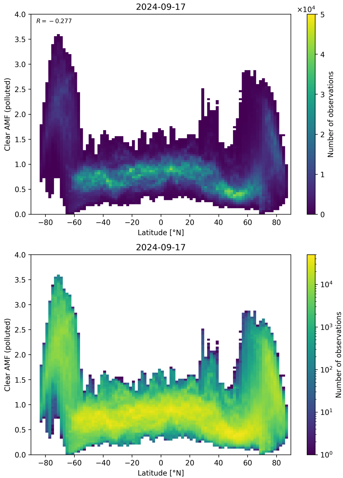
Figure 145: Scatter density plot of “Latitude” against “Clear AMF (polluted)” for 2024-09-17 to 2024-09-18.
