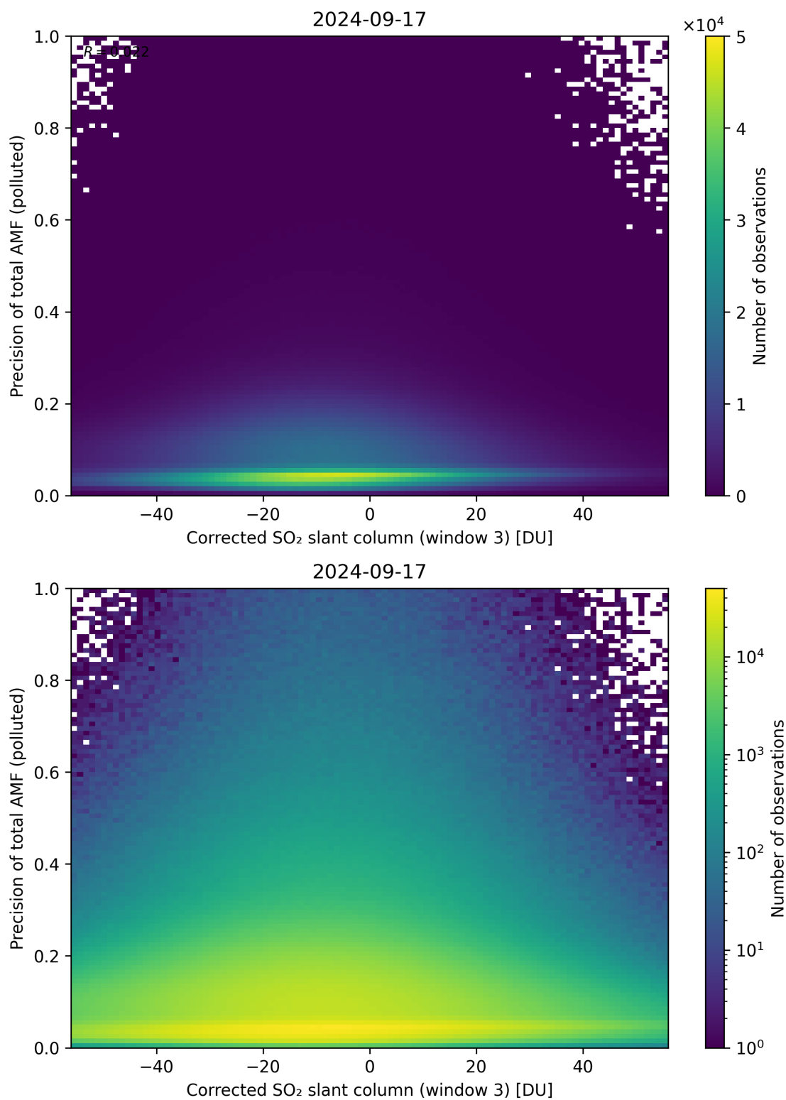
Figure 211: Scatter density plot of “Corrected SO 2 slant column (window 3)” against “Precision of total AMF (polluted)” for 2024-09-17 to 2024-09-18.
