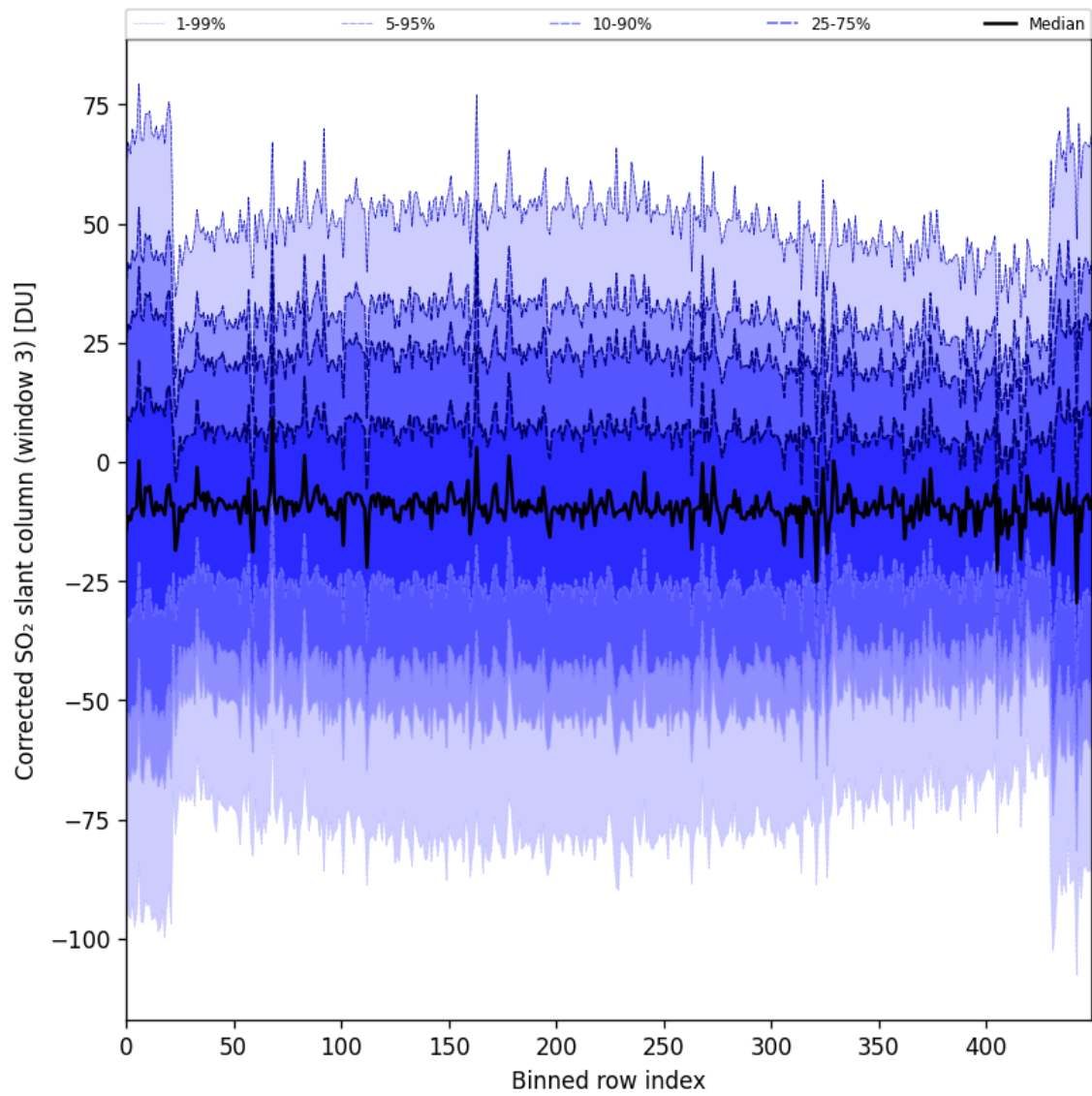
Figure 89: Along track statistics of “Corrected SO 2 slant column (window 3)” for 2024-09-17 to 2024-09-18
