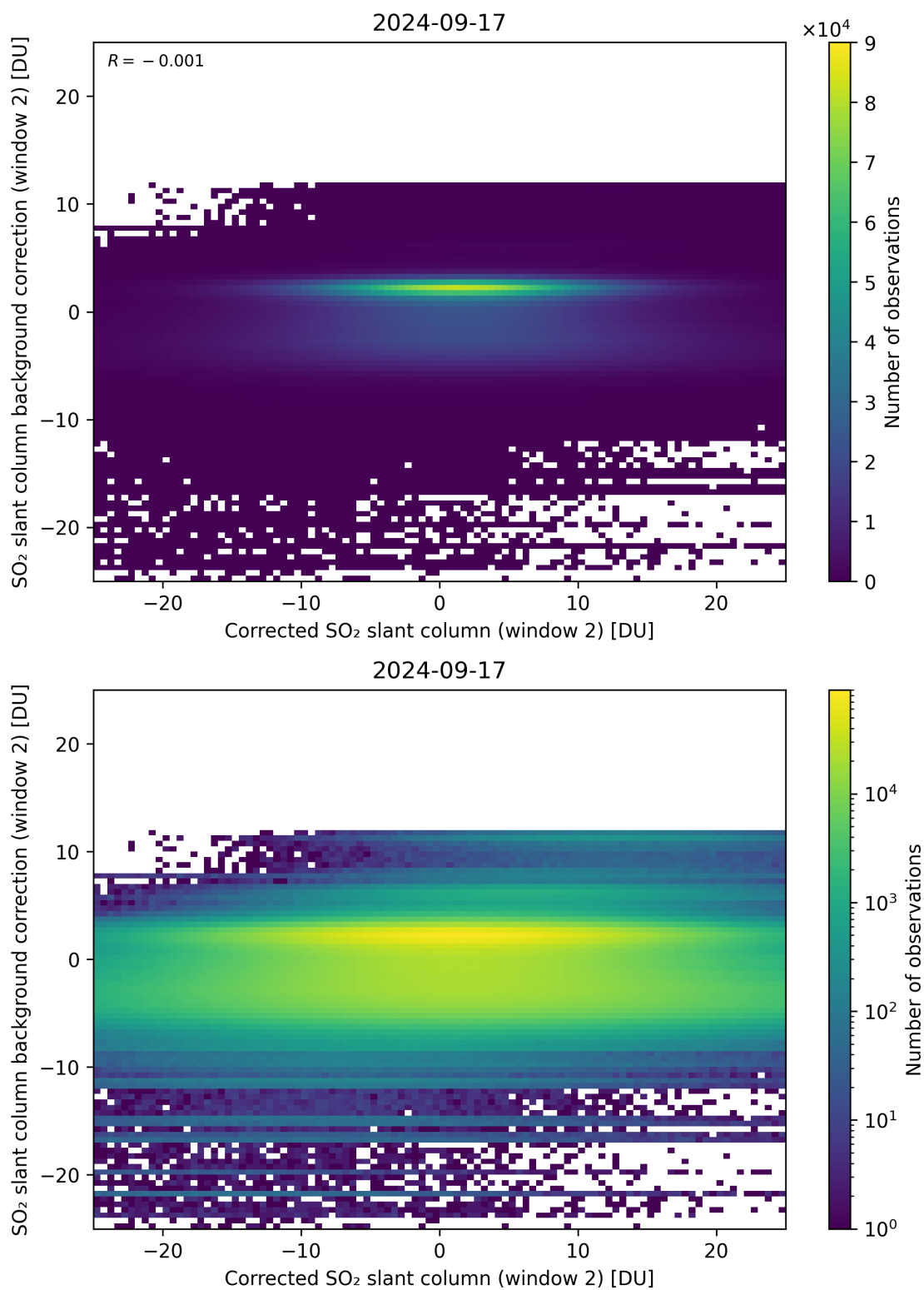
Figure 194: Scatter density plot of “Corrected SO 2 slant column (window 2)” against “SO 2 slant column background correction (window 2)” for 2024-09-17 to 2024-09-18.
