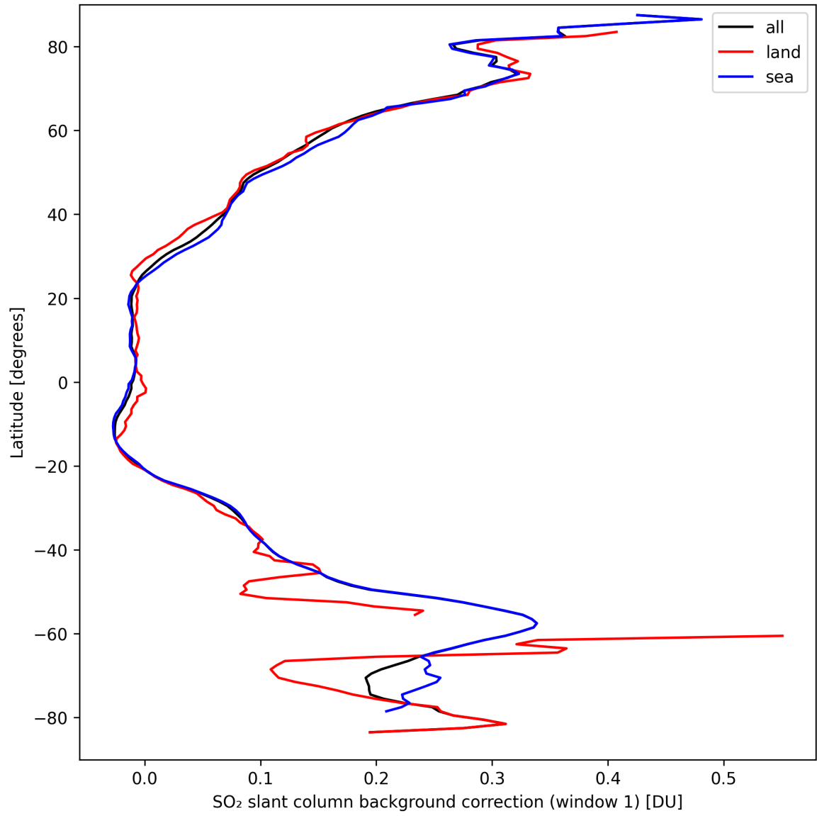
Figure 36: Zonal average of “SO 2 slant column background correction (window 1)” for 2024-09-17 to 2024-09-18.
