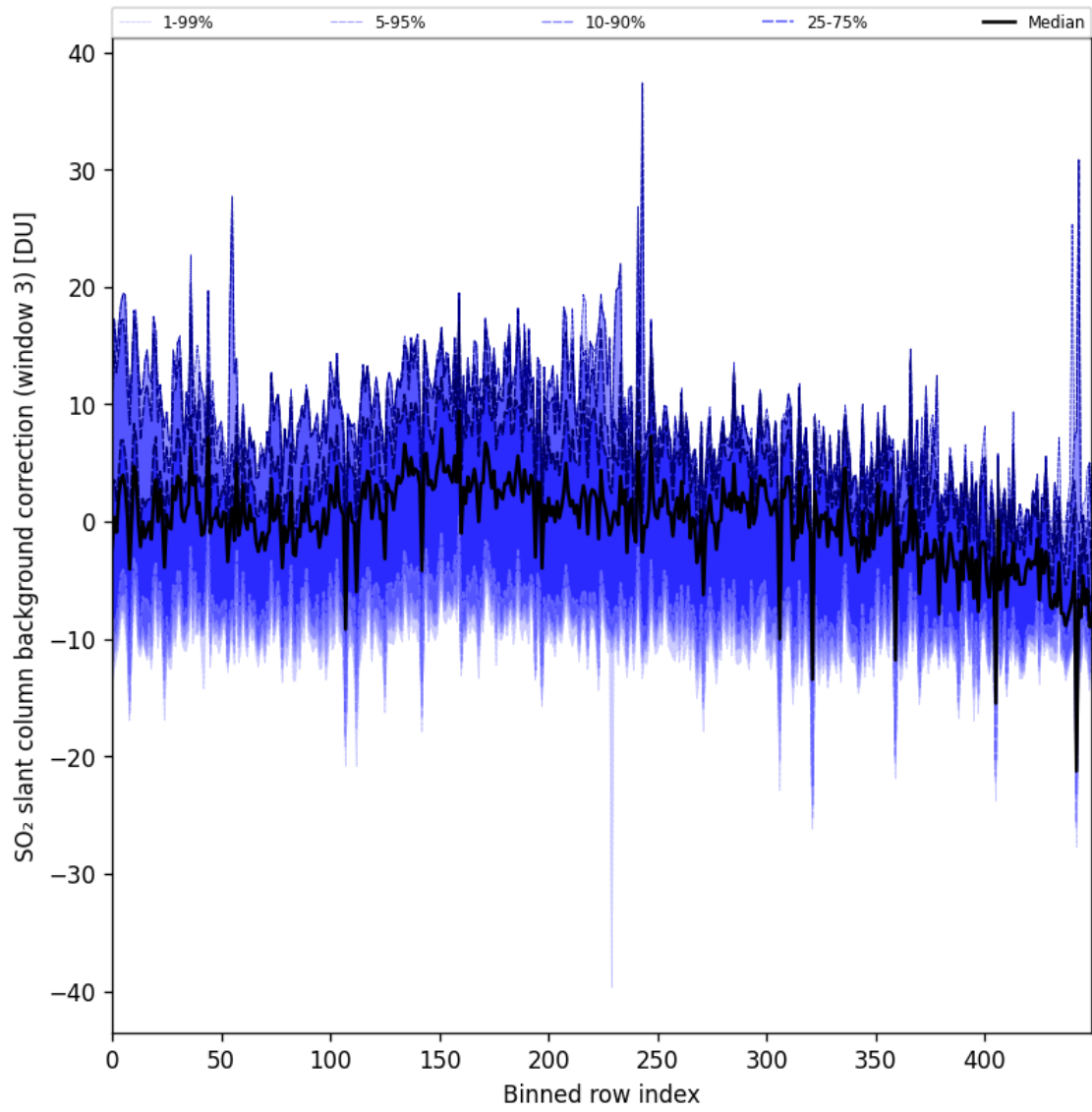
Figure 90: Along track statistics of “SO 2 slant column background correction (window 3)” for 2024-09-17 to 2024-09-18
