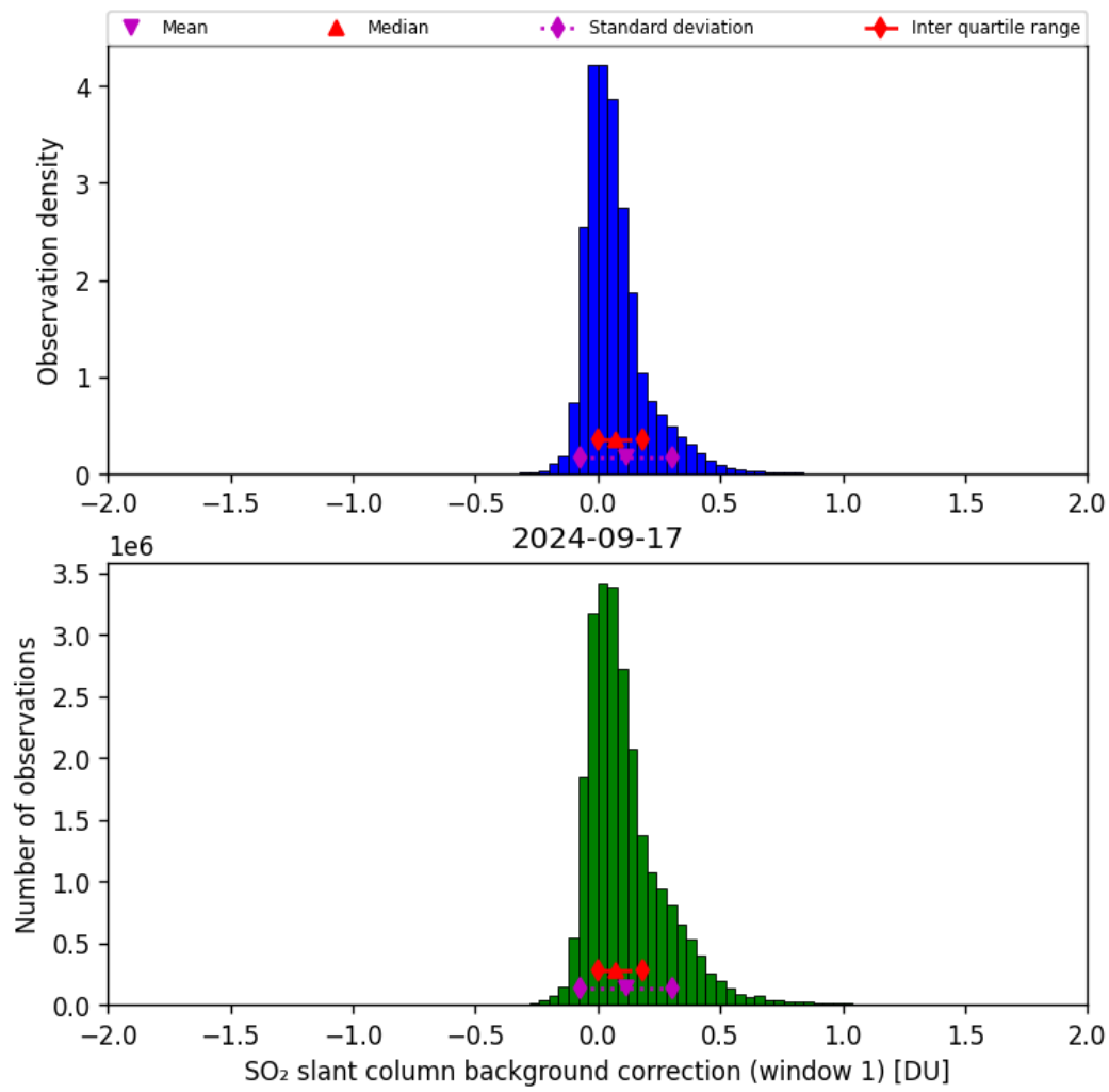
Figure 59: Histogram of “SO 2 slant column background correction (window 1)” for 2024-09-17 to 2024-09-18
