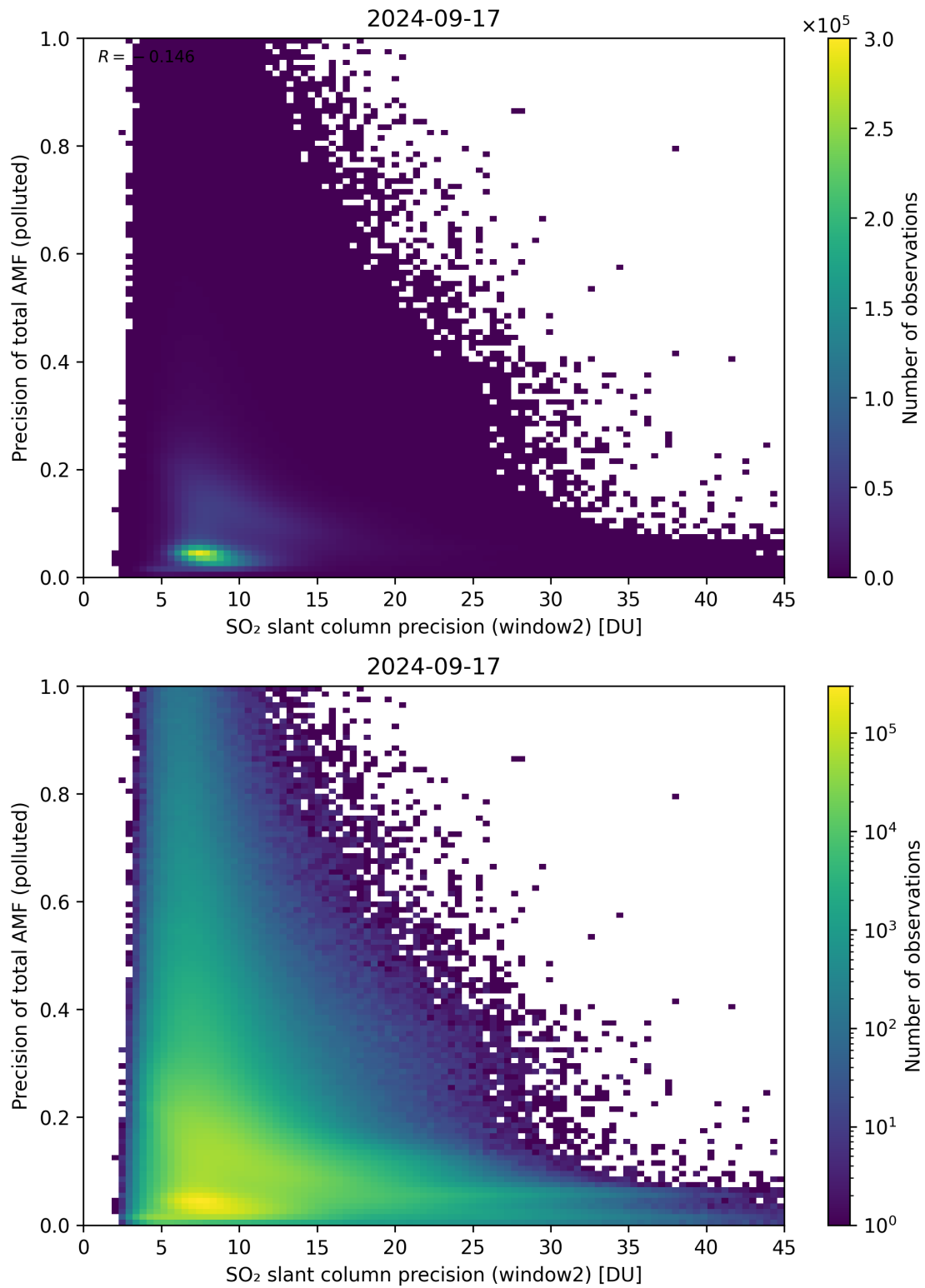
Figure 252: Scatter density plot of “SO 2 slant column precision (window2)” against “Precision of total AMF (polluted)” for 2024-09-17 to 2024-09-18.
