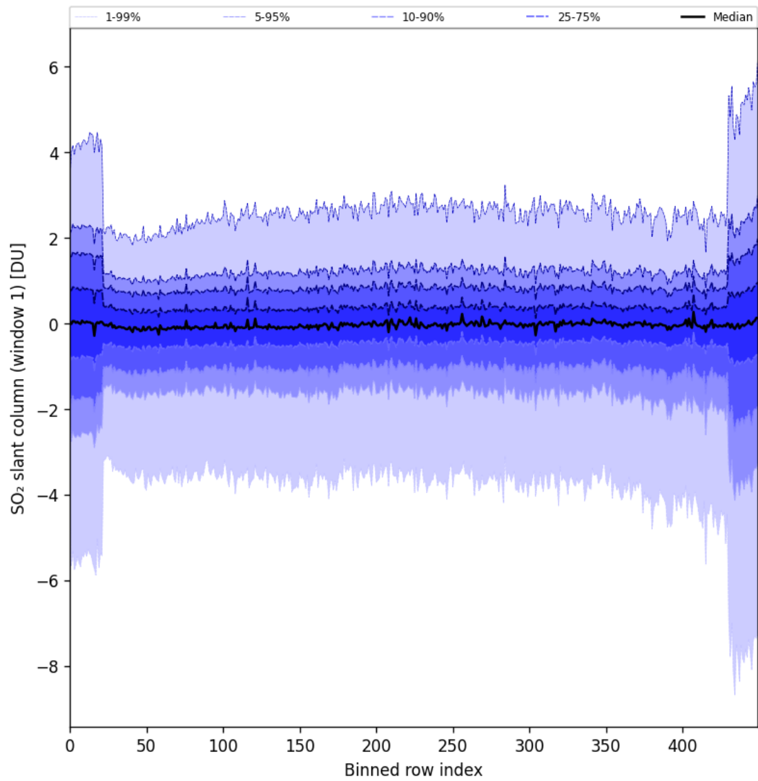
Figure 79: Along track statistics of “SO 2 slant column (window 1)” for 2024-09-17 to 2024-09-18
