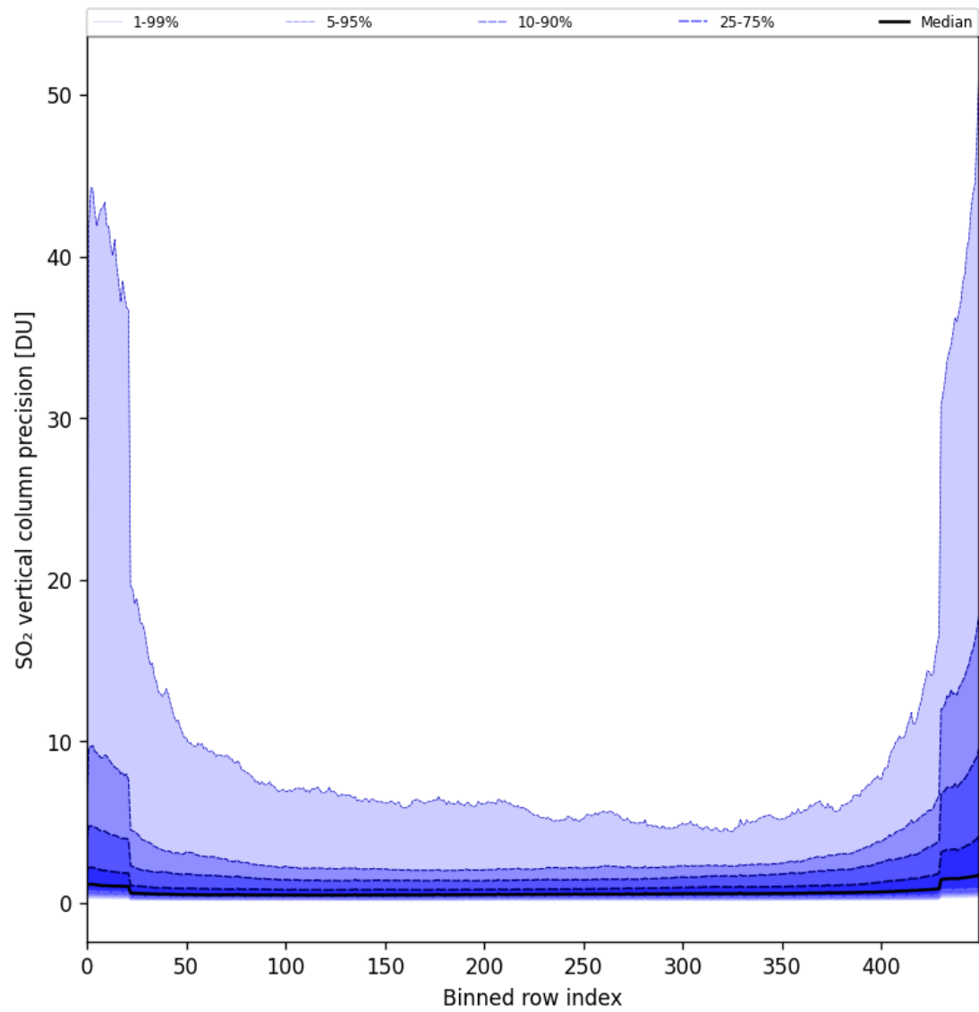
Figure 77: Along track statistics of “SO 2 vertical column precision” for 2024-09-17 to 2024-09-18
