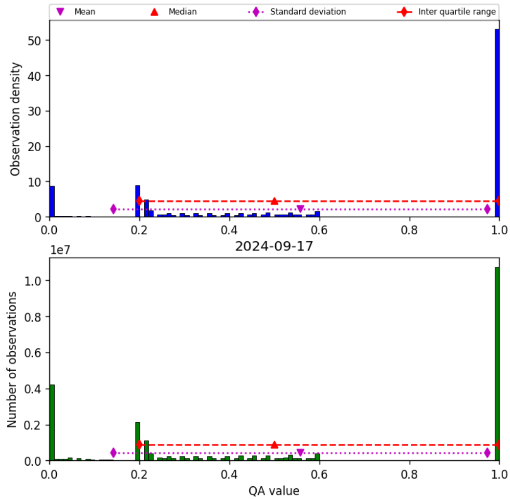
Figure 52: Histogram of “QA value” for 2024-09-17 to 2024-09-18
