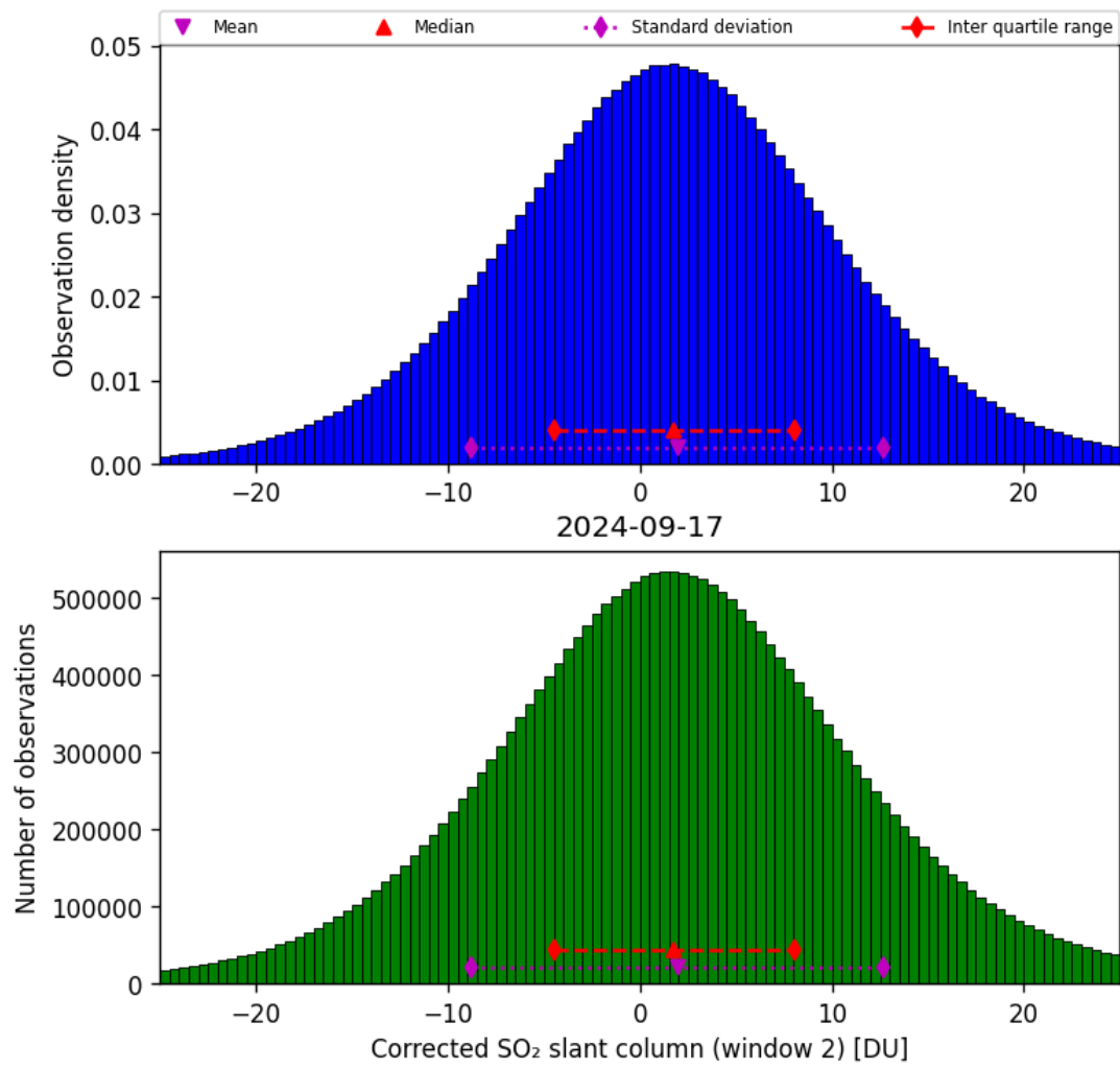
Figure 62: Histogram of “Corrected SO 2 slant column (window 2)” for 2024-09-17 to 2024-09-18
