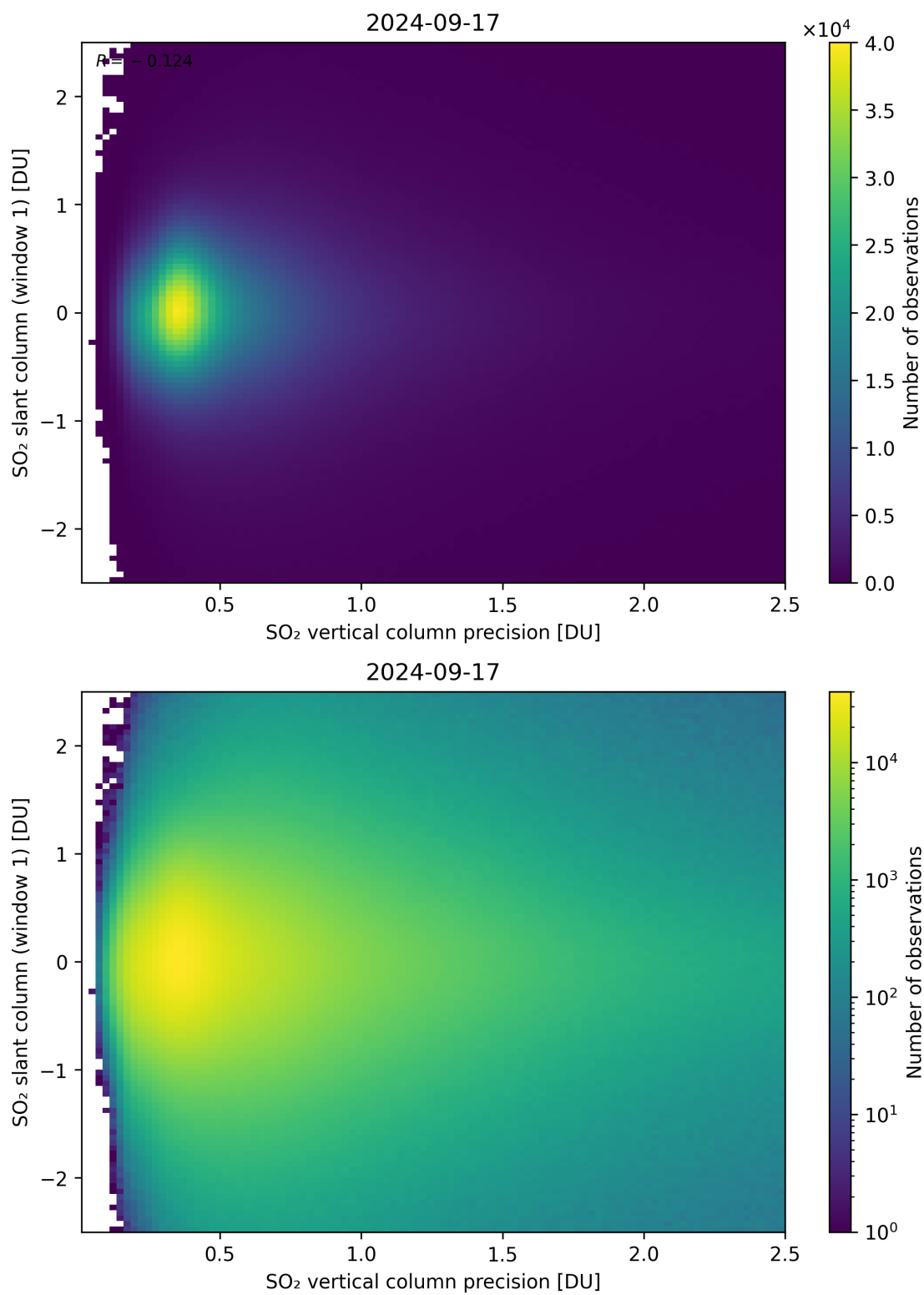
Figure 289: Scatter density plot of “SO 2 vertical column precision” against “SO 2 slant column (window 1)” for 2024-09-17 to 2024-09-18.
