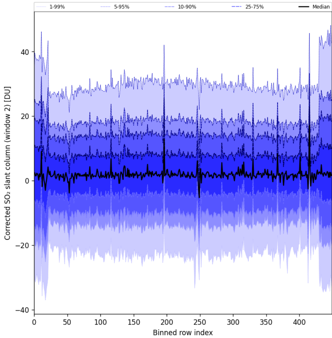
Figure 85: Along track statistics of "Corrected SO 2 slant column (window 2)" for 2024-09-17 to 2024-09-18
