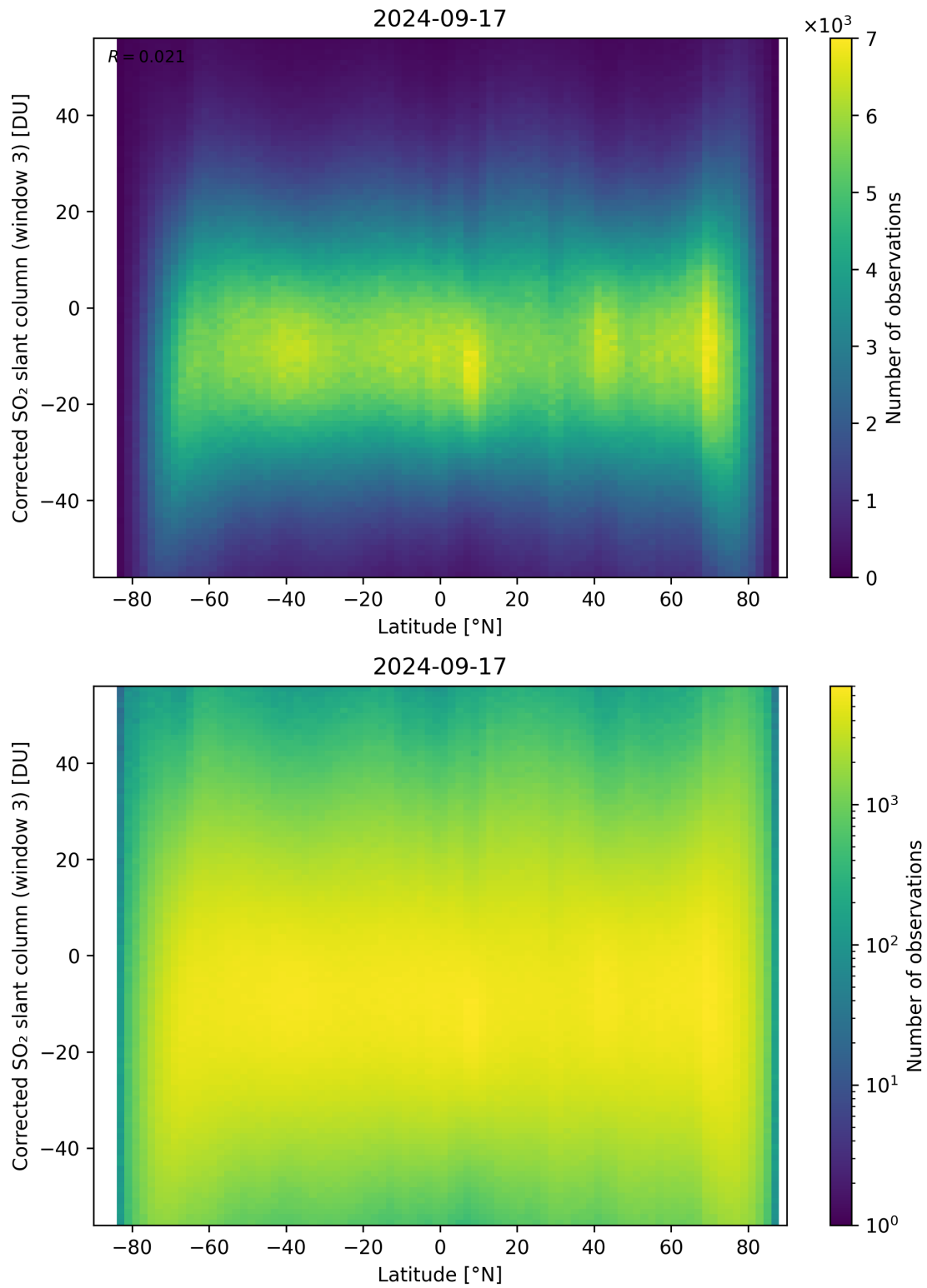
Figure 148: Scatter density plot of “Latitude” against “Corrected SO 2 slant column (window 3)” for 2024-09-17 to 2024-09-18.
