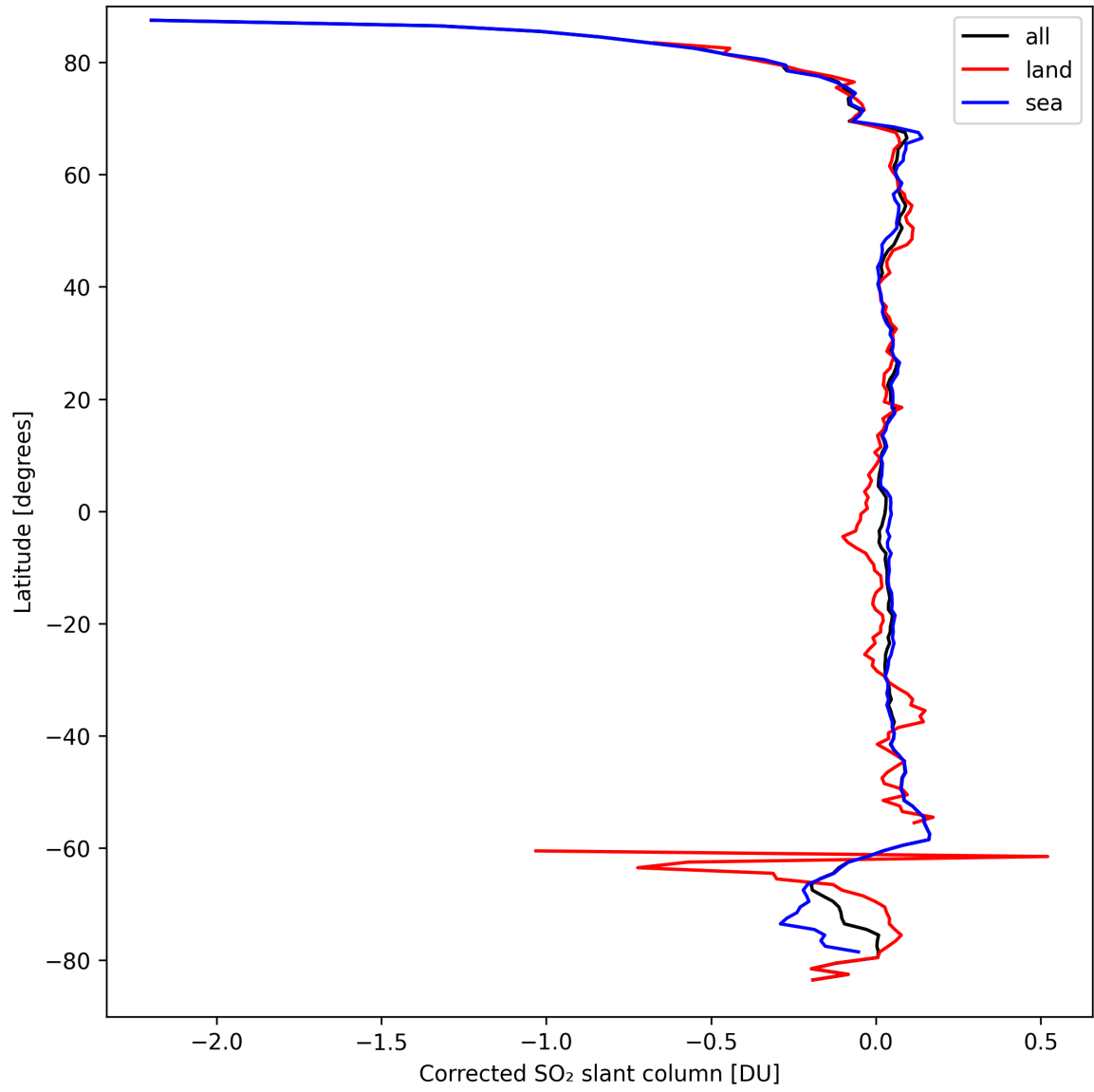
Figure 32: Zonal average of “Corrected SO 2 slant column” for 2024-09-17 to 2024-09-18.
