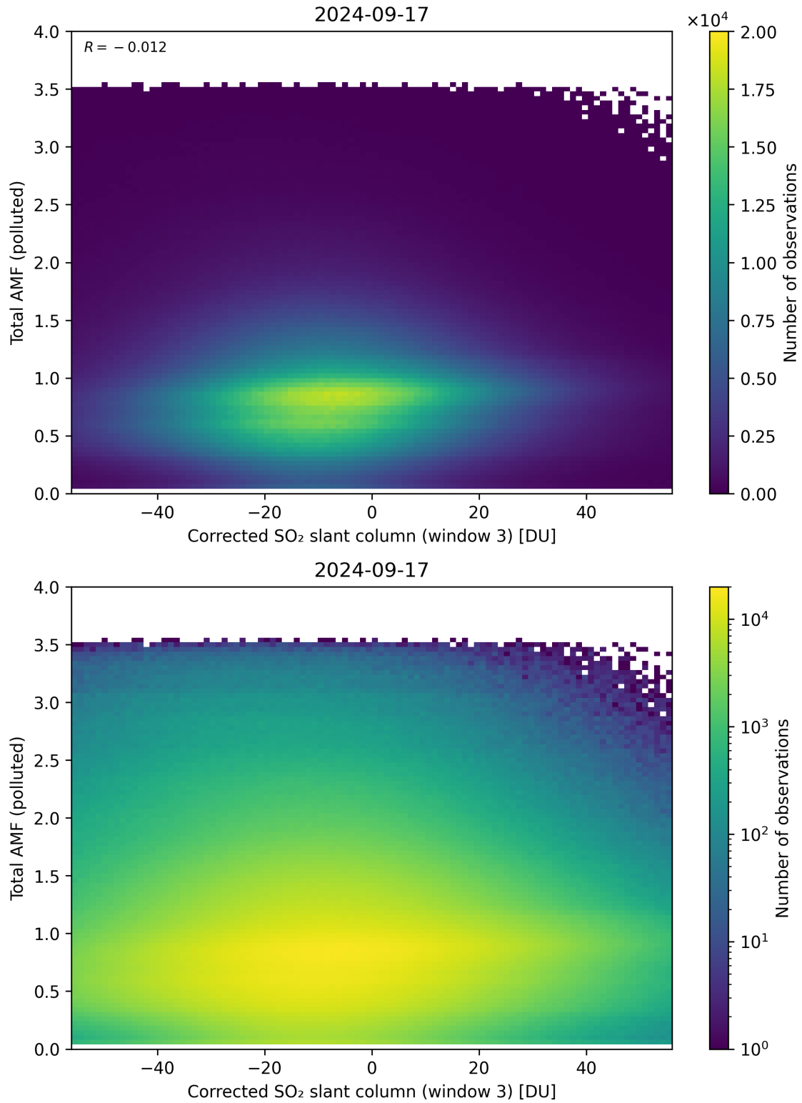
Figure 210: Scatter density plot of “Corrected SO 2 slant column (window 3)” against “Total AMF (polluted)” for 2024-09-17 to 2024-09-18.
