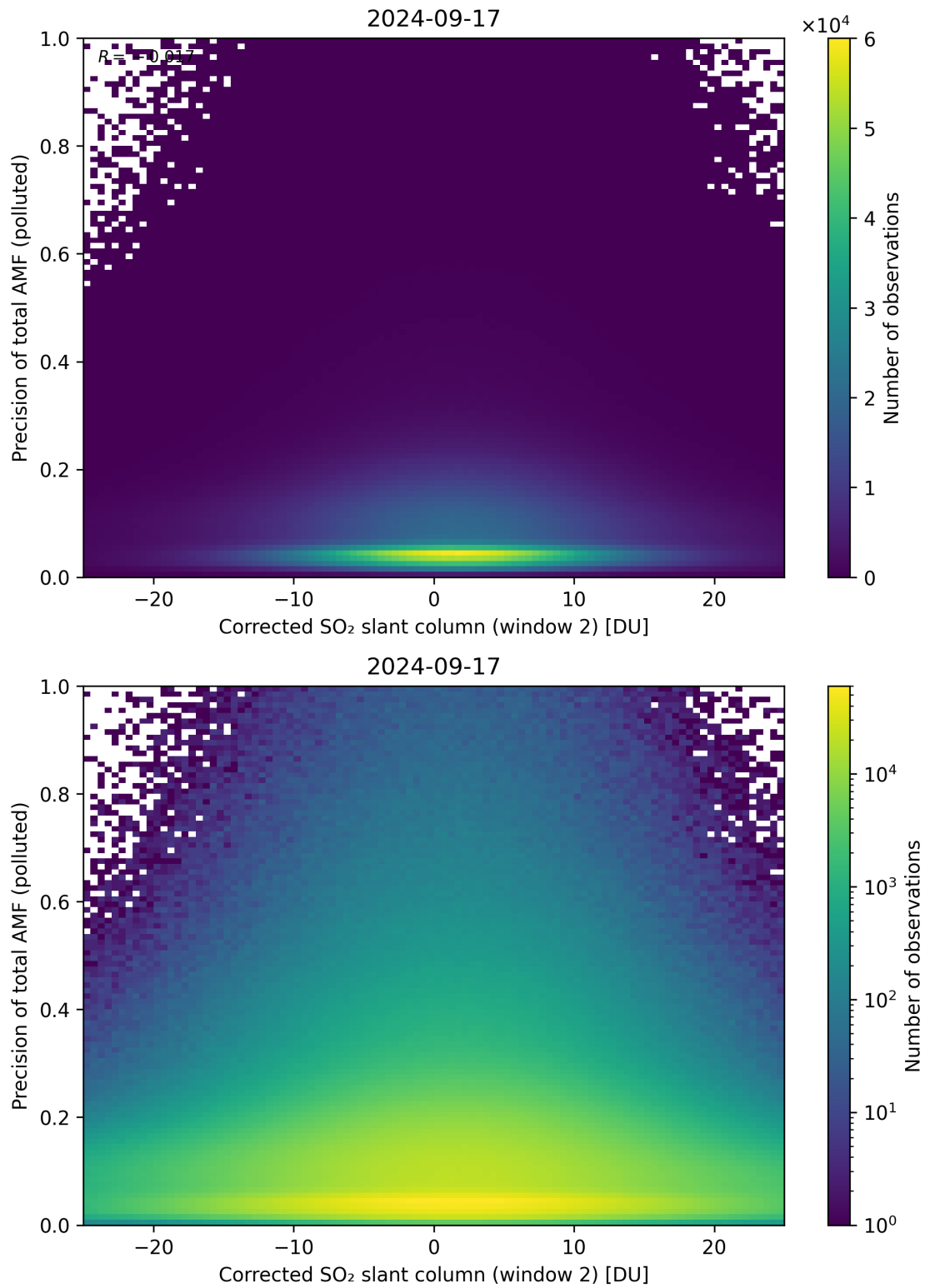
Figure 204: Scatter density plot of “Corrected SO 2 slant column (window 2)” against “Precision of total AMF (polluted)” for 2024-09-17 to 2024-09-18.
