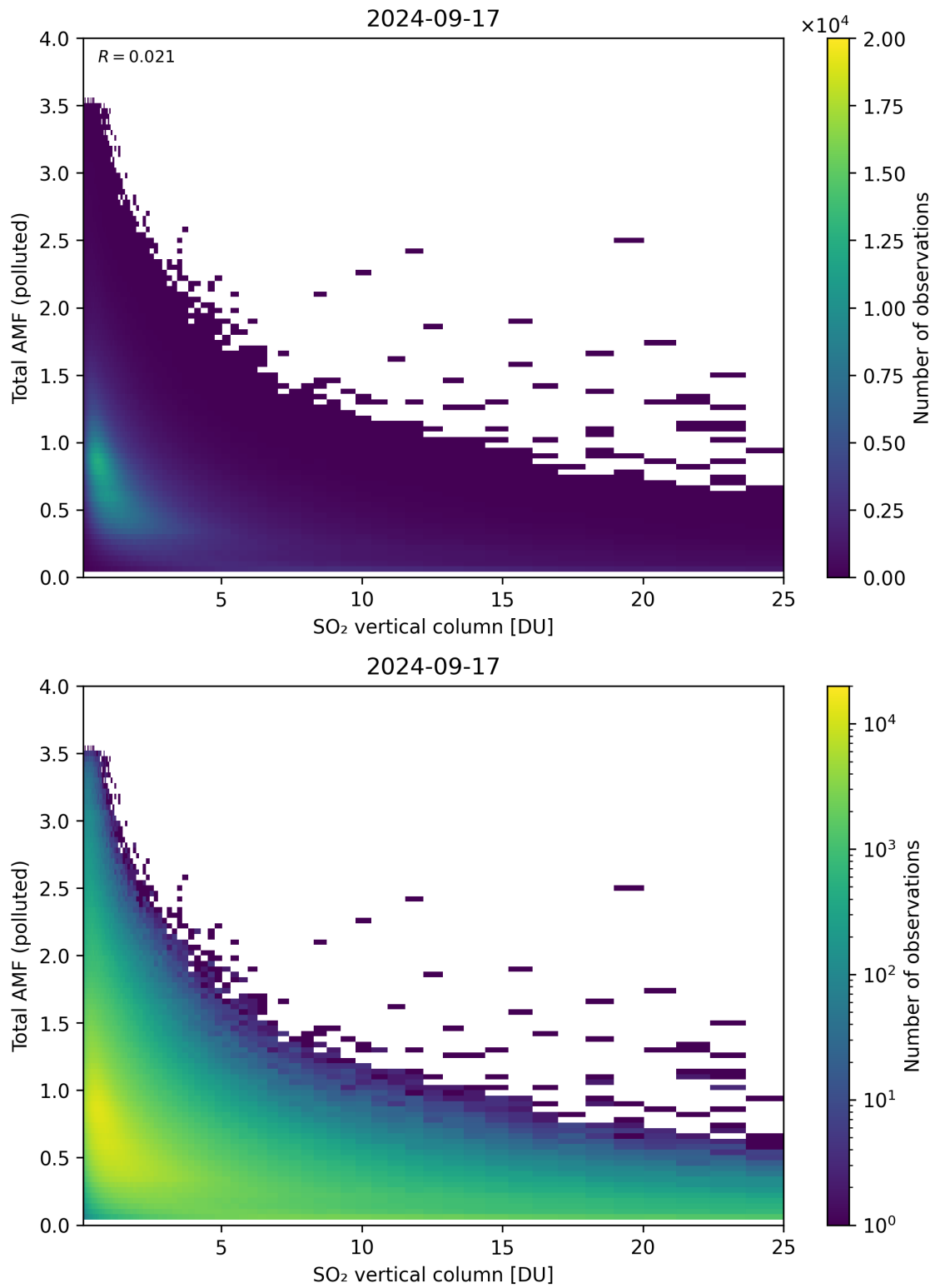
Figure 305: Scatter density plot of “SO 2 vertical column” against “Total AMF (polluted)” for 2024-09-17 to 2024-09-18.
