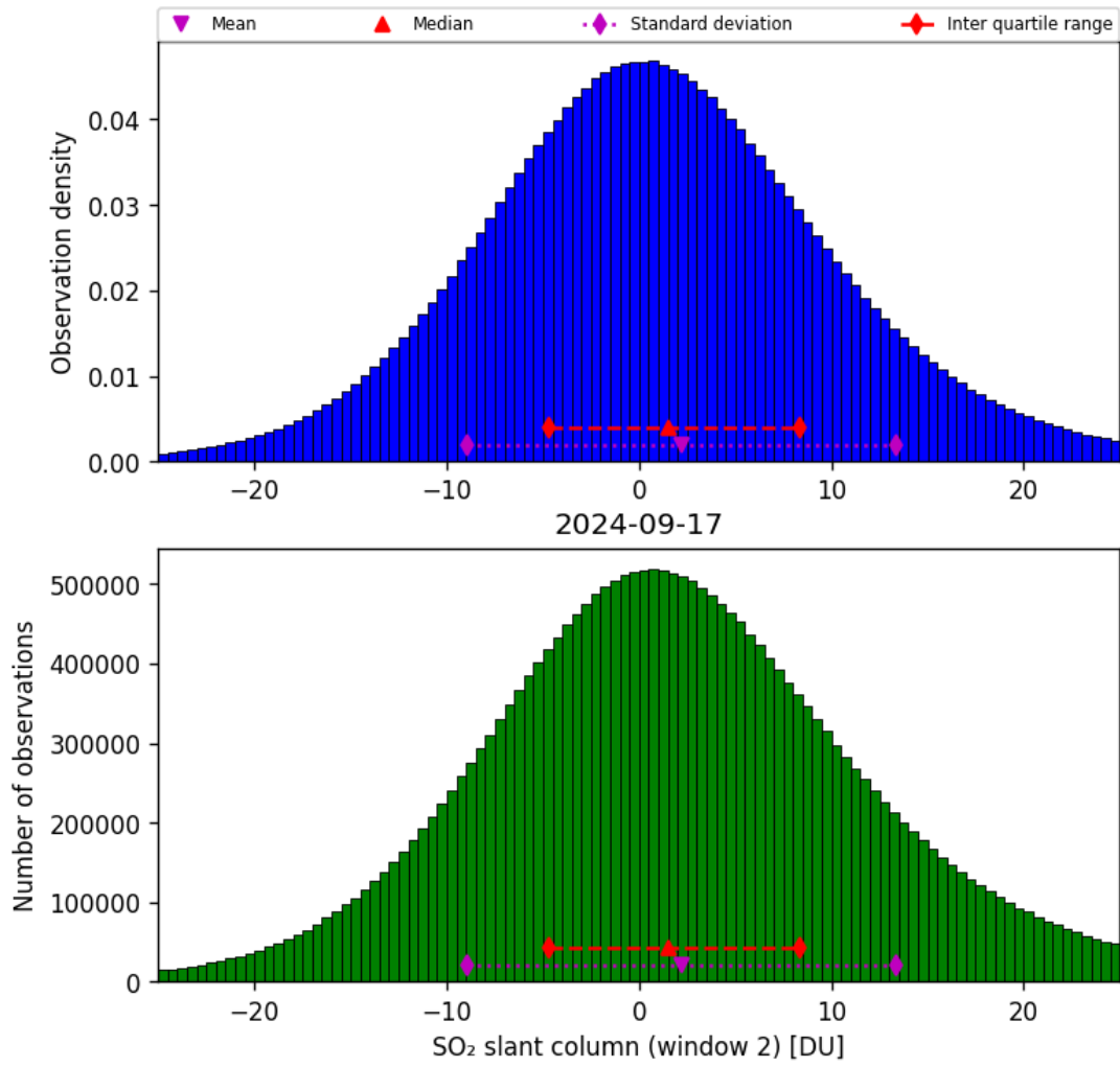
Figure 60: Histogram of “SO 2 slant column (window 2)” for 2024-09-17 to 2024-09-18
