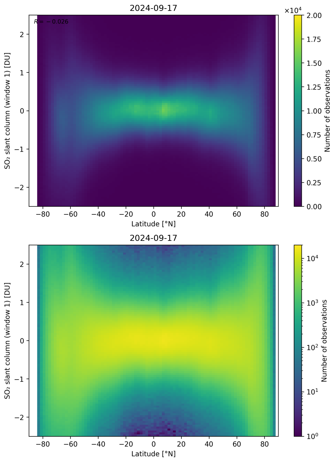
Figure 149: Scatter density plot of “Latitude” against “SO 2 slant column (window 1)” for 2024-09-17 to 2024-09-18.
