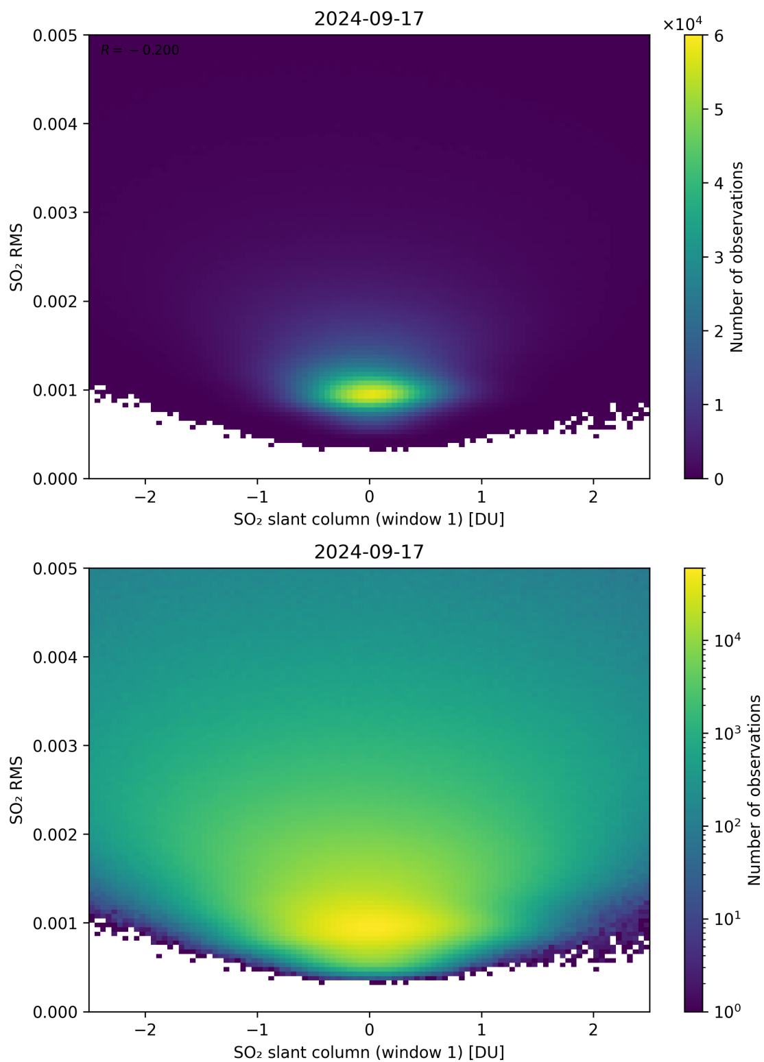
Figure 217: Scatter density plot of “SO 2 slant column (window 1)” against “SO 2 RMS” for 2024-09-17 to 2024-09-18.
