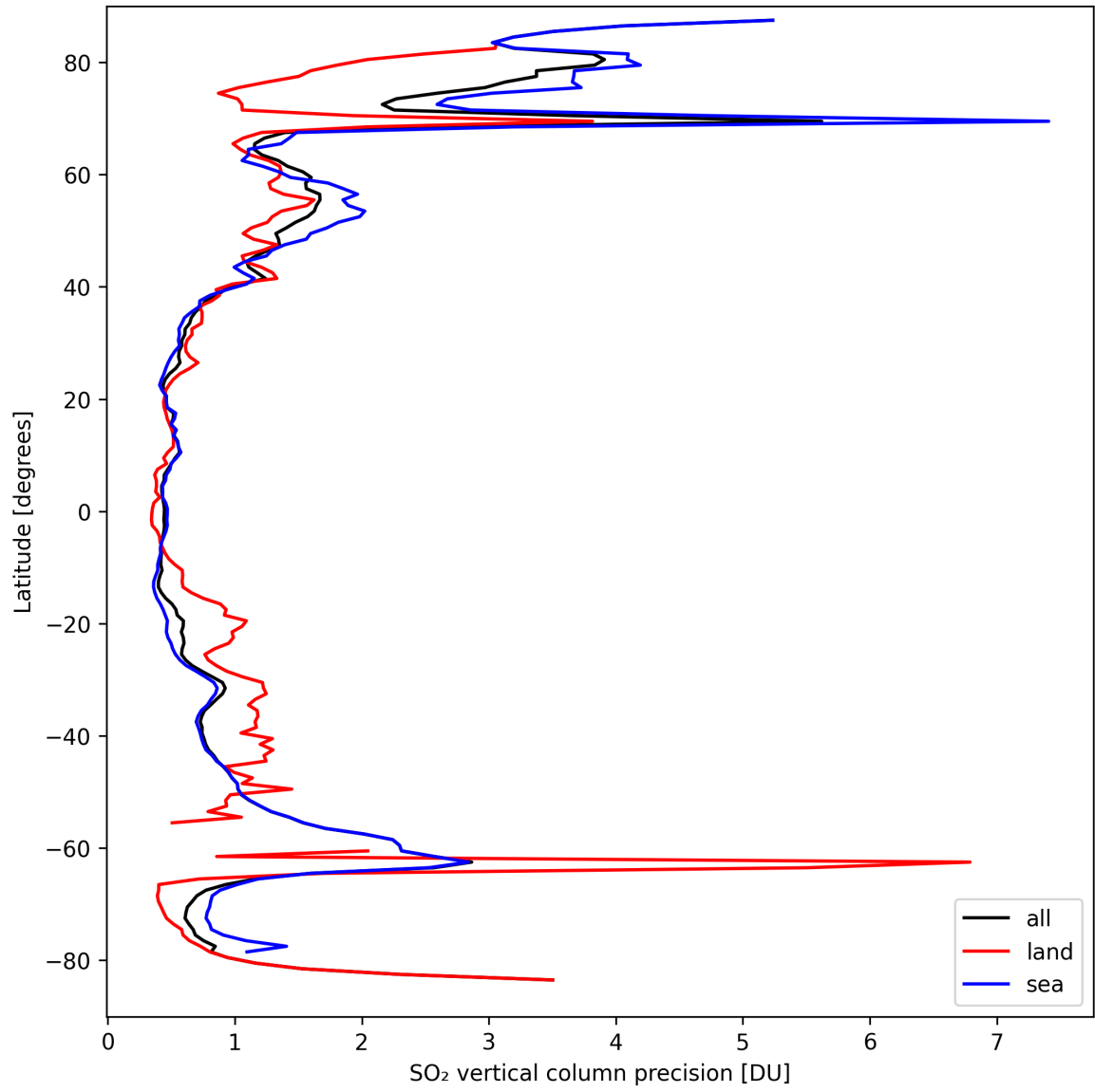
Figure 31: Zonal average of “SO 2 vertical column precision” for 2024-09-17 to 2024-09-18.
