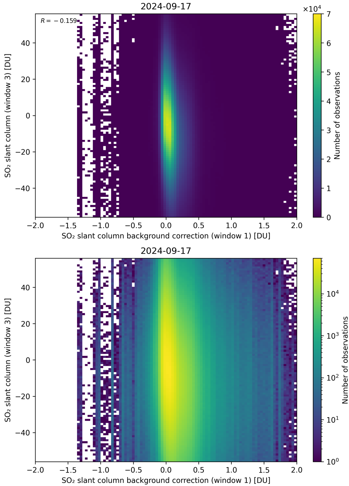
Figure 107: Scatter density plot of “SO 2 slant column background correction (window 1)” against “SO 2 slant column (window 3)” for 2024-09-17 to 2024-09-18.
