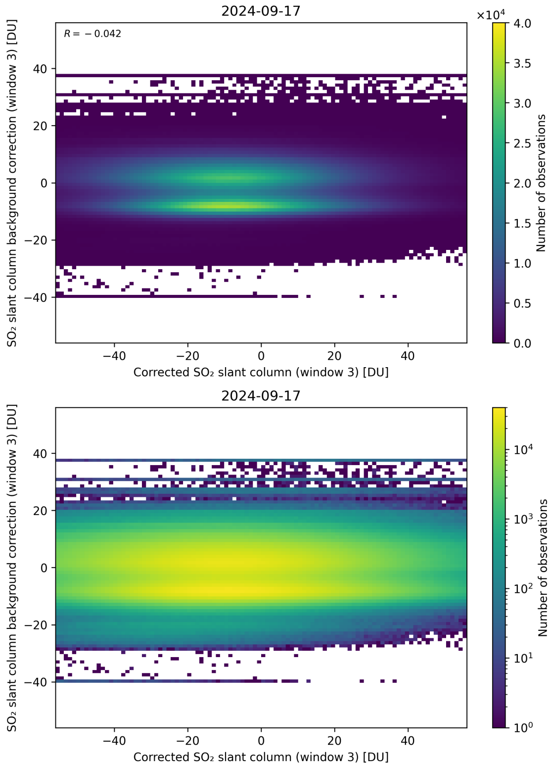
Figure 205: Scatter density plot of “Corrected SO 2 slant column (window 3)” against “SO 2 slant column background correction (window 3)” for 2024-09-17 to 2024-09-18.
