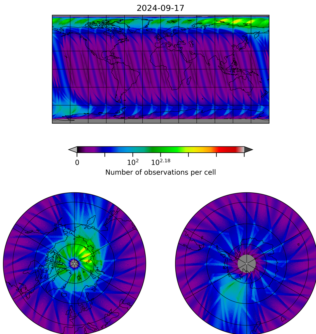
Figure 28: Map of the number of observations for 2024-09-17 to 2024-09-18
