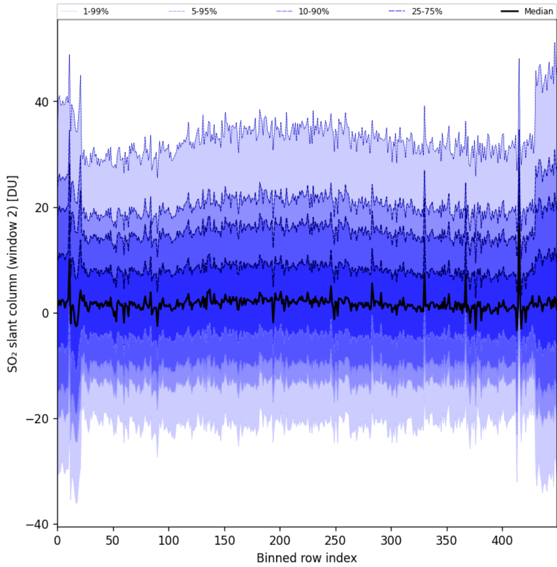
Figure 83: Along track statistics of “SO 2 slant column (window 2)” for 2024-09-17 to 2024-09-18
