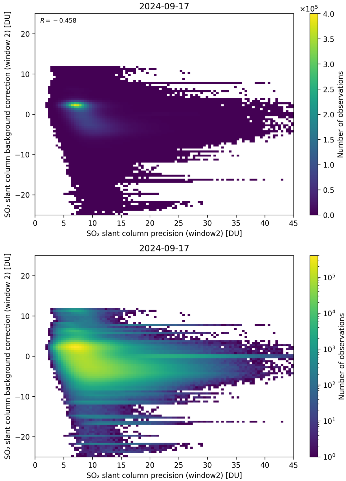
Figure 241: Scatter density plot of “SO 2 slant column precision (window2)” against “SO 2 slant column background correction (window 2)” for 2024-09-17 to 2024-09-18.
