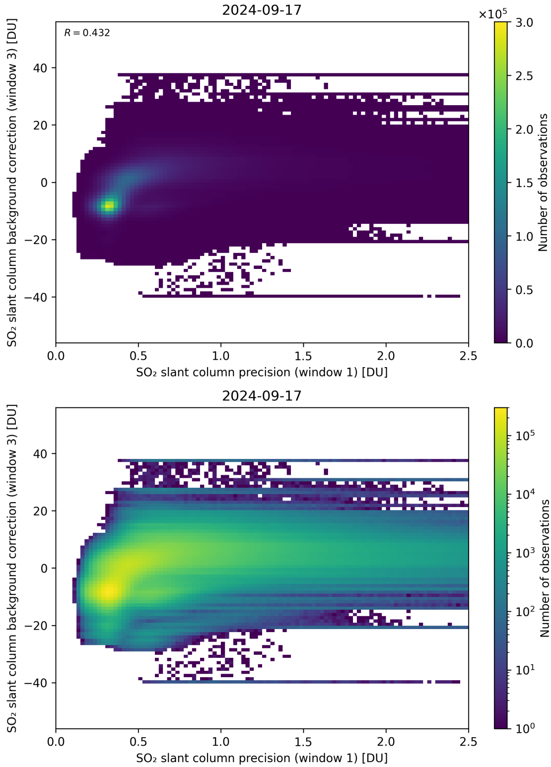
Figure 220: Scatter density plot of “SO 2 slant column precision (window 1)” against “SO 2 slant column background correction (window 3)” for 2024-09-17 to 2024-09-18.
