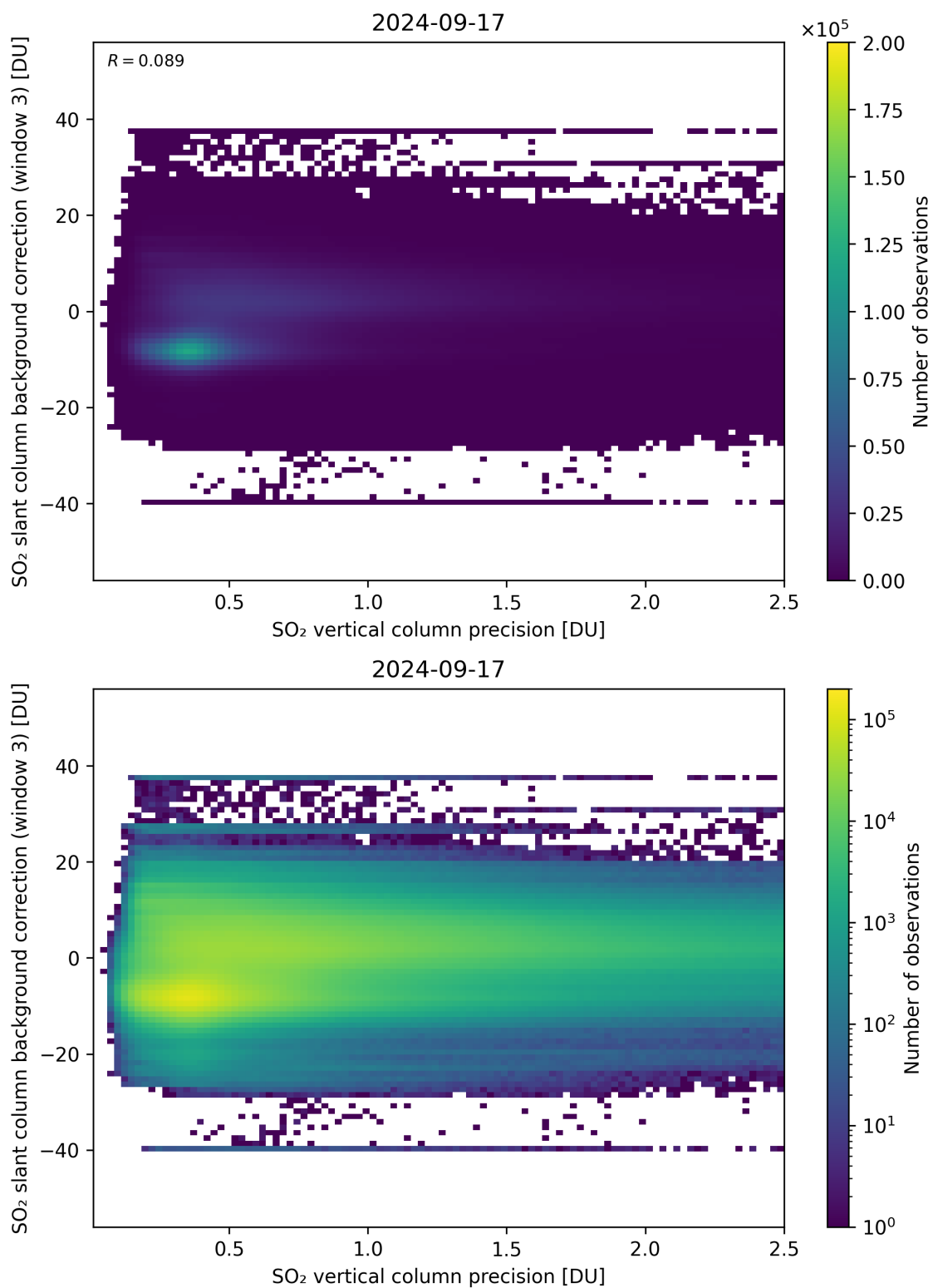
Figure 281: Scatter density plot of “SO 2 vertical column precision” against “SO 2 slant column background correction (window 3)” for 2024-09-17 to 2024-09-18.
