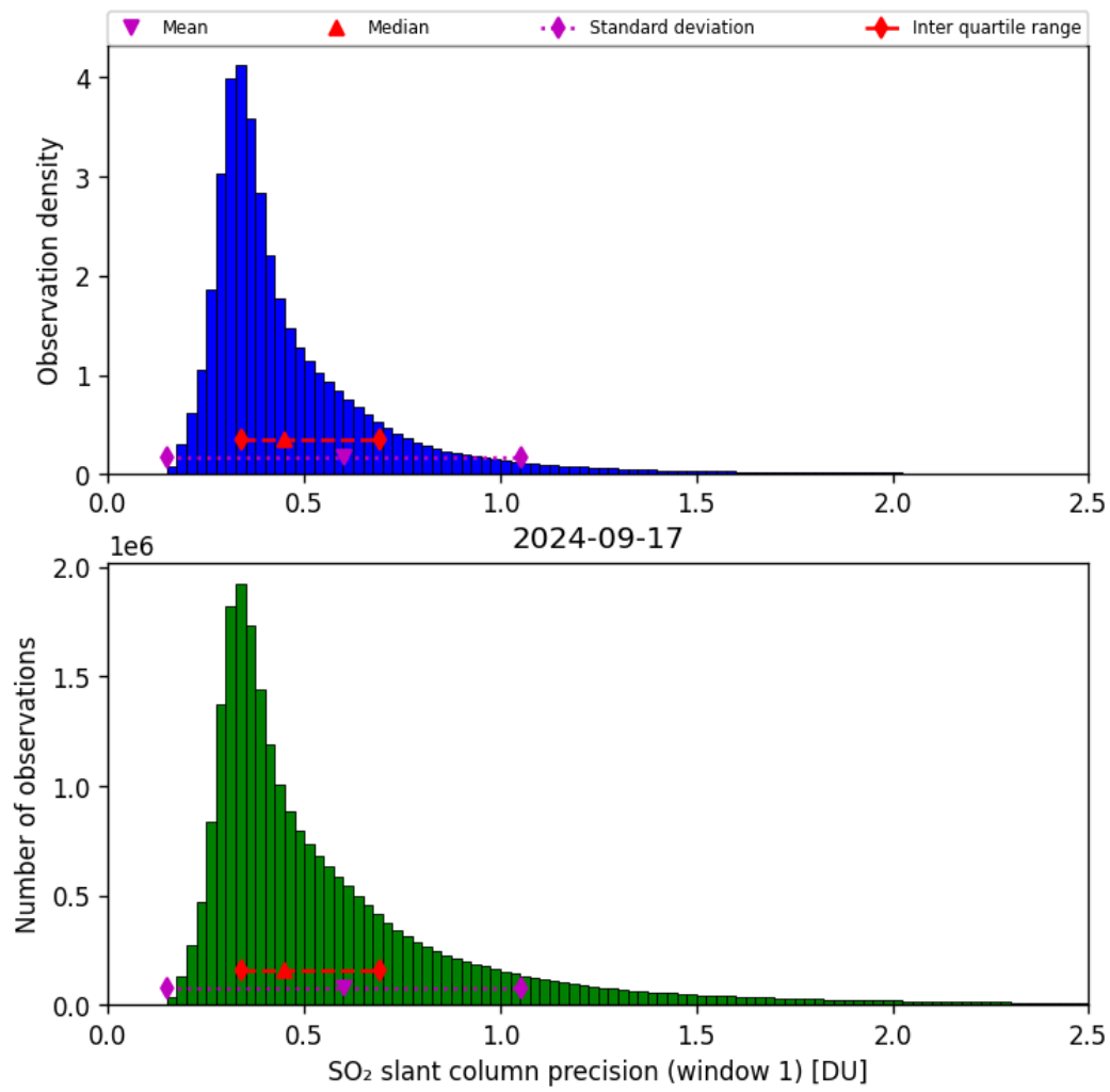
Figure 57: Histogram of “SO 2 slant column precision (window 1)” for 2024-09-17 to 2024-09-18
