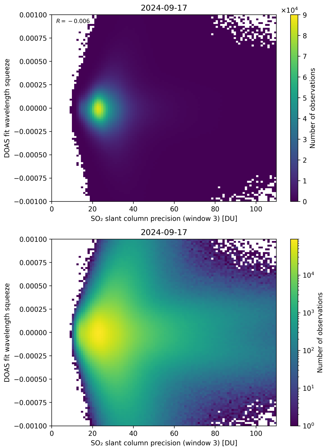
Figure 259: Scatter density plot of “SO 2 slant column precision (window 3)” against “DOAS fit wavelength squeeze” for 2024-09-17 to 2024-09-18.
