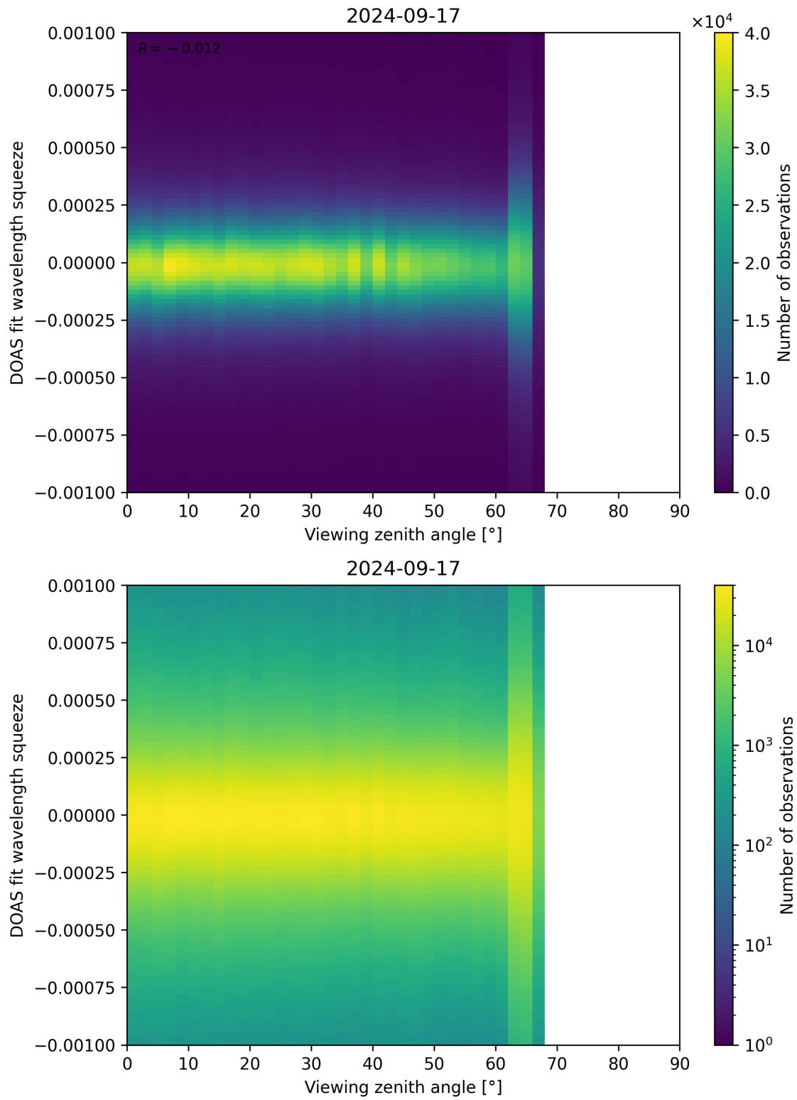
Figure 312: Scatter density plot of “Viewing zenith angle” against “DOAS fit wavelength squeeze” for 2024-09-17 to 2024-09-18.
