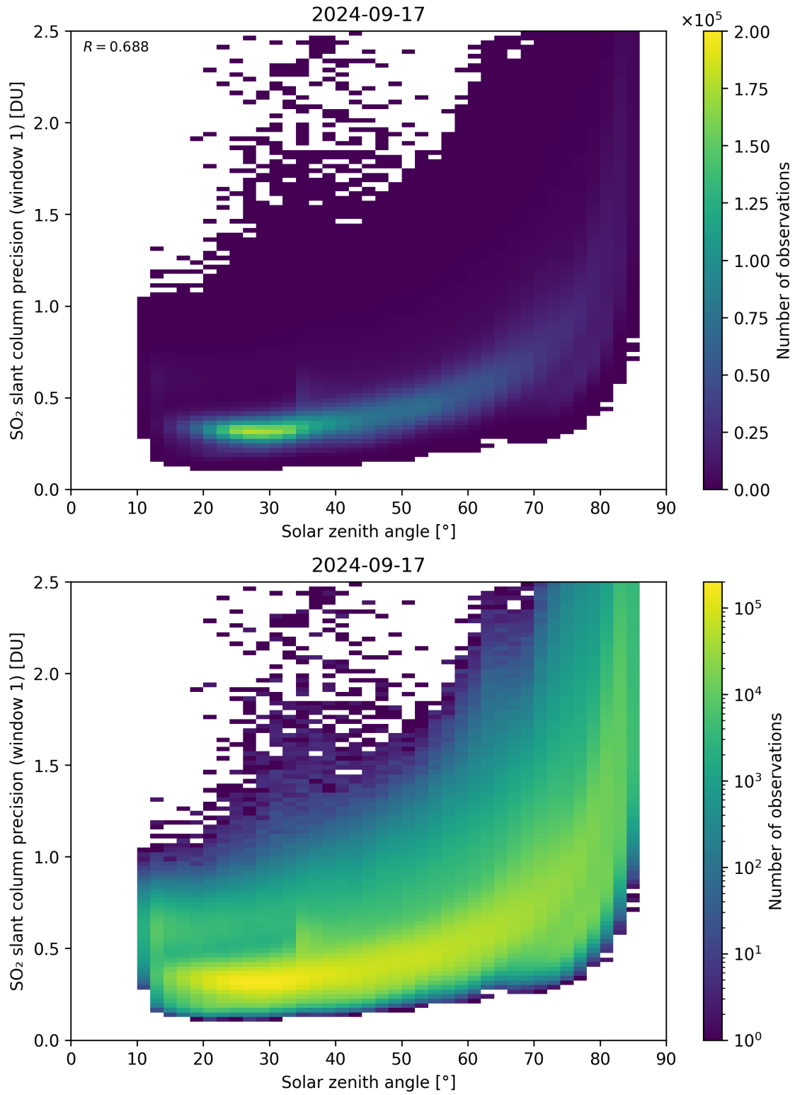
Figure 170: Scatter density plot of “Solar zenith angle” against “SO 2 slant column precision (window 1)” for 2024-09-17 to 2024-09-18.
