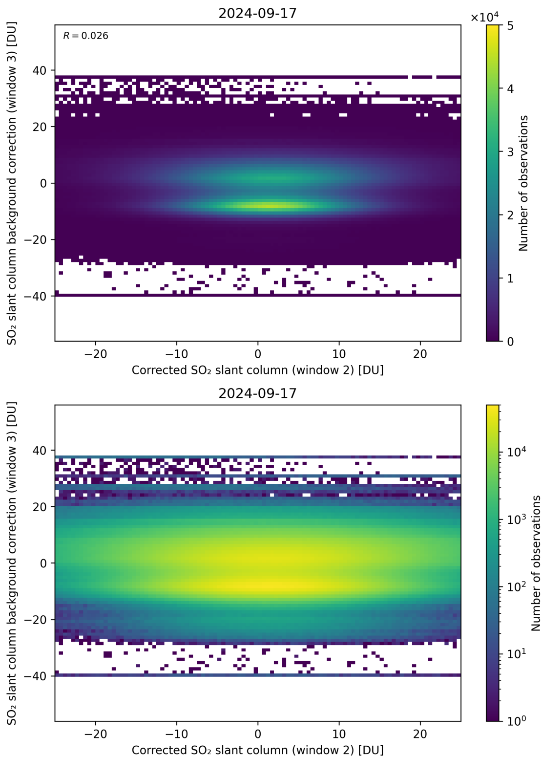
Figure 195: Scatter density plot of “Corrected SO 2 slant column (window 2)” against “SO 2 slant column background correction (window 3)” for 2024-09-17 to 2024-09-18.
