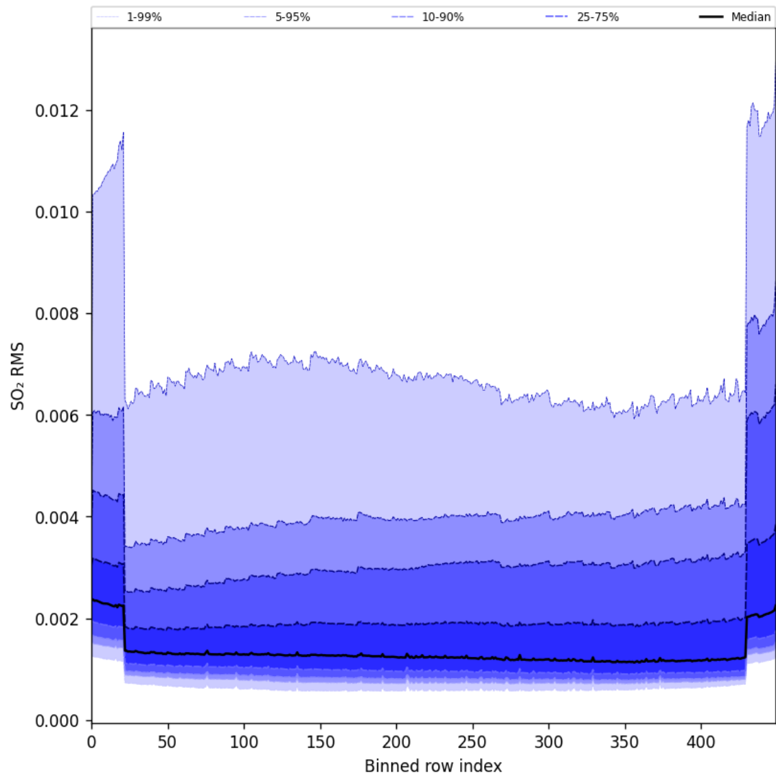
Figure 93: Along track statistics of “SO 2 RMS” for 2024-09-17 to 2024-09-18
