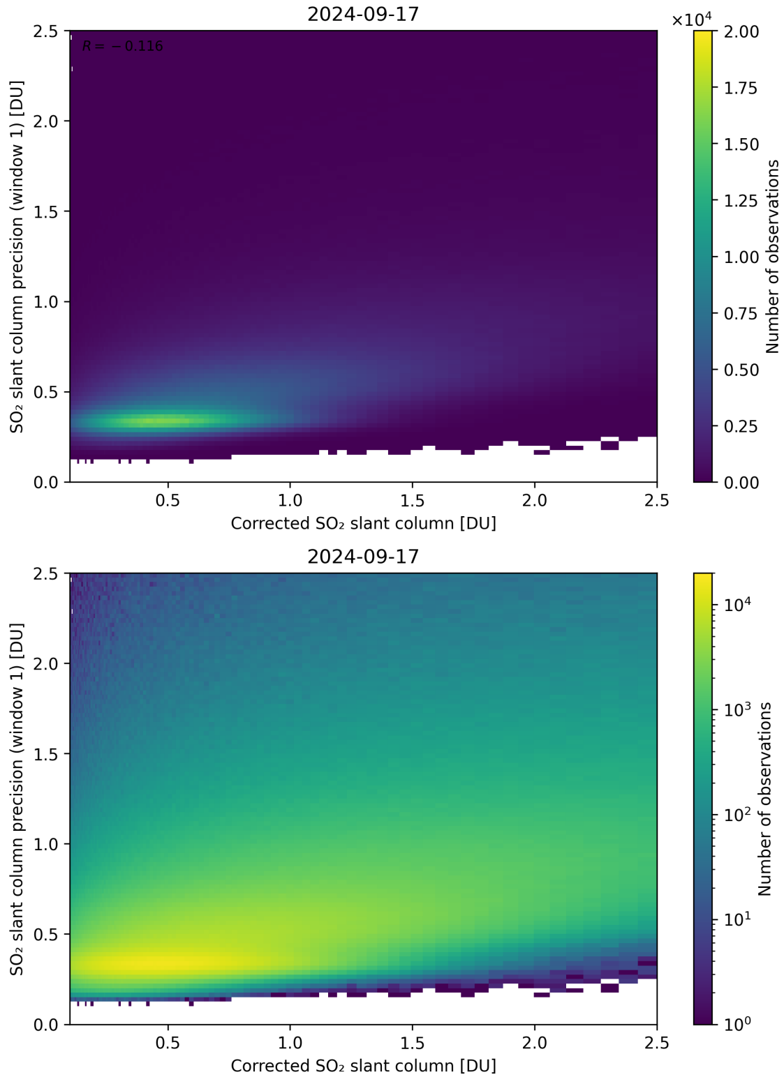
Figure 188: Scatter density plot of “Corrected SO 2 slant column” against “SO 2 slant column precision (window 1)” for 2024-09-17 to 2024-09-18.
