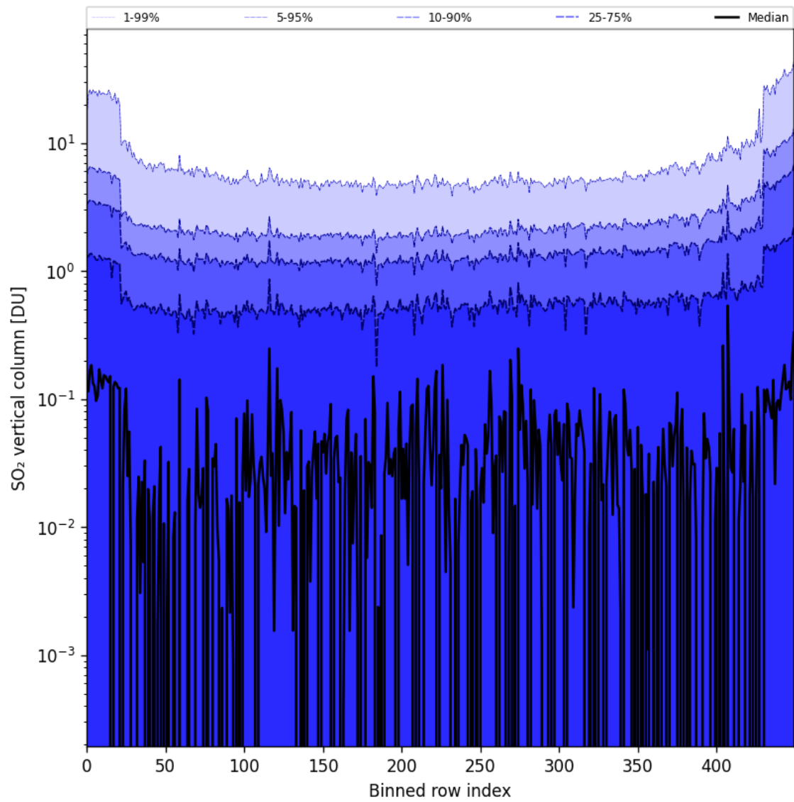
Figure 76: Along track statistics of “SO 2 vertical column” for 2024-09-17 to 2024-09-18
