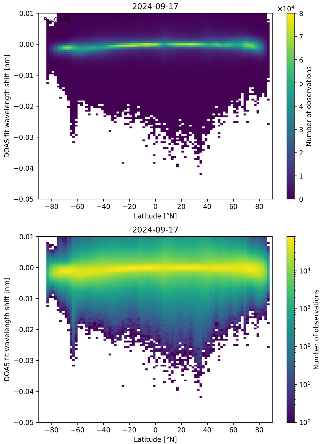
Figure 142: Scatter density plot of “Latitude” against “DOAS fit wavelength shift” for 2024-09-17 to 2024-09-18.
