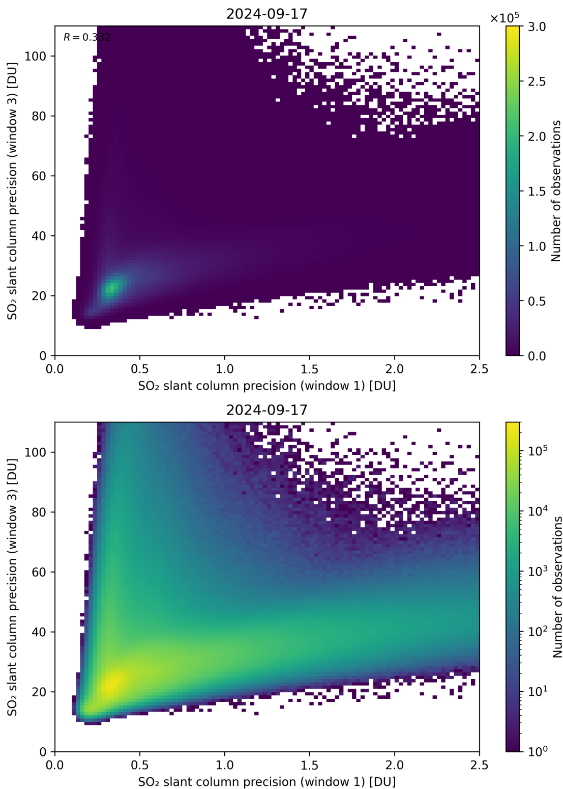
Figure 229: Scatter density plot of “SO 2 slant column precision (window 1)” against “SO 2 slant column precision (window 3)” for 2024-09-17 to 2024-09-18.
