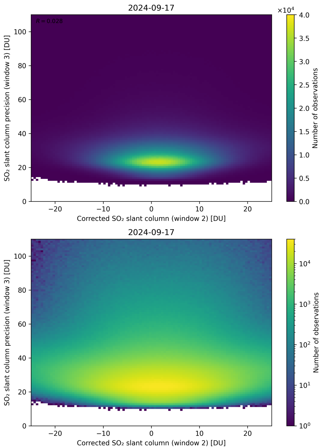
Figure 202: Scatter density plot of “Corrected SO 2 slant column (window 2)” against “SO 2 slant column precision (window 3)” for 2024-09-17 to 2024-09-18.
