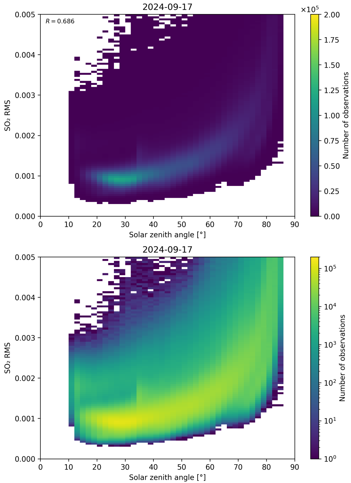
Figure 163: Scatter density plot of “Solar zenith angle” against “SO 2 RMS” for 2024-09-17 to 2024-09-18.
