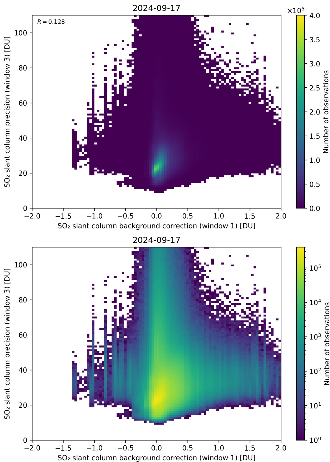
Figure 108: Scatter density plot of “SO 2 slant column background correction (window 1)” against “SO 2 slant column precision (window 3)” for 2024-09-17 to 2024-09-18.
