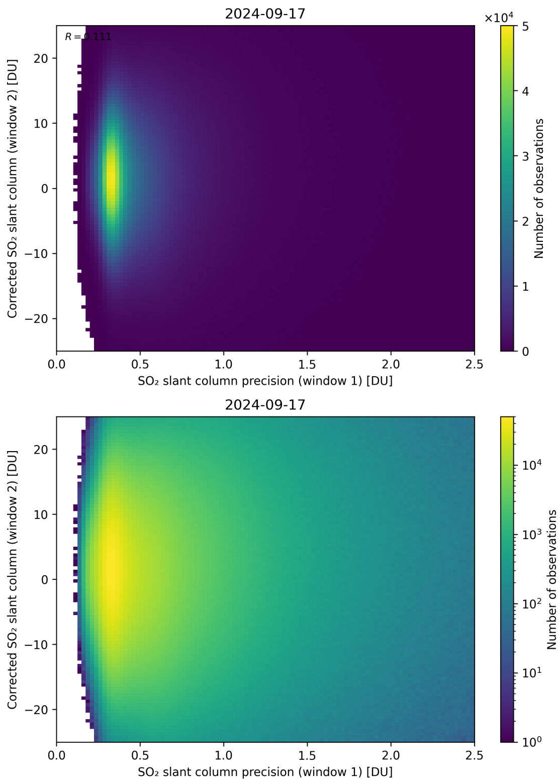
Figure 225: Scatter density plot of “SO 2 slant column precision (window 1)” against “Corrected SO 2 slant column (window 2)” for 2024-09-17 to 2024-09-18.
