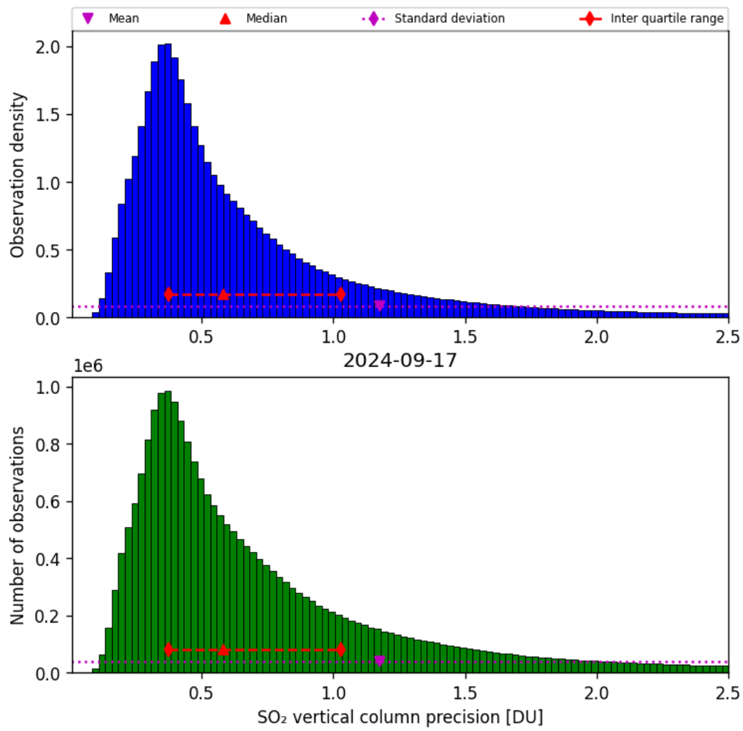
Figure 54: Histogram of “SO 2 vertical column precision” for 2024-09-17 to 2024-09-18
