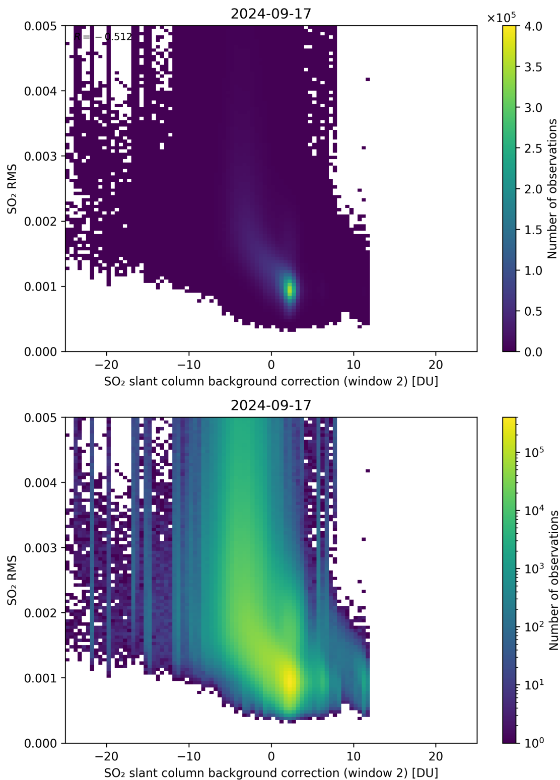
Figure 114: Scatter density plot of “SO 2 slant column background correction (window 2)” against “SO 2 RMS” for 2024-09-17 to 2024-09-18.
