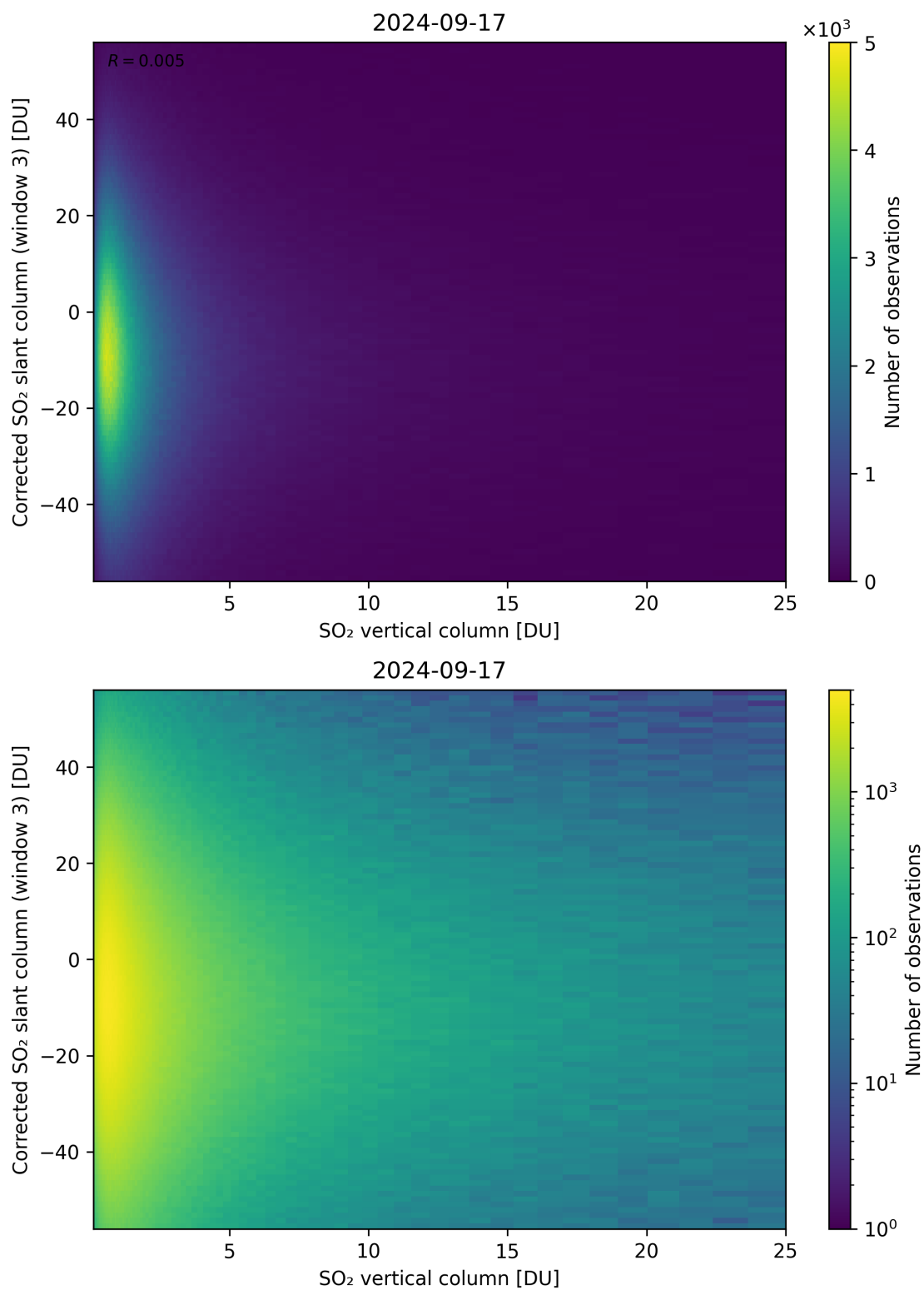
Figure 299: Scatter density plot of “SO 2 vertical column” against “Corrected SO 2 slant column (window 3)” for 2024-09-17 to 2024-09-18.
