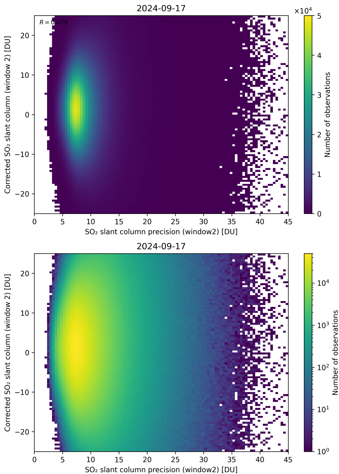
Figure 247: Scatter density plot of “SO 2 slant column precision (window2)” against “Corrected SO 2 slant column (window 2)” for 2024-09-17 to 2024-09-18.
