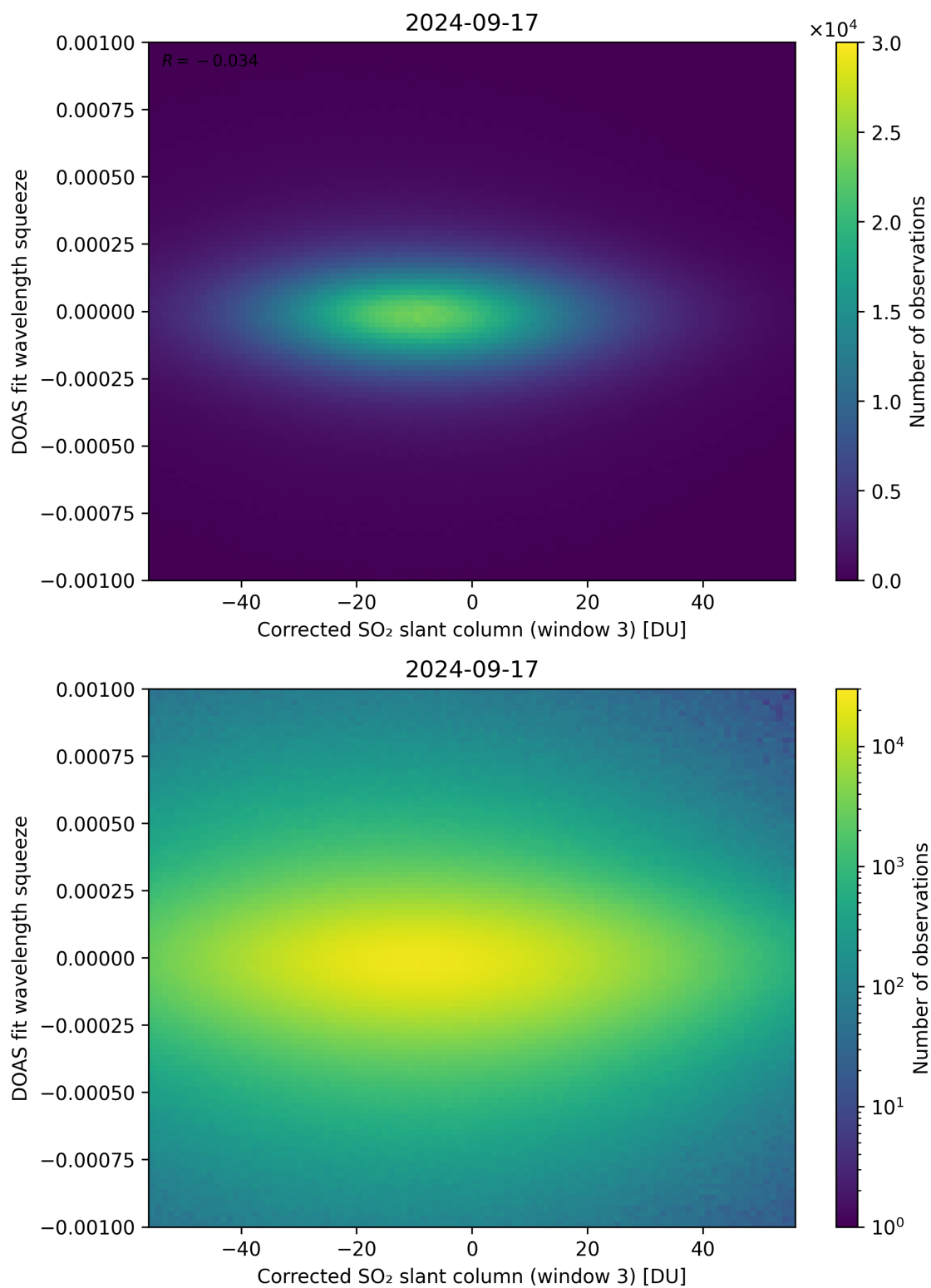
Figure 207: Scatter density plot of “Corrected SO 2 slant column (window 3)” against “DOAS fit wavelength squeeze” for 2024-09-17 to 2024-09-18.
