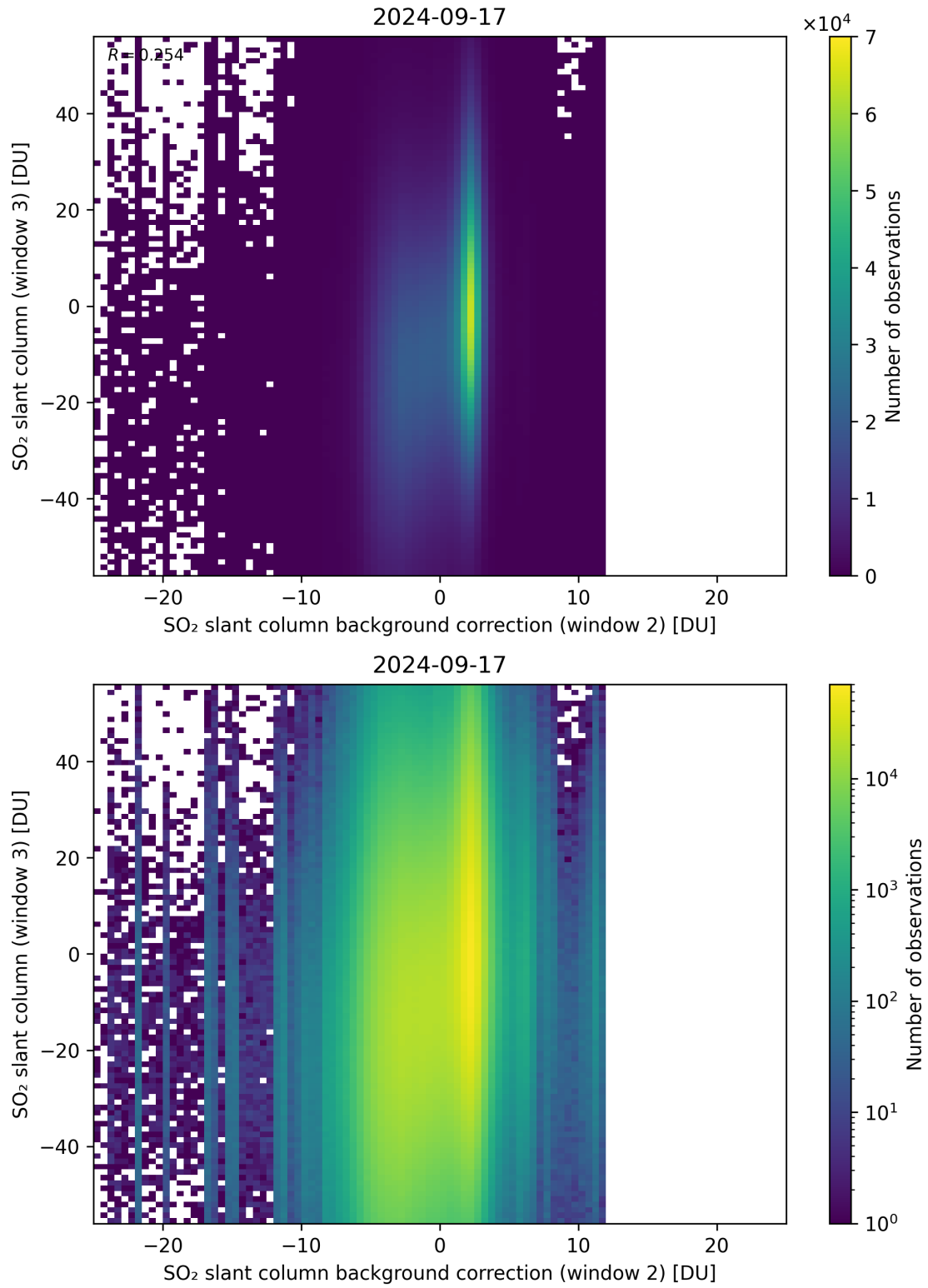
Figure 117: Scatter density plot of “SO 2 slant column background correction (window 2)” against “SO 2 slant column (window 3)” for 2024-09-17 to 2024-09-18.
