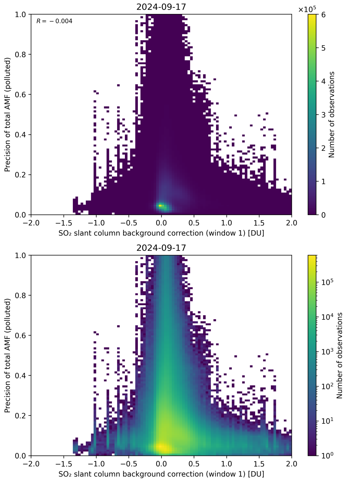
Figure 110: Scatter density plot of “SO 2 slant column background correction (window 1)” against “Precision of total AMF (polluted)” for 2024-09-17 to 2024-09-18.
