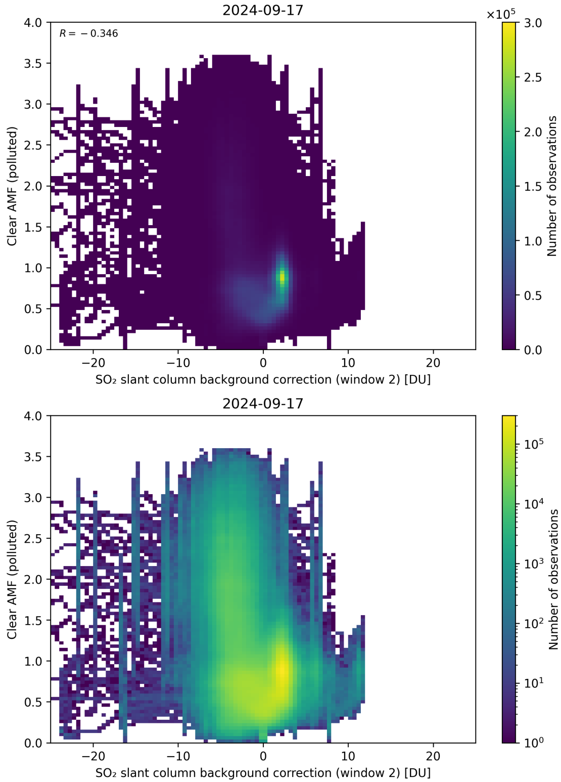
Figure 115: Scatter density plot of “SO 2 slant column background correction (window 2)” against “Clear AMF (polluted)” for 2024-09-17 to 2024-09-18.
