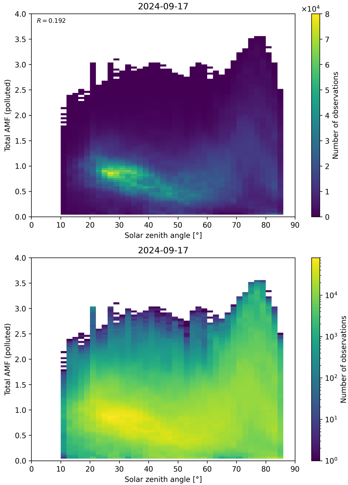
Figure 174: Scatter density plot of “Solar zenith angle” against “Total AMF (polluted)” for 2024-09-17 to 2024-09-18.
