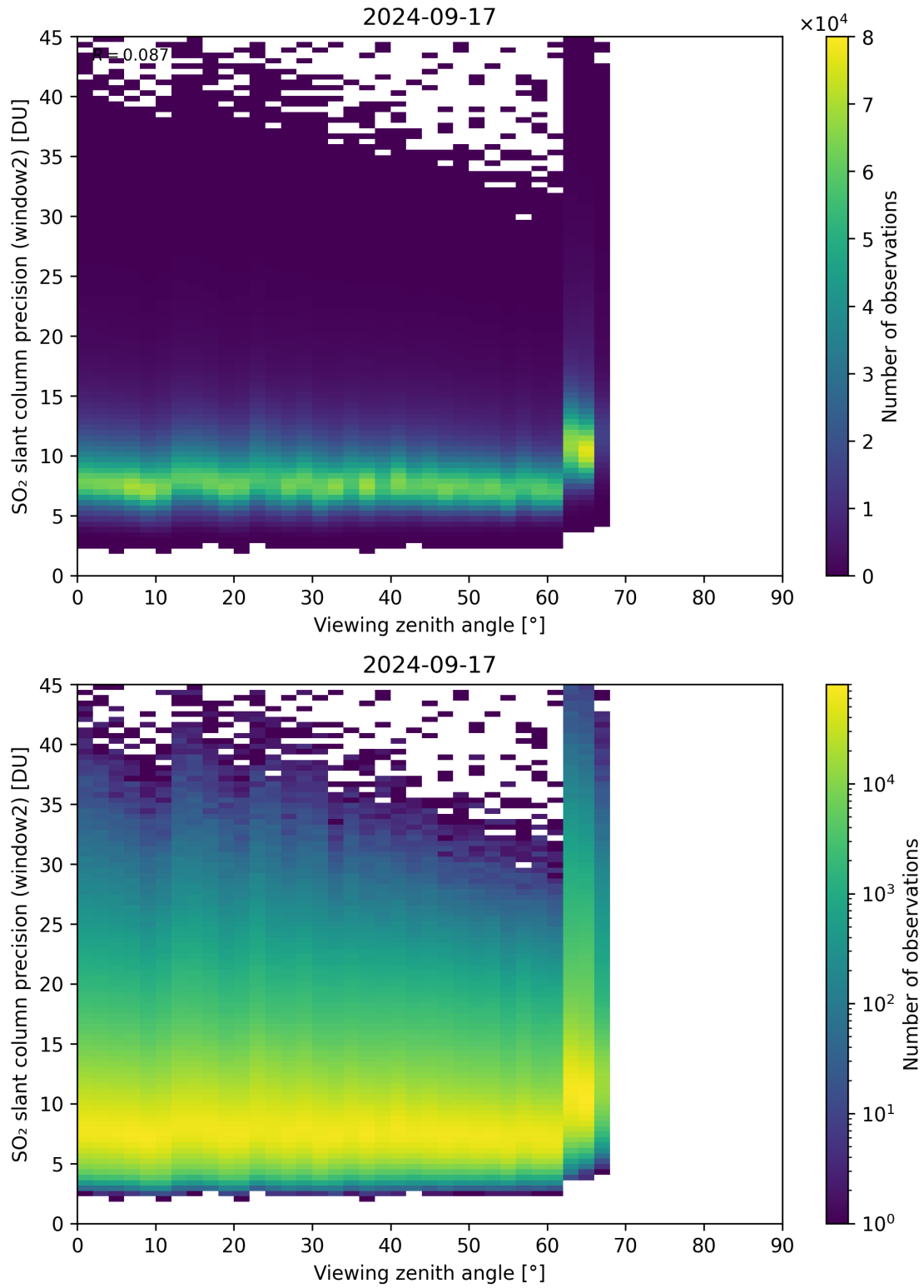
Figure 322: Scatter density plot of “Viewing zenith angle” against “SO 2 slant column precision (window2)” for 2024-09-17 to 2024-09-18.
