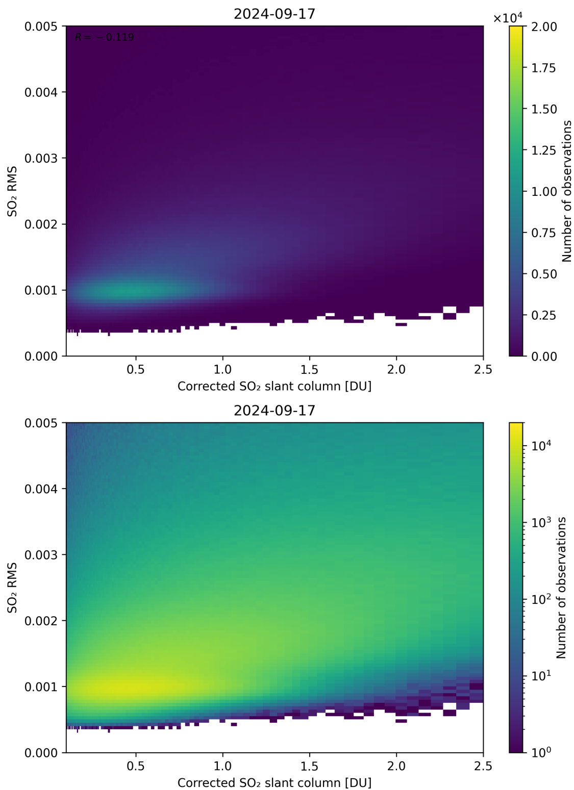
Figure 183: Scatter density plot of “Corrected SO 2 slant column” against “SO 2 RMS” for 2024-09-17 to 2024-09-18.
