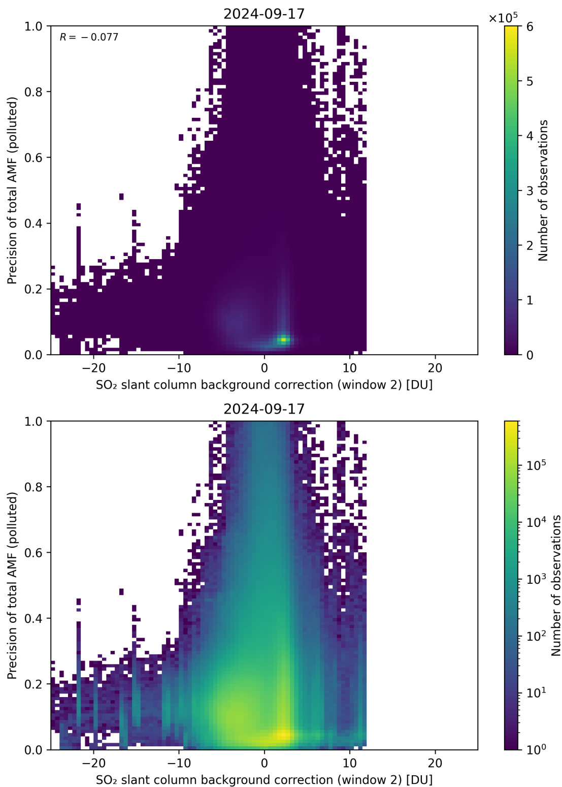
Figure 120: Scatter density plot of “SO 2 slant column background correction (window 2)” against “Precision of total AMF (polluted)” for 2024-09-17 to 2024-09-18.
