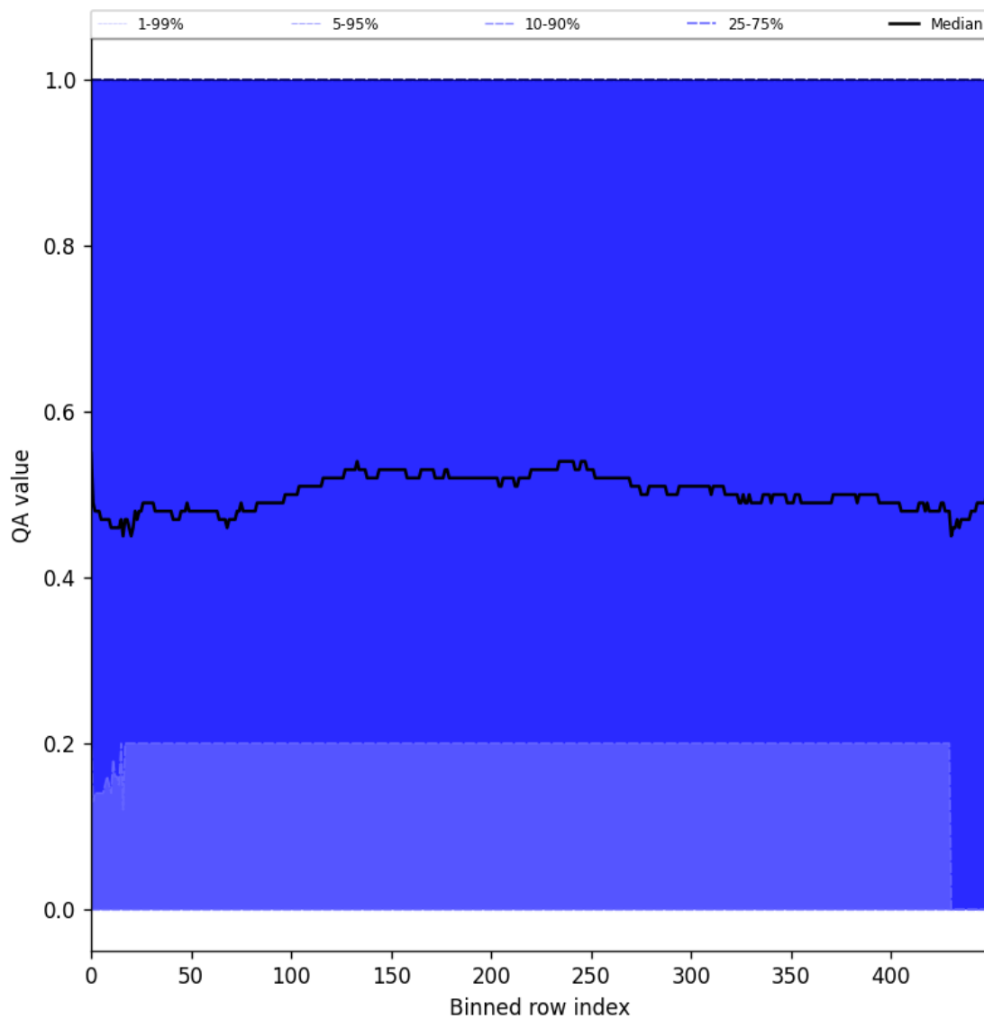
Figure 75: Along track statistics of “QA value” for 2024-09-17 to 2024-09-18
