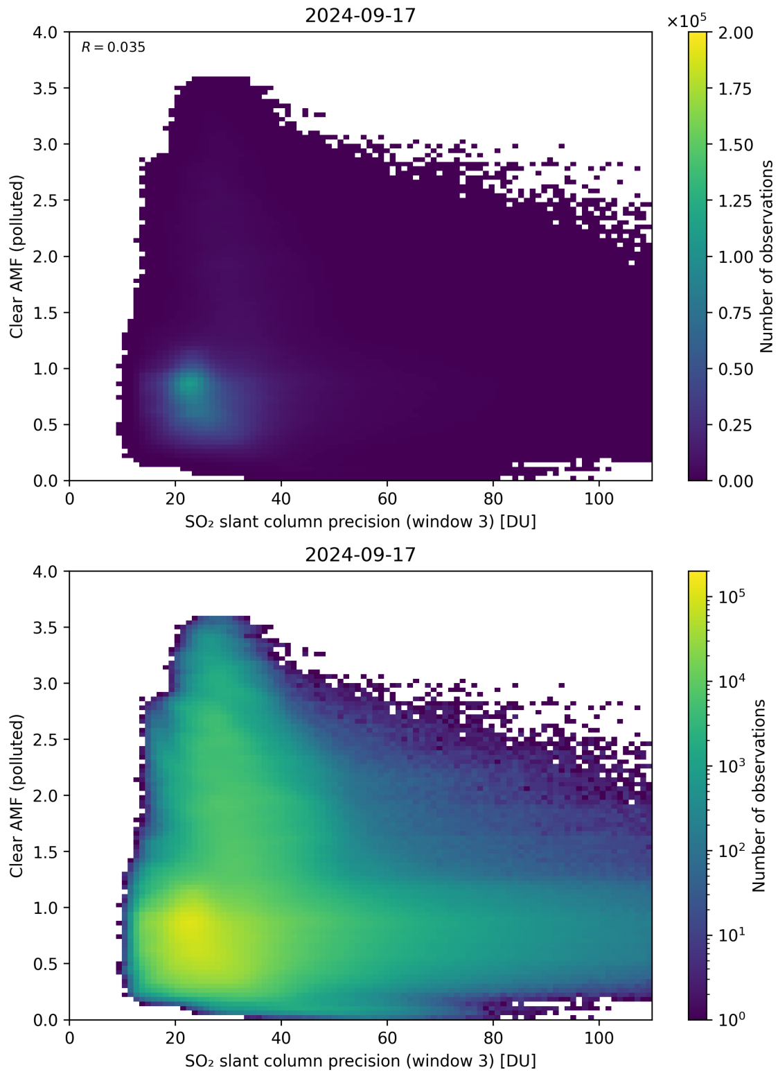
Figure 261: Scatter density plot of “SO 2 slant column precision (window 3)” against “Clear AMF (polluted)” for 2024-09-17 to 2024-09-18.
