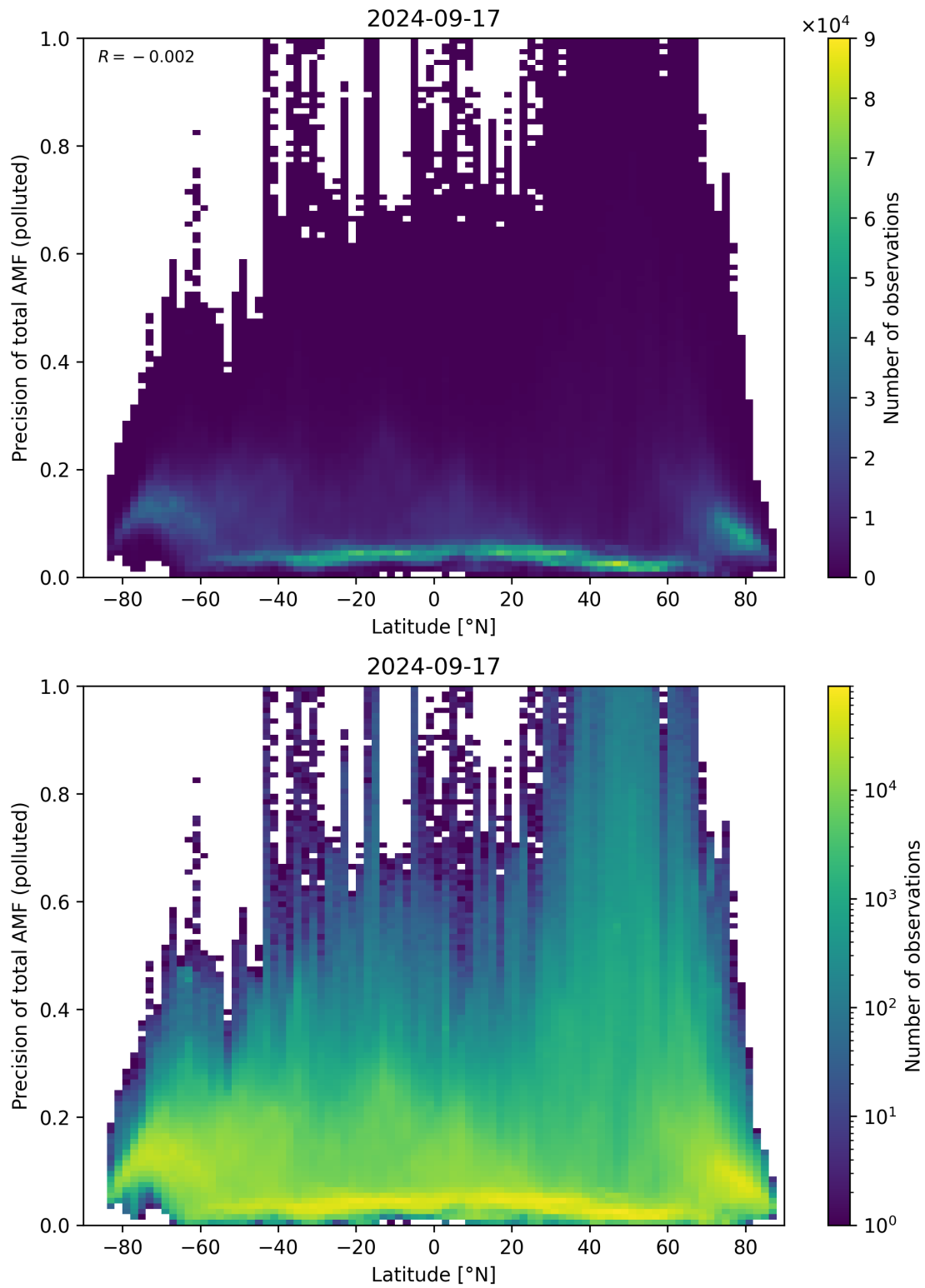
Figure 155: Scatter density plot of “Latitude” against “Precision of total AMF (polluted)” for 2024-09-17 to 2024-09-18.
