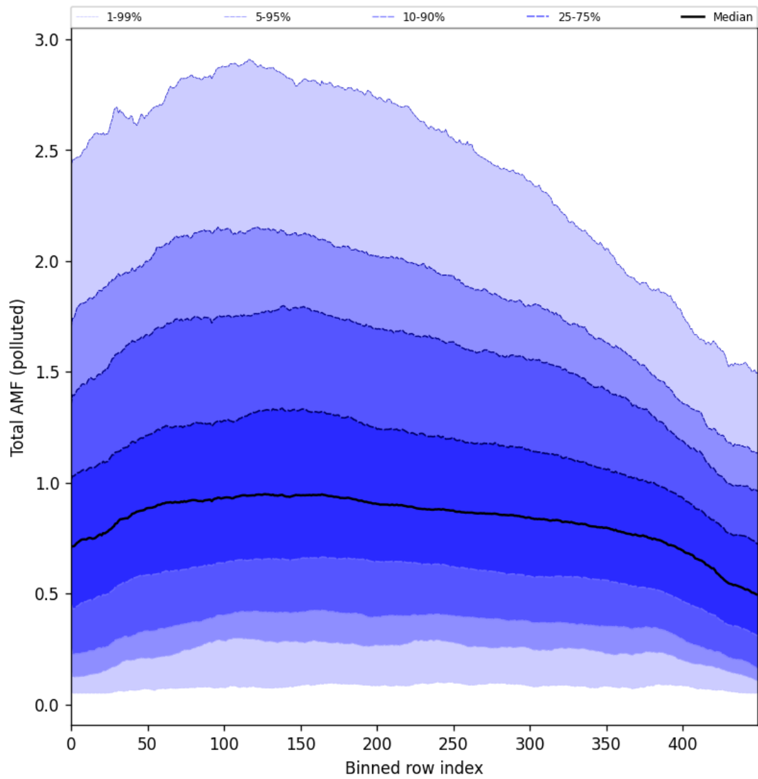
Figure 94: Along track statistics of “Total AMF (polluted)” for 2024-09-17 to 2024-09-18
