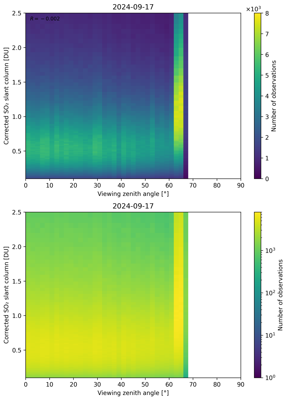
Figure 317: Scatter density plot of “Viewing zenith angle” against “Corrected SO 2 slant column” for 2024-09-17 to 2024-09-18.
