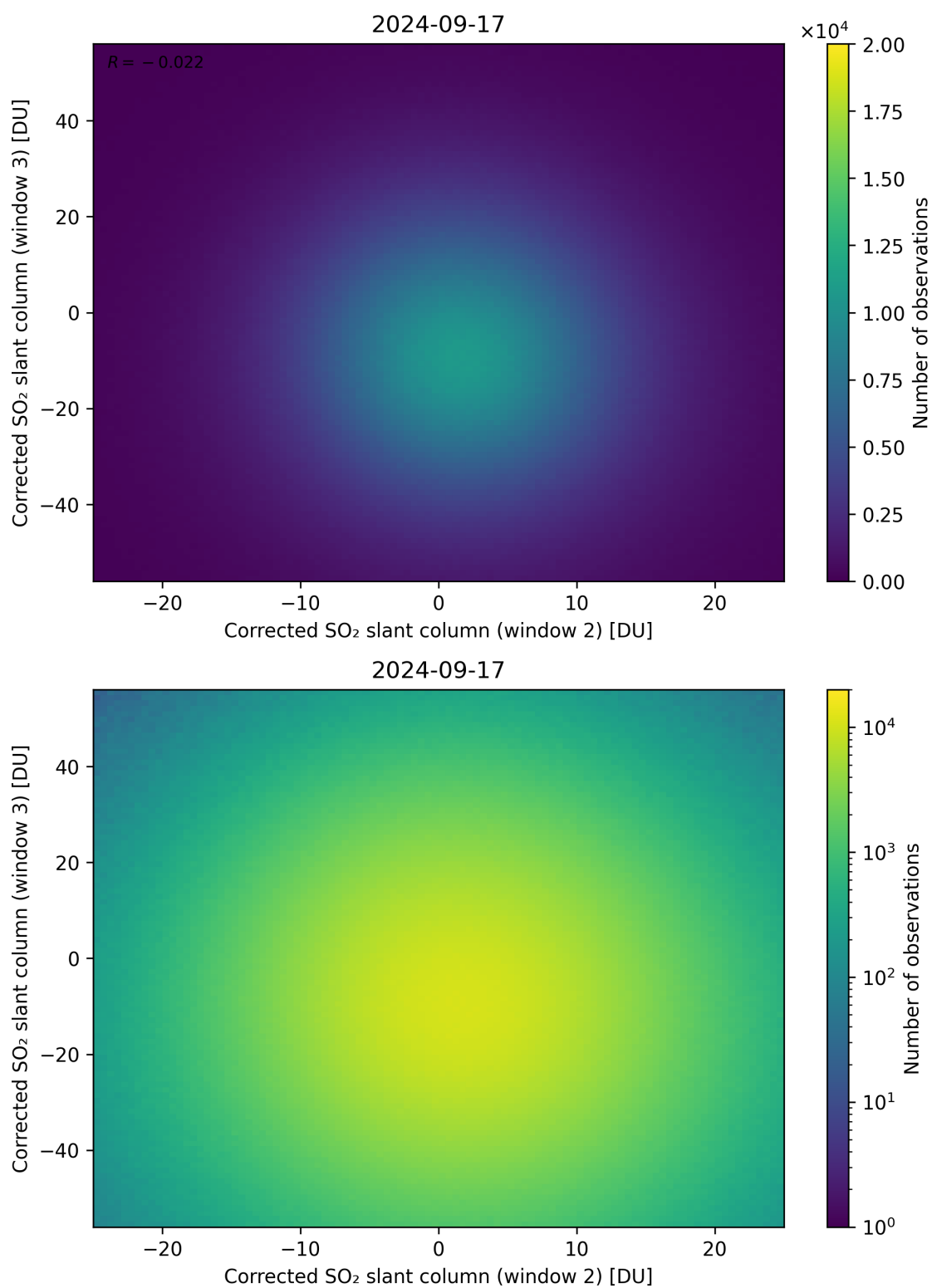
Figure 200: Scatter density plot of “Corrected SO 2 slant column (window 2)” against “Corrected SO 2 slant column (window 3)” for 2024-09-17 to 2024-09-18.
