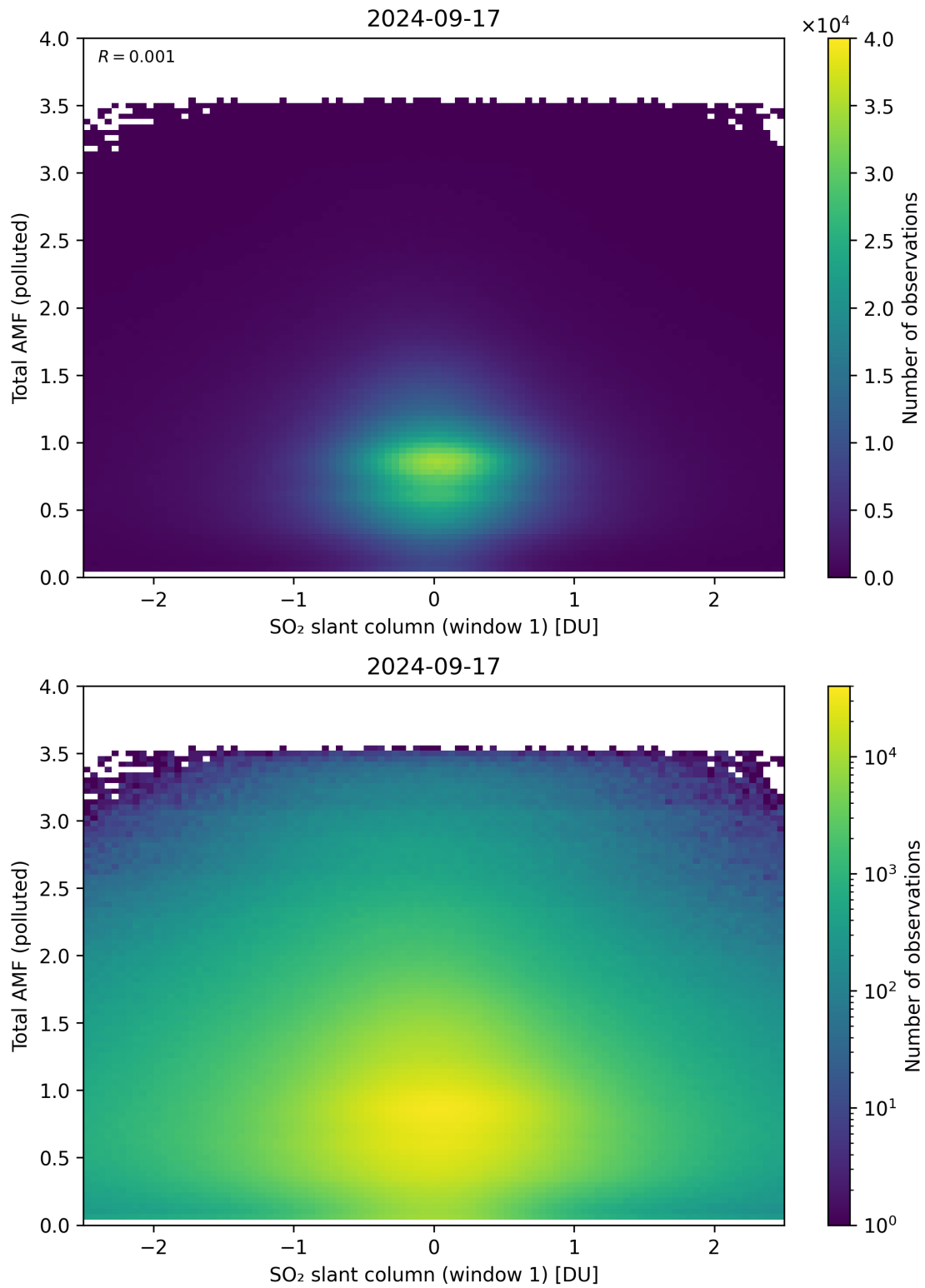
Figure 239: Scatter density plot of “SO 2 slant column (window 1)” against “Total AMF (polluted)” for 2024-09-17 to 2024-09-18.
