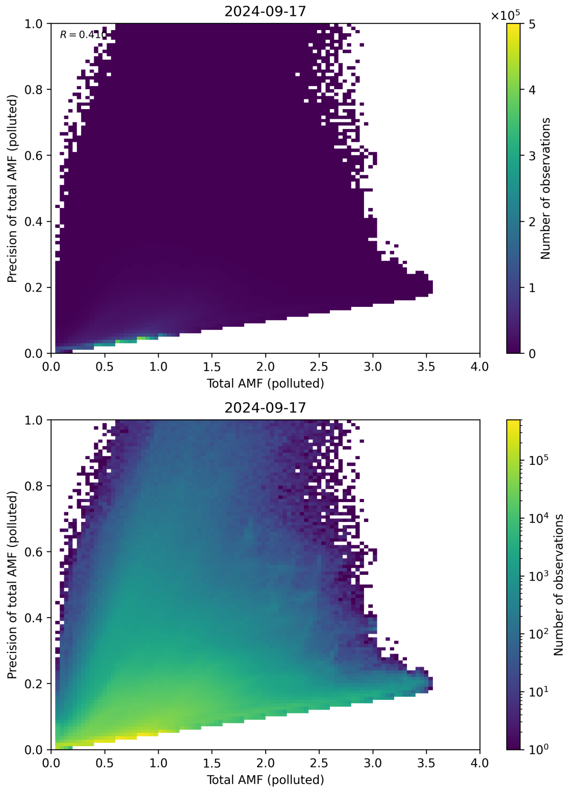
Figure 272: Scatter density plot of “Total AMF (polluted)” against “Precision of total AMF (polluted)” for 2024-09-17 to 2024-09-18.
