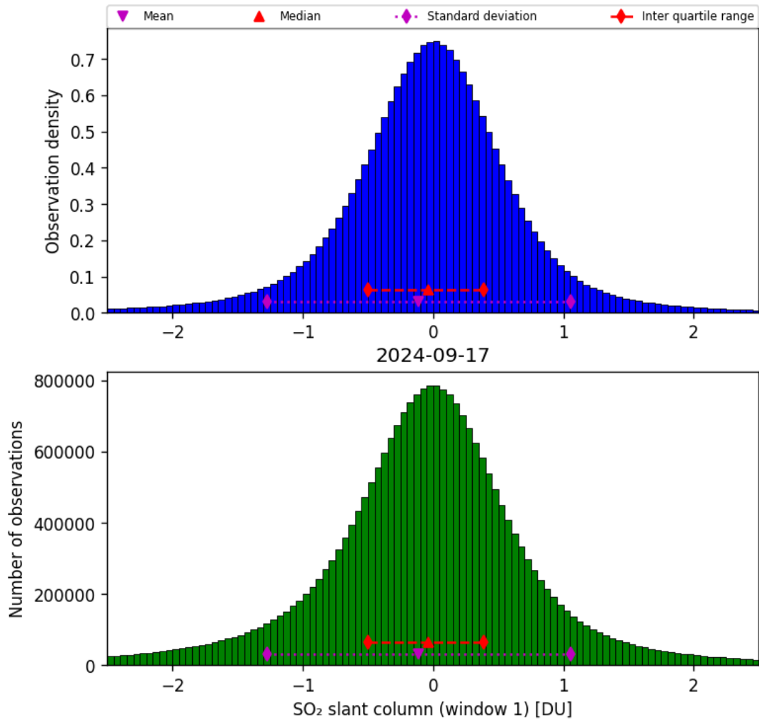
Figure 56: Histogram of “SO 2 slant column (window 1)” for 2024-09-17 to 2024-09-18
