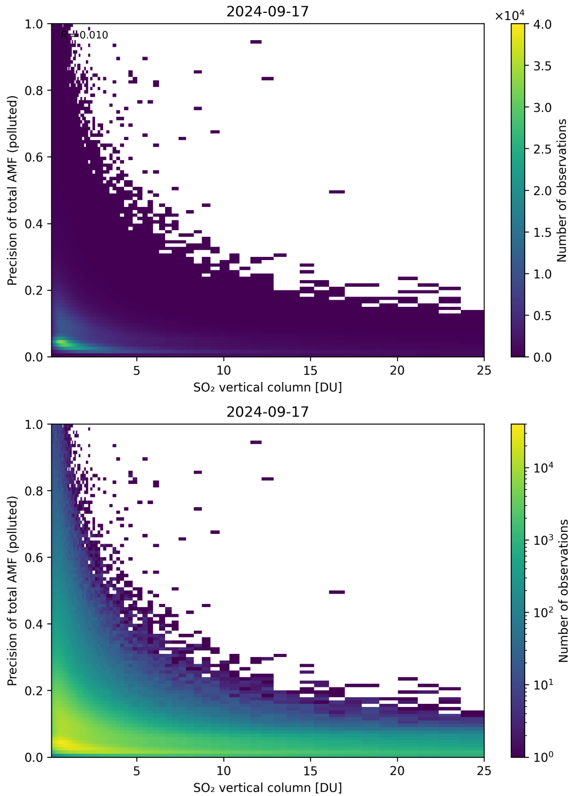
Figure 306: Scatter density plot of “SO 2 vertical column” against “Precision of total AMF (polluted)” for 2024-09-17 to 2024-09-18.
