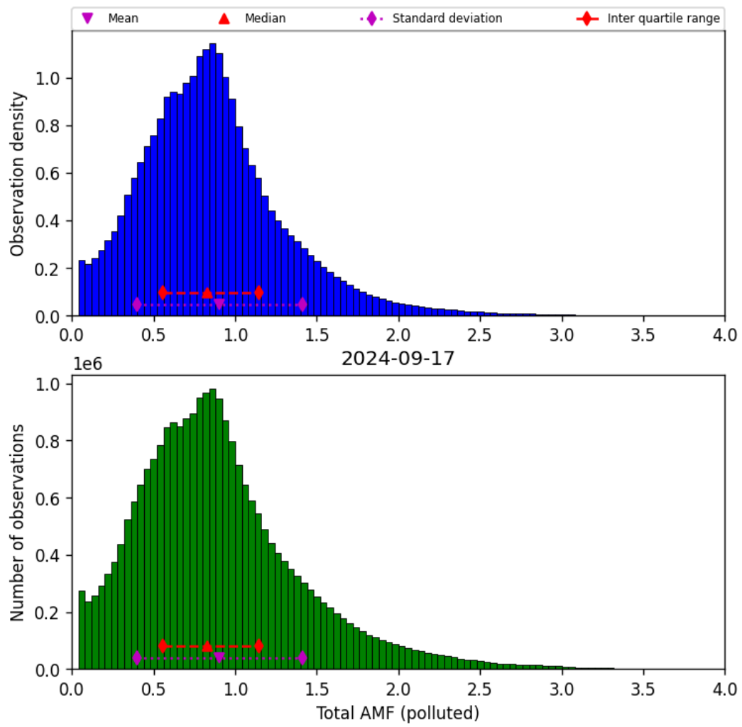
Figure 71: Histogram of “Total AMF (polluted)” for 2024-09-17 to 2024-09-18
