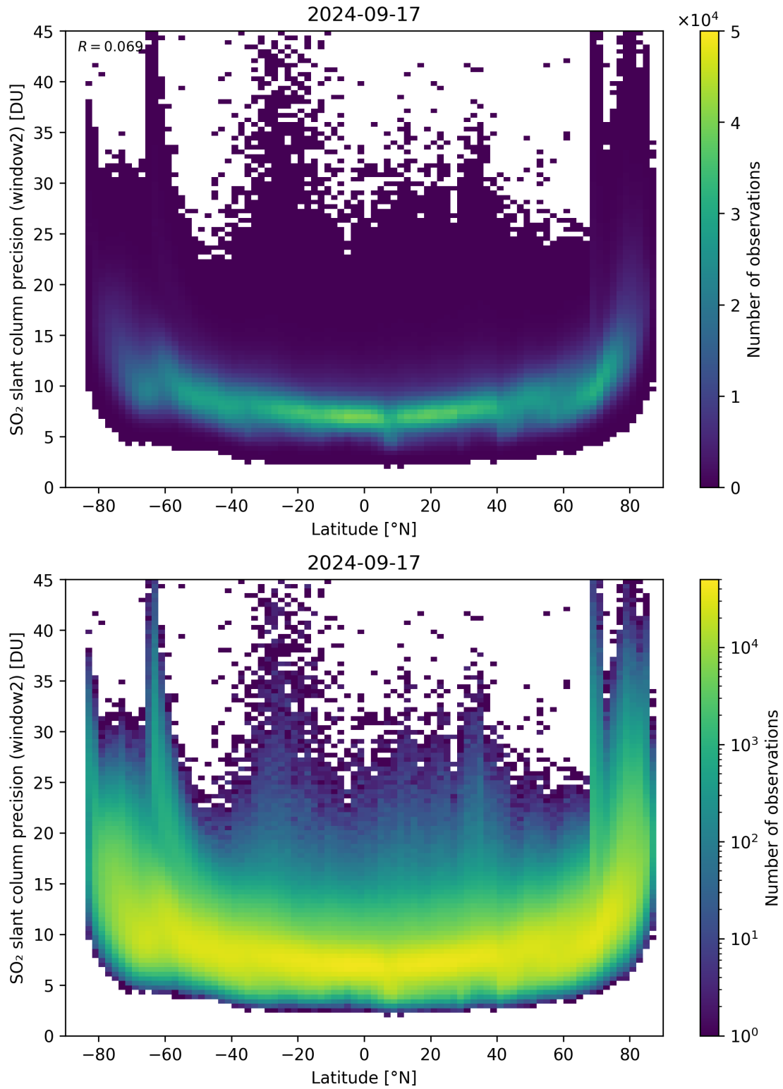
Figure 151: Scatter density plot of “Latitude” against “SO 2 slant column precision (window2)” for 2024-09-17 to 2024-09-18.
