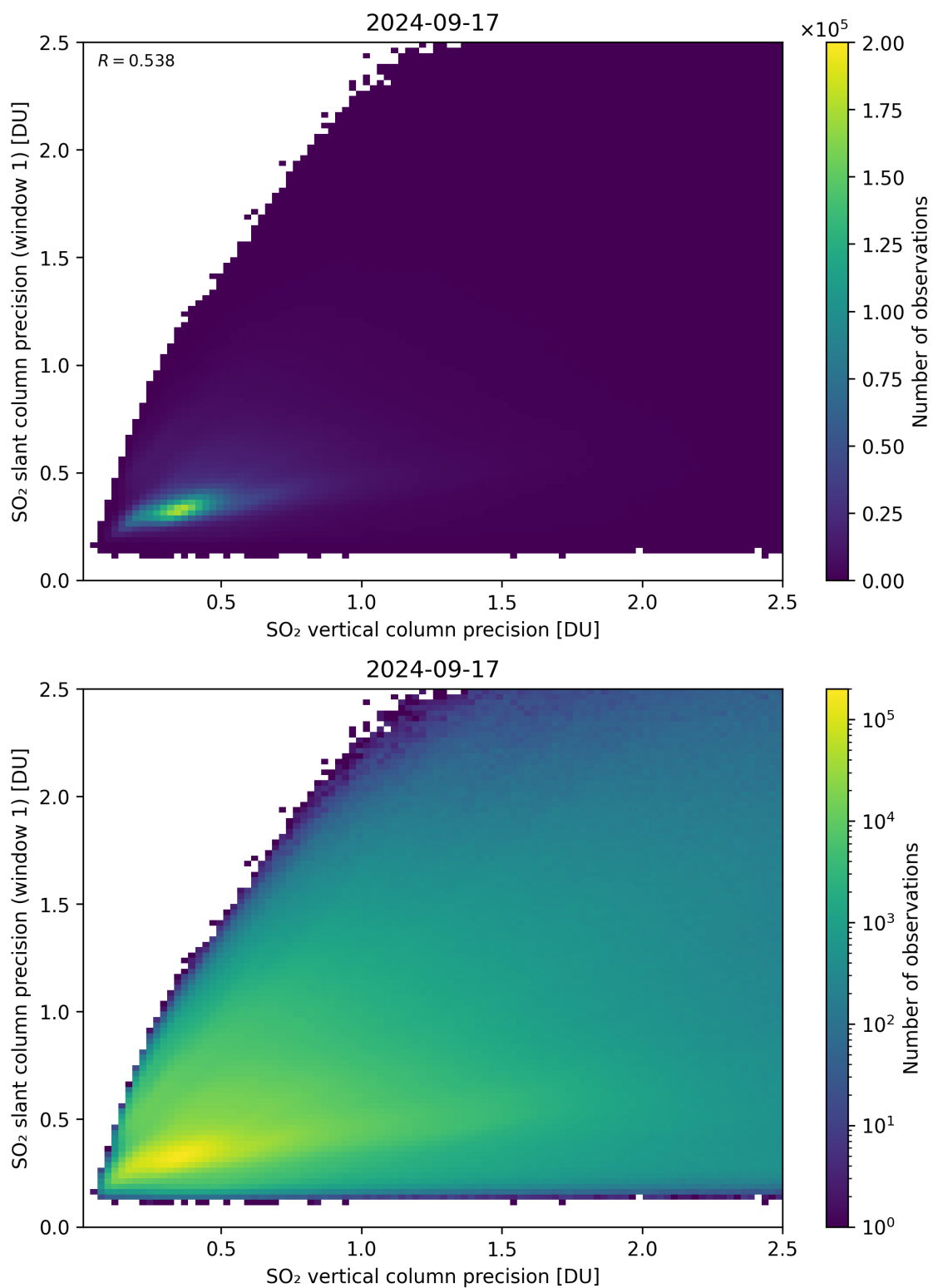
Figure 290: Scatter density plot of “SO 2 vertical column precision” against “SO 2 slant column precision (window 1)” for 2024-09-17 to 2024-09-18.
