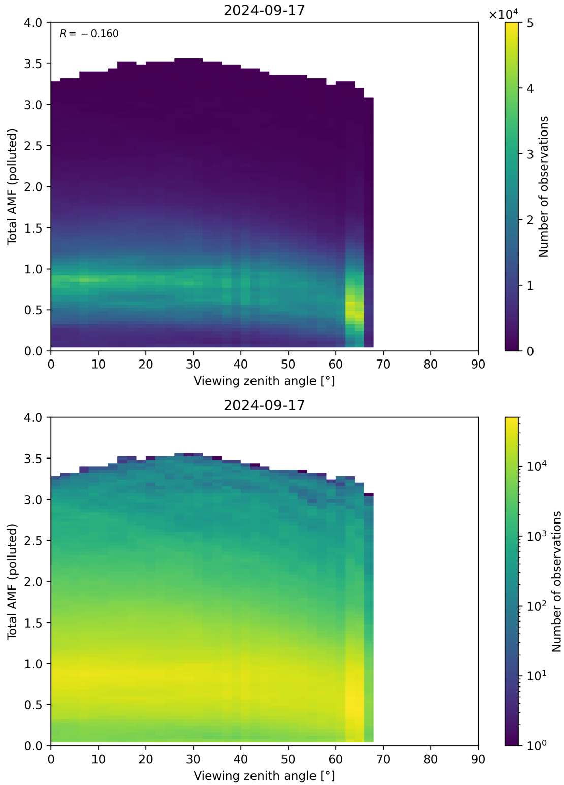
Figure 325: Scatter density plot of “Viewing zenith angle” against “Total AMF (polluted)” for 2024-09-17 to 2024-09-18.
