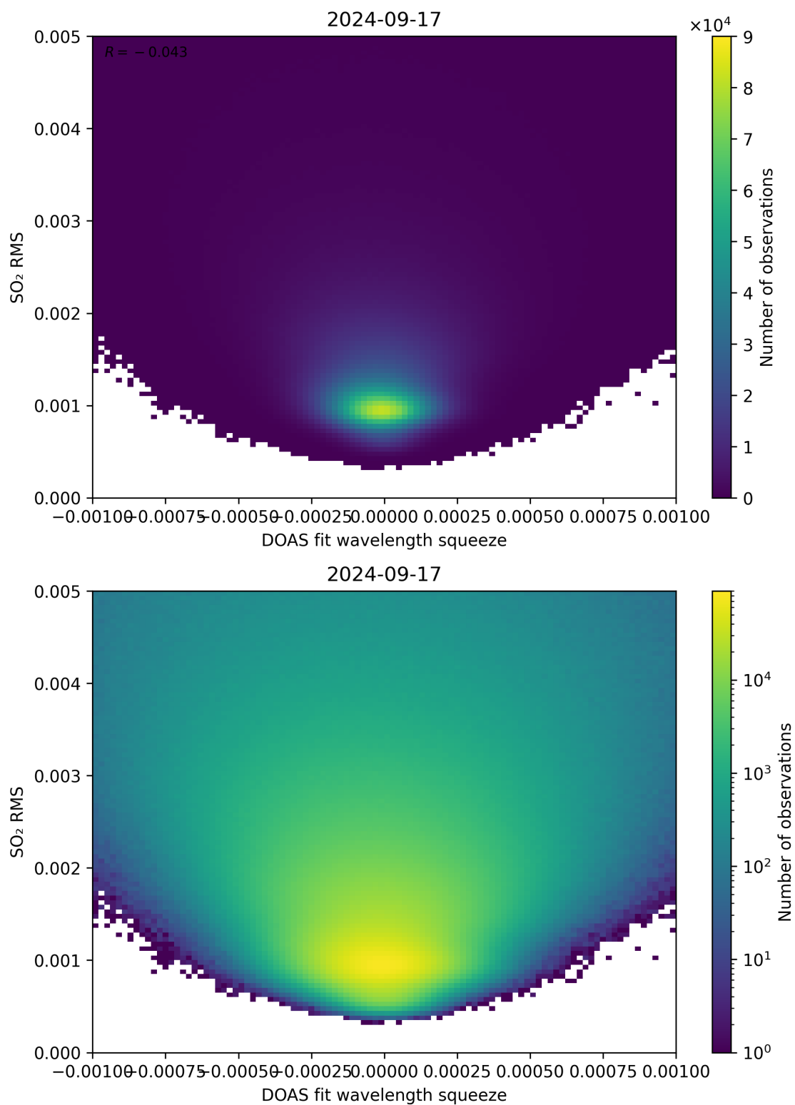
Figure 132: Scatter density plot of “DOAS fit wavelength squeeze” against “SO 2 RMS” for 2024-09-17 to 2024-09-18.
