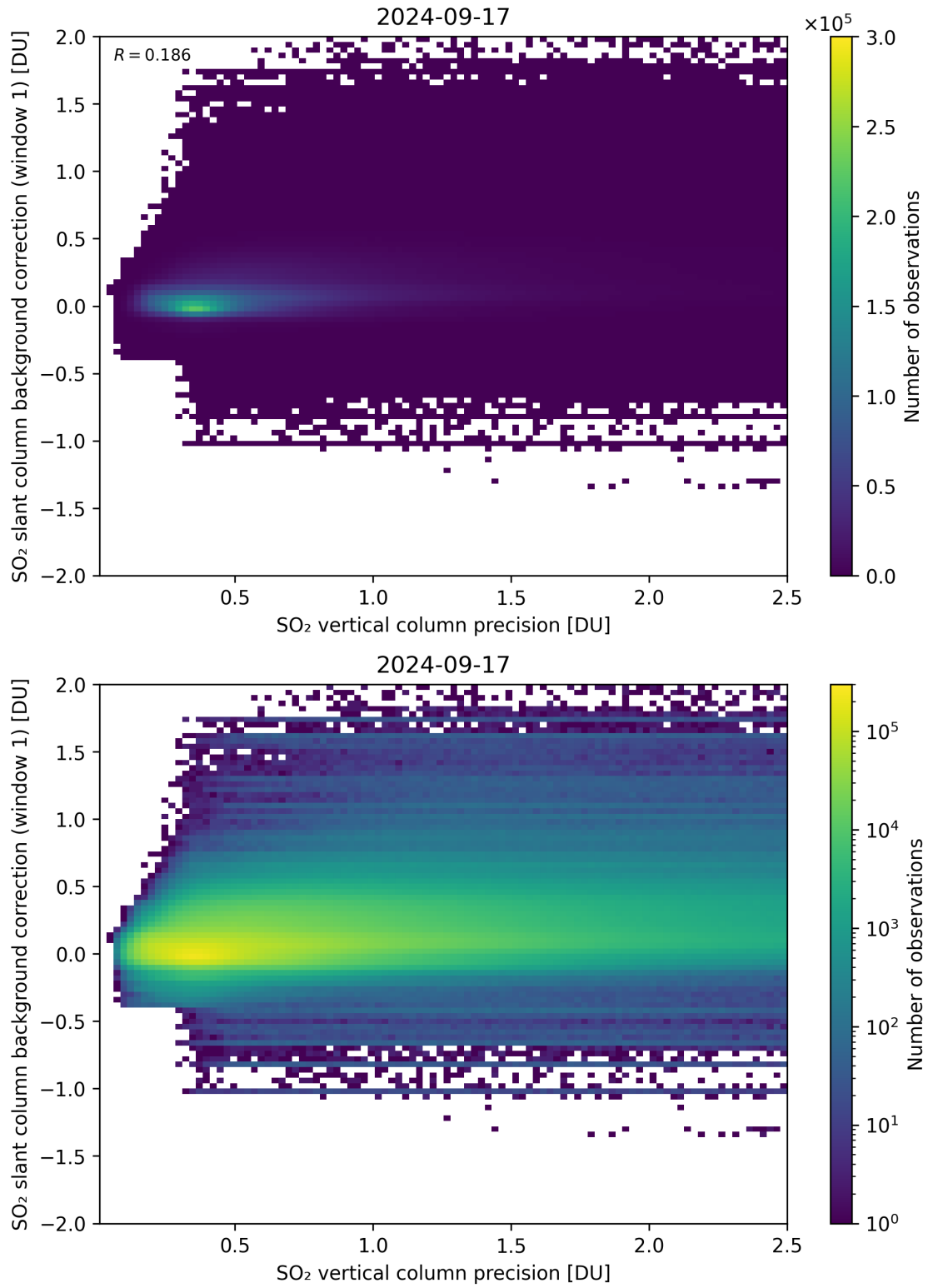
Figure 279: Scatter density plot of “SO 2 vertical column precision” against “SO 2 slant column background correction (window 1)” for 2024-09-17 to 2024-09-18.
