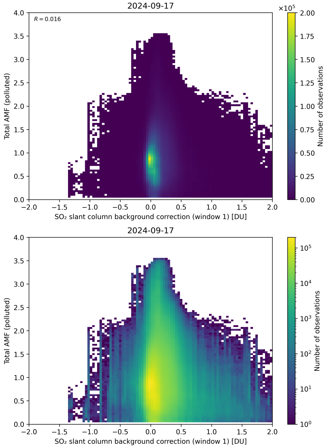
Figure 109: Scatter density plot of “SO 2 slant column background correction (window 1)” against “Total AMF (polluted)” for 2024-09-17 to 2024-09-18.
