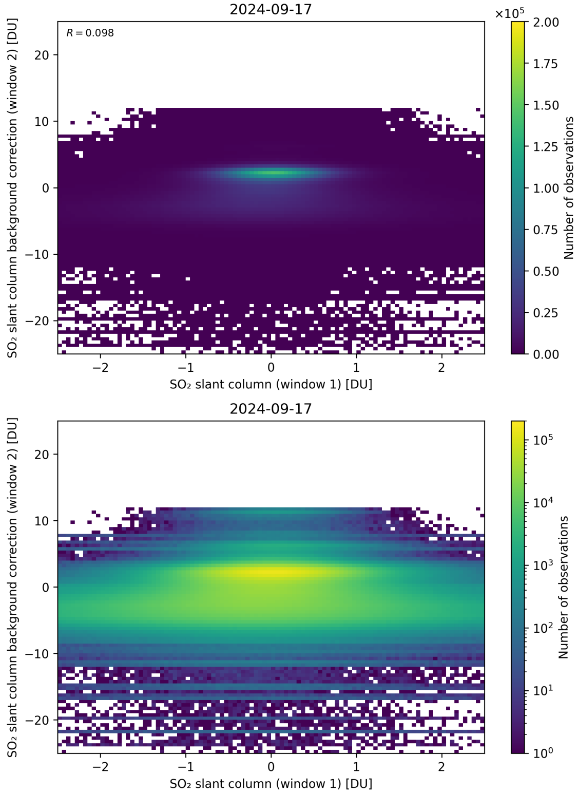
Figure 213: Scatter density plot of “SO 2 slant column (window 1)” against “SO 2 slant column background correction (window 2)” for 2024-09-17 to 2024-09-18.
