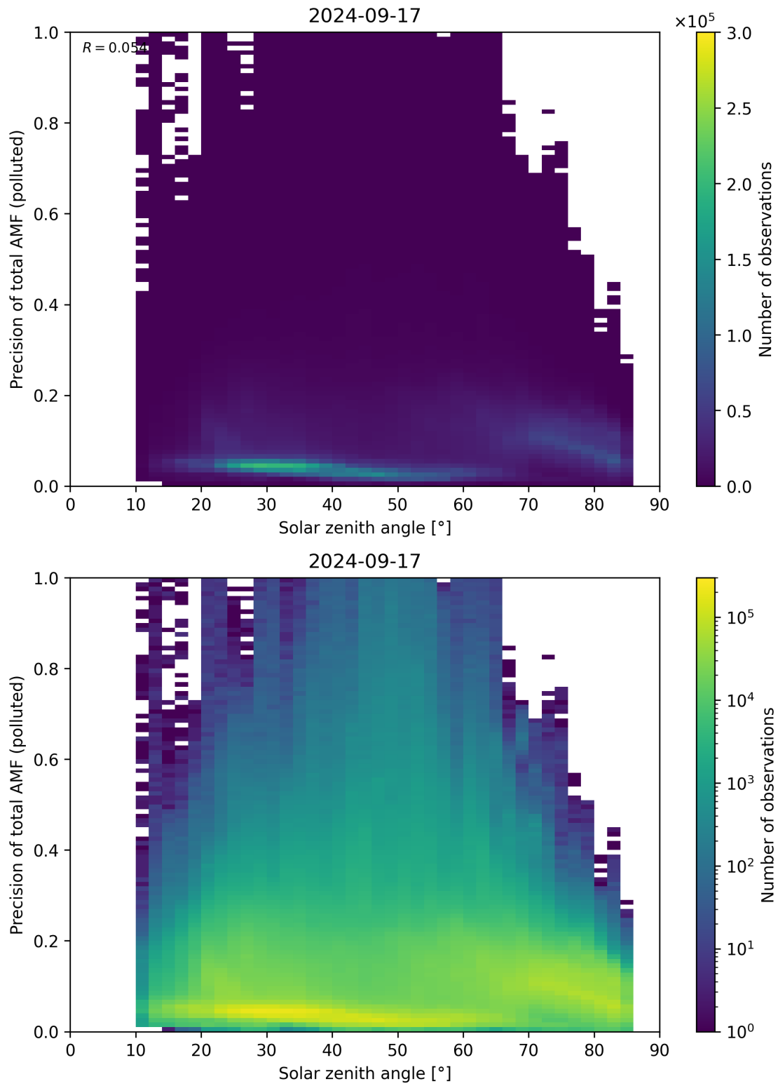
Figure 175: Scatter density plot of “Solar zenith angle” against “Precision of total AMF (polluted)” for 2024-09-17 to 2024-09-18.
