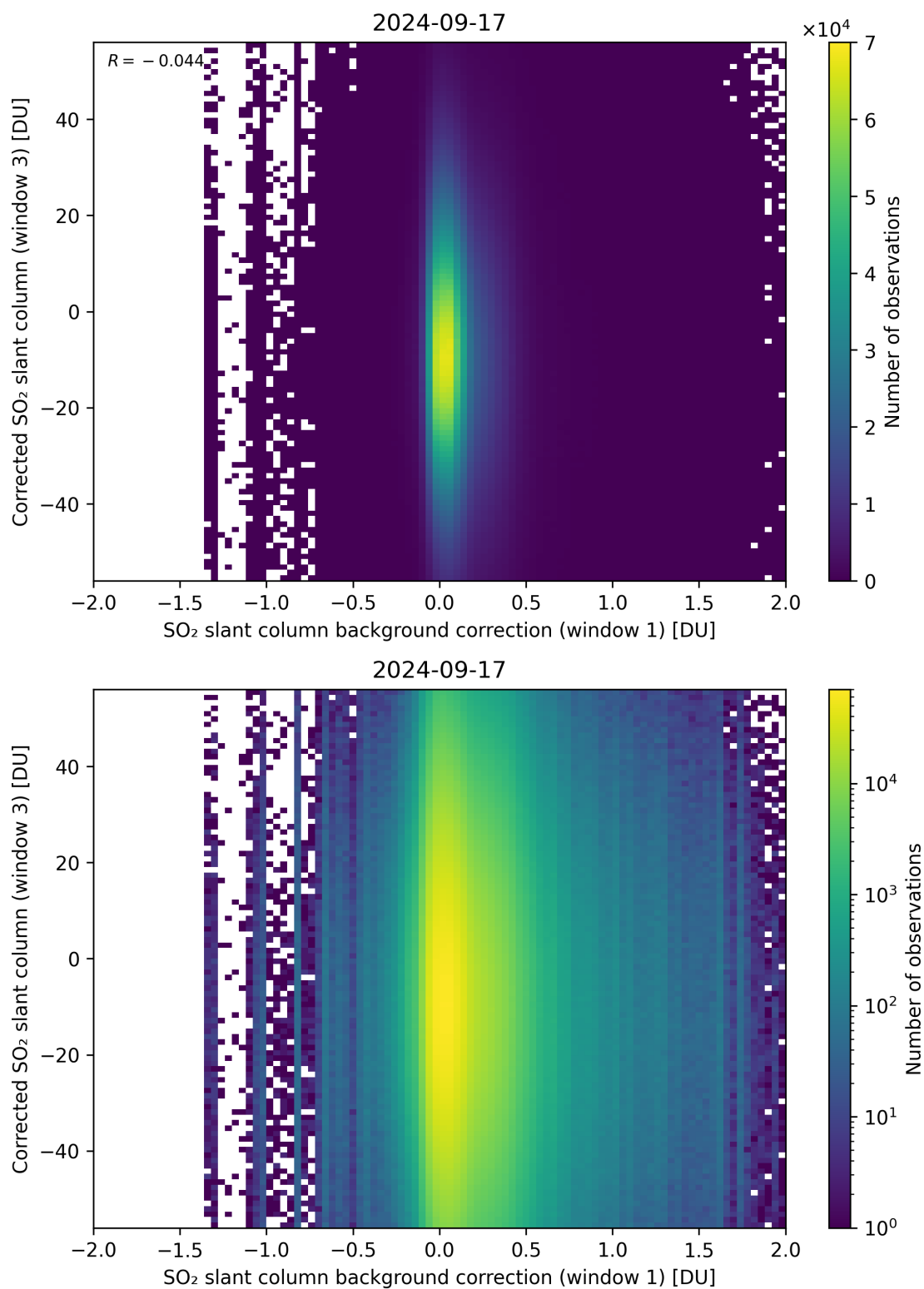
Figure 105: Scatter density plot of “SO 2 slant column background correction (window 1)” against “Corrected SO 2 slant column (window 3)” for 2024-09-17 to 2024-09-18.
