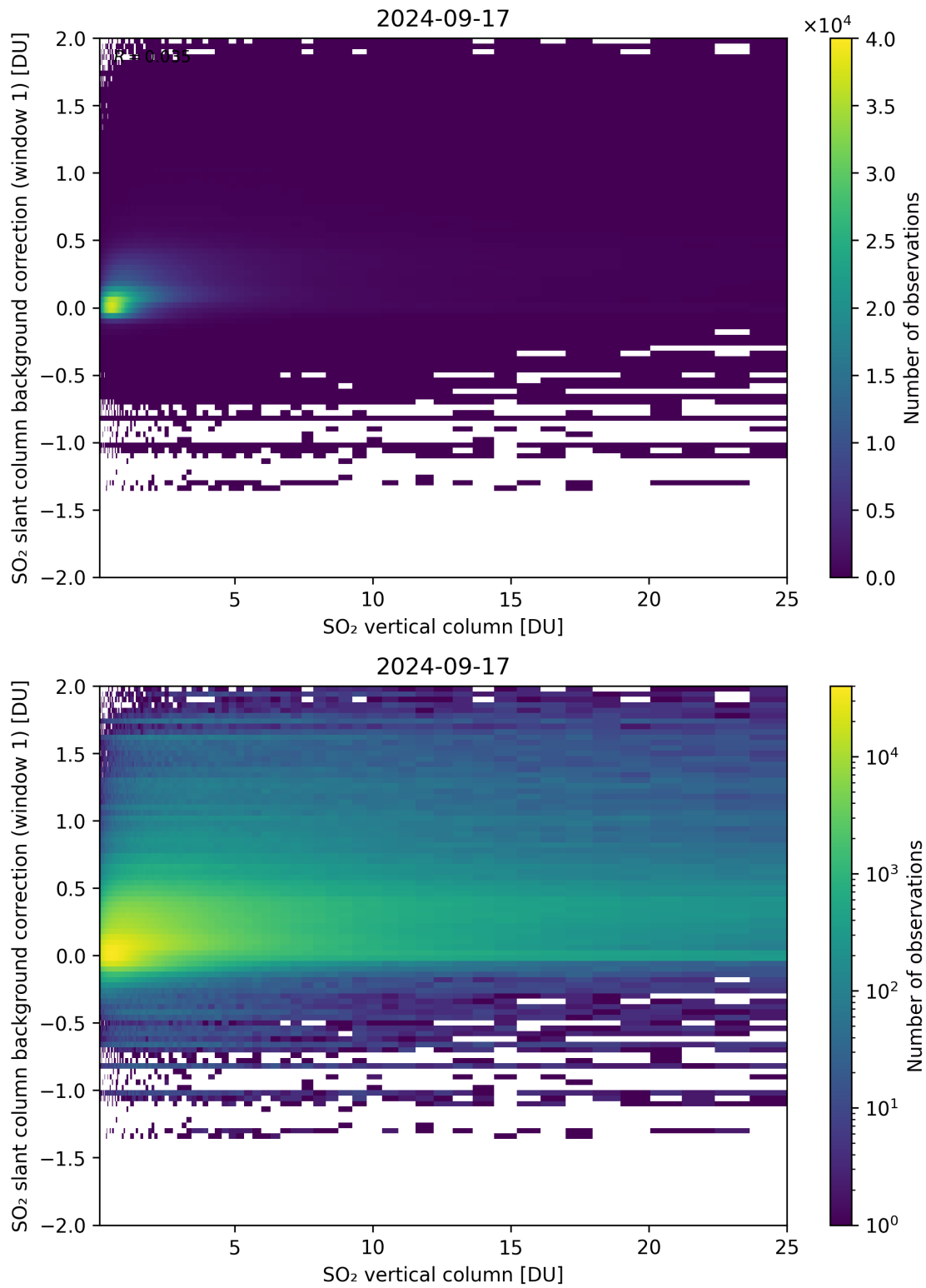
Figure 273: Scatter density plot of “SO 2 vertical column” against “SO 2 slant column background correction (window 1)” for 2024-09-17 to 2024-09-18.
