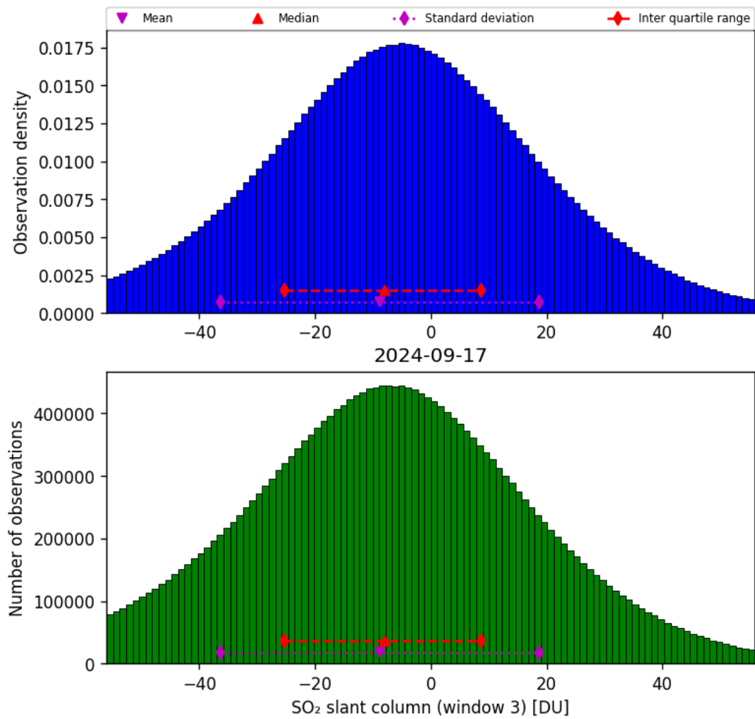
Figure 64: Histogram of “SO 2 slant column (window 3)” for 2024-09-17 to 2024-09-18
