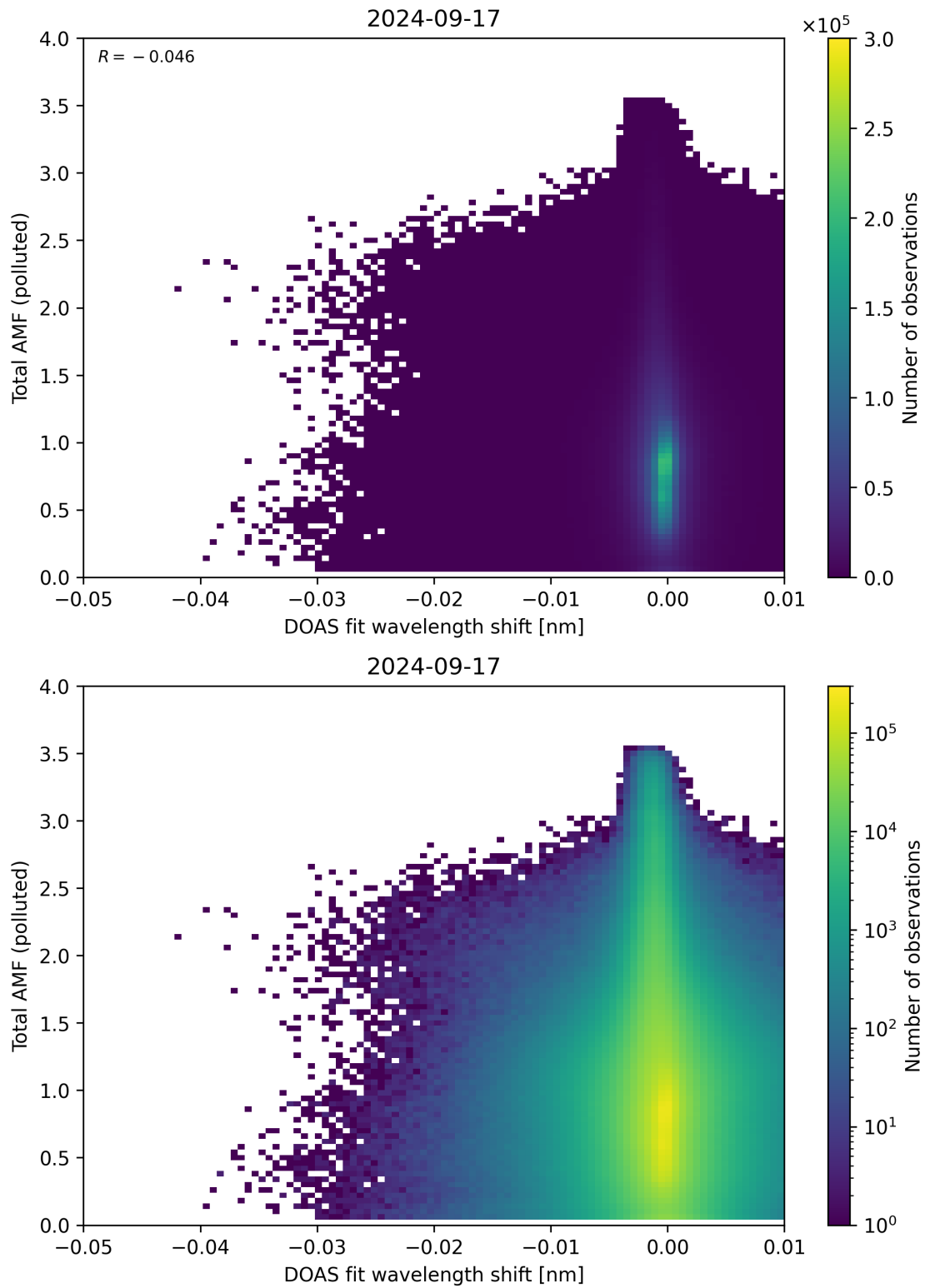
Figure 130: Scatter density plot of “DOAS fit wavelength shift” against “Total AMF (polluted)” for 2024-09-17 to 2024-09-18.
