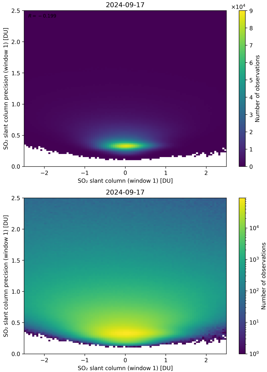
Figure 235: Scatter density plot of “SO 2 slant column (window 1)” against “SO 2 slant column precision (window 1)” for 2024-09-17 to 2024-09-18.
