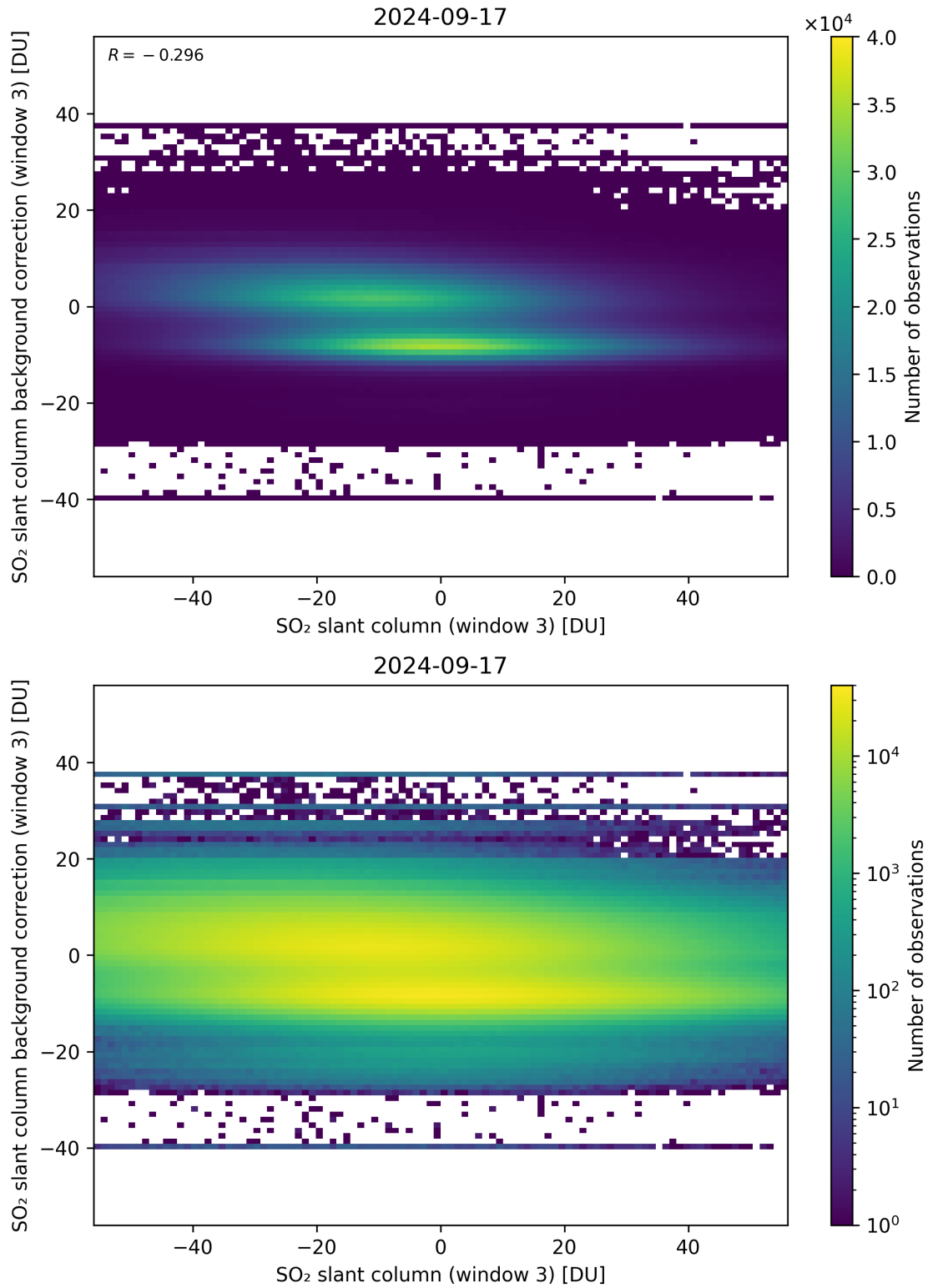
Figure 253: Scatter density plot of “SO 2 slant column (window 3)” against “SO 2 slant column background correction (window 3)” for 2024-09-17 to 2024-09-18.
