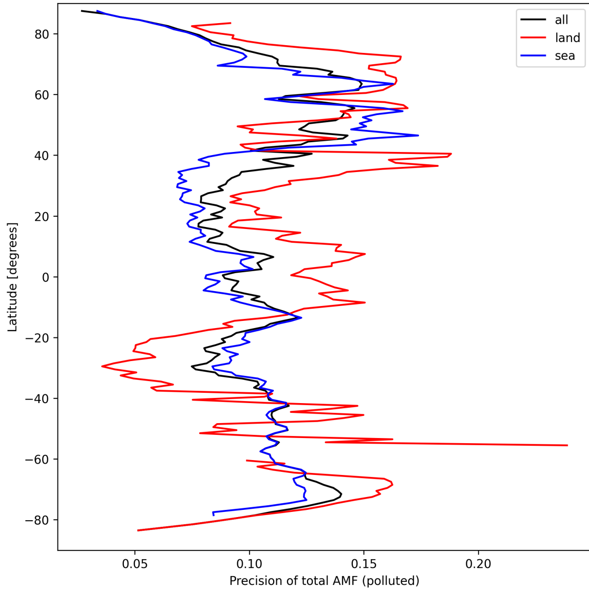
Figure 49: Zonal average of “Precision of total AMF (polluted)” for 2024-09-17 to 2024-09-18.
