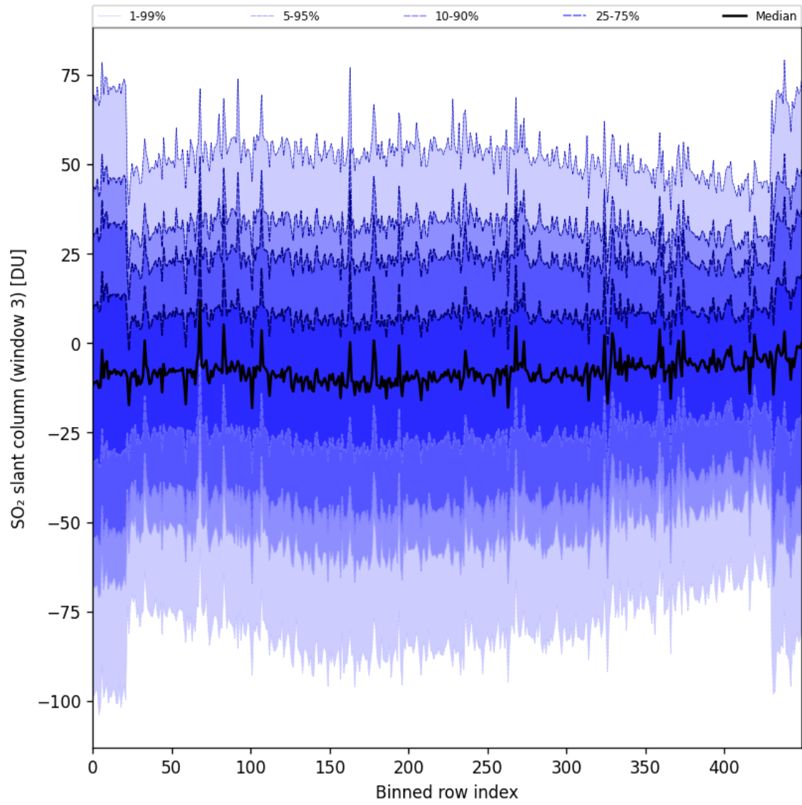
Figure 87: Along track statistics of “SO 2 slant column (window 3)” for 2024-09-17 to 2024-09-18
