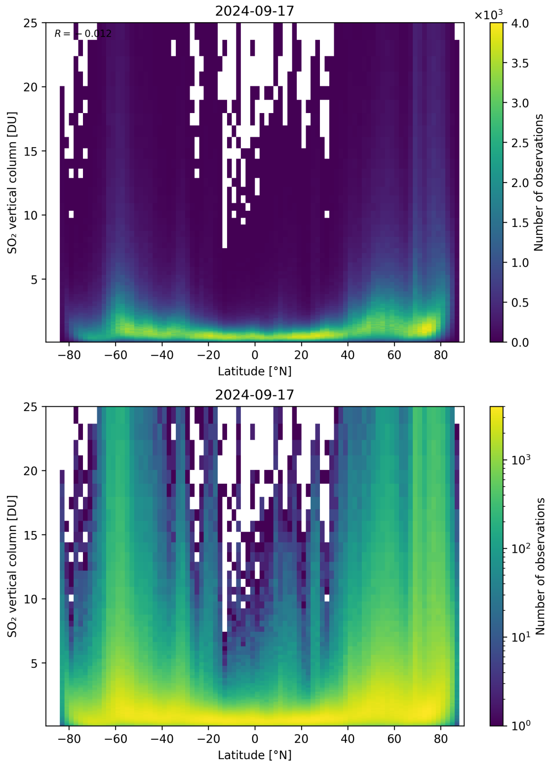
Figure 156: Scatter density plot of “Latitude” against “SO 2 vertical column” for 2024-09-17 to 2024-09-18.
