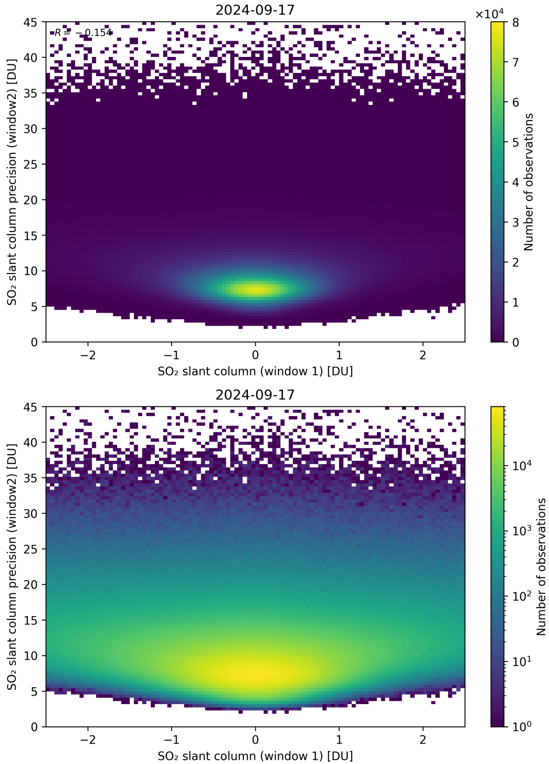
Figure 236: Scatter density plot of “SO 2 slant column (window 1)” against “SO 2 slant column precision (window2)” for 2024-09-17 to 2024-09-18.
