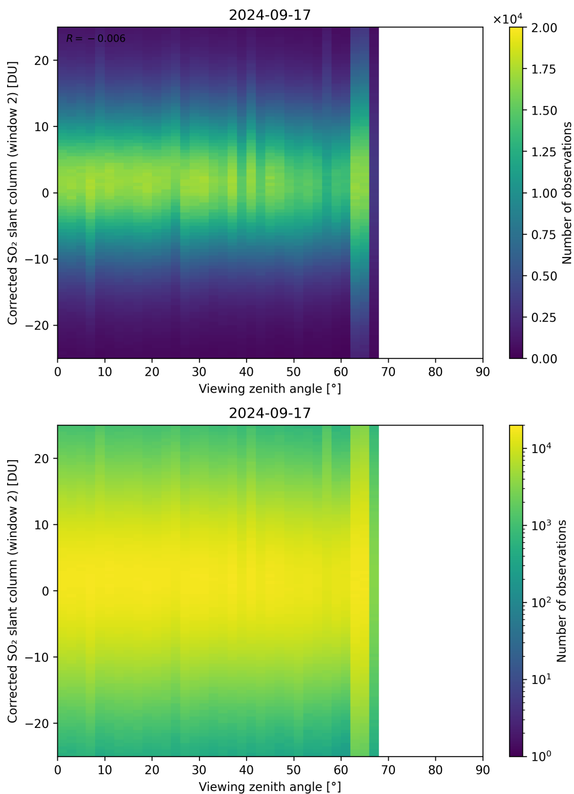
Figure 318: Scatter density plot of “Viewing zenith angle” against “Corrected SO 2 slant column (window 2)” for 2024-09-17 to 2024-09-18.
