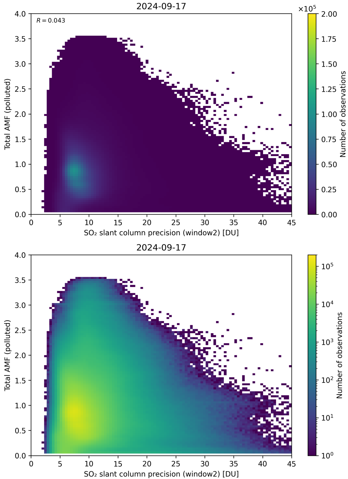
Figure 251: Scatter density plot of “SO 2 slant column precision (window2)” against “Total AMF (polluted)” for 2024-09-17 to 2024-09-18.
