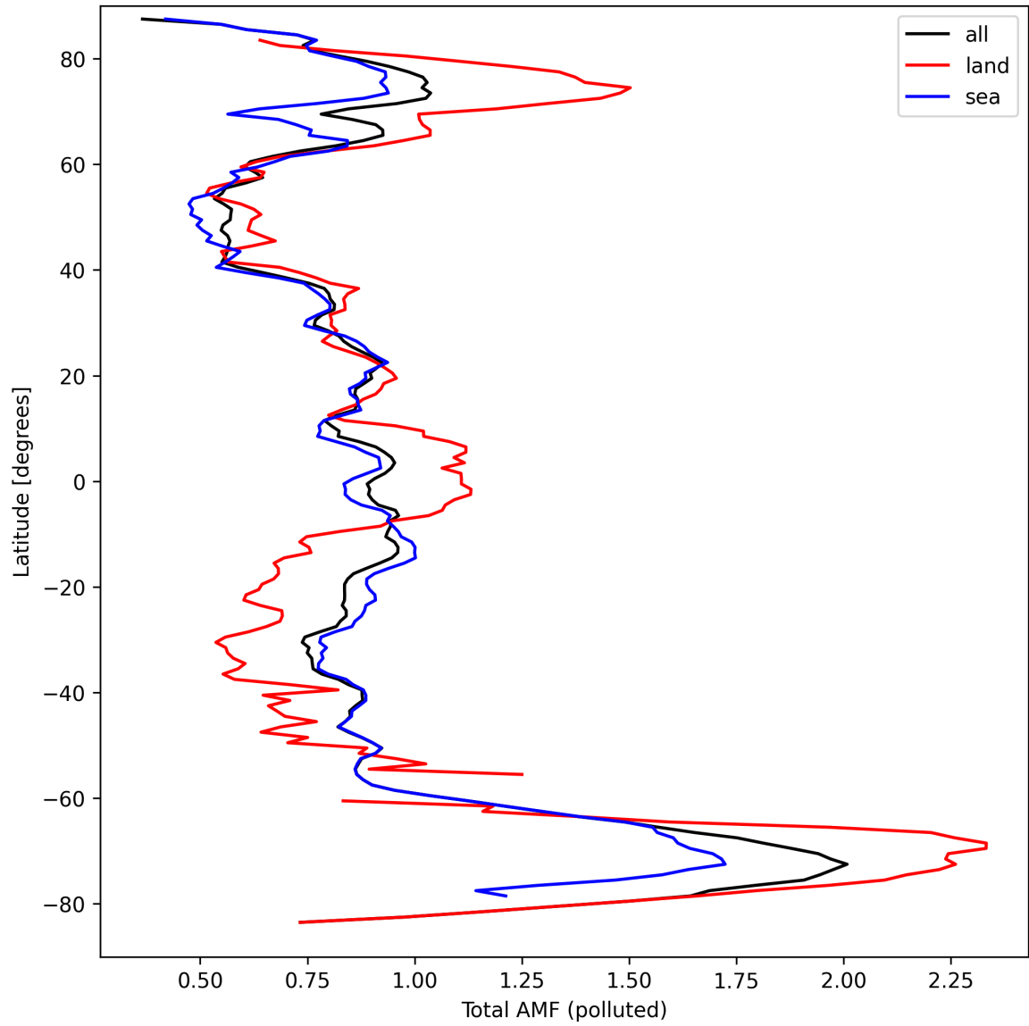
Figure 48: Zonal average of “Total AMF (polluted)” for 2024-09-17 to 2024-09-18.
