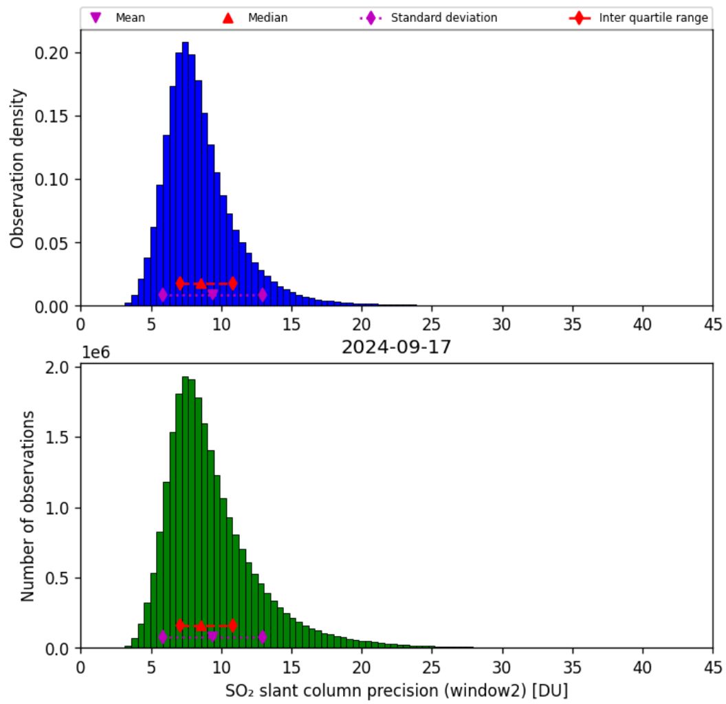
Figure 61: Histogram of “SO 2 slant column precision (window2)” for 2024-09-17 to 2024-09-18
