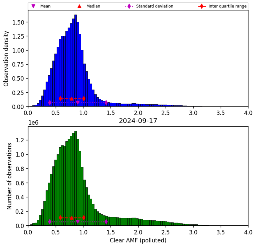
Figure 73: Histogram of “Clear AMF (polluted)” for 2024-09-17 to 2024-09-18
