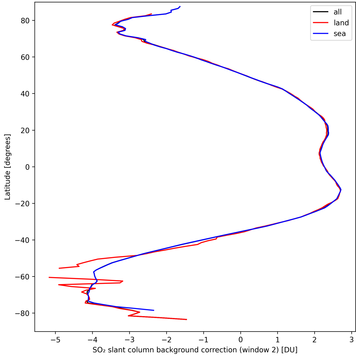
Figure 40: Zonal average of “SO 2 slant column background correction (window 2)” for 2024-09-17 to 2024-09-18.
