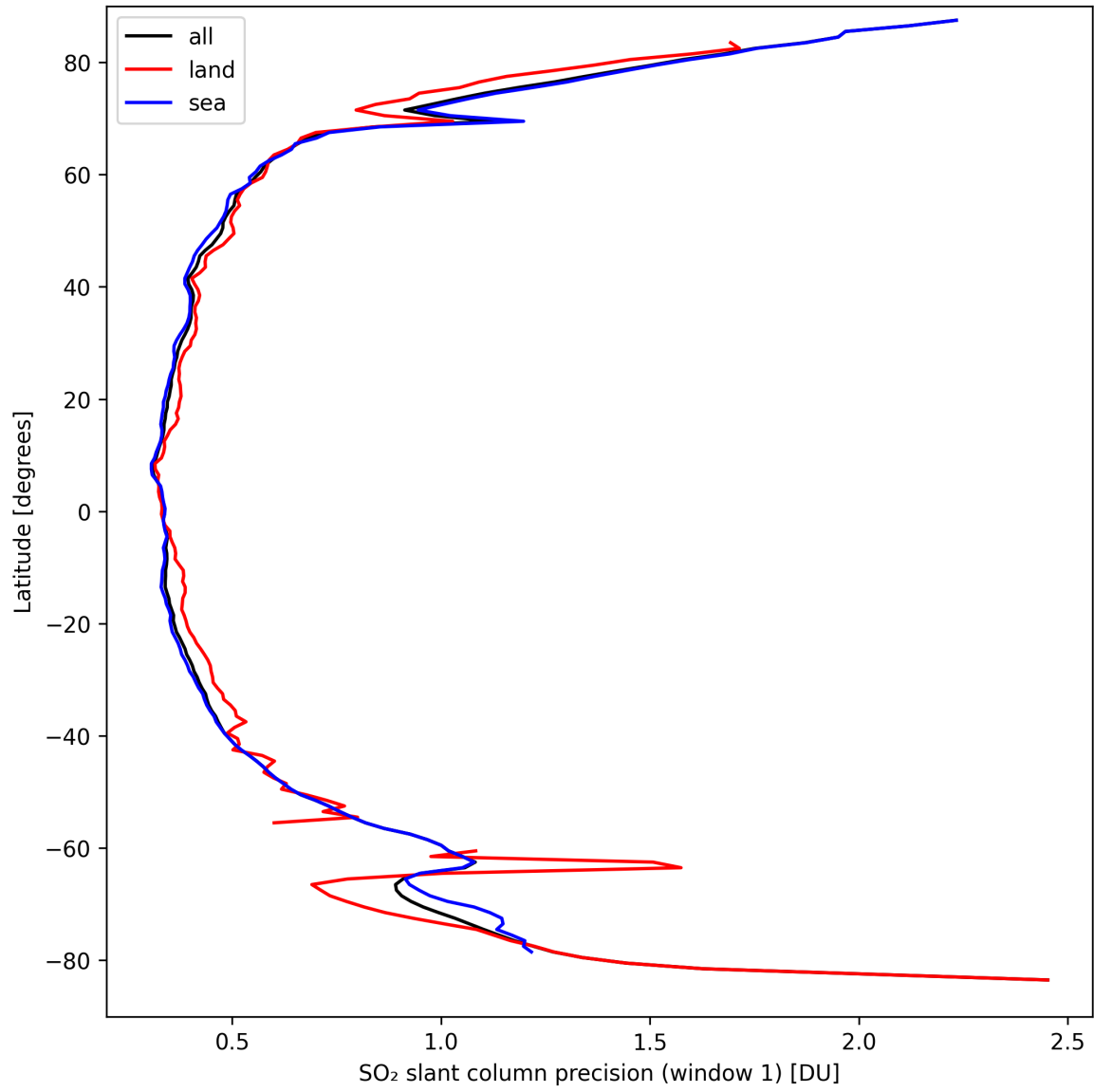
Figure 34: Zonal average of “SO 2 slant column precision (window 1)” for 2024-09-17 to 2024-09-18.
