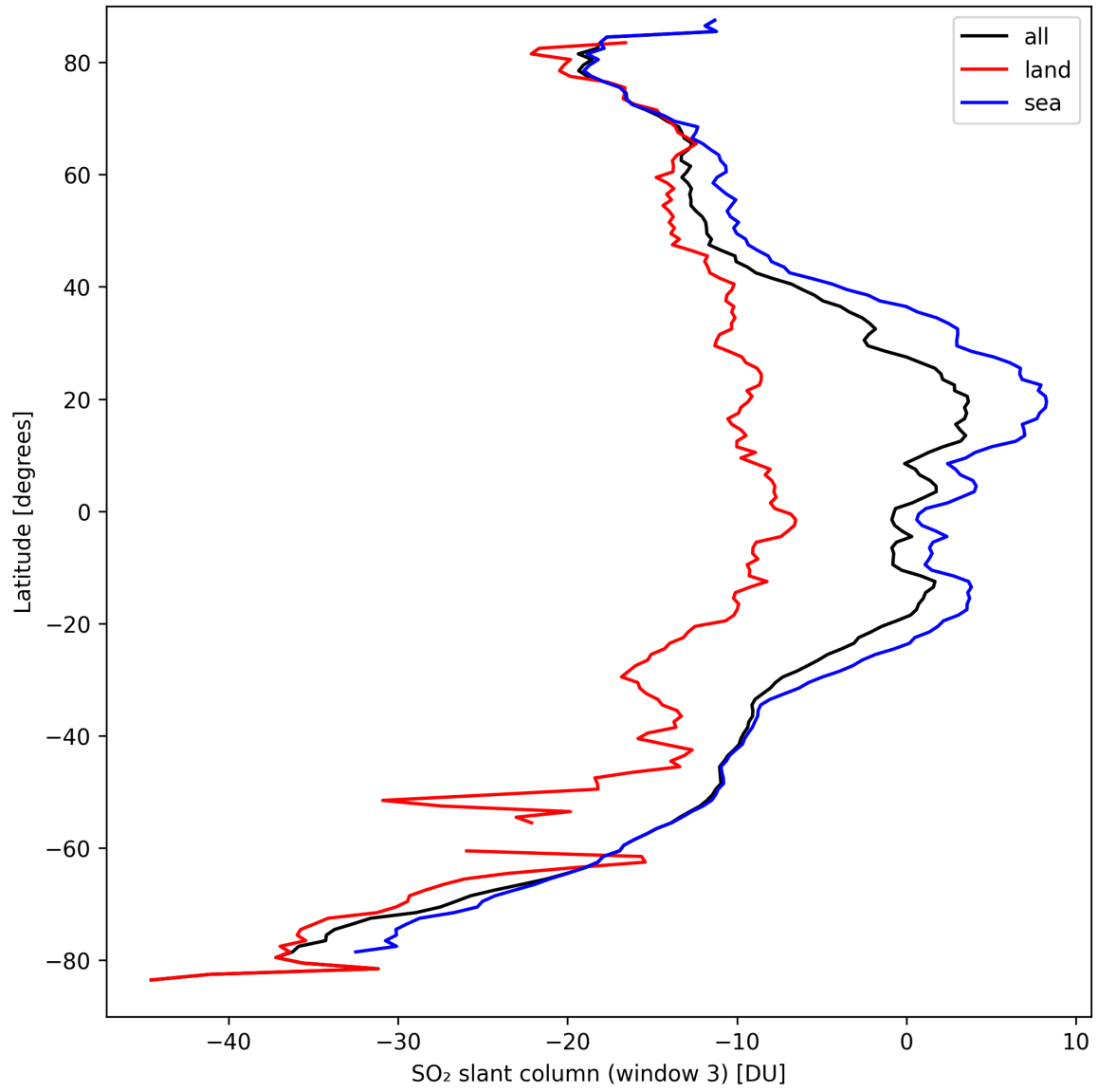
Figure 41: Zonal average of “SO 2 slant column (window 3)” for 2024-09-17 to 2024-09-18.
