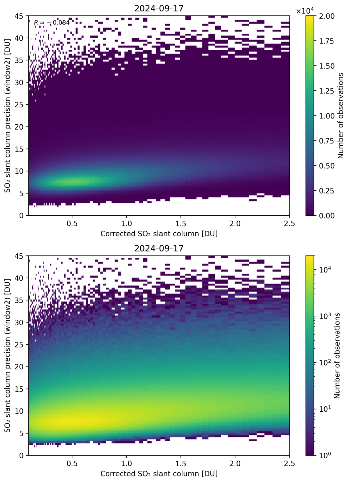
Figure 189: Scatter density plot of “Corrected SO 2 slant column” against “SO 2 slant column precision (window2)” for 2024-09-17 to 2024-09-18.
