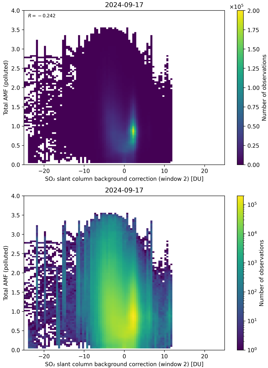
Figure 119: Scatter density plot of “SO 2 slant column background correction (window 2)” against “Total AMF (polluted)” for 2024-09-17 to 2024-09-18.
