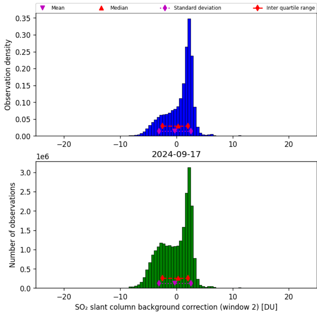
Figure 63: Histogram of “SO 2 slant column background correction (window 2)” for 2024-09-17 to 2024-09-18
