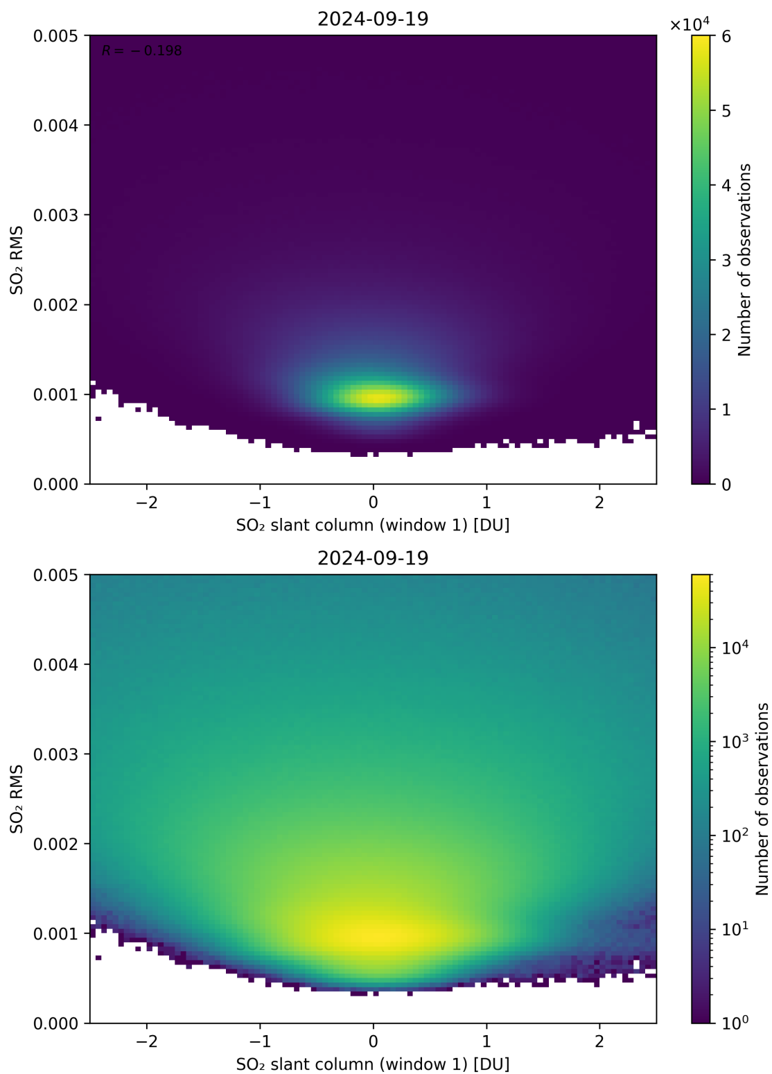
Figure 217: Scatter density plot of “SO 2 slant column (window 1)” against “SO 2 RMS” for 2024-09-18 to 2024-09-20.
