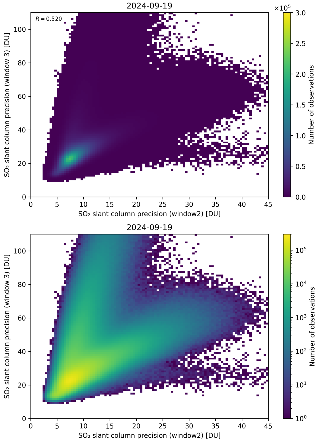
Figure 250: Scatter density plot of “SO 2 slant column precision (window2)” against “SO 2 slant column precision (window 3)” for 2024-09-18 to 2024-09-20.
