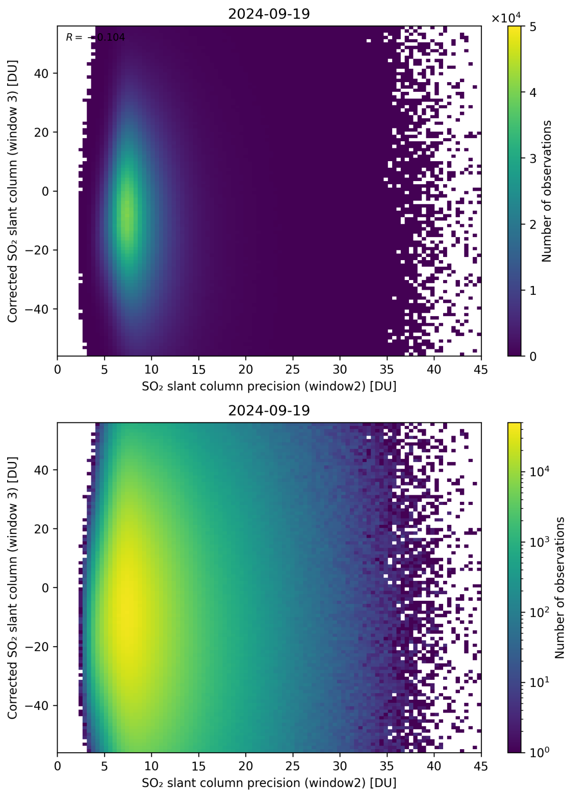
Figure 248: Scatter density plot of “SO 2 slant column precision (window2)” against “Corrected SO 2 slant column (window 3)” for 2024-09-18 to 2024-09-20.
