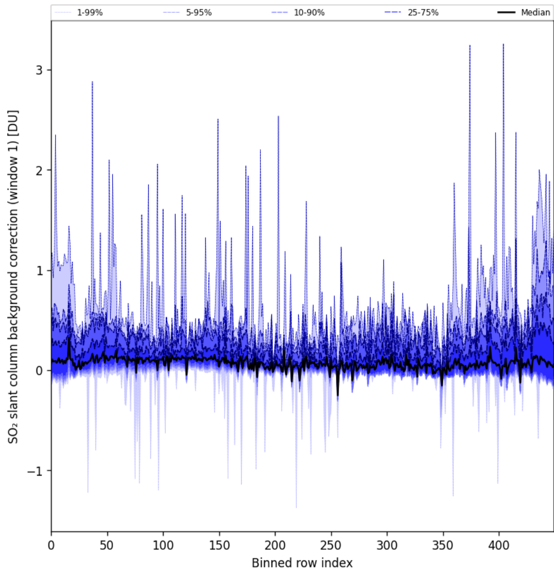
Figure 82: Along track statistics of “SO 2 slant column background correction (window 1)” for 2024-09-18 to 2024-09-20
