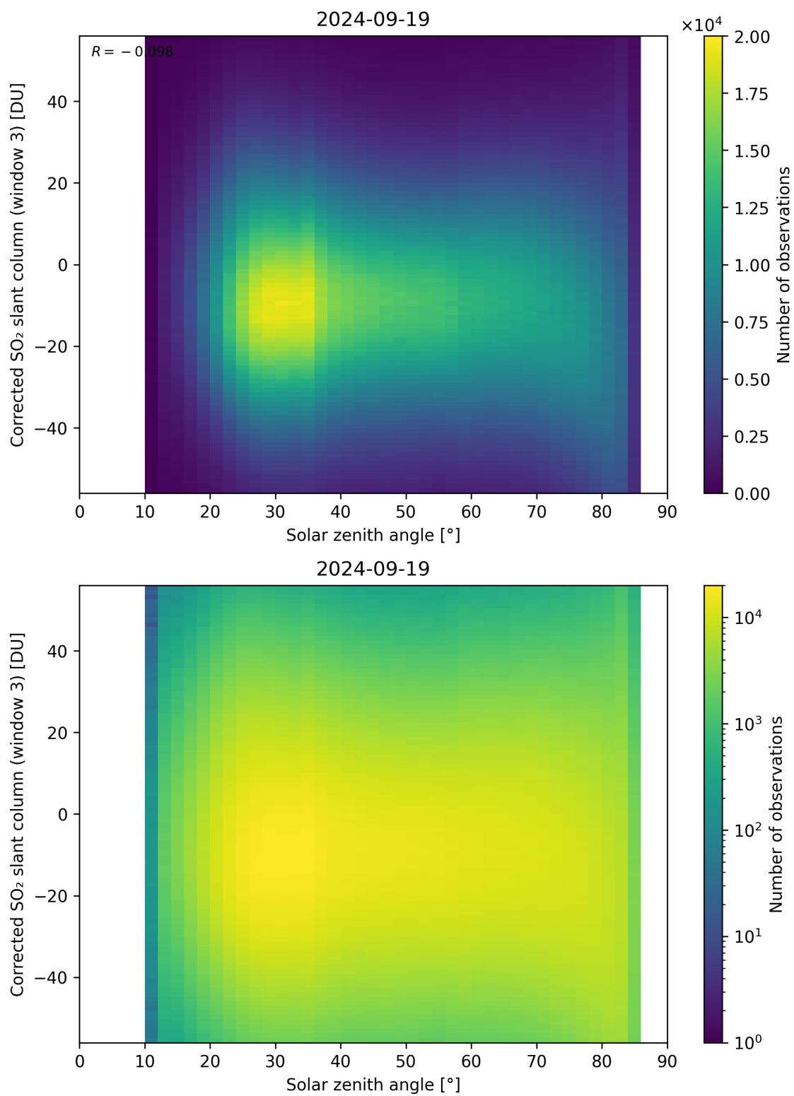
Figure 168: Scatter density plot of “Solar zenith angle” against “Corrected SO 2 slant column (window 3)” for 2024-09-18 to 2024-09-20.
