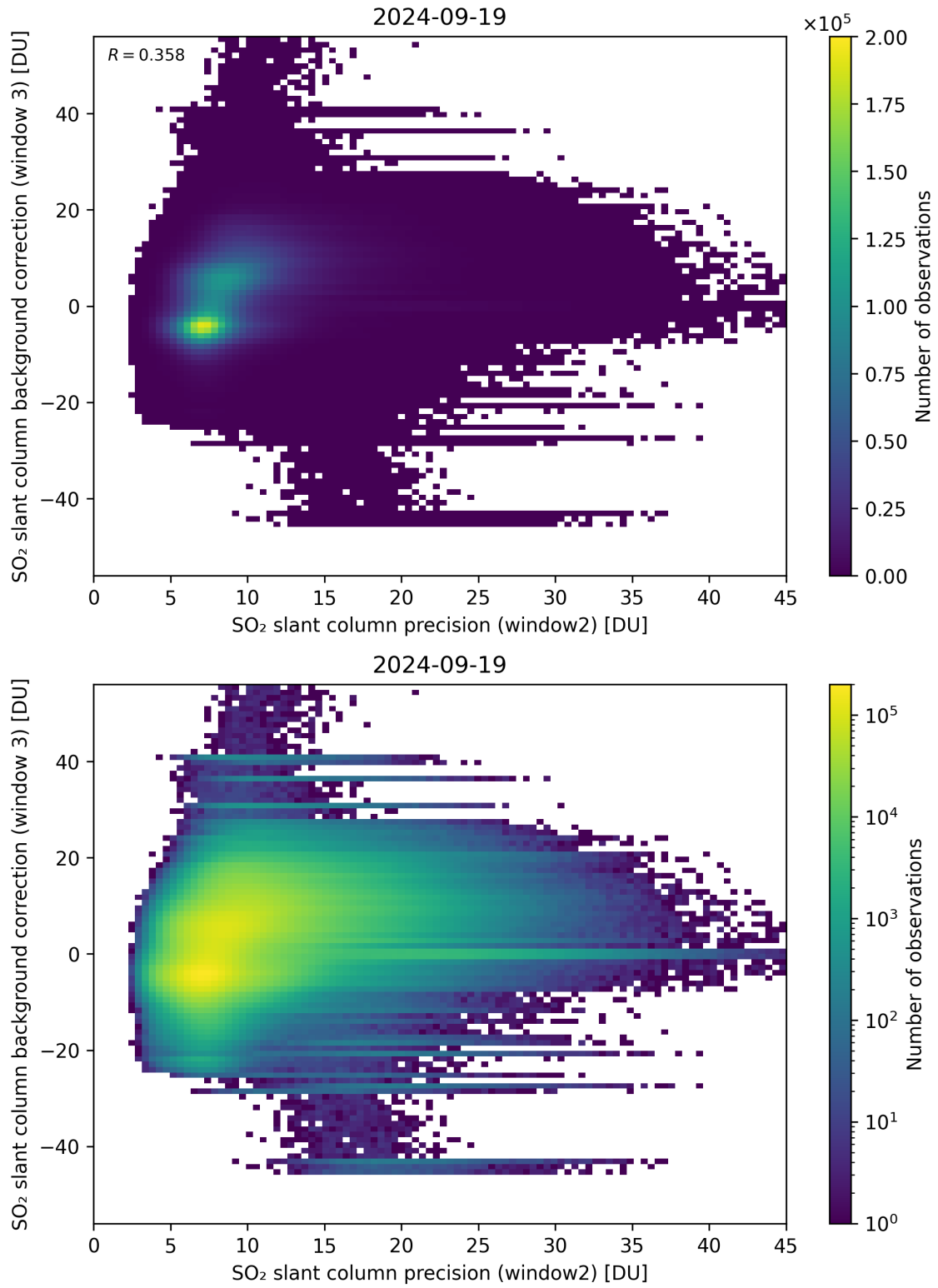
Figure 242: Scatter density plot of “SO 2 slant column precision (window2)” against “SO 2 slant column background correction (window 3)” for 2024-09-18 to 2024-09-20.
