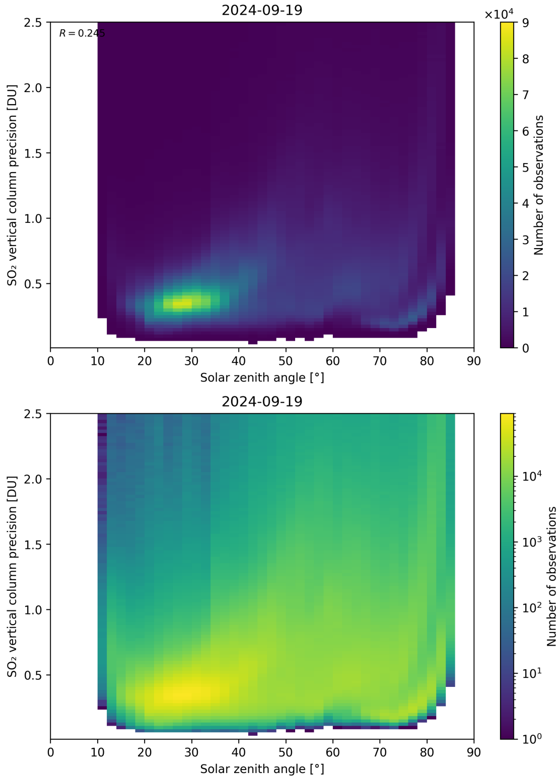
Figure 177: Scatter density plot of “Solar zenith angle” against “SO 2 vertical column precision” for 2024-09-18 to 2024-09-20.
