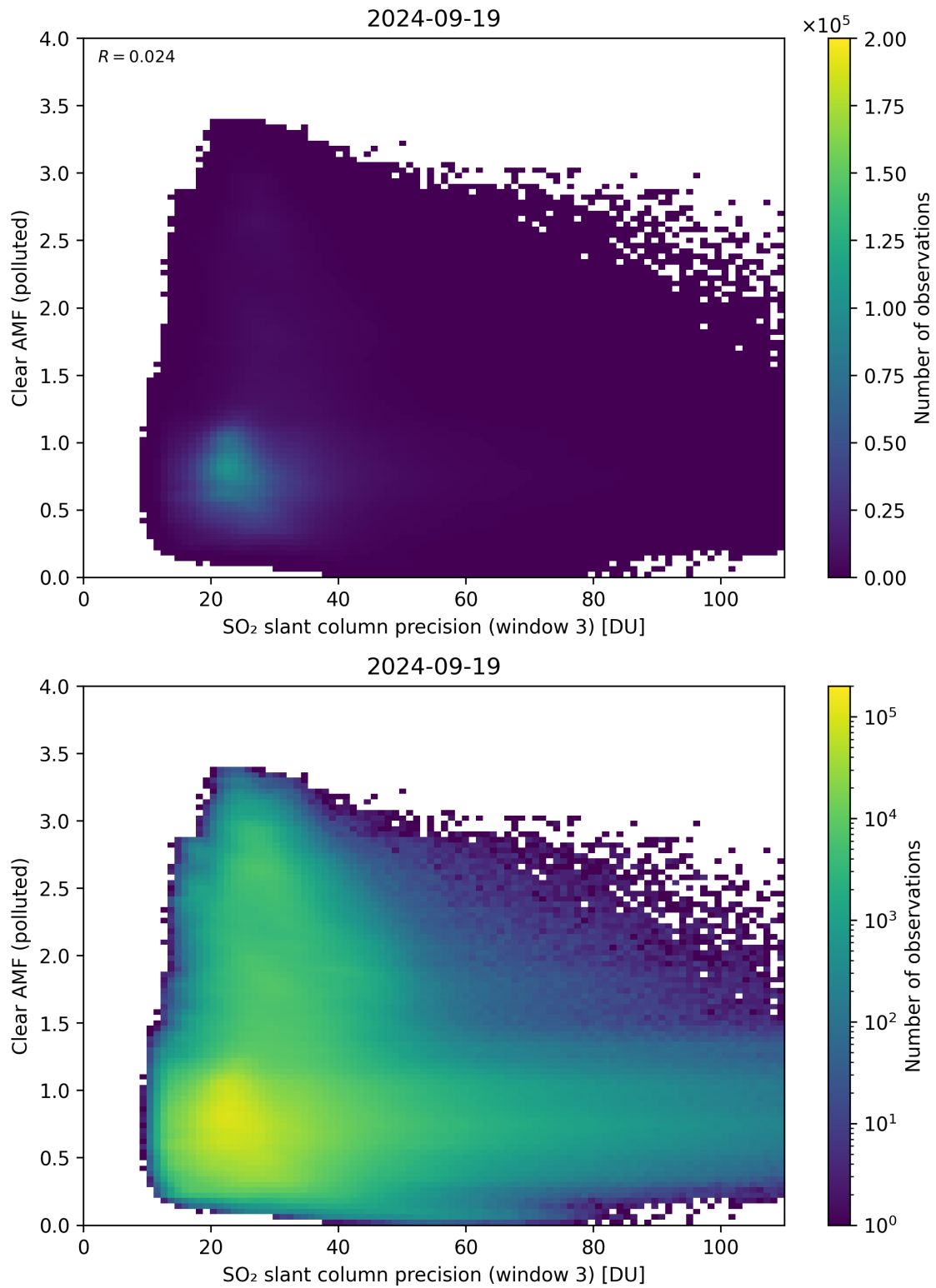
Figure 261: Scatter density plot of “SO 2 slant column precision (window 3)” against “Clear AMF (polluted)” for 2024-09-18 to 2024-09-20.
