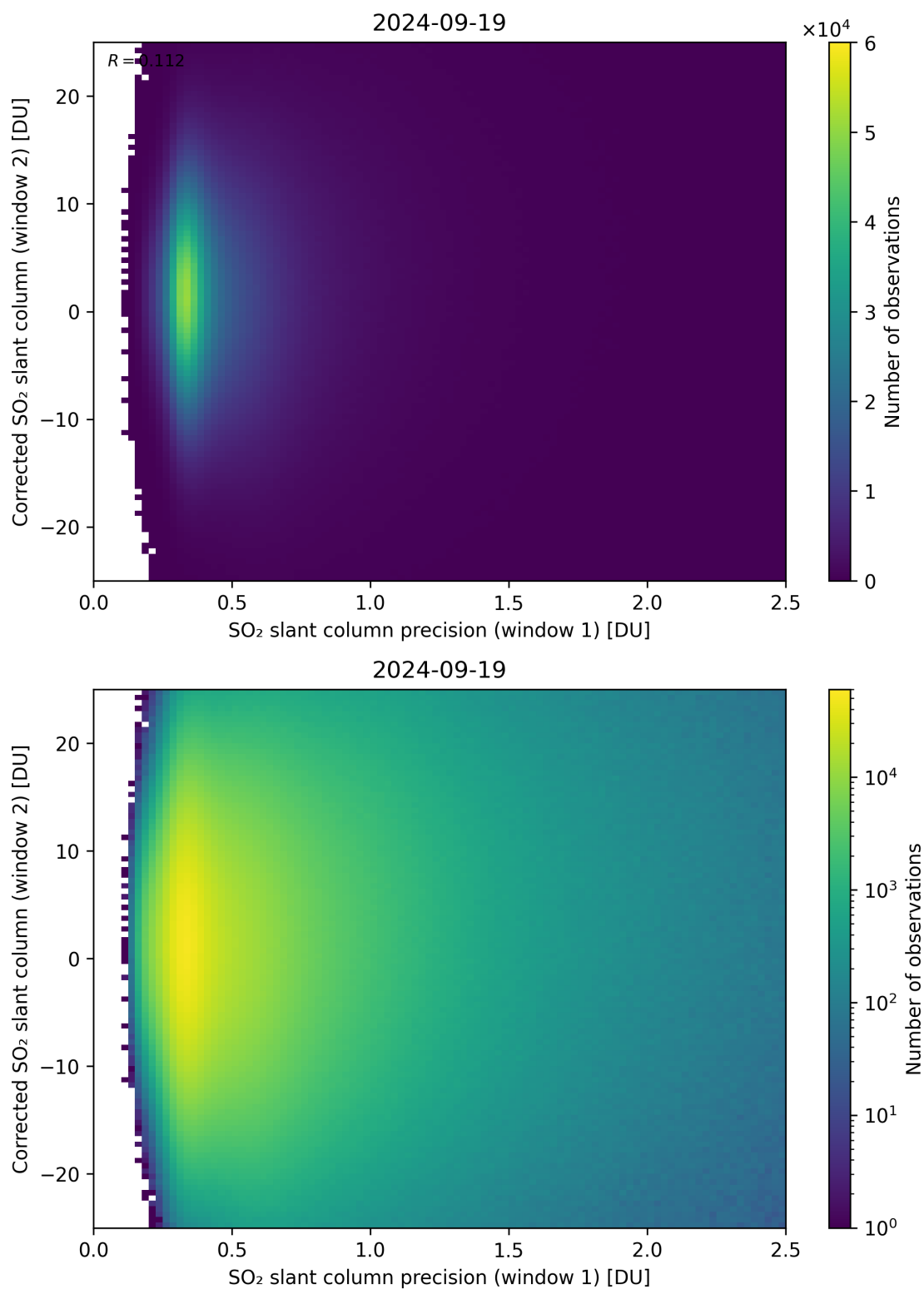
Figure 225: Scatter density plot of “SO 2 slant column precision (window 1)” against “Corrected SO 2 slant column (window 2)” for 2024-09-18 to 2024-09-20.
