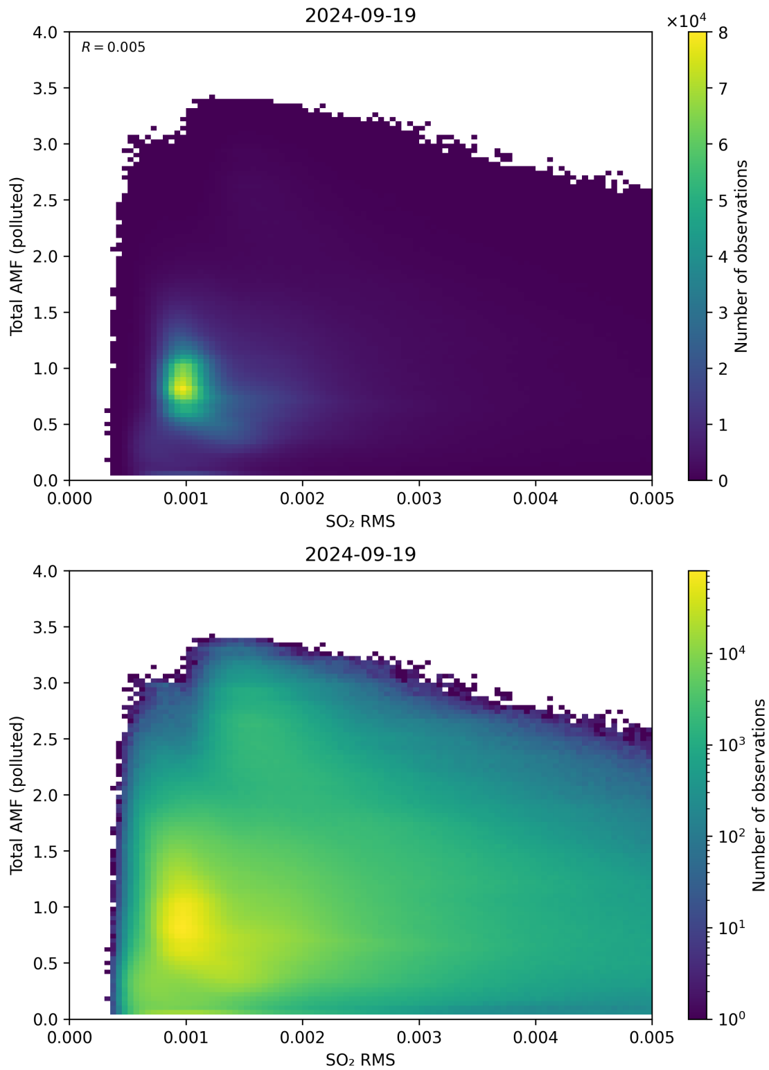
Figure 137: Scatter density plot of “SO 2 RMS” against “Total AMF (polluted)” for 2024-09-18 to 2024-09-20.
