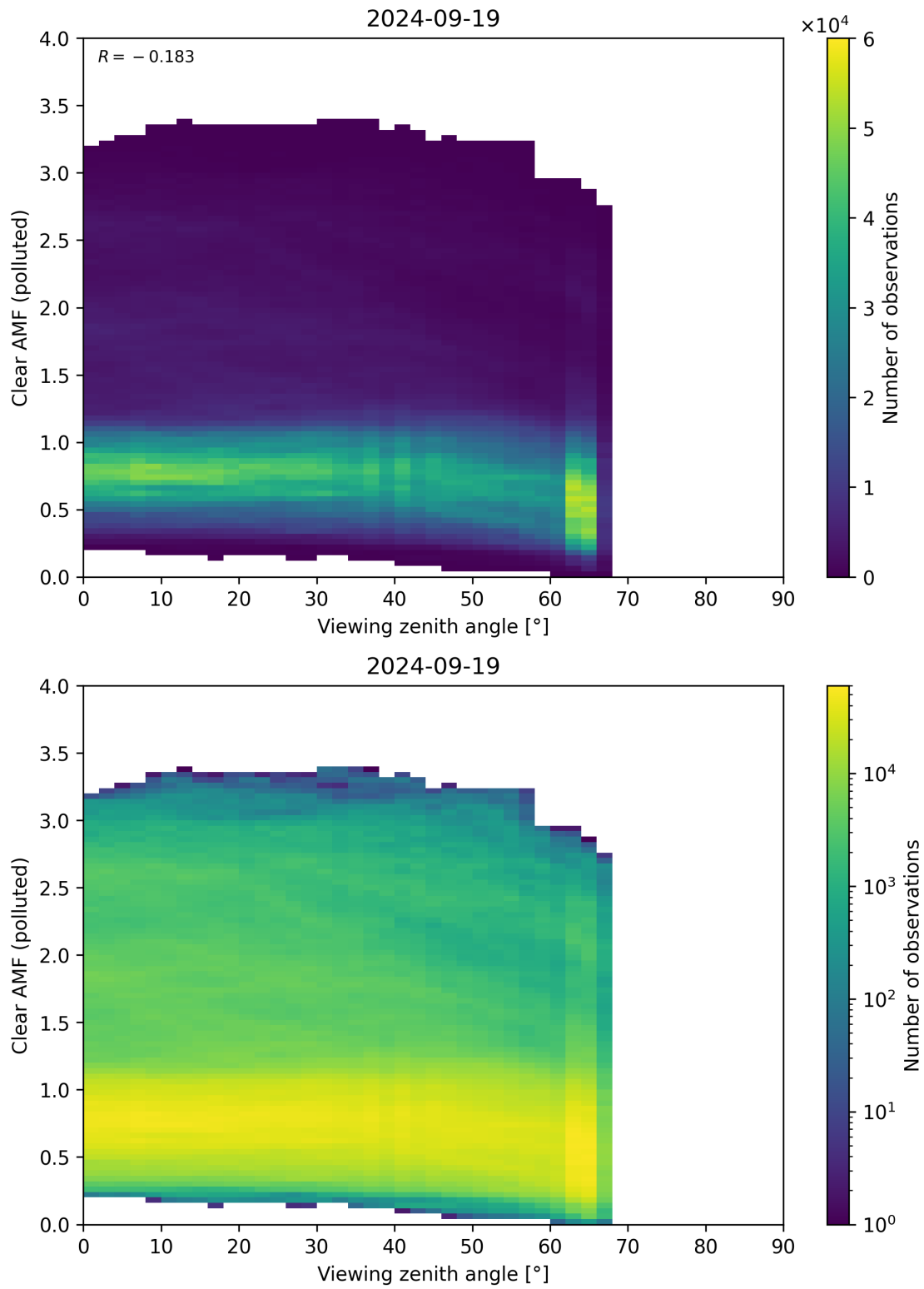
Figure 316: Scatter density plot of “Viewing zenith angle” against “Clear AMF (polluted)” for 2024-09-18 to 2024-09-20.
