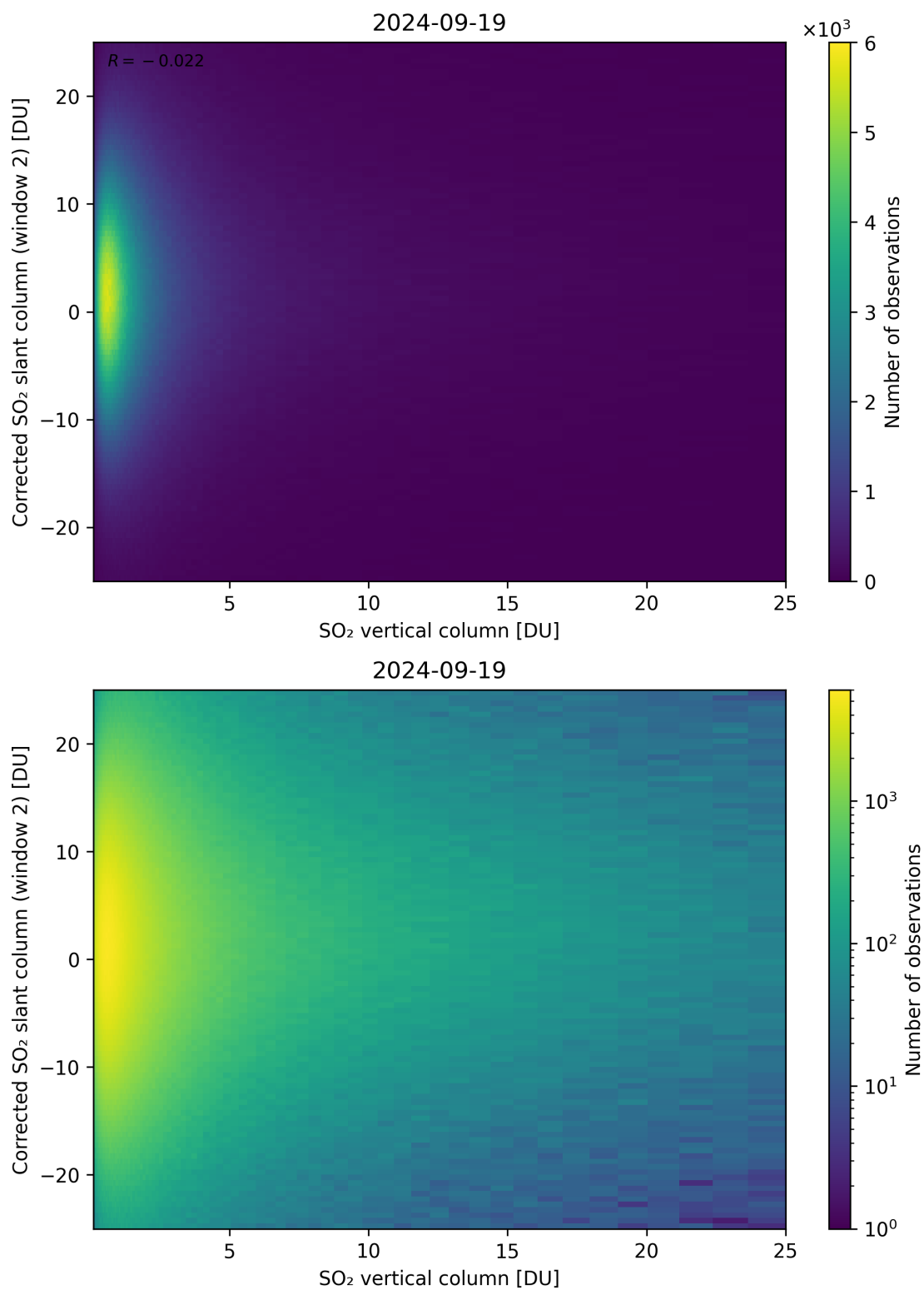
Figure 298: Scatter density plot of “SO 2 vertical column” against “Corrected SO 2 slant column (window 2)” for 2024-09-18 to 2024-09-20.
