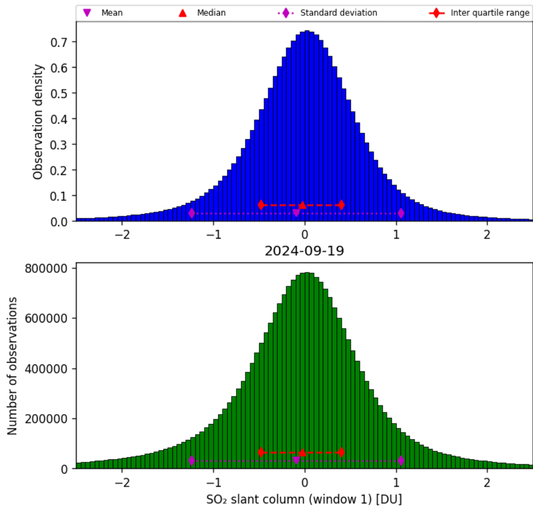
Figure 56: Histogram of “SO 2 slant column (window 1)” for 2024-09-18 to 2024-09-20
