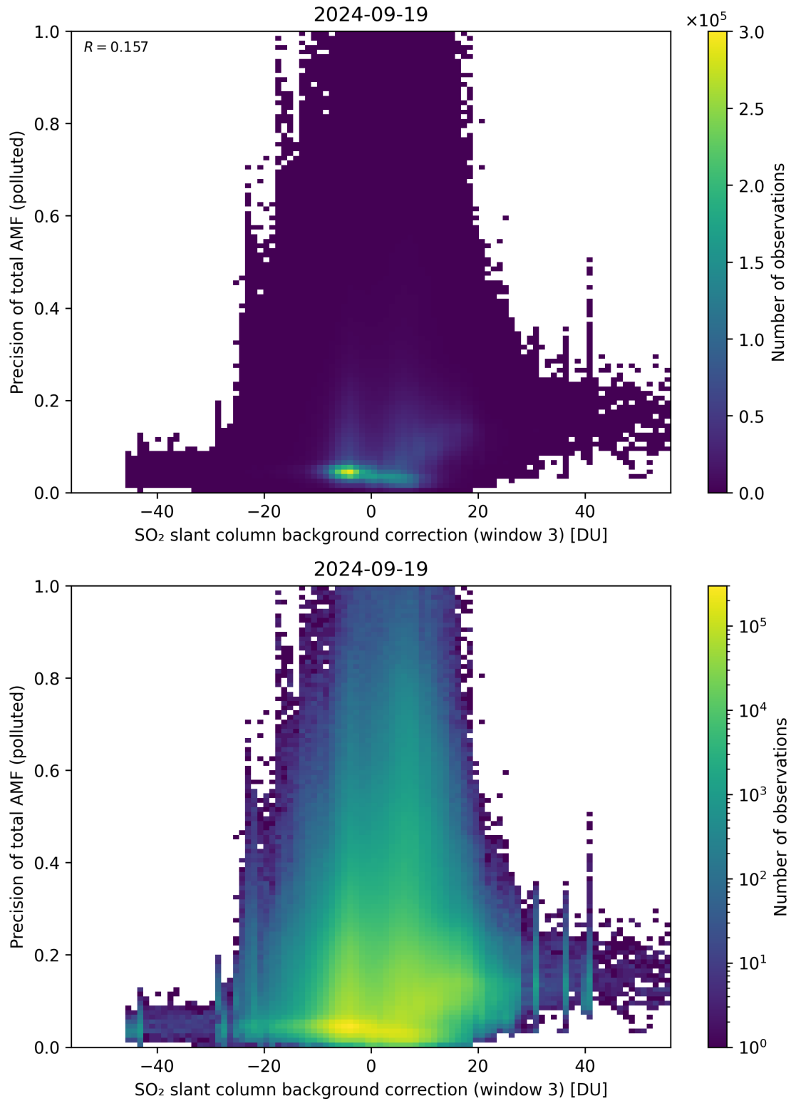
Figure 126: Scatter density plot of “SO 2 slant column background correction (window 3)” against “Precision of total AMF (polluted)” for 2024-09-18 to 2024-09-20.
