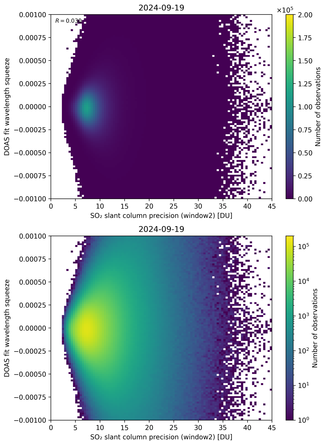
Figure 244: Scatter density plot of “SO 2 slant column precision (window2)” against “DOAS fit wavelength squeeze” for 2024-09-18 to 2024-09-20.
