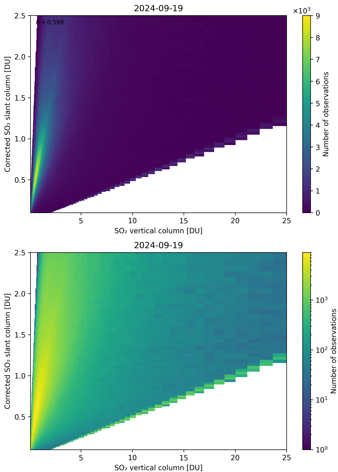
Figure 297: Scatter density plot of “SO 2 vertical column” against “Corrected SO 2 slant column” for 2024-09-18 to 2024-09-20.
