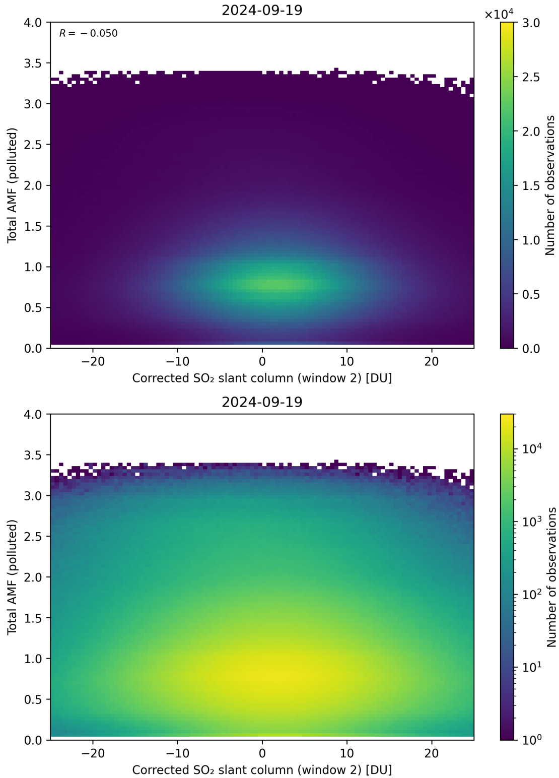
Figure 203: Scatter density plot of “Corrected SO 2 slant column (window 2)” against “Total AMF (polluted)” for 2024-09-18 to 2024-09-20.
