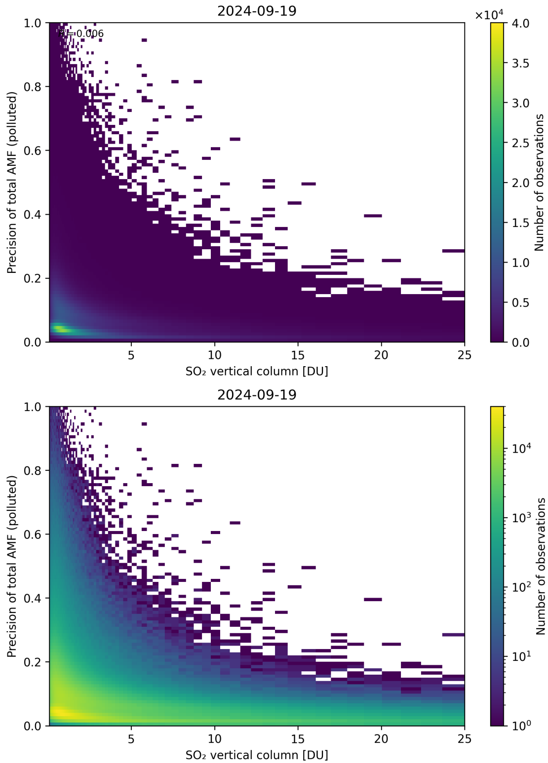
Figure 306: Scatter density plot of “SO 2 vertical column” against “Precision of total AMF (polluted)” for 2024-09-18 to 2024-09-20.
