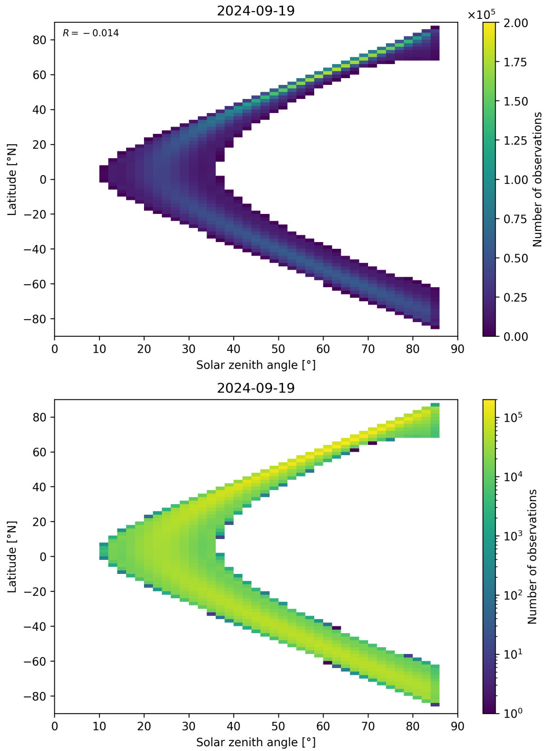
Figure 164: Scatter density plot of “Solar zenith angle” against “Latitude” for 2024-09-18 to 2024-09-20.
