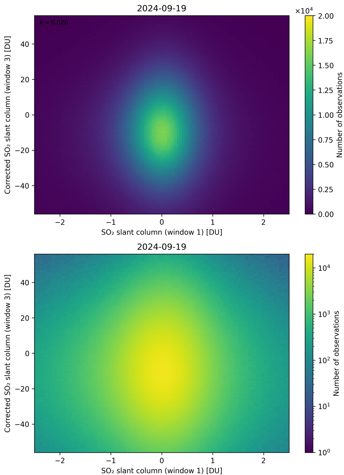
Figure 234: Scatter density plot of “SO 2 slant column (window 1)” against “Corrected SO 2 slant column (window 3)” for 2024-09-18 to 2024-09-20.
