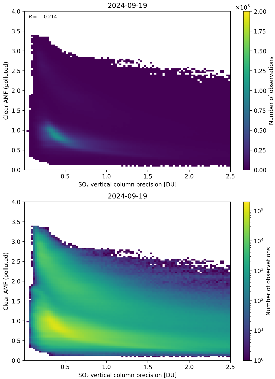
Figure 285: Scatter density plot of “SO 2 vertical column precision” against “Clear AMF (polluted)” for 2024-09-18 to 2024-09-20.
