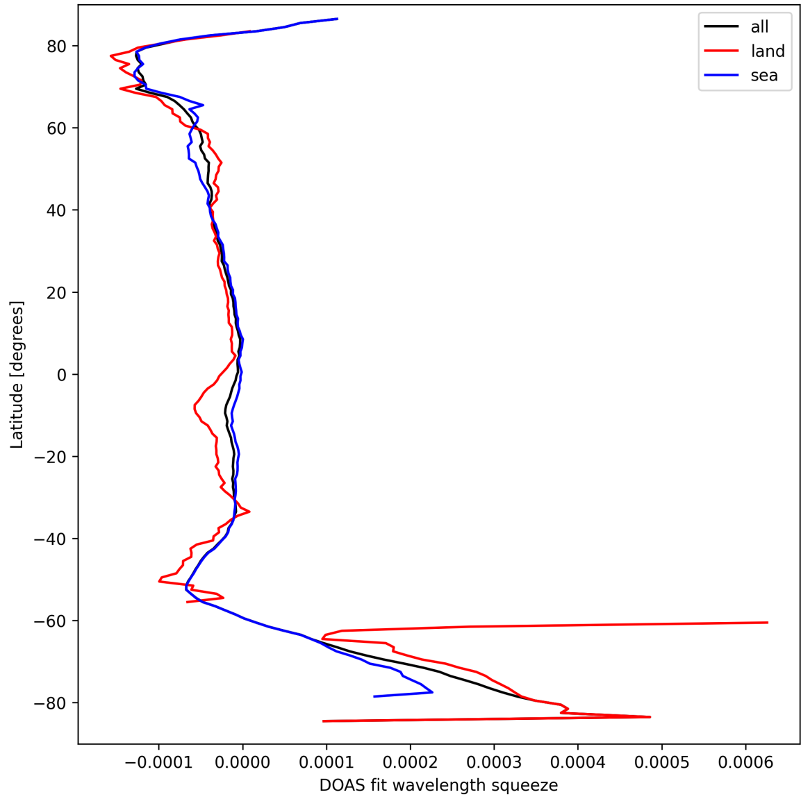
Figure 46: Zonal average of “DOAS fit wavelength squeeze” for 2024-09-18 to 2024-09-20.
