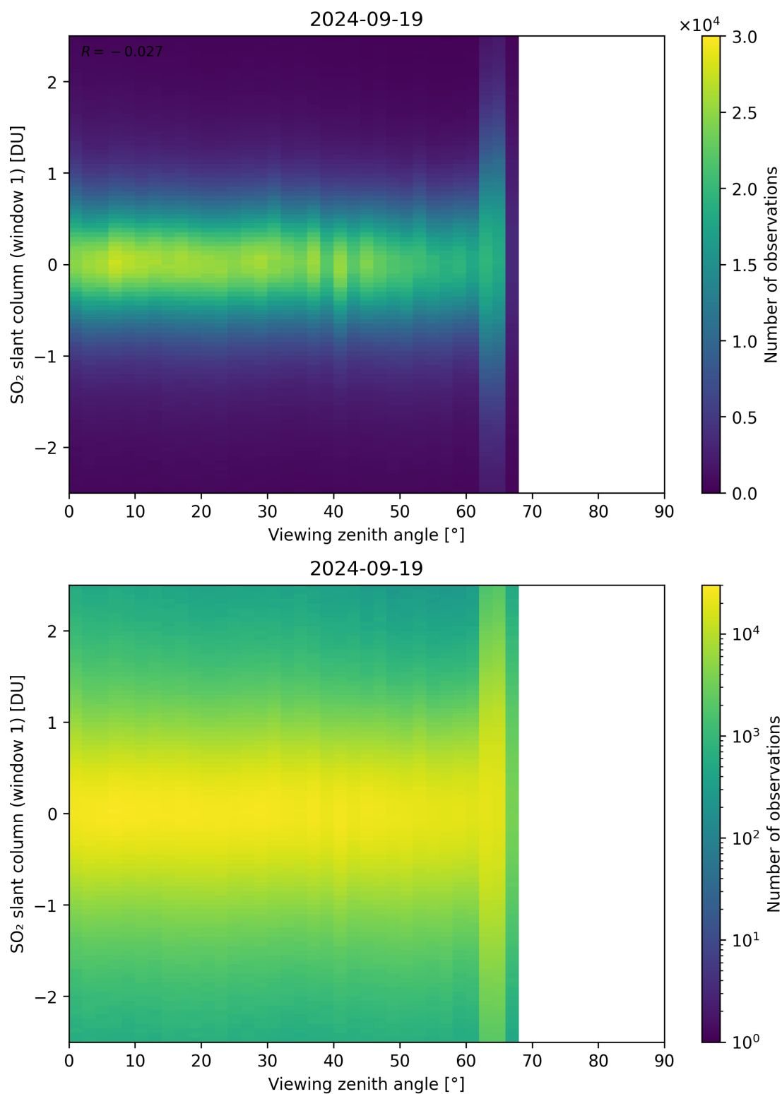
Figure 320: Scatter density plot of “Viewing zenith angle” against “SO 2 slant column (window 1)” for 2024-09-18 to 2024-09-20.
