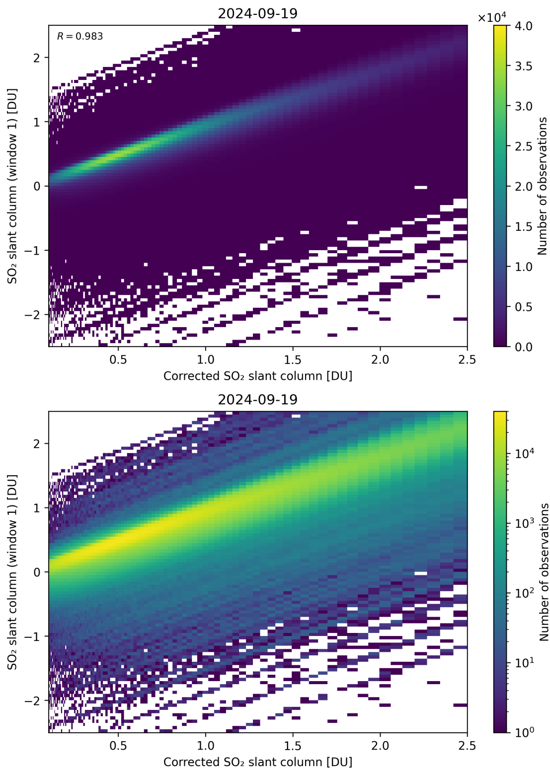
Figure 187: Scatter density plot of “Corrected SO 2 slant column” against “SO 2 slant column (window 1)” for 2024-09-18 to 2024-09-20.
