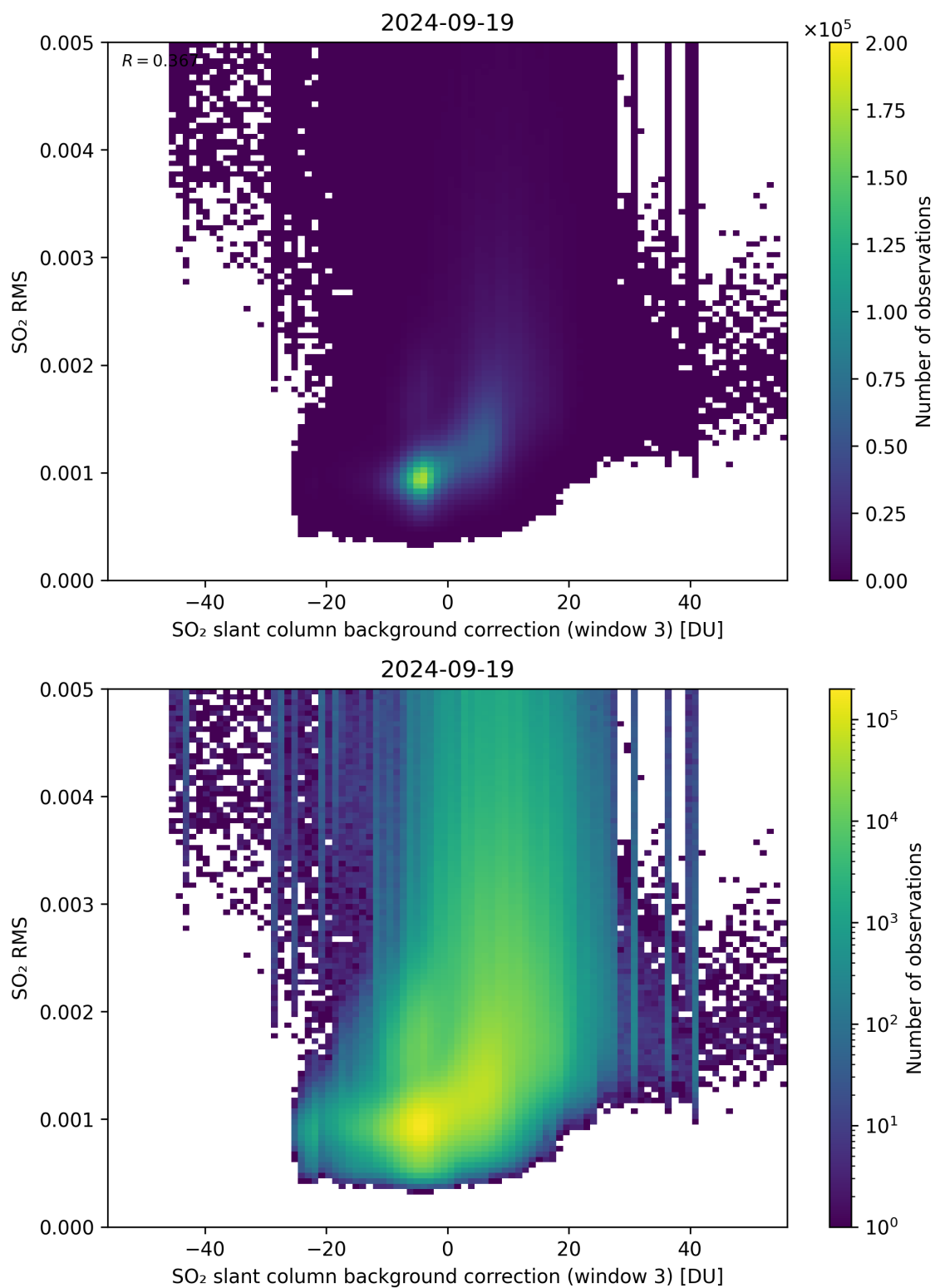
Figure 123: Scatter density plot of “SO 2 slant column background correction (window 3)” against “SO 2 RMS” for 2024-09-18 to 2024-09-20.
