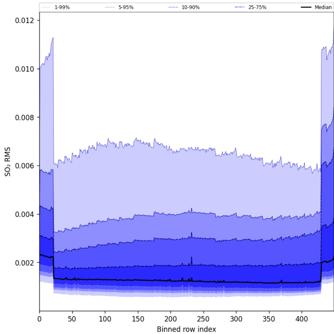
Figure 93: Along track statistics of “SO 2 RMS” for 2024-09-18 to 2024-09-20
