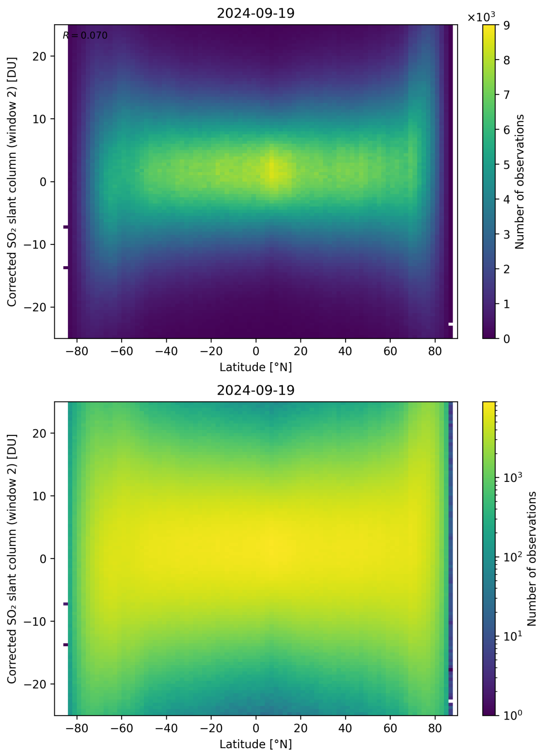
Figure 147: Scatter density plot of “Latitude” against “Corrected SO 2 slant column (window 2)” for 2024-09-18 to 2024-09-20.
