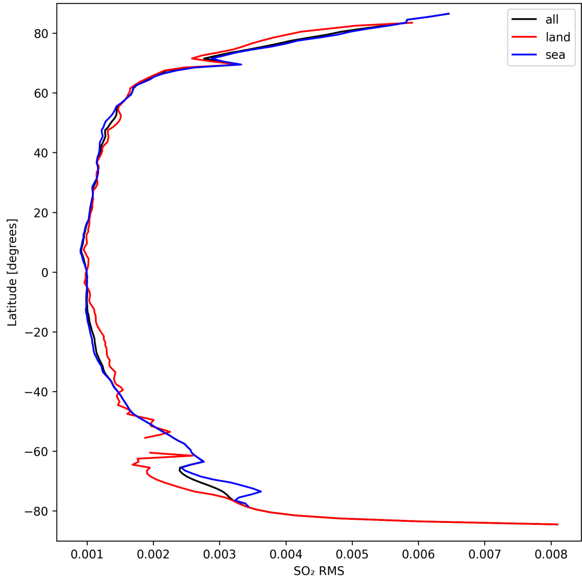
Figure 47: Zonal average of “SO 2 RMS” for 2024-09-18 to 2024-09-20.
