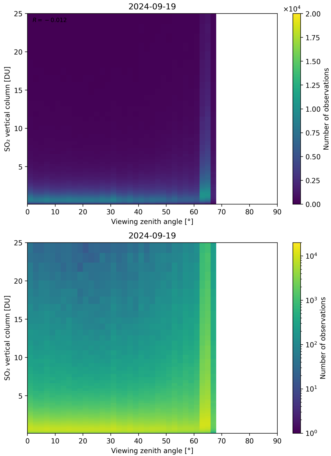
Figure 327: Scatter density plot of “Viewing zenith angle” against “SO 2 vertical column” for 2024-09-18 to 2024-09-20.
