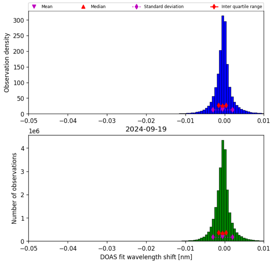
Figure 68: Histogram of “DOAS fit wavelength shift” for 2024-09-18 to 2024-09-20
