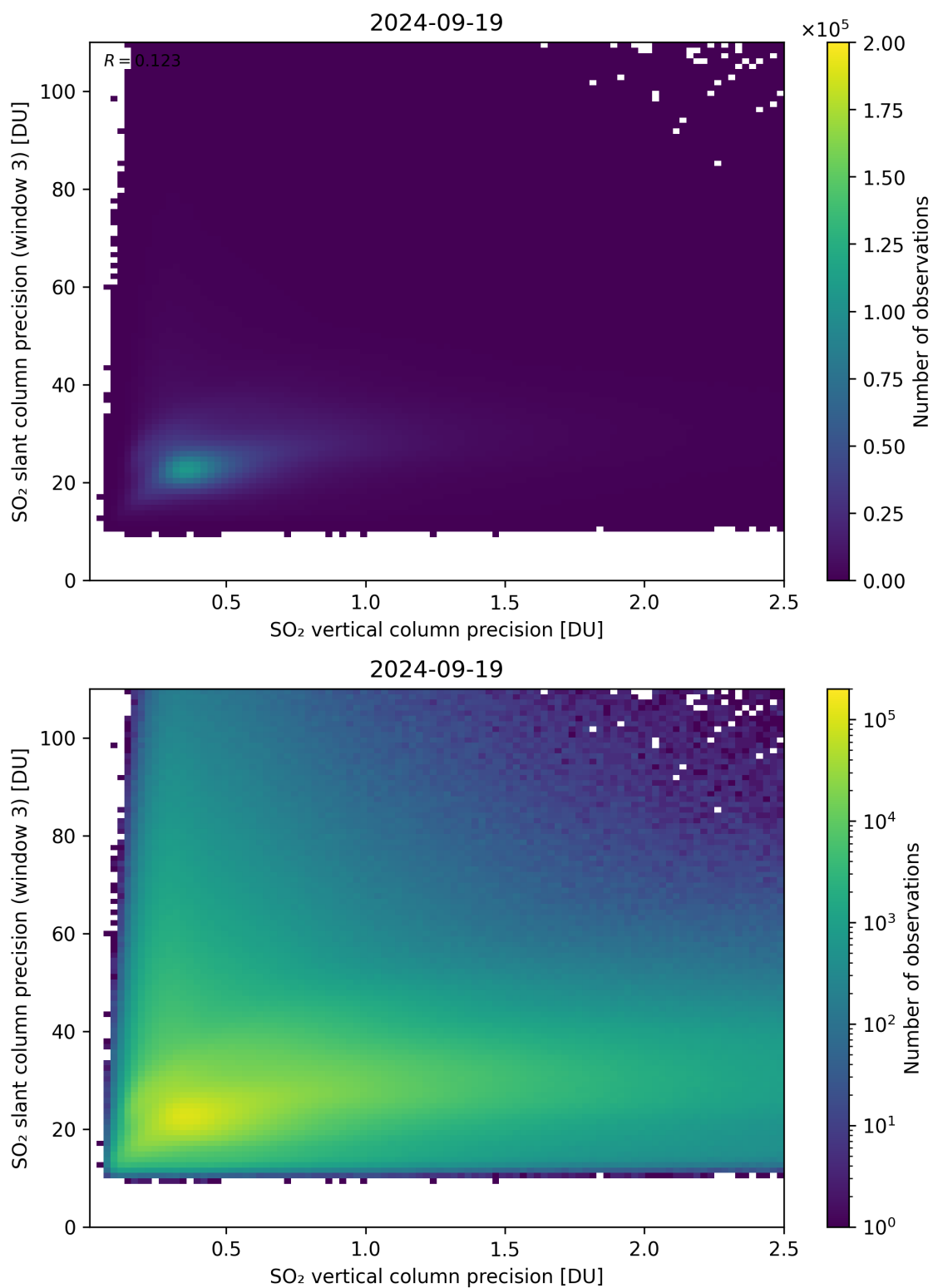
Figure 293: Scatter density plot of “SO 2 vertical column precision” against “SO 2 slant column precision (window 3)” for 2024-09-18 to 2024-09-20.
