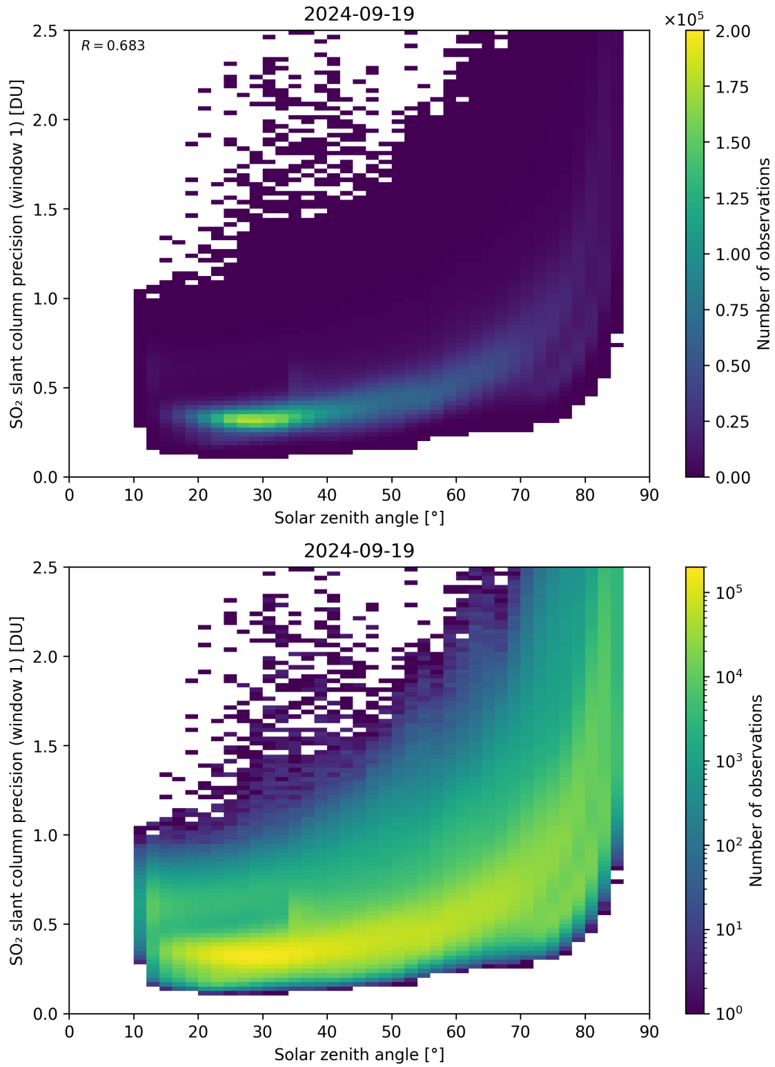
Figure 170: Scatter density plot of “Solar zenith angle” against “SO 2 slant column precision (window 1)” for 2024-09-18 to 2024-09-20.
