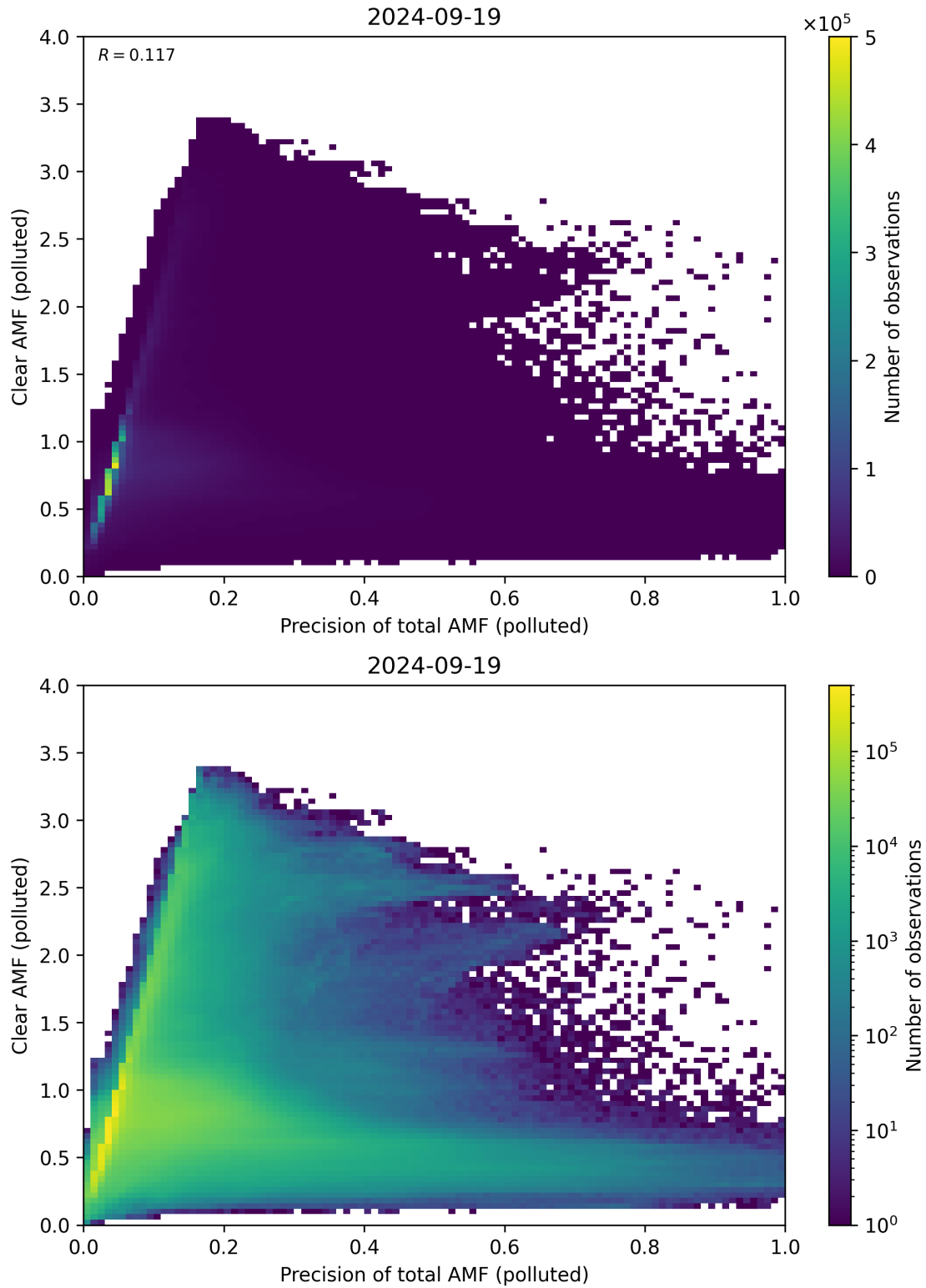
Figure 270: Scatter density plot of “Precision of total AMF (polluted)” against “Clear AMF (polluted)” for 2024-09-18 to 2024-09-20.
