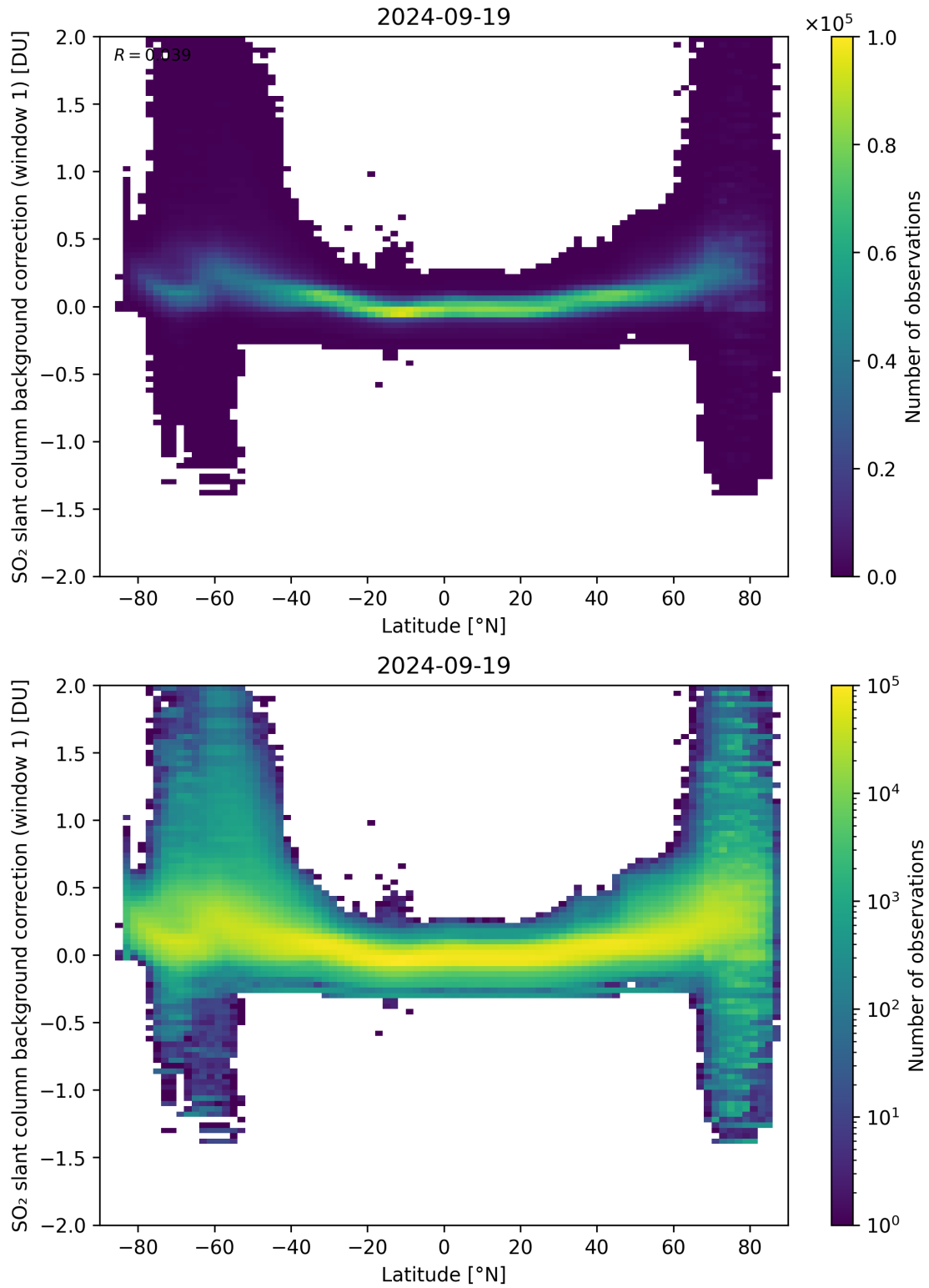
Figure 139: Scatter density plot of “Latitude” against “SO 2 slant column background correction (window 1)” for 2024-09-18 to 2024-09-20.
