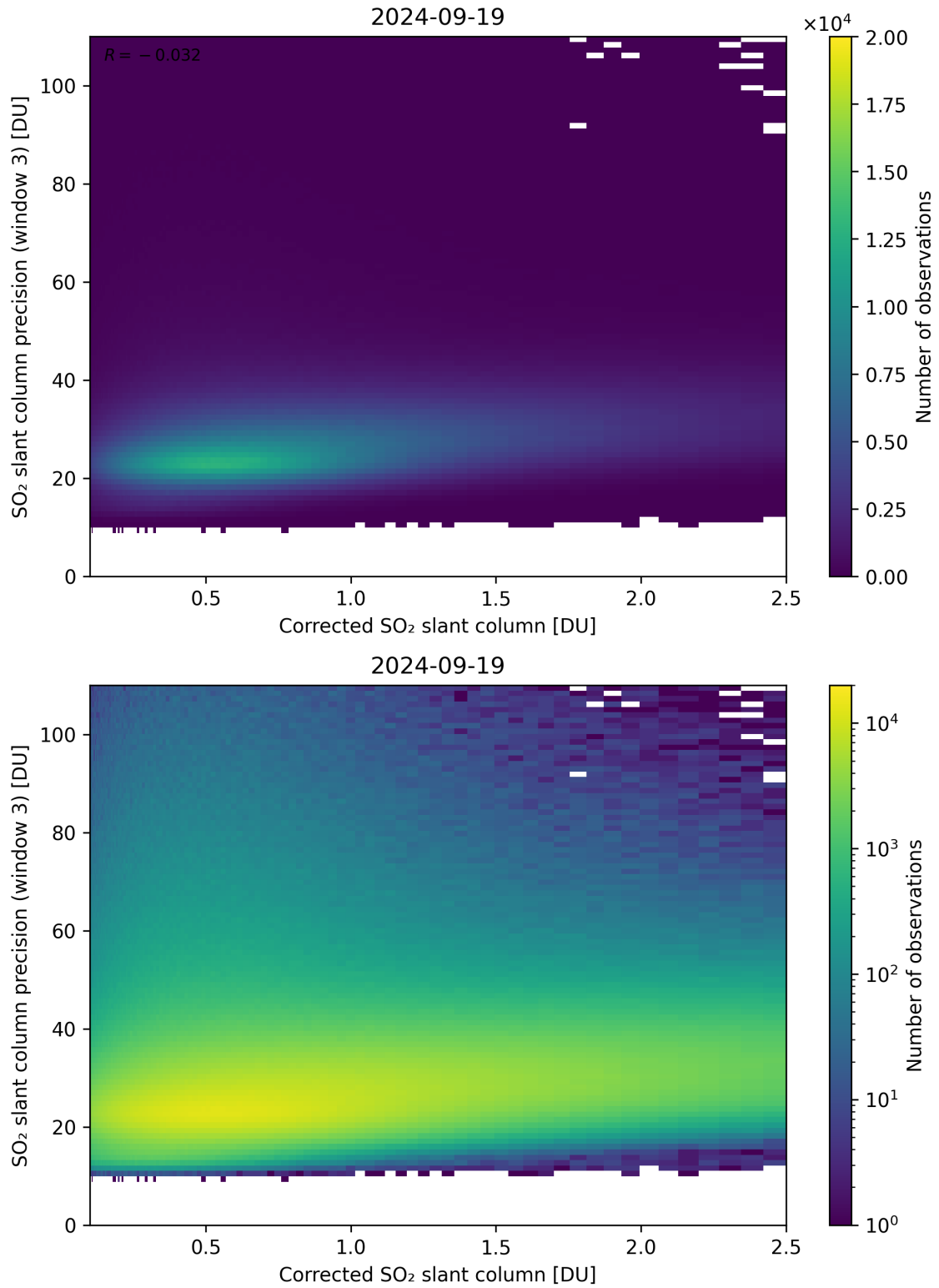
Figure 191: Scatter density plot of “Corrected SO 2 slant column” against “SO 2 slant column precision (window 3)” for 2024-09-18 to 2024-09-20.
