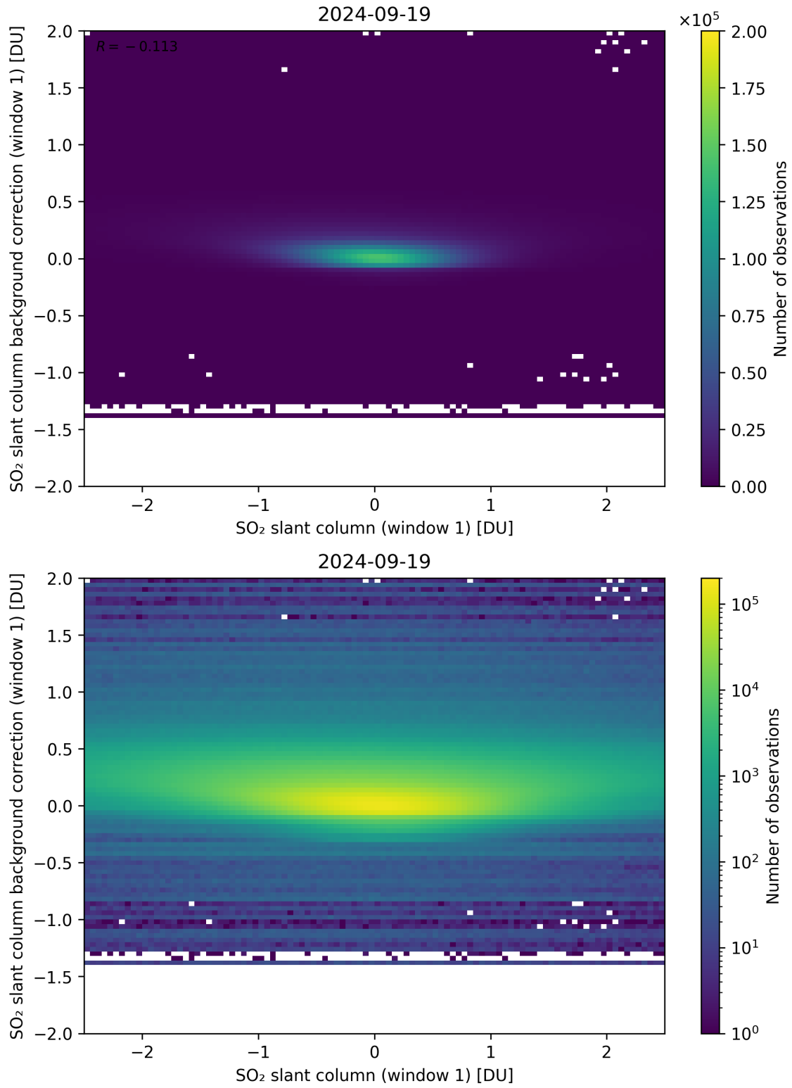
Figure 212: Scatter density plot of “SO 2 slant column (window 1)” against “SO 2 slant column background correction (window 1)” for 2024-09-18 to 2024-09-20.
