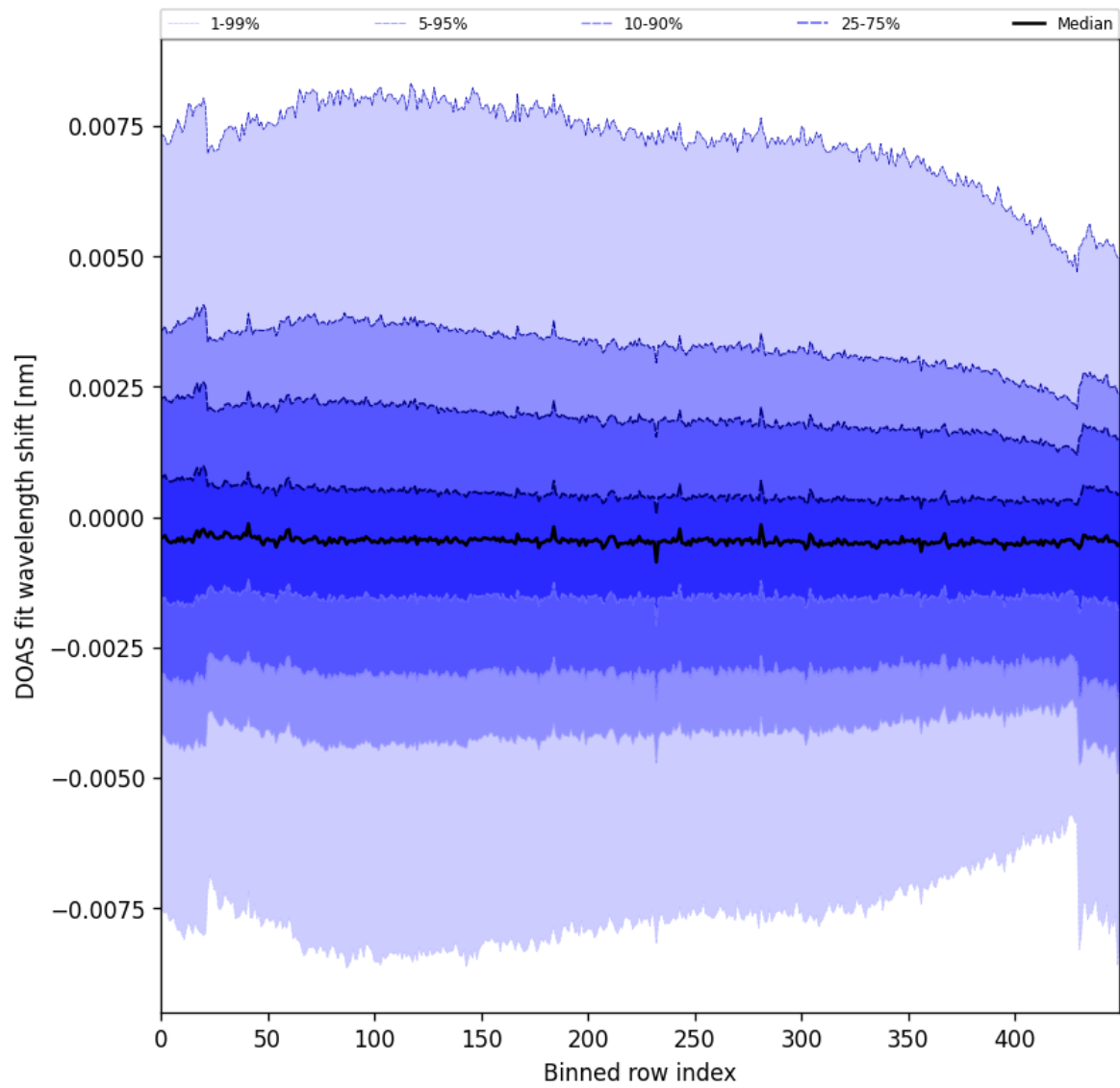
Figure 91: Along track statistics of “DOAS fit wavelength shift” for 2024-09-18 to 2024-09-20
