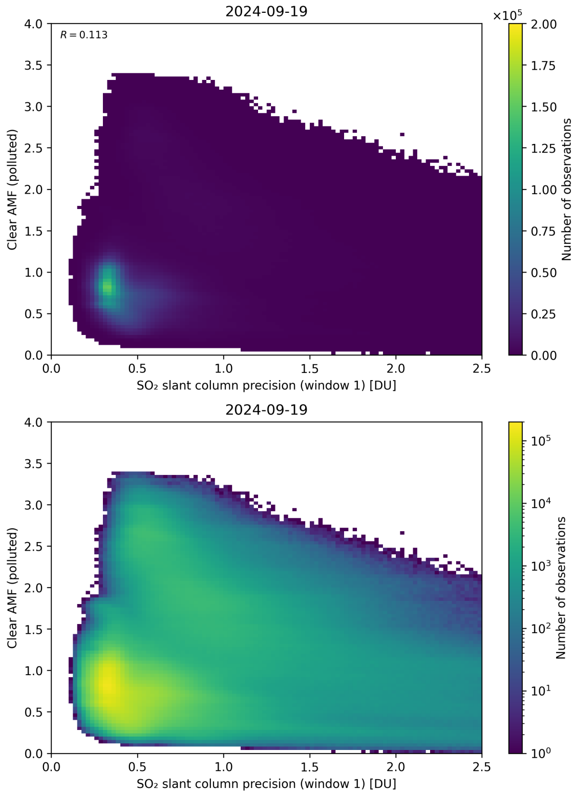
Figure 224: Scatter density plot of “SO 2 slant column precision (window 1)” against “Clear AMF (polluted)” for 2024-09-18 to 2024-09-20.
