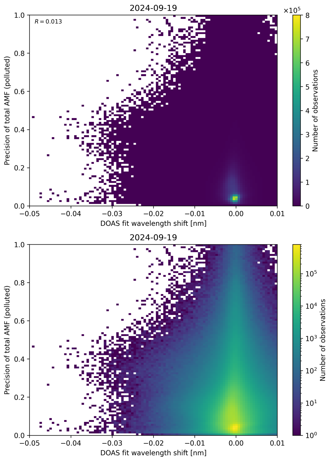
Figure 131: Scatter density plot of “DOAS fit wavelength shift” against “Precision of total AMF (polluted)” for 2024-09-18 to 2024-09-20.
