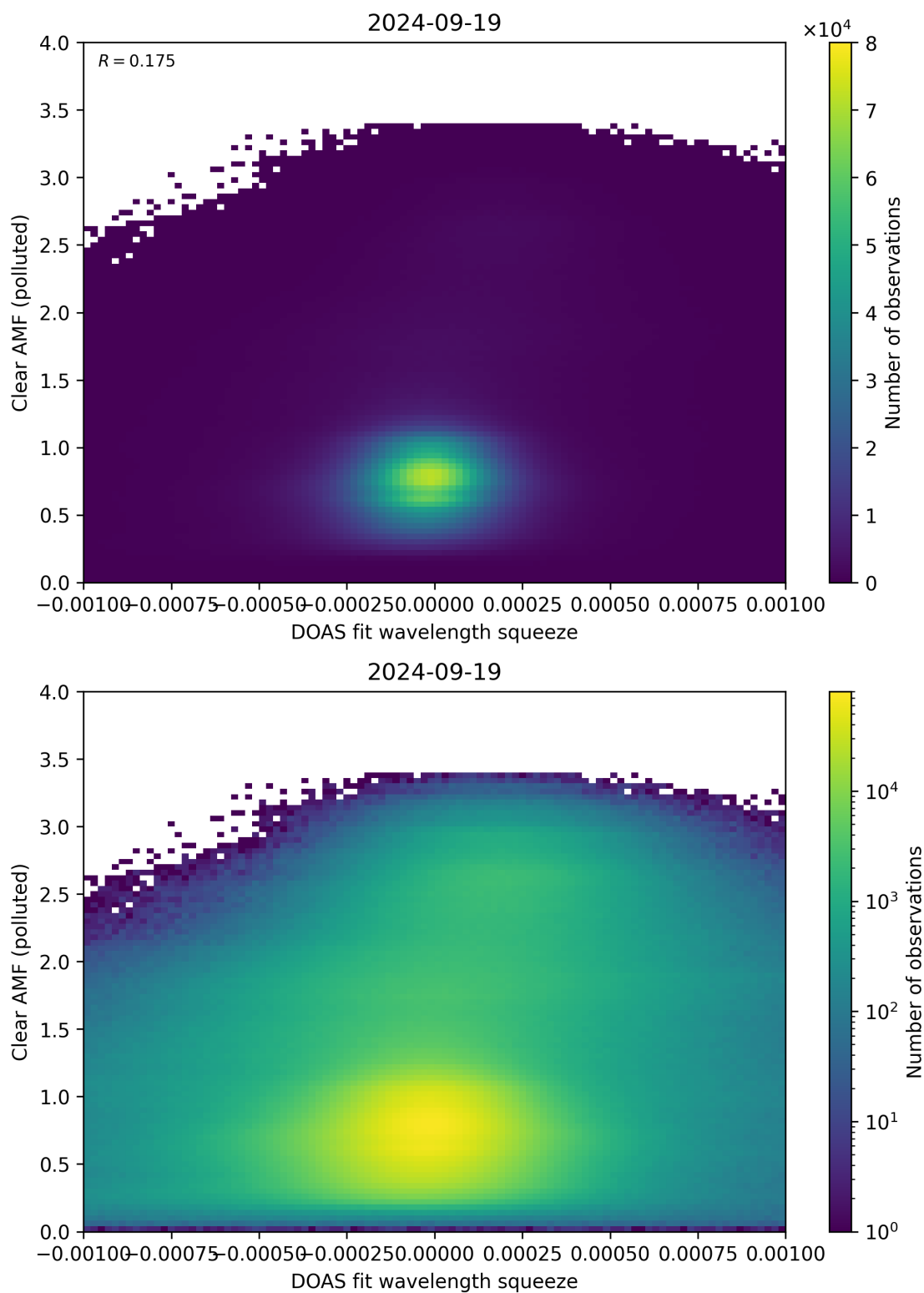
Figure 133: Scatter density plot of “DOAS fit wavelength squeeze” against “Clear AMF (polluted)” for 2024-09-18 to 2024-09-20.
