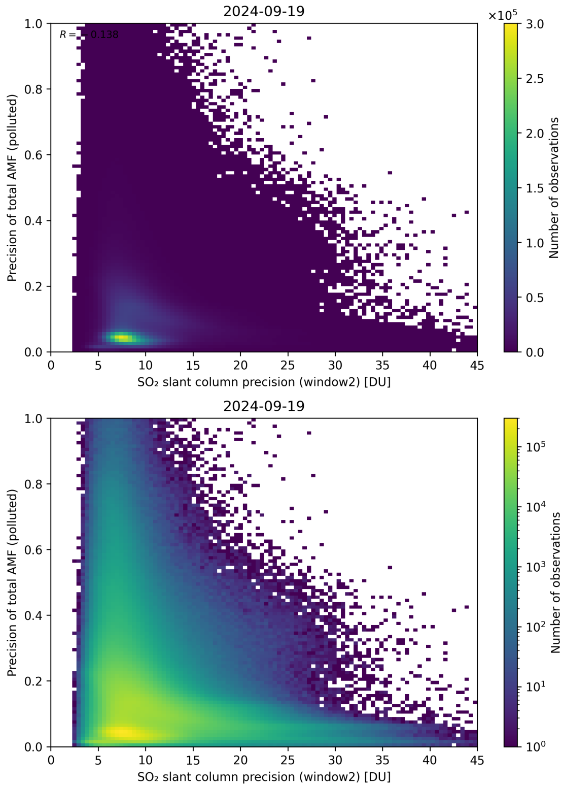
Figure 252: Scatter density plot of “SO 2 slant column precision (window2)” against “Precision of total AMF (polluted)” for 2024-09-18 to 2024-09-20.
