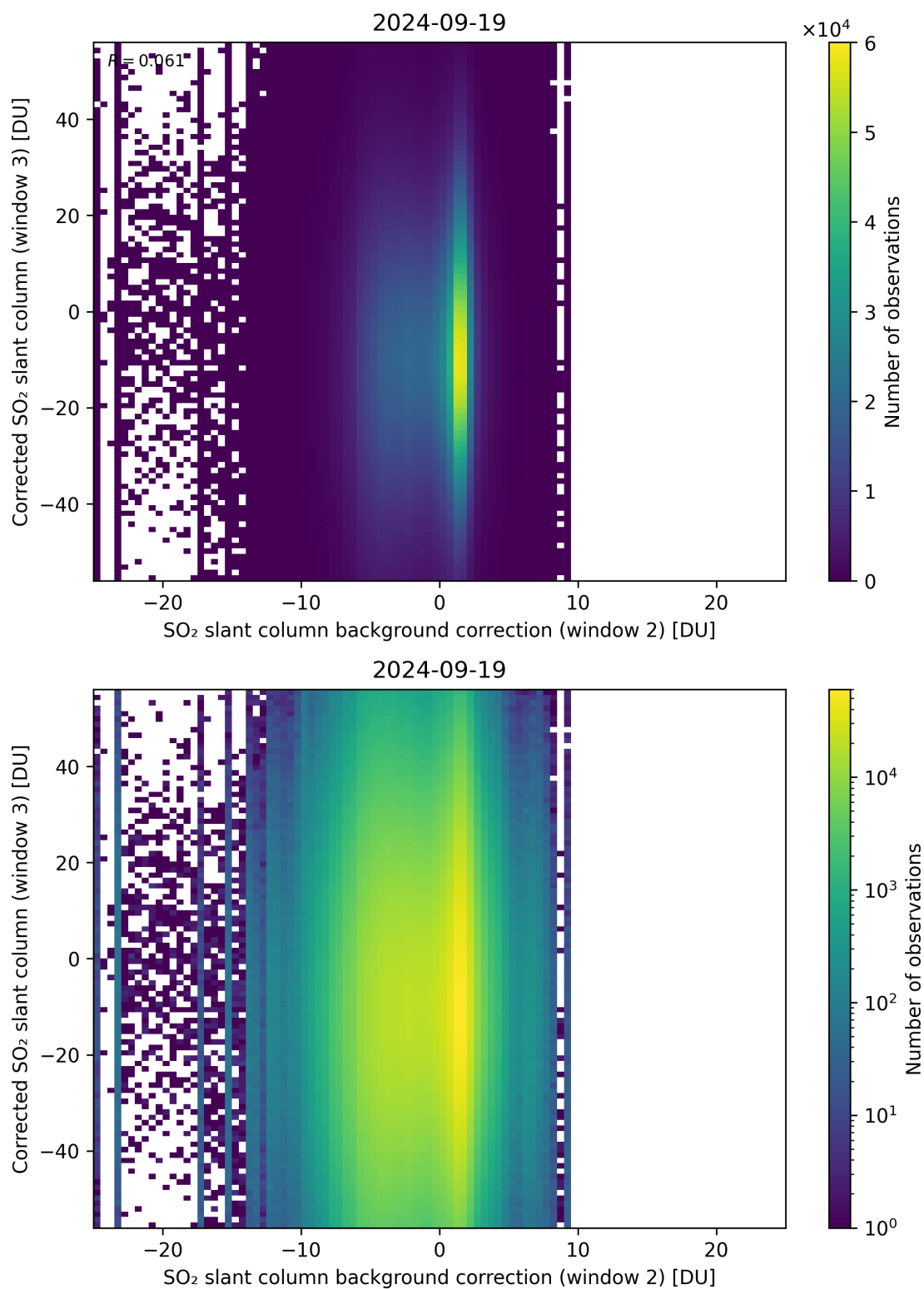
Figure 116: Scatter density plot of “SO 2 slant column background correction (window 2)” against “Corrected SO 2 slant column (window 3)” for 2024-09-18 to 2024-09-20.
