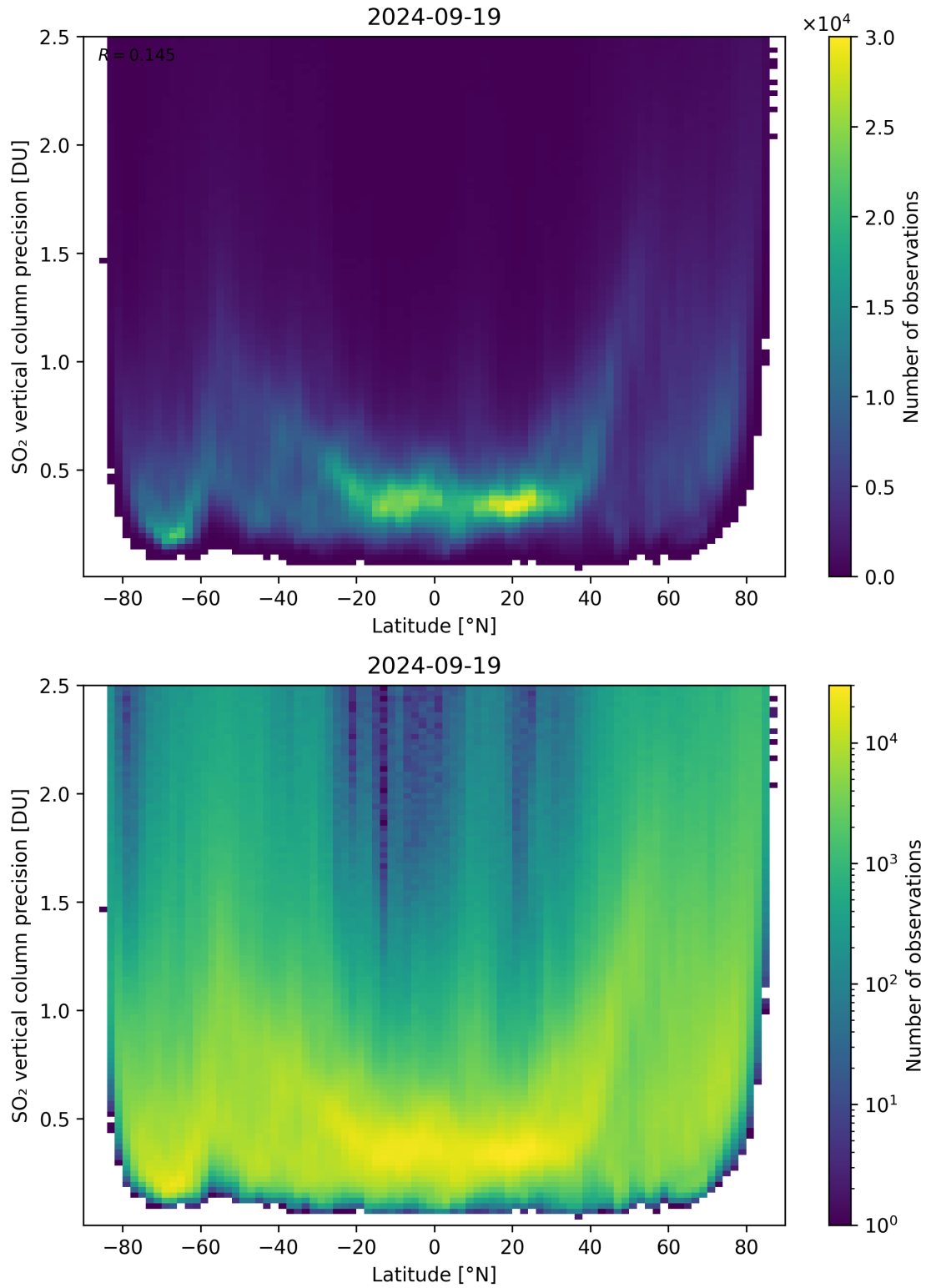
Figure 157: Scatter density plot of “Latitude” against “SO 2 vertical column precision” for 2024-09-18 to 2024-09-20.
