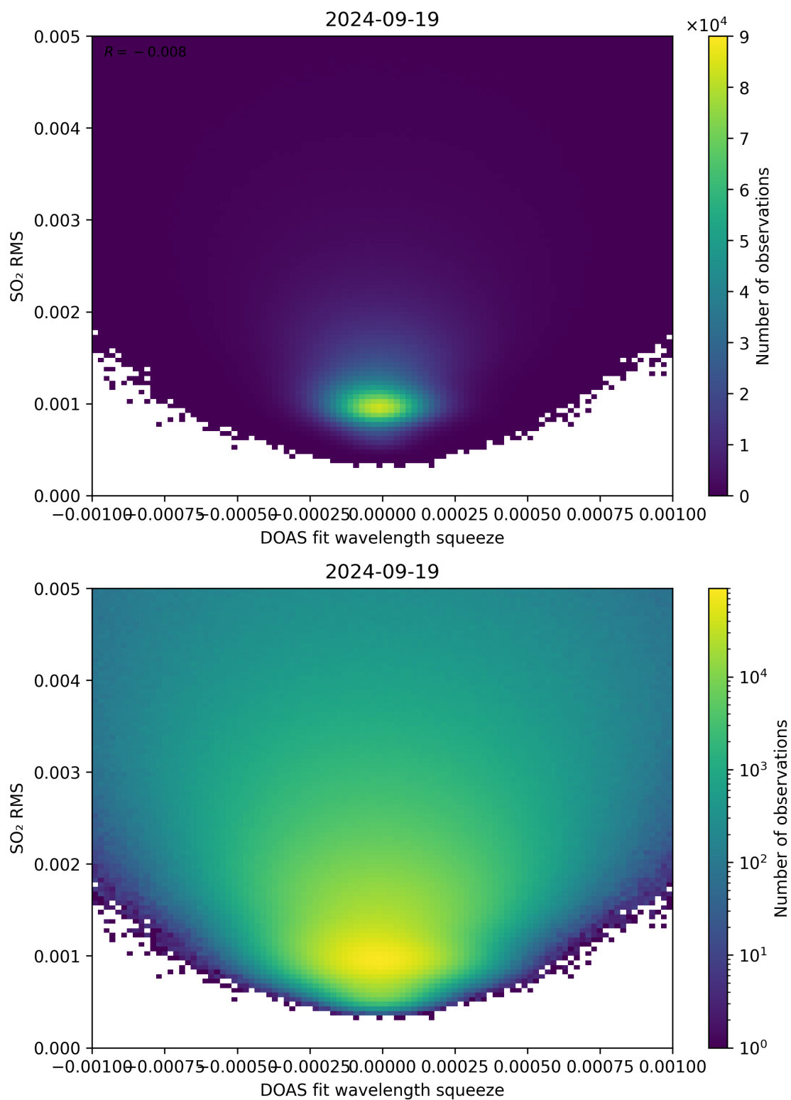
Figure 132: Scatter density plot of “DOAS fit wavelength squeeze” against “SO 2 RMS” for 2024-09-18 to 2024-09-20.
