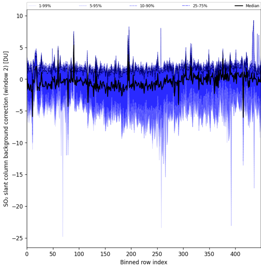
Figure 86: Along track statistics of “SO 2 slant column background correction (window 2)” for 2024-09-18 to 2024-09-20
