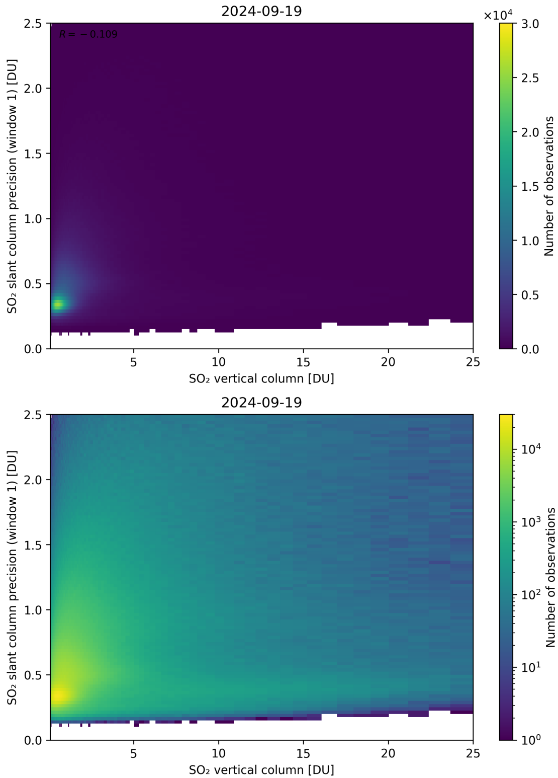
Figure 301: Scatter density plot of “SO 2 vertical column” against “SO 2 slant column precision (window 1)” for 2024-09-18 to 2024-09-20.
