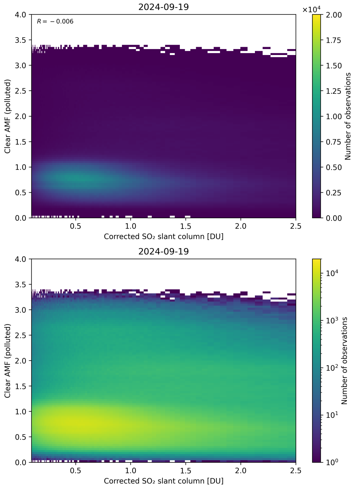
Figure 184: Scatter density plot of “Corrected SO 2 slant column” against “Clear AMF (polluted)” for 2024-09-18 to 2024-09-20.
