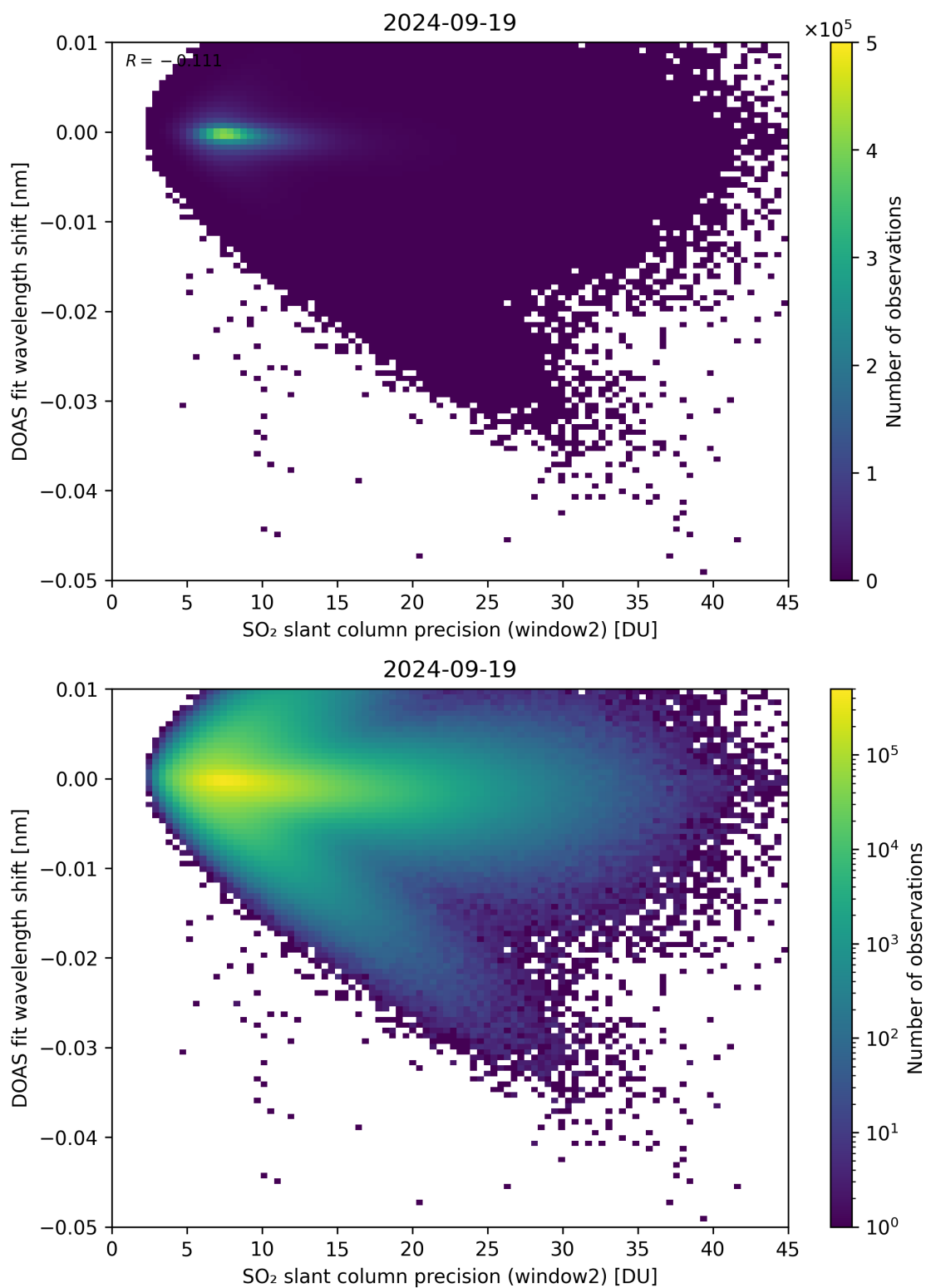
Figure 243: Scatter density plot of “SO 2 slant column precision (window2)” against “DOAS fit wavelength shift” for 2024-09-18 to 2024-09-20.
