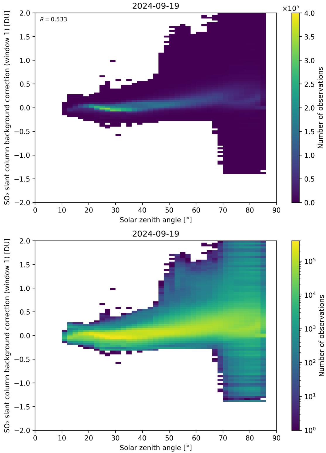
Figure 158: Scatter density plot of “Solar zenith angle” against “SO 2 slant column background correction (window 1)” for 2024-09-18 to 2024-09-20.
