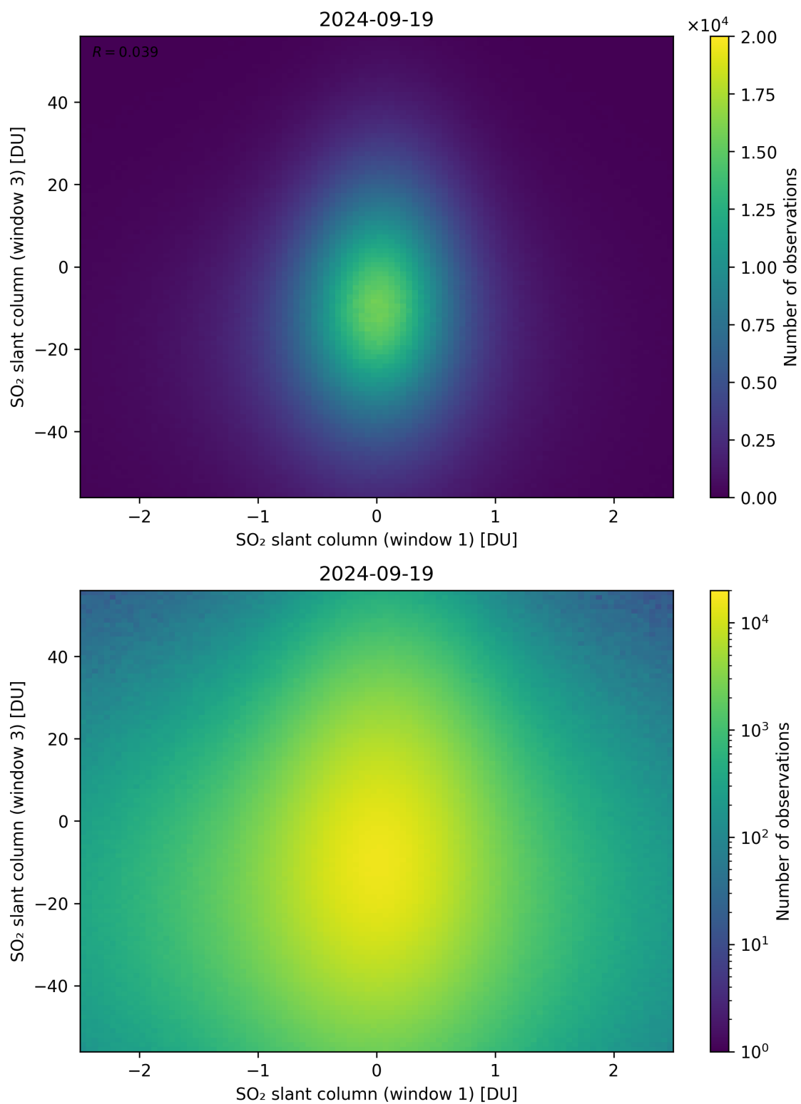
Figure 237: Scatter density plot of “SO 2 slant column (window 1)” against “SO 2 slant column (window 3)” for 2024-09-18 to 2024-09-20.
