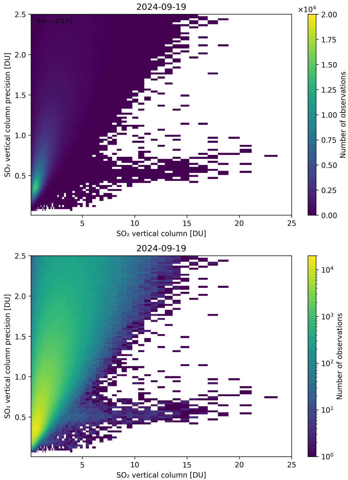
Figure 307: Scatter density plot of “SO 2 vertical column” against “SO 2 vertical column precision” for 2024-09-18 to 2024-09-20.
