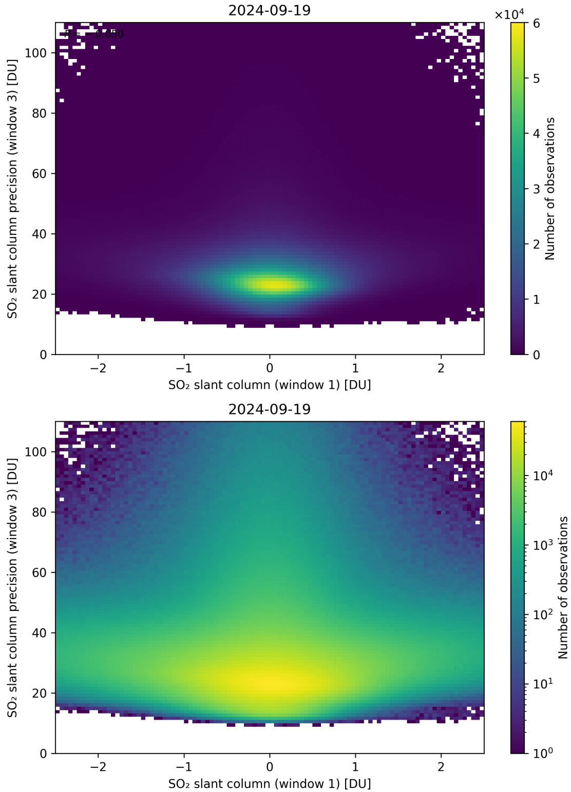
Figure 238: Scatter density plot of “SO 2 slant column (window 1)” against “SO 2 slant column precision (window 3)” for 2024-09-18 to 2024-09-20.
