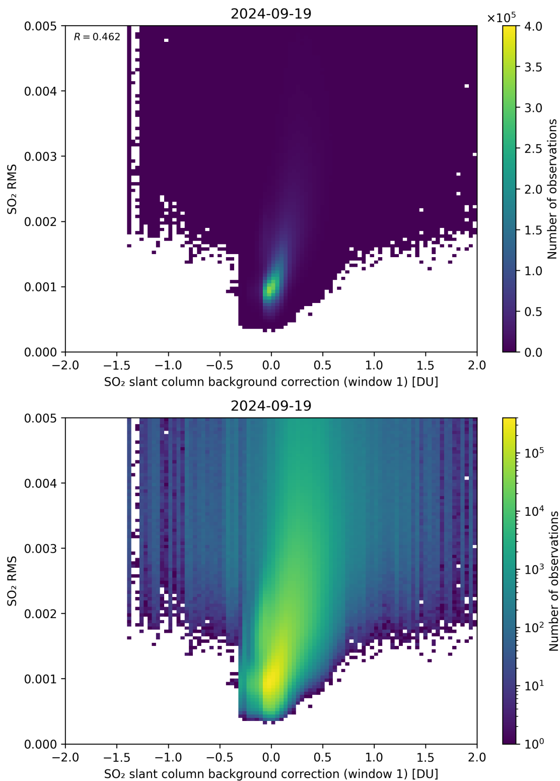
Figure 102: Scatter density plot of “SO 2 slant column background correction (window 1)” against “SO 2 RMS” for 2024-09-18 to 2024-09-20.
