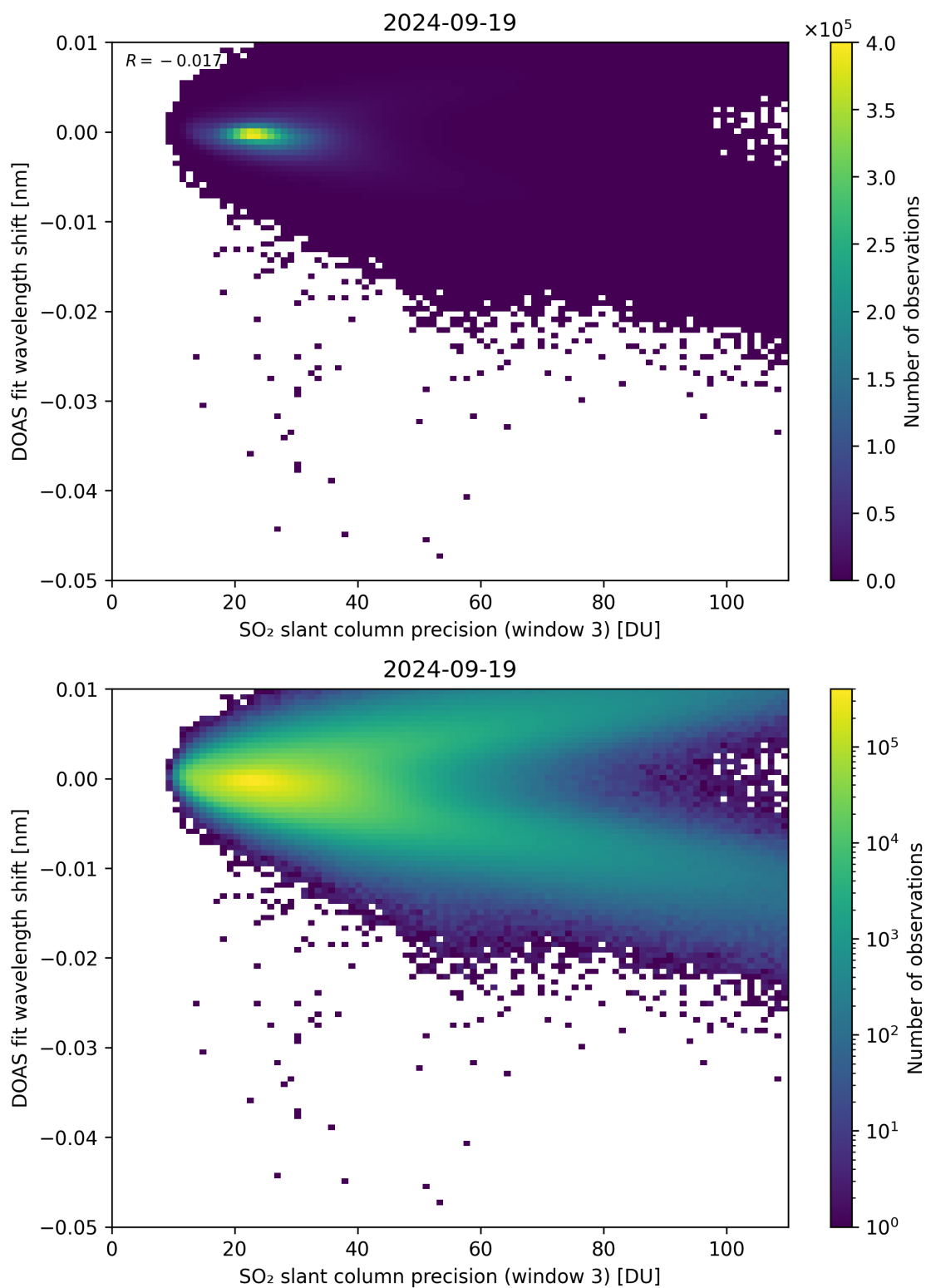
Figure 258: Scatter density plot of “SO 2 slant column precision (window 3)” against “DOAS fit wavelength shift” for 2024-09-18 to 2024-09-20.
