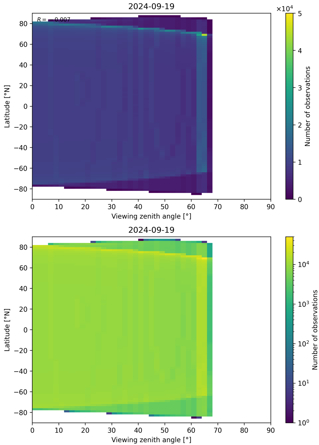
Figure 314: Scatter density plot of “Viewing zenith angle” against “Latitude” for 2024-09-18 to 2024-09-20.
