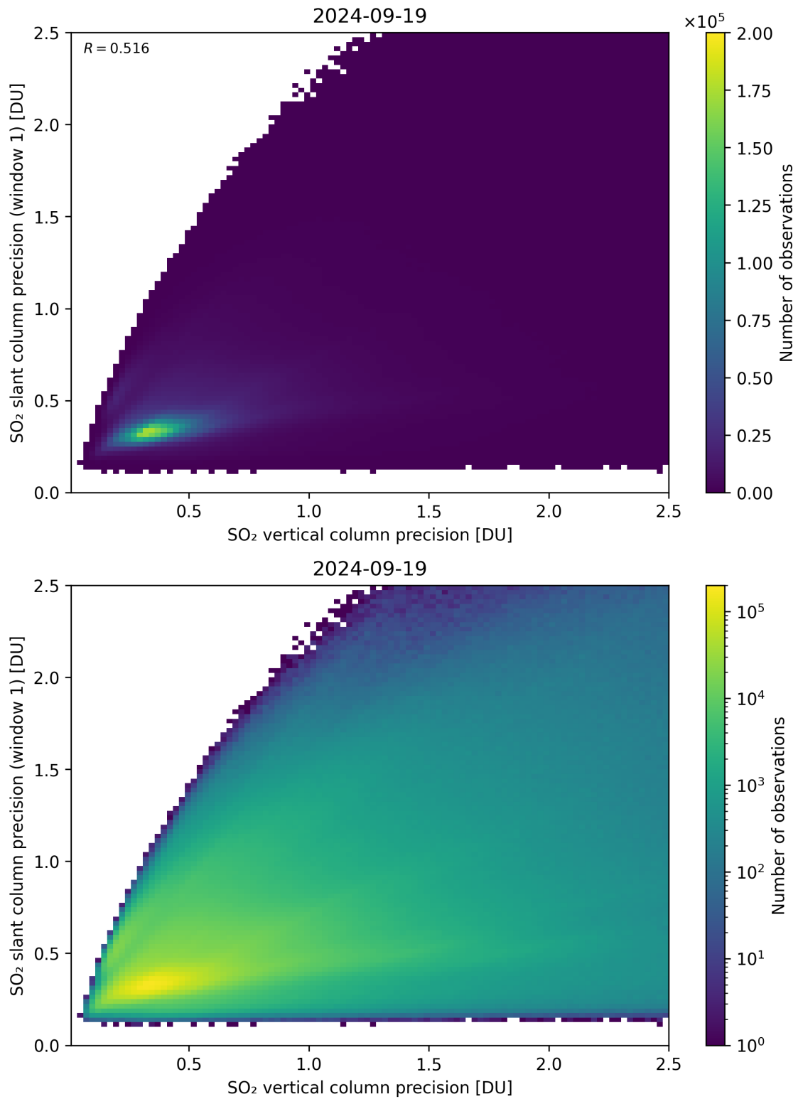
Figure 290: Scatter density plot of “SO 2 vertical column precision” against “SO 2 slant column precision (window 1)” for 2024-09-18 to 2024-09-20.
