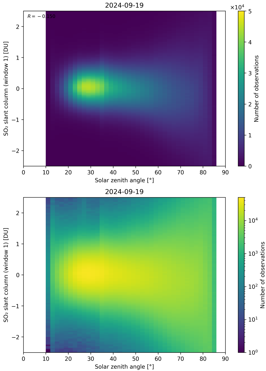
Figure 169: Scatter density plot of “Solar zenith angle” against “SO 2 slant column (window 1)” for 2024-09-18 to 2024-09-20.
