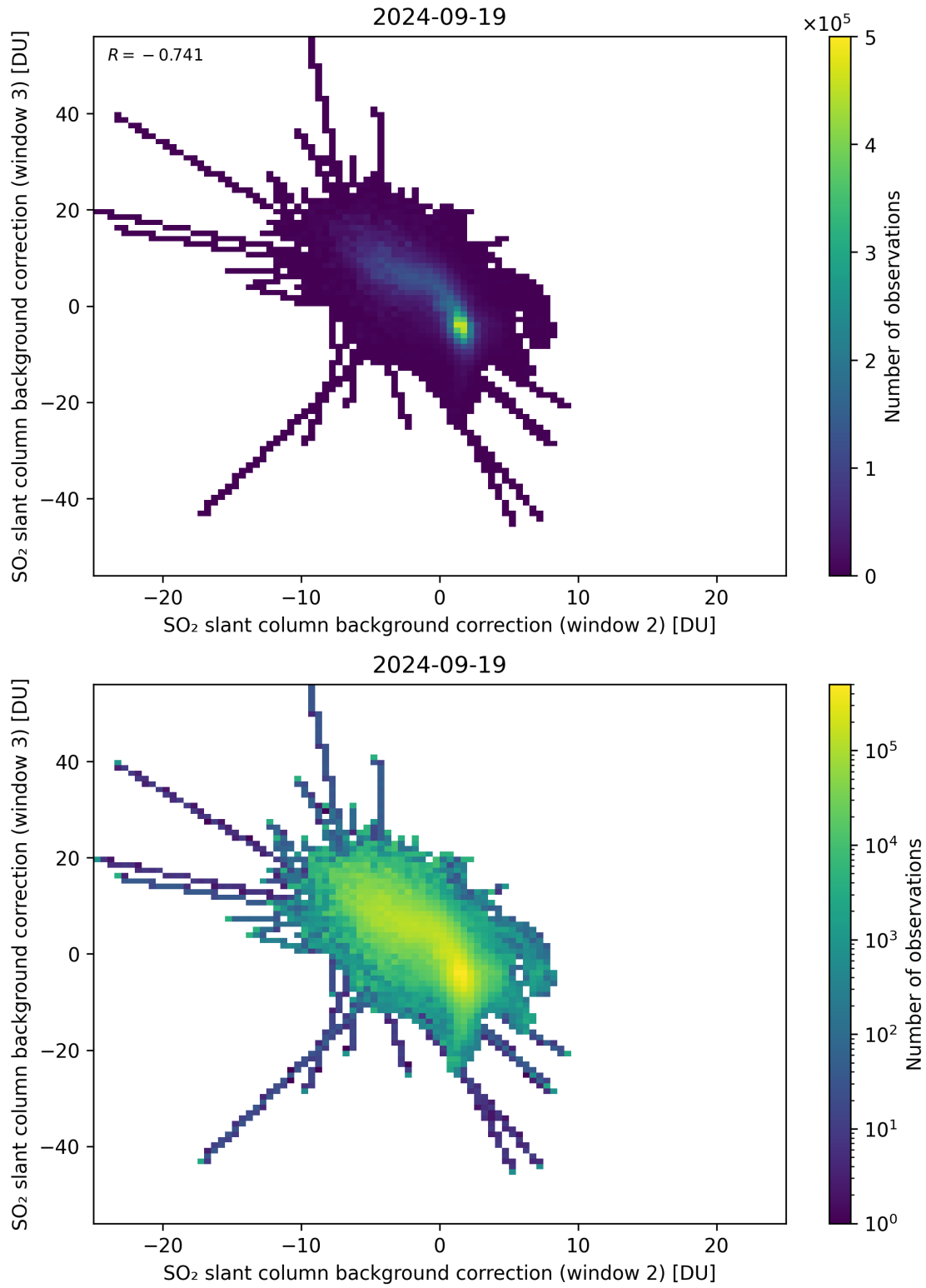
Figure 111: Scatter density plot of “SO 2 slant column background correction (window 2)” against “SO 2 slant column background correction (window 3)” for 2024-09-18 to 2024-09-20.
