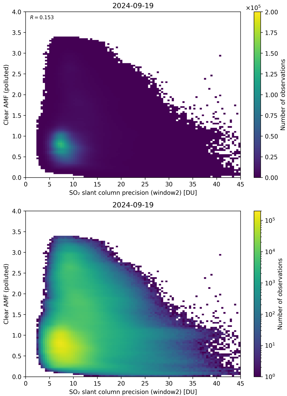
Figure 246: Scatter density plot of “SO 2 slant column precision (window2)” against “Clear AMF (polluted)” for 2024-09-18 to 2024-09-20.
