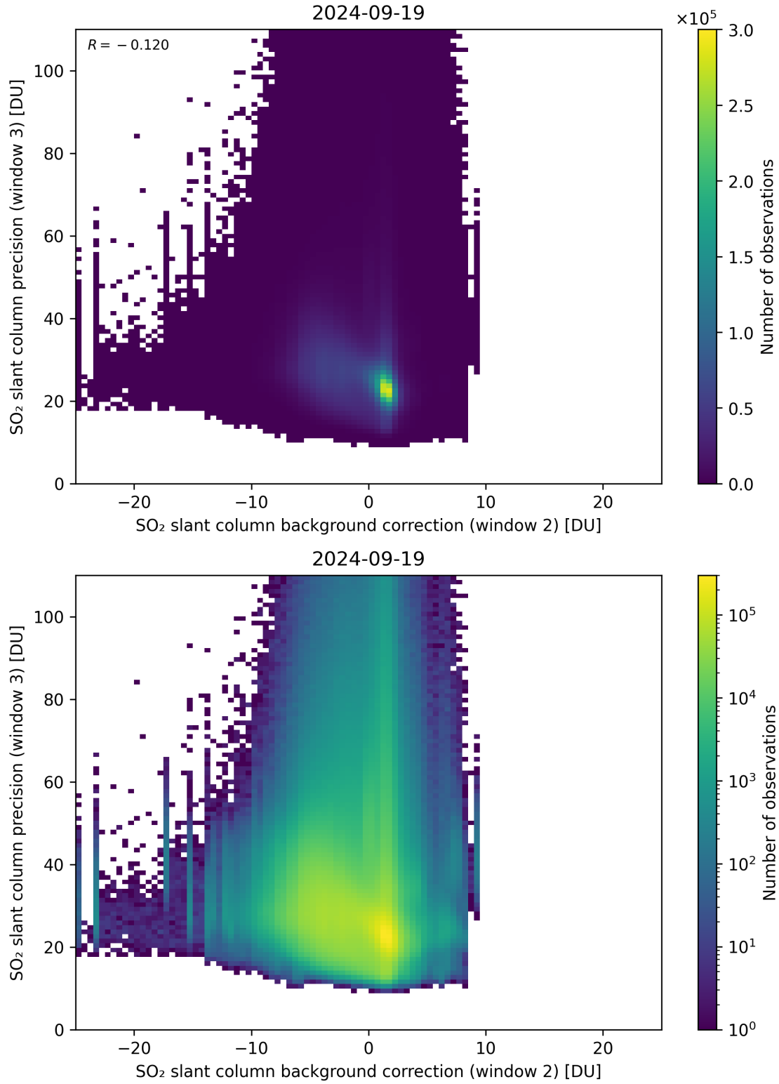
Figure 118: Scatter density plot of “SO 2 slant column background correction (window 2)” against “SO 2 slant column precision (window 3)” for 2024-09-18 to 2024-09-20.
