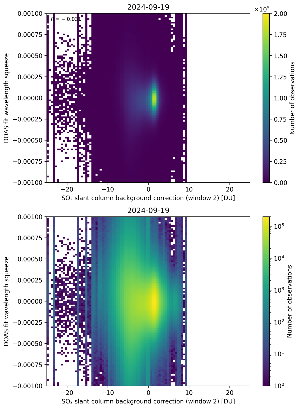
Figure 113: Scatter density plot of “SO 2 slant column background correction (window 2)” against “DOAS fit wavelength squeeze” for 2024-09-18 to 2024-09-20.
