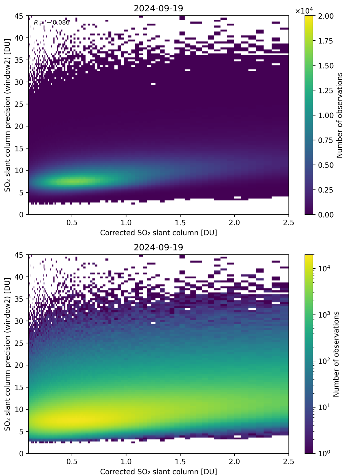
Figure 189: Scatter density plot of “Corrected SO 2 slant column” against “SO 2 slant column precision (window2)” for 2024-09-18 to 2024-09-20.
