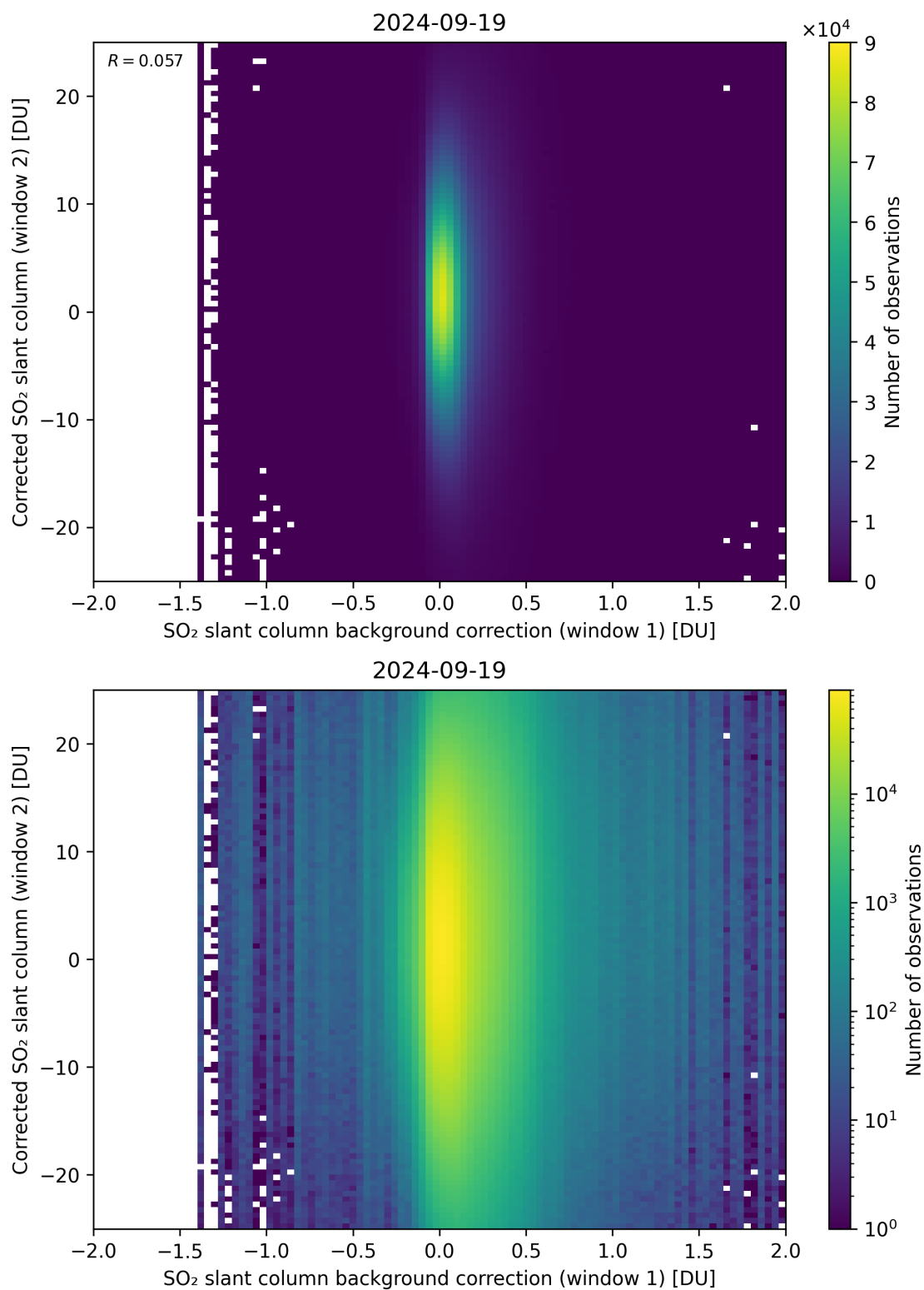
Figure 104: Scatter density plot of “SO 2 slant column background correction (window 1)” against “Corrected SO 2 slant column (window 2)” for 2024-09-18 to 2024-09-20.
