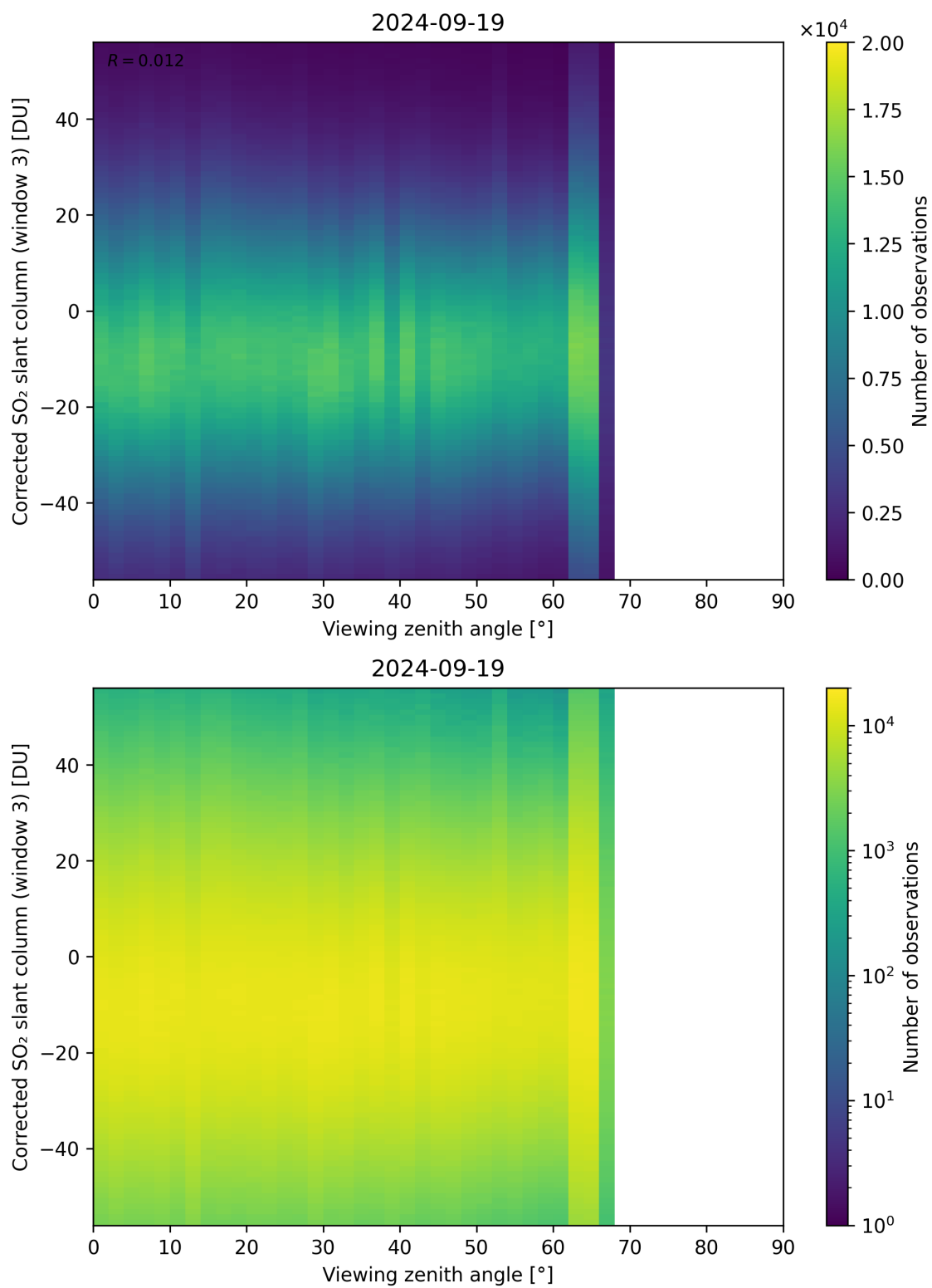
Figure 319: Scatter density plot of “Viewing zenith angle” against “Corrected SO 2 slant column (window 3)” for 2024-09-18 to 2024-09-20.
