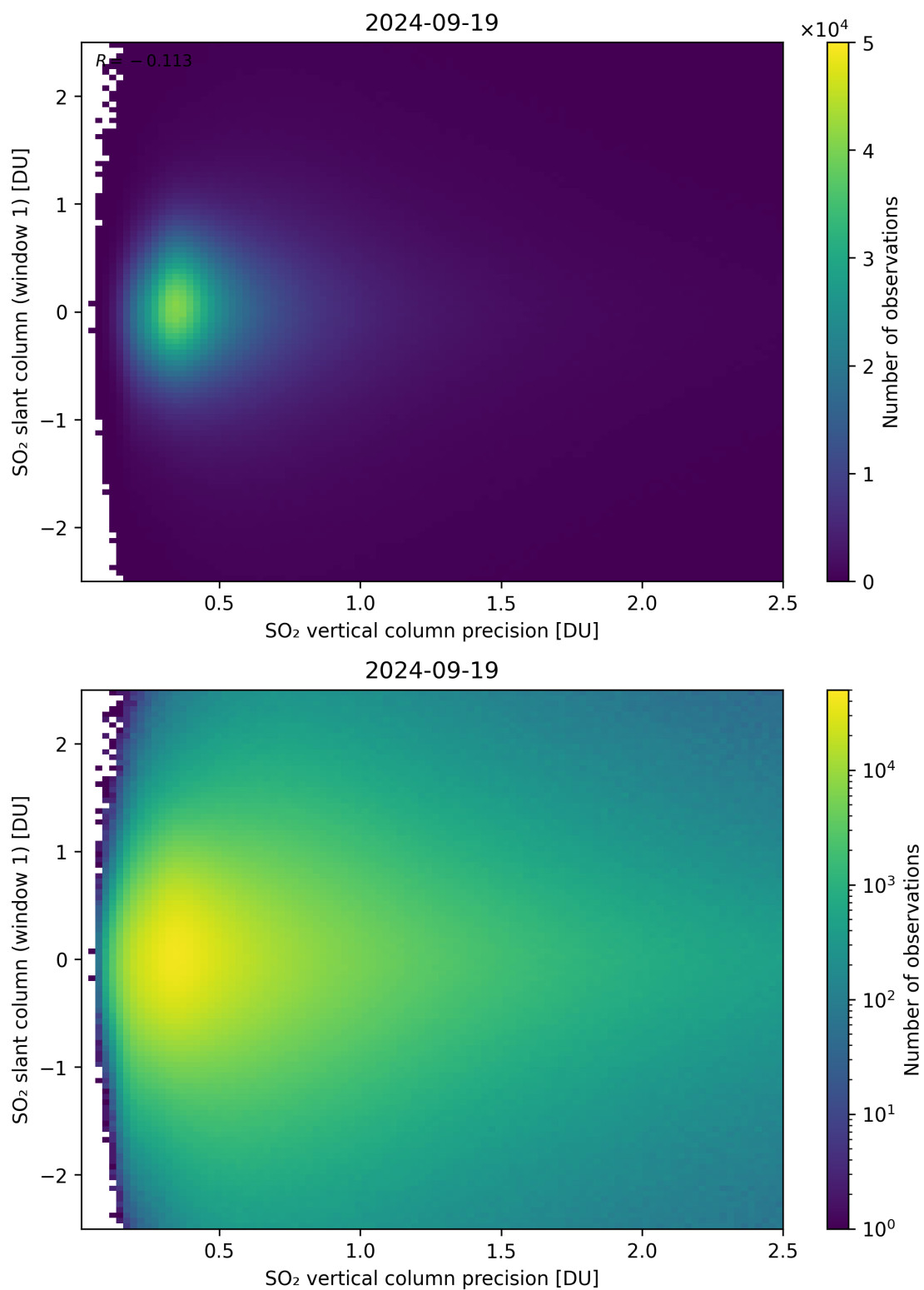
Figure 289: Scatter density plot of “SO 2 vertical column precision” against “SO 2 slant column (window 1)” for 2024-09-18 to 2024-09-20.
