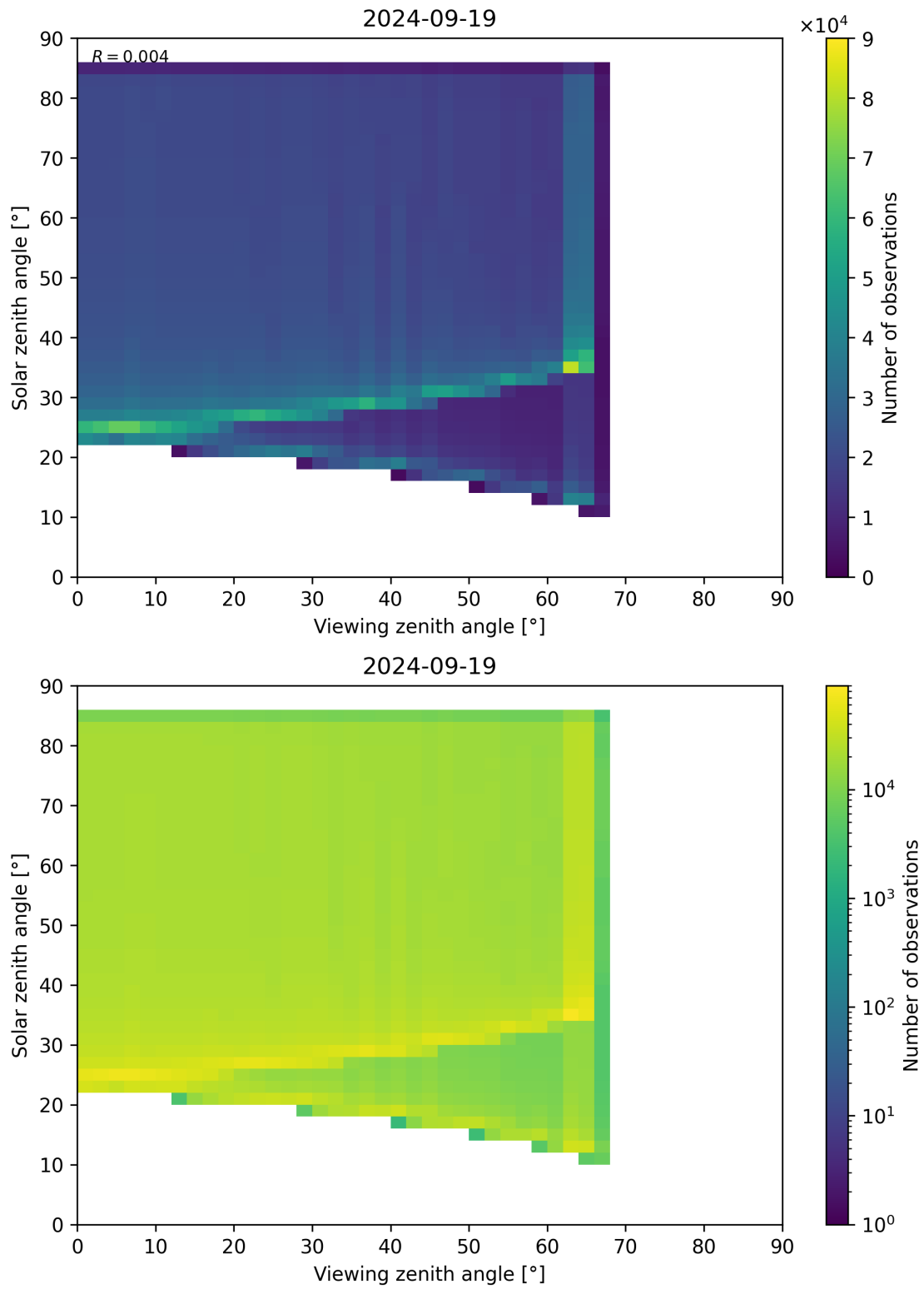
Figure 315: Scatter density plot of “Viewing zenith angle” against “Solar zenith angle” for 2024-09-18 to 2024-09-20.
