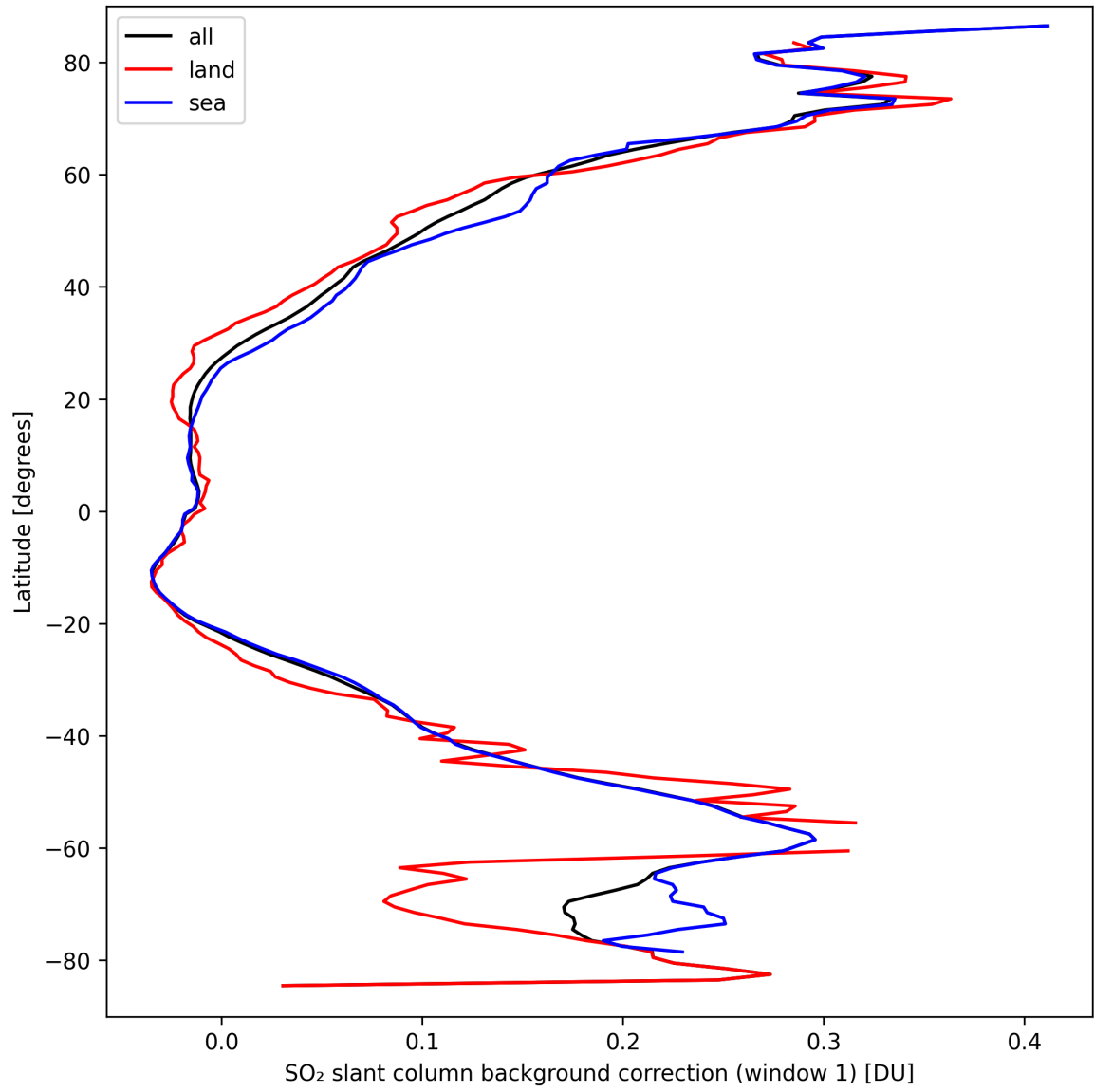
Figure 36: Zonal average of “SO 2 slant column background correction (window 1)” for 2024-09-18 to 2024-09-20.
