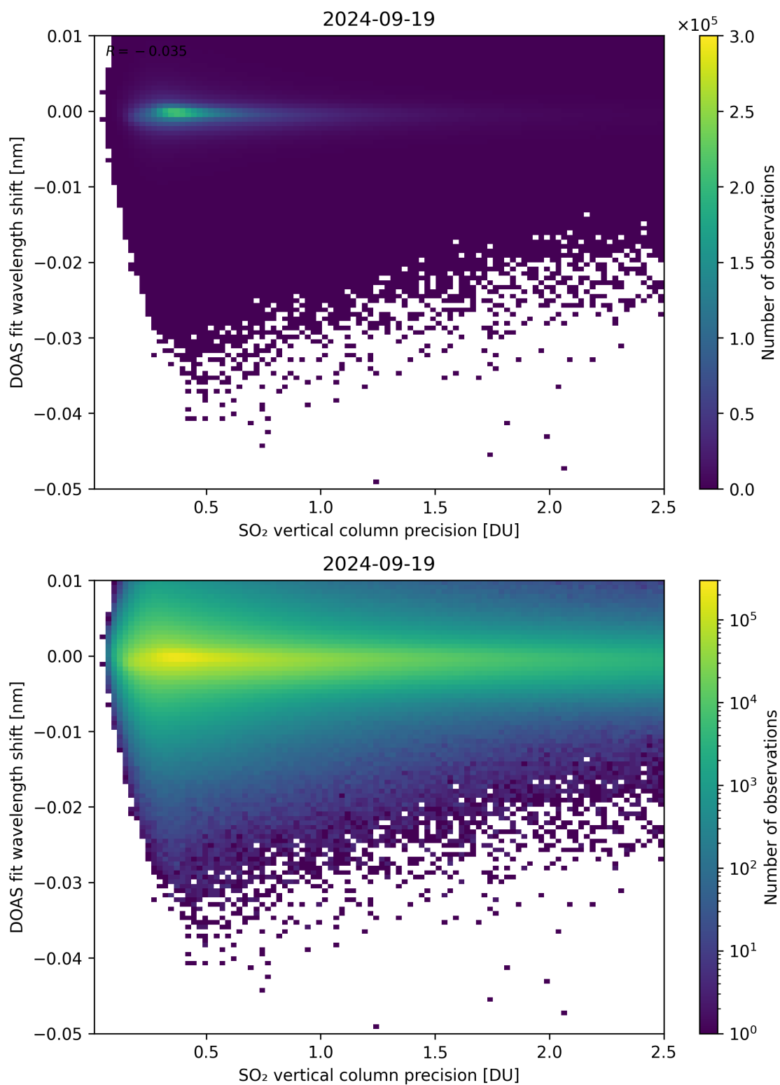
Figure 282: Scatter density plot of “SO 2 vertical column precision” against “DOAS fit wavelength shift” for 2024-09-18 to 2024-09-20.
