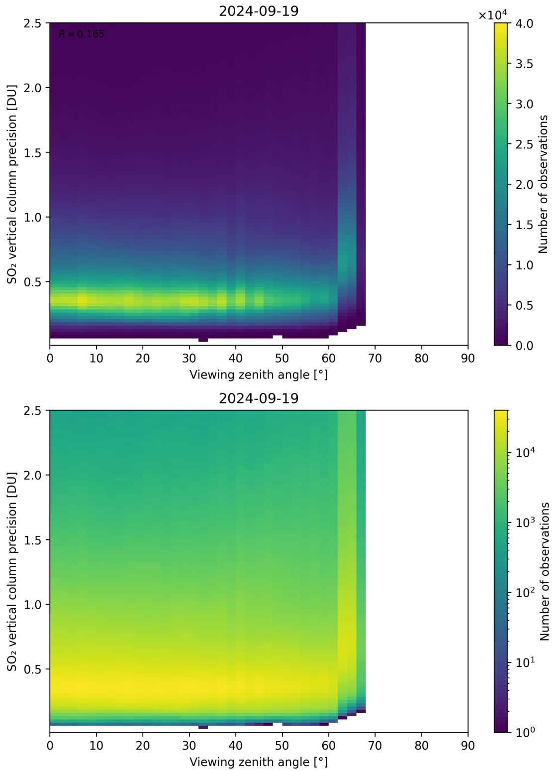
Figure 328: Scatter density plot of “Viewing zenith angle” against “SO 2 vertical column precision” for 2024-09-18 to 2024-09-20.
