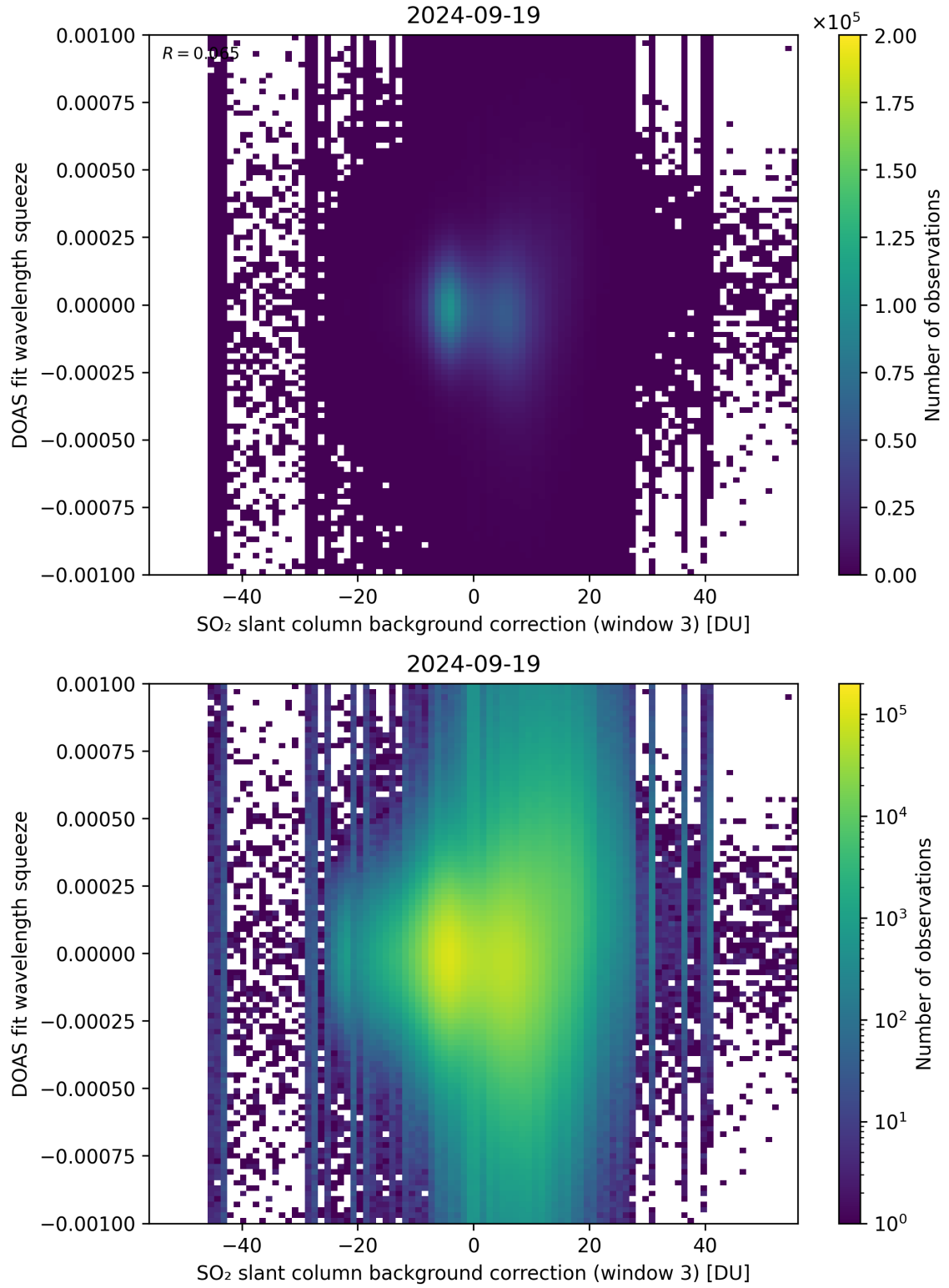
Figure 122: Scatter density plot of “SO 2 slant column background correction (window 3)” against “DOAS fit wavelength squeeze” for 2024-09-18 to 2024-09-20.
