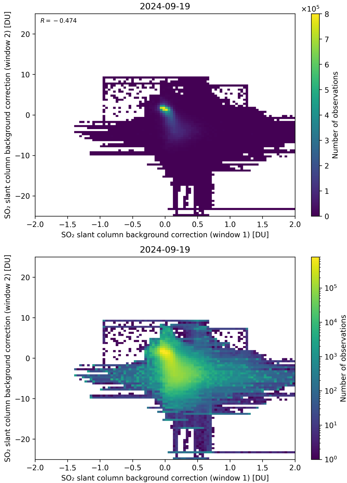
Figure 98: Scatter density plot of “SO 2 slant column background correction (window 1)” against “SO 2 slant column background correction (window 2)” for 2024-09-18 to 2024-09-20.
