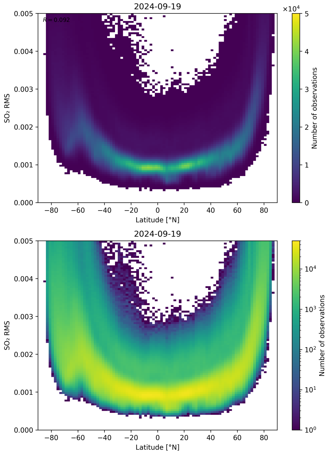
Figure 144: Scatter density plot of “Latitude” against “SO 2 RMS” for 2024-09-18 to 2024-09-20.
