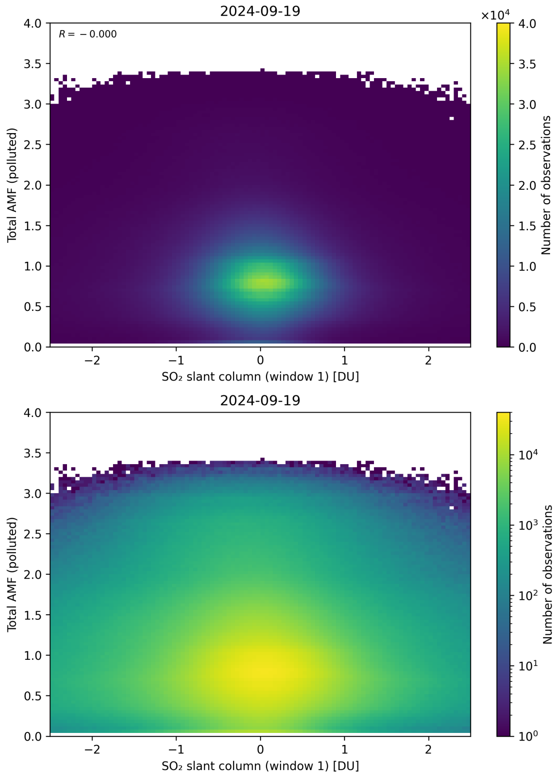
Figure 239: Scatter density plot of “SO 2 slant column (window 1)” against “Total AMF (polluted)” for 2024-09-18 to 2024-09-20.
