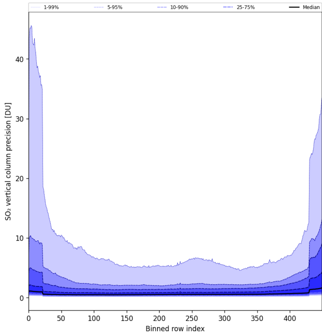
Figure 77: Along track statistics of “SO 2 vertical column precision” for 2024-09-18 to 2024-09-20
