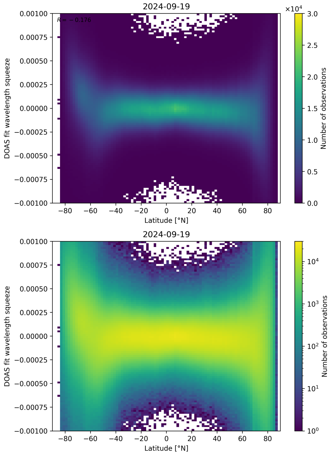
Figure 143: Scatter density plot of “Latitude” against “DOAS fit wavelength squeeze” for 2024-09-18 to 2024-09-20.
