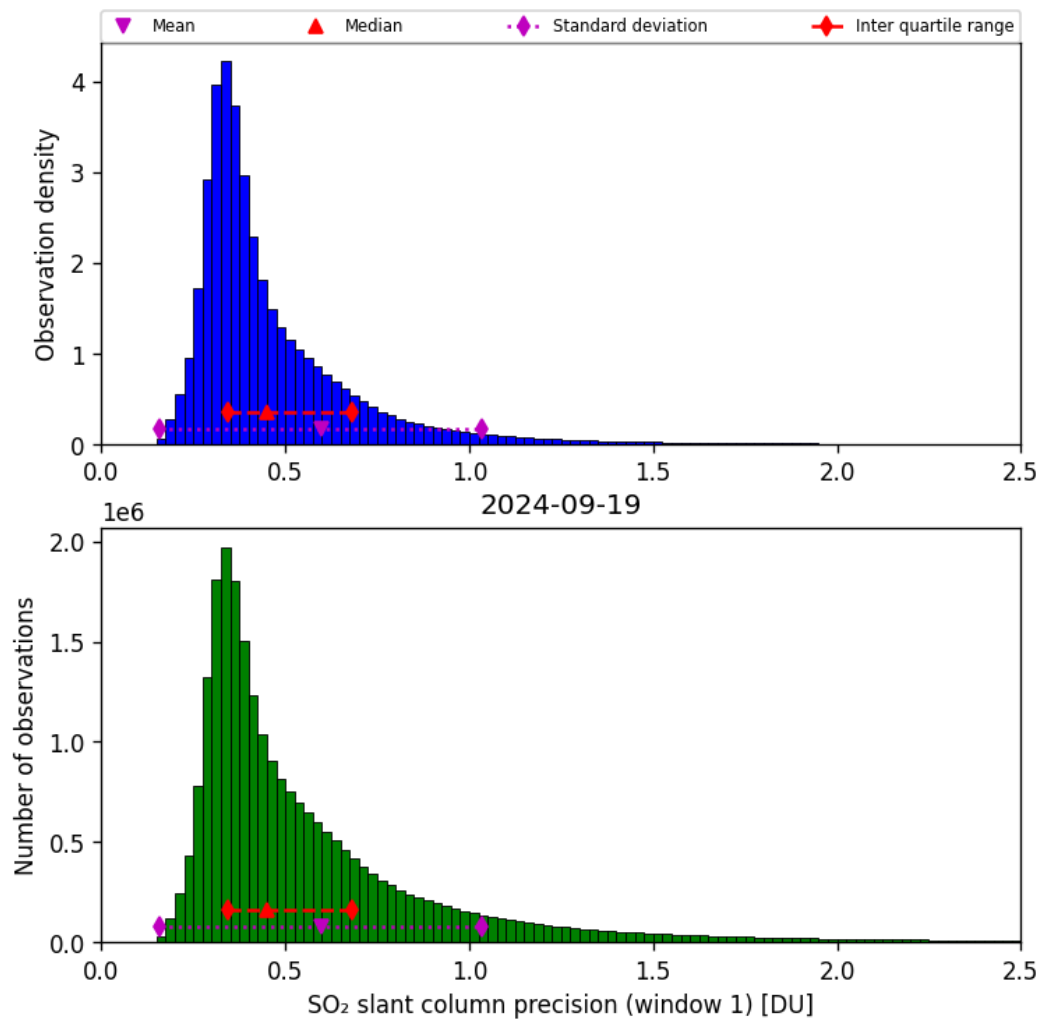
Figure 57: Histogram of “SO 2 slant column precision (window 1)” for 2024-09-18 to 2024-09-20
