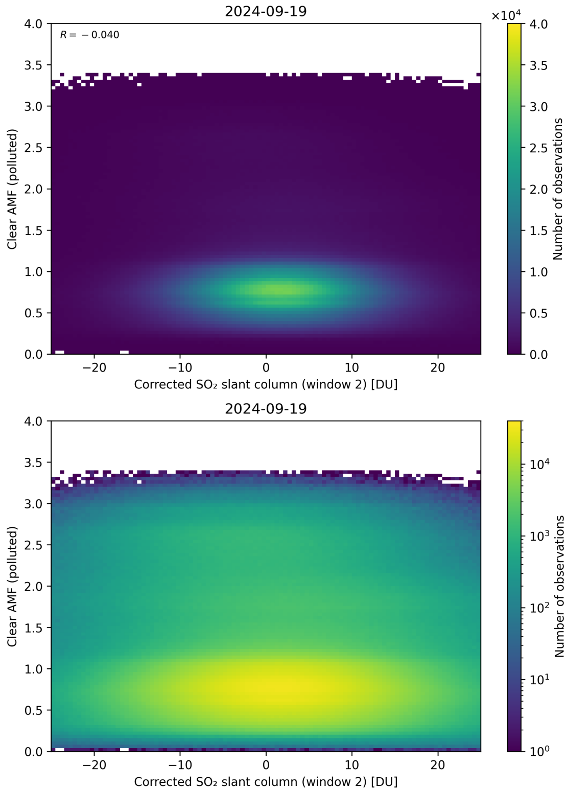
Figure 199: Scatter density plot of “Corrected SO 2 slant column (window 2)” against “Clear AMF (polluted)” for 2024-09-18 to 2024-09-20.
