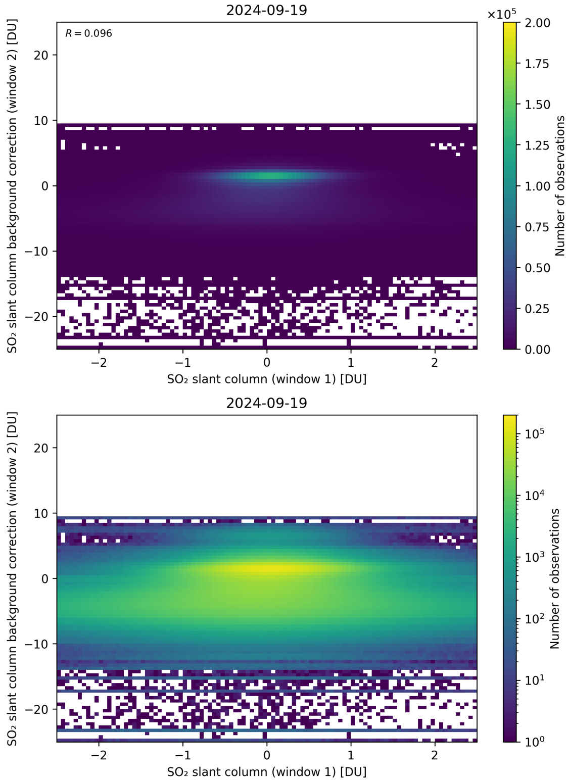
Figure 213: Scatter density plot of “SO 2 slant column (window 1)” against “SO 2 slant column background correction (window 2)” for 2024-09-18 to 2024-09-20.
