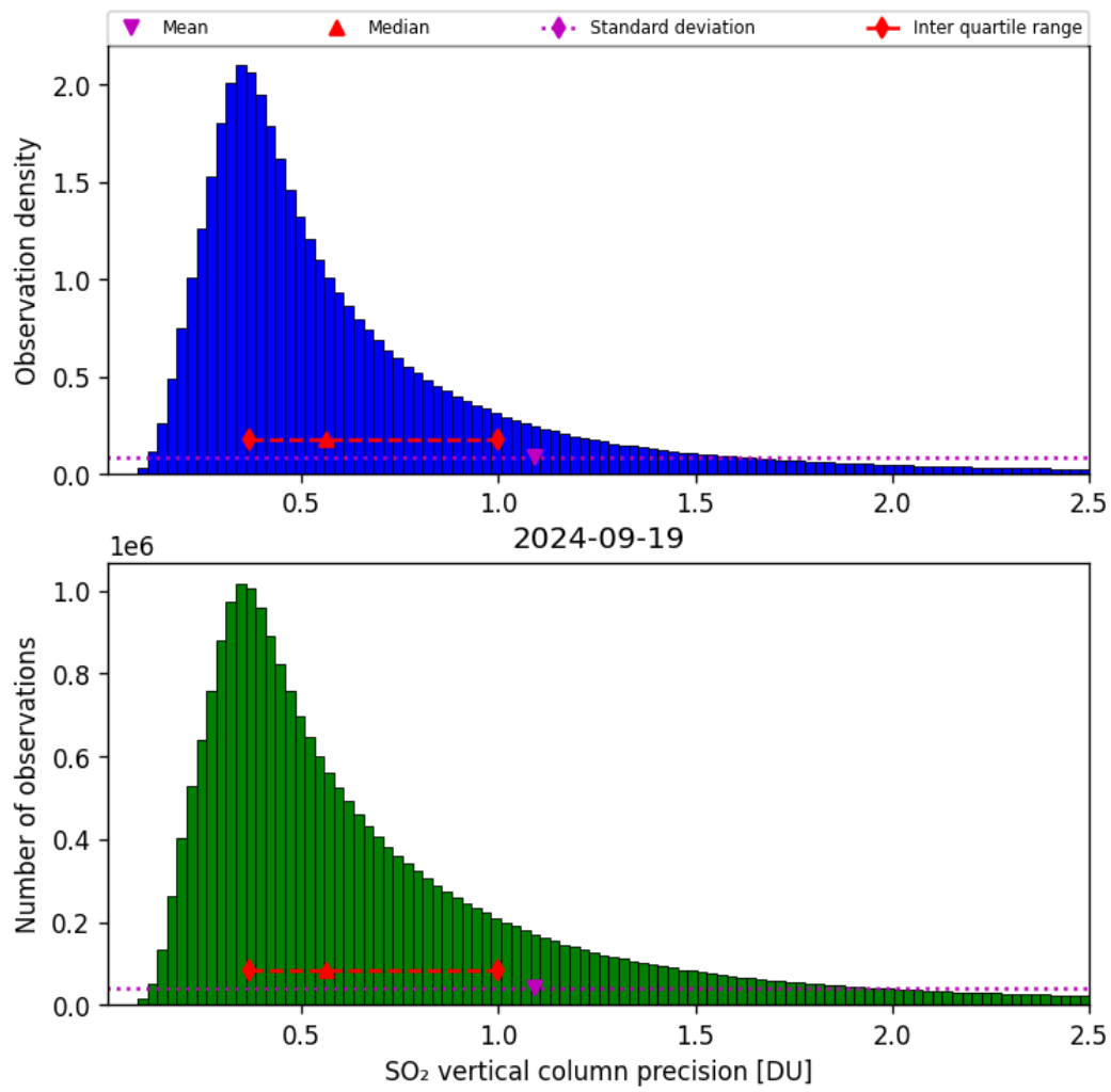
Figure 54: Histogram of “SO 2 vertical column precision” for 2024-09-18 to 2024-09-20
