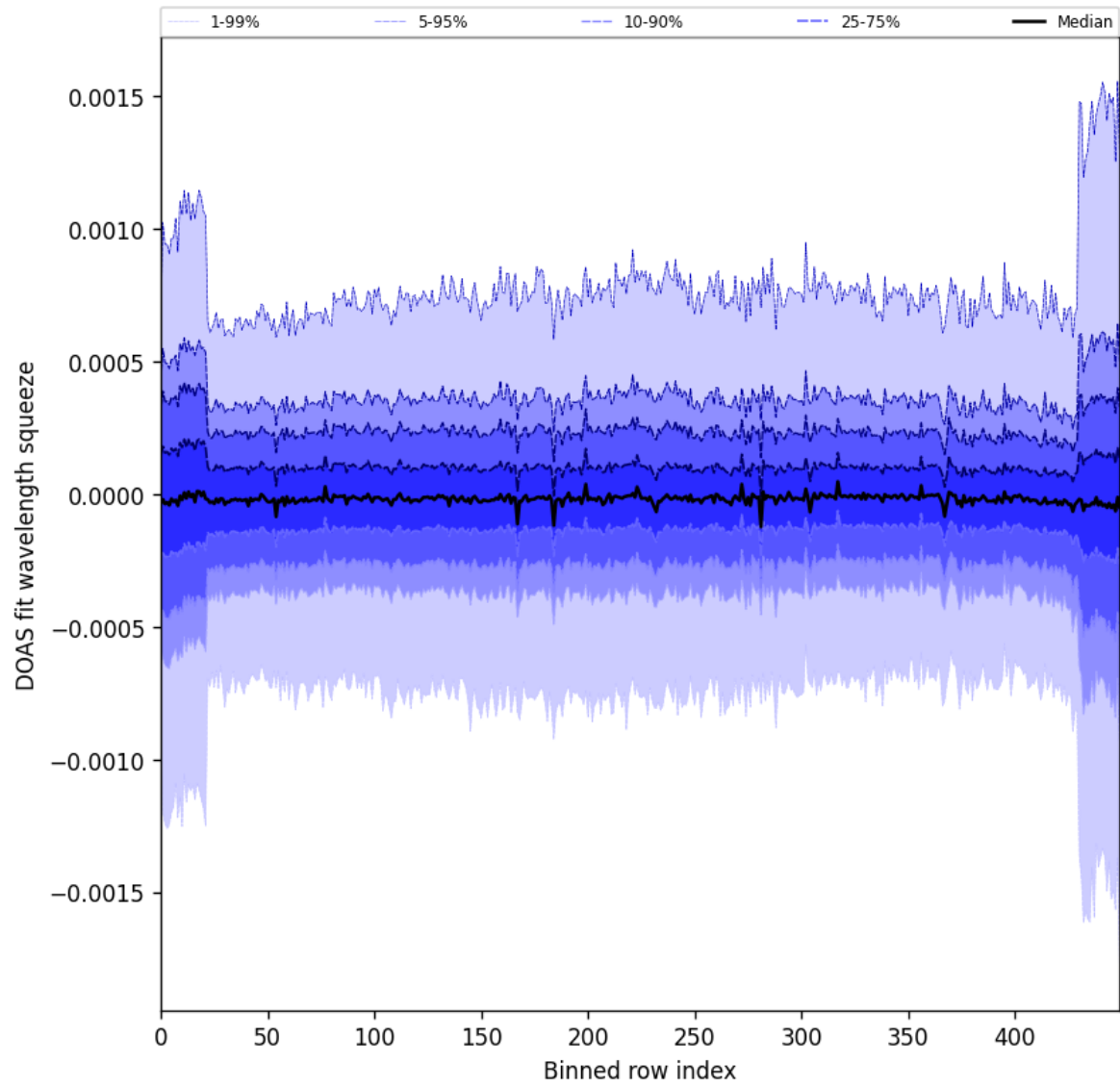
Figure 92: Along track statistics of “DOAS fit wavelength squeeze” for 2024-09-18 to 2024-09-20
