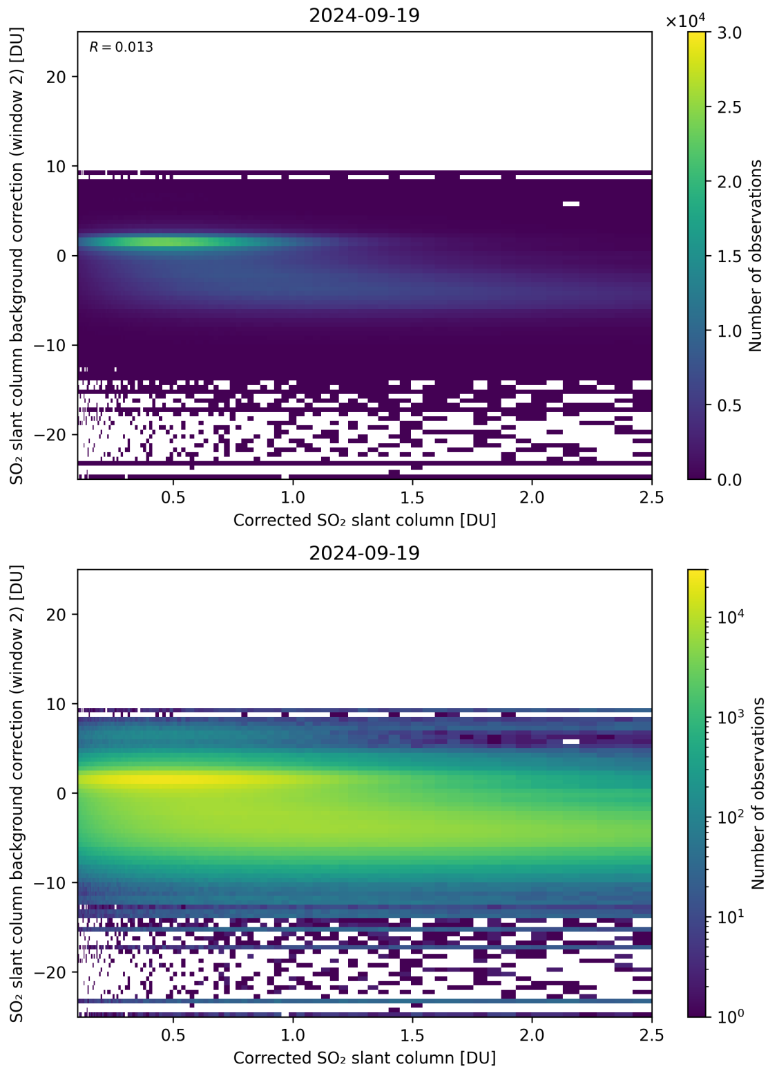
Figure 179: Scatter density plot of “Corrected SO 2 slant column” against “SO 2 slant column background correction (window 2)” for 2024-09-18 to 2024-09-20.
