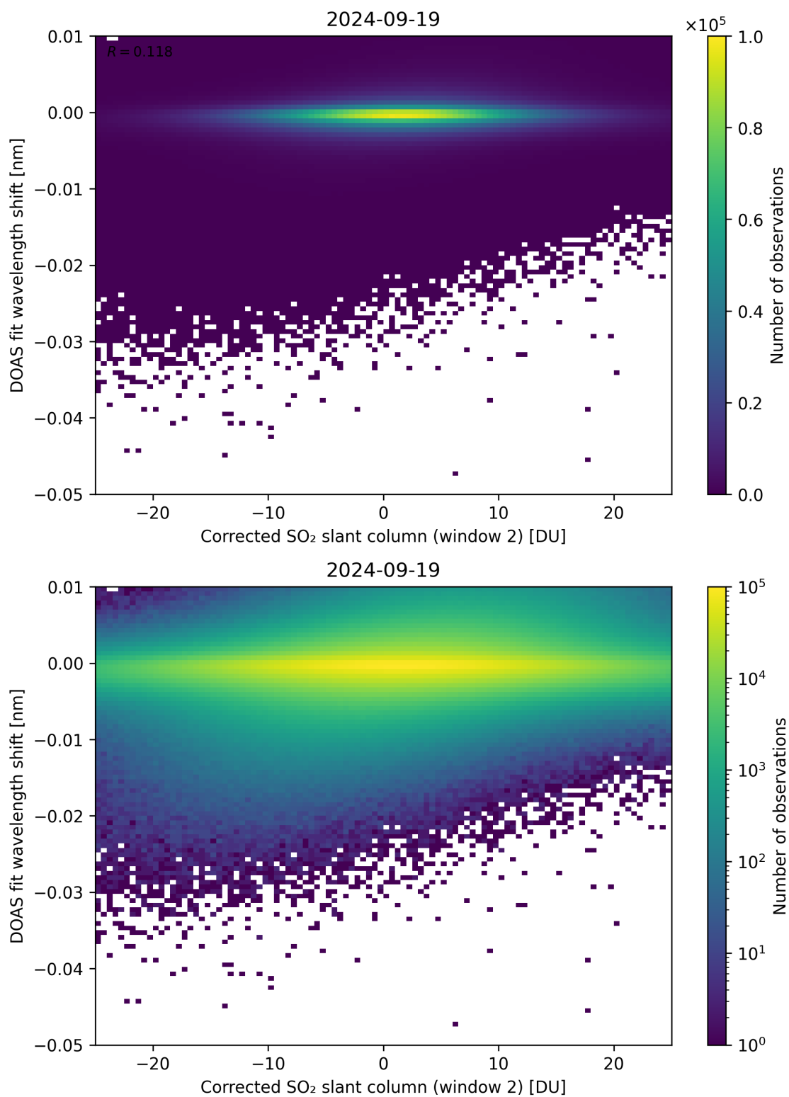
Figure 196: Scatter density plot of “Corrected SO 2 slant column (window 2)” against “DOAS fit wavelength shift” for 2024-09-18 to 2024-09-20.
