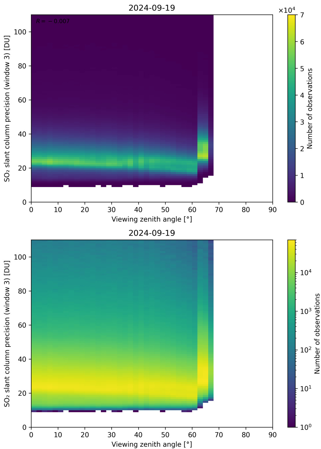
Figure 324: Scatter density plot of “Viewing zenith angle” against “SO 2 slant column precision (window 3)” for 2024-09-18 to 2024-09-20.
