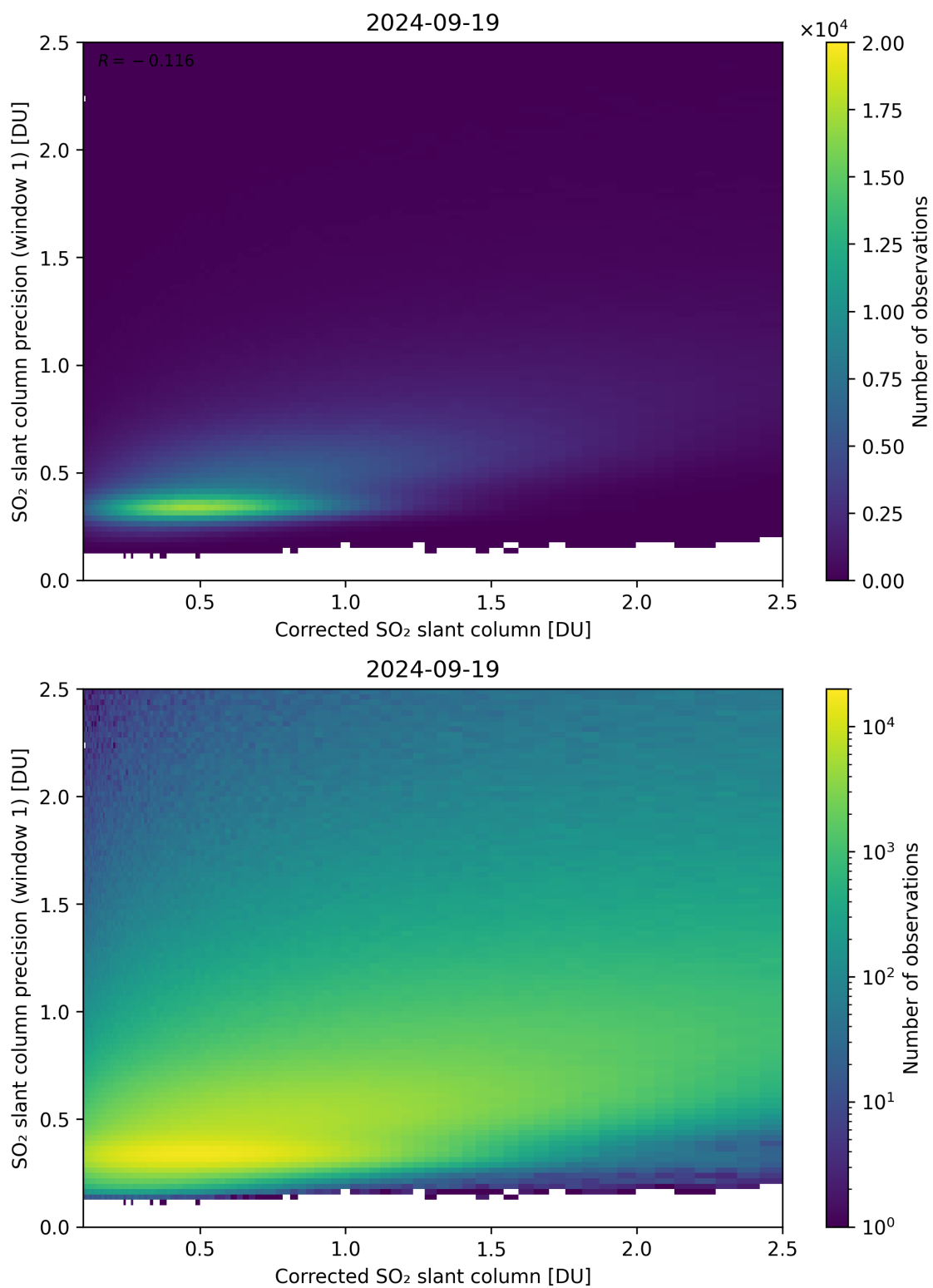
Figure 188: Scatter density plot of “Corrected SO 2 slant column” against “SO 2 slant column precision (window 1)” for 2024-09-18 to 2024-09-20.
