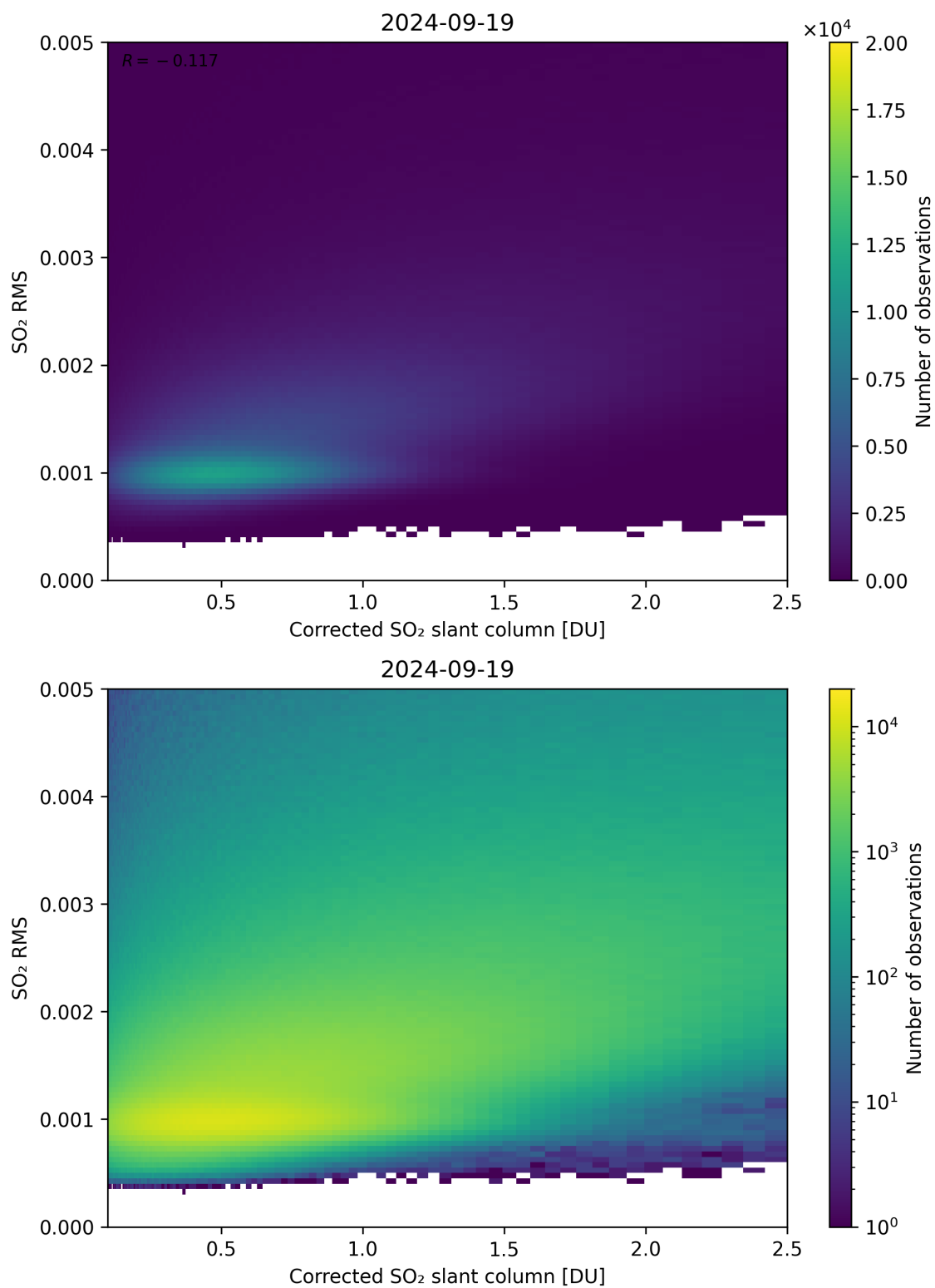
Figure 183: Scatter density plot of “Corrected SO 2 slant column” against “SO 2 RMS” for 2024-09-18 to 2024-09-20.
