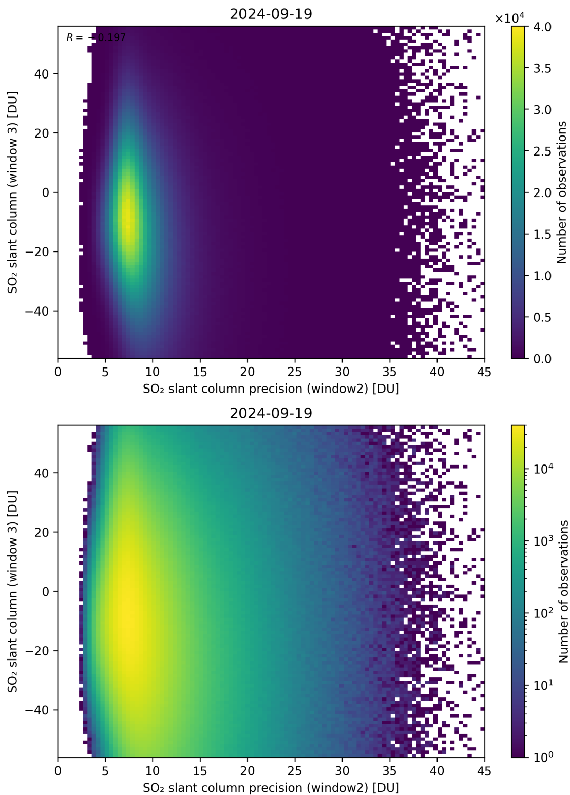
Figure 249: Scatter density plot of “SO 2 slant column precision (window2)” against “SO 2 slant column (window 3)” for 2024-09-18 to 2024-09-20.
