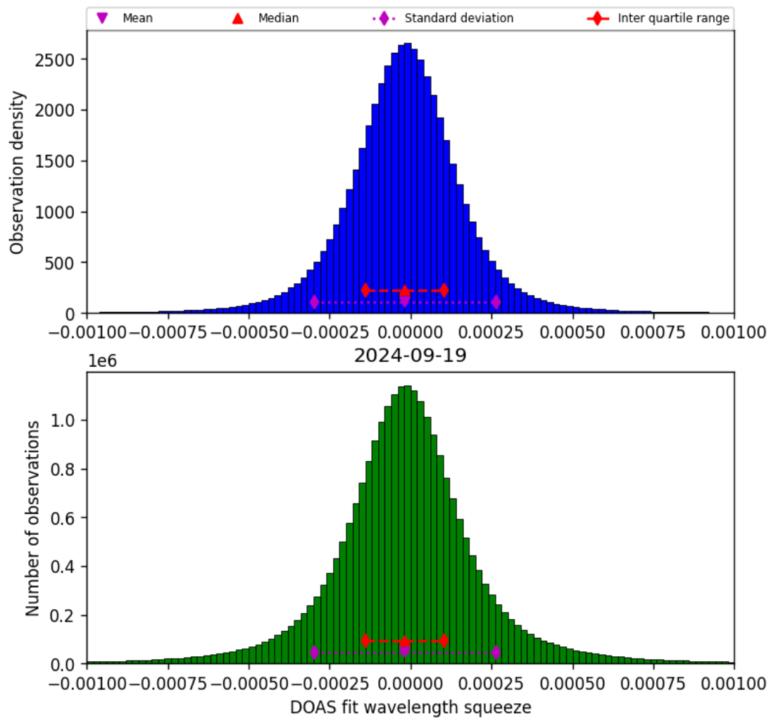
Figure 69: Histogram of “DOAS fit wavelength squeeze” for 2024-09-18 to 2024-09-20
