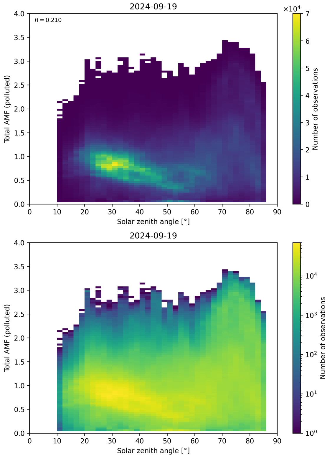
Figure 174: Scatter density plot of “Solar zenith angle” against “Total AMF (polluted)” for 2024-09-18 to 2024-09-20.
