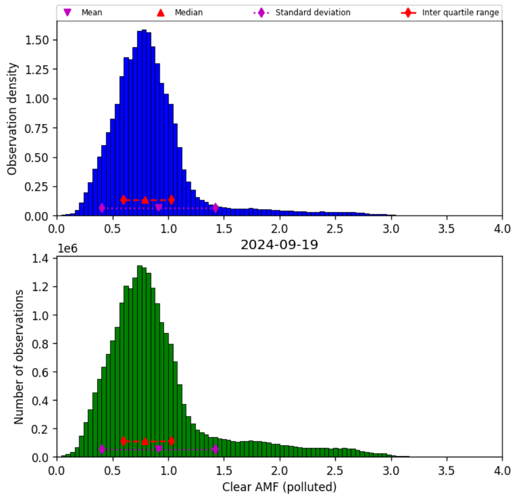
Figure 73: Histogram of “Clear AMF (polluted)” for 2024-09-18 to 2024-09-20
