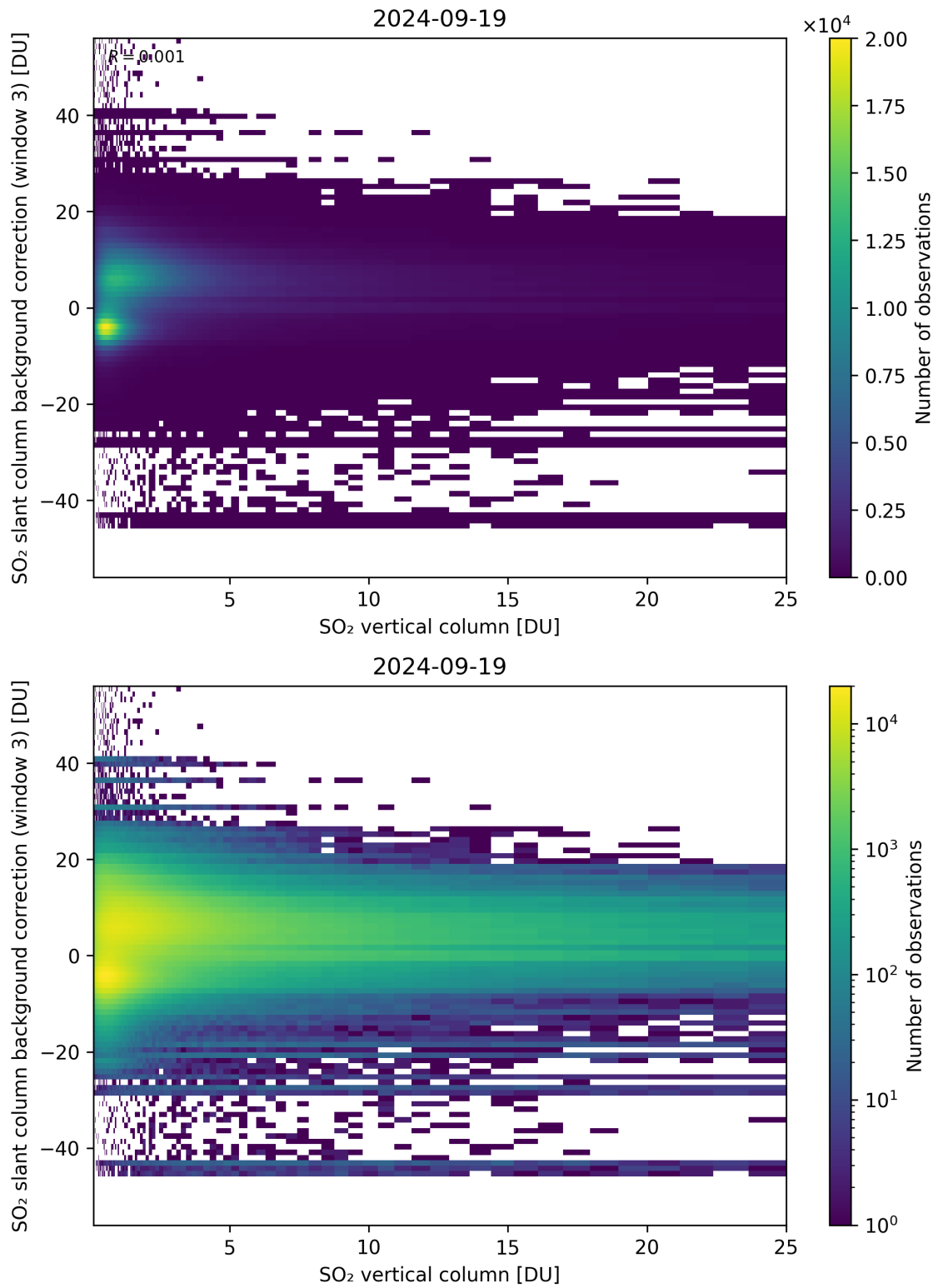
Figure 275: Scatter density plot of “SO 2 vertical column” against “SO 2 slant column background correction (window 3)” for 2024-09-18 to 2024-09-20.
