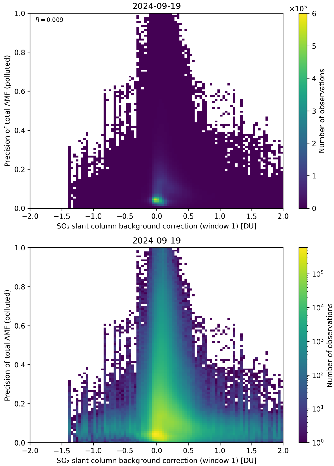
Figure 110: Scatter density plot of “SO 2 slant column background correction (window 1)” against “Precision of total AMF (polluted)” for 2024-09-18 to 2024-09-20.
