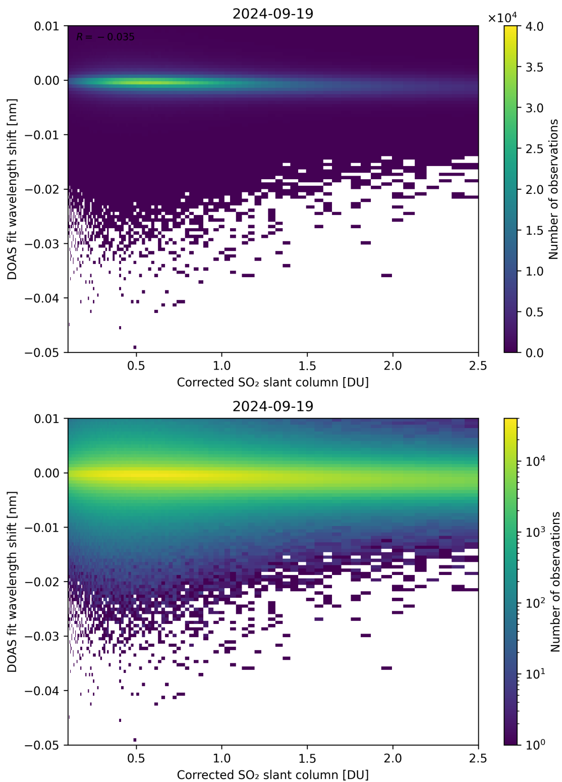
Figure 181: Scatter density plot of “Corrected SO 2 slant column” against “DOAS fit wavelength shift” for 2024-09-18 to 2024-09-20.
