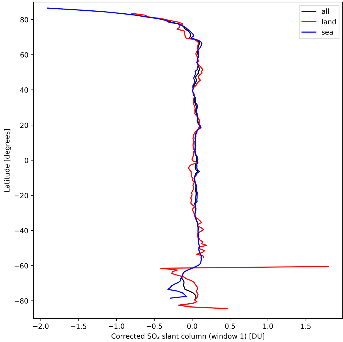
Figure 35: Zonal average of “Corrected SO 2 slant column (window 1)” for 2024-09-18 to 2024-09-20.
