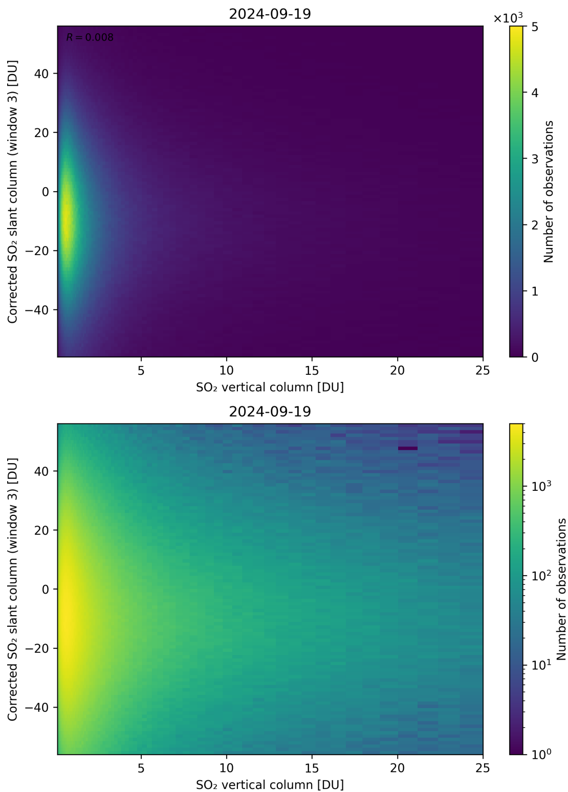
Figure 299: Scatter density plot of “SO 2 vertical column” against “Corrected SO 2 slant column (window 3)” for 2024-09-18 to 2024-09-20.
