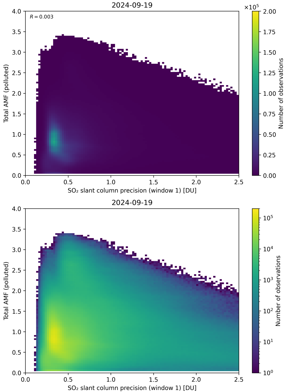
Figure 230: Scatter density plot of “SO 2 slant column precision (window 1)” against “Total AMF (polluted)” for 2024-09-18 to 2024-09-20.
