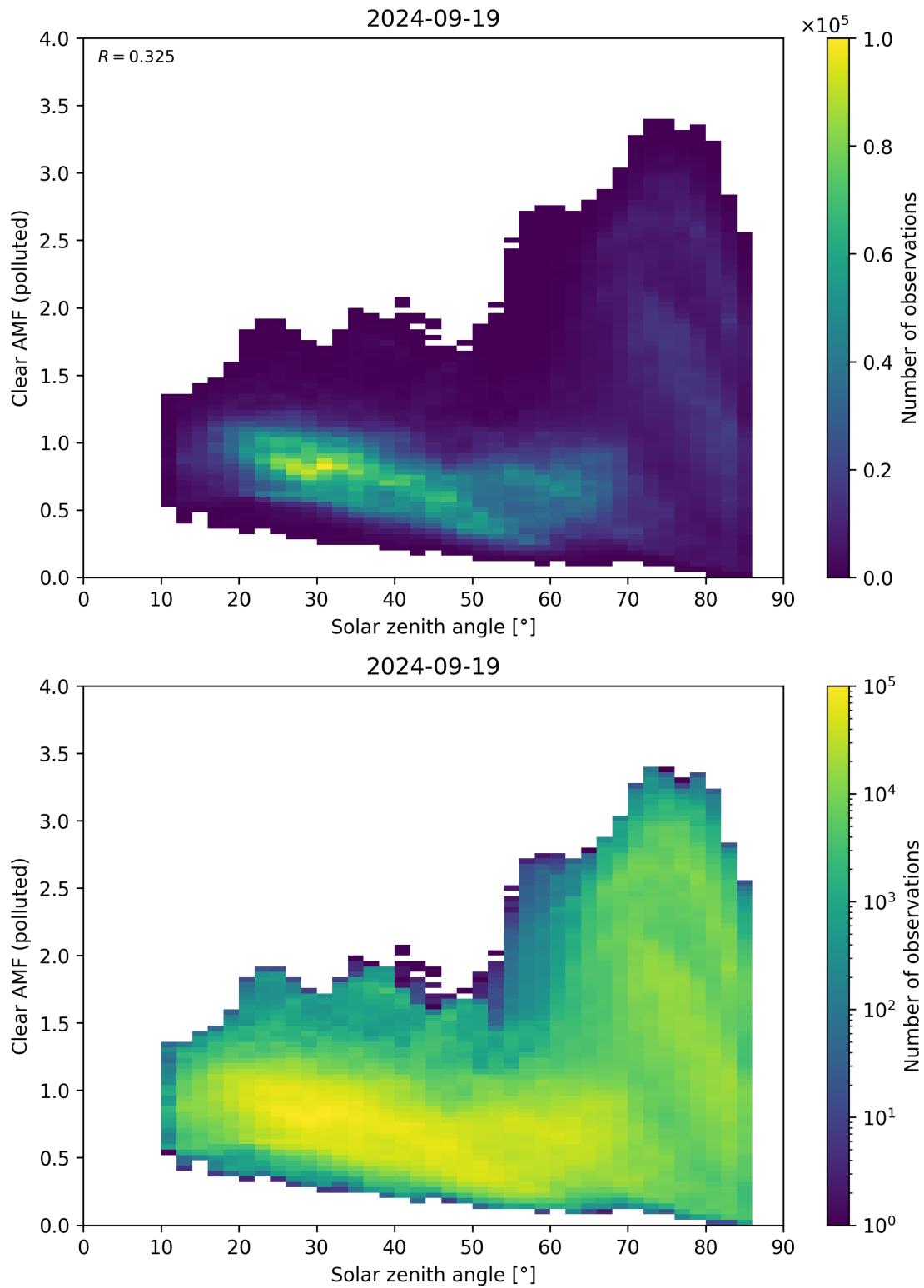
Figure 165: Scatter density plot of “Solar zenith angle” against “Clear AMF (polluted)” for 2024-09-18 to 2024-09-20.
