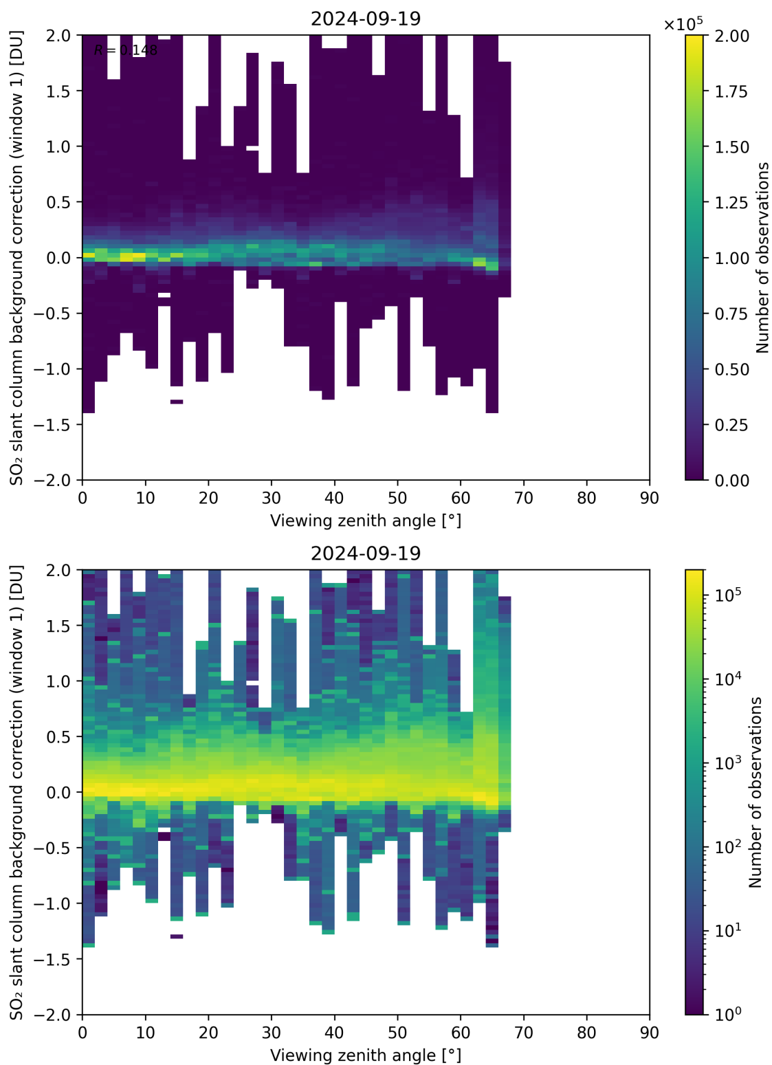
Figure 308: Scatter density plot of “Viewing zenith angle” against “SO 2 slant column background correction (window 1)” for 2024-09-18 to 2024-09-20.
