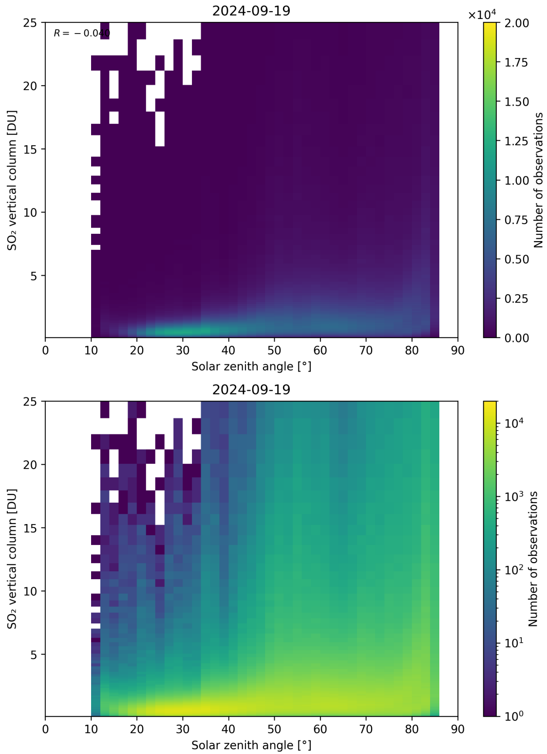
Figure 176: Scatter density plot of “Solar zenith angle” against “SO 2 vertical column” for 2024-09-18 to 2024-09-20.
