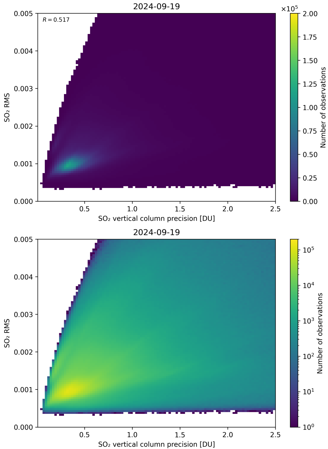
Figure 284: Scatter density plot of “SO 2 vertical column precision” against “SO 2 RMS” for 2024-09-18 to 2024-09-20.
