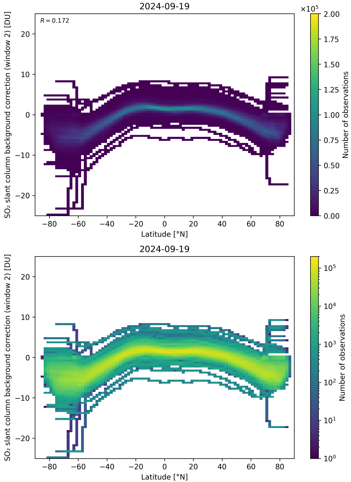
Figure 140: Scatter density plot of “Latitude” against “SO 2 slant column background correction (window 2)” for 2024-09-18 to 2024-09-20.
