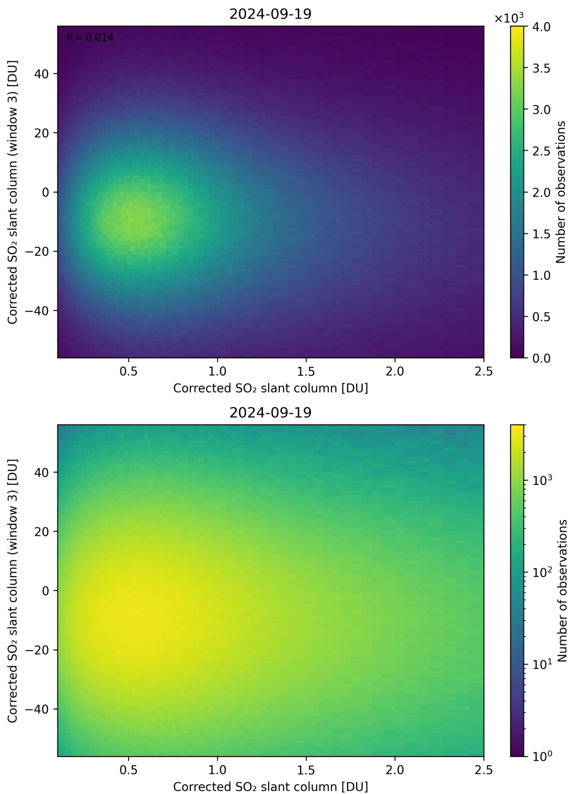
Figure 186: Scatter density plot of “Corrected SO 2 slant column” against “Corrected SO 2 slant column (window 3)” for 2024-09-18 to 2024-09-20.
