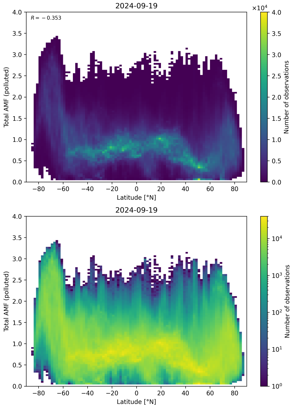
Figure 154: Scatter density plot of “Latitude” against “Total AMF (polluted)” for 2024-09-18 to 2024-09-20.
