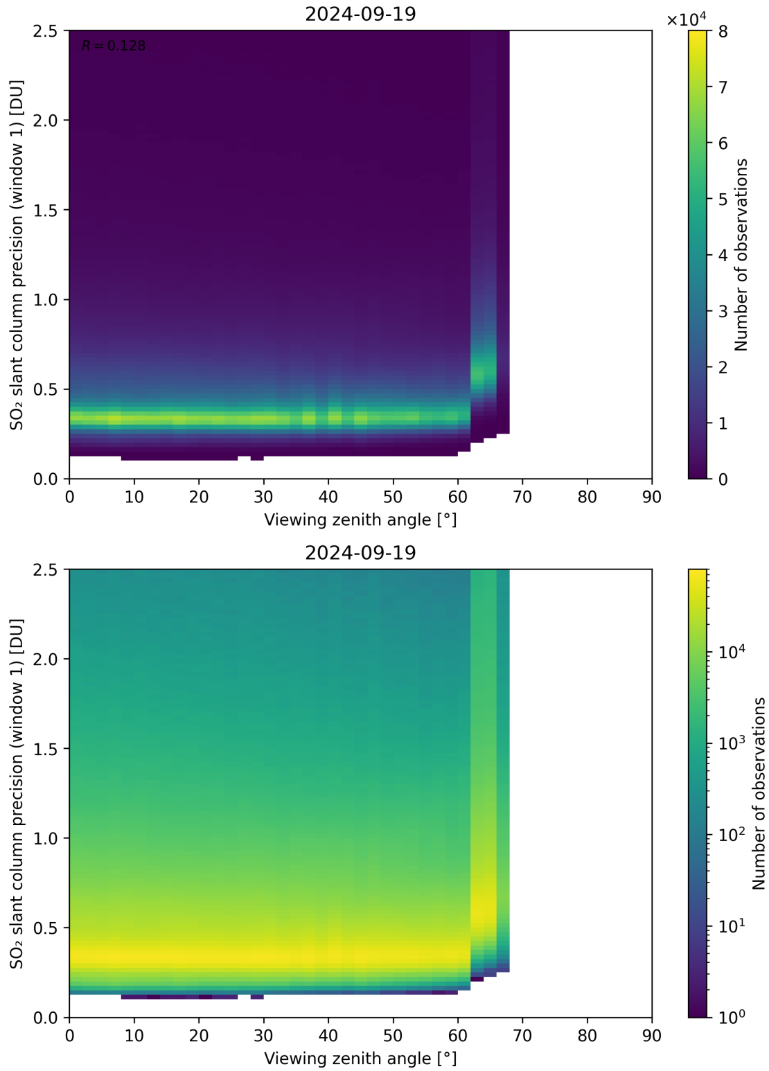
Figure 321: Scatter density plot of “Viewing zenith angle” against “SO 2 slant column precision (window 1)” for 2024-09-18 to 2024-09-20.
