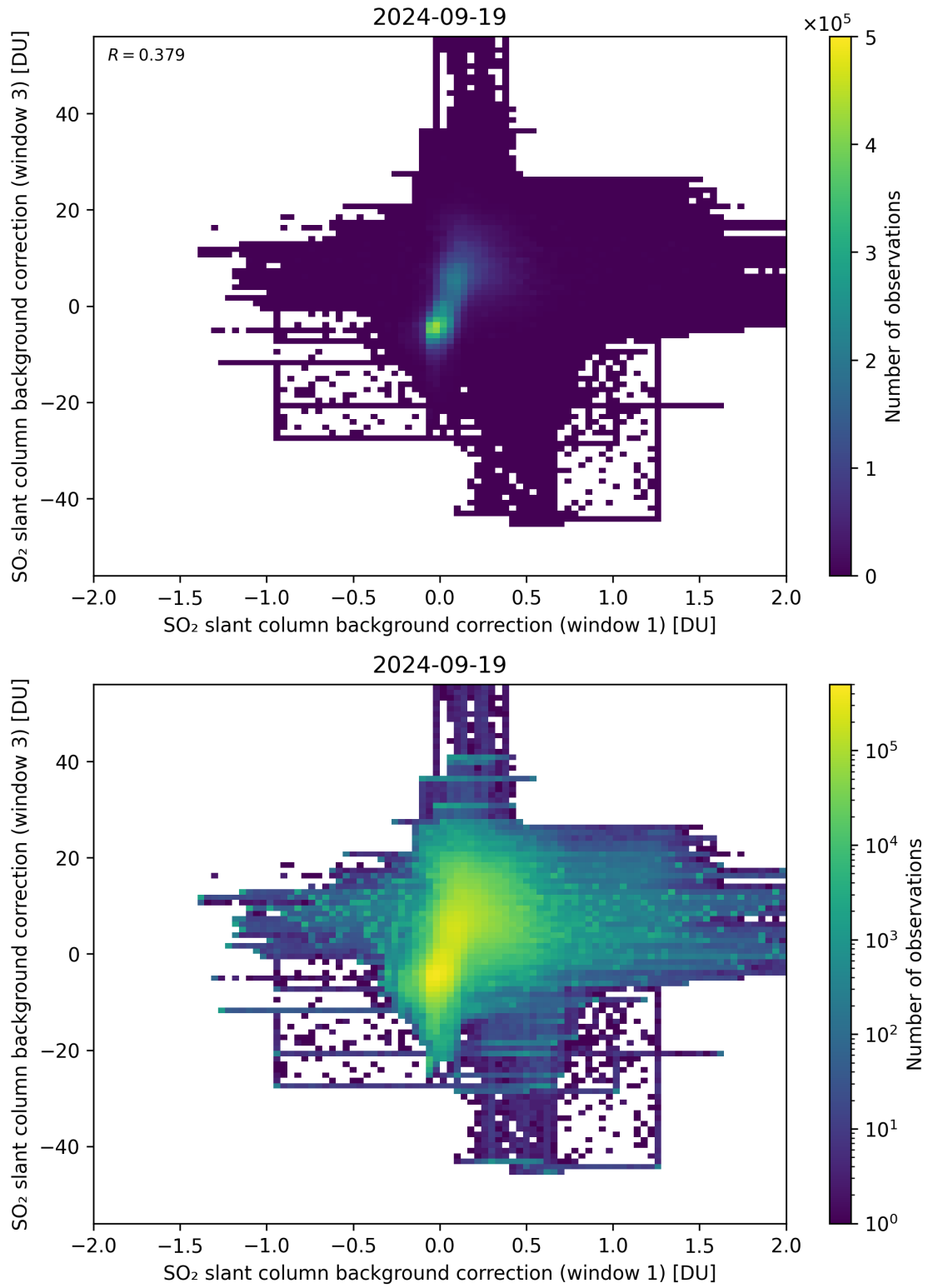
Figure 99: Scatter density plot of “SO 2 slant column background correction (window 1)” against “SO 2 slant column background correction (window 3)” for 2024-09-18 to 2024-09-20.
