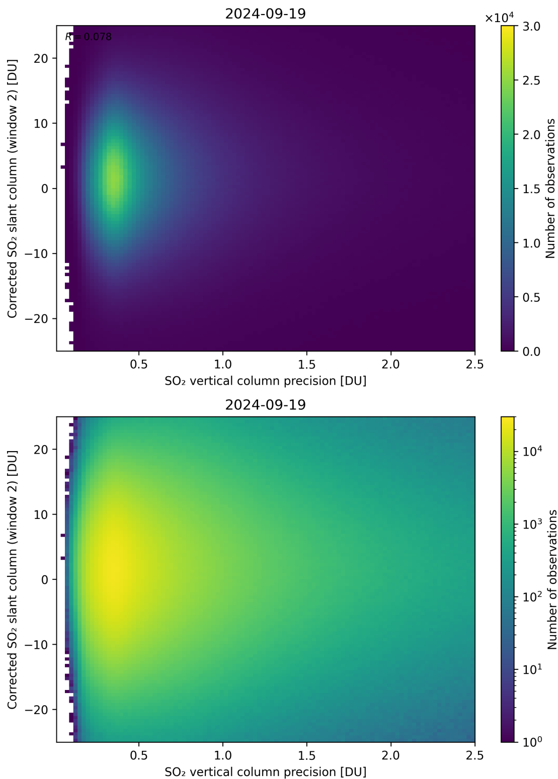
Figure 287: Scatter density plot of “SO 2 vertical column precision” against “Corrected SO 2 slant column (window 2)” for 2024-09-18 to 2024-09-20.
