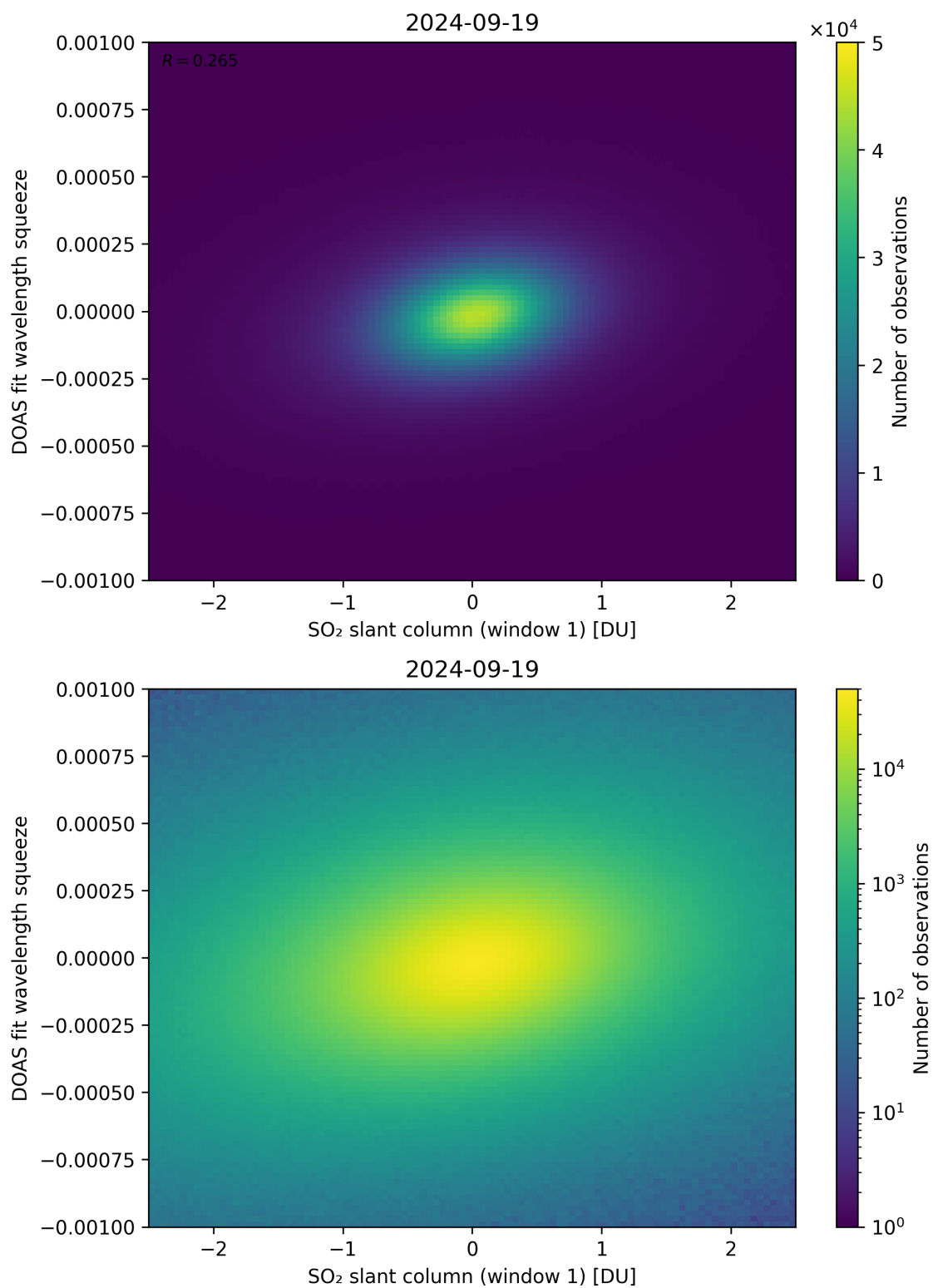
Figure 216: Scatter density plot of “SO 2 slant column (window 1)” against “DOAS fit wavelength squeeze” for 2024-09-18 to 2024-09-20.
