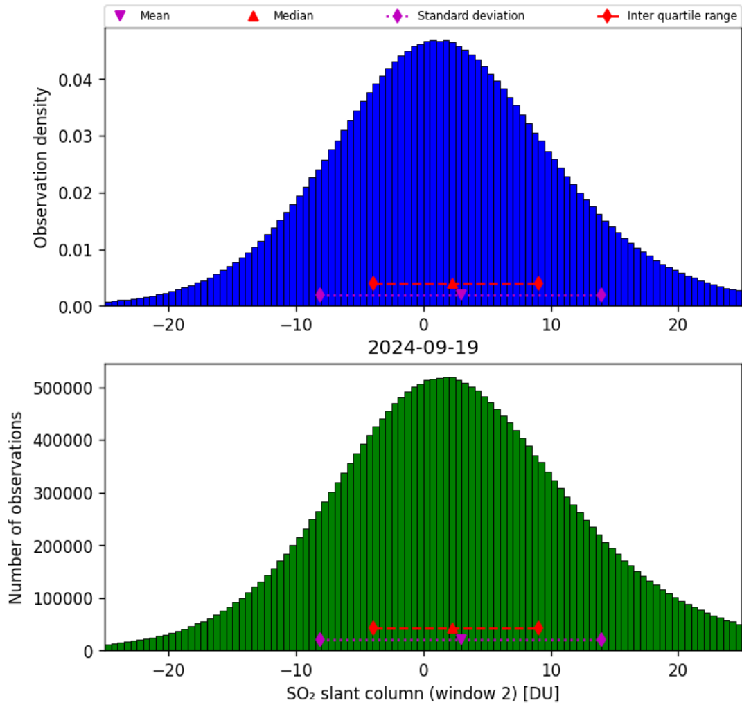
Figure 60: Histogram of “SO 2 slant column (window 2)” for 2024-09-18 to 2024-09-20
