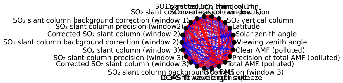
Figure 1: Map of correlation graph for 2024-09-18 to 2024-09-20.
