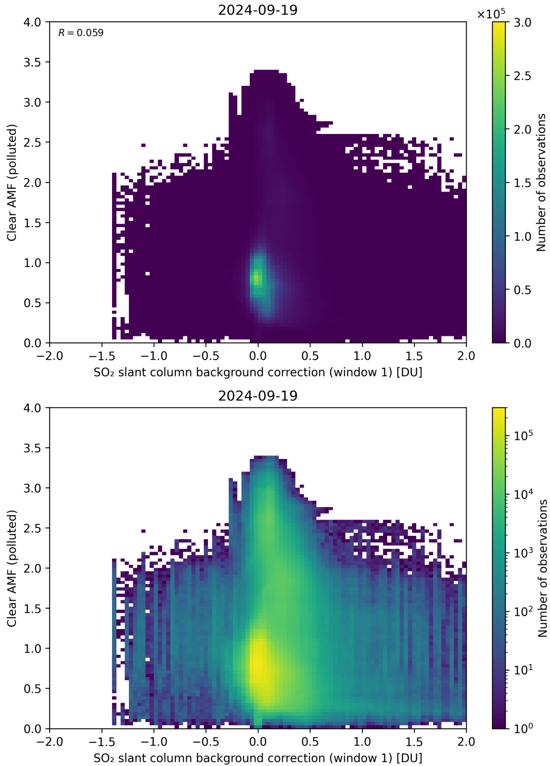
Figure 103: Scatter density plot of “SO 2 slant column background correction (window 1)” against “Clear AMF (polluted)” for 2024-09-18 to 2024-09-20.
