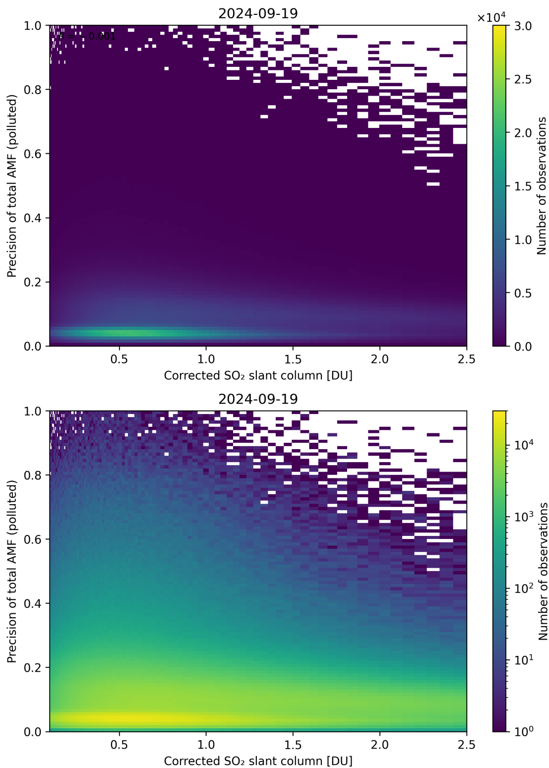
Figure 193: Scatter density plot of “Corrected SO 2 slant column” against “Precision of total AMF (polluted)” for 2024-09-18 to 2024-09-20.
