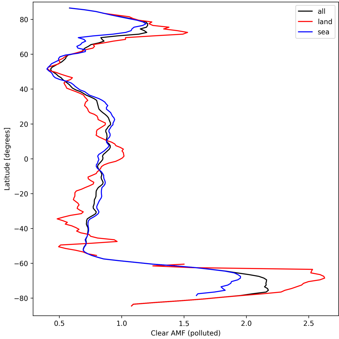
Figure 50: Zonal average of “Clear AMF (polluted)” for 2024-09-18 to 2024-09-20.
