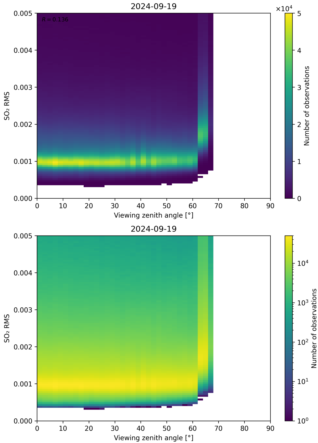
Figure 313: Scatter density plot of “Viewing zenith angle” against “SO 2 RMS” for 2024-09-18 to 2024-09-20.
