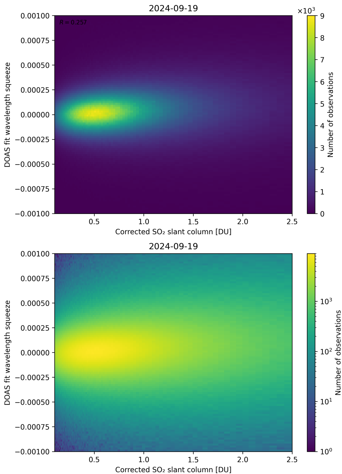
Figure 182: Scatter density plot of “Corrected SO 2 slant column” against “DOAS fit wavelength squeeze” for 2024-09-18 to 2024-09-20.
