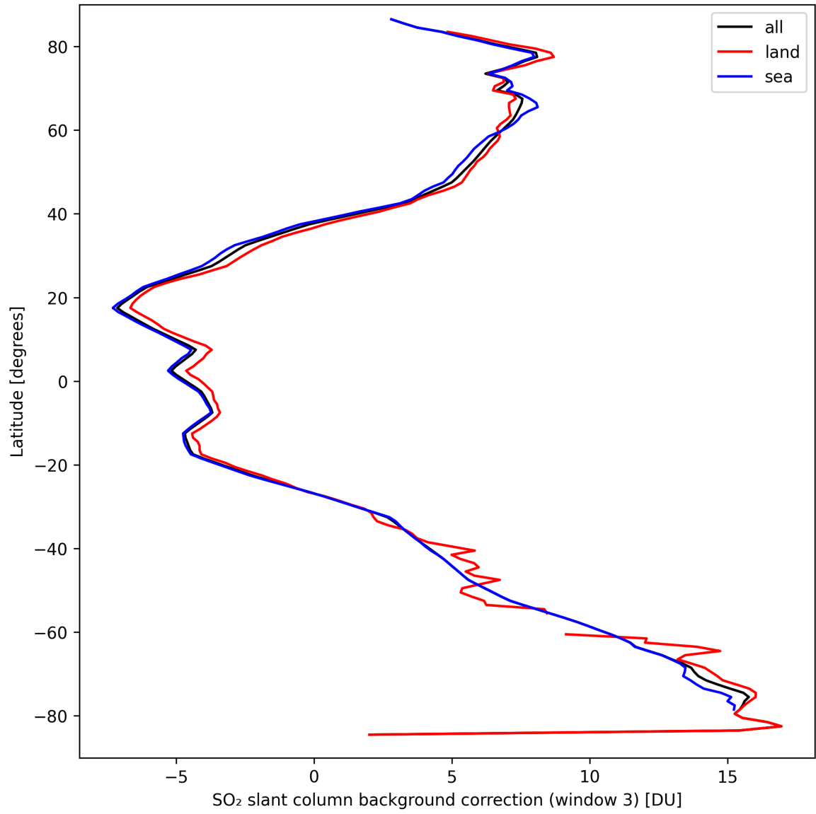
Figure 44: Zonal average of “SO 2 slant column background correction (window 3)” for 2024-09-18 to 2024-09-20.
