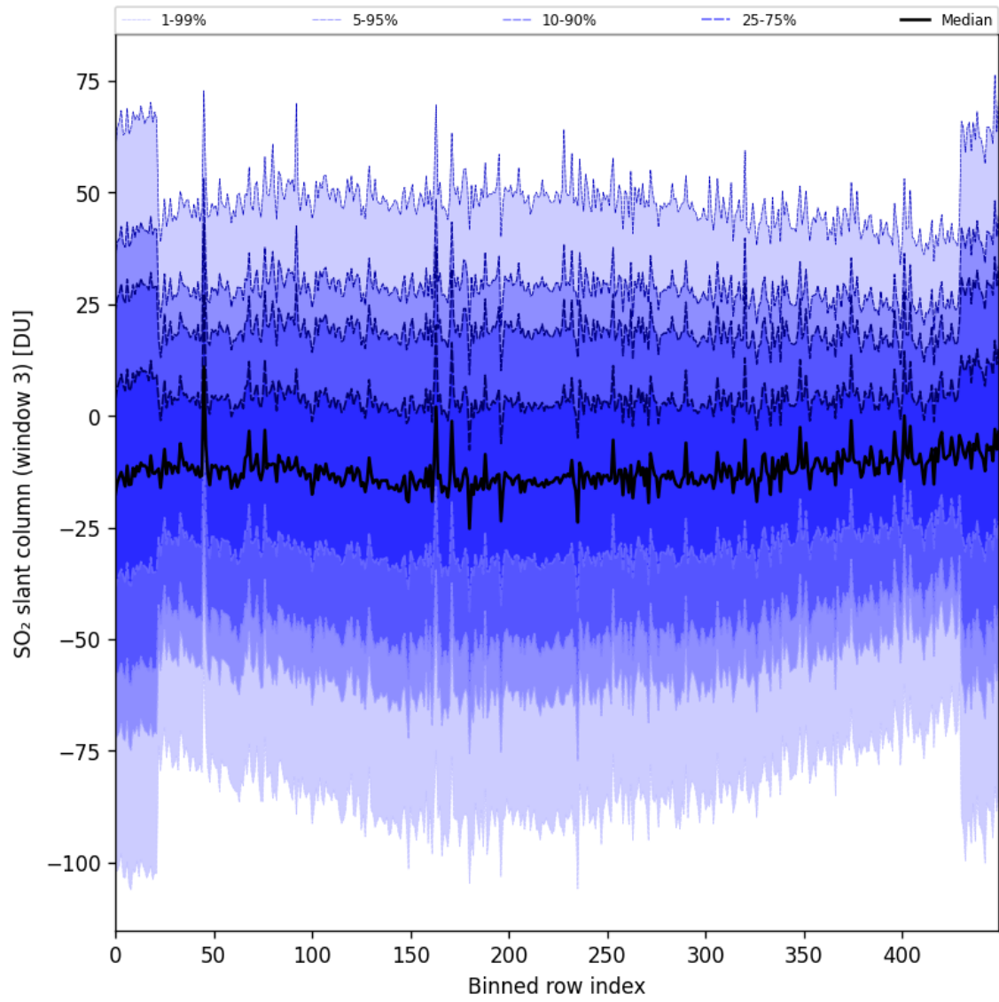
Figure 87: Along track statistics of “SO 2 slant column (window 3)” for 2024-09-18 to 2024-09-20
