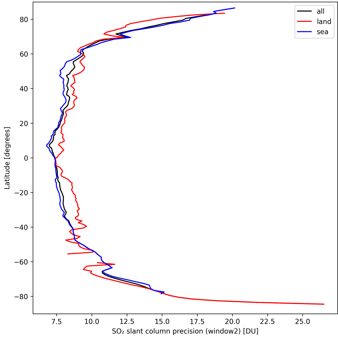
Figure 38: Zonal average of “SO 2 slant column precision (window2)” for 2024-09-18 to 2024-09-20.
