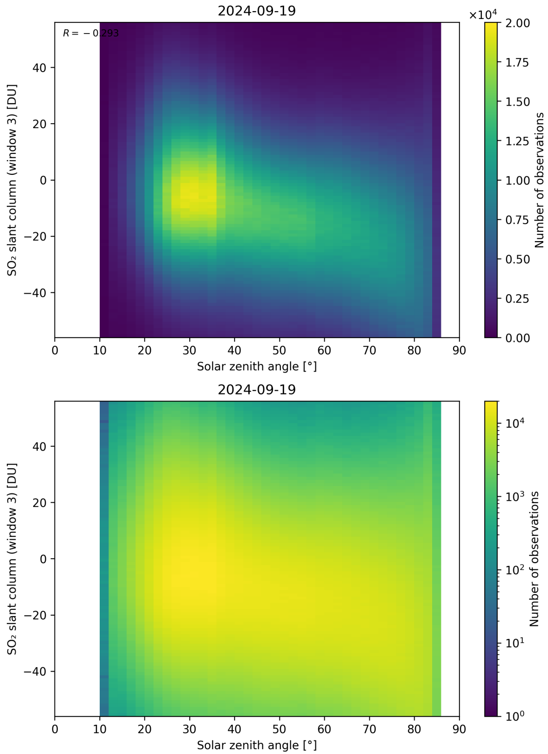
Figure 172: Scatter density plot of “Solar zenith angle” against “SO 2 slant column (window 3)” for 2024-09-18 to 2024-09-20.
