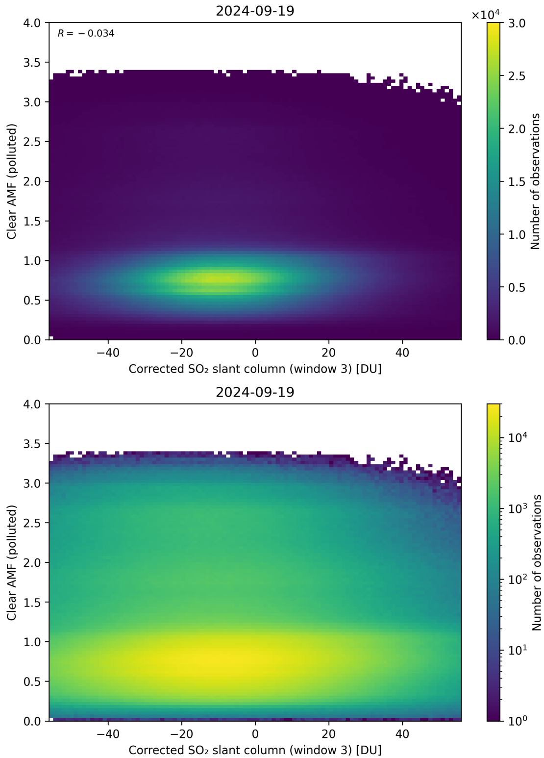
Figure 209: Scatter density plot of “Corrected SO 2 slant column (window 3)” against “Clear AMF (polluted)” for 2024-09-18 to 2024-09-20.
