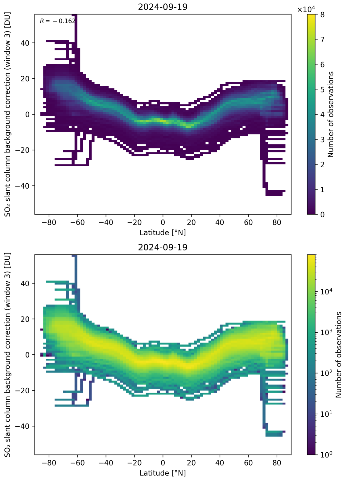
Figure 141: Scatter density plot of “Latitude” against “SO 2 slant column background correction (window 3)” for 2024-09-18 to 2024-09-20.
