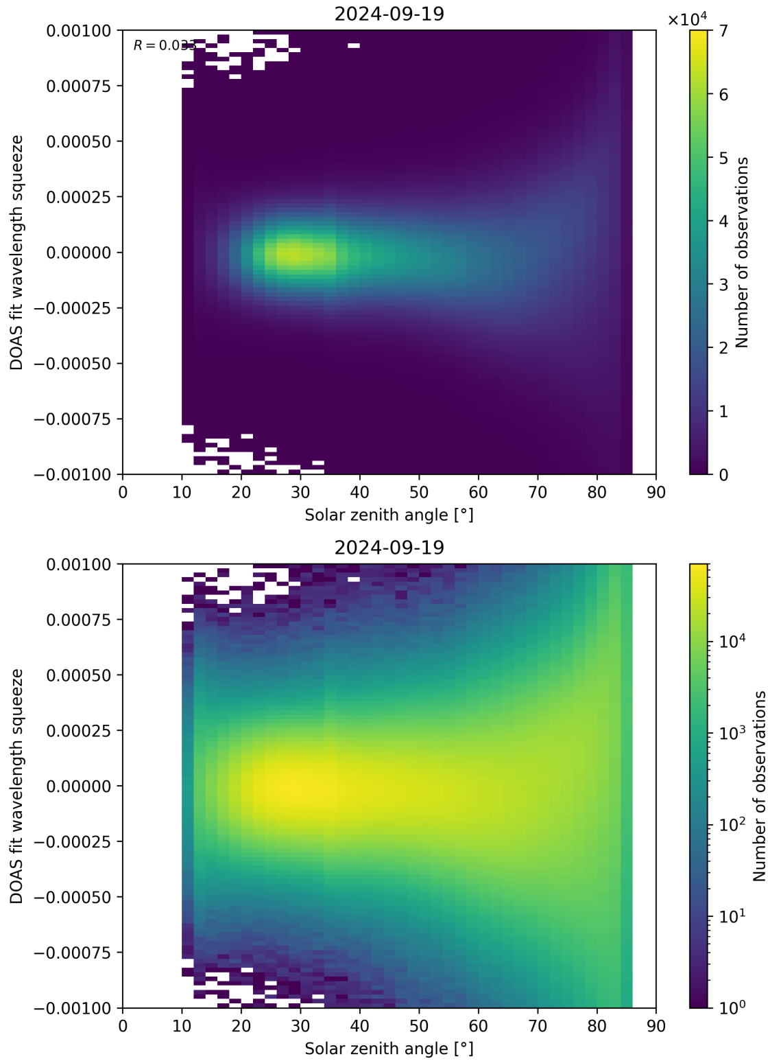
Figure 162: Scatter density plot of “Solar zenith angle” against “DOAS fit wavelength squeeze” for 2024-09-18 to 2024-09-20.
