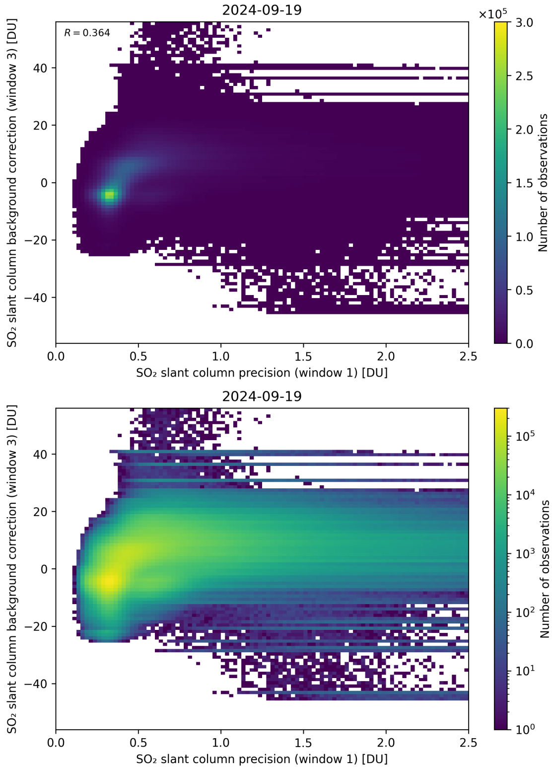
Figure 220: Scatter density plot of “SO 2 slant column precision (window 1)” against “SO 2 slant column background correction (window 3)” for 2024-09-18 to 2024-09-20.
