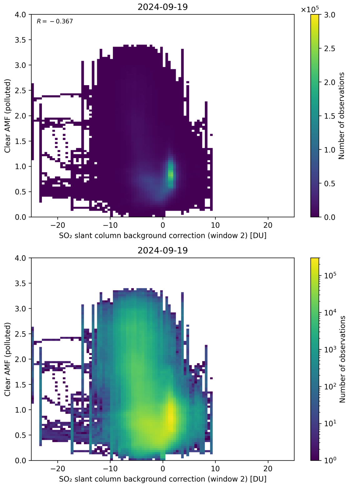
Figure 115: Scatter density plot of “SO 2 slant column background correction (window 2)” against “Clear AMF (polluted)” for 2024-09-18 to 2024-09-20.
