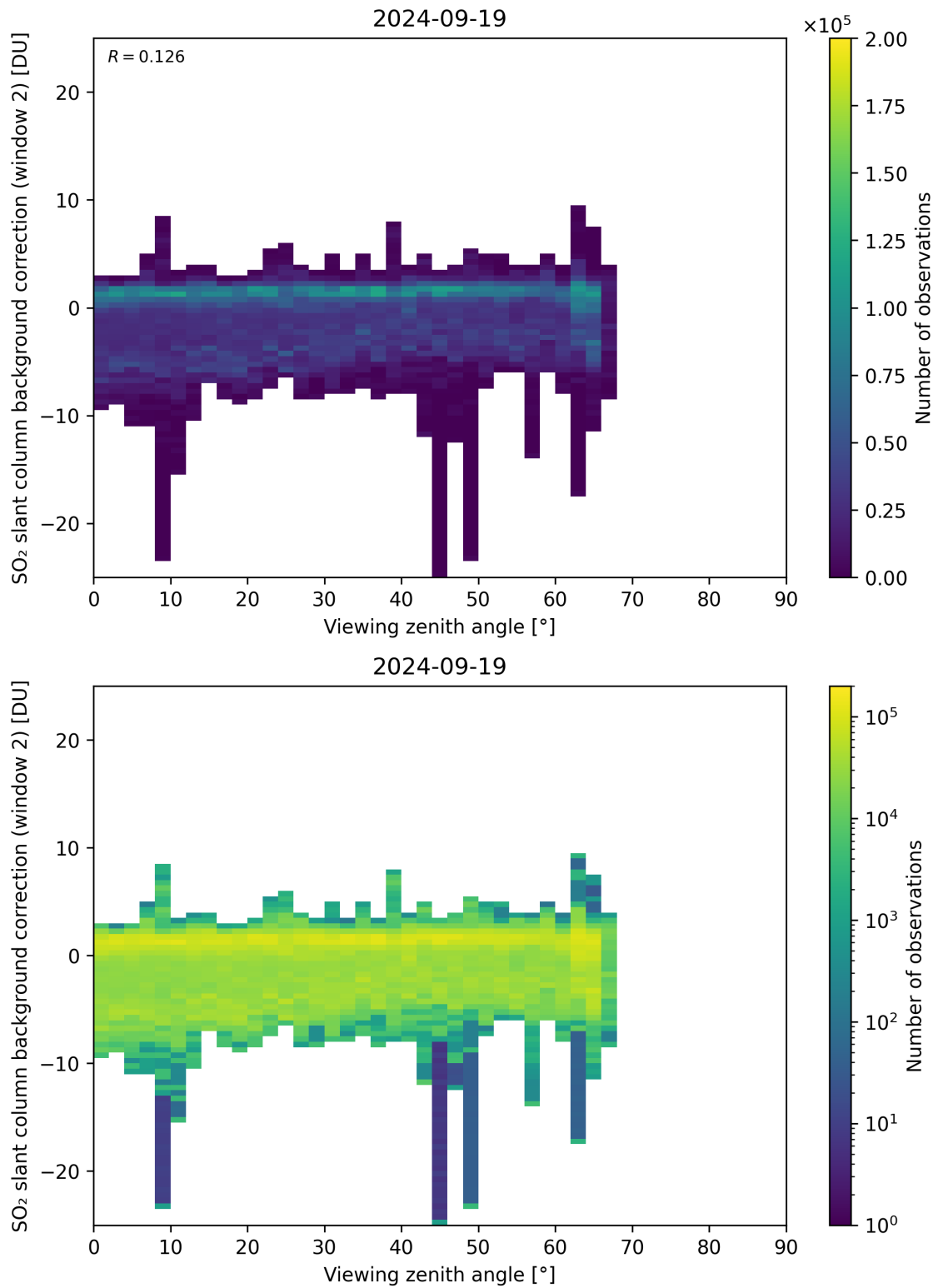
Figure 309: Scatter density plot of “Viewing zenith angle” against “SO 2 slant column background correction (window 2)” for 2024-09-18 to 2024-09-20.
