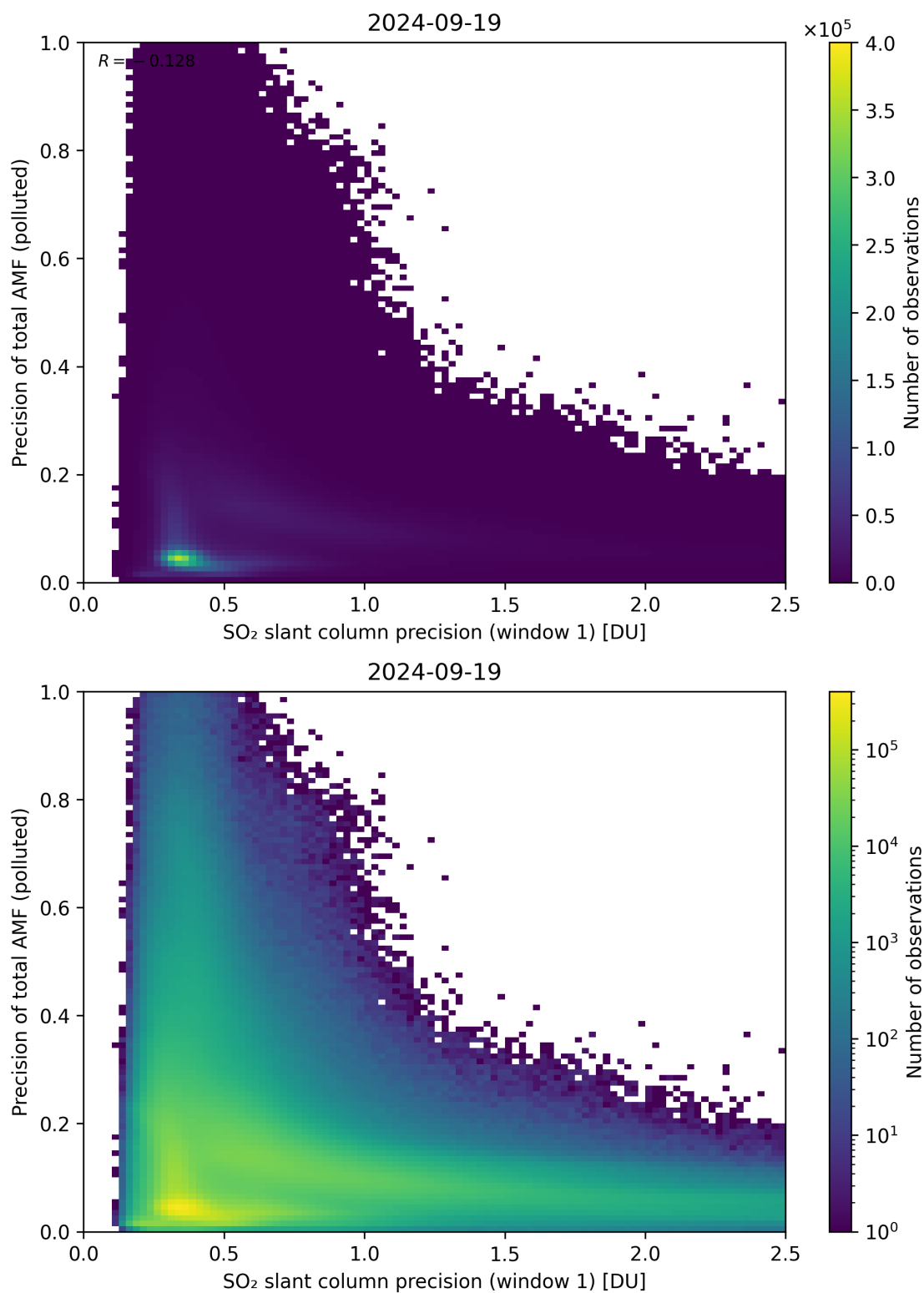
Figure 231: Scatter density plot of “SO 2 slant column precision (window 1)” against “Precision of total AMF (polluted)” for 2024-09-18 to 2024-09-20.
