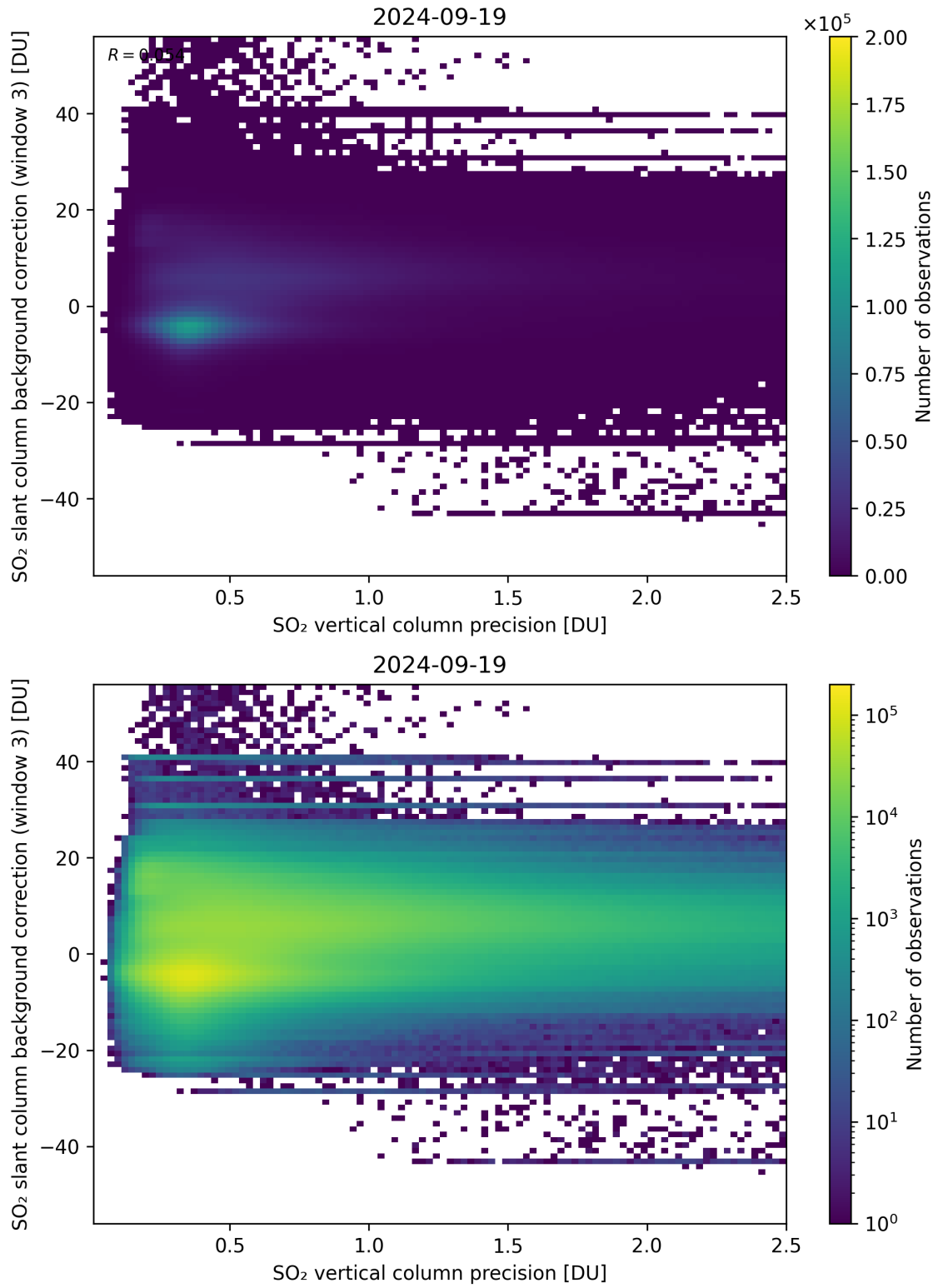
Figure 281: Scatter density plot of “SO 2 vertical column precision” against “SO 2 slant column background correction (window 3)” for 2024-09-18 to 2024-09-20.
