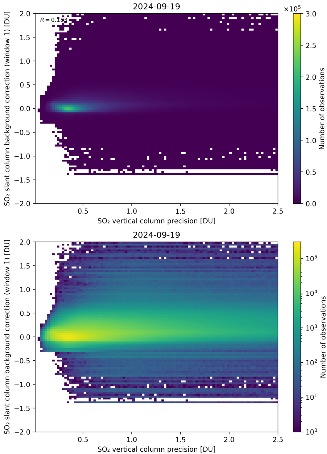
Figure 279: Scatter density plot of “SO 2 vertical column precision” against “SO 2 slant column background correction (window 1)” for 2024-09-18 to 2024-09-20.
