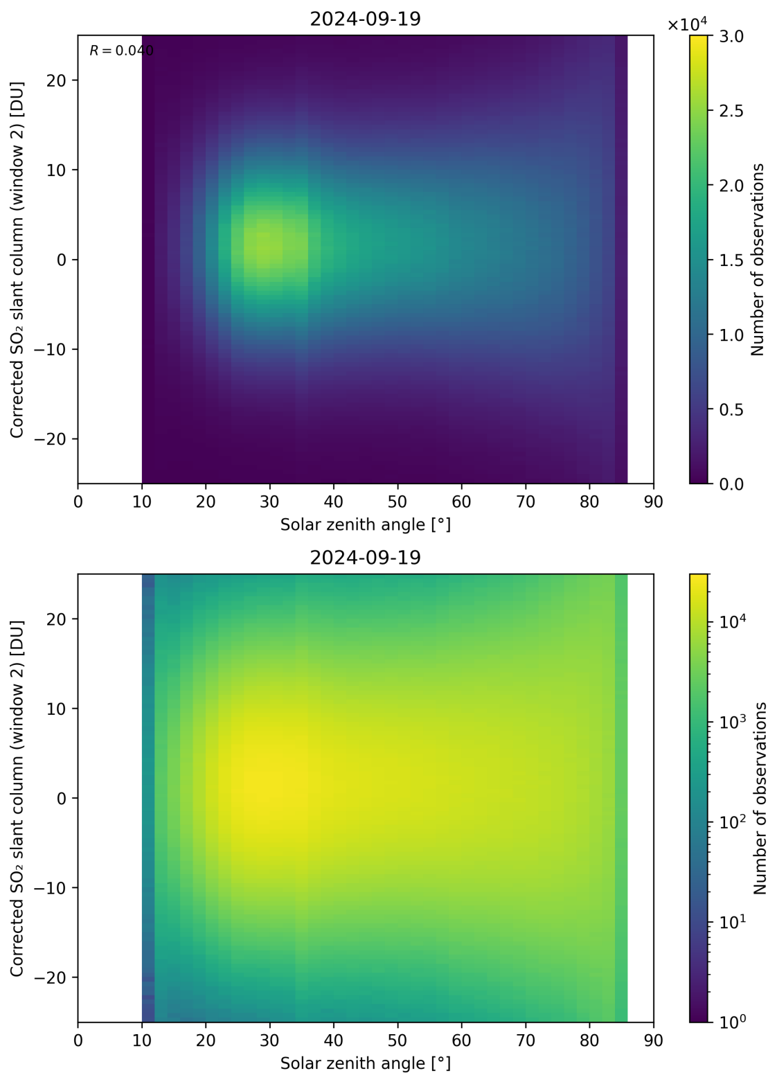
Figure 167: Scatter density plot of “Solar zenith angle” against “Corrected SO 2 slant column (window 2)” for 2024-09-18 to 2024-09-20.
