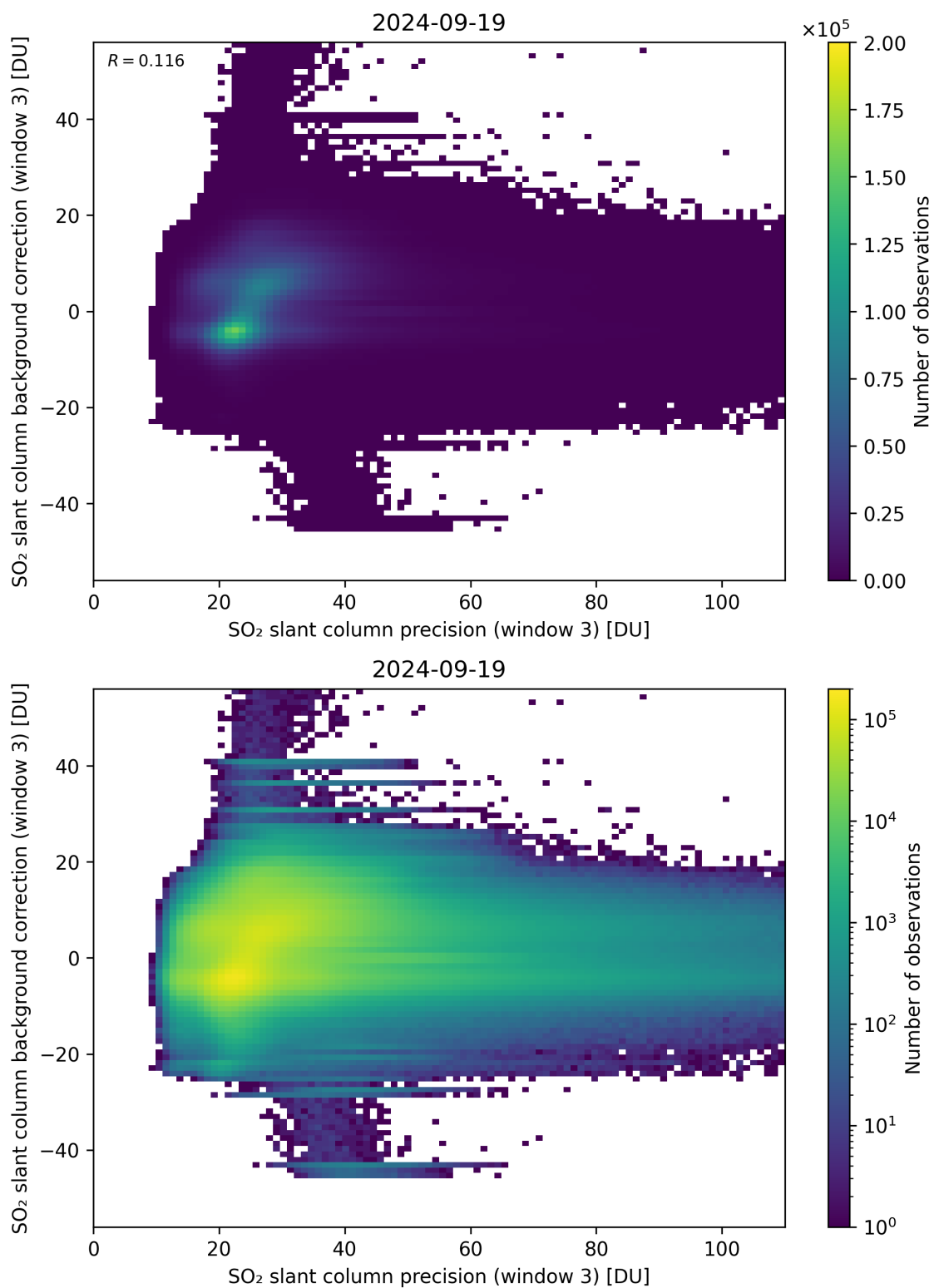
Figure 257: Scatter density plot of “SO 2 slant column precision (window 3)” against “SO 2 slant column background correction (window 3)” for 2024-09-18 to 2024-09-20.
