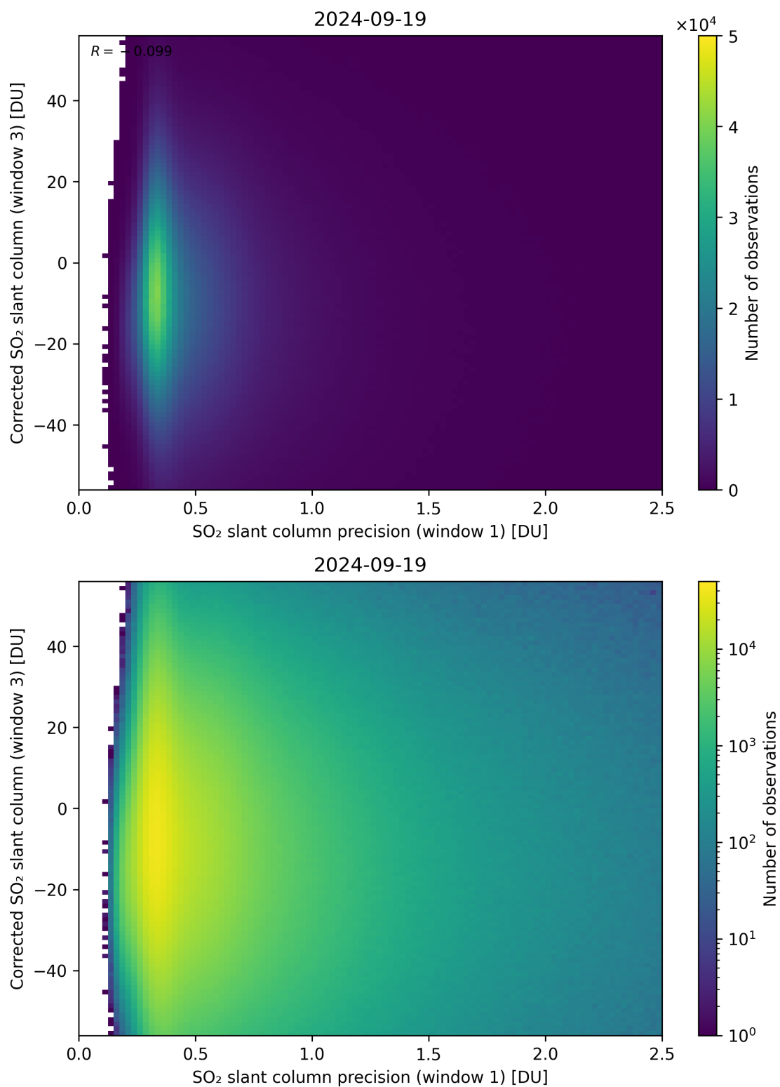
Figure 226: Scatter density plot of “SO 2 slant column precision (window 1)” against “Corrected SO 2 slant column (window 3)” for 2024-09-18 to 2024-09-20.
