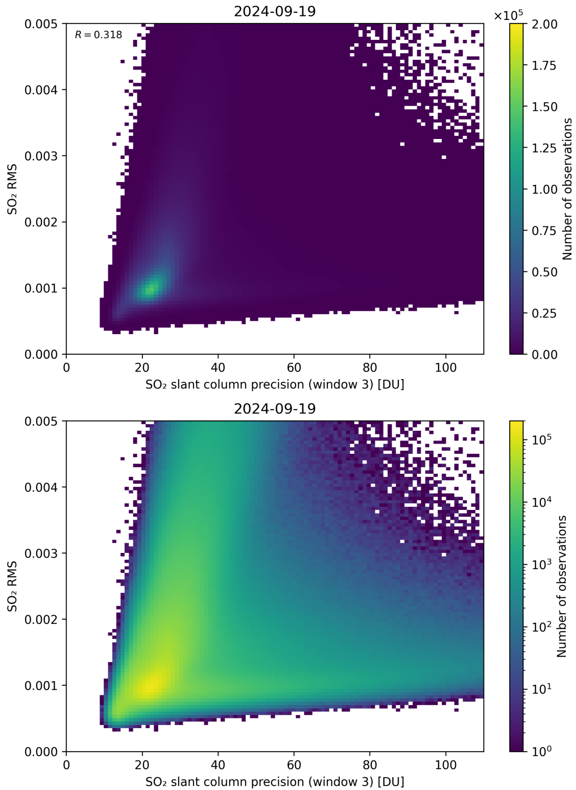
Figure 260: Scatter density plot of “SO 2 slant column precision (window 3)” against “SO 2 RMS” for 2024-09-18 to 2024-09-20.
