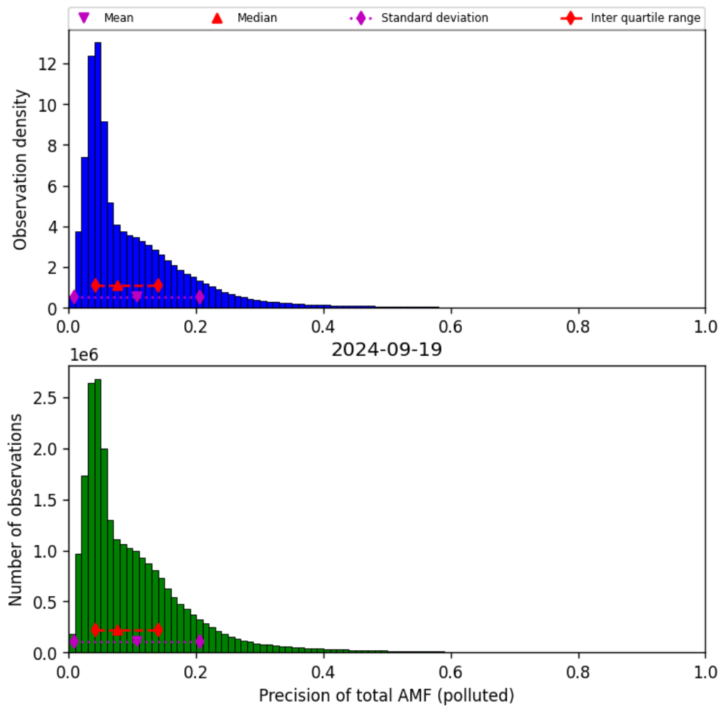
Figure 72: Histogram of “Precision of total AMF (polluted)” for 2024-09-18 to 2024-09-20
