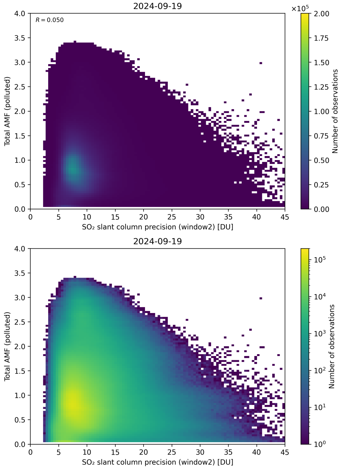
Figure 251: Scatter density plot of “SO 2 slant column precision (window2)” against “Total AMF (polluted)” for 2024-09-18 to 2024-09-20.
