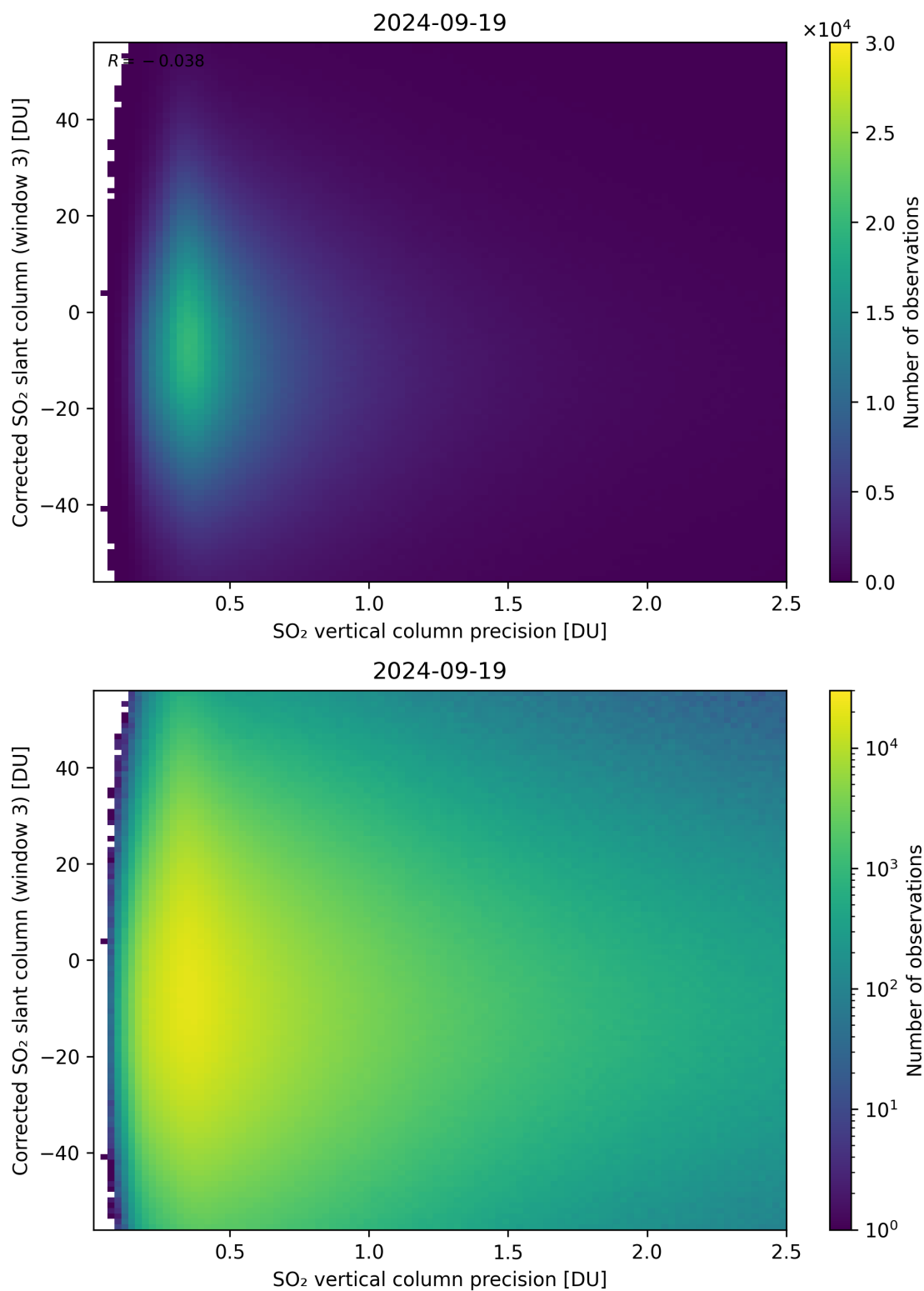
Figure 288: Scatter density plot of “SO 2 vertical column precision” against “Corrected SO 2 slant column (window 3)” for 2024-09-18 to 2024-09-20.
