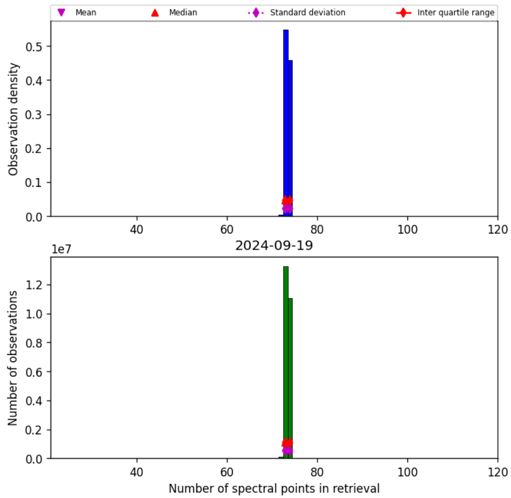
Figure 74: Histogram of “Number of spectral points in retrieval” for 2024-09-18 to 2024-09-20
