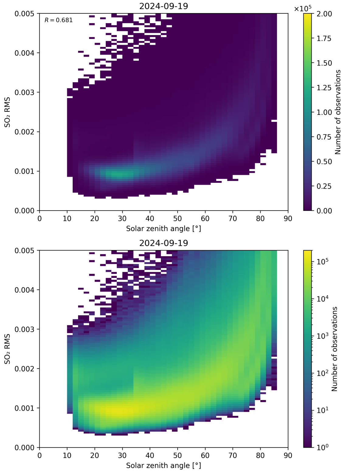
Figure 163: Scatter density plot of “Solar zenith angle” against “SO 2 RMS” for 2024-09-18 to 2024-09-20.
