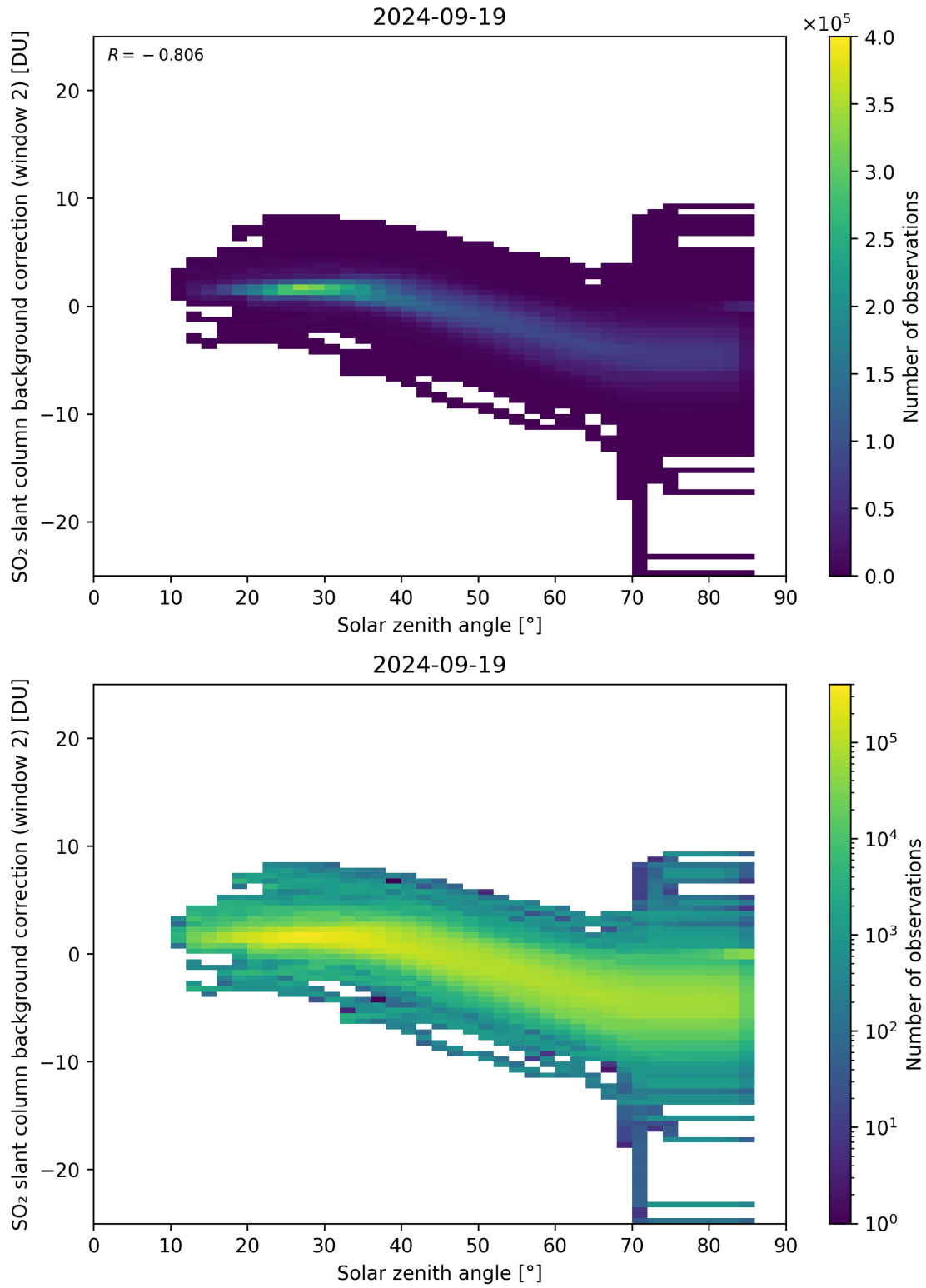
Figure 159: Scatter density plot of “Solar zenith angle” against “SO 2 slant column background correction (window 2)” for 2024-09-18 to 2024-09-20.
