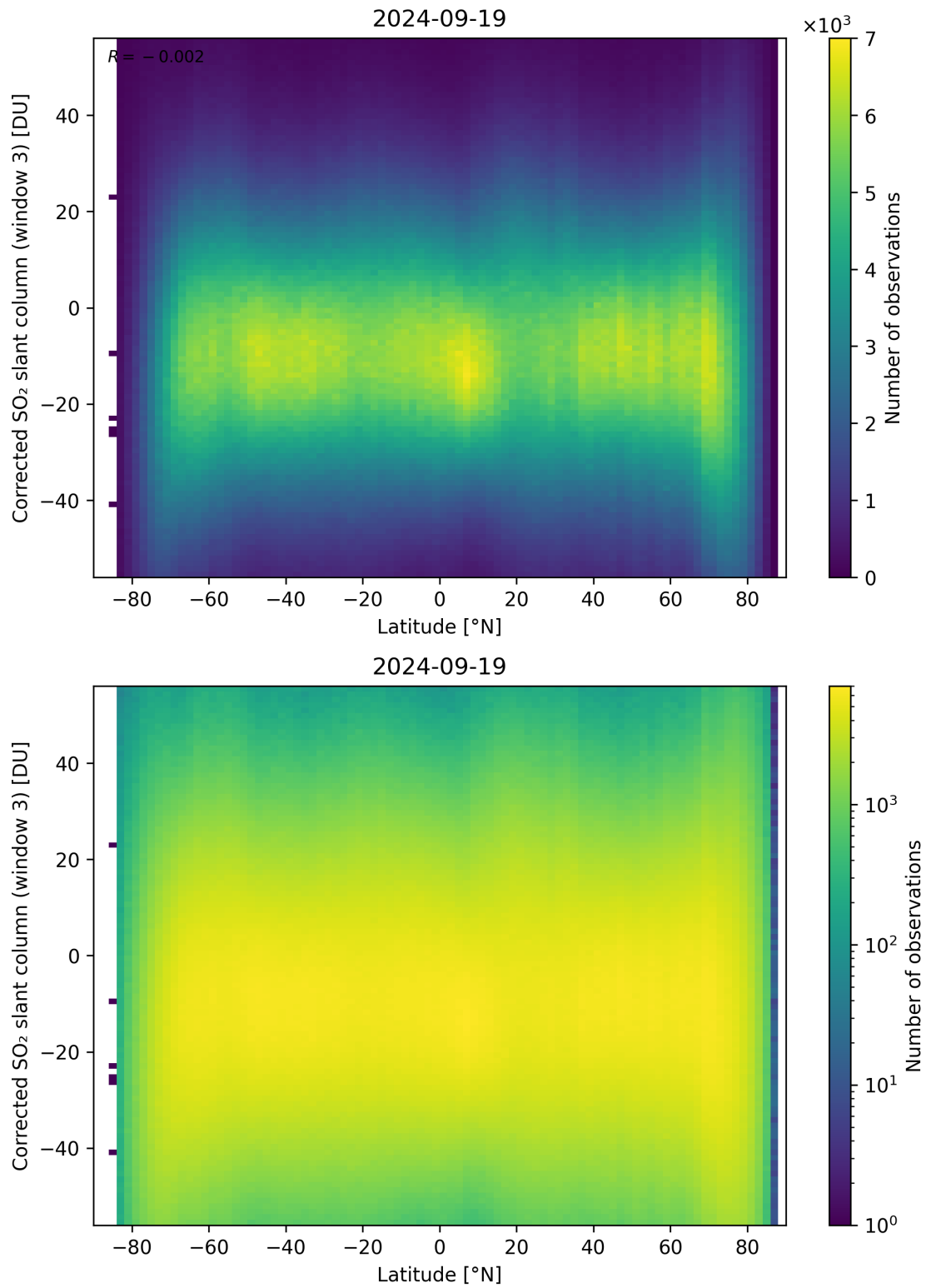
Figure 148: Scatter density plot of “Latitude” against “Corrected SO 2 slant column (window 3)” for 2024-09-18 to 2024-09-20.
