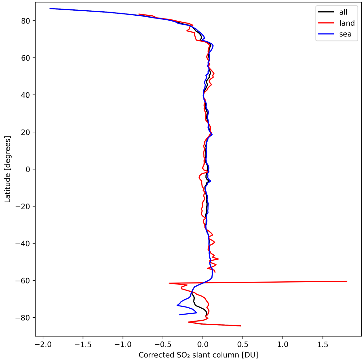
Figure 32: Zonal average of “Corrected SO 2 slant column” for 2024-09-18 to 2024-09-20.
