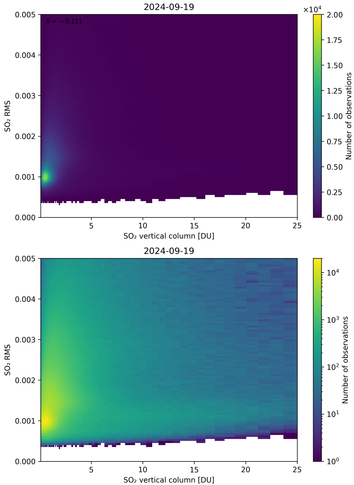
Figure 278: Scatter density plot of “SO 2 vertical column” against “SO 2 RMS” for 2024-09-18 to 2024-09-20.
