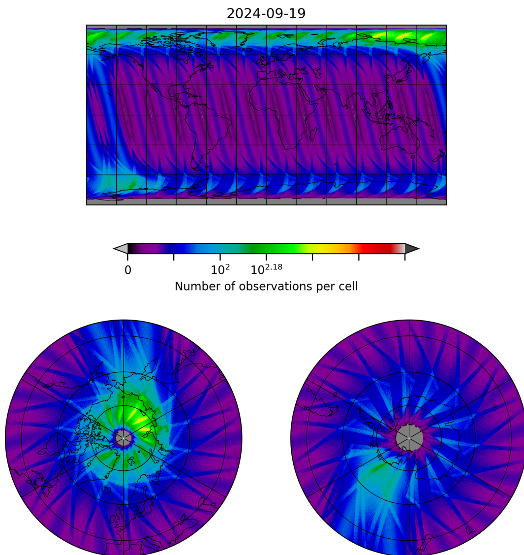
Figure 28: Map of the number of observations for 2024-09-18 to 2024-09-20
