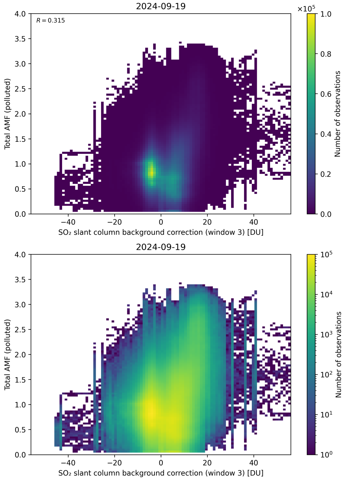
Figure 125: Scatter density plot of “SO 2 slant column background correction (window 3)” against “Total AMF (polluted)” for 2024-09-18 to 2024-09-20.
