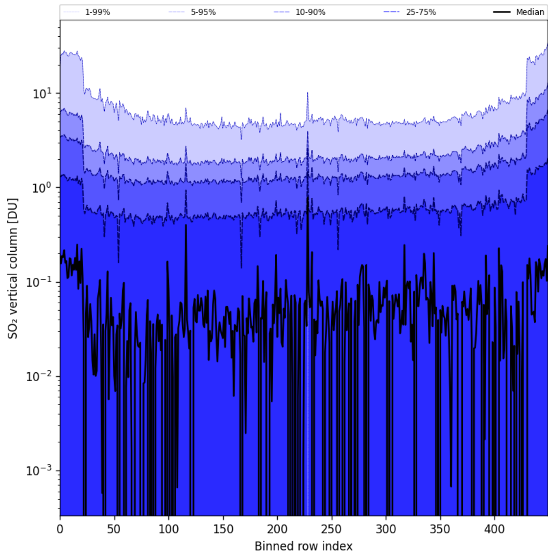
Figure 76: Along track statistics of “SO 2 vertical column” for 2024-09-18 to 2024-09-20
