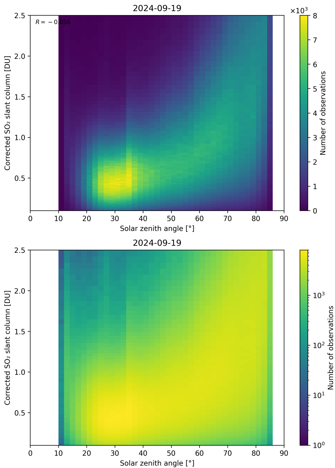
Figure 166: Scatter density plot of “Solar zenith angle” against “Corrected SO 2 slant column” for 2024-09-18 to 2024-09-20.
