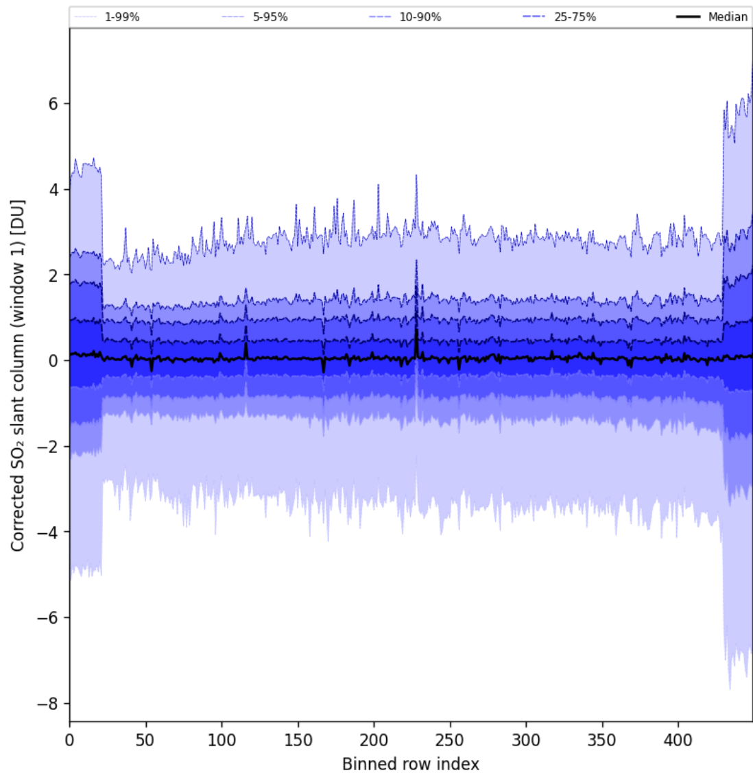
Figure 81: Along track statistics of “Corrected SO 2 slant column (window 1)” for 2024-09-18 to 2024-09-20
