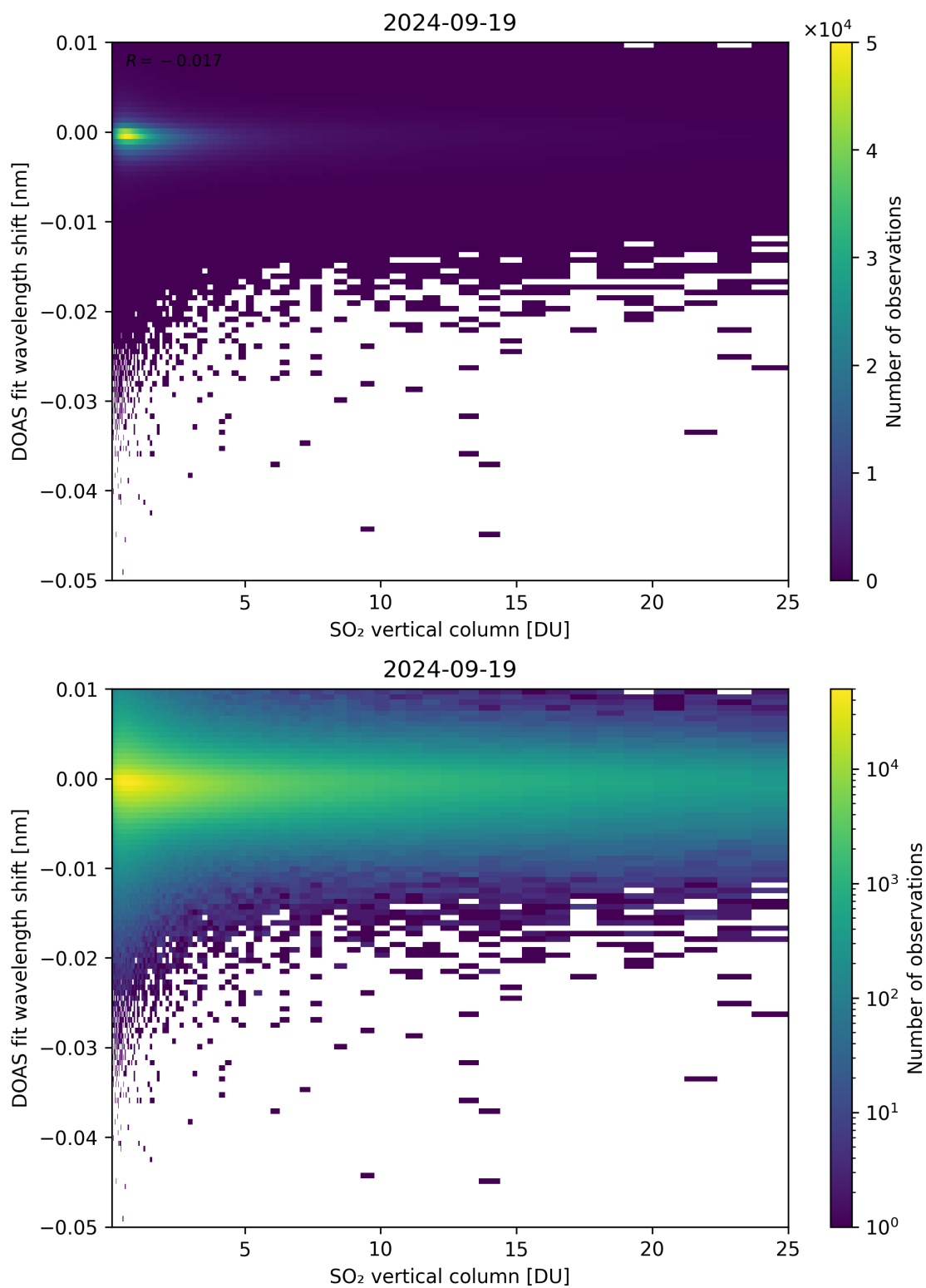
Figure 276: Scatter density plot of “SO 2 vertical column” against “DOAS fit wavelength shift” for 2024-09-18 to 2024-09-20.
