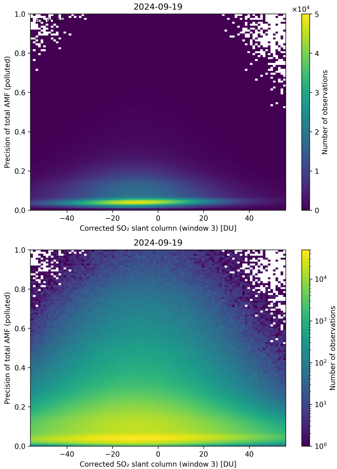
Figure 211: Scatter density plot of “Corrected SO 2 slant column (window 3)” against “Precision of total AMF (polluted)” for 2024-09-18 to 2024-09-20.
