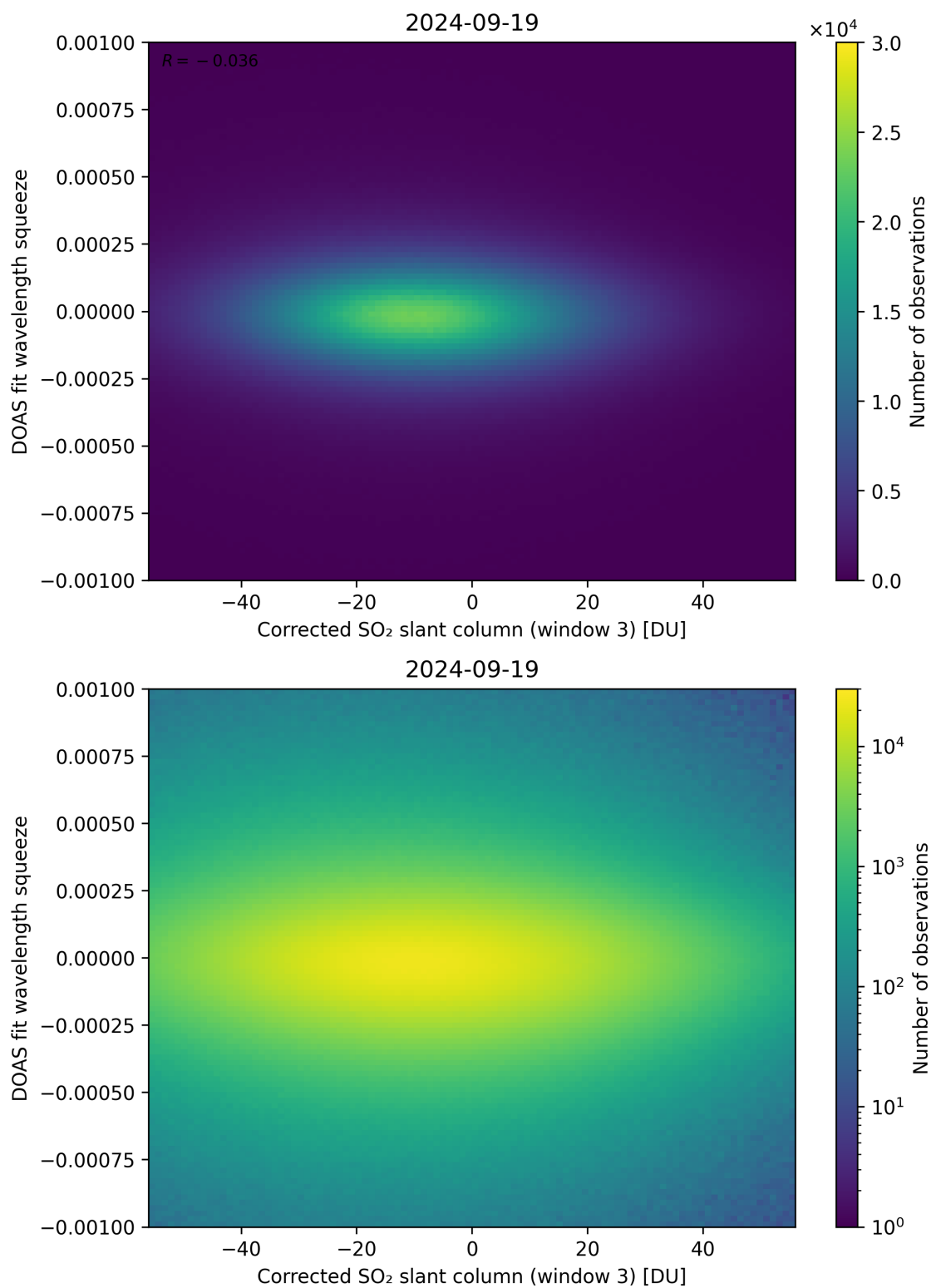
Figure 207: Scatter density plot of “Corrected SO 2 slant column (window 3)” against “DOAS fit wavelength squeeze” for 2024-09-18 to 2024-09-20.
