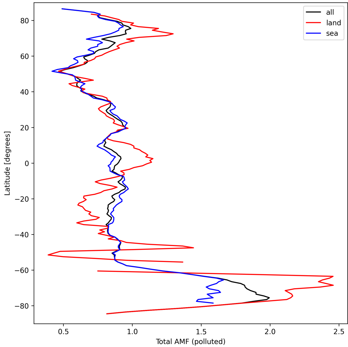
Figure 48: Zonal average of “Total AMF (polluted)” for 2024-09-18 to 2024-09-20.
