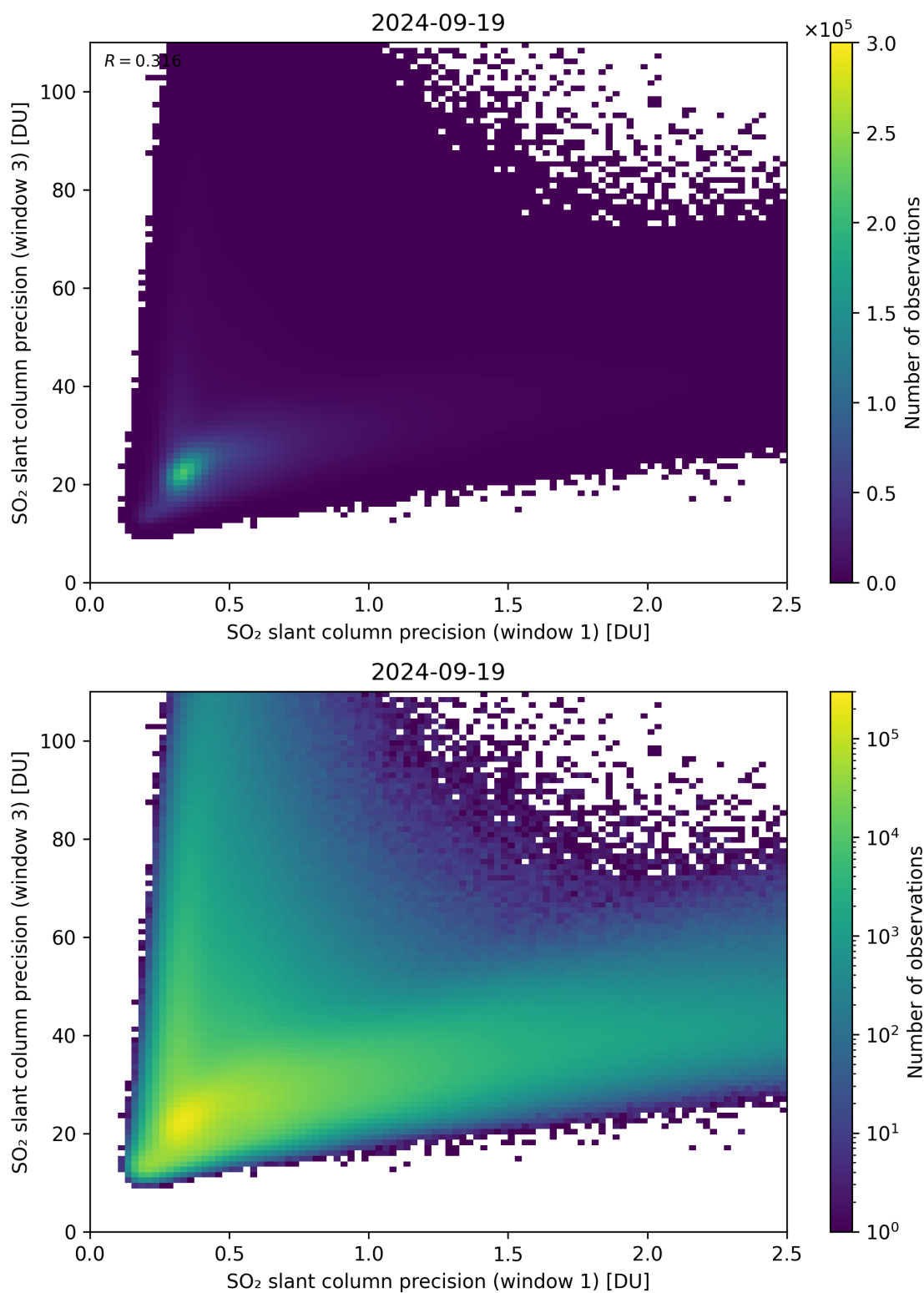
Figure 229: Scatter density plot of “SO 2 slant column precision (window 1)” against “SO 2 slant column precision (window 3)” for 2024-09-18 to 2024-09-20.
