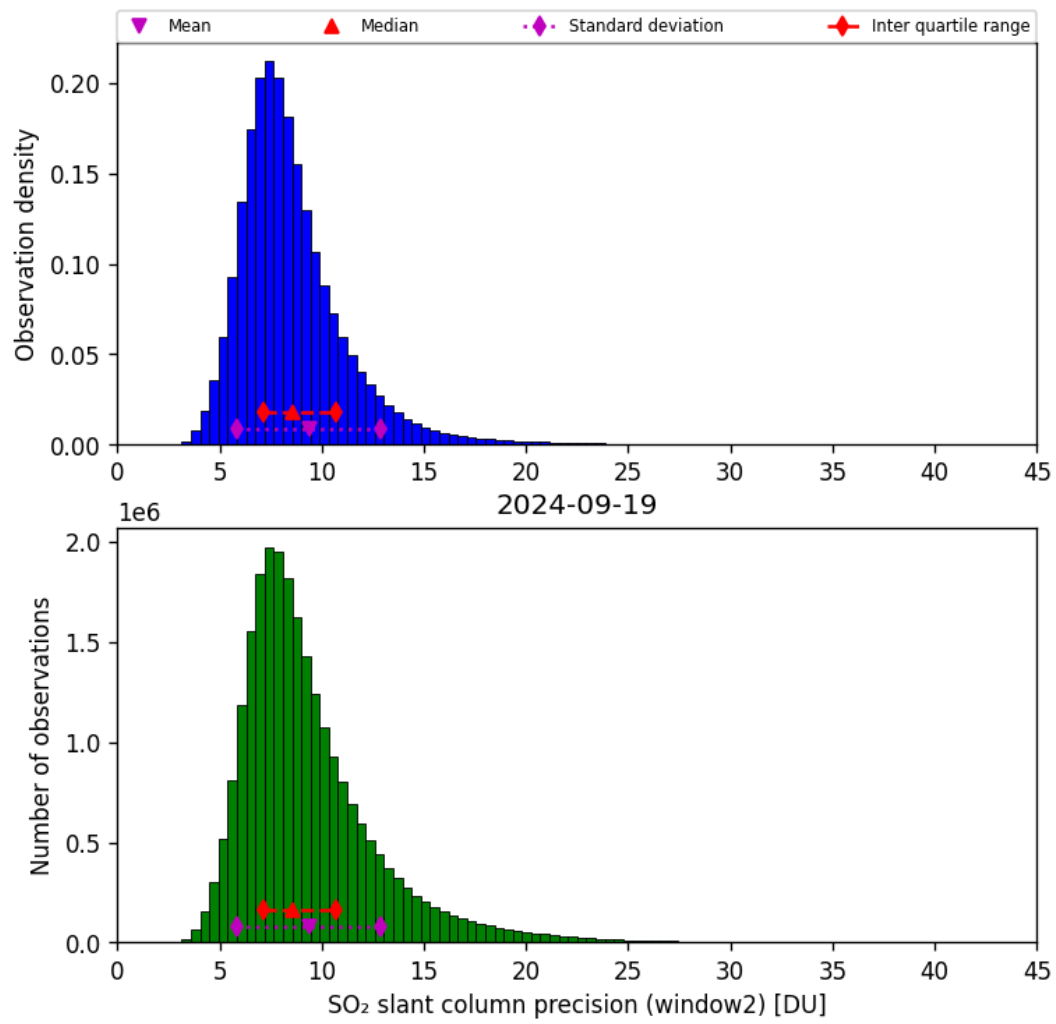
Figure 61: Histogram of “SO 2 slant column precision (window2)” for 2024-09-18 to 2024-09-20
