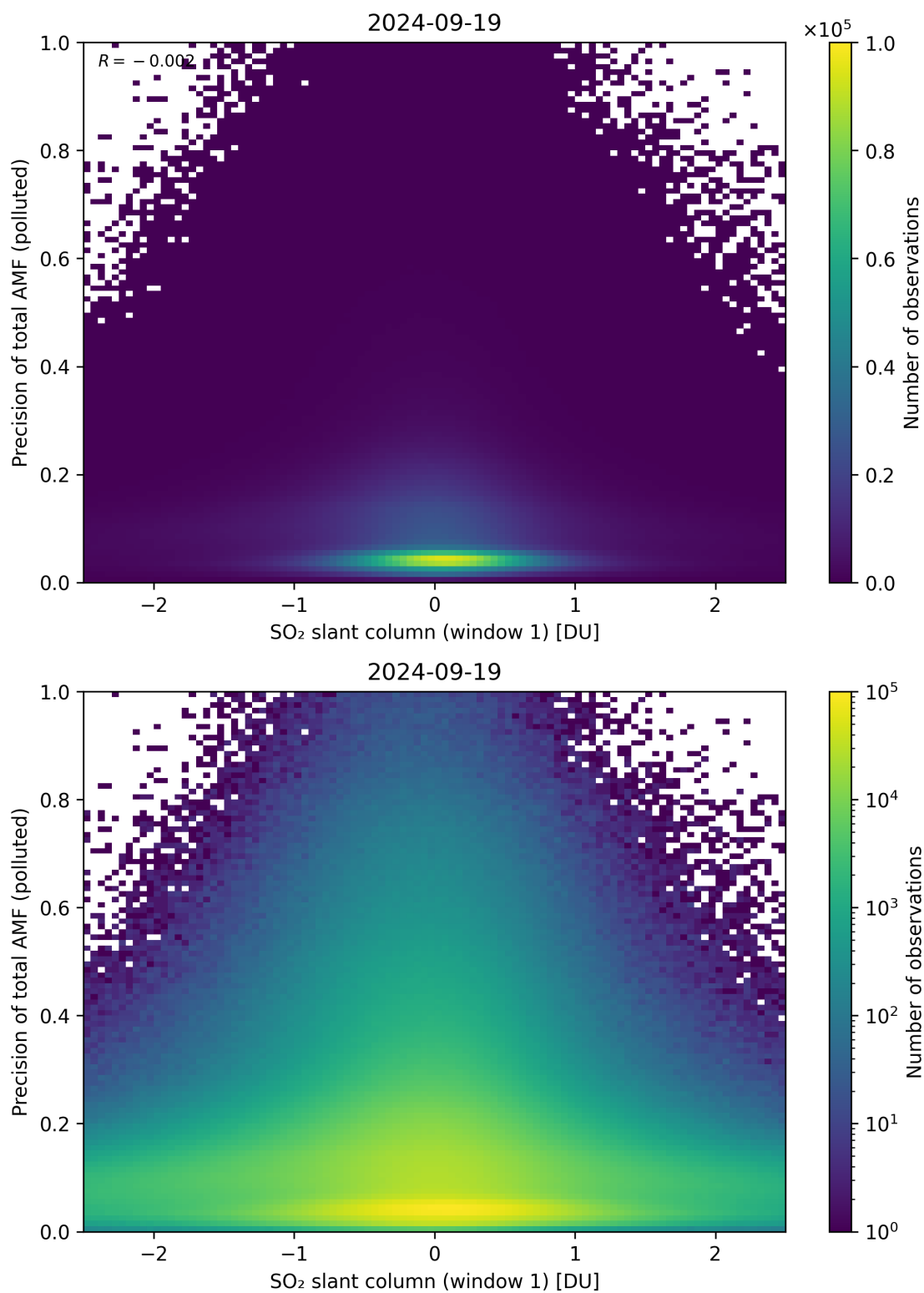
Figure 240: Scatter density plot of “SO 2 slant column (window 1)” against “Precision of total AMF (polluted)” for 2024-09-18 to 2024-09-20.
