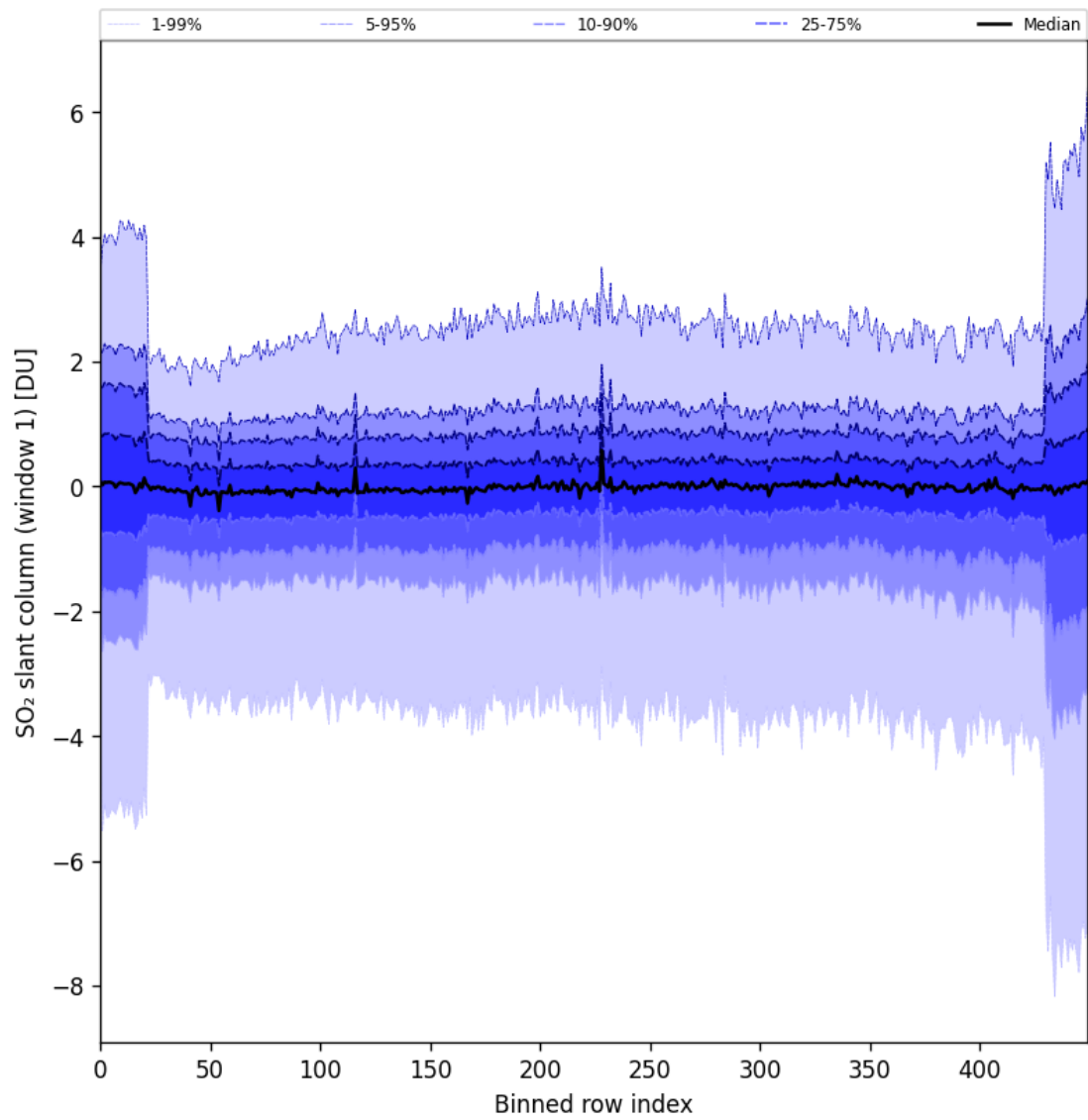
Figure 79: Along track statistics of “SO 2 slant column (window 1)” for 2024-09-18 to 2024-09-20
