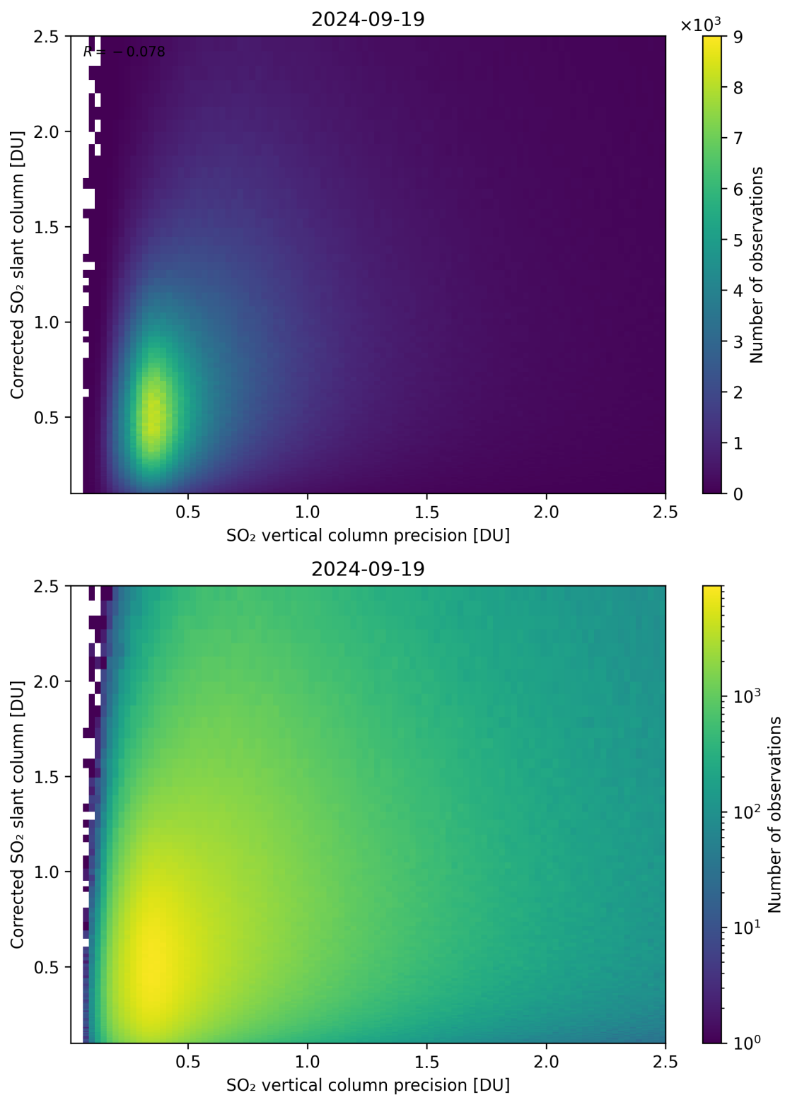
Figure 286: Scatter density plot of “SO 2 vertical column precision” against “Corrected SO 2 slant column” for 2024-09-18 to 2024-09-20.
