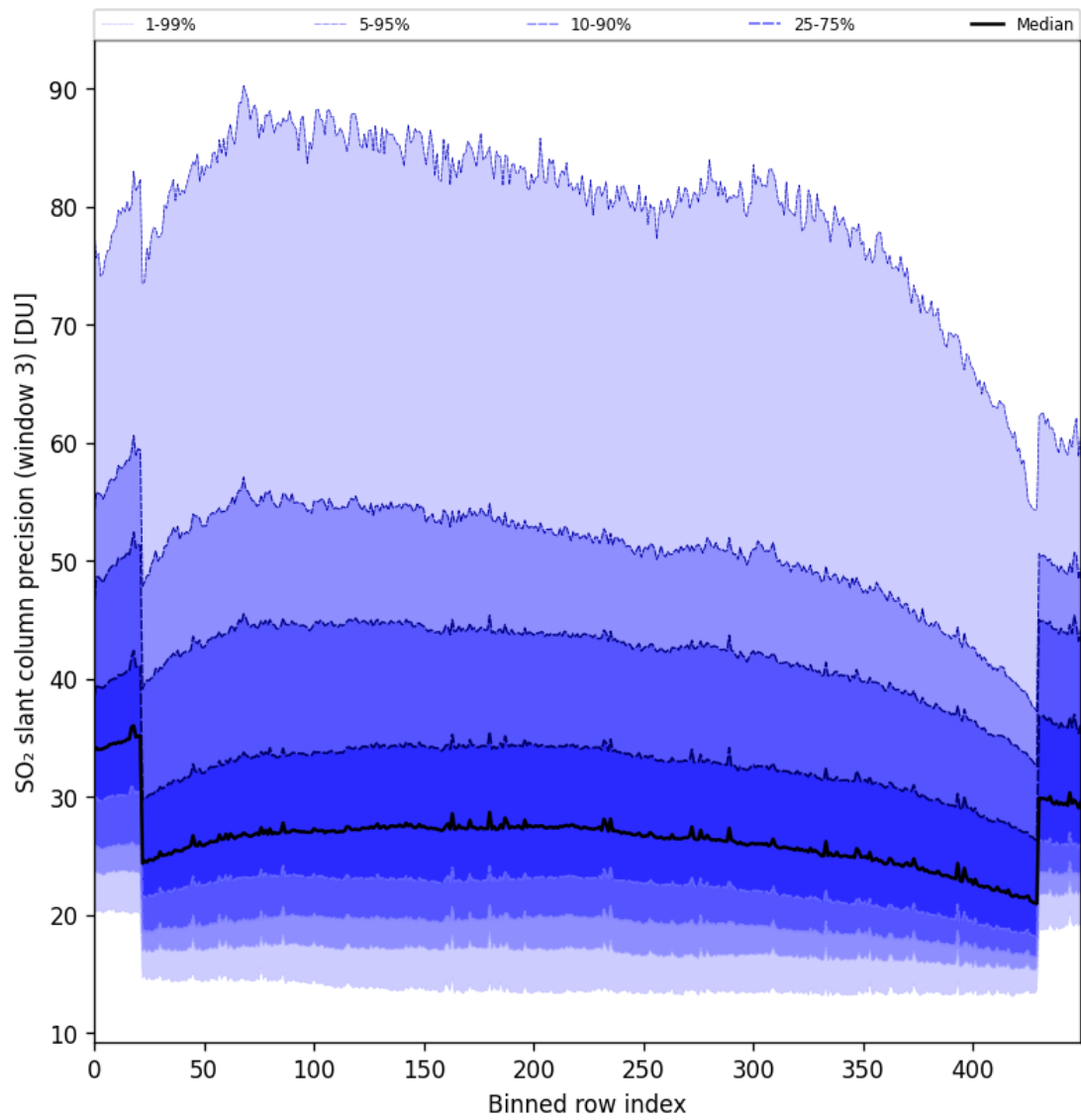
Figure 88: Along track statistics of “SO 2 slant column precision (window 3)” for 2024-09-18 to 2024-09-20
