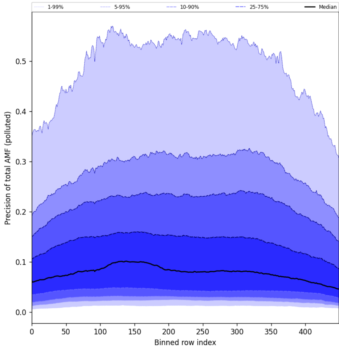
Figure 95: Along track statistics of “Precision of total AMF (polluted)” for 2024-09-18 to 2024-09-20
