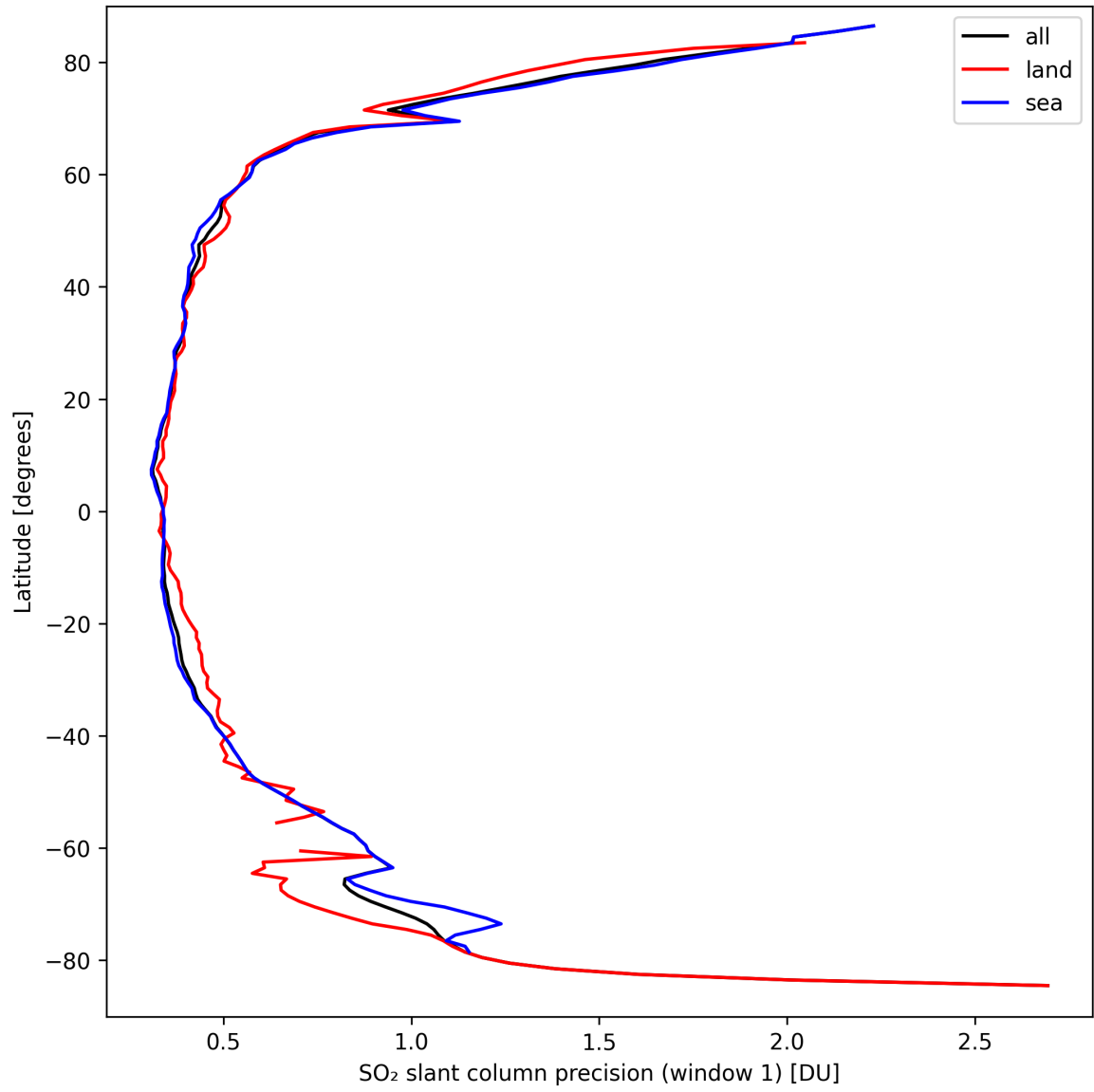
Figure 34: Zonal average of “SO 2 slant column precision (window 1)” for 2024-09-18 to 2024-09-20.
