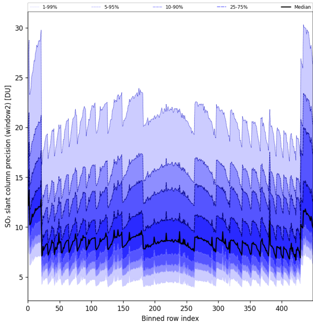
Figure 84: Along track statistics of “SO 2 slant column precision (window2)” for 2024-09-18 to 2024-09-20
