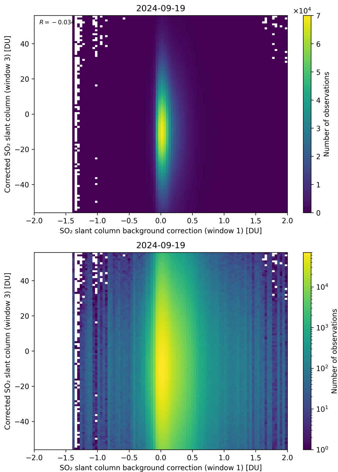
Figure 105: Scatter density plot of “SO 2 slant column background correction (window 1)” against “Corrected SO 2 slant column (window 3)” for 2024-09-18 to 2024-09-20.
