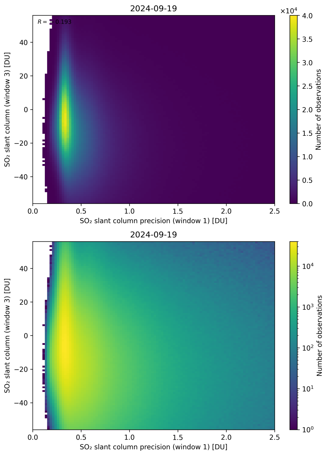
Figure 228: Scatter density plot of “SO 2 slant column precision (window 1)” against “SO 2 slant column (window 3)” for 2024-09-18 to 2024-09-20.
