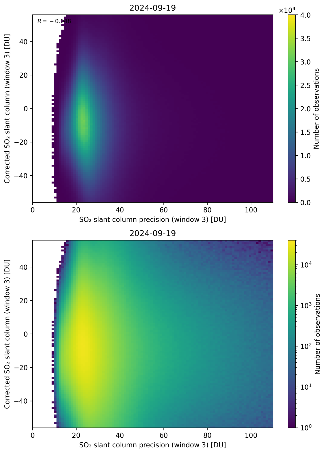
Figure 262: Scatter density plot of “SO 2 slant column precision (window 3)” against “Corrected SO 2 slant column (window 3)” for 2024-09-18 to 2024-09-20.
