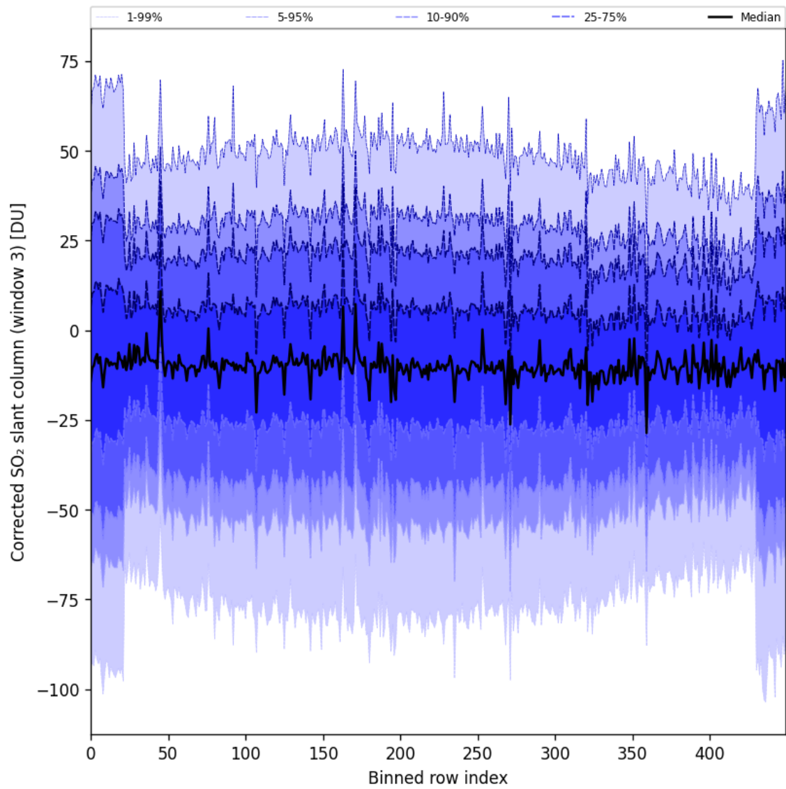
Figure 89: Along track statistics of "Corrected SO 2 slant column (window 3)" for 2024-09-18 to 2024-09-20
