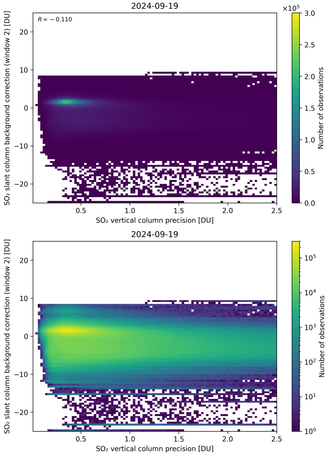
Figure 280: Scatter density plot of “SO 2 vertical column precision” against “SO 2 slant column background correction (window 2)” for 2024-09-18 to 2024-09-20.
