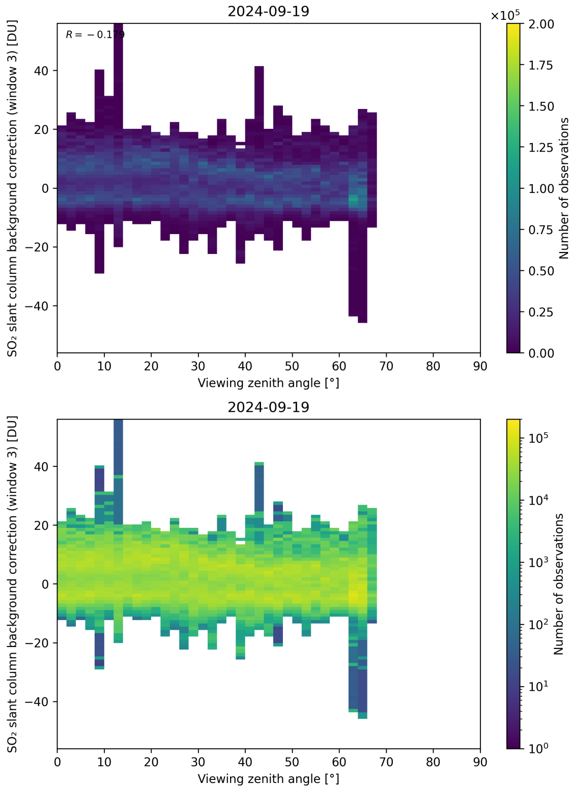
Figure 310: Scatter density plot of “Viewing zenith angle” against “SO 2 slant column background correction (window 3)” for 2024-09-18 to 2024-09-20.
