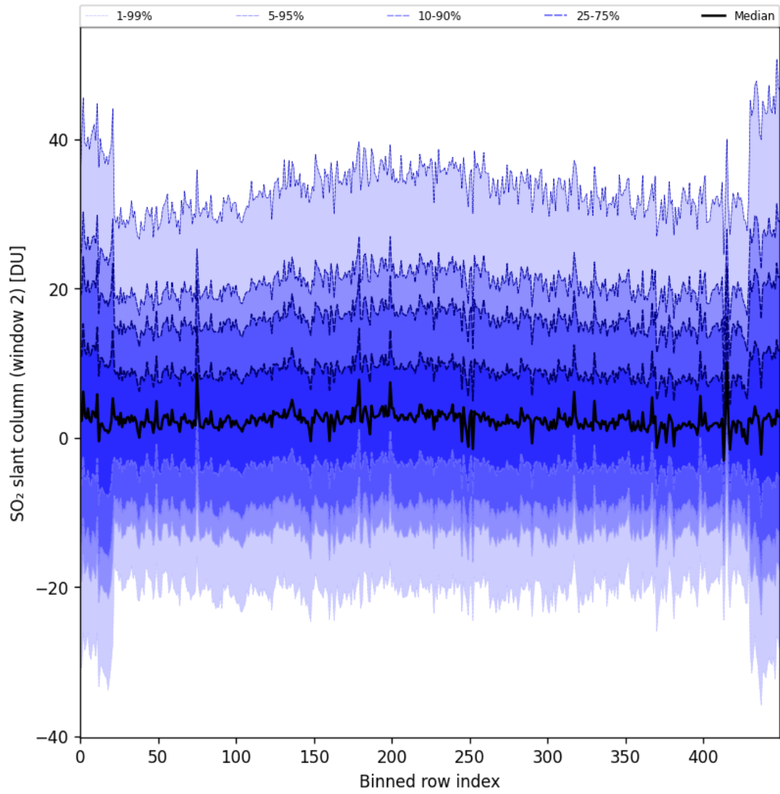
Figure 83: Along track statistics of “SO 2 slant column (window 2)” for 2024-09-18 to 2024-09-20
