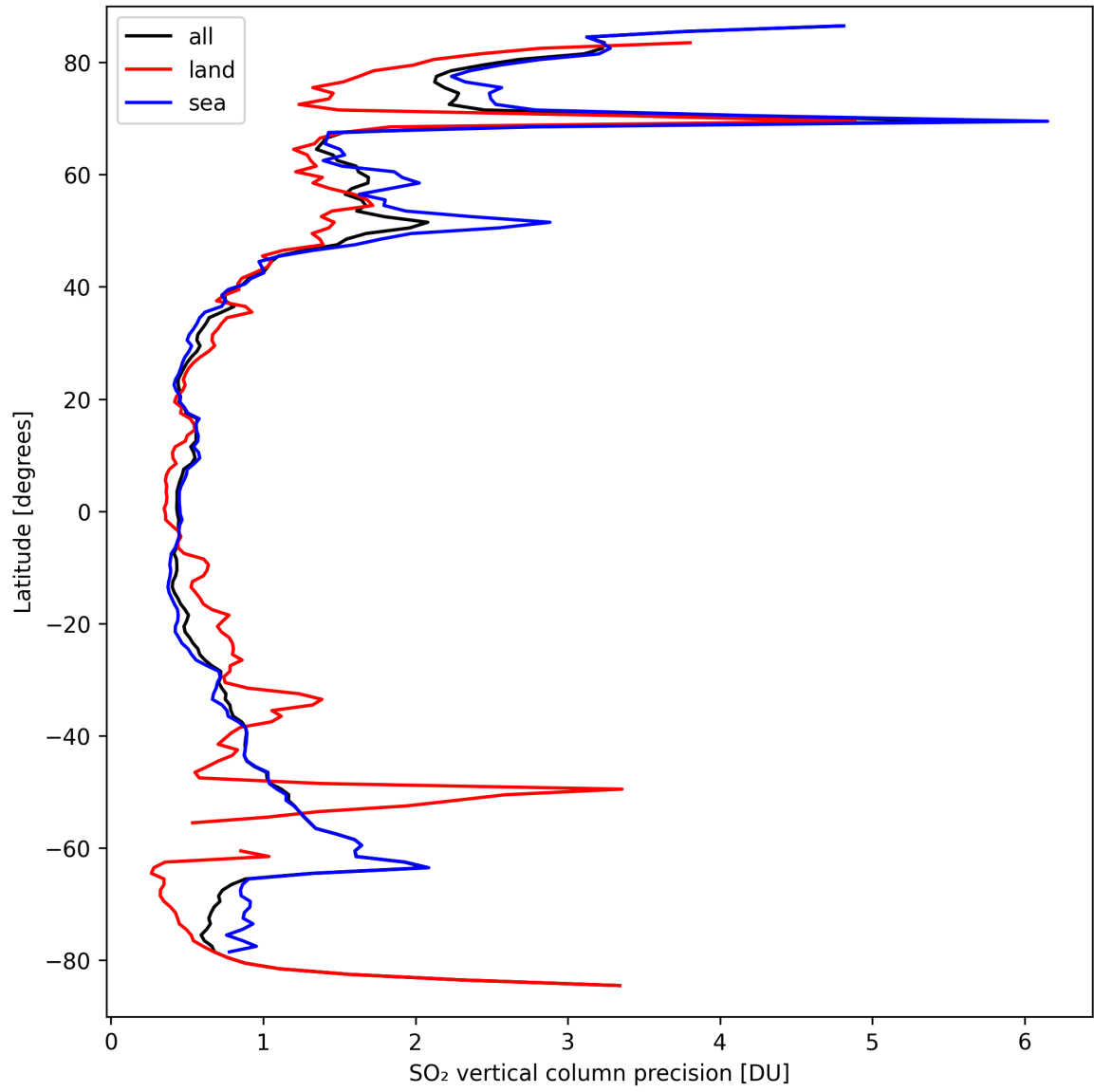
Figure 31: Zonal average of “SO 2 vertical column precision” for 2024-09-18 to 2024-09-20.
