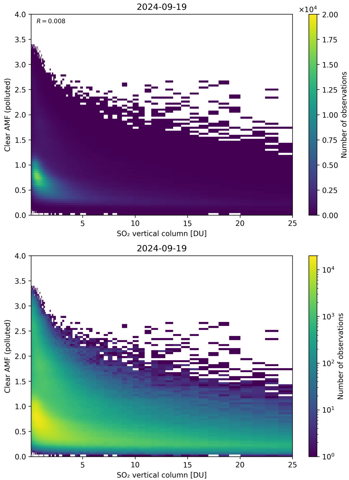
Figure 296: Scatter density plot of “SO 2 vertical column” against “Clear AMF (polluted)” for 2024-09-18 to 2024-09-20.
