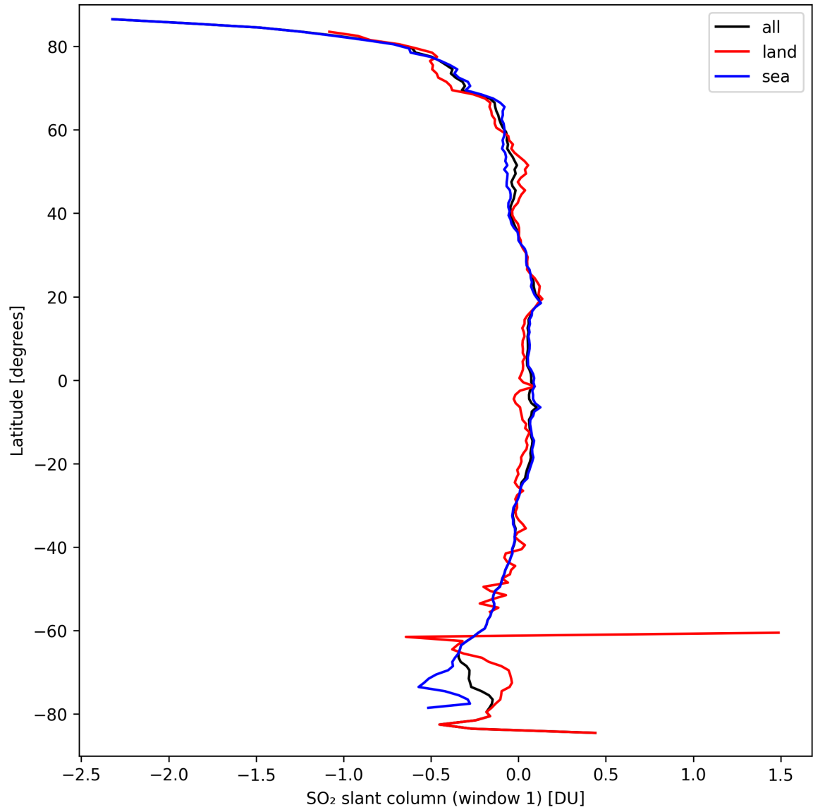
Figure 33: Zonal average of “SO 2 slant column (window 1)” for 2024-09-18 to 2024-09-20.
