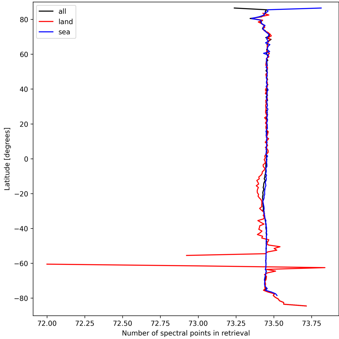
Figure 51: Zonal average of “Number of spectral points in retrieval” for 2024-09-18 to 2024-09-20.
