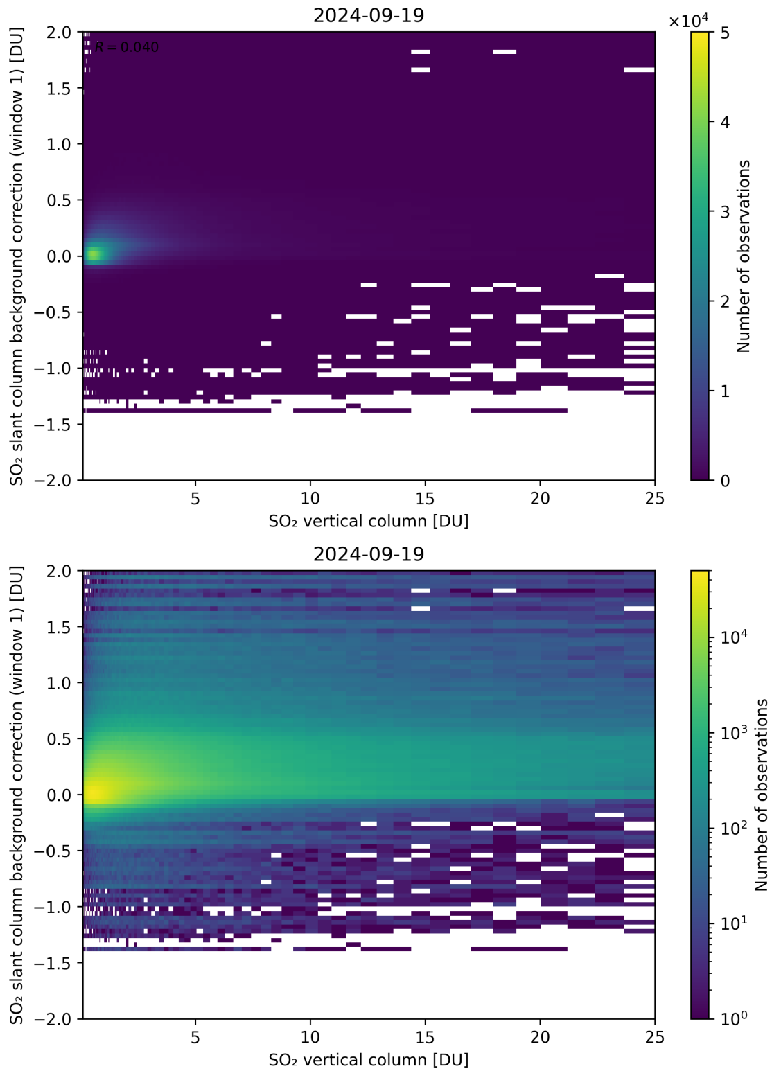
Figure 273: Scatter density plot of “SO 2 vertical column” against “SO 2 slant column background correction (window 1)” for 2024-09-18 to 2024-09-20.
