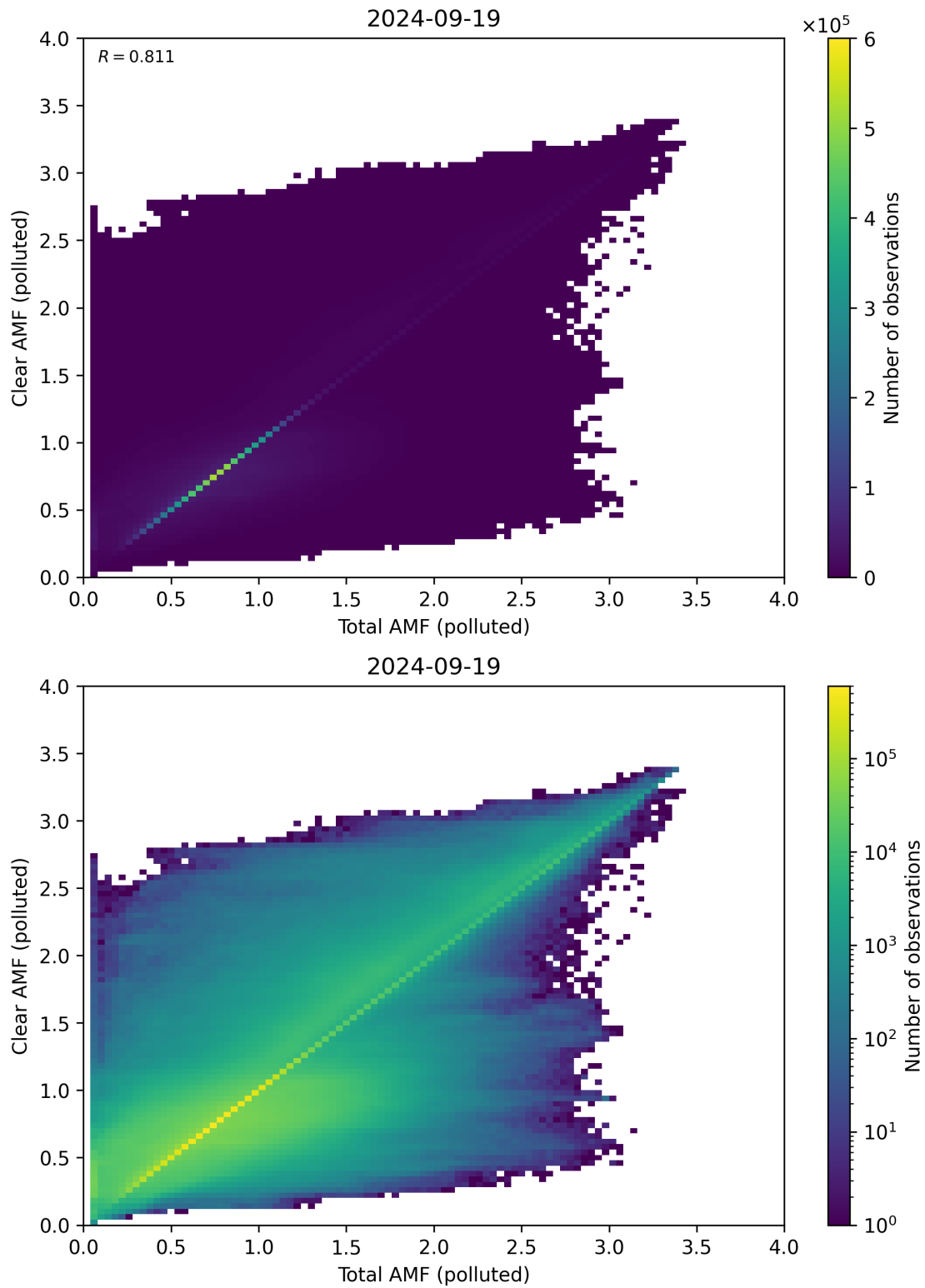
Figure 271: Scatter density plot of “Total AMF (polluted)” against “Clear AMF (polluted)” for 2024-09-18 to 2024-09-20.
