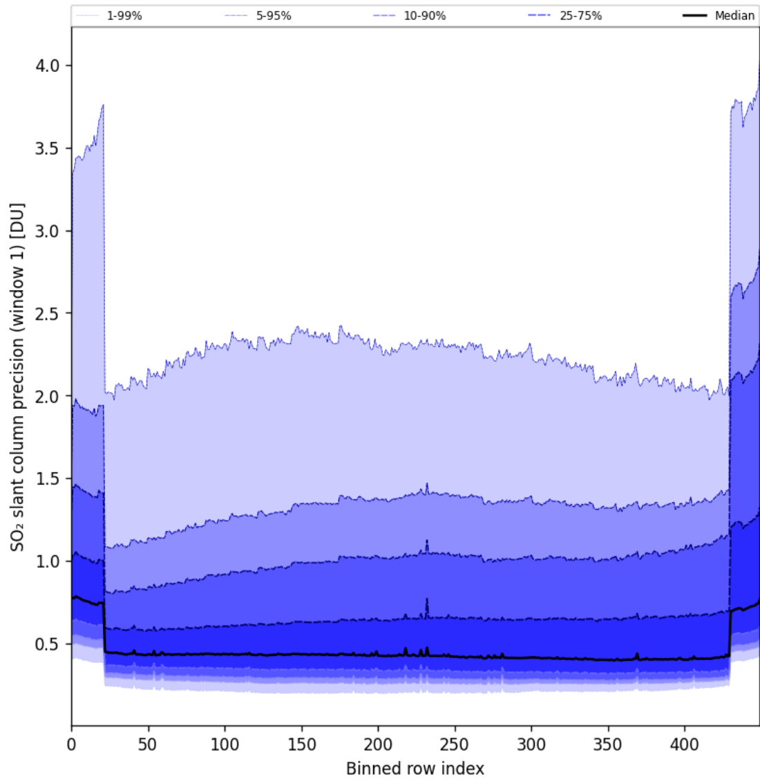
Figure 80: Along track statistics of “SO 2 slant column precision (window 1)” for 2024-09-18 to 2024-09-20
