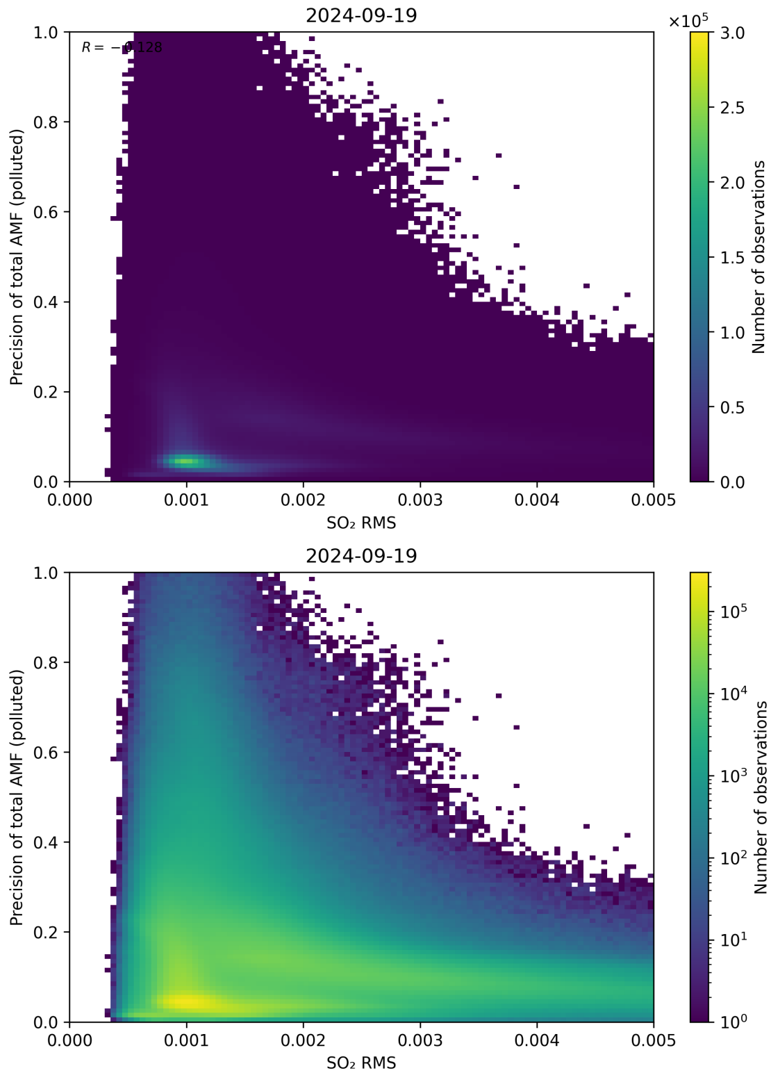
Figure 138: Scatter density plot of “SO 2 RMS” against “Precision of total AMF (polluted)” for 2024-09-18 to 2024-09-20.
