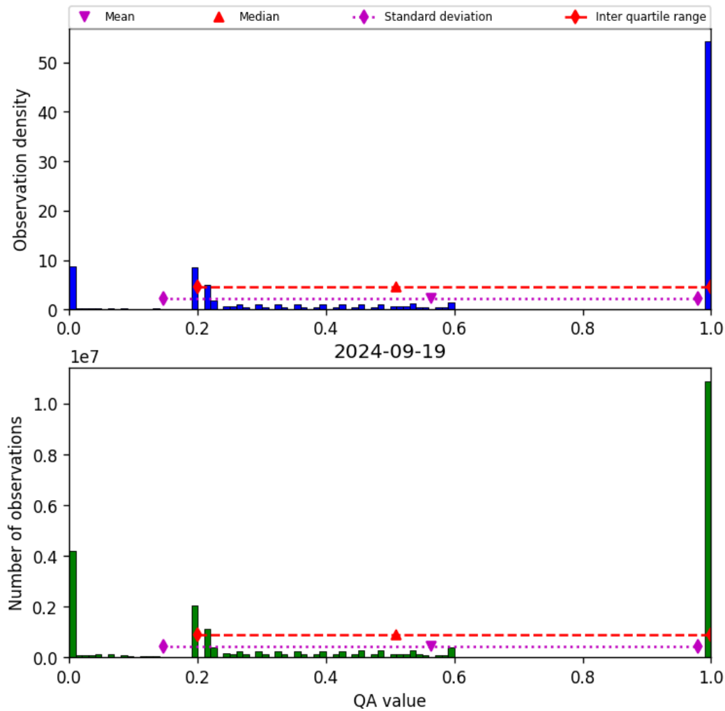
Figure 52: Histogram of “QA value” for 2024-09-18 to 2024-09-20
