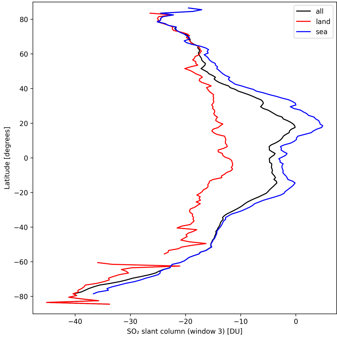
Figure 41: Zonal average of “SO 2 slant column (window 3)” for 2024-09-18 to 2024-09-20.
