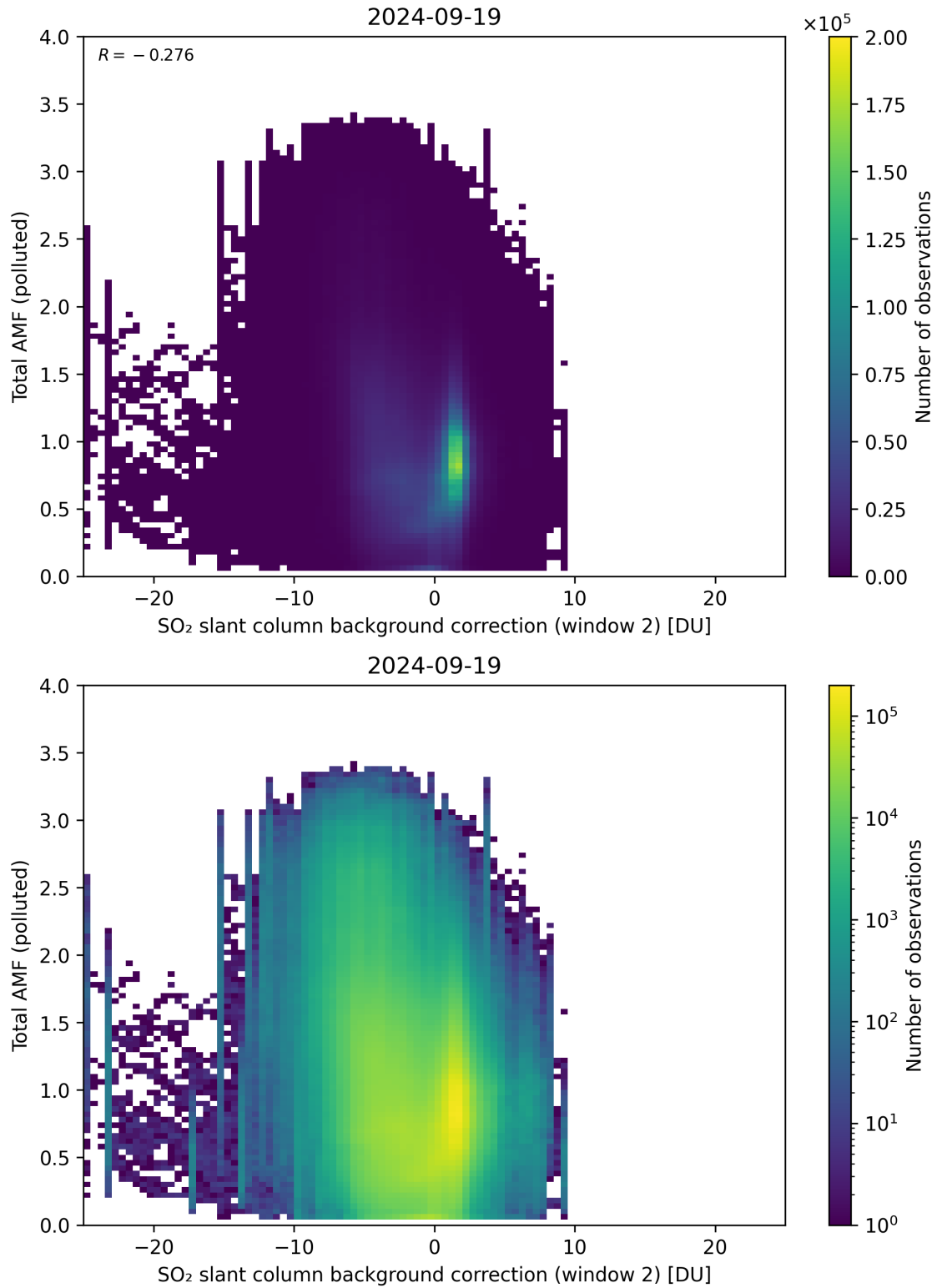
Figure 119: Scatter density plot of “SO 2 slant column background correction (window 2)” against “Total AMF (polluted)” for 2024-09-18 to 2024-09-20.
