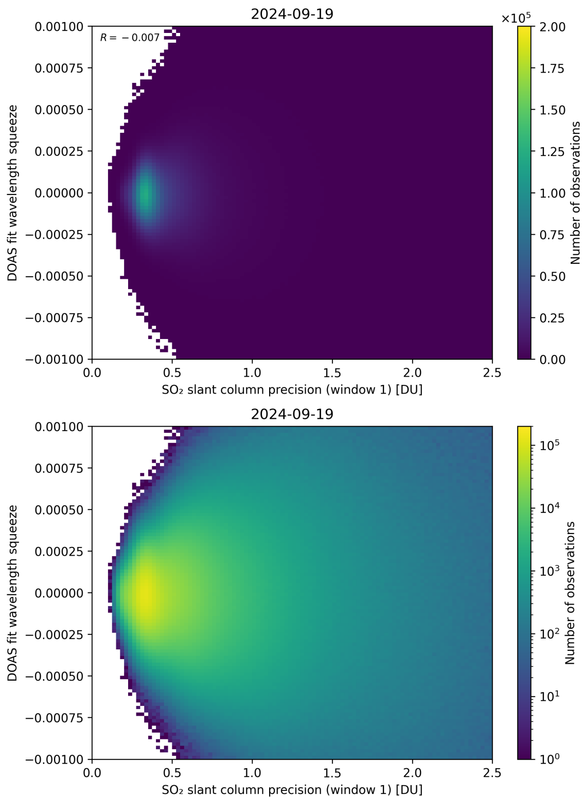
Figure 222: Scatter density plot of “SO 2 slant column precision (window 1)” against “DOAS fit wavelength squeeze” for 2024-09-18 to 2024-09-20.
