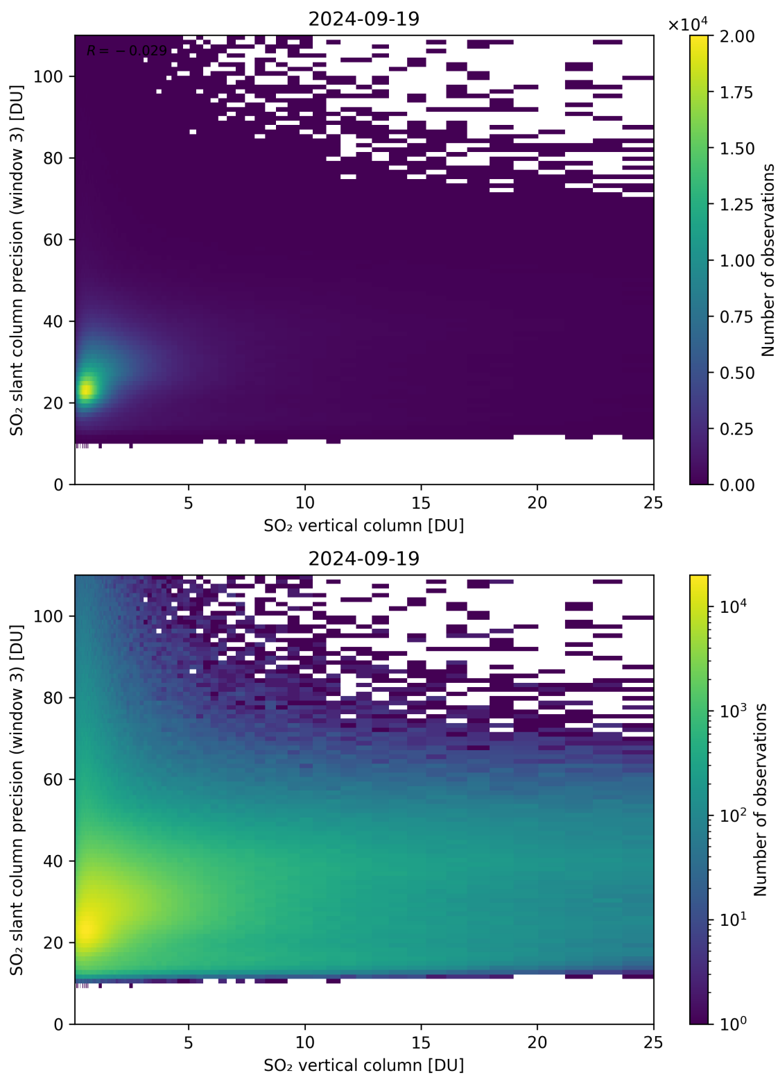
Figure 304: Scatter density plot of “SO 2 vertical column” against “SO 2 slant column precision (window 3)” for 2024-09-18 to 2024-09-20.
