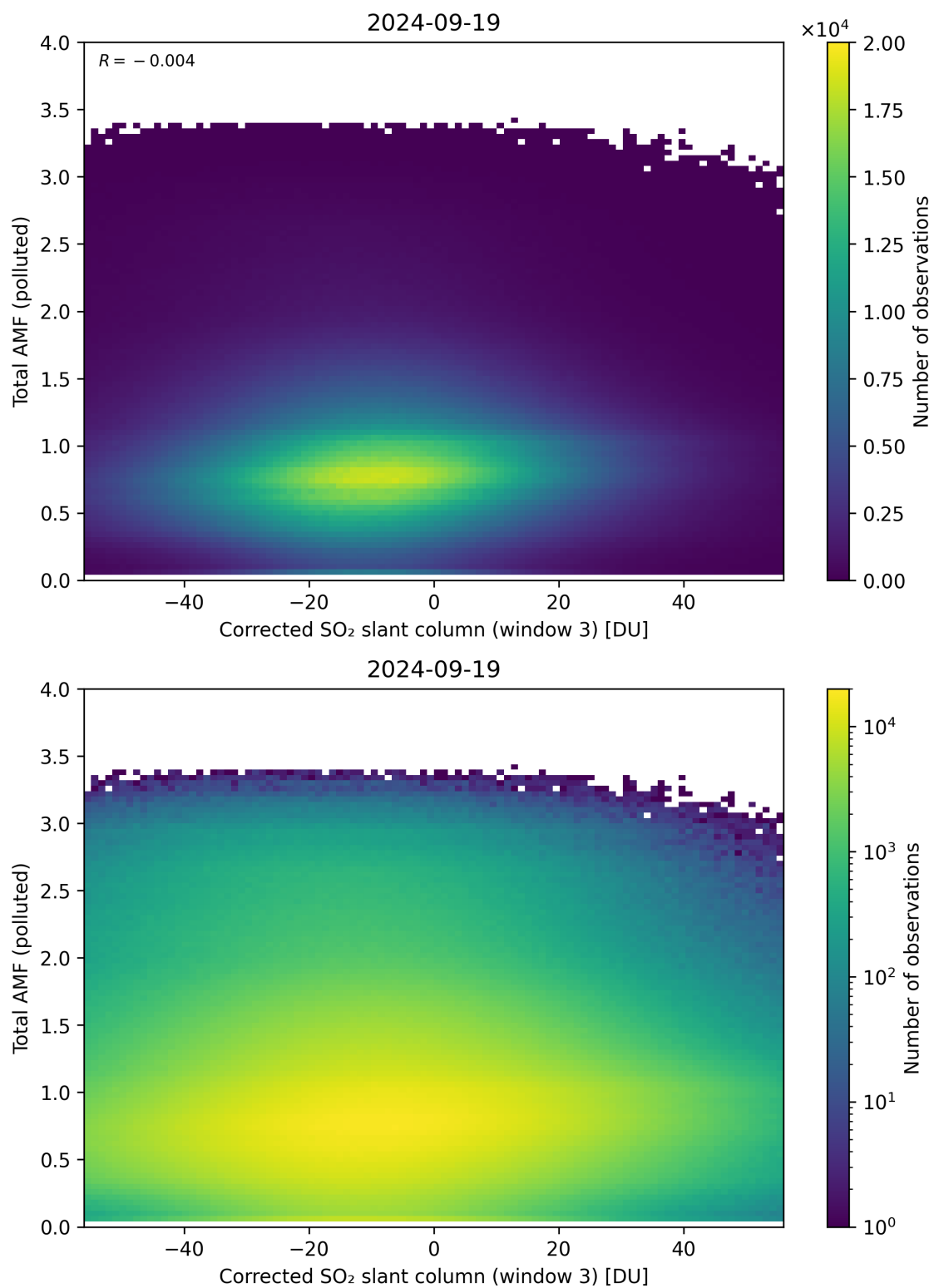
Figure 210: Scatter density plot of “Corrected SO 2 slant column (window 3)” against “Total AMF (polluted)” for 2024-09-18 to 2024-09-20.
