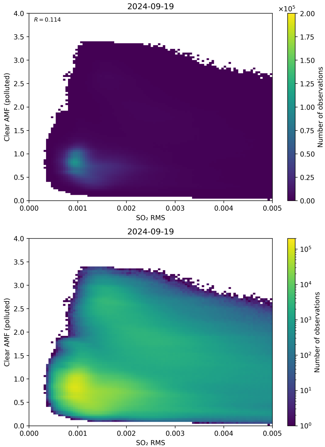
Figure 136: Scatter density plot of “SO 2 RMS” against “Clear AMF (polluted)” for 2024-09-18 to 2024-09-20.
