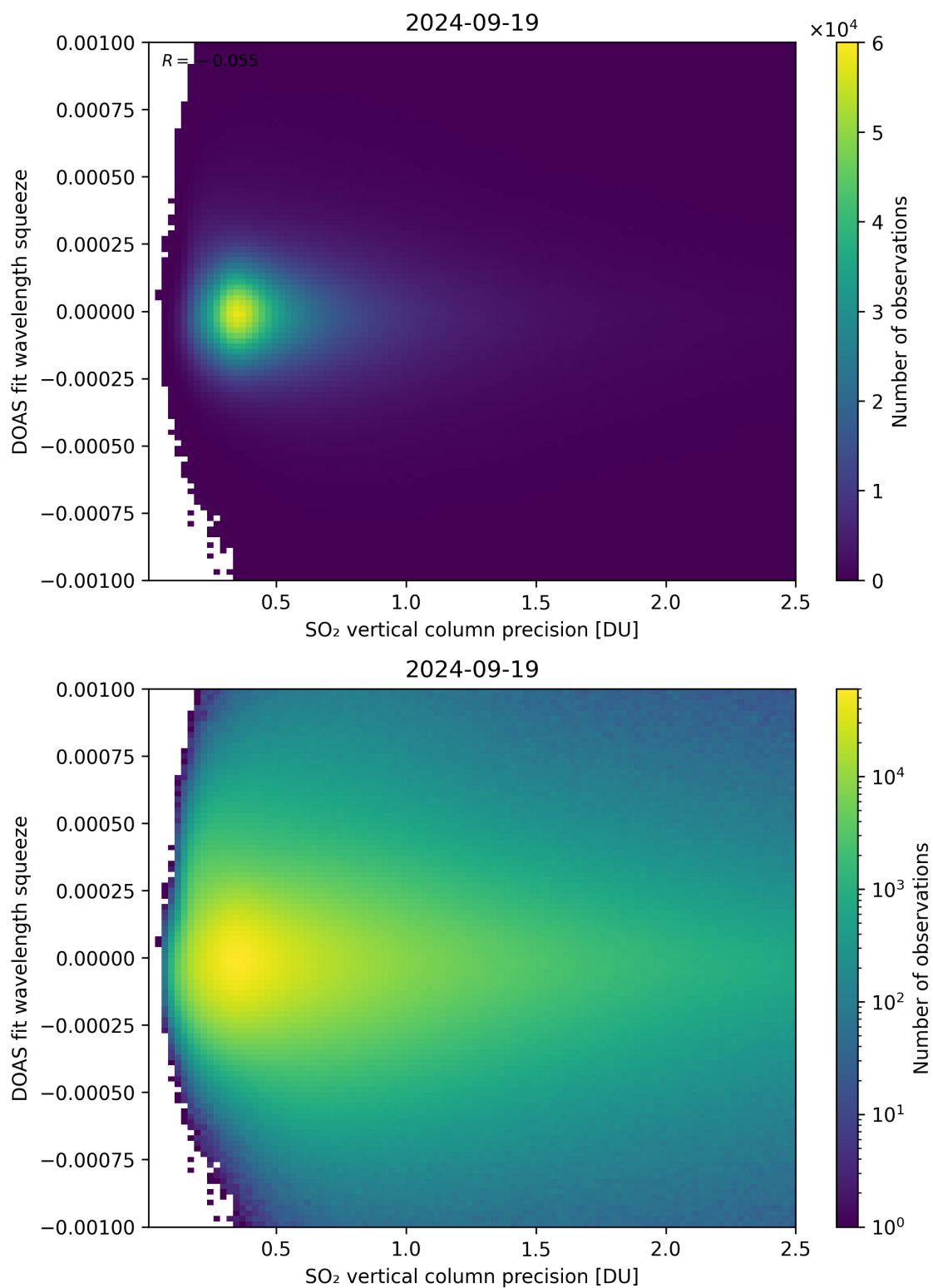
Figure 283: Scatter density plot of “SO 2 vertical column precision” against “DOAS fit wavelength squeeze” for 2024-09-18 to 2024-09-20.
