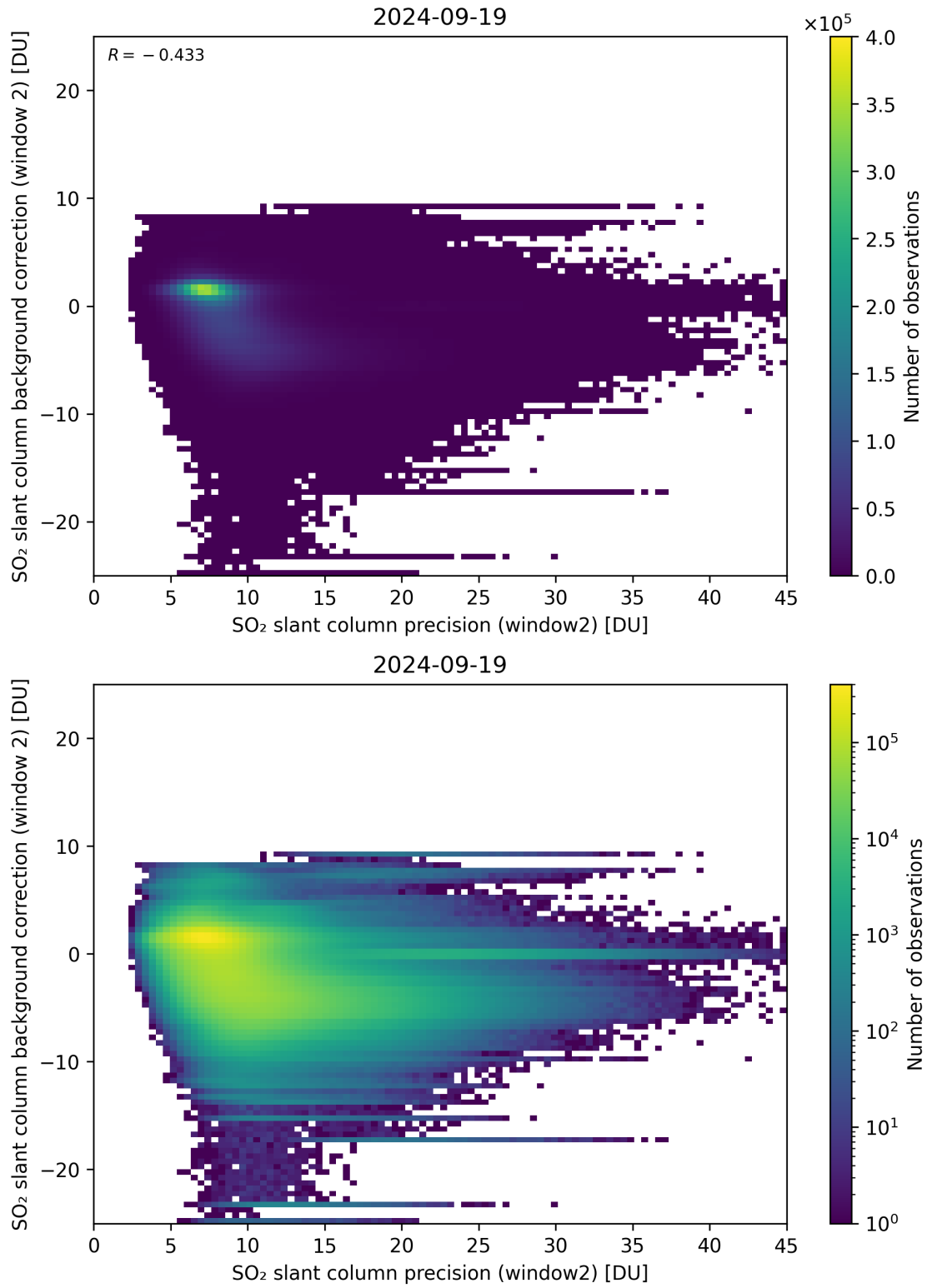
Figure 241: Scatter density plot of “SO 2 slant column precision (window2)” against “SO 2 slant column background correction (window 2)” for 2024-09-18 to 2024-09-20.
