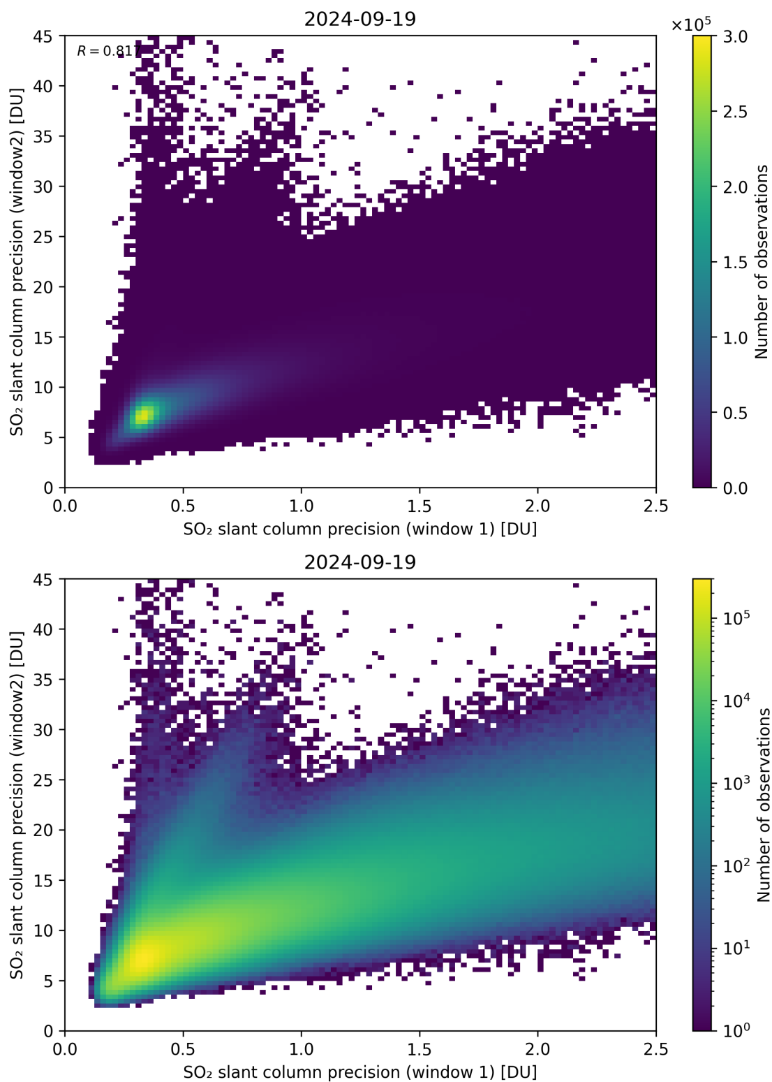
Figure 227: Scatter density plot of “SO 2 slant column precision (window 1)” against “SO 2 slant column precision (window2)” for 2024-09-18 to 2024-09-20.
