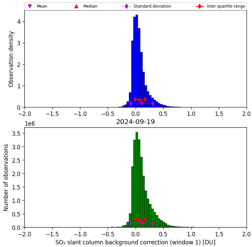
Figure 59: Histogram of “SO 2 slant column background correction (window 1)” for 2024-09-18 to 2024-09-20
