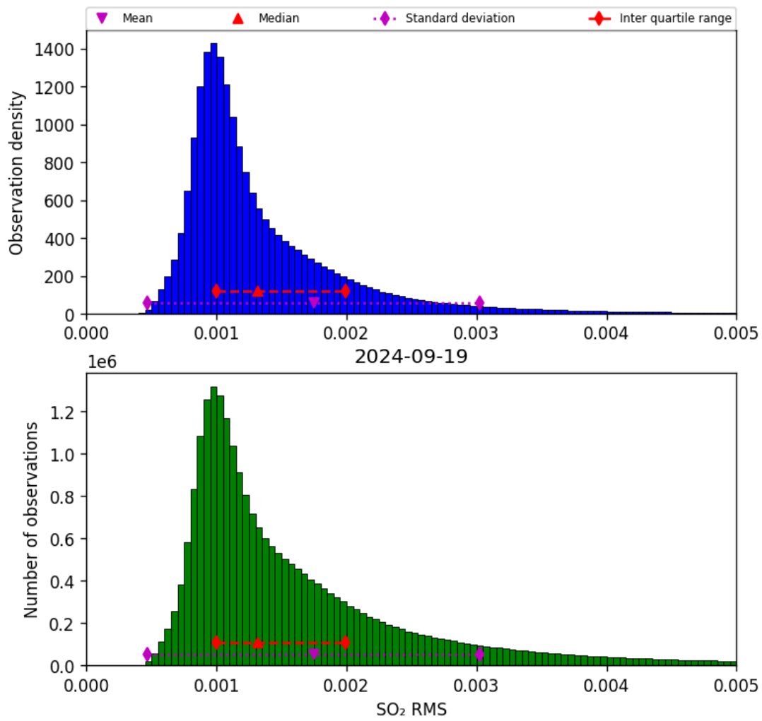
Figure 70: Histogram of “SO 2 RMS” for 2024-09-18 to 2024-09-20
