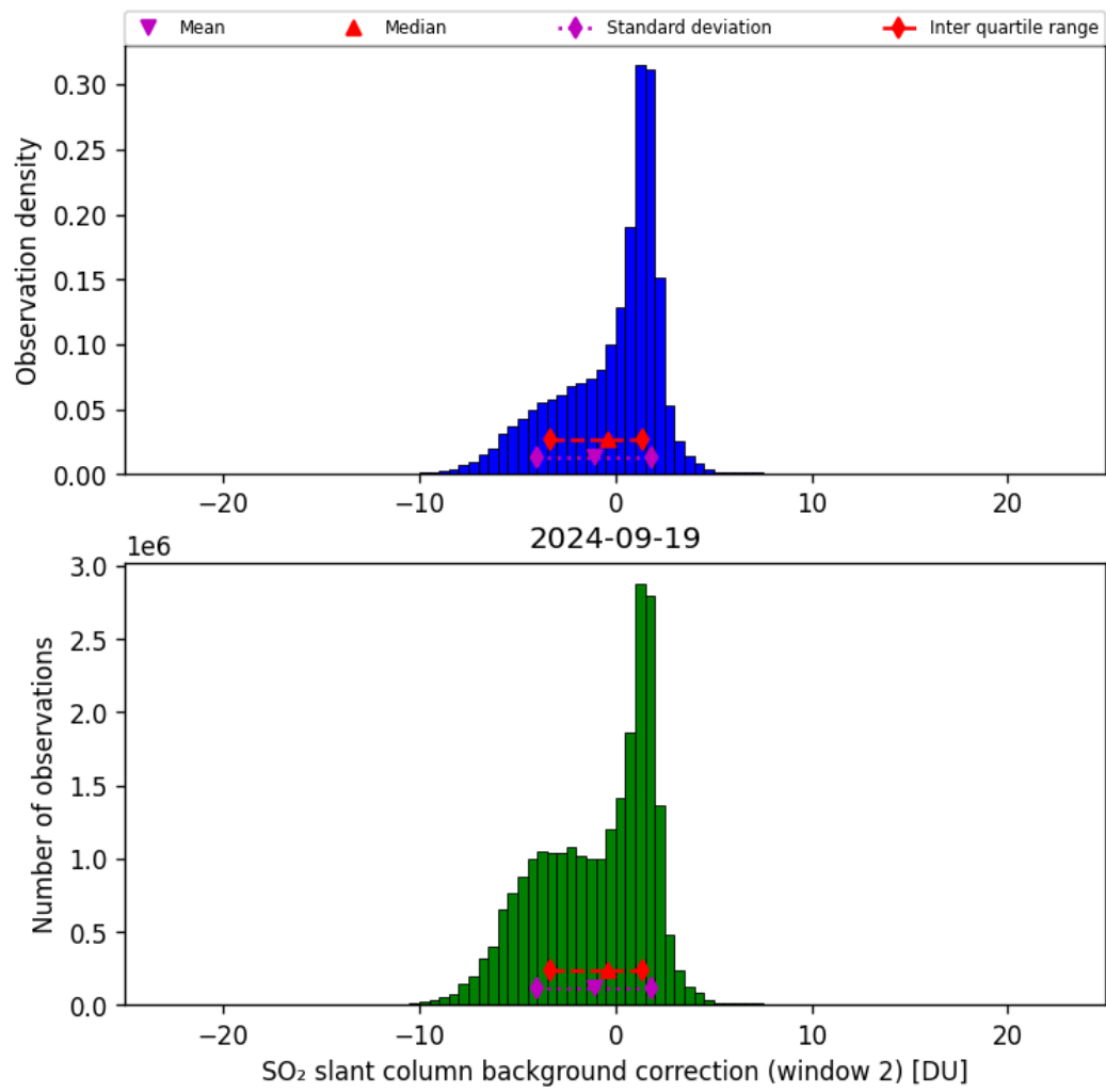
Figure 63: Histogram of “SO 2 slant column background correction (window 2)” for 2024-09-18 to 2024-09-20
