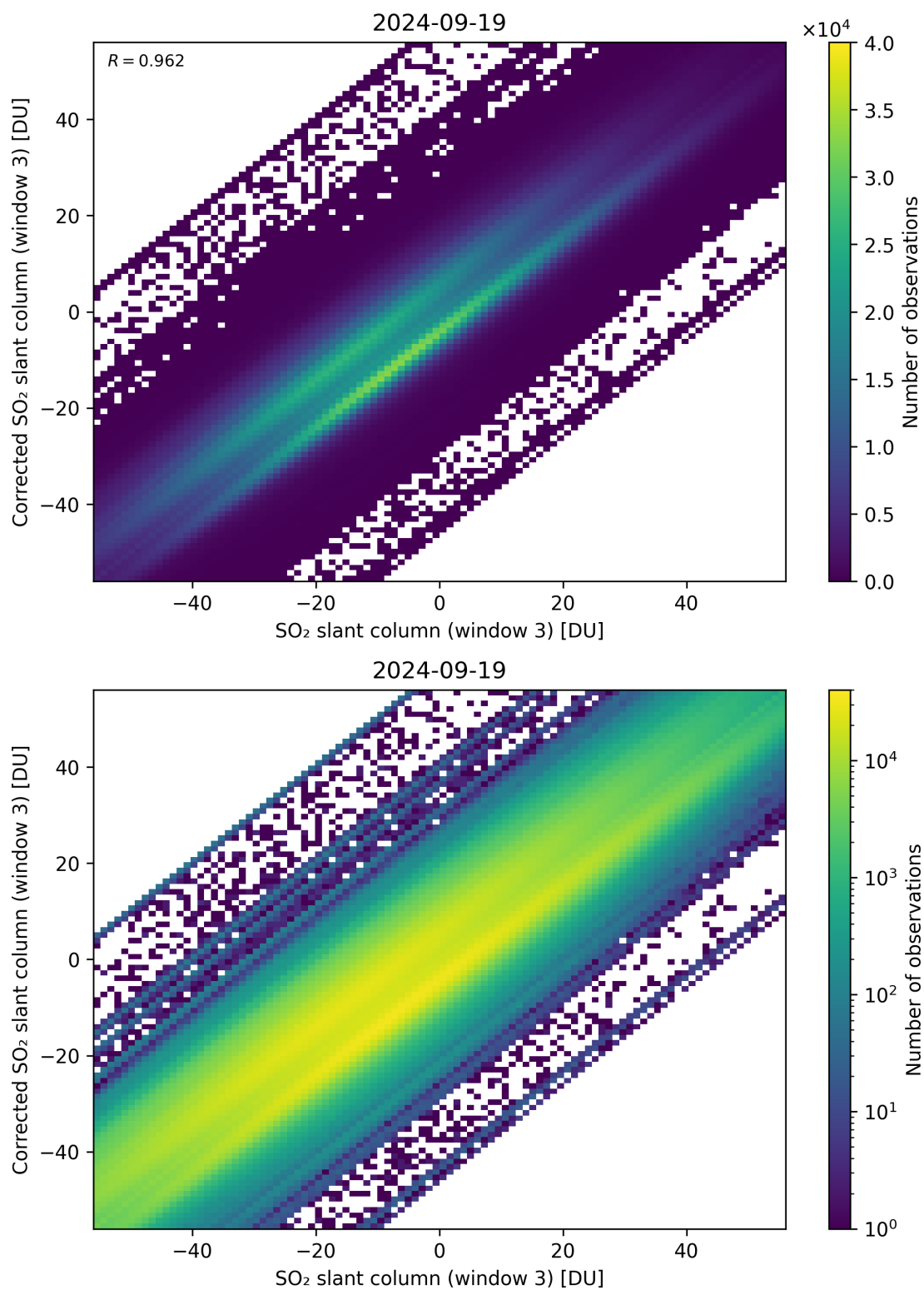
Figure 266: Scatter density plot of “SO 2 slant column (window 3)” against “Corrected SO 2 slant column (window 3)” for 2024-09-18 to 2024-09-20.
