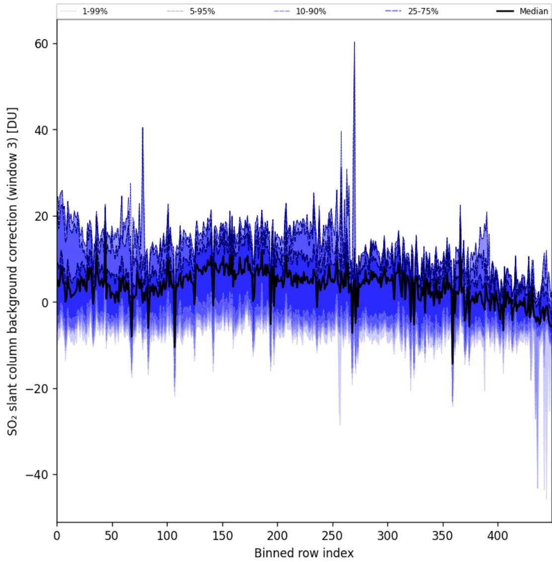
Figure 90: Along track statistics of “SO 2 slant column background correction (window 3)” for 2024-09-18 to 2024-09-20
