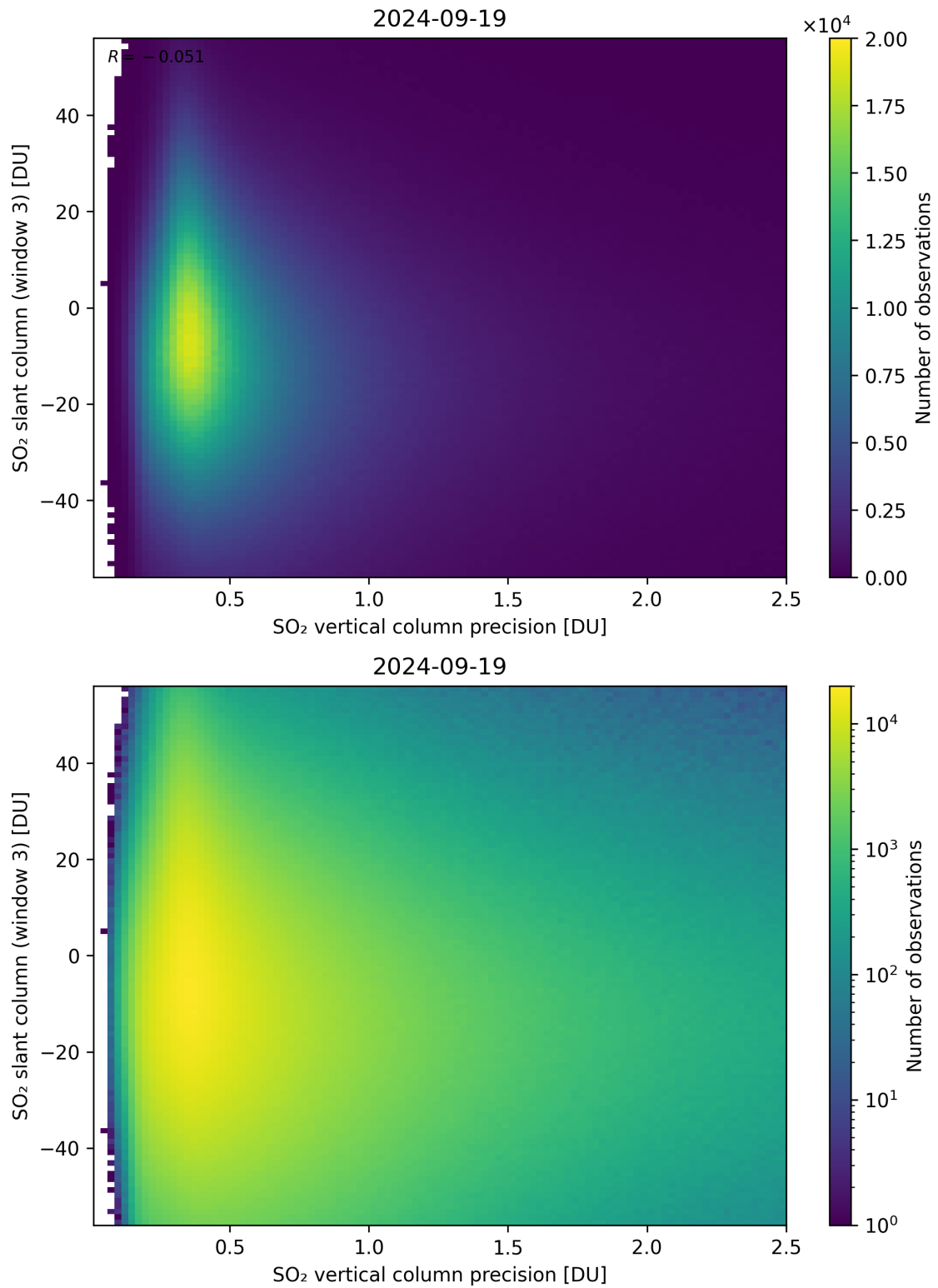
Figure 292: Scatter density plot of “SO 2 vertical column precision” against “SO 2 slant column (window 3)” for 2024-09-18 to 2024-09-20.
