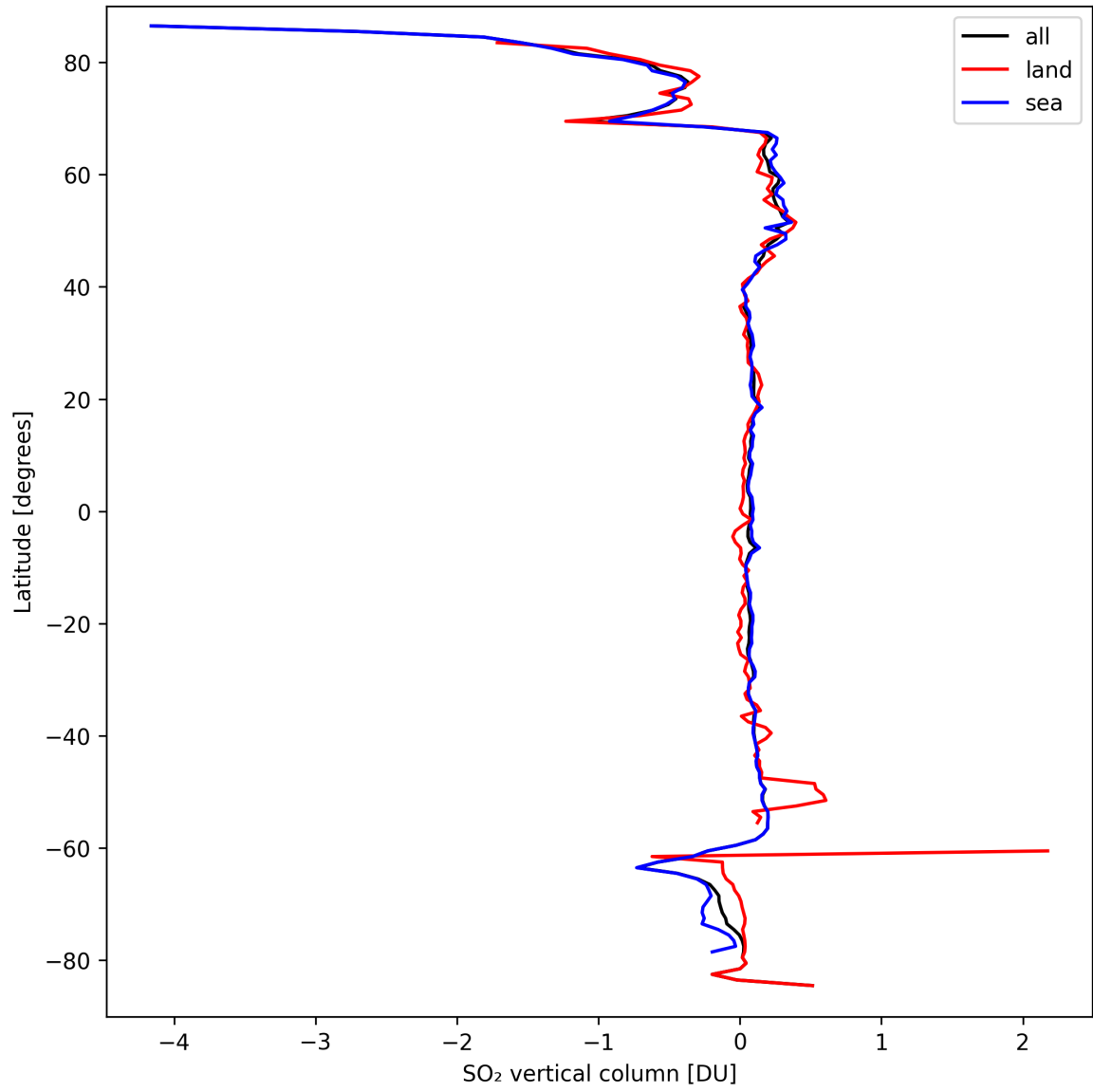
Figure 30: Zonal average of “SO 2 vertical column” for 2024-09-18 to 2024-09-20.
