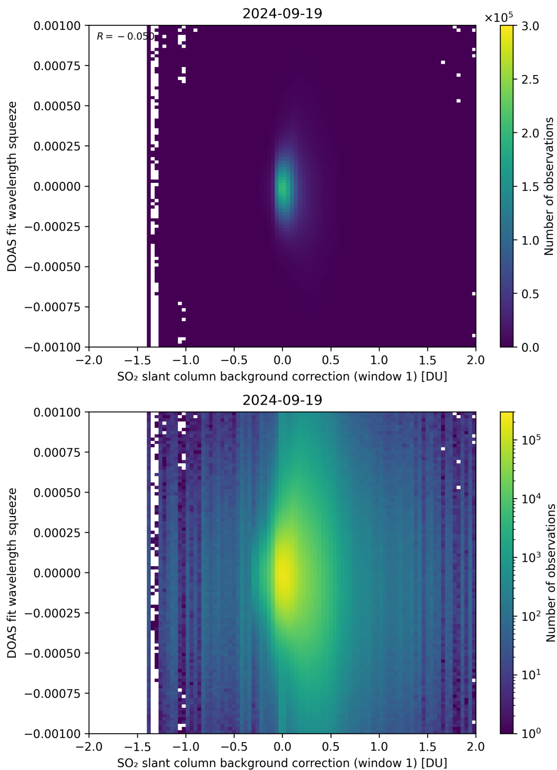
Figure 101: Scatter density plot of “SO 2 slant column background correction (window 1)” against “DOAS fit wavelength squeeze” for 2024-09-18 to 2024-09-20.
