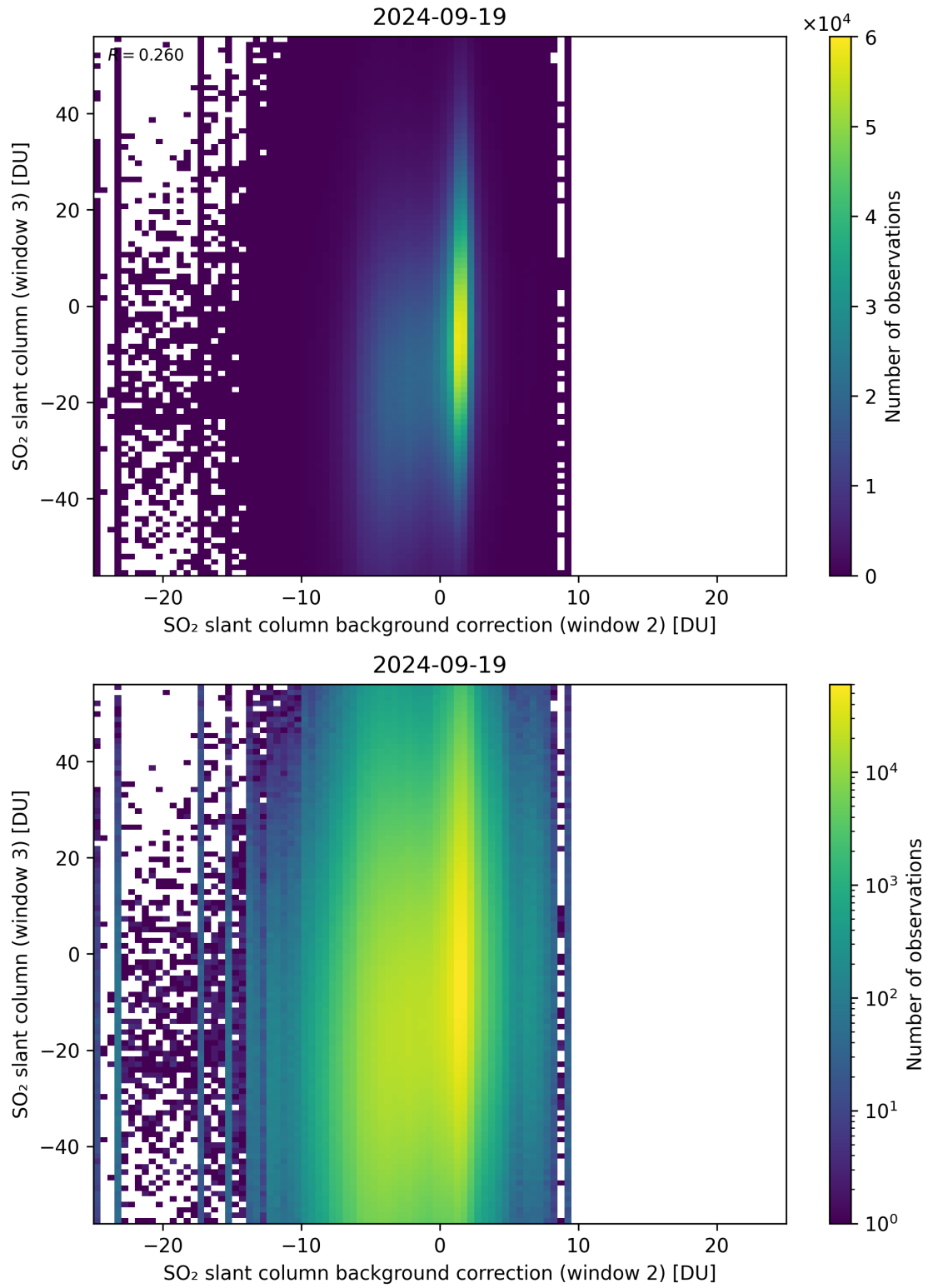
Figure 117: Scatter density plot of “SO 2 slant column background correction (window 2)” against “SO 2 slant column (window 3)” for 2024-09-18 to 2024-09-20.
