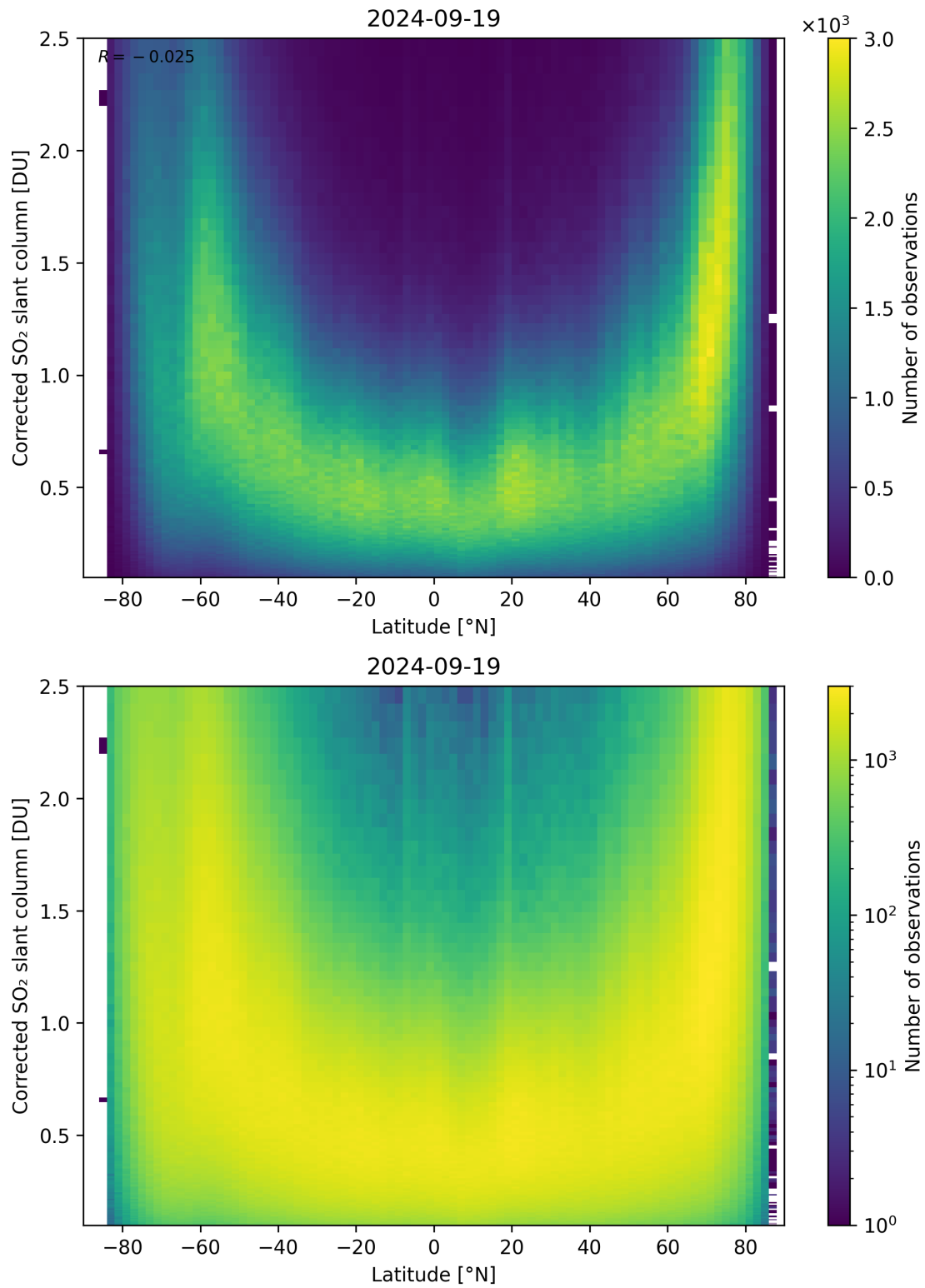
Figure 146: Scatter density plot of “Latitude” against “Corrected SO 2 slant column” for 2024-09-18 to 2024-09-20.
