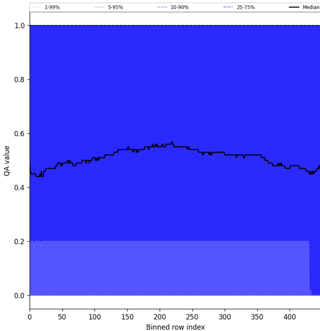
Figure 75: Along track statistics of “QA value” for 2024-09-18 to 2024-09-20
