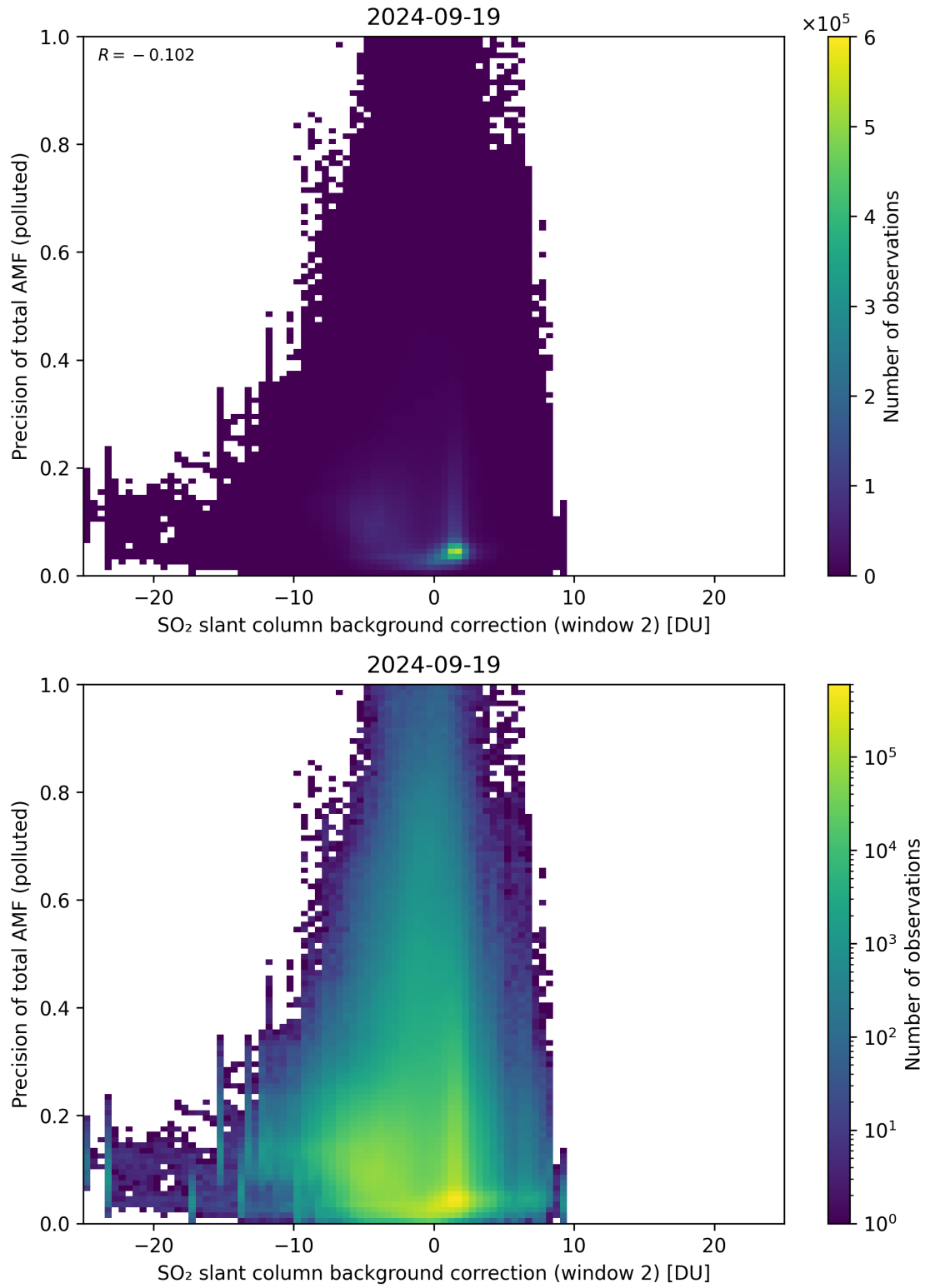
Figure 120: Scatter density plot of “SO 2 slant column background correction (window 2)” against “Precision of total AMF (polluted)” for 2024-09-18 to 2024-09-20.
