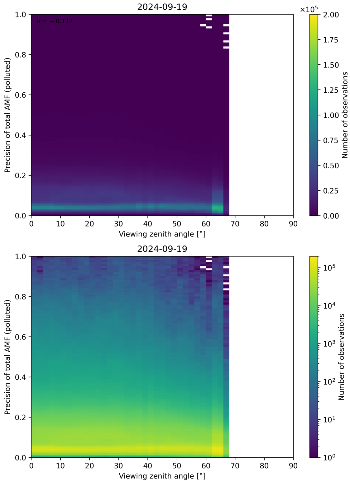
Figure 326: Scatter density plot of “Viewing zenith angle” against “Precision of total AMF (polluted)” for 2024-09-18 to 2024-09-20.
