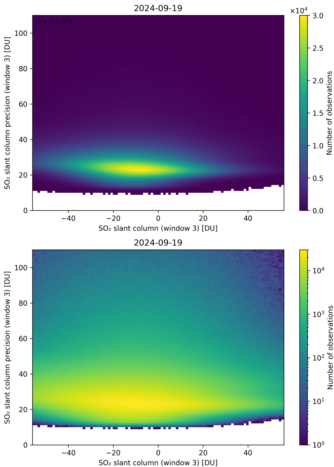
Figure 267: Scatter density plot of “SO 2 slant column (window 3)” against “SO 2 slant column precision (window 3)” for 2024-09-18 to 2024-09-20.
