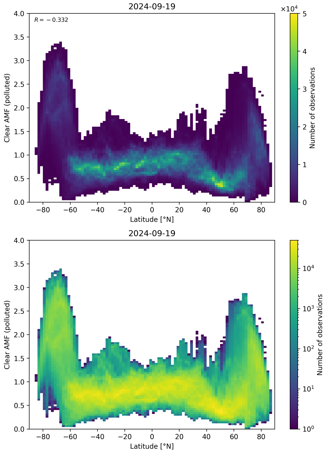
Figure 145: Scatter density plot of “Latitude” against “Clear AMF (polluted)” for 2024-09-18 to 2024-09-20.
