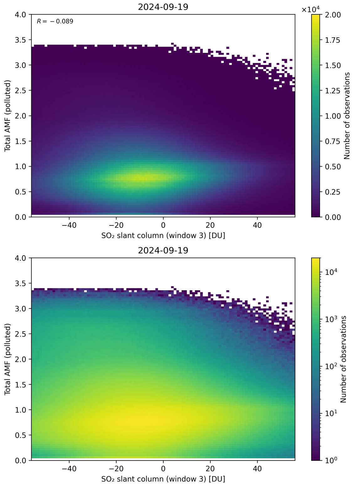
Figure 268: Scatter density plot of “SO 2 slant column (window 3)” against “Total AMF (polluted)” for 2024-09-18 to 2024-09-20.
