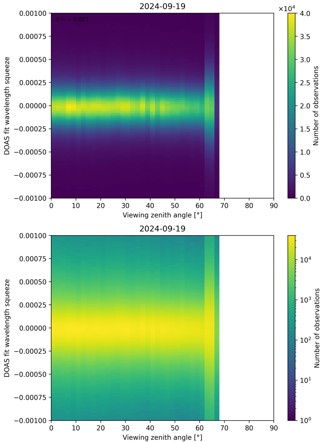
Figure 312: Scatter density plot of “Viewing zenith angle” against “DOAS fit wavelength squeeze” for 2024-09-18 to 2024-09-20.
