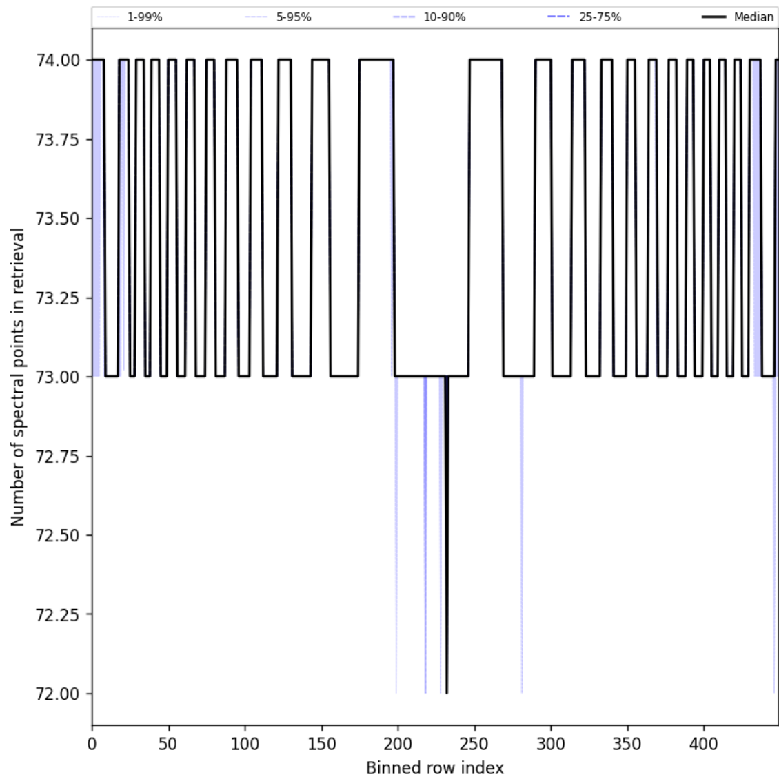
Figure 97: Along track statistics of “Number of spectral points in retrieval” for 2024-09-18 to 2024-09-20
