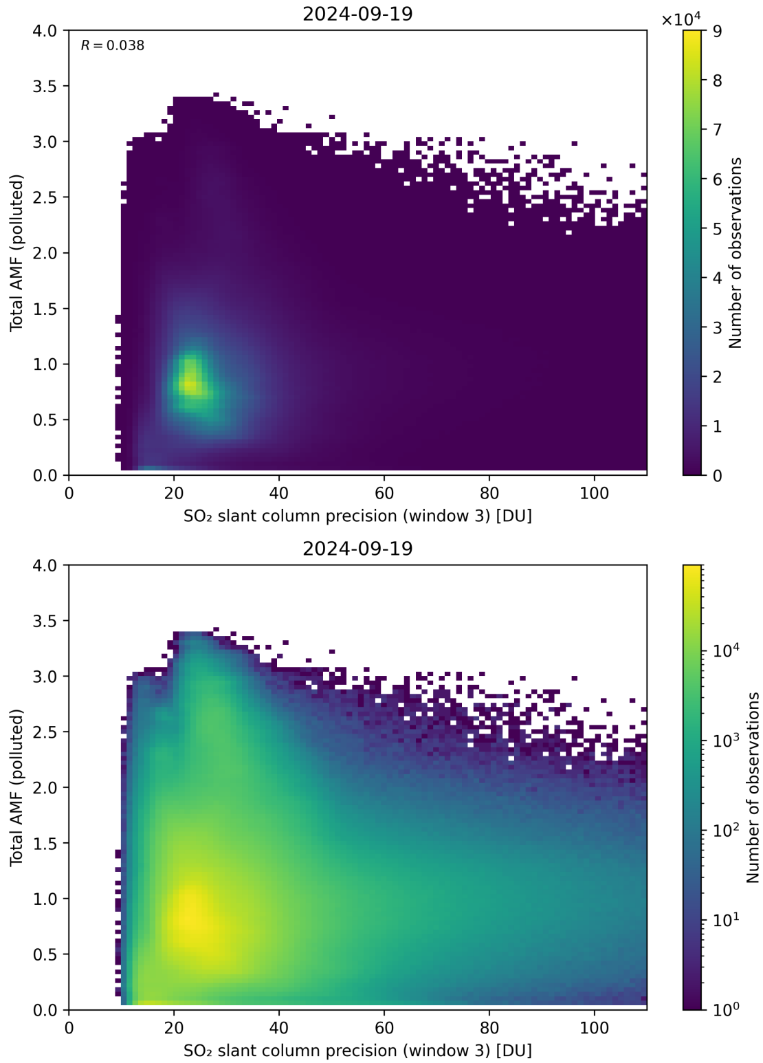
Figure 263: Scatter density plot of “SO 2 slant column precision (window 3)” against “Total AMF (polluted)” for 2024-09-18 to 2024-09-20.
