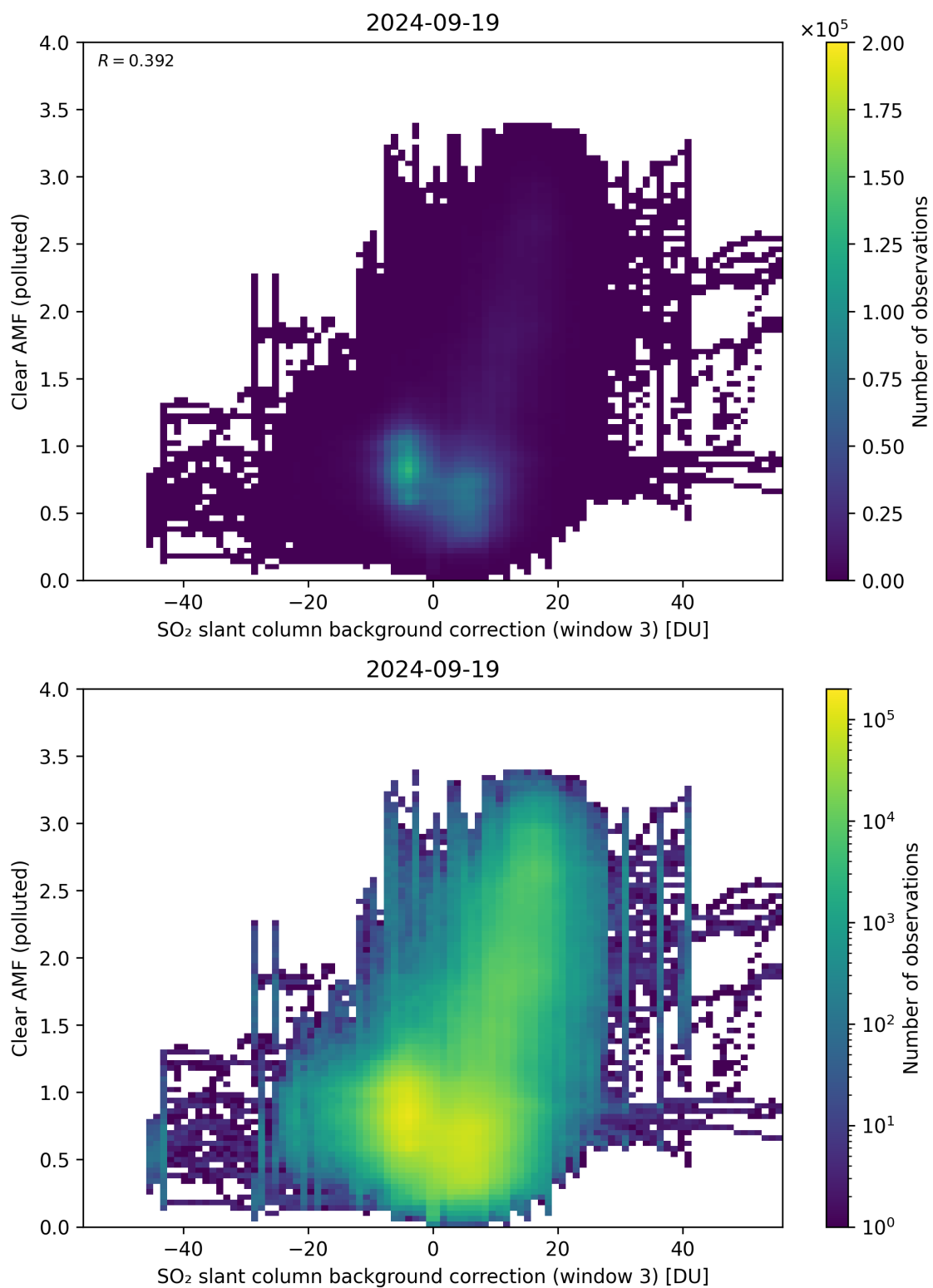
Figure 124: Scatter density plot of “SO 2 slant column background correction (window 3)” against “Clear AMF (polluted)” for 2024-09-18 to 2024-09-20.
