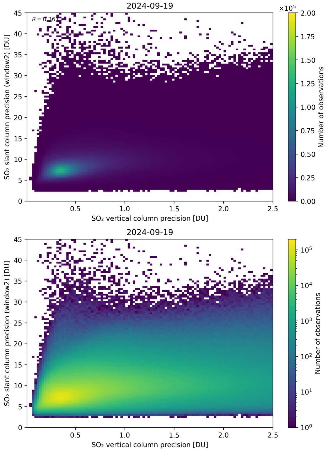
Figure 291: Scatter density plot of “SO 2 vertical column precision” against “SO 2 slant column precision (window2)” for 2024-09-18 to 2024-09-20.
