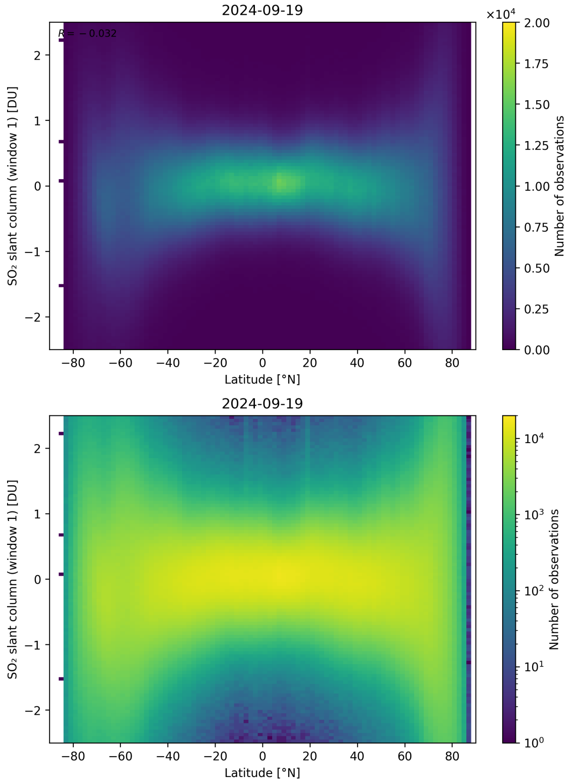
Figure 149: Scatter density plot of “Latitude” against “SO 2 slant column (window 1)” for 2024-09-18 to 2024-09-20.
