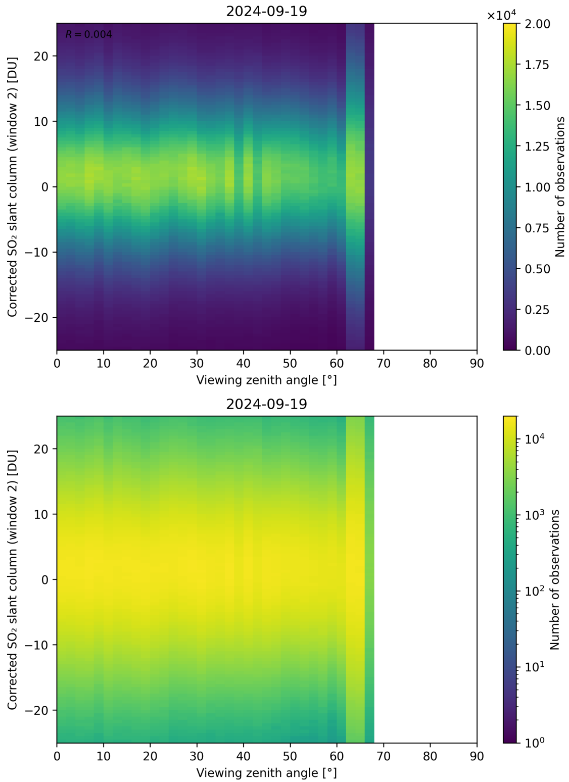
Figure 318: Scatter density plot of “Viewing zenith angle” against “Corrected SO 2 slant column (window 2)” for 2024-09-18 to 2024-09-20.
