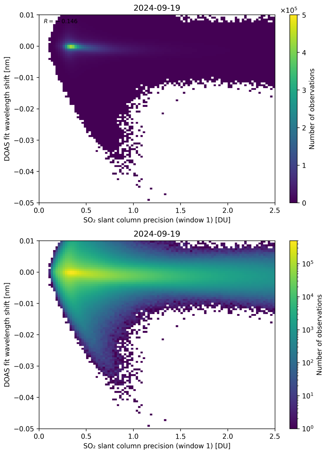
Figure 221: Scatter density plot of “SO 2 slant column precision (window 1)” against “DOAS fit wavelength shift” for 2024-09-18 to 2024-09-20.
