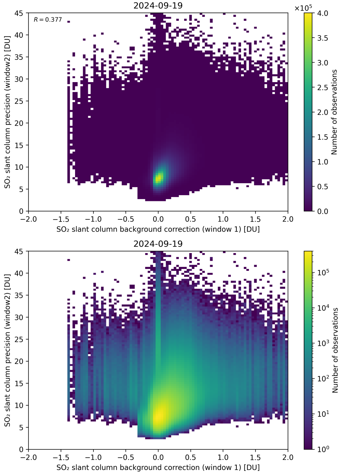
Figure 106: Scatter density plot of “SO 2 slant column background correction (window 1)” against “SO 2 slant column precision (window2)” for 2024-09-18 to 2024-09-20.
