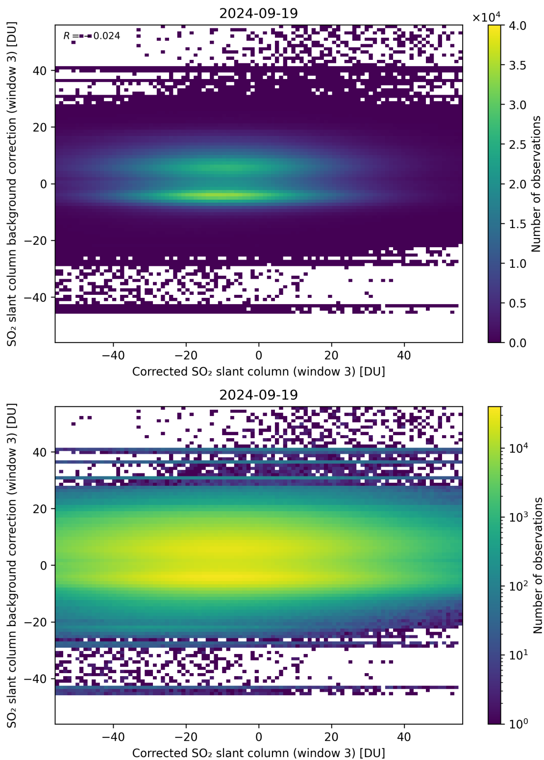
Figure 205: Scatter density plot of “Corrected SO 2 slant column (window 3)” against “SO 2 slant column background correction (window 3)” for 2024-09-18 to 2024-09-20.
