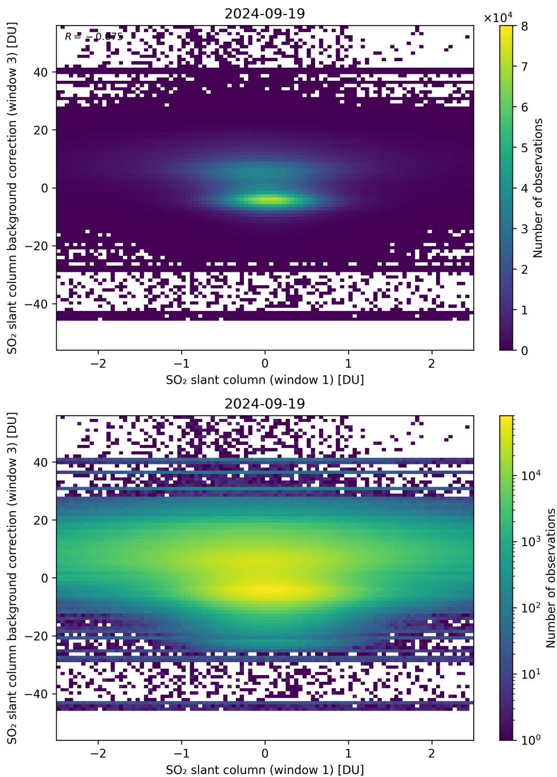
Figure 214: Scatter density plot of “SO 2 slant column (window 1)” against “SO 2 slant column background correction (window 3)” for 2024-09-18 to 2024-09-20.
