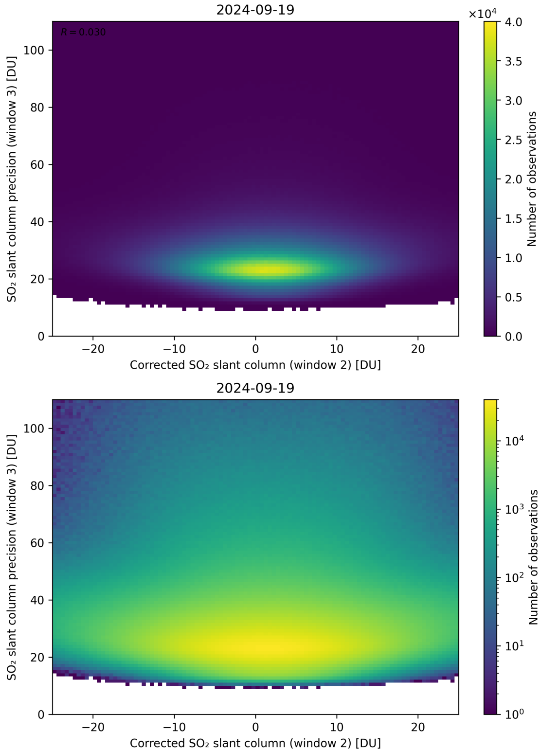
Figure 202: Scatter density plot of “Corrected SO 2 slant column (window 2)” against “SO 2 slant column precision (window 3)” for 2024-09-18 to 2024-09-20.
