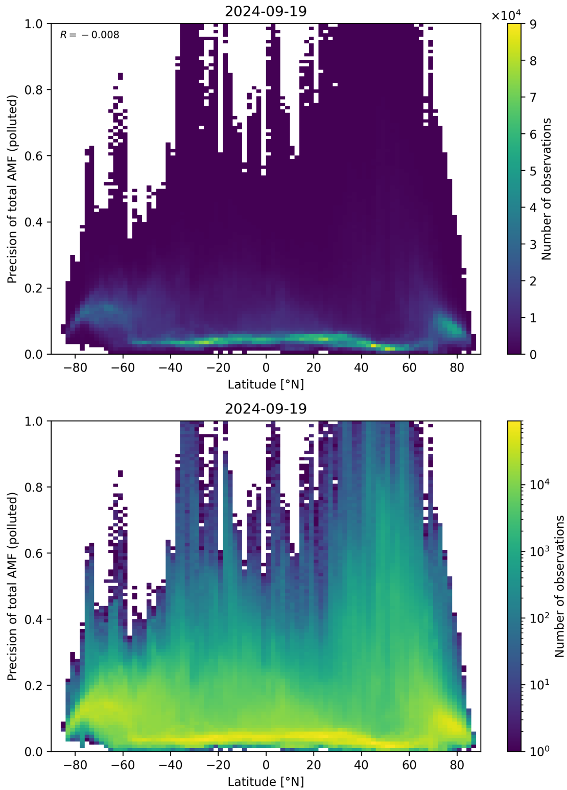
Figure 155: Scatter density plot of “Latitude” against “Precision of total AMF (polluted)” for 2024-09-18 to 2024-09-20.
