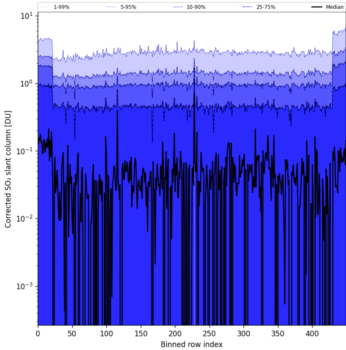
Figure 78: Along track statistics of “Corrected SO 2 slant column” for 2024-09-18 to 2024-09-20
