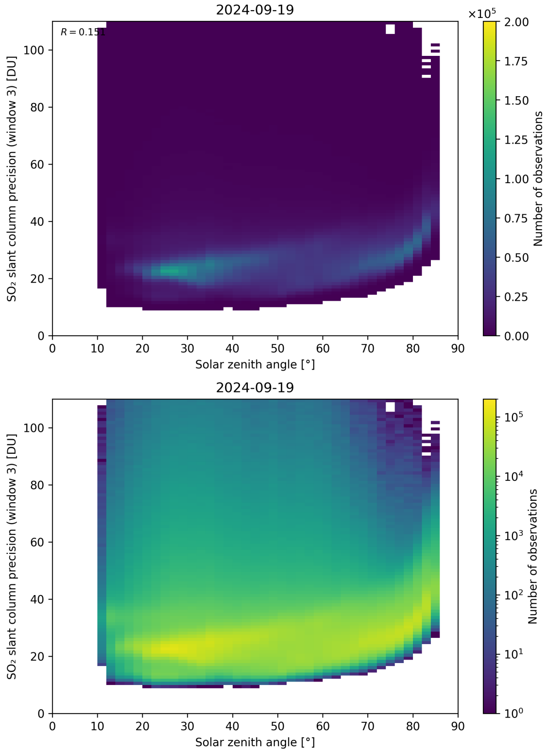
Figure 173: Scatter density plot of “Solar zenith angle” against “SO 2 slant column precision (window 3)” for 2024-09-18 to 2024-09-20.
