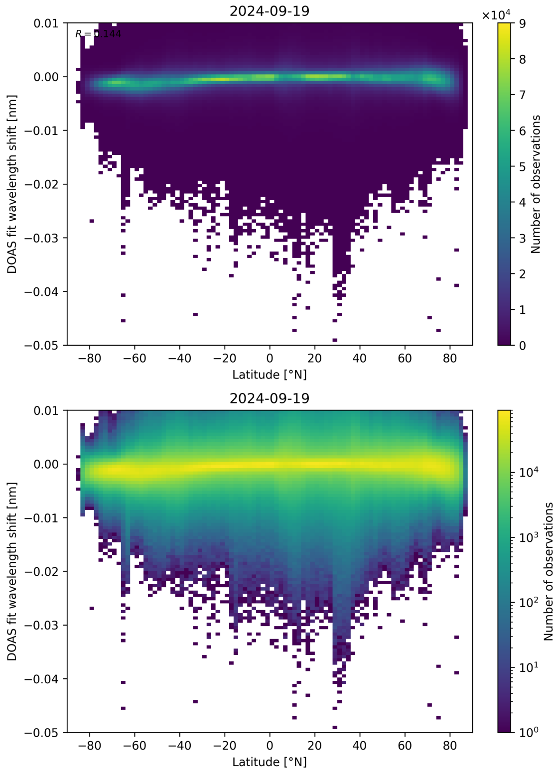
Figure 142: Scatter density plot of “Latitude” against “DOAS fit wavelength shift” for 2024-09-18 to 2024-09-20.
