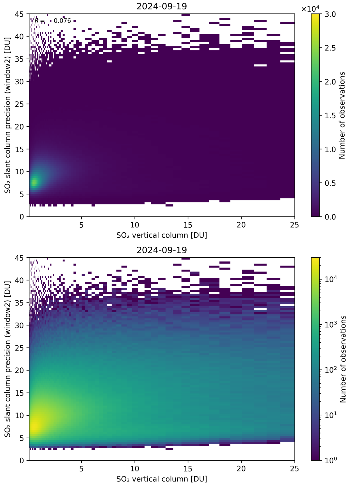
Figure 302: Scatter density plot of “SO 2 vertical column” against “SO 2 slant column precision (window2)” for 2024-09-18 to 2024-09-20.
