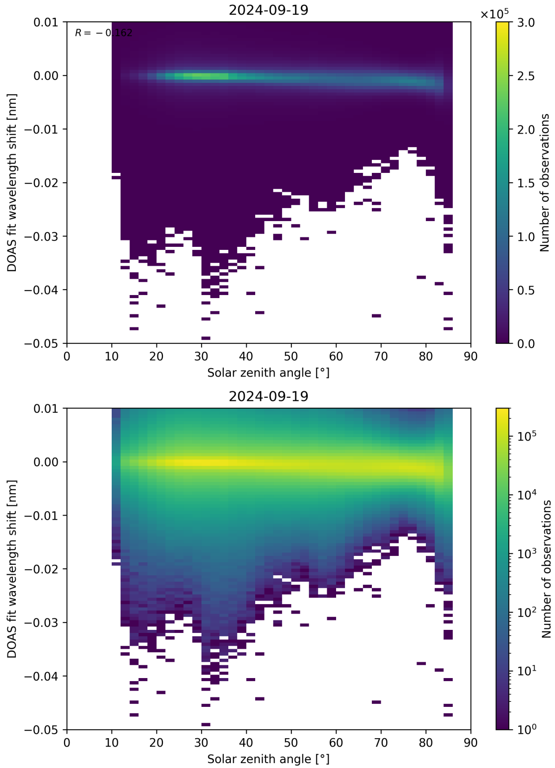
Figure 161: Scatter density plot of “Solar zenith angle” against “DOAS fit wavelength shift” for 2024-09-18 to 2024-09-20.
