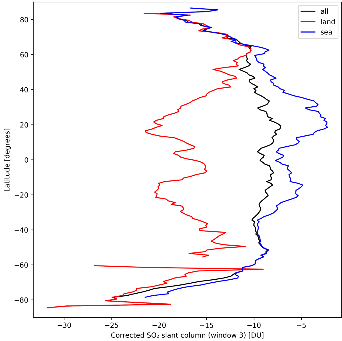
Figure 43: Zonal average of “Corrected SO 2 slant column (window 3)” for 2024-09-18 to 2024-09-20.
