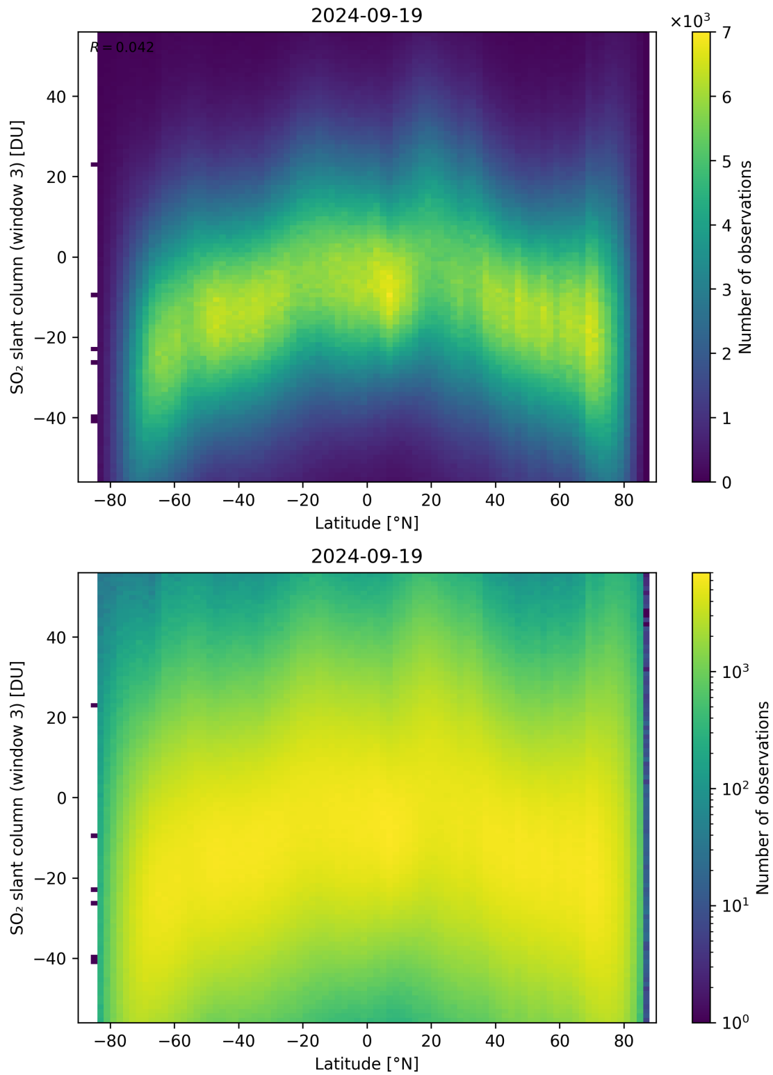
Figure 152: Scatter density plot of “Latitude” against “SO 2 slant column (window 3)” for 2024-09-18 to 2024-09-20.
