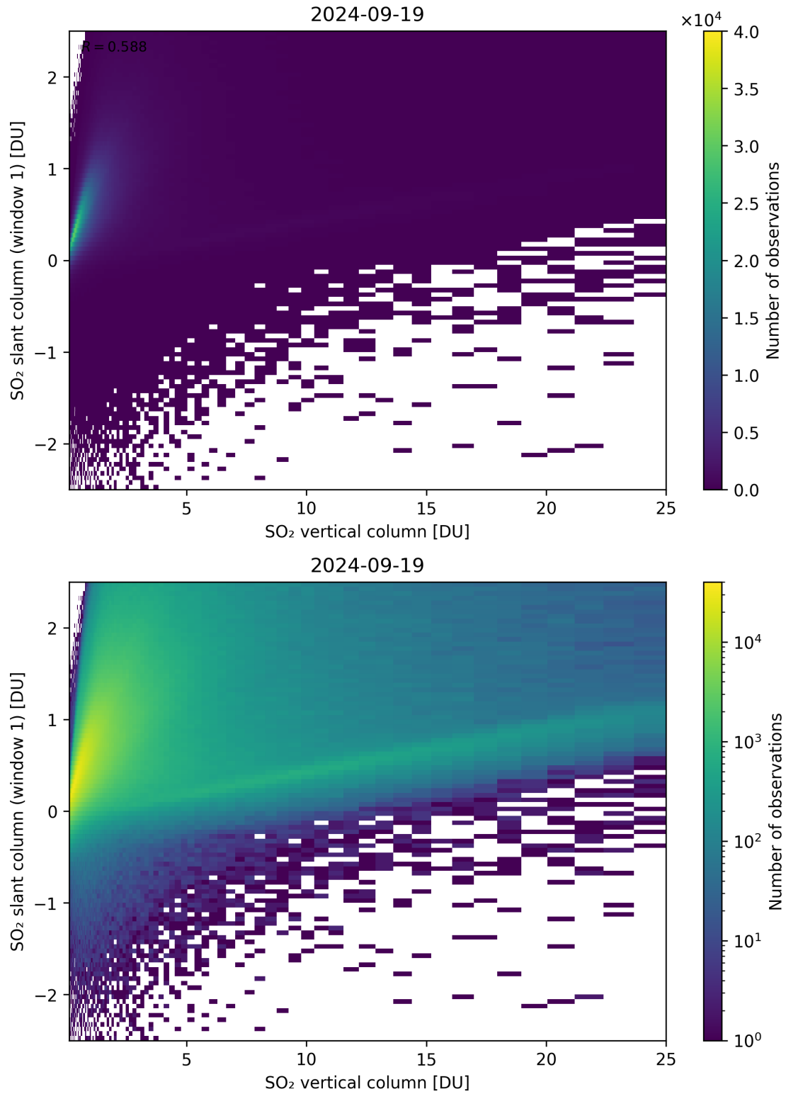
Figure 300: Scatter density plot of “SO 2 vertical column” against “SO 2 slant column (window 1)” for 2024-09-18 to 2024-09-20.
