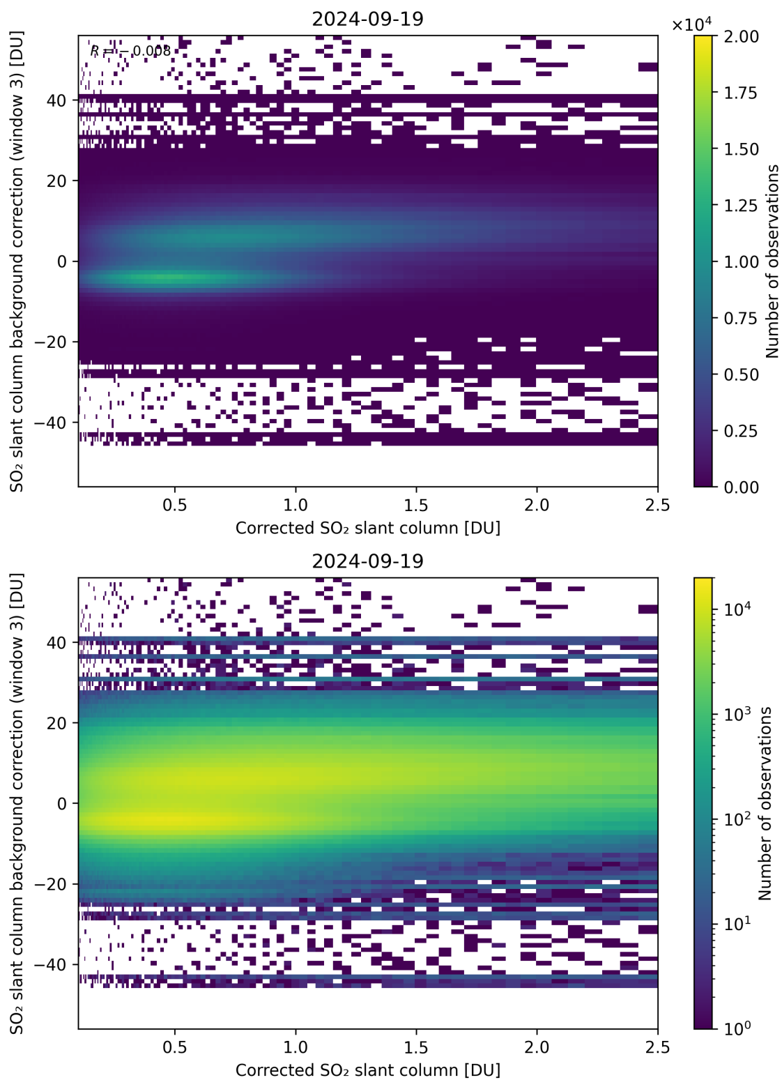
Figure 180: Scatter density plot of “Corrected SO 2 slant column” against “SO 2 slant column background correction (window 3)” for 2024-09-18 to 2024-09-20.
