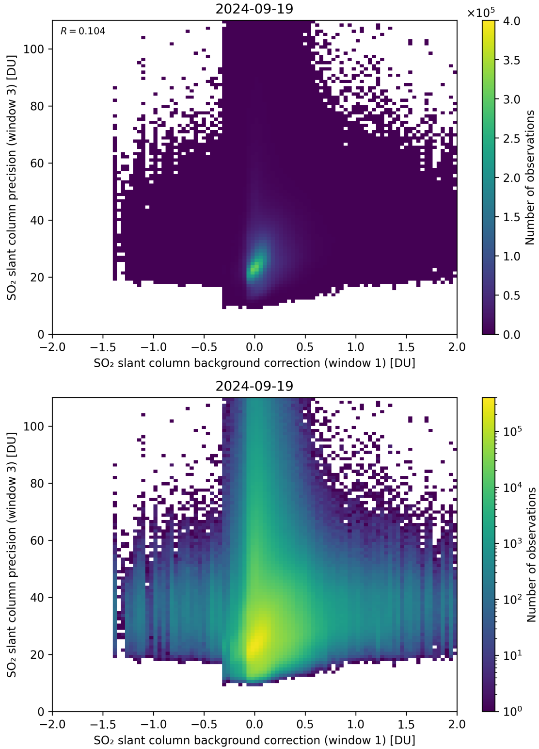
Figure 108: Scatter density plot of “SO 2 slant column background correction (window 1)” against “SO 2 slant column precision (window 3)” for 2024-09-18 to 2024-09-20.
