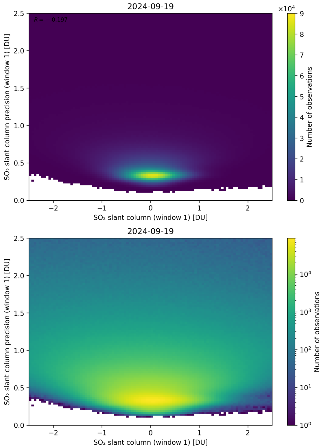
Figure 235: Scatter density plot of “SO 2 slant column (window 1)” against “SO 2 slant column precision (window 1)” for 2024-09-18 to 2024-09-20.
