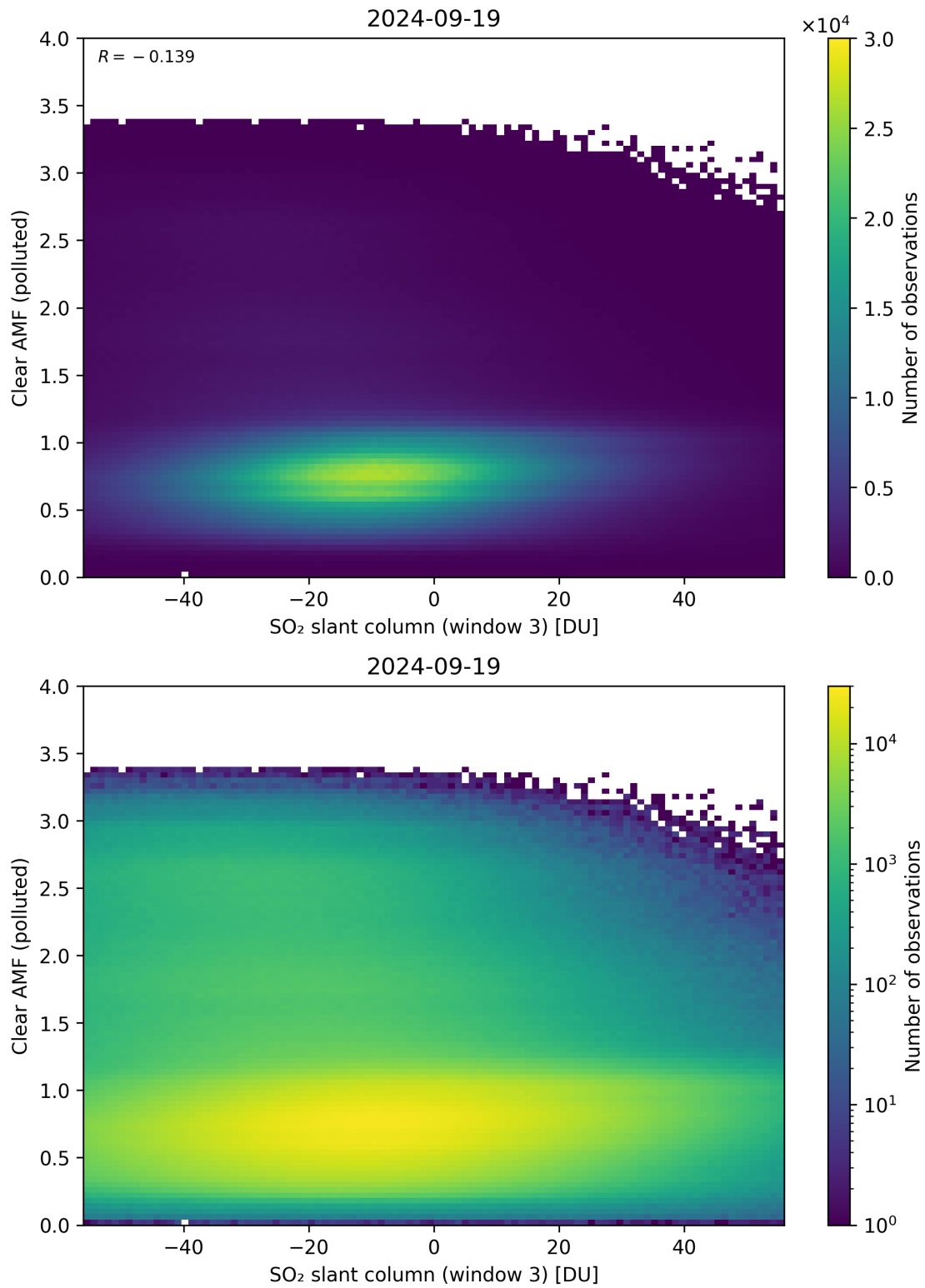
Figure 265: Scatter density plot of “SO 2 slant column (window 3)” against “Clear AMF (polluted)” for 2024-09-18 to 2024-09-20.
