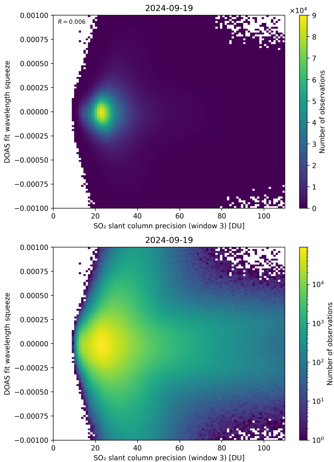
Figure 259: Scatter density plot of “SO 2 slant column precision (window 3)” against “DOAS fit wavelength squeeze” for 2024-09-18 to 2024-09-20.
