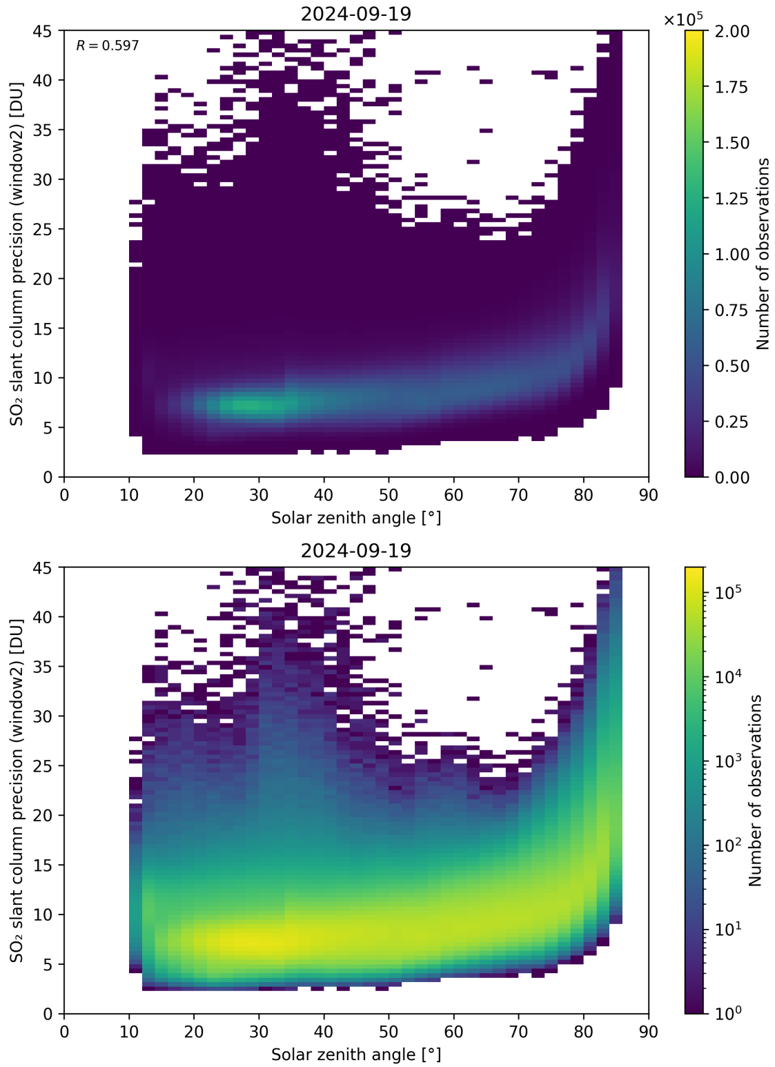
Figure 171: Scatter density plot of “Solar zenith angle” against “SO 2 slant column precision (window2)” for 2024-09-18 to 2024-09-20.
