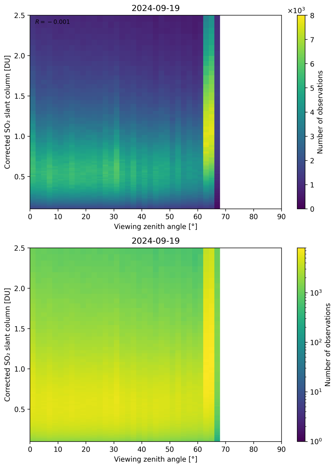
Figure 317: Scatter density plot of “Viewing zenith angle” against “Corrected SO 2 slant column” for 2024-09-18 to 2024-09-20.
