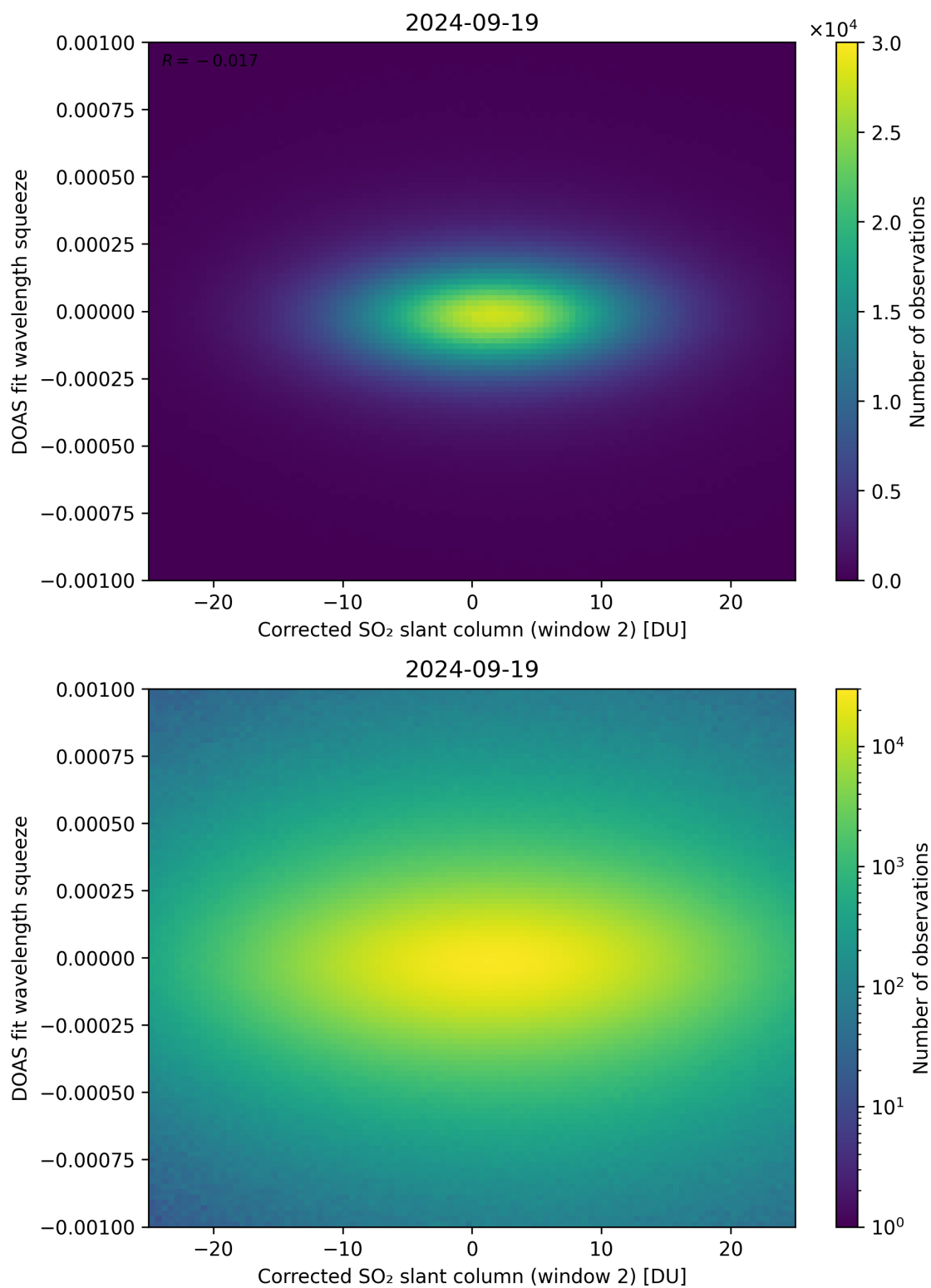
Figure 197: Scatter density plot of “Corrected SO 2 slant column (window 2)” against “DOAS fit wavelength squeeze” for 2024-09-18 to 2024-09-20.
