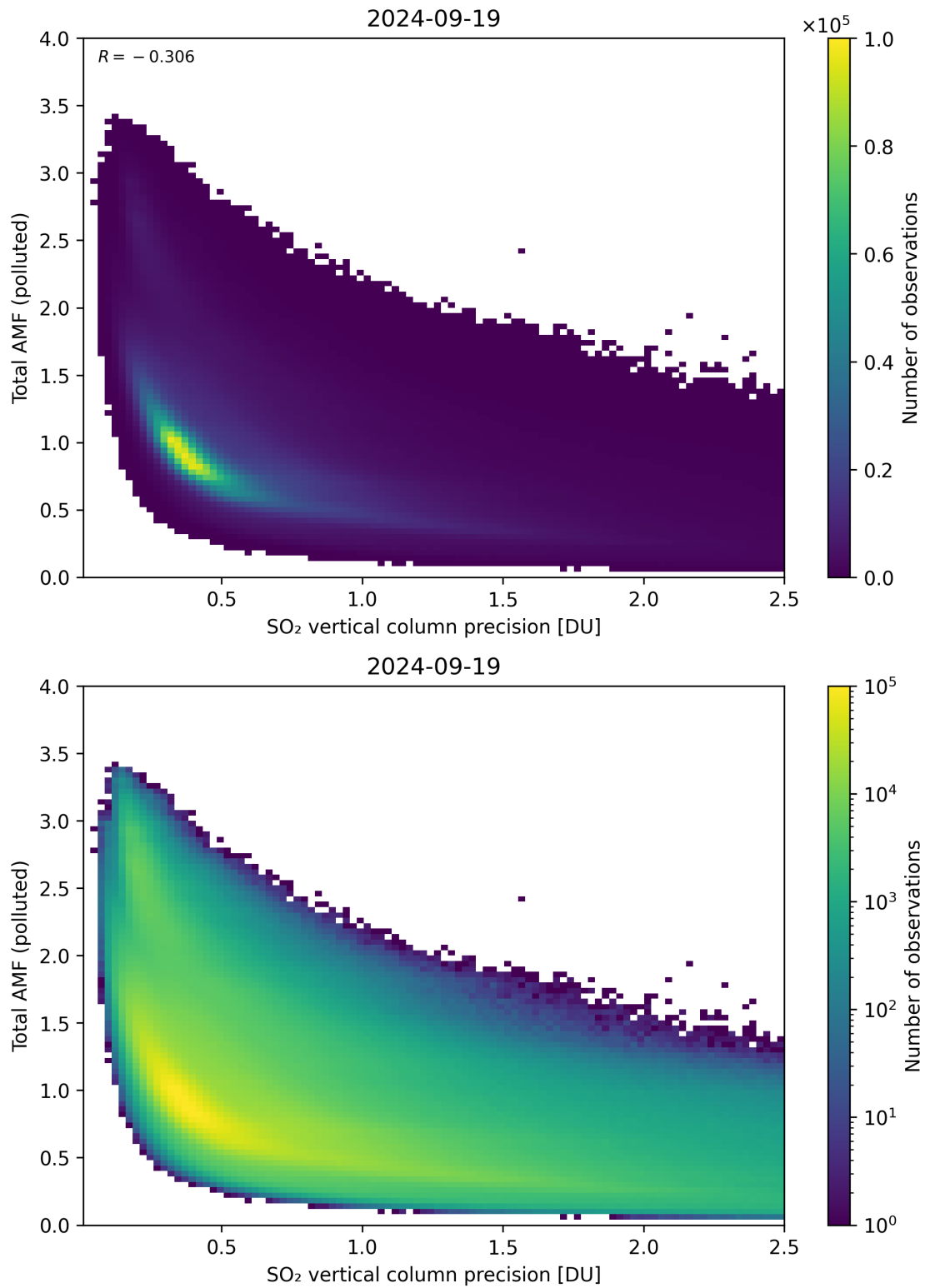
Figure 294: Scatter density plot of “SO 2 vertical column precision” against “Total AMF (polluted)” for 2024-09-18 to 2024-09-20.
