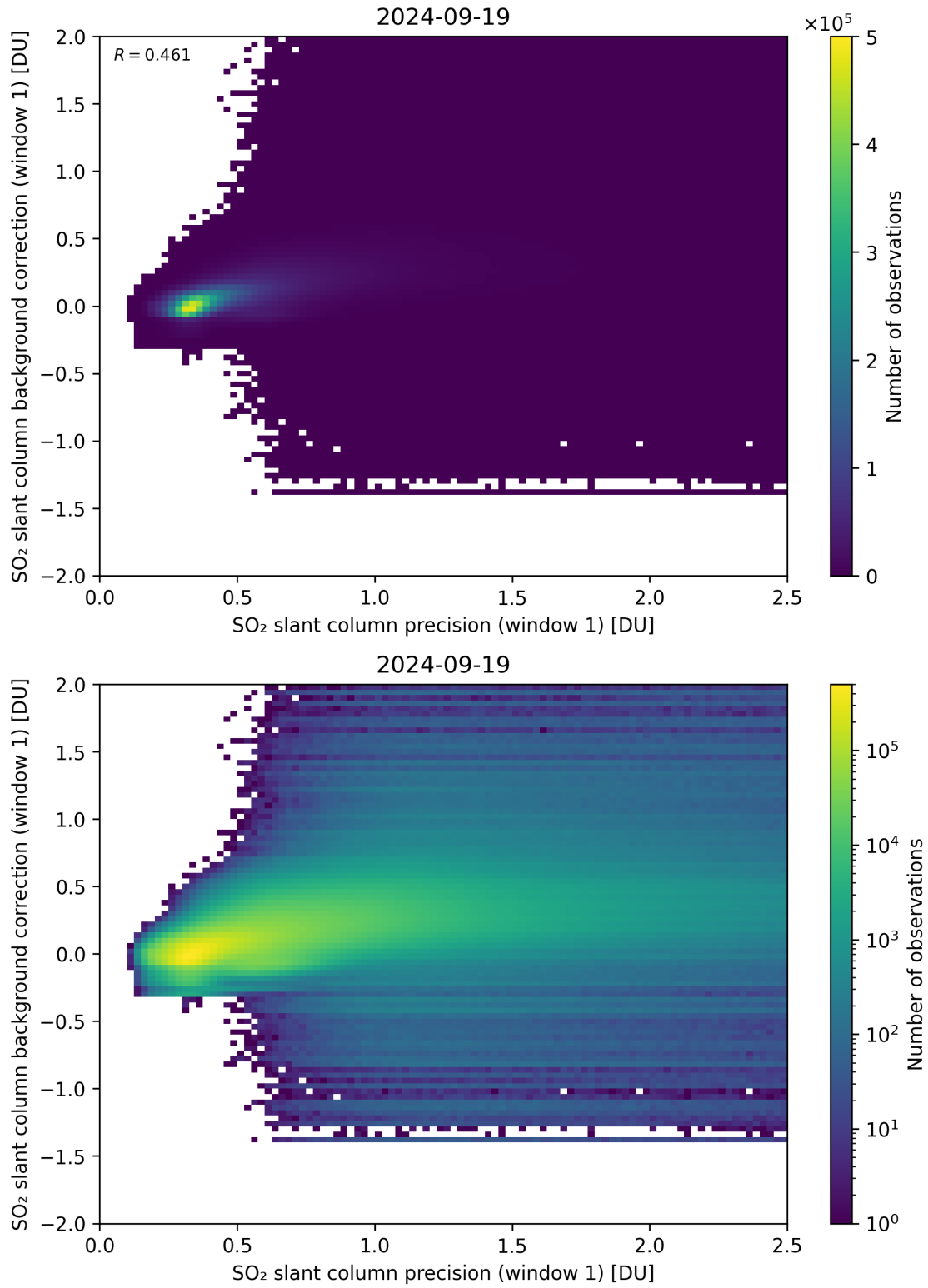
Figure 218: Scatter density plot of “SO 2 slant column precision (window 1)” against “SO 2 slant column background correction (window 1)” for 2024-09-18 to 2024-09-20.
