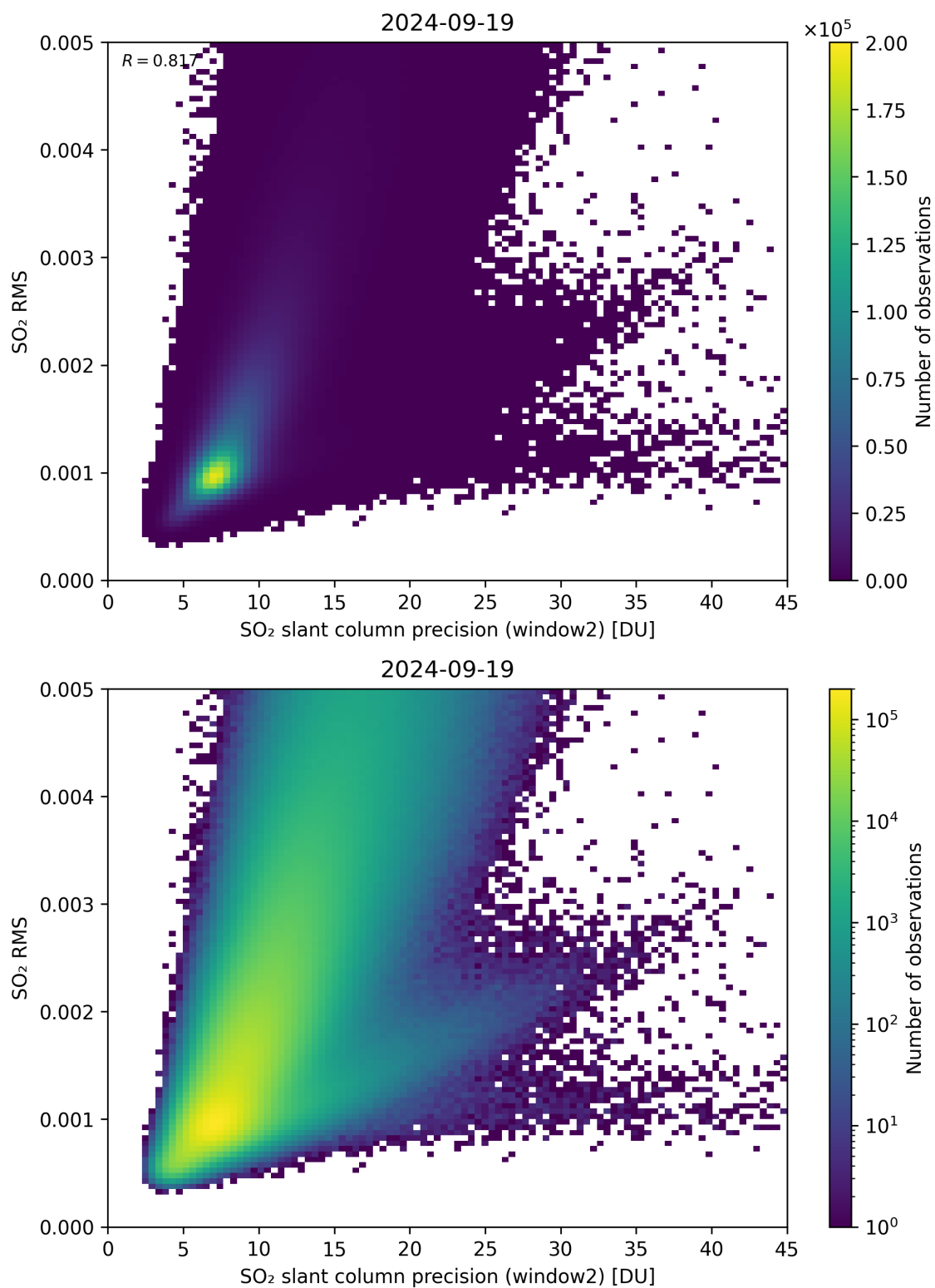
Figure 245: Scatter density plot of “SO 2 slant column precision (window2)” against “SO 2 RMS” for 2024-09-18 to 2024-09-20.
