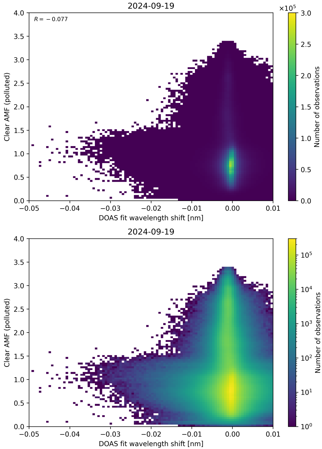
Figure 129: Scatter density plot of “DOAS fit wavelength shift” against “Clear AMF (polluted)” for 2024-09-18 to 2024-09-20.
