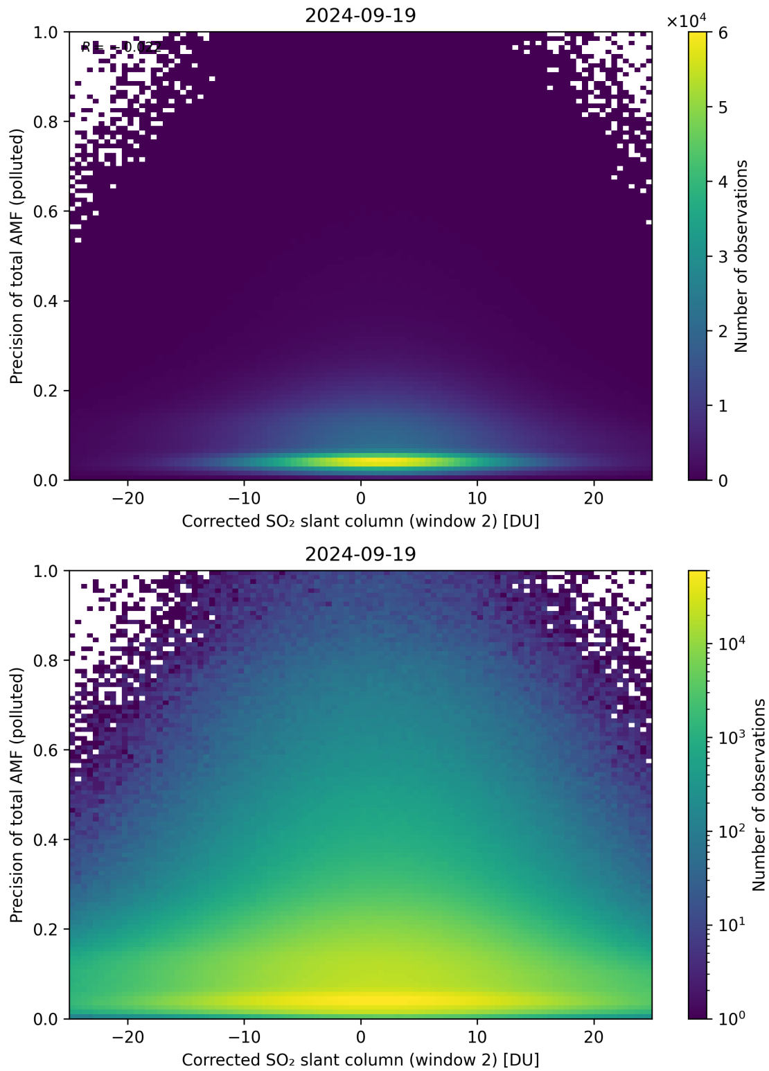
Figure 204: Scatter density plot of “Corrected SO 2 slant column (window 2)” against “Precision of total AMF (polluted)” for 2024-09-18 to 2024-09-20.
