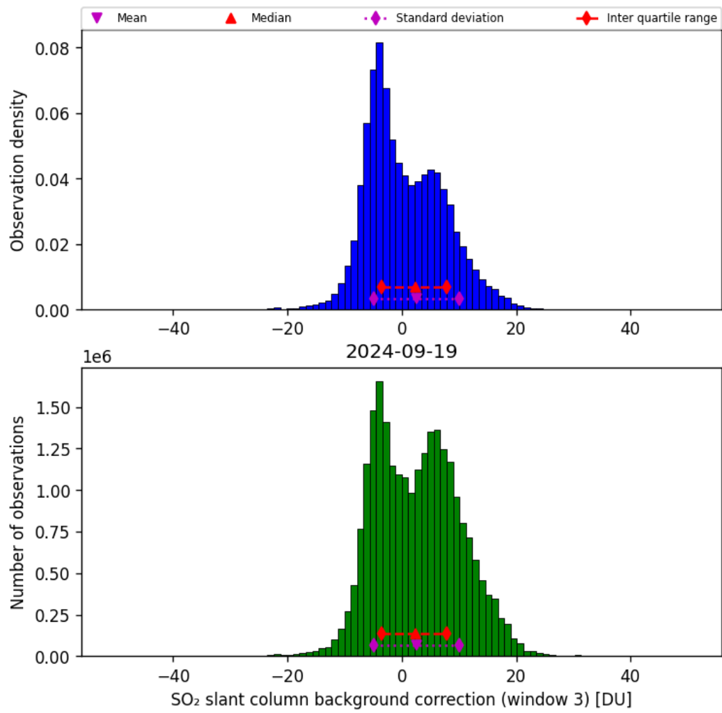
Figure 67: Histogram of “SO 2 slant column background correction (window 3)” for 2024-09-18 to 2024-09-20
