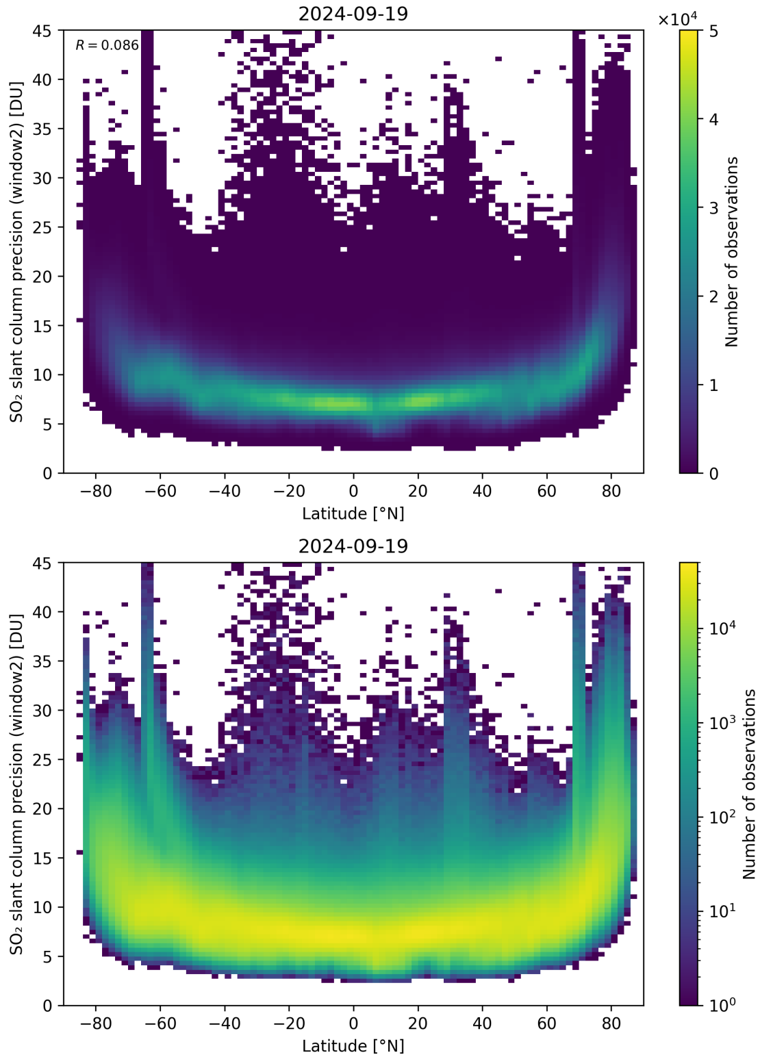
Figure 151: Scatter density plot of “Latitude” against “SO 2 slant column precision (window2)” for 2024-09-18 to 2024-09-20.
