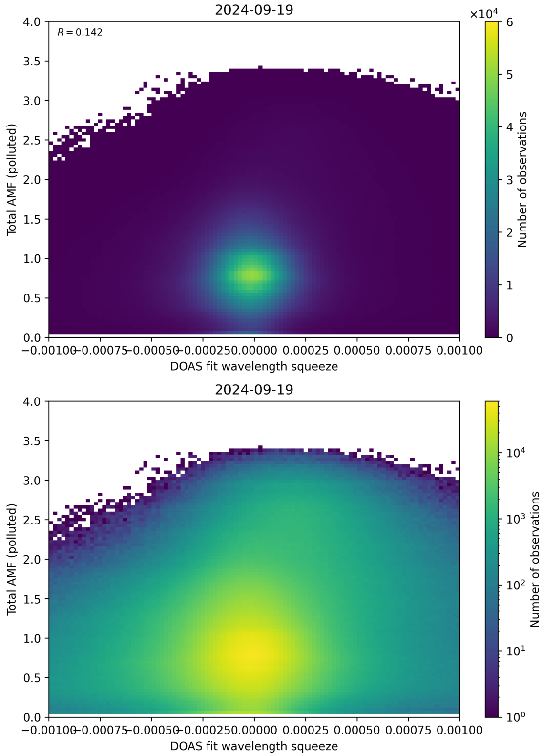
Figure 134: Scatter density plot of “DOAS fit wavelength squeeze” against “Total AMF (polluted)” for 2024-09-18 to 2024-09-20.
