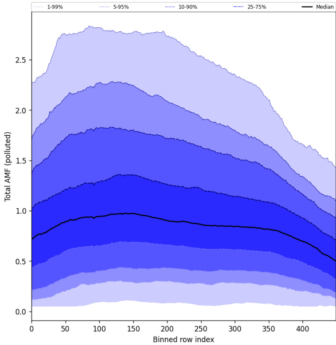
Figure 94: Along track statistics of “Total AMF (polluted)” for 2024-09-18 to 2024-09-20
