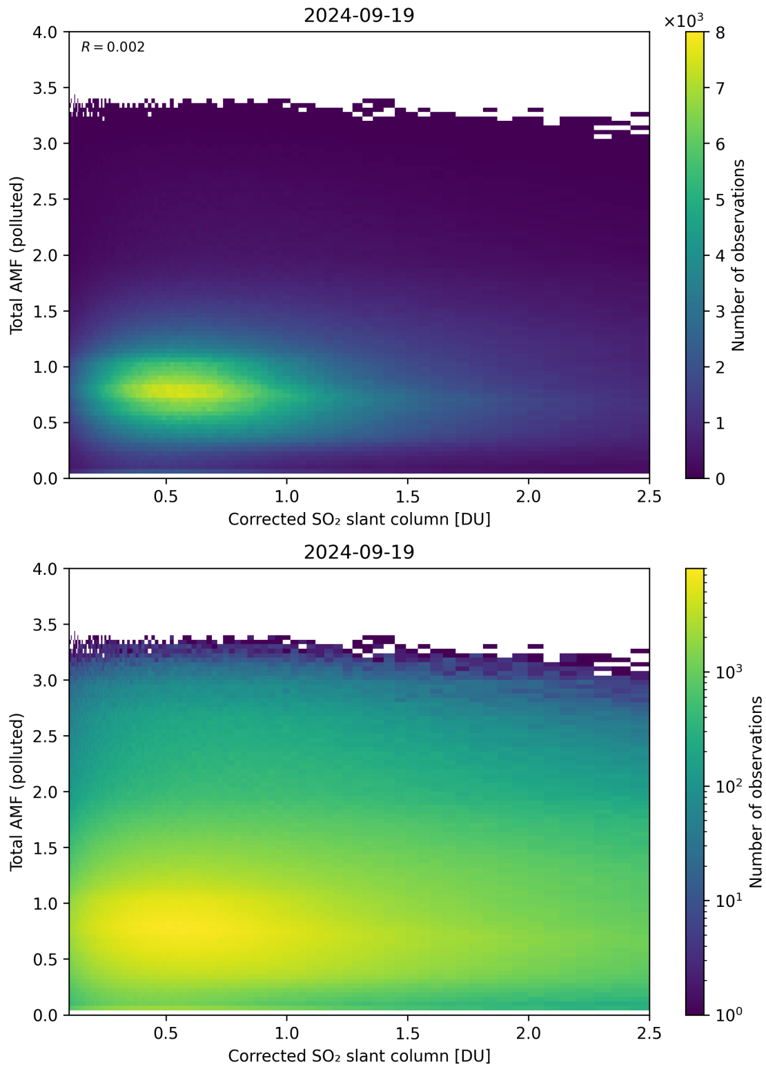
Figure 192: Scatter density plot of “Corrected SO 2 slant column” against “Total AMF (polluted)” for 2024-09-18 to 2024-09-20.
