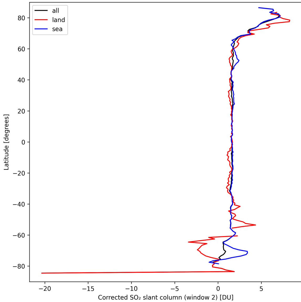
Figure 39: Zonal average of “Corrected SO 2 slant column (window 2)” for 2024-09-18 to 2024-09-20.
