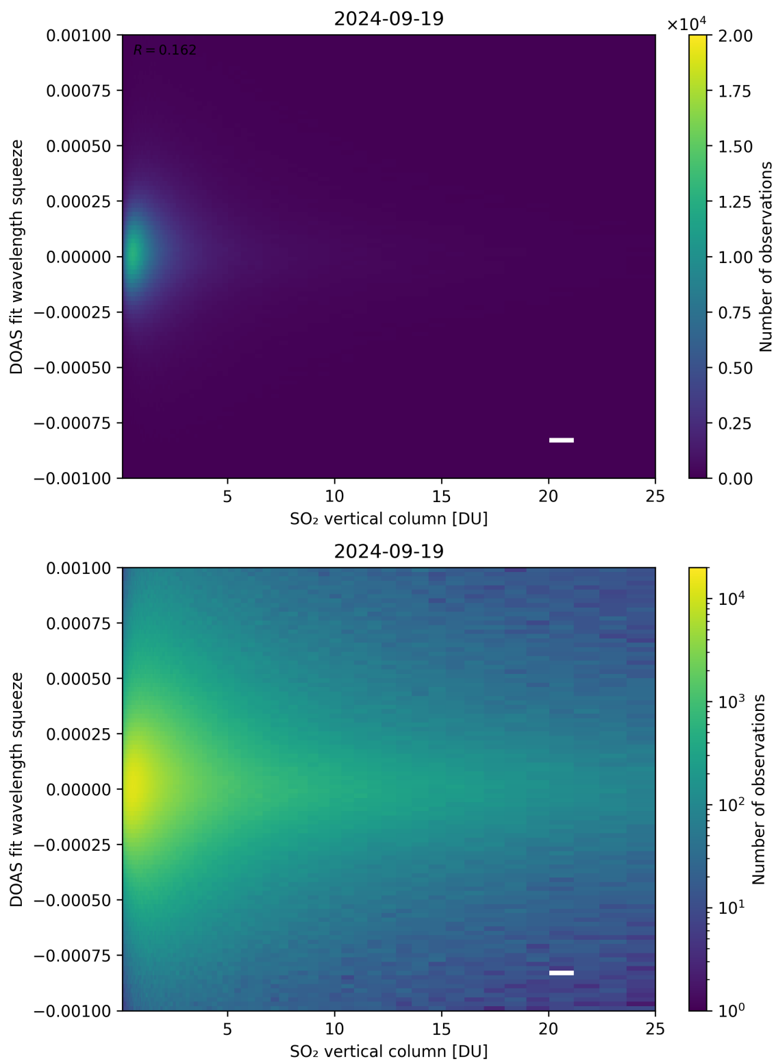
Figure 277: Scatter density plot of “SO 2 vertical column” against “DOAS fit wavelength squeeze” for 2024-09-18 to 2024-09-20.
