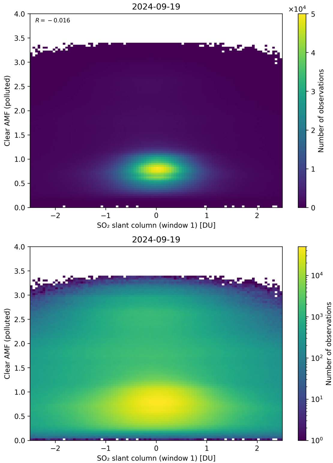
Figure 232: Scatter density plot of “SO 2 slant column (window 1)” against “Clear AMF (polluted)” for 2024-09-18 to 2024-09-20.
