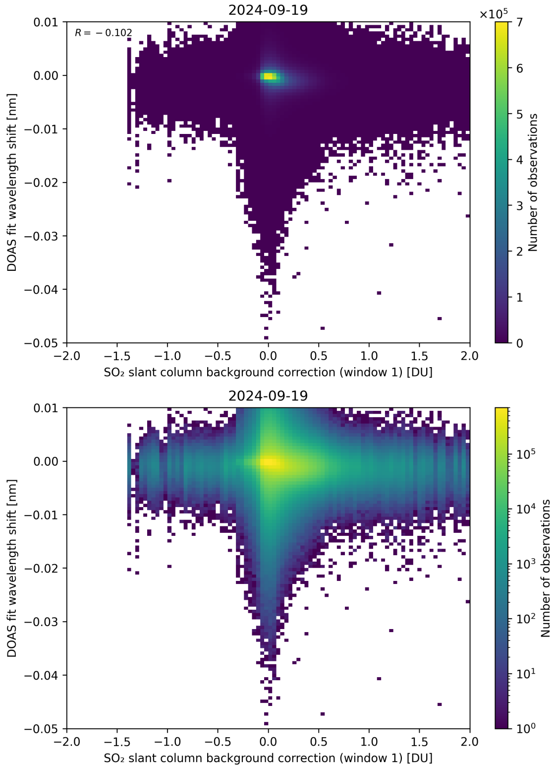
Figure 100: Scatter density plot of “SO 2 slant column background correction (window 1)” against “DOAS fit wavelength shift” for 2024-09-18 to 2024-09-20.
