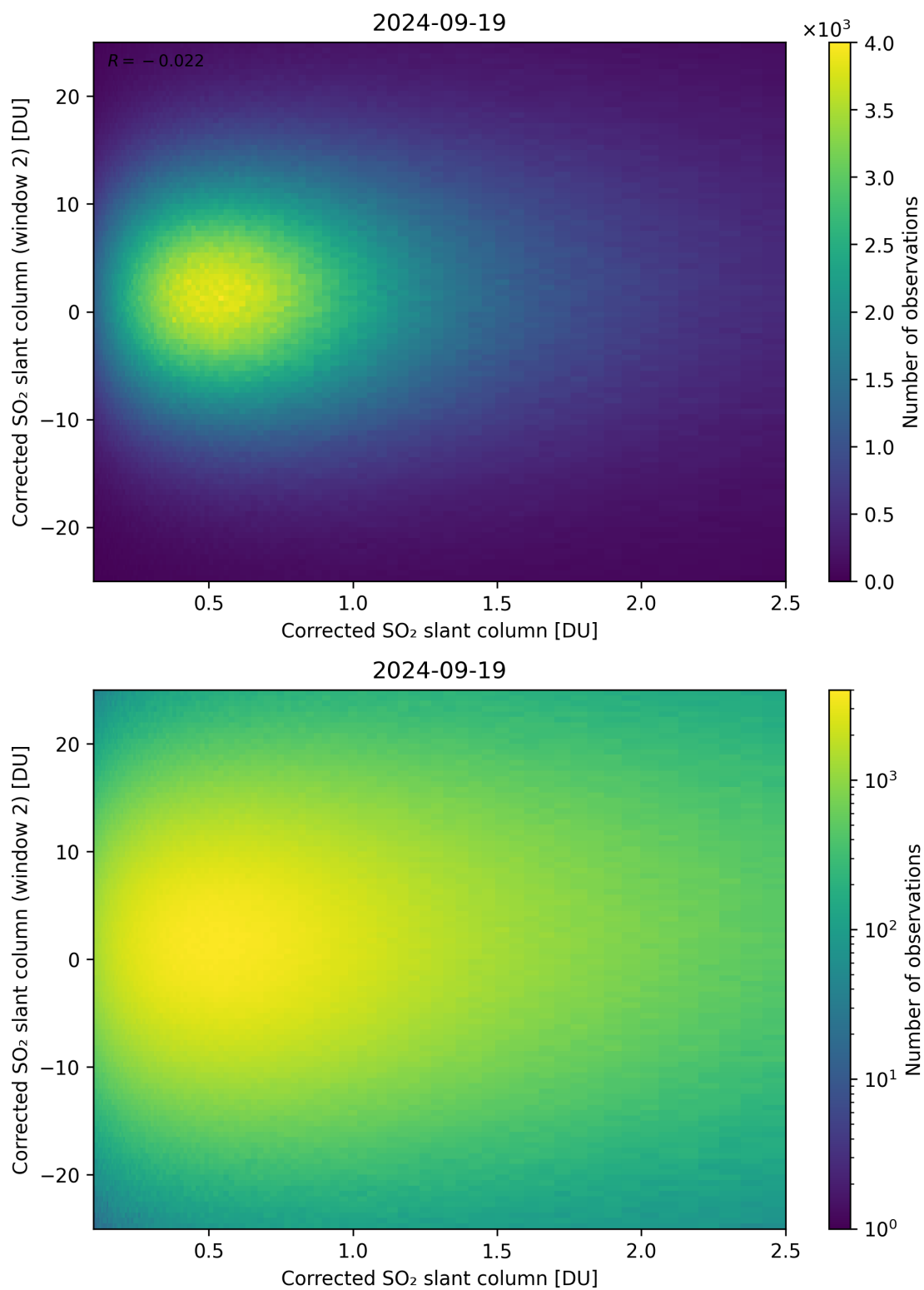
Figure 185: Scatter density plot of “Corrected SO 2 slant column” against “Corrected SO 2 slant column (window 2)” for 2024-09-18 to 2024-09-20.
