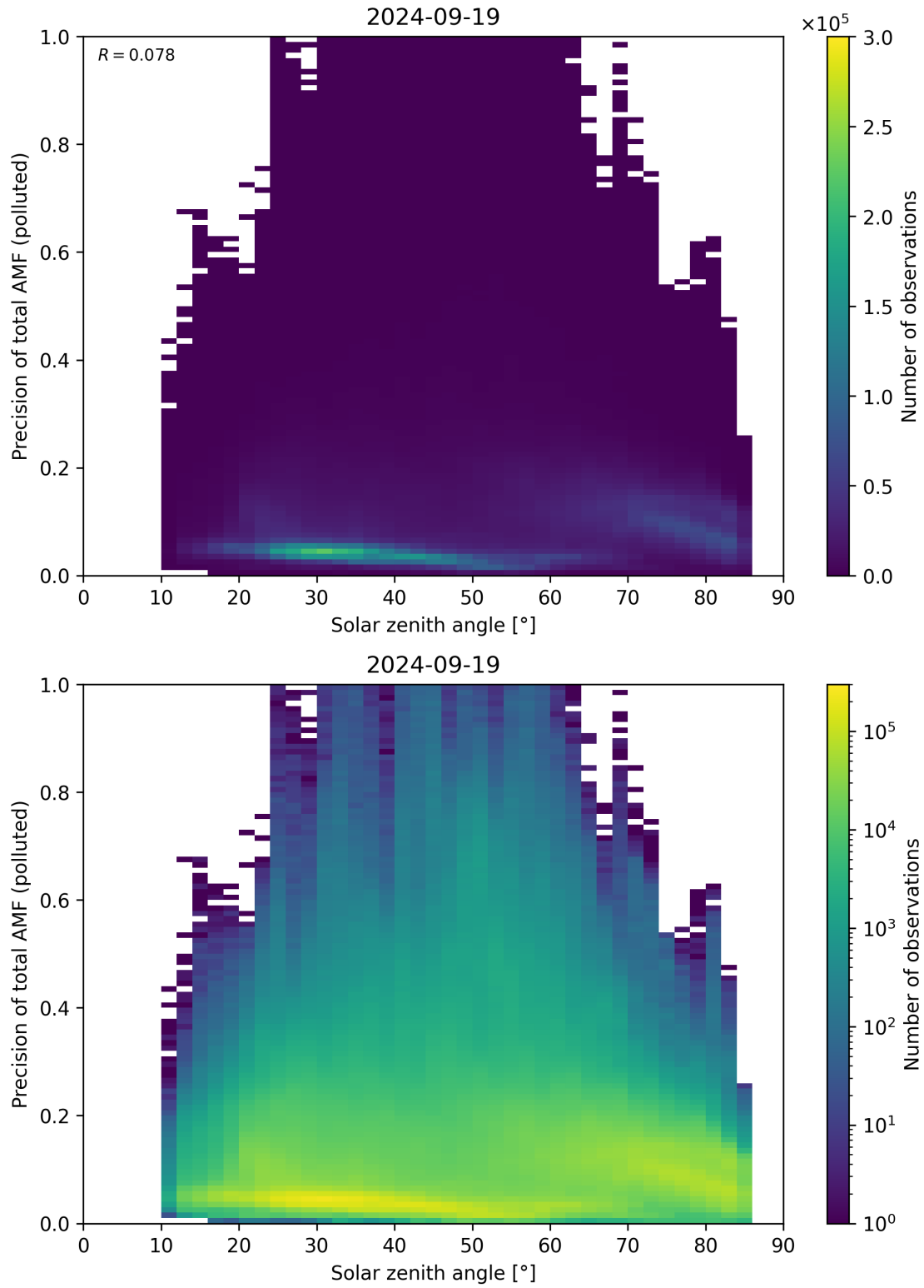
Figure 175: Scatter density plot of “Solar zenith angle” against “Precision of total AMF (polluted)” for 2024-09-18 to 2024-09-20.
