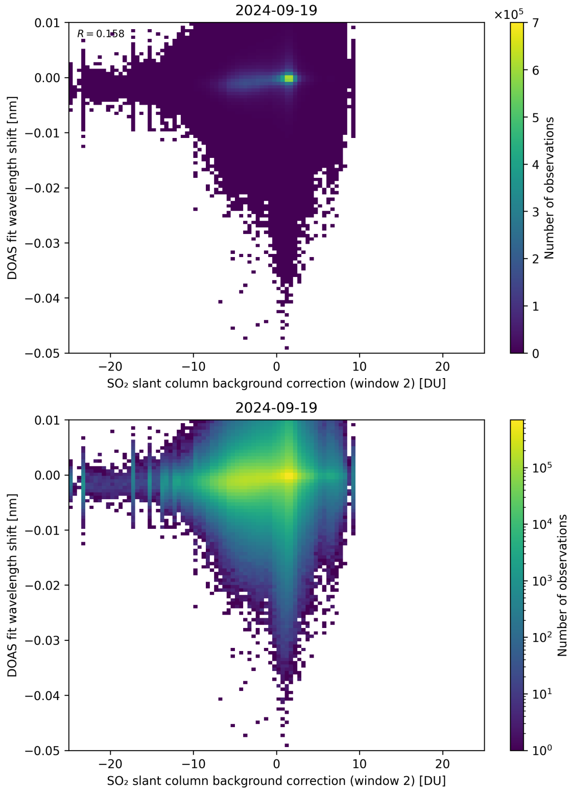
Figure 112: Scatter density plot of “SO 2 slant column background correction (window 2)” against “DOAS fit wavelength shift” for 2024-09-18 to 2024-09-20.
