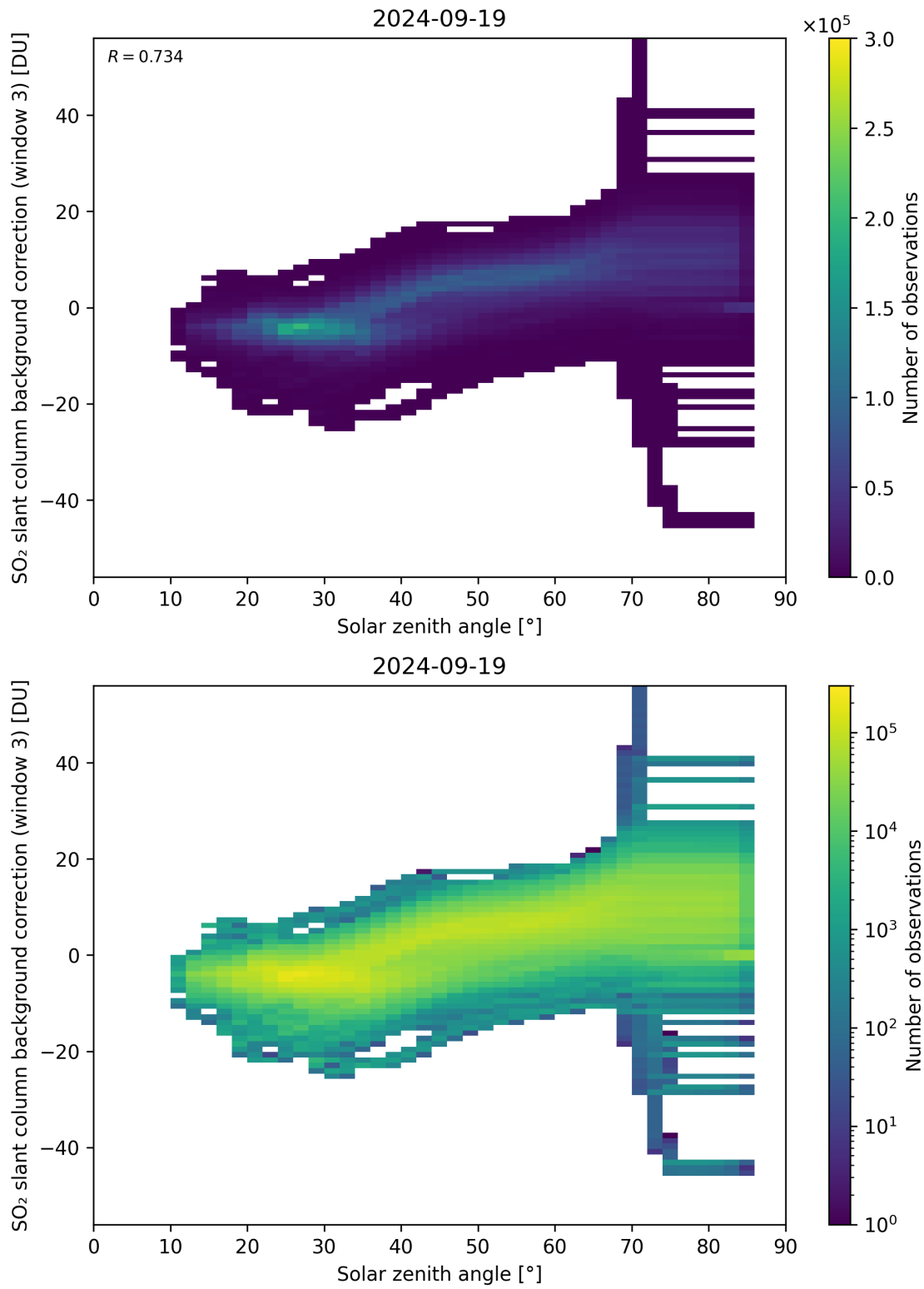
Figure 160: Scatter density plot of “Solar zenith angle” against “SO 2 slant column background correction (window 3)” for 2024-09-18 to 2024-09-20.
