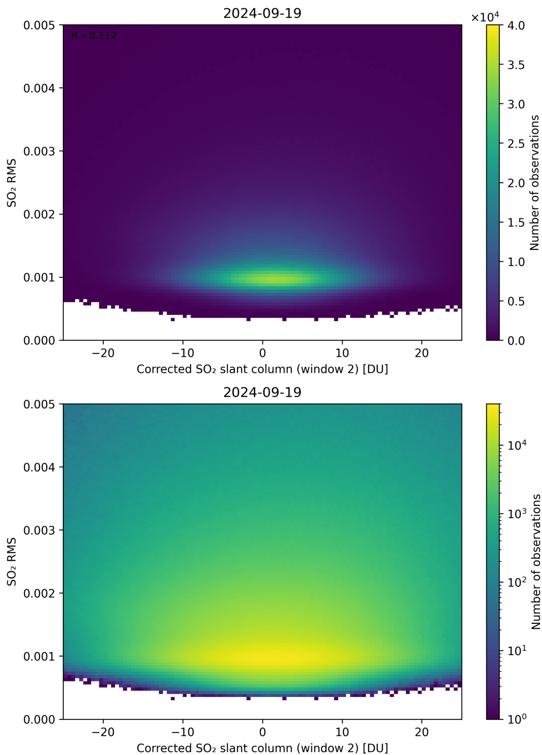
Figure 198: Scatter density plot of “Corrected SO 2 slant column (window 2)” against “SO 2 RMS” for 2024-09-18 to 2024-09-20.
