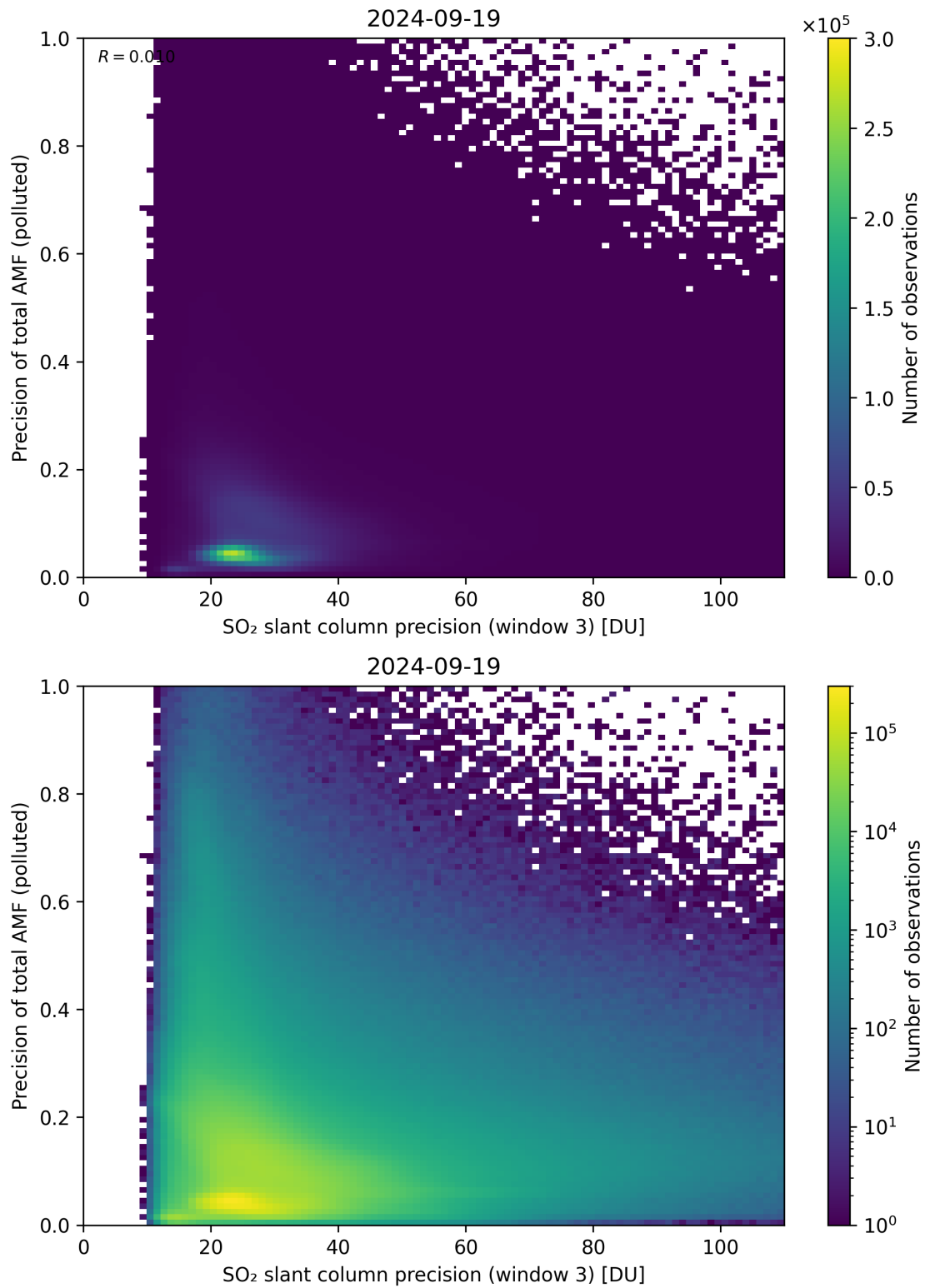
Figure 264: Scatter density plot of “SO 2 slant column precision (window 3)” against “Precision of total AMF (polluted)” for 2024-09-18 to 2024-09-20.
