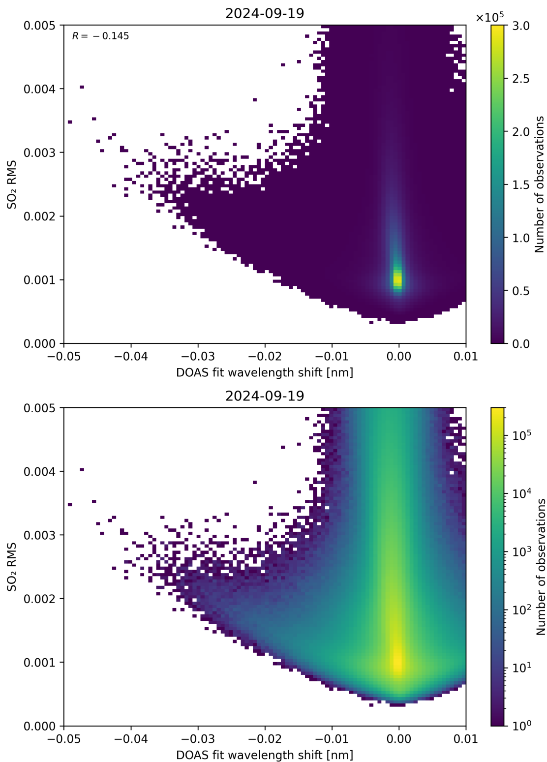
Figure 128: Scatter density plot of “DOAS fit wavelength shift” against “SO 2 RMS” for 2024-09-18 to 2024-09-20.
