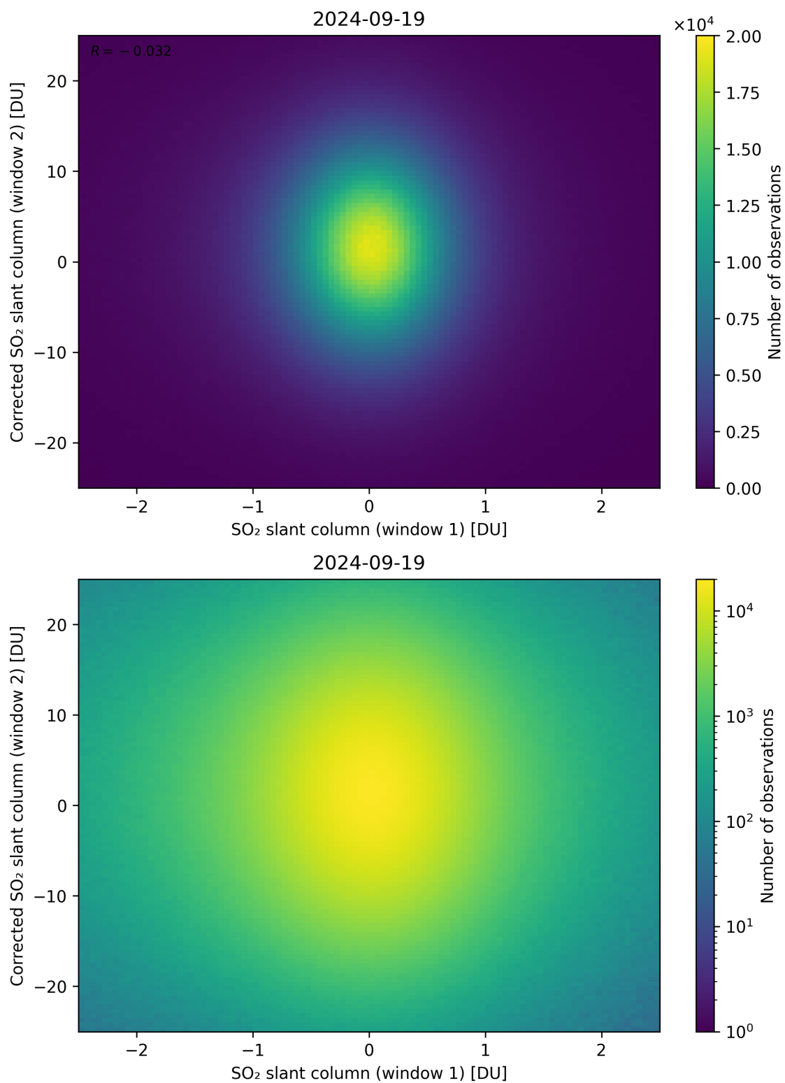
Figure 233: Scatter density plot of “SO 2 slant column (window 1)” against “Corrected SO 2 slant column (window 2)” for 2024-09-18 to 2024-09-20.
