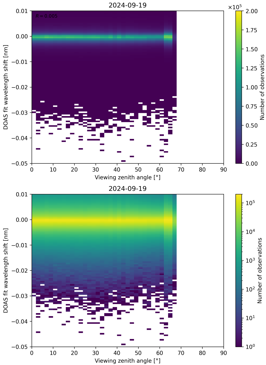
Figure 311: Scatter density plot of “Viewing zenith angle” against “DOAS fit wavelength shift” for 2024-09-18 to 2024-09-20.
