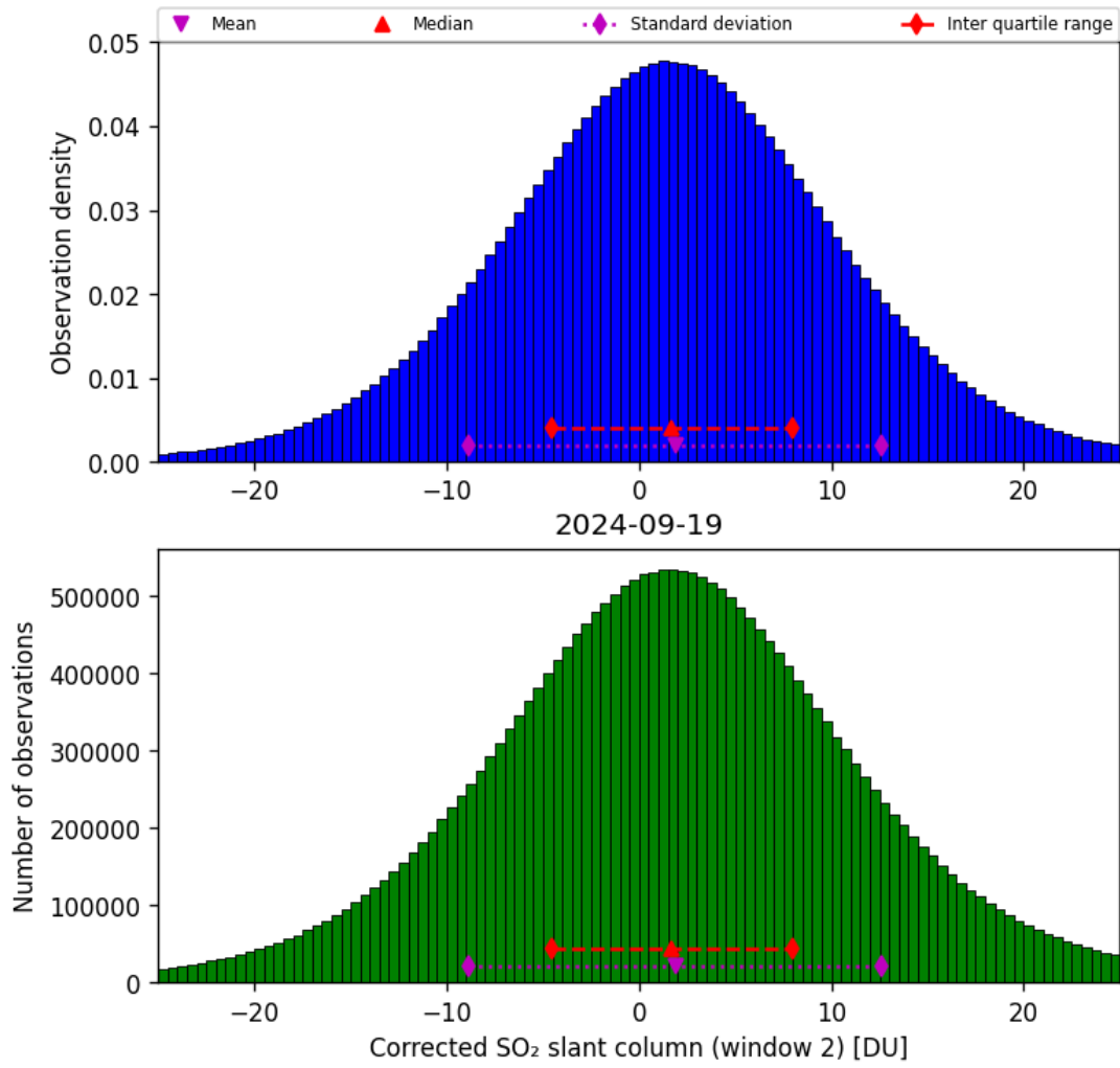
Figure 62: Histogram of “Corrected SO 2 slant column (window 2)” for 2024-09-18 to 2024-09-20
