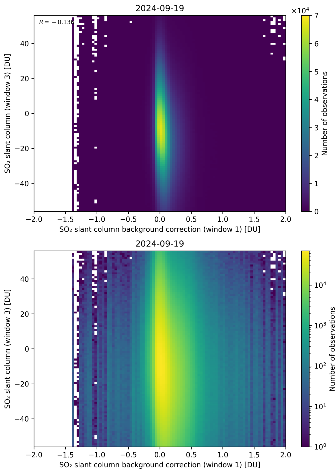
Figure 107: Scatter density plot of “SO 2 slant column background correction (window 1)” against “SO 2 slant column (window 3)” for 2024-09-18 to 2024-09-20.
