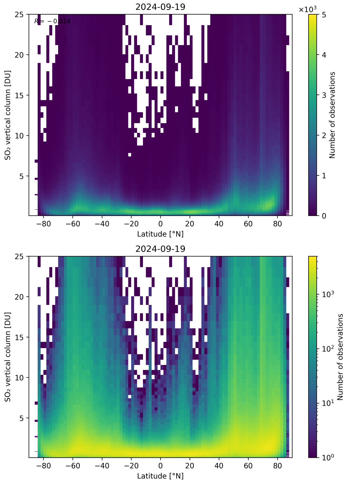
Figure 156: Scatter density plot of “Latitude” against “SO 2 vertical column” for 2024-09-18 to 2024-09-20.
