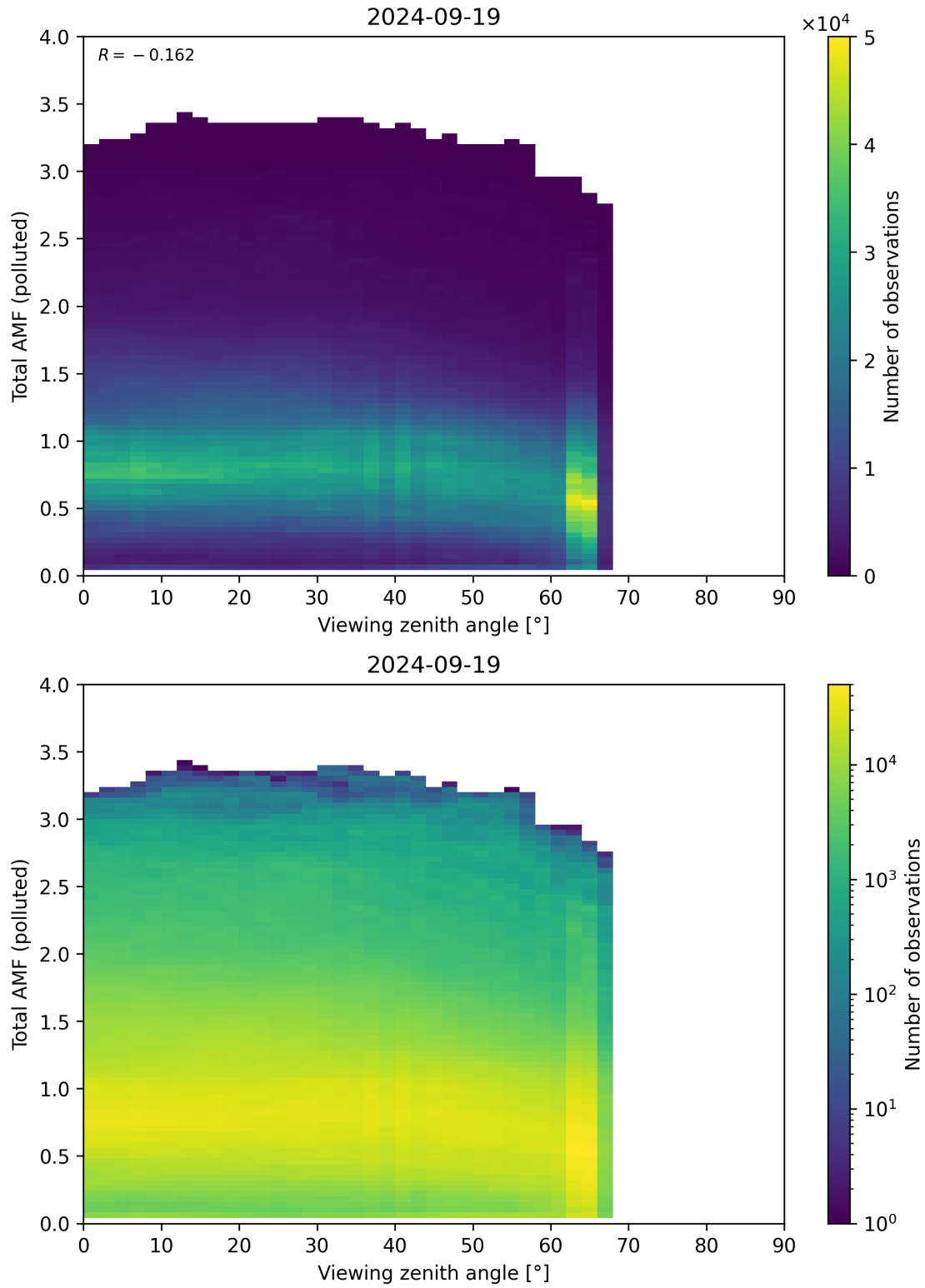
Figure 325: Scatter density plot of “Viewing zenith angle” against “Total AMF (polluted)” for 2024-09-18 to 2024-09-20.
