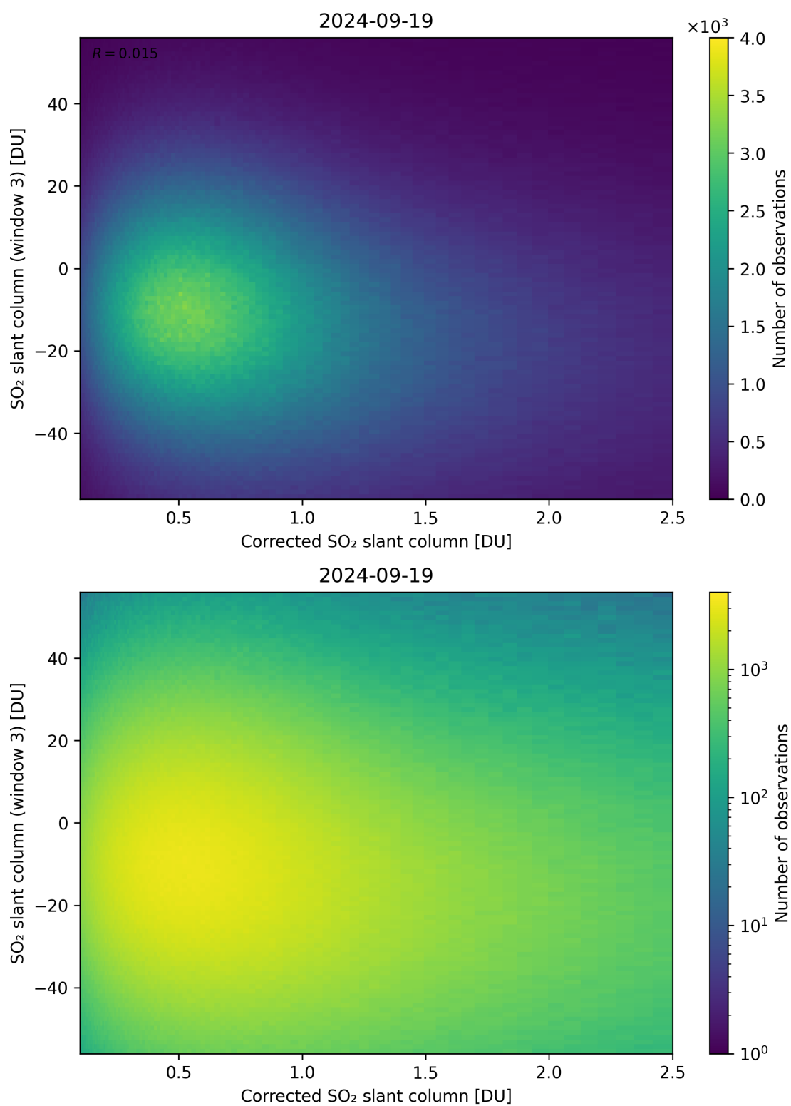
Figure 190: Scatter density plot of “Corrected SO 2 slant column” against “SO 2 slant column (window 3)” for 2024-09-18 to 2024-09-20.
