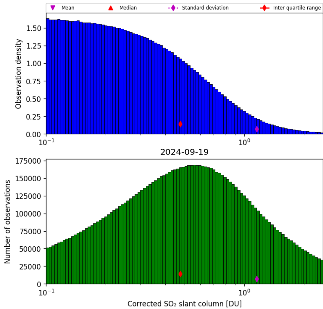
Figure 55: Histogram of “Corrected SO 2 slant column” for 2024-09-18 to 2024-09-20
