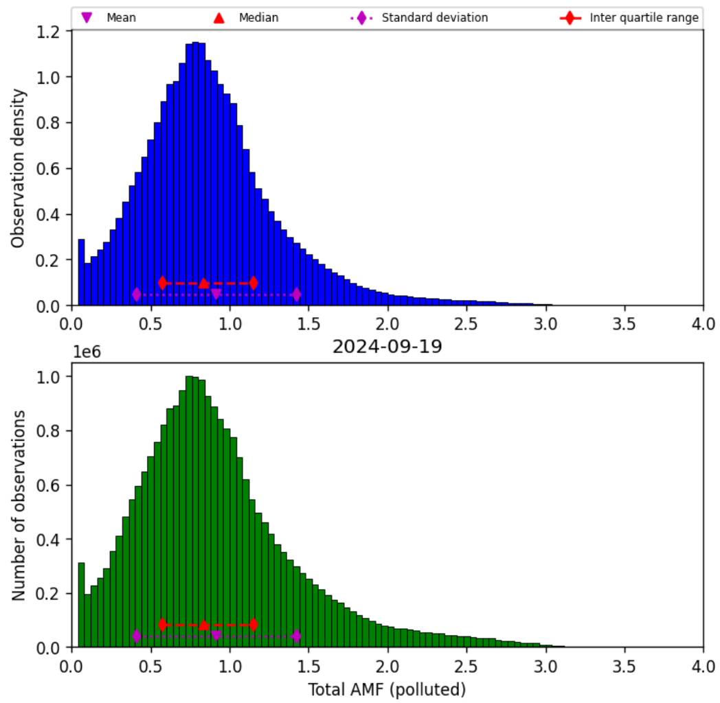
Figure 71: Histogram of “Total AMF (polluted)” for 2024-09-18 to 2024-09-20
