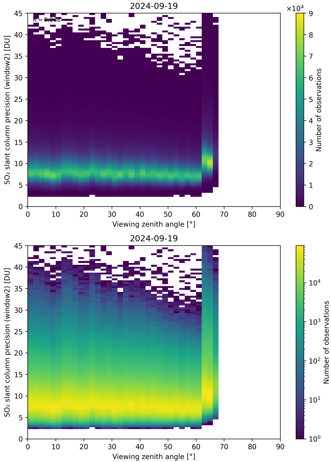
Figure 322: Scatter density plot of “Viewing zenith angle” against “SO 2 slant column precision (window2)” for 2024-09-18 to 2024-09-20.
