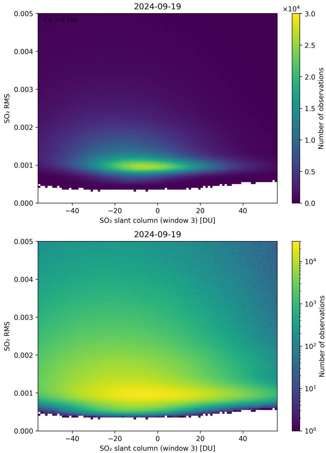
Figure 256: Scatter density plot of “SO 2 slant column (window 3)” against “SO 2 RMS” for 2024-09-18 to 2024-09-20.
