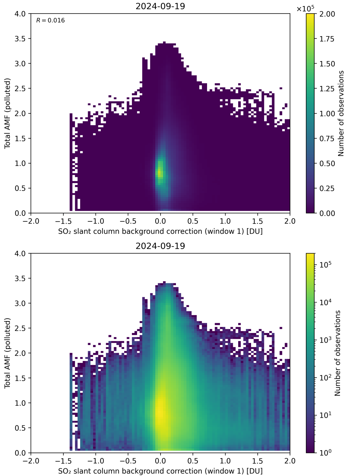
Figure 109: Scatter density plot of “SO 2 slant column background correction (window 1)” against “Total AMF (polluted)” for 2024-09-18 to 2024-09-20.
