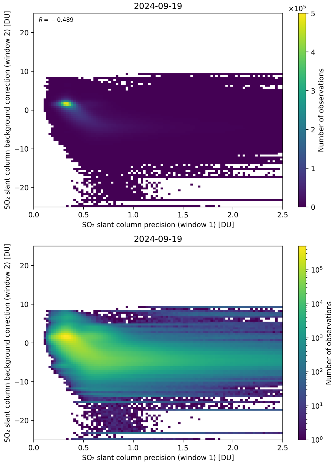
Figure 219: Scatter density plot of “SO 2 slant column precision (window 1)” against “SO 2 slant column background correction (window 2)” for 2024-09-18 to 2024-09-20.
