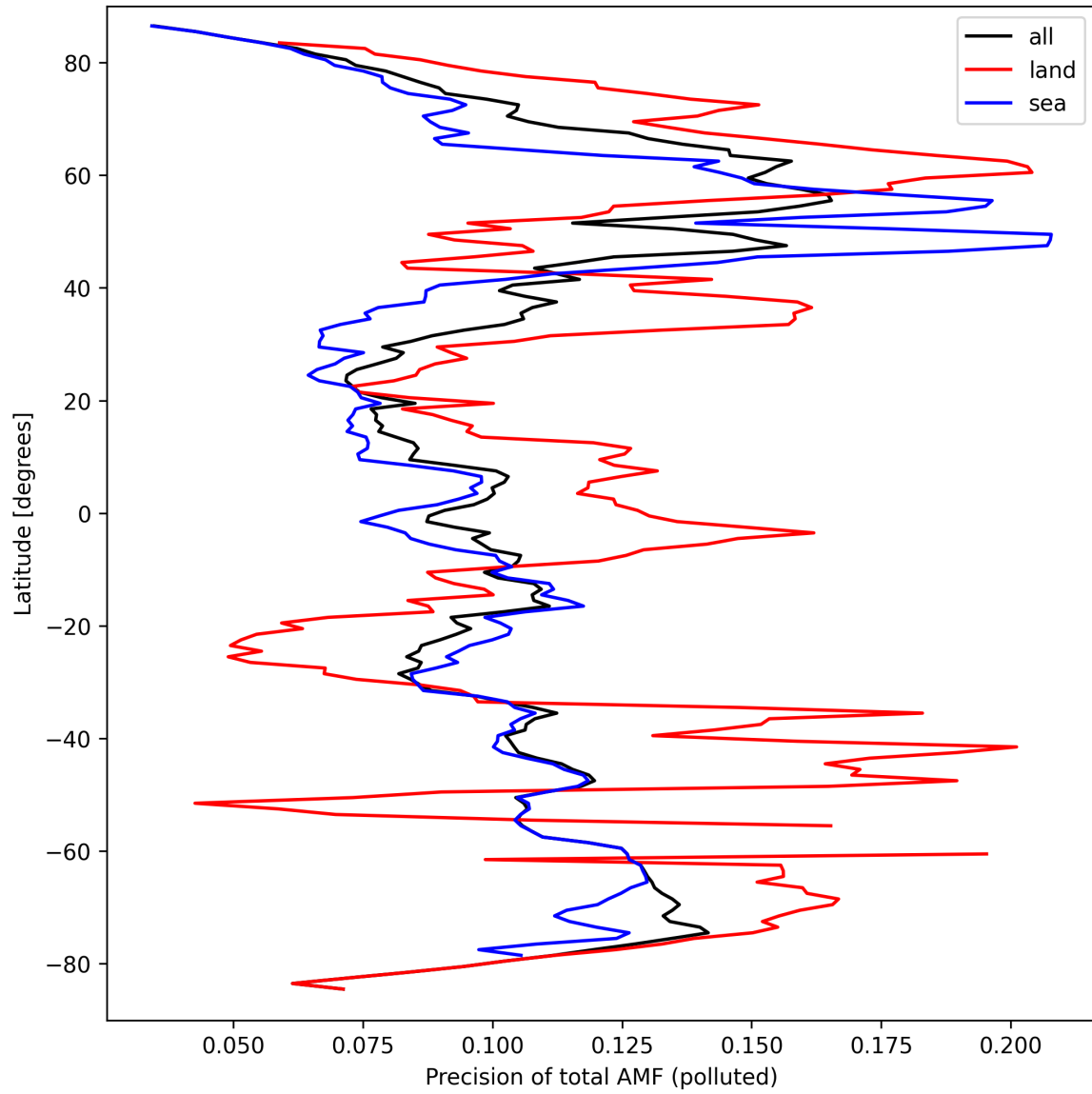
Figure 49: Zonal average of “Precision of total AMF (polluted)” for 2024-09-18 to 2024-09-20.
