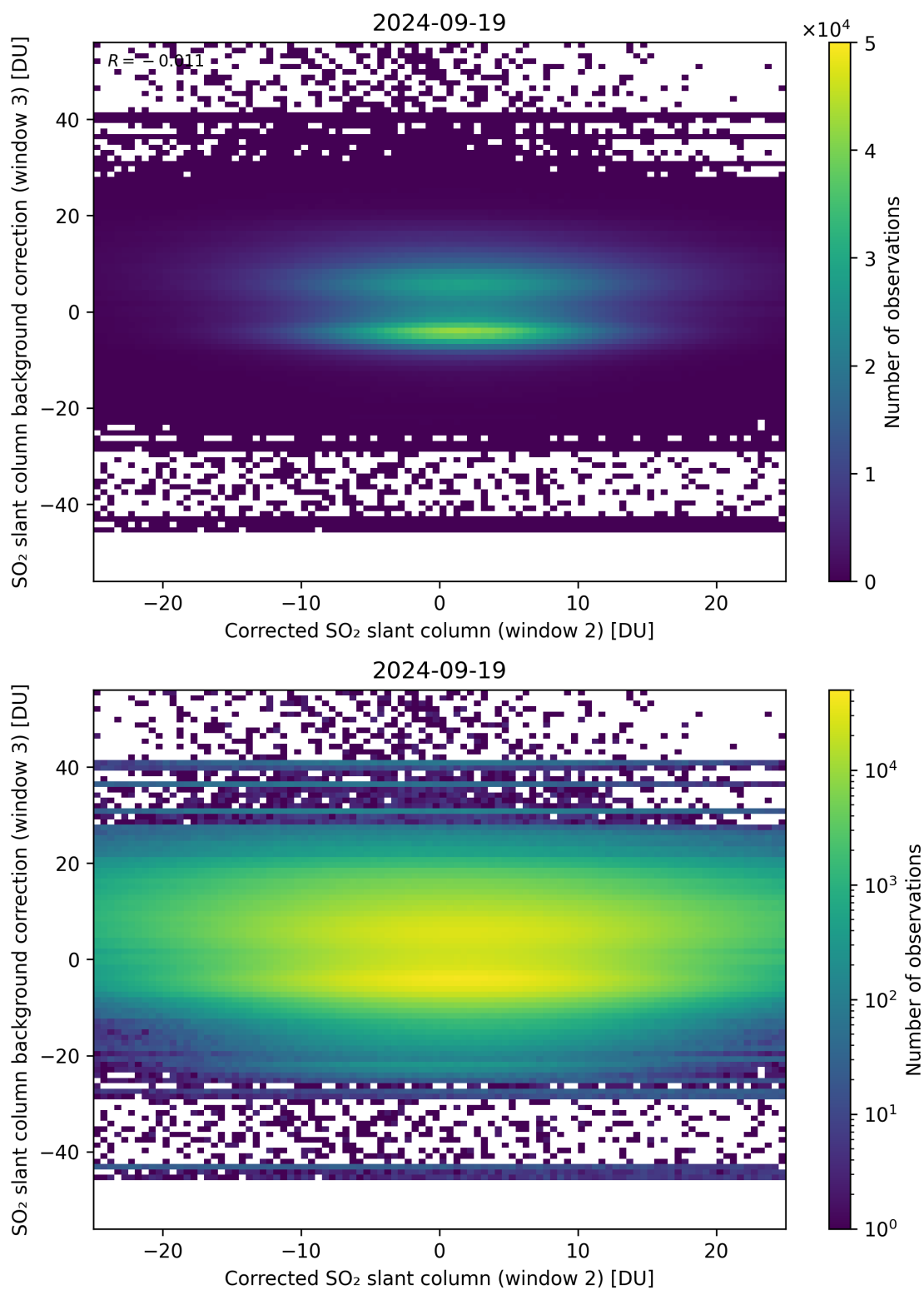
Figure 195: Scatter density plot of “Corrected SO 2 slant column (window 2)” against “SO 2 slant column background correction (window 3)” for 2024-09-18 to 2024-09-20.
