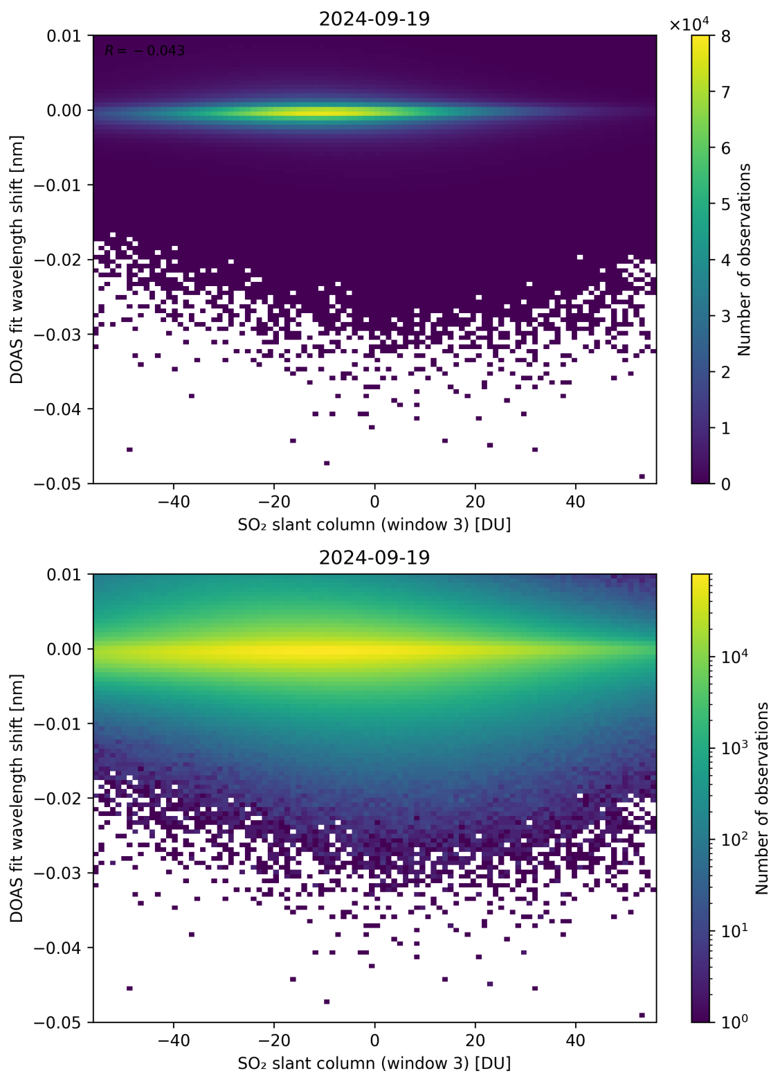
Figure 254: Scatter density plot of “SO 2 slant column (window 3)” against “DOAS fit wavelength shift” for 2024-09-18 to 2024-09-20.
