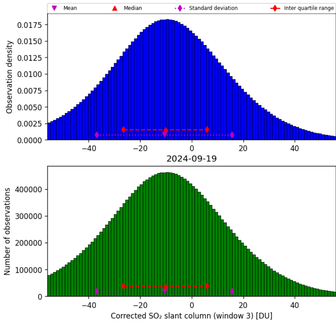
Figure 66: Histogram of “Corrected SO 2 slant column (window 3)” for 2024-09-18 to 2024-09-20
