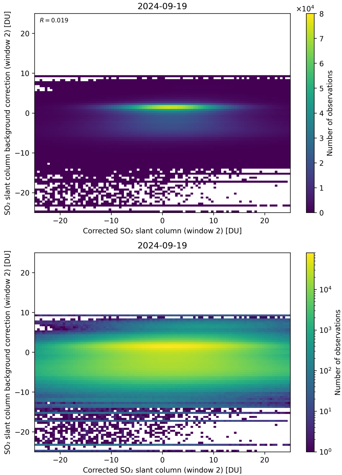
Figure 194: Scatter density plot of “Corrected SO 2 slant column (window 2)” against “SO 2 slant column background correction (window 2)” for 2024-09-18 to 2024-09-20.
