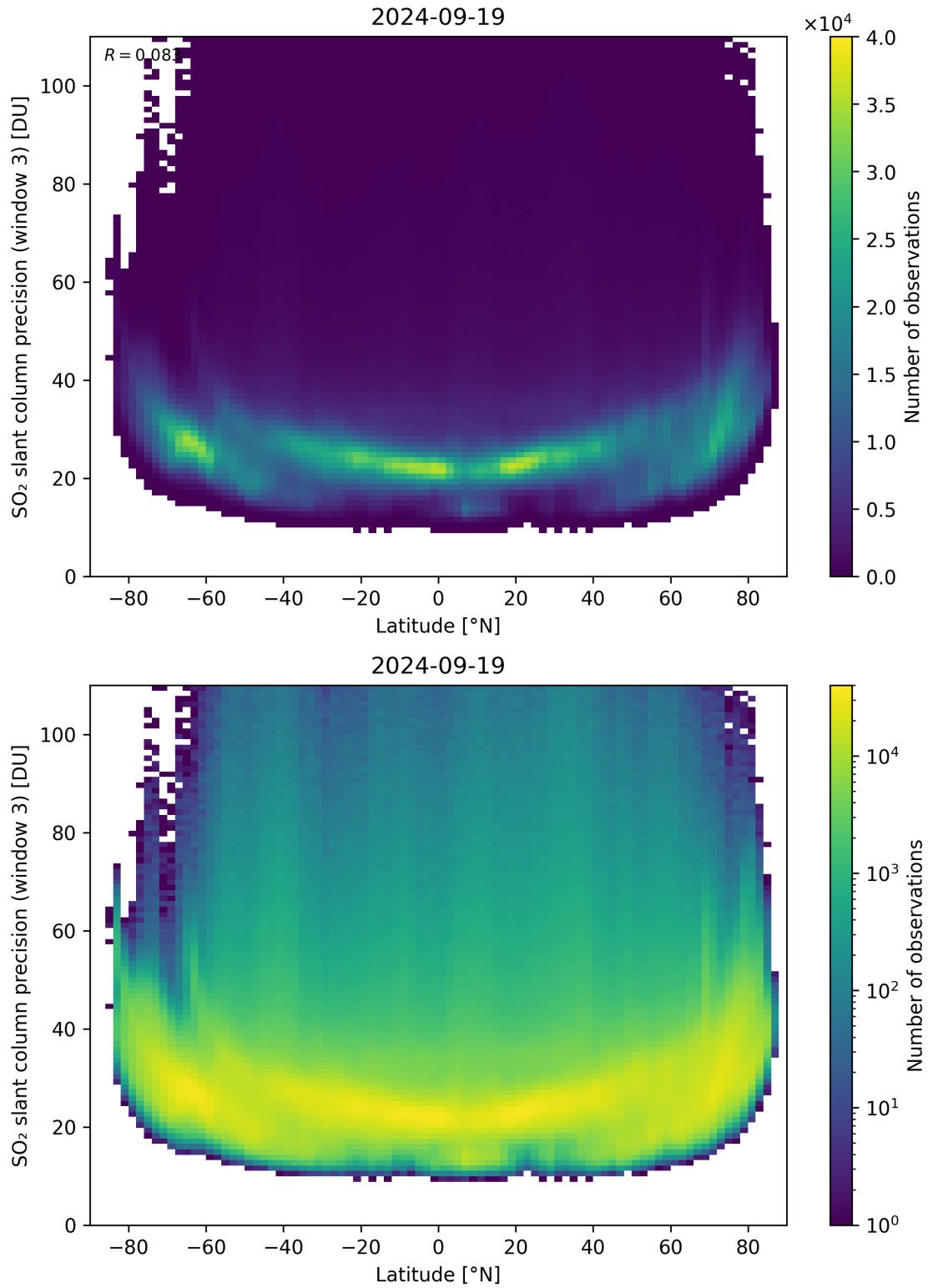
Figure 153: Scatter density plot of “Latitude” against “SO 2 slant column precision (window 3)” for 2024-09-18 to 2024-09-20.
