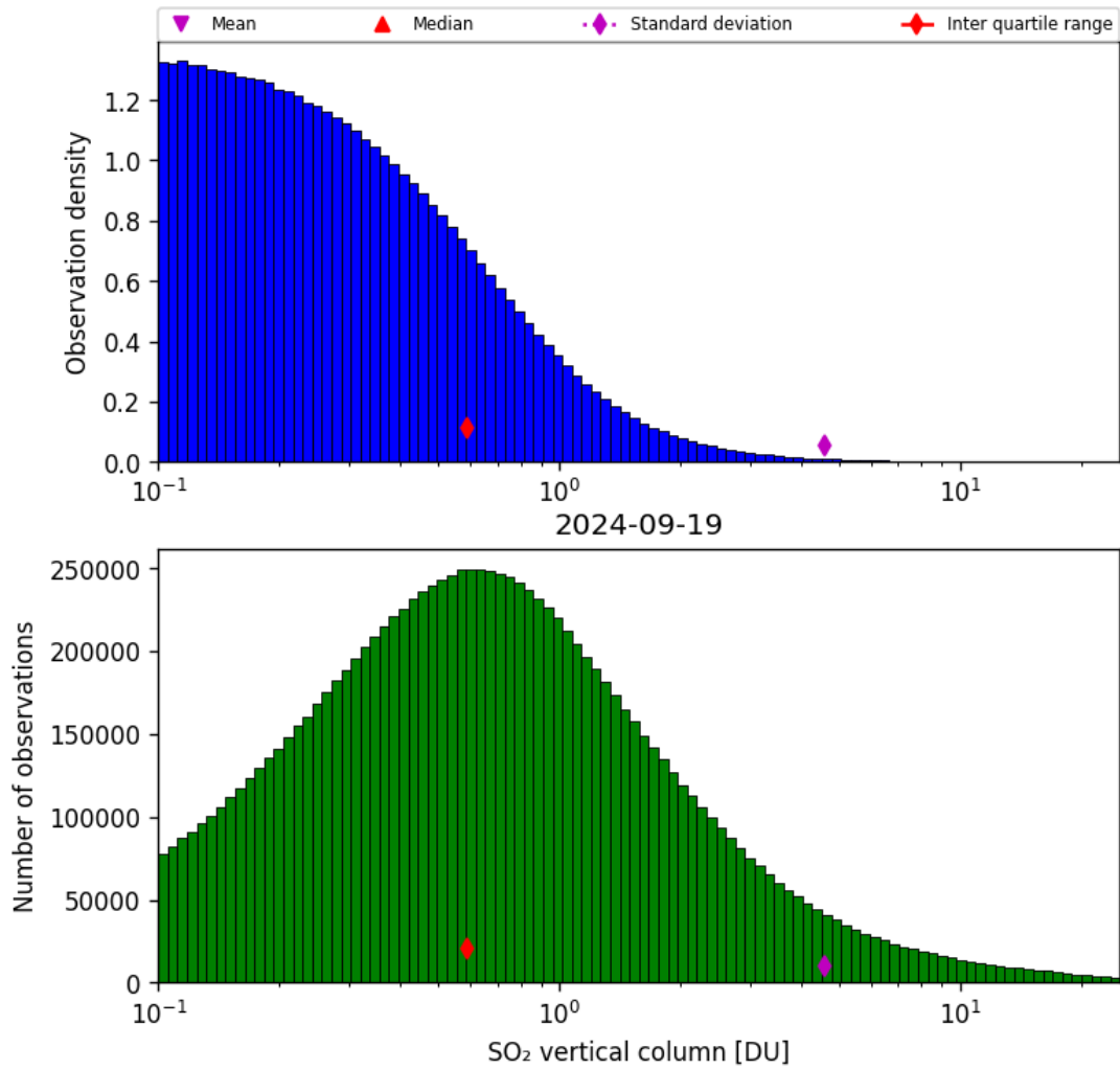
Figure 53: Histogram of “SO 2 vertical column” for 2024-09-18 to 2024-09-20
