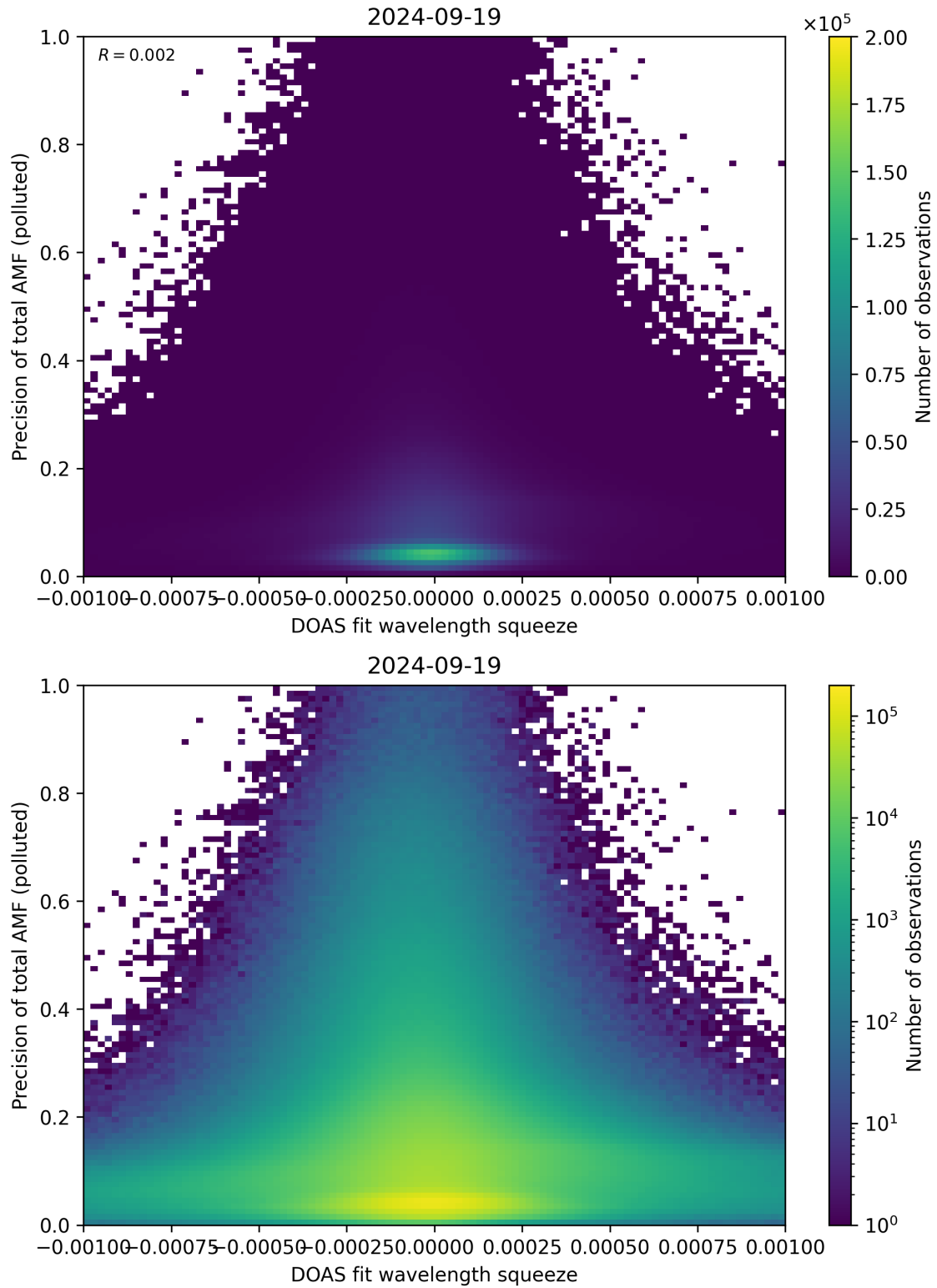
Figure 135: Scatter density plot of “DOAS fit wavelength squeeze” against “Precision of total AMF (polluted)” for 2024-09-18 to 2024-09-20.
