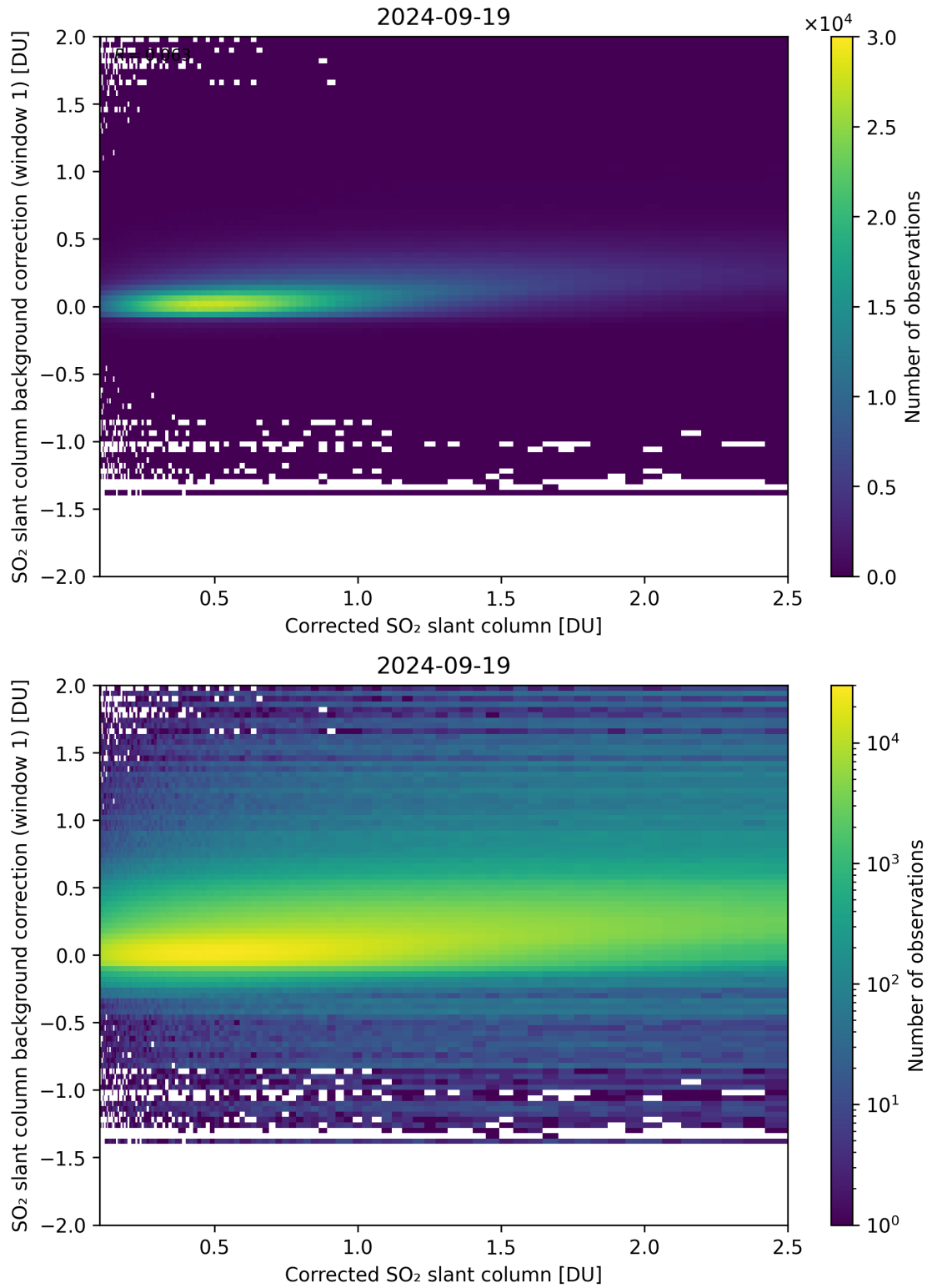
Figure 178: Scatter density plot of “Corrected SO 2 slant column” against “SO 2 slant column background correction (window 1)” for 2024-09-18 to 2024-09-20.
