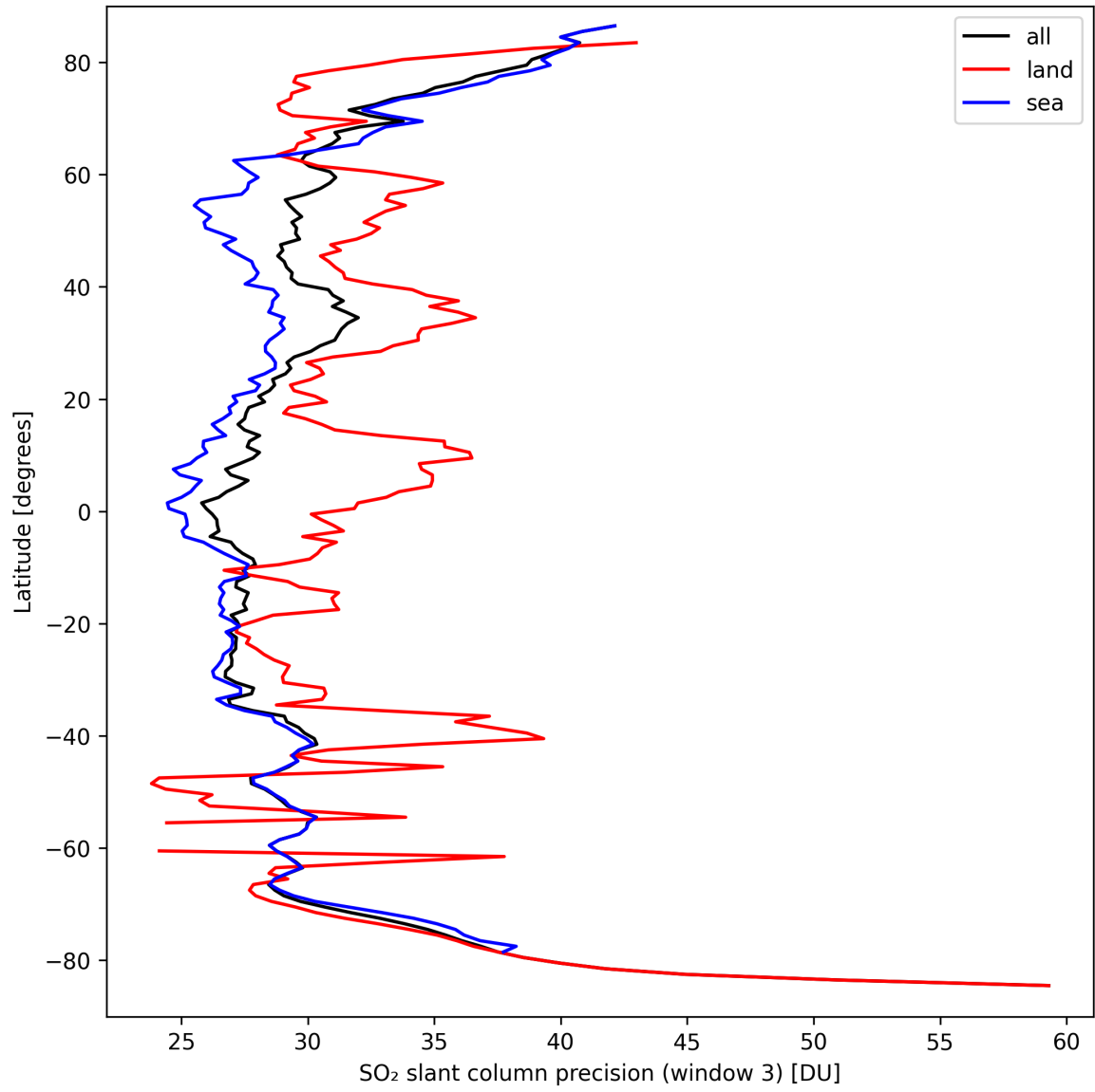
Figure 42: Zonal average of “SO 2 slant column precision (window 3)” for 2024-09-18 to 2024-09-20.
