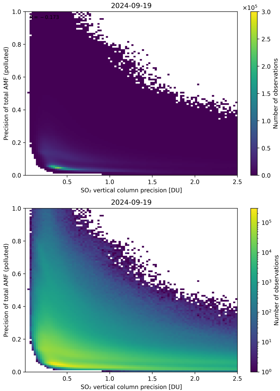
Figure 295: Scatter density plot of “SO 2 vertical column precision” against “Precision of total AMF (polluted)” for 2024-09-18 to 2024-09-20.
