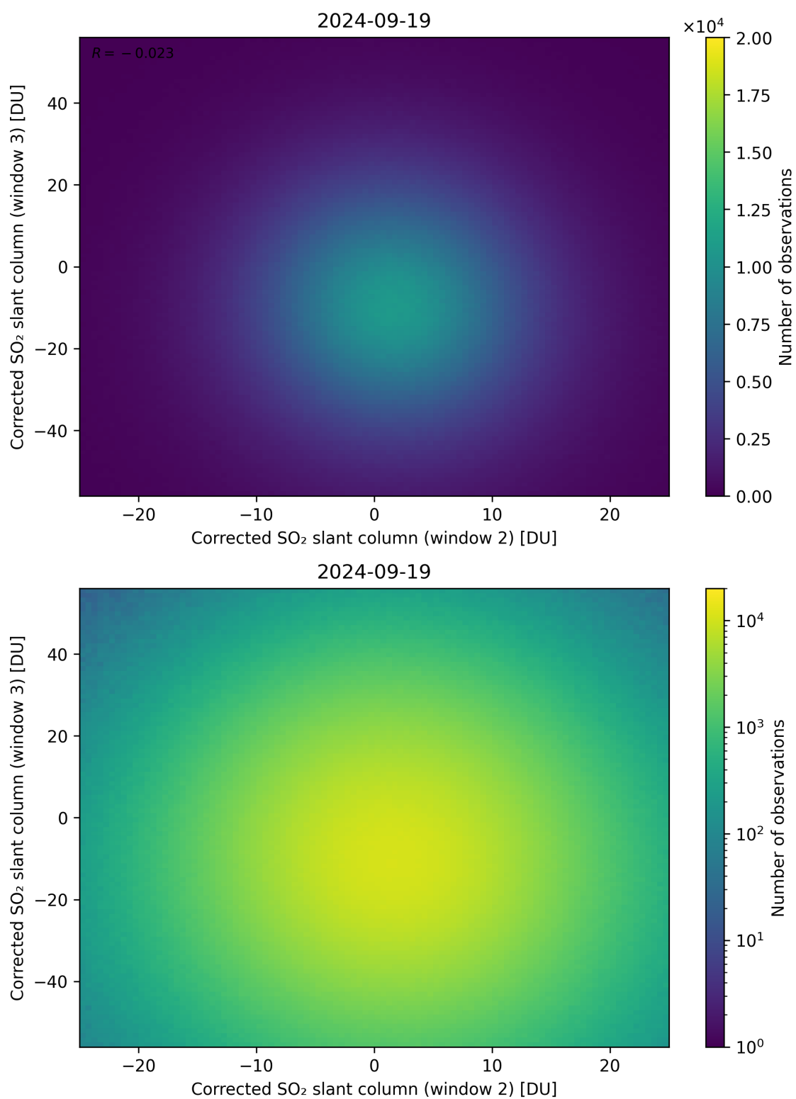
Figure 200: Scatter density plot of “Corrected SO 2 slant column (window 2)” against “Corrected SO 2 slant column (window 3)” for 2024-09-18 to 2024-09-20.
