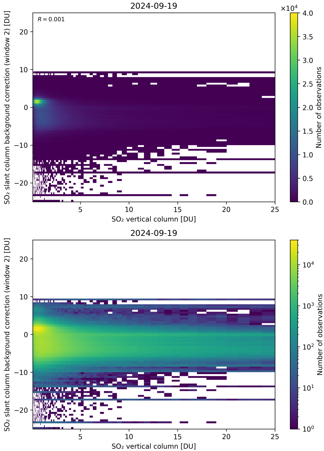
Figure 274: Scatter density plot of “SO 2 vertical column” against “SO 2 slant column background correction (window 2)” for 2024-09-18 to 2024-09-20.
