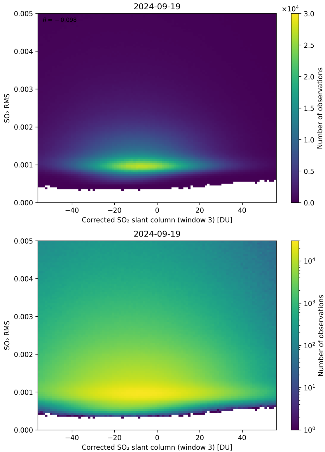
Figure 208: Scatter density plot of “Corrected SO 2 slant column (window 3)” against “SO 2 RMS” for 2024-09-18 to 2024-09-20.
