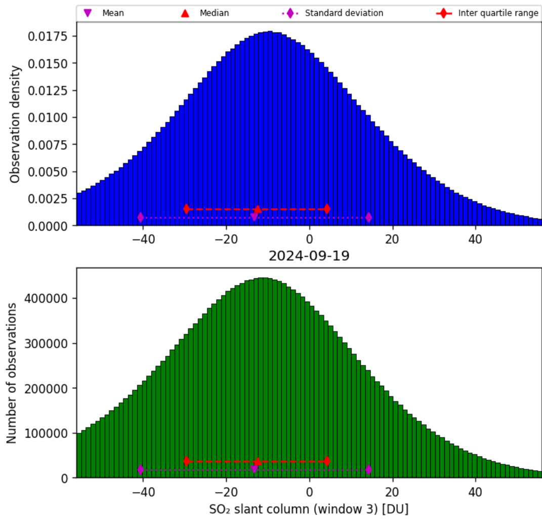
Figure 64: Histogram of “SO 2 slant column (window 3)” for 2024-09-18 to 2024-09-20
