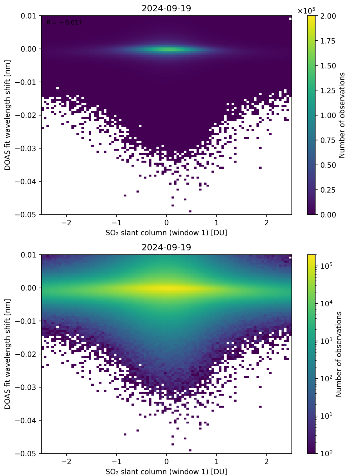
Figure 215: Scatter density plot of “SO 2 slant column (window 1)” against “DOAS fit wavelength shift” for 2024-09-18 to 2024-09-20.
