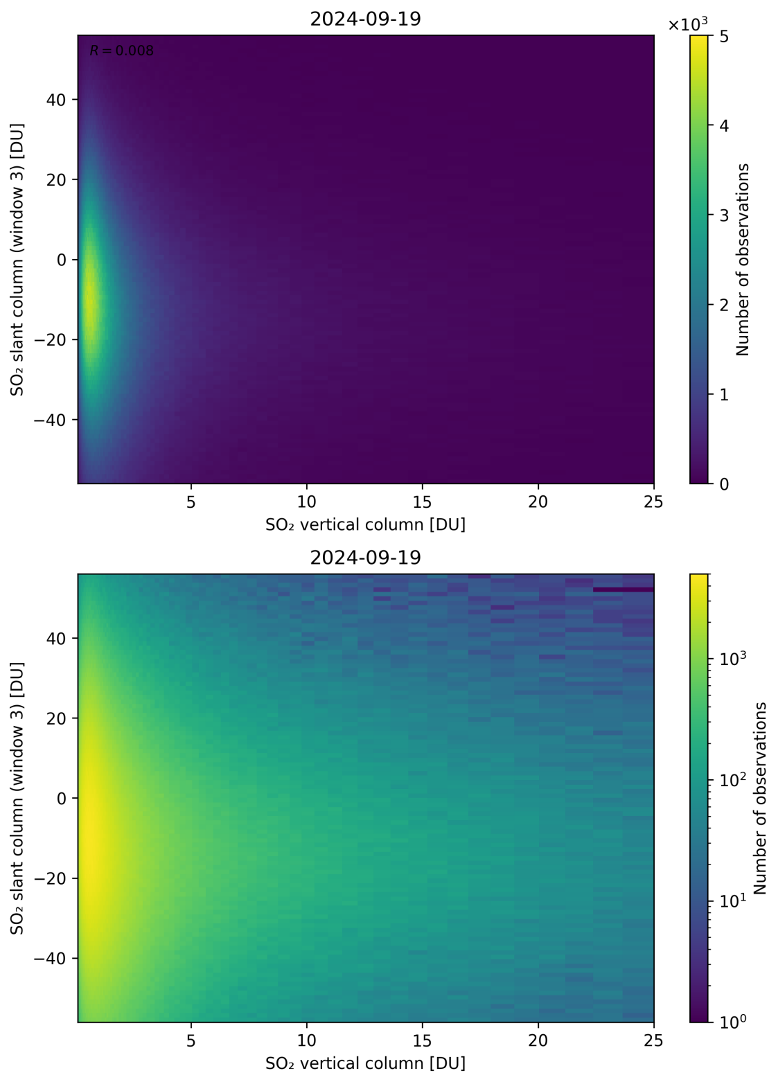
Figure 303: Scatter density plot of “SO 2 vertical column” against “SO 2 slant column (window 3)” for 2024-09-18 to 2024-09-20.
