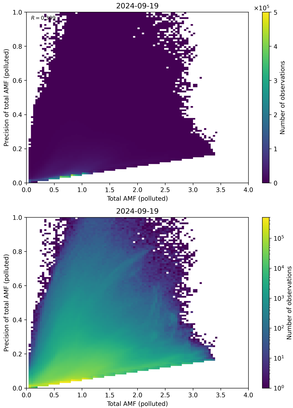
Figure 272: Scatter density plot of “Total AMF (polluted)” against “Precision of total AMF (polluted)” for 2024-09-18 to 2024-09-20.
