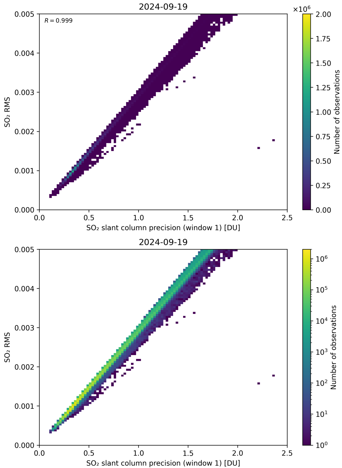
Figure 223: Scatter density plot of “SO 2 slant column precision (window 1)” against “SO 2 RMS” for 2024-09-18 to 2024-09-20.
