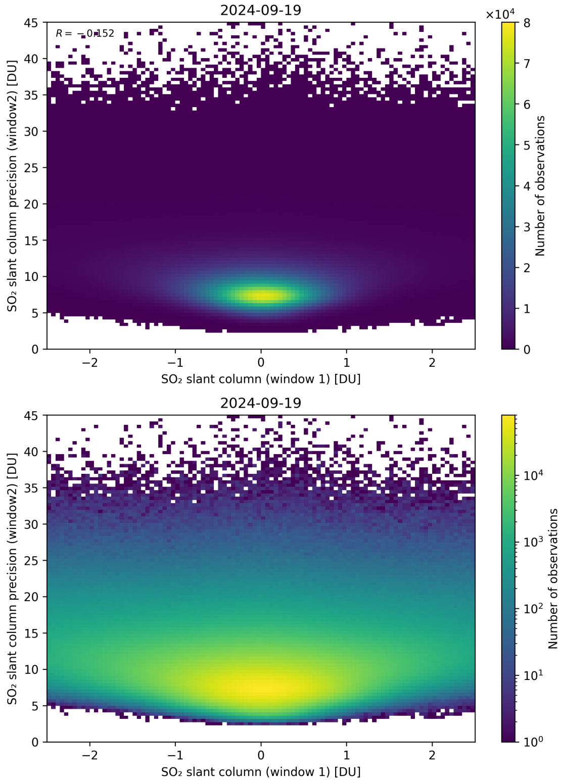
Figure 236: Scatter density plot of “SO 2 slant column (window 1)” against “SO 2 slant column precision (window2)” for 2024-09-18 to 2024-09-20.
