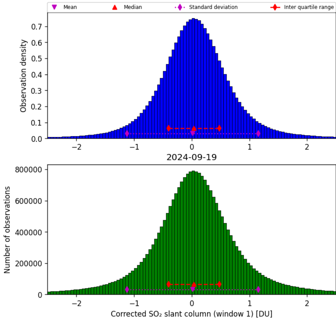
Figure 58: Histogram of “Corrected SO 2 slant column (window 1)” for 2024-09-18 to 2024-09-20
