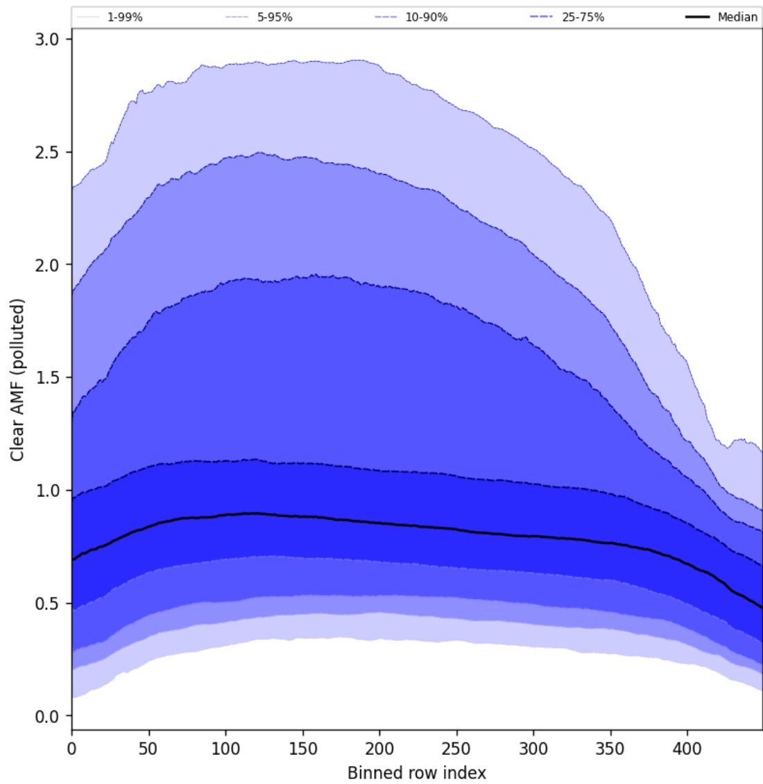
Figure 96: Along track statistics of “Clear AMF (polluted)” for 2024-09-18 to 2024-09-20
