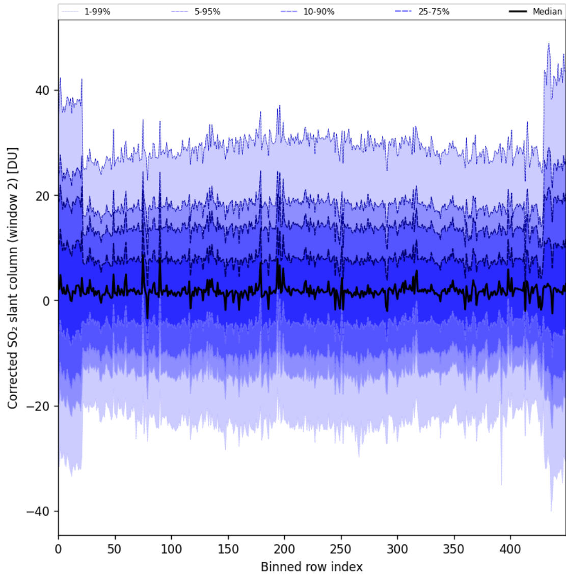
Figure 85: Along track statistics of “Corrected SO 2 slant column (window 2)” for 2024-09-18 to 2024-09-20
