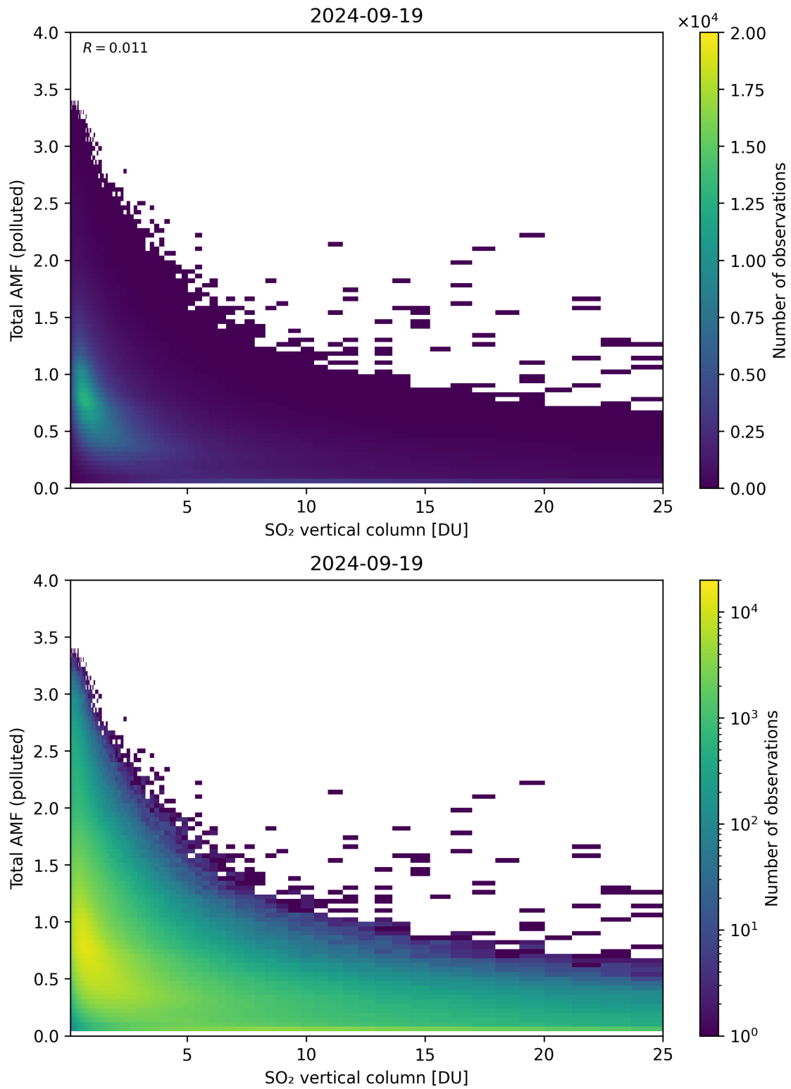
Figure 305: Scatter density plot of “SO 2 vertical column” against “Total AMF (polluted)” for 2024-09-18 to 2024-09-20.
