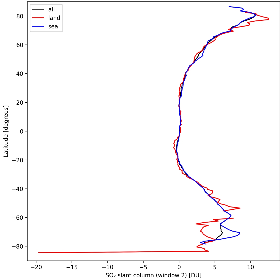
Figure 37: Zonal average of “SO 2 slant column (window 2)” for 2024-09-18 to 2024-09-20.
