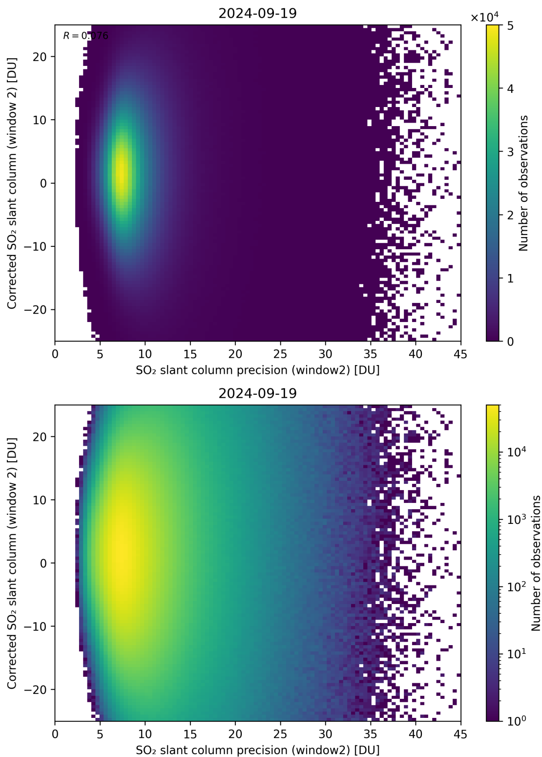
Figure 247: Scatter density plot of “SO 2 slant column precision (window2)” against “Corrected SO 2 slant column (window 2)” for 2024-09-18 to 2024-09-20.
