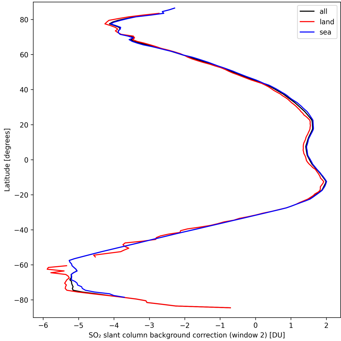
Figure 40: Zonal average of “SO 2 slant column background correction (window 2)” for 2024-09-18 to 2024-09-20.
