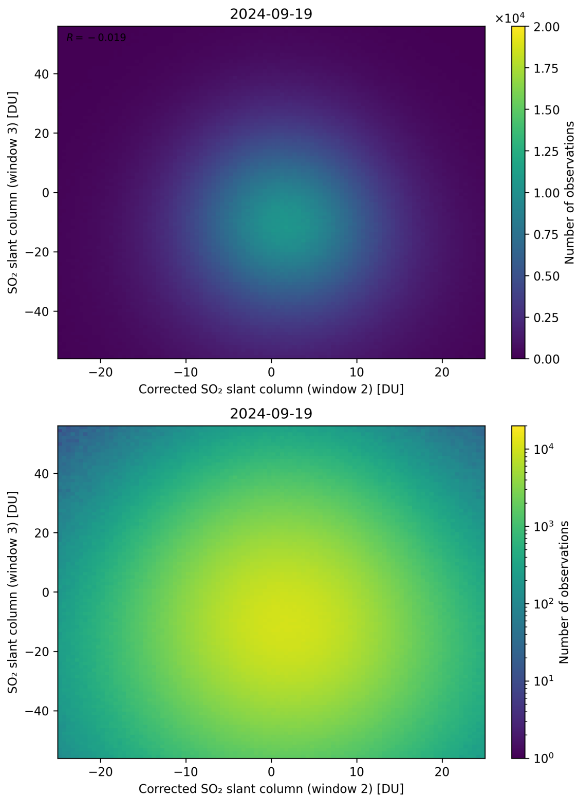
Figure 201: Scatter density plot of “Corrected SO 2 slant column (window 2)” against “SO 2 slant column (window 3)” for 2024-09-18 to 2024-09-20.
