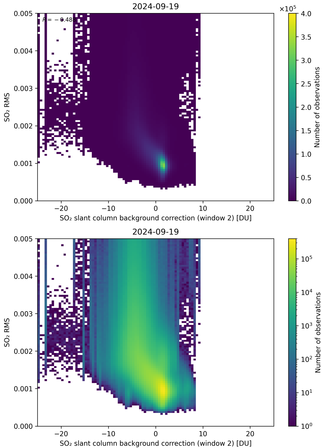
Figure 114: Scatter density plot of “SO 2 slant column background correction (window 2)” against “SO 2 RMS” for 2024-09-18 to 2024-09-20.
