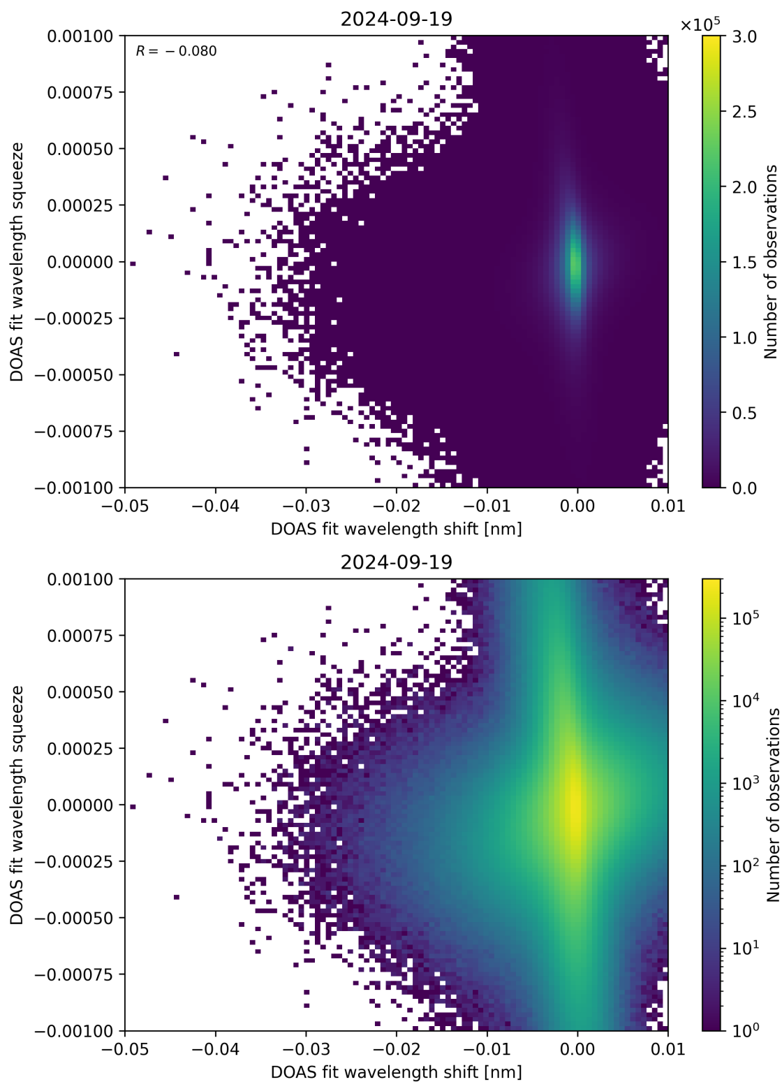
Figure 127: Scatter density plot of “DOAS fit wavelength shift” against “DOAS fit wavelength squeeze” for 2024-09-18 to 2024-09-20.
