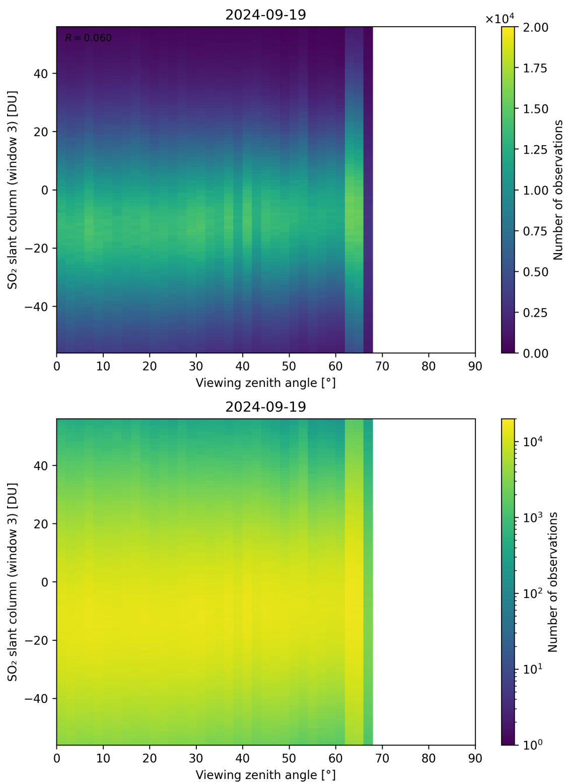
Figure 323: Scatter density plot of “Viewing zenith angle” against “SO 2 slant column (window 3)” for 2024-09-18 to 2024-09-20.
