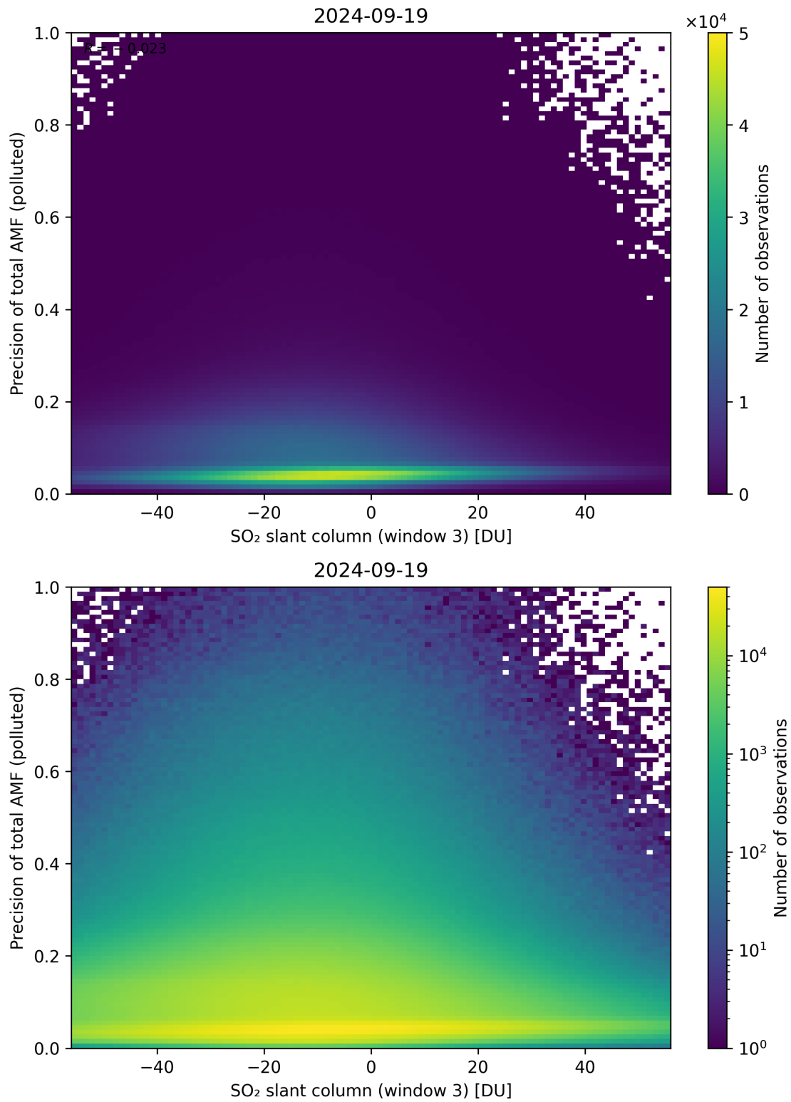
Figure 269: Scatter density plot of “SO 2 slant column (window 3)” against “Precision of total AMF (polluted)” for 2024-09-18 to 2024-09-20.
