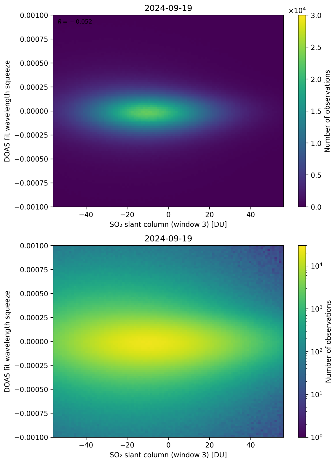
Figure 255: Scatter density plot of “SO 2 slant column (window 3)” against “DOAS fit wavelength squeeze” for 2024-09-18 to 2024-09-20.
