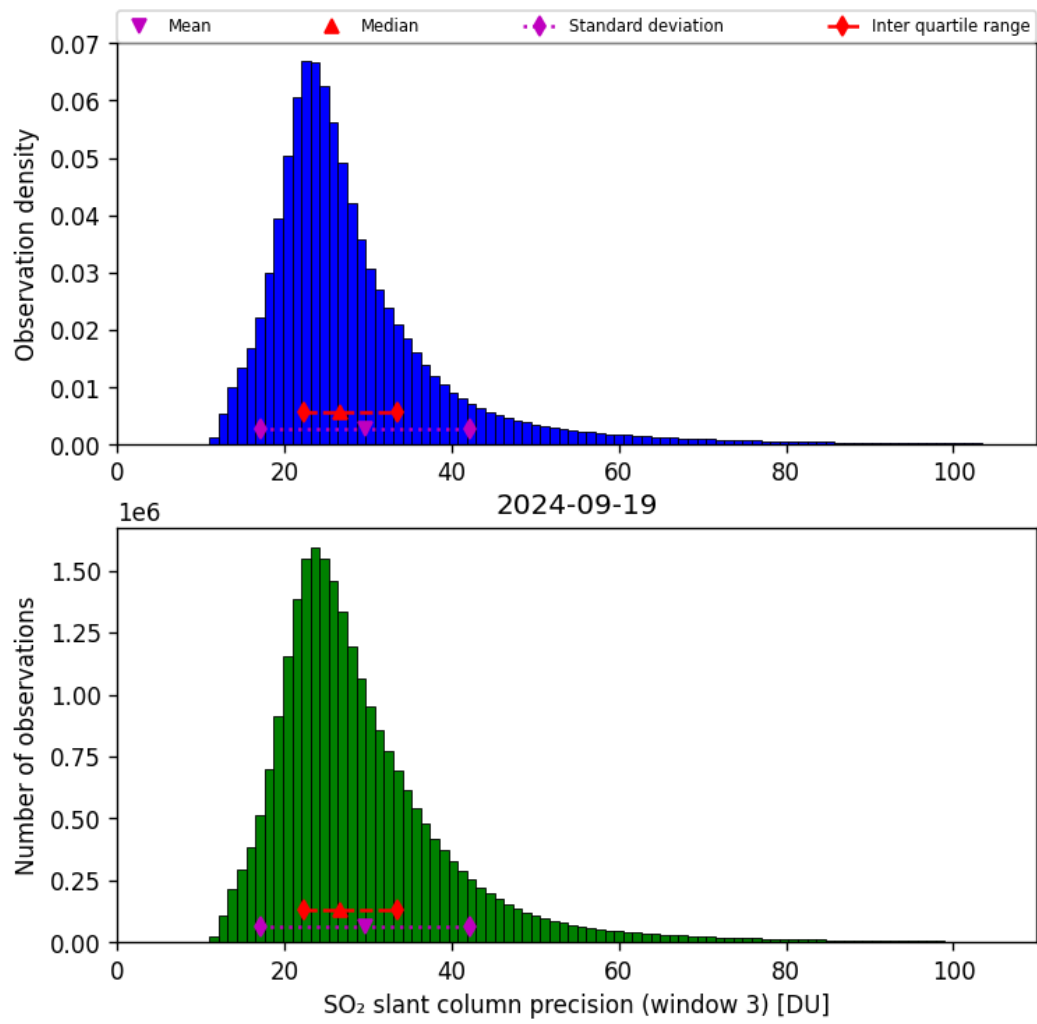
Figure 65: Histogram of “SO 2 slant column precision (window 3)” for 2024-09-18 to 2024-09-20
