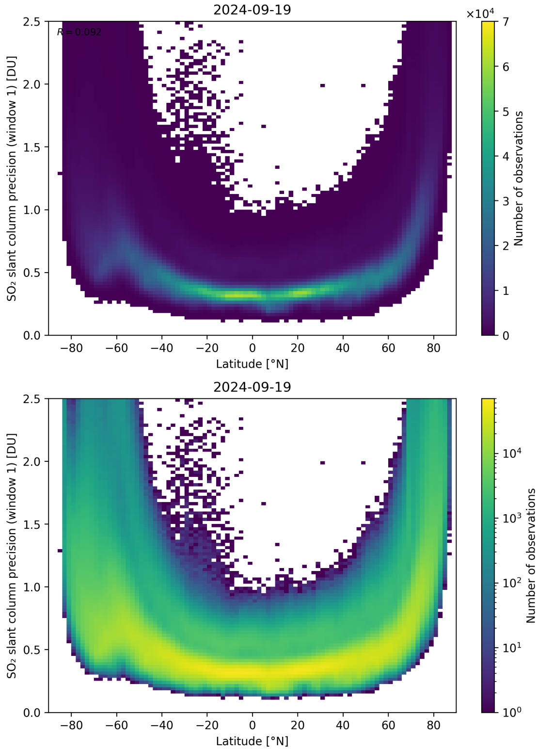
Figure 150: Scatter density plot of “Latitude” against “SO 2 slant column precision (window 1)” for 2024-09-18 to 2024-09-20.
