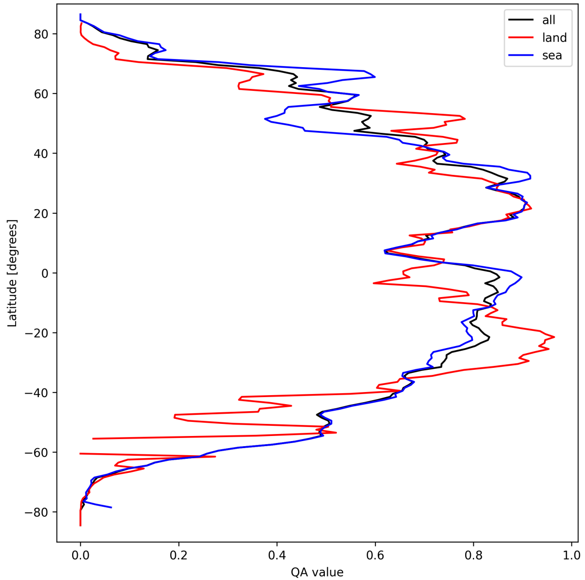
Figure 29: Zonal average of “QA value” for 2024-09-18 to 2024-09-20.
