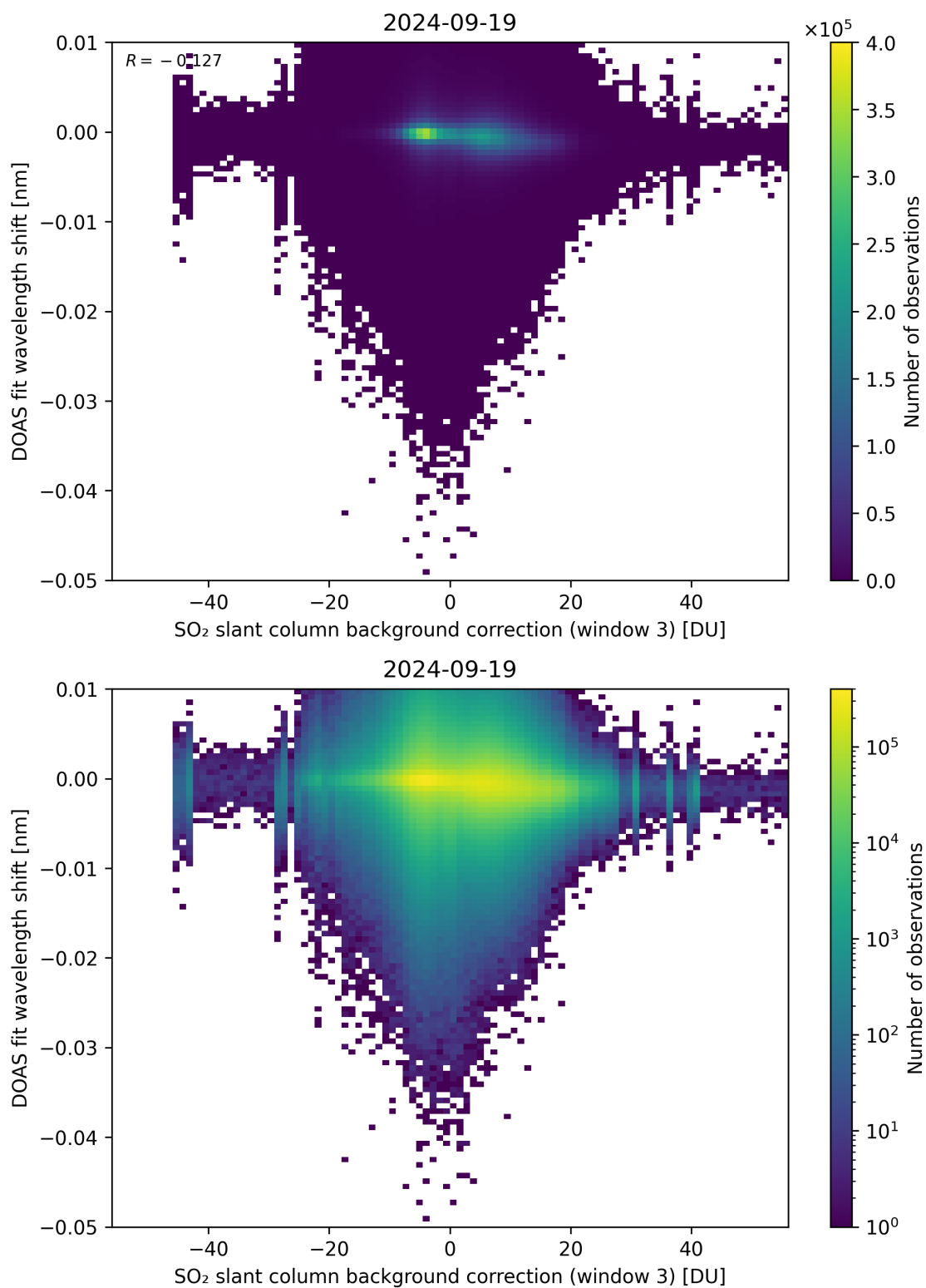
Figure 121: Scatter density plot of “SO 2 slant column background correction (window 3)” against “DOAS fit wavelength shift” for 2024-09-18 to 2024-09-20.
