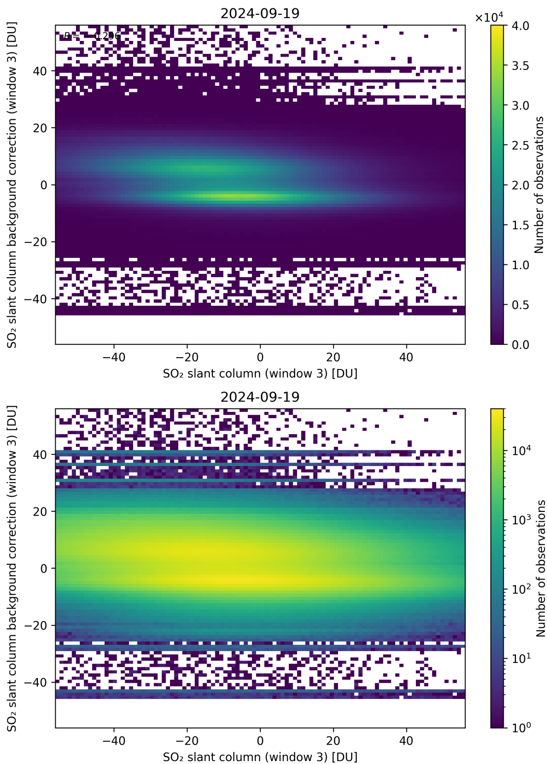
Figure 253: Scatter density plot of “SO 2 slant column (window 3)” against “SO 2 slant column background correction (window 3)” for 2024-09-18 to 2024-09-20.
