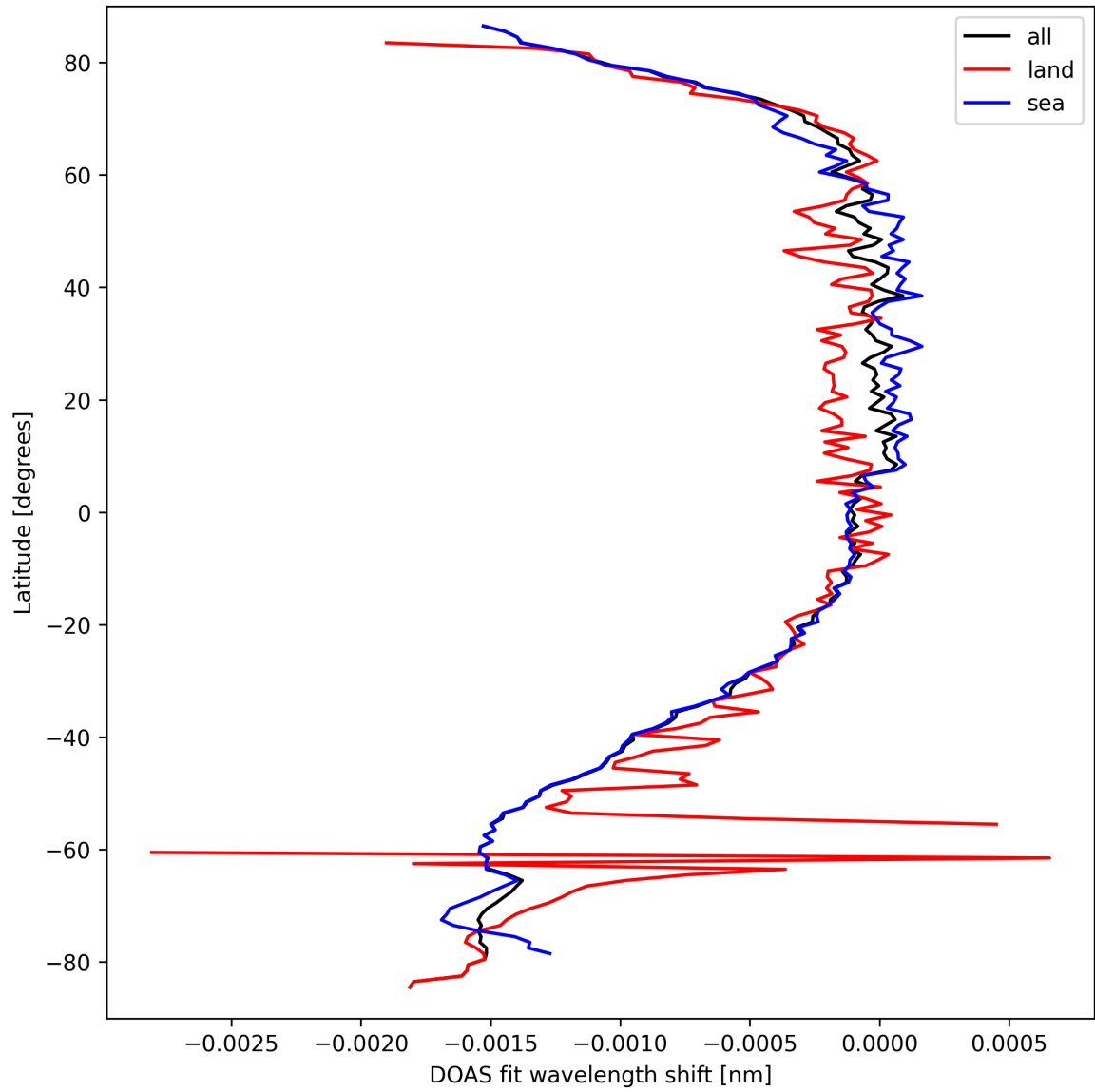
Figure 45: Zonal average of “DOAS fit wavelength shift” for 2024-09-18 to 2024-09-20.
