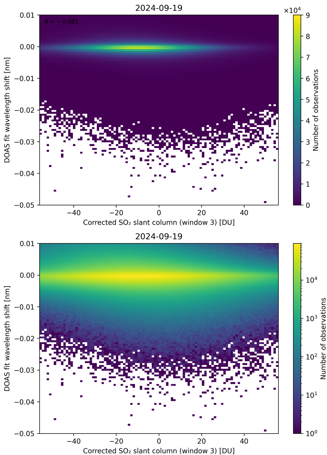
Figure 206: Scatter density plot of “Corrected SO 2 slant column (window 3)” against “DOAS fit wavelength shift” for 2024-09-18 to 2024-09-20.
