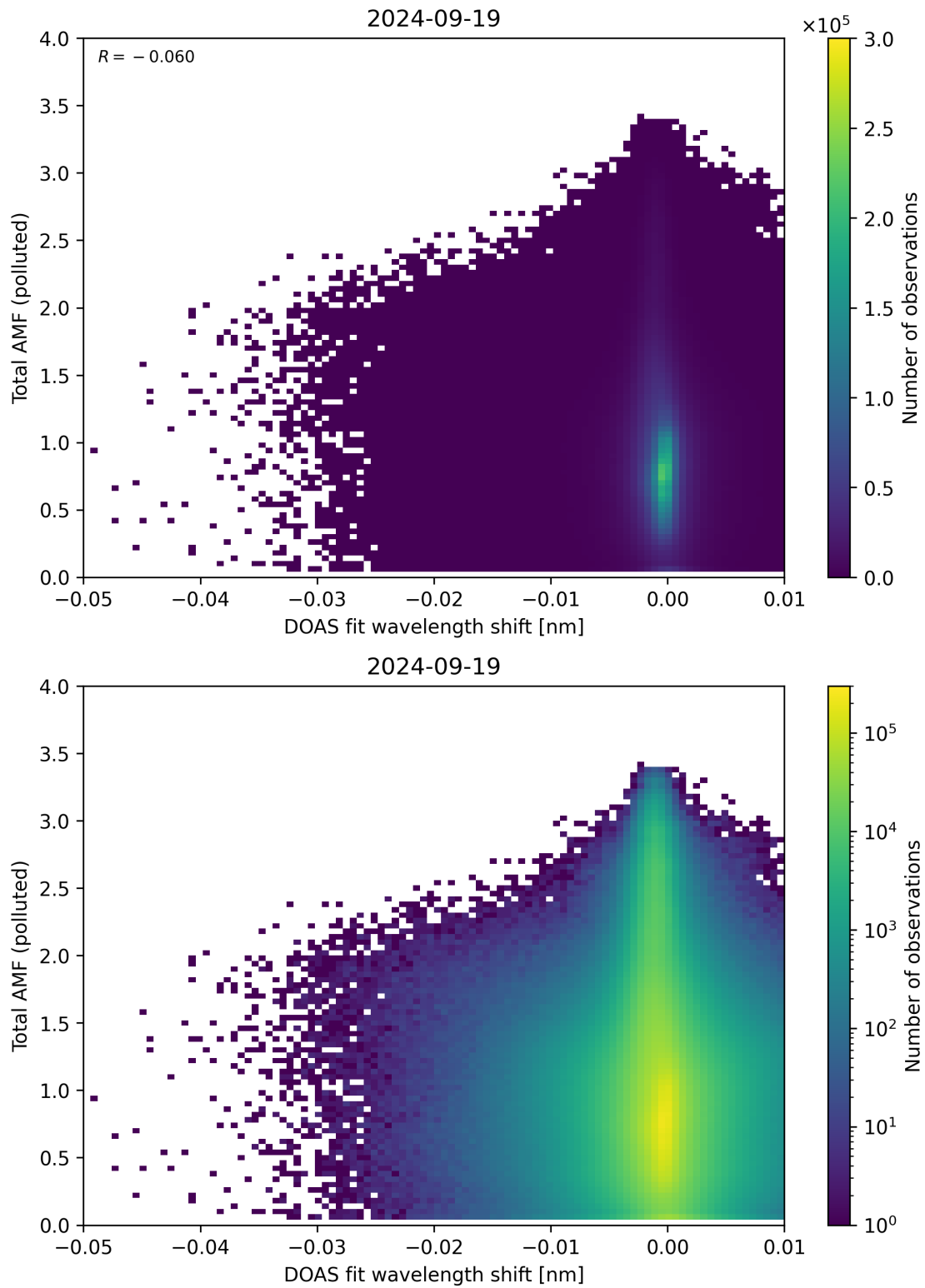
Figure 130: Scatter density plot of “DOAS fit wavelength shift” against “Total AMF (polluted)” for 2024-09-18 to 2024-09-20.
