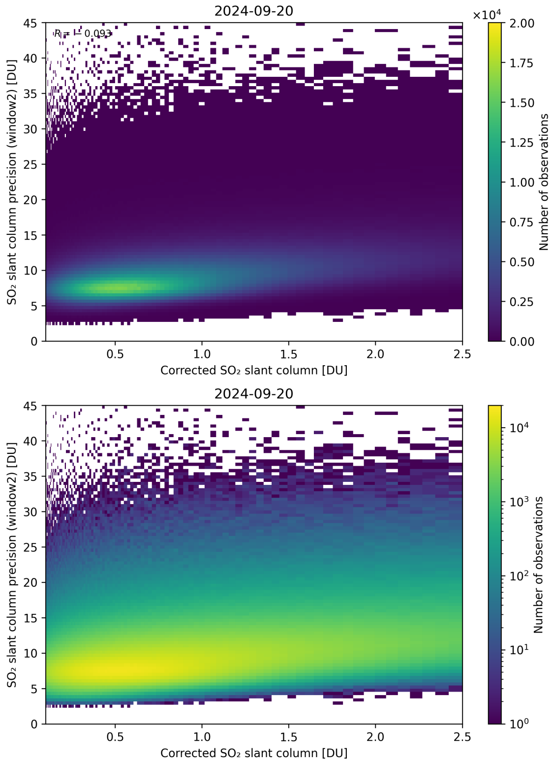
Figure 189: Scatter density plot of “Corrected SO 2 slant column” against “SO 2 slant column precision (window2)” for 2024-09-19 to 2024-09-21.
