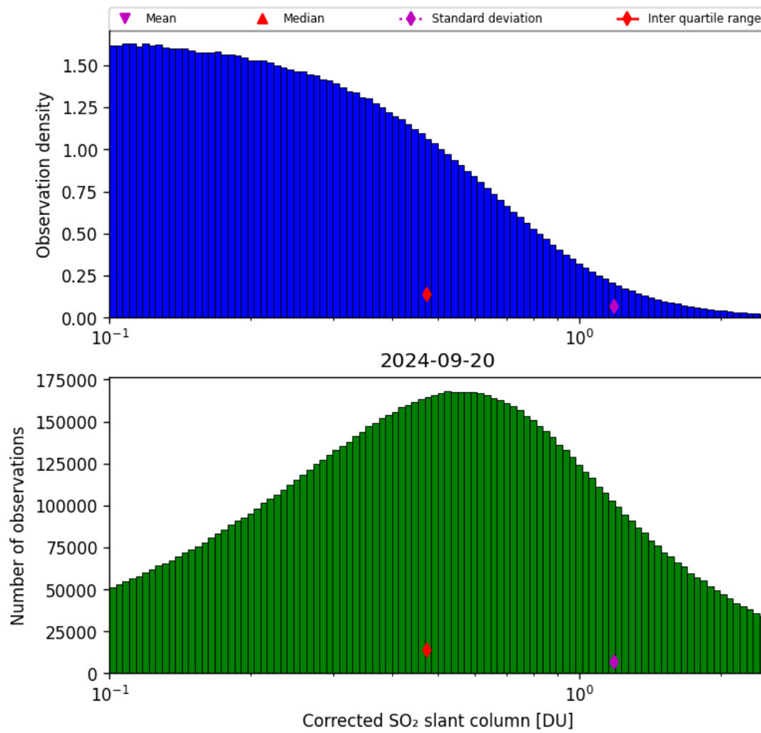
Figure 55: Histogram of "Corrected SO 2 slant column" for 2024-09-19 to 2024-09-21
