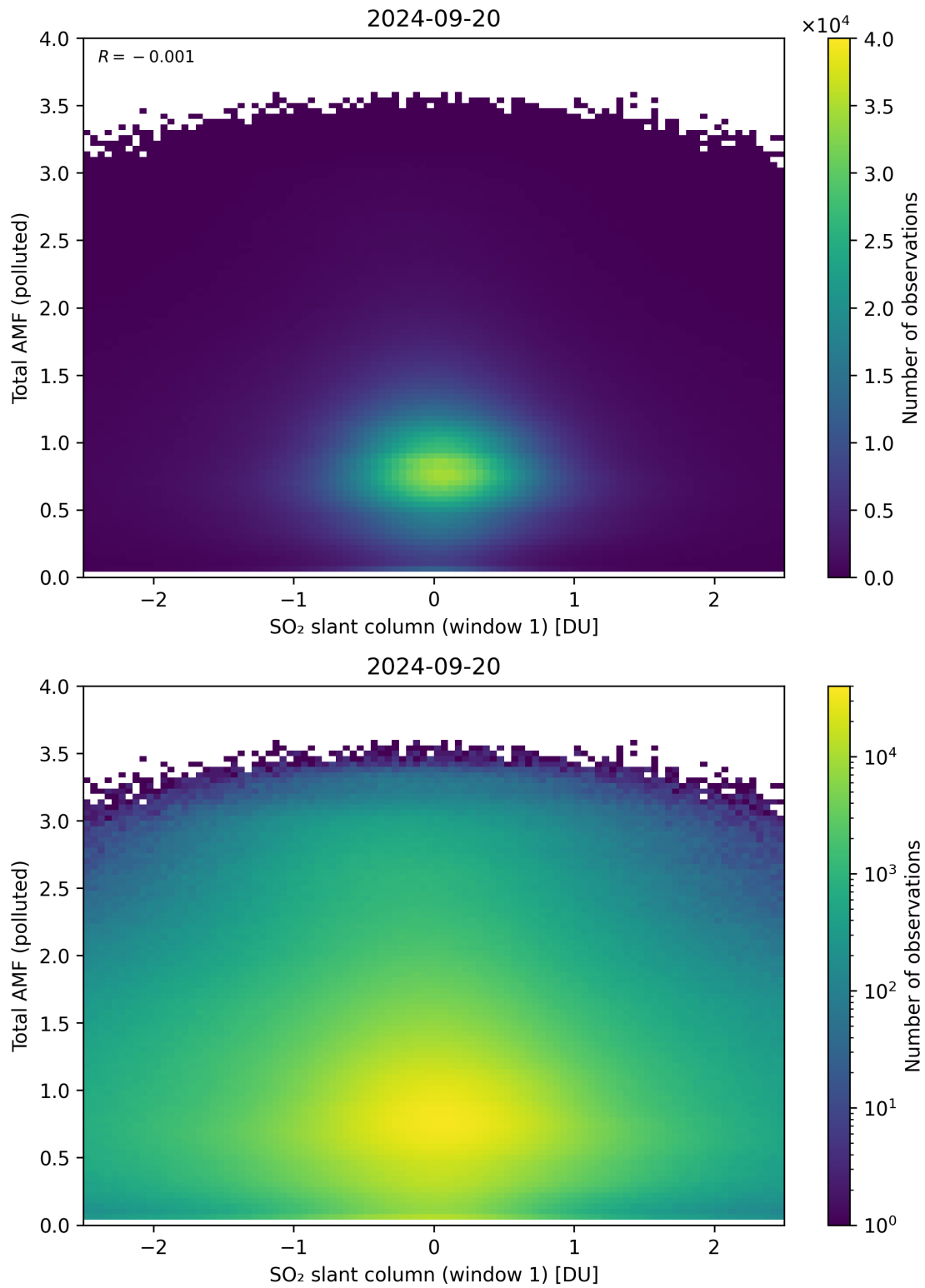
Figure 239: Scatter density plot of “SO 2 slant column (window 1)” against “Total AMF (polluted)” for 2024-09-19 to 2024-09-21.
