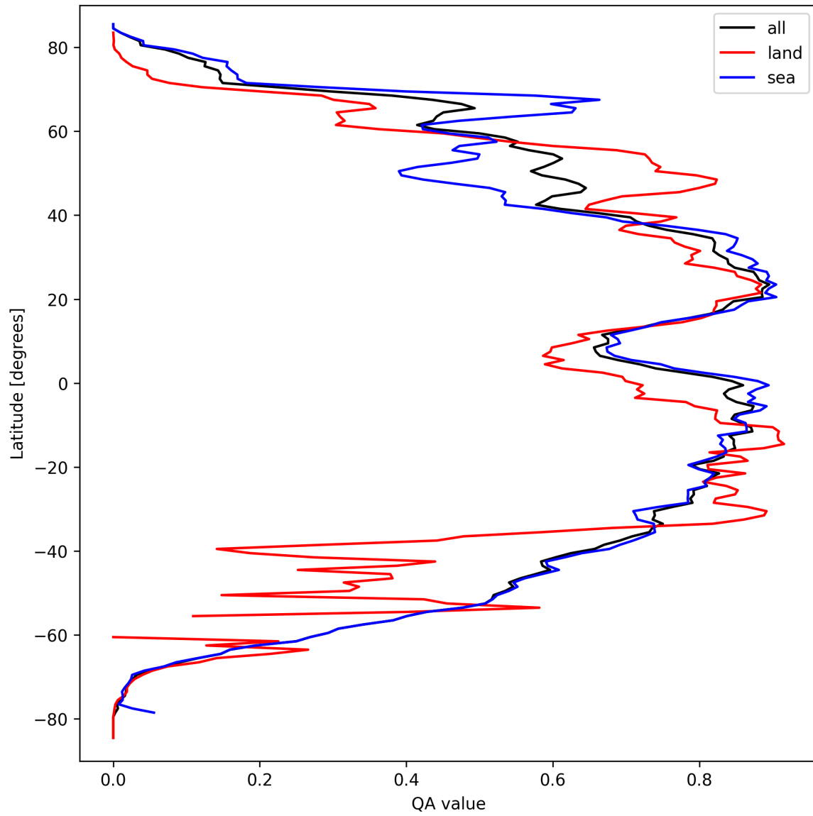
Figure 29: Zonal average of “QA value” for 2024-09-19 to 2024-09-21.
