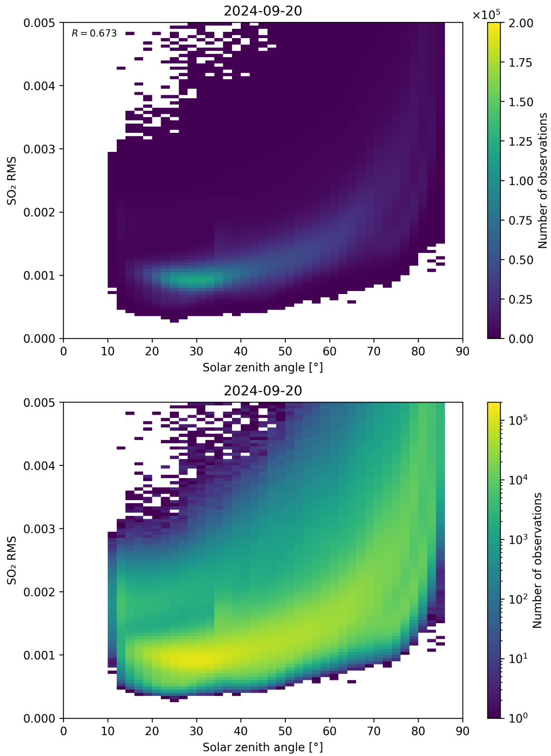
Figure 163: Scatter density plot of “Solar zenith angle” against “SO 2 RMS” for 2024-09-19 to 2024-09-21.
