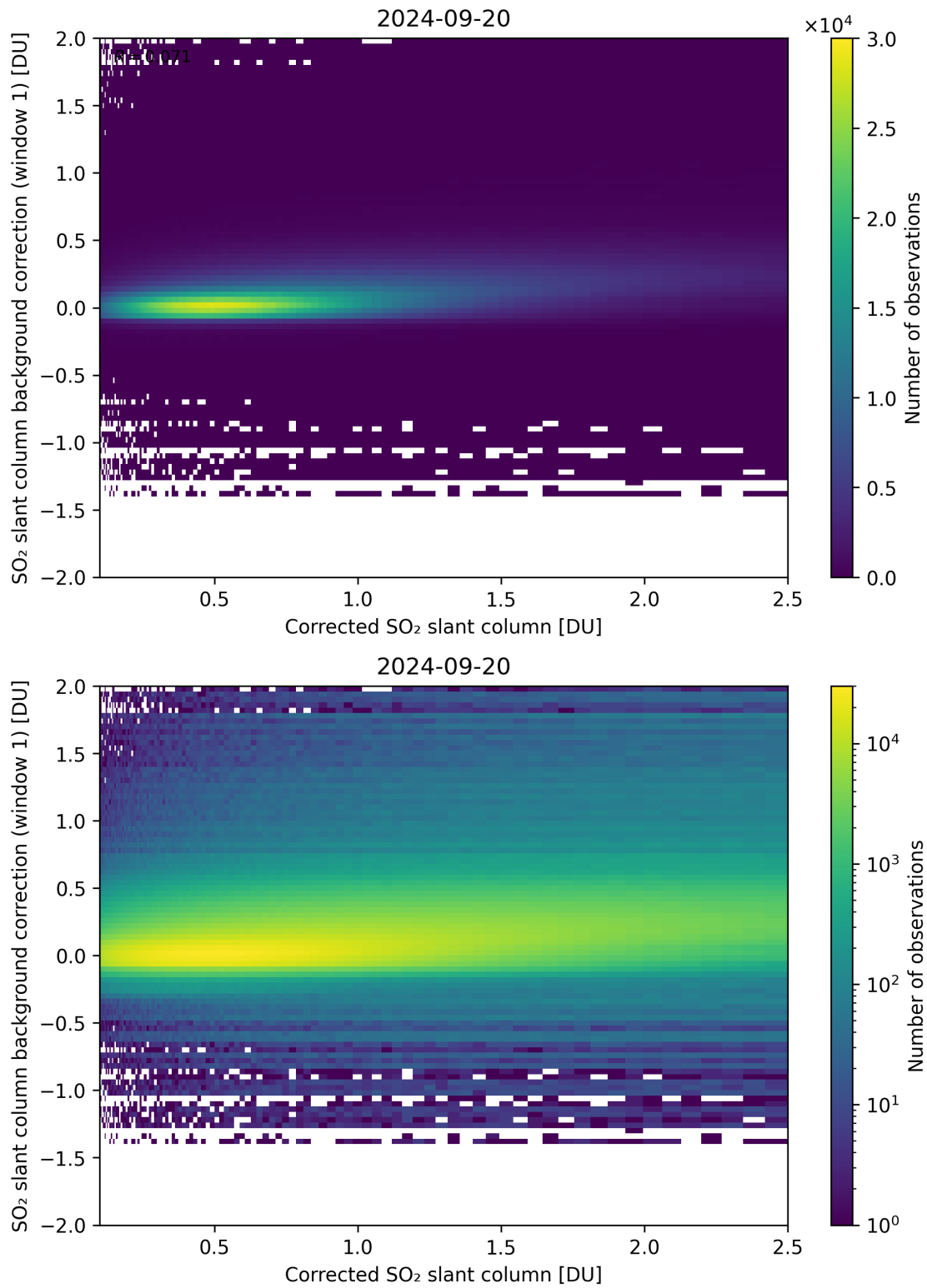
Figure 178: Scatter density plot of “Corrected SO 2 slant column” against “SO 2 slant column background correction (window 1)” for 2024-09-19 to 2024-09-21.
