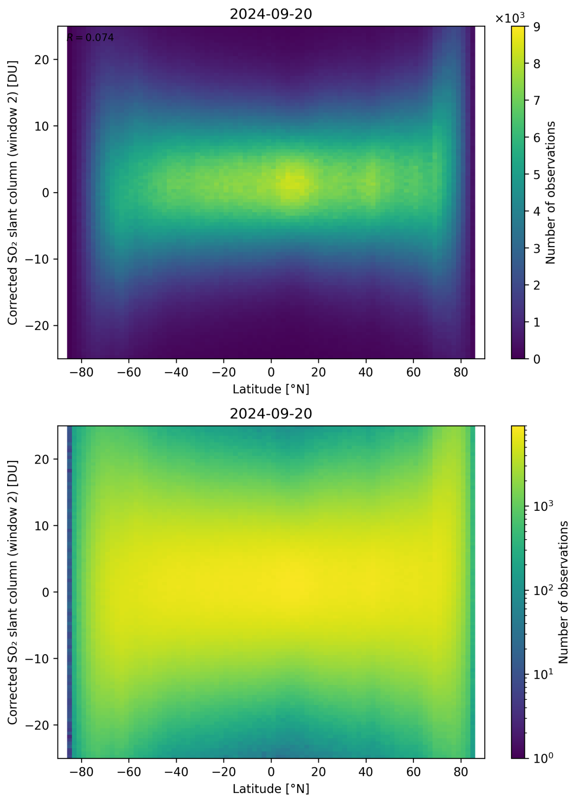
Figure 147: Scatter density plot of “Latitude” against “Corrected SO 2 slant column (window 2)” for 2024-09-19 to 2024-09-21.
