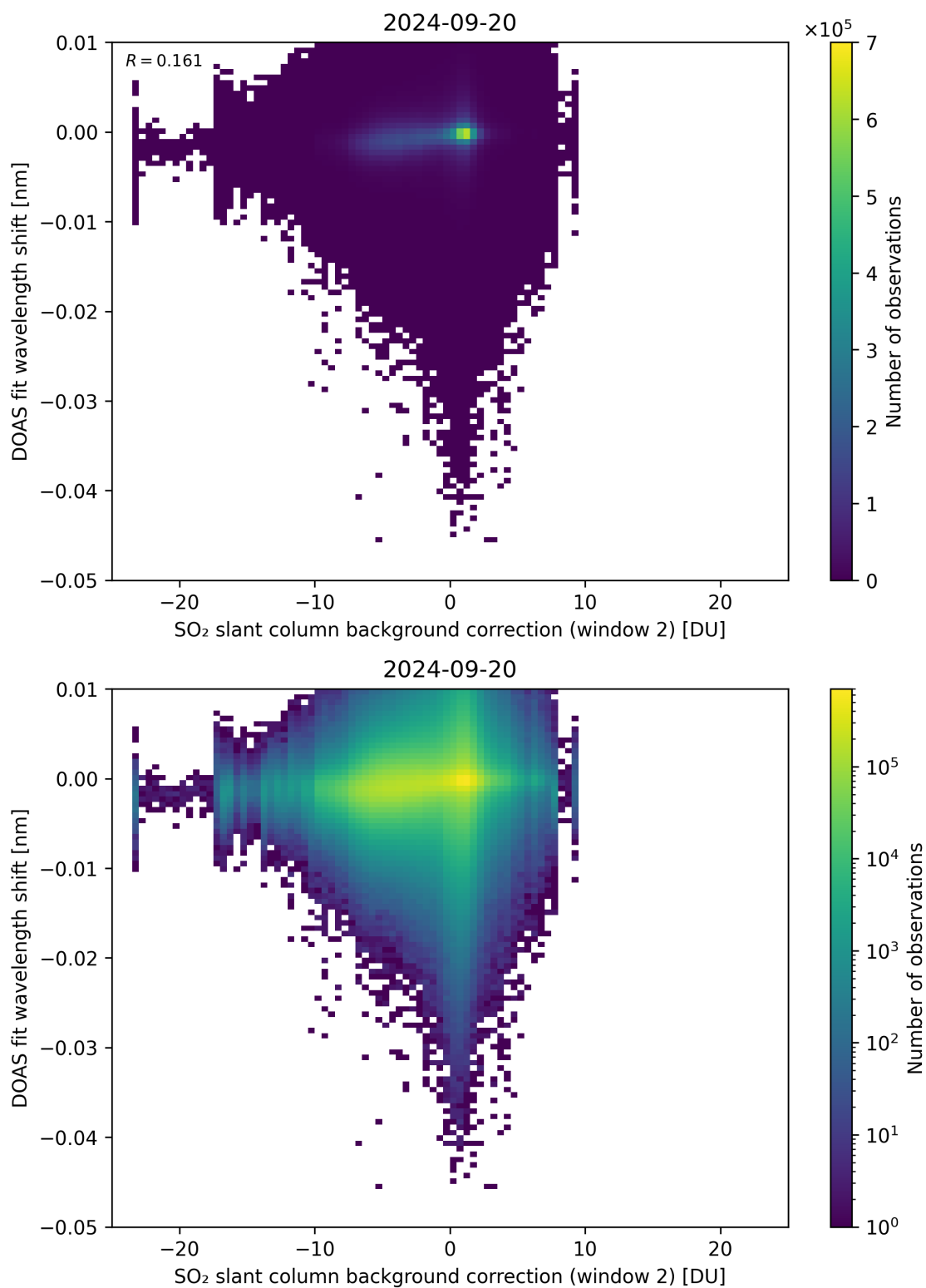
Figure 112: Scatter density plot of “SO 2 slant column background correction (window 2)” against “DOAS fit wavelength shift” for 2024-09-19 to 2024-09-21.
