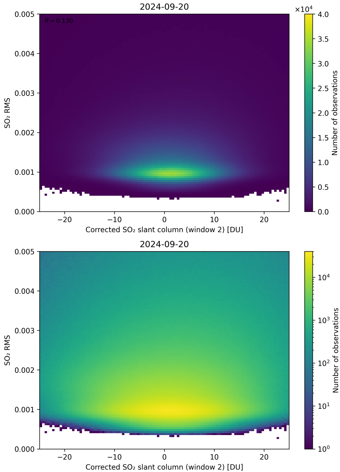
Figure 198: Scatter density plot of “Corrected SO 2 slant column (window 2)” against “SO 2 RMS” for 2024-09-19 to 2024-09-21.
