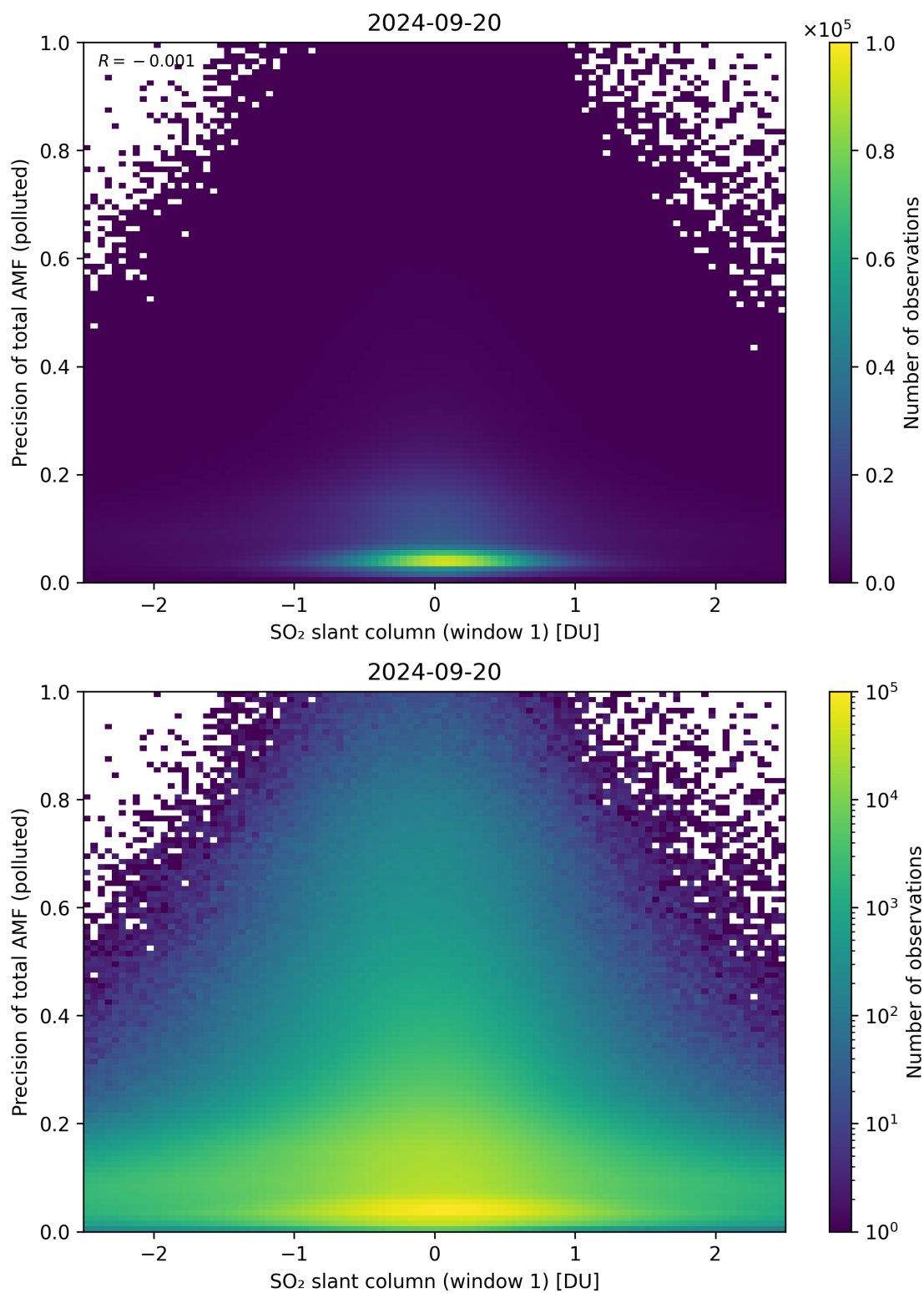
Figure 240: Scatter density plot of “SO 2 slant column (window 1)” against “Precision of total AMF (polluted)” for 2024-09-19 to 2024-09-21.
