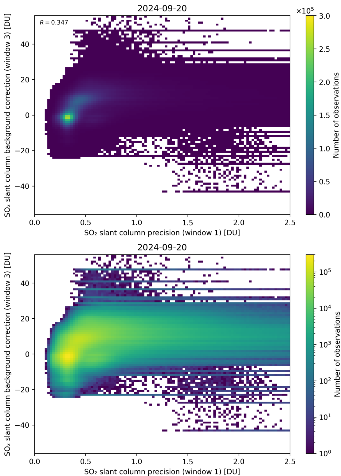
Figure 220: Scatter density plot of “SO 2 slant column precision (window 1)” against “SO 2 slant column background correction (window 3)” for 2024-09-19 to 2024-09-21.
