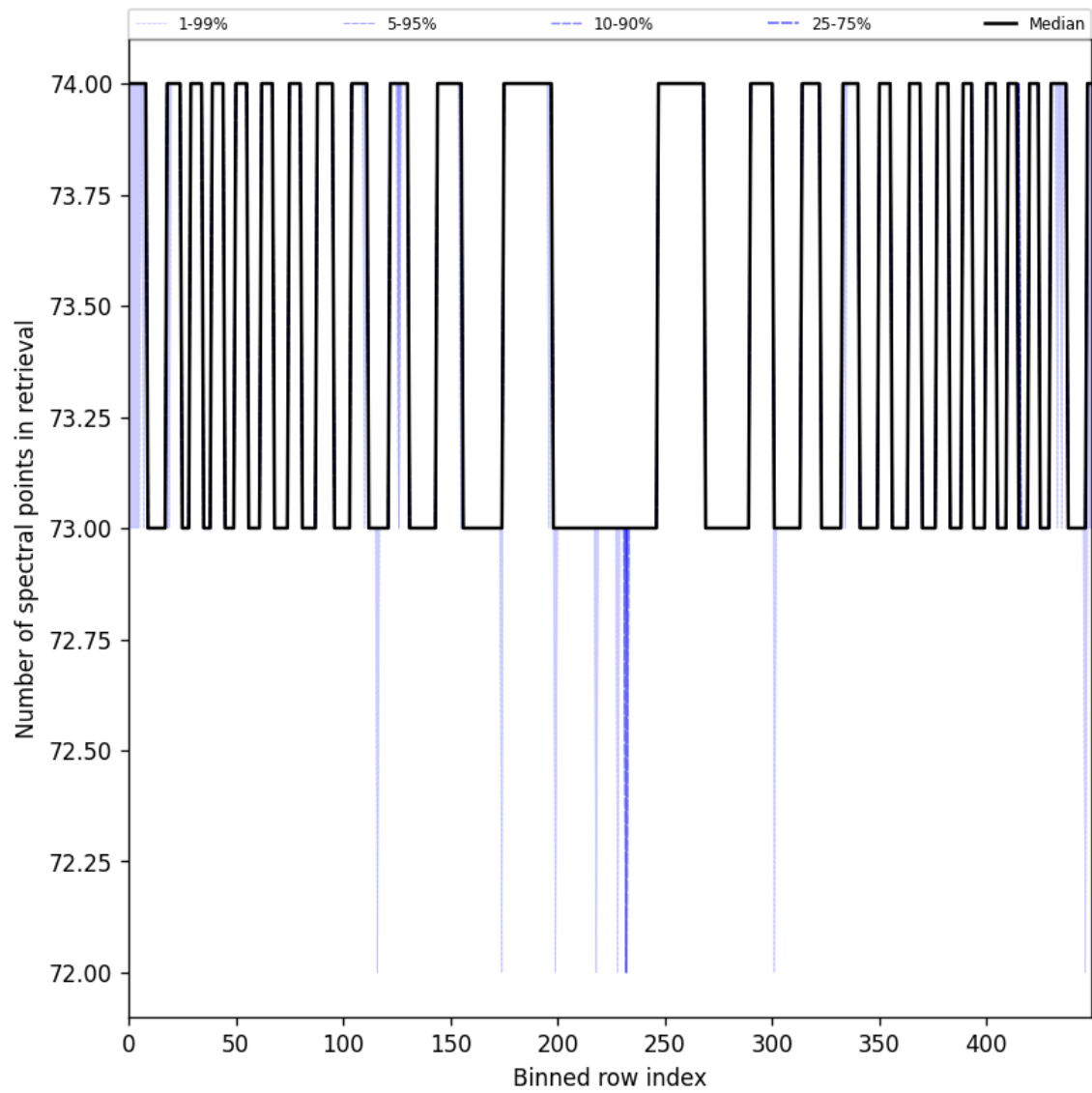
Figure 97: Along track statistics of “Number of spectral points in retrieval” for 2024-09-19 to 2024-09-21
