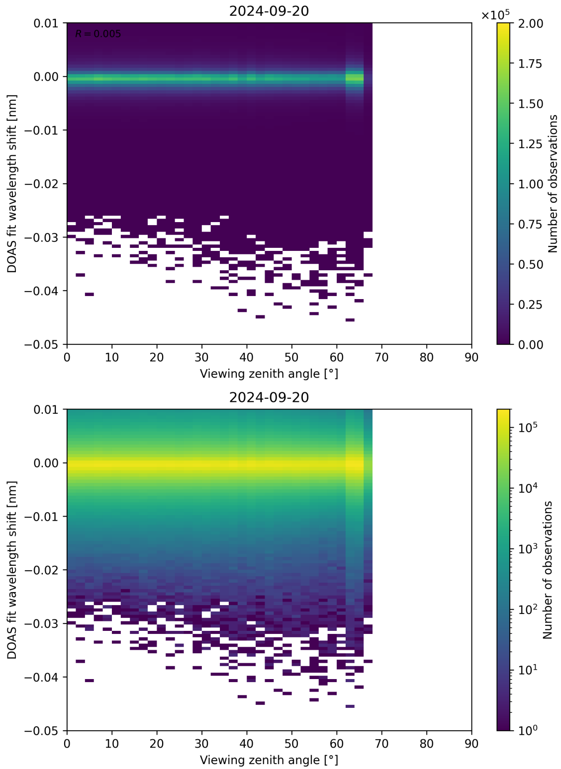
Figure 311: Scatter density plot of “Viewing zenith angle” against “DOAS fit wavelength shift” for 2024-09-19 to 2024-09-21.
