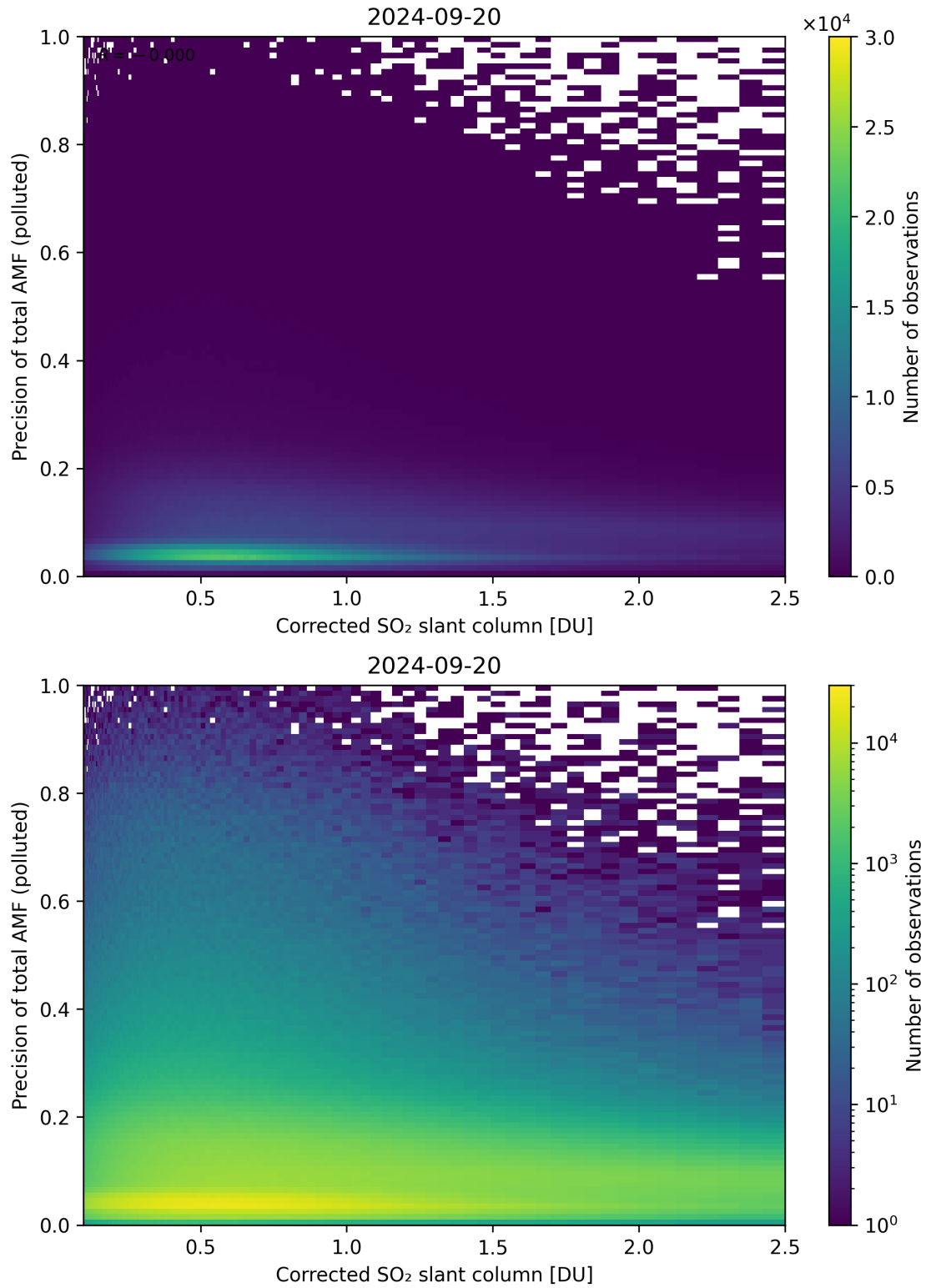
Figure 193: Scatter density plot of “Corrected SO 2 slant column” against “Precision of total AMF (polluted)” for 2024-09-19 to 2024-09-21.
