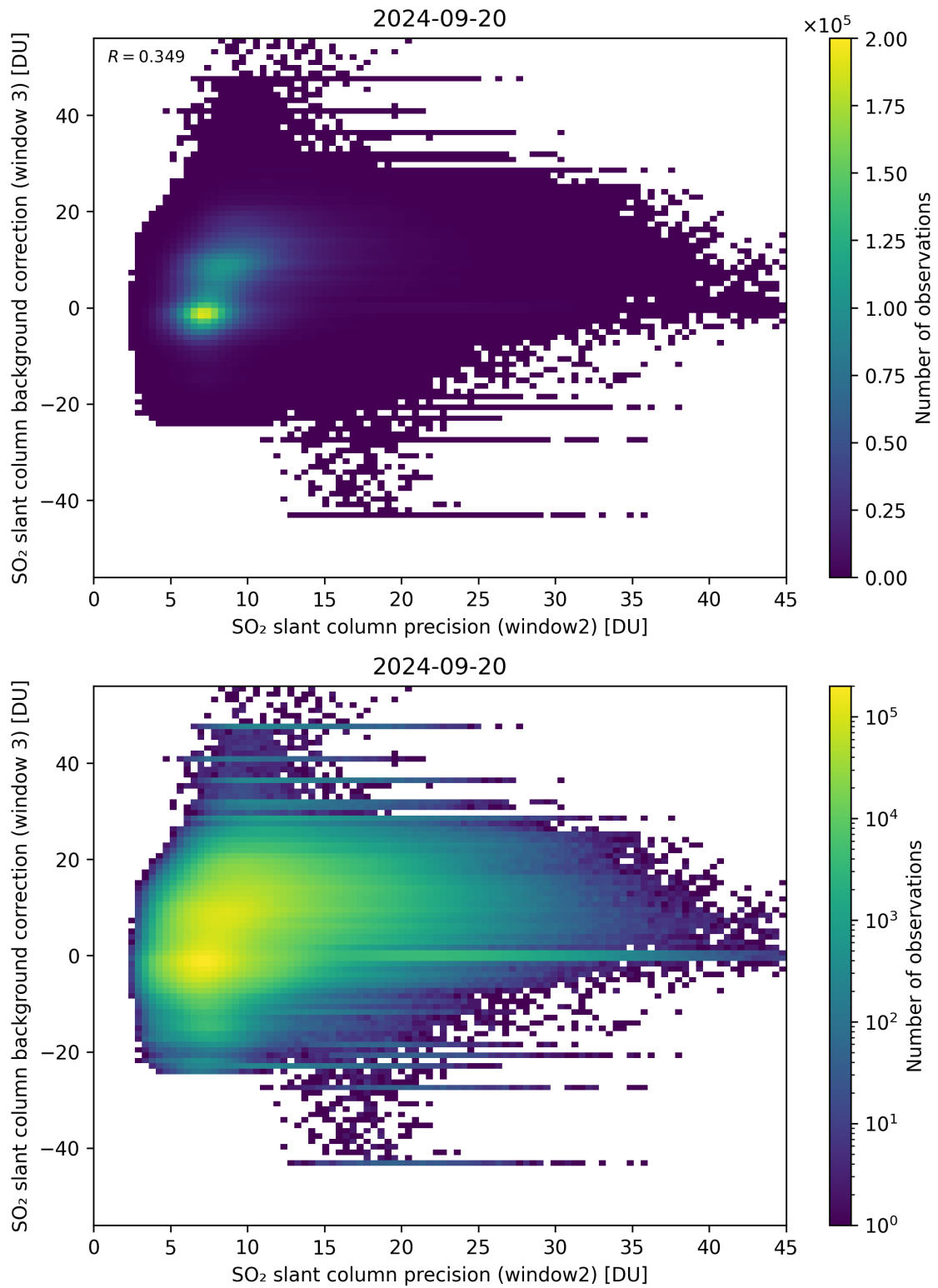
Figure 242: Scatter density plot of “SO 2 slant column precision (window2)” against “SO 2 slant column background correction (window 3)” for 2024-09-19 to 2024-09-21.
