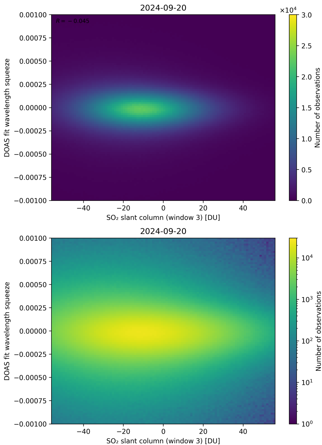
Figure 255: Scatter density plot of “SO 2 slant column (window 3)” against “DOAS fit wavelength squeeze” for 2024-09-19 to 2024-09-21.
