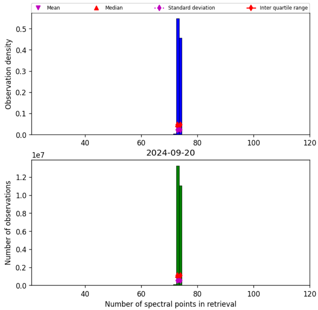
Figure 74: Histogram of “Number of spectral points in retrieval” for 2024-09-19 to 2024-09-21
