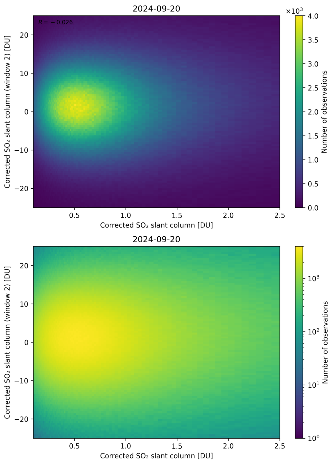
Figure 185: Scatter density plot of “Corrected SO 2 slant column” against “Corrected SO 2 slant column (window 2)” for 2024-09-19 to 2024-09-21.
