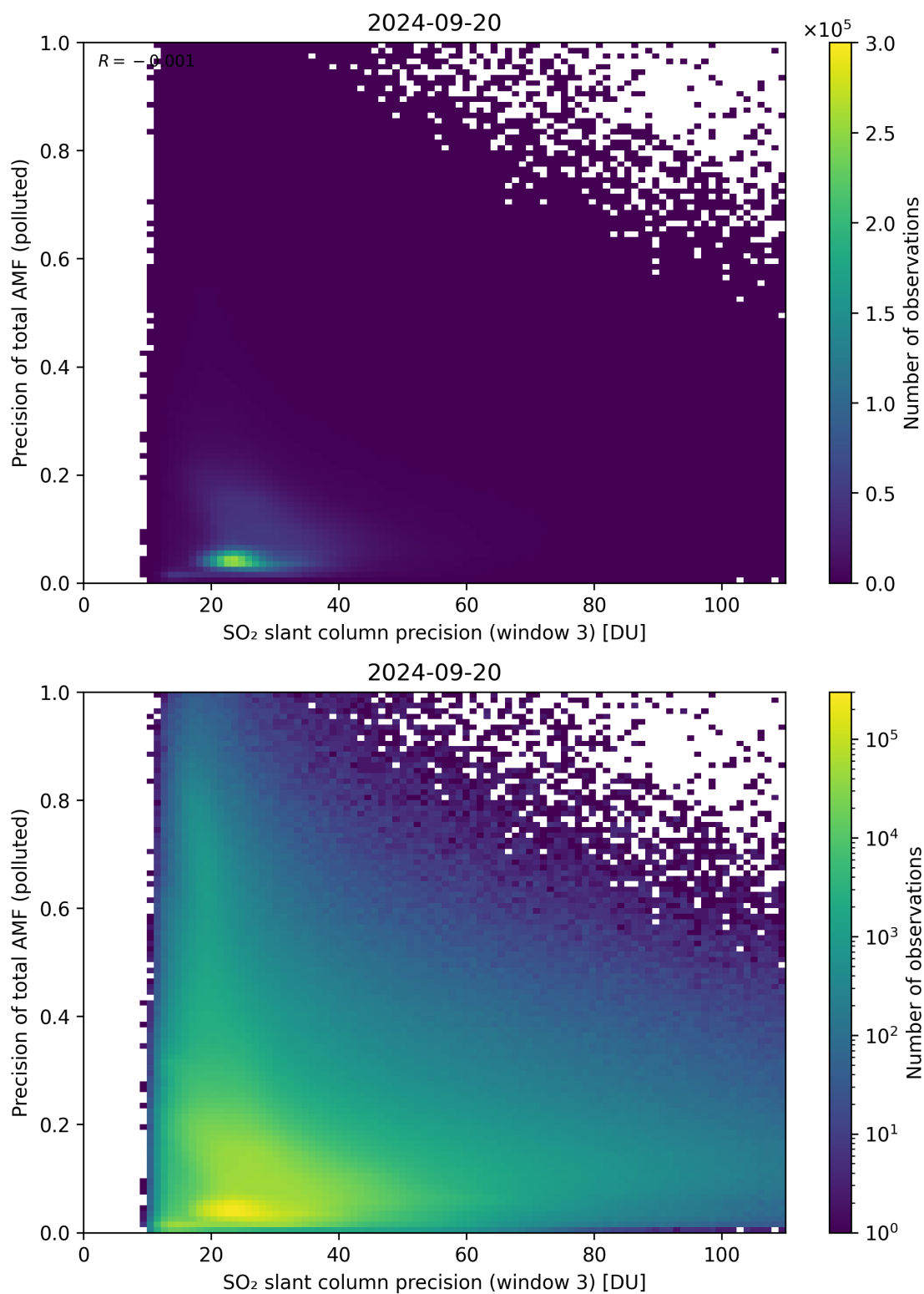
Figure 264: Scatter density plot of “SO 2 slant column precision (window 3)” against “Precision of total AMF (polluted)” for 2024-09-19 to 2024-09-21.
