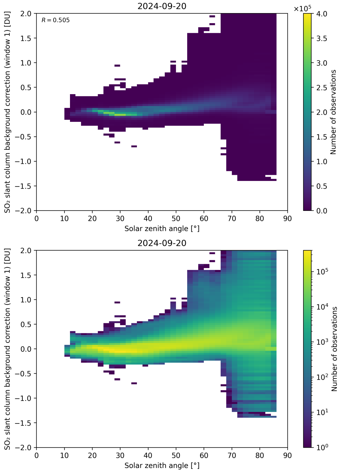
Figure 158: Scatter density plot of “Solar zenith angle” against “SO 2 slant column background correction (window 1)” for 2024-09-19 to 2024-09-21.
