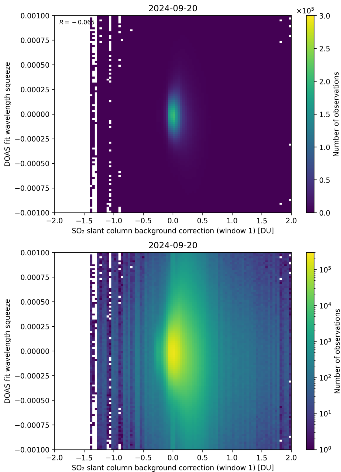
Figure 101: Scatter density plot of “SO 2 slant column background correction (window 1)” against “DOAS fit wavelength squeeze” for 2024-09-19 to 2024-09-21.
