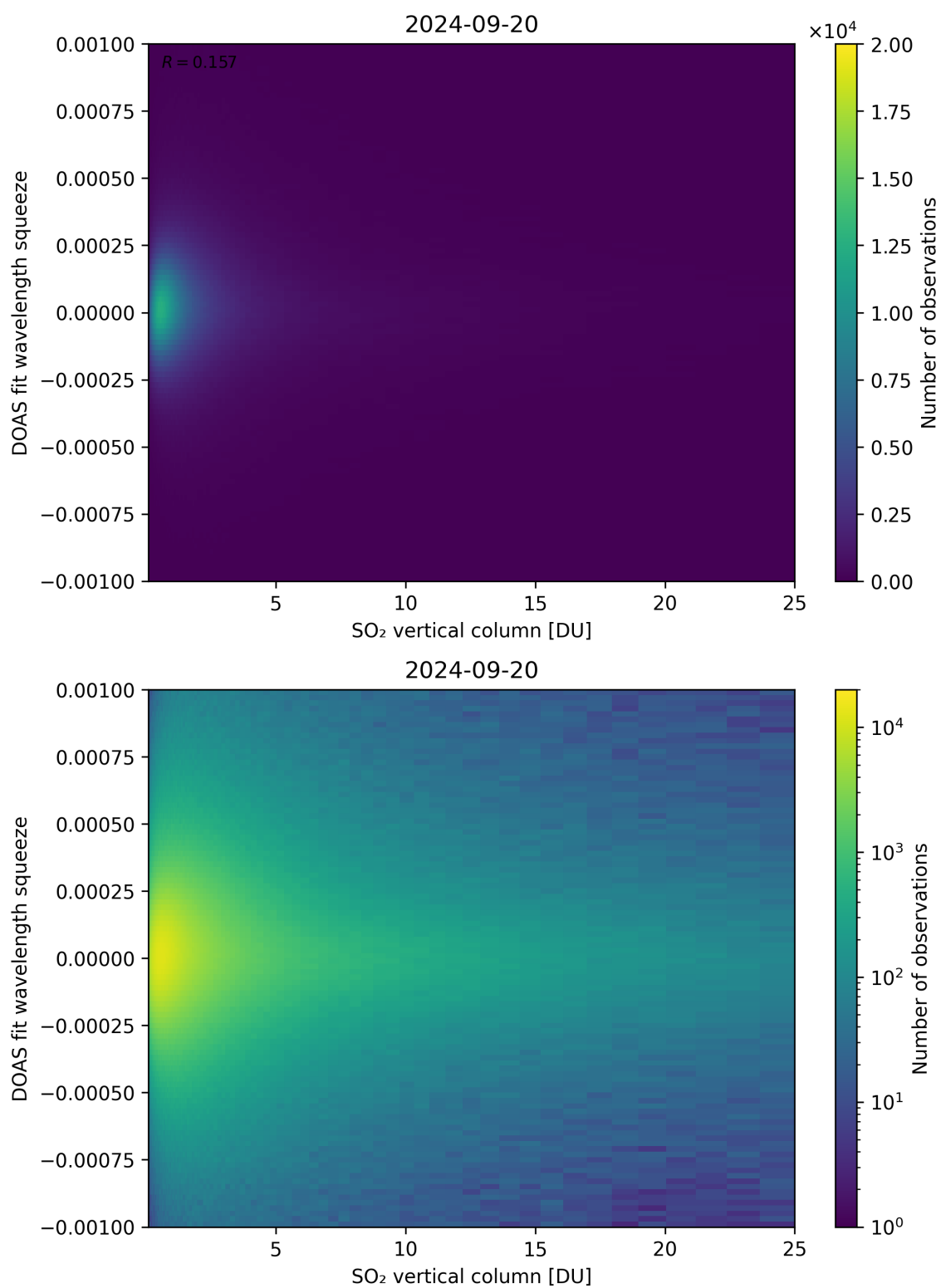
Figure 277: Scatter density plot of “SO 2 vertical column” against “DOAS fit wavelength squeeze” for 2024-09-19 to 2024-09-21.
