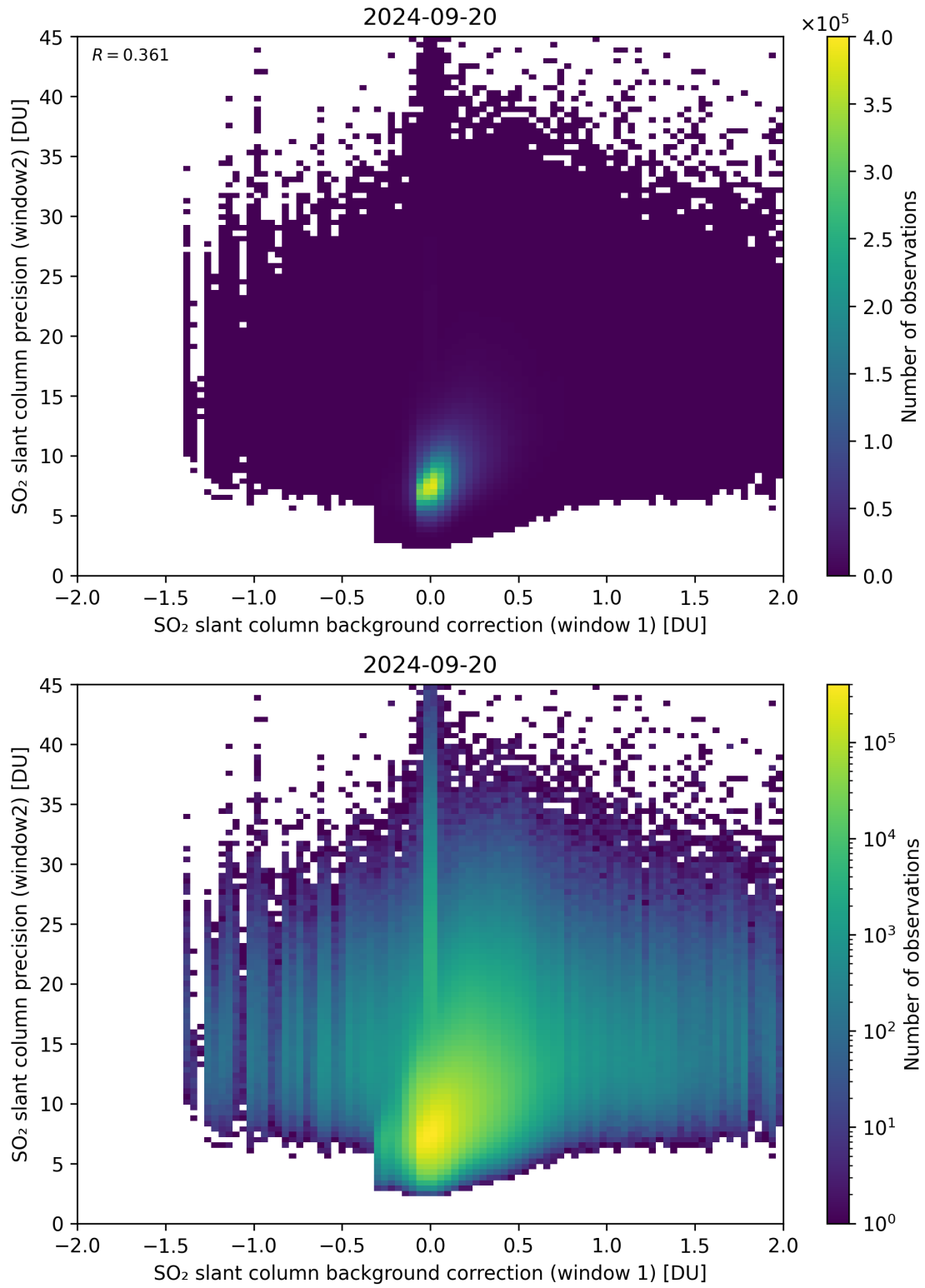
Figure 106: Scatter density plot of “SO 2 slant column background correction (window 1)” against “SO 2 slant column precision (window2)” for 2024-09-19 to 2024-09-21.
