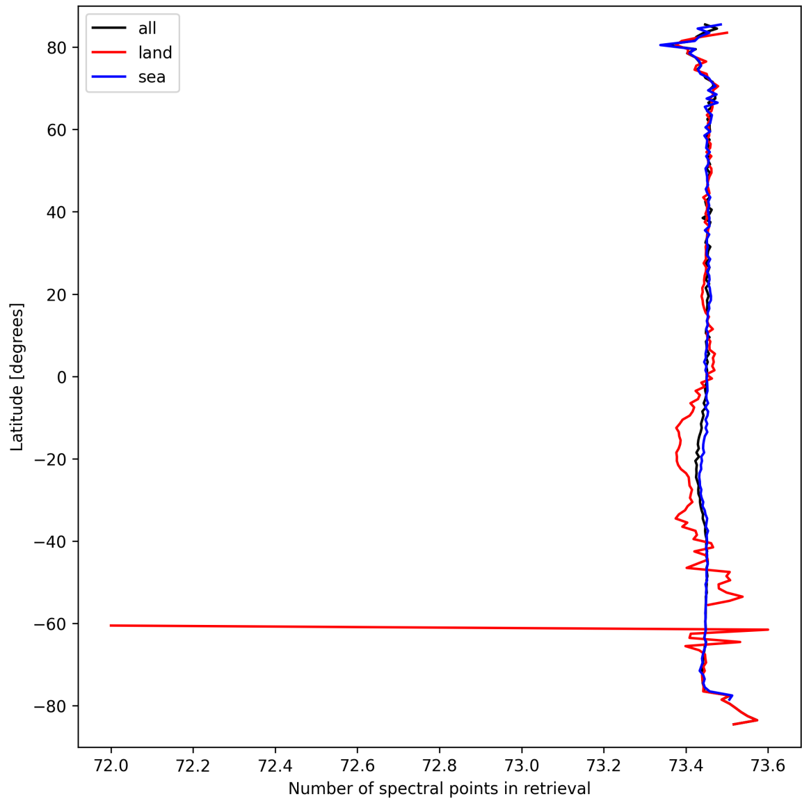
Figure 51: Zonal average of “Number of spectral points in retrieval” for 2024-09-19 to 2024-09-21.
