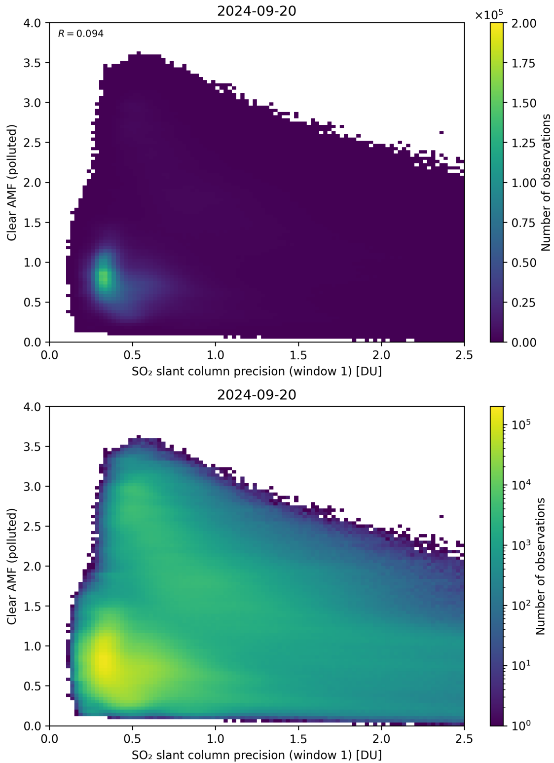
Figure 224: Scatter density plot of “SO 2 slant column precision (window 1)” against “Clear AMF (polluted)” for 2024-09-19 to 2024-09-21.
