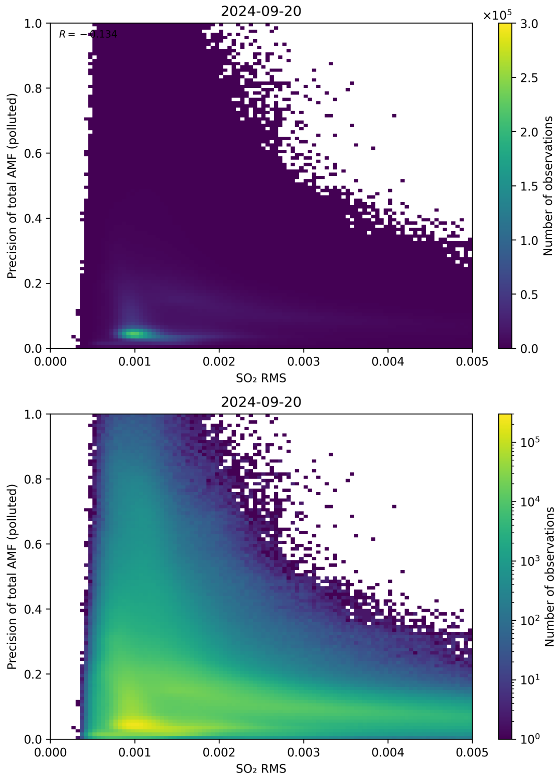
Figure 138: Scatter density plot of “SO 2 RMS” against “Precision of total AMF (polluted)” for 2024-09-19 to 2024-09-21.
