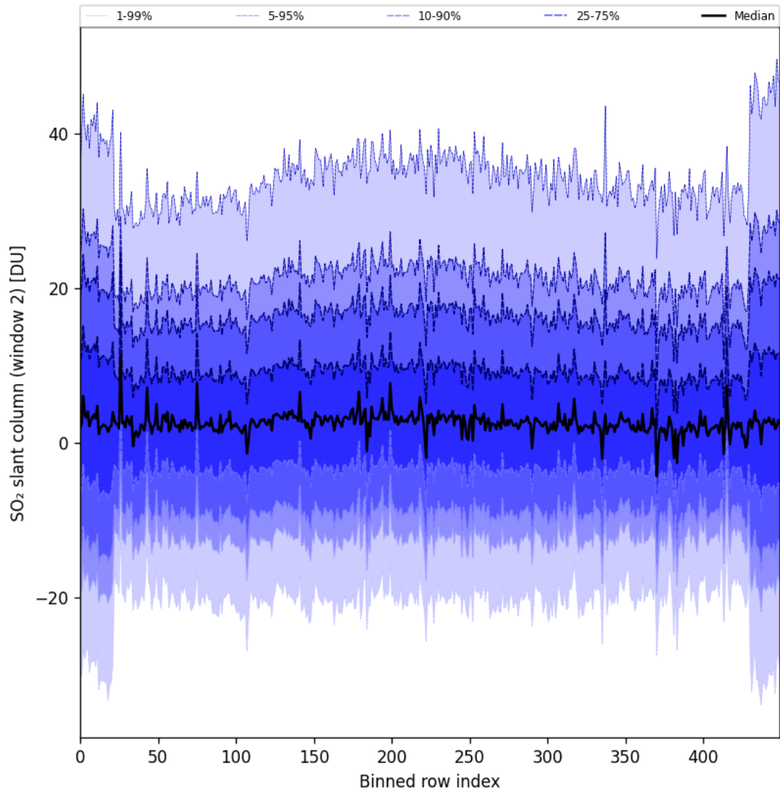
Figure 83: Along track statistics of “SO 2 slant column (window 2)” for 2024-09-19 to 2024-09-21
