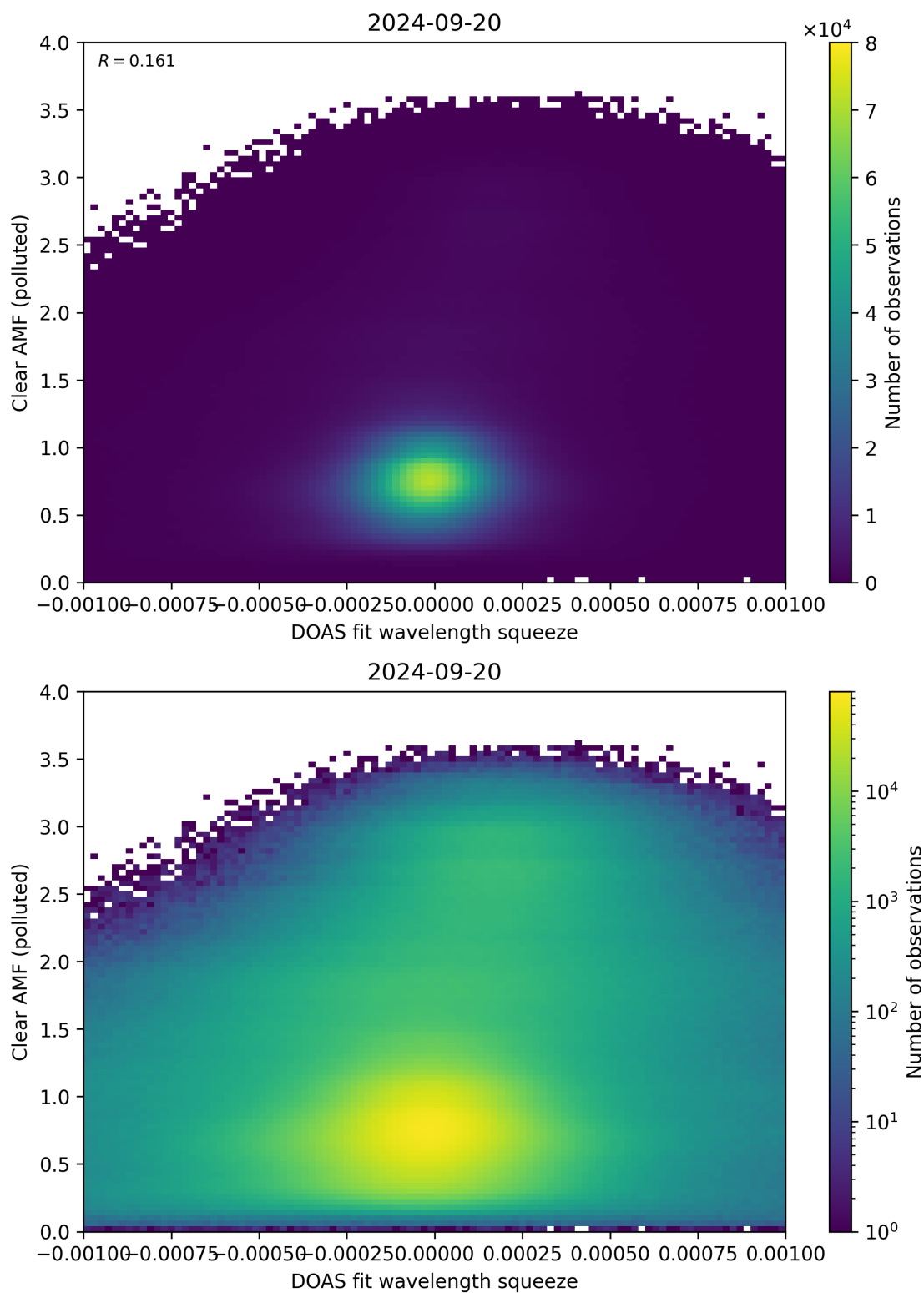
Figure 133: Scatter density plot of “DOAS fit wavelength squeeze” against “Clear AMF (polluted)” for 2024-09-19 to 2024-09-21.
