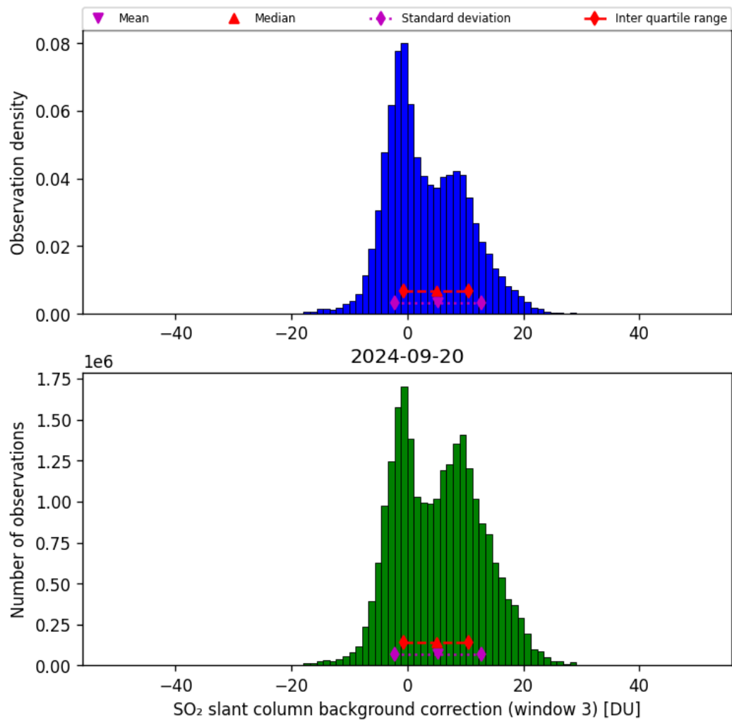
Figure 67: Histogram of “SO 2 slant column background correction (window 3)” for 2024-09-19 to 2024-09-21
