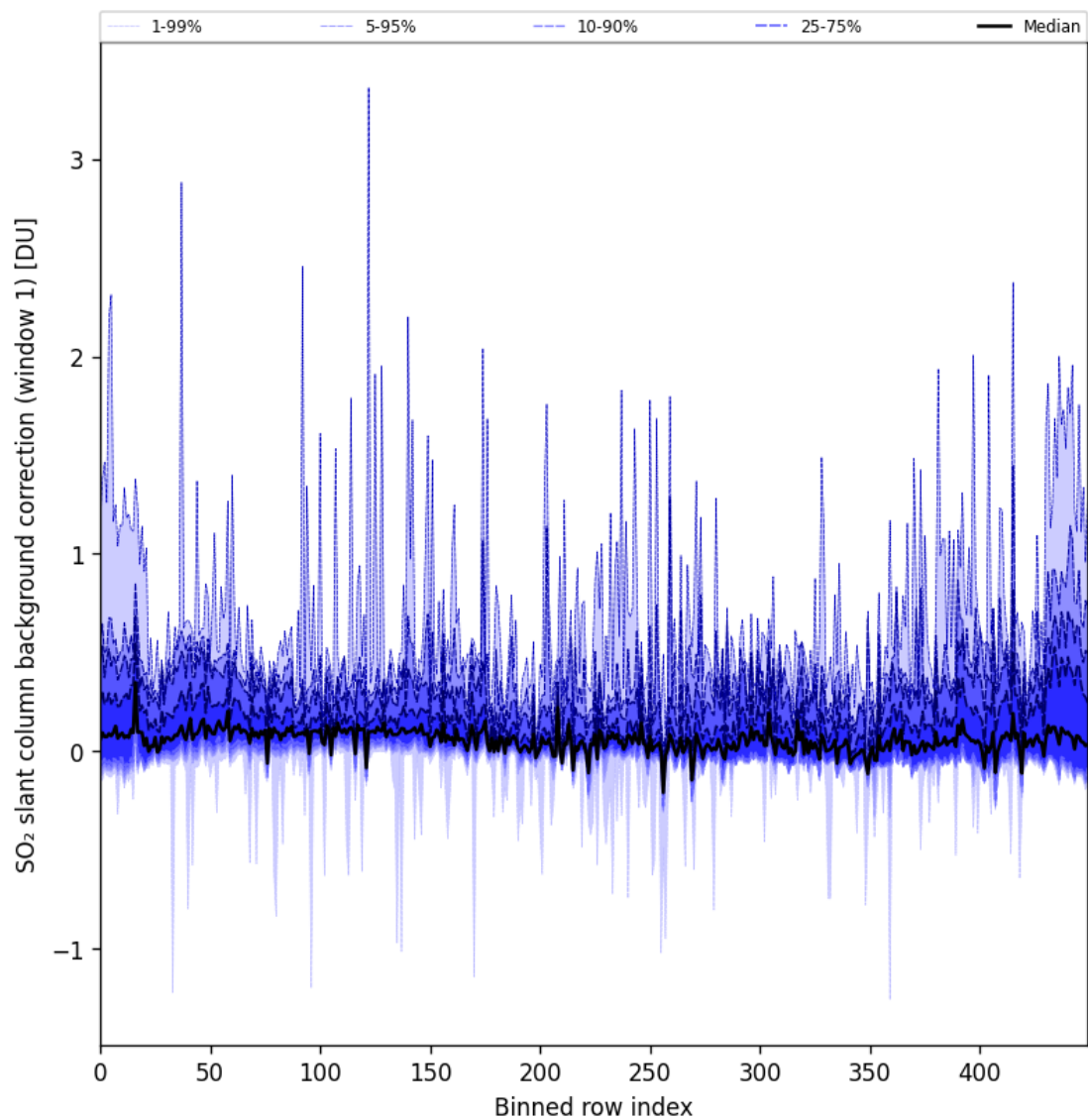
Figure 82: Along track statistics of “SO 2 slant column background correction (window 1)” for 2024-09-19 to 2024-09-21
