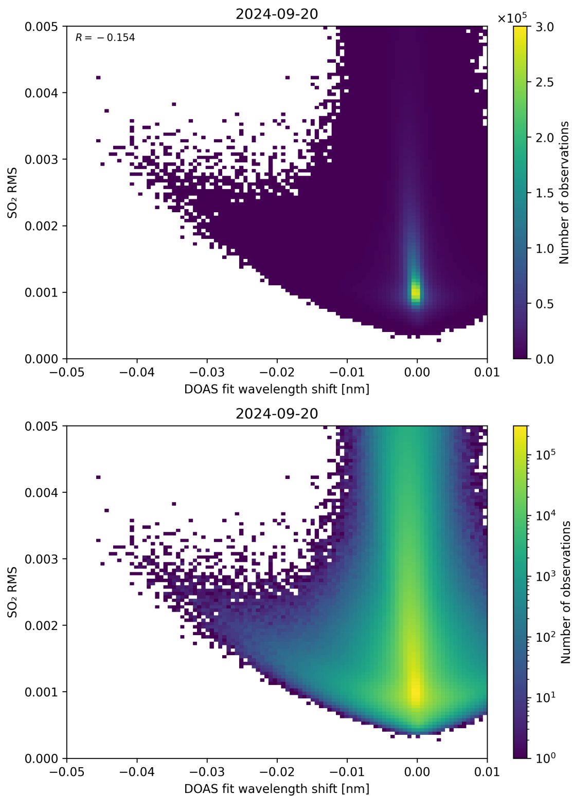
Figure 128: Scatter density plot of “DOAS fit wavelength shift” against “SO 2 RMS” for 2024-09-19 to 2024-09-21.
