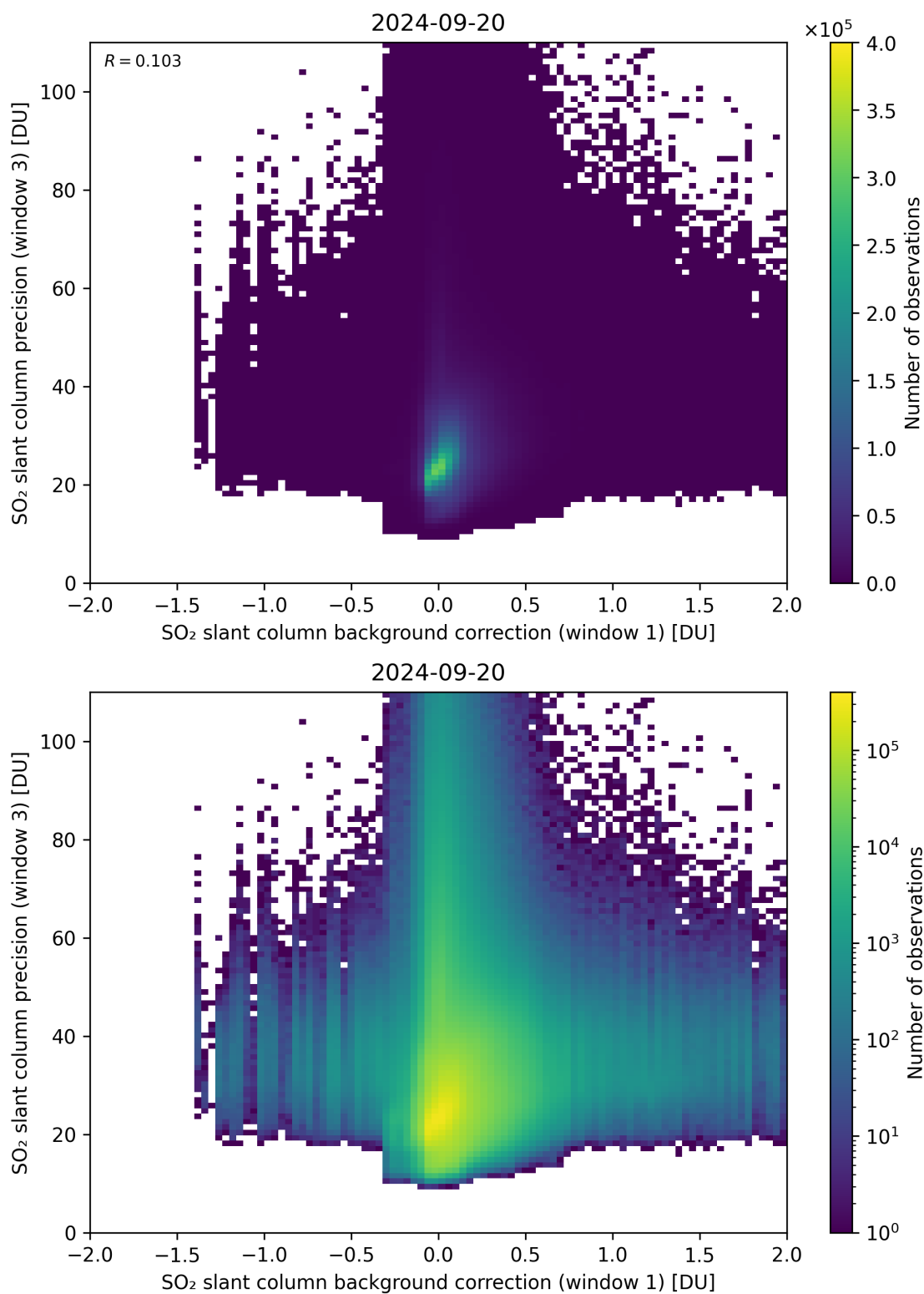
Figure 108: Scatter density plot of “SO 2 slant column background correction (window 1)” against “SO 2 slant column precision (window 3)” for 2024-09-19 to 2024-09-21.
