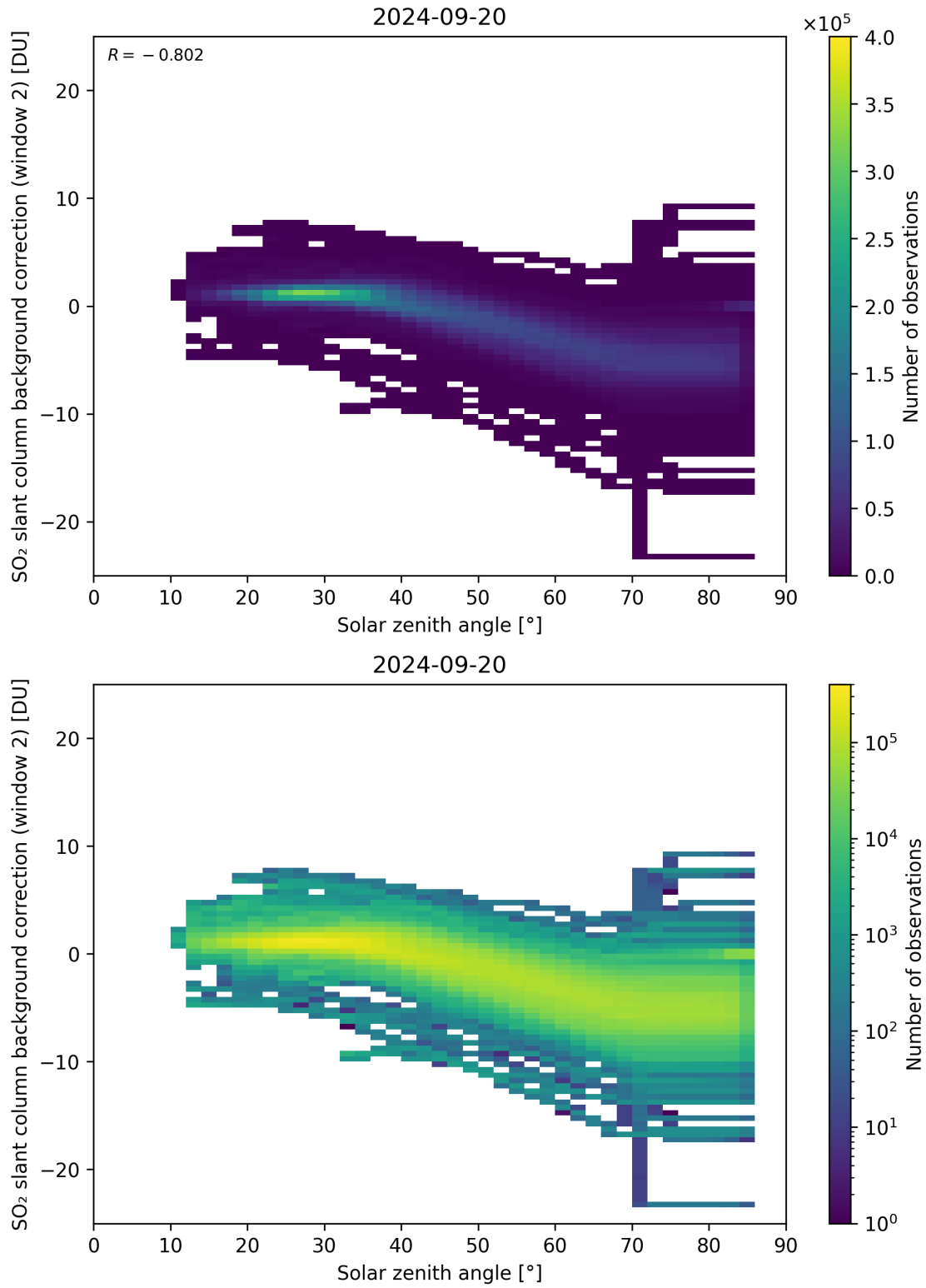
Figure 159: Scatter density plot of “Solar zenith angle” against “SO 2 slant column background correction (window 2)” for 2024-09-19 to 2024-09-21.
