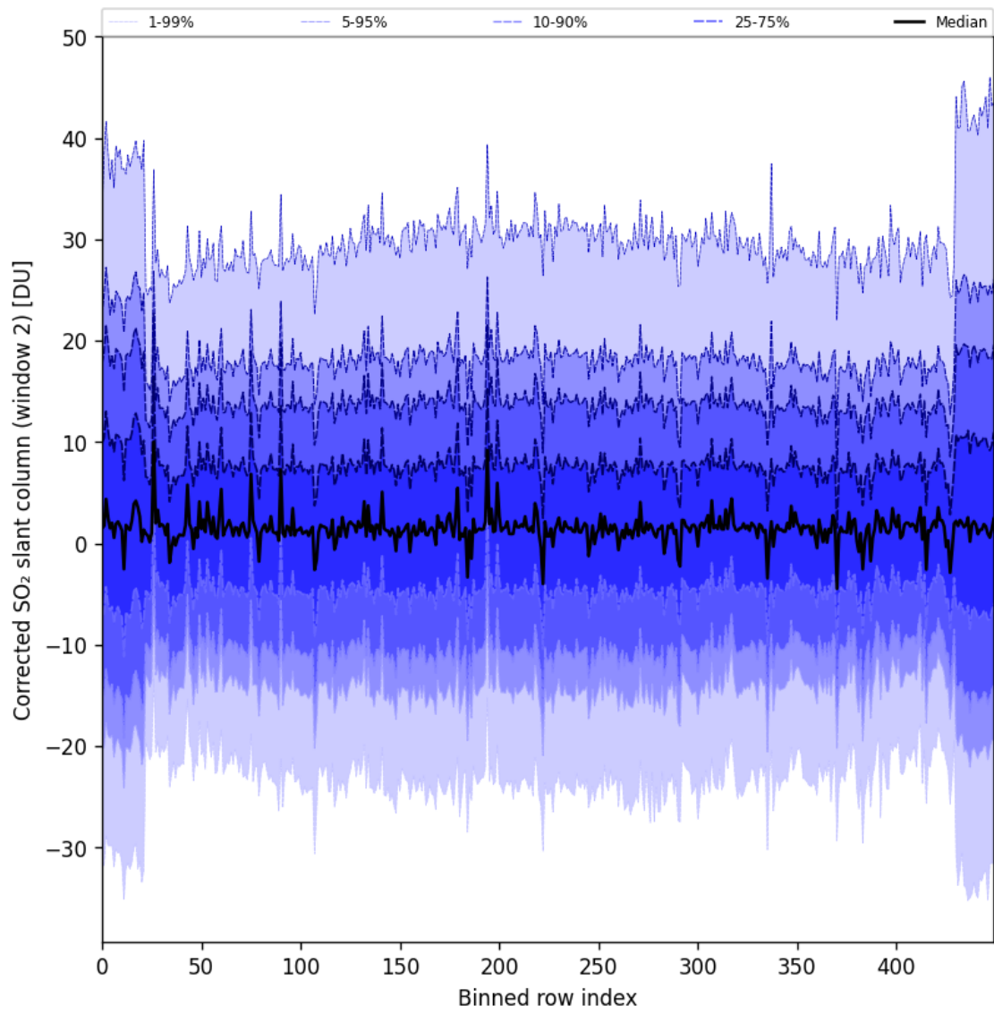
Figure 85: Along track statistics of “Corrected SO 2 slant column (window 2)” for 2024-09-19 to 2024-09-21
