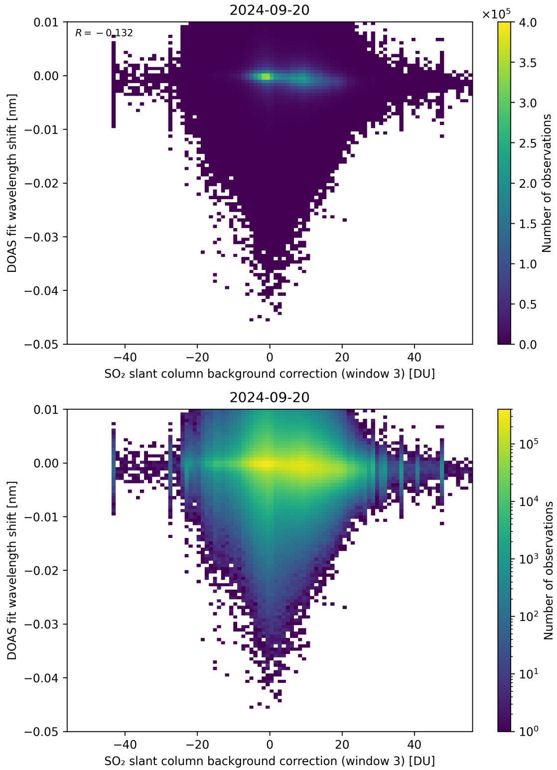
Figure 121: Scatter density plot of “SO 2 slant column background correction (window 3)” against “DOAS fit wavelength shift” for 2024-09-19 to 2024-09-21.
