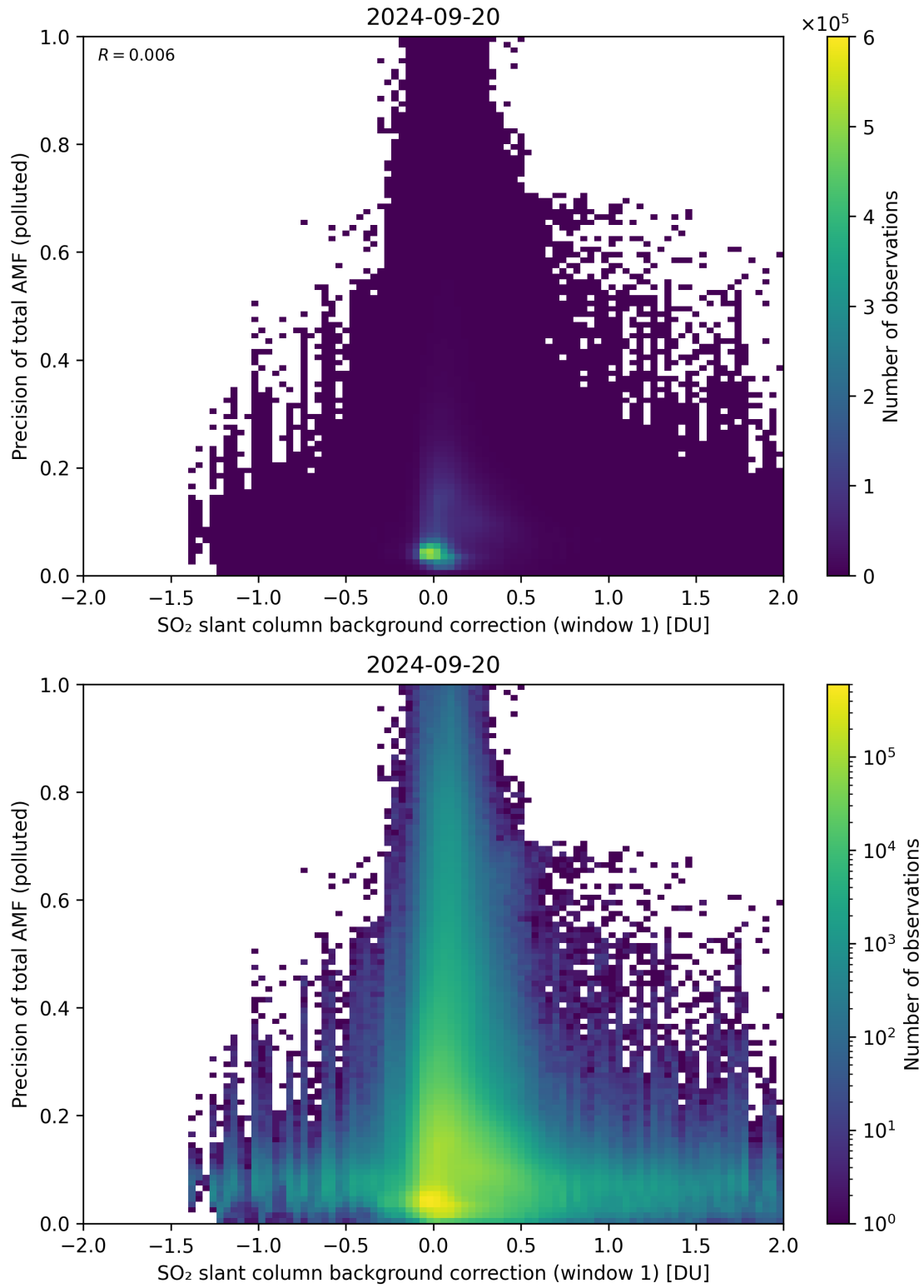
Figure 110: Scatter density plot of “SO 2 slant column background correction (window 1)” against “Precision of total AMF (polluted)” for 2024-09-19 to 2024-09-21.
