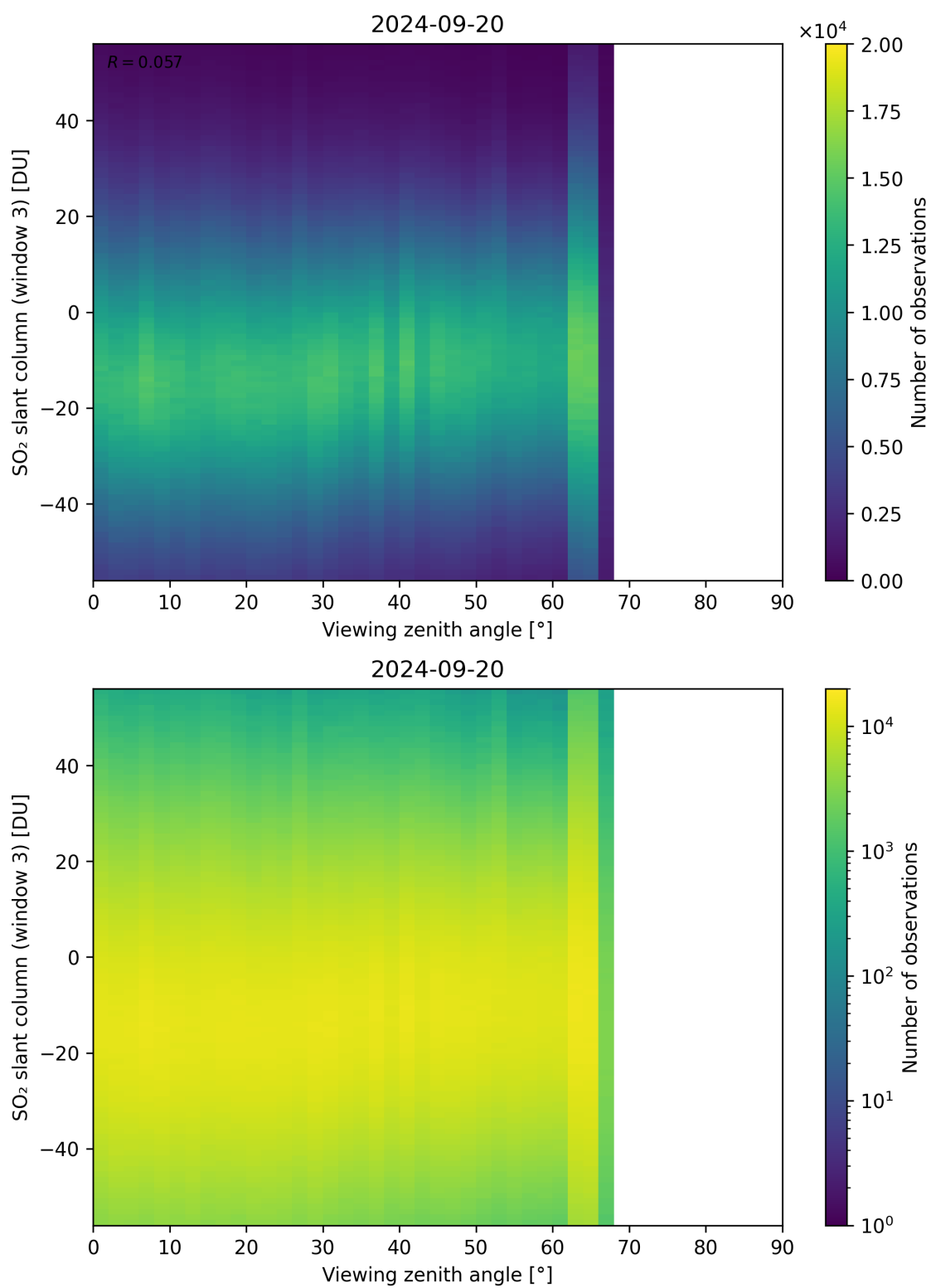
Figure 323: Scatter density plot of “Viewing zenith angle” against “SO 2 slant column (window 3)” for 2024-09-19 to 2024-09-21.
