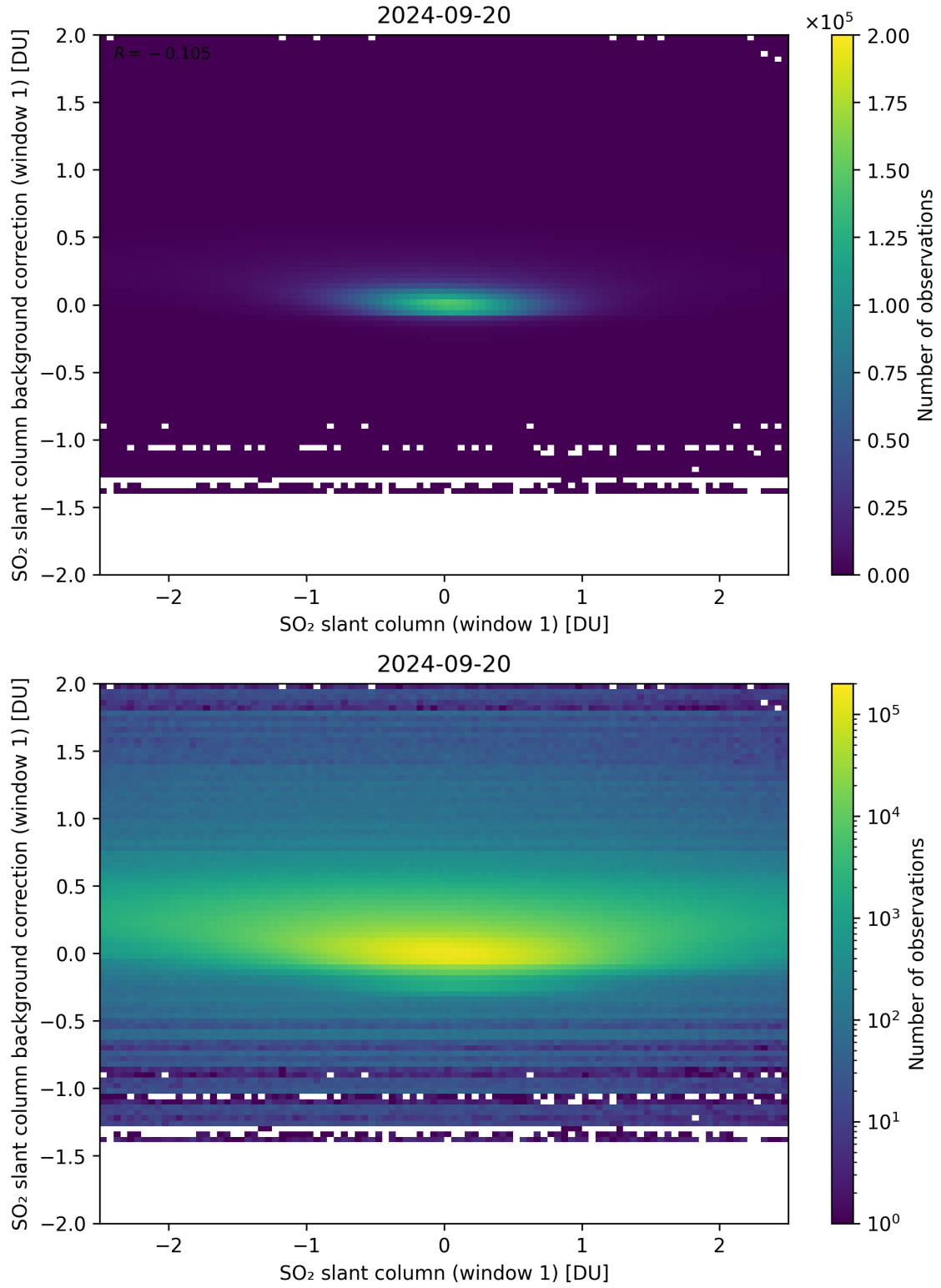
Figure 212: Scatter density plot of “SO 2 slant column (window 1)” against “SO 2 slant column background correction (window 1)” for 2024-09-19 to 2024-09-21.
