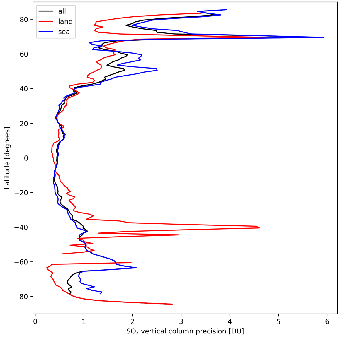
Figure 31: Zonal average of “SO 2 vertical column precision” for 2024-09-19 to 2024-09-21.
