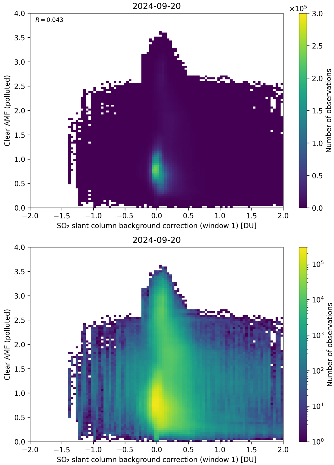
Figure 103: Scatter density plot of “SO 2 slant column background correction (window 1)” against “Clear AMF (polluted)” for 2024-09-19 to 2024-09-21.
