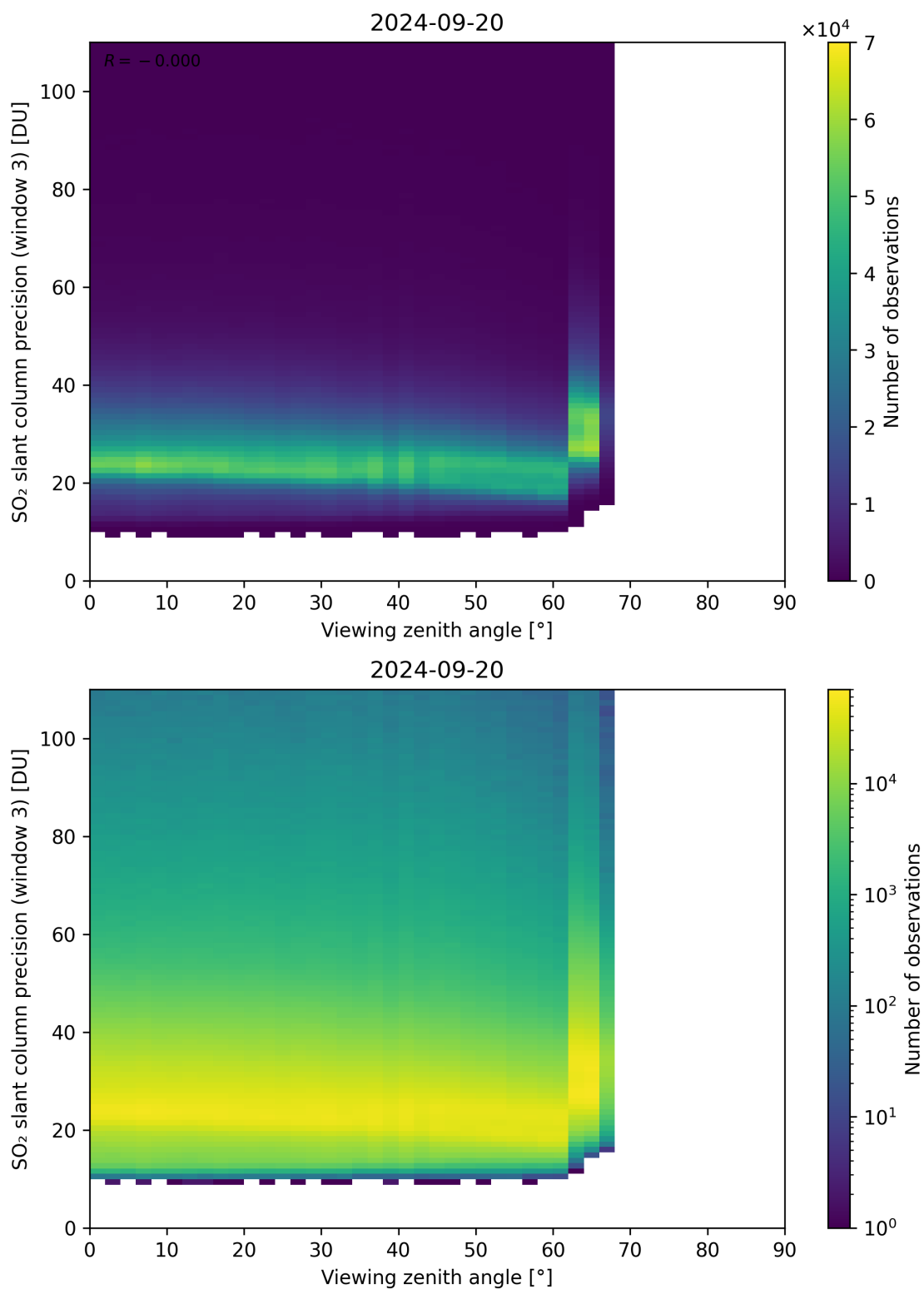
Figure 324: Scatter density plot of “Viewing zenith angle” against “SO 2 slant column precision (window 3)” for 2024-09-19 to 2024-09-21.
