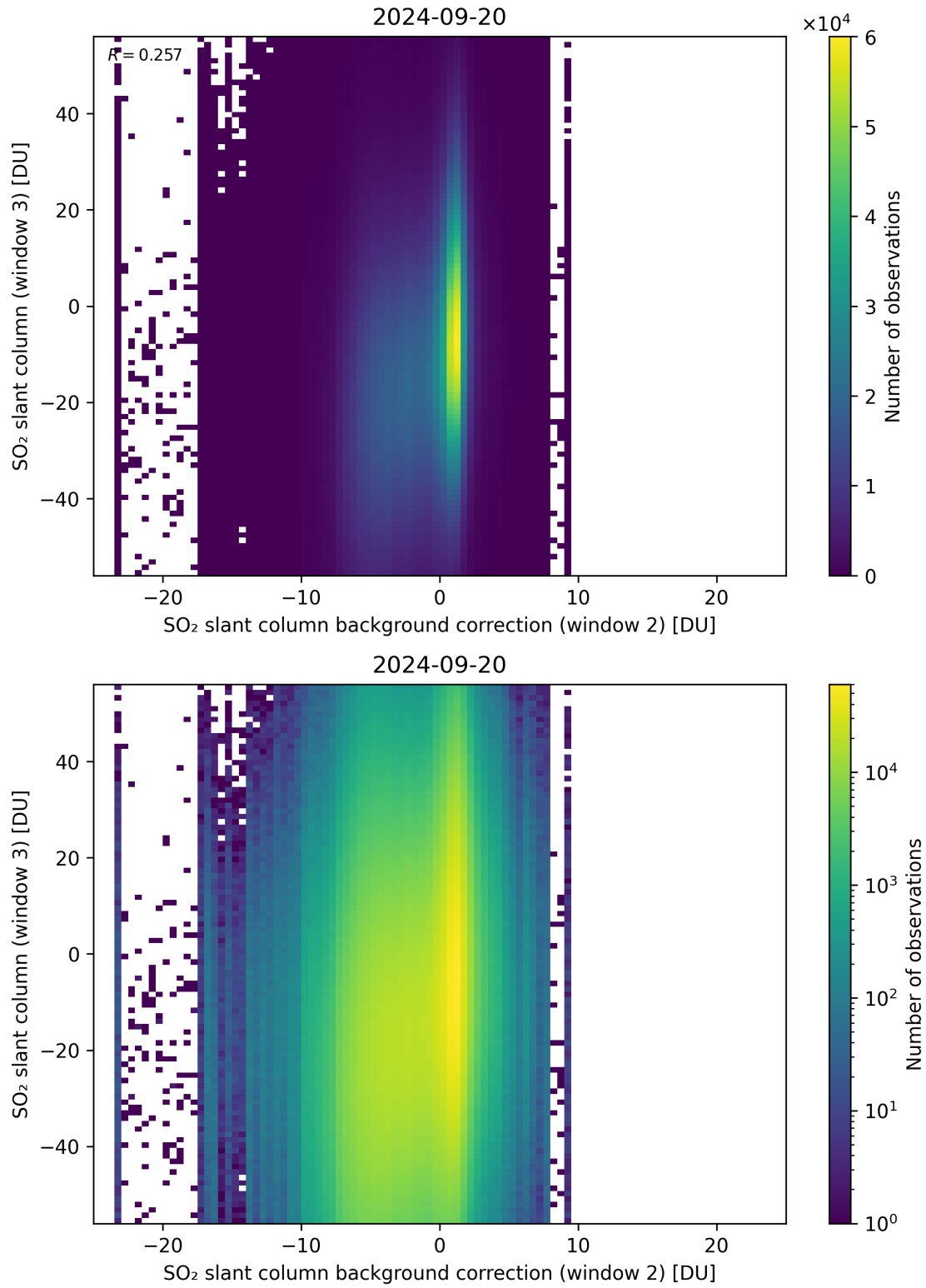
Figure 117: Scatter density plot of “SO 2 slant column background correction (window 2)” against “SO 2 slant column (window 3)” for 2024-09-19 to 2024-09-21.
