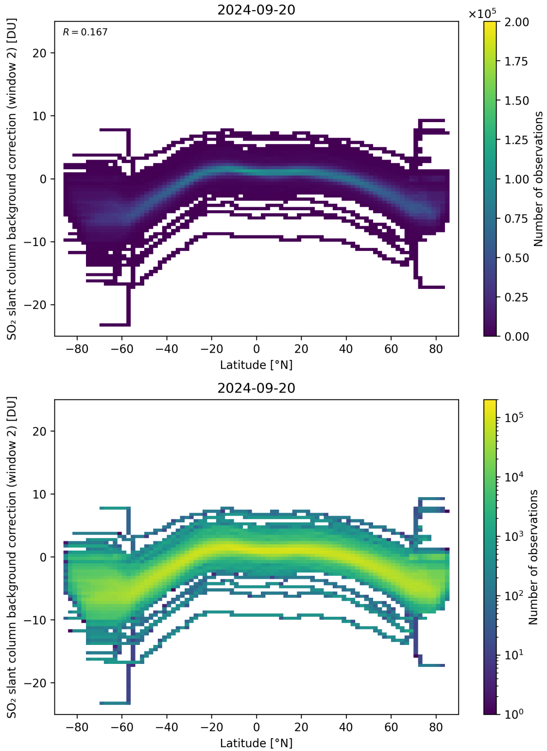
Figure 140: Scatter density plot of “Latitude” against “SO 2 slant column background correction (window 2)” for 2024-09-19 to 2024-09-21.
