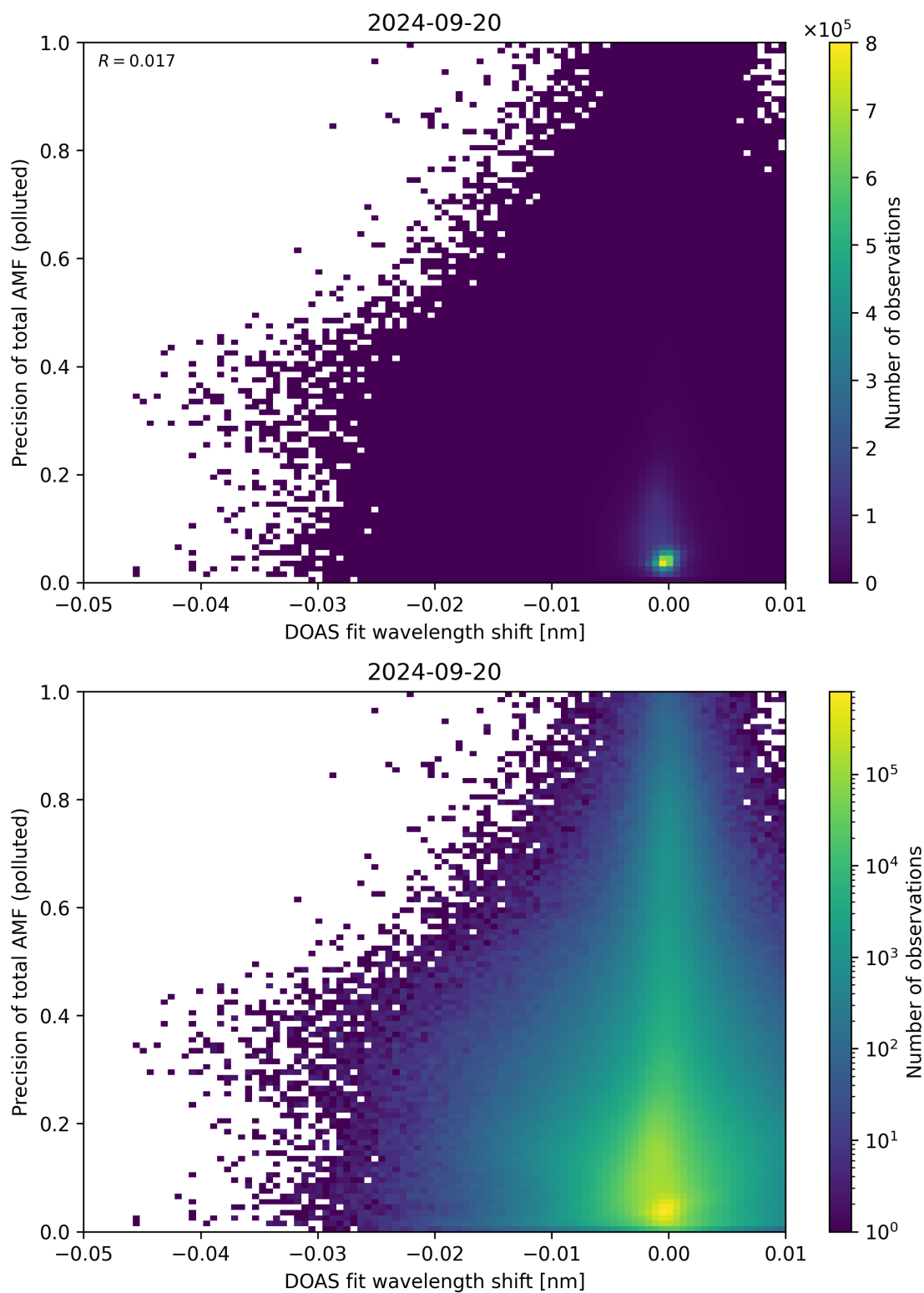
Figure 131: Scatter density plot of “DOAS fit wavelength shift” against “Precision of total AMF (polluted)” for 2024-09-19 to 2024-09-21.
