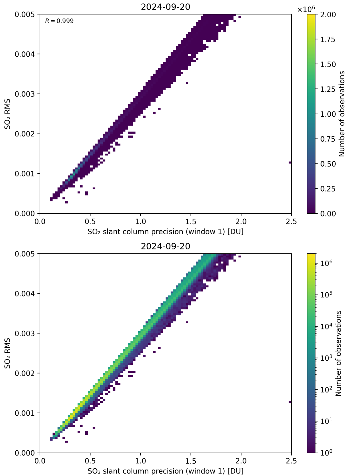
Figure 223: Scatter density plot of “SO 2 slant column precision (window 1)” against “SO 2 RMS” for 2024-09-19 to 2024-09-21.
