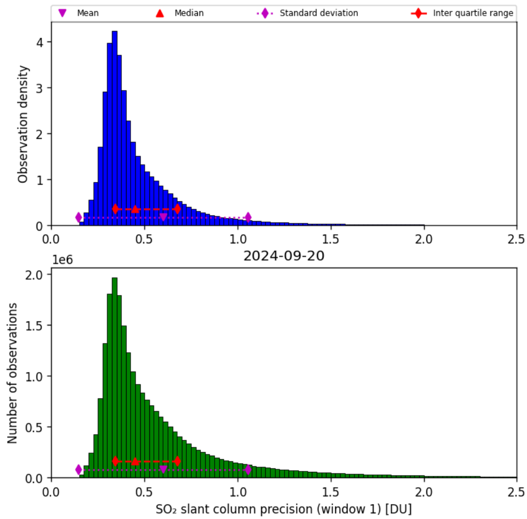
Figure 57: Histogram of “SO 2 slant column precision (window 1)” for 2024-09-19 to 2024-09-21
