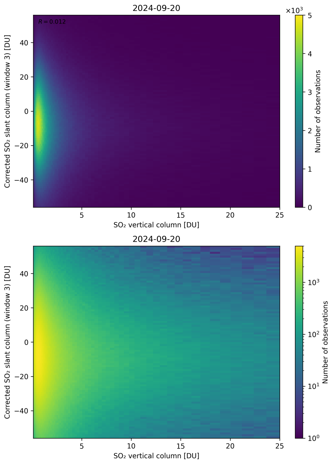
Figure 299: Scatter density plot of “SO 2 vertical column” against “Corrected SO 2 slant column (window 3)” for 2024-09-19 to 2024-09-21.
