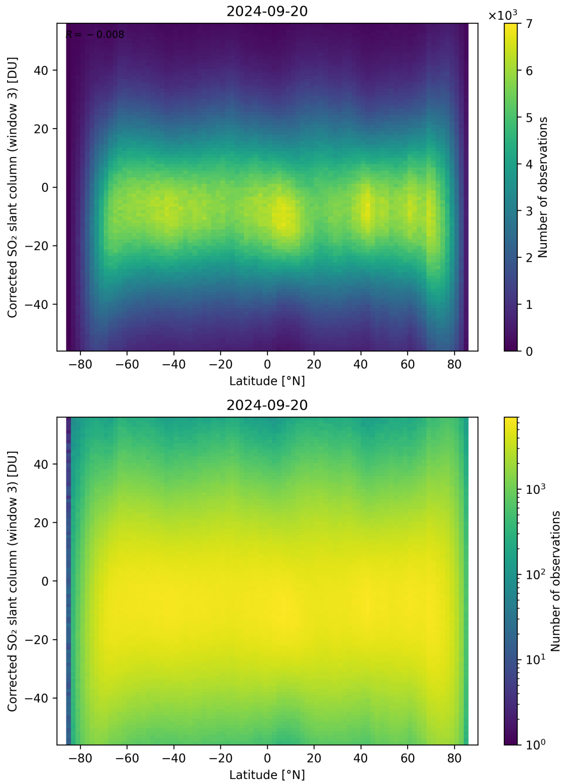
Figure 148: Scatter density plot of “Latitude” against “Corrected SO 2 slant column (window 3)” for 2024-09-19 to 2024-09-21.
