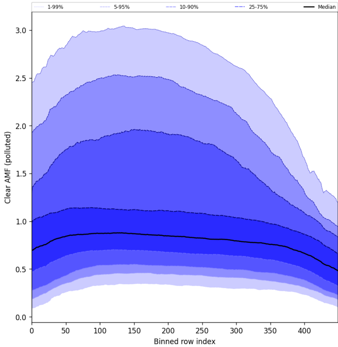
Figure 96: Along track statistics of “Clear AMF (polluted)” for 2024-09-19 to 2024-09-21
