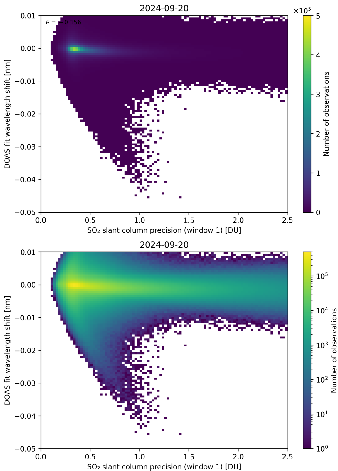
Figure 221: Scatter density plot of “SO 2 slant column precision (window 1)” against “DOAS fit wavelength shift” for 2024-09-19 to 2024-09-21.
