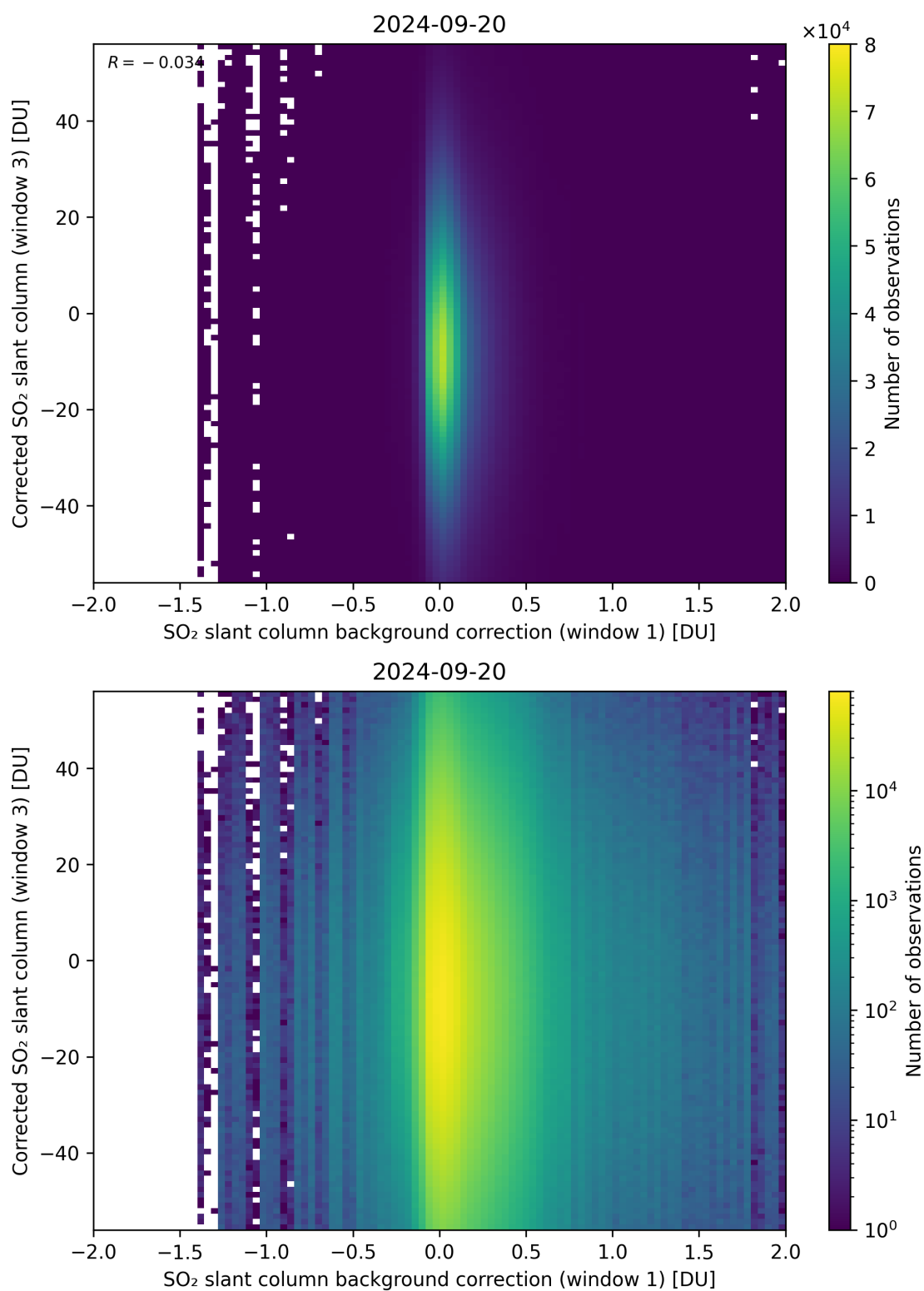
Figure 105: Scatter density plot of “SO 2 slant column background correction (window 1)” against “Corrected SO 2 slant column (window 3)” for 2024-09-19 to 2024-09-21.
