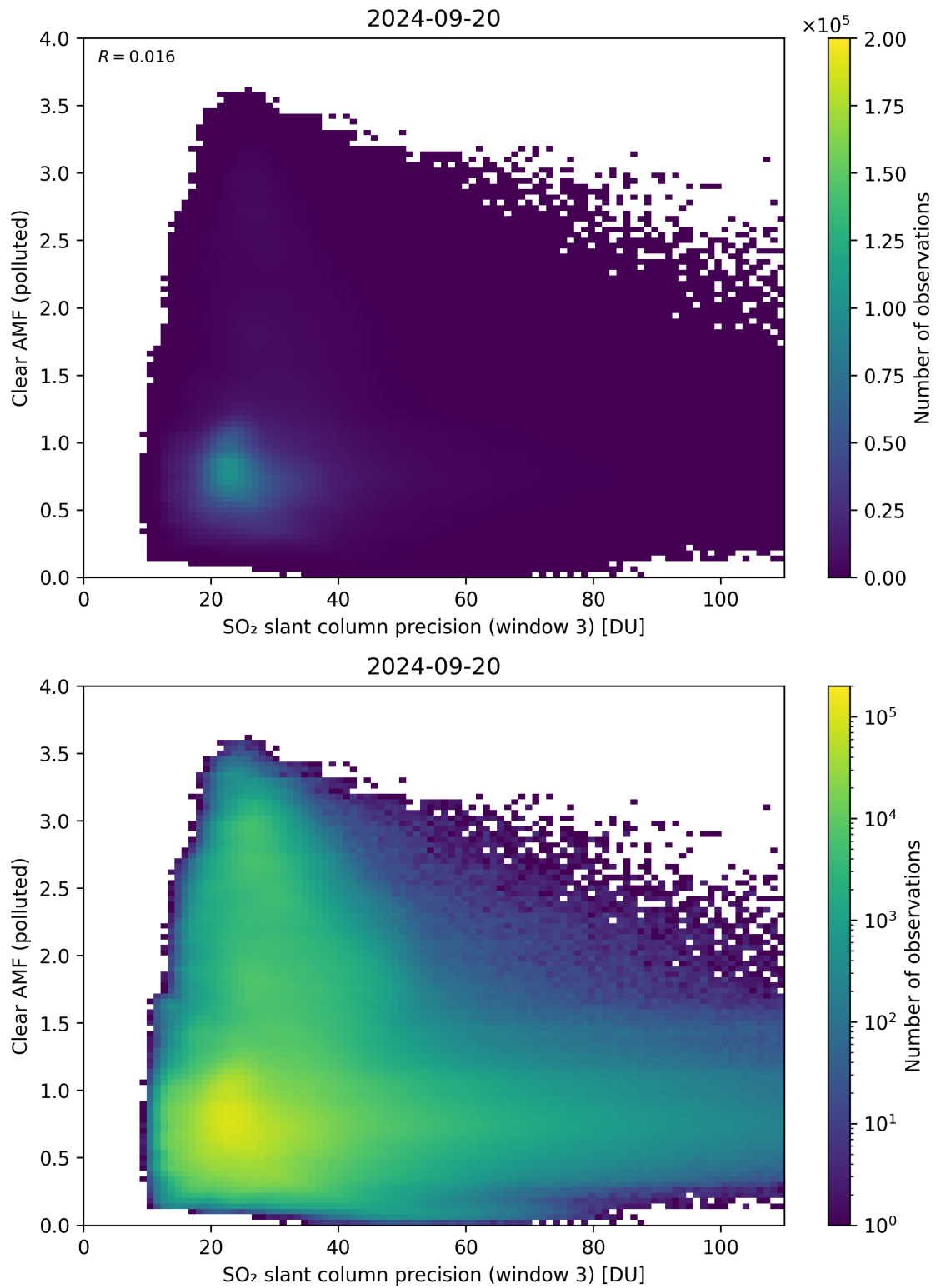
Figure 261: Scatter density plot of “SO 2 slant column precision (window 3)” against “Clear AMF (polluted)” for 2024-09-19 to 2024-09-21.
