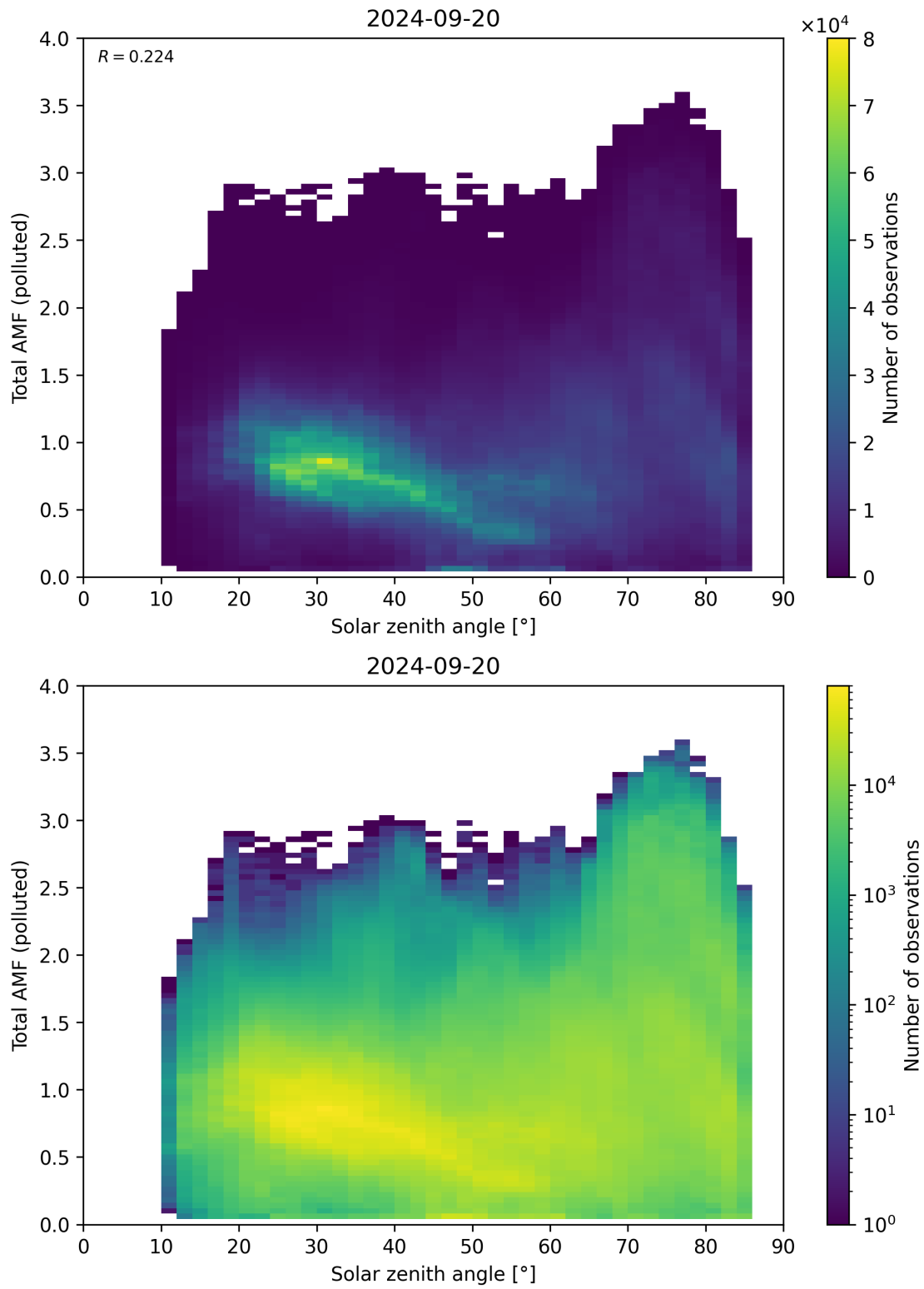
Figure 174: Scatter density plot of “Solar zenith angle” against “Total AMF (polluted)” for 2024-09-19 to 2024-09-21.
