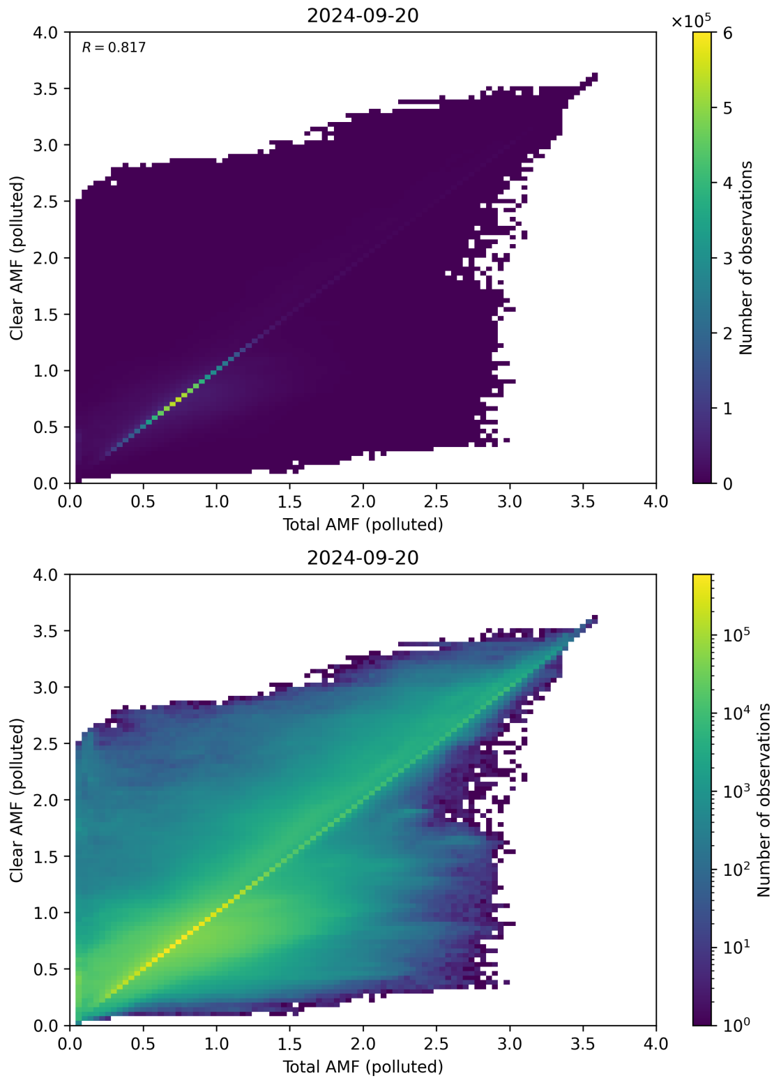
Figure 271: Scatter density plot of “Total AMF (polluted)” against “Clear AMF (polluted)” for 2024-09-19 to 2024-09-21.
