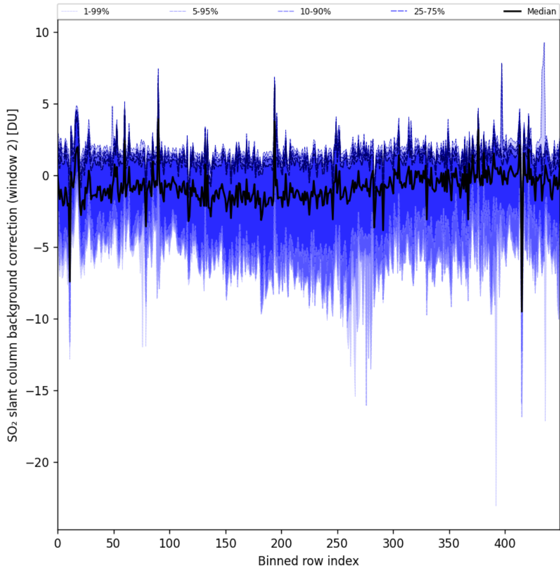
Figure 86: Along track statistics of “SO 2 slant column background correction (window 2)” for 2024-09-19 to 2024-09-21
