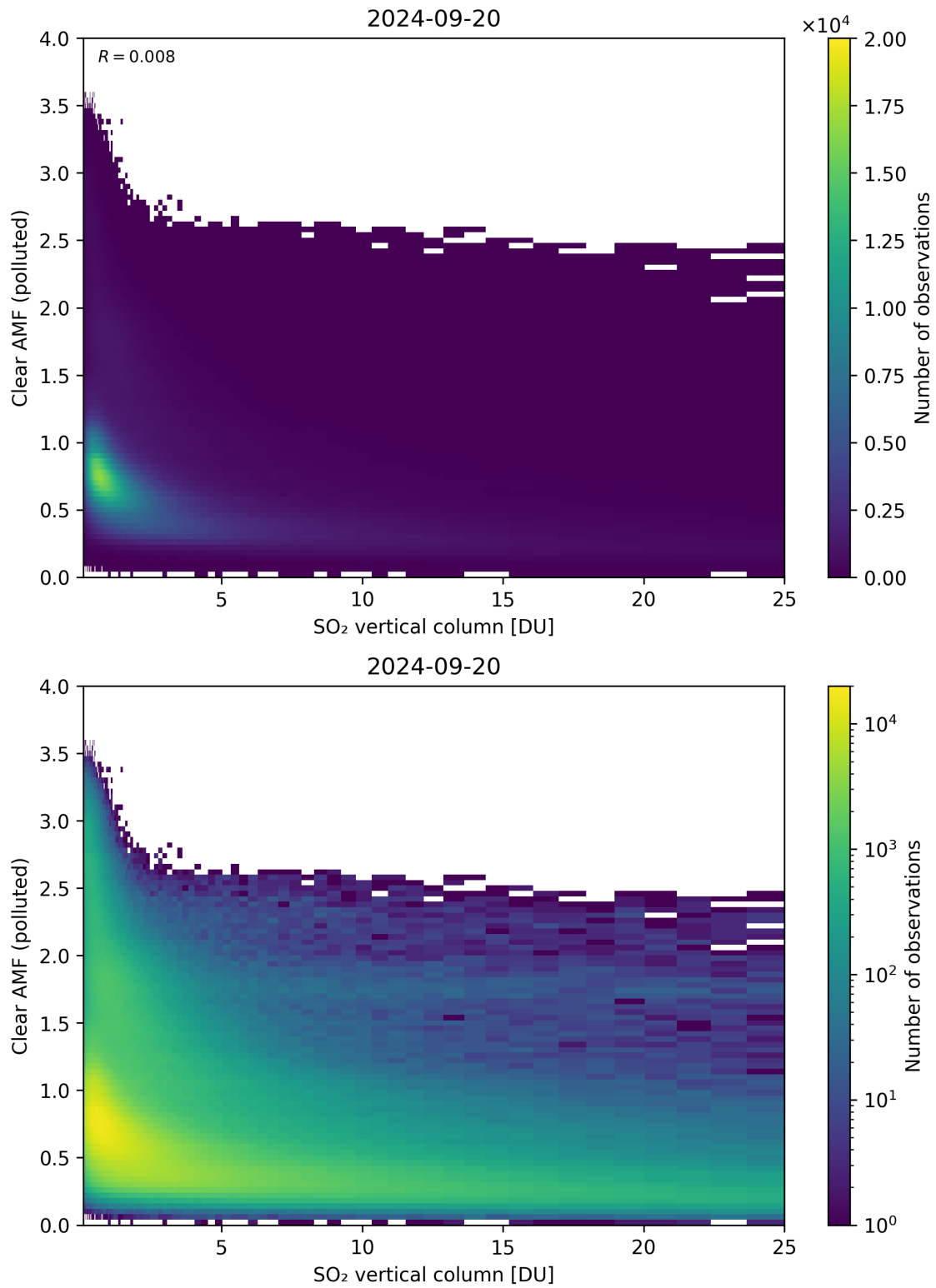
Figure 296: Scatter density plot of “SO 2 vertical column” against “Clear AMF (polluted)” for 2024-09-19 to 2024-09-21.
