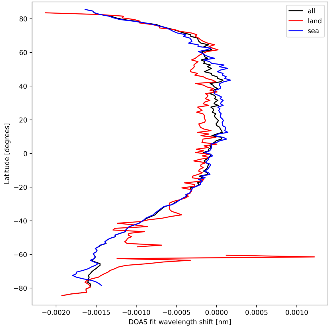
Figure 45: Zonal average of “DOAS fit wavelength shift” for 2024-09-19 to 2024-09-21.
