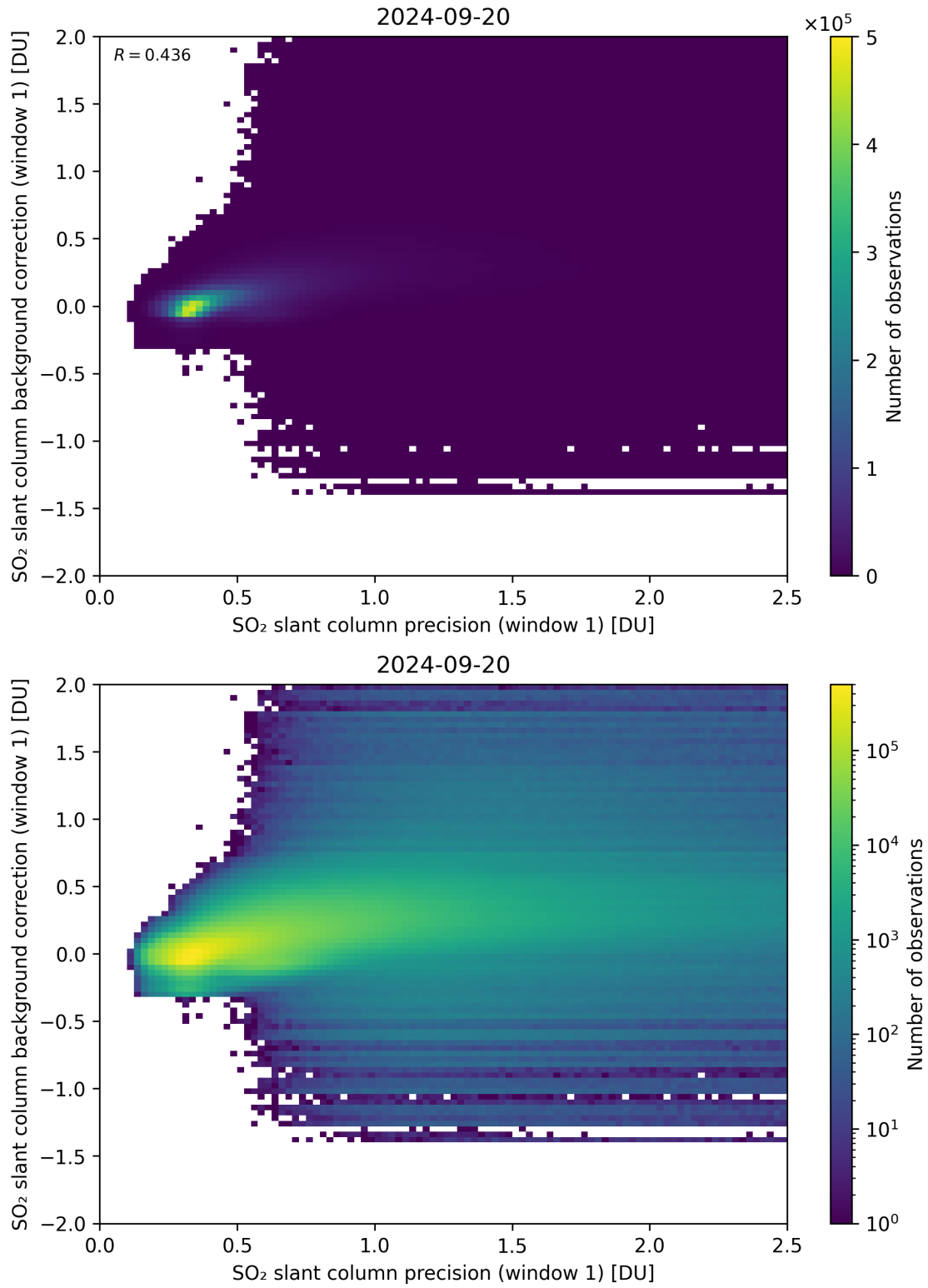
Figure 218: Scatter density plot of “SO 2 slant column precision (window 1)” against “SO 2 slant column background correction (window 1)” for 2024-09-19 to 2024-09-21.
