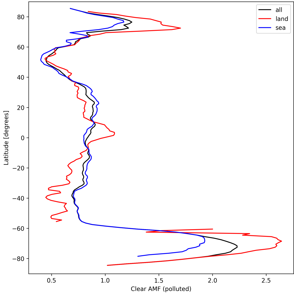
Figure 50: Zonal average of “Clear AMF (polluted)” for 2024-09-19 to 2024-09-21.
