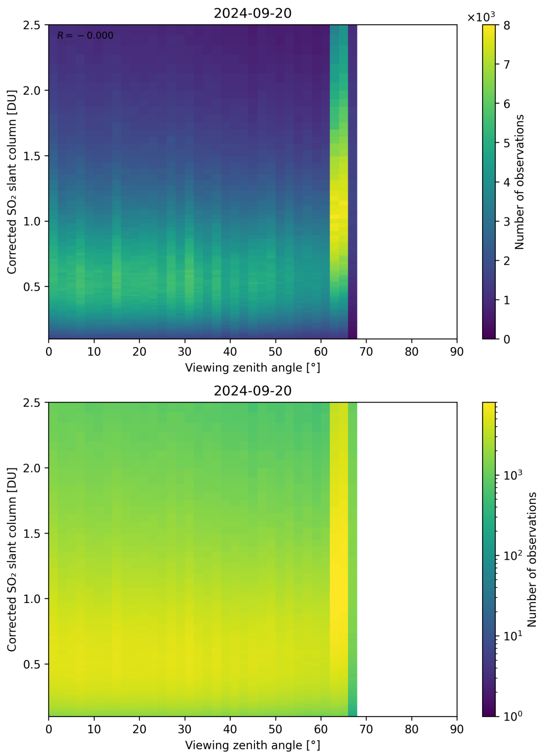
Figure 317: Scatter density plot of “Viewing zenith angle” against “Corrected SO 2 slant column” for 2024-09-19 to 2024-09-21.
