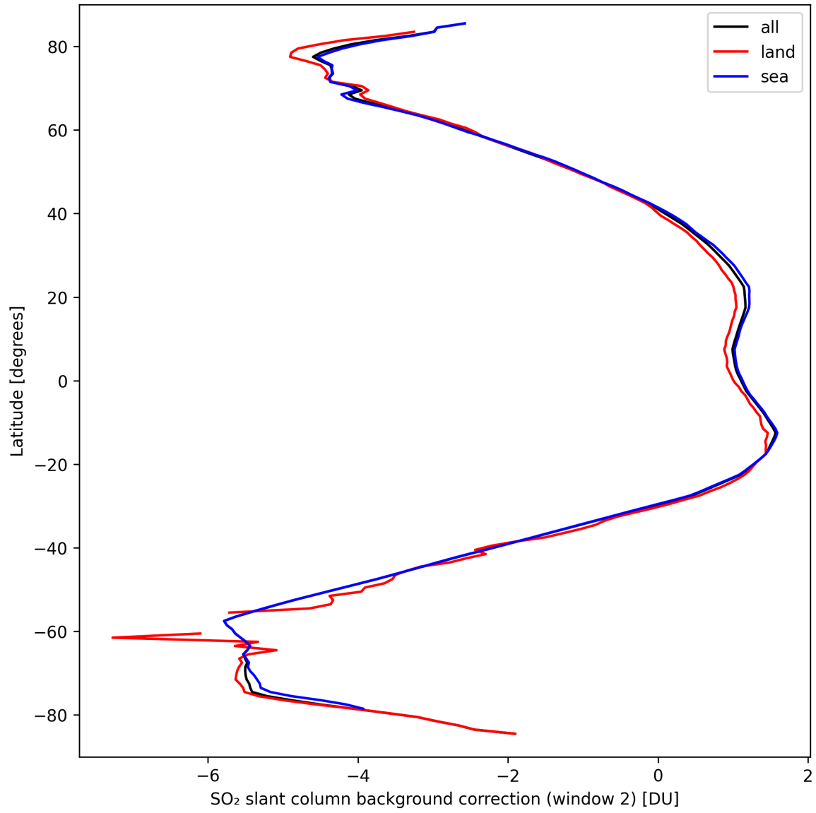
Figure 40: Zonal average of “SO 2 slant column background correction (window 2)” for 2024-09-19 to 2024-09-21.
