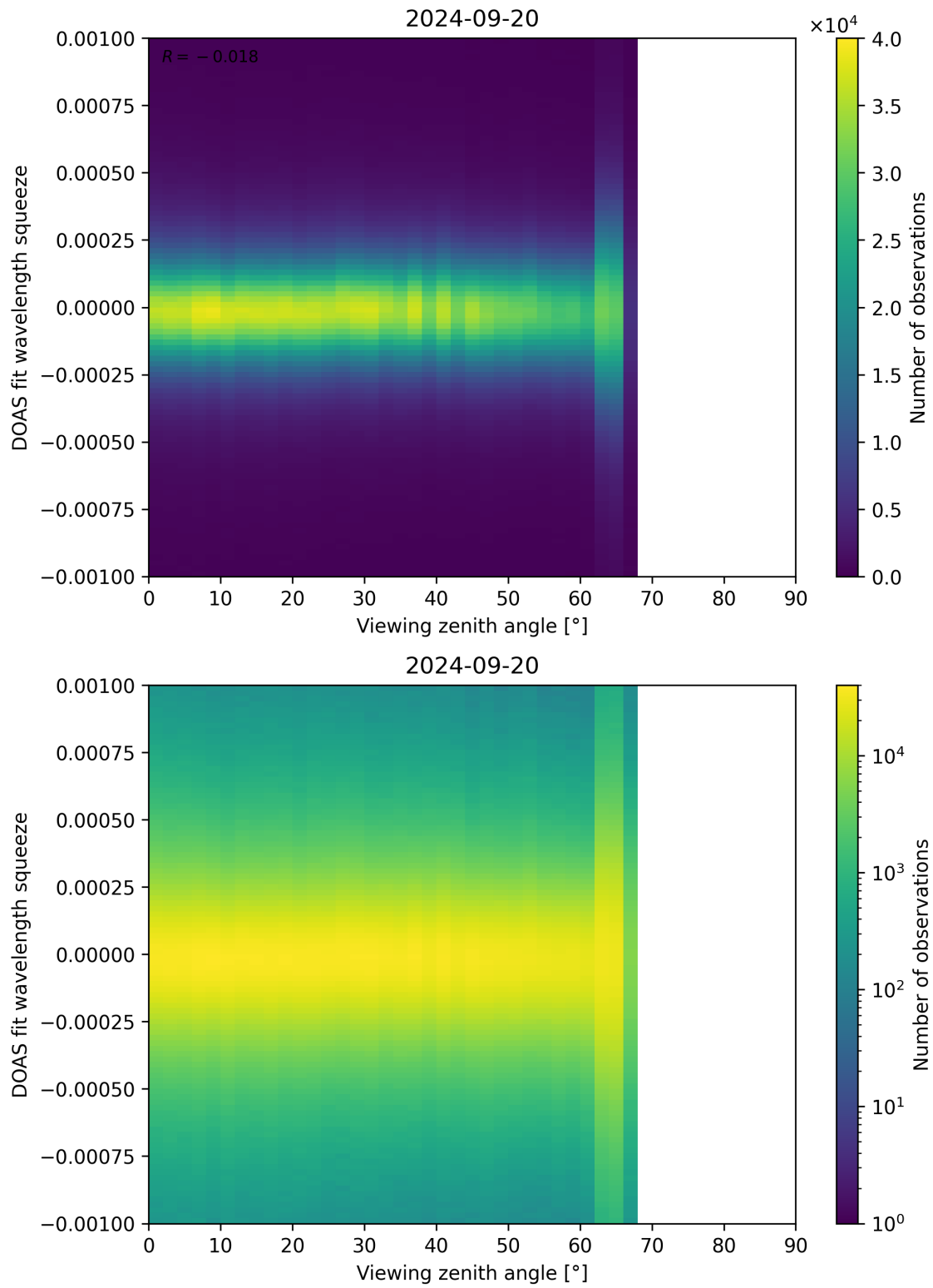
Figure 312: Scatter density plot of “Viewing zenith angle” against “DOAS fit wavelength squeeze” for 2024-09-19 to 2024-09-21.
