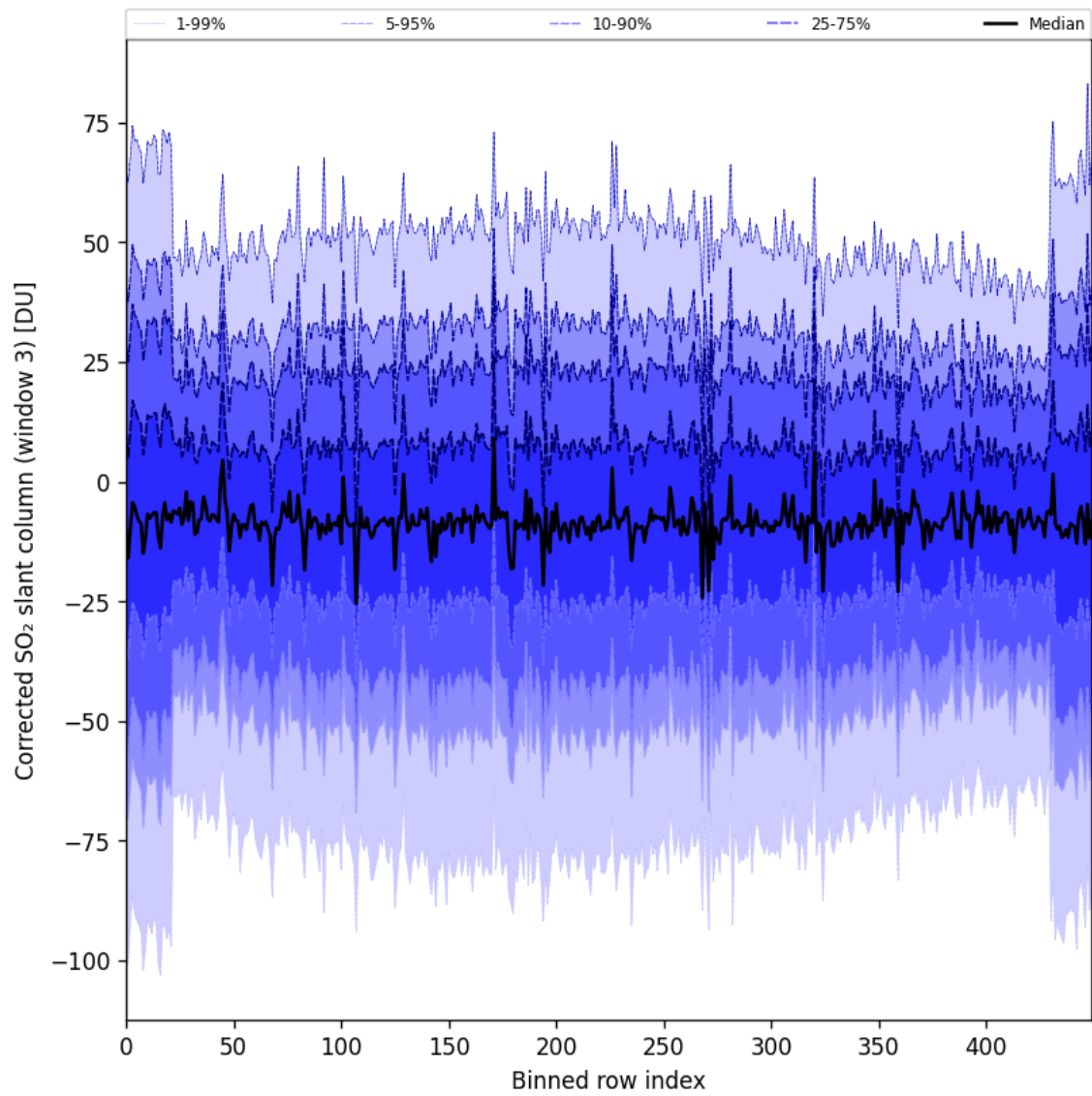
Figure 89: Along track statistics of “Corrected SO 2 slant column (window 3)” for 2024-09-19 to 2024-09-21
