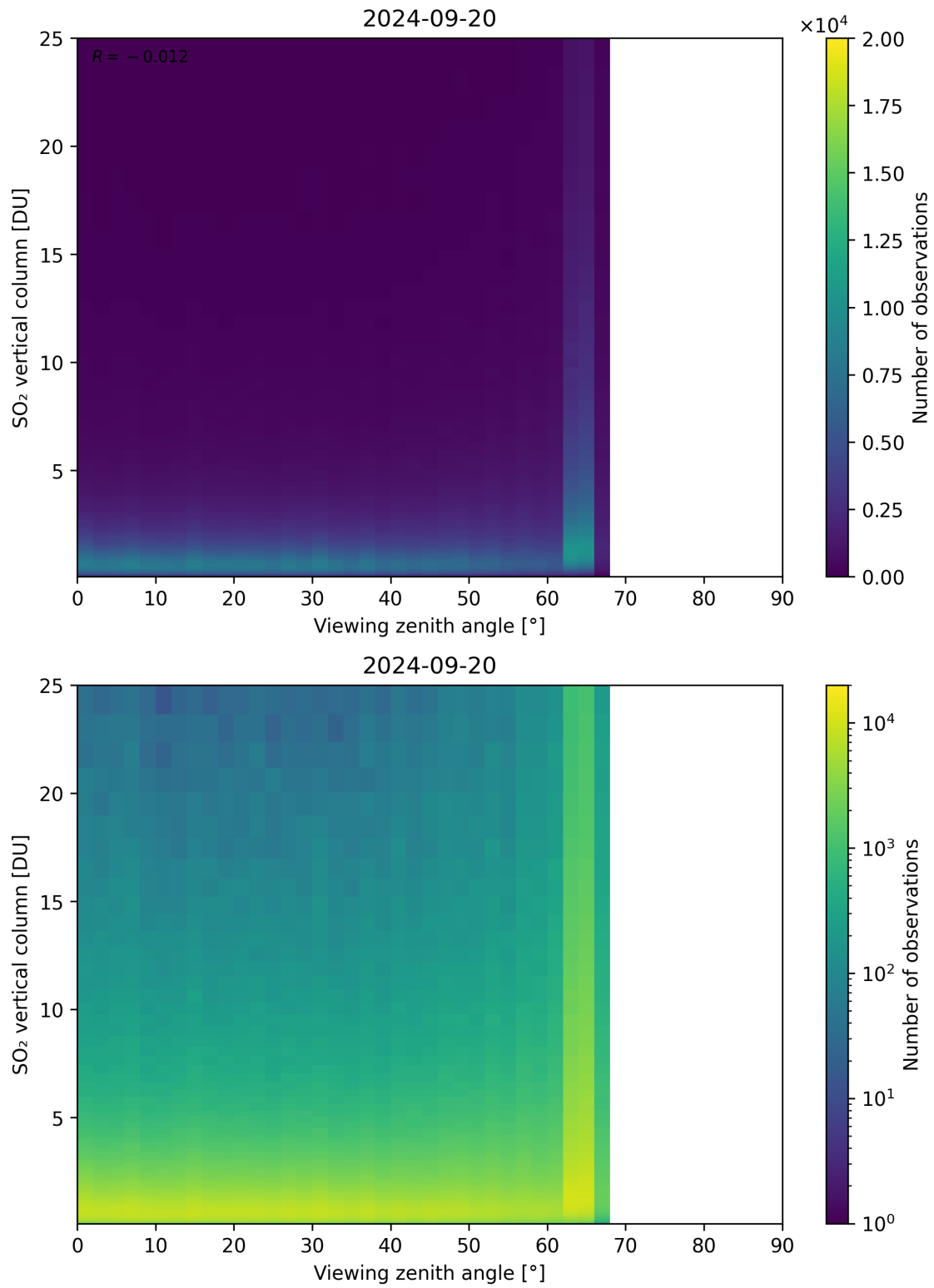
Figure 327: Scatter density plot of “Viewing zenith angle” against “SO 2 vertical column” for 2024-09-19 to 2024-09-21.
