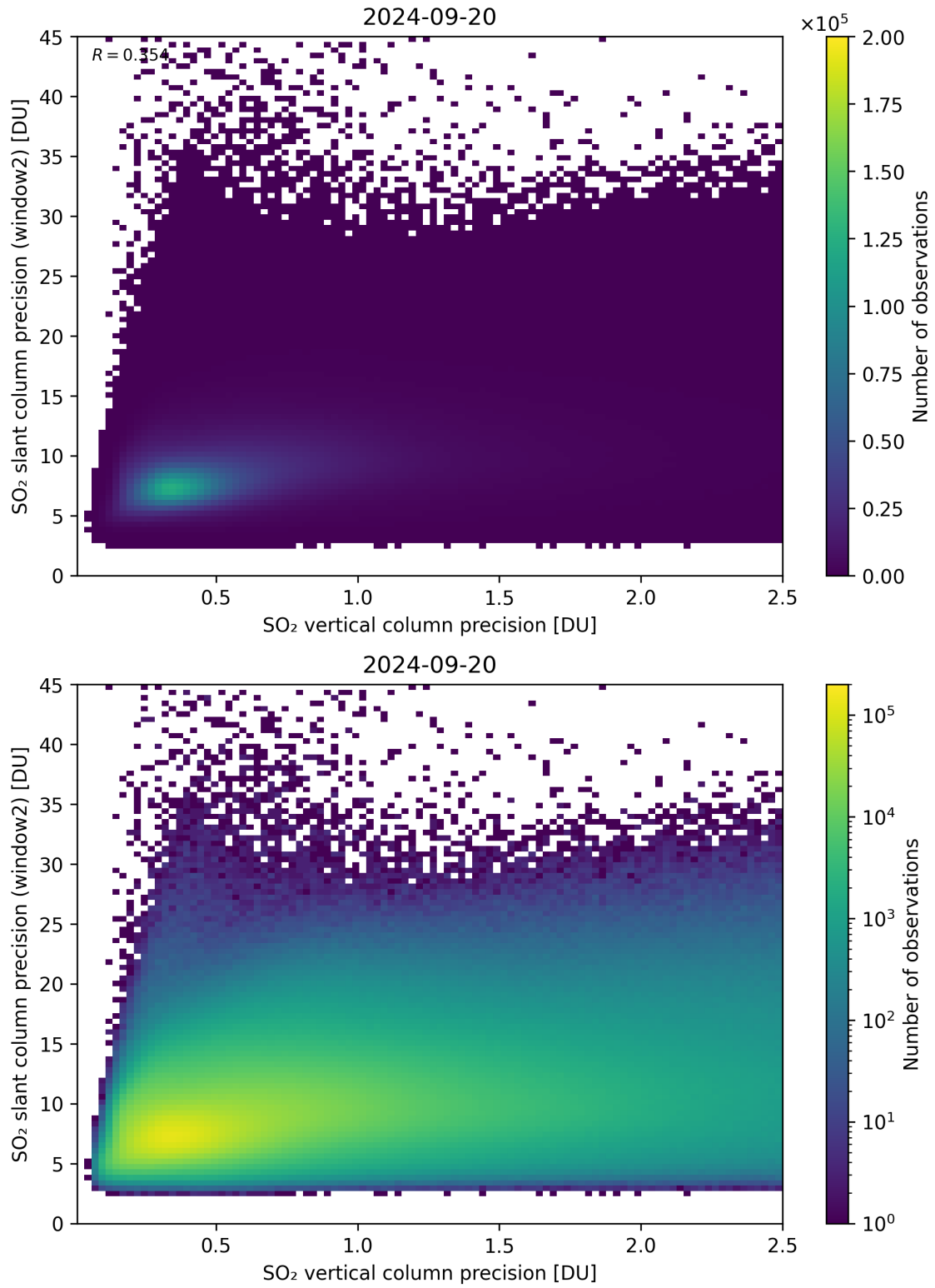
Figure 291: Scatter density plot of “SO 2 vertical column precision” against “SO 2 slant column precision (window2)” for 2024-09-19 to 2024-09-21.
