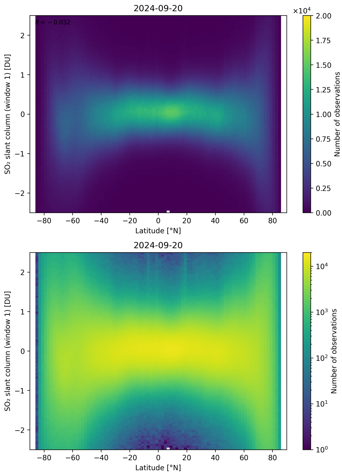
Figure 149: Scatter density plot of “Latitude” against “SO 2 slant column (window 1)” for 2024-09-19 to 2024-09-21.
