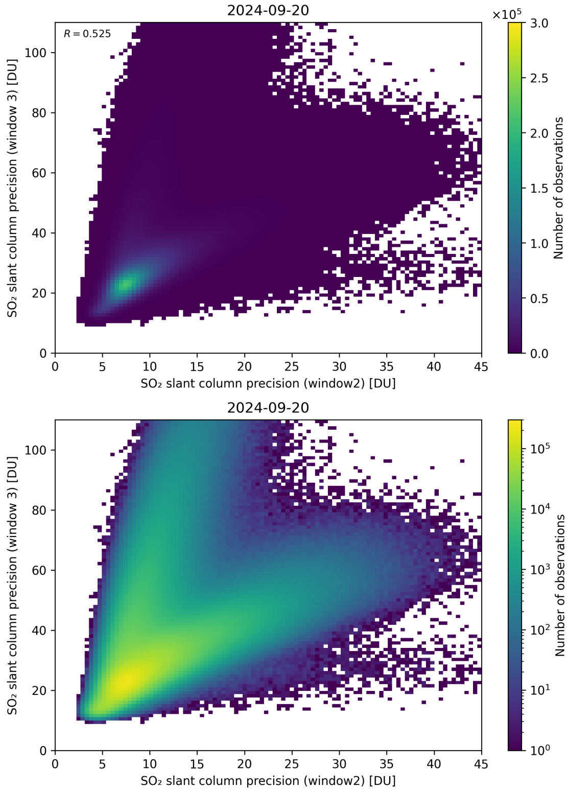
Figure 250: Scatter density plot of “SO 2 slant column precision (window2)” against “SO 2 slant column precision (window 3)” for 2024-09-19 to 2024-09-21.
