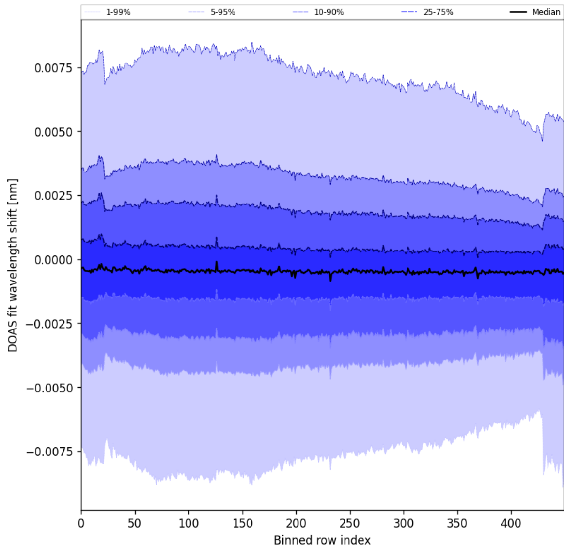
Figure 91: Along track statistics of “DOAS fit wavelength shift” for 2024-09-19 to 2024-09-21
