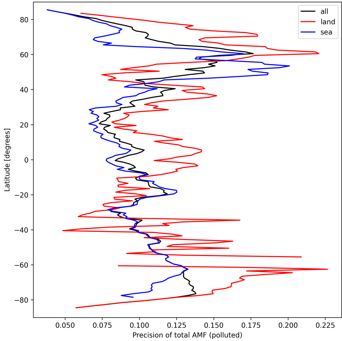
Figure 49: Zonal average of “Precision of total AMF (polluted)” for 2024-09-19 to 2024-09-21.
