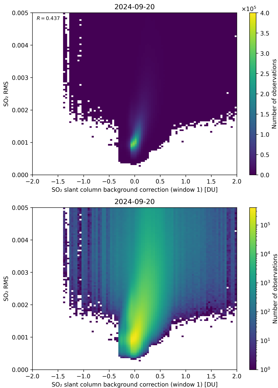
Figure 102: Scatter density plot of “SO 2 slant column background correction (window 1)” against “SO 2 RMS” for 2024-09-19 to 2024-09-21.
