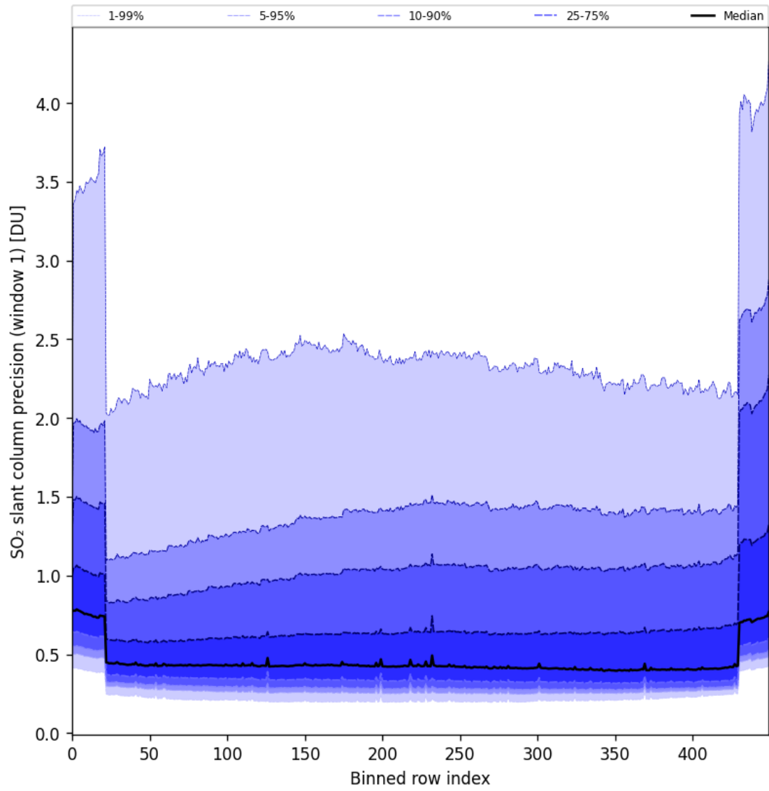
Figure 80: Along track statistics of “SO 2 slant column precision (window 1)” for 2024-09-19 to 2024-09-21
