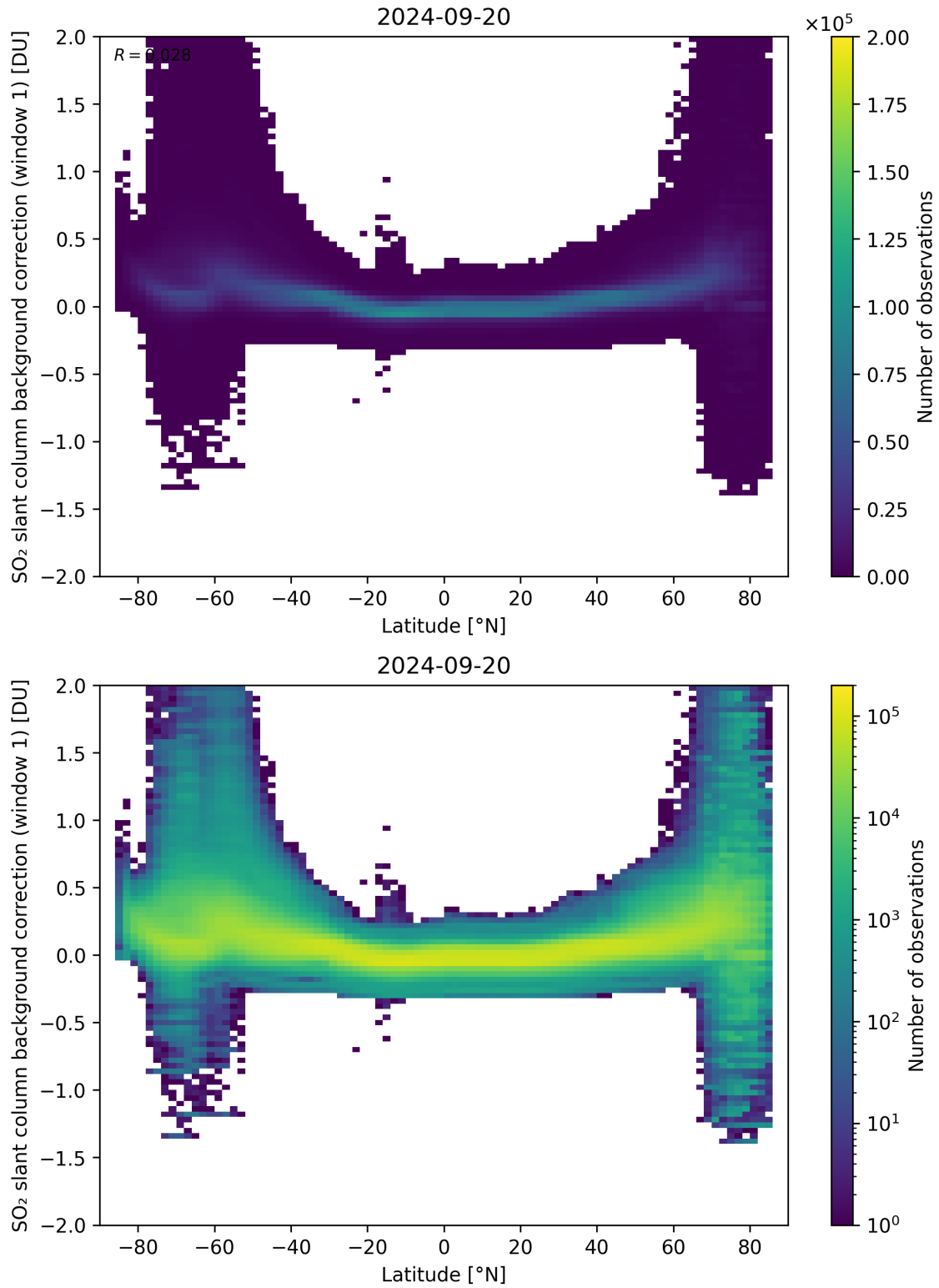
Figure 139: Scatter density plot of “Latitude” against “SO 2 slant column background correction (window 1)” for 2024-09-19 to 2024-09-21.
