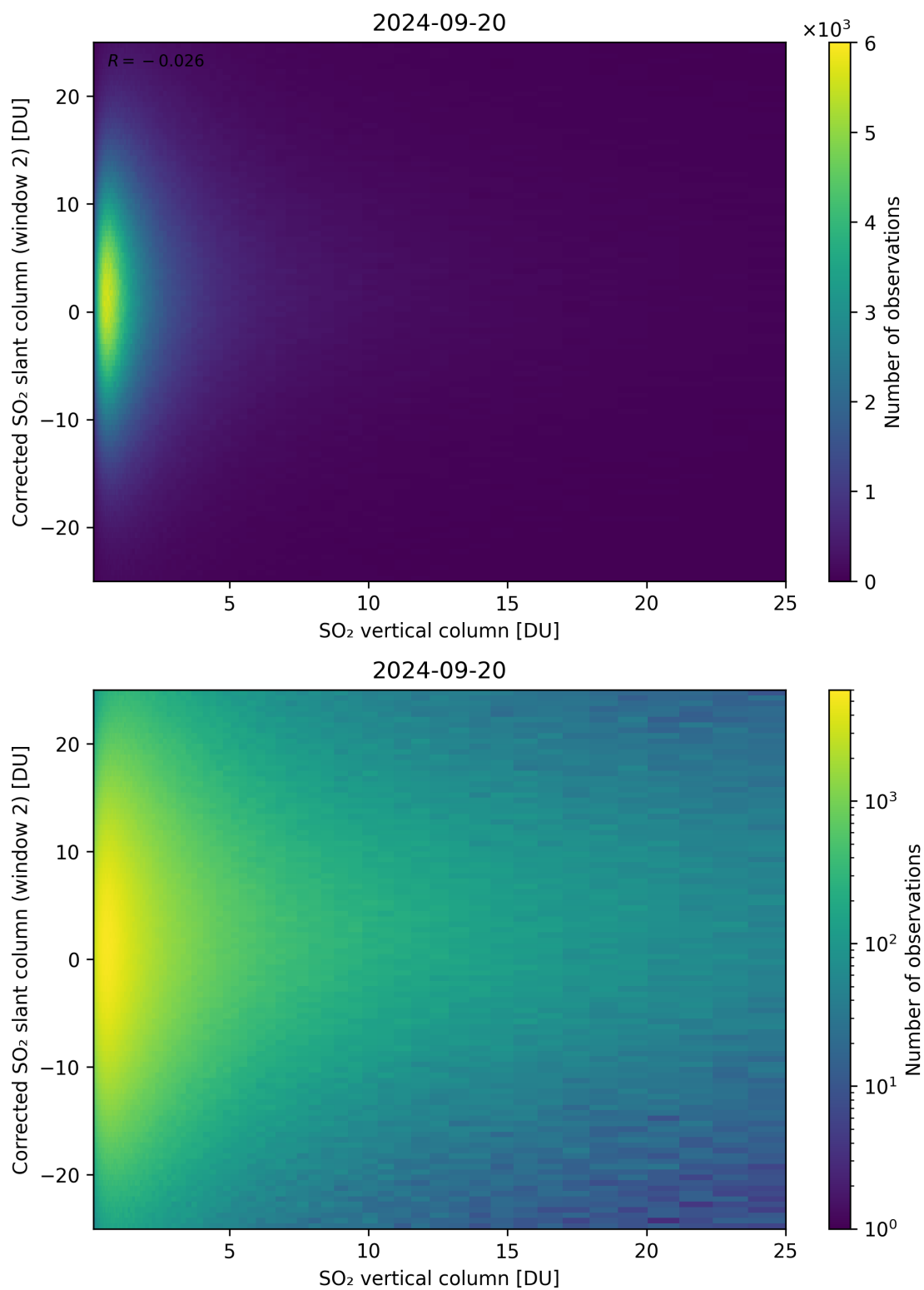
Figure 298: Scatter density plot of “SO 2 vertical column” against “Corrected SO 2 slant column (window 2)” for 2024-09-19 to 2024-09-21.
