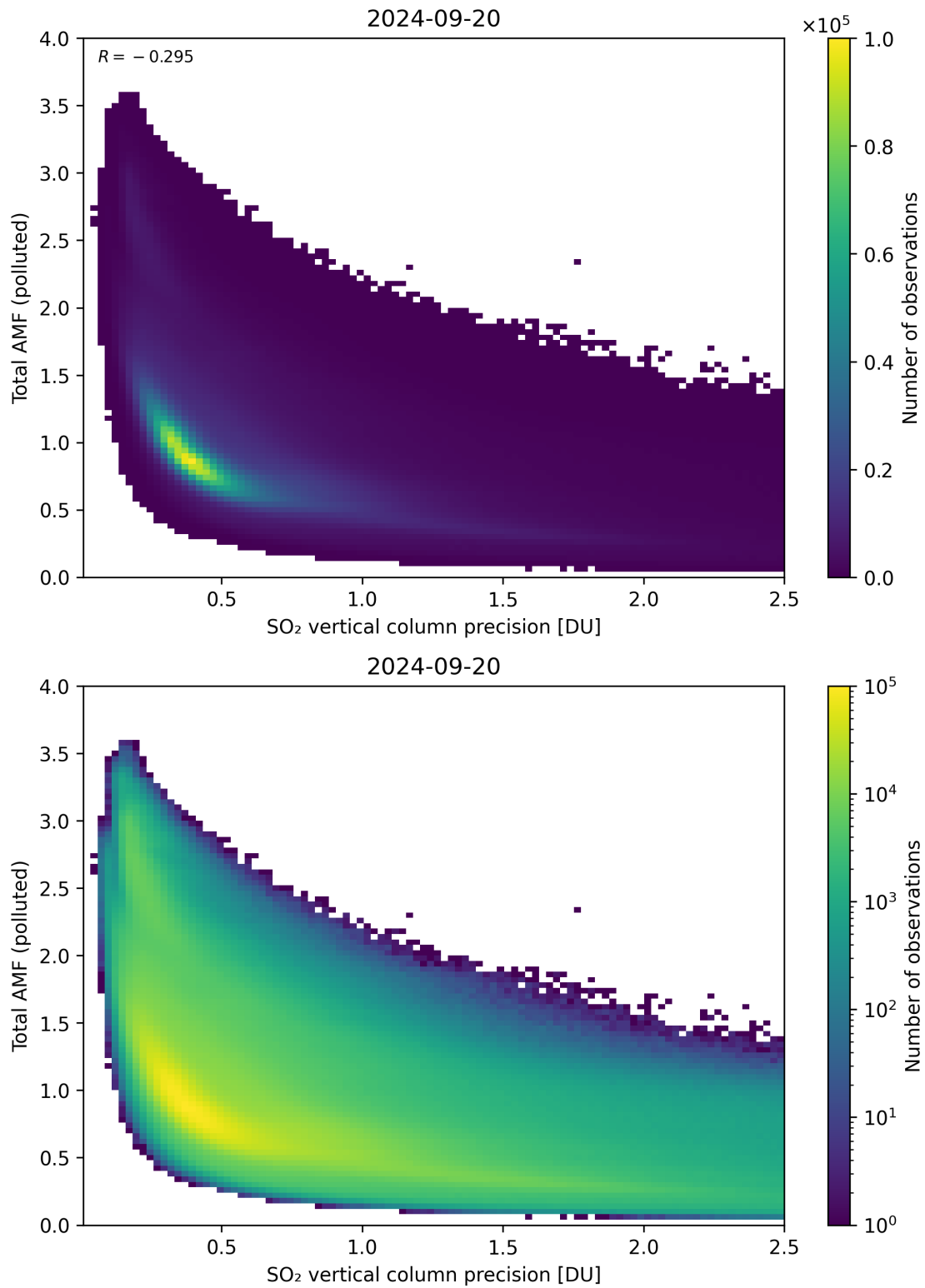
Figure 294: Scatter density plot of “SO 2 vertical column precision” against “Total AMF (polluted)” for 2024-09-19 to 2024-09-21.
