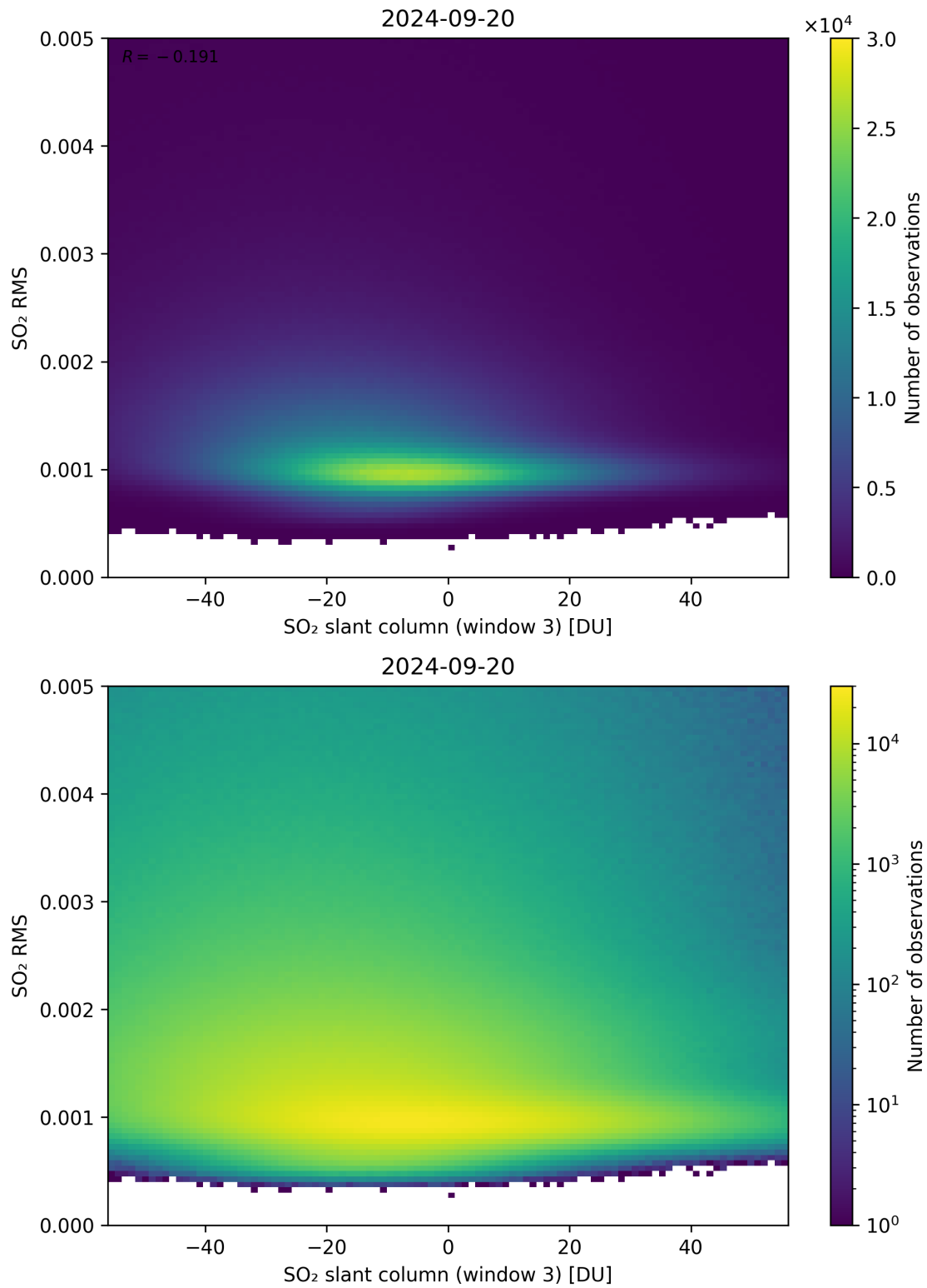
Figure 256: Scatter density plot of “SO 2 slant column (window 3)” against “SO 2 RMS” for 2024-09-19 to 2024-09-21.
