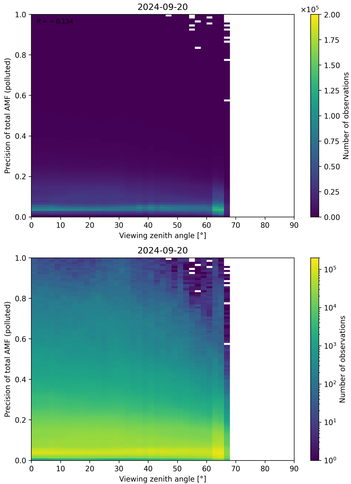
Figure 326: Scatter density plot of “Viewing zenith angle” against “Precision of total AMF (polluted)” for 2024-09-19 to 2024-09-21.
