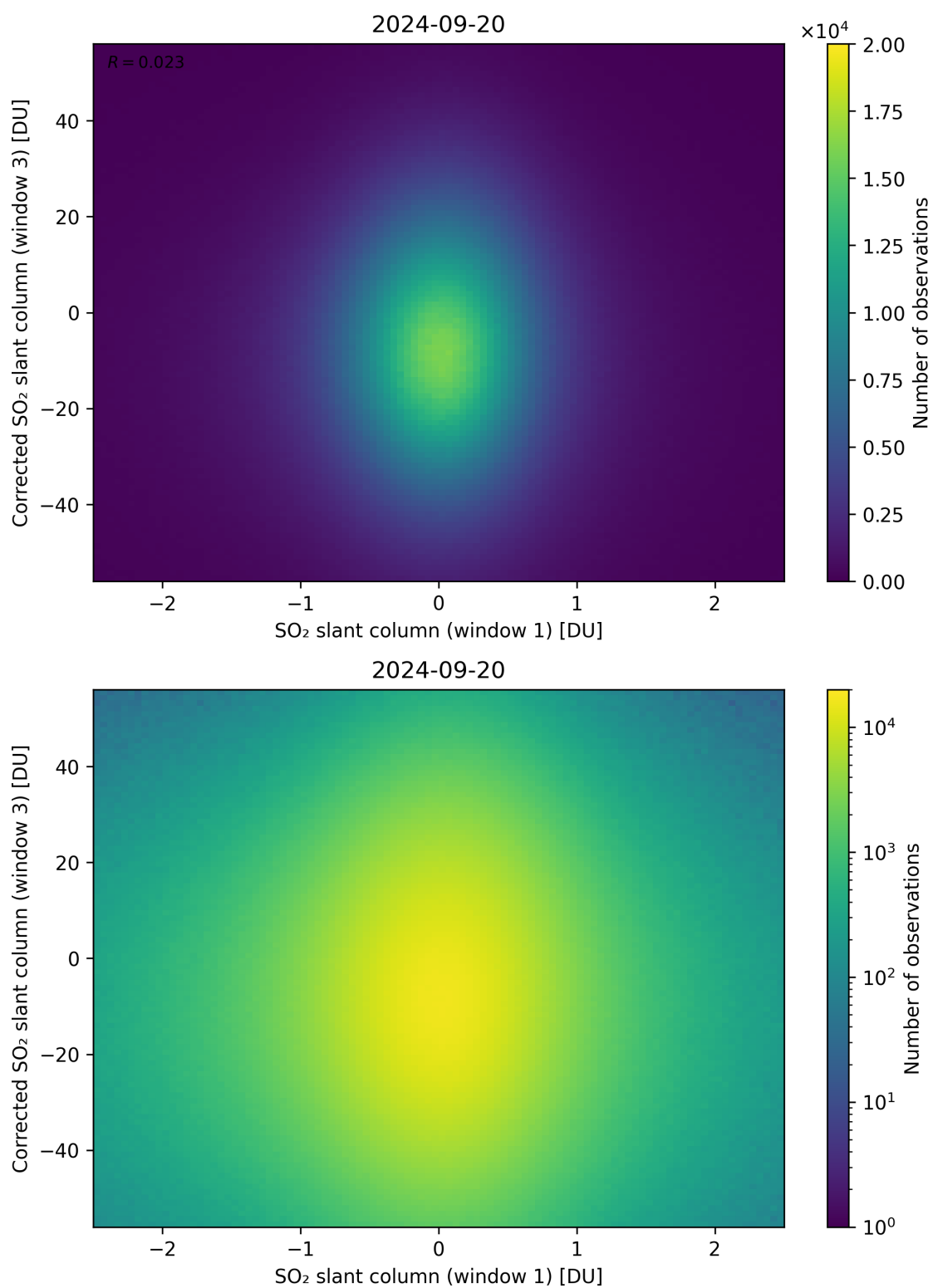
Figure 234: Scatter density plot of “SO 2 slant column (window 1)” against “Corrected SO 2 slant column (window 3)” for 2024-09-19 to 2024-09-21.
