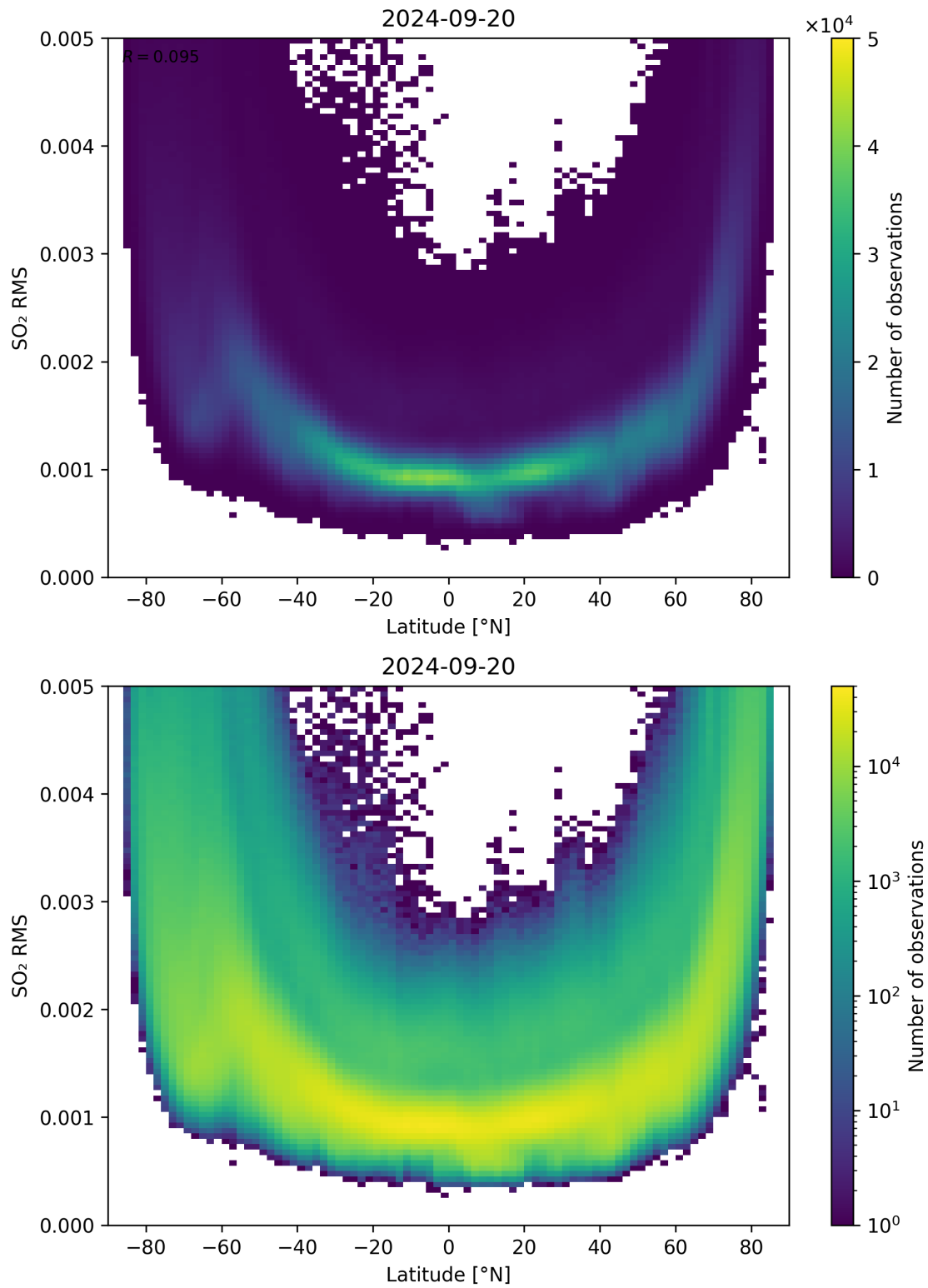
Figure 144: Scatter density plot of “Latitude” against “SO 2 RMS” for 2024-09-19 to 2024-09-21.
