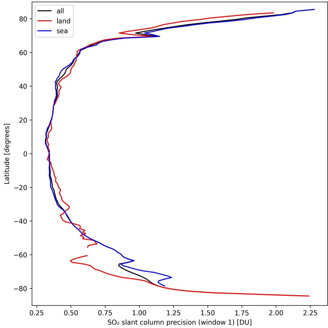
Figure 34: Zonal average of “SO 2 slant column precision (window 1)” for 2024-09-19 to 2024-09-21.
