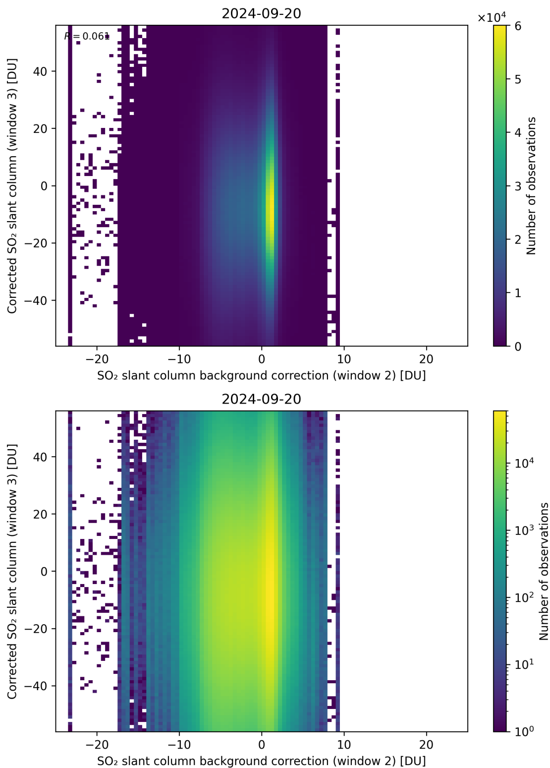
Figure 116: Scatter density plot of “SO 2 slant column background correction (window 2)” against “Corrected SO 2 slant column (window 3)” for 2024-09-19 to 2024-09-21.
