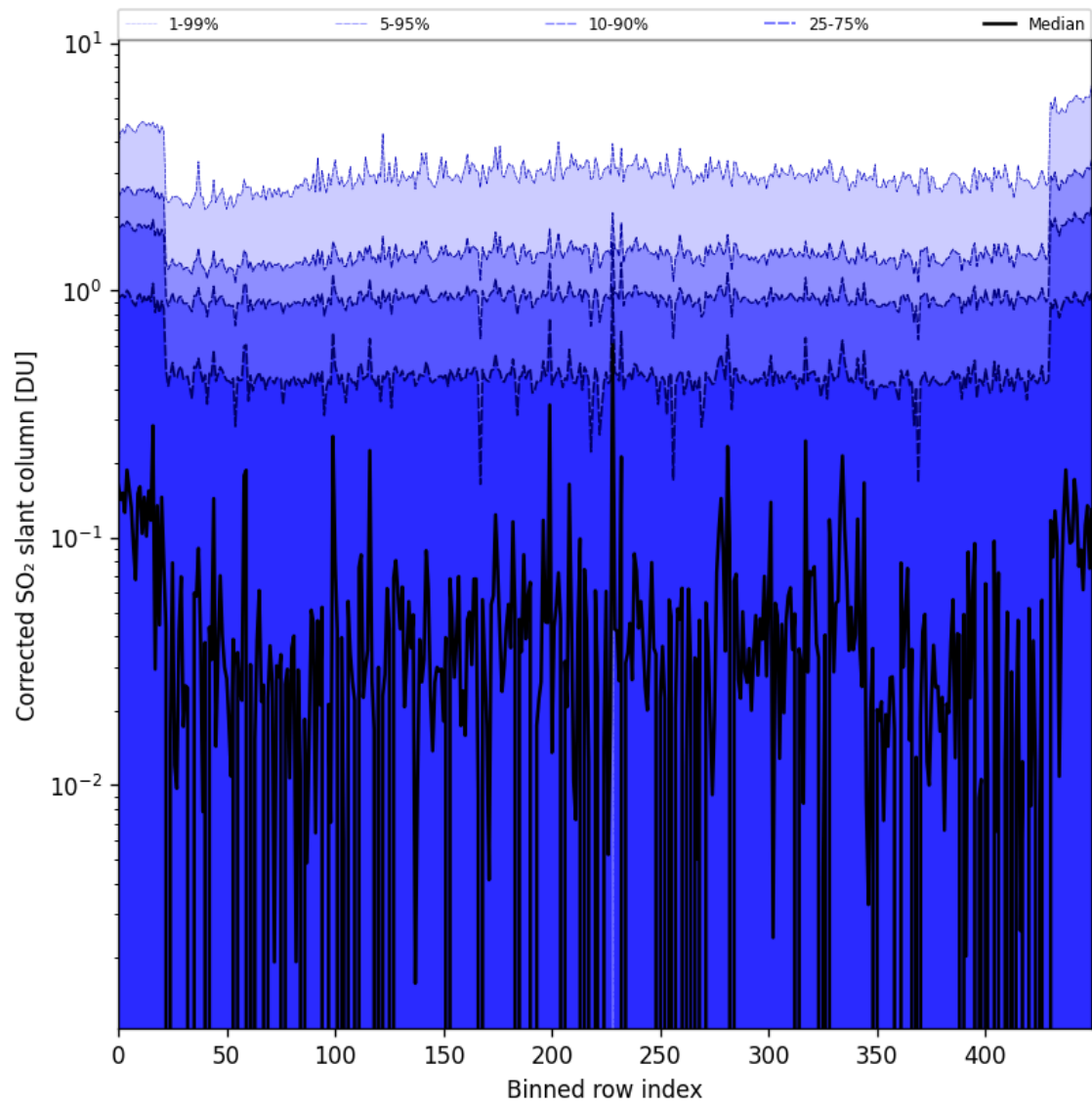
Figure 78: Along track statistics of “Corrected SO 2 slant column” for 2024-09-19 to 2024-09-21
