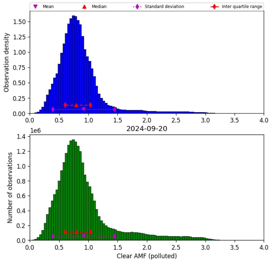
Figure 73: Histogram of “Clear AMF (polluted)” for 2024-09-19 to 2024-09-21
