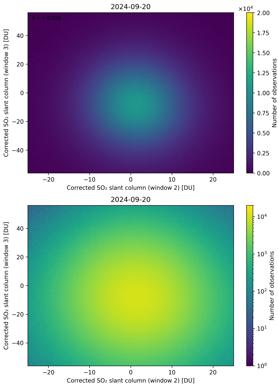
Figure 200: Scatter density plot of “Corrected SO 2 slant column (window 2)” against “Corrected SO 2 slant column (window 3)” for 2024-09-19 to 2024-09-21.
