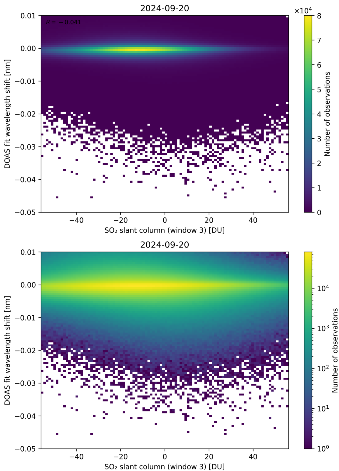
Figure 254: Scatter density plot of “SO 2 slant column (window 3)” against “DOAS fit wavelength shift” for 2024-09-19 to 2024-09-21.
