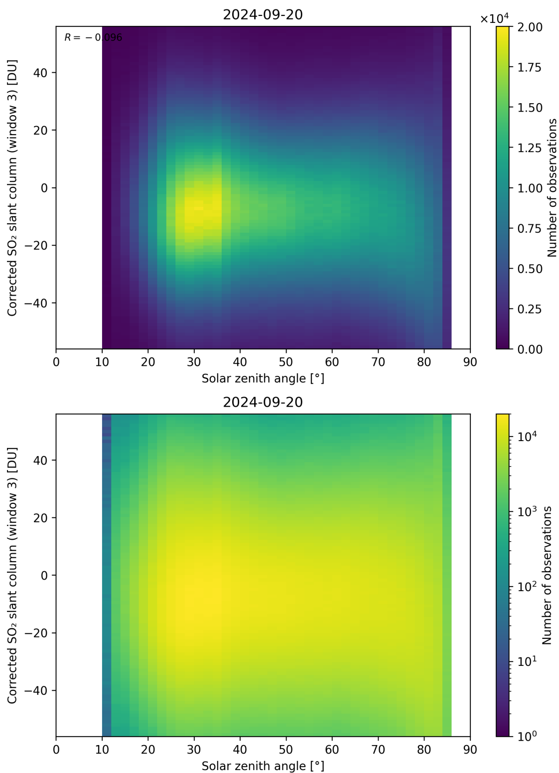
Figure 168: Scatter density plot of “Solar zenith angle” against “Corrected SO 2 slant column (window 3)” for 2024-09-19 to 2024-09-21.
