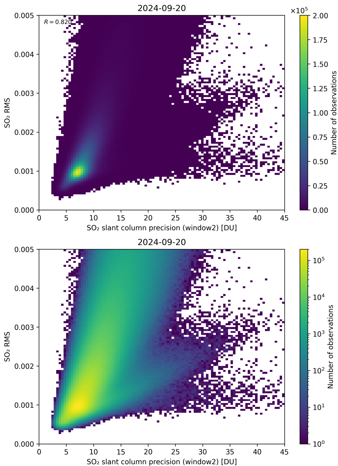
Figure 245: Scatter density plot of “SO 2 slant column precision (window2)” against “SO 2 RMS” for 2024-09-19 to 2024-09-21.
