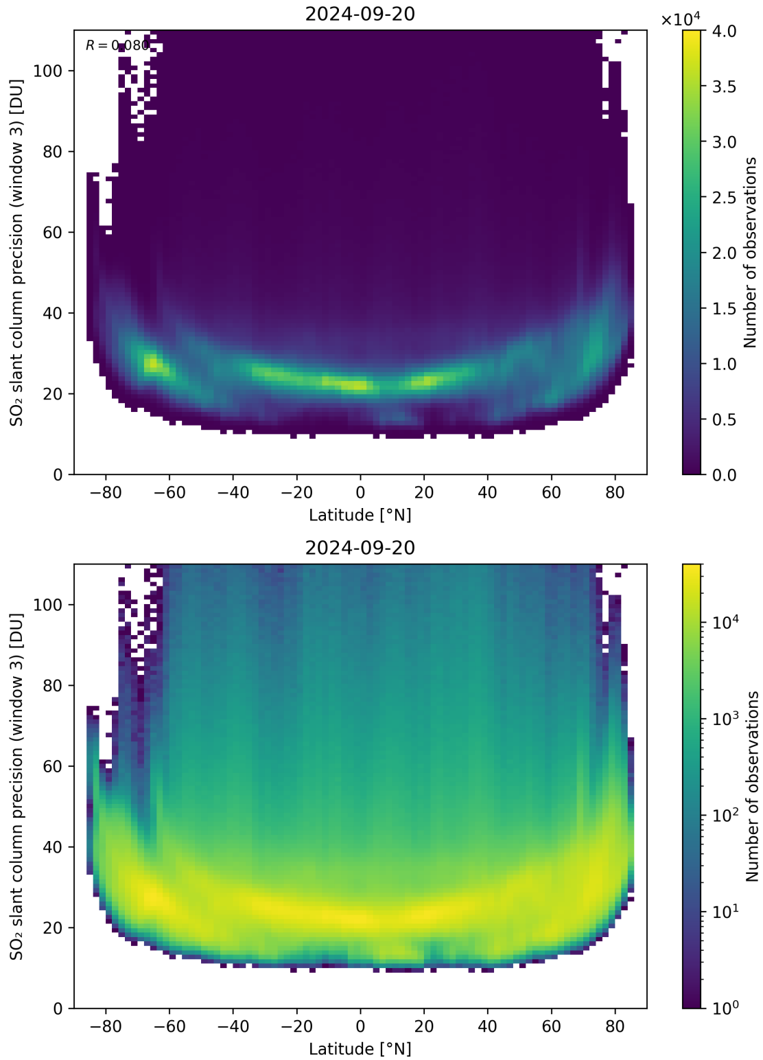
Figure 153: Scatter density plot of “Latitude” against “SO 2 slant column precision (window 3)” for 2024-09-19 to 2024-09-21.
