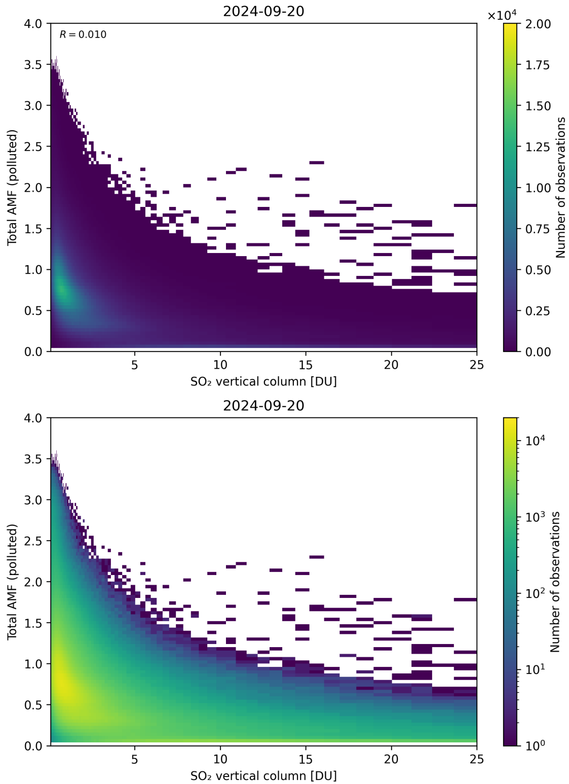
Figure 305: Scatter density plot of “SO 2 vertical column” against “Total AMF (polluted)” for 2024-09-19 to 2024-09-21.
