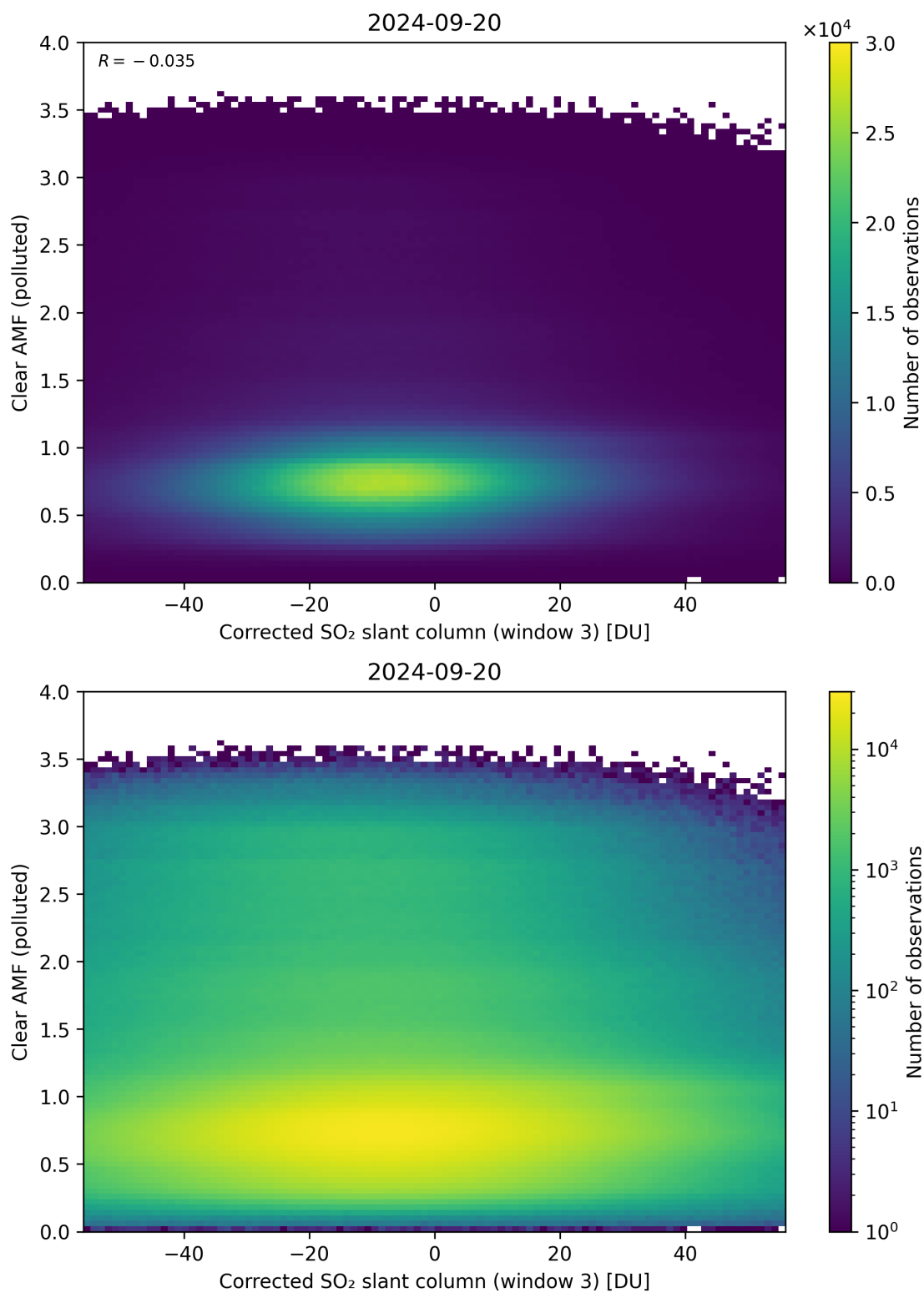
Figure 209: Scatter density plot of “Corrected SO 2 slant column (window 3)” against “Clear AMF (polluted)” for 2024-09-19 to 2024-09-21.
