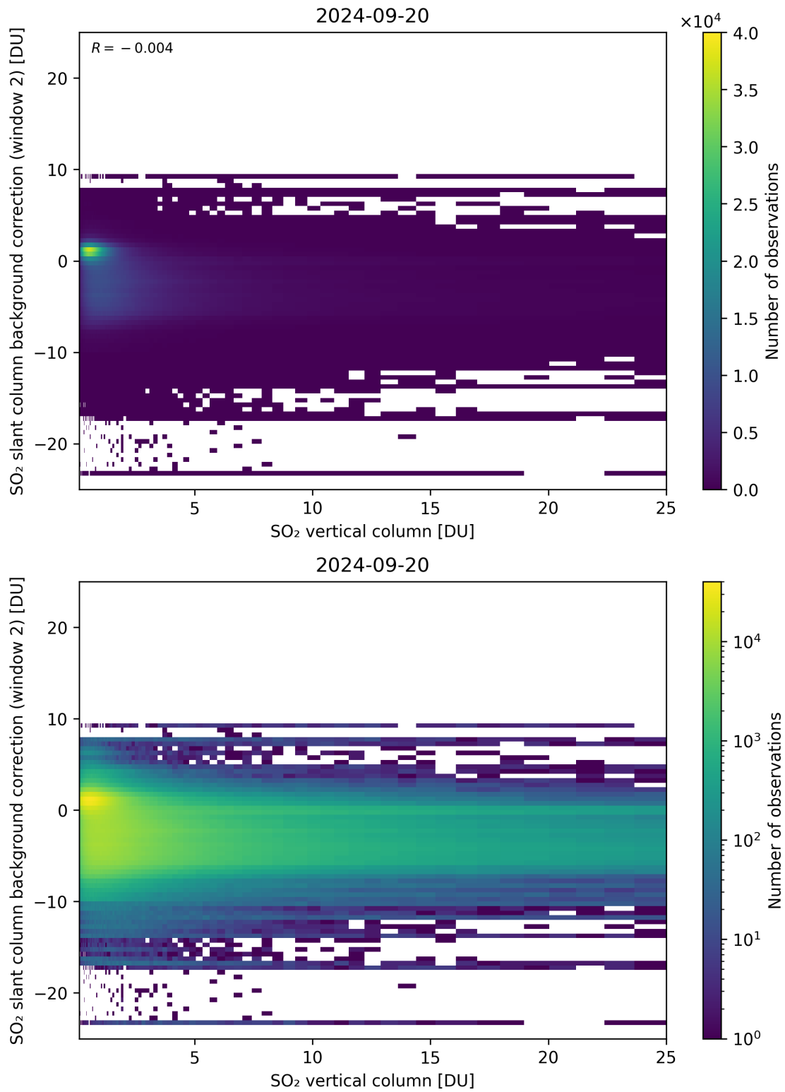
Figure 274: Scatter density plot of “SO 2 vertical column” against “SO 2 slant column background correction (window 2)” for 2024-09-19 to 2024-09-21.
