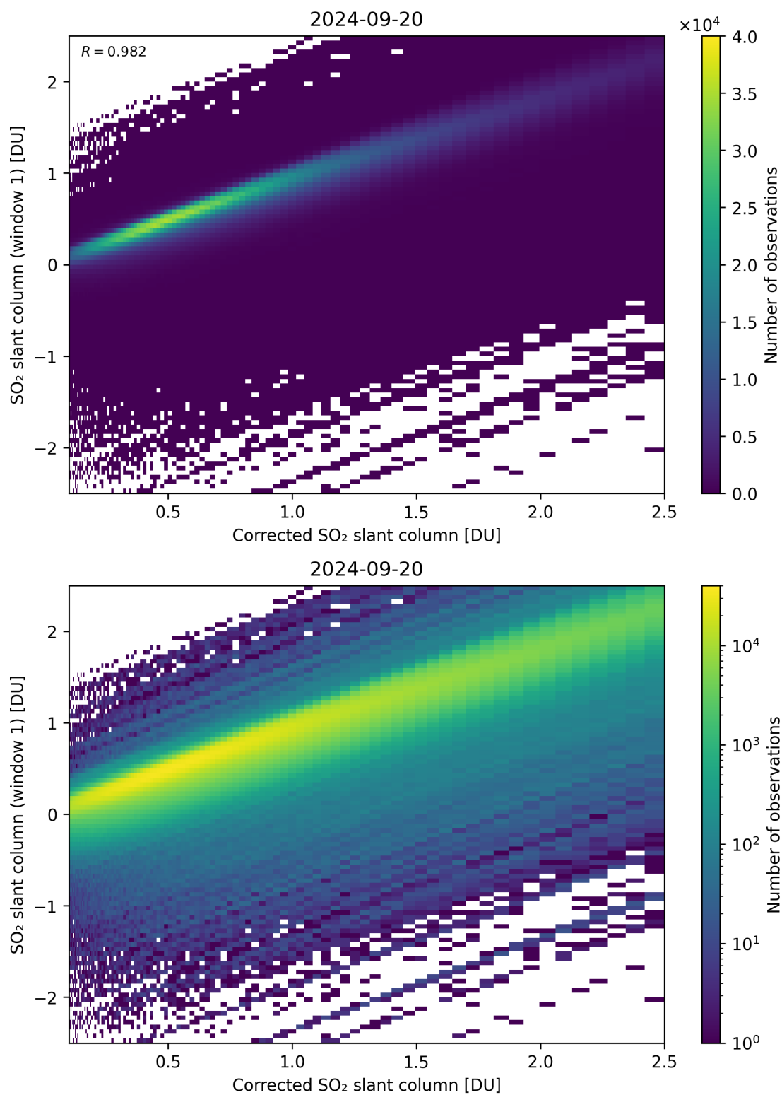
Figure 187: Scatter density plot of “Corrected SO 2 slant column” against “SO 2 slant column (window 1)” for 2024-09-19 to 2024-09-21.
