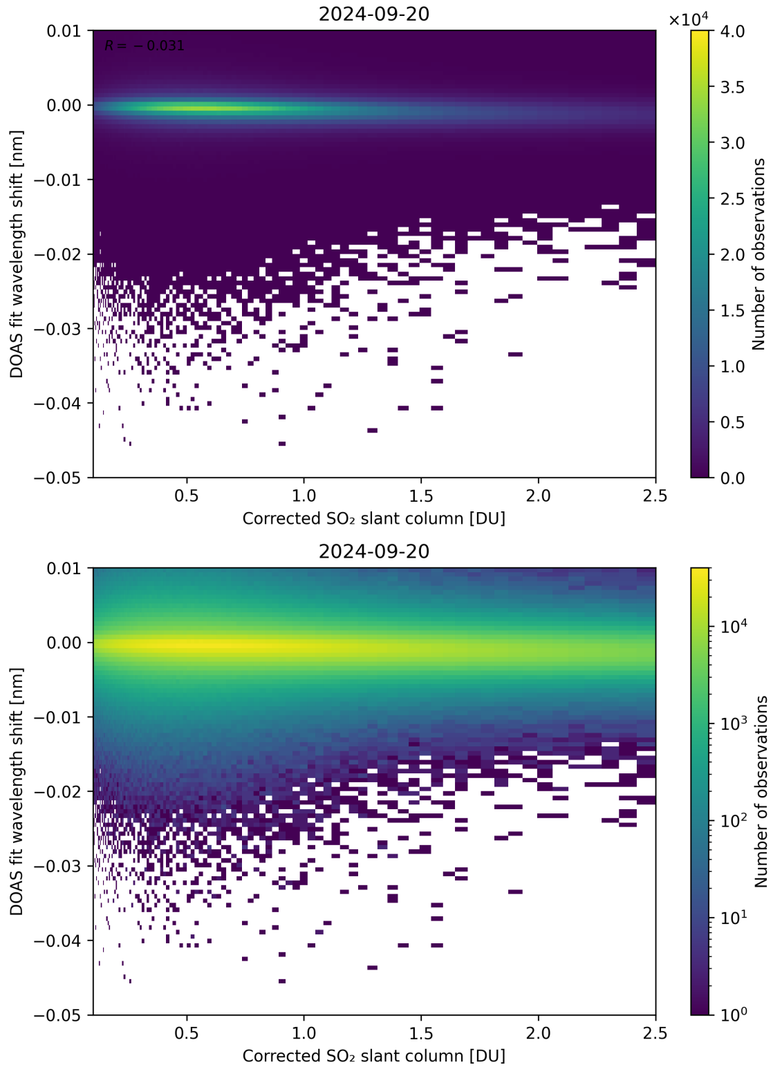
Figure 181: Scatter density plot of “Corrected SO 2 slant column” against “DOAS fit wavelength shift” for 2024-09-19 to 2024-09-21.
