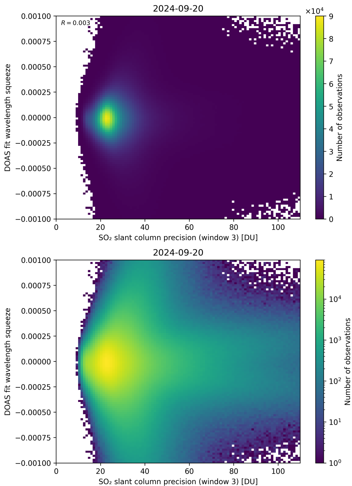
Figure 259: Scatter density plot of “SO 2 slant column precision (window 3)” against “DOAS fit wavelength squeeze” for 2024-09-19 to 2024-09-21.
