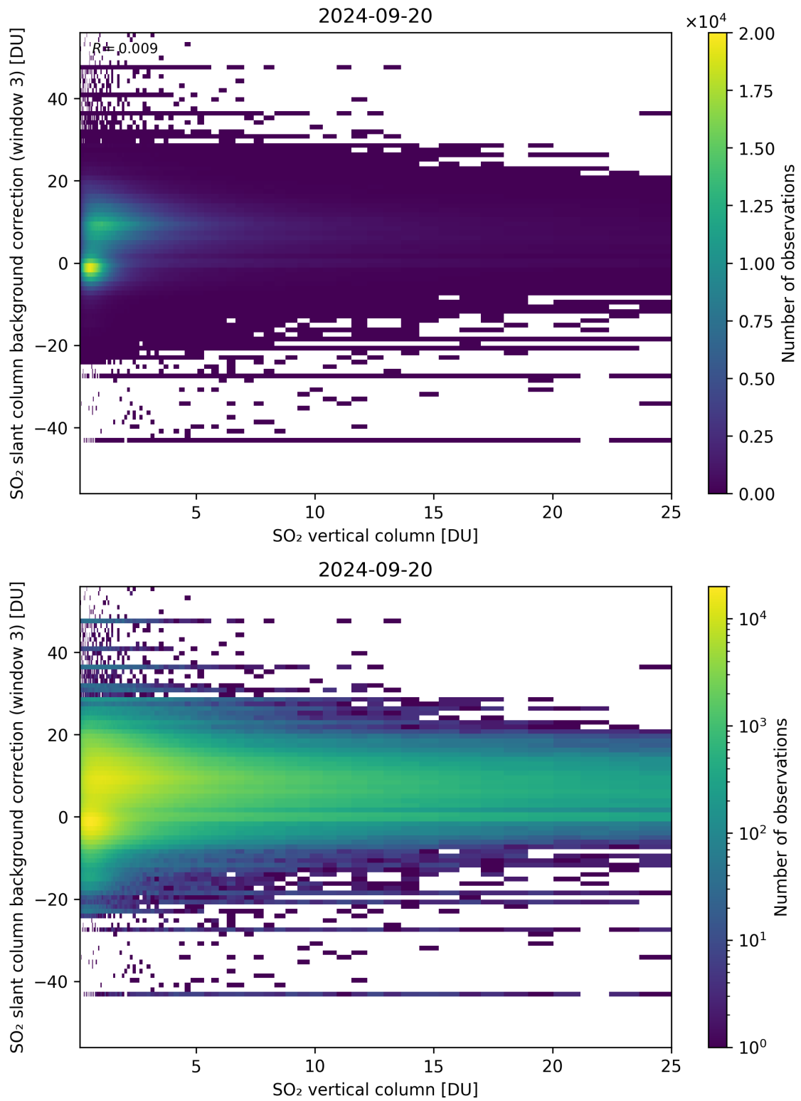
Figure 275: Scatter density plot of “SO 2 vertical column” against “SO 2 slant column background correction (window 3)” for 2024-09-19 to 2024-09-21.
