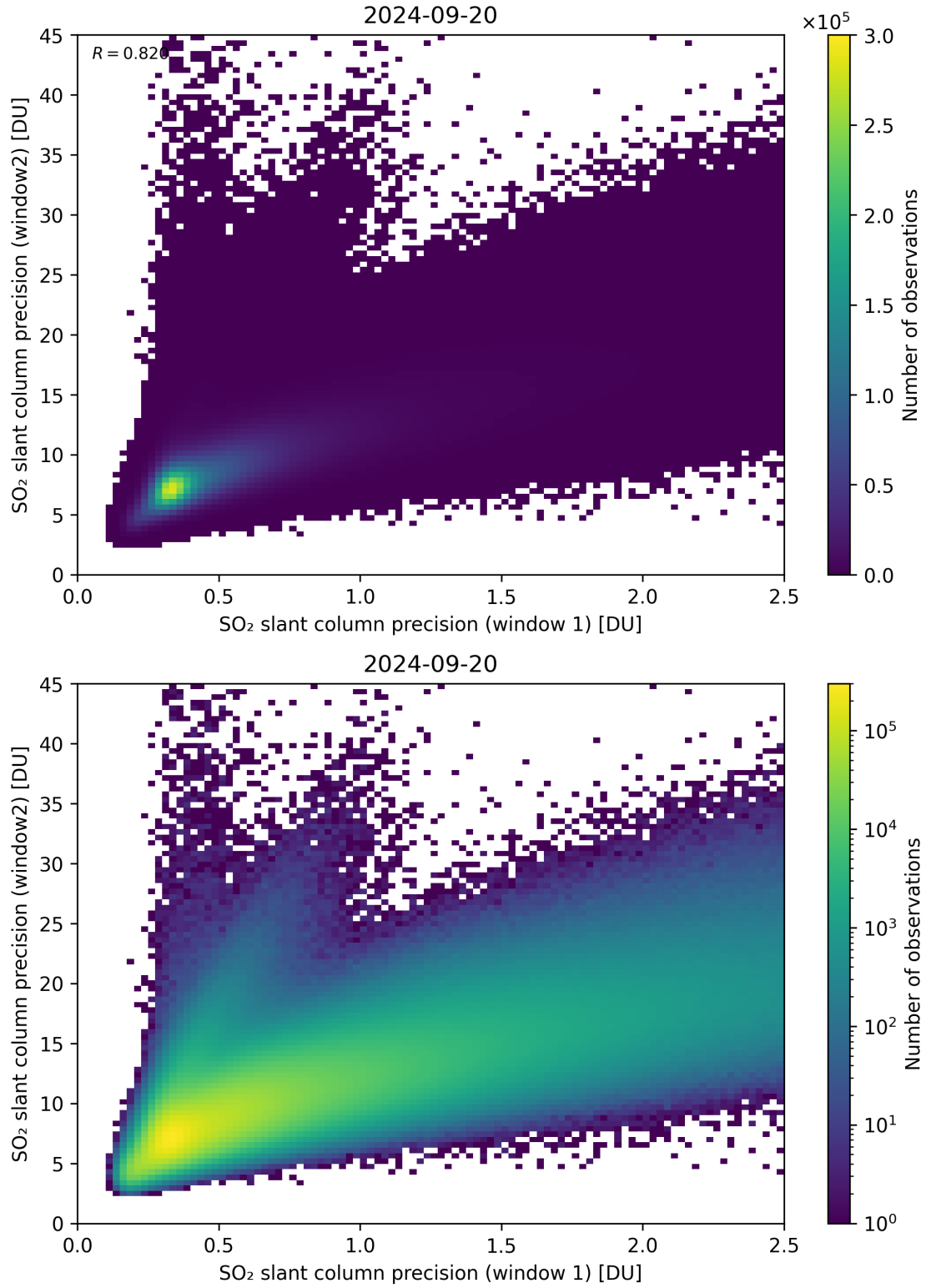
Figure 227: Scatter density plot of “SO 2 slant column precision (window 1)” against “SO 2 slant column precision (window2)” for 2024-09-19 to 2024-09-21.
