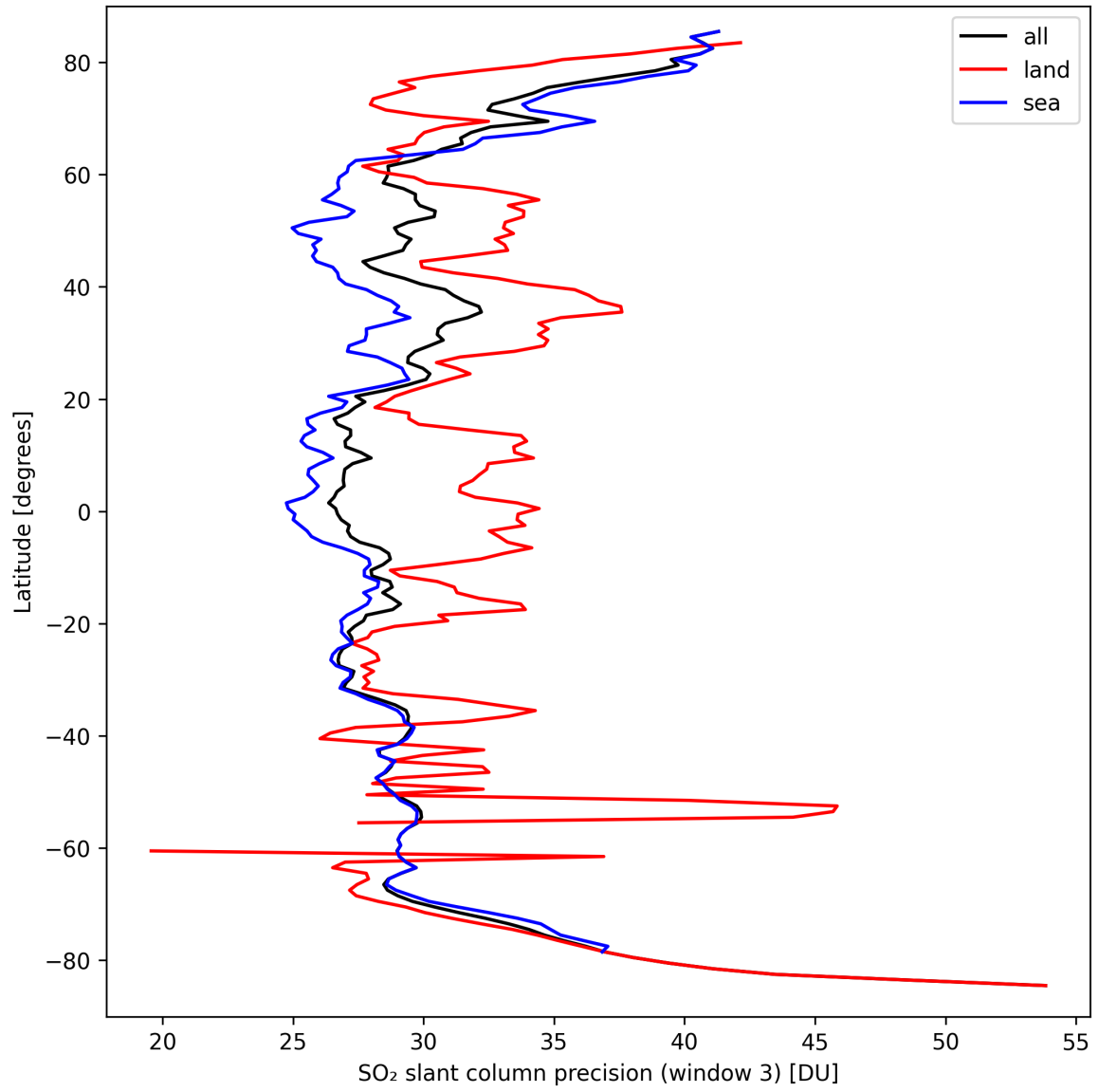
Figure 42: Zonal average of “SO 2 slant column precision (window 3)” for 2024-09-19 to 2024-09-21.
