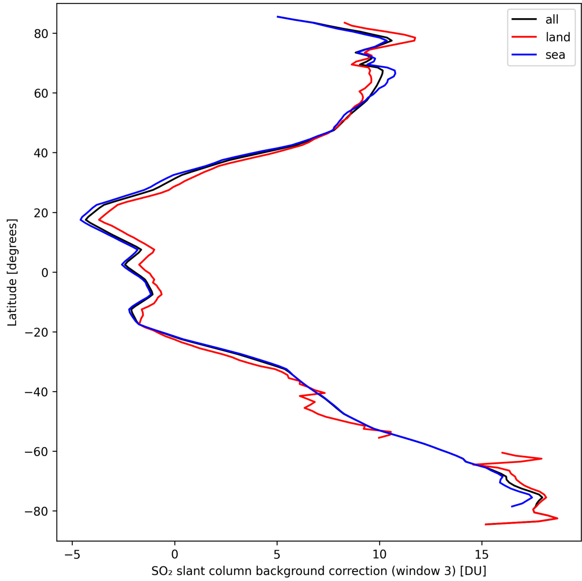
Figure 44: Zonal average of “SO 2 slant column background correction (window 3)” for 2024-09-19 to 2024-09-21.
