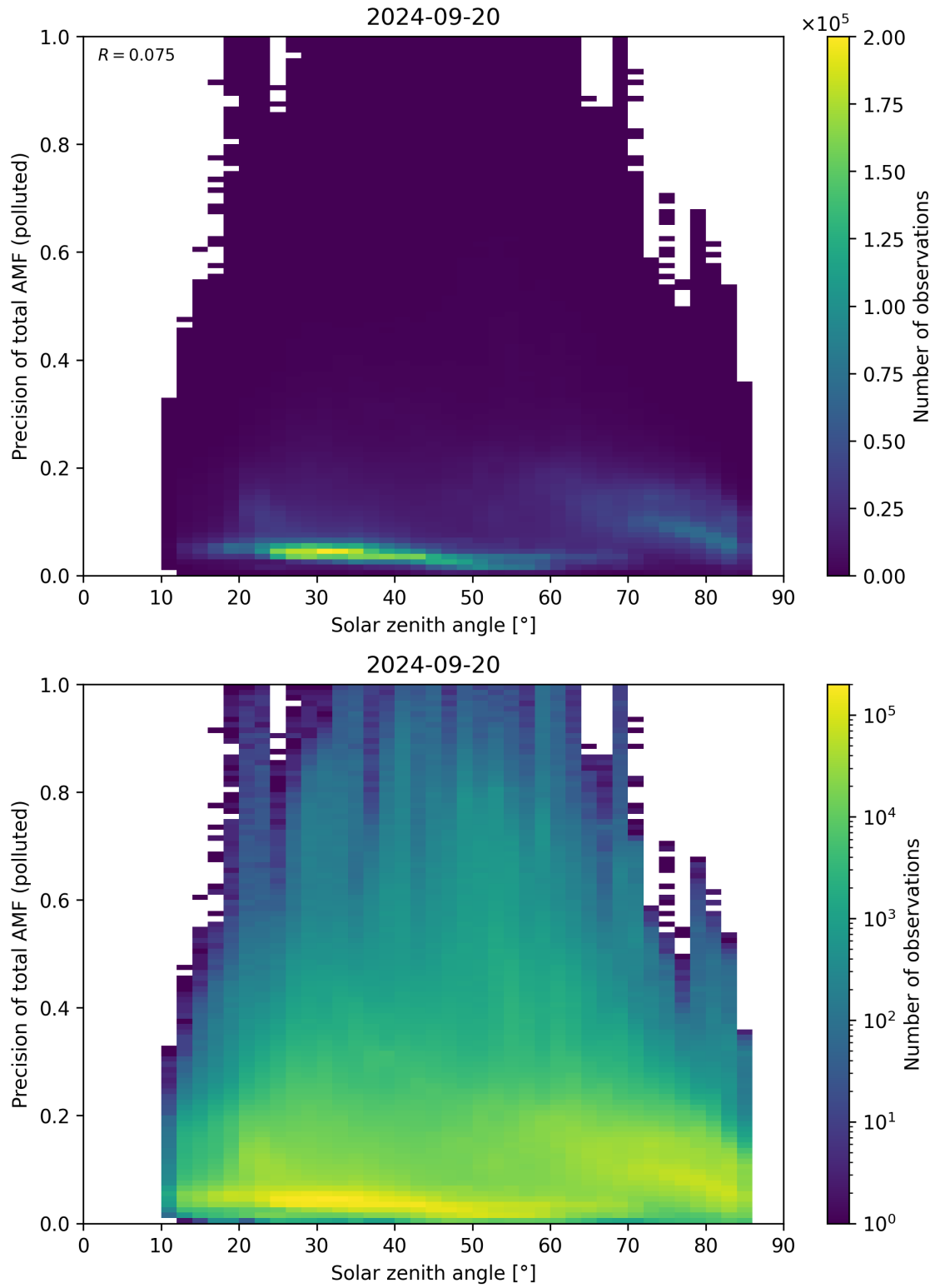
Figure 175: Scatter density plot of “Solar zenith angle” against “Precision of total AMF (polluted)” for 2024-09-19 to 2024-09-21.
