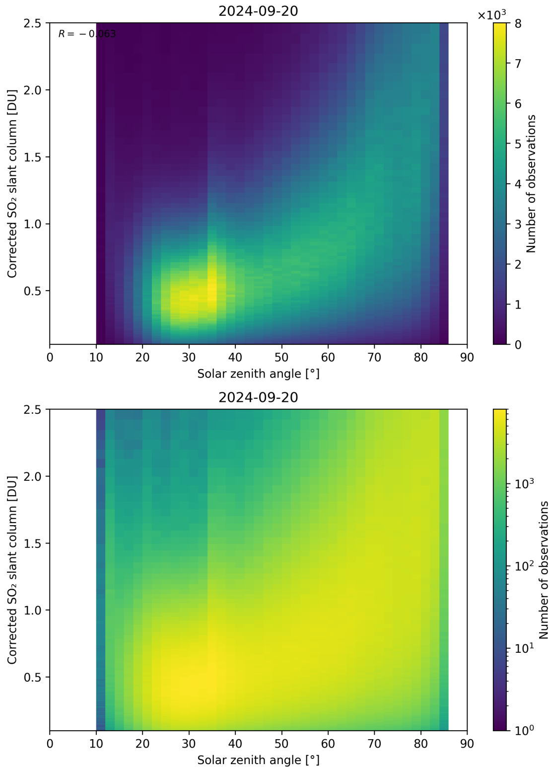
Figure 166: Scatter density plot of “Solar zenith angle” against “Corrected SO 2 slant column” for 2024-09-19 to 2024-09-21.
