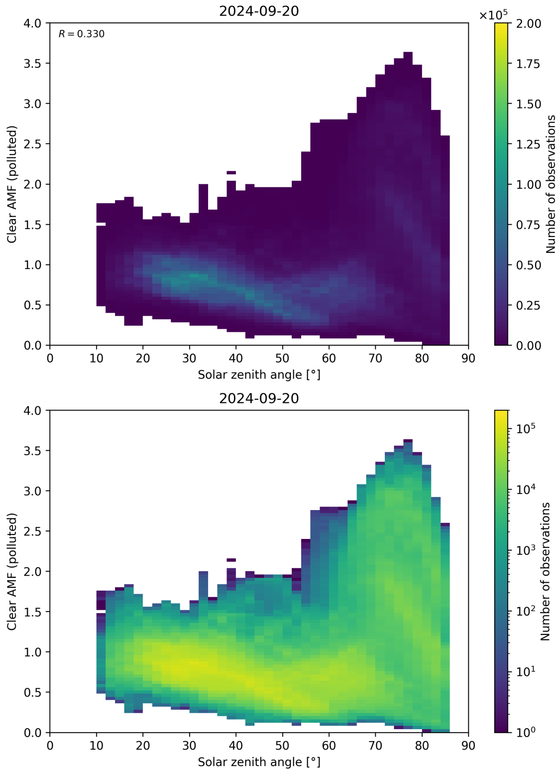
Figure 165: Scatter density plot of “Solar zenith angle” against “Clear AMF (polluted)” for 2024-09-19 to 2024-09-21.
