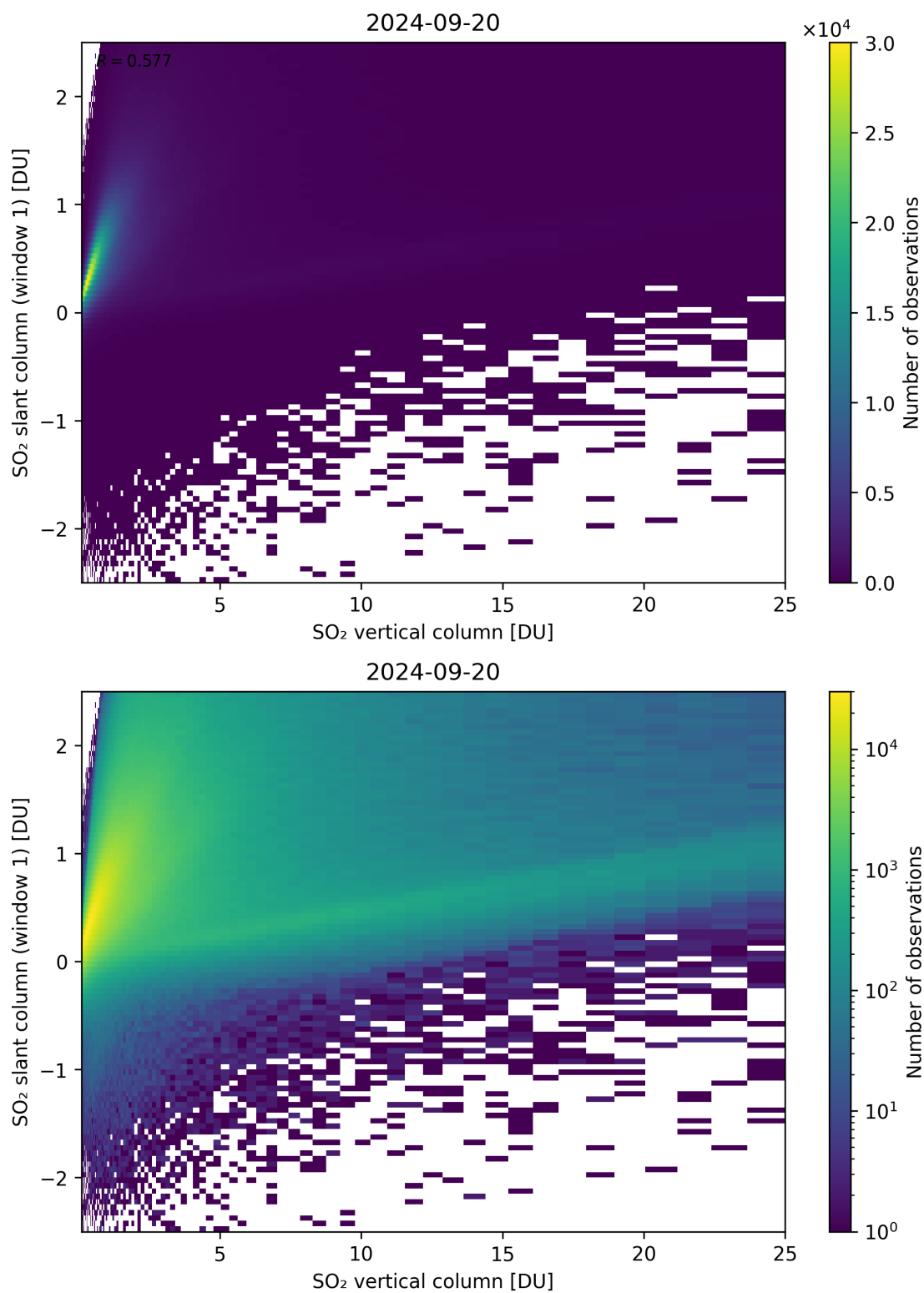
Figure 300: Scatter density plot of “SO 2 vertical column” against “SO 2 slant column (window 1)” for 2024-09-19 to 2024-09-21.
