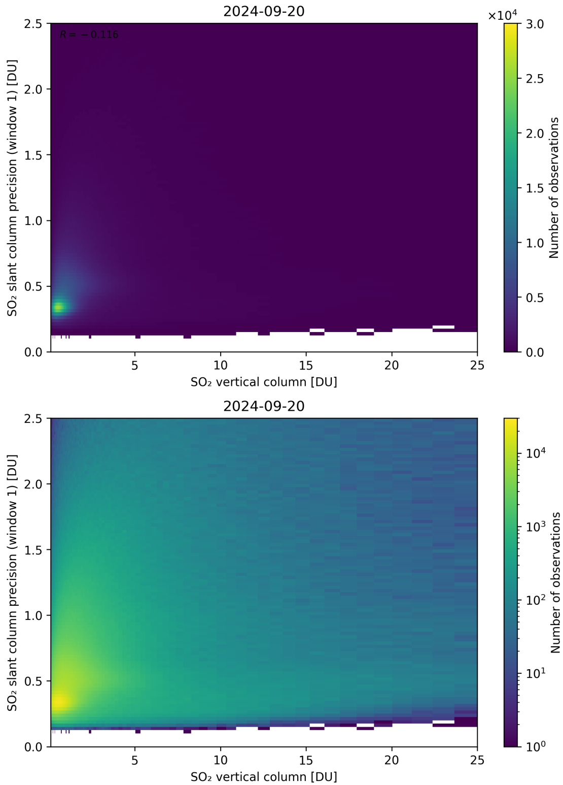
Figure 301: Scatter density plot of “SO 2 vertical column” against “SO 2 slant column precision (window 1)” for 2024-09-19 to 2024-09-21.
