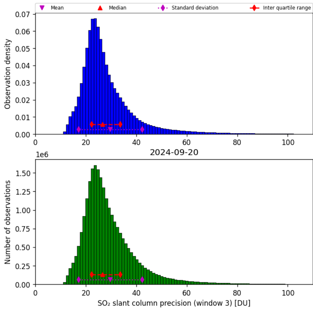
Figure 65: Histogram of “SO 2 slant column precision (window 3)” for 2024-09-19 to 2024-09-21
