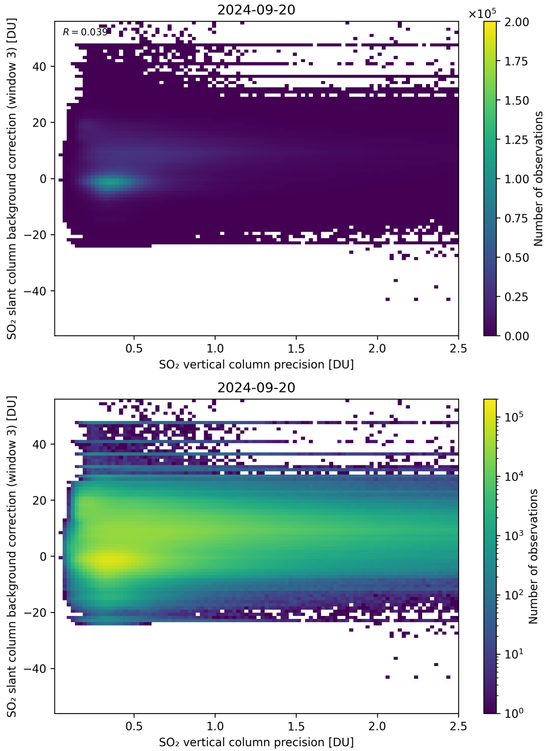
Figure 281: Scatter density plot of “SO 2 vertical column precision” against “SO 2 slant column background correction (window 3)” for 2024-09-19 to 2024-09-21.
