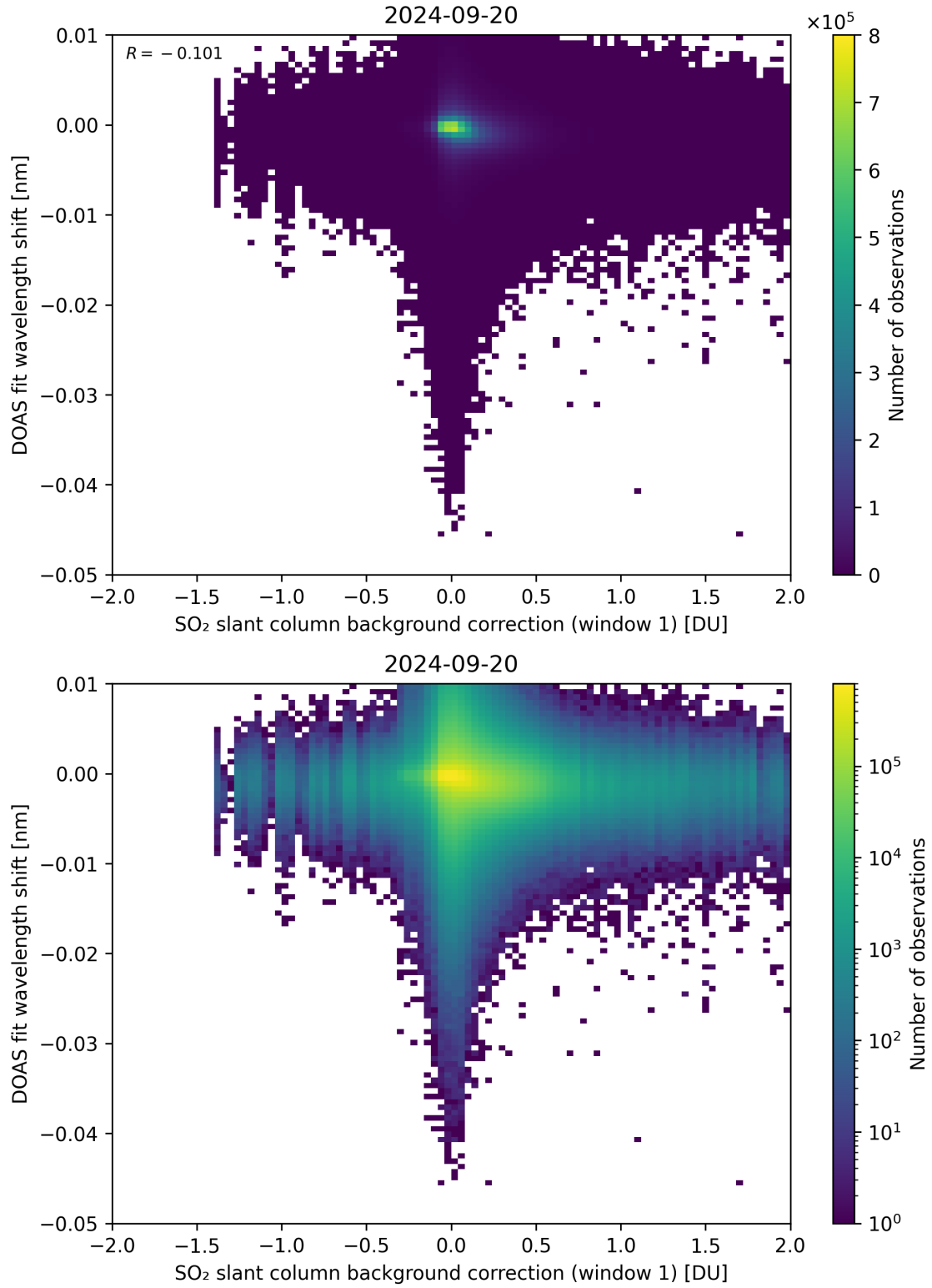
Figure 100: Scatter density plot of “SO 2 slant column background correction (window 1)” against “DOAS fit wavelength shift” for 2024-09-19 to 2024-09-21.
