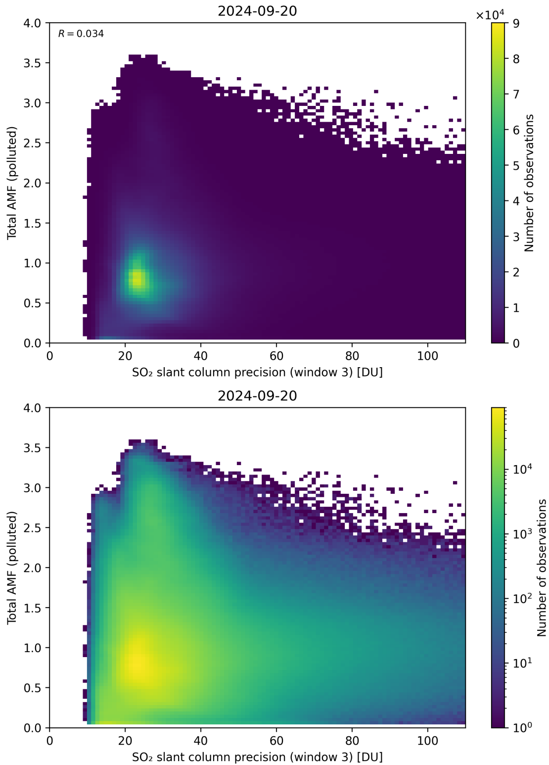
Figure 263: Scatter density plot of “SO 2 slant column precision (window 3)” against “Total AMF (polluted)” for 2024-09-19 to 2024-09-21.
