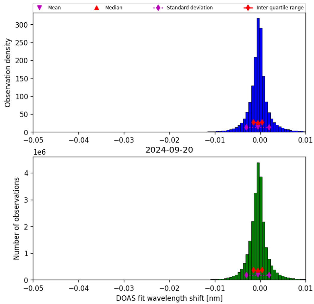
Figure 68: Histogram of “DOAS fit wavelength shift” for 2024-09-19 to 2024-09-21
