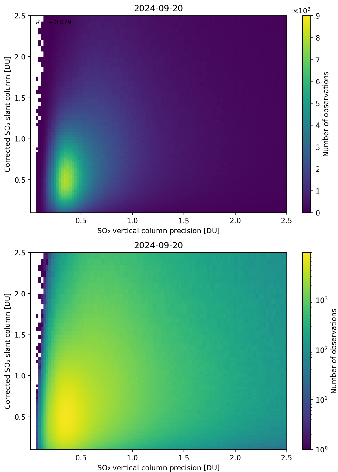
Figure 286: Scatter density plot of “SO 2 vertical column precision” against “Corrected SO 2 slant column” for 2024-09-19 to 2024-09-21.
