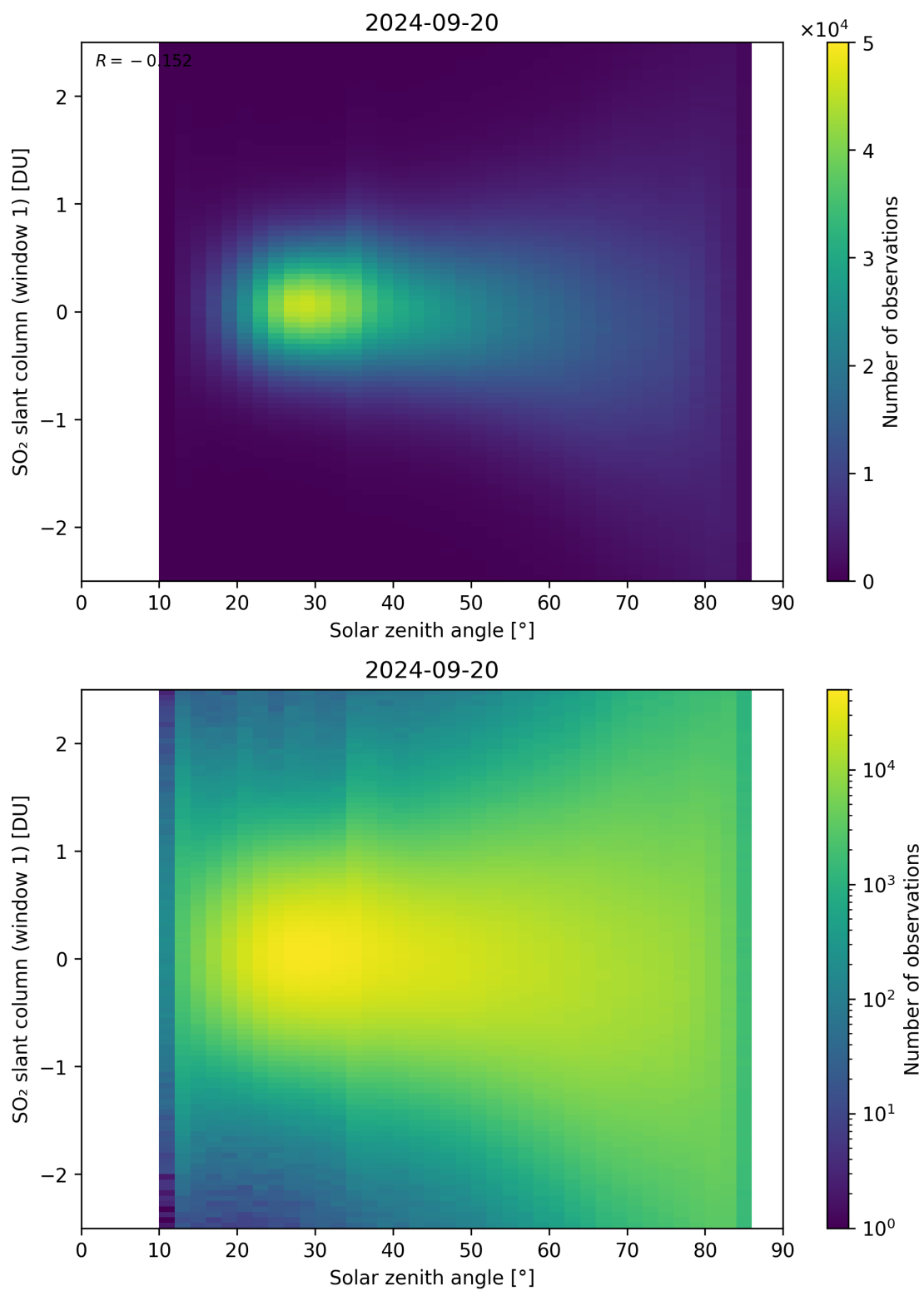
Figure 169: Scatter density plot of “Solar zenith angle” against “SO 2 slant column (window 1)” for 2024-09-19 to 2024-09-21.
