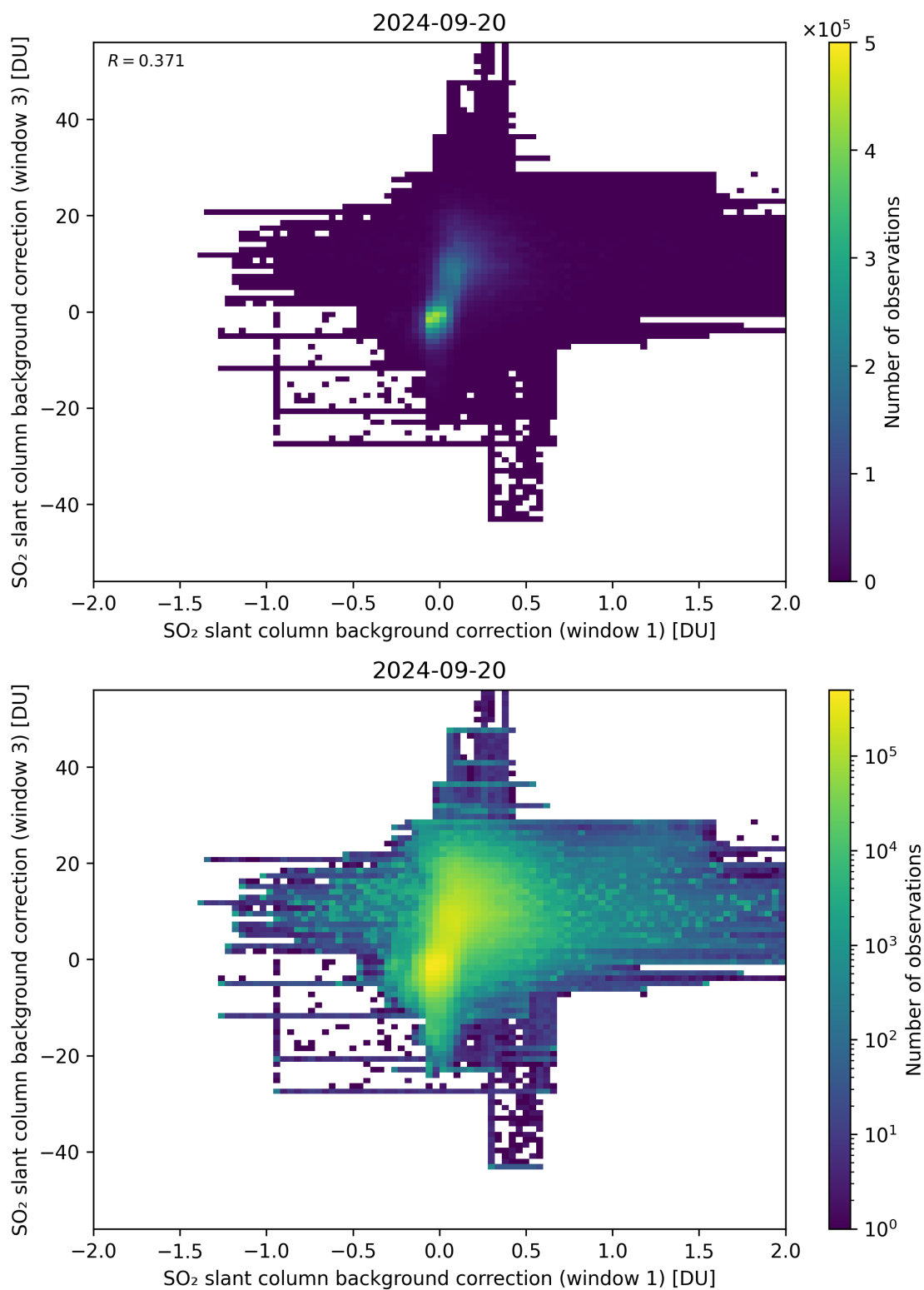
Figure 99: Scatter density plot of “SO 2 slant column background correction (window 1)” against “SO 2 slant column background correction (window 3)” for 2024-09-19 to 2024-09-21.
