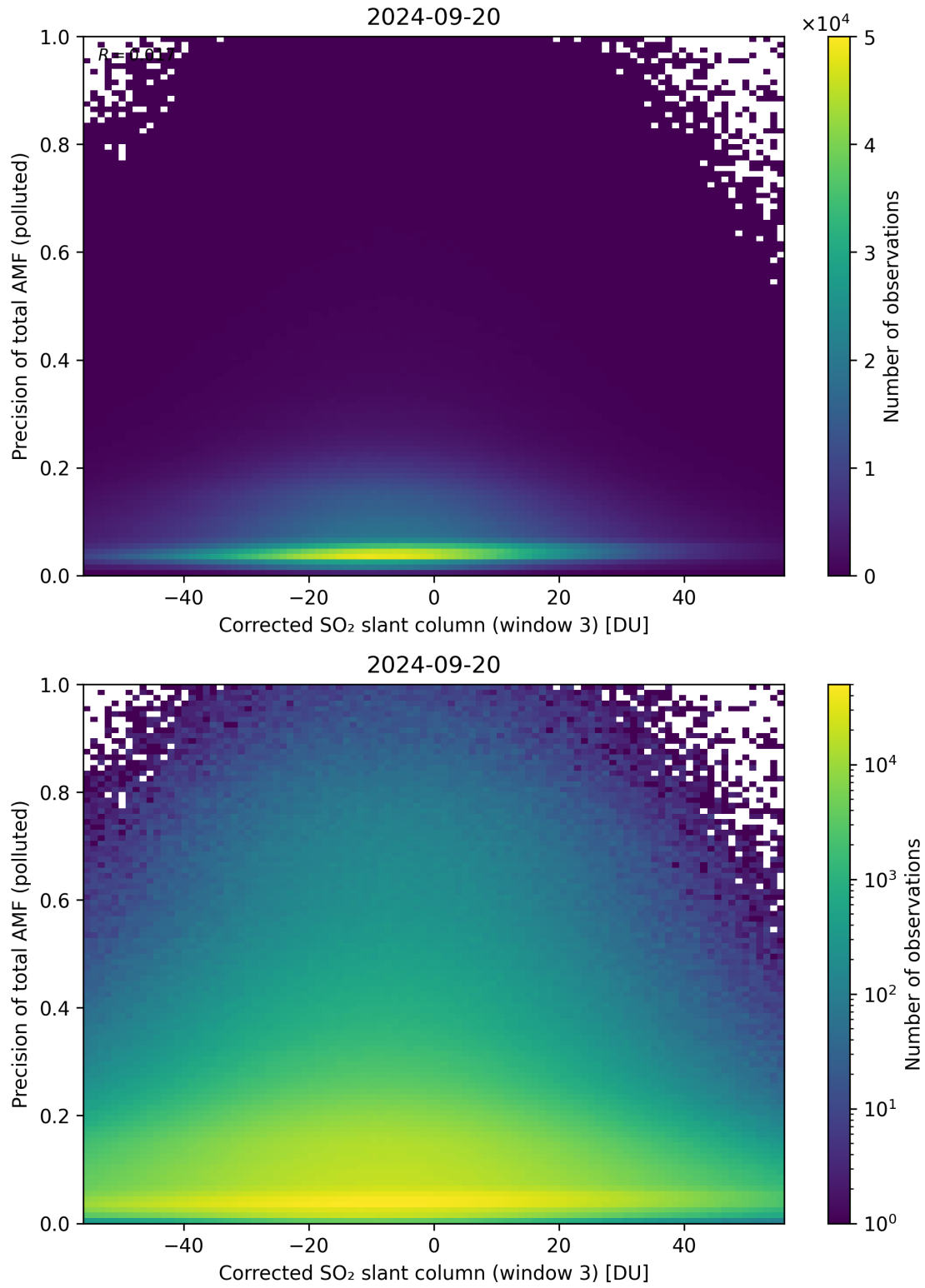
Figure 211: Scatter density plot of “Corrected SO 2 slant column (window 3)” against “Precision of total AMF (polluted)” for 2024-09-19 to 2024-09-21.
