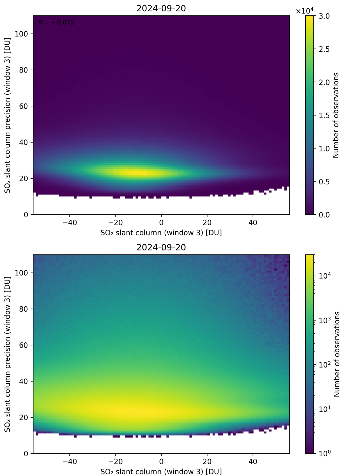
Figure 267: Scatter density plot of “SO 2 slant column (window 3)” against “SO 2 slant column precision (window 3)” for 2024-09-19 to 2024-09-21.
