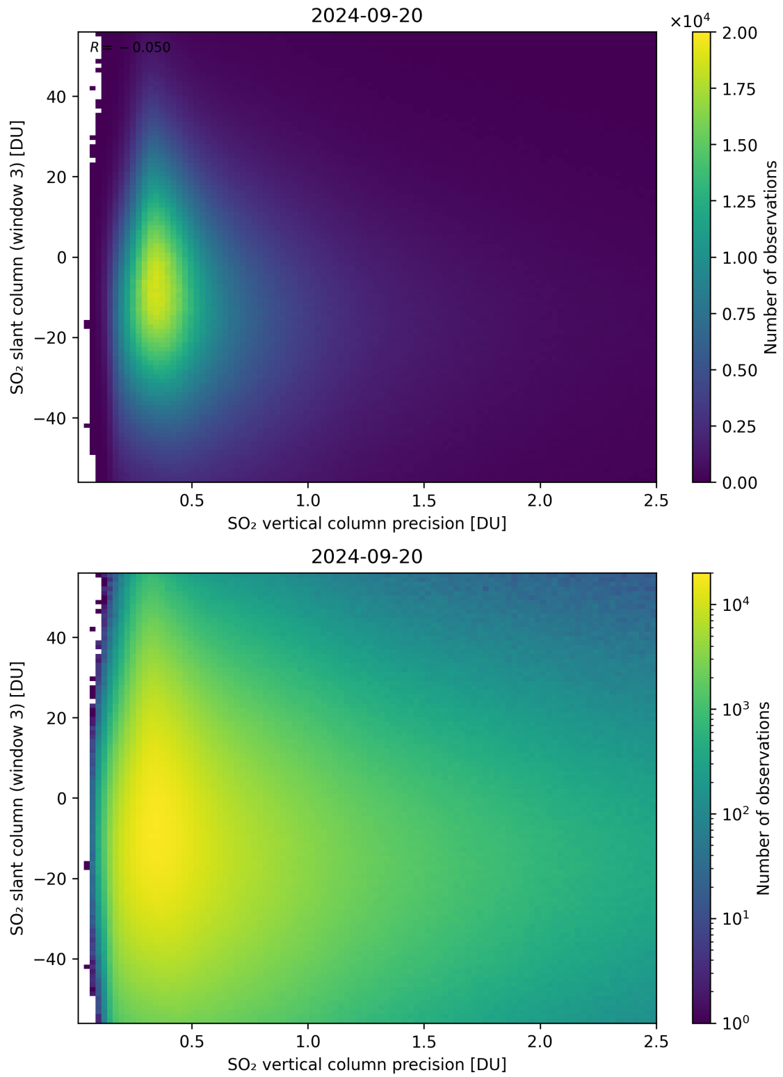
Figure 292: Scatter density plot of “SO 2 vertical column precision” against “SO 2 slant column (window 3)” for 2024-09-19 to 2024-09-21.
