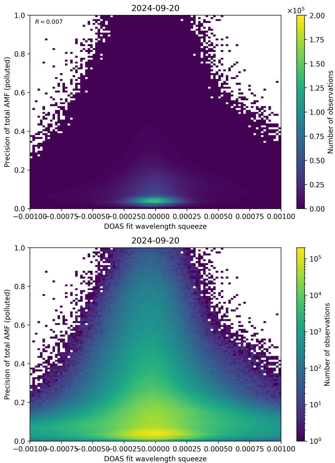
Figure 135: Scatter density plot of “DOAS fit wavelength squeeze” against “Precision of total AMF (polluted)” for 2024-09-19 to 2024-09-21.
