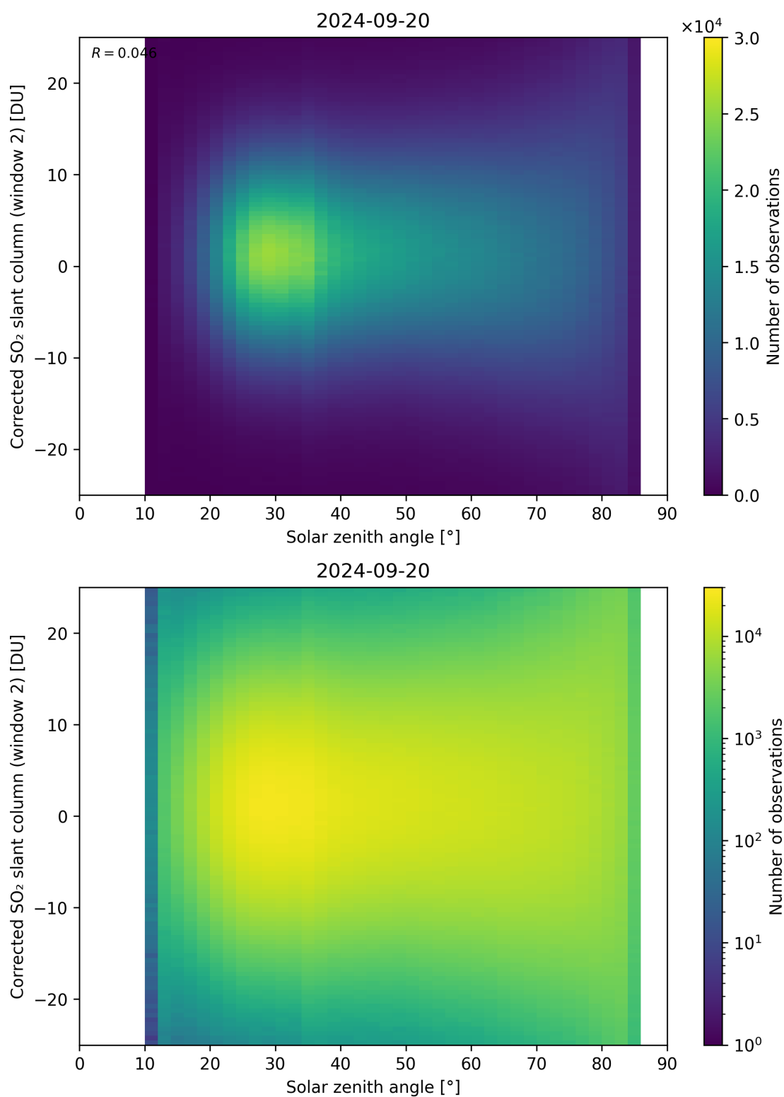
Figure 167: Scatter density plot of “Solar zenith angle” against “Corrected SO 2 slant column (window 2)” for 2024-09-19 to 2024-09-21.
