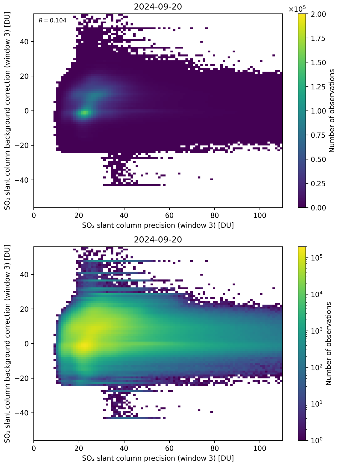
Figure 257: Scatter density plot of “SO 2 slant column precision (window 3)” against “SO 2 slant column background correction (window 3)” for 2024-09-19 to 2024-09-21.
