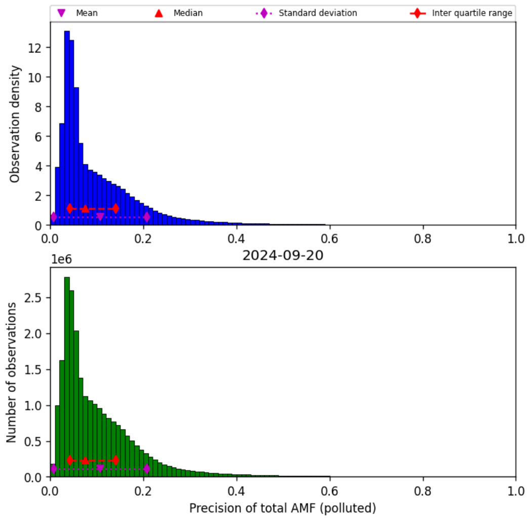
Figure 72: Histogram of “Precision of total AMF (polluted)” for 2024-09-19 to 2024-09-21
