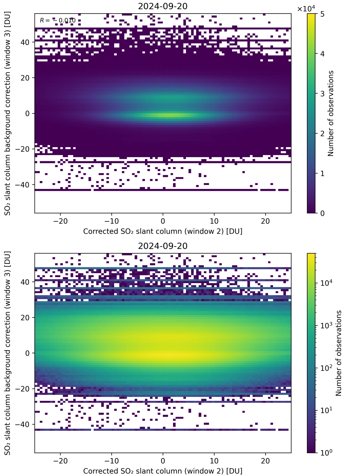
Figure 195: Scatter density plot of “Corrected SO 2 slant column (window 2)” against “SO 2 slant column background correction (window 3)” for 2024-09-19 to 2024-09-21.
