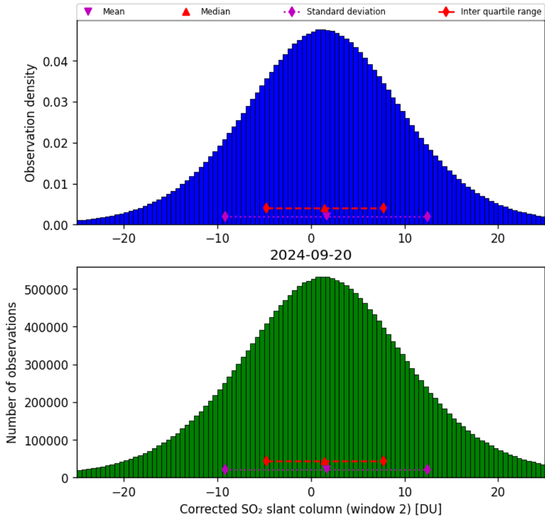
Figure 62: Histogram of “Corrected SO 2 slant column (window 2)” for 2024-09-19 to 2024-09-21
