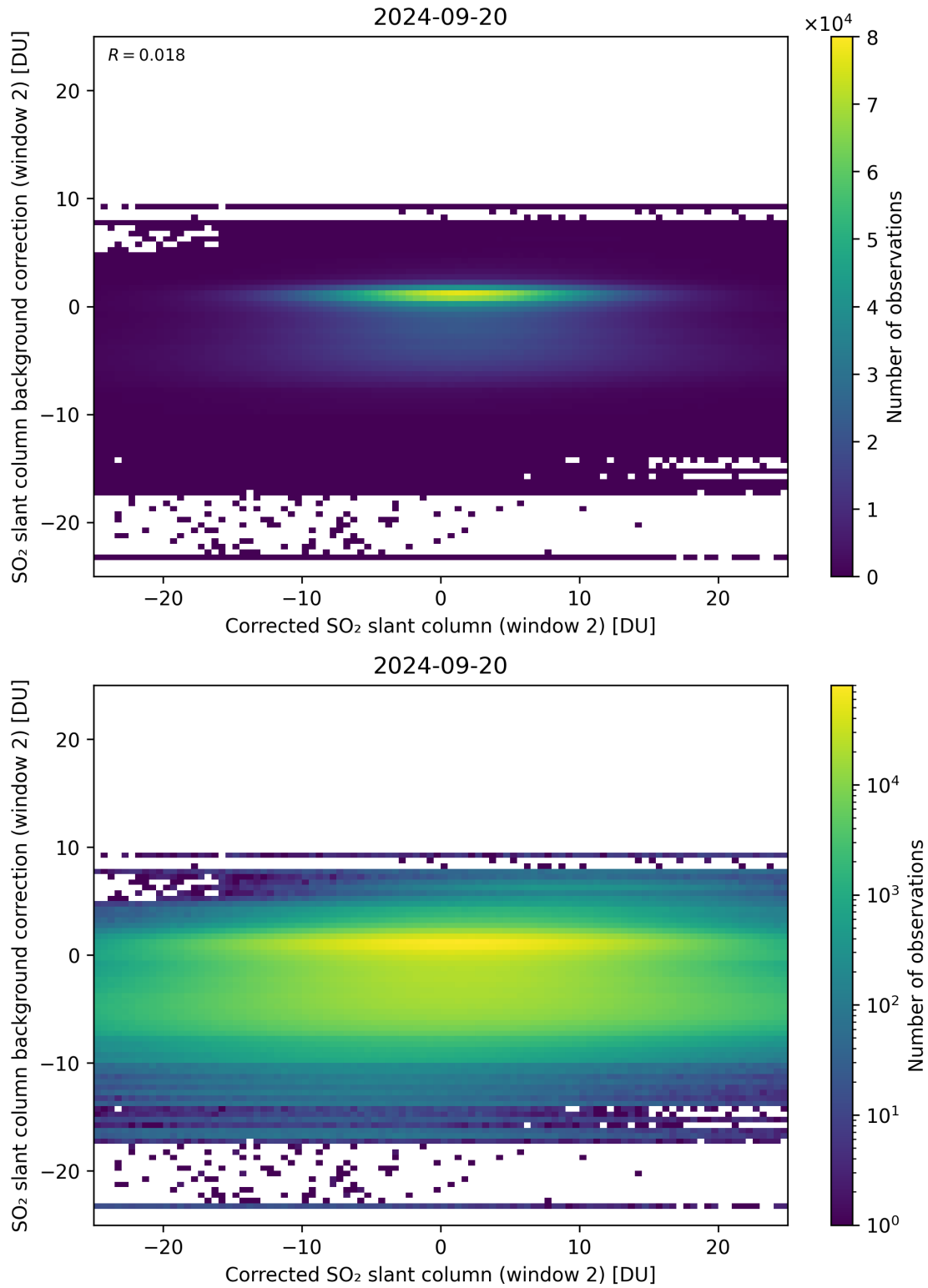
Figure 194: Scatter density plot of “Corrected SO 2 slant column (window 2)” against “SO 2 slant column background correction (window 2)” for 2024-09-19 to 2024-09-21.
