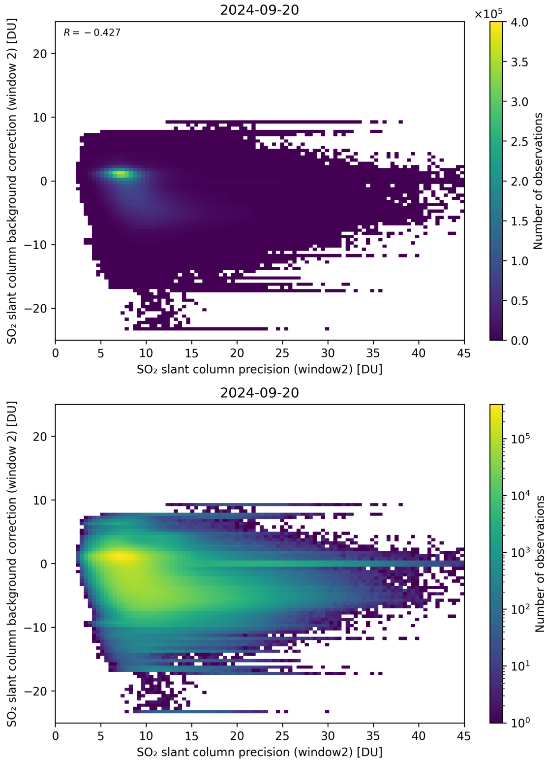
Figure 241: Scatter density plot of “SO 2 slant column precision (window2)” against “SO 2 slant column background correction (window 2)” for 2024-09-19 to 2024-09-21.
