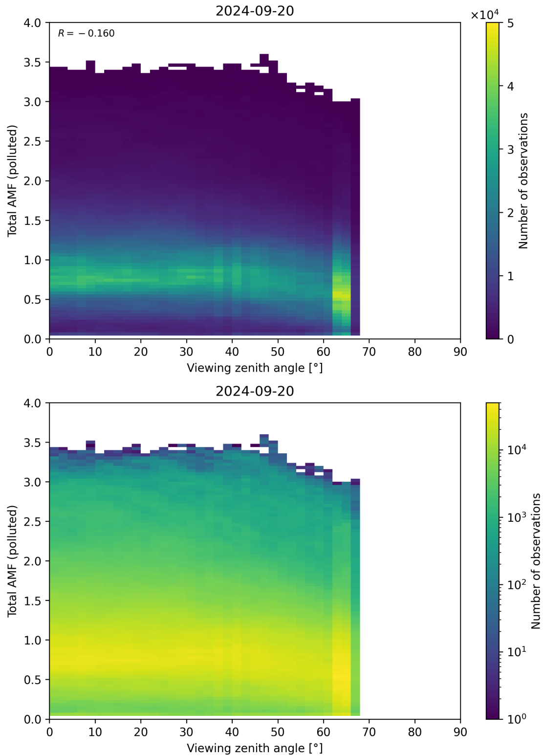
Figure 325: Scatter density plot of “Viewing zenith angle” against “Total AMF (polluted)” for 2024-09-19 to 2024-09-21.
