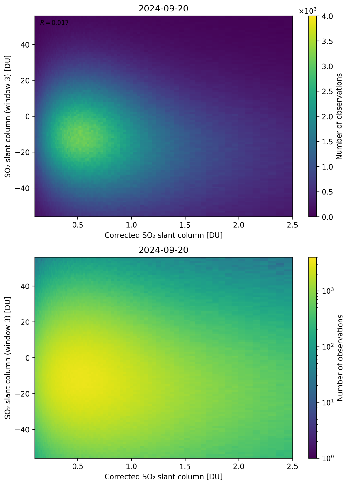
Figure 190: Scatter density plot of “Corrected SO 2 slant column” against “SO 2 slant column (window 3)” for 2024-09-19 to 2024-09-21.
