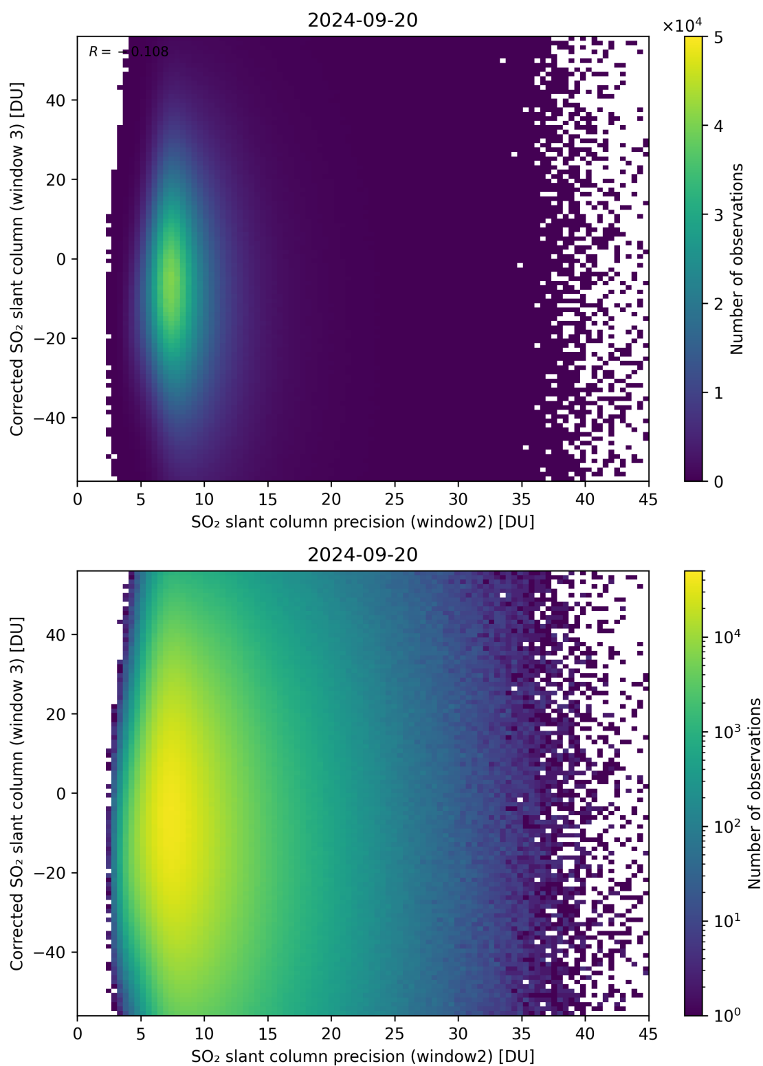
Figure 248: Scatter density plot of “SO 2 slant column precision (window2)” against “Corrected SO 2 slant column (window 3)” for 2024-09-19 to 2024-09-21.
