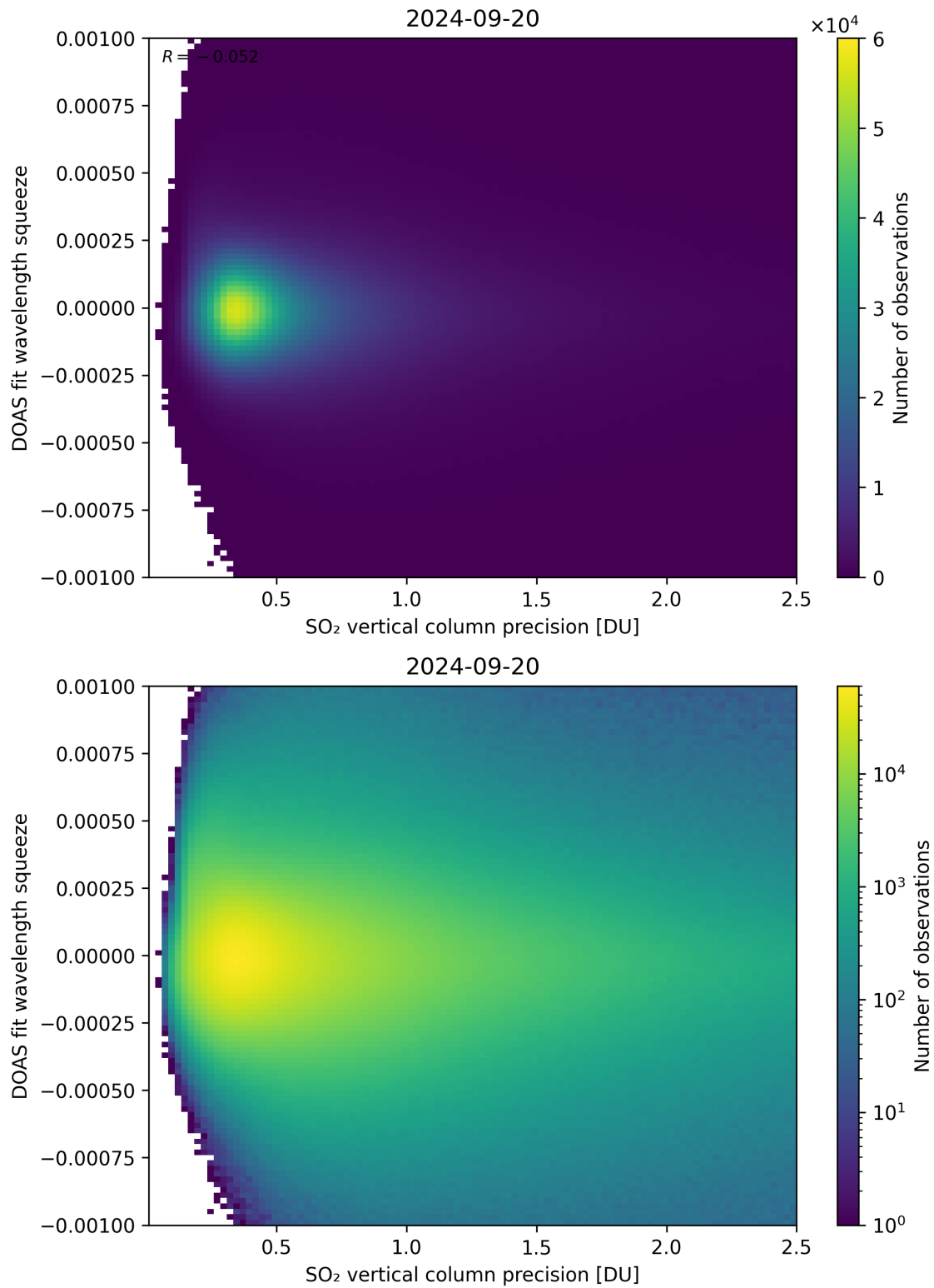
Figure 283: Scatter density plot of “SO 2 vertical column precision” against “DOAS fit wavelength squeeze” for 2024-09-19 to 2024-09-21.
