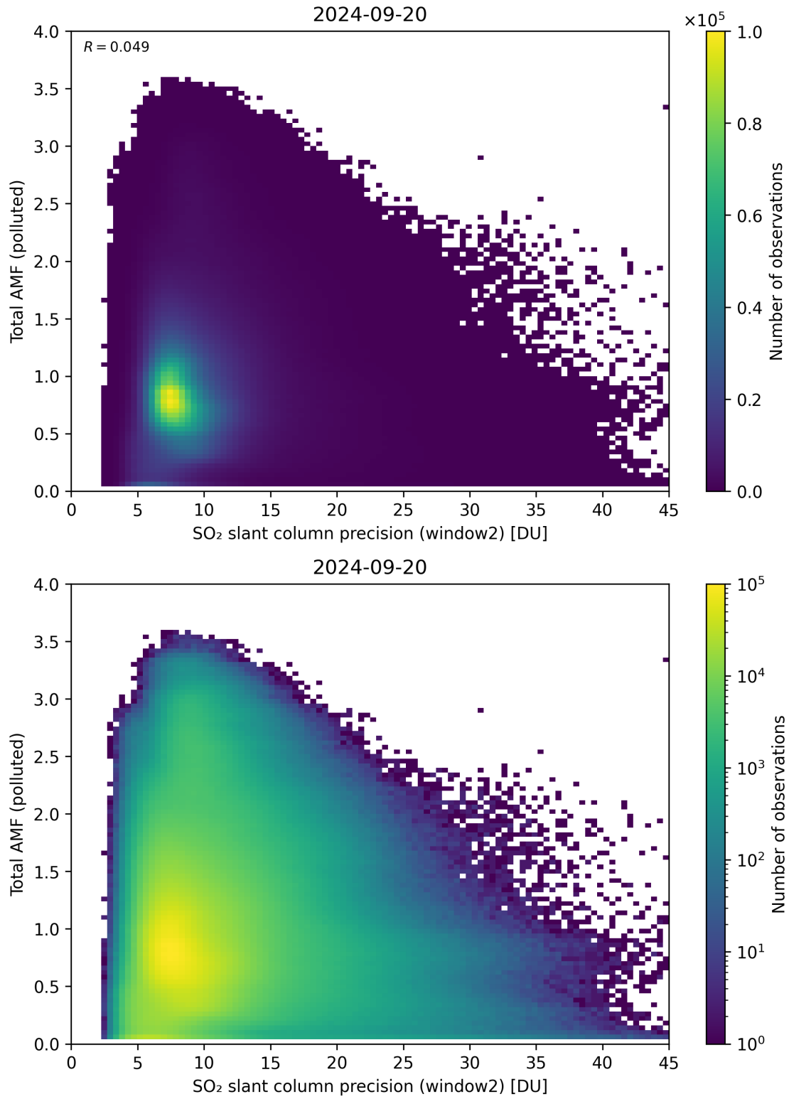
Figure 251: Scatter density plot of “SO 2 slant column precision (window2)” against “Total AMF (polluted)” for 2024-09-19 to 2024-09-21.
