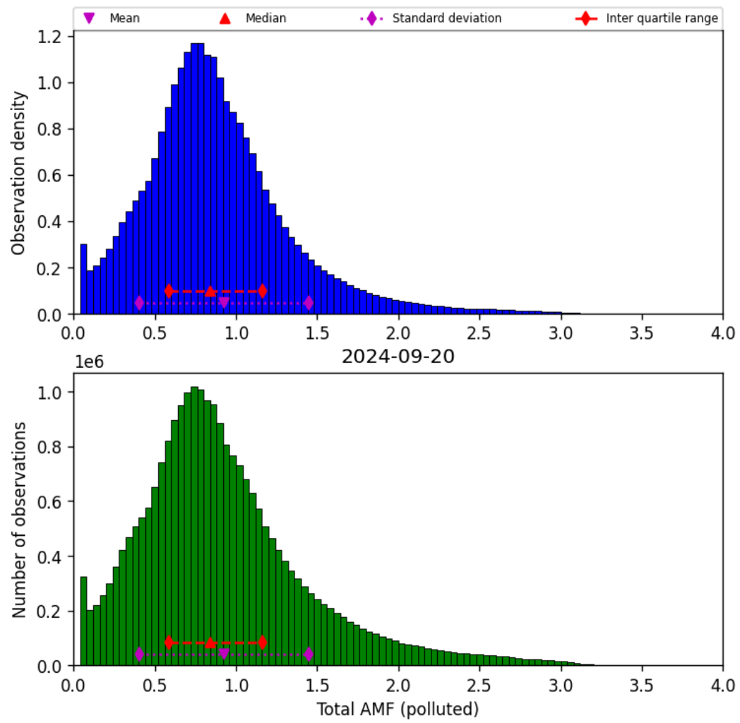
Figure 71: Histogram of “Total AMF (polluted)” for 2024-09-19 to 2024-09-21
