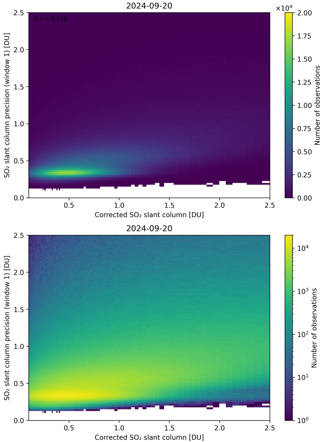
Figure 188: Scatter density plot of “Corrected SO 2 slant column” against “SO 2 slant column precision (window 1)” for 2024-09-19 to 2024-09-21.
