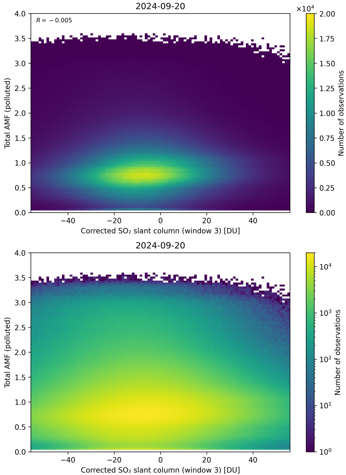
Figure 210: Scatter density plot of “Corrected SO 2 slant column (window 3)” against “Total AMF (polluted)” for 2024-09-19 to 2024-09-21.
