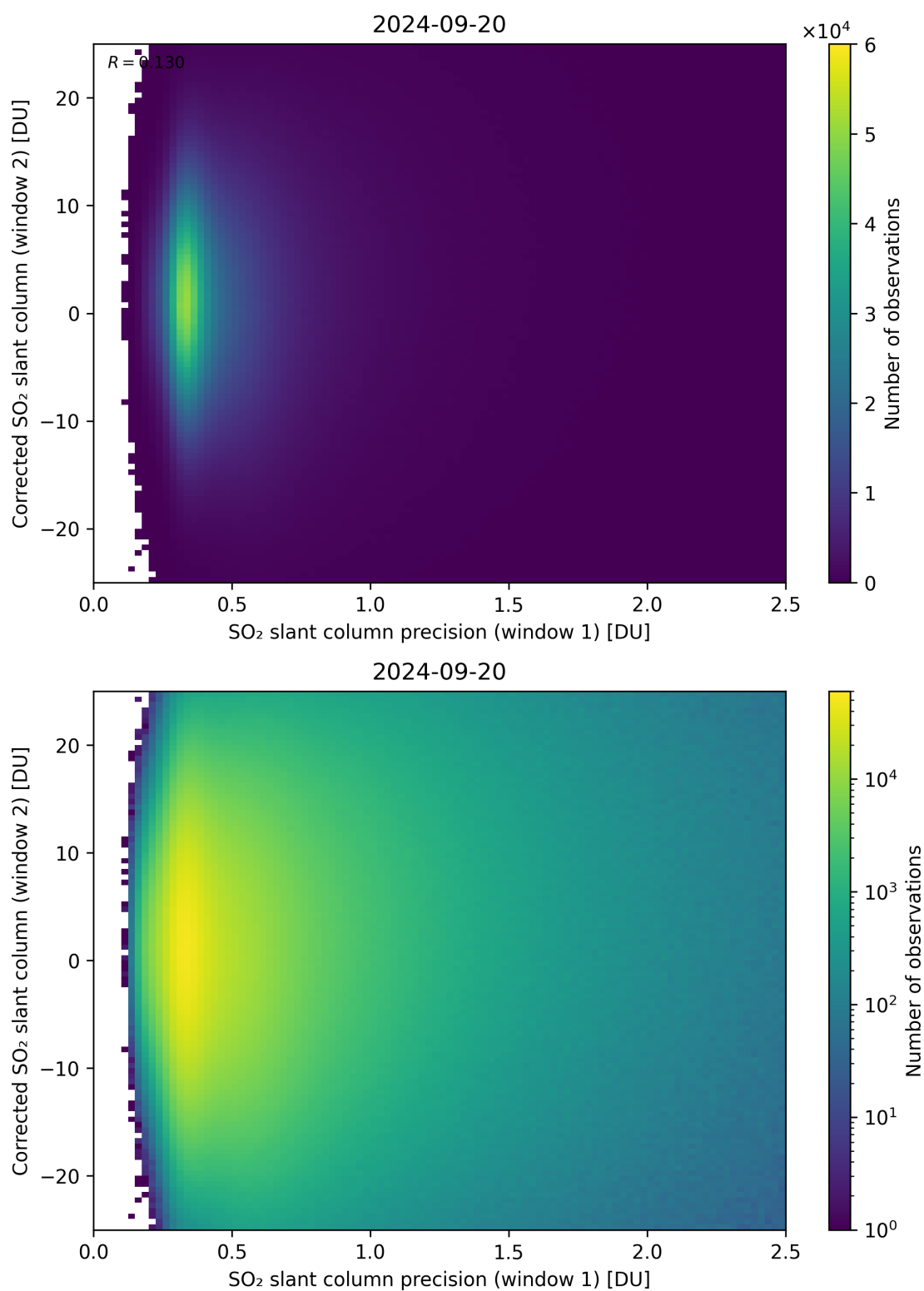
Figure 225: Scatter density plot of “SO 2 slant column precision (window 1)” against “Corrected SO 2 slant column (window 2)” for 2024-09-19 to 2024-09-21.
