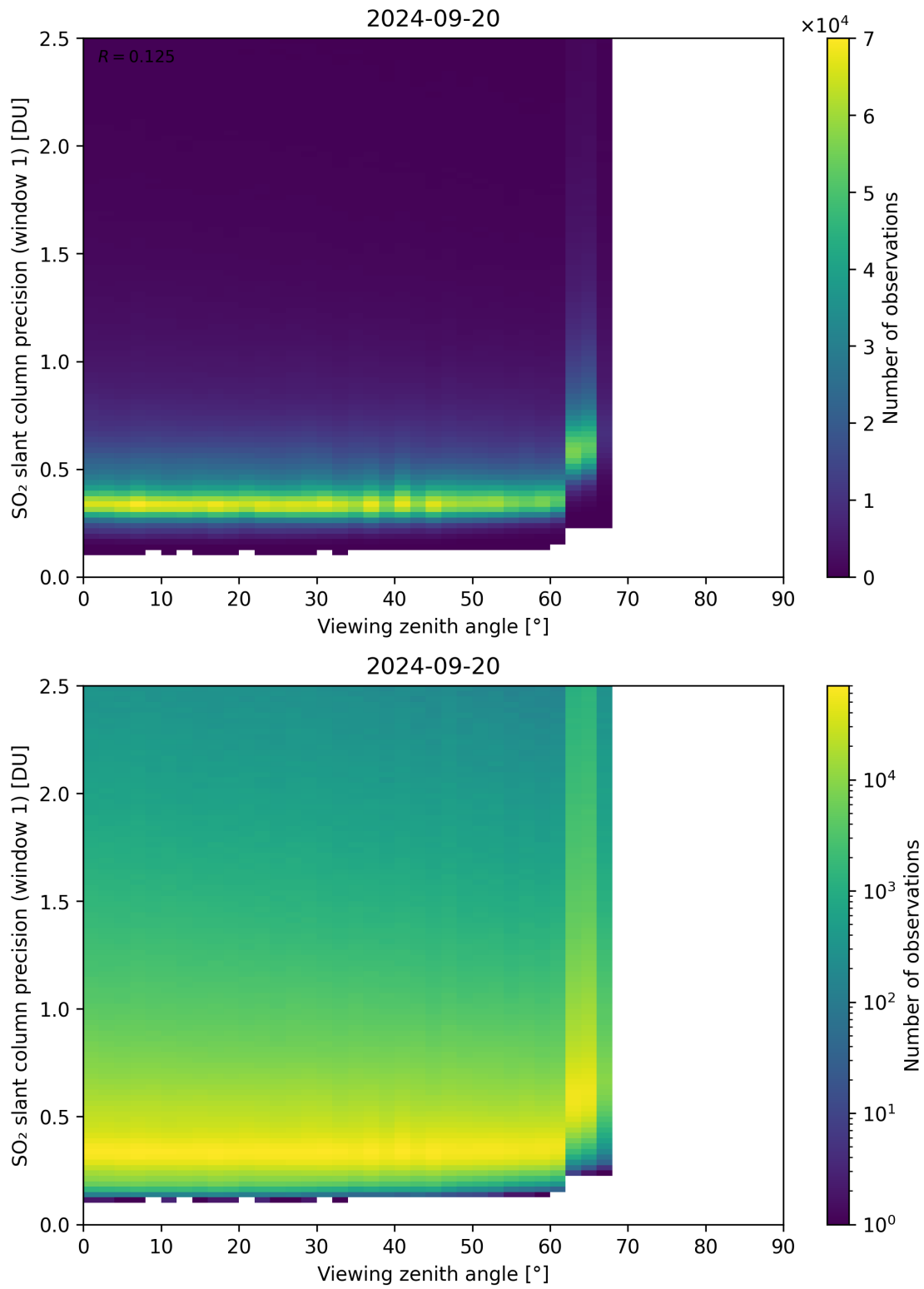
Figure 321: Scatter density plot of “Viewing zenith angle” against “SO 2 slant column precision (window 1)” for 2024-09-19 to 2024-09-21.
