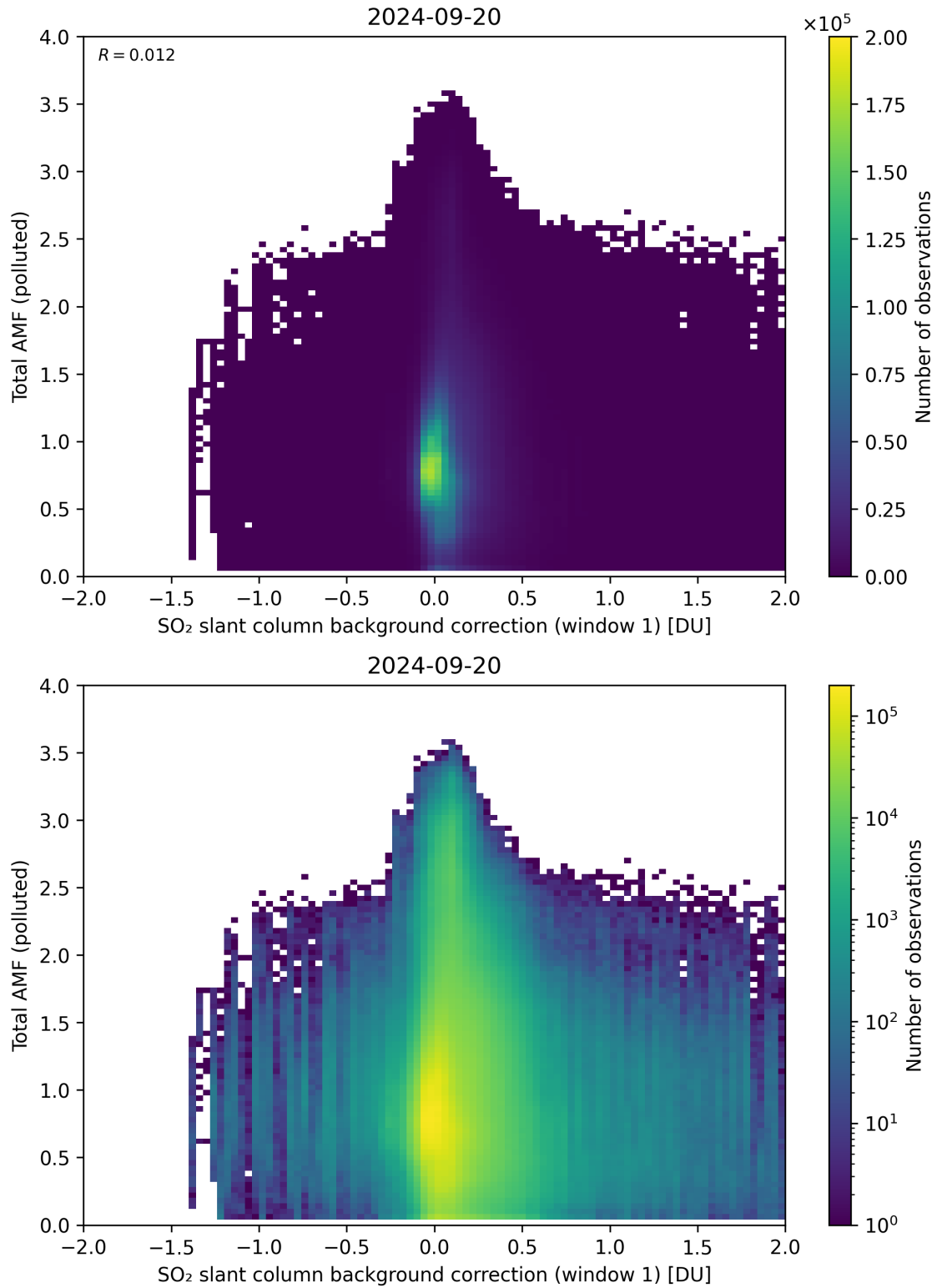
Figure 109: Scatter density plot of “SO 2 slant column background correction (window 1)” against “Total AMF (polluted)” for 2024-09-19 to 2024-09-21.
