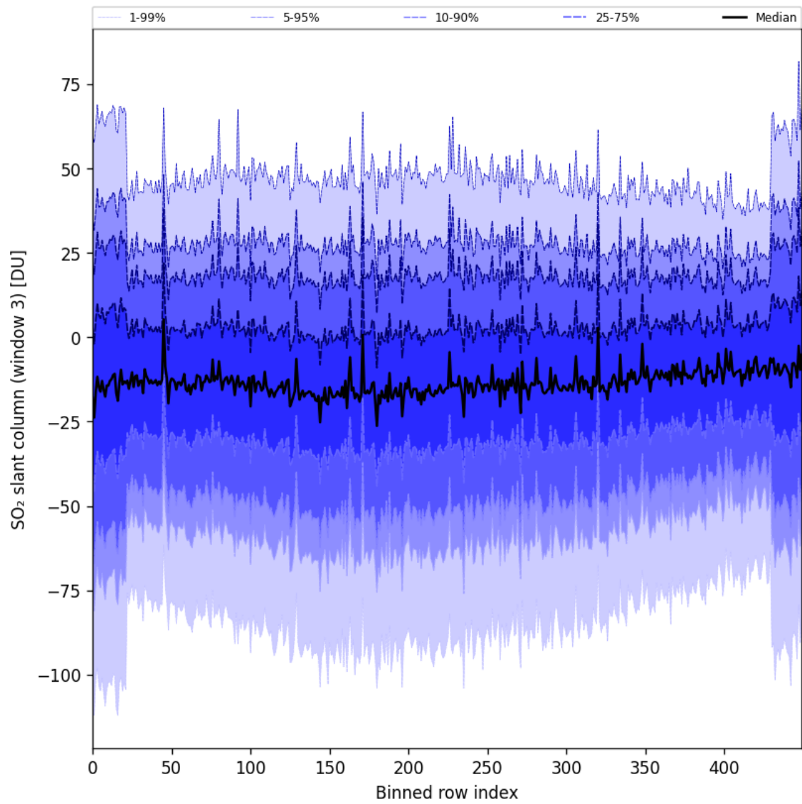
Figure 87: Along track statistics of “SO 2 slant column (window 3)” for 2024-09-19 to 2024-09-21
