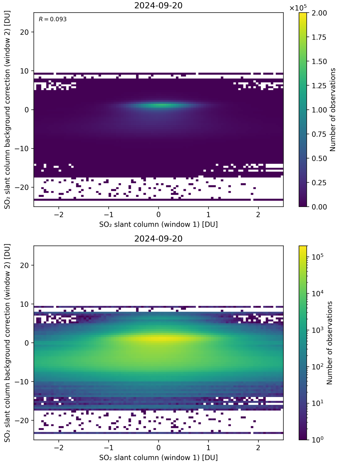
Figure 213: Scatter density plot of “SO 2 slant column (window 1)” against “SO 2 slant column background correction (window 2)” for 2024-09-19 to 2024-09-21.
