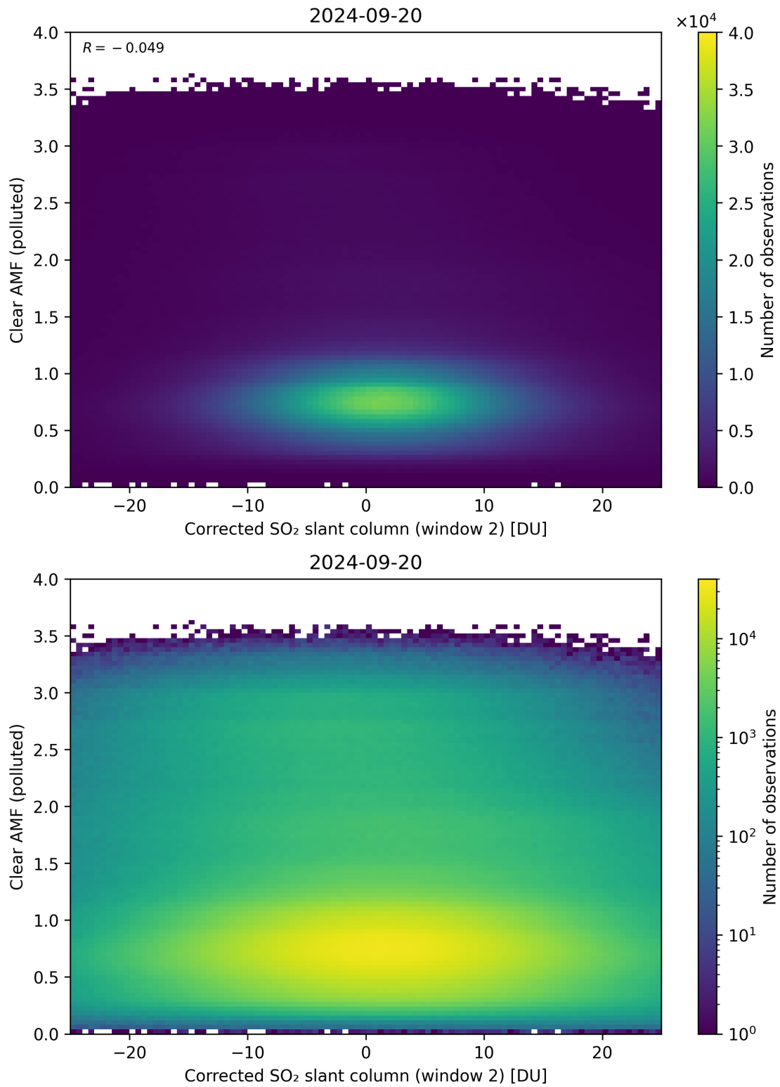
Figure 199: Scatter density plot of “Corrected SO 2 slant column (window 2)” against “Clear AMF (polluted)” for 2024-09-19 to 2024-09-21.
