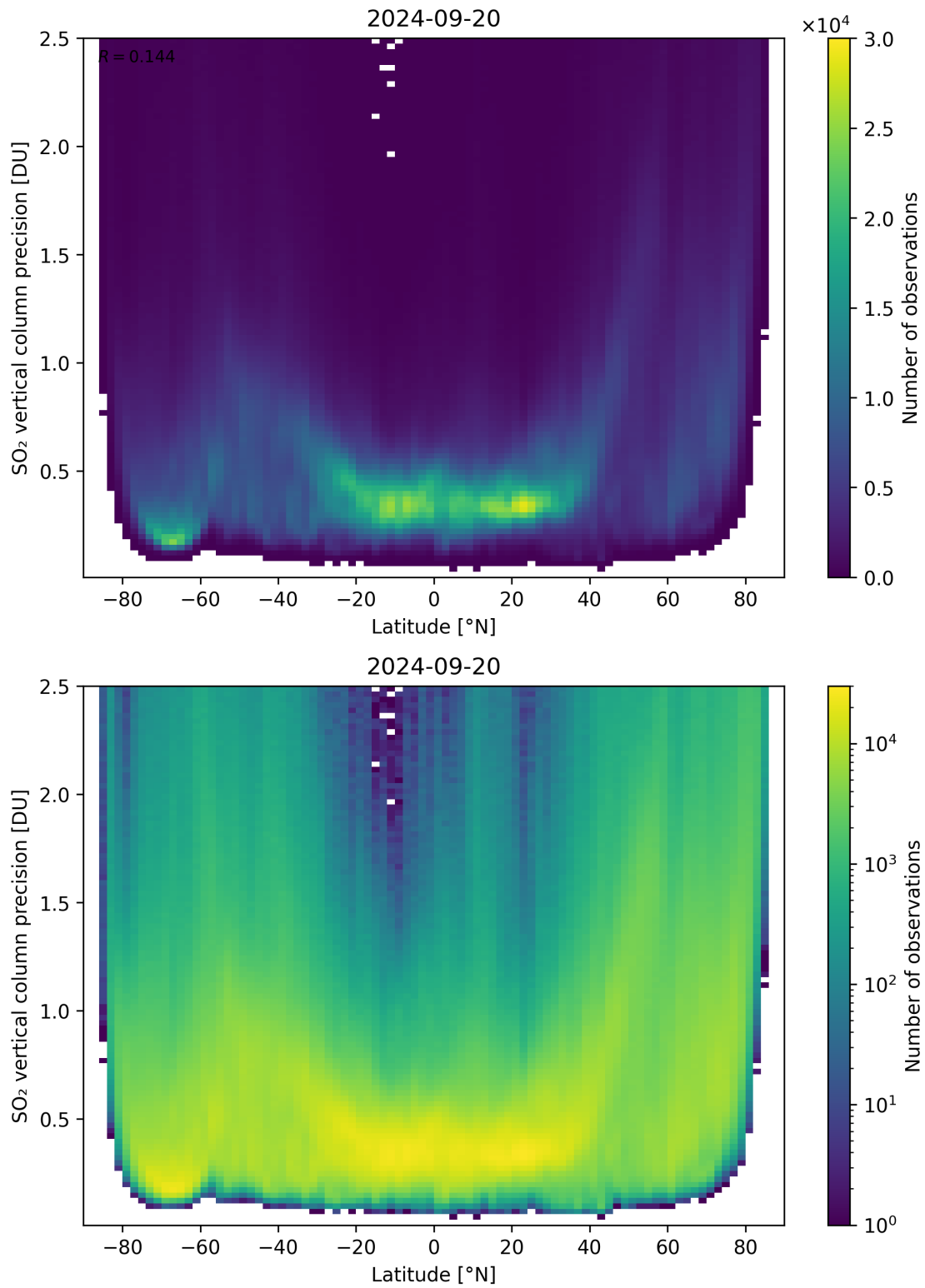
Figure 157: Scatter density plot of “Latitude” against “SO 2 vertical column precision” for 2024-09-19 to 2024-09-21.
