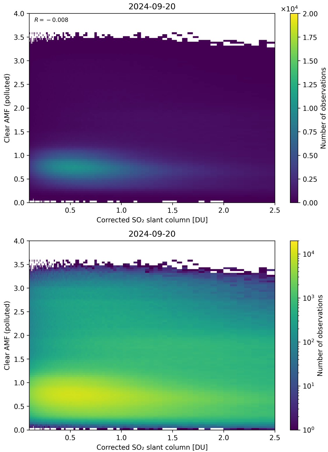
Figure 184: Scatter density plot of “Corrected SO 2 slant column” against “Clear AMF (polluted)” for 2024-09-19 to 2024-09-21.
