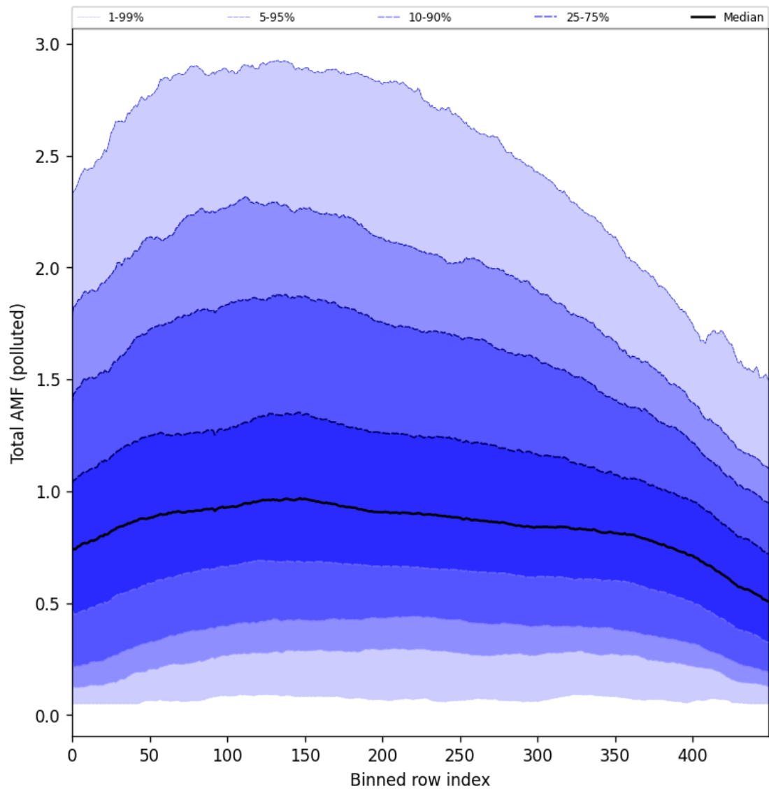
Figure 94: Along track statistics of “Total AMF (polluted)” for 2024-09-19 to 2024-09-21
