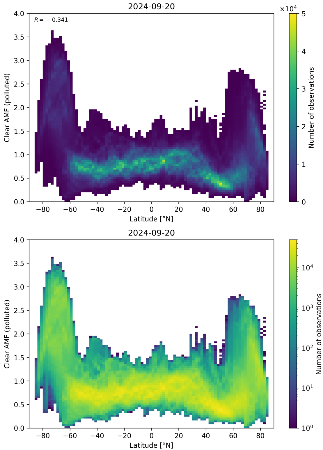
Figure 145: Scatter density plot of “Latitude” against “Clear AMF (polluted)” for 2024-09-19 to 2024-09-21.
