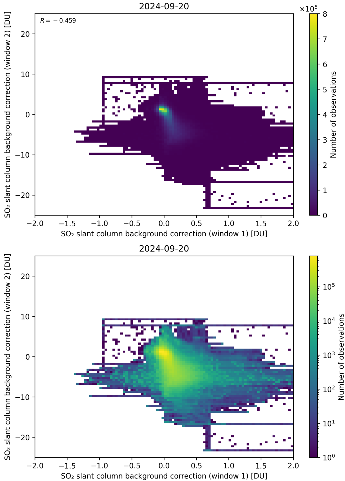
Figure 98: Scatter density plot of “SO 2 slant column background correction (window 1)” against “SO 2 slant column background correction (window 2)” for 2024-09-19 to 2024-09-21.
