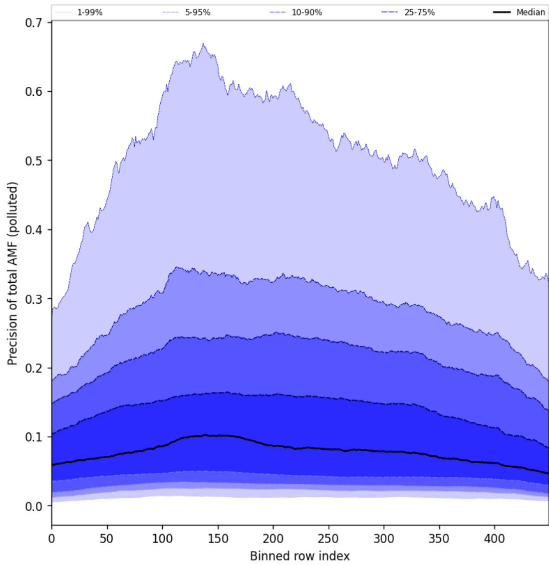
Figure 95: Along track statistics of “Precision of total AMF (polluted)” for 2024-09-19 to 2024-09-21
