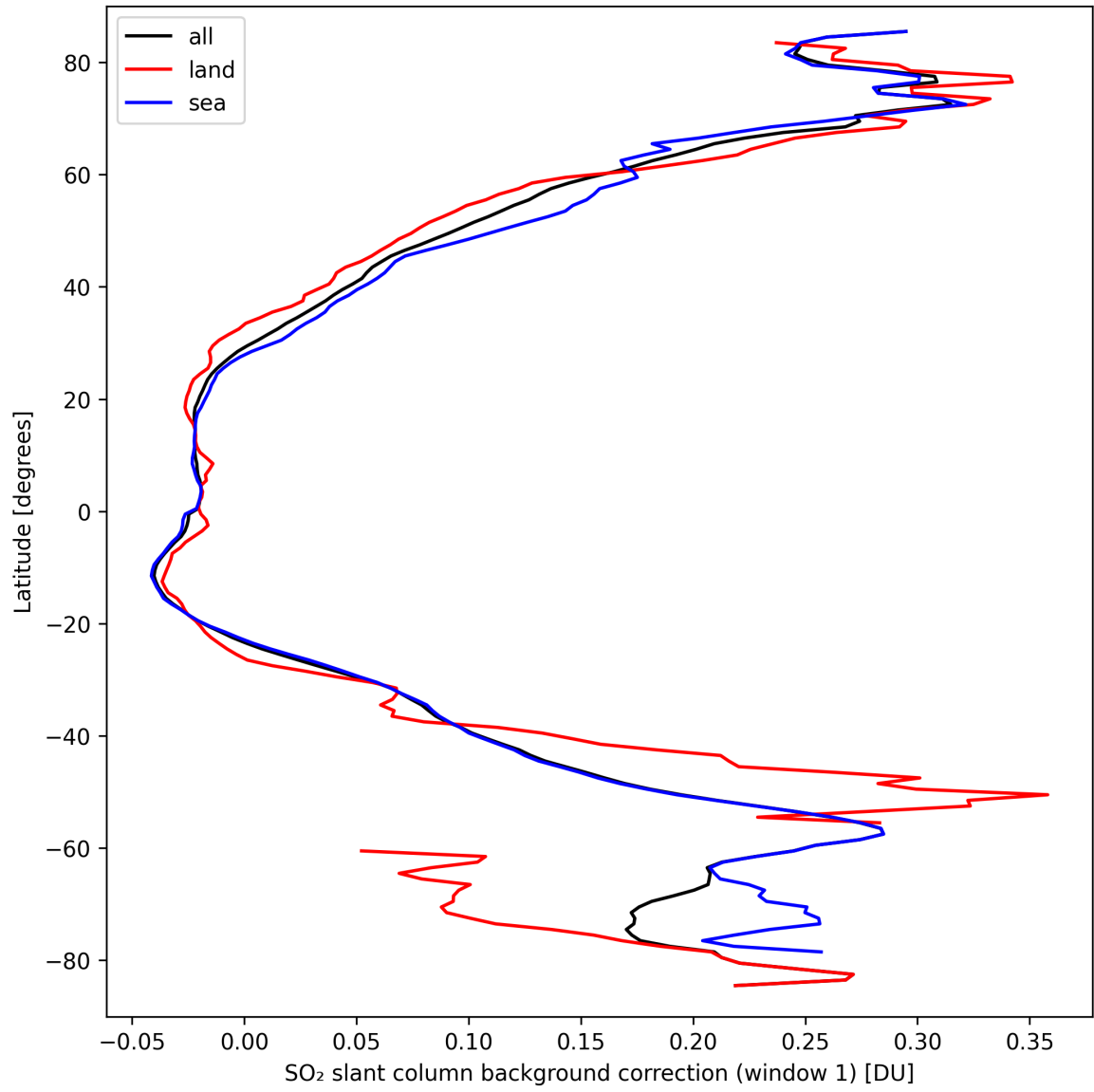
Figure 36: Zonal average of “SO 2 slant column background correction (window 1)” for 2024-09-19 to 2024-09-21.
