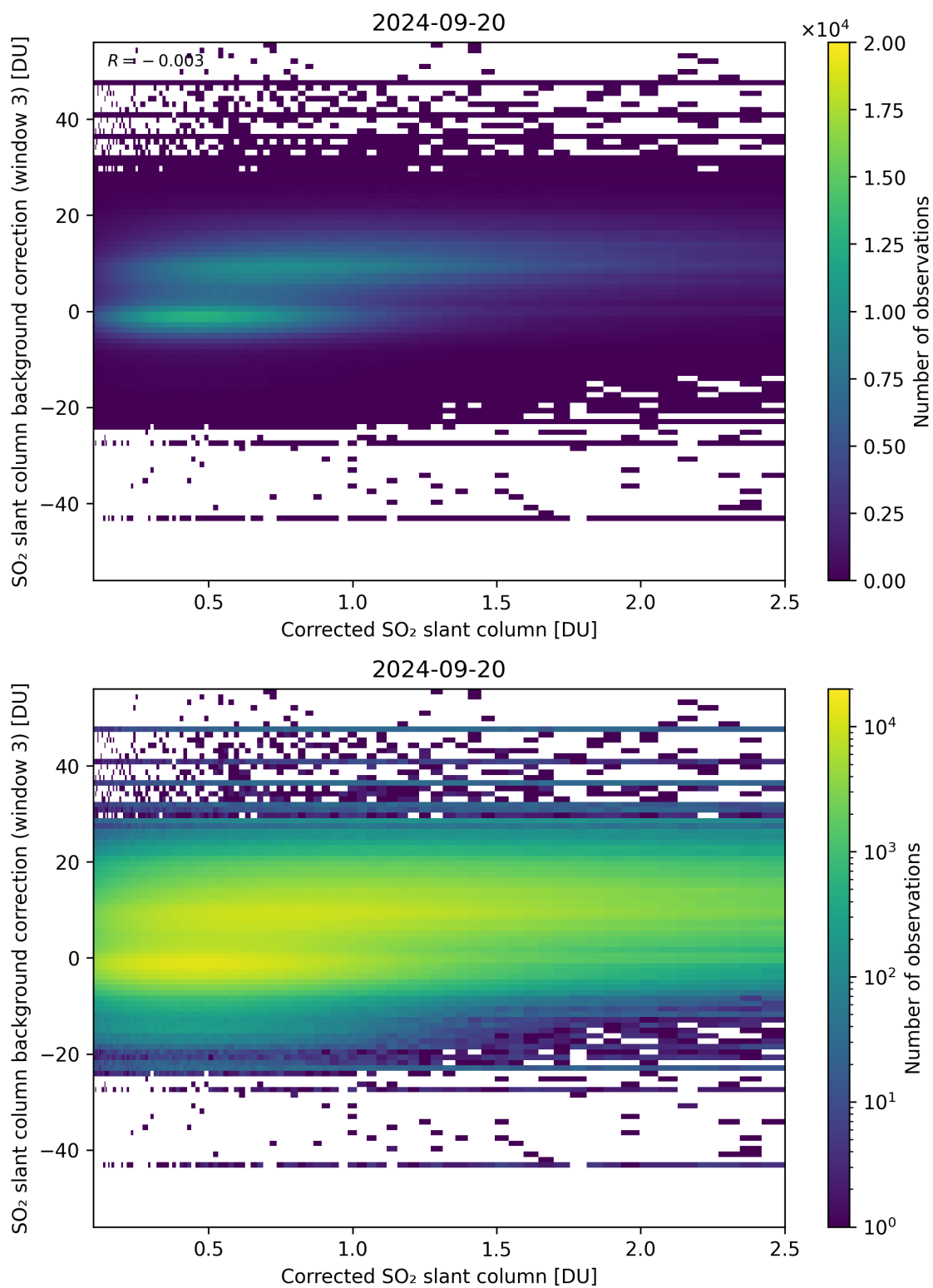
Figure 180: Scatter density plot of “Corrected SO 2 slant column” against “SO 2 slant column background correction (window 3)” for 2024-09-19 to 2024-09-21.
