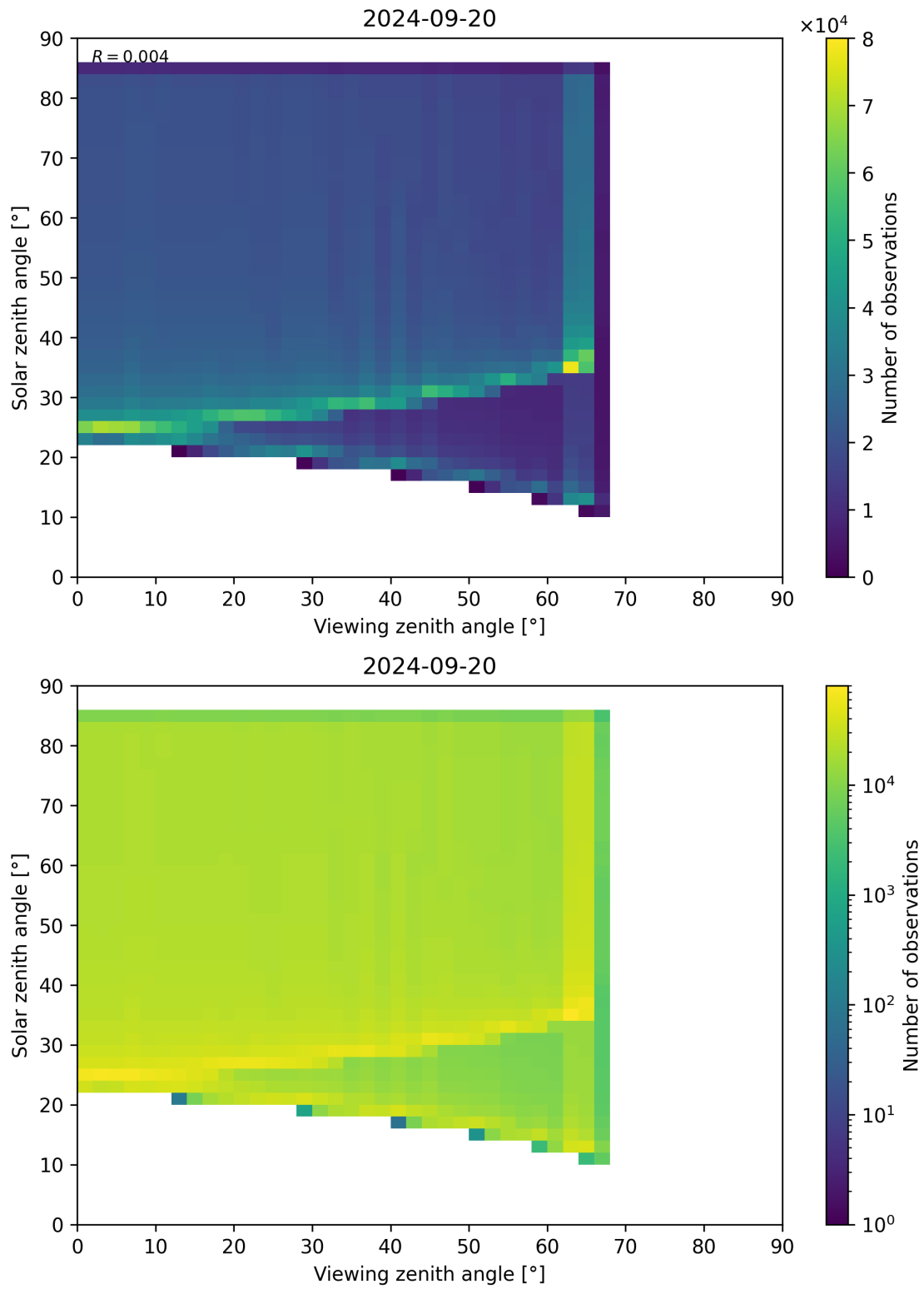
Figure 315: Scatter density plot of “Viewing zenith angle” against “Solar zenith angle” for 2024-09-19 to 2024-09-21.
