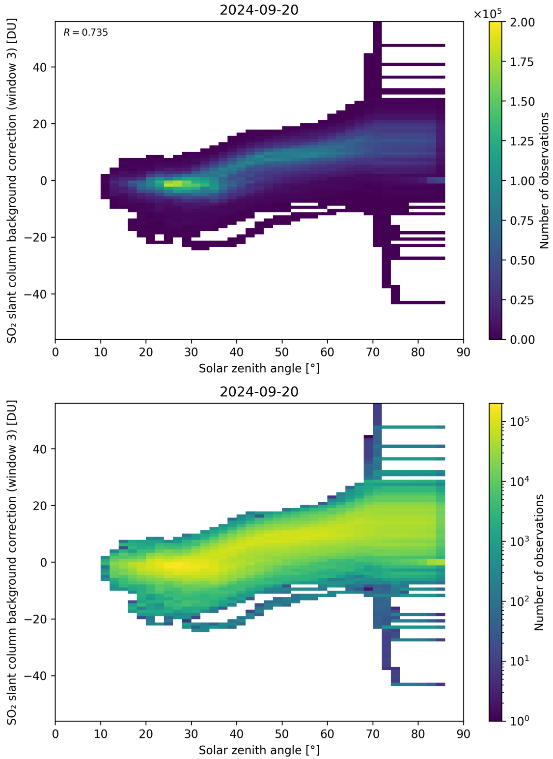
Figure 160: Scatter density plot of “Solar zenith angle” against “SO 2 slant column background correction (window 3)” for 2024-09-19 to 2024-09-21.
