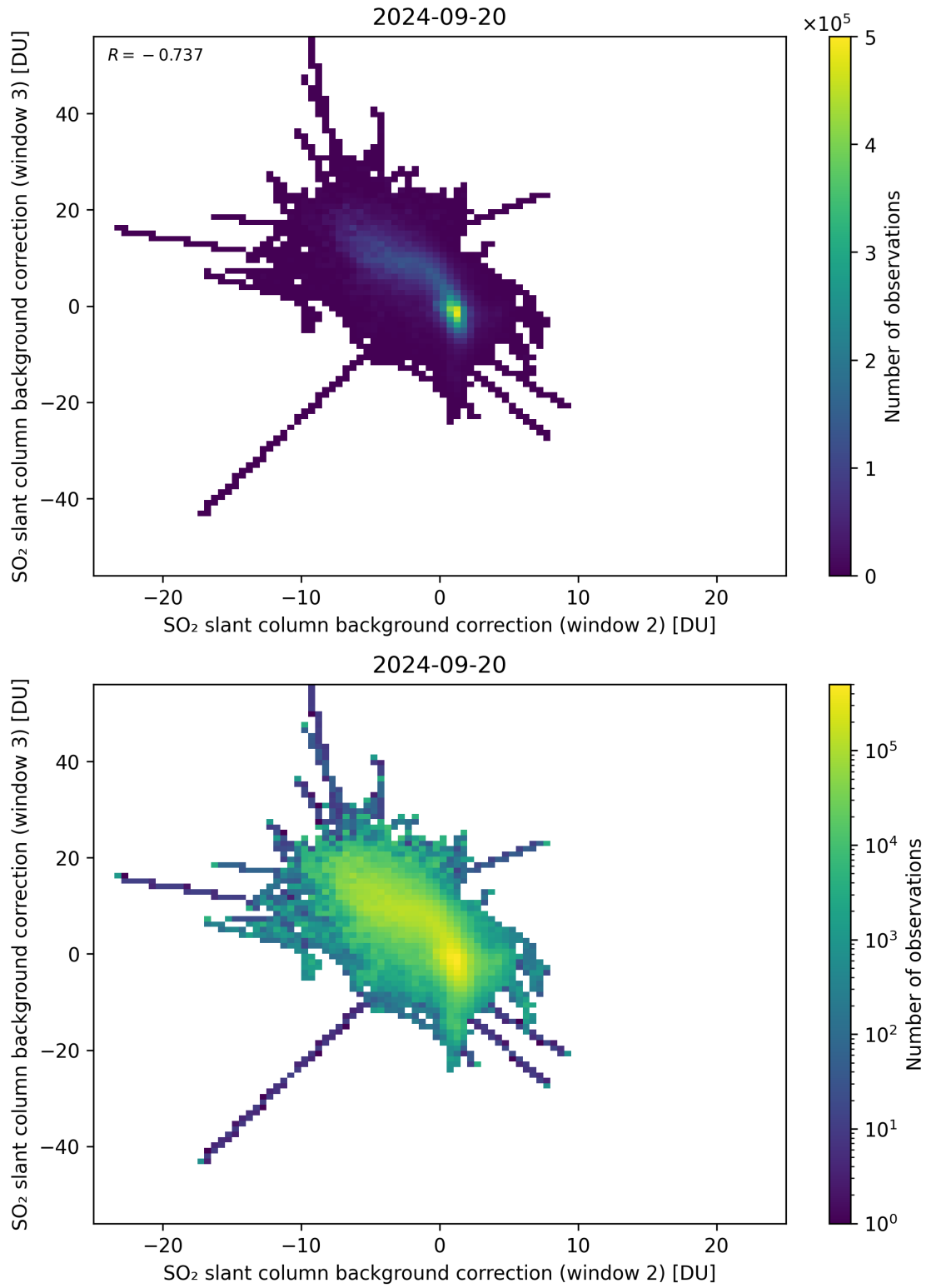
Figure 111: Scatter density plot of “SO 2 slant column background correction (window 2)” against “SO 2 slant column background correction (window 3)” for 2024-09-19 to 2024-09-21.
