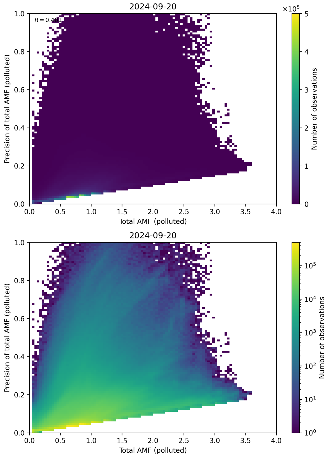
Figure 272: Scatter density plot of “Total AMF (polluted)” against “Precision of total AMF (polluted)” for 2024-09-19 to 2024-09-21.
