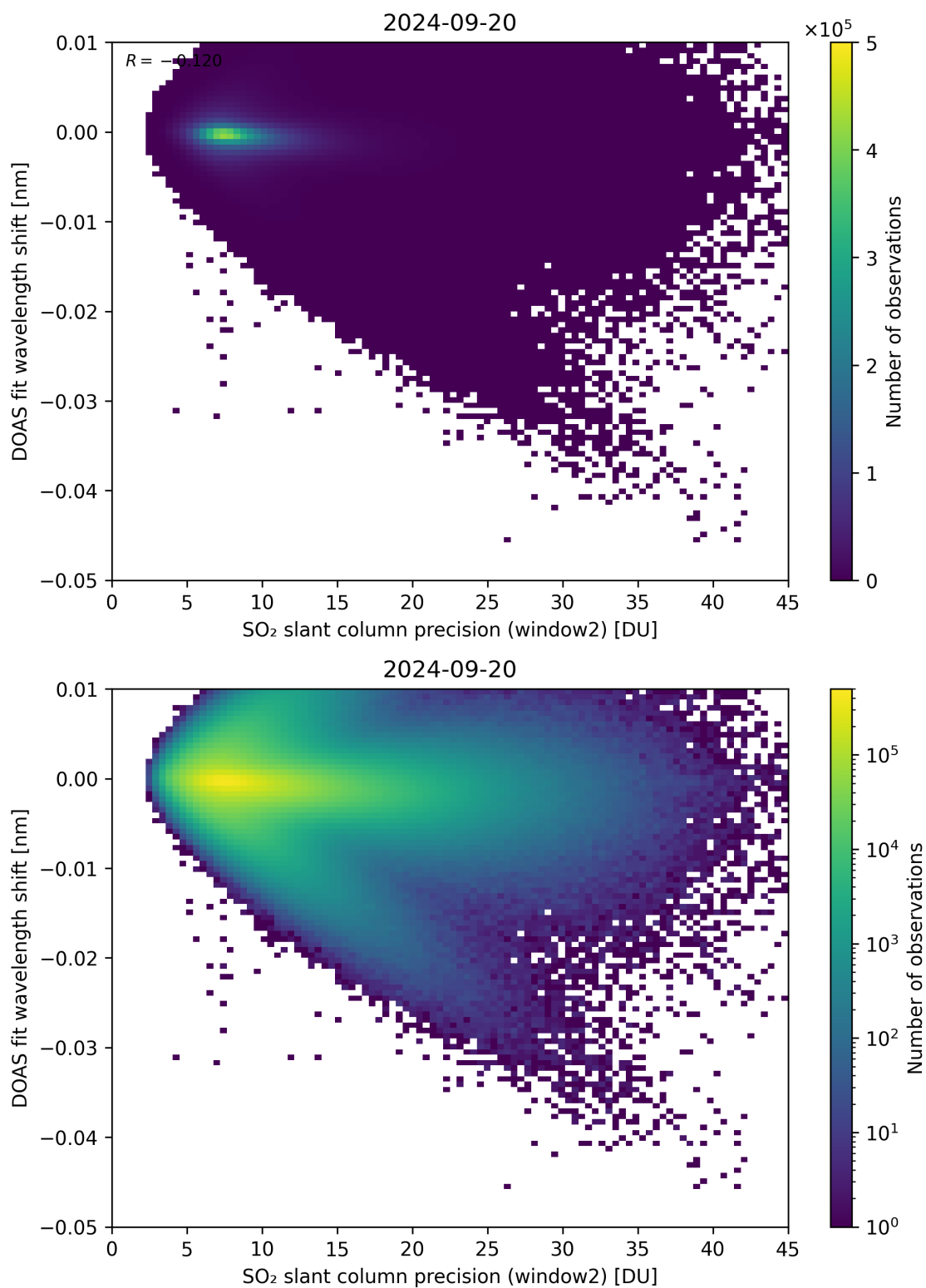
Figure 243: Scatter density plot of “SO 2 slant column precision (window2)” against “DOAS fit wavelength shift” for 2024-09-19 to 2024-09-21.
