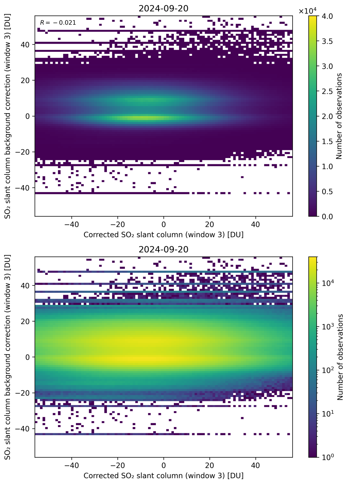
Figure 205: Scatter density plot of “Corrected SO 2 slant column (window 3)” against “SO 2 slant column background correction (window 3)” for 2024-09-19 to 2024-09-21.
