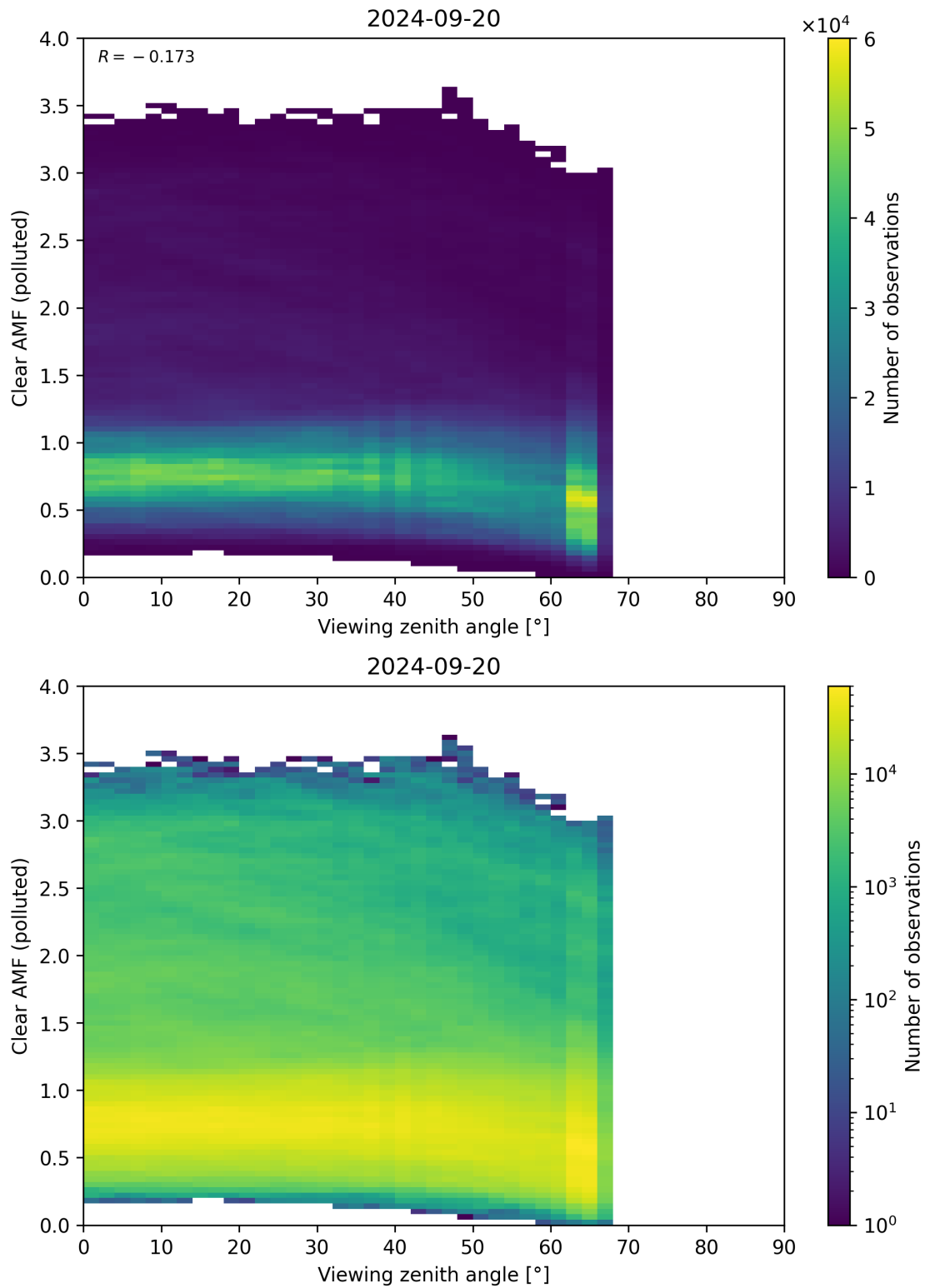
Figure 316: Scatter density plot of “Viewing zenith angle” against “Clear AMF (polluted)” for 2024-09-19 to 2024-09-21.
