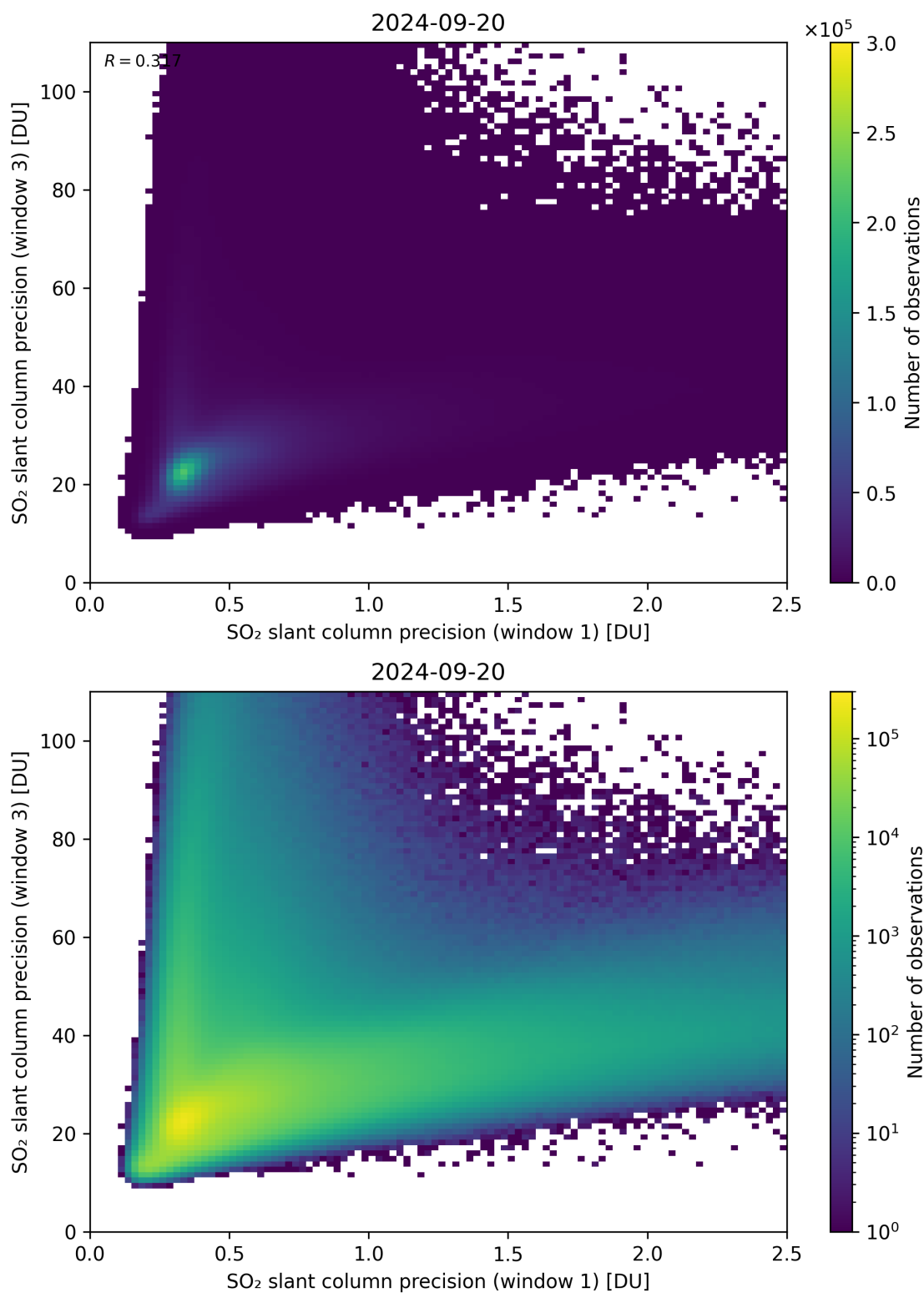
Figure 229: Scatter density plot of “SO 2 slant column precision (window 1)” against “SO 2 slant column precision (window 3)” for 2024-09-19 to 2024-09-21.
