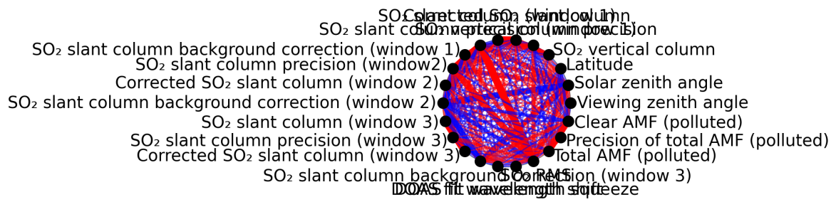
Figure 1: Map of correlation graph for 2024-09-19 to 2024-09-21.
