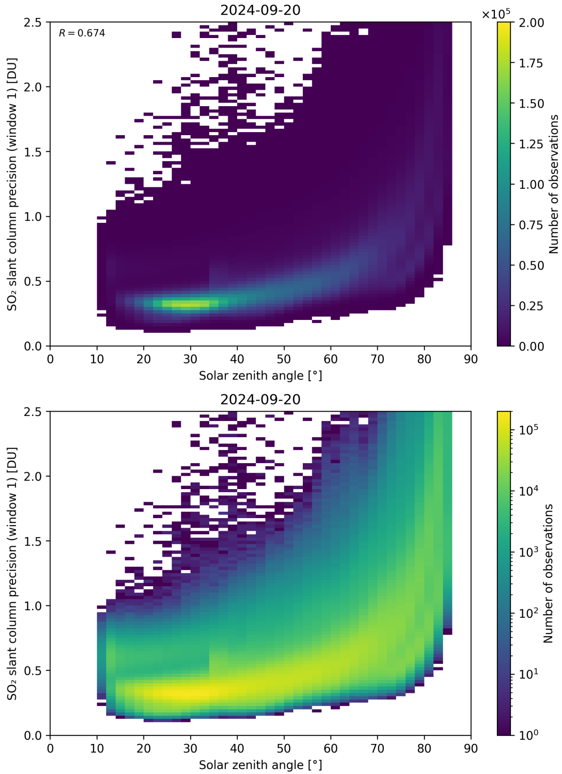
Figure 170: Scatter density plot of “Solar zenith angle” against “SO 2 slant column precision (window 1)” for 2024-09-19 to 2024-09-21.
