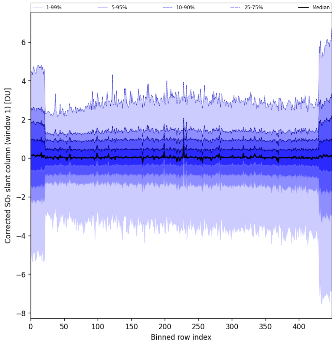
Figure 81: Along track statistics of “Corrected SO 2 slant column (window 1)” for 2024-09-19 to 2024-09-21
