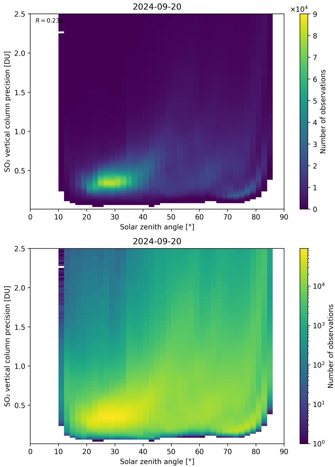
Figure 177: Scatter density plot of “Solar zenith angle” against “SO 2 vertical column precision” for 2024-09-19 to 2024-09-21.
