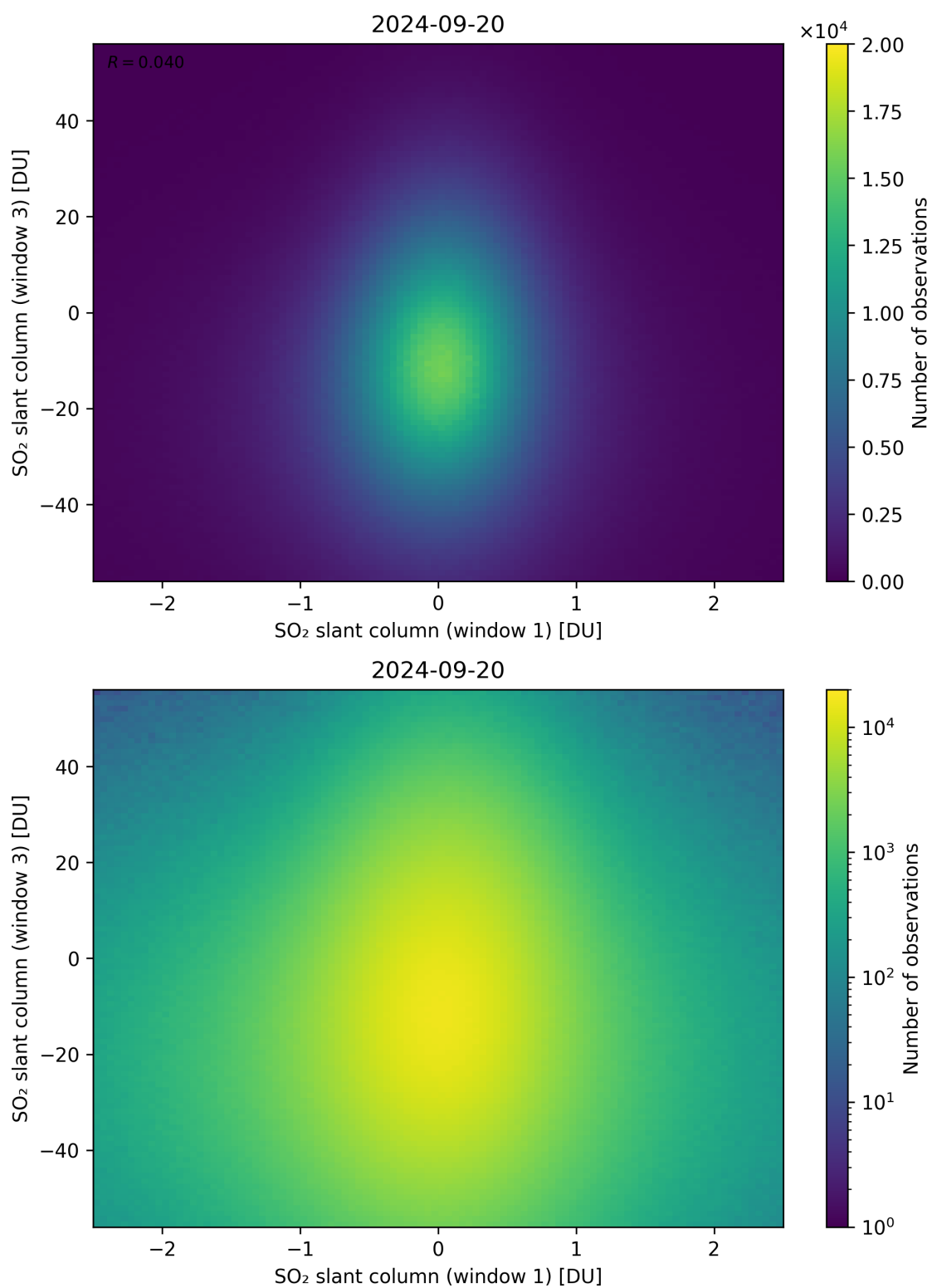
Figure 237: Scatter density plot of “SO 2 slant column (window 1)” against “SO 2 slant column (window 3)” for 2024-09-19 to 2024-09-21.
