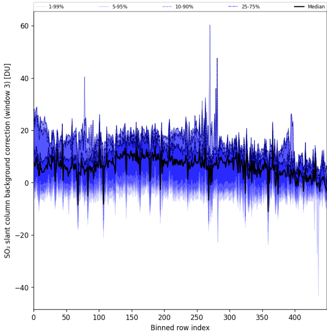
Figure 90: Along track statistics of “SO 2 slant column background correction (window 3)” for 2024-09-19 to 2024-09-21
