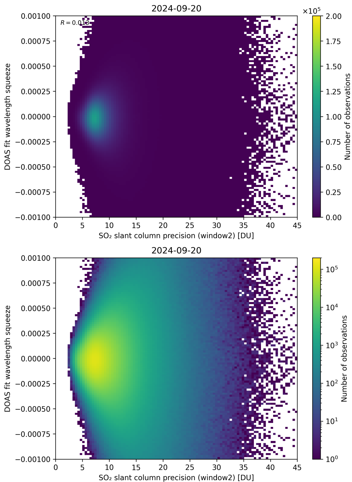
Figure 244: Scatter density plot of “SO 2 slant column precision (window2)” against “DOAS fit wavelength squeeze” for 2024-09-19 to 2024-09-21.
