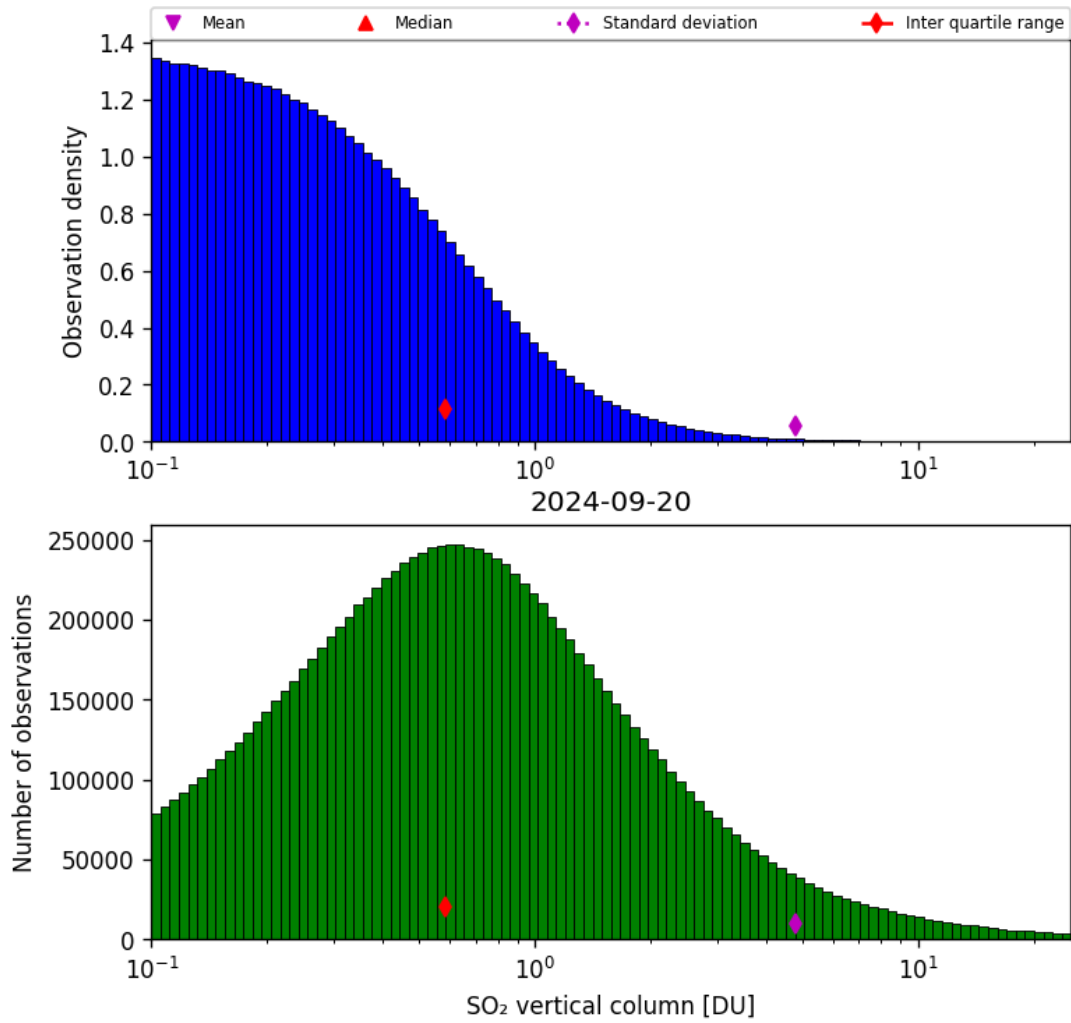
Figure 53: Histogram of “SO 2 vertical column” for 2024-09-19 to 2024-09-21
