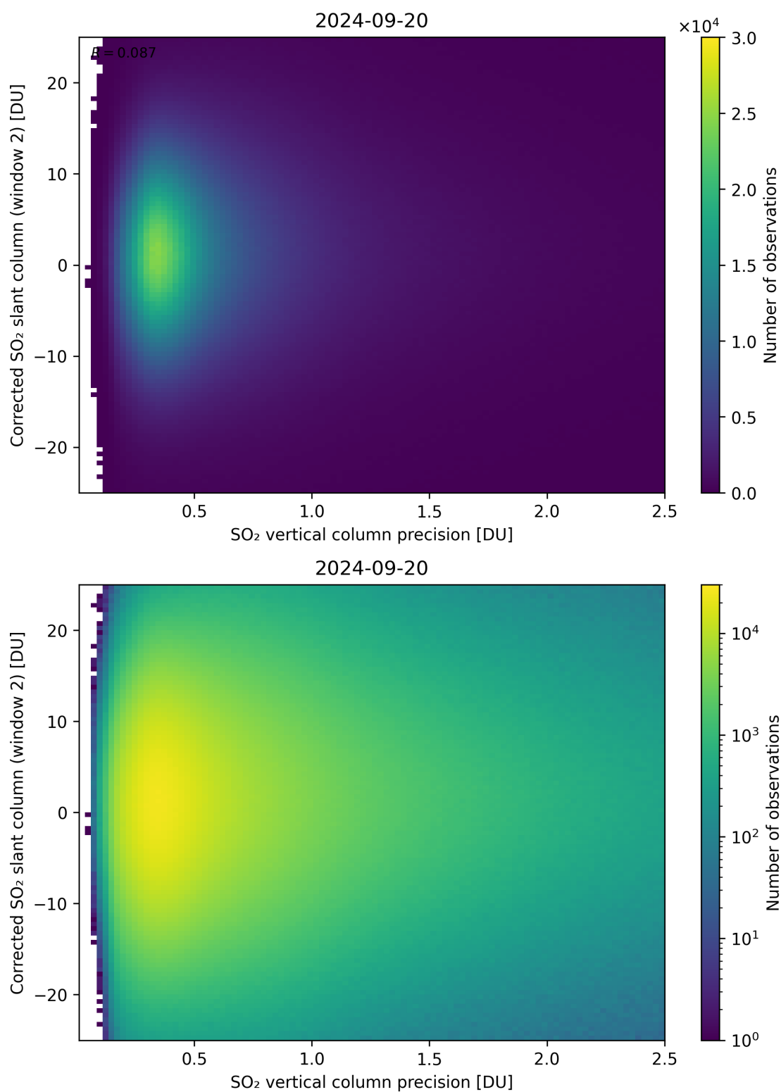
Figure 287: Scatter density plot of “SO 2 vertical column precision” against “Corrected SO 2 slant column (window 2)” for 2024-09-19 to 2024-09-21.
