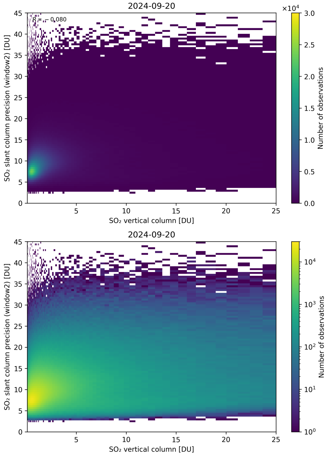
Figure 302: Scatter density plot of “SO 2 vertical column” against “SO 2 slant column precision (window2)” for 2024-09-19 to 2024-09-21.
