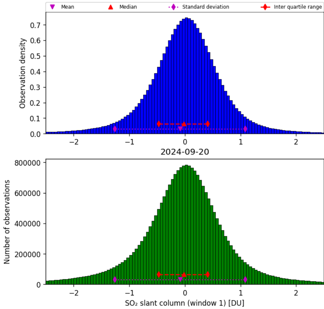
Figure 56: Histogram of “SO 2 slant column (window 1)” for 2024-09-19 to 2024-09-21
