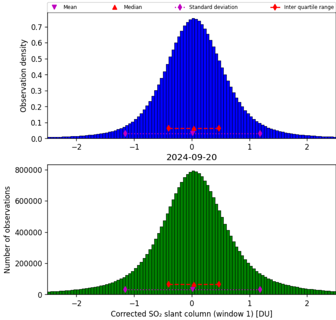
Figure 58: Histogram of “Corrected SO 2 slant column (window 1)” for 2024-09-19 to 2024-09-21
