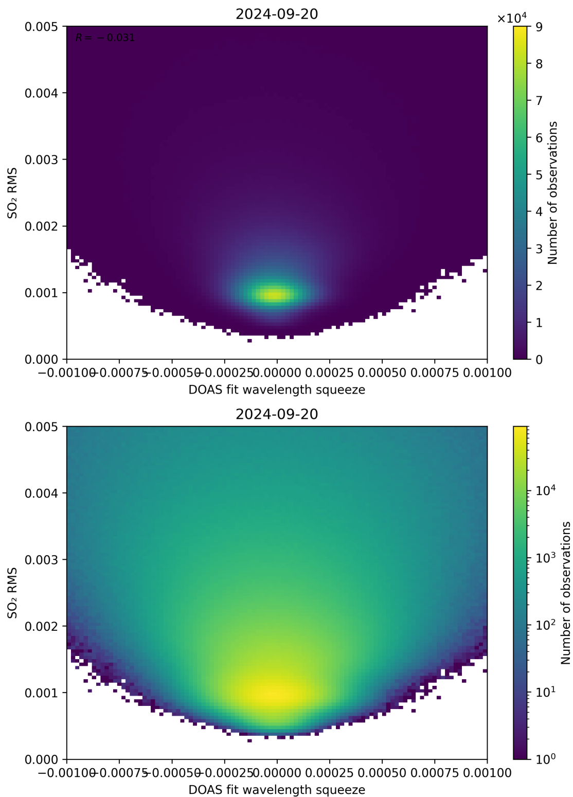
Figure 132: Scatter density plot of “DOAS fit wavelength squeeze” against “SO 2 RMS” for 2024-09-19 to 2024-09-21.
