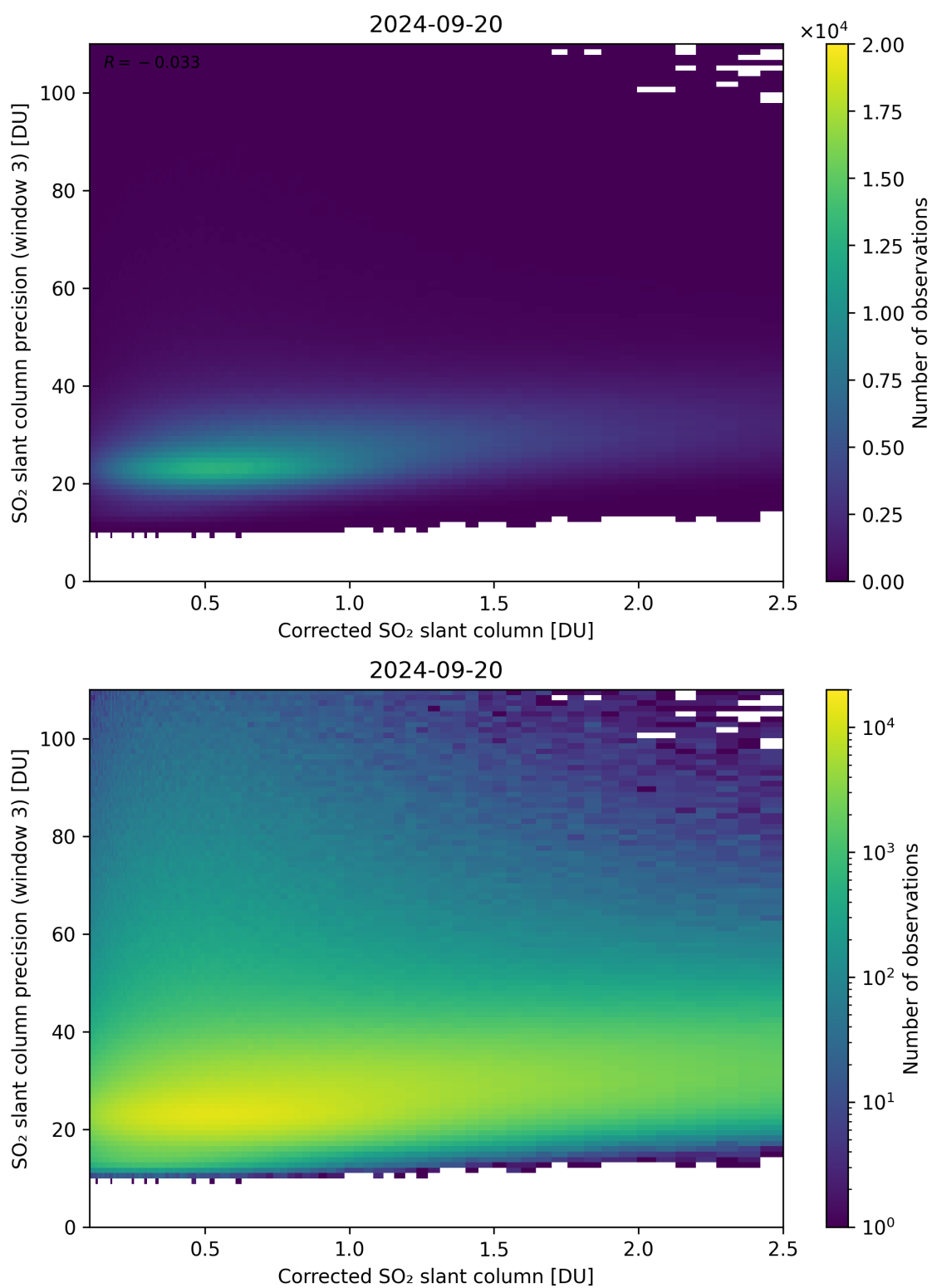
Figure 191: Scatter density plot of “Corrected SO 2 slant column” against “SO 2 slant column precision (window 3)” for 2024-09-19 to 2024-09-21.
