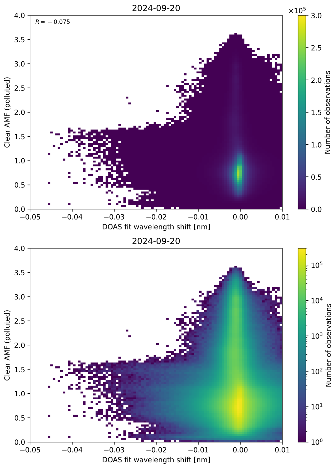
Figure 129: Scatter density plot of “DOAS fit wavelength shift” against “Clear AMF (polluted)” for 2024-09-19 to 2024-09-21.
