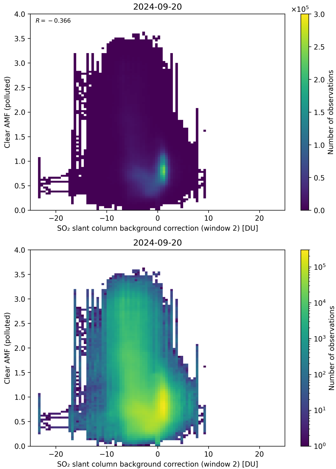
Figure 115: Scatter density plot of “SO 2 slant column background correction (window 2)” against “Clear AMF (polluted)” for 2024-09-19 to 2024-09-21.
