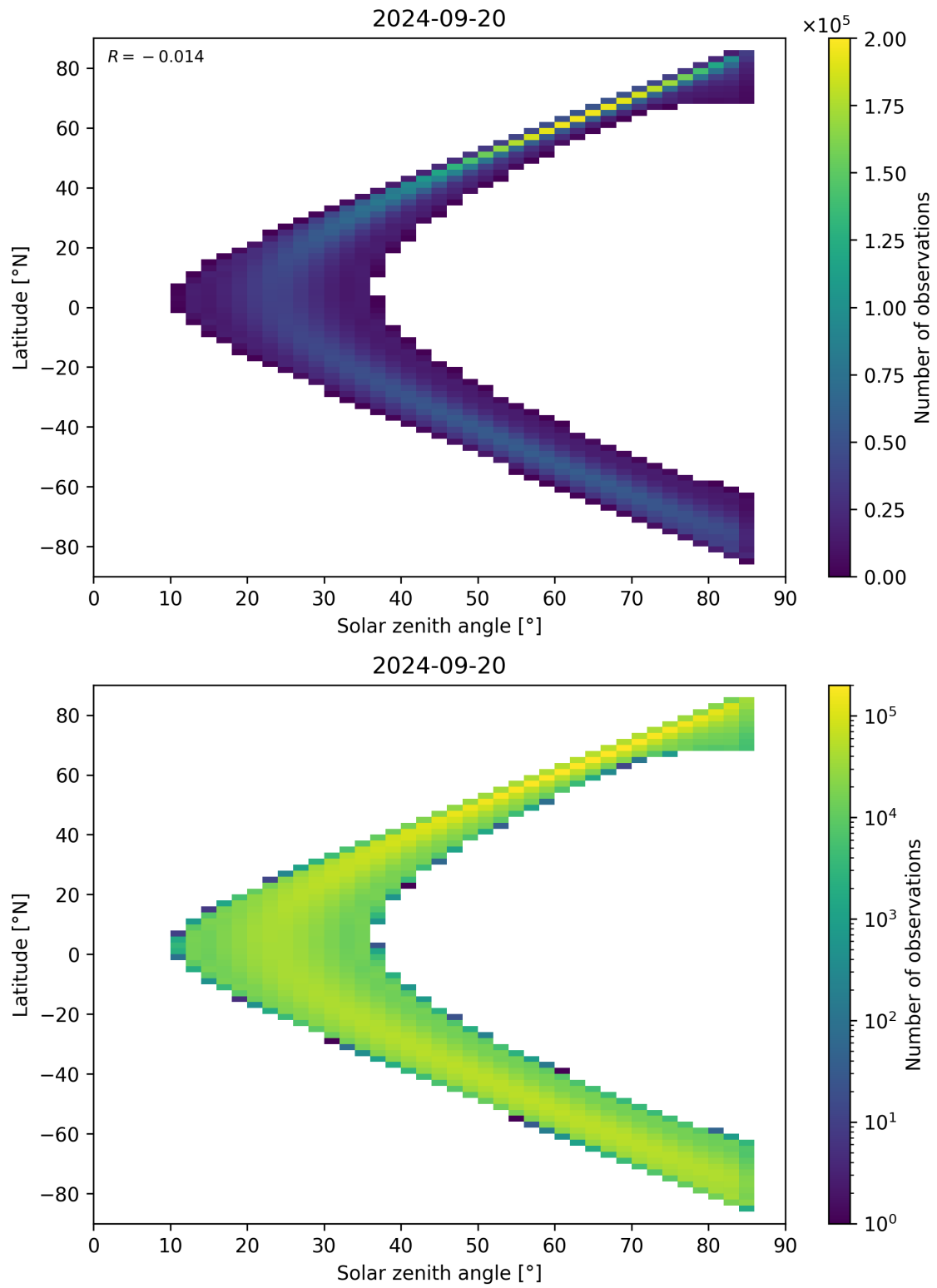
Figure 164: Scatter density plot of “Solar zenith angle” against “Latitude” for 2024-09-19 to 2024-09-21.
