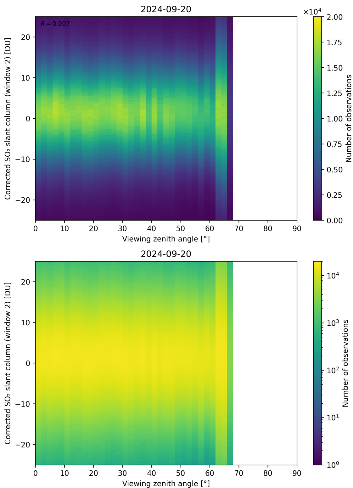
Figure 318: Scatter density plot of “Viewing zenith angle” against “Corrected SO 2 slant column (window 2)” for 2024-09-19 to 2024-09-21.
