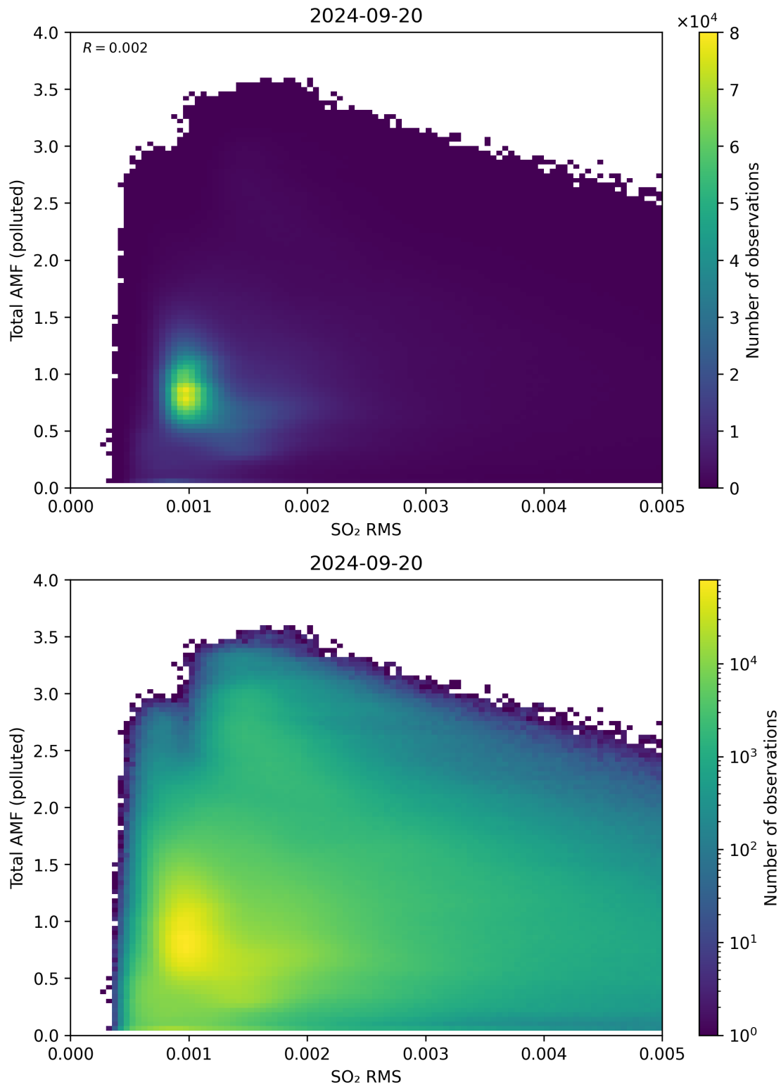
Figure 137: Scatter density plot of “SO 2 RMS” against “Total AMF (polluted)” for 2024-09-19 to 2024-09-21.
