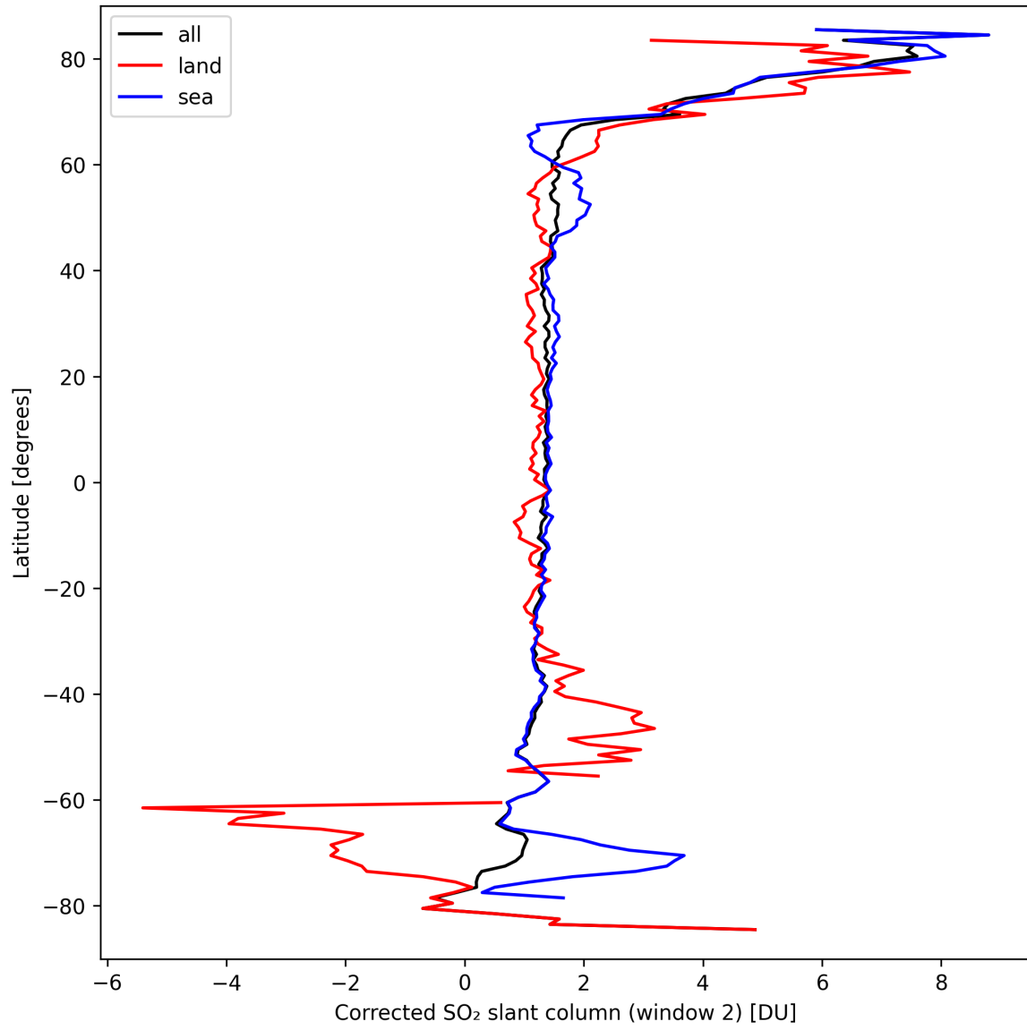
Figure 39: Zonal average of “Corrected SO 2 slant column (window 2)” for 2024-09-19 to 2024-09-21.
