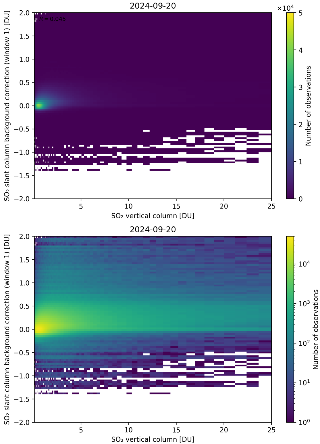
Figure 273: Scatter density plot of “SO 2 vertical column” against “SO 2 slant column background correction (window 1)” for 2024-09-19 to 2024-09-21.
