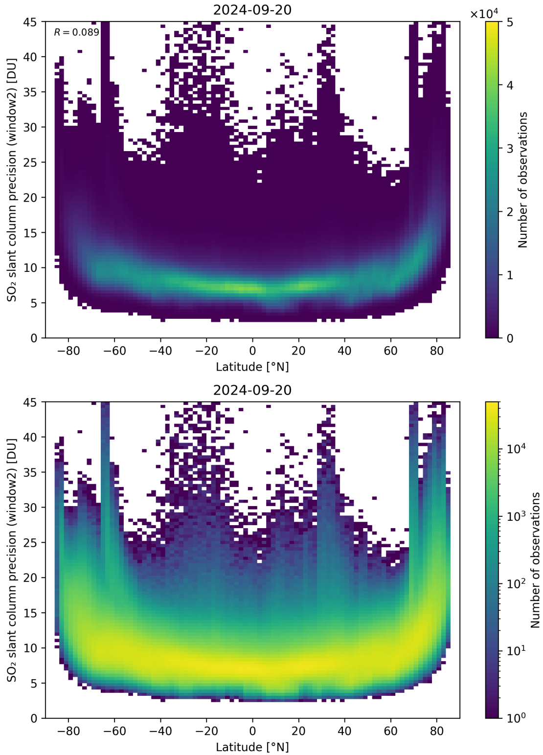
Figure 151: Scatter density plot of “Latitude” against “SO 2 slant column precision (window2)” for 2024-09-19 to 2024-09-21.
