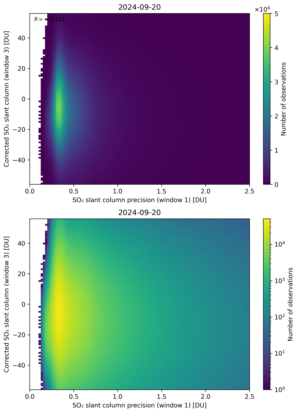
Figure 226: Scatter density plot of “SO 2 slant column precision (window 1)” against “Corrected SO 2 slant column (window 3)” for 2024-09-19 to 2024-09-21.
