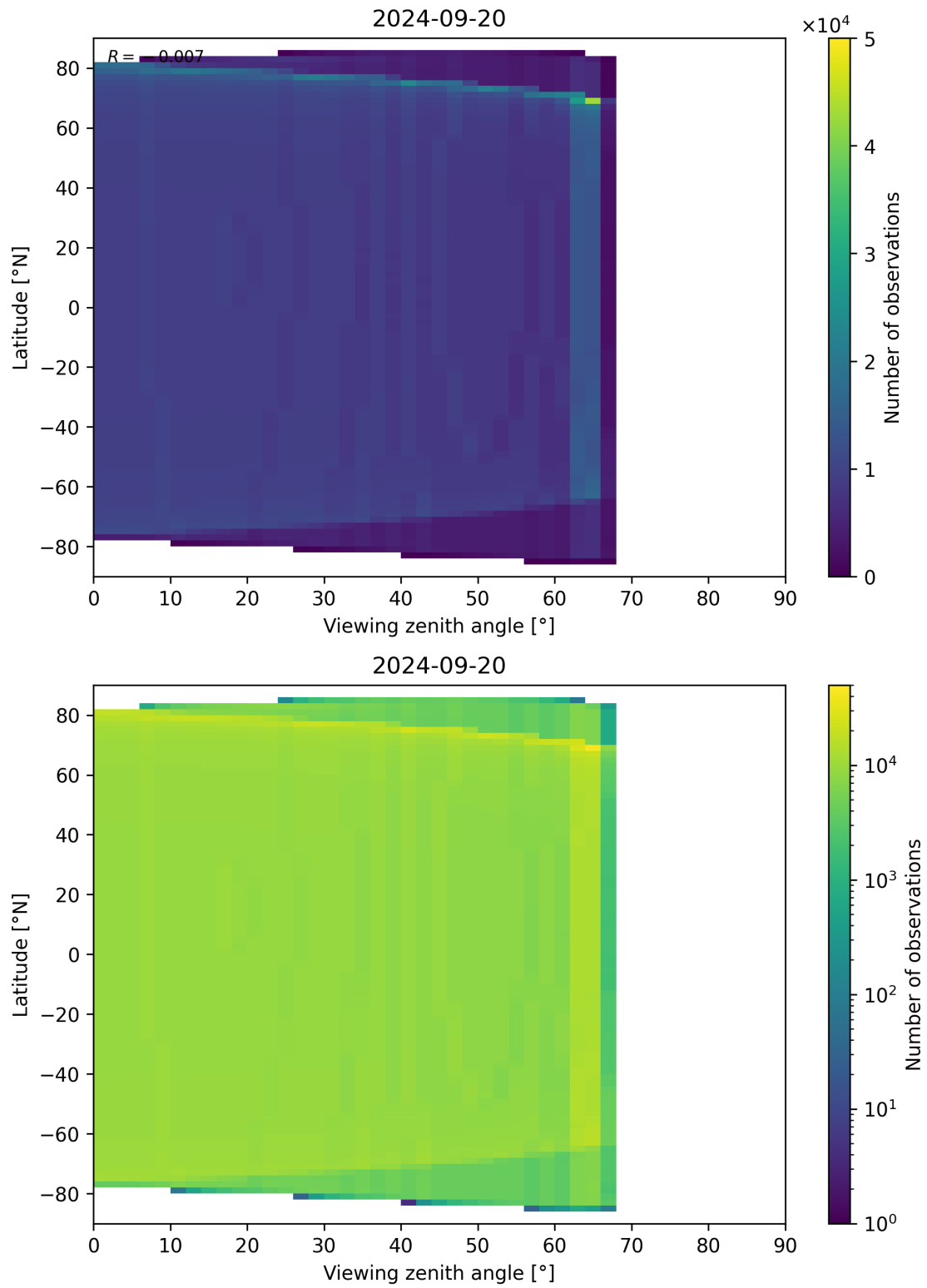
Figure 314: Scatter density plot of “Viewing zenith angle” against “Latitude” for 2024-09-19 to 2024-09-21.
