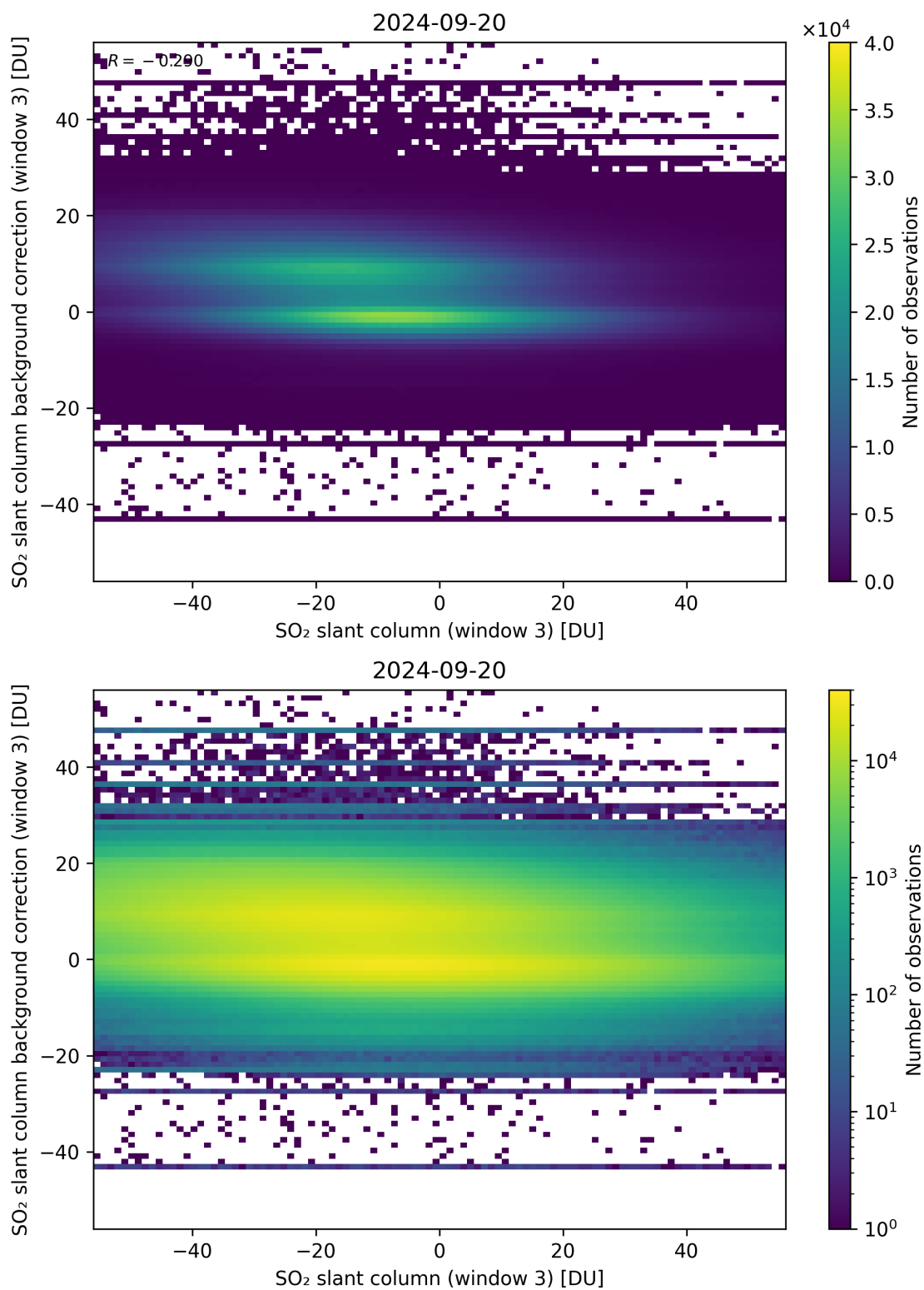
Figure 253: Scatter density plot of “SO 2 slant column (window 3)” against “SO 2 slant column background correction (window 3)” for 2024-09-19 to 2024-09-21.
