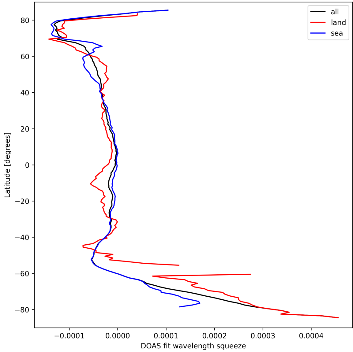
Figure 46: Zonal average of "DOAS fit wavelength squeeze" for 2024-09-19 to 2024-09-21.
