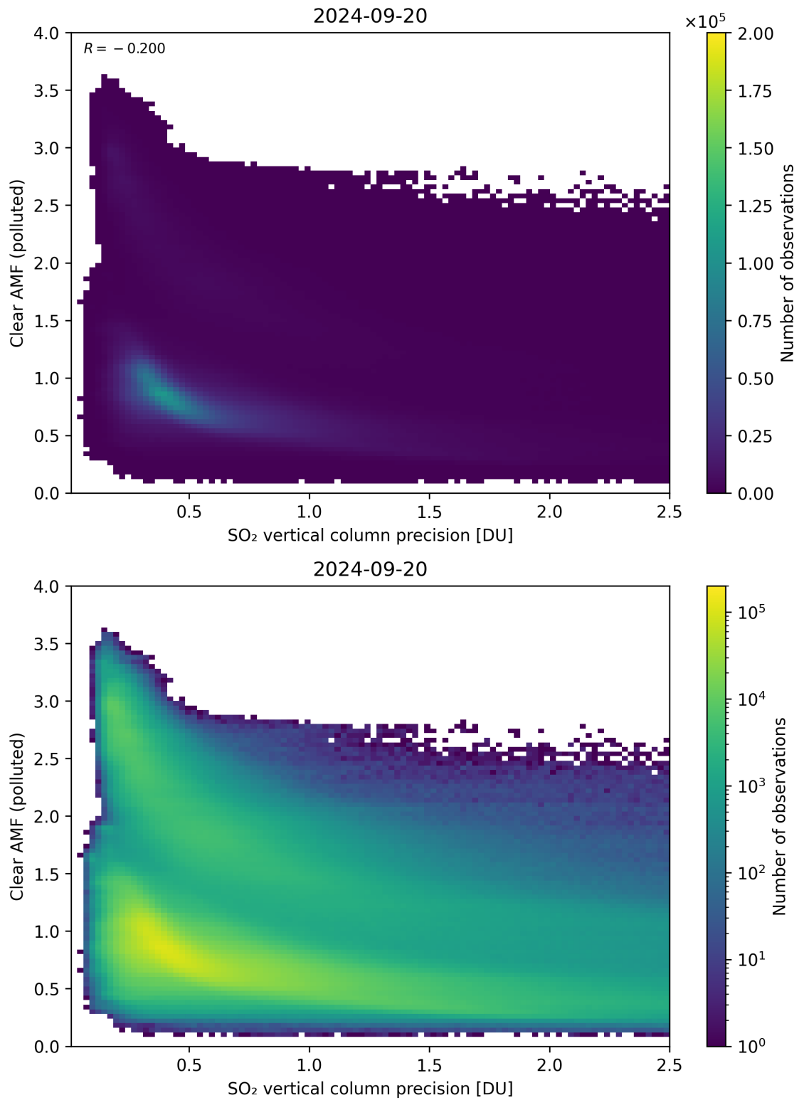
Figure 285: Scatter density plot of “SO 2 vertical column precision” against “Clear AMF (polluted)” for 2024-09-19 to 2024-09-21.
