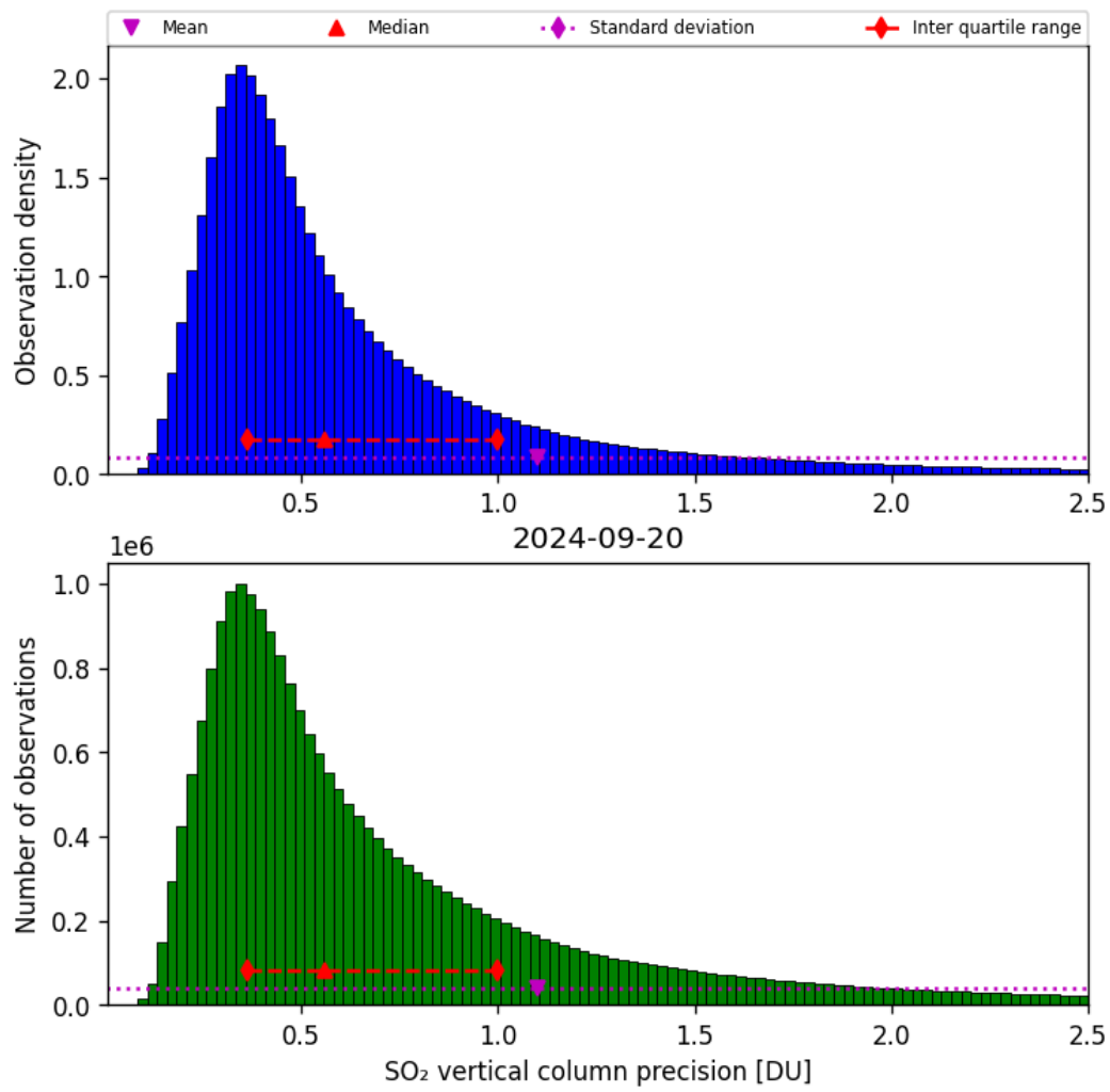
Figure 54: Histogram of “SO 2 vertical column precision” for 2024-09-19 to 2024-09-21
