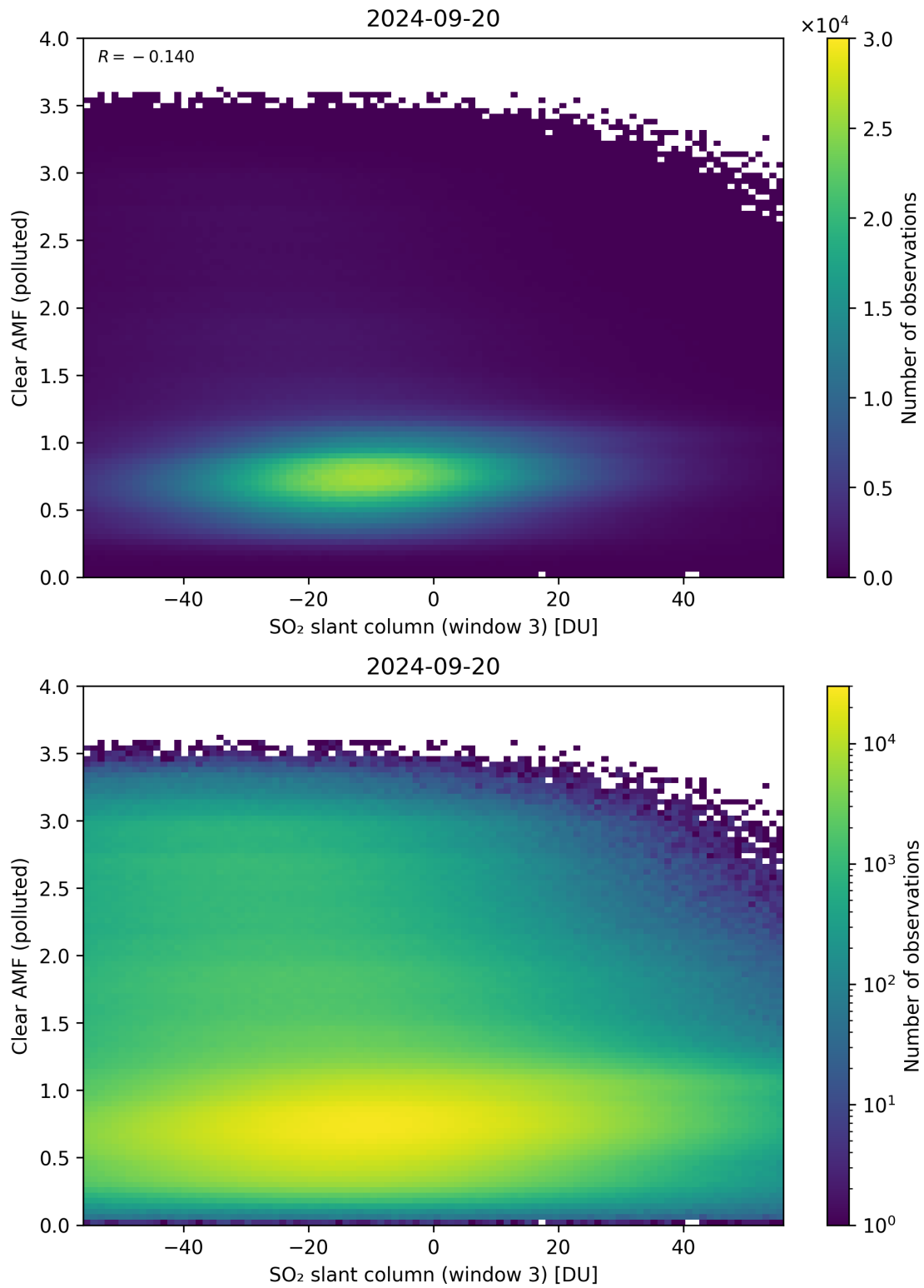
Figure 265: Scatter density plot of “SO 2 slant column (window 3)” against “Clear AMF (polluted)” for 2024-09-19 to 2024-09-21.
