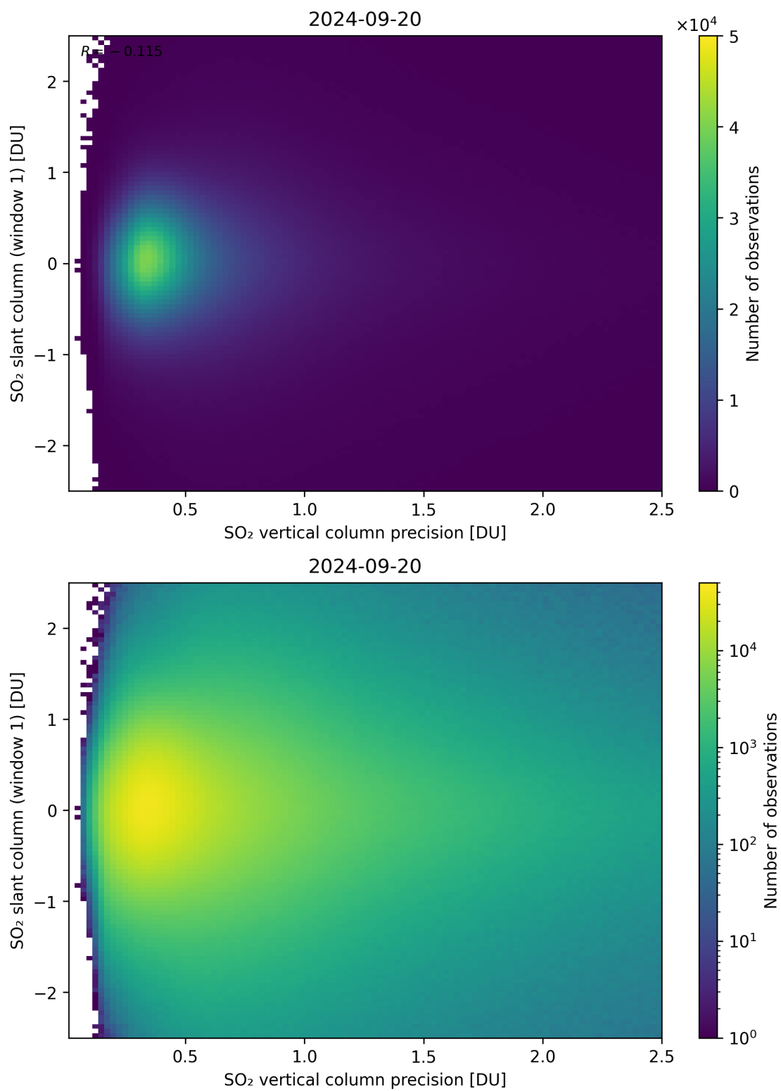
Figure 289: Scatter density plot of “SO 2 vertical column precision” against “SO 2 slant column (window 1)” for 2024-09-19 to 2024-09-21.
