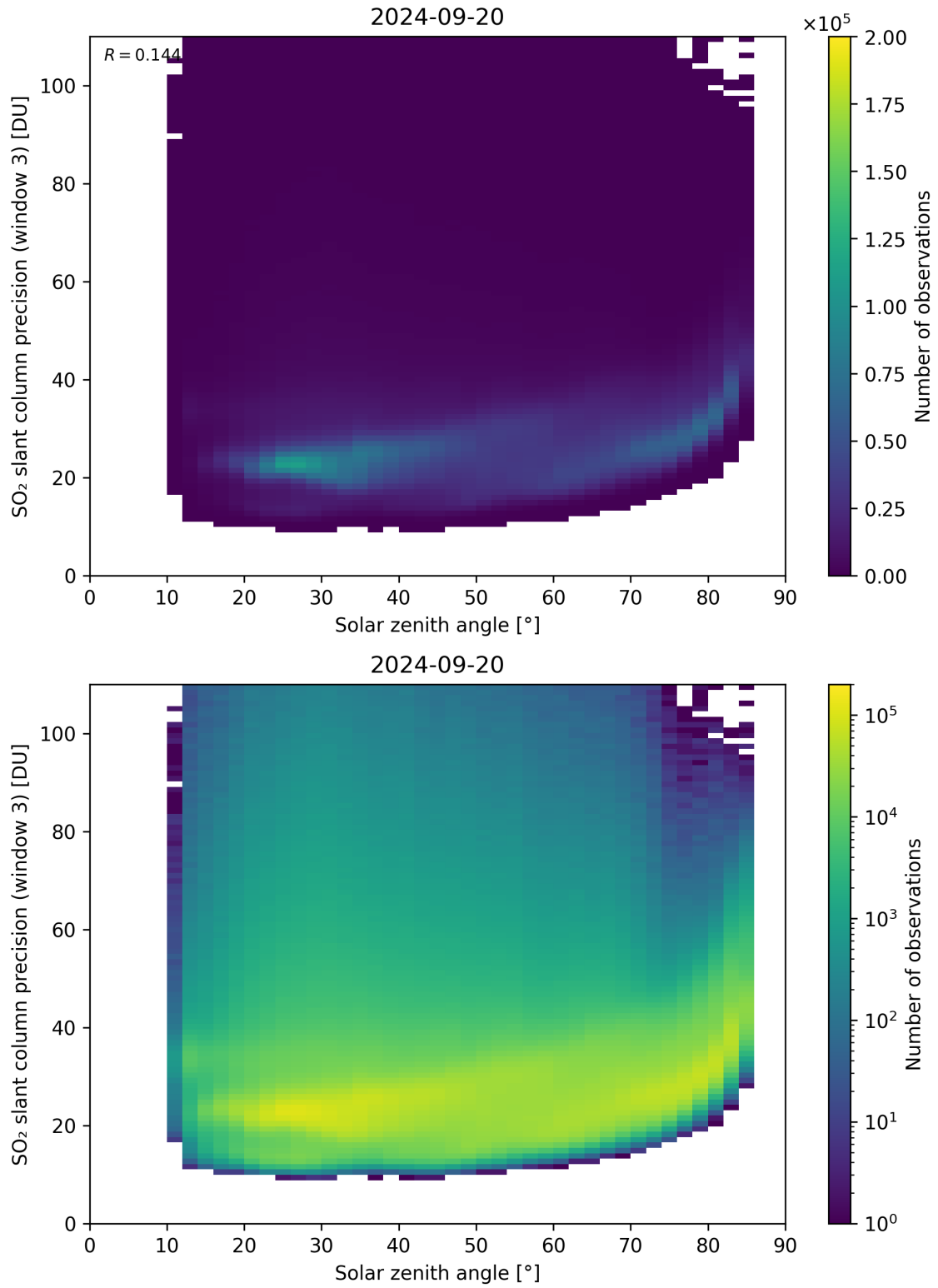
Figure 173: Scatter density plot of “Solar zenith angle” against “SO 2 slant column precision (window 3)” for 2024-09-19 to 2024-09-21.
