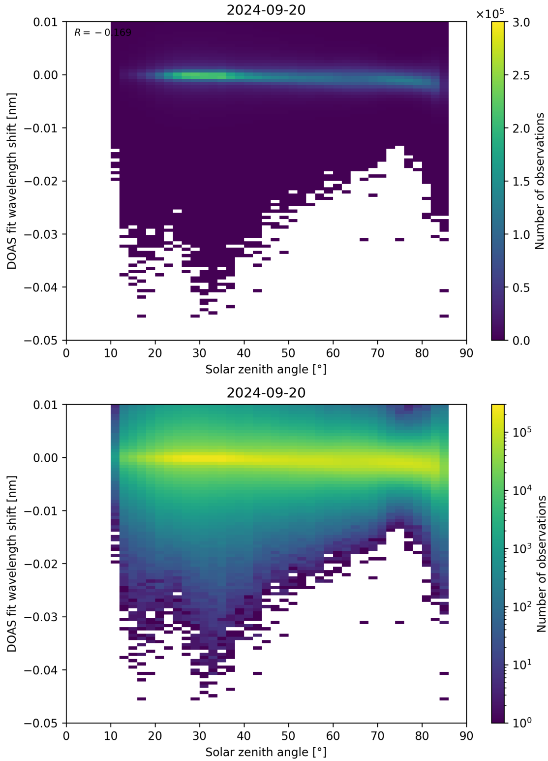
Figure 161: Scatter density plot of “Solar zenith angle” against “DOAS fit wavelength shift” for 2024-09-19 to 2024-09-21.
