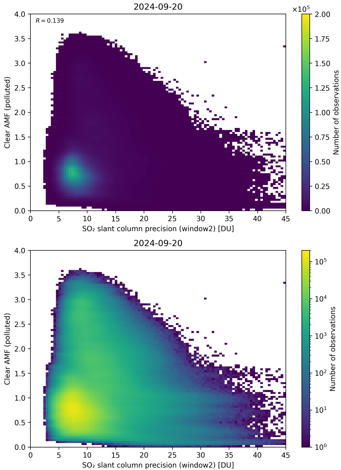
Figure 246: Scatter density plot of “SO 2 slant column precision (window2)” against “Clear AMF (polluted)” for 2024-09-19 to 2024-09-21.
