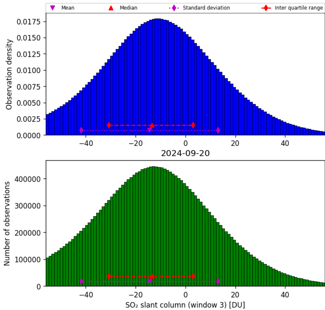
Figure 64: Histogram of “SO 2 slant column (window 3)” for 2024-09-19 to 2024-09-21
