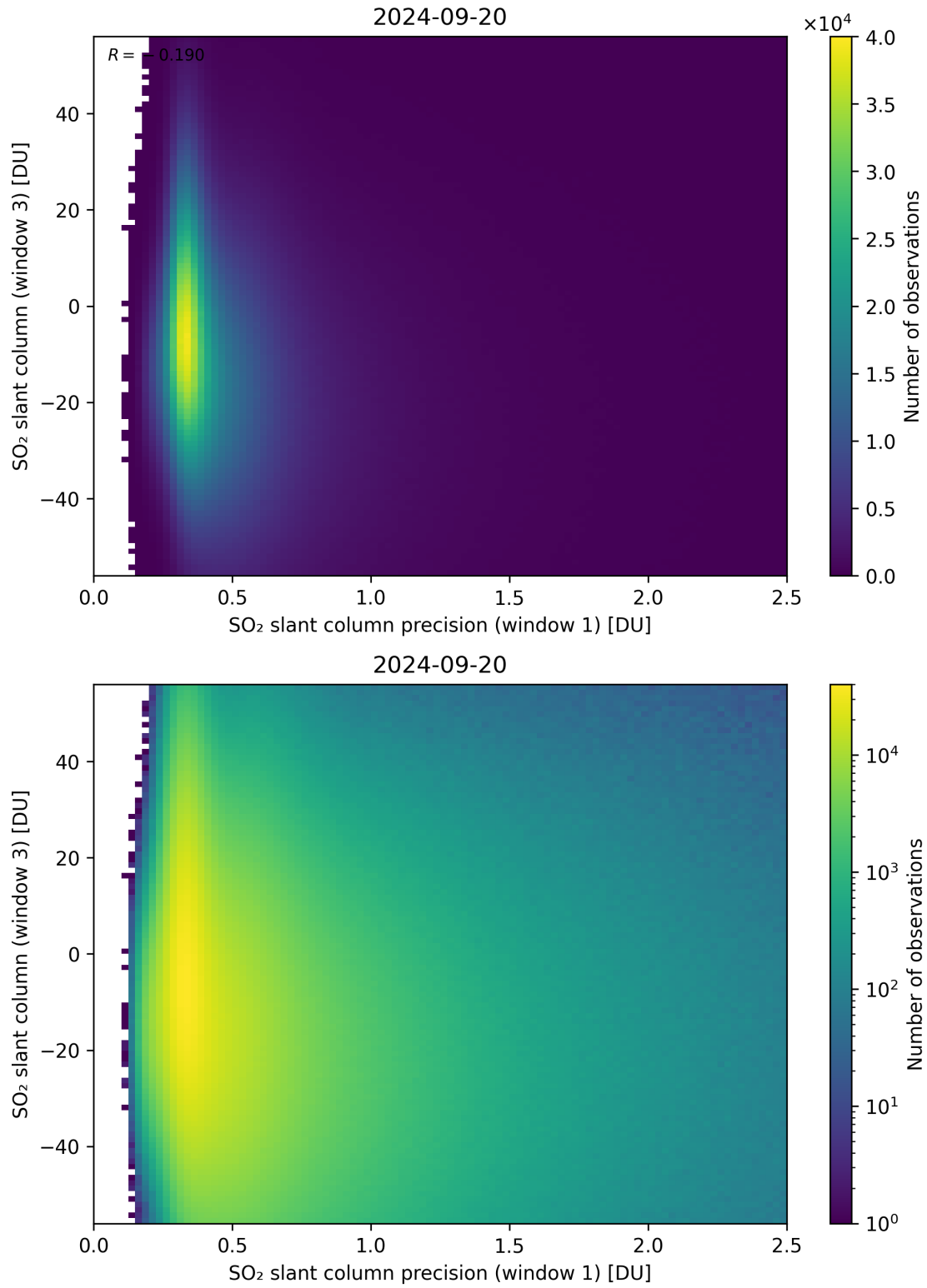
Figure 228: Scatter density plot of “SO 2 slant column precision (window 1)” against “SO 2 slant column (window 3)” for 2024-09-19 to 2024-09-21.
