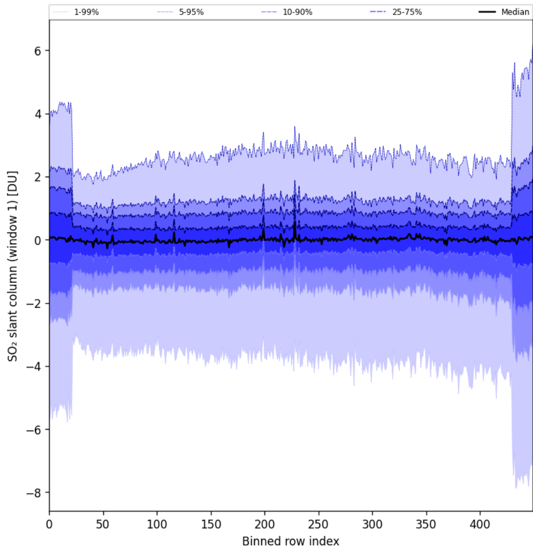
Figure 79: Along track statistics of “SO 2 slant column (window 1)” for 2024-09-19 to 2024-09-21
