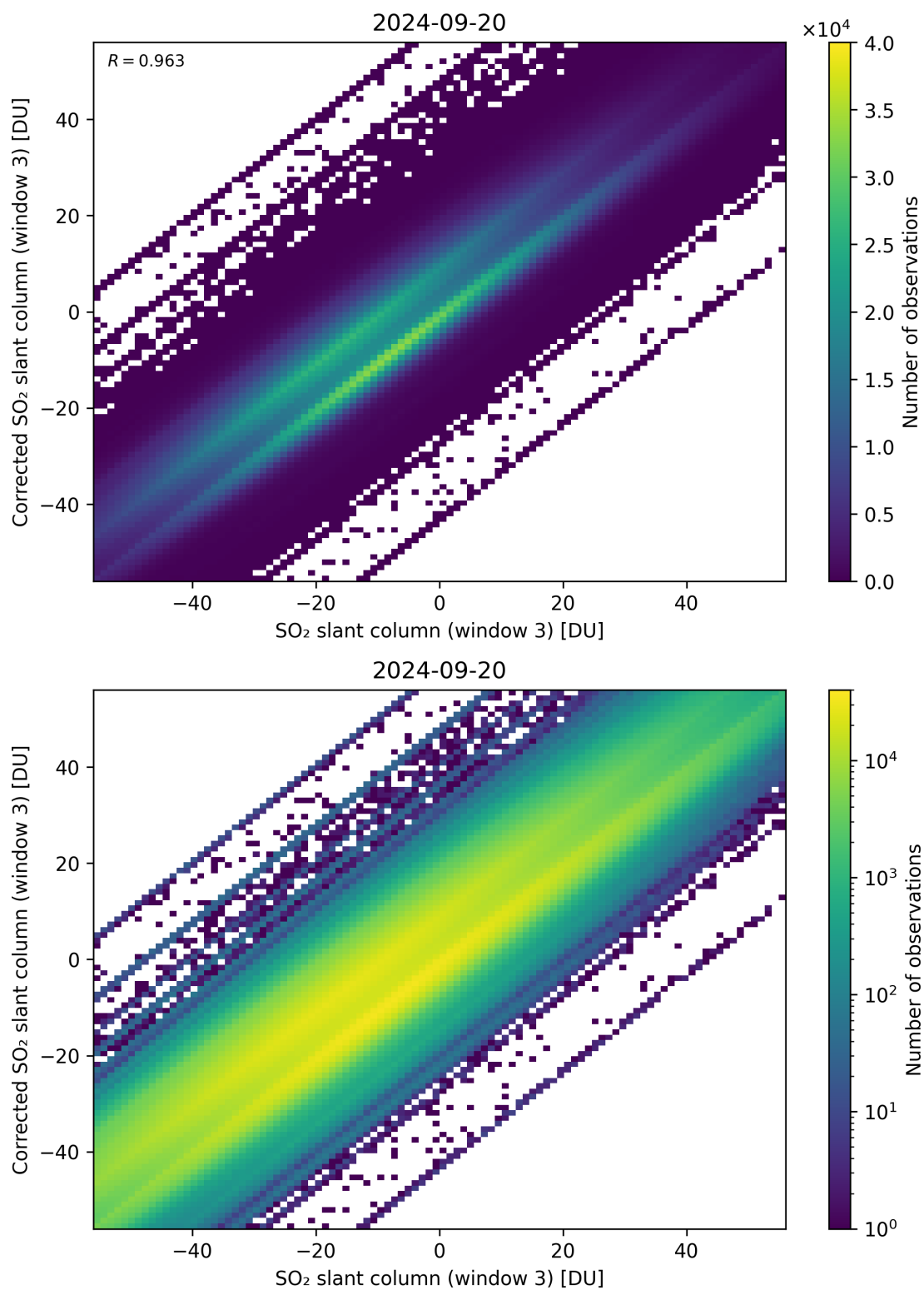
Figure 266: Scatter density plot of “SO 2 slant column (window 3)” against “Corrected SO 2 slant column (window 3)” for 2024-09-19 to 2024-09-21.
