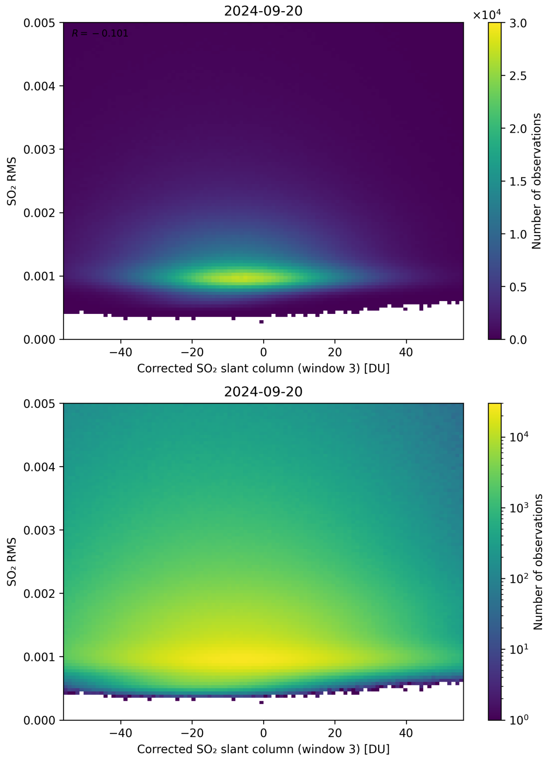
Figure 208: Scatter density plot of “Corrected SO 2 slant column (window 3)” against “SO 2 RMS” for 2024-09-19 to 2024-09-21.
