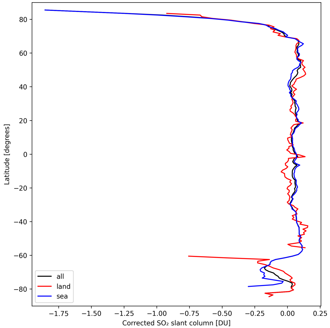
Figure 32: Zonal average of “Corrected SO 2 slant column” for 2024-09-19 to 2024-09-21.
