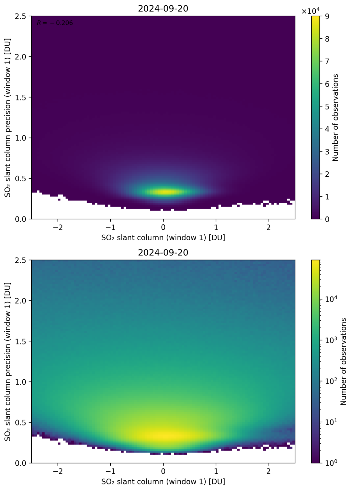
Figure 235: Scatter density plot of “SO 2 slant column (window 1)” against “SO 2 slant column precision (window 1)” for 2024-09-19 to 2024-09-21.
