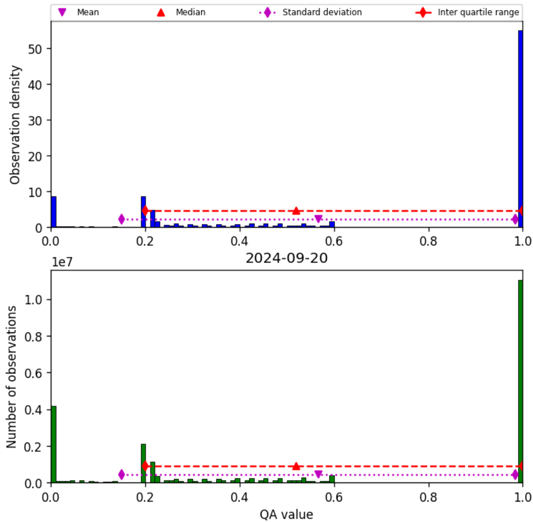
Figure 52: Histogram of “QA value” for 2024-09-19 to 2024-09-21
