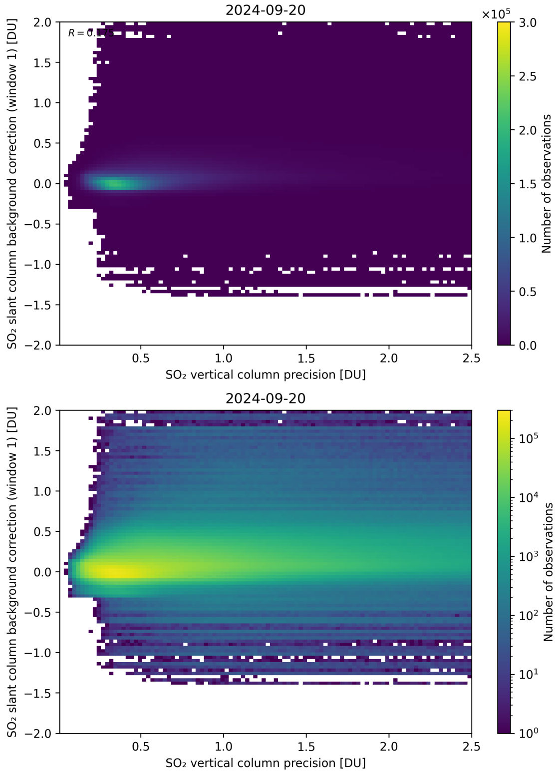
Figure 279: Scatter density plot of “SO 2 vertical column precision” against “SO 2 slant column background correction (window 1)” for 2024-09-19 to 2024-09-21.
