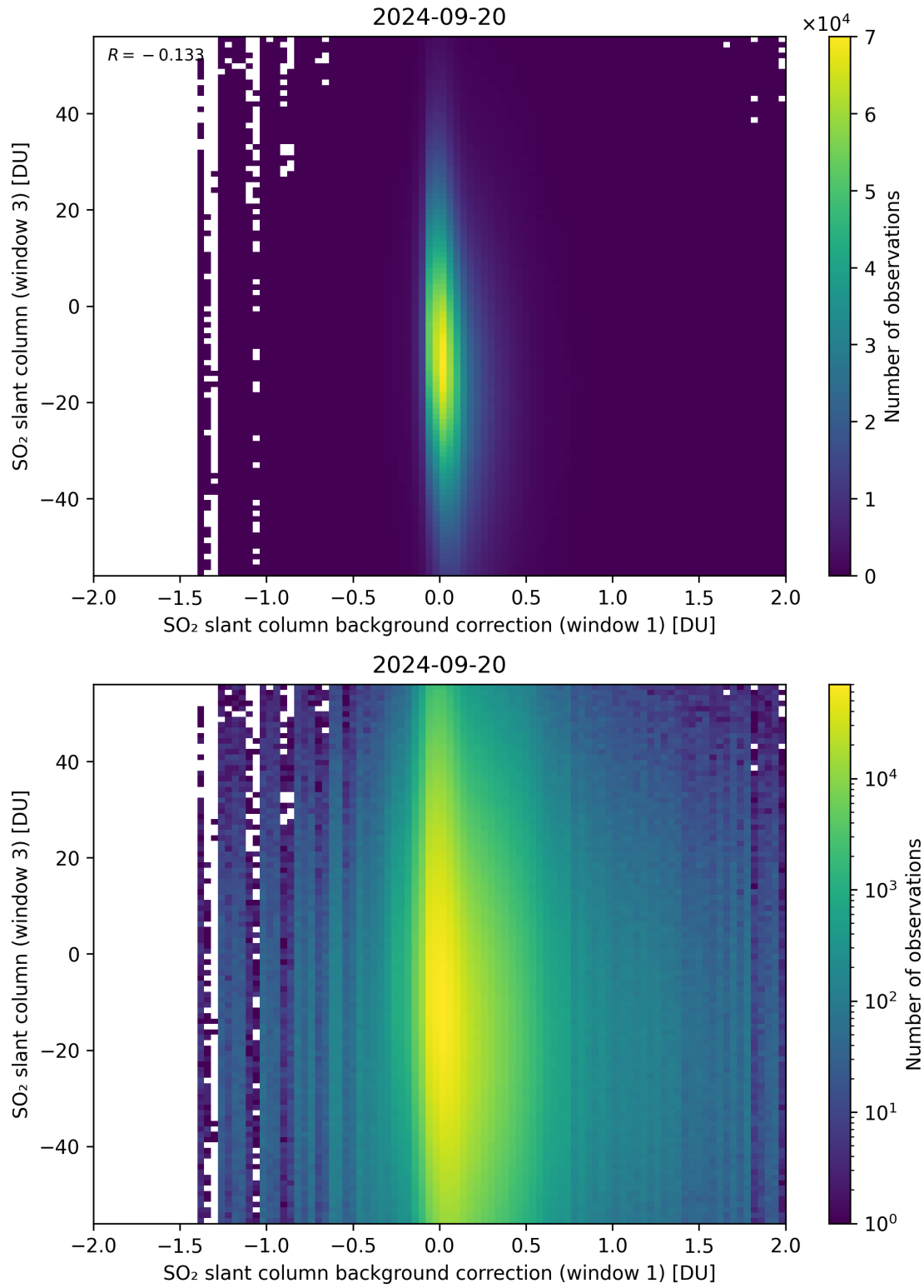
Figure 107: Scatter density plot of “SO 2 slant column background correction (window 1)” against “SO 2 slant column (window 3)” for 2024-09-19 to 2024-09-21.
