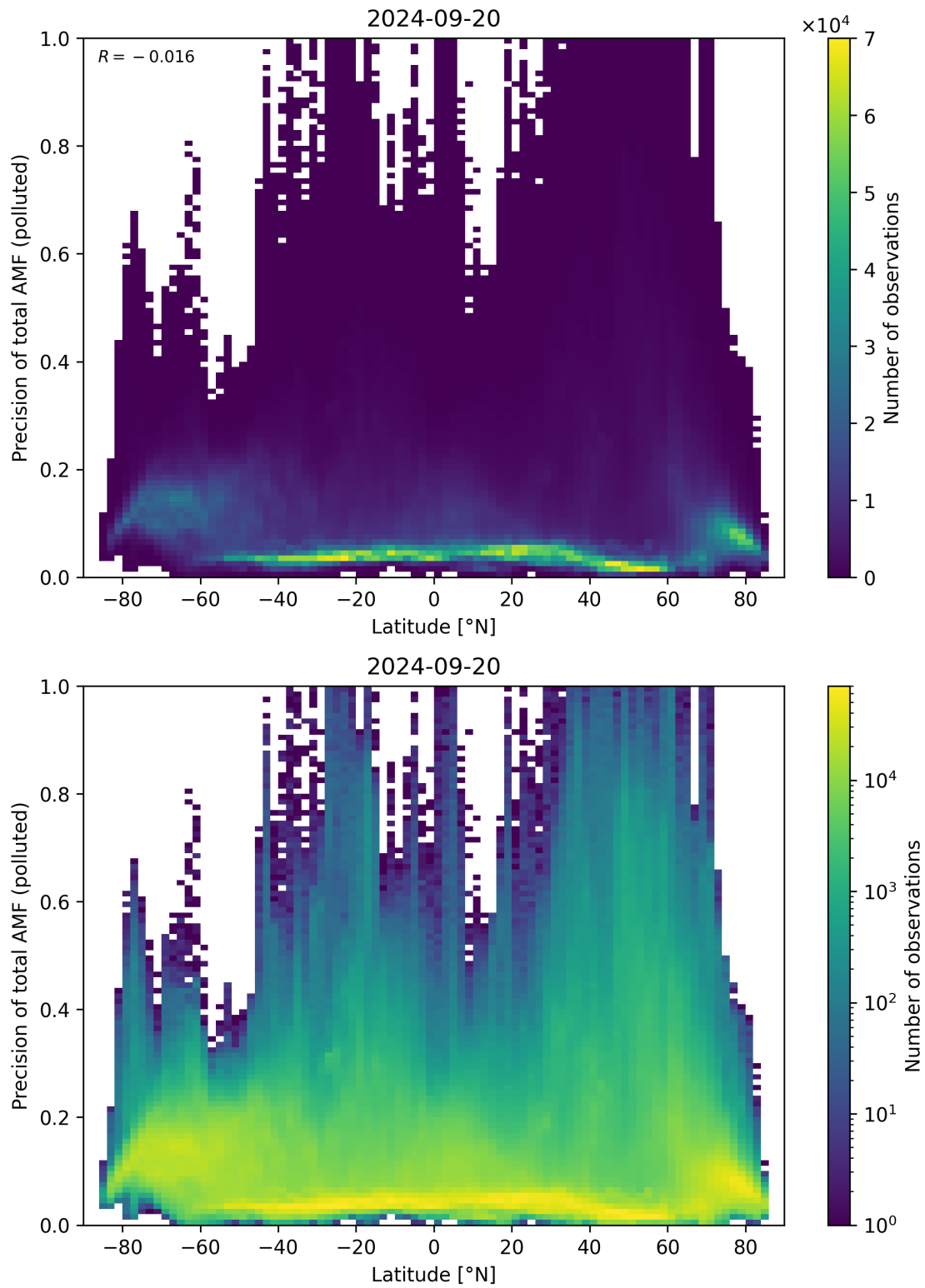
Figure 155: Scatter density plot of “Latitude” against “Precision of total AMF (polluted)” for 2024-09-19 to 2024-09-21.
