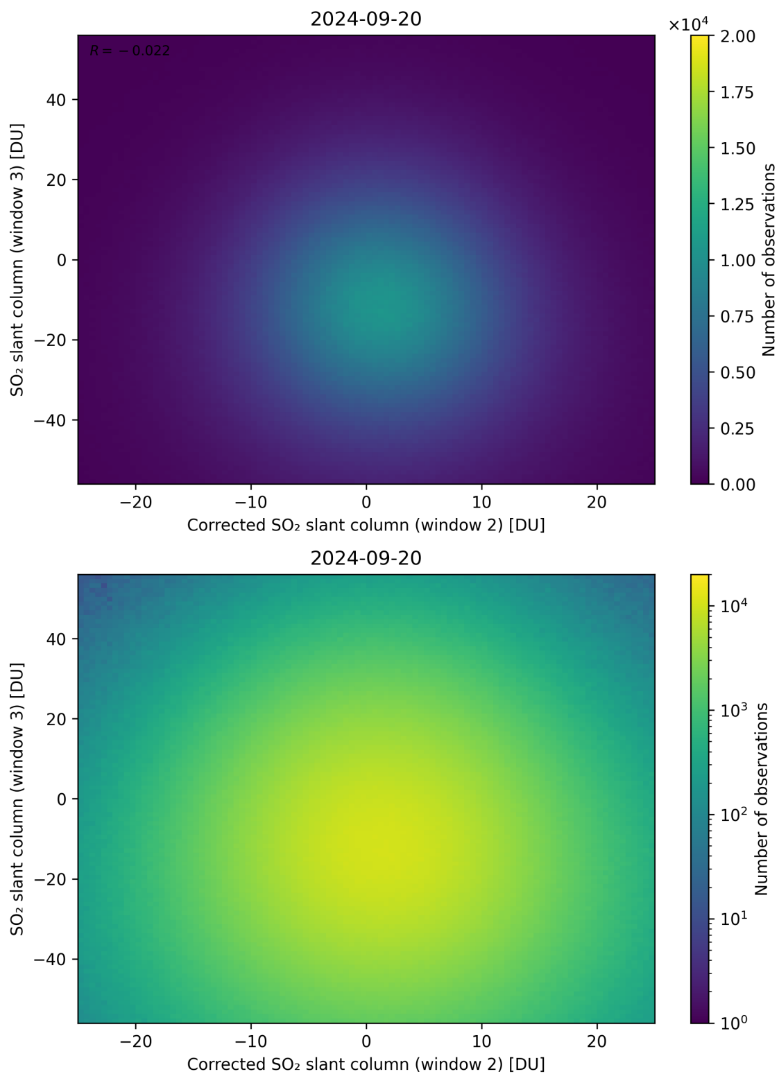
Figure 201: Scatter density plot of “Corrected SO 2 slant column (window 2)” against “SO 2 slant column (window 3)” for 2024-09-19 to 2024-09-21.
