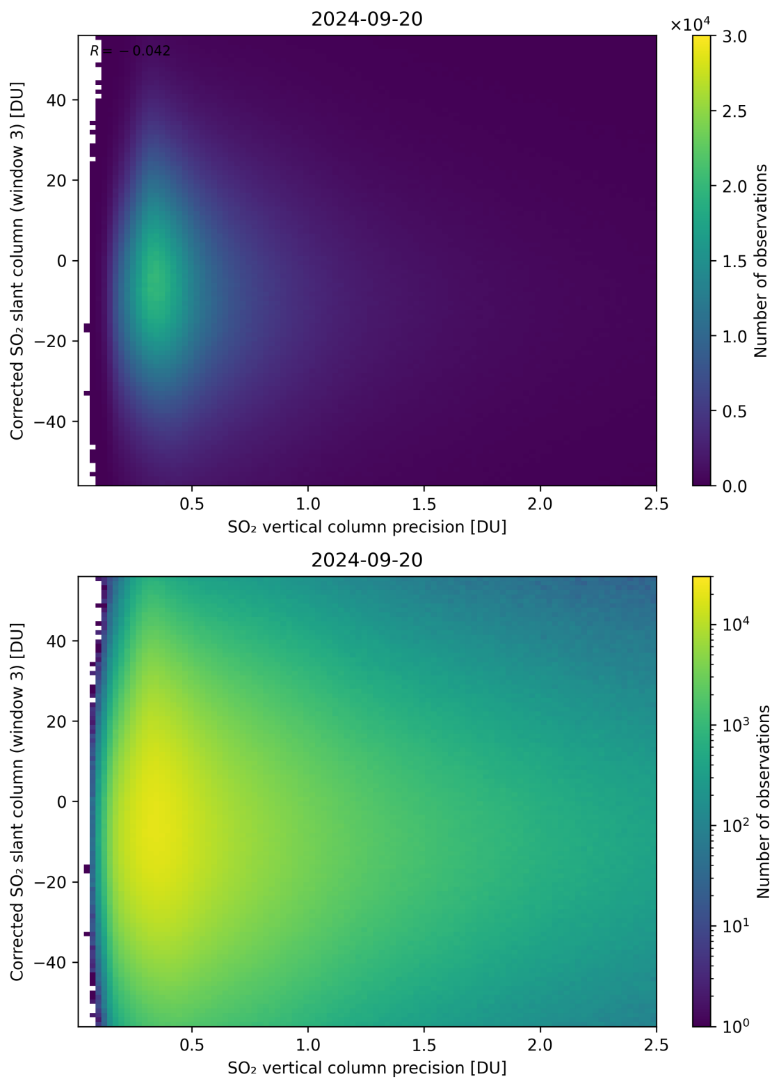
Figure 288: Scatter density plot of “SO 2 vertical column precision” against “Corrected SO 2 slant column (window 3)” for 2024-09-19 to 2024-09-21.
