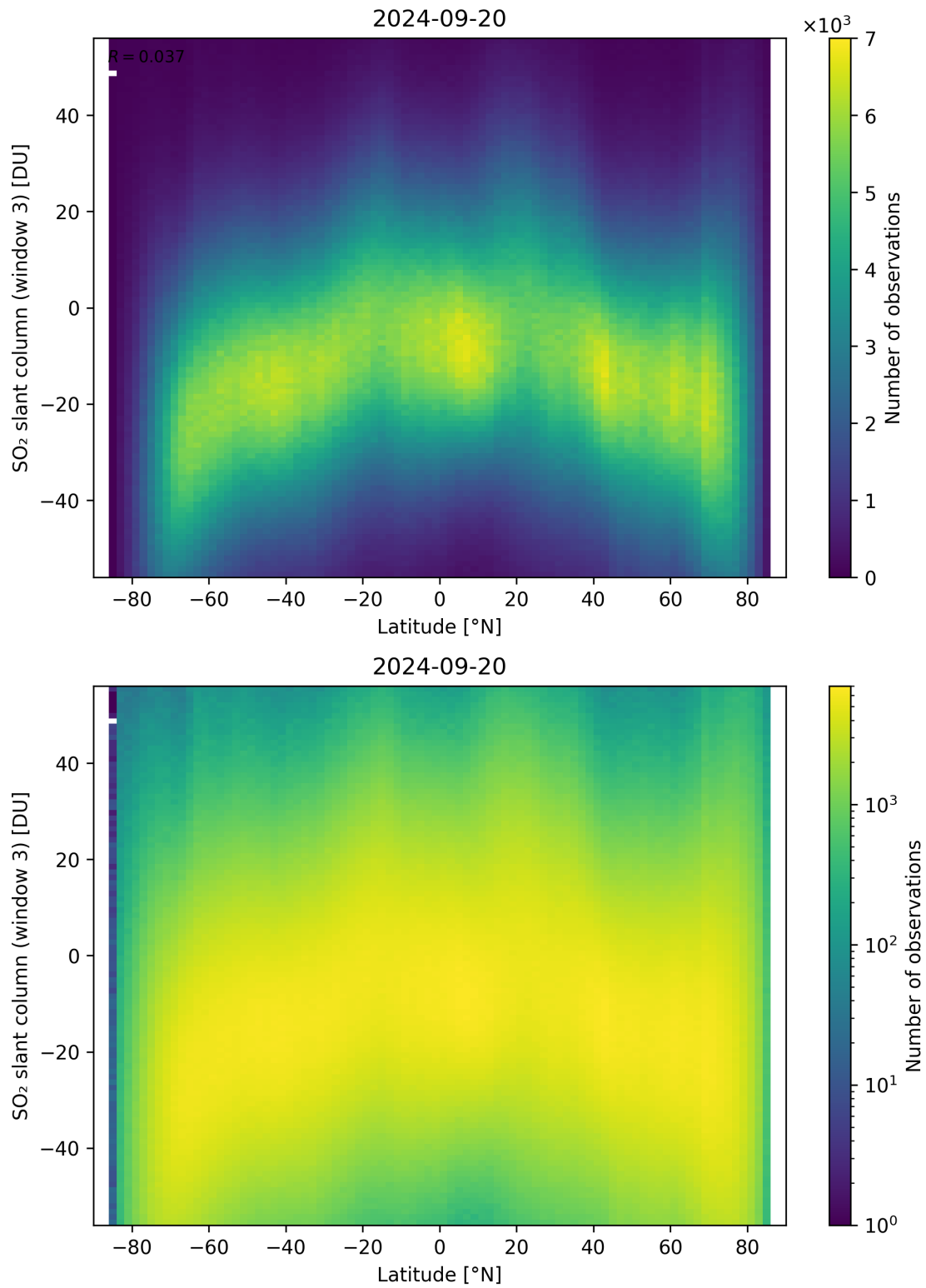
Figure 152: Scatter density plot of “Latitude” against “SO 2 slant column (window 3)” for 2024-09-19 to 2024-09-21.
