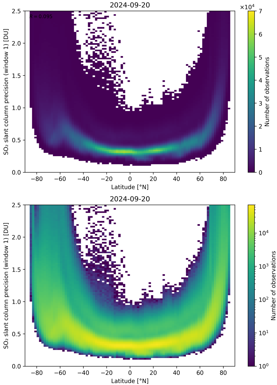
Figure 150: Scatter density plot of “Latitude” against “SO 2 slant column precision (window 1)” for 2024-09-19 to 2024-09-21.
