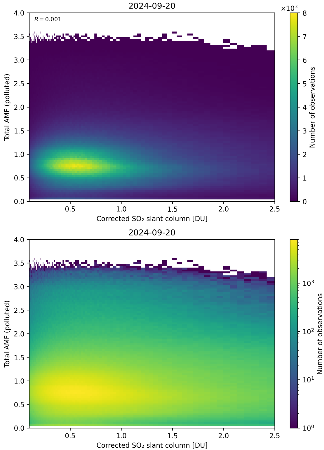
Figure 192: Scatter density plot of “Corrected SO 2 slant column” against “Total AMF (polluted)” for 2024-09-19 to 2024-09-21.
