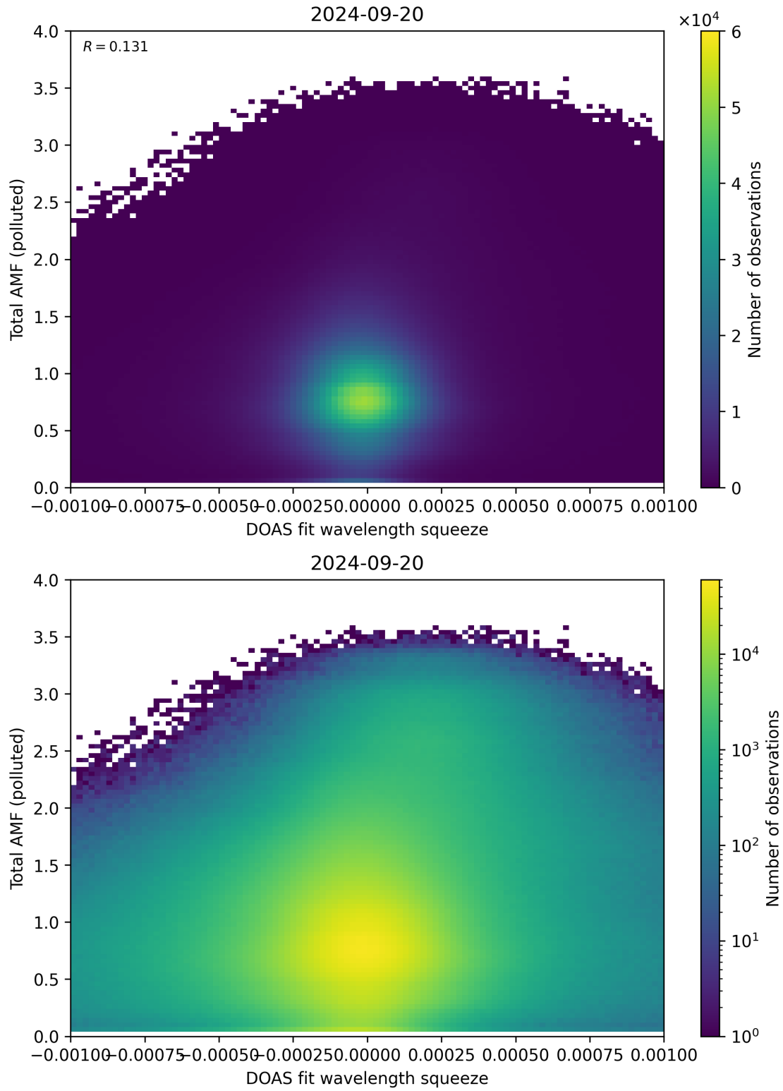
Figure 134: Scatter density plot of “DOAS fit wavelength squeeze” against “Total AMF (polluted)” for 2024-09-19 to 2024-09-21.
