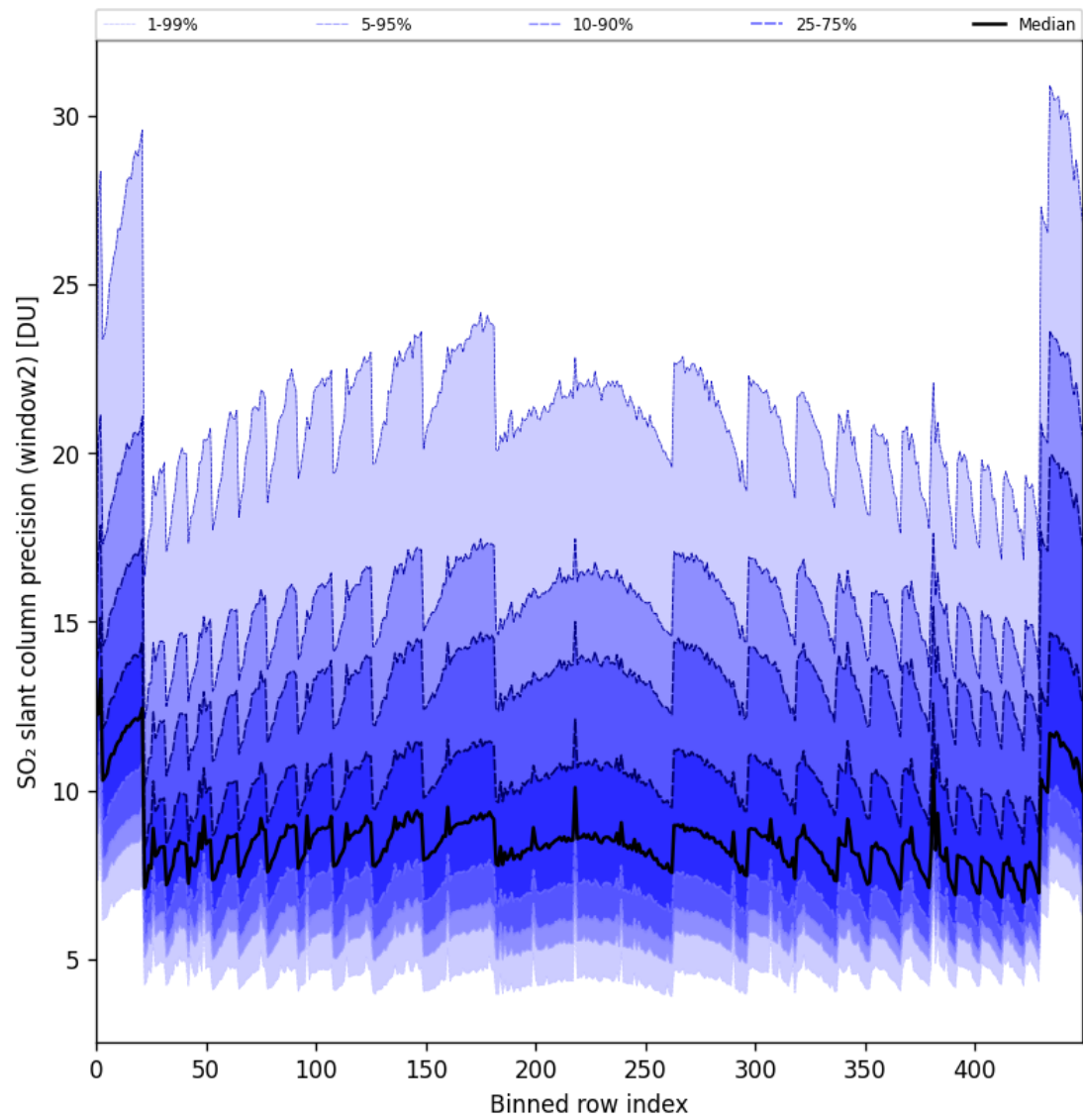
Figure 84: Along track statistics of “SO 2 slant column precision (window2)” for 2024-09-19 to 2024-09-21
