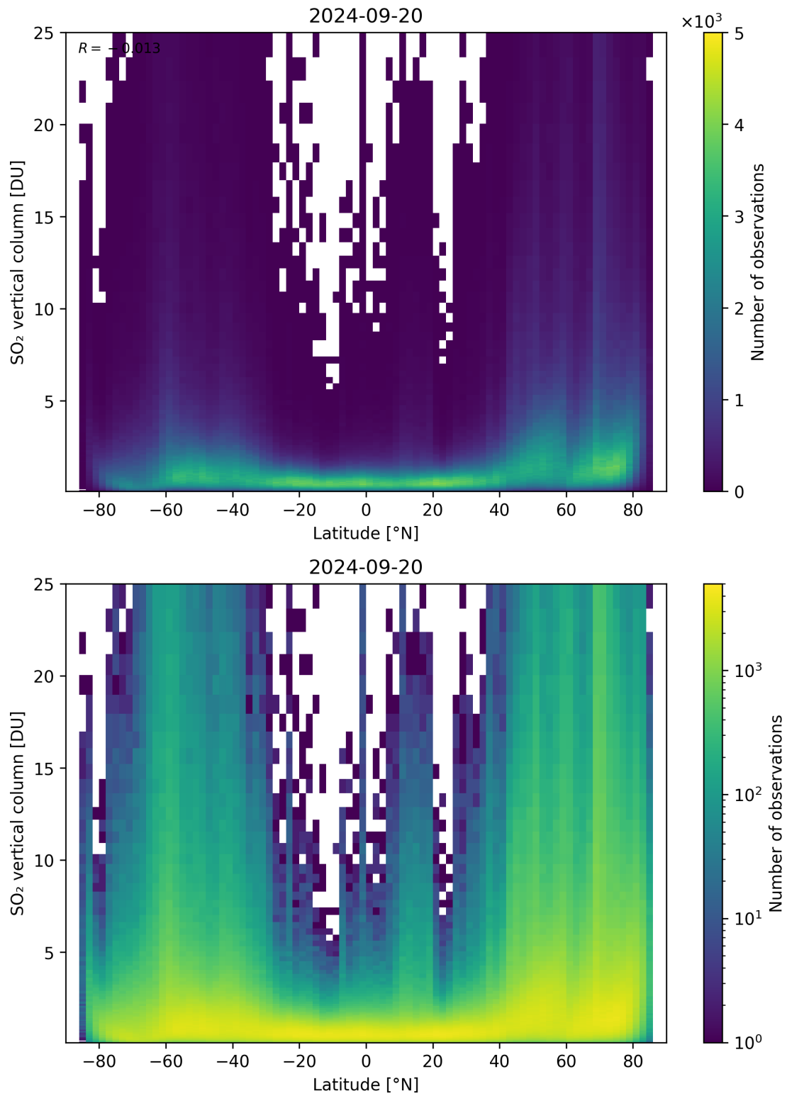
Figure 156: Scatter density plot of “Latitude” against “SO 2 vertical column” for 2024-09-19 to 2024-09-21.
