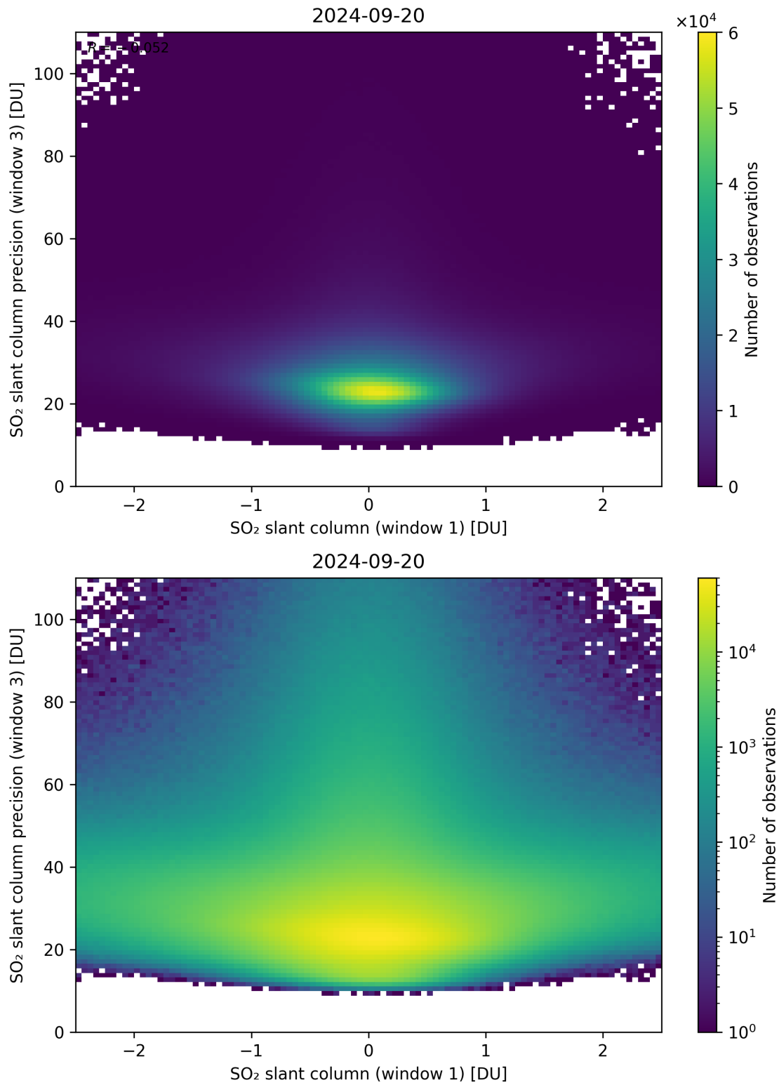
Figure 238: Scatter density plot of “SO 2 slant column (window 1)” against “SO 2 slant column precision (window 3)” for 2024-09-19 to 2024-09-21.
