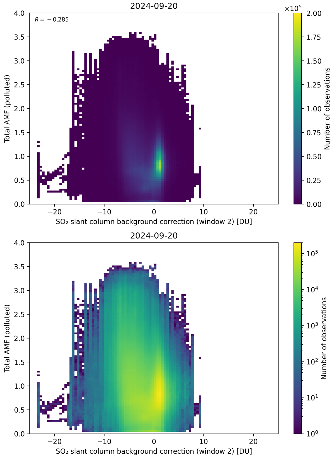
Figure 119: Scatter density plot of “SO 2 slant column background correction (window 2)” against “Total AMF (polluted)” for 2024-09-19 to 2024-09-21.
