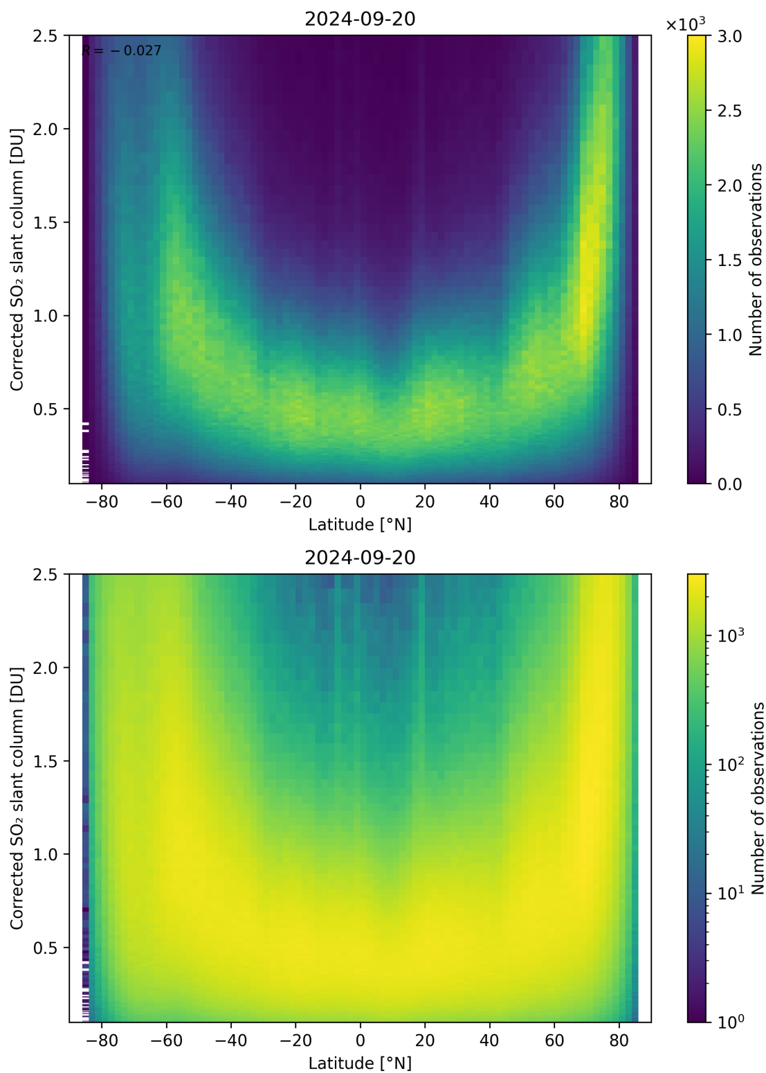
Figure 146: Scatter density plot of “Latitude” against “Corrected SO 2 slant column” for 2024-09-19 to 2024-09-21.
