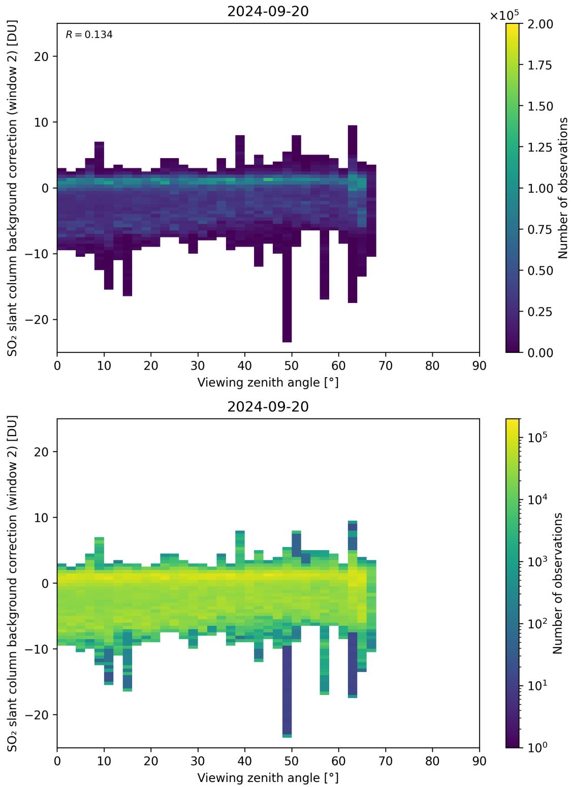
Figure 309: Scatter density plot of “Viewing zenith angle” against “SO 2 slant column background correction (window 2)” for 2024-09-19 to 2024-09-21.
