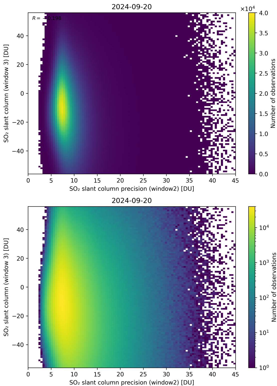
Figure 249: Scatter density plot of “SO 2 slant column precision (window2)” against “SO 2 slant column (window 3)” for 2024-09-19 to 2024-09-21.
