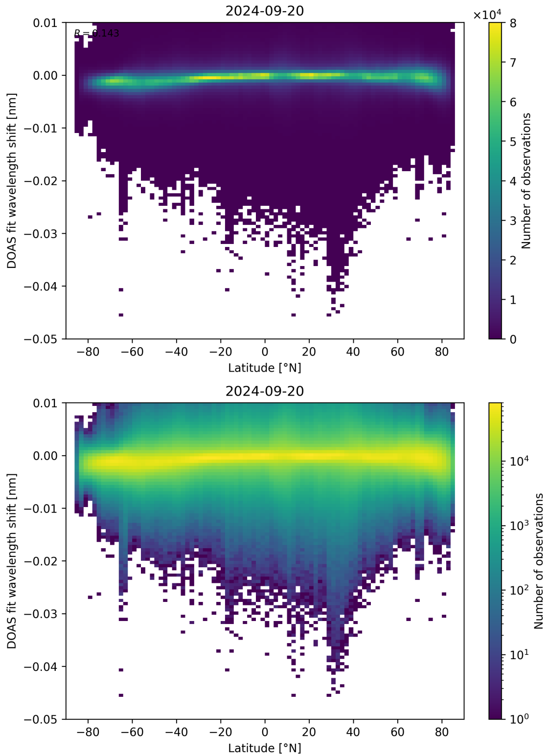
Figure 142: Scatter density plot of “Latitude” against “DOAS fit wavelength shift” for 2024-09-19 to 2024-09-21.
