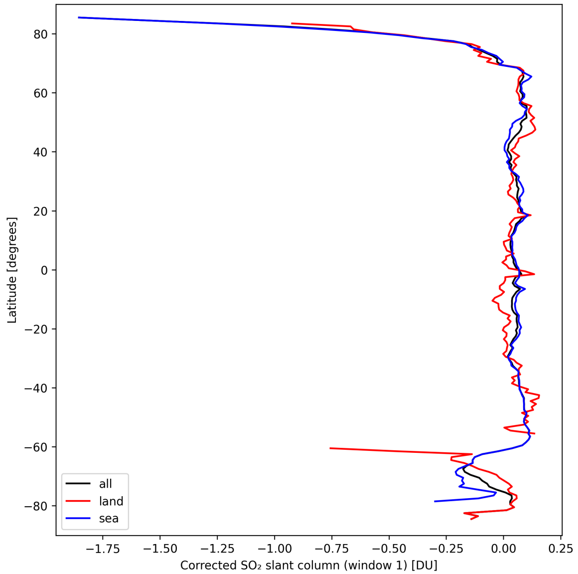
Figure 35: Zonal average of “Corrected SO 2 slant column (window 1)” for 2024-09-19 to 2024-09-21.
