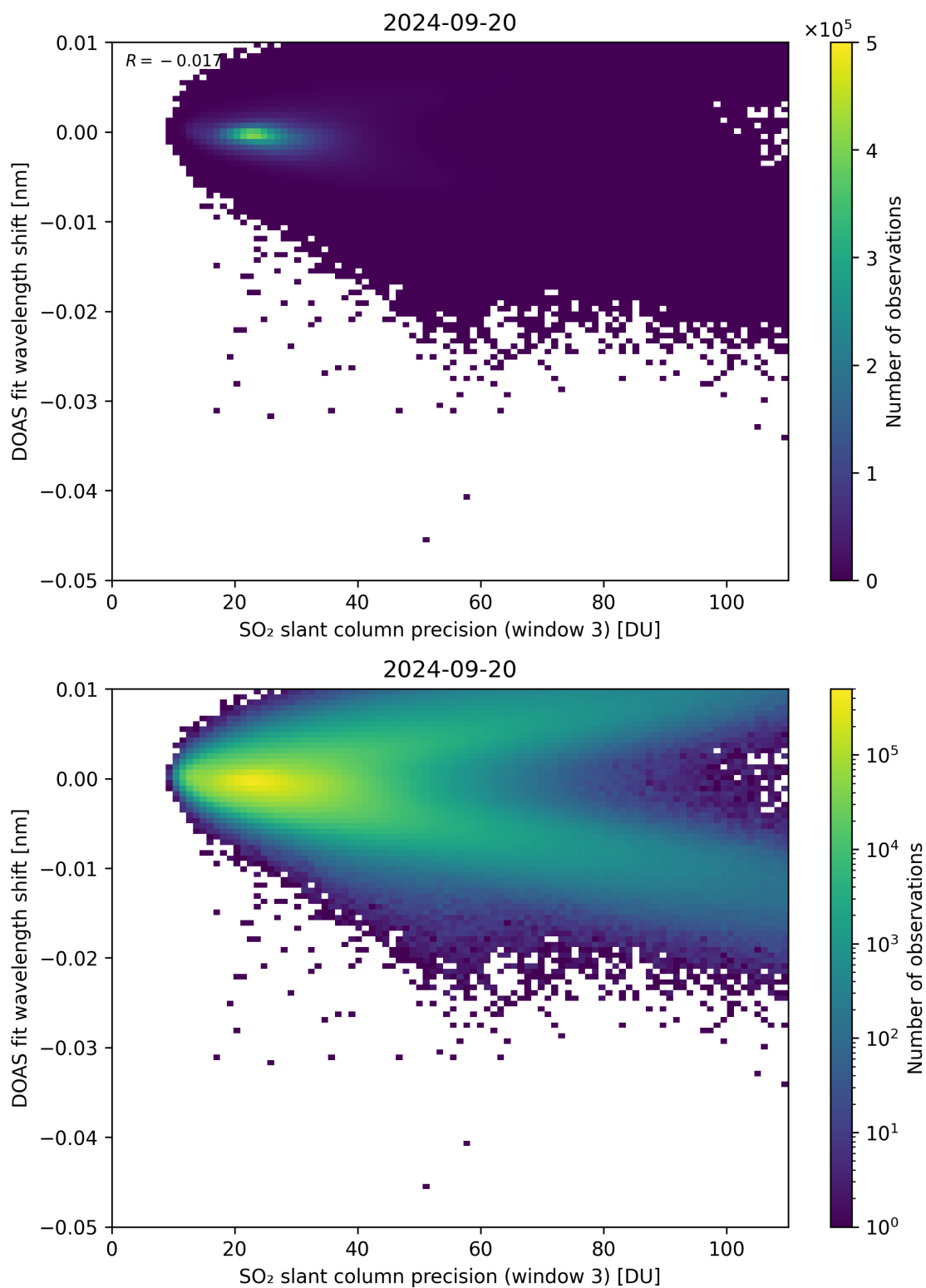
Figure 258: Scatter density plot of “SO 2 slant column precision (window 3)” against “DOAS fit wavelength shift” for 2024-09-19 to 2024-09-21.
