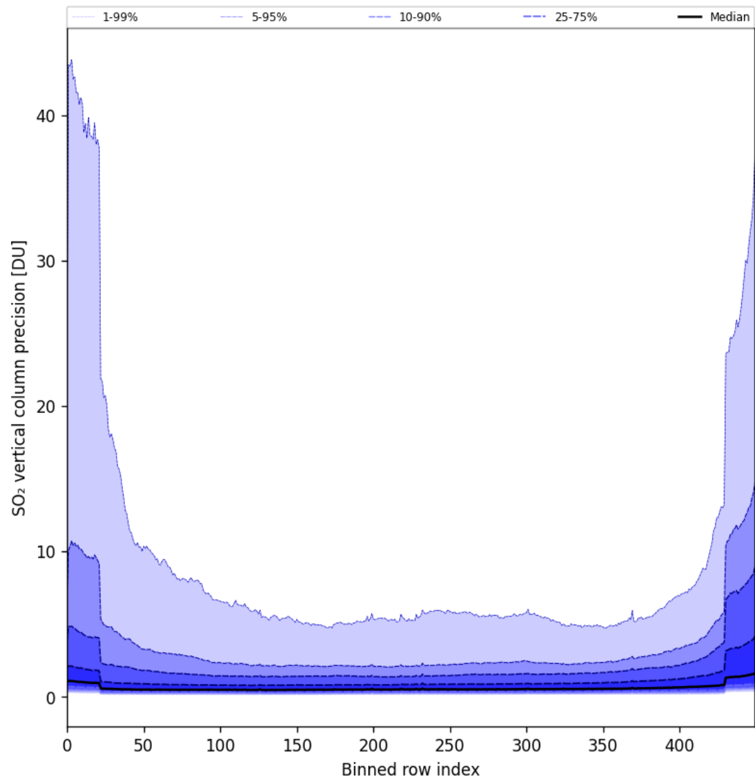
Figure 77: Along track statistics of “SO 2 vertical column precision” for 2024-09-19 to 2024-09-21
