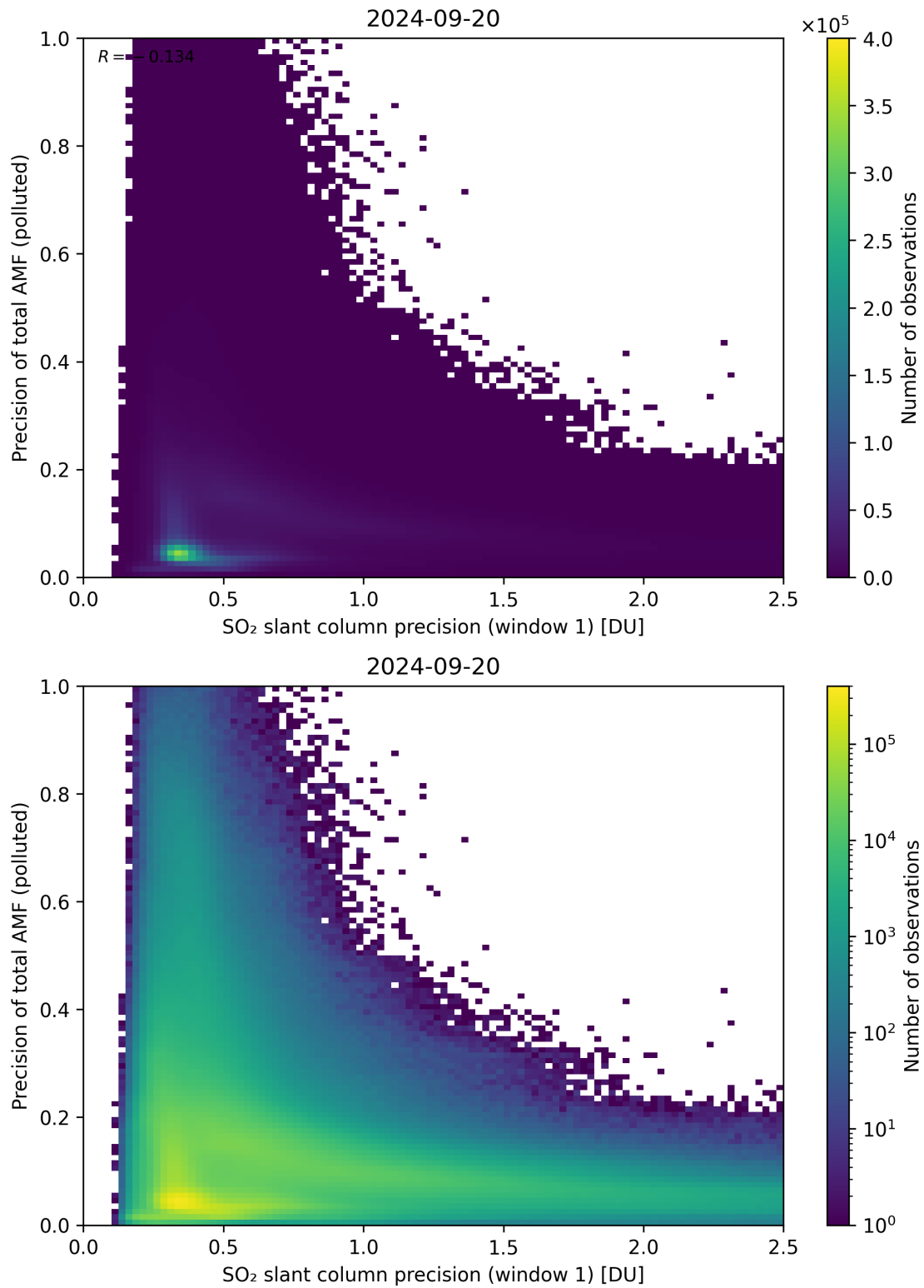
Figure 231: Scatter density plot of “SO 2 slant column precision (window 1)” against “Precision of total AMF (polluted)” for 2024-09-19 to 2024-09-21.
