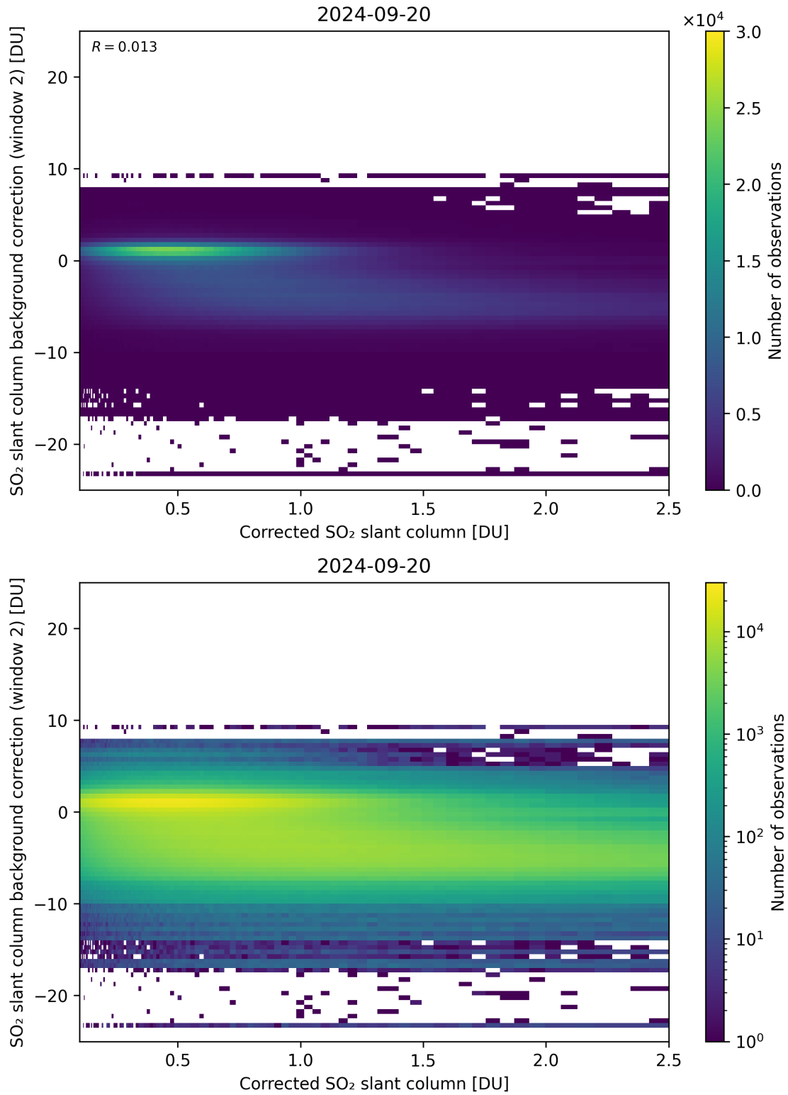
Figure 179: Scatter density plot of “Corrected SO 2 slant column” against “SO 2 slant column background correction (window 2)” for 2024-09-19 to 2024-09-21.
