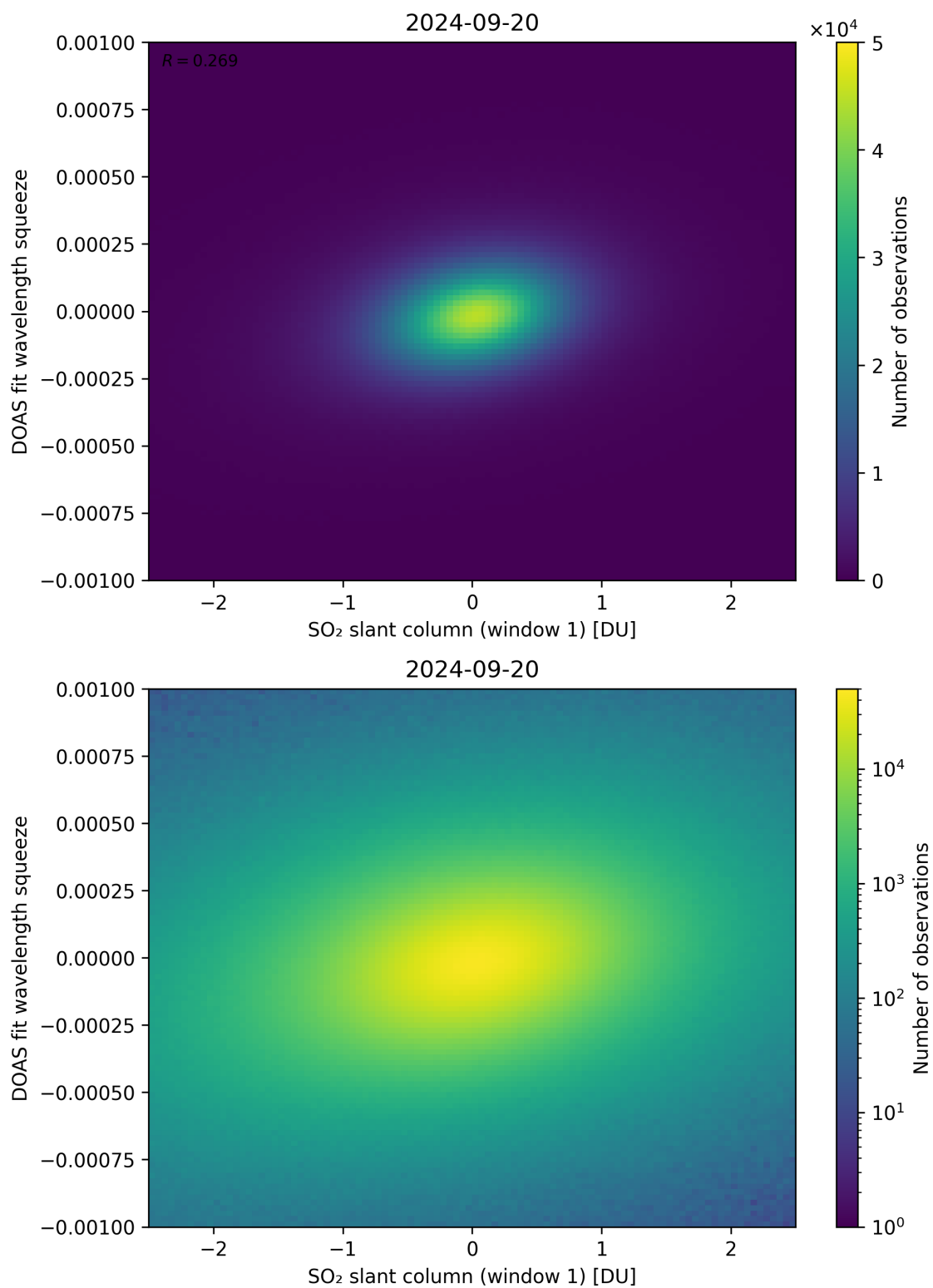
Figure 216: Scatter density plot of “SO 2 slant column (window 1)” against “DOAS fit wavelength squeeze” for 2024-09-19 to 2024-09-21.
