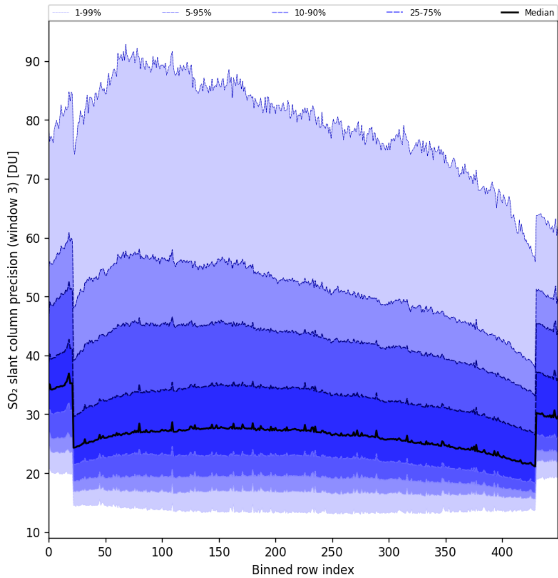
Figure 88: Along track statistics of “SO 2 slant column precision (window 3)” for 2024-09-19 to 2024-09-21
