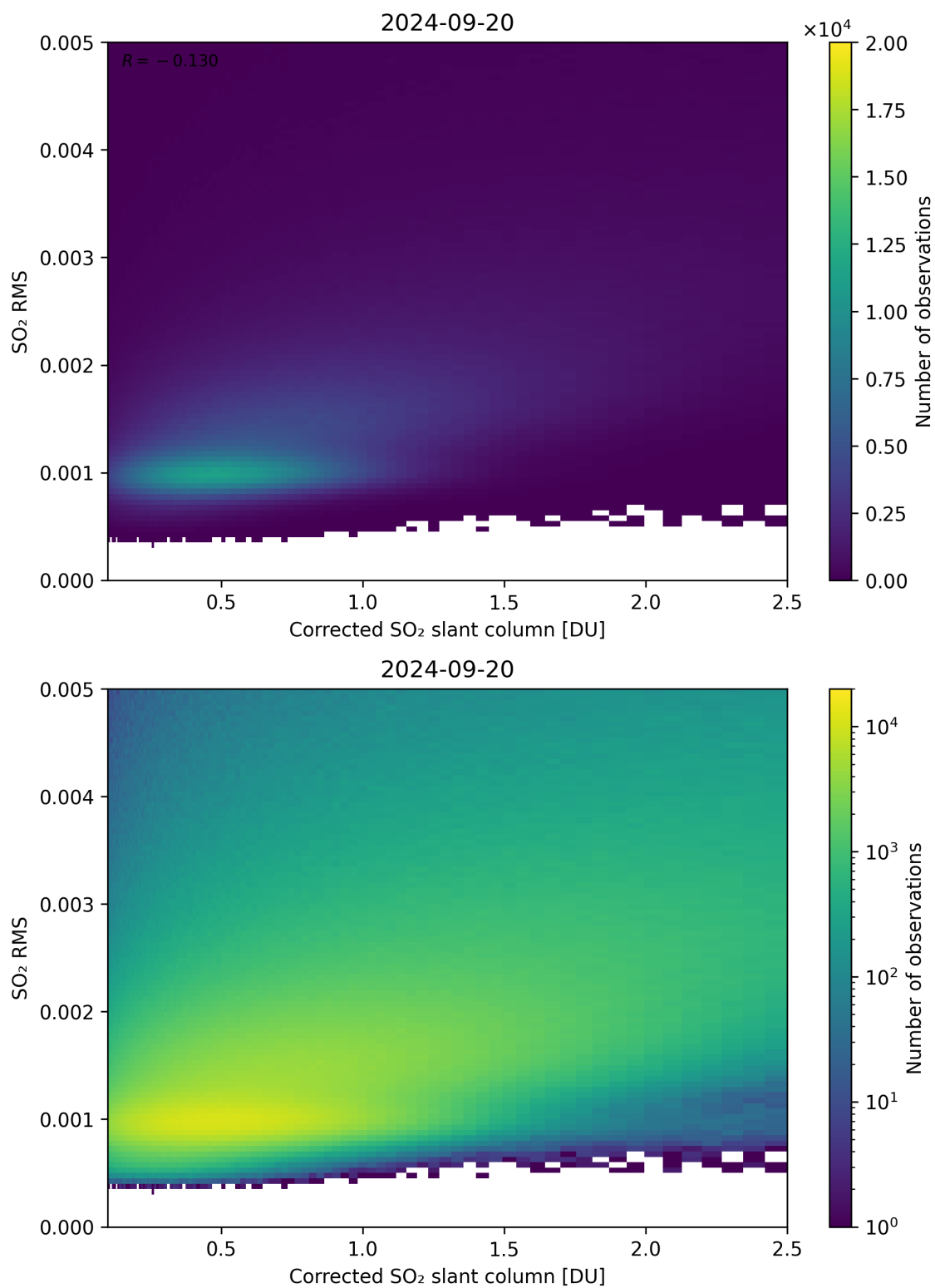
Figure 183: Scatter density plot of “Corrected SO 2 slant column” against “SO 2 RMS” for 2024-09-19 to 2024-09-21.
