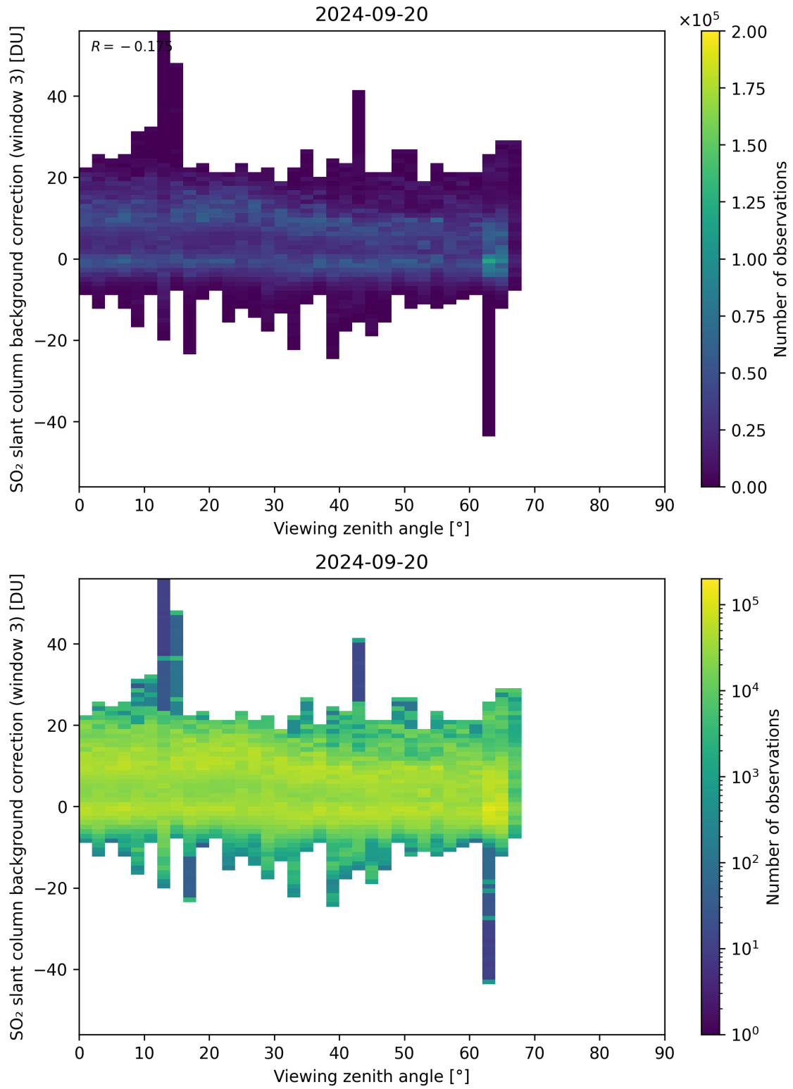
Figure 310: Scatter density plot of “Viewing zenith angle” against “SO 2 slant column background correction (window 3)” for 2024-09-19 to 2024-09-21.
