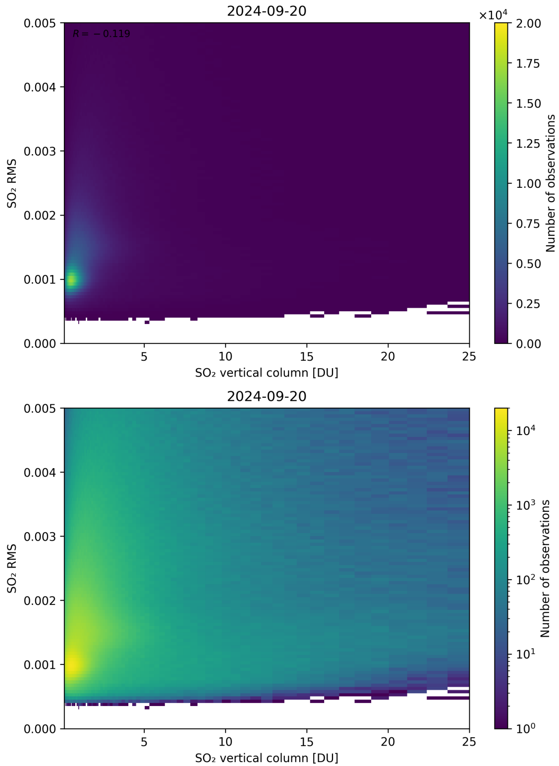
Figure 278: Scatter density plot of “SO 2 vertical column” against “SO 2 RMS” for 2024-09-19 to 2024-09-21.
