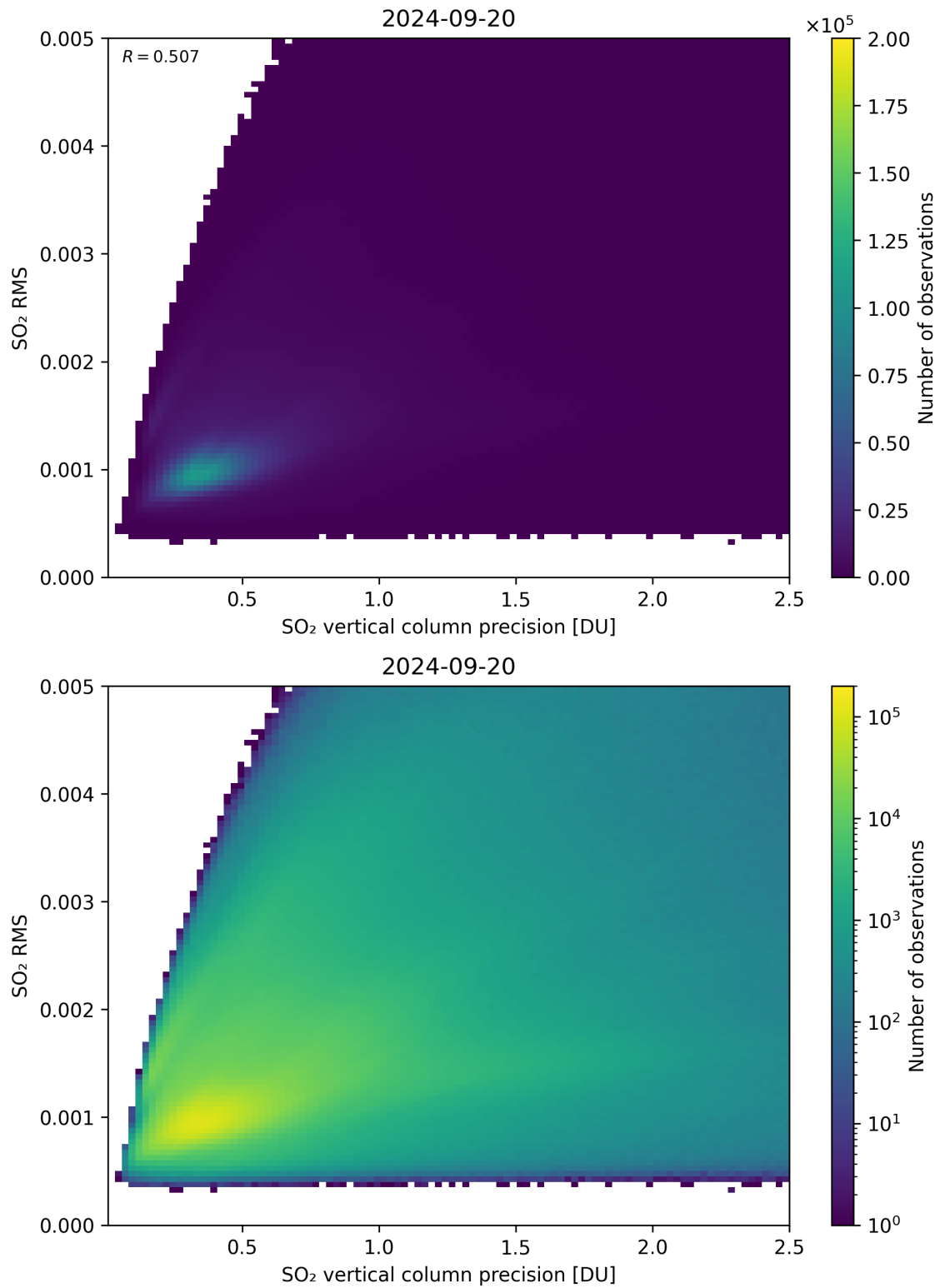
Figure 284: Scatter density plot of “SO 2 vertical column precision” against “SO 2 RMS” for 2024-09-19 to 2024-09-21.
