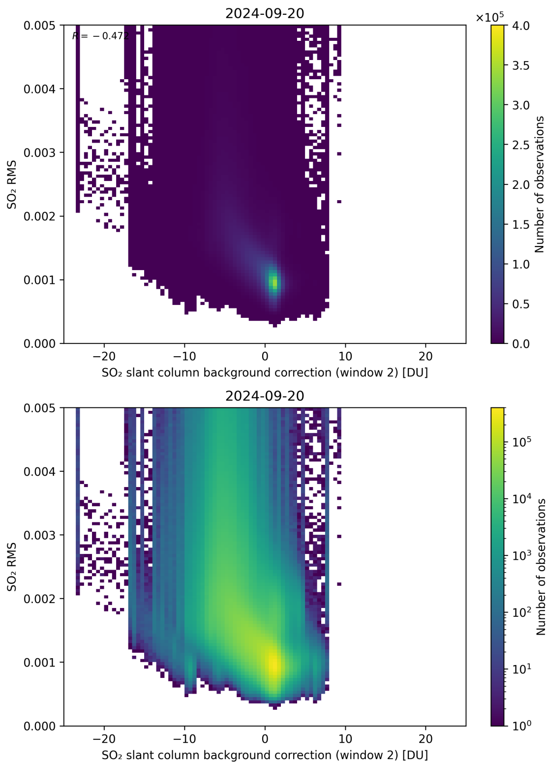
Figure 114: Scatter density plot of “SO 2 slant column background correction (window 2)” against “SO 2 RMS” for 2024-09-19 to 2024-09-21.
