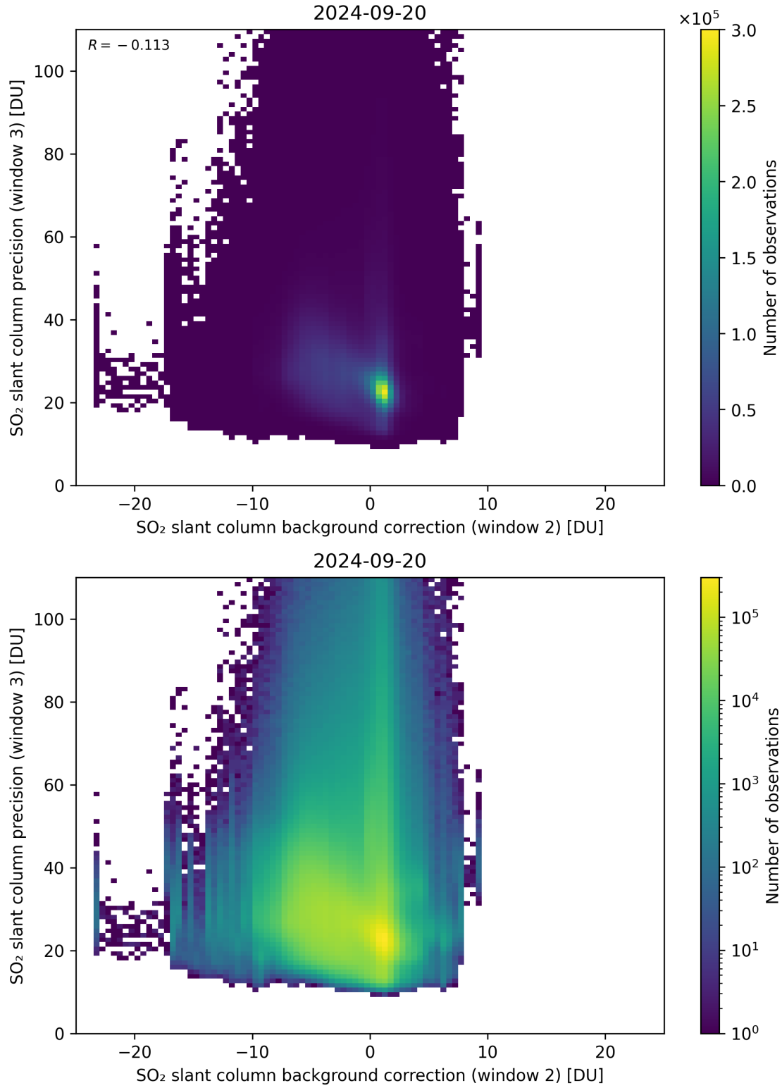
Figure 118: Scatter density plot of “SO 2 slant column background correction (window 2)” against “SO 2 slant column precision (window 3)” for 2024-09-19 to 2024-09-21.
