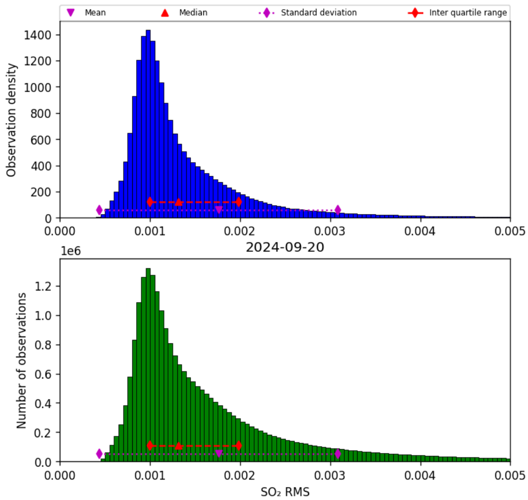
Figure 70: Histogram of “SO 2 RMS” for 2024-09-19 to 2024-09-21
