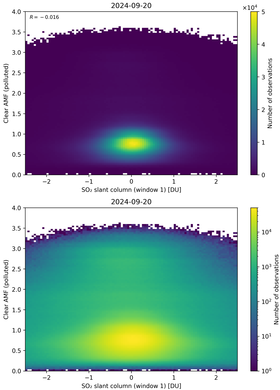
Figure 232: Scatter density plot of “SO 2 slant column (window 1)” against “Clear AMF (polluted)” for 2024-09-19 to 2024-09-21.
