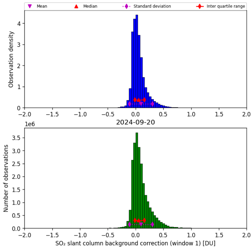
Figure 59: Histogram of “SO 2 slant column background correction (window 1)” for 2024-09-19 to 2024-09-21
