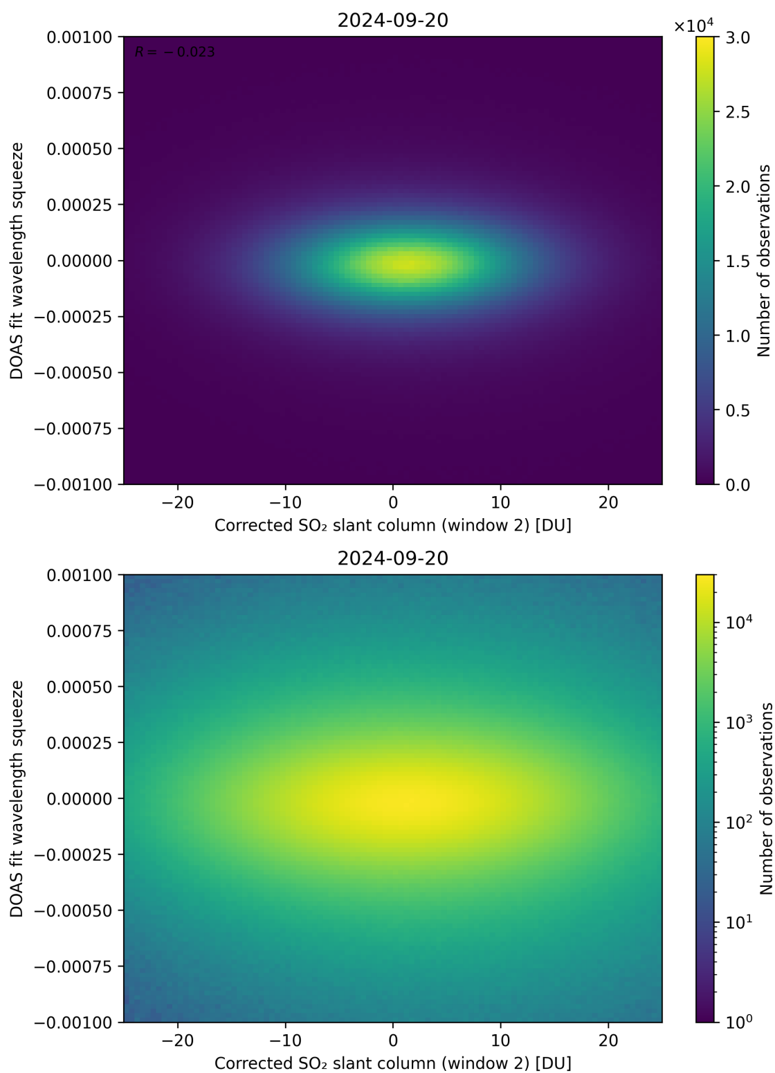
Figure 197: Scatter density plot of “Corrected SO 2 slant column (window 2)” against “DOAS fit wavelength squeeze” for 2024-09-19 to 2024-09-21.
