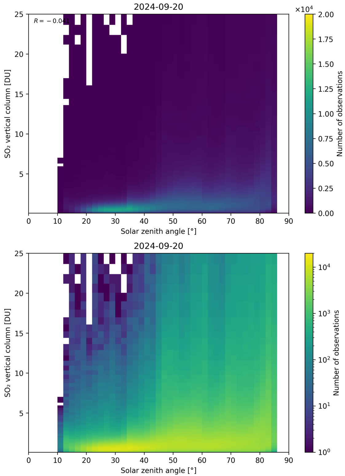
Figure 176: Scatter density plot of “Solar zenith angle” against “SO 2 vertical column” for 2024-09-19 to 2024-09-21.
