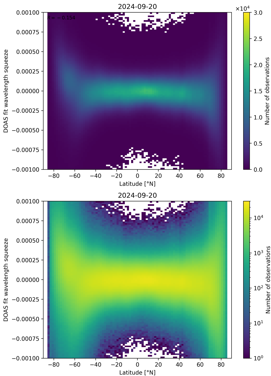
Figure 143: Scatter density plot of “Latitude” against “DOAS fit wavelength squeeze” for 2024-09-19 to 2024-09-21.
