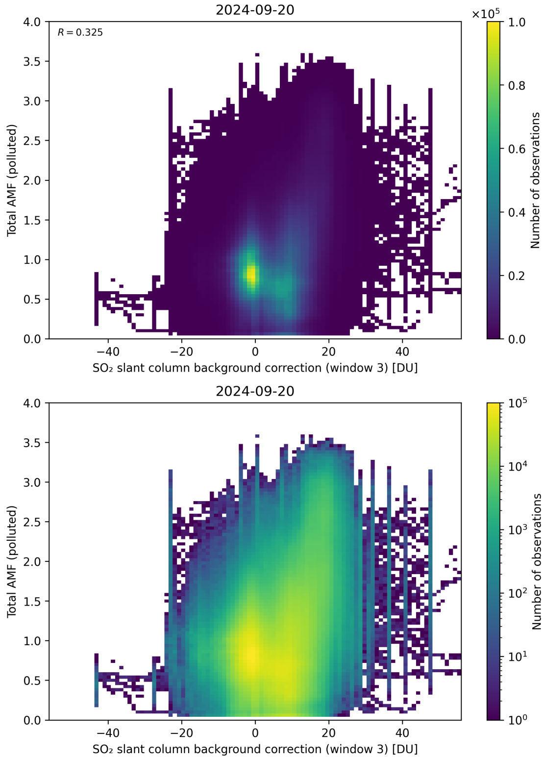
Figure 125: Scatter density plot of “SO 2 slant column background correction (window 3)” against “Total AMF (polluted)” for 2024-09-19 to 2024-09-21.
