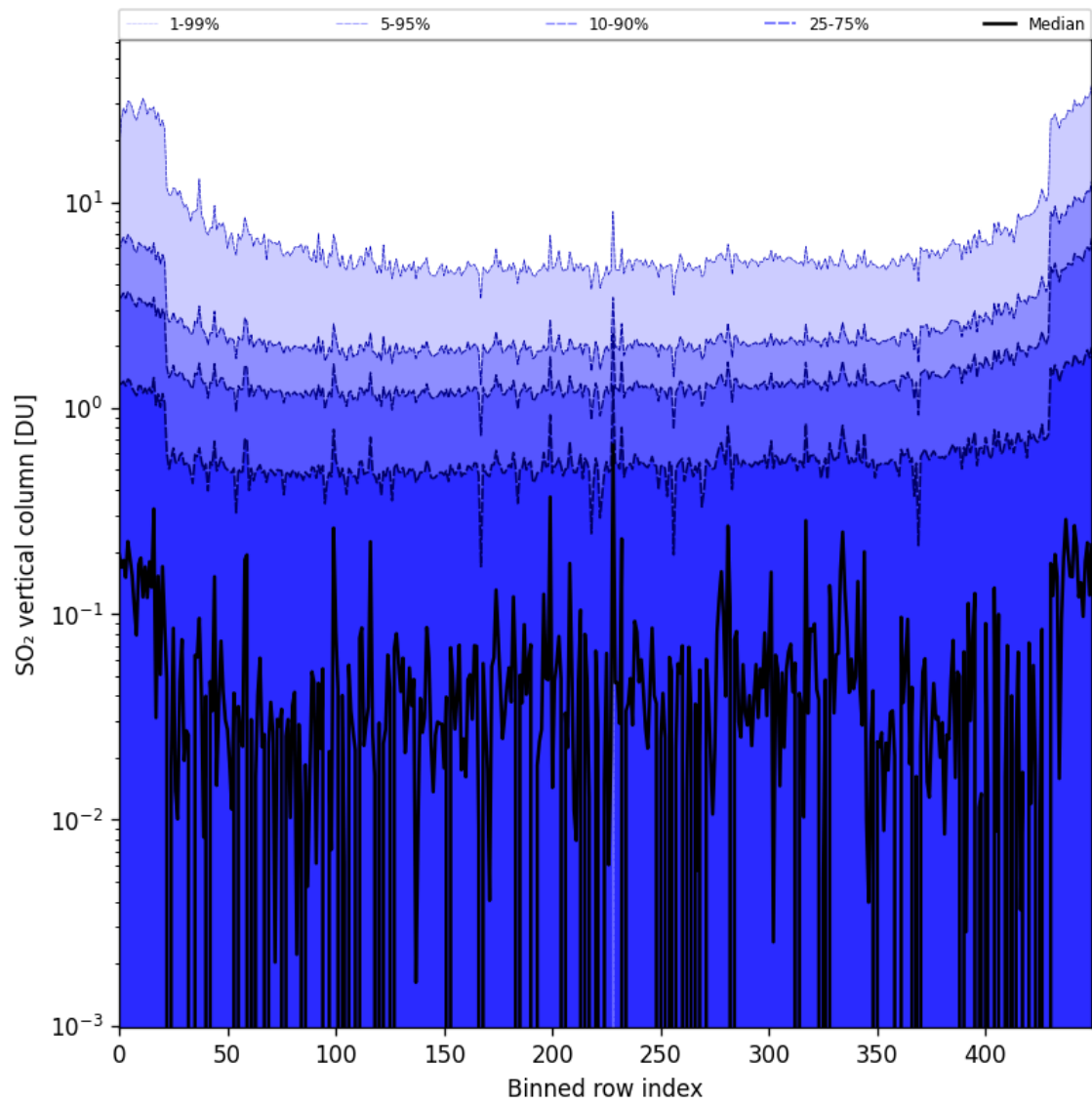
Figure 76: Along track statistics of “SO 2 vertical column” for 2024-09-19 to 2024-09-21
