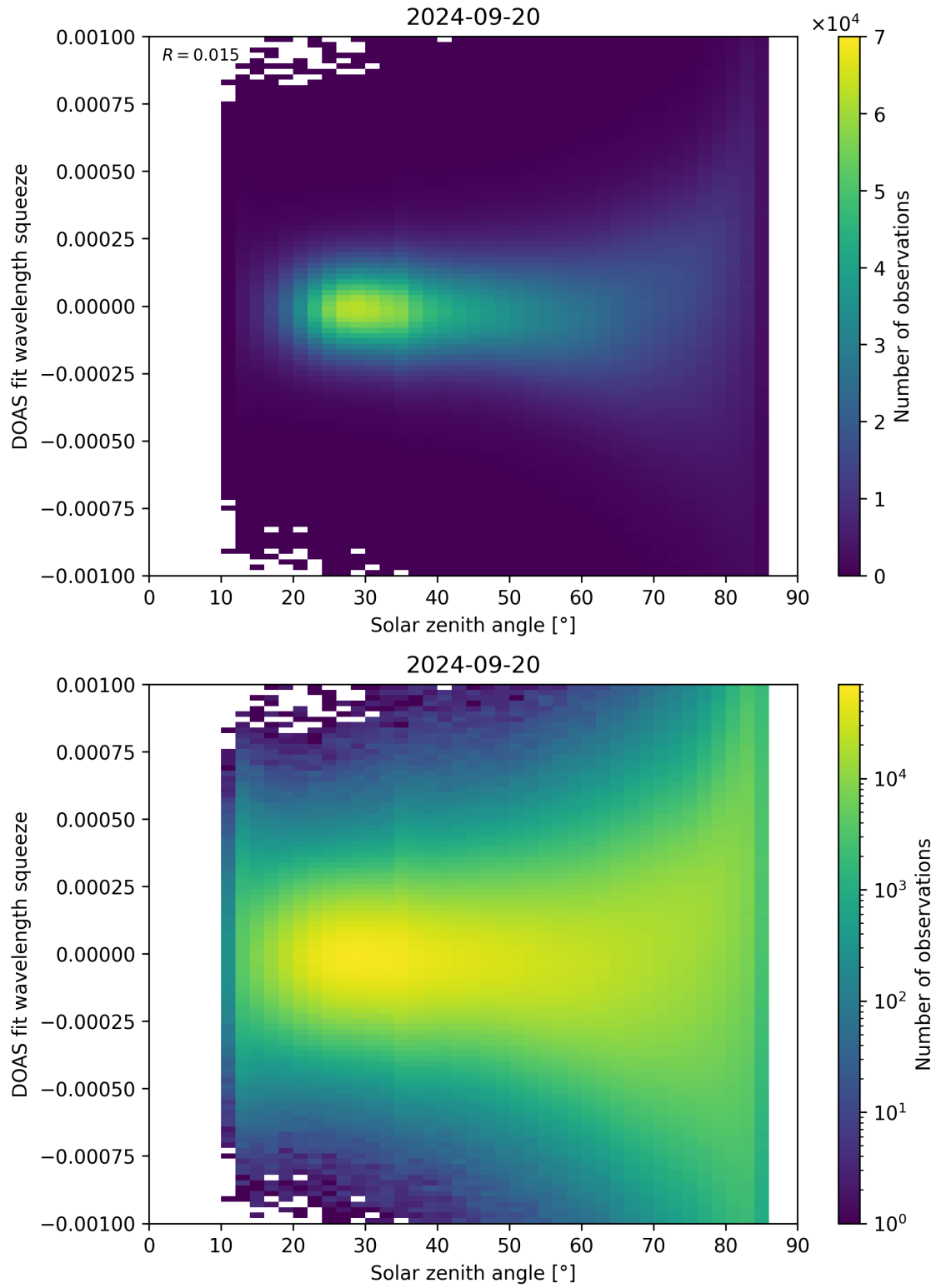
Figure 162: Scatter density plot of “Solar zenith angle” against “DOAS fit wavelength squeeze” for 2024-09-19 to 2024-09-21.
