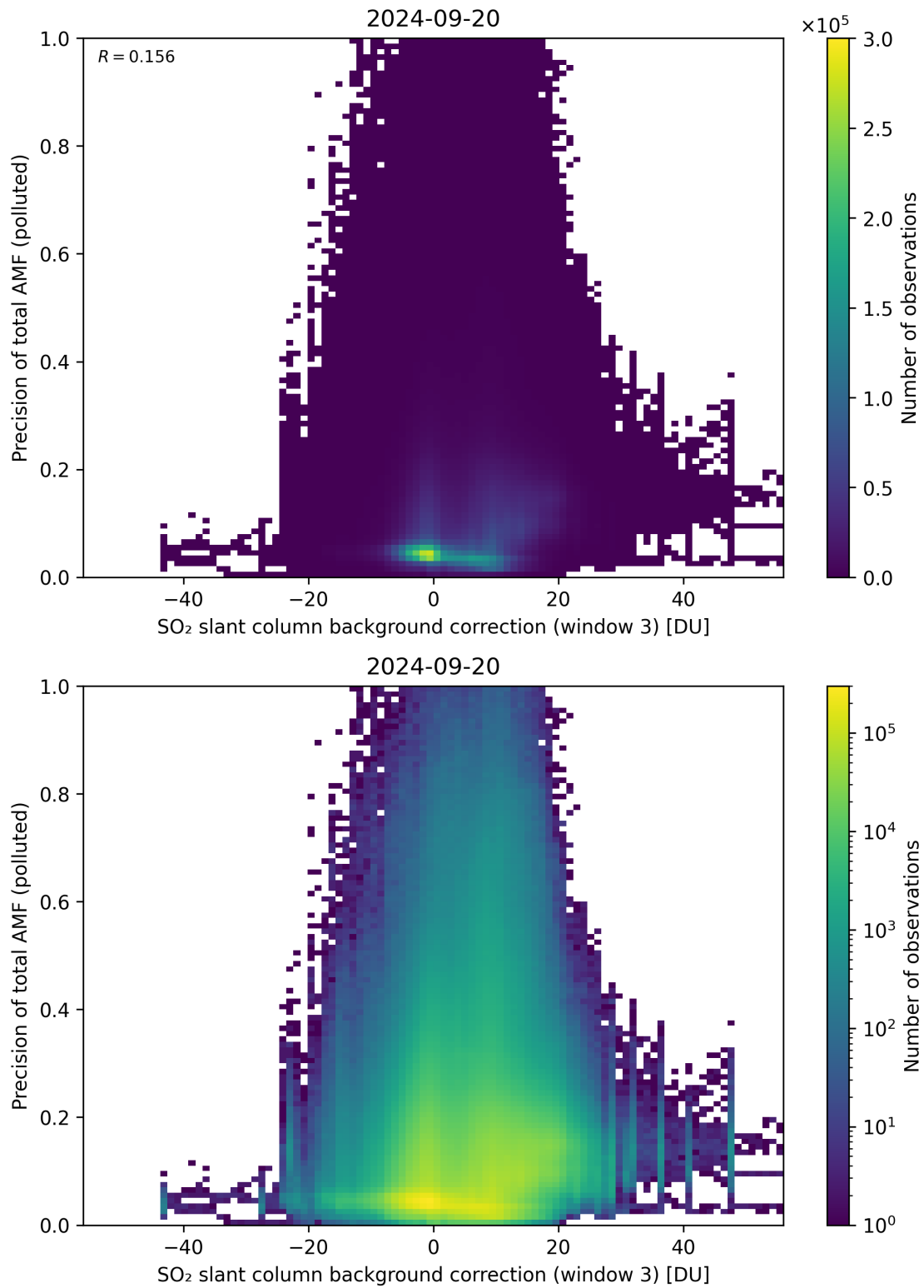
Figure 126: Scatter density plot of “SO 2 slant column background correction (window 3)” against “Precision of total AMF (polluted)” for 2024-09-19 to 2024-09-21.
