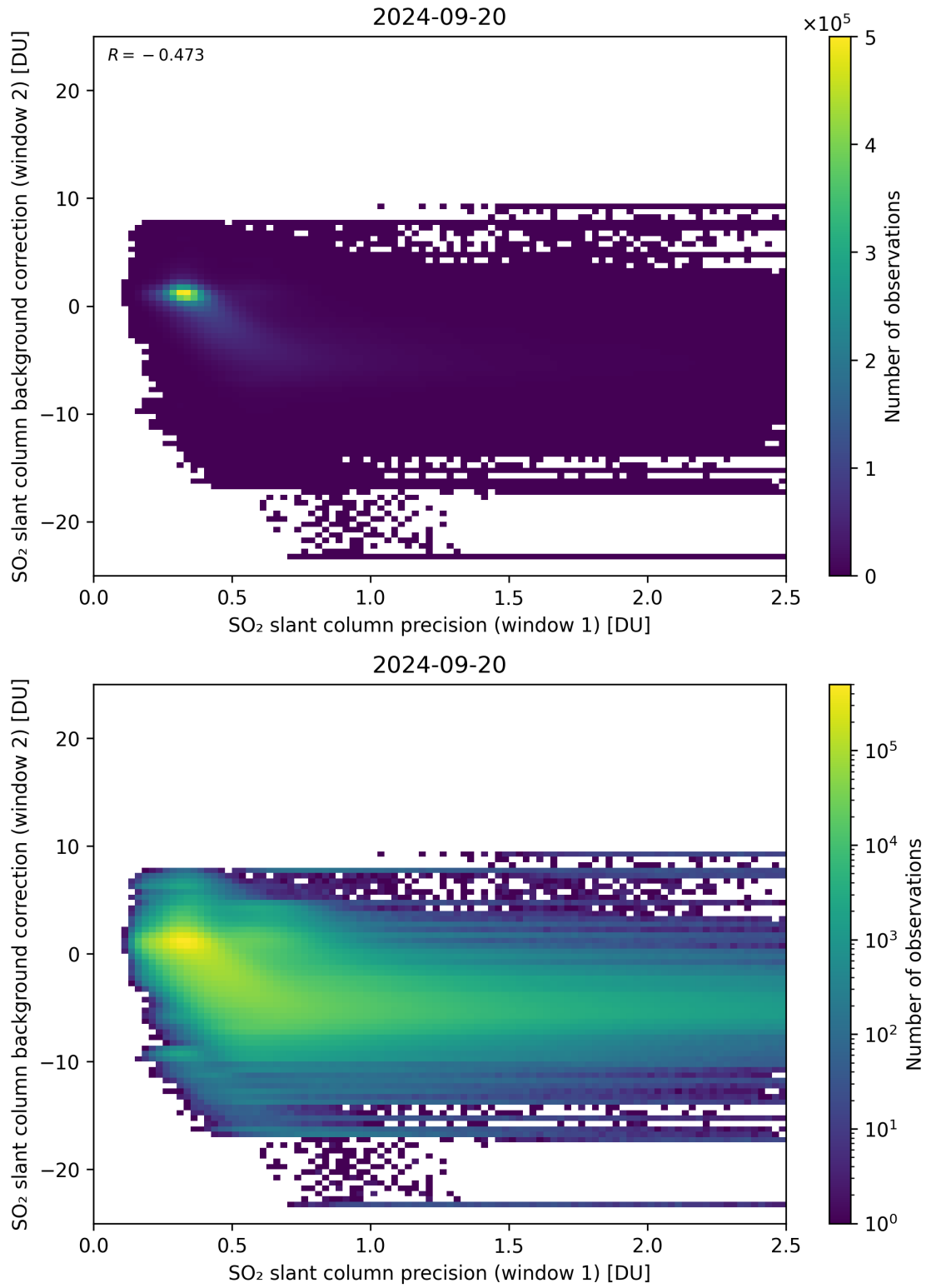
Figure 219: Scatter density plot of “SO 2 slant column precision (window 1)” against “SO 2 slant column background correction (window 2)” for 2024-09-19 to 2024-09-21.
