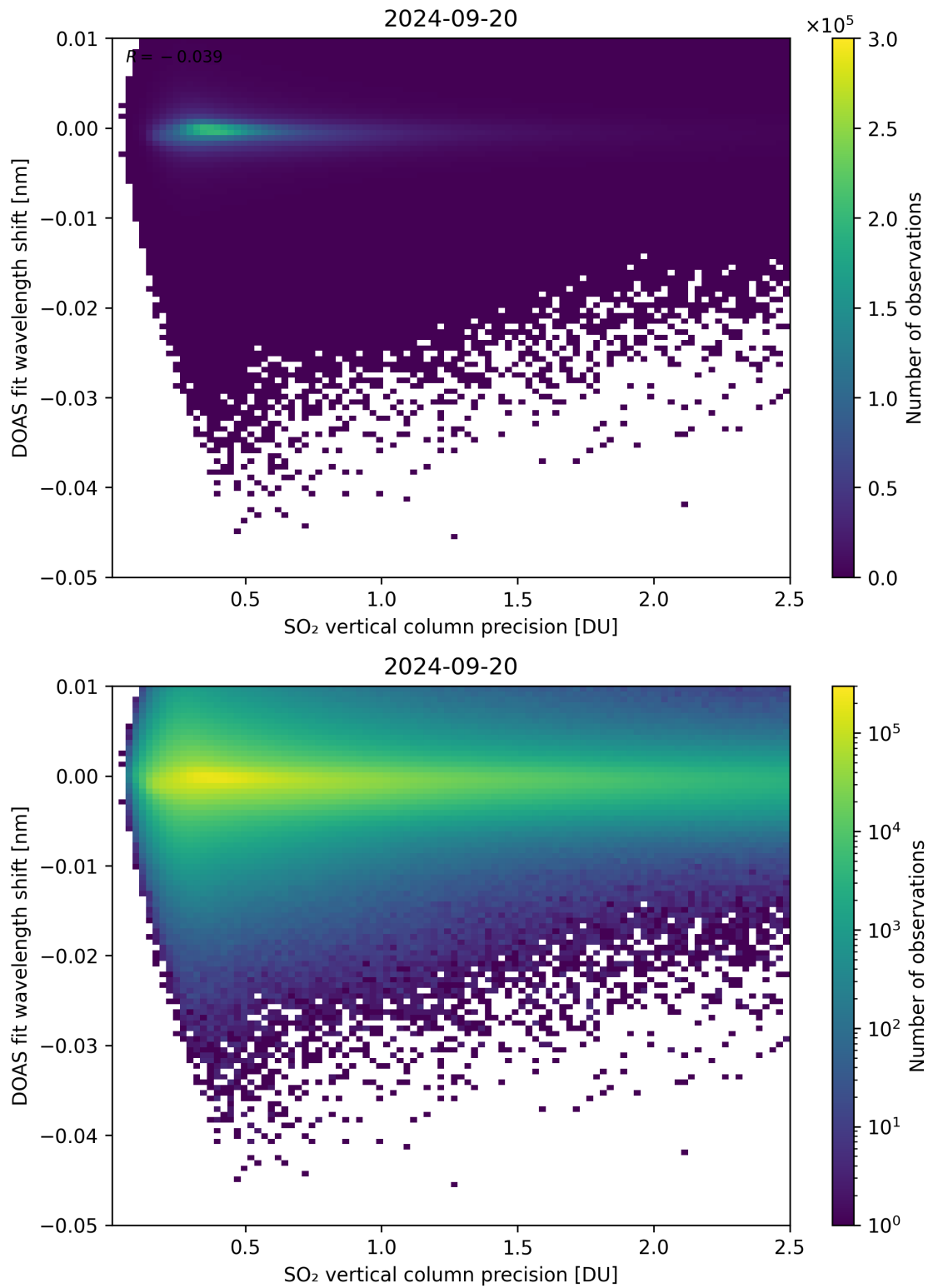
Figure 282: Scatter density plot of “SO 2 vertical column precision” against “DOAS fit wavelength shift” for 2024-09-19 to 2024-09-21.
