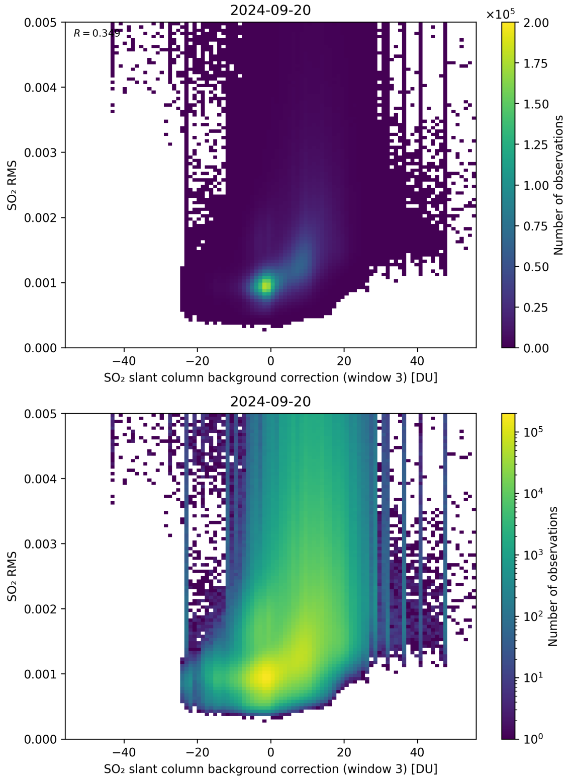
Figure 123: Scatter density plot of “SO 2 slant column background correction (window 3)” against “SO 2 RMS” for 2024-09-19 to 2024-09-21.
