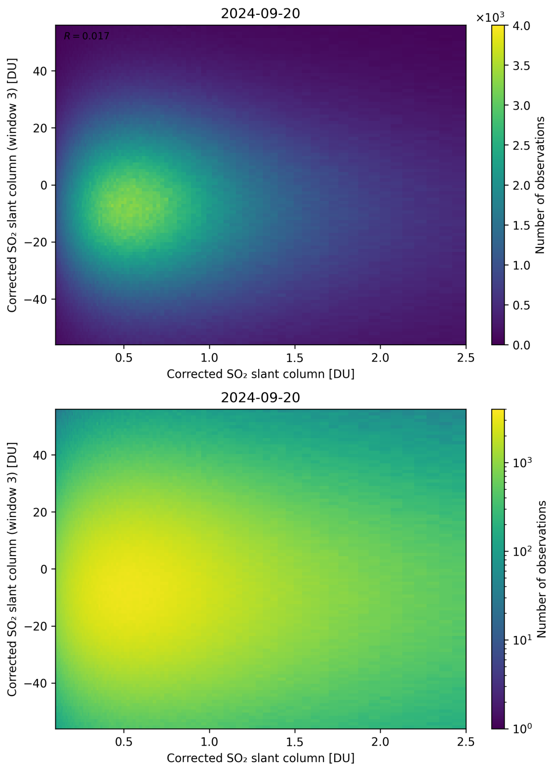
Figure 186: Scatter density plot of “Corrected SO 2 slant column” against “Corrected SO 2 slant column (window 3)” for 2024-09-19 to 2024-09-21.
