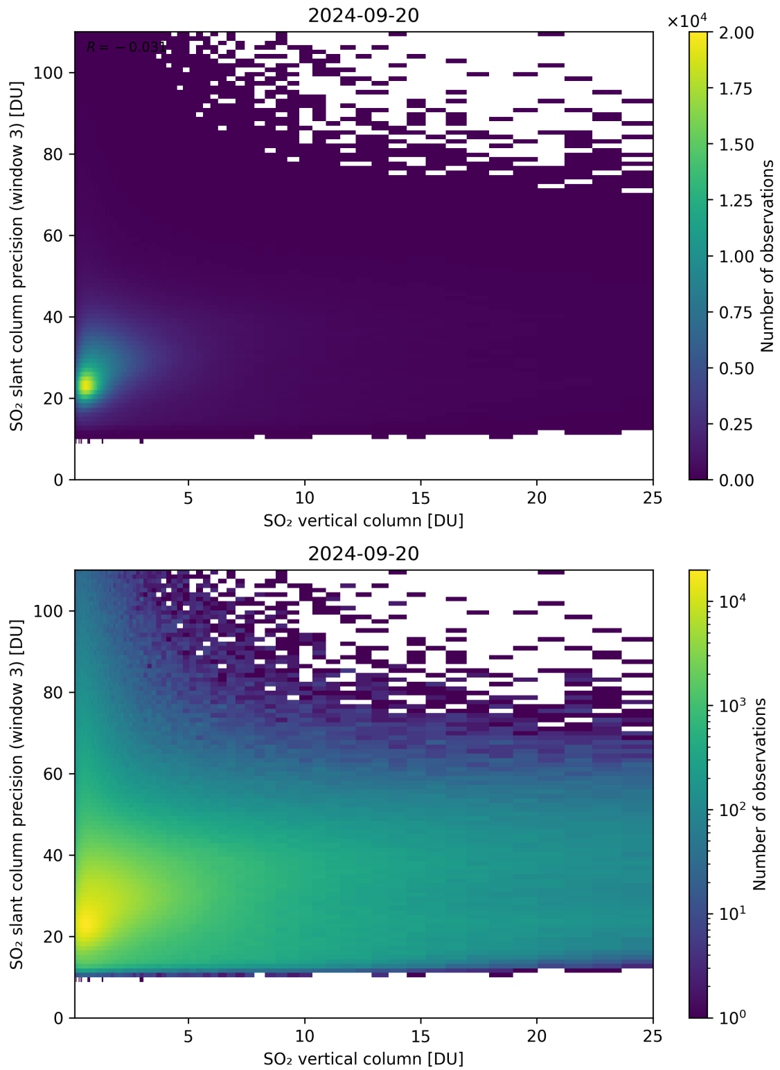
Figure 304: Scatter density plot of “SO 2 vertical column” against “SO 2 slant column precision (window 3)” for 2024-09-19 to 2024-09-21.
