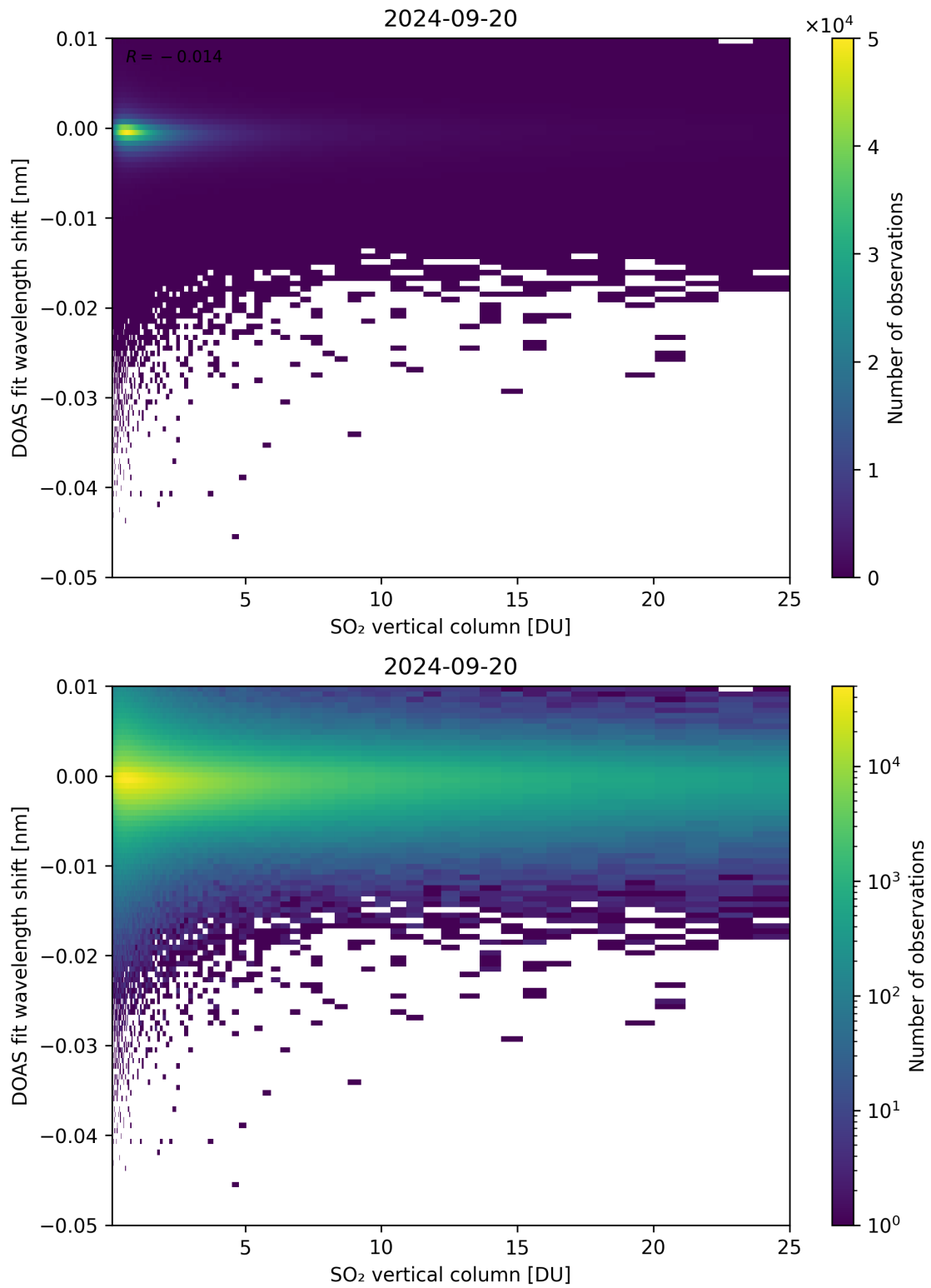
Figure 276: Scatter density plot of “SO 2 vertical column” against “DOAS fit wavelength shift” for 2024-09-19 to 2024-09-21.
