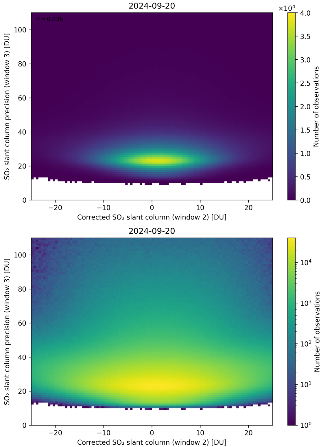
Figure 202: Scatter density plot of “Corrected SO 2 slant column (window 2)” against “SO 2 slant column precision (window 3)” for 2024-09-19 to 2024-09-21.
