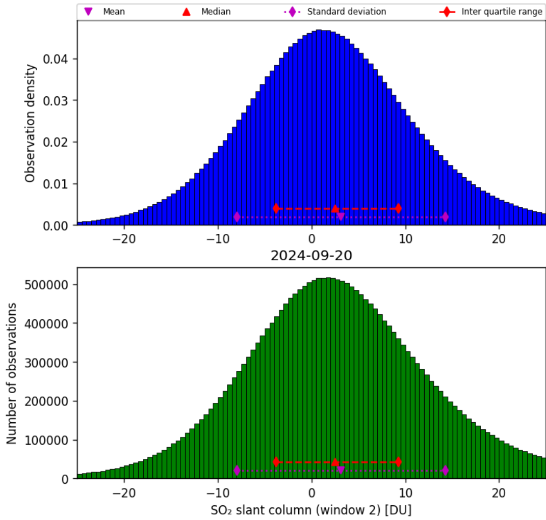
Figure 60: Histogram of “SO 2 slant column (window 2)” for 2024-09-19 to 2024-09-21
