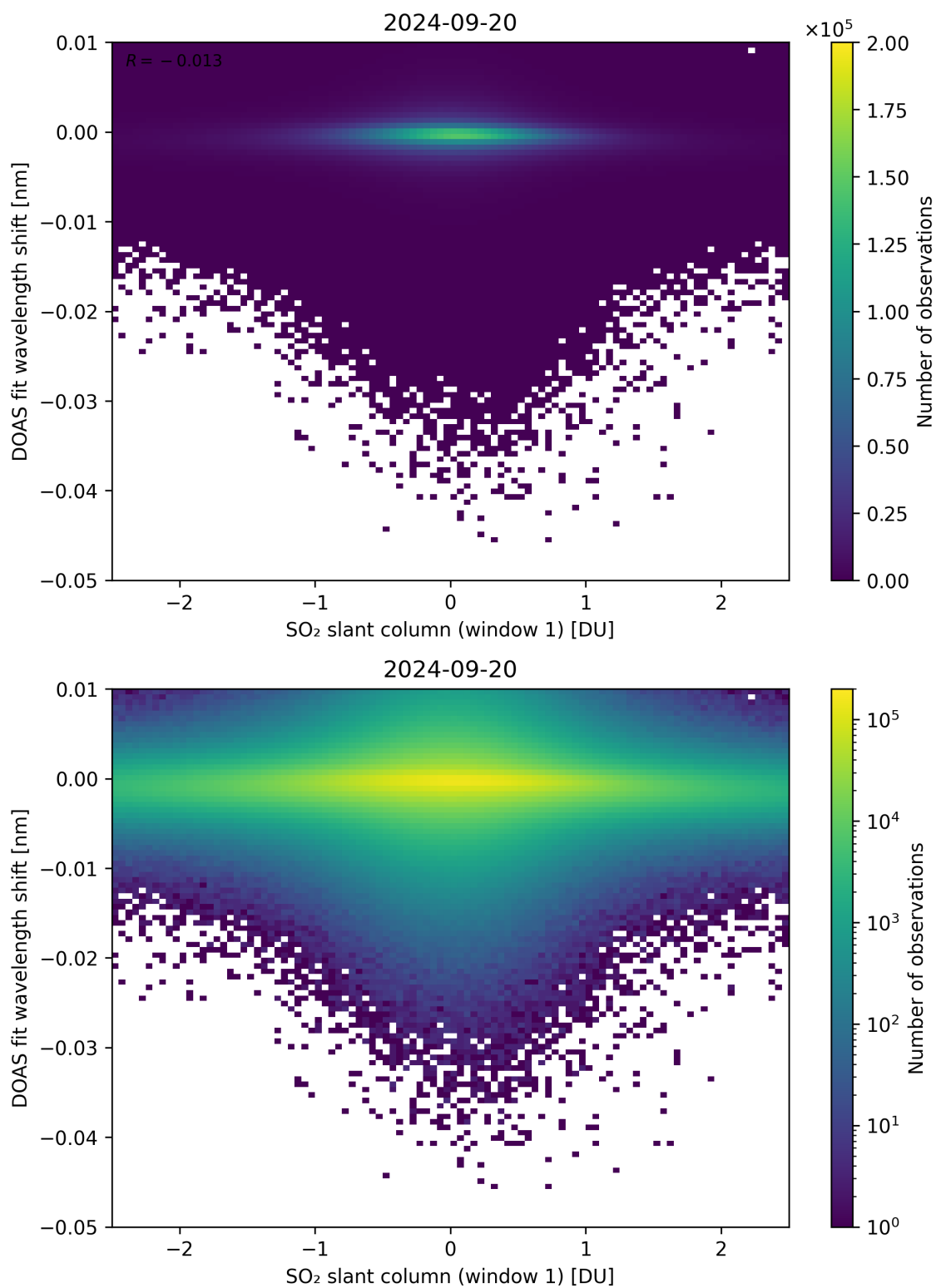
Figure 215: Scatter density plot of “SO 2 slant column (window 1)” against “DOAS fit wavelength shift” for 2024-09-19 to 2024-09-21.
