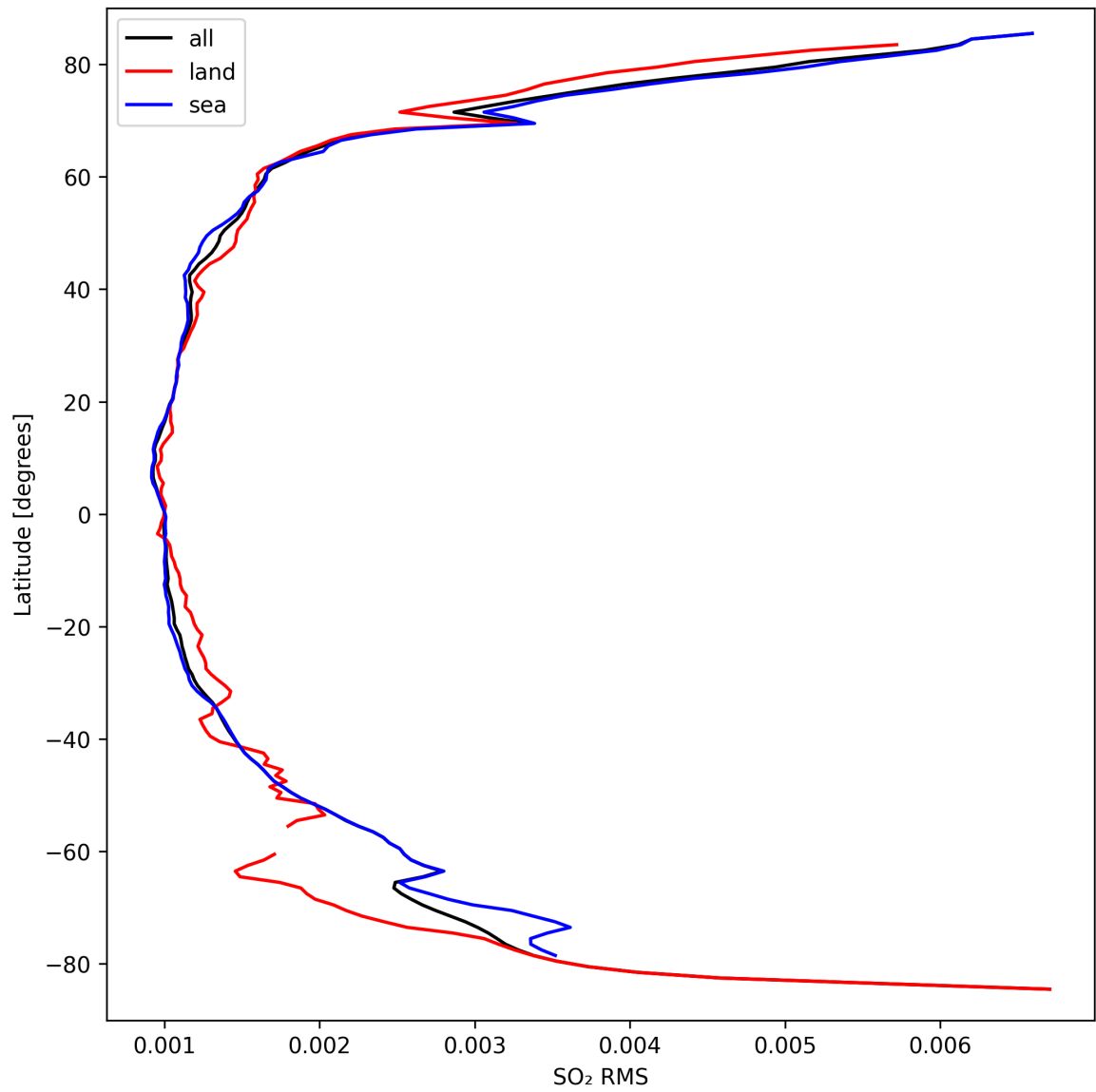
Figure 47: Zonal average of “SO 2 RMS” for 2024-09-19 to 2024-09-21.
