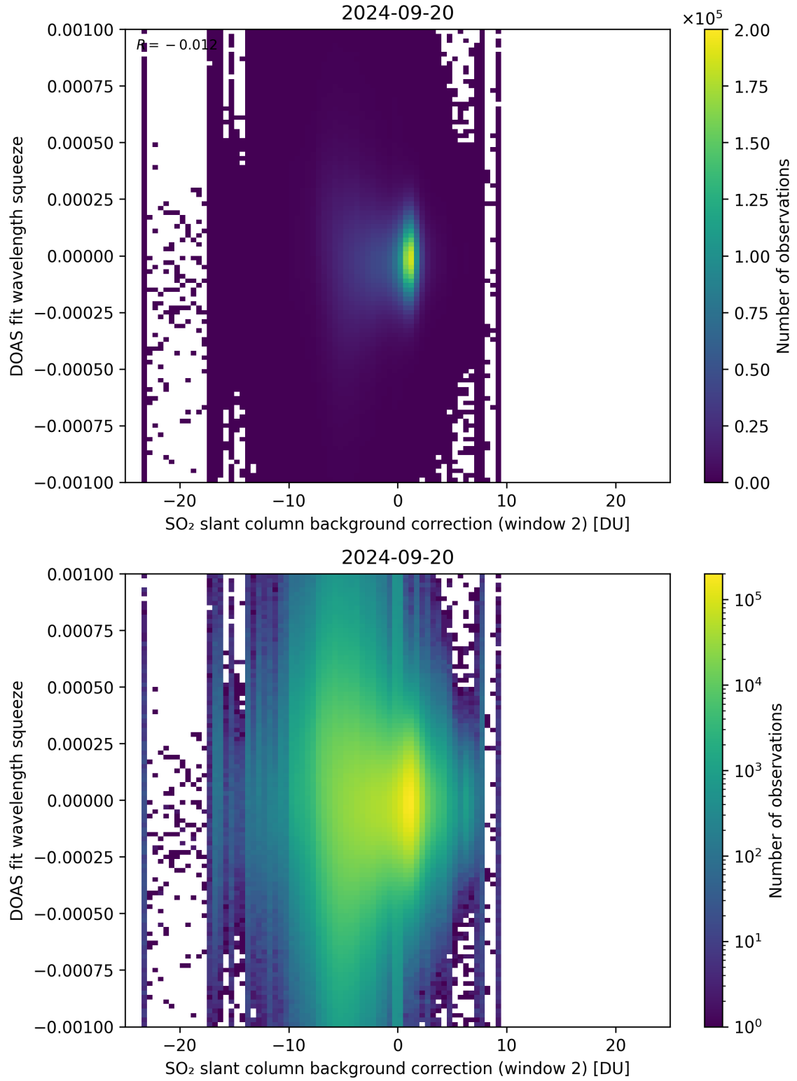
Figure 113: Scatter density plot of “SO 2 slant column background correction (window 2)” against “DOAS fit wavelength squeeze” for 2024-09-19 to 2024-09-21.
