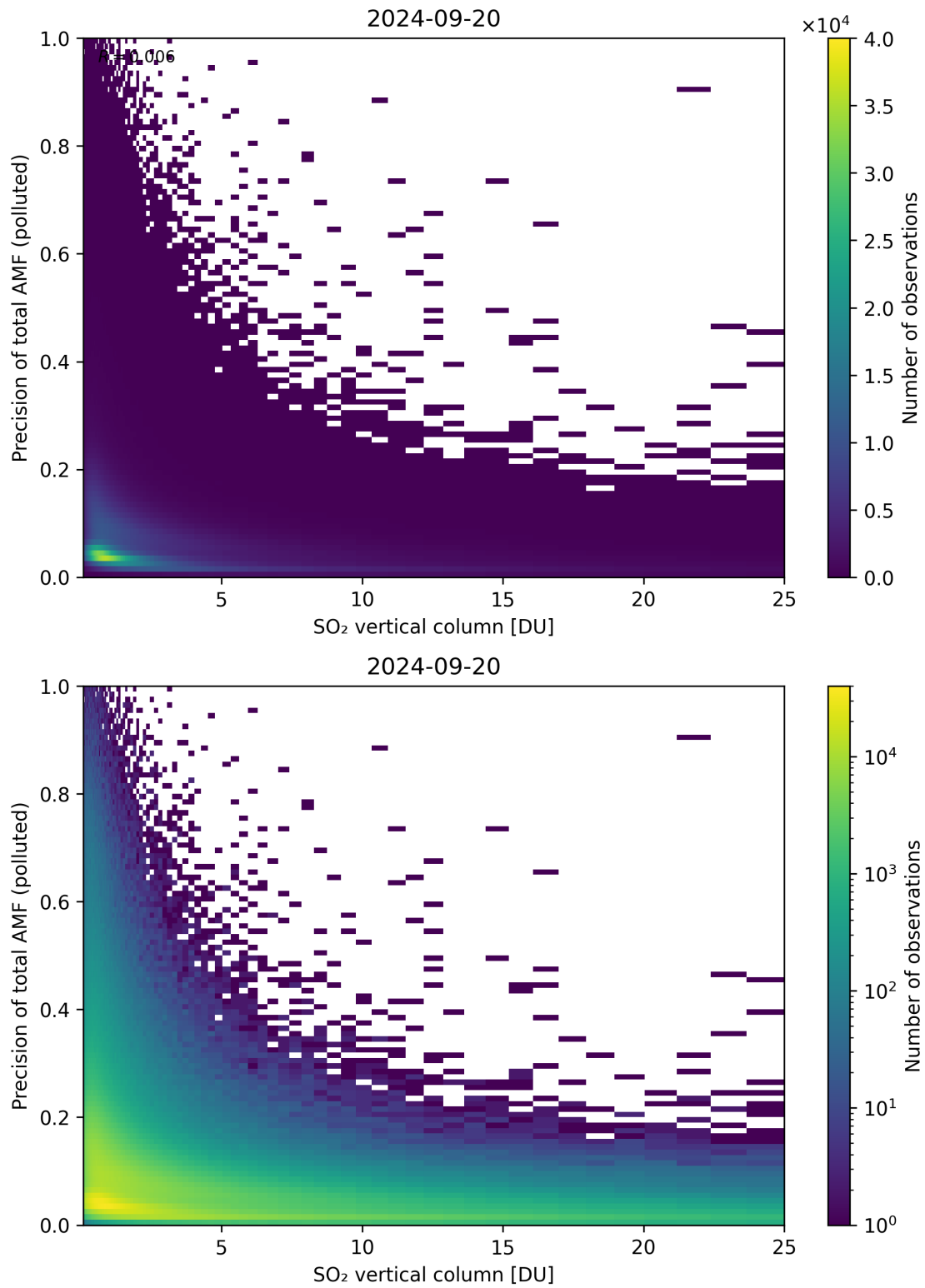
Figure 306: Scatter density plot of “SO 2 vertical column” against “Precision of total AMF (polluted)” for 2024-09-19 to 2024-09-21.
