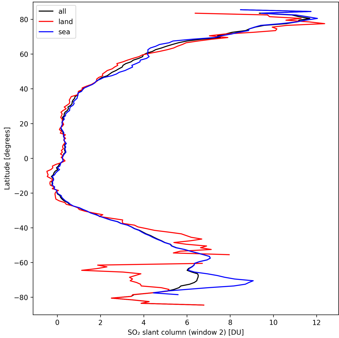
Figure 37: Zonal average of “SO 2 slant column (window 2)” for 2024-09-19 to 2024-09-21.
