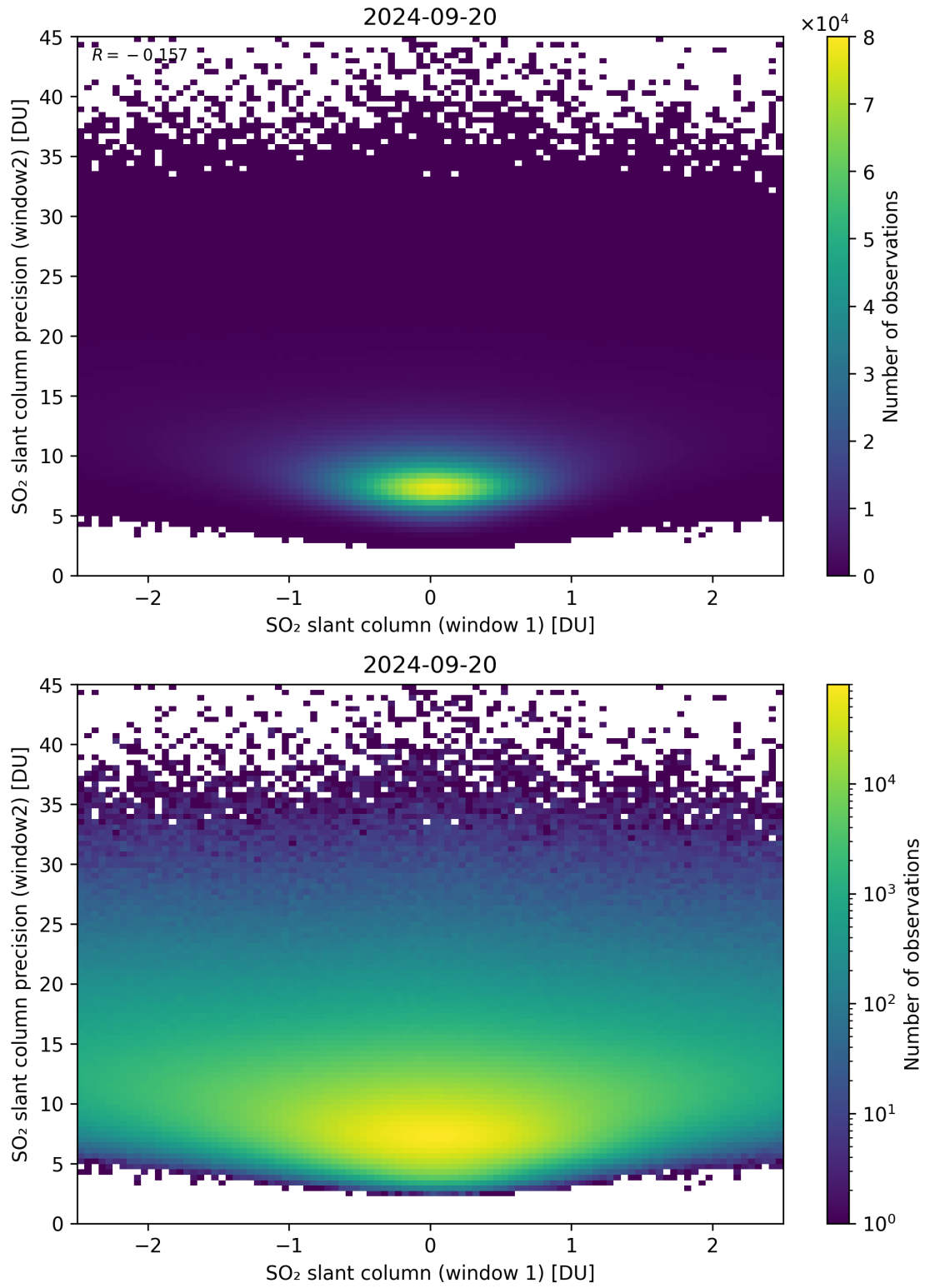
Figure 236: Scatter density plot of “SO 2 slant column (window 1)” against “SO 2 slant column precision (window2)” for 2024-09-19 to 2024-09-21.
