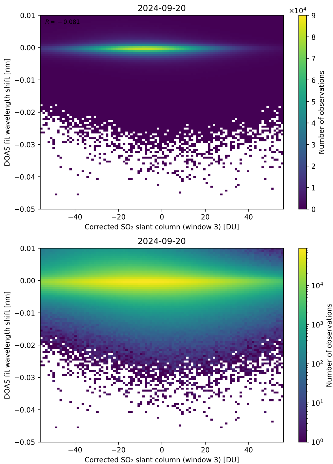
Figure 206: Scatter density plot of “Corrected SO 2 slant column (window 3)” against “DOAS fit wavelength shift” for 2024-09-19 to 2024-09-21.
