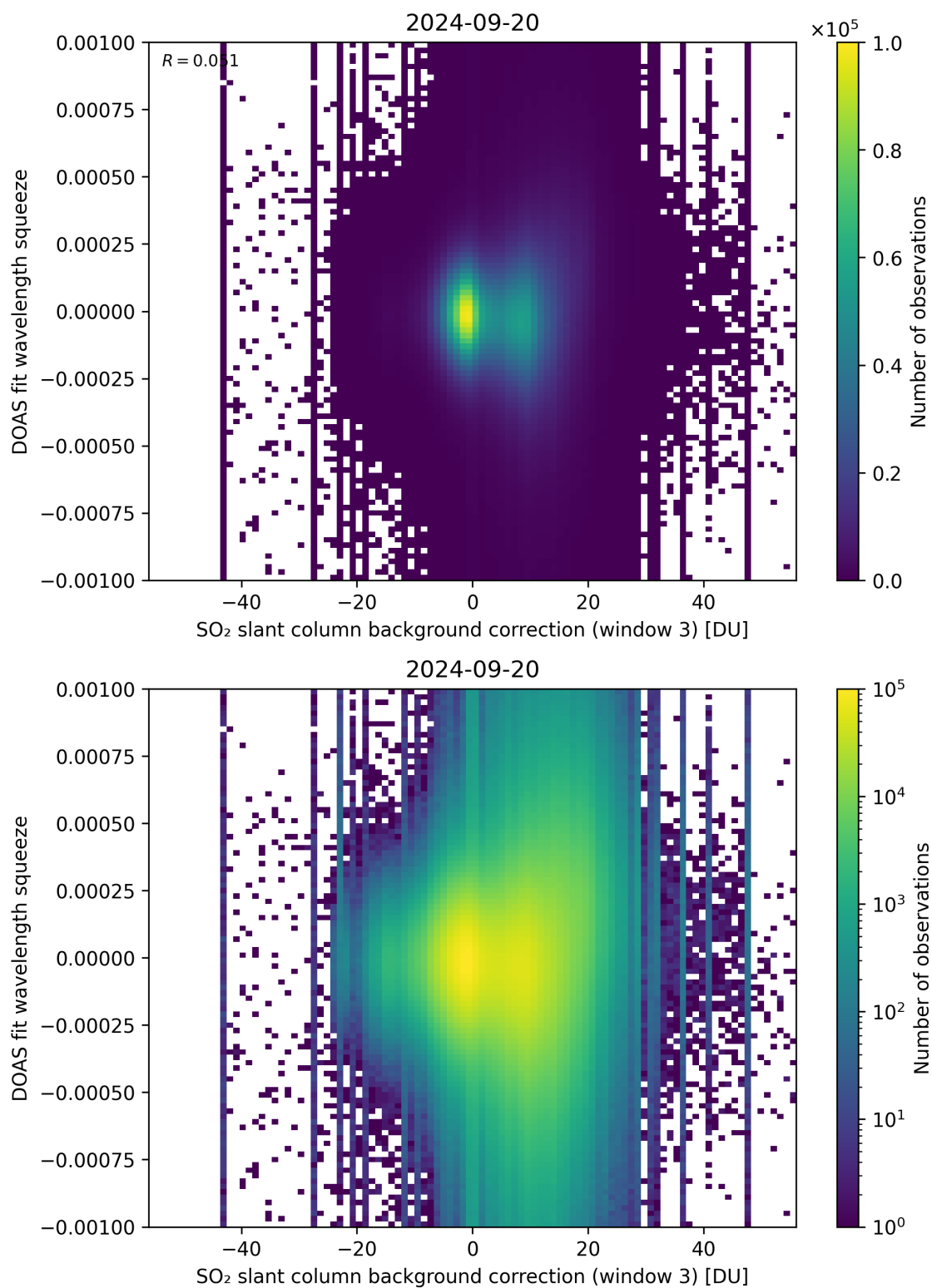
Figure 122: Scatter density plot of “SO 2 slant column background correction (window 3)” against “DOAS fit wavelength squeeze” for 2024-09-19 to 2024-09-21.
