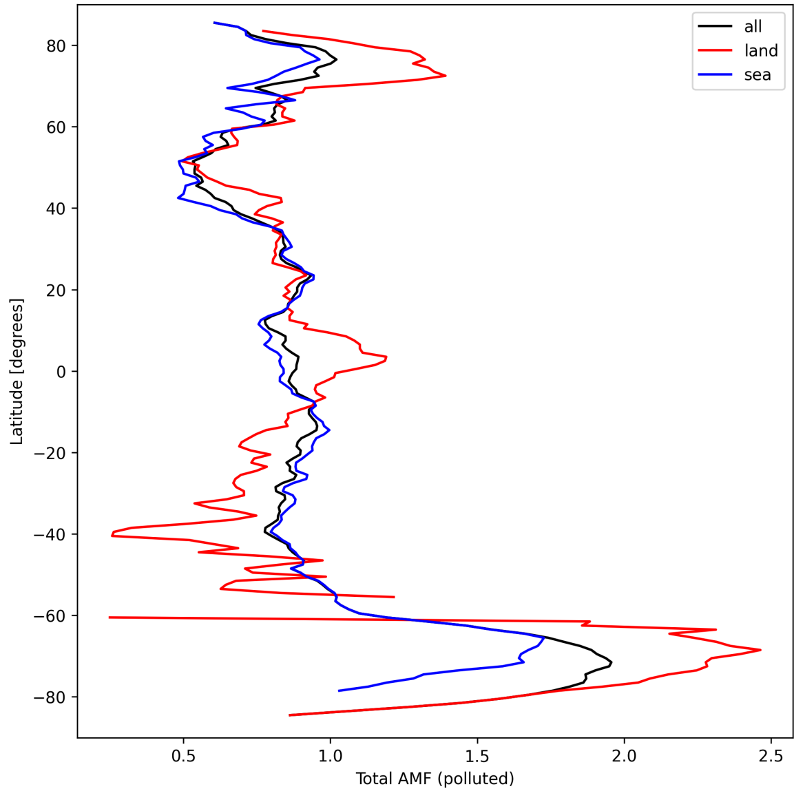
Figure 48: Zonal average of “Total AMF (polluted)” for 2024-09-19 to 2024-09-21.
