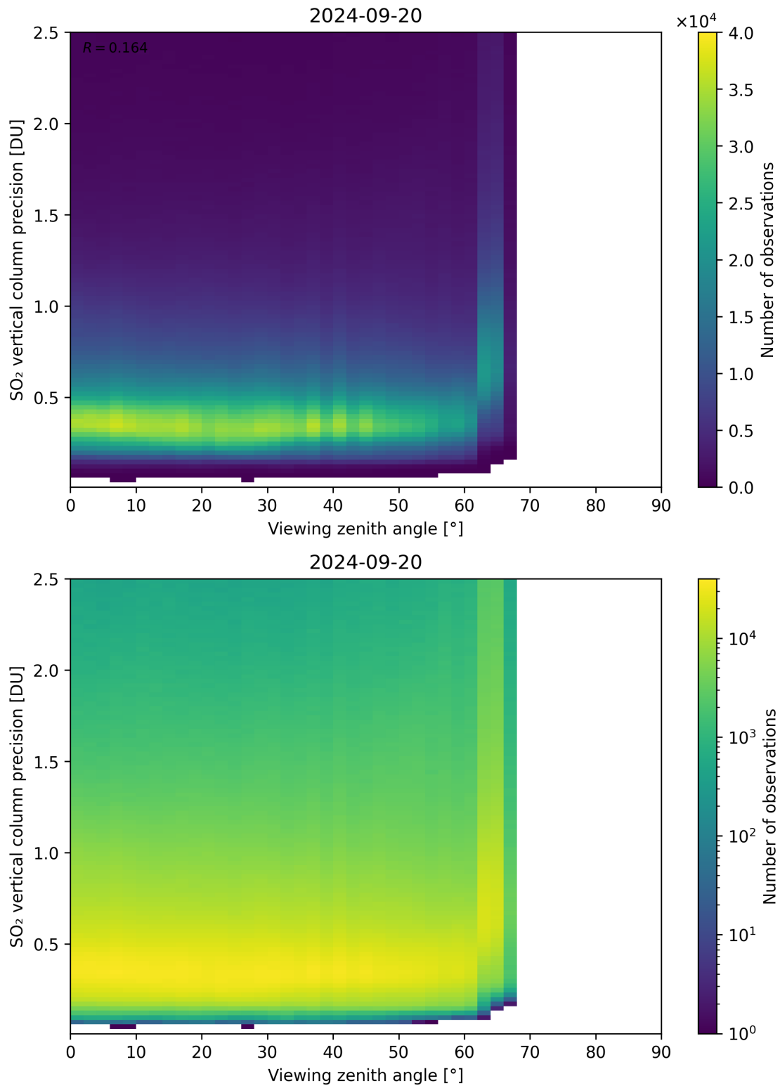
Figure 328: Scatter density plot of “Viewing zenith angle” against “SO 2 vertical column precision” for 2024-09-19 to 2024-09-21.
